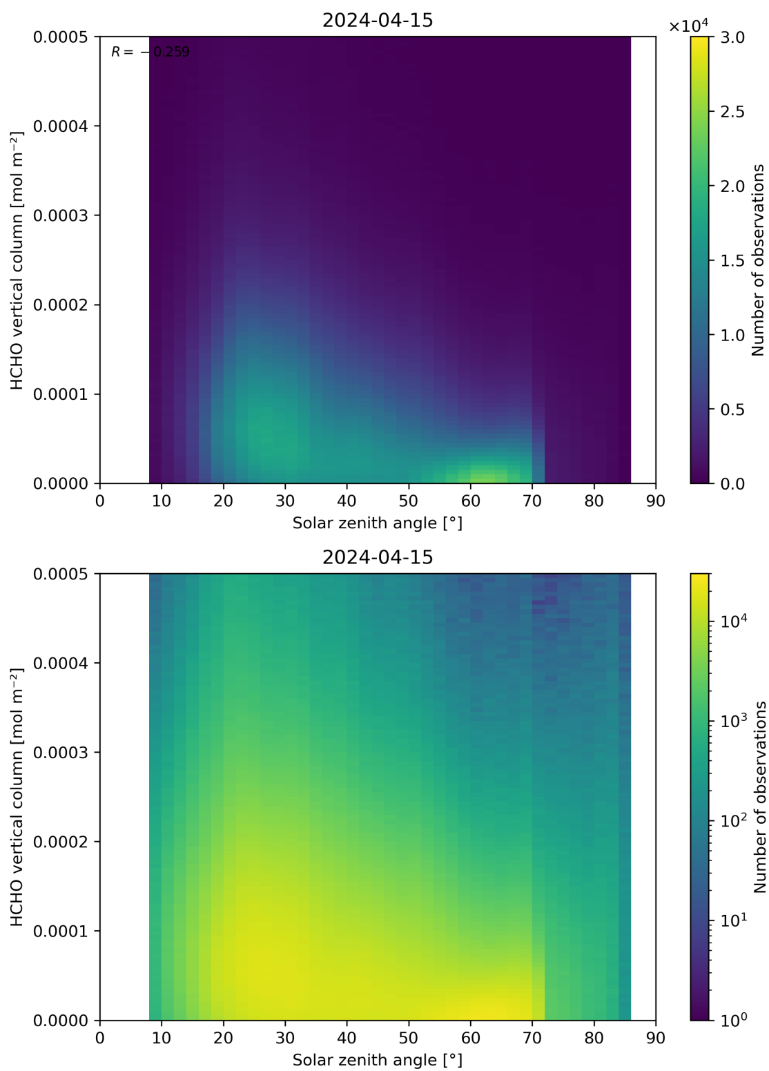
Figure 177: Scatter density plot of “Solar zenith angle” against “HCHO vertical column” for 2024-04-15 to 2024-04-16.
