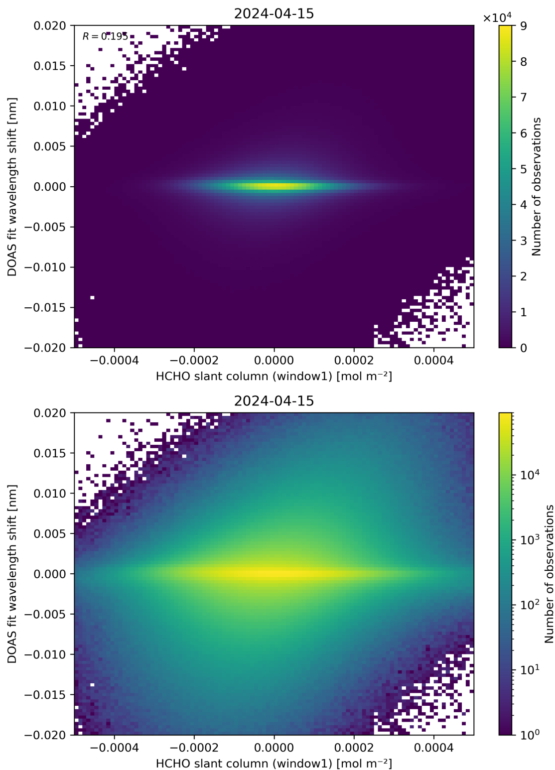
Figure 79: Scatter density plot of “HCHO slant column (window1)” against “DOAS fit wavelength shift” for 2024-04-15 to 2024-04-16.
