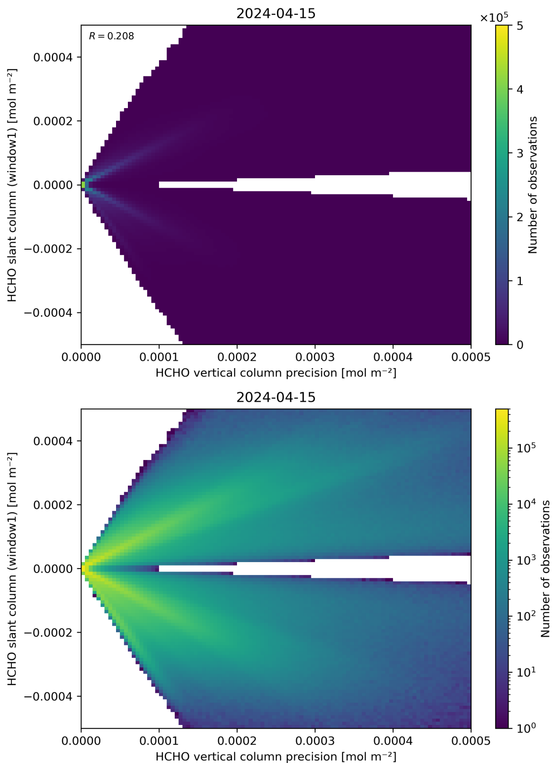
Figure 142: Scatter density plot of “HCHO vertical column precision” against “HCHO slant column (window1)” for 2024-04-15 to 2024-04-16.
