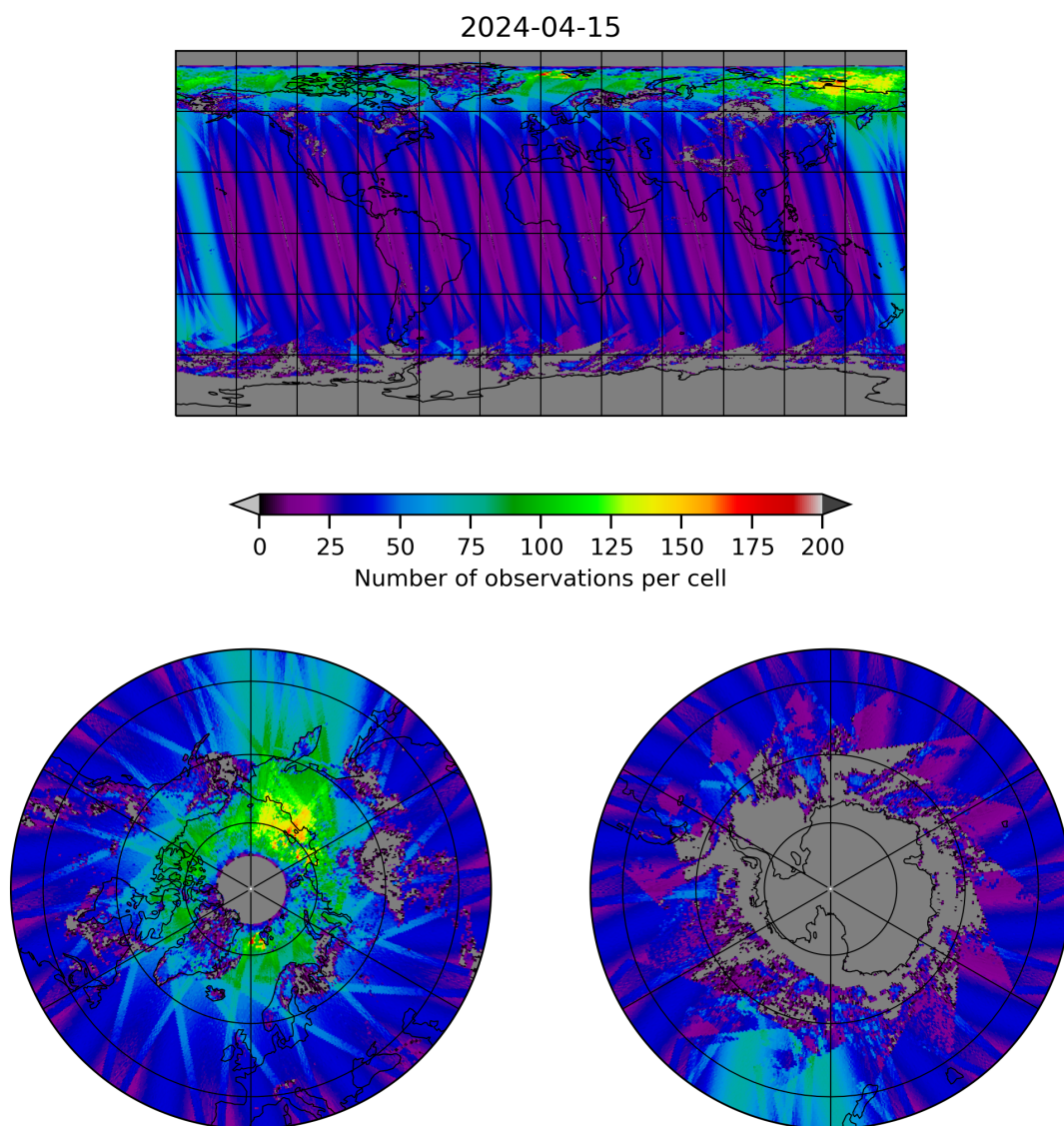
Figure 19: Map of the number of observations for 2024-04-15 to 2024-04-16
