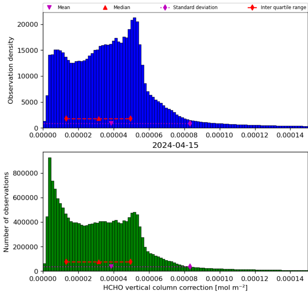
Figure 37: Histogram of “HCHO vertical column correction” for 2024-04-15 to 2024-04-16
