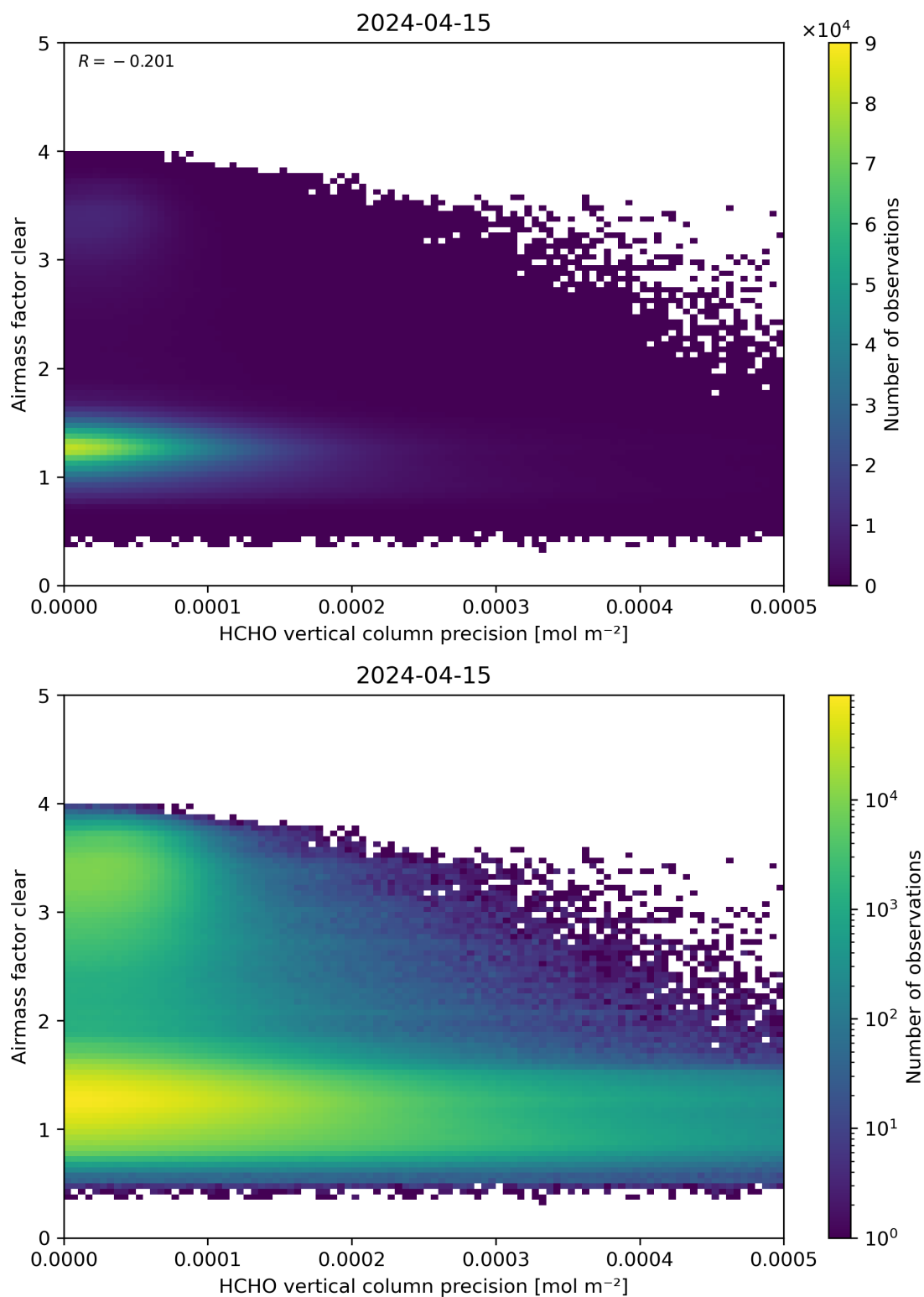
Figure 139: Scatter density plot of “HCHO vertical column precision” against “Airmass factor clear” for 2024-04-15 to 2024-04-16.
