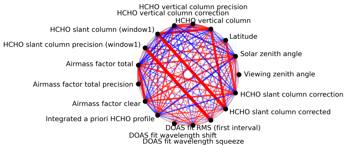
Figure 1: Map of correlation graph for 2024-04-15 to 2024-04-16.
