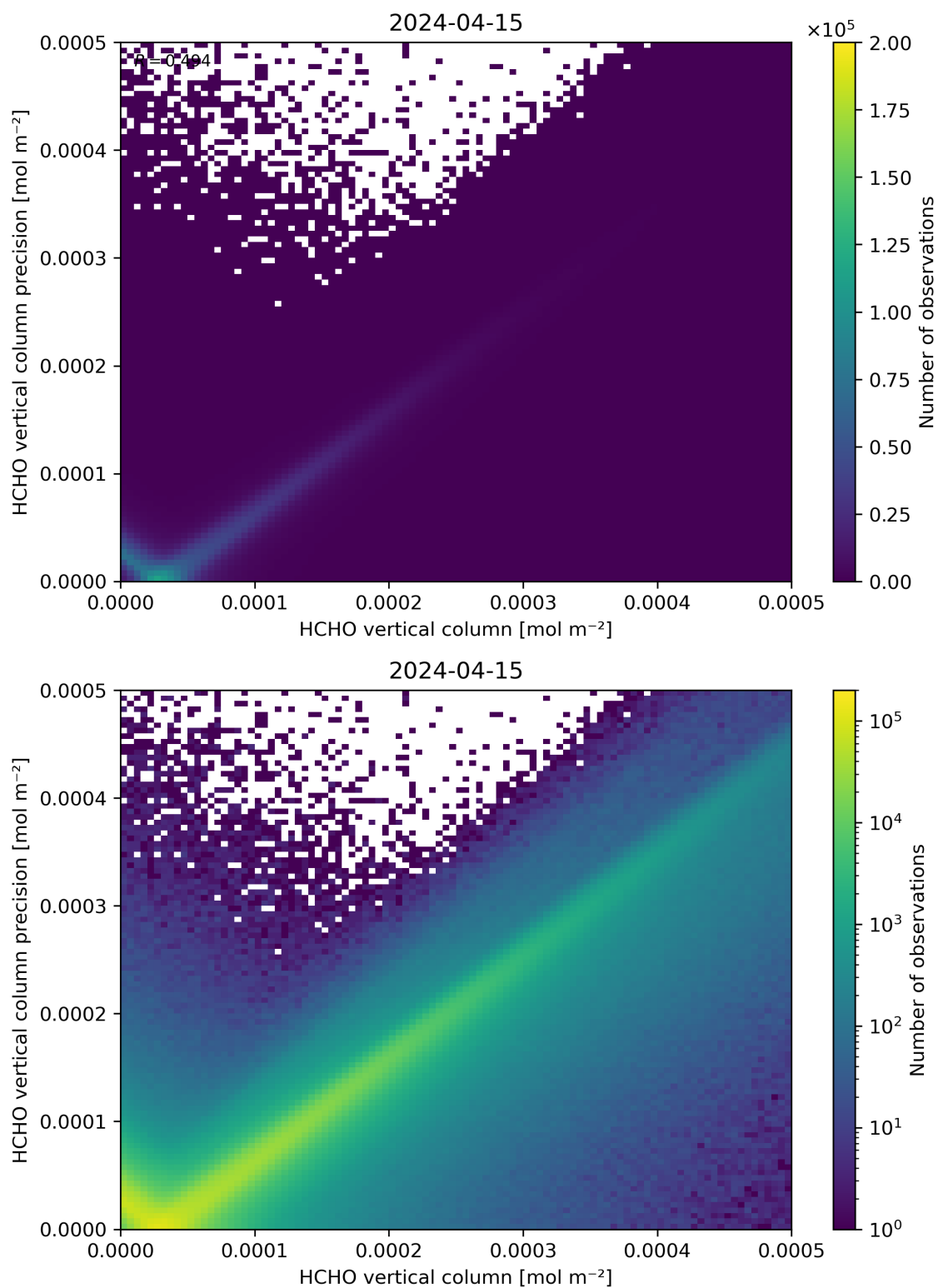
Figure 134: Scatter density plot of “HCHO vertical column” against “HCHO vertical column precision” for 2024-04-15 to 2024-04-16.
