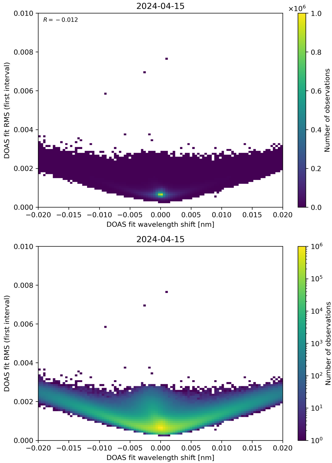
Figure 64: Scatter density plot of “DOAS fit wavelength shift” against “DOAS fit RMS (first interval)” for 2024-04-15 to 2024-04-16.
