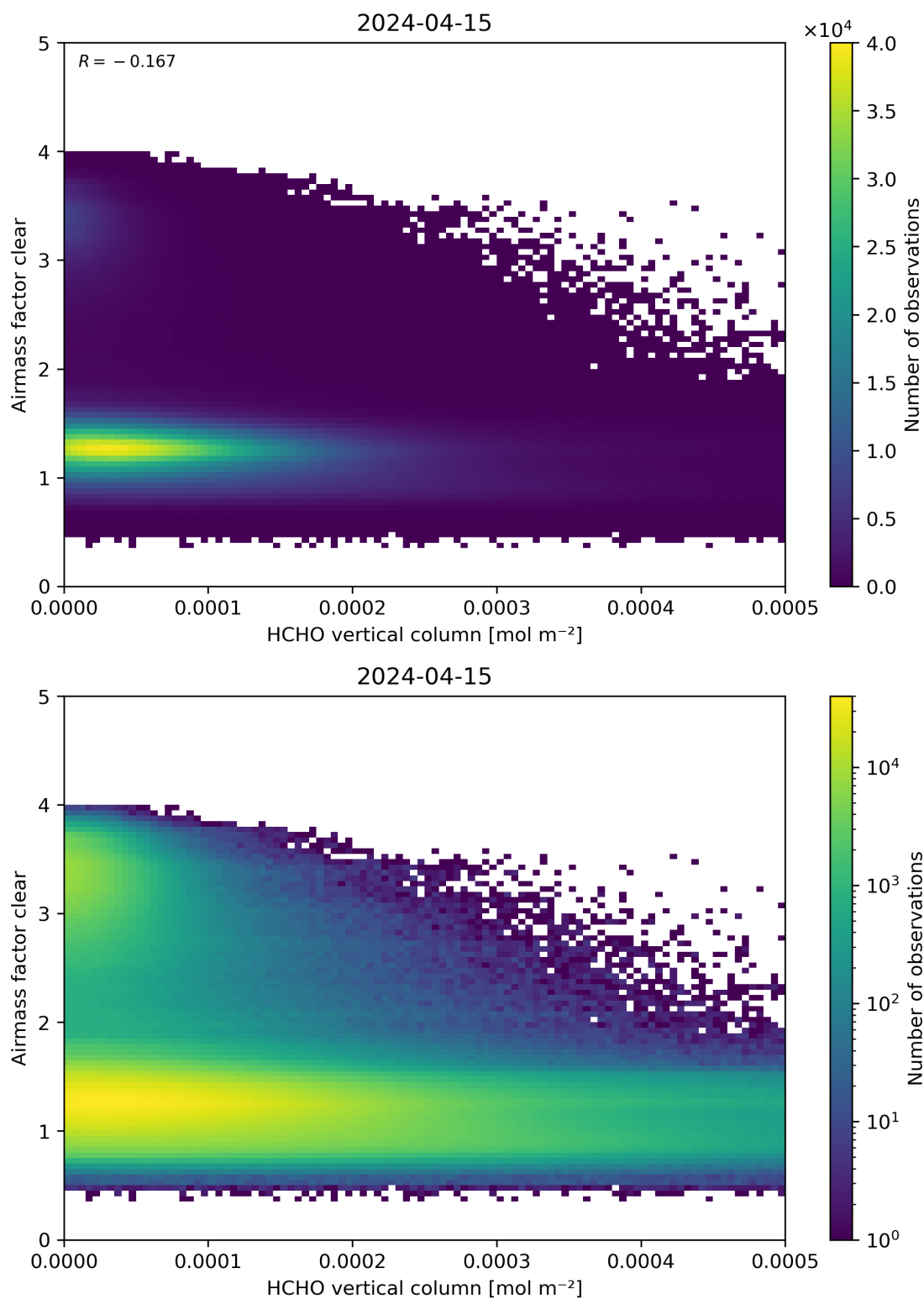
Figure 126: Scatter density plot of “HCHO vertical column” against “Airmass factor clear” for 2024-04-15 to 2024-04-16.
