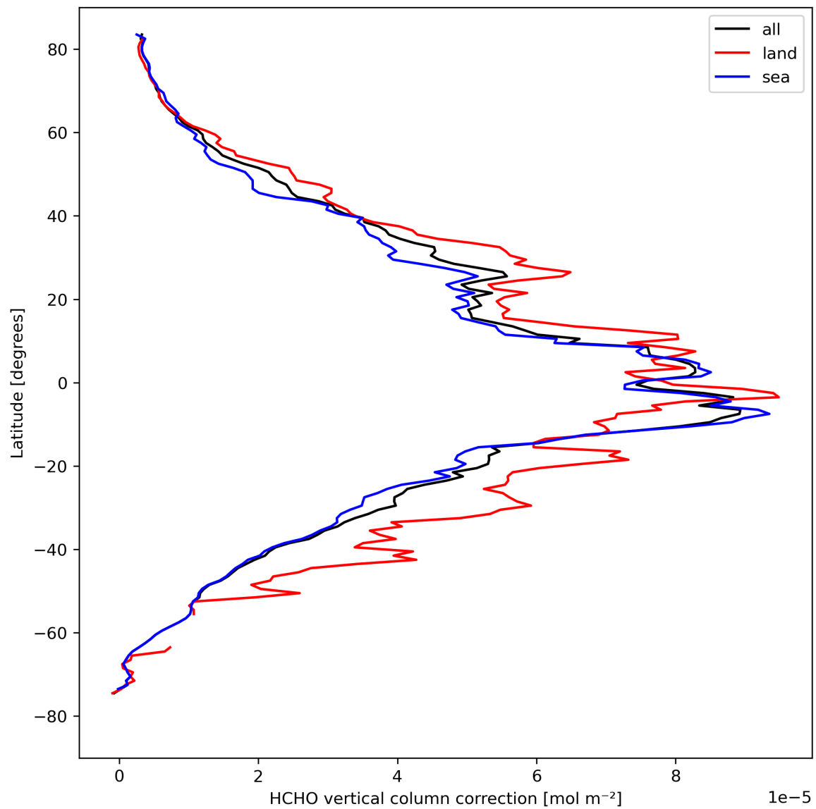
Figure 23: Zonal average of “HCHO vertical column correction” for 2024-04-15 to 2024-04-16.
