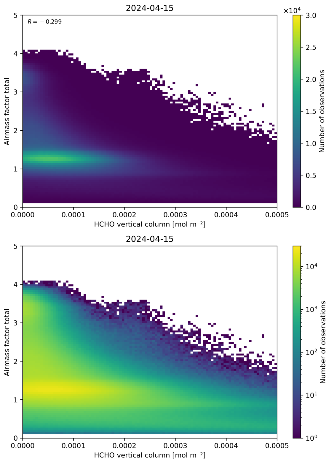
Figure 131: Scatter density plot of “HCHO vertical column” against “Airmass factor total” for 2024-04-15 to 2024-04-16.
