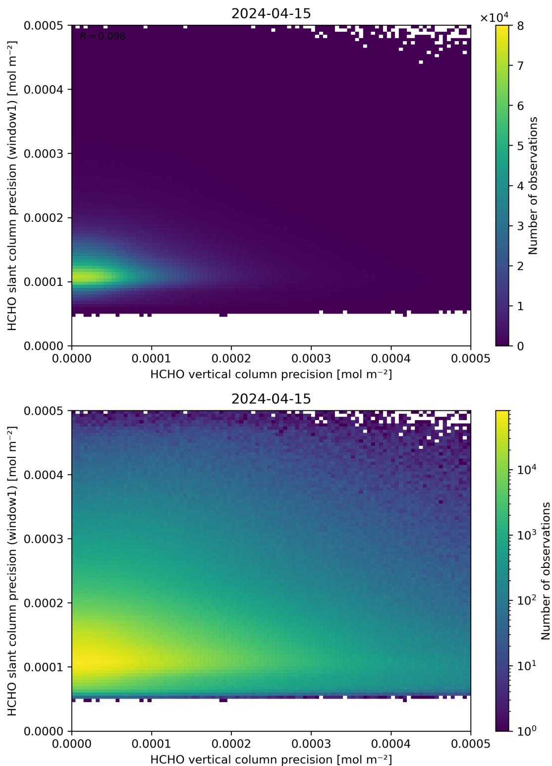
Figure 143: Scatter density plot of “HCHO vertical column precision” against “HCHO slant column precision (window1)” for 2024-04-15 to 2024-04-16.
