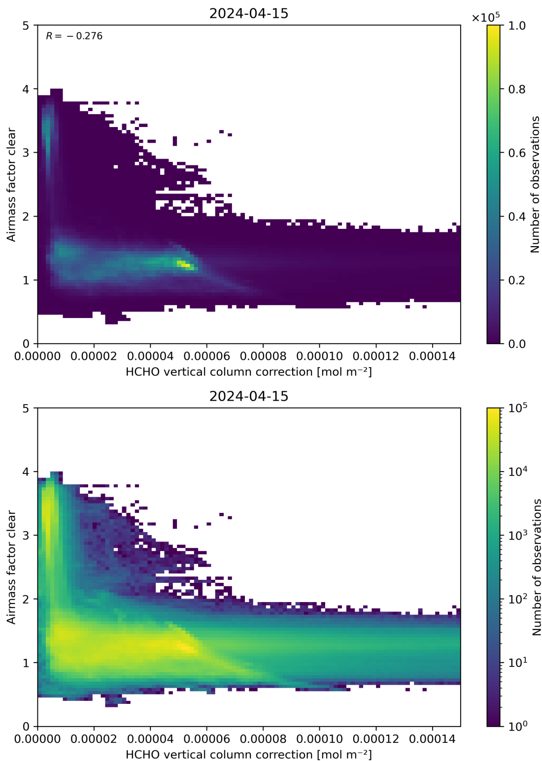
Figure 115: Scatter density plot of “HCHO vertical column correction” against “Airmass factor clear” for 2024-04-15 to 2024-04-16.
