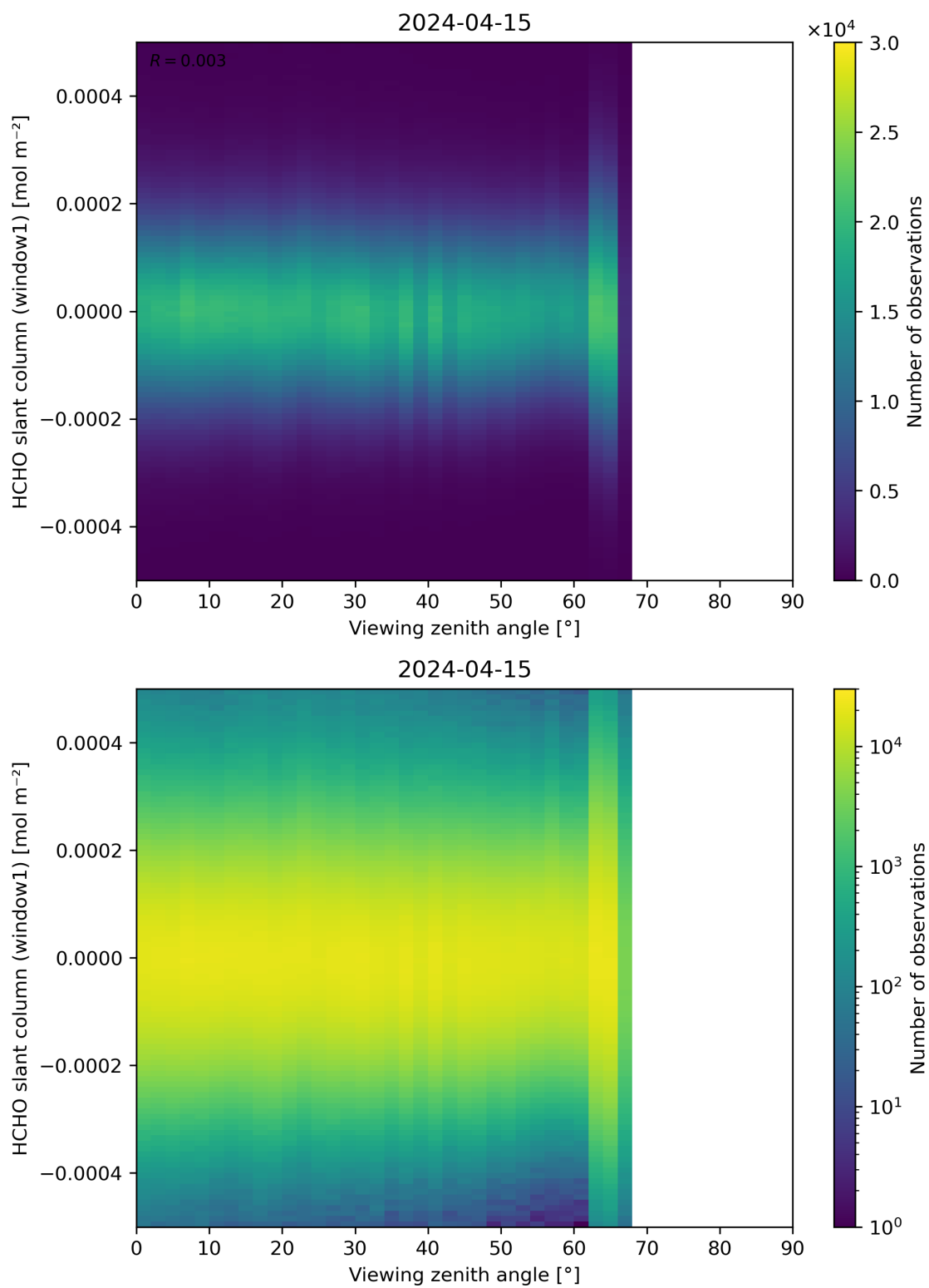
Figure 188: Scatter density plot of “Viewing zenith angle” against “HCHO slant column (window1)” for 2024-04-15 to 2024-04-16.
