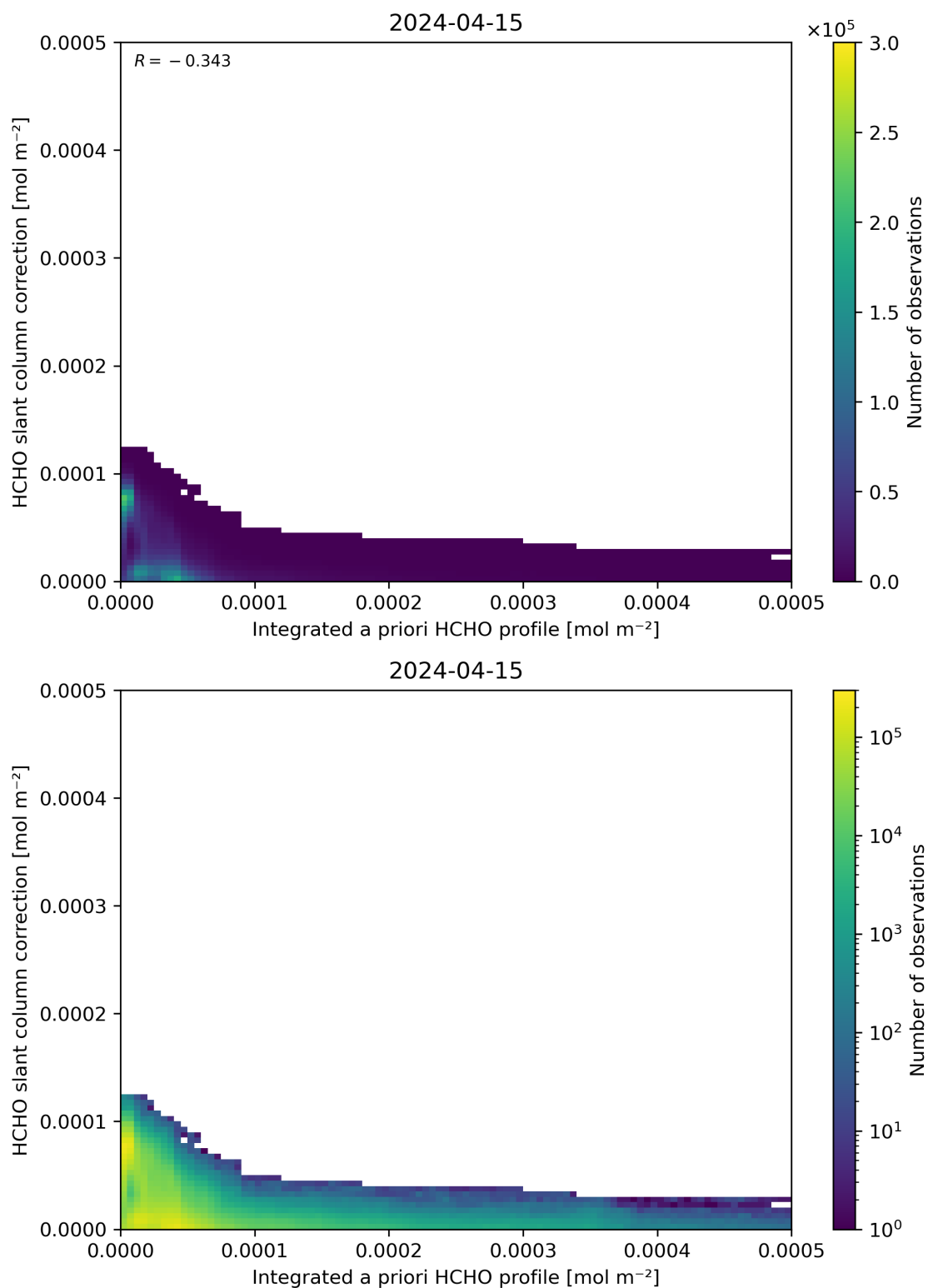
Figure 152: Scatter density plot of “Integrated a priori HCHO profile” against “HCHO slant column correction” for 2024-04-15 to 2024-04-16.
