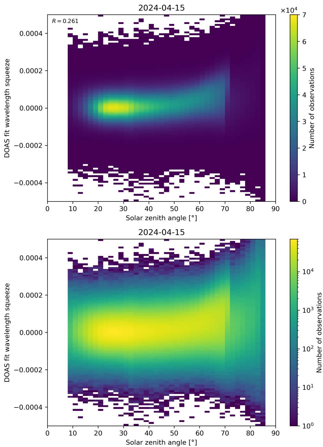
Figure 169: Scatter density plot of “Solar zenith angle” against “DOAS fit wavelength squeeze” for 2024-04-15 to 2024-04-16.
