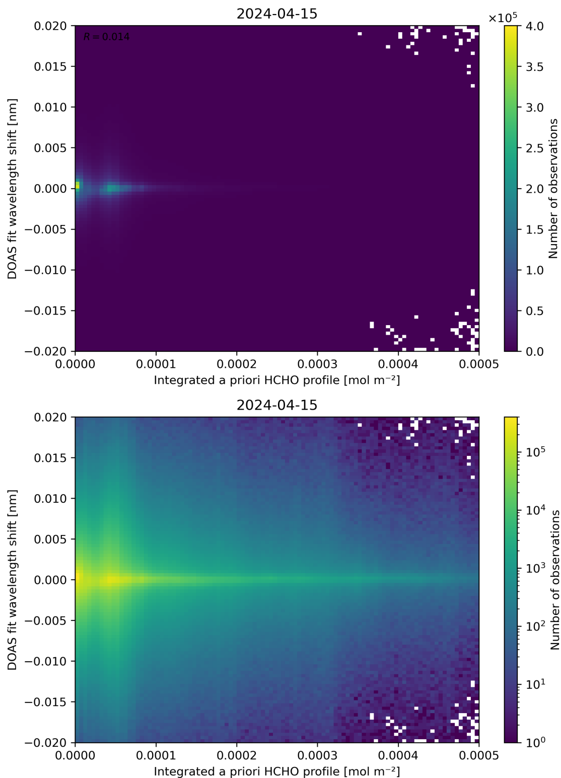
Figure 149: Scatter density plot of “Integrated a priori HCHO profile” against “DOAS fit wavelength shift” for 2024-04-15 to 2024-04-16.
