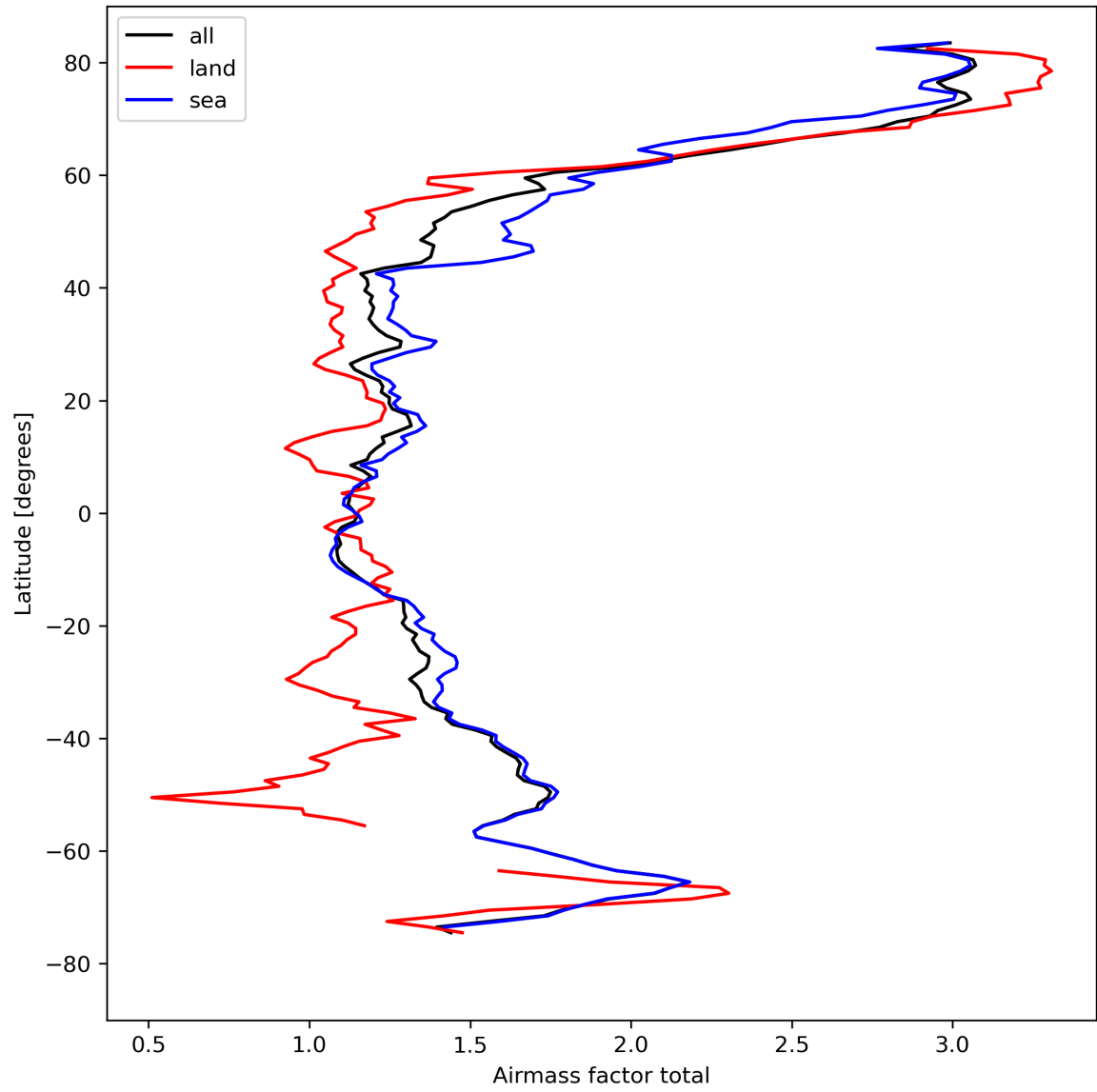
Figure 26: Zonal average of “Airmass factor total” for 2024-04-15 to 2024-04-16.
