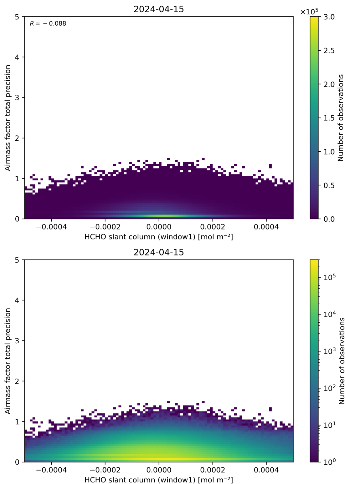
Figure 86: Scatter density plot of “HCHO slant column (window1)” against “Airmass factor total precision” for 2024-04-15 to 2024-04-16.
