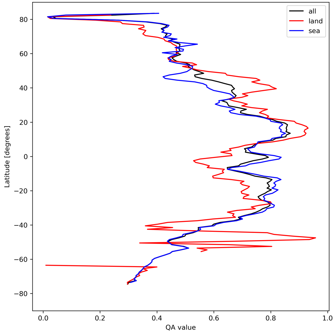
Figure 20: Zonal average of “QA value” for 2024-04-15 to 2024-04-16.
