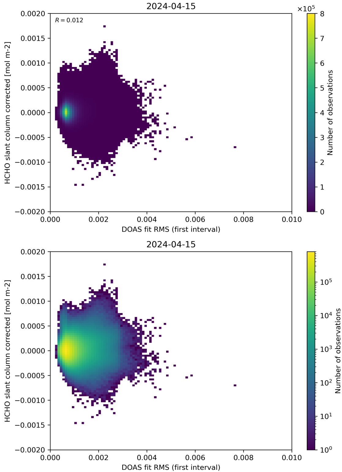
Figure 62: Scatter density plot of “DOAS fit RMS (first interval)” against “HCHO slant column corrected” for 2024-04-15 to 2024-04-16.
