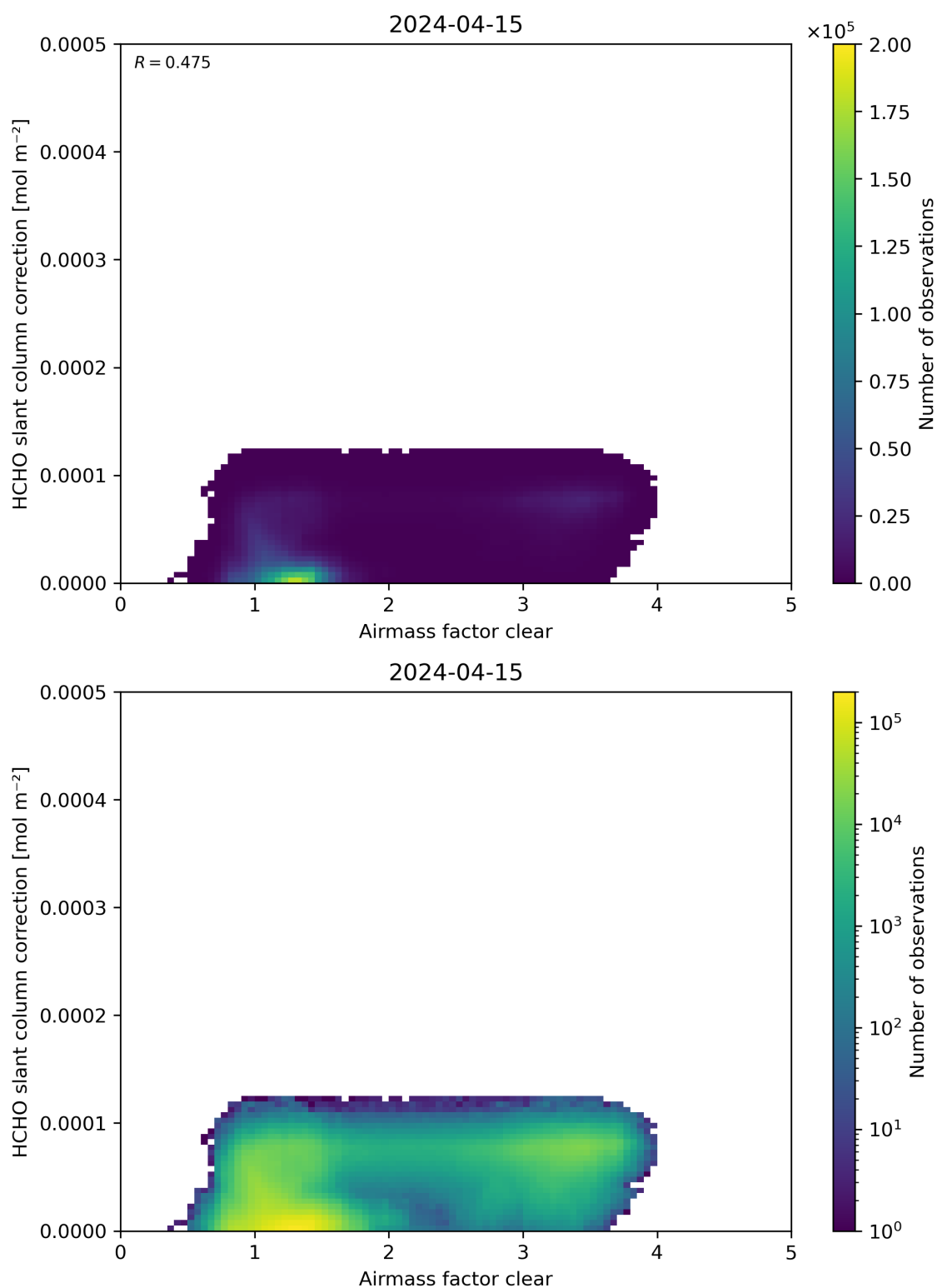
Figure 75: Scatter density plot of “Airmass factor clear” against “HCHO slant column correction” for 2024-04-15 to 2024-04-16.
