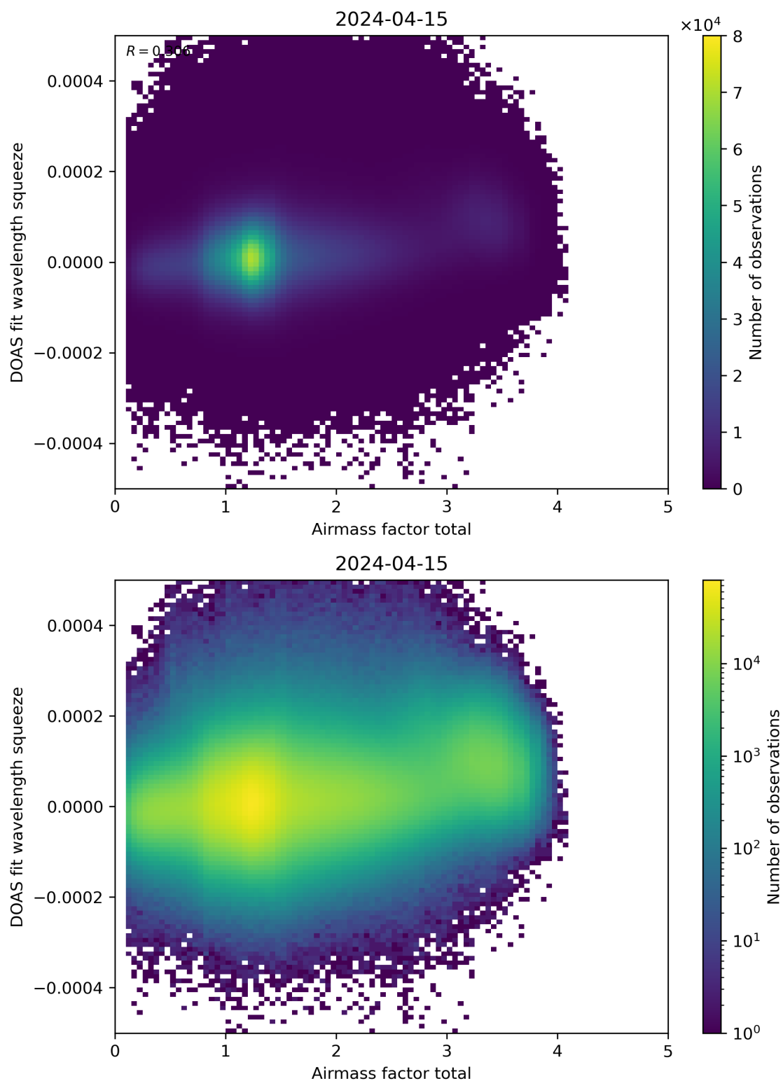
Figure 99: Scatter density plot of “Airmass factor total” against “DOAS fit wavelength squeeze” for 2024-04-15 to 2024-04-16.
