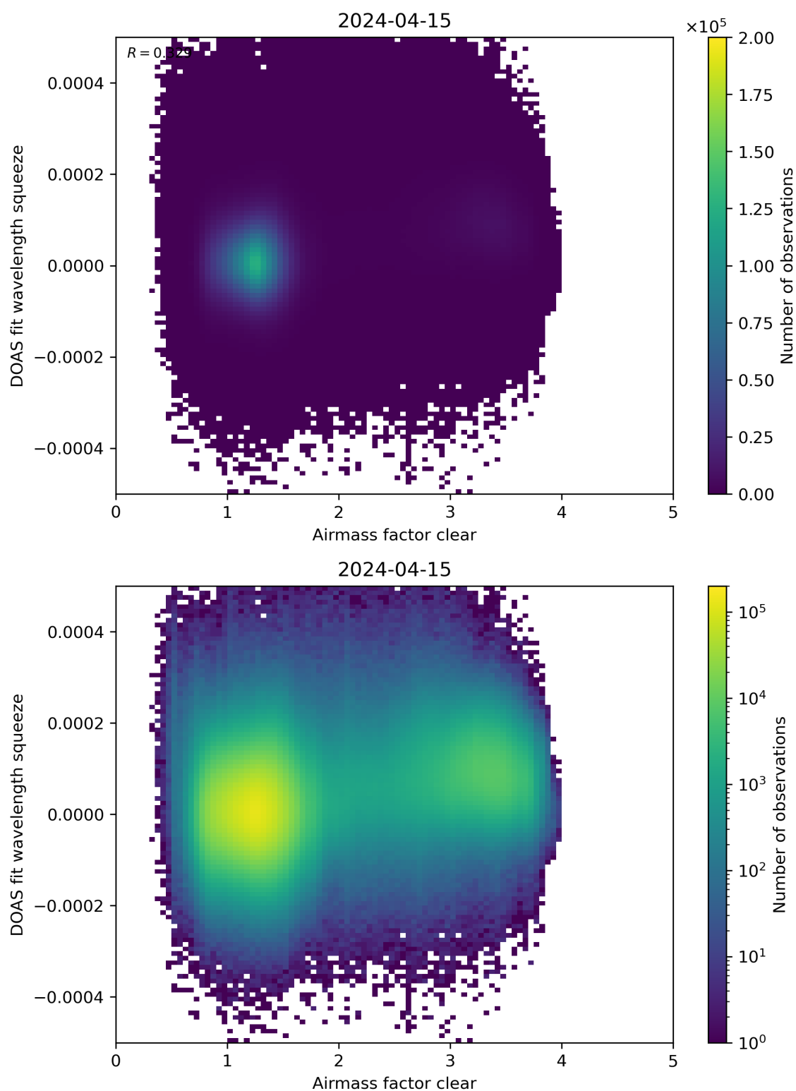
Figure 73: Scatter density plot of “Airmass factor clear” against “DOAS fit wavelength squeeze” for 2024-04-15 to 2024-04-16.
