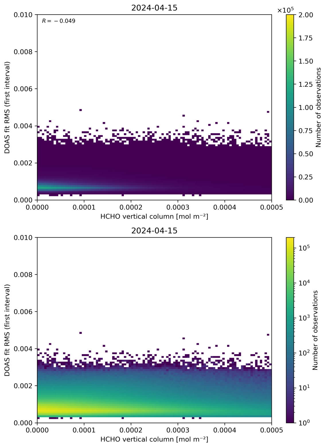
Figure 123: Scatter density plot of “HCHO vertical column” against “DOAS fit RMS (first interval)” for 2024-04-15 to 2024-04-16.
