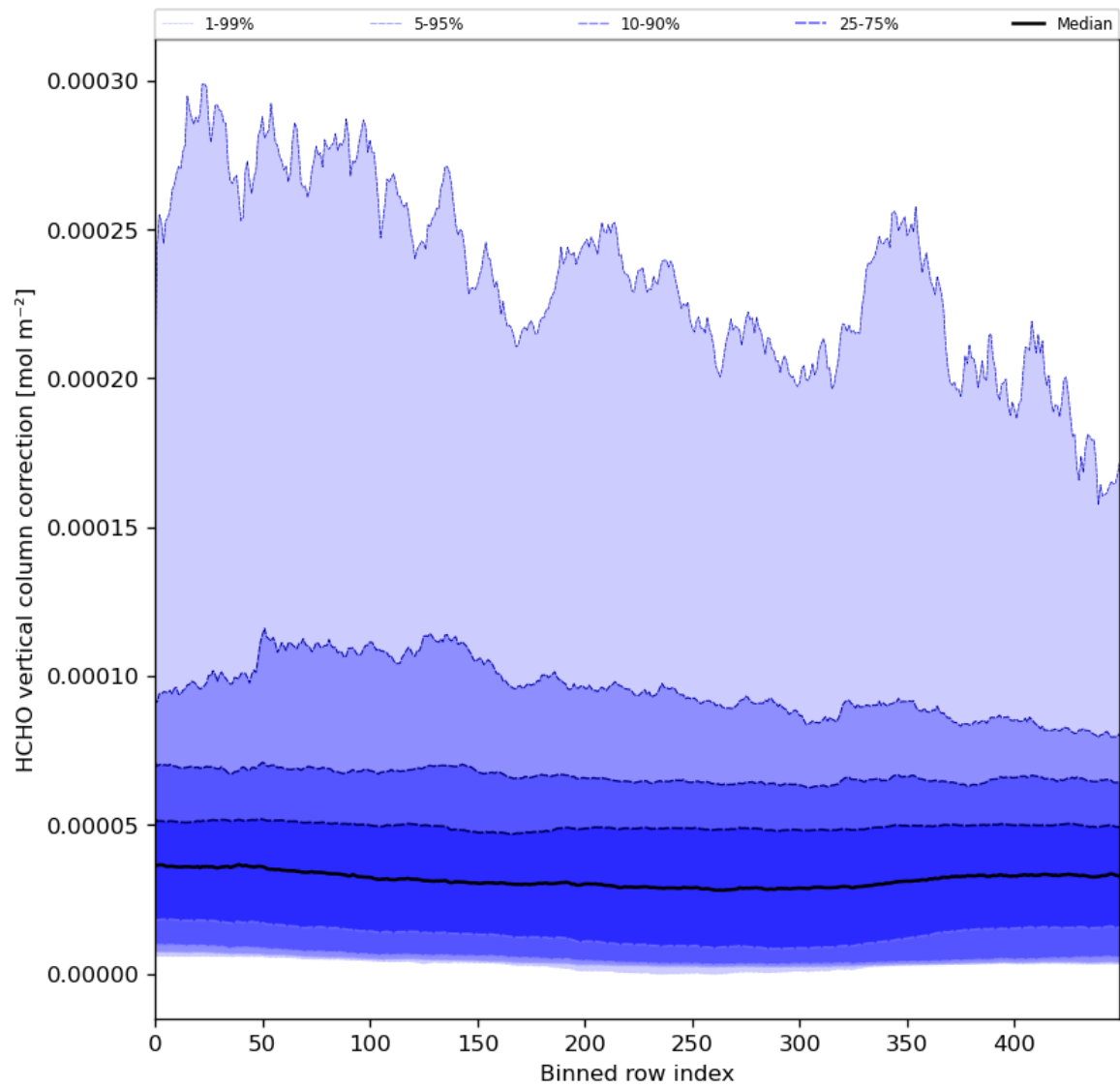
Figure 51: Along track statistics of “HCHO vertical column correction” for 2024-04-15 to 2024-04-16
