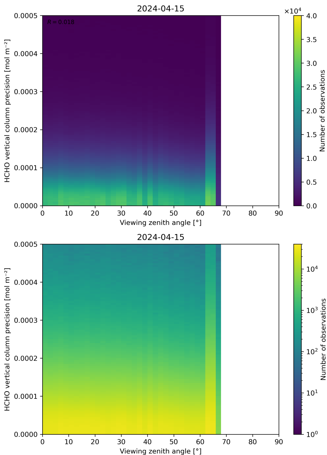
Figure 194: Scatter density plot of “Viewing zenith angle” against “HCHO vertical column precision” for 2024-04-15 to 2024-04-16.
