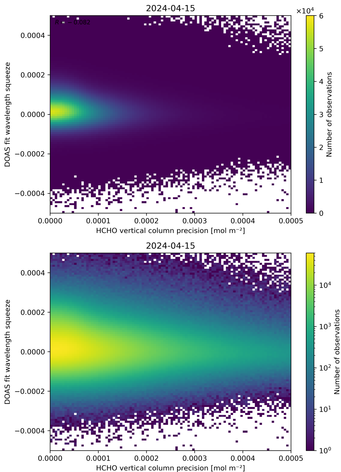
Figure 138: Scatter density plot of “HCHO vertical column precision” against “DOAS fit wavelength squeeze” for 2024-04-15 to 2024-04-16.
