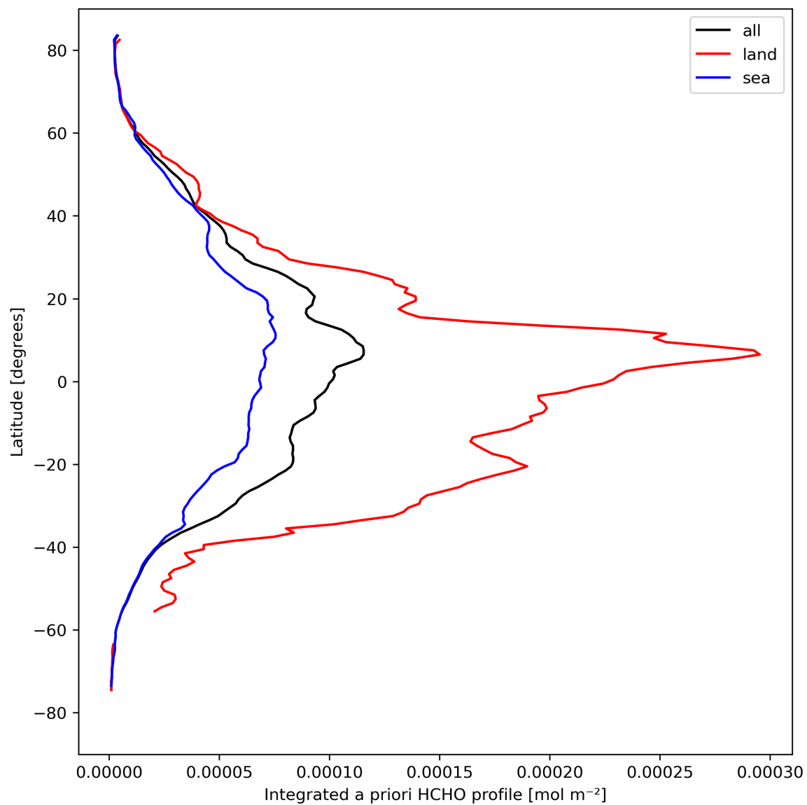
Figure 29: Zonal average of “Integrated a priori HCHO profile” for 2024-04-15 to 2024-04-16.
