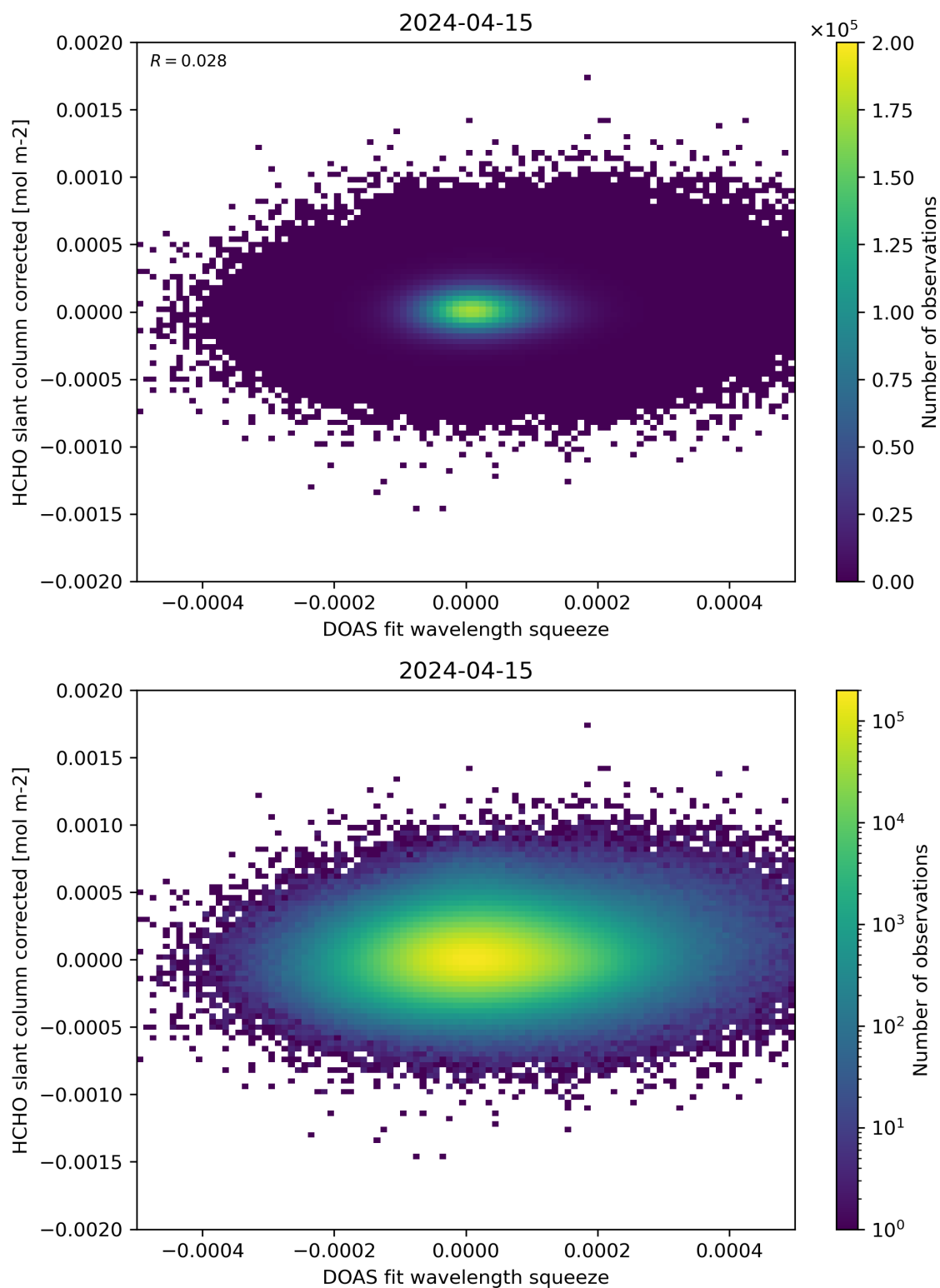
Figure 69: Scatter density plot of “DOAS fit wavelength squeeze” against “HCHO slant column corrected” for 2024-04-15 to 2024-04-16.
