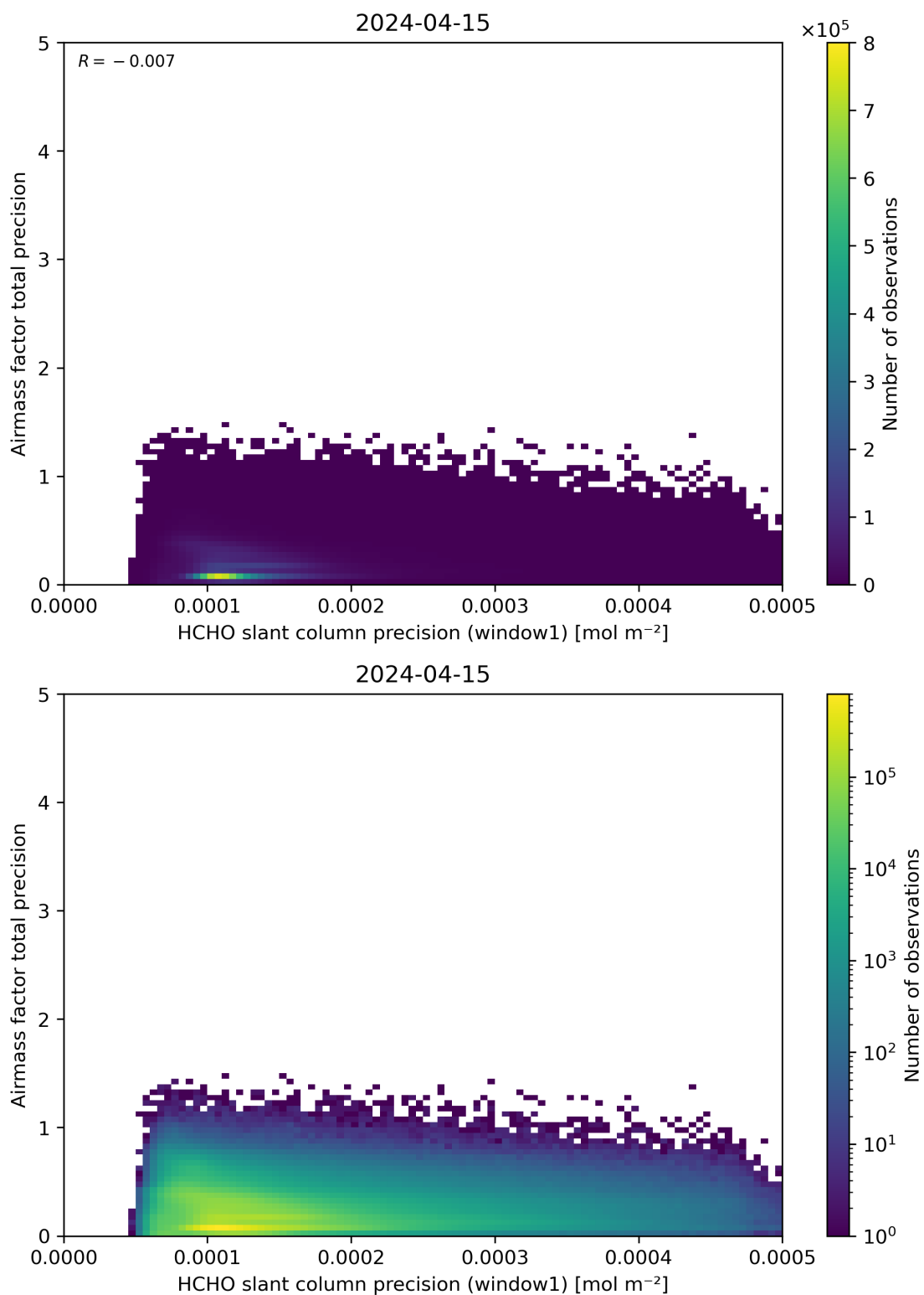
Figure 95: Scatter density plot of “HCHO slant column precision (window1)” against “Airmass factor total precision” for 2024-04-15 to 2024-04-16.
