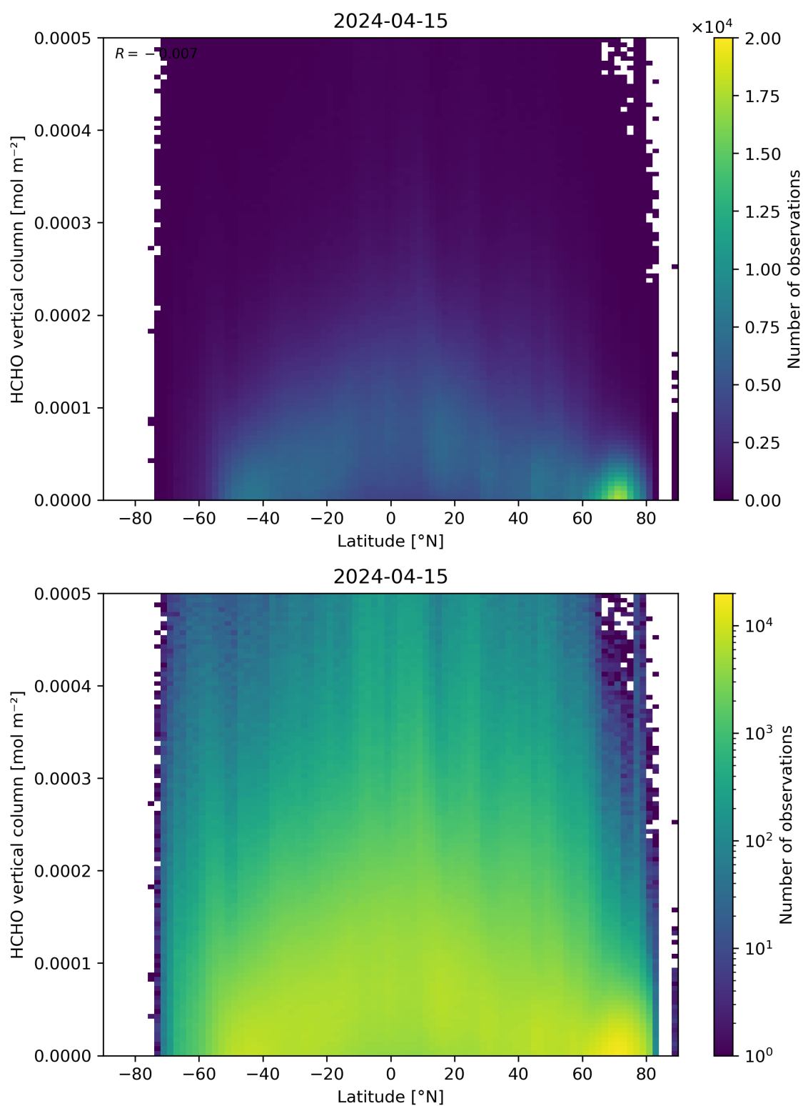
Figure 163: Scatter density plot of “Latitude” against “HCHO vertical column” for 2024-04-15 to 2024-04-16.
