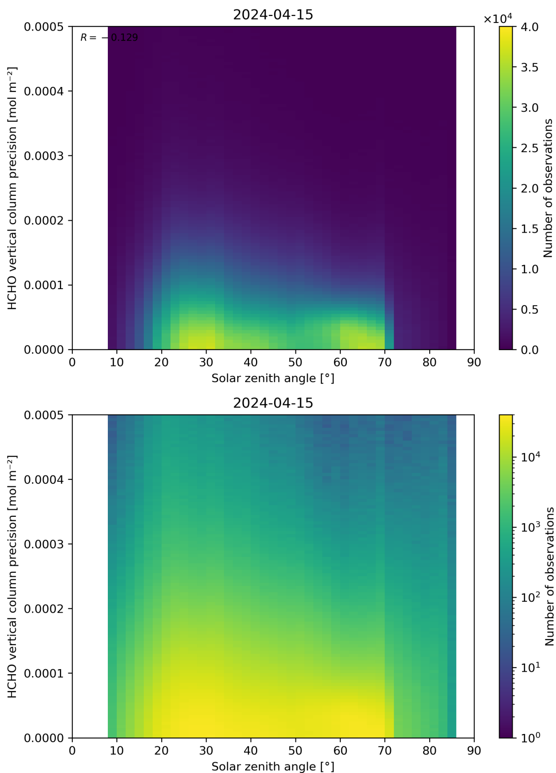
Figure 179: Scatter density plot of “Solar zenith angle” against “HCHO vertical column precision” for 2024-04-15 to 2024-04-16.
