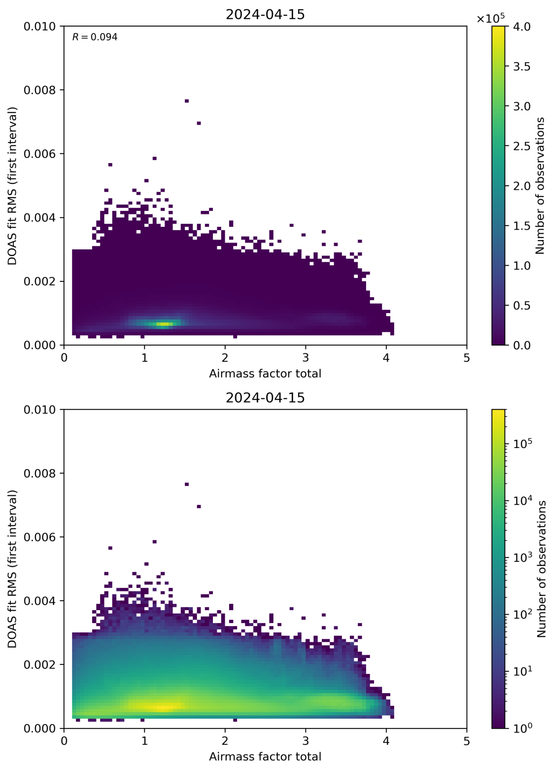
Figure 97: Scatter density plot of “Airmass factor total” against “DOAS fit RMS (first interval)” for 2024-04-15 to 2024-04-16.
