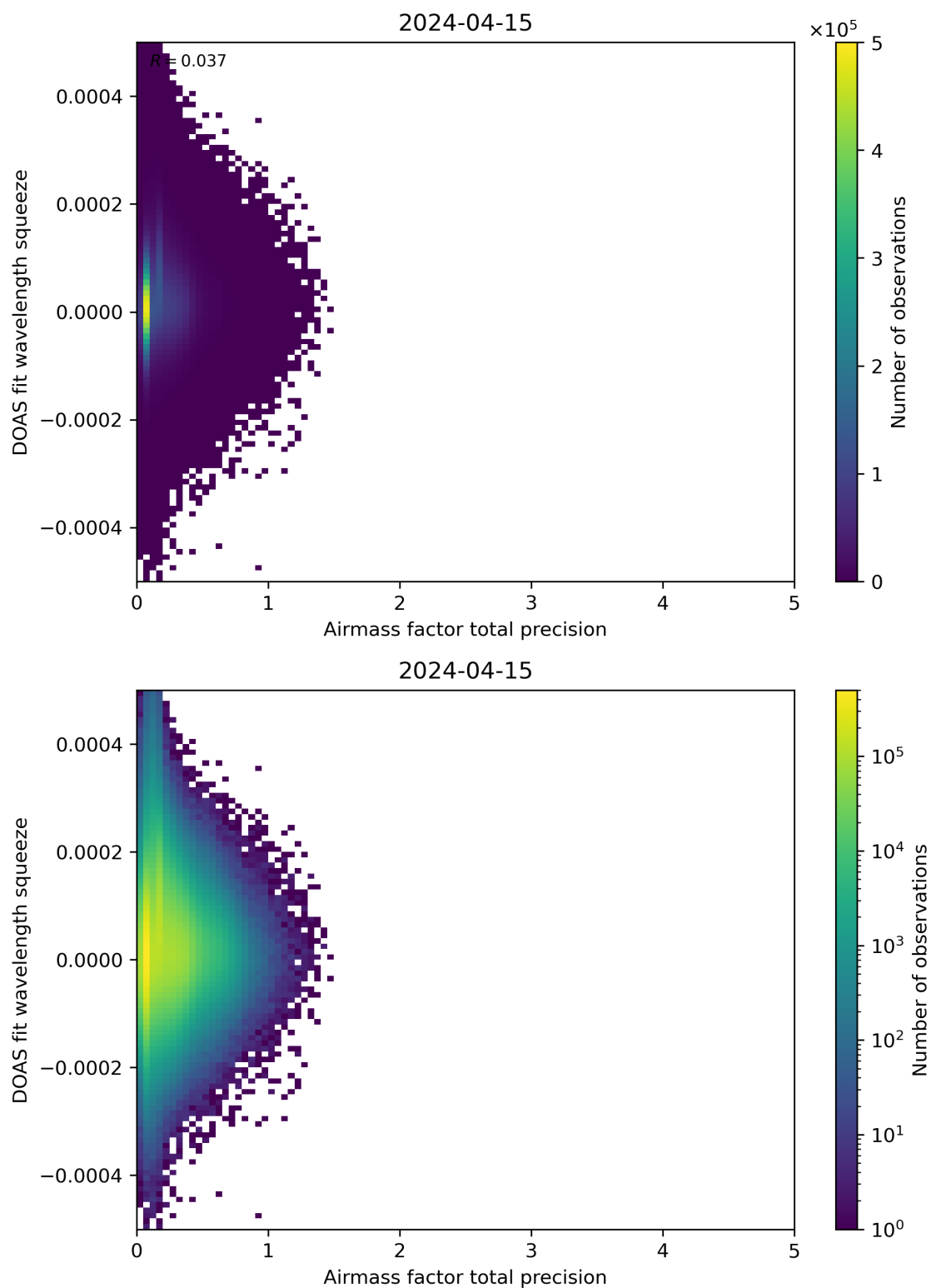
Figure 107: Scatter density plot of “Airmass factor total precision” against “DOAS fit wavelength squeeze” for 2024-04-15 to 2024-04-16.
