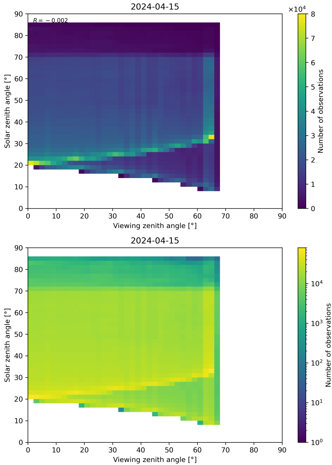
Figure 197: Scatter density plot of “Viewing zenith angle” against “Solar zenith angle” for 2024-04-15 to 2024-04-16.
