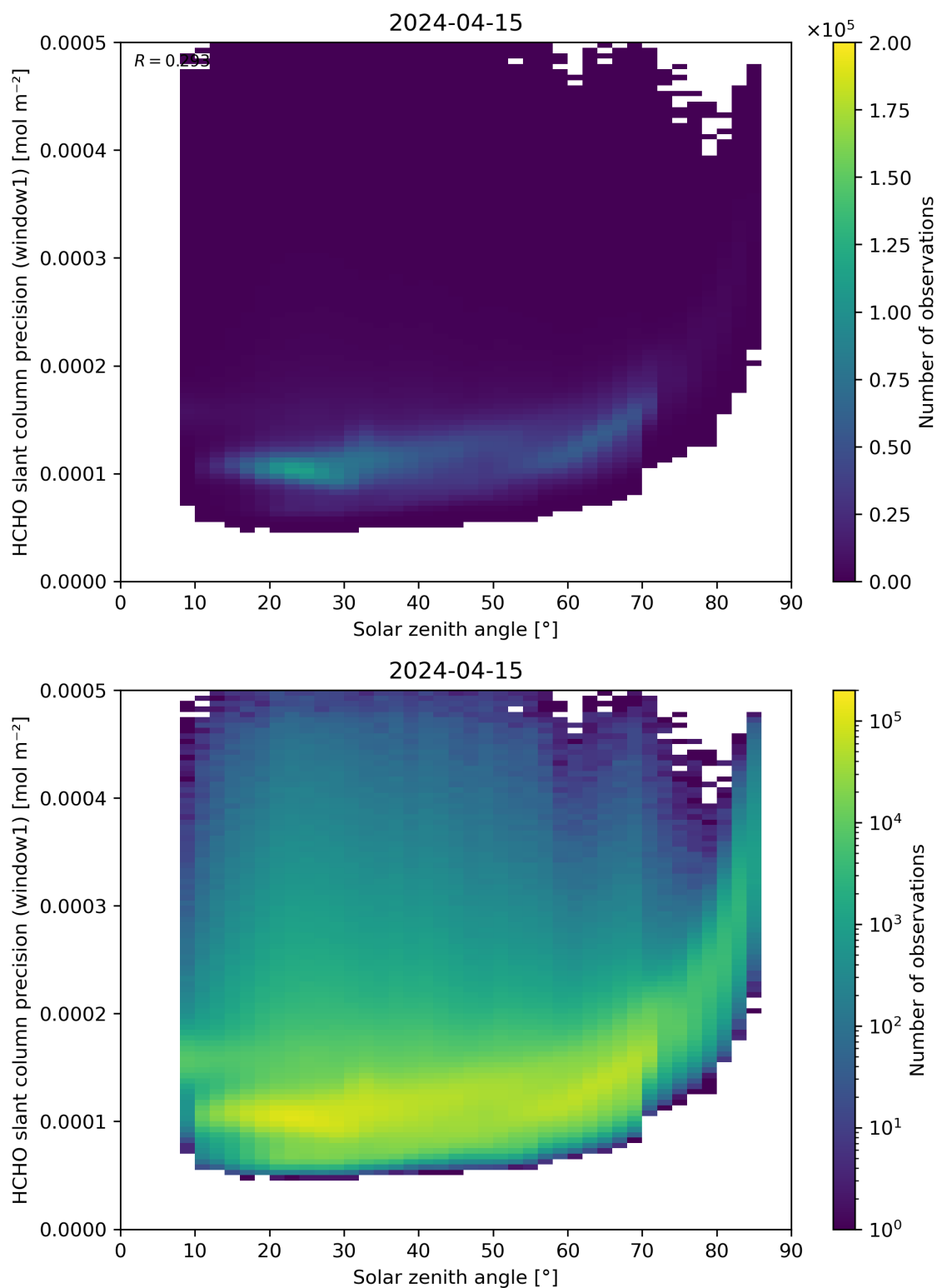
Figure 174: Scatter density plot of “Solar zenith angle” against “HCHO slant column precision (window1)” for 2024-04-15 to 2024-04-16.
