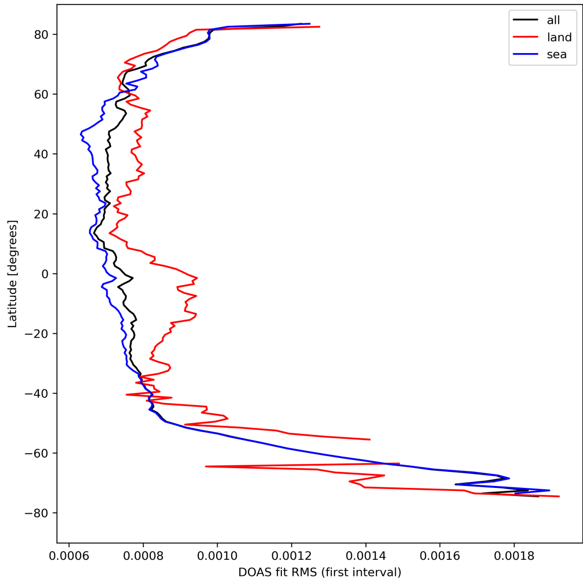
Figure 32: Zonal average of “DOAS fit RMS (first interval)” for 2024-04-15 to 2024-04-16.
