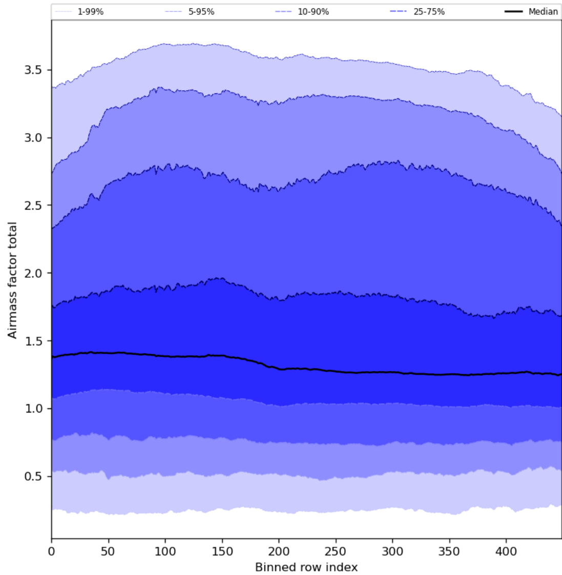
Figure 54: Along track statistics of “Airmass factor total” for 2024-04-15 to 2024-04-16
