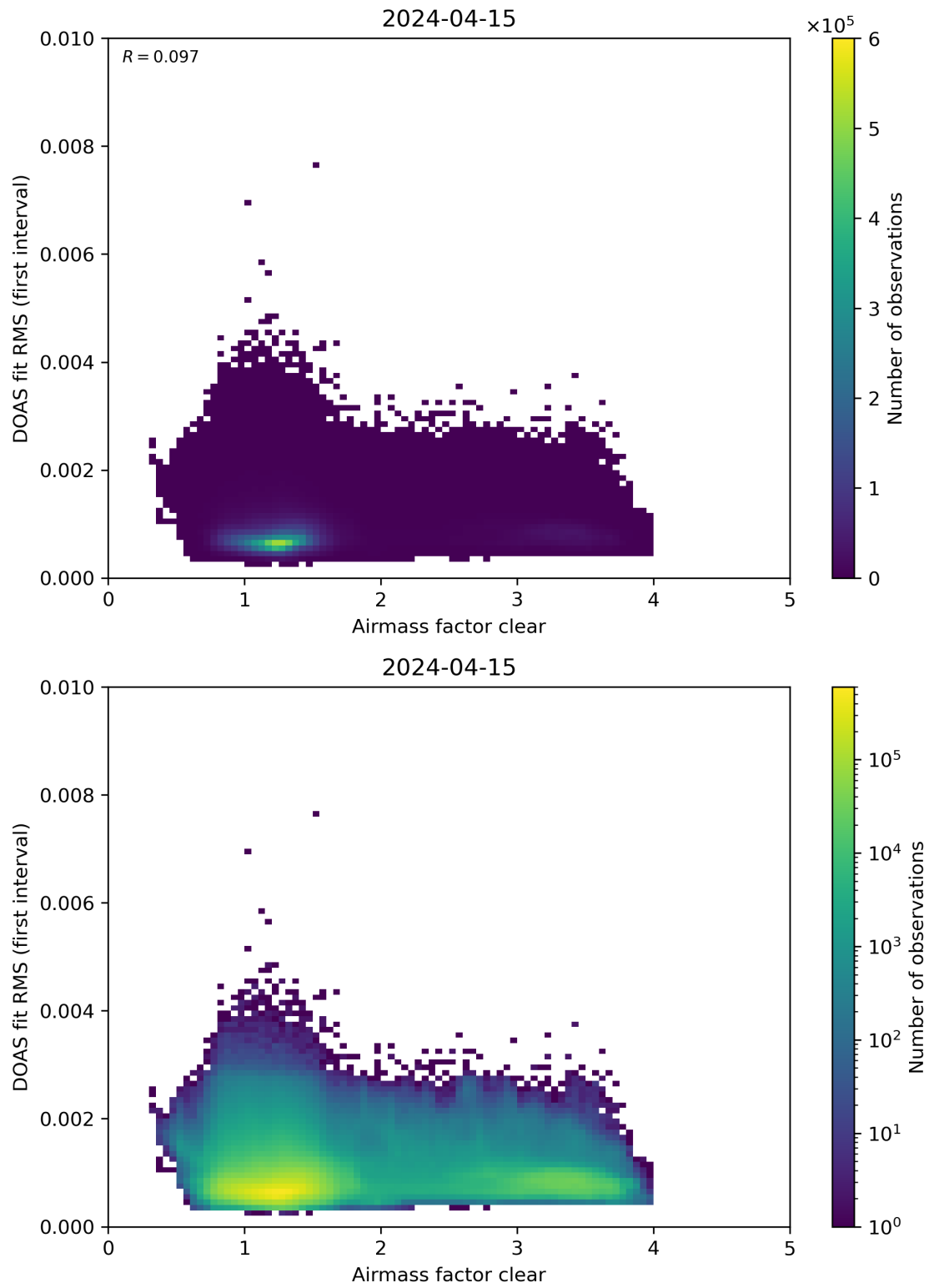
Figure 71: Scatter density plot of “Airmass factor clear” against “DOAS fit RMS (first interval)” for 2024-04-15 to 2024-04-16.
