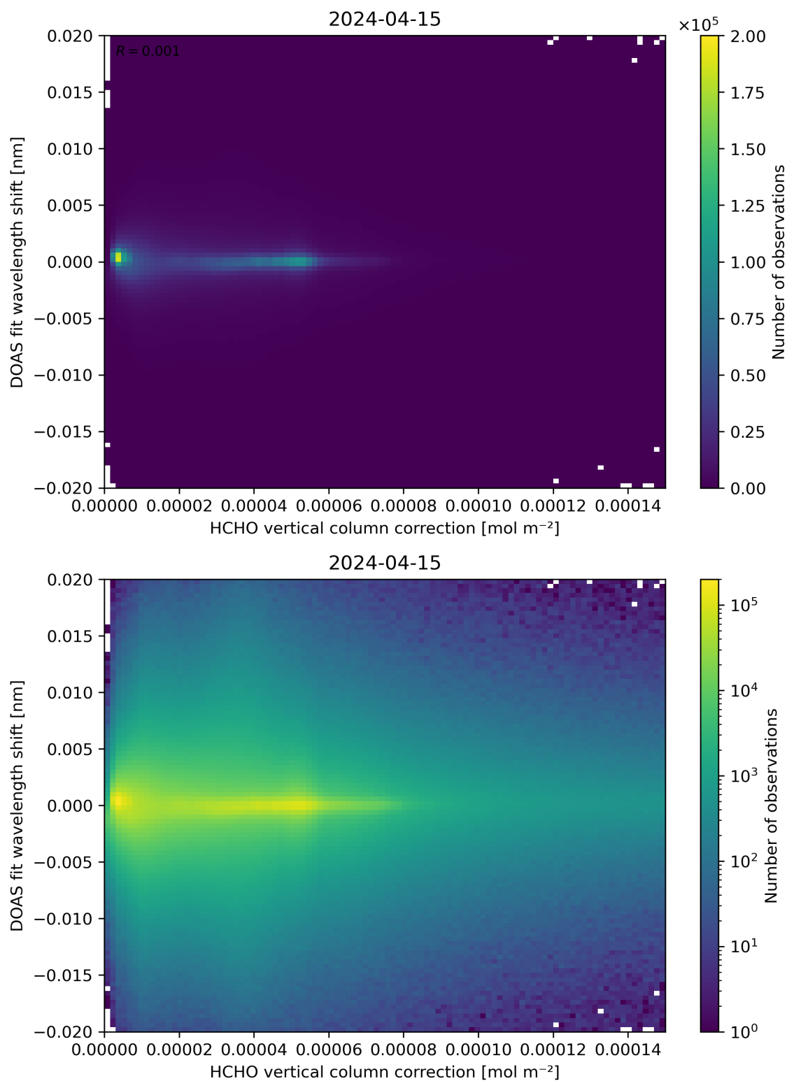
Figure 113: Scatter density plot of “HCHO vertical column correction” against “DOAS fit wavelength shift” for 2024-04-15 to 2024-04-16.
