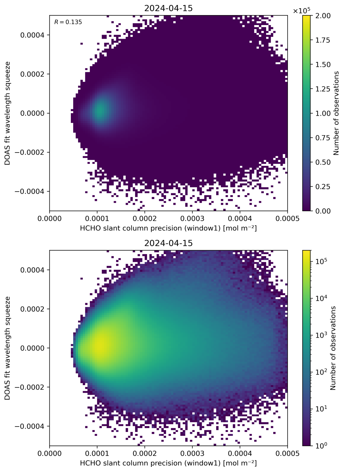
Figure 90: Scatter density plot of “HCHO slant column precision (window1)” against “DOAS fit wavelength squeeze” for 2024-04-15 to 2024-04-16.
