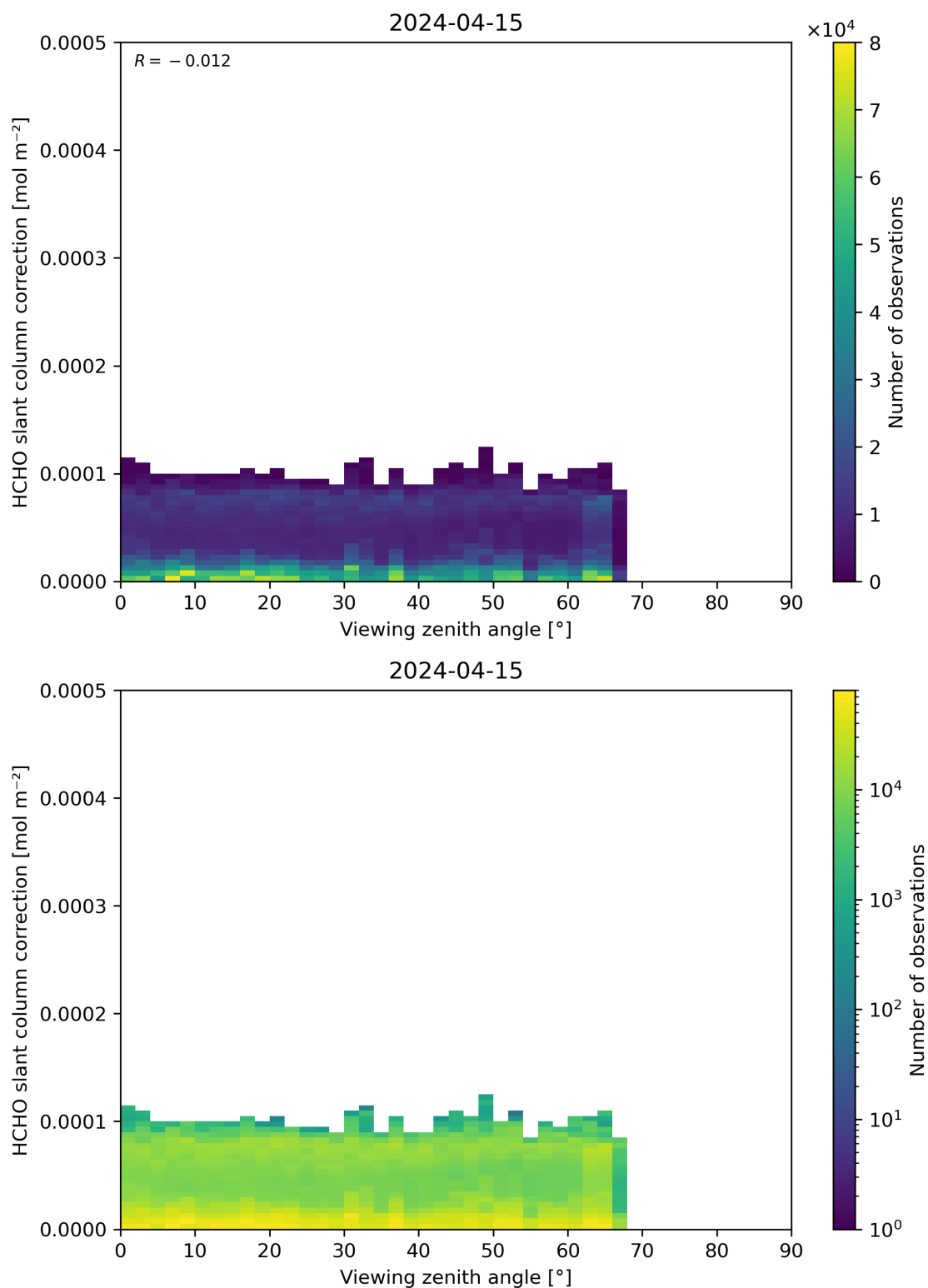
Figure 187: Scatter density plot of “Viewing zenith angle” against “HCHO slant column correction” for 2024-04-15 to 2024-04-16.
