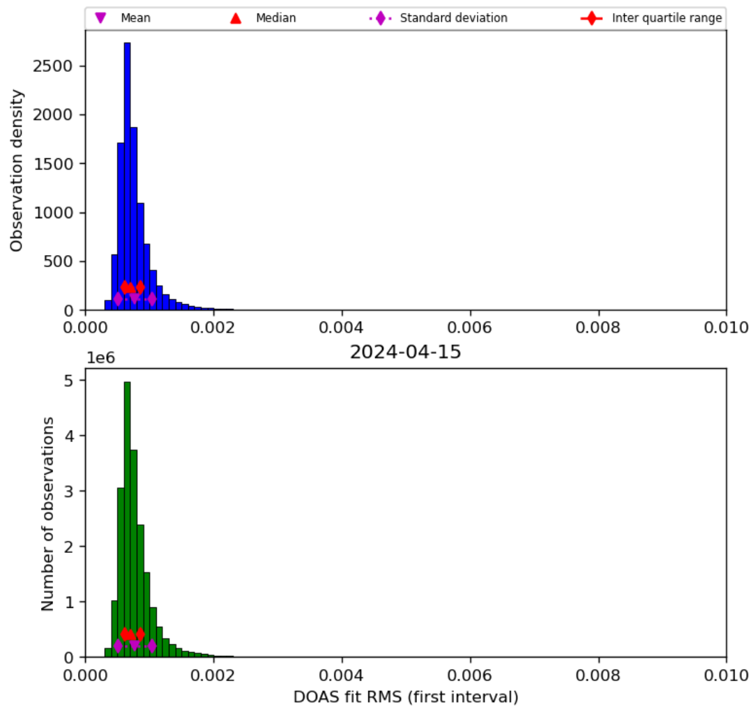
Figure 46: Histogram of “DOAS fit RMS (first interval)” for 2024-04-15 to 2024-04-16
