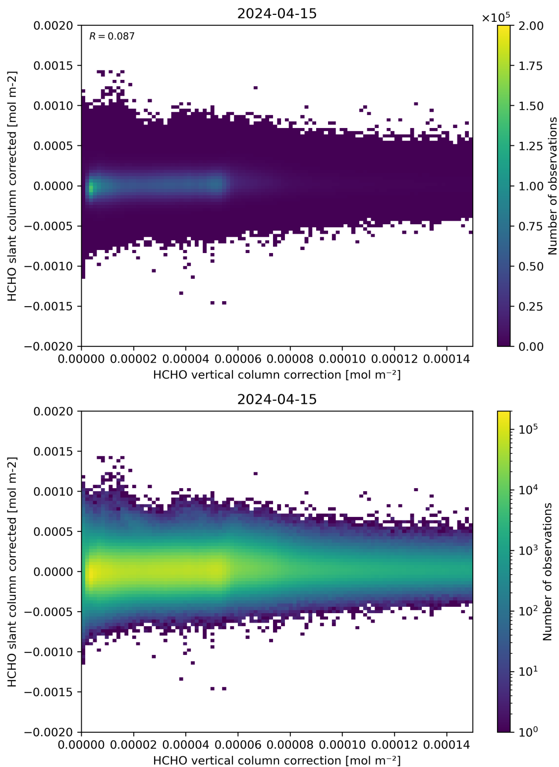
Figure 116: Scatter density plot of “HCHO vertical column correction” against “HCHO slant column corrected” for 2024-04-15 to 2024-04-16.
