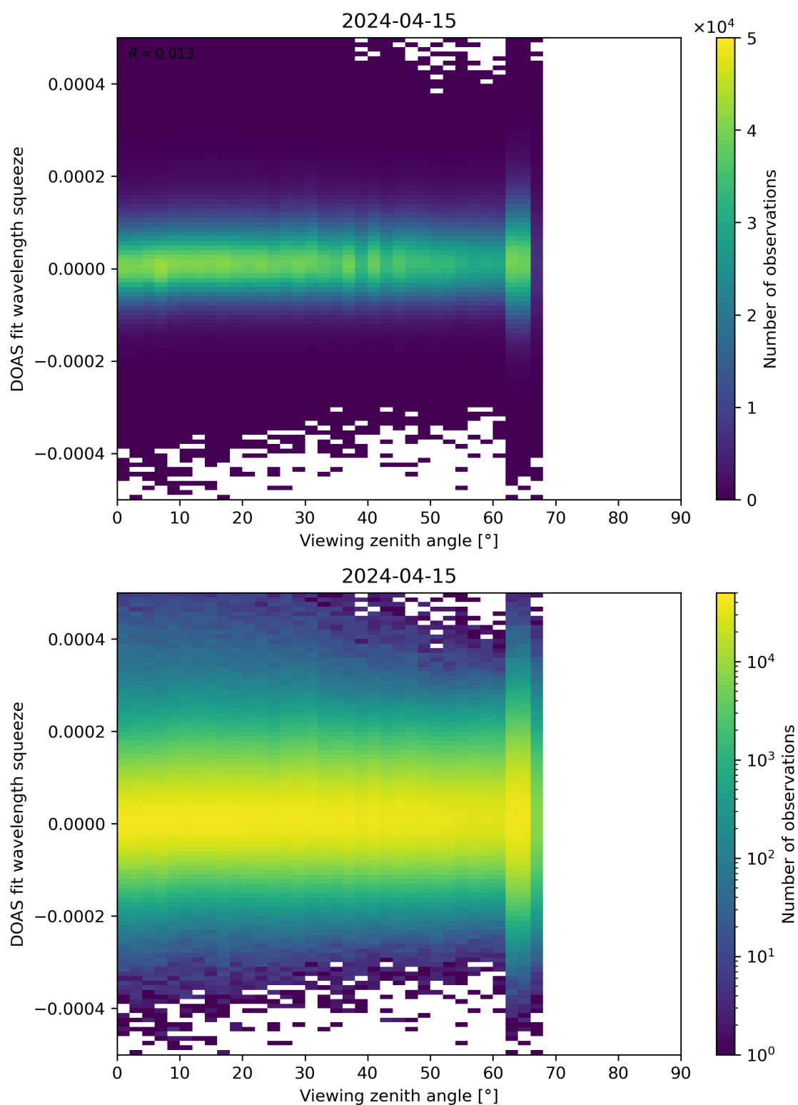
Figure 184: Scatter density plot of “Viewing zenith angle” against “DOAS fit wavelength squeeze” for 2024-04-15 to 2024-04-16.
