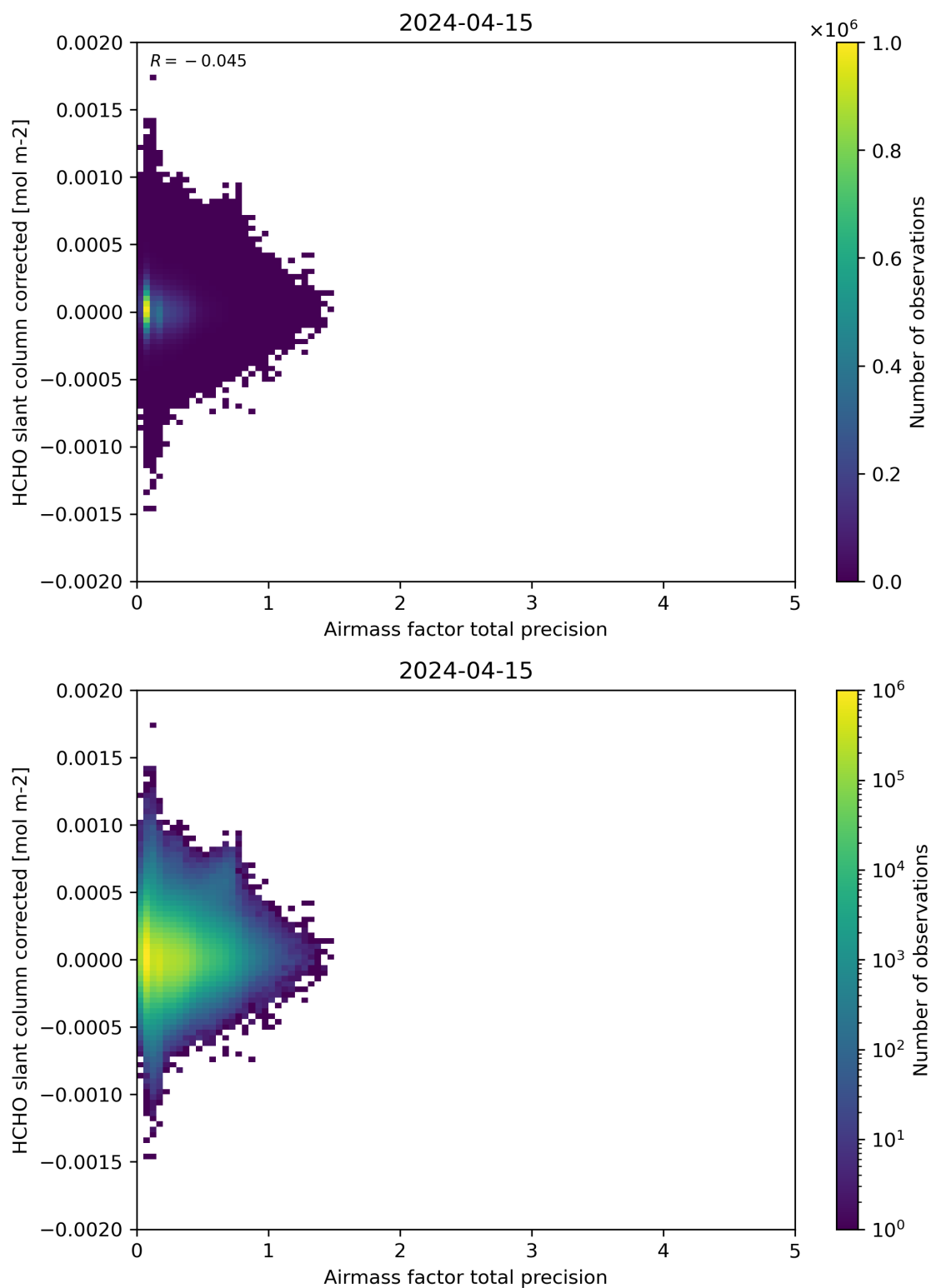
Figure 109: Scatter density plot of “Airmass factor total precision” against “HCHO slant column corrected” for 2024-04-15 to 2024-04-16.
