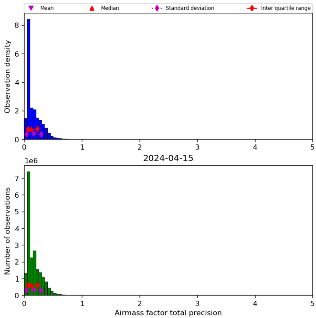
Figure 41: Histogram of “Airmass factor total precision” for 2024-04-15 to 2024-04-16
