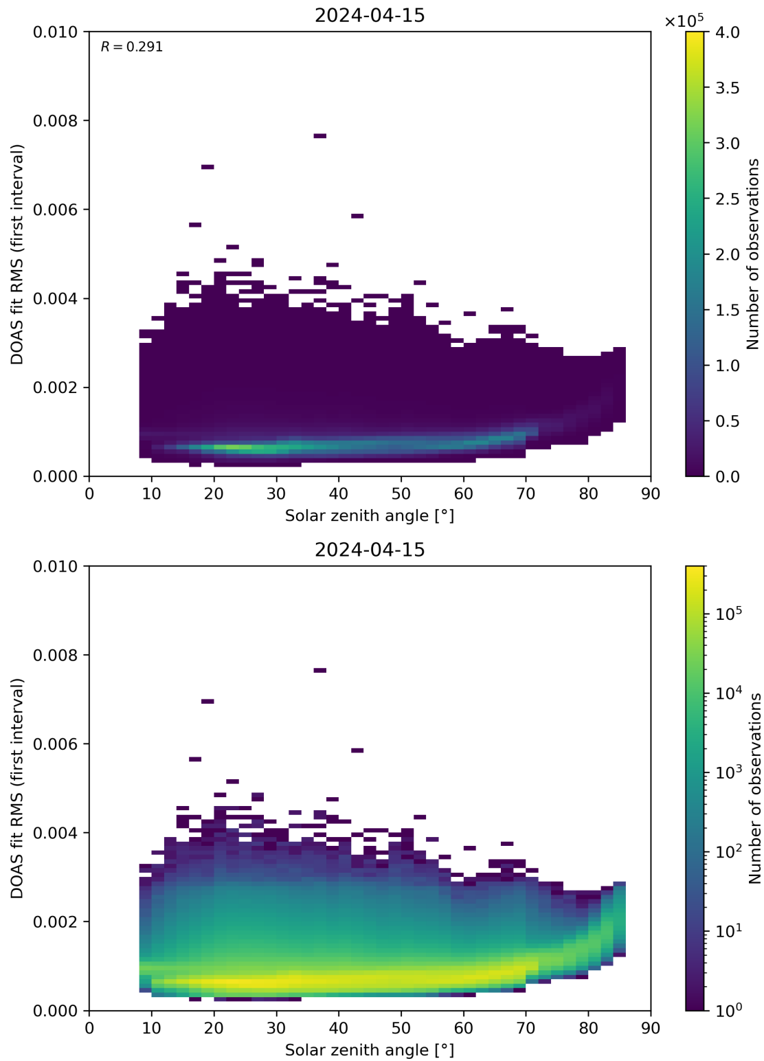
Figure 167: Scatter density plot of “Solar zenith angle” against “DOAS fit RMS (first interval)” for 2024-04-15 to 2024-04-16.
