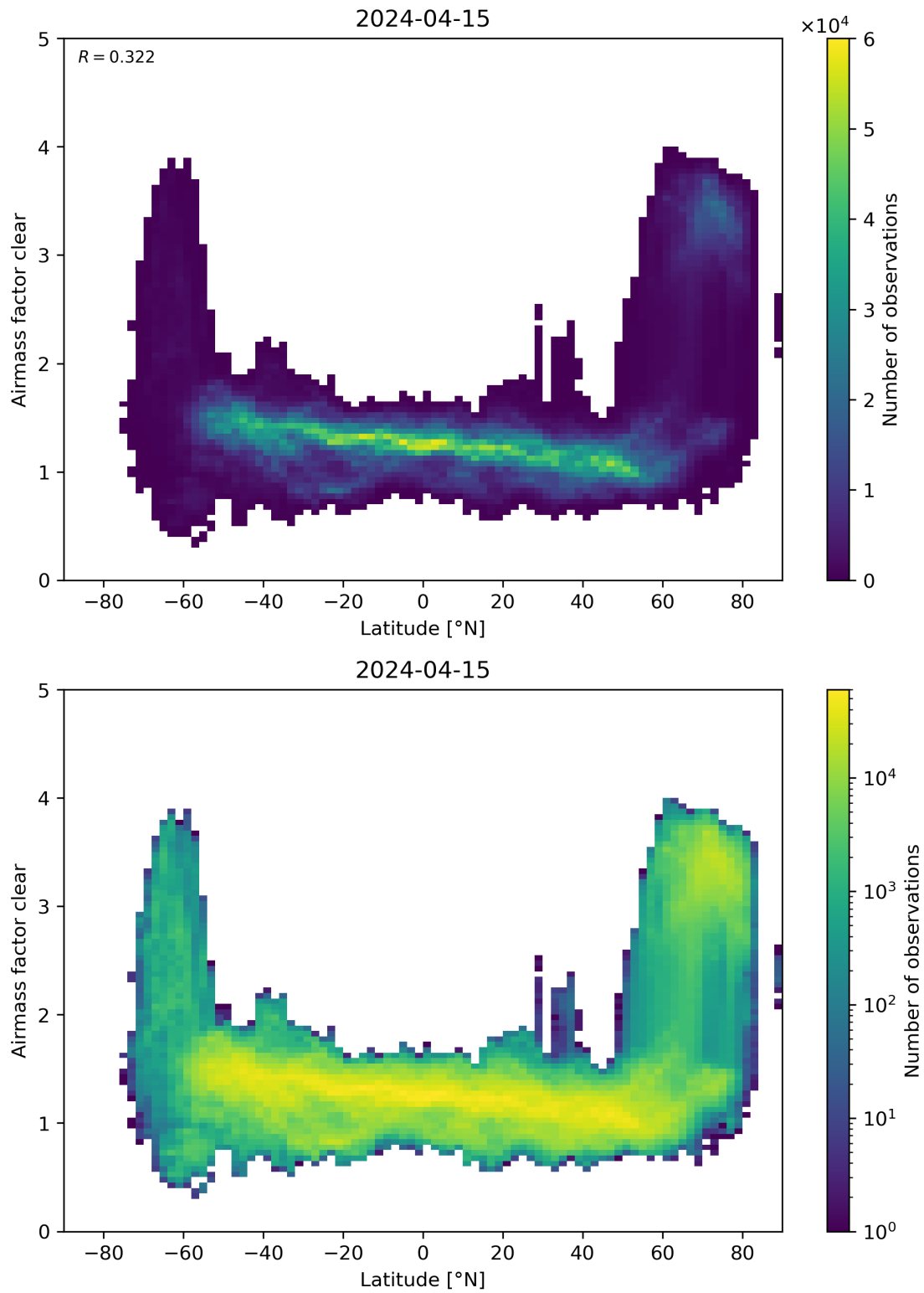
Figure 156: Scatter density plot of “Latitude” against “Airmass factor clear” for 2024-04-15 to 2024-04-16.
