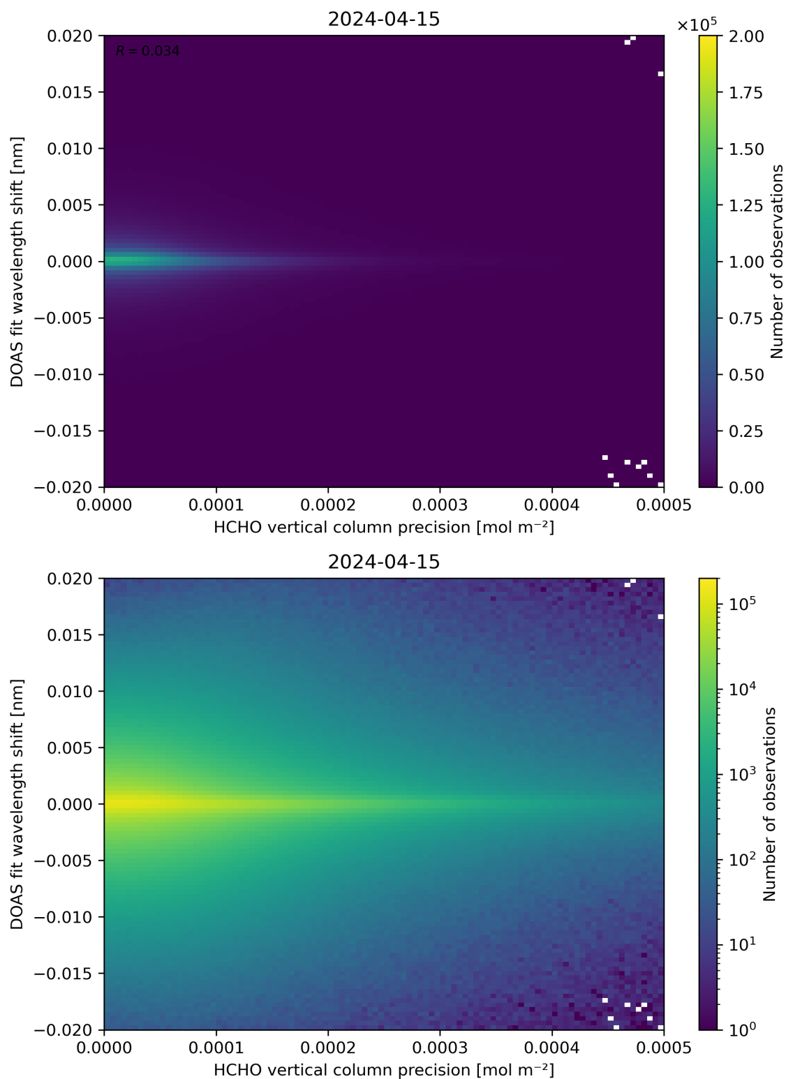
Figure 137: Scatter density plot of “HCHO vertical column precision” against “DOAS fit wavelength shift” for 2024-04-15 to 2024-04-16.
