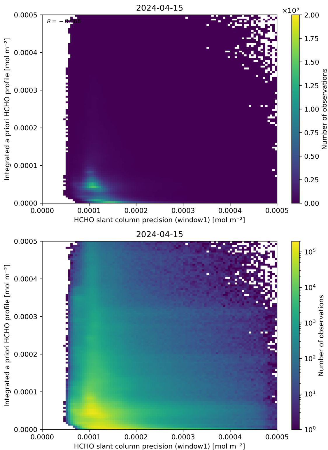
Figure 96: Scatter density plot of “HCHO slant column precision (window1)” against “Integrated a priori HCHO profile” for 2024-04-15 to 2024-04-16.
