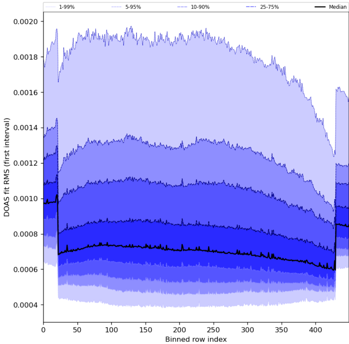
Figure 60: Along track statistics of “DOAS fit RMS (first interval)” for 2024-04-15 to 2024-04-16
