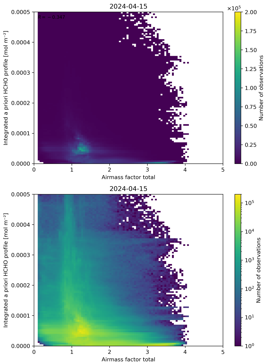
Figure 104: Scatter density plot of “Airmass factor total” against “Integrated a priori HCHO profile” for 2024-04-15 to 2024-04-16.
