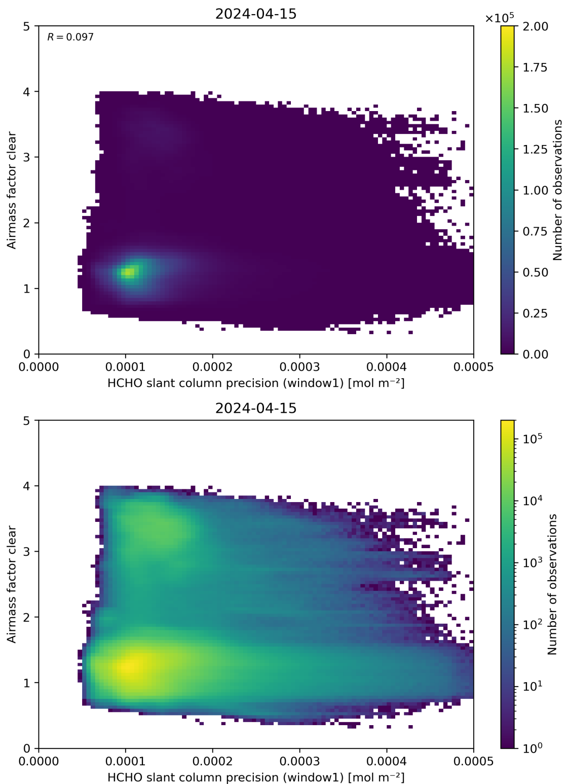
Figure 91: Scatter density plot of “HCHO slant column precision (window1)” against “Airmass factor clear” for 2024-04-15 to 2024-04-16.
