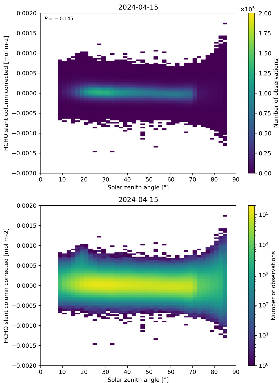
Figure 171: Scatter density plot of “Solar zenith angle” against “HCHO slant column corrected” for 2024-04-15 to 2024-04-16.
