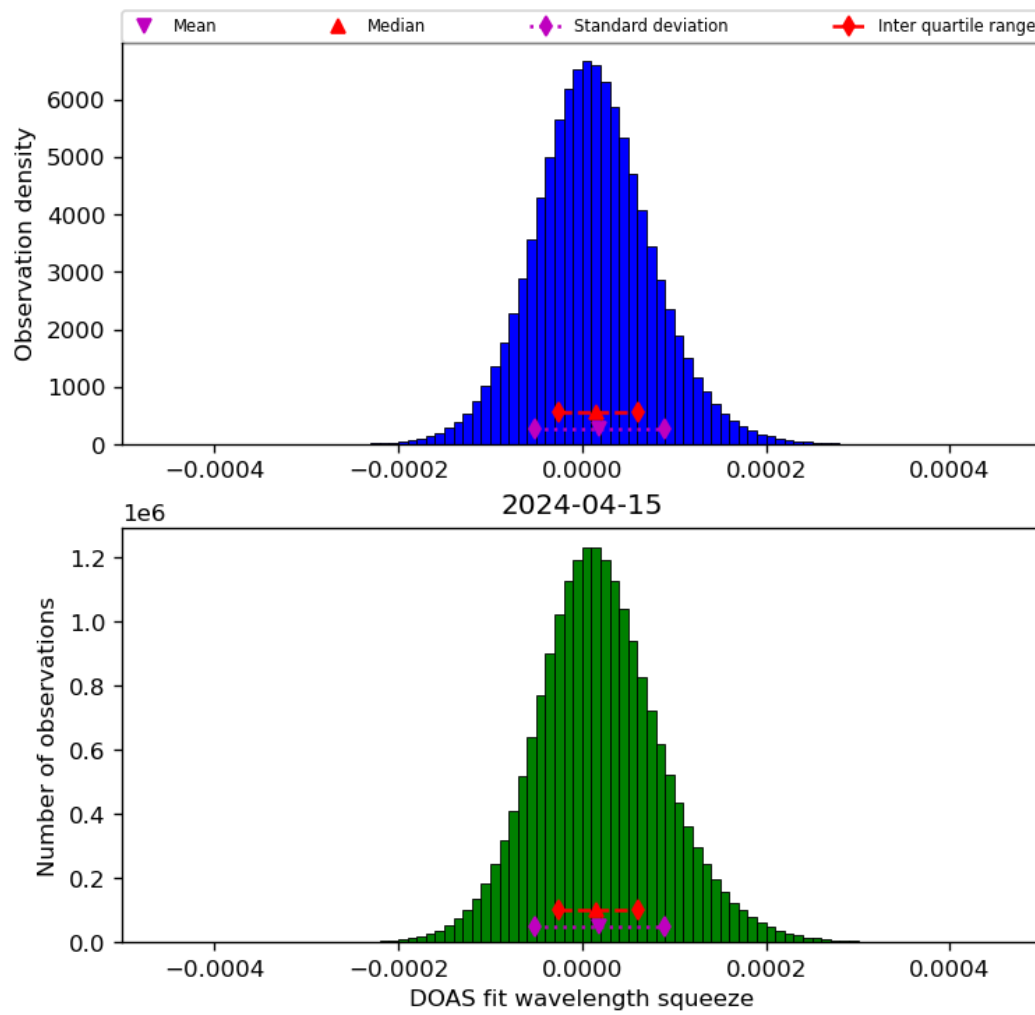
Figure 45: Histogram of “DOAS fit wavelength squeeze” for 2024-04-15 to 2024-04-16
