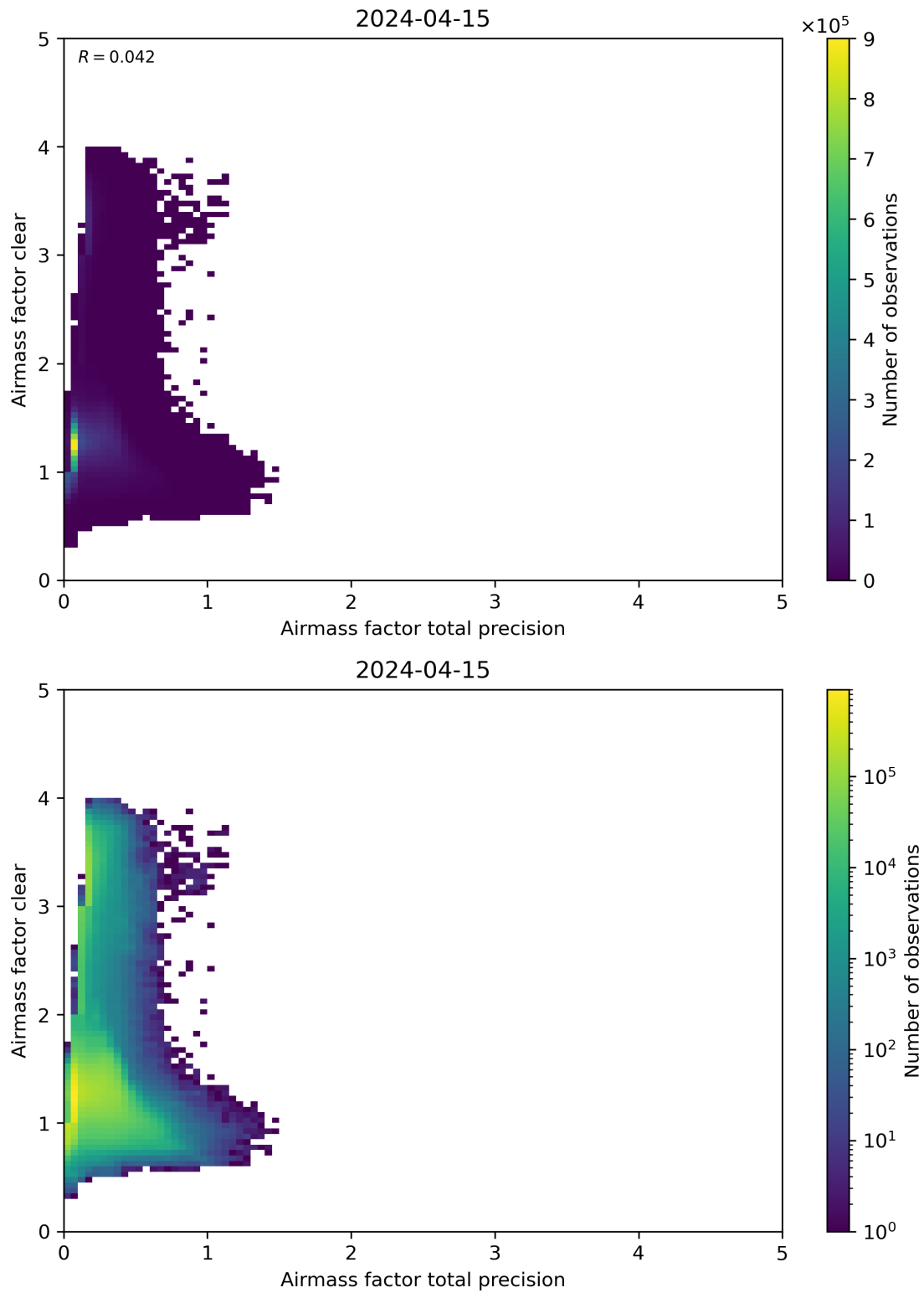
Figure 108: Scatter density plot of “Airmass factor total precision” against “Airmass factor clear” for 2024-04-15 to 2024-04-16.
