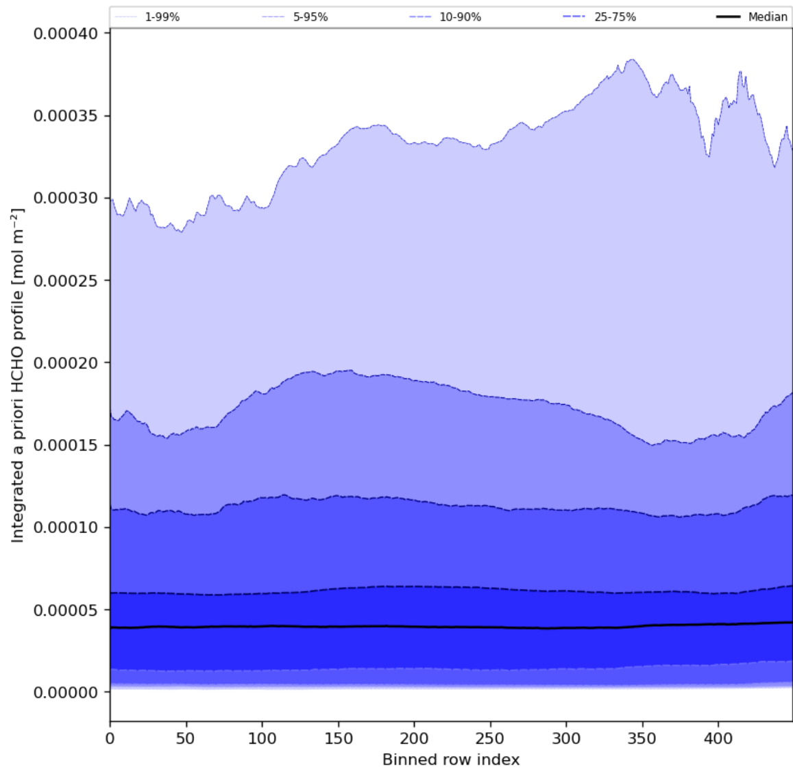
Figure 57: Along track statistics of “Integrated a priori HCHO profile” for 2024-04-15 to 2024-04-16
