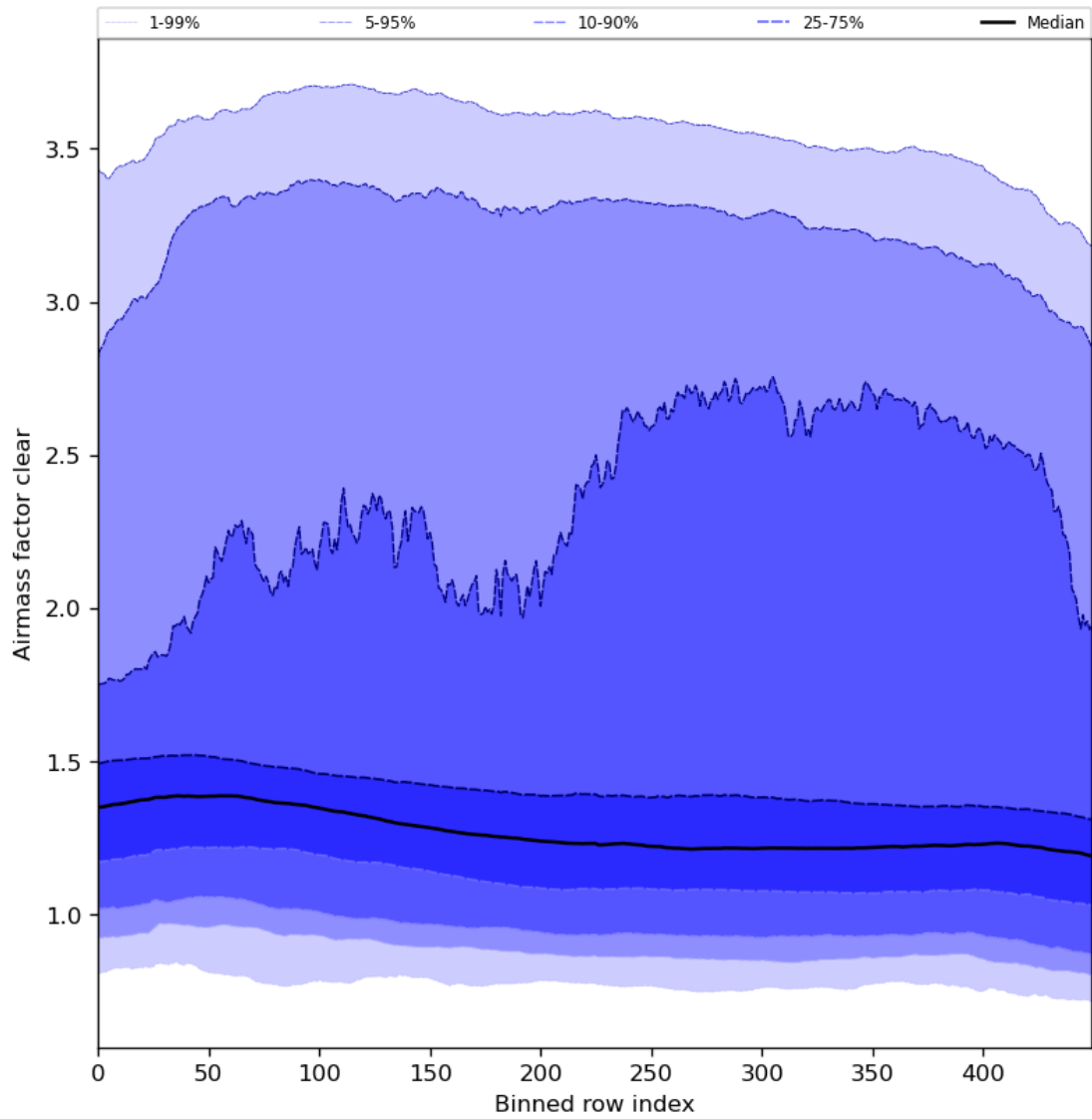
Figure 56: Along track statistics of “Airmass factor clear” for 2024-04-15 to 2024-04-16
