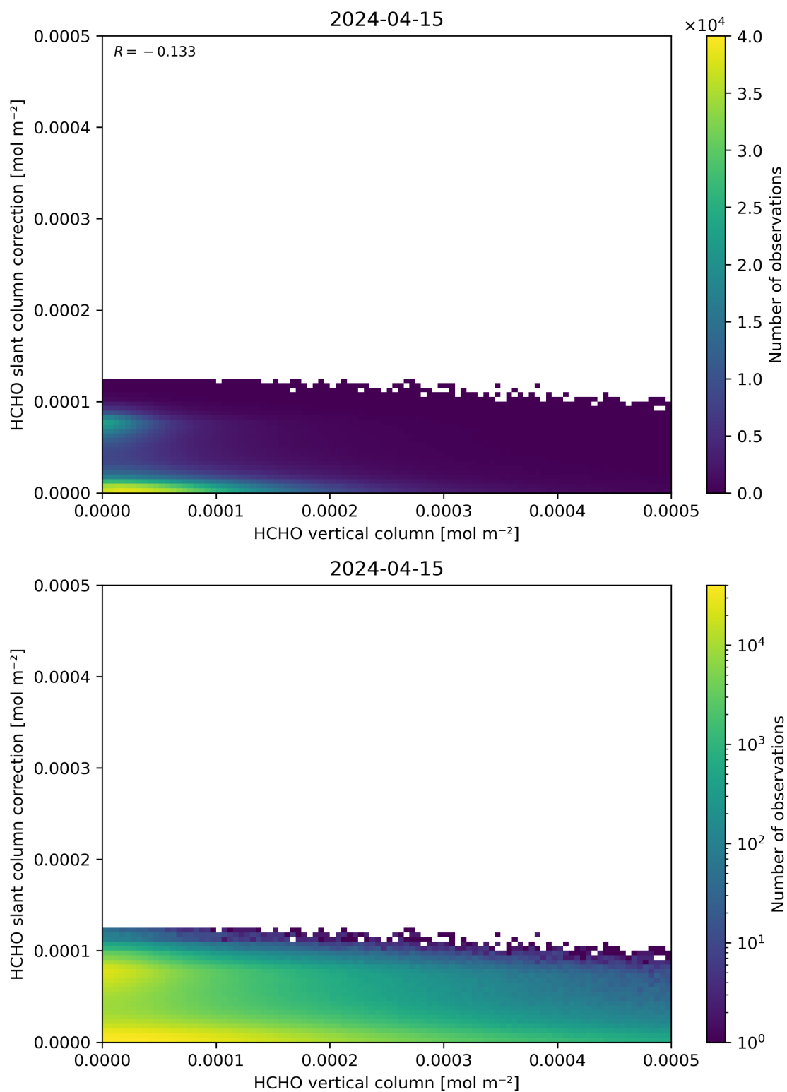
Figure 128: Scatter density plot of “HCHO vertical column” against “HCHO slant column correction” for 2024-04-15 to 2024-04-16.
