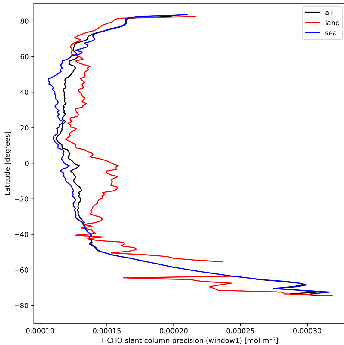
Figure 25: Zonal average of “HCHO slant column precision (window1)” for 2024-04-15 to 2024-04-16.
