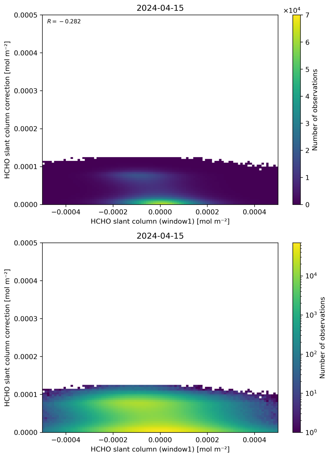
Figure 83: Scatter density plot of “HCHO slant column (window1)” against “HCHO slant column correction” for 2024-04-15 to 2024-04-16.
