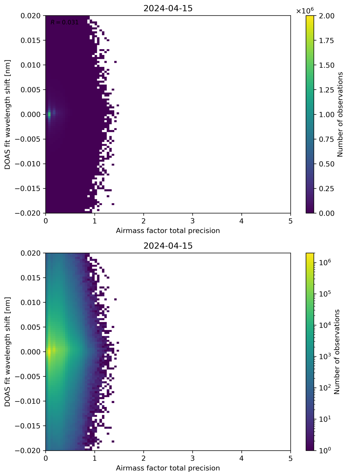
Figure 106: Scatter density plot of “Airmass factor total precision” against “DOAS fit wavelength shift” for 2024-04-15 to 2024-04-16.
