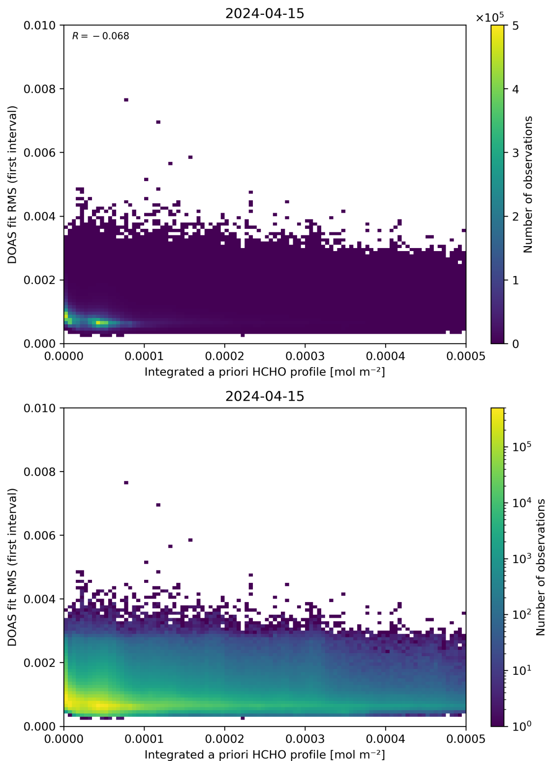
Figure 148: Scatter density plot of “Integrated a priori HCHO profile” against “DOAS fit RMS (first interval)” for 2024-04-15 to 2024-04-16.
