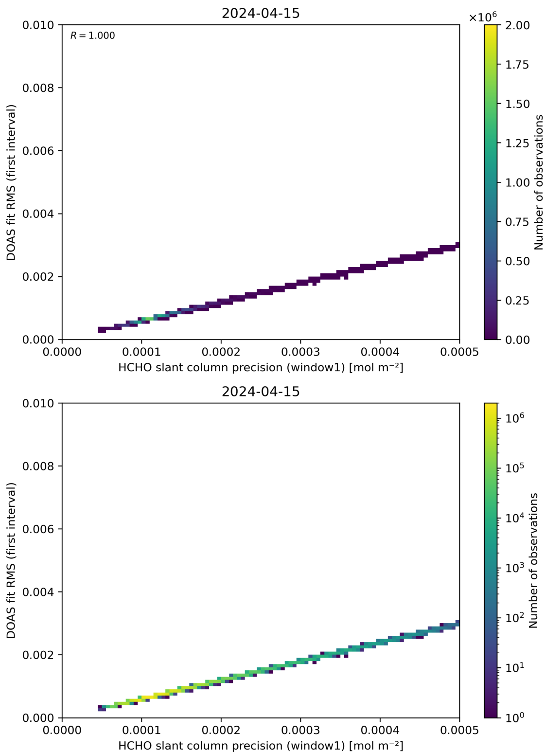
Figure 88: Scatter density plot of “HCHO slant column precision (window1)” against “DOAS fit RMS (first interval)” for 2024-04-15 to 2024-04-16.
