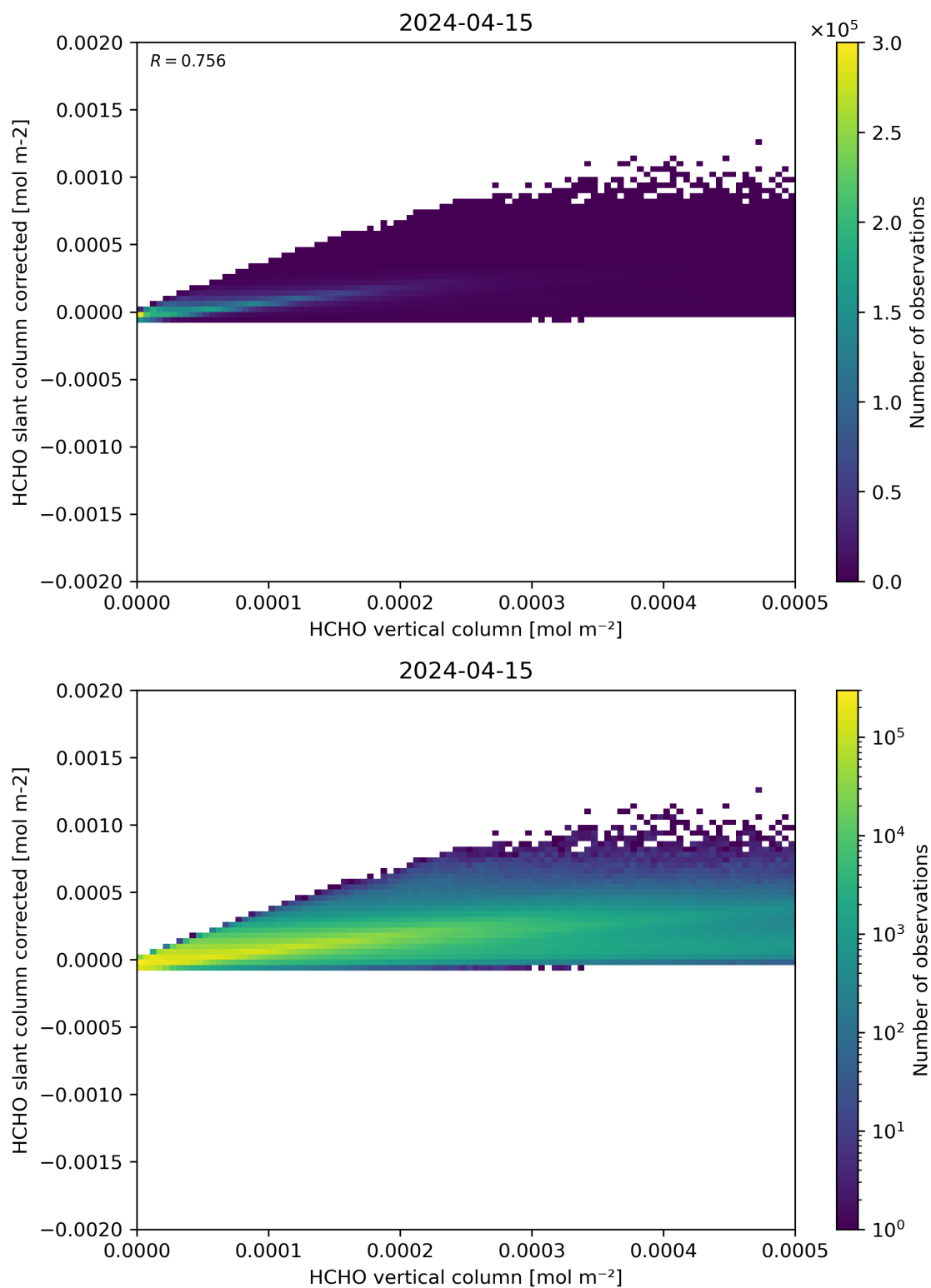
Figure 127: Scatter density plot of “HCHO vertical column” against “HCHO slant column corrected” for 2024-04-15 to 2024-04-16.
