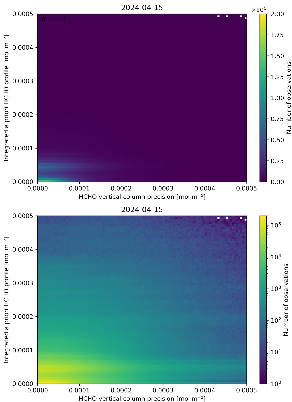
Figure 147: Scatter density plot of “HCHO vertical column precision” against “Integrated a priori HCHO profile” for 2024-04-15 to 2024-04-16.
