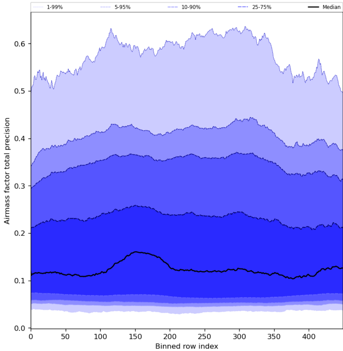
Figure 55: Along track statistics of “Airmass factor total precision” for 2024-04-15 to 2024-04-16
