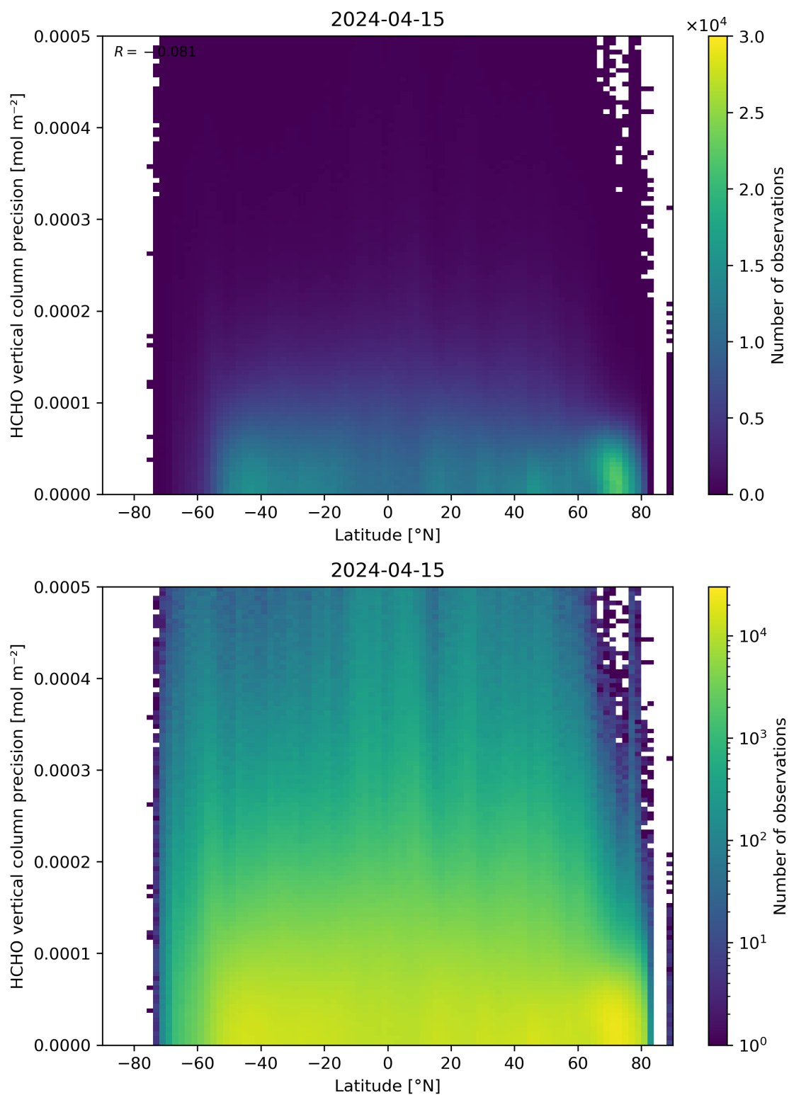
Figure 165: Scatter density plot of “Latitude” against “HCHO vertical column precision” for 2024-04-15 to 2024-04-16.
