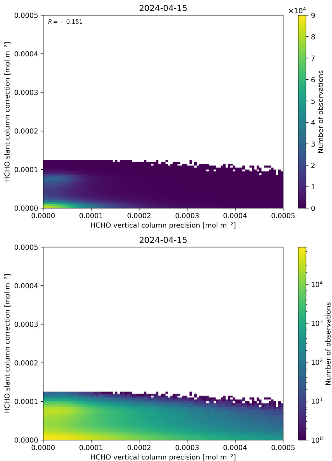
Figure 141: Scatter density plot of “HCHO vertical column precision” against “HCHO slant column correction” for 2024-04-15 to 2024-04-16.
