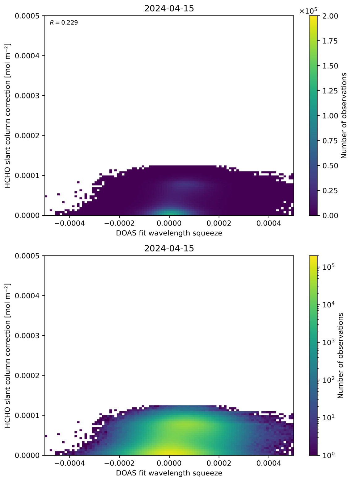
Figure 70: Scatter density plot of “DOAS fit wavelength squeeze” against “HCHO slant column correction” for 2024-04-15 to 2024-04-16.
