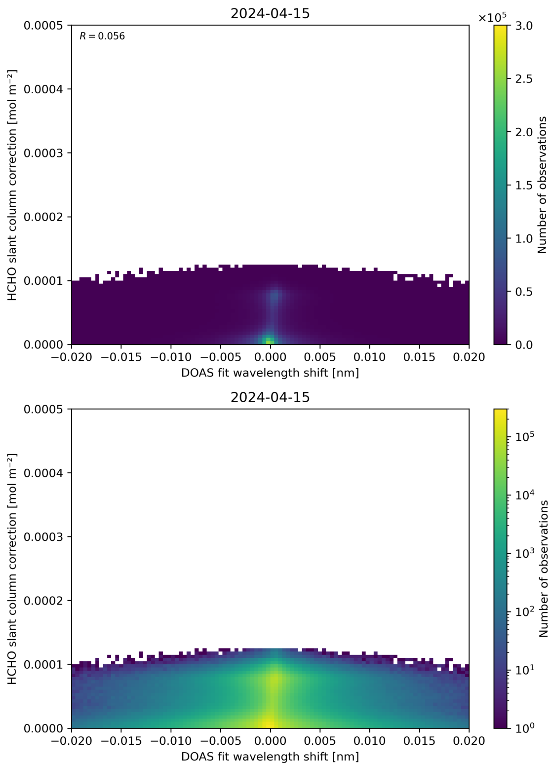
Figure 67: Scatter density plot of “DOAS fit wavelength shift” against “HCHO slant column correction” for 2024-04-15 to 2024-04-16.
