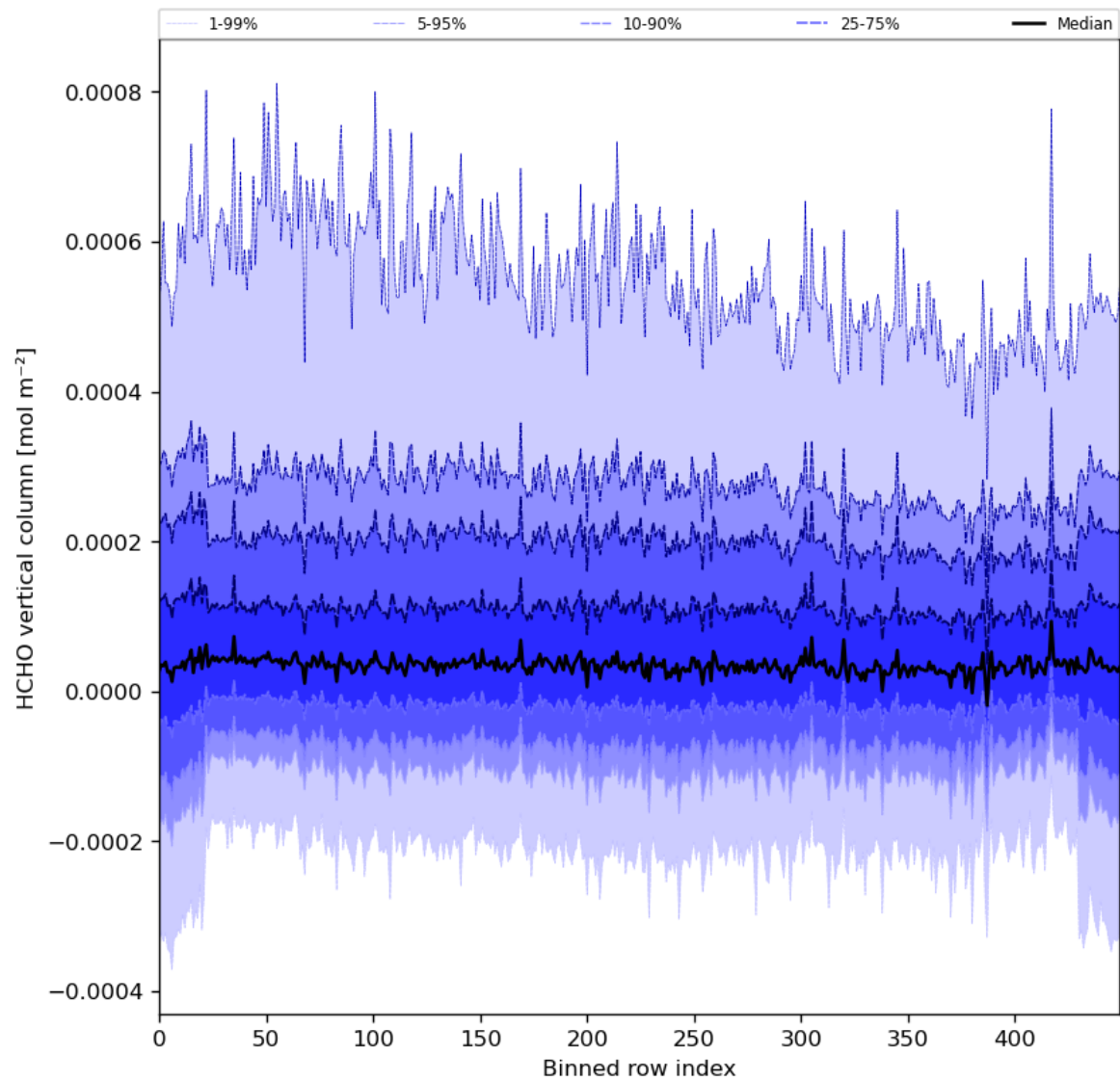
Figure 49: Along track statistics of “HCHO vertical column” for 2024-04-15 to 2024-04-16
