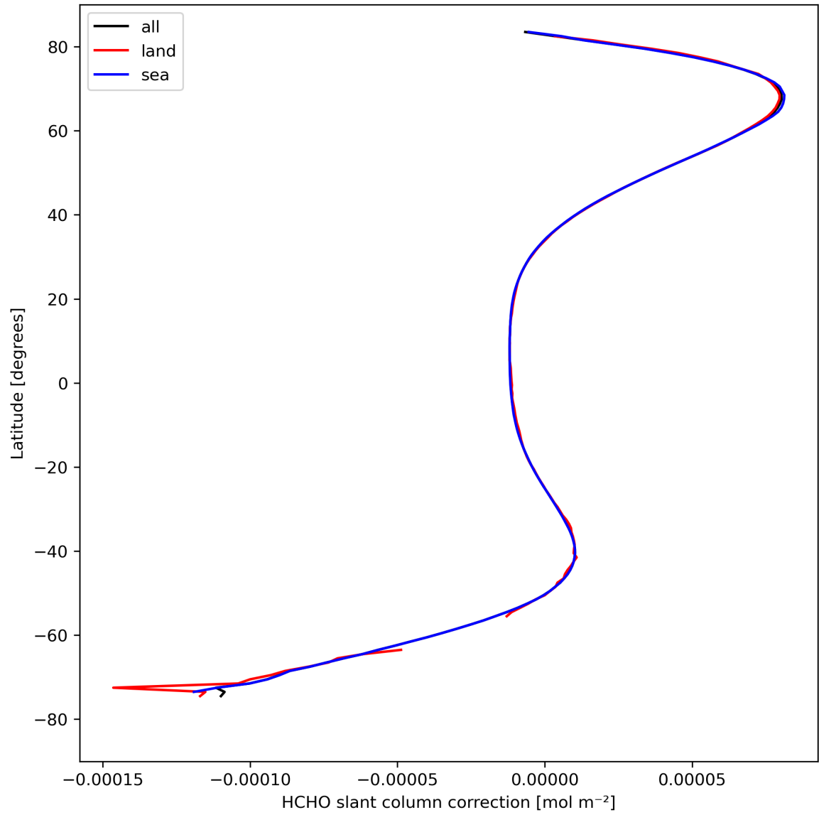
Figure 33: Zonal average of "HCHO slant column correction" for 2024-04-15 to 2024-04-16.
