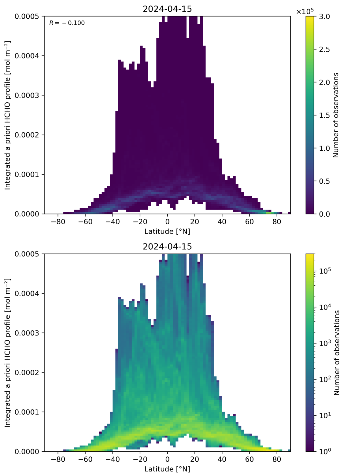
Figure 166: Scatter density plot of “Latitude” against “Integrated a priori HCHO profile” for 2024-04-15 to 2024-04-16.
