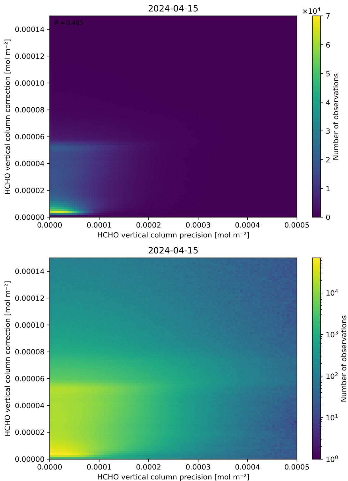
Figure 146: Scatter density plot of “HCHO vertical column precision” against “HCHO vertical column correction” for 2024-04-15 to 2024-04-16.
