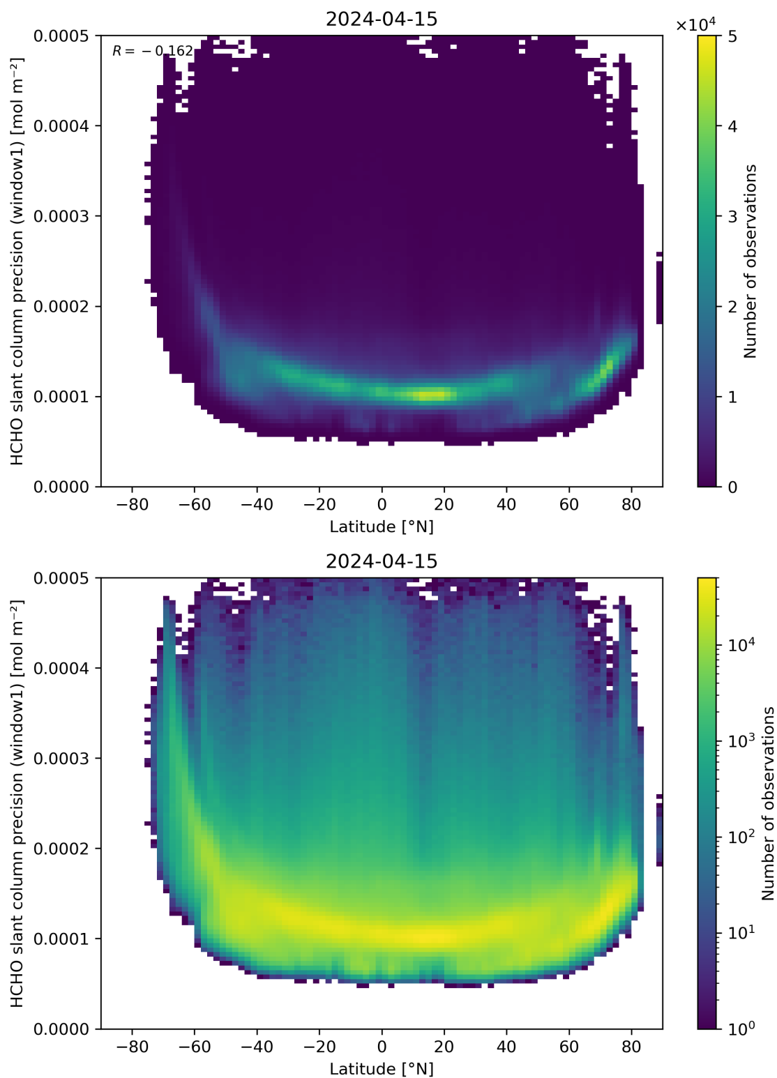
Figure 160: Scatter density plot of “Latitude” against “HCHO slant column precision (window1)” for 2024-04-15 to 2024-04-16.
