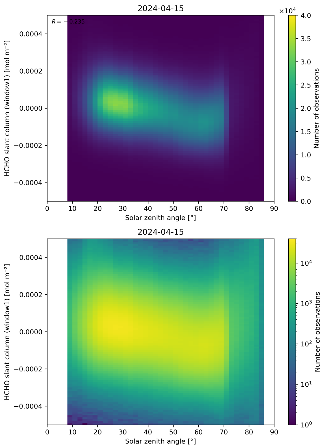
Figure 173: Scatter density plot of “Solar zenith angle” against “HCHO slant column (window1)” for 2024-04-15 to 2024-04-16.
