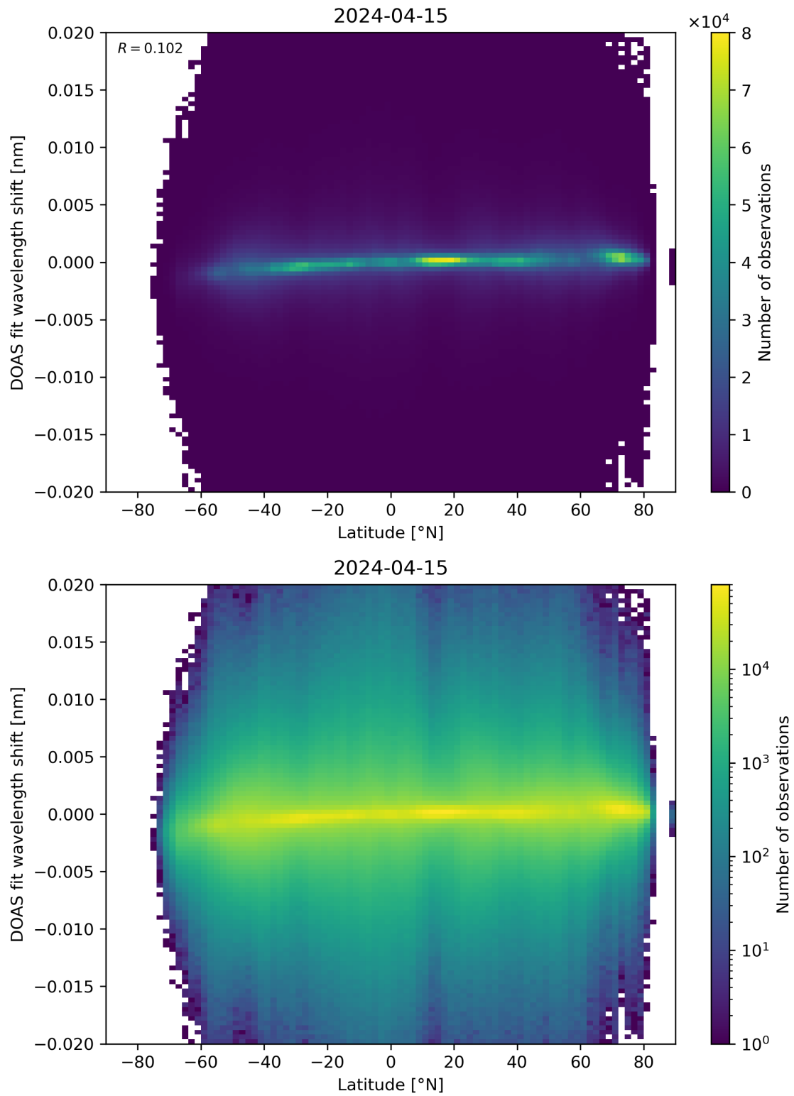
Figure 154: Scatter density plot of “Latitude” against “DOAS fit wavelength shift” for 2024-04-15 to 2024-04-16.
