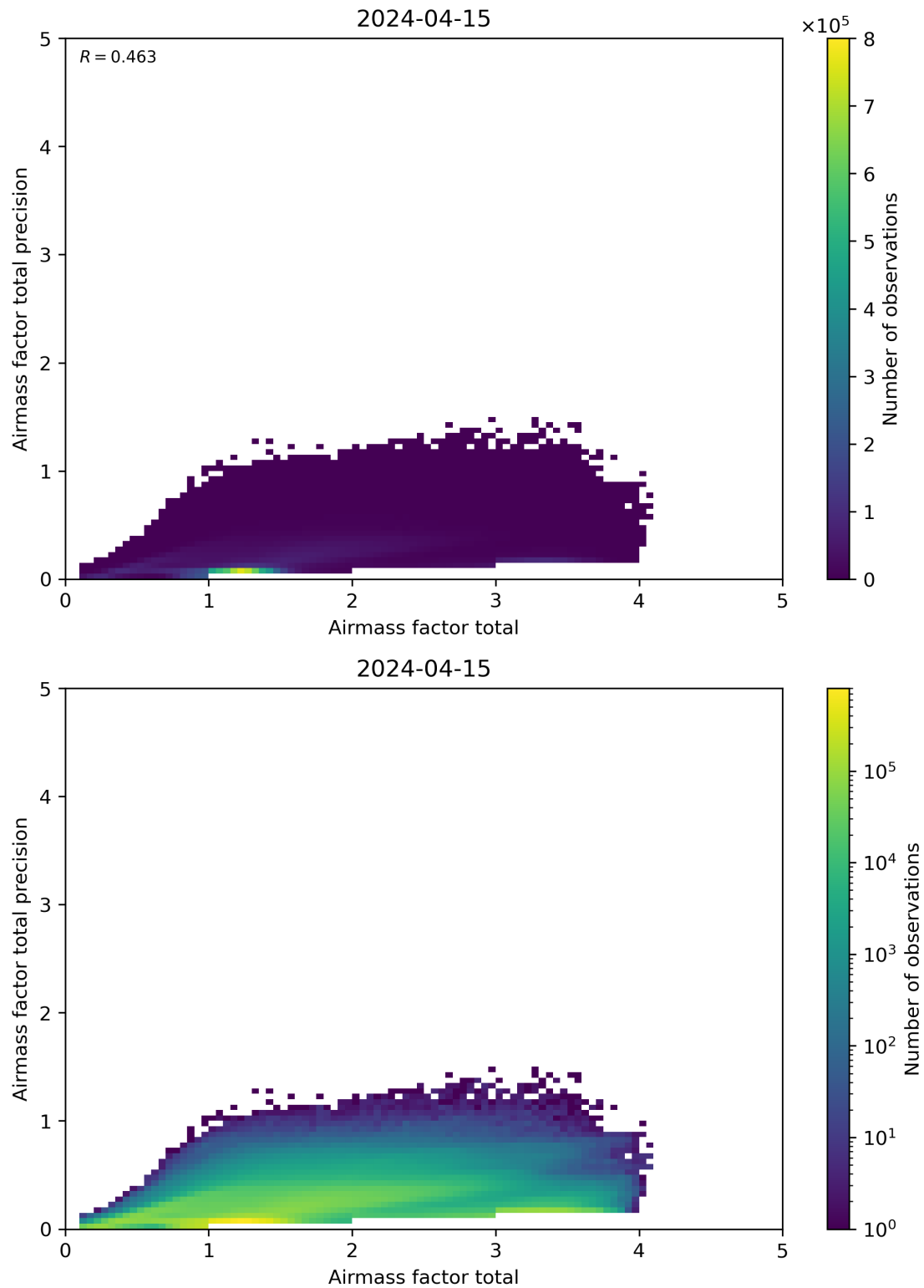
Figure 103: Scatter density plot of “Airmass factor total” against “Airmass factor total precision” for 2024-04-15 to 2024-04-16.
