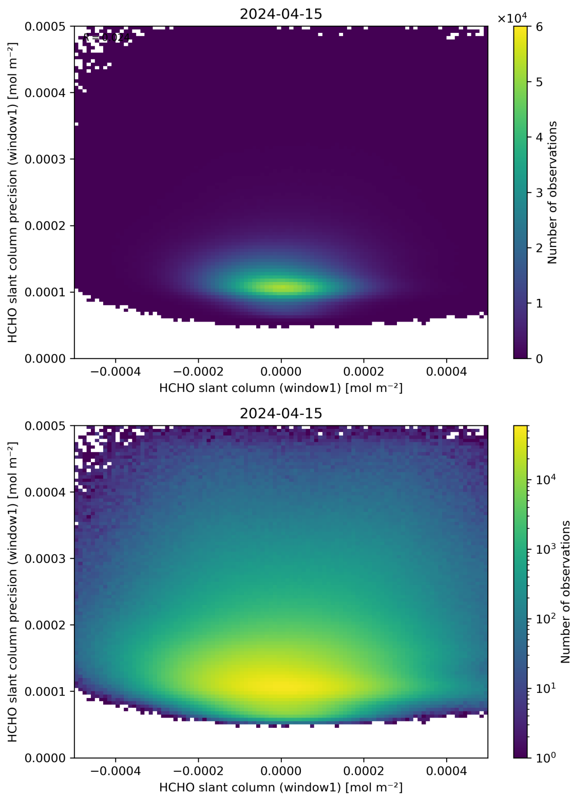
Figure 84: Scatter density plot of “HCHO slant column (window1)” against “HCHO slant column precision (window1)” for 2024-04-15 to 2024-04-16.
