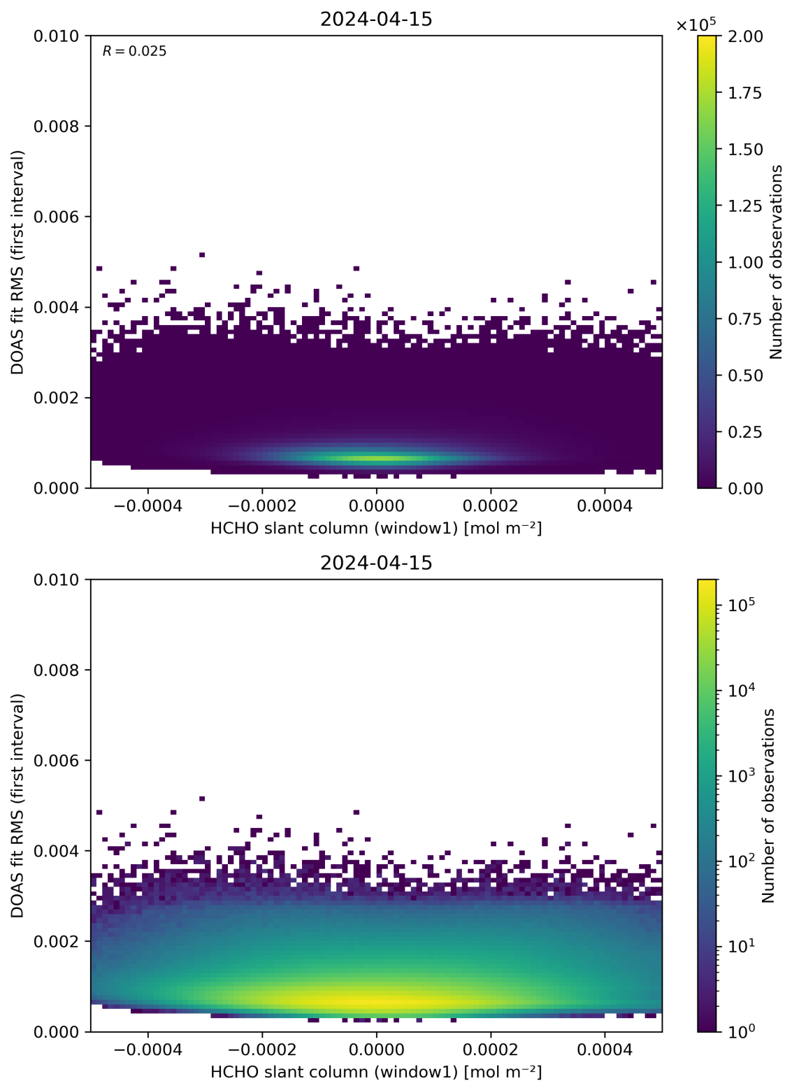
Figure 78: Scatter density plot of “HCHO slant column (window1)” against “DOAS fit RMS (first interval)” for 2024-04-15 to 2024-04-16.
