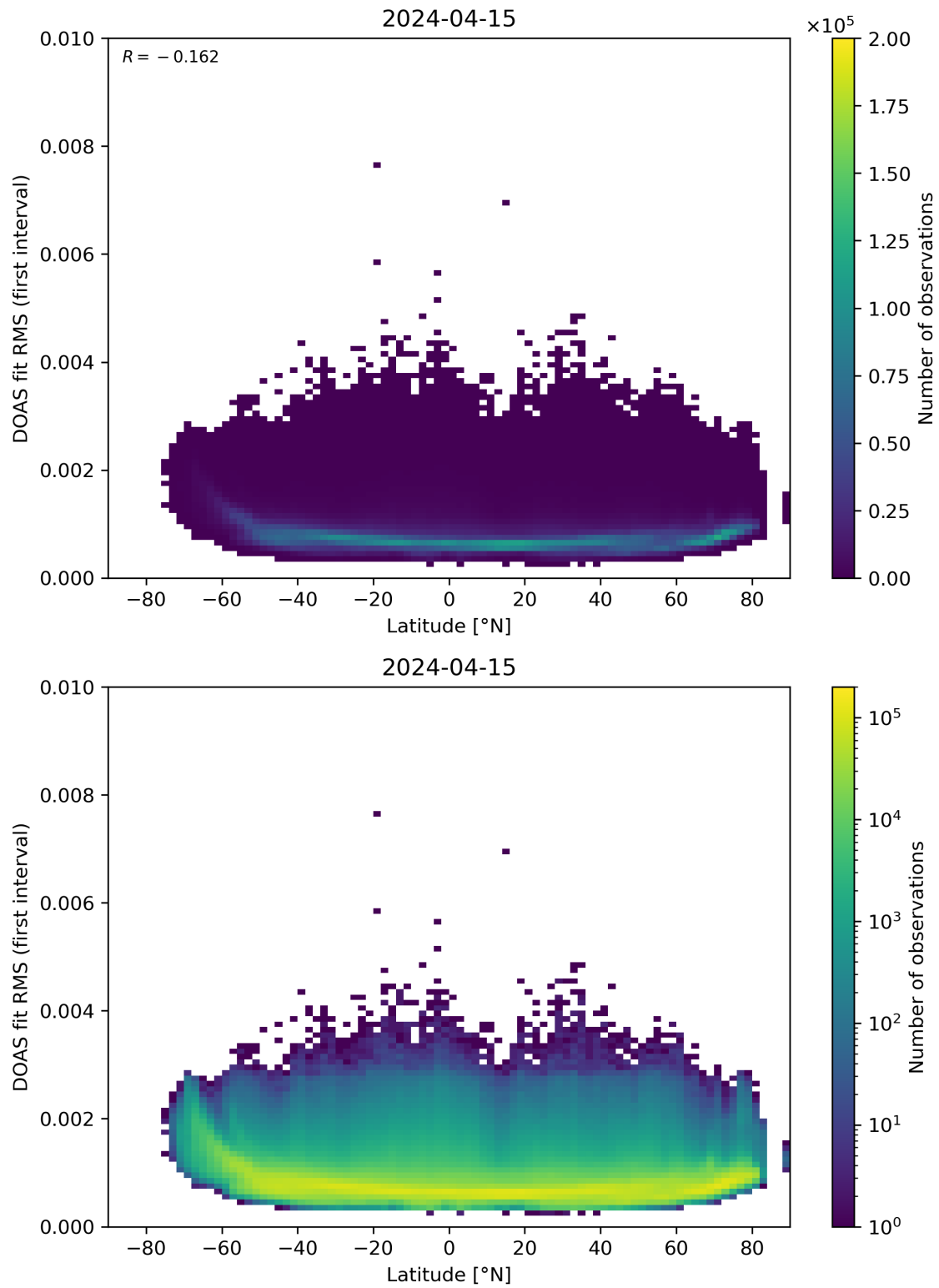
Figure 153: Scatter density plot of “Latitude” against “DOAS fit RMS (first interval)” for 2024-04-15 to 2024-04-16.
