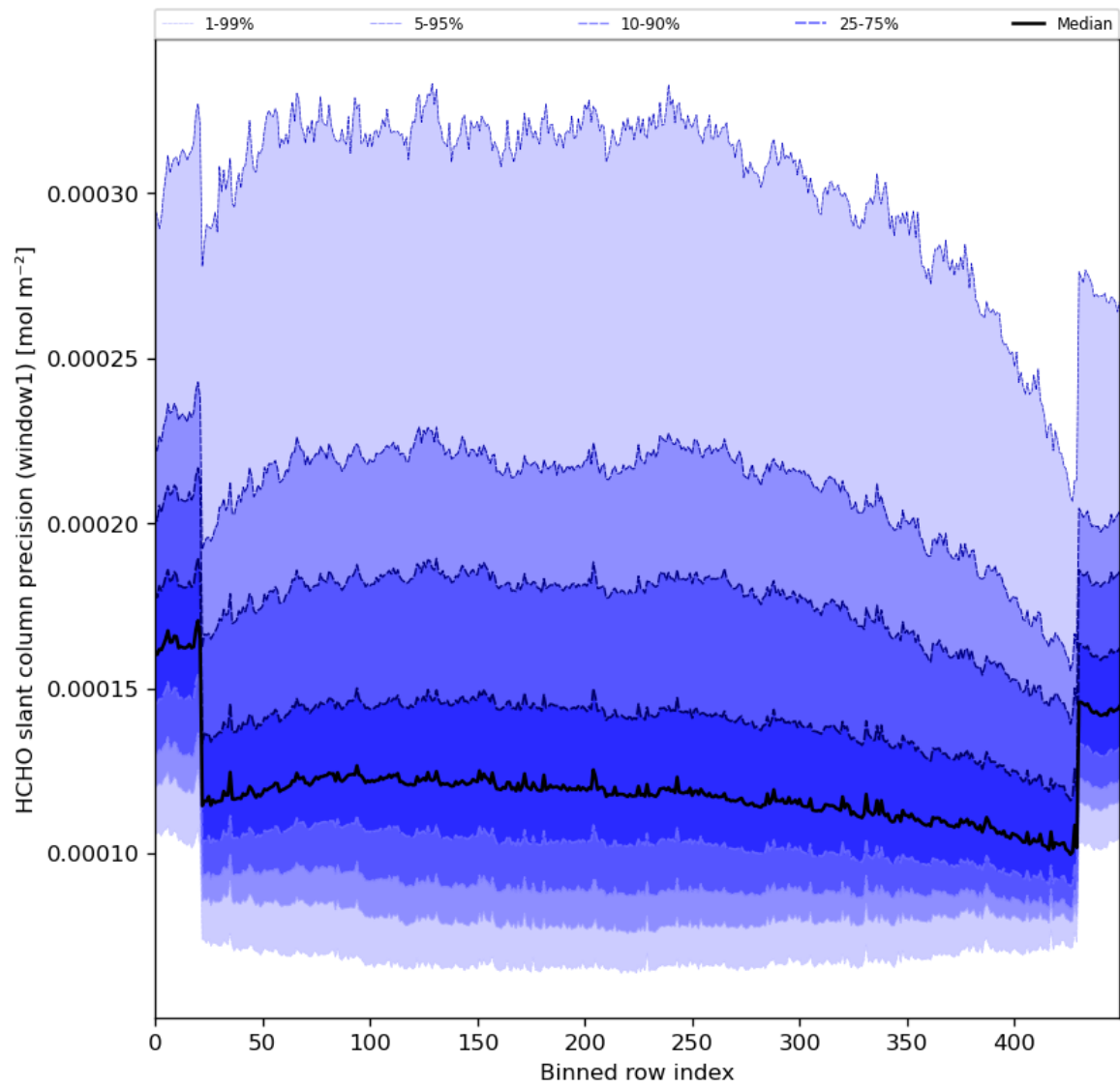
Figure 53: Along track statistics of “HCHO slant column precision (window1)” for 2024-04-15 to 2024-04-16
