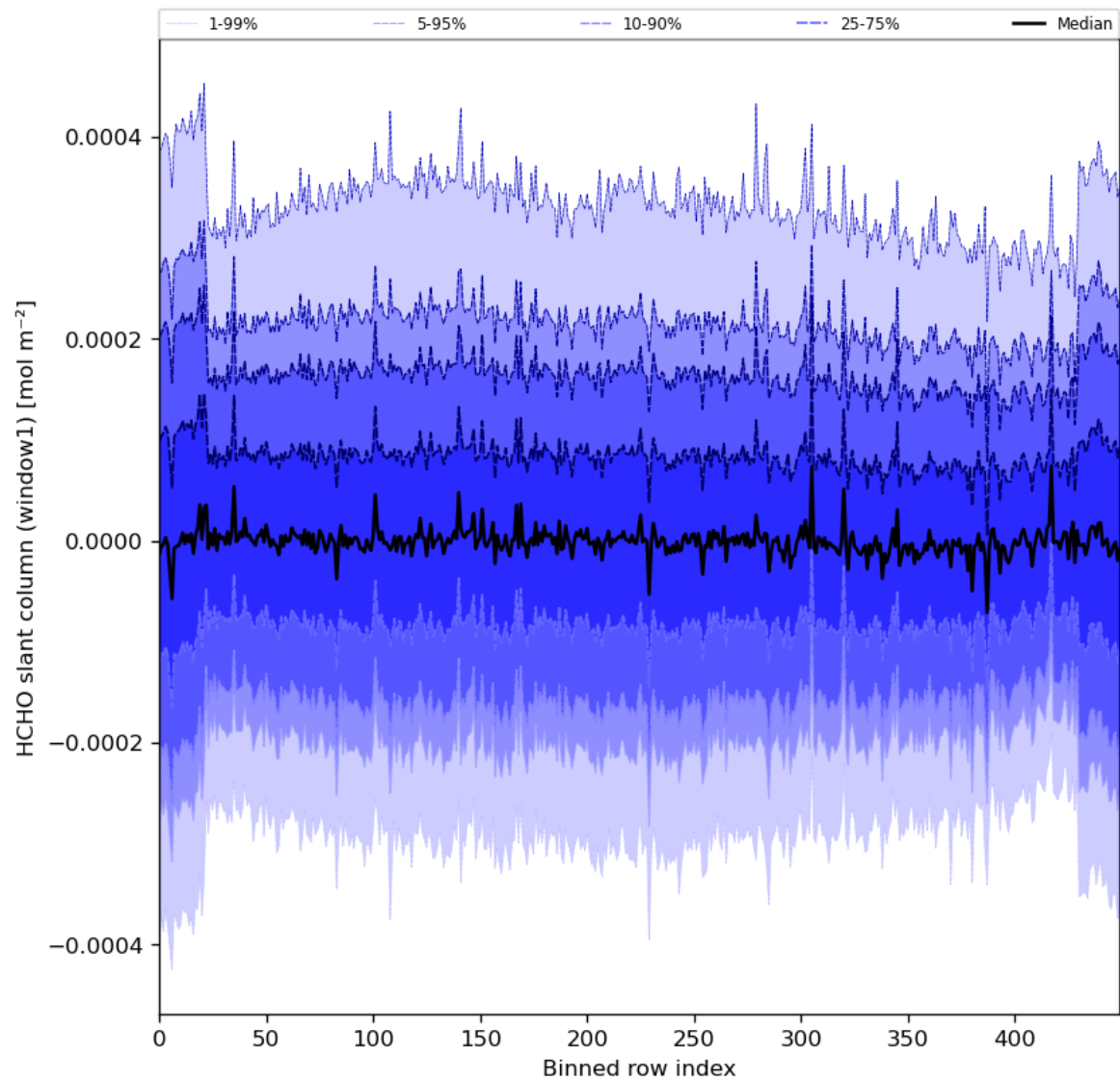
Figure 52: Along track statistics of “HCHO slant column (window1)” for 2024-04-15 to 2024-04-16
