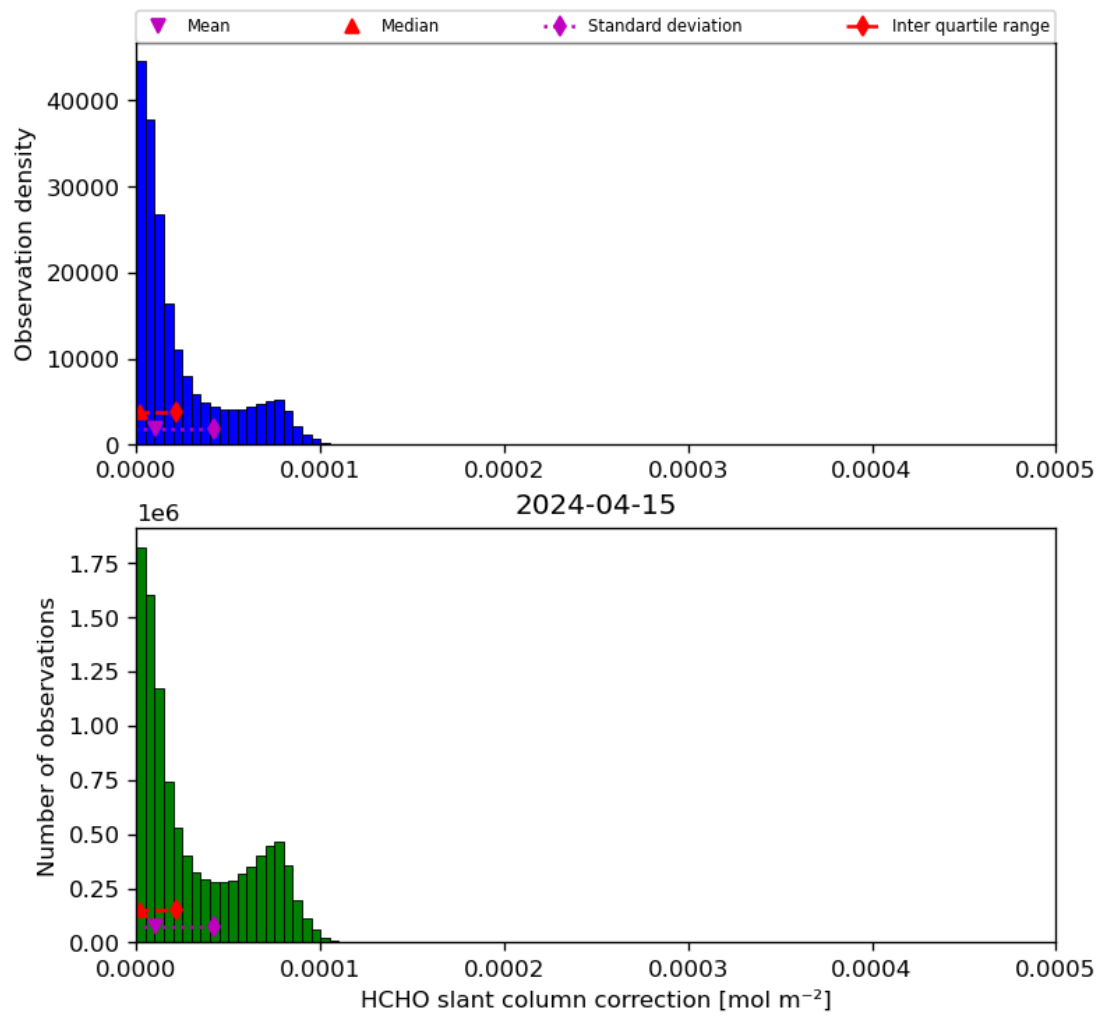
Figure 47: Histogram of “HCHO slant column correction” for 2024-04-15 to 2024-04-16
