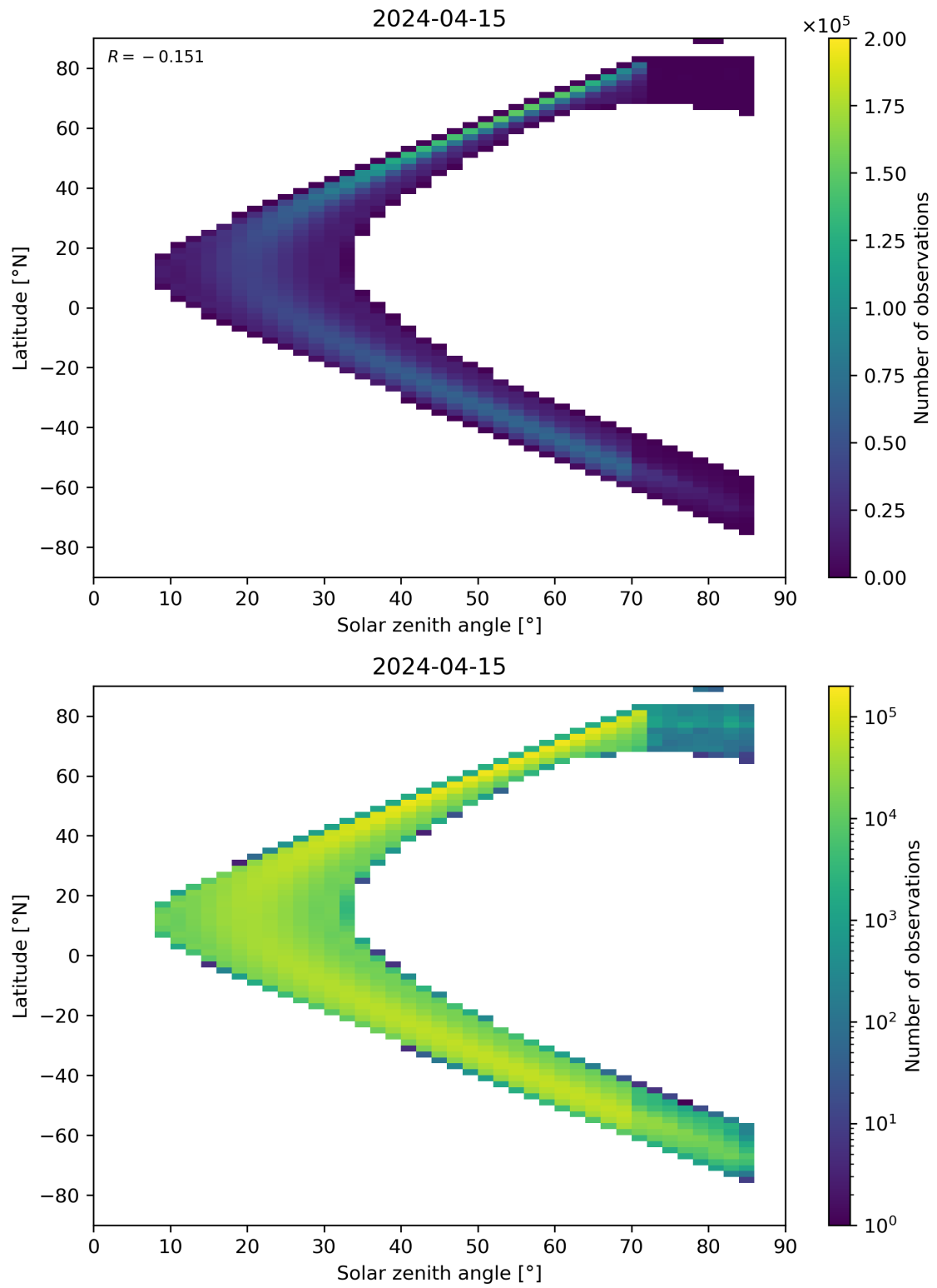
Figure 181: Scatter density plot of “Solar zenith angle” against “Latitude” for 2024-04-15 to 2024-04-16.
