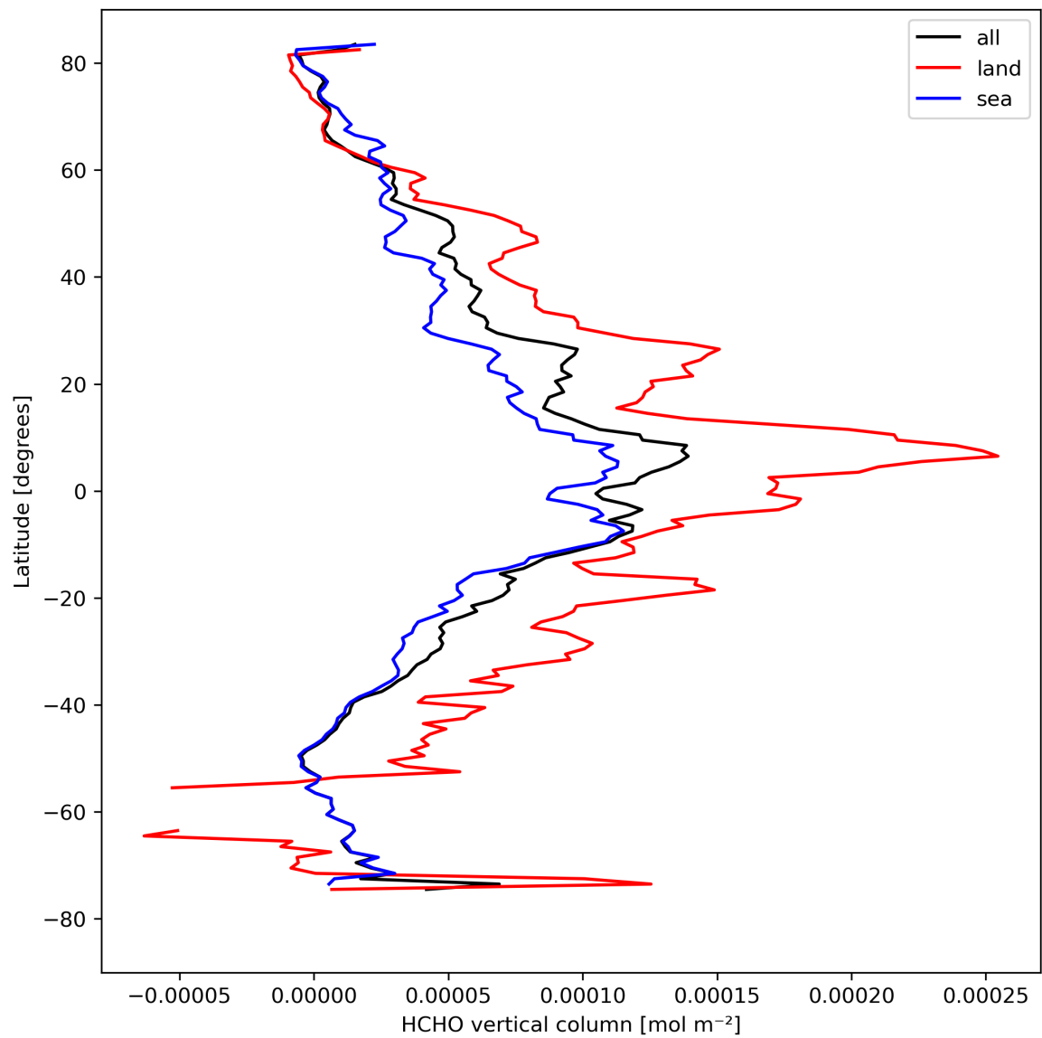
Figure 21: Zonal average of “HCHO vertical column” for 2024-04-15 to 2024-04-16.
