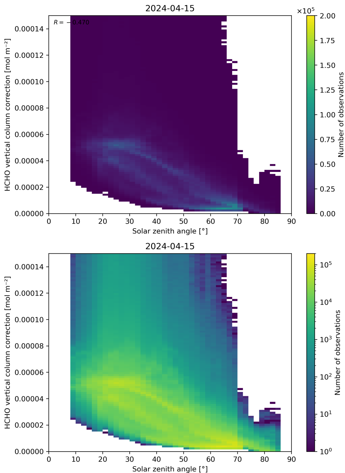
Figure 178: Scatter density plot of “Solar zenith angle” against “HCHO vertical column correction” for 2024-04-15 to 2024-04-16.
