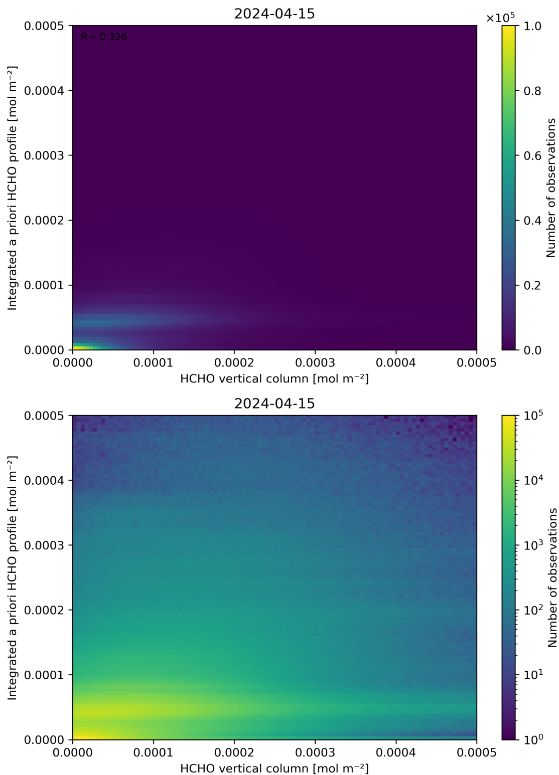
Figure 135: Scatter density plot of “HCHO vertical column” against “Integrated a priori HCHO profile” for 2024-04-15 to 2024-04-16.
