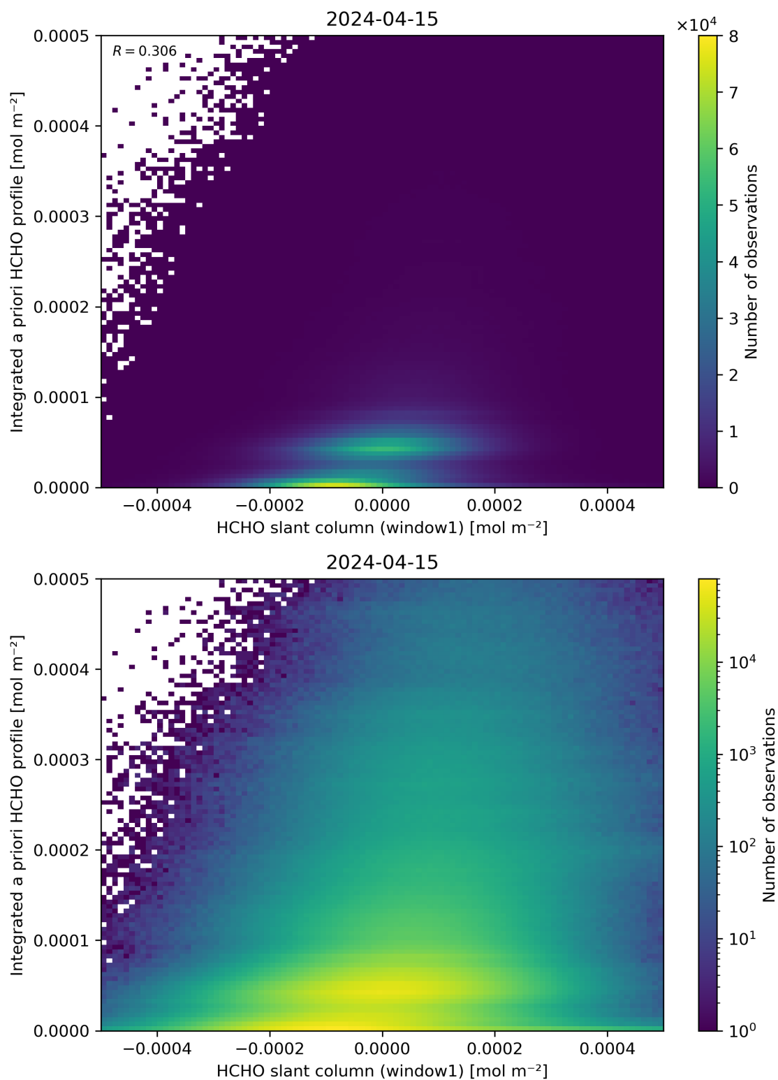
Figure 87: Scatter density plot of “HCHO slant column (window1)” against “Integrated a priori HCHO profile” for 2024-04-15 to 2024-04-16.
