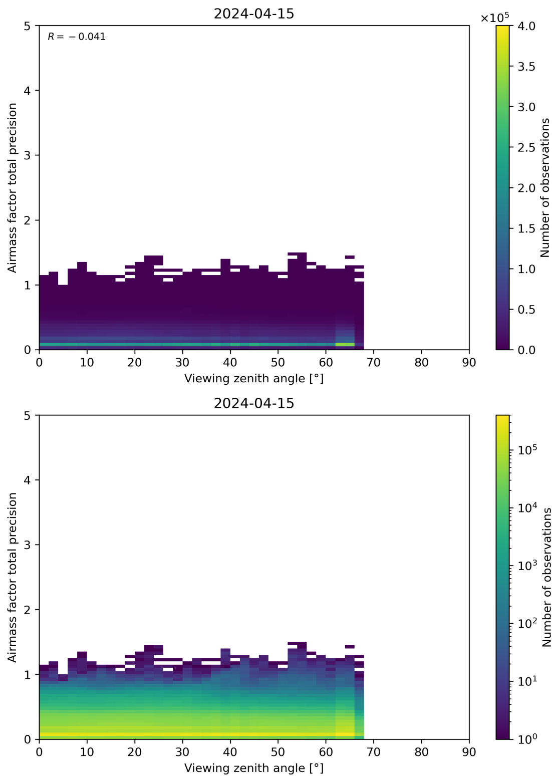
Figure 191: Scatter density plot of “Viewing zenith angle” against “Airmass factor total precision” for 2024-04-15 to 2024-04-16.
