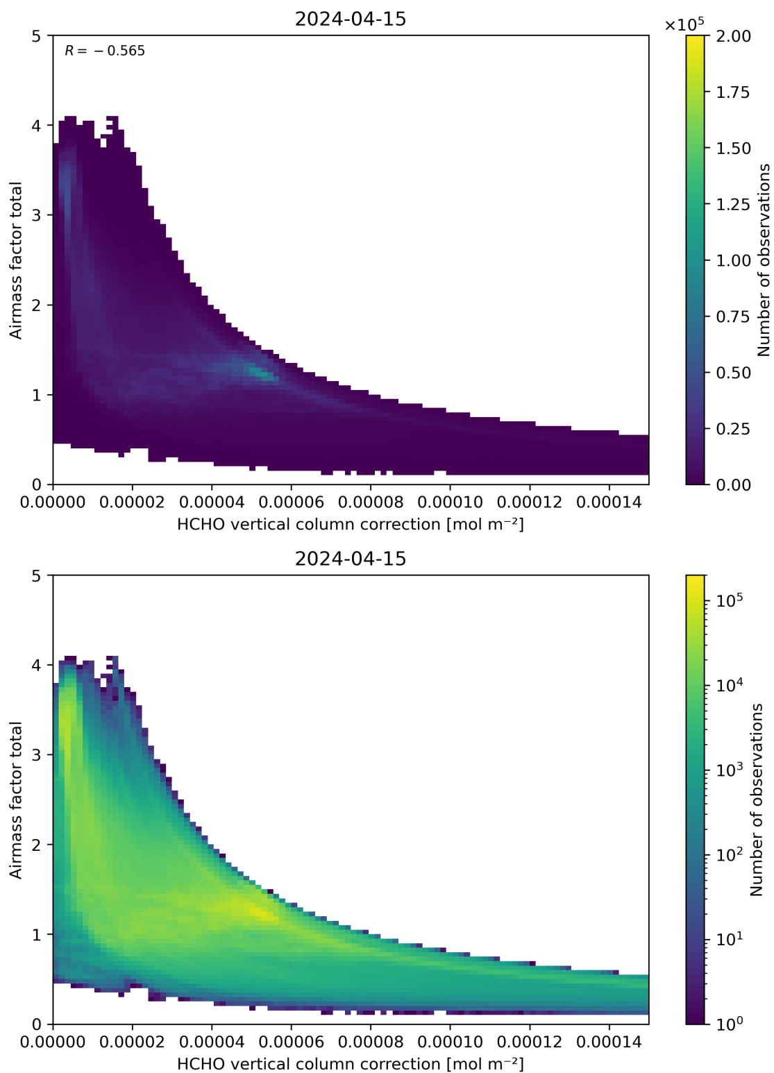
Figure 120: Scatter density plot of “HCHO vertical column correction” against “Airmass factor total” for 2024-04-15 to 2024-04-16.
