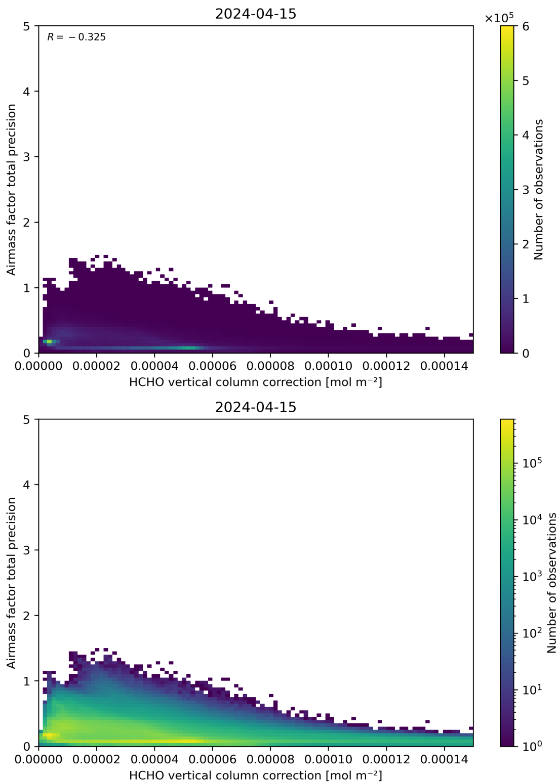
Figure 121: Scatter density plot of “HCHO vertical column correction” against “Airmass factor total precision” for 2024-04-15 to 2024-04-16.
