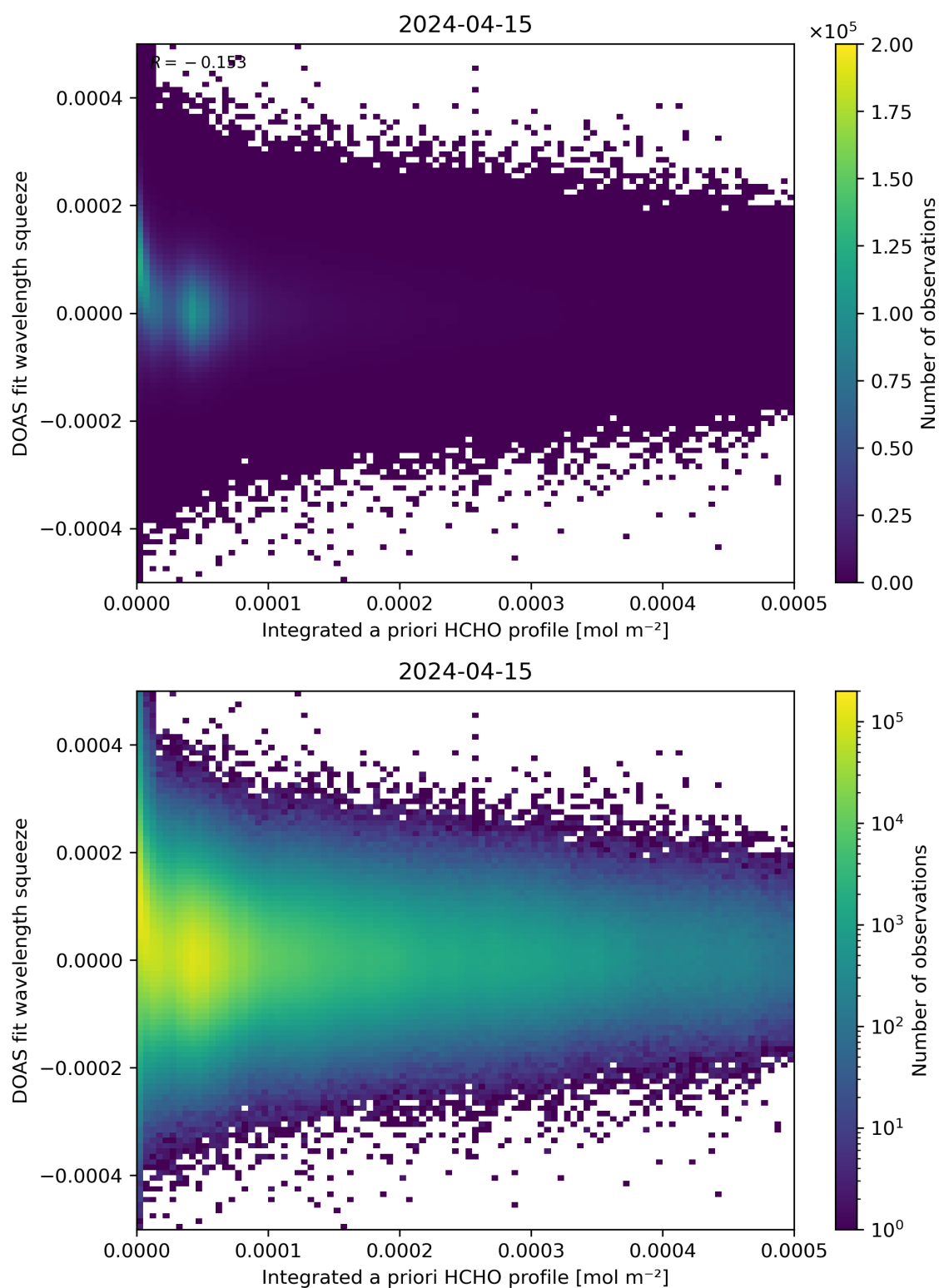
Figure 150: Scatter density plot of “Integrated a priori HCHO profile” against “DOAS fit wavelength squeeze” for 2024-04-15 to 2024-04-16.
