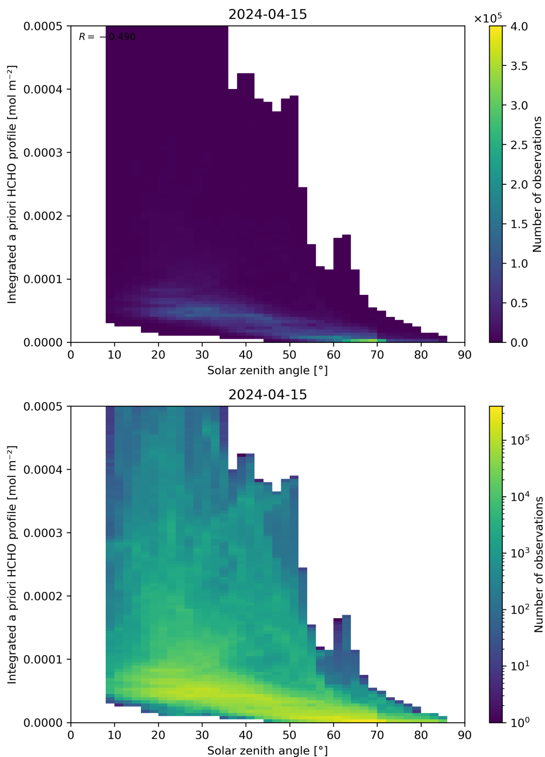
Figure 180: Scatter density plot of “Solar zenith angle” against “Integrated a priori HCHO profile” for 2024-04-15 to 2024-04-16.
