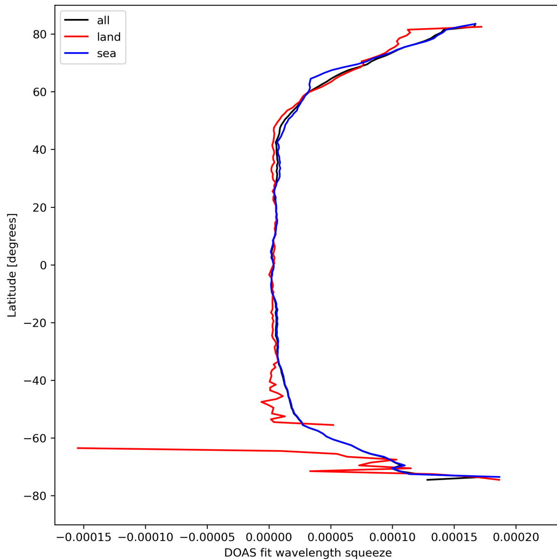
Figure 31: Zonal average of “DOAS fit wavelength squeeze” for 2024-04-15 to 2024-04-16.
