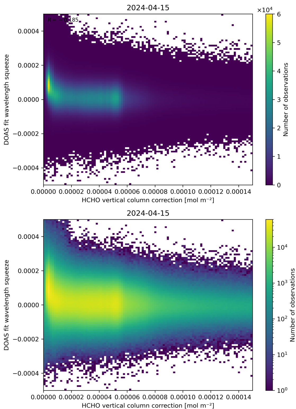
Figure 114: Scatter density plot of “HCHO vertical column correction” against “DOAS fit wavelength squeeze” for 2024-04-15 to 2024-04-16.
