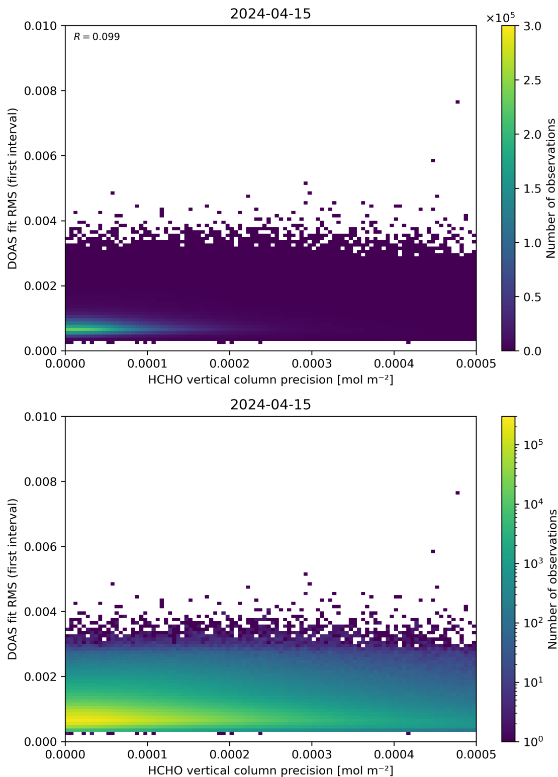
Figure 136: Scatter density plot of “HCHO vertical column precision” against “DOAS fit RMS (first interval)” for 2024-04-15 to 2024-04-16.
