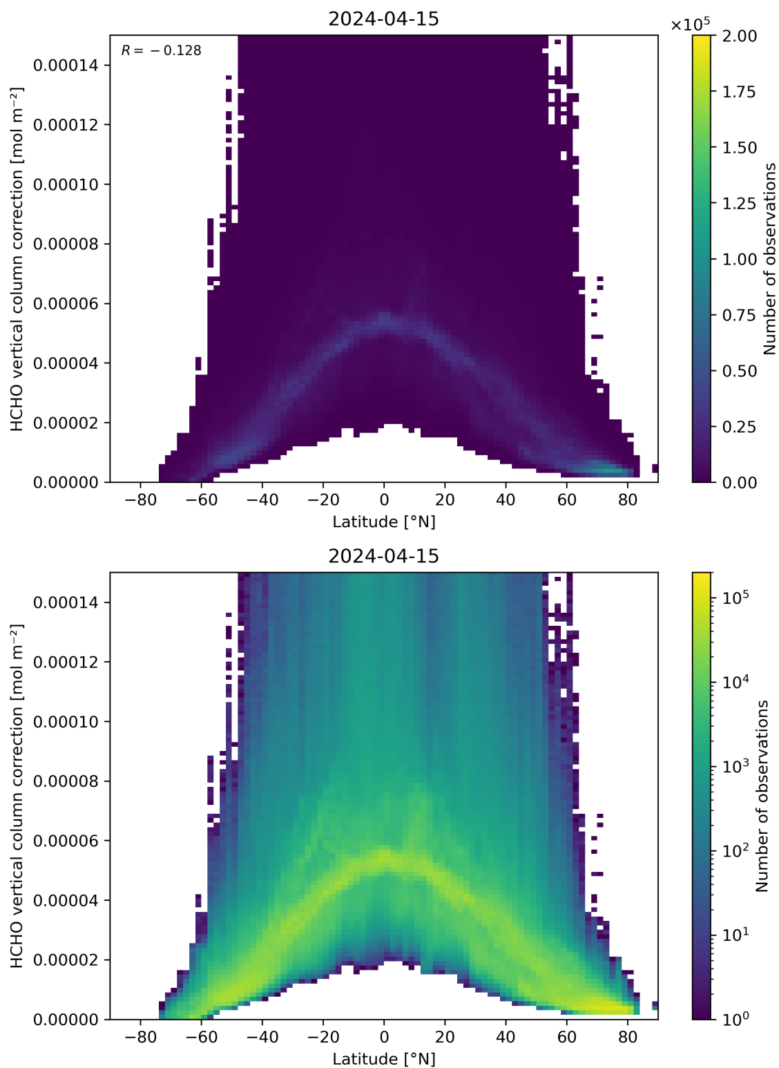
Figure 164: Scatter density plot of “Latitude” against “HCHO vertical column correction” for 2024-04-15 to 2024-04-16.
