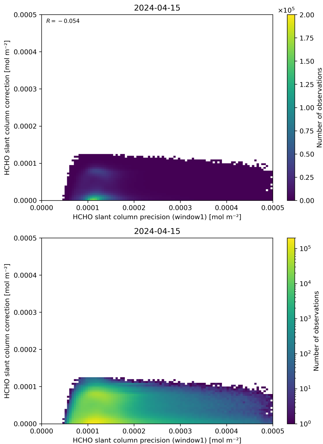
Figure 93: Scatter density plot of “HCHO slant column precision (window1)” against “HCHO slant column correction” for 2024-04-15 to 2024-04-16.
