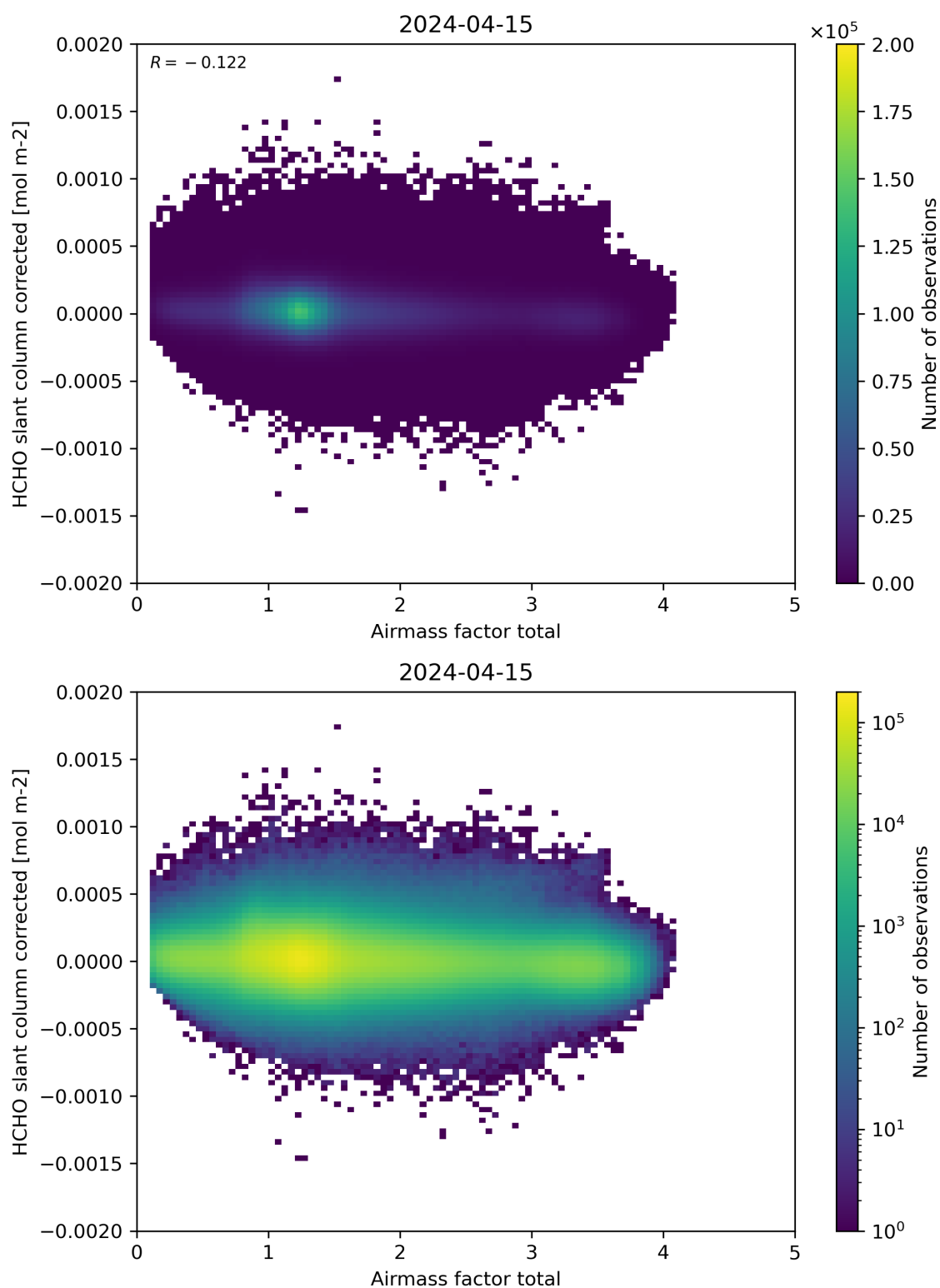
Figure 101: Scatter density plot of “Airmass factor total” against “HCHO slant column corrected” for 2024-04-15 to 2024-04-16.
