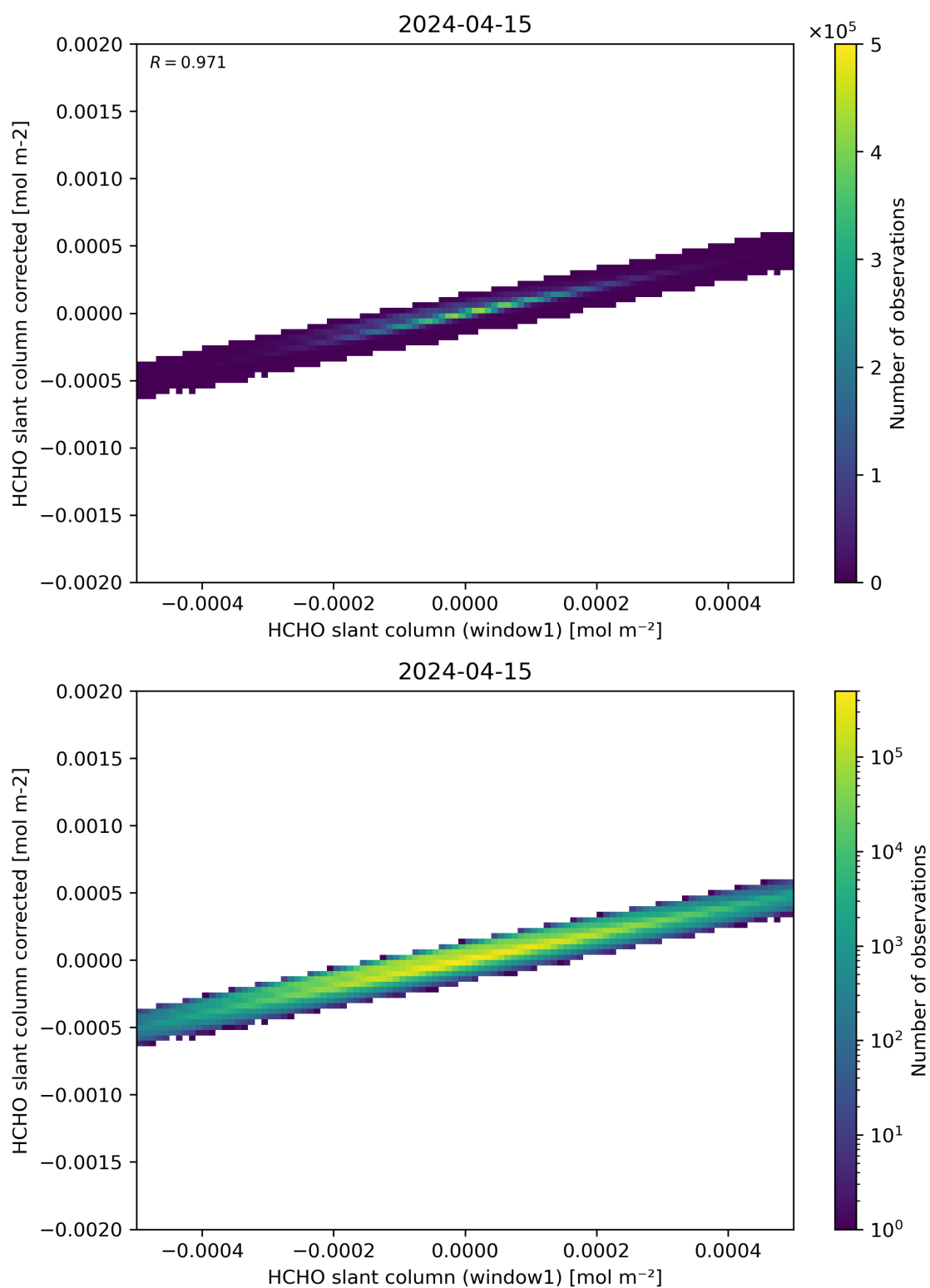
Figure 82: Scatter density plot of “HCHO slant column (window1)” against “HCHO slant column corrected” for 2024-04-15 to 2024-04-16.
