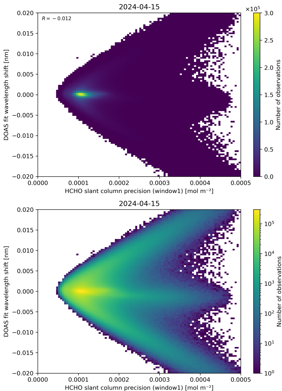
Figure 89: Scatter density plot of “HCHO slant column precision (window1)” against “DOAS fit wavelength shift” for 2024-04-15 to 2024-04-16.
