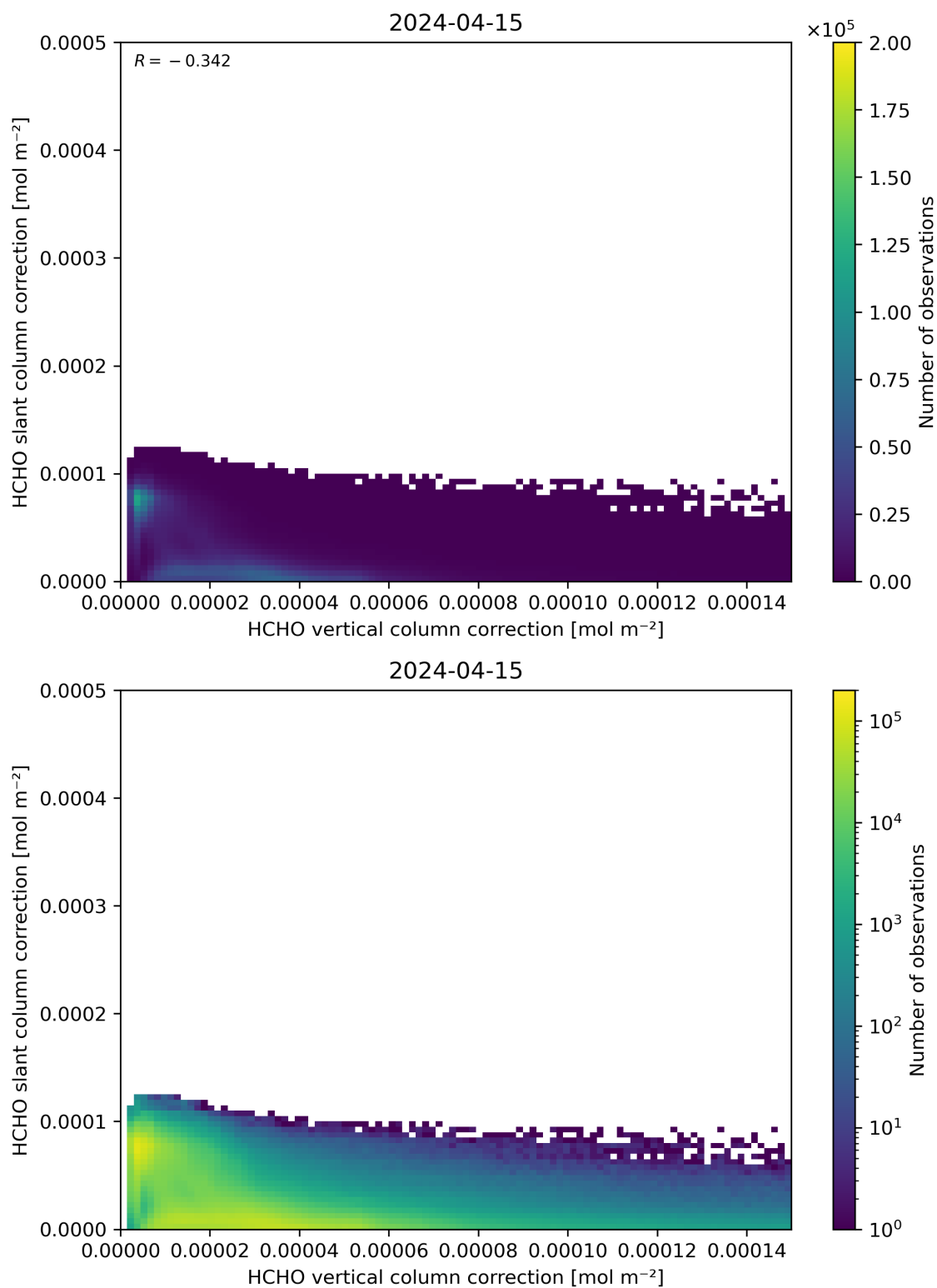
Figure 117: Scatter density plot of “HCHO vertical column correction” against “HCHO slant column correction” for 2024-04-15 to 2024-04-16.
