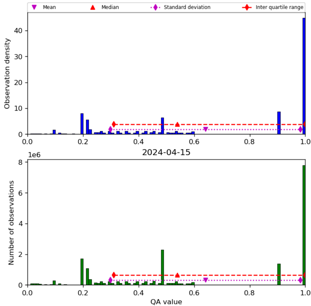
Figure 34: Histogram of “QA value” for 2024-04-15 to 2024-04-16
