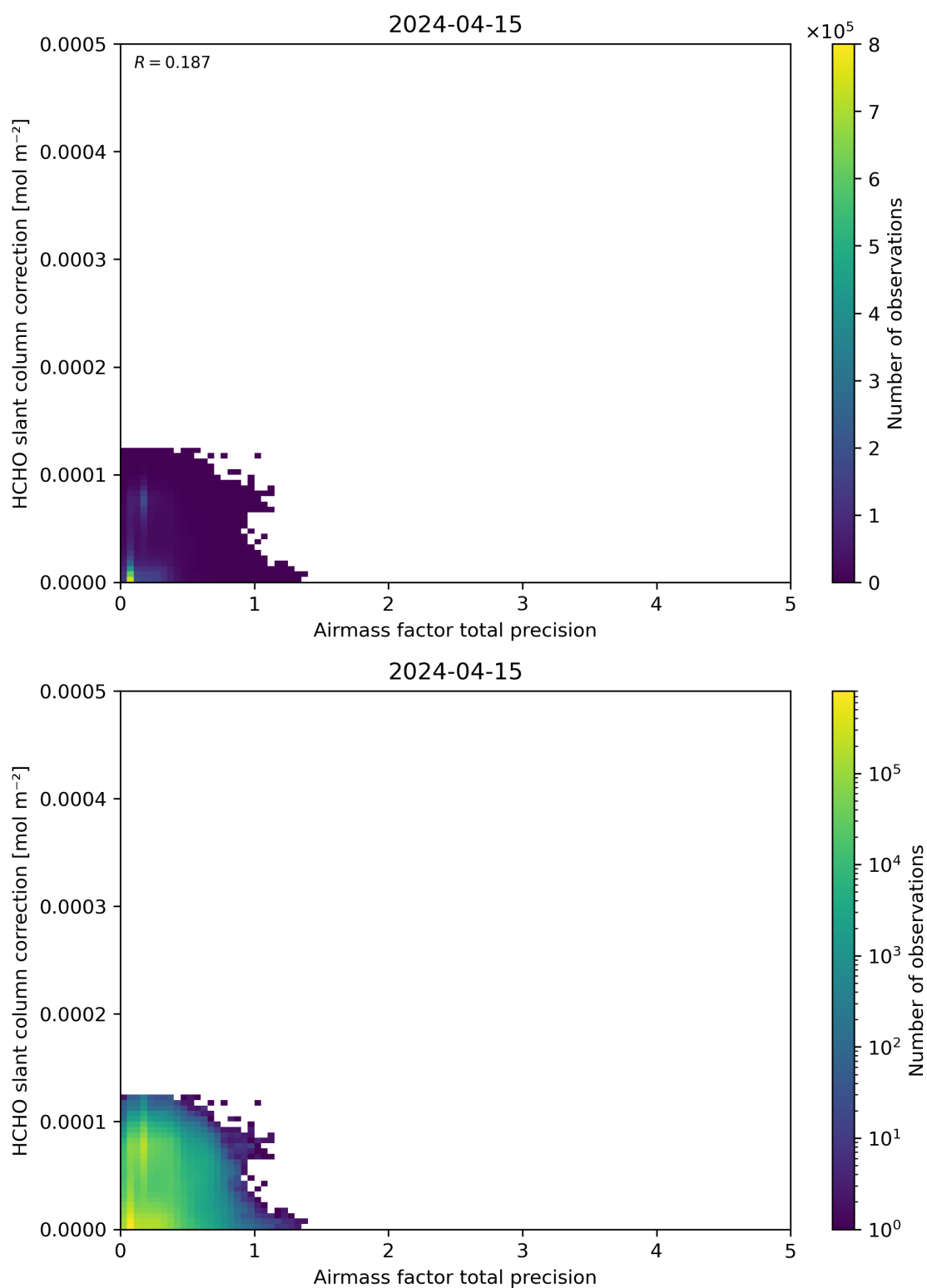
Figure 110: Scatter density plot of “Airmass factor total precision” against “HCHO slant column correction” for 2024-04-15 to 2024-04-16.
