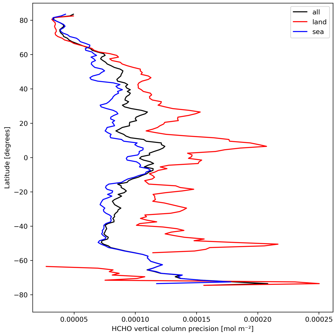
Figure 22: Zonal average of “HCHO vertical column precision” for 2024-04-15 to 2024-04-16.
