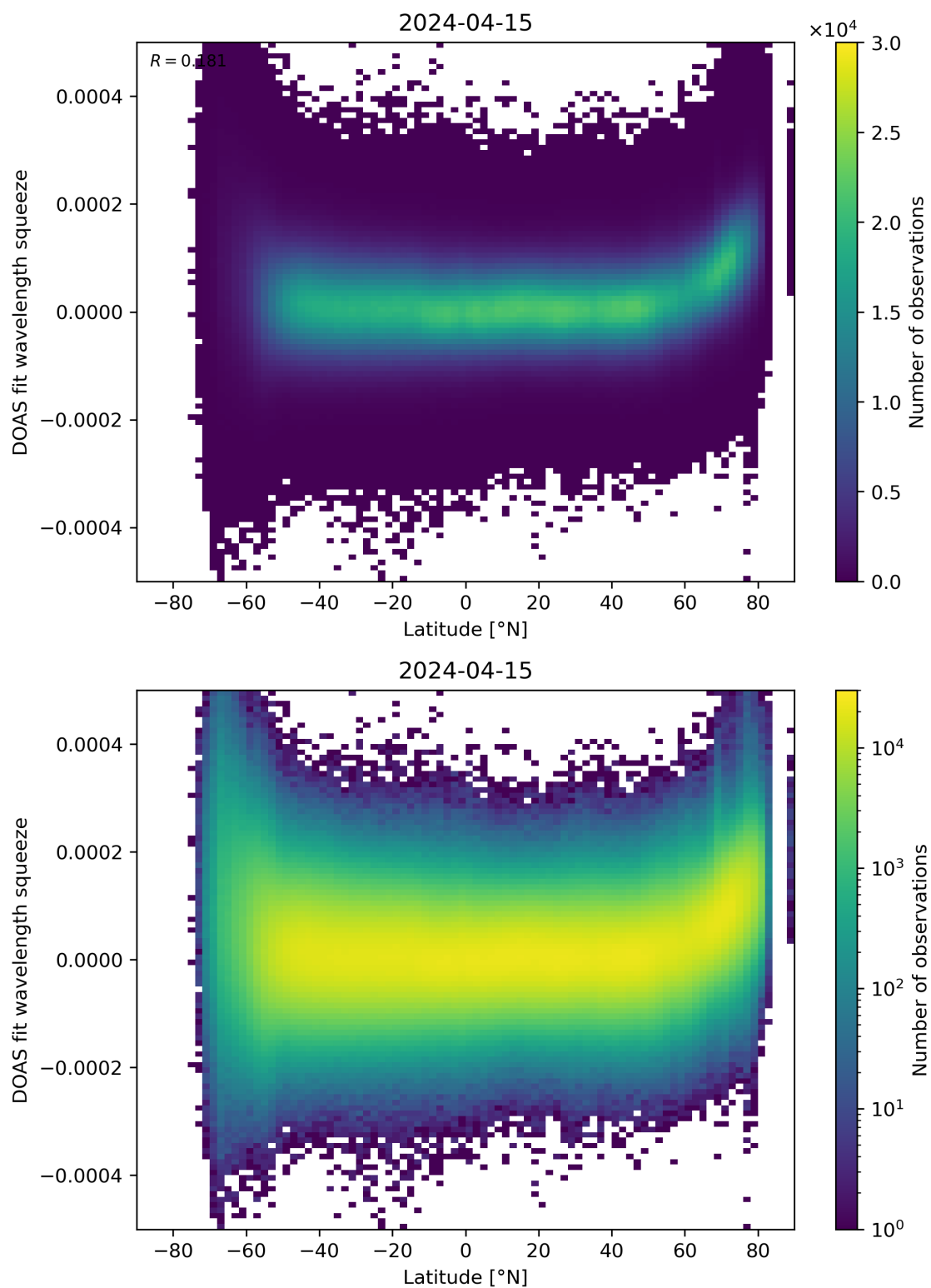
Figure 155: Scatter density plot of “Latitude” against “DOAS fit wavelength squeeze” for 2024-04-15 to 2024-04-16.
