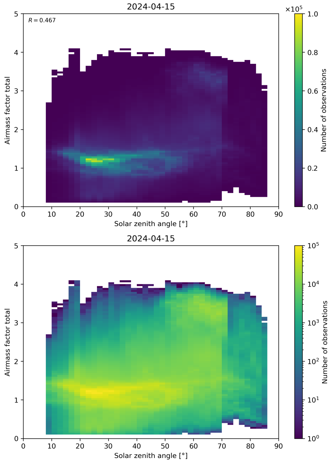
Figure 175: Scatter density plot of “Solar zenith angle” against “Airmass factor total” for 2024-04-15 to 2024-04-16.
