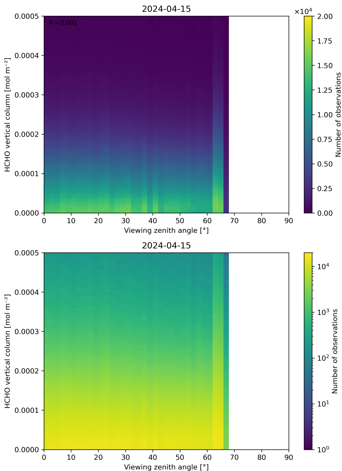
Figure 192: Scatter density plot of “Viewing zenith angle” against “HCHO vertical column” for 2024-04-15 to 2024-04-16.
