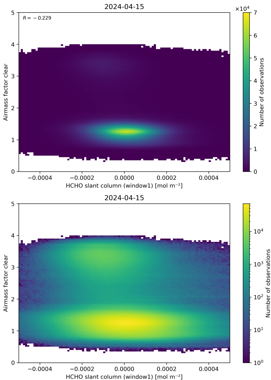
Figure 81: Scatter density plot of “HCHO slant column (window1)” against “Airmass factor clear” for 2024-04-15 to 2024-04-16.
