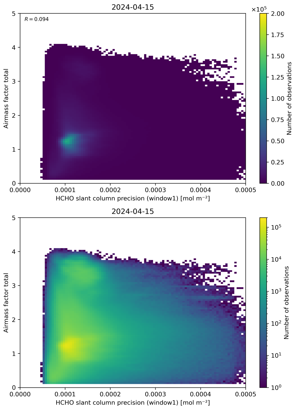
Figure 94: Scatter density plot of “HCHO slant column precision (window1)” against “Airmass factor total” for 2024-04-15 to 2024-04-16.
