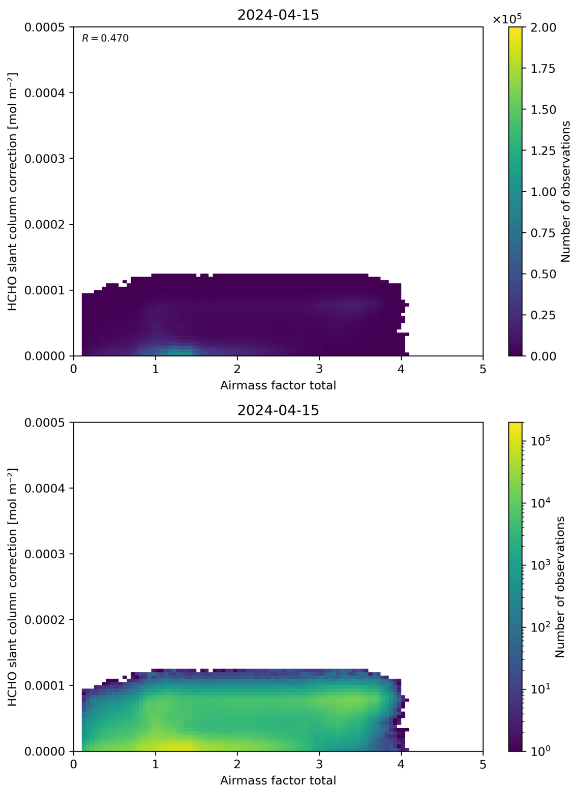
Figure 102: Scatter density plot of “Airmass factor total” against “HCHO slant column correction” for 2024-04-15 to 2024-04-16.
