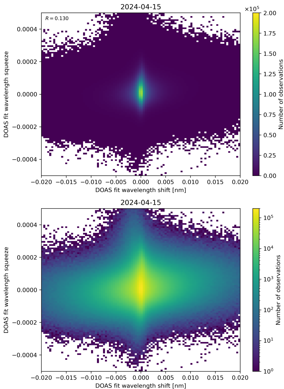
Figure 65: Scatter density plot of “DOAS fit wavelength shift” against “DOAS fit wavelength squeeze” for 2024-04-15 to 2024-04-16.
