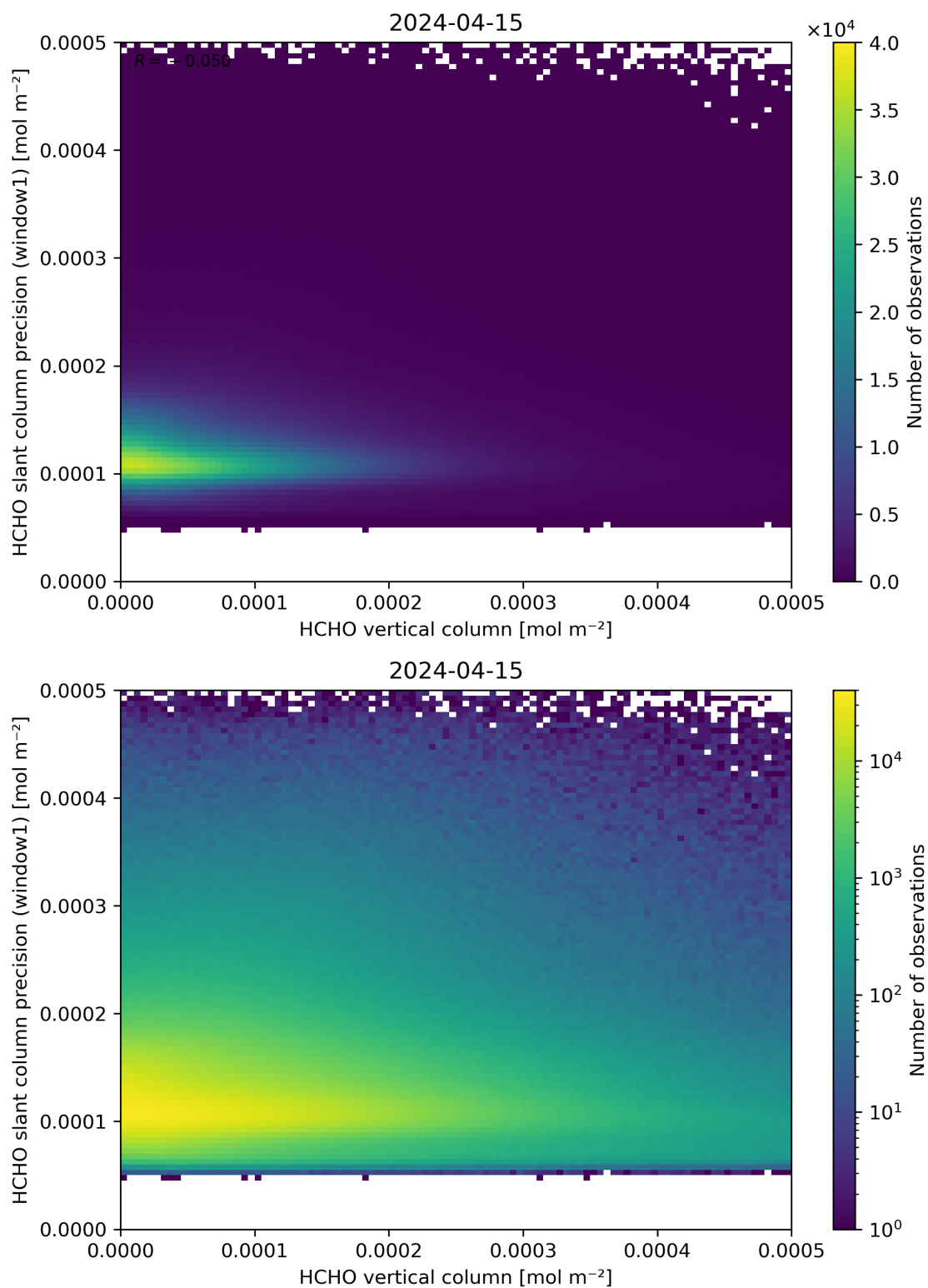
Figure 130: Scatter density plot of “HCHO vertical column” against “HCHO slant column precision (window1)” for 2024-04-15 to 2024-04-16.
