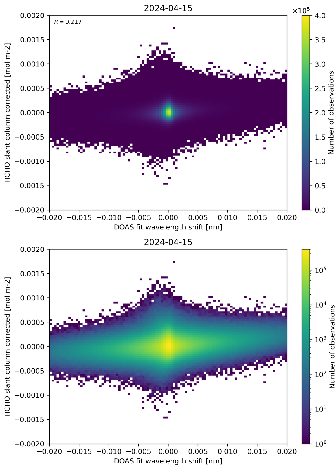
Figure 66: Scatter density plot of “DOAS fit wavelength shift” against “HCHO slant column corrected” for 2024-04-15 to 2024-04-16.
