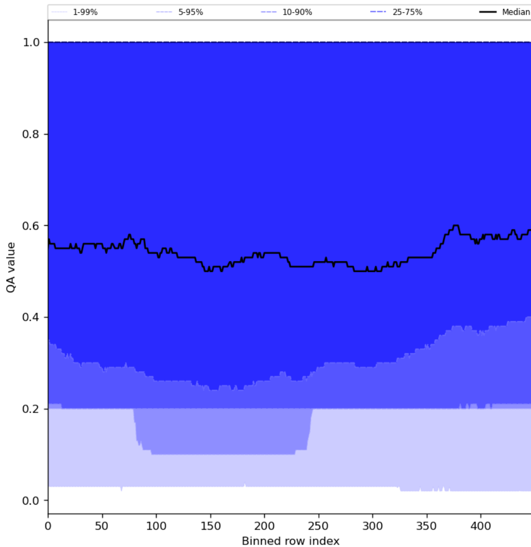
Figure 48: Along track statistics of “QA value” for 2024-04-15 to 2024-04-16
