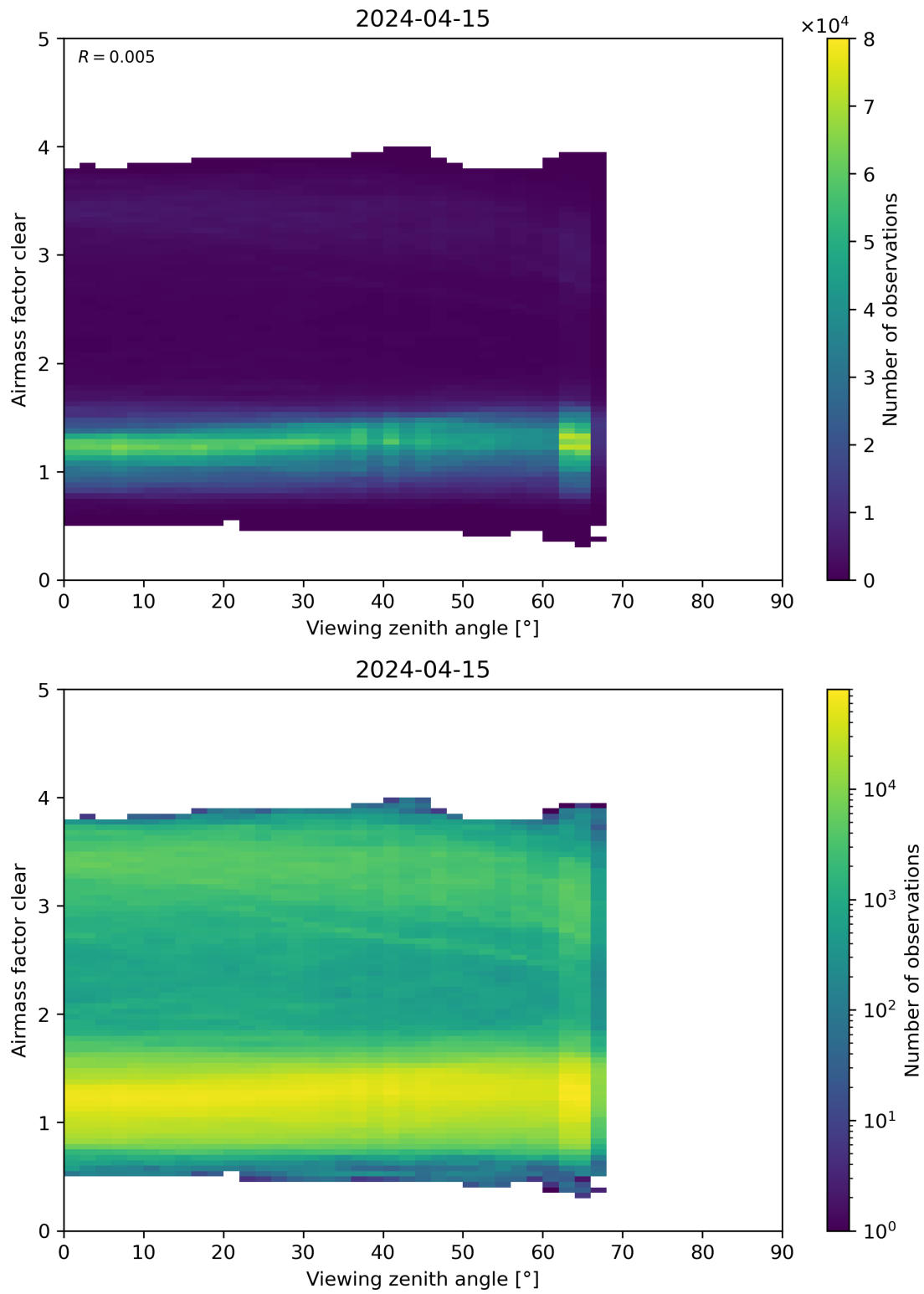
Figure 185: Scatter density plot of “Viewing zenith angle” against “Airmass factor clear” for 2024-04-15 to 2024-04-16.
