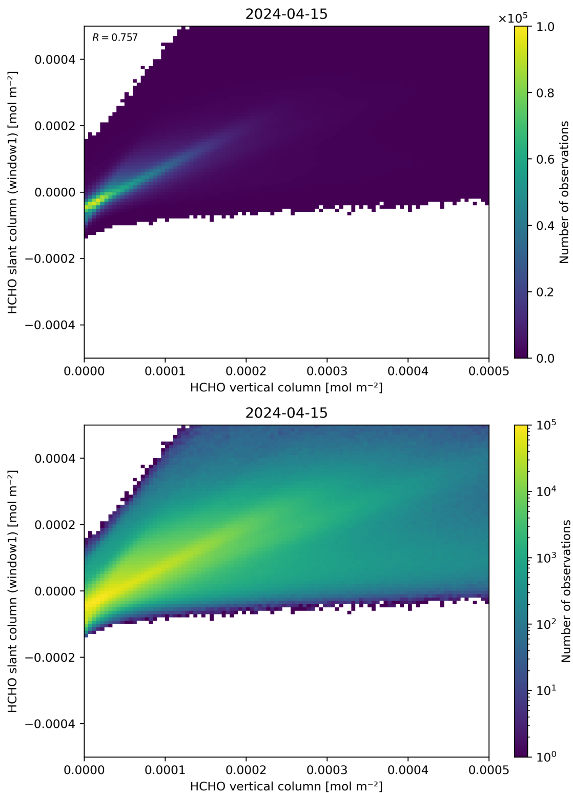
Figure 129: Scatter density plot of “HCHO vertical column” against “HCHO slant column (window1)” for 2024-04-15 to 2024-04-16.
