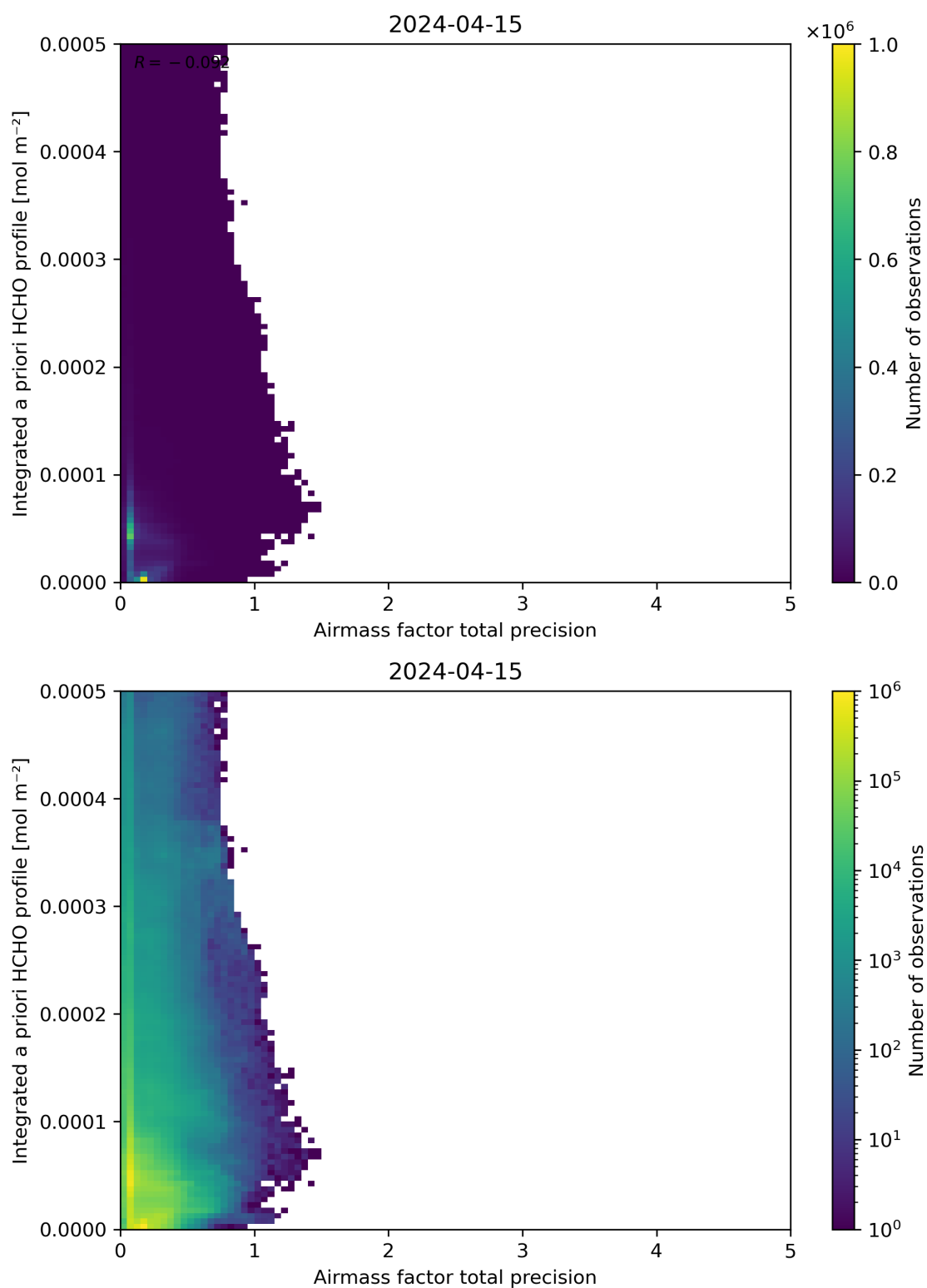
Figure 111: Scatter density plot of “Airmass factor total precision” against “Integrated a priori HCHO profile” for 2024-04-15 to 2024-04-16.
