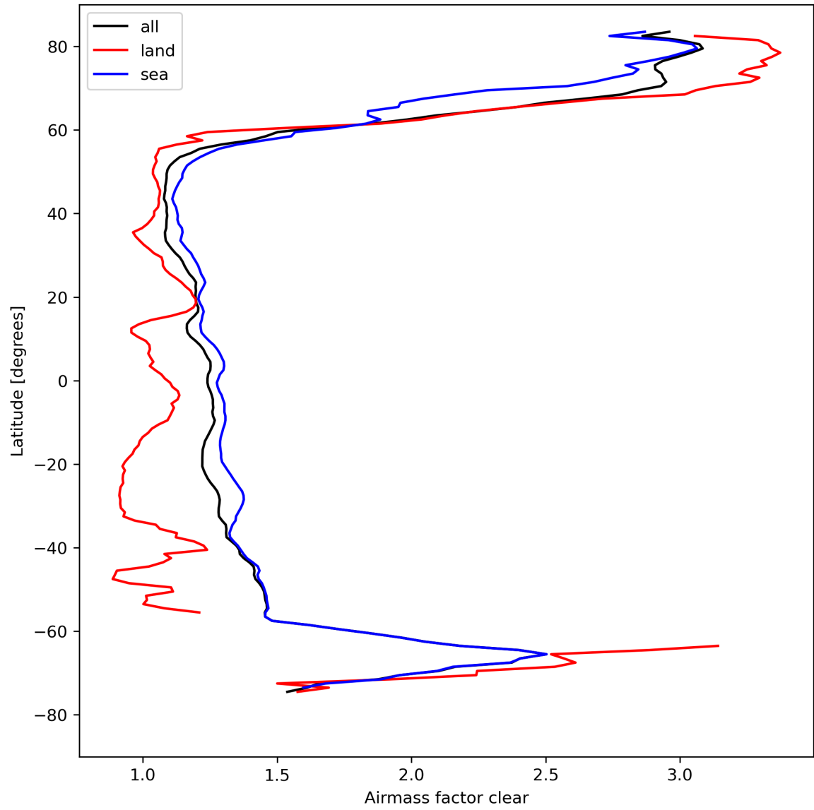
Figure 28: Zonal average of “Airmass factor clear” for 2024-04-15 to 2024-04-16.
