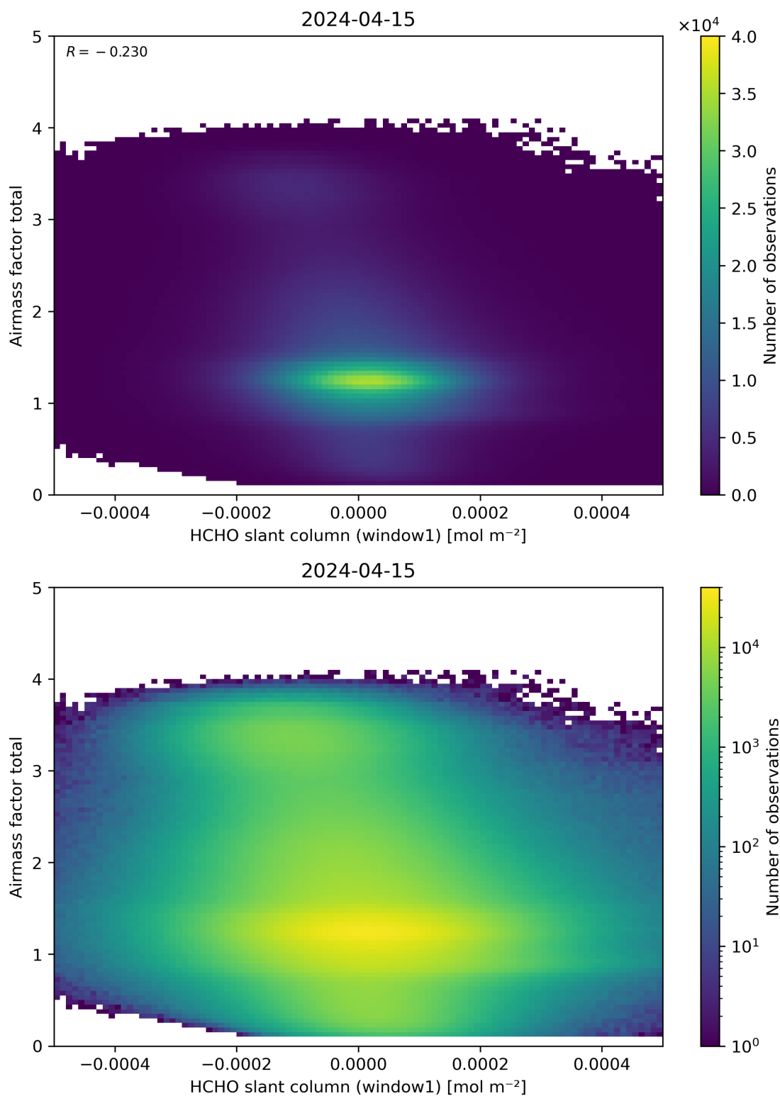
Figure 85: Scatter density plot of “HCHO slant column (window1)” against “Airmass factor total” for 2024-04-15 to 2024-04-16.
