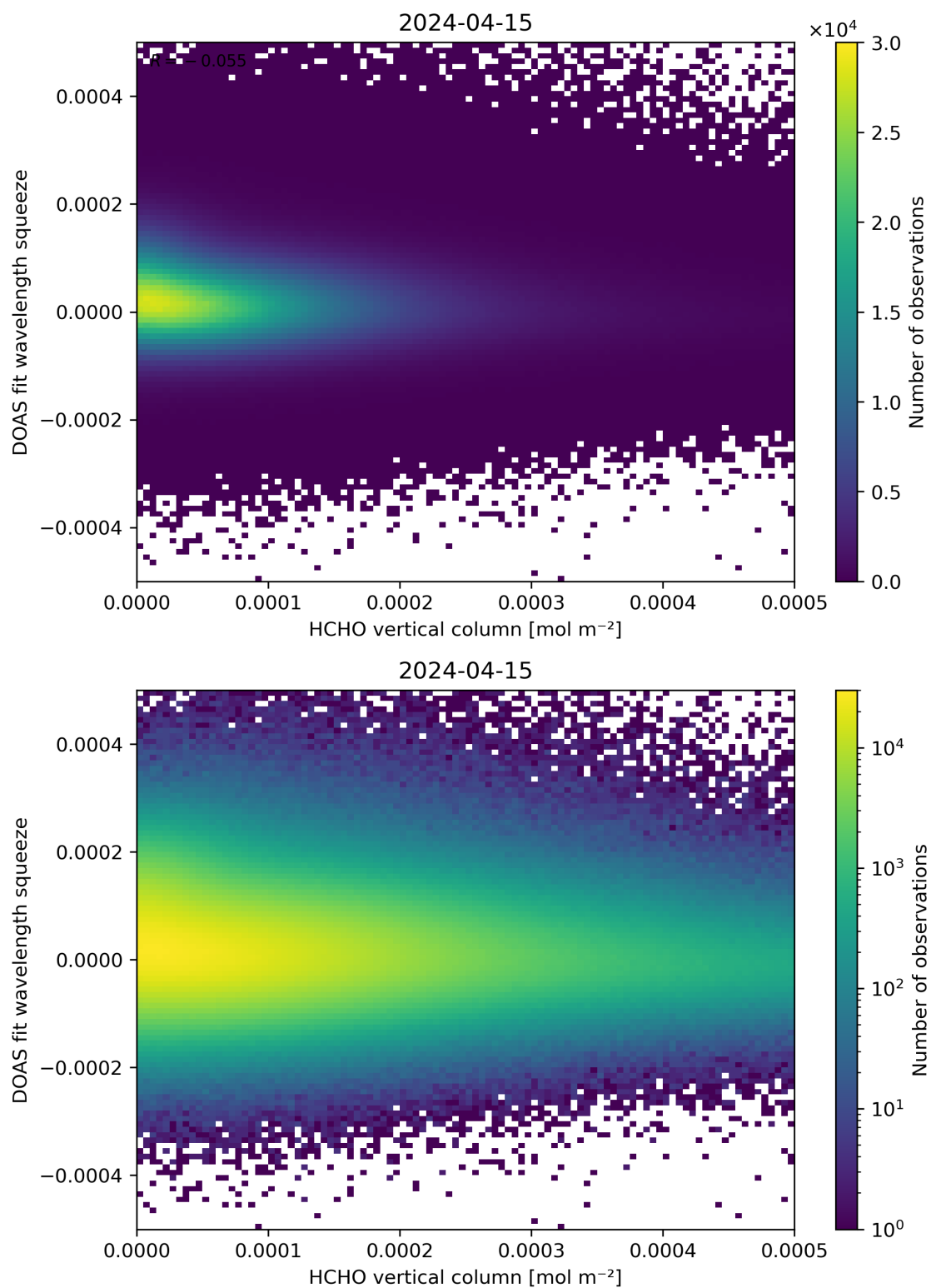
Figure 125: Scatter density plot of “HCHO vertical column” against “DOAS fit wavelength squeeze” for 2024-04-15 to 2024-04-16.
