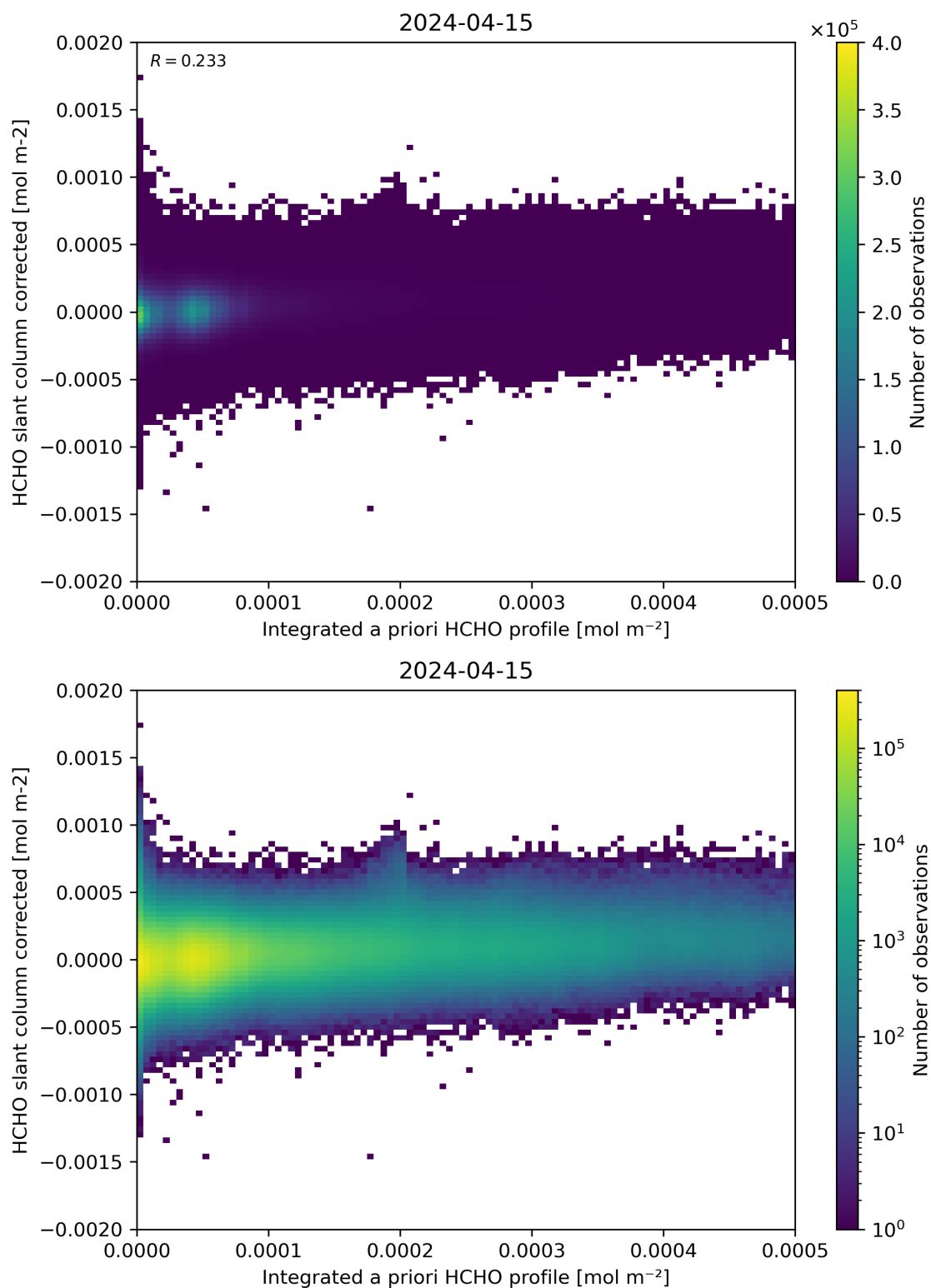
Figure 151: Scatter density plot of “Integrated a priori HCHO profile” against “HCHO slant column corrected” for 2024-04-15 to 2024-04-16.
