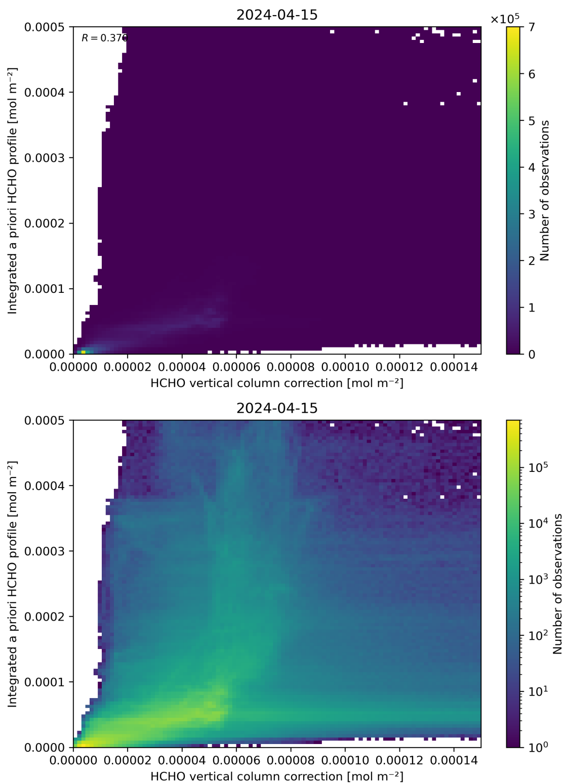
Figure 122: Scatter density plot of “HCHO vertical column correction” against “Integrated a priori HCHO profile” for 2024-04-15 to 2024-04-16.
