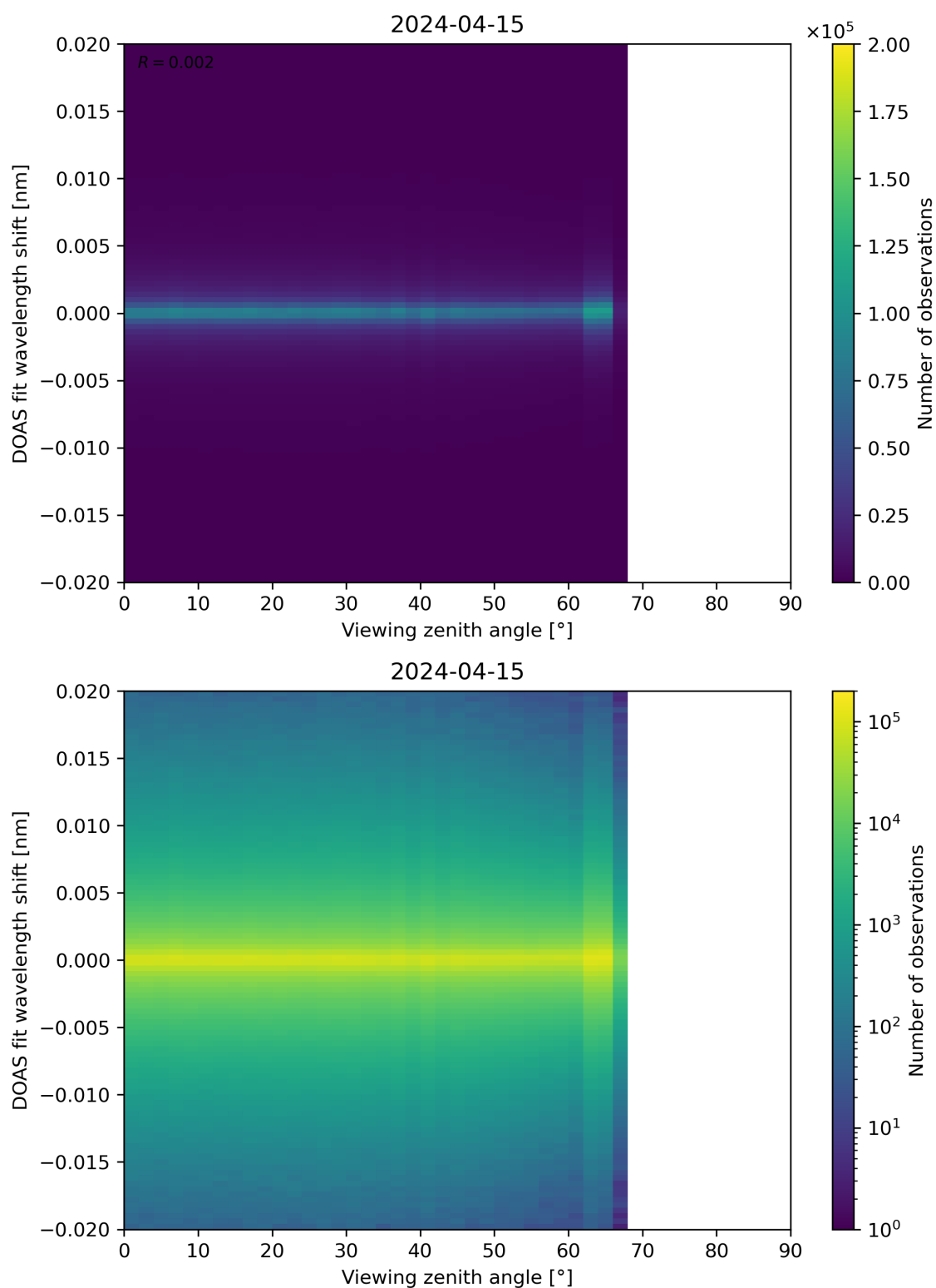
Figure 183: Scatter density plot of “Viewing zenith angle” against “DOAS fit wavelength shift” for 2024-04-15 to 2024-04-16.
