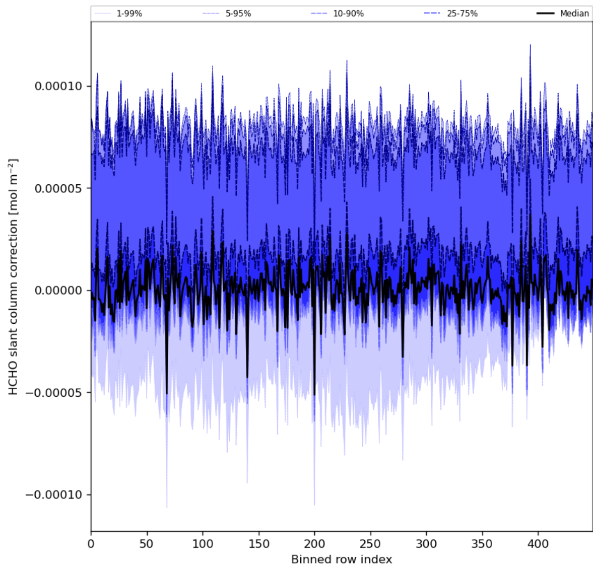
Figure 61: Along track statistics of “HCHO slant column correction” for 2024-04-15 to 2024-04-16
