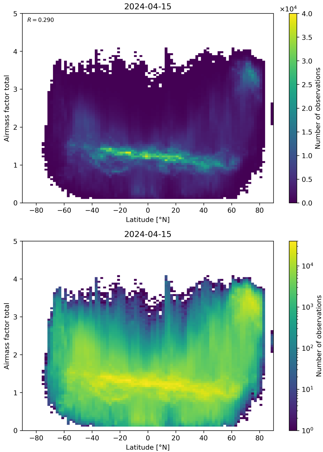
Figure 161: Scatter density plot of “Latitude” against “Airmass factor total” for 2024-04-15 to 2024-04-16.
