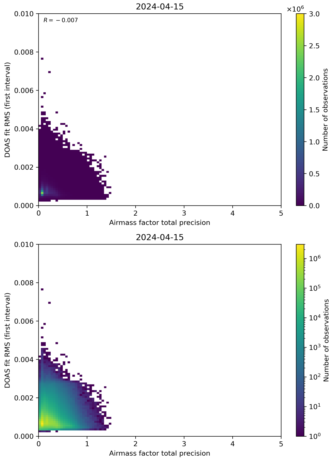
Figure 105: Scatter density plot of “Airmass factor total precision” against “DOAS fit RMS (first interval)” for 2024-04-15 to 2024-04-16.
