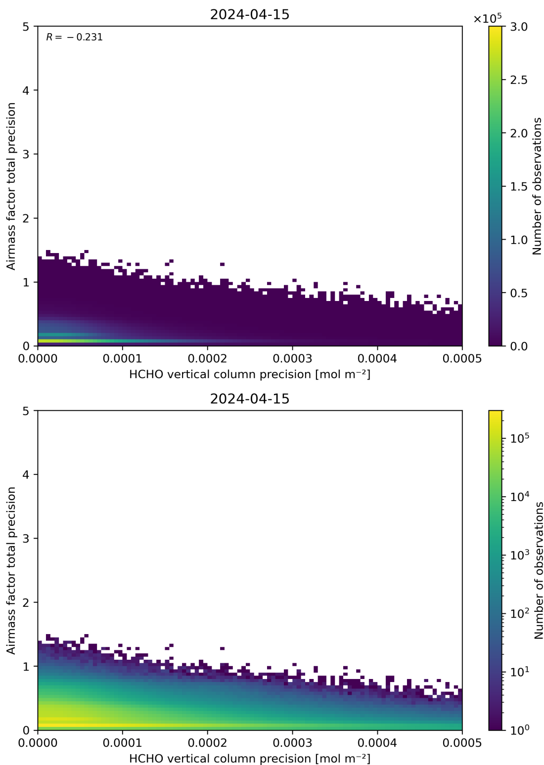
Figure 145: Scatter density plot of “HCHO vertical column precision” against “Airmass factor total precision” for 2024-04-15 to 2024-04-16.
