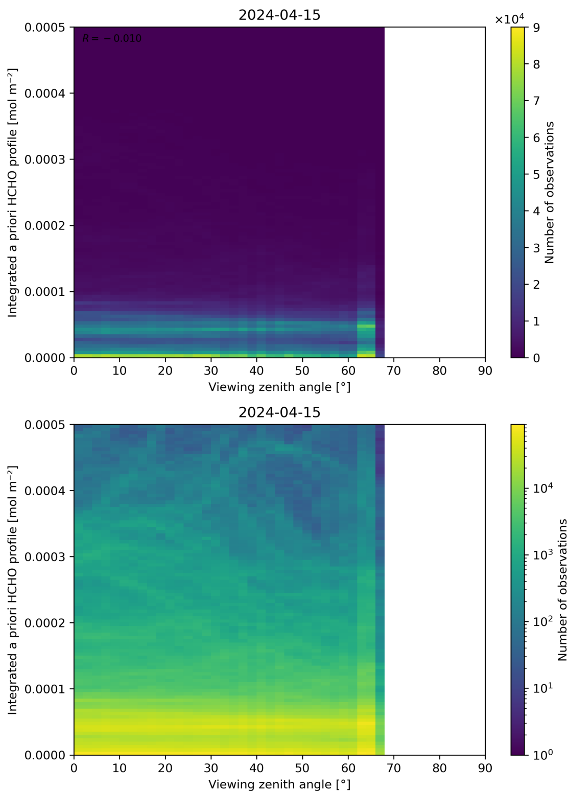
Figure 195: Scatter density plot of “Viewing zenith angle” against “Integrated a priori HCHO profile” for 2024-04-15 to 2024-04-16.
