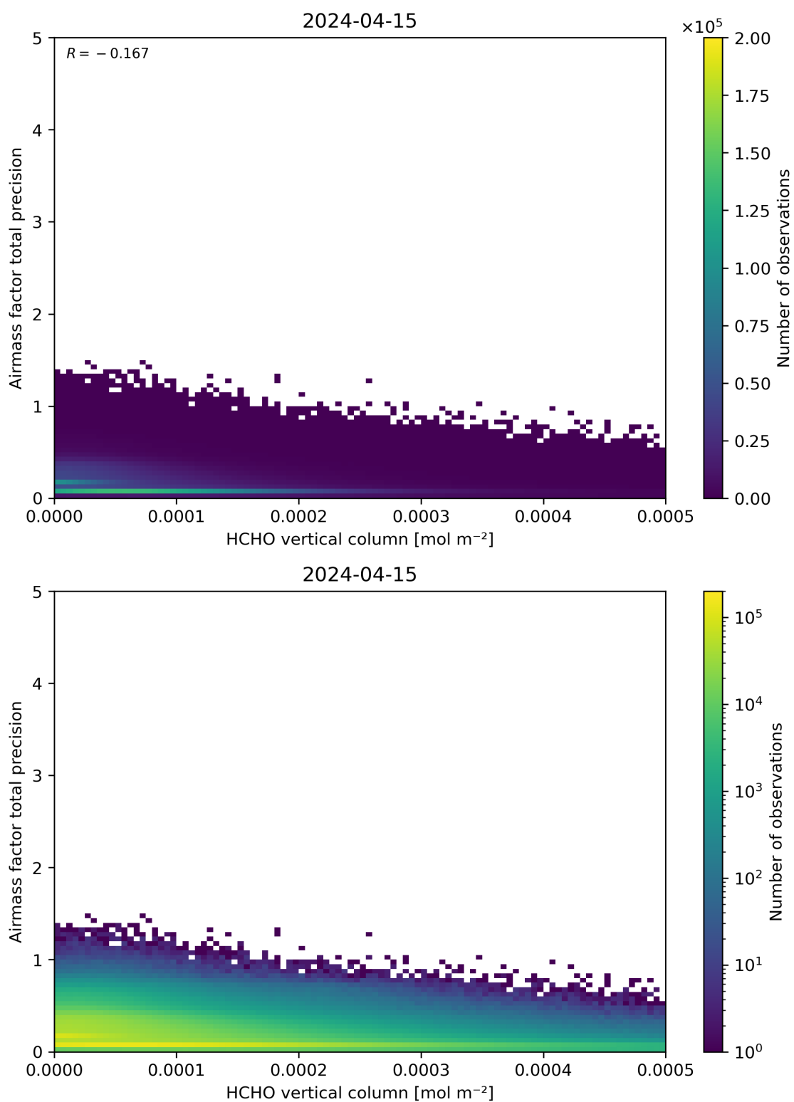
Figure 132: Scatter density plot of “HCHO vertical column” against “Airmass factor total precision” for 2024-04-15 to 2024-04-16.
