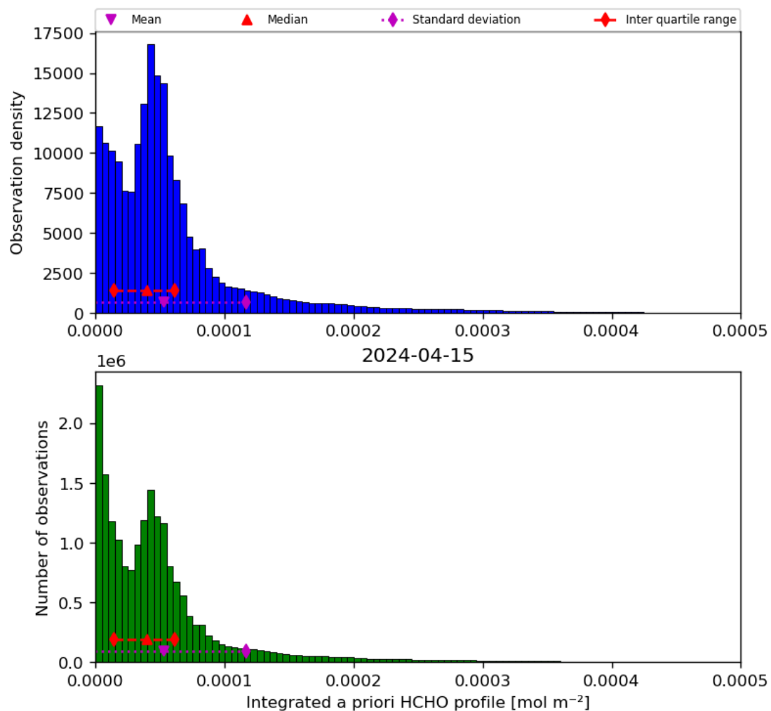
Figure 43: Histogram of “Integrated a priori HCHO profile” for 2024-04-15 to 2024-04-16
