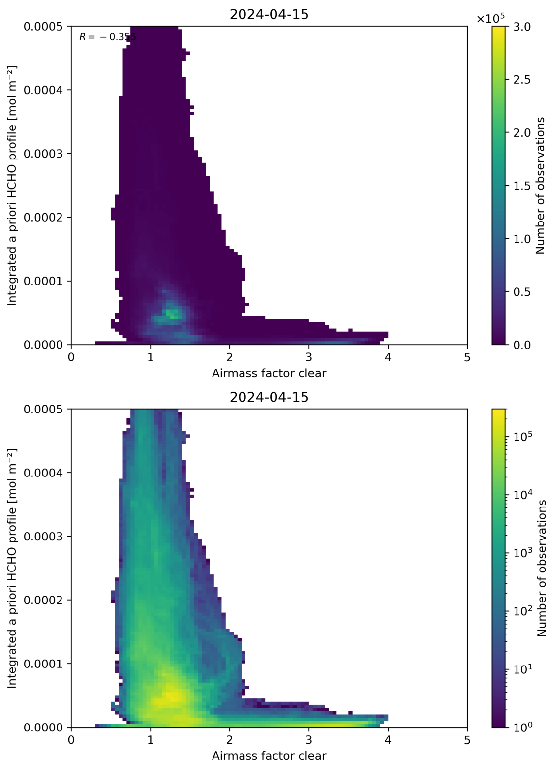
Figure 76: Scatter density plot of “Airmass factor clear” against “Integrated a priori HCHO profile” for 2024-04-15 to 2024-04-16.
