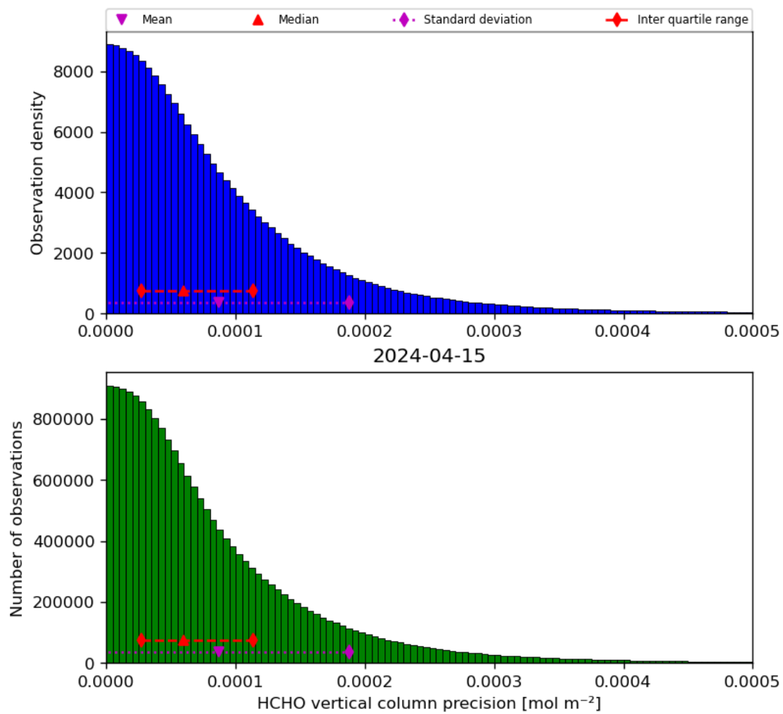
Figure 36: Histogram of “HCHO vertical column precision” for 2024-04-15 to 2024-04-16
