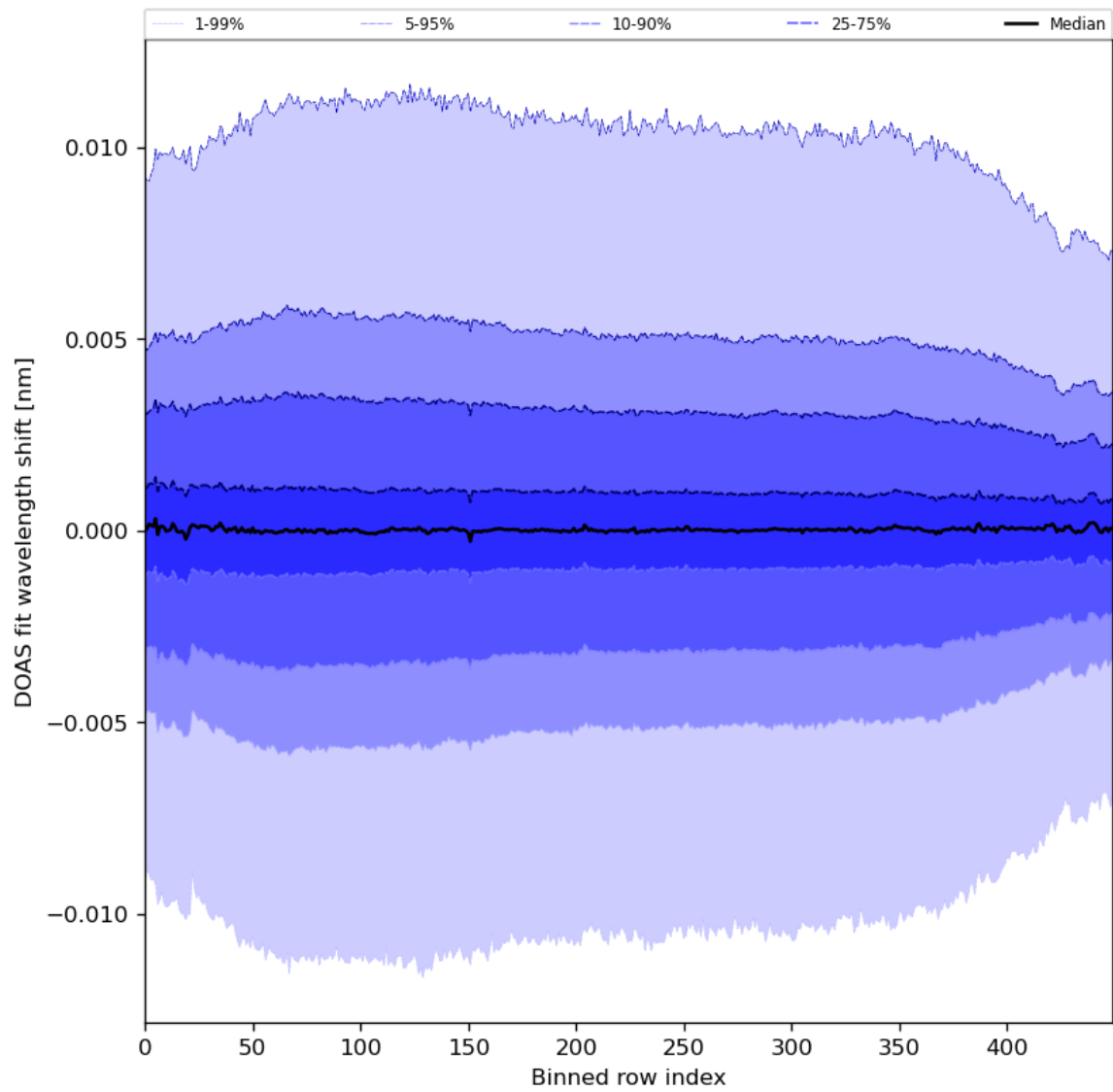
Figure 58: Along track statistics of “DOAS fit wavelength shift” for 2024-04-15 to 2024-04-16
