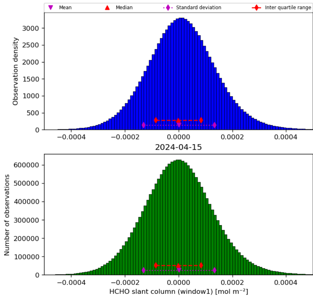
Figure 38: Histogram of “HCHO slant column (window1)” for 2024-04-15 to 2024-04-16
