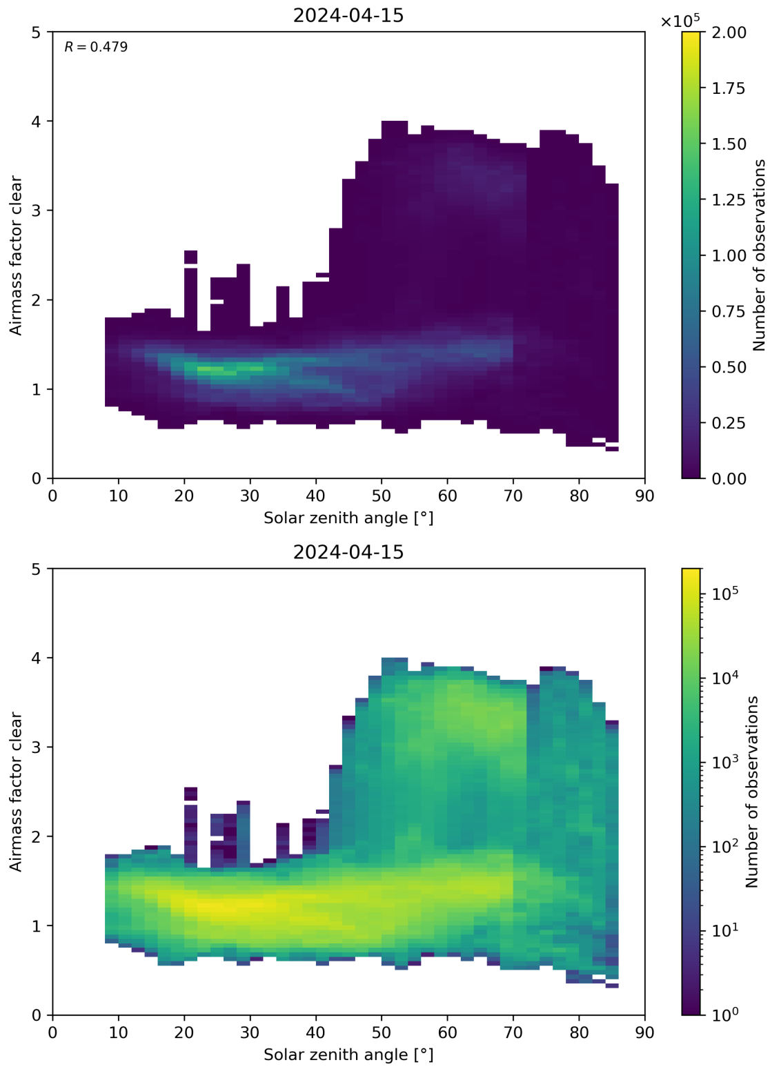
Figure 170: Scatter density plot of “Solar zenith angle” against “Airmass factor clear” for 2024-04-15 to 2024-04-16.
