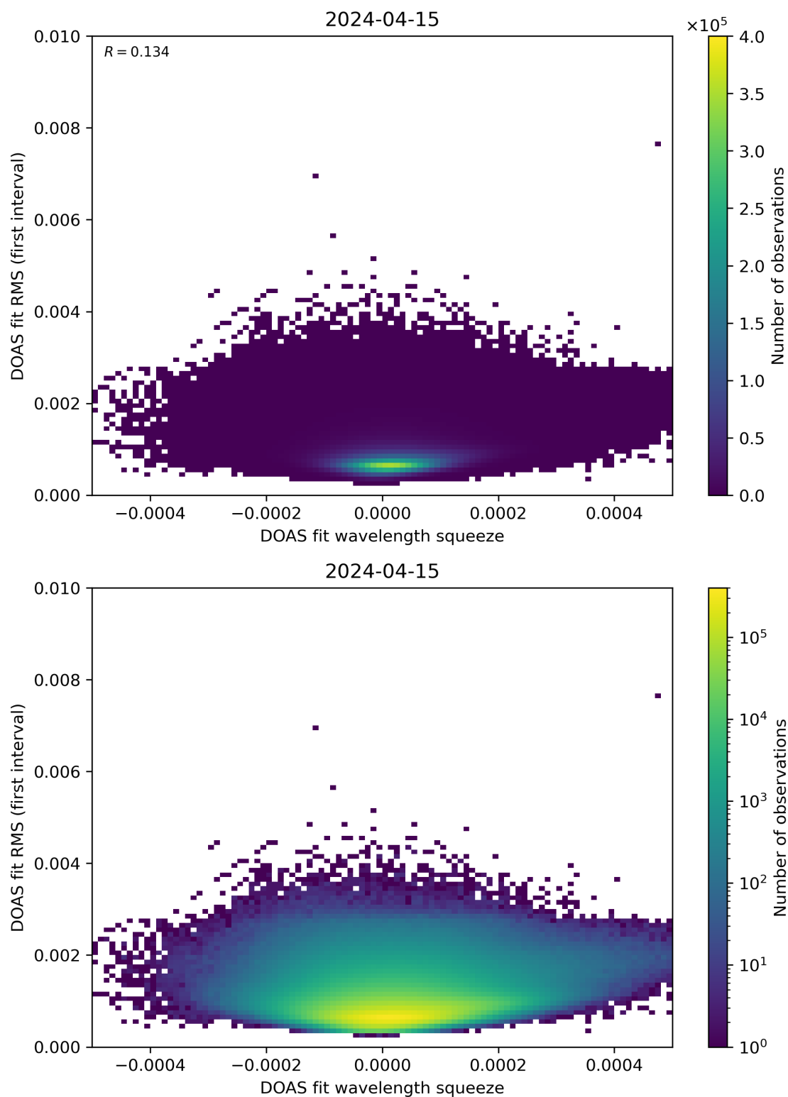
Figure 68: Scatter density plot of “DOAS fit wavelength squeeze” against “DOAS fit RMS (first interval)” for 2024-04-15 to 2024-04-16.
