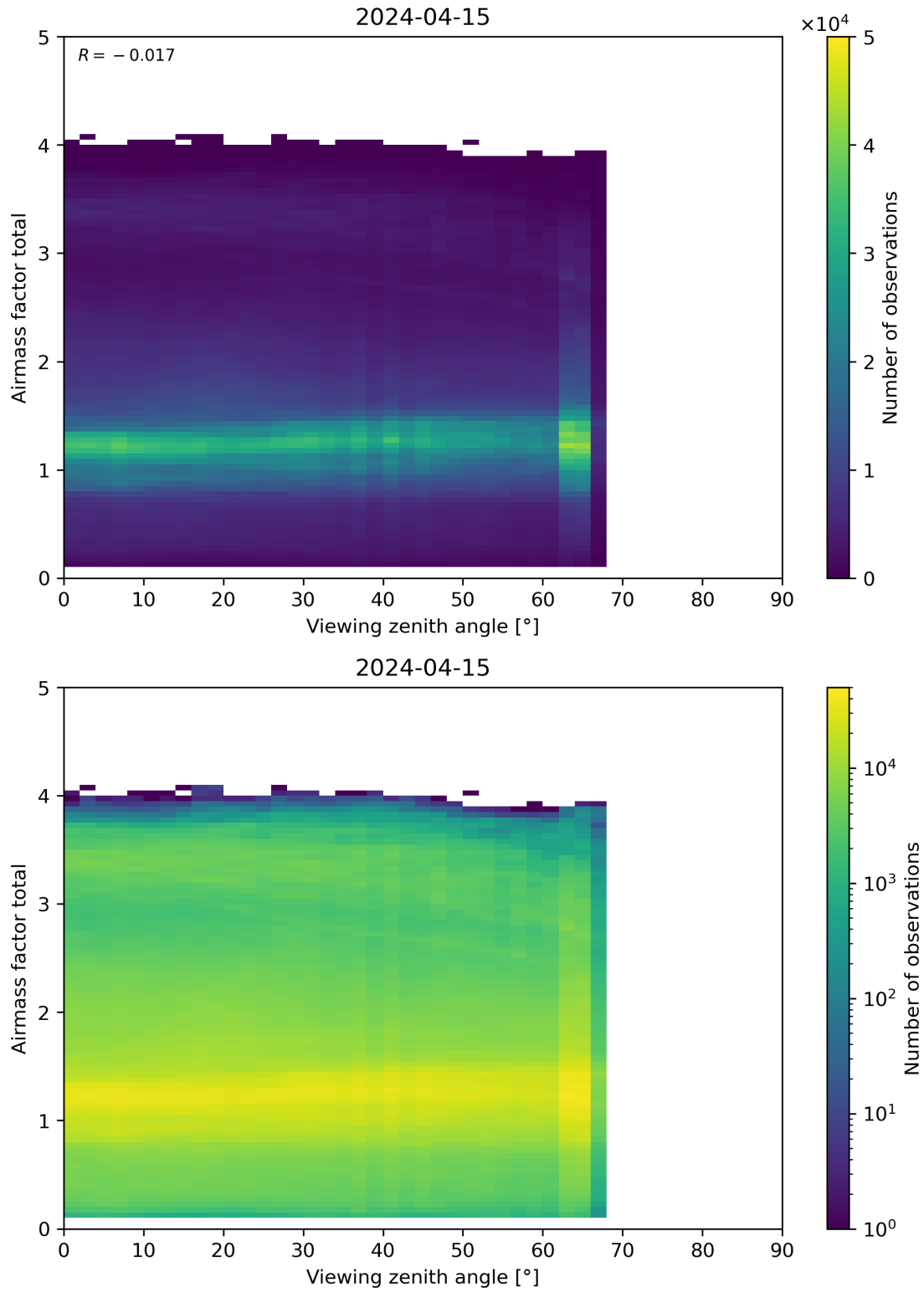
Figure 190: Scatter density plot of “Viewing zenith angle” against “Airmass factor total” for 2024-04-15 to 2024-04-16.
