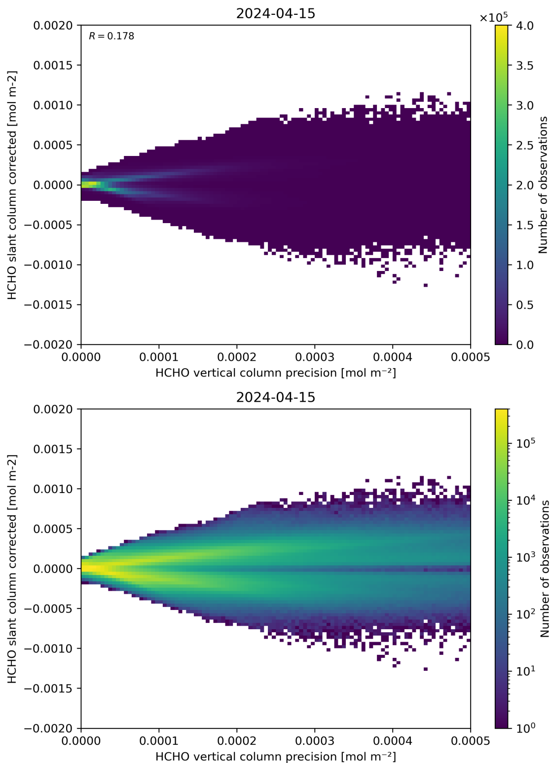
Figure 140: Scatter density plot of “HCHO vertical column precision” against “HCHO slant column corrected” for 2024-04-15 to 2024-04-16.
