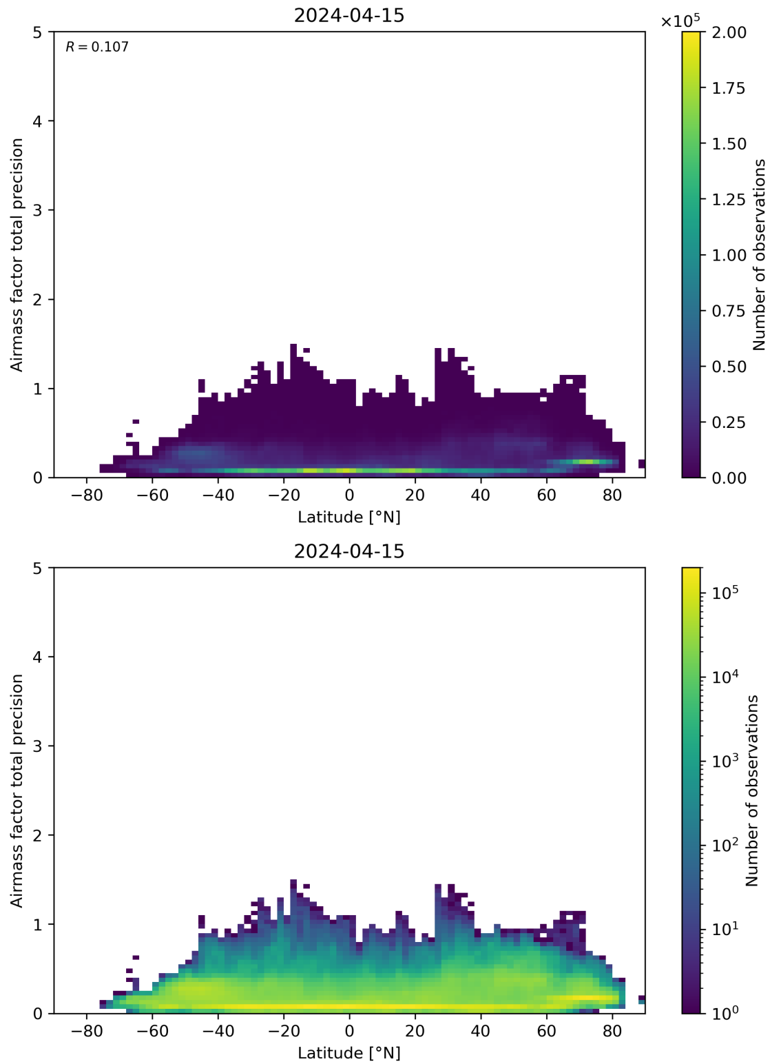
Figure 162: Scatter density plot of “Latitude” against “Airmass factor total precision” for 2024-04-15 to 2024-04-16.
