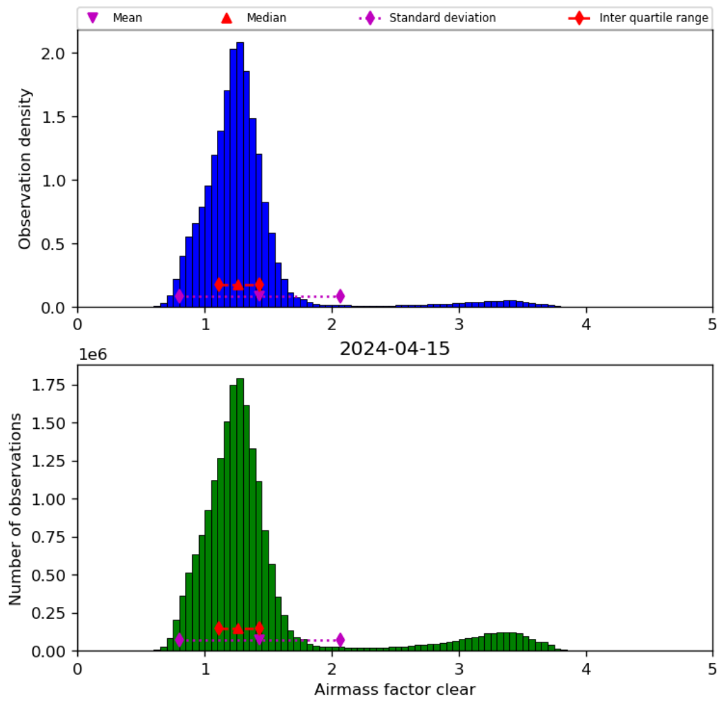
Figure 42: Histogram of “Airmass factor clear” for 2024-04-15 to 2024-04-16
