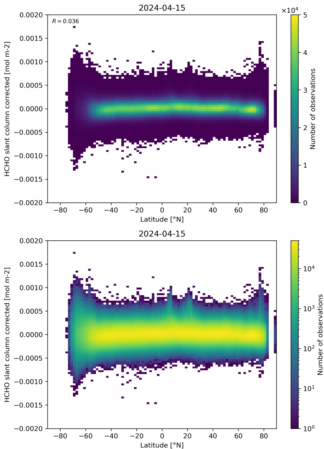
Figure 157: Scatter density plot of “Latitude” against “HCHO slant column corrected” for 2024-04-15 to 2024-04-16.
