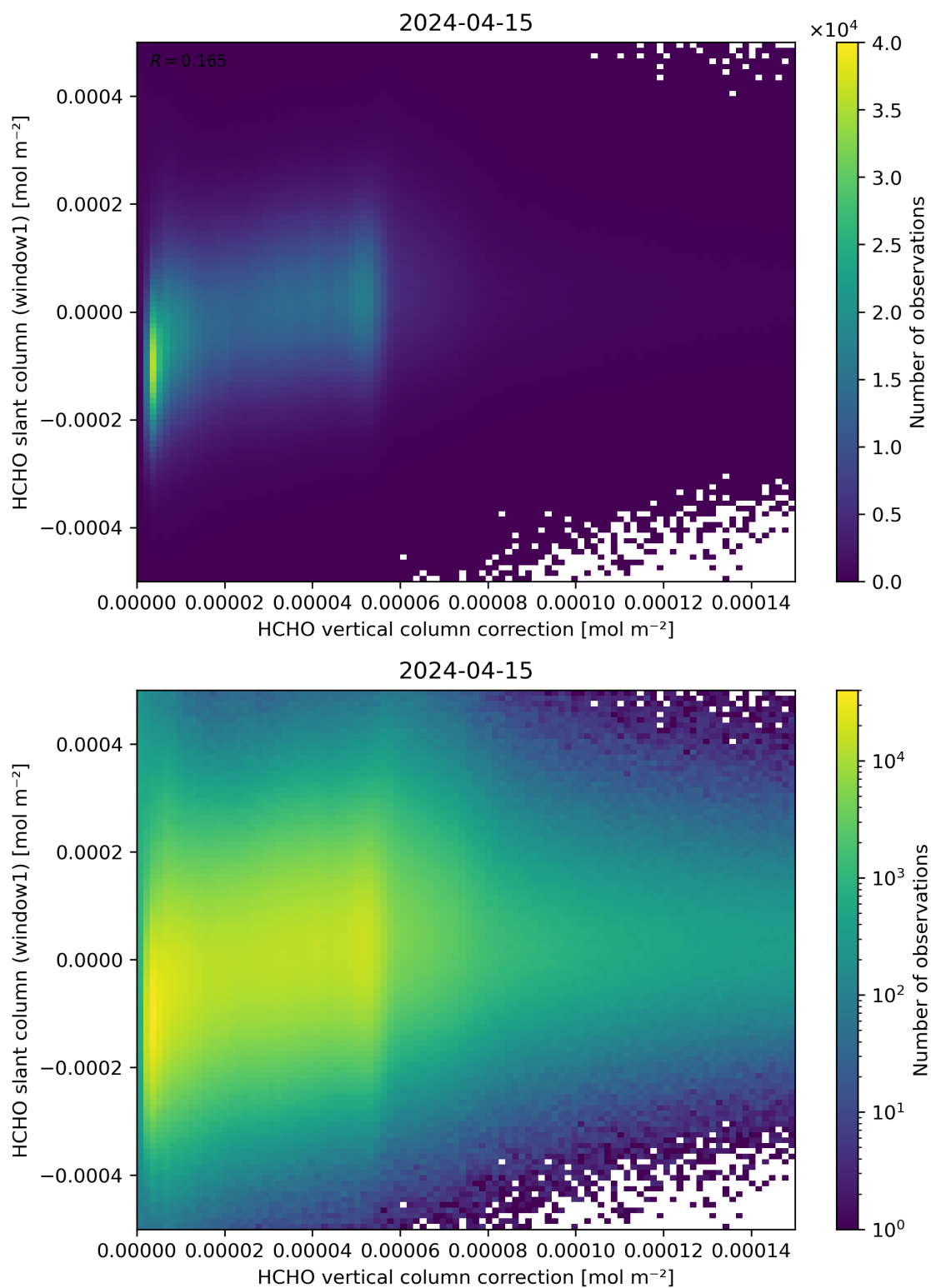
Figure 118: Scatter density plot of “HCHO vertical column correction” against “HCHO slant column (window1)” for 2024-04-15 to 2024-04-16.
