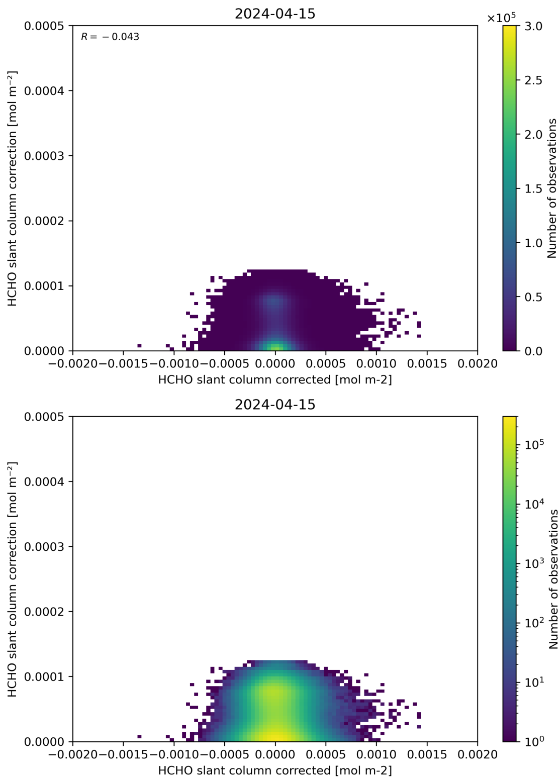
Figure 77: Scatter density plot of “HCHO slant column corrected” against “HCHO slant column correction” for 2024-04-15 to 2024-04-16.
