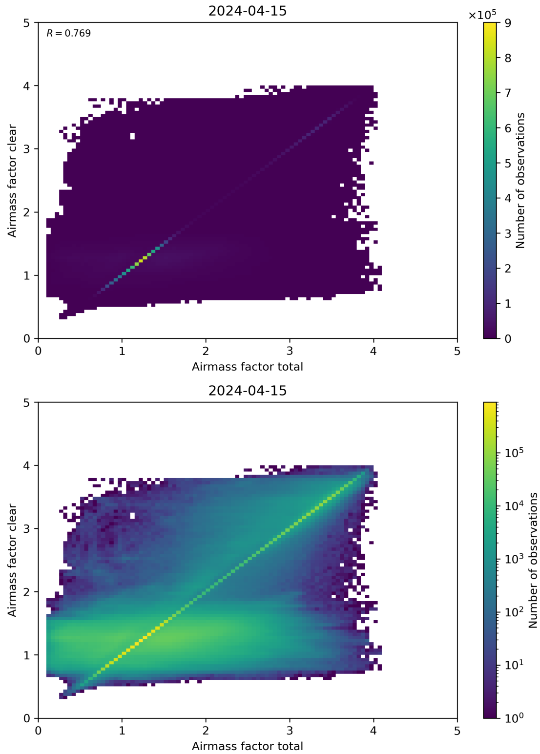
Figure 100: Scatter density plot of “Airmass factor total” against “Airmass factor clear” for 2024-04-15 to 2024-04-16.
