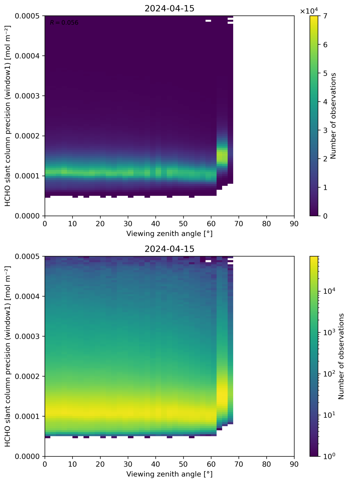
Figure 189: Scatter density plot of “Viewing zenith angle” against “HCHO slant column precision (window1)” for 2024-04-15 to 2024-04-16.
