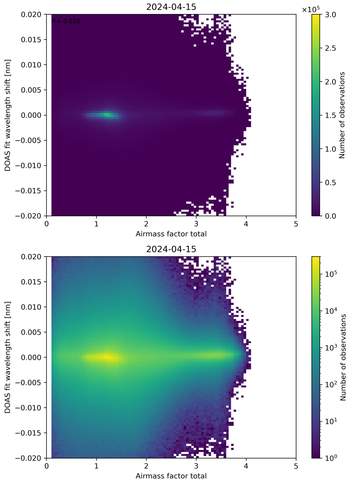
Figure 98: Scatter density plot of “Airmass factor total” against “DOAS fit wavelength shift” for 2024-04-15 to 2024-04-16.
