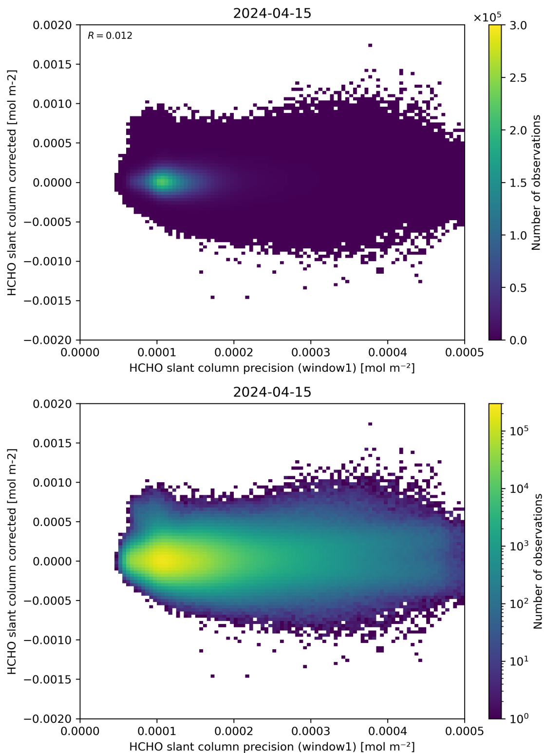
Figure 92: Scatter density plot of “HCHO slant column precision (window1)” against “HCHO slant column corrected” for 2024-04-15 to 2024-04-16.
