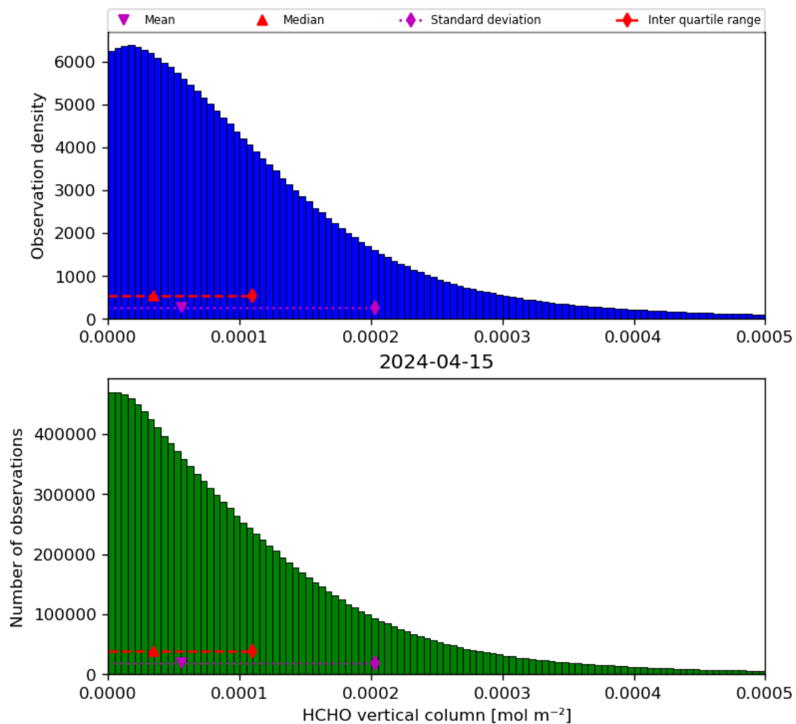
Figure 35: Histogram of “HCHO vertical column” for 2024-04-15 to 2024-04-16
