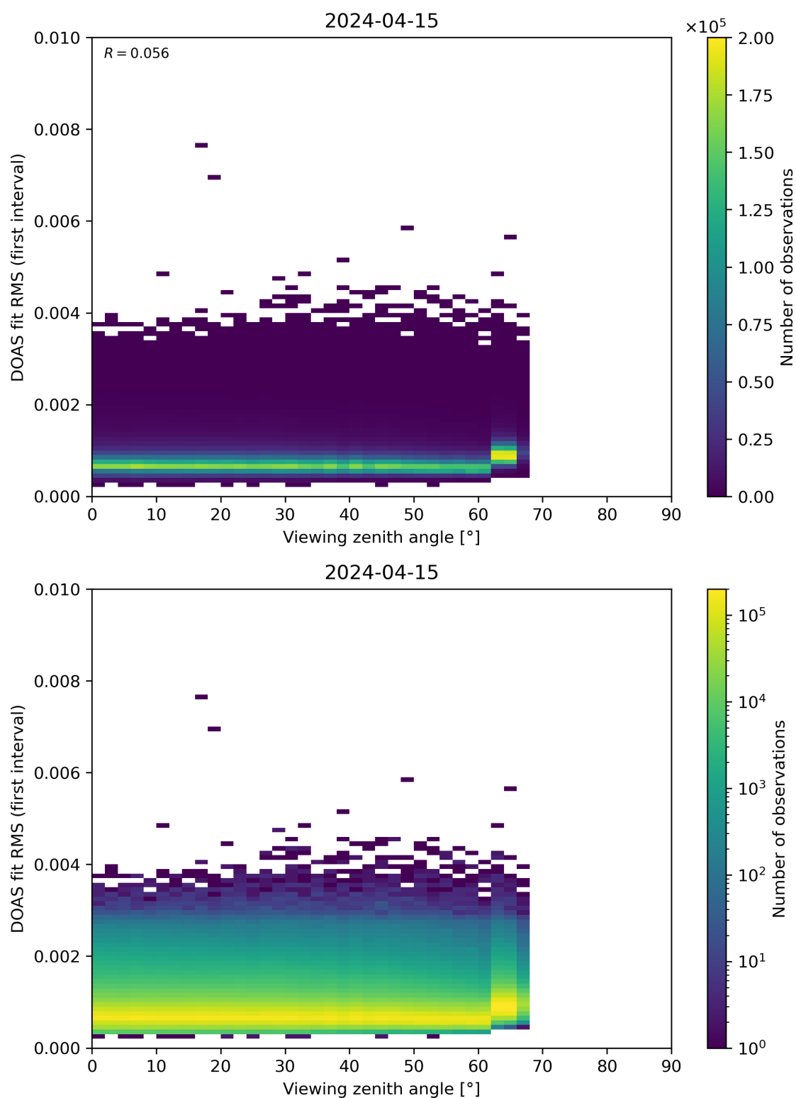
Figure 182: Scatter density plot of “Viewing zenith angle” against “DOAS fit RMS (first interval)” for 2024-04-15 to 2024-04-16.
