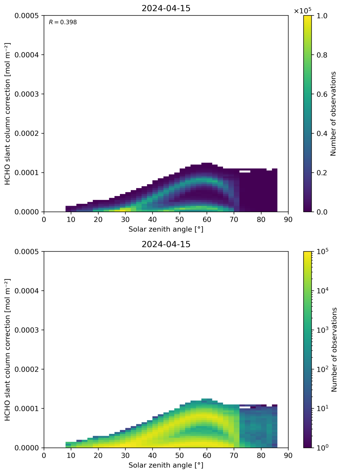
Figure 172: Scatter density plot of “Solar zenith angle” against “HCHO slant column correction” for 2024-04-15 to 2024-04-16.
