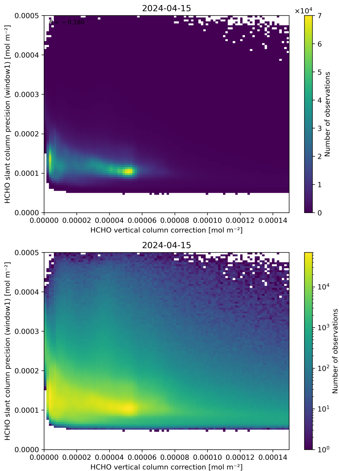
Figure 119: Scatter density plot of “HCHO vertical column correction” against “HCHO slant column precision (window1)” for 2024-04-15 to 2024-04-16.
