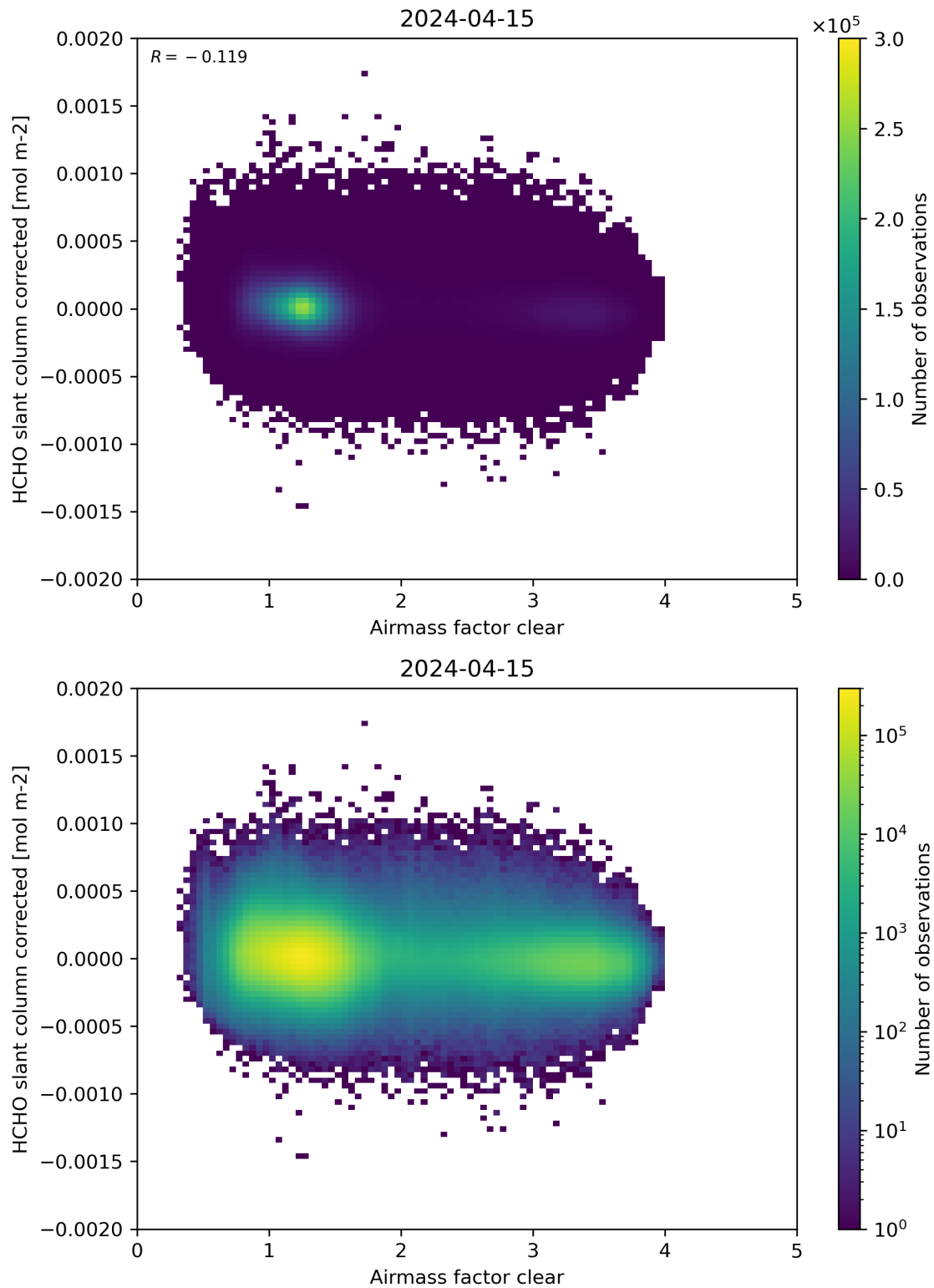
Figure 74: Scatter density plot of “Airmass factor clear” against “HCHO slant column corrected” for 2024-04-15 to 2024-04-16.
