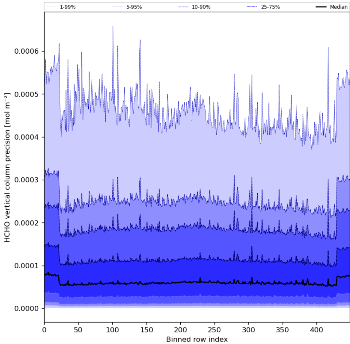
Figure 50: Along track statistics of “HCHO vertical column precision” for 2024-04-15 to 2024-04-16
