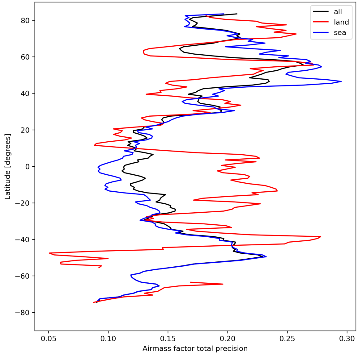
Figure 27: Zonal average of “Airmass factor total precision” for 2024-04-15 to 2024-04-16.
