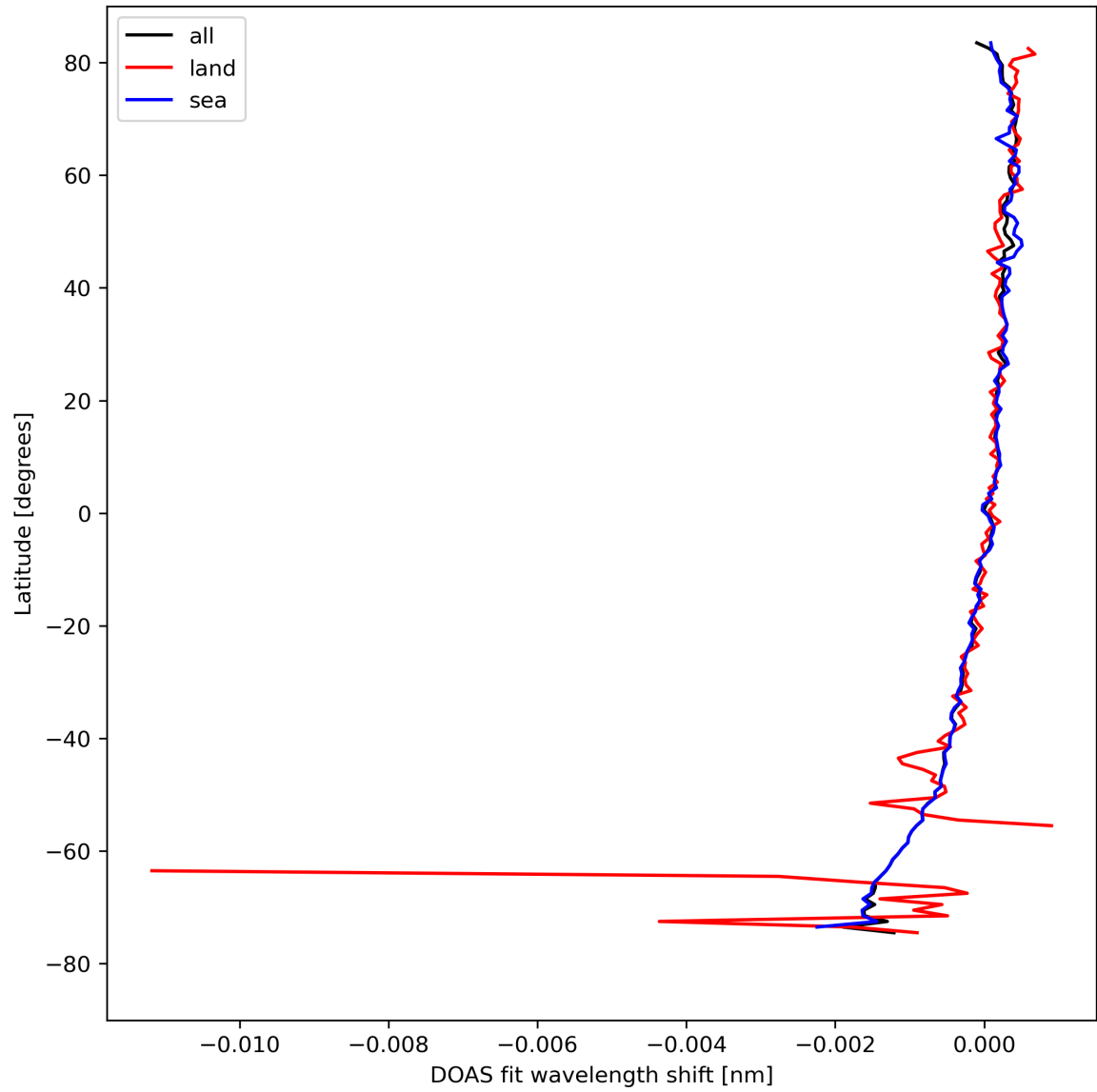
Figure 30: Zonal average of “DOAS fit wavelength shift” for 2024-04-15 to 2024-04-16.
