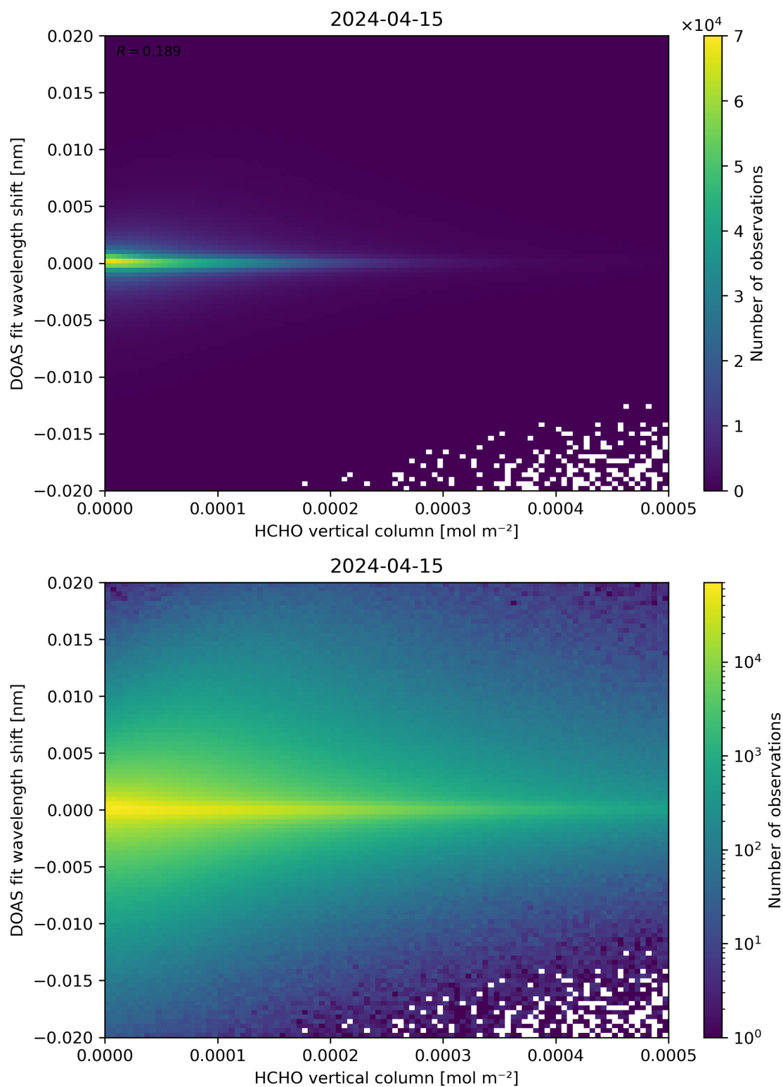
Figure 124: Scatter density plot of “HCHO vertical column” against “DOAS fit wavelength shift” for 2024-04-15 to 2024-04-16.
