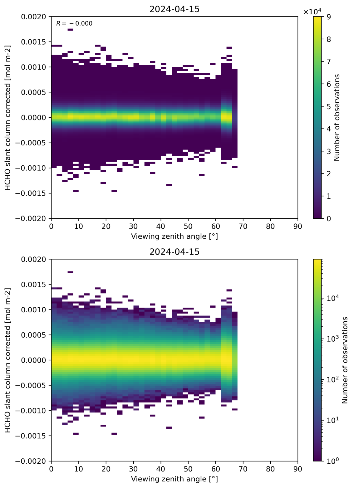
Figure 186: Scatter density plot of “Viewing zenith angle” against “HCHO slant column corrected” for 2024-04-15 to 2024-04-16.
