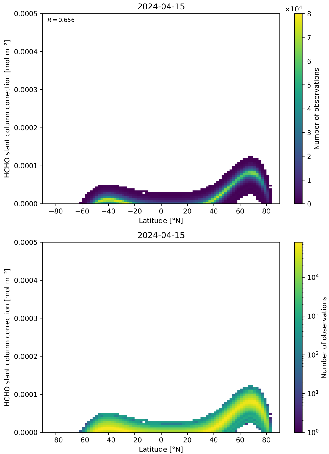
Figure 158: Scatter density plot of “Latitude” against “HCHO slant column correction” for 2024-04-15 to 2024-04-16.
