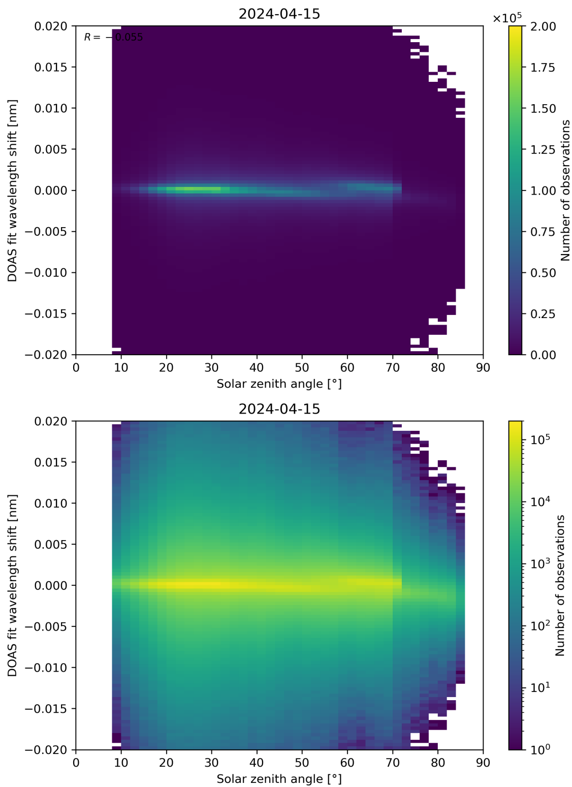
Figure 168: Scatter density plot of “Solar zenith angle” against “DOAS fit wavelength shift” for 2024-04-15 to 2024-04-16.
