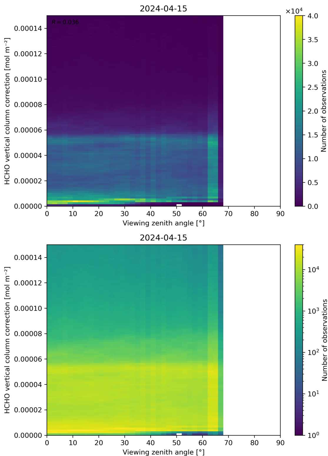
Figure 193: Scatter density plot of “Viewing zenith angle” against “HCHO vertical column correction” for 2024-04-15 to 2024-04-16.
