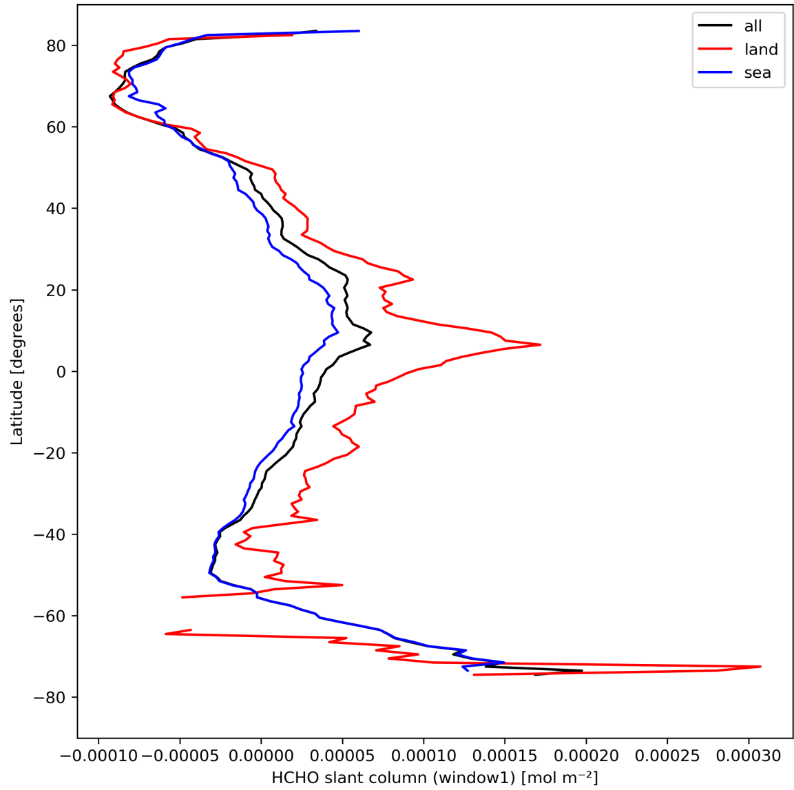
Figure 24: Zonal average of “HCHO slant column (window1)” for 2024-04-15 to 2024-04-16.
