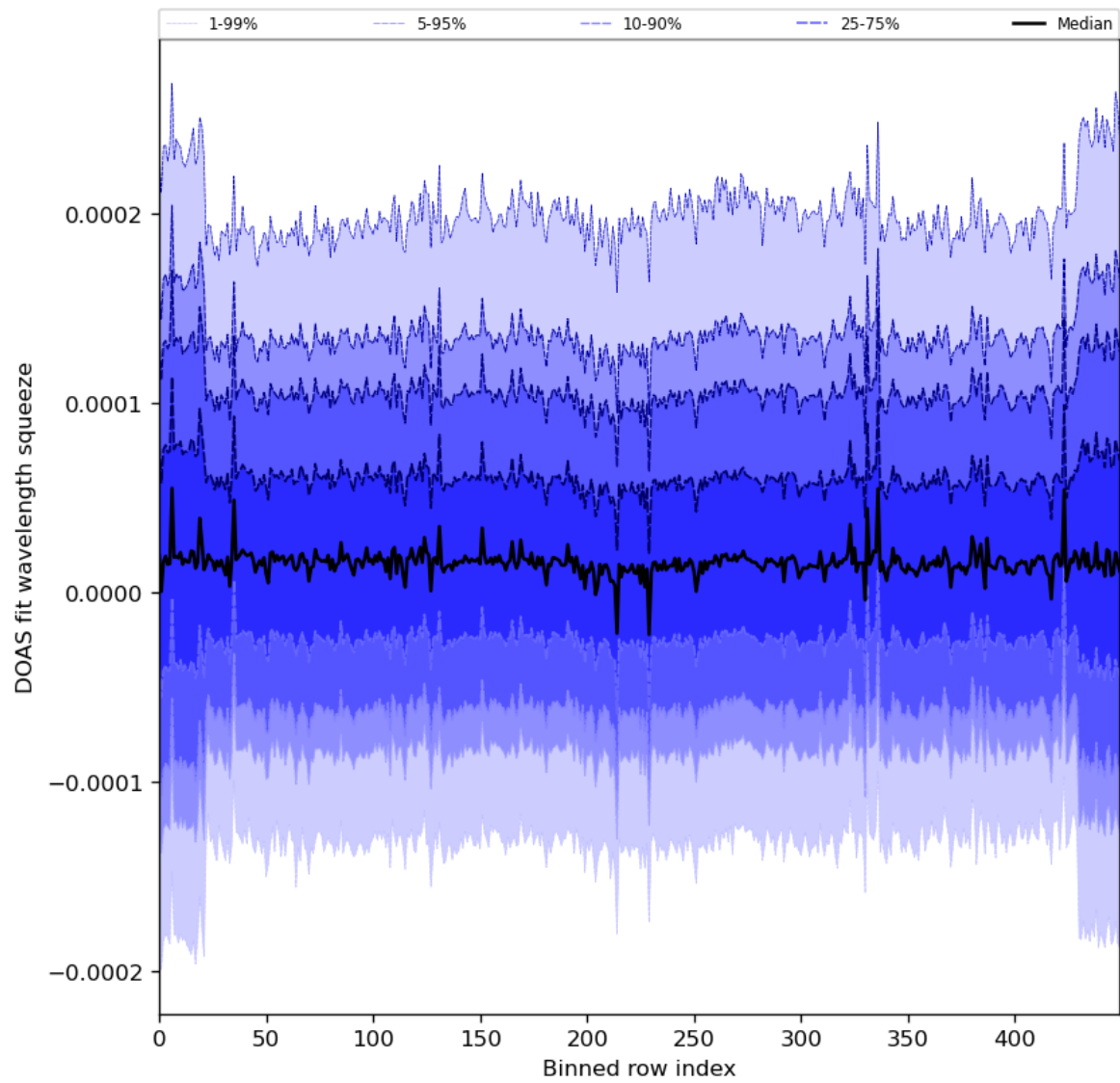
Figure 59: Along track statistics of “DOAS fit wavelength squeeze” for 2024-04-15 to 2024-04-16
