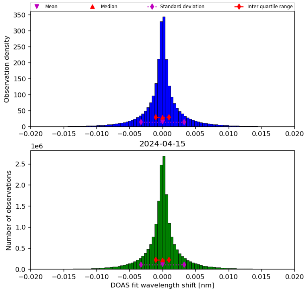
Figure 44: Histogram of “DOAS fit wavelength shift” for 2024-04-15 to 2024-04-16
