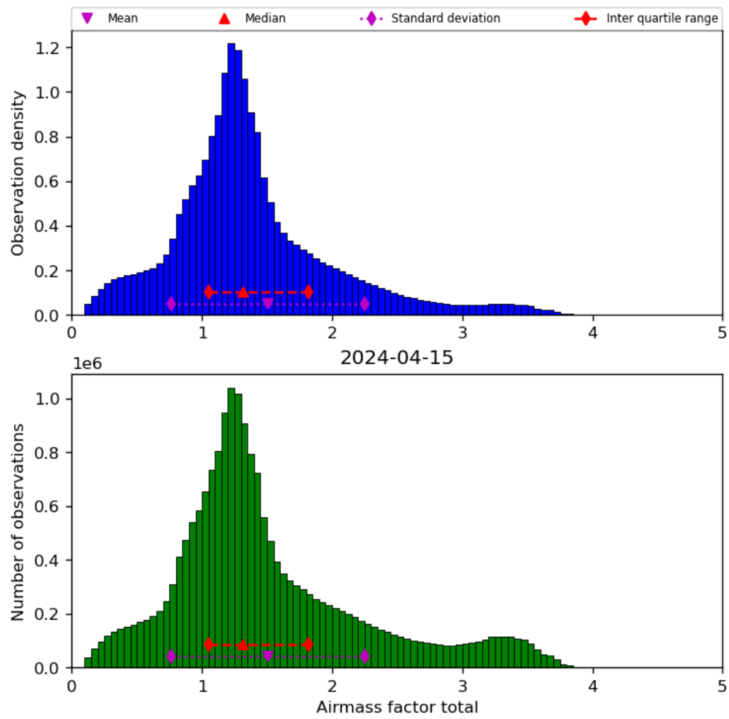
Figure 40: Histogram of “Airmass factor total” for 2024-04-15 to 2024-04-16
