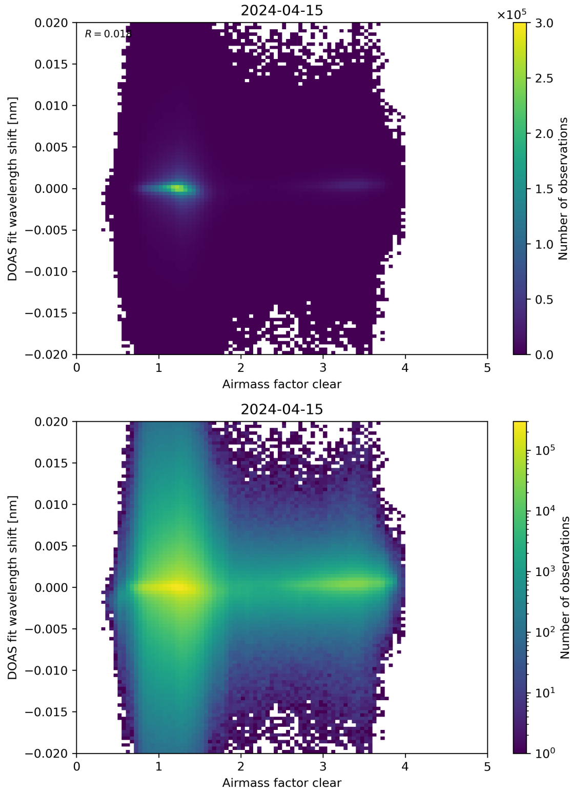
Figure 72: Scatter density plot of “Airmass factor clear” against “DOAS fit wavelength shift” for 2024-04-15 to 2024-04-16.
