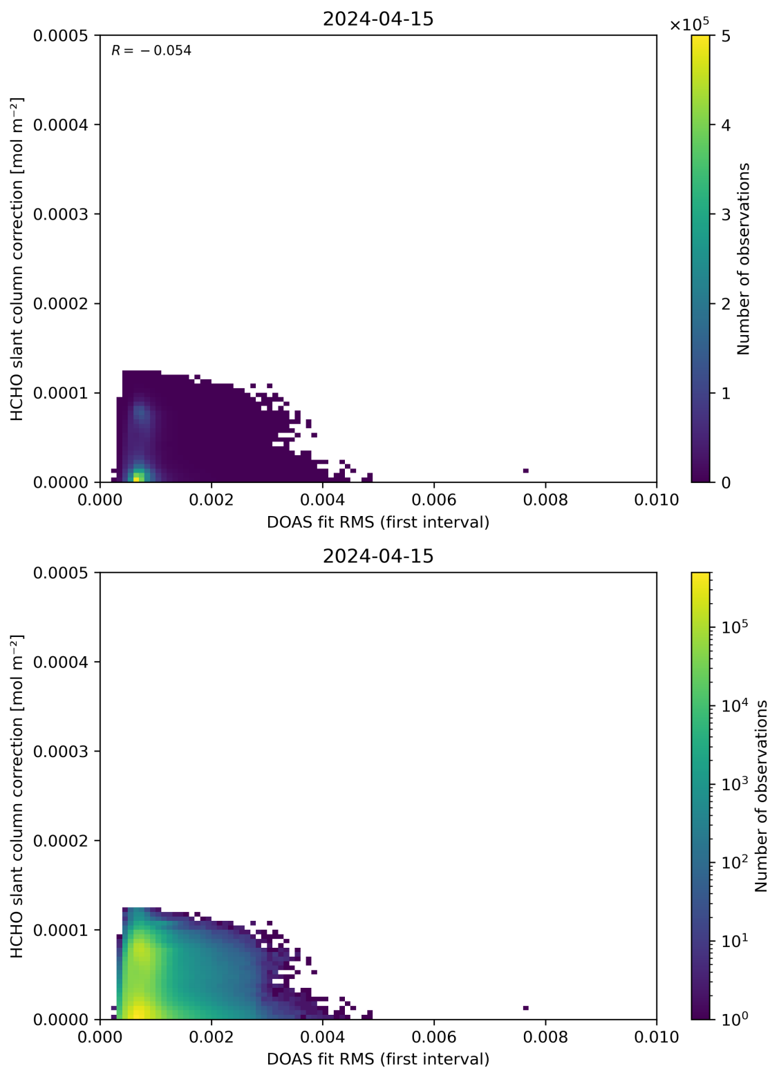
Figure 63: Scatter density plot of “DOAS fit RMS (first interval)” against “HCHO slant column correction” for 2024-04-15 to 2024-04-16.
