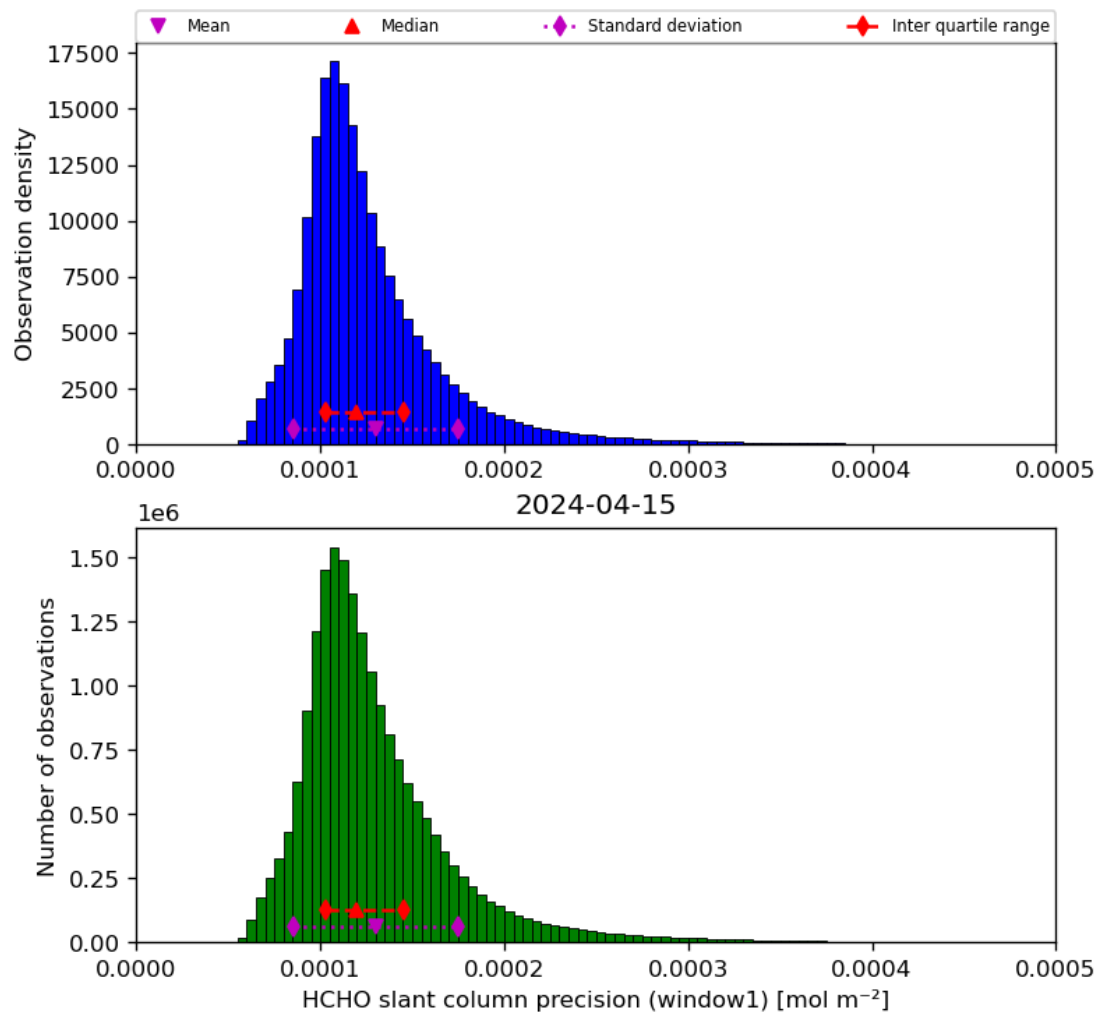
Figure 39: Histogram of “HCHO slant column precision (window1)” for 2024-04-15 to 2024-04-16
