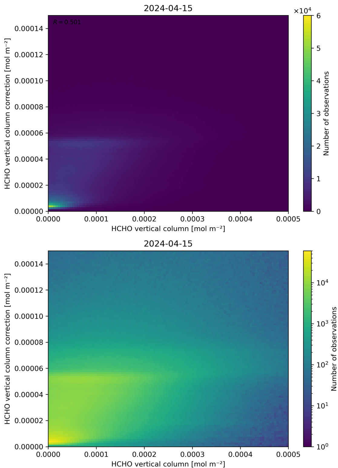
Figure 133: Scatter density plot of “HCHO vertical column” against “HCHO vertical column correction” for 2024-04-15 to 2024-04-16.
