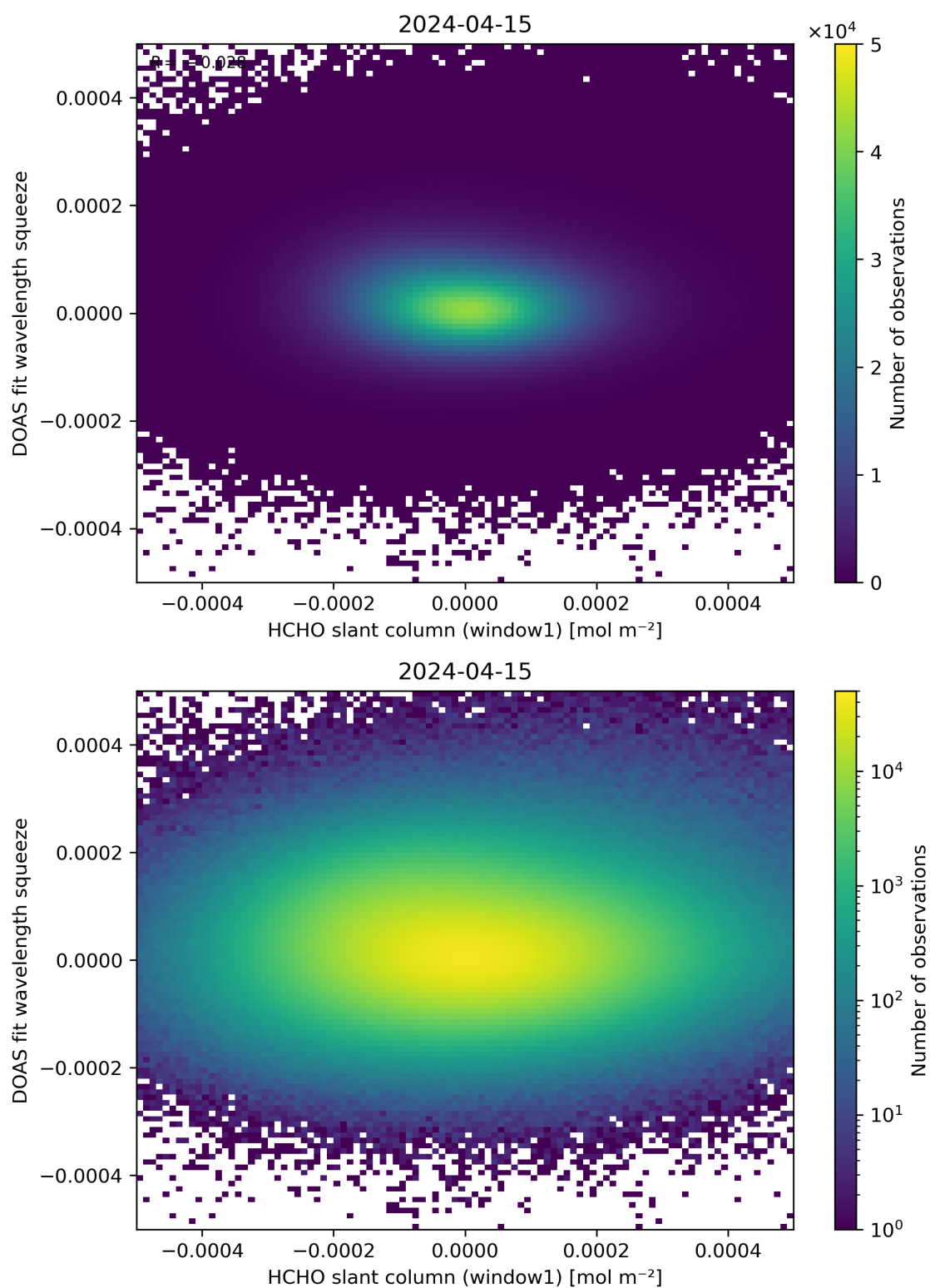
Figure 80: Scatter density plot of “HCHO slant column (window1)” against “DOAS fit wavelength squeeze” for 2024-04-15 to 2024-04-16.
