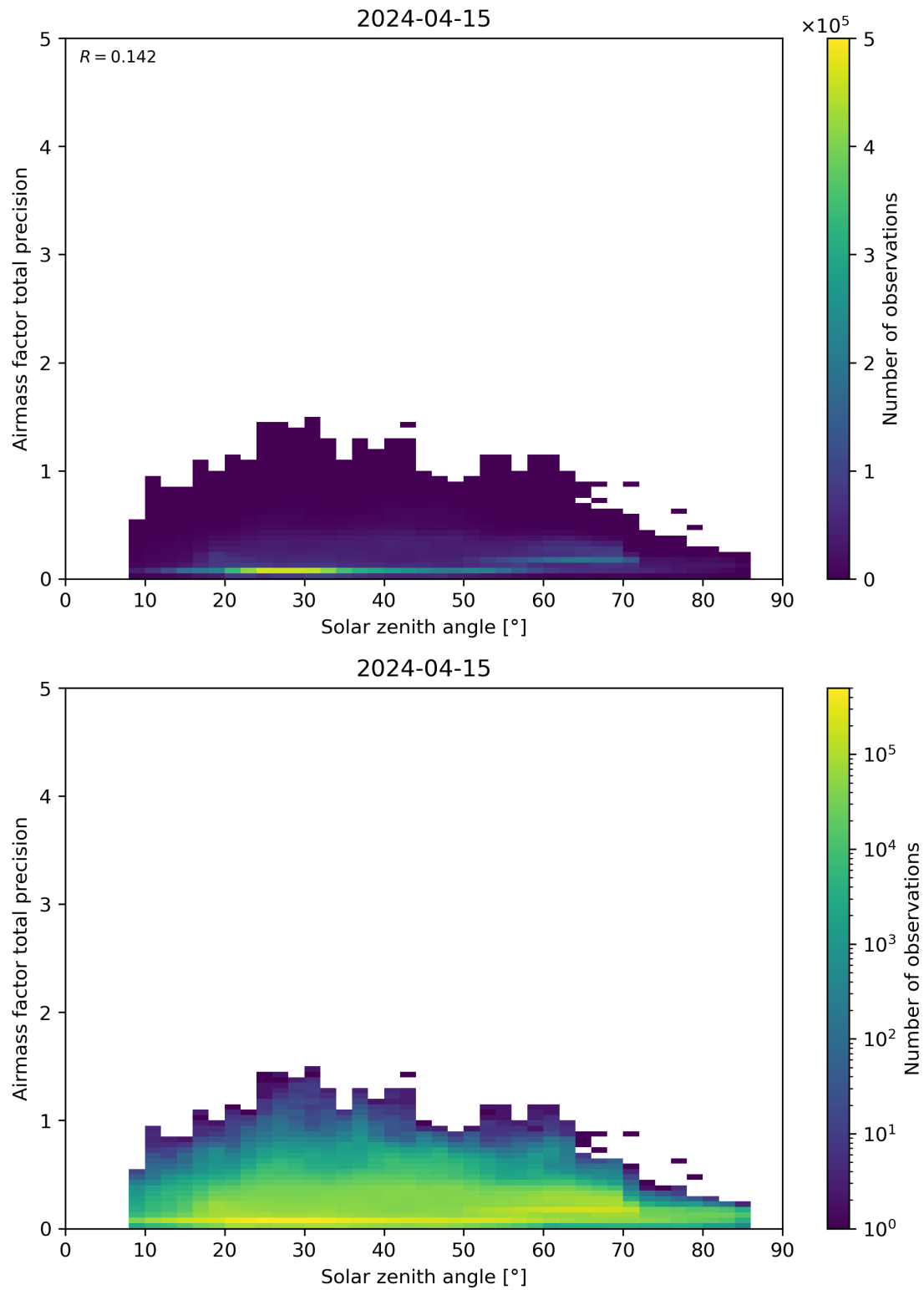
Figure 176: Scatter density plot of “Solar zenith angle” against “Airmass factor total precision” for 2024-04-15 to 2024-04-16.
