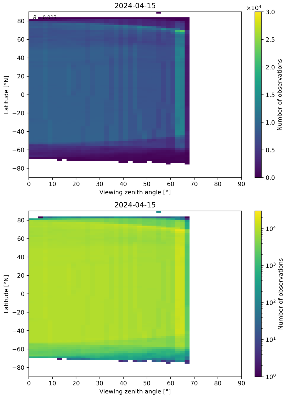
Figure 196: Scatter density plot of “Viewing zenith angle” against “Latitude” for 2024-04-15 to 2024-04-16.
