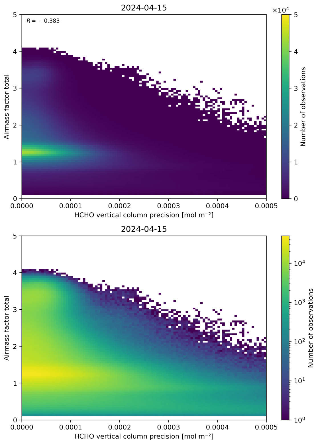
Figure 144: Scatter density plot of “HCHO vertical column precision” against “Airmass factor total” for 2024-04-15 to 2024-04-16.
