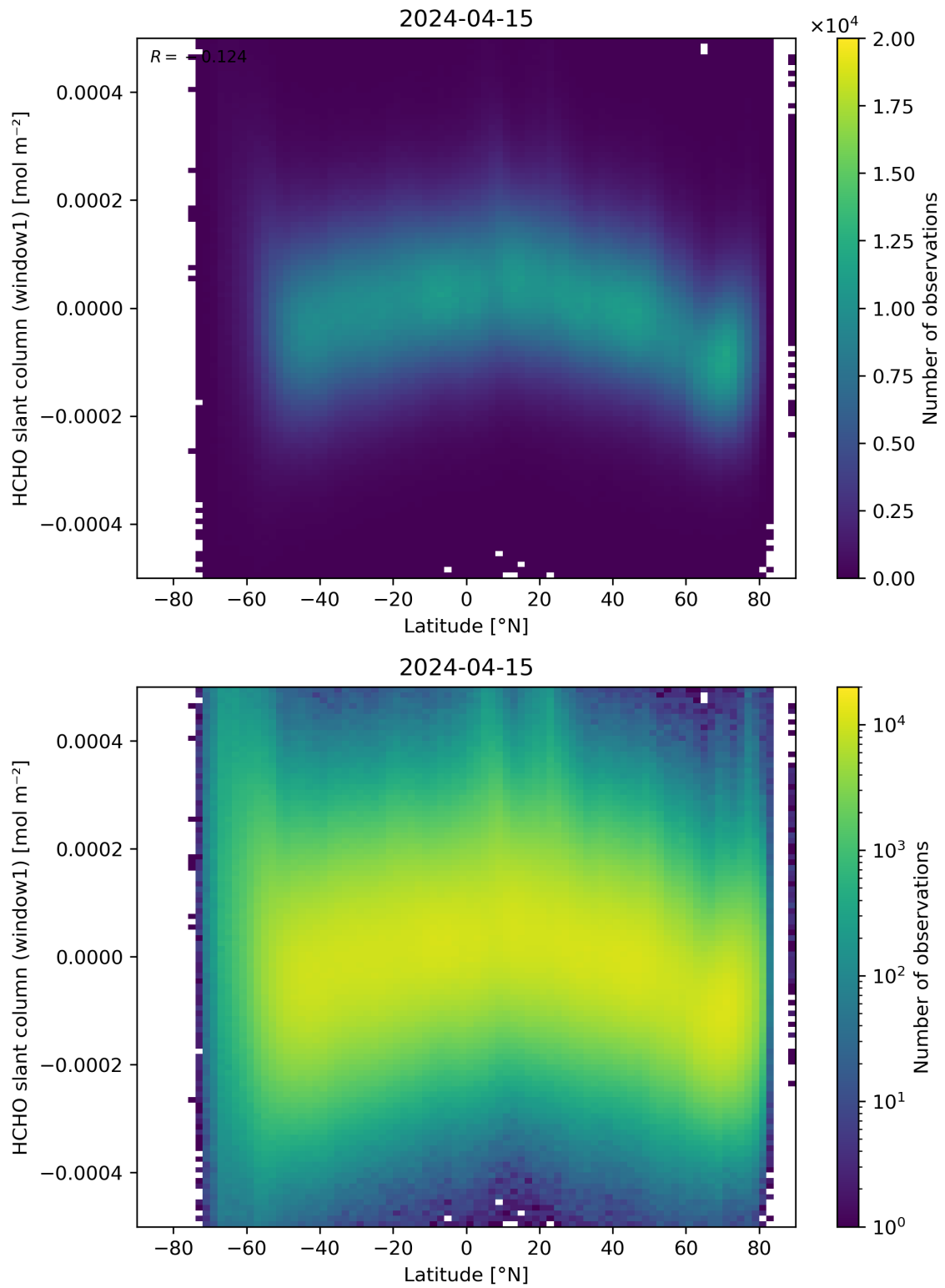
Figure 159: Scatter density plot of “Latitude” against “HCHO slant column (window1)” for 2024-04-15 to 2024-04-16.
