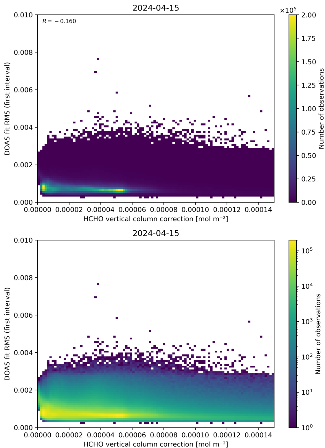
Figure 112: Scatter density plot of “HCHO vertical column correction” against “DOAS fit RMS (first interval)” for 2024-04-15 to 2024-04-16.
