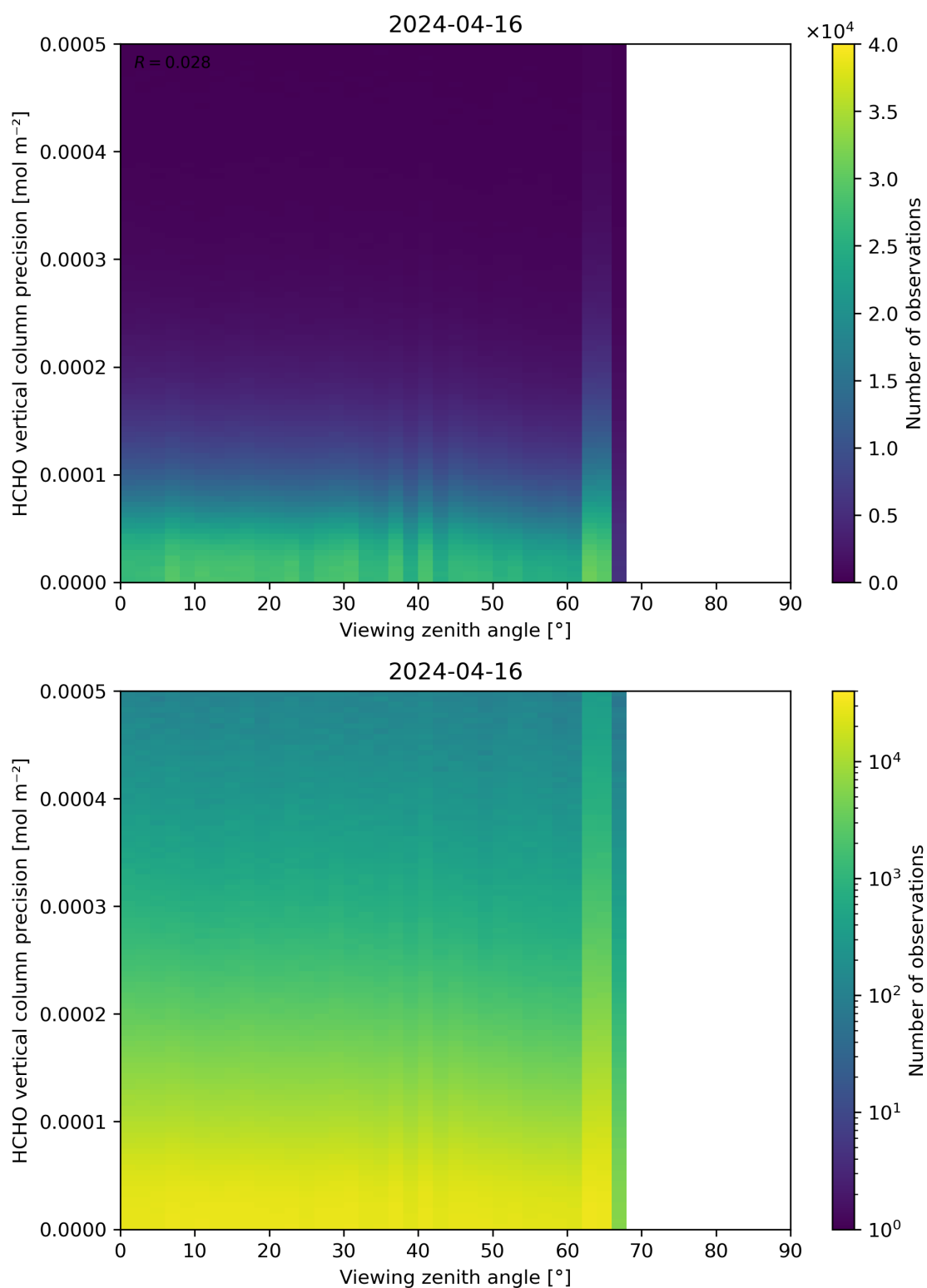
Figure 194: Scatter density plot of “Viewing zenith angle” against “HCHO vertical column precision” for 2024-04-16 to 2024-04-17.
