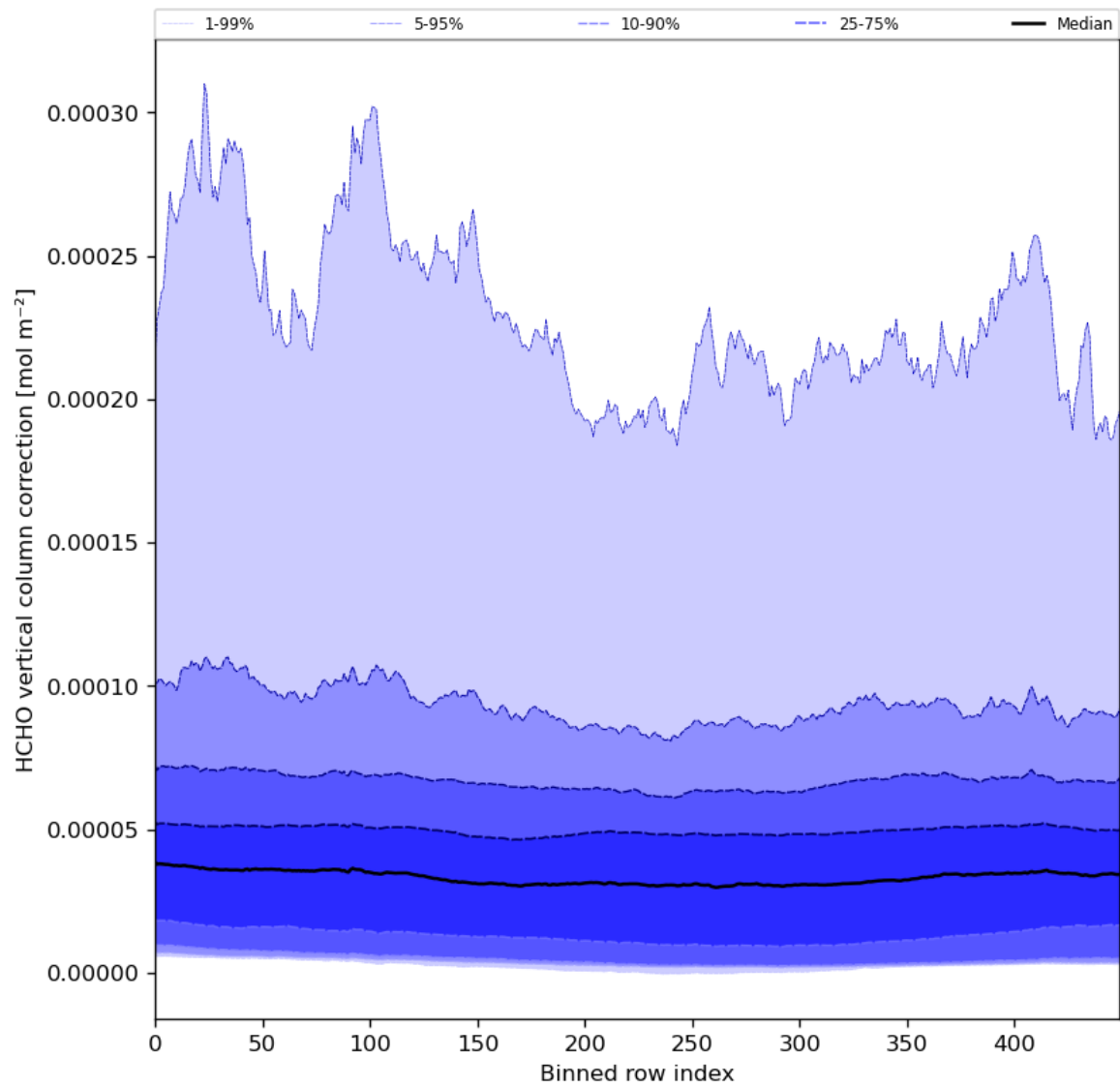
Figure 51: Along track statistics of “HCHO vertical column correction” for 2024-04-16 to 2024-04-17
