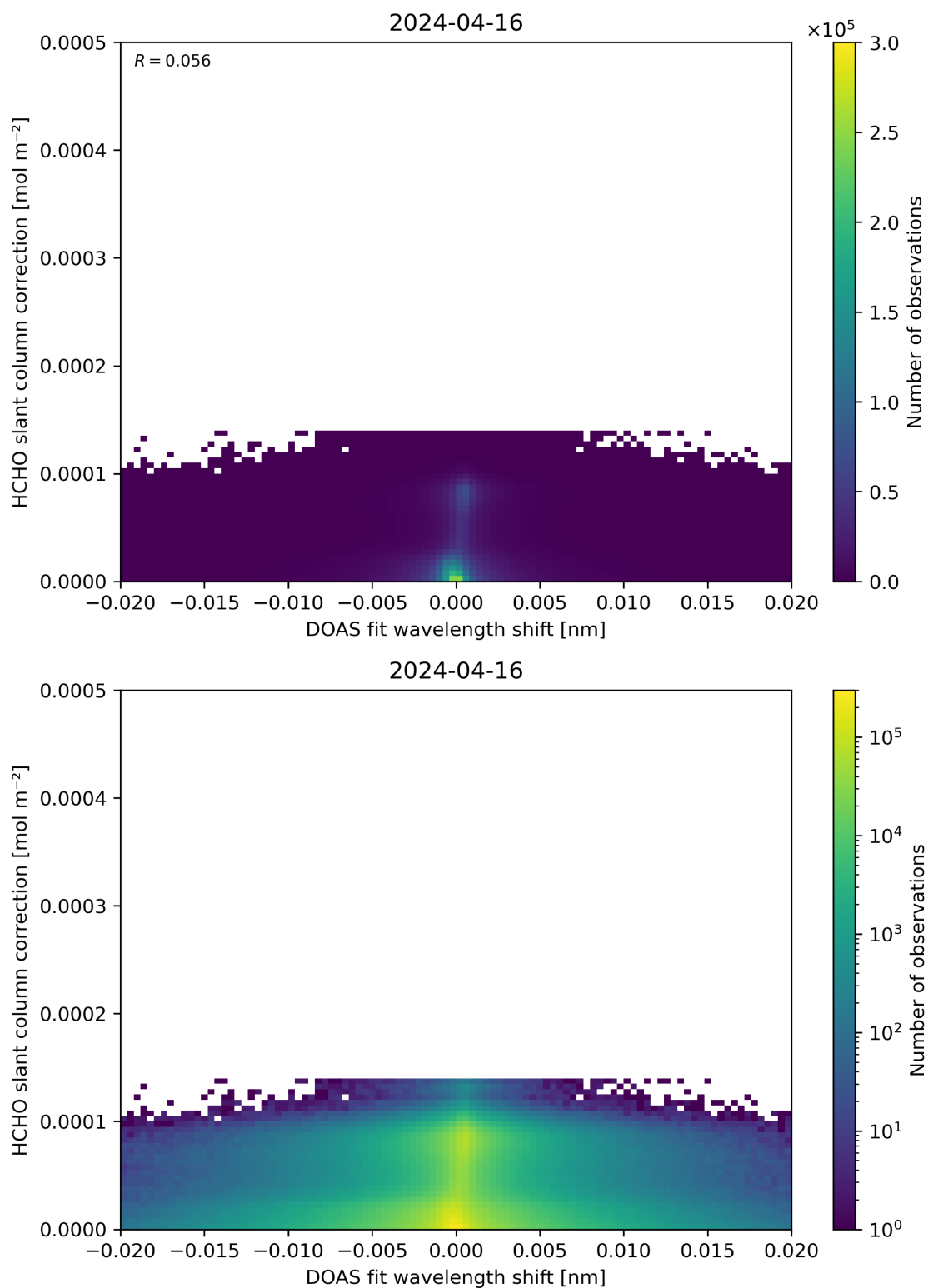
Figure 67: Scatter density plot of “DOAS fit wavelength shift” against “HCHO slant column correction” for 2024-04-16 to 2024-04-17.
