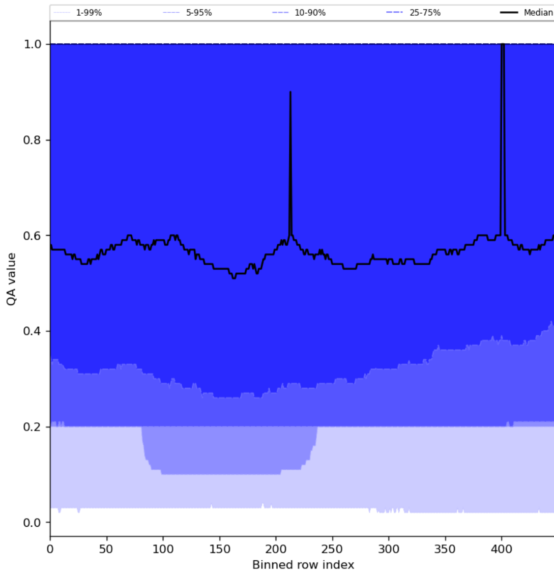
Figure 48: Along track statistics of “QA value” for 2024-04-16 to 2024-04-17
