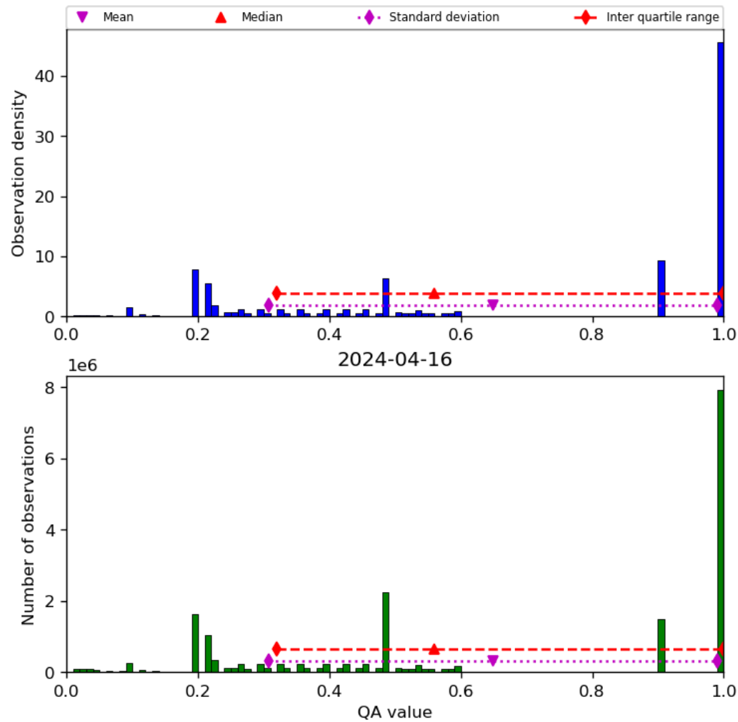
Figure 34: Histogram of “QA value” for 2024-04-16 to 2024-04-17
