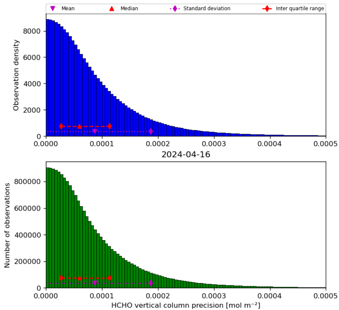
Figure 36: Histogram of “HCHO vertical column precision” for 2024-04-16 to 2024-04-17
