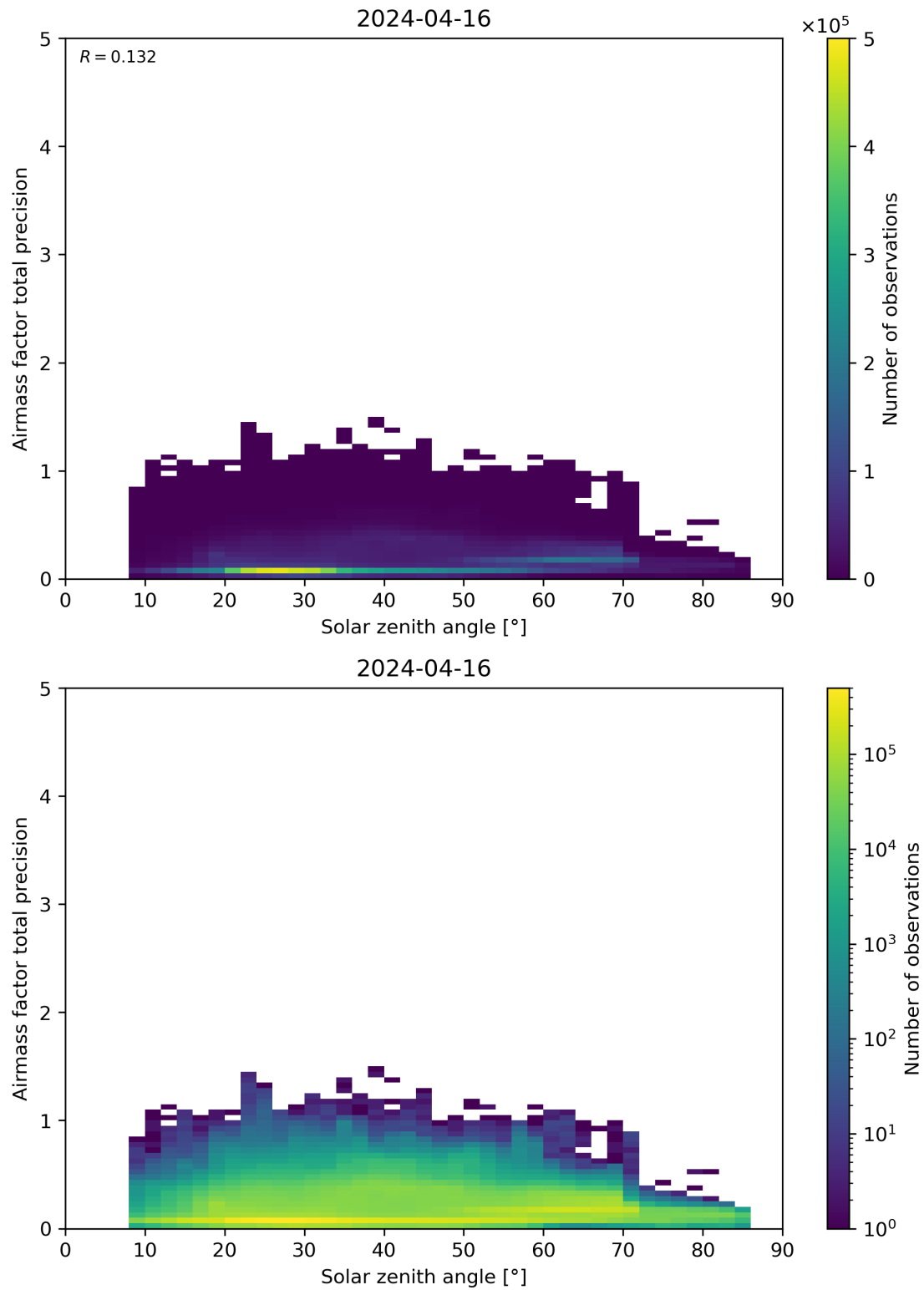
Figure 176: Scatter density plot of “Solar zenith angle” against “Airmass factor total precision” for 2024-04-16 to 2024-04-17.
