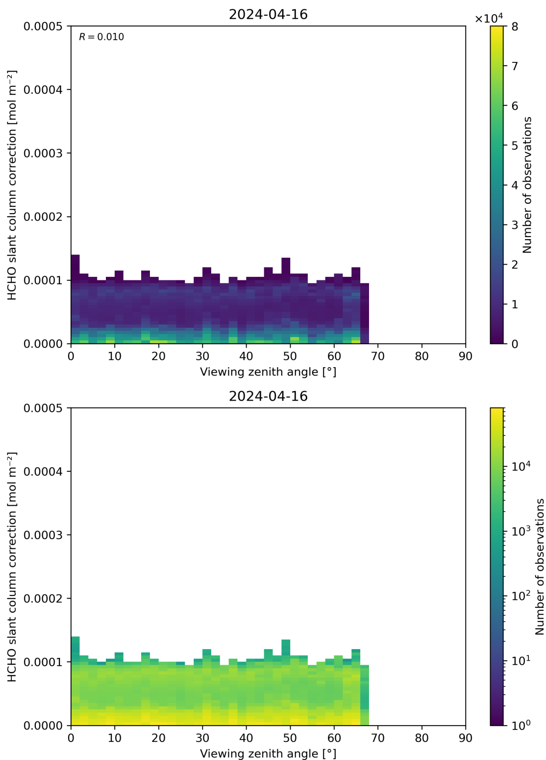
Figure 187: Scatter density plot of “Viewing zenith angle” against “HCHO slant column correction” for 2024-04-16 to 2024-04-17.
