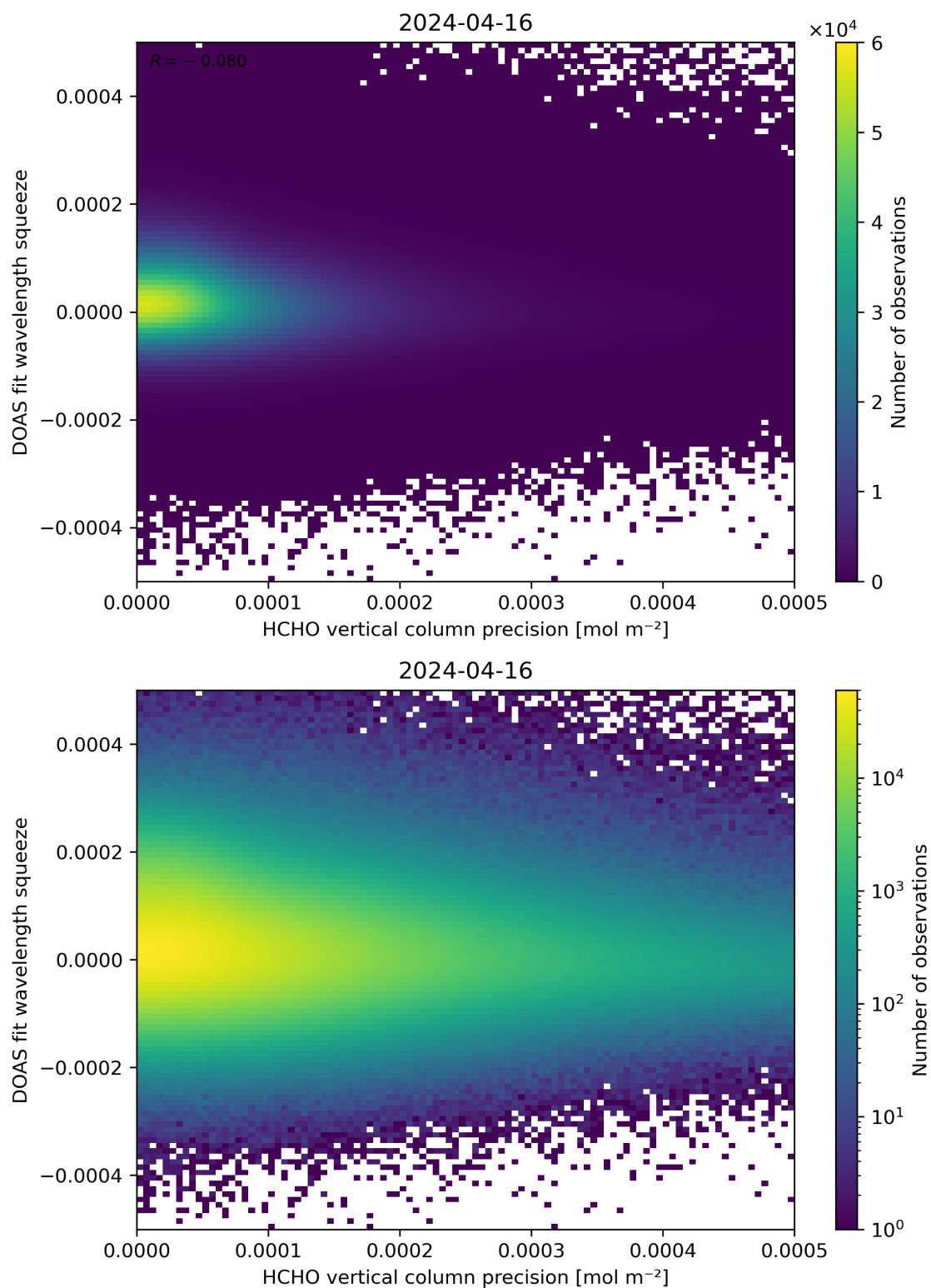
Figure 138: Scatter density plot of “HCHO vertical column precision” against “DOAS fit wavelength squeeze” for 2024-04-16 to 2024-04-17.
