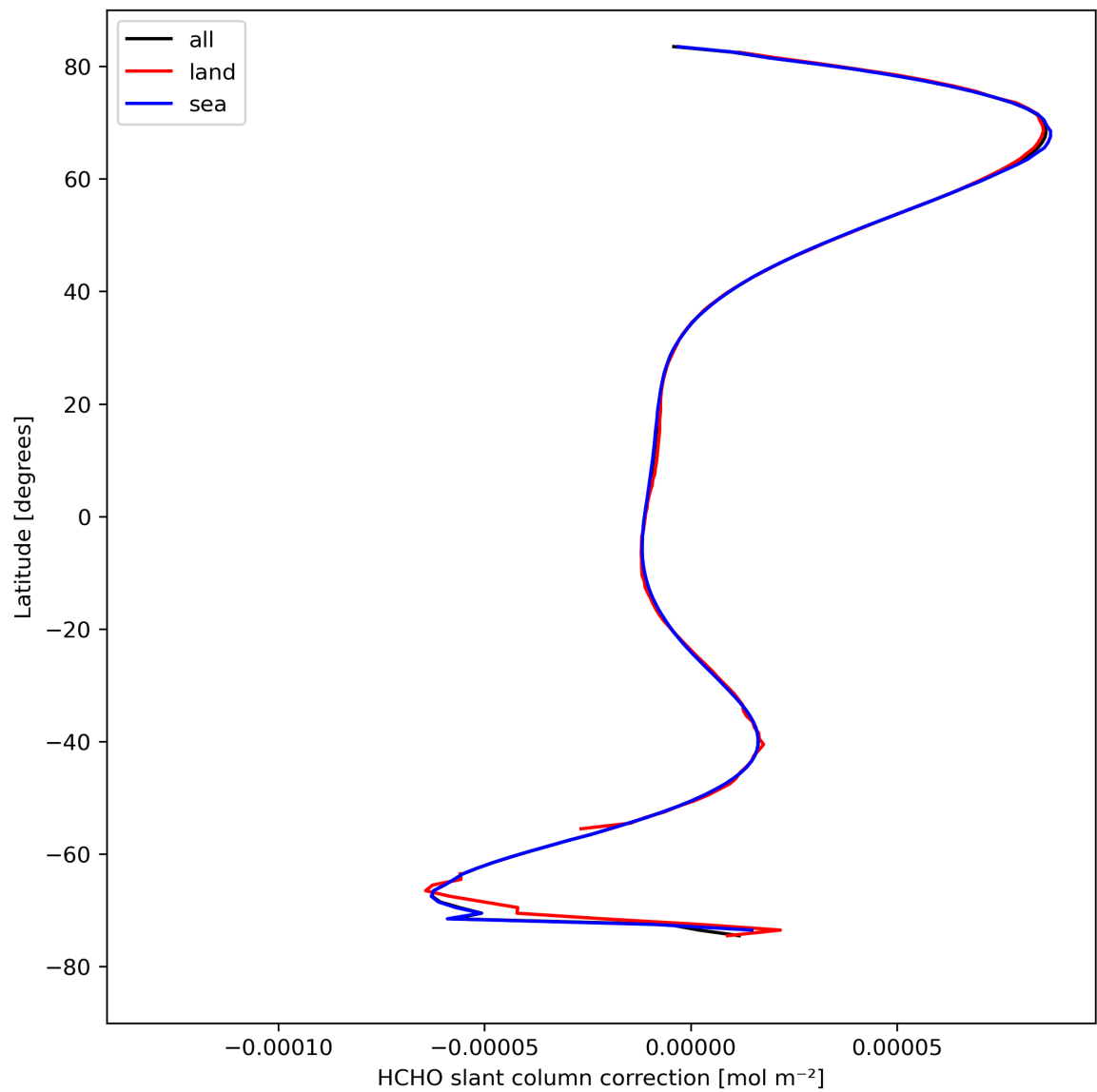
Figure 33: Zonal average of “HCHO slant column correction” for 2024-04-16 to 2024-04-17.
