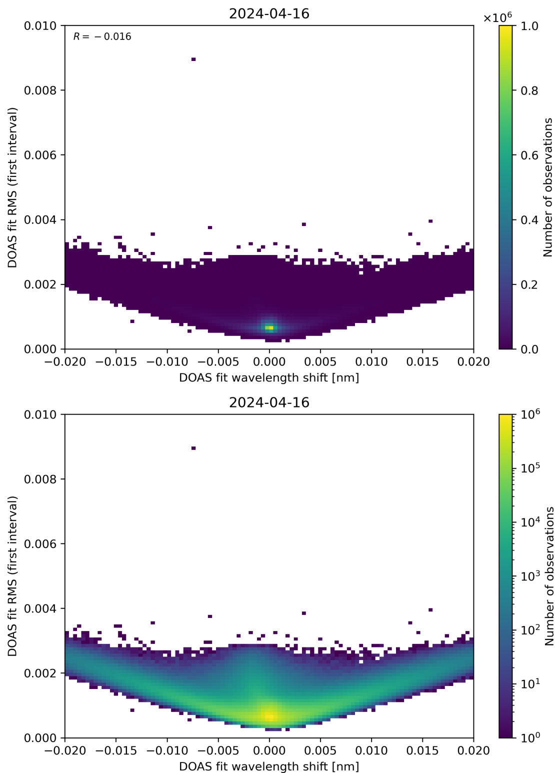
Figure 64: Scatter density plot of “DOAS fit wavelength shift” against “DOAS fit RMS (first interval)” for 2024-04-16 to 2024-04-17.
