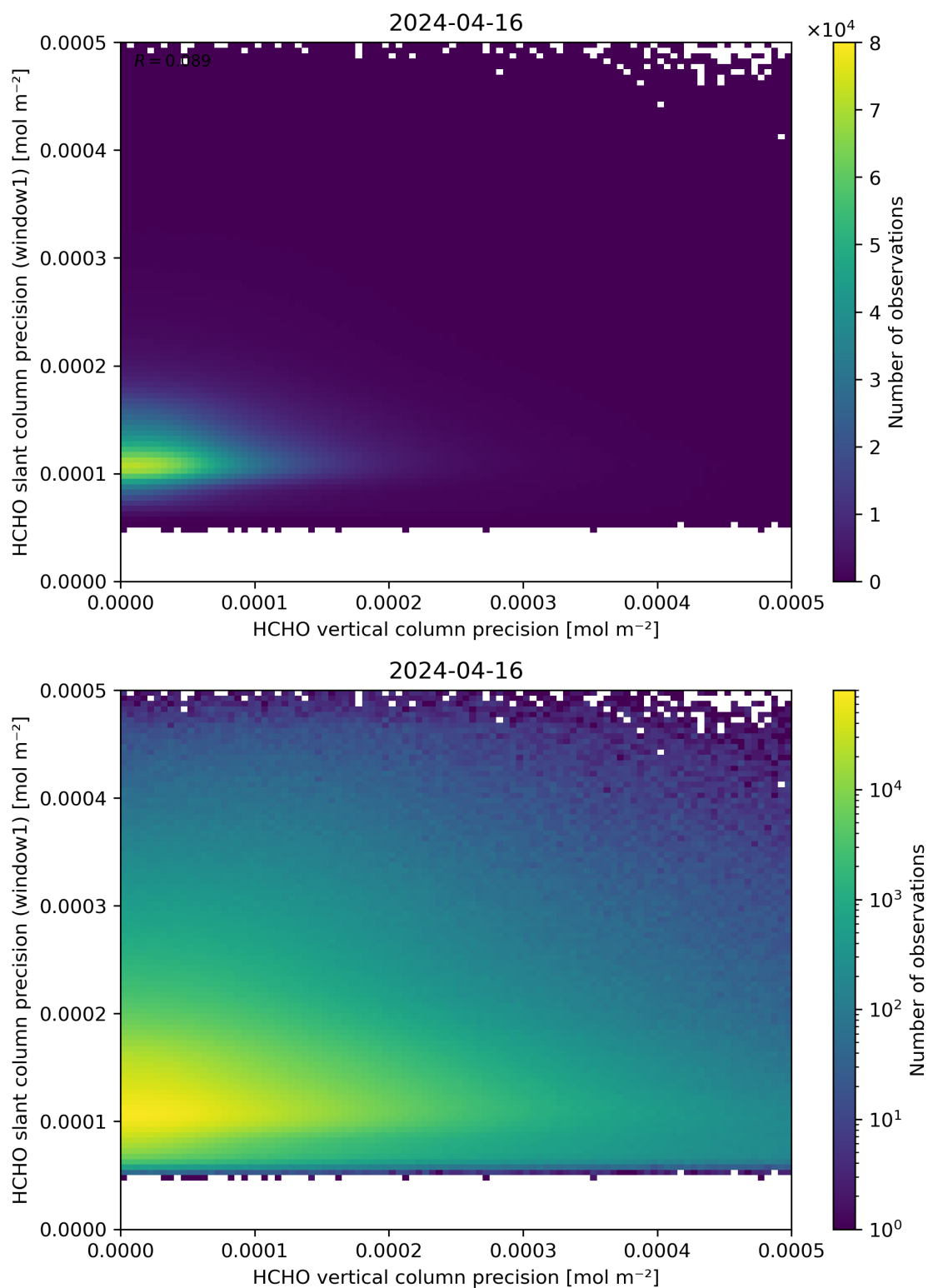
Figure 143: Scatter density plot of “HCHO vertical column precision” against “HCHO slant column precision (window1)” for 2024-04-16 to 2024-04-17.
