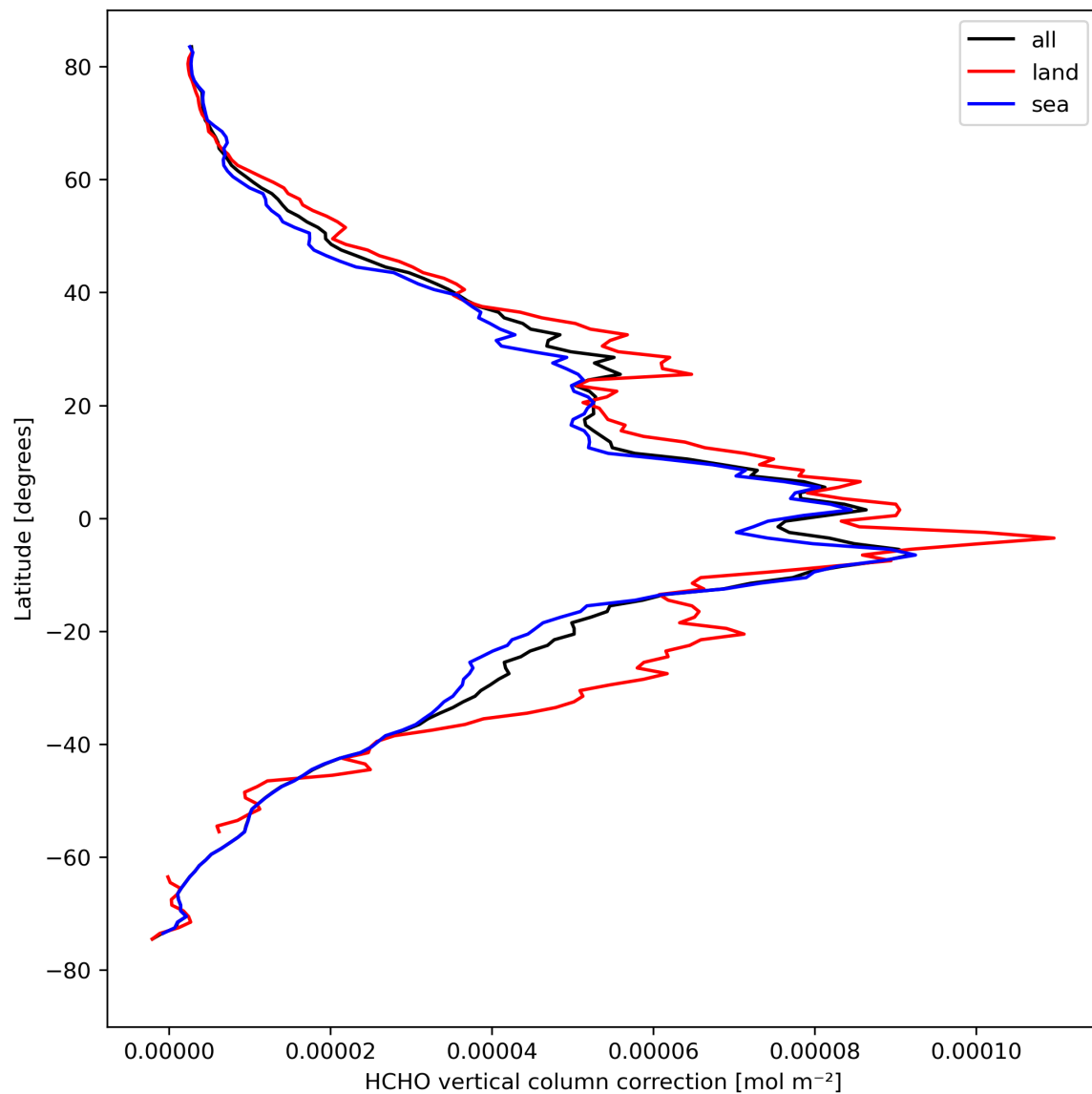
Figure 23: Zonal average of “HCHO vertical column correction” for 2024-04-16 to 2024-04-17.
