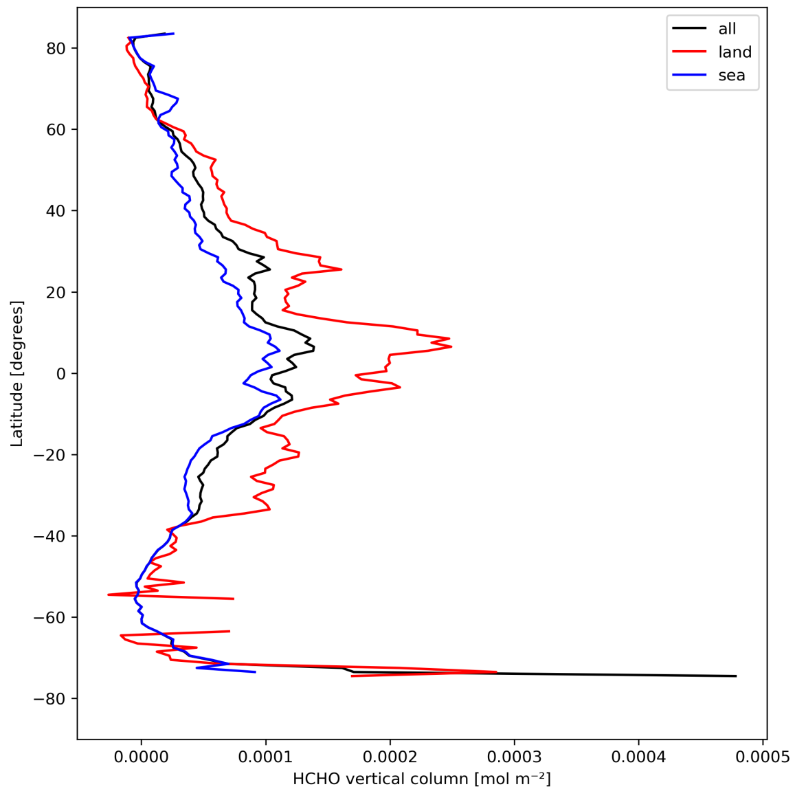
Figure 21: Zonal average of “HCHO vertical column” for 2024-04-16 to 2024-04-17.
