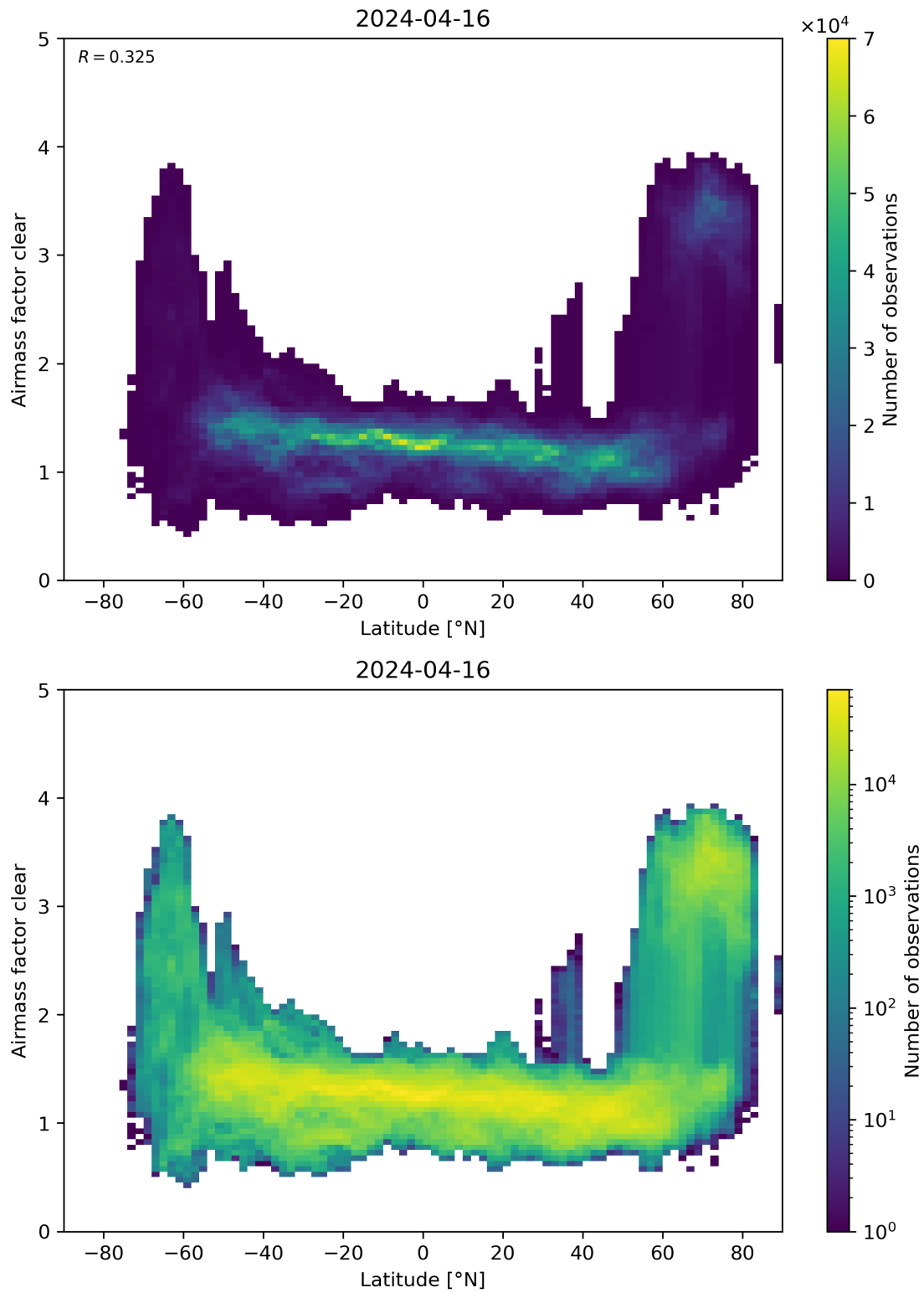
Figure 156: Scatter density plot of “Latitude” against “Airmass factor clear” for 2024-04-16 to 2024-04-17.
