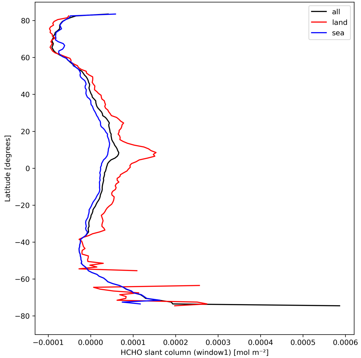
Figure 24: Zonal average of “HCHO slant column (window1)” for 2024-04-16 to 2024-04-17.
