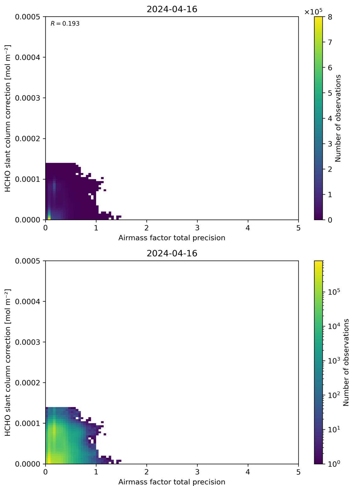
Figure 110: Scatter density plot of “Airmass factor total precision” against “HCHO slant column correction” for 2024-04-16 to 2024-04-17.
