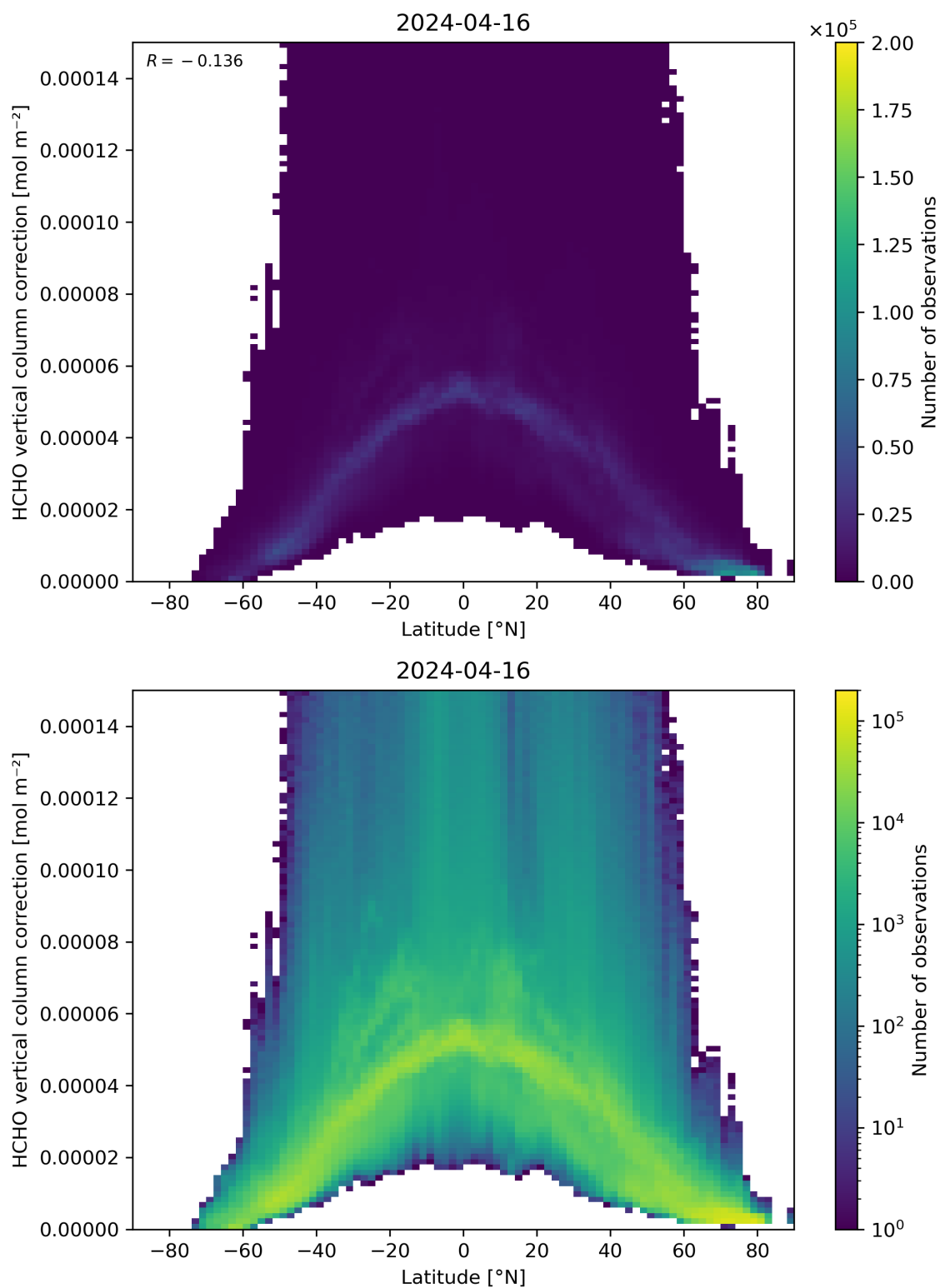
Figure 164: Scatter density plot of “Latitude” against “HCHO vertical column correction” for 2024-04-16 to 2024-04-17.
