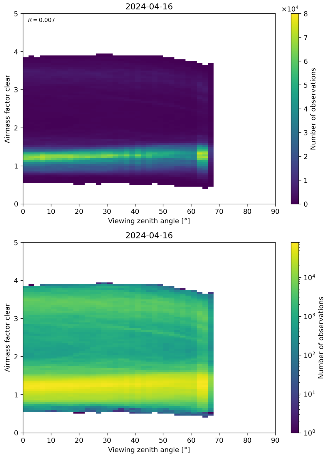
Figure 185: Scatter density plot of “Viewing zenith angle” against “Airmass factor clear” for 2024-04-16 to 2024-04-17.
