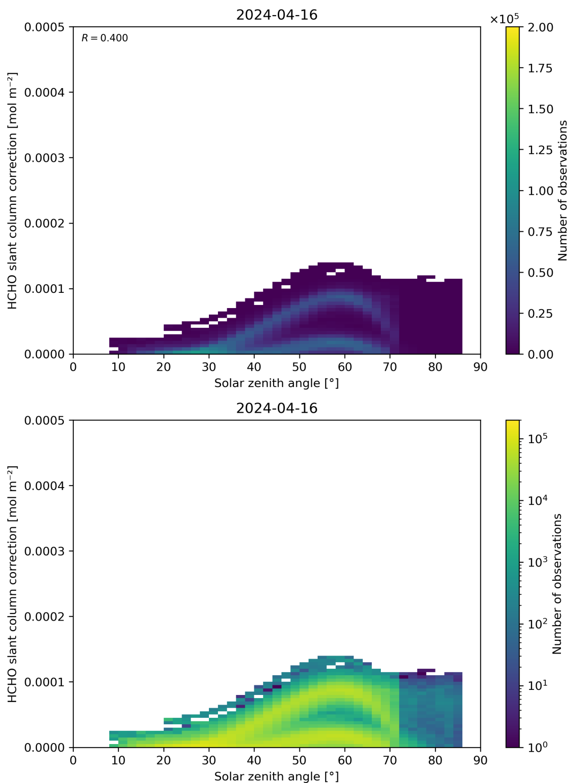
Figure 172: Scatter density plot of “Solar zenith angle” against “HCHO slant column correction” for 2024-04-16 to 2024-04-17.
