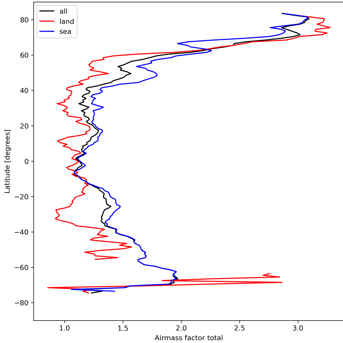
Figure 26: Zonal average of “Airmass factor total” for 2024-04-16 to 2024-04-17.
