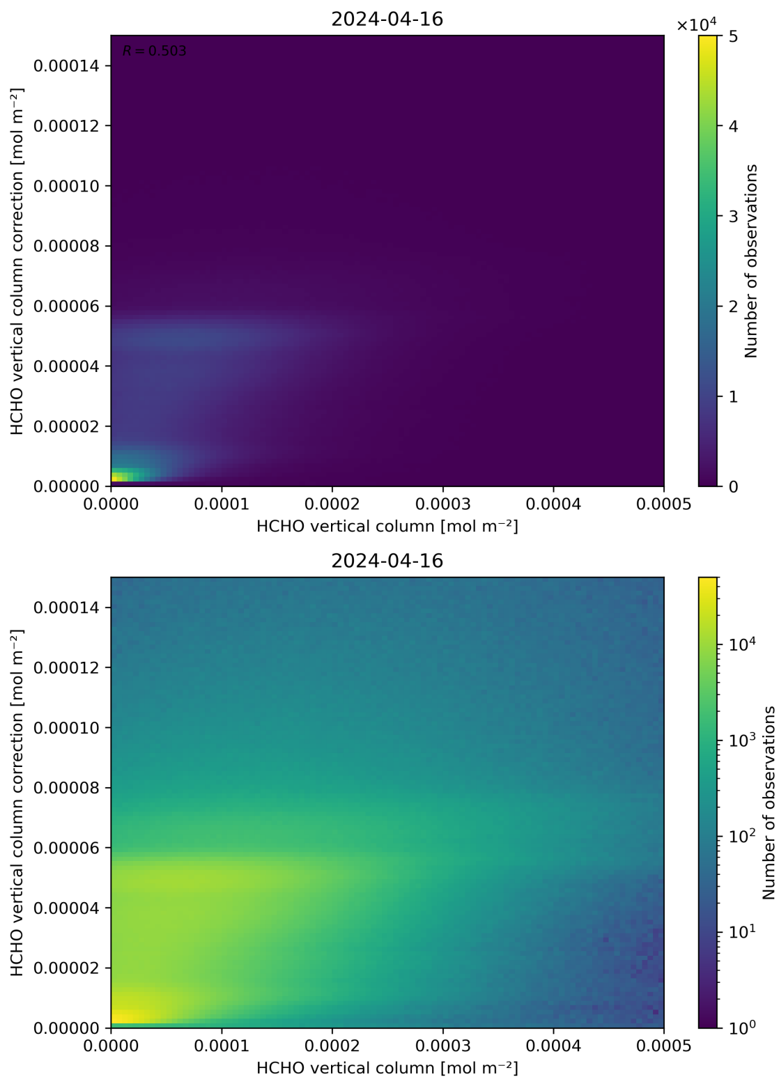
Figure 133: Scatter density plot of “HCHO vertical column” against “HCHO vertical column correction” for 2024-04-16 to 2024-04-17.
