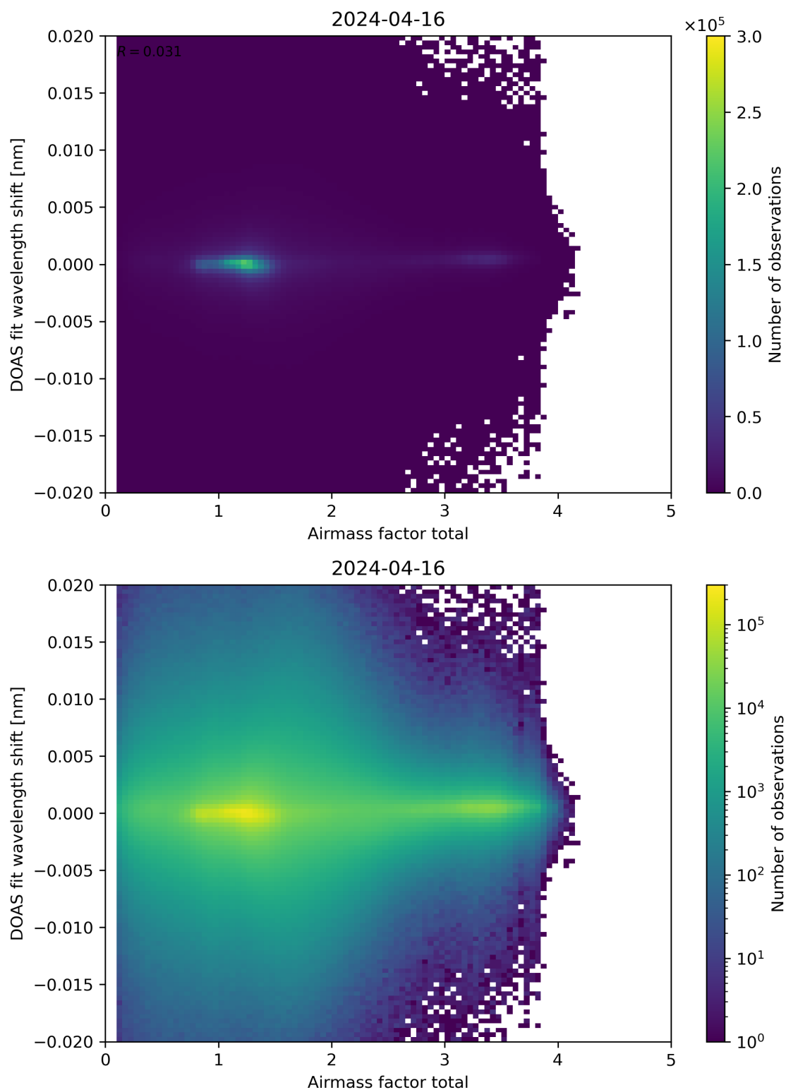
Figure 98: Scatter density plot of “Airmass factor total” against “DOAS fit wavelength shift” for 2024-04-16 to 2024-04-17.
