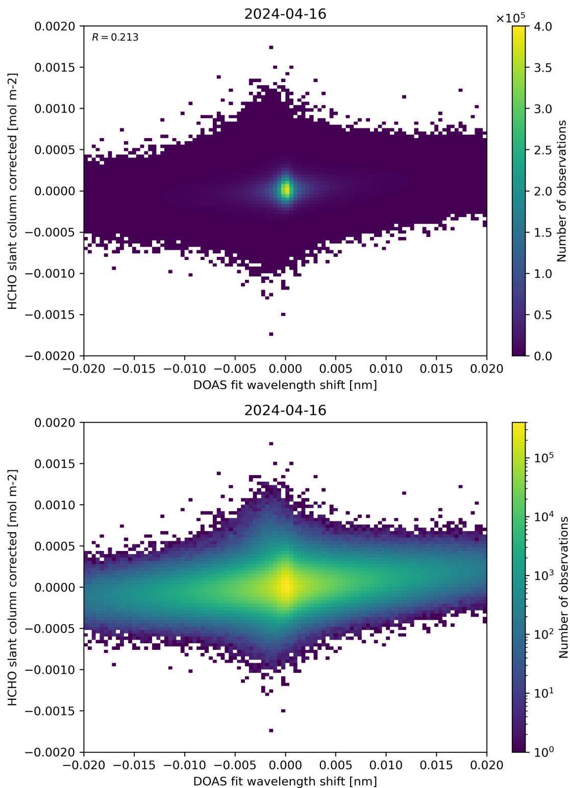
Figure 66: Scatter density plot of “DOAS fit wavelength shift” against “HCHO slant column corrected” for 2024-04-16 to 2024-04-17.
