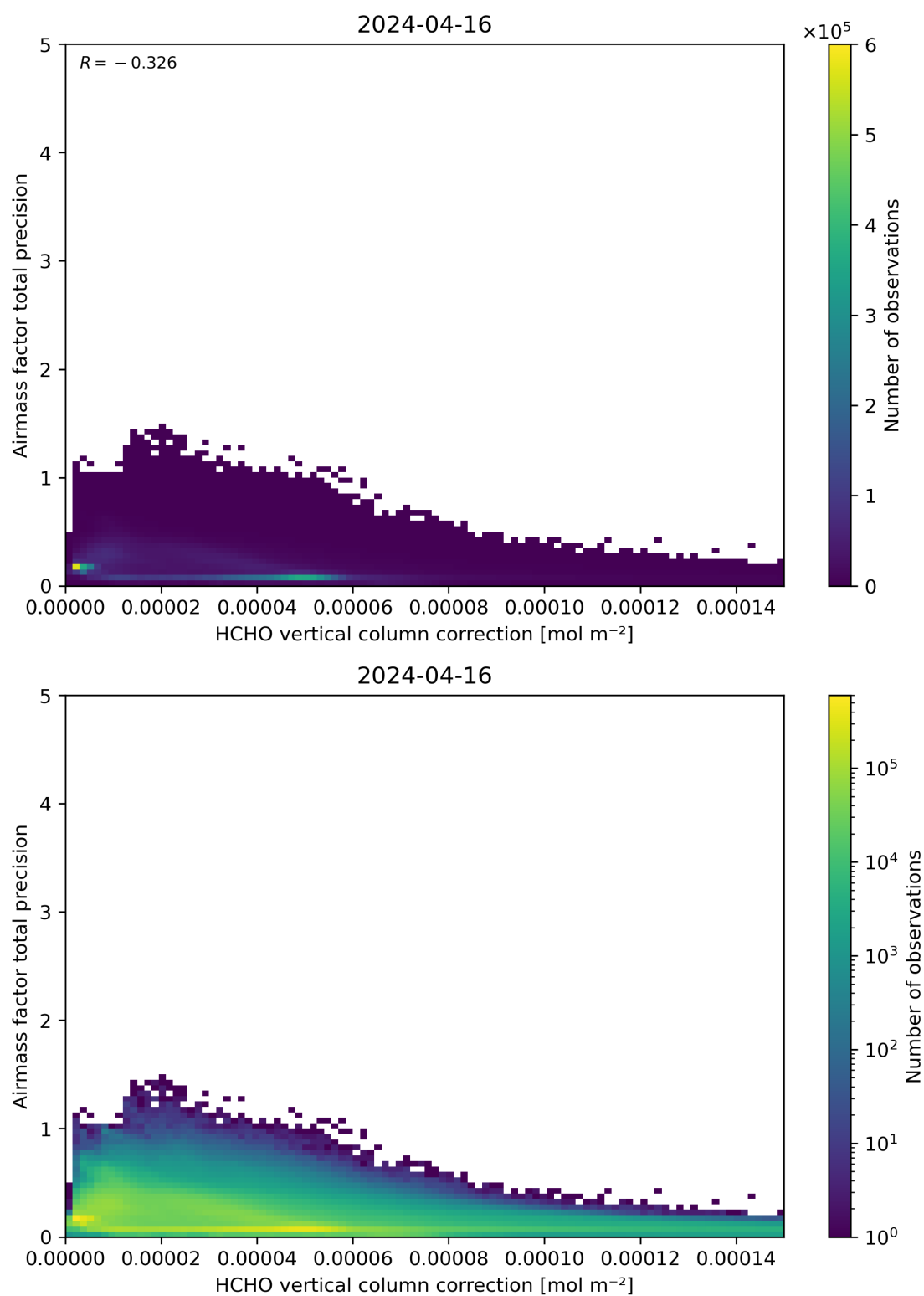
Figure 121: Scatter density plot of “HCHO vertical column correction” against “Airmass factor total precision” for 2024-04-16 to 2024-04-17.
