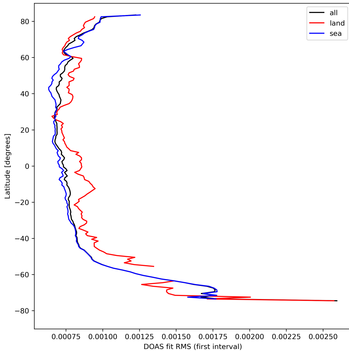
Figure 32: Zonal average of “DOAS fit RMS (first interval)” for 2024-04-16 to 2024-04-17.
