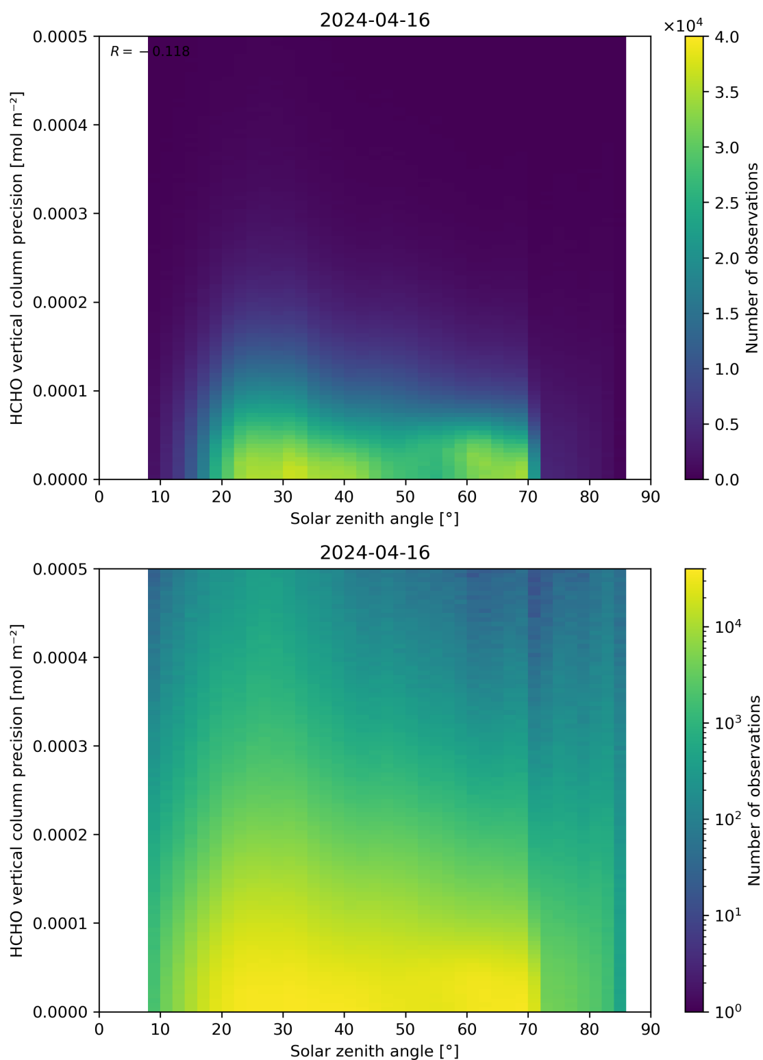
Figure 179: Scatter density plot of “Solar zenith angle” against “HCHO vertical column precision” for 2024-04-16 to 2024-04-17.
