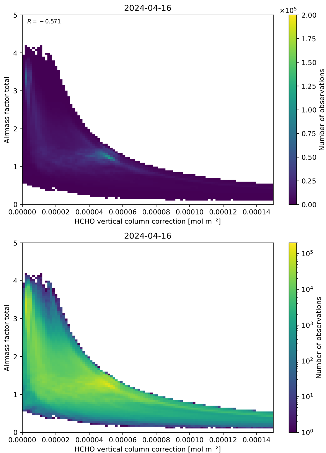
Figure 120: Scatter density plot of “HCHO vertical column correction” against “Airmass factor total” for 2024-04-16 to 2024-04-17.
