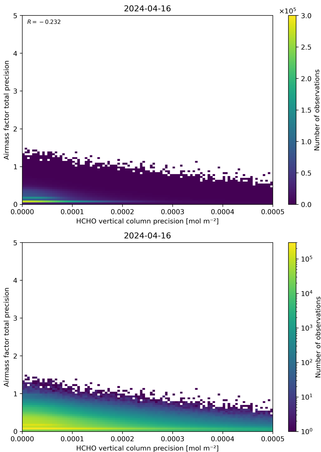
Figure 145: Scatter density plot of “HCHO vertical column precision” against “Airmass factor total precision” for 2024-04-16 to 2024-04-17.
