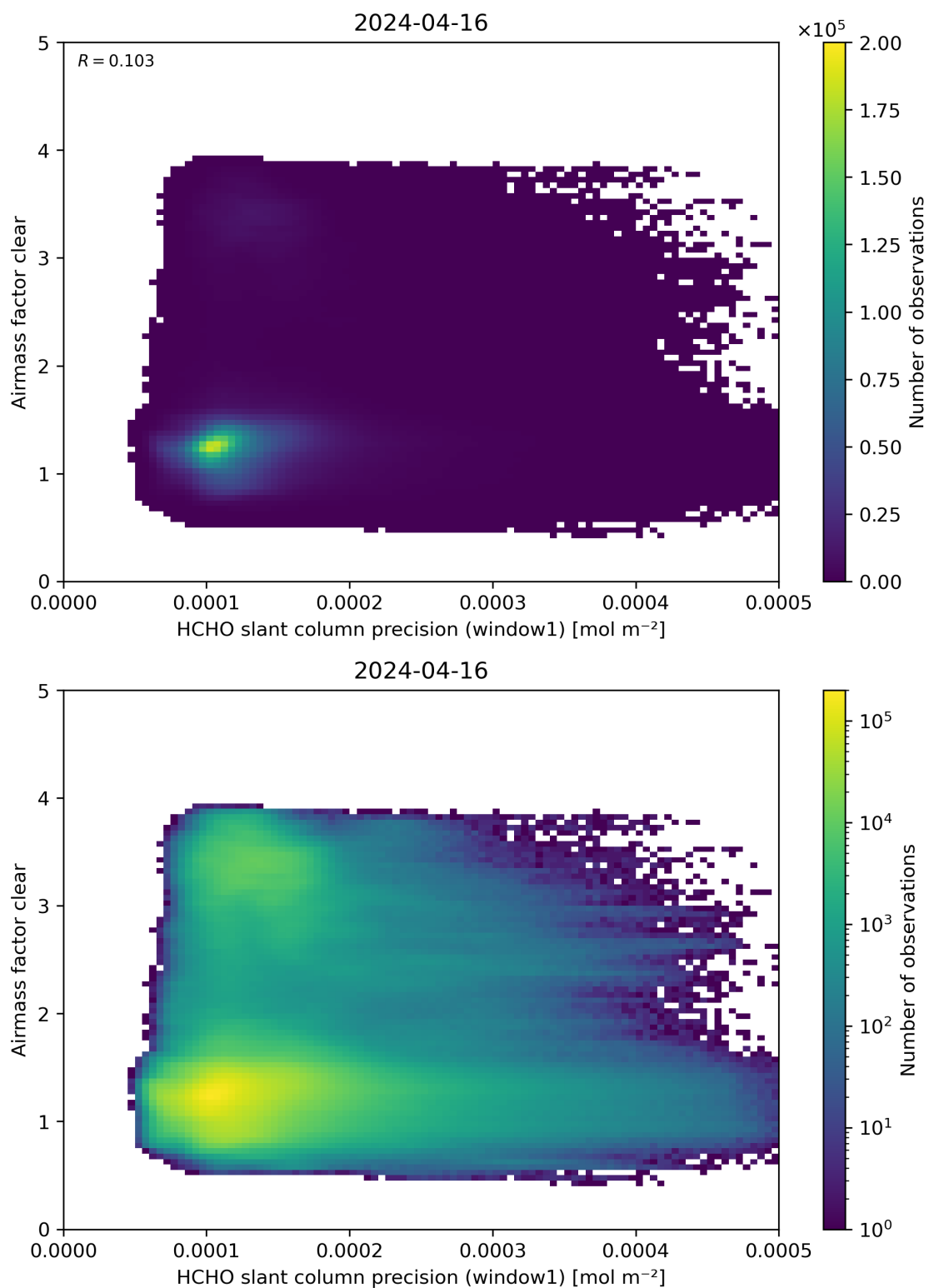
Figure 91: Scatter density plot of “HCHO slant column precision (window1)” against “Airmass factor clear” for 2024-04-16 to 2024-04-17.
