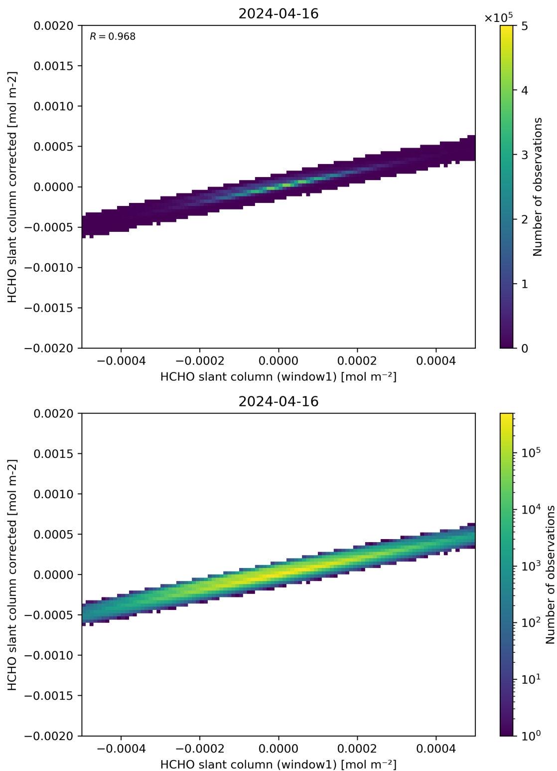
Figure 82: Scatter density plot of “HCHO slant column (window1)” against “HCHO slant column corrected” for 2024-04-16 to 2024-04-17.
