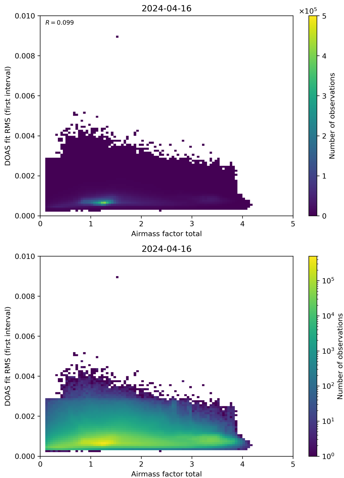
Figure 97: Scatter density plot of “Airmass factor total” against “DOAS fit RMS (first interval)” for 2024-04-16 to 2024-04-17.
