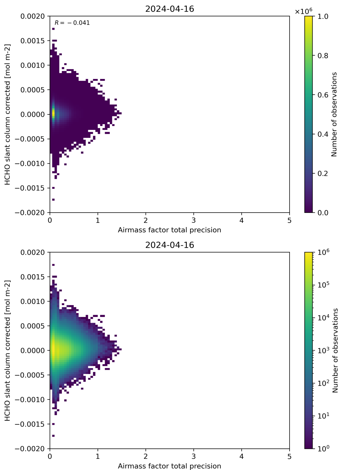
Figure 109: Scatter density plot of “Airmass factor total precision” against “HCHO slant column corrected” for 2024-04-16 to 2024-04-17.
