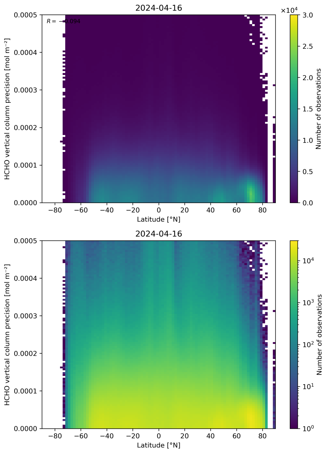
Figure 165: Scatter density plot of “Latitude” against “HCHO vertical column precision” for 2024-04-16 to 2024-04-17.
