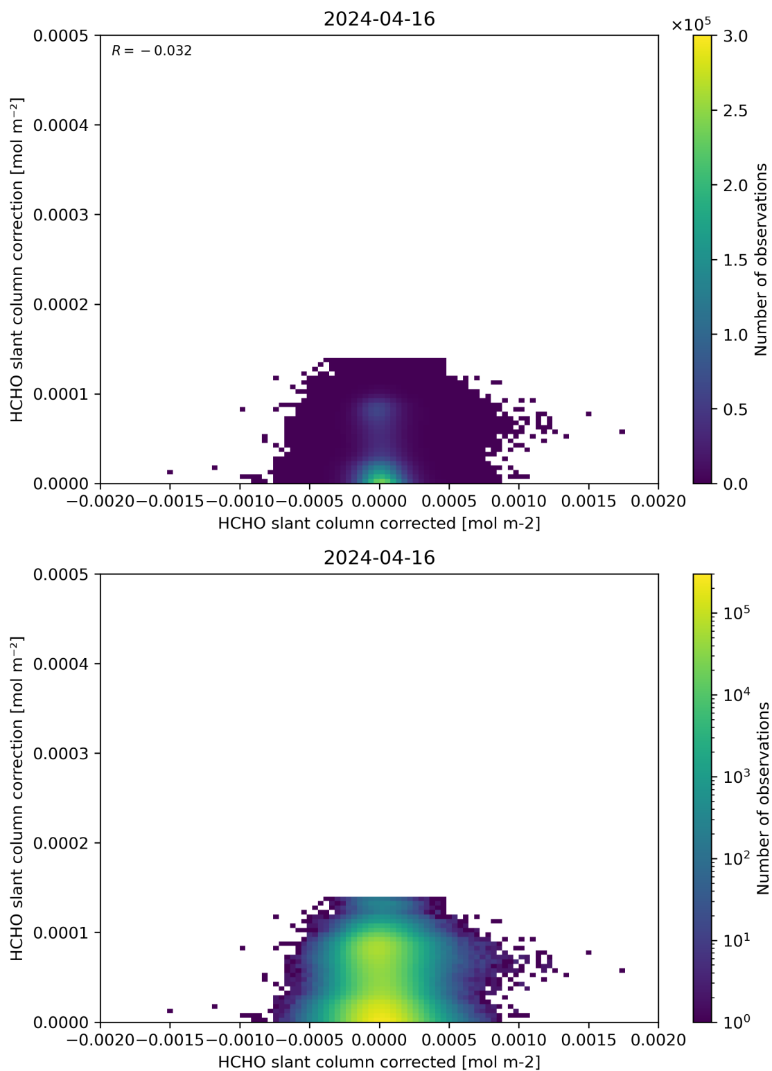
Figure 77: Scatter density plot of “HCHO slant column corrected” against “HCHO slant column correction” for 2024-04-16 to 2024-04-17.
