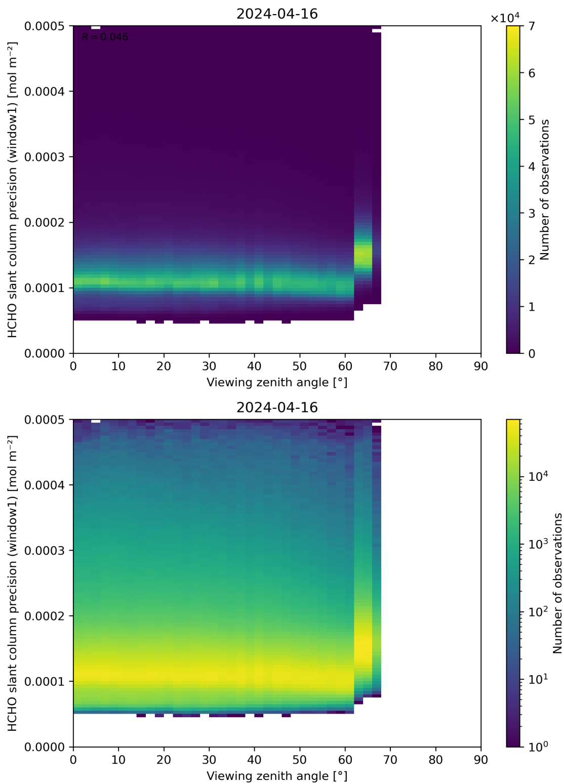
Figure 189: Scatter density plot of “Viewing zenith angle” against “HCHO slant column precision (window1)” for 2024-04-16 to 2024-04-17.
