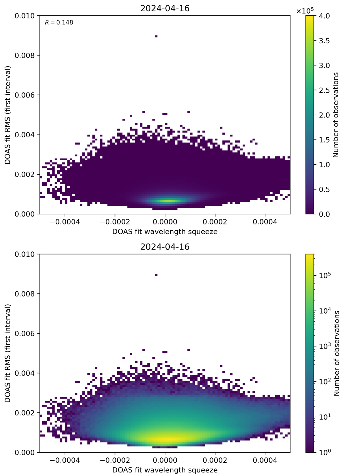
Figure 68: Scatter density plot of “DOAS fit wavelength squeeze” against “DOAS fit RMS (first interval)” for 2024-04-16 to 2024-04-17.
