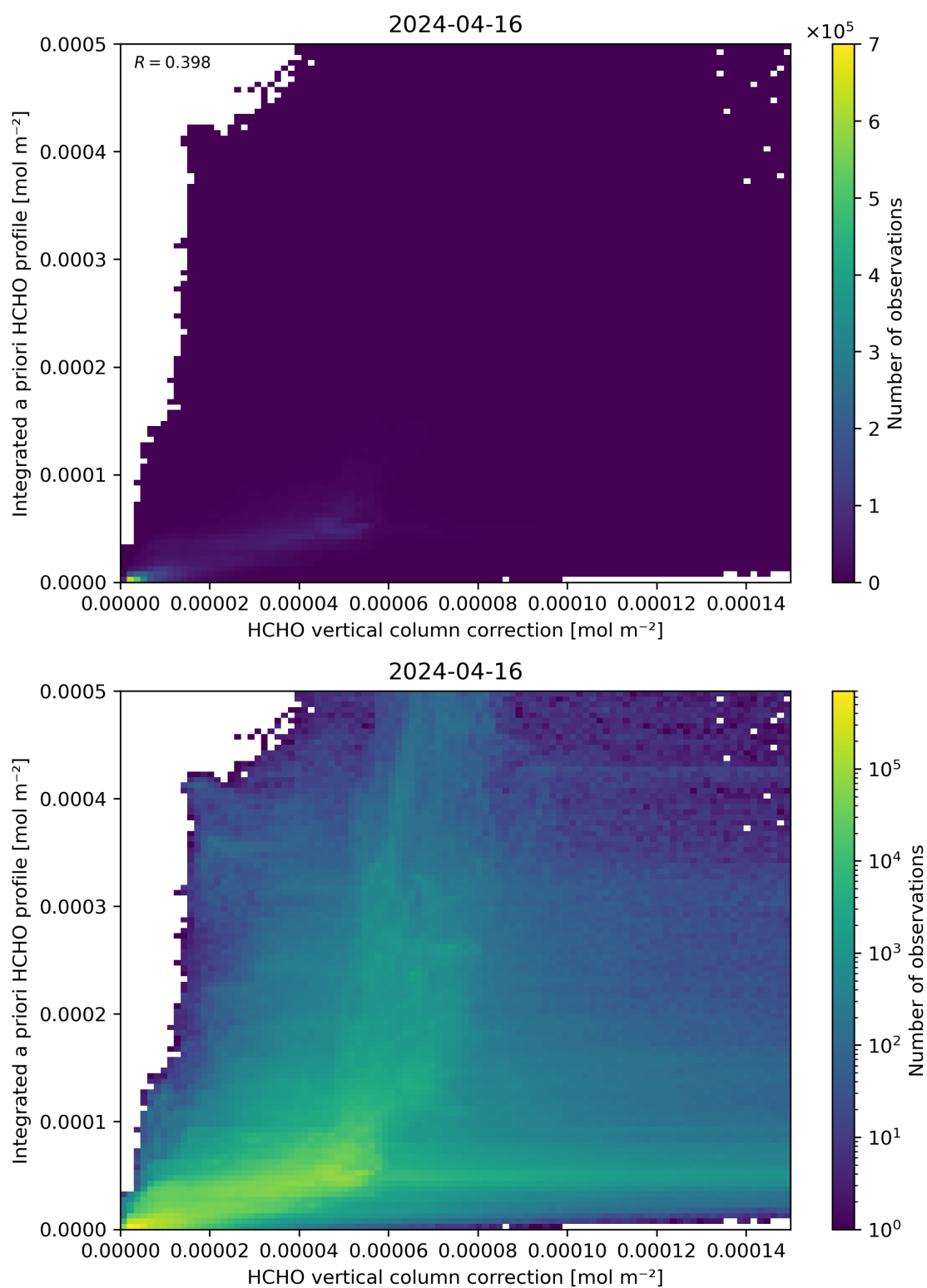
Figure 122: Scatter density plot of “HCHO vertical column correction” against “Integrated a priori HCHO profile” for 2024-04-16 to 2024-04-17.
