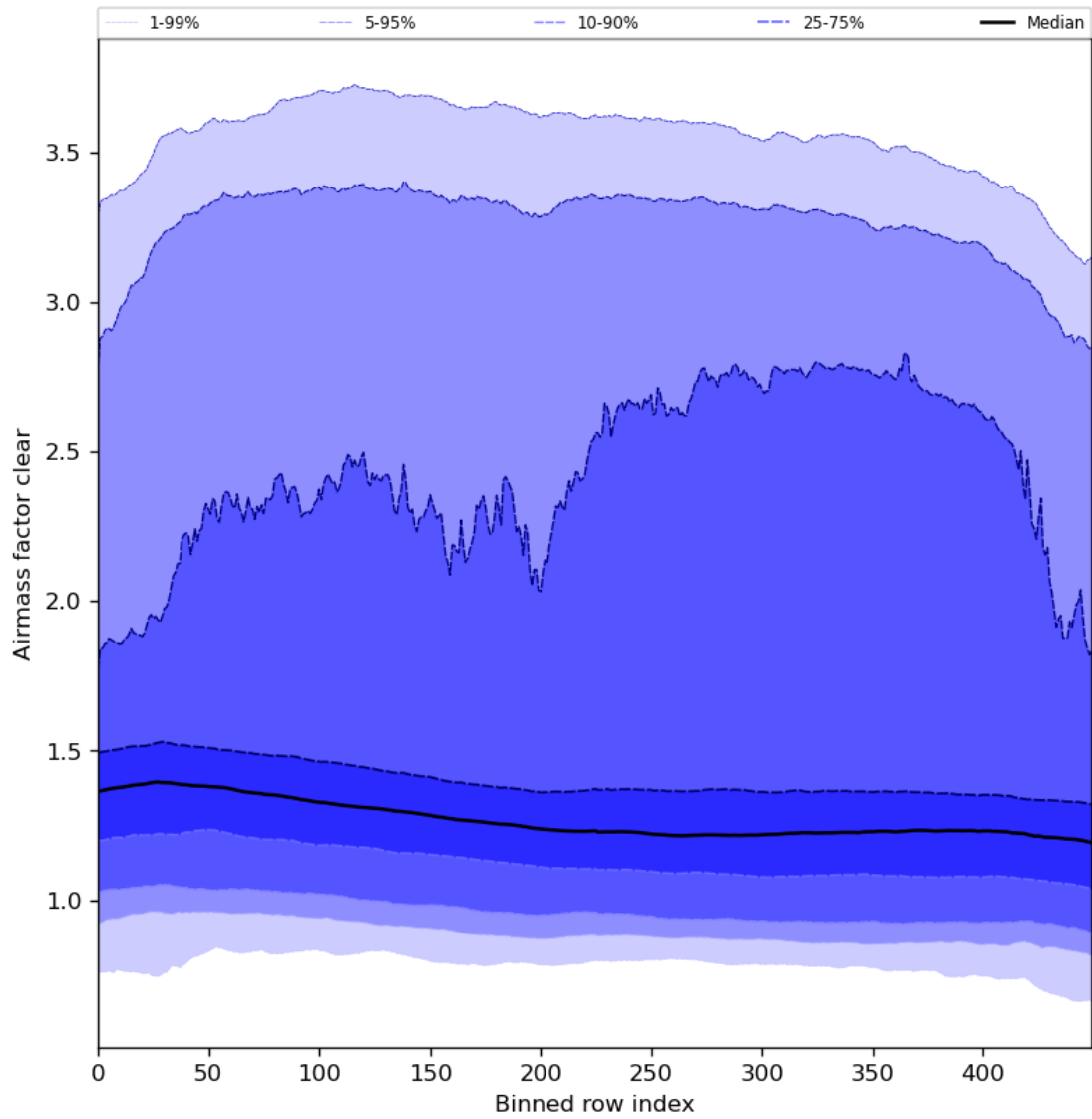
Figure 56: Along track statistics of “Airmass factor clear” for 2024-04-16 to 2024-04-17
