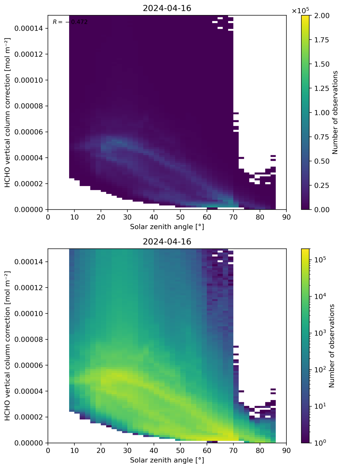
Figure 178: Scatter density plot of “Solar zenith angle” against “HCHO vertical column correction” for 2024-04-16 to 2024-04-17.
