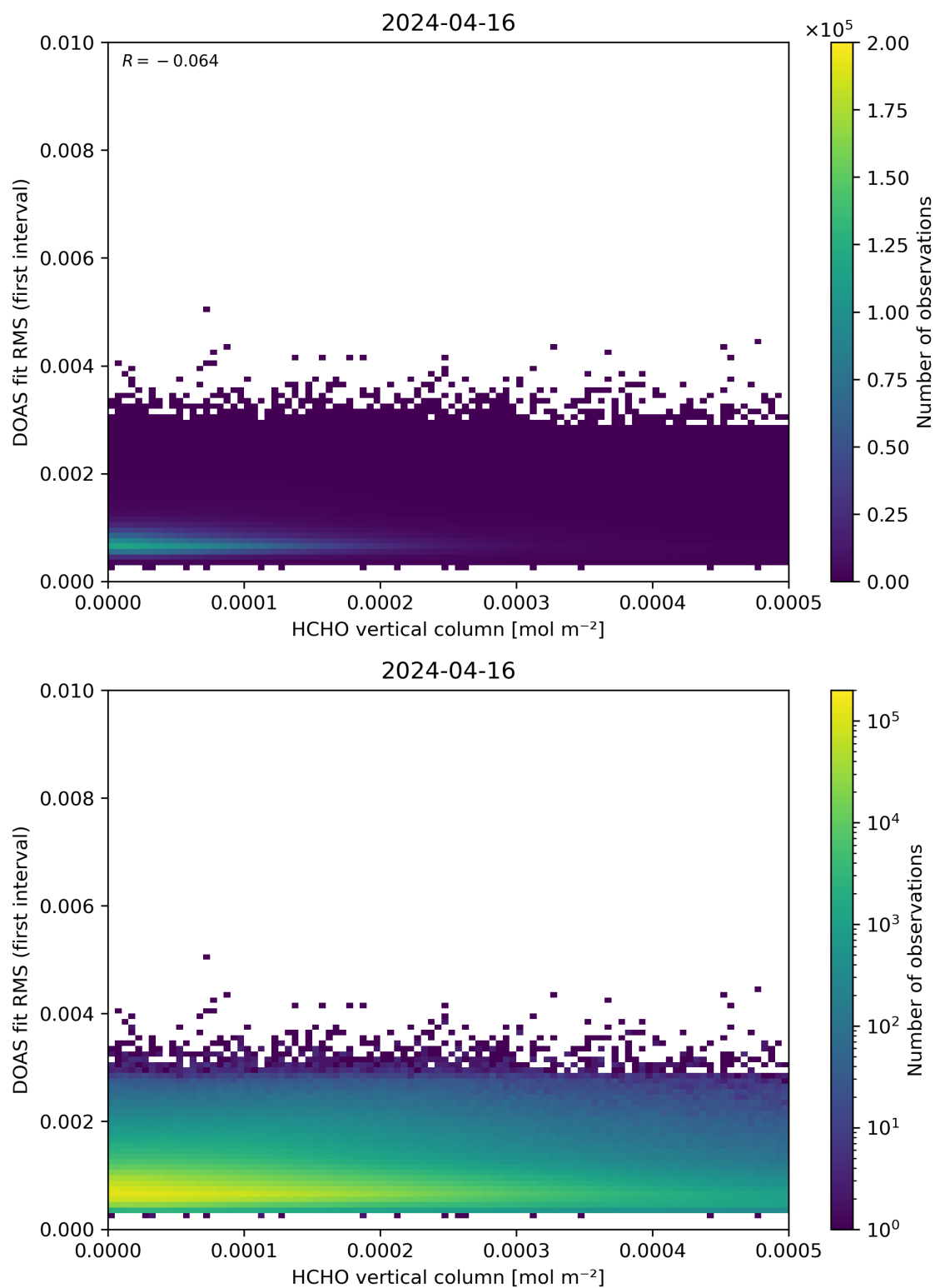
Figure 123: Scatter density plot of “HCHO vertical column” against “DOAS fit RMS (first interval)” for 2024-04-16 to 2024-04-17.
