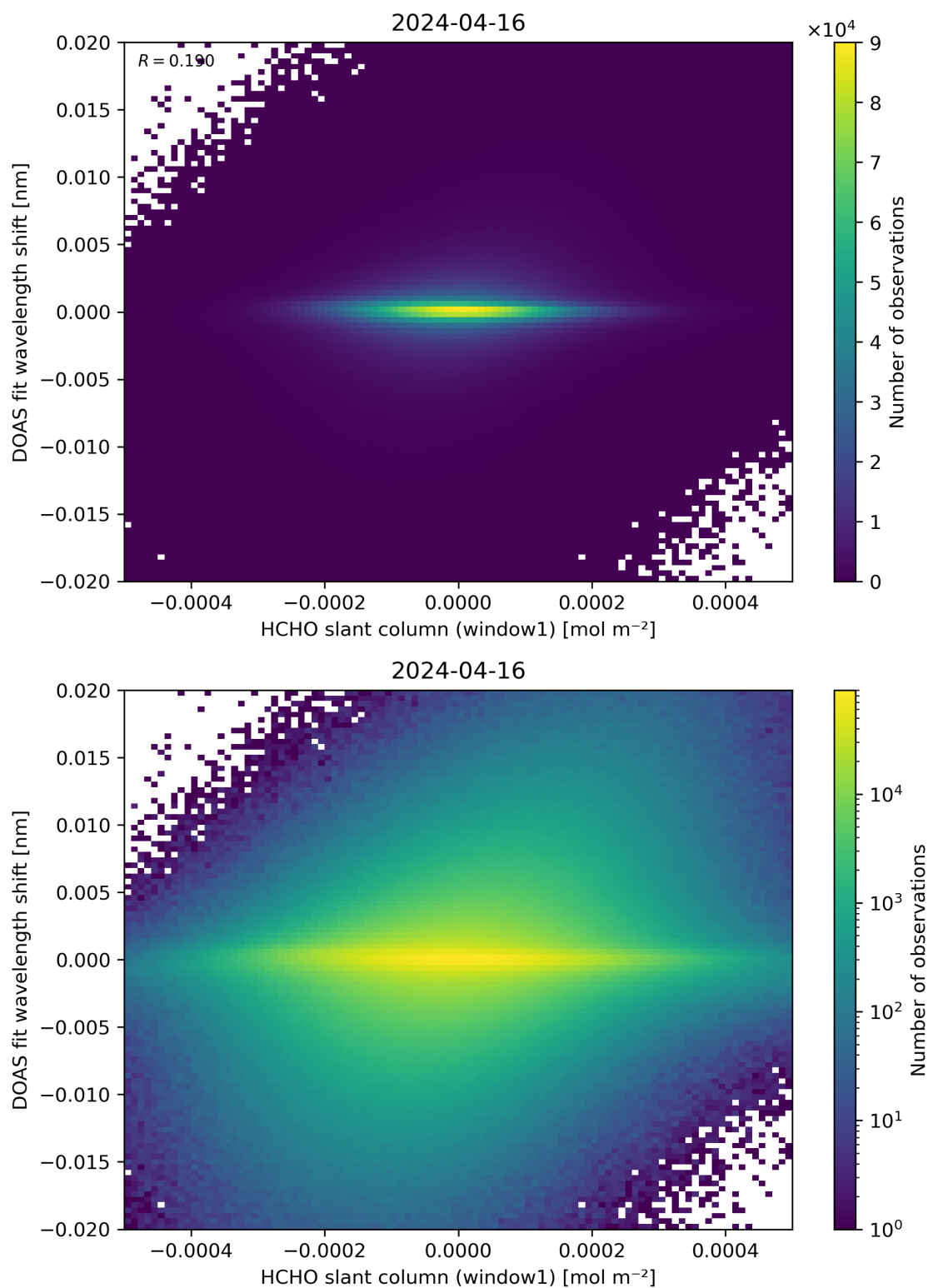
Figure 79: Scatter density plot of “HCHO slant column (window1)” against “DOAS fit wavelength shift” for 2024-04-16 to 2024-04-17.
