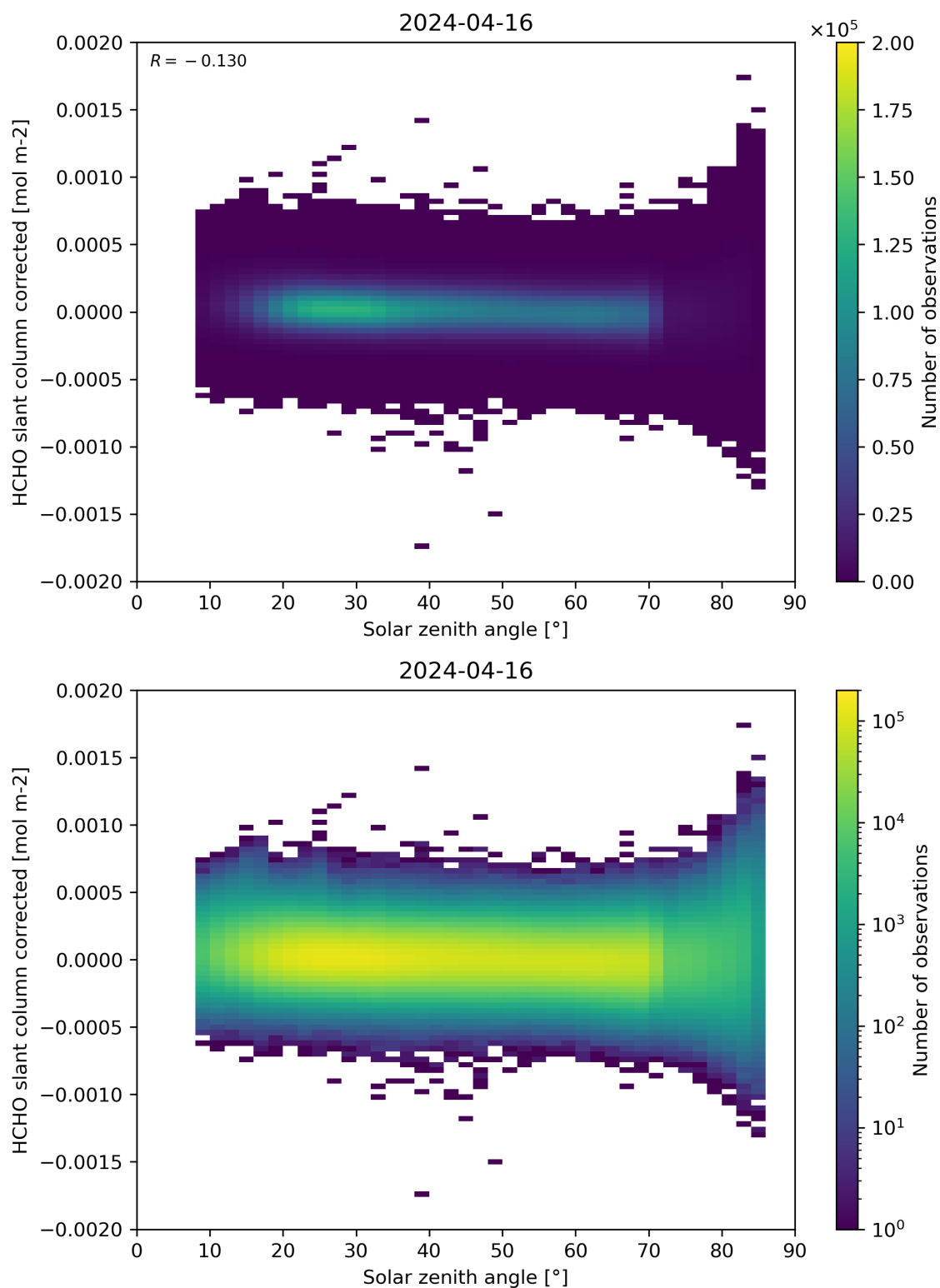
Figure 171: Scatter density plot of “Solar zenith angle” against “HCHO slant column corrected” for 2024-04-16 to 2024-04-17.
