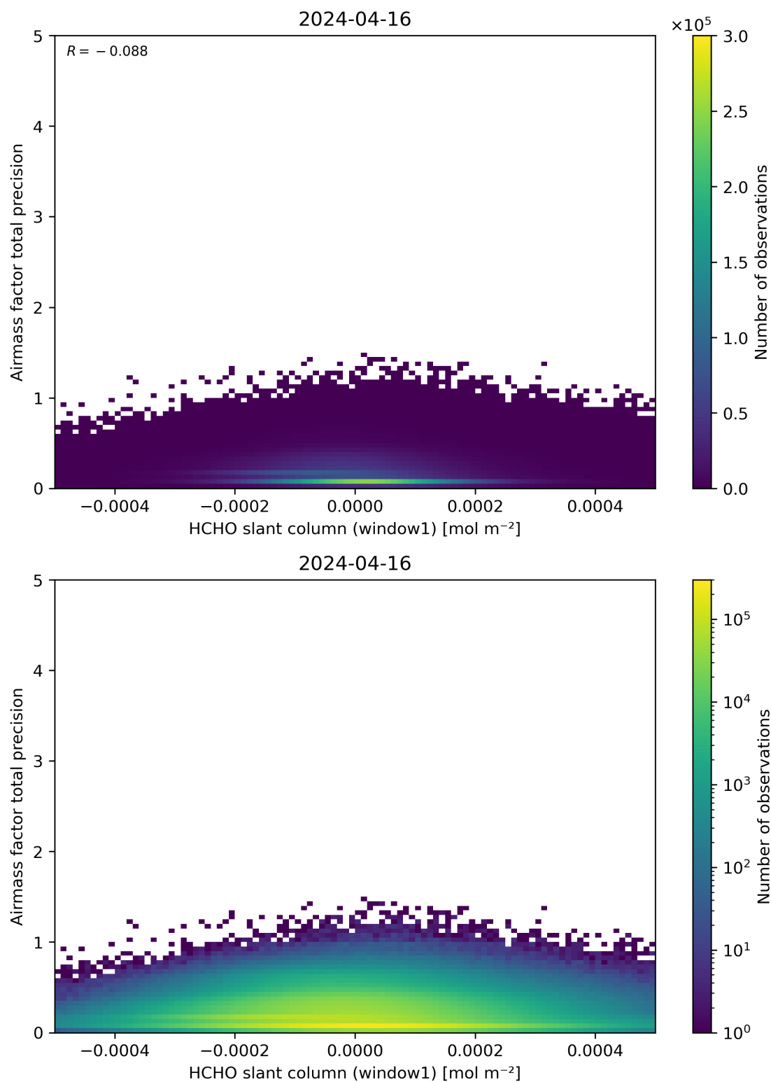
Figure 86: Scatter density plot of “HCHO slant column (window1)” against “Airmass factor total precision” for 2024-04-16 to 2024-04-17.
