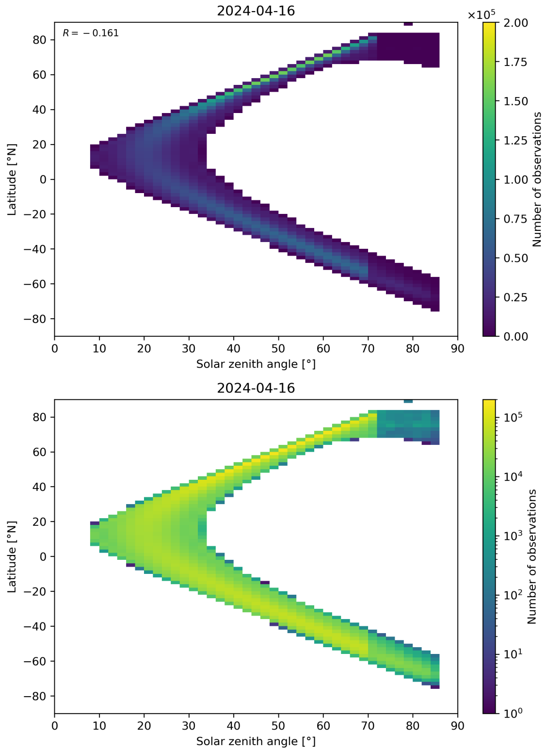
Figure 181: Scatter density plot of “Solar zenith angle” against “Latitude” for 2024-04-16 to 2024-04-17.
