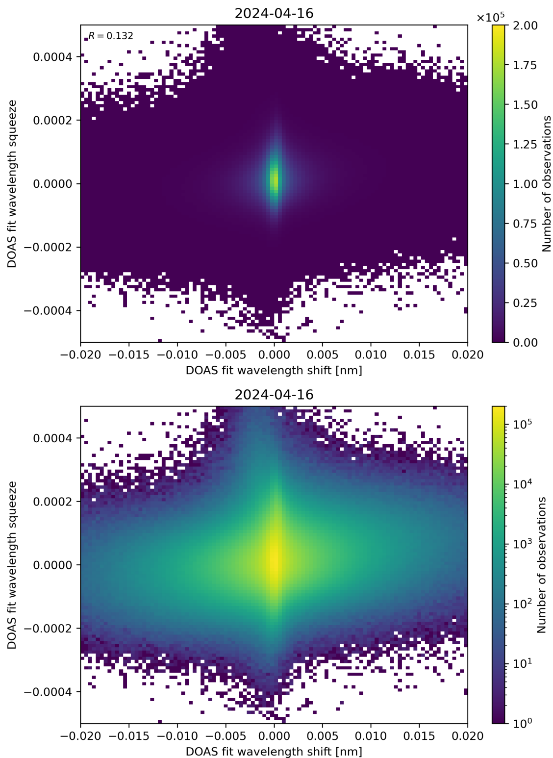
Figure 65: Scatter density plot of “DOAS fit wavelength shift” against “DOAS fit wavelength squeeze” for 2024-04-16 to 2024-04-17.
