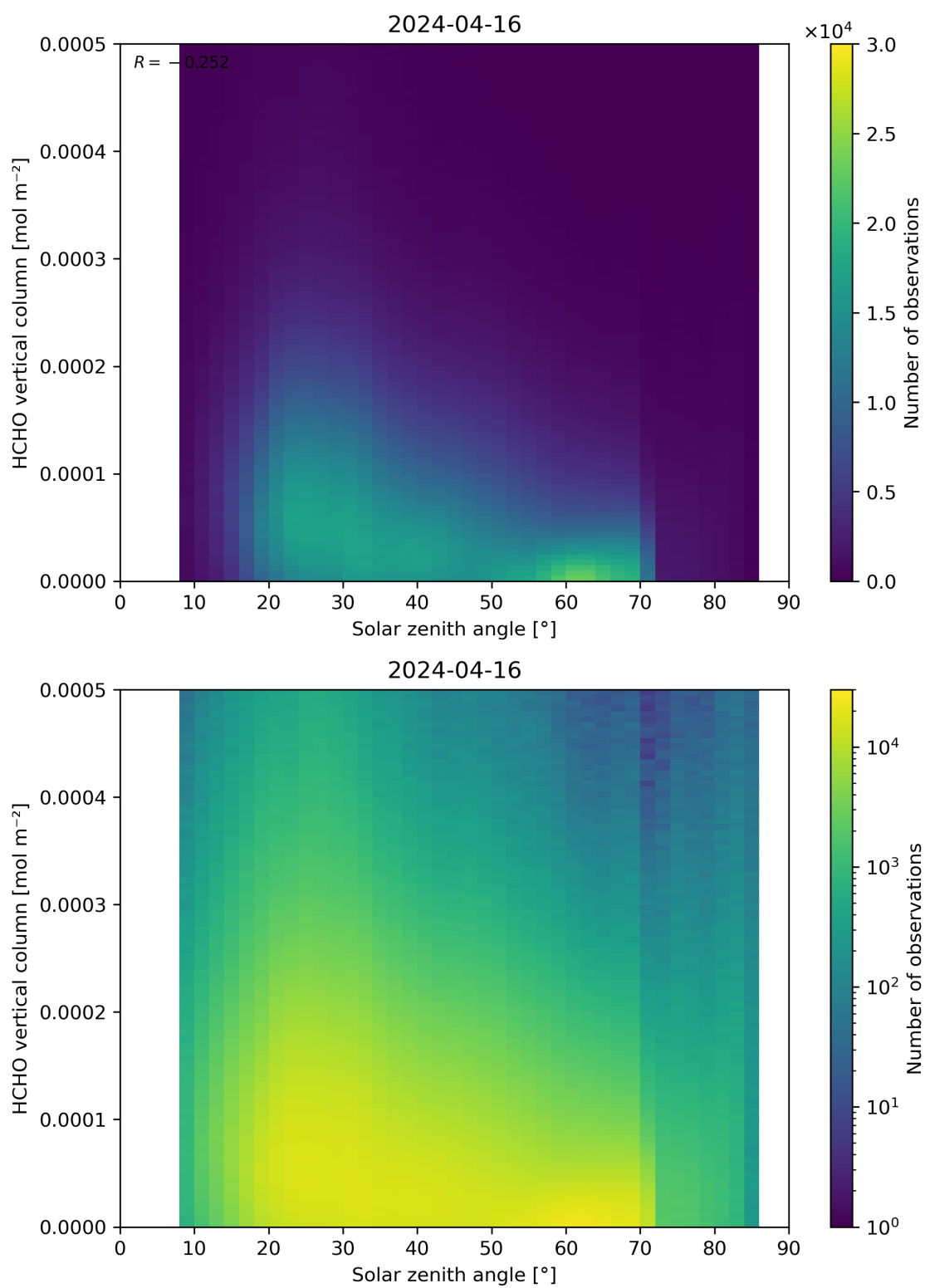
Figure 177: Scatter density plot of “Solar zenith angle” against “HCHO vertical column” for 2024-04-16 to 2024-04-17.
