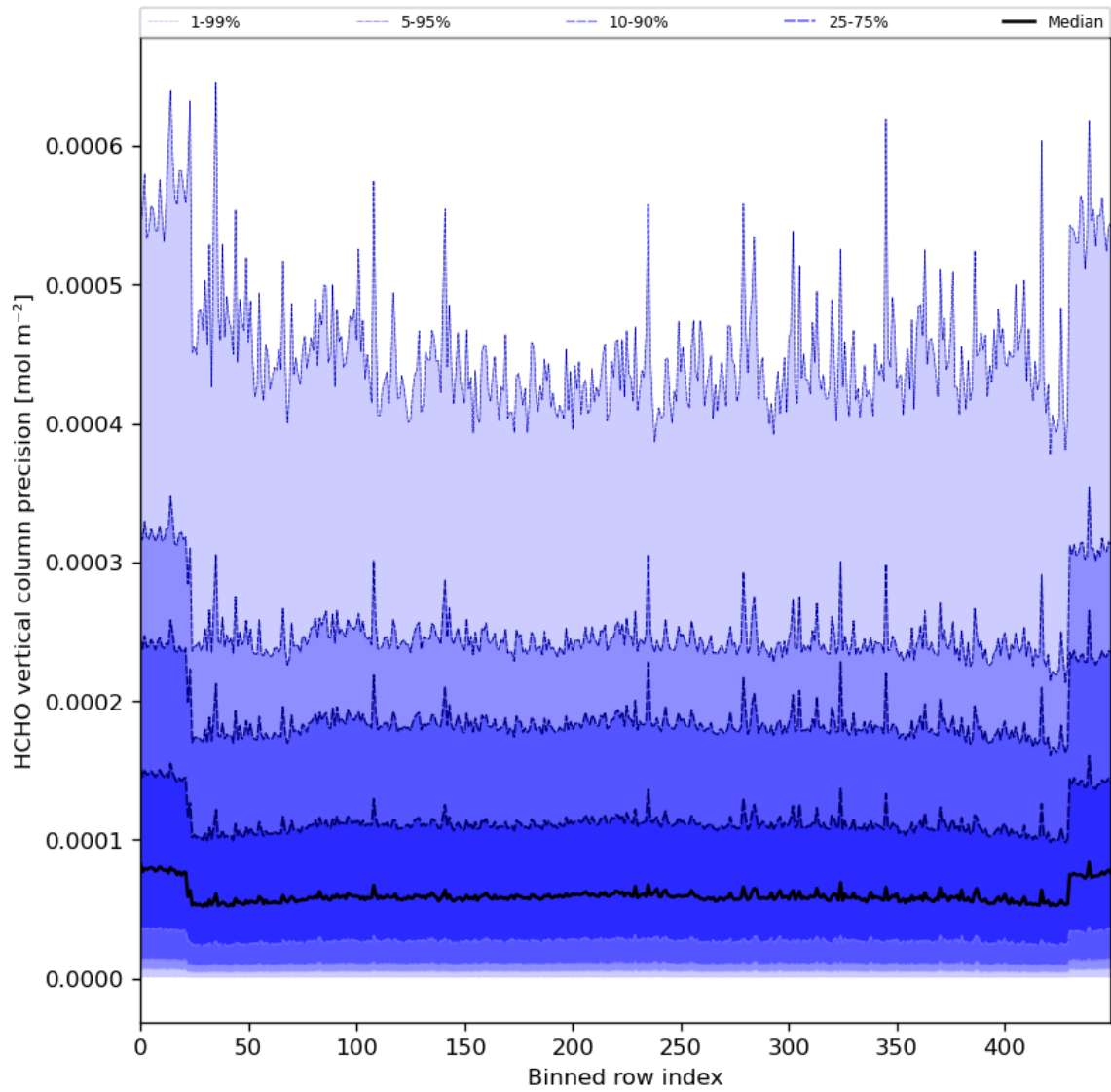
Figure 50: Along track statistics of “HCHO vertical column precision” for 2024-04-16 to 2024-04-17
