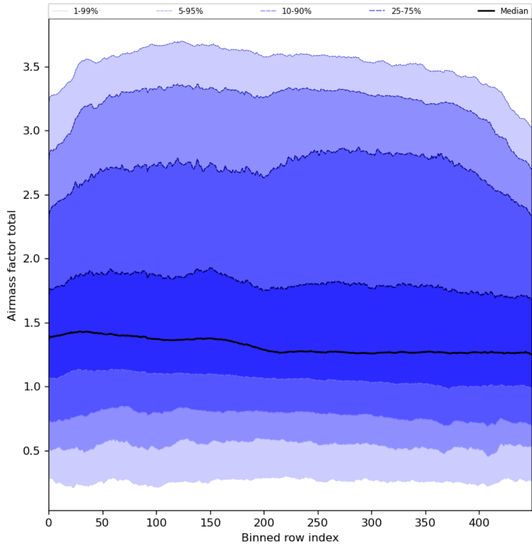
Figure 54: Along track statistics of “Airmass factor total” for 2024-04-16 to 2024-04-17
