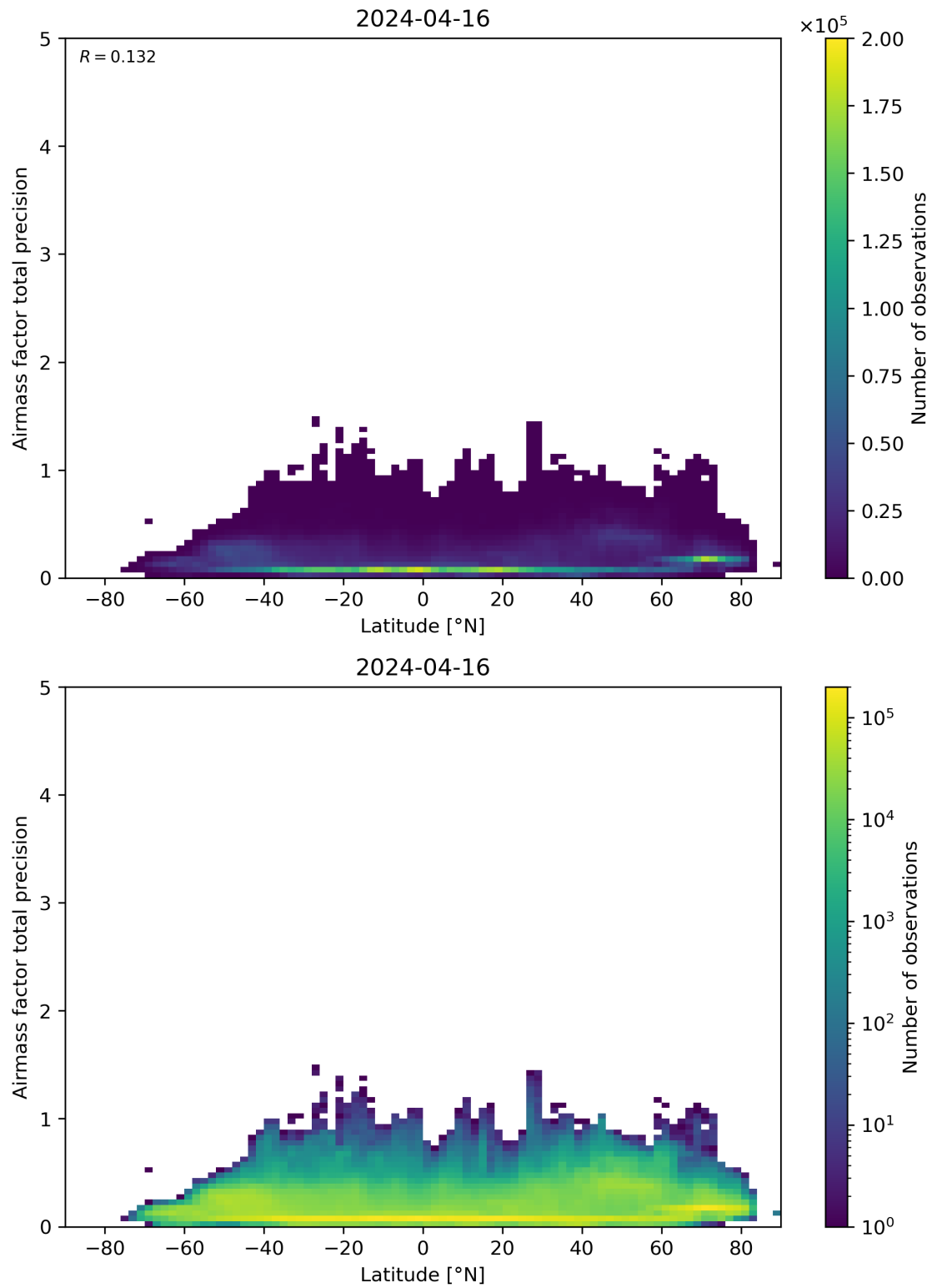
Figure 162: Scatter density plot of “Latitude” against “Airmass factor total precision” for 2024-04-16 to 2024-04-17.
