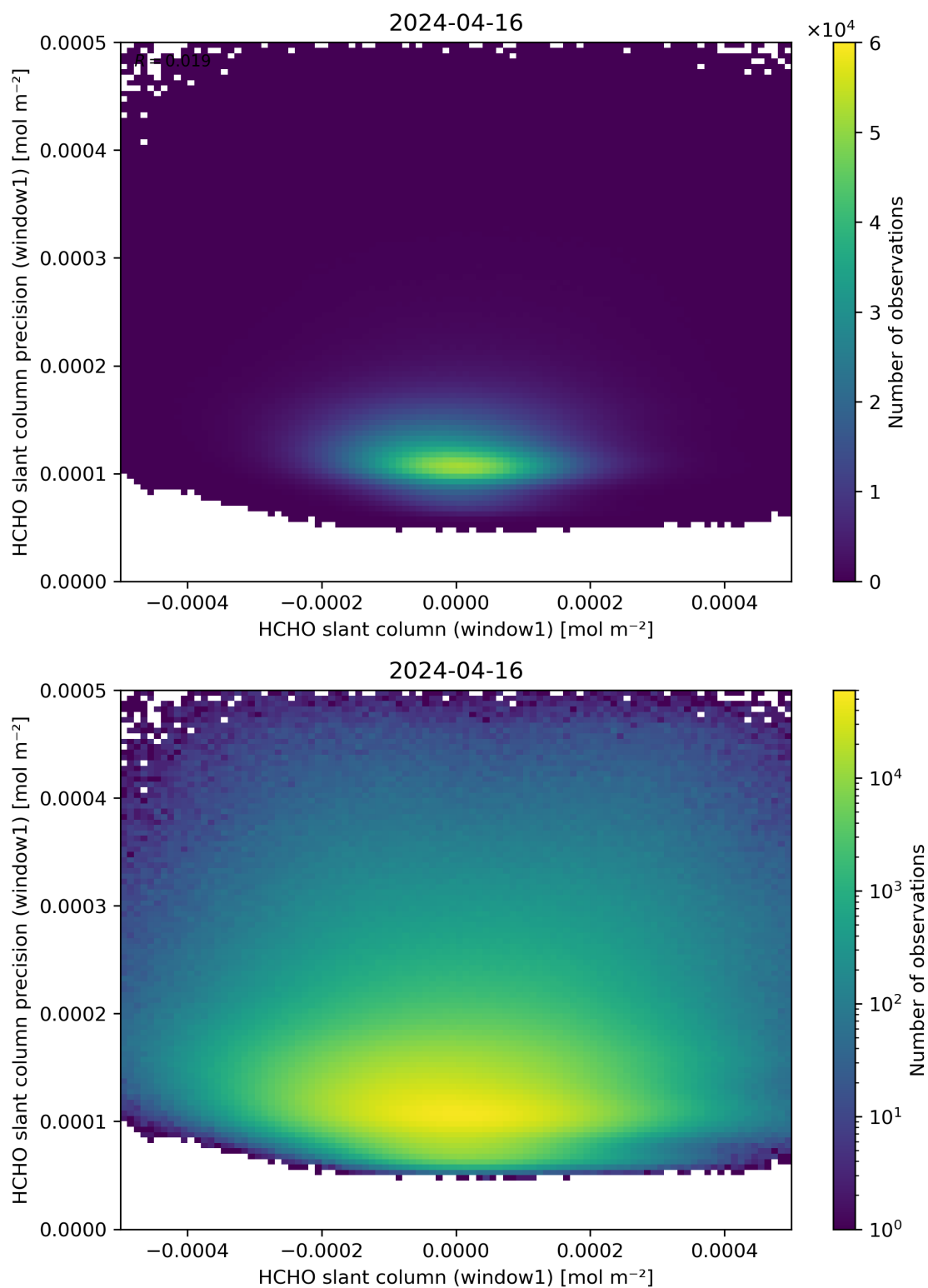
Figure 84: Scatter density plot of “HCHO slant column (window1)” against “HCHO slant column precision (window1)” for 2024-04-16 to 2024-04-17.
