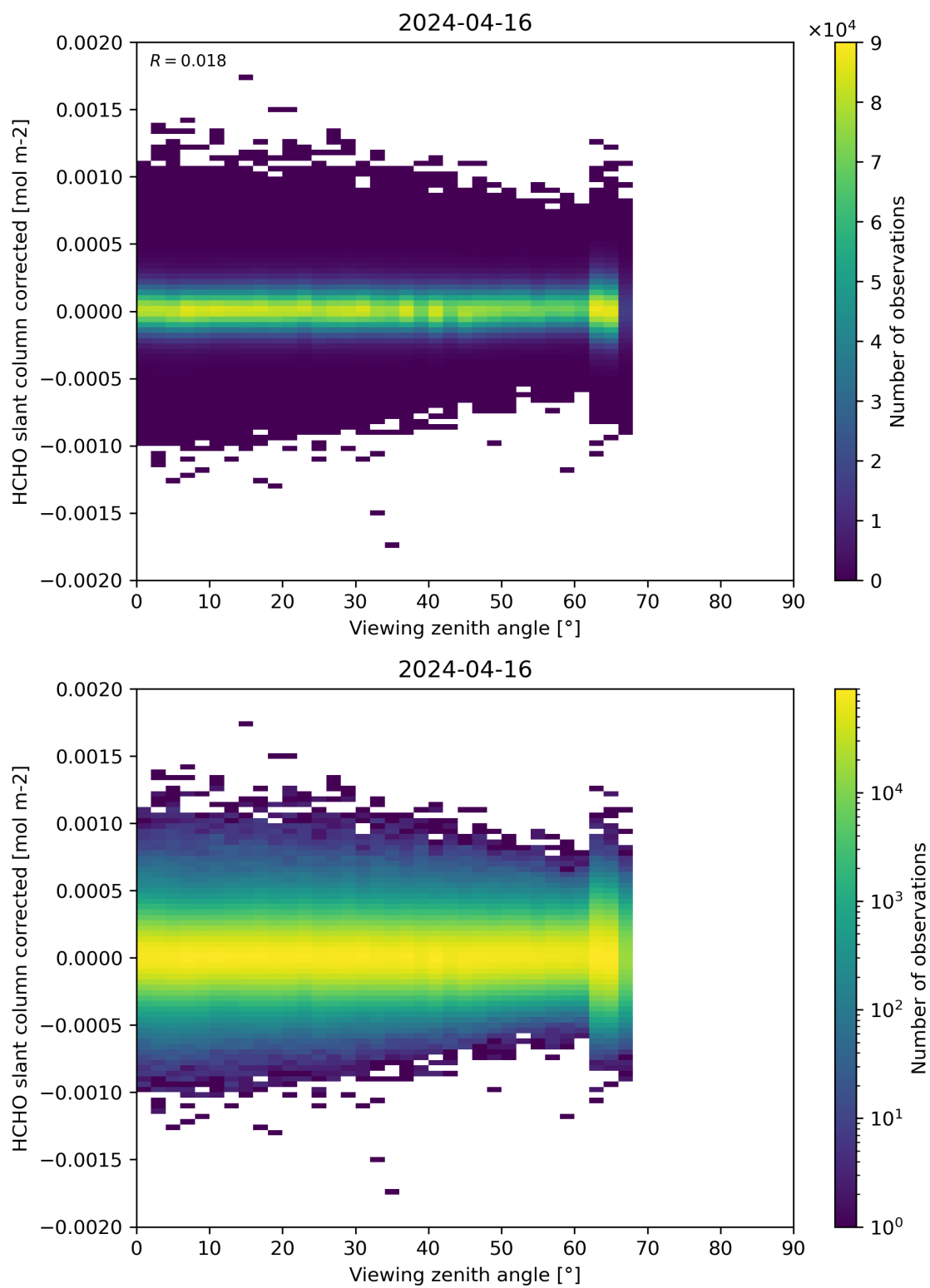
Figure 186: Scatter density plot of “Viewing zenith angle” against “HCHO slant column corrected” for 2024-04-16 to 2024-04-17.
