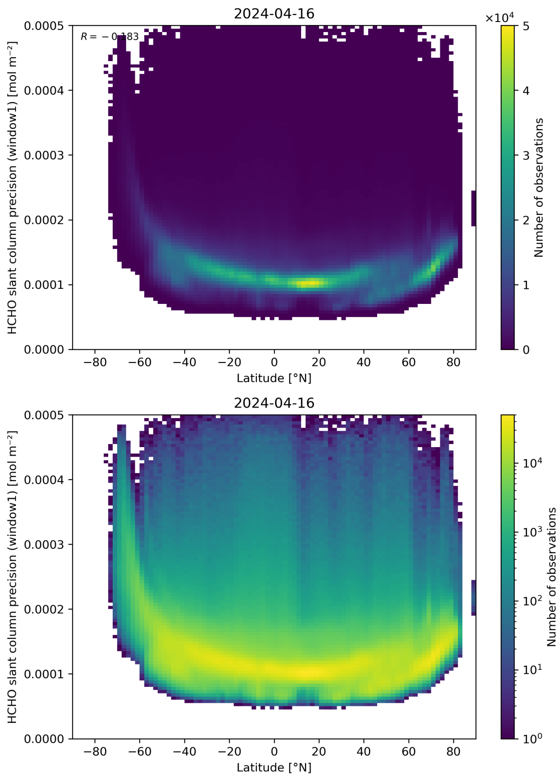
Figure 160: Scatter density plot of “Latitude” against “HCHO slant column precision (window1)” for 2024-04-16 to 2024-04-17.
