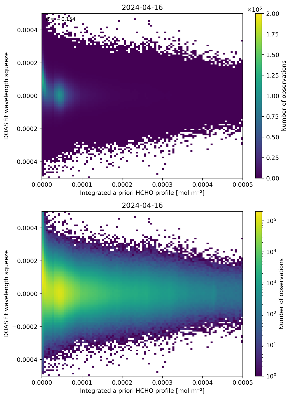
Figure 150: Scatter density plot of “Integrated a priori HCHO profile” against “DOAS fit wavelength squeeze” for 2024-04-16 to 2024-04-17.
