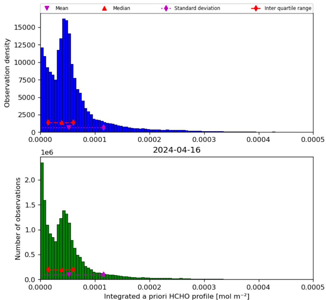
Figure 43: Histogram of “Integrated a priori HCHO profile” for 2024-04-16 to 2024-04-17
