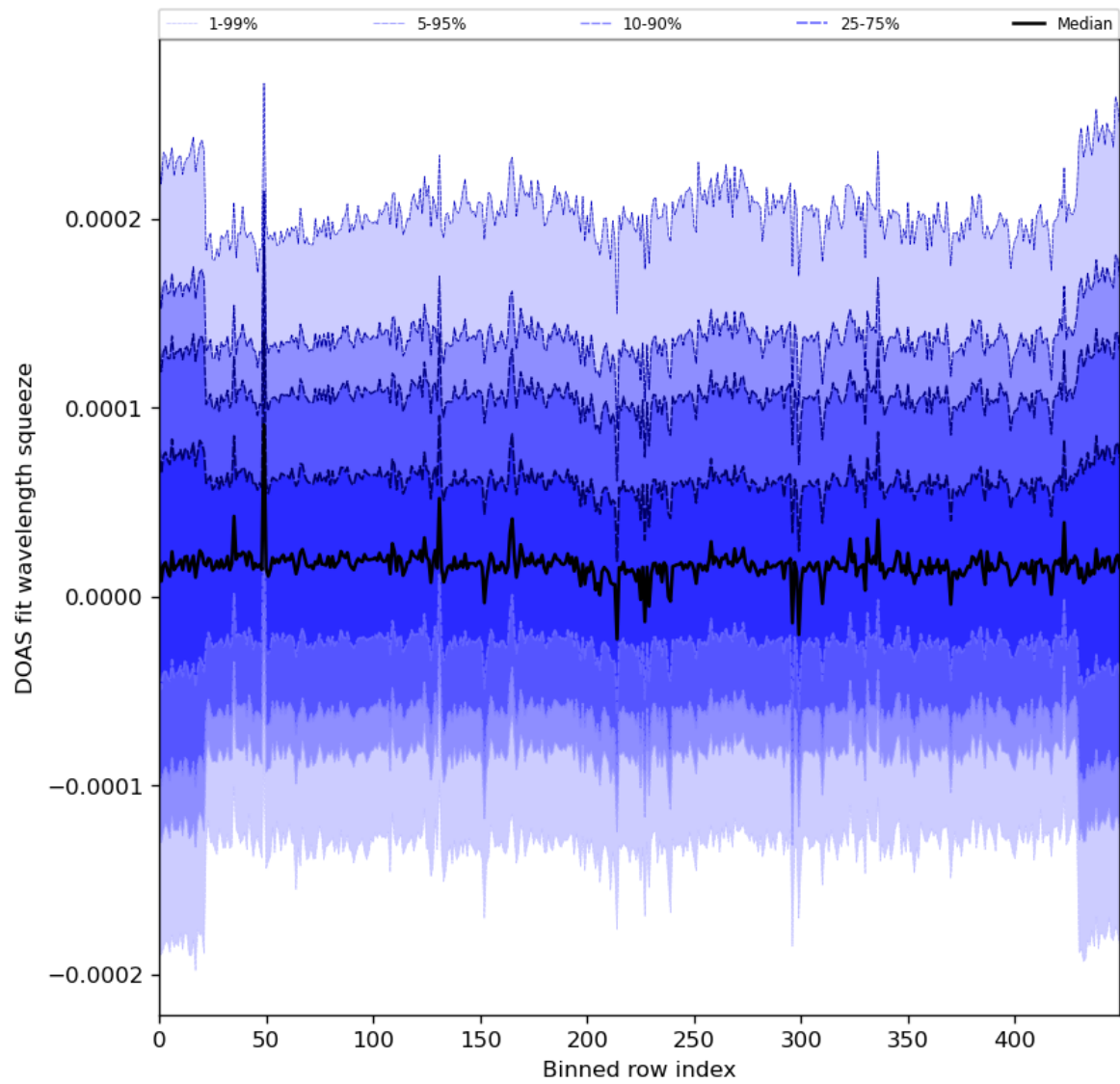
Figure 59: Along track statistics of “DOAS fit wavelength squeeze” for 2024-04-16 to 2024-04-17
