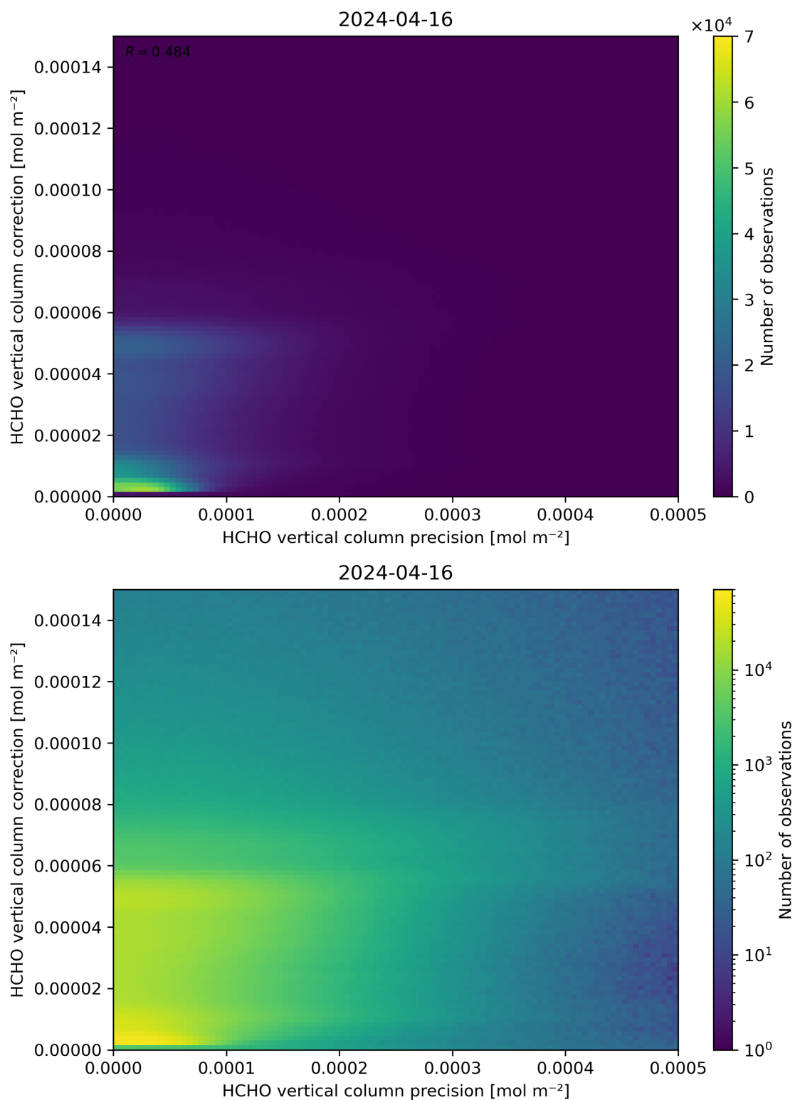
Figure 146: Scatter density plot of “HCHO vertical column precision” against “HCHO vertical column correction” for 2024-04-16 to 2024-04-17.
