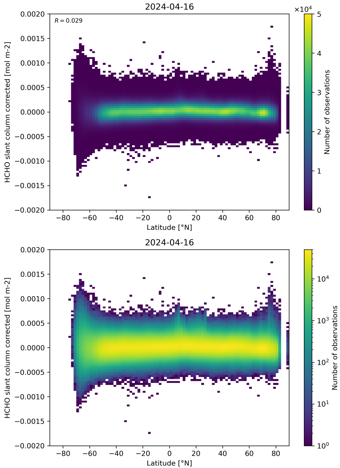
Figure 157: Scatter density plot of “Latitude” against “HCHO slant column corrected” for 2024-04-16 to 2024-04-17.
