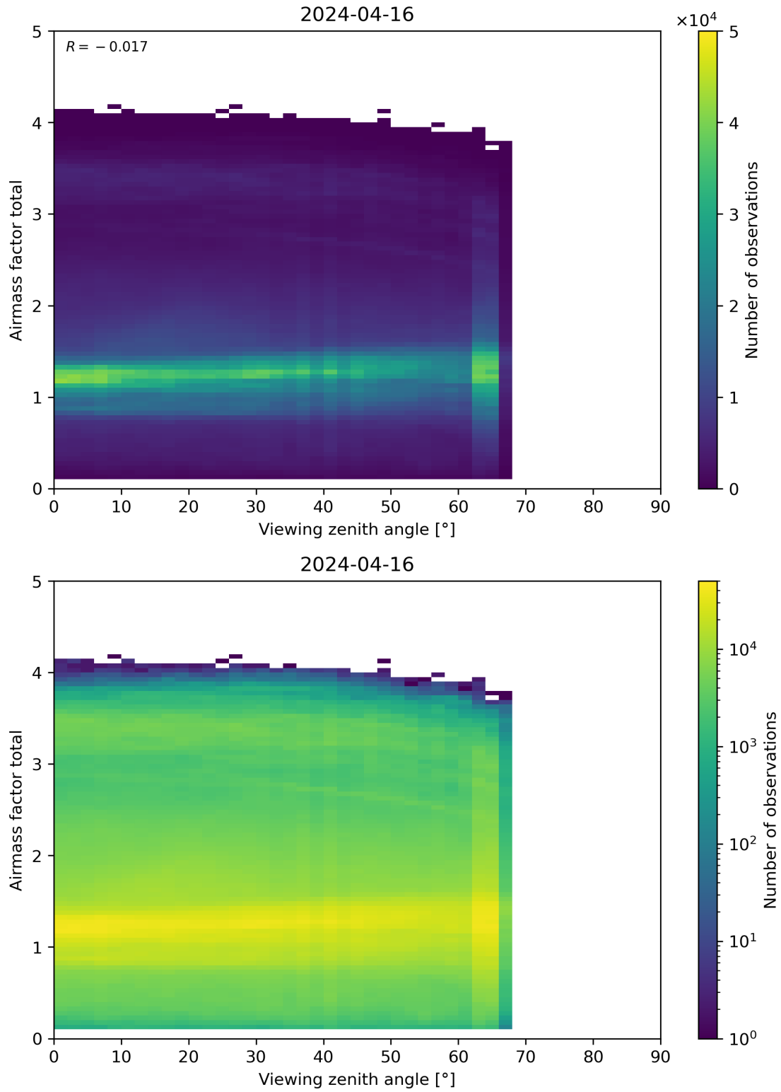
Figure 190: Scatter density plot of “Viewing zenith angle” against “Airmass factor total” for 2024-04-16 to 2024-04-17.
