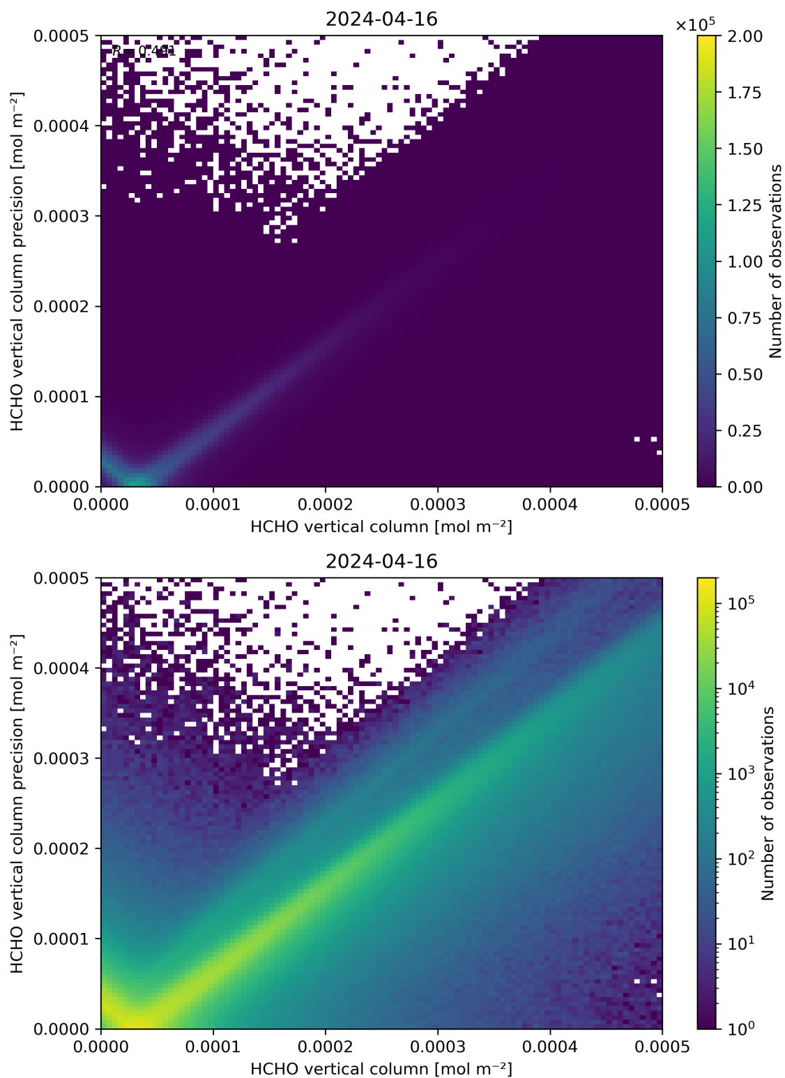
Figure 134: Scatter density plot of “HCHO vertical column” against “HCHO vertical column precision” for 2024-04-16 to 2024-04-17.
