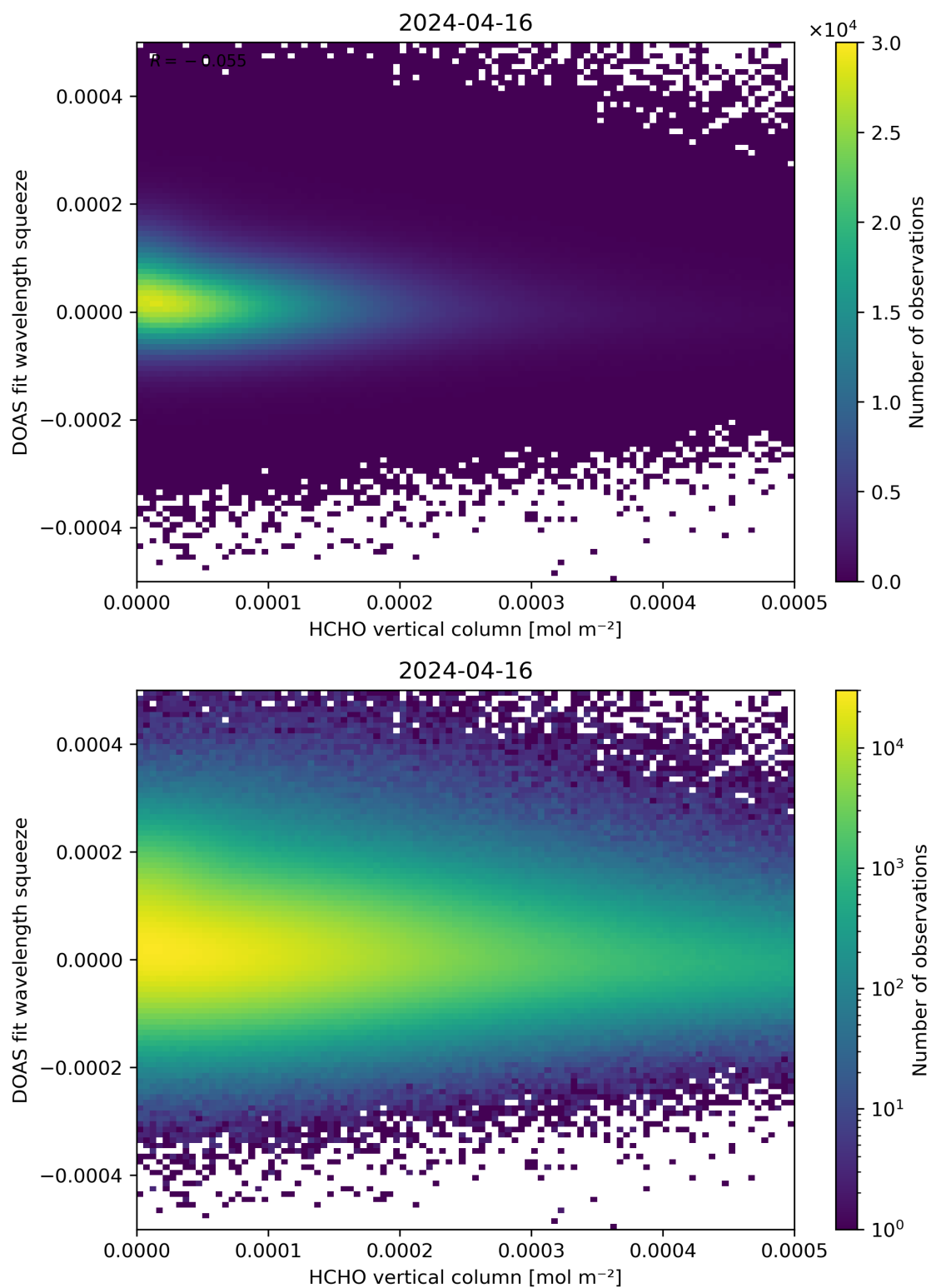
Figure 125: Scatter density plot of “HCHO vertical column” against “DOAS fit wavelength squeeze” for 2024-04-16 to 2024-04-17.
