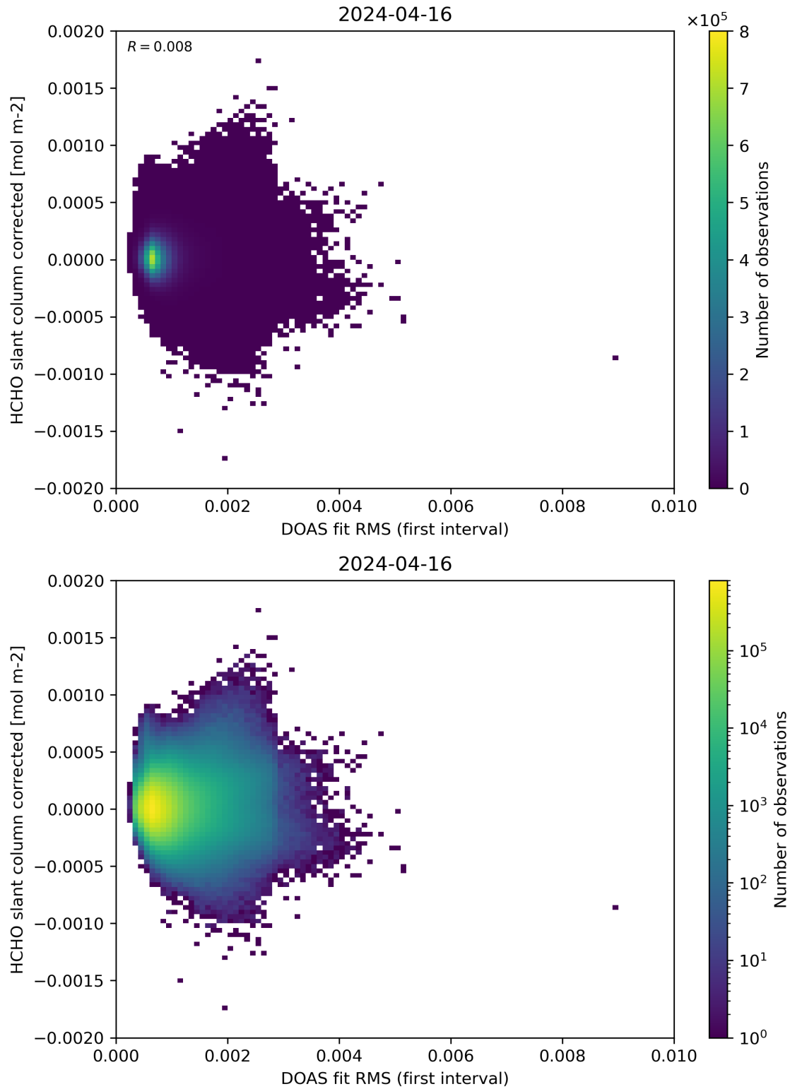
Figure 62: Scatter density plot of “DOAS fit RMS (first interval)” against “HCHO slant column corrected” for 2024-04-16 to 2024-04-17.
