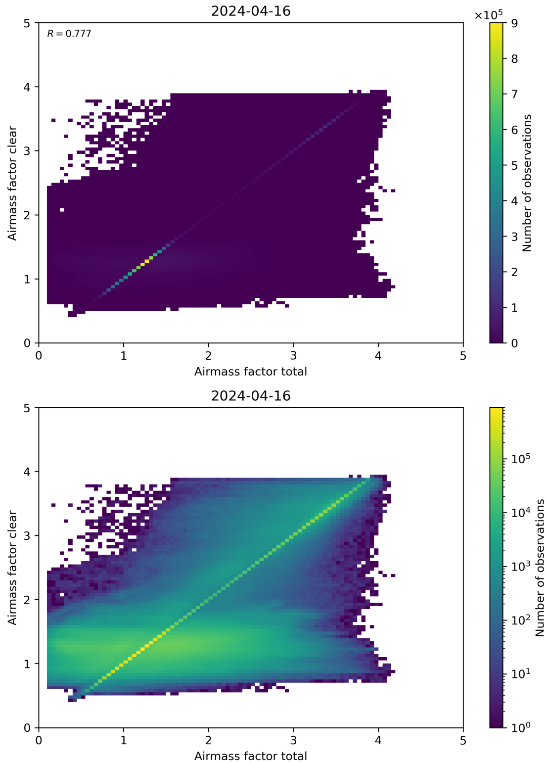
Figure 100: Scatter density plot of “Airmass factor total” against “Airmass factor clear” for 2024-04-16 to 2024-04-17.
