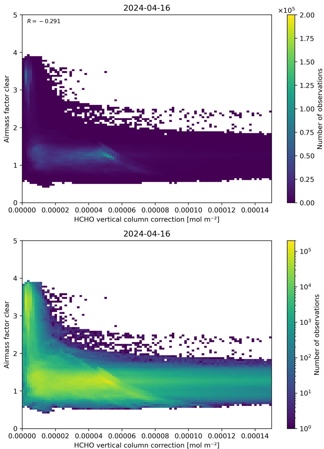
Figure 115: Scatter density plot of “HCHO vertical column correction” against “Airmass factor clear” for 2024-04-16 to 2024-04-17.
