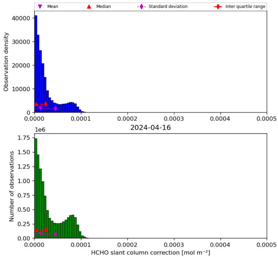
Figure 47: Histogram of “HCHO slant column correction” for 2024-04-16 to 2024-04-17
