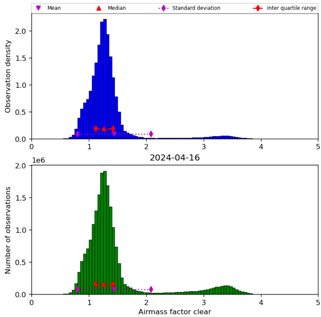
Figure 42: Histogram of “Airmass factor clear” for 2024-04-16 to 2024-04-17
