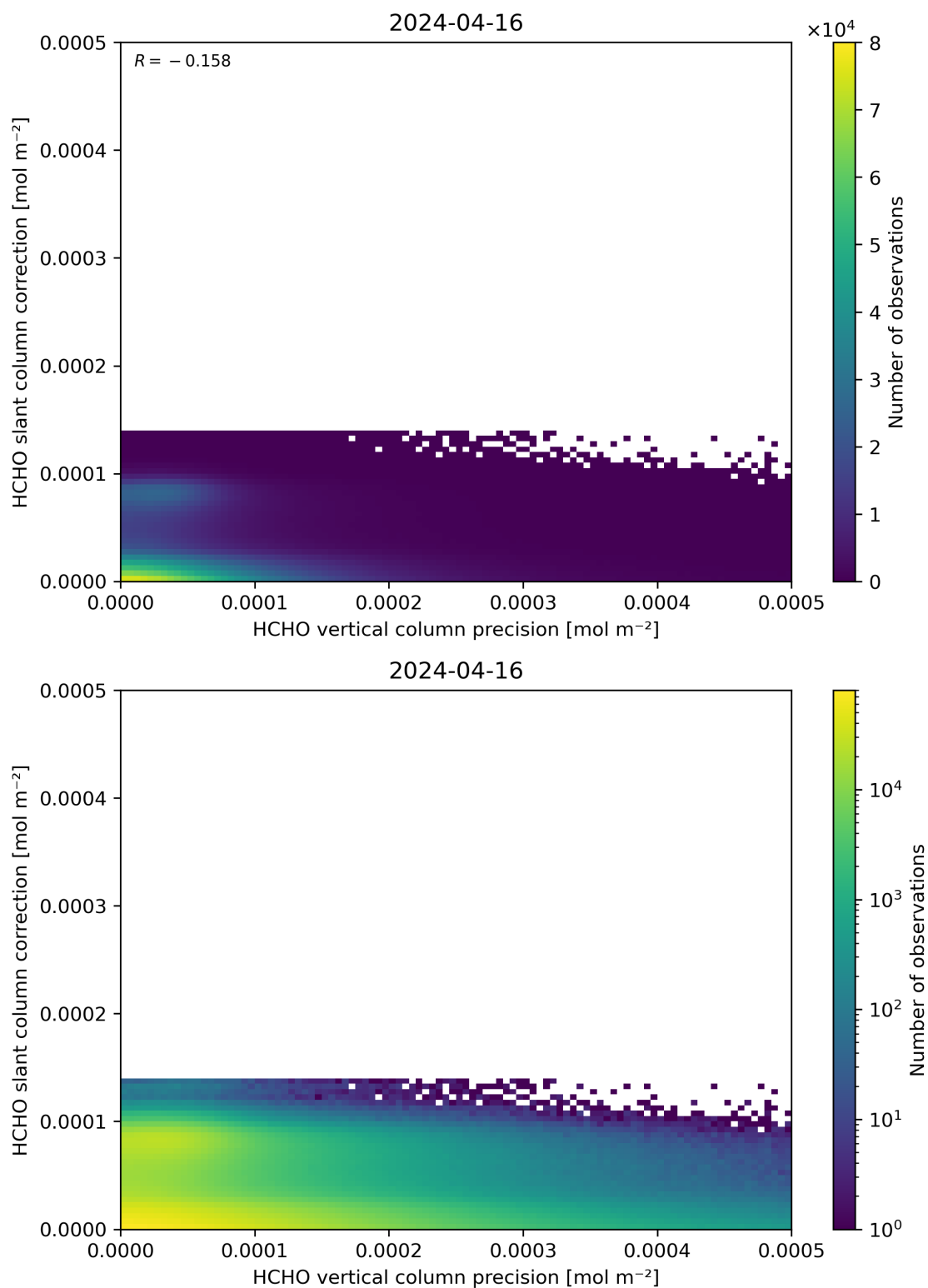
Figure 141: Scatter density plot of “HCHO vertical column precision” against “HCHO slant column correction” for 2024-04-16 to 2024-04-17.
