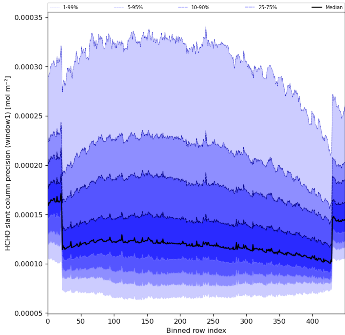
Figure 53: Along track statistics of “HCHO slant column precision (window1)” for 2024-04-16 to 2024-04-17
