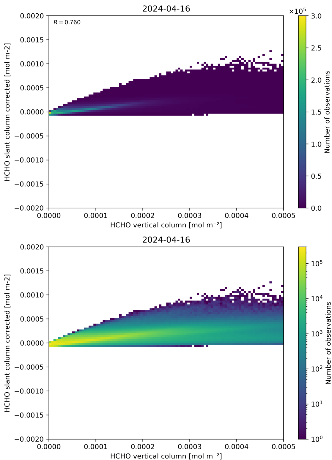
Figure 127: Scatter density plot of “HCHO vertical column” against “HCHO slant column corrected” for 2024-04-16 to 2024-04-17.
