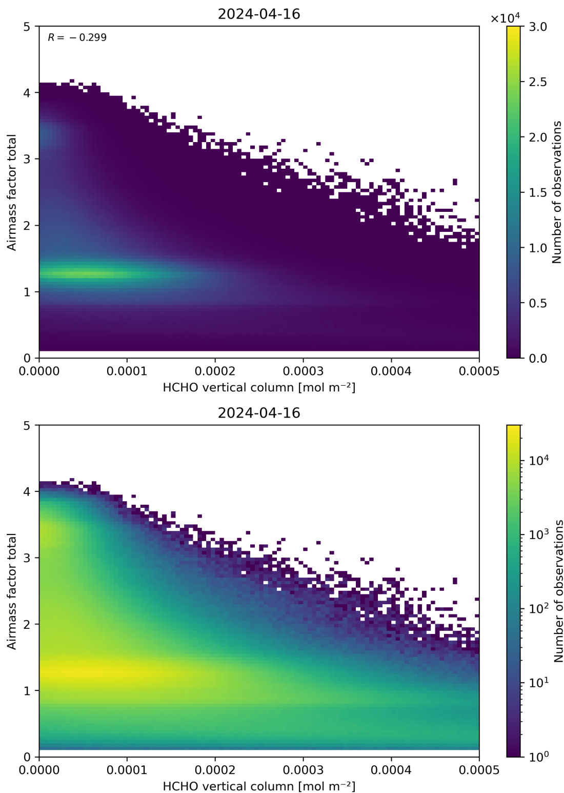
Figure 131: Scatter density plot of “HCHO vertical column” against “Airmass factor total” for 2024-04-16 to 2024-04-17.
