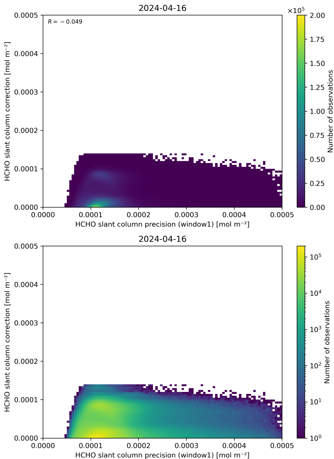
Figure 93: Scatter density plot of “HCHO slant column precision (window1)” against “HCHO slant column correction” for 2024-04-16 to 2024-04-17.
