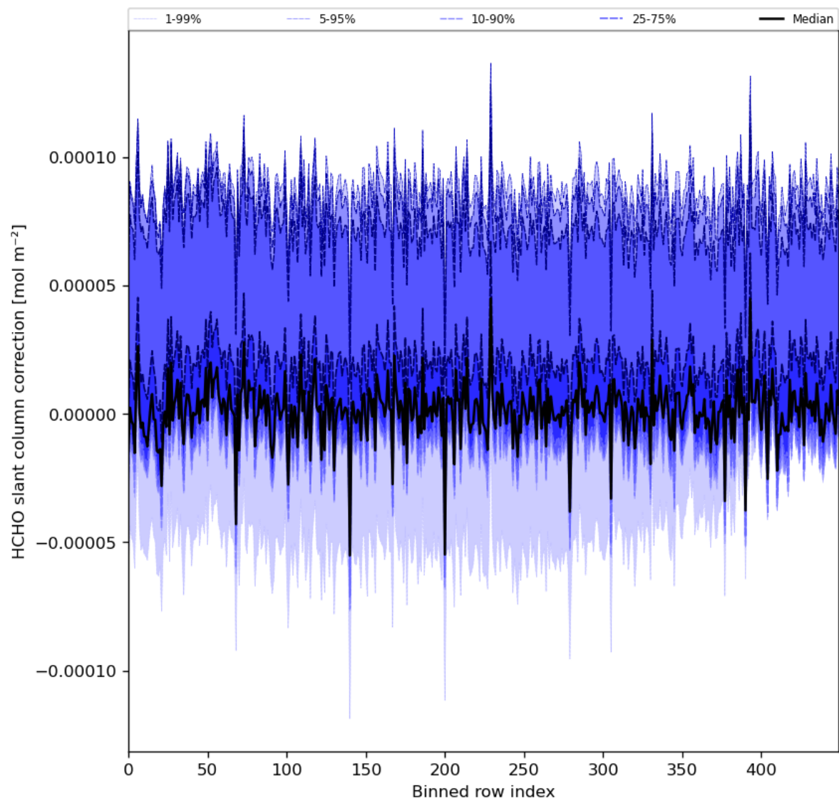
Figure 61: Along track statistics of “HCHO slant column correction” for 2024-04-16 to 2024-04-17
