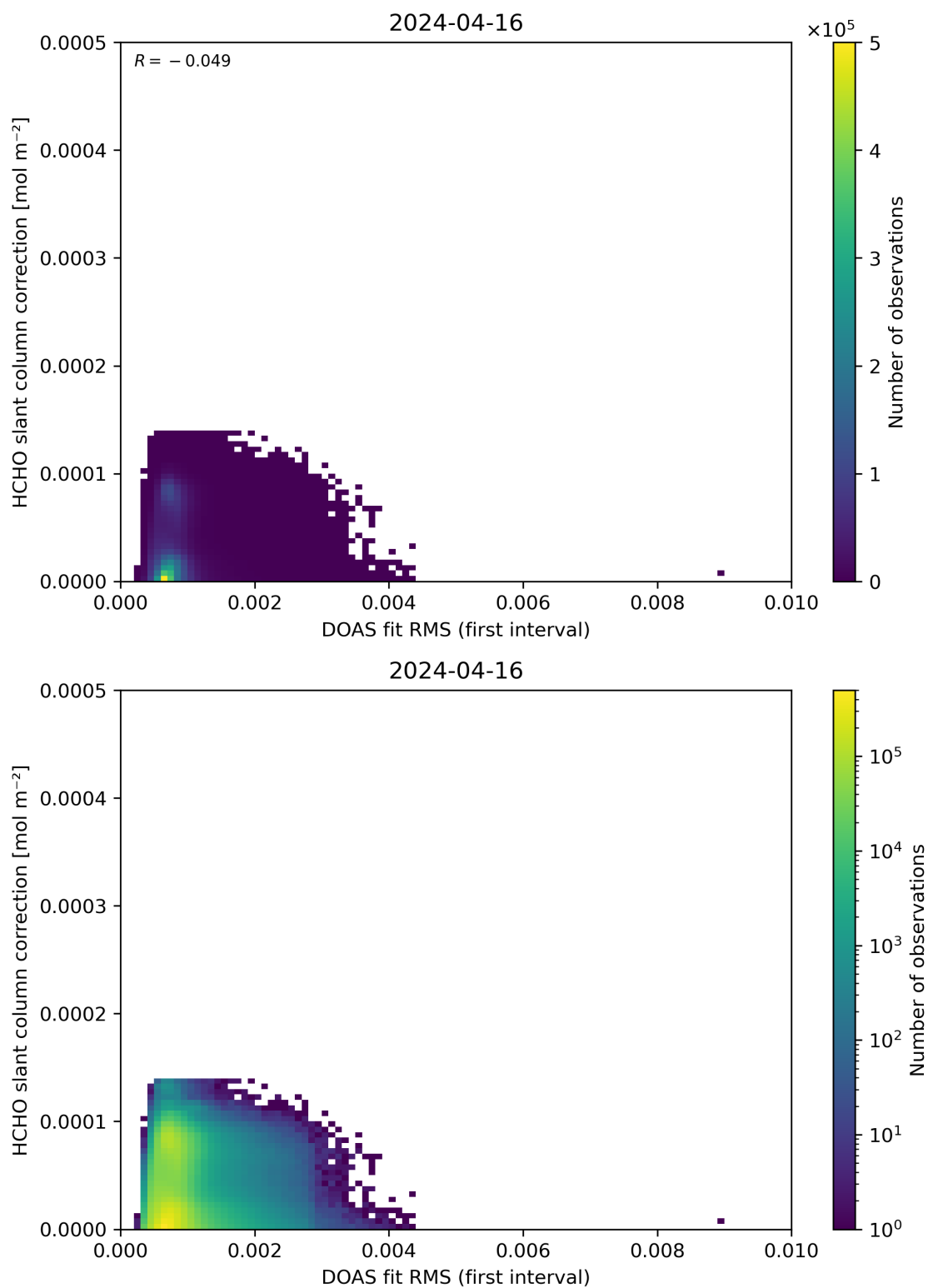
Figure 63: Scatter density plot of “DOAS fit RMS (first interval)” against “HCHO slant column correction” for 2024-04-16 to 2024-04-17.
