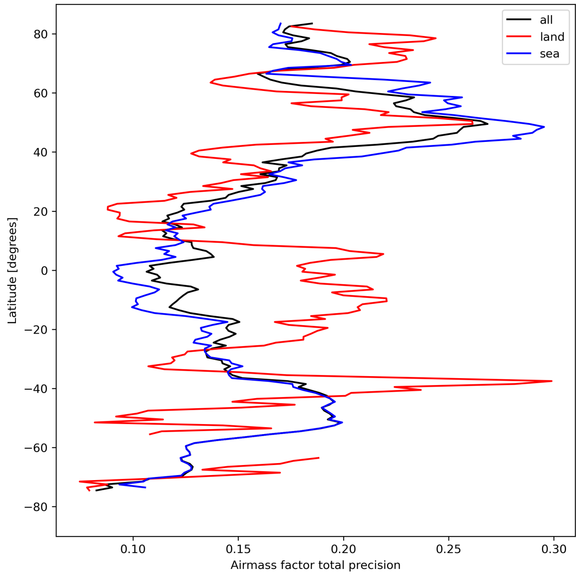
Figure 27: Zonal average of “Airmass factor total precision” for 2024-04-16 to 2024-04-17.
