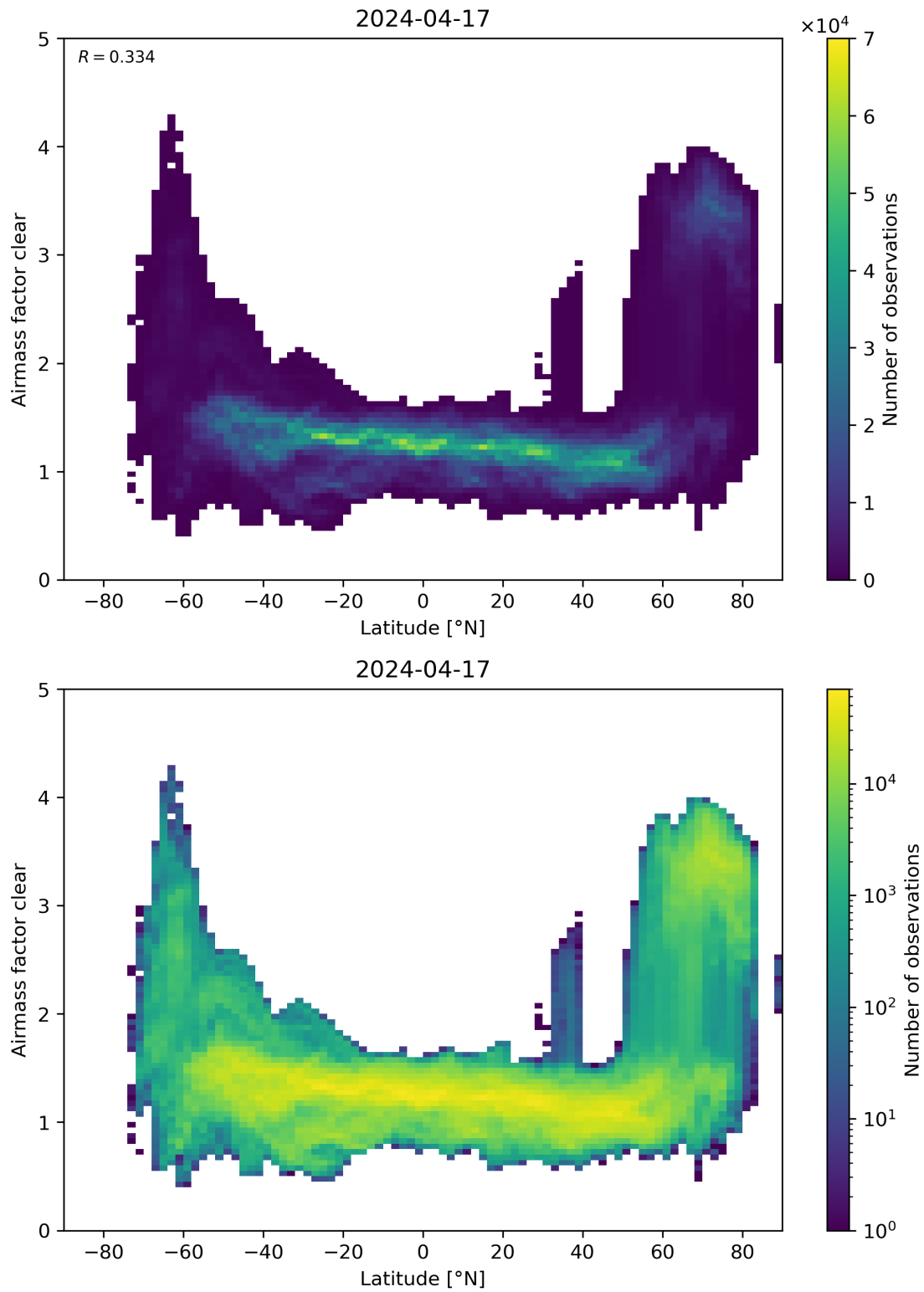
Figure 156: Scatter density plot of “Latitude” against “Airmass factor clear” for 2024-04-16 to 2024-04-18.
