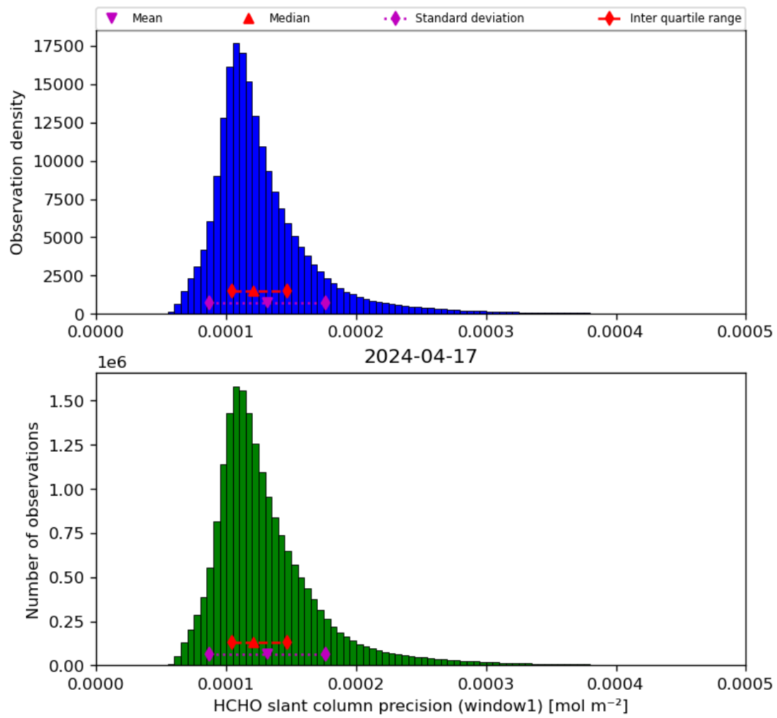
Figure 39: Histogram of “HCHO slant column precision (window1)” for 2024-04-16 to 2024-04-18
