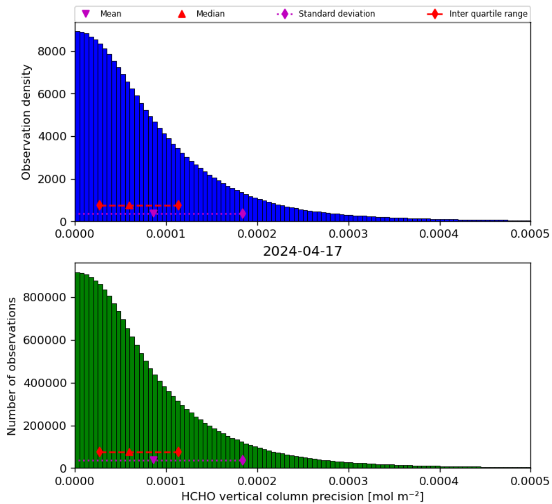
Figure 36: Histogram of “HCHO vertical column precision” for 2024-04-16 to 2024-04-18
