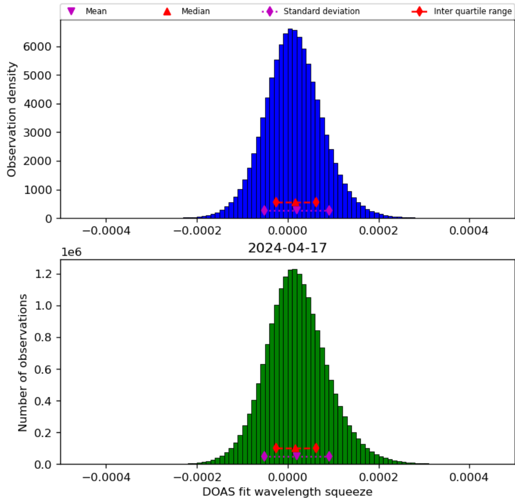
Figure 45: Histogram of “DOAS fit wavelength squeeze” for 2024-04-16 to 2024-04-18
