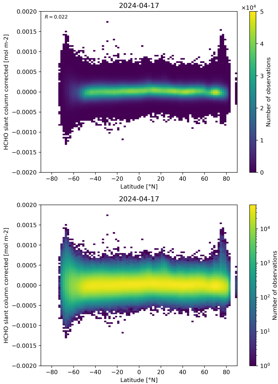
Figure 157: Scatter density plot of “Latitude” against “HCHO slant column corrected” for 2024-04-16 to 2024-04-18.
