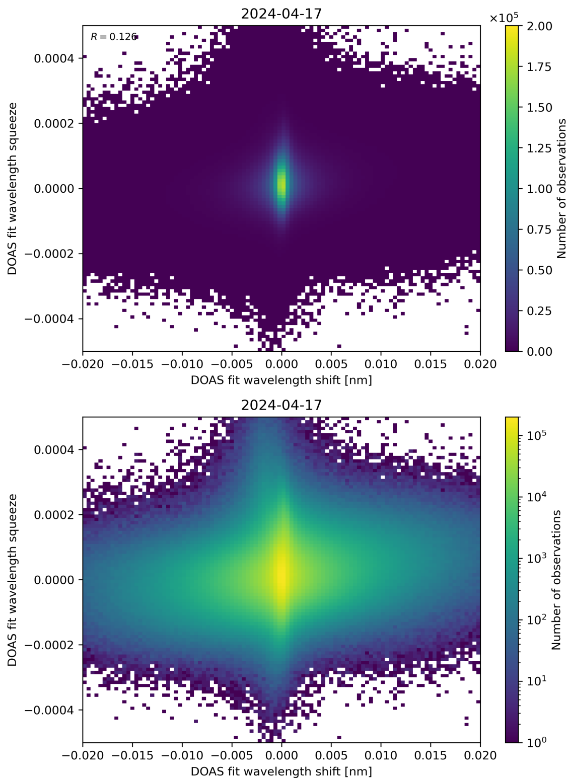
Figure 65: Scatter density plot of “DOAS fit wavelength shift” against “DOAS fit wavelength squeeze” for 2024-04-16 to 2024-04-18.
