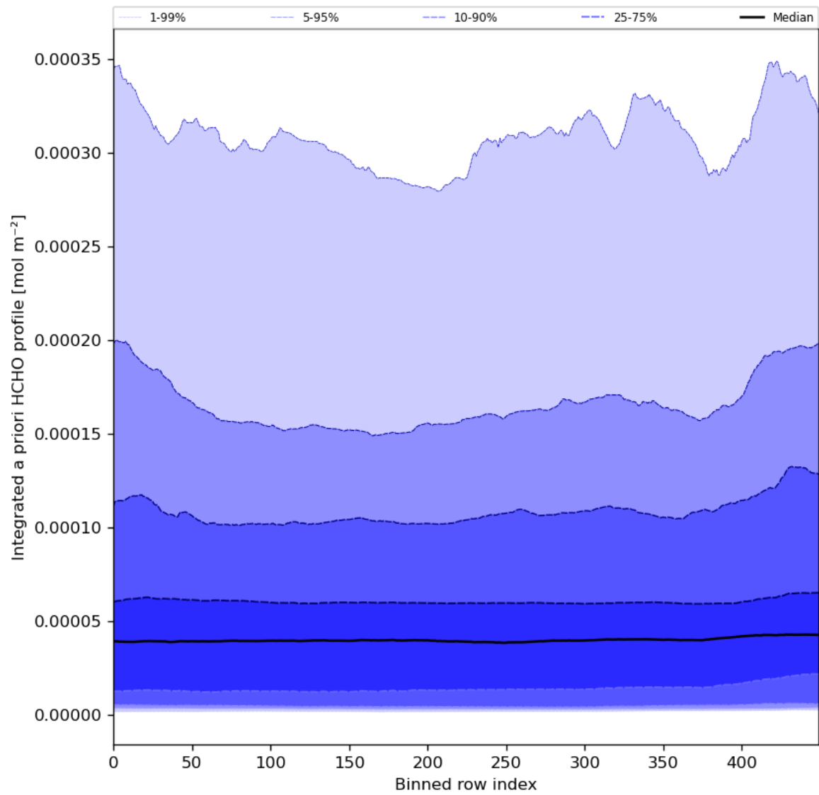
Figure 57: Along track statistics of "Integrated a priori HCHO profile" for 2024-04-16 to 2024-04-18
