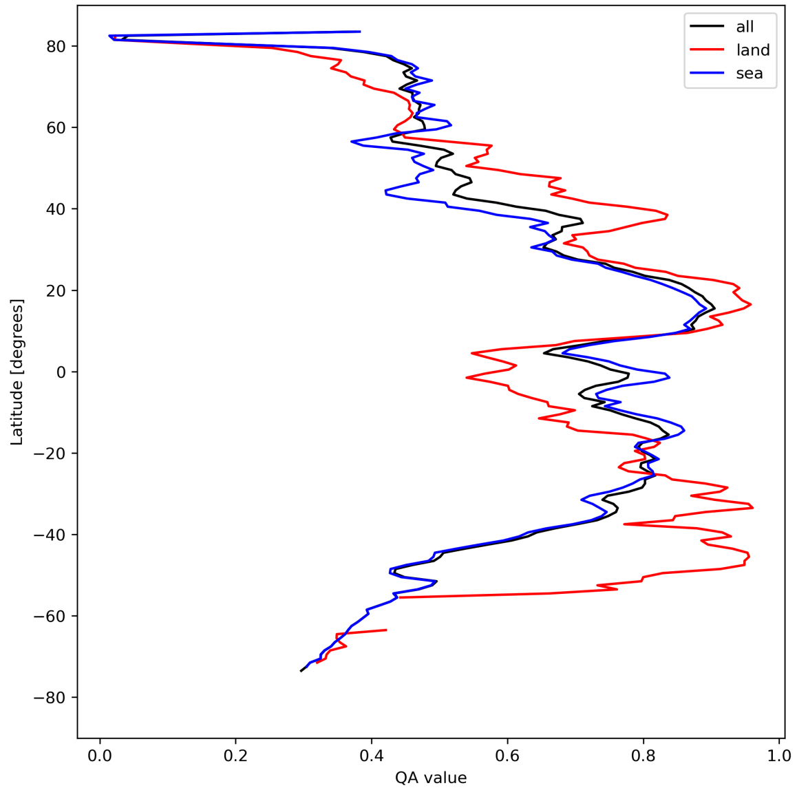
Figure 20: Zonal average of “QA value” for 2024-04-16 to 2024-04-18.
