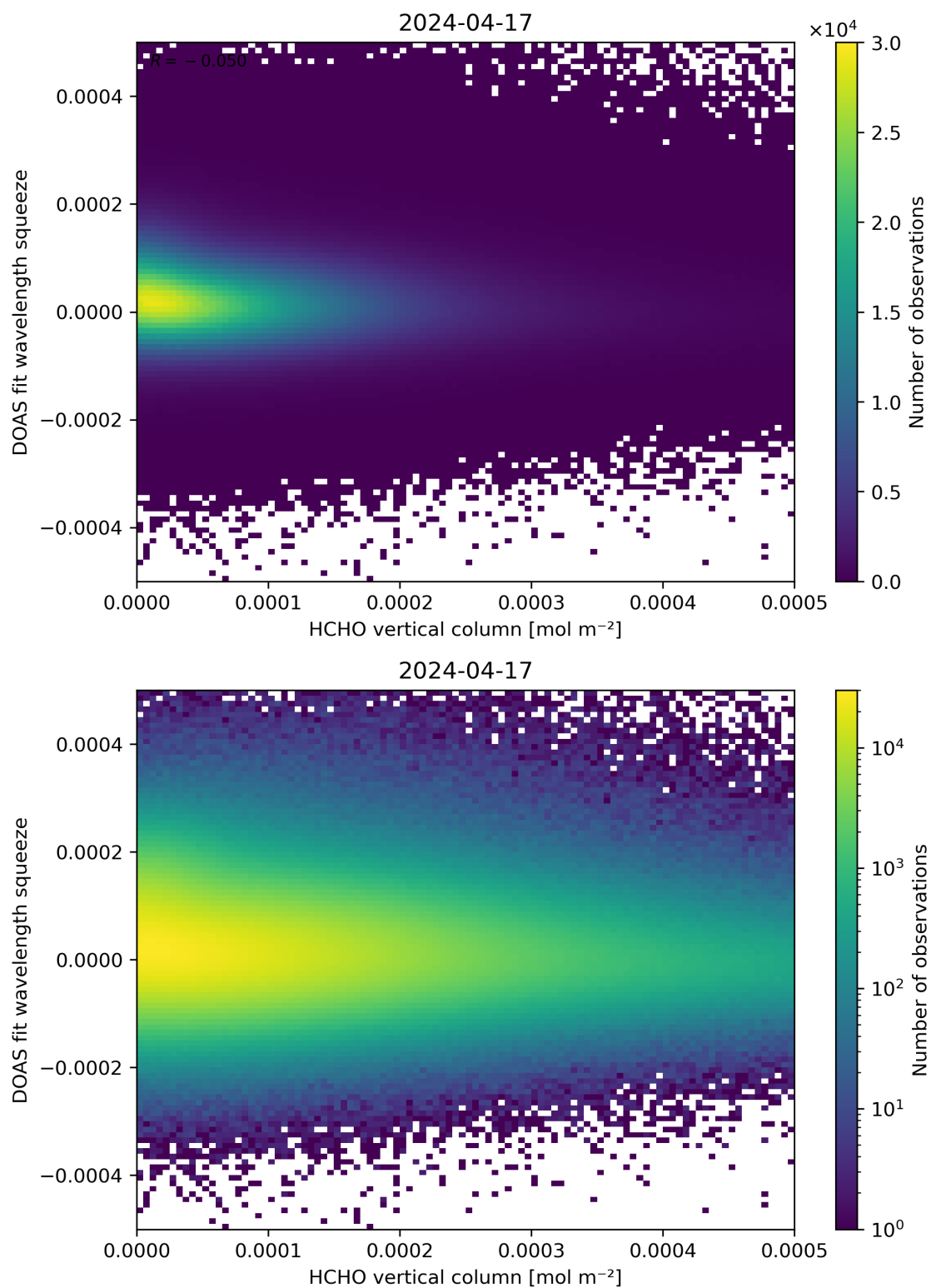
Figure 125: Scatter density plot of “HCHO vertical column” against “DOAS fit wavelength squeeze” for 2024-04-16 to 2024-04-18.
