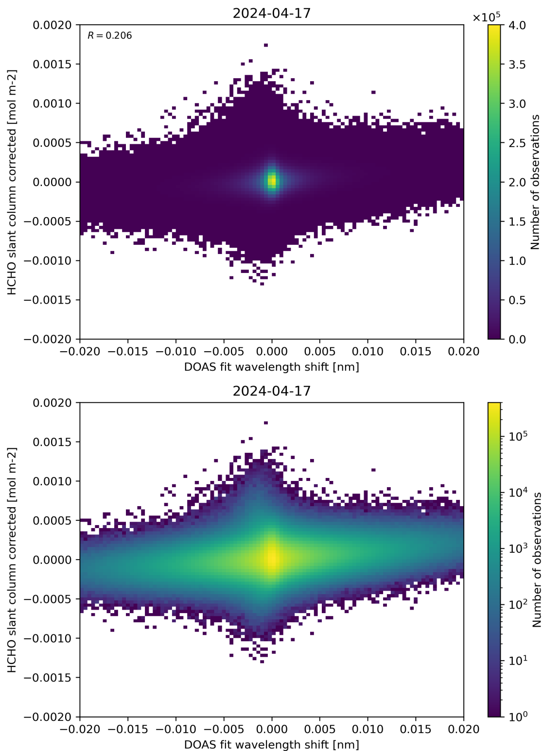
Figure 66: Scatter density plot of “DOAS fit wavelength shift” against “HCHO slant column corrected” for 2024-04-16 to 2024-04-18.
