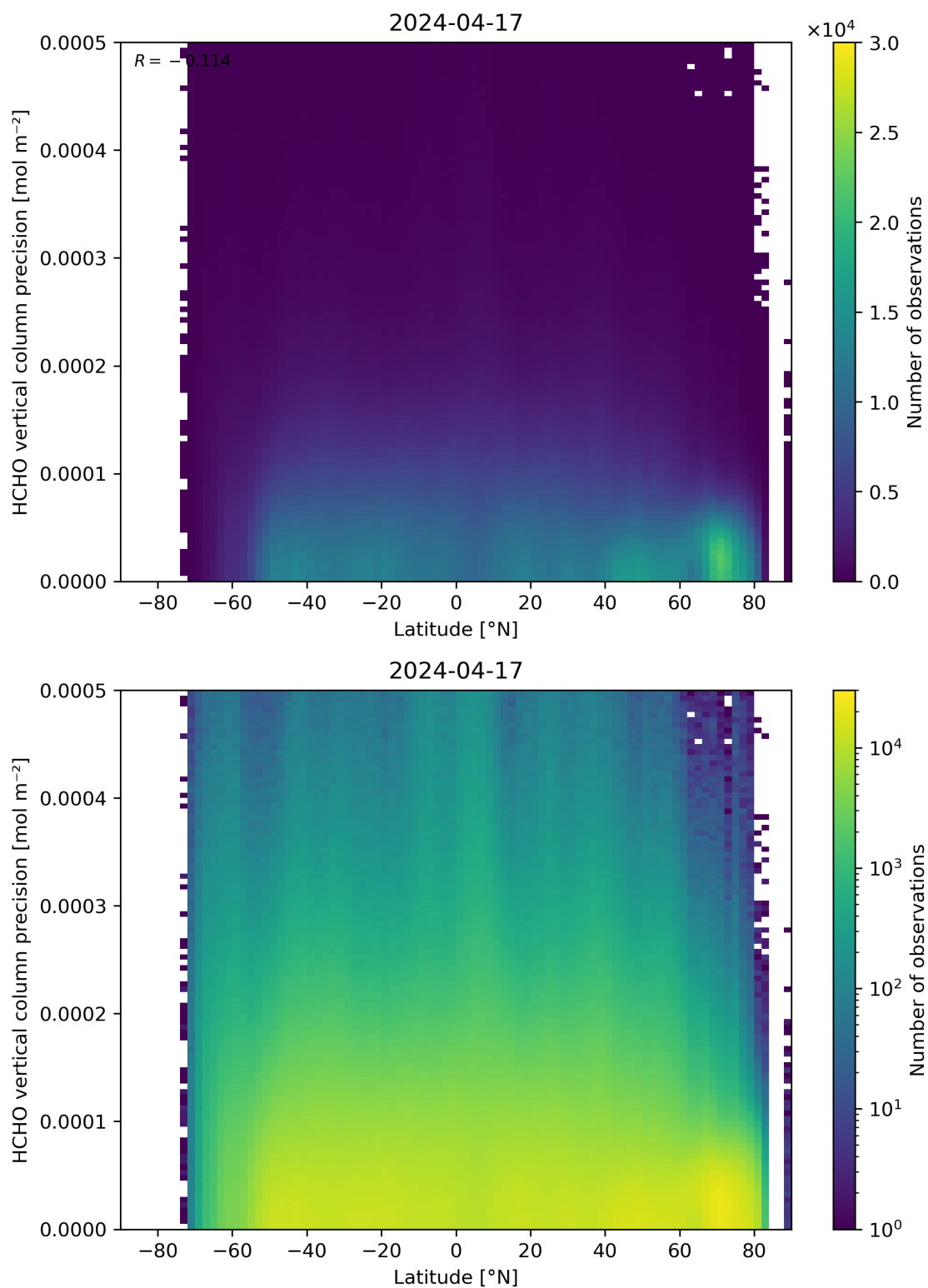
Figure 165: Scatter density plot of “Latitude” against “HCHO vertical column precision” for 2024-04-16 to 2024-04-18.
