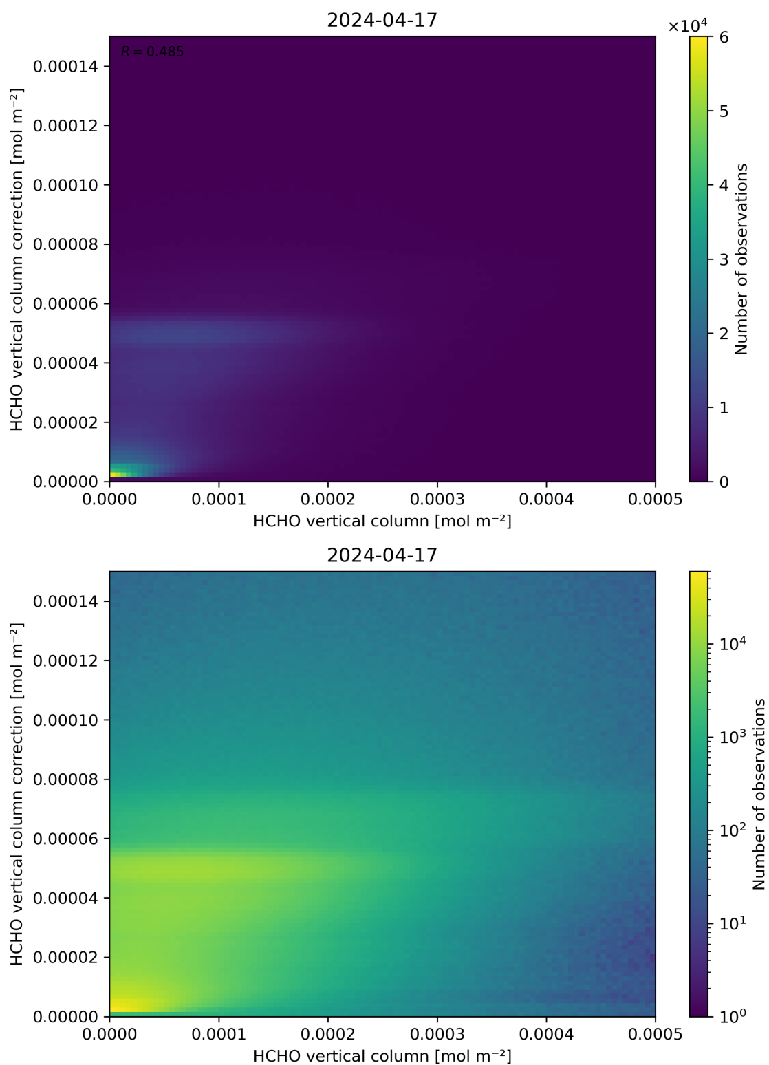
Figure 133: Scatter density plot of “HCHO vertical column” against “HCHO vertical column correction” for 2024-04-16 to 2024-04-18.
