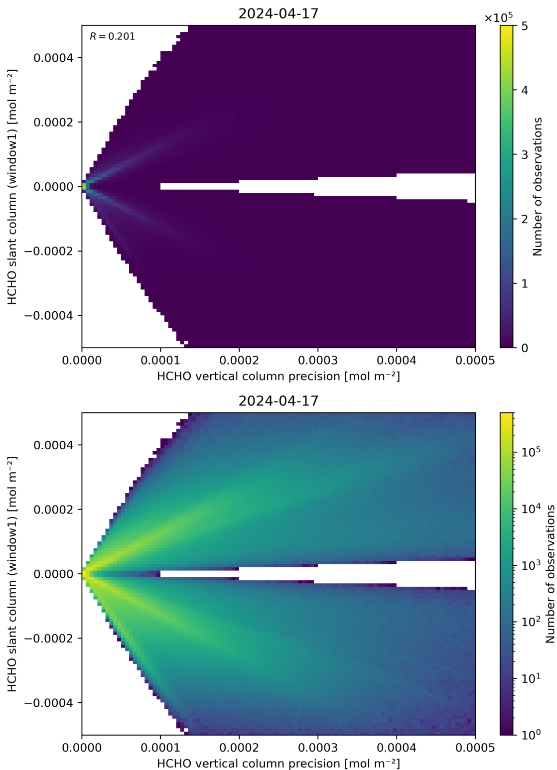
Figure 142: Scatter density plot of “HCHO vertical column precision” against “HCHO slant column (window1)” for 2024-04-16 to 2024-04-18.
