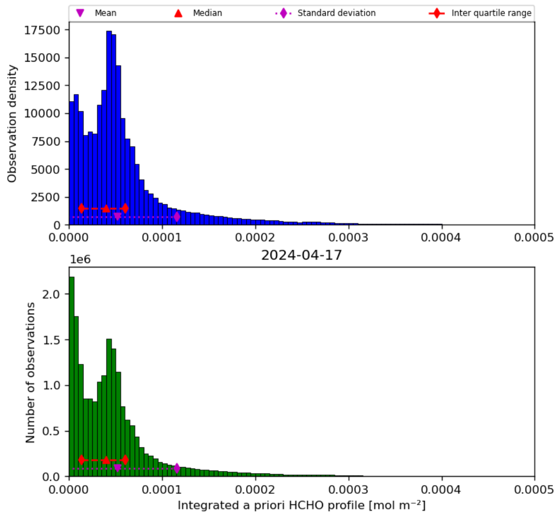
Figure 43: Histogram of “Integrated a priori HCHO profile” for 2024-04-16 to 2024-04-18
