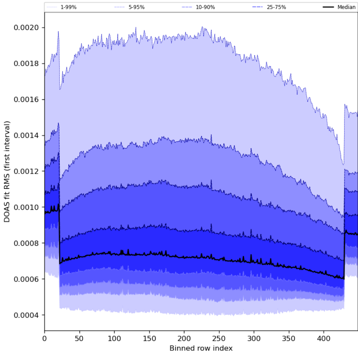
Figure 60: Along track statistics of “DOAS fit RMS (first interval)” for 2024-04-16 to 2024-04-18
