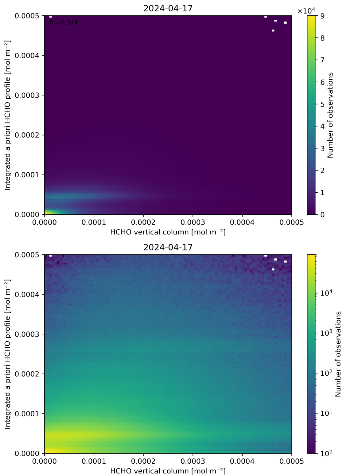
Figure 135: Scatter density plot of “HCHO vertical column” against “Integrated a priori HCHO profile” for 2024-04-16 to 2024-04-18.
