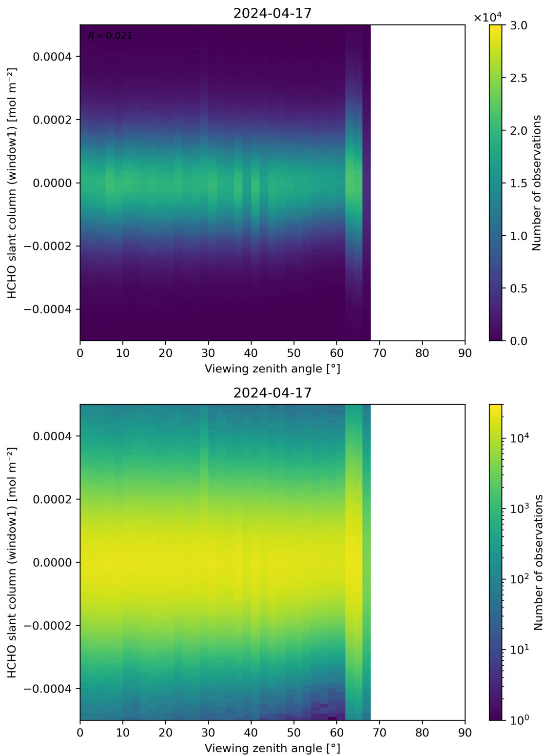
Figure 188: Scatter density plot of “Viewing zenith angle” against “HCHO slant column (window1)” for 2024-04-16 to 2024-04-18.
