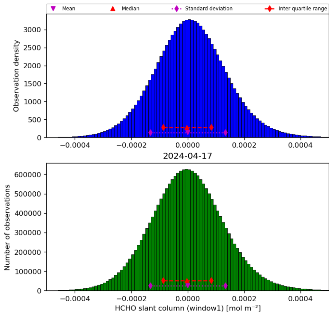
Figure 38: Histogram of “HCHO slant column (window1)” for 2024-04-16 to 2024-04-18
