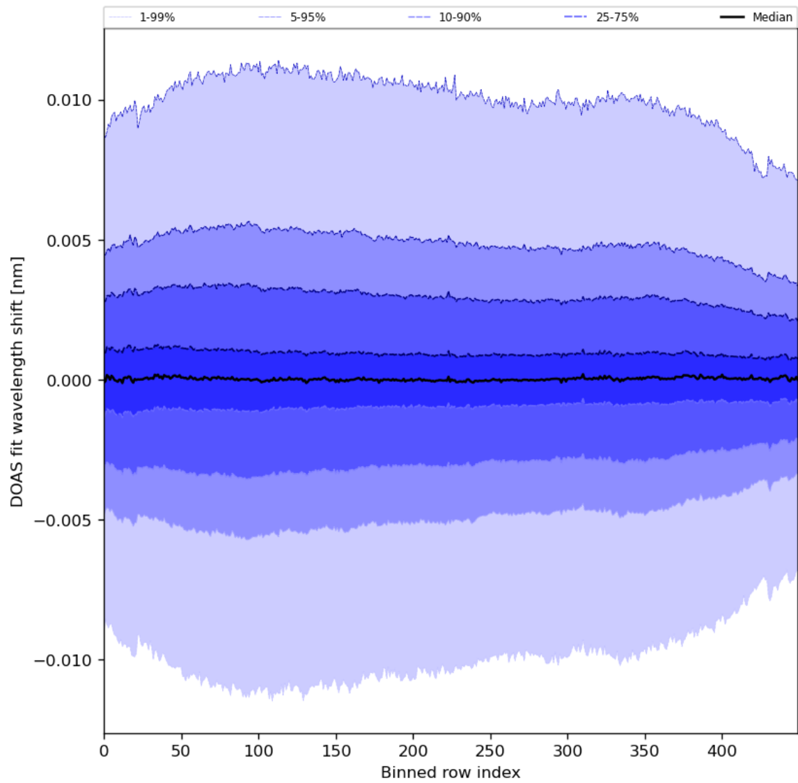
Figure 58: Along track statistics of “DOAS fit wavelength shift” for 2024-04-16 to 2024-04-18
