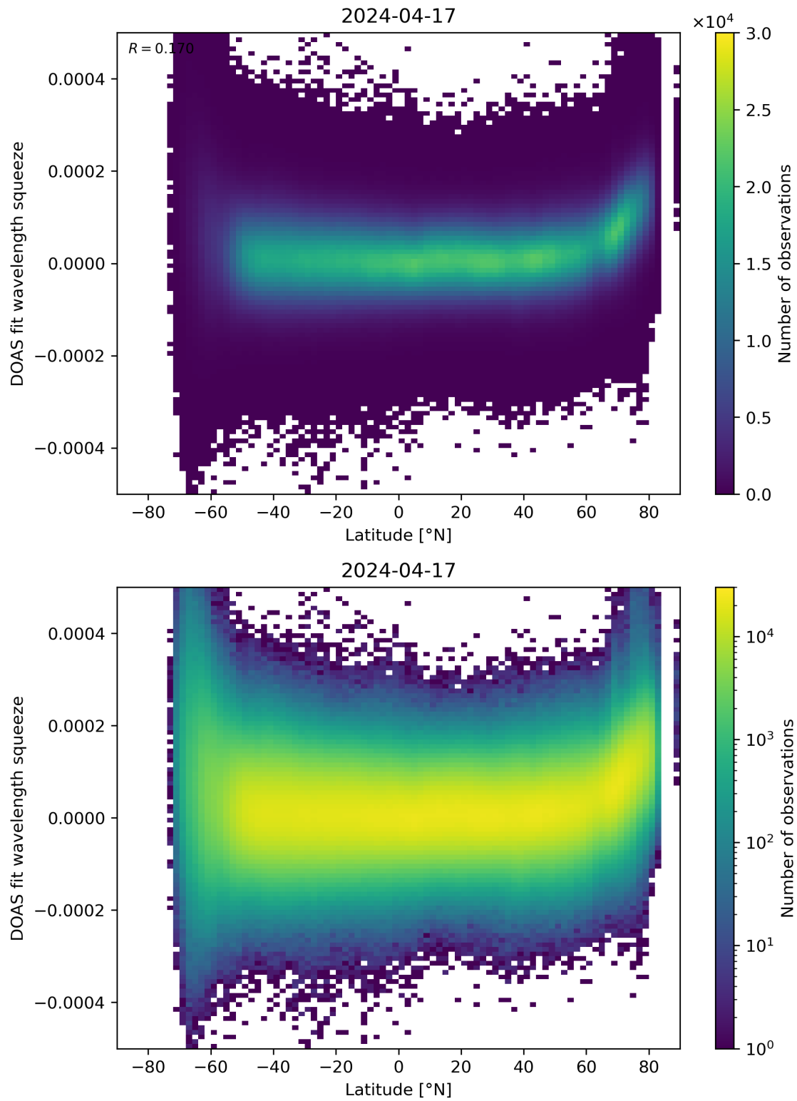
Figure 155: Scatter density plot of “Latitude” against “DOAS fit wavelength squeeze” for 2024-04-16 to 2024-04-18.
