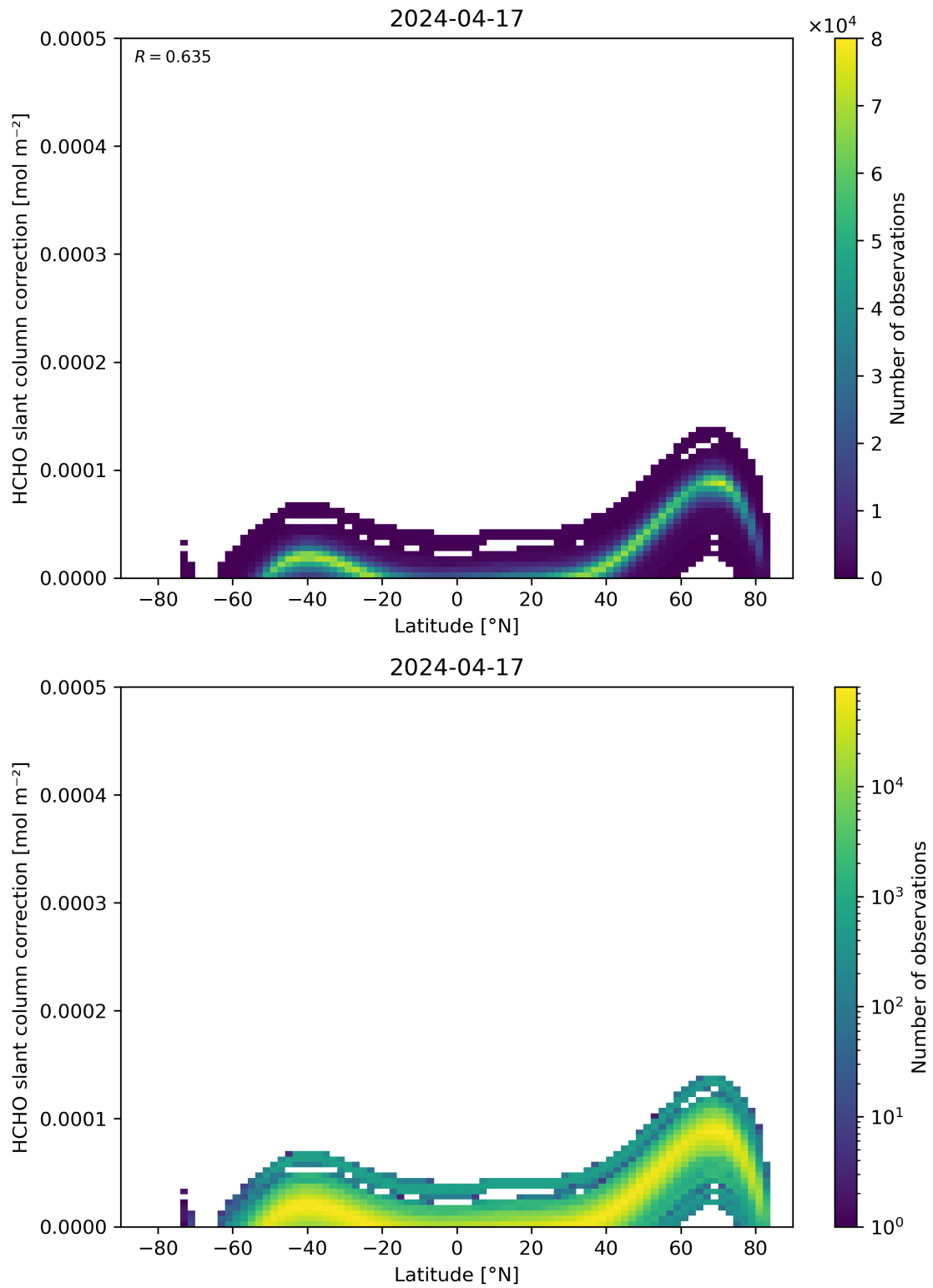
Figure 158: Scatter density plot of “Latitude” against “HCHO slant column correction” for 2024-04-16 to 2024-04-18.
