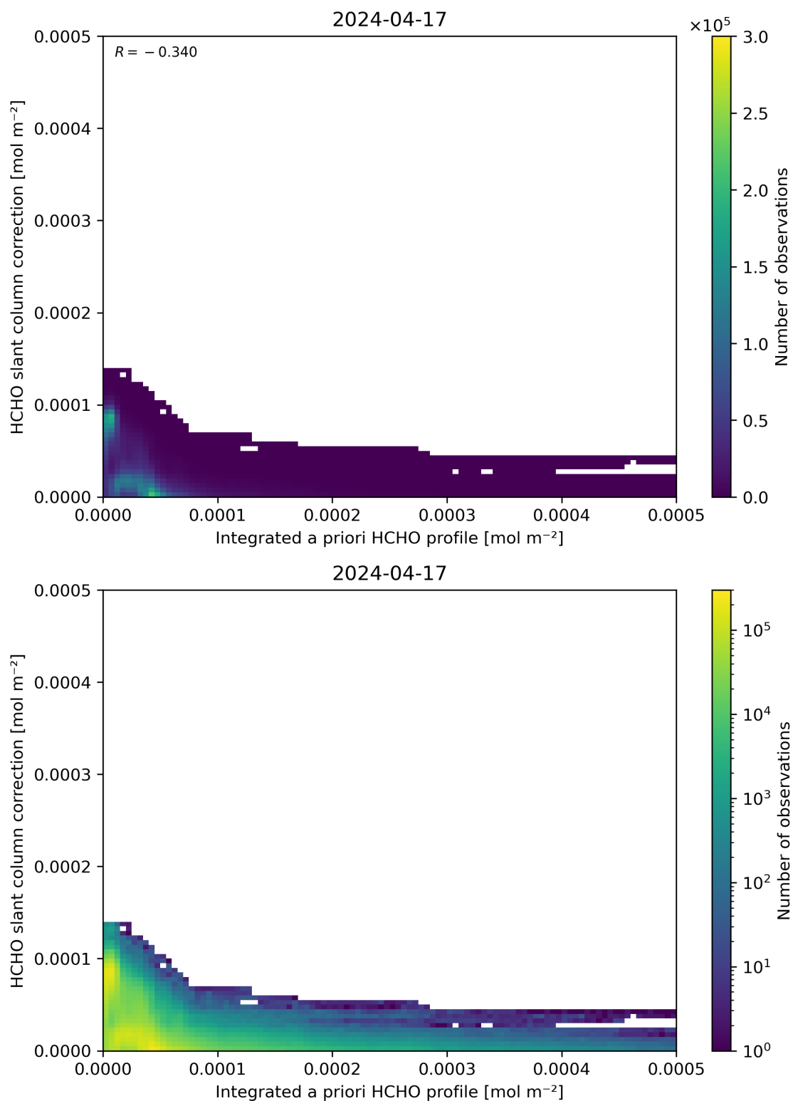
Figure 152: Scatter density plot of “Integrated a priori HCHO profile” against “HCHO slant column correction” for 2024-04-16 to 2024-04-18.
