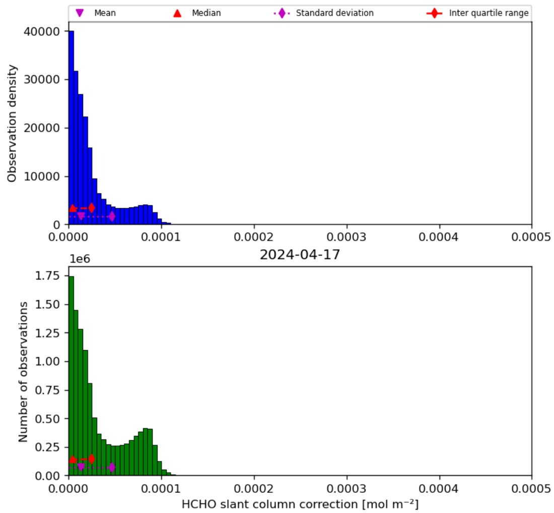
Figure 47: Histogram of “HCHO slant column correction” for 2024-04-16 to 2024-04-18
