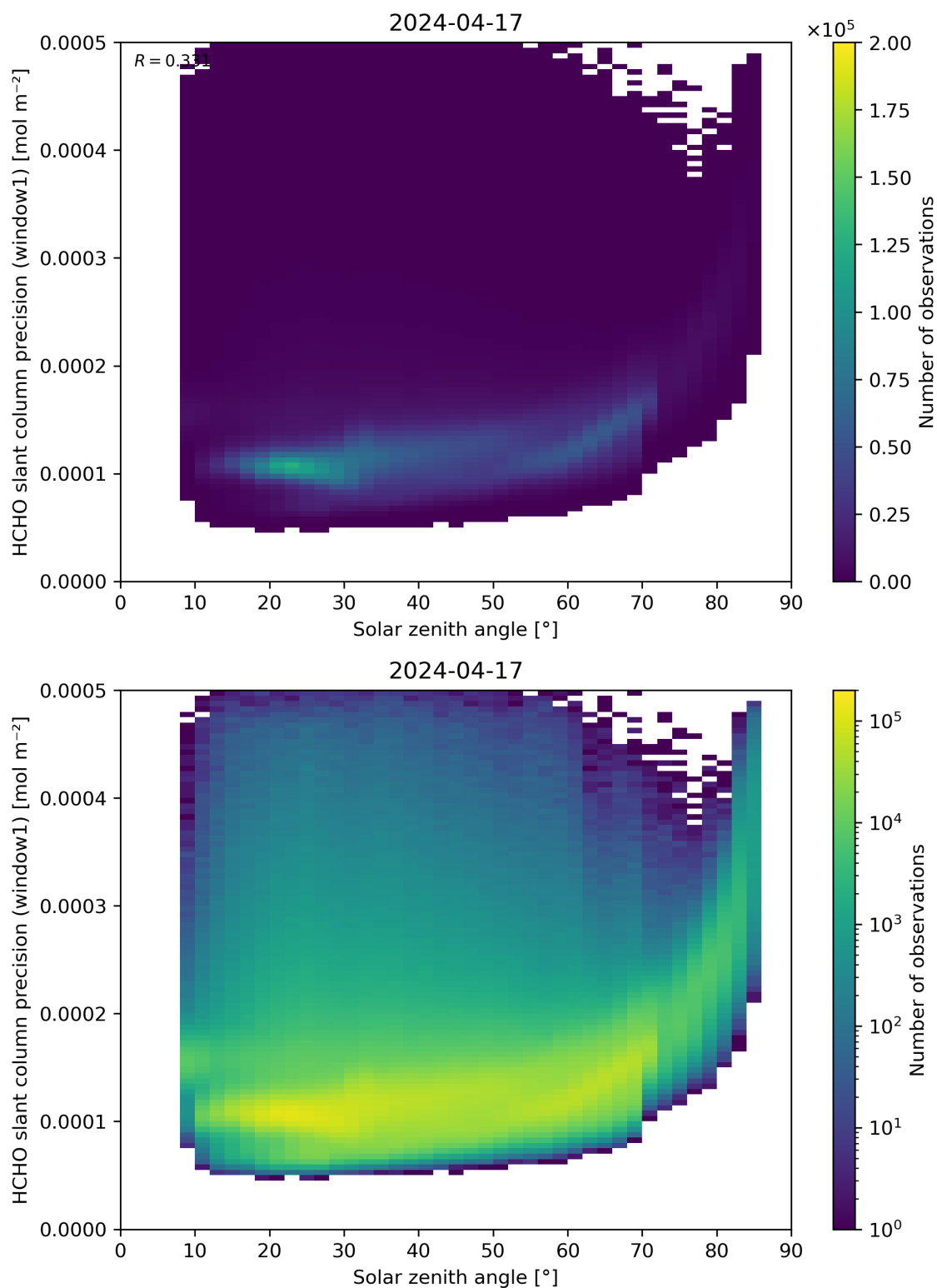
Figure 174: Scatter density plot of “Solar zenith angle” against “HCHO slant column precision (window1)” for 2024-04-16 to 2024-04-18.
