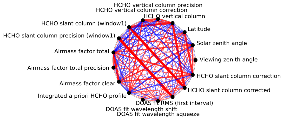
Figure 1: Map of correlation graph for 2024-04-16 to 2024-04-18.
