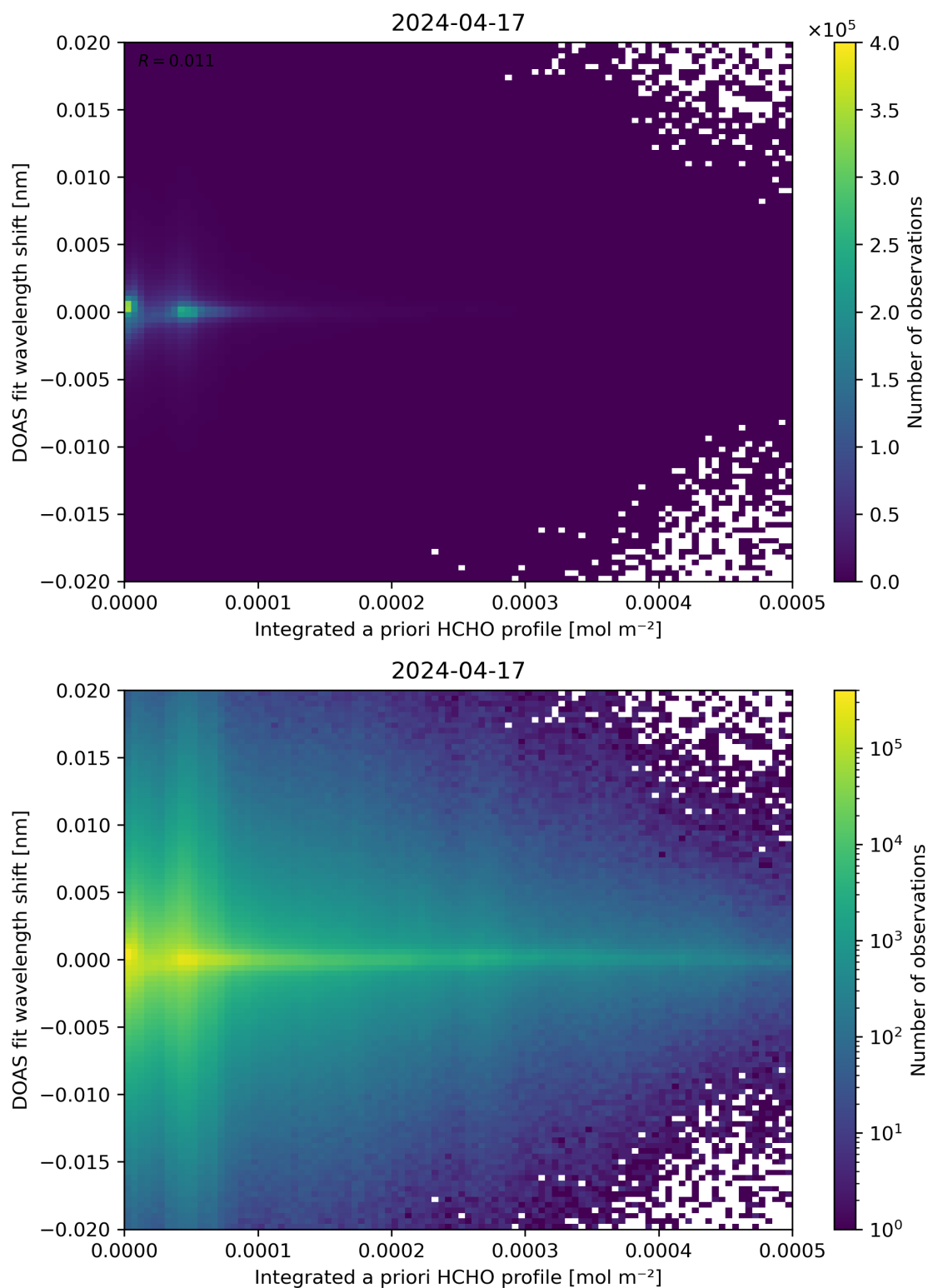
Figure 149: Scatter density plot of “Integrated a priori HCHO profile” against “DOAS fit wavelength shift” for 2024-04-16 to 2024-04-18.
