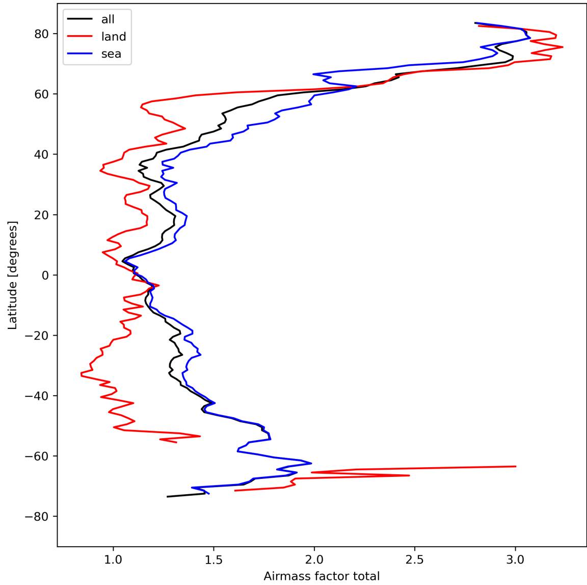
Figure 26: Zonal average of “Airmass factor total” for 2024-04-16 to 2024-04-18.
