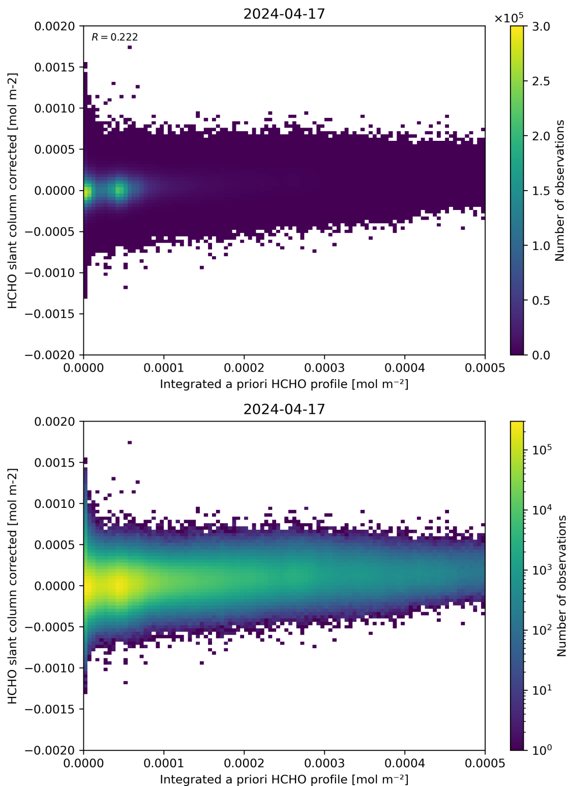
Figure 151: Scatter density plot of “Integrated a priori HCHO profile” against “HCHO slant column corrected” for 2024-04-16 to 2024-04-18.
