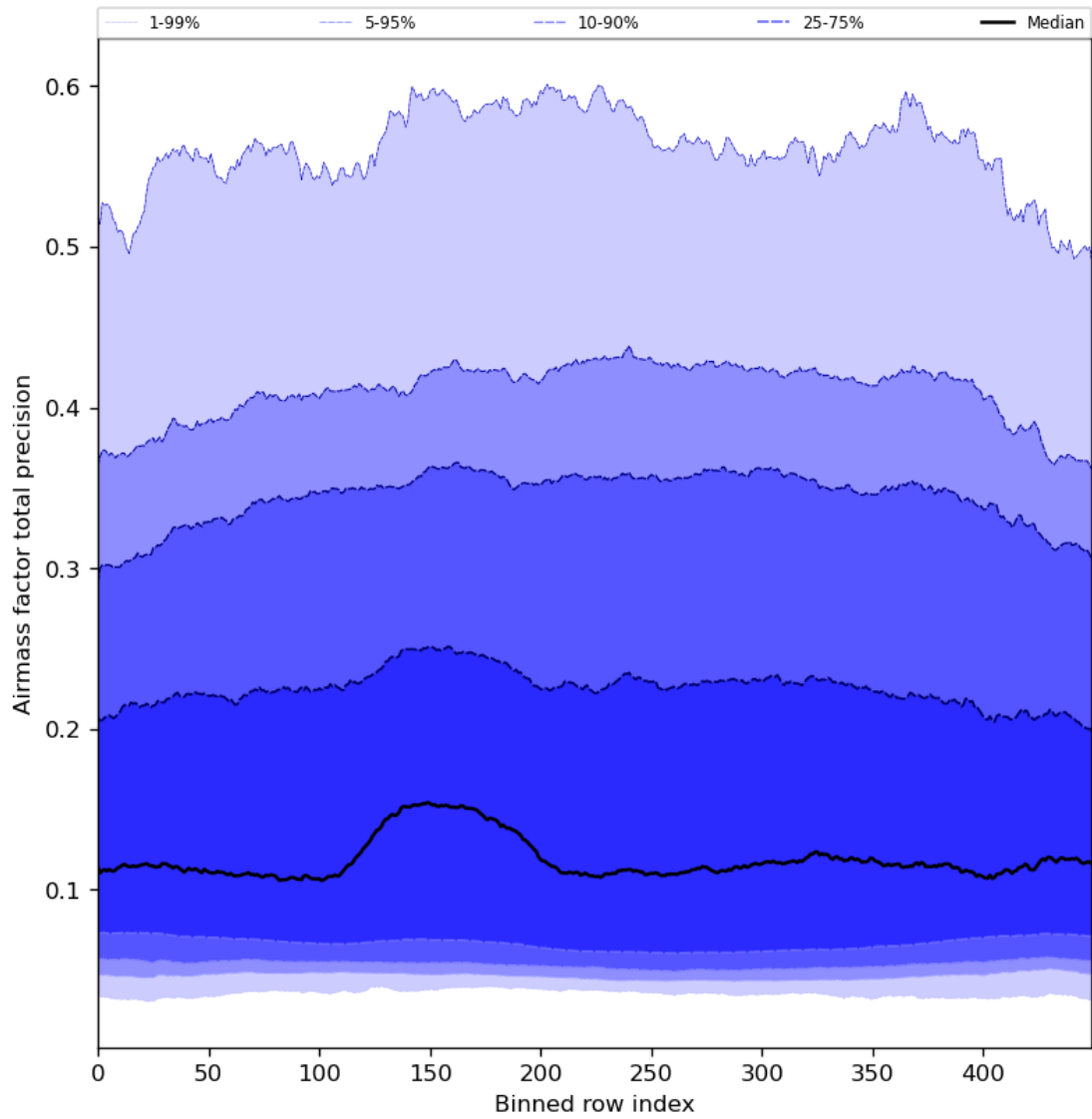
Figure 55: Along track statistics of “Airmass factor total precision” for 2024-04-16 to 2024-04-18
