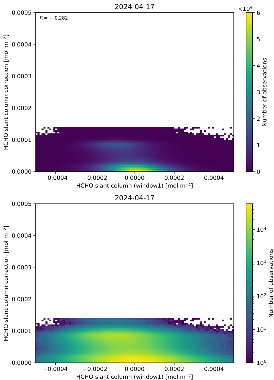
Figure 83: Scatter density plot of “HCHO slant column (window1)” against “HCHO slant column correction” for 2024-04-16 to 2024-04-18.
