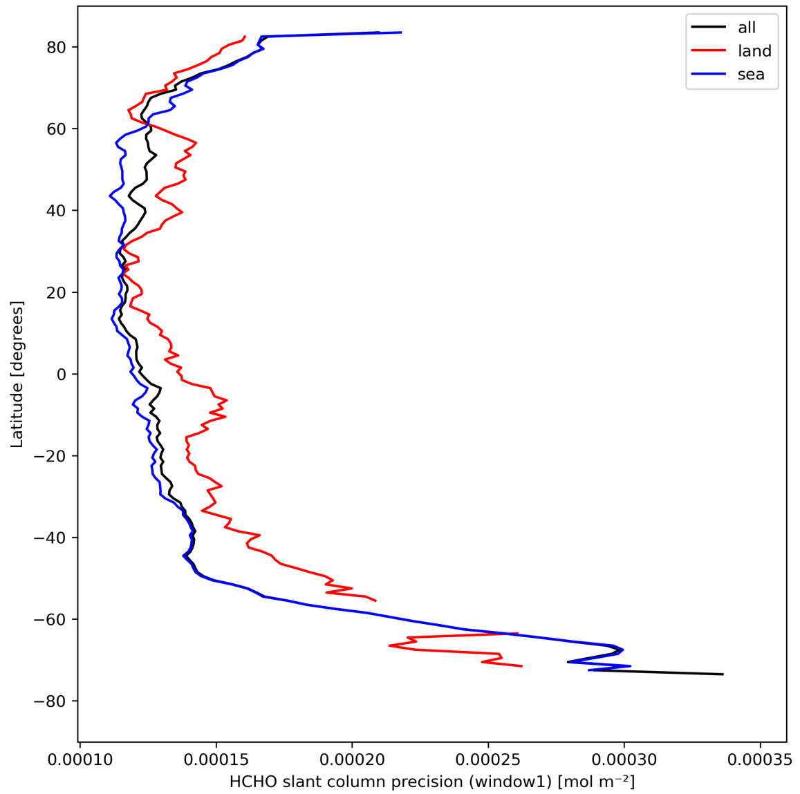
Figure 25: Zonal average of “HCHO slant column precision (window1)” for 2024-04-16 to 2024-04-18.
