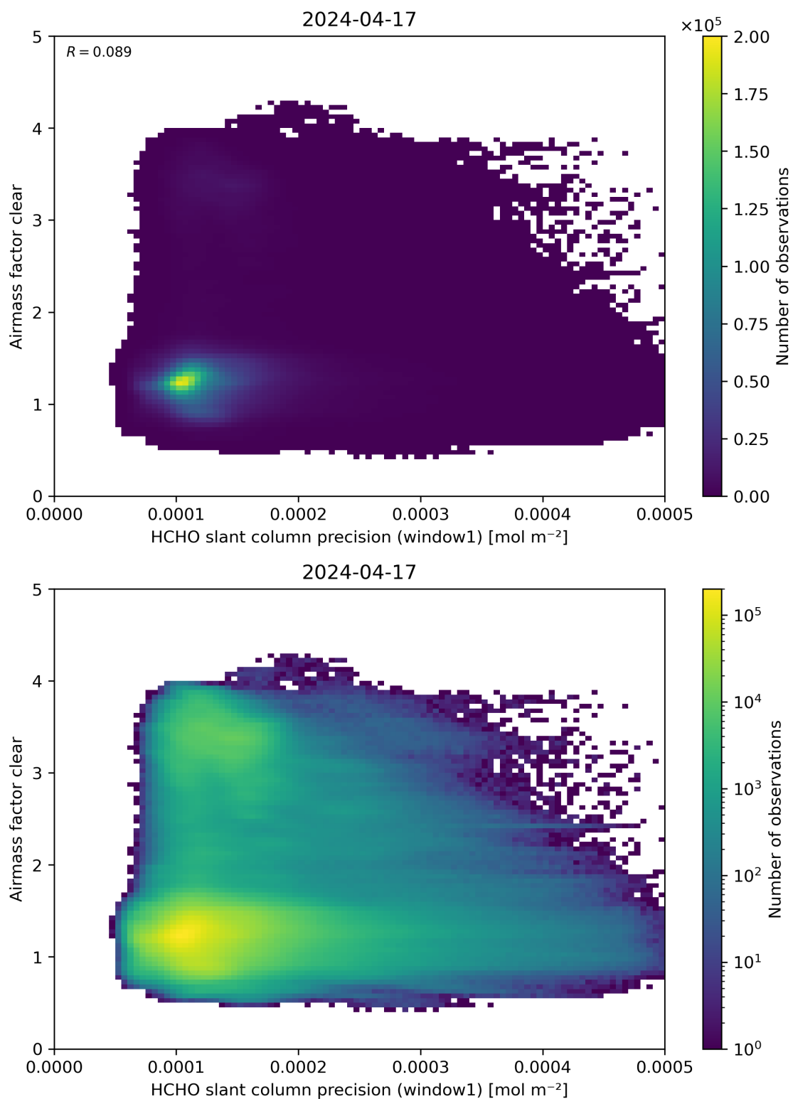
Figure 91: Scatter density plot of “HCHO slant column precision (window1)” against “Airmass factor clear” for 2024-04-16 to 2024-04-18.
