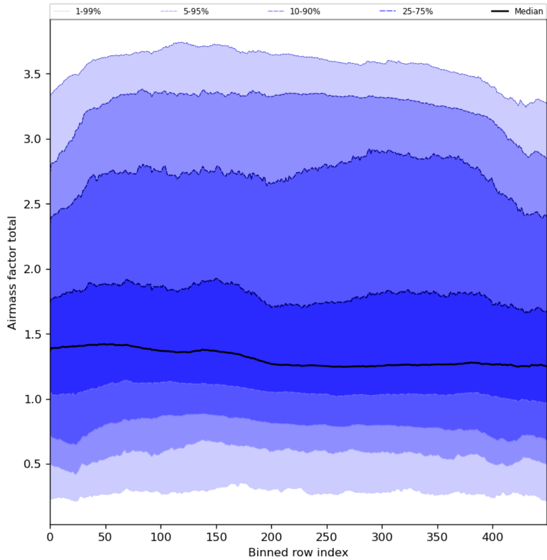
Figure 54: Along track statistics of “Airmass factor total” for 2024-04-16 to 2024-04-18
