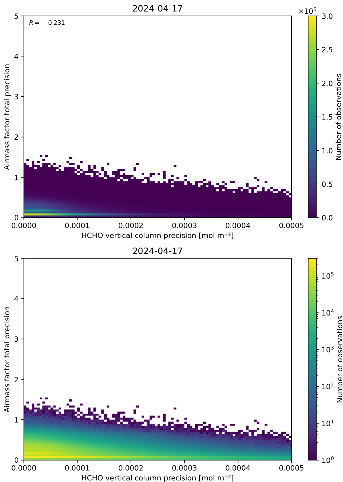
Figure 145: Scatter density plot of “HCHO vertical column precision” against “Airmass factor total precision” for 2024-04-16 to 2024-04-18.
