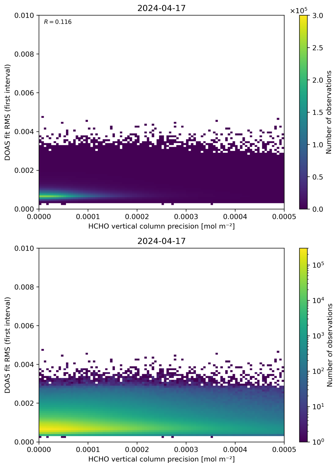
Figure 136: Scatter density plot of “HCHO vertical column precision” against “DOAS fit RMS (first interval)” for 2024-04-16 to 2024-04-18.
