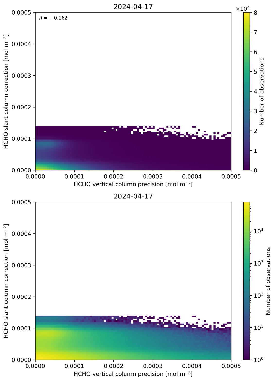
Figure 141: Scatter density plot of “HCHO vertical column precision” against “HCHO slant column correction” for 2024-04-16 to 2024-04-18.
