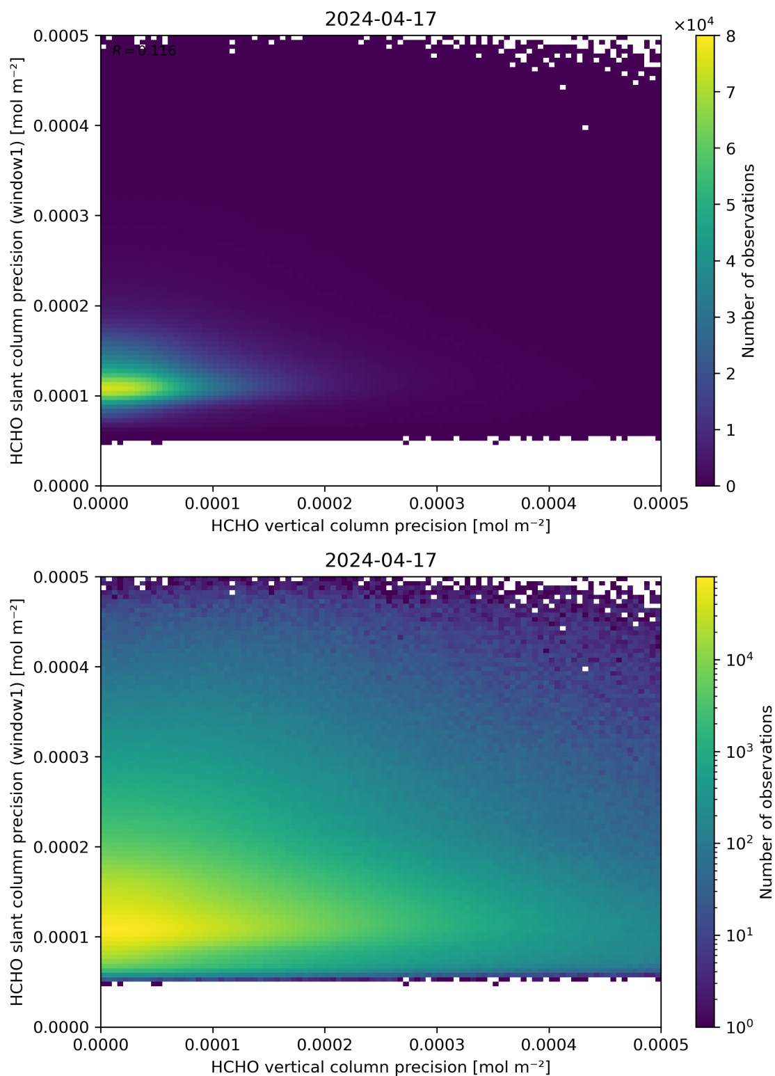
Figure 143: Scatter density plot of “HCHO vertical column precision” against “HCHO slant column precision (window1)” for 2024-04-16 to 2024-04-18.
