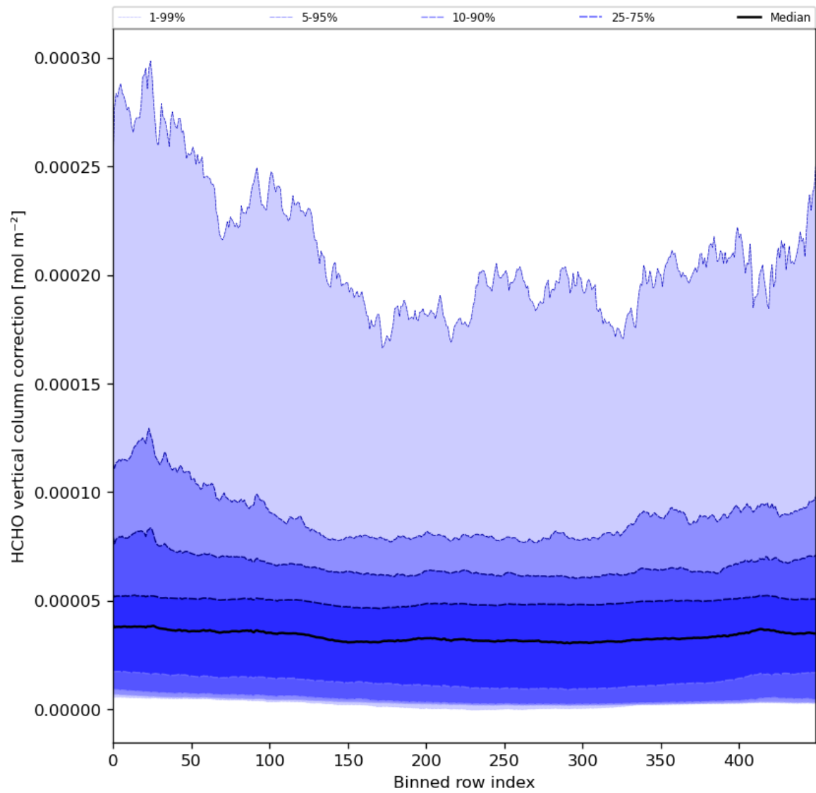
Figure 51: Along track statistics of “HCHO vertical column correction” for 2024-04-16 to 2024-04-18
