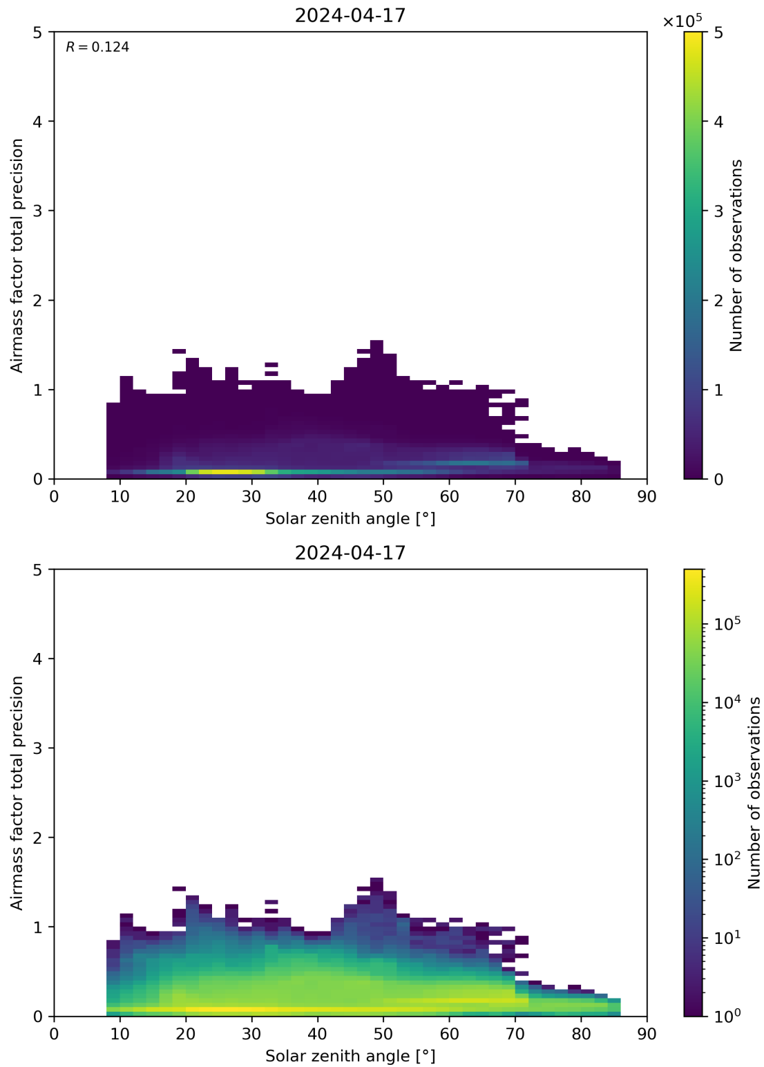
Figure 176: Scatter density plot of “Solar zenith angle” against “Airmass factor total precision” for 2024-04-16 to 2024-04-18.
