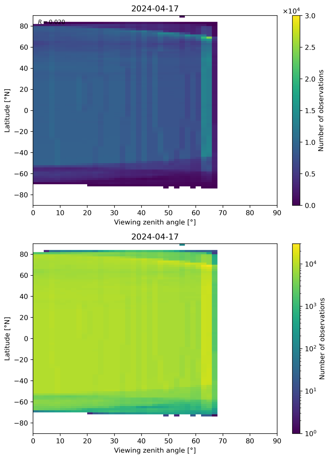
Figure 196: Scatter density plot of “Viewing zenith angle” against “Latitude” for 2024-04-16 to 2024-04-18.
