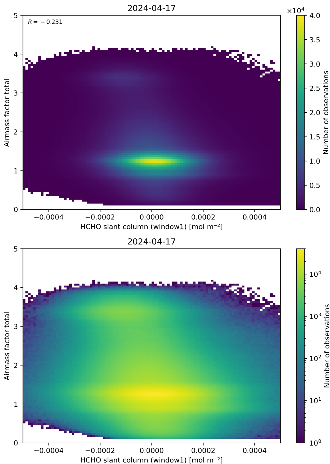
Figure 85: Scatter density plot of “HCHO slant column (window1)” against “Airmass factor total” for 2024-04-16 to 2024-04-18.
