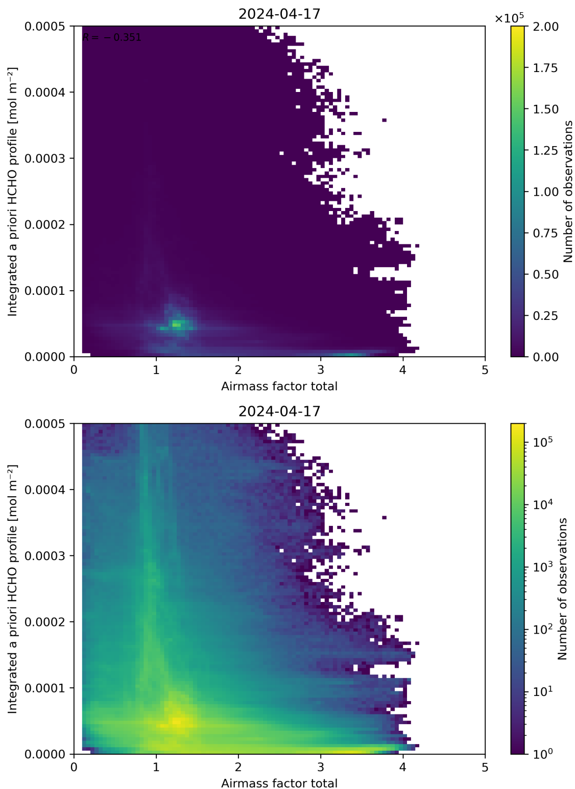
Figure 104: Scatter density plot of “Airmass factor total” against “Integrated a priori HCHO profile” for 2024-04-16 to 2024-04-18.
