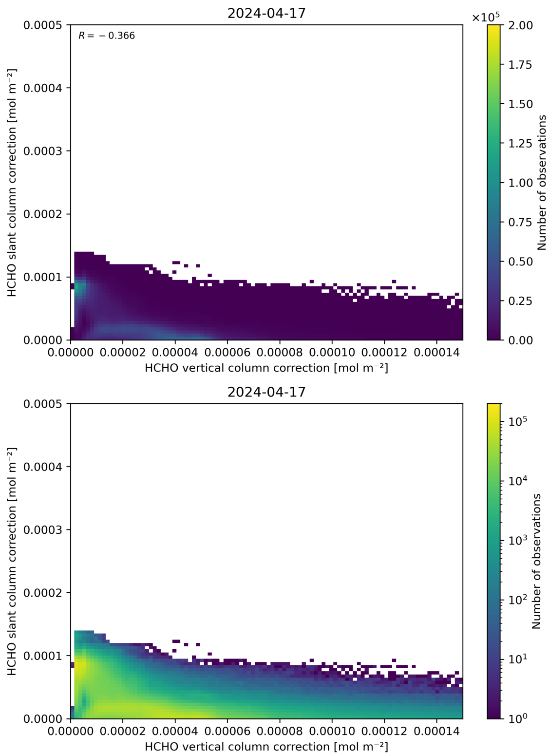
Figure 117: Scatter density plot of “HCHO vertical column correction” against “HCHO slant column correction” for 2024-04-16 to 2024-04-18.
