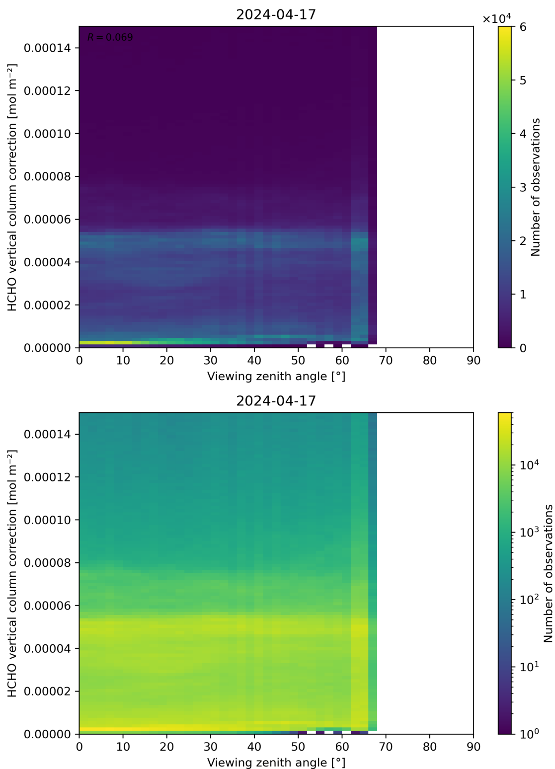
Figure 193: Scatter density plot of “Viewing zenith angle” against “HCHO vertical column correction” for 2024-04-16 to 2024-04-18.
