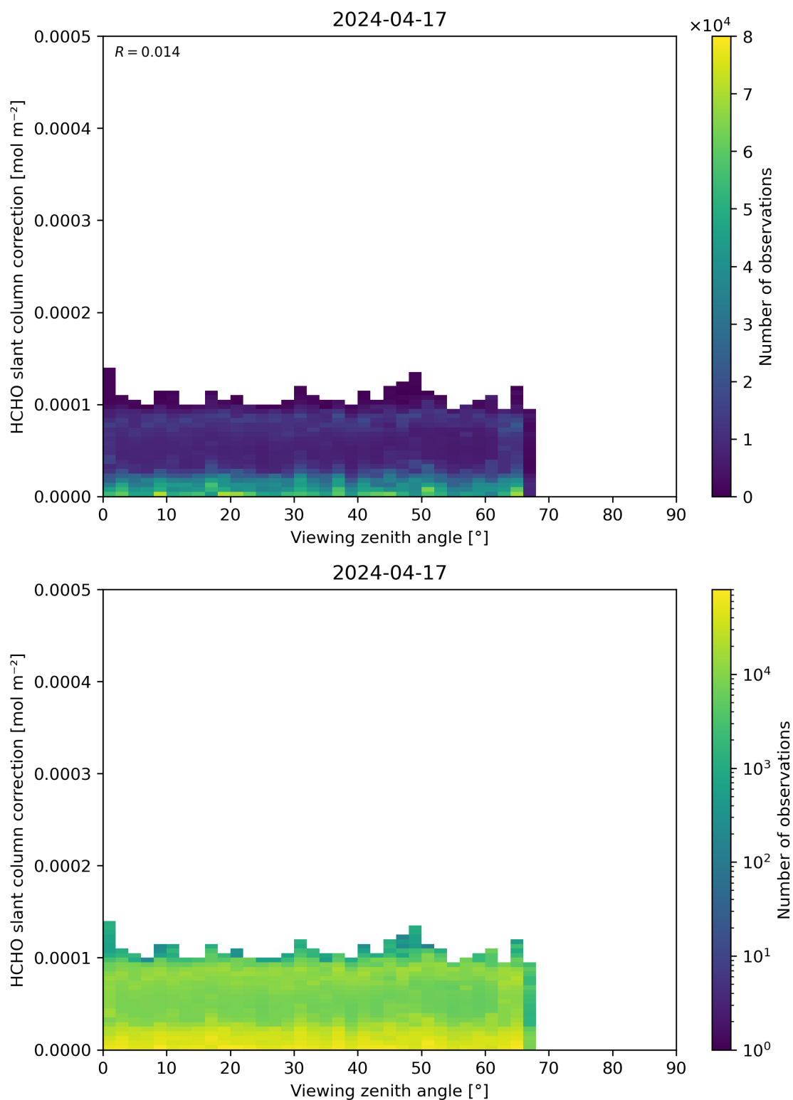
Figure 187: Scatter density plot of “Viewing zenith angle” against “HCHO slant column correction” for 2024-04-16 to 2024-04-18.
