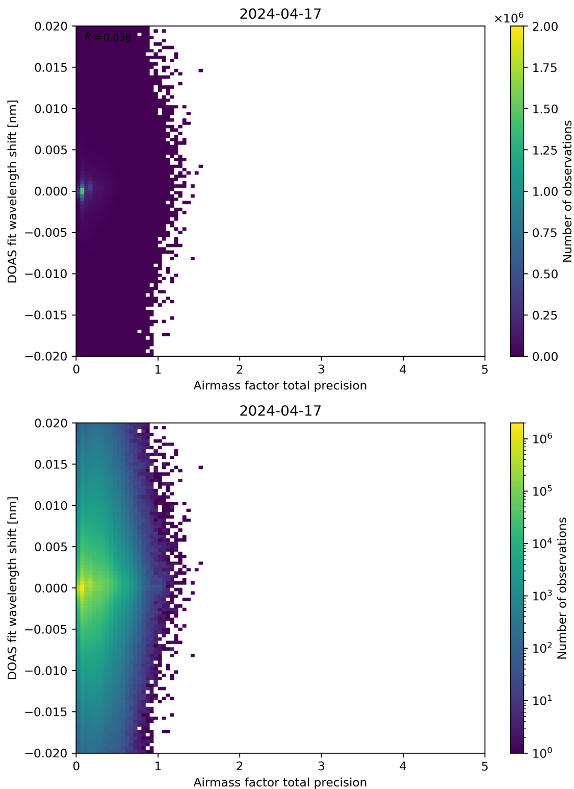
Figure 106: Scatter density plot of “Airmass factor total precision” against “DOAS fit wavelength shift” for 2024-04-16 to 2024-04-18.
