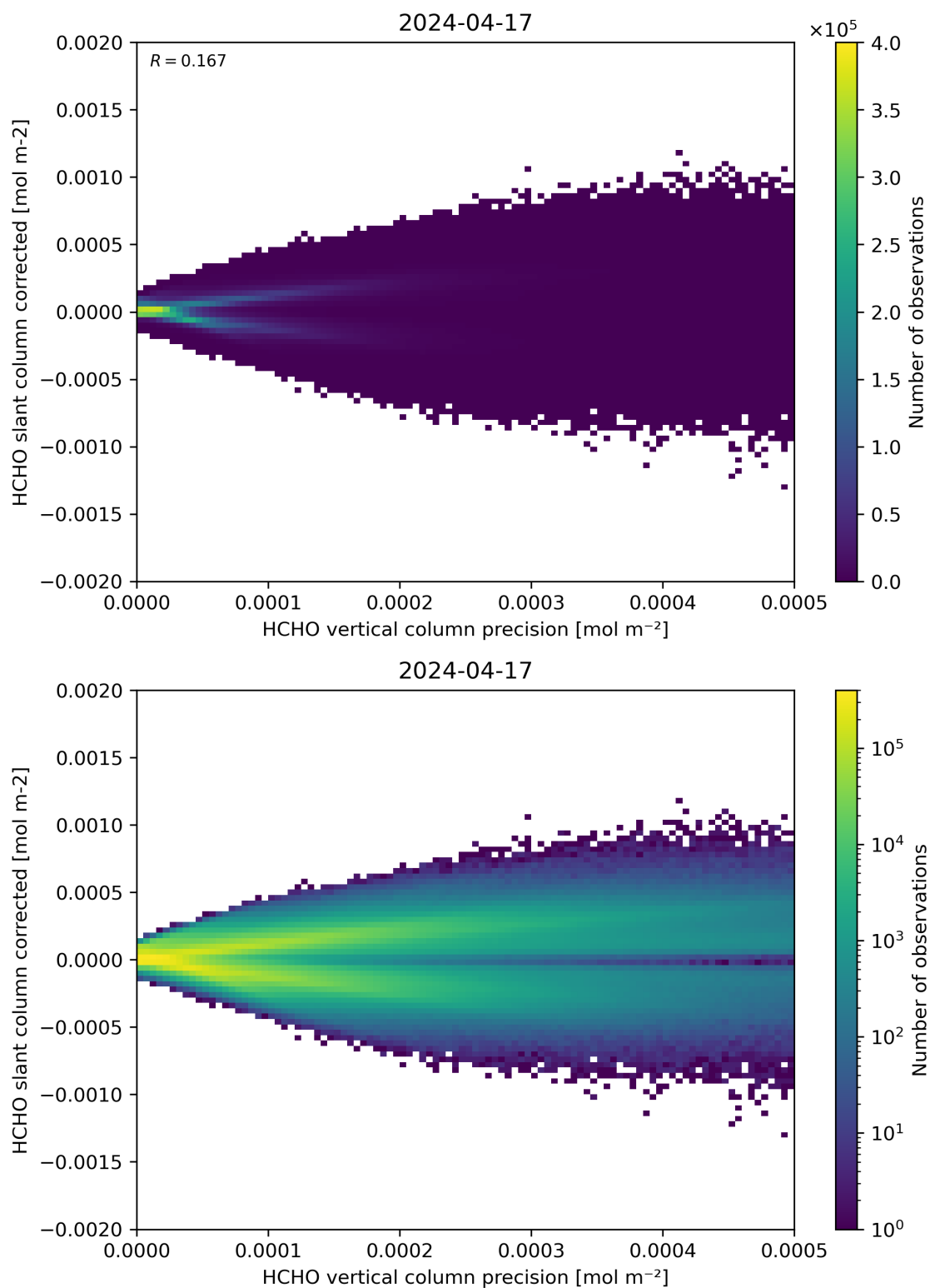
Figure 140: Scatter density plot of “HCHO vertical column precision” against “HCHO slant column corrected” for 2024-04-16 to 2024-04-18.
