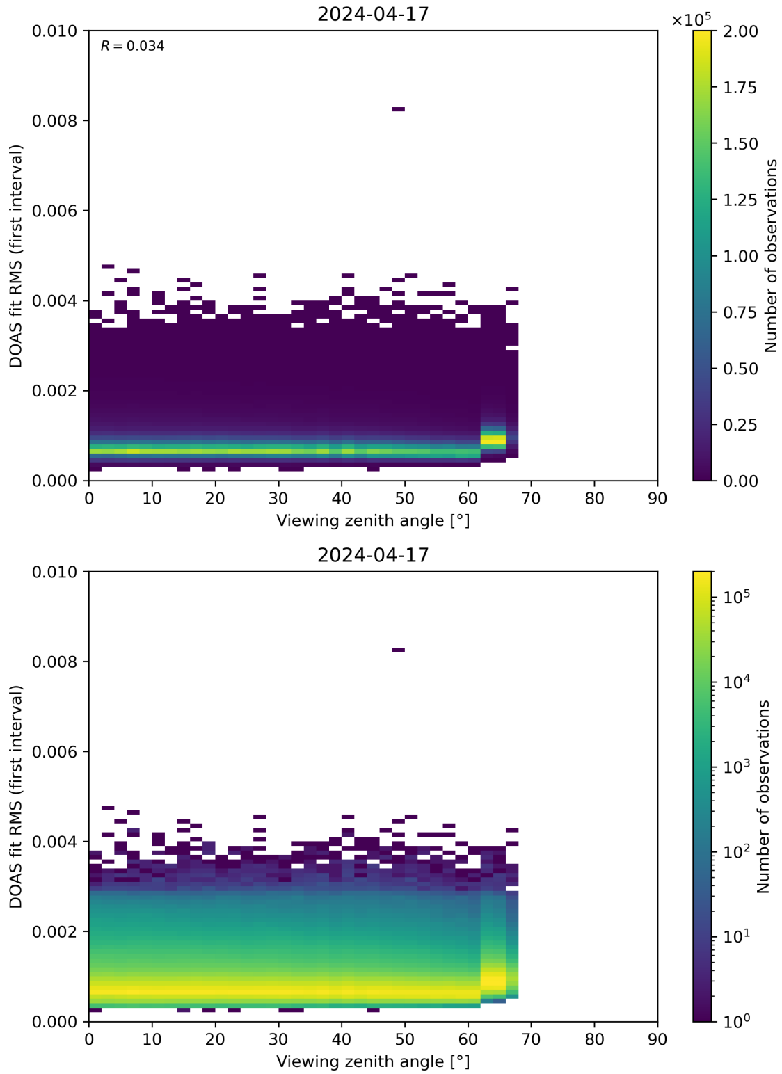
Figure 182: Scatter density plot of “Viewing zenith angle” against “DOAS fit RMS (first interval)” for 2024-04-16 to 2024-04-18.
