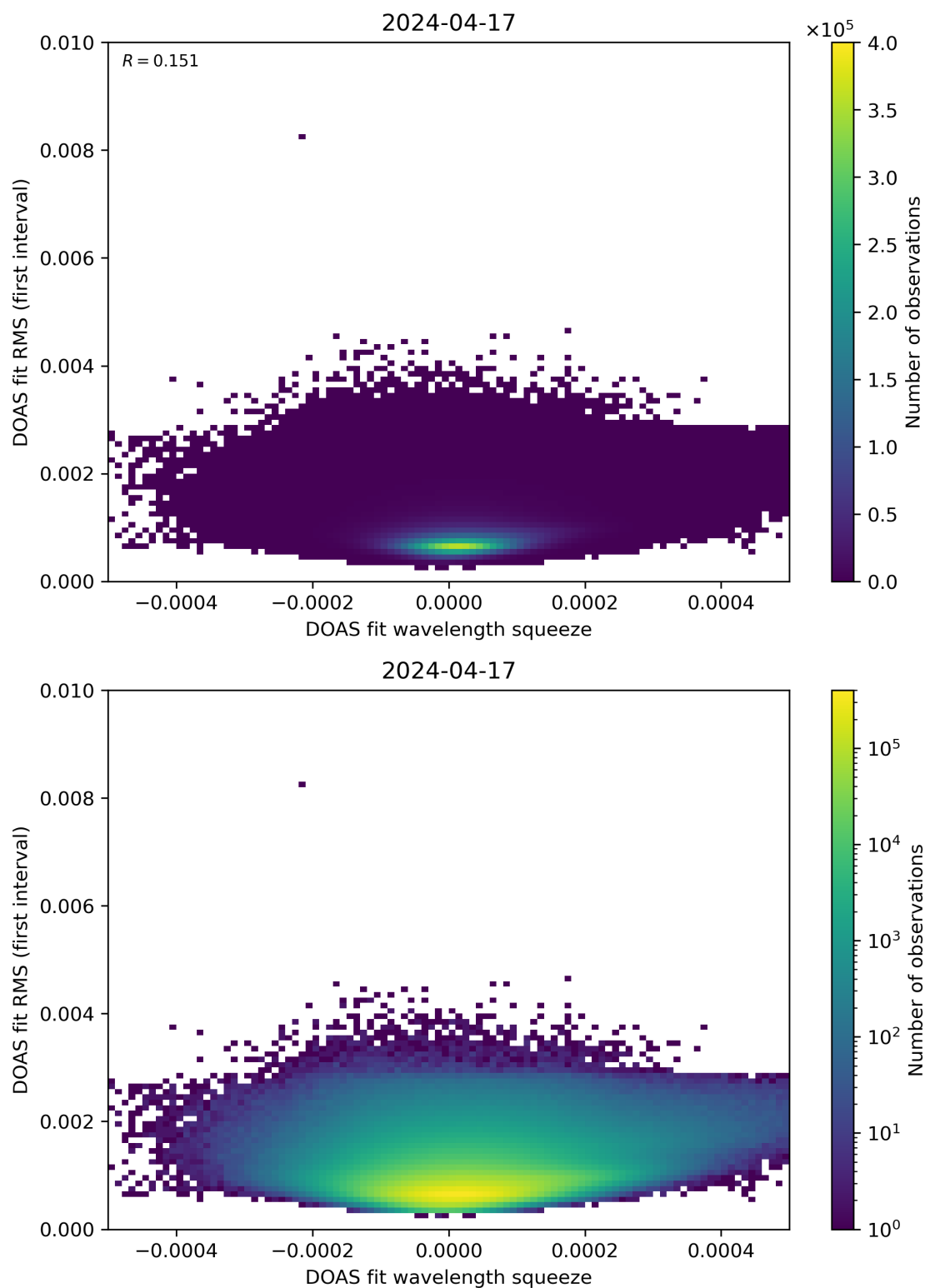
Figure 68: Scatter density plot of “DOAS fit wavelength squeeze” against “DOAS fit RMS (first interval)” for 2024-04-16 to 2024-04-18.
