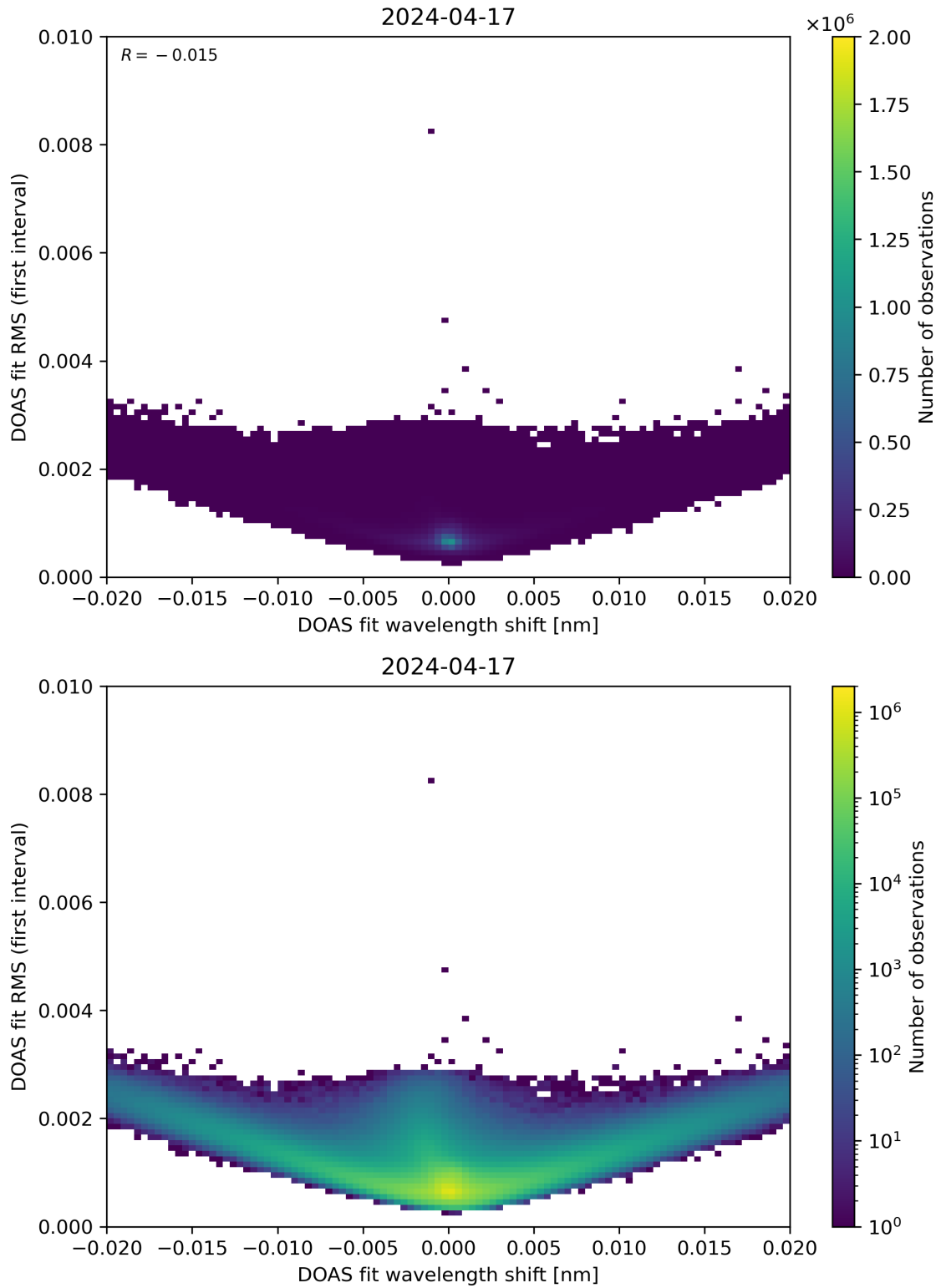
Figure 64: Scatter density plot of “DOAS fit wavelength shift” against “DOAS fit RMS (first interval)” for 2024-04-16 to 2024-04-18.
