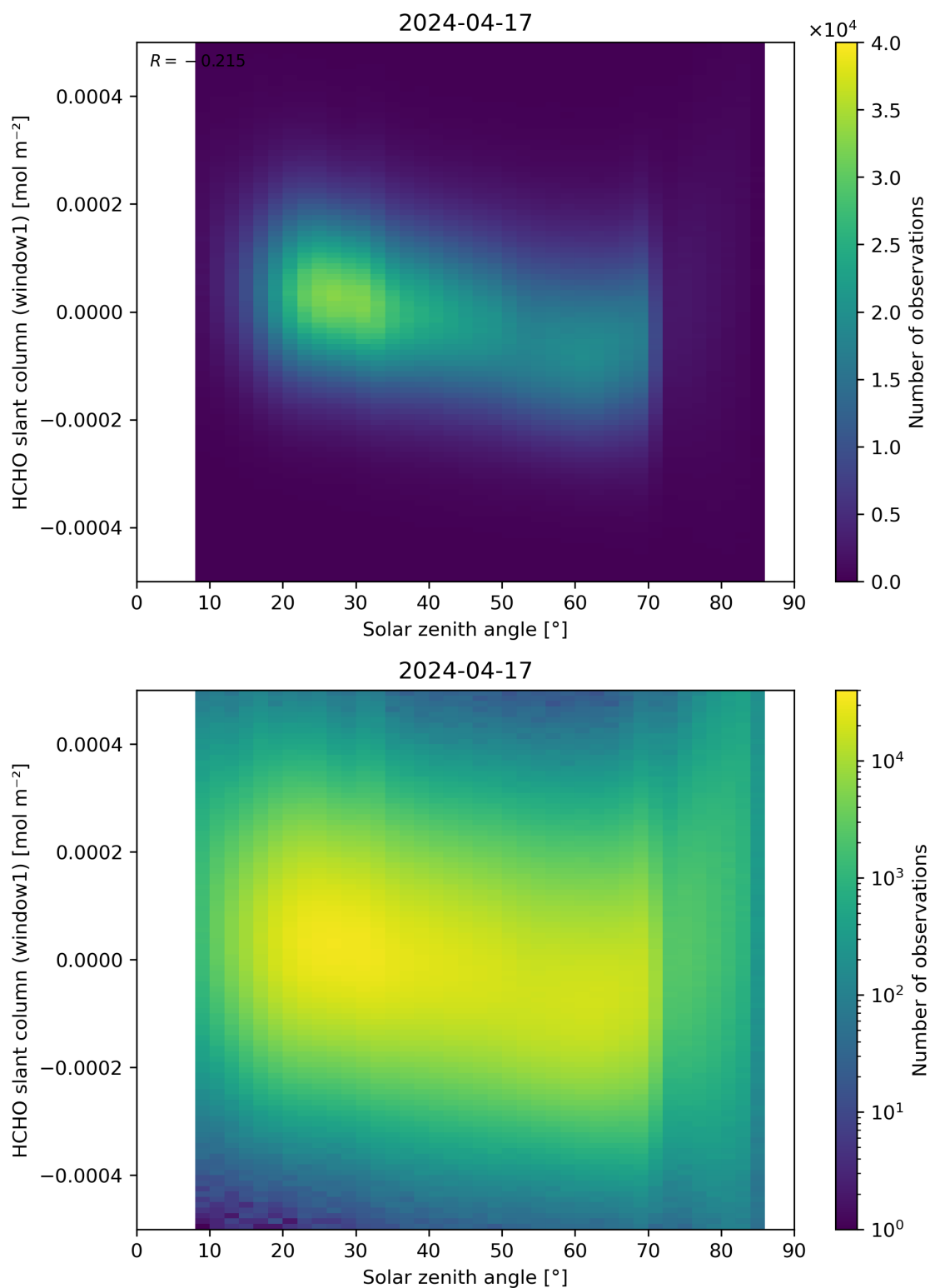
Figure 173: Scatter density plot of “Solar zenith angle” against “HCHO slant column (window1)” for 2024-04-16 to 2024-04-18.
