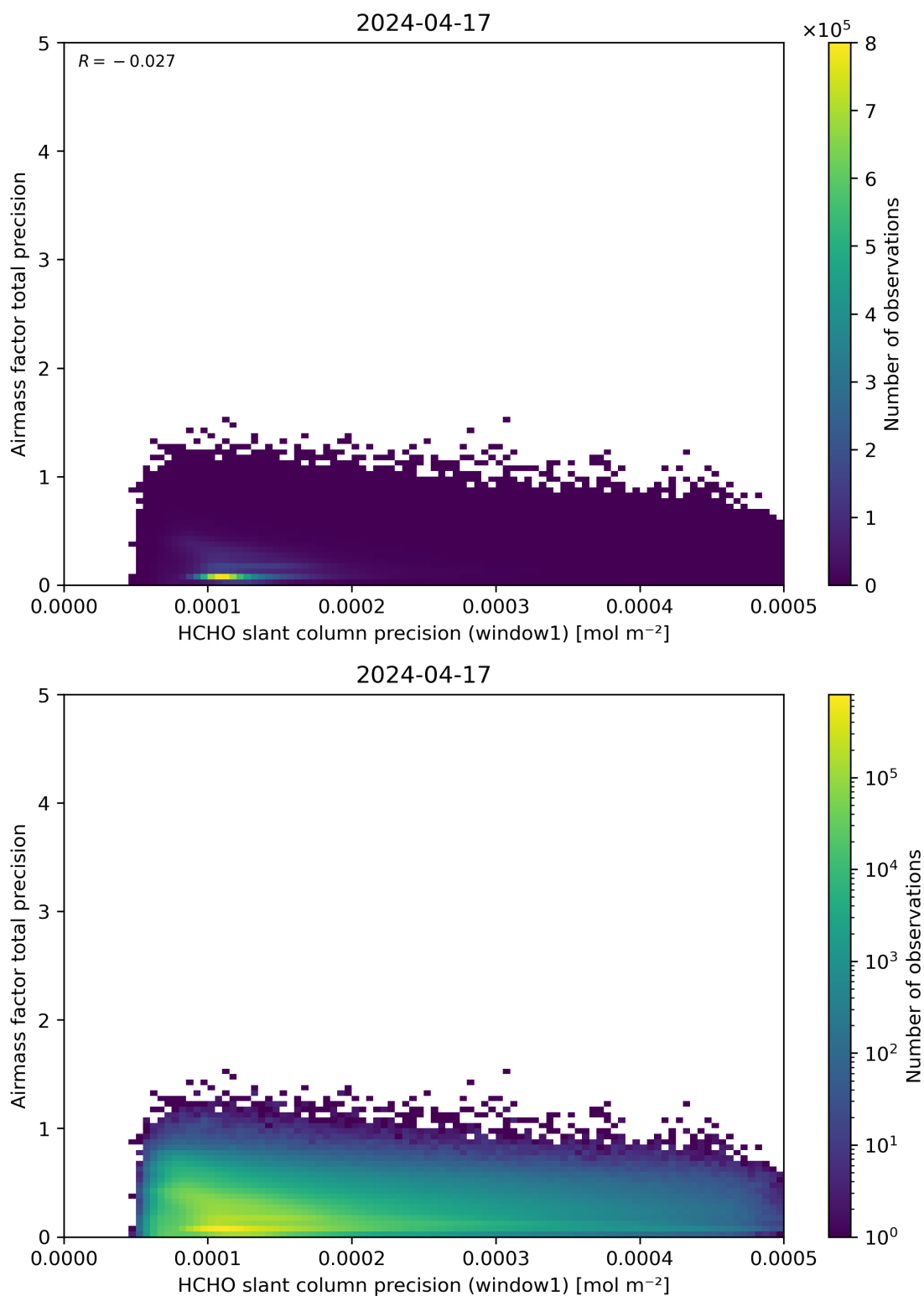
Figure 95: Scatter density plot of “HCHO slant column precision (window1)” against “Airmass factor total precision” for 2024-04-16 to 2024-04-18.
