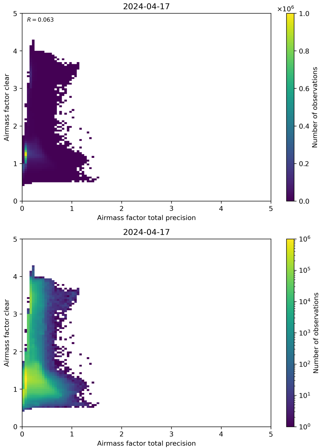
Figure 108: Scatter density plot of “Airmass factor total precision” against “Airmass factor clear” for 2024-04-16 to 2024-04-18.
