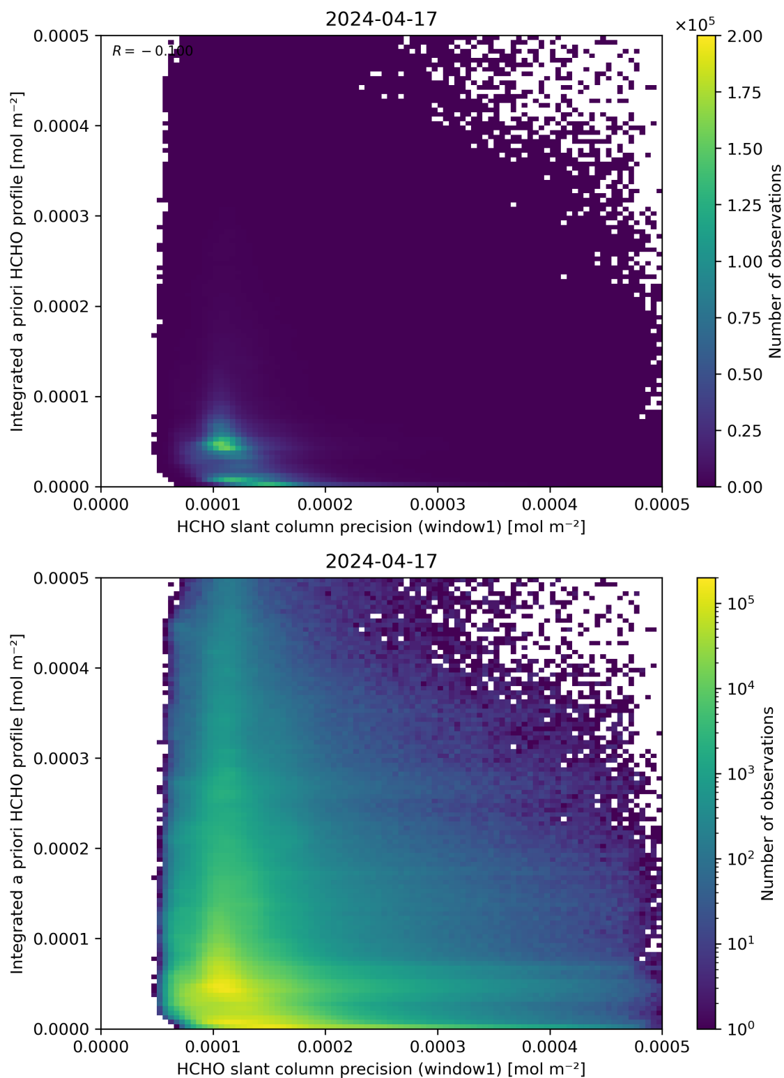
Figure 96: Scatter density plot of “HCHO slant column precision (window1)” against “Integrated a priori HCHO profile” for 2024-04-16 to 2024-04-18.
