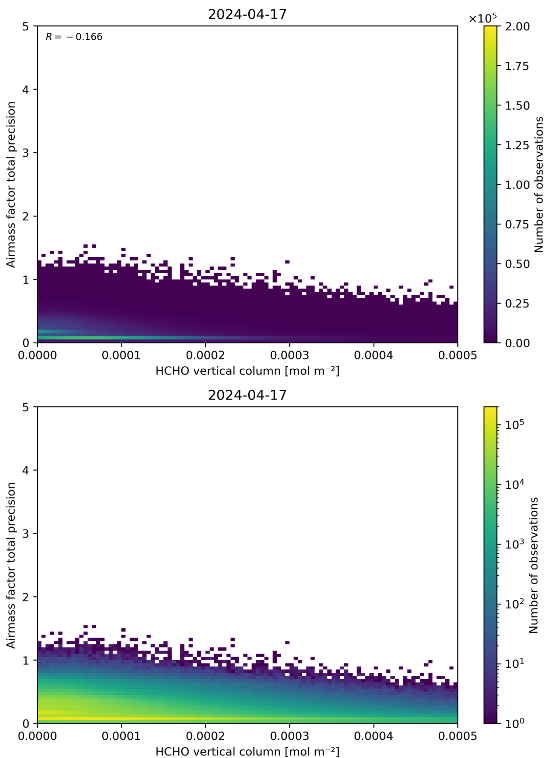
Figure 132: Scatter density plot of “HCHO vertical column” against “Airmass factor total precision” for 2024-04-16 to 2024-04-18.
