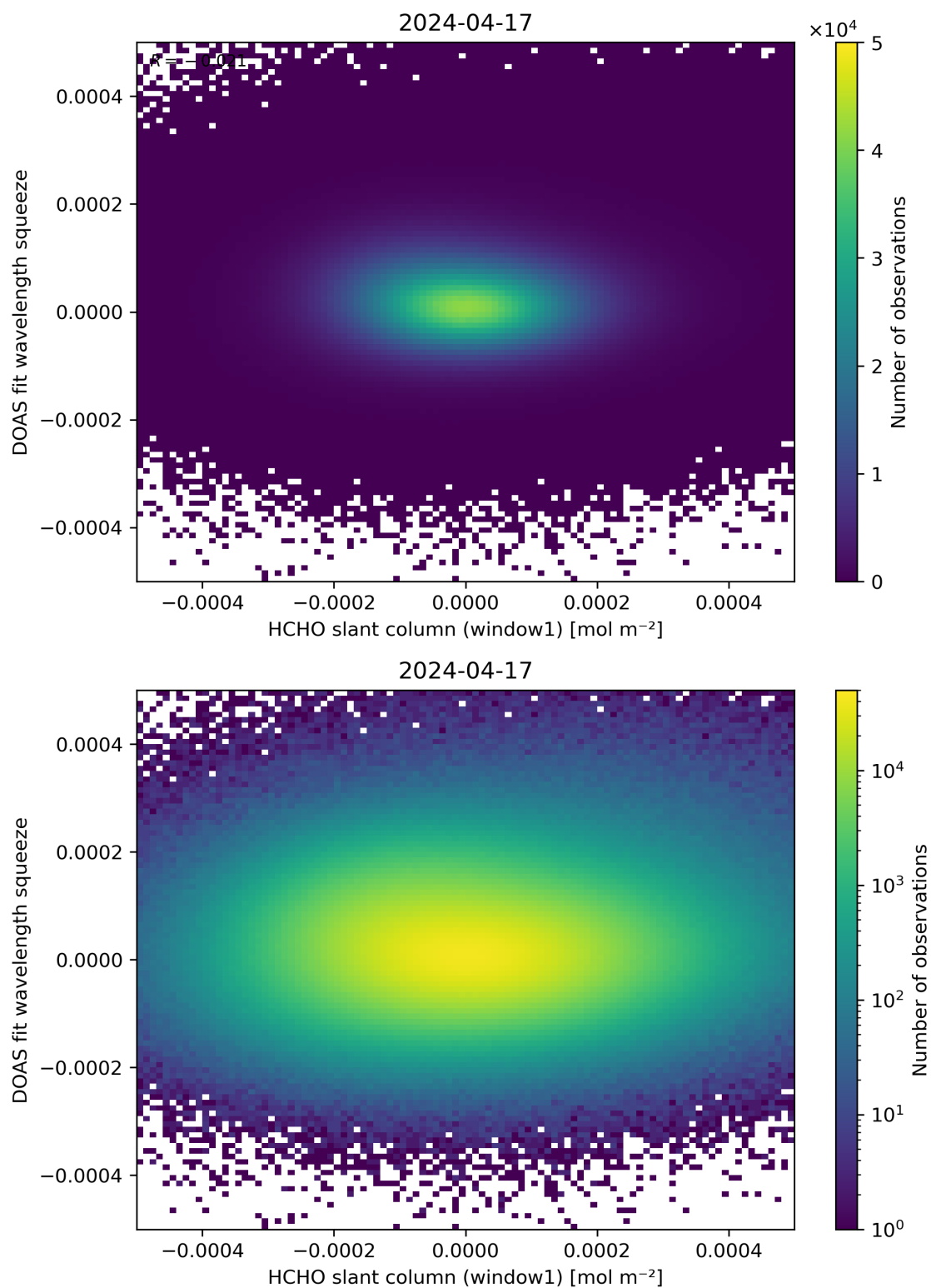
Figure 80: Scatter density plot of “HCHO slant column (window1)” against “DOAS fit wavelength squeeze” for 2024-04-16 to 2024-04-18.
