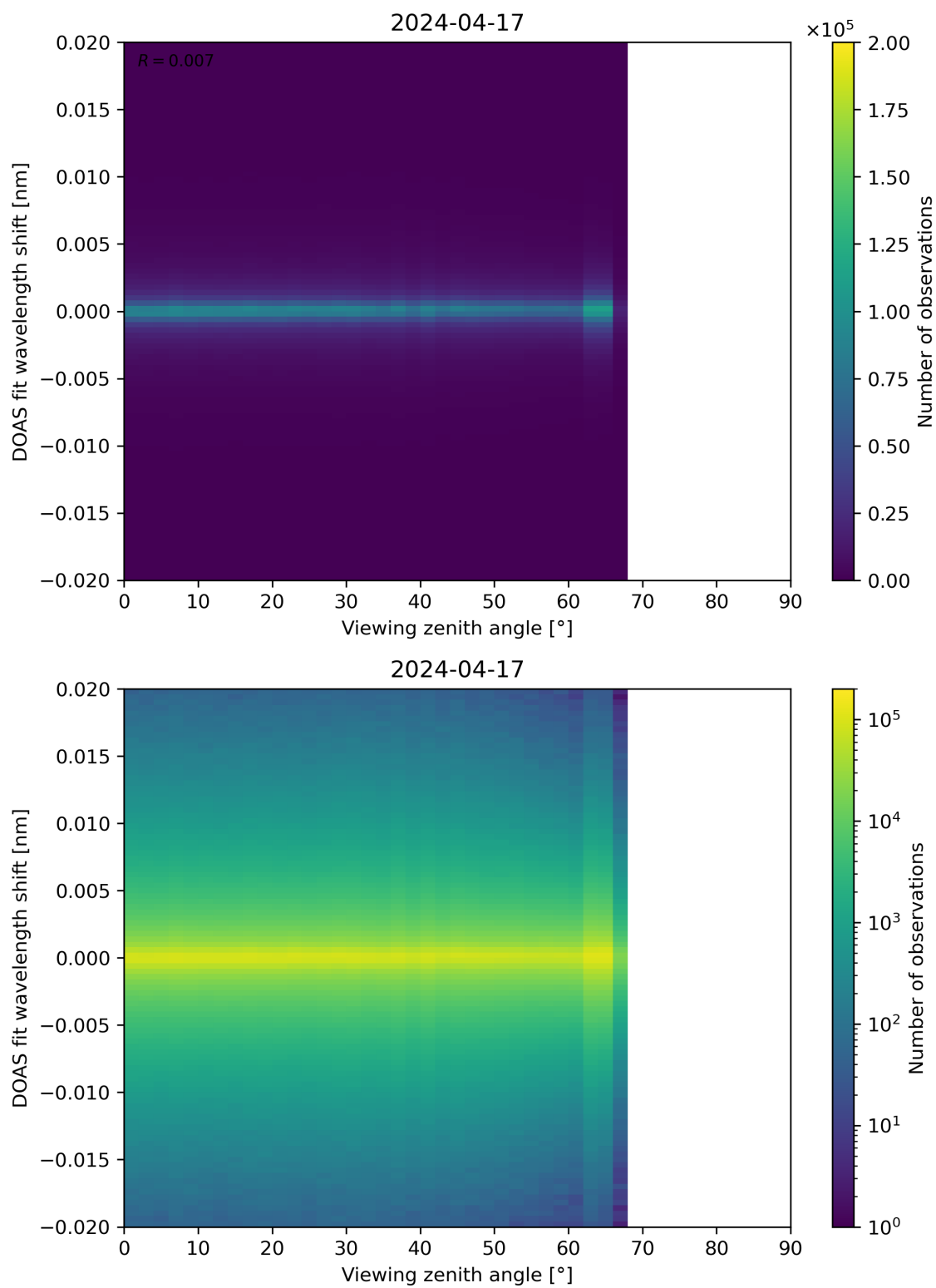
Figure 183: Scatter density plot of “Viewing zenith angle” against “DOAS fit wavelength shift” for 2024-04-16 to 2024-04-18.
