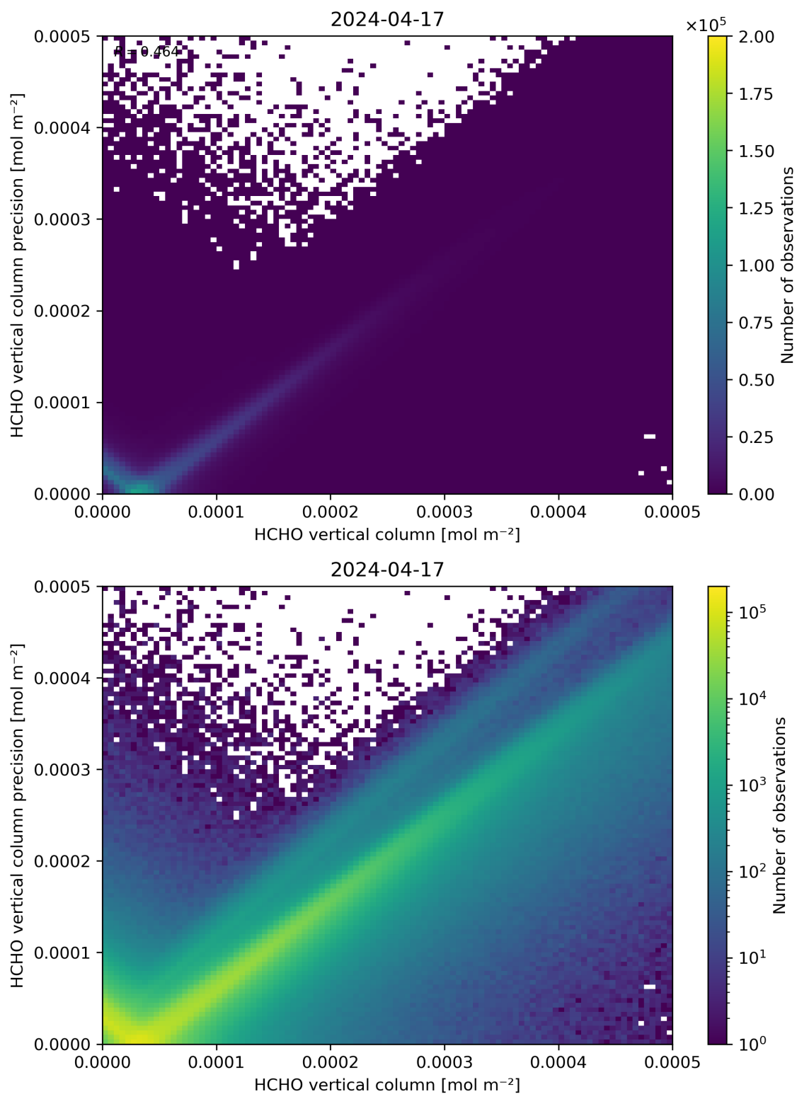
Figure 134: Scatter density plot of “HCHO vertical column” against “HCHO vertical column precision” for 2024-04-16 to 2024-04-18.
