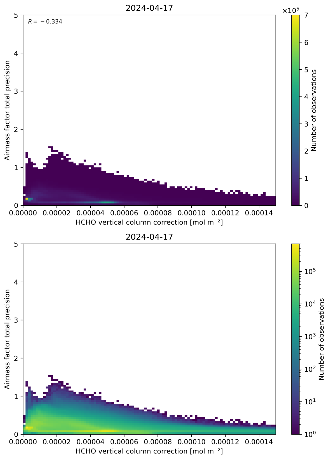
Figure 121: Scatter density plot of “HCHO vertical column correction” against “Airmass factor total precision” for 2024-04-16 to 2024-04-18.
