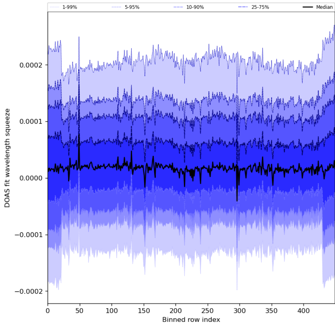
Figure 59: Along track statistics of “DOAS fit wavelength squeeze” for 2024-04-16 to 2024-04-18
