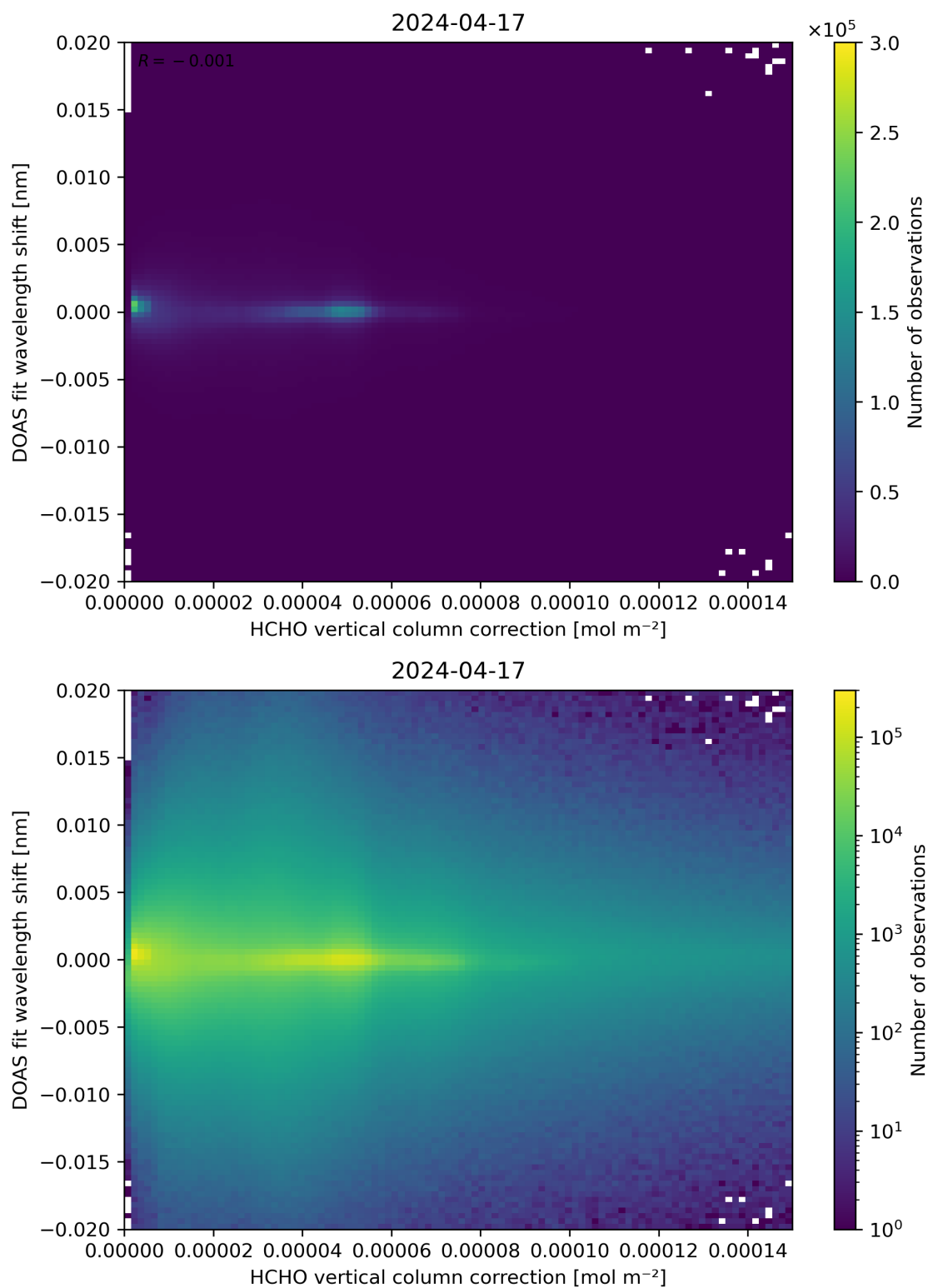
Figure 113: Scatter density plot of “HCHO vertical column correction” against “DOAS fit wavelength shift” for 2024-04-16 to 2024-04-18.
