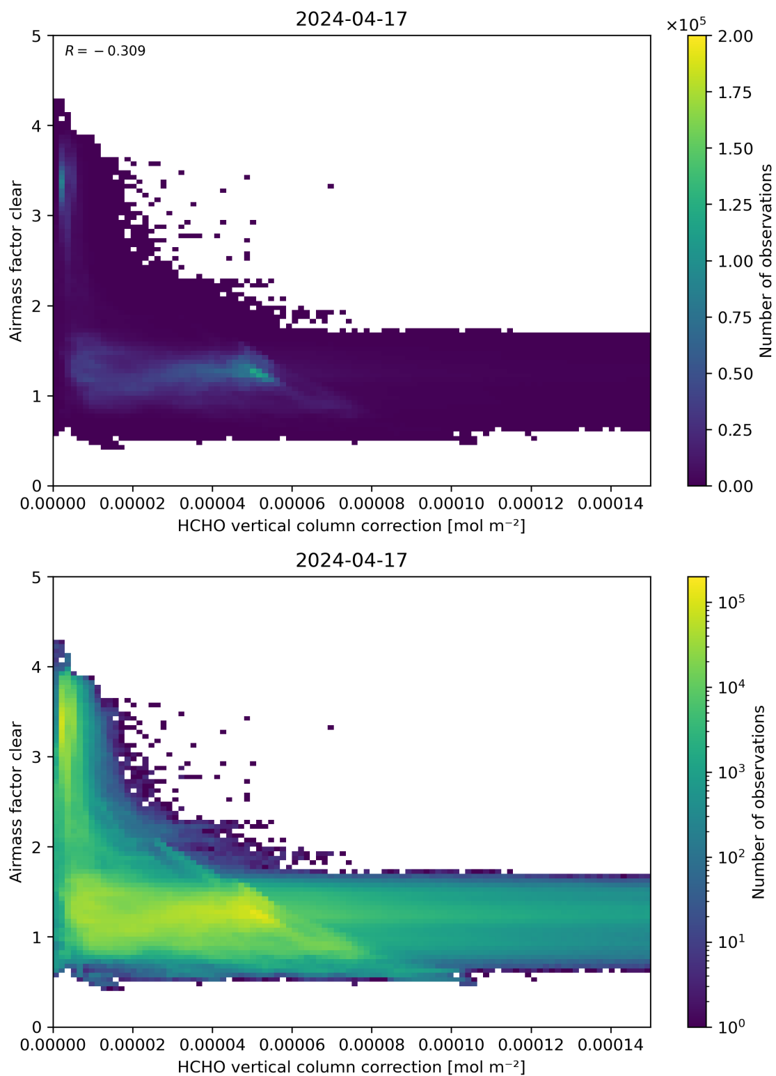
Figure 115: Scatter density plot of “HCHO vertical column correction” against “Airmass factor clear” for 2024-04-16 to 2024-04-18.
