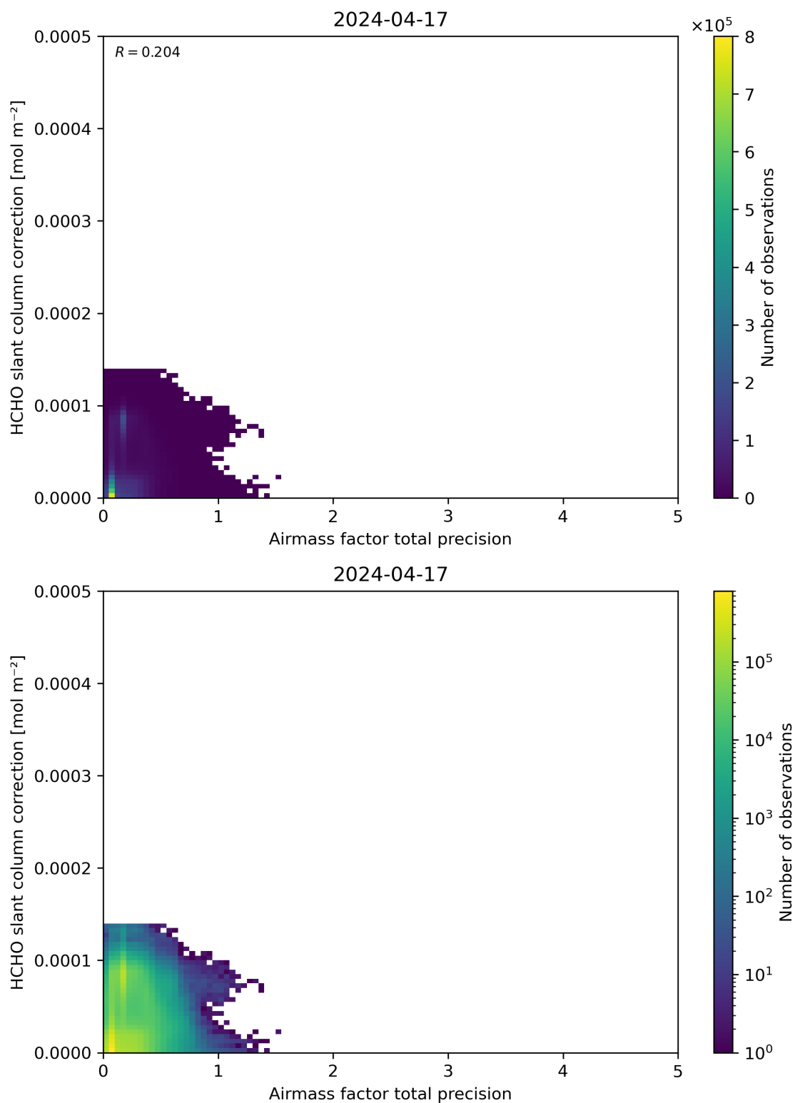
Figure 110: Scatter density plot of “Airmass factor total precision” against “HCHO slant column correction” for 2024-04-16 to 2024-04-18.
