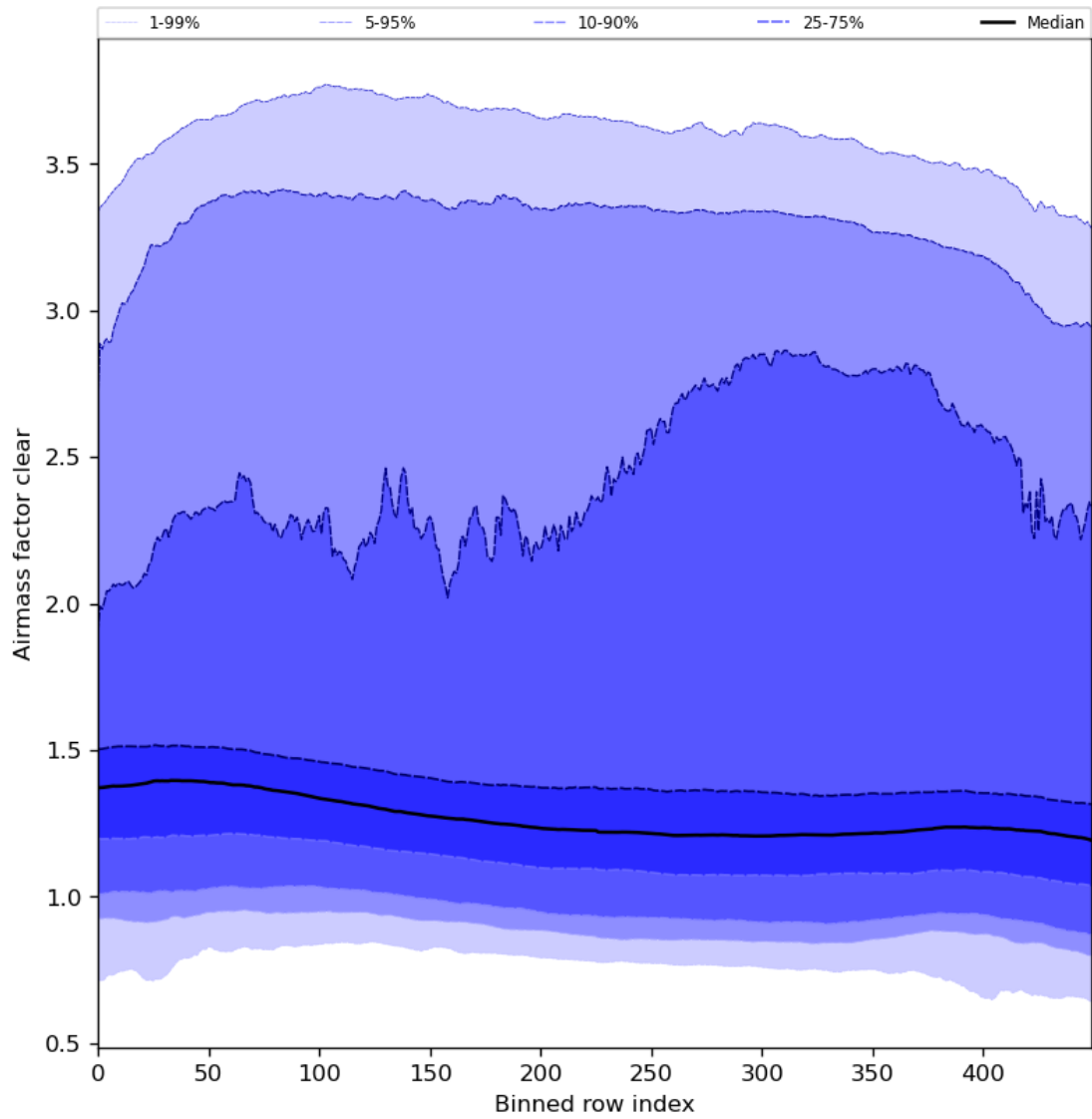
Figure 56: Along track statistics of “Airmass factor clear” for 2024-04-16 to 2024-04-18
