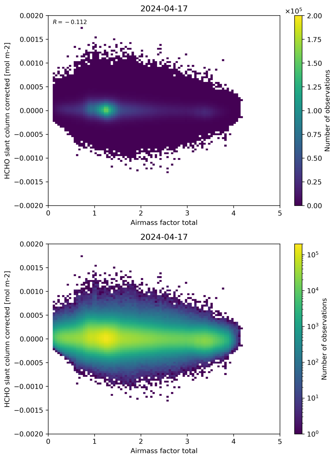
Figure 101: Scatter density plot of “Airmass factor total” against “HCHO slant column corrected” for 2024-04-16 to 2024-04-18.
