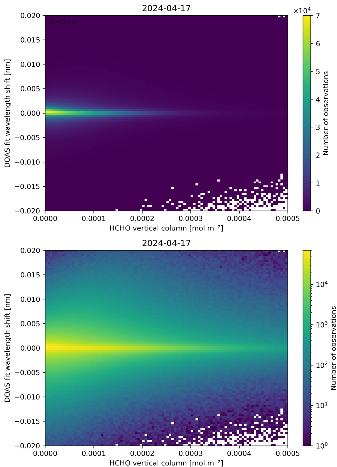
Figure 124: Scatter density plot of “HCHO vertical column” against “DOAS fit wavelength shift” for 2024-04-16 to 2024-04-18.
