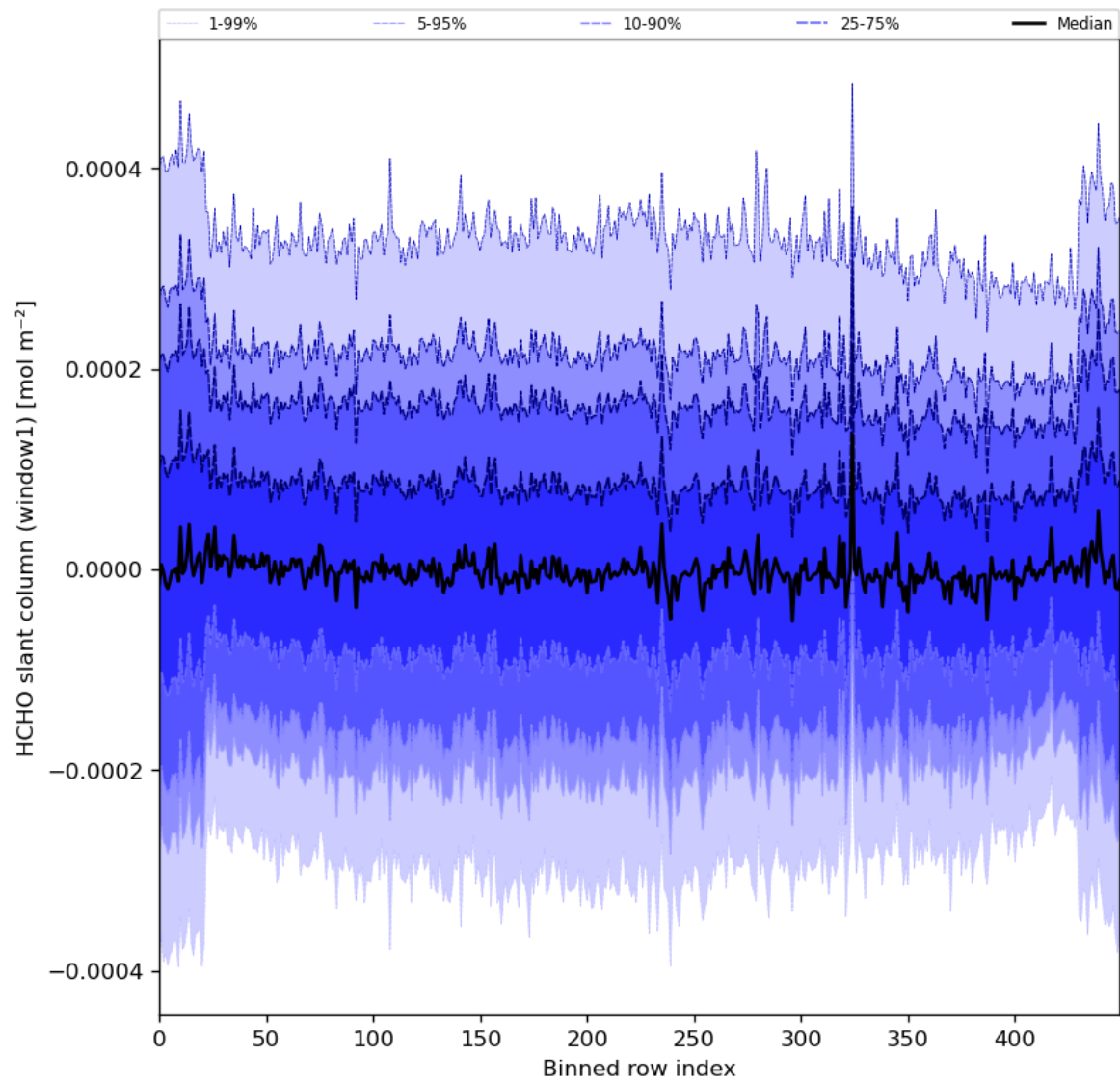
Figure 52: Along track statistics of “HCHO slant column (window1)” for 2024-04-16 to 2024-04-18
