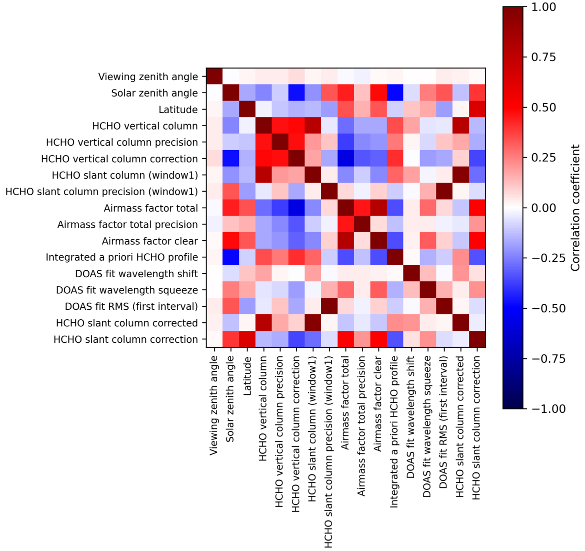
Figure 2: Map of correlation matrix for 2024-04-16 to 2024-04-18.
