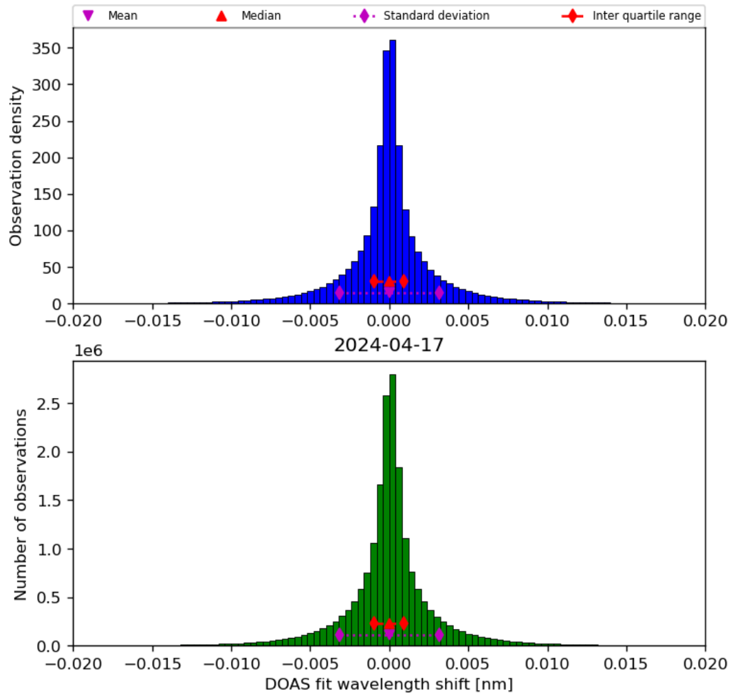
Figure 44: Histogram of “DOAS fit wavelength shift” for 2024-04-16 to 2024-04-18
