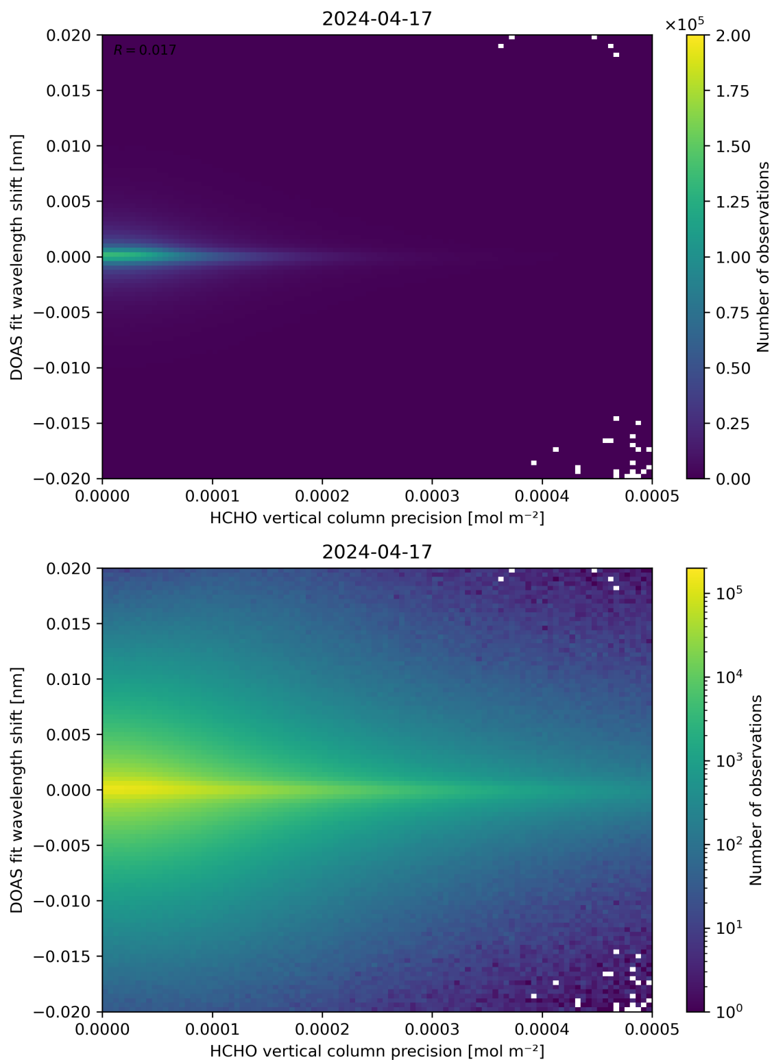
Figure 137: Scatter density plot of “HCHO vertical column precision” against “DOAS fit wavelength shift” for 2024-04-16 to 2024-04-18.
