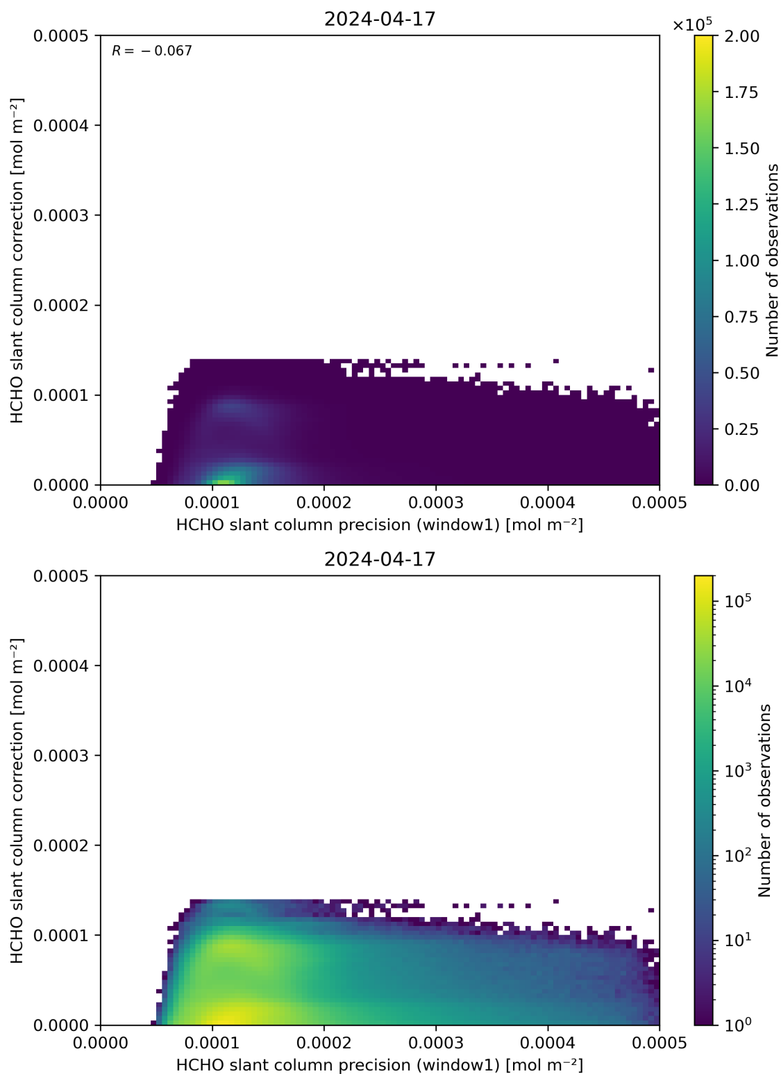
Figure 93: Scatter density plot of “HCHO slant column precision (window1)” against “HCHO slant column correction” for 2024-04-16 to 2024-04-18.
