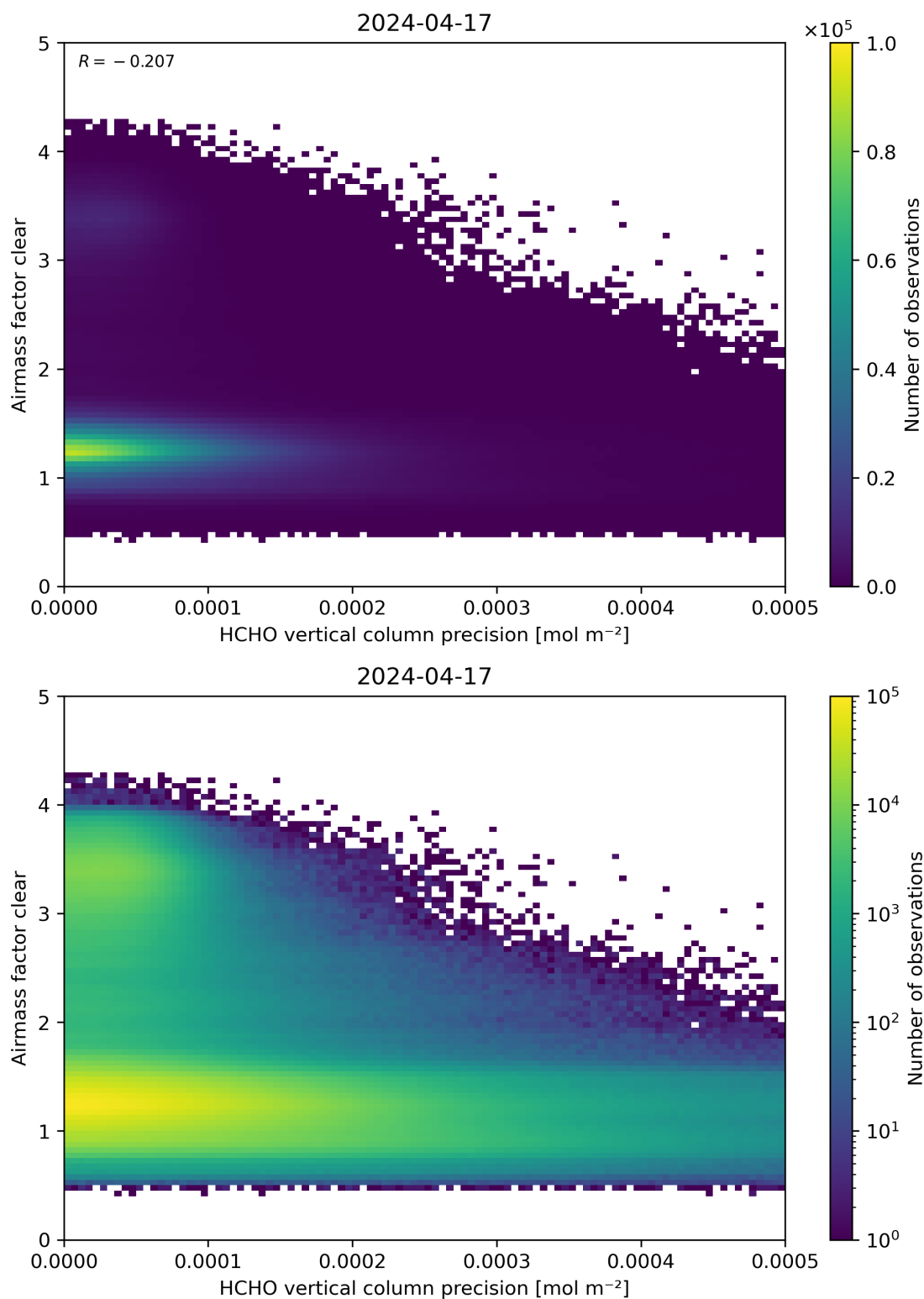
Figure 139: Scatter density plot of “HCHO vertical column precision” against “Airmass factor clear” for 2024-04-16 to 2024-04-18.
