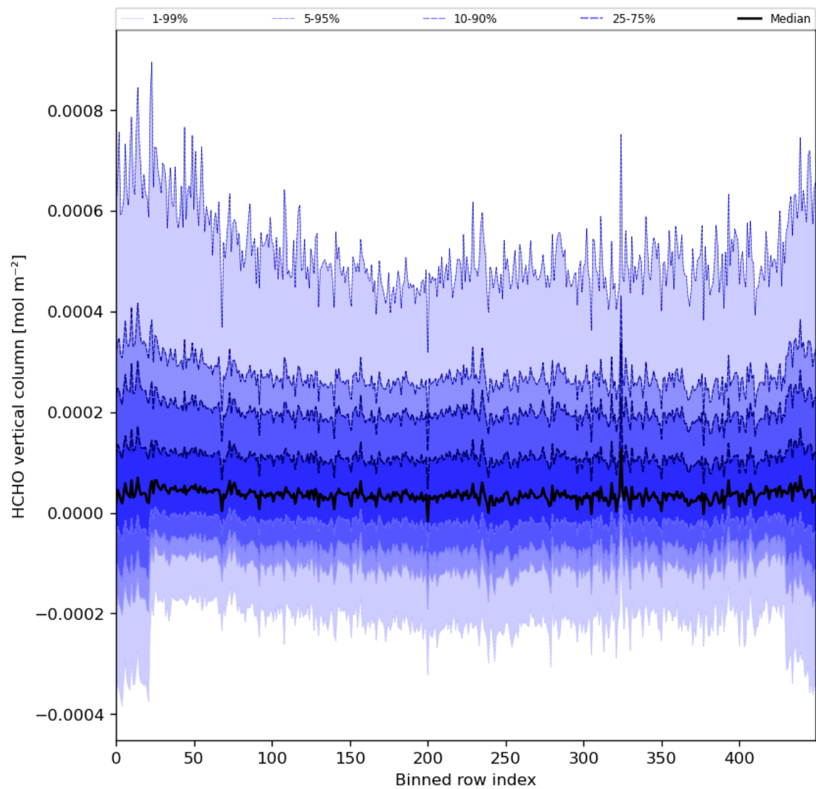
Figure 49: Along track statistics of “HCHO vertical column” for 2024-04-16 to 2024-04-18
