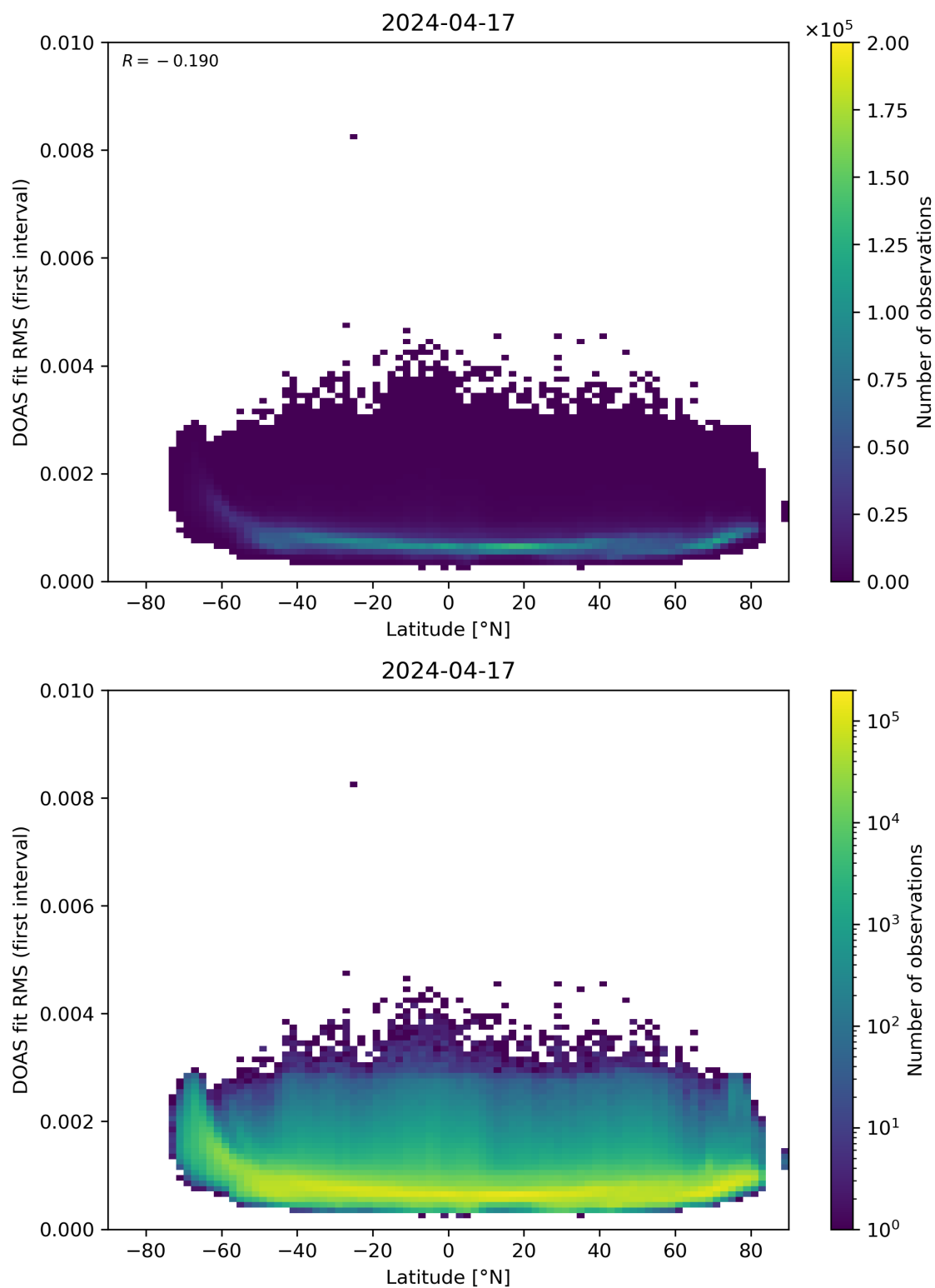
Figure 153: Scatter density plot of “Latitude” against “DOAS fit RMS (first interval)” for 2024-04-16 to 2024-04-18.
