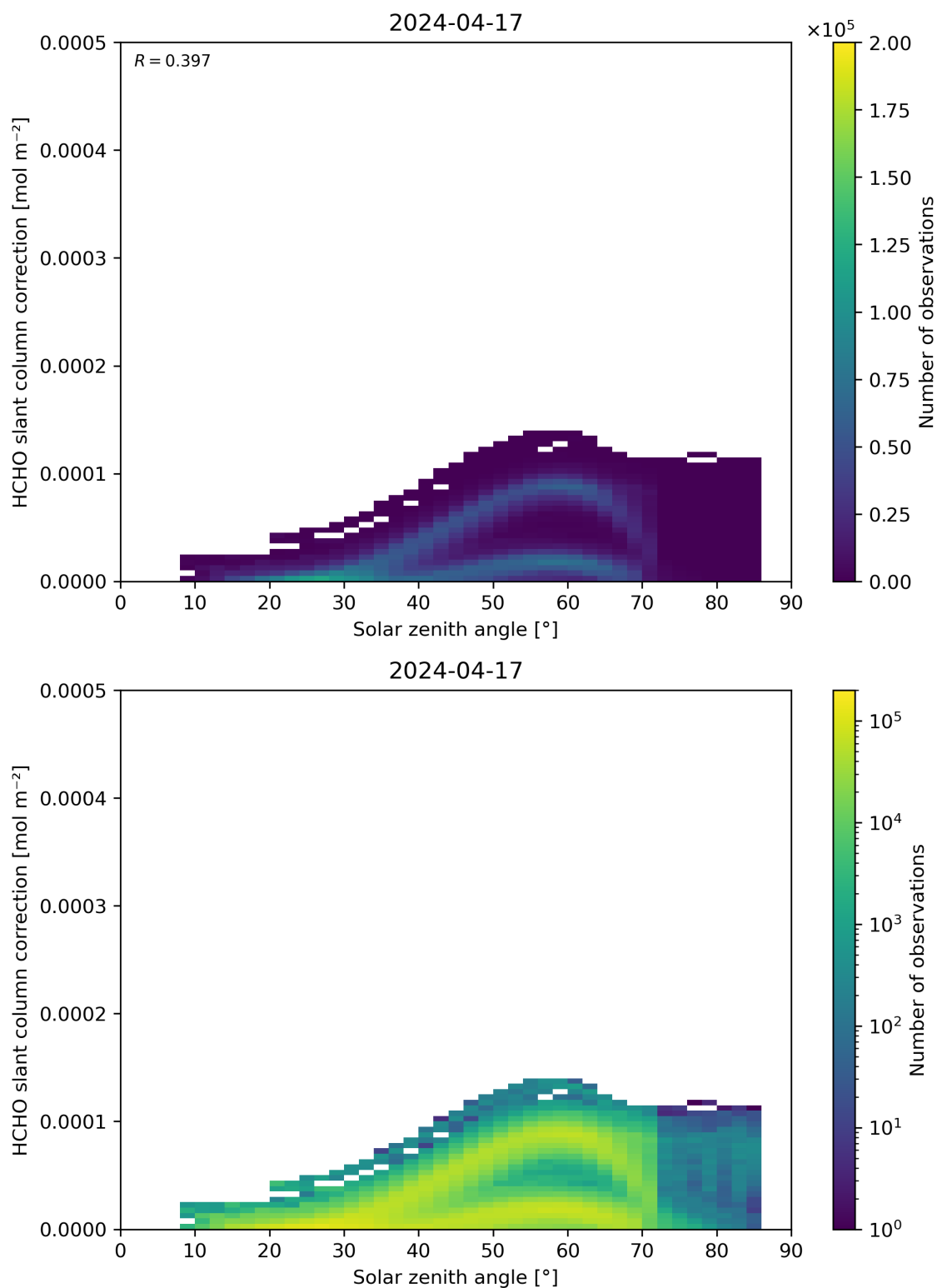
Figure 172: Scatter density plot of “Solar zenith angle” against “HCHO slant column correction” for 2024-04-16 to 2024-04-18.
