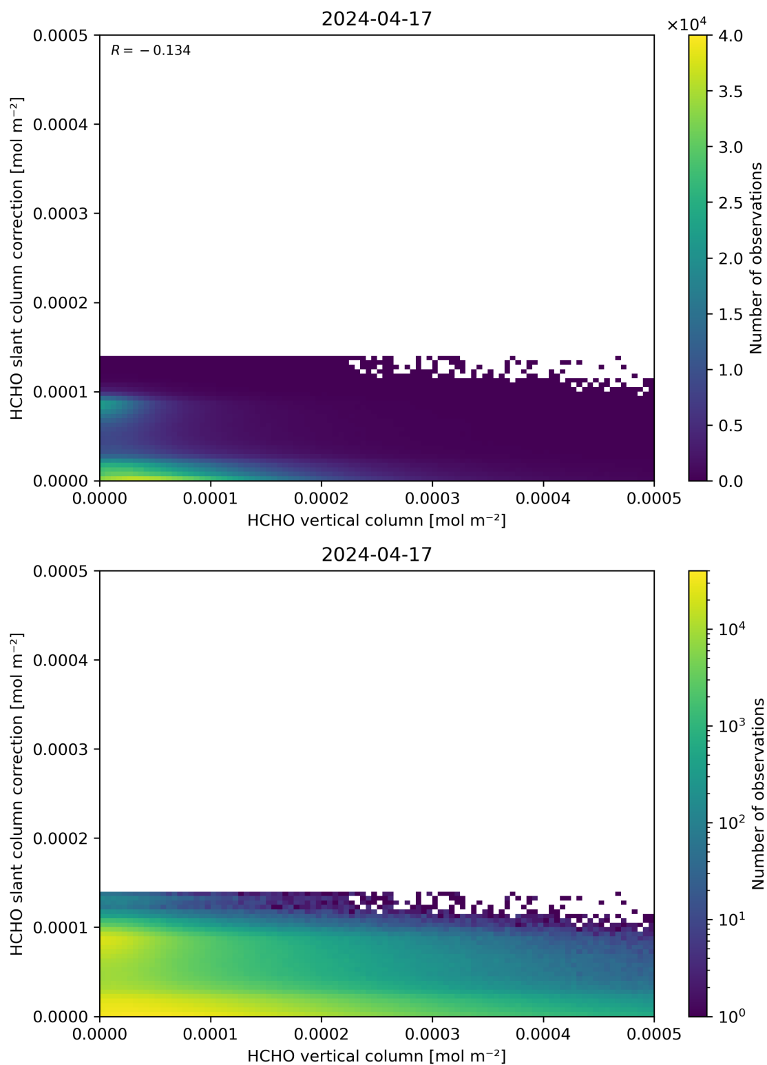
Figure 128: Scatter density plot of “HCHO vertical column” against “HCHO slant column correction” for 2024-04-16 to 2024-04-18.
