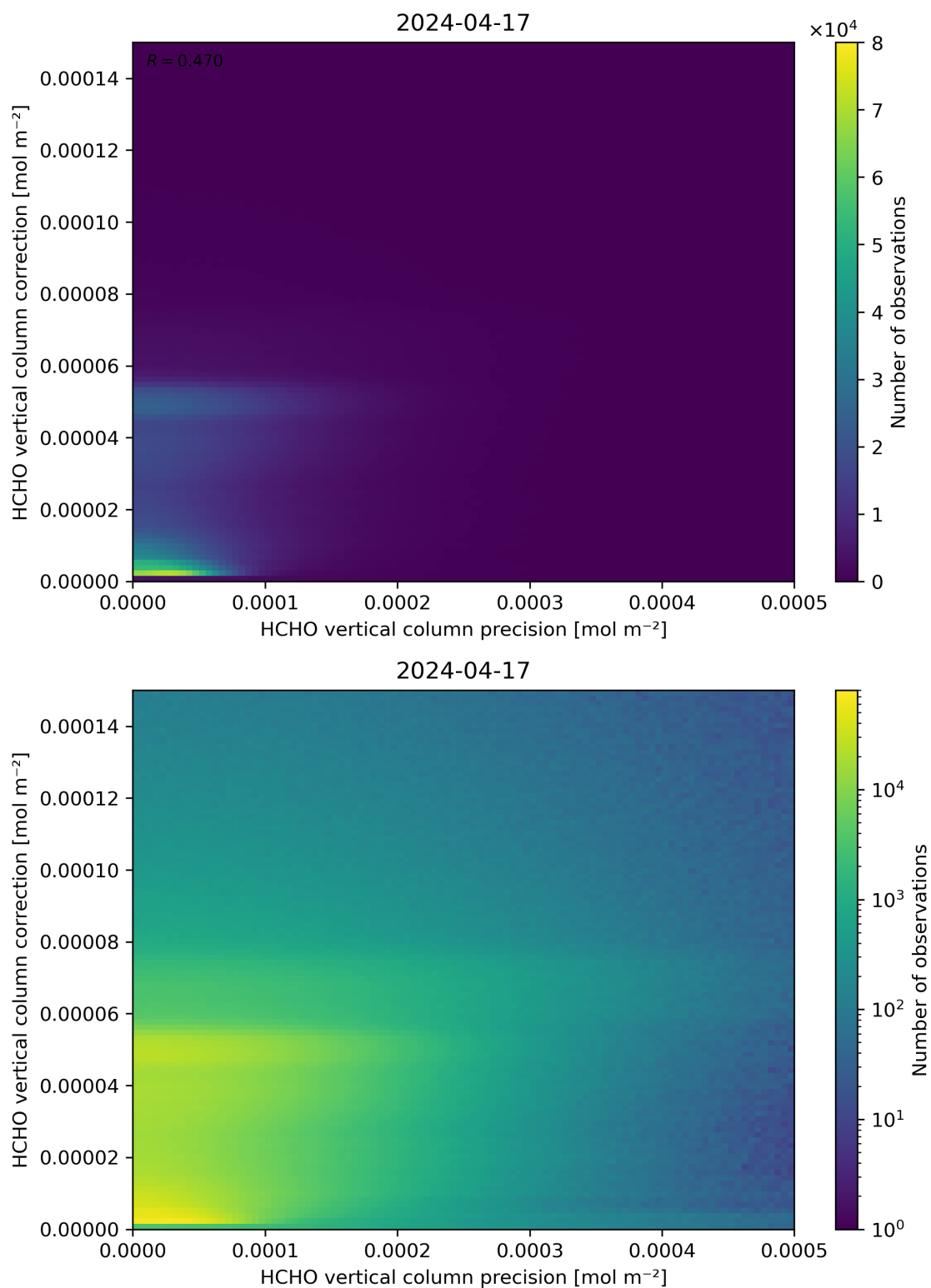
Figure 146: Scatter density plot of “HCHO vertical column precision” against “HCHO vertical column correction” for 2024-04-16 to 2024-04-18.
