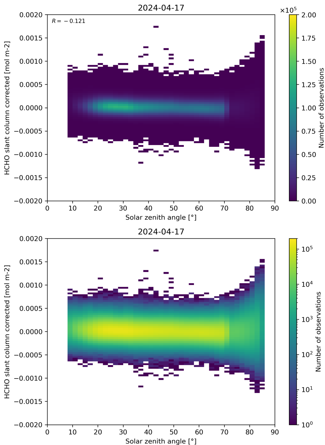
Figure 171: Scatter density plot of “Solar zenith angle” against “HCHO slant column corrected” for 2024-04-16 to 2024-04-18.
