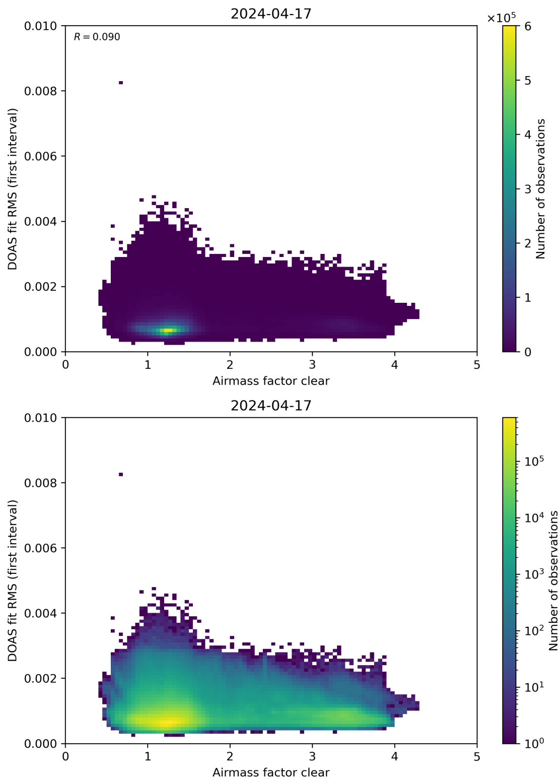
Figure 71: Scatter density plot of “Airmass factor clear” against “DOAS fit RMS (first interval)” for 2024-04-16 to 2024-04-18.
