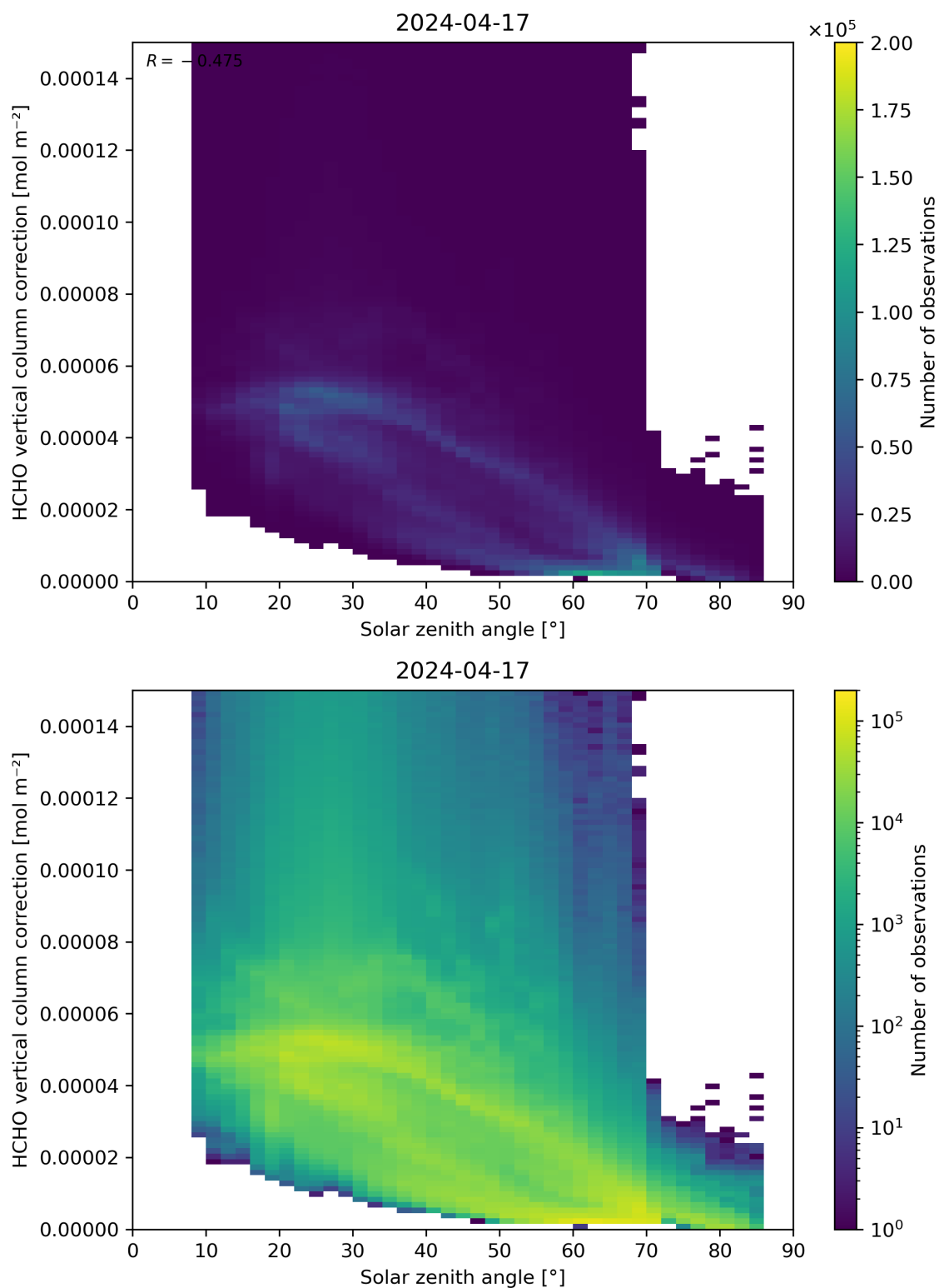
Figure 178: Scatter density plot of “Solar zenith angle” against “HCHO vertical column correction” for 2024-04-16 to 2024-04-18.
