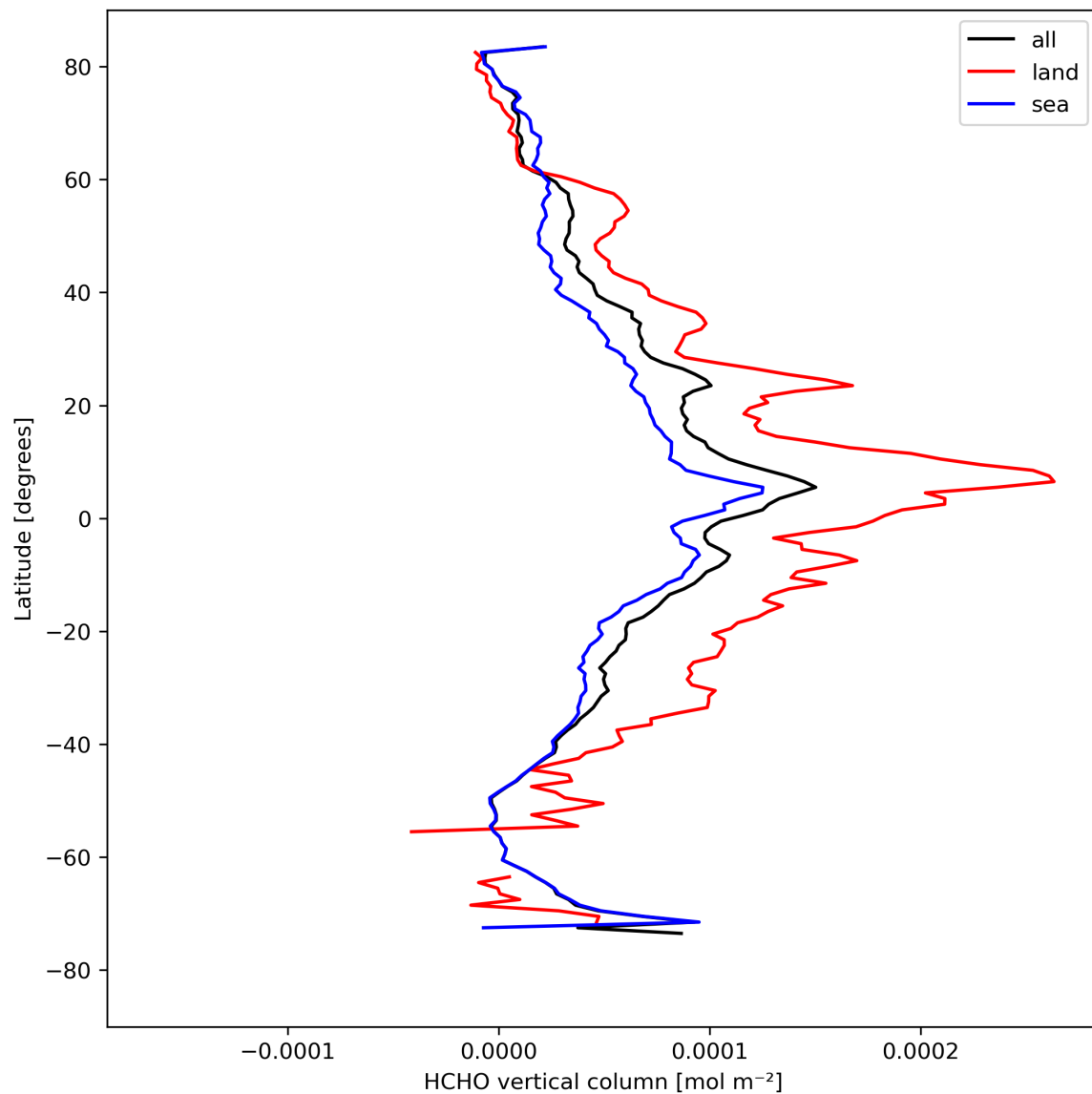
Figure 21: Zonal average of “HCHO vertical column” for 2024-04-16 to 2024-04-18.
