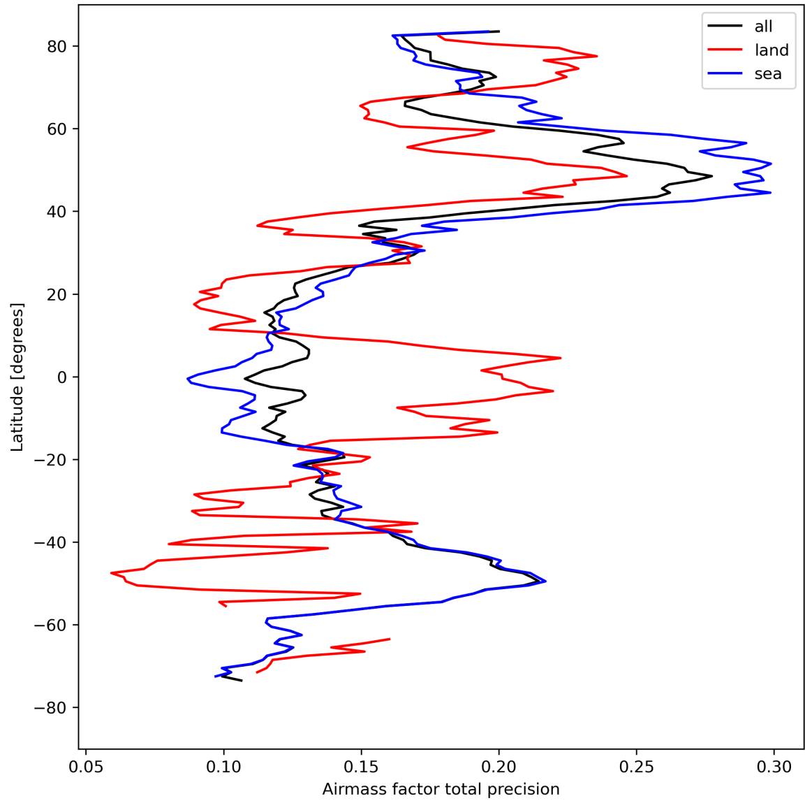
Figure 27: Zonal average of “Airmass factor total precision” for 2024-04-16 to 2024-04-18.
