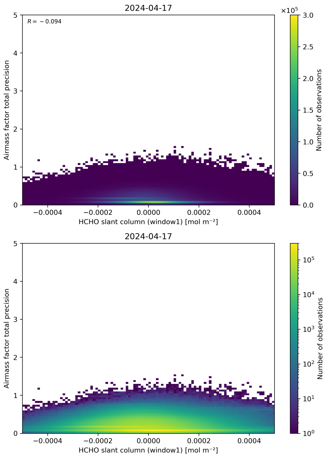
Figure 86: Scatter density plot of “HCHO slant column (window1)” against “Airmass factor total precision” for 2024-04-16 to 2024-04-18.
