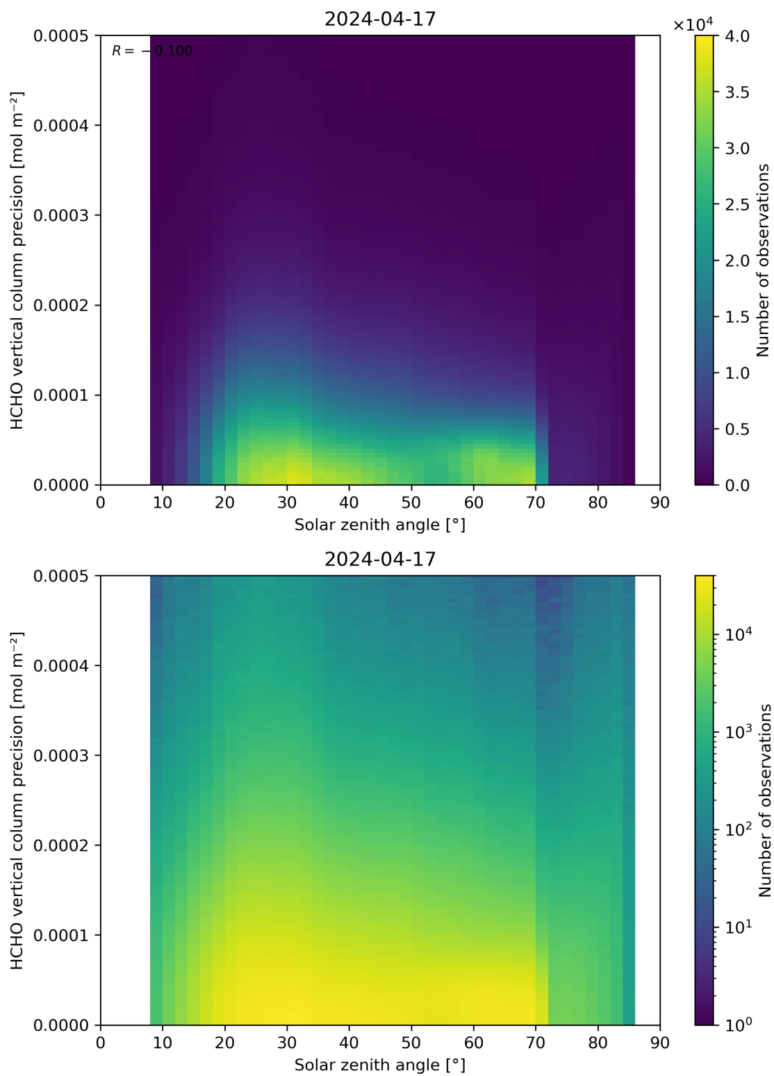
Figure 179: Scatter density plot of “Solar zenith angle” against “HCHO vertical column precision” for 2024-04-16 to 2024-04-18.
