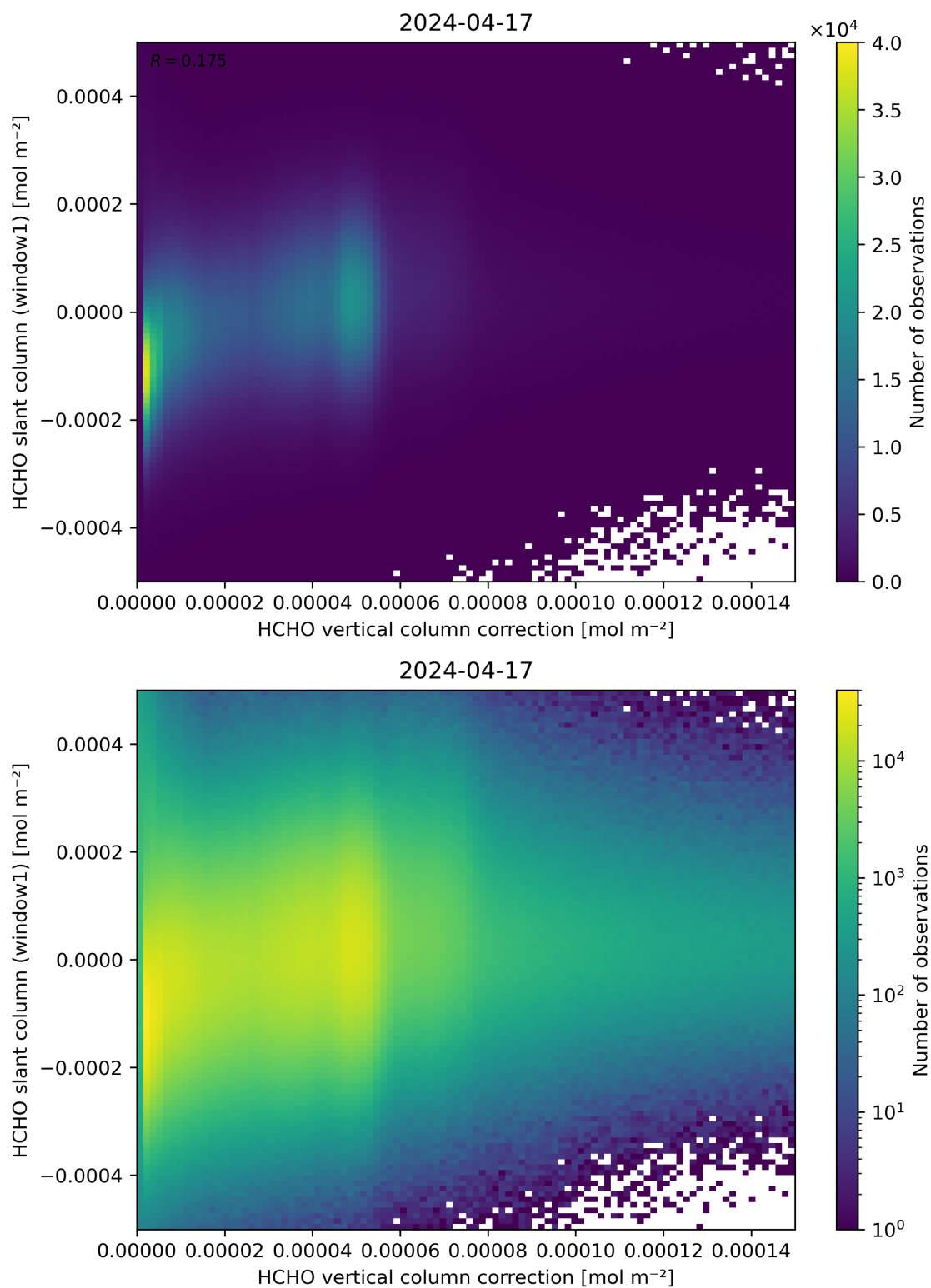
Figure 118: Scatter density plot of “HCHO vertical column correction” against “HCHO slant column (window1)” for 2024-04-16 to 2024-04-18.
