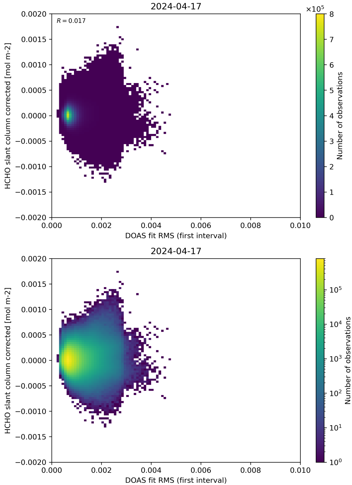
Figure 62: Scatter density plot of “DOAS fit RMS (first interval)” against “HCHO slant column corrected” for 2024-04-16 to 2024-04-18.
