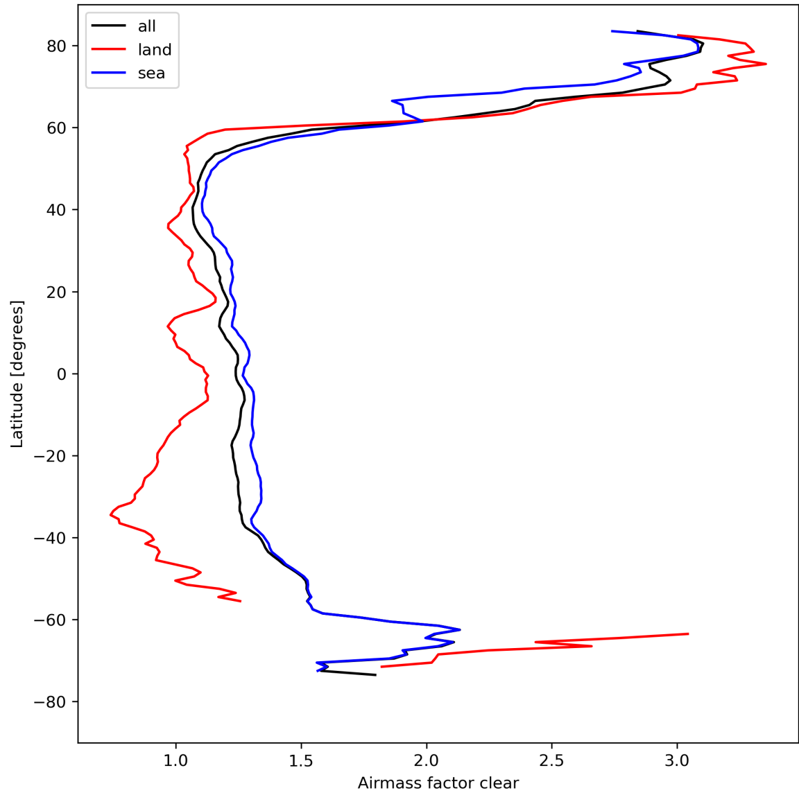
Figure 28: Zonal average of “Airmass factor clear” for 2024-04-16 to 2024-04-18.
