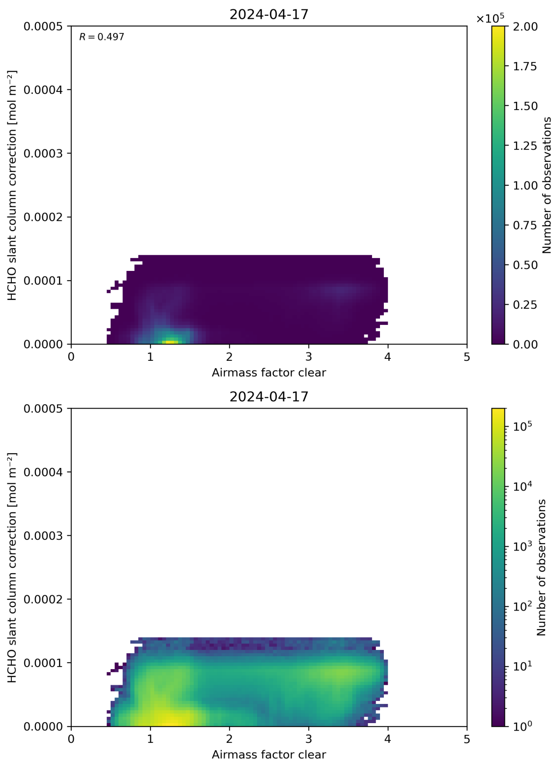
Figure 75: Scatter density plot of “Airmass factor clear” against “HCHO slant column correction” for 2024-04-16 to 2024-04-18.
