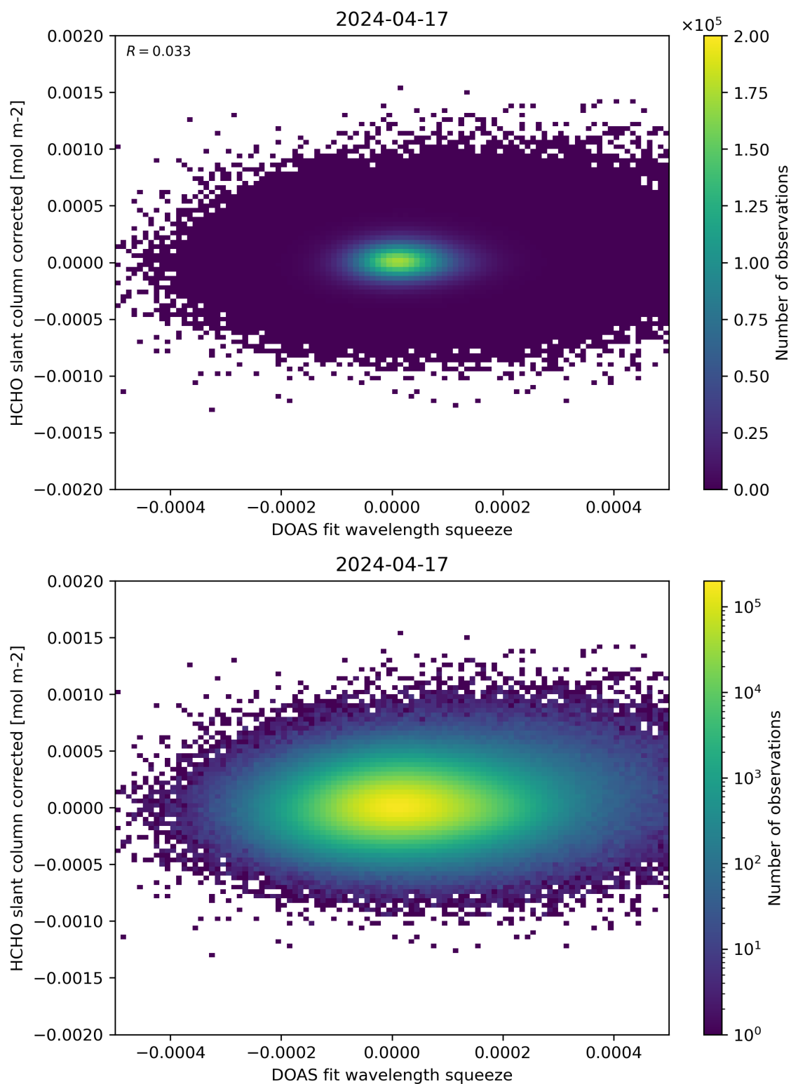
Figure 69: Scatter density plot of “DOAS fit wavelength squeeze” against “HCHO slant column corrected” for 2024-04-16 to 2024-04-18.
