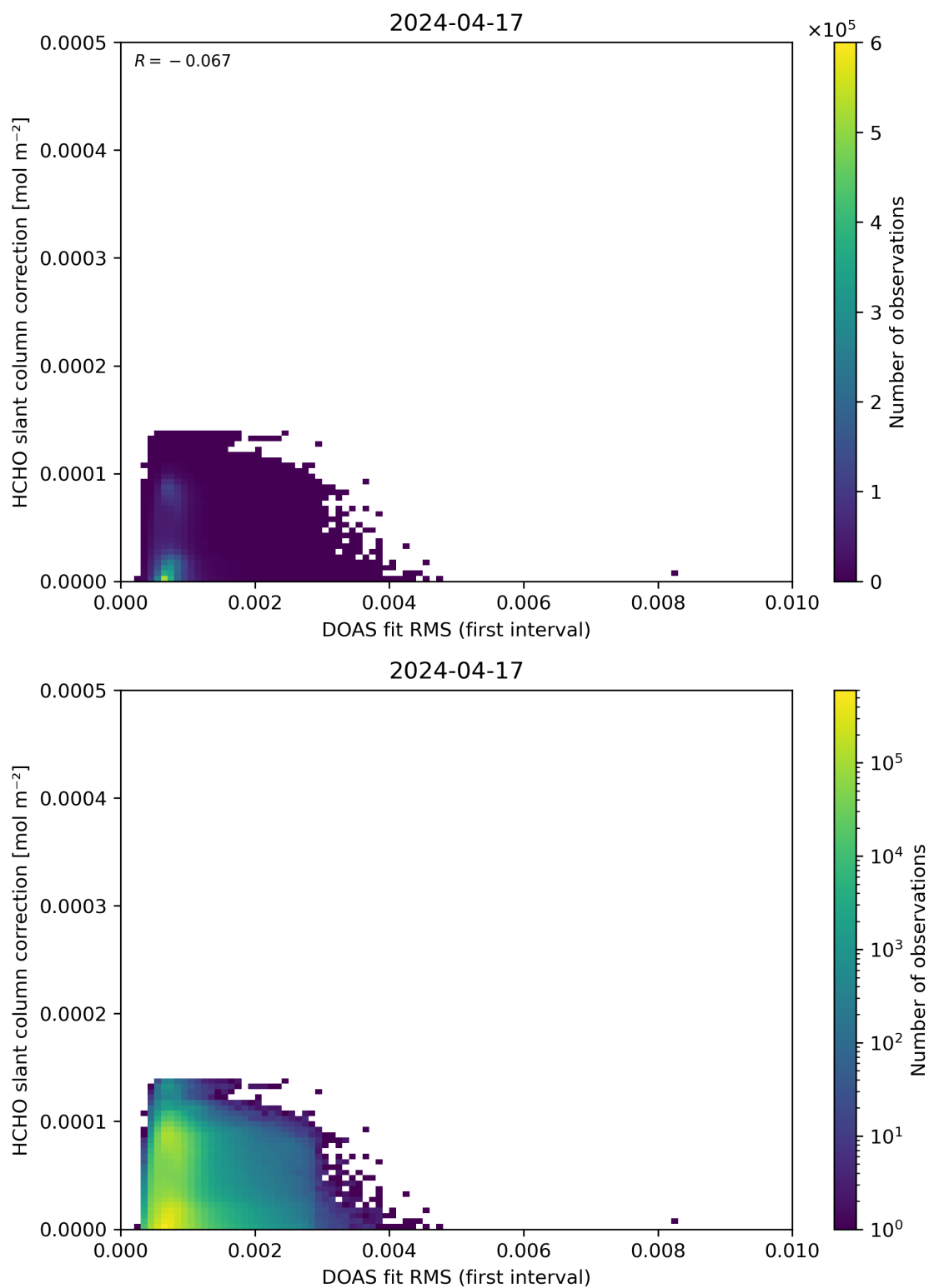
Figure 63: Scatter density plot of “DOAS fit RMS (first interval)” against “HCHO slant column correction” for 2024-04-16 to 2024-04-18.
