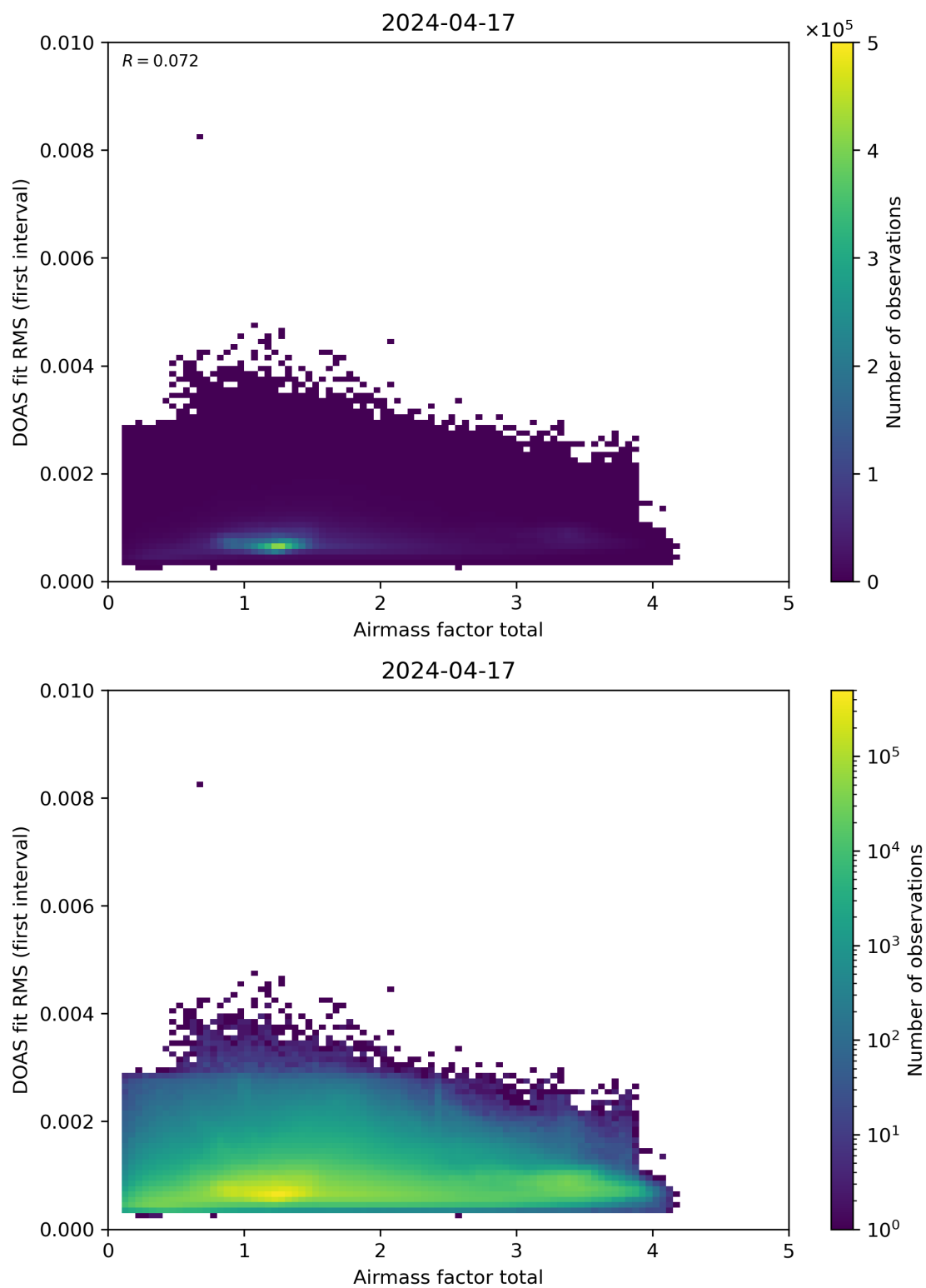
Figure 97: Scatter density plot of “Airmass factor total” against “DOAS fit RMS (first interval)” for 2024-04-16 to 2024-04-18.
