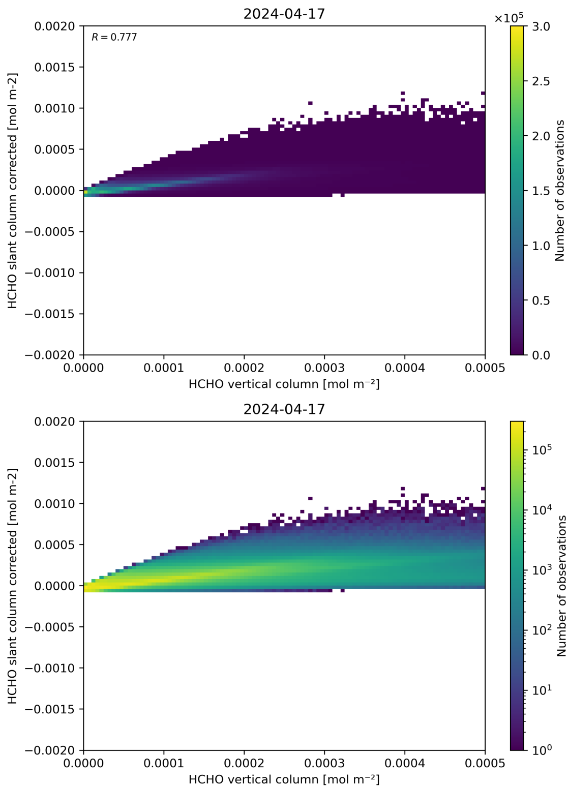
Figure 127: Scatter density plot of “HCHO vertical column” against “HCHO slant column corrected” for 2024-04-16 to 2024-04-18.
