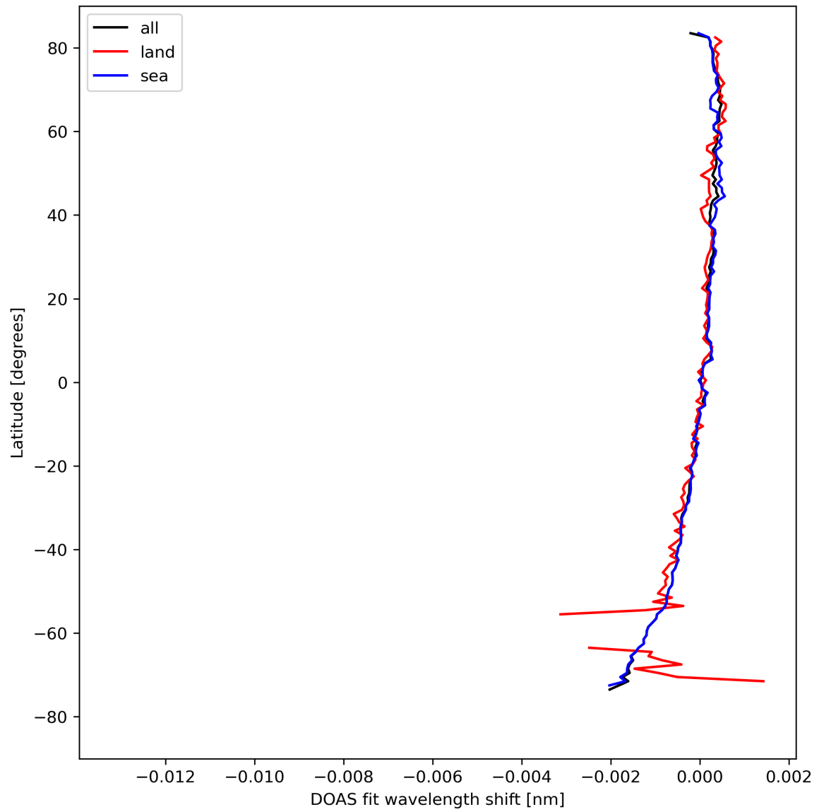
Figure 30: Zonal average of “DOAS fit wavelength shift” for 2024-04-16 to 2024-04-18.
