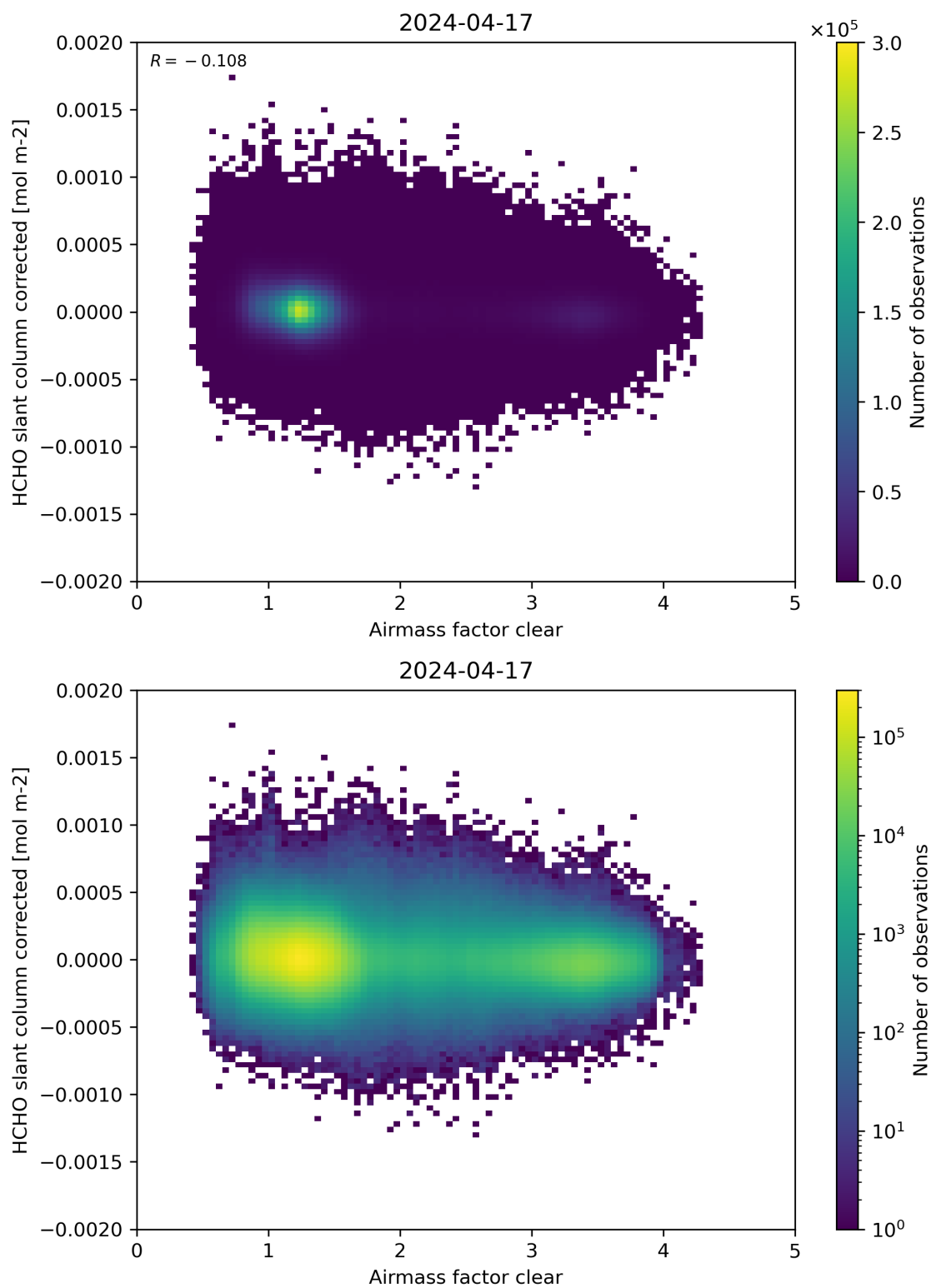
Figure 74: Scatter density plot of “Airmass factor clear” against “HCHO slant column corrected” for 2024-04-16 to 2024-04-18.
