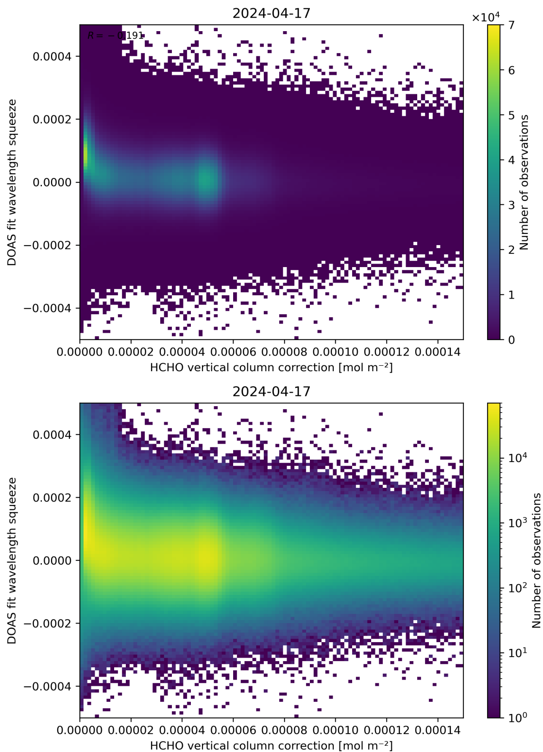
Figure 114: Scatter density plot of “HCHO vertical column correction” against “DOAS fit wavelength squeeze” for 2024-04-16 to 2024-04-18.
