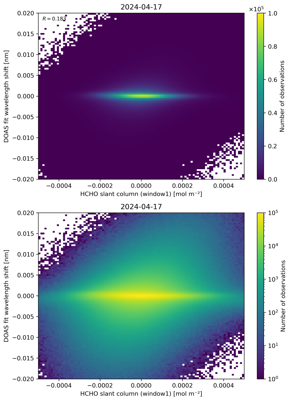
Figure 79: Scatter density plot of “HCHO slant column (window1)” against “DOAS fit wavelength shift” for 2024-04-16 to 2024-04-18.
