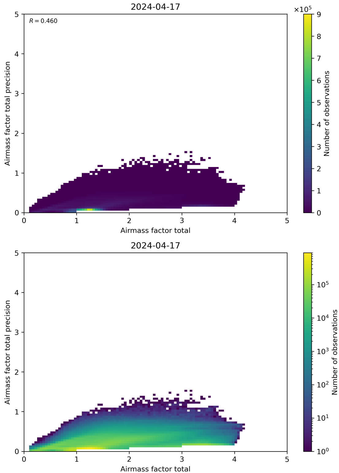
Figure 103: Scatter density plot of “Airmass factor total” against “Airmass factor total precision” for 2024-04-16 to 2024-04-18.
