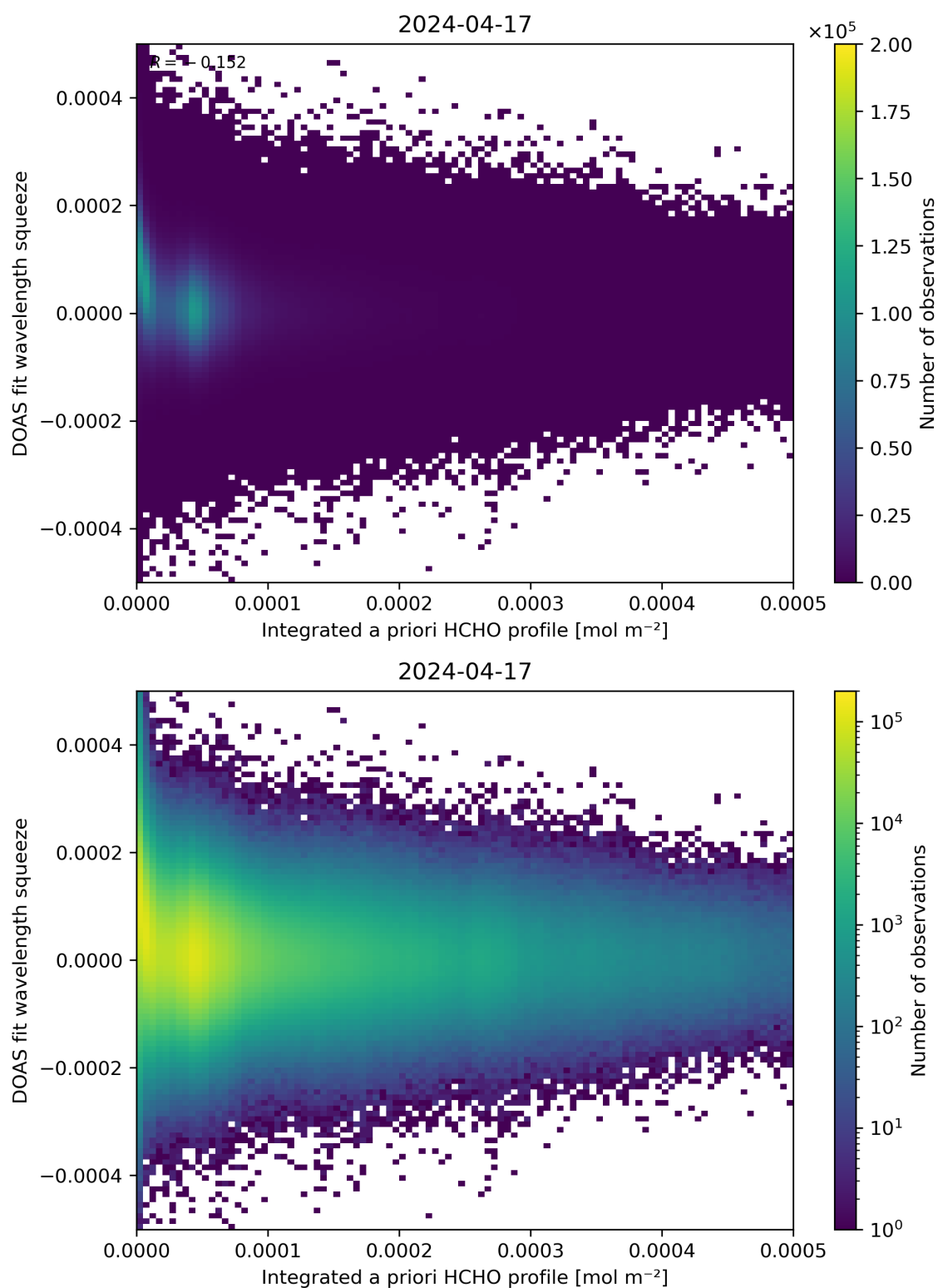
Figure 150: Scatter density plot of “Integrated a priori HCHO profile” against “DOAS fit wavelength squeeze” for 2024-04-16 to 2024-04-18.
