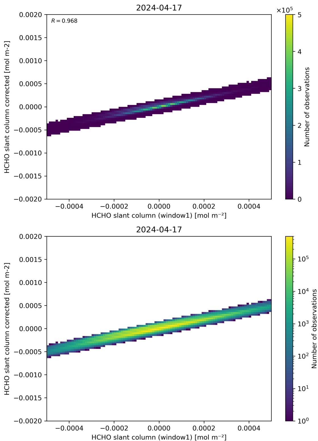
Figure 82: Scatter density plot of “HCHO slant column (window1)” against “HCHO slant column corrected” for 2024-04-16 to 2024-04-18.
