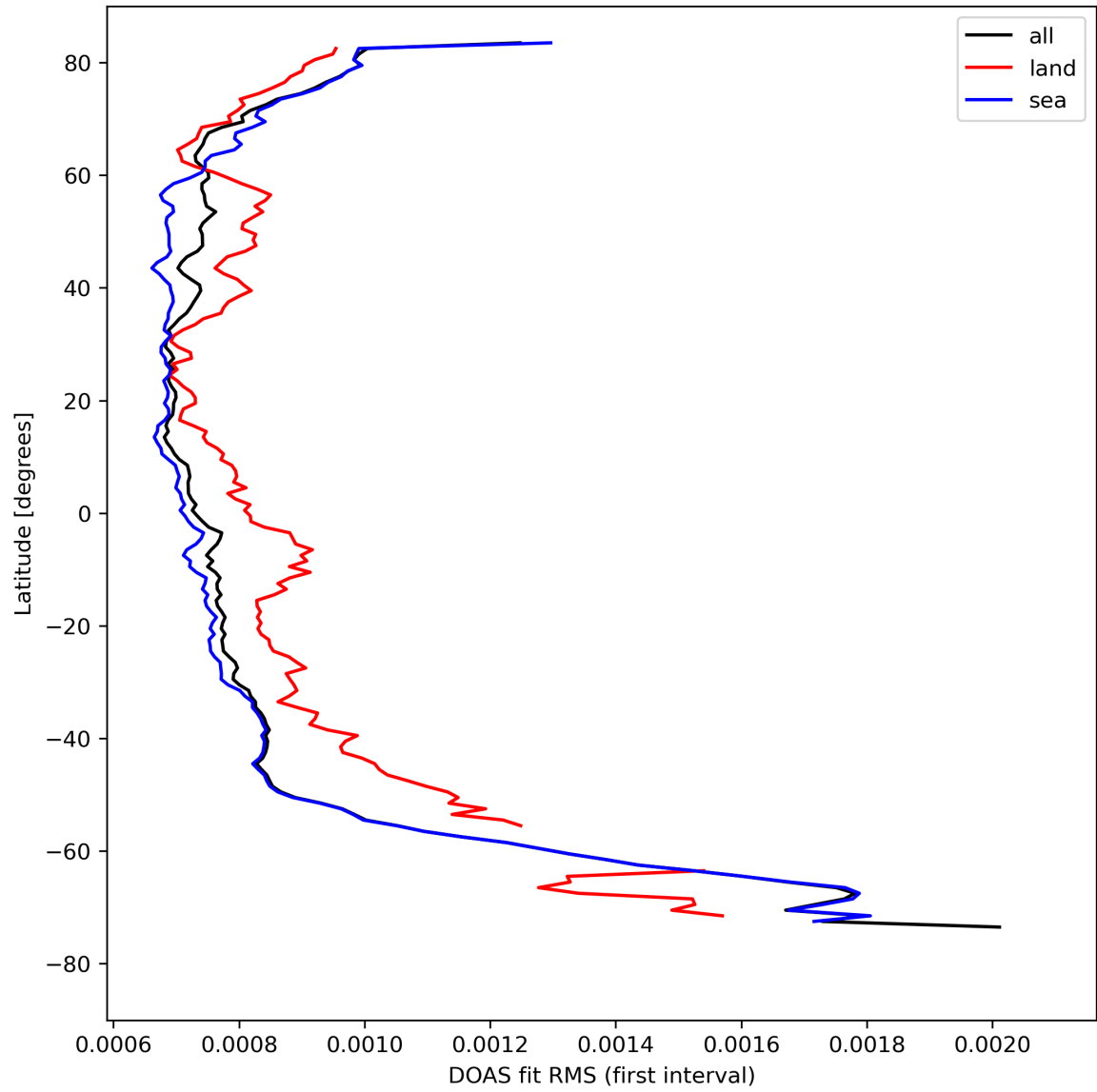
Figure 32: Zonal average of “DOAS fit RMS (first interval)” for 2024-04-16 to 2024-04-18.
