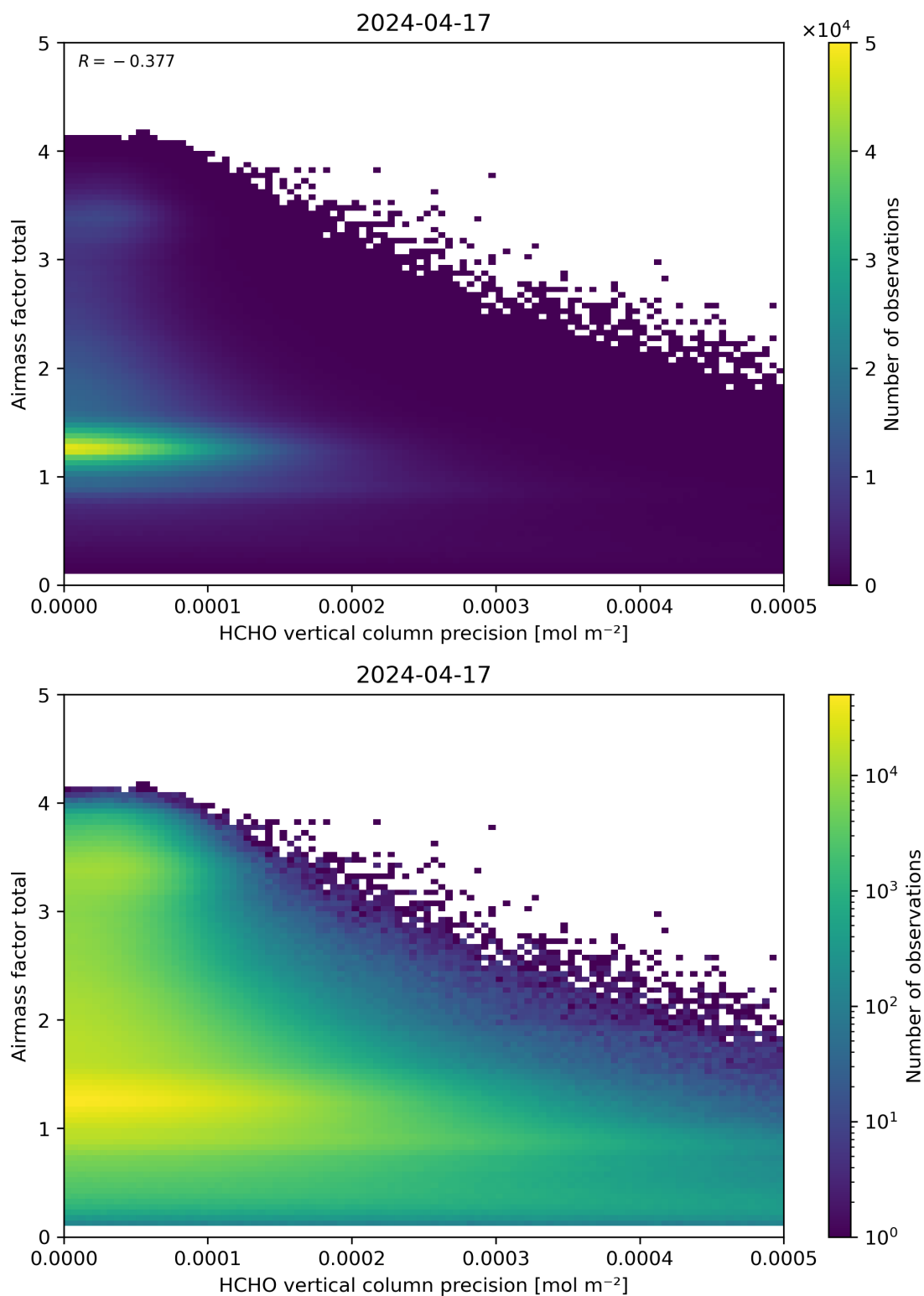
Figure 144: Scatter density plot of “HCHO vertical column precision” against “Airmass factor total” for 2024-04-16 to 2024-04-18.
