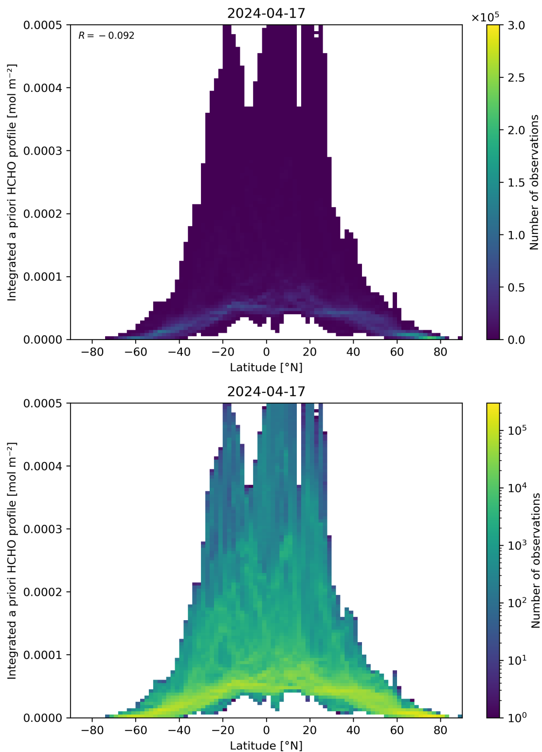
Figure 166: Scatter density plot of “Latitude” against “Integrated a priori HCHO profile” for 2024-04-16 to 2024-04-18.
