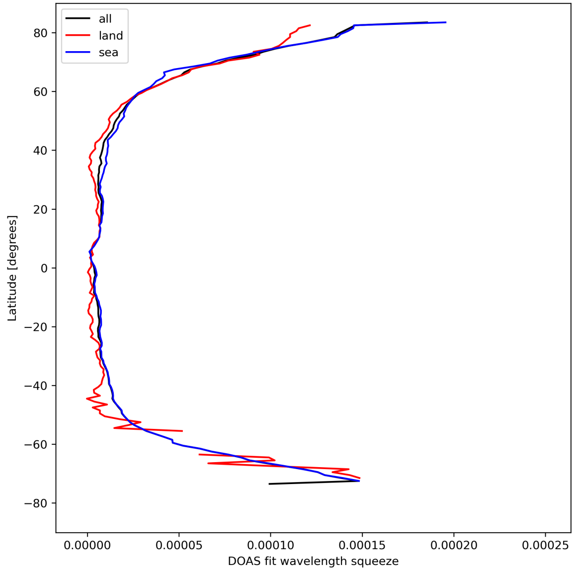
Figure 31: Zonal average of “DOAS fit wavelength squeeze” for 2024-04-16 to 2024-04-18.
