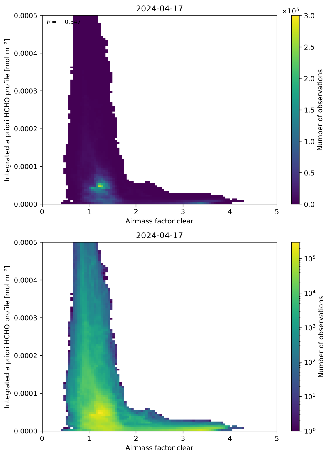
Figure 76: Scatter density plot of “Airmass factor clear” against “Integrated a priori HCHO profile” for 2024-04-16 to 2024-04-18.
