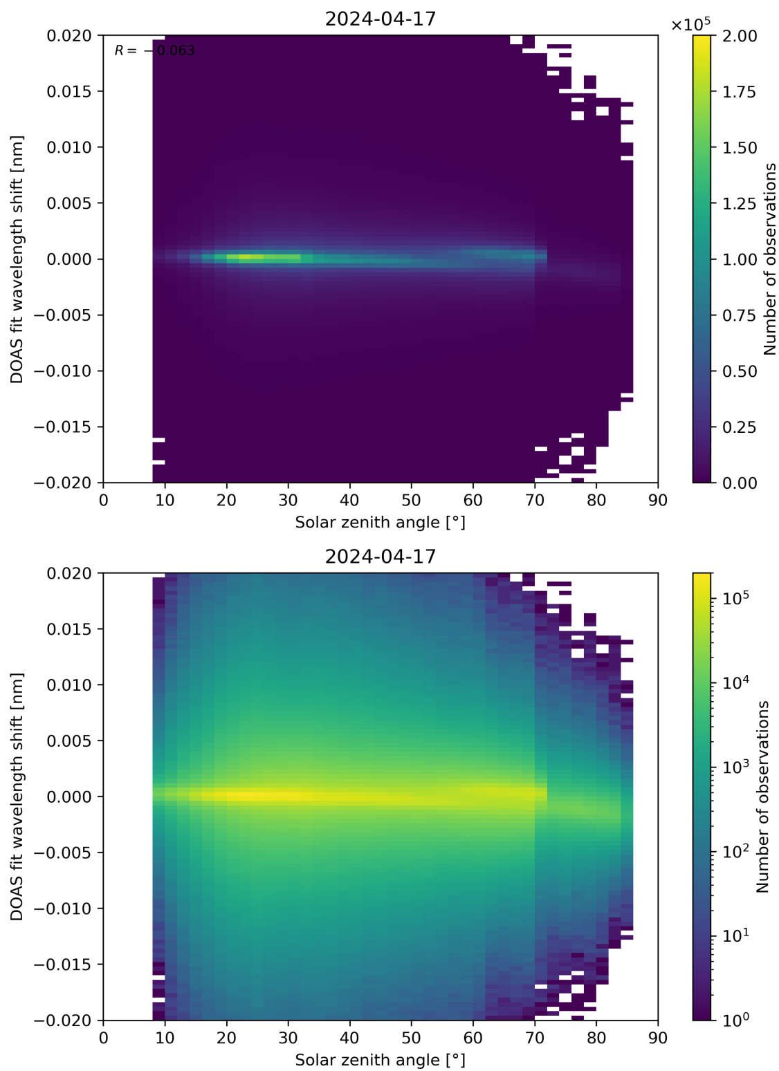
Figure 168: Scatter density plot of “Solar zenith angle” against “DOAS fit wavelength shift” for 2024-04-16 to 2024-04-18.
