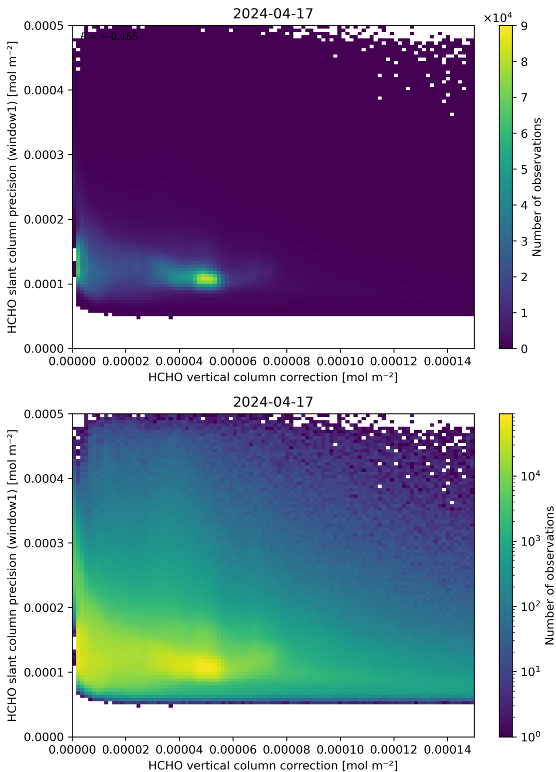
Figure 119: Scatter density plot of “HCHO vertical column correction” against “HCHO slant column precision (window1)” for 2024-04-16 to 2024-04-18.
