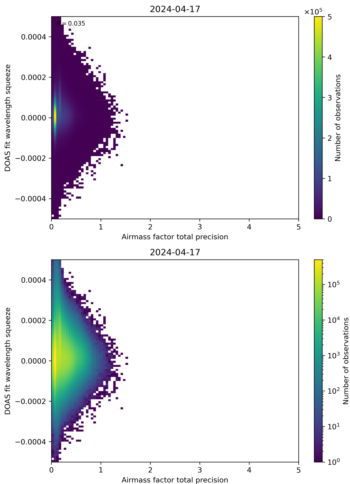
Figure 107: Scatter density plot of “Airmass factor total precision” against “DOAS fit wavelength squeeze” for 2024-04-16 to 2024-04-18.
