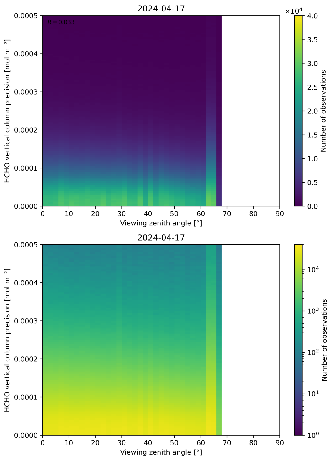
Figure 194: Scatter density plot of “Viewing zenith angle” against “HCHO vertical column precision” for 2024-04-16 to 2024-04-18.
