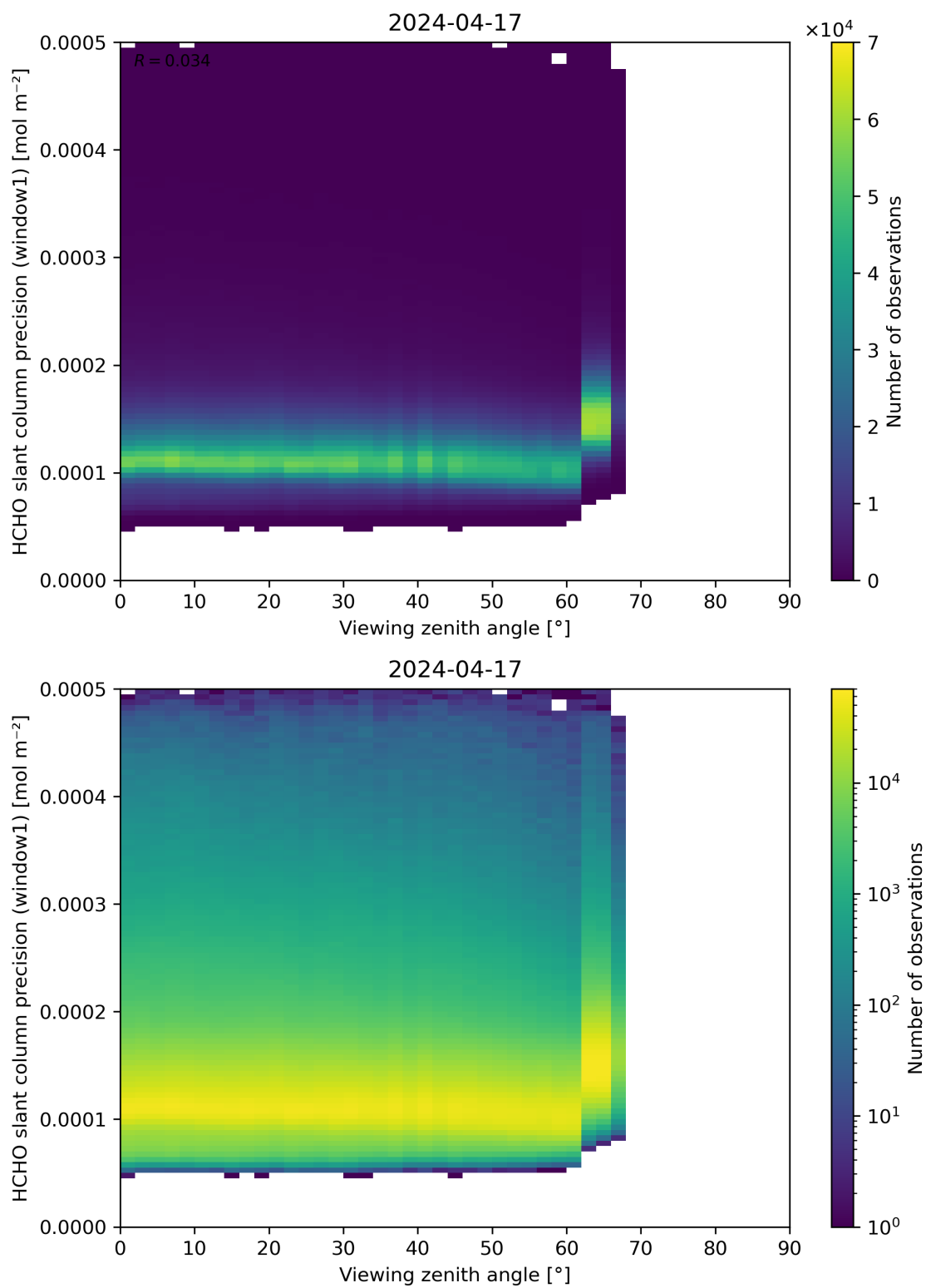
Figure 189: Scatter density plot of “Viewing zenith angle” against “HCHO slant column precision (window1)” for 2024-04-16 to 2024-04-18.
