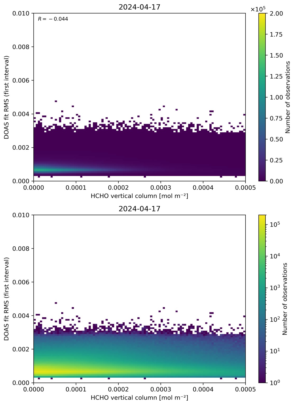
Figure 123: Scatter density plot of “HCHO vertical column” against “DOAS fit RMS (first interval)” for 2024-04-16 to 2024-04-18.
