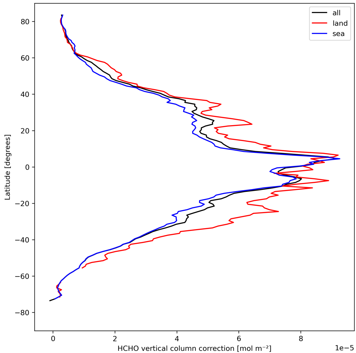
Figure 23: Zonal average of “HCHO vertical column correction” for 2024-04-16 to 2024-04-18.
