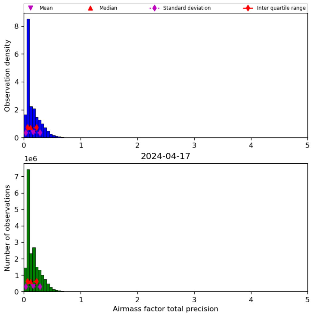
Figure 41: Histogram of “Airmass factor total precision” for 2024-04-16 to 2024-04-18
