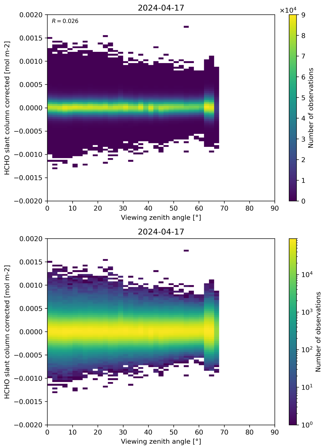
Figure 186: Scatter density plot of “Viewing zenith angle” against “HCHO slant column corrected” for 2024-04-16 to 2024-04-18.
