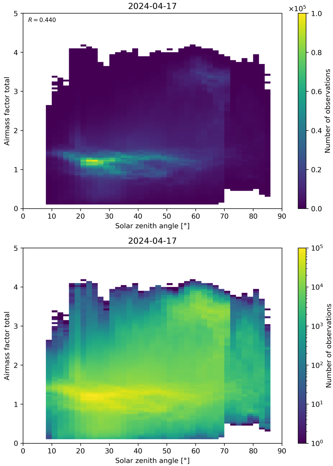
Figure 175: Scatter density plot of “Solar zenith angle” against “Airmass factor total” for 2024-04-16 to 2024-04-18.
