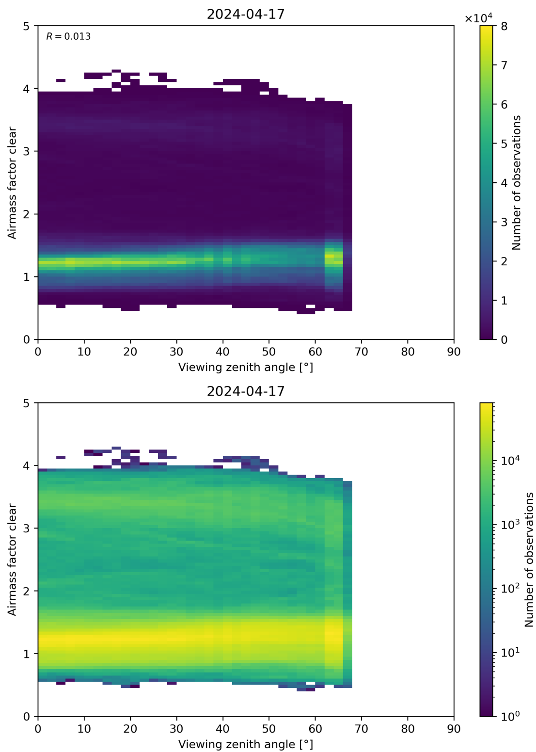
Figure 185: Scatter density plot of “Viewing zenith angle” against “Airmass factor clear” for 2024-04-16 to 2024-04-18.
