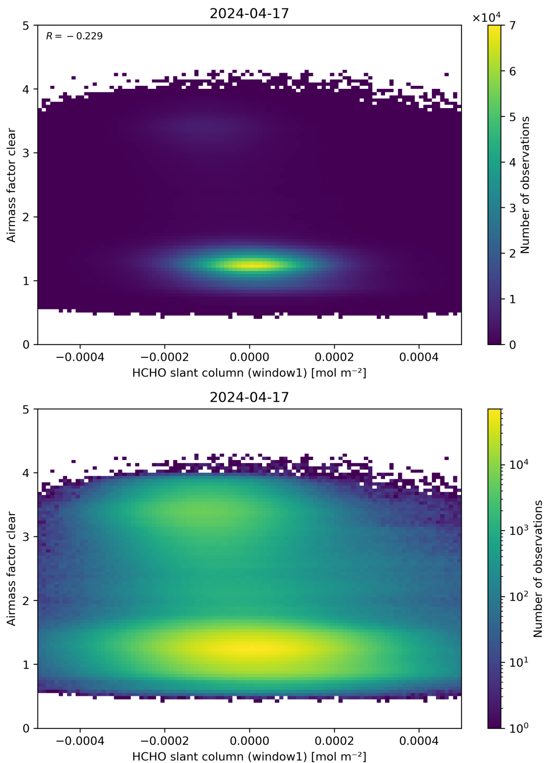
Figure 81: Scatter density plot of “HCHO slant column (window1)” against “Airmass factor clear” for 2024-04-16 to 2024-04-18.
