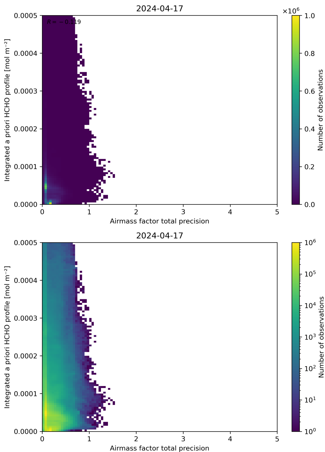
Figure 111: Scatter density plot of “Airmass factor total precision” against “Integrated a priori HCHO profile” for 2024-04-16 to 2024-04-18.
