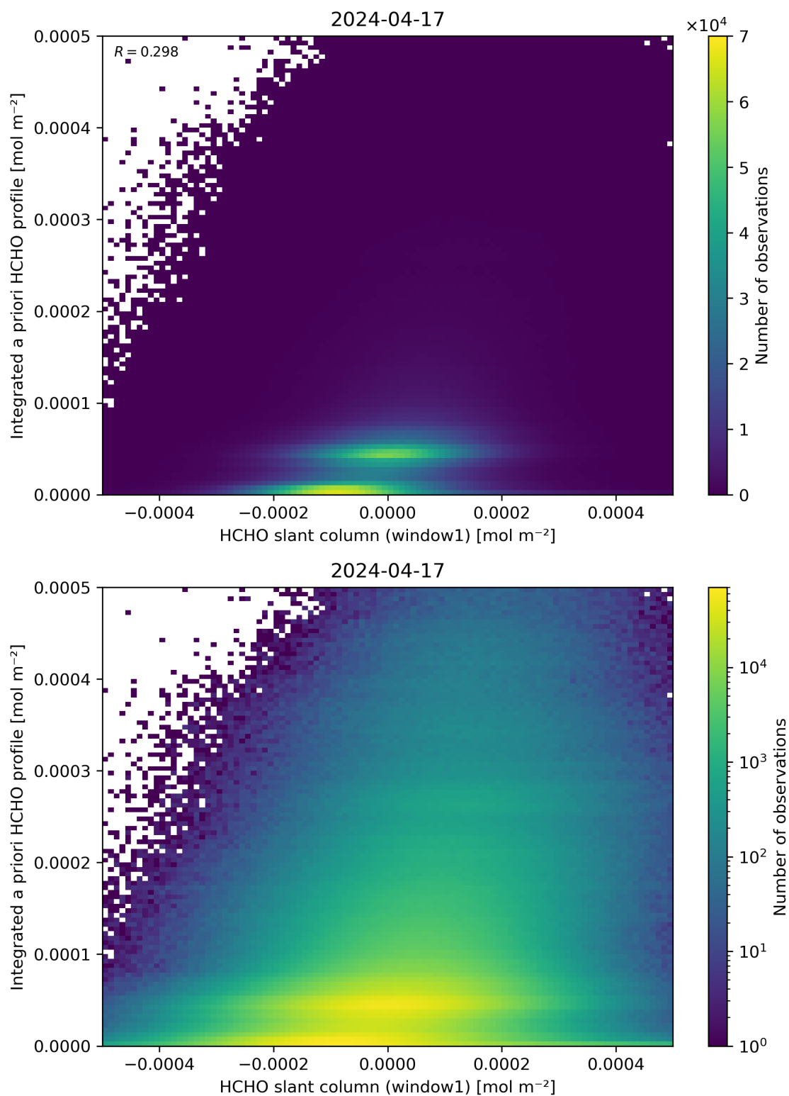
Figure 87: Scatter density plot of “HCHO slant column (window1)” against “Integrated a priori HCHO profile” for 2024-04-16 to 2024-04-18.
