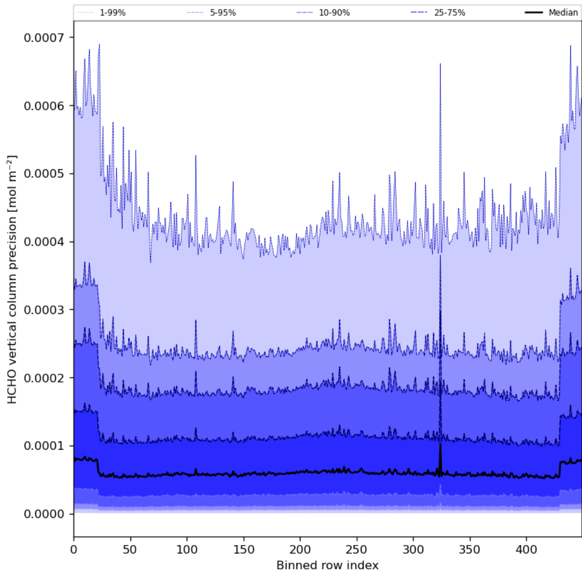
Figure 50: Along track statistics of "HCHO vertical column precision" for 2024-04-16 to 2024-04-18
