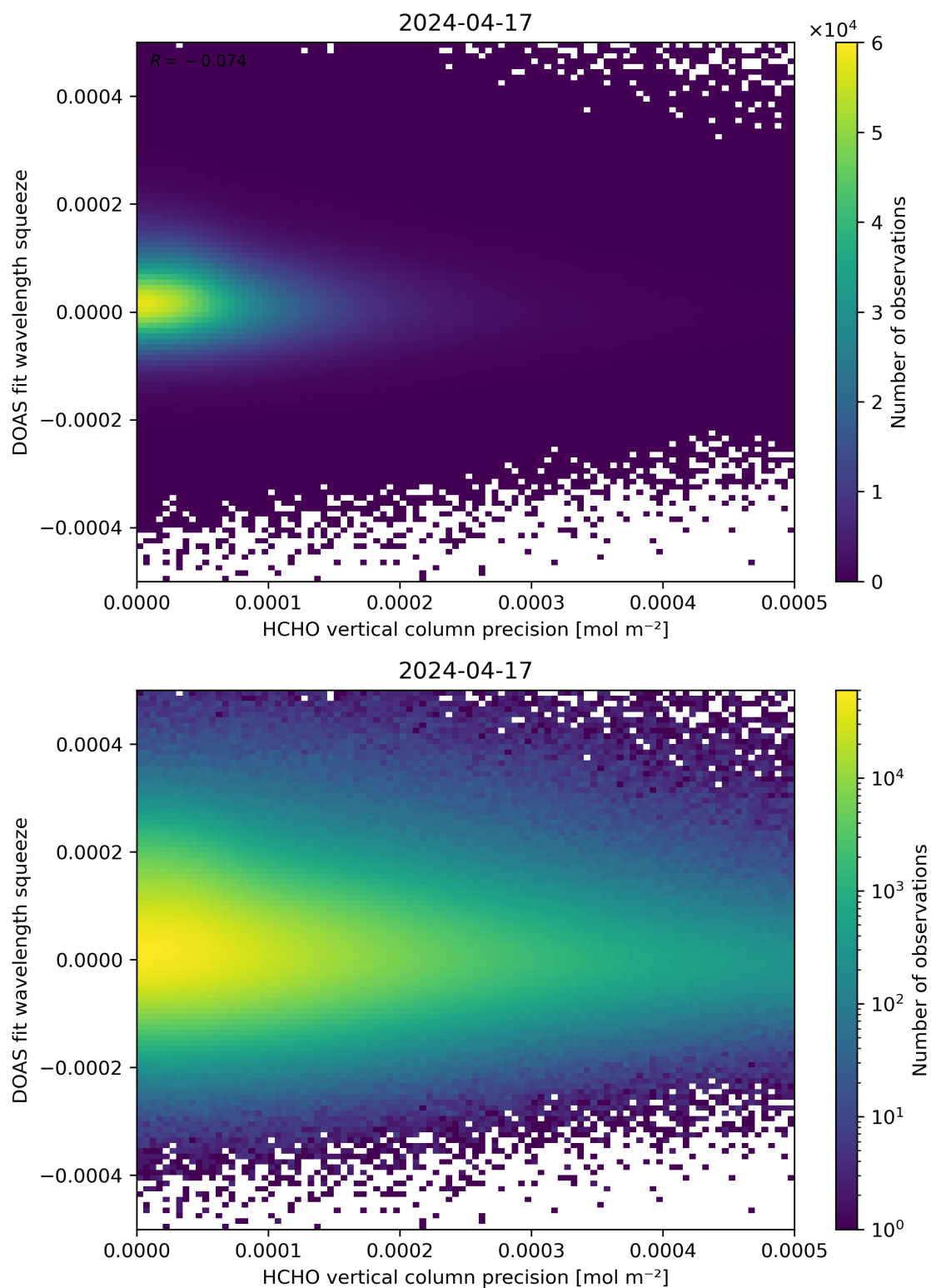
Figure 138: Scatter density plot of “HCHO vertical column precision” against “DOAS fit wavelength squeeze” for 2024-04-16 to 2024-04-18.
