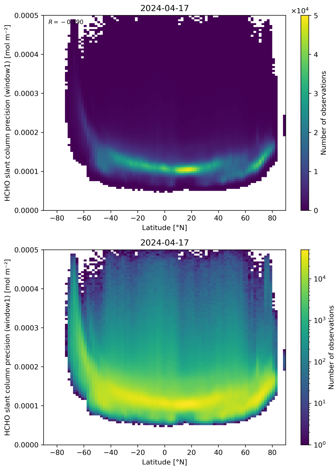
Figure 160: Scatter density plot of “Latitude” against “HCHO slant column precision (window1)” for 2024-04-16 to 2024-04-18.
