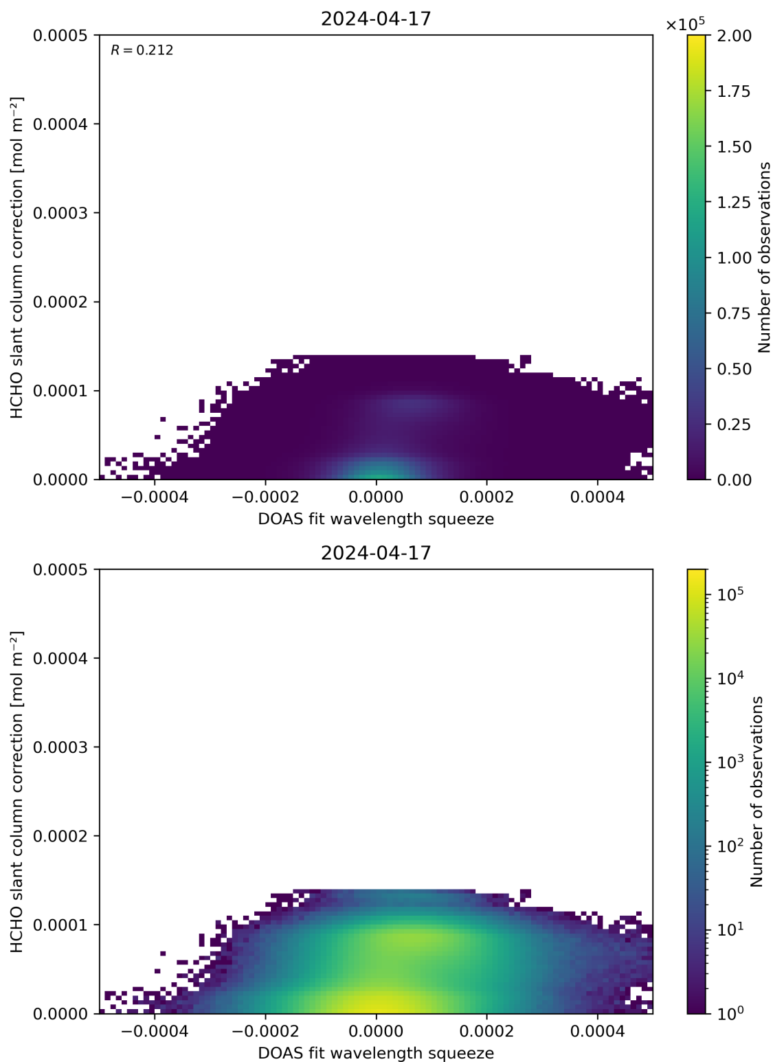
Figure 70: Scatter density plot of “DOAS fit wavelength squeeze” against “HCHO slant column correction” for 2024-04-16 to 2024-04-18.
