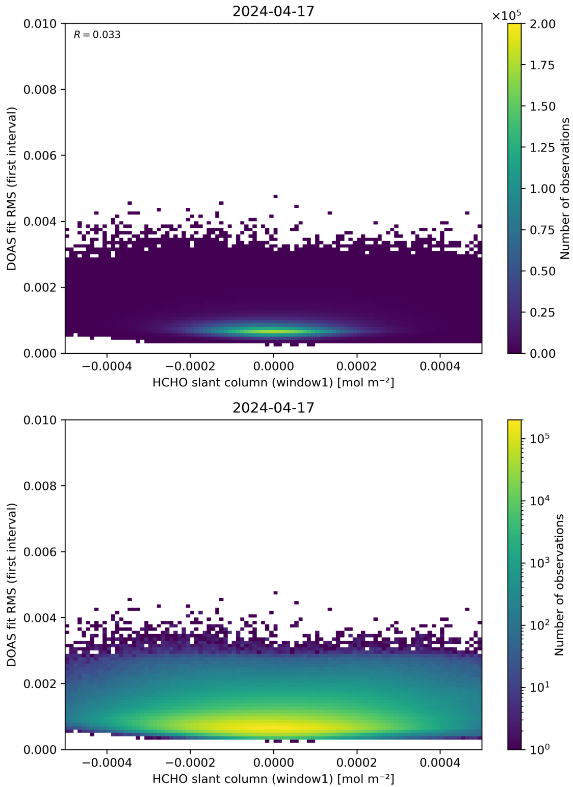
Figure 78: Scatter density plot of “HCHO slant column (window1)” against “DOAS fit RMS (first interval)” for 2024-04-16 to 2024-04-18.
