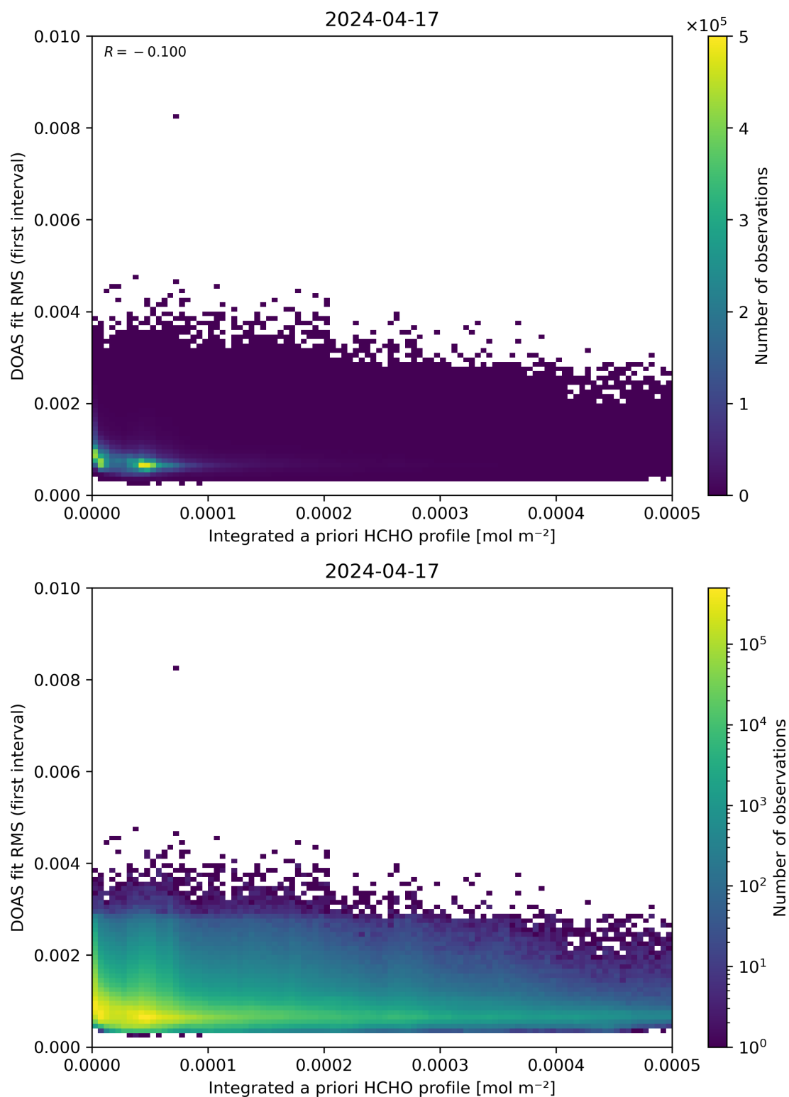
Figure 148: Scatter density plot of “Integrated a priori HCHO profile” against “DOAS fit RMS (first interval)” for 2024-04-16 to 2024-04-18.
