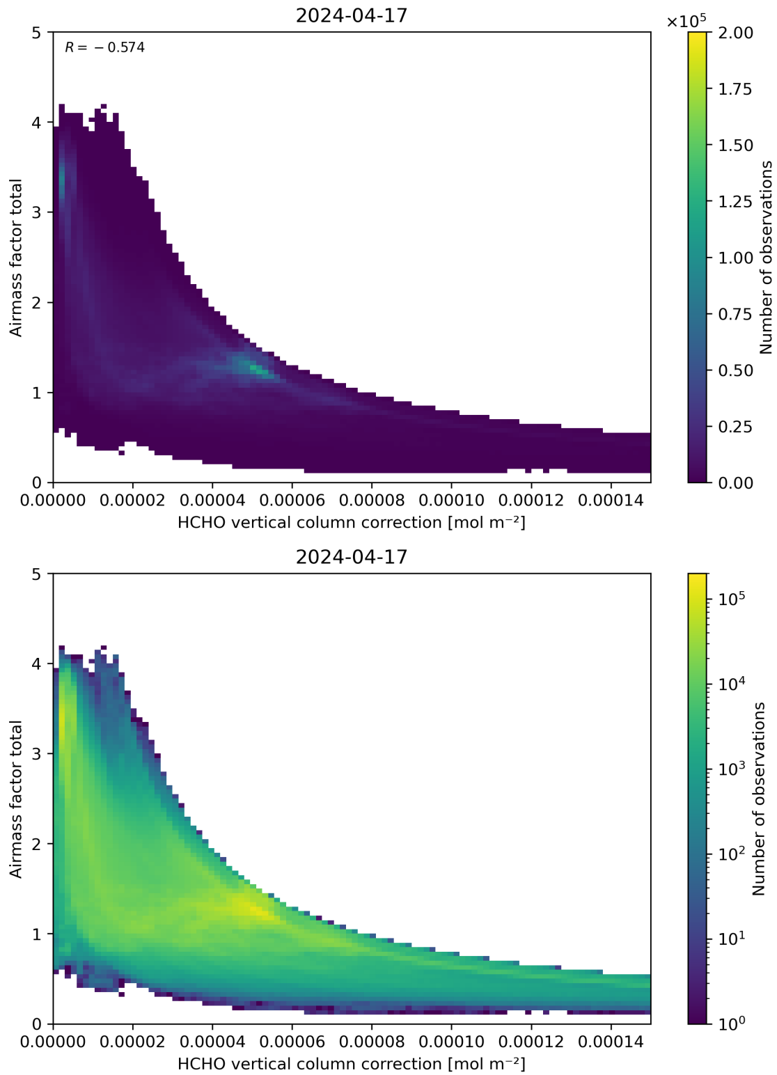
Figure 120: Scatter density plot of “HCHO vertical column correction” against “Airmass factor total” for 2024-04-16 to 2024-04-18.
