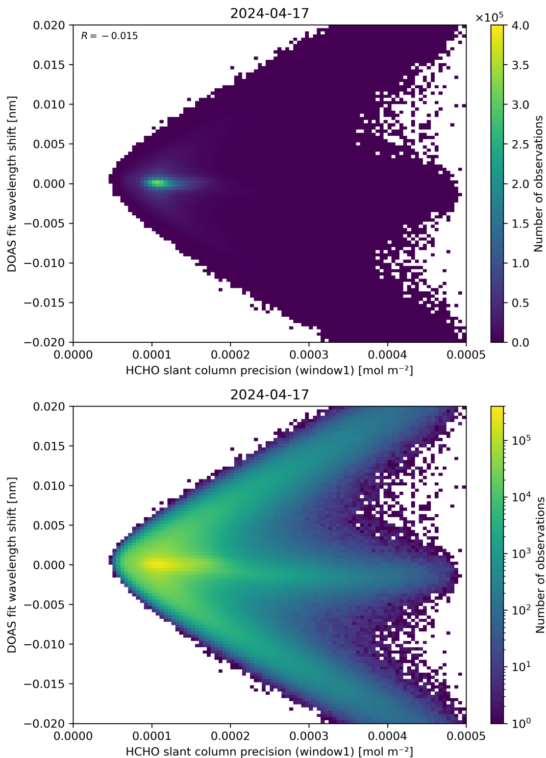
Figure 89: Scatter density plot of “HCHO slant column precision (window1)” against “DOAS fit wavelength shift” for 2024-04-16 to 2024-04-18.
