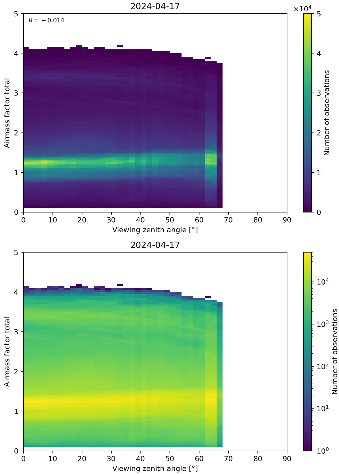
Figure 190: Scatter density plot of “Viewing zenith angle” against “Airmass factor total” for 2024-04-16 to 2024-04-18.
