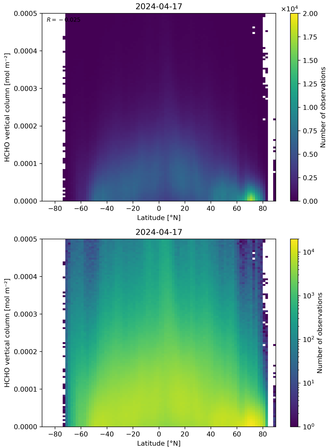
Figure 163: Scatter density plot of “Latitude” against “HCHO vertical column” for 2024-04-16 to 2024-04-18.
