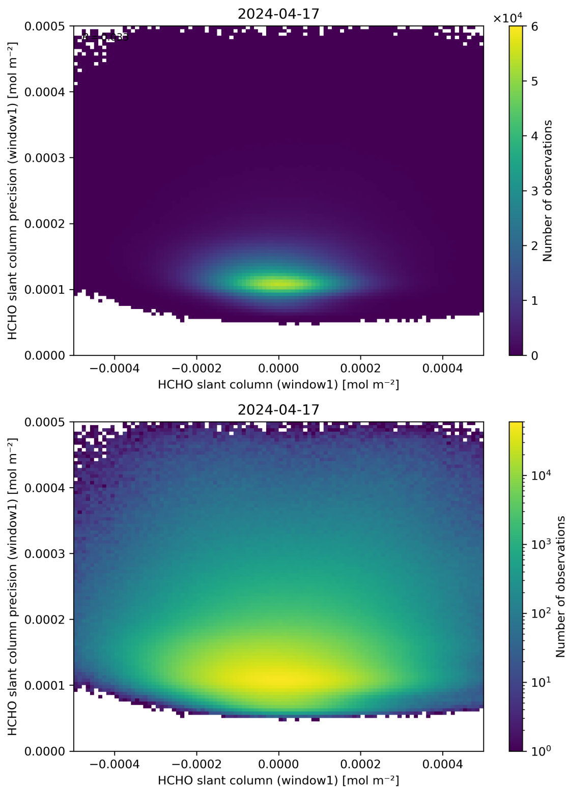
Figure 84: Scatter density plot of “HCHO slant column (window1)” against “HCHO slant column precision (window1)” for 2024-04-16 to 2024-04-18.
