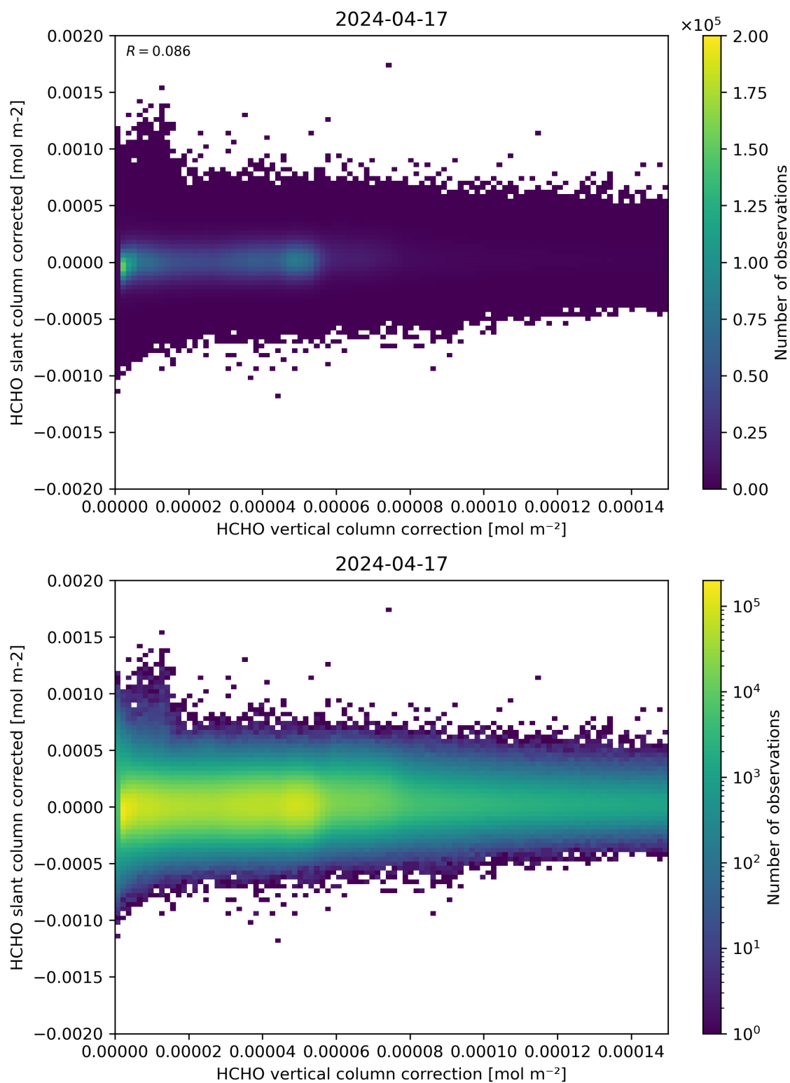
Figure 116: Scatter density plot of “HCHO vertical column correction” against “HCHO slant column corrected” for 2024-04-16 to 2024-04-18.
