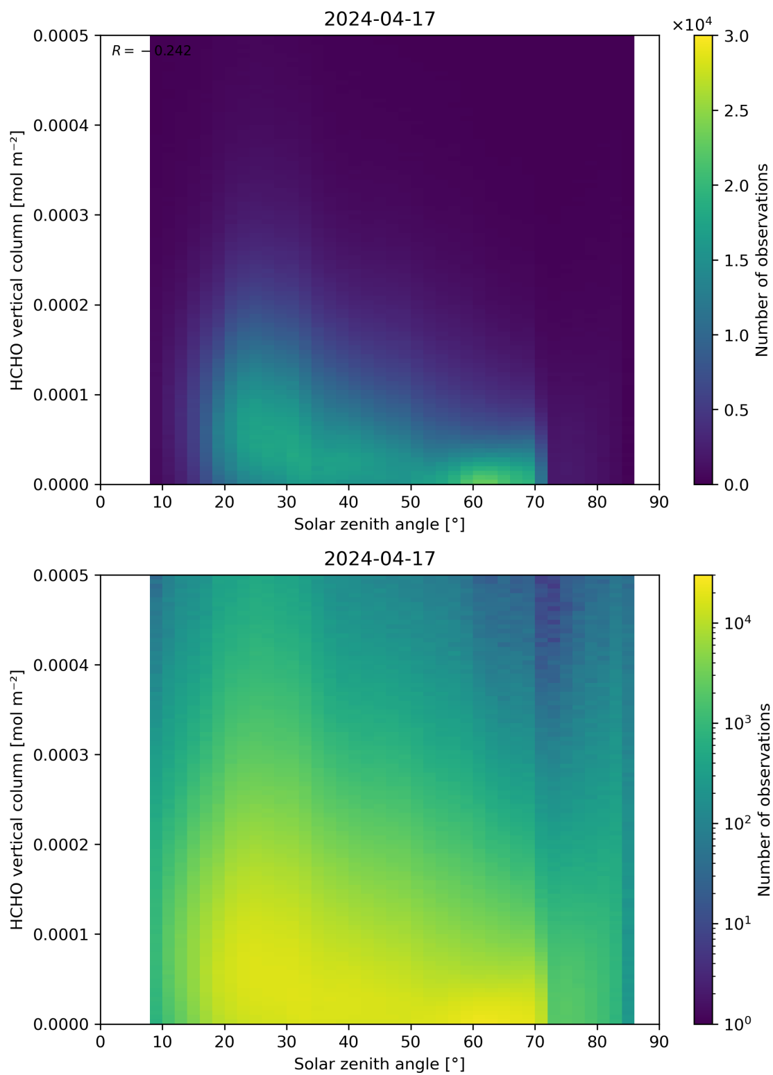
Figure 177: Scatter density plot of “Solar zenith angle” against “HCHO vertical column” for 2024-04-16 to 2024-04-18.
