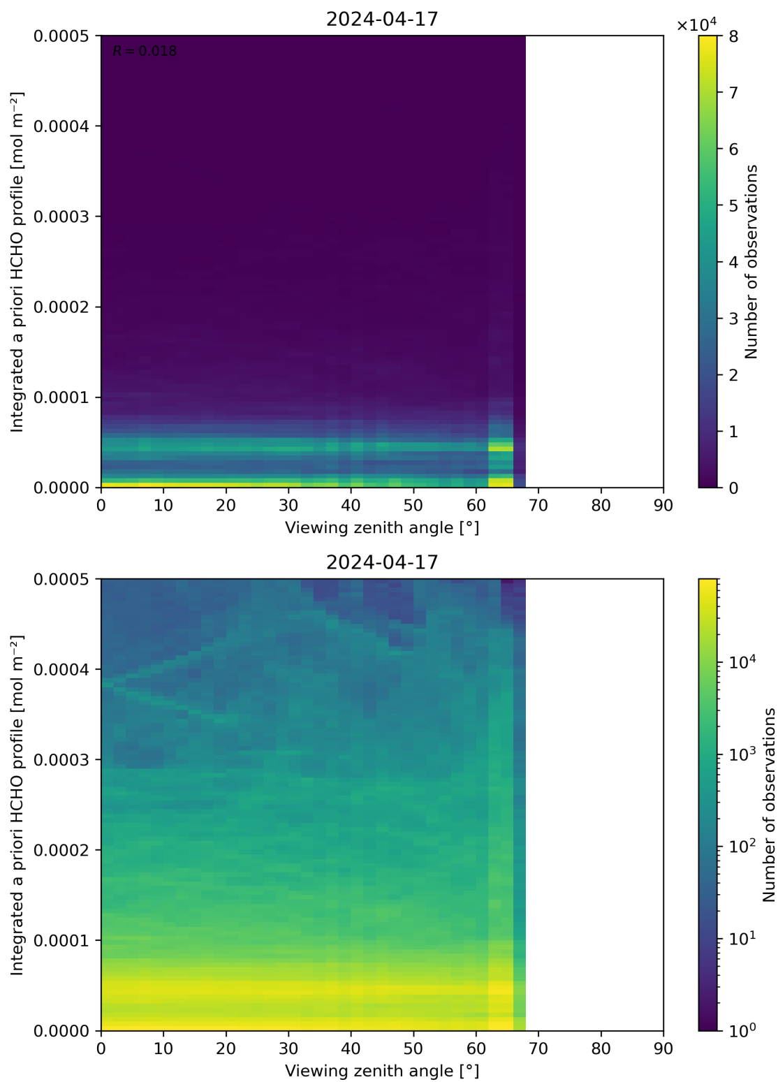
Figure 195: Scatter density plot of “Viewing zenith angle” against “Integrated a priori HCHO profile” for 2024-04-16 to 2024-04-18.
