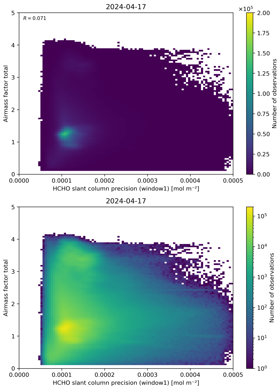
Figure 94: Scatter density plot of “HCHO slant column precision (window1)” against “Airmass factor total” for 2024-04-16 to 2024-04-18.
