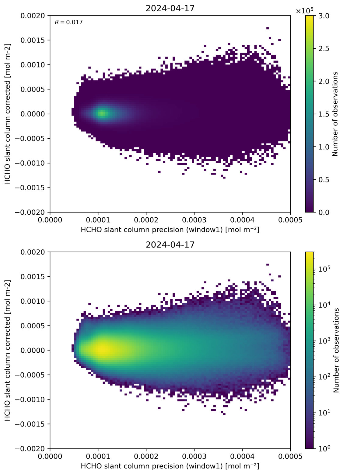
Figure 92: Scatter density plot of “HCHO slant column precision (window1)” against “HCHO slant column corrected” for 2024-04-16 to 2024-04-18.
