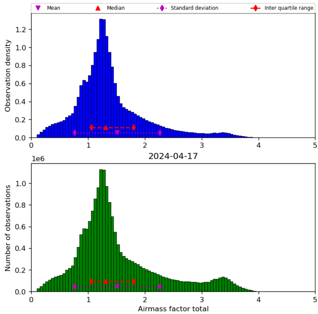
Figure 40: Histogram of “Airmass factor total” for 2024-04-16 to 2024-04-18
