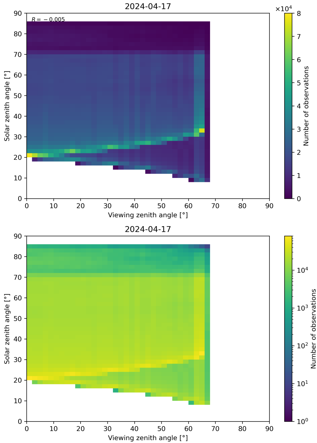
Figure 197: Scatter density plot of “Viewing zenith angle” against “Solar zenith angle” for 2024-04-16 to 2024-04-18.
