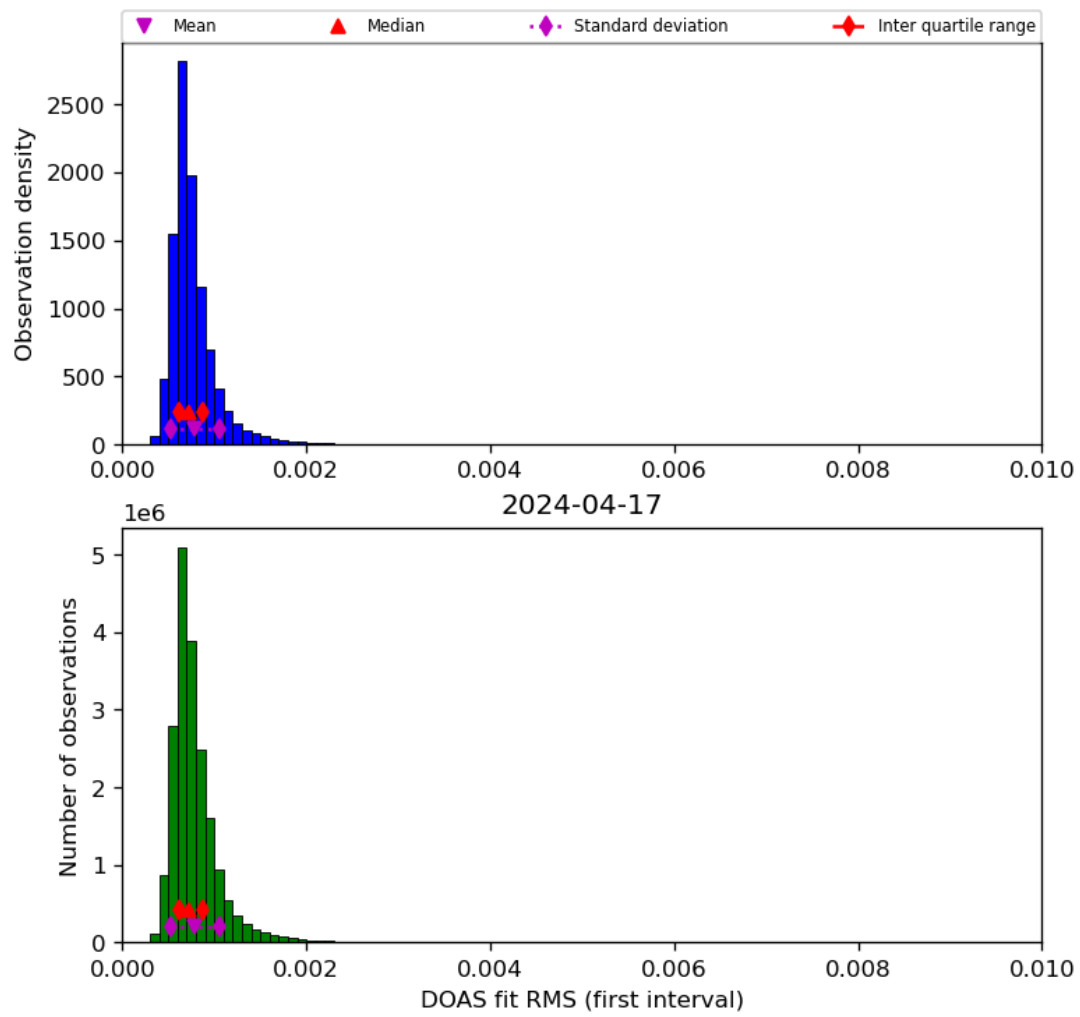
Figure 46: Histogram of “DOAS fit RMS (first interval)” for 2024-04-16 to 2024-04-18
