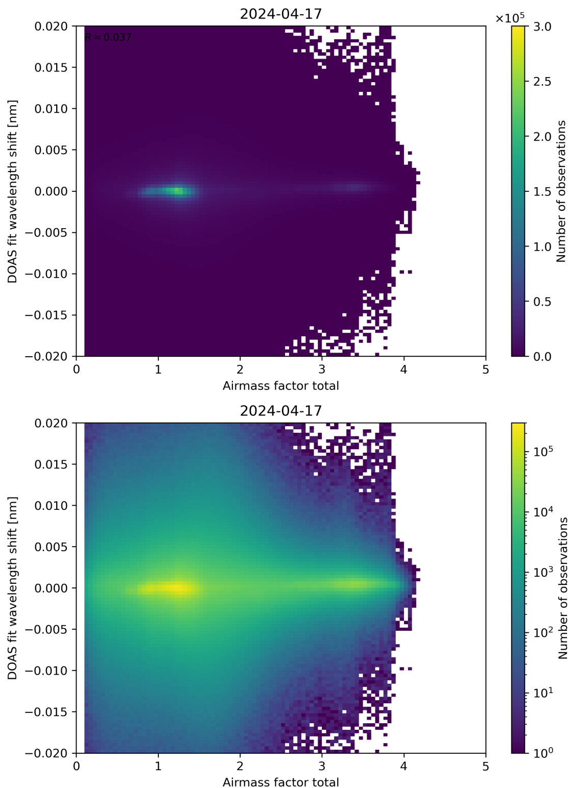
Figure 98: Scatter density plot of “Airmass factor total” against “DOAS fit wavelength shift” for 2024-04-16 to 2024-04-18.
