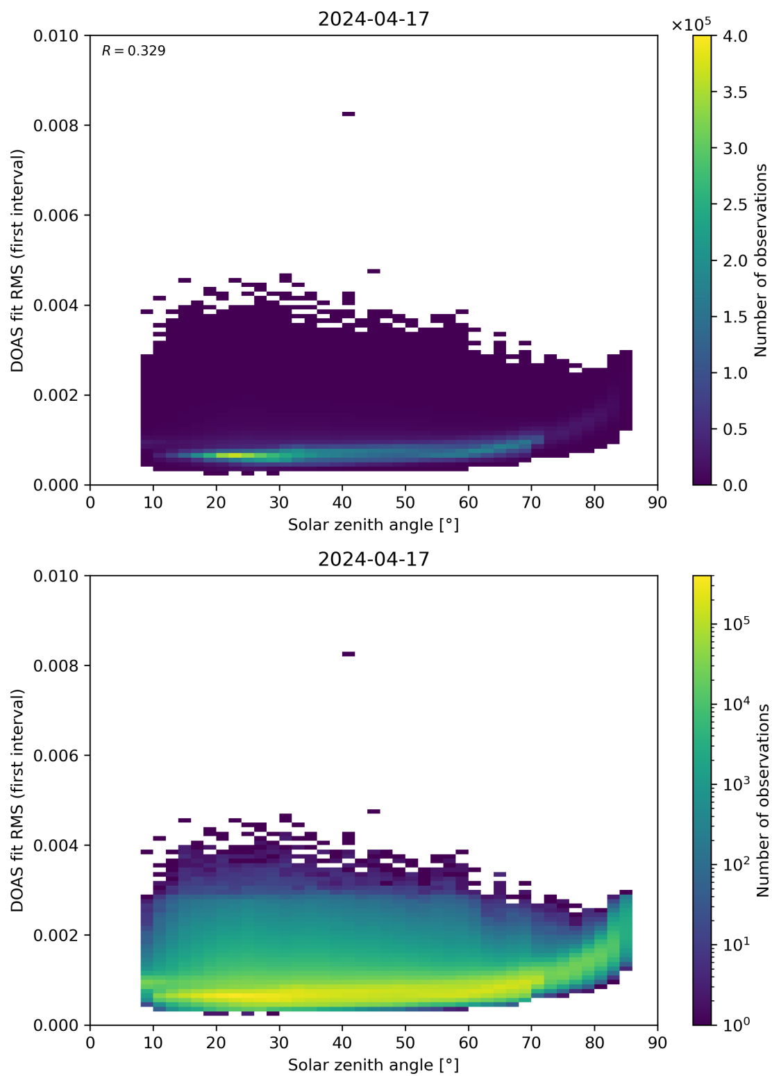
Figure 167: Scatter density plot of “Solar zenith angle” against “DOAS fit RMS (first interval)” for 2024-04-16 to 2024-04-18.
