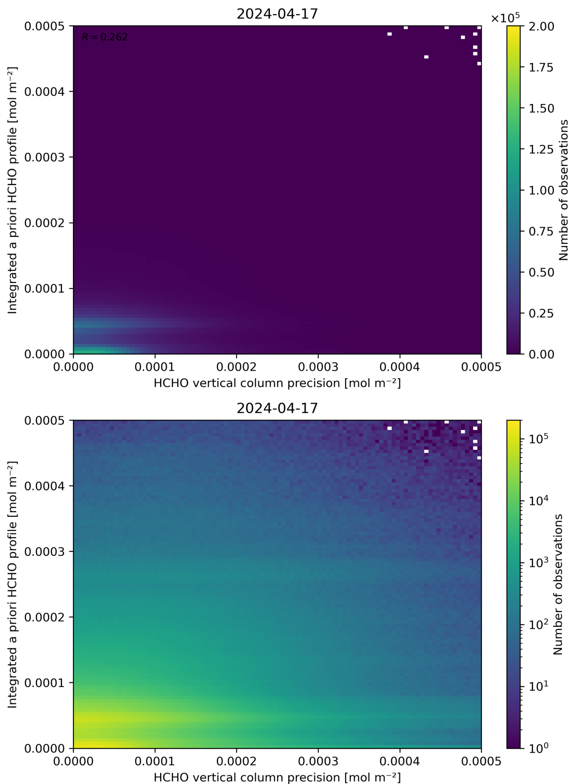
Figure 147: Scatter density plot of “HCHO vertical column precision” against “Integrated a priori HCHO profile” for 2024-04-16 to 2024-04-18.
