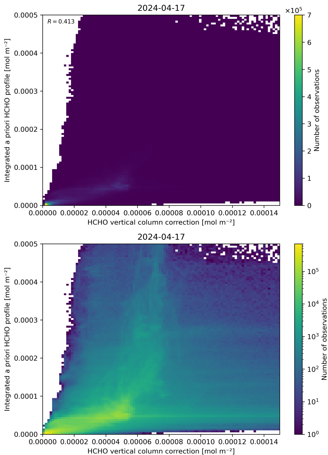
Figure 122: Scatter density plot of “HCHO vertical column correction” against “Integrated a priori HCHO profile” for 2024-04-16 to 2024-04-18.
