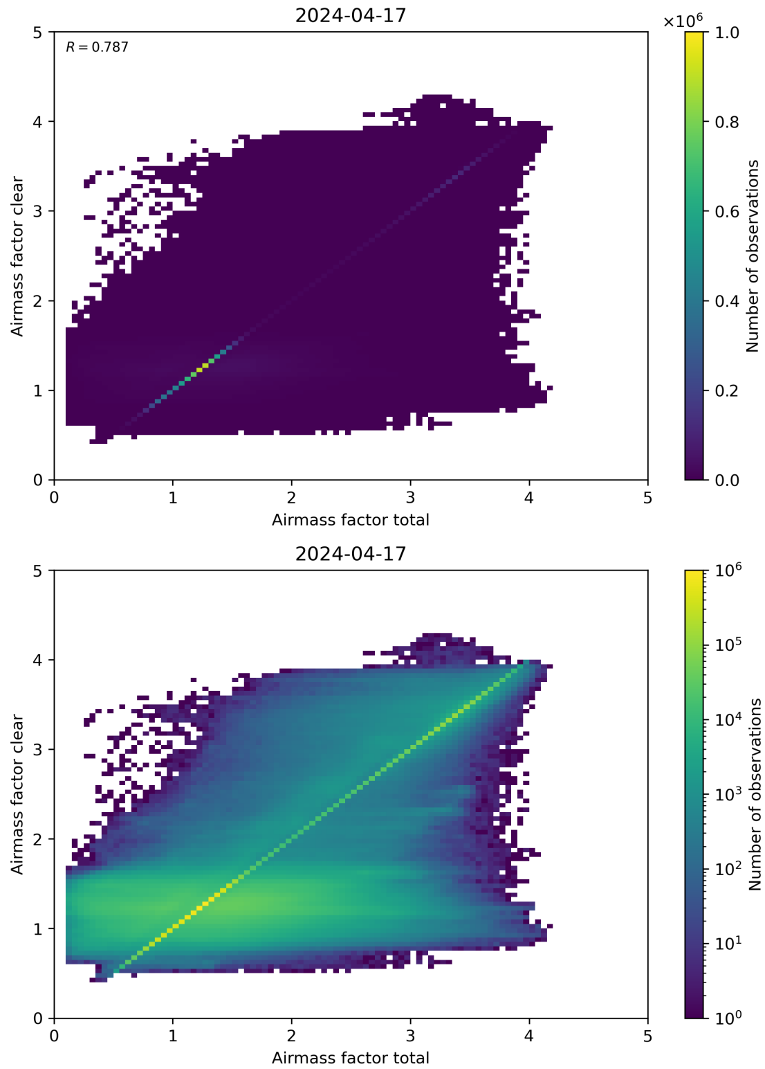
Figure 100: Scatter density plot of “Airmass factor total” against “Airmass factor clear” for 2024-04-16 to 2024-04-18.
