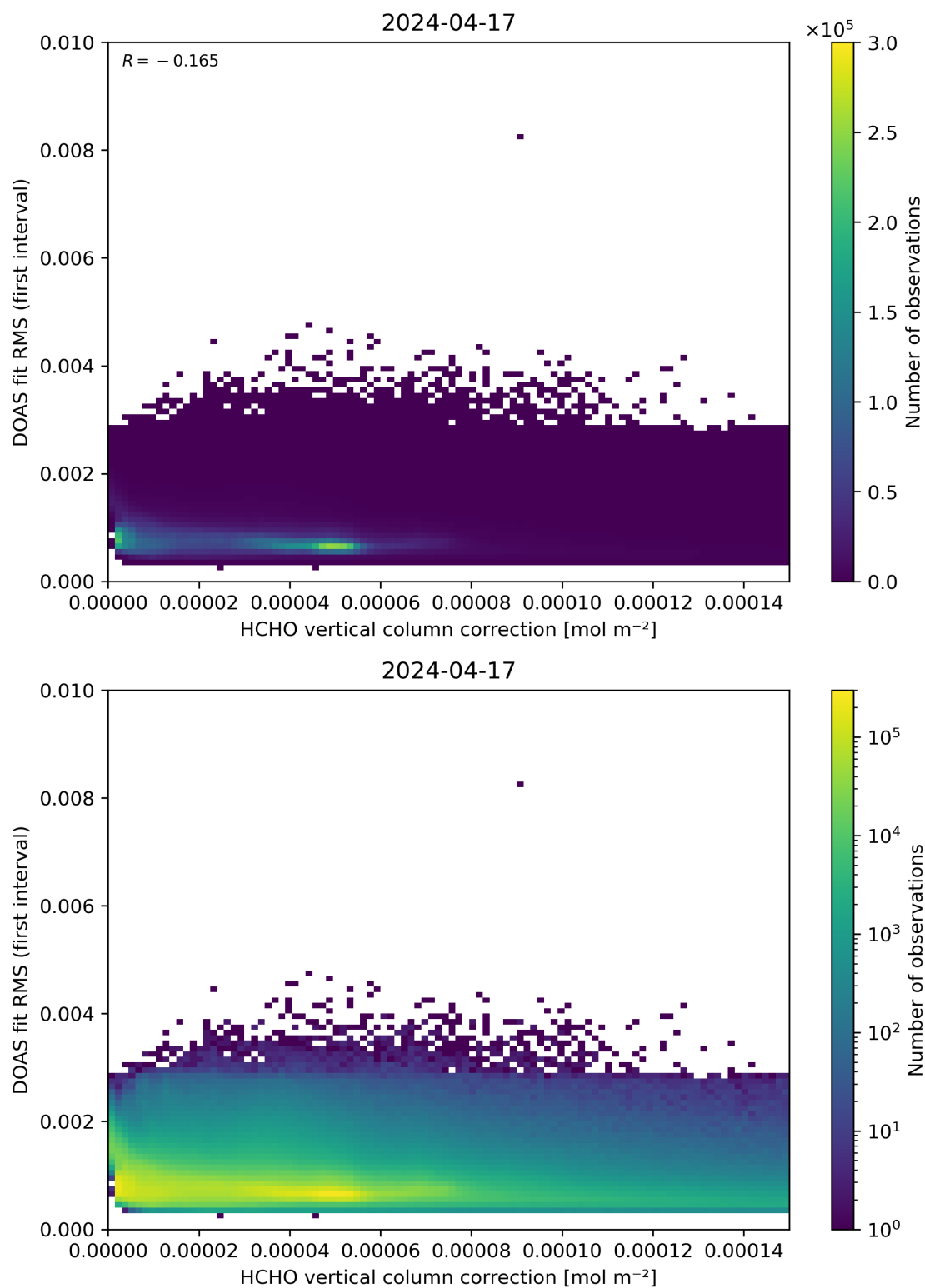
Figure 112: Scatter density plot of “HCHO vertical column correction” against “DOAS fit RMS (first interval)” for 2024-04-16 to 2024-04-18.
