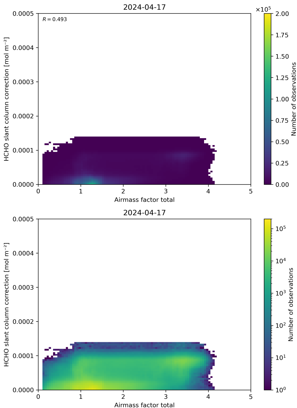
Figure 102: Scatter density plot of “Airmass factor total” against “HCHO slant column correction” for 2024-04-16 to 2024-04-18.
