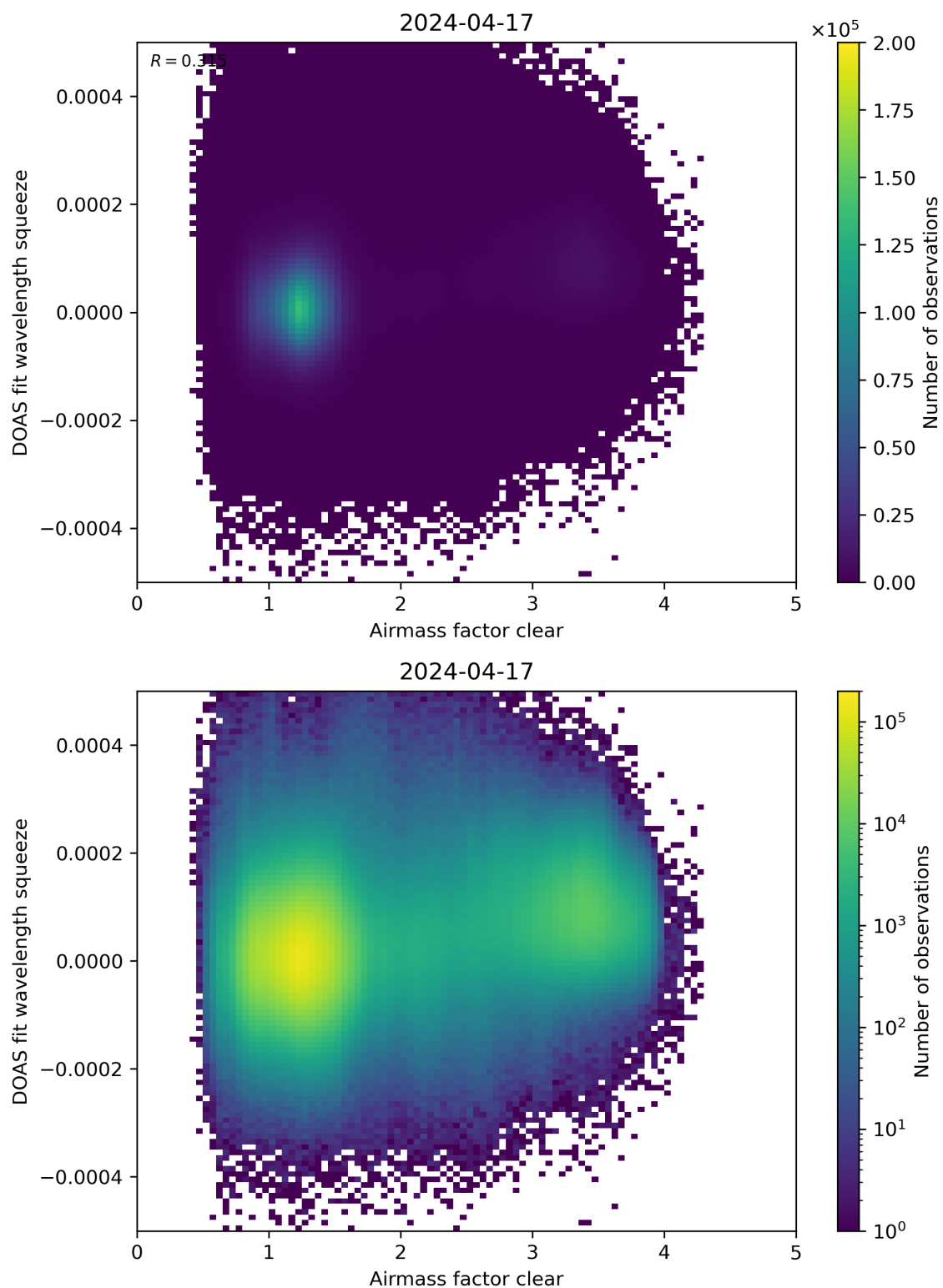
Figure 73: Scatter density plot of “Airmass factor clear” against “DOAS fit wavelength squeeze” for 2024-04-16 to 2024-04-18.
