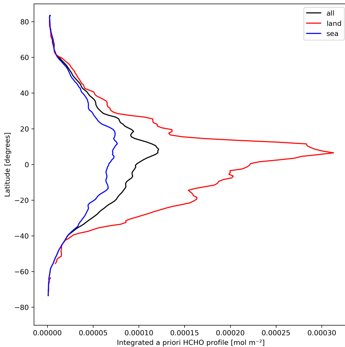
Figure 29: Zonal average of “Integrated a priori HCHO profile” for 2024-04-16 to 2024-04-18.
