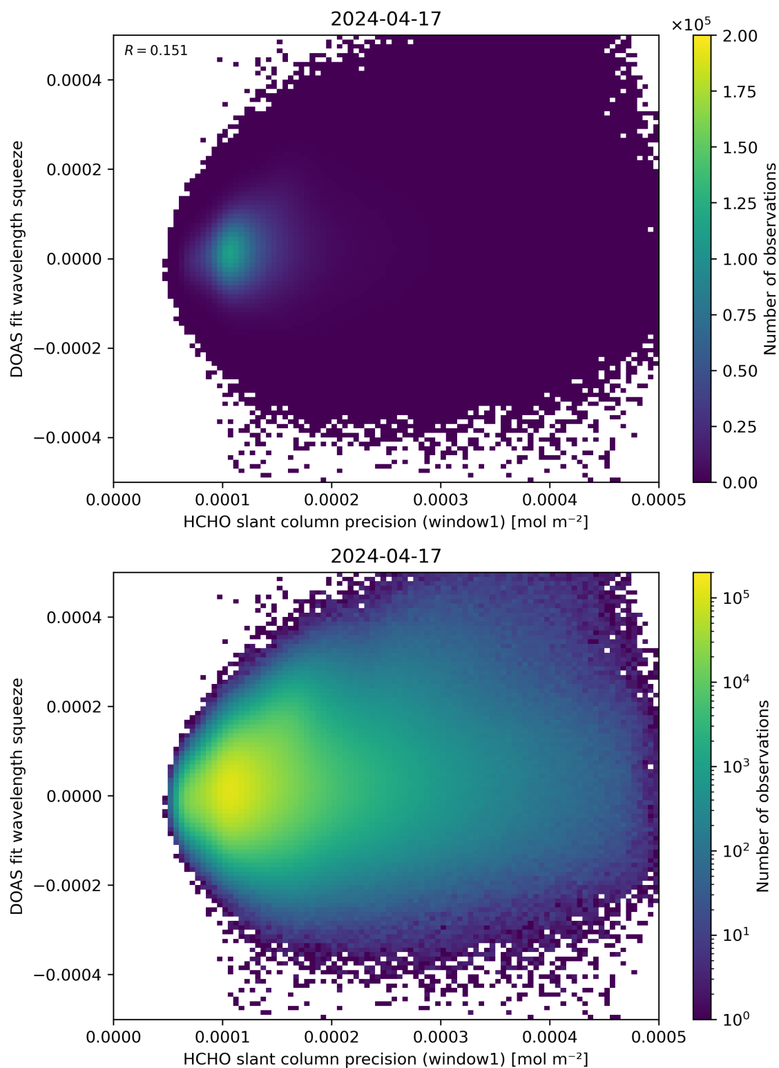
Figure 90: Scatter density plot of “HCHO slant column precision (window1)” against “DOAS fit wavelength squeeze” for 2024-04-16 to 2024-04-18.
