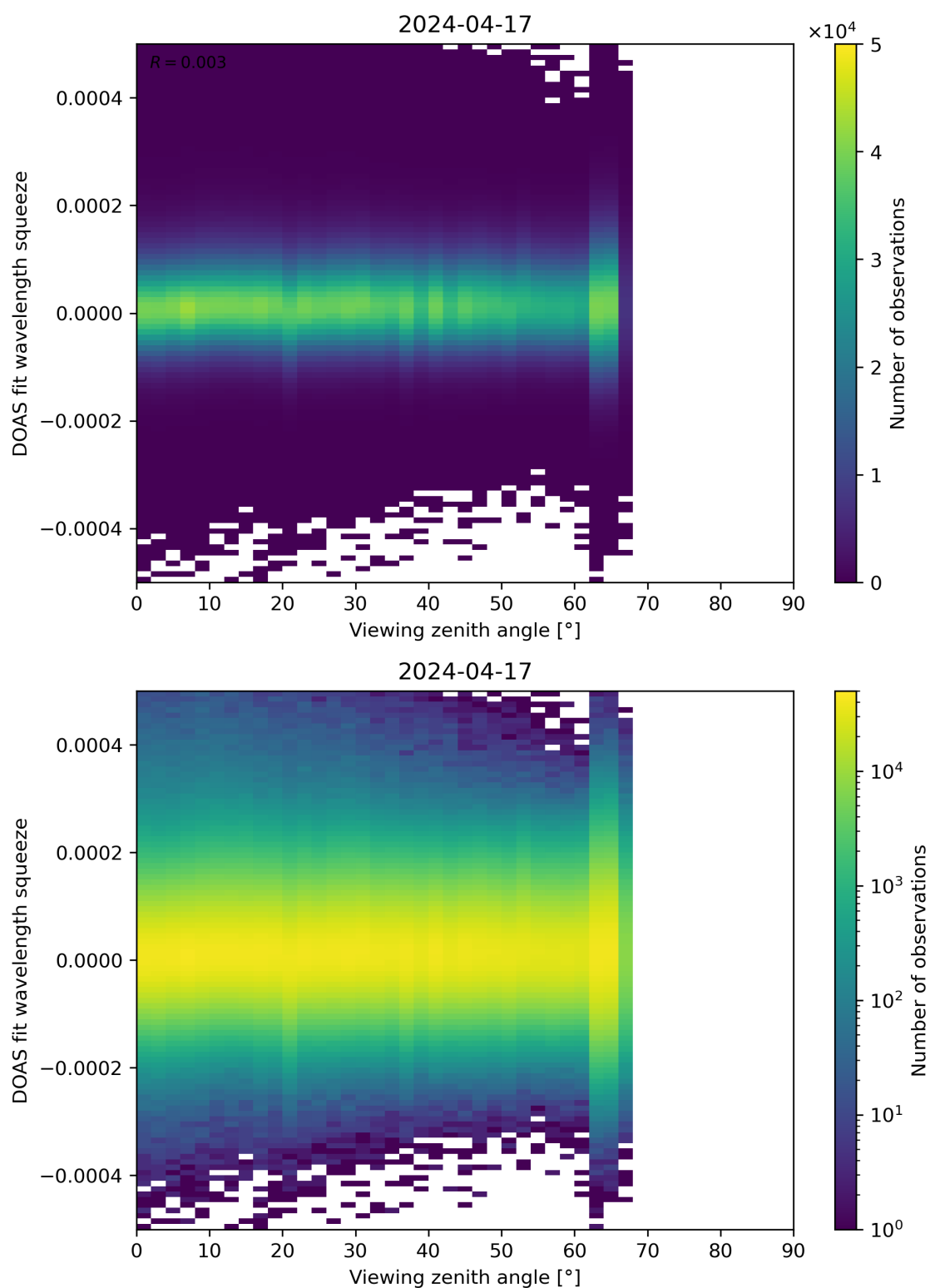
Figure 184: Scatter density plot of “Viewing zenith angle” against “DOAS fit wavelength squeeze” for 2024-04-16 to 2024-04-18.
