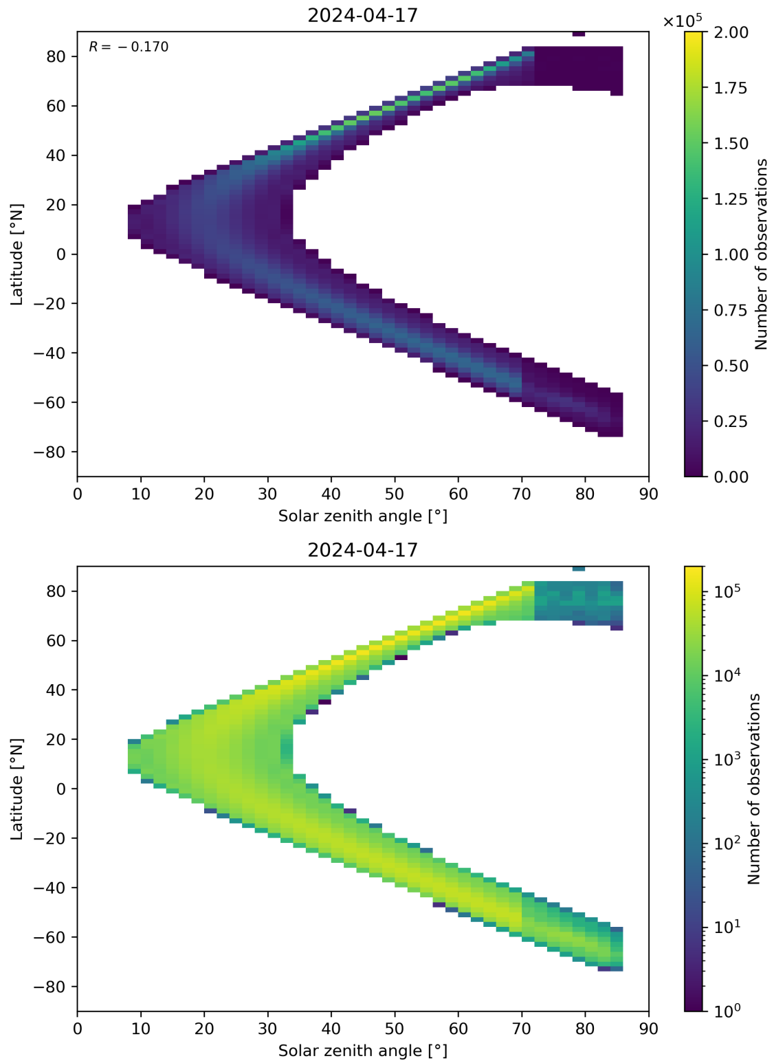
Figure 181: Scatter density plot of “Solar zenith angle” against “Latitude” for 2024-04-16 to 2024-04-18.
