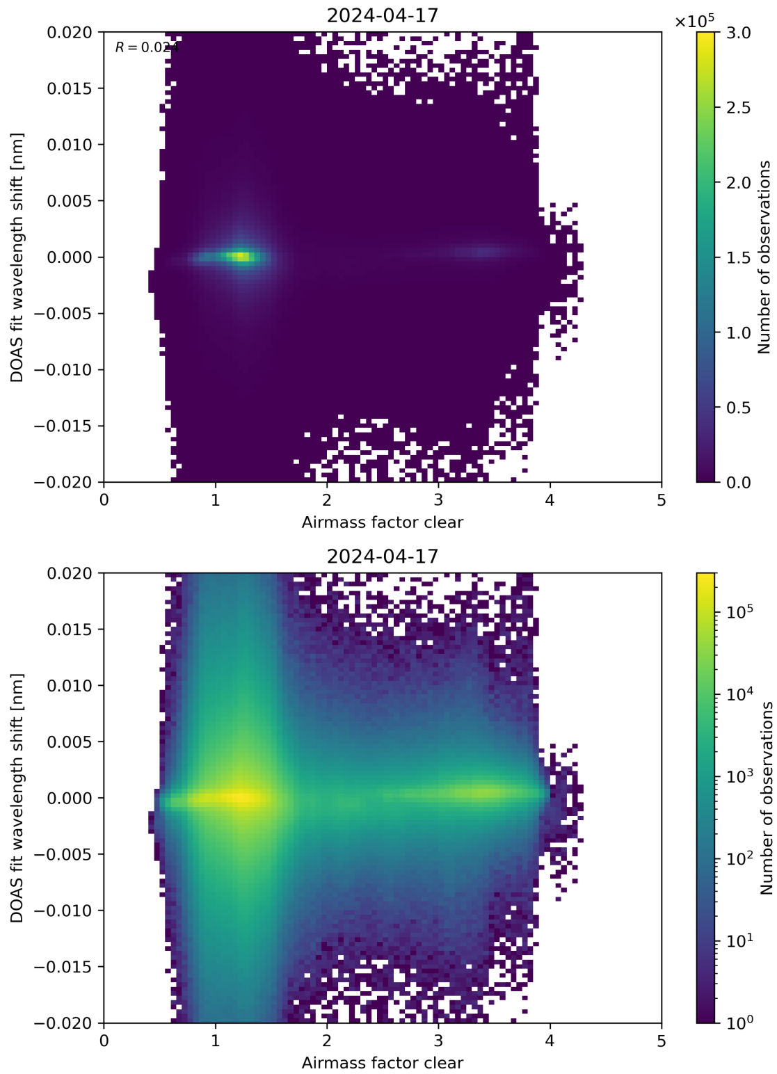
Figure 72: Scatter density plot of “Airmass factor clear” against “DOAS fit wavelength shift” for 2024-04-16 to 2024-04-18.
