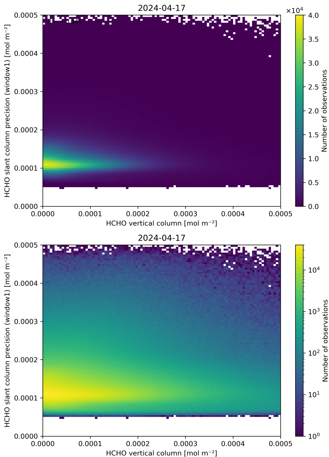
Figure 130: Scatter density plot of “HCHO vertical column” against “HCHO slant column precision (window1)” for 2024-04-16 to 2024-04-18.
