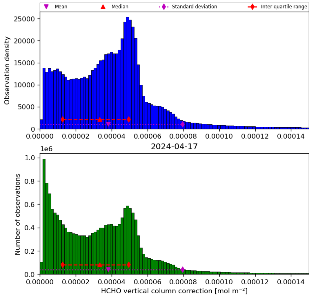
Figure 37: Histogram of “HCHO vertical column correction” for 2024-04-16 to 2024-04-18
