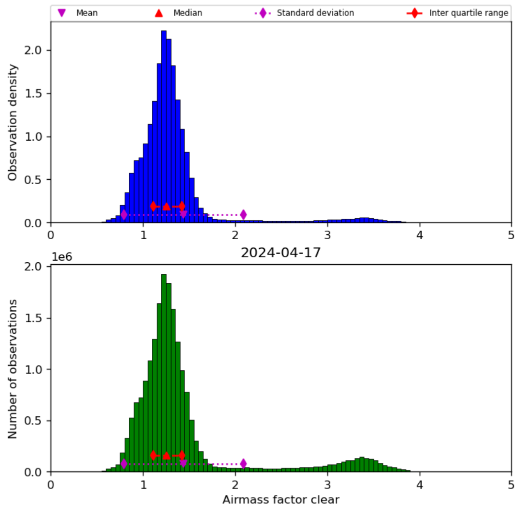
Figure 42: Histogram of “Airmass factor clear” for 2024-04-16 to 2024-04-18
