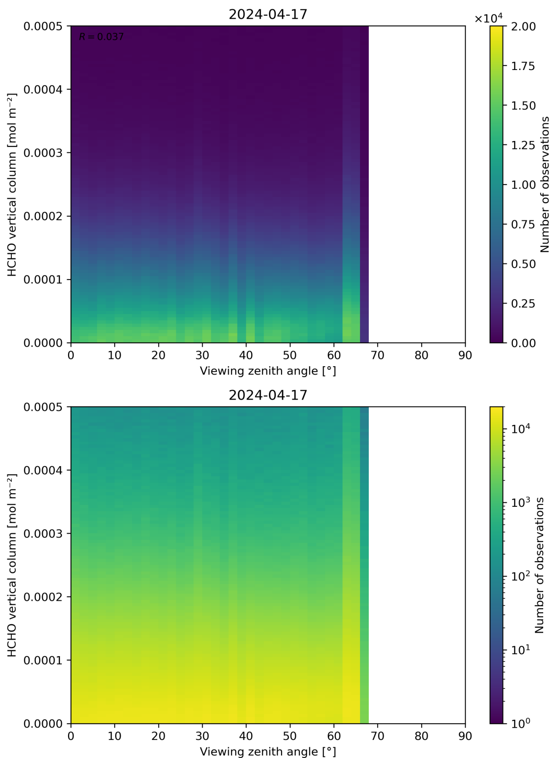
Figure 192: Scatter density plot of “Viewing zenith angle” against “HCHO vertical column” for 2024-04-16 to 2024-04-18.
