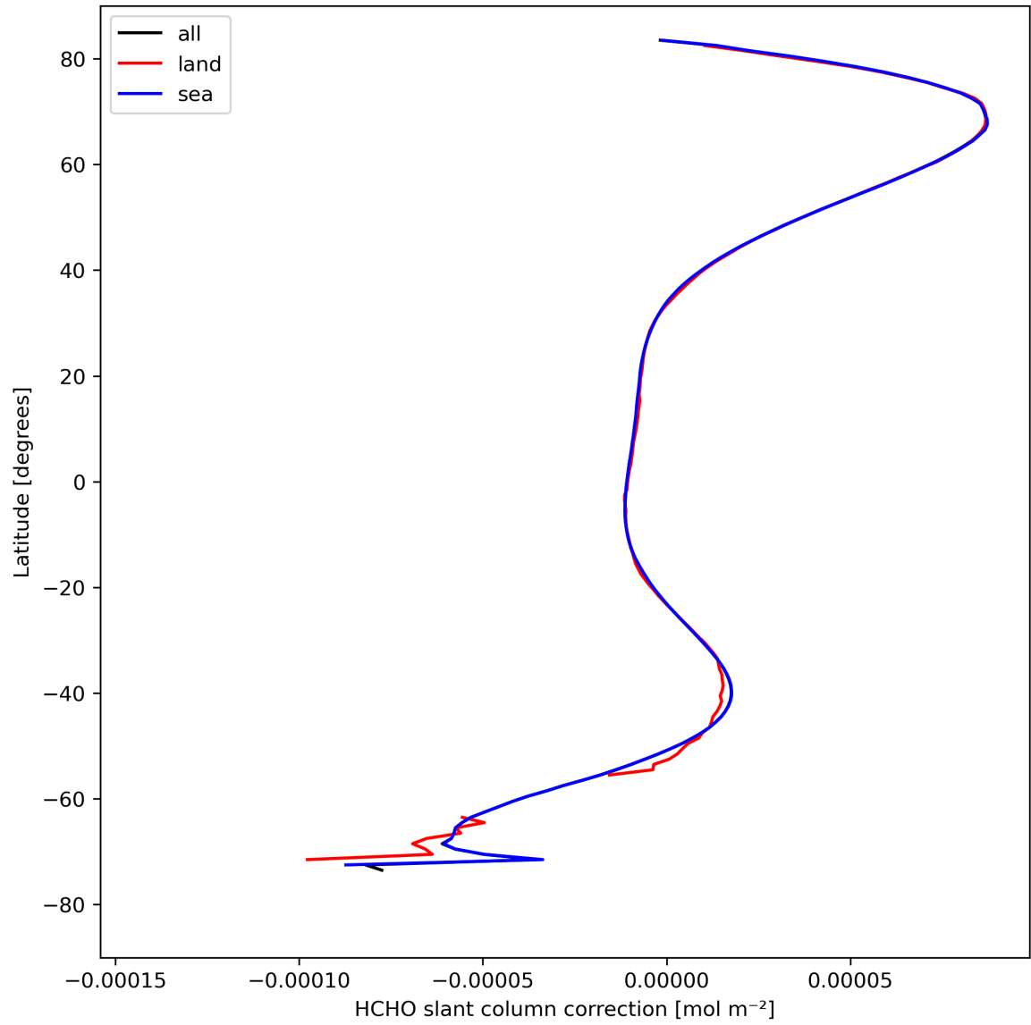
Figure 33: Zonal average of “HCHO slant column correction” for 2024-04-16 to 2024-04-18.
