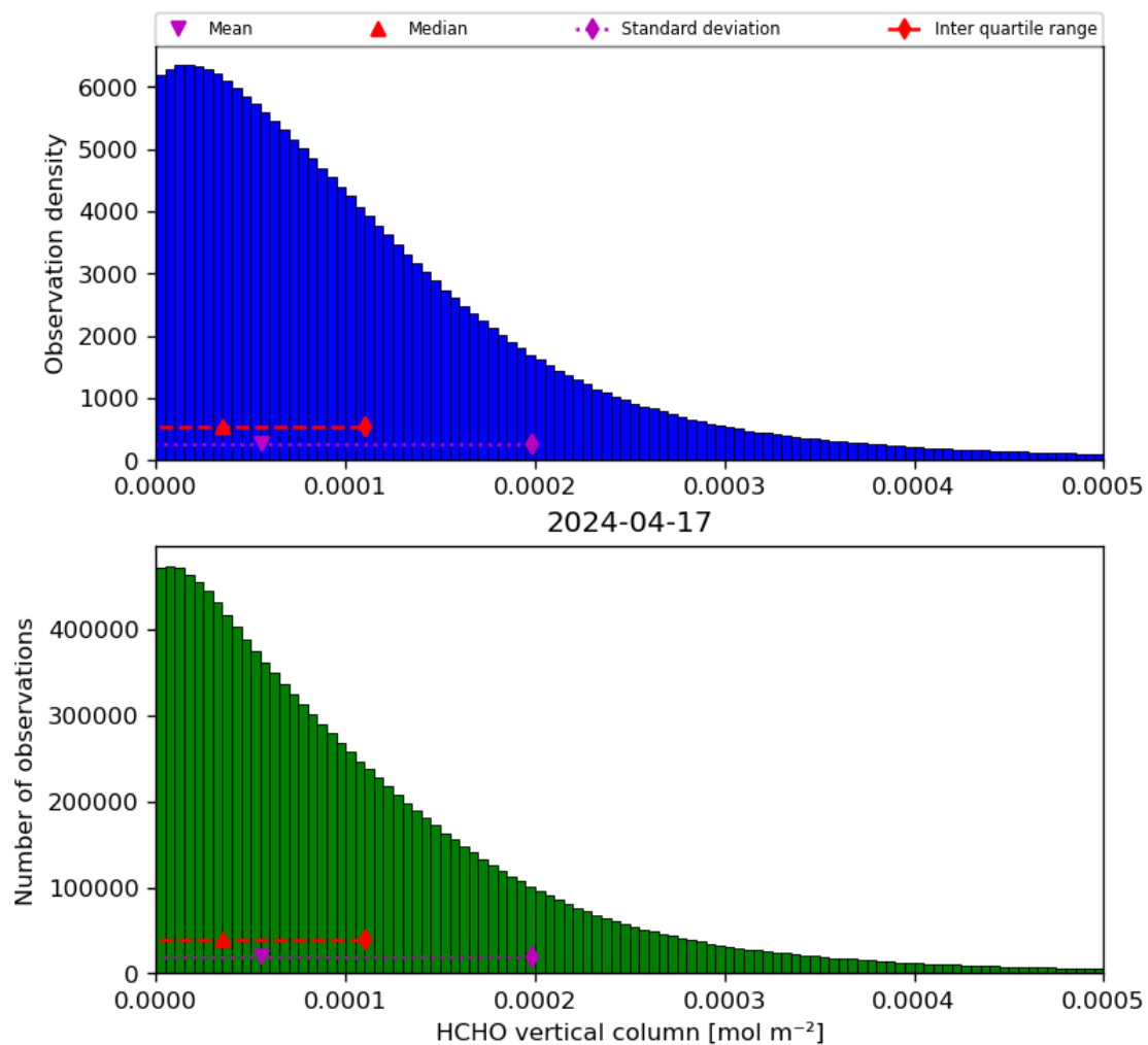
Figure 35: Histogram of “HCHO vertical column” for 2024-04-16 to 2024-04-18
