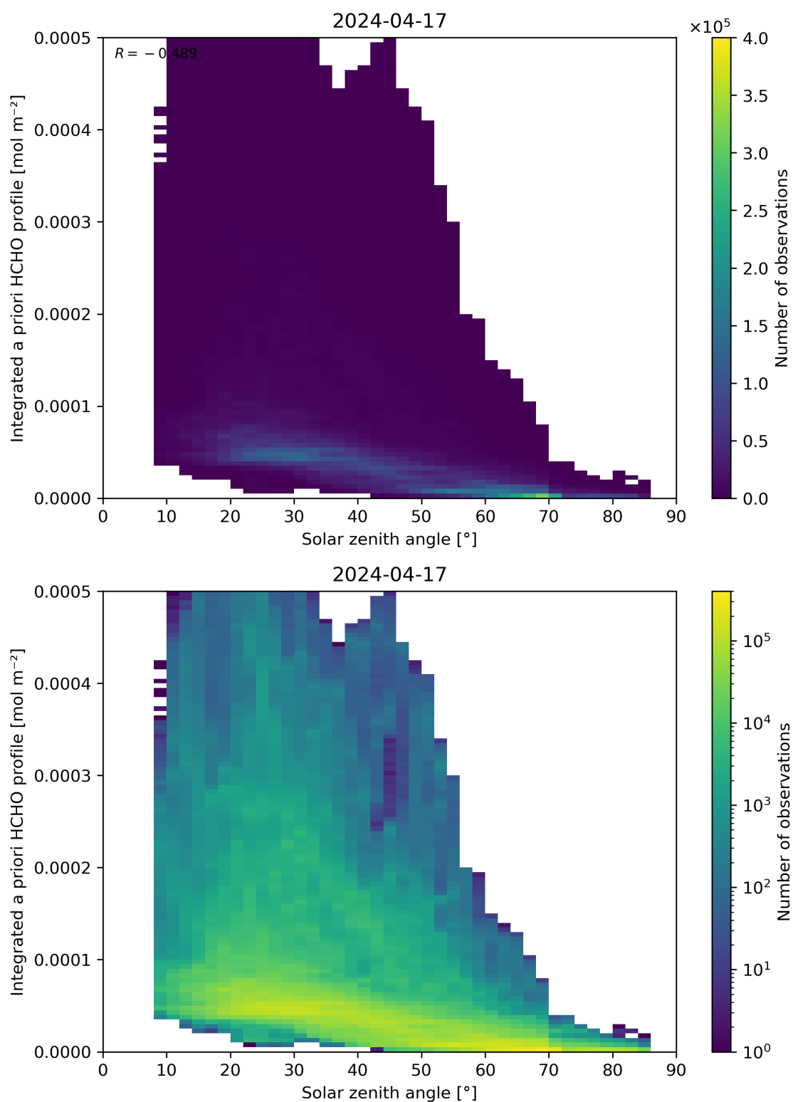
Figure 180: Scatter density plot of “Solar zenith angle” against “Integrated a priori HCHO profile” for 2024-04-16 to 2024-04-18.
