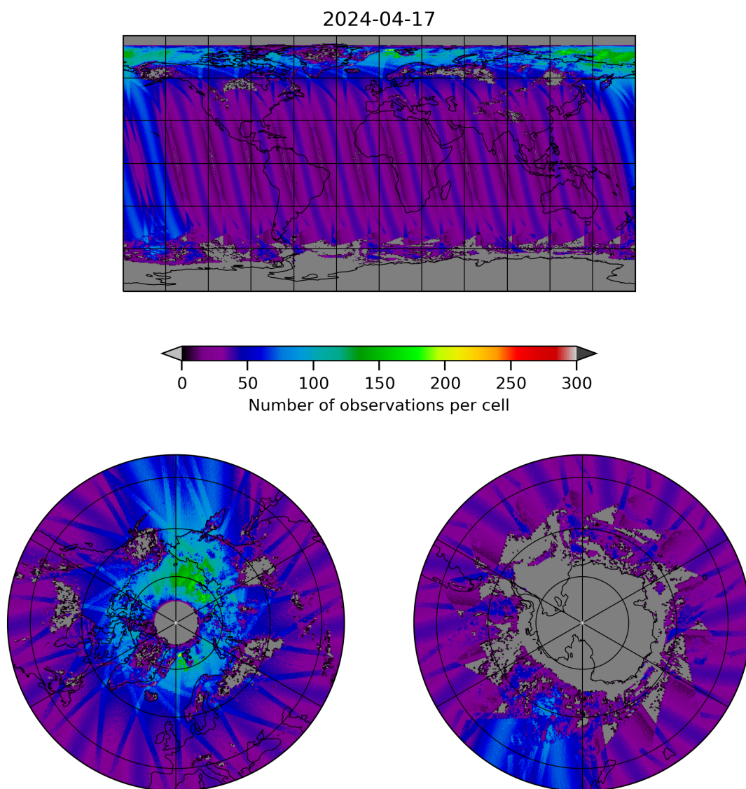
Figure 19: Map of the number of observations for 2024-04-16 to 2024-04-18
