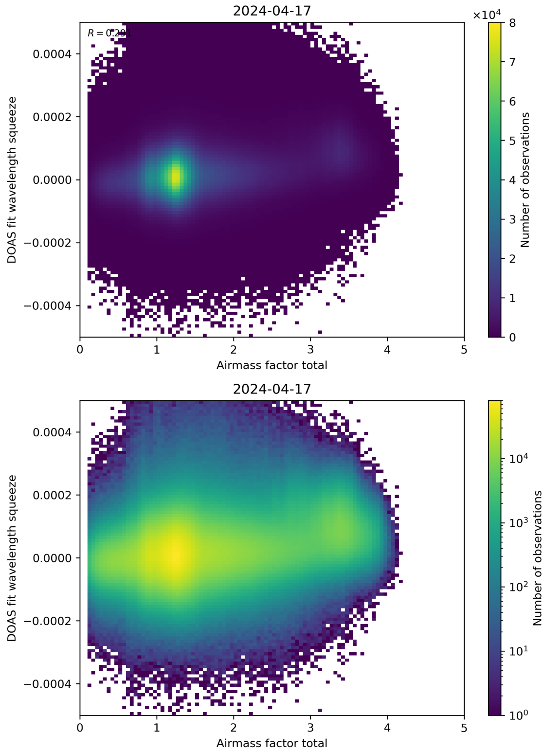
Figure 99: Scatter density plot of “Airmass factor total” against “DOAS fit wavelength squeeze” for 2024-04-16 to 2024-04-18.
