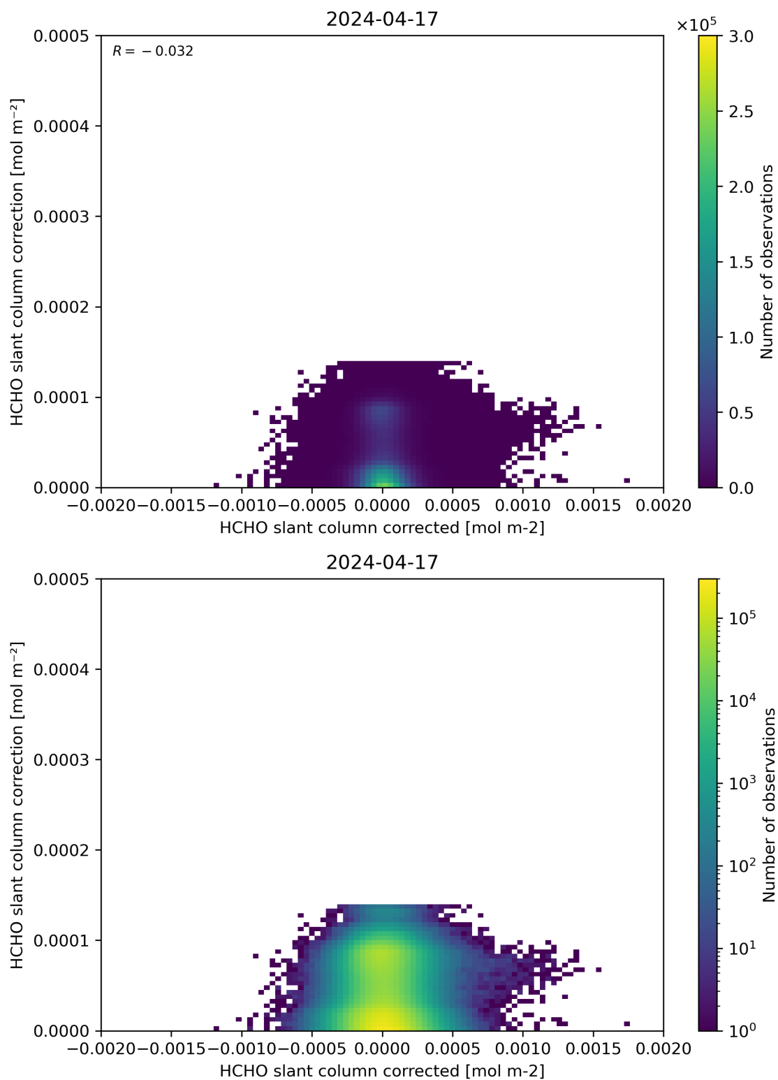
Figure 77: Scatter density plot of “HCHO slant column corrected” against “HCHO slant column correction” for 2024-04-16 to 2024-04-18.
