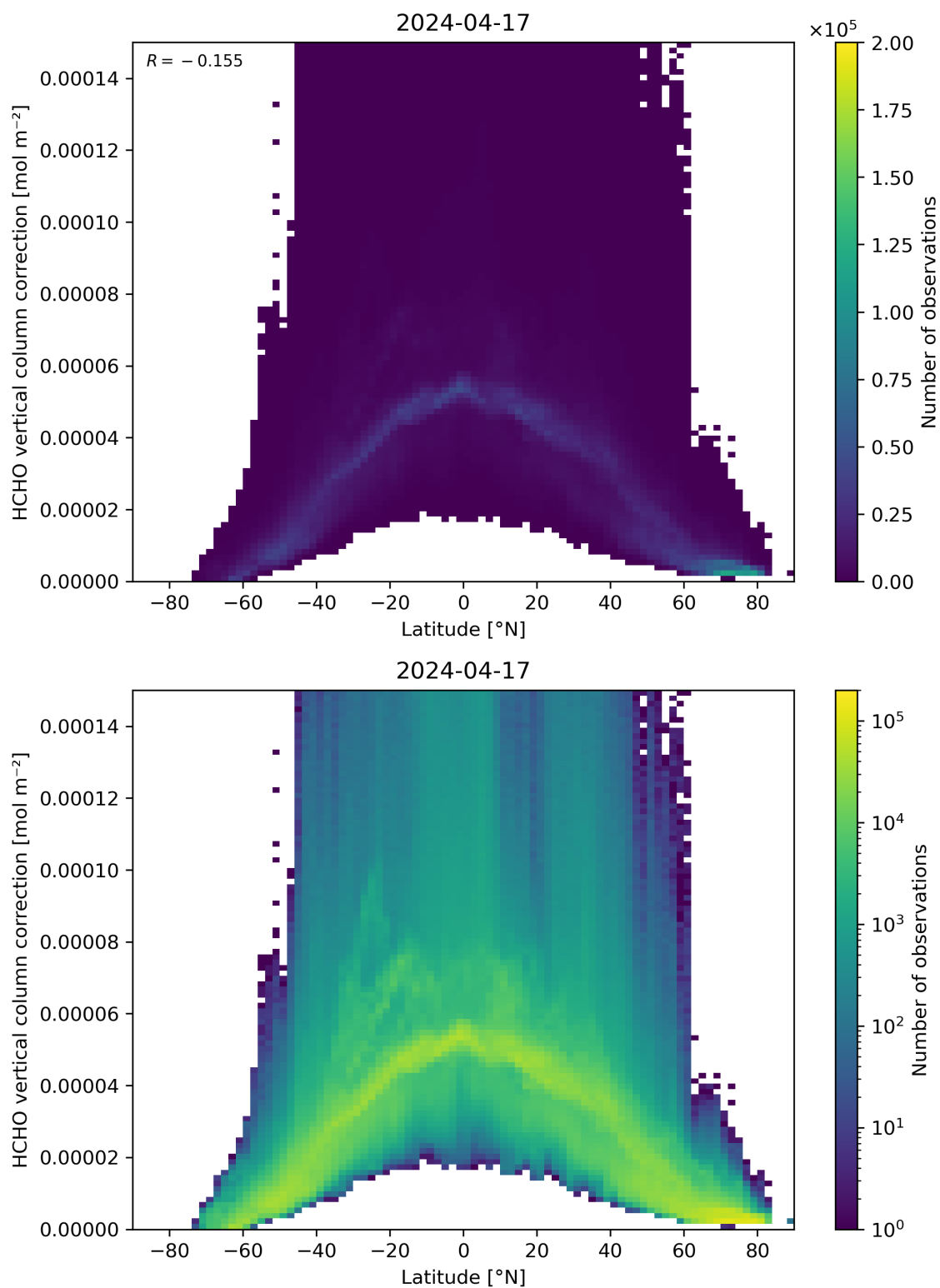
Figure 164: Scatter density plot of “Latitude” against “HCHO vertical column correction” for 2024-04-16 to 2024-04-18.
