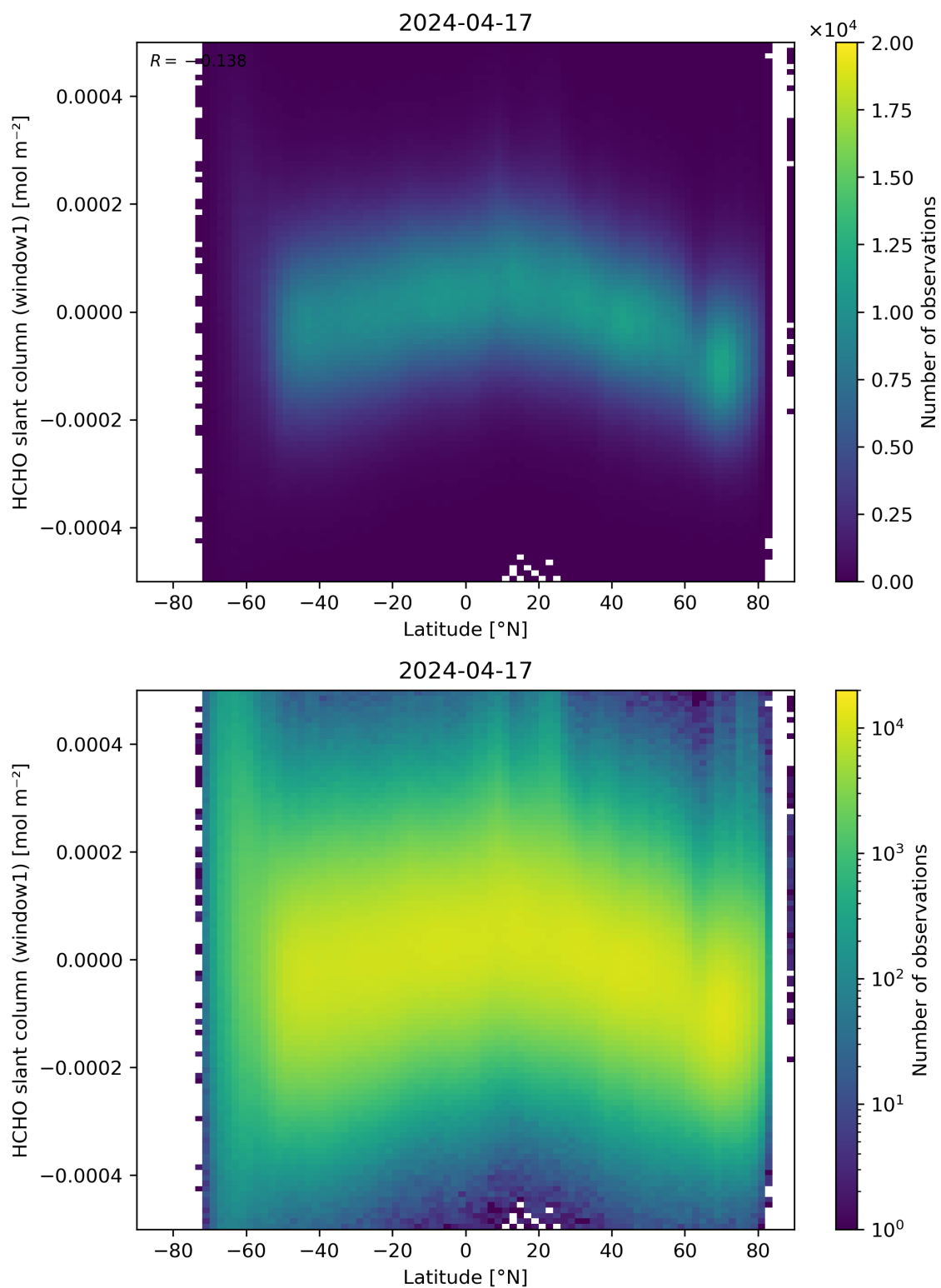
Figure 159: Scatter density plot of “Latitude” against “HCHO slant column (window1)” for 2024-04-16 to 2024-04-18.
