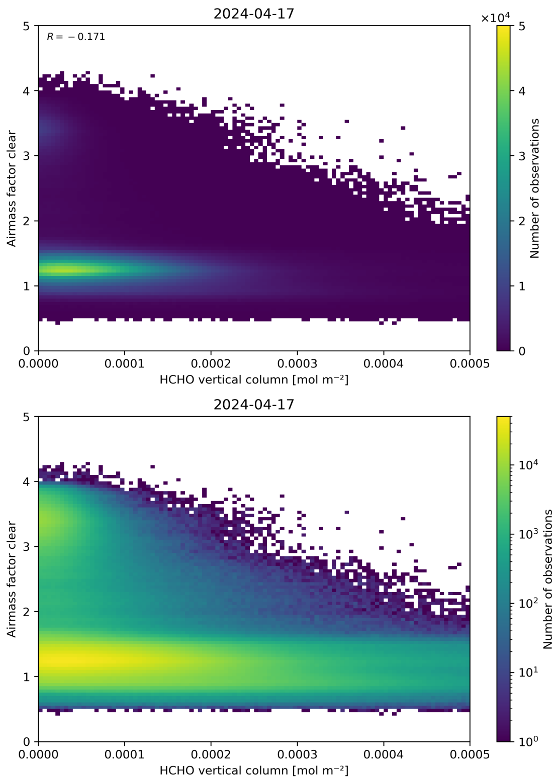
Figure 126: Scatter density plot of “HCHO vertical column” against “Airmass factor clear” for 2024-04-16 to 2024-04-18.
