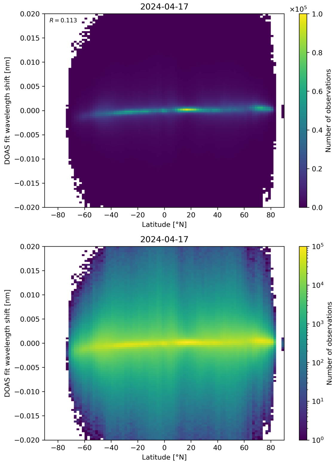
Figure 154: Scatter density plot of “Latitude” against “DOAS fit wavelength shift” for 2024-04-16 to 2024-04-18.
