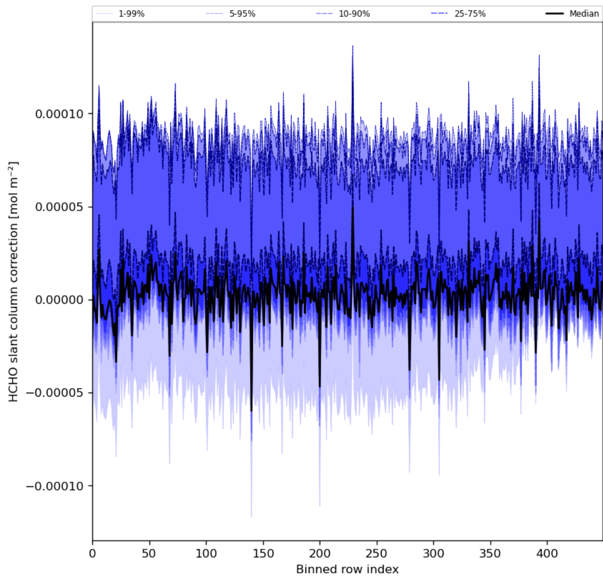
Figure 61: Along track statistics of “HCHO slant column correction” for 2024-04-16 to 2024-04-18
