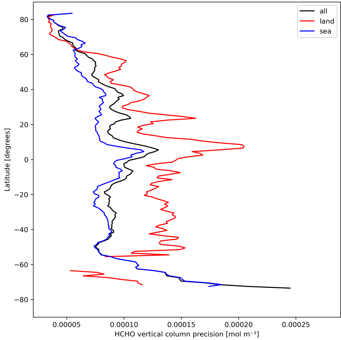
Figure 22: Zonal average of “HCHO vertical column precision” for 2024-04-16 to 2024-04-18.
