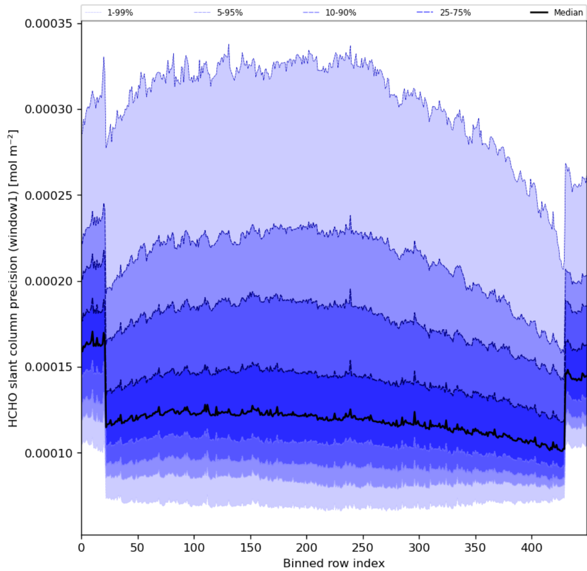
Figure 53: Along track statistics of “HCHO slant column precision (window1)” for 2024-04-16 to 2024-04-18
