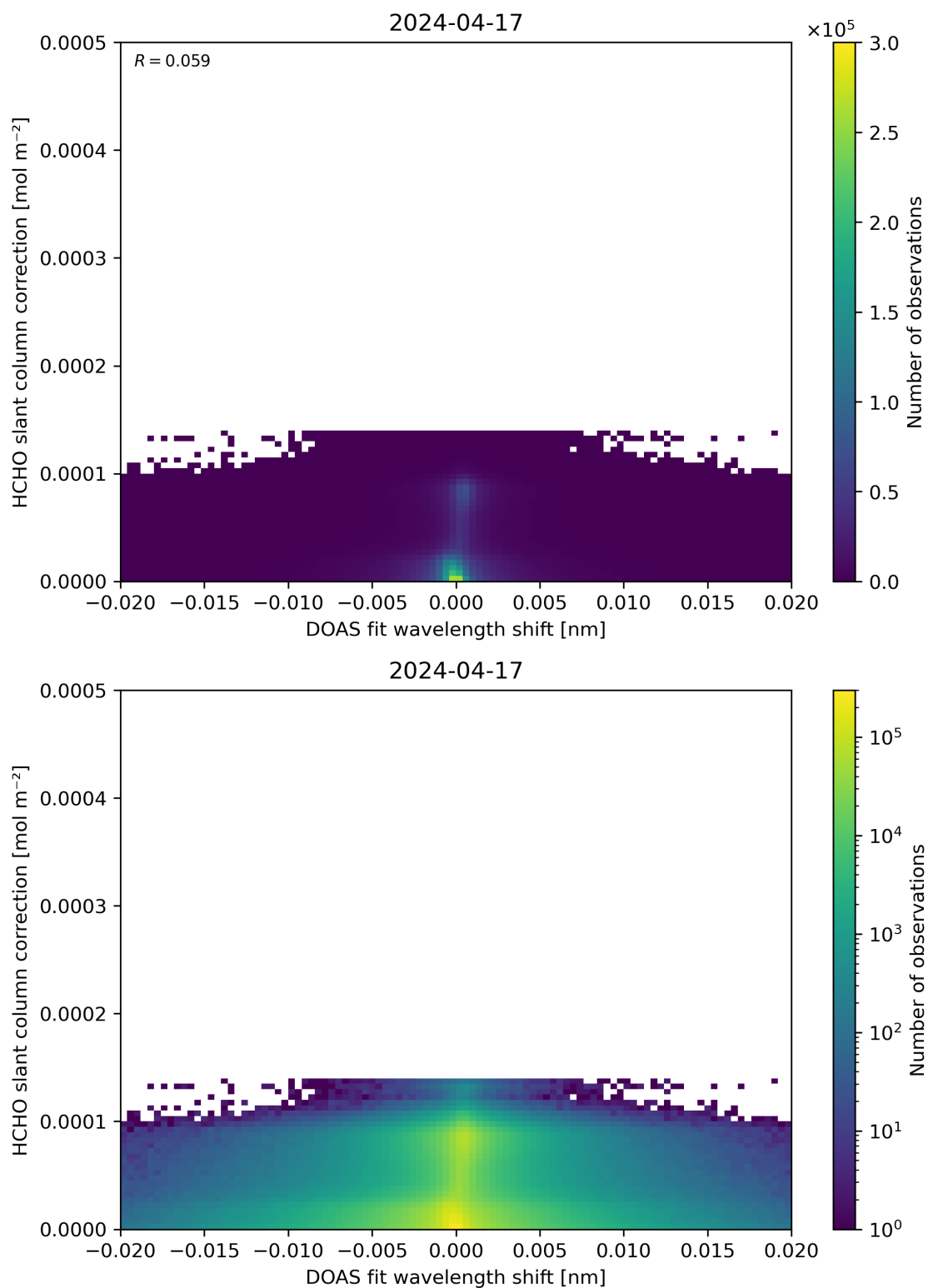
Figure 67: Scatter density plot of “DOAS fit wavelength shift” against “HCHO slant column correction” for 2024-04-16 to 2024-04-18.
