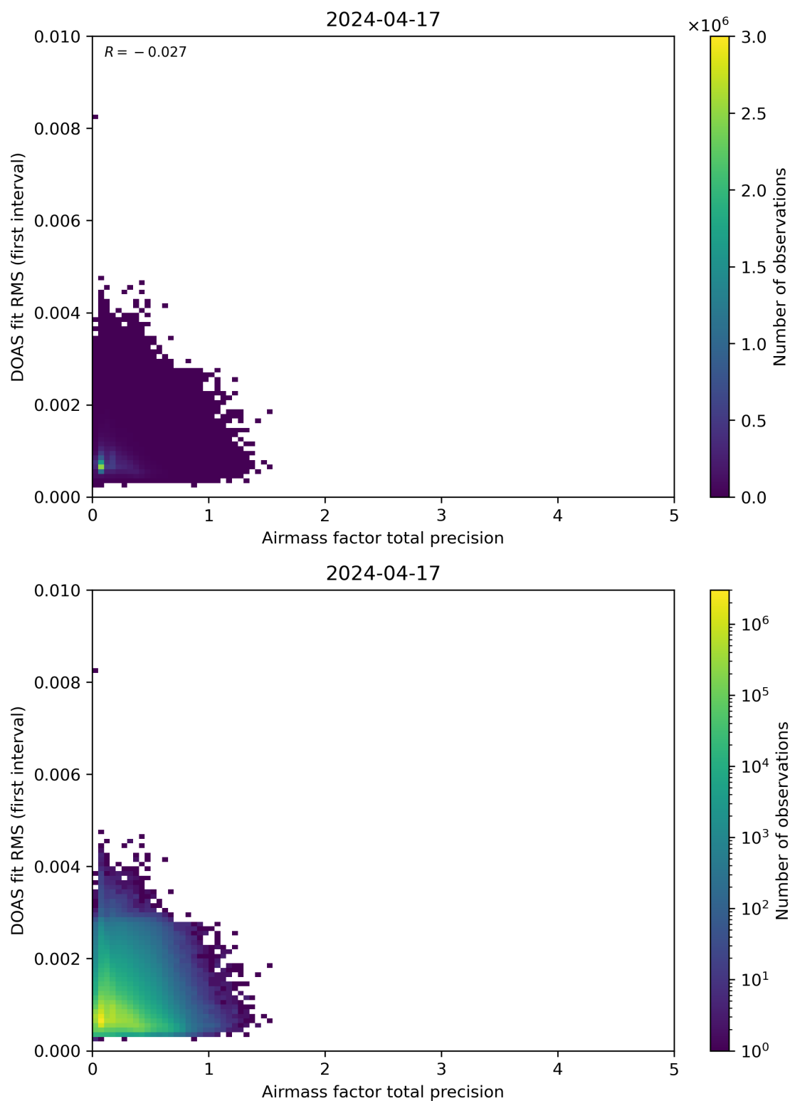
Figure 105: Scatter density plot of “Airmass factor total precision” against “DOAS fit RMS (first interval)” for 2024-04-16 to 2024-04-18.
