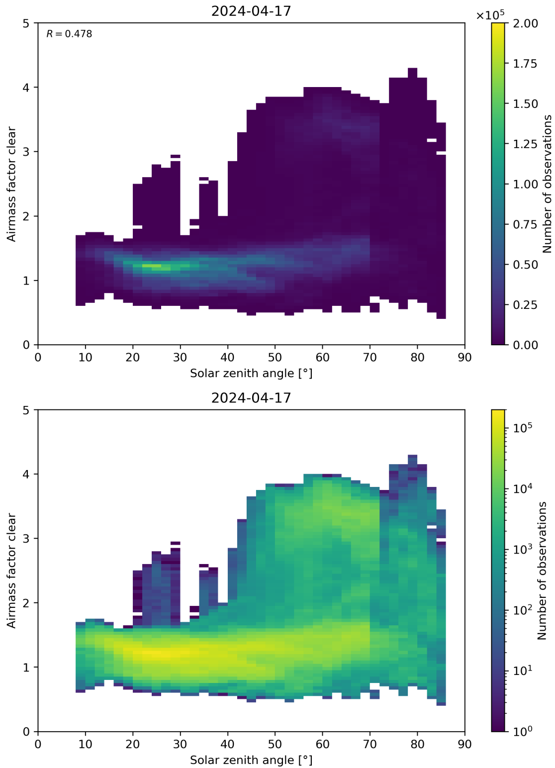
Figure 170: Scatter density plot of “Solar zenith angle” against “Airmass factor clear” for 2024-04-16 to 2024-04-18.
