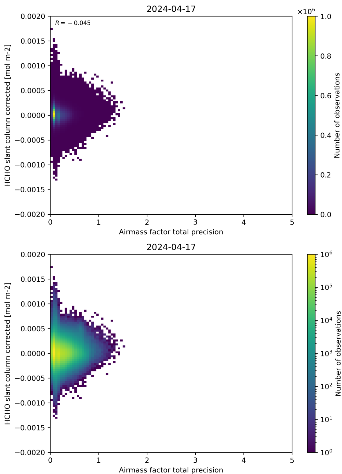
Figure 109: Scatter density plot of “Airmass factor total precision” against “HCHO slant column corrected” for 2024-04-16 to 2024-04-18.
