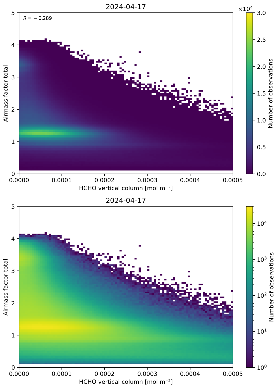
Figure 131: Scatter density plot of “HCHO vertical column” against “Airmass factor total” for 2024-04-16 to 2024-04-18.
