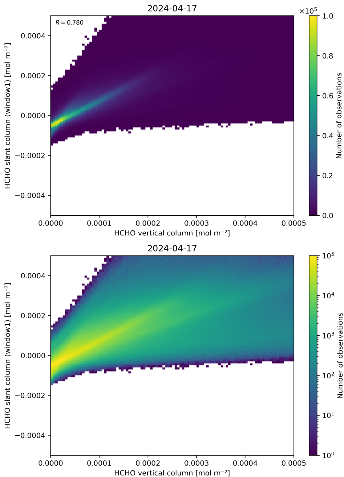
Figure 129: Scatter density plot of “HCHO vertical column” against “HCHO slant column (window1)” for 2024-04-16 to 2024-04-18.
