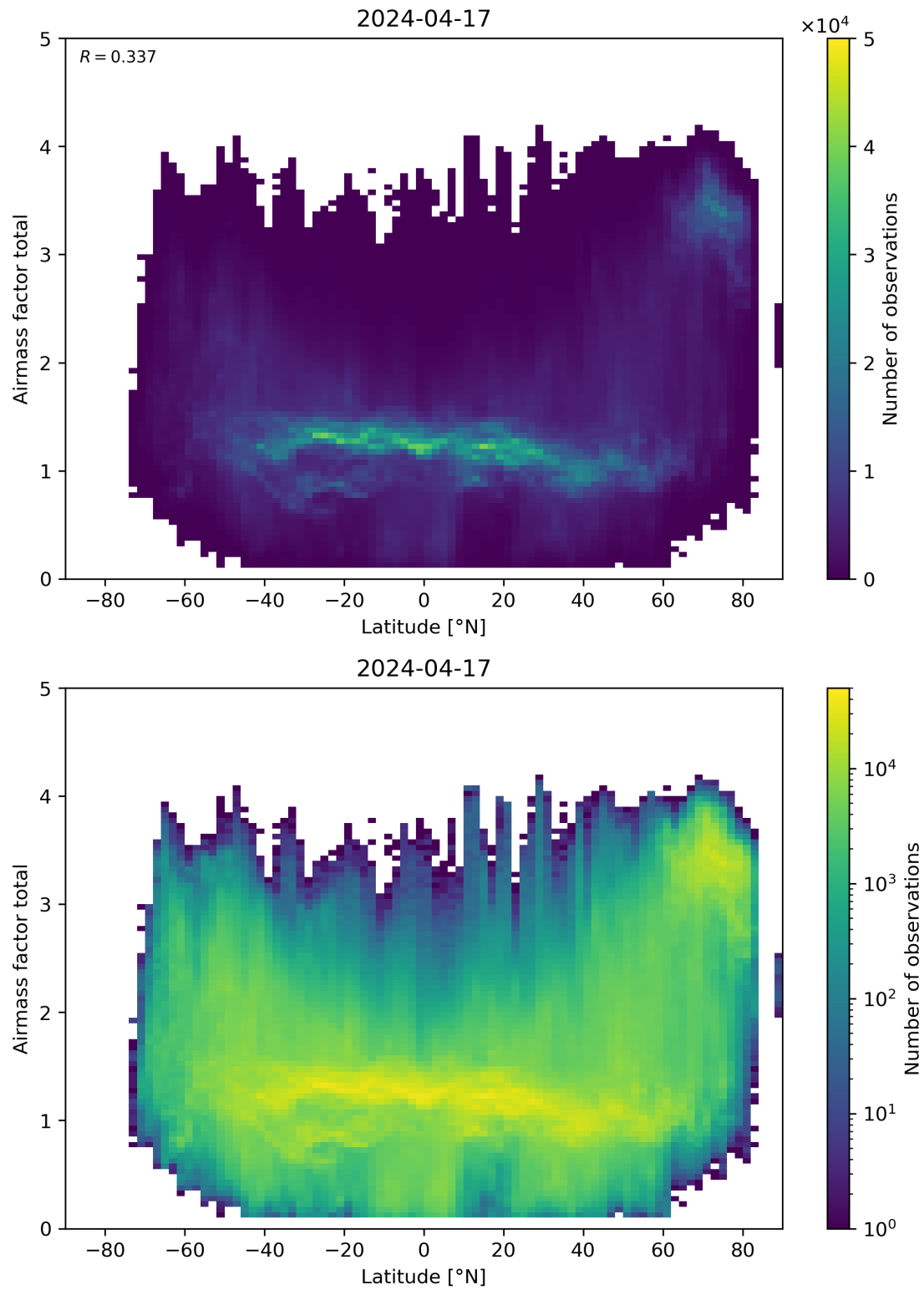
Figure 161: Scatter density plot of “Latitude” against “Airmass factor total” for 2024-04-16 to 2024-04-18.
