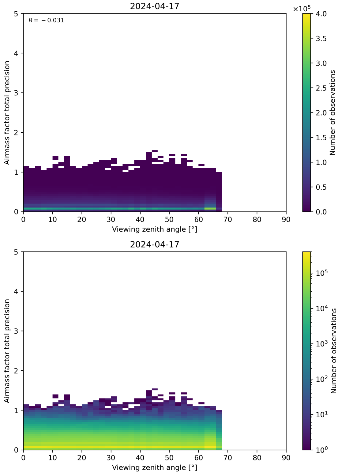
Figure 191: Scatter density plot of “Viewing zenith angle” against “Airmass factor total precision” for 2024-04-16 to 2024-04-18.
