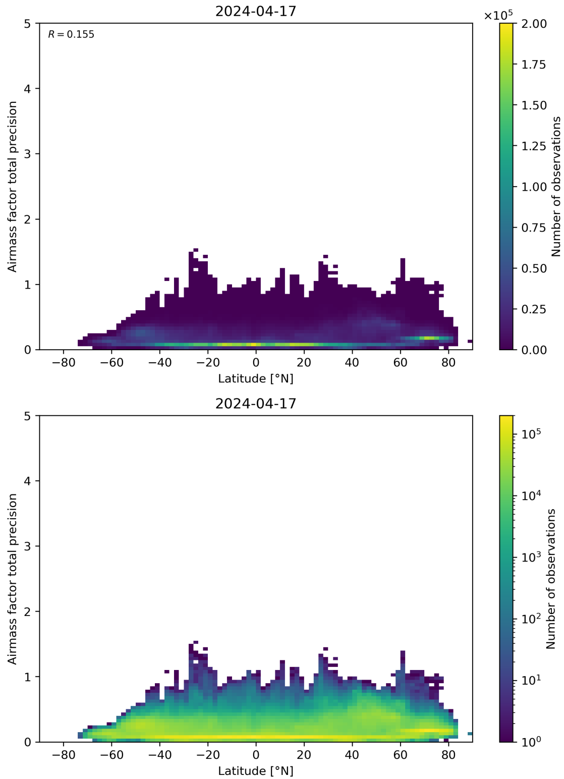
Figure 162: Scatter density plot of “Latitude” against “Airmass factor total precision” for 2024-04-16 to 2024-04-18.
