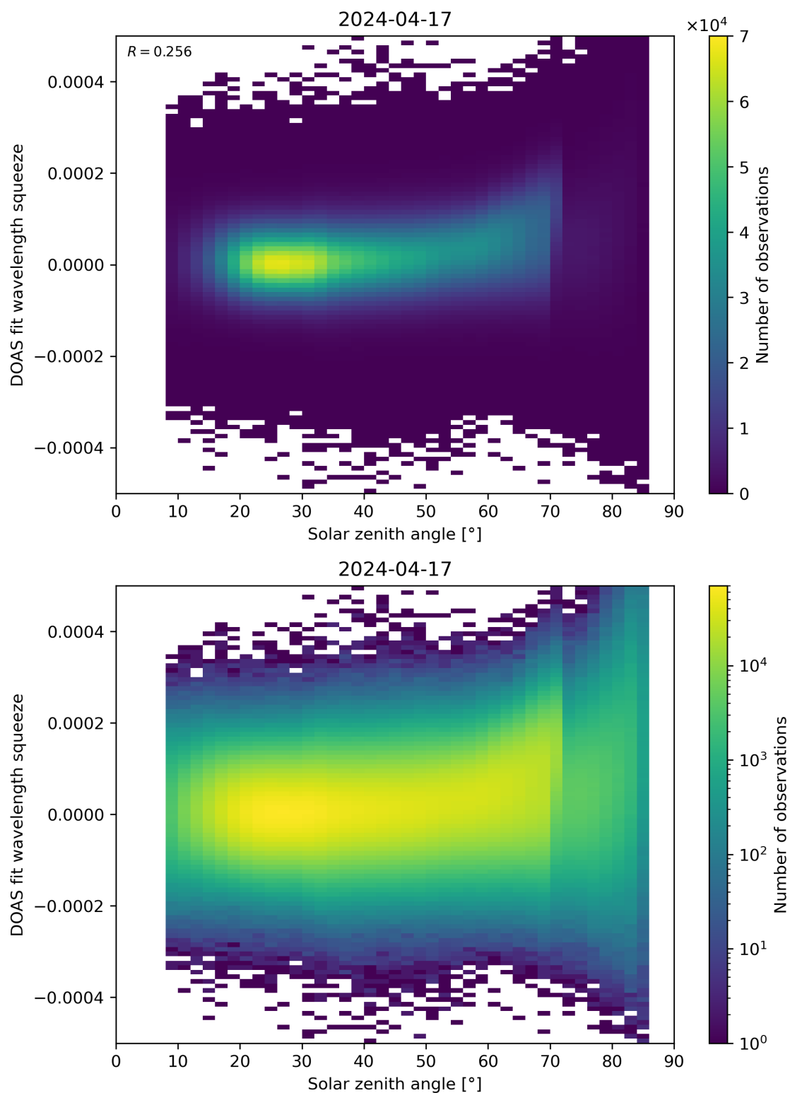
Figure 169: Scatter density plot of “Solar zenith angle” against “DOAS fit wavelength squeeze” for 2024-04-16 to 2024-04-18.
