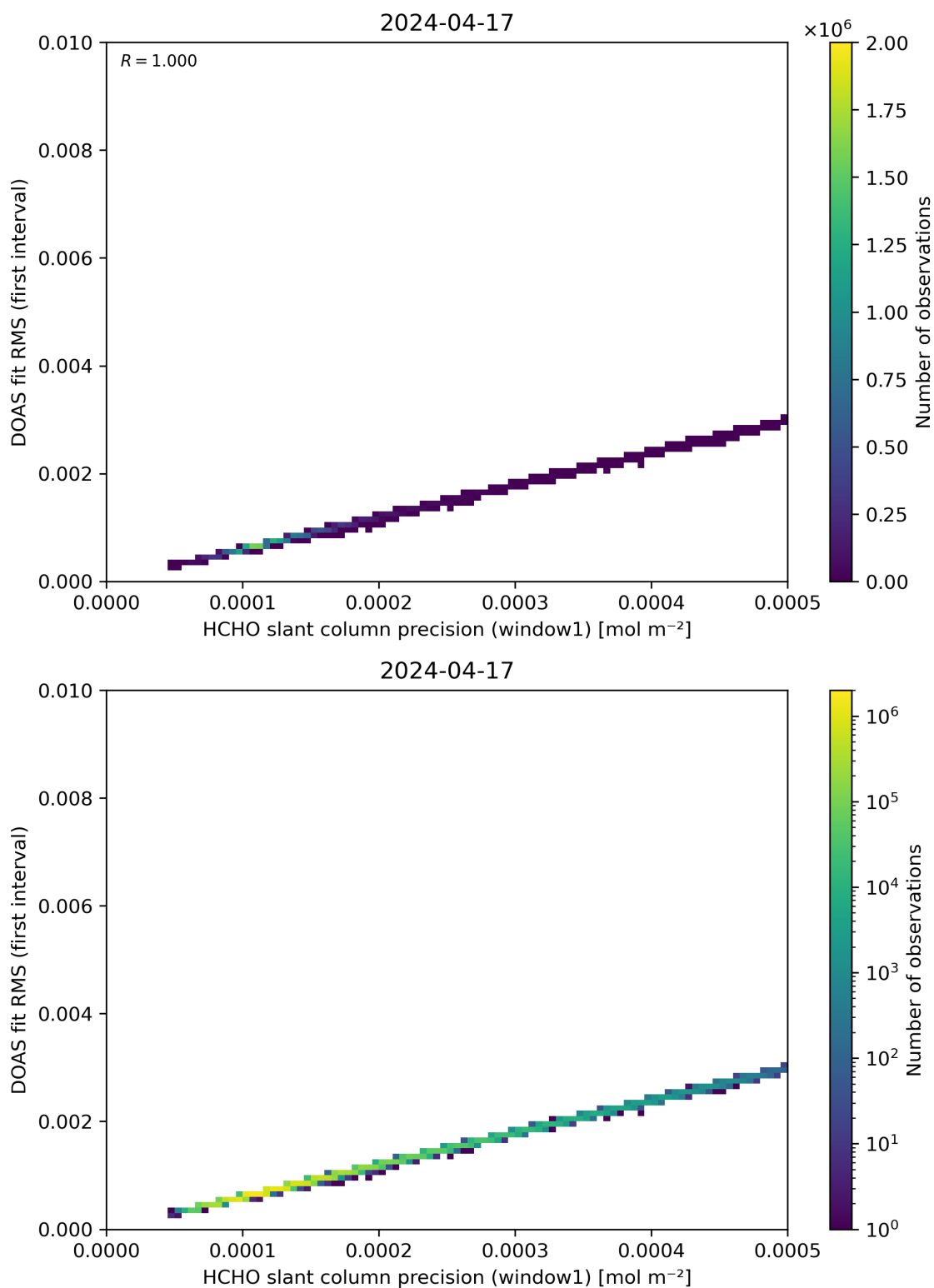
Figure 88: Scatter density plot of “HCHO slant column precision (window1)” against “DOAS fit RMS (first interval)” for 2024-04-16 to 2024-04-18.
