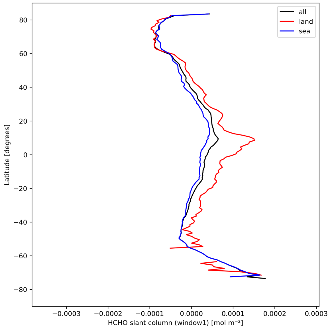
Figure 24: Zonal average of “HCHO slant column (window1)” for 2024-04-16 to 2024-04-18.
