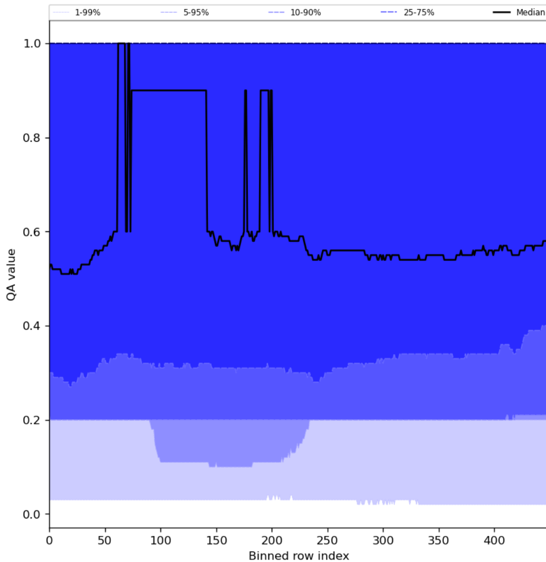
Figure 48: Along track statistics of “QA value” for 2024-04-16 to 2024-04-18
