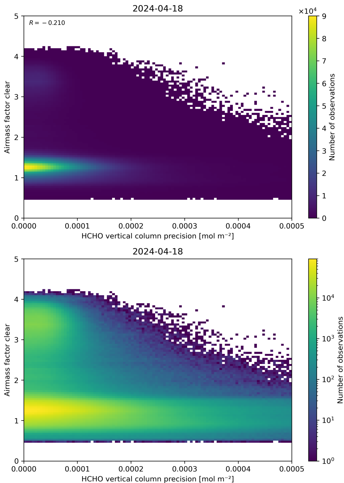
Figure 139: Scatter density plot of “HCHO vertical column precision” against “Airmass factor clear” for 2024-04-17 to 2024-04-19.
