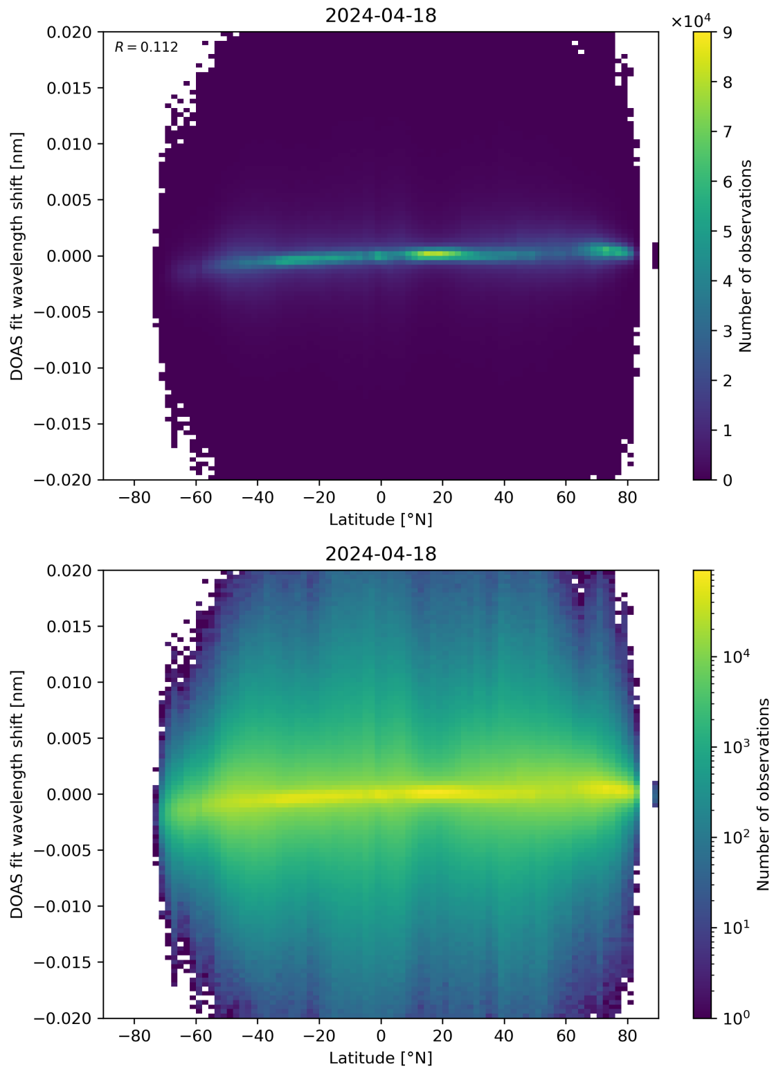
Figure 154: Scatter density plot of “Latitude” against “DOAS fit wavelength shift” for 2024-04-17 to 2024-04-19.
