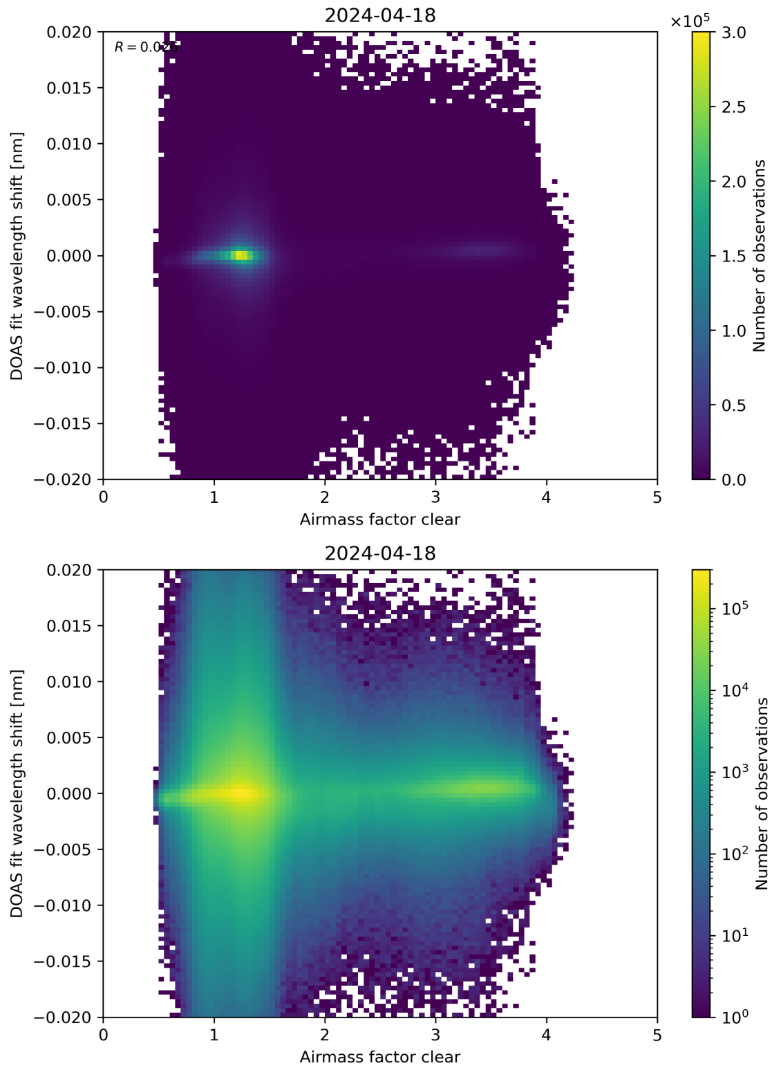
Figure 72: Scatter density plot of “Airmass factor clear” against “DOAS fit wavelength shift” for 2024-04-17 to 2024-04-19.
