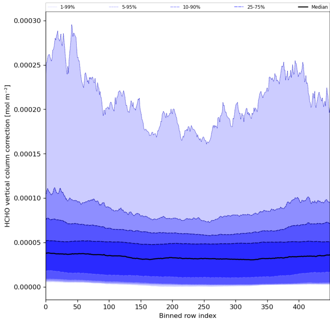
Figure 51: Along track statistics of “HCHO vertical column correction” for 2024-04-17 to 2024-04-19
