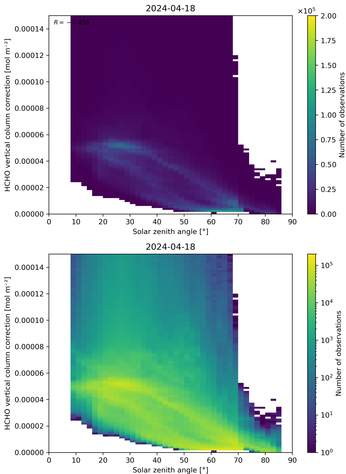
Figure 178: Scatter density plot of “Solar zenith angle” against “HCHO vertical column correction” for 2024-04-17 to 2024-04-19.
