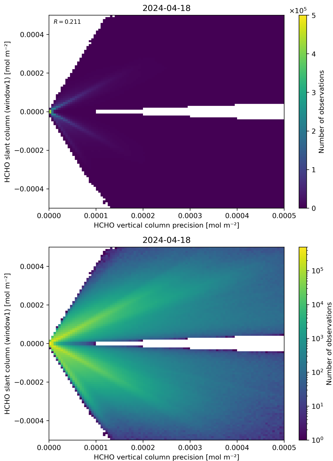
Figure 142: Scatter density plot of “HCHO vertical column precision” against “HCHO slant column (window1)” for 2024-04-17 to 2024-04-19.
