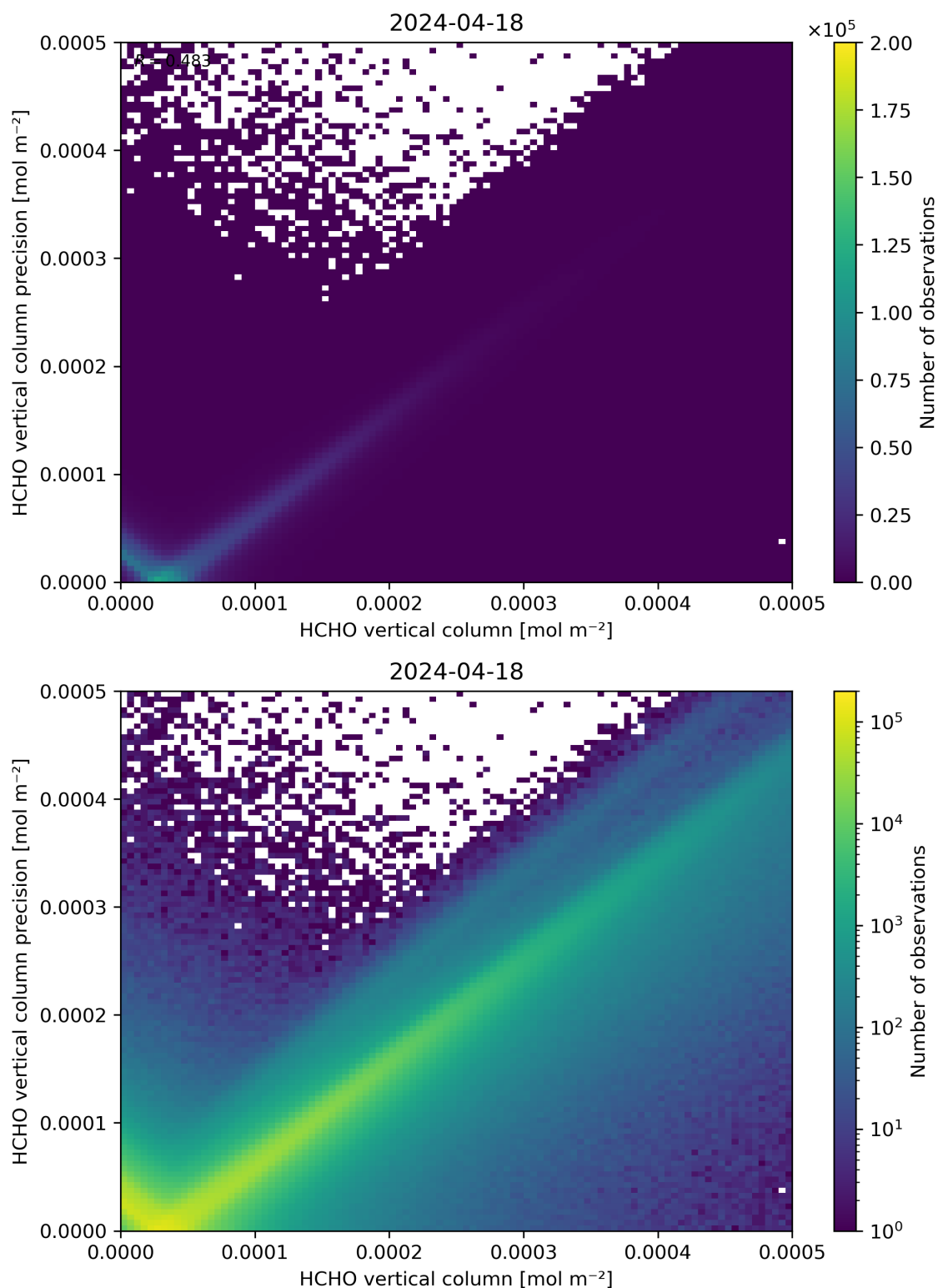
Figure 134: Scatter density plot of “HCHO vertical column” against “HCHO vertical column precision” for 2024-04-17 to 2024-04-19.
