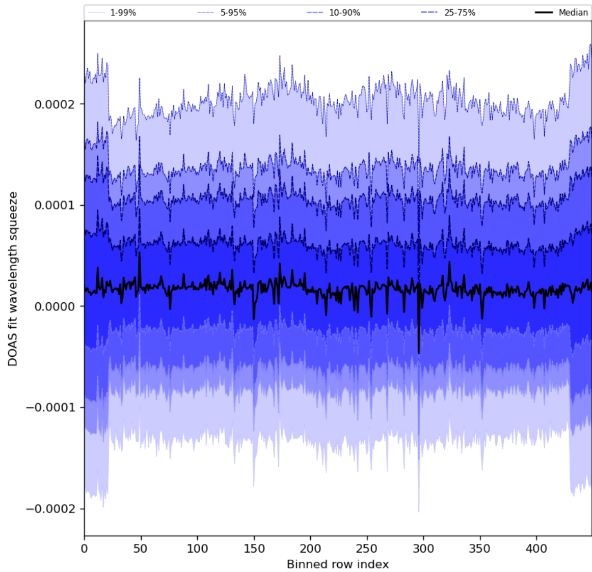
Figure 59: Along track statistics of “DOAS fit wavelength squeeze” for 2024-04-17 to 2024-04-19
