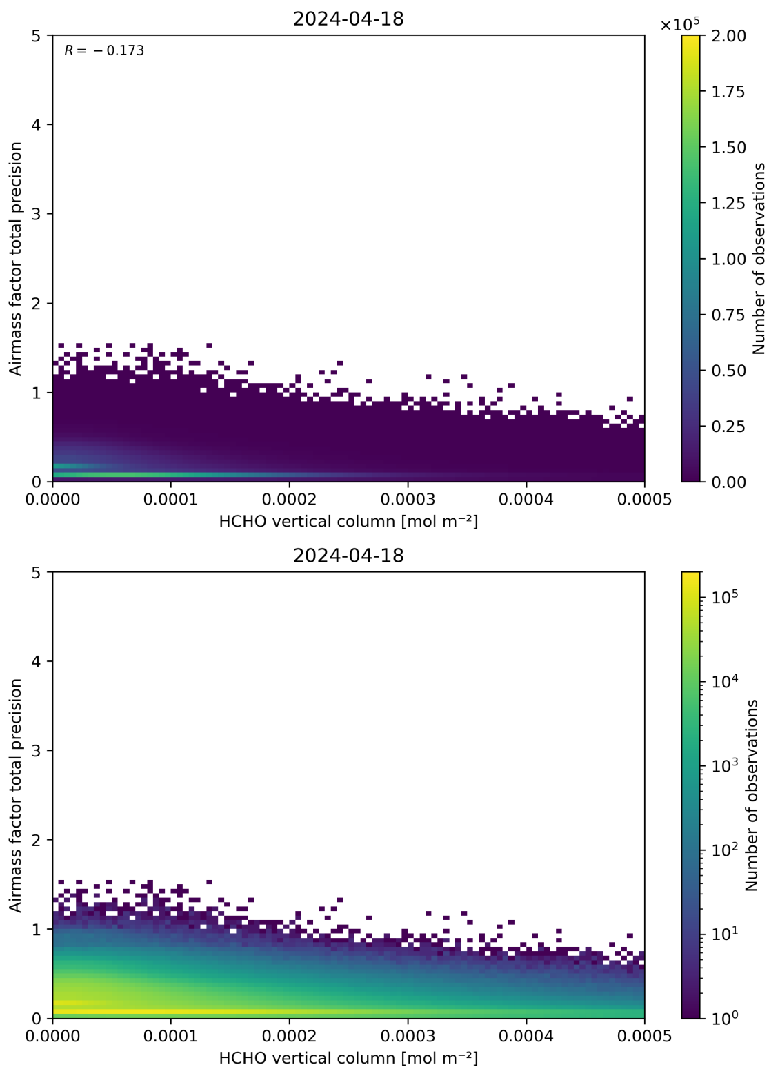
Figure 132: Scatter density plot of “HCHO vertical column” against “Airmass factor total precision” for 2024-04-17 to 2024-04-19.
