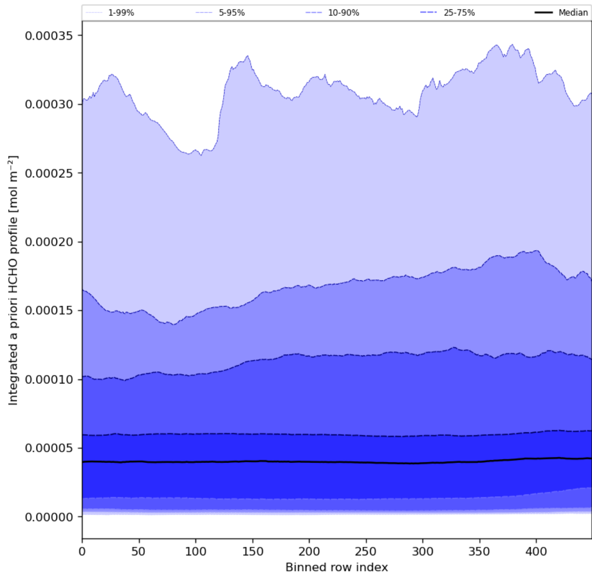
Figure 57: Along track statistics of “Integrated a priori HCHO profile” for 2024-04-17 to 2024-04-19
