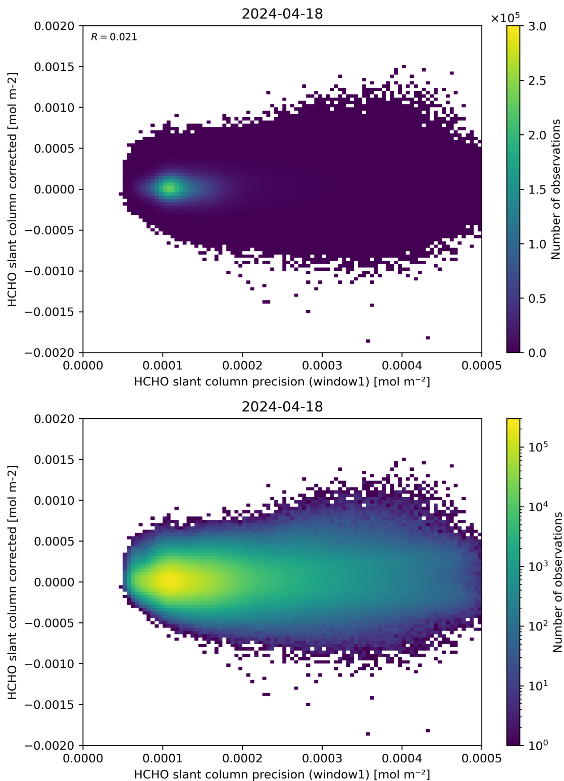
Figure 92: Scatter density plot of “HCHO slant column precision (window1)” against “HCHO slant column corrected” for 2024-04-17 to 2024-04-19.
