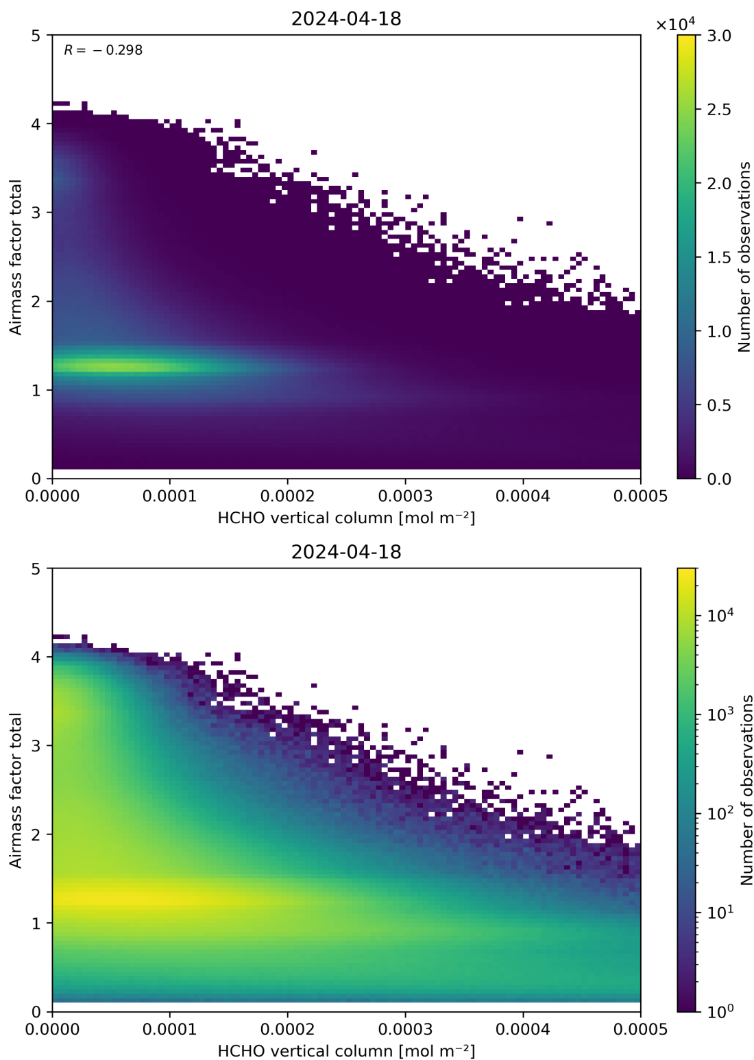
Figure 131: Scatter density plot of “HCHO vertical column” against “Airmass factor total” for 2024-04-17 to 2024-04-19.
