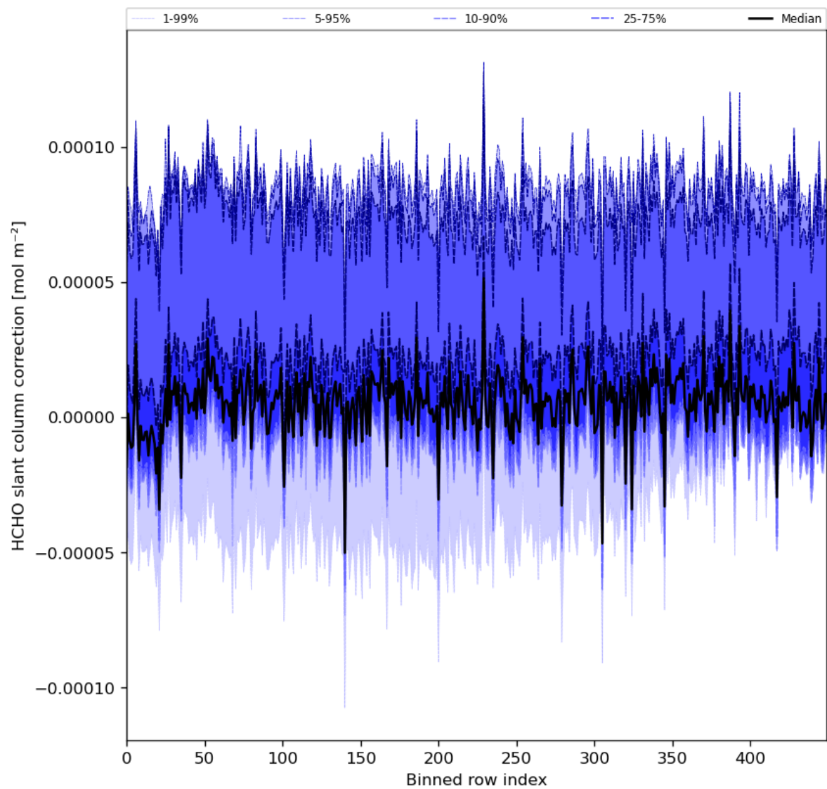
Figure 61: Along track statistics of “HCHO slant column correction” for 2024-04-17 to 2024-04-19
