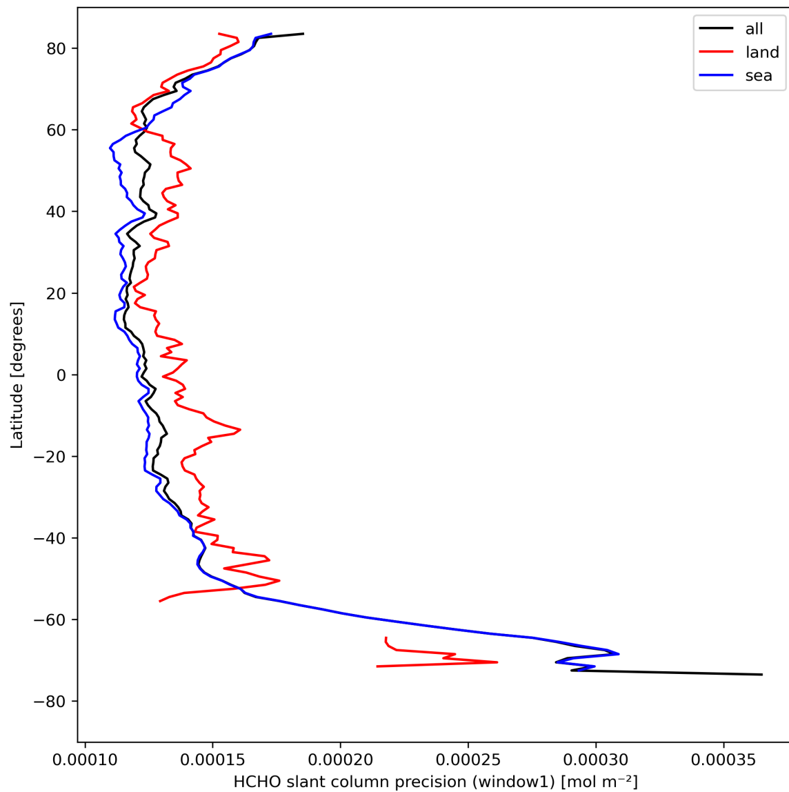
Figure 25: Zonal average of “HCHO slant column precision (window1)” for 2024-04-17 to 2024-04-19.
