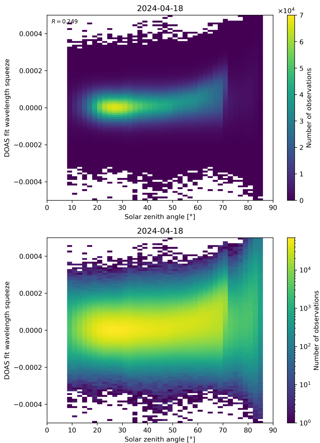
Figure 169: Scatter density plot of “Solar zenith angle” against “DOAS fit wavelength squeeze” for 2024-04-17 to 2024-04-19.
