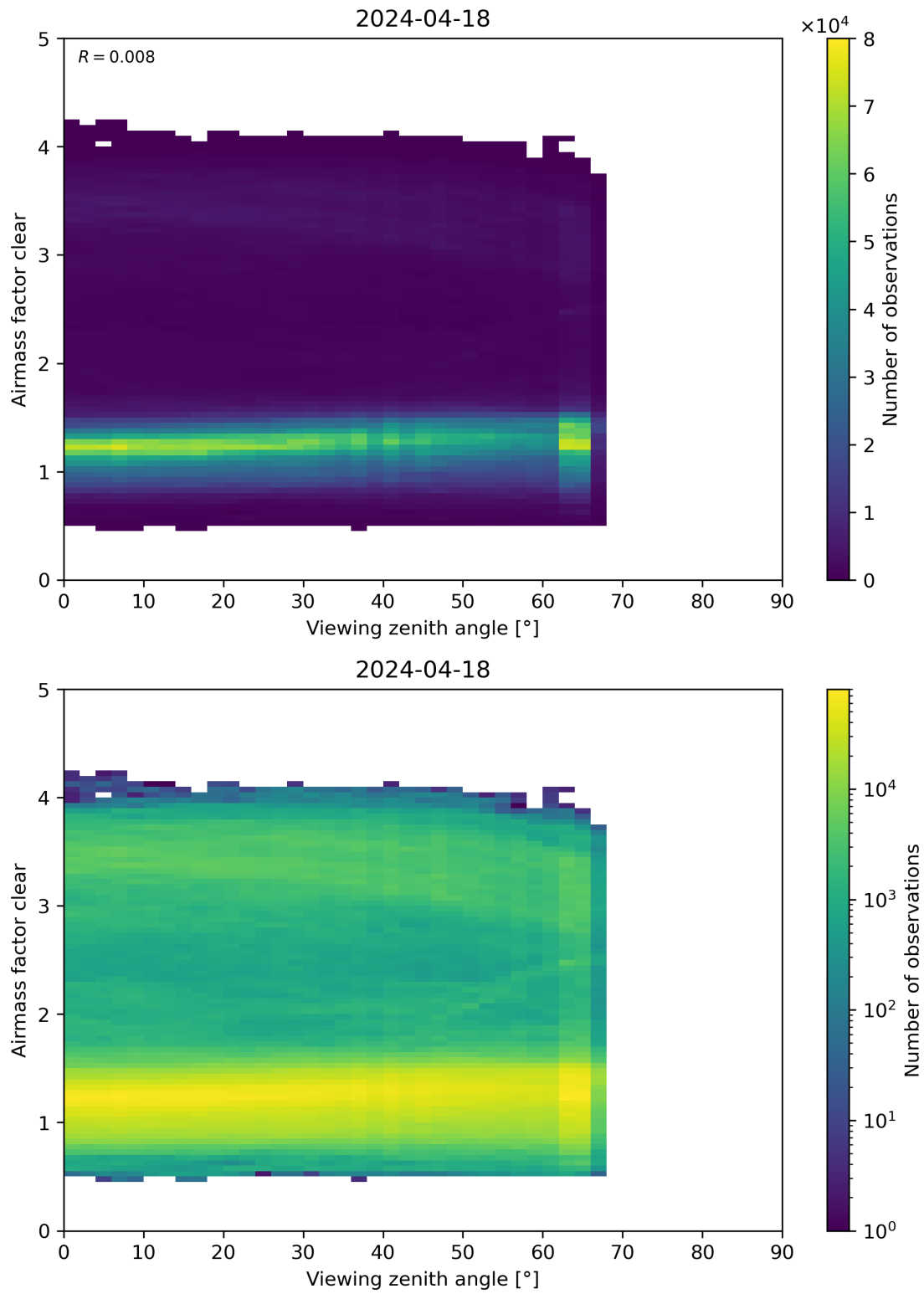
Figure 185: Scatter density plot of “Viewing zenith angle” against “Airmass factor clear” for 2024-04-17 to 2024-04-19.
