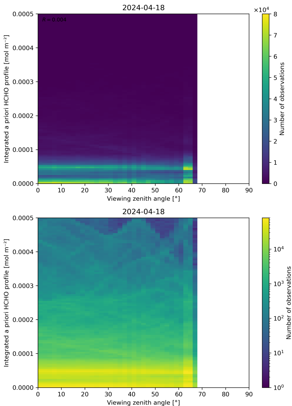
Figure 195: Scatter density plot of “Viewing zenith angle” against “Integrated a priori HCHO profile” for 2024-04-17 to 2024-04-19.
