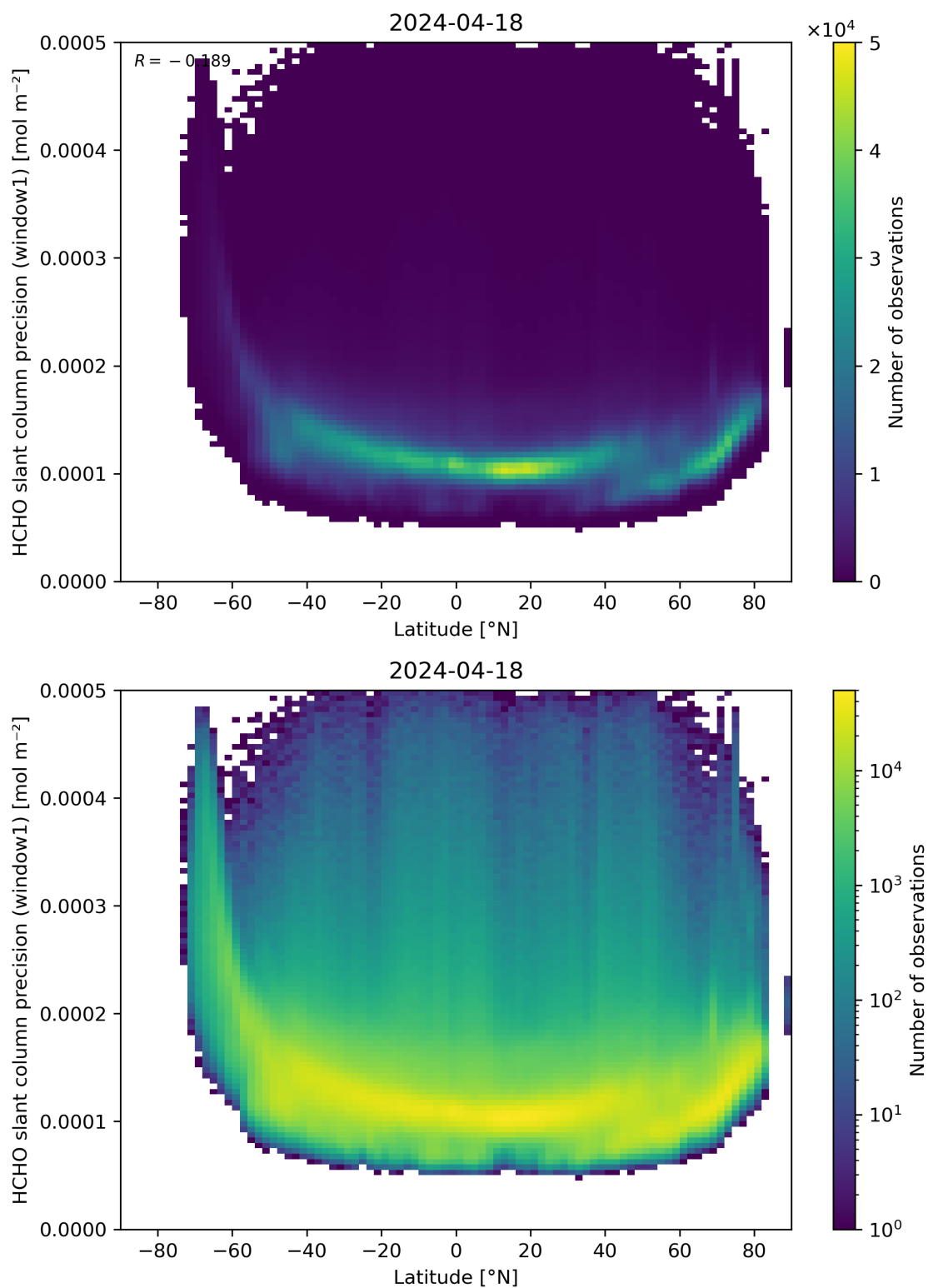
Figure 160: Scatter density plot of “Latitude” against “HCHO slant column precision (window1)” for 2024-04-17 to 2024-04-19.
