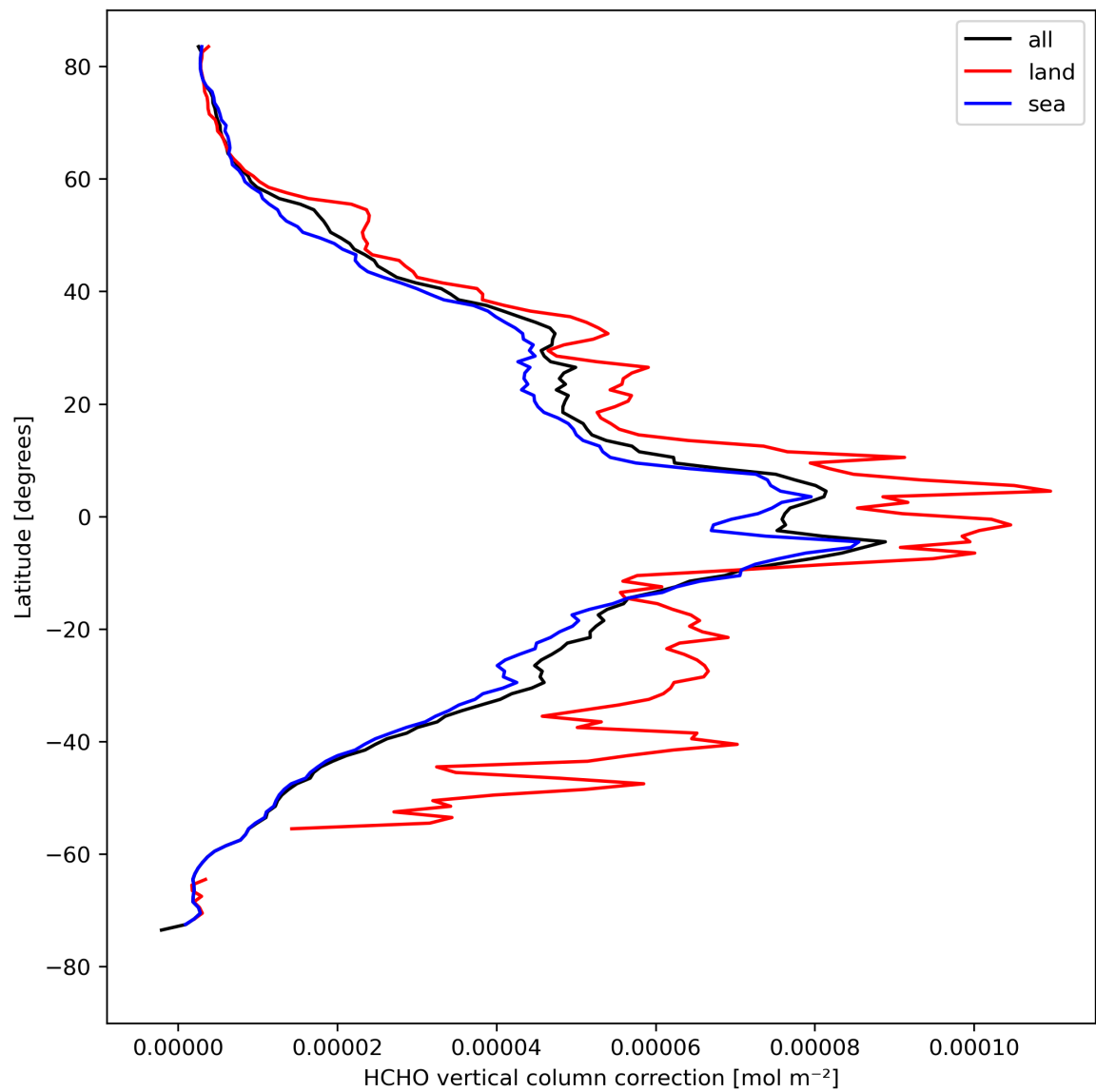
Figure 23: Zonal average of “HCHO vertical column correction” for 2024-04-17 to 2024-04-19.
