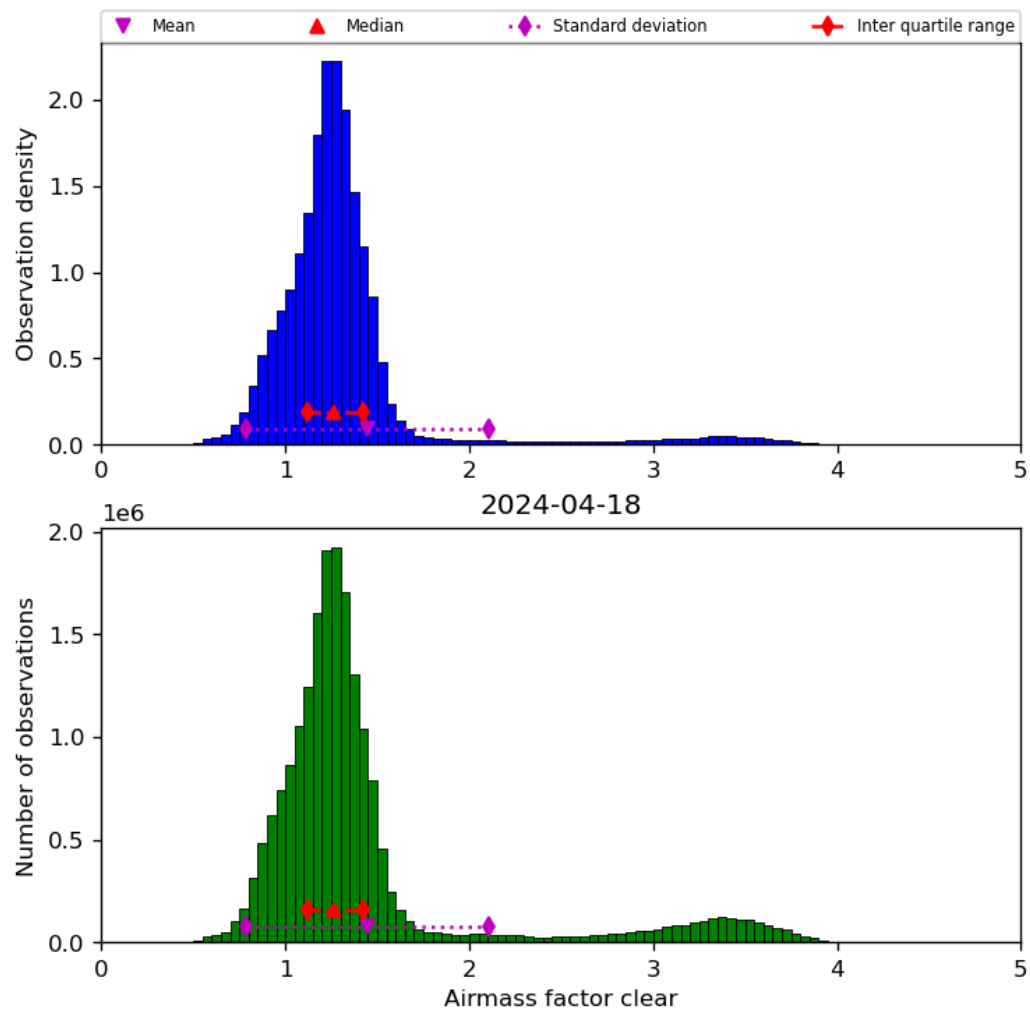
Figure 42: Histogram of “Airmass factor clear” for 2024-04-17 to 2024-04-19
