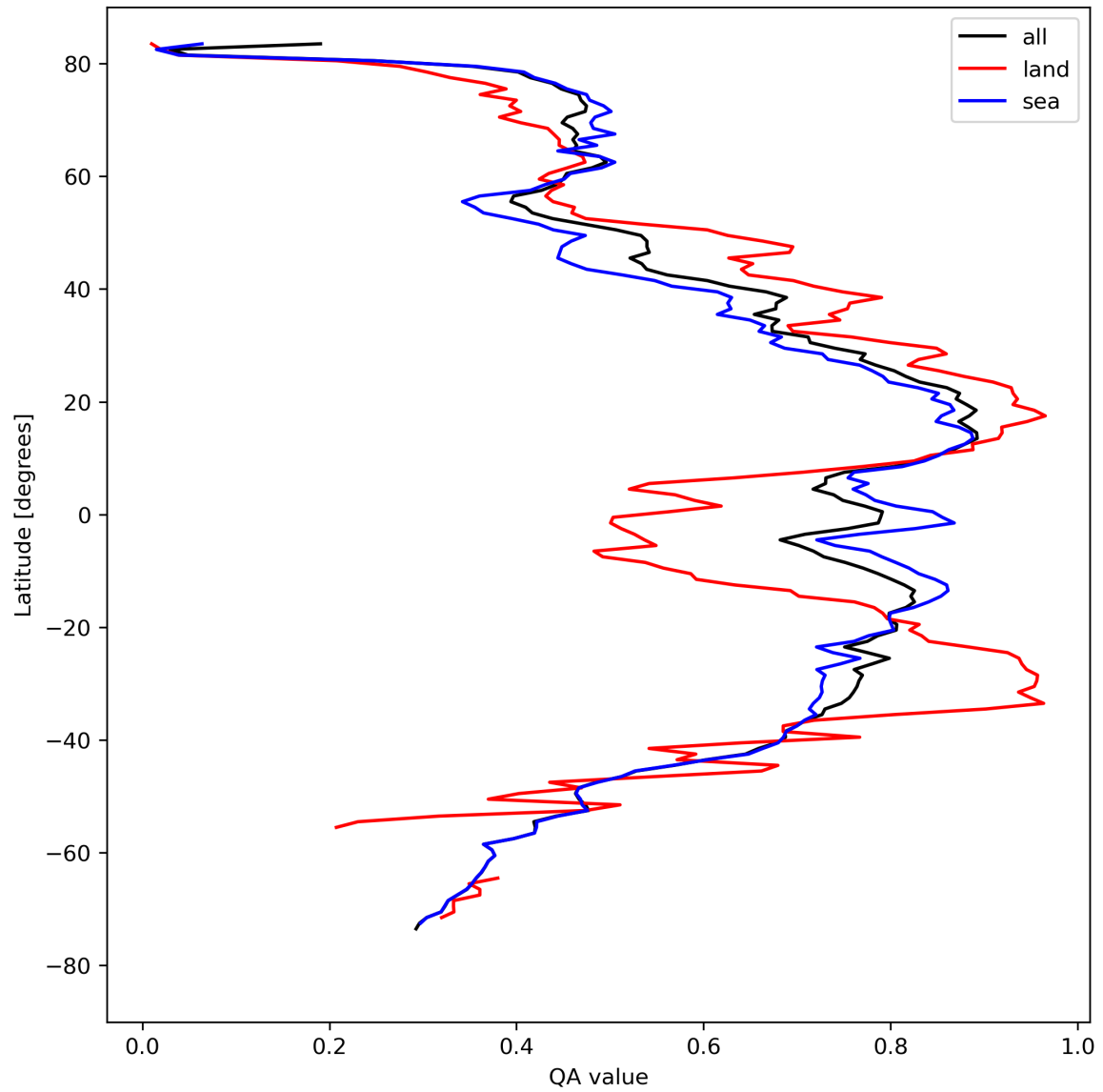
Figure 20: Zonal average of “QA value” for 2024-04-17 to 2024-04-19.
