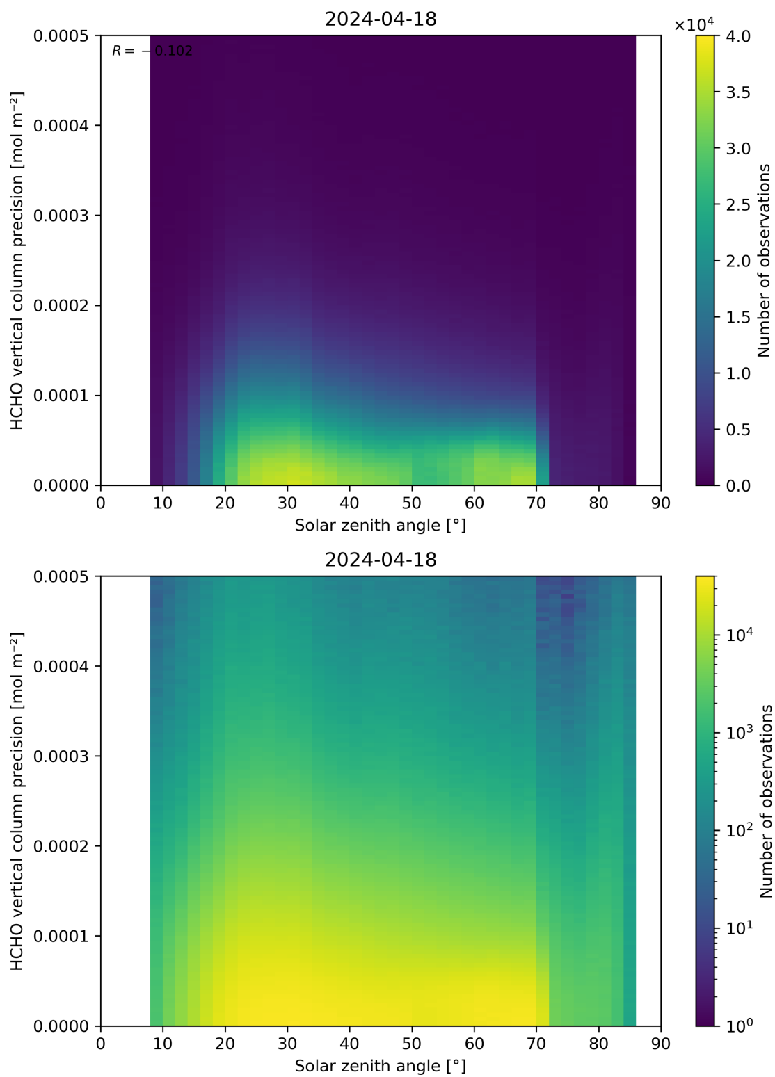
Figure 179: Scatter density plot of “Solar zenith angle” against “HCHO vertical column precision” for 2024-04-17 to 2024-04-19.
