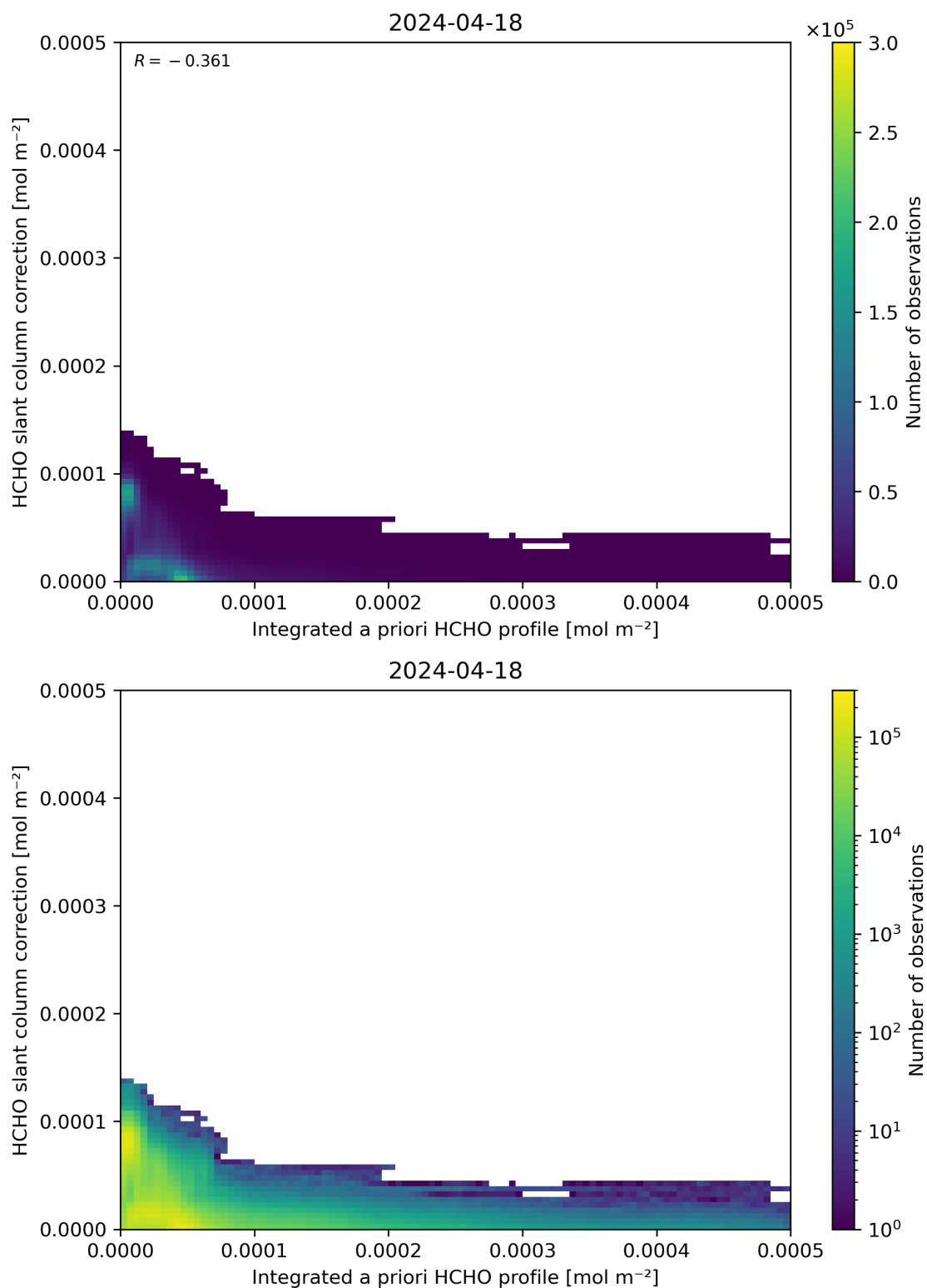
Figure 152: Scatter density plot of “Integrated a priori HCHO profile” against “HCHO slant column correction” for 2024-04-17 to 2024-04-19.
