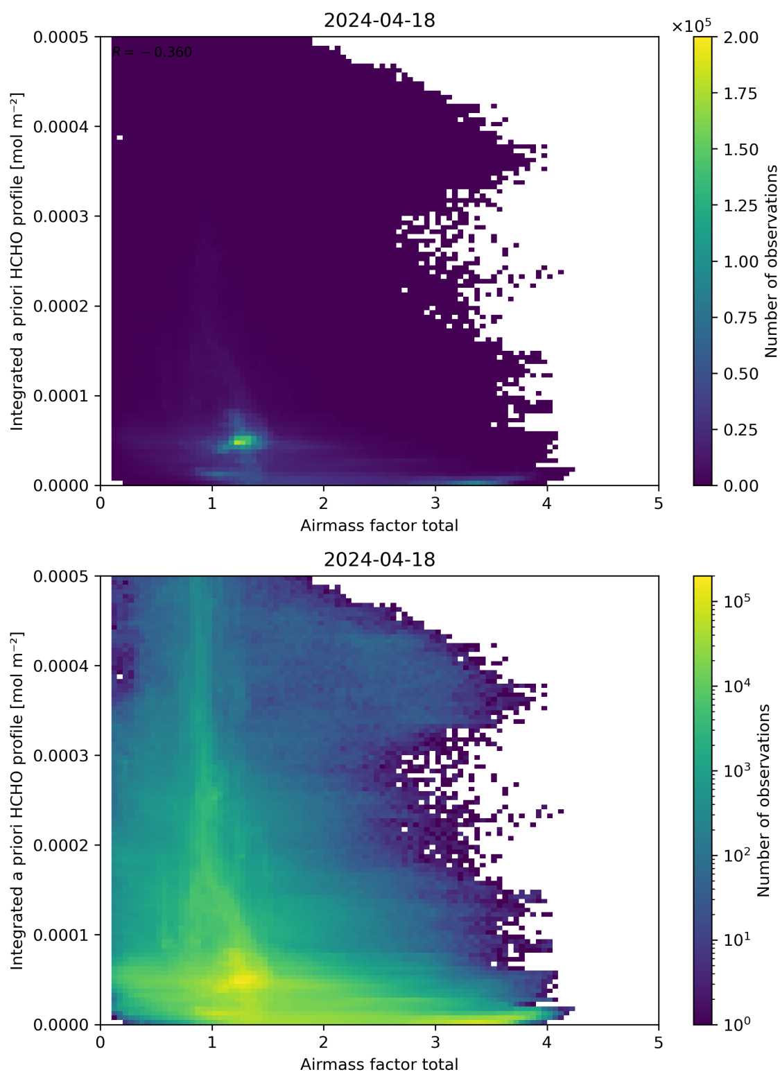
Figure 104: Scatter density plot of “Airmass factor total” against “Integrated a priori HCHO profile” for 2024-04-17 to 2024-04-19.
