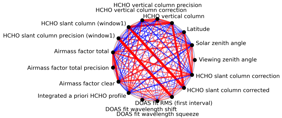
Figure 1: Map of correlation graph for 2024-04-17 to 2024-04-19.
