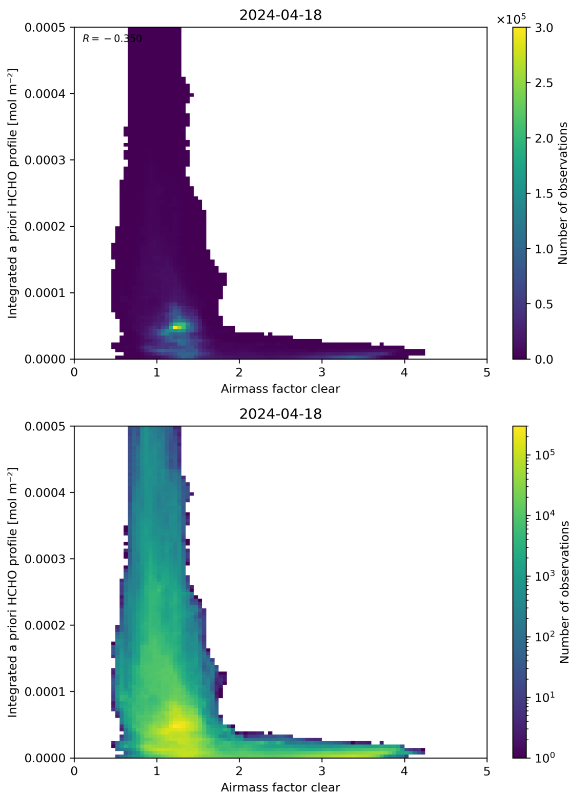
Figure 76: Scatter density plot of “Airmass factor clear” against “Integrated a priori HCHO profile” for 2024-04-17 to 2024-04-19.
