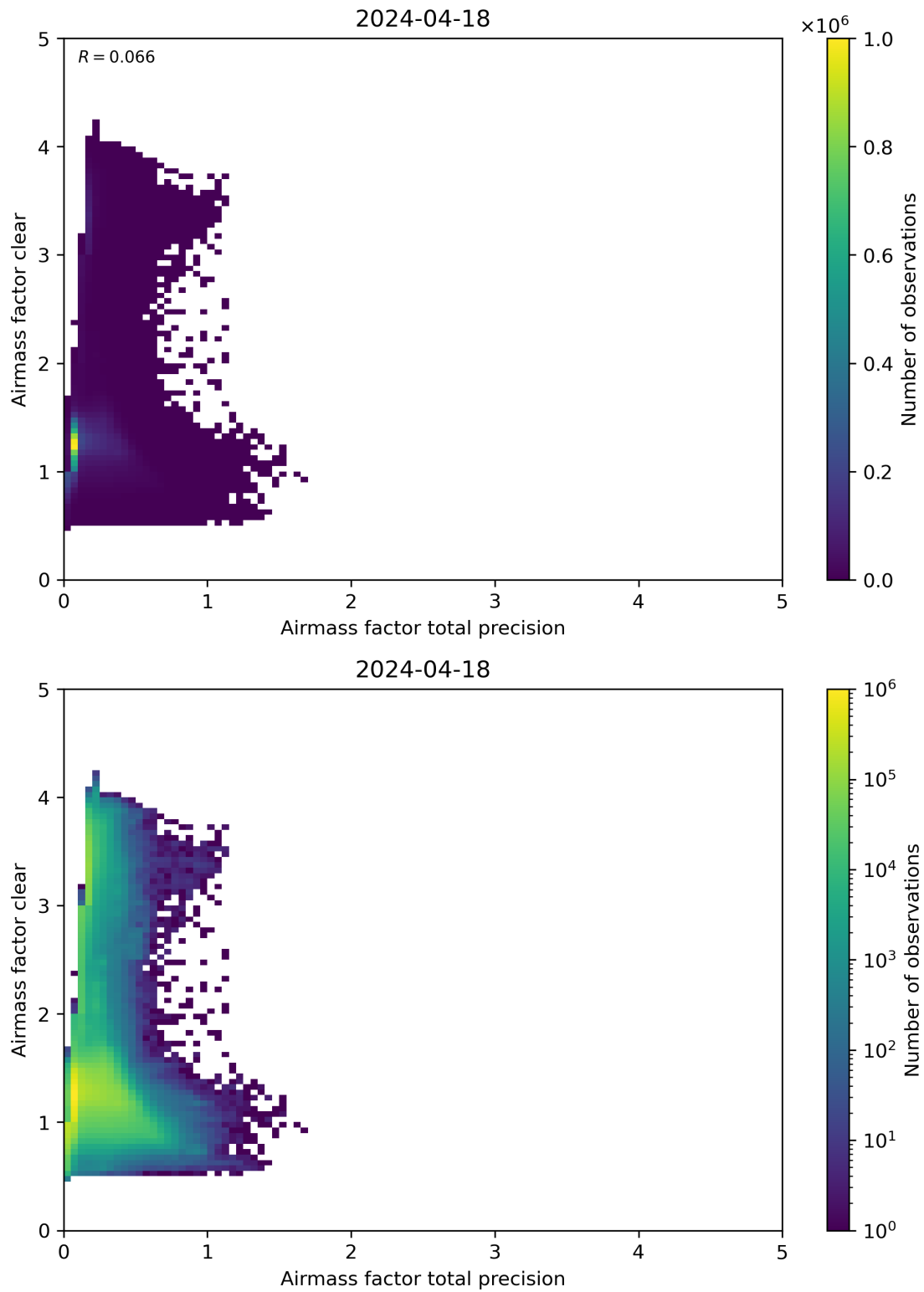
Figure 108: Scatter density plot of “Airmass factor total precision” against “Airmass factor clear” for 2024-04-17 to 2024-04-19.
