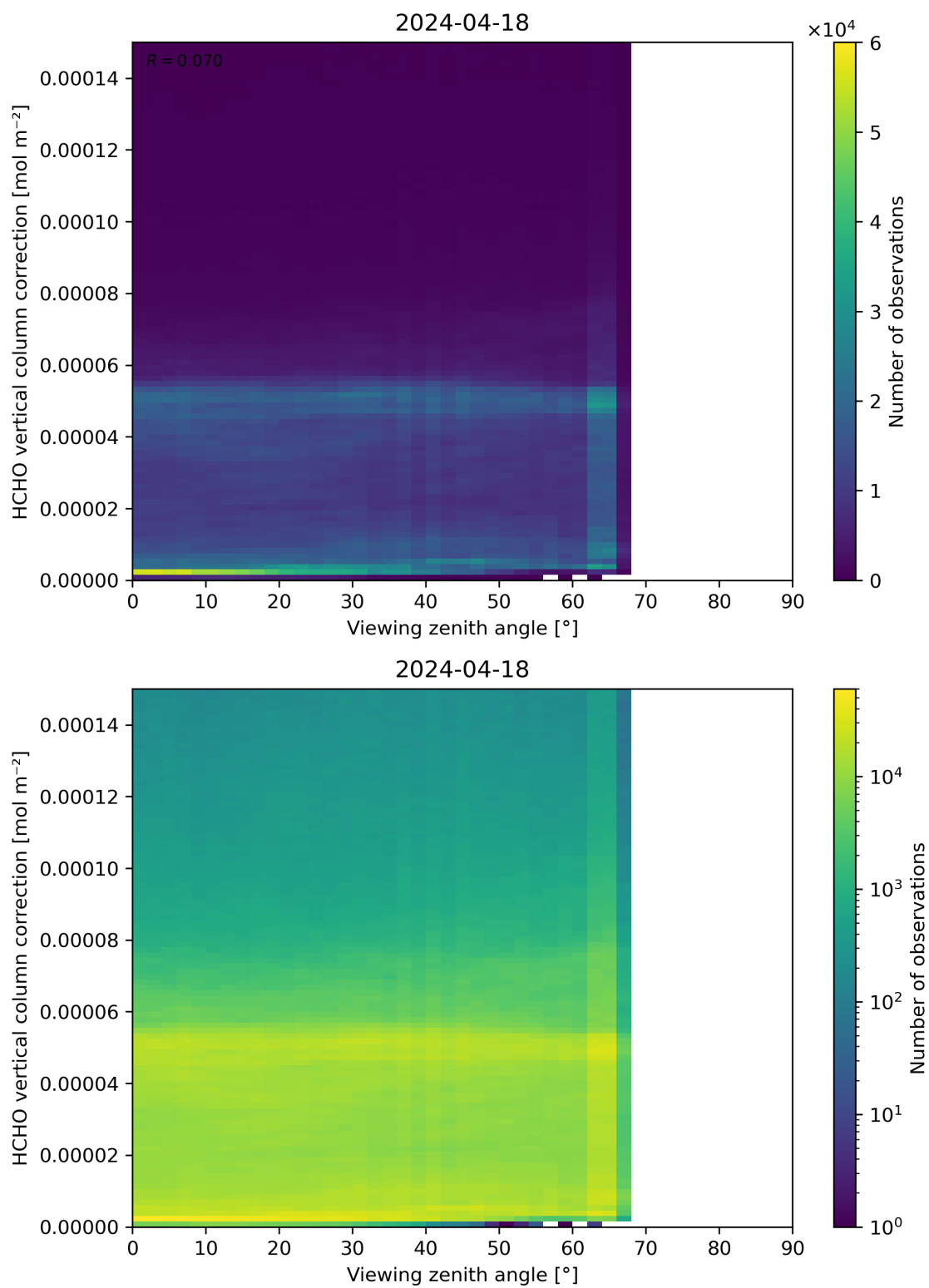
Figure 193: Scatter density plot of “Viewing zenith angle” against “HCHO vertical column correction” for 2024-04-17 to 2024-04-19.
