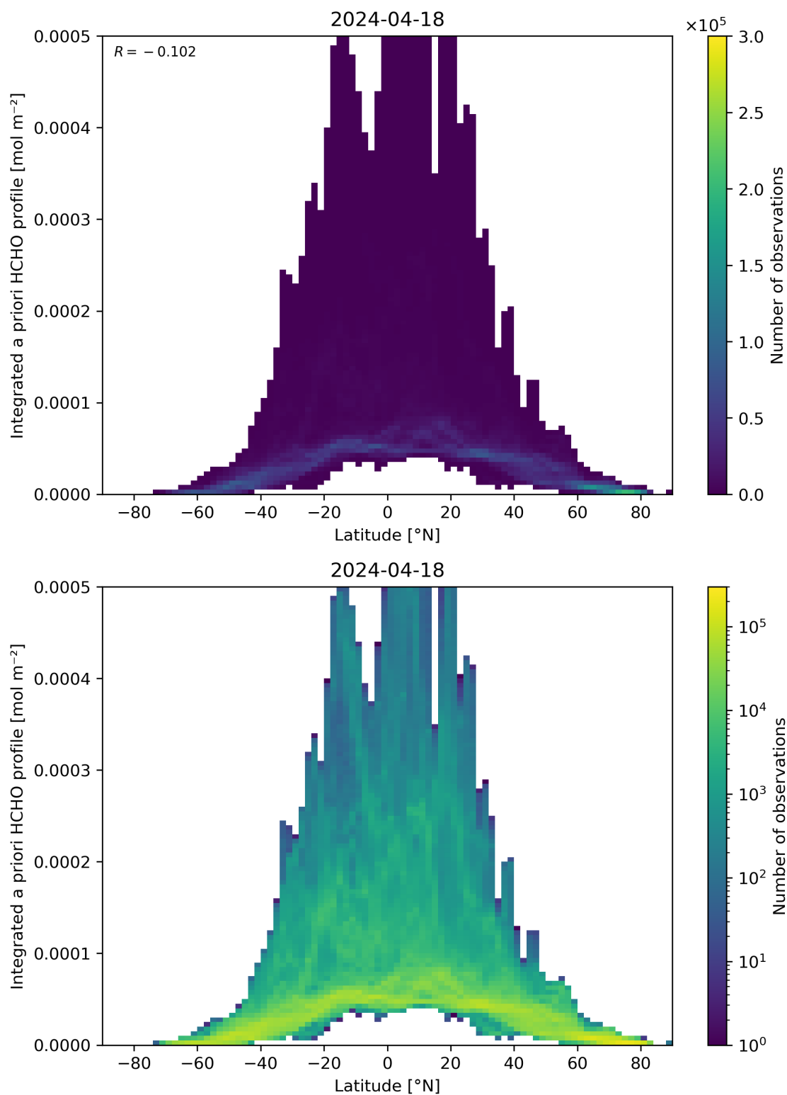
Figure 166: Scatter density plot of “Latitude” against “Integrated a priori HCHO profile” for 2024-04-17 to 2024-04-19.
