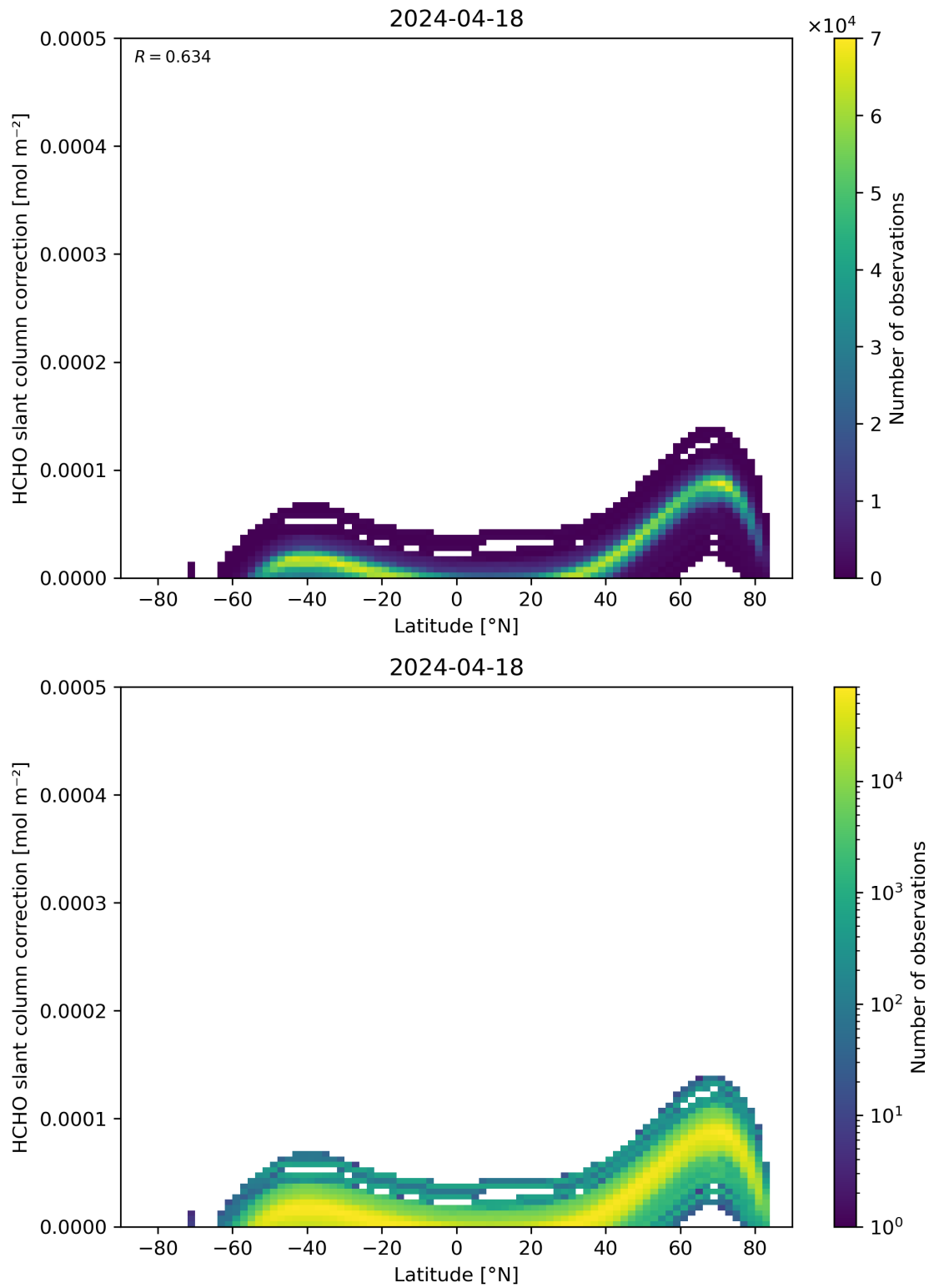
Figure 158: Scatter density plot of “Latitude” against “HCHO slant column correction” for 2024-04-17 to 2024-04-19.
