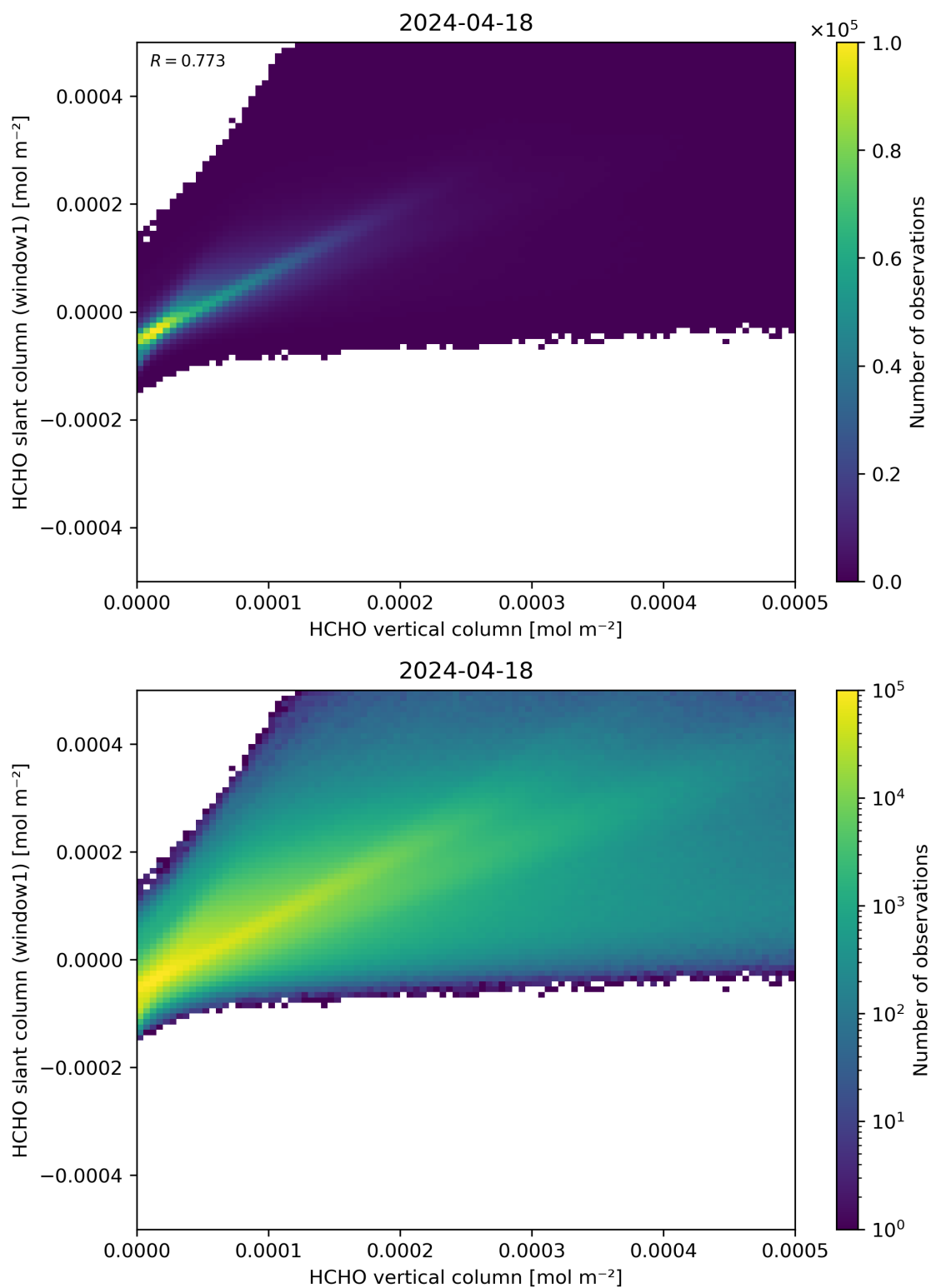
Figure 129: Scatter density plot of “HCHO vertical column” against “HCHO slant column (window1)” for 2024-04-17 to 2024-04-19.
