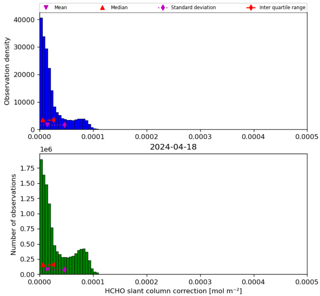
Figure 47: Histogram of “HCHO slant column correction” for 2024-04-17 to 2024-04-19
