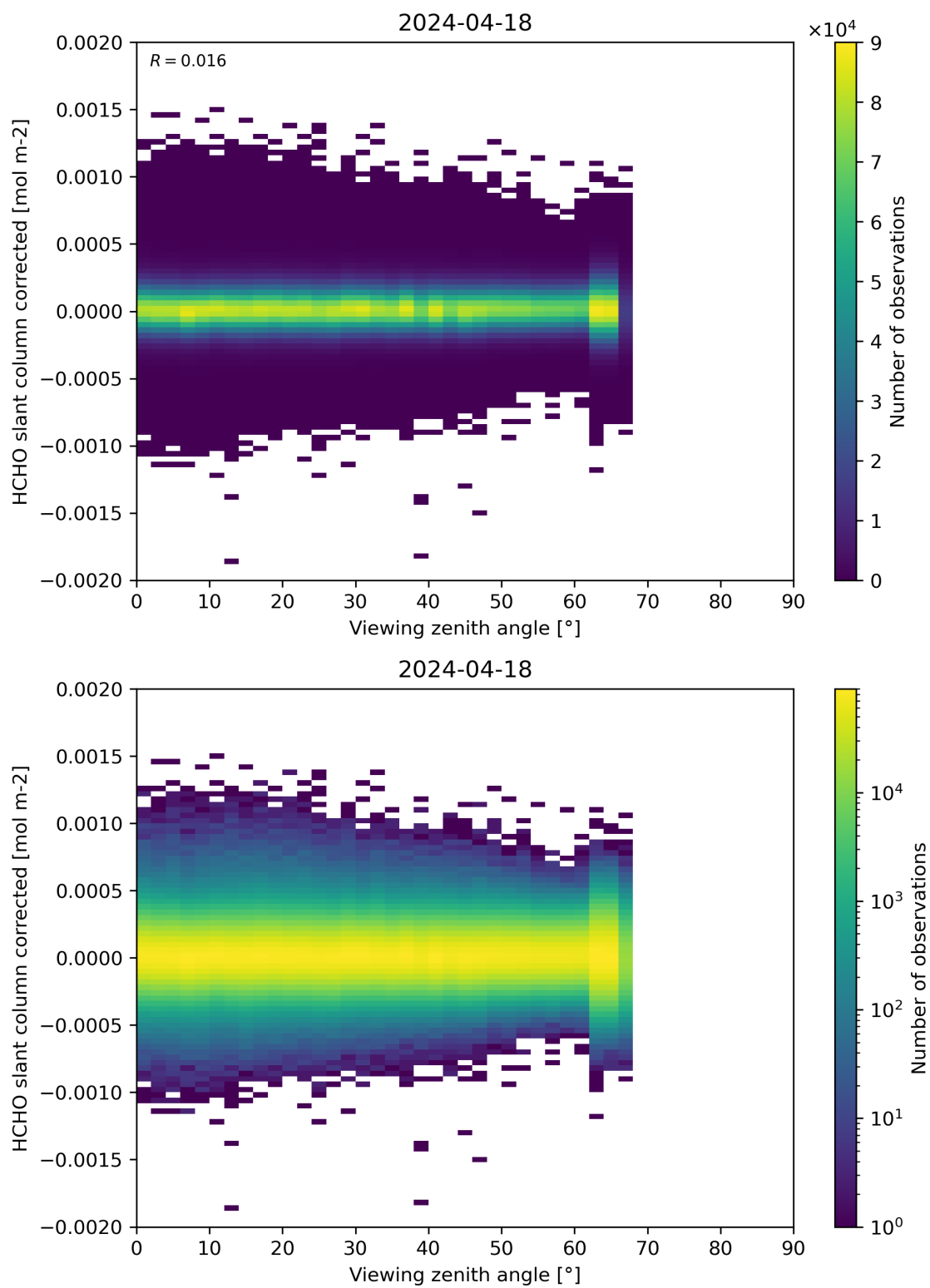
Figure 186: Scatter density plot of “Viewing zenith angle” against “HCHO slant column corrected” for 2024-04-17 to 2024-04-19.
