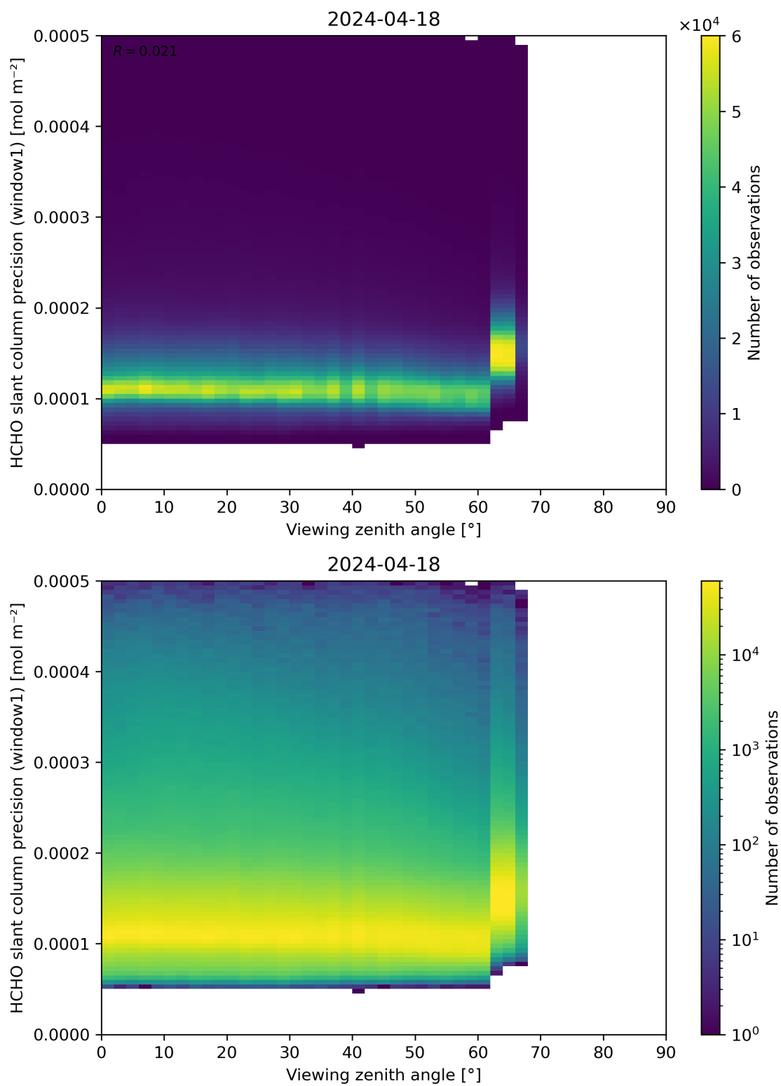
Figure 189: Scatter density plot of “Viewing zenith angle” against “HCHO slant column precision (window1)” for 2024-04-17 to 2024-04-19.
