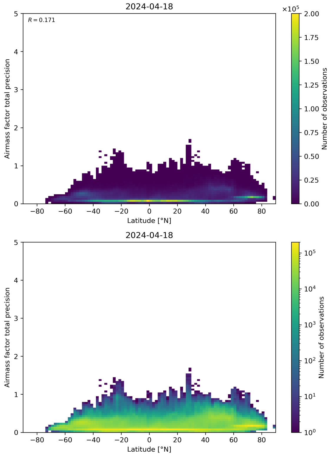
Figure 162: Scatter density plot of “Latitude” against “Airmass factor total precision” for 2024-04-17 to 2024-04-19.
