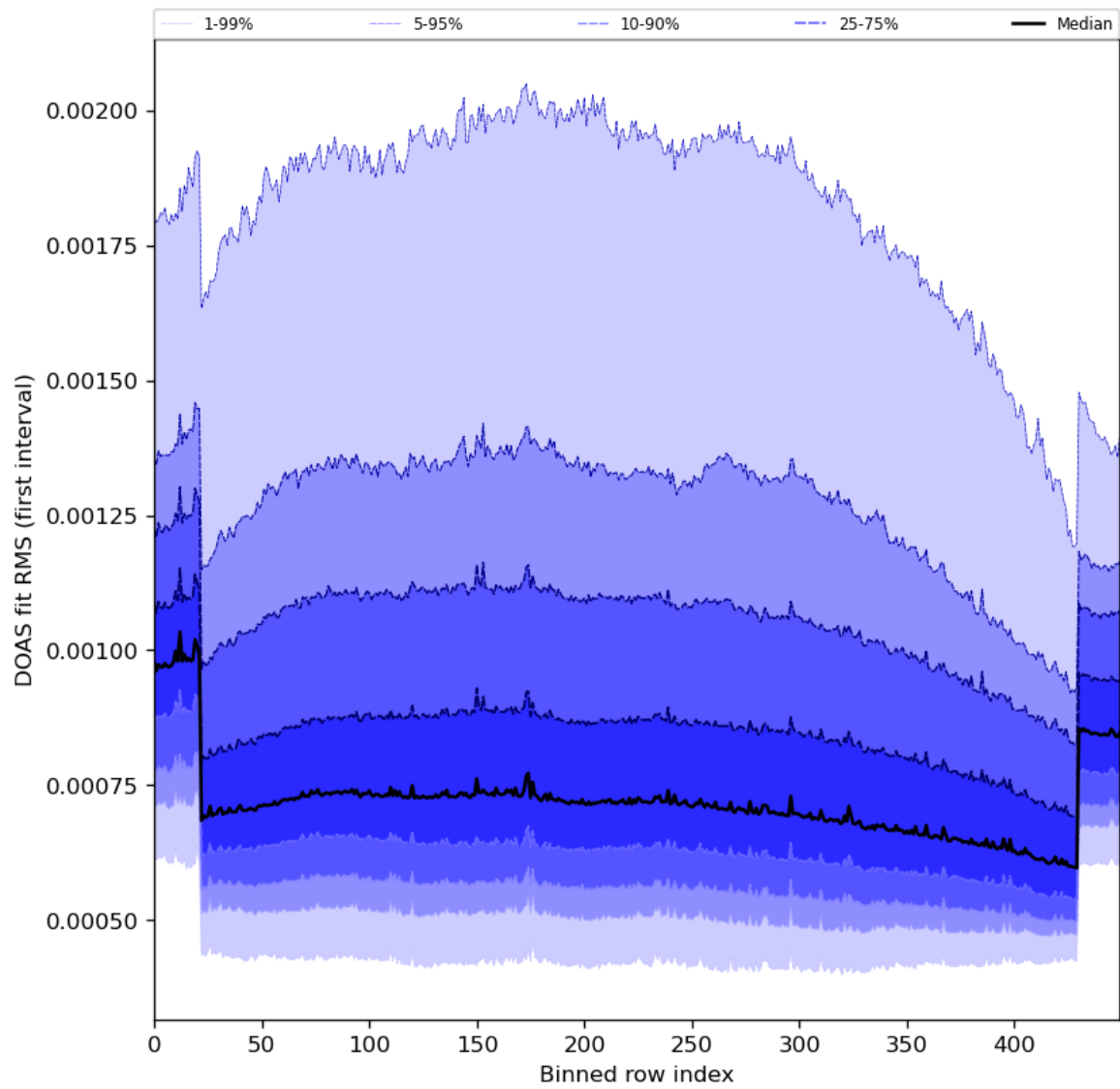
Figure 60: Along track statistics of “DOAS fit RMS (first interval)” for 2024-04-17 to 2024-04-19
