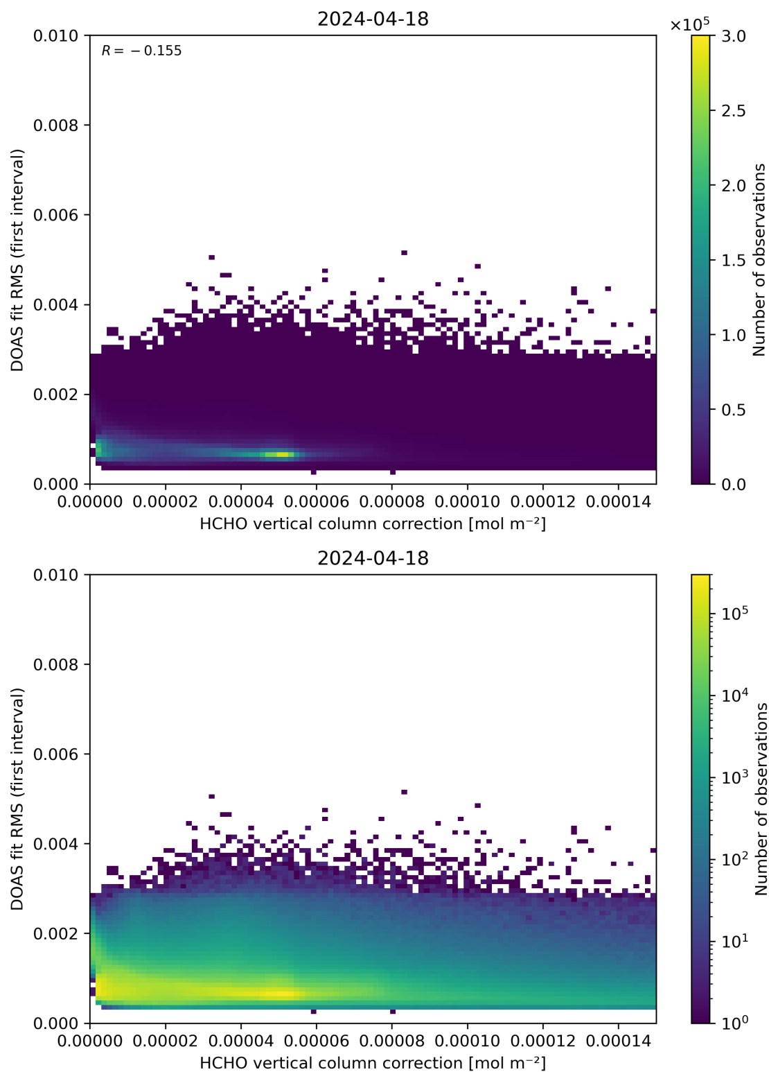
Figure 112: Scatter density plot of “HCHO vertical column correction” against “DOAS fit RMS (first interval)” for 2024-04-17 to 2024-04-19.
