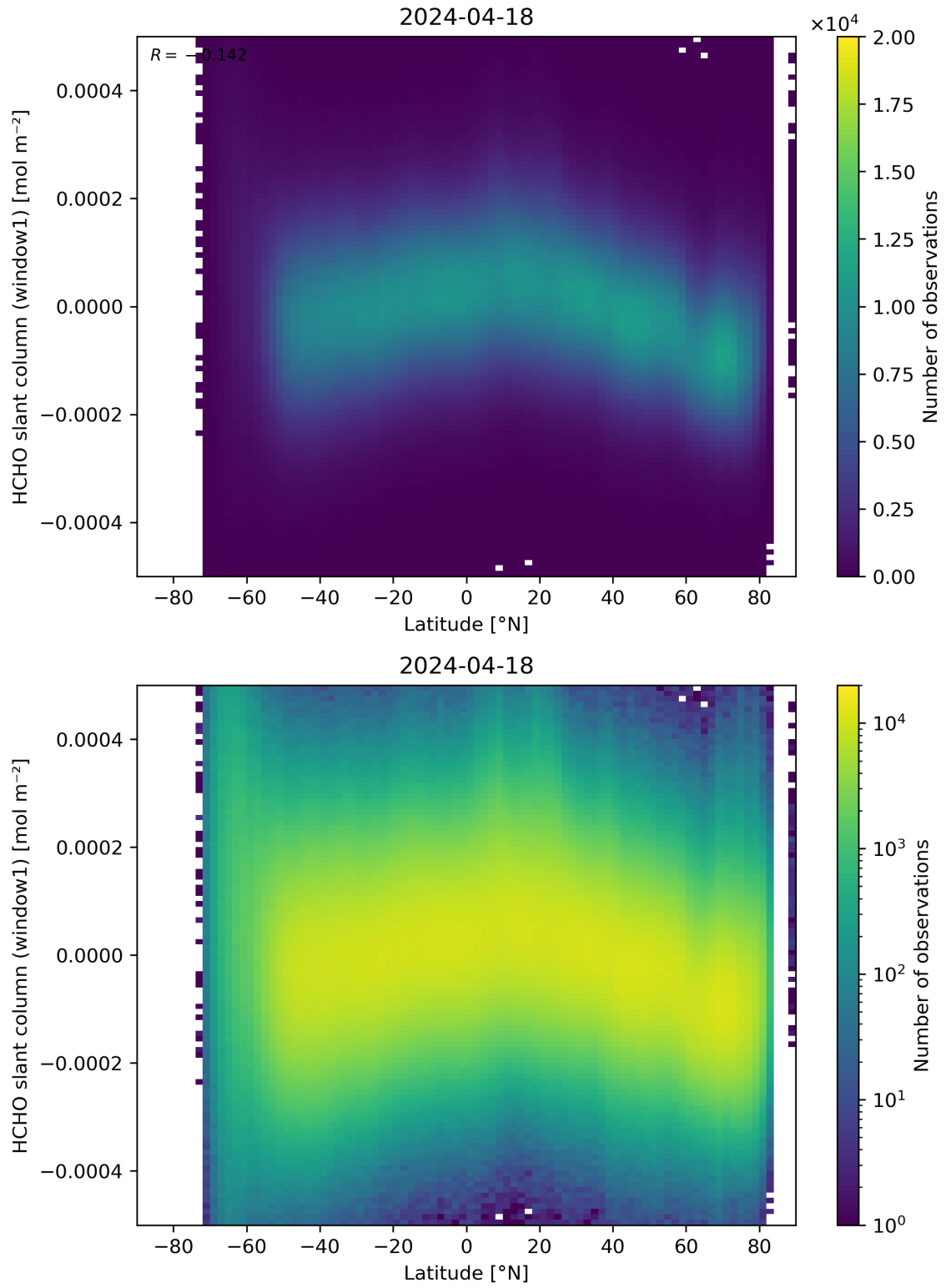
Figure 159: Scatter density plot of “Latitude” against “HCHO slant column (window1)” for 2024-04-17 to 2024-04-19.
