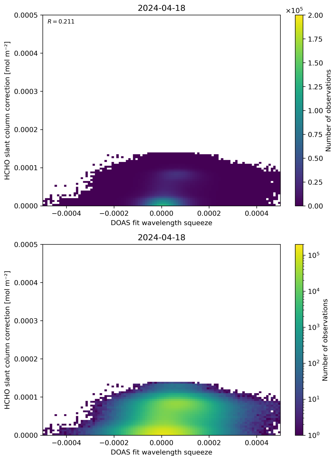
Figure 70: Scatter density plot of “DOAS fit wavelength squeeze” against “HCHO slant column correction” for 2024-04-17 to 2024-04-19.
