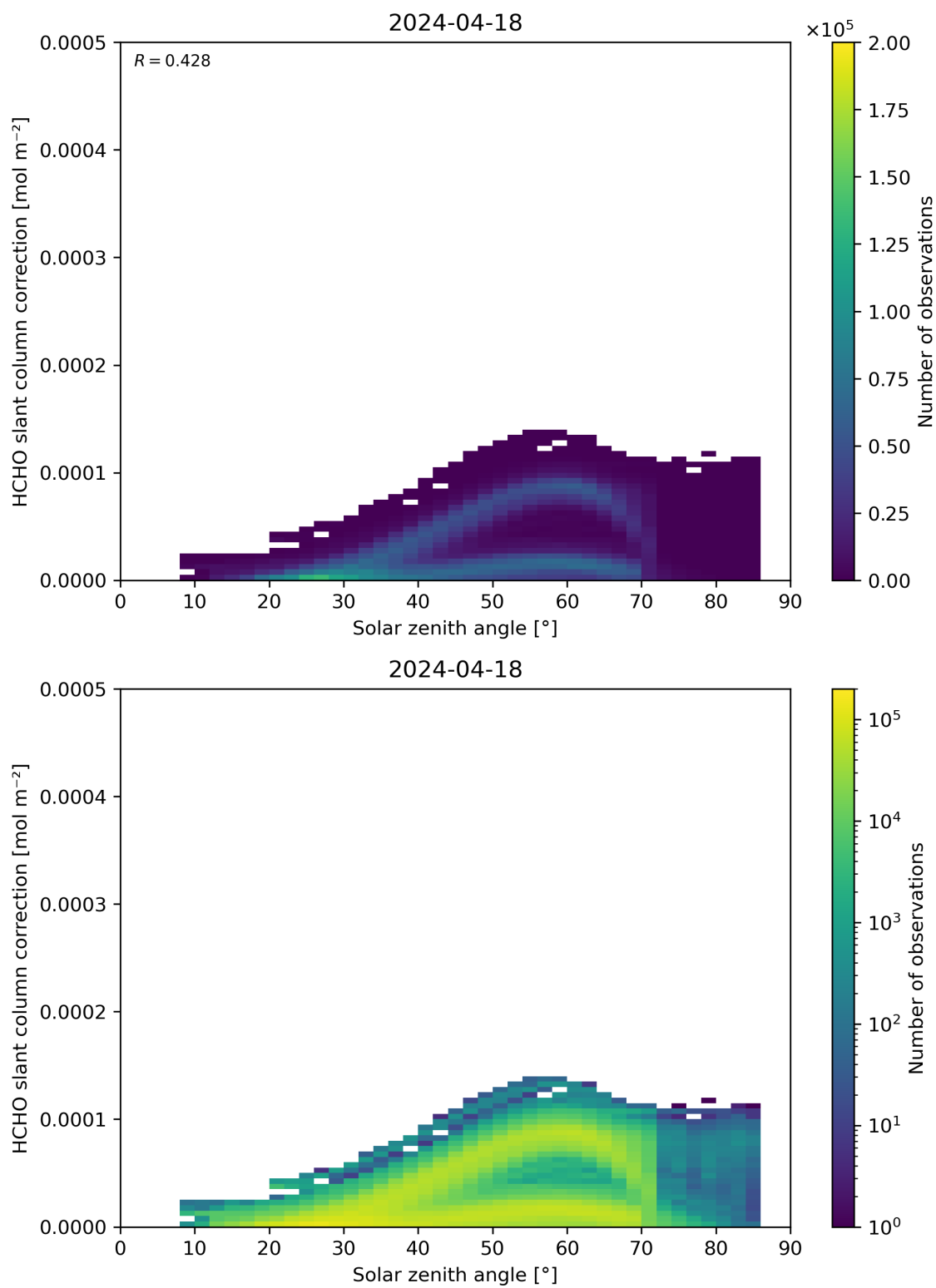
Figure 172: Scatter density plot of “Solar zenith angle” against “HCHO slant column correction” for 2024-04-17 to 2024-04-19.
