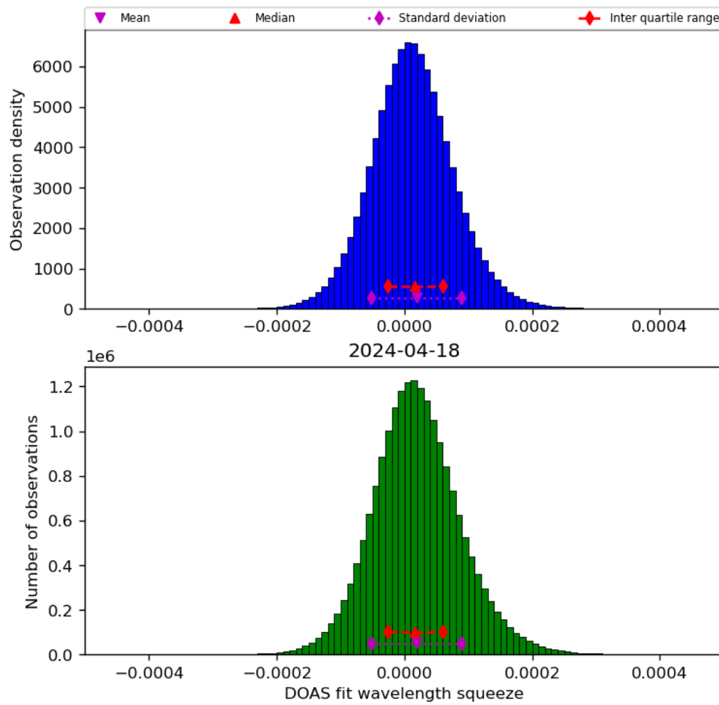
Figure 45: Histogram of “DOAS fit wavelength squeeze” for 2024-04-17 to 2024-04-19
