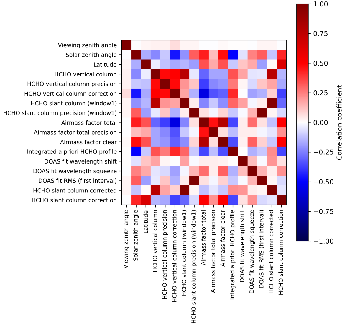
Figure 2: Map of correlation matrix for 2024-04-17 to 2024-04-19.
