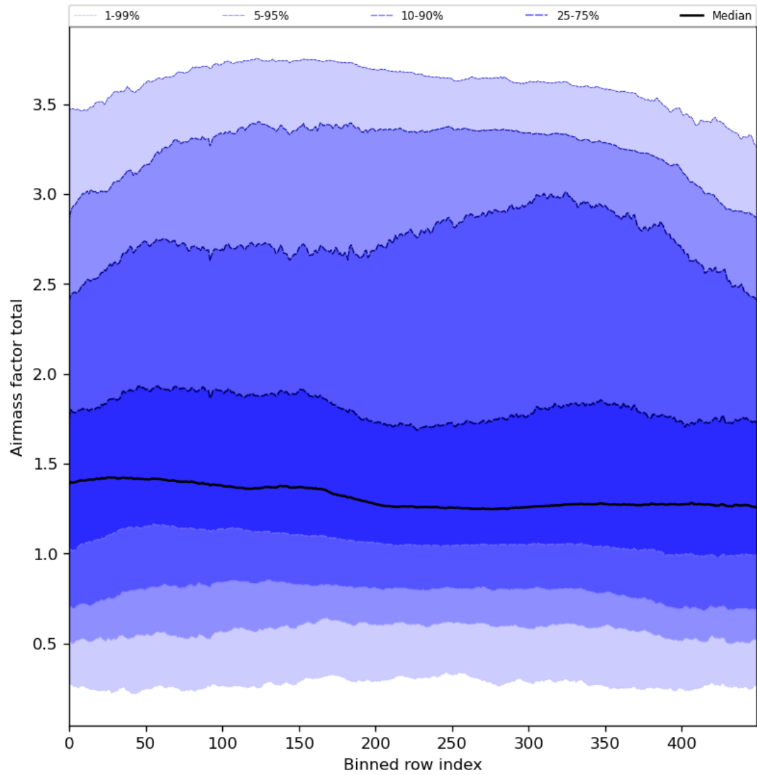
Figure 54: Along track statistics of “Airmass factor total” for 2024-04-17 to 2024-04-19
