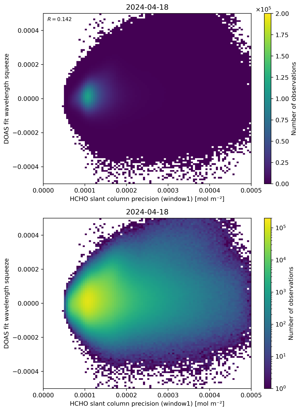
Figure 90: Scatter density plot of “HCHO slant column precision (window1)” against “DOAS fit wavelength squeeze” for 2024-04-17 to 2024-04-19.
