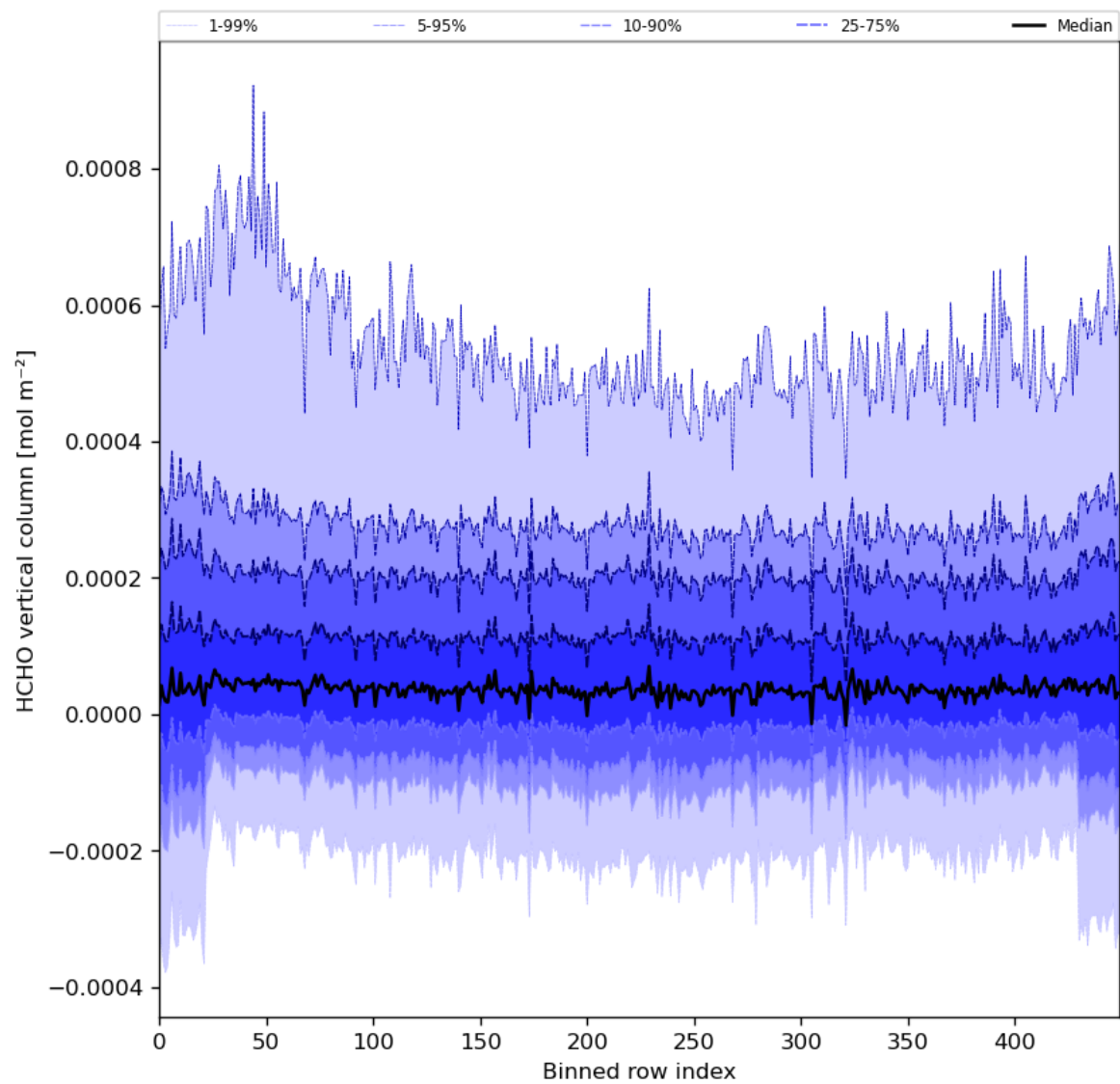
Figure 49: Along track statistics of “HCHO vertical column” for 2024-04-17 to 2024-04-19
