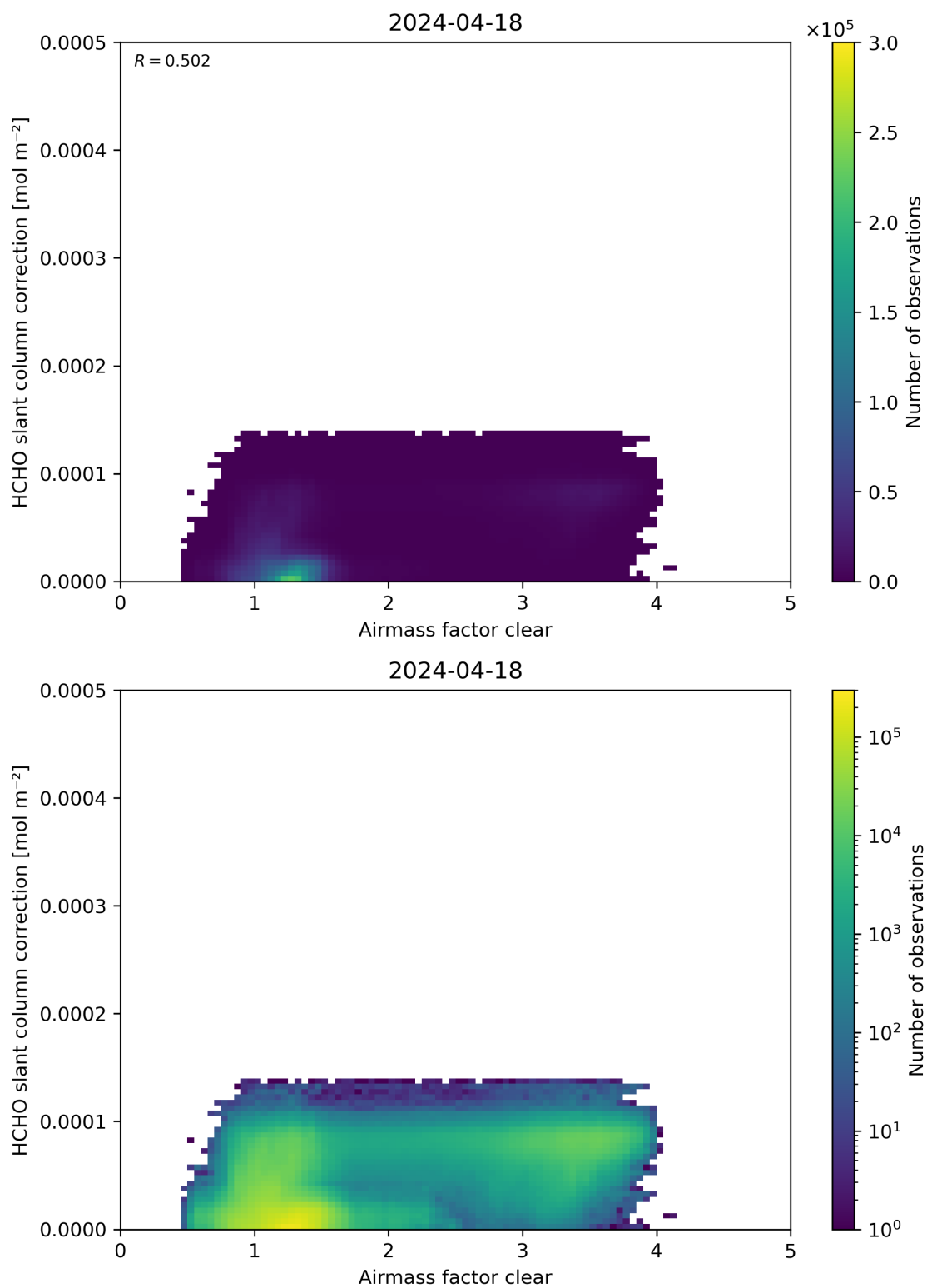
Figure 75: Scatter density plot of “Airmass factor clear” against “HCHO slant column correction” for 2024-04-17 to 2024-04-19.
