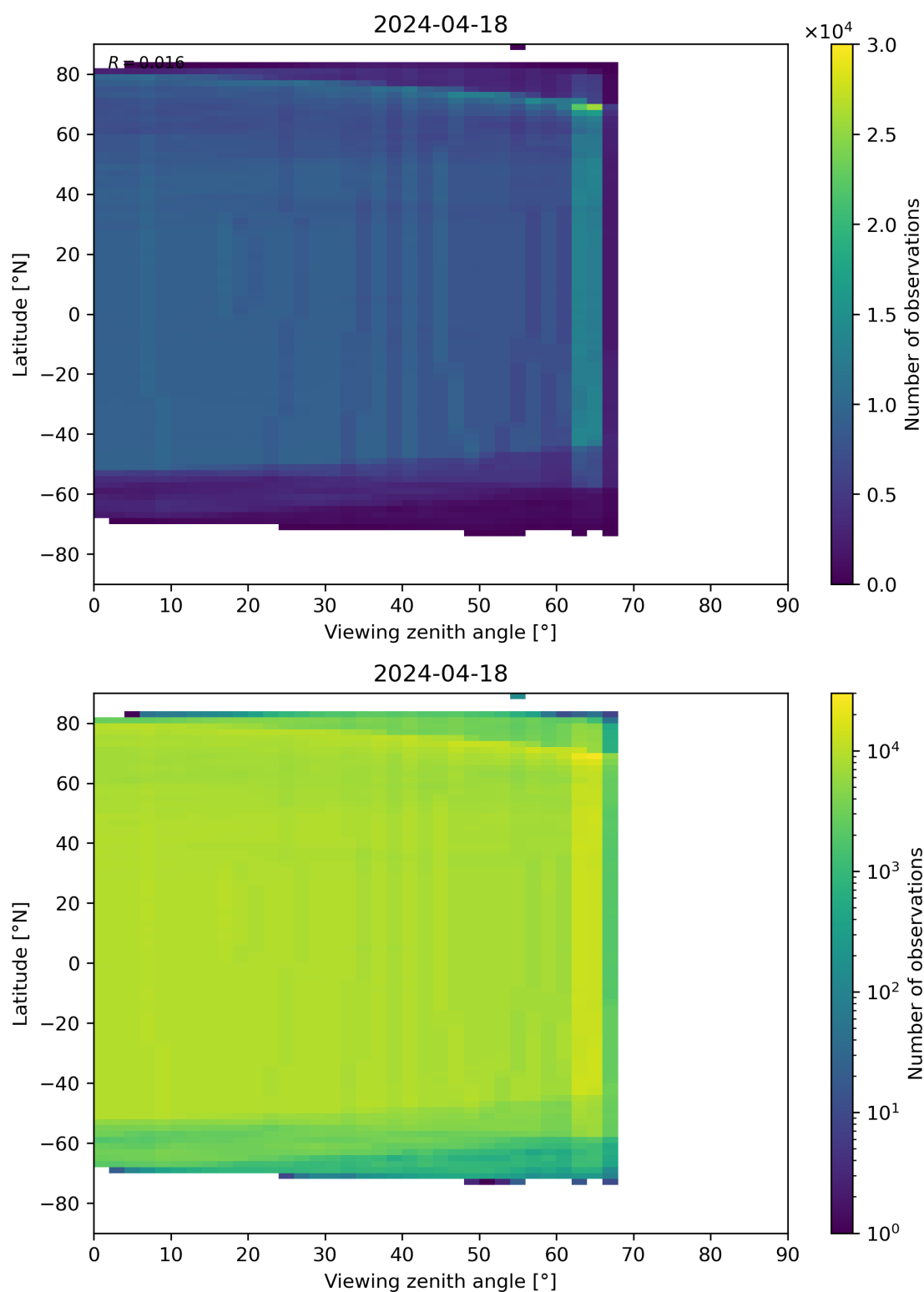
Figure 196: Scatter density plot of “Viewing zenith angle” against “Latitude” for 2024-04-17 to 2024-04-19.
