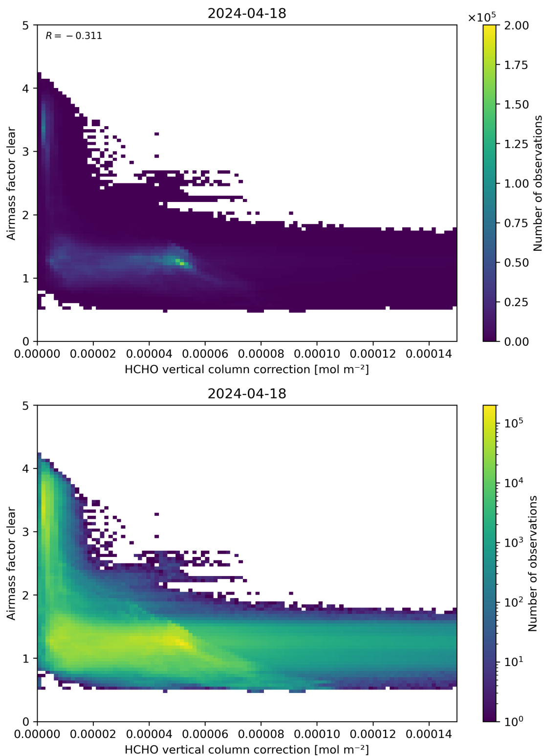
Figure 115: Scatter density plot of “HCHO vertical column correction” against “Airmass factor clear” for 2024-04-17 to 2024-04-19.
