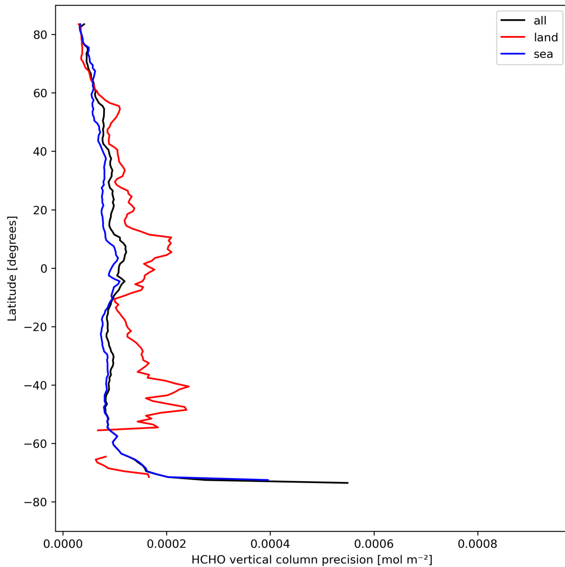
Figure 22: Zonal average of “HCHO vertical column precision” for 2024-04-17 to 2024-04-19.
