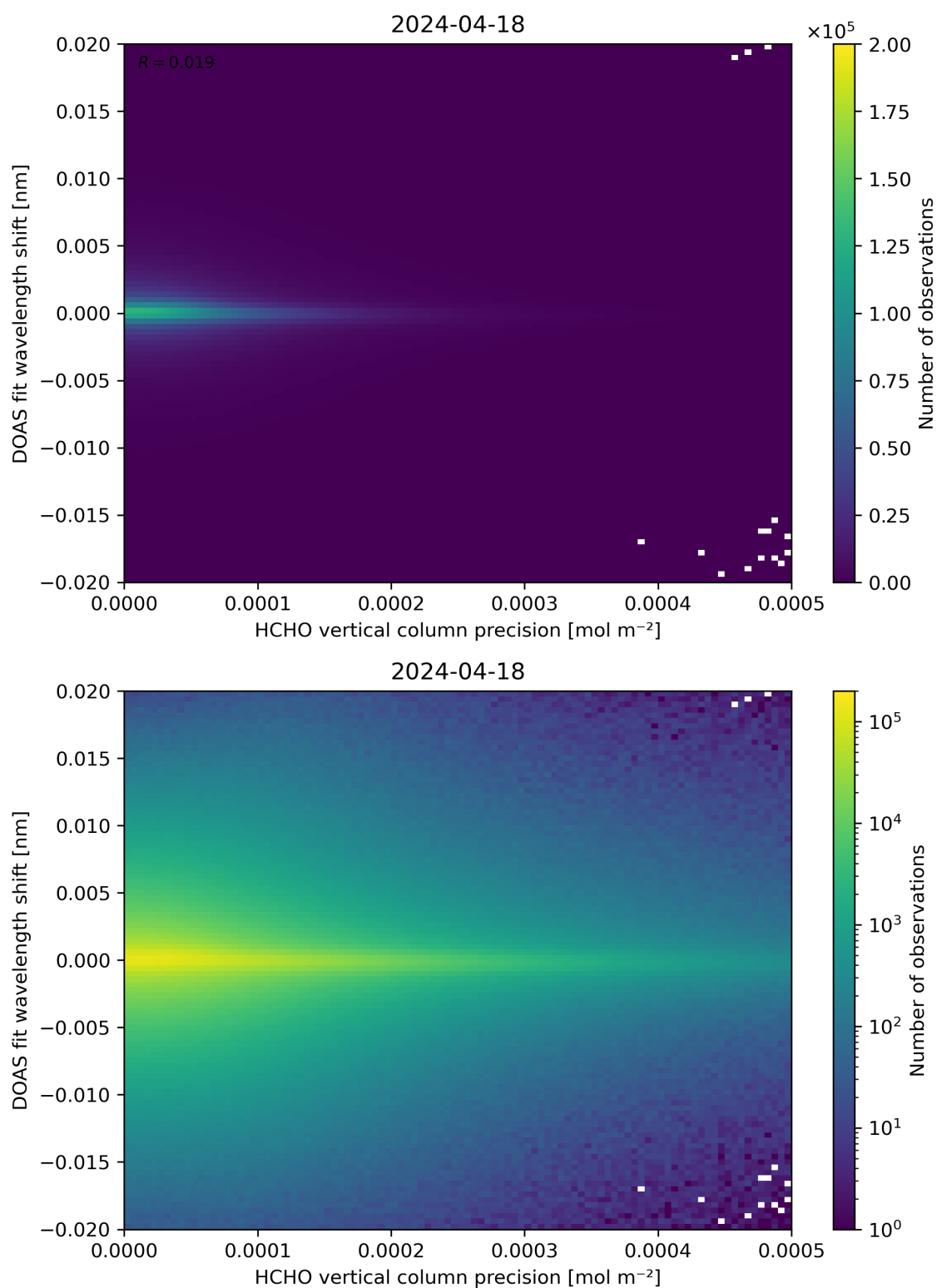
Figure 137: Scatter density plot of “HCHO vertical column precision” against “DOAS fit wavelength shift” for 2024-04-17 to 2024-04-19.
