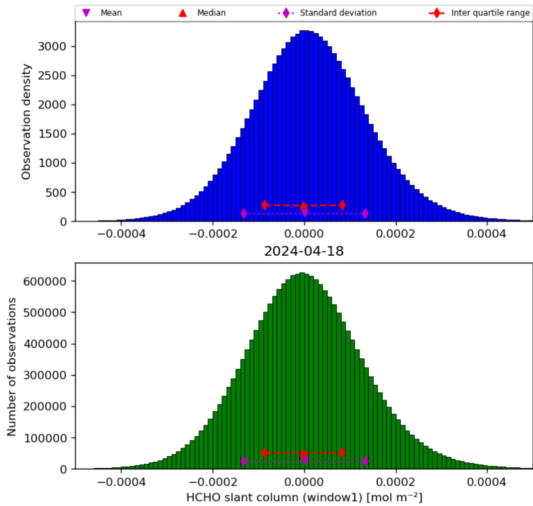
Figure 38: Histogram of “HCHO slant column (window1)” for 2024-04-17 to 2024-04-19
