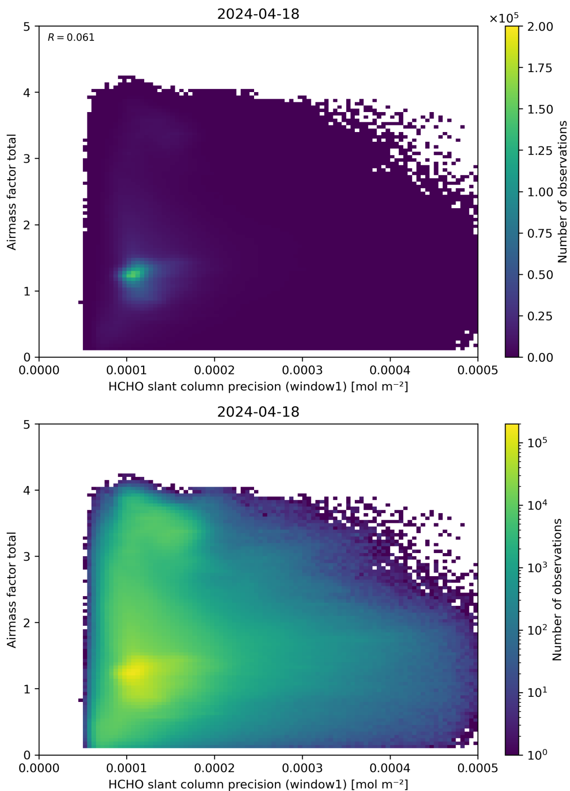
Figure 94: Scatter density plot of “HCHO slant column precision (window1)” against “Airmass factor total” for 2024-04-17 to 2024-04-19.
