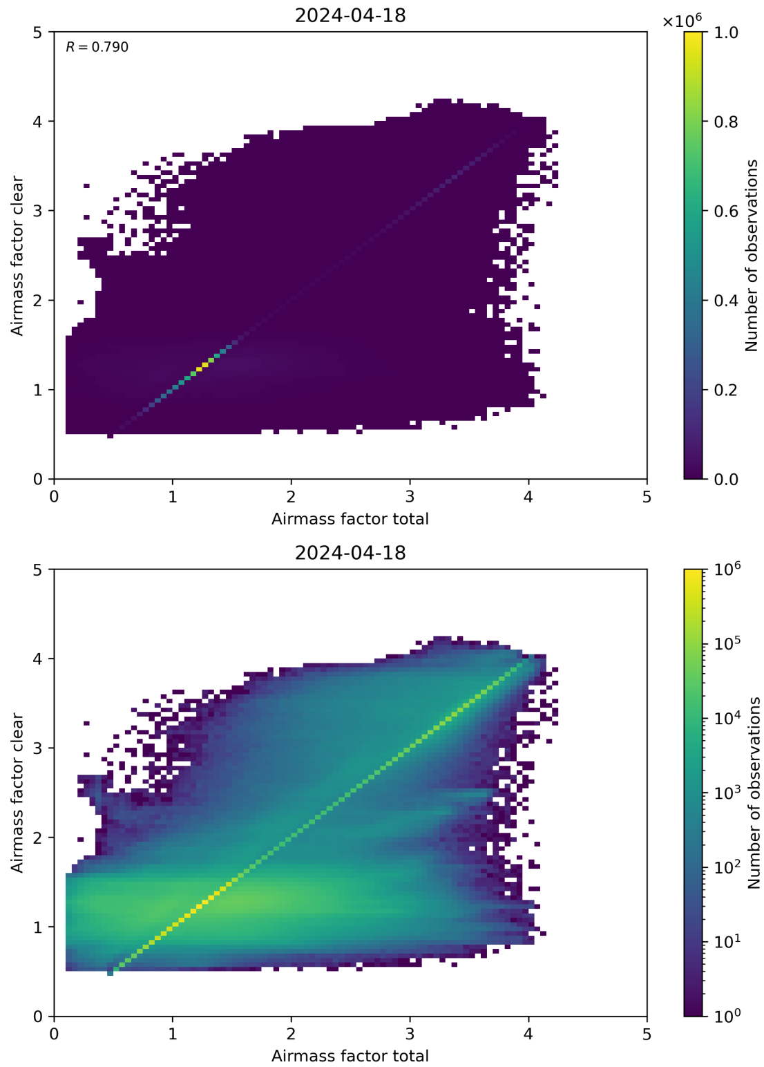
Figure 100: Scatter density plot of “Airmass factor total” against “Airmass factor clear” for 2024-04-17 to 2024-04-19.
