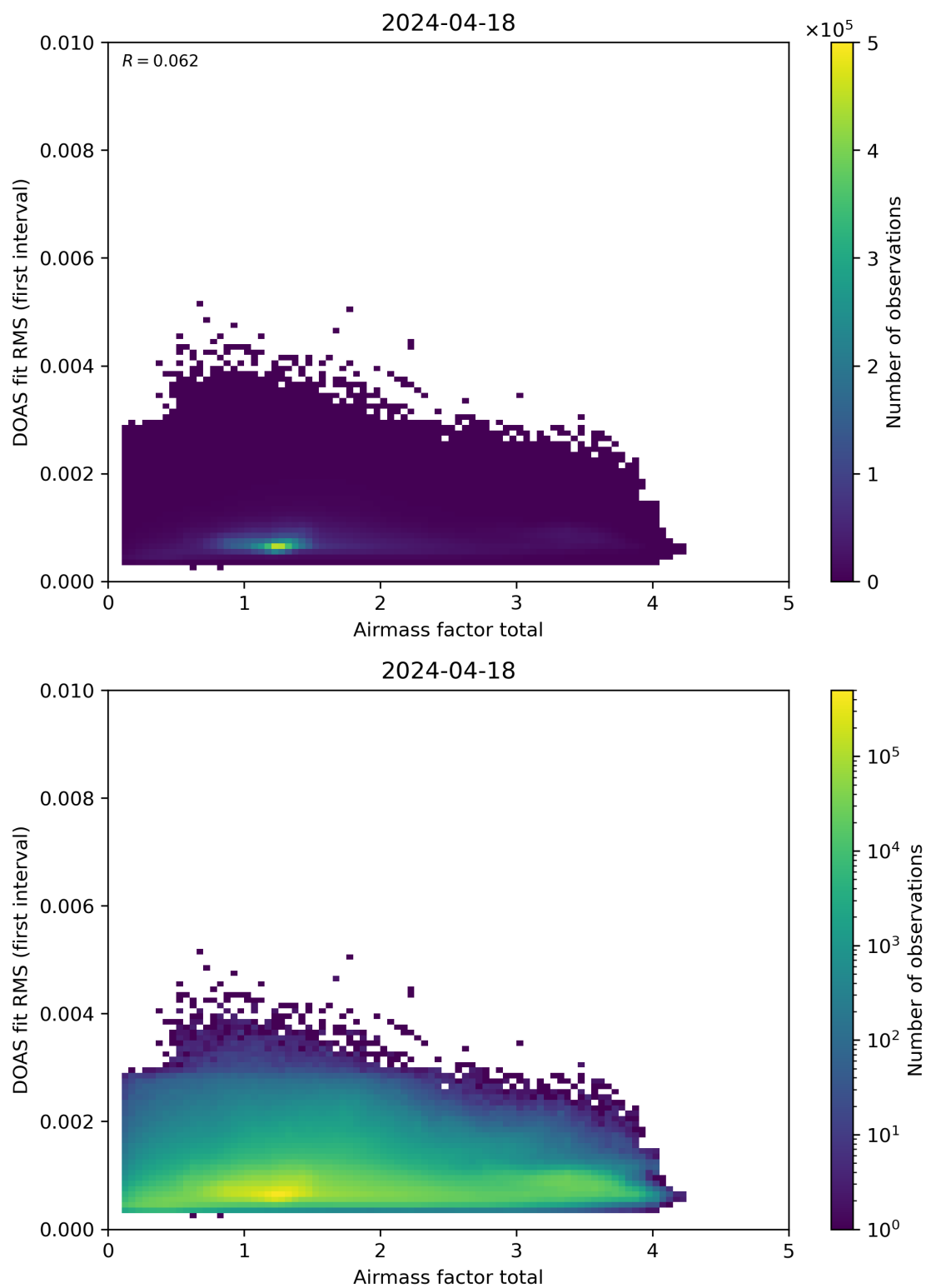
Figure 97: Scatter density plot of “Airmass factor total” against “DOAS fit RMS (first interval)” for 2024-04-17 to 2024-04-19.
