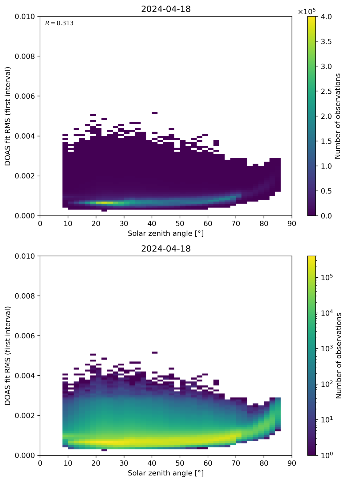
Figure 167: Scatter density plot of “Solar zenith angle” against “DOAS fit RMS (first interval)” for 2024-04-17 to 2024-04-19.
