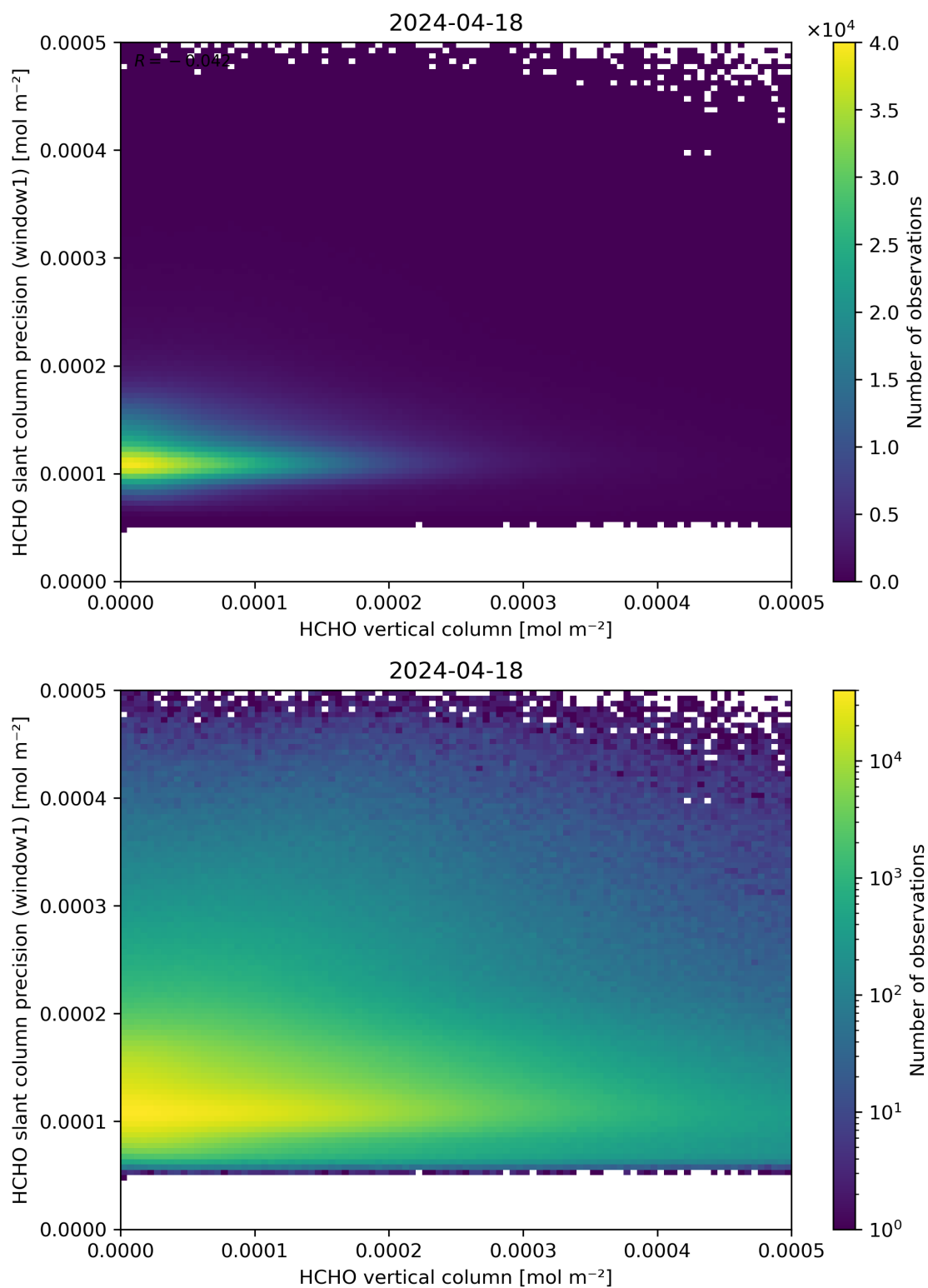
Figure 130: Scatter density plot of “HCHO vertical column” against “HCHO slant column precision (window1)” for 2024-04-17 to 2024-04-19.
