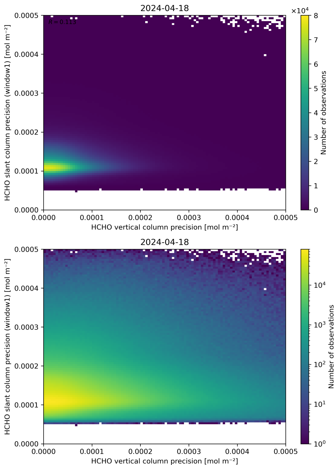
Figure 143: Scatter density plot of “HCHO vertical column precision” against “HCHO slant column precision (window1)” for 2024-04-17 to 2024-04-19.
