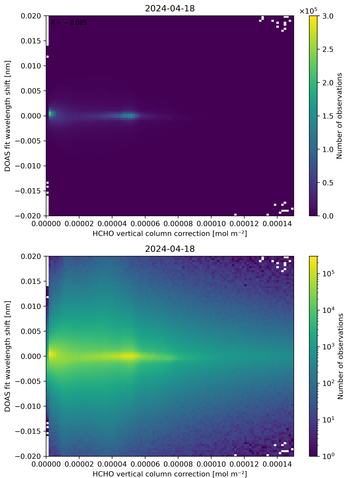
Figure 113: Scatter density plot of “HCHO vertical column correction” against “DOAS fit wavelength shift” for 2024-04-17 to 2024-04-19.
