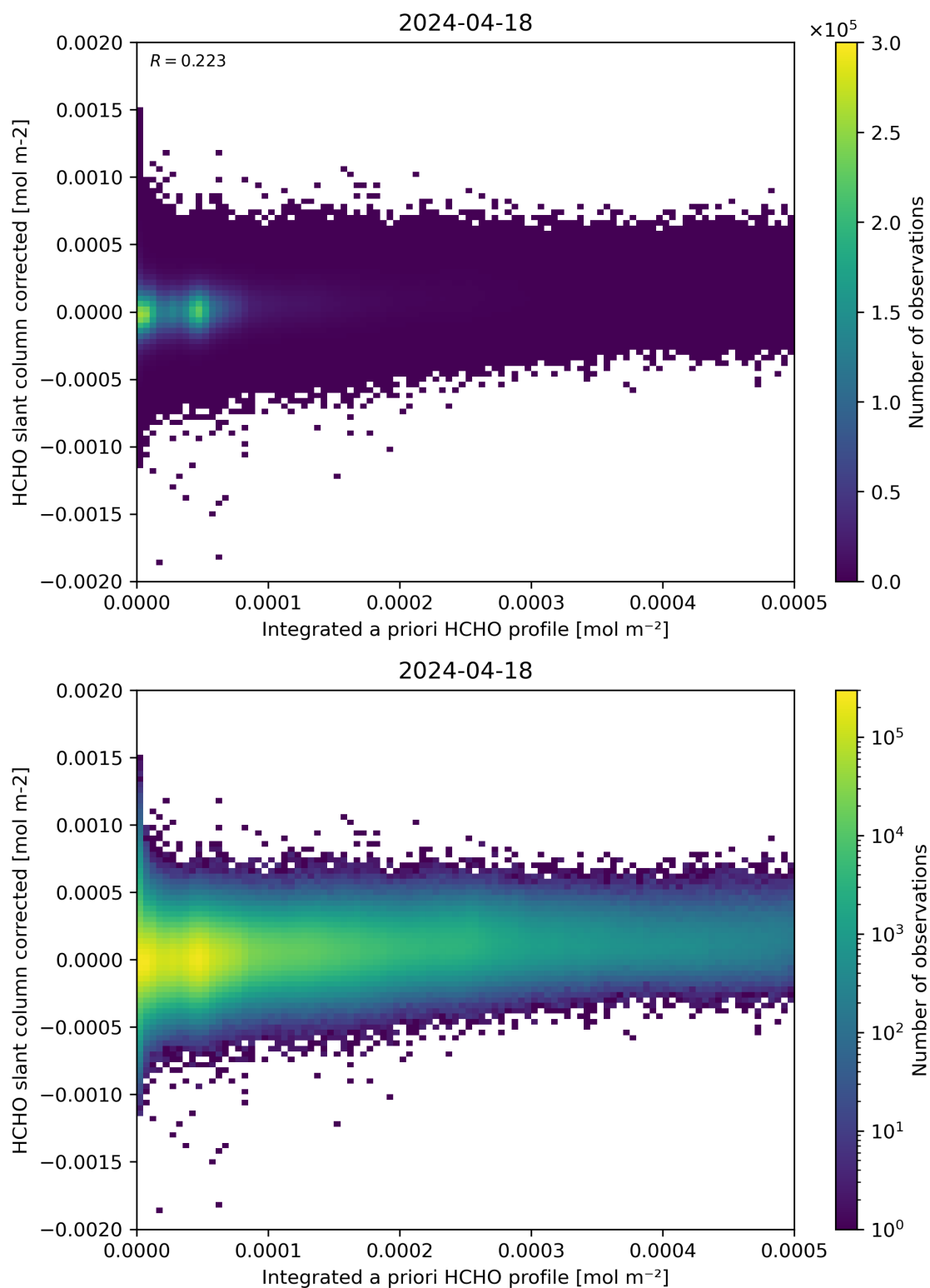
Figure 151: Scatter density plot of “Integrated a priori HCHO profile” against “HCHO slant column corrected” for 2024-04-17 to 2024-04-19.
