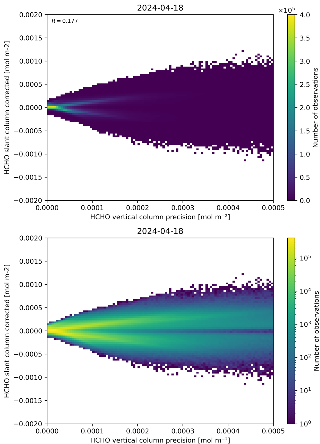
Figure 140: Scatter density plot of “HCHO vertical column precision” against “HCHO slant column corrected” for 2024-04-17 to 2024-04-19.
