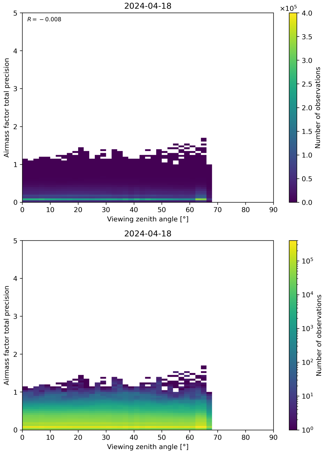
Figure 191: Scatter density plot of “Viewing zenith angle” against “Airmass factor total precision” for 2024-04-17 to 2024-04-19.
