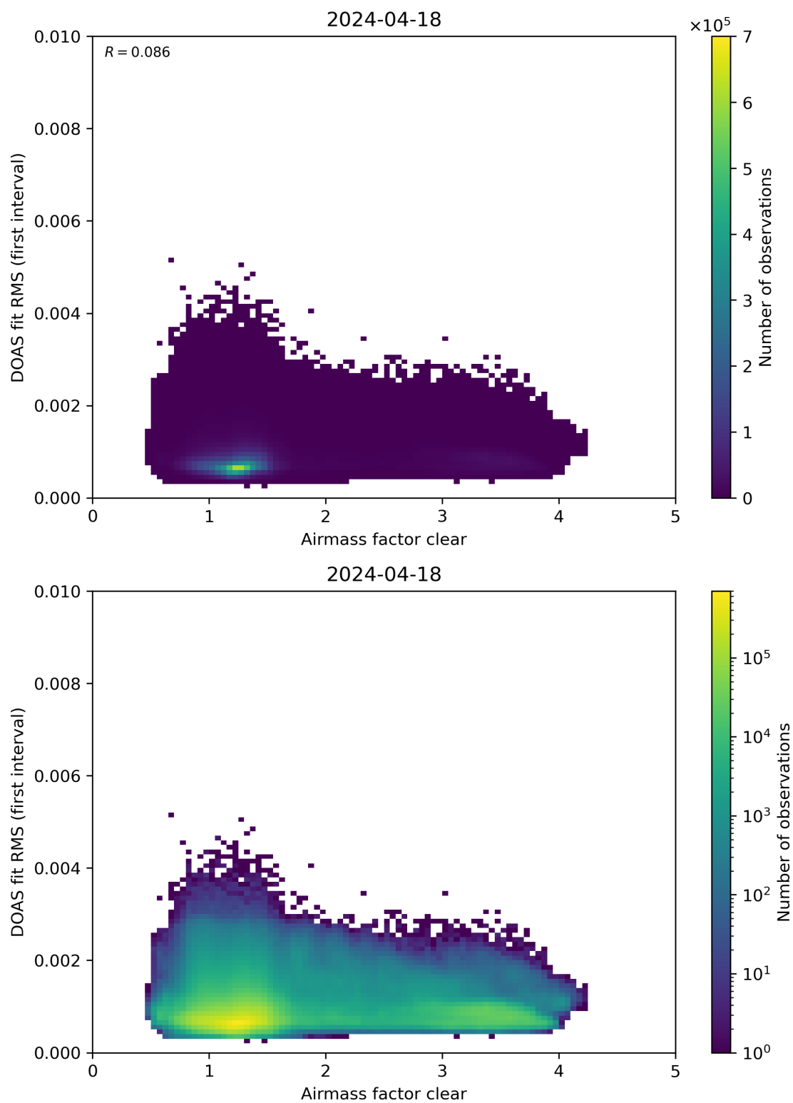
Figure 71: Scatter density plot of “Airmass factor clear” against “DOAS fit RMS (first interval)” for 2024-04-17 to 2024-04-19.
