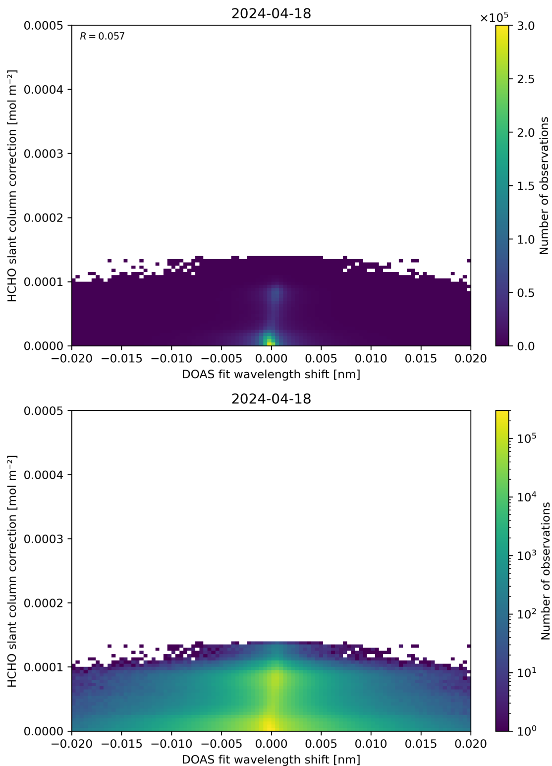
Figure 67: Scatter density plot of “DOAS fit wavelength shift” against “HCHO slant column correction” for 2024-04-17 to 2024-04-19.
