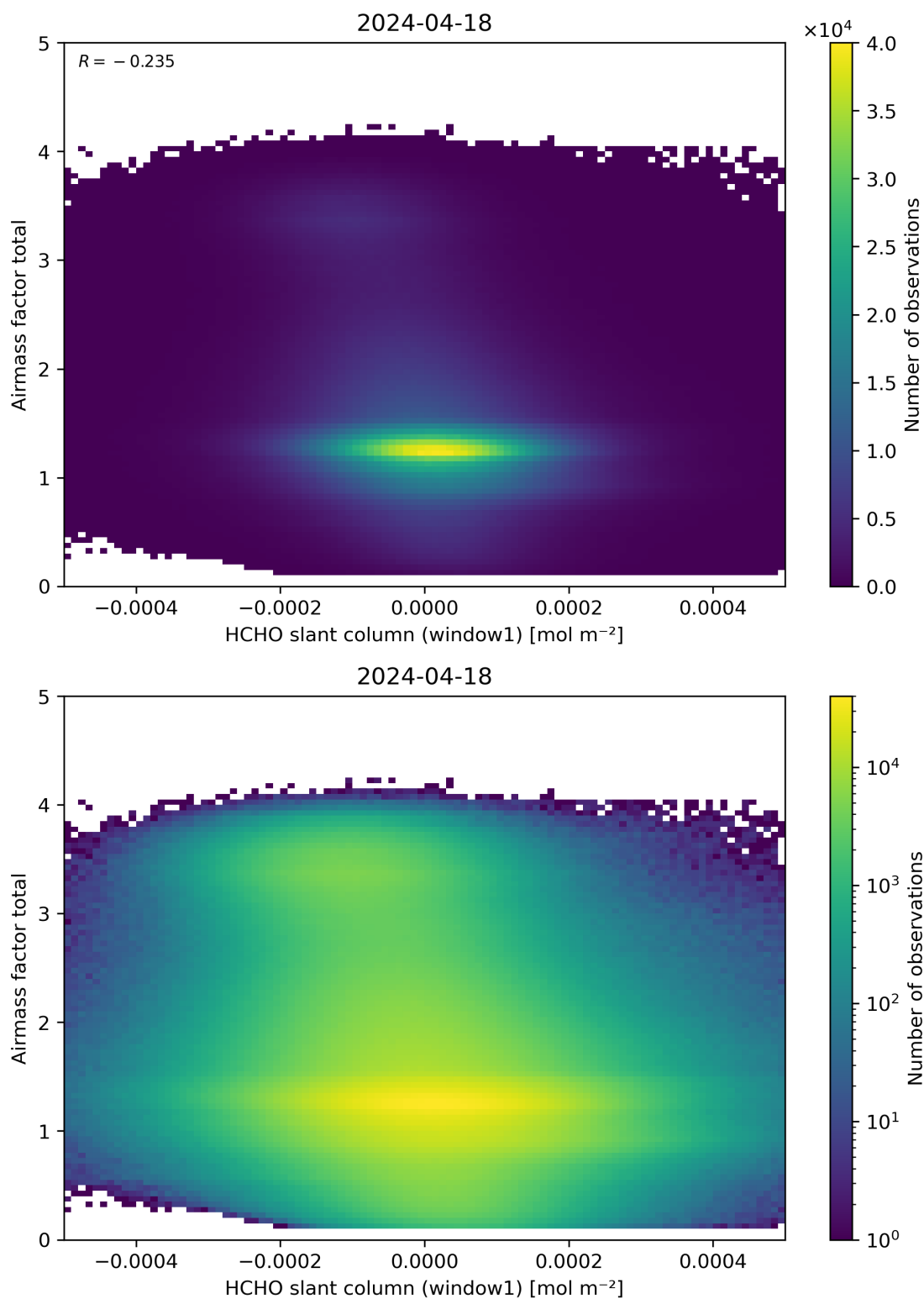
Figure 85: Scatter density plot of “HCHO slant column (window1)” against “Airmass factor total” for 2024-04-17 to 2024-04-19.
