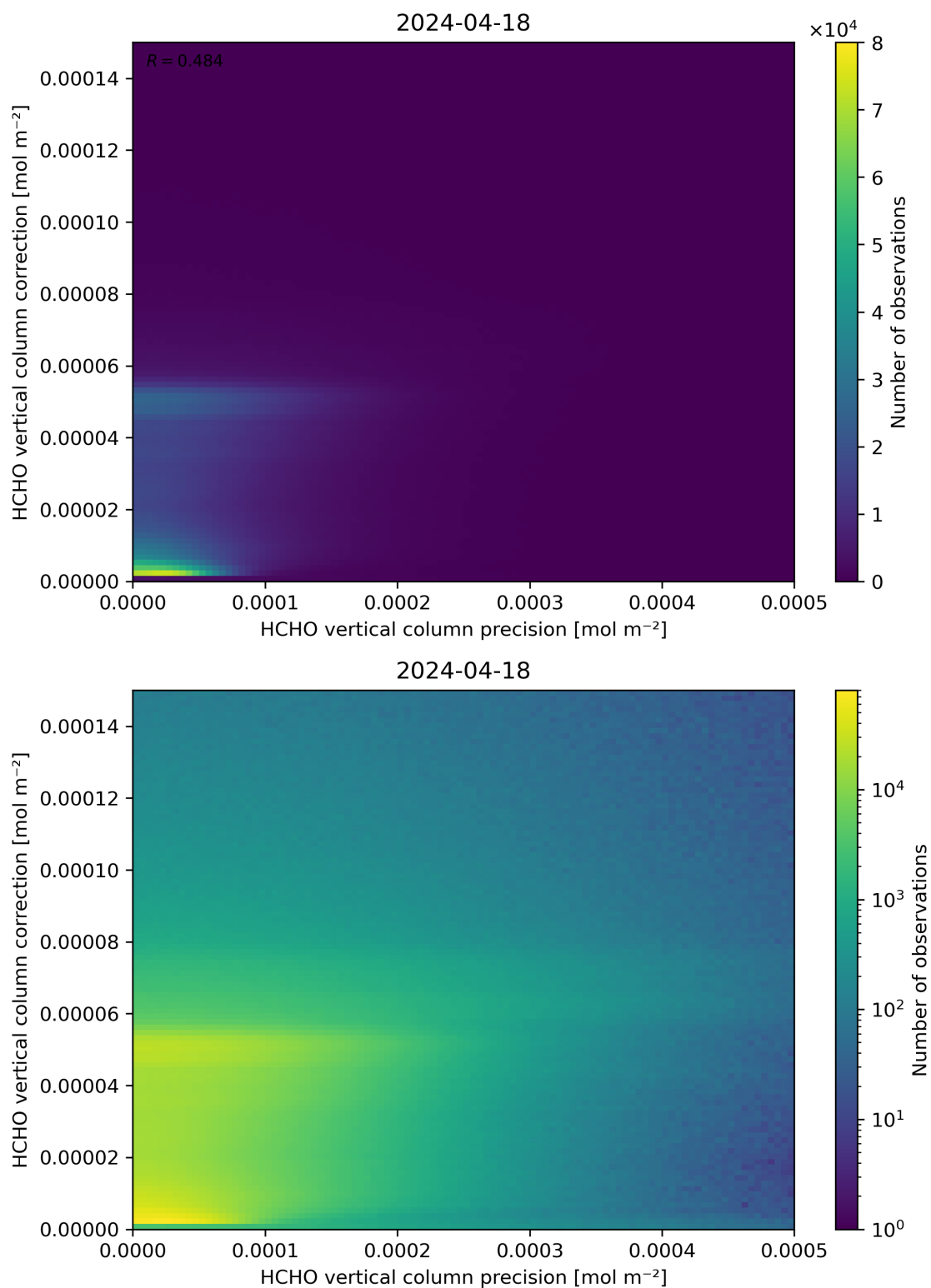
Figure 146: Scatter density plot of “HCHO vertical column precision” against “HCHO vertical column correction” for 2024-04-17 to 2024-04-19.
