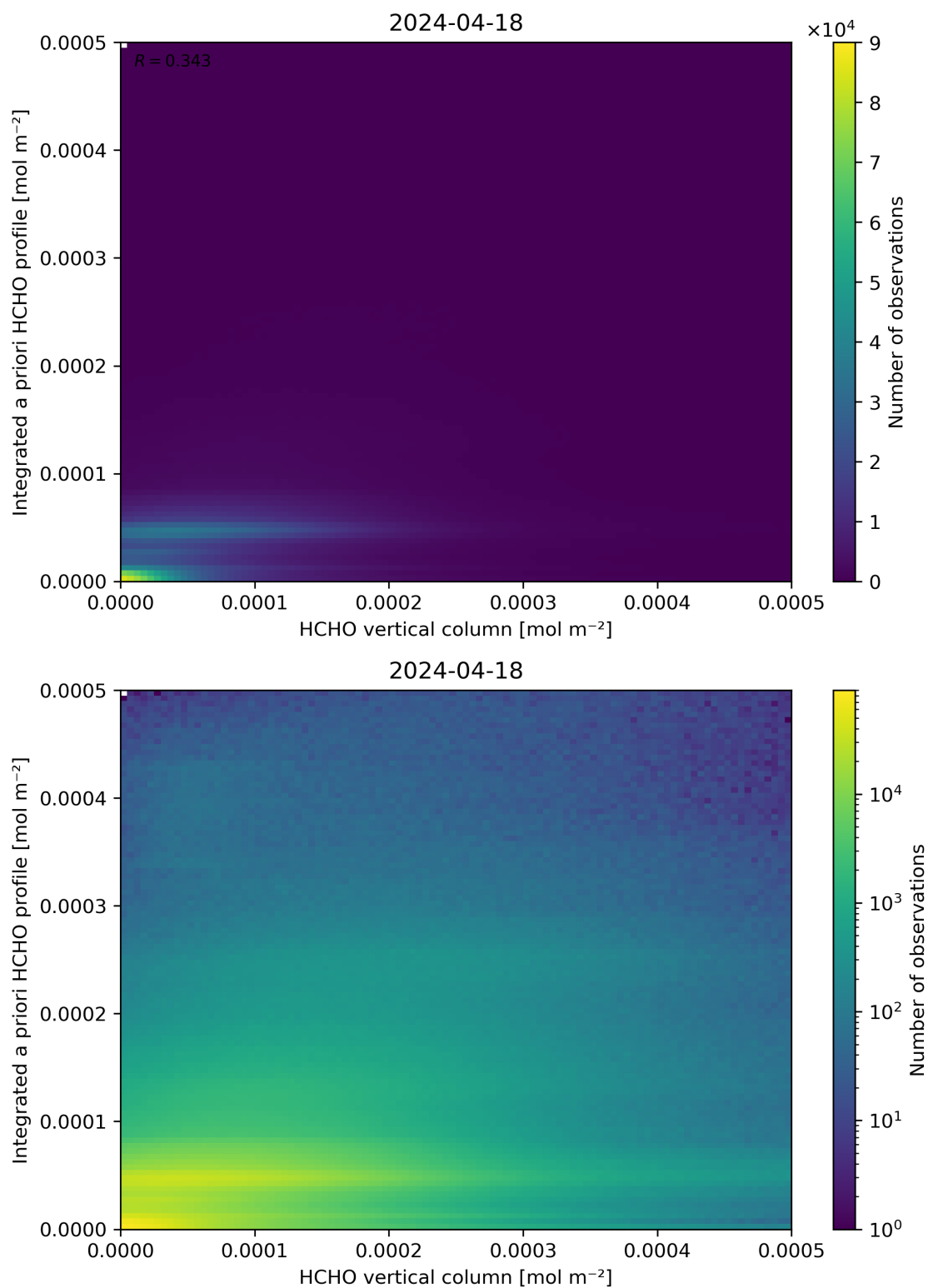
Figure 135: Scatter density plot of “HCHO vertical column” against “Integrated a priori HCHO profile” for 2024-04-17 to 2024-04-19.
