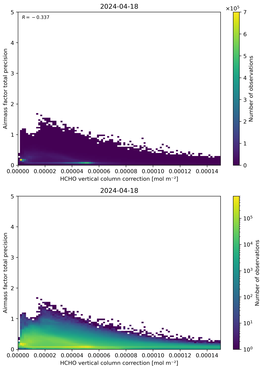
Figure 121: Scatter density plot of “HCHO vertical column correction” against “Airmass factor total precision” for 2024-04-17 to 2024-04-19.
