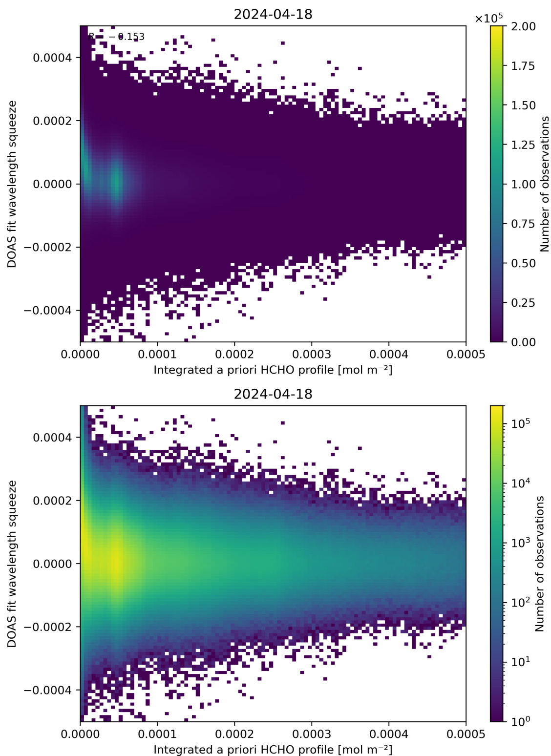
Figure 150: Scatter density plot of “Integrated a priori HCHO profile” against “DOAS fit wavelength squeeze” for 2024-04-17 to 2024-04-19.
