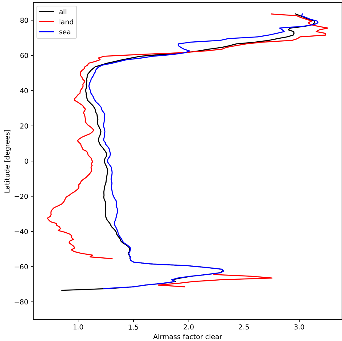
Figure 28: Zonal average of “Airmass factor clear” for 2024-04-17 to 2024-04-19.
