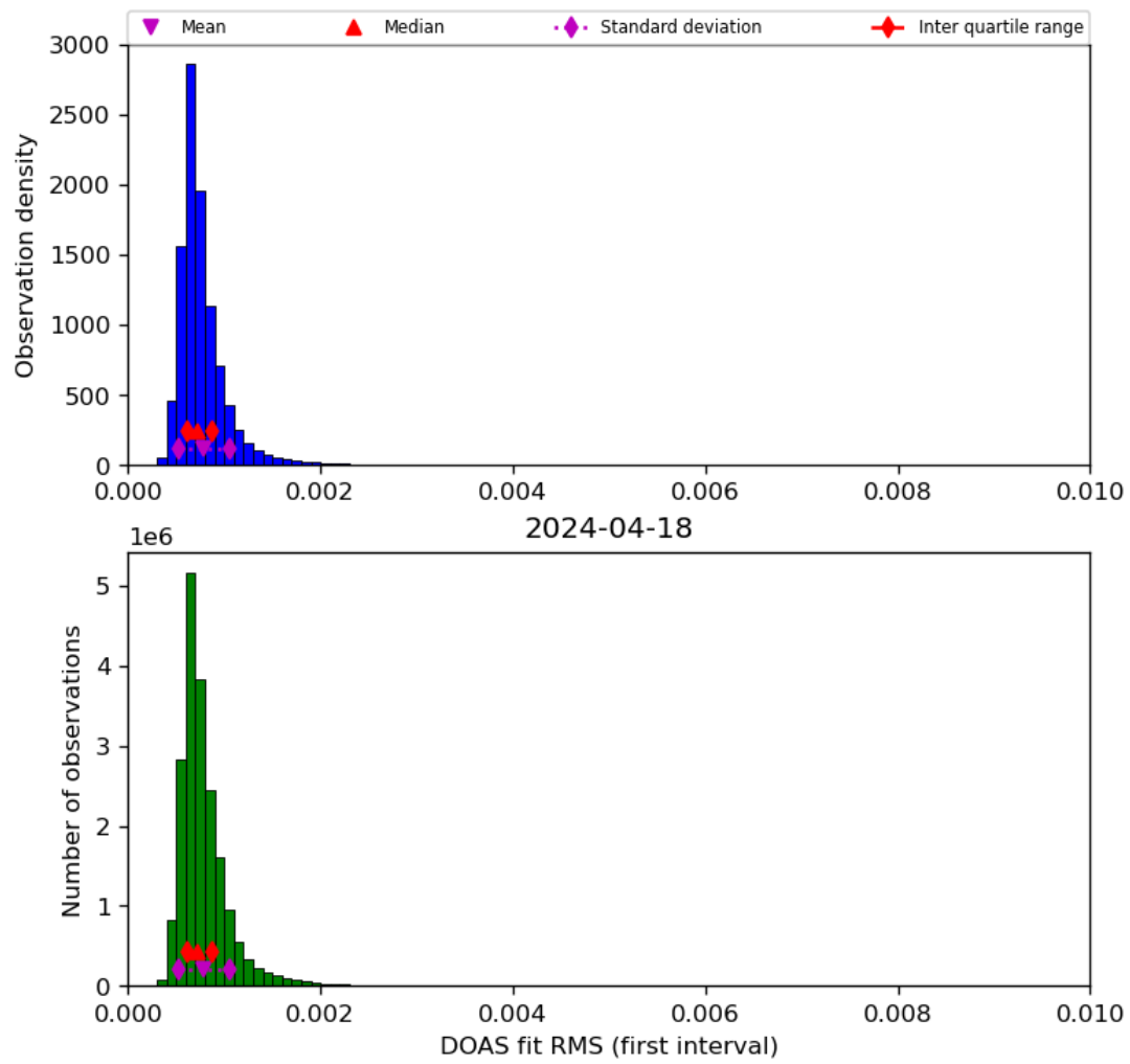
Figure 46: Histogram of “DOAS fit RMS (first interval)” for 2024-04-17 to 2024-04-19
