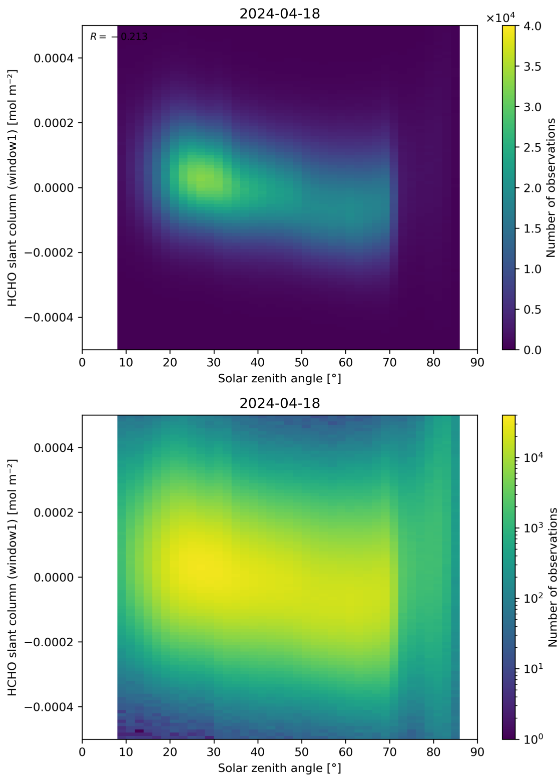
Figure 173: Scatter density plot of “Solar zenith angle” against “HCHO slant column (window1)” for 2024-04-17 to 2024-04-19.
