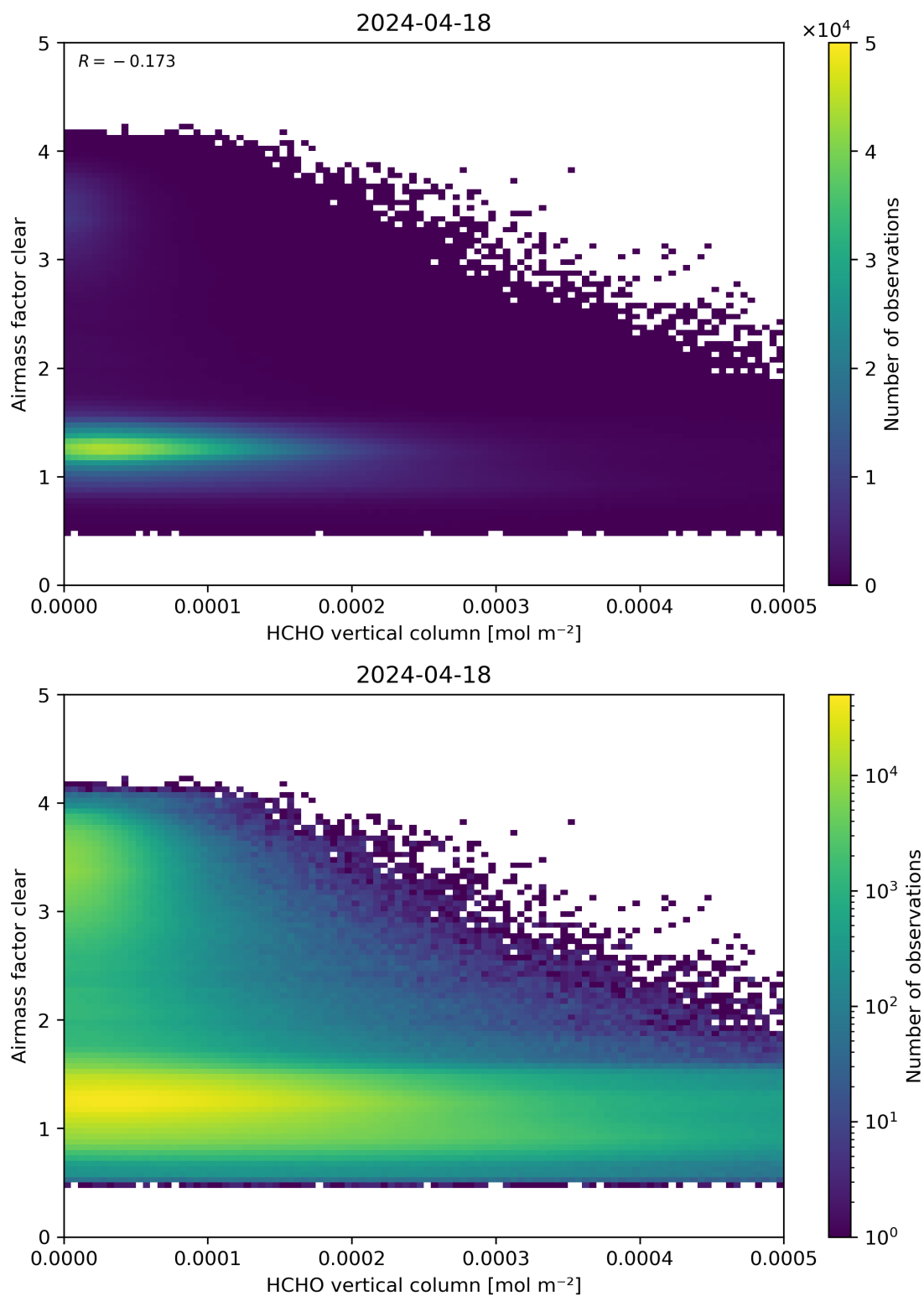
Figure 126: Scatter density plot of “HCHO vertical column” against “Airmass factor clear” for 2024-04-17 to 2024-04-19.
