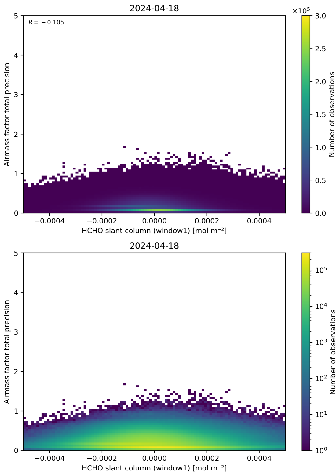
Figure 86: Scatter density plot of “HCHO slant column (window1)” against “Airmass factor total precision” for 2024-04-17 to 2024-04-19.
