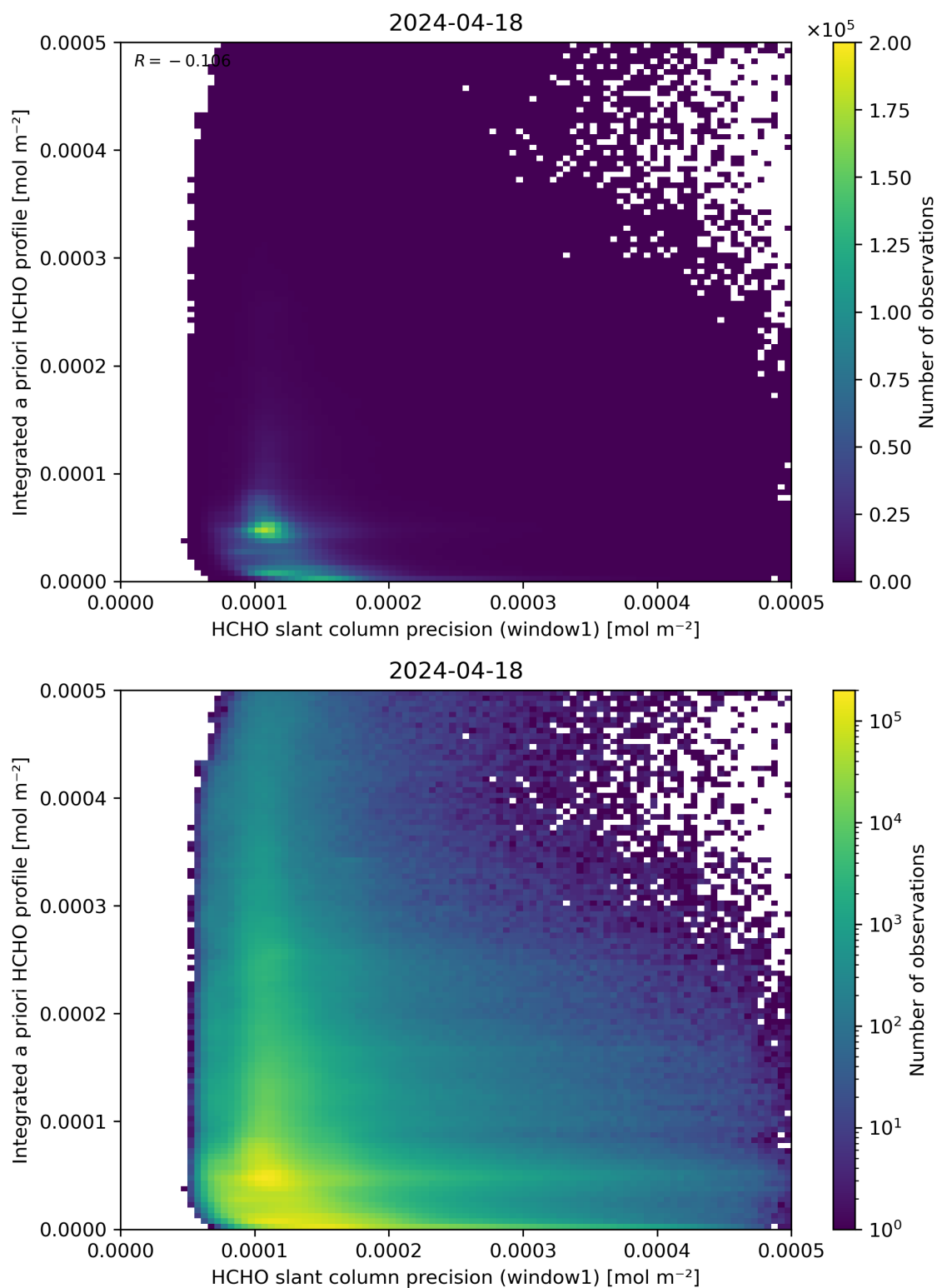
Figure 96: Scatter density plot of “HCHO slant column precision (window1)” against “Integrated a priori HCHO profile” for 2024-04-17 to 2024-04-19.
