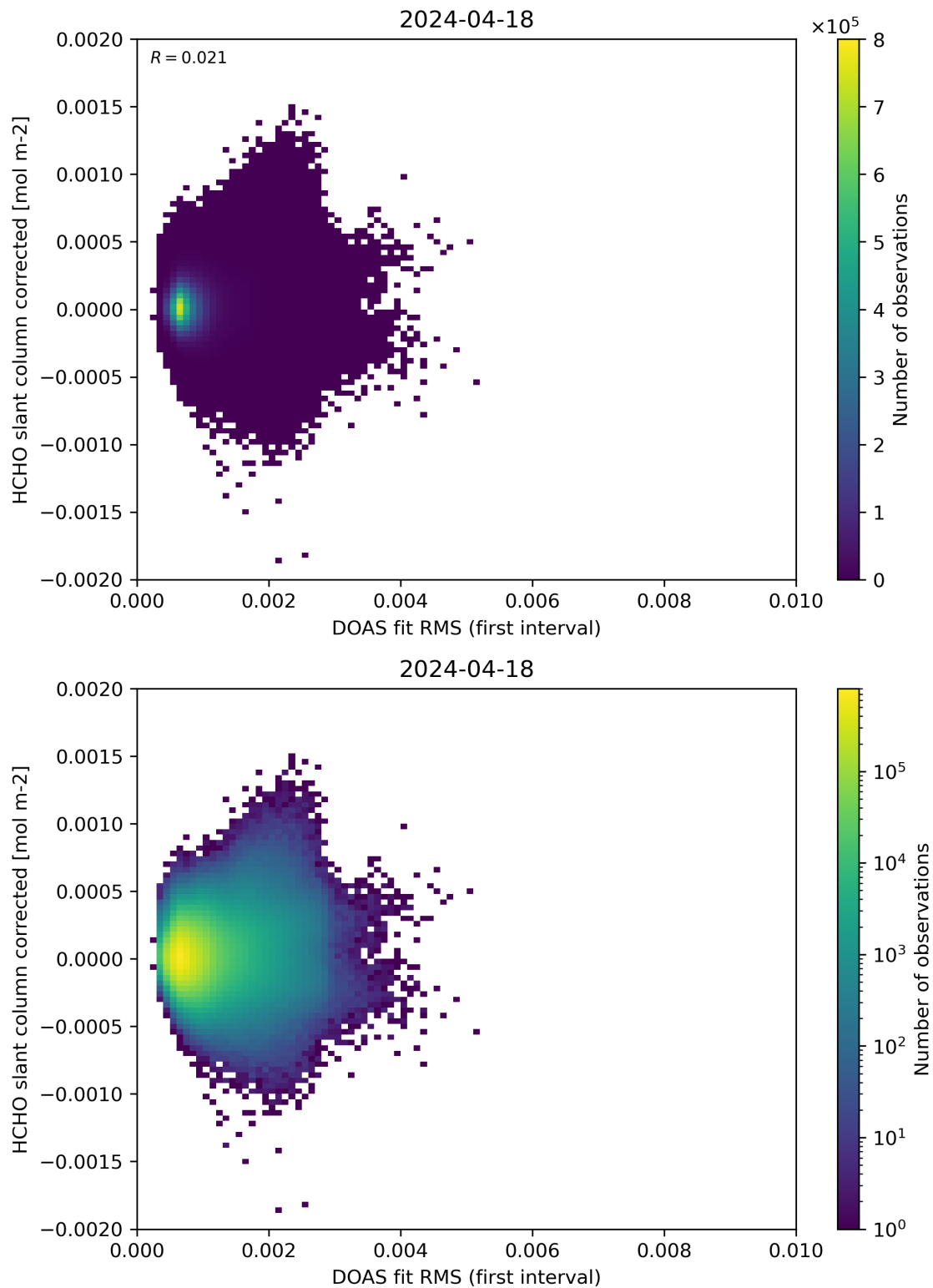
Figure 62: Scatter density plot of “DOAS fit RMS (first interval)” against “HCHO slant column corrected” for 2024-04-17 to 2024-04-19.
