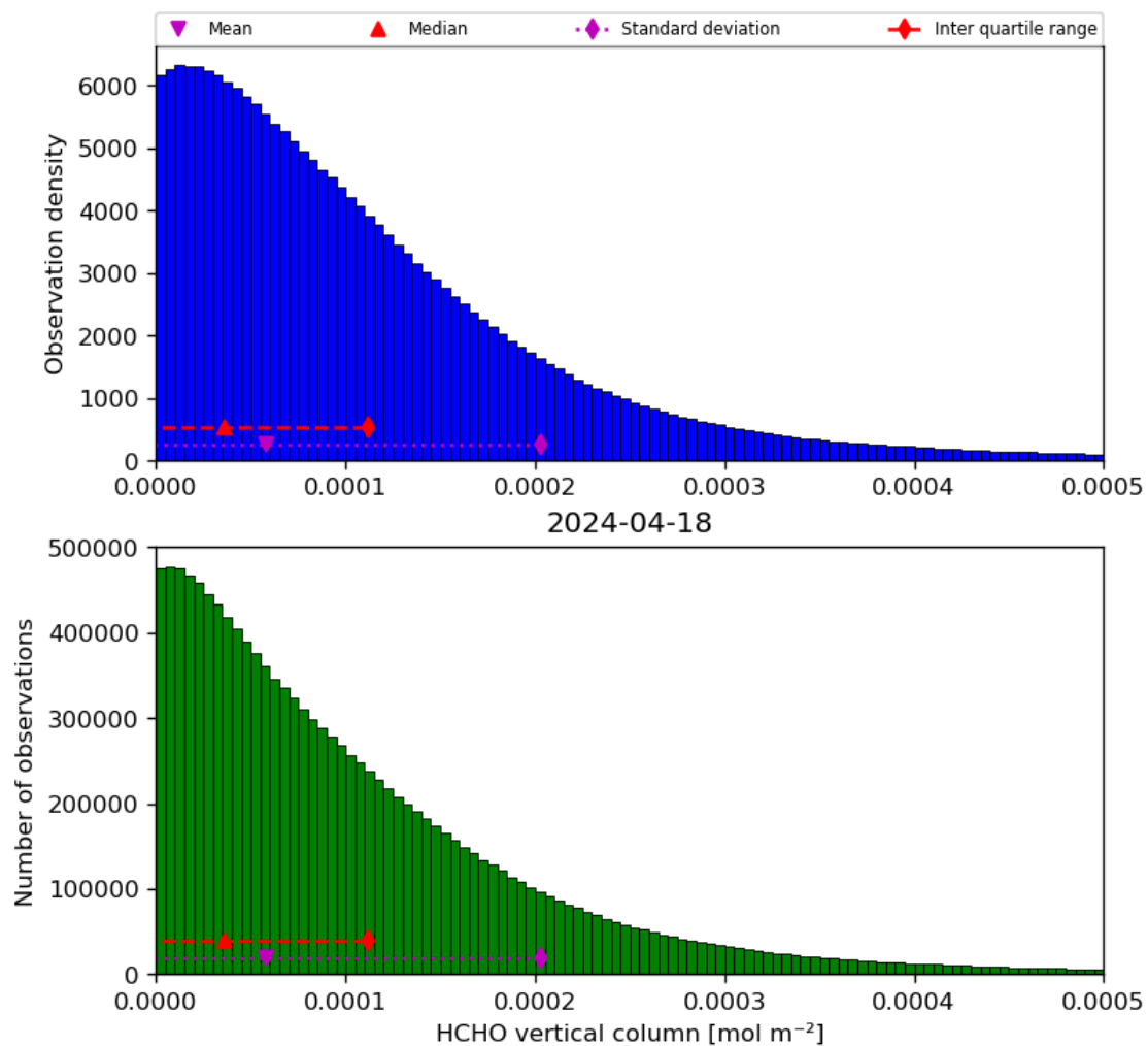
Figure 35: Histogram of “HCHO vertical column” for 2024-04-17 to 2024-04-19
