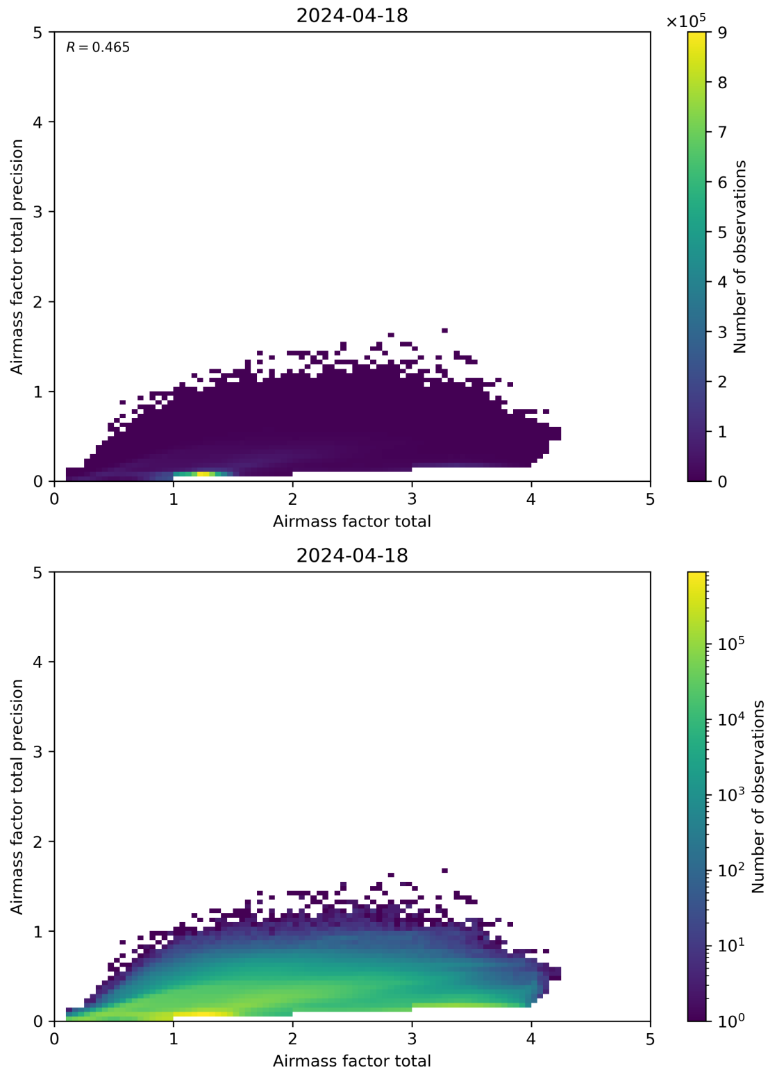
Figure 103: Scatter density plot of “Airmass factor total” against “Airmass factor total precision” for 2024-04-17 to 2024-04-19.
