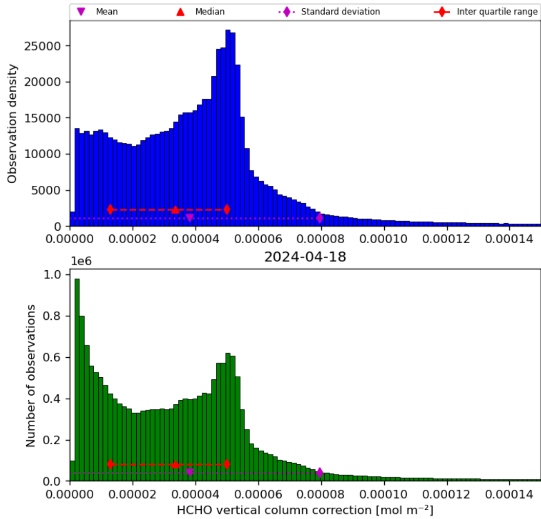
Figure 37: Histogram of “HCHO vertical column correction” for 2024-04-17 to 2024-04-19
