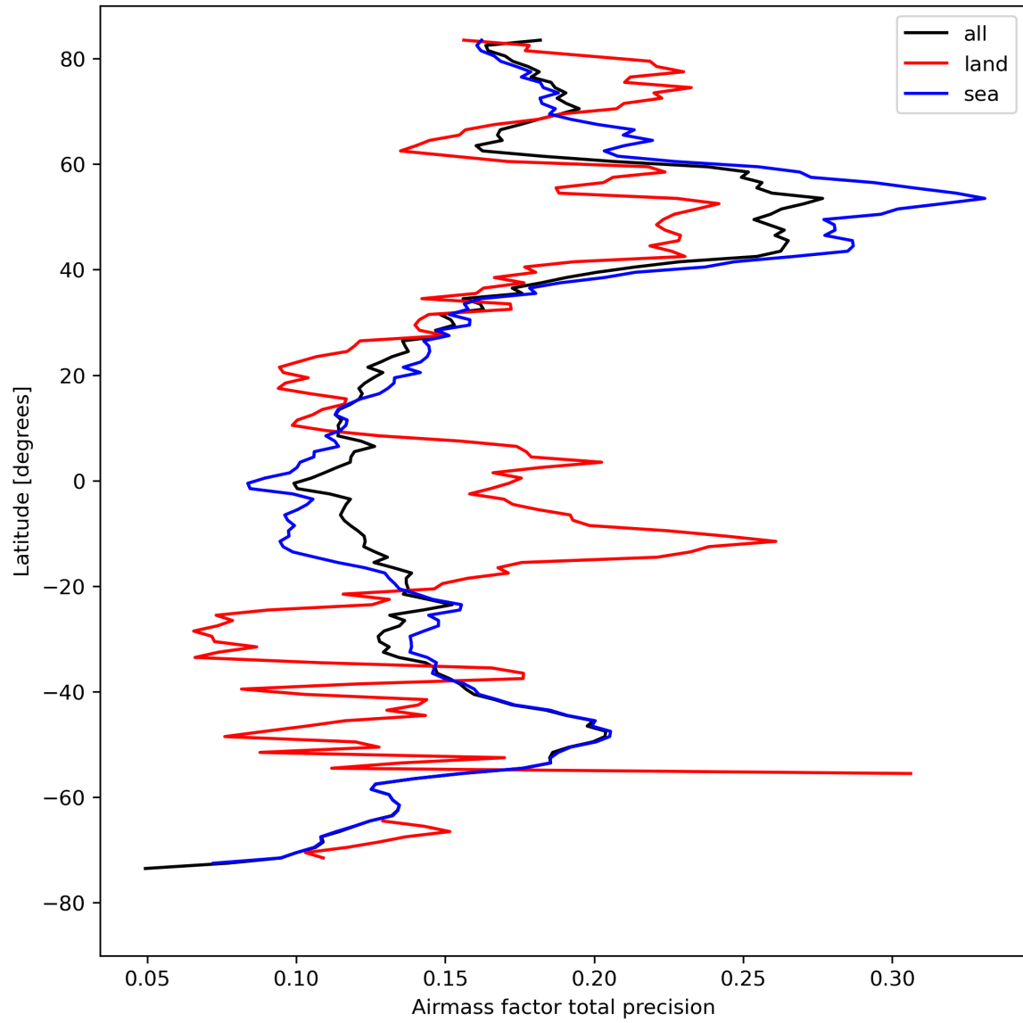
Figure 27: Zonal average of “Airmass factor total precision” for 2024-04-17 to 2024-04-19.
