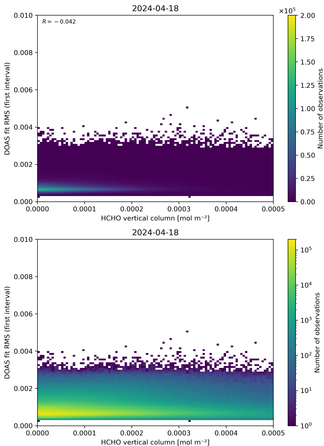
Figure 123: Scatter density plot of “HCHO vertical column” against “DOAS fit RMS (first interval)” for 2024-04-17 to 2024-04-19.
