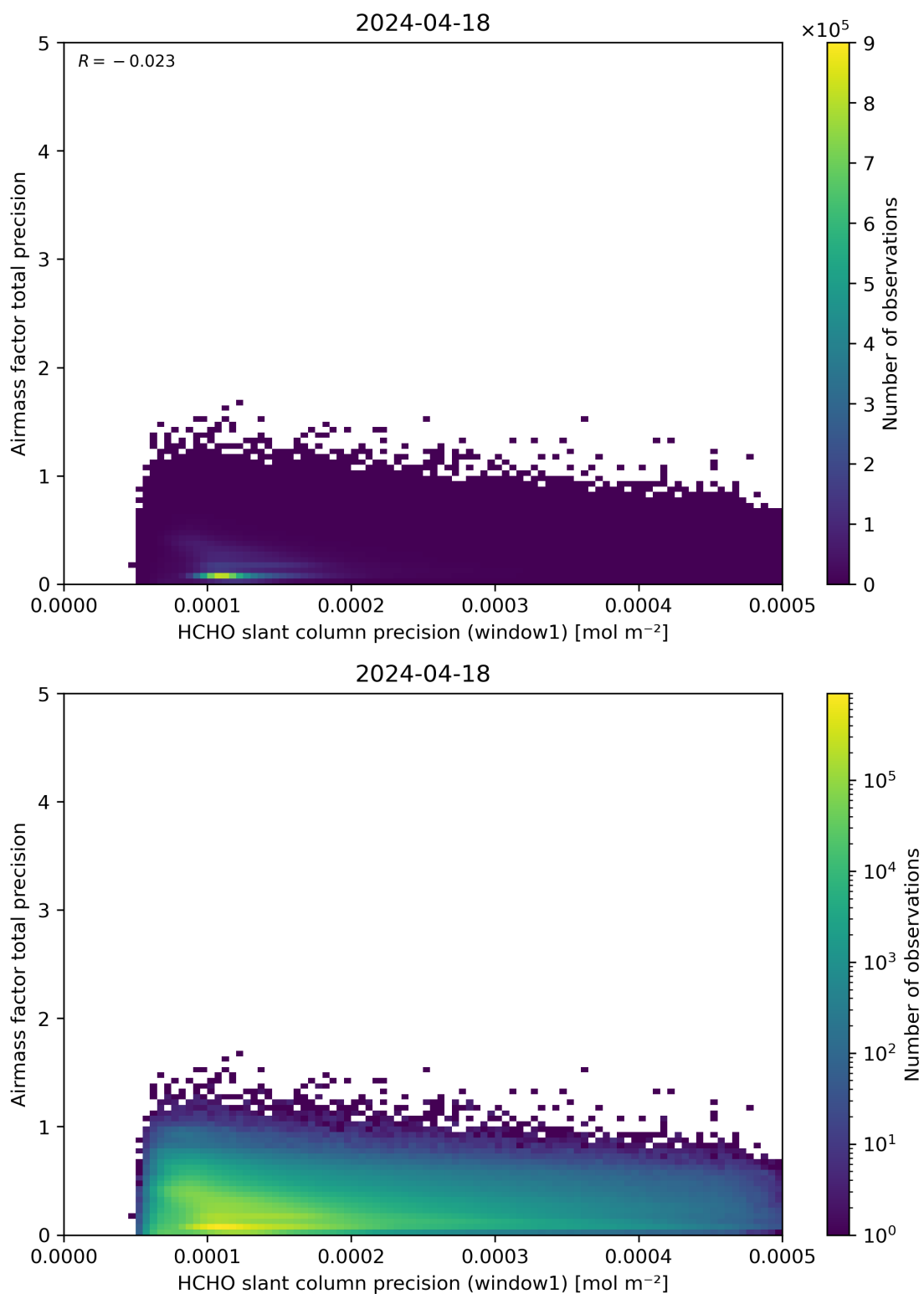
Figure 95: Scatter density plot of “HCHO slant column precision (window1)” against “Airmass factor total precision” for 2024-04-17 to 2024-04-19.
