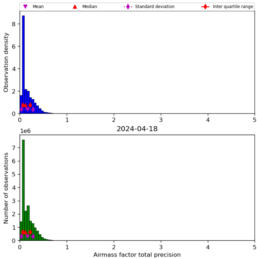
Figure 41: Histogram of "Airmass factor total precision" for 2024-04-17 to 2024-04-19
