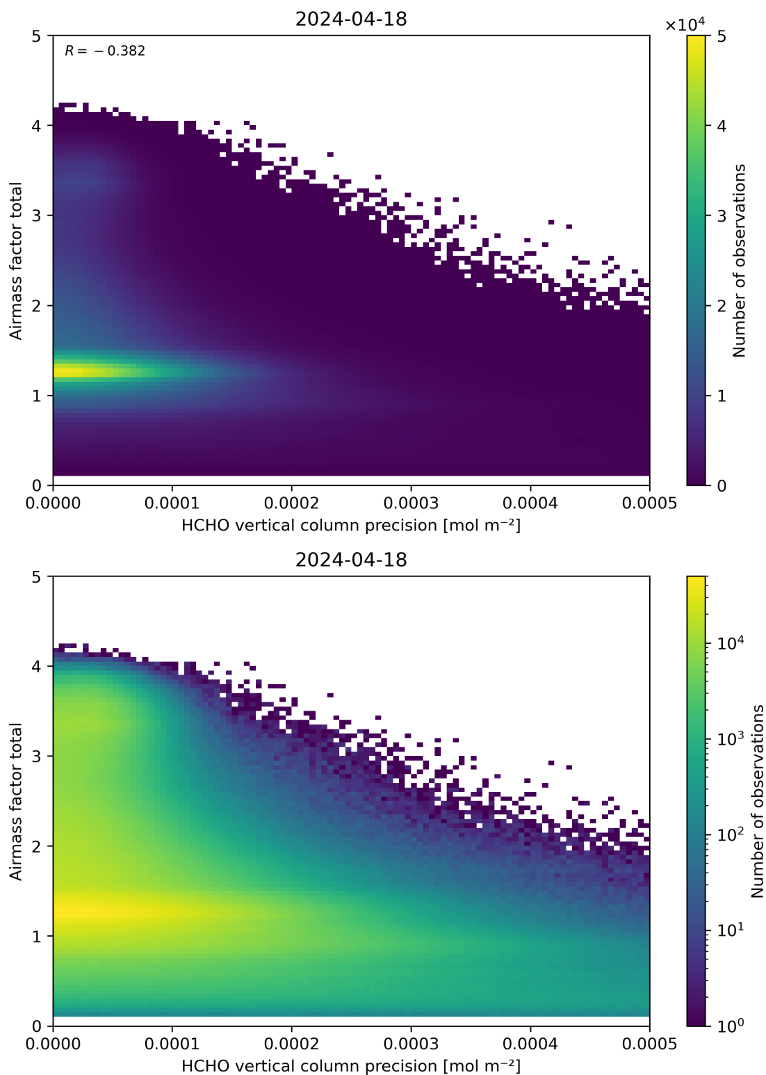
Figure 144: Scatter density plot of “HCHO vertical column precision” against “Airmass factor total” for 2024-04-17 to 2024-04-19.
