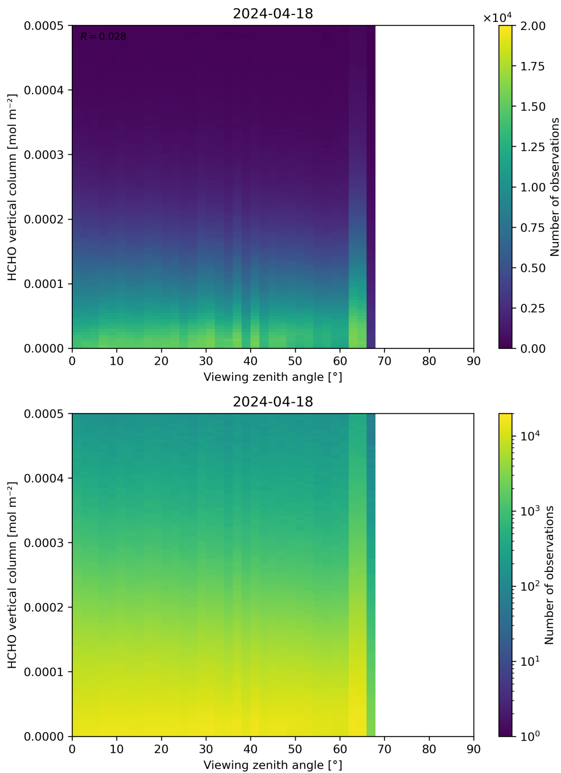
Figure 192: Scatter density plot of “Viewing zenith angle” against “HCHO vertical column” for 2024-04-17 to 2024-04-19.
