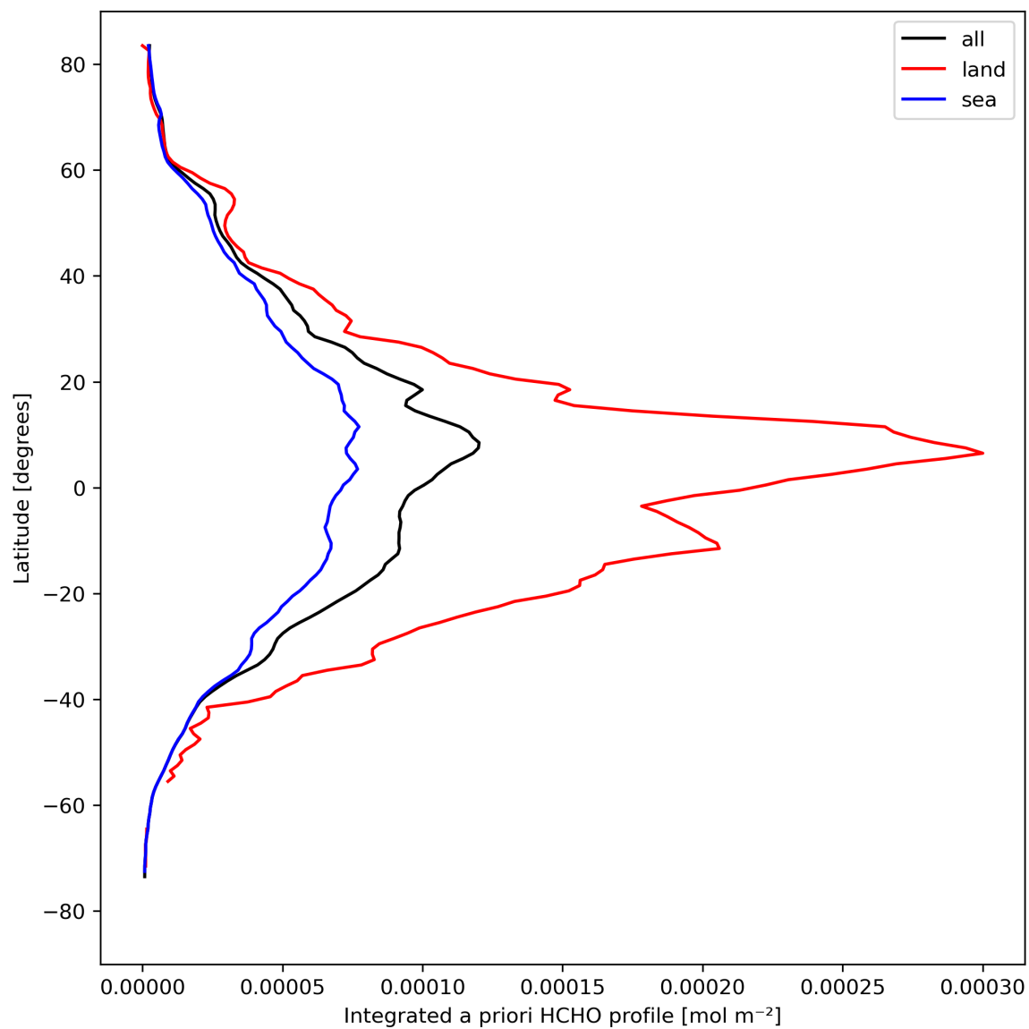
Figure 29: Zonal average of “Integrated a priori HCHO profile” for 2024-04-17 to 2024-04-19.
