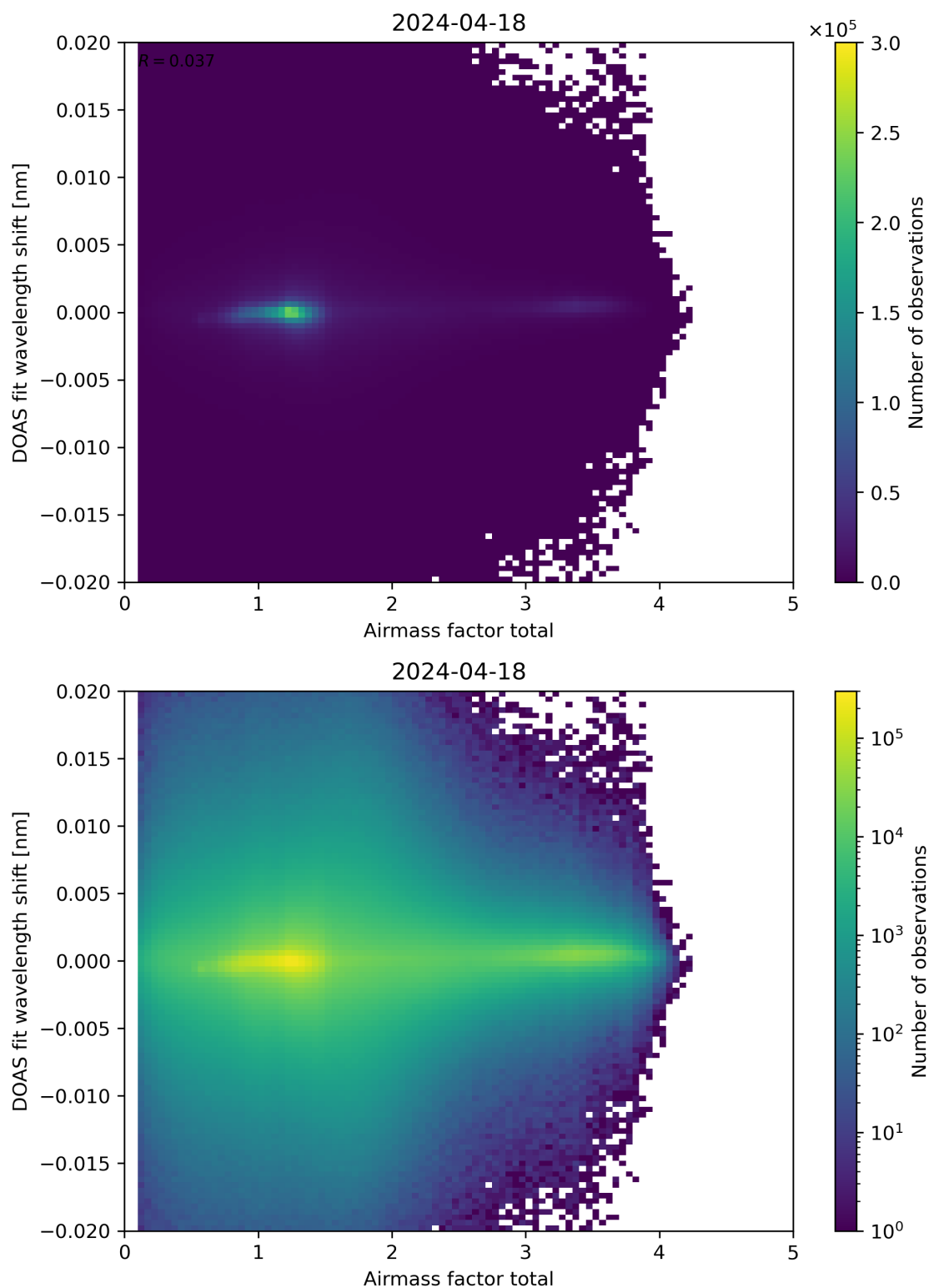
Figure 98: Scatter density plot of “Airmass factor total” against “DOAS fit wavelength shift” for 2024-04-17 to 2024-04-19.
