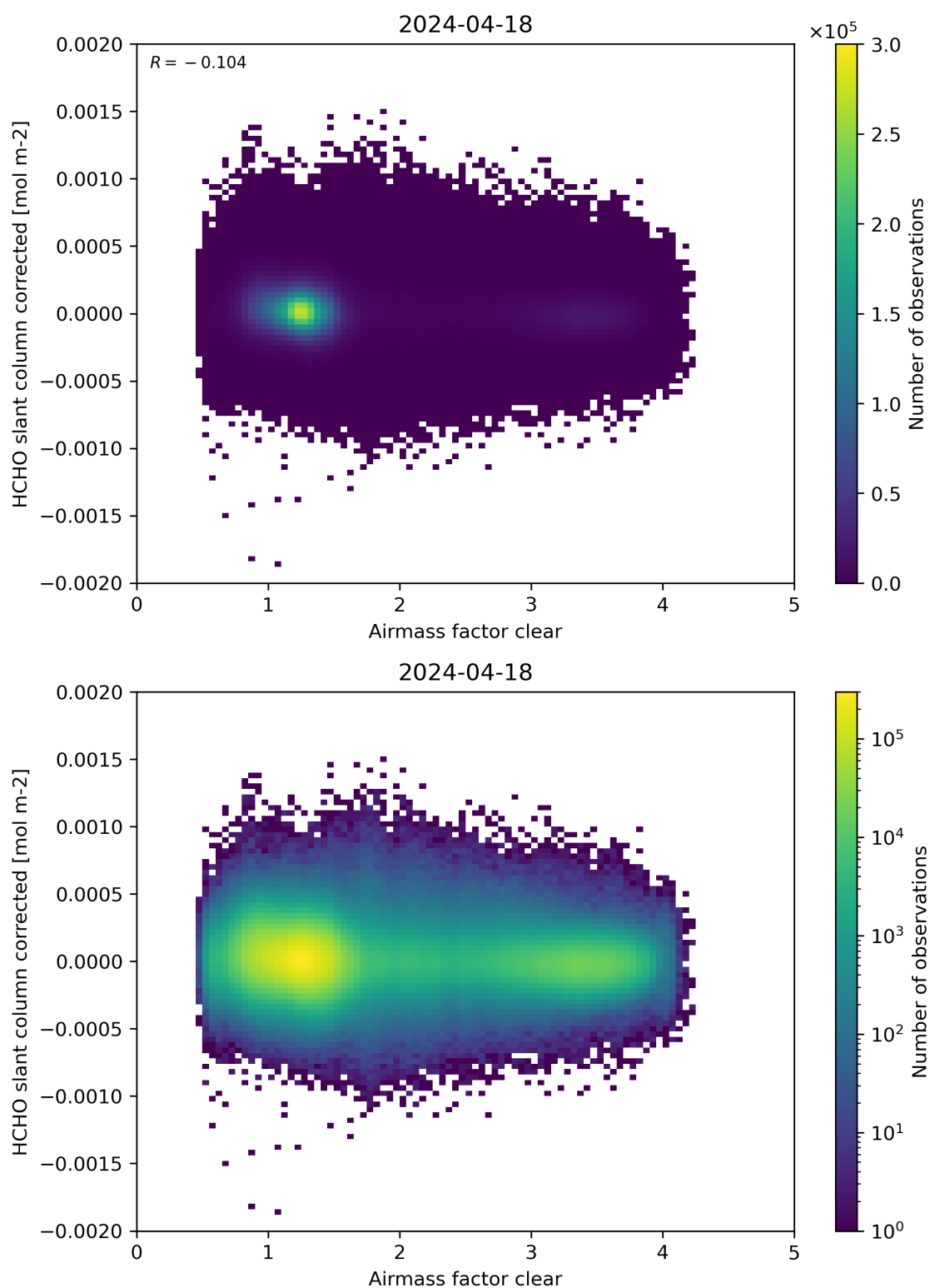
Figure 74: Scatter density plot of “Airmass factor clear” against “HCHO slant column corrected” for 2024-04-17 to 2024-04-19.
