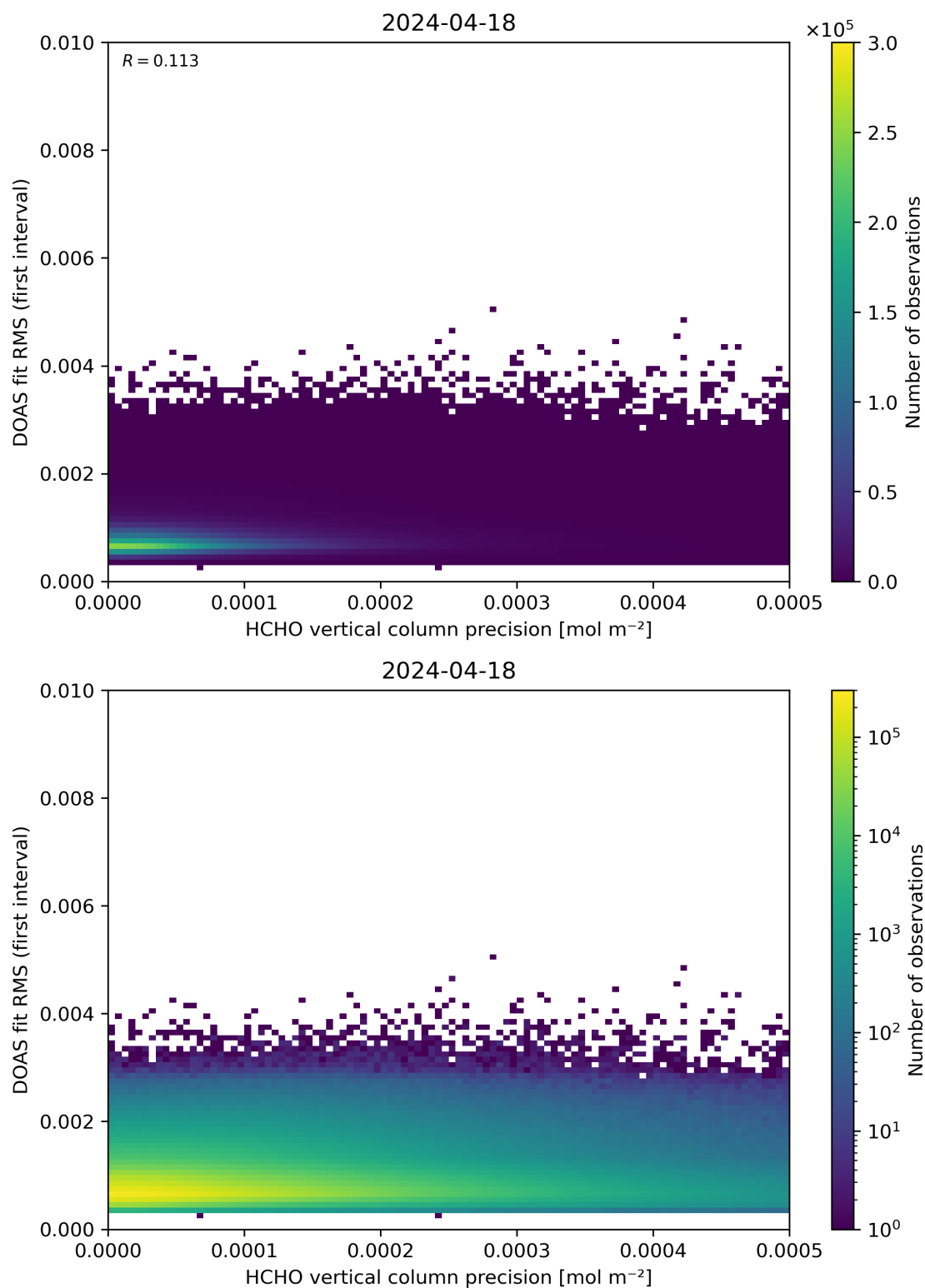
Figure 136: Scatter density plot of “HCHO vertical column precision” against “DOAS fit RMS (first interval)” for 2024-04-17 to 2024-04-19.
