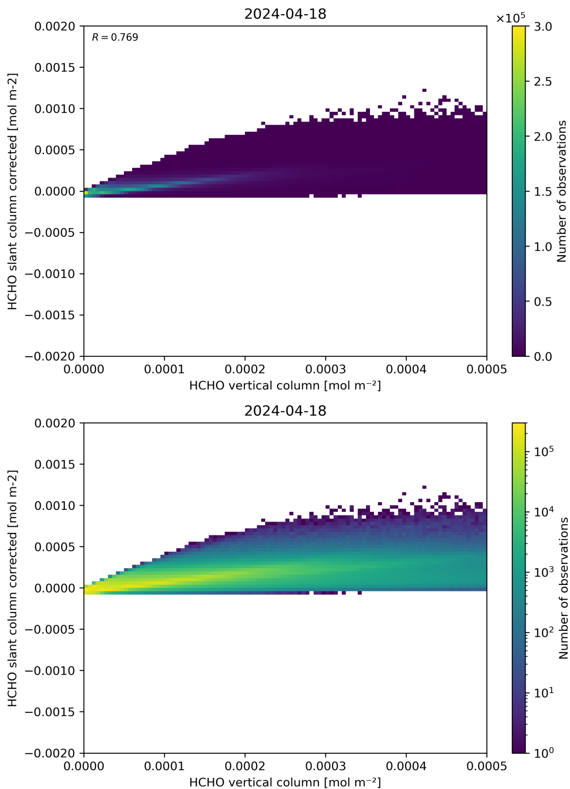
Figure 127: Scatter density plot of “HCHO vertical column” against “HCHO slant column corrected” for 2024-04-17 to 2024-04-19.
