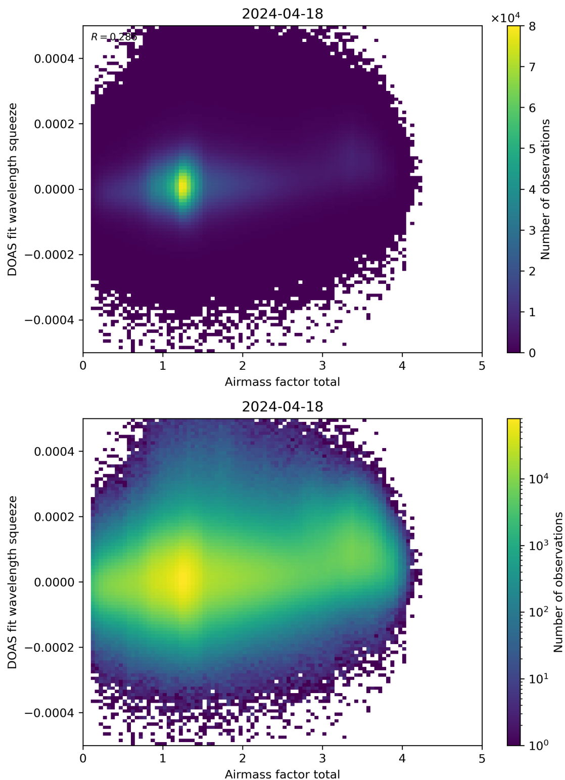
Figure 99: Scatter density plot of “Airmass factor total” against “DOAS fit wavelength squeeze” for 2024-04-17 to 2024-04-19.
