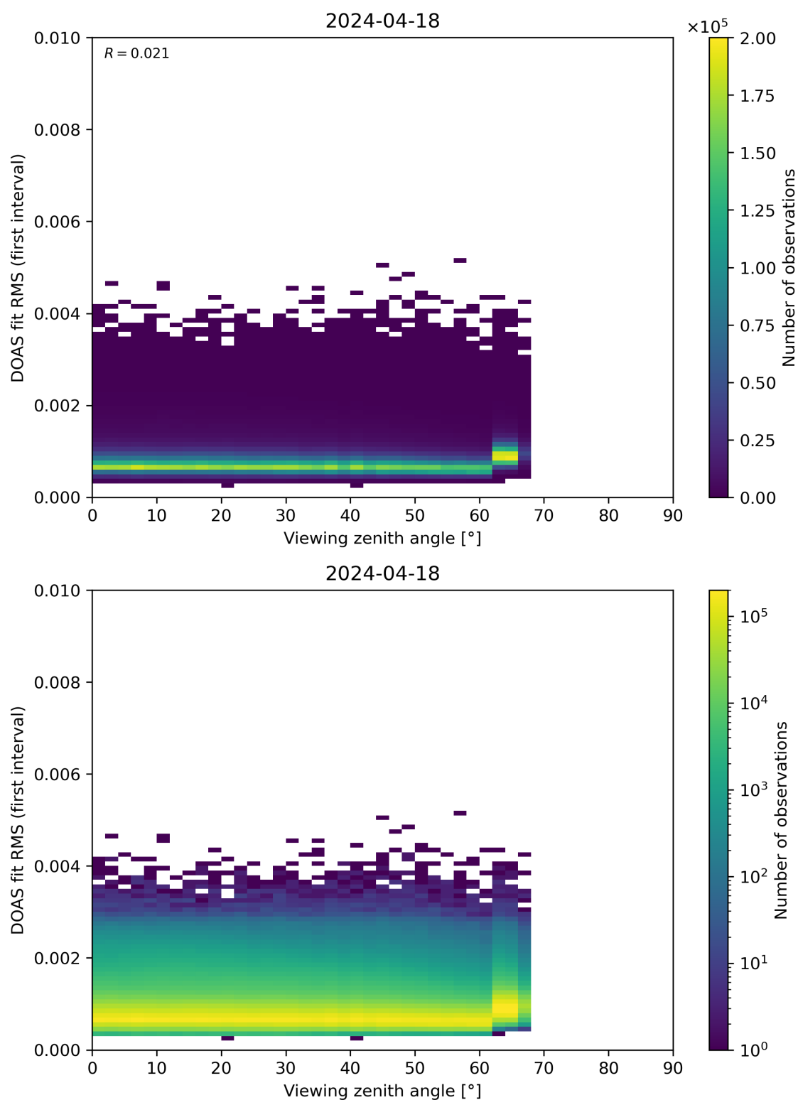
Figure 182: Scatter density plot of “Viewing zenith angle” against “DOAS fit RMS (first interval)” for 2024-04-17 to 2024-04-19.
