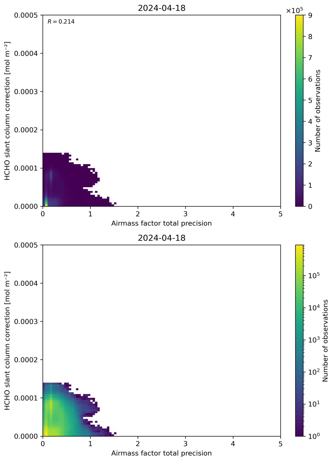
Figure 110: Scatter density plot of “Airmass factor total precision” against “HCHO slant column correction” for 2024-04-17 to 2024-04-19.
