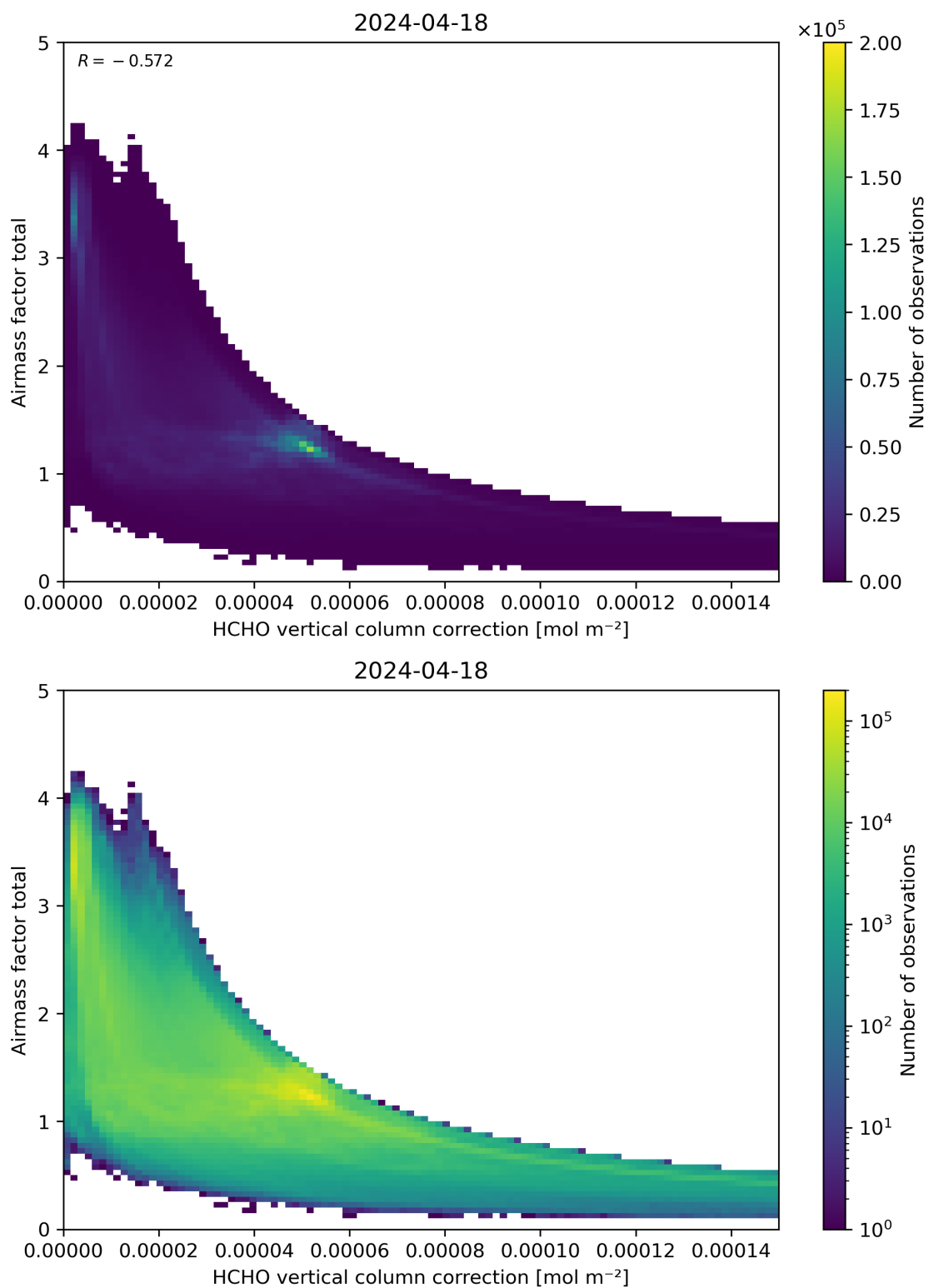
Figure 120: Scatter density plot of “HCHO vertical column correction” against “Airmass factor total” for 2024-04-17 to 2024-04-19.
