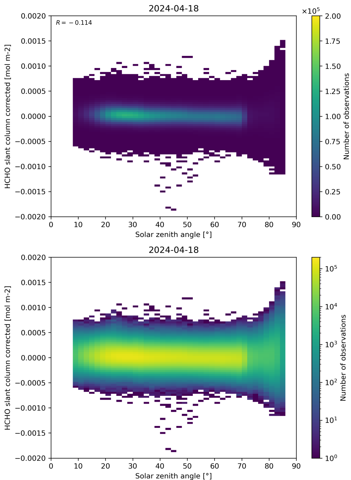
Figure 171: Scatter density plot of “Solar zenith angle” against “HCHO slant column corrected” for 2024-04-17 to 2024-04-19.
