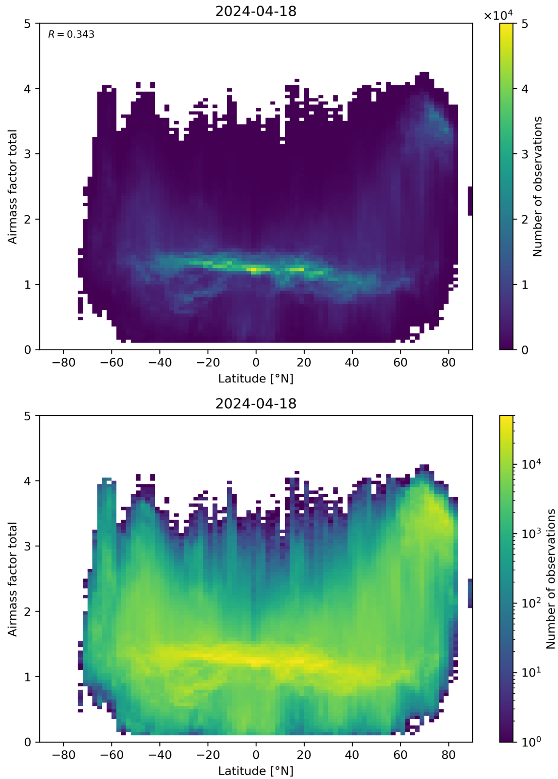
Figure 161: Scatter density plot of “Latitude” against “Airmass factor total” for 2024-04-17 to 2024-04-19.
