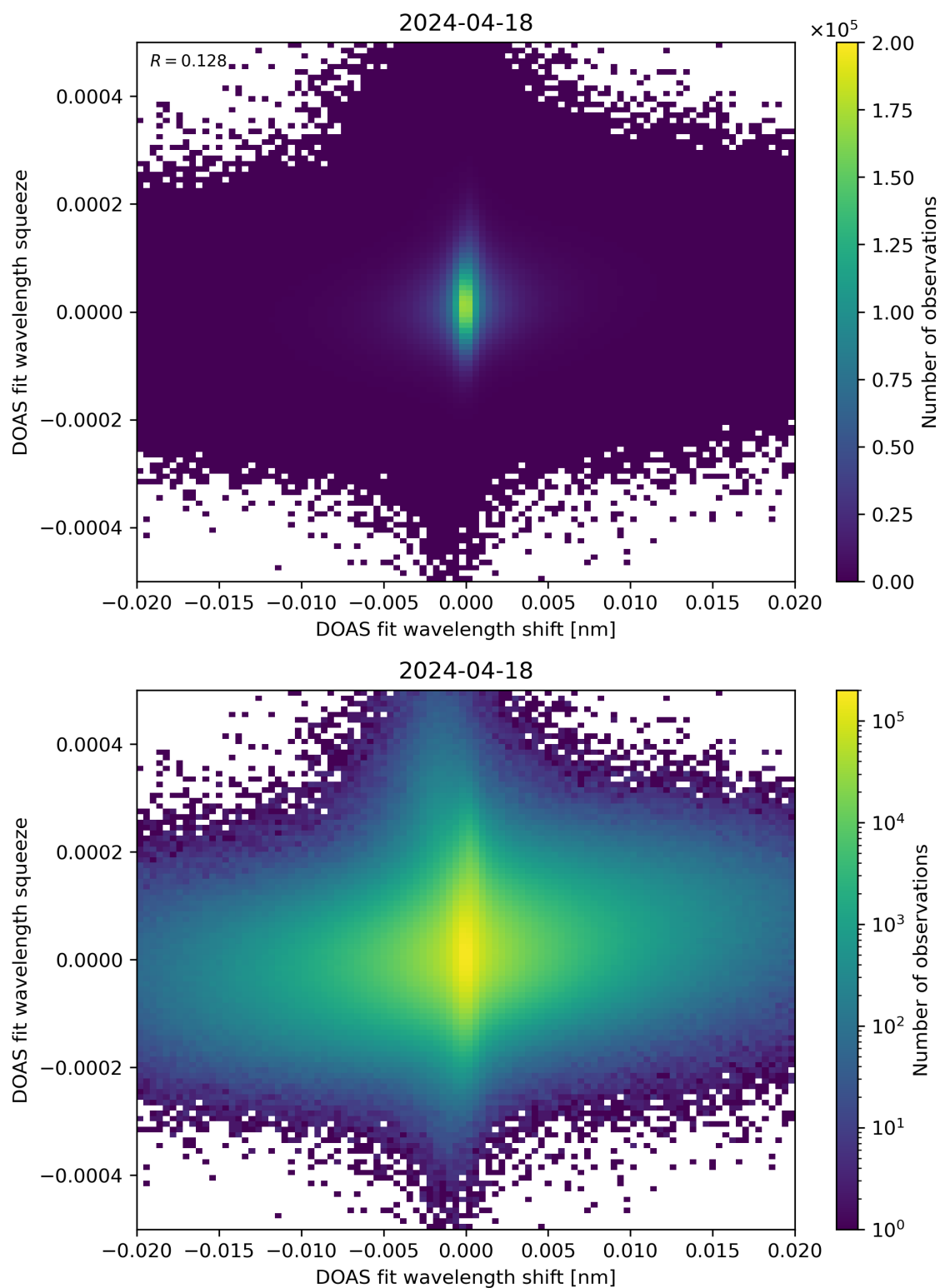
Figure 65: Scatter density plot of “DOAS fit wavelength shift” against “DOAS fit wavelength squeeze” for 2024-04-17 to 2024-04-19.
