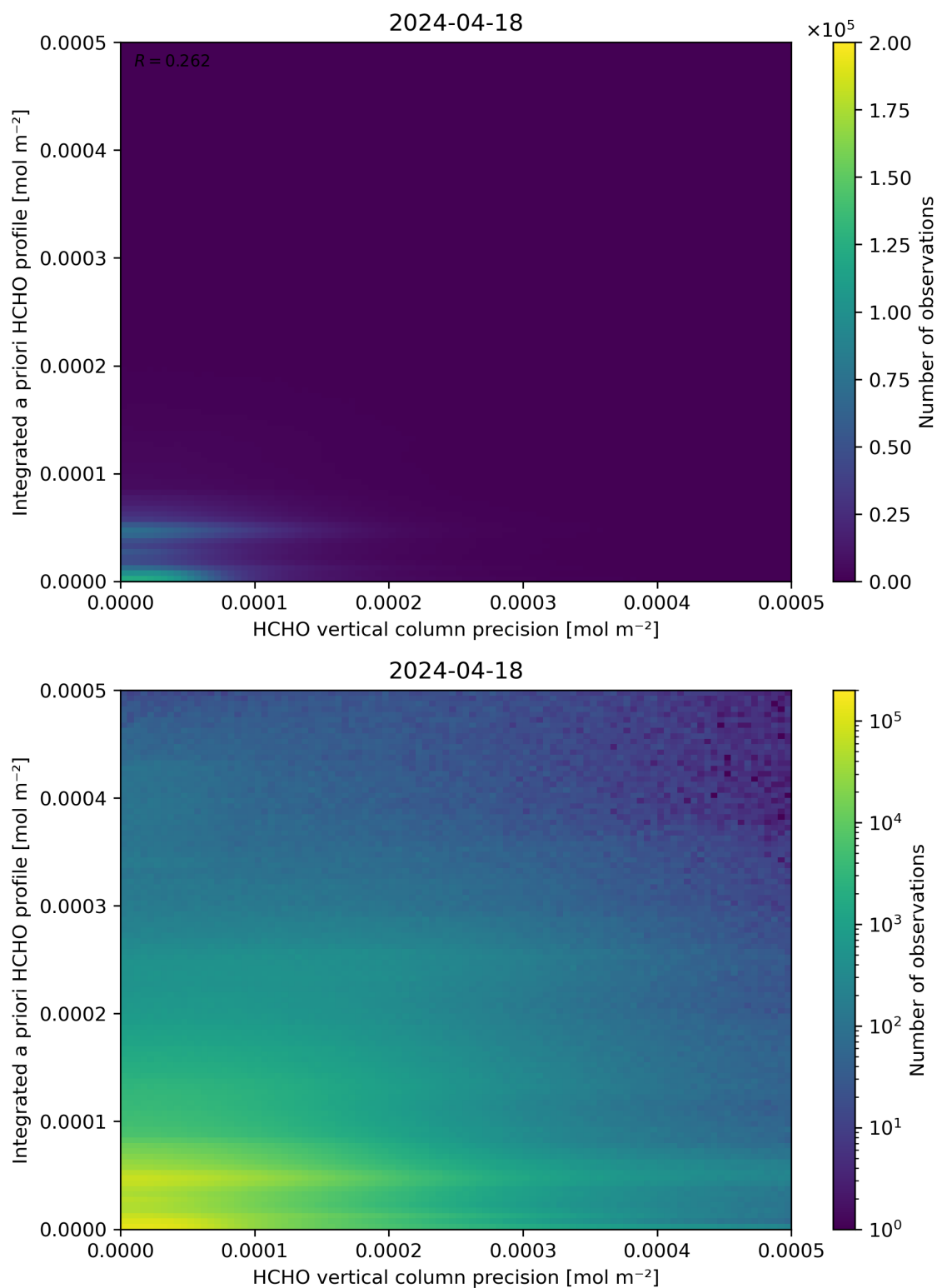
Figure 147: Scatter density plot of “HCHO vertical column precision” against “Integrated a priori HCHO profile” for 2024-04-17 to 2024-04-19.
