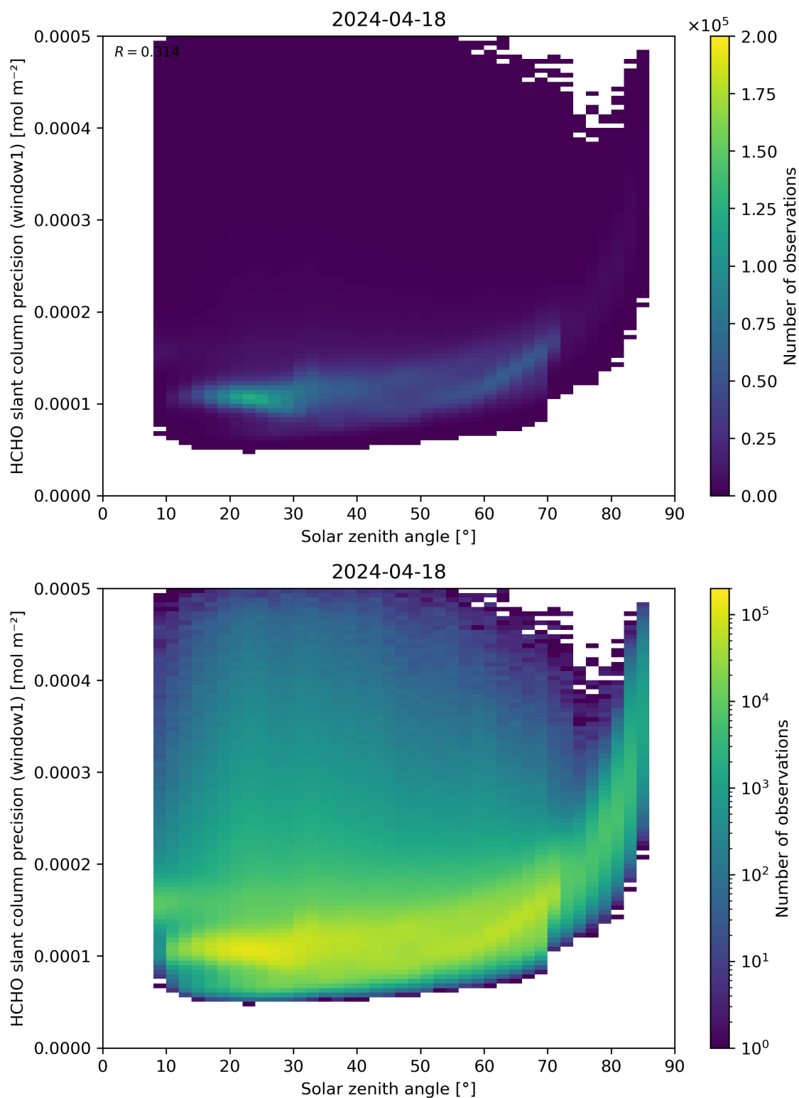
Figure 174: Scatter density plot of “Solar zenith angle” against “HCHO slant column precision (window1)” for 2024-04-17 to 2024-04-19.
