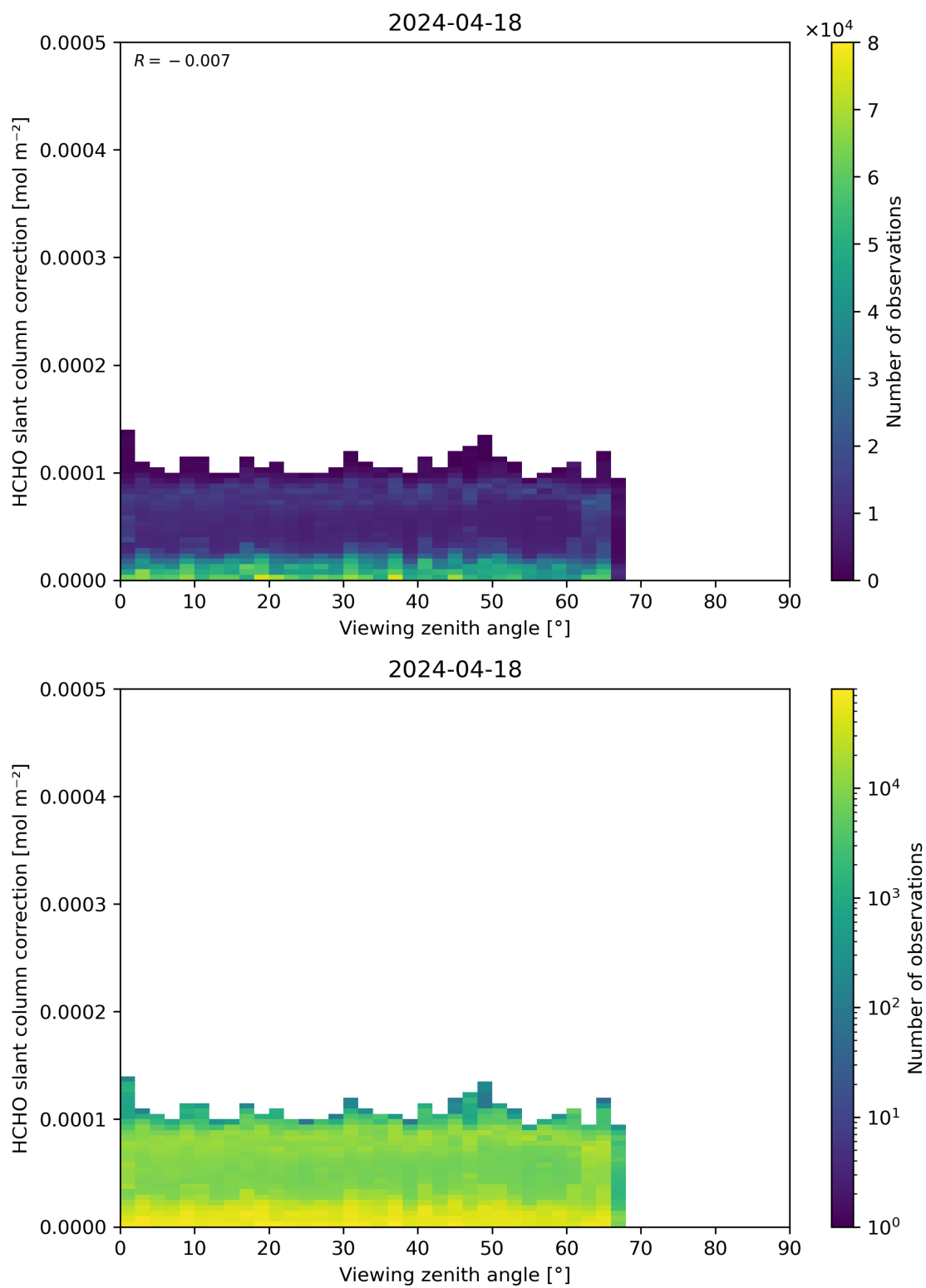
Figure 187: Scatter density plot of “Viewing zenith angle” against “HCHO slant column correction” for 2024-04-17 to 2024-04-19.
