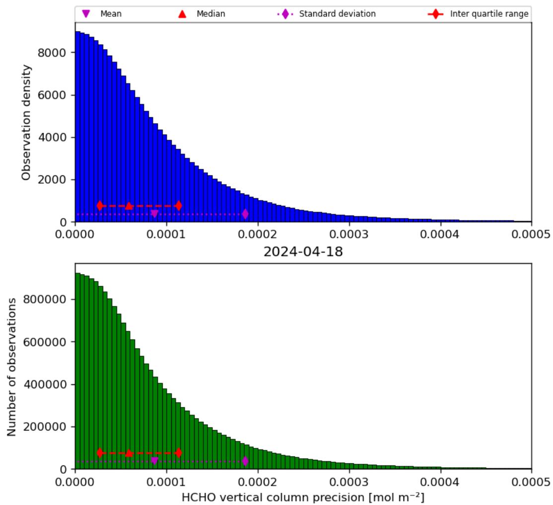
Figure 36: Histogram of “HCHO vertical column precision” for 2024-04-17 to 2024-04-19
