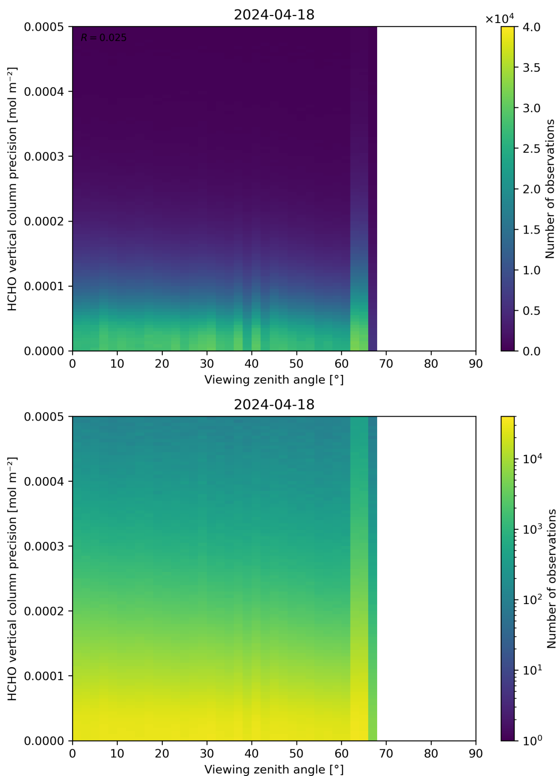
Figure 194: Scatter density plot of “Viewing zenith angle” against “HCHO vertical column precision” for 2024-04-17 to 2024-04-19.
