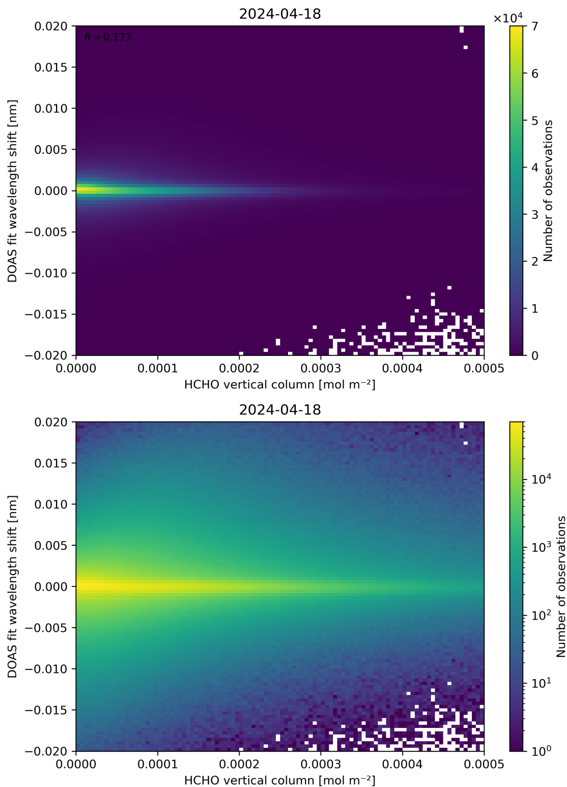
Figure 124: Scatter density plot of “HCHO vertical column” against “DOAS fit wavelength shift” for 2024-04-17 to 2024-04-19.
