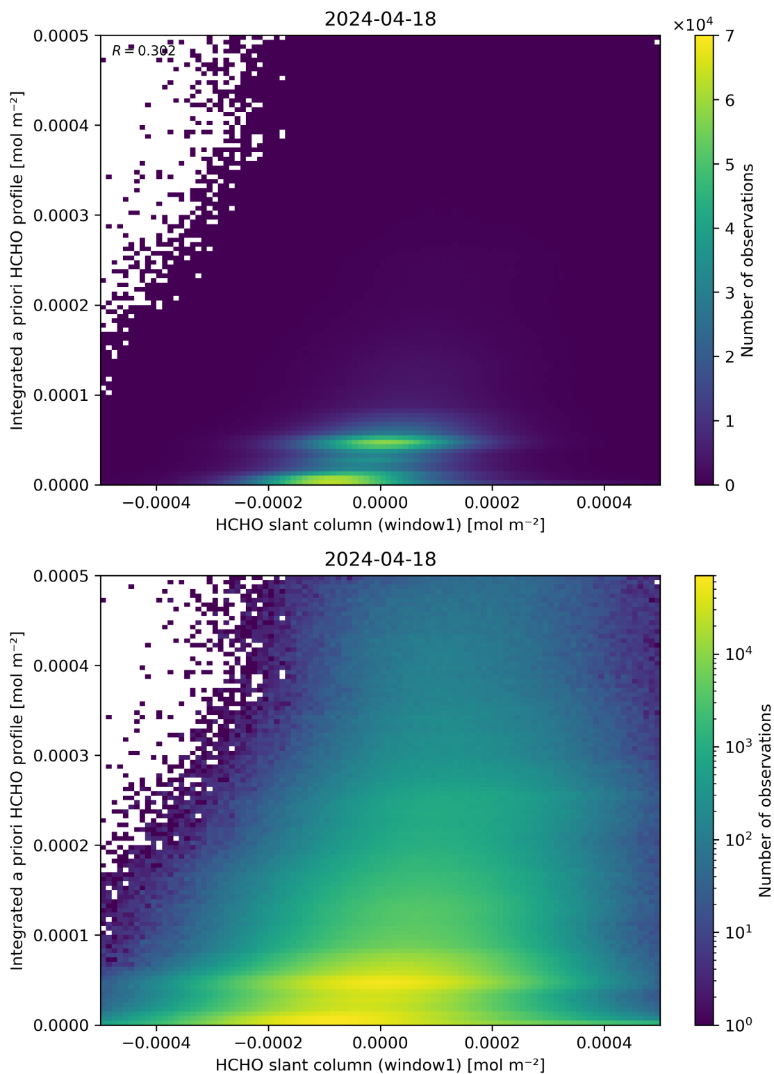
Figure 87: Scatter density plot of “HCHO slant column (window1)” against “Integrated a priori HCHO profile” for 2024-04-17 to 2024-04-19.
