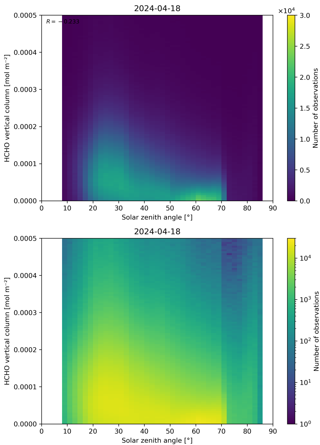
Figure 177: Scatter density plot of “Solar zenith angle” against “HCHO vertical column” for 2024-04-17 to 2024-04-19.
