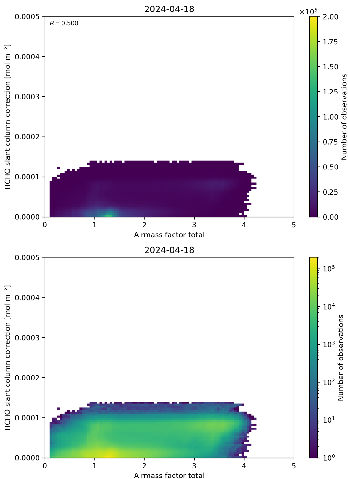
Figure 102: Scatter density plot of “Airmass factor total” against “HCHO slant column correction” for 2024-04-17 to 2024-04-19.
