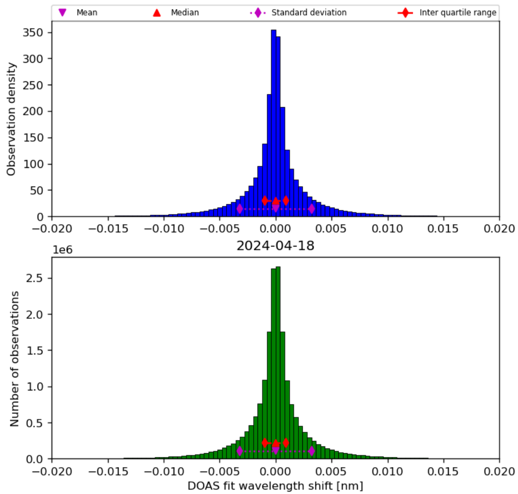
Figure 44: Histogram of “DOAS fit wavelength shift” for 2024-04-17 to 2024-04-19
