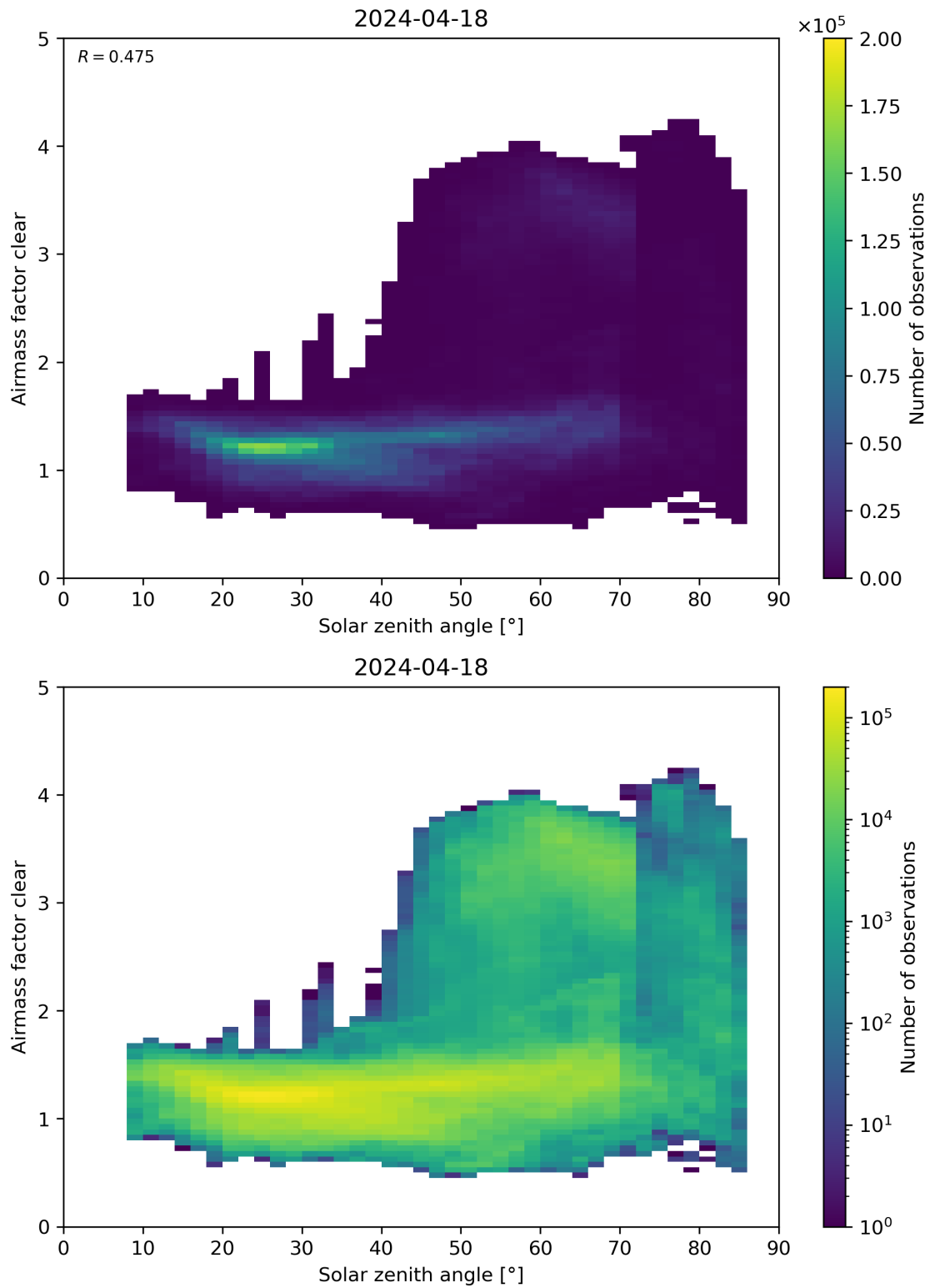
Figure 170: Scatter density plot of “Solar zenith angle” against “Airmass factor clear” for 2024-04-17 to 2024-04-19.
