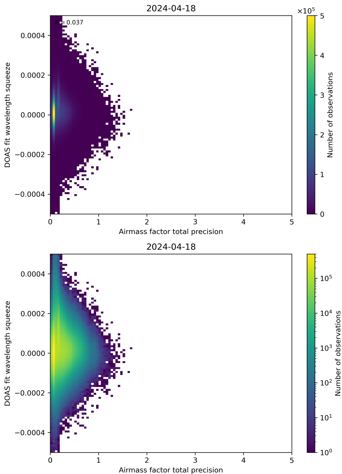
Figure 107: Scatter density plot of “Airmass factor total precision” against “DOAS fit wavelength squeeze” for 2024-04-17 to 2024-04-19.
