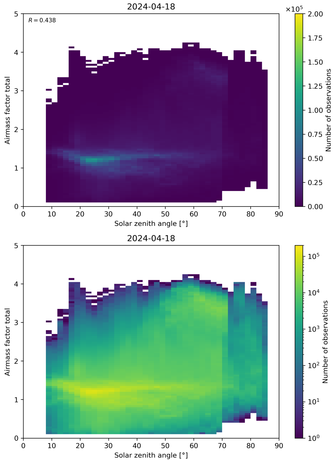
Figure 175: Scatter density plot of “Solar zenith angle” against “Airmass factor total” for 2024-04-17 to 2024-04-19.
