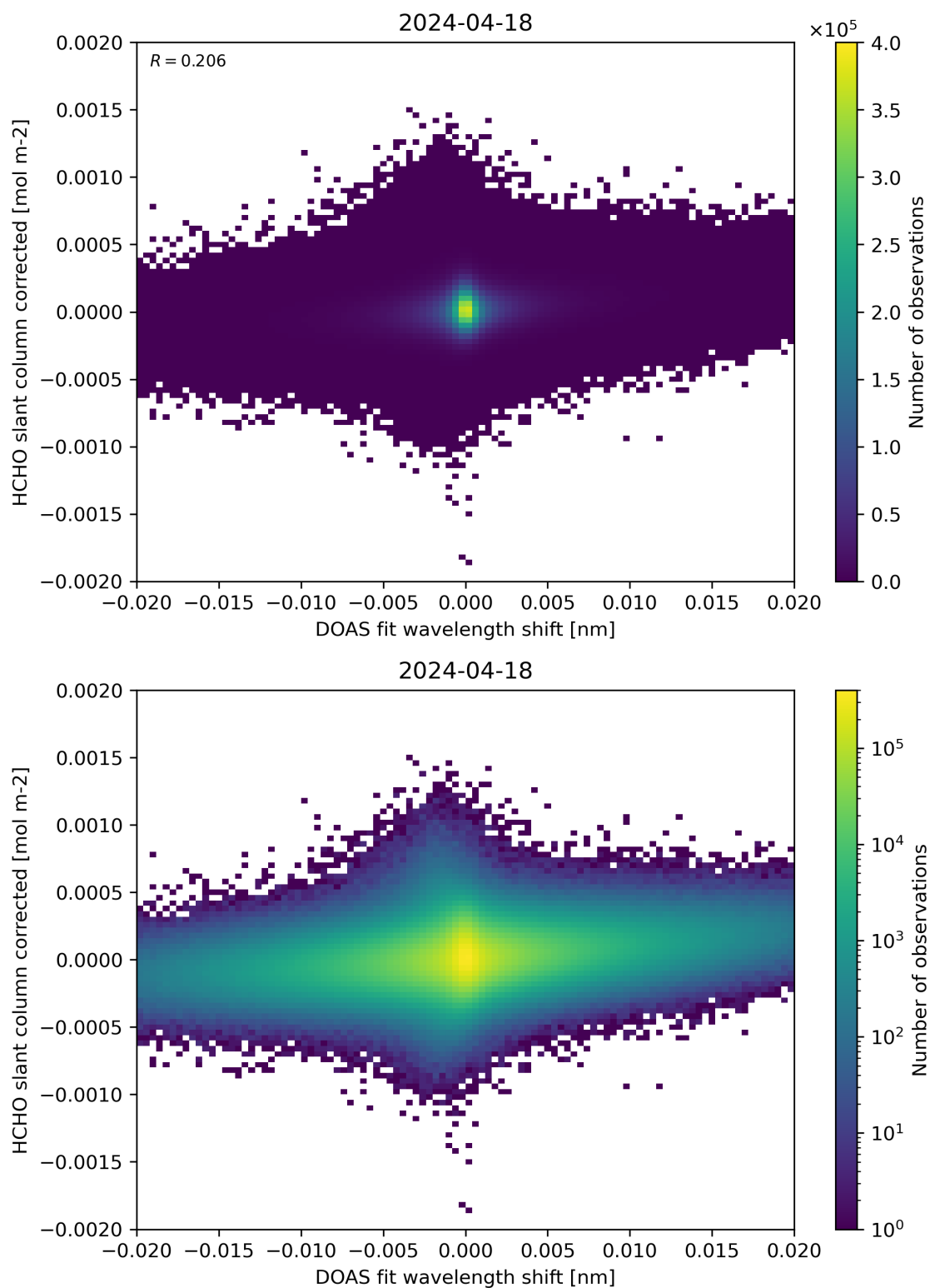
Figure 66: Scatter density plot of “DOAS fit wavelength shift” against “HCHO slant column corrected” for 2024-04-17 to 2024-04-19.
