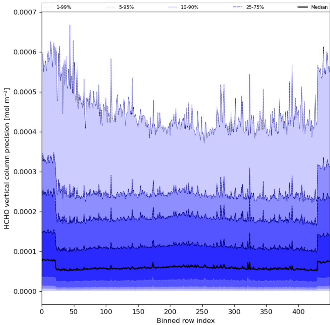
Figure 50: Along track statistics of “HCHO vertical column precision” for 2024-04-17 to 2024-04-19
