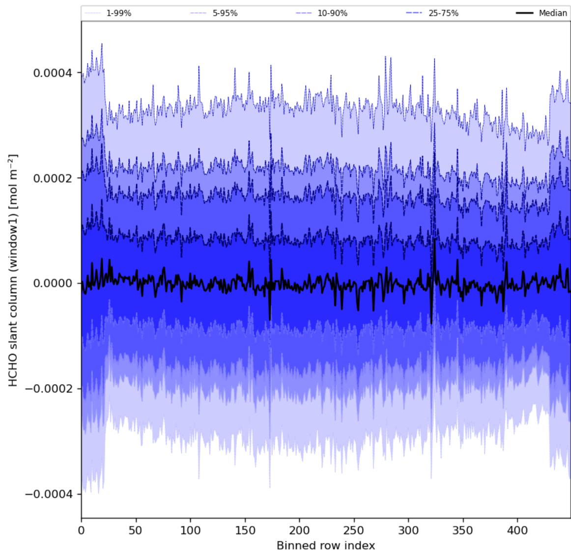
Figure 52: Along track statistics of “HCHO slant column (window1)” for 2024-04-17 to 2024-04-19
