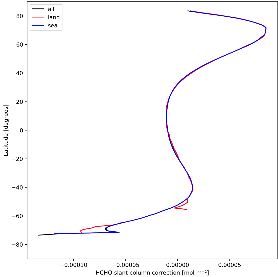
Figure 33: Zonal average of “HCHO slant column correction” for 2024-04-17 to 2024-04-19.
