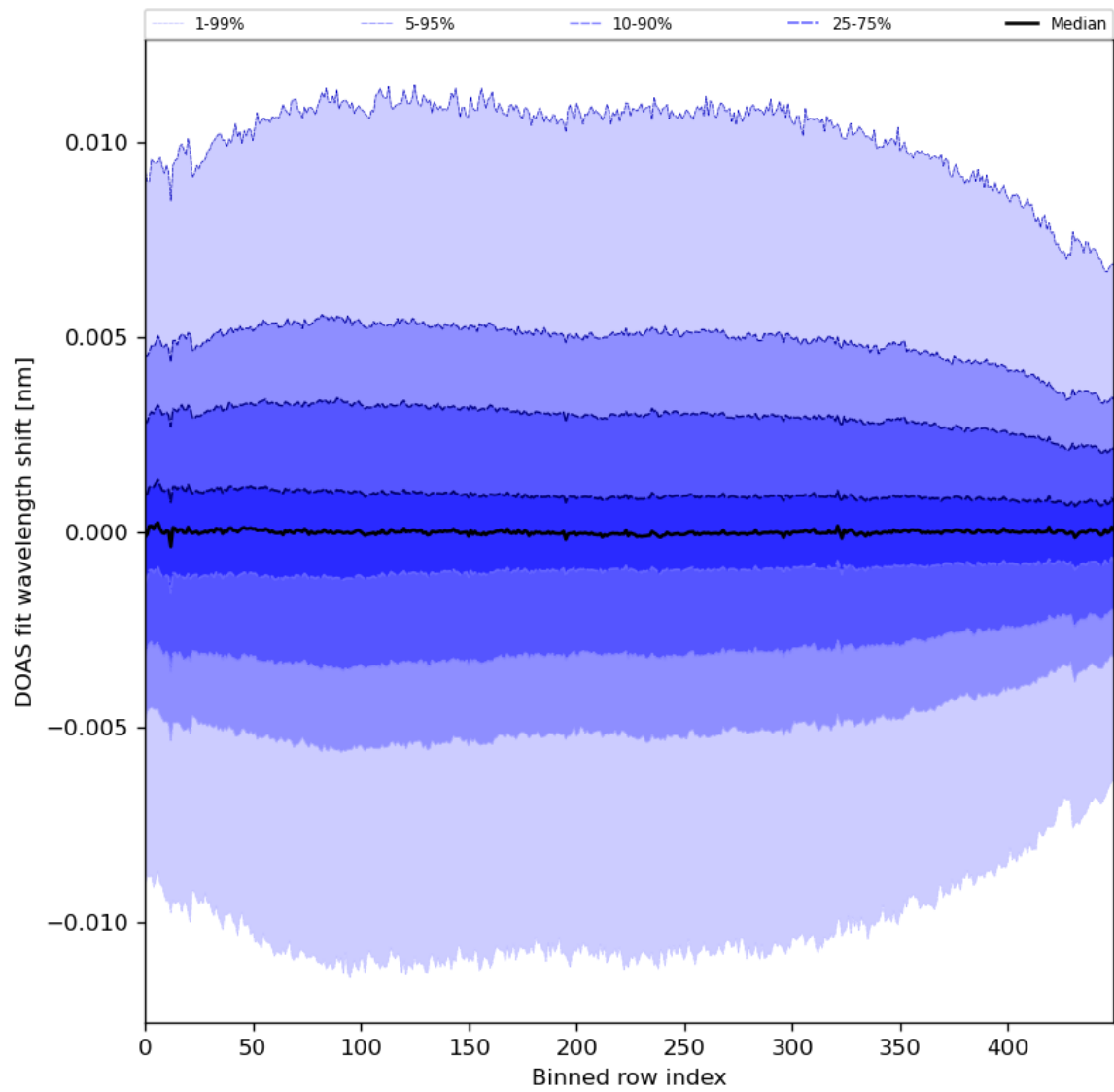
Figure 58: Along track statistics of “DOAS fit wavelength shift” for 2024-04-17 to 2024-04-19
