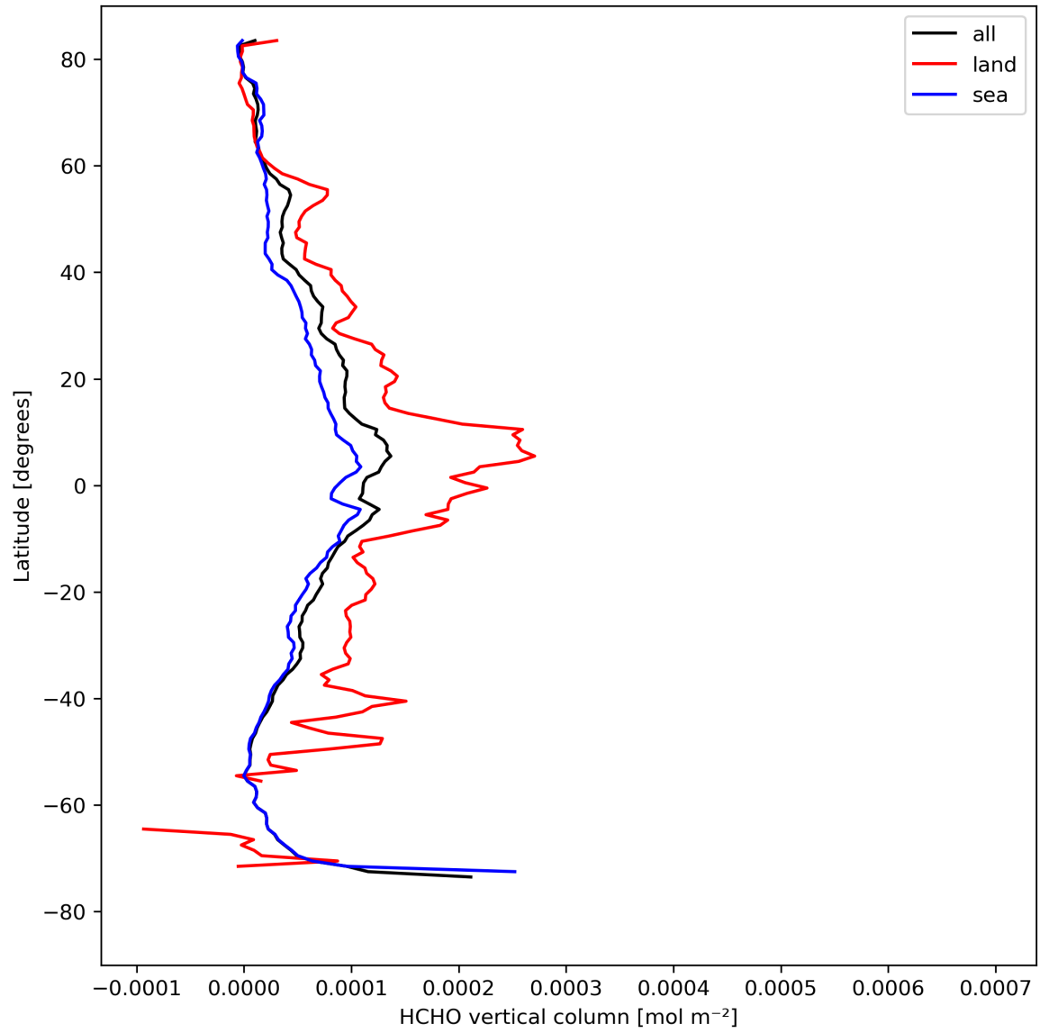
Figure 21: Zonal average of “HCHO vertical column” for 2024-04-17 to 2024-04-19.
