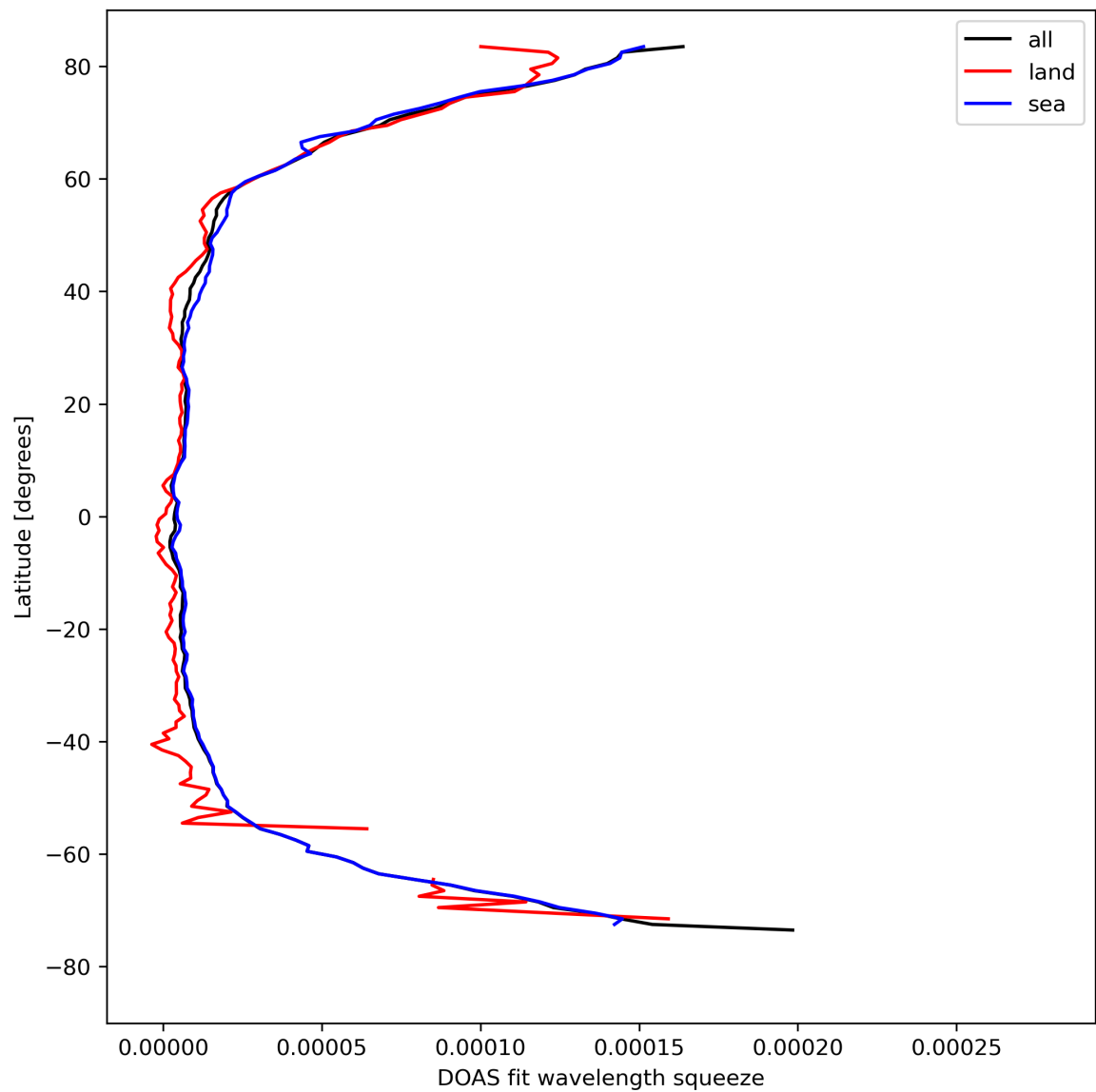
Figure 31: Zonal average of “DOAS fit wavelength squeeze” for 2024-04-17 to 2024-04-19.
