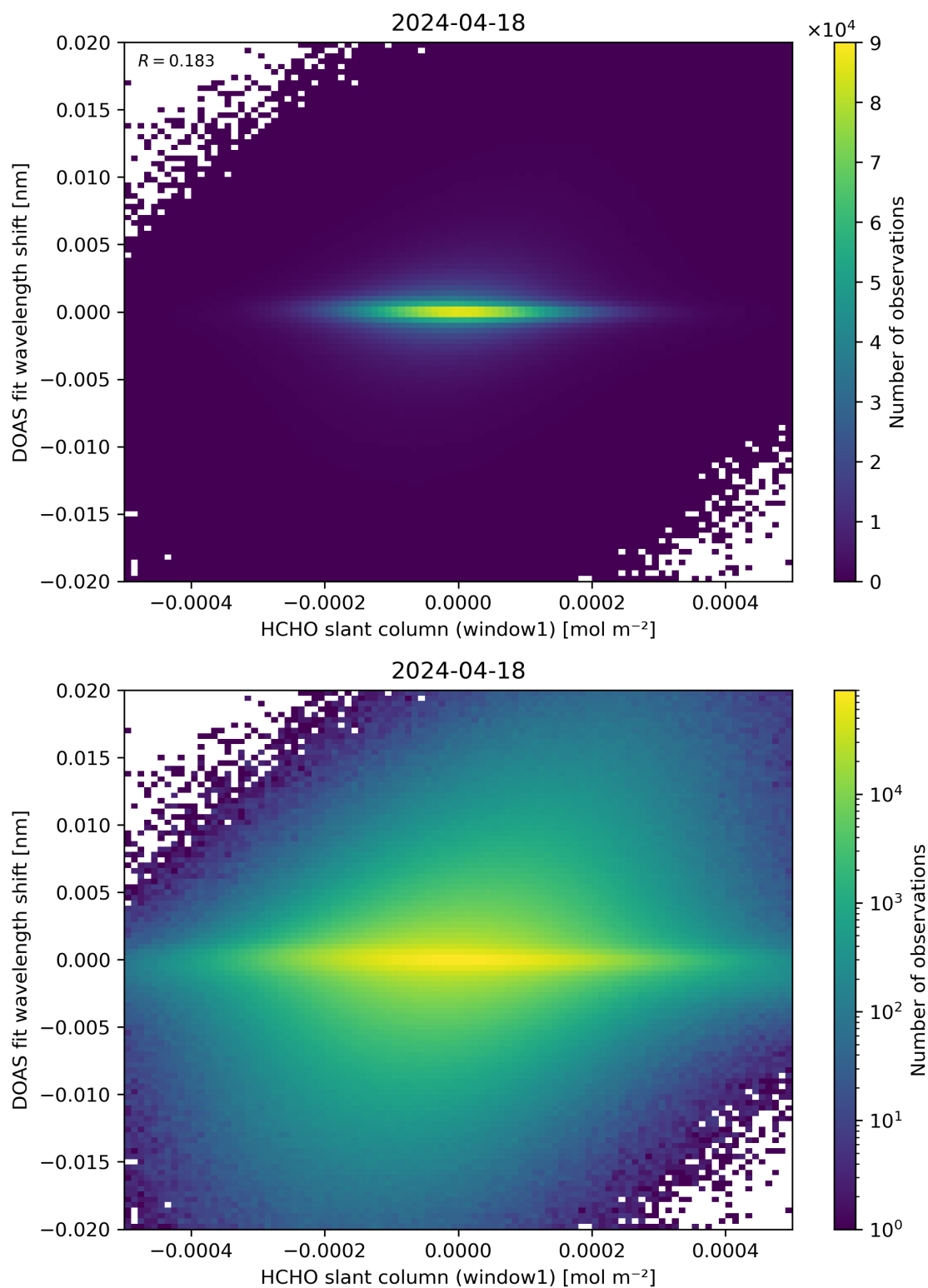
Figure 79: Scatter density plot of “HCHO slant column (window1)” against “DOAS fit wavelength shift” for 2024-04-17 to 2024-04-19.
