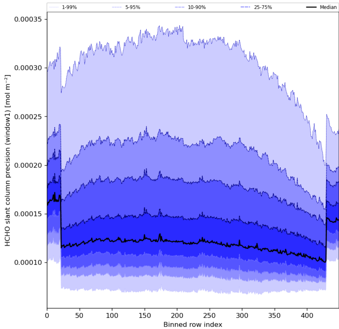
Figure 53: Along track statistics of “HCHO slant column precision (window1)” for 2024-04-17 to 2024-04-19
