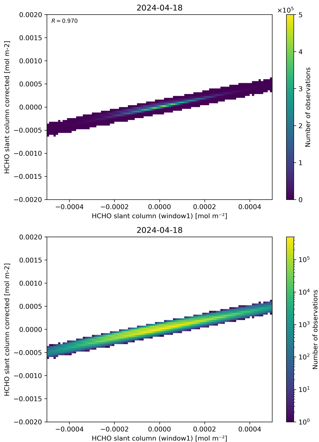
Figure 82: Scatter density plot of “HCHO slant column (window1)” against “HCHO slant column corrected” for 2024-04-17 to 2024-04-19.
