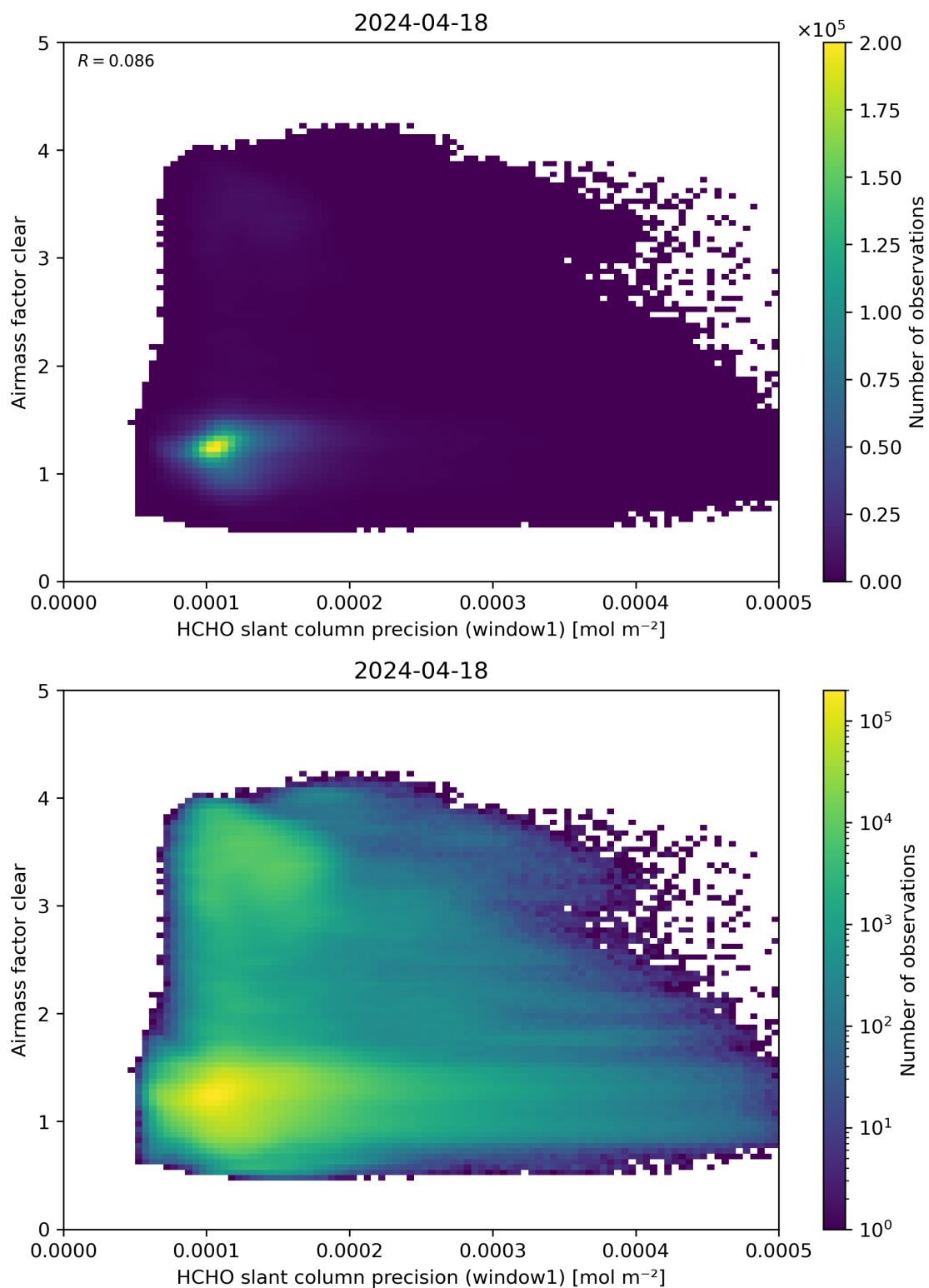
Figure 91: Scatter density plot of “HCHO slant column precision (window1)” against “Airmass factor clear” for 2024-04-17 to 2024-04-19.
