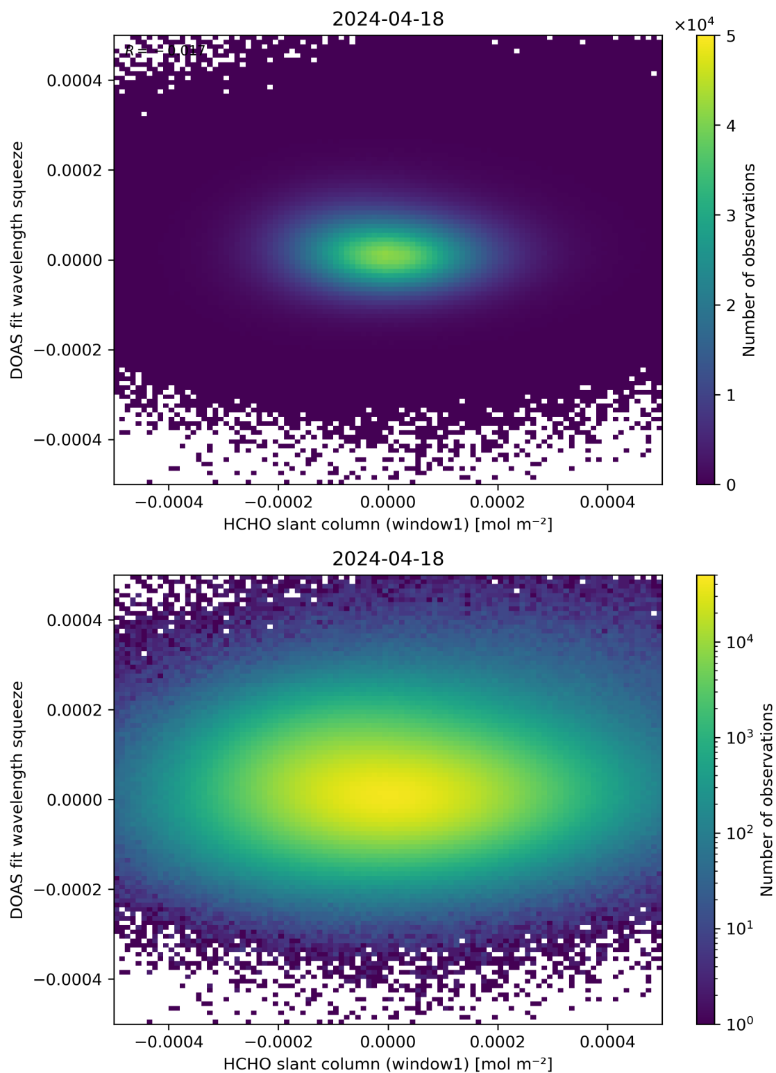
Figure 80: Scatter density plot of “HCHO slant column (window1)” against “DOAS fit wavelength squeeze” for 2024-04-17 to 2024-04-19.
