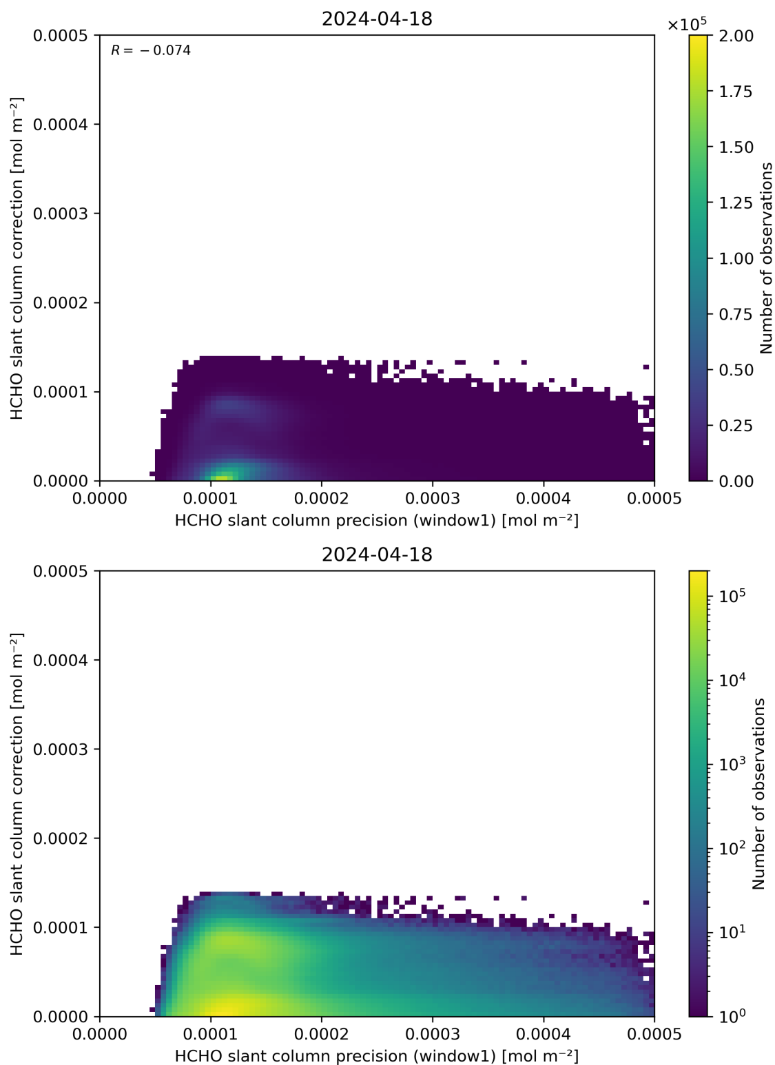
Figure 93: Scatter density plot of “HCHO slant column precision (window1)” against “HCHO slant column correction” for 2024-04-17 to 2024-04-19.
