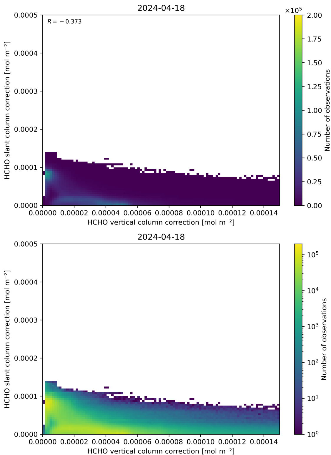
Figure 117: Scatter density plot of “HCHO vertical column correction” against “HCHO slant column correction” for 2024-04-17 to 2024-04-19.
