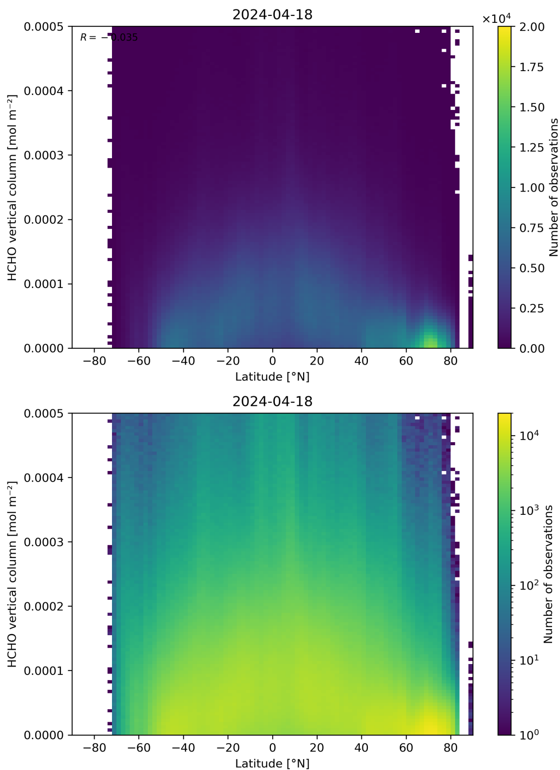
Figure 163: Scatter density plot of “Latitude” against “HCHO vertical column” for 2024-04-17 to 2024-04-19.
