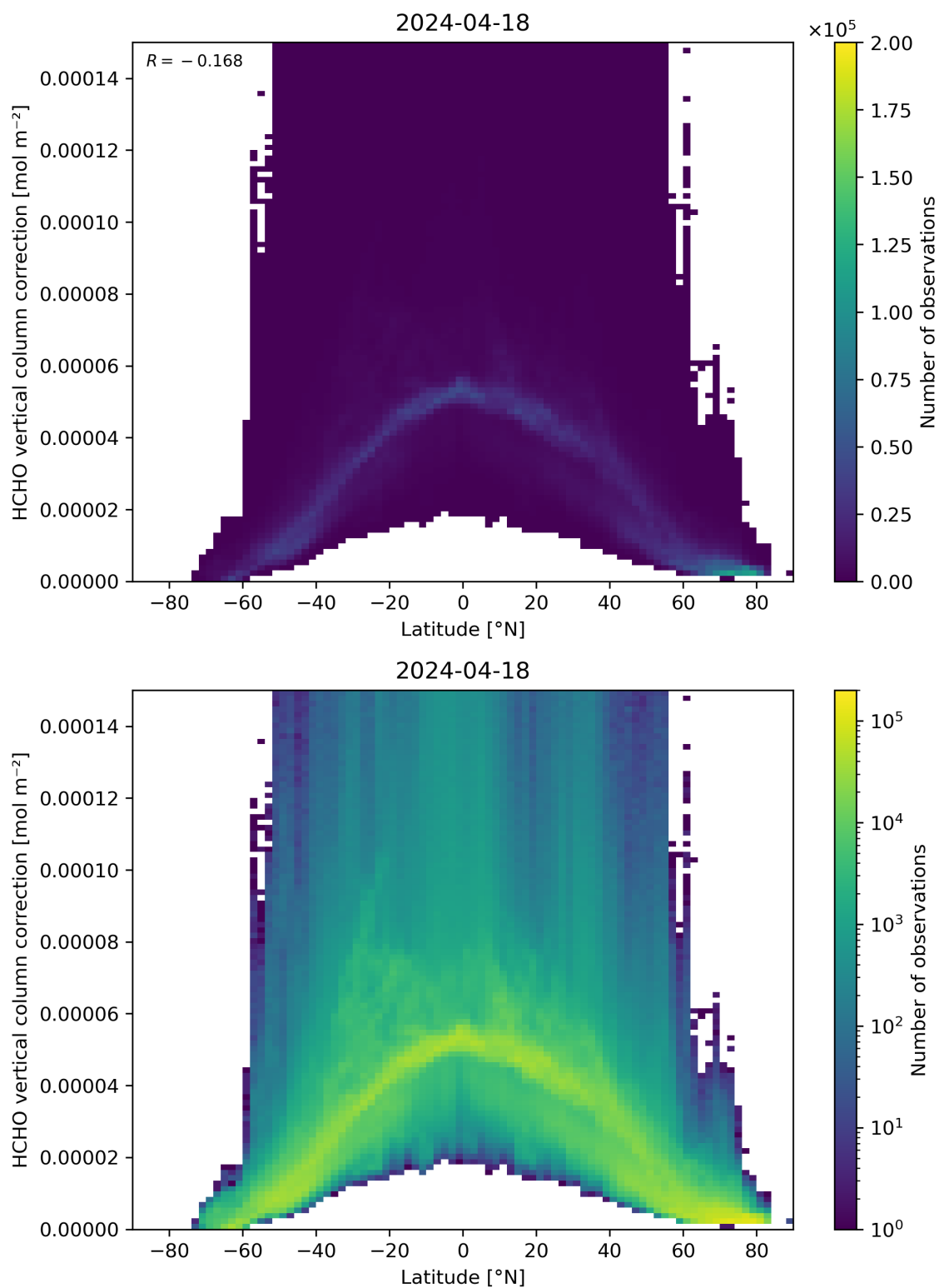
Figure 164: Scatter density plot of “Latitude” against “HCHO vertical column correction” for 2024-04-17 to 2024-04-19.
