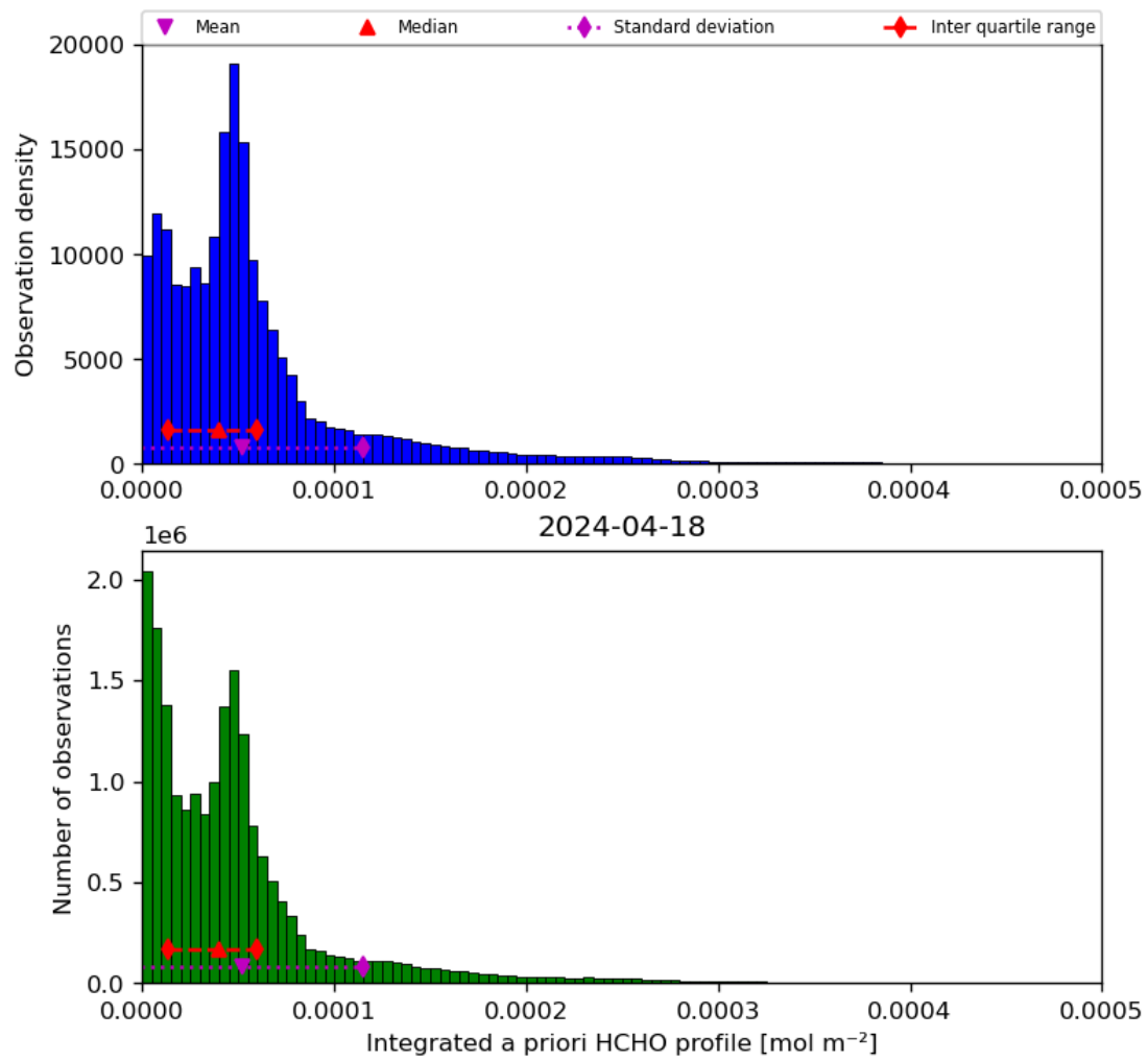
Figure 43: Histogram of “Integrated a priori HCHO profile” for 2024-04-17 to 2024-04-19
