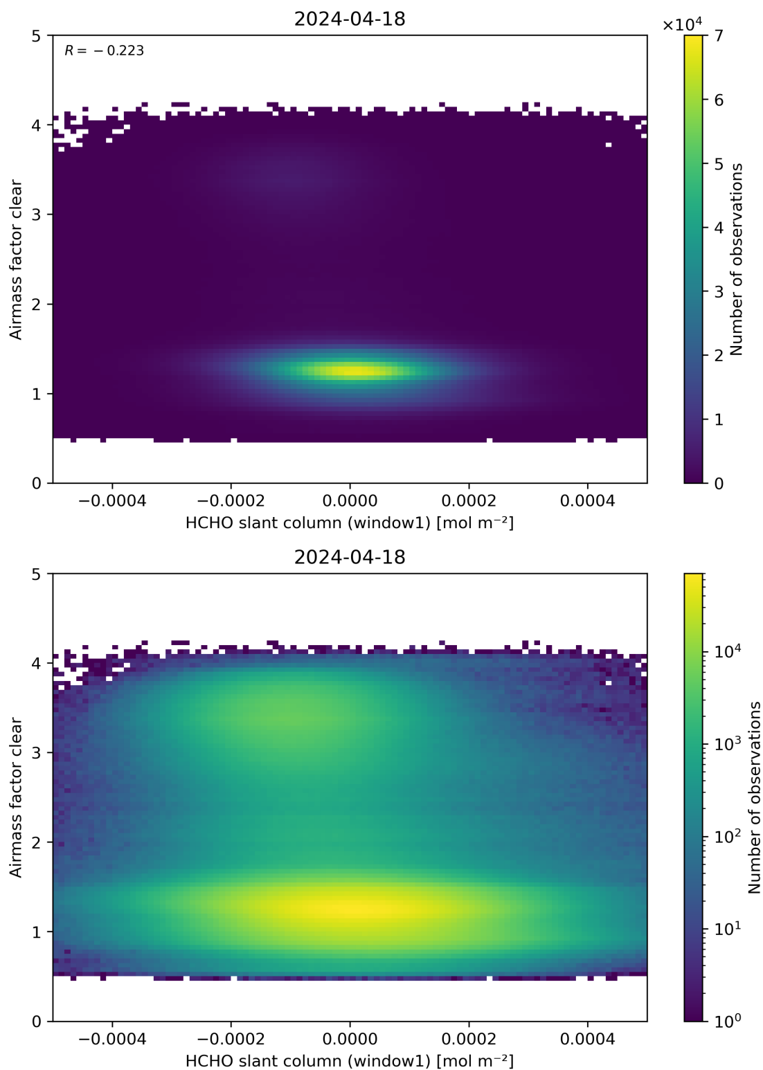
Figure 81: Scatter density plot of “HCHO slant column (window1)” against “Airmass factor clear” for 2024-04-17 to 2024-04-19.
