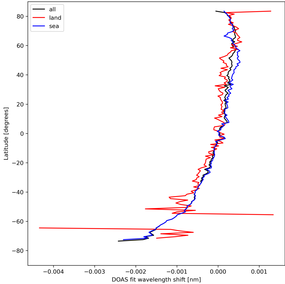
Figure 30: Zonal average of “DOAS fit wavelength shift” for 2024-04-17 to 2024-04-19.
