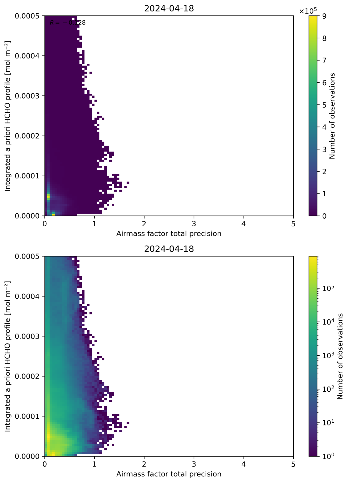
Figure 111: Scatter density plot of “Airmass factor total precision” against “Integrated a priori HCHO profile” for 2024-04-17 to 2024-04-19.
