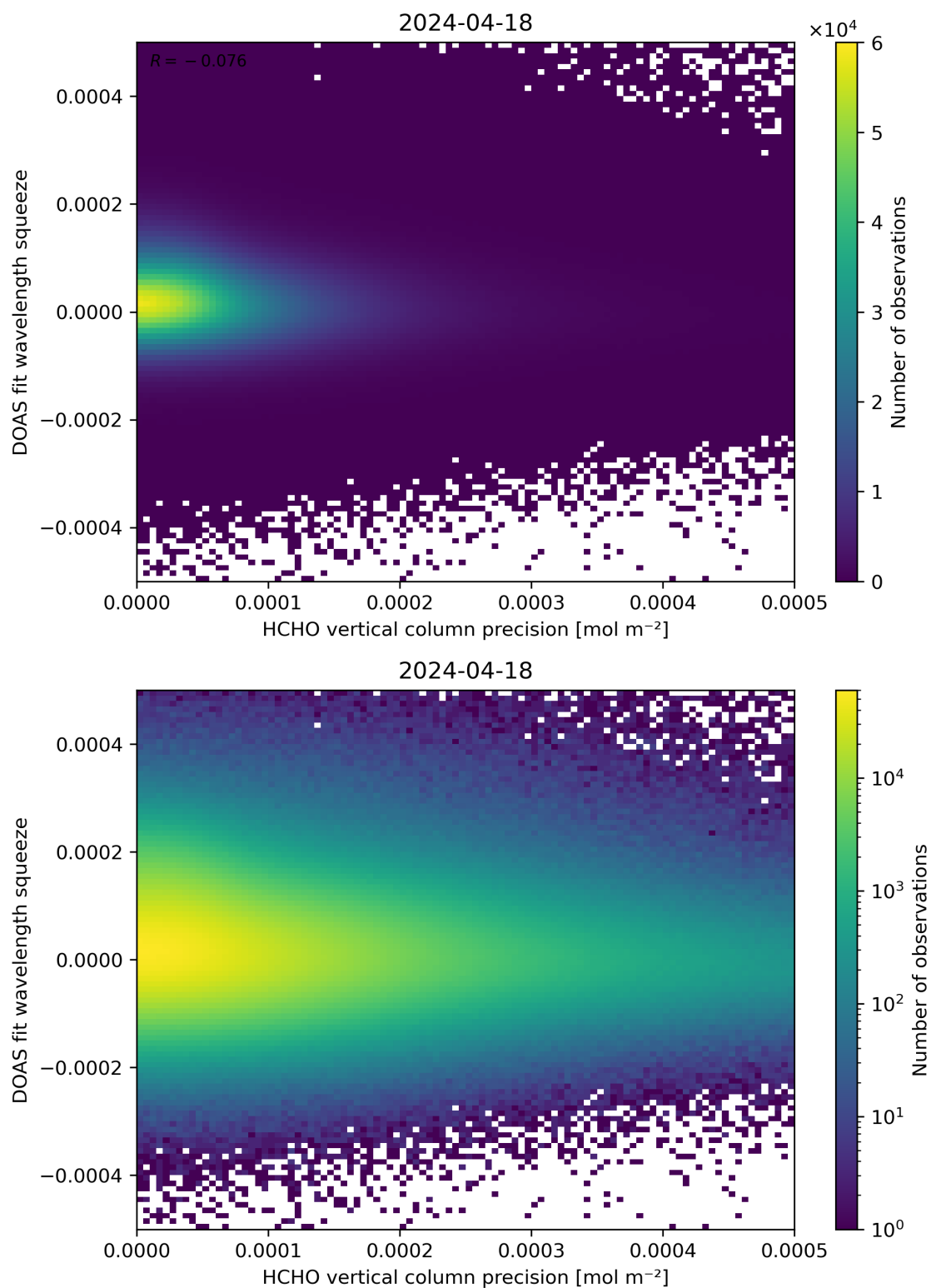
Figure 138: Scatter density plot of “HCHO vertical column precision” against “DOAS fit wavelength squeeze” for 2024-04-17 to 2024-04-19.
