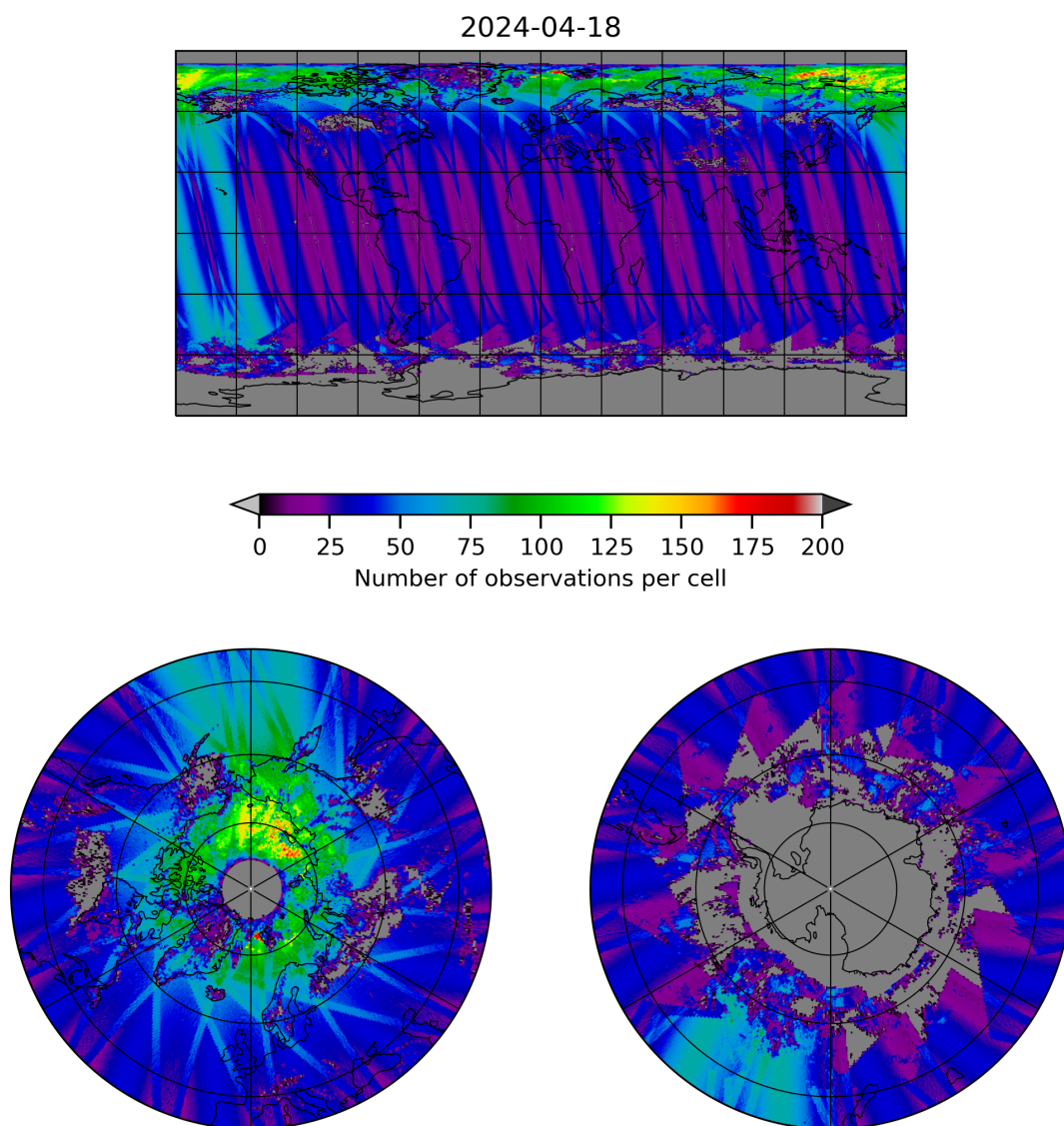
Figure 19: Map of the number of observations for 2024-04-17 to 2024-04-19
