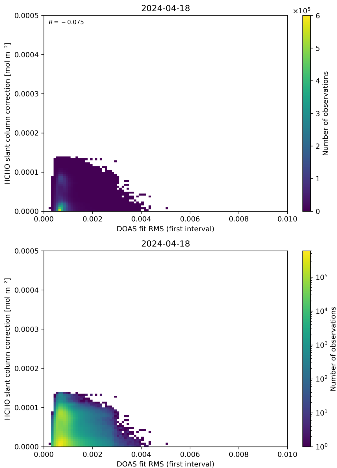
Figure 63: Scatter density plot of “DOAS fit RMS (first interval)” against “HCHO slant column correction” for 2024-04-17 to 2024-04-19.
