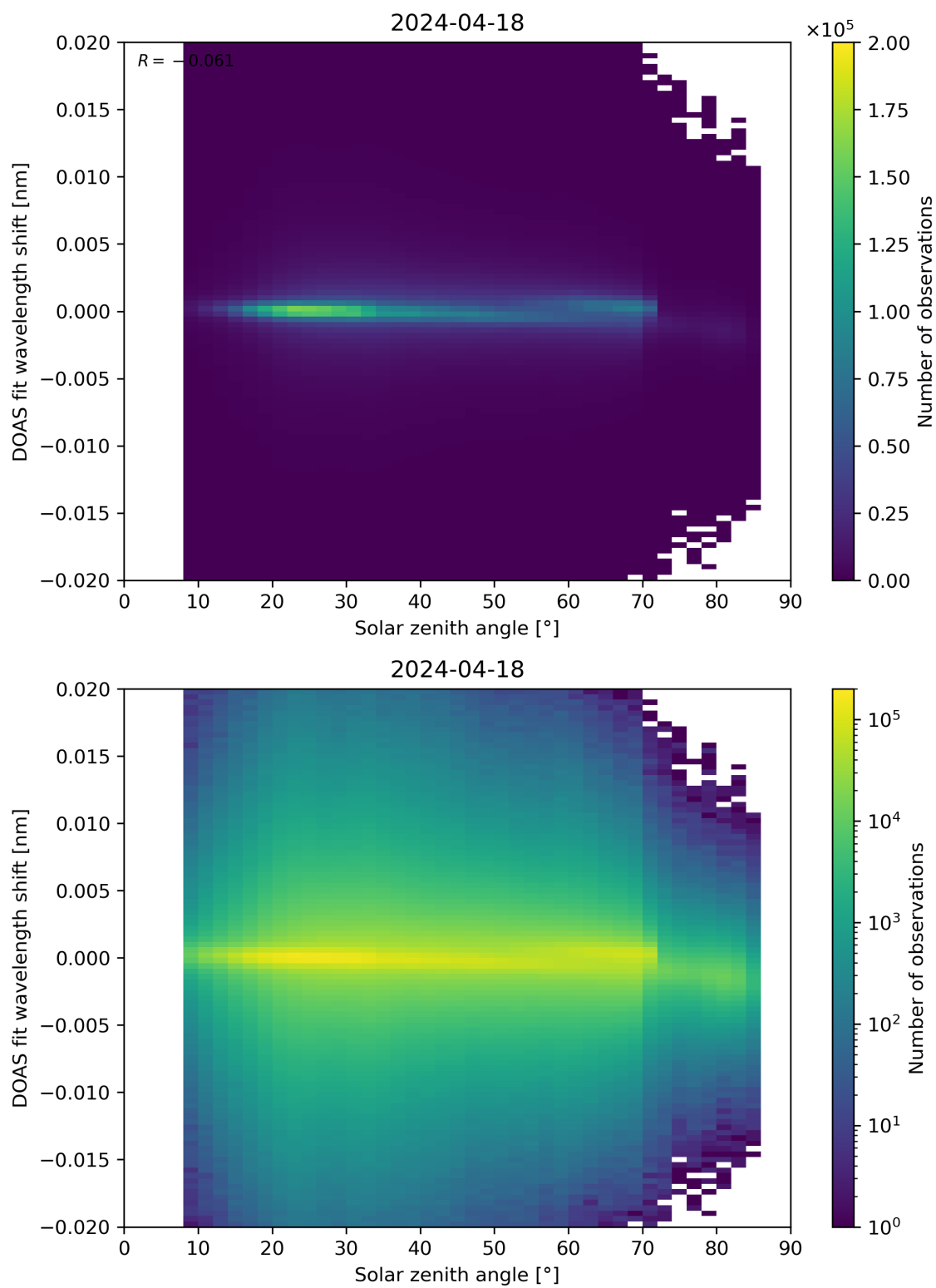
Figure 168: Scatter density plot of “Solar zenith angle” against “DOAS fit wavelength shift” for 2024-04-17 to 2024-04-19.
