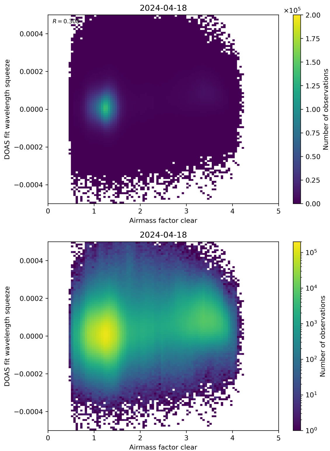
Figure 73: Scatter density plot of “Airmass factor clear” against “DOAS fit wavelength squeeze” for 2024-04-17 to 2024-04-19.
