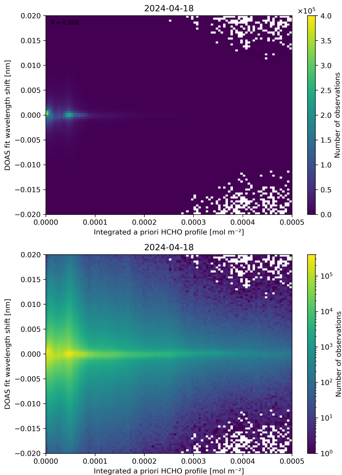
Figure 149: Scatter density plot of “Integrated a priori HCHO profile” against “DOAS fit wavelength shift” for 2024-04-17 to 2024-04-19.
