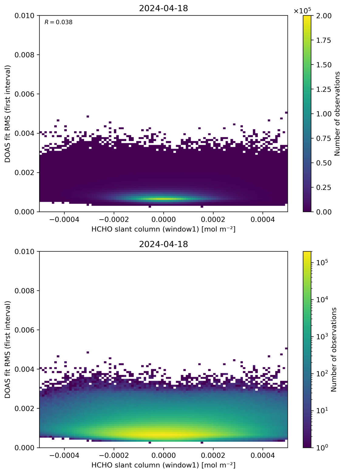
Figure 78: Scatter density plot of “HCHO slant column (window1)” against “DOAS fit RMS (first interval)” for 2024-04-17 to 2024-04-19.
