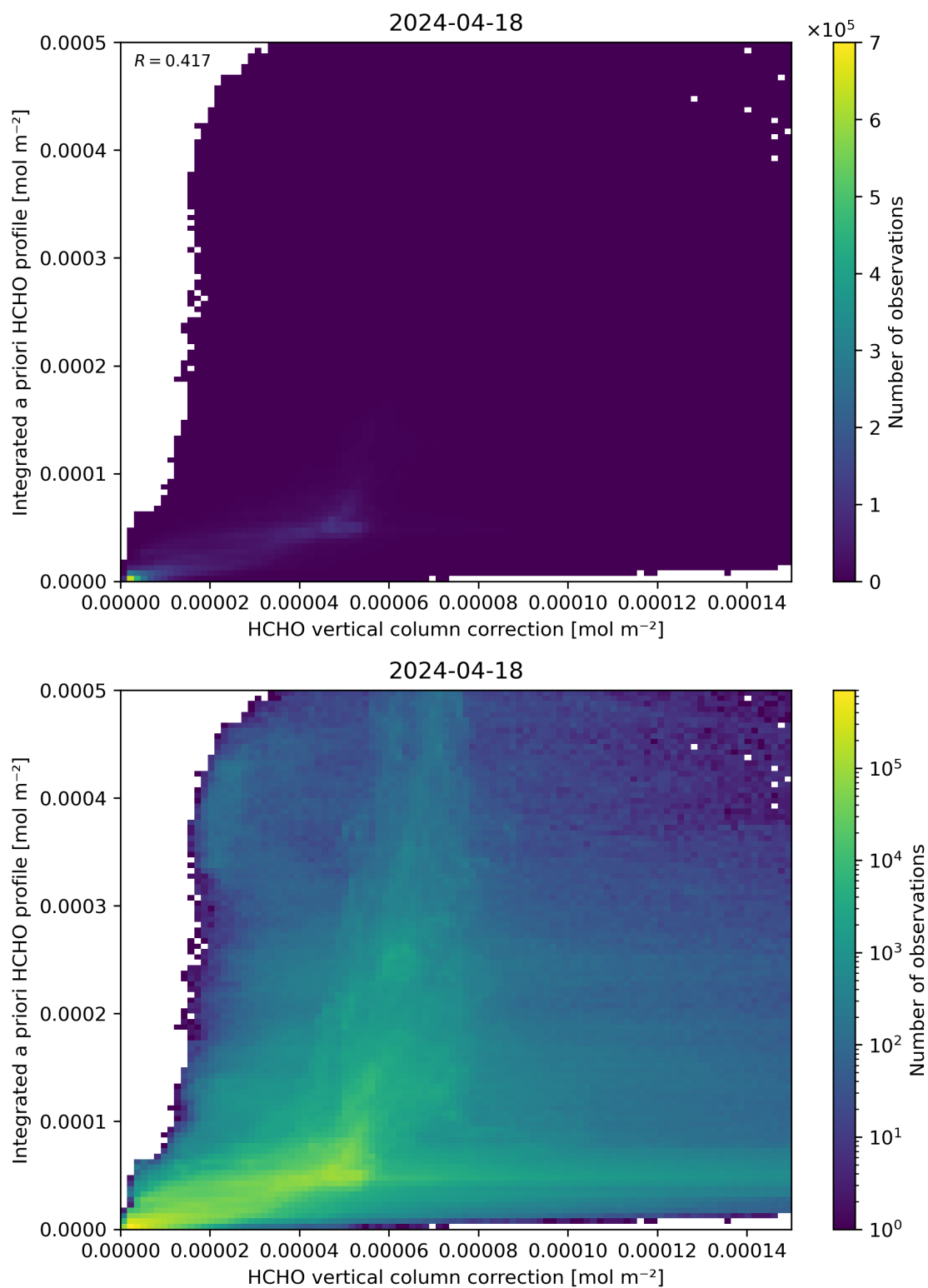
Figure 122: Scatter density plot of “HCHO vertical column correction” against “Integrated a priori HCHO profile” for 2024-04-17 to 2024-04-19.
