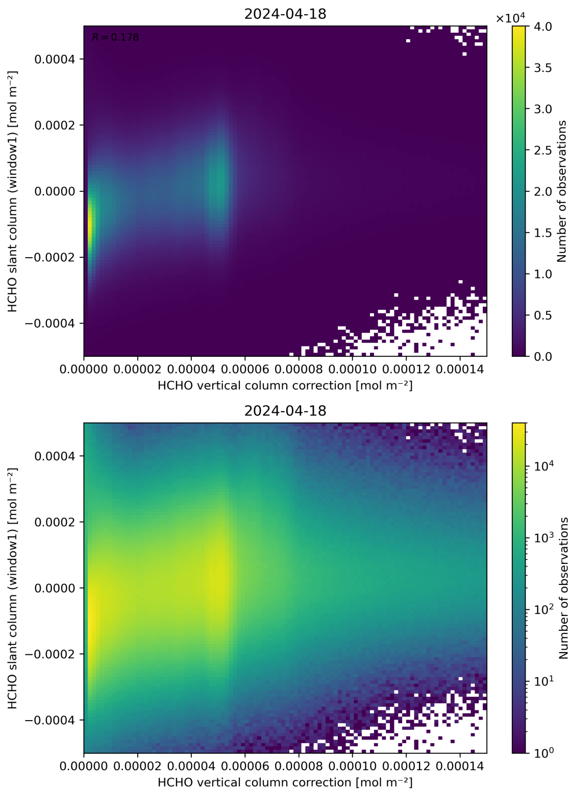
Figure 118: Scatter density plot of “HCHO vertical column correction” against “HCHO slant column (window1)” for 2024-04-17 to 2024-04-19.
