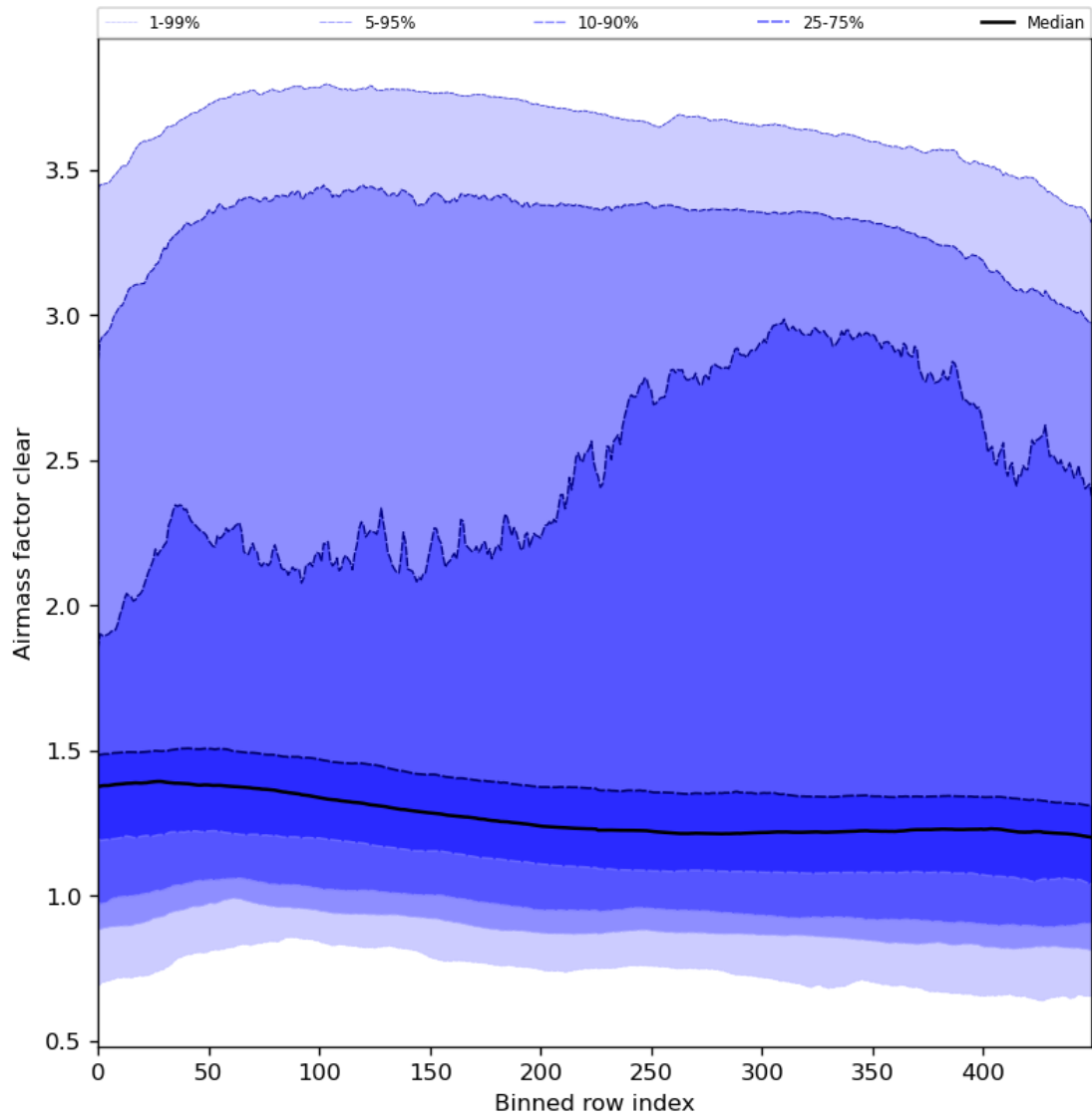
Figure 56: Along track statistics of “Airmass factor clear” for 2024-04-17 to 2024-04-19
