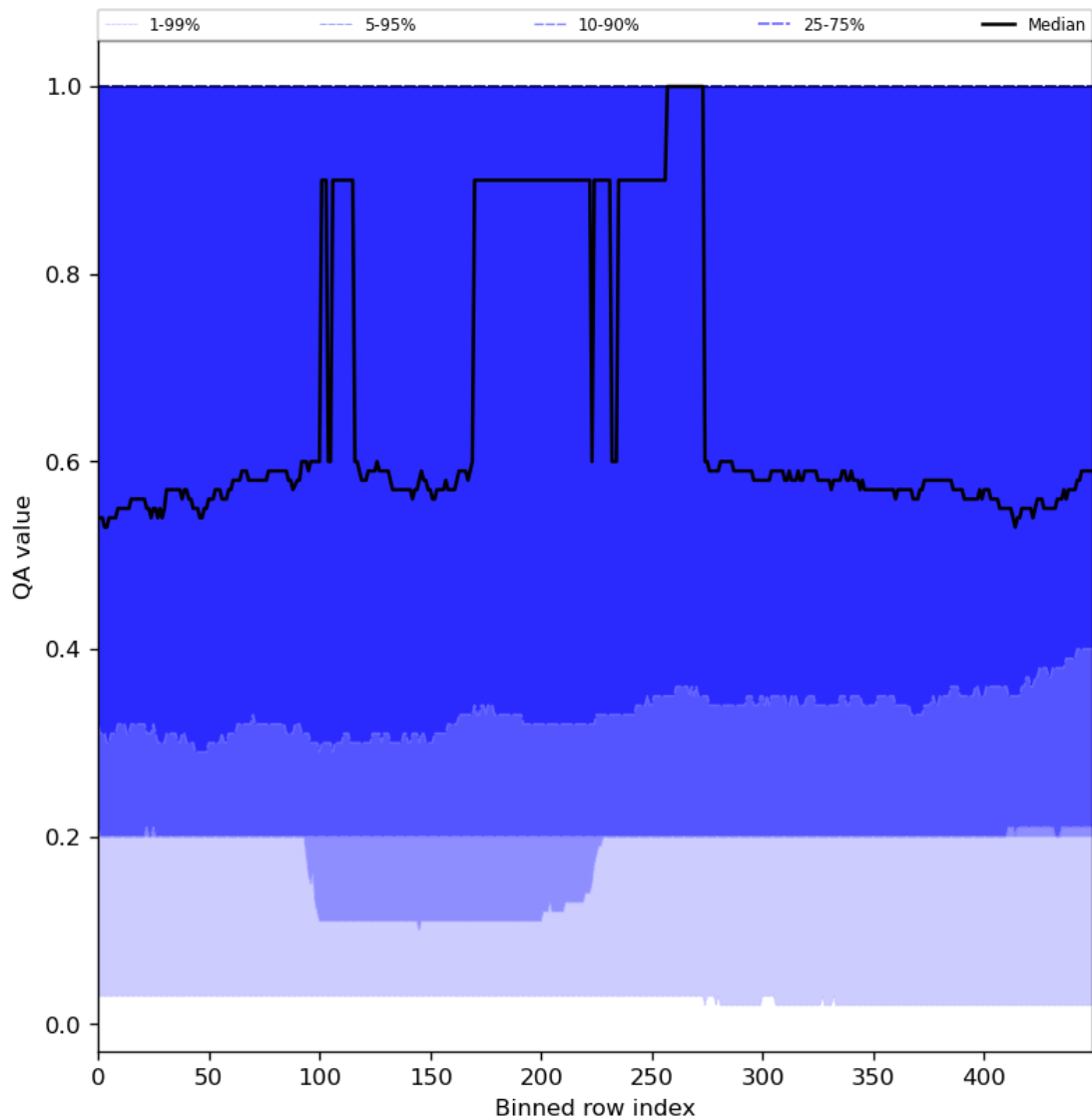
Figure 48: Along track statistics of “QA value” for 2024-04-17 to 2024-04-19
