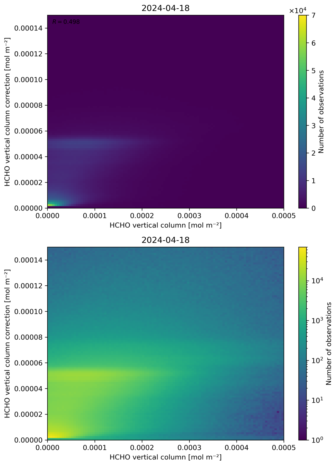
Figure 133: Scatter density plot of “HCHO vertical column” against “HCHO vertical column correction” for 2024-04-17 to 2024-04-19.
