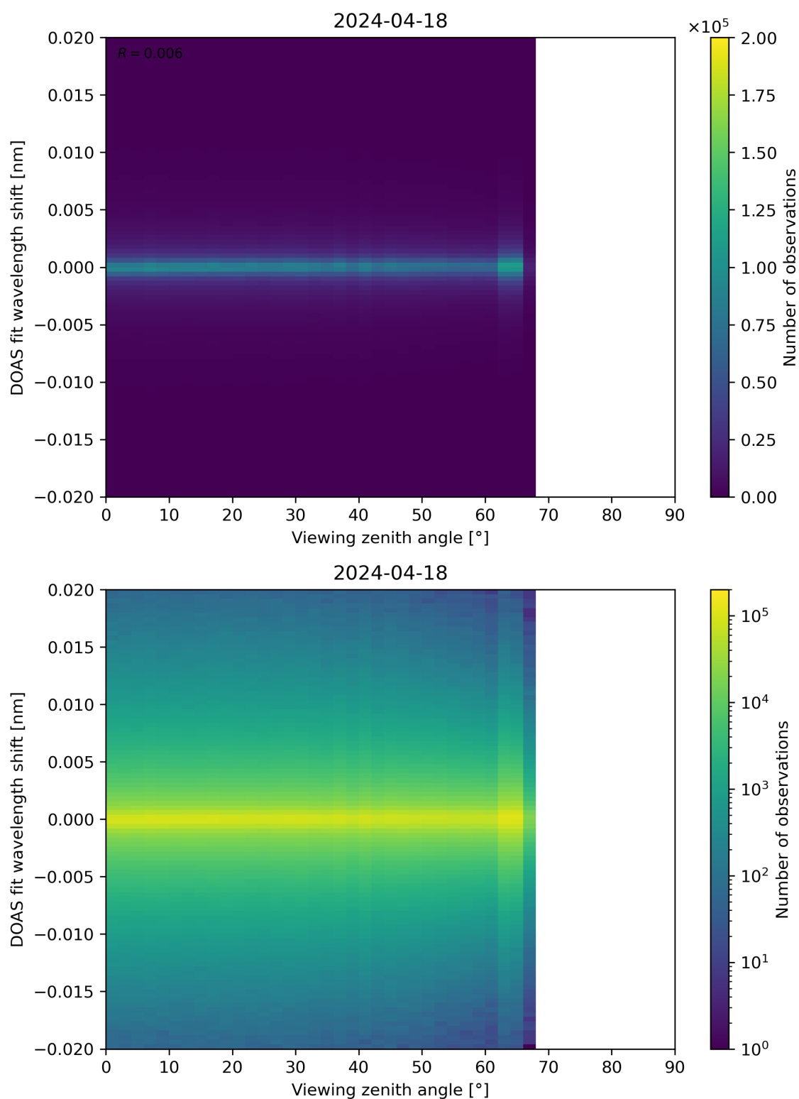
Figure 183: Scatter density plot of “Viewing zenith angle” against “DOAS fit wavelength shift” for 2024-04-17 to 2024-04-19.
