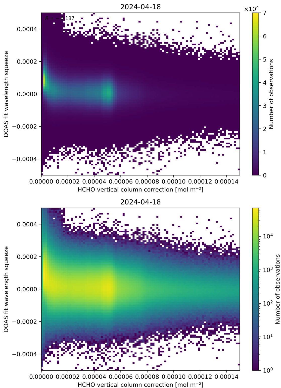
Figure 114: Scatter density plot of “HCHO vertical column correction” against “DOAS fit wavelength squeeze” for 2024-04-17 to 2024-04-19.
