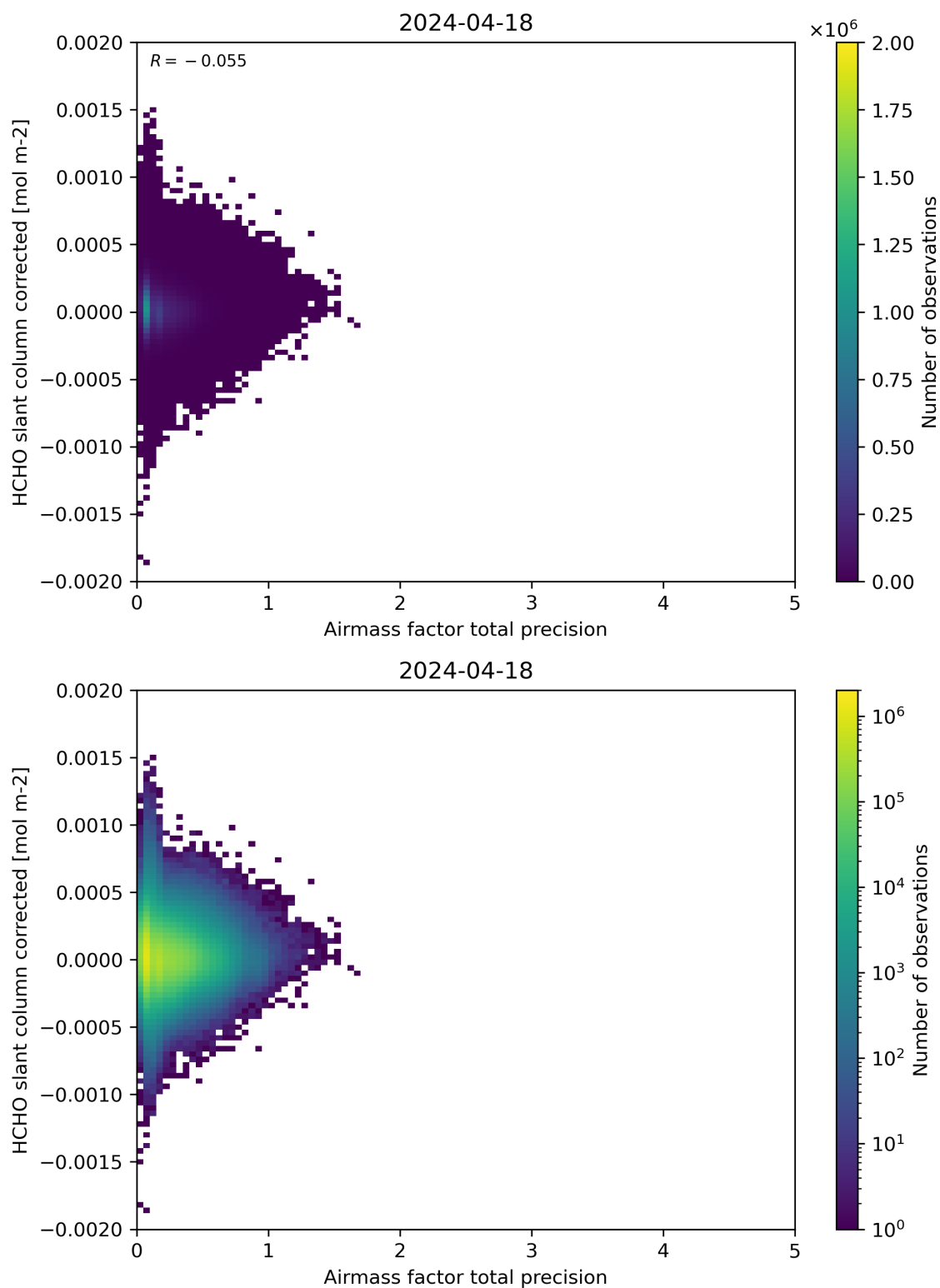
Figure 109: Scatter density plot of “Airmass factor total precision” against “HCHO slant column corrected” for 2024-04-17 to 2024-04-19.
