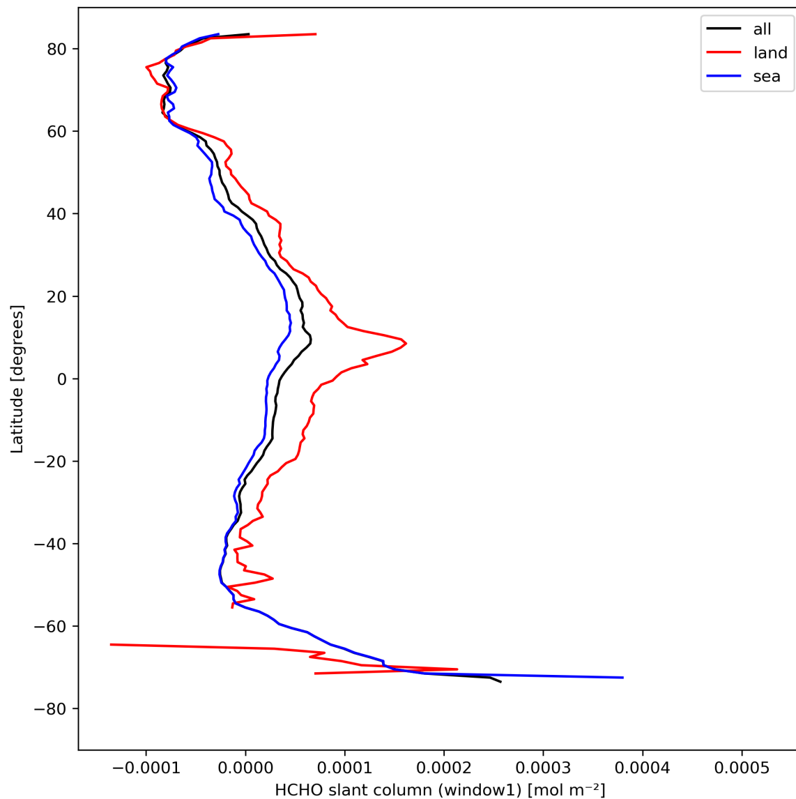
Figure 24: Zonal average of “HCHO slant column (window1)” for 2024-04-17 to 2024-04-19.
