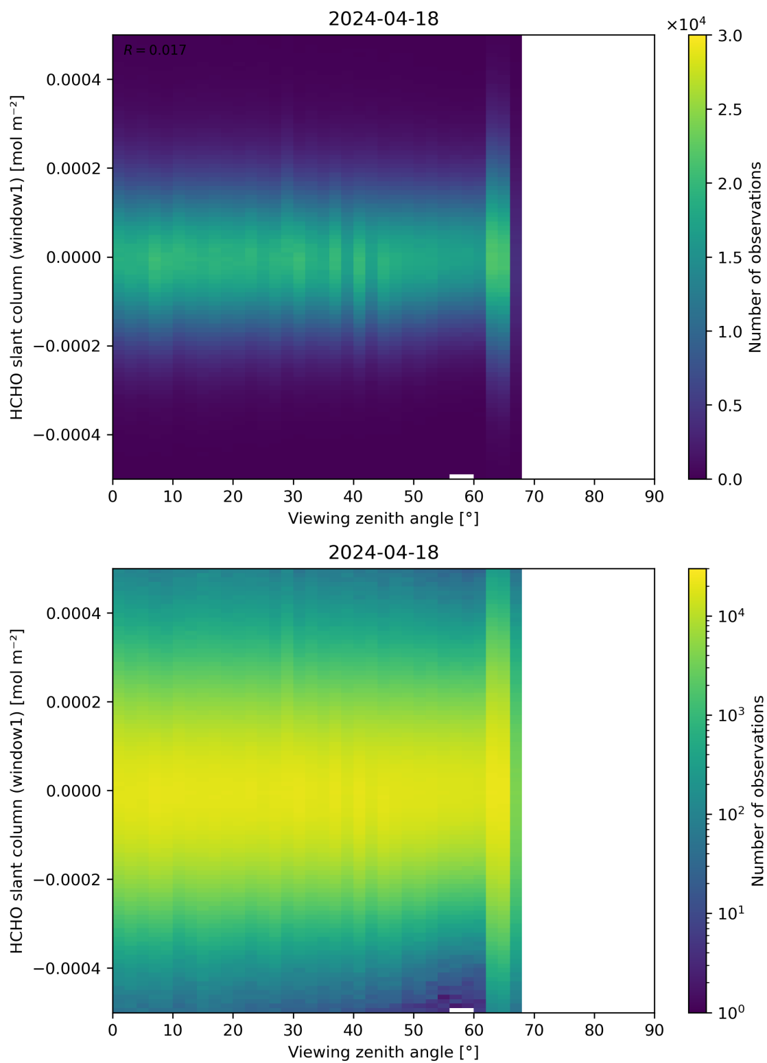
Figure 188: Scatter density plot of “Viewing zenith angle” against “HCHO slant column (window1)” for 2024-04-17 to 2024-04-19.
