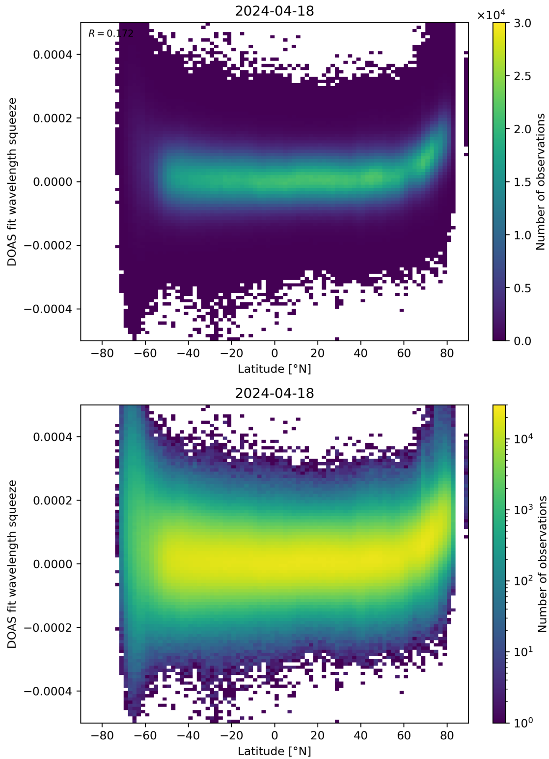
Figure 155: Scatter density plot of “Latitude” against “DOAS fit wavelength squeeze” for 2024-04-17 to 2024-04-19.
