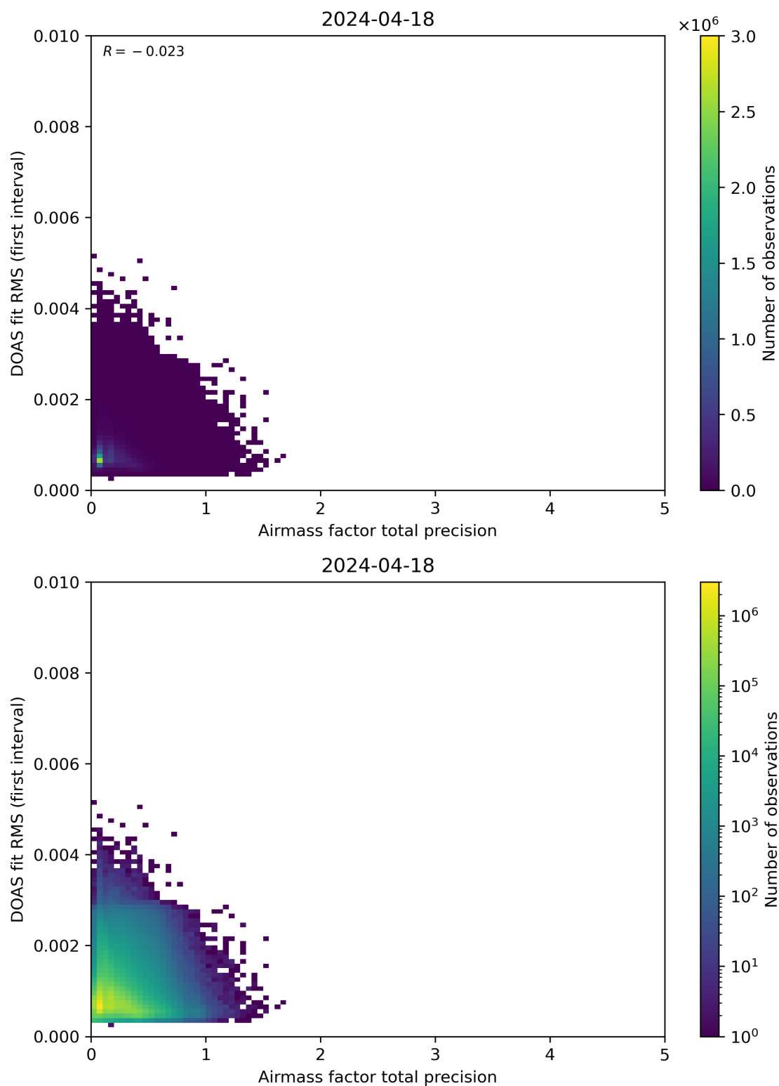
Figure 105: Scatter density plot of “Airmass factor total precision” against “DOAS fit RMS (first interval)” for 2024-04-17 to 2024-04-19.
