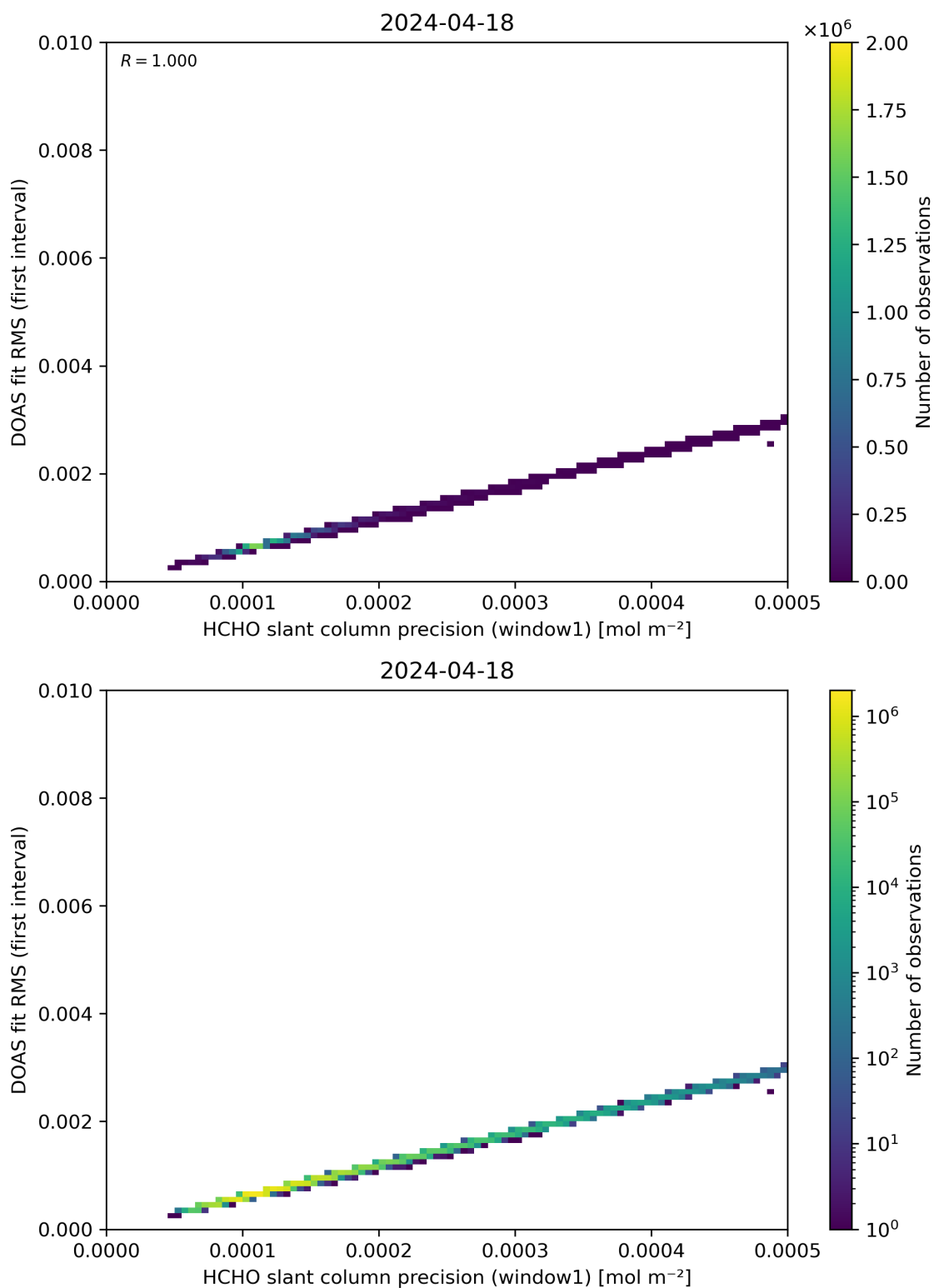
Figure 88: Scatter density plot of “HCHO slant column precision (window1)” against “DOAS fit RMS (first interval)” for 2024-04-17 to 2024-04-19.
