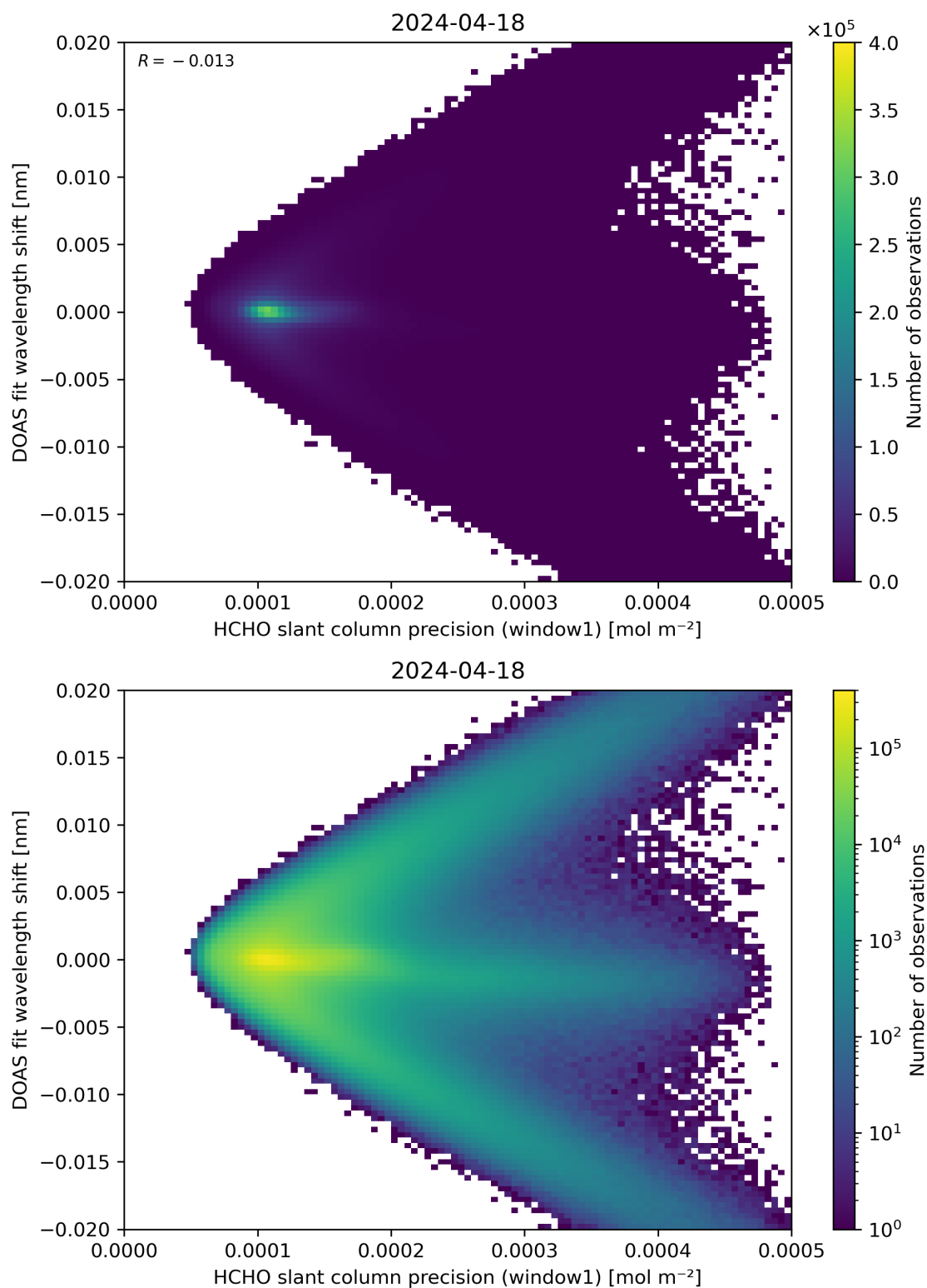
Figure 89: Scatter density plot of “HCHO slant column precision (window1)” against “DOAS fit wavelength shift” for 2024-04-17 to 2024-04-19.
