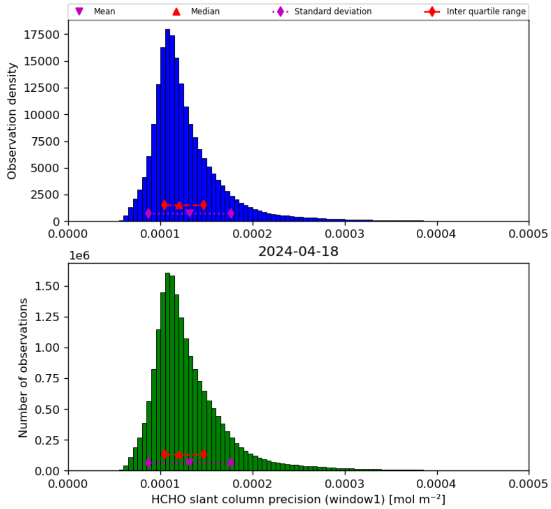
Figure 39: Histogram of “HCHO slant column precision (window1)” for 2024-04-17 to 2024-04-19
