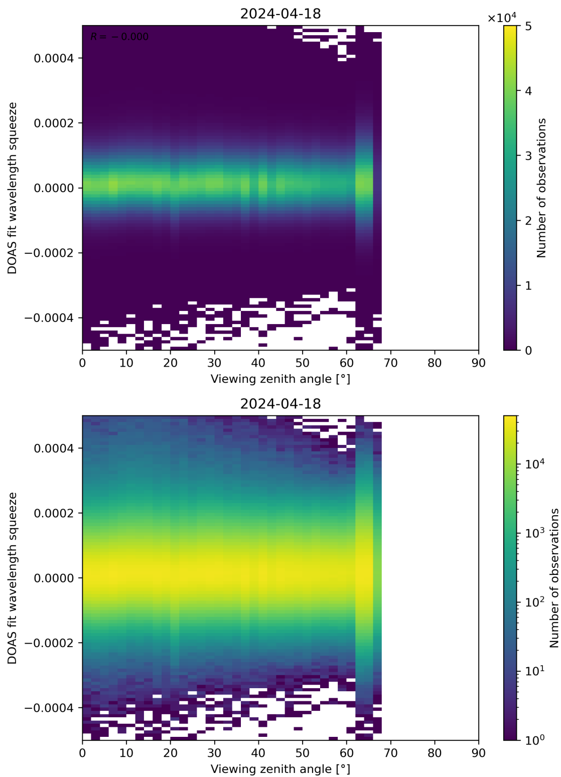
Figure 184: Scatter density plot of “Viewing zenith angle” against “DOAS fit wavelength squeeze” for 2024-04-17 to 2024-04-19.
