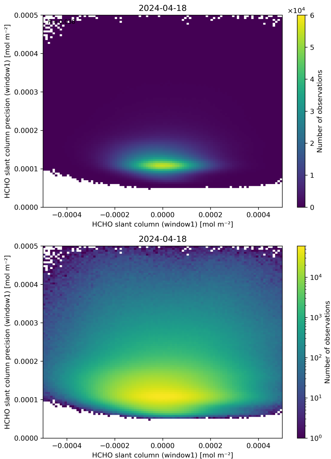
Figure 84: Scatter density plot of “HCHO slant column (window1)” against “HCHO slant column precision (window1)” for 2024-04-17 to 2024-04-19.
