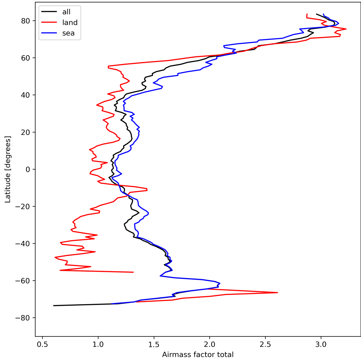
Figure 26: Zonal average of “Airmass factor total” for 2024-04-17 to 2024-04-19.
