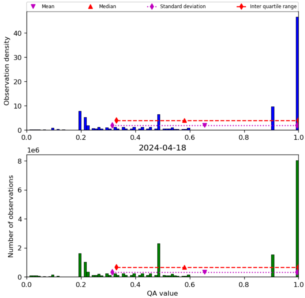
Figure 34: Histogram of “QA value” for 2024-04-17 to 2024-04-19
