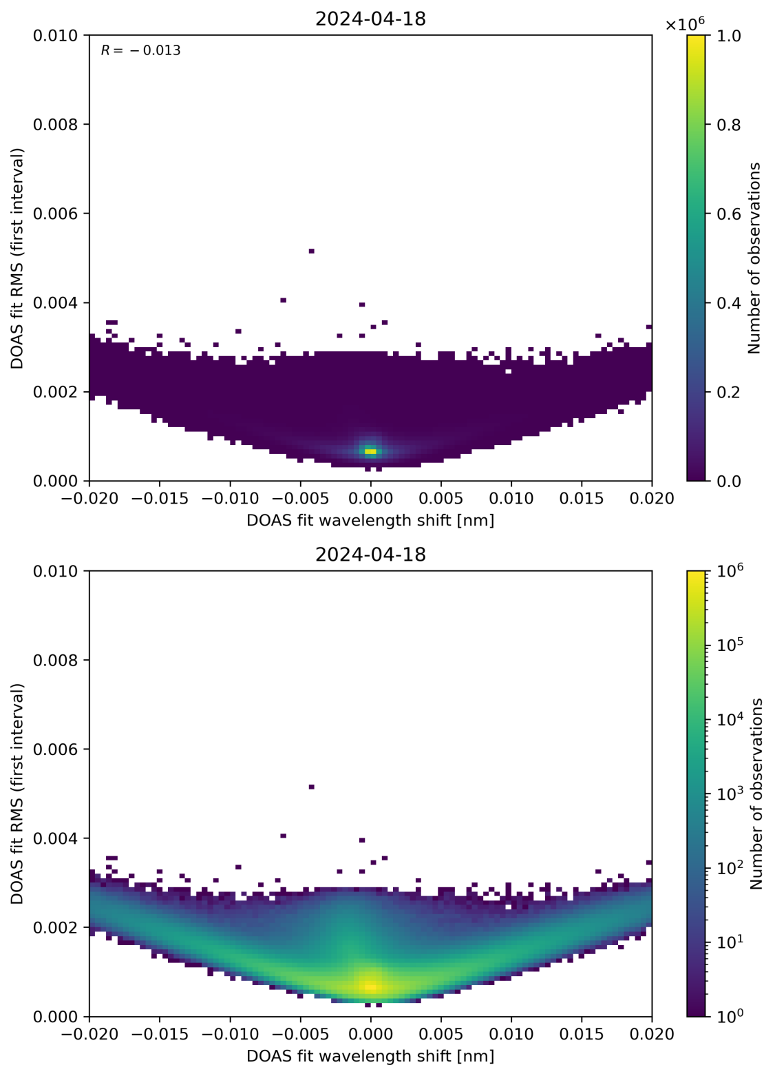
Figure 64: Scatter density plot of “DOAS fit wavelength shift” against “DOAS fit RMS (first interval)” for 2024-04-17 to 2024-04-19.
