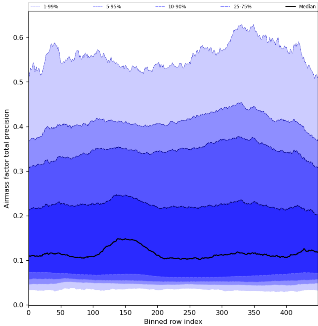
Figure 55: Along track statistics of “Airmass factor total precision” for 2024-04-17 to 2024-04-19
