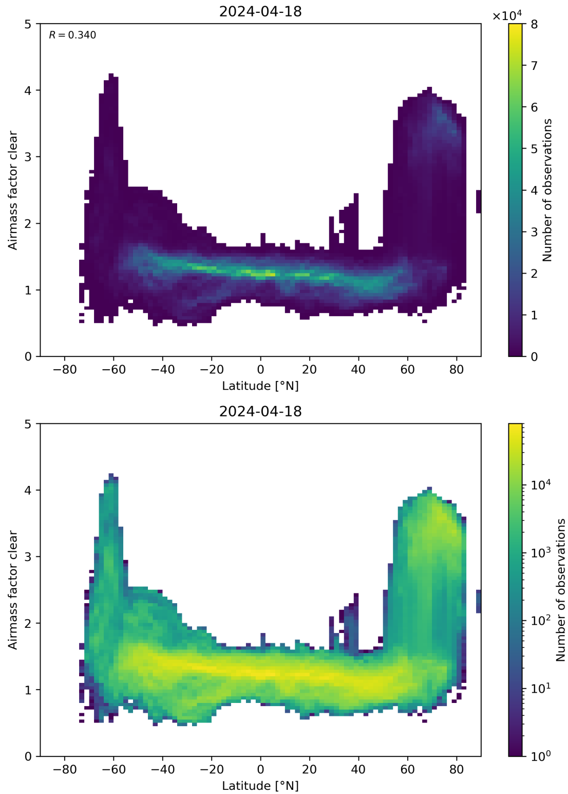
Figure 156: Scatter density plot of “Latitude” against “Airmass factor clear” for 2024-04-17 to 2024-04-19.
