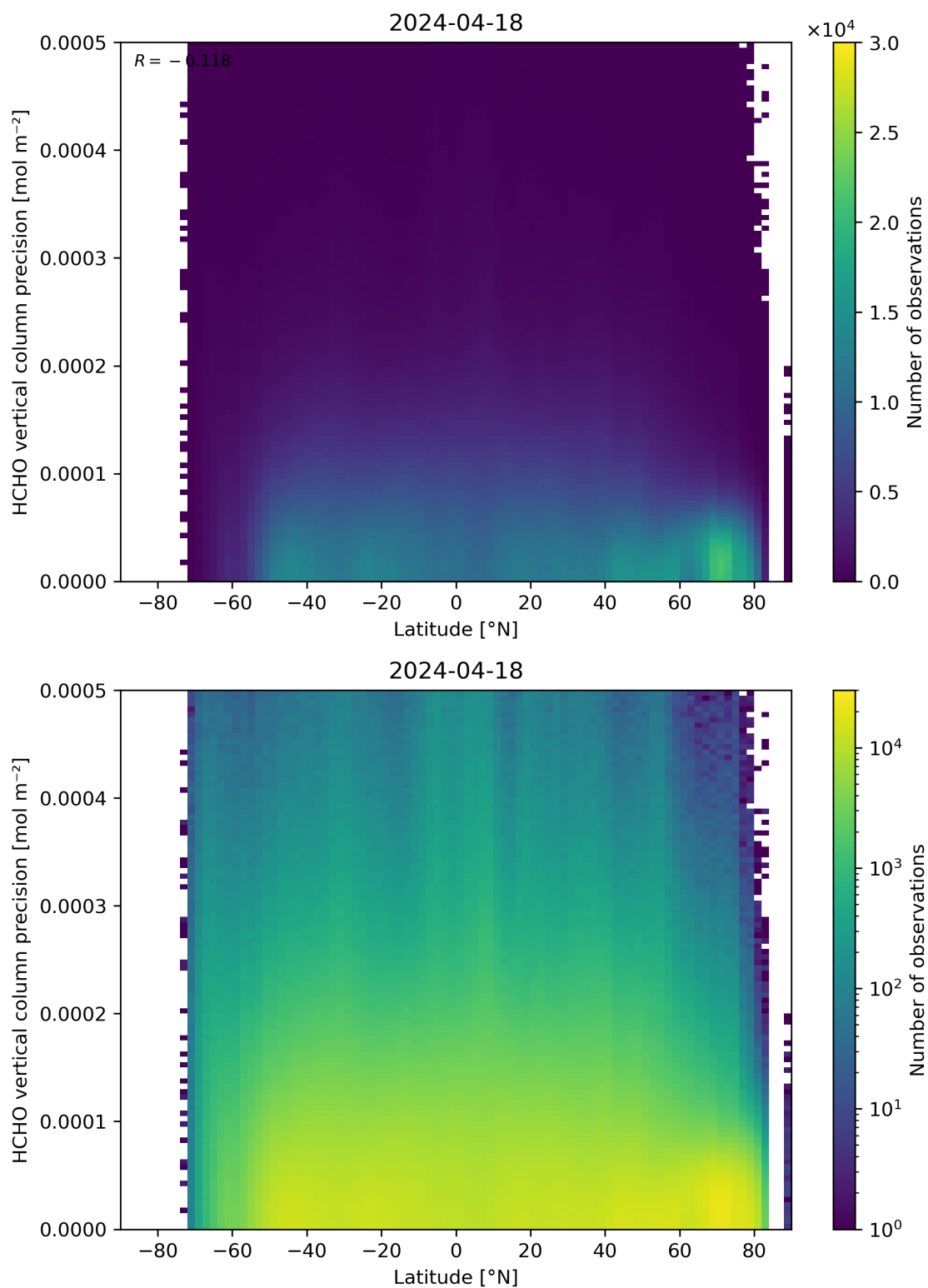
Figure 165: Scatter density plot of “Latitude” against “HCHO vertical column precision” for 2024-04-17 to 2024-04-19.
