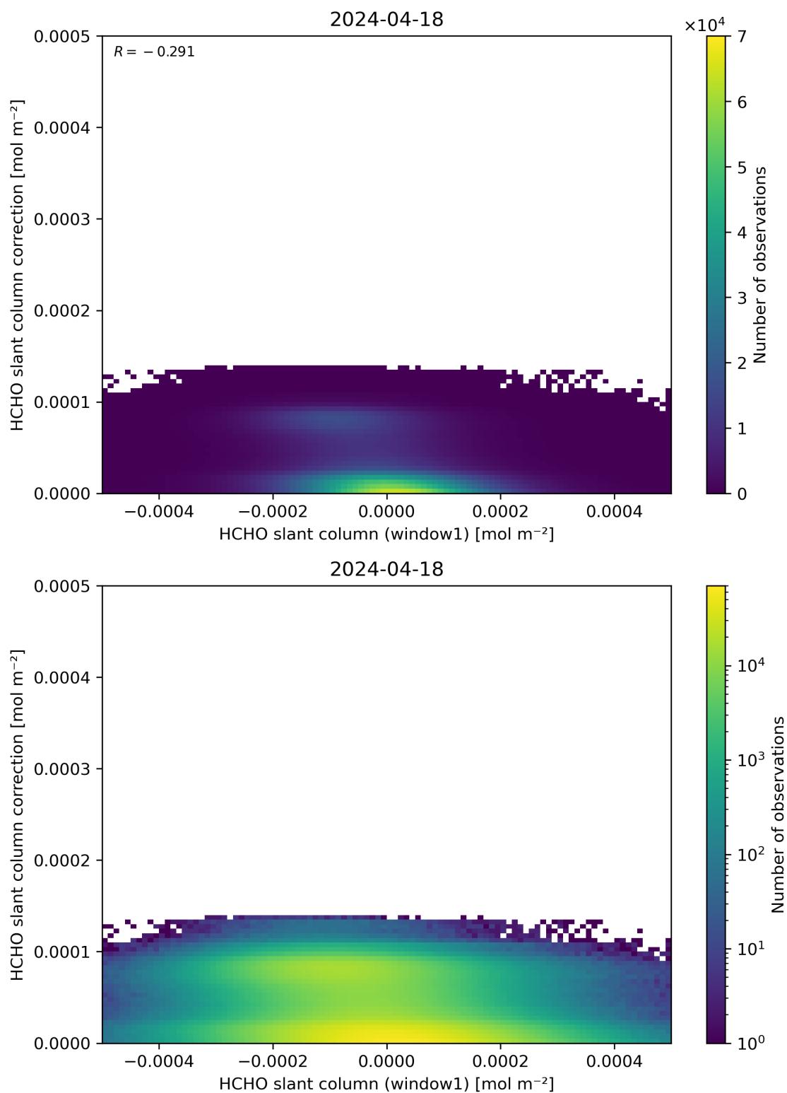
Figure 83: Scatter density plot of “HCHO slant column (window1)” against “HCHO slant column correction” for 2024-04-17 to 2024-04-19.
