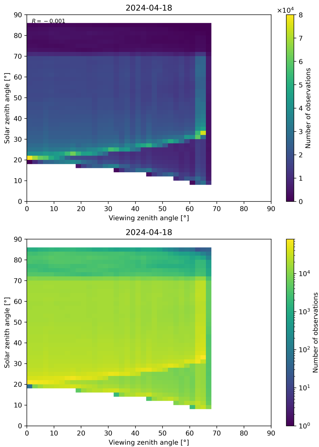
Figure 197: Scatter density plot of “Viewing zenith angle” against “Solar zenith angle” for 2024-04-17 to 2024-04-19.
