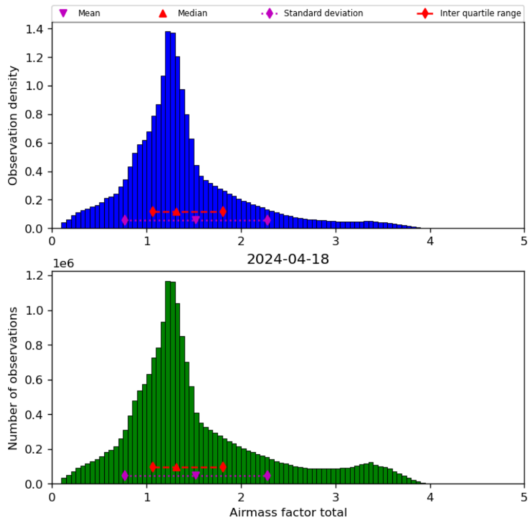
Figure 40: Histogram of “Airmass factor total” for 2024-04-17 to 2024-04-19
