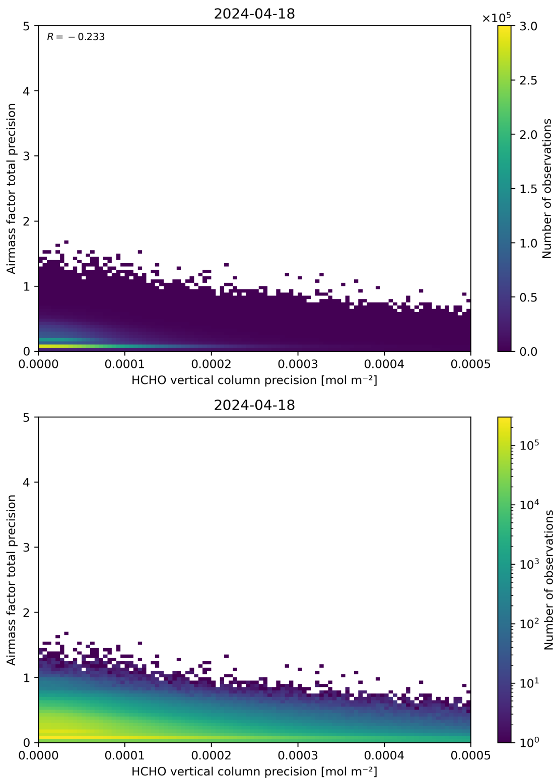
Figure 145: Scatter density plot of “HCHO vertical column precision” against “Airmass factor total precision” for 2024-04-17 to 2024-04-19.
