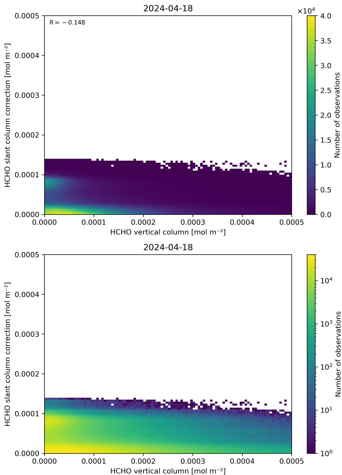
Figure 128: Scatter density plot of “HCHO vertical column” against “HCHO slant column correction” for 2024-04-17 to 2024-04-19.
