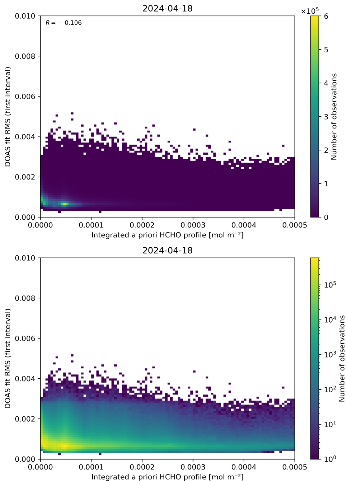
Figure 148: Scatter density plot of “Integrated a priori HCHO profile” against “DOAS fit RMS (first interval)” for 2024-04-17 to 2024-04-19.
