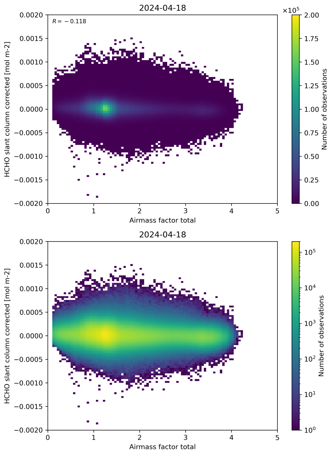
Figure 101: Scatter density plot of “Airmass factor total” against “HCHO slant column corrected” for 2024-04-17 to 2024-04-19.
