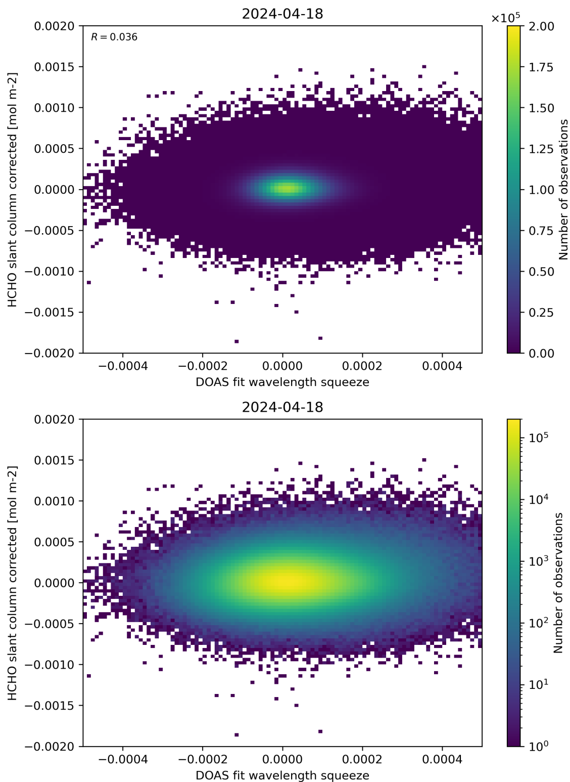
Figure 69: Scatter density plot of “DOAS fit wavelength squeeze” against “HCHO slant column corrected” for 2024-04-17 to 2024-04-19.
