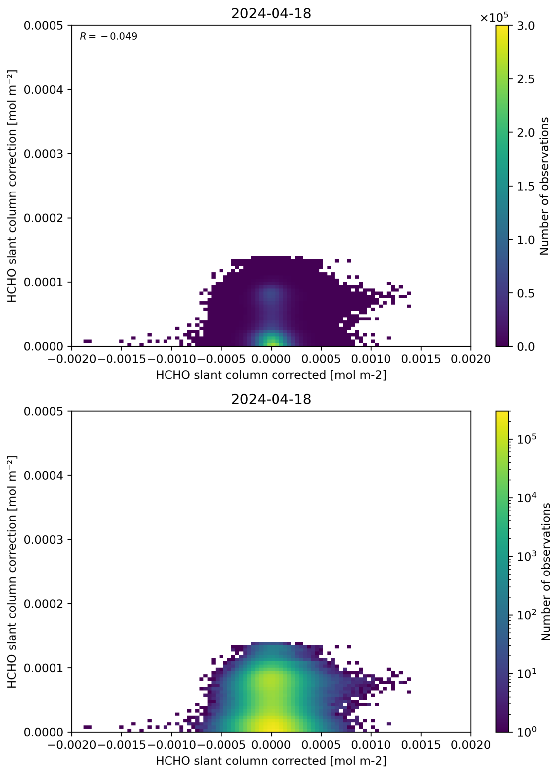
Figure 77: Scatter density plot of “HCHO slant column corrected” against “HCHO slant column correction” for 2024-04-17 to 2024-04-19.
