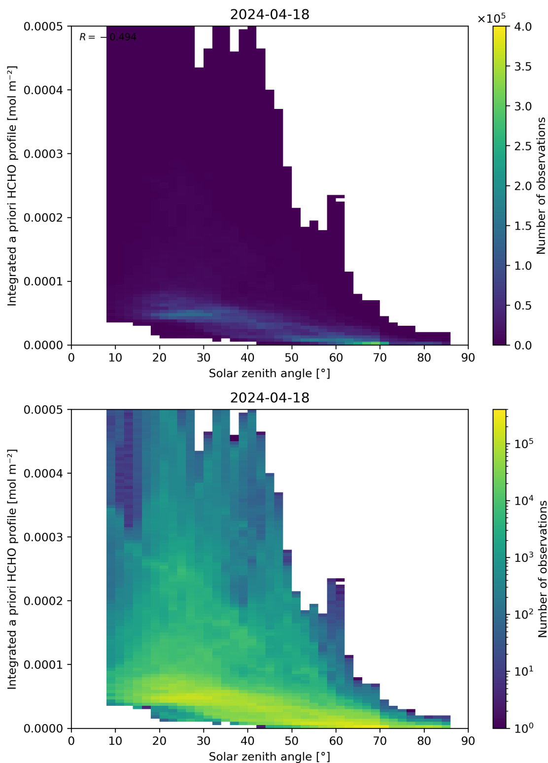
Figure 180: Scatter density plot of “Solar zenith angle” against “Integrated a priori HCHO profile” for 2024-04-17 to 2024-04-19.
