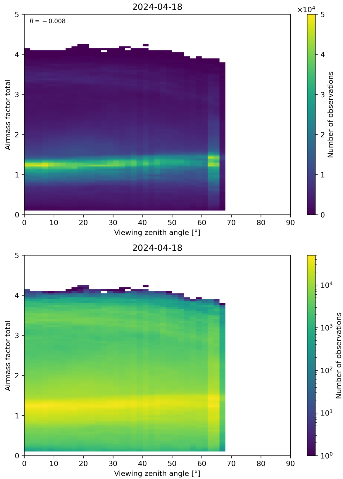
Figure 190: Scatter density plot of “Viewing zenith angle” against “Airmass factor total” for 2024-04-17 to 2024-04-19.
