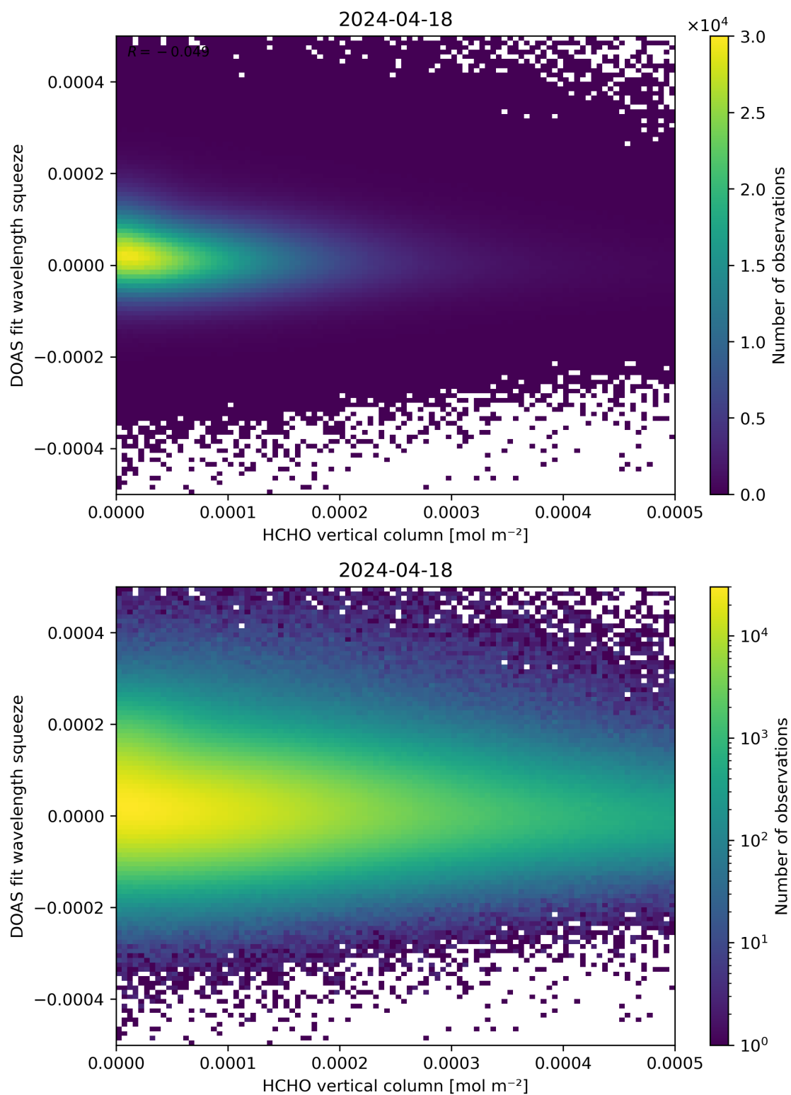
Figure 125: Scatter density plot of “HCHO vertical column” against “DOAS fit wavelength squeeze” for 2024-04-17 to 2024-04-19.
