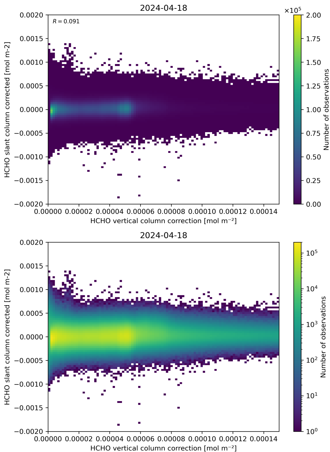
Figure 116: Scatter density plot of “HCHO vertical column correction” against “HCHO slant column corrected” for 2024-04-17 to 2024-04-19.
