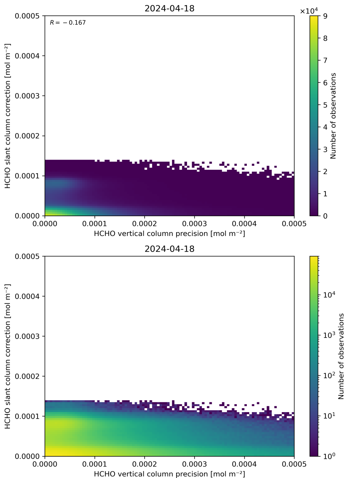
Figure 141: Scatter density plot of “HCHO vertical column precision” against “HCHO slant column correction” for 2024-04-17 to 2024-04-19.
