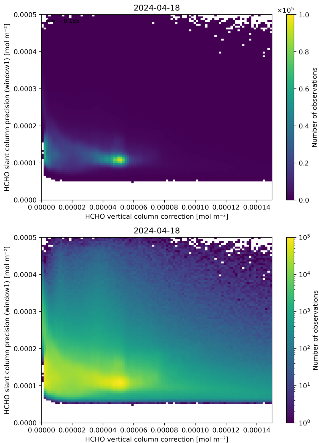
Figure 119: Scatter density plot of “HCHO vertical column correction” against “HCHO slant column precision (window1)” for 2024-04-17 to 2024-04-19.
