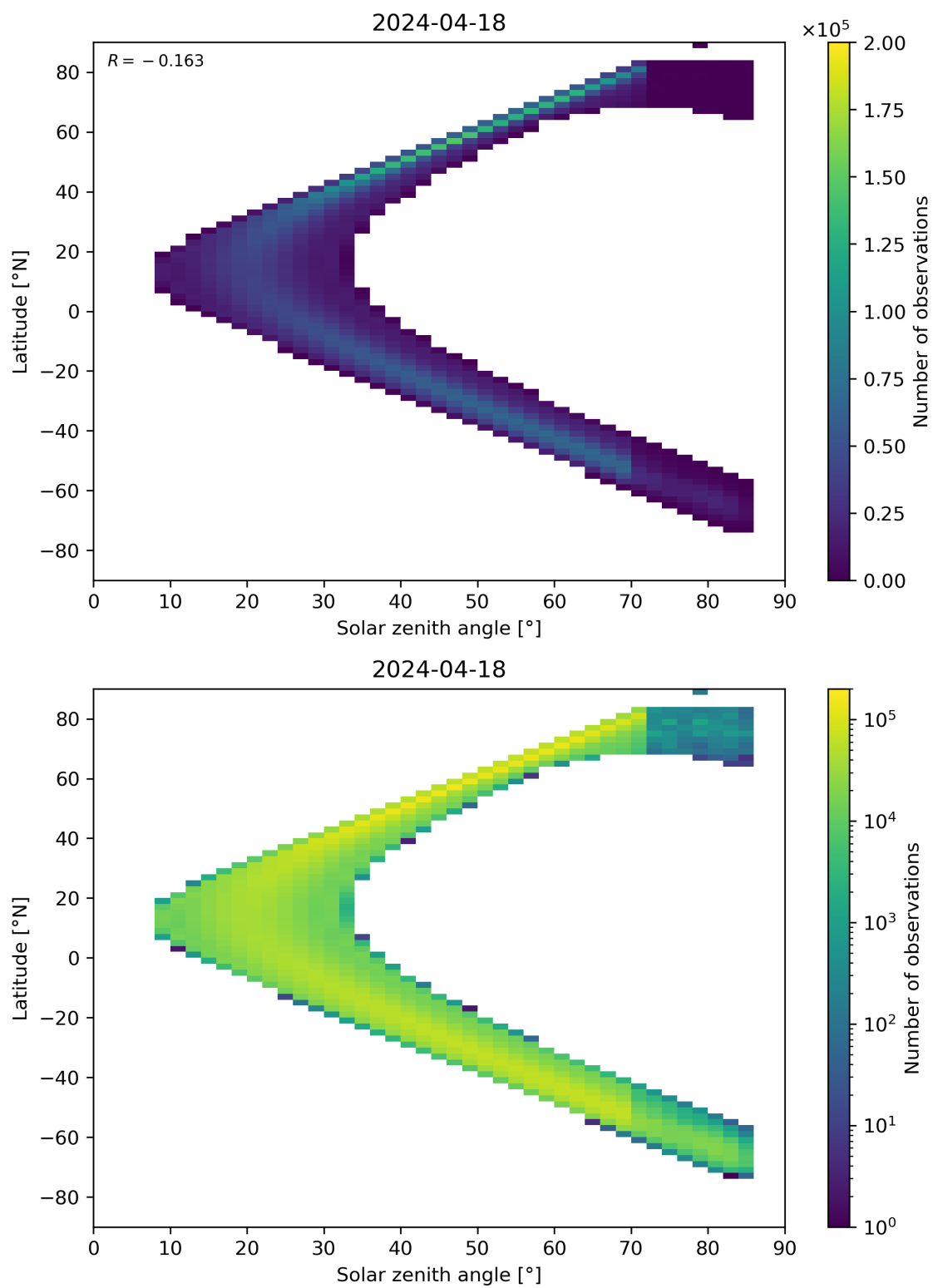
Figure 181: Scatter density plot of “Solar zenith angle” against “Latitude” for 2024-04-17 to 2024-04-19.
