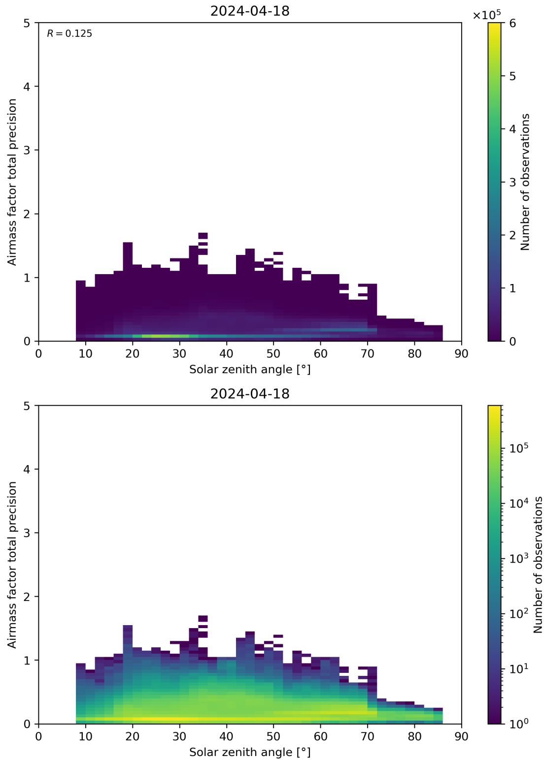
Figure 176: Scatter density plot of “Solar zenith angle” against “Airmass factor total precision” for 2024-04-17 to 2024-04-19.
