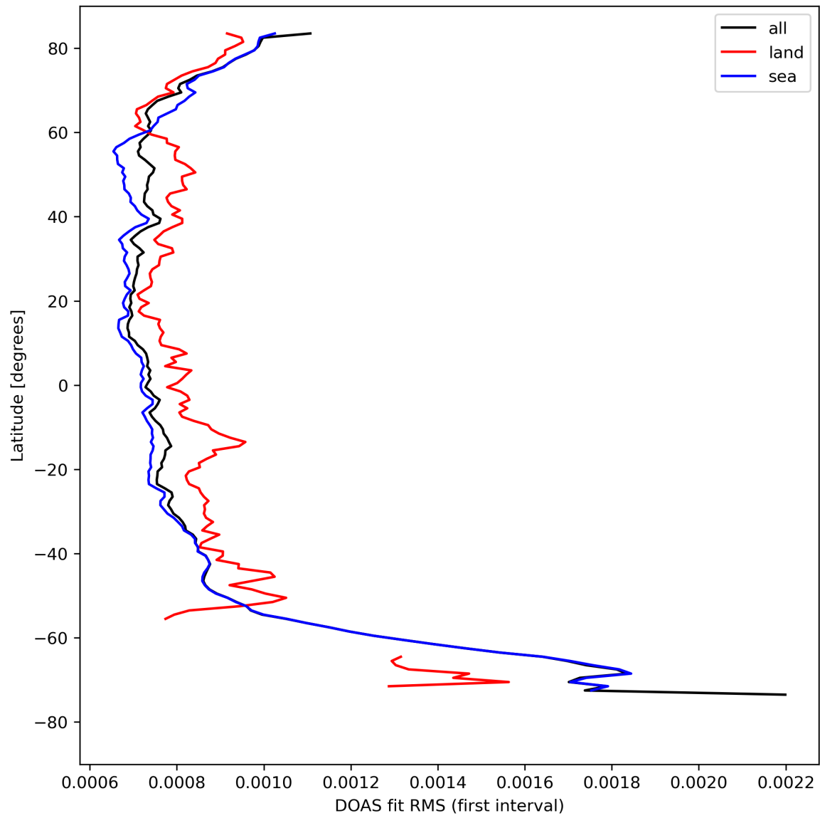
Figure 32: Zonal average of “DOAS fit RMS (first interval)” for 2024-04-17 to 2024-04-19.
