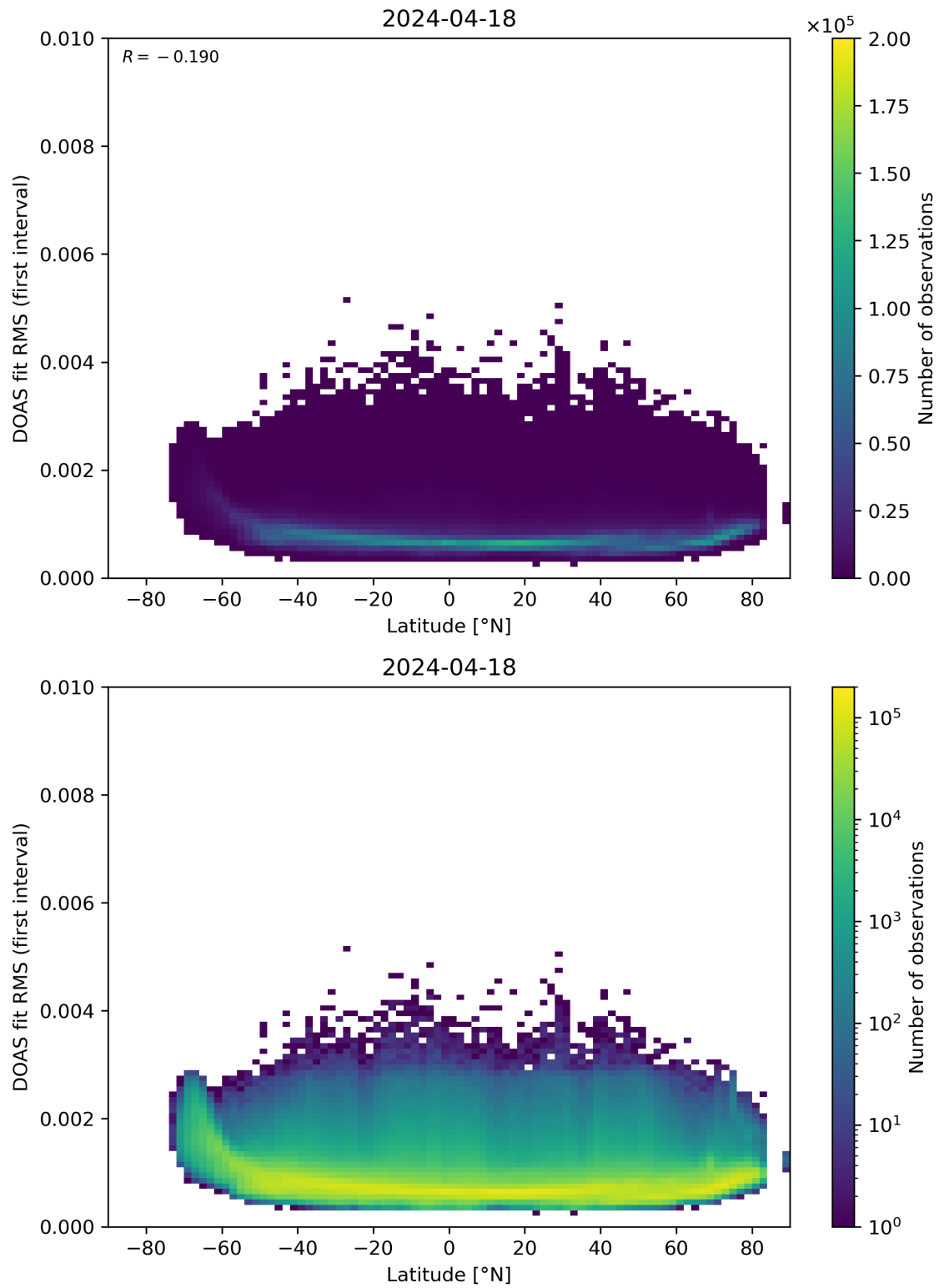
Figure 153: Scatter density plot of “Latitude” against “DOAS fit RMS (first interval)” for 2024-04-17 to 2024-04-19.
