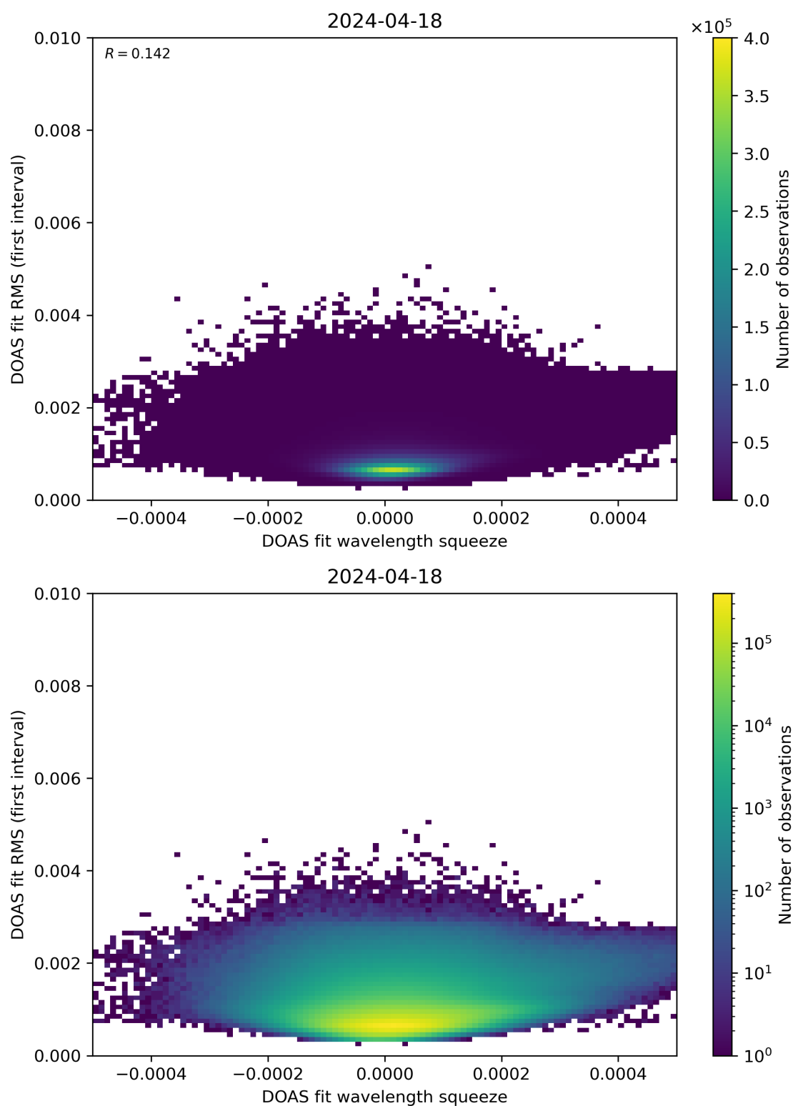
Figure 68: Scatter density plot of “DOAS fit wavelength squeeze” against “DOAS fit RMS (first interval)” for 2024-04-17 to 2024-04-19.
