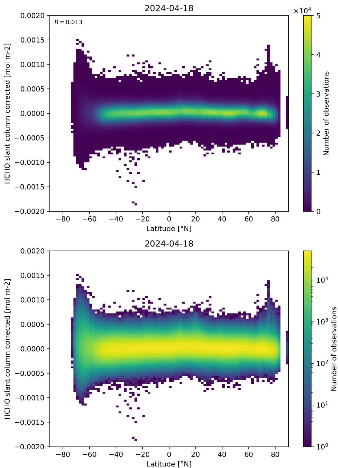
Figure 157: Scatter density plot of “Latitude” against “HCHO slant column corrected” for 2024-04-17 to 2024-04-19.
