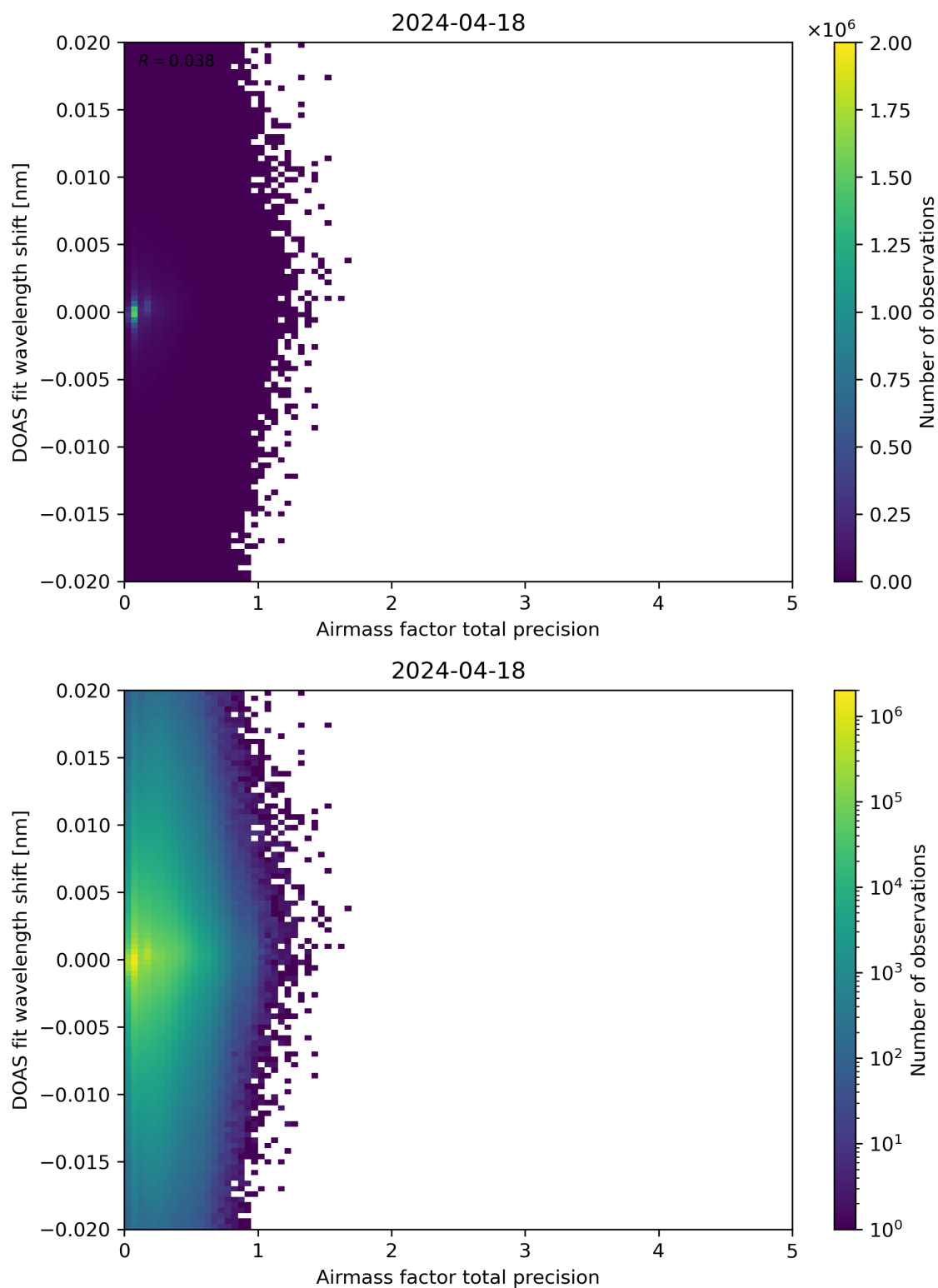
Figure 106: Scatter density plot of “Airmass factor total precision” against “DOAS fit wavelength shift” for 2024-04-17 to 2024-04-19.
