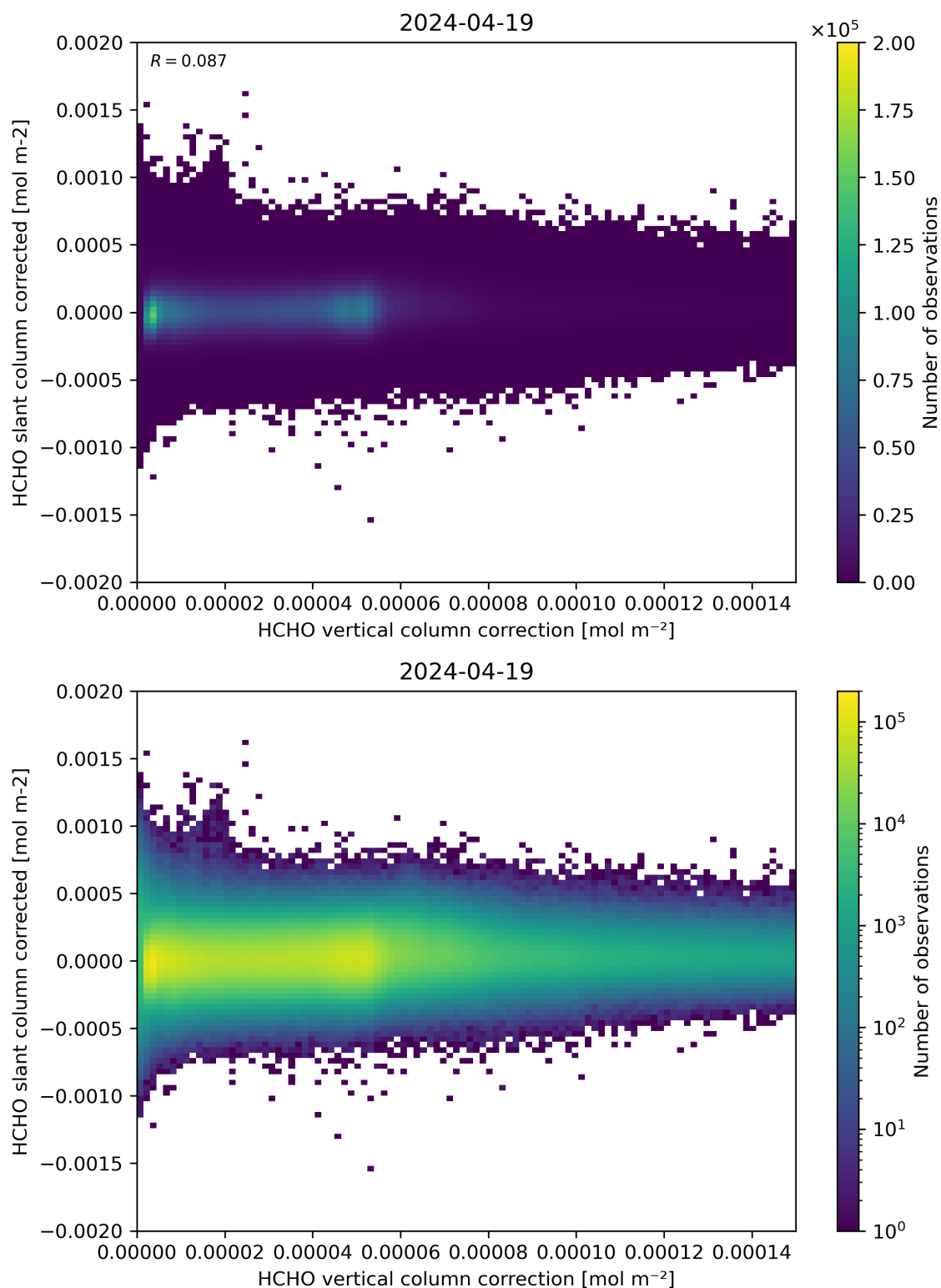
Figure 116: Scatter density plot of “HCHO vertical column correction” against “HCHO slant column corrected” for 2024-04-18 to 2024-04-20.
