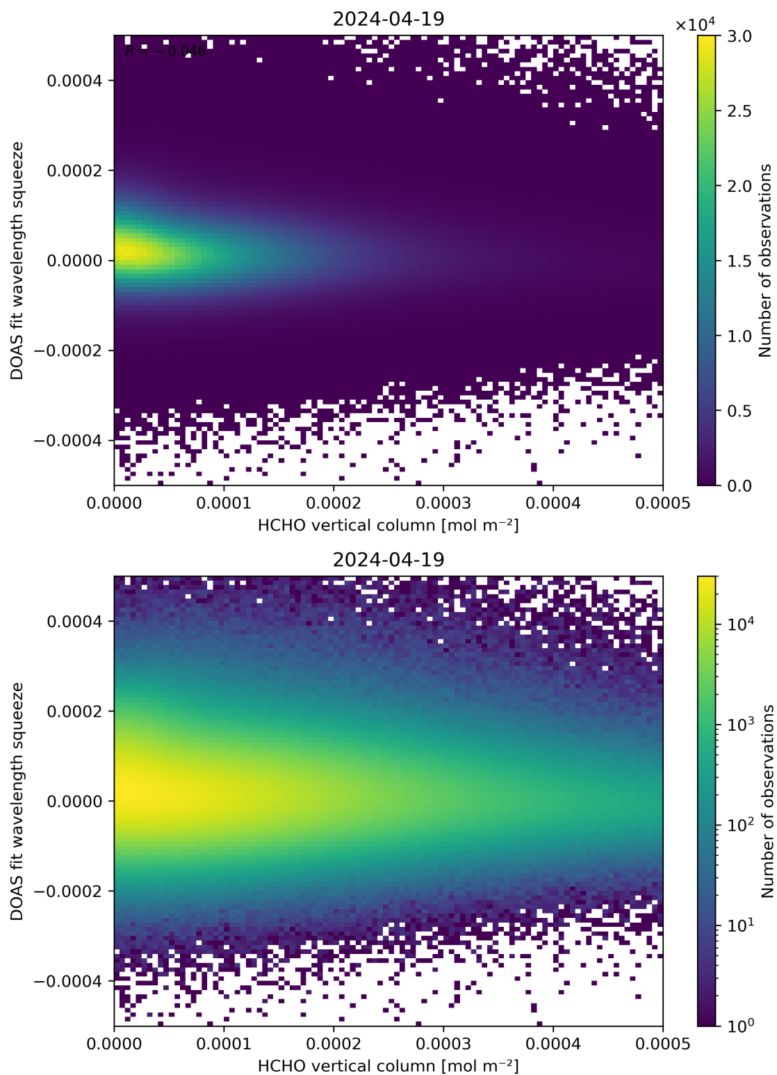
Figure 125: Scatter density plot of “HCHO vertical column” against “DOAS fit wavelength squeeze” for 2024-04-18 to 2024-04-20.
