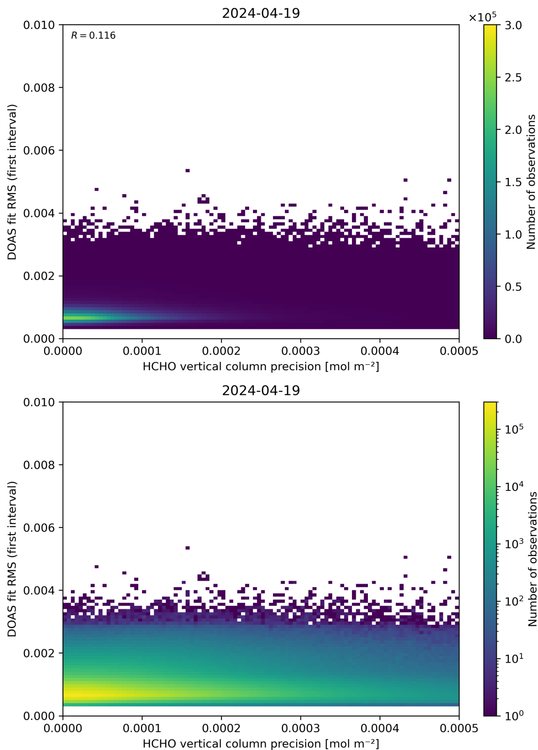
Figure 136: Scatter density plot of “HCHO vertical column precision” against “DOAS fit RMS (first interval)” for 2024-04-18 to 2024-04-20.
