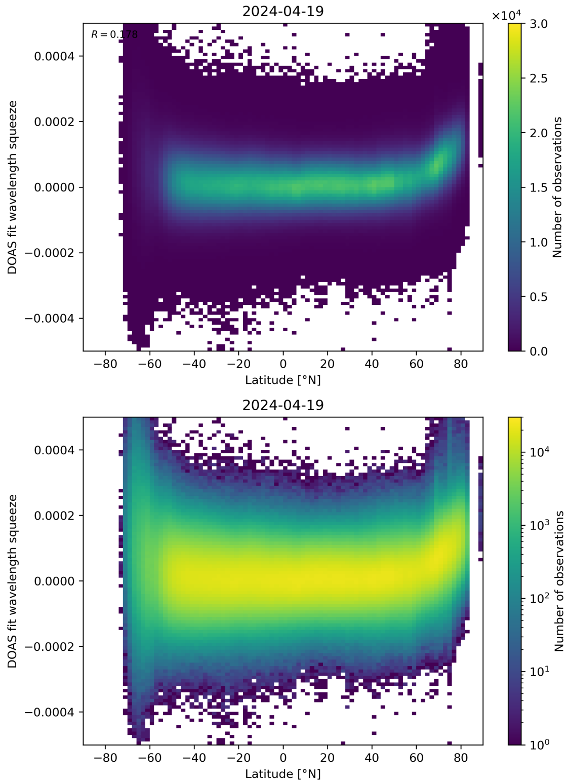
Figure 155: Scatter density plot of “Latitude” against “DOAS fit wavelength squeeze” for 2024-04-18 to 2024-04-20.
