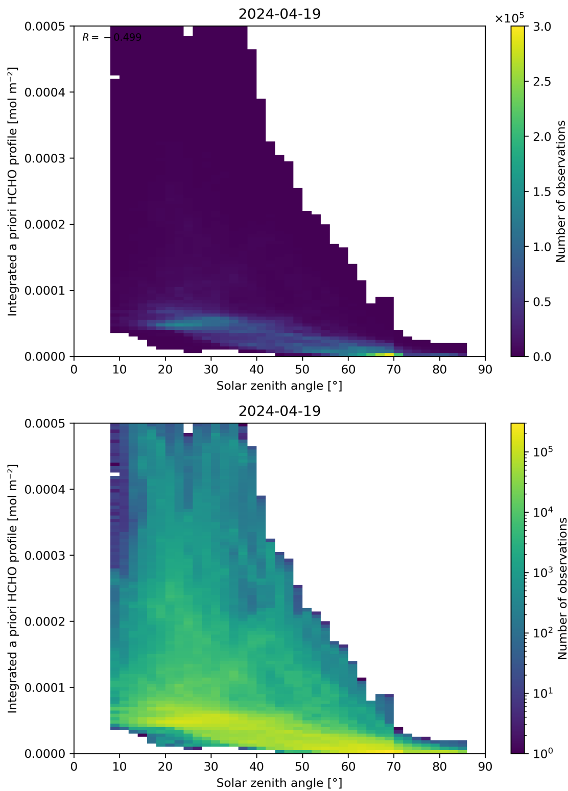
Figure 180: Scatter density plot of “Solar zenith angle” against “Integrated a priori HCHO profile” for 2024-04-18 to 2024-04-20.
