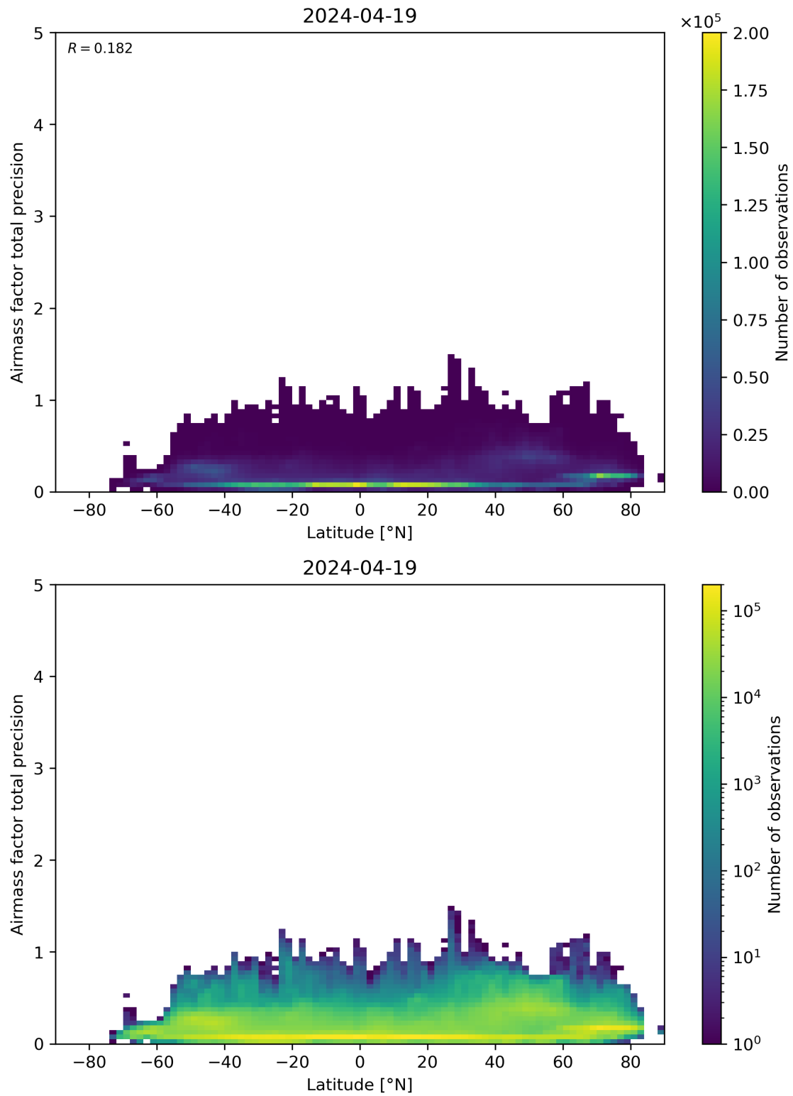
Figure 162: Scatter density plot of “Latitude” against “Airmass factor total precision” for 2024-04-18 to 2024-04-20.
