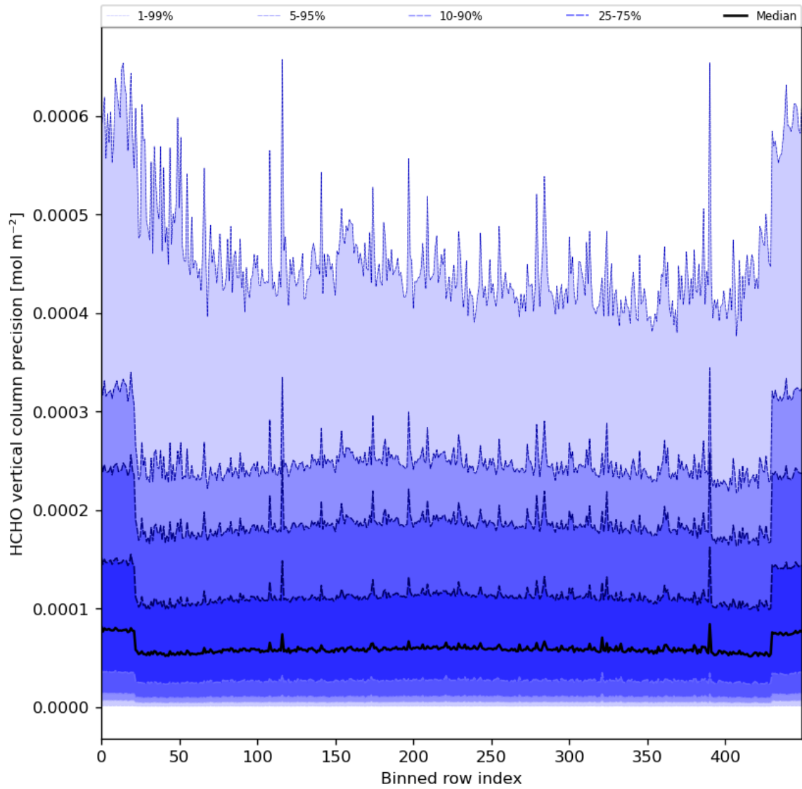
Figure 50: Along track statistics of “HCHO vertical column precision” for 2024-04-18 to 2024-04-20
