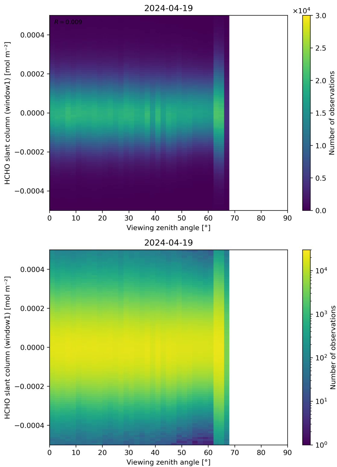
Figure 188: Scatter density plot of “Viewing zenith angle” against “HCHO slant column (window1)” for 2024-04-18 to 2024-04-20.
