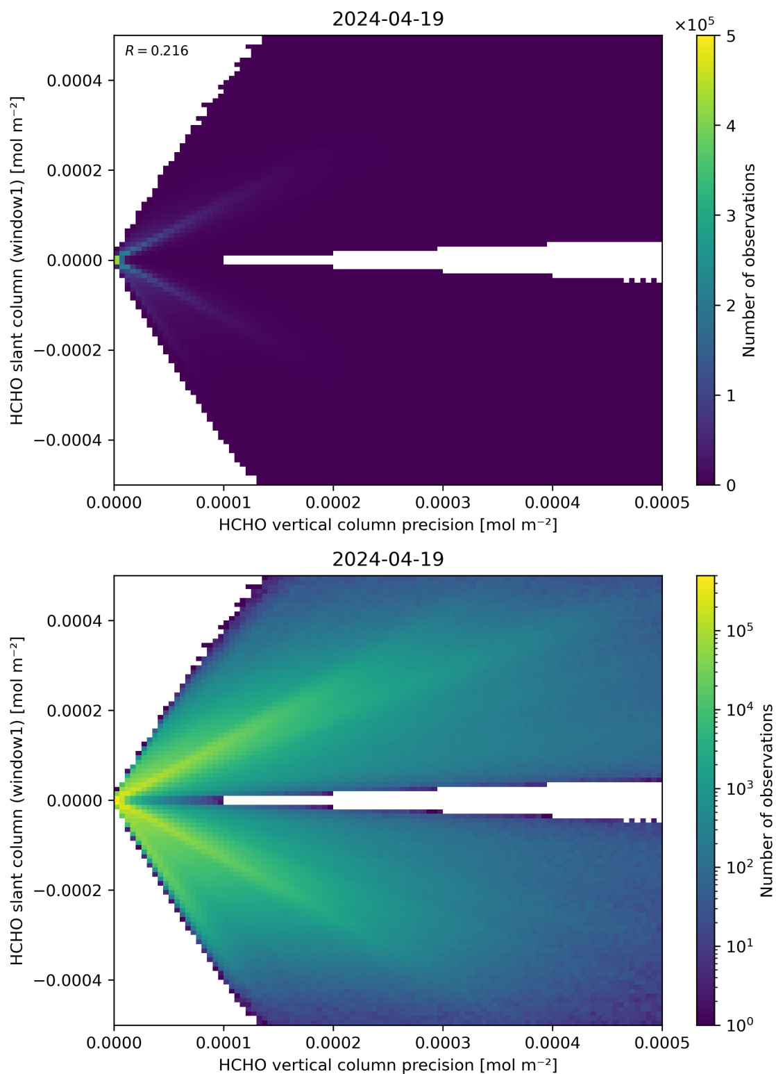
Figure 142: Scatter density plot of “HCHO vertical column precision” against “HCHO slant column (window1)” for 2024-04-18 to 2024-04-20.
