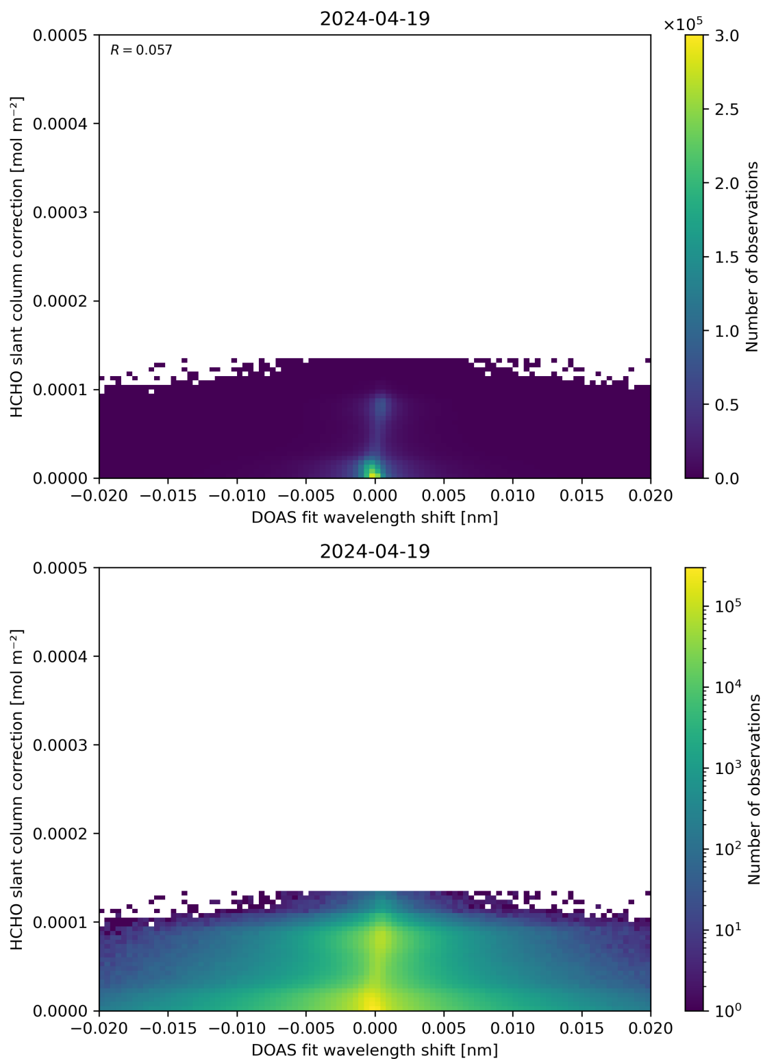
Figure 67: Scatter density plot of “DOAS fit wavelength shift” against “HCHO slant column correction” for 2024-04-18 to 2024-04-20.
