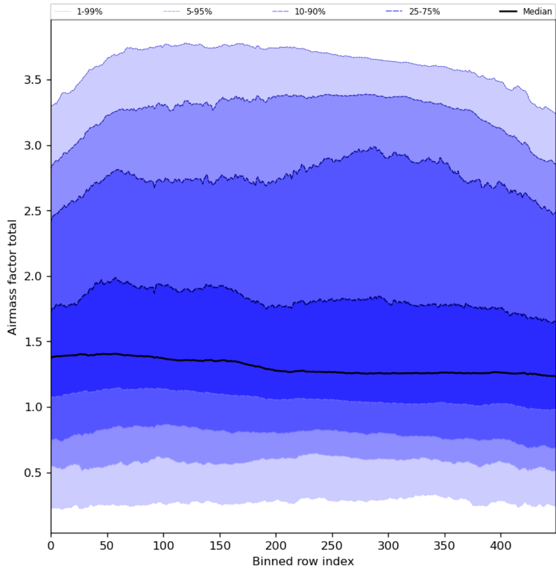
Figure 54: Along track statistics of “Airmass factor total” for 2024-04-18 to 2024-04-20
