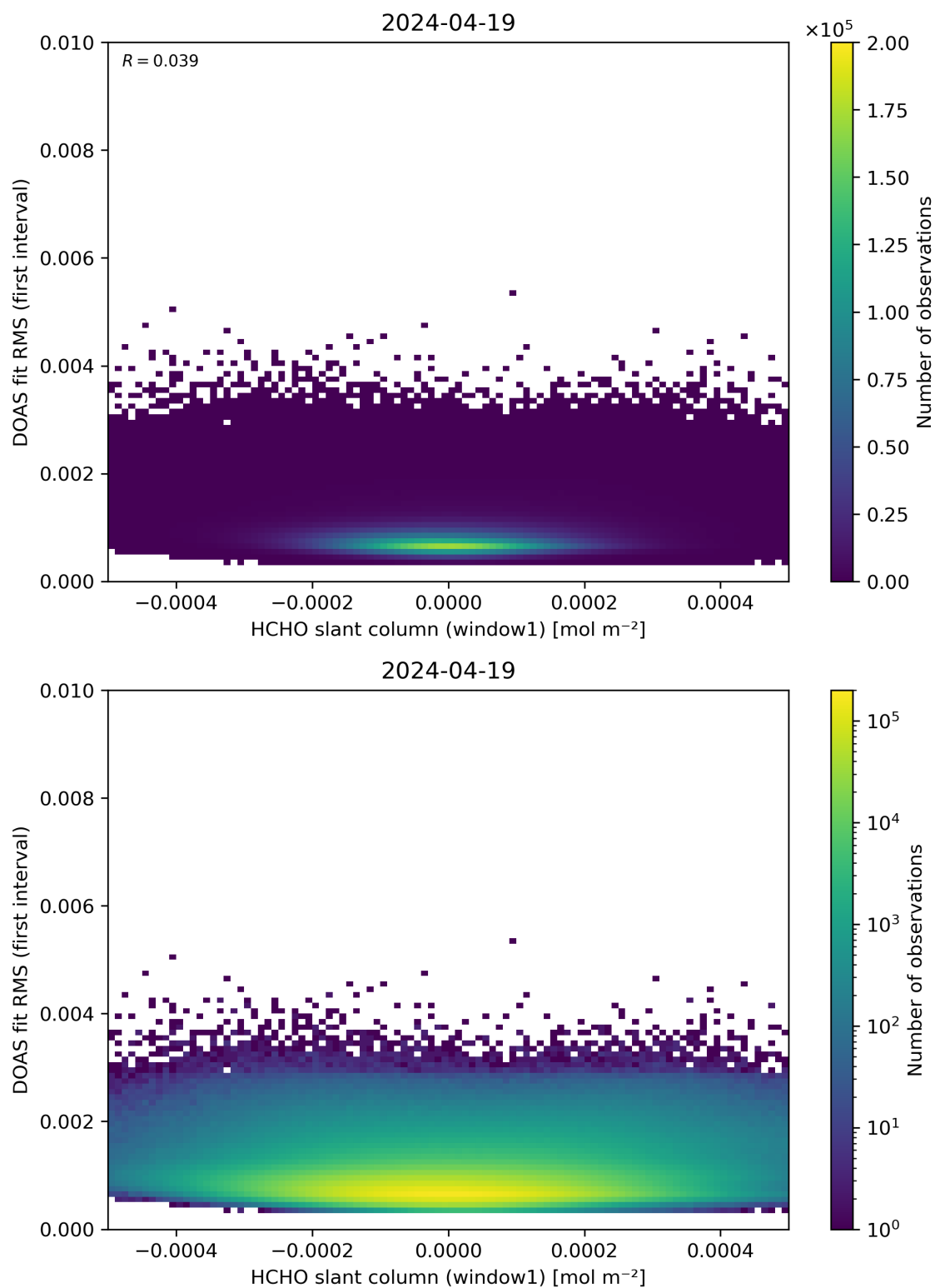
Figure 78: Scatter density plot of “HCHO slant column (window1)” against “DOAS fit RMS (first interval)” for 2024-04-18 to 2024-04-20.
