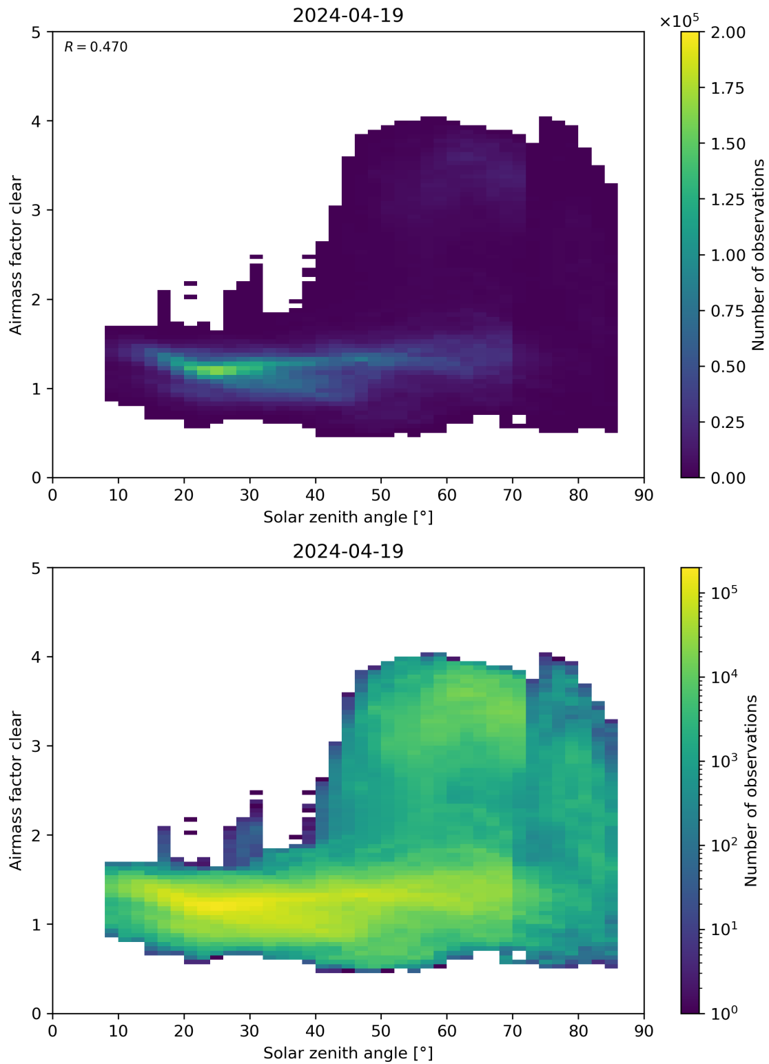
Figure 170: Scatter density plot of “Solar zenith angle” against “Airmass factor clear” for 2024-04-18 to 2024-04-20.
