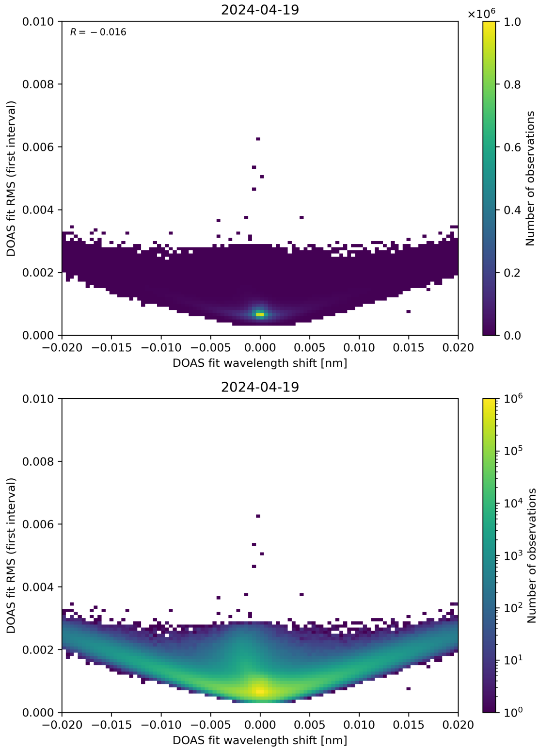
Figure 64: Scatter density plot of “DOAS fit wavelength shift” against “DOAS fit RMS (first interval)” for 2024-04-18 to 2024-04-20.
