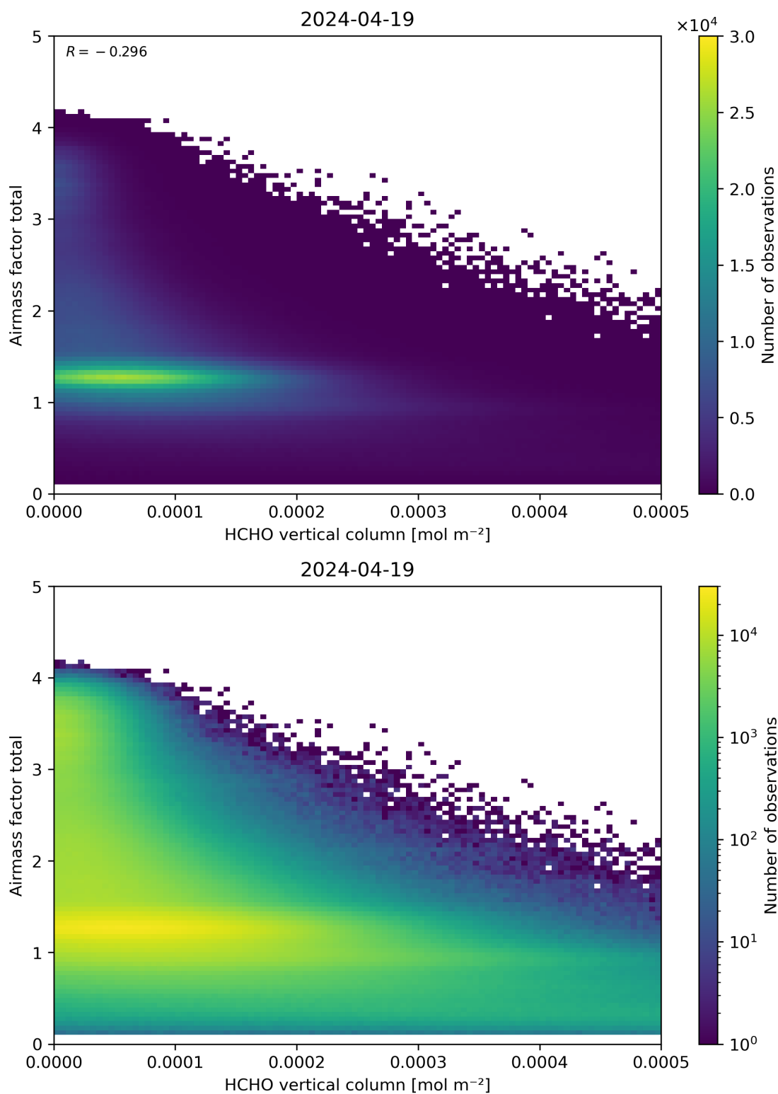
Figure 131: Scatter density plot of “HCHO vertical column” against “Airmass factor total” for 2024-04-18 to 2024-04-20.
