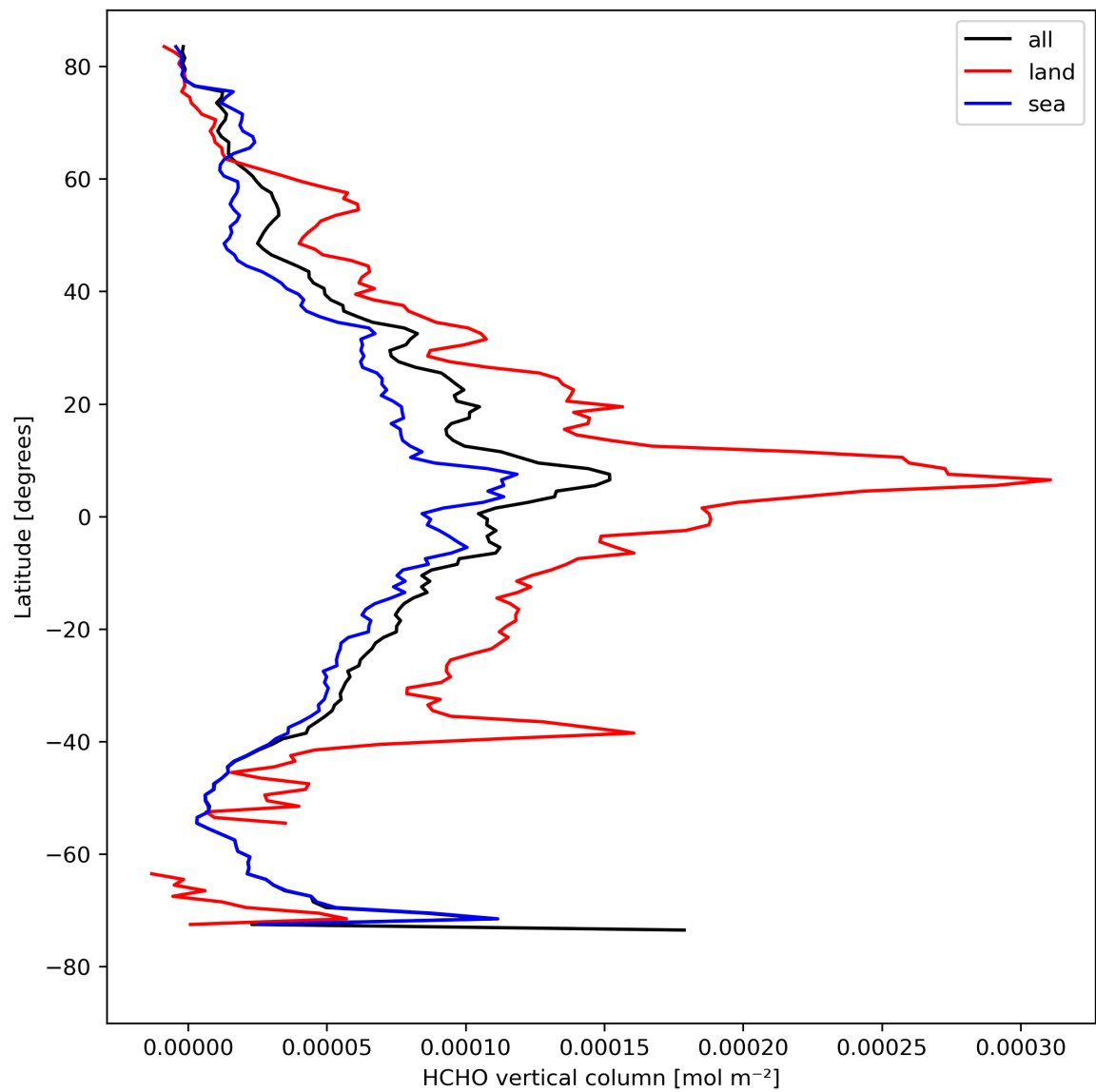
Figure 21: Zonal average of “HCHO vertical column” for 2024-04-18 to 2024-04-20.
