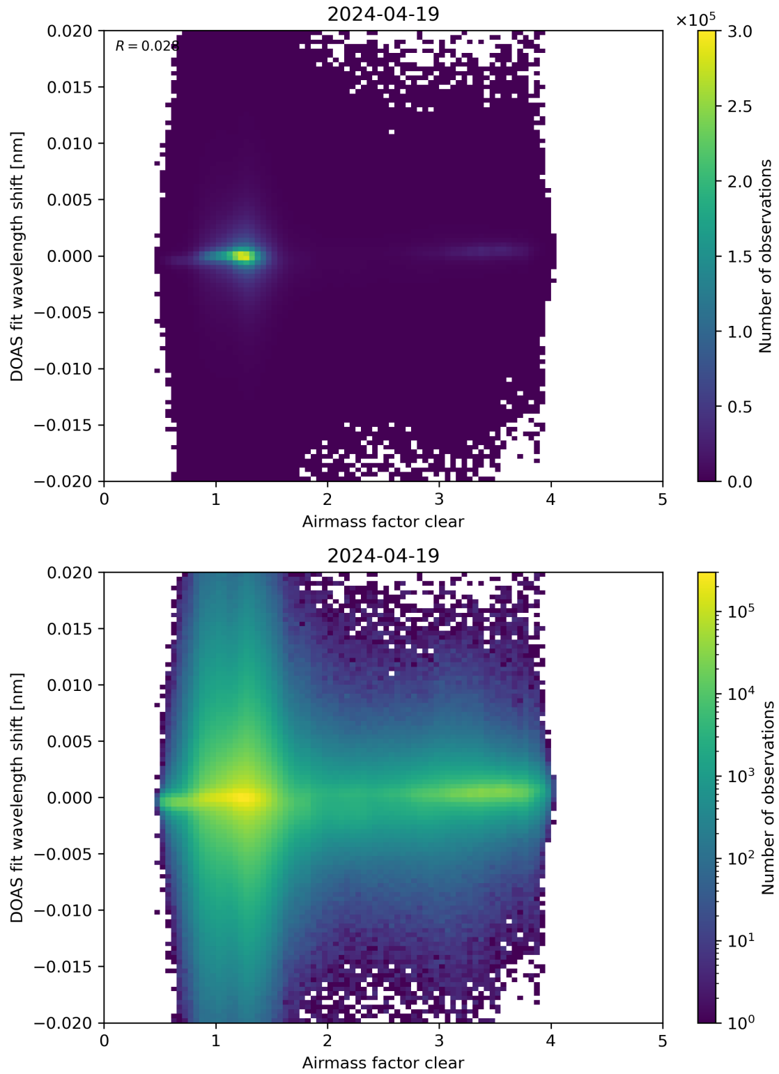
Figure 72: Scatter density plot of “Airmass factor clear” against “DOAS fit wavelength shift” for 2024-04-18 to 2024-04-20.
