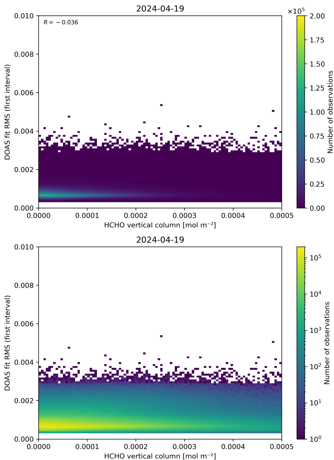
Figure 123: Scatter density plot of “HCHO vertical column” against “DOAS fit RMS (first interval)” for 2024-04-18 to 2024-04-20.
