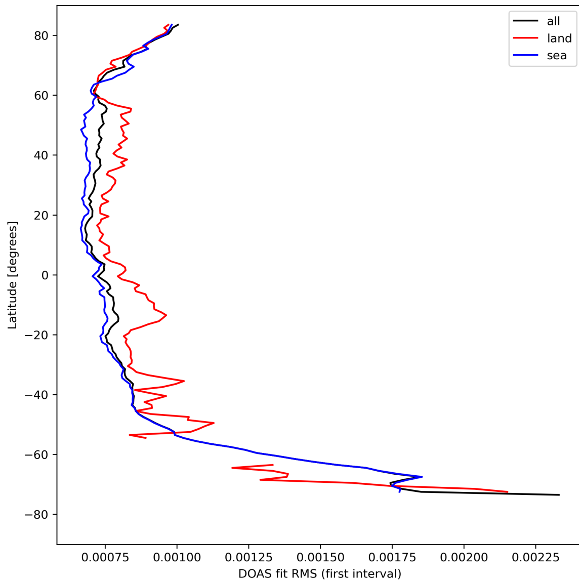
Figure 32: Zonal average of “DOAS fit RMS (first interval)” for 2024-04-18 to 2024-04-20.
