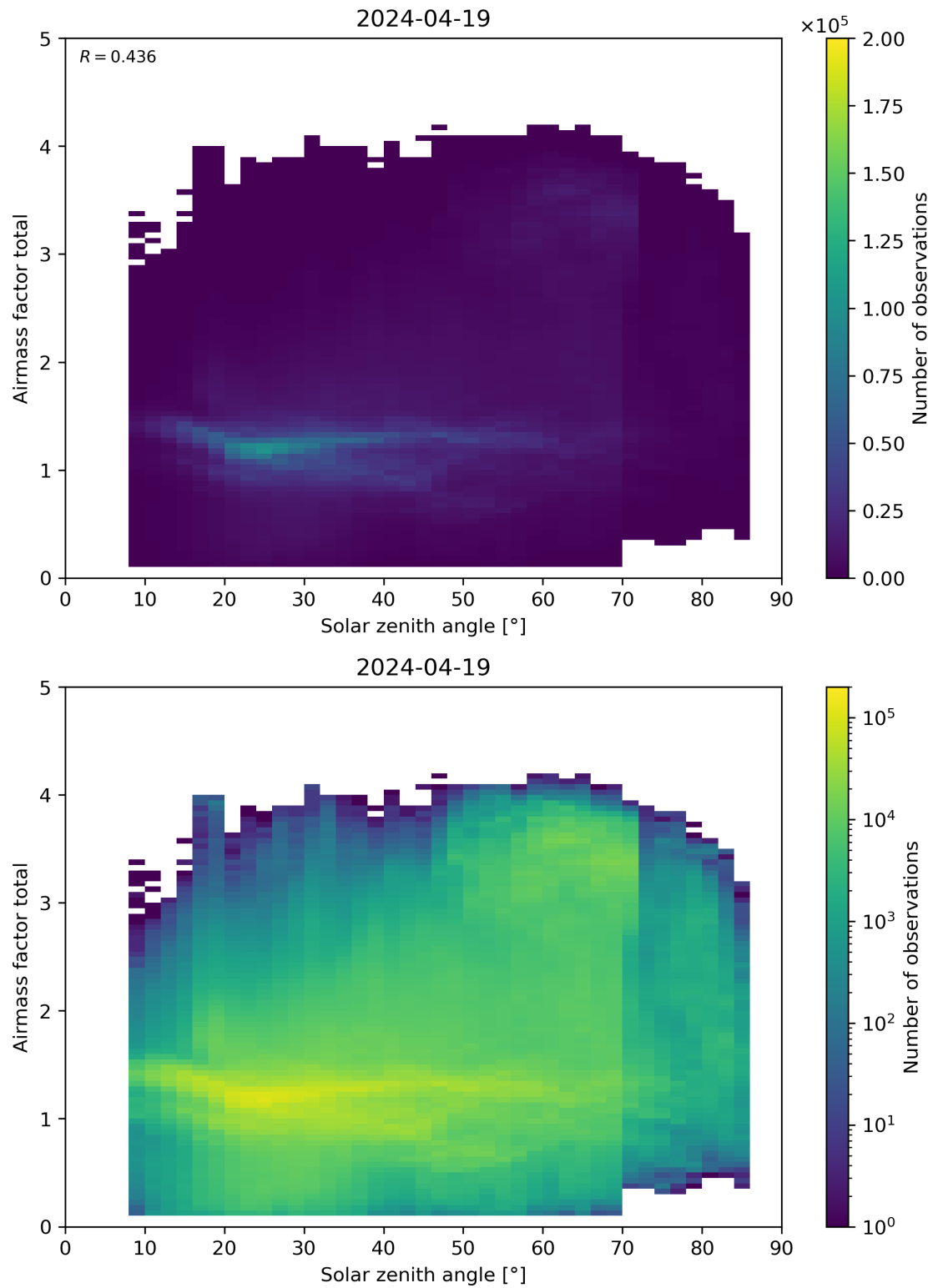
Figure 175: Scatter density plot of “Solar zenith angle” against “Airmass factor total” for 2024-04-18 to 2024-04-20.
