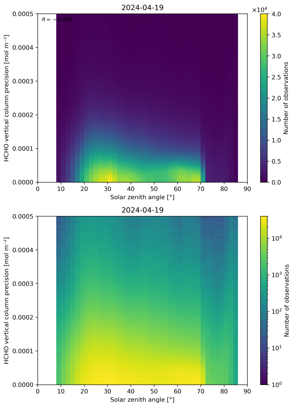
Figure 179: Scatter density plot of “Solar zenith angle” against “HCHO vertical column precision” for 2024-04-18 to 2024-04-20.
