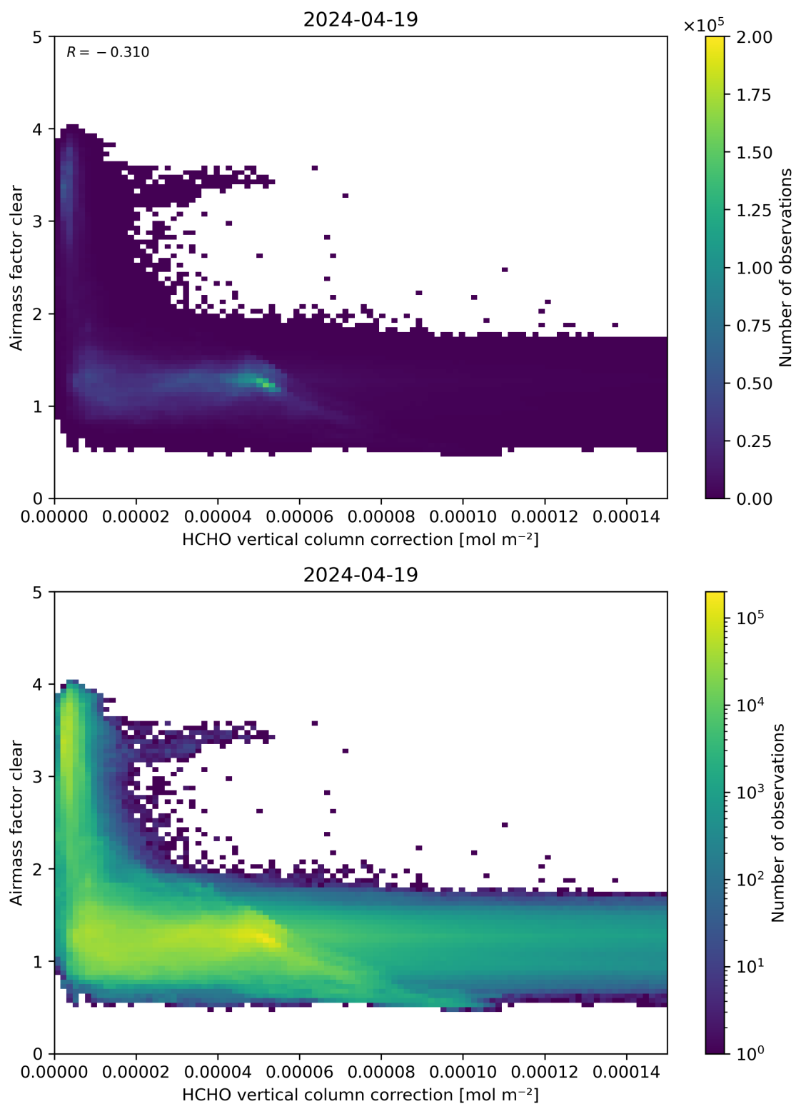
Figure 115: Scatter density plot of “HCHO vertical column correction” against “Airmass factor clear” for 2024-04-18 to 2024-04-20.
