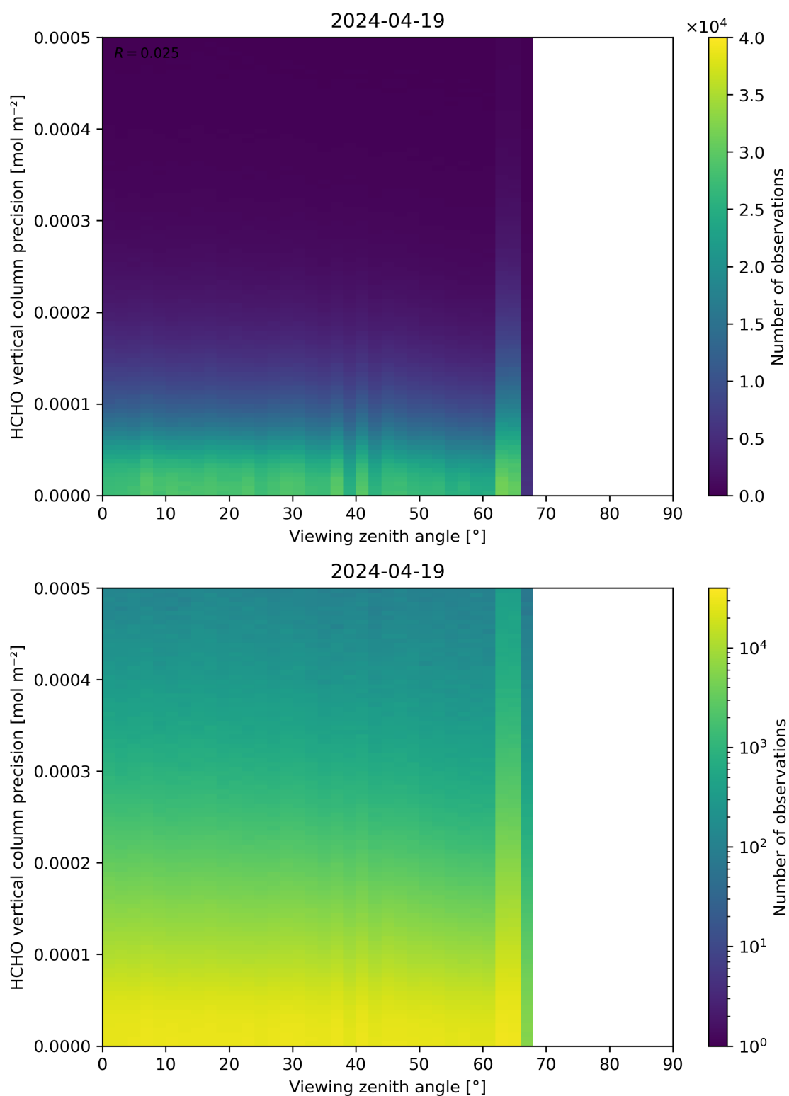
Figure 194: Scatter density plot of “Viewing zenith angle” against “HCHO vertical column precision” for 2024-04-18 to 2024-04-20.
