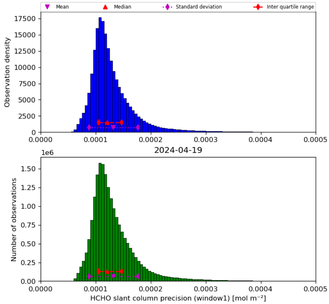
Figure 39: Histogram of “HCHO slant column precision (window1)” for 2024-04-18 to 2024-04-20
