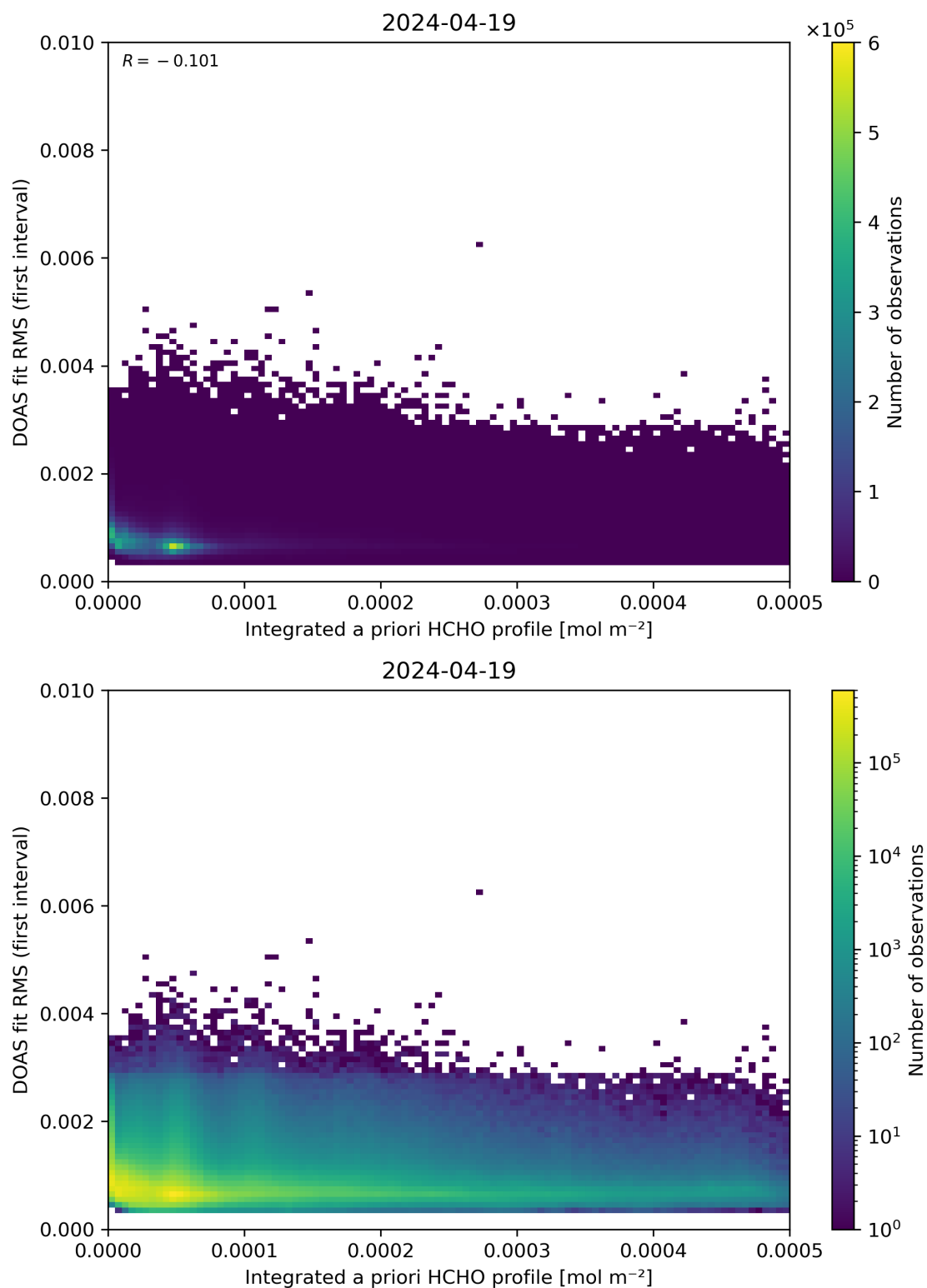
Figure 148: Scatter density plot of “Integrated a priori HCHO profile” against “DOAS fit RMS (first interval)” for 2024-04-18 to 2024-04-20.
