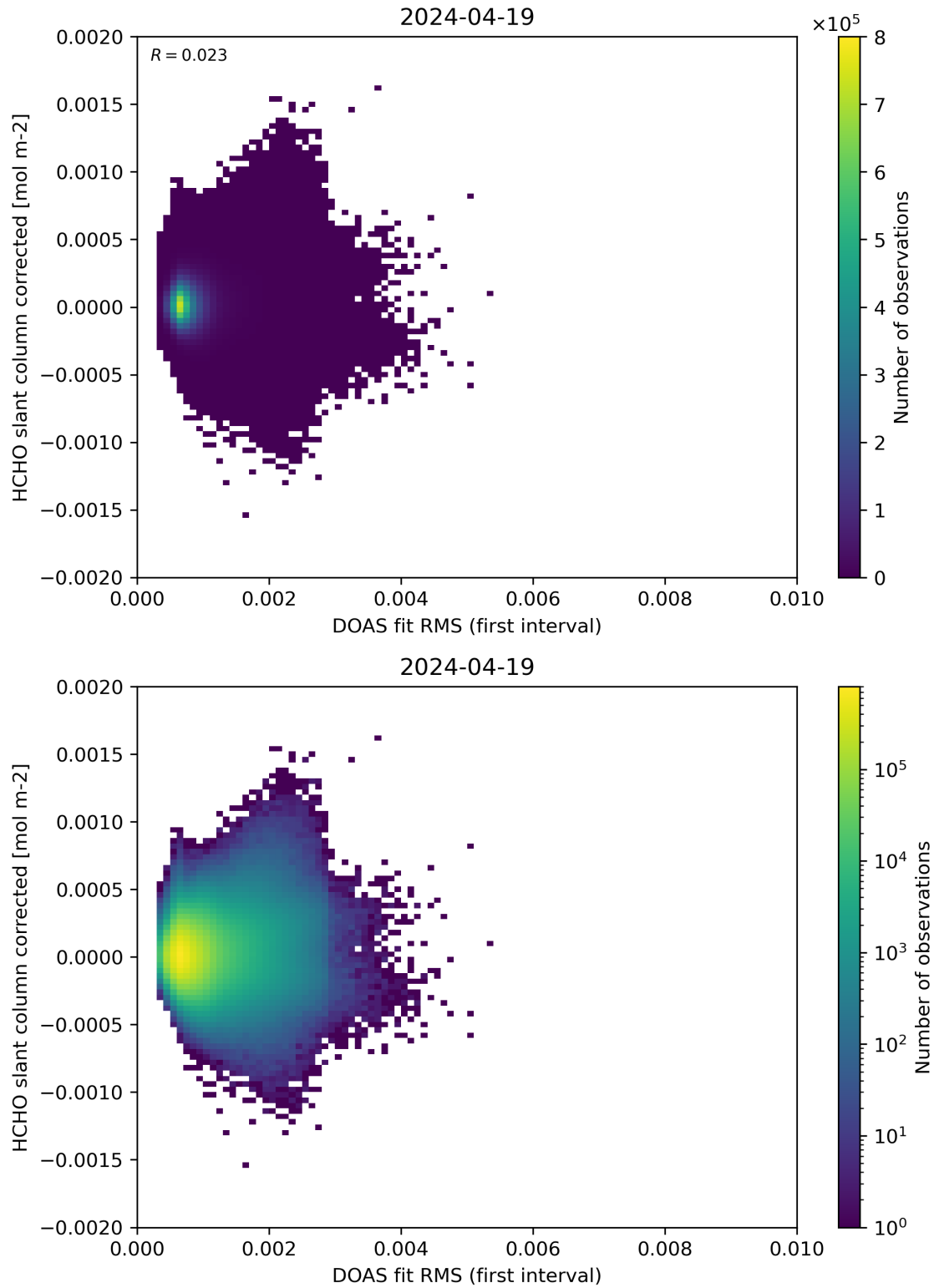
Figure 62: Scatter density plot of “DOAS fit RMS (first interval)” against “HCHO slant column corrected” for 2024-04-18 to 2024-04-20.
