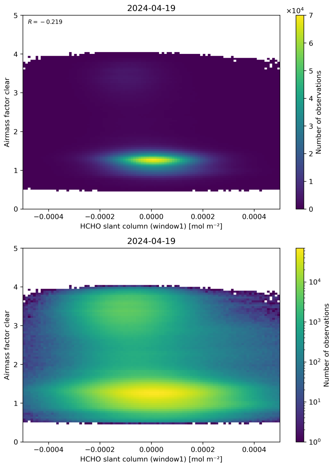
Figure 81: Scatter density plot of “HCHO slant column (window1)” against “Airmass factor clear” for 2024-04-18 to 2024-04-20.
