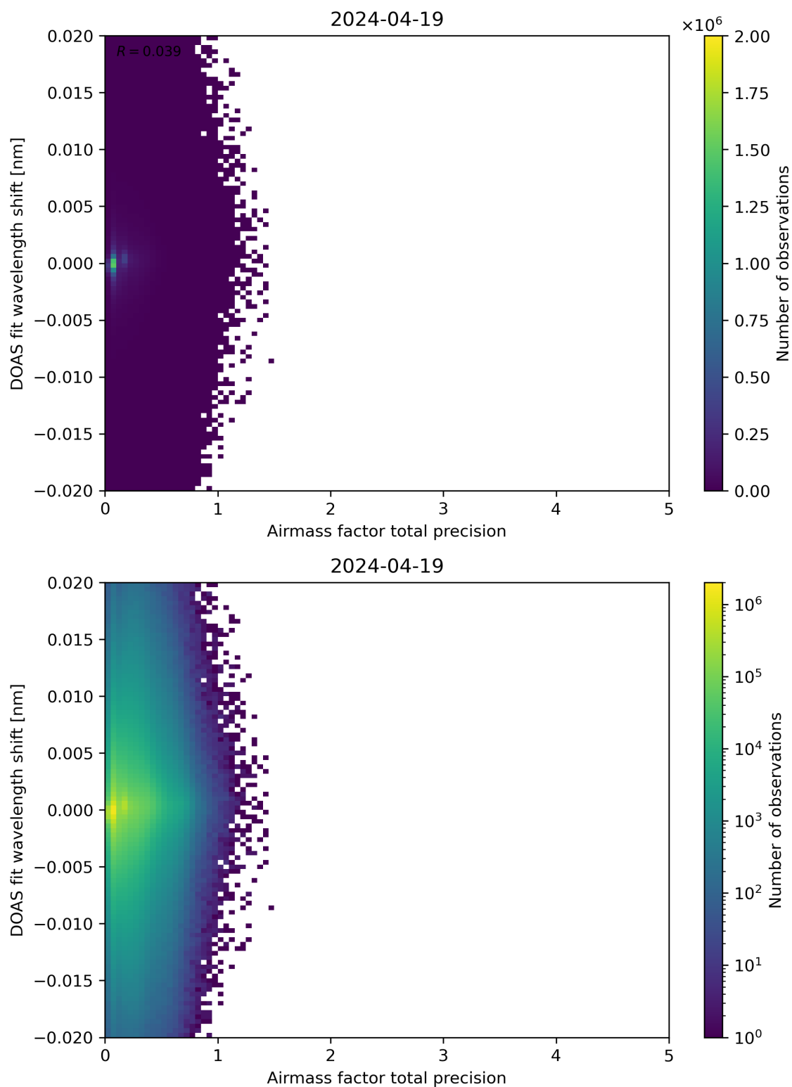
Figure 106: Scatter density plot of “Airmass factor total precision” against “DOAS fit wavelength shift” for 2024-04-18 to 2024-04-20.
