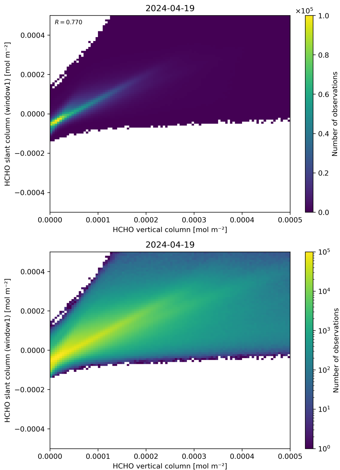
Figure 129: Scatter density plot of “HCHO vertical column” against “HCHO slant column (window1)” for 2024-04-18 to 2024-04-20.
