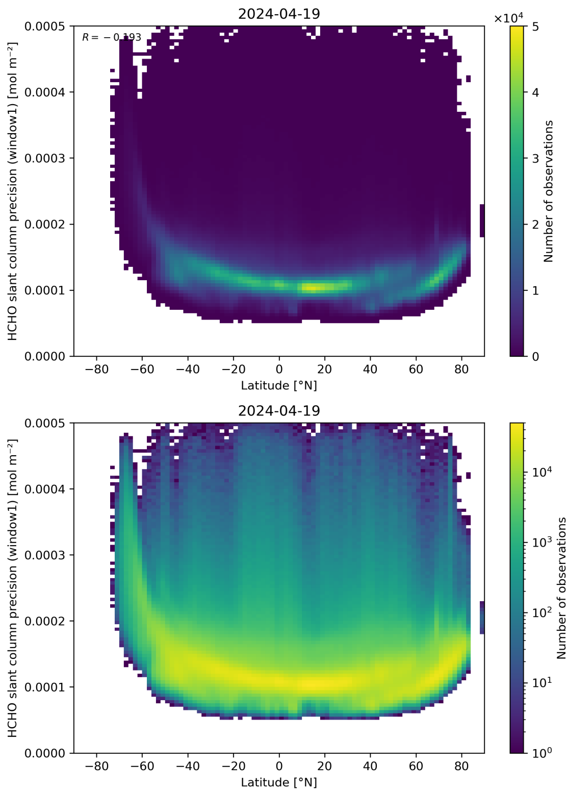
Figure 160: Scatter density plot of “Latitude” against “HCHO slant column precision (window1)” for 2024-04-18 to 2024-04-20.
