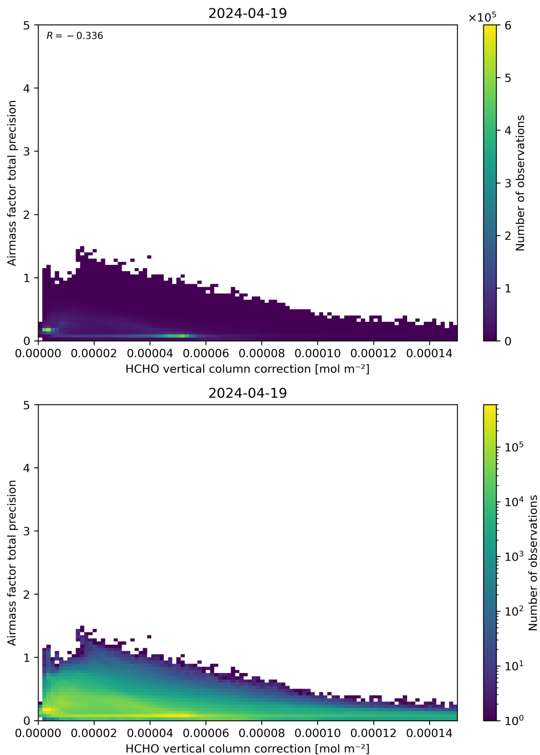
Figure 121: Scatter density plot of “HCHO vertical column correction” against “Airmass factor total precision” for 2024-04-18 to 2024-04-20.
