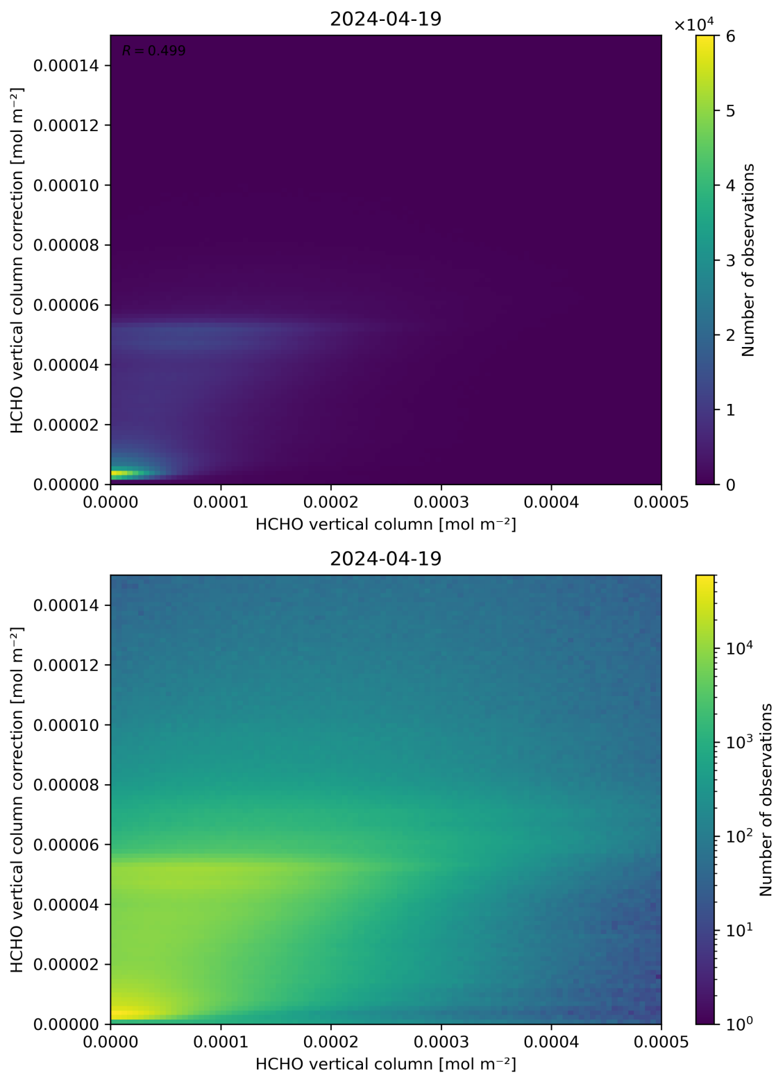
Figure 133: Scatter density plot of “HCHO vertical column” against “HCHO vertical column correction” for 2024-04-18 to 2024-04-20.
