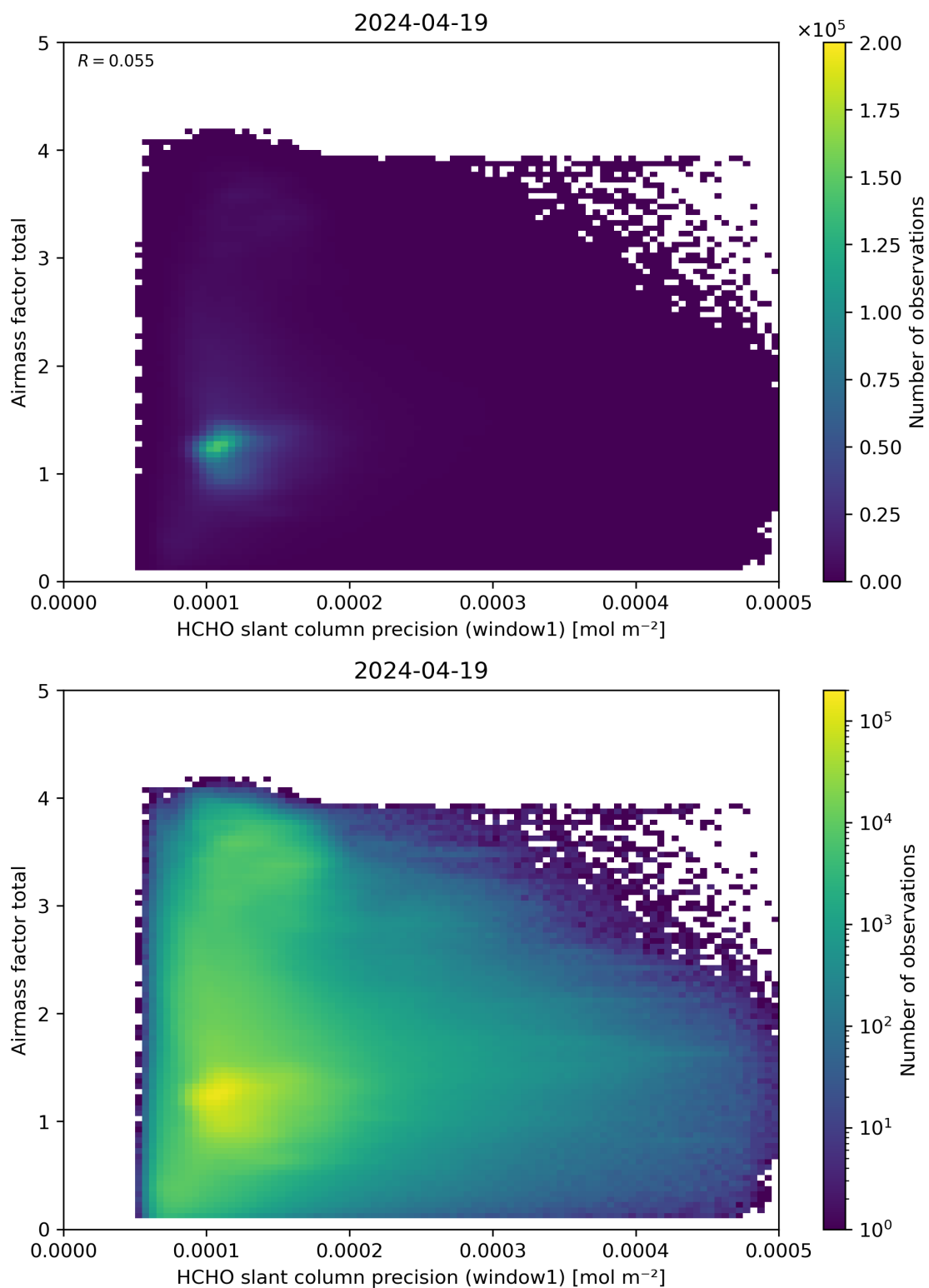
Figure 94: Scatter density plot of “HCHO slant column precision (window1)” against “Airmass factor total” for 2024-04-18 to 2024-04-20.
