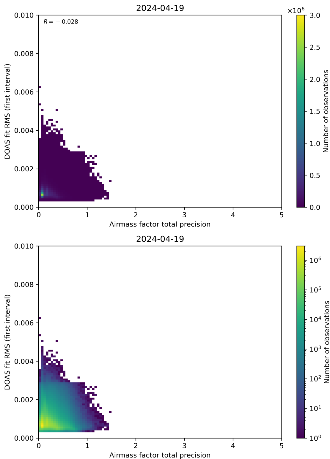
Figure 105: Scatter density plot of “Airmass factor total precision” against “DOAS fit RMS (first interval)” for 2024-04-18 to 2024-04-20.
