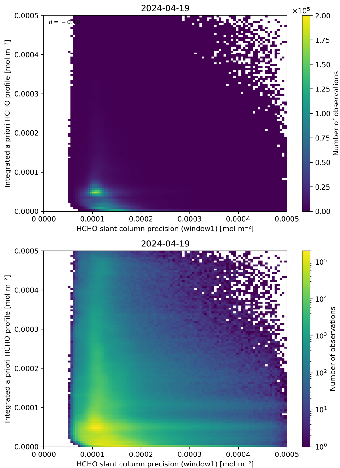
Figure 96: Scatter density plot of “HCHO slant column precision (window1)” against “Integrated a priori HCHO profile” for 2024-04-18 to 2024-04-20.
