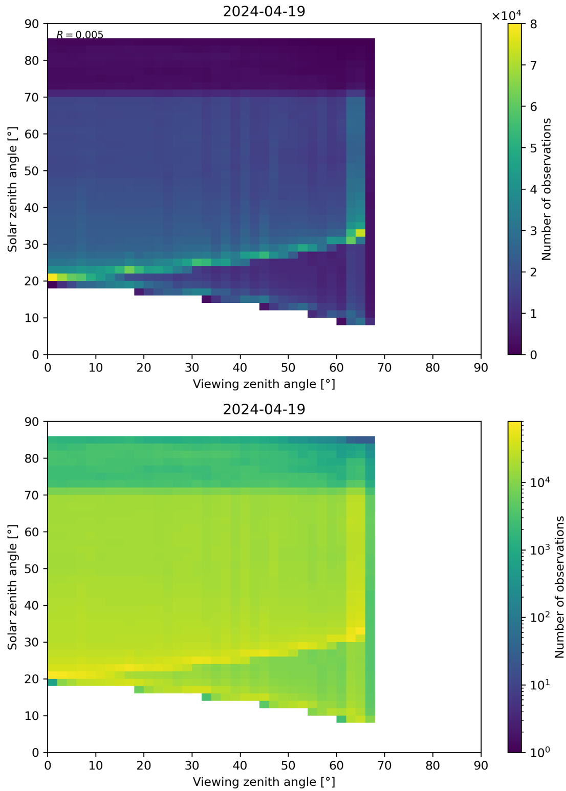
Figure 197: Scatter density plot of “Viewing zenith angle” against “Solar zenith angle” for 2024-04-18 to 2024-04-20.
