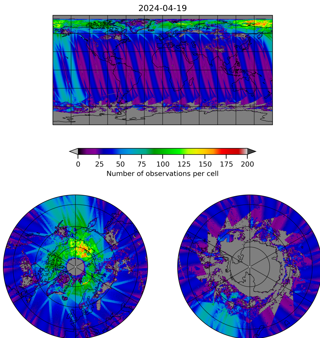
Figure 19: Map of the number of observations for 2024-04-18 to 2024-04-20
