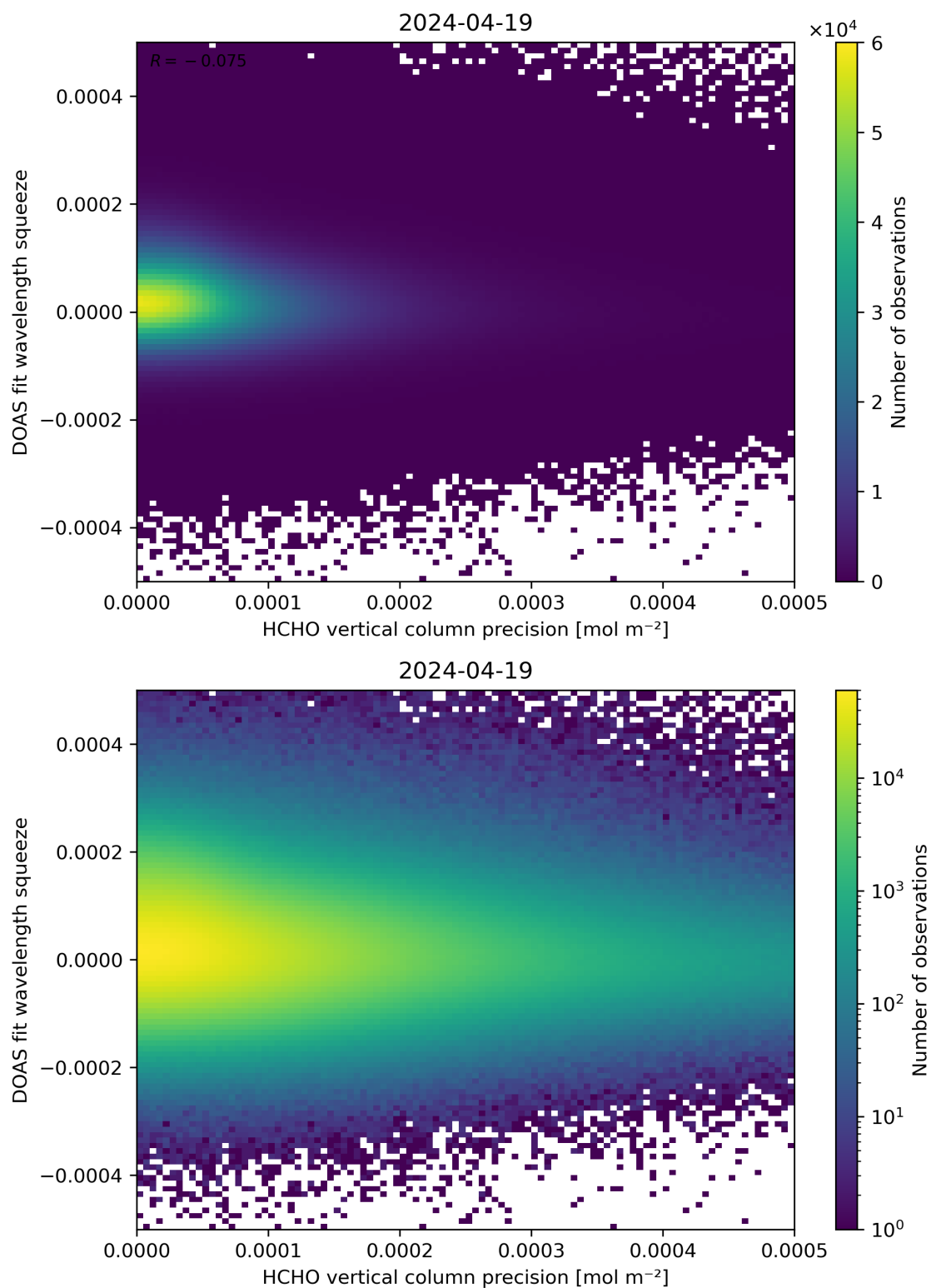
Figure 138: Scatter density plot of “HCHO vertical column precision” against “DOAS fit wavelength squeeze” for 2024-04-18 to 2024-04-20.
