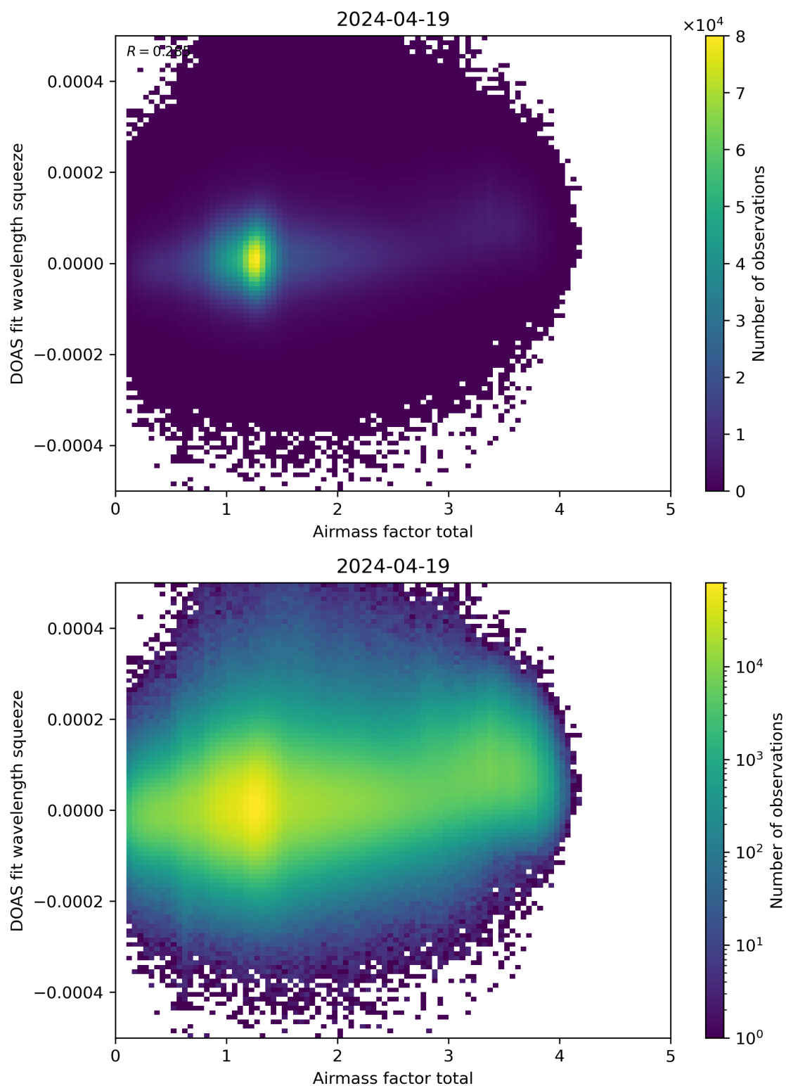
Figure 99: Scatter density plot of “Airmass factor total” against “DOAS fit wavelength squeeze” for 2024-04-18 to 2024-04-20.
