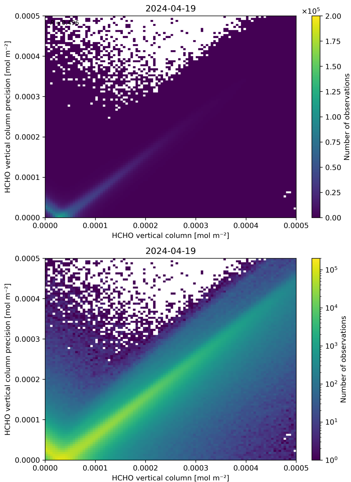
Figure 134: Scatter density plot of “HCHO vertical column” against “HCHO vertical column precision” for 2024-04-18 to 2024-04-20.
