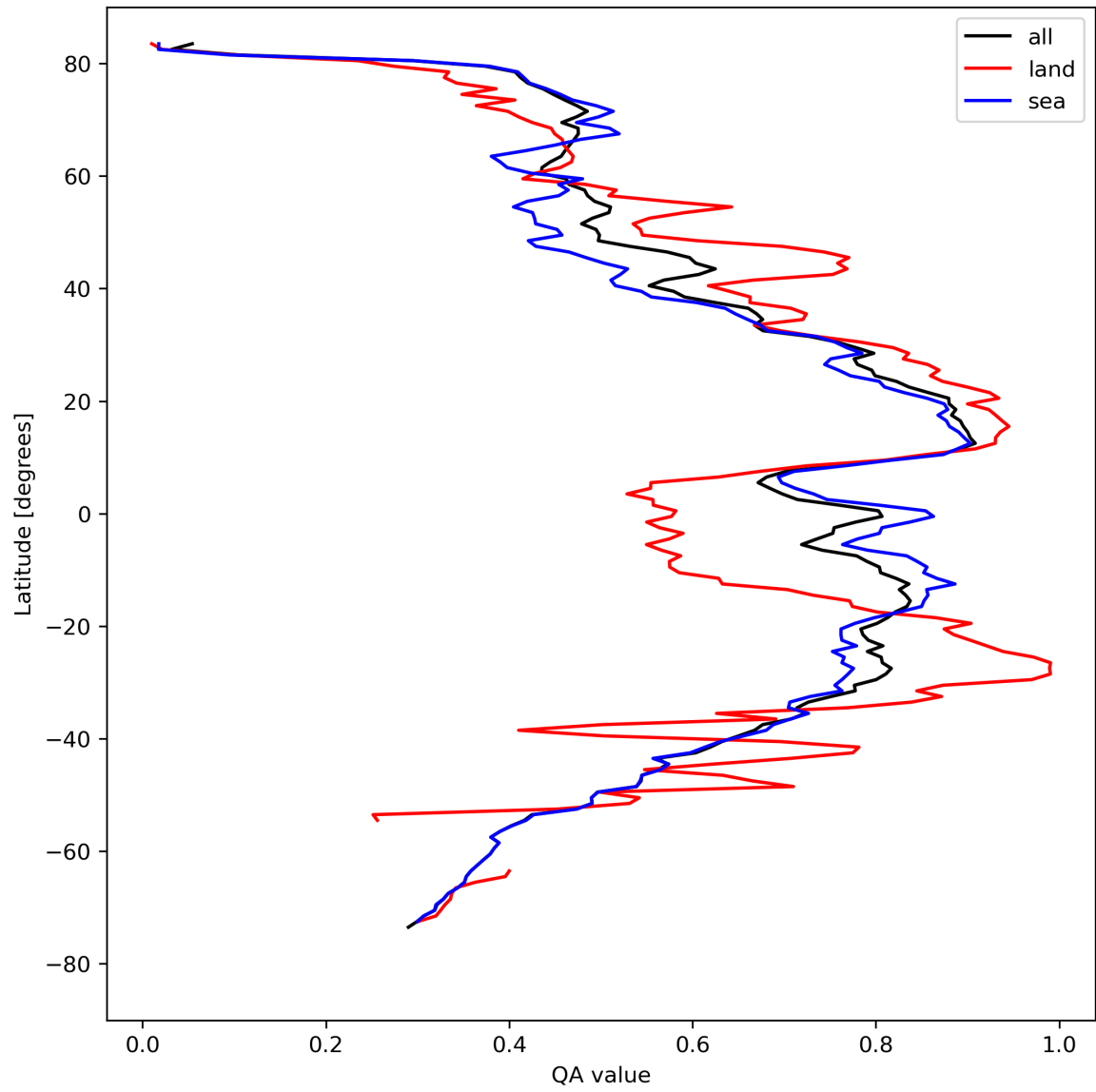
Figure 20: Zonal average of “QA value” for 2024-04-18 to 2024-04-20.
