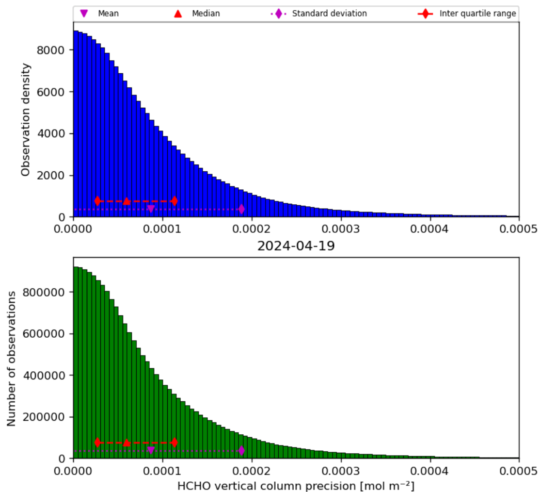
Figure 36: Histogram of “HCHO vertical column precision” for 2024-04-18 to 2024-04-20
