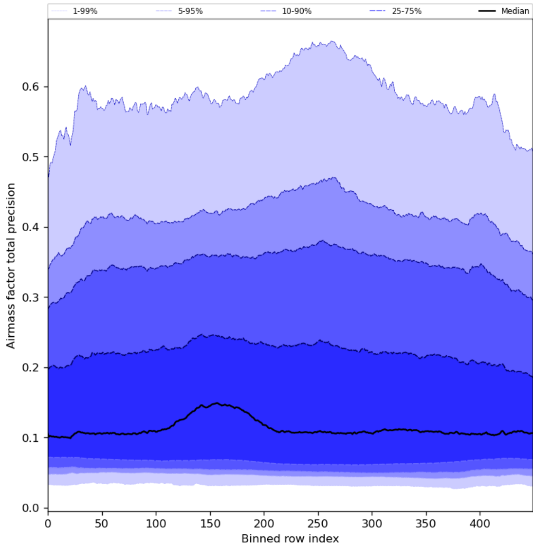
Figure 55: Along track statistics of “Airmass factor total precision” for 2024-04-18 to 2024-04-20
