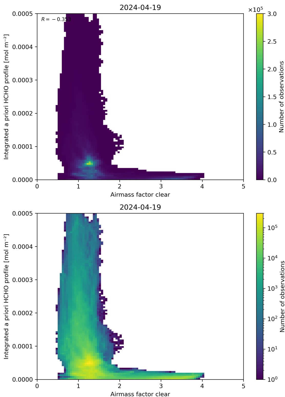
Figure 76: Scatter density plot of “Airmass factor clear” against “Integrated a priori HCHO profile” for 2024-04-18 to 2024-04-20.
