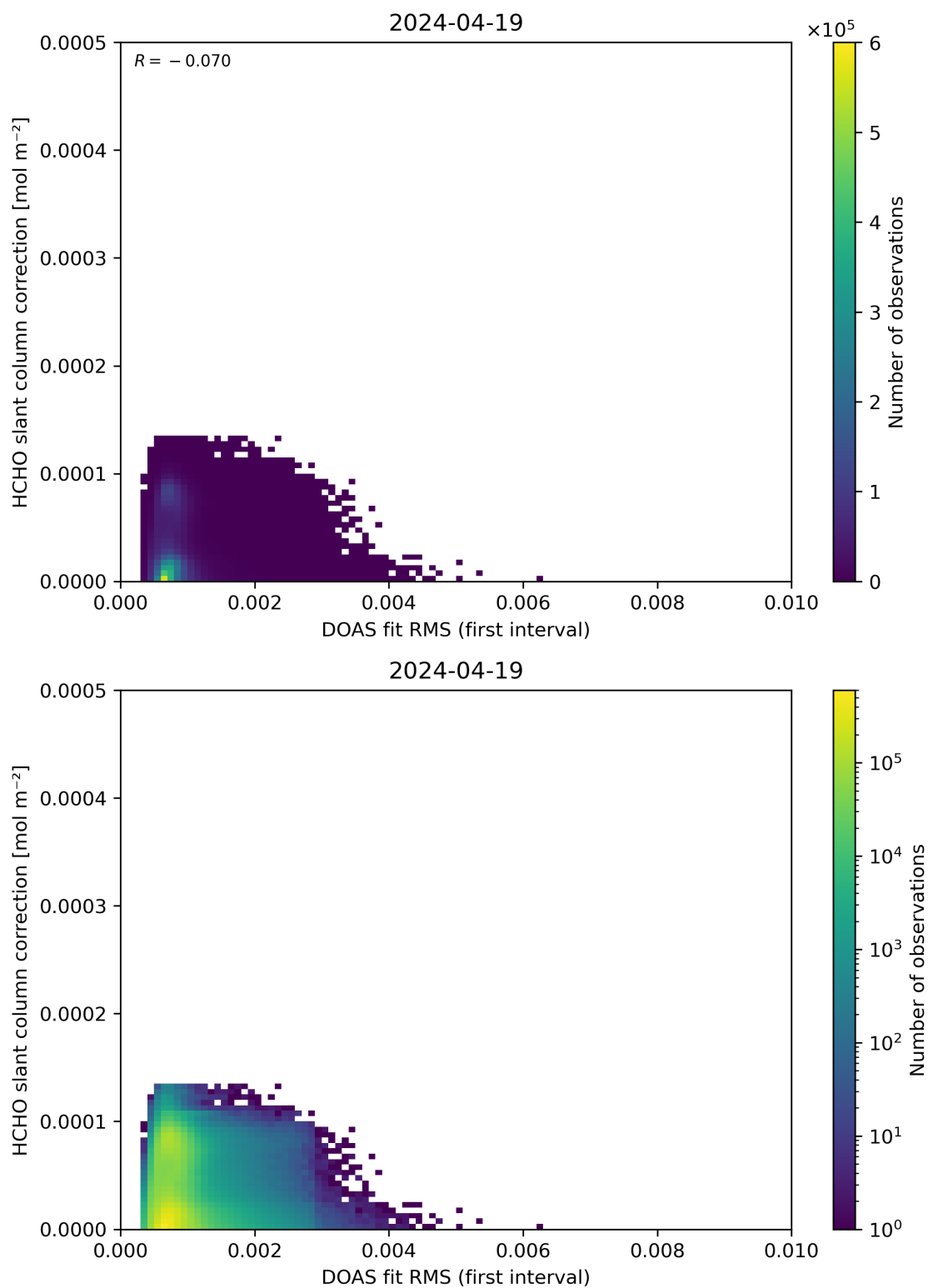
Figure 63: Scatter density plot of “DOAS fit RMS (first interval)” against “HCHO slant column correction” for 2024-04-18 to 2024-04-20.
