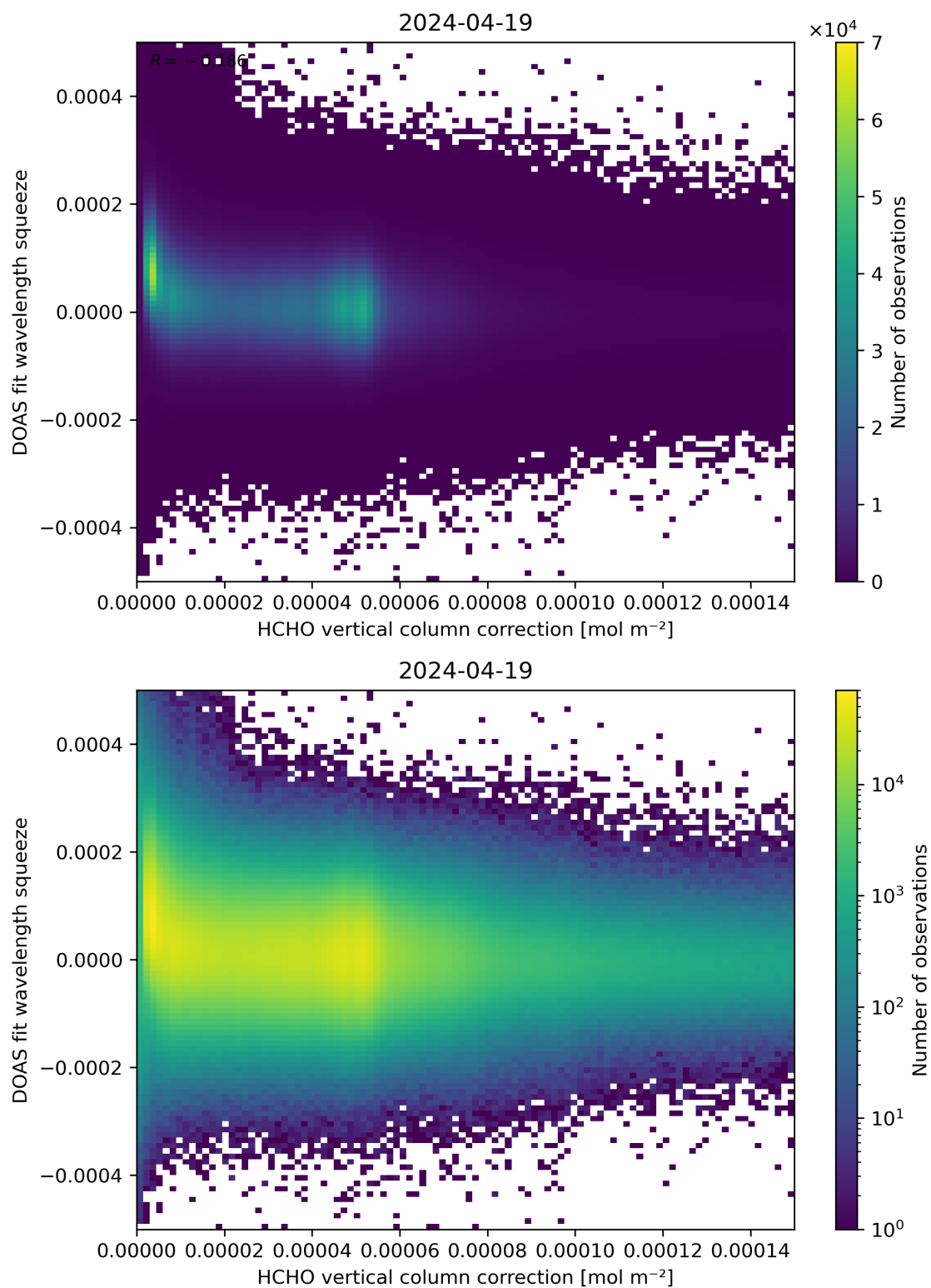
Figure 114: Scatter density plot of “HCHO vertical column correction” against “DOAS fit wavelength squeeze” for 2024-04-18 to 2024-04-20.
