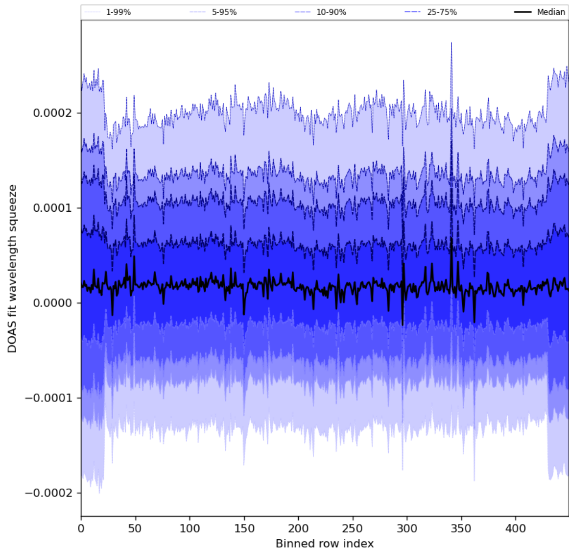
Figure 59: Along track statistics of “DOAS fit wavelength squeeze” for 2024-04-18 to 2024-04-20
