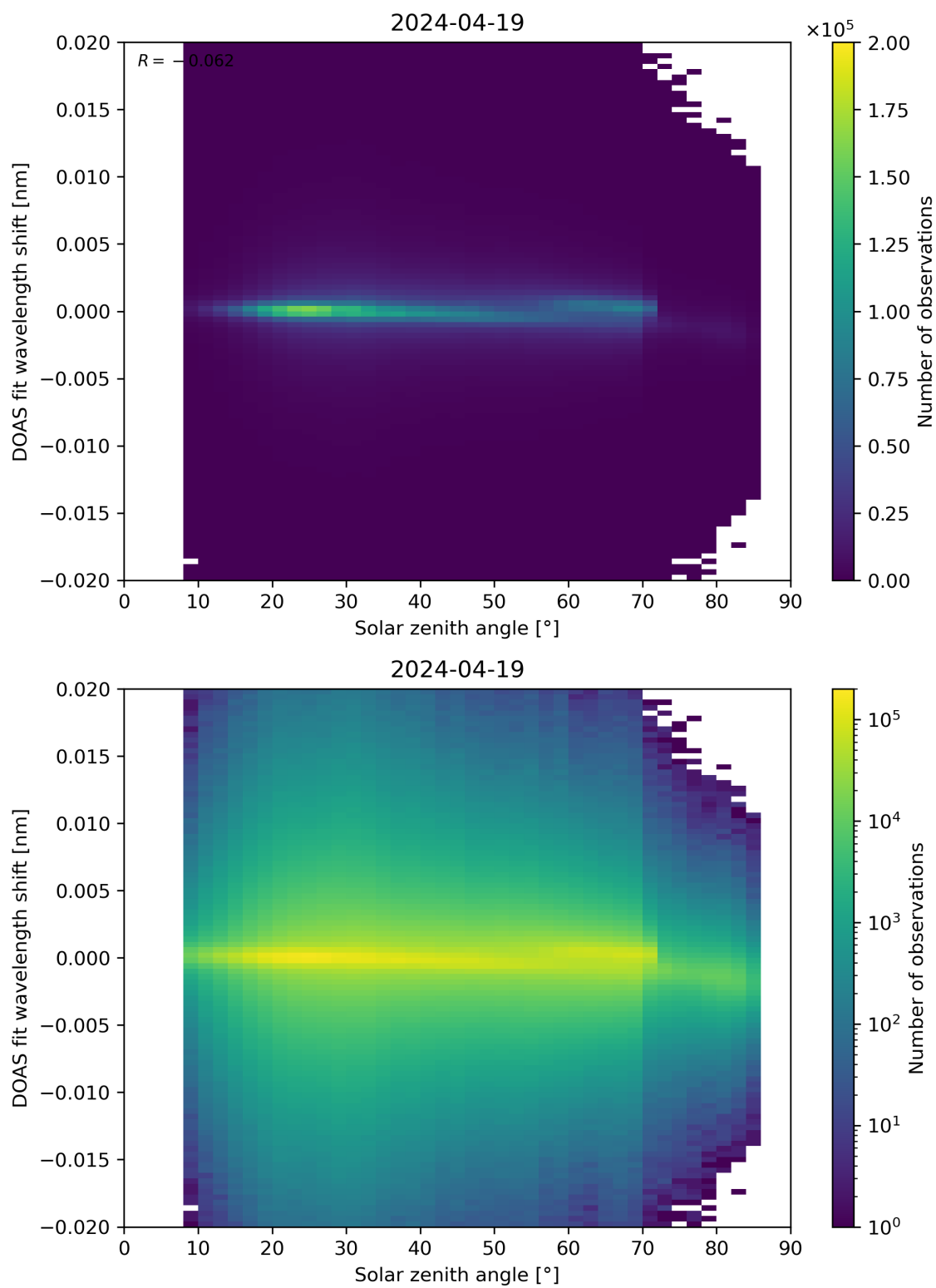
Figure 168: Scatter density plot of “Solar zenith angle” against “DOAS fit wavelength shift” for 2024-04-18 to 2024-04-20.
