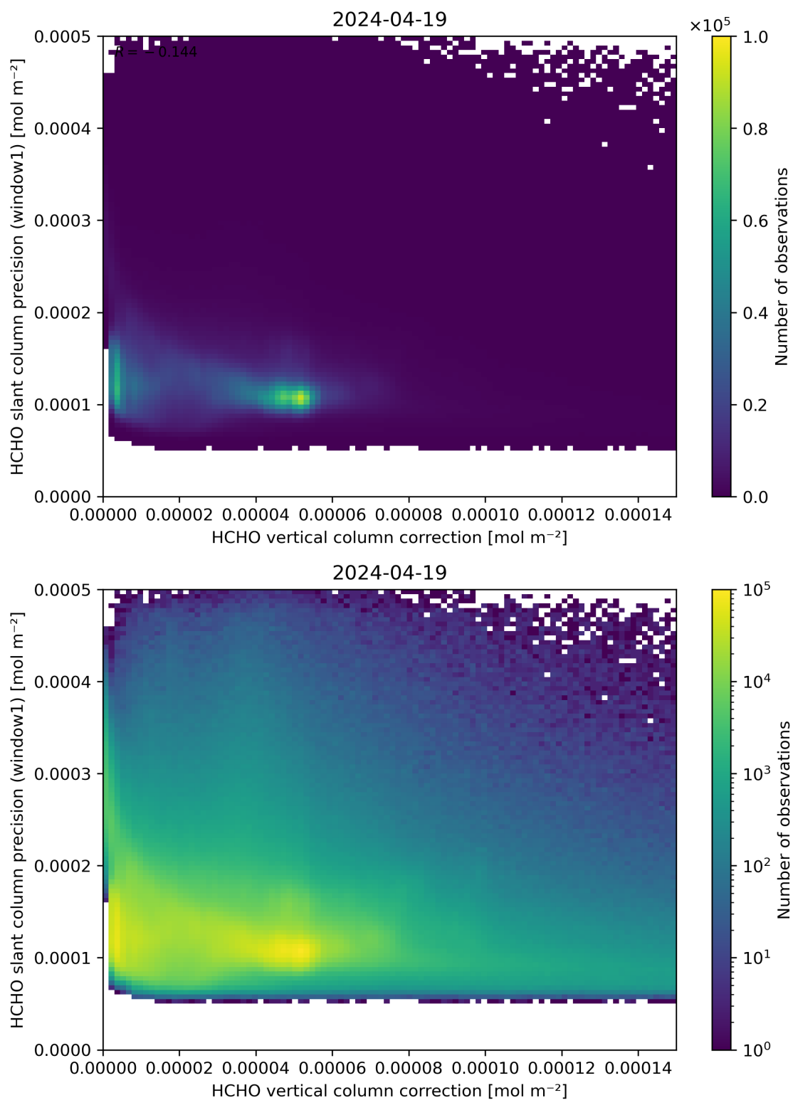
Figure 119: Scatter density plot of “HCHO vertical column correction” against “HCHO slant column precision (window1)” for 2024-04-18 to 2024-04-20.
