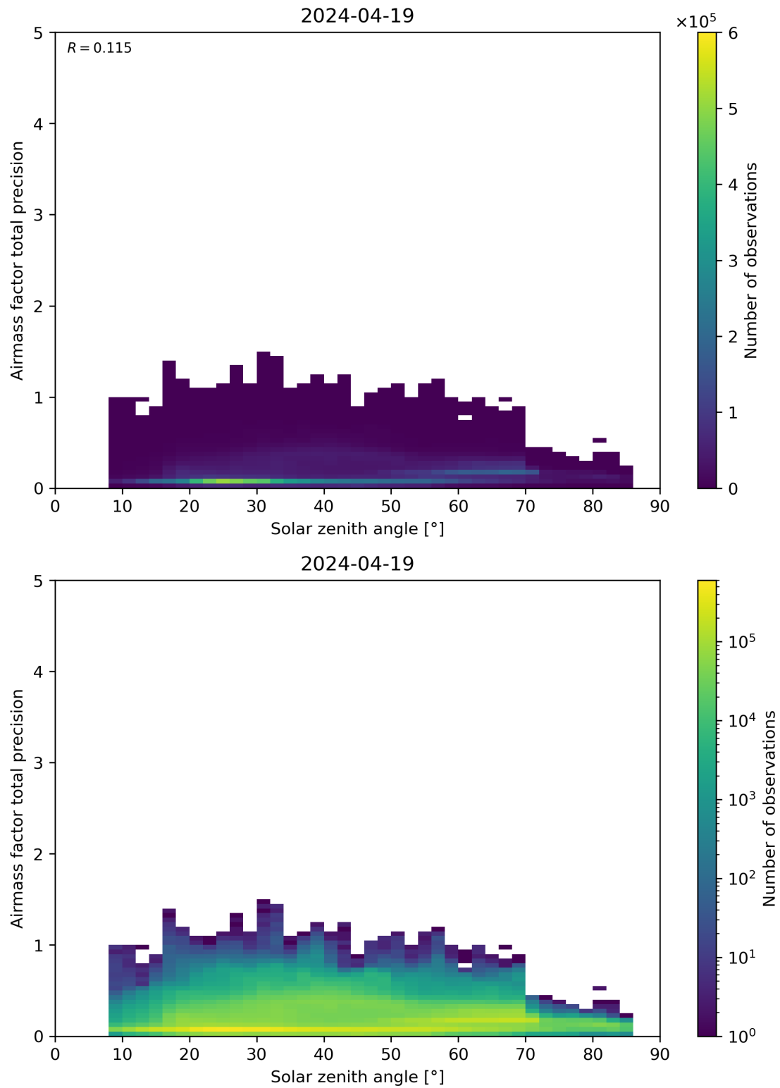
Figure 176: Scatter density plot of “Solar zenith angle” against “Airmass factor total precision” for 2024-04-18 to 2024-04-20.
