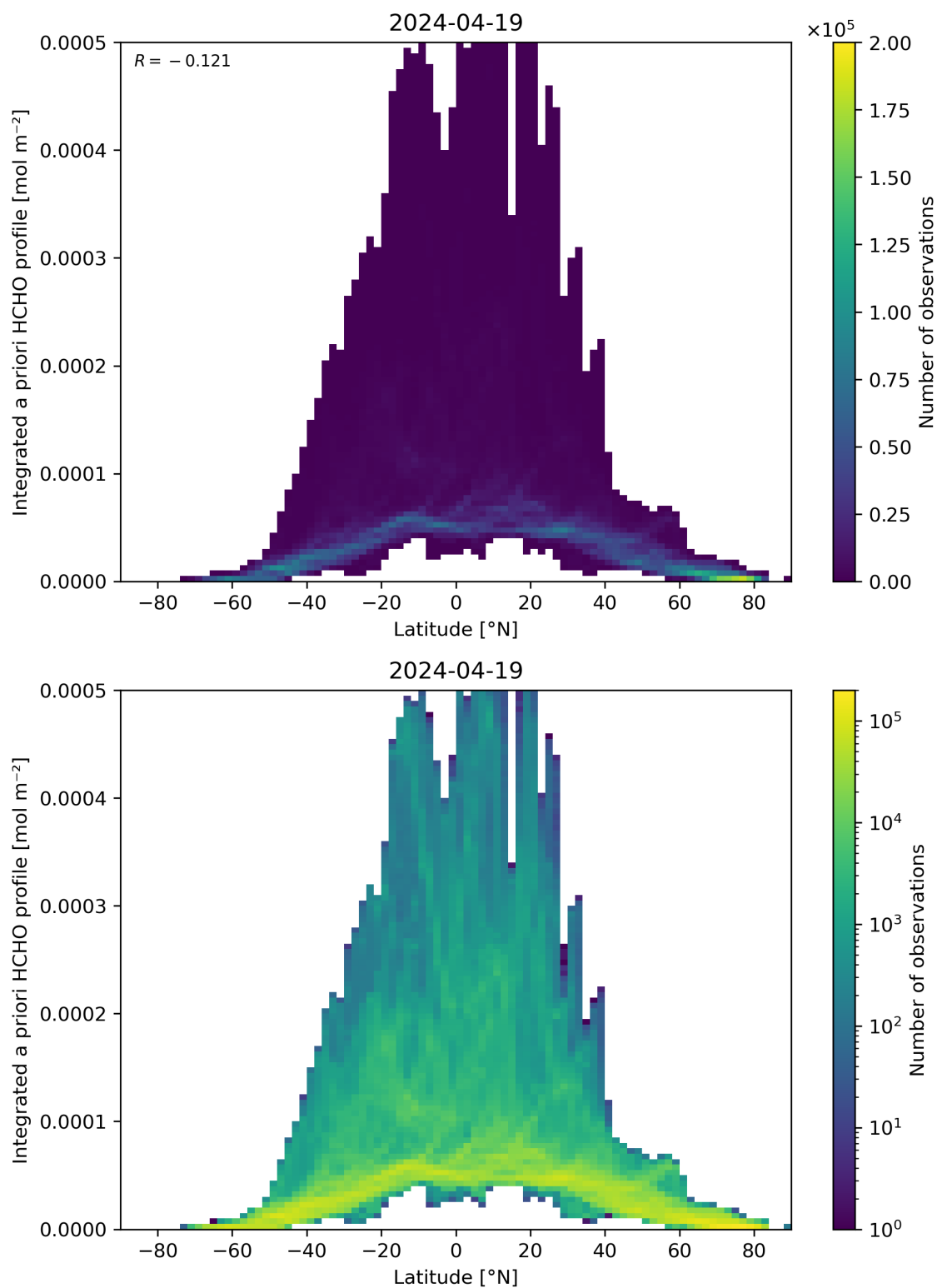
Figure 166: Scatter density plot of “Latitude” against “Integrated a priori HCHO profile” for 2024-04-18 to 2024-04-20.
