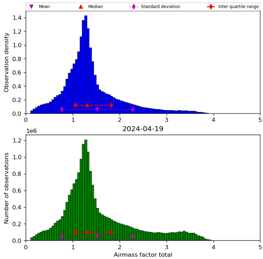
Figure 40: Histogram of “Airmass factor total” for 2024-04-18 to 2024-04-20
