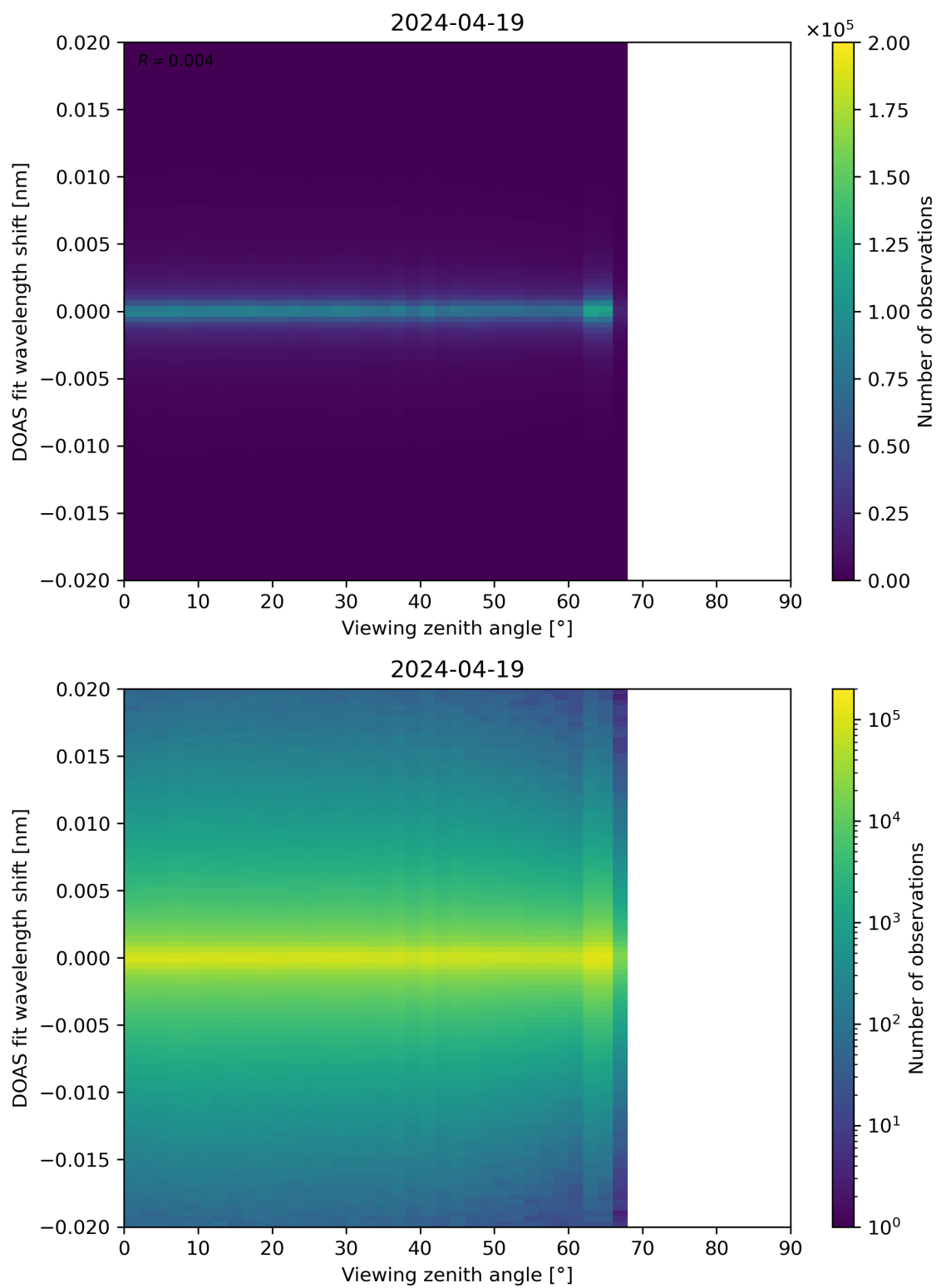
Figure 183: Scatter density plot of “Viewing zenith angle” against “DOAS fit wavelength shift” for 2024-04-18 to 2024-04-20.
