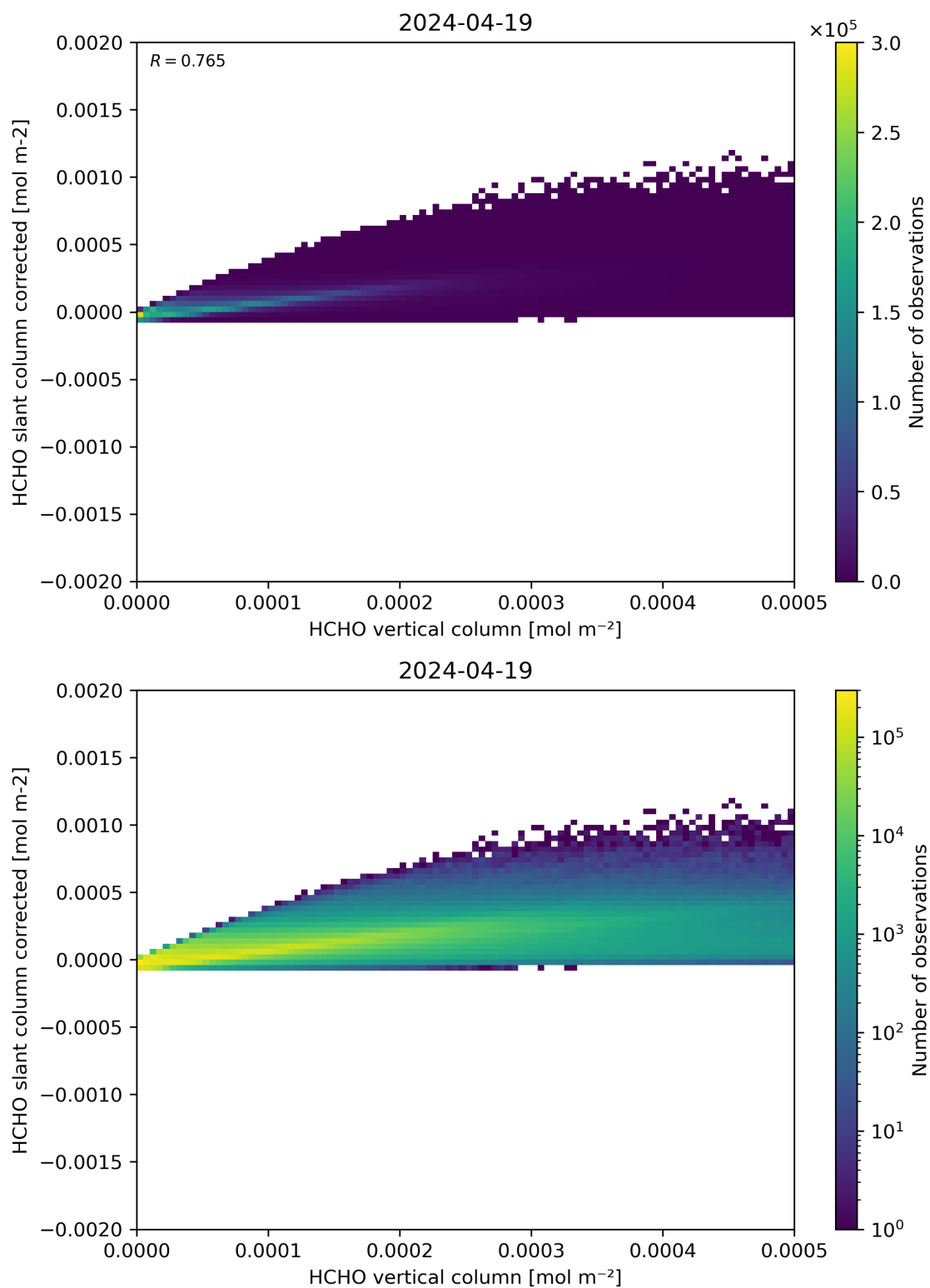
Figure 127: Scatter density plot of “HCHO vertical column” against “HCHO slant column corrected” for 2024-04-18 to 2024-04-20.
