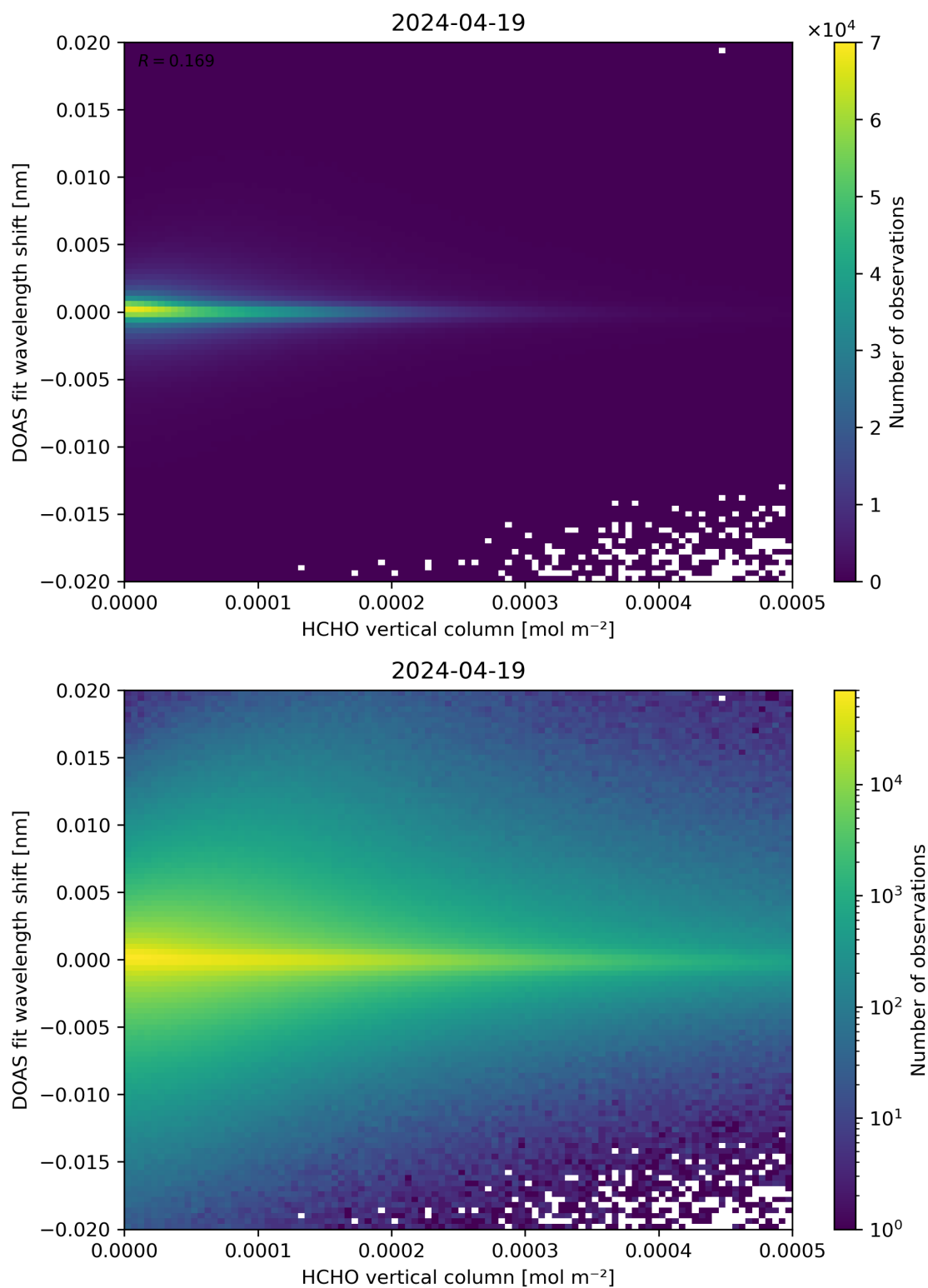
Figure 124: Scatter density plot of “HCHO vertical column” against “DOAS fit wavelength shift” for 2024-04-18 to 2024-04-20.
