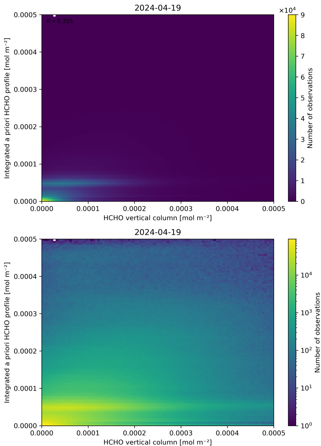
Figure 135: Scatter density plot of “HCHO vertical column” against “Integrated a priori HCHO profile” for 2024-04-18 to 2024-04-20.
