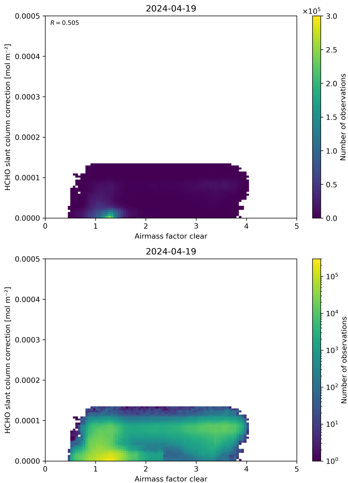
Figure 75: Scatter density plot of “Airmass factor clear” against “HCHO slant column correction” for 2024-04-18 to 2024-04-20.
