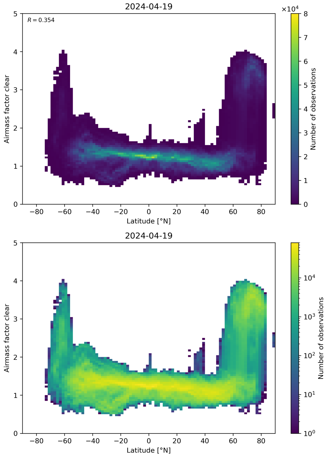
Figure 156: Scatter density plot of “Latitude” against “Airmass factor clear” for 2024-04-18 to 2024-04-20.
