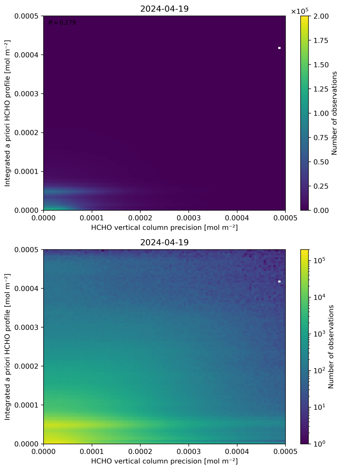
Figure 147: Scatter density plot of “HCHO vertical column precision” against “Integrated a priori HCHO profile” for 2024-04-18 to 2024-04-20.
