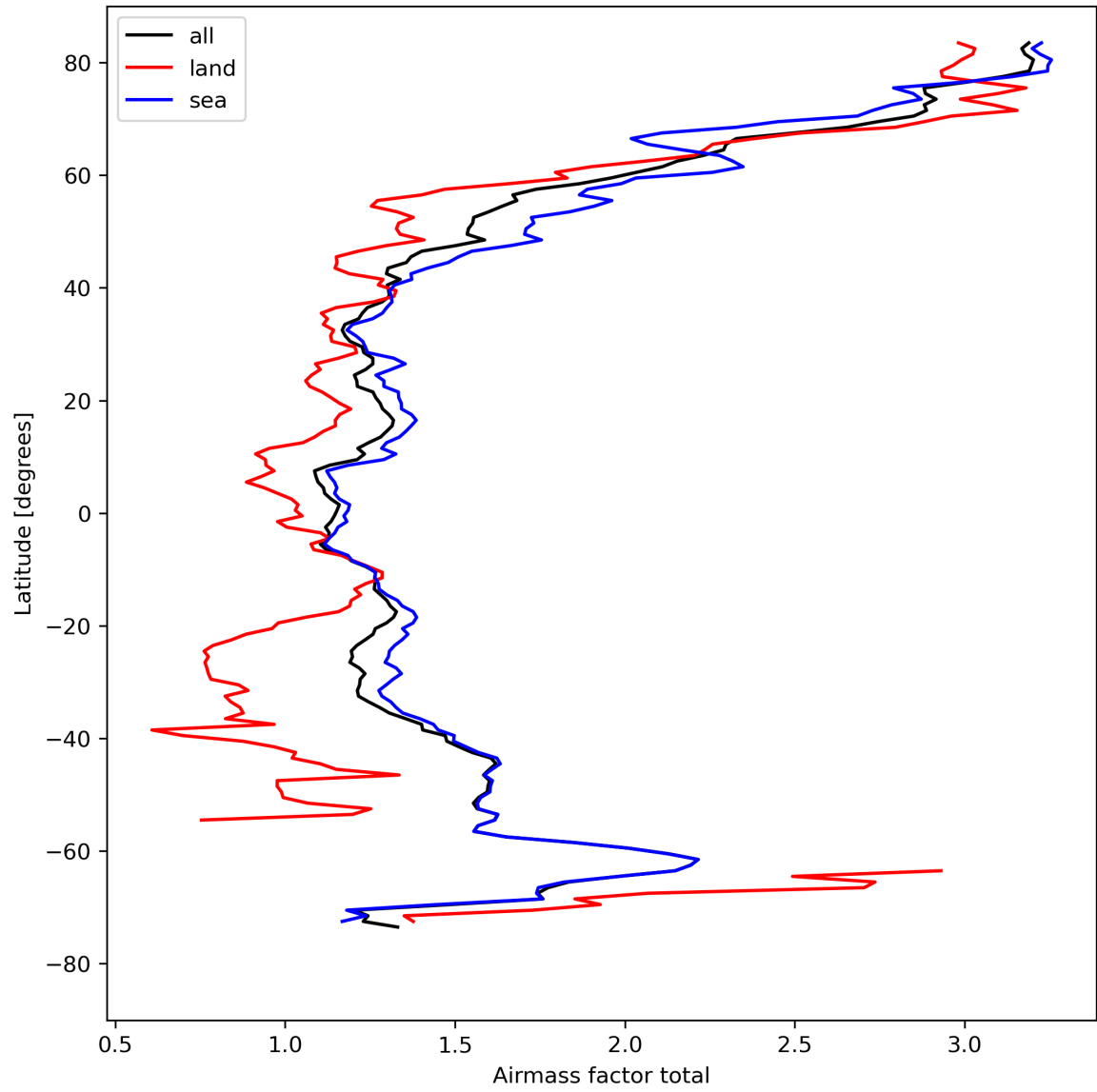
Figure 26: Zonal average of “Airmass factor total” for 2024-04-18 to 2024-04-20.
