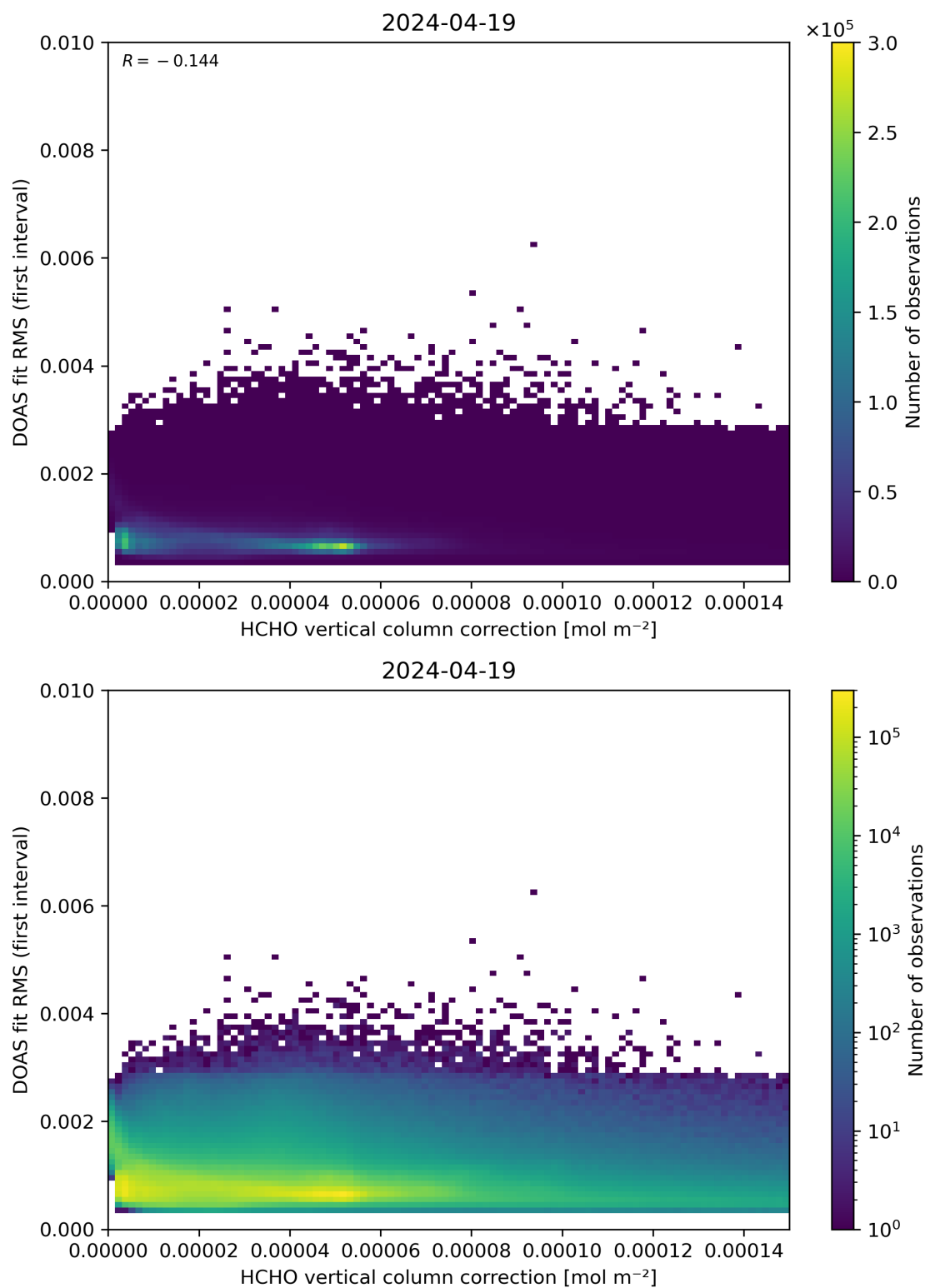
Figure 112: Scatter density plot of “HCHO vertical column correction” against “DOAS fit RMS (first interval)” for 2024-04-18 to 2024-04-20.
