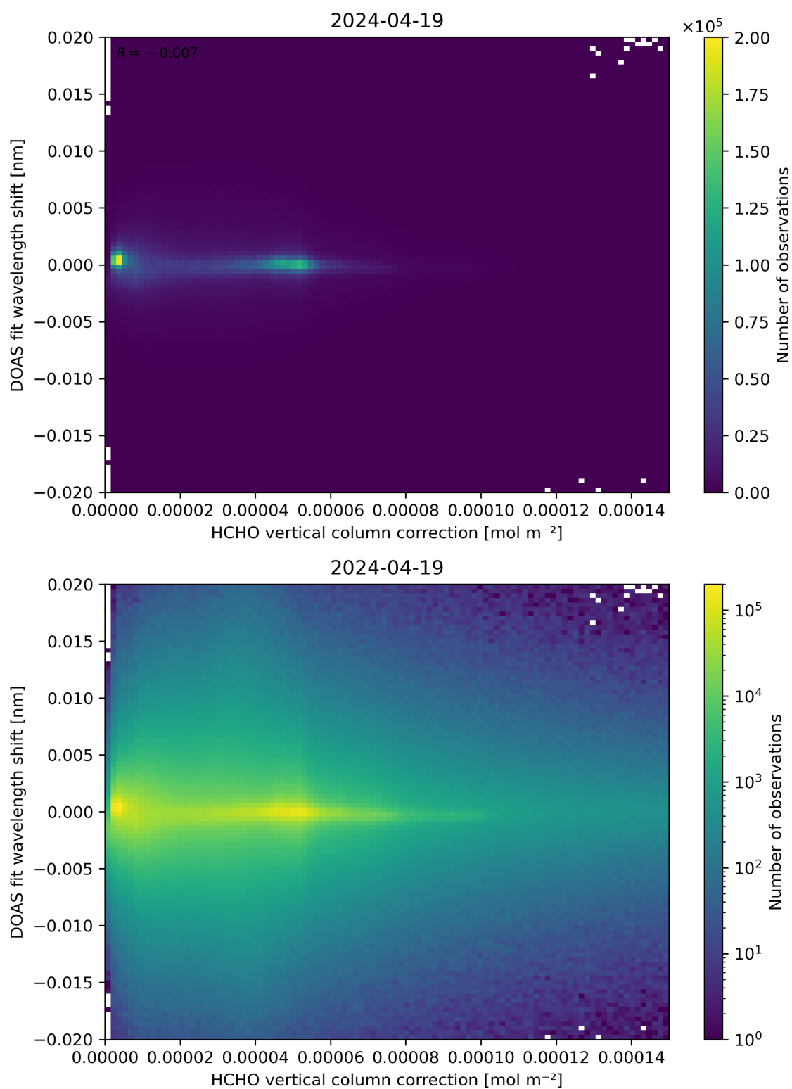
Figure 113: Scatter density plot of “HCHO vertical column correction” against “DOAS fit wavelength shift” for 2024-04-18 to 2024-04-20.
