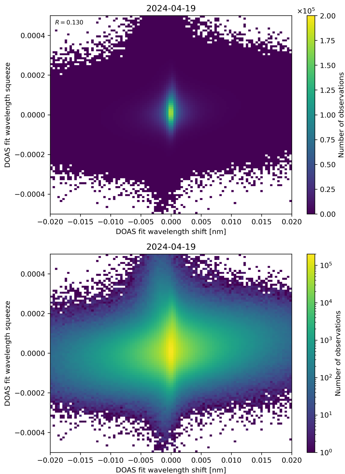
Figure 65: Scatter density plot of “DOAS fit wavelength shift” against “DOAS fit wavelength squeeze” for 2024-04-18 to 2024-04-20.
