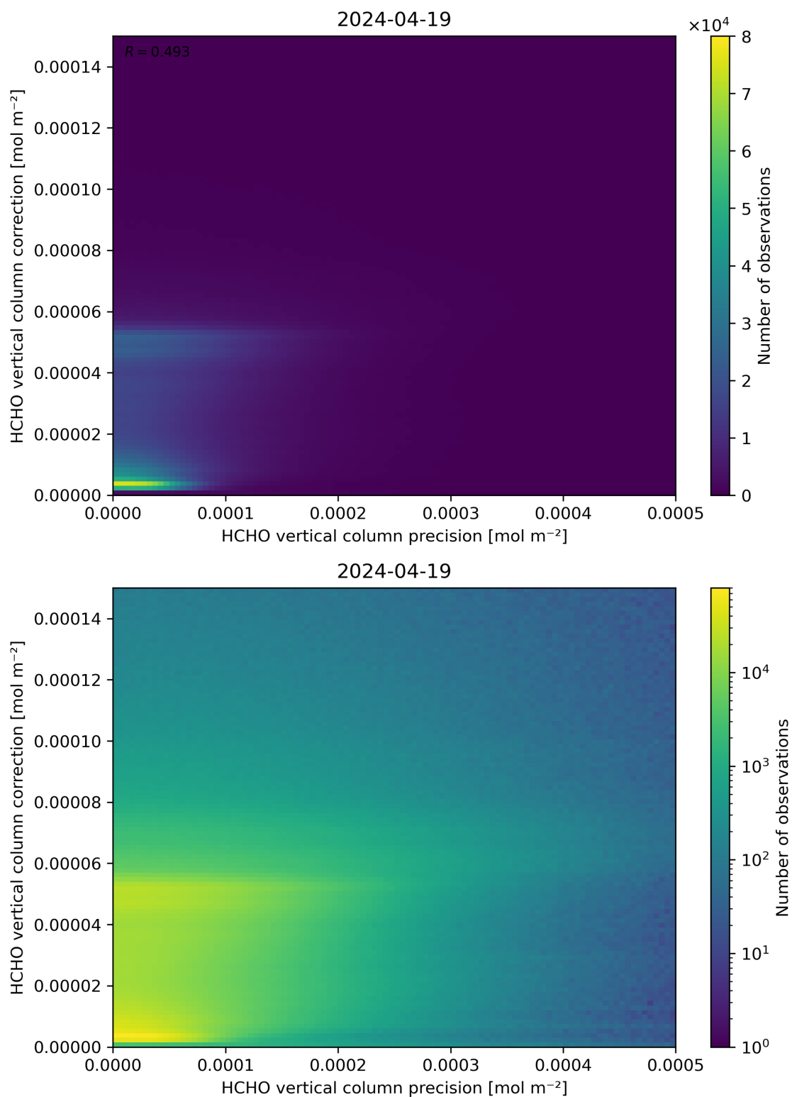
Figure 146: Scatter density plot of “HCHO vertical column precision” against “HCHO vertical column correction” for 2024-04-18 to 2024-04-20.
