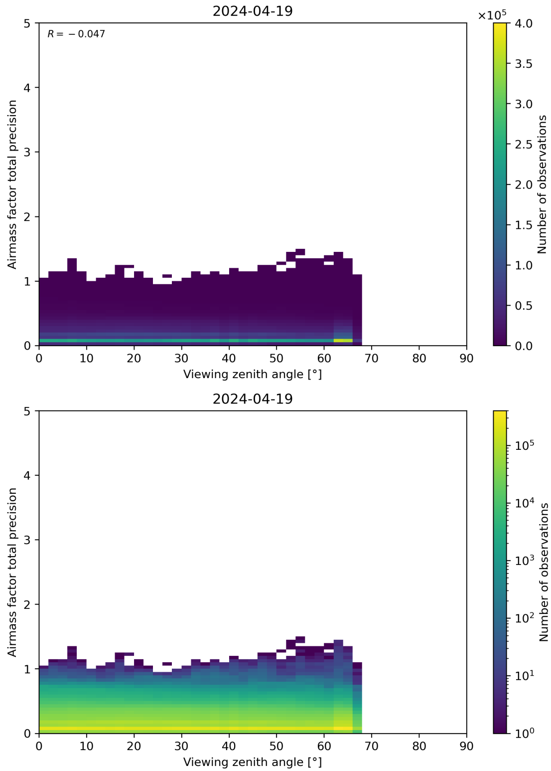
Figure 191: Scatter density plot of “Viewing zenith angle” against “Airmass factor total precision” for 2024-04-18 to 2024-04-20.
