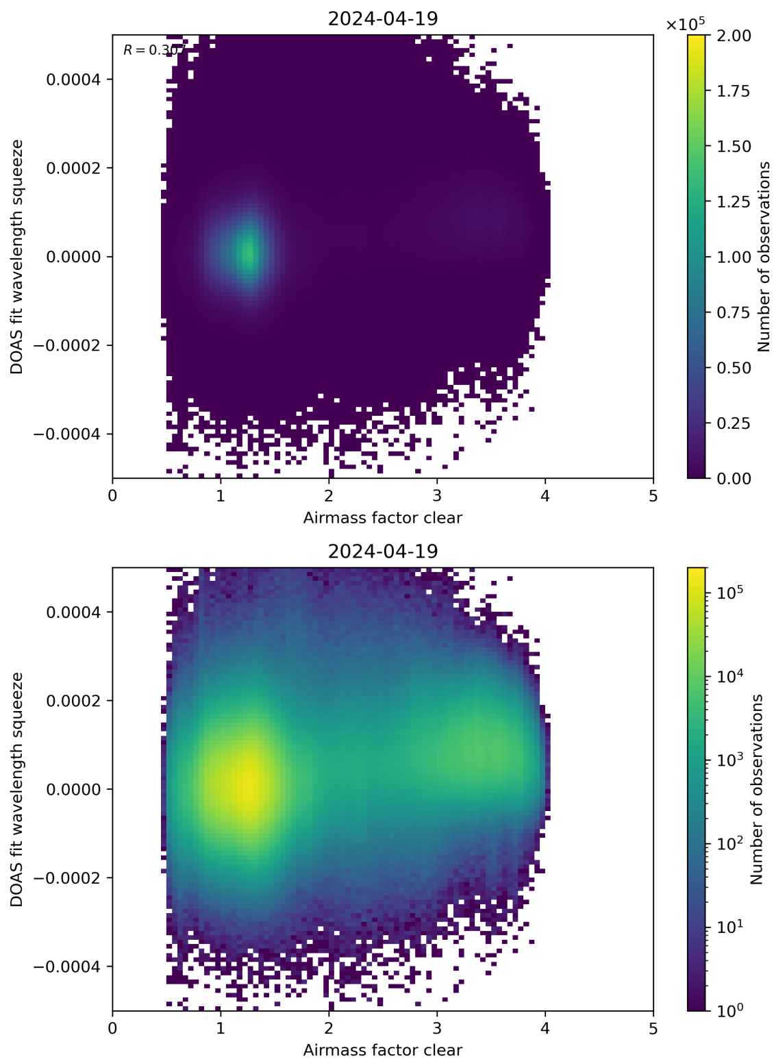
Figure 73: Scatter density plot of “Airmass factor clear” against “DOAS fit wavelength squeeze” for 2024-04-18 to 2024-04-20.
