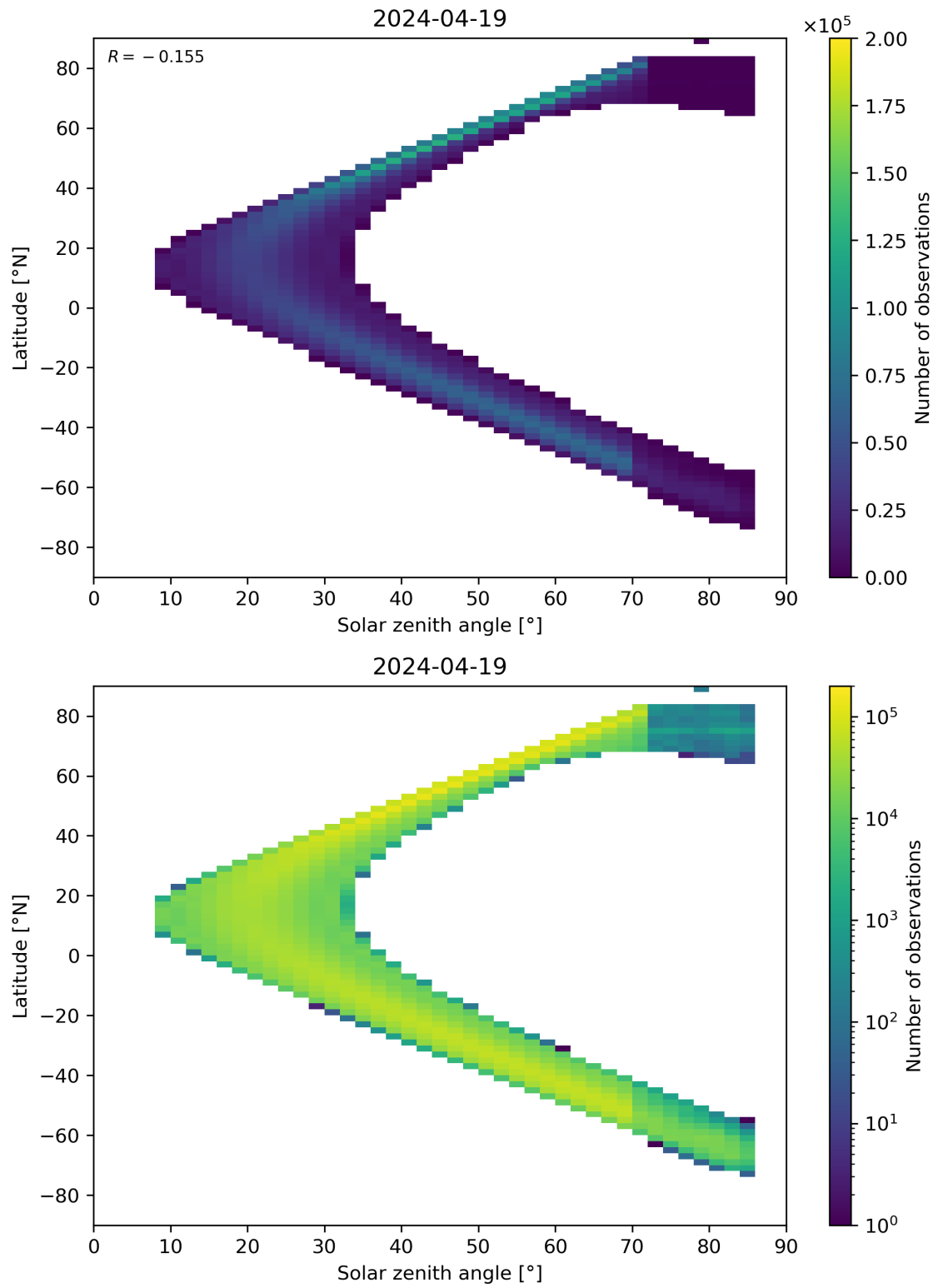
Figure 181: Scatter density plot of “Solar zenith angle” against “Latitude” for 2024-04-18 to 2024-04-20.
