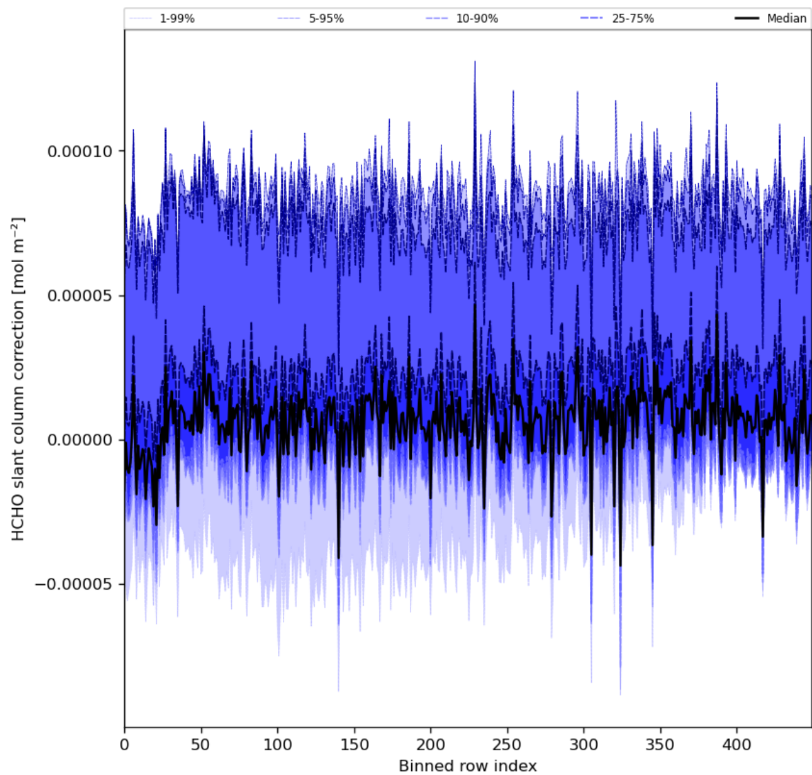
Figure 61: Along track statistics of “HCHO slant column correction” for 2024-04-18 to 2024-04-20
