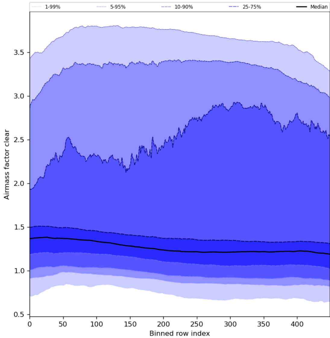
Figure 56: Along track statistics of “Airmass factor clear” for 2024-04-18 to 2024-04-20
