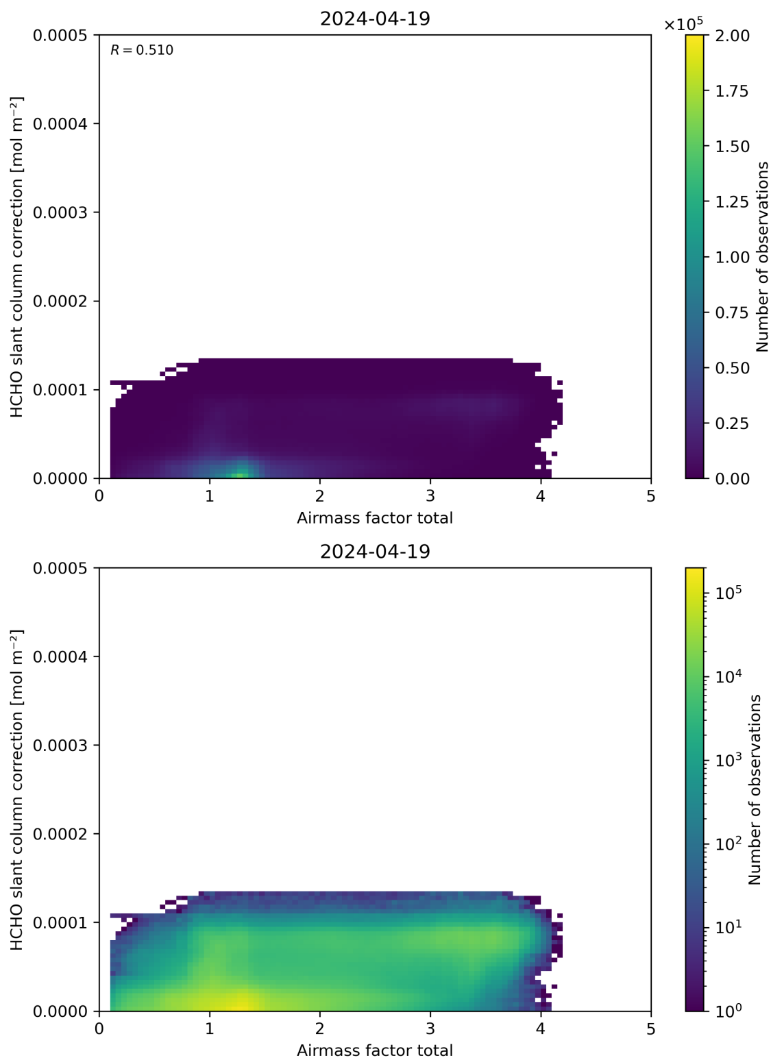
Figure 102: Scatter density plot of “Airmass factor total” against “HCHO slant column correction” for 2024-04-18 to 2024-04-20.
