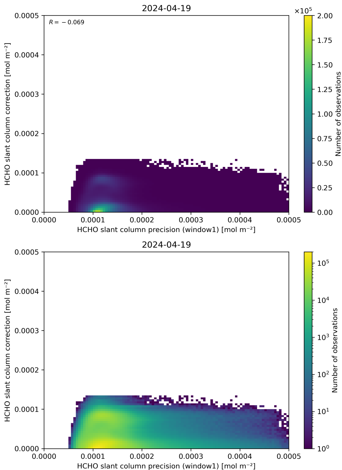
Figure 93: Scatter density plot of “HCHO slant column precision (window1)” against “HCHO slant column correction” for 2024-04-18 to 2024-04-20.
