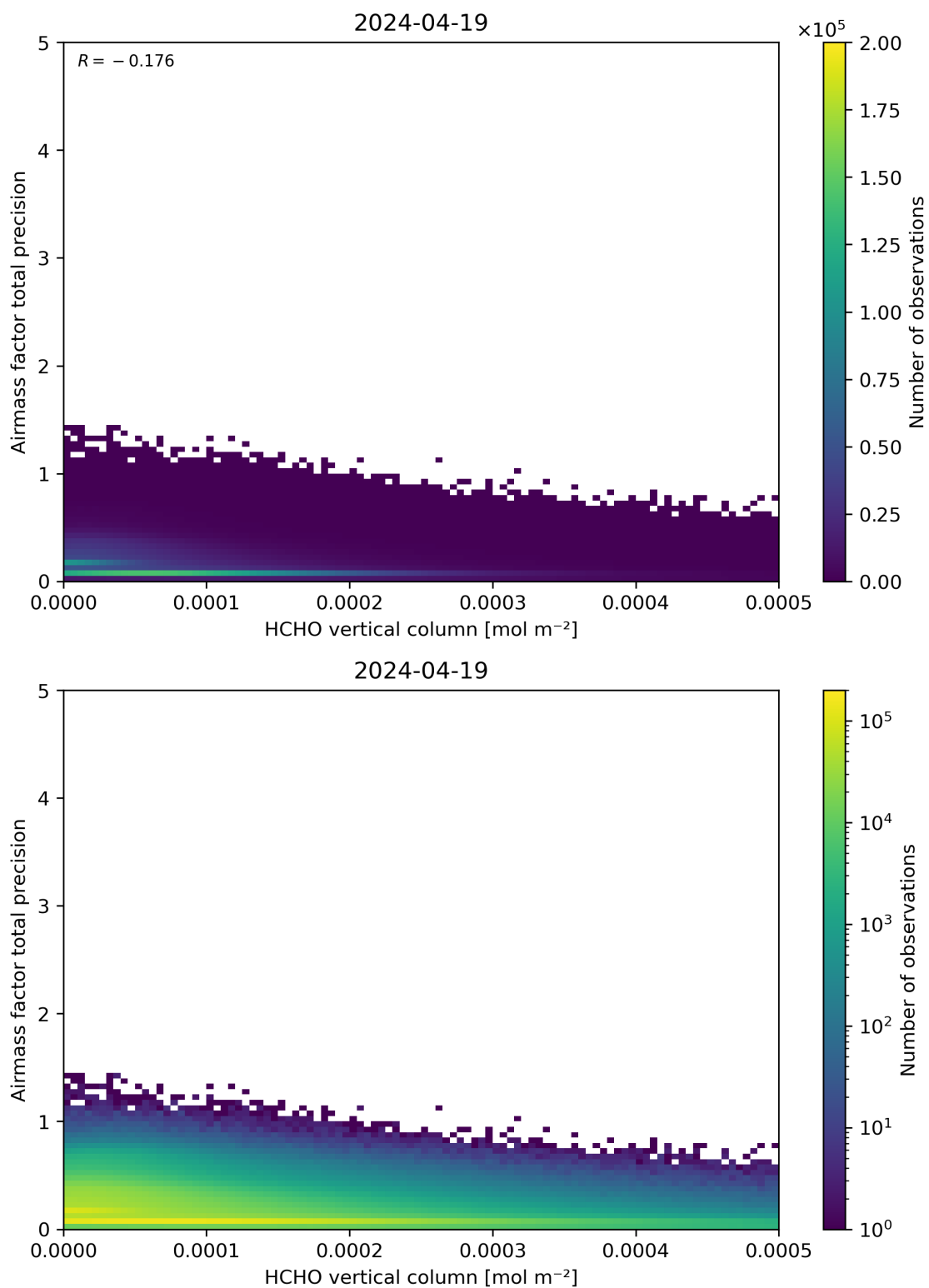
Figure 132: Scatter density plot of “HCHO vertical column” against “Airmass factor total precision” for 2024-04-18 to 2024-04-20.
