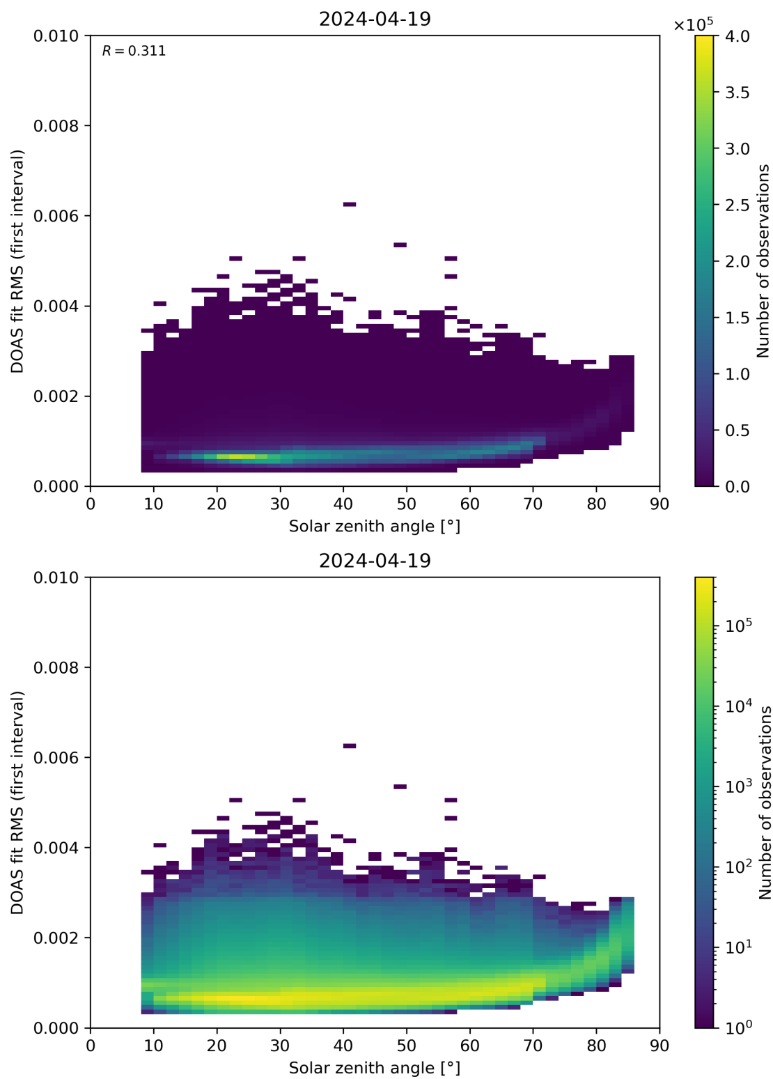
Figure 167: Scatter density plot of “Solar zenith angle” against “DOAS fit RMS (first interval)” for 2024-04-18 to 2024-04-20.
