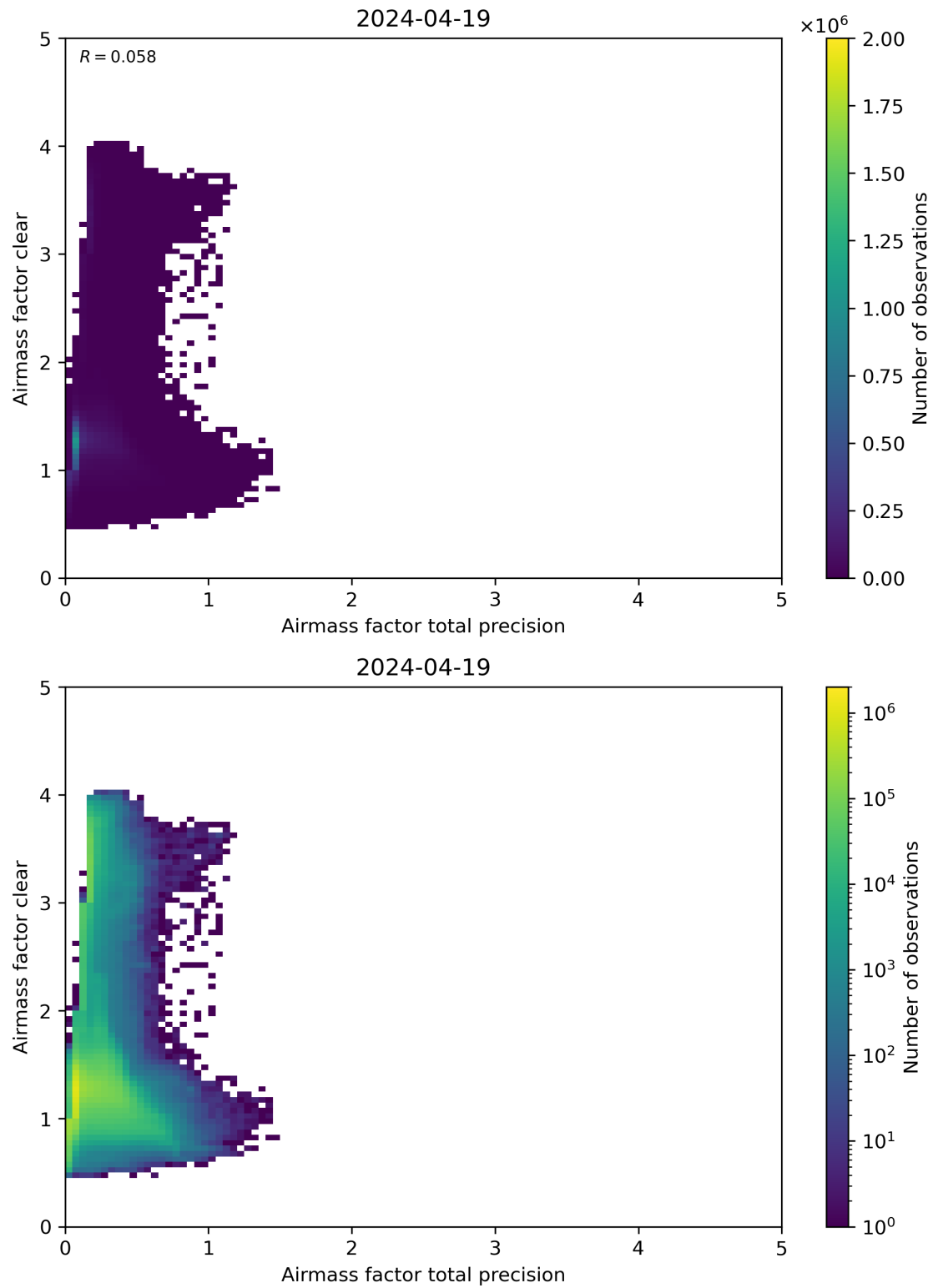
Figure 108: Scatter density plot of “Airmass factor total precision” against “Airmass factor clear” for 2024-04-18 to 2024-04-20.
