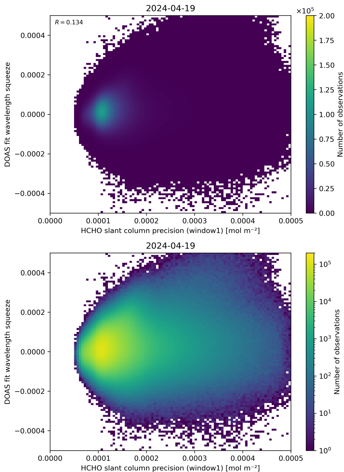
Figure 90: Scatter density plot of “HCHO slant column precision (window1)” against “DOAS fit wavelength squeeze” for 2024-04-18 to 2024-04-20.
