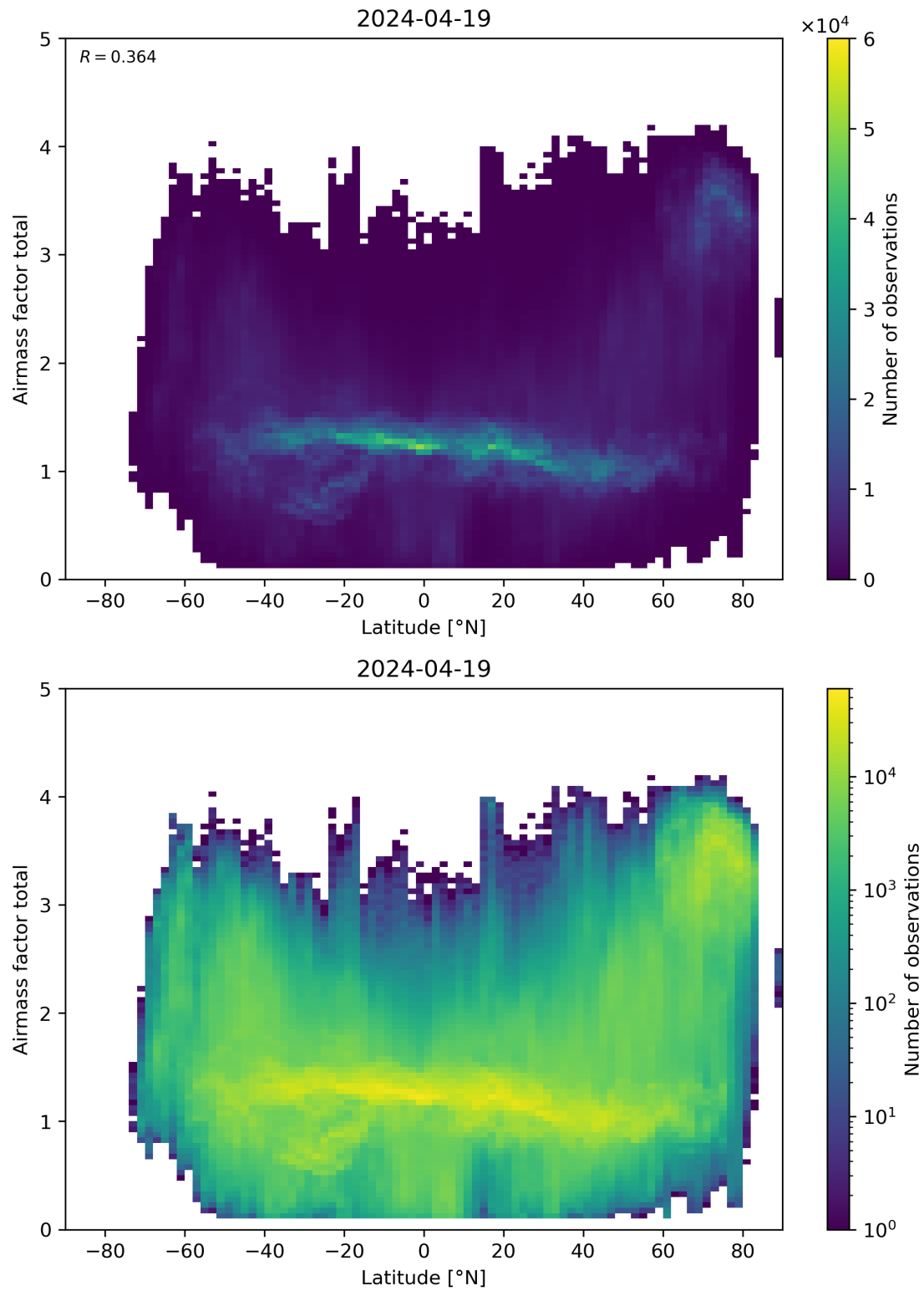
Figure 161: Scatter density plot of “Latitude” against “Airmass factor total” for 2024-04-18 to 2024-04-20.
