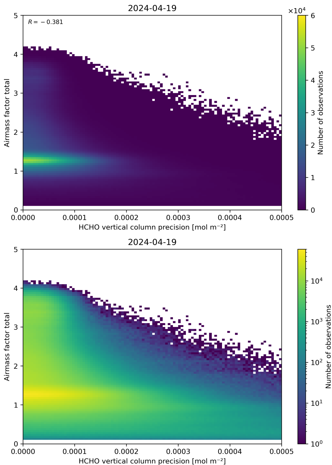
Figure 144: Scatter density plot of “HCHO vertical column precision” against “Airmass factor total” for 2024-04-18 to 2024-04-20.
