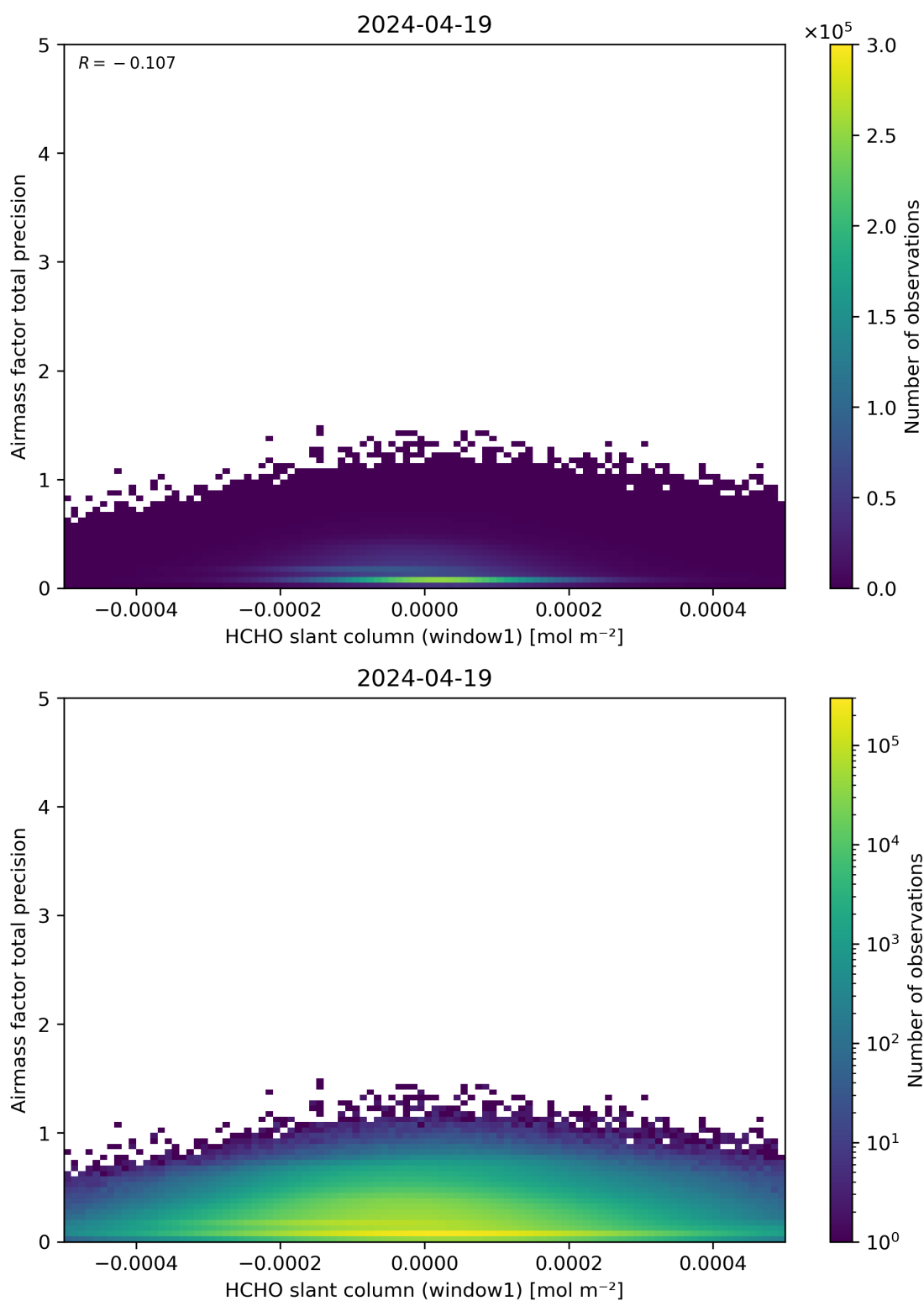
Figure 86: Scatter density plot of “HCHO slant column (window1)” against “Airmass factor total precision” for 2024-04-18 to 2024-04-20.
