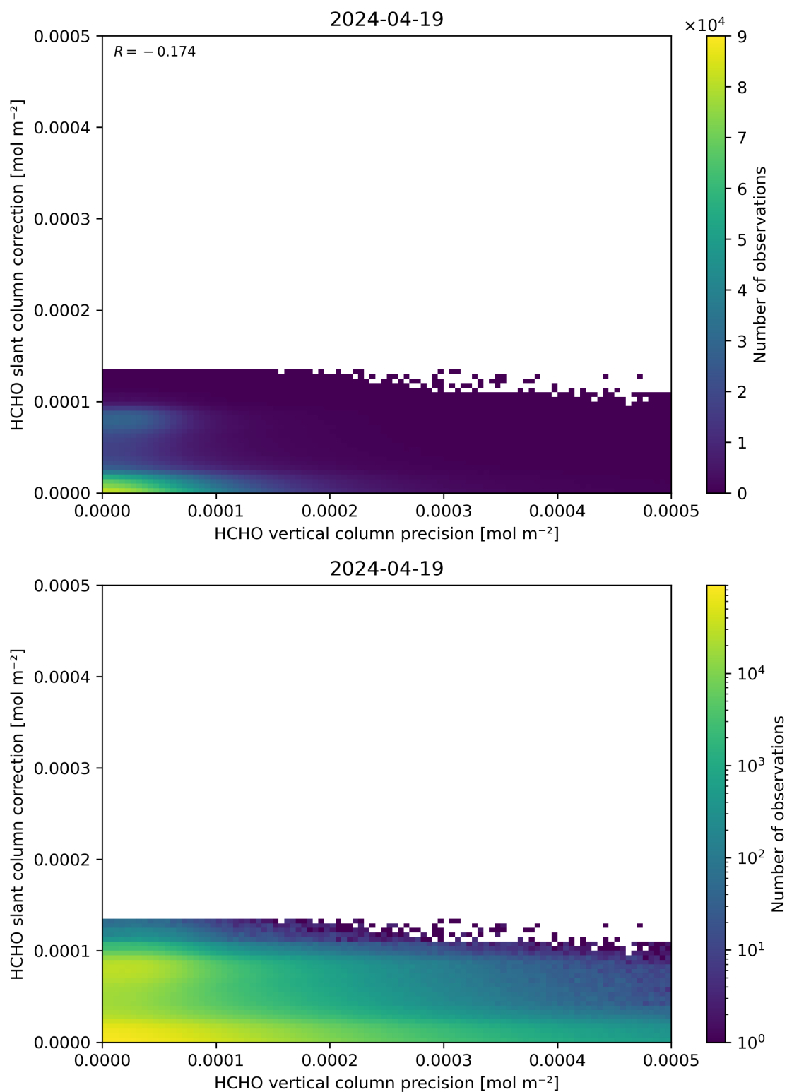
Figure 141: Scatter density plot of “HCHO vertical column precision” against “HCHO slant column correction” for 2024-04-18 to 2024-04-20.
