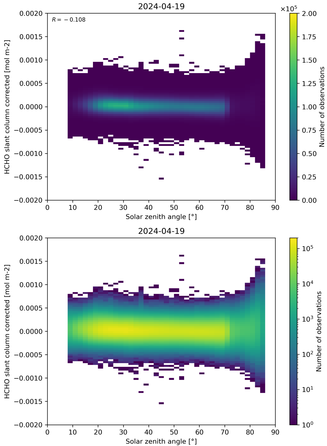
Figure 171: Scatter density plot of “Solar zenith angle” against “HCHO slant column corrected” for 2024-04-18 to 2024-04-20.
