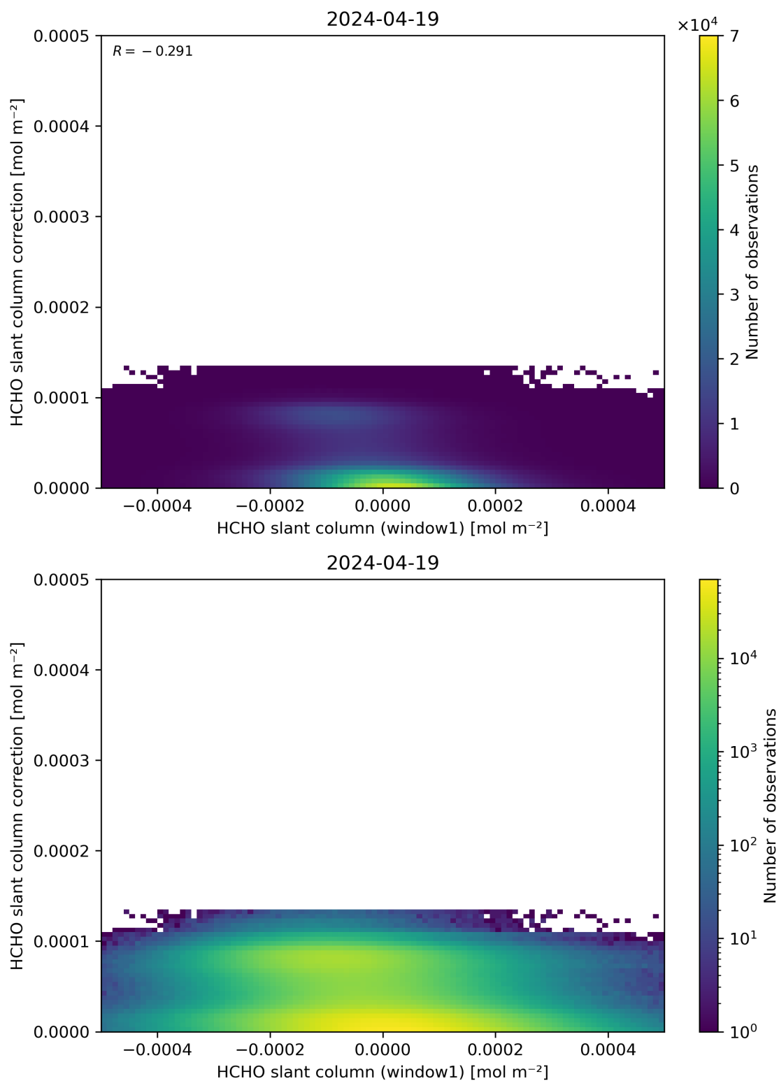
Figure 83: Scatter density plot of “HCHO slant column (window1)” against “HCHO slant column correction” for 2024-04-18 to 2024-04-20.
