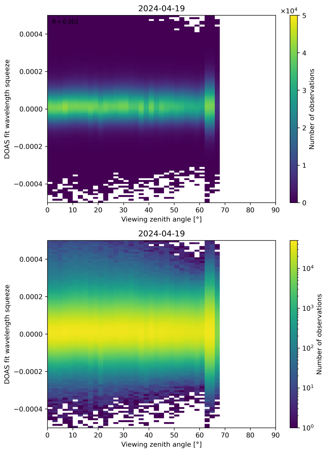
Figure 184: Scatter density plot of “Viewing zenith angle” against “DOAS fit wavelength squeeze” for 2024-04-18 to 2024-04-20.
