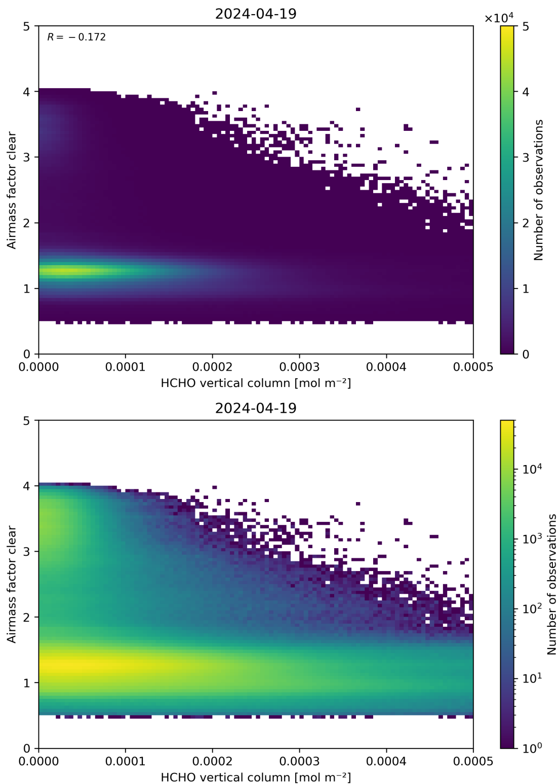
Figure 126: Scatter density plot of “HCHO vertical column” against “Airmass factor clear” for 2024-04-18 to 2024-04-20.
