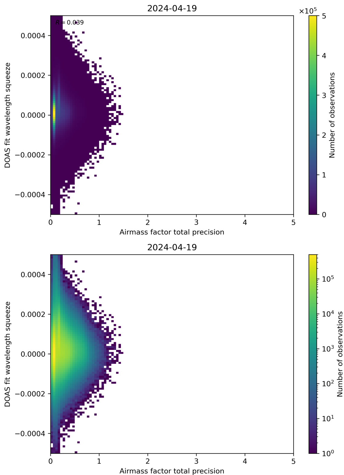
Figure 107: Scatter density plot of “Airmass factor total precision” against “DOAS fit wavelength squeeze” for 2024-04-18 to 2024-04-20.
