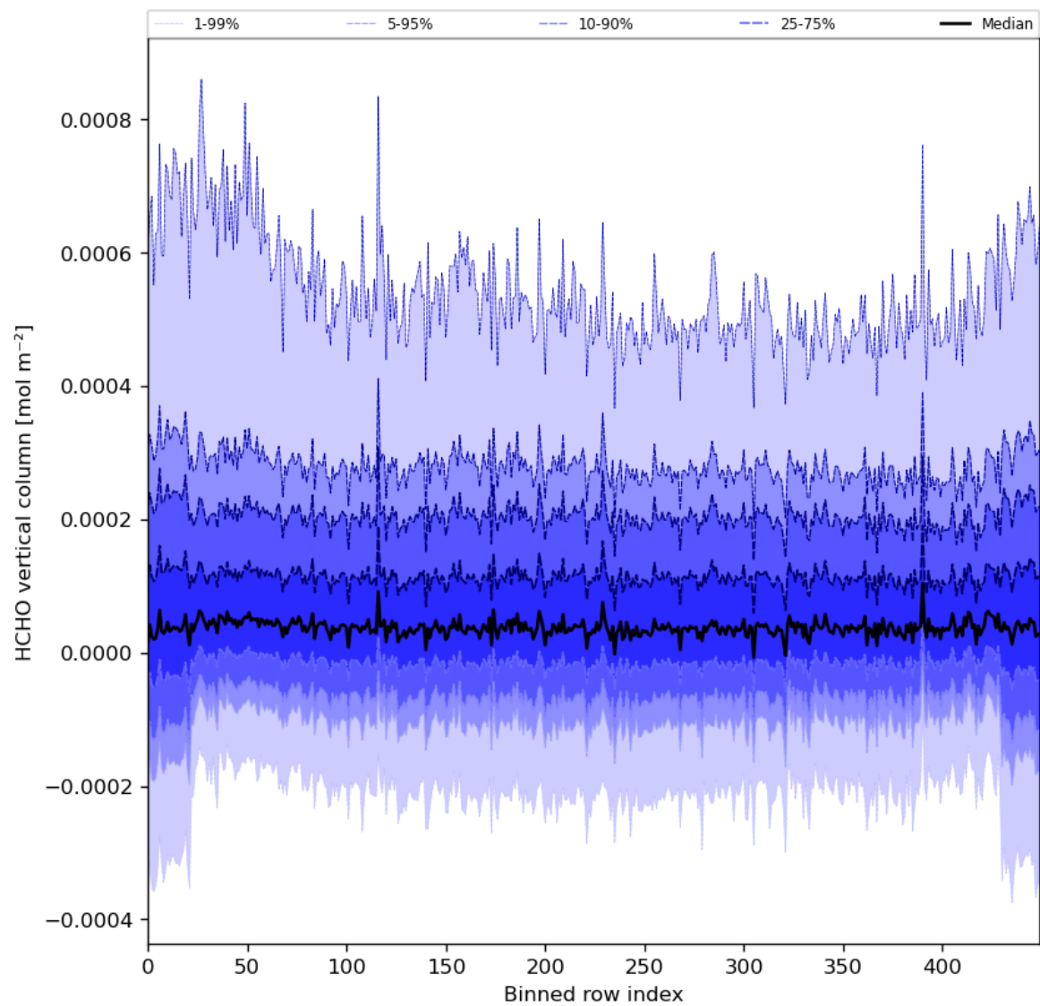
Figure 49: Along track statistics of “HCHO vertical column” for 2024-04-18 to 2024-04-20
