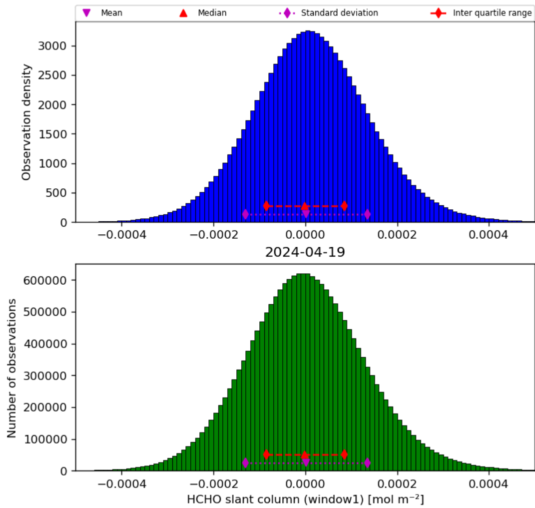
Figure 38: Histogram of “HCHO slant column (window1)” for 2024-04-18 to 2024-04-20
