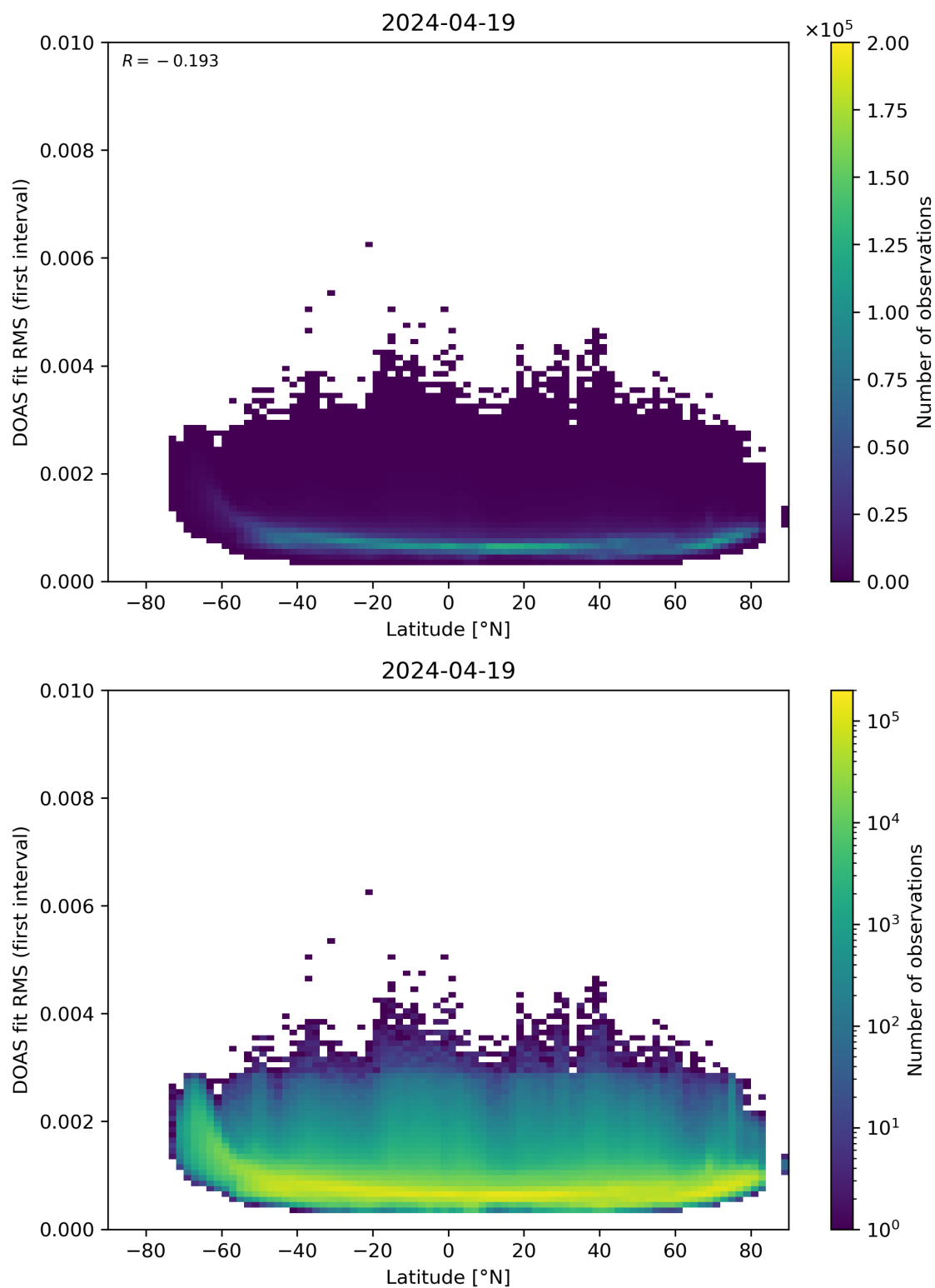
Figure 153: Scatter density plot of “Latitude” against “DOAS fit RMS (first interval)” for 2024-04-18 to 2024-04-20.
