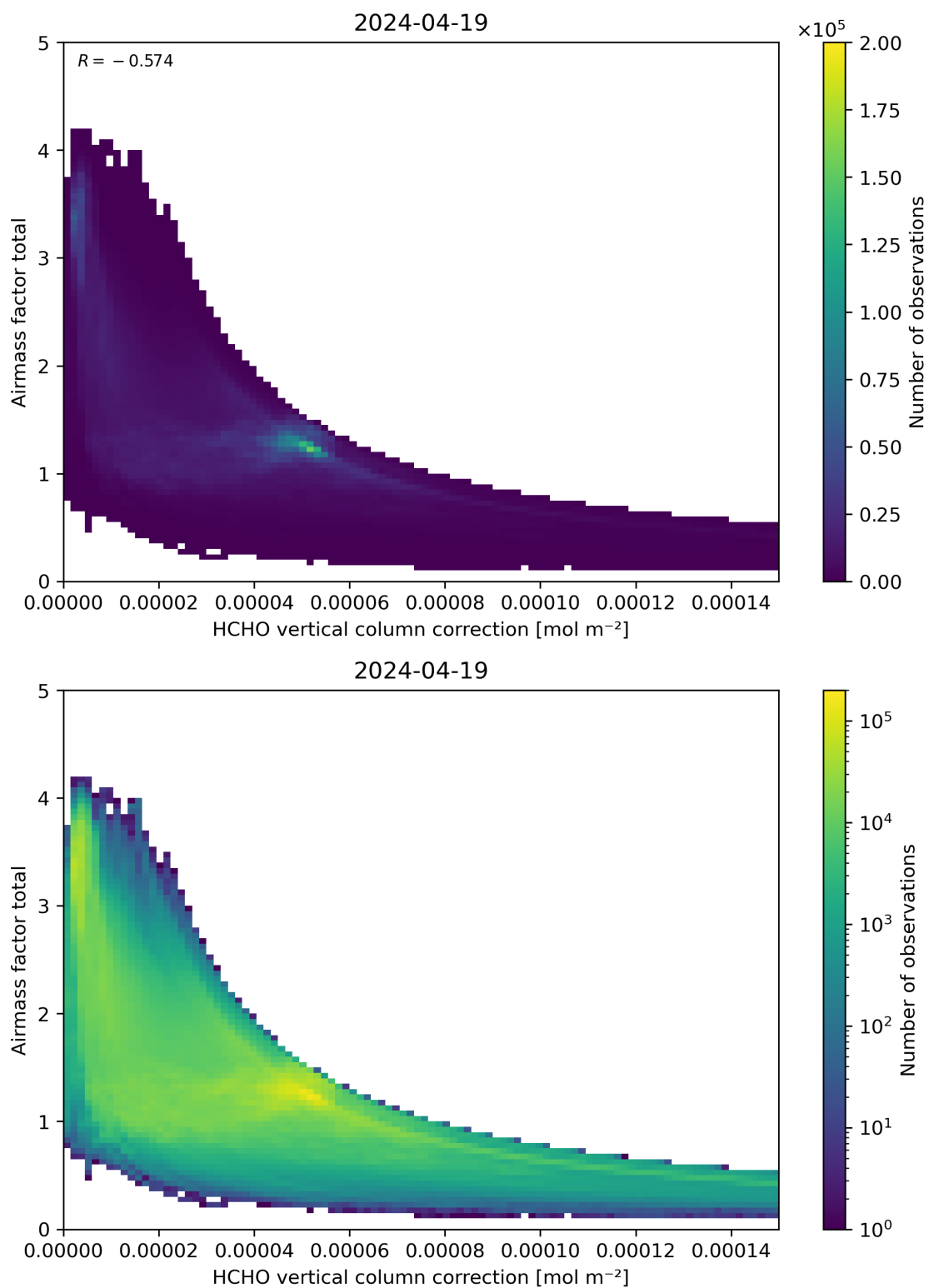
Figure 120: Scatter density plot of “HCHO vertical column correction” against “Airmass factor total” for 2024-04-18 to 2024-04-20.
