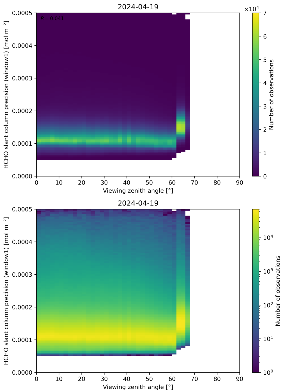
Figure 189: Scatter density plot of “Viewing zenith angle” against “HCHO slant column precision (window1)” for 2024-04-18 to 2024-04-20.
