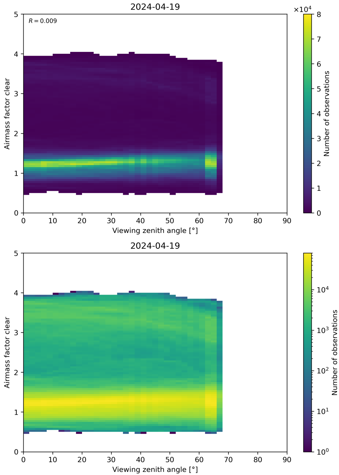
Figure 185: Scatter density plot of “Viewing zenith angle” against “Airmass factor clear” for 2024-04-18 to 2024-04-20.
