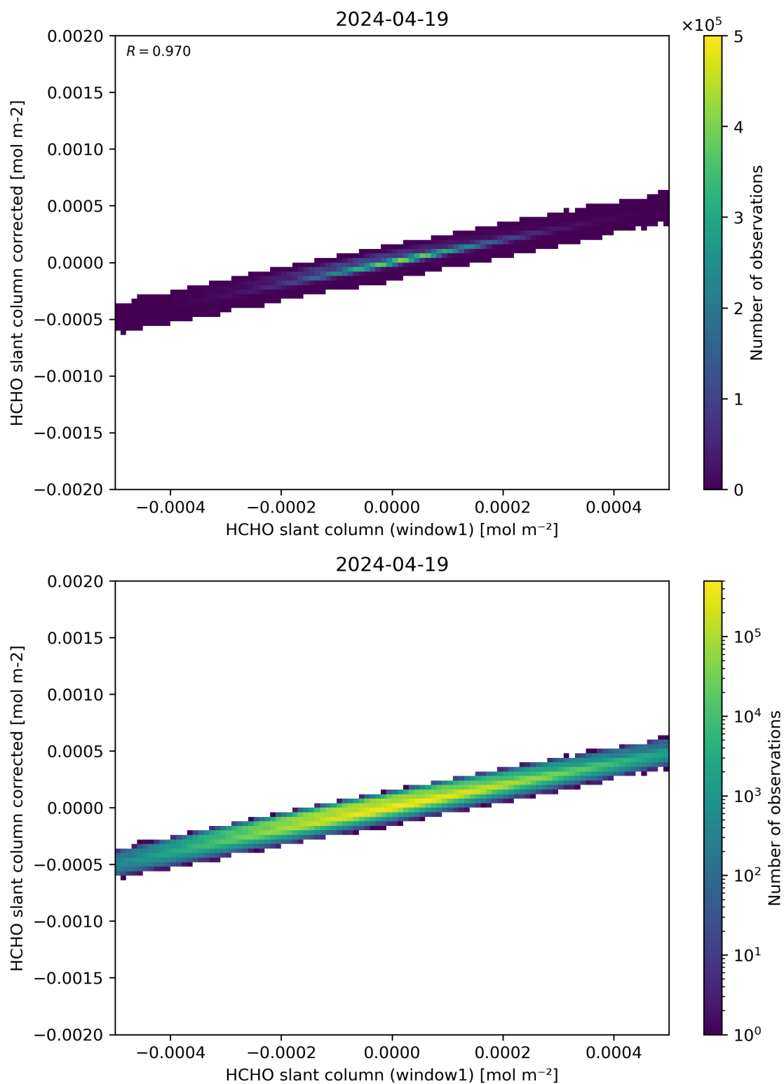
Figure 82: Scatter density plot of “HCHO slant column (window1)” against “HCHO slant column corrected” for 2024-04-18 to 2024-04-20.
