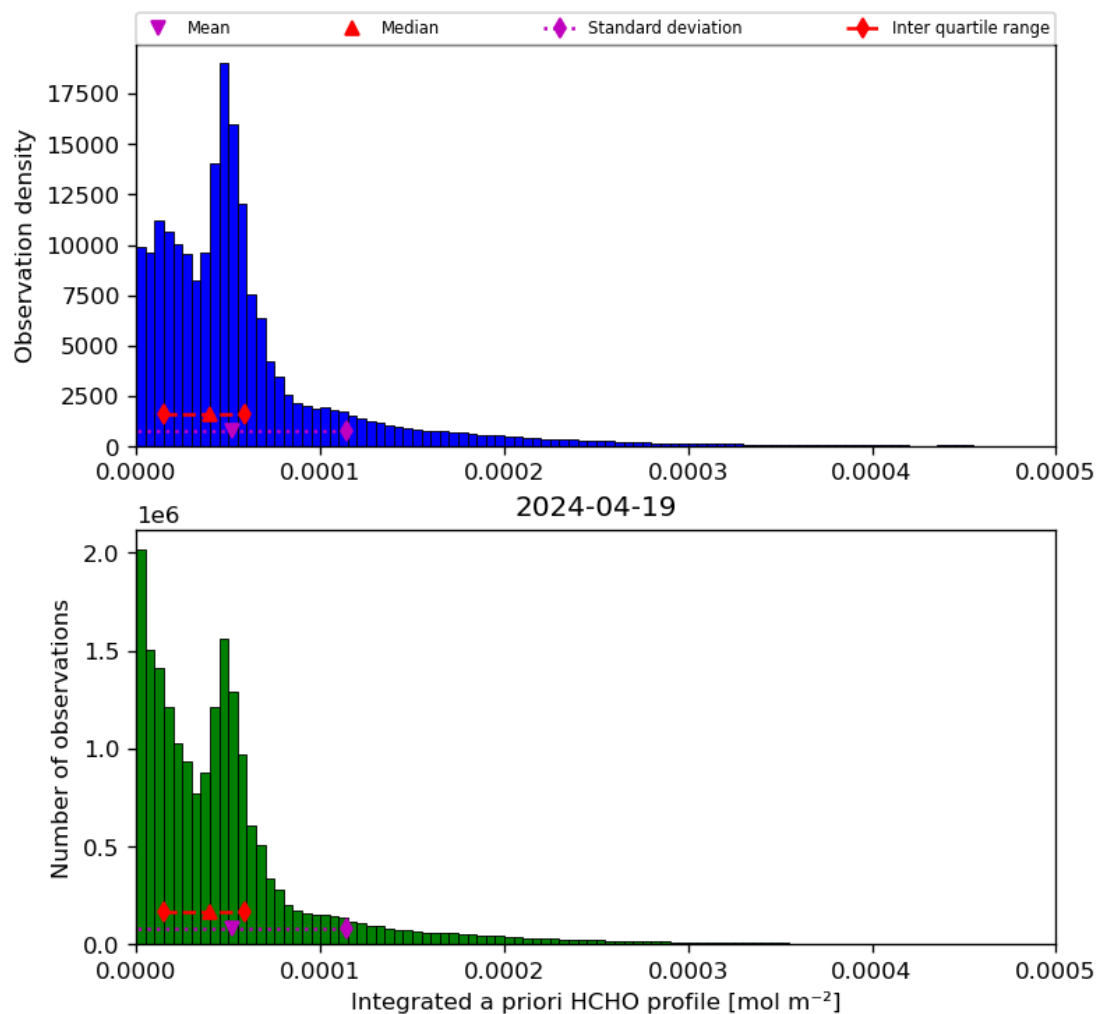
Figure 43: Histogram of “Integrated a priori HCHO profile” for 2024-04-18 to 2024-04-20
