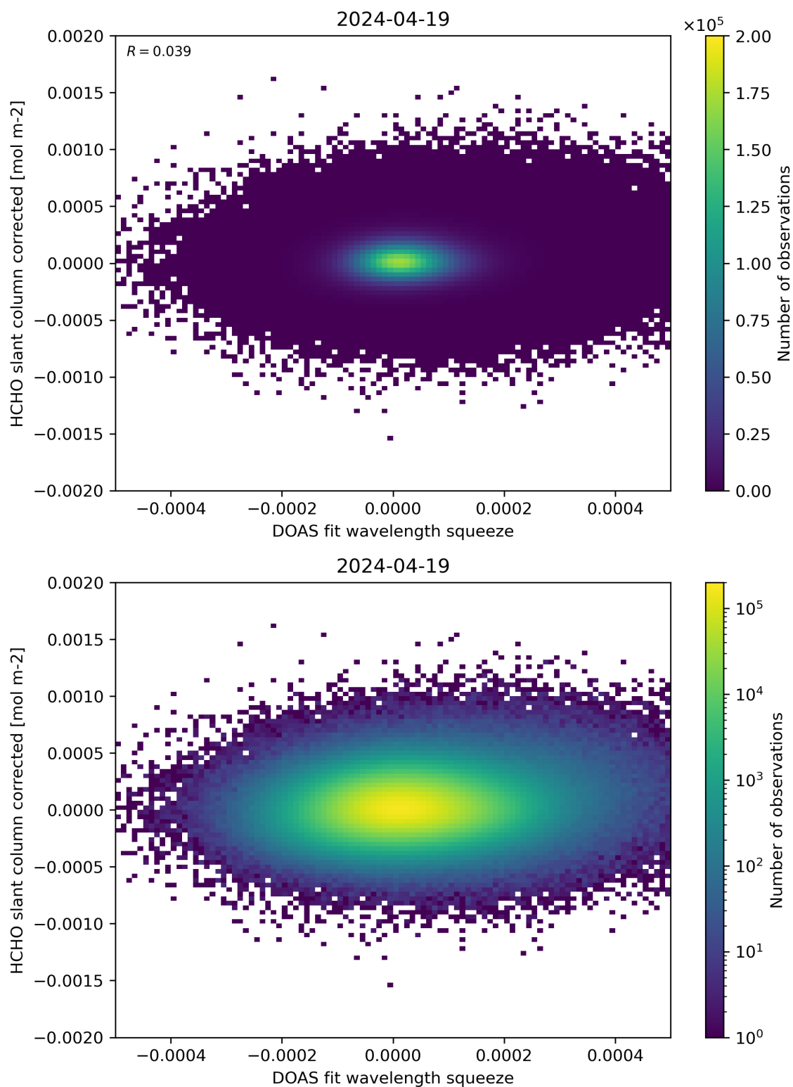
Figure 69: Scatter density plot of “DOAS fit wavelength squeeze” against “HCHO slant column corrected” for 2024-04-18 to 2024-04-20.
