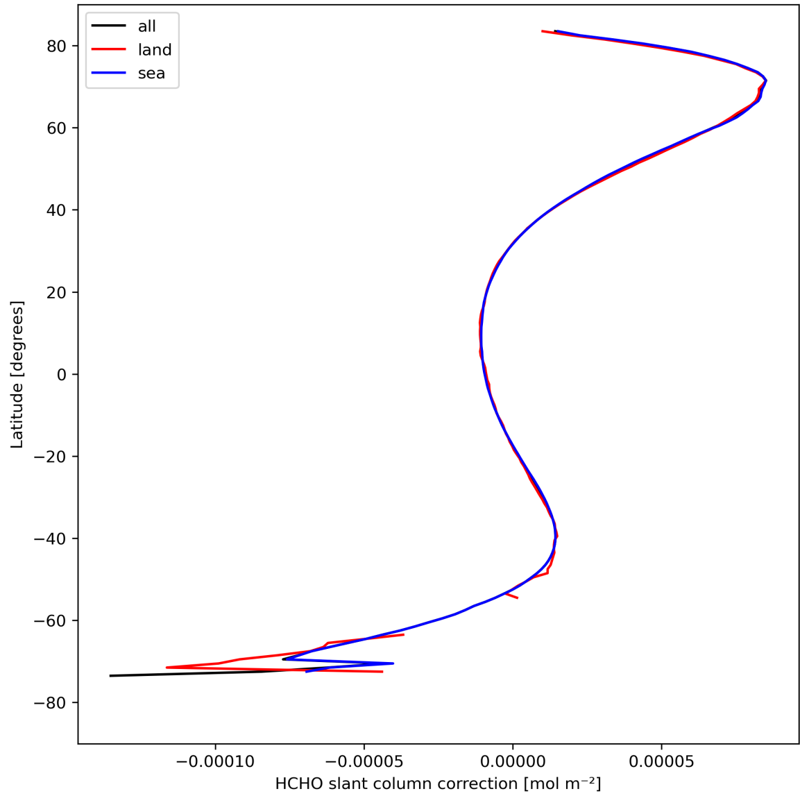
Figure 33: Zonal average of “HCHO slant column correction” for 2024-04-18 to 2024-04-20.
