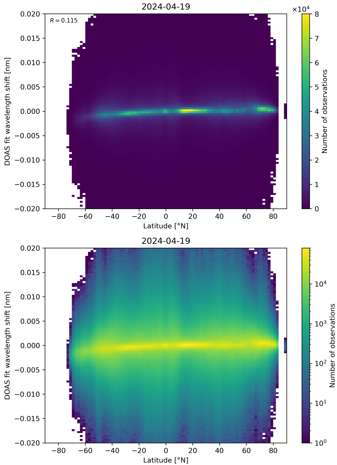
Figure 154: Scatter density plot of “Latitude” against “DOAS fit wavelength shift” for 2024-04-18 to 2024-04-20.
