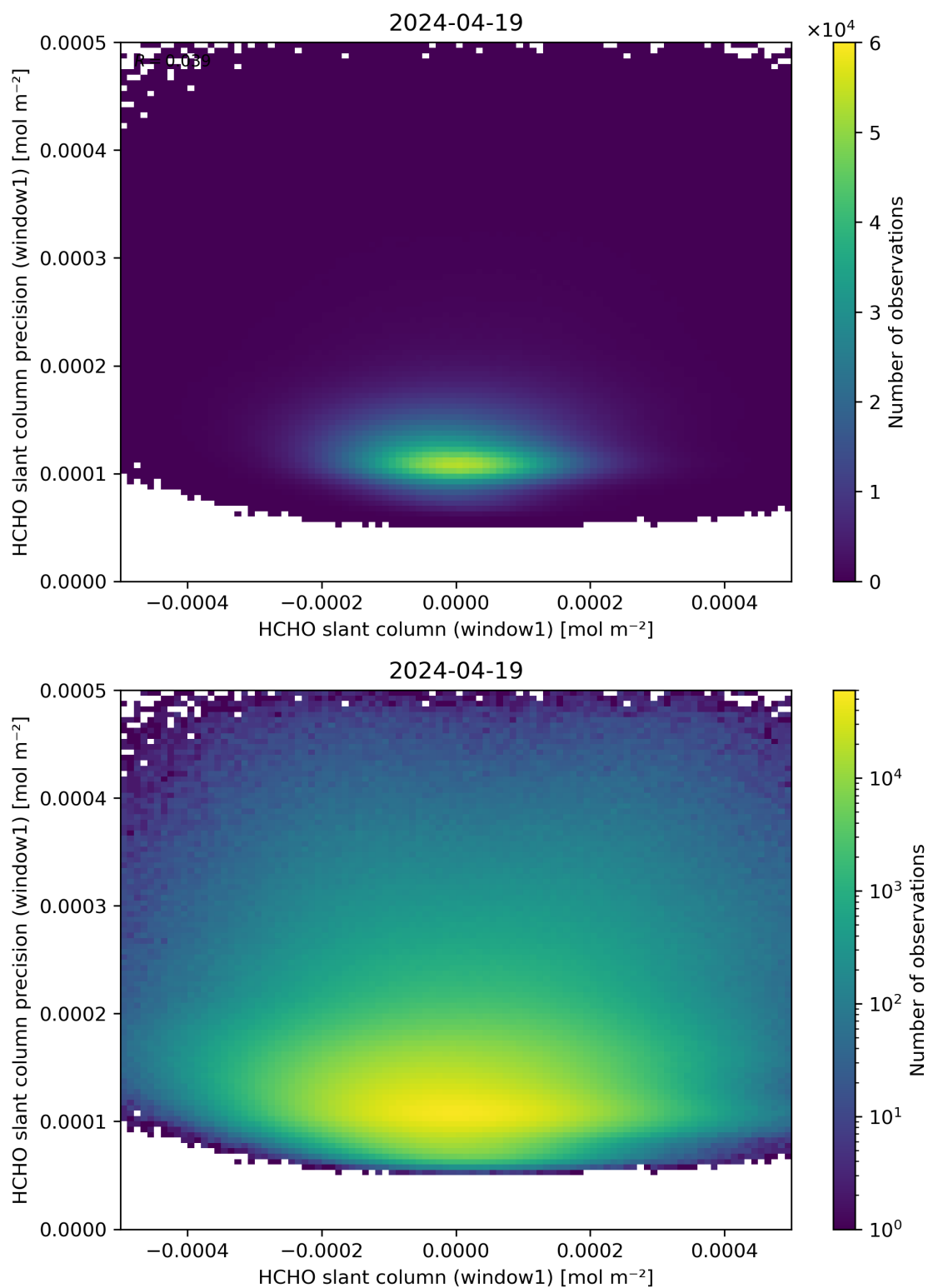
Figure 84: Scatter density plot of “HCHO slant column (window1)” against “HCHO slant column precision (window1)” for 2024-04-18 to 2024-04-20.
