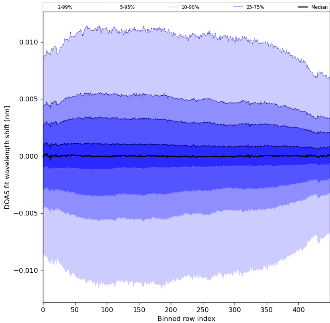
Figure 58: Along track statistics of “DOAS fit wavelength shift” for 2024-04-18 to 2024-04-20
