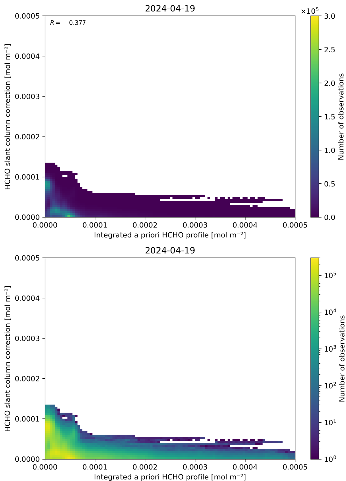
Figure 152: Scatter density plot of “Integrated a priori HCHO profile” against “HCHO slant column correction” for 2024-04-18 to 2024-04-20.
