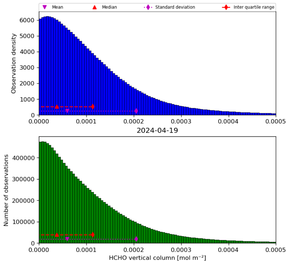
Figure 35: Histogram of “HCHO vertical column” for 2024-04-18 to 2024-04-20
