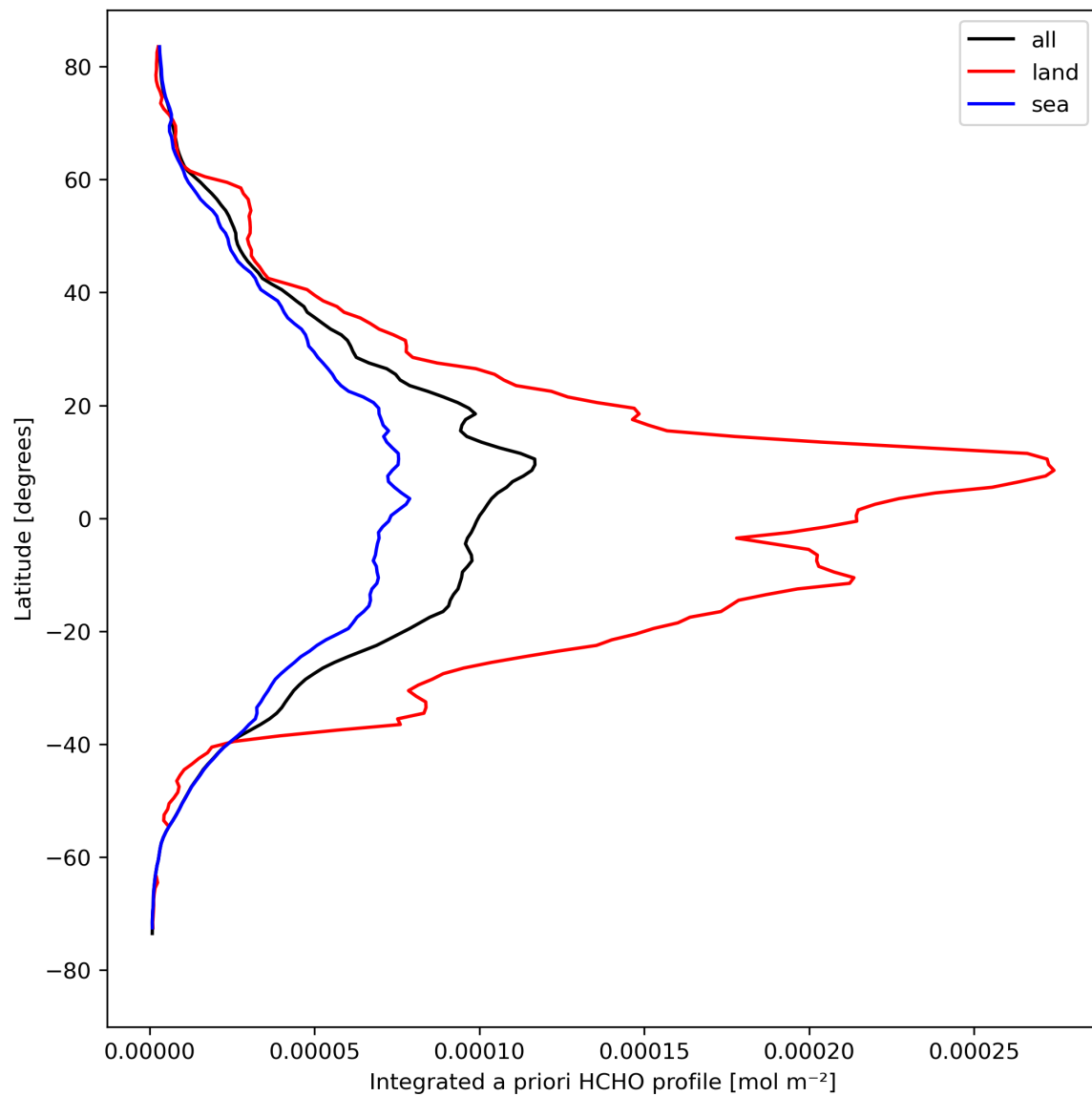
Figure 29: Zonal average of “Integrated a priori HCHO profile” for 2024-04-18 to 2024-04-20.
