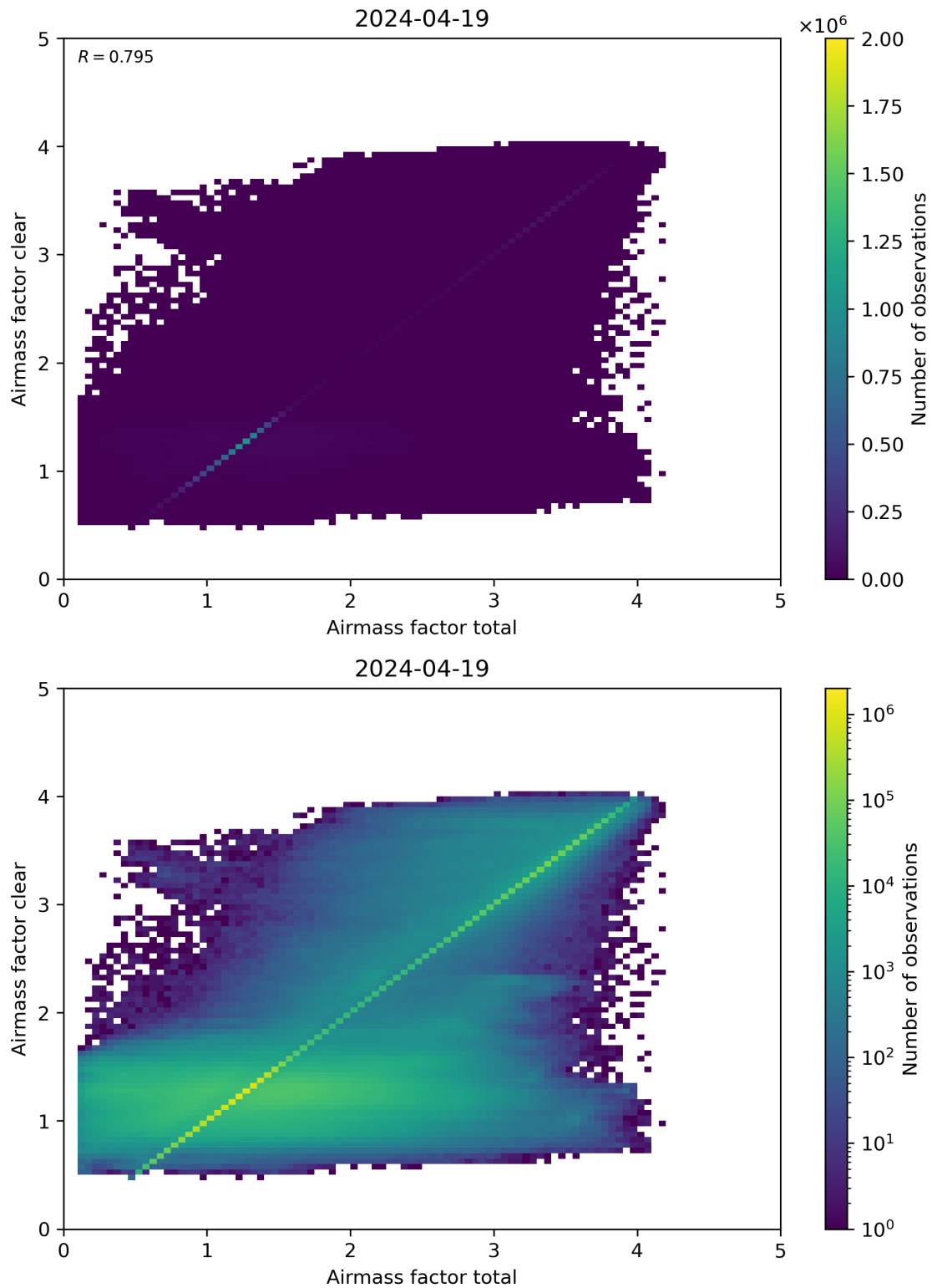
Figure 100: Scatter density plot of “Airmass factor total” against “Airmass factor clear” for 2024-04-18 to 2024-04-20.
