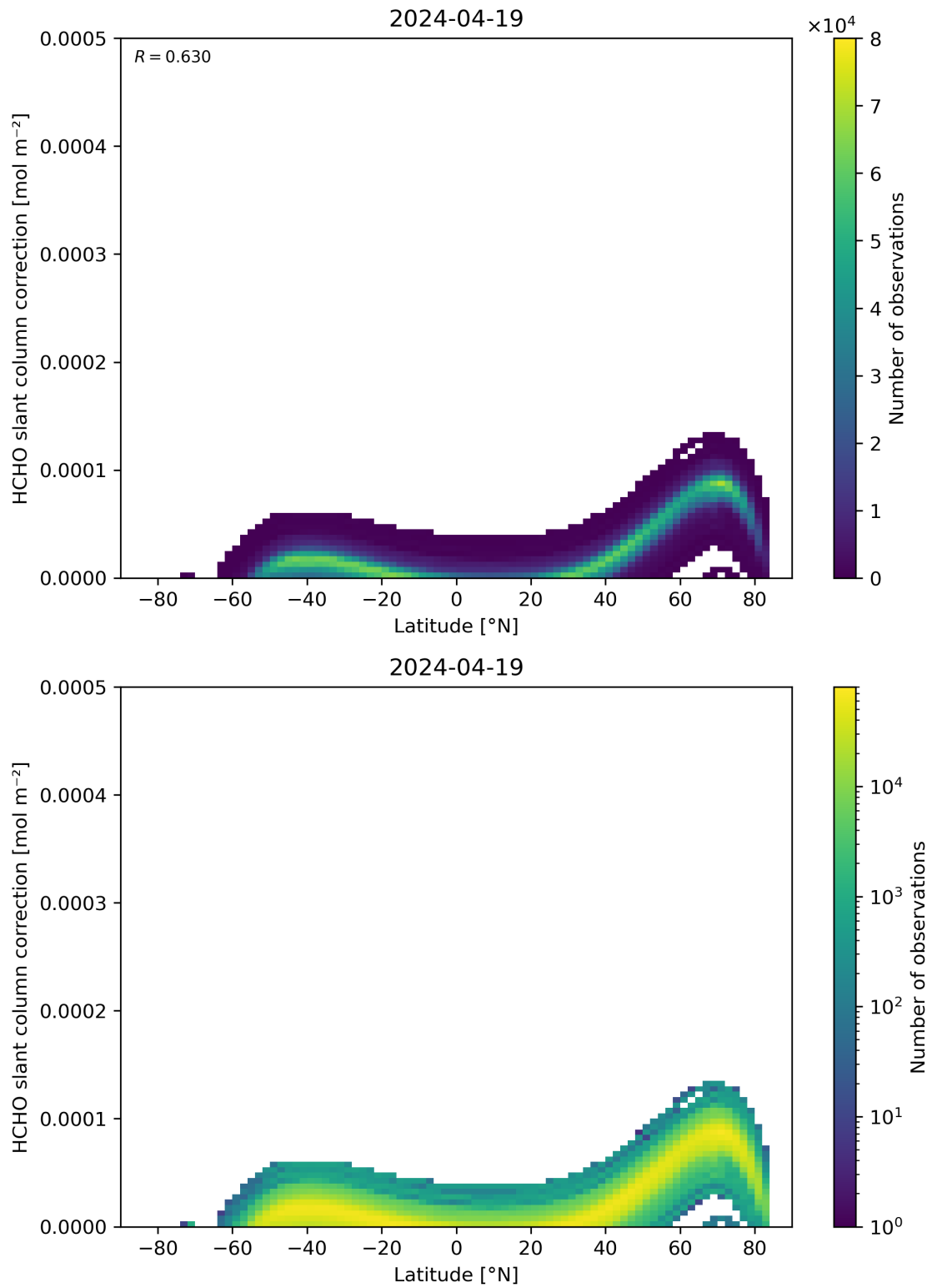
Figure 158: Scatter density plot of “Latitude” against “HCHO slant column correction” for 2024-04-18 to 2024-04-20.
