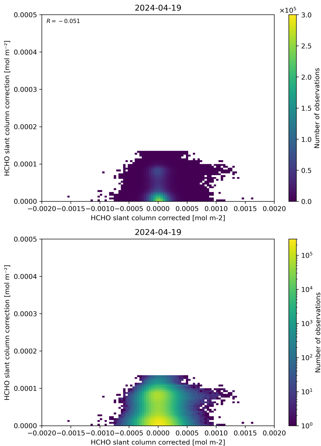
Figure 77: Scatter density plot of “HCHO slant column corrected” against “HCHO slant column correction” for 2024-04-18 to 2024-04-20.
