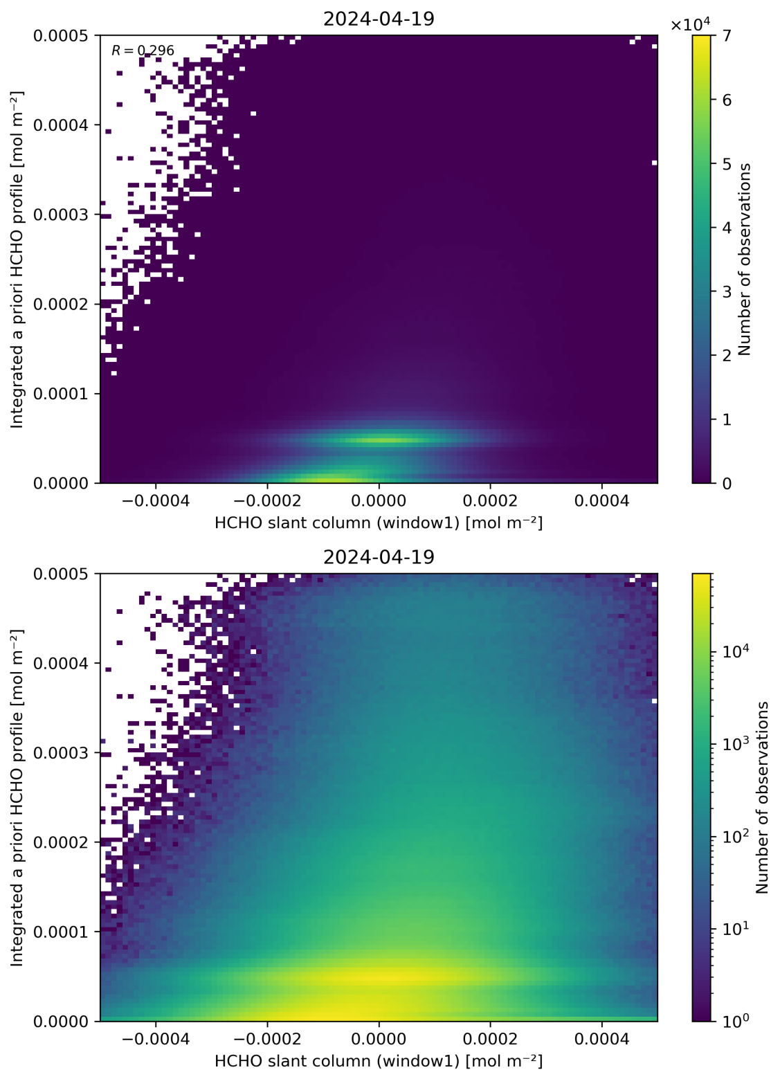
Figure 87: Scatter density plot of “HCHO slant column (window1)” against “Integrated a priori HCHO profile” for 2024-04-18 to 2024-04-20.
