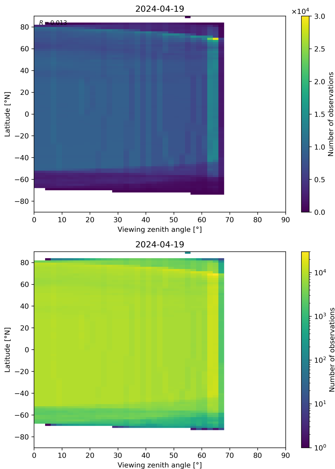
Figure 196: Scatter density plot of “Viewing zenith angle” against “Latitude” for 2024-04-18 to 2024-04-20.
