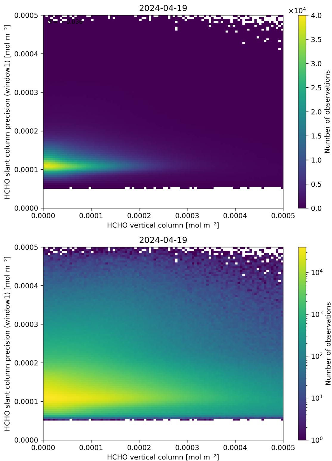
Figure 130: Scatter density plot of “HCHO vertical column” against “HCHO slant column precision (window1)” for 2024-04-18 to 2024-04-20.
