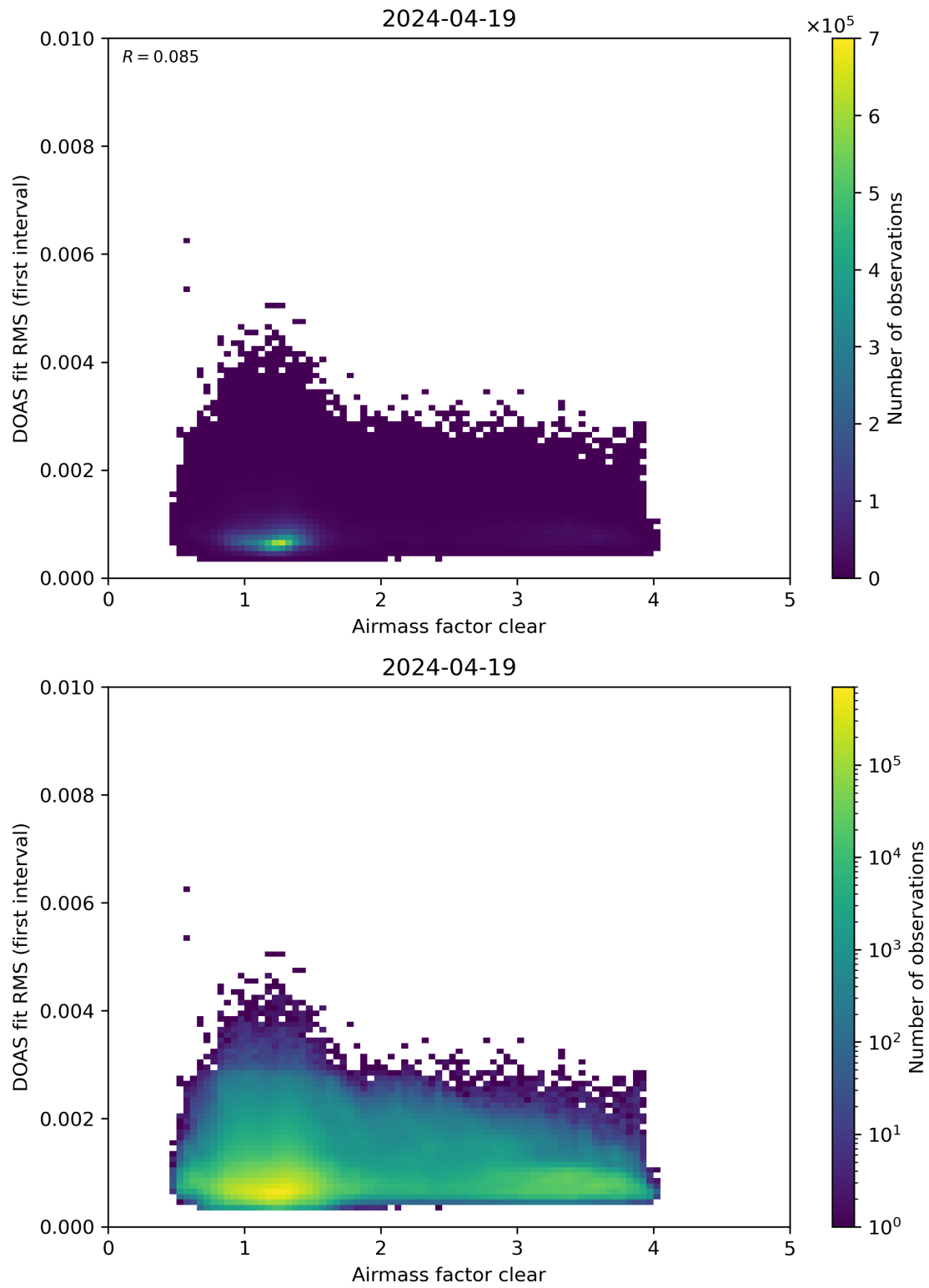
Figure 71: Scatter density plot of “Airmass factor clear” against “DOAS fit RMS (first interval)” for 2024-04-18 to 2024-04-20.
