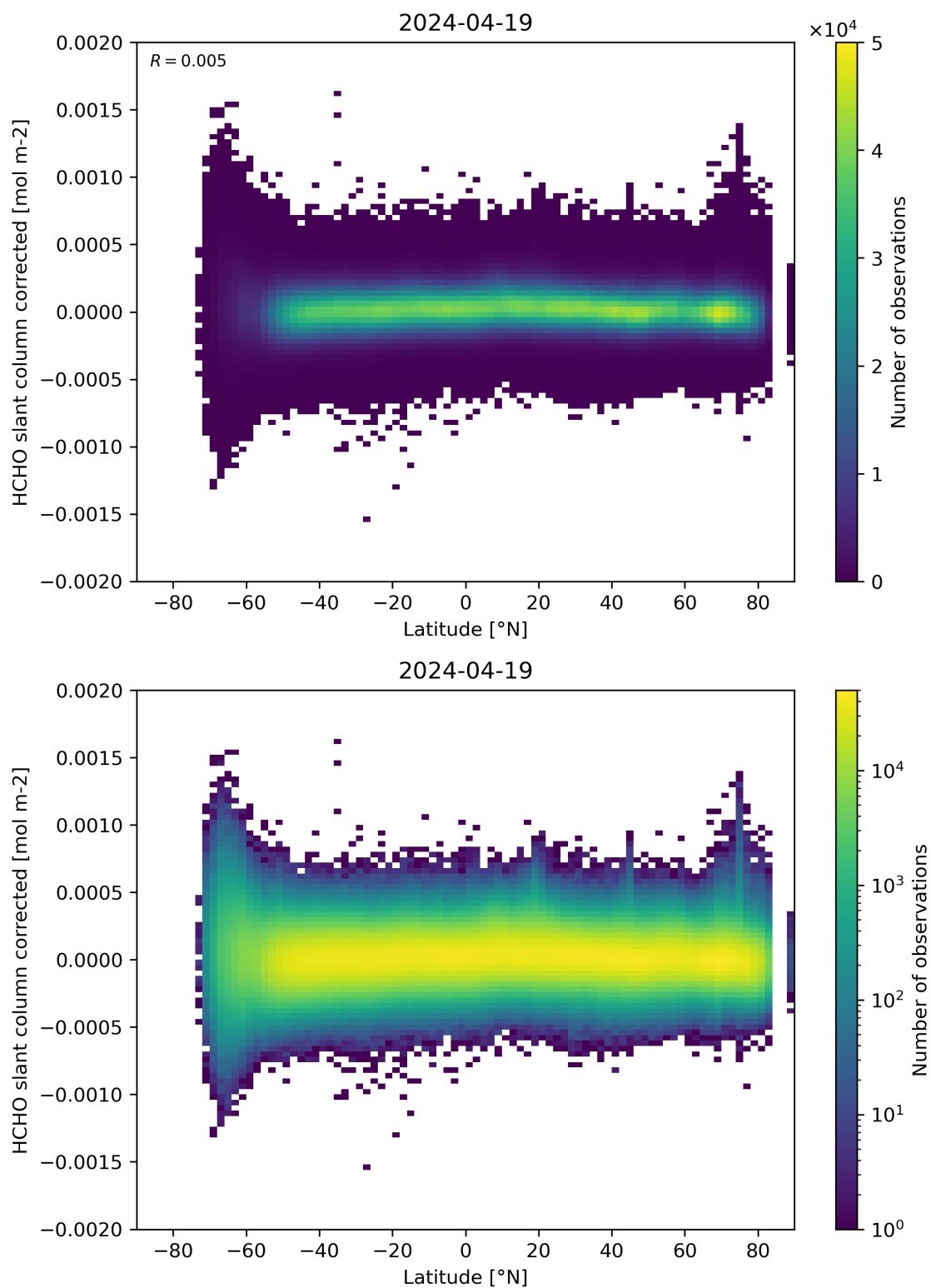
Figure 157: Scatter density plot of “Latitude” against “HCHO slant column corrected” for 2024-04-18 to 2024-04-20.
