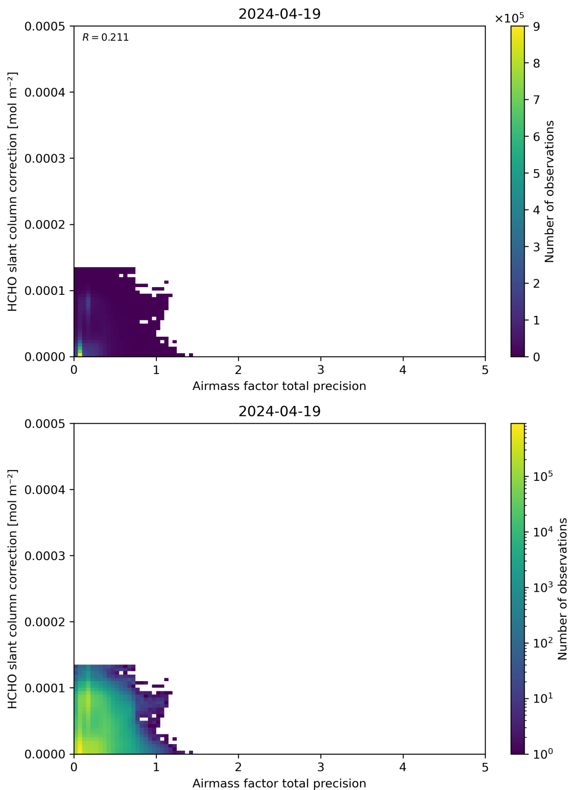
Figure 110: Scatter density plot of “Airmass factor total precision” against “HCHO slant column correction” for 2024-04-18 to 2024-04-20.
