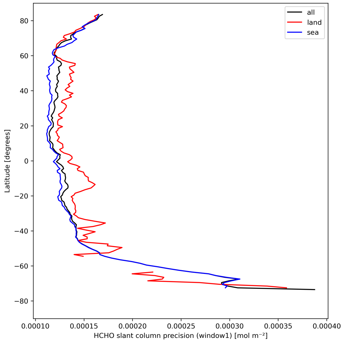
Figure 25: Zonal average of “HCHO slant column precision (window1)” for 2024-04-18 to 2024-04-20.
