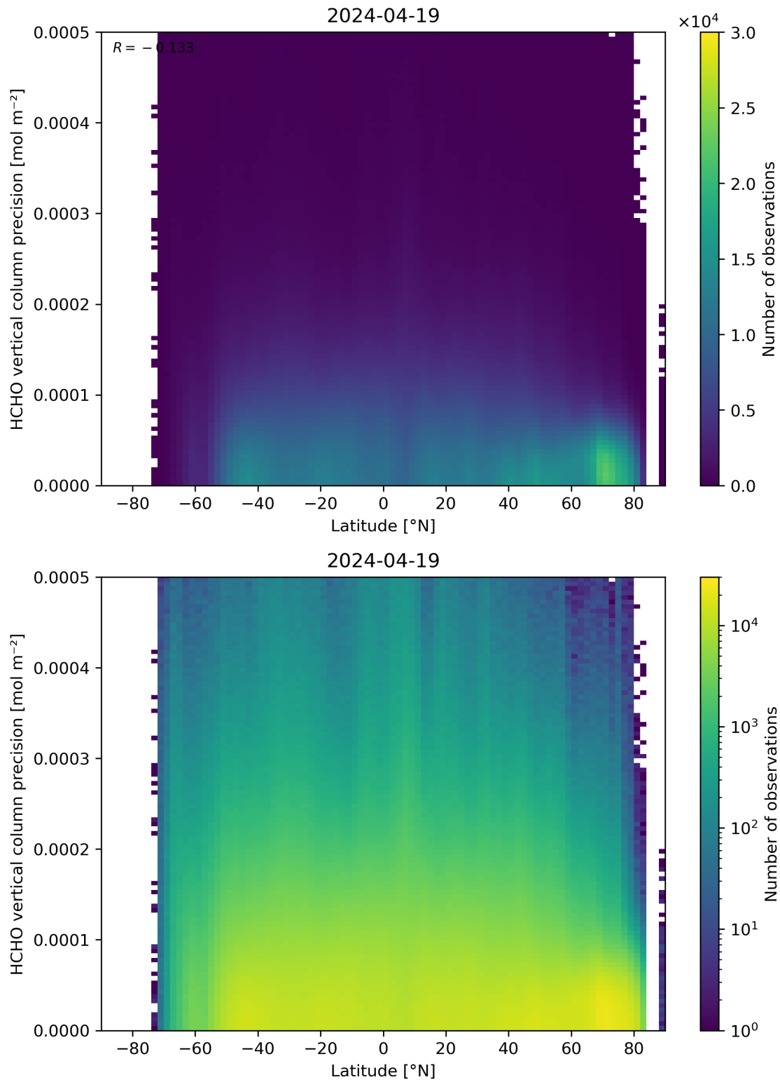
Figure 165: Scatter density plot of “Latitude” against “HCHO vertical column precision” for 2024-04-18 to 2024-04-20.
