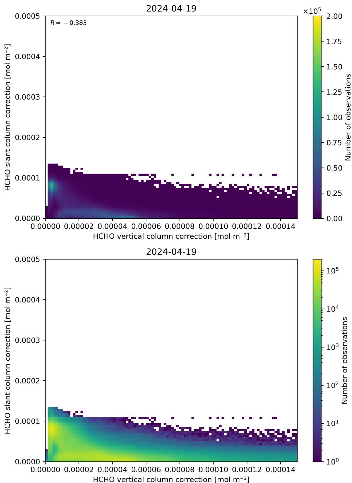
Figure 117: Scatter density plot of “HCHO vertical column correction” against “HCHO slant column correction” for 2024-04-18 to 2024-04-20.
