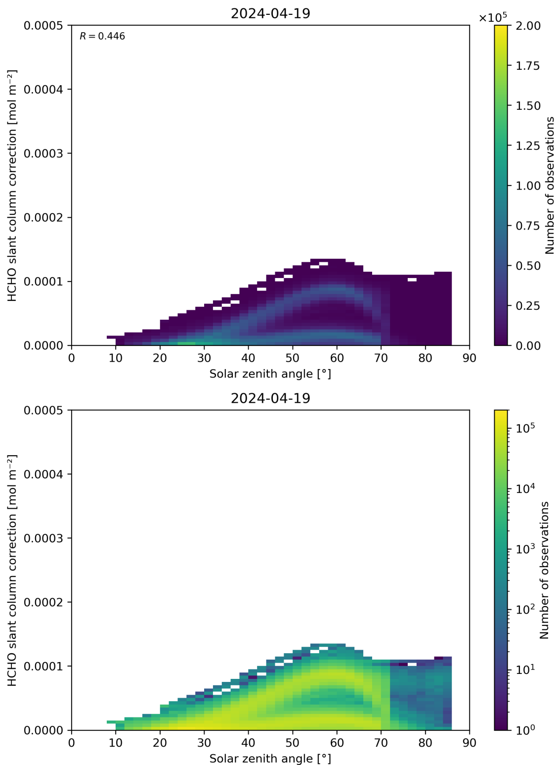
Figure 172: Scatter density plot of “Solar zenith angle” against “HCHO slant column correction” for 2024-04-18 to 2024-04-20.
