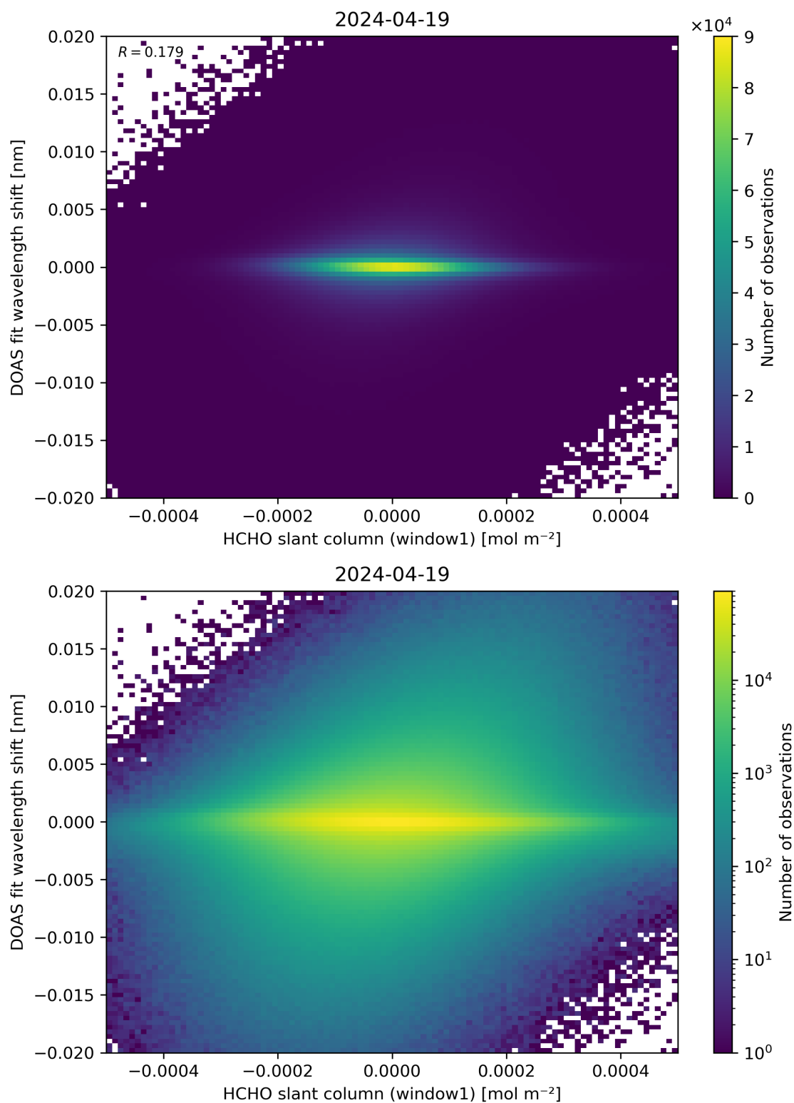
Figure 79: Scatter density plot of “HCHO slant column (window1)” against “DOAS fit wavelength shift” for 2024-04-18 to 2024-04-20.
