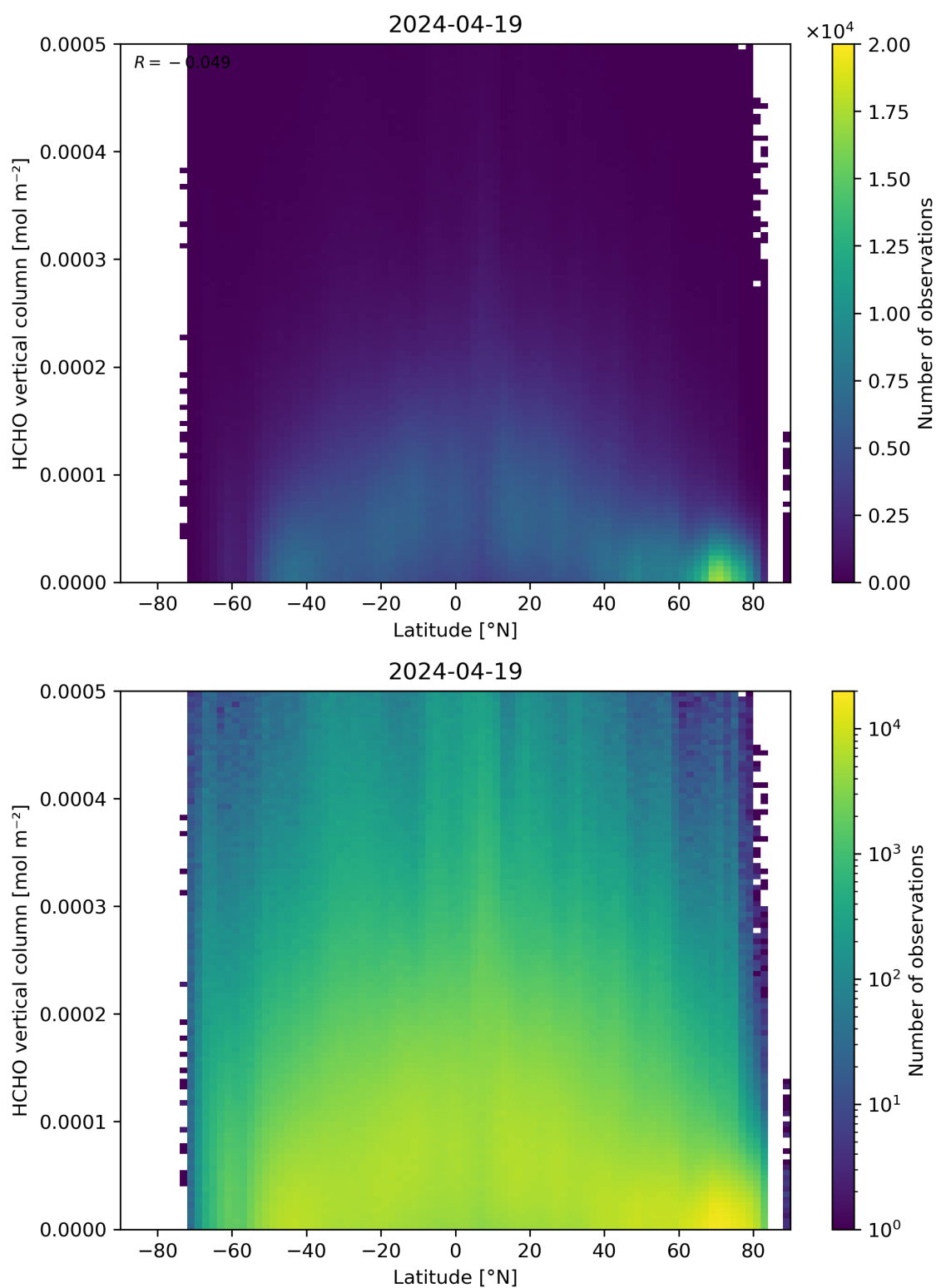
Figure 163: Scatter density plot of “Latitude” against “HCHO vertical column” for 2024-04-18 to 2024-04-20.
