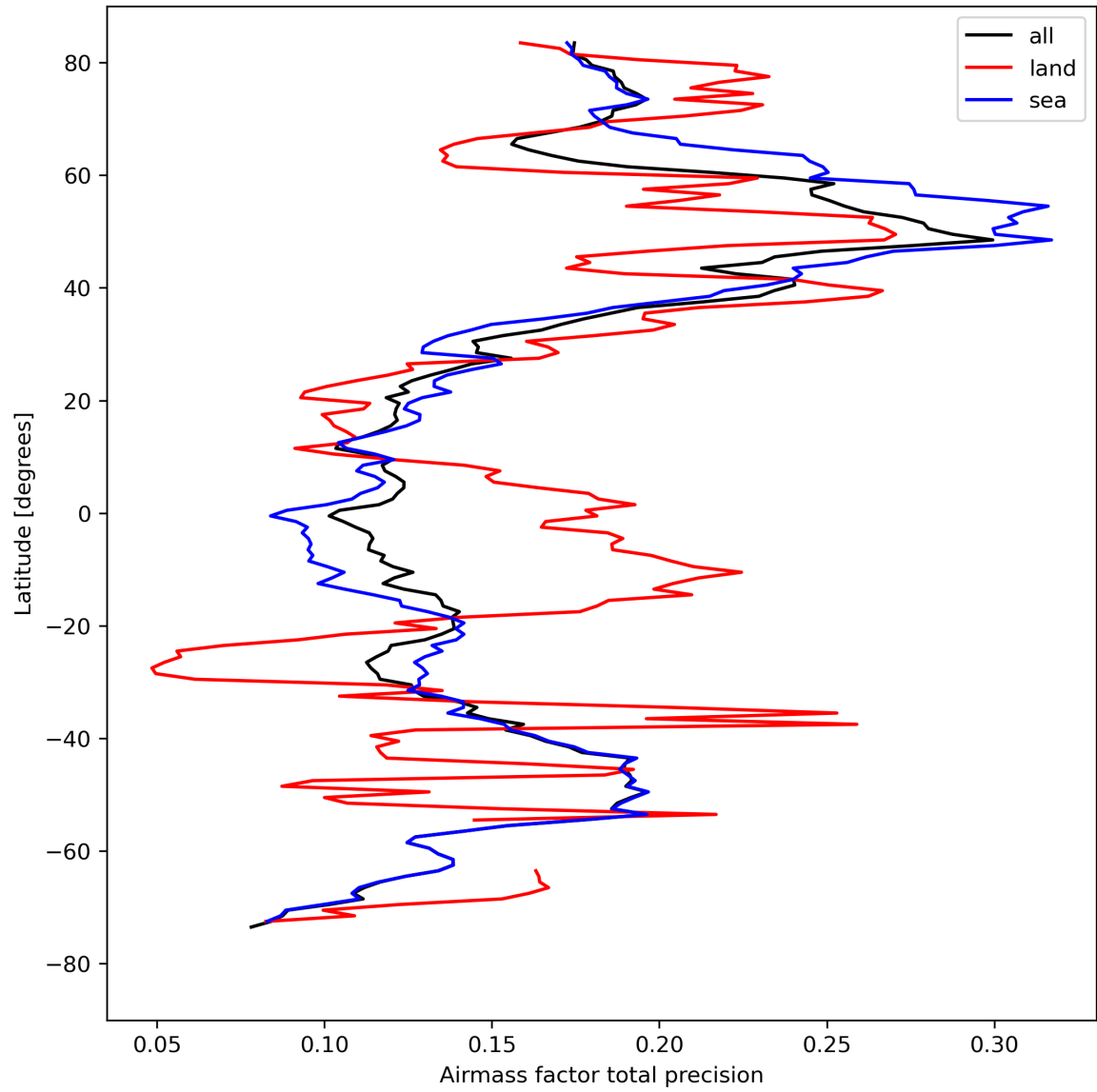
Figure 27: Zonal average of “Airmass factor total precision” for 2024-04-18 to 2024-04-20.
