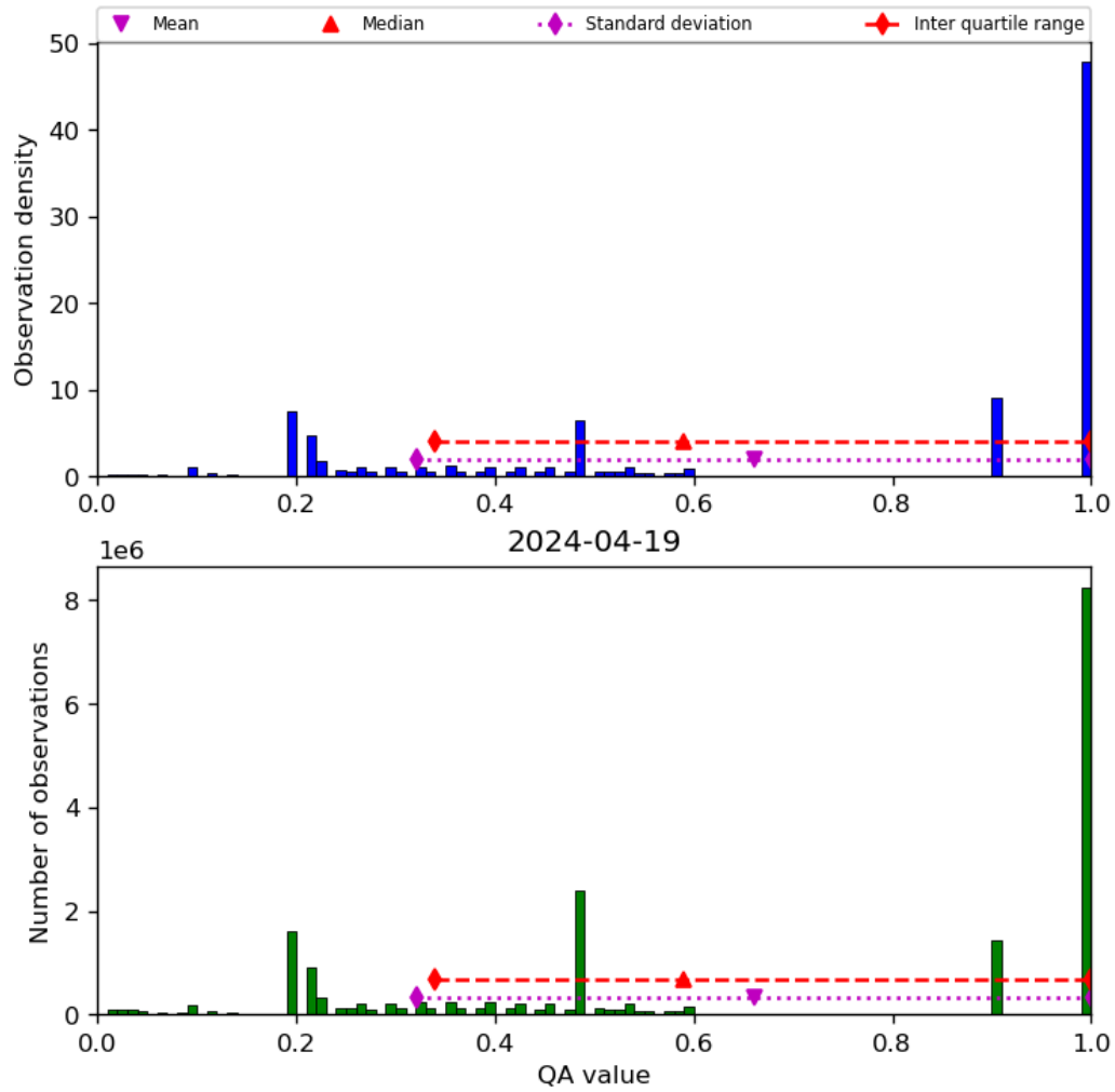
Figure 34: Histogram of “QA value” for 2024-04-18 to 2024-04-20
