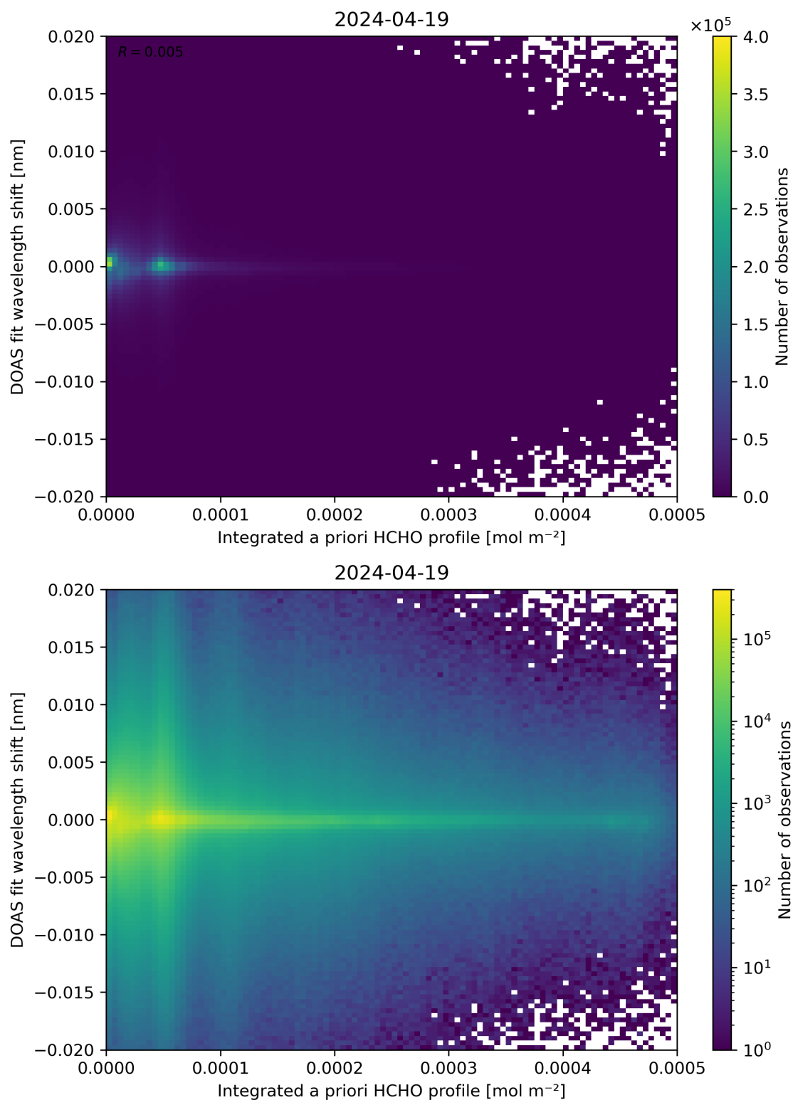
Figure 149: Scatter density plot of “Integrated a priori HCHO profile” against “DOAS fit wavelength shift” for 2024-04-18 to 2024-04-20.
