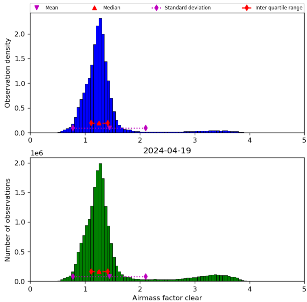
Figure 42: Histogram of “Airmass factor clear” for 2024-04-18 to 2024-04-20
