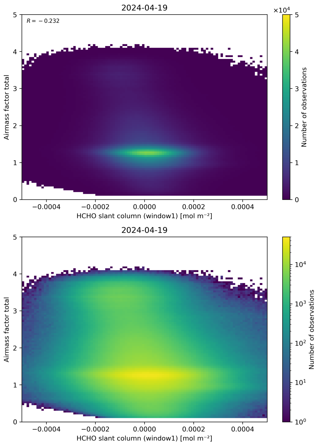
Figure 85: Scatter density plot of “HCHO slant column (window1)” against “Airmass factor total” for 2024-04-18 to 2024-04-20.
