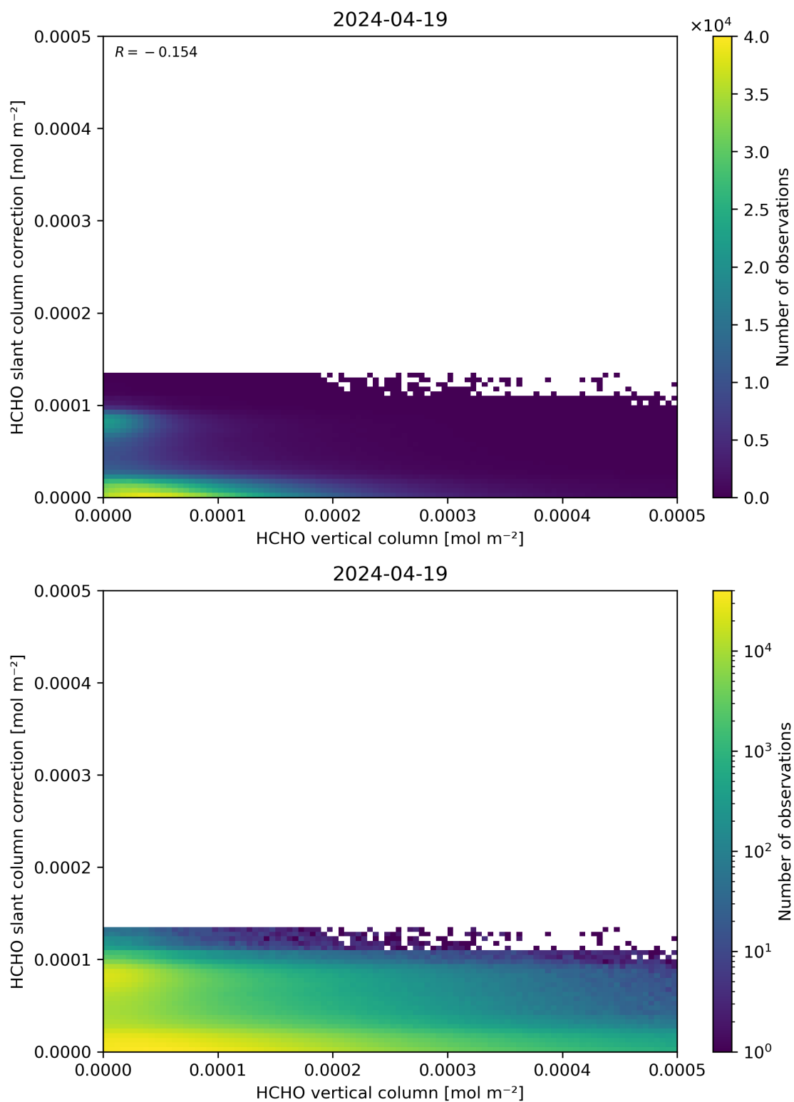
Figure 128: Scatter density plot of “HCHO vertical column” against “HCHO slant column correction” for 2024-04-18 to 2024-04-20.
