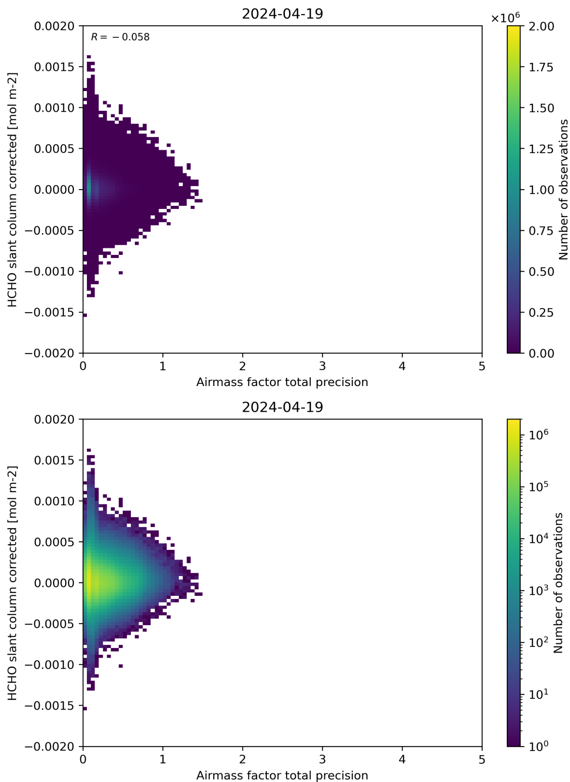
Figure 109: Scatter density plot of “Airmass factor total precision” against “HCHO slant column corrected” for 2024-04-18 to 2024-04-20.
