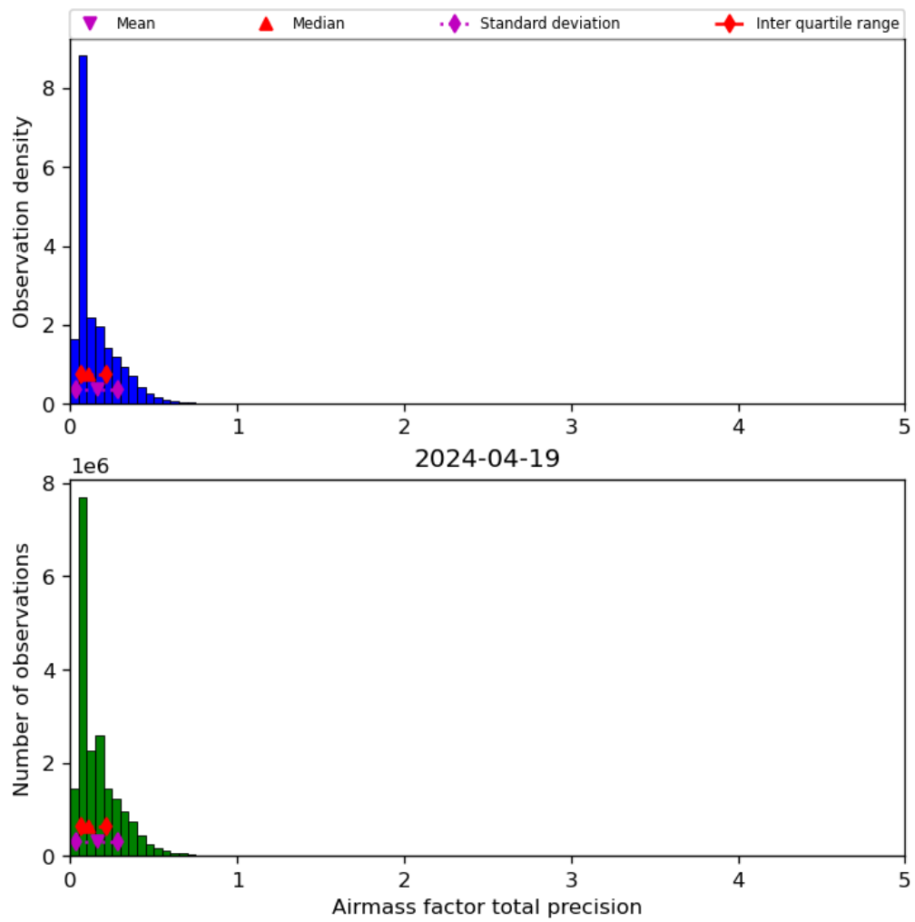
Figure 41: Histogram of "Airmass factor total precision" for 2024-04-18 to 2024-04-20
