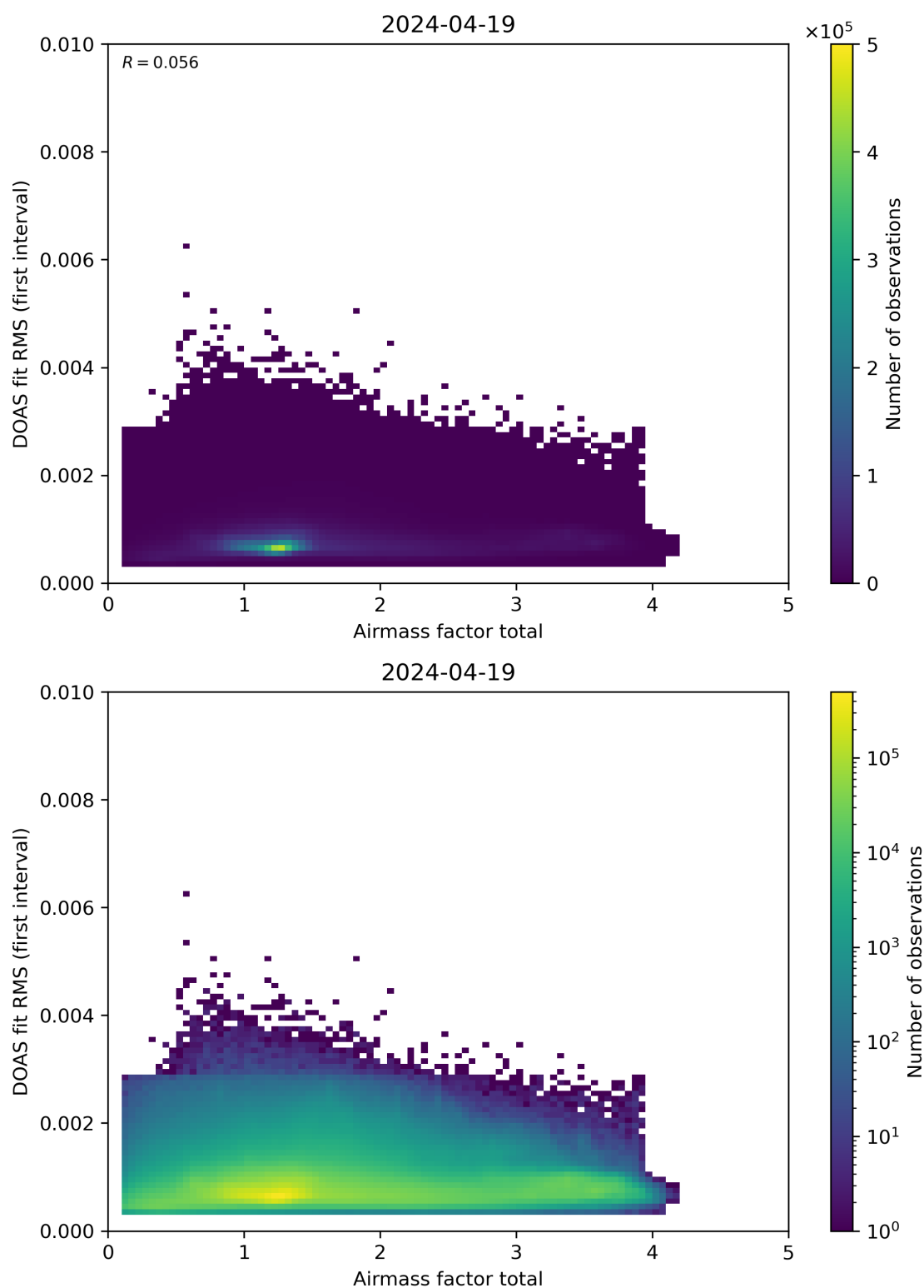
Figure 97: Scatter density plot of “Airmass factor total” against “DOAS fit RMS (first interval)” for 2024-04-18 to 2024-04-20.
