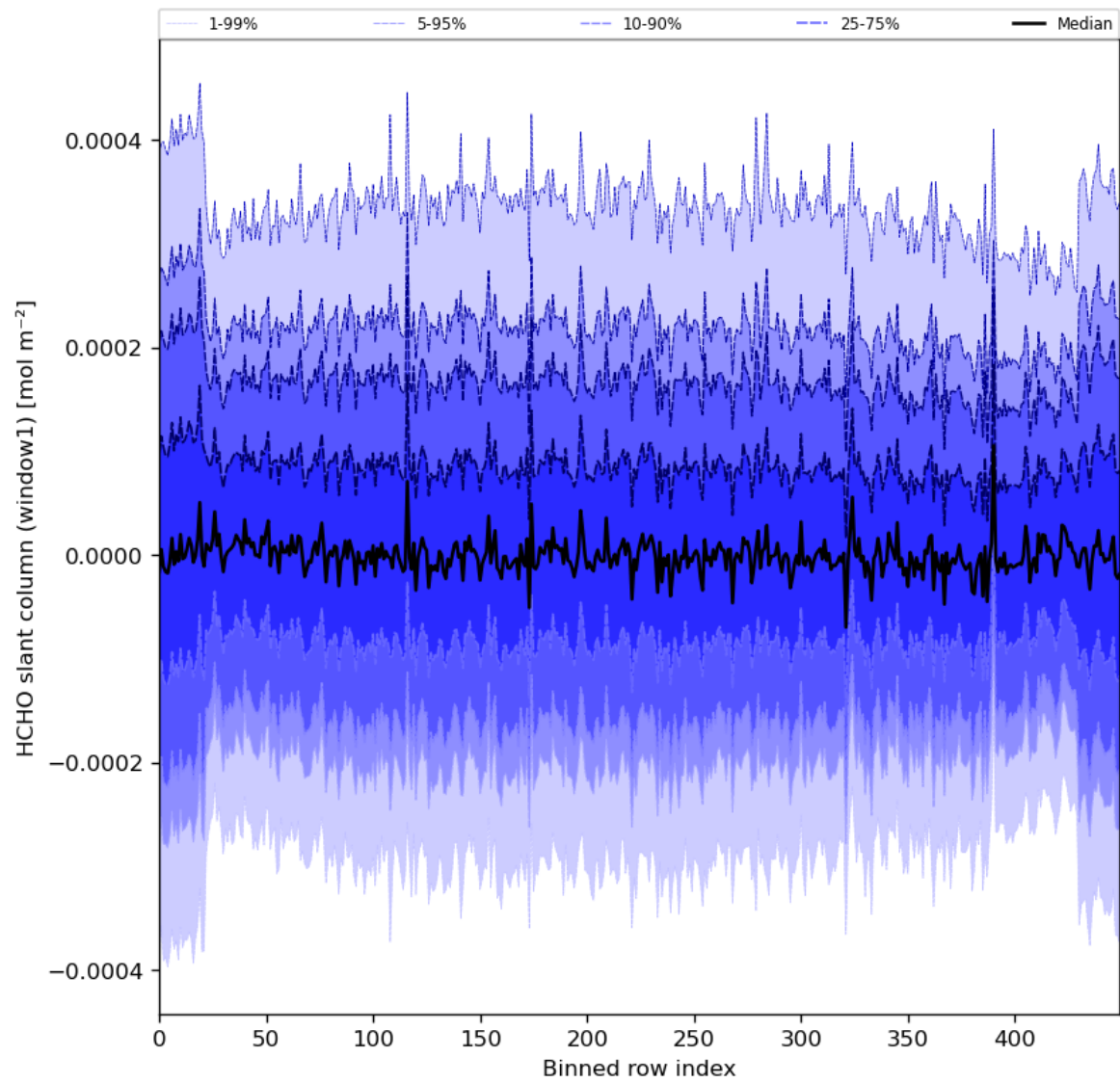
Figure 52: Along track statistics of “HCHO slant column (window1)” for 2024-04-18 to 2024-04-20
