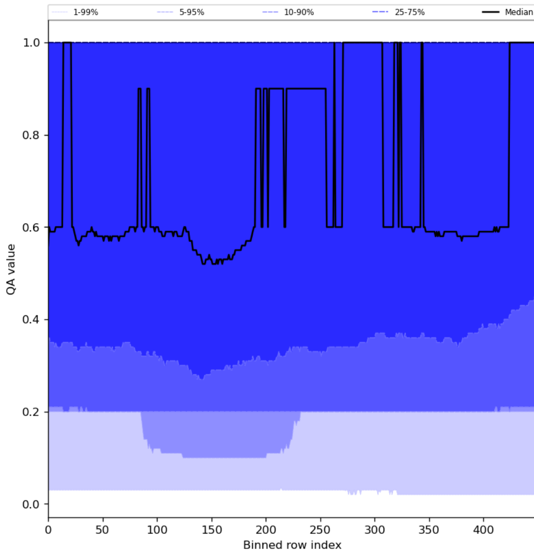
Figure 48: Along track statistics of “QA value” for 2024-04-18 to 2024-04-20
