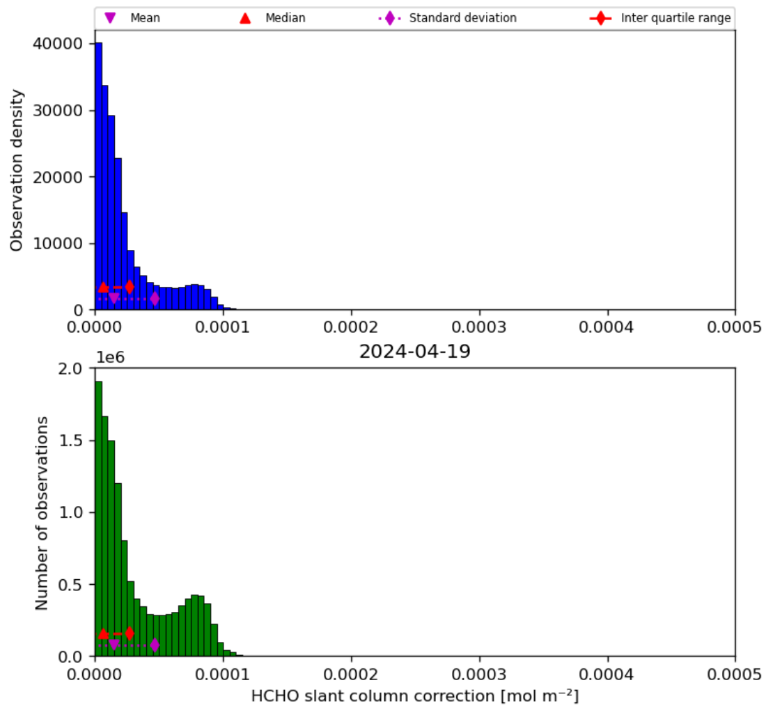
Figure 47: Histogram of “HCHO slant column correction” for 2024-04-18 to 2024-04-20
