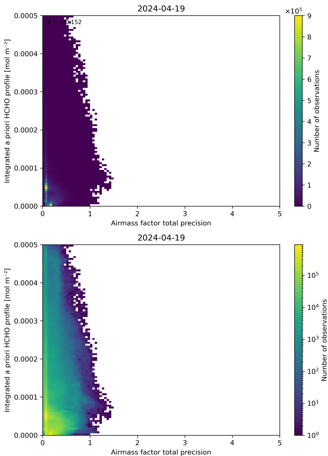
Figure 111: Scatter density plot of “Airmass factor total precision” against “Integrated a priori HCHO profile” for 2024-04-18 to 2024-04-20.
