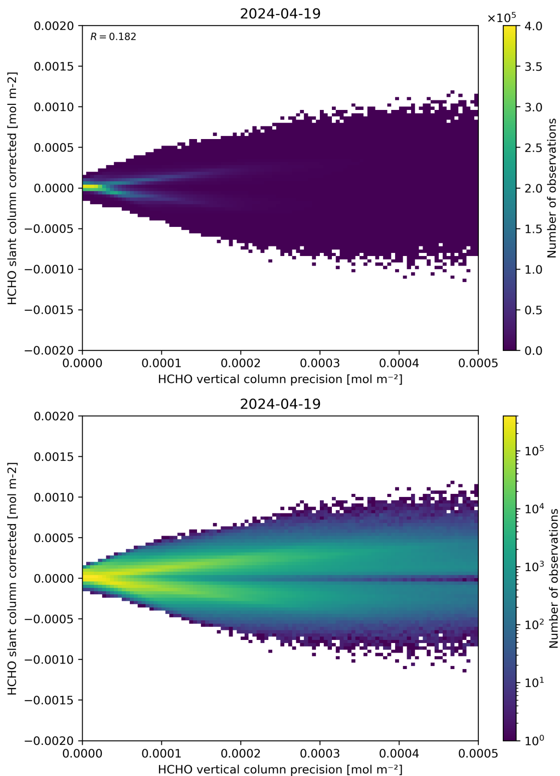
Figure 140: Scatter density plot of “HCHO vertical column precision” against “HCHO slant column corrected” for 2024-04-18 to 2024-04-20.
