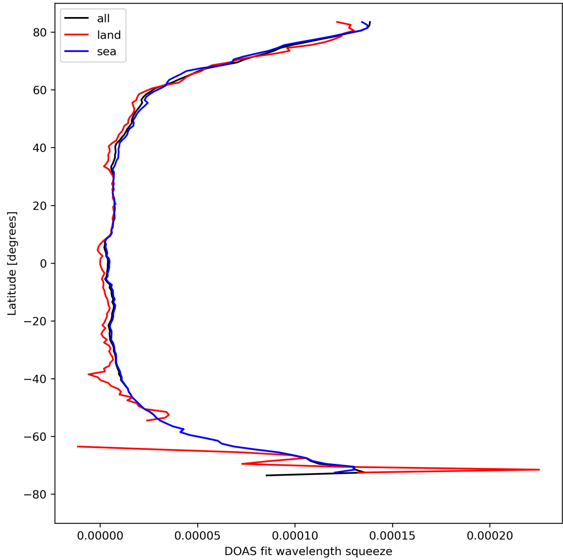
Figure 31: Zonal average of “DOAS fit wavelength squeeze” for 2024-04-18 to 2024-04-20.
