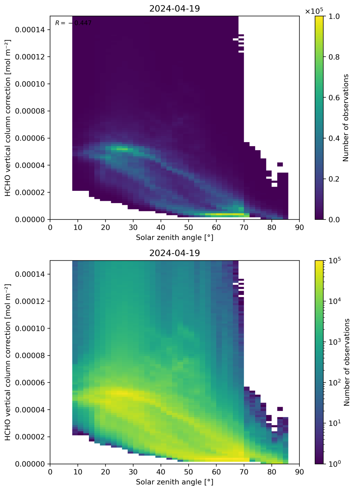
Figure 178: Scatter density plot of “Solar zenith angle” against “HCHO vertical column correction” for 2024-04-18 to 2024-04-20.
