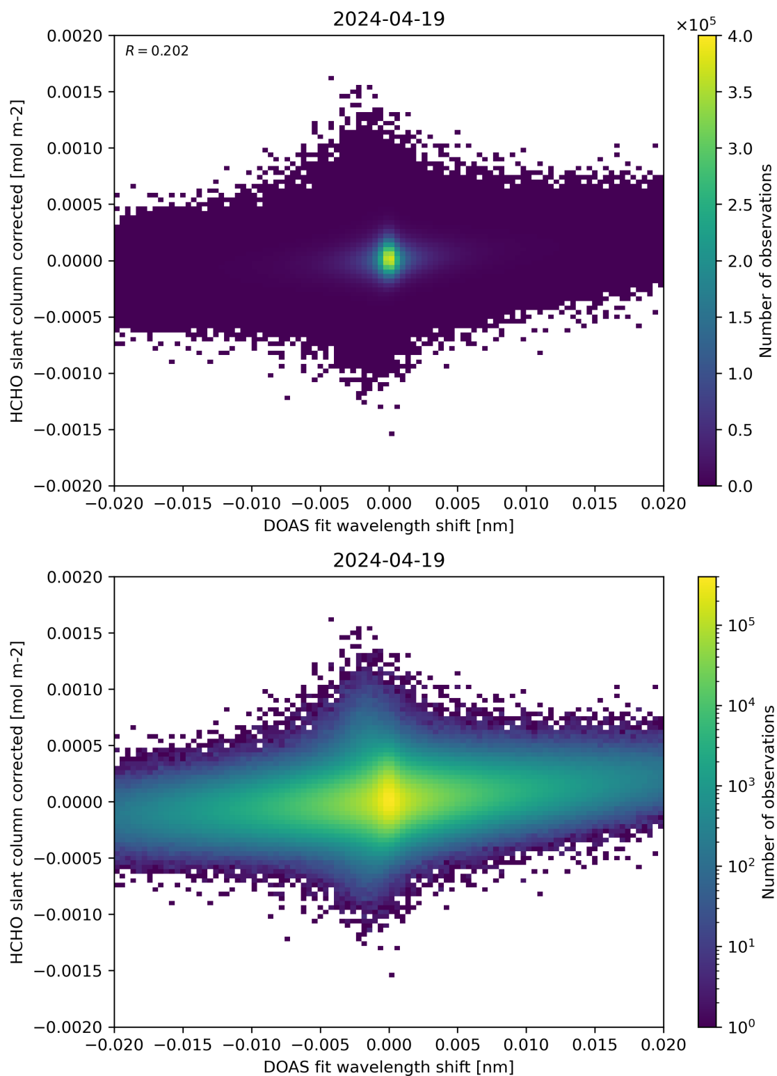
Figure 66: Scatter density plot of “DOAS fit wavelength shift” against “HCHO slant column corrected” for 2024-04-18 to 2024-04-20.
