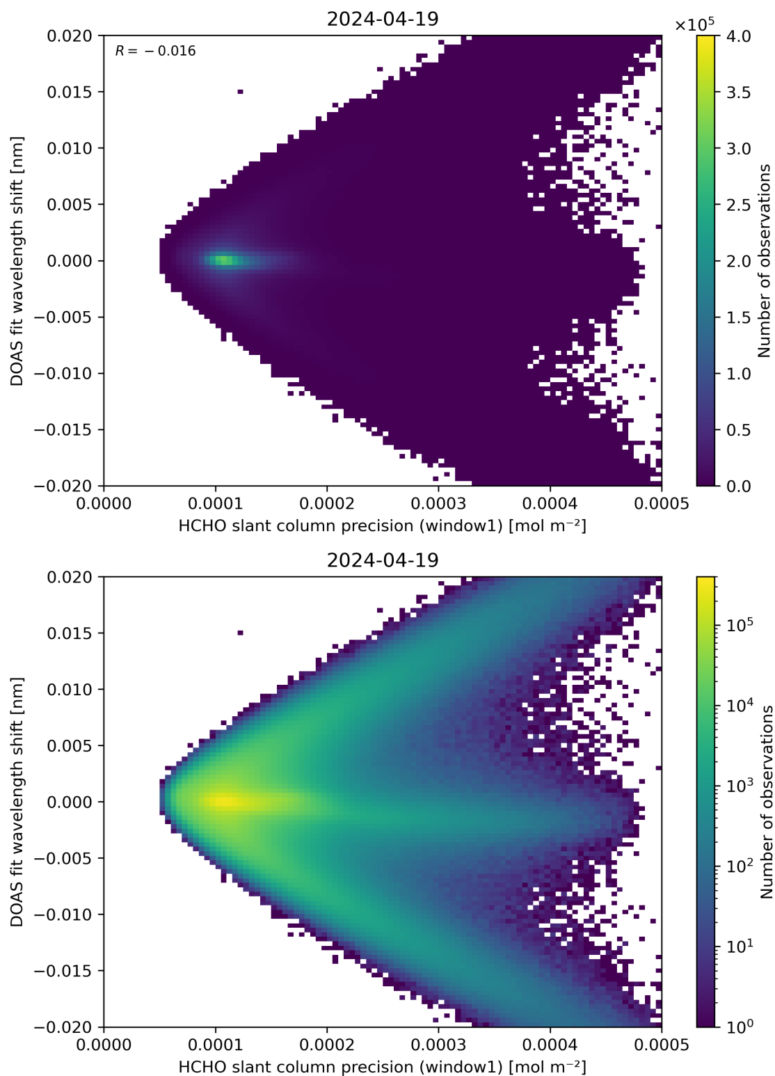
Figure 89: Scatter density plot of “HCHO slant column precision (window1)” against “DOAS fit wavelength shift” for 2024-04-18 to 2024-04-20.
