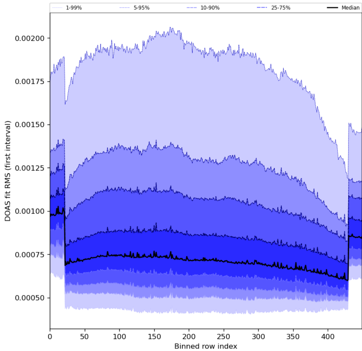
Figure 60: Along track statistics of “DOAS fit RMS (first interval)” for 2024-04-18 to 2024-04-20
