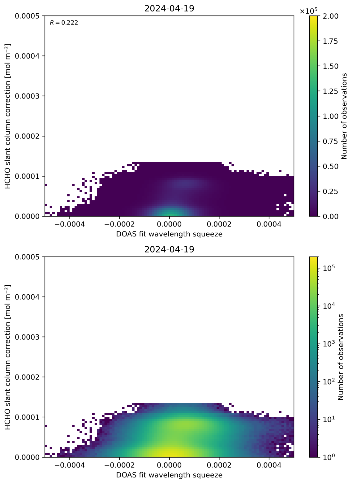
Figure 70: Scatter density plot of “DOAS fit wavelength squeeze” against “HCHO slant column correction” for 2024-04-18 to 2024-04-20.
