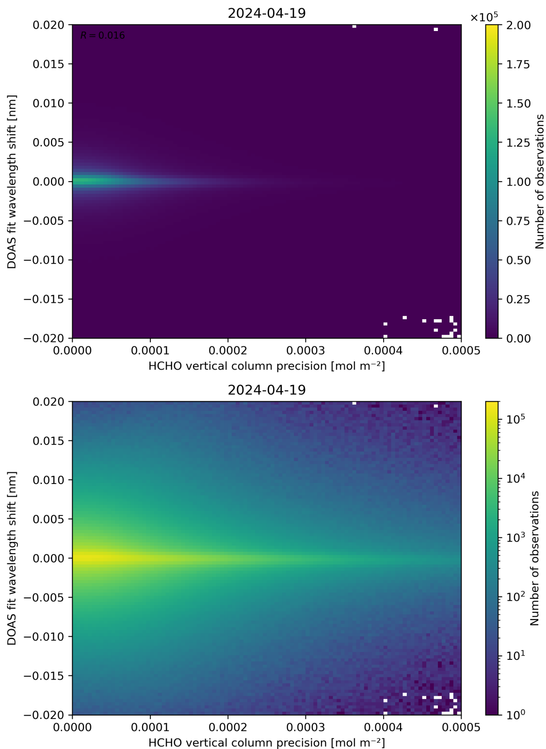
Figure 137: Scatter density plot of “HCHO vertical column precision” against “DOAS fit wavelength shift” for 2024-04-18 to 2024-04-20.
