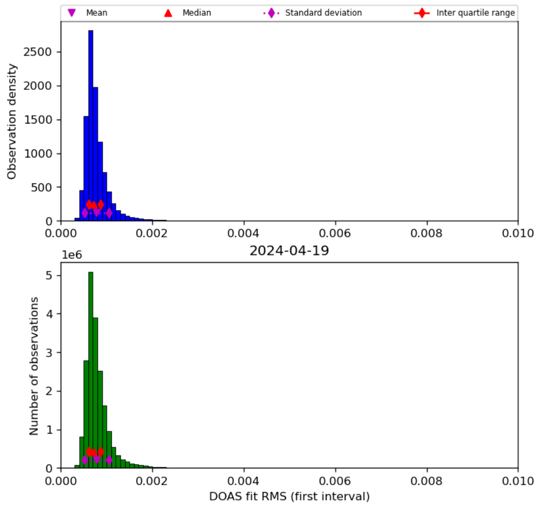
Figure 46: Histogram of “DOAS fit RMS (first interval)” for 2024-04-18 to 2024-04-20
