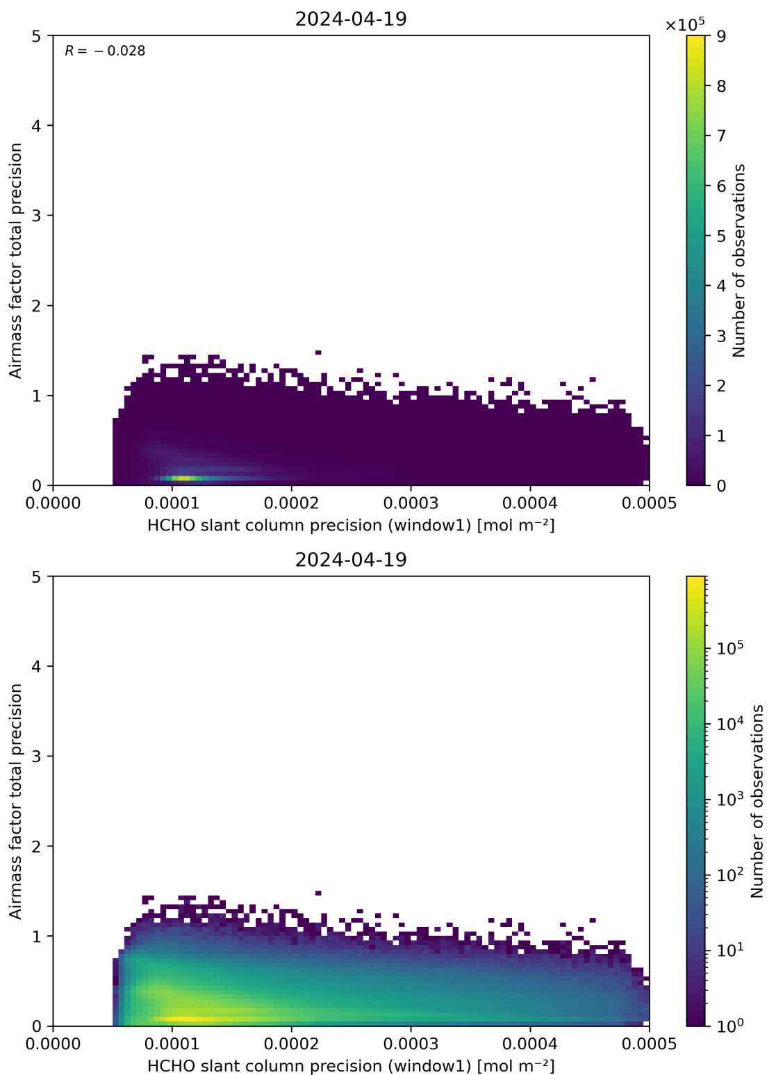
Figure 95: Scatter density plot of “HCHO slant column precision (window1)” against “Airmass factor total precision” for 2024-04-18 to 2024-04-20.
