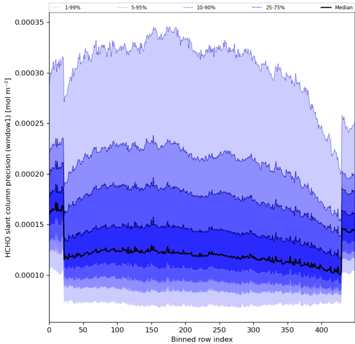
Figure 53: Along track statistics of “HCHO slant column precision (window1)” for 2024-04-18 to 2024-04-20
