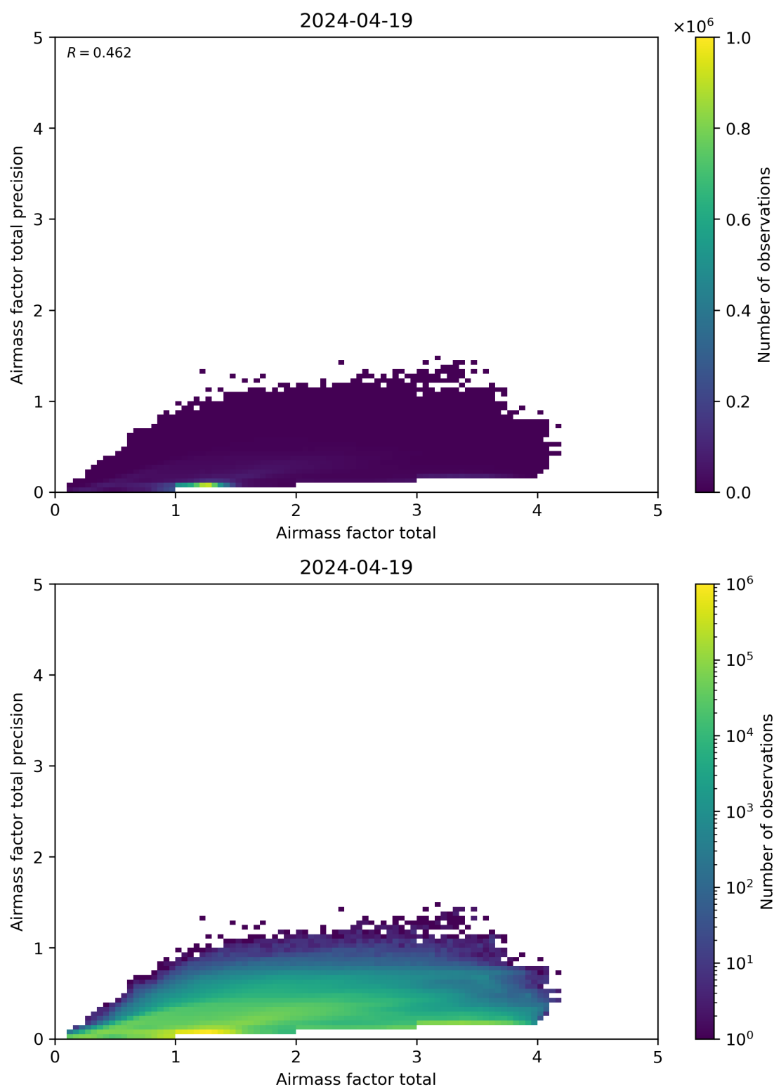
Figure 103: Scatter density plot of “Airmass factor total” against “Airmass factor total precision” for 2024-04-18 to 2024-04-20.
