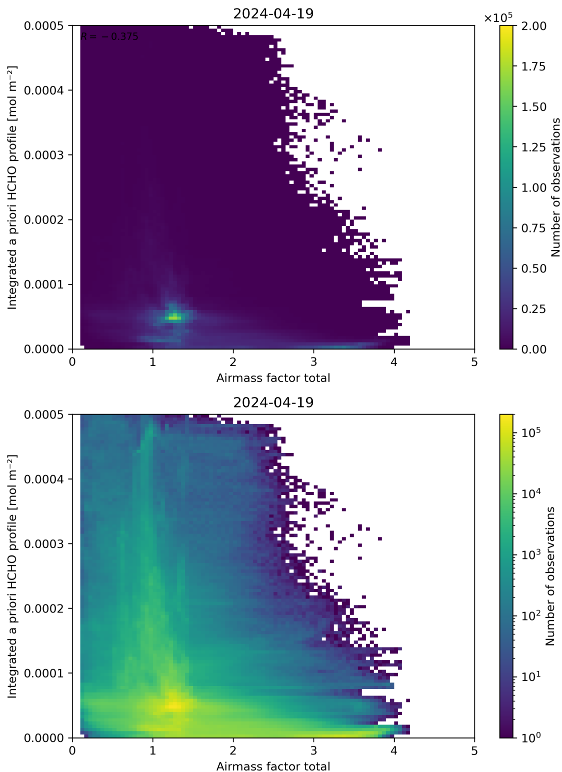
Figure 104: Scatter density plot of “Air mass factor total” against “Integrated a priori HCHO profile” for 2024-04-18 to 2024-04-20.
