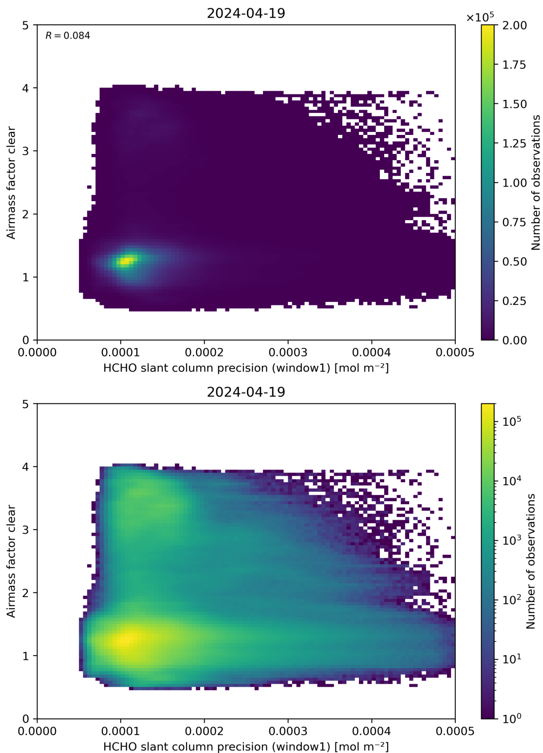
Figure 91: Scatter density plot of “HCHO slant column precision (window1)” against “Airmass factor clear” for 2024-04-18 to 2024-04-20.
