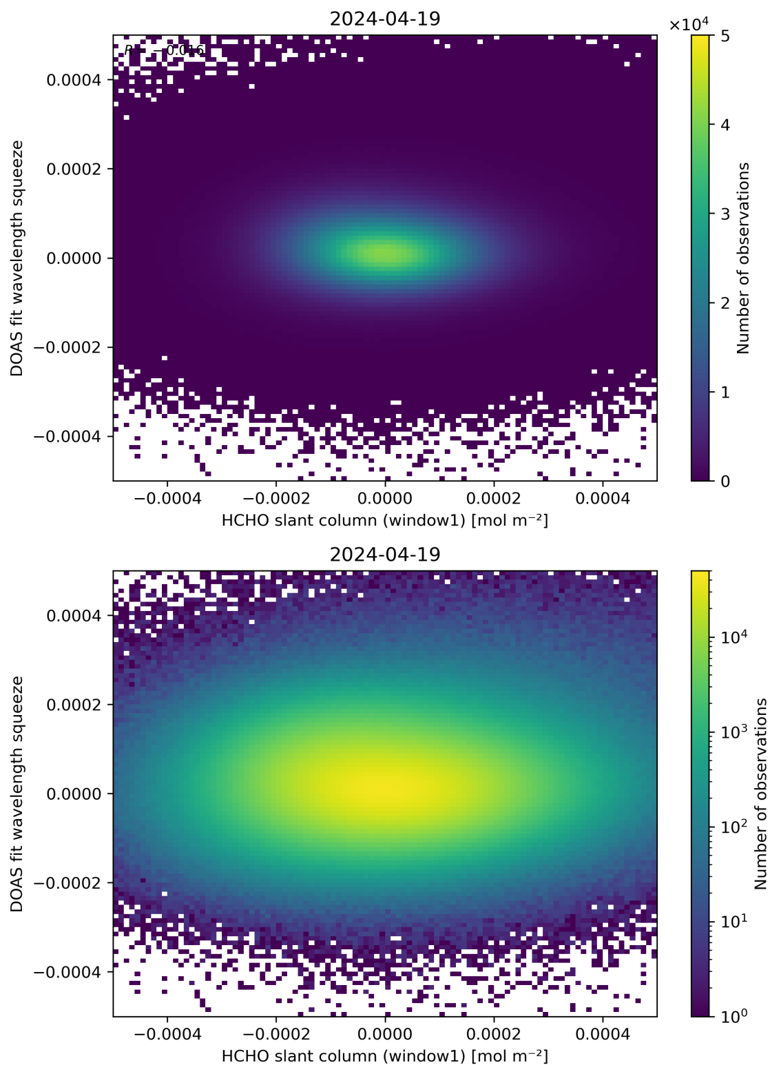
Figure 80: Scatter density plot of “HCHO slant column (window1)” against “DOAS fit wavelength squeeze” for 2024-04-18 to 2024-04-20.
