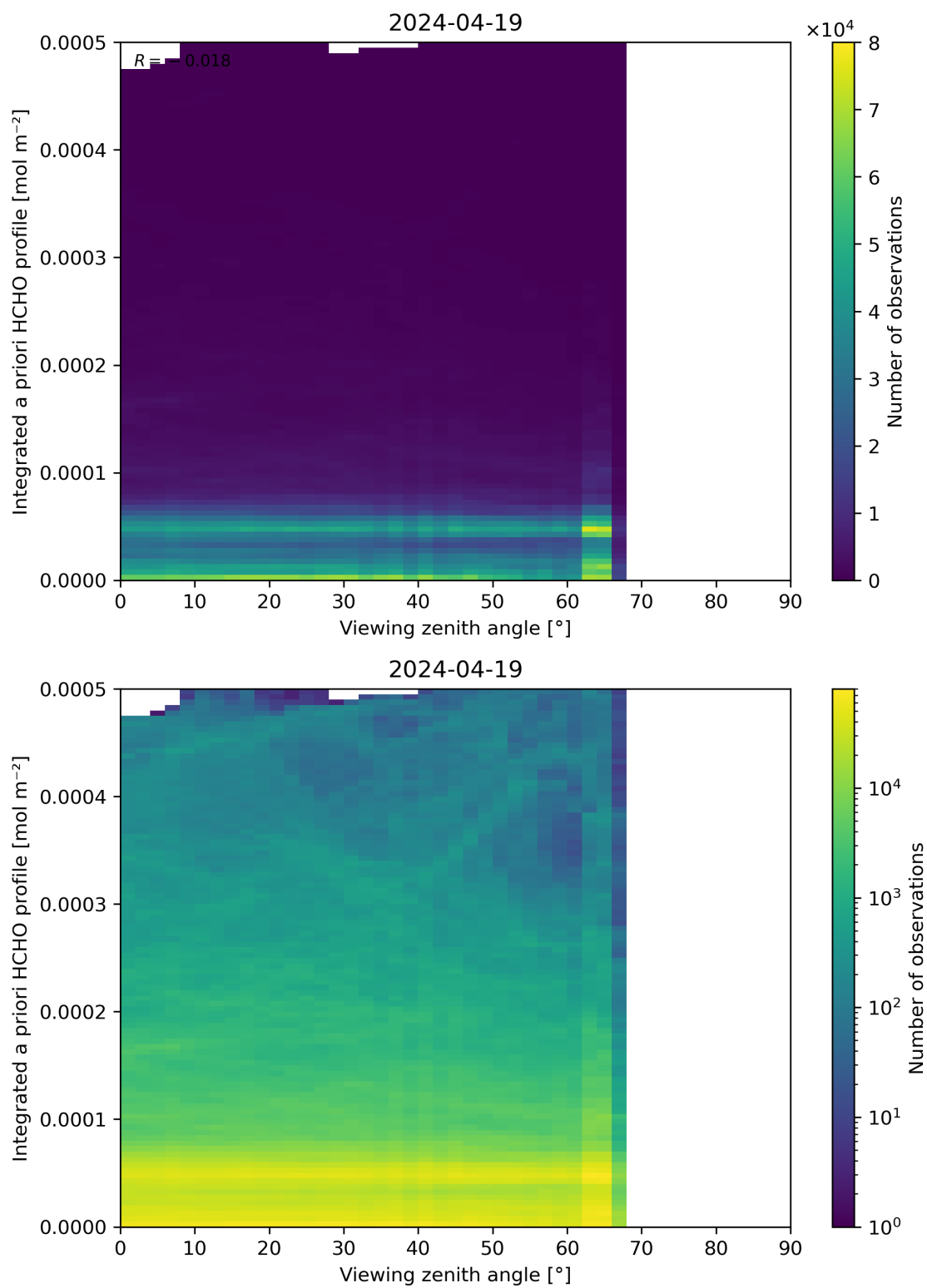
Figure 195: Scatter density plot of “Viewing zenith angle” against “Integrated a priori HCHO profile” for 2024-04-18 to 2024-04-20.
