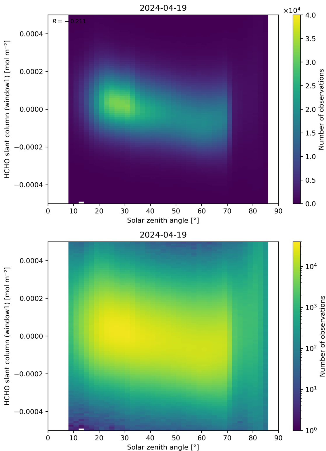
Figure 173: Scatter density plot of “Solar zenith angle” against “HCHO slant column (window1)” for 2024-04-18 to 2024-04-20.
