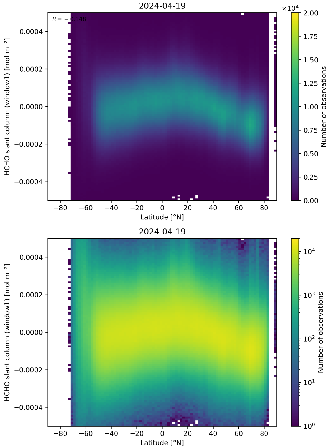
Figure 159: Scatter density plot of “Latitude” against “HCHO slant column (window1)” for 2024-04-18 to 2024-04-20.
