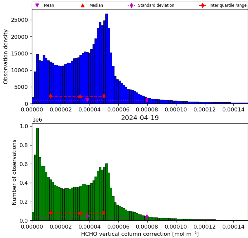
Figure 37: Histogram of “HCHO vertical column correction” for 2024-04-18 to 2024-04-20
