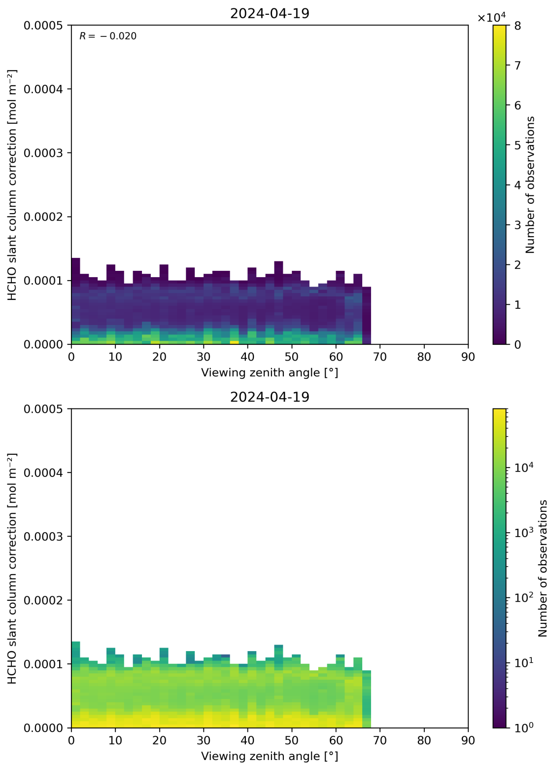
Figure 187: Scatter density plot of “Viewing zenith angle” against “HCHO slant column correction” for 2024-04-18 to 2024-04-20.
