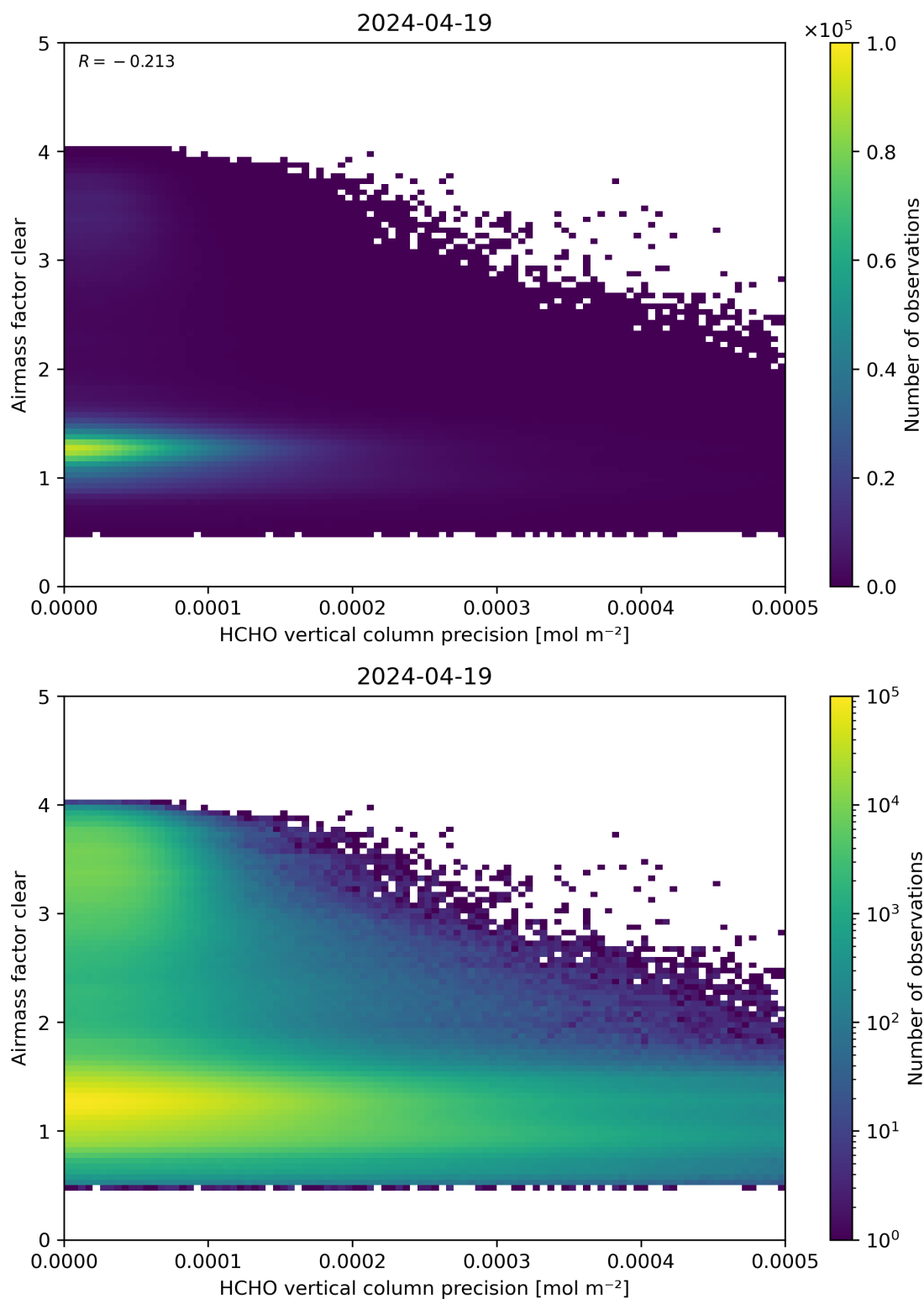
Figure 139: Scatter density plot of “HCHO vertical column precision” against “Airmass factor clear” for 2024-04-18 to 2024-04-20.
