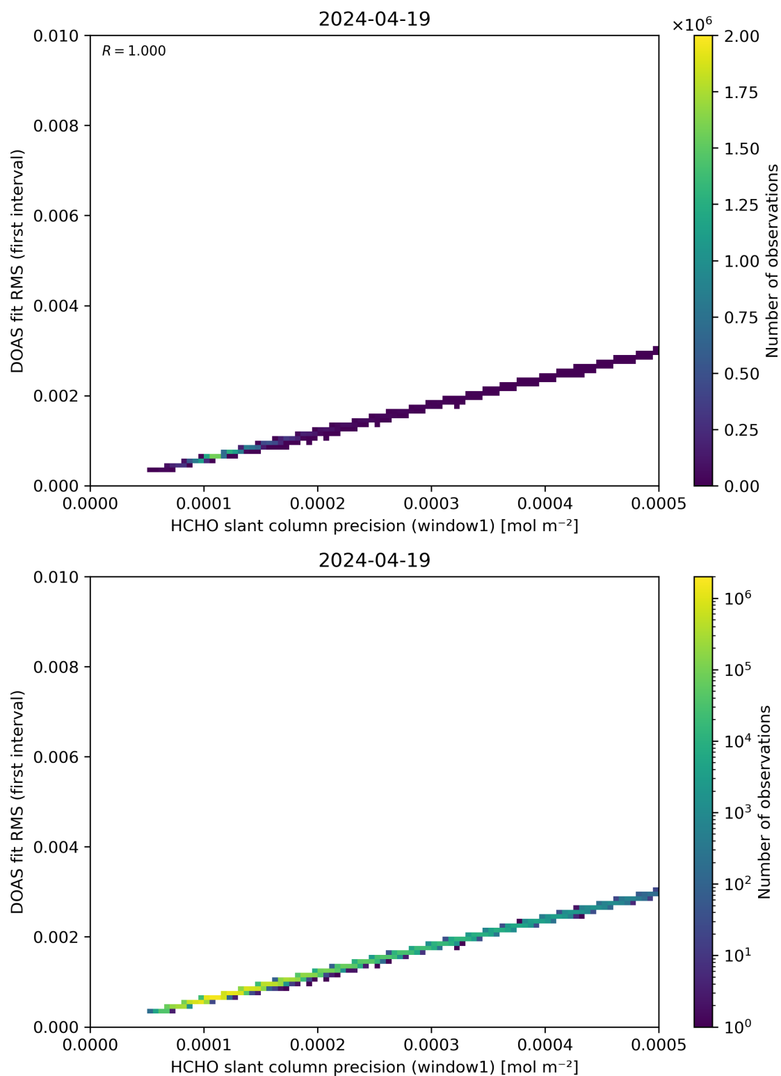
Figure 88: Scatter density plot of “HCHO slant column precision (window1)” against “DOAS fit RMS (first interval)” for 2024-04-18 to 2024-04-20.
