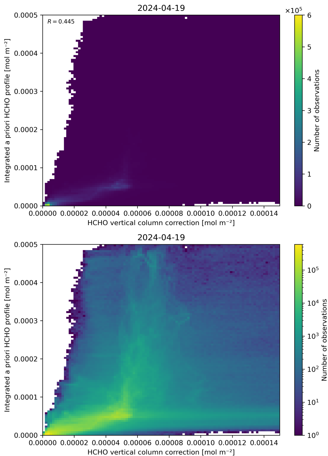
Figure 122: Scatter density plot of “HCHO vertical column correction” against “Integrated a priori HCHO profile” for 2024-04-18 to 2024-04-20.
