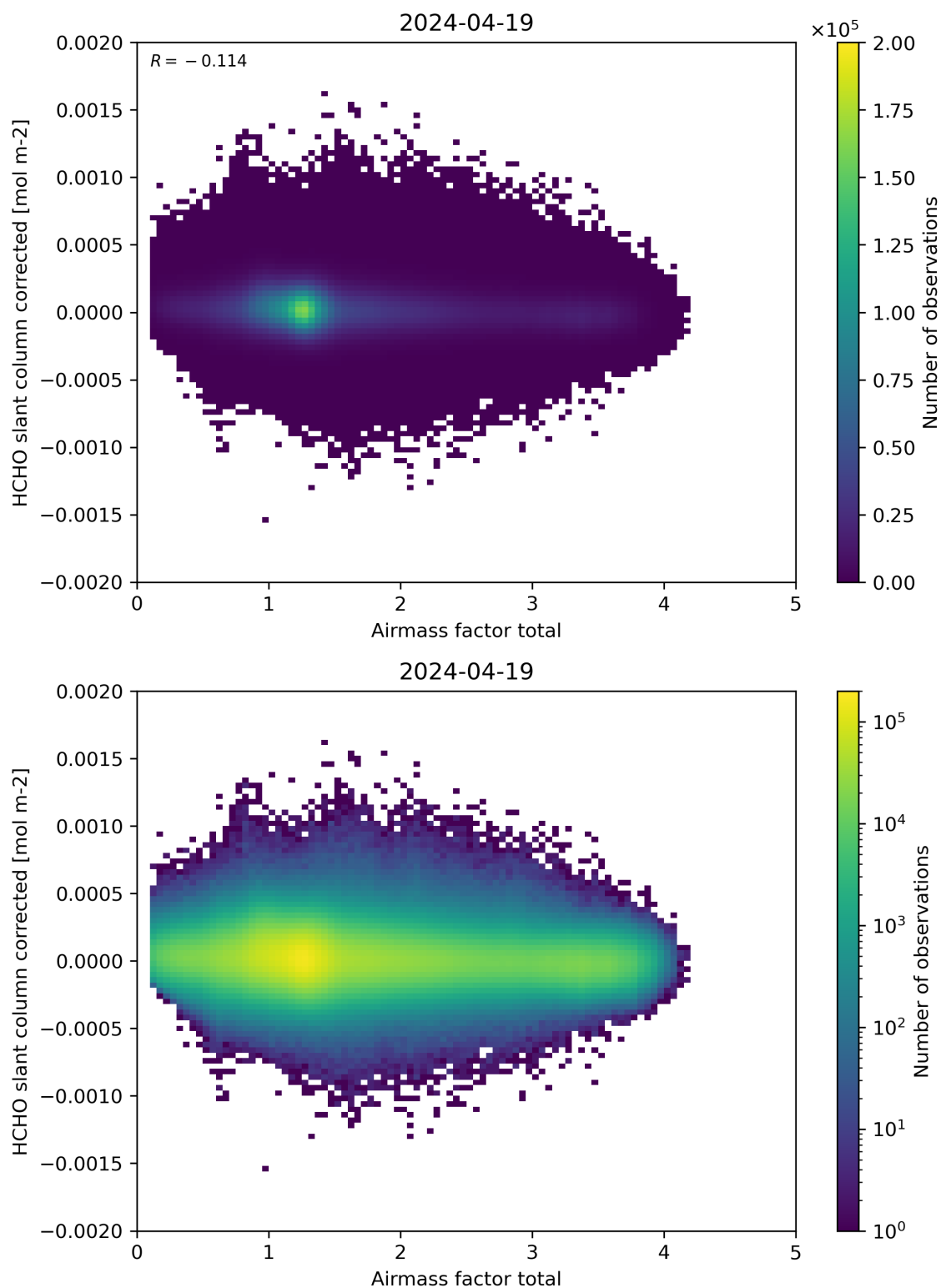
Figure 101: Scatter density plot of “Airmass factor total” against “HCHO slant column corrected” for 2024-04-18 to 2024-04-20.
