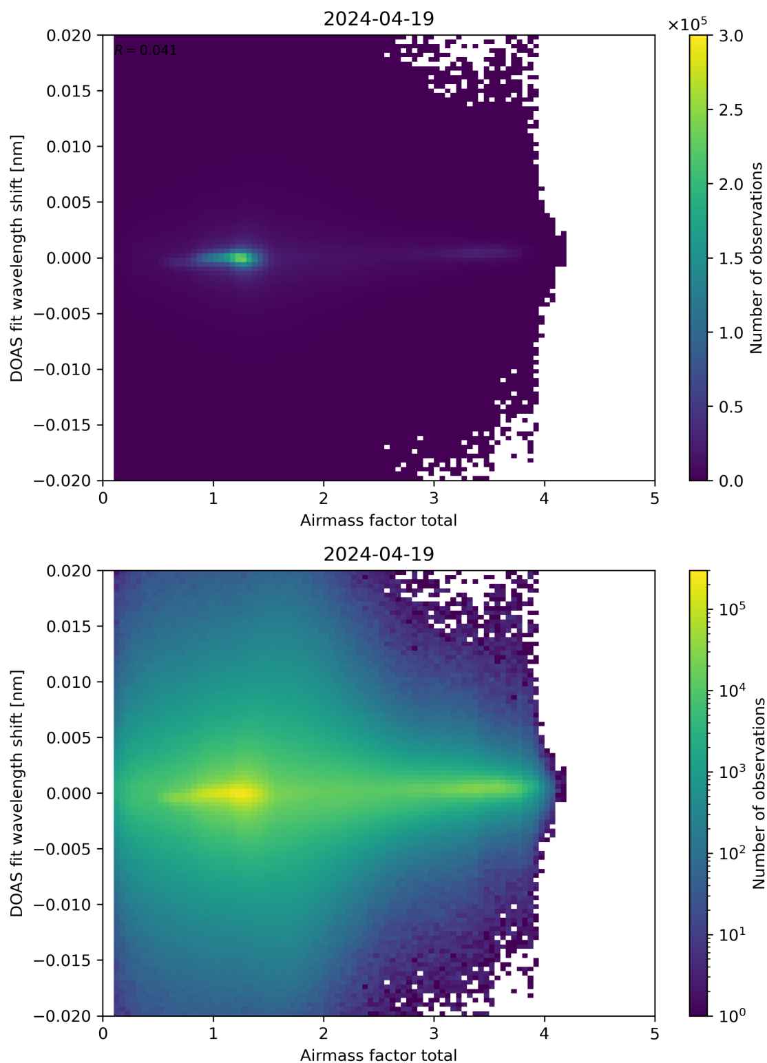
Figure 98: Scatter density plot of “Airmass factor total” against “DOAS fit wavelength shift” for 2024-04-18 to 2024-04-20.
