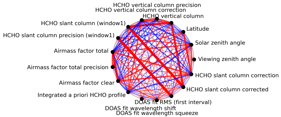
Figure 1: Map of correlation graph for 2024-04-18 to 2024-04-20.
