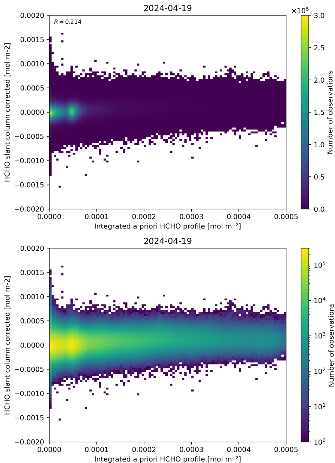
Figure 151: Scatter density plot of “Integrated a priori HCHO profile” against “HCHO slant column corrected” for 2024-04-18 to 2024-04-20.
