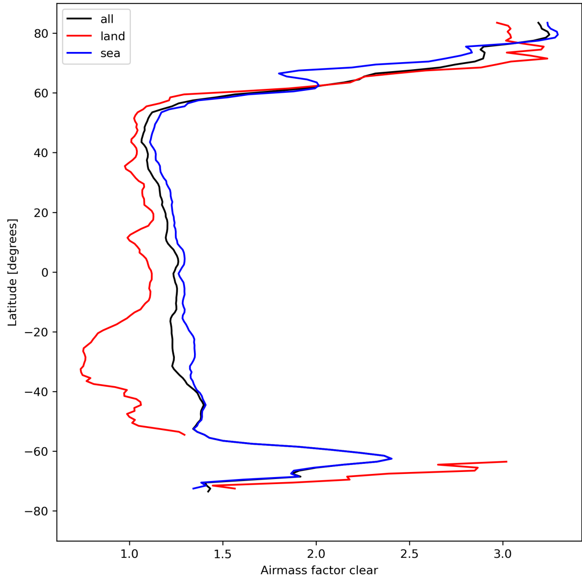
Figure 28: Zonal average of “Airmass factor clear” for 2024-04-18 to 2024-04-20.
