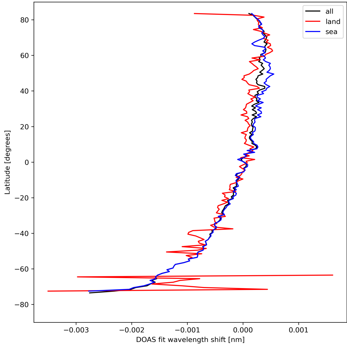
Figure 30: Zonal average of “DOAS fit wavelength shift” for 2024-04-18 to 2024-04-20.
