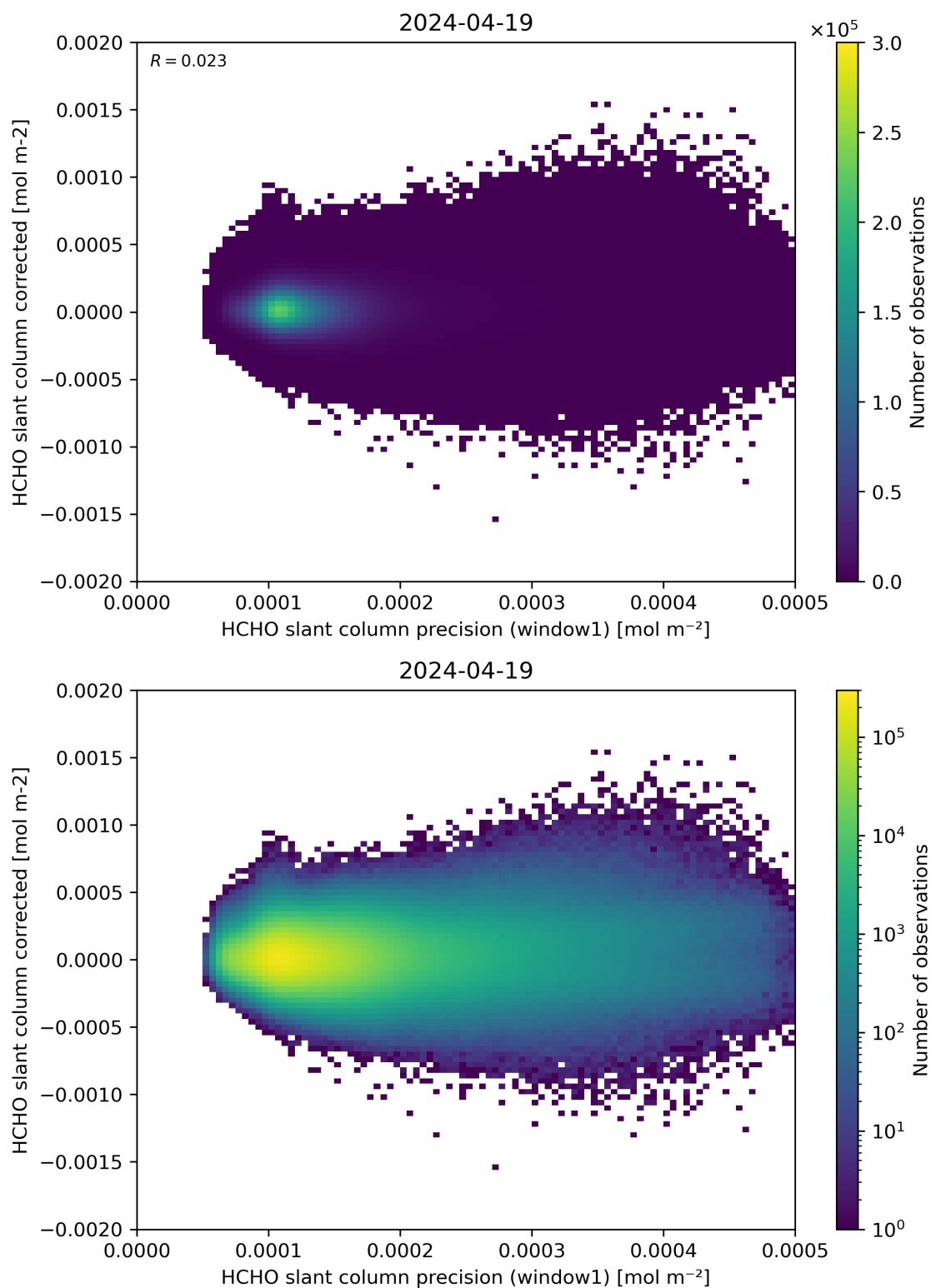
Figure 92: Scatter density plot of “HCHO slant column precision (window1)” against “HCHO slant column corrected” for 2024-04-18 to 2024-04-20.
