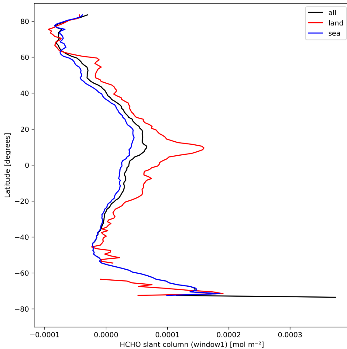
Figure 24: Zonal average of “HCHO slant column (window1)” for 2024-04-18 to 2024-04-20.
