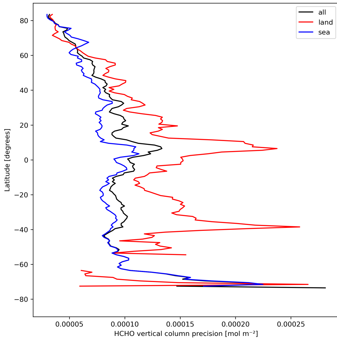
Figure 22: Zonal average of “HCHO vertical column precision” for 2024-04-18 to 2024-04-20.
