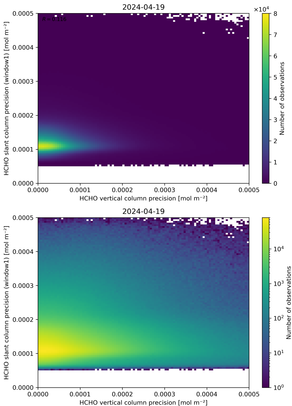
Figure 143: Scatter density plot of “HCHO vertical column precision” against “HCHO slant column precision (window1)” for 2024-04-18 to 2024-04-20.
