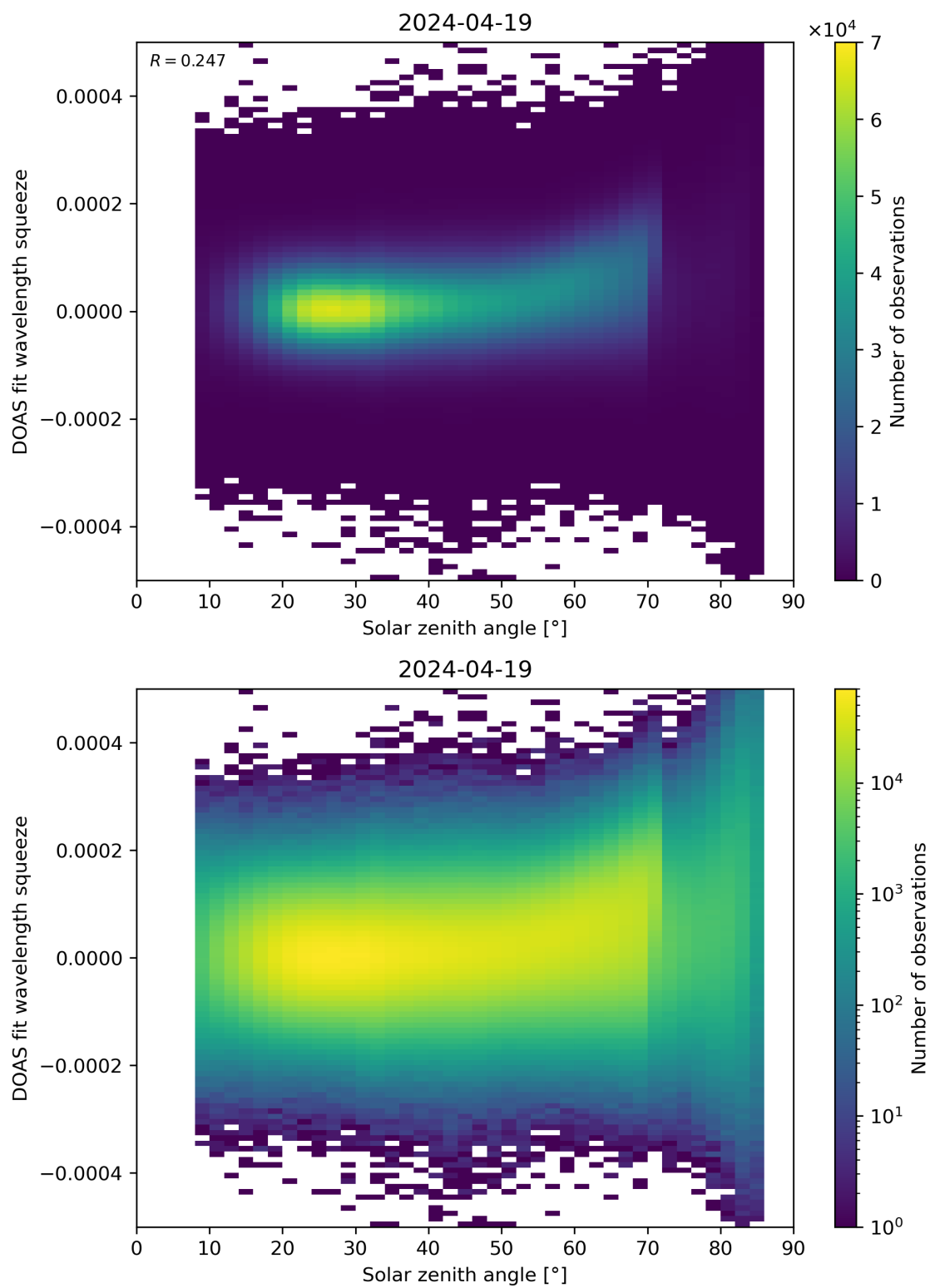
Figure 169: Scatter density plot of “Solar zenith angle” against “DOAS fit wavelength squeeze” for 2024-04-18 to 2024-04-20.
