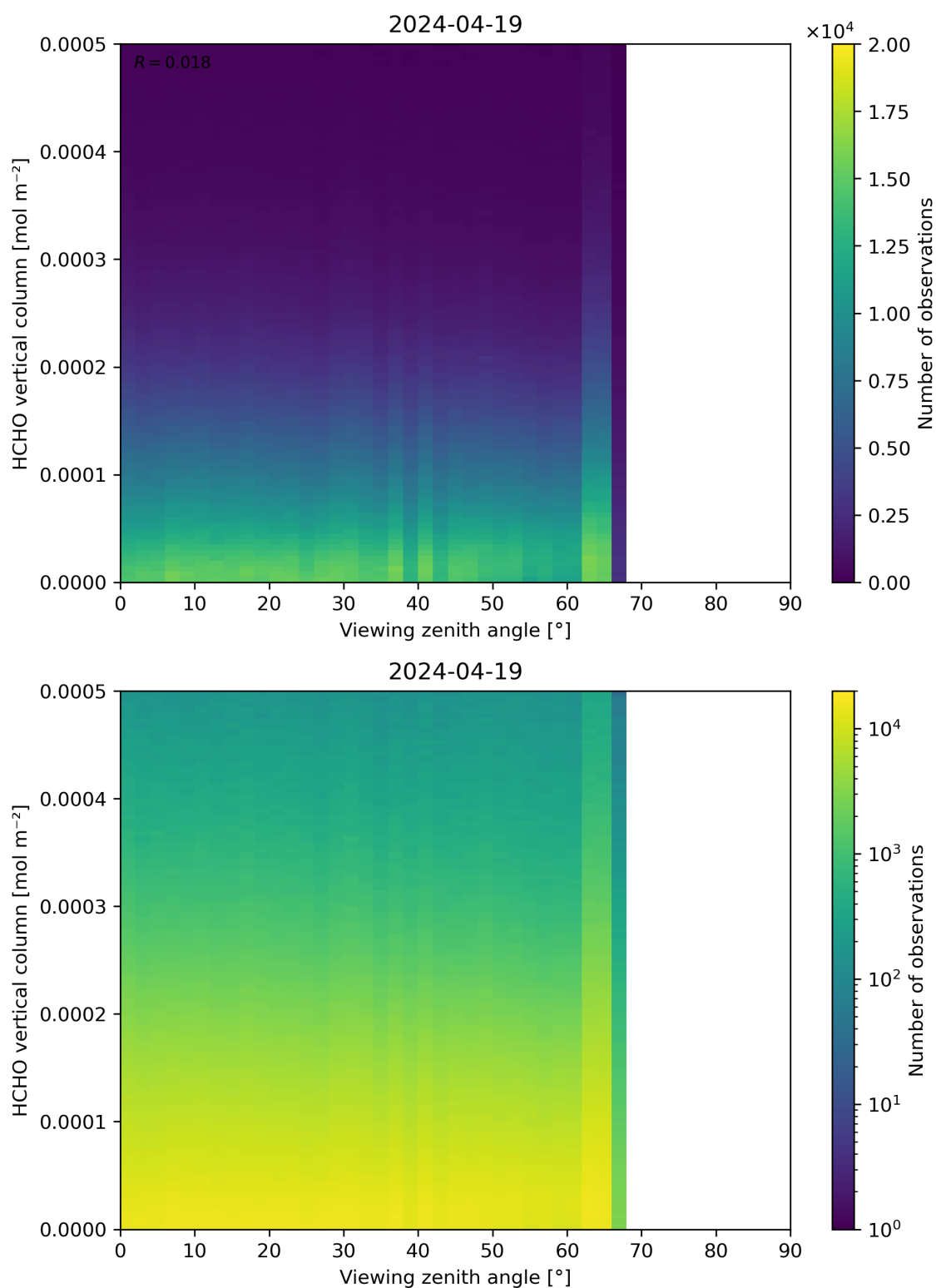
Figure 192: Scatter density plot of “Viewing zenith angle” against “HCHO vertical column” for 2024-04-18 to 2024-04-20.
