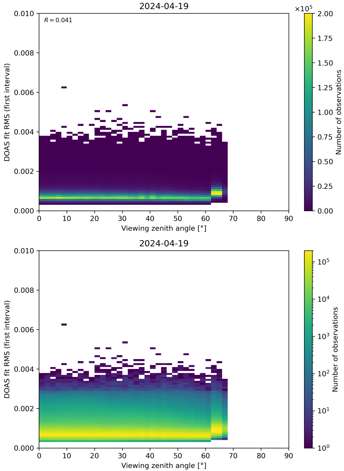
Figure 182: Scatter density plot of “Viewing zenith angle” against “DOAS fit RMS (first interval)” for 2024-04-18 to 2024-04-20.
