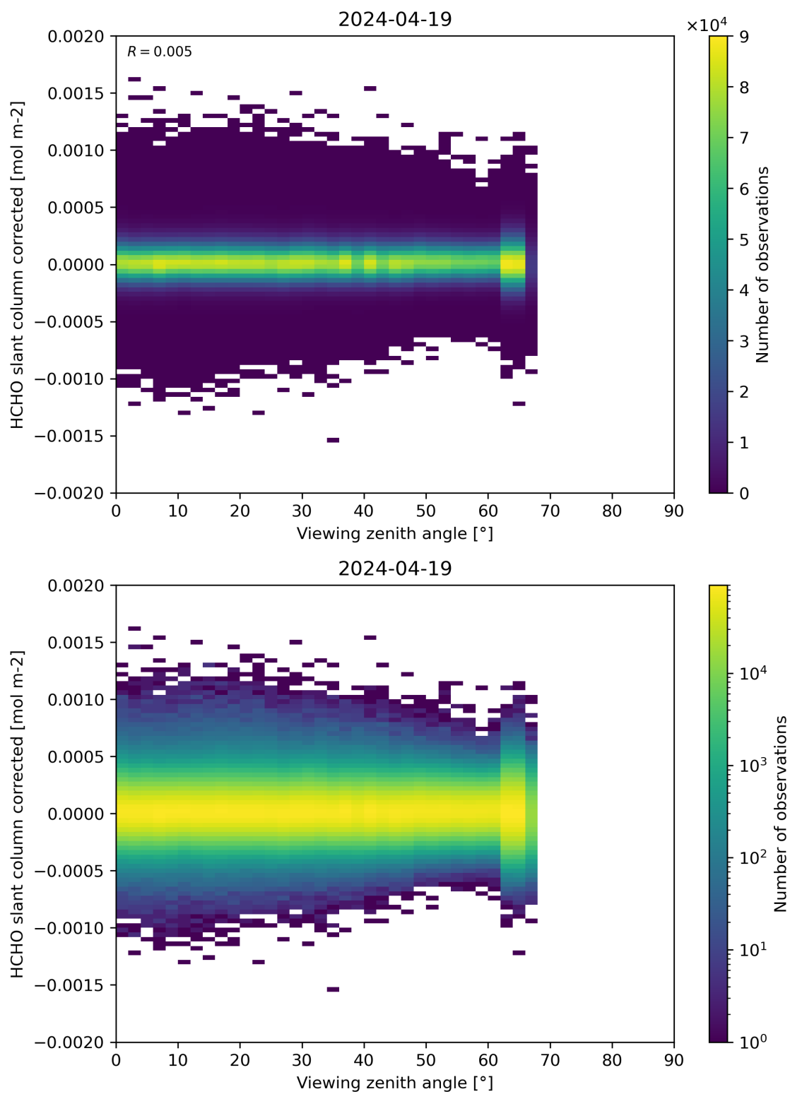
Figure 186: Scatter density plot of “Viewing zenith angle” against “HCHO slant column corrected” for 2024-04-18 to 2024-04-20.
