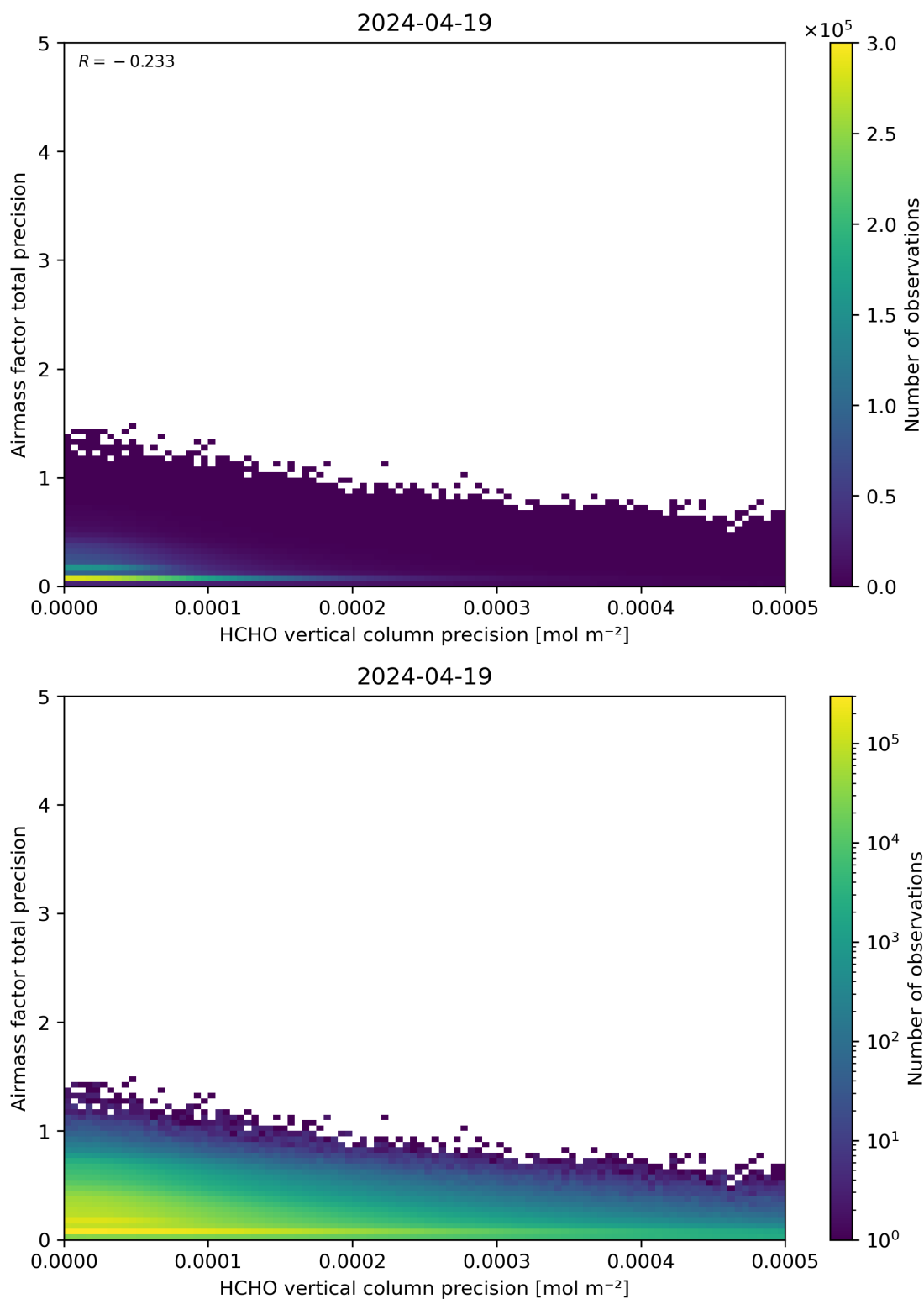
Figure 145: Scatter density plot of “HCHO vertical column precision” against “Airmass factor total precision” for 2024-04-18 to 2024-04-20.
