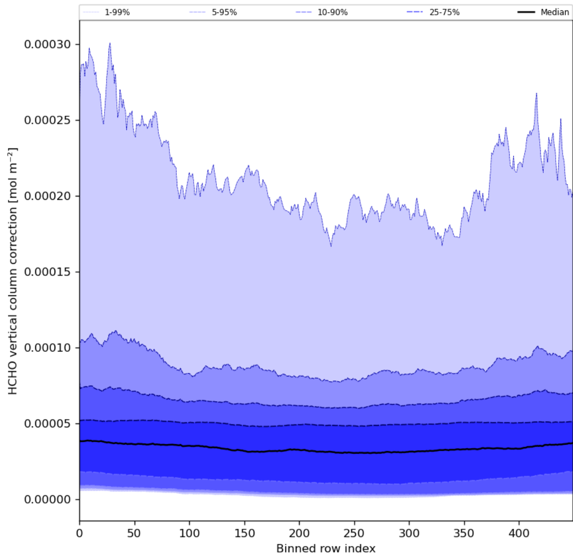
Figure 51: Along track statistics of “HCHO vertical column correction” for 2024-04-18 to 2024-04-20
