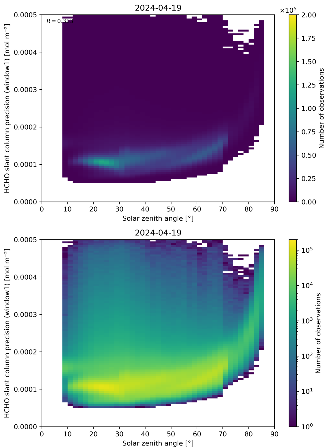
Figure 174: Scatter density plot of “Solar zenith angle” against “HCHO slant column precision (window1)” for 2024-04-18 to 2024-04-20.
