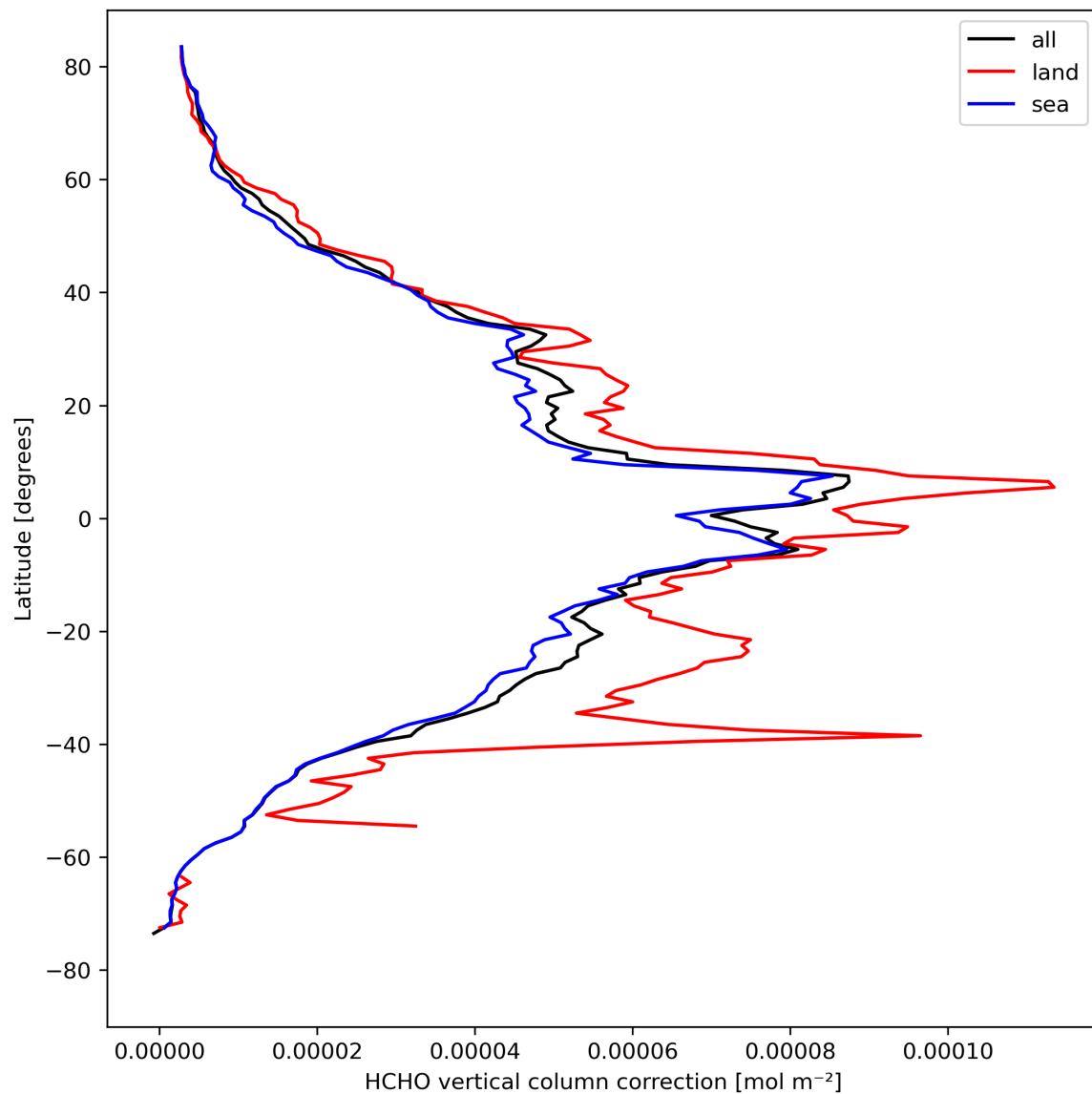
Figure 23: Zonal average of “HCHO vertical column correction” for 2024-04-18 to 2024-04-20.
