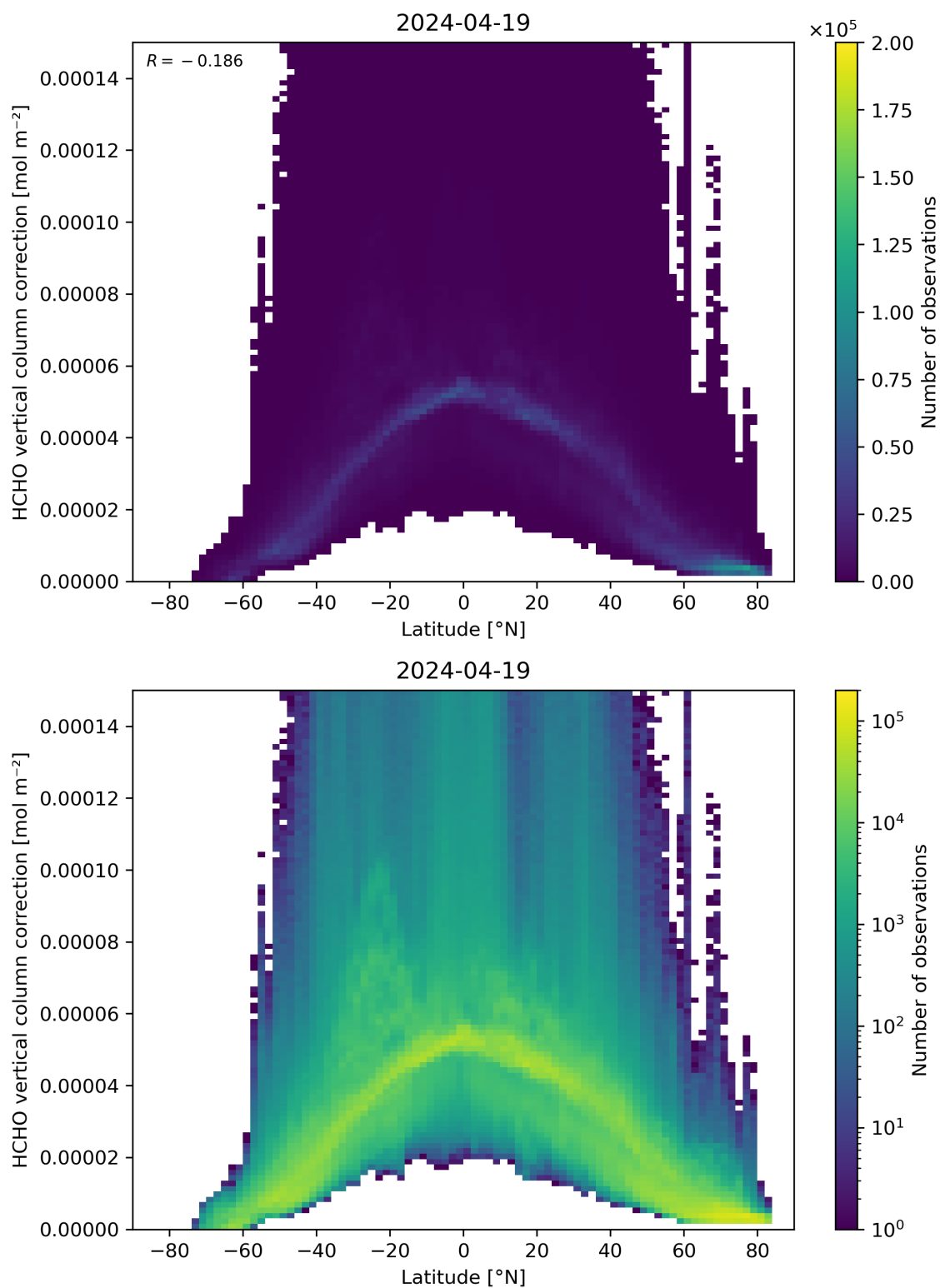
Figure 164: Scatter density plot of “Latitude” against “HCHO vertical column correction” for 2024-04-18 to 2024-04-20.
