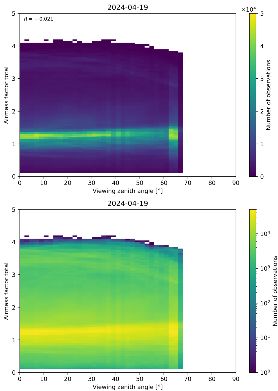
Figure 190: Scatter density plot of “Viewing zenith angle” against “Airmass factor total” for 2024-04-18 to 2024-04-20.
