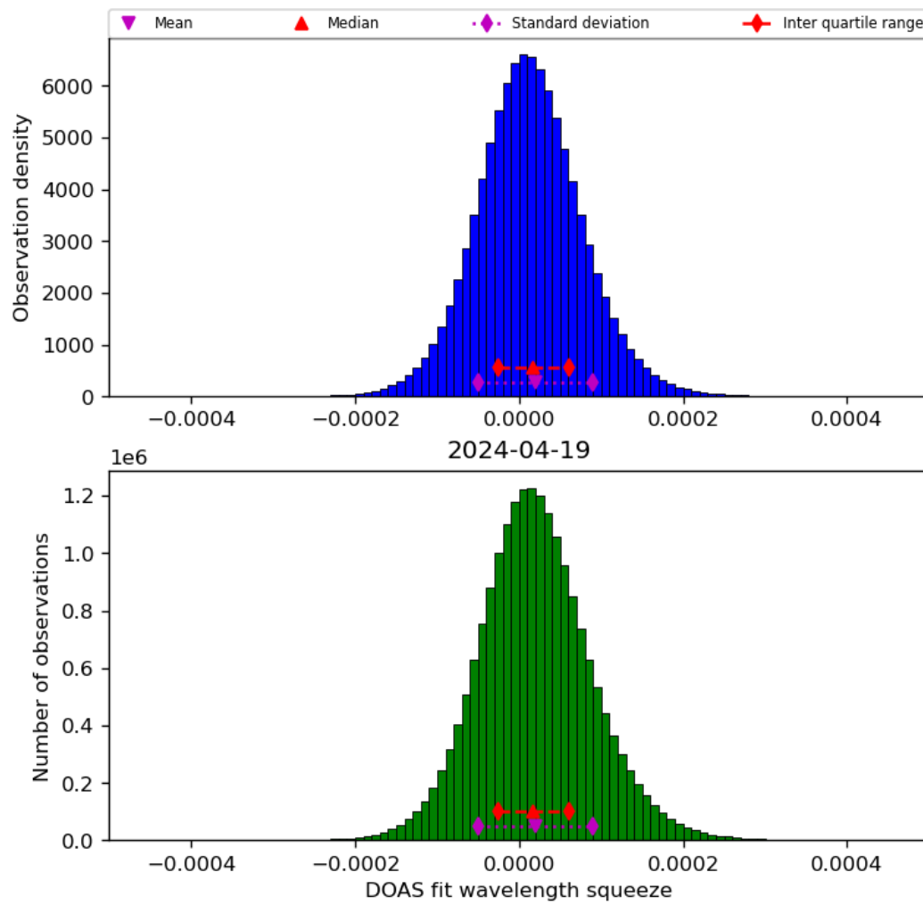
Figure 45: Histogram of “DOAS fit wavelength squeeze” for 2024-04-18 to 2024-04-20
