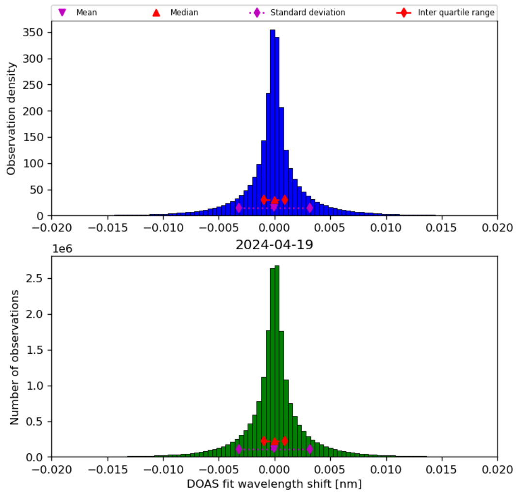
Figure 44: Histogram of “DOAS fit wavelength shift” for 2024-04-18 to 2024-04-20
