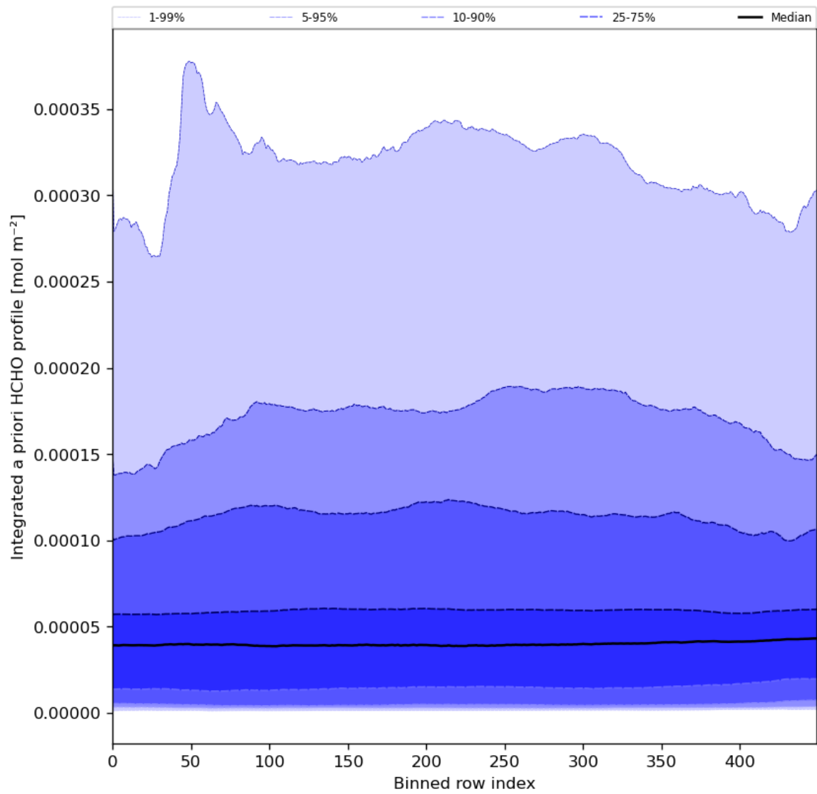
Figure 57: Along track statistics of "Integrated a priori HCHO profile" for 2024-04-18 to 2024-04-20
