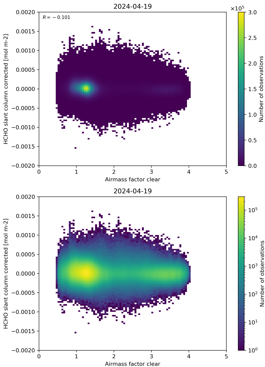
Figure 74: Scatter density plot of “Airmass factor clear” against “HCHO slant column corrected” for 2024-04-18 to 2024-04-20.
