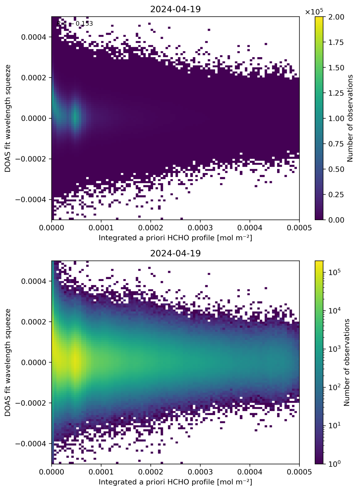
Figure 150: Scatter density plot of “Integrated a priori HCHO profile” against “DOAS fit wavelength squeeze” for 2024-04-18 to 2024-04-20.
