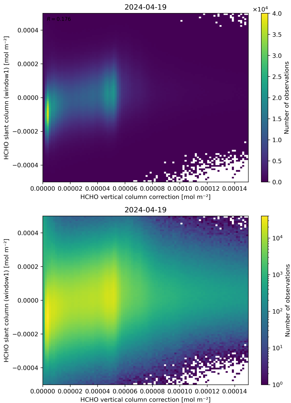
Figure 118: Scatter density plot of “HCHO vertical column correction” against “HCHO slant column (window1)” for 2024-04-18 to 2024-04-20.
