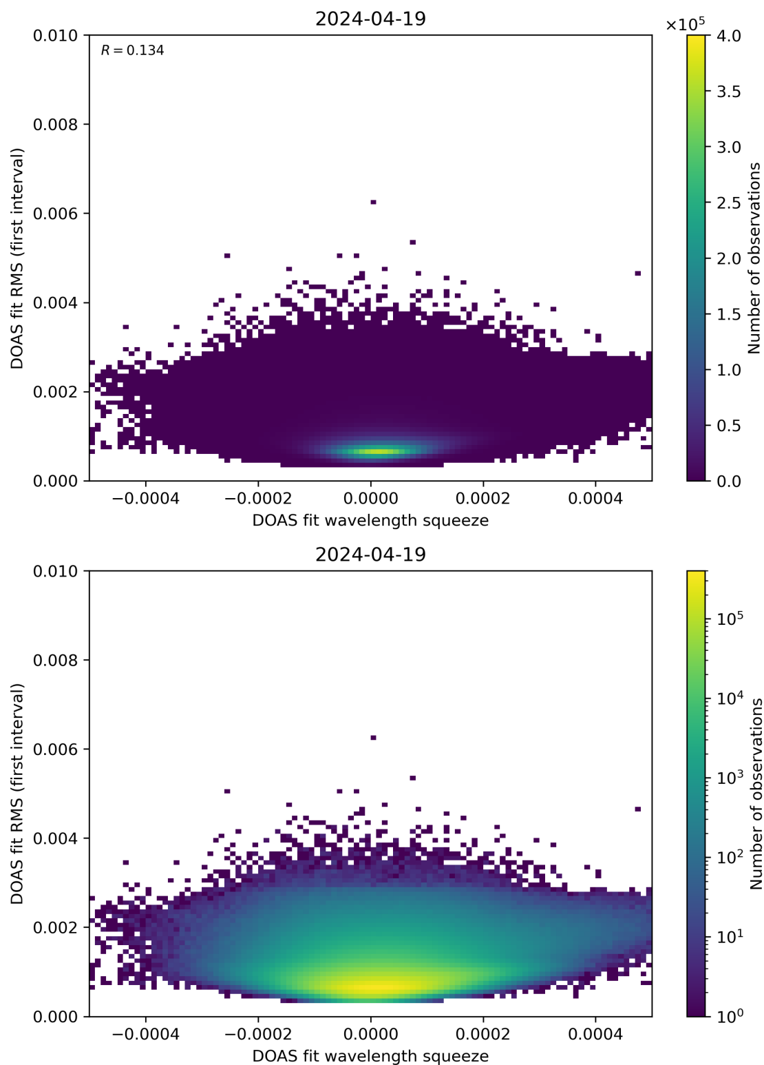
Figure 68: Scatter density plot of “DOAS fit wavelength squeeze” against “DOAS fit RMS (first interval)” for 2024-04-18 to 2024-04-20.
