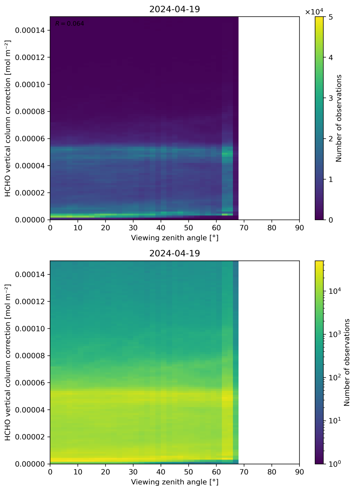
Figure 193: Scatter density plot of “Viewing zenith angle” against “HCHO vertical column correction” for 2024-04-18 to 2024-04-20.
