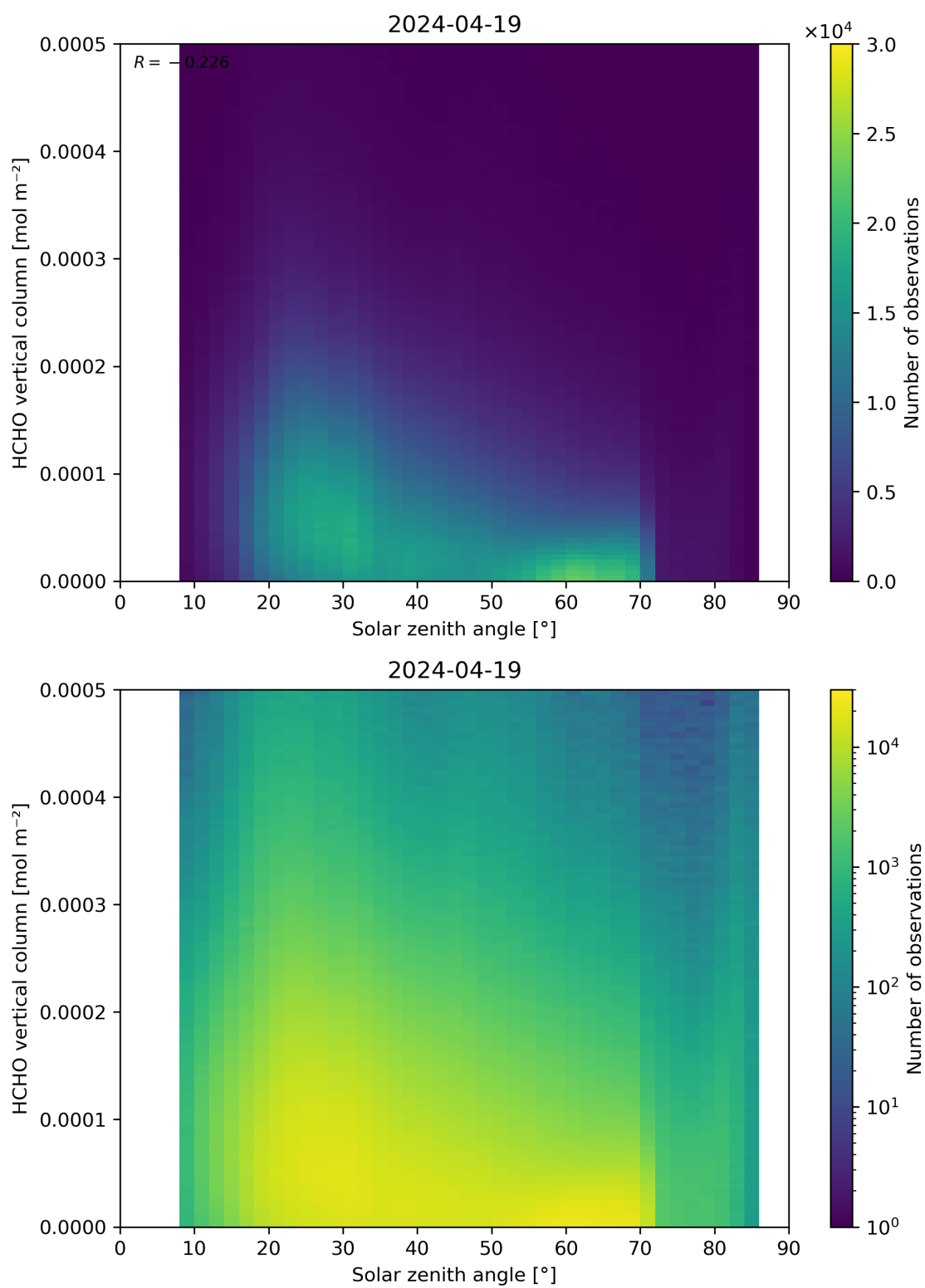
Figure 177: Scatter density plot of “Solar zenith angle” against “HCHO vertical column” for 2024-04-18 to 2024-04-20.
