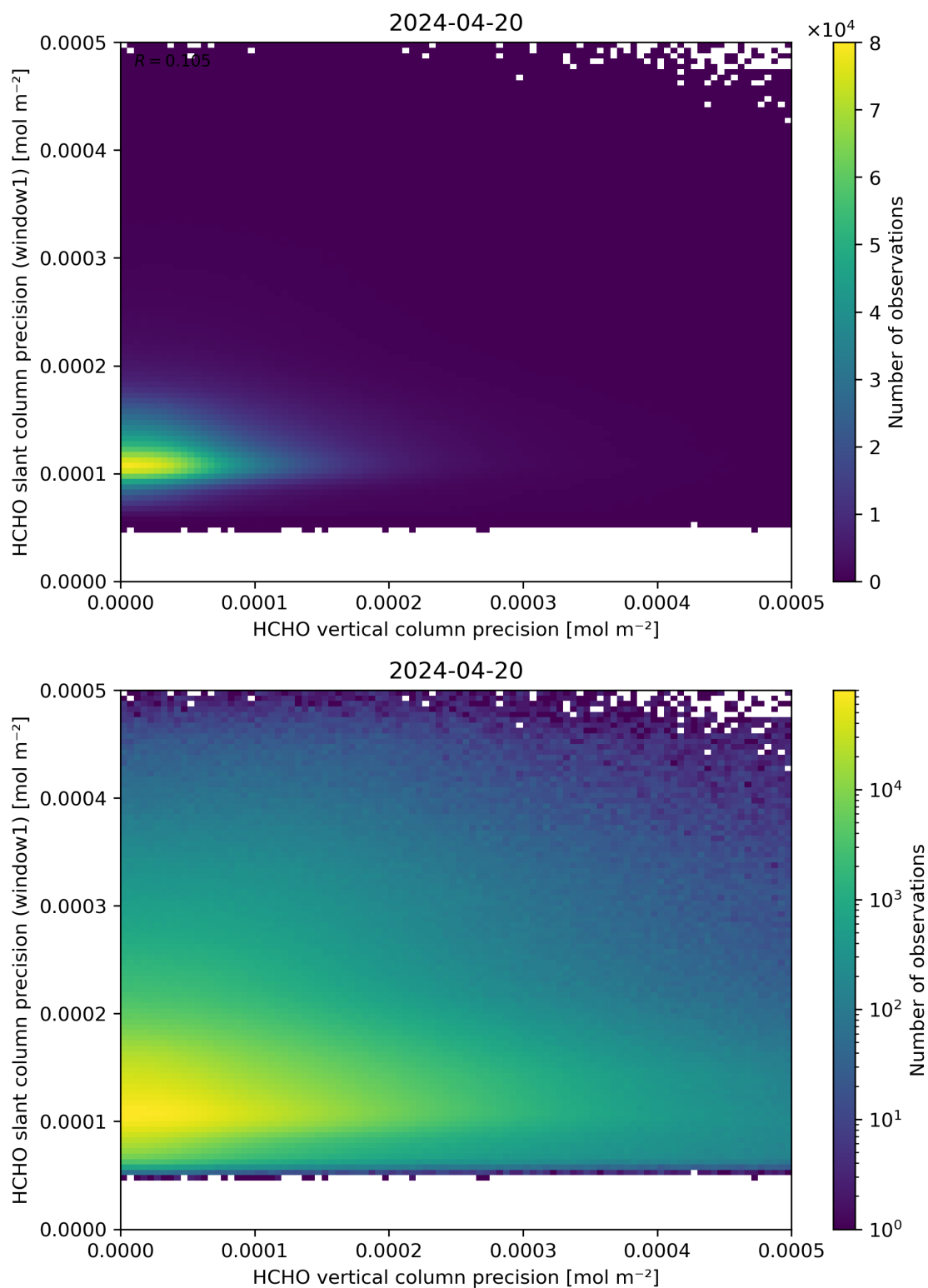
Figure 143: Scatter density plot of “HCHO vertical column precision” against “HCHO slant column precision (window1)” for 2024-04-19 to 2024-04-21.
