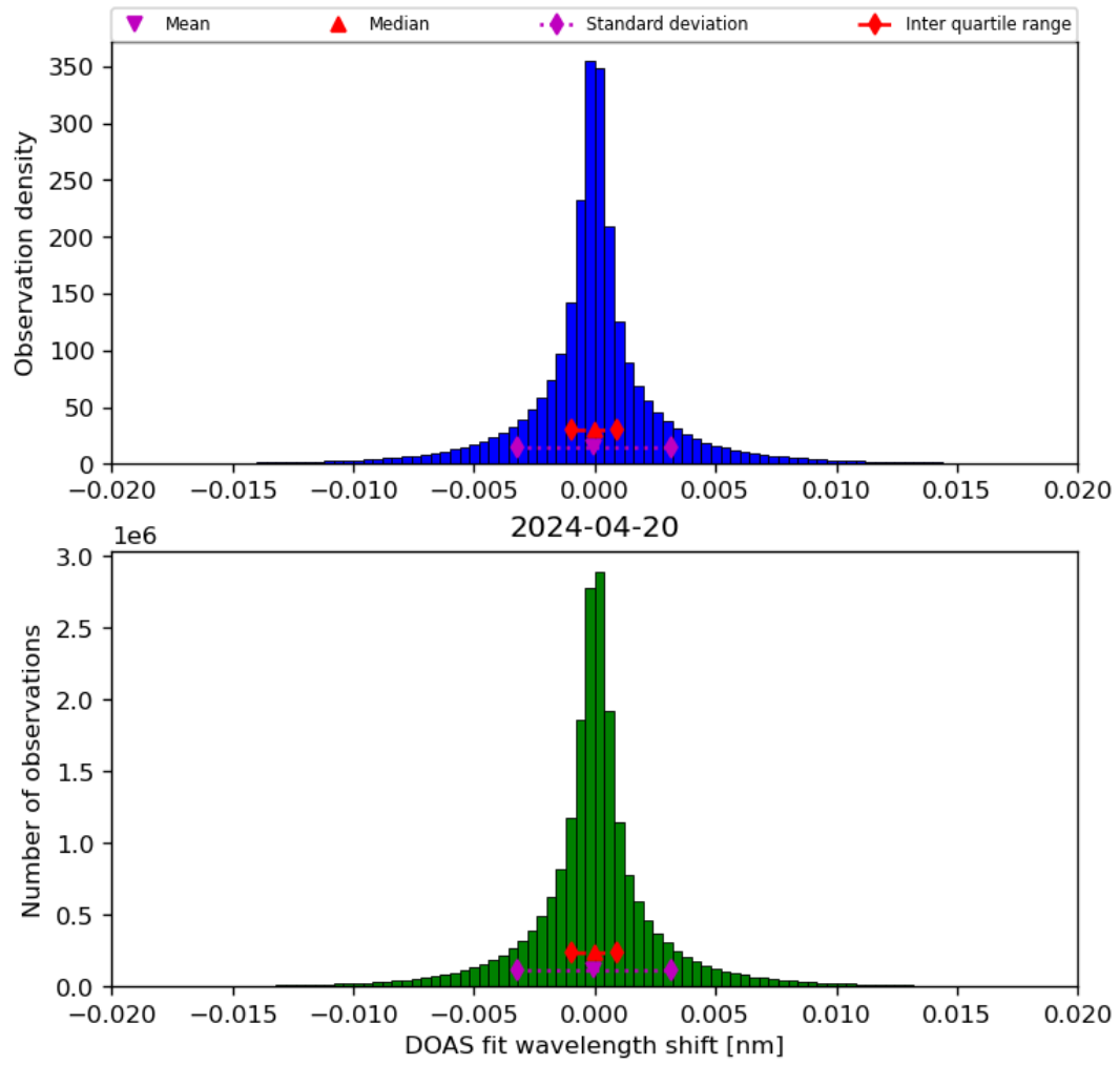
Figure 44: Histogram of “DOAS fit wavelength shift” for 2024-04-19 to 2024-04-21
