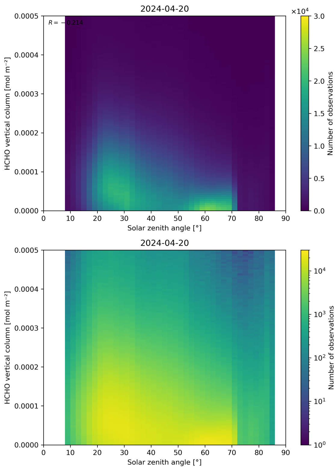
Figure 177: Scatter density plot of “Solar zenith angle” against “HCHO vertical column” for 2024-04-19 to 2024-04-21.
