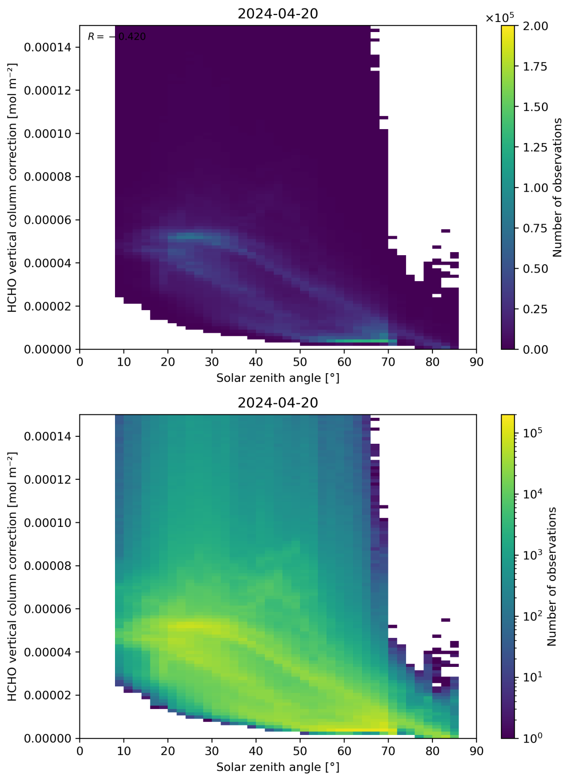
Figure 178: Scatter density plot of “Solar zenith angle” against “HCHO vertical column correction” for 2024-04-19 to 2024-04-21.
