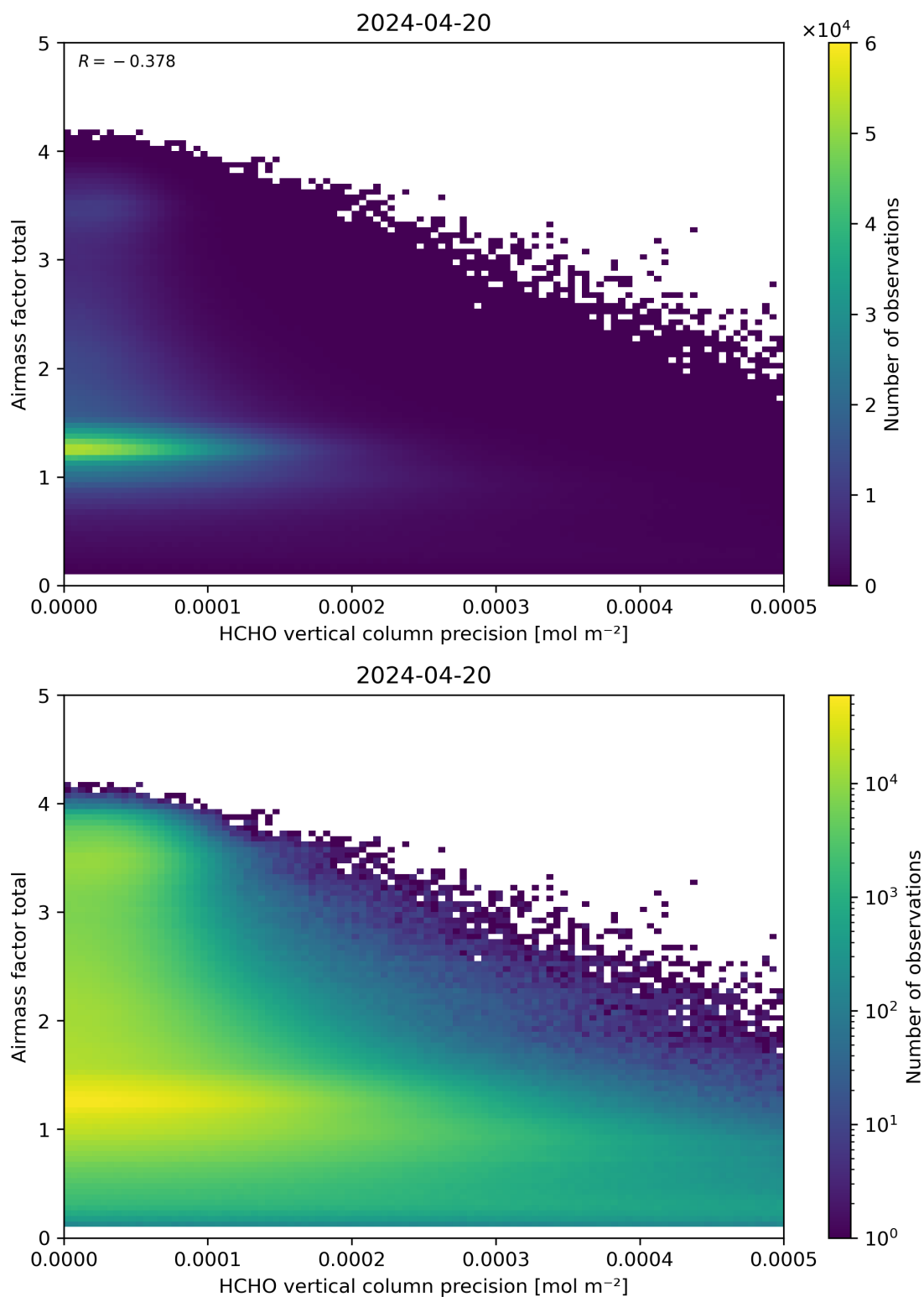
Figure 144: Scatter density plot of “HCHO vertical column precision” against “Airmass factor total” for 2024-04-19 to 2024-04-21.
