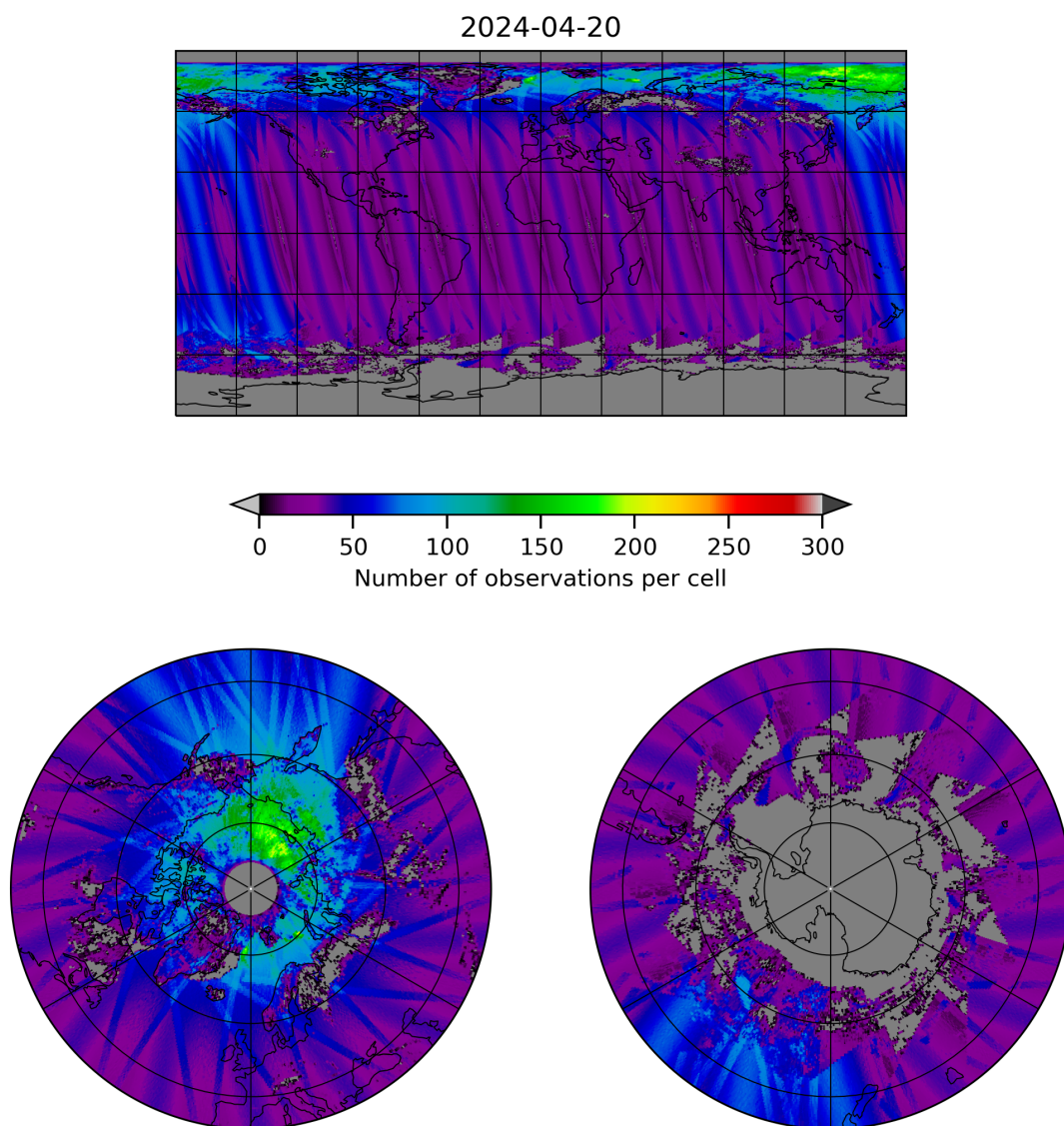
Figure 19: Map of the number of observations for 2024-04-19 to 2024-04-21
