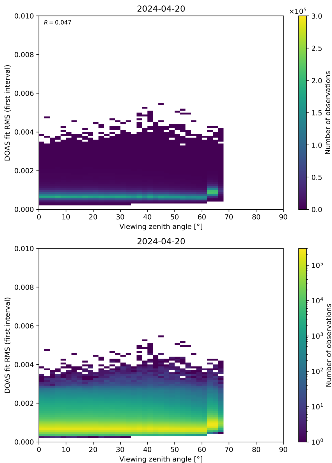
Figure 182: Scatter density plot of “Viewing zenith angle” against “DOAS fit RMS (first interval)” for 2024-04-19 to 2024-04-21.
