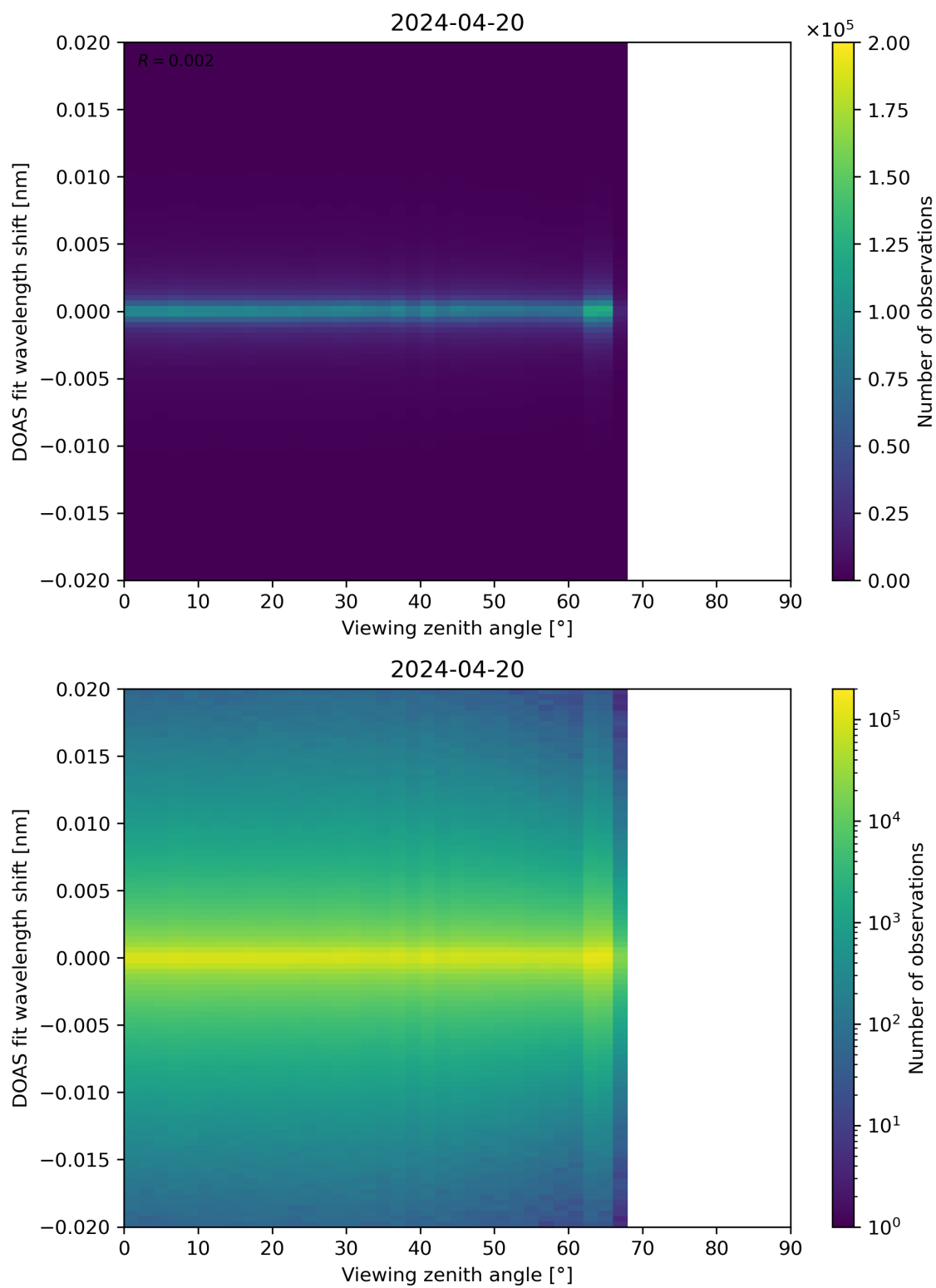
Figure 183: Scatter density plot of “Viewing zenith angle” against “DOAS fit wavelength shift” for 2024-04-19 to 2024-04-21.
