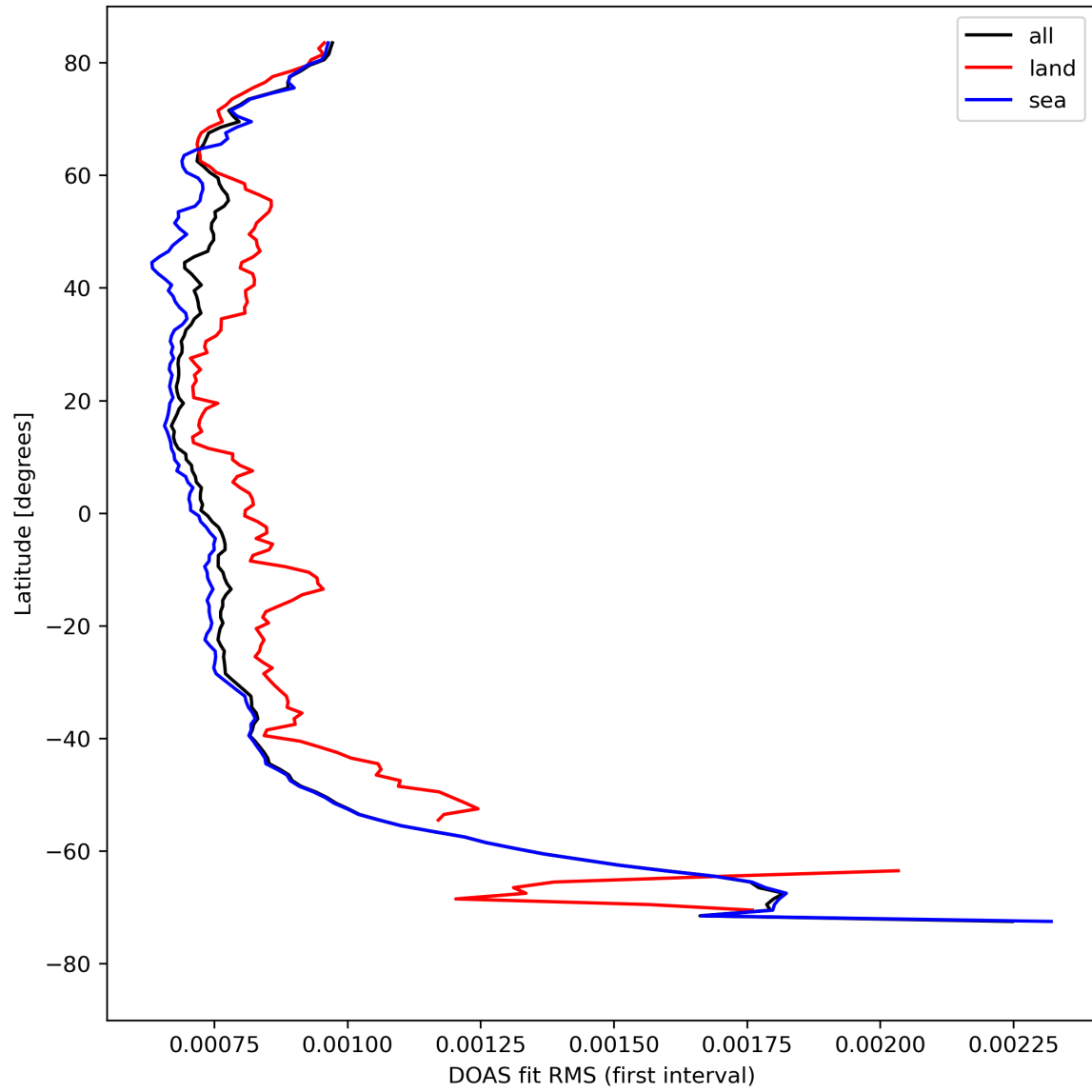
Figure 32: Zonal average of “DOAS fit RMS (first interval)” for 2024-04-19 to 2024-04-21.
