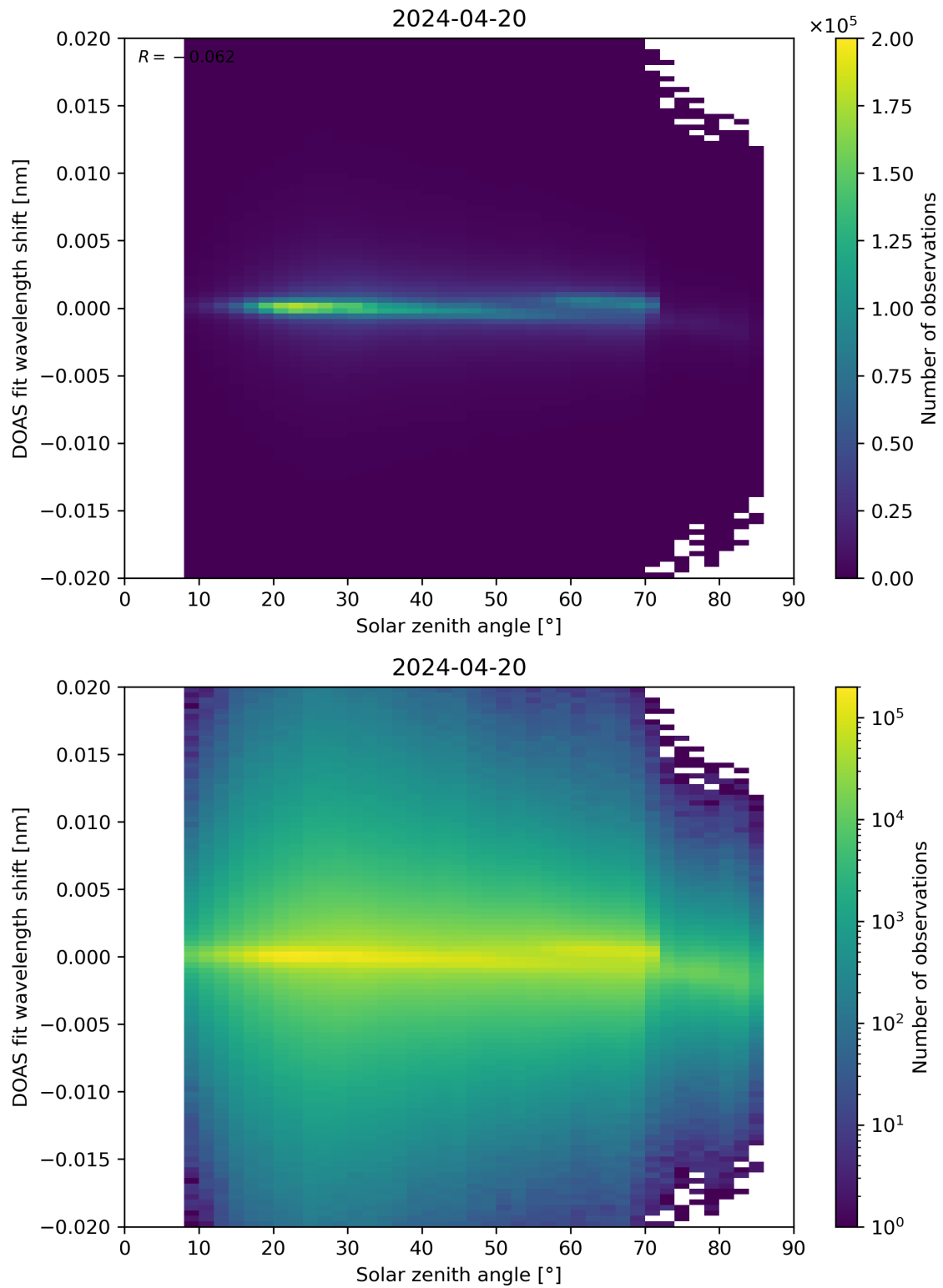
Figure 168: Scatter density plot of “Solar zenith angle” against “DOAS fit wavelength shift” for 2024-04-19 to 2024-04-21.
