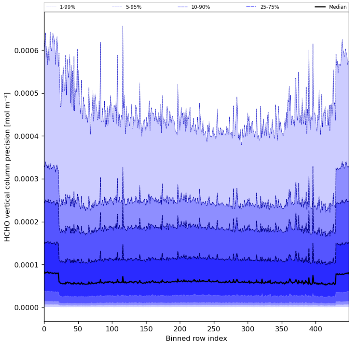
Figure 50: Along track statistics of “HCHO vertical column precision” for 2024-04-19 to 2024-04-21
