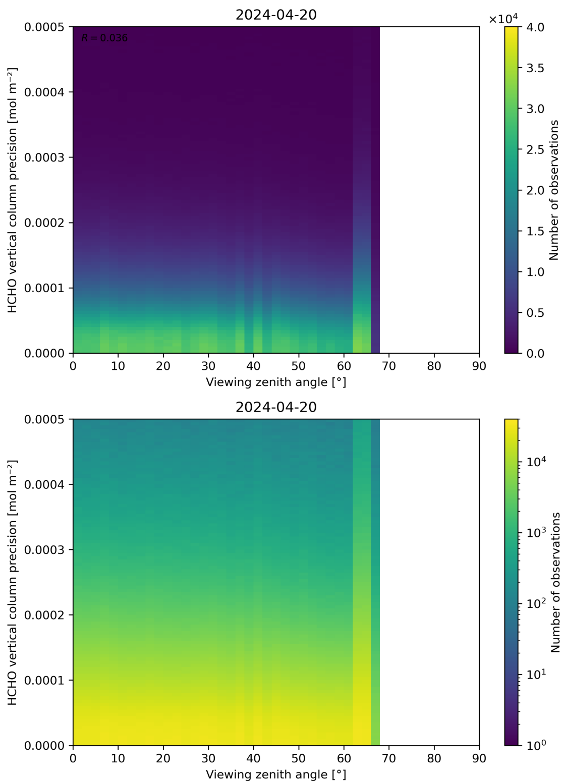
Figure 194: Scatter density plot of “Viewing zenith angle” against “HCHO vertical column precision” for 2024-04-19 to 2024-04-21.
