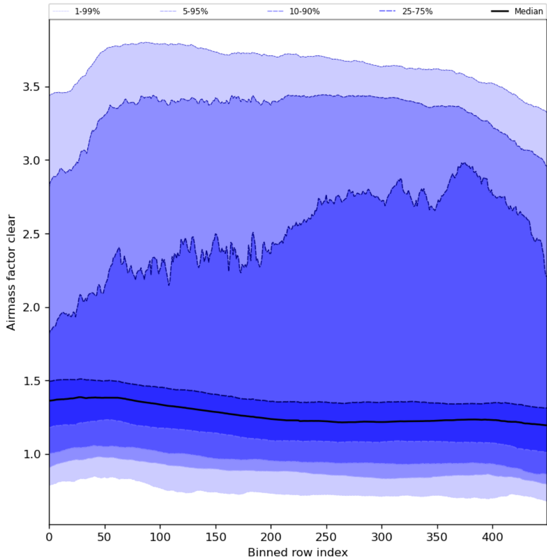
Figure 56: Along track statistics of “Airmass factor clear” for 2024-04-19 to 2024-04-21
