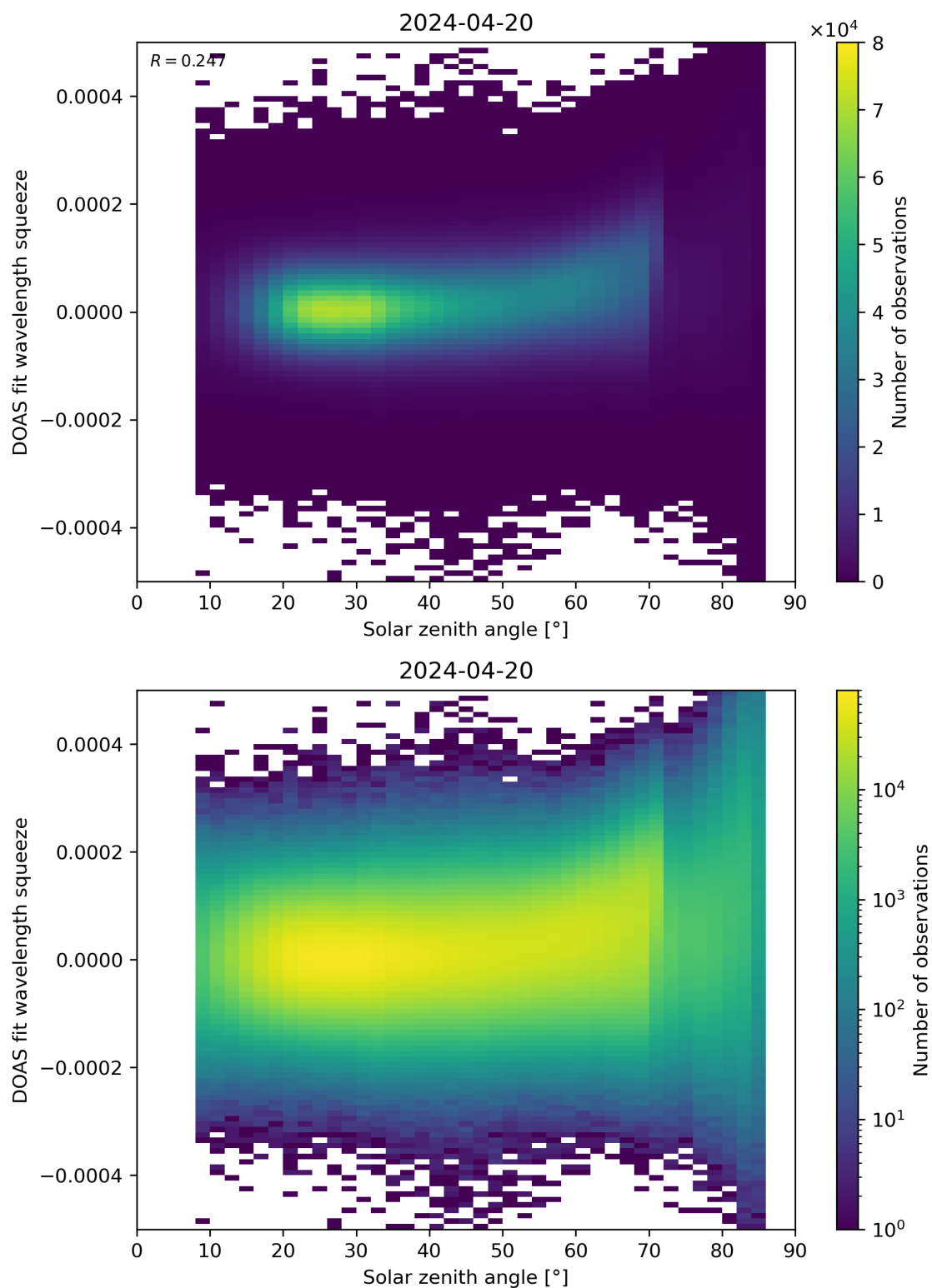
Figure 169: Scatter density plot of “Solar zenith angle” against “DOAS fit wavelength squeeze” for 2024-04-19 to 2024-04-21.
