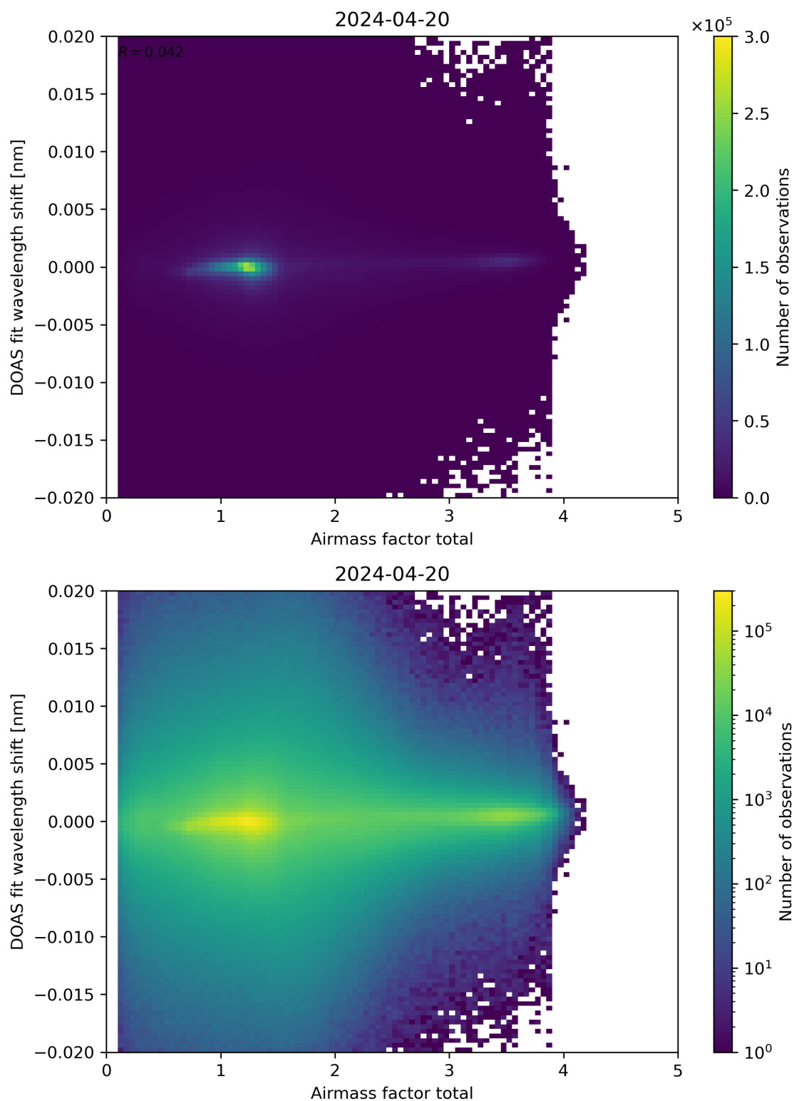
Figure 98: Scatter density plot of “Airmass factor total” against “DOAS fit wavelength shift” for 2024-04-19 to 2024-04-21.
