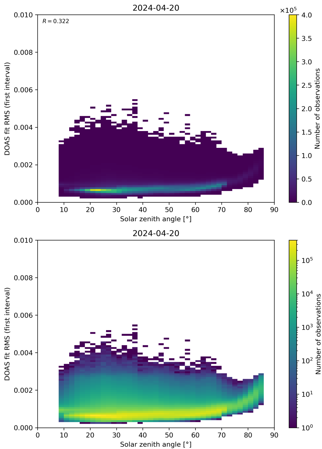
Figure 167: Scatter density plot of “Solar zenith angle” against “DOAS fit RMS (first interval)” for 2024-04-19 to 2024-04-21.
