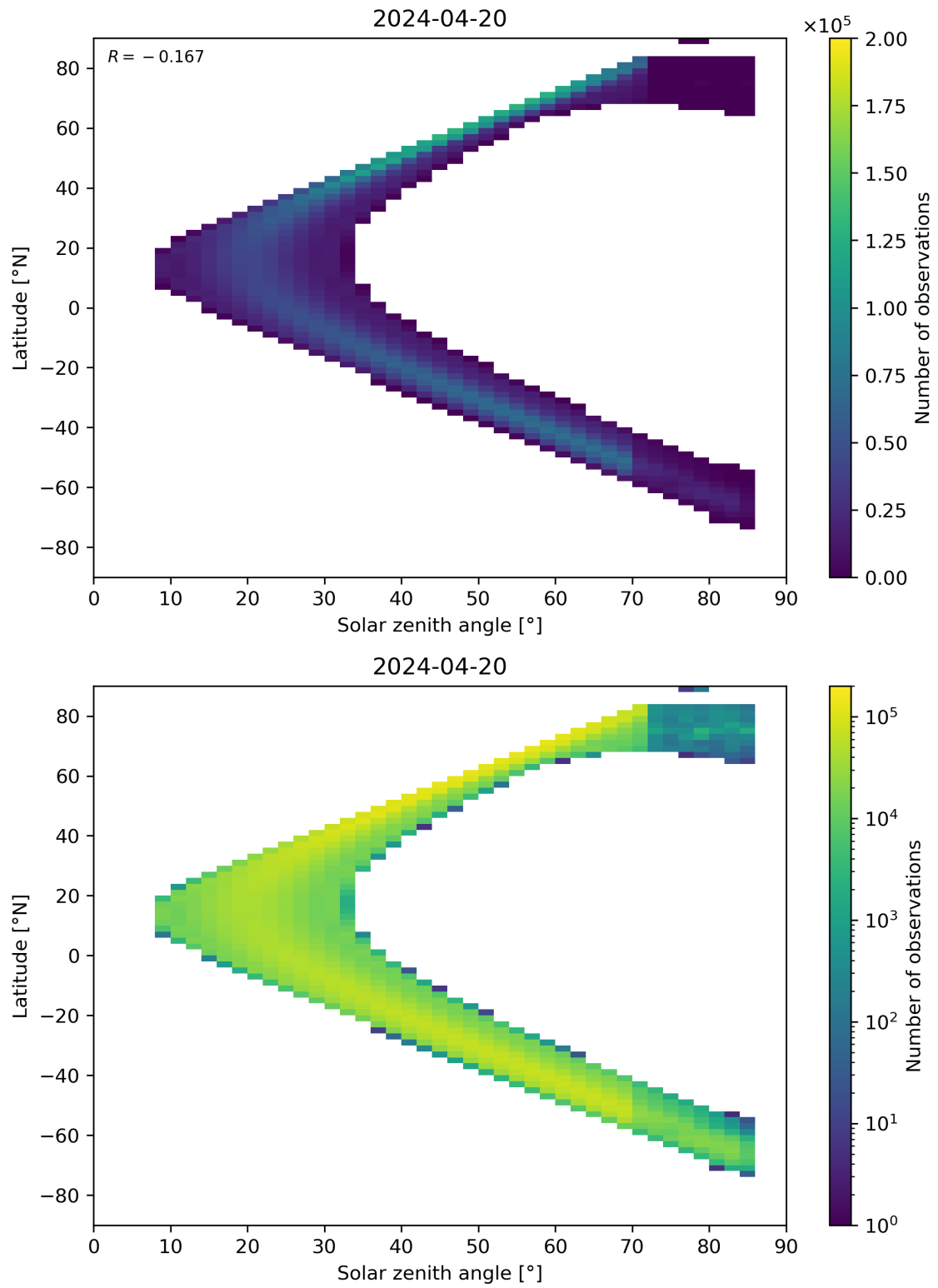
Figure 181: Scatter density plot of “Solar zenith angle” against “Latitude” for 2024-04-19 to 2024-04-21.
