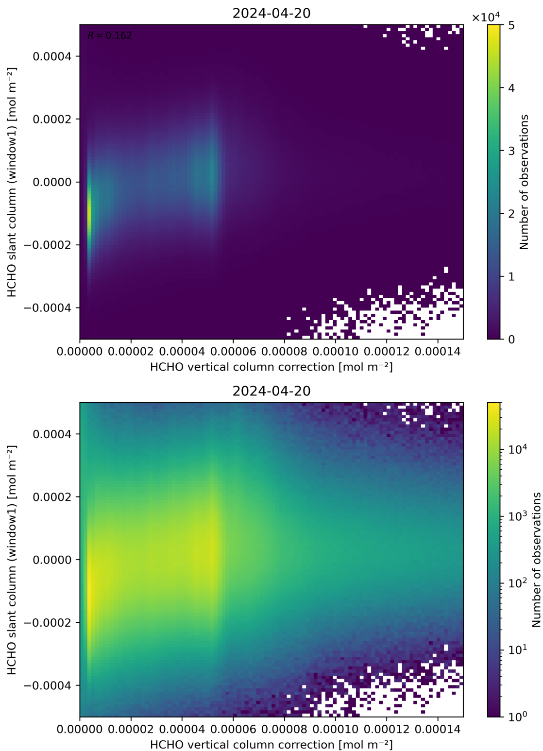
Figure 118: Scatter density plot of “HCHO vertical column correction” against “HCHO slant column (window1)” for 2024-04-19 to 2024-04-21.
