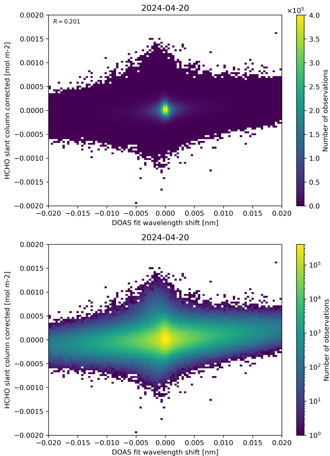
Figure 66: Scatter density plot of “DOAS fit wavelength shift” against “HCHO slant column corrected” for 2024-04-19 to 2024-04-21.
