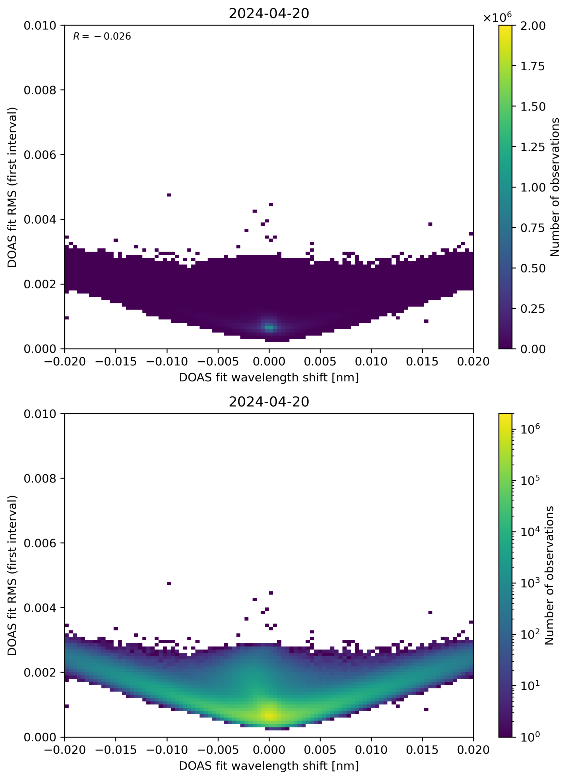
Figure 64: Scatter density plot of “DOAS fit wavelength shift” against “DOAS fit RMS (first interval)” for 2024-04-19 to 2024-04-21.
