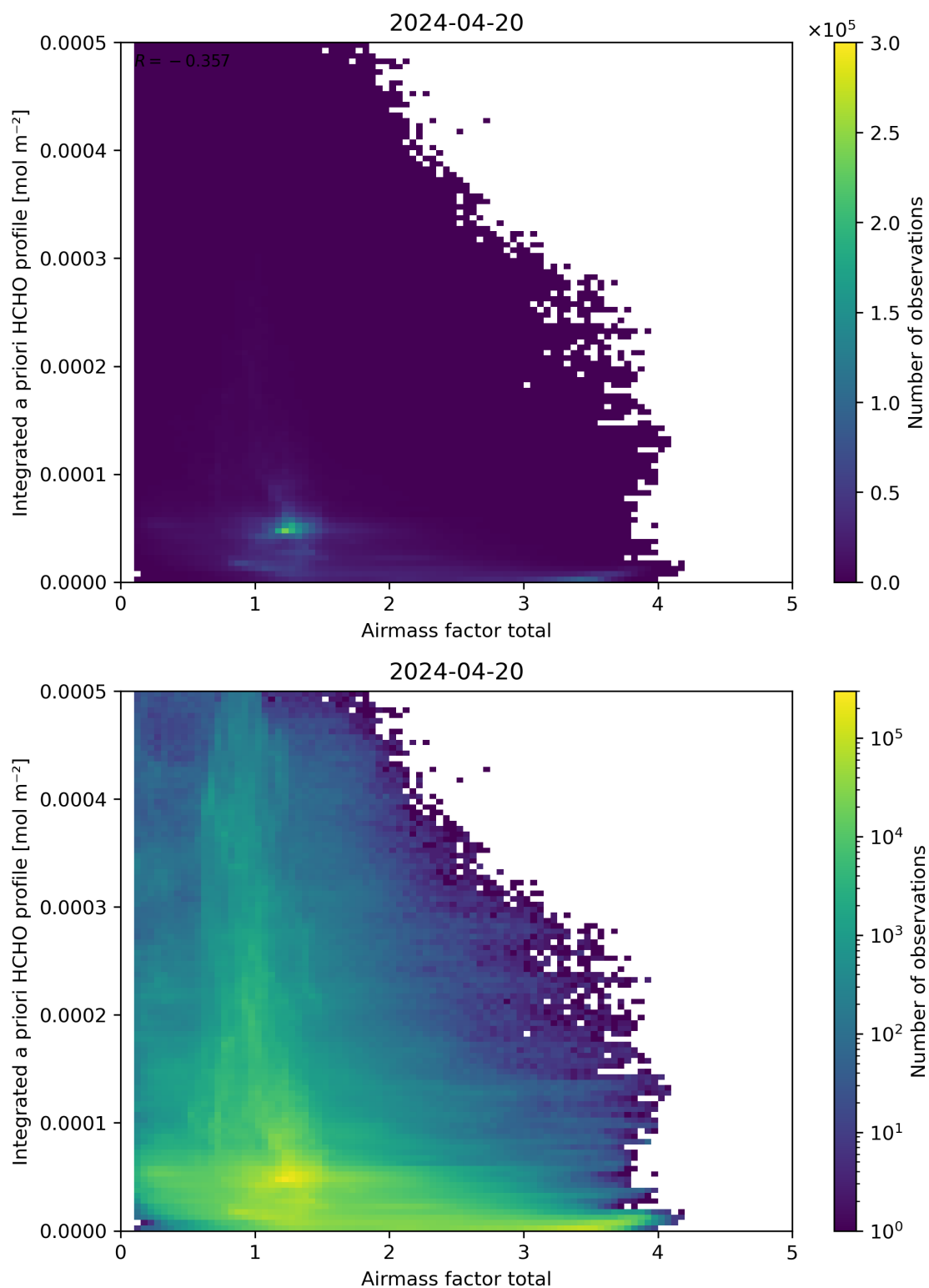
Figure 104: Scatter density plot of “Air mass factor total” against “Integrated a priori HCHO profile” for 2024-04-19 to 2024-04-21.
