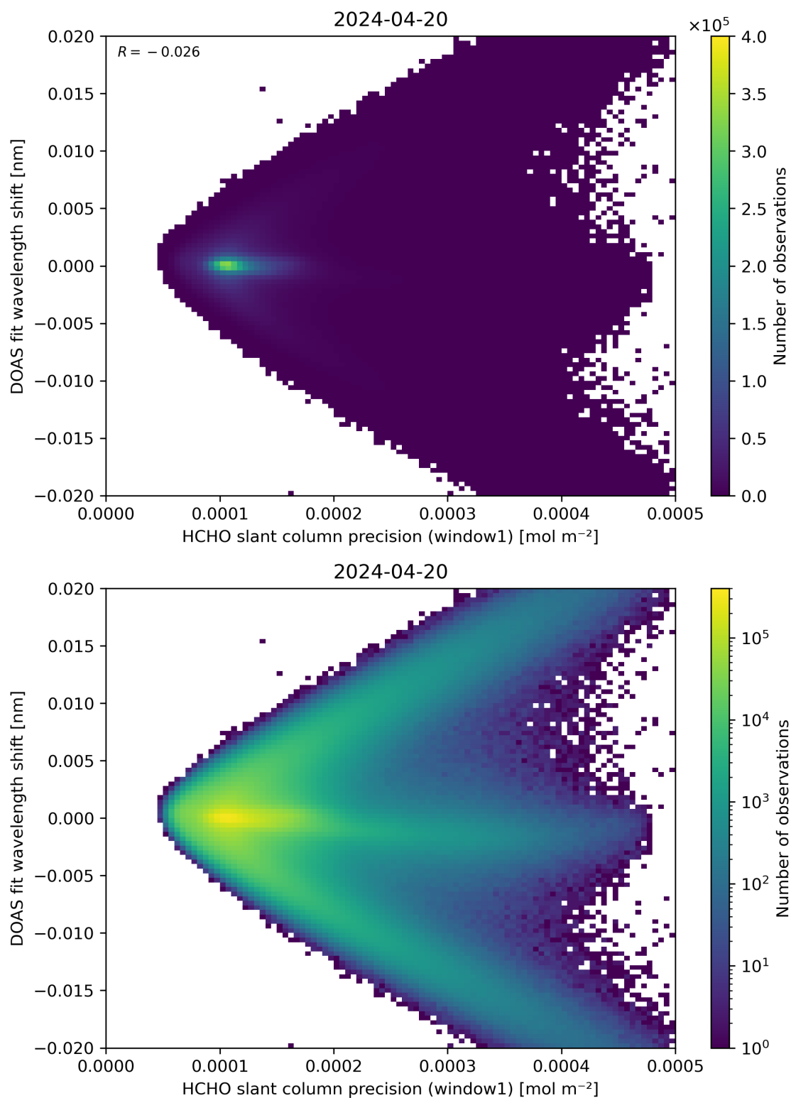
Figure 89: Scatter density plot of “HCHO slant column precision (window1)” against “DOAS fit wavelength shift” for 2024-04-19 to 2024-04-21.
