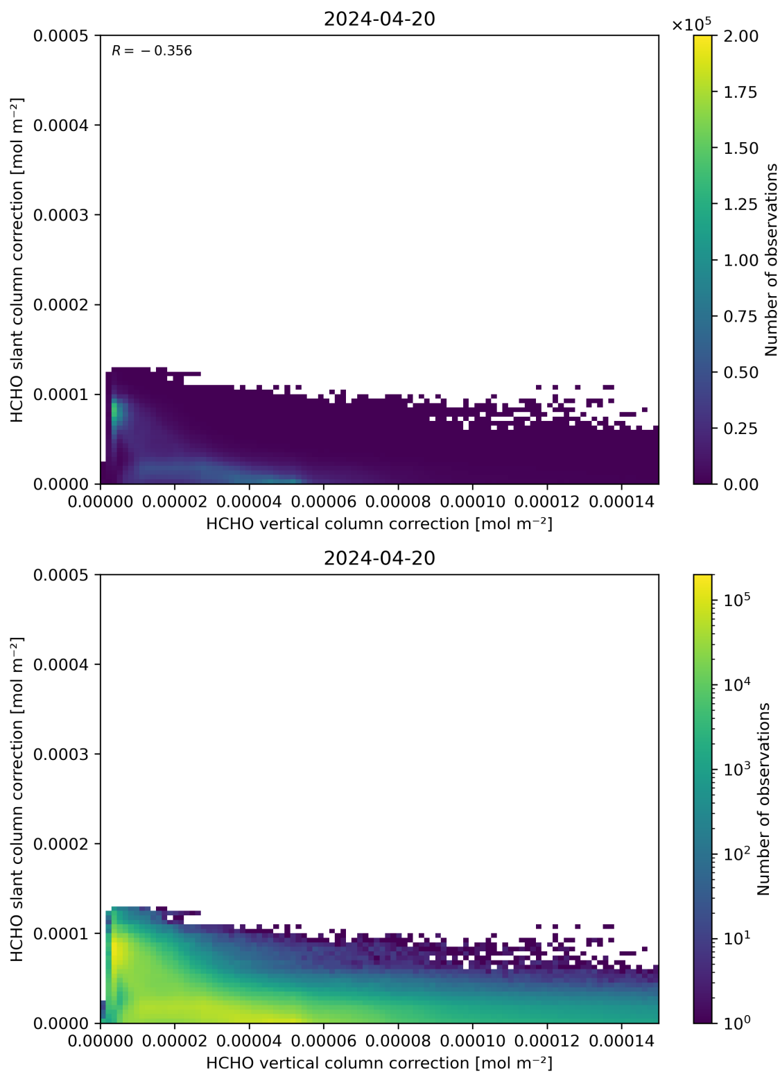
Figure 117: Scatter density plot of “HCHO vertical column correction” against “HCHO slant column correction” for 2024-04-19 to 2024-04-21.
