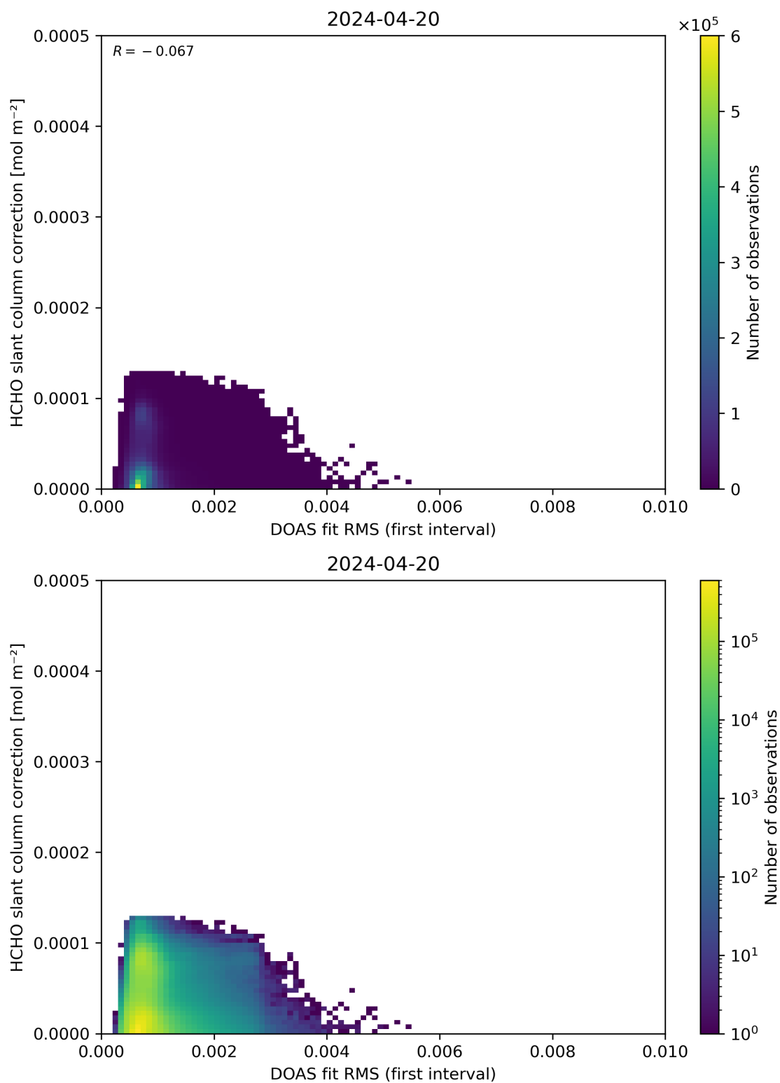
Figure 63: Scatter density plot of “DOAS fit RMS (first interval)” against “HCHO slant column correction” for 2024-04-19 to 2024-04-21.
