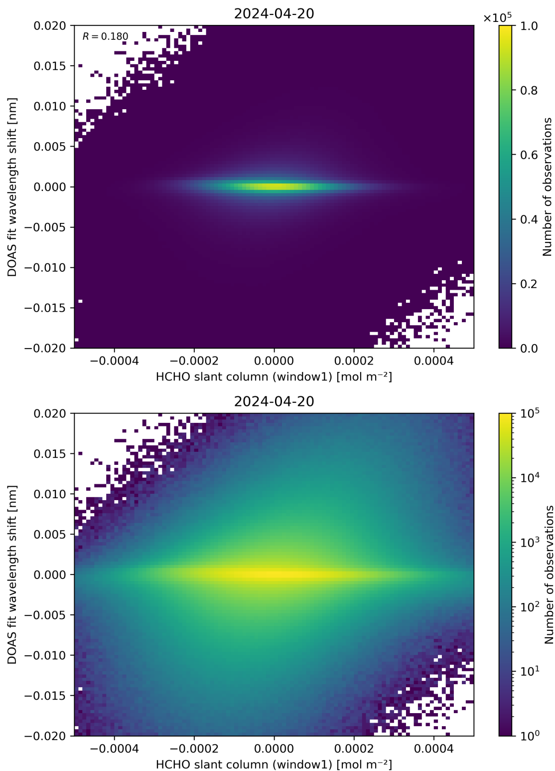
Figure 79: Scatter density plot of “HCHO slant column (window1)” against “DOAS fit wavelength shift” for 2024-04-19 to 2024-04-21.
