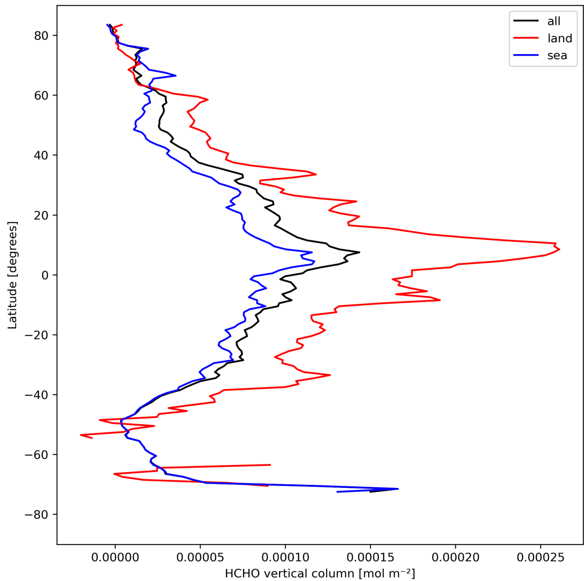
Figure 21: Zonal average of “HCHO vertical column” for 2024-04-19 to 2024-04-21.
