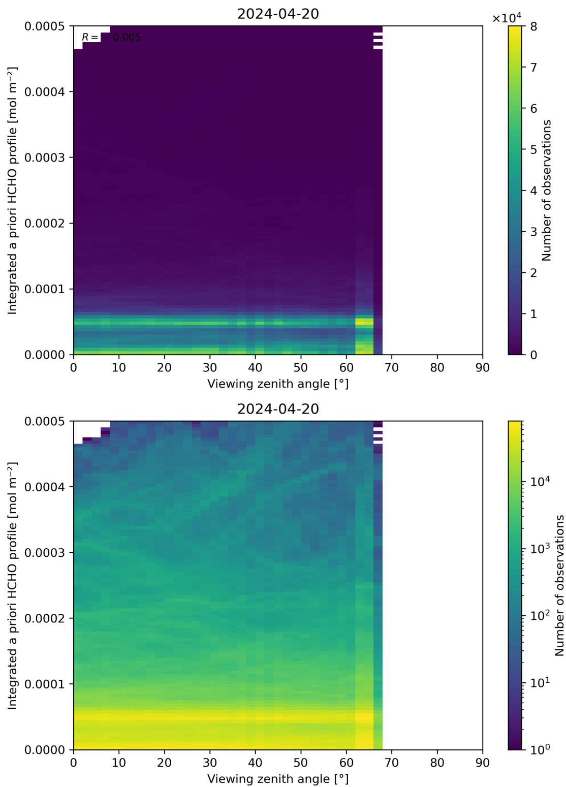
Figure 195: Scatter density plot of “Viewing zenith angle” against “Integrated a priori HCHO profile” for 2024-04-19 to 2024-04-21.
