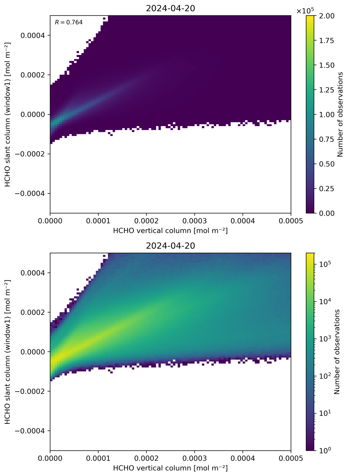
Figure 129: Scatter density plot of “HCHO vertical column” against “HCHO slant column (window1)” for 2024-04-19 to 2024-04-21.
