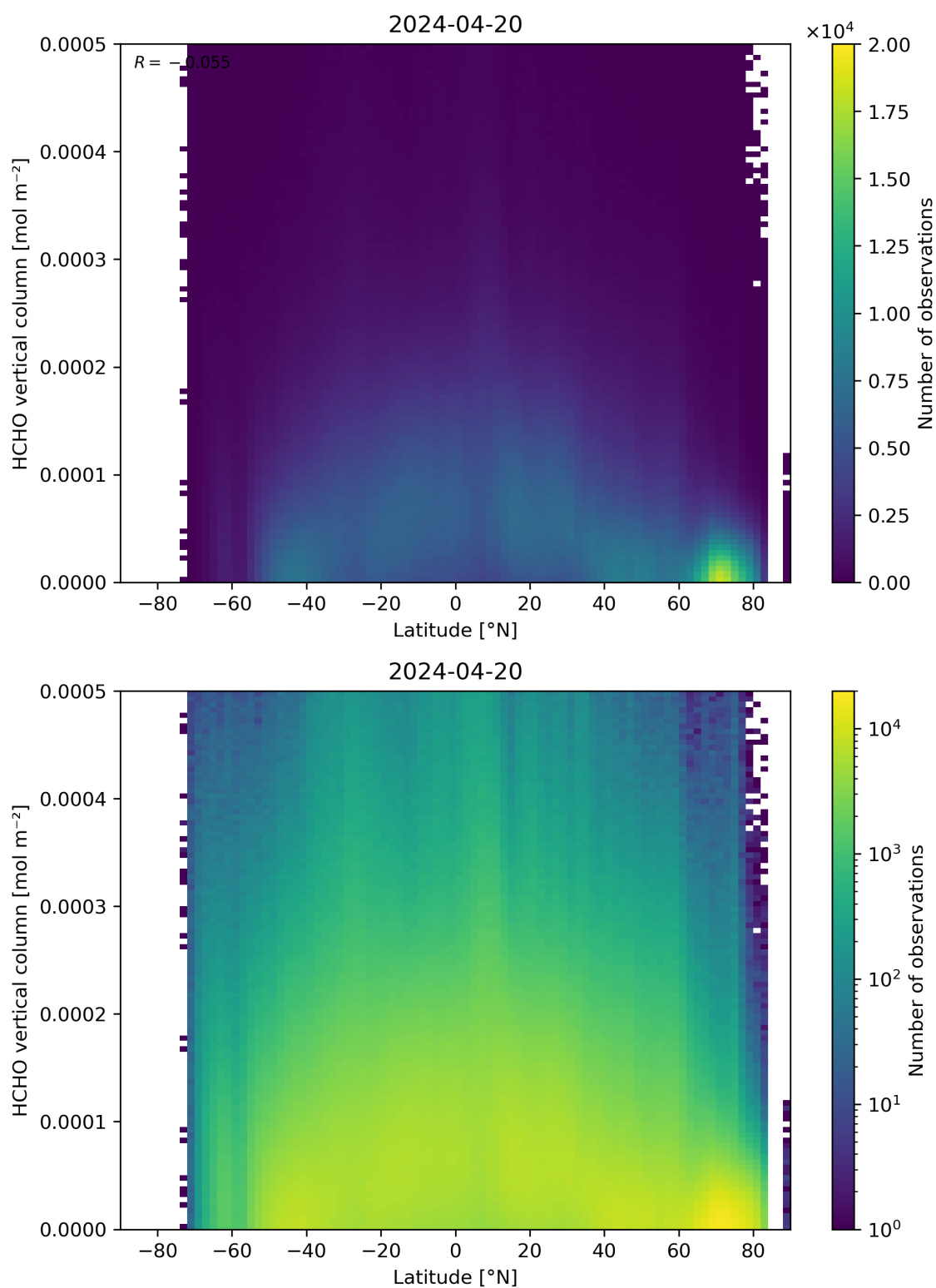
Figure 163: Scatter density plot of “Latitude” against “HCHO vertical column” for 2024-04-19 to 2024-04-21.
