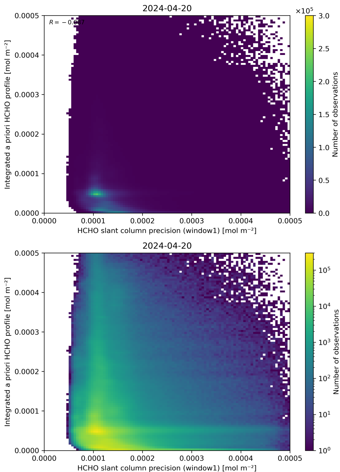
Figure 96: Scatter density plot of “HCHO slant column precision (window1)” against “Integrated a priori HCHO profile” for 2024-04-19 to 2024-04-21.
