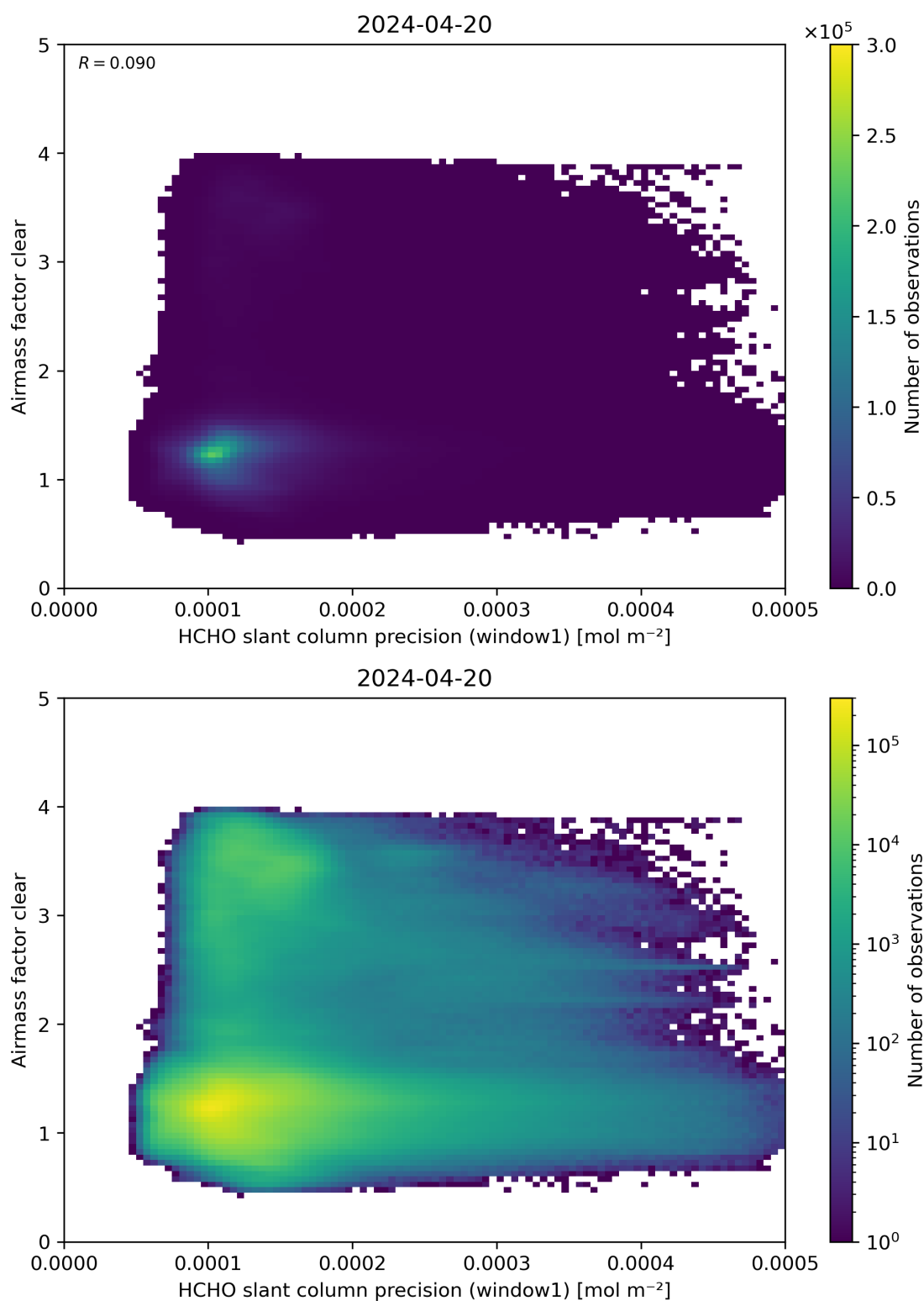
Figure 91: Scatter density plot of “HCHO slant column precision (window1)” against “Airmass factor clear” for 2024-04-19 to 2024-04-21.
