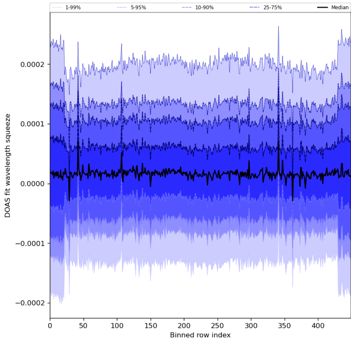
Figure 59: Along track statistics of “DOAS fit wavelength squeeze” for 2024-04-19 to 2024-04-21
