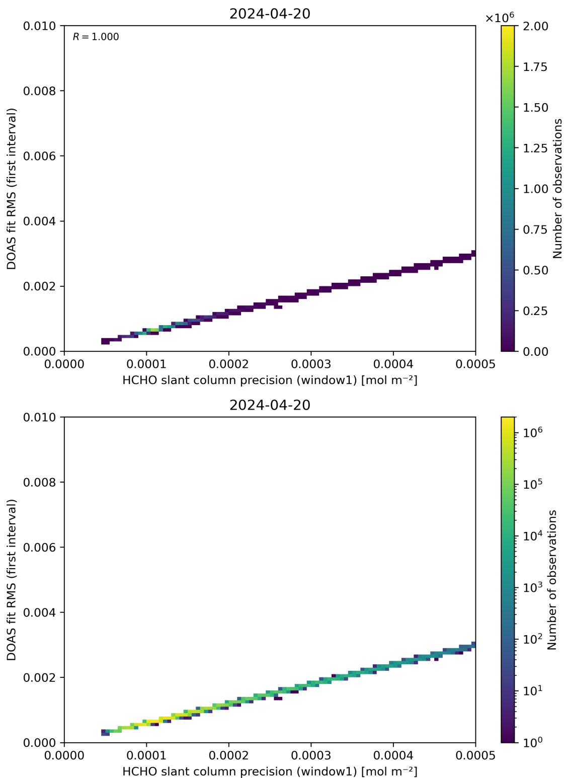
Figure 88: Scatter density plot of “HCHO slant column precision (window1)” against “DOAS fit RMS (first interval)” for 2024-04-19 to 2024-04-21.
