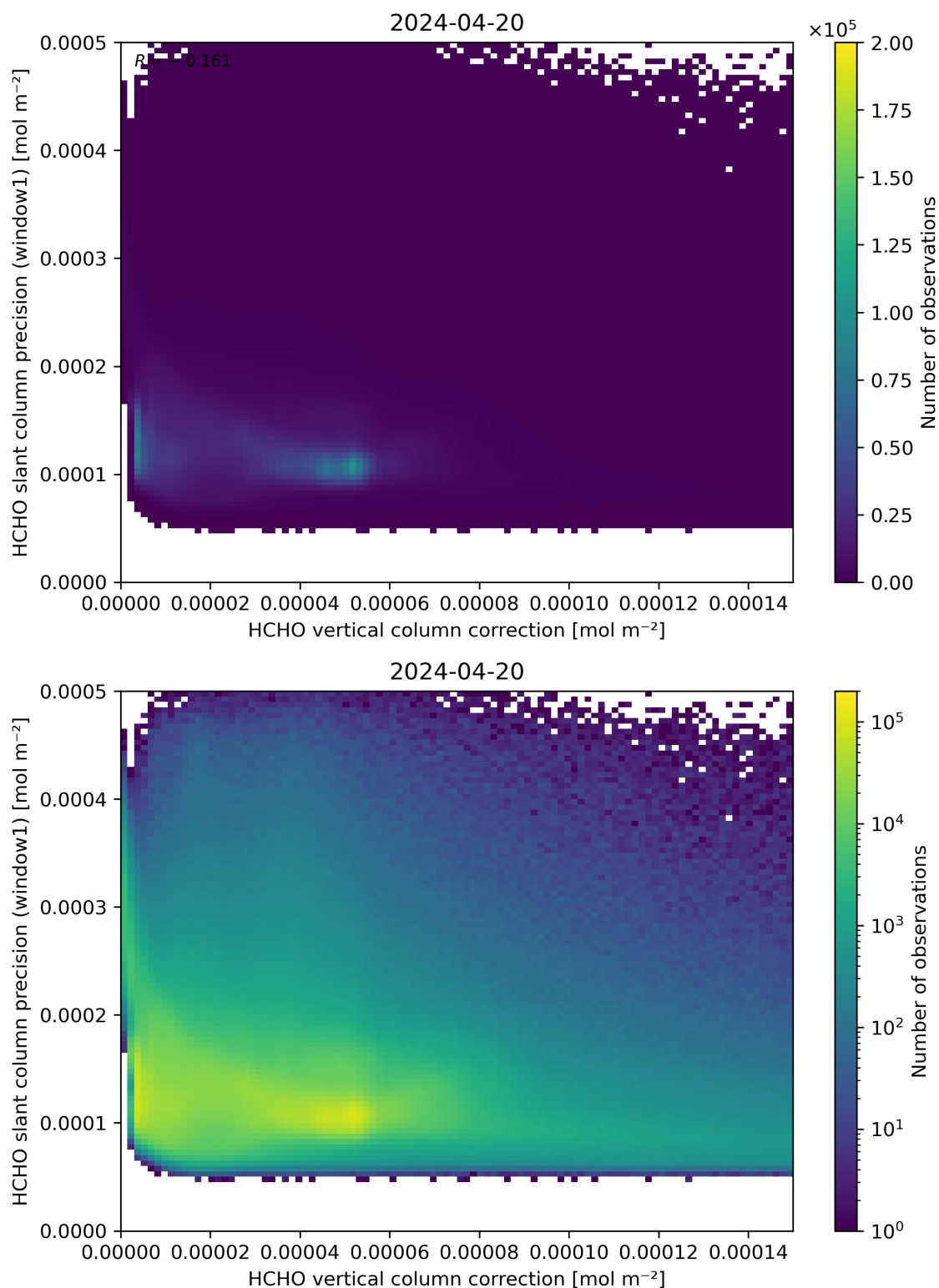
Figure 119: Scatter density plot of “HCHO vertical column correction” against “HCHO slant column precision (window1)” for 2024-04-19 to 2024-04-21.
