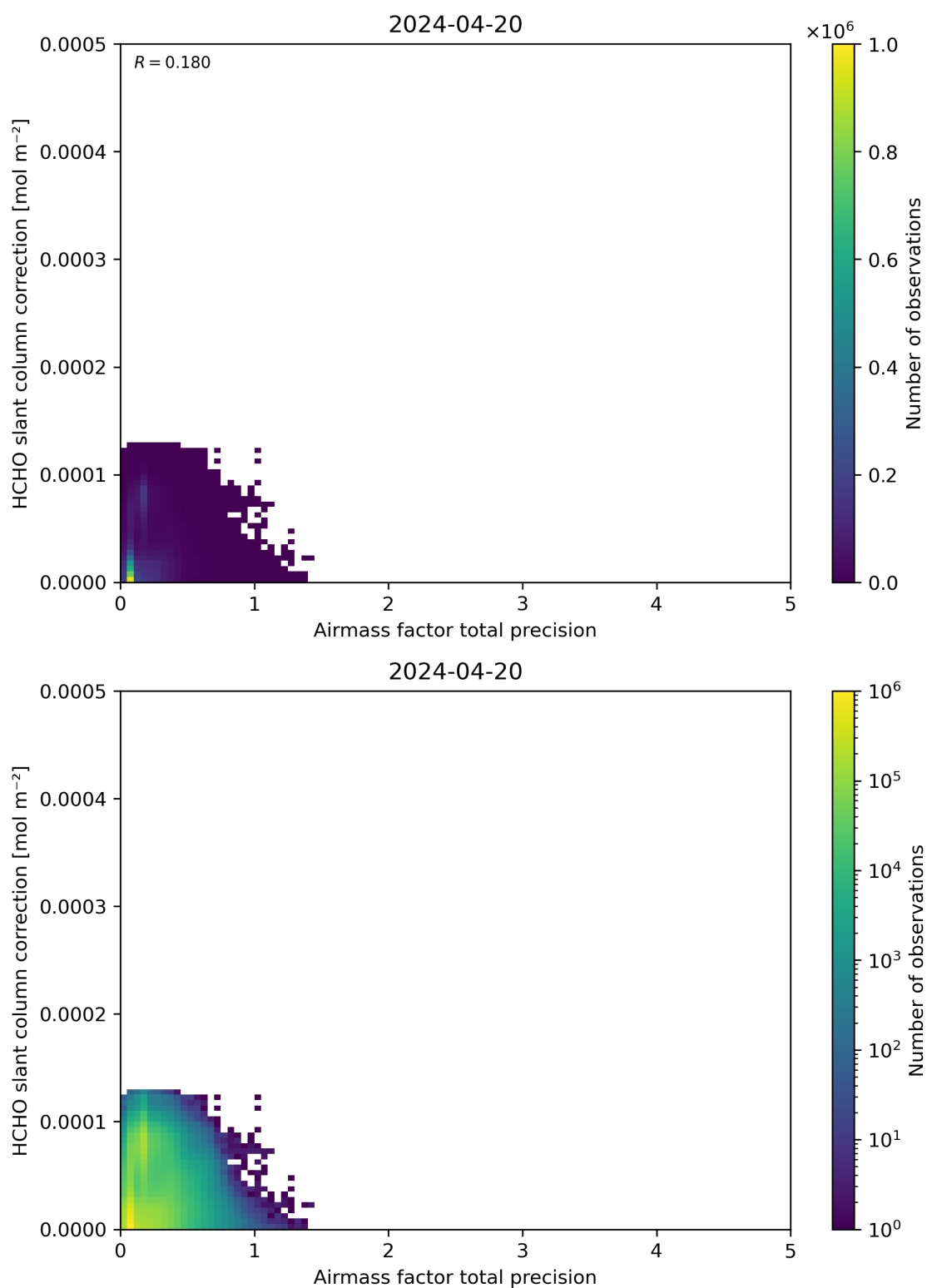
Figure 110: Scatter density plot of “Airmass factor total precision” against “HCHO slant column correction” for 2024-04-19 to 2024-04-21.
