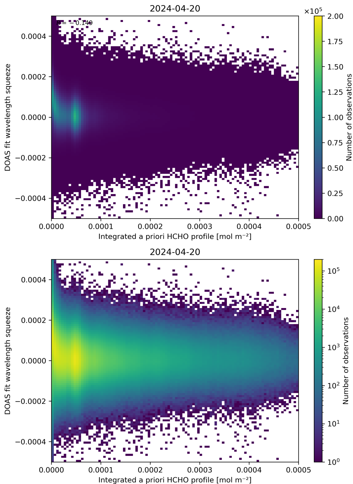
Figure 150: Scatter density plot of “Integrated a priori HCHO profile” against “DOAS fit wavelength squeeze” for 2024-04-19 to 2024-04-21.
