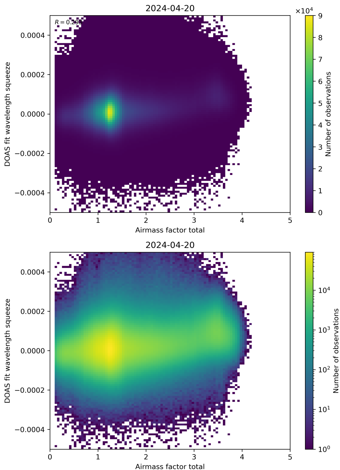
Figure 99: Scatter density plot of “Airmass factor total” against “DOAS fit wavelength squeeze” for 2024-04-19 to 2024-04-21.
