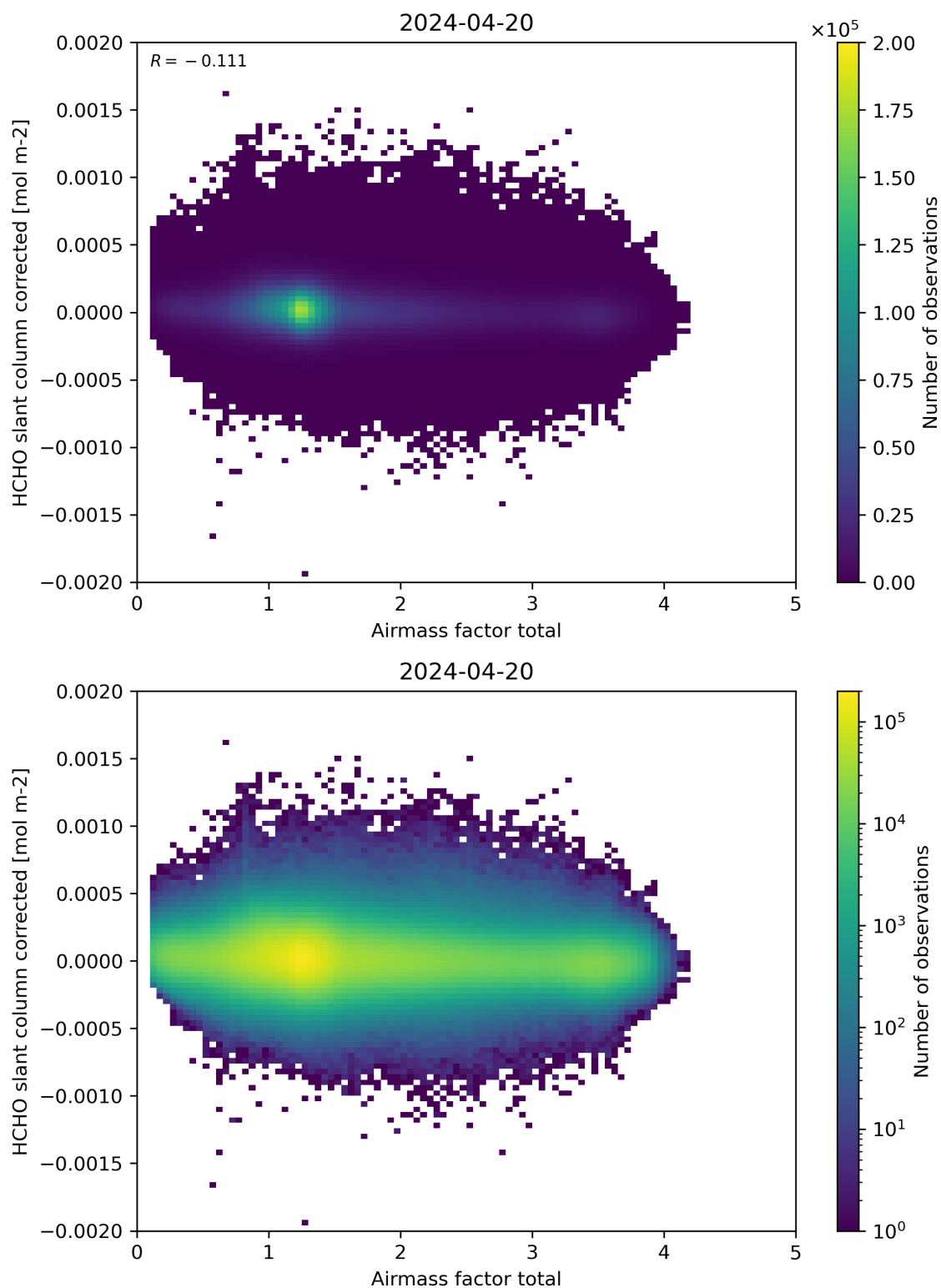
Figure 101: Scatter density plot of “Airmass factor total” against “HCHO slant column corrected” for 2024-04-19 to 2024-04-21.
