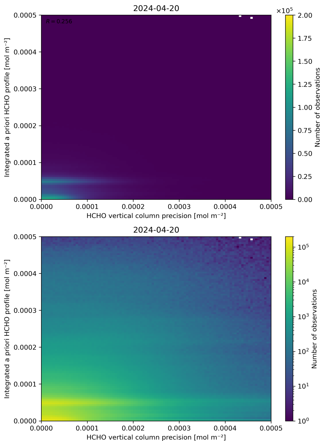
Figure 147: Scatter density plot of “HCHO vertical column precision” against “Integrated a priori HCHO profile” for 2024-04-19 to 2024-04-21.
