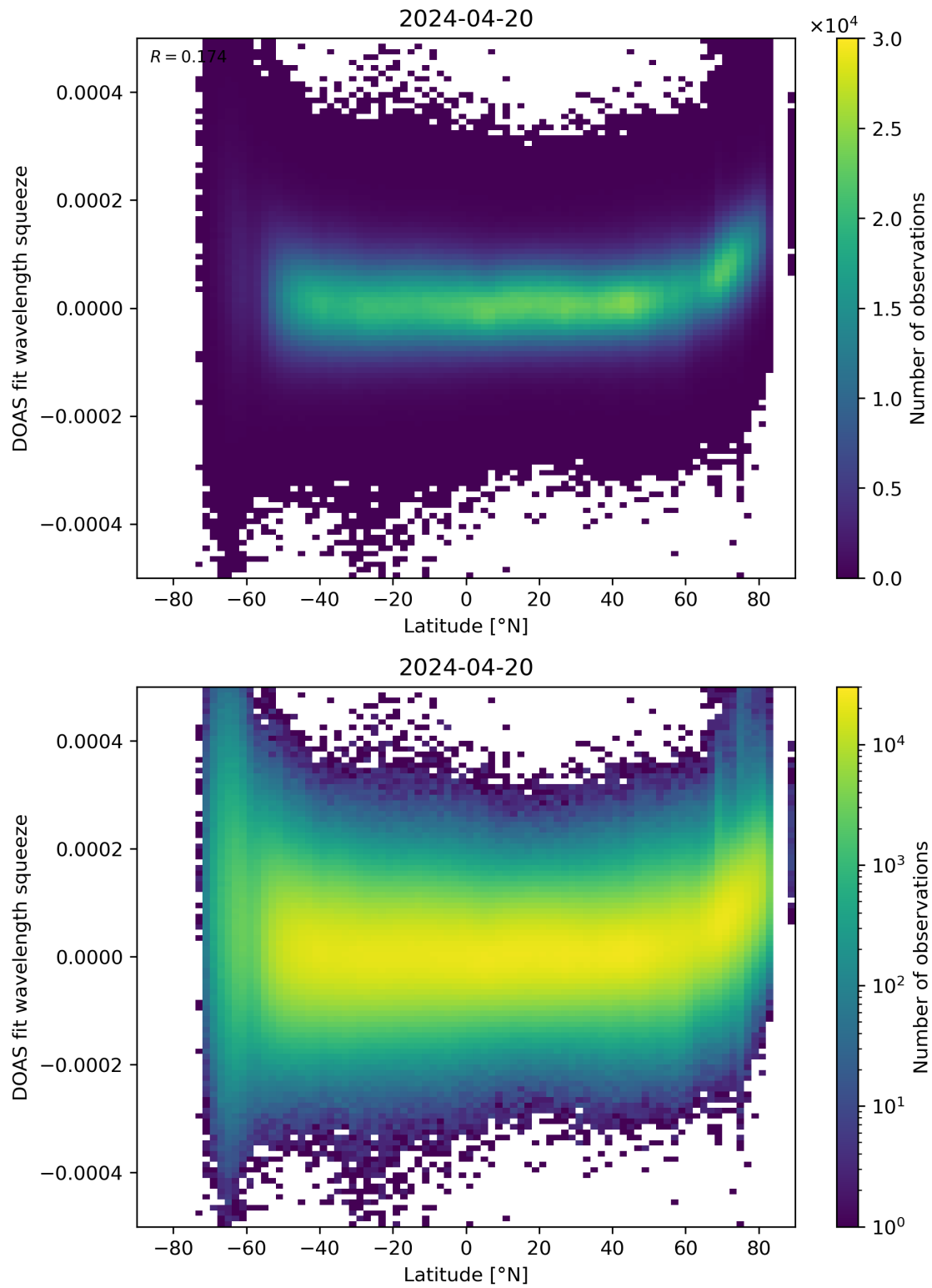
Figure 155: Scatter density plot of “Latitude” against “DOAS fit wavelength squeeze” for 2024-04-19 to 2024-04-21.
