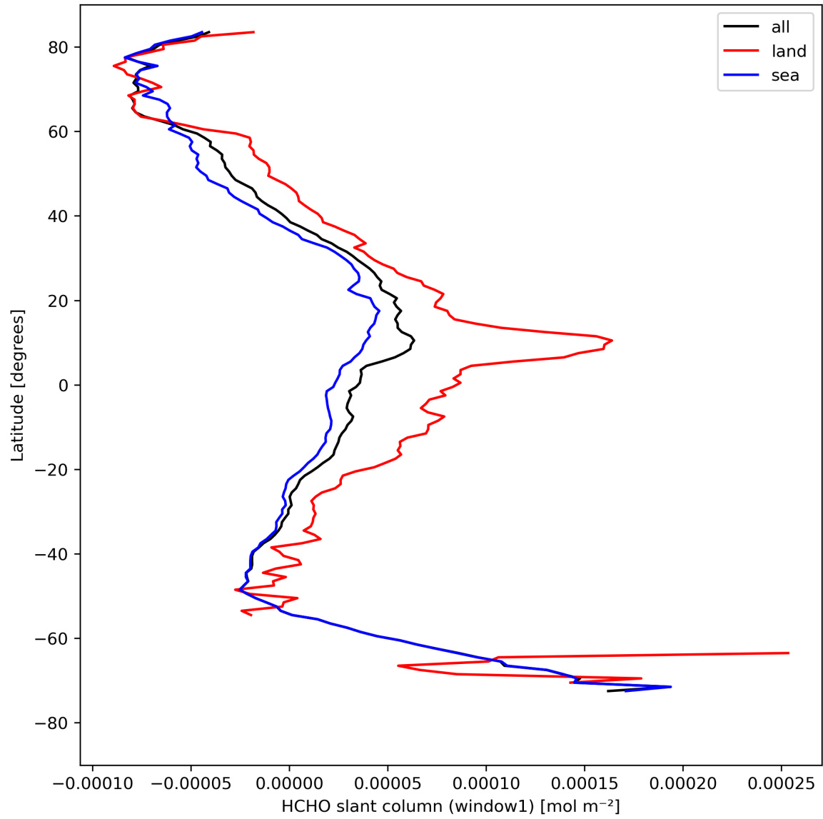
Figure 24: Zonal average of “HCHO slant column (window1)” for 2024-04-19 to 2024-04-21.
