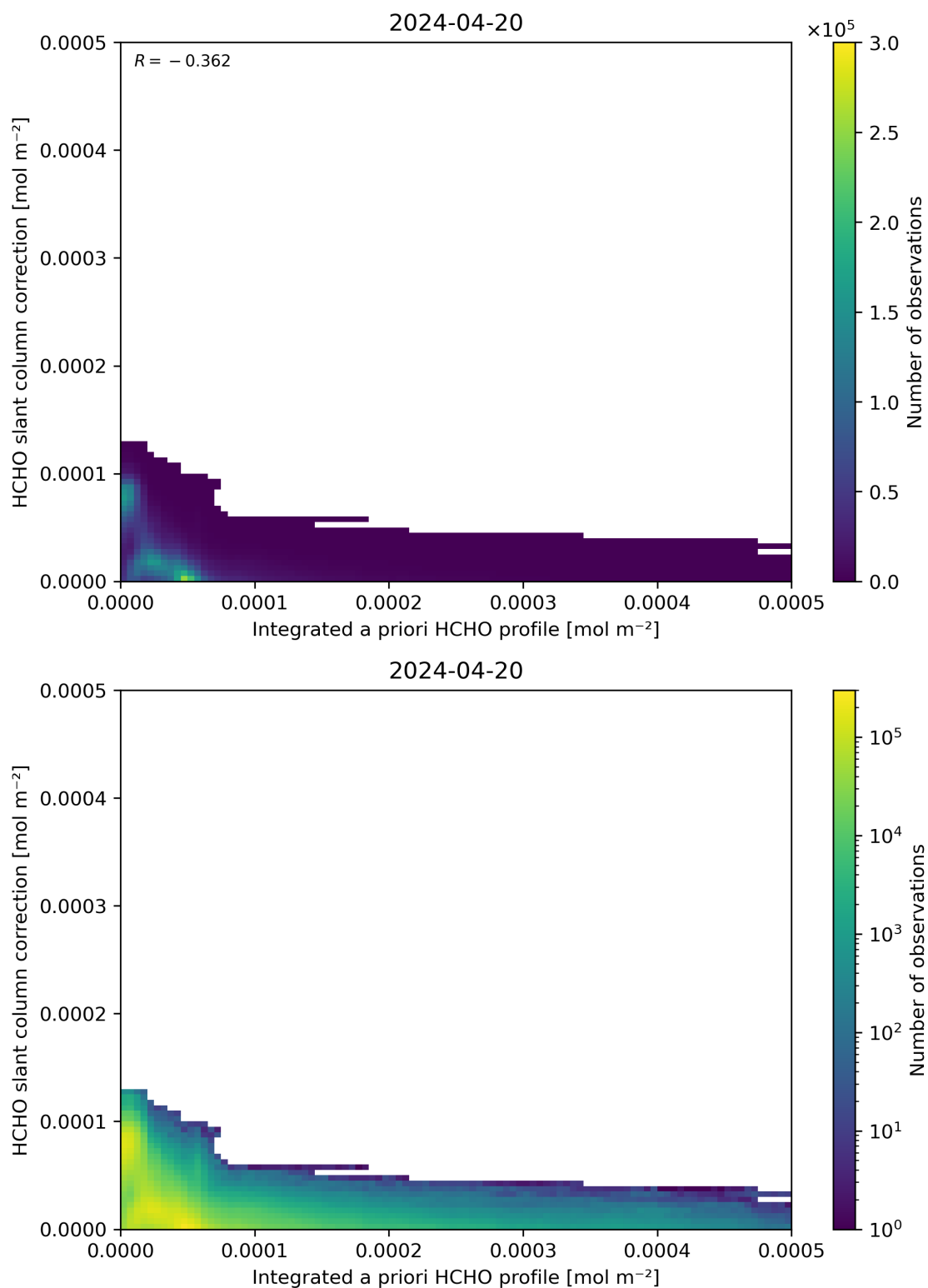
Figure 152: Scatter density plot of “Integrated a priori HCHO profile” against “HCHO slant column correction” for 2024-04-19 to 2024-04-21.
