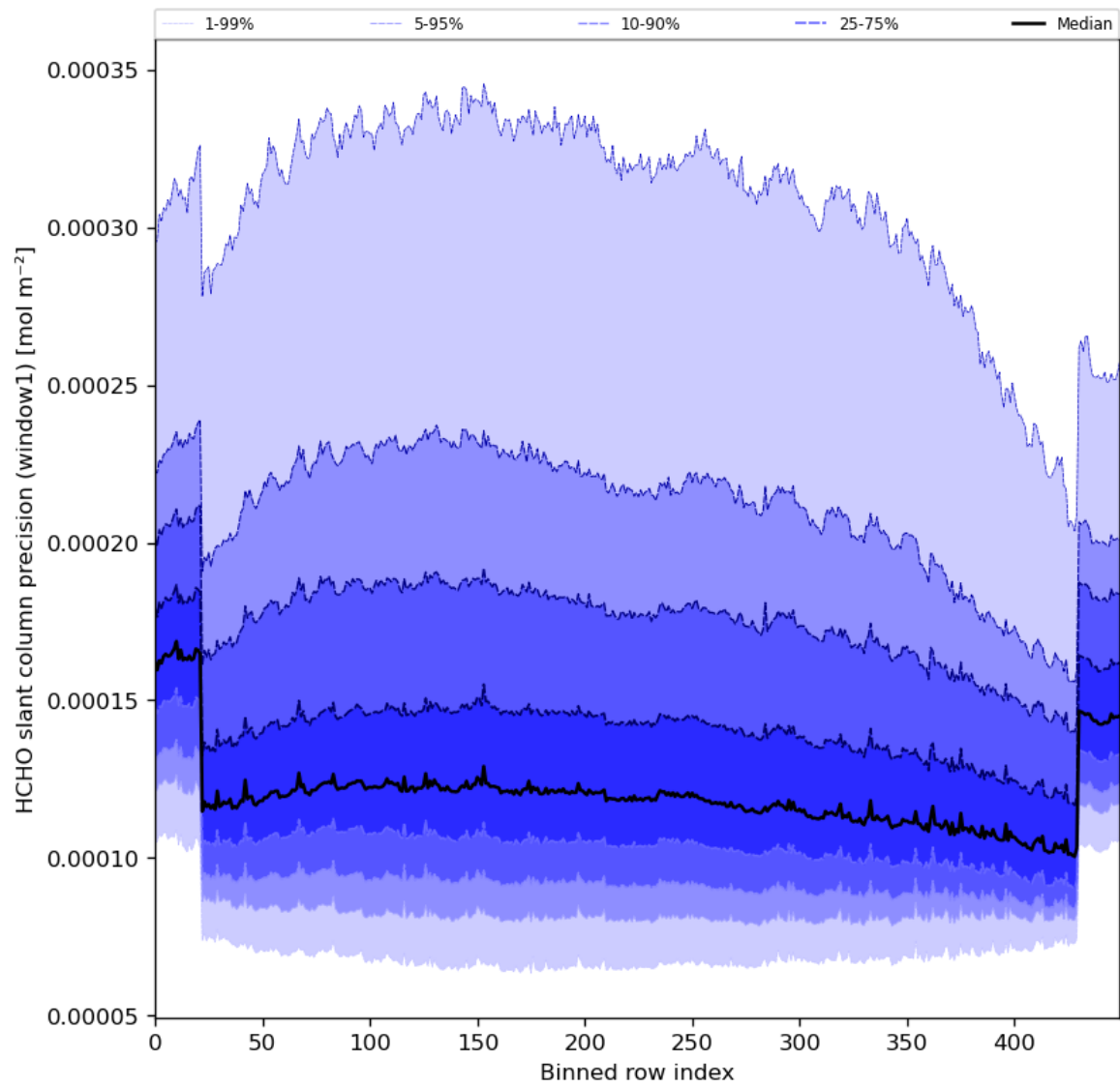
Figure 53: Along track statistics of “HCHO slant column precision (window1)” for 2024-04-19 to 2024-04-21
