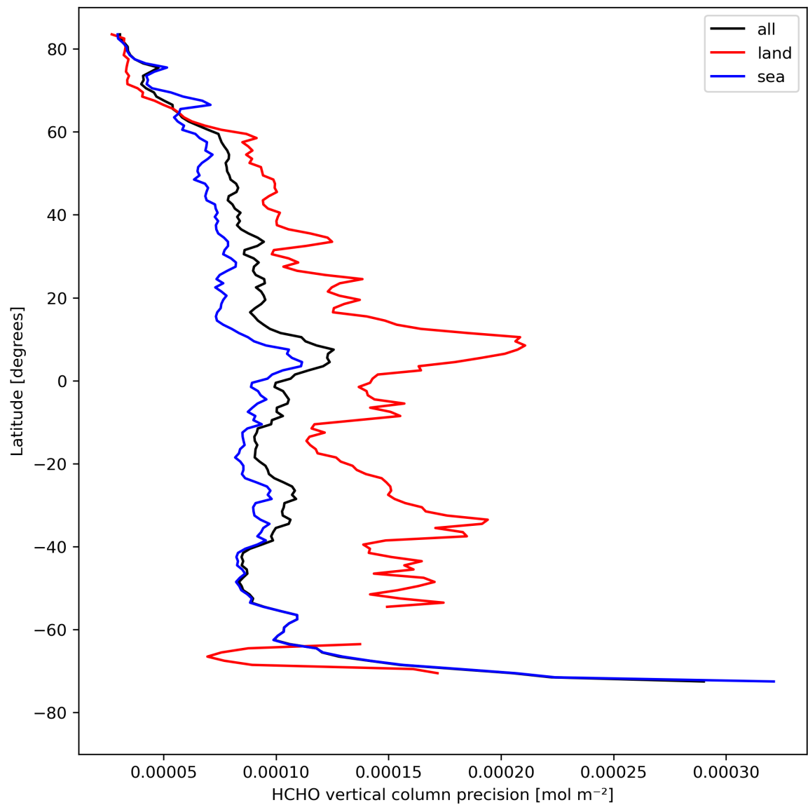
Figure 22: Zonal average of “HCHO vertical column precision” for 2024-04-19 to 2024-04-21.
