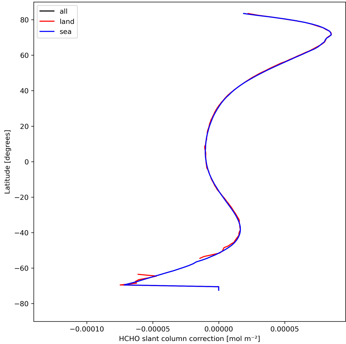
Figure 33: Zonal average of “HCHO slant column correction” for 2024-04-19 to 2024-04-21.
