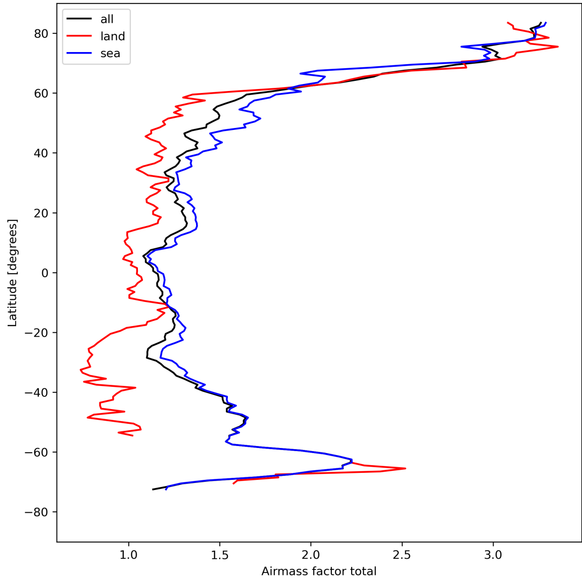
Figure 26: Zonal average of “Airmass factor total” for 2024-04-19 to 2024-04-21.
