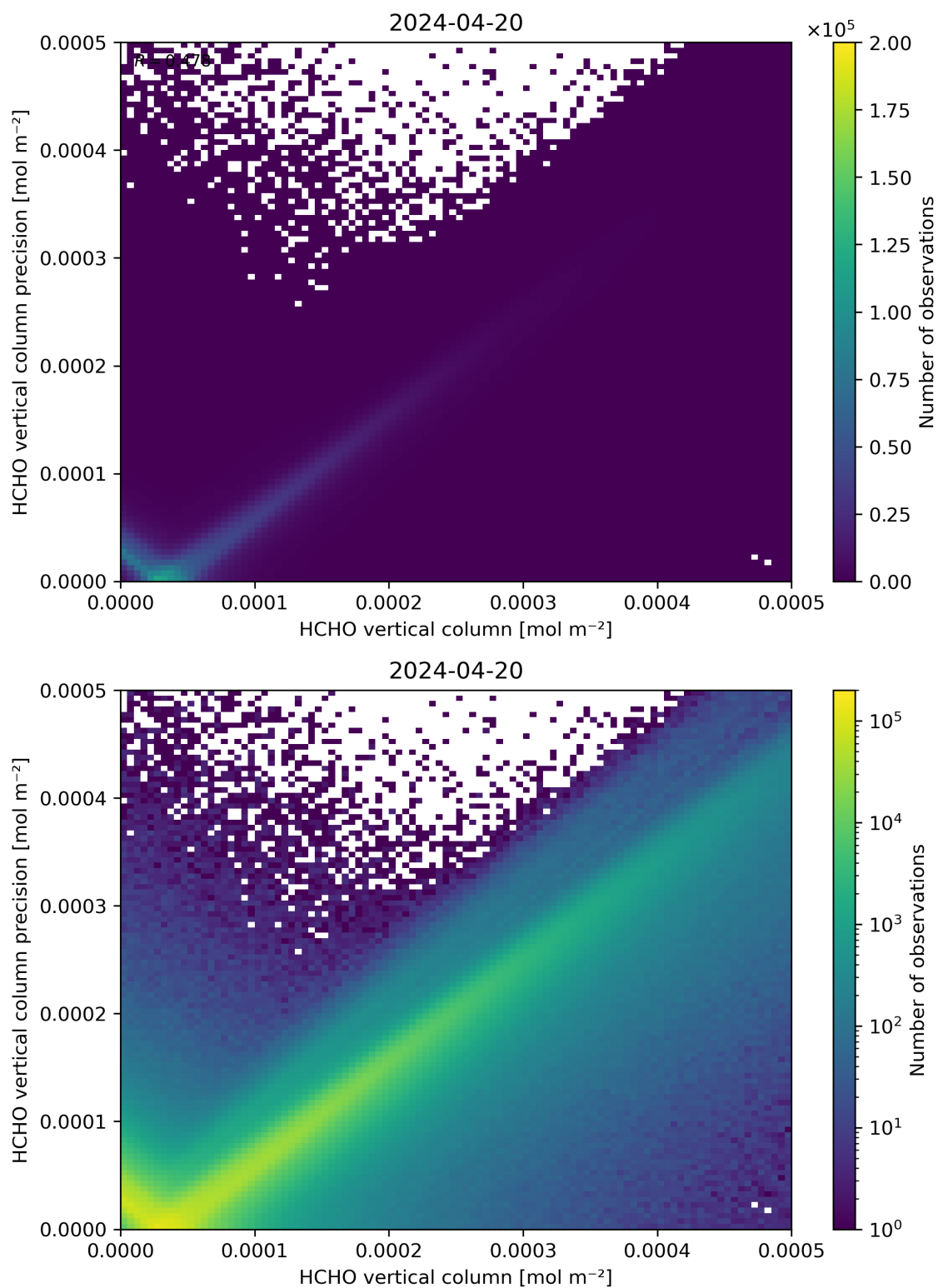
Figure 134: Scatter density plot of “HCHO vertical column” against “HCHO vertical column precision” for 2024-04-19 to 2024-04-21.
