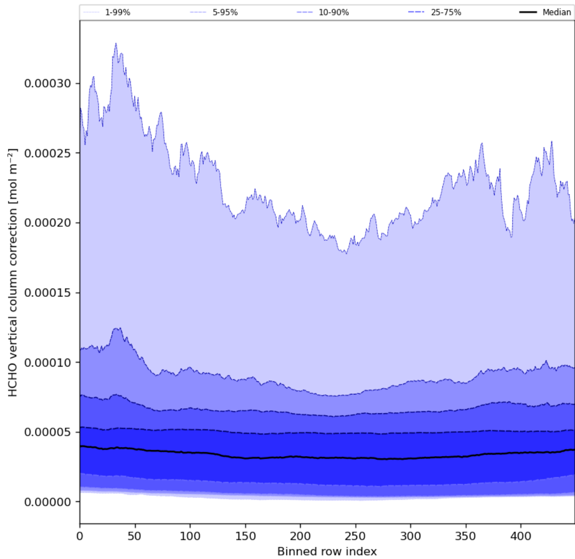
Figure 51: Along track statistics of “HCHO vertical column correction” for 2024-04-19 to 2024-04-21
