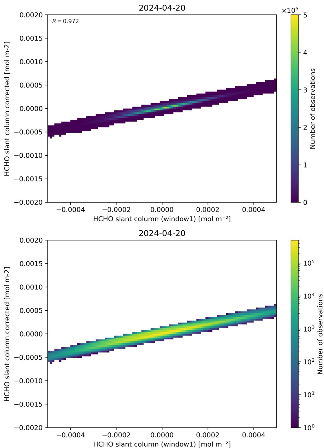
Figure 82: Scatter density plot of “HCHO slant column (window1)” against “HCHO slant column corrected” for 2024-04-19 to 2024-04-21.
