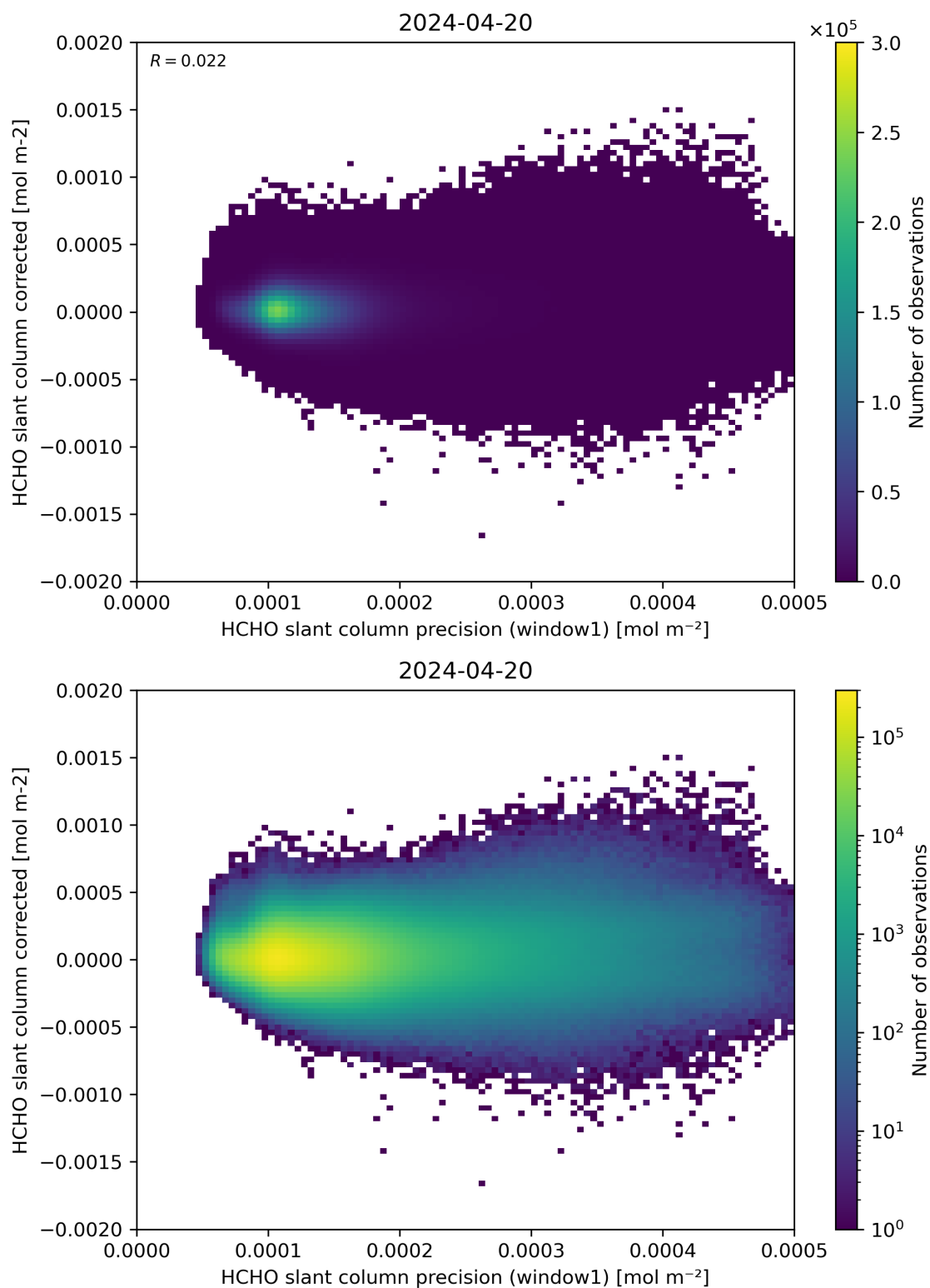
Figure 92: Scatter density plot of “HCHO slant column precision (window1)” against “HCHO slant column corrected” for 2024-04-19 to 2024-04-21.
