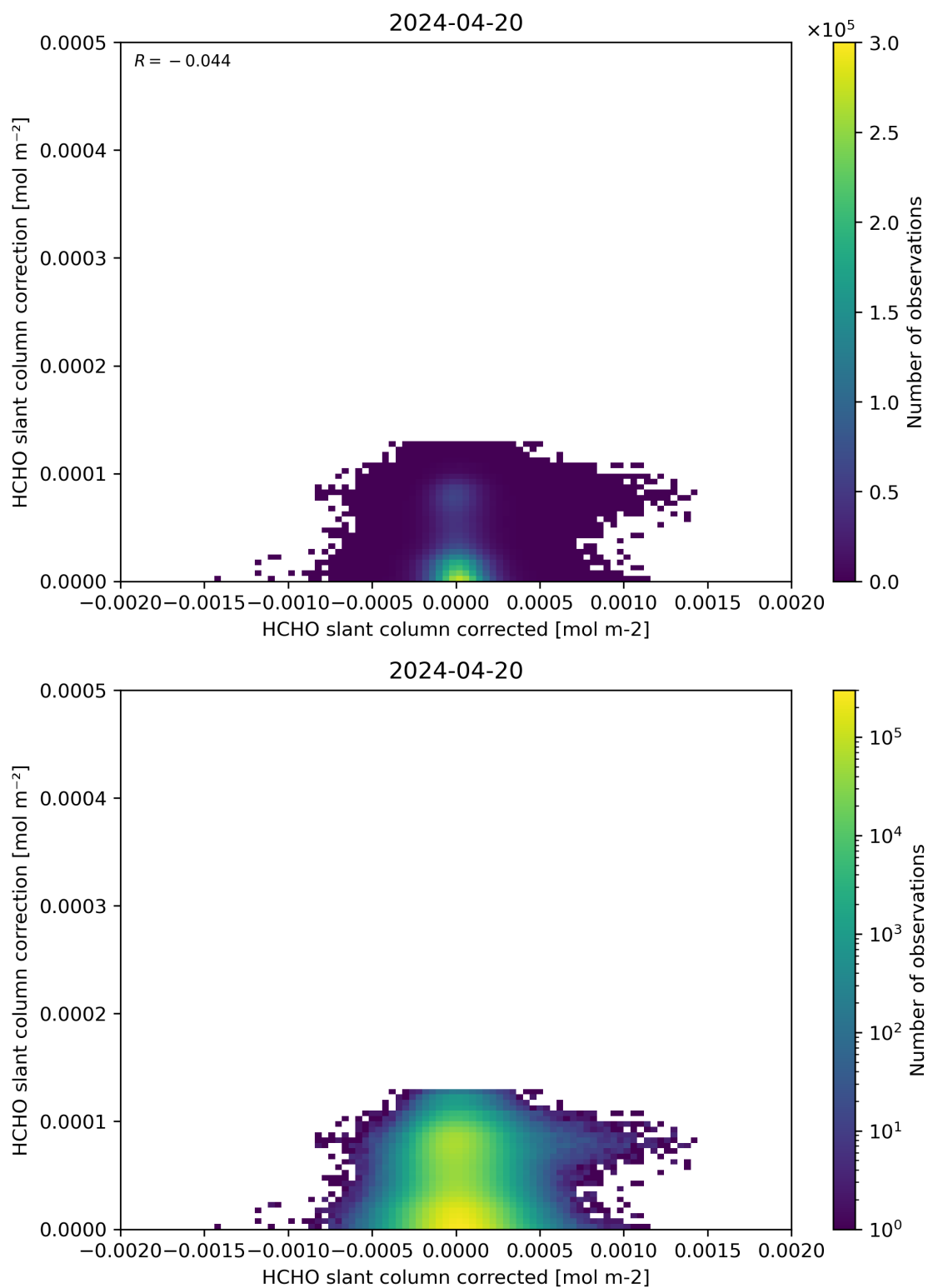
Figure 77: Scatter density plot of “HCHO slant column corrected” against “HCHO slant column correction” for 2024-04-19 to 2024-04-21.
