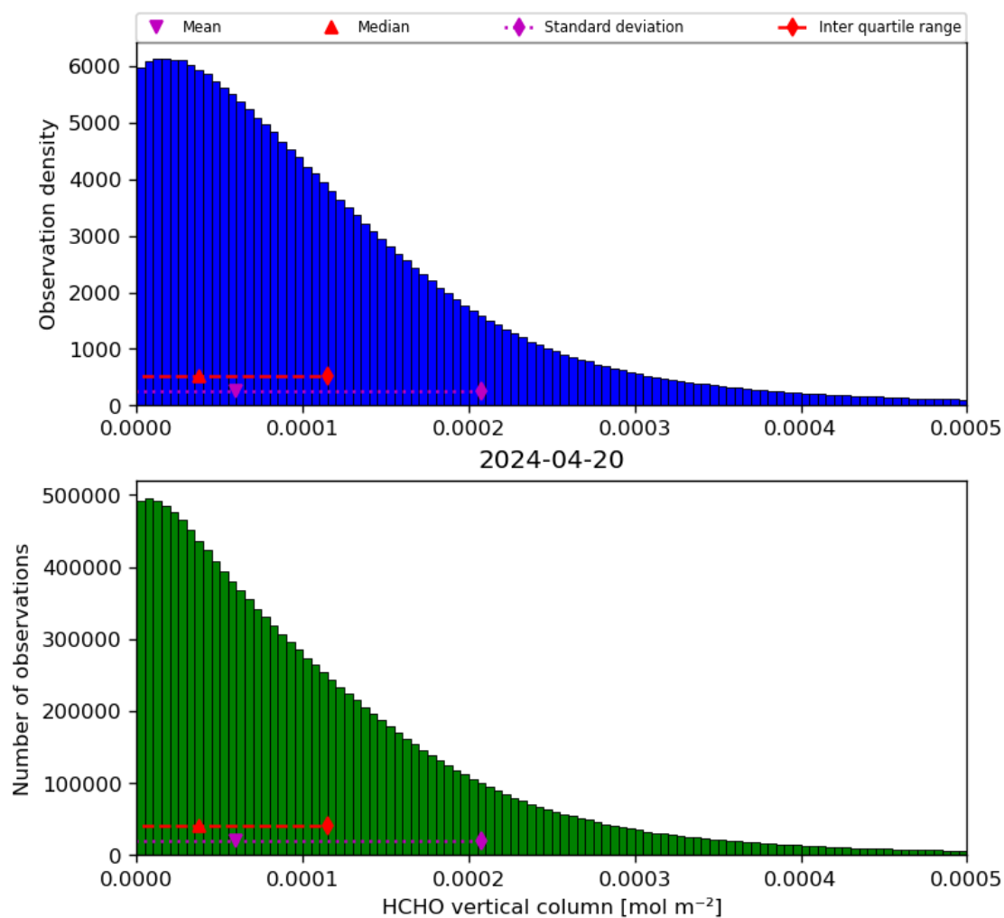
Figure 35: Histogram of “HCHO vertical column” for 2024-04-19 to 2024-04-21
