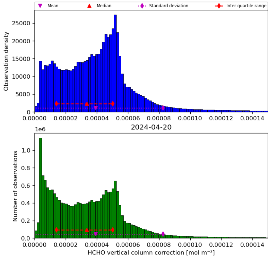
Figure 37: Histogram of “HCHO vertical column correction” for 2024-04-19 to 2024-04-21
