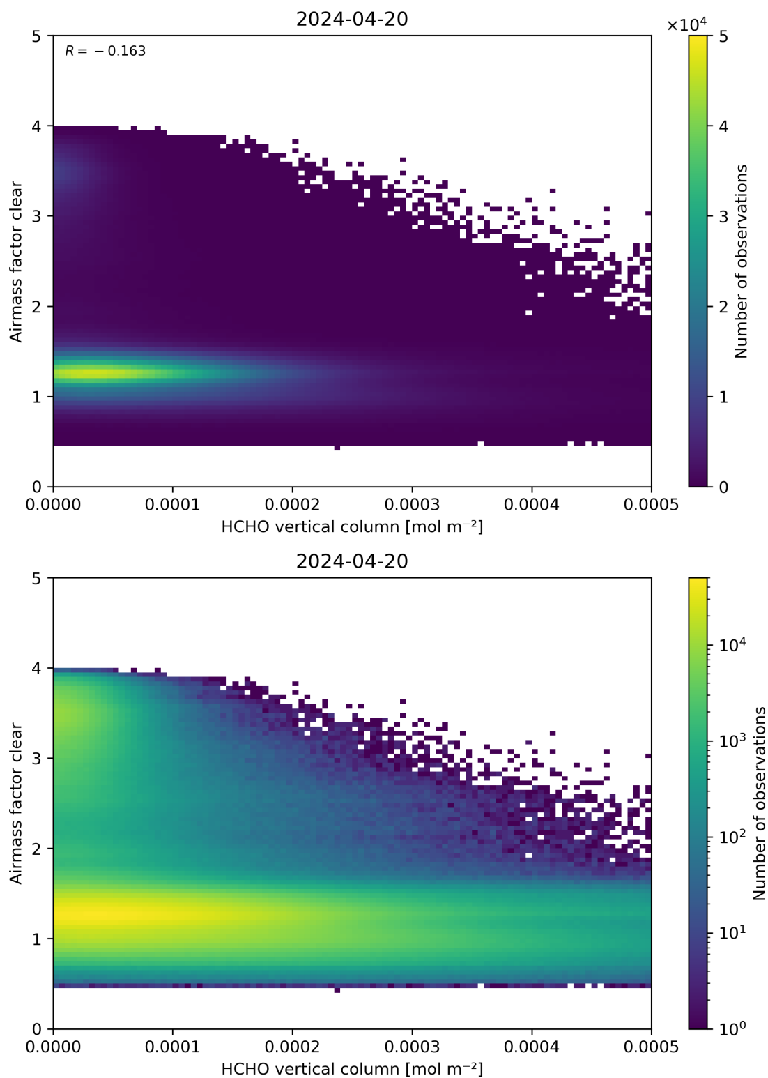
Figure 126: Scatter density plot of “HCHO vertical column” against “Airmass factor clear” for 2024-04-19 to 2024-04-21.
