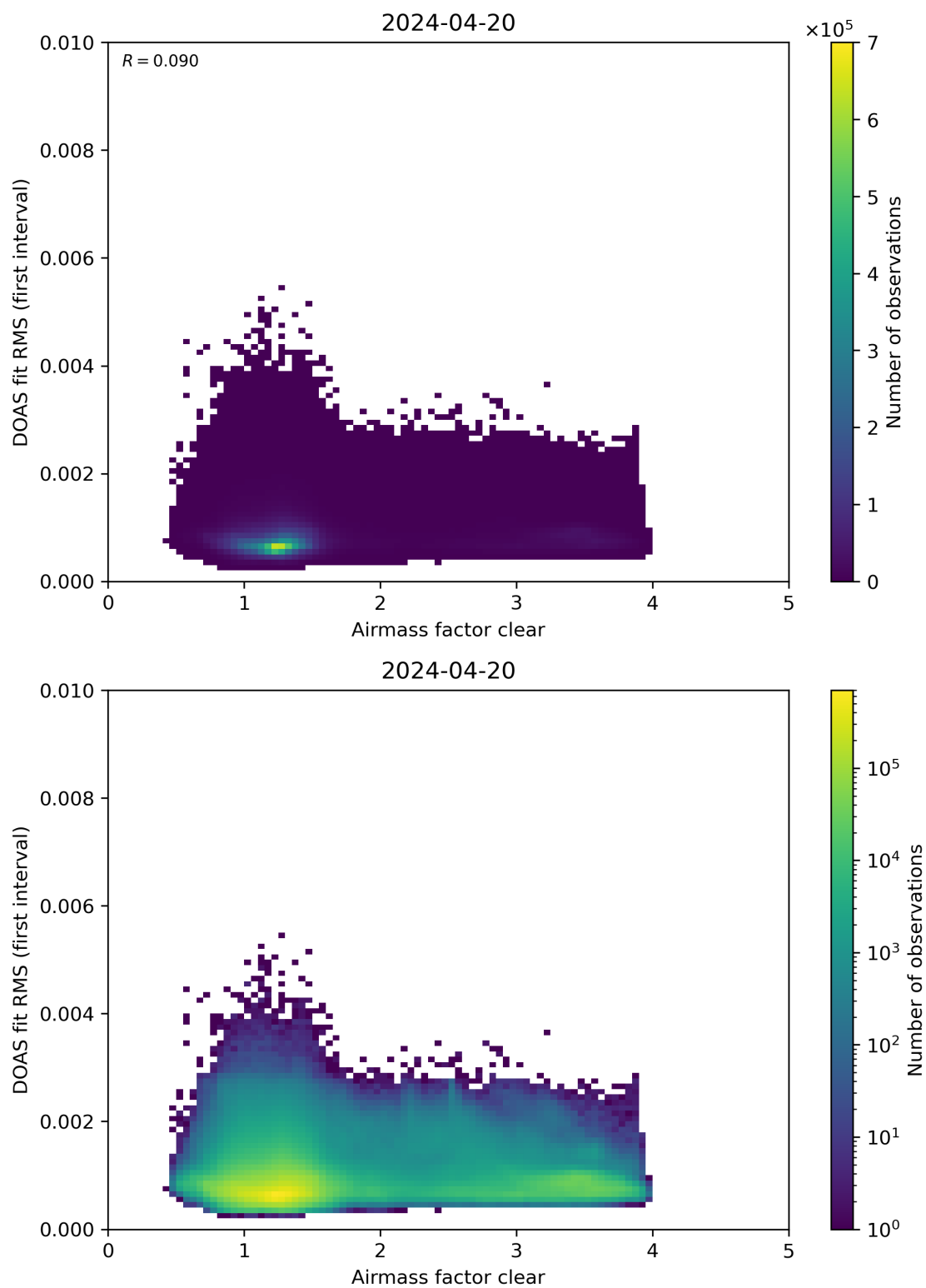
Figure 71: Scatter density plot of “Airmass factor clear” against “DOAS fit RMS (first interval)” for 2024-04-19 to 2024-04-21.
