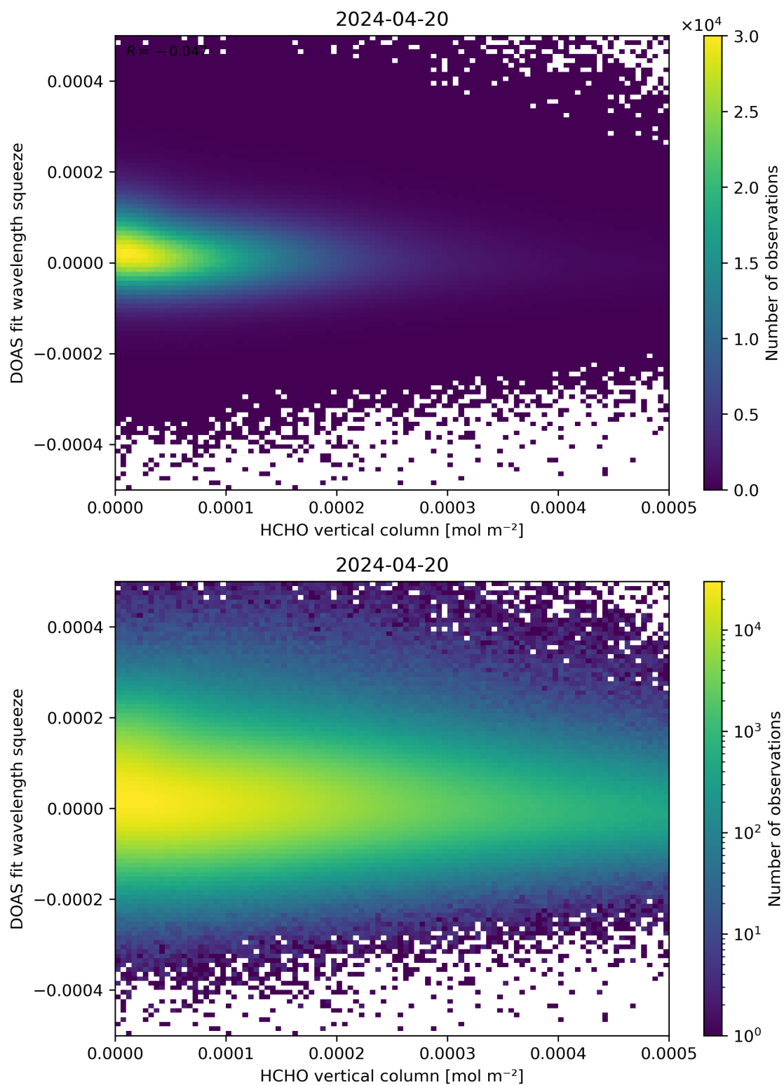
Figure 125: Scatter density plot of “HCHO vertical column” against “DOAS fit wavelength squeeze” for 2024-04-19 to 2024-04-21.
