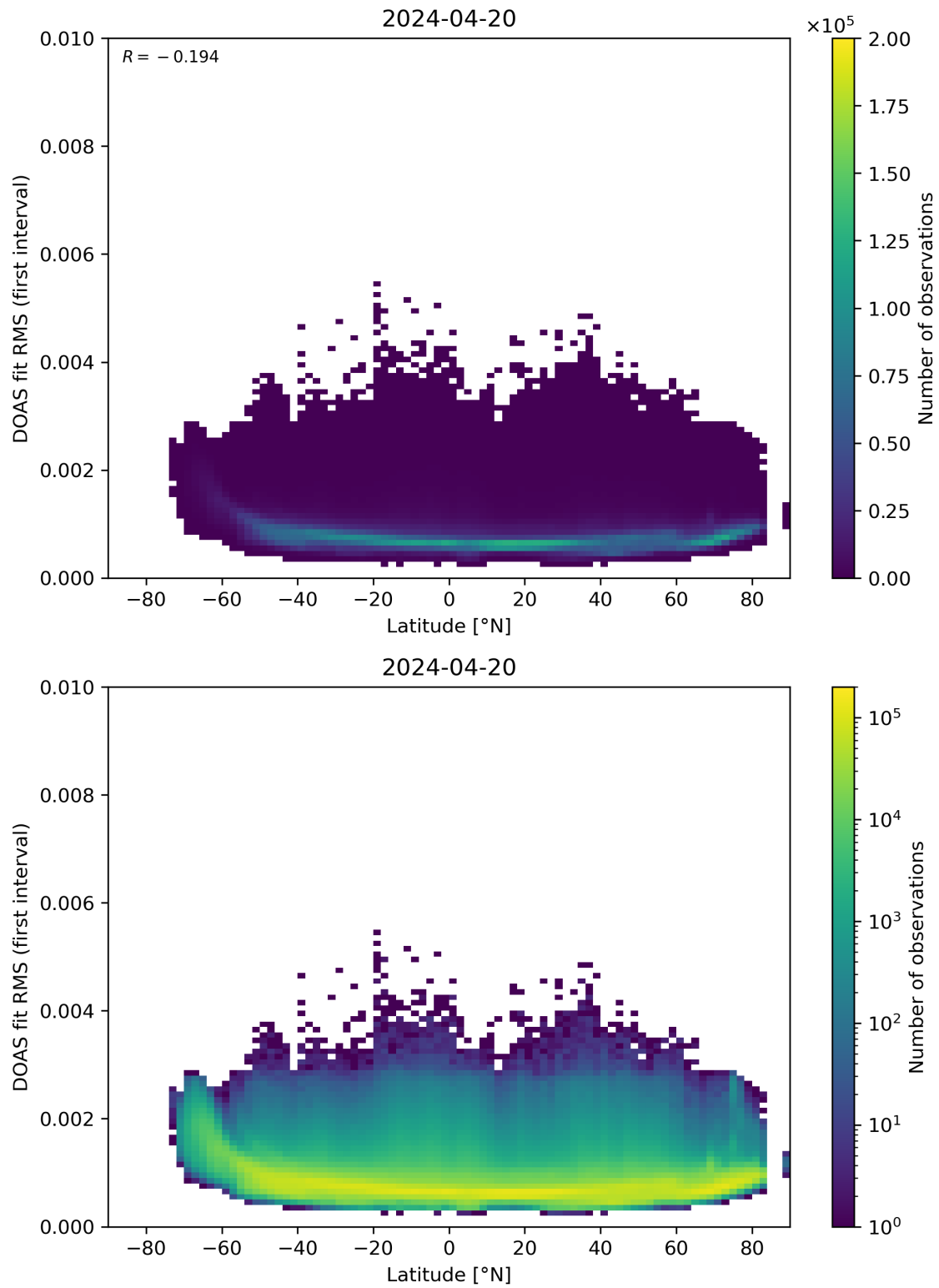
Figure 153: Scatter density plot of “Latitude” against “DOAS fit RMS (first interval)” for 2024-04-19 to 2024-04-21.
