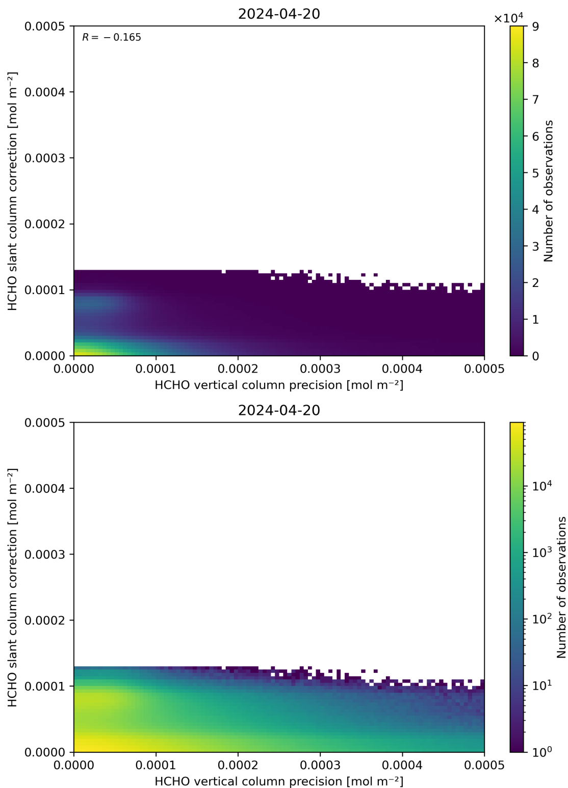
Figure 141: Scatter density plot of “HCHO vertical column precision” against “HCHO slant column correction” for 2024-04-19 to 2024-04-21.
