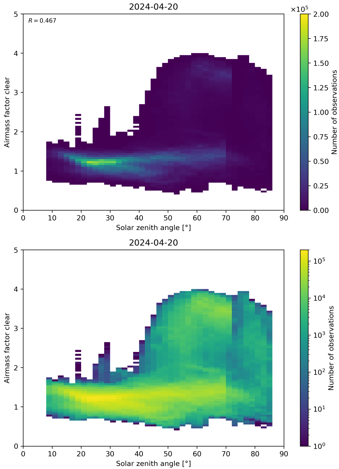
Figure 170: Scatter density plot of “Solar zenith angle” against “Airmass factor clear” for 2024-04-19 to 2024-04-21.
