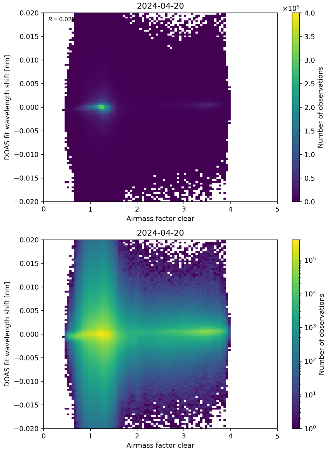
Figure 72: Scatter density plot of “Airmass factor clear” against “DOAS fit wavelength shift” for 2024-04-19 to 2024-04-21.
