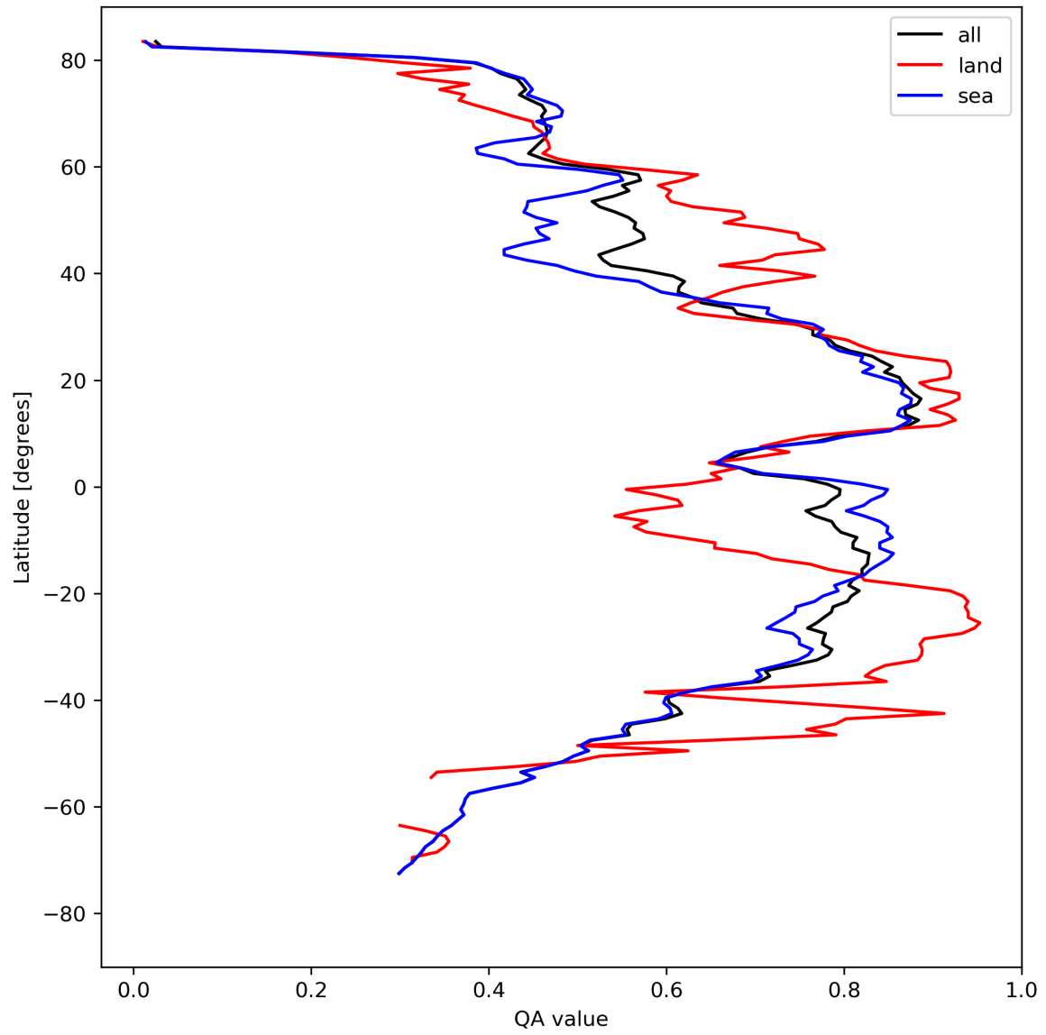
Figure 20: Zonal average of “QA value” for 2024-04-19 to 2024-04-21.
