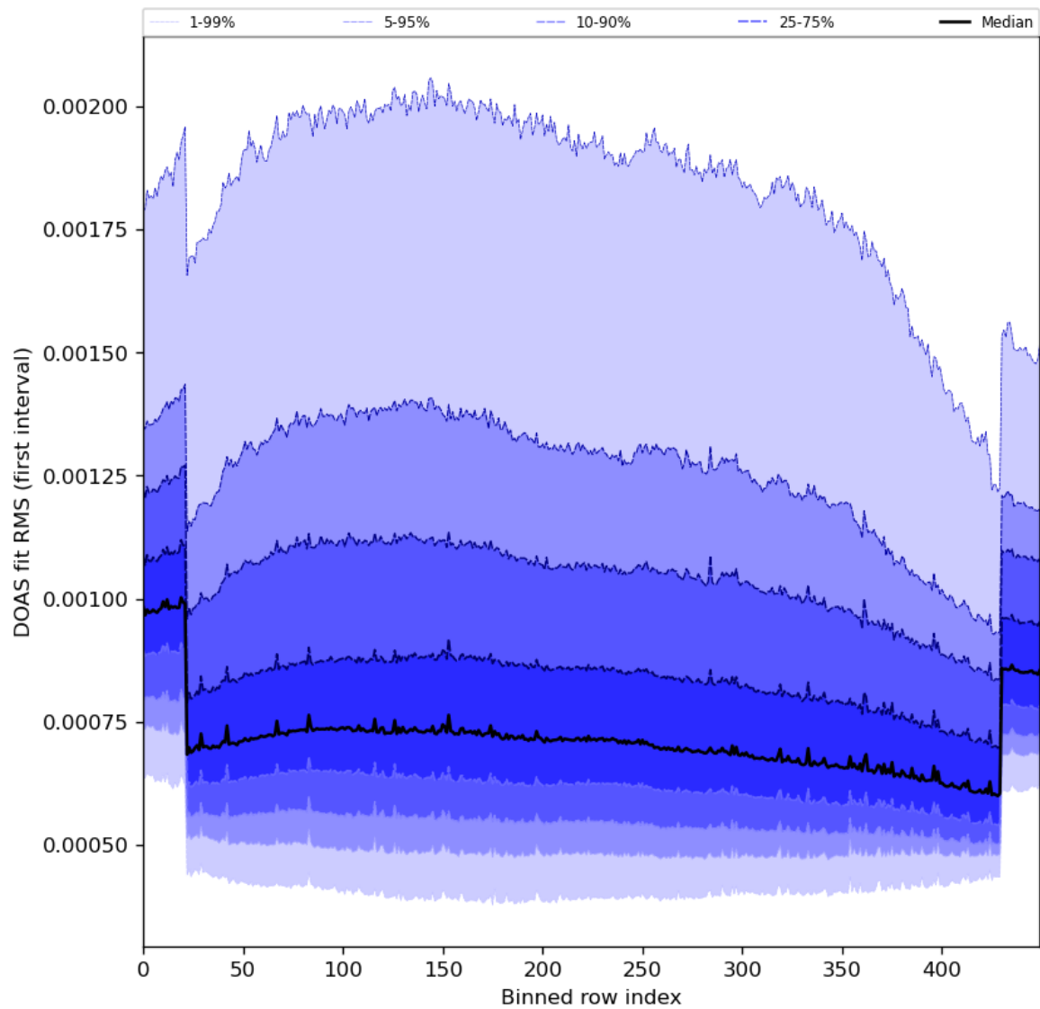
Figure 60: Along track statistics of “DOAS fit RMS (first interval)” for 2024-04-19 to 2024-04-21
