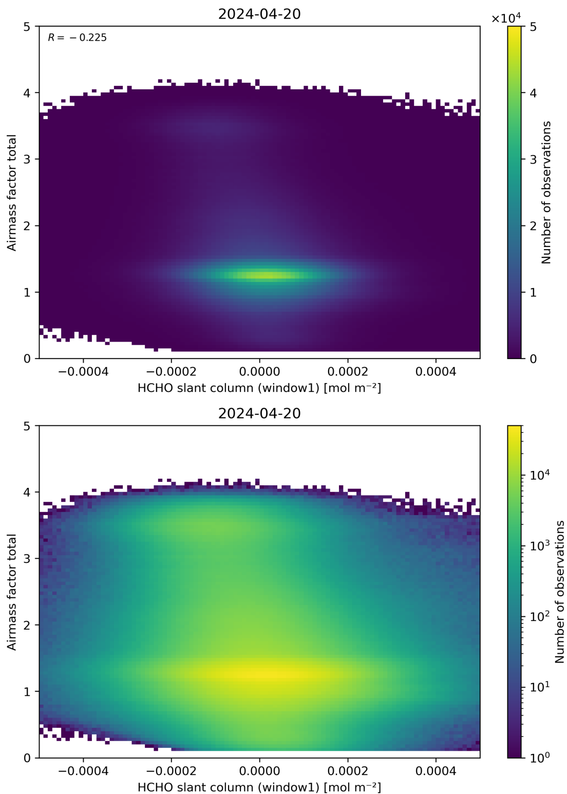
Figure 85: Scatter density plot of “HCHO slant column (window1)” against “Airmass factor total” for 2024-04-19 to 2024-04-21.
