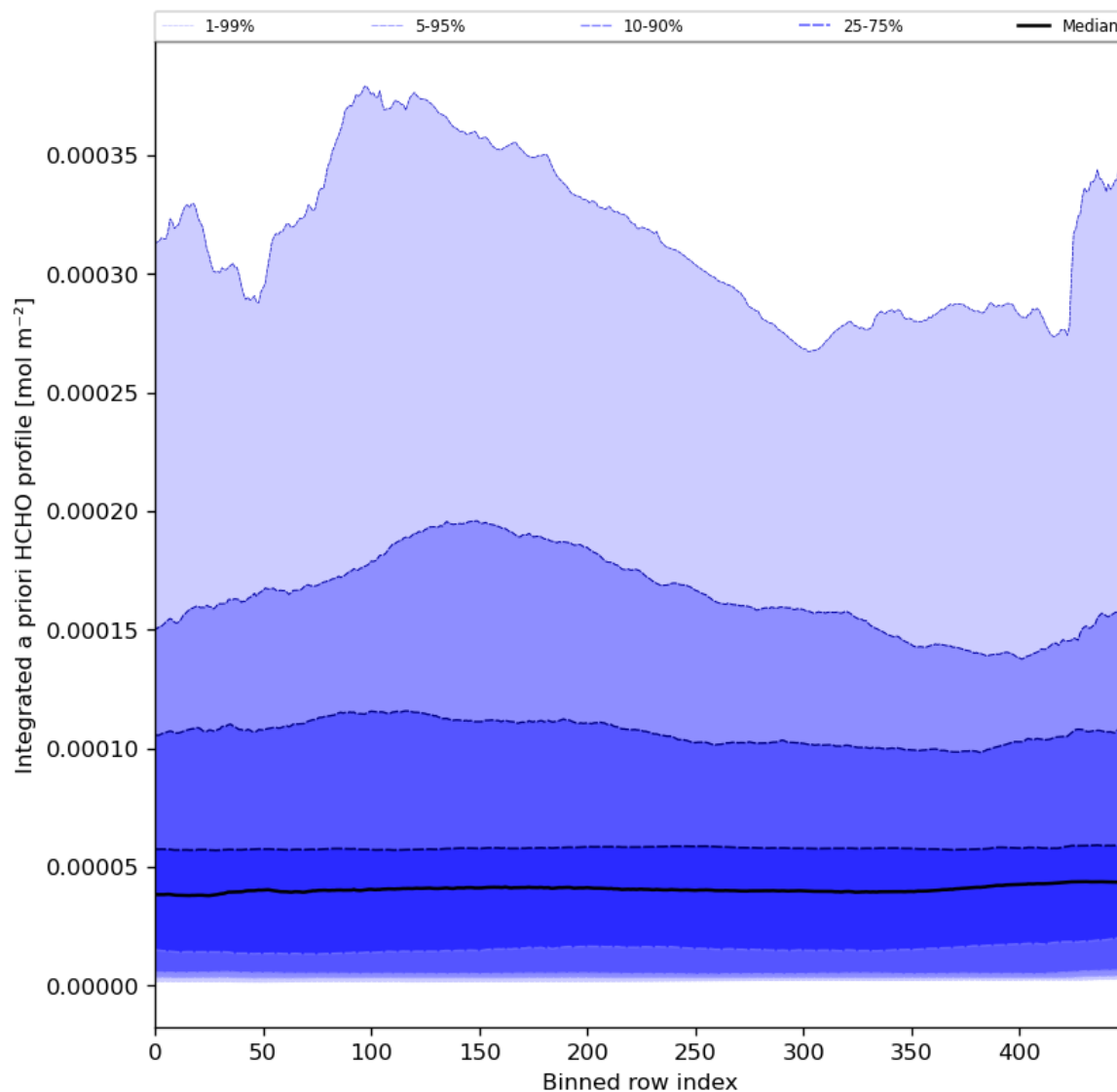
Figure 57: Along track statistics of “Integrated a priori HCHO profile” for 2024-04-19 to 2024-04-21
