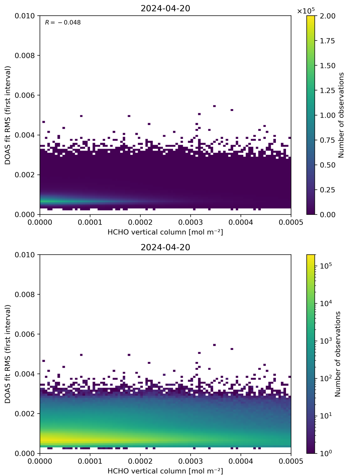
Figure 123: Scatter density plot of “HCHO vertical column” against “DOAS fit RMS (first interval)” for 2024-04-19 to 2024-04-21.
