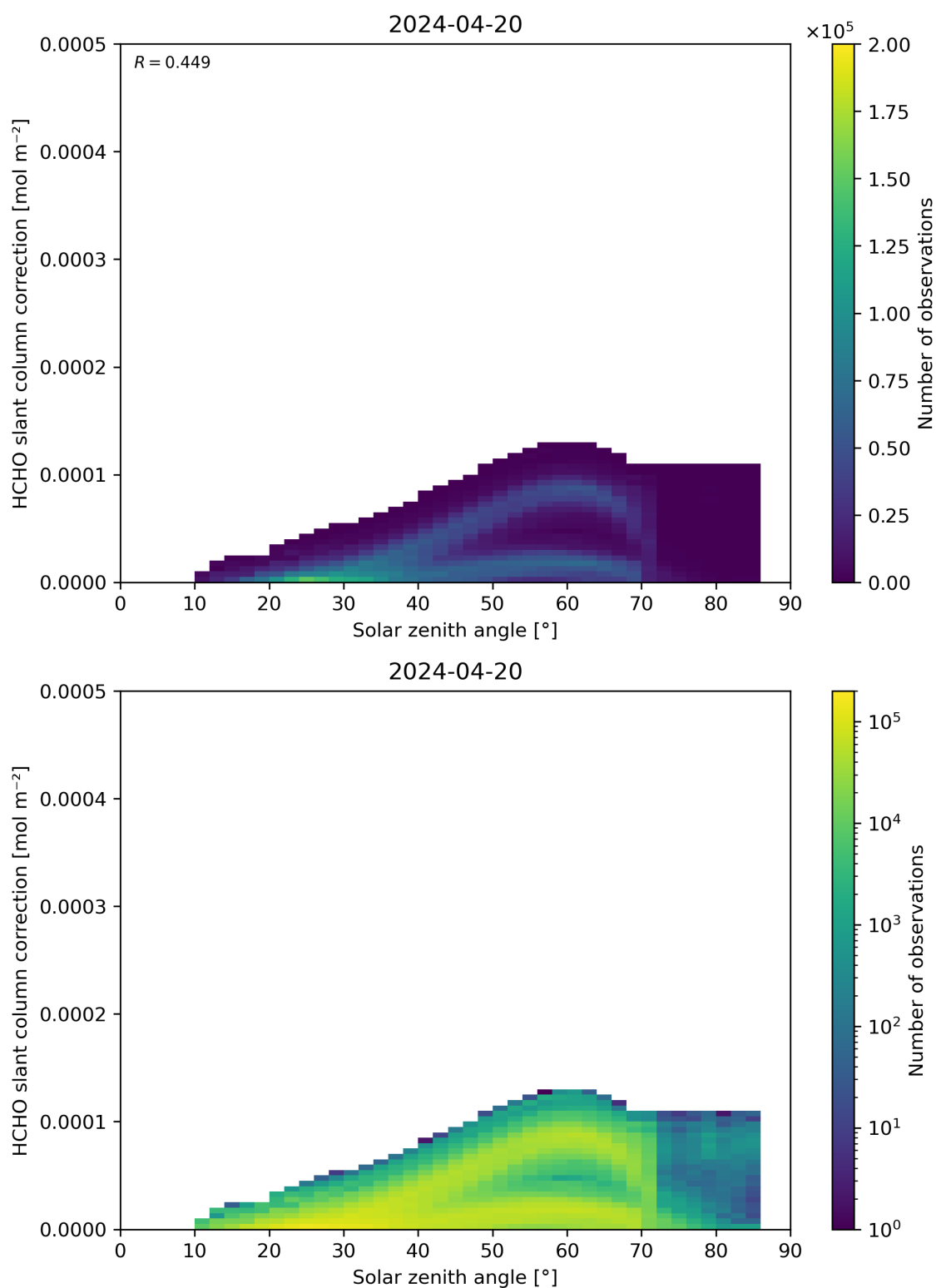
Figure 172: Scatter density plot of “Solar zenith angle” against “HCHO slant column correction” for 2024-04-19 to 2024-04-21.
