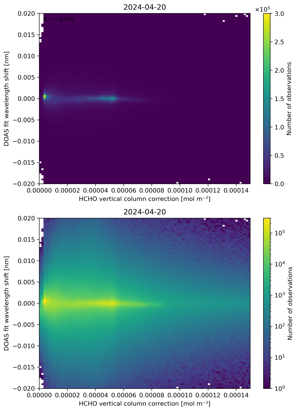
Figure 113: Scatter density plot of “HCHO vertical column correction” against “DOAS fit wavelength shift” for 2024-04-19 to 2024-04-21.
