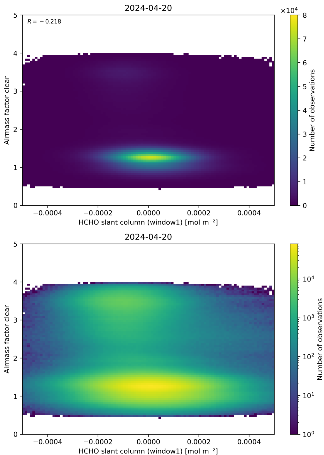
Figure 81: Scatter density plot of “HCHO slant column (window1)” against “Airmass factor clear” for 2024-04-19 to 2024-04-21.
