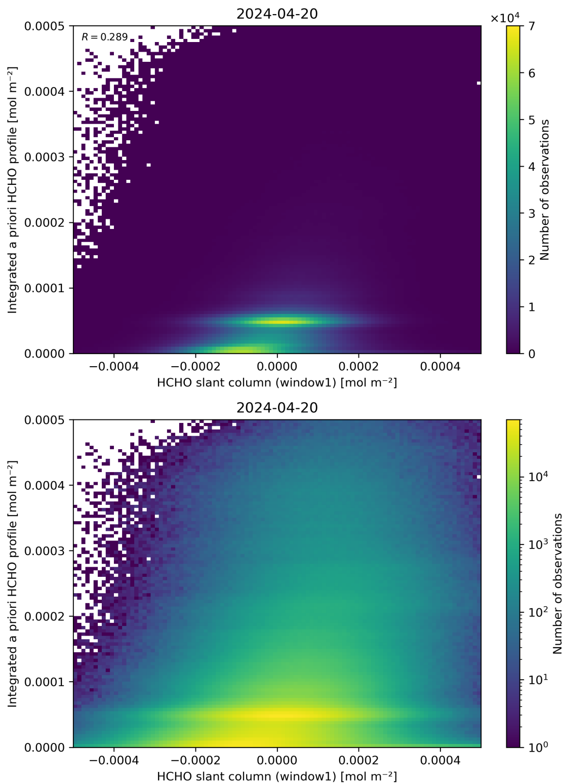
Figure 87: Scatter density plot of “HCHO slant column (window1)” against “Integrated a priori HCHO profile” for 2024-04-19 to 2024-04-21.
