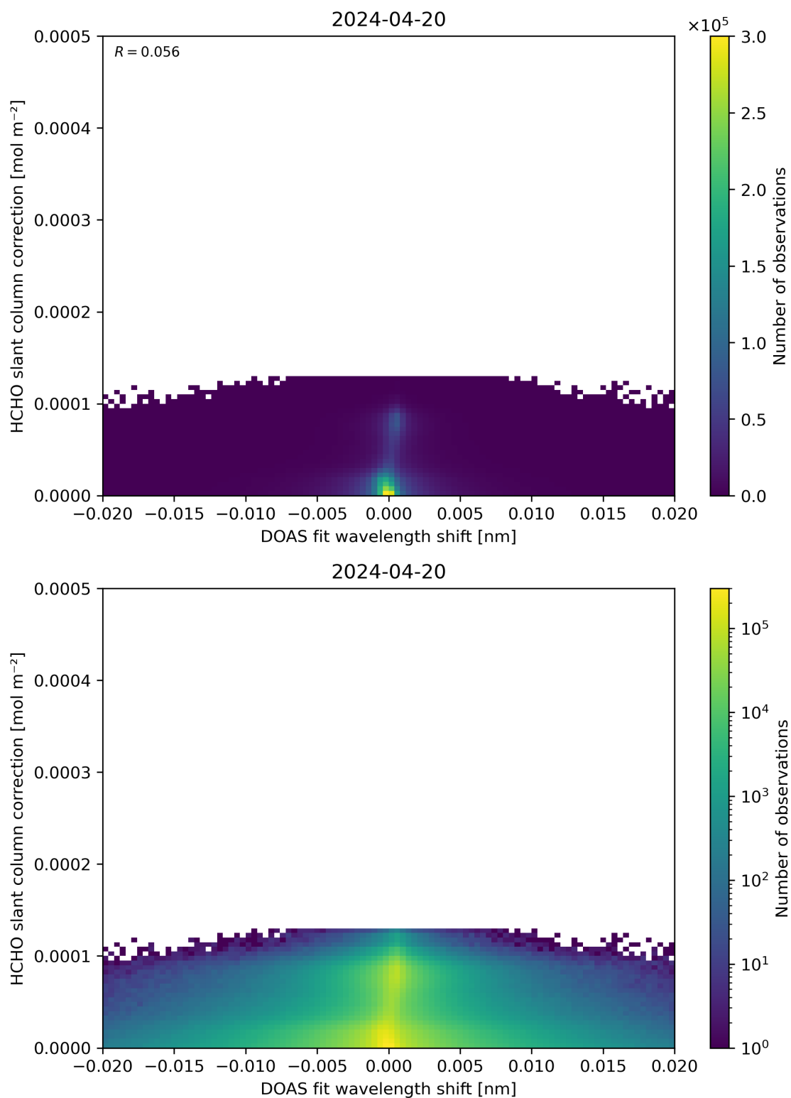
Figure 67: Scatter density plot of “DOAS fit wavelength shift” against “HCHO slant column correction” for 2024-04-19 to 2024-04-21.
