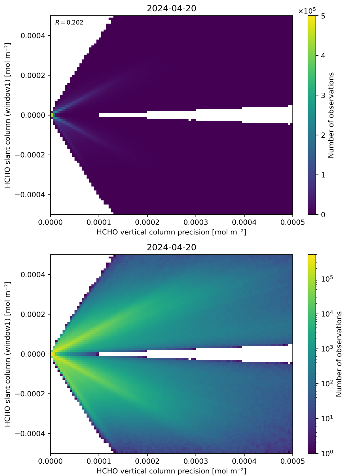
Figure 142: Scatter density plot of “HCHO vertical column precision” against “HCHO slant column (window1)” for 2024-04-19 to 2024-04-21.
