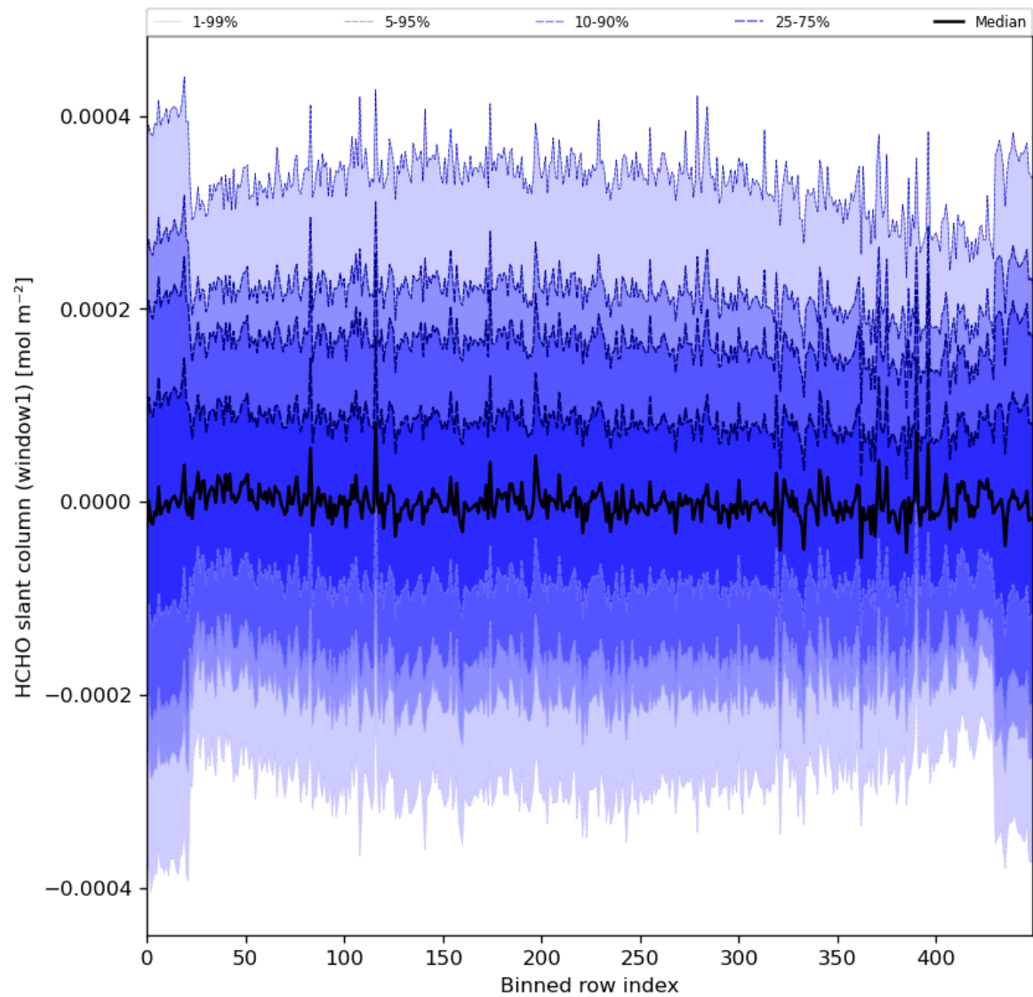
Figure 52: Along track statistics of “HCHO slant column (window1)” for 2024-04-19 to 2024-04-21
