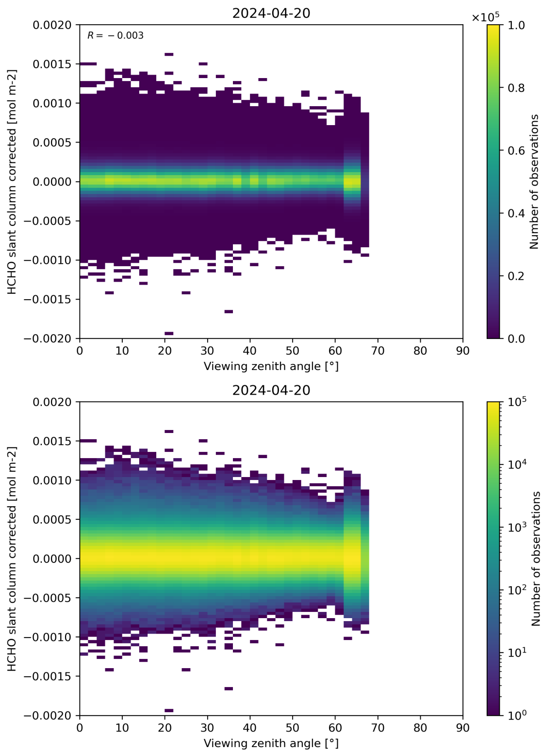
Figure 186: Scatter density plot of “Viewing zenith angle” against “HCHO slant column corrected” for 2024-04-19 to 2024-04-21.
