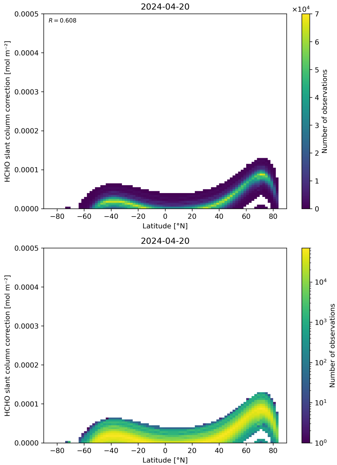
Figure 158: Scatter density plot of “Latitude” against “HCHO slant column correction” for 2024-04-19 to 2024-04-21.
