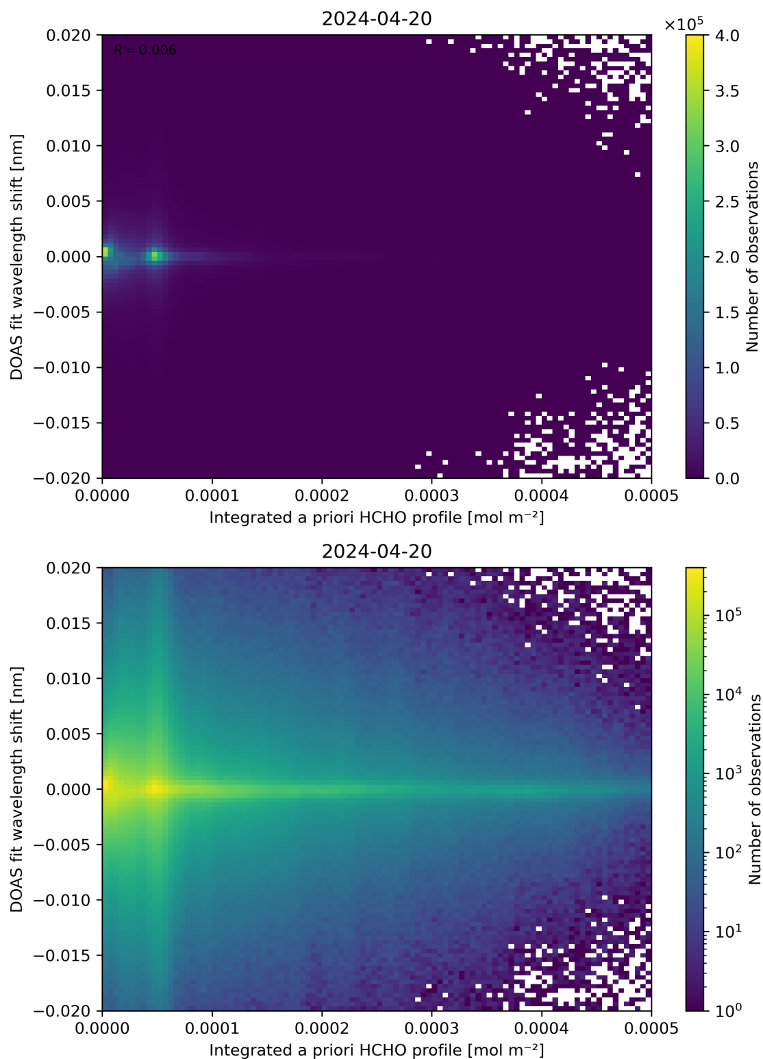
Figure 149: Scatter density plot of “Integrated a priori HCHO profile” against “DOAS fit wavelength shift” for 2024-04-19 to 2024-04-21.
