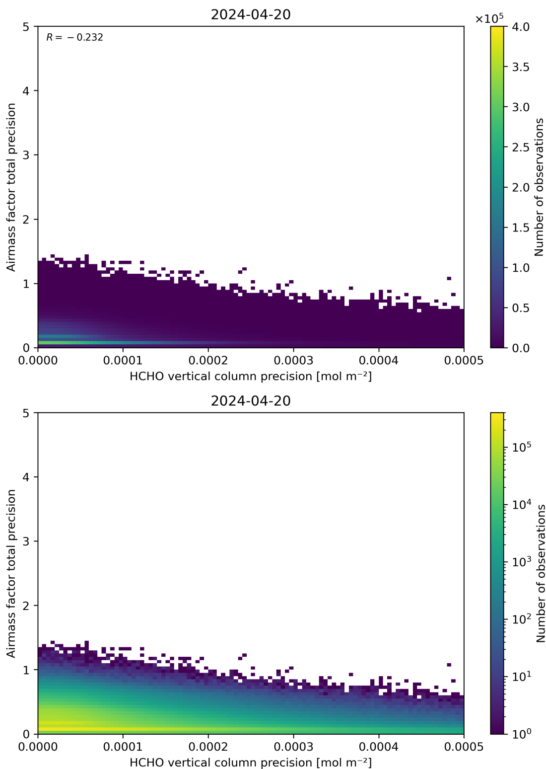
Figure 145: Scatter density plot of “HCHO vertical column precision” against “Airmass factor total precision” for 2024-04-19 to 2024-04-21.
