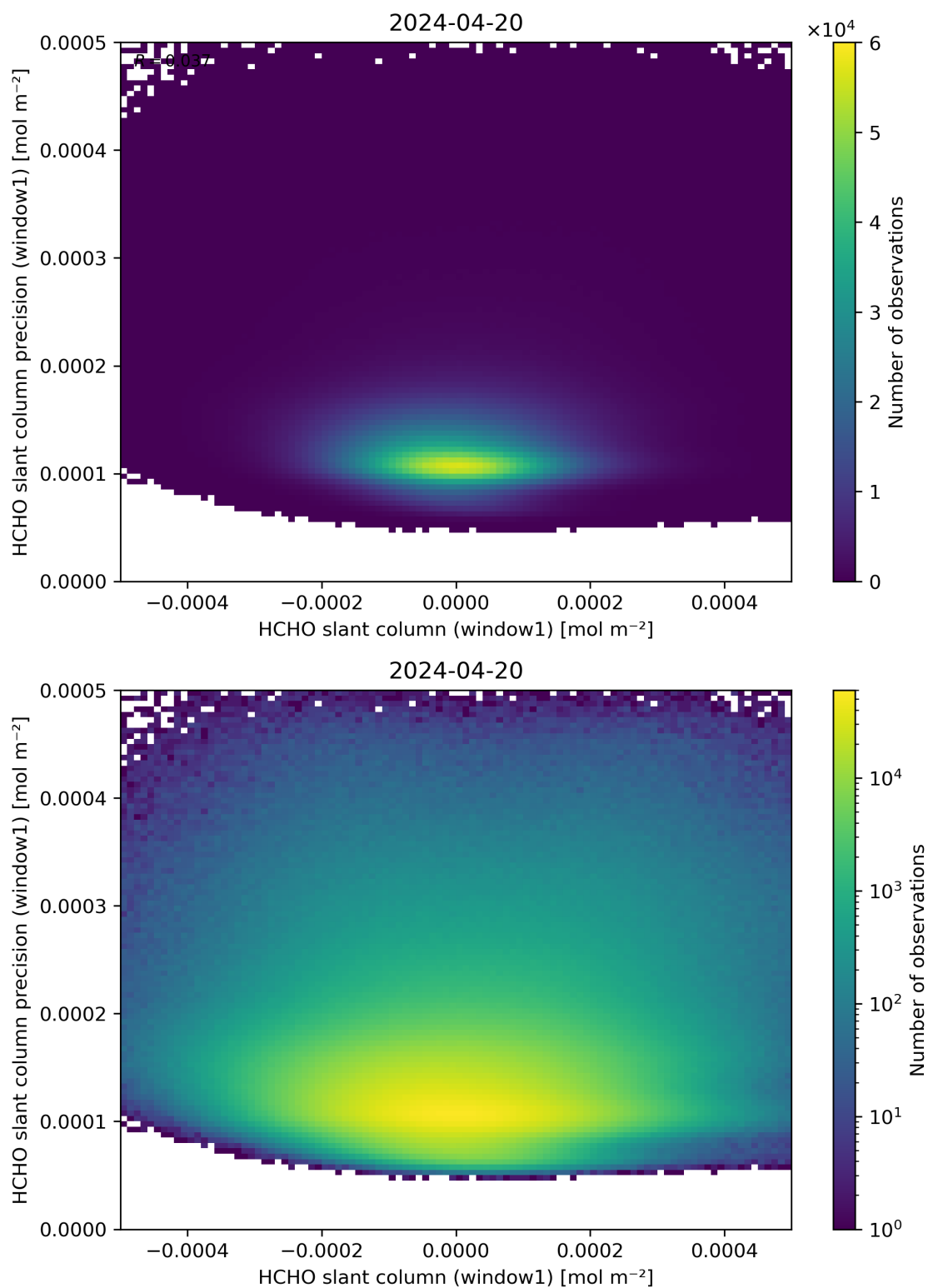
Figure 84: Scatter density plot of “HCHO slant column (window1)” against “HCHO slant column precision (window1)” for 2024-04-19 to 2024-04-21.
