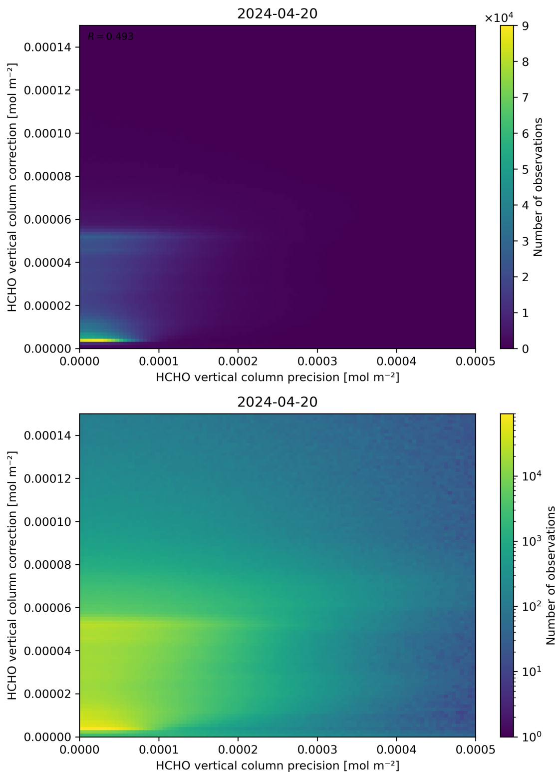
Figure 146: Scatter density plot of “HCHO vertical column precision” against “HCHO vertical column correction” for 2024-04-19 to 2024-04-21.
