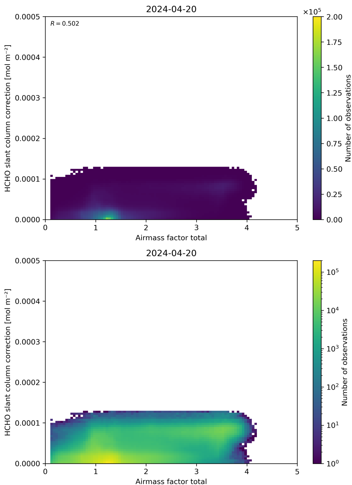
Figure 102: Scatter density plot of “Airmass factor total” against “HCHO slant column correction” for 2024-04-19 to 2024-04-21.
