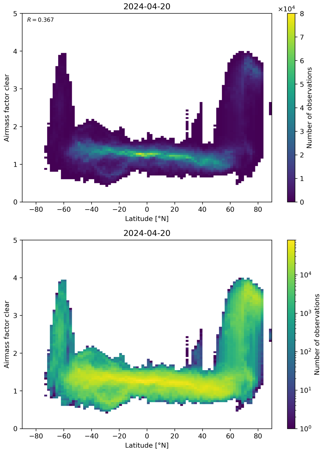
Figure 156: Scatter density plot of “Latitude” against “Airmass factor clear” for 2024-04-19 to 2024-04-21.
