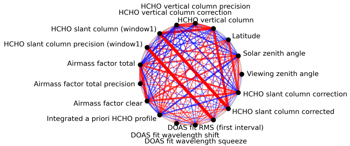
Figure 1: Map of correlation graph for 2024-04-19 to 2024-04-21.
