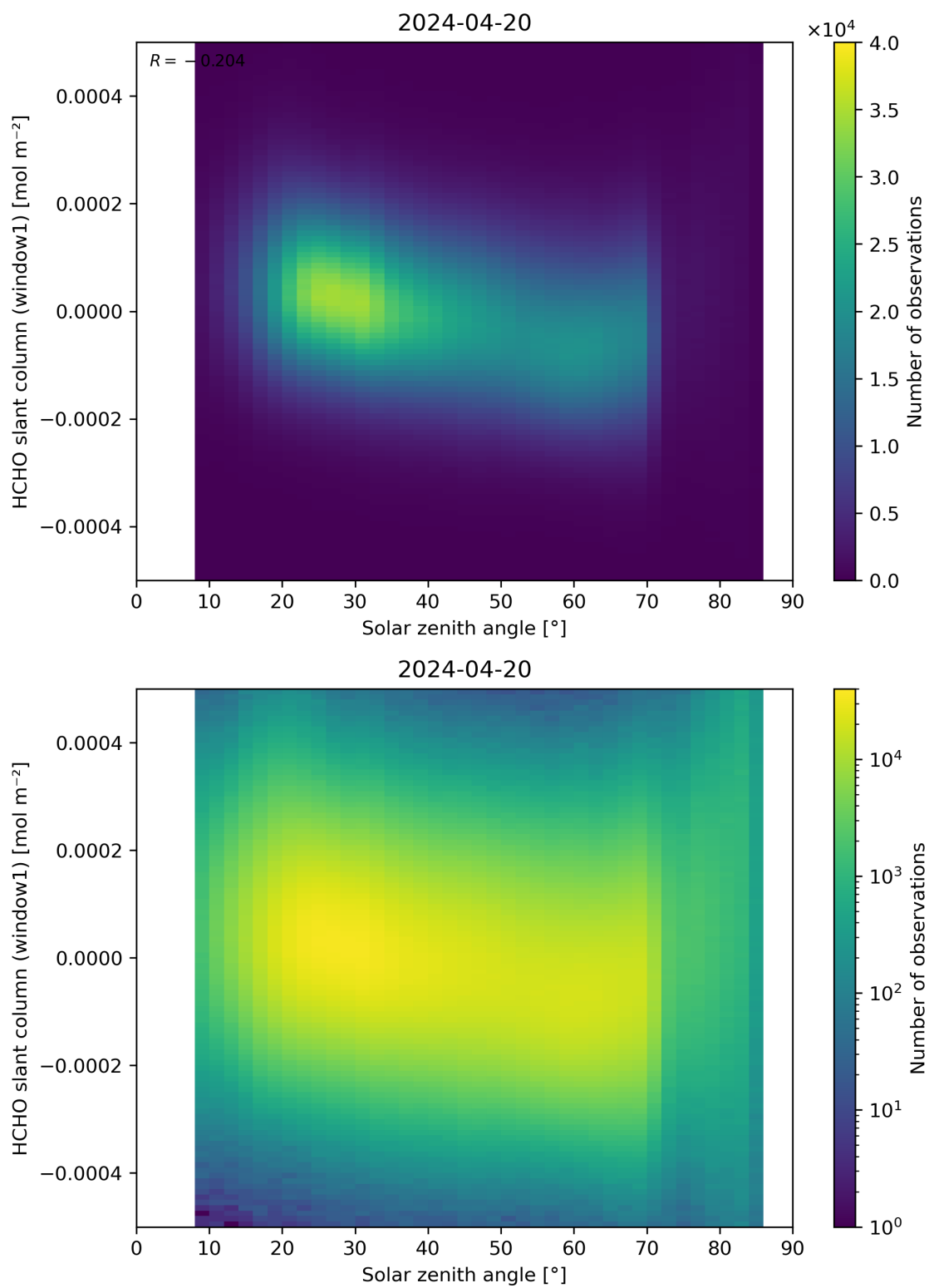
Figure 173: Scatter density plot of “Solar zenith angle” against “HCHO slant column (window1)” for 2024-04-19 to 2024-04-21.
