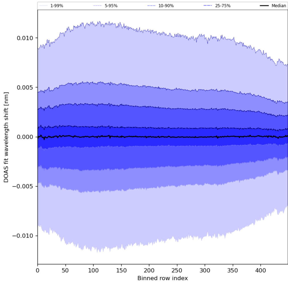
Figure 58: Along track statistics of “DOAS fit wavelength shift” for 2024-04-19 to 2024-04-21
