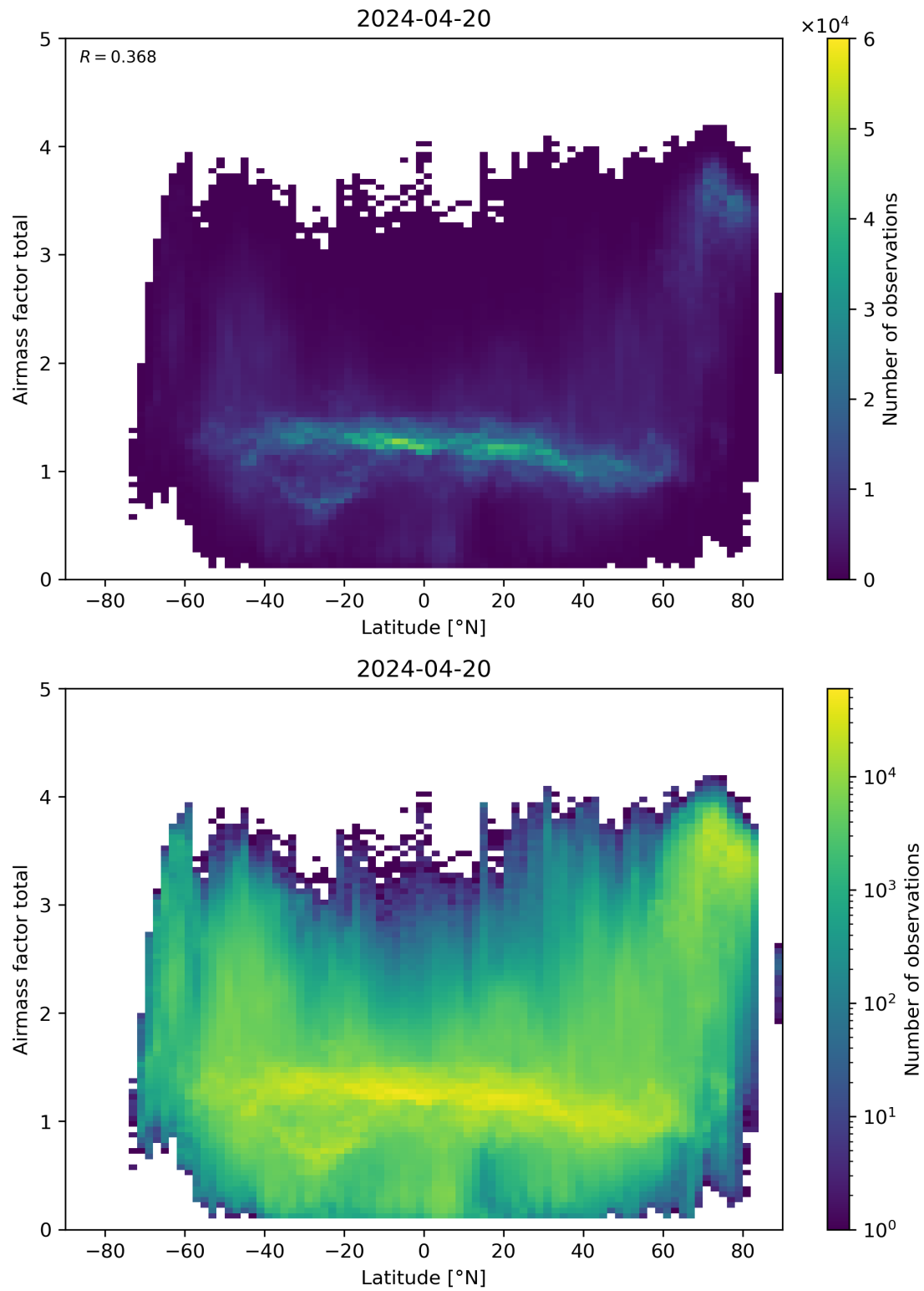
Figure 161: Scatter density plot of “Latitude” against “Airmass factor total” for 2024-04-19 to 2024-04-21.
