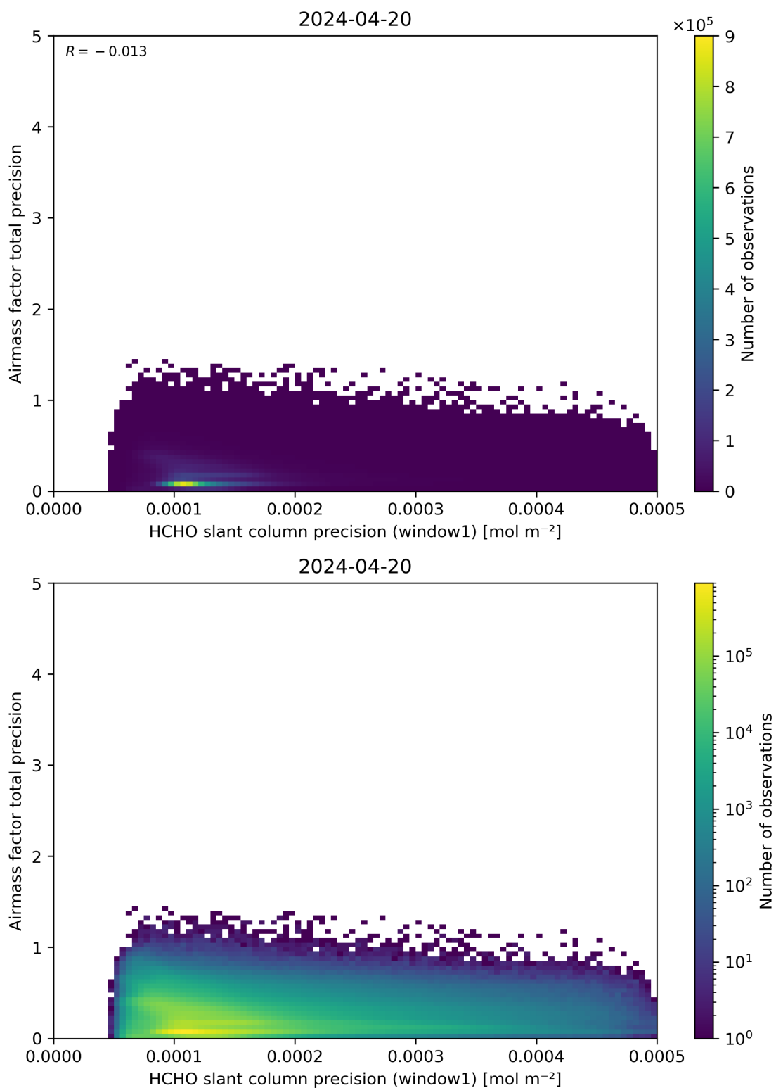
Figure 95: Scatter density plot of “HCHO slant column precision (window1)” against “Airmass factor total precision” for 2024-04-19 to 2024-04-21.
