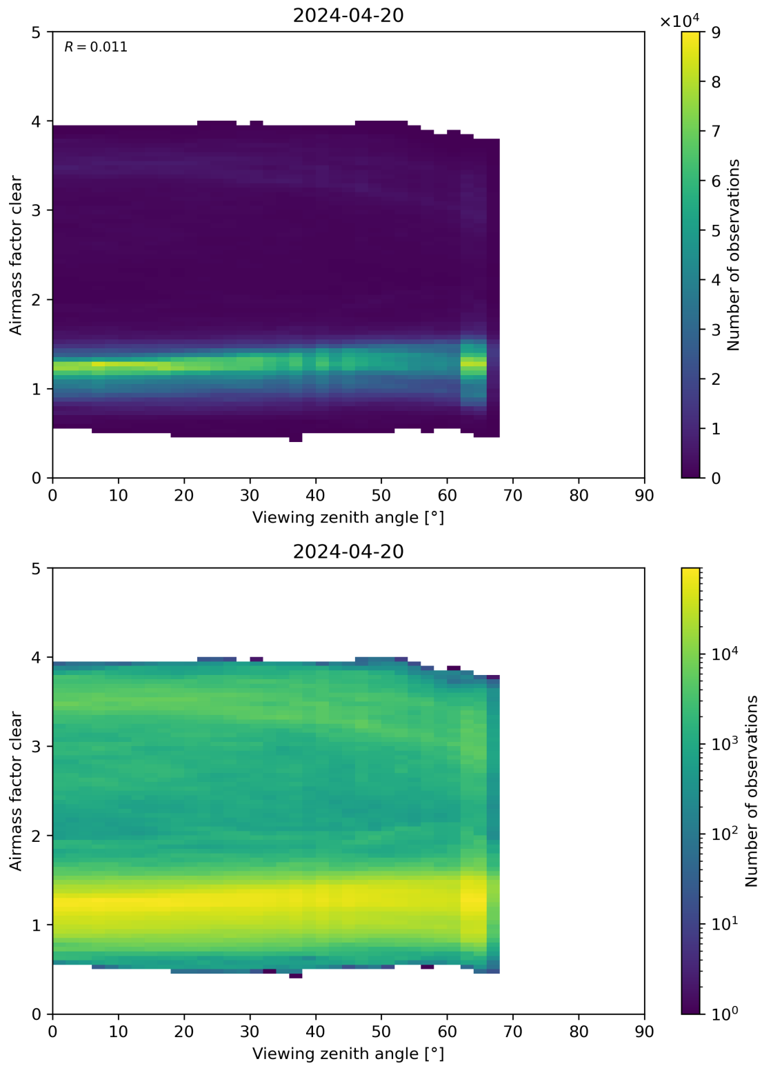
Figure 185: Scatter density plot of “Viewing zenith angle” against “Airmass factor clear” for 2024-04-19 to 2024-04-21.
