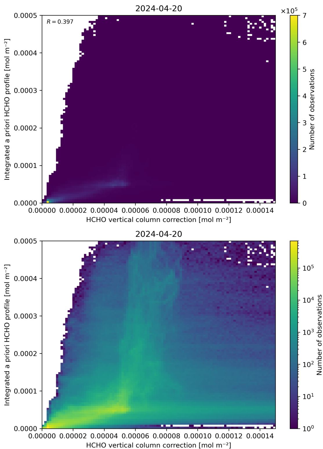
Figure 122: Scatter density plot of “HCHO vertical column correction” against “Integrated a priori HCHO profile” for 2024-04-19 to 2024-04-21.
