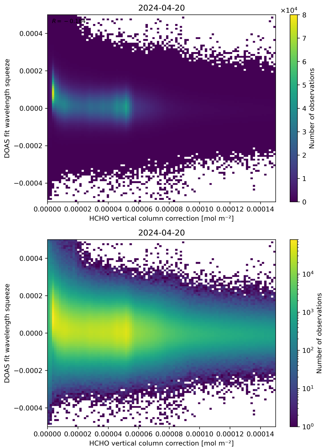
Figure 114: Scatter density plot of “HCHO vertical column correction” against “DOAS fit wavelength squeeze” for 2024-04-19 to 2024-04-21.
