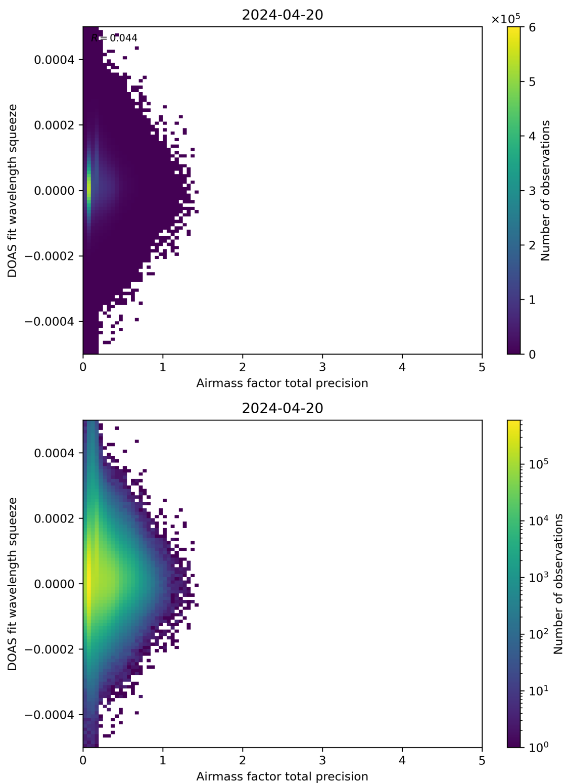
Figure 107: Scatter density plot of “Airmass factor total precision” against “DOAS fit wavelength squeeze” for 2024-04-19 to 2024-04-21.
