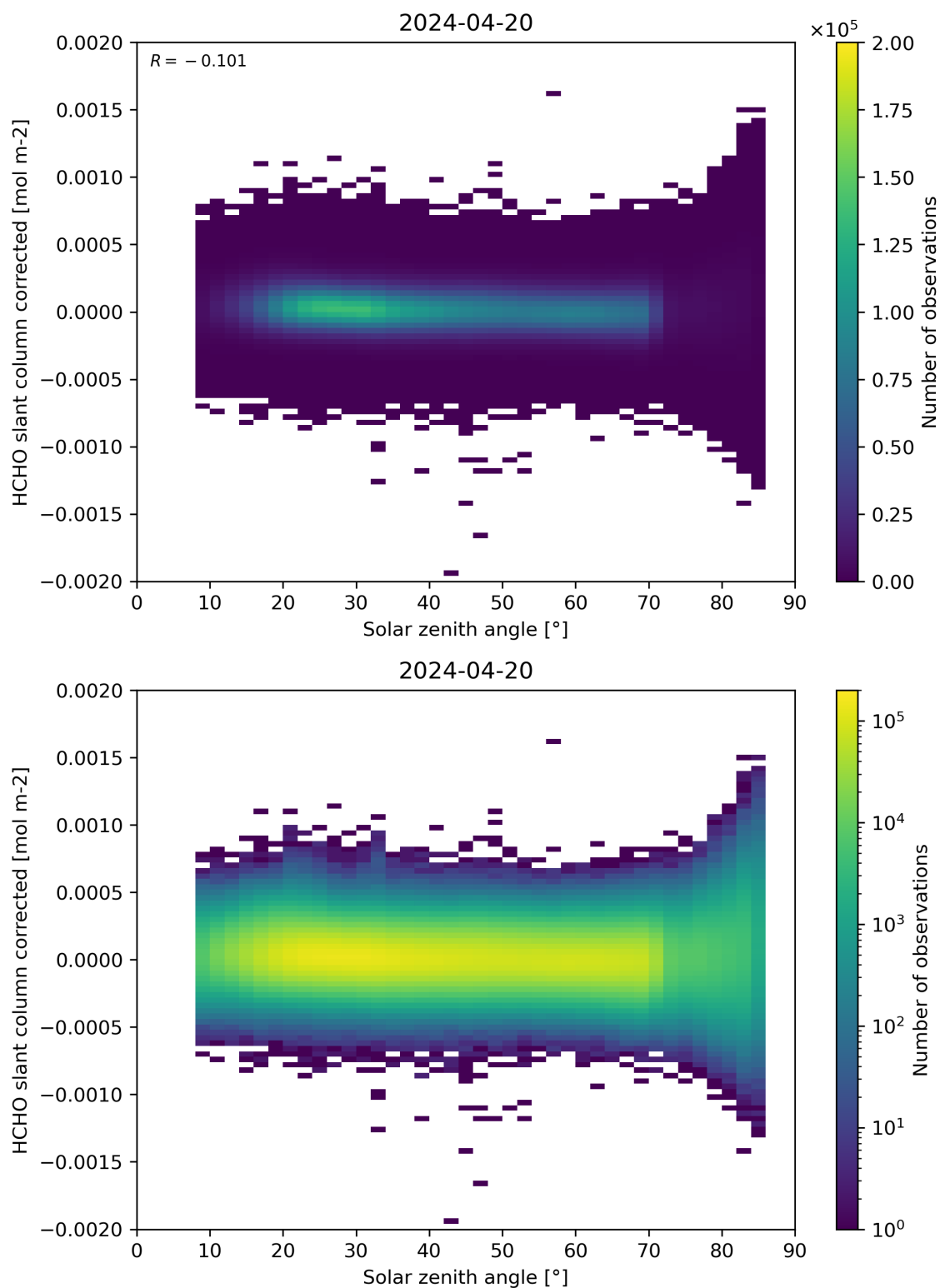
Figure 171: Scatter density plot of “Solar zenith angle” against “HCHO slant column corrected” for 2024-04-19 to 2024-04-21.
