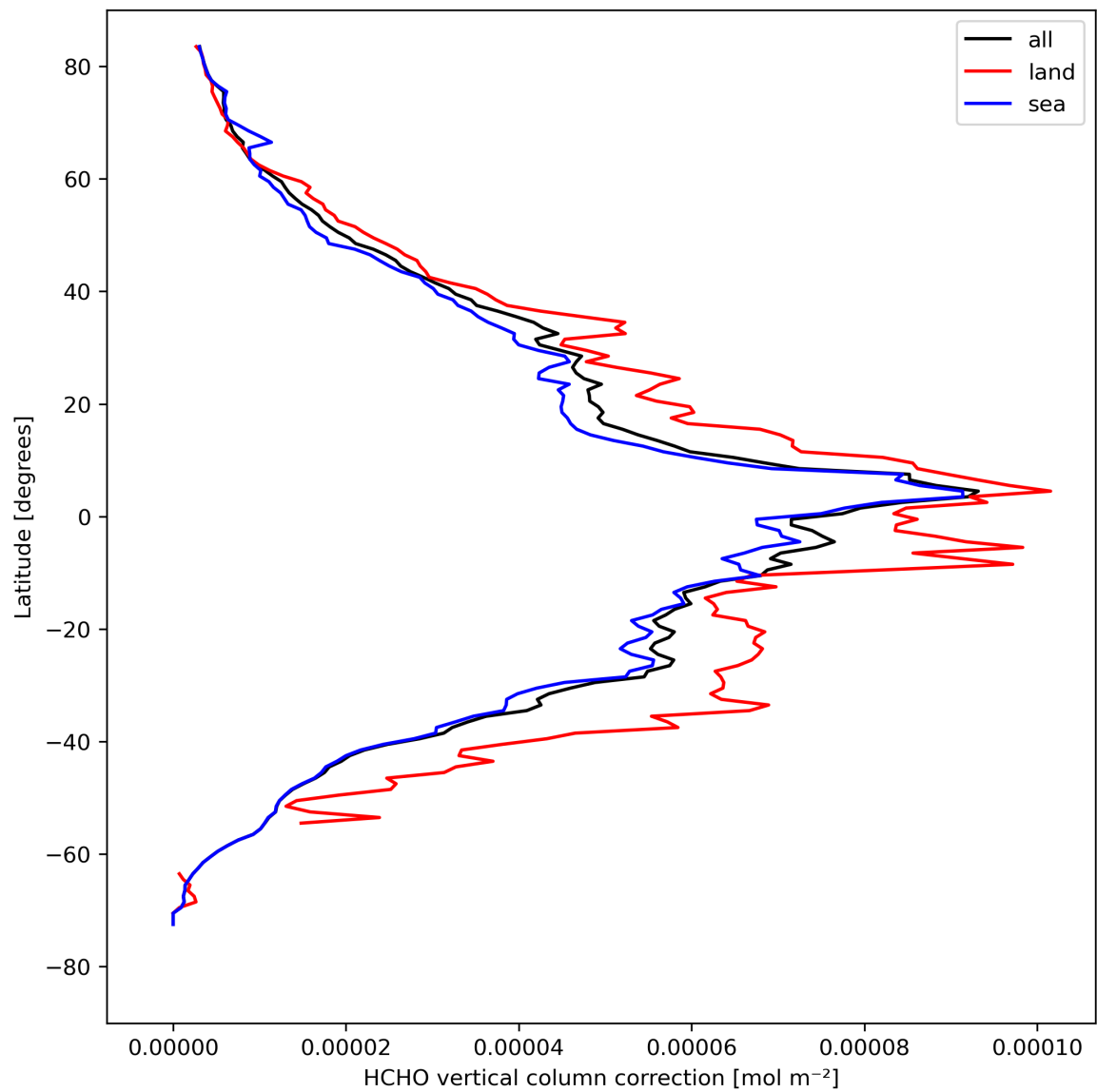
Figure 23: Zonal average of “HCHO vertical column correction” for 2024-04-19 to 2024-04-21.
