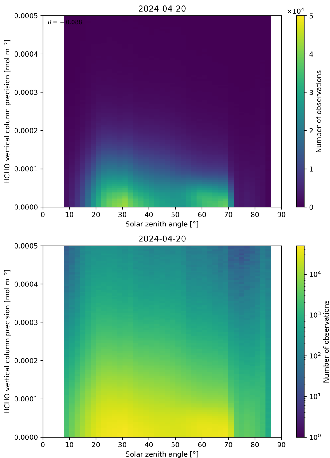
Figure 179: Scatter density plot of “Solar zenith angle” against “HCHO vertical column precision” for 2024-04-19 to 2024-04-21.
