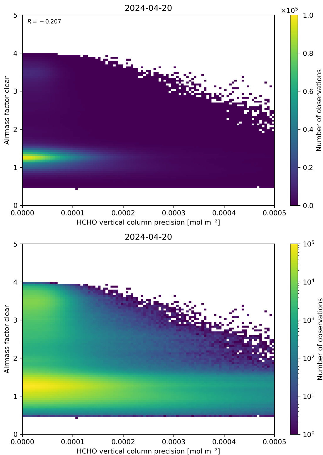
Figure 139: Scatter density plot of “HCHO vertical column precision” against “Airmass factor clear” for 2024-04-19 to 2024-04-21.
