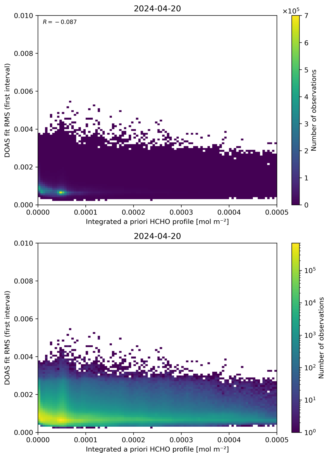
Figure 148: Scatter density plot of “Integrated a priori HCHO profile” against “DOAS fit RMS (first interval)” for 2024-04-19 to 2024-04-21.
