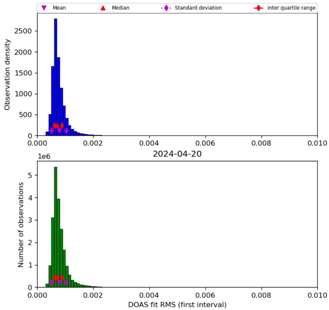
Figure 46: Histogram of “DOAS fit RMS (first interval)” for 2024-04-19 to 2024-04-21
