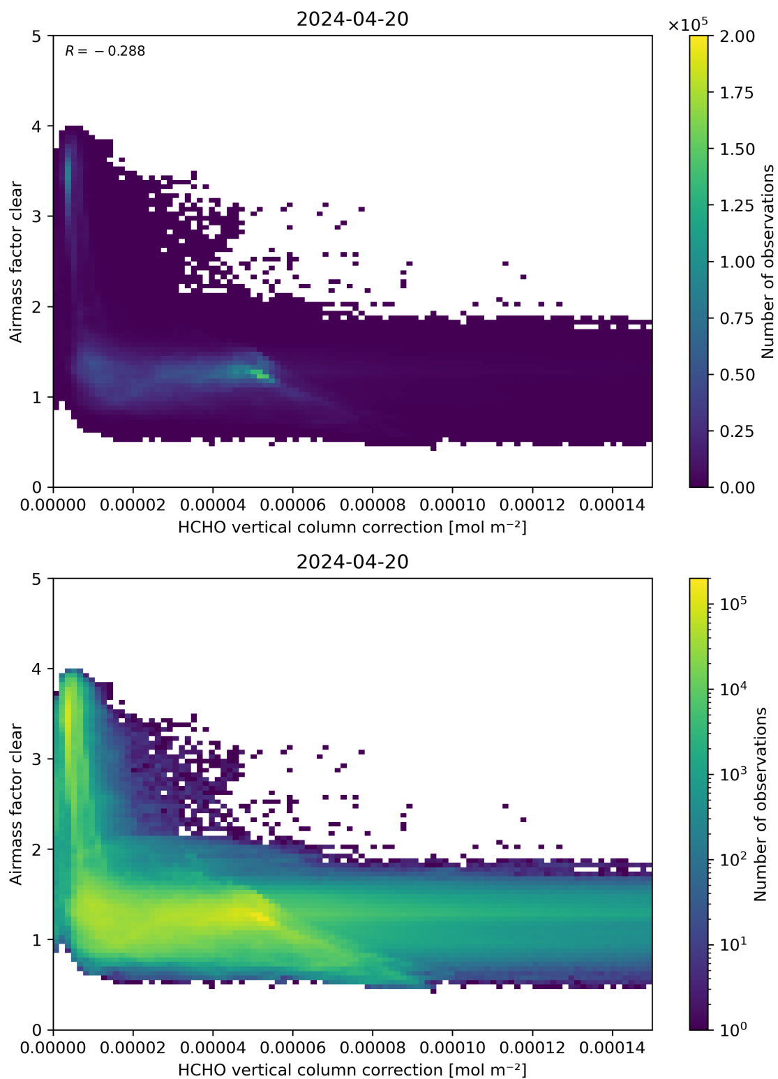
Figure 115: Scatter density plot of “HCHO vertical column correction” against “Airmass factor clear” for 2024-04-19 to 2024-04-21.
