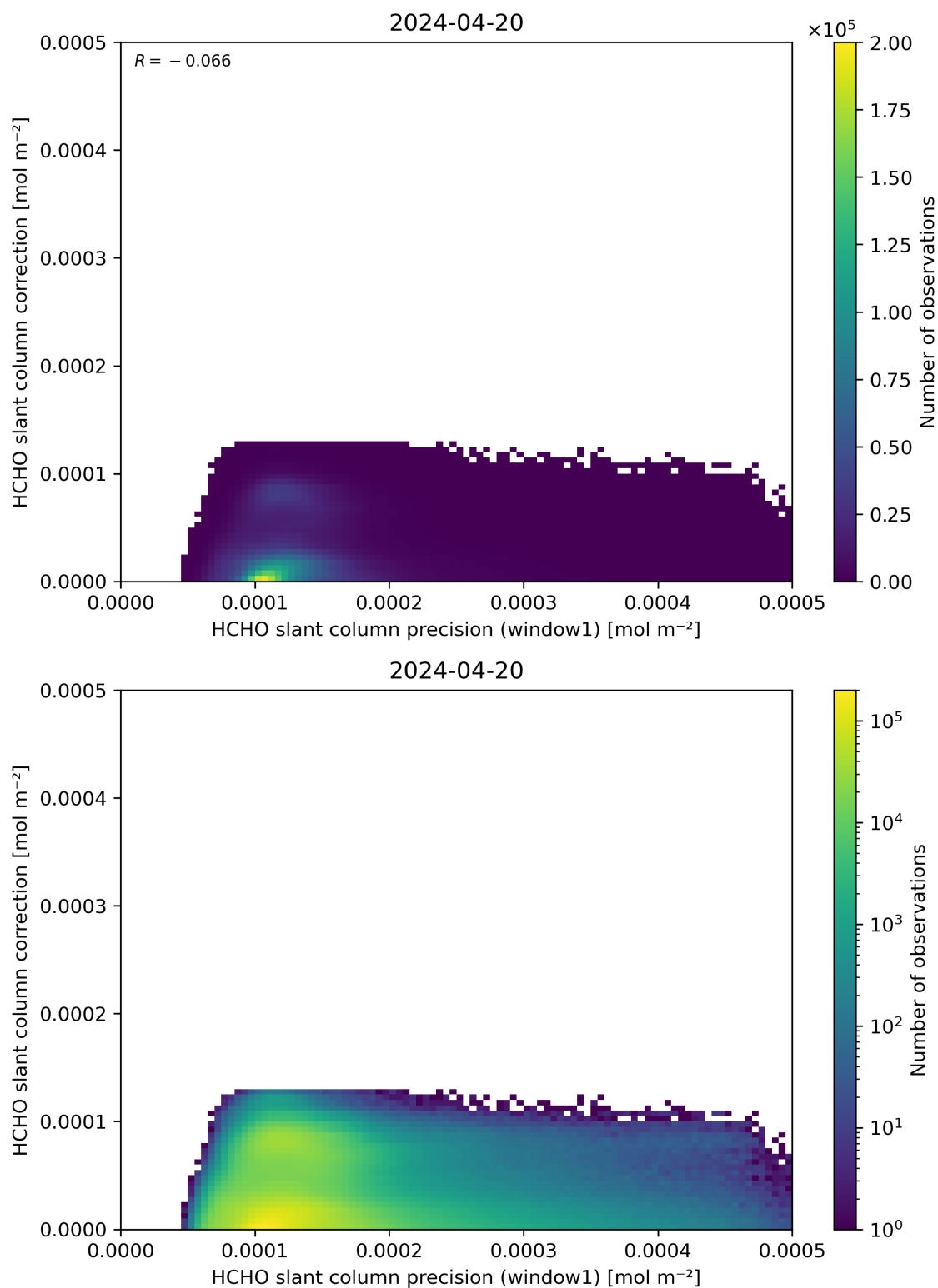
Figure 93: Scatter density plot of “HCHO slant column precision (window1)” against “HCHO slant column correction” for 2024-04-19 to 2024-04-21.
