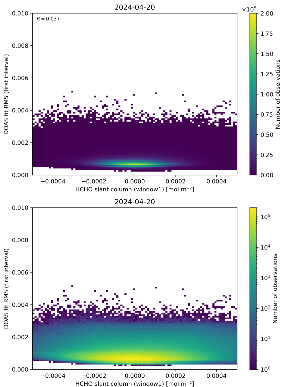
Figure 78: Scatter density plot of “HCHO slant column (window1)” against “DOAS fit RMS (first interval)” for 2024-04-19 to 2024-04-21.
