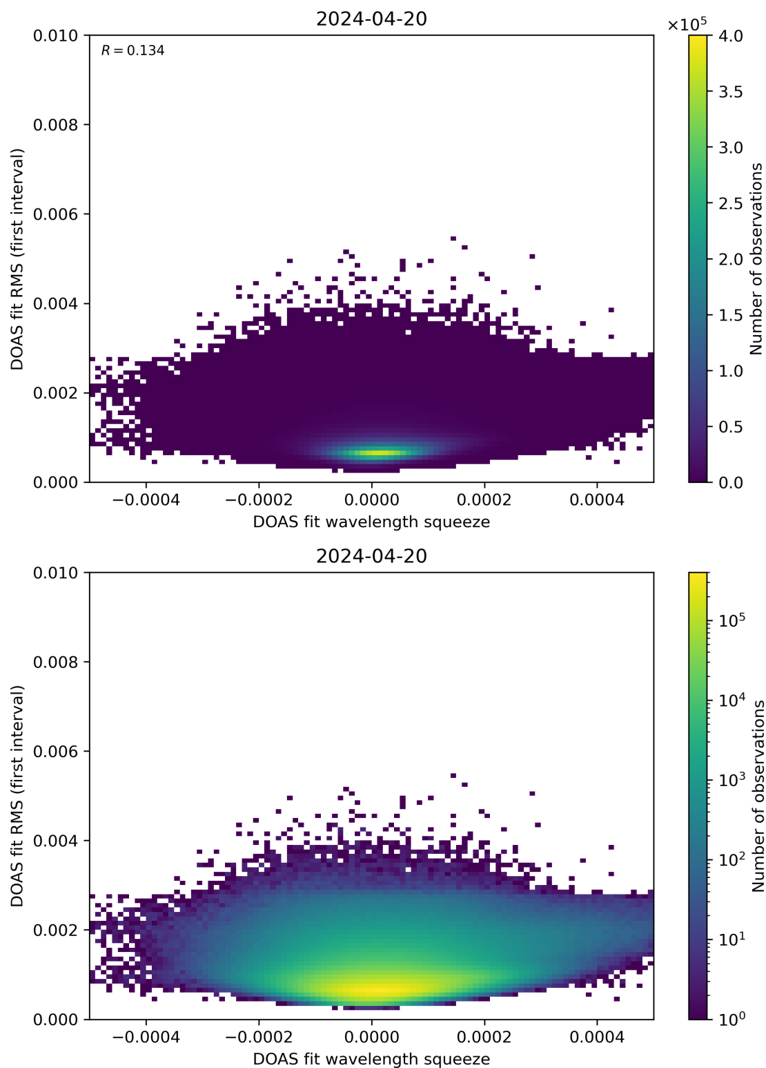
Figure 68: Scatter density plot of “DOAS fit wavelength squeeze” against “DOAS fit RMS (first interval)” for 2024-04-19 to 2024-04-21.
