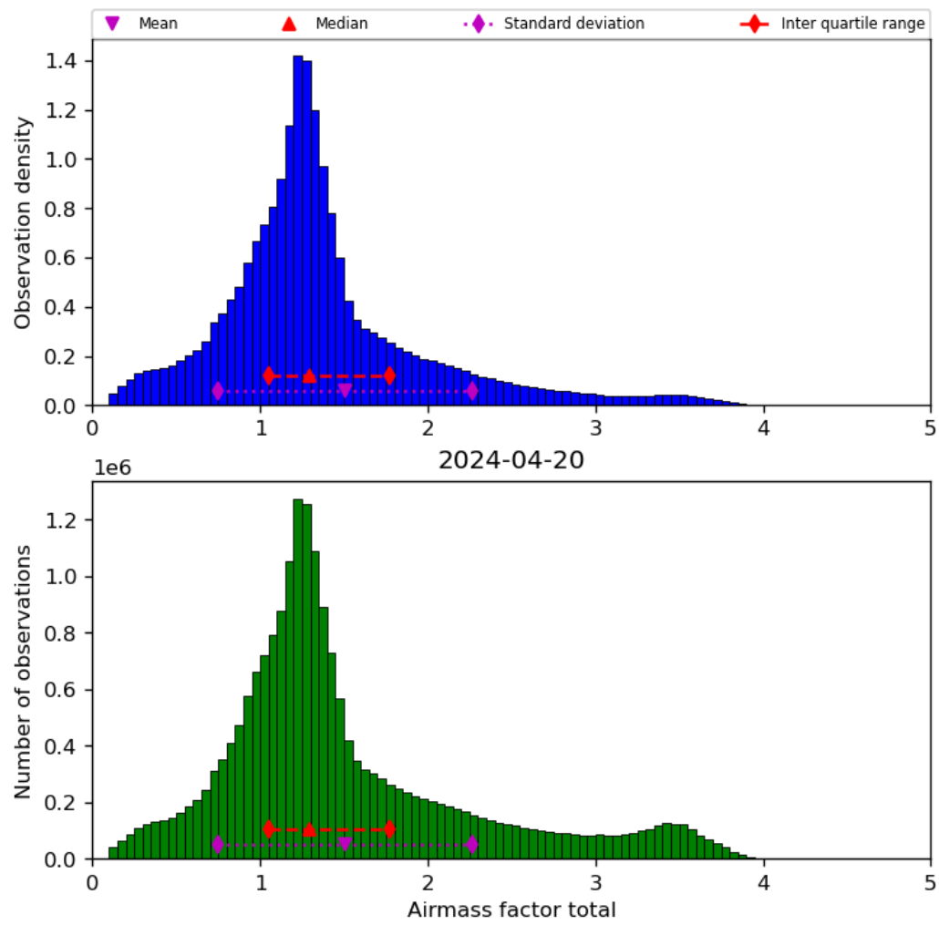
Figure 40: Histogram of “Airmass factor total” for 2024-04-19 to 2024-04-21
