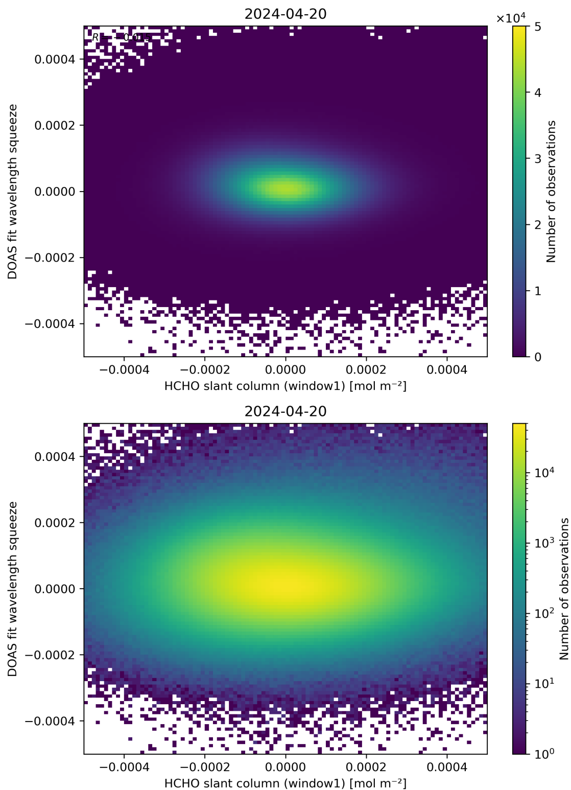
Figure 80: Scatter density plot of “HCHO slant column (window1)” against “DOAS fit wavelength squeeze” for 2024-04-19 to 2024-04-21.
