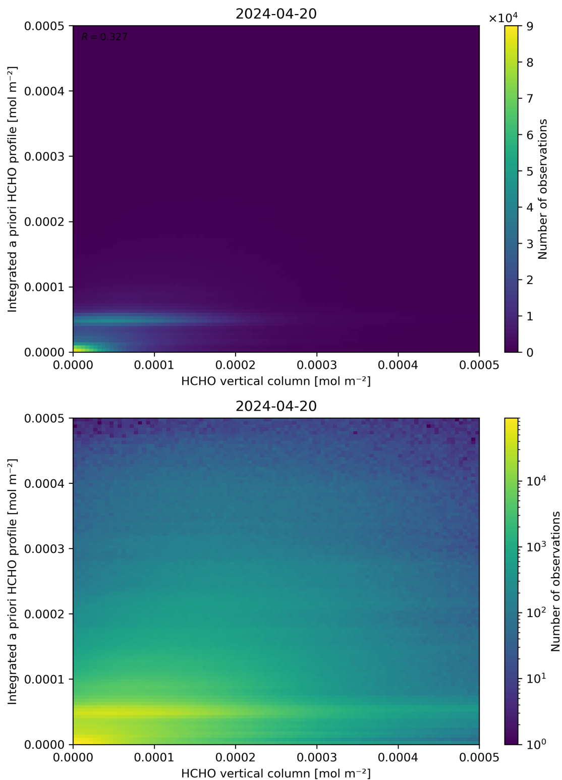
Figure 135: Scatter density plot of “HCHO vertical column” against “Integrated a priori HCHO profile” for 2024-04-19 to 2024-04-21.
