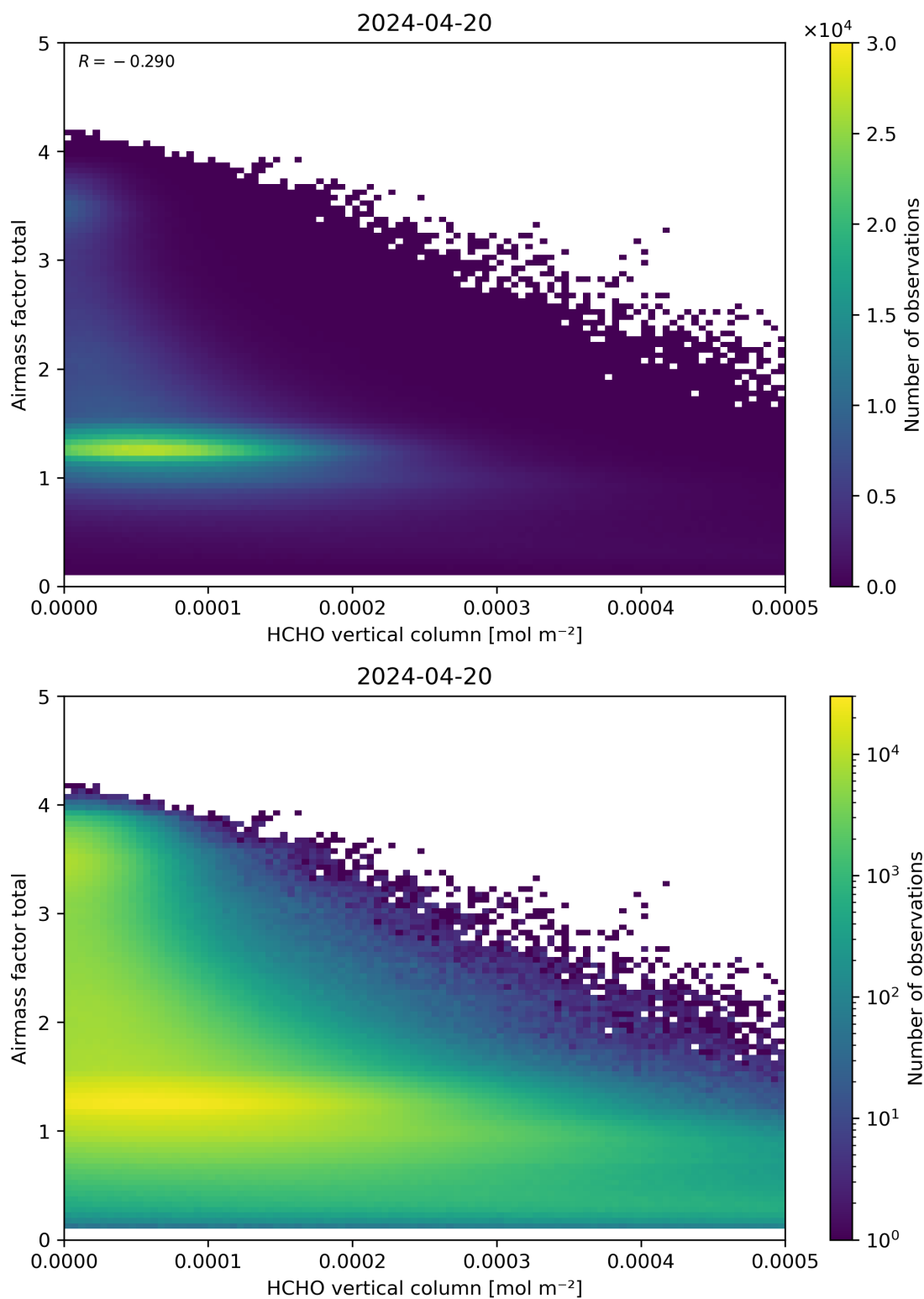
Figure 131: Scatter density plot of “HCHO vertical column” against “Airmass factor total” for 2024-04-19 to 2024-04-21.
