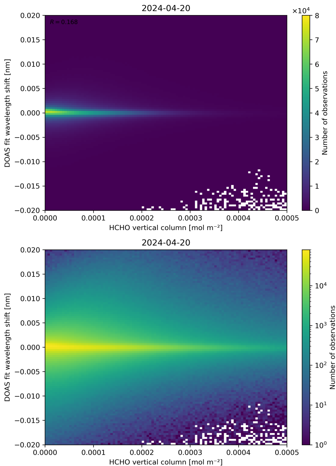
Figure 124: Scatter density plot of “HCHO vertical column” against “DOAS fit wavelength shift” for 2024-04-19 to 2024-04-21.
