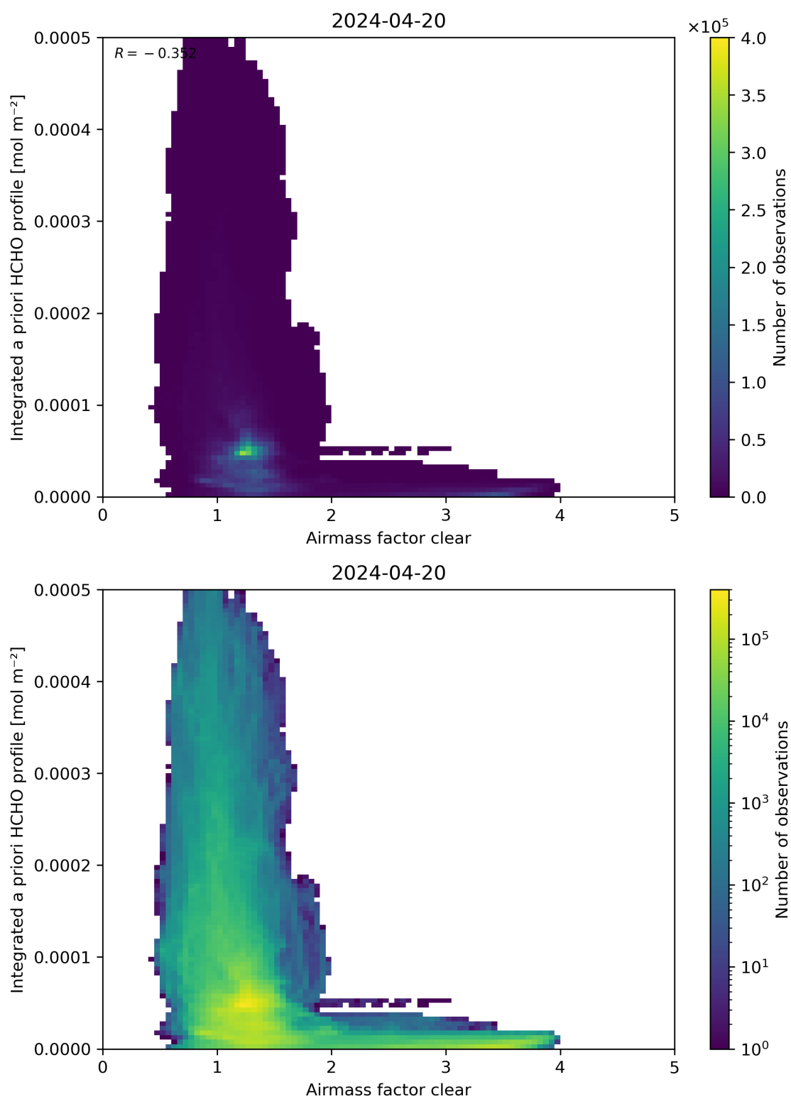
Figure 76: Scatter density plot of “Airmass factor clear” against “Integrated a priori HCHO profile” for 2024-04-19 to 2024-04-21.
