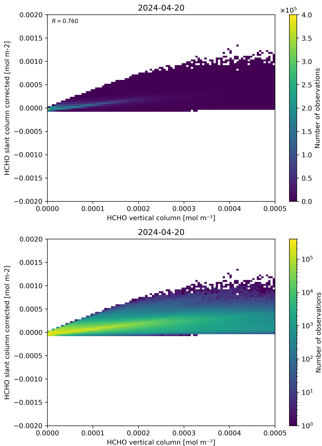
Figure 127: Scatter density plot of “HCHO vertical column” against “HCHO slant column corrected” for 2024-04-19 to 2024-04-21.
