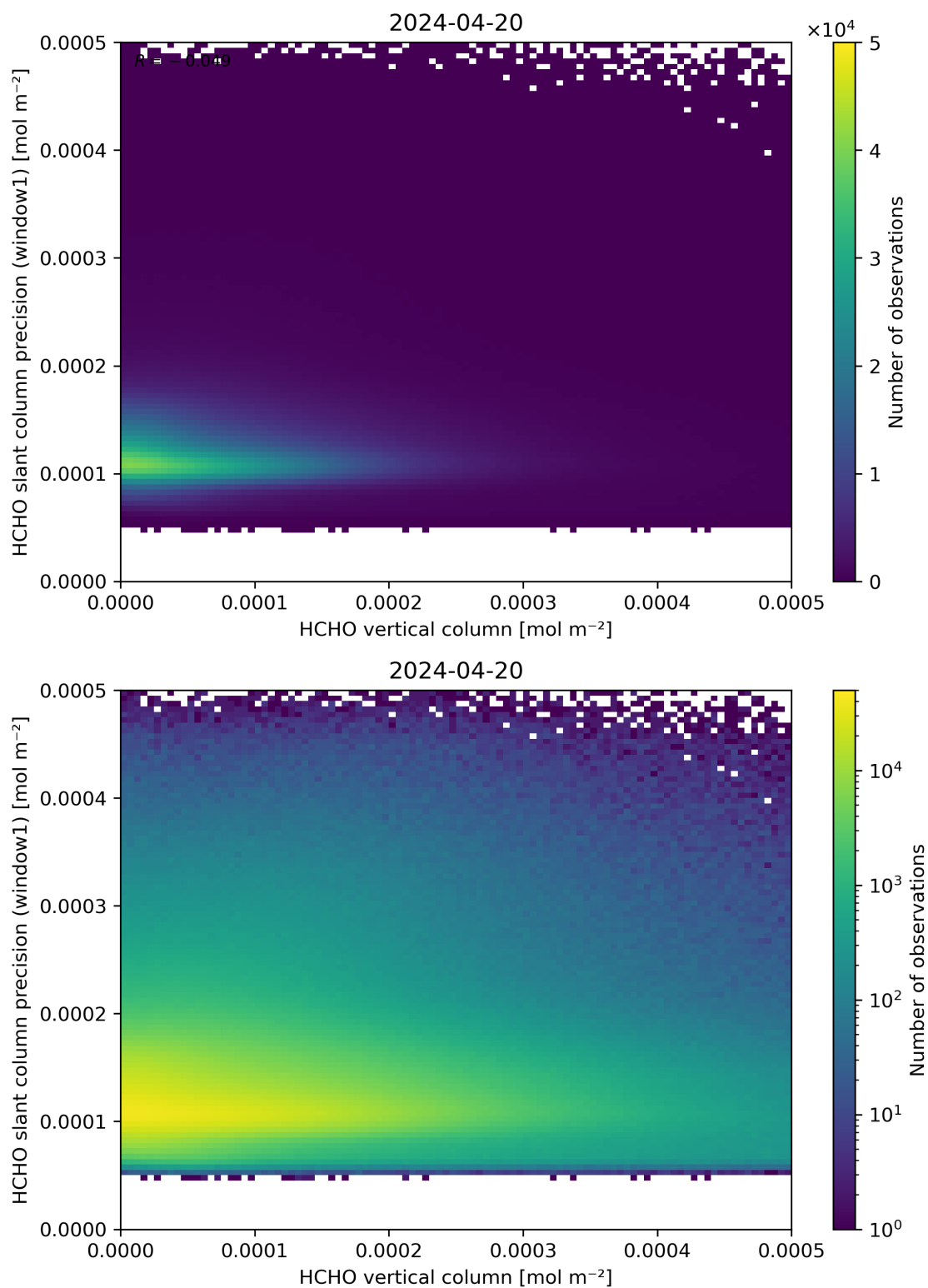
Figure 130: Scatter density plot of “HCHO vertical column” against “HCHO slant column precision (window1)” for 2024-04-19 to 2024-04-21.
