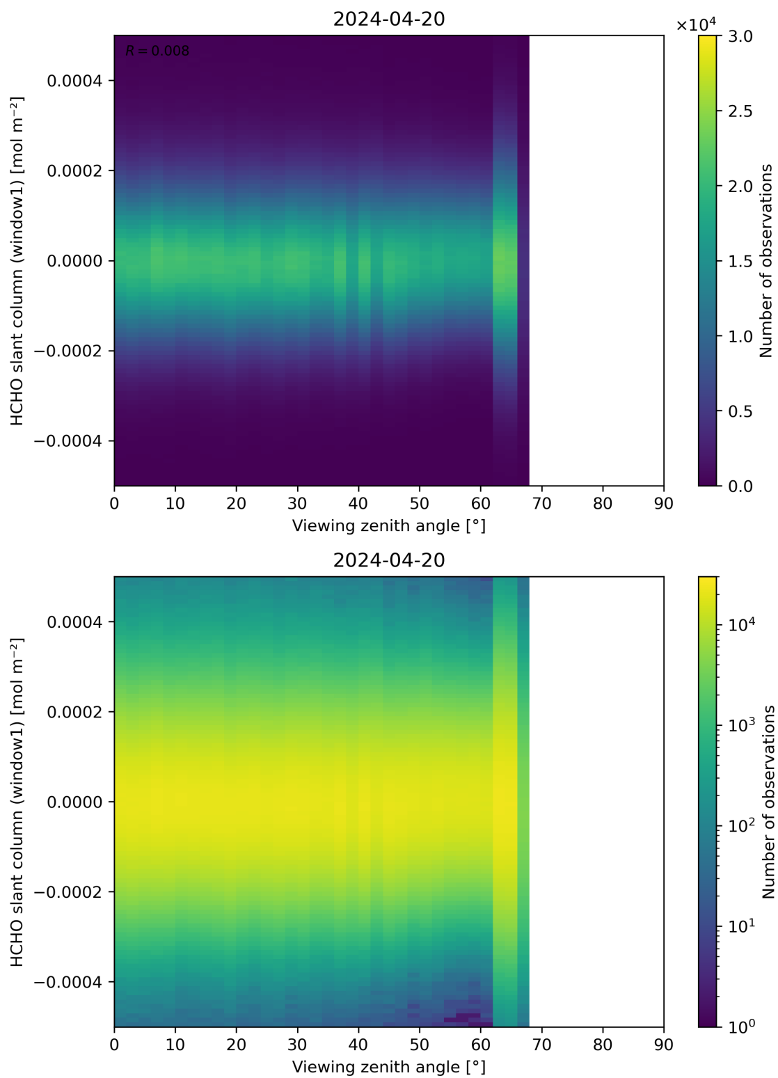
Figure 188: Scatter density plot of “Viewing zenith angle” against “HCHO slant column (window1)” for 2024-04-19 to 2024-04-21.
