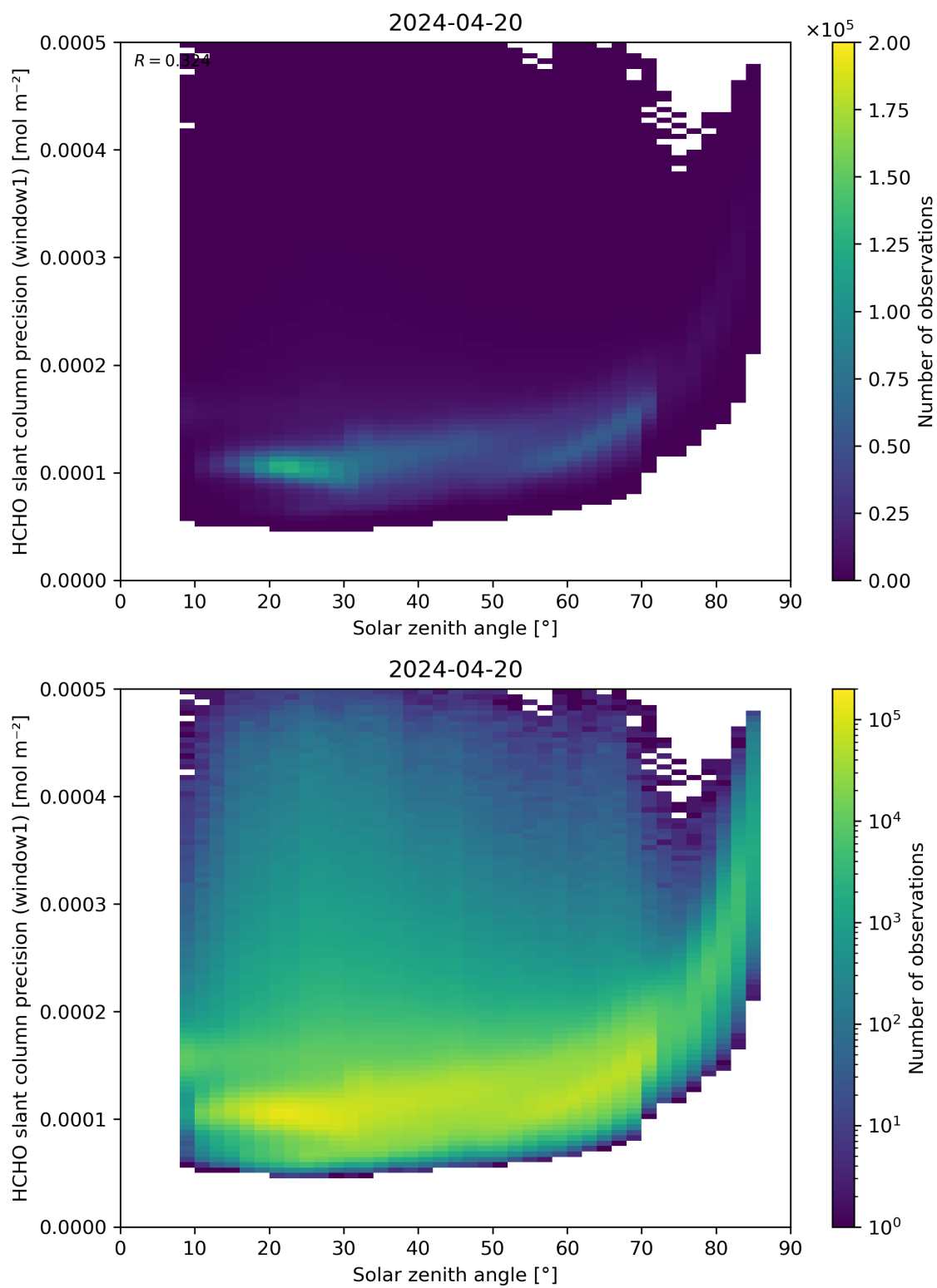
Figure 174: Scatter density plot of “Solar zenith angle” against “HCHO slant column precision (window1)” for 2024-04-19 to 2024-04-21.
