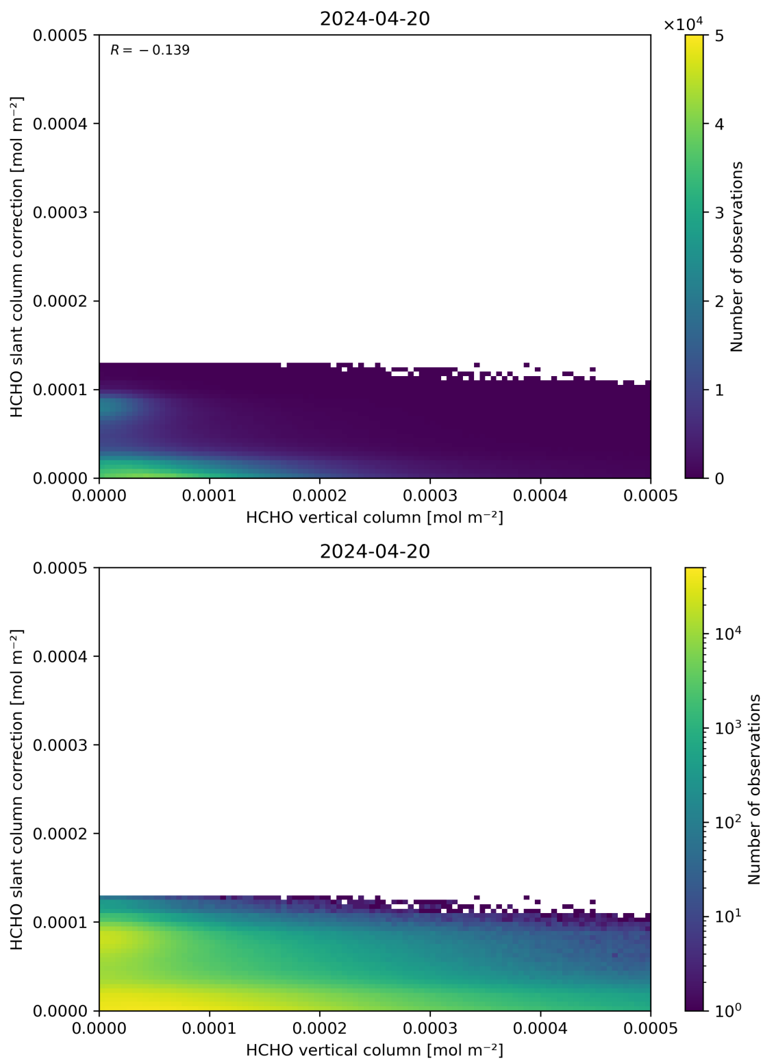
Figure 128: Scatter density plot of “HCHO vertical column” against “HCHO slant column correction” for 2024-04-19 to 2024-04-21.
