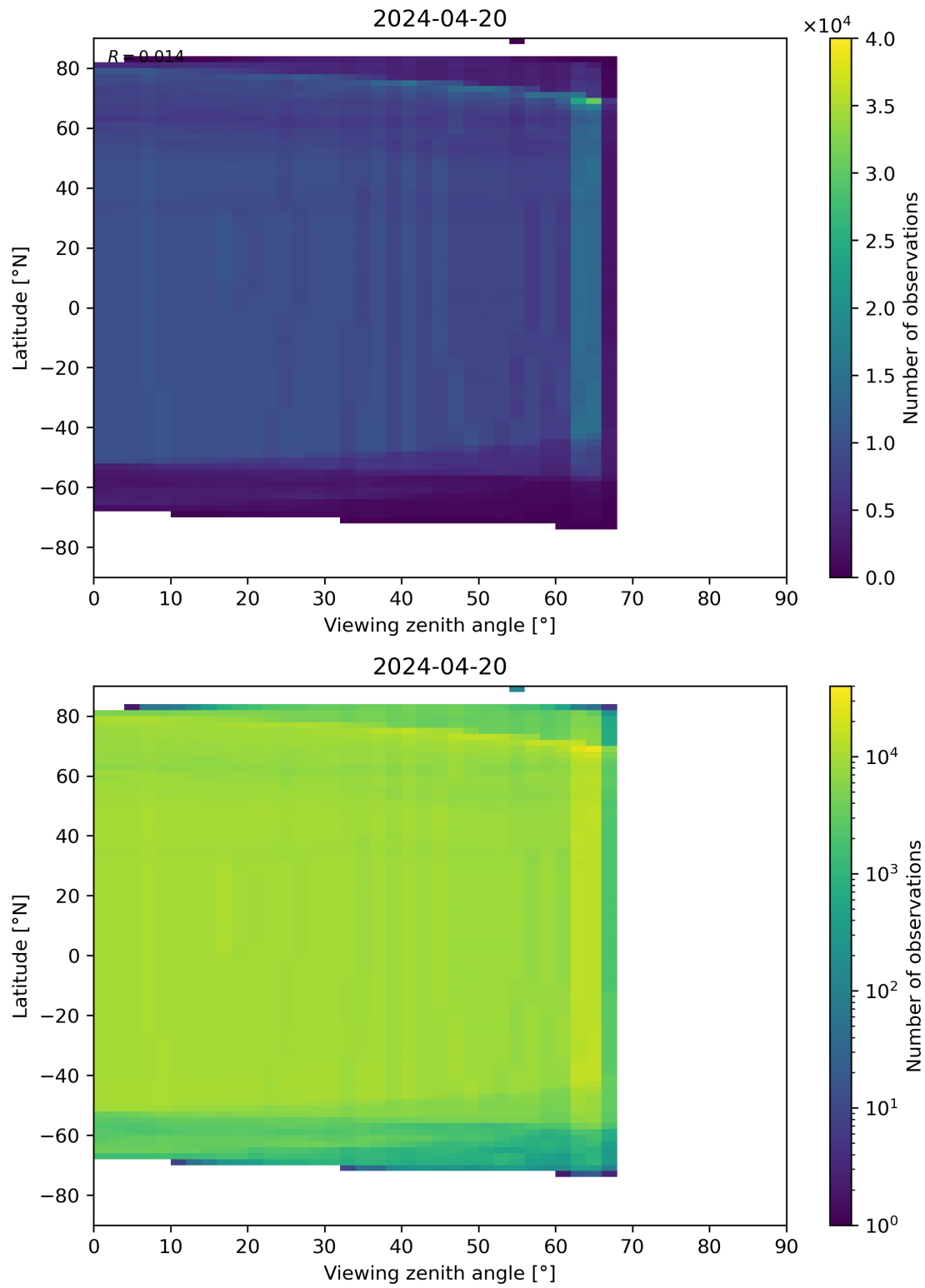
Figure 196: Scatter density plot of “Viewing zenith angle” against “Latitude” for 2024-04-19 to 2024-04-21.
