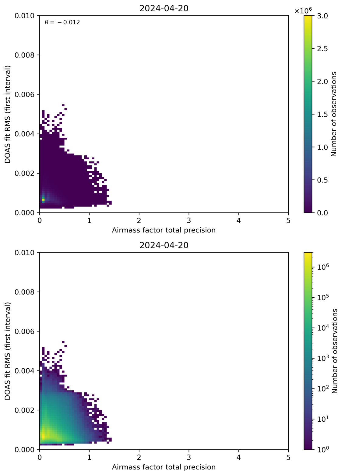
Figure 105: Scatter density plot of “Airmass factor total precision” against “DOAS fit RMS (first interval)” for 2024-04-19 to 2024-04-21.
