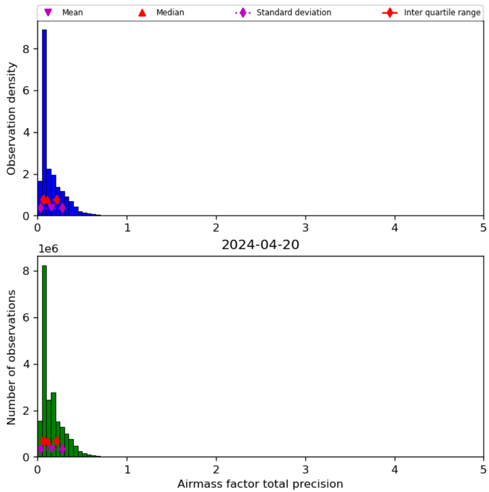
Figure 41: Histogram of “Airmass factor total precision” for 2024-04-19 to 2024-04-21
