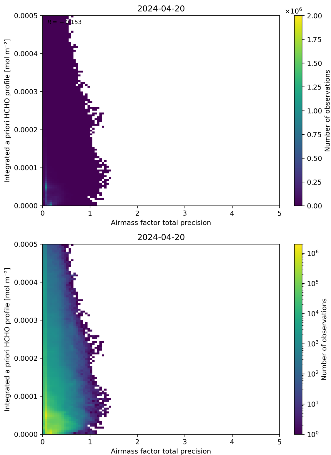
Figure 111: Scatter density plot of “Airmass factor total precision” against “Integrated a priori HCHO profile” for 2024-04-19 to 2024-04-21.
