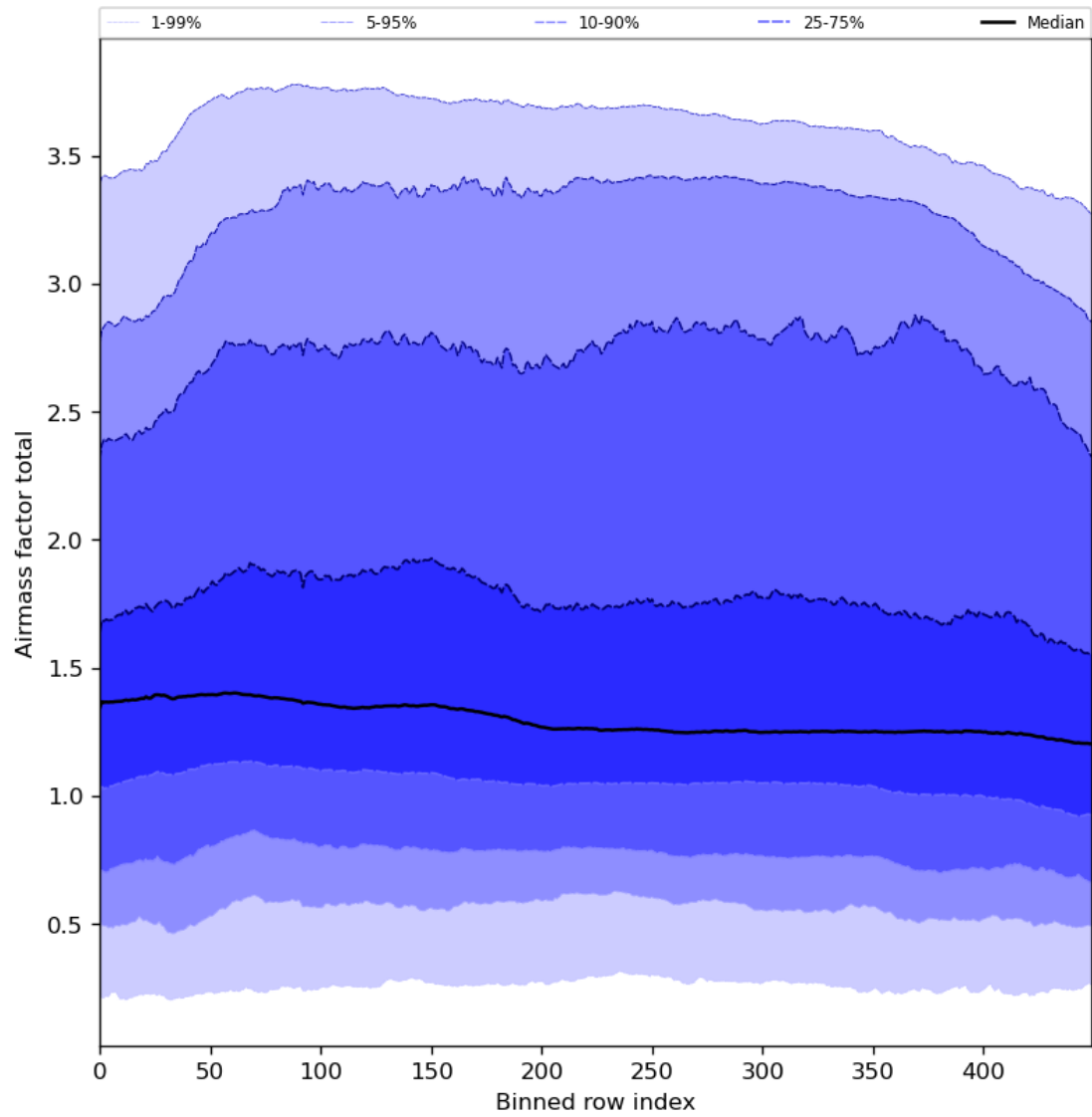
Figure 54: Along track statistics of “Airmass factor total” for 2024-04-19 to 2024-04-21
