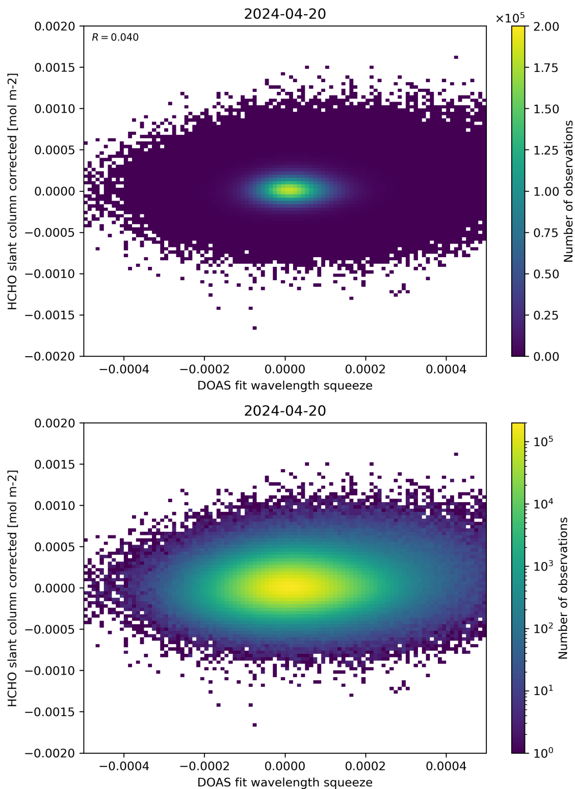
Figure 69: Scatter density plot of “DOAS fit wavelength squeeze” against “HCHO slant column corrected” for 2024-04-19 to 2024-04-21.
