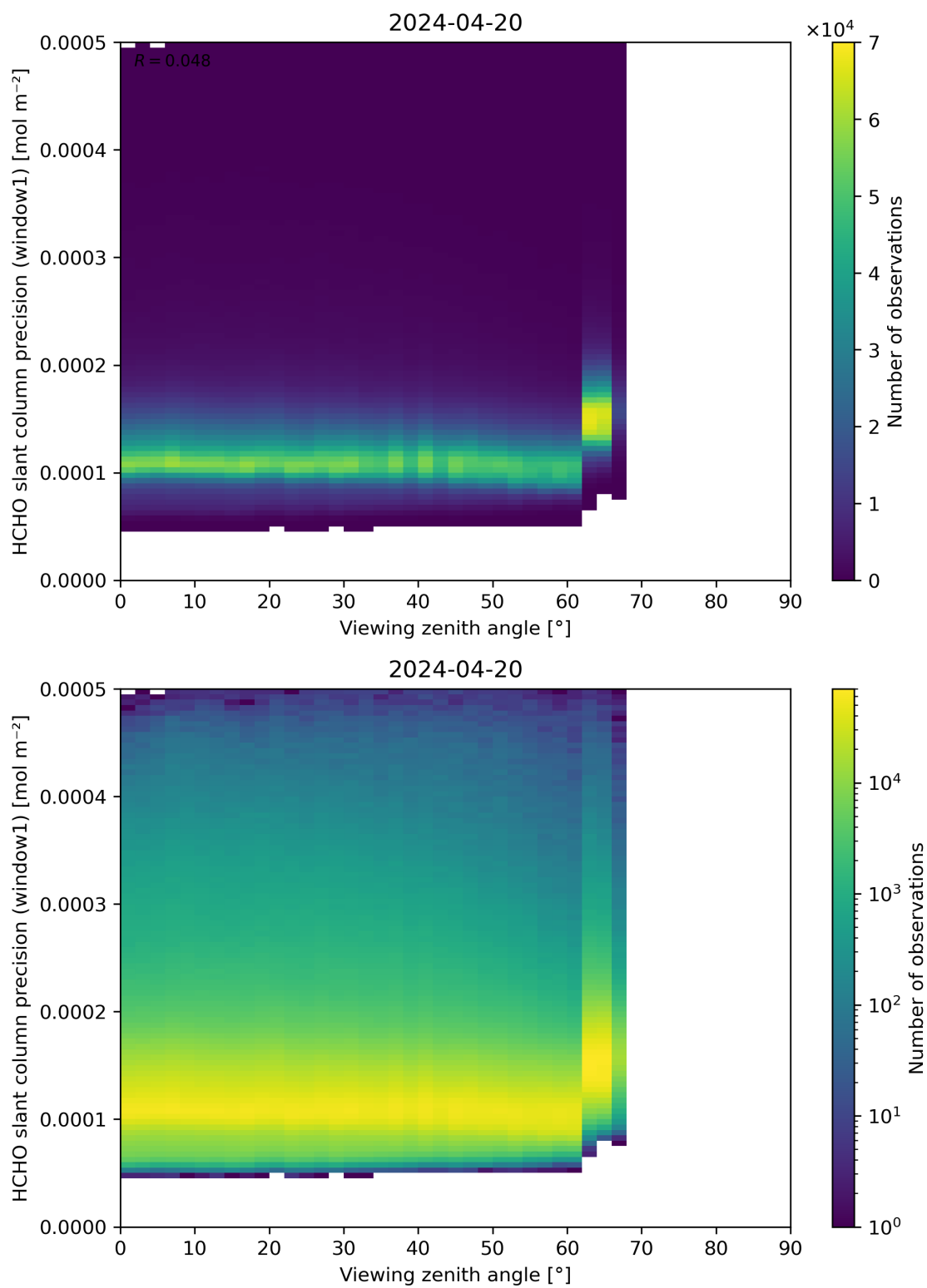
Figure 189: Scatter density plot of “Viewing zenith angle” against “HCHO slant column precision (window1)” for 2024-04-19 to 2024-04-21.
