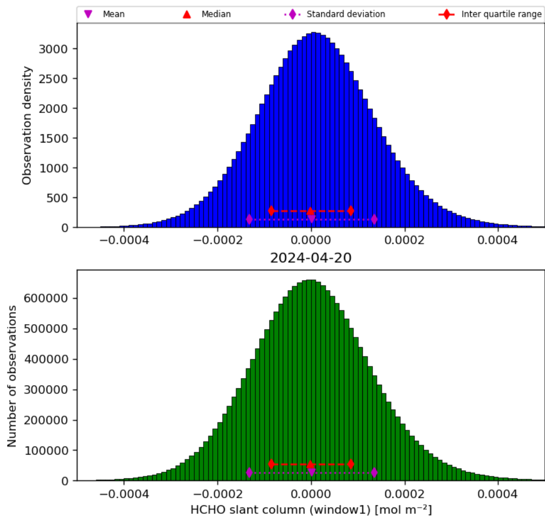
Figure 38: Histogram of “HCHO slant column (window1)” for 2024-04-19 to 2024-04-21
