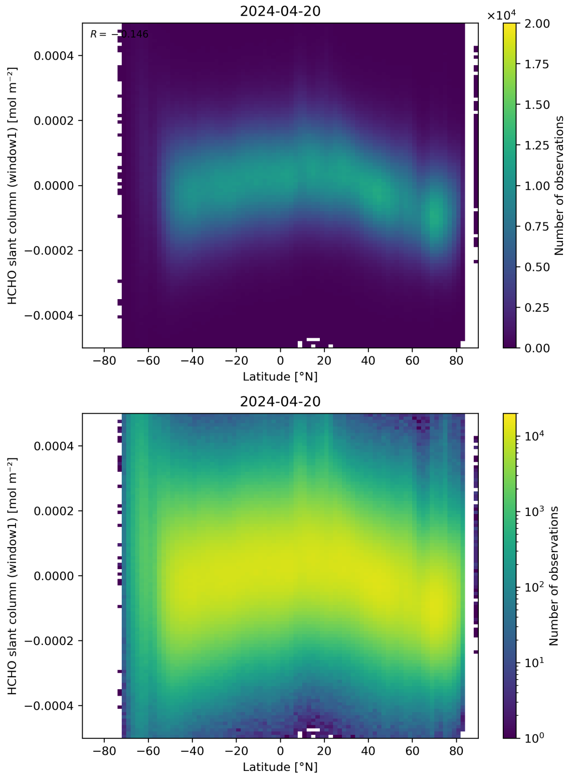
Figure 159: Scatter density plot of “Latitude” against “HCHO slant column (window1)” for 2024-04-19 to 2024-04-21.
