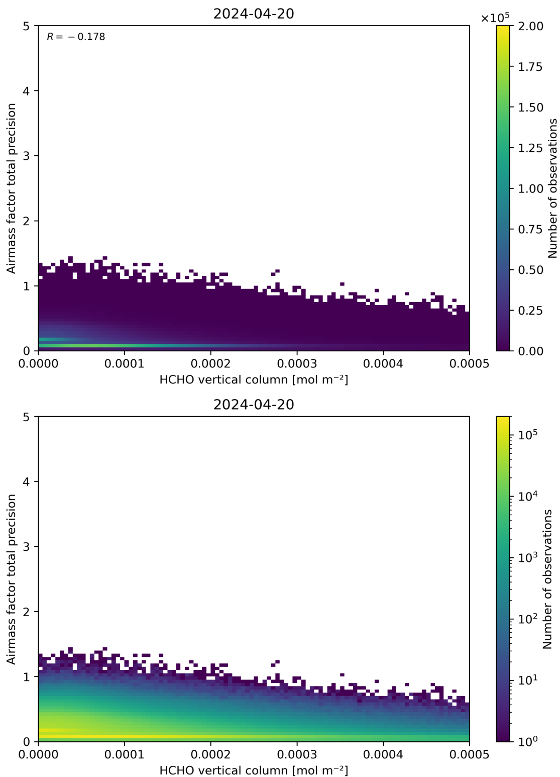
Figure 132: Scatter density plot of “HCHO vertical column” against “Airmass factor total precision” for 2024-04-19 to 2024-04-21.
