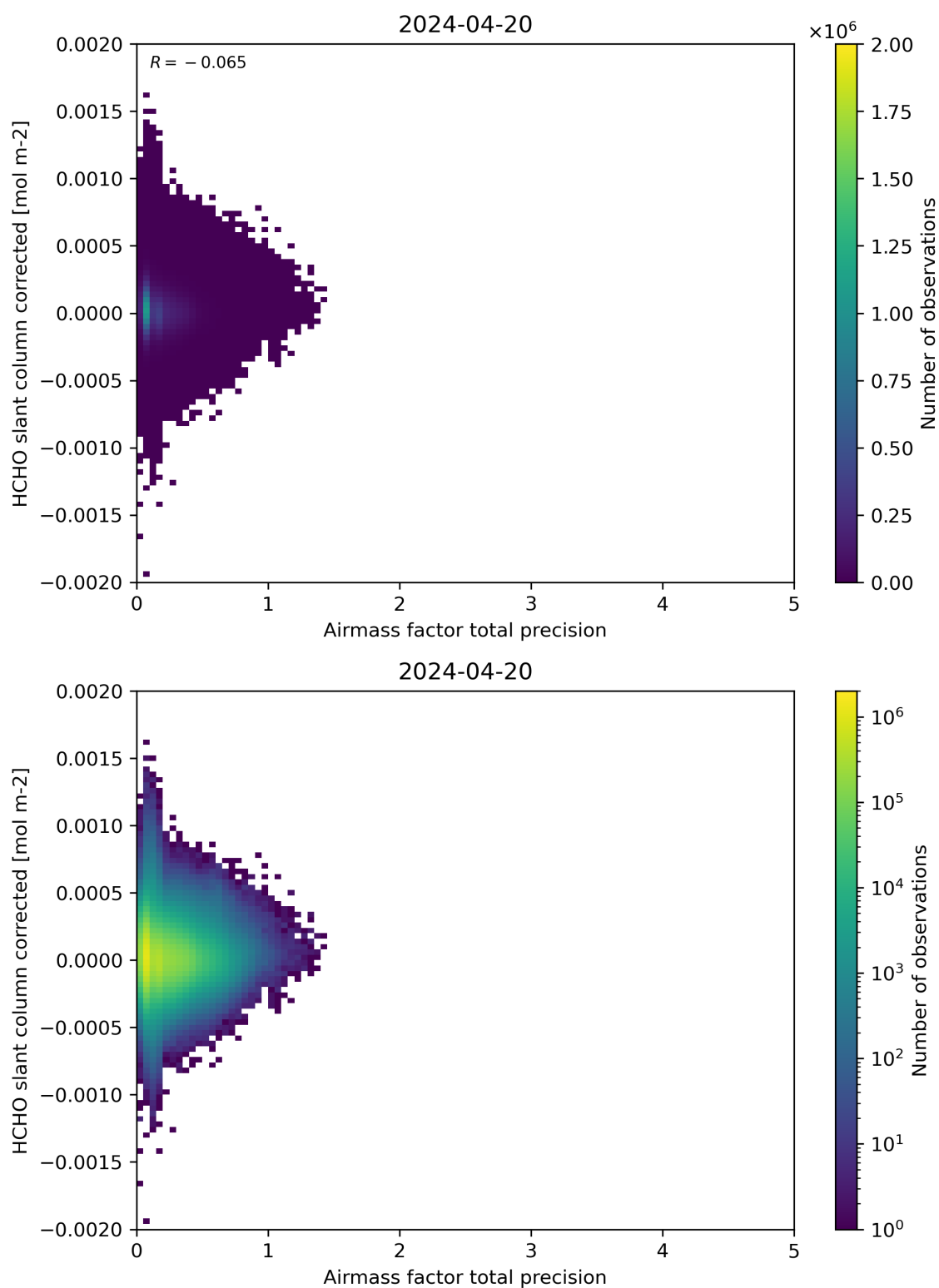
Figure 109: Scatter density plot of “Airmass factor total precision” against “HCHO slant column corrected” for 2024-04-19 to 2024-04-21.
