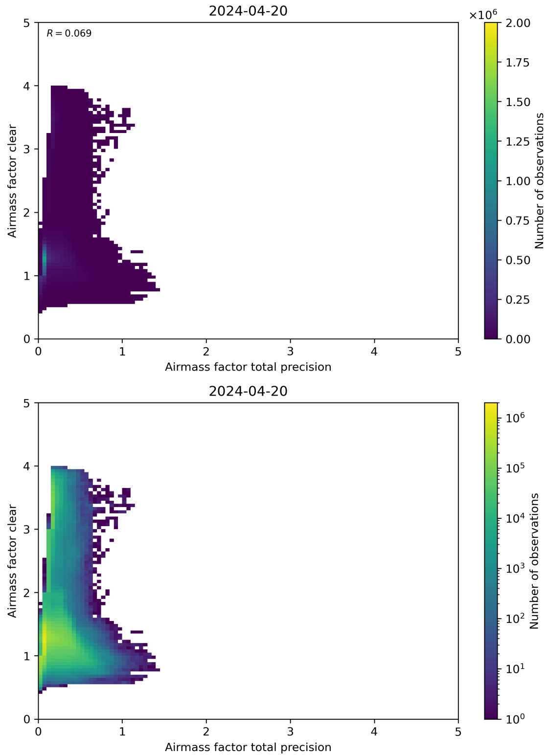
Figure 108: Scatter density plot of “Airmass factor total precision” against “Airmass factor clear” for 2024-04-19 to 2024-04-21.
