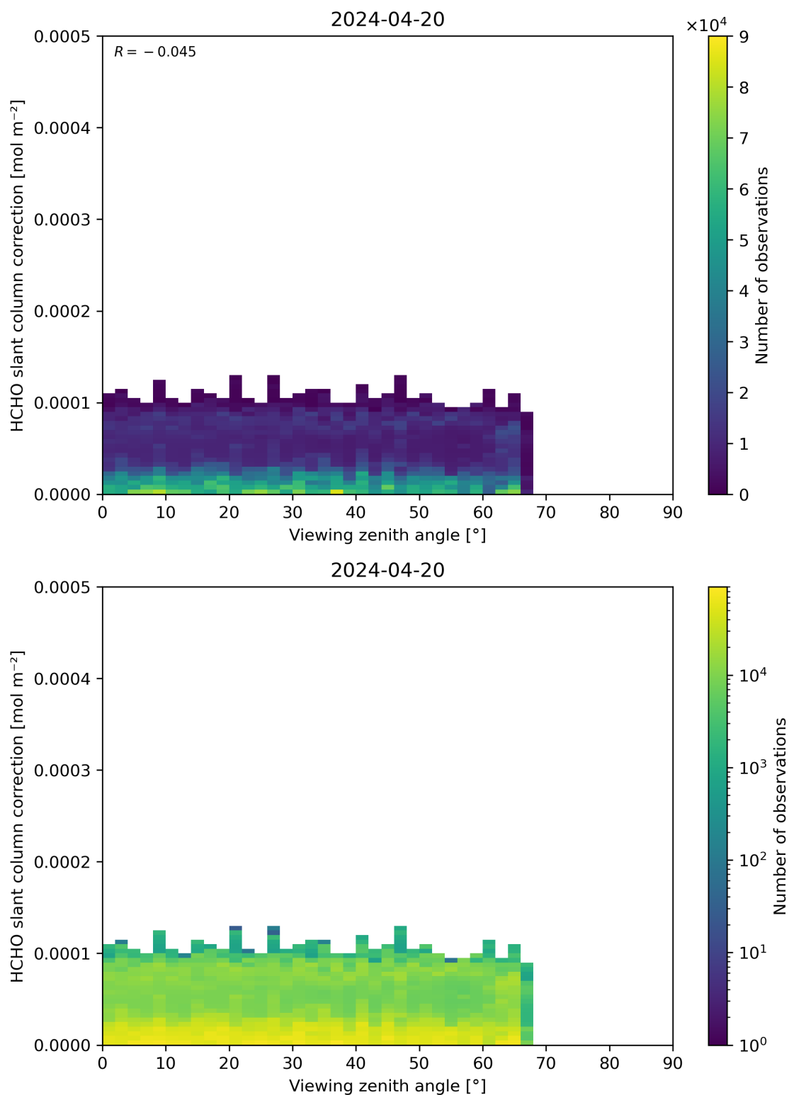
Figure 187: Scatter density plot of “Viewing zenith angle” against “HCHO slant column correction” for 2024-04-19 to 2024-04-21.
