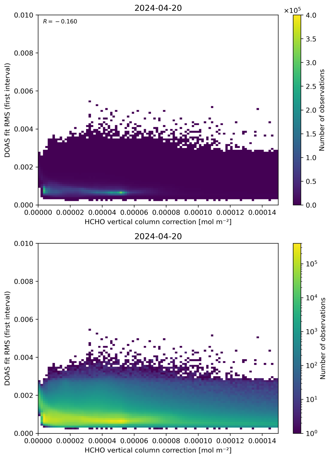
Figure 112: Scatter density plot of “HCHO vertical column correction” against “DOAS fit RMS (first interval)” for 2024-04-19 to 2024-04-21.
