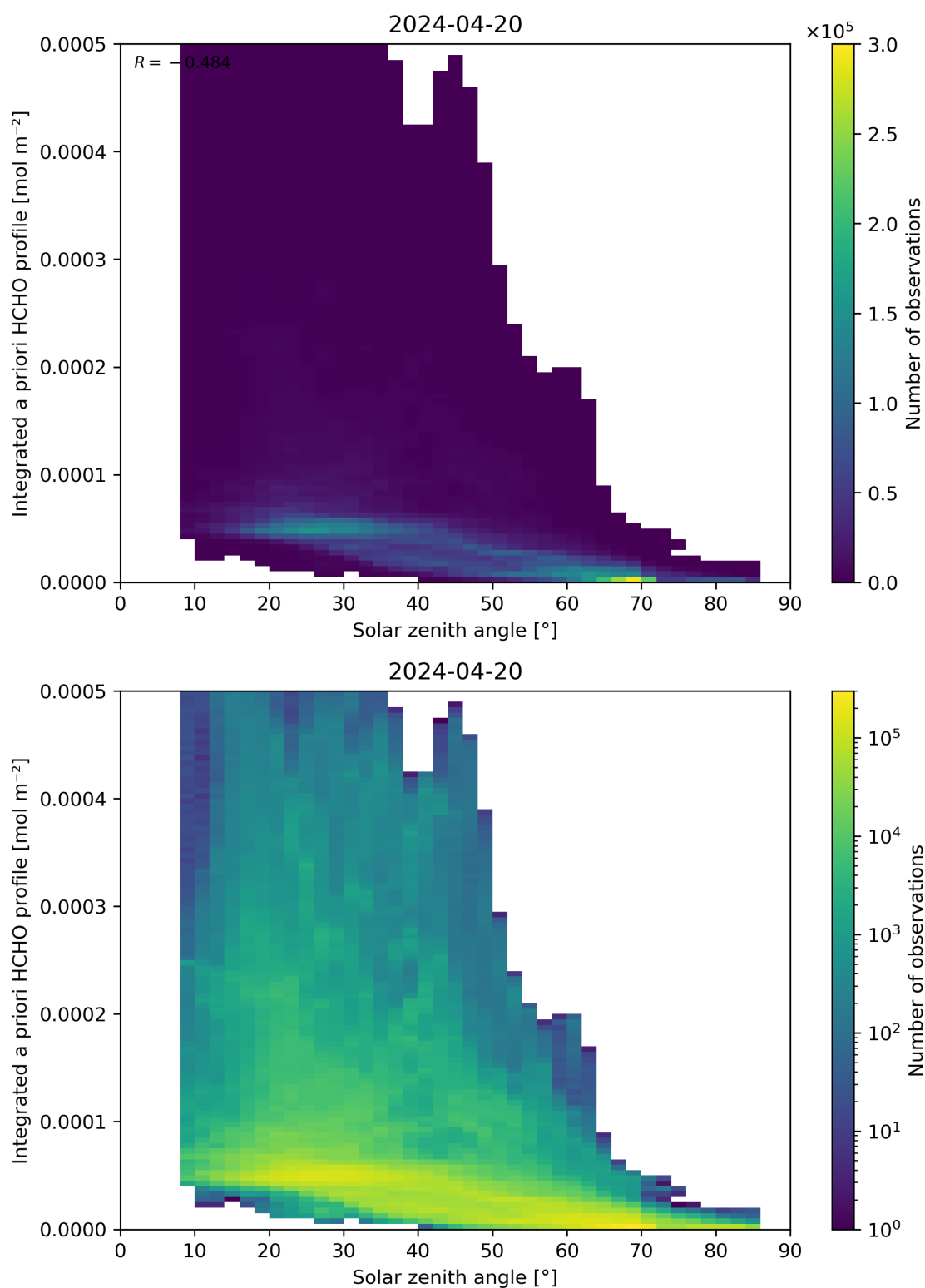
Figure 180: Scatter density plot of “Solar zenith angle” against “Integrated a priori HCHO profile” for 2024-04-19 to 2024-04-21.
