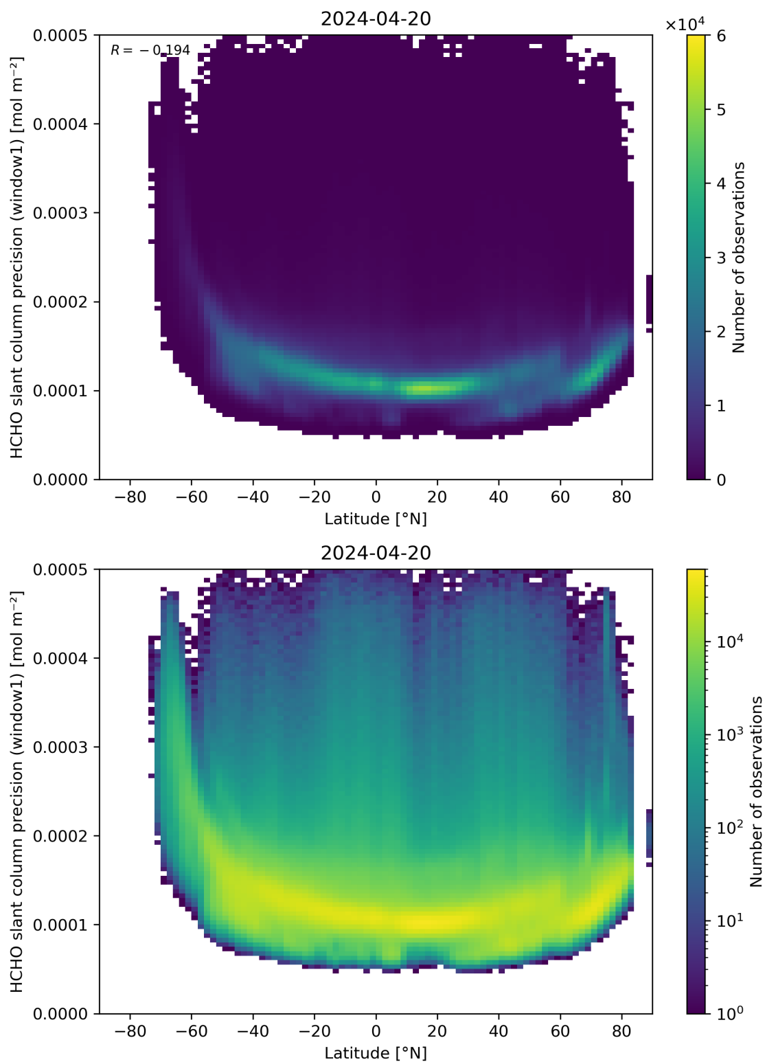
Figure 160: Scatter density plot of “Latitude” against “HCHO slant column precision (window1)” for 2024-04-19 to 2024-04-21.
