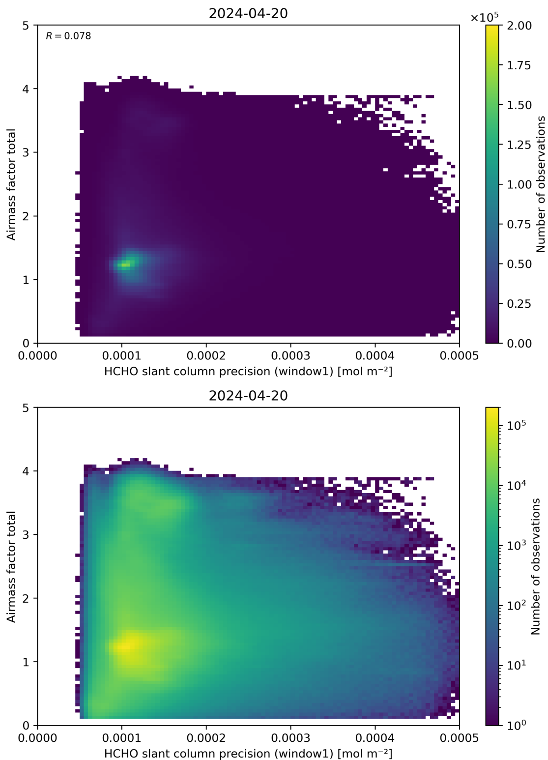
Figure 94: Scatter density plot of “HCHO slant column precision (window1)” against “Airmass factor total” for 2024-04-19 to 2024-04-21.
