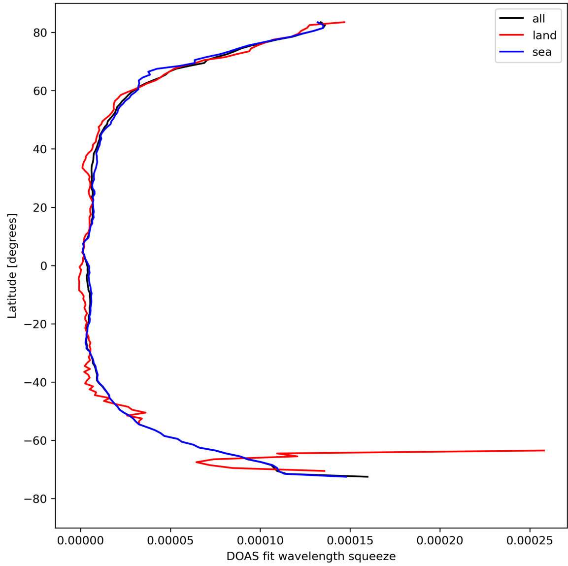
Figure 31: Zonal average of “DOAS fit wavelength squeeze” for 2024-04-19 to 2024-04-21.
