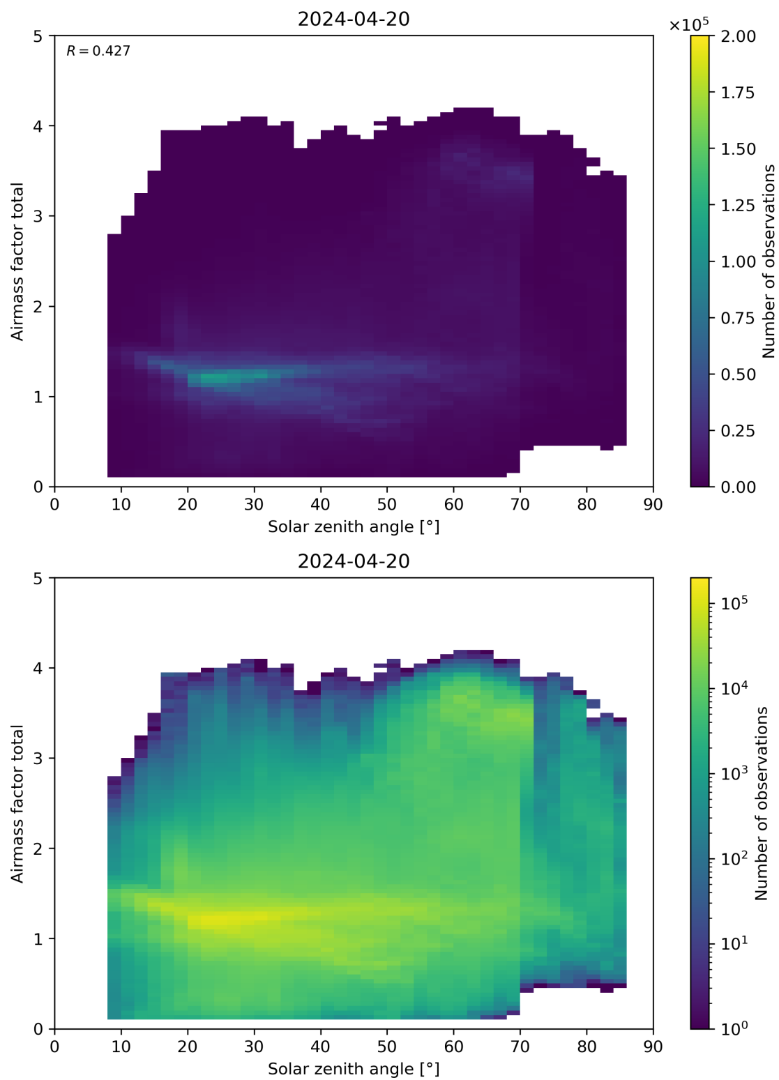
Figure 175: Scatter density plot of “Solar zenith angle” against “Airmass factor total” for 2024-04-19 to 2024-04-21.
