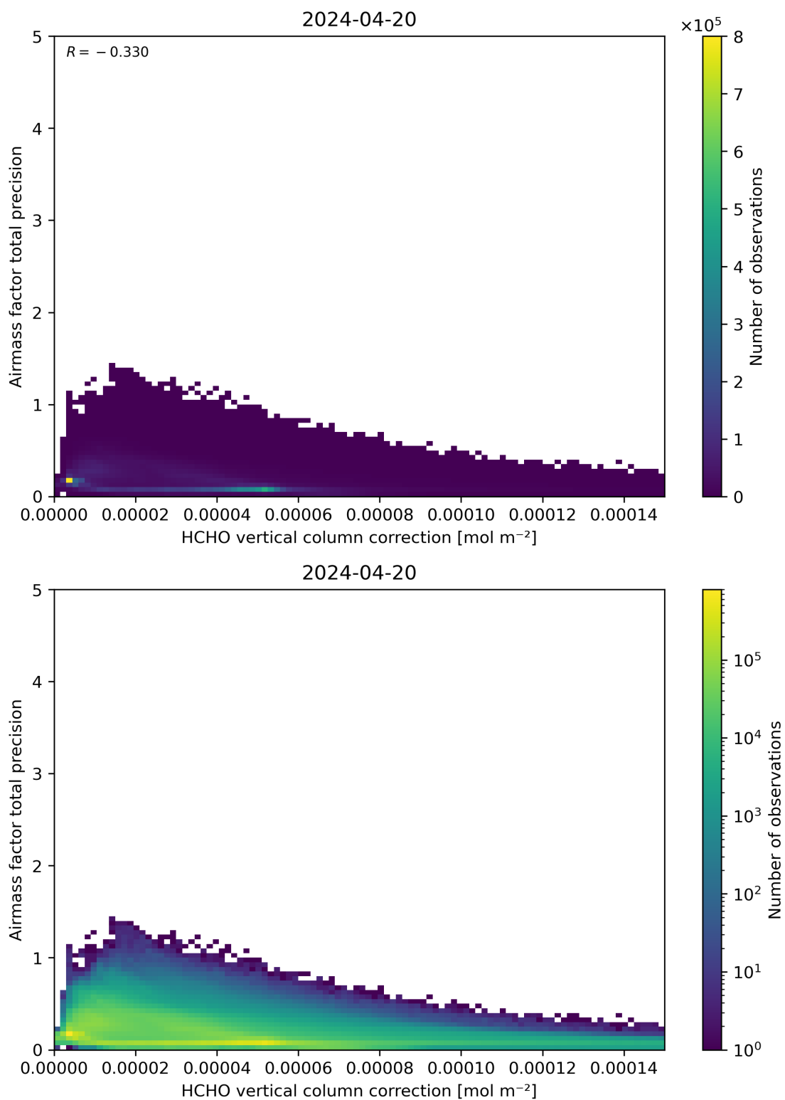
Figure 121: Scatter density plot of “HCHO vertical column correction” against “Airmass factor total precision” for 2024-04-19 to 2024-04-21.
