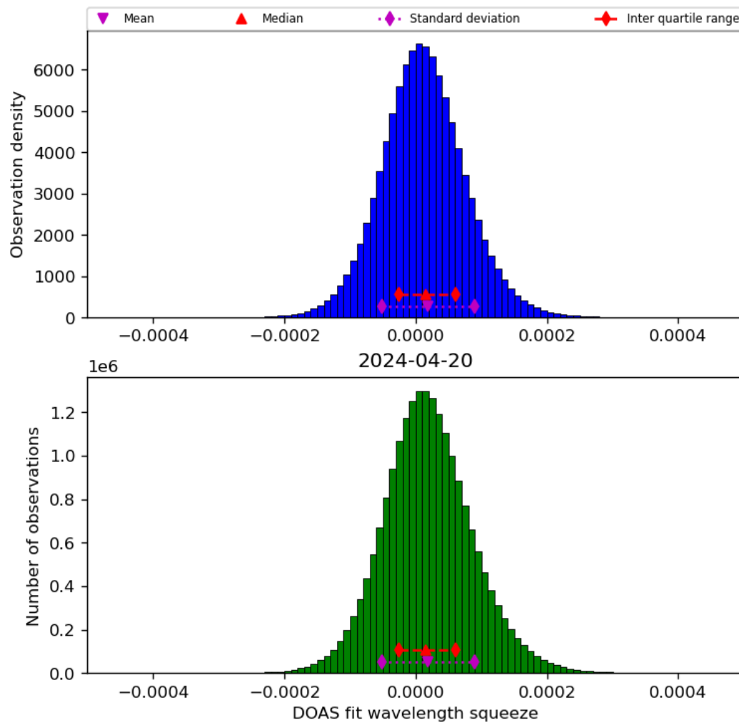
Figure 45: Histogram of “DOAS fit wavelength squeeze” for 2024-04-19 to 2024-04-21
