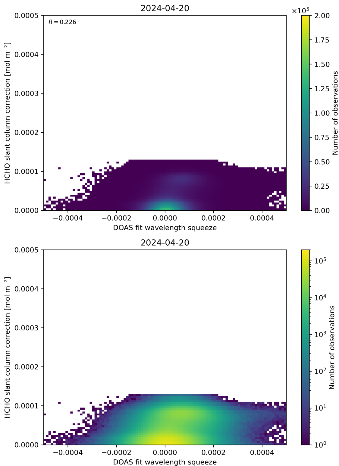
Figure 70: Scatter density plot of “DOAS fit wavelength squeeze” against “HCHO slant column correction” for 2024-04-19 to 2024-04-21.
