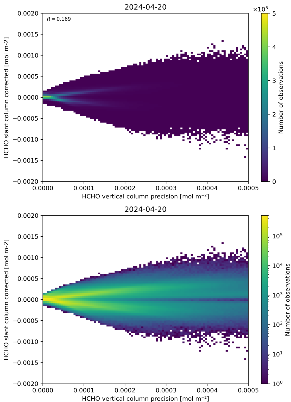
Figure 140: Scatter density plot of “HCHO vertical column precision” against “HCHO slant column corrected” for 2024-04-19 to 2024-04-21.
