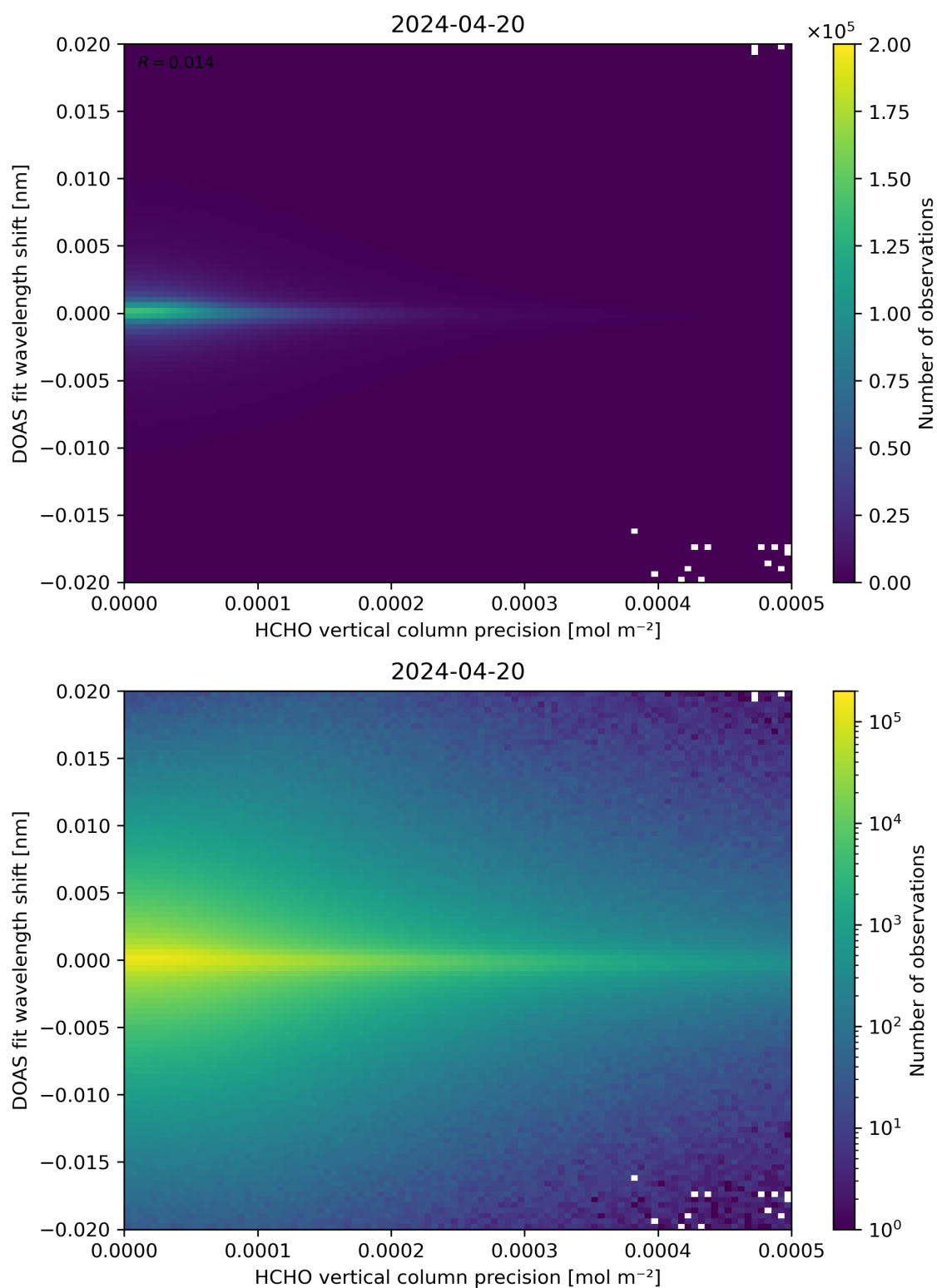
Figure 137: Scatter density plot of “HCHO vertical column precision” against “DOAS fit wavelength shift” for 2024-04-19 to 2024-04-21.
