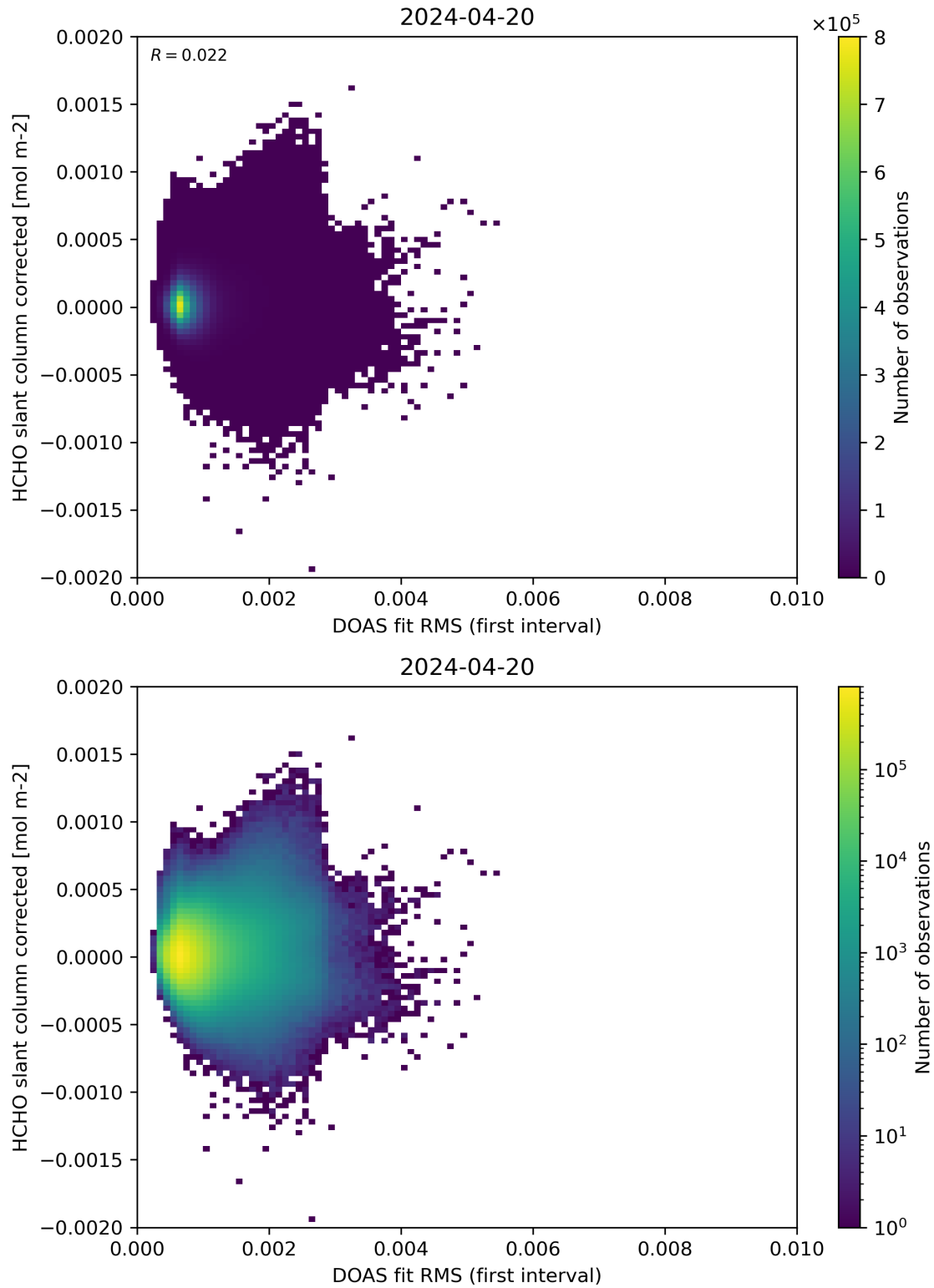
Figure 62: Scatter density plot of “DOAS fit RMS (first interval)” against “HCHO slant column corrected” for 2024-04-19 to 2024-04-21.
