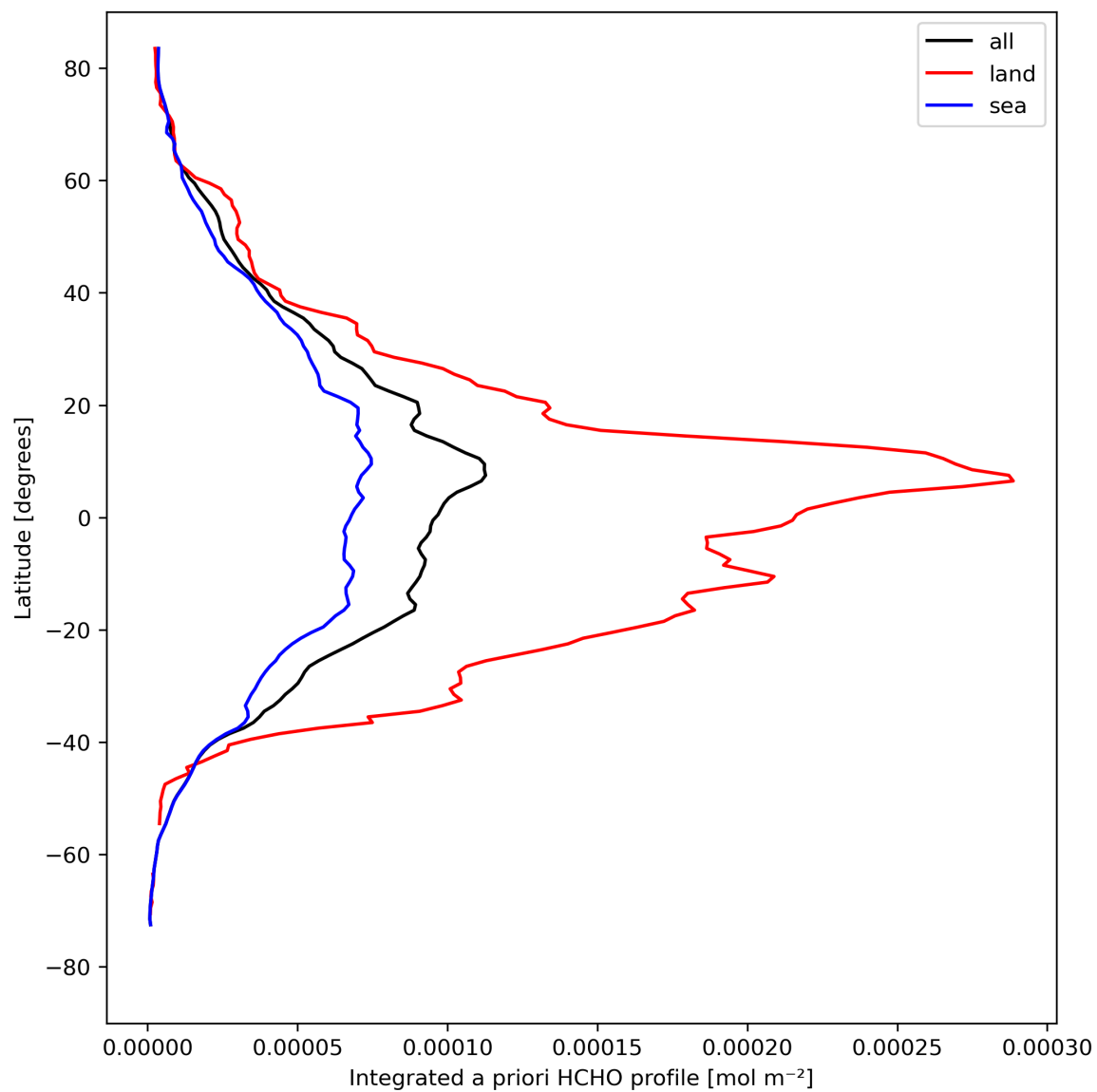
Figure 29: Zonal average of “Integrated a priori HCHO profile” for 2024-04-19 to 2024-04-21.
