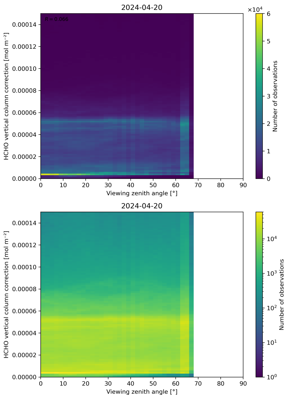
Figure 193: Scatter density plot of “Viewing zenith angle” against “HCHO vertical column correction” for 2024-04-19 to 2024-04-21.
