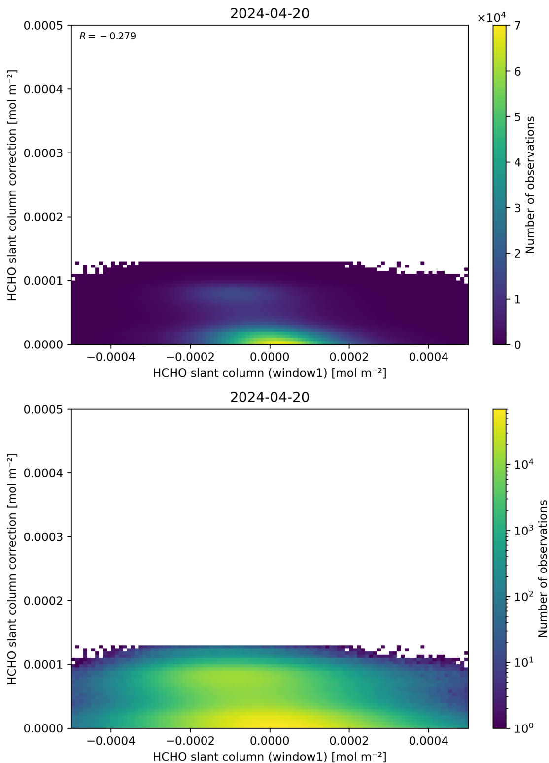
Figure 83: Scatter density plot of “HCHO slant column (window1)” against “HCHO slant column correction” for 2024-04-19 to 2024-04-21.
