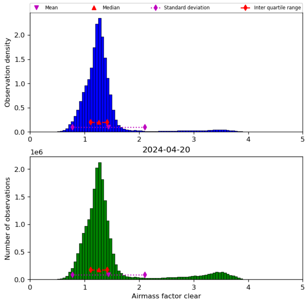
Figure 42: Histogram of “Airmass factor clear” for 2024-04-19 to 2024-04-21
