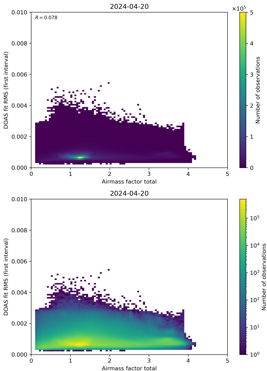
Figure 97: Scatter density plot of “Airmass factor total” against “DOAS fit RMS (first interval)” for 2024-04-19 to 2024-04-21.
