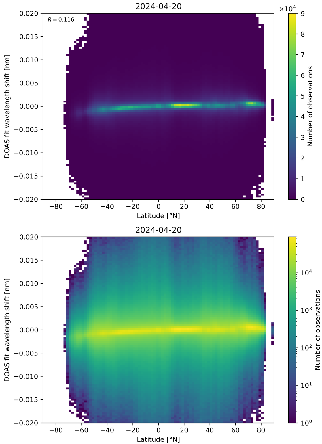
Figure 154: Scatter density plot of “Latitude” against “DOAS fit wavelength shift” for 2024-04-19 to 2024-04-21.
