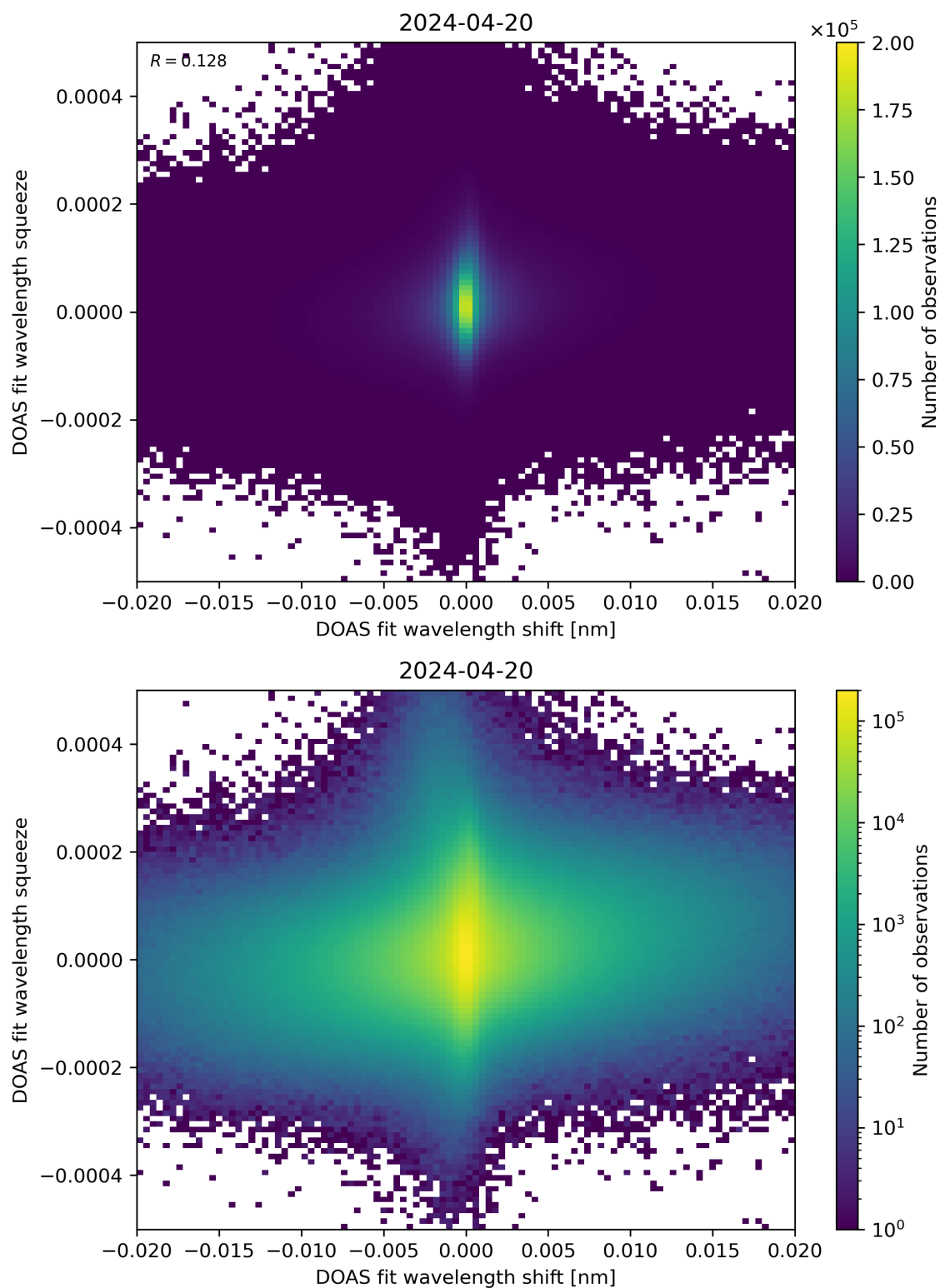
Figure 65: Scatter density plot of “DOAS fit wavelength shift” against “DOAS fit wavelength squeeze” for 2024-04-19 to 2024-04-21.
