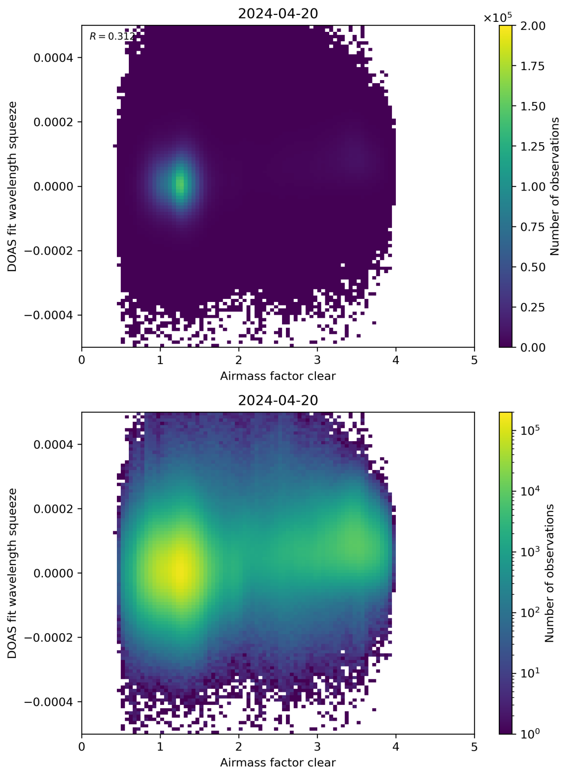
Figure 73: Scatter density plot of “Airmass factor clear” against “DOAS fit wavelength squeeze” for 2024-04-19 to 2024-04-21.
