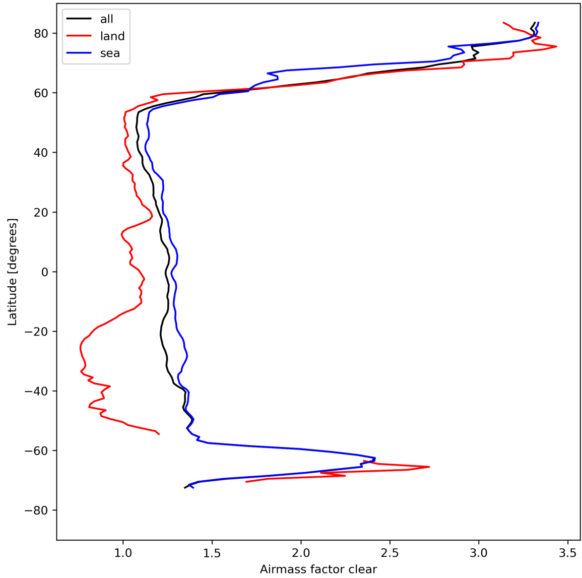
Figure 28: Zonal average of “Airmass factor clear” for 2024-04-19 to 2024-04-21.
