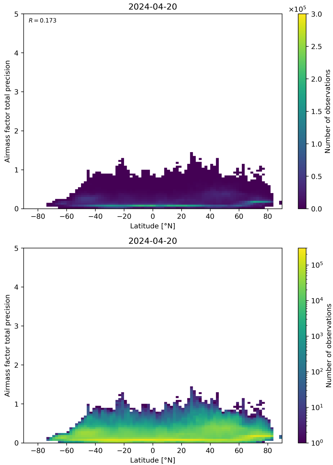
Figure 162: Scatter density plot of “Latitude” against “Airmass factor total precision” for 2024-04-19 to 2024-04-21.
