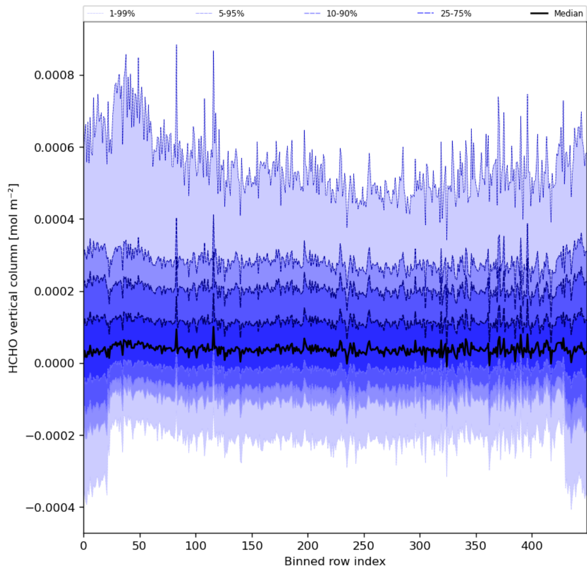
Figure 49: Along track statistics of “HCHO vertical column” for 2024-04-19 to 2024-04-21
