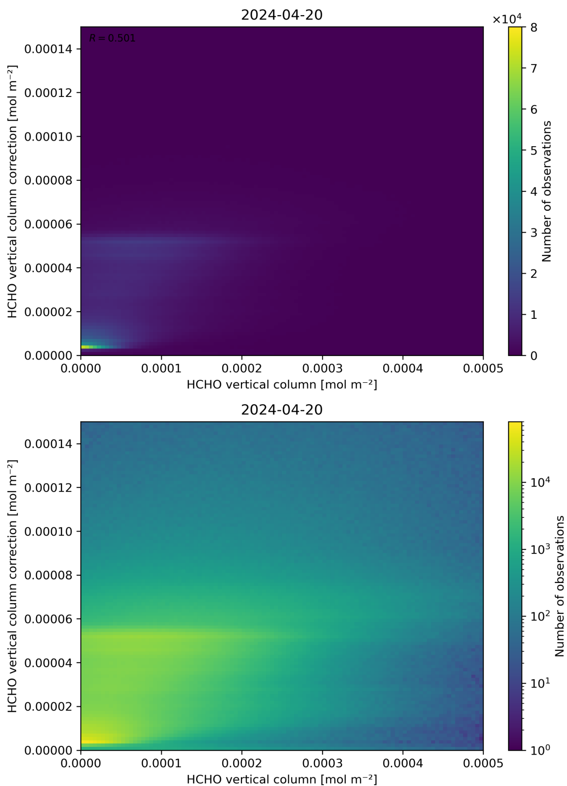
Figure 133: Scatter density plot of “HCHO vertical column” against “HCHO vertical column correction” for 2024-04-19 to 2024-04-21.
