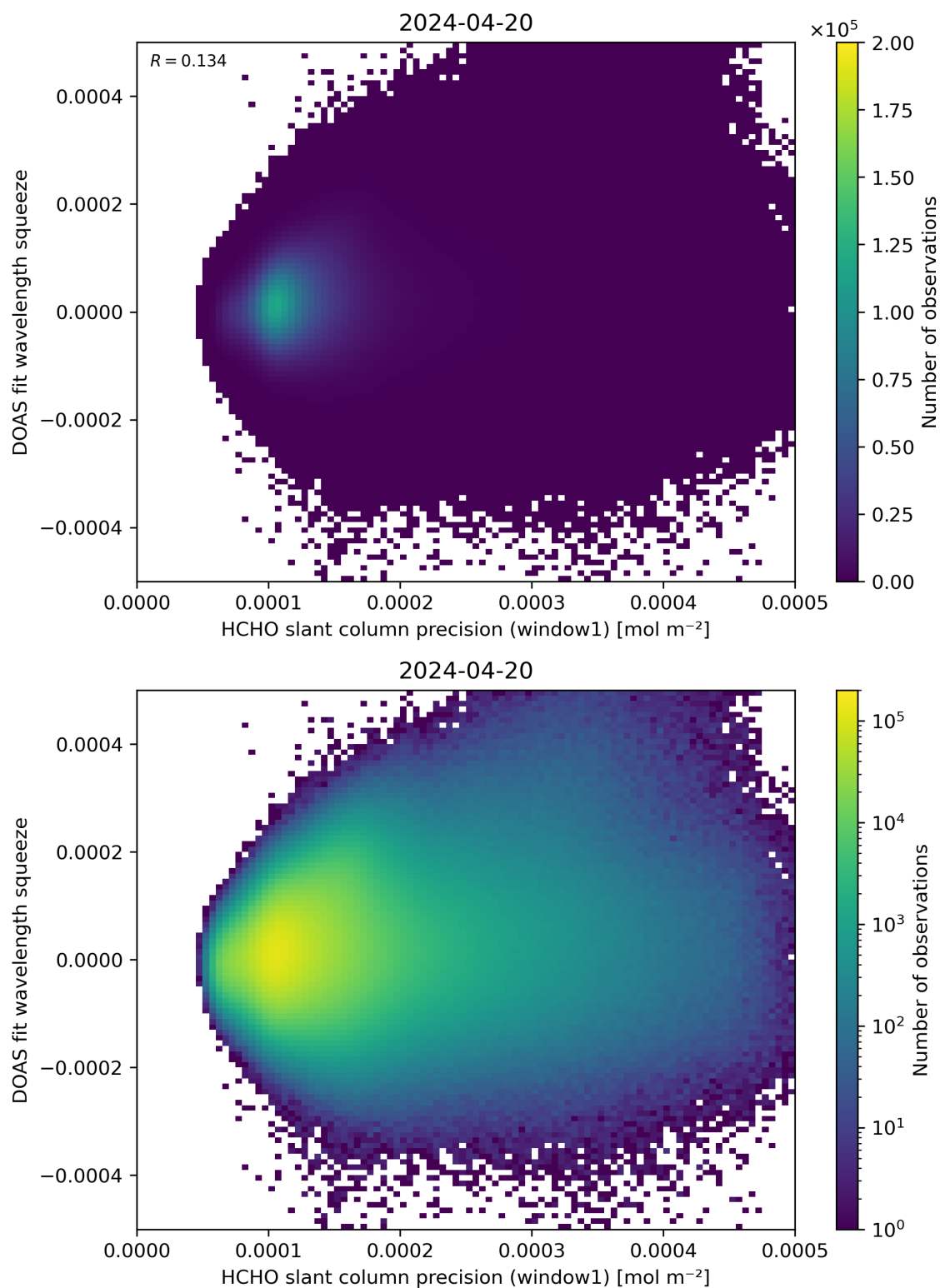
Figure 90: Scatter density plot of “HCHO slant column precision (window1)” against “DOAS fit wavelength squeeze” for 2024-04-19 to 2024-04-21.
