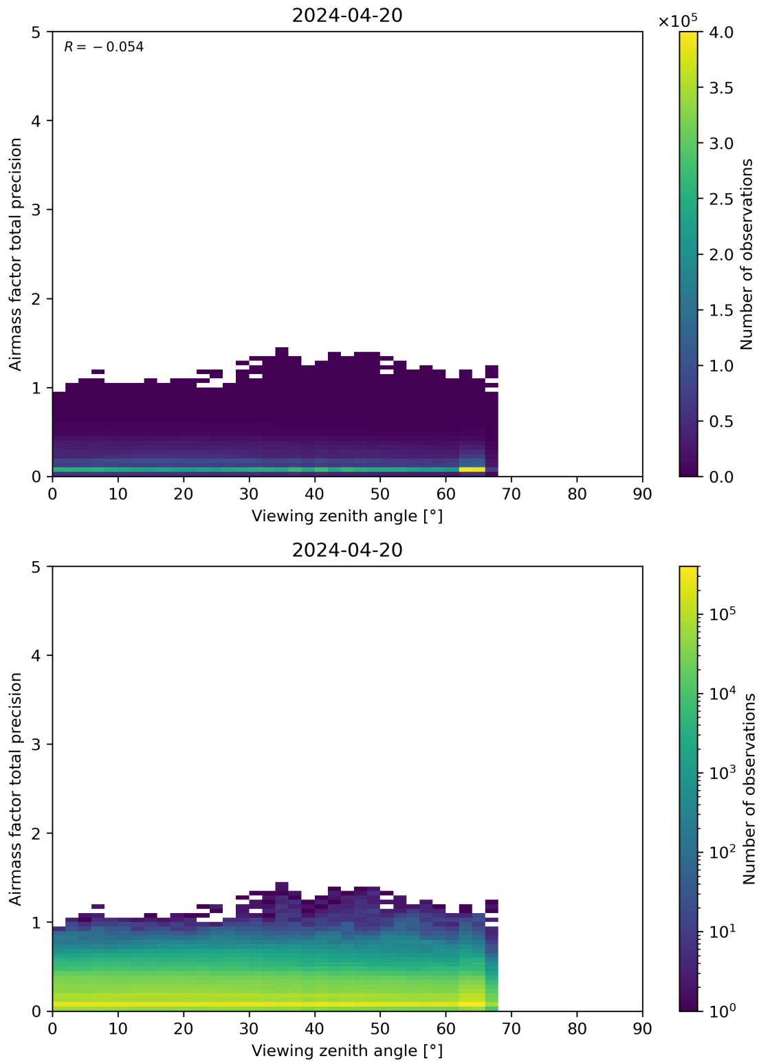
Figure 191: Scatter density plot of “Viewing zenith angle” against “Airmass factor total precision” for 2024-04-19 to 2024-04-21.
