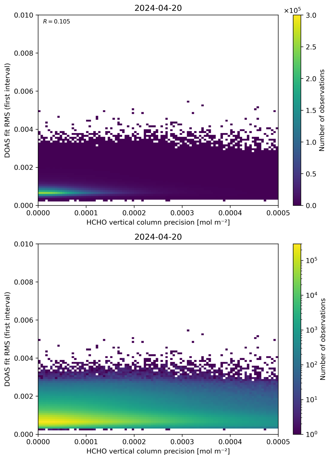
Figure 136: Scatter density plot of “HCHO vertical column precision” against “DOAS fit RMS (first interval)” for 2024-04-19 to 2024-04-21.
