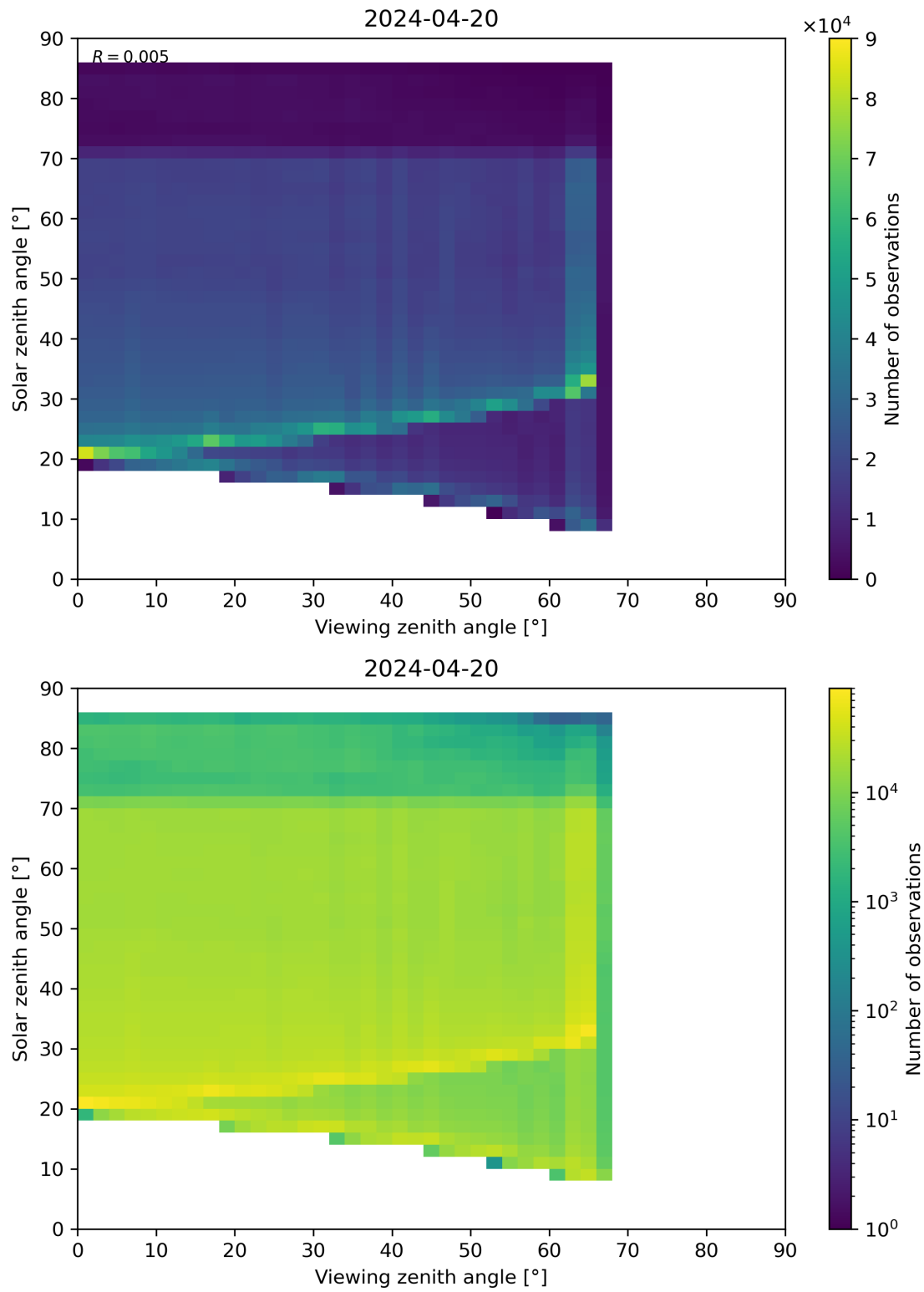
Figure 197: Scatter density plot of “Viewing zenith angle” against “Solar zenith angle” for 2024-04-19 to 2024-04-21.
