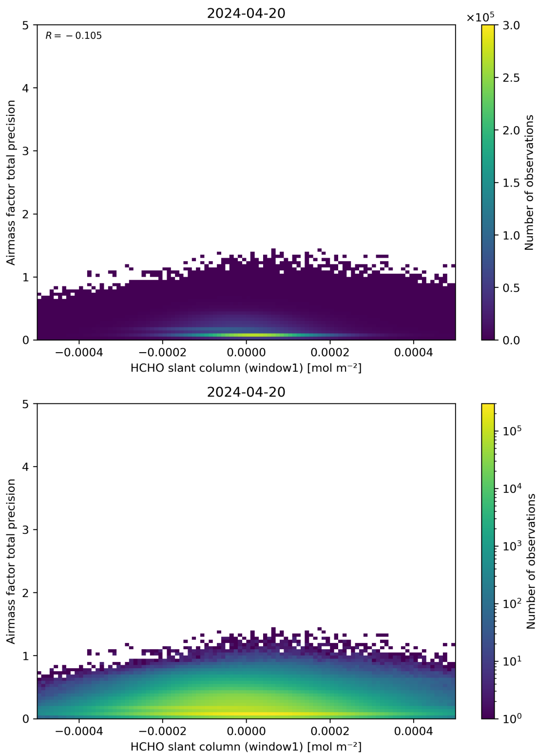
Figure 86: Scatter density plot of “HCHO slant column (window1)” against “Airmass factor total precision” for 2024-04-19 to 2024-04-21.
