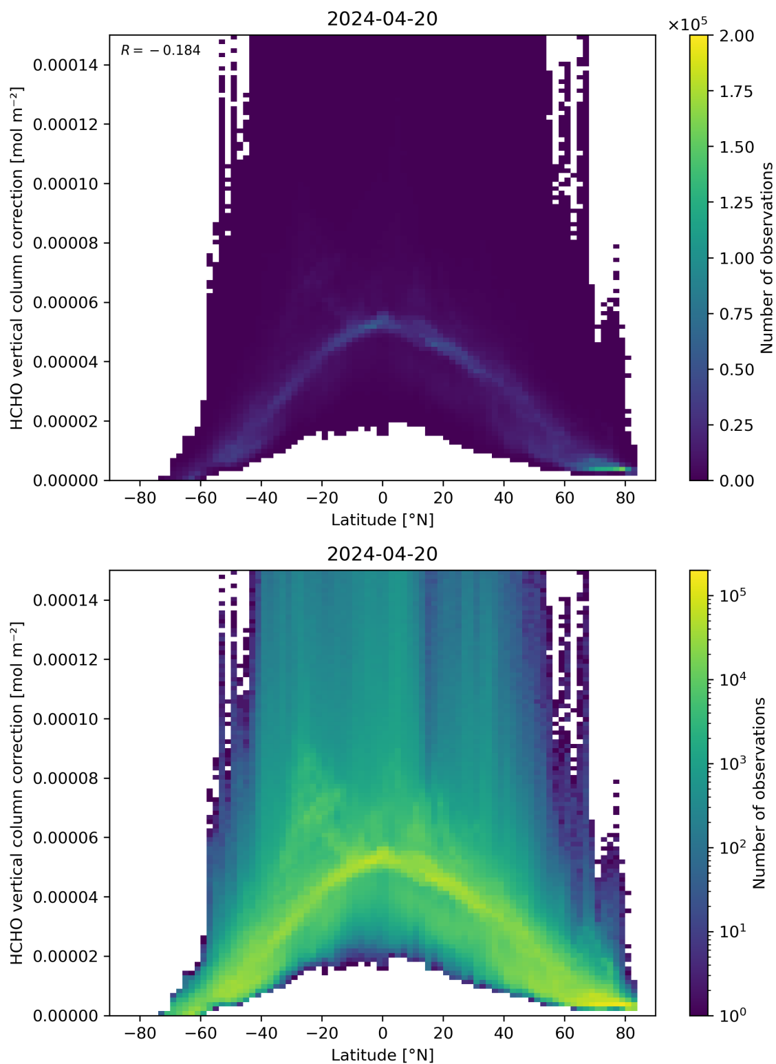
Figure 164: Scatter density plot of “Latitude” against “HCHO vertical column correction” for 2024-04-19 to 2024-04-21.
