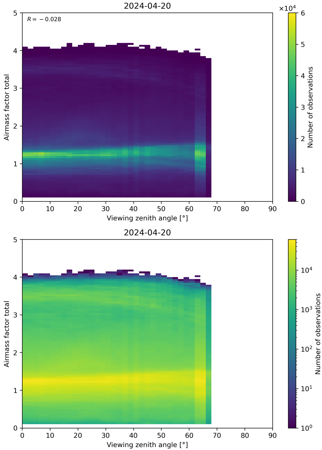
Figure 190: Scatter density plot of “Viewing zenith angle” against “Airmass factor total” for 2024-04-19 to 2024-04-21.
