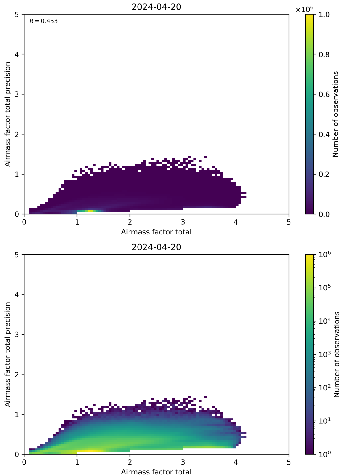
Figure 103: Scatter density plot of “Airmass factor total” against “Airmass factor total precision” for 2024-04-19 to 2024-04-21.
