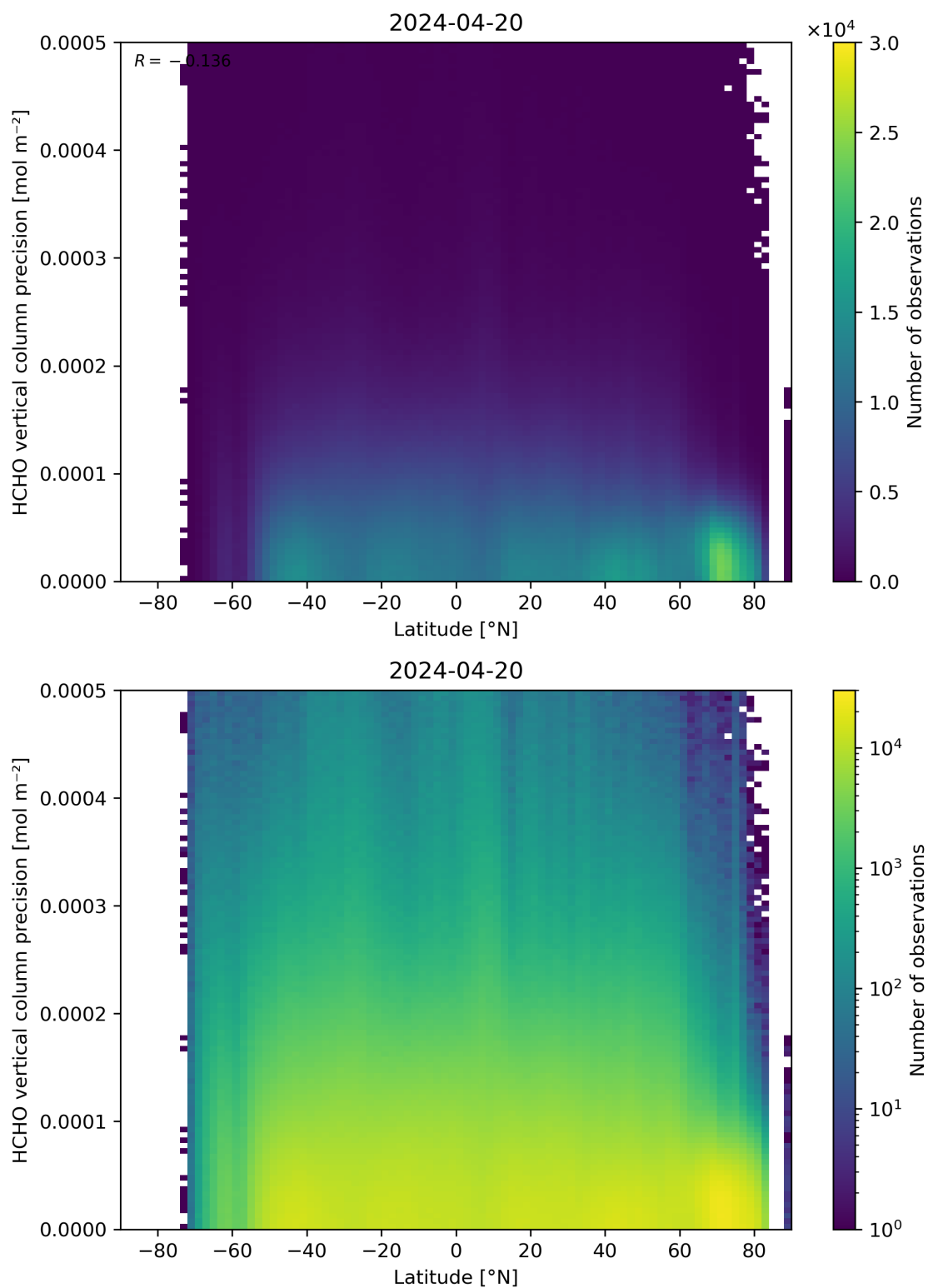
Figure 165: Scatter density plot of “Latitude” against “HCHO vertical column precision” for 2024-04-19 to 2024-04-21.
