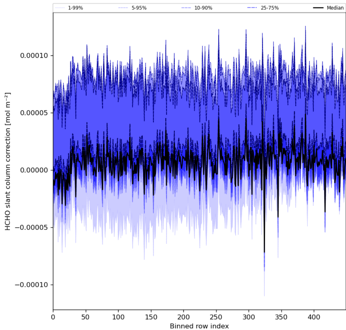
Figure 61: Along track statistics of “HCHO slant column correction” for 2024-04-19 to 2024-04-21
