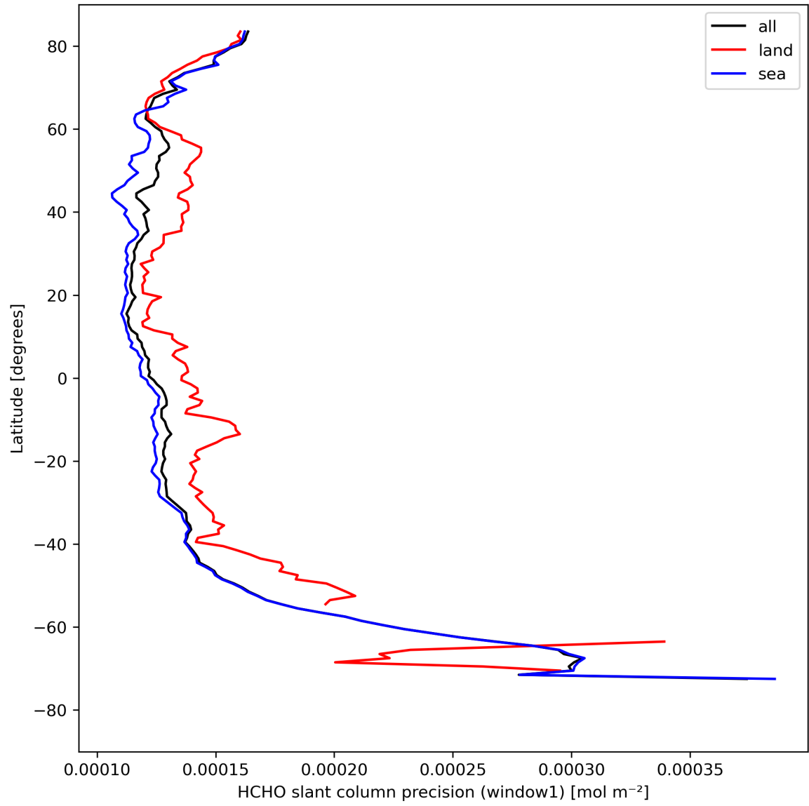
Figure 25: Zonal average of “HCHO slant column precision (window1)” for 2024-04-19 to 2024-04-21.
