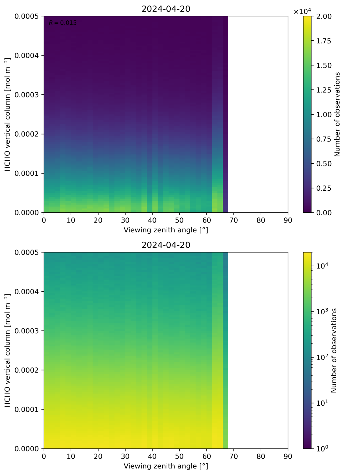
Figure 192: Scatter density plot of “Viewing zenith angle” against “HCHO vertical column” for 2024-04-19 to 2024-04-21.
