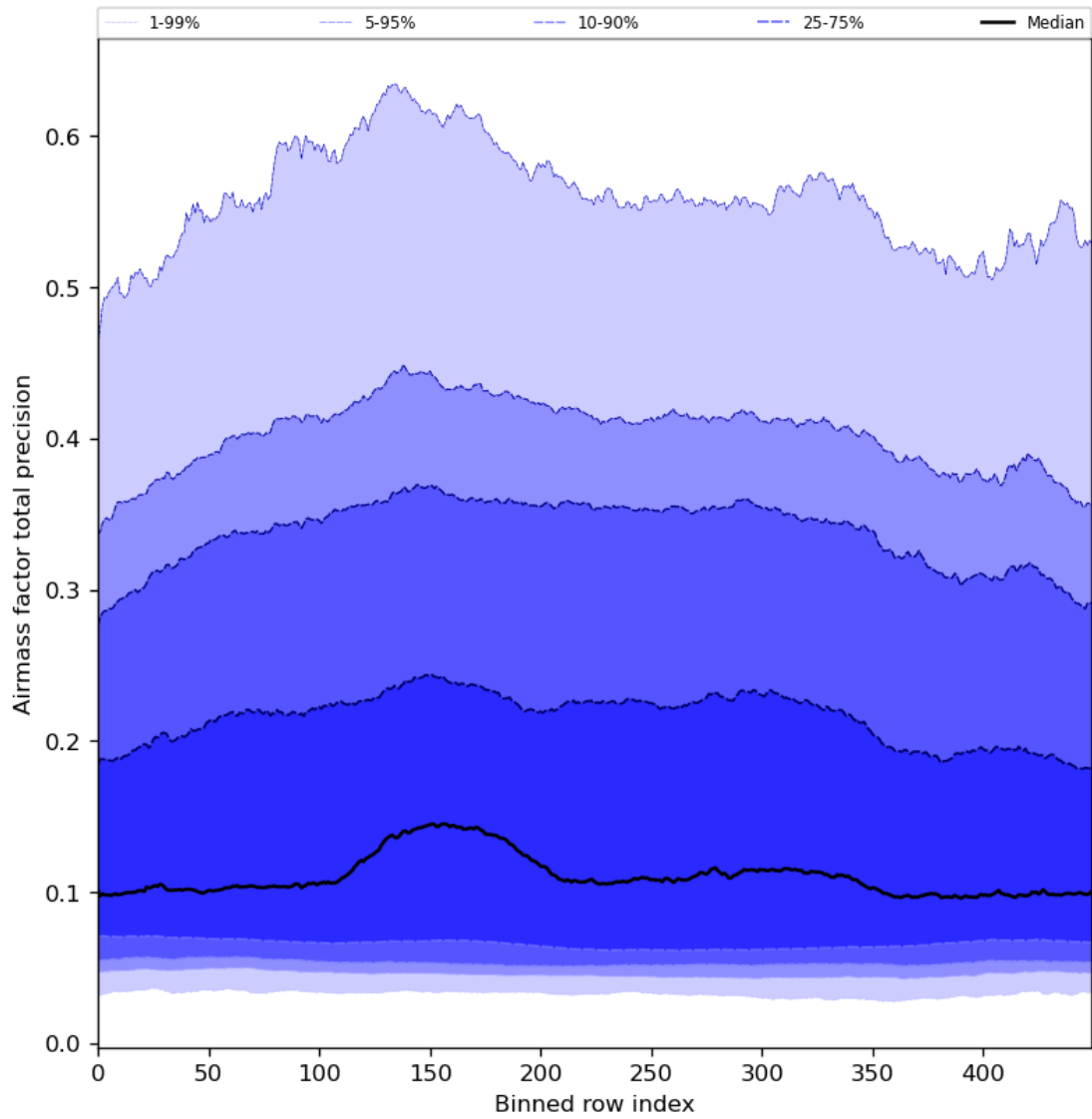
Figure 55: Along track statistics of “Airmass factor total precision” for 2024-04-19 to 2024-04-21
