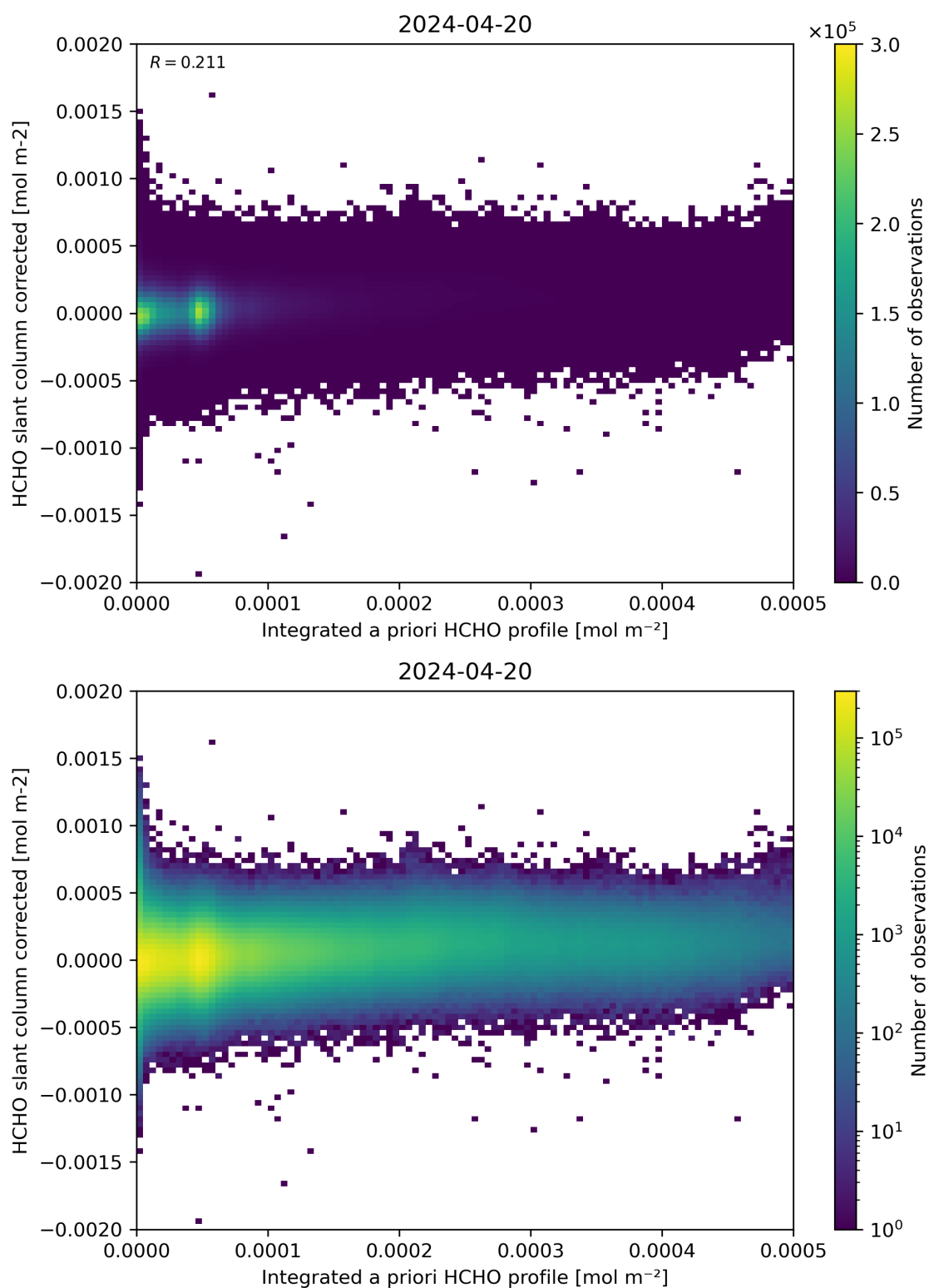
Figure 151: Scatter density plot of “Integrated a priori HCHO profile” against “HCHO slant column corrected” for 2024-04-19 to 2024-04-21.
