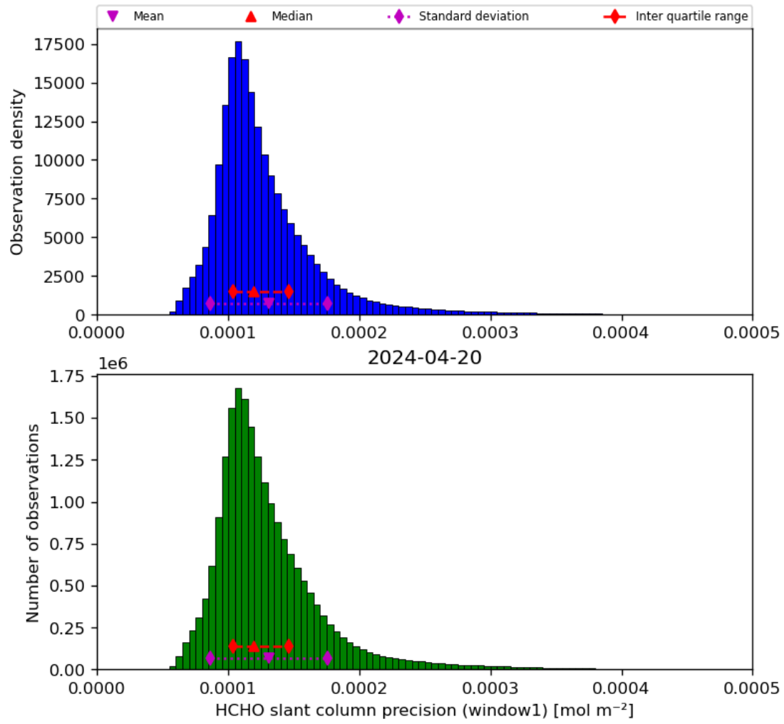
Figure 39: Histogram of “HCHO slant column precision (window1)” for 2024-04-19 to 2024-04-21
