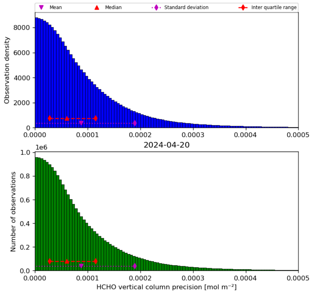
Figure 36: Histogram of “HCHO vertical column precision” for 2024-04-19 to 2024-04-21
