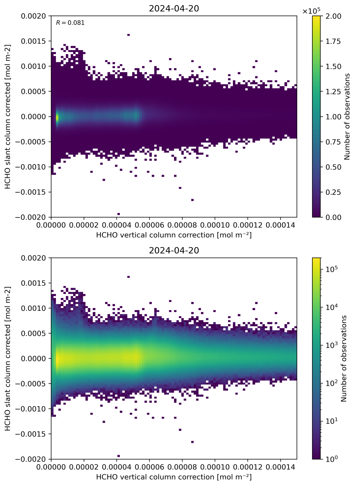
Figure 116: Scatter density plot of “HCHO vertical column correction” against “HCHO slant column corrected” for 2024-04-19 to 2024-04-21.
