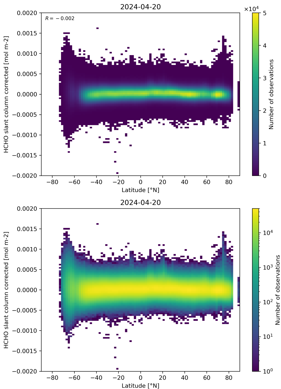
Figure 157: Scatter density plot of “Latitude” against “HCHO slant column corrected” for 2024-04-19 to 2024-04-21.
