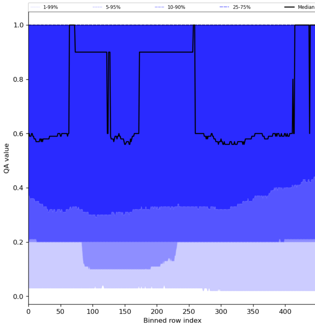
Figure 48: Along track statistics of “QA value” for 2024-04-19 to 2024-04-21
