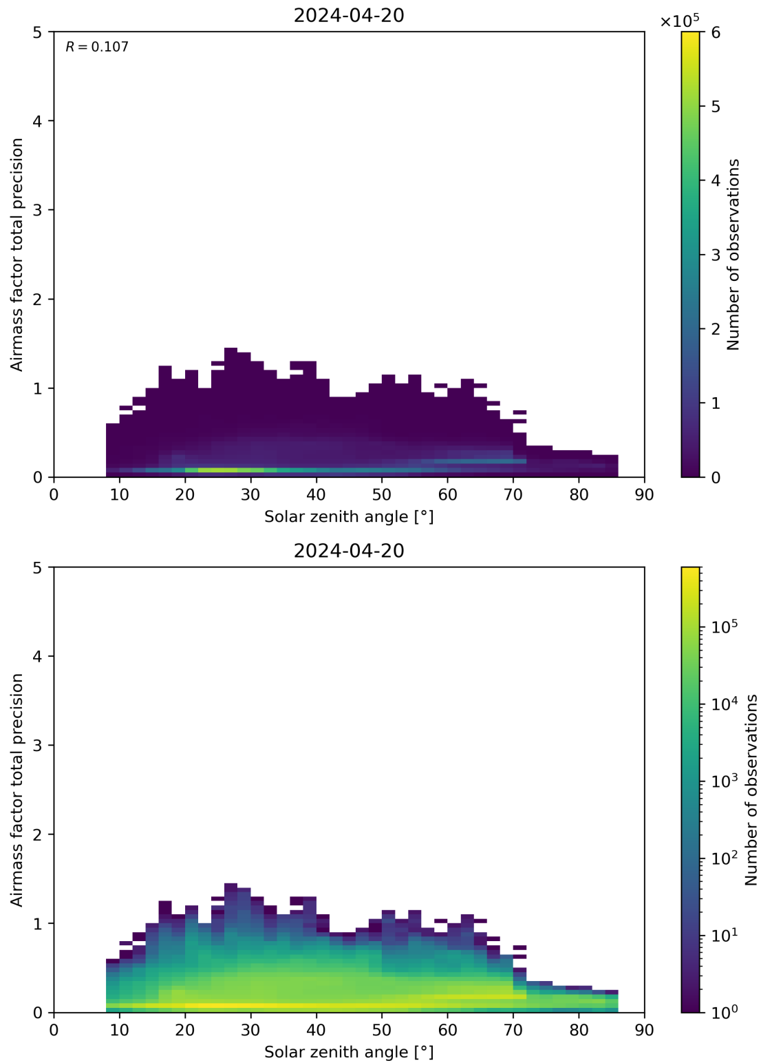
Figure 176: Scatter density plot of “Solar zenith angle” against “Airmass factor total precision” for 2024-04-19 to 2024-04-21.
