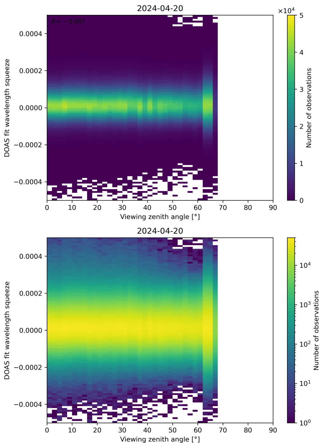
Figure 184: Scatter density plot of “Viewing zenith angle” against “DOAS fit wavelength squeeze” for 2024-04-19 to 2024-04-21.
