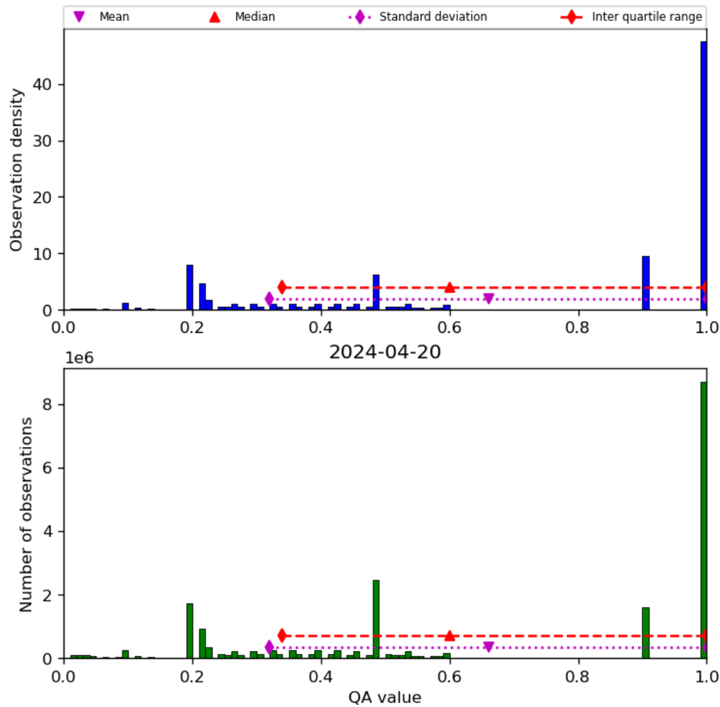
Figure 34: Histogram of “QA value” for 2024-04-19 to 2024-04-21
