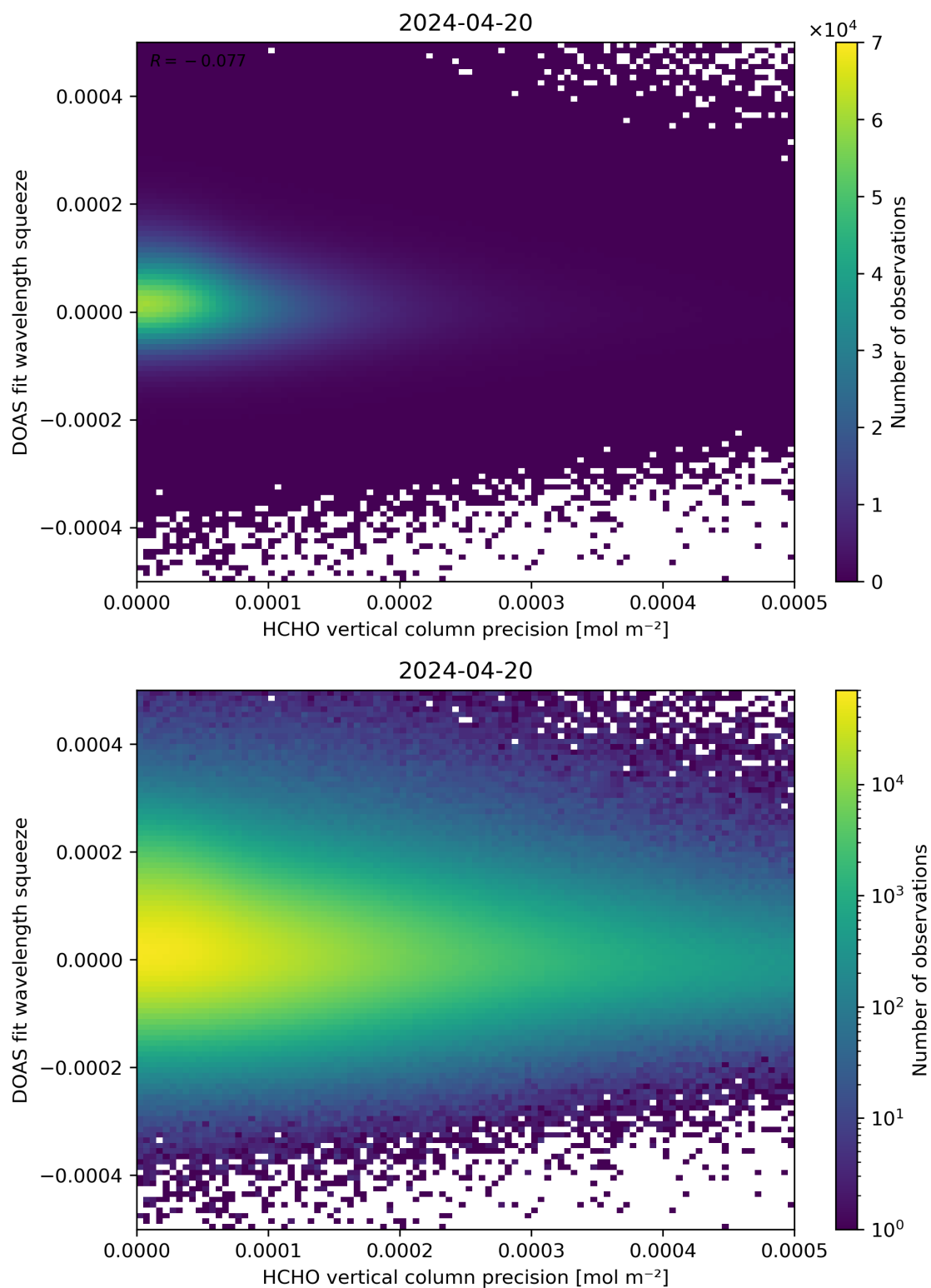
Figure 138: Scatter density plot of “HCHO vertical column precision” against “DOAS fit wavelength squeeze” for 2024-04-19 to 2024-04-21.
