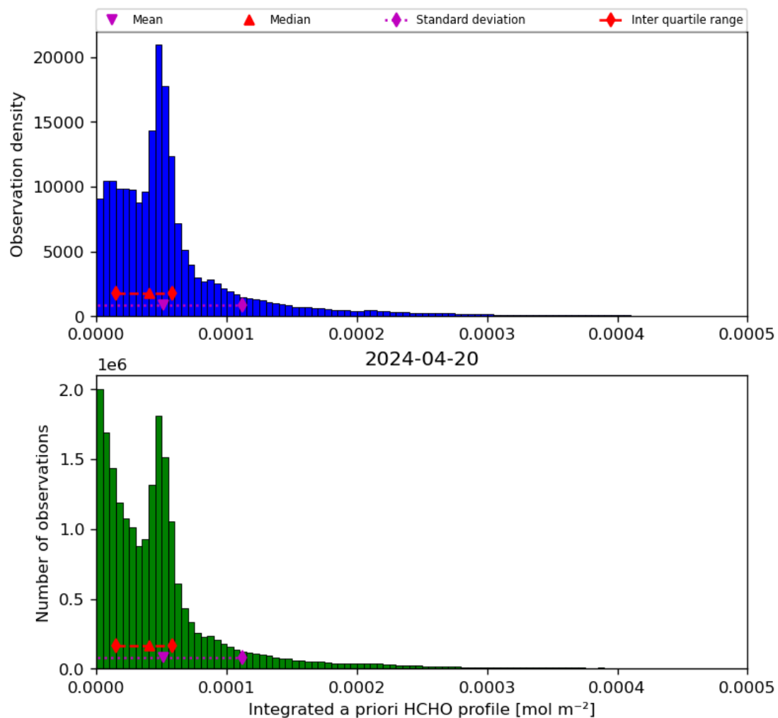
Figure 43: Histogram of “Integrated a priori HCHO profile” for 2024-04-19 to 2024-04-21
