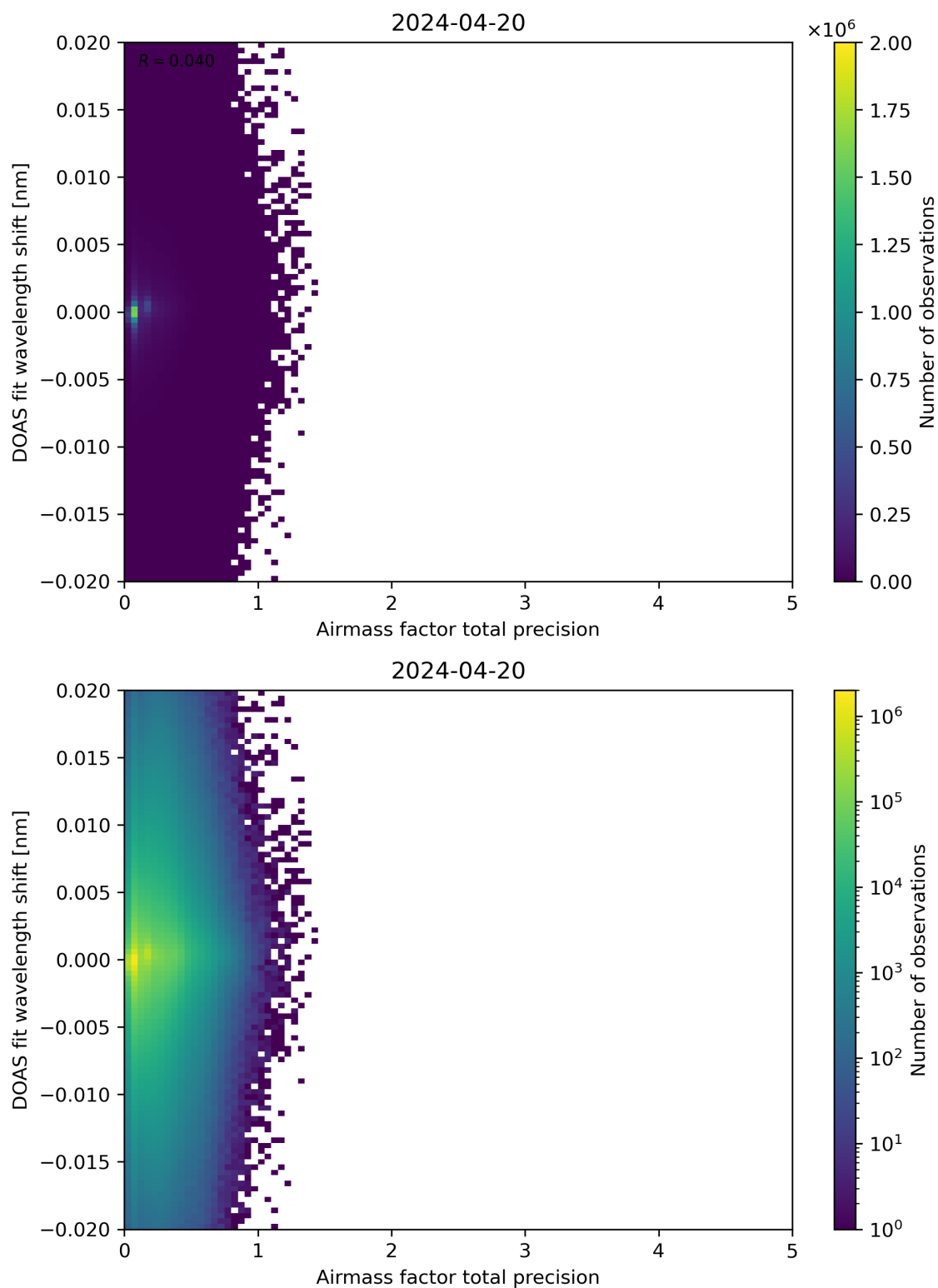
Figure 106: Scatter density plot of “Airmass factor total precision” against “DOAS fit wavelength shift” for 2024-04-19 to 2024-04-21.
