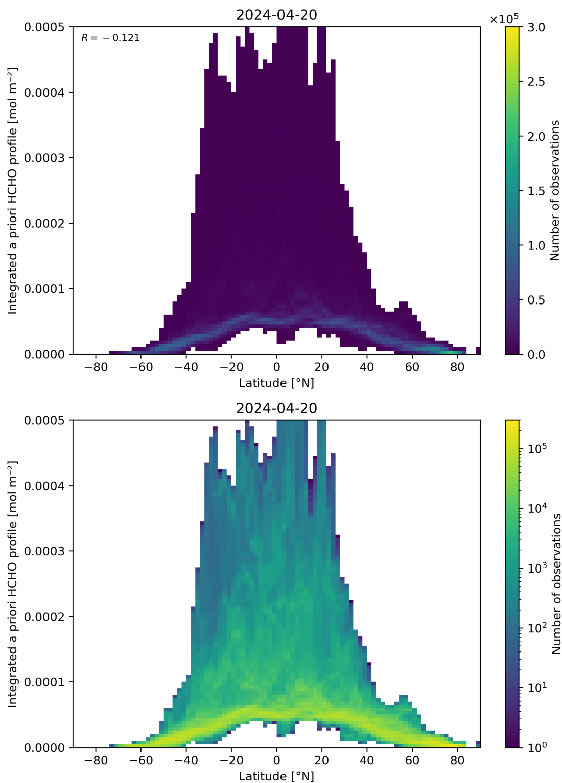
Figure 166: Scatter density plot of “Latitude” against “Integrated a priori HCHO profile” for 2024-04-19 to 2024-04-21.
