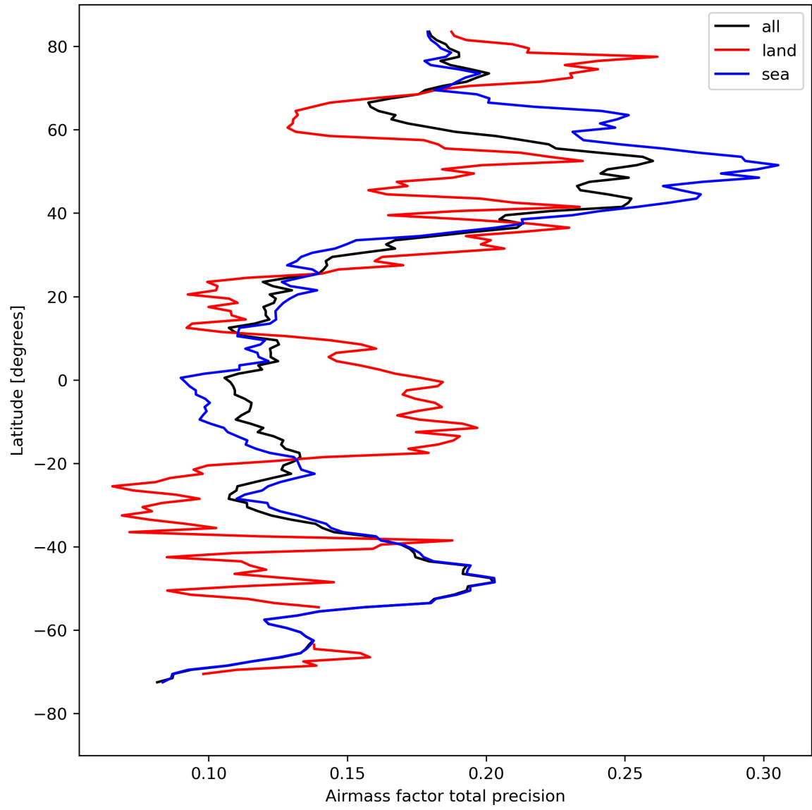
Figure 27: Zonal average of “Airmass factor total precision” for 2024-04-19 to 2024-04-21.
