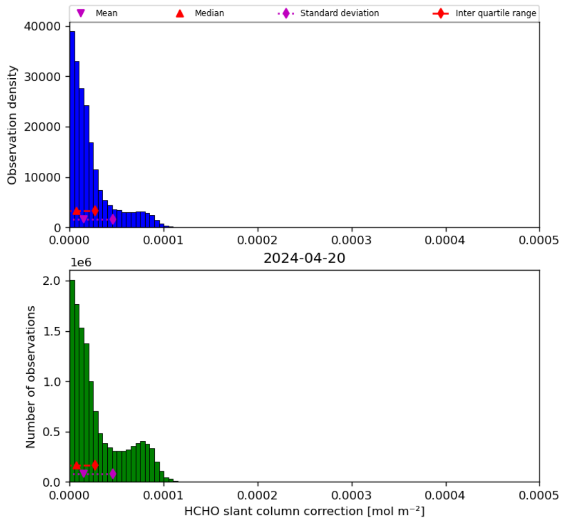
Figure 47: Histogram of “HCHO slant column correction” for 2024-04-19 to 2024-04-21
