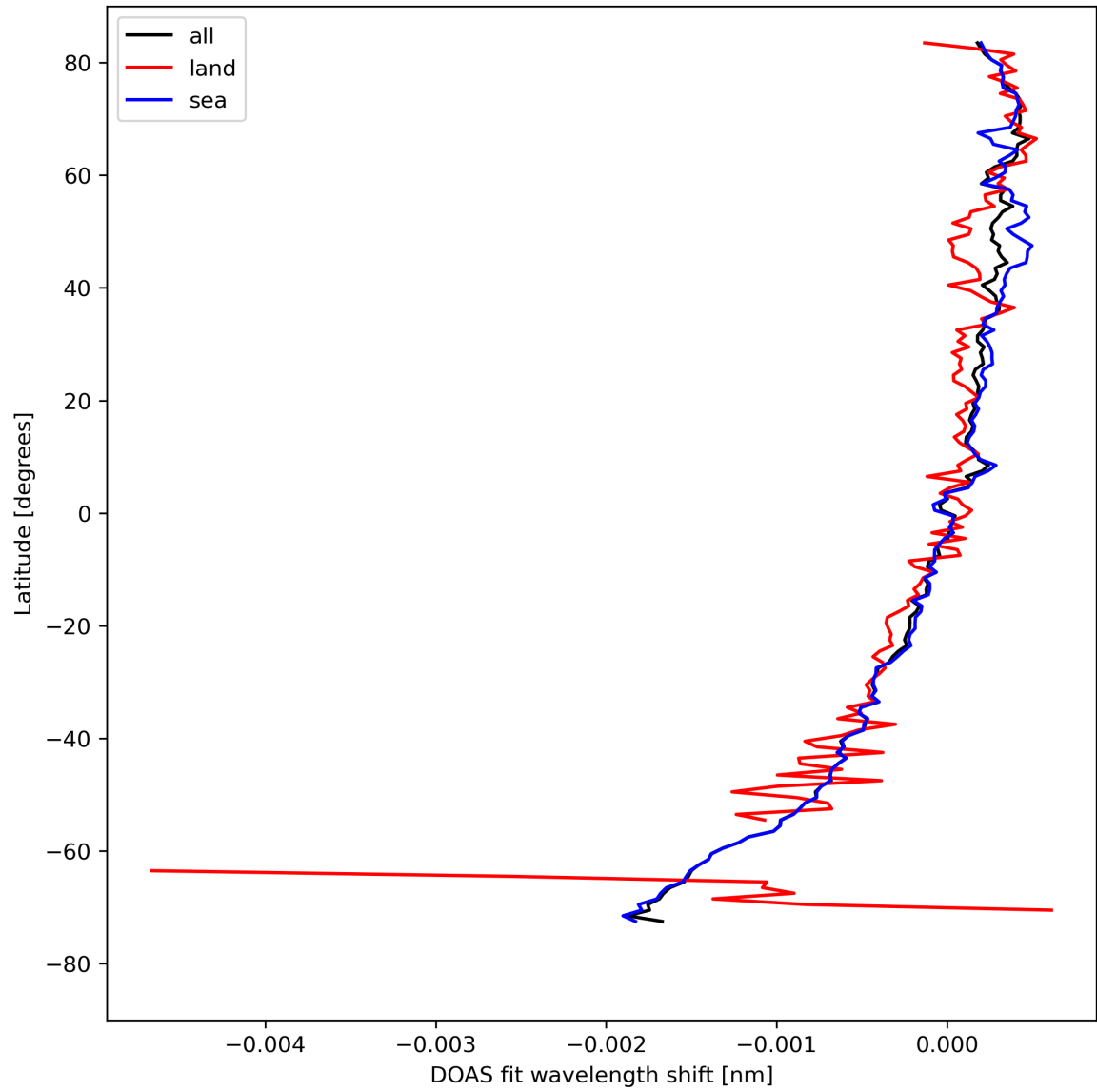
Figure 30: Zonal average of “DOAS fit wavelength shift” for 2024-04-19 to 2024-04-21.
