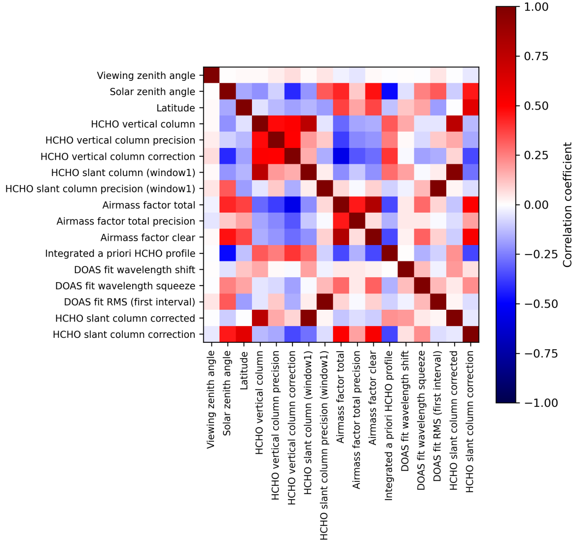
Figure 2: Map of correlation matrix for 2024-04-19 to 2024-04-21.
