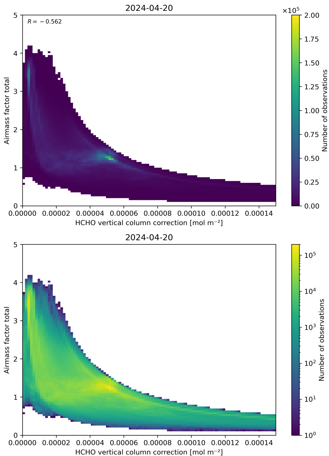
Figure 120: Scatter density plot of “HCHO vertical column correction” against “Airmass factor total” for 2024-04-19 to 2024-04-21.
