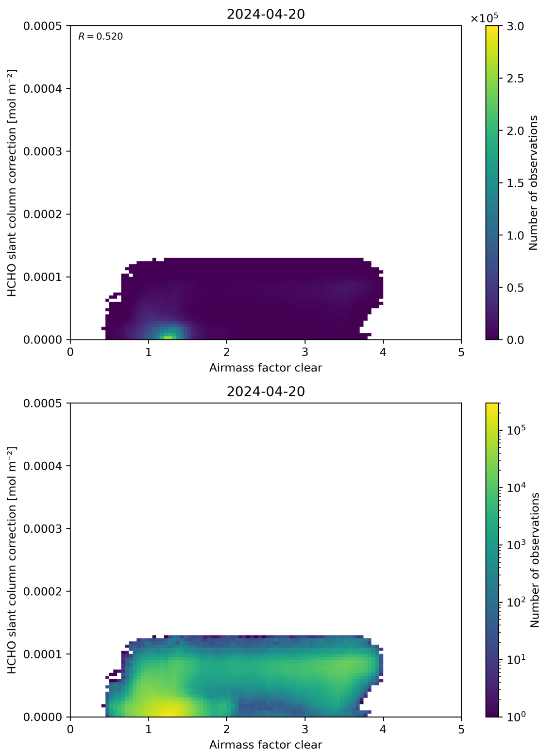
Figure 75: Scatter density plot of “Airmass factor clear” against “HCHO slant column correction” for 2024-04-19 to 2024-04-21.
