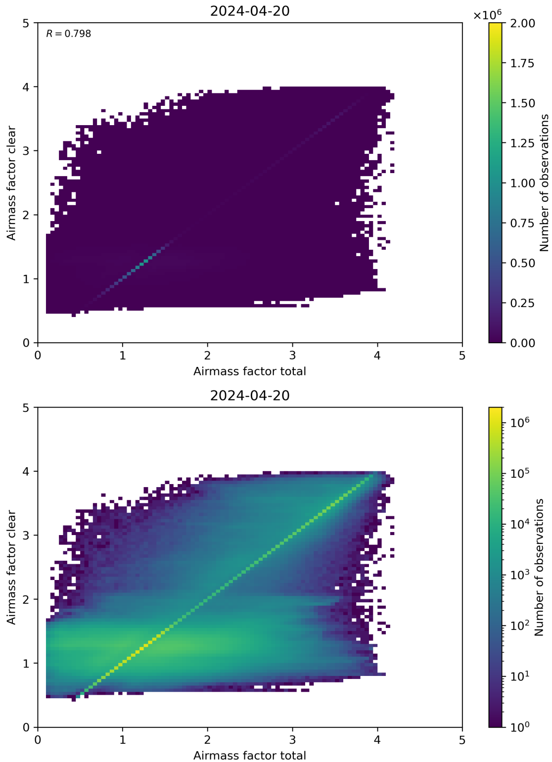
Figure 100: Scatter density plot of “Airmass factor total” against “Airmass factor clear” for 2024-04-19 to 2024-04-21.
