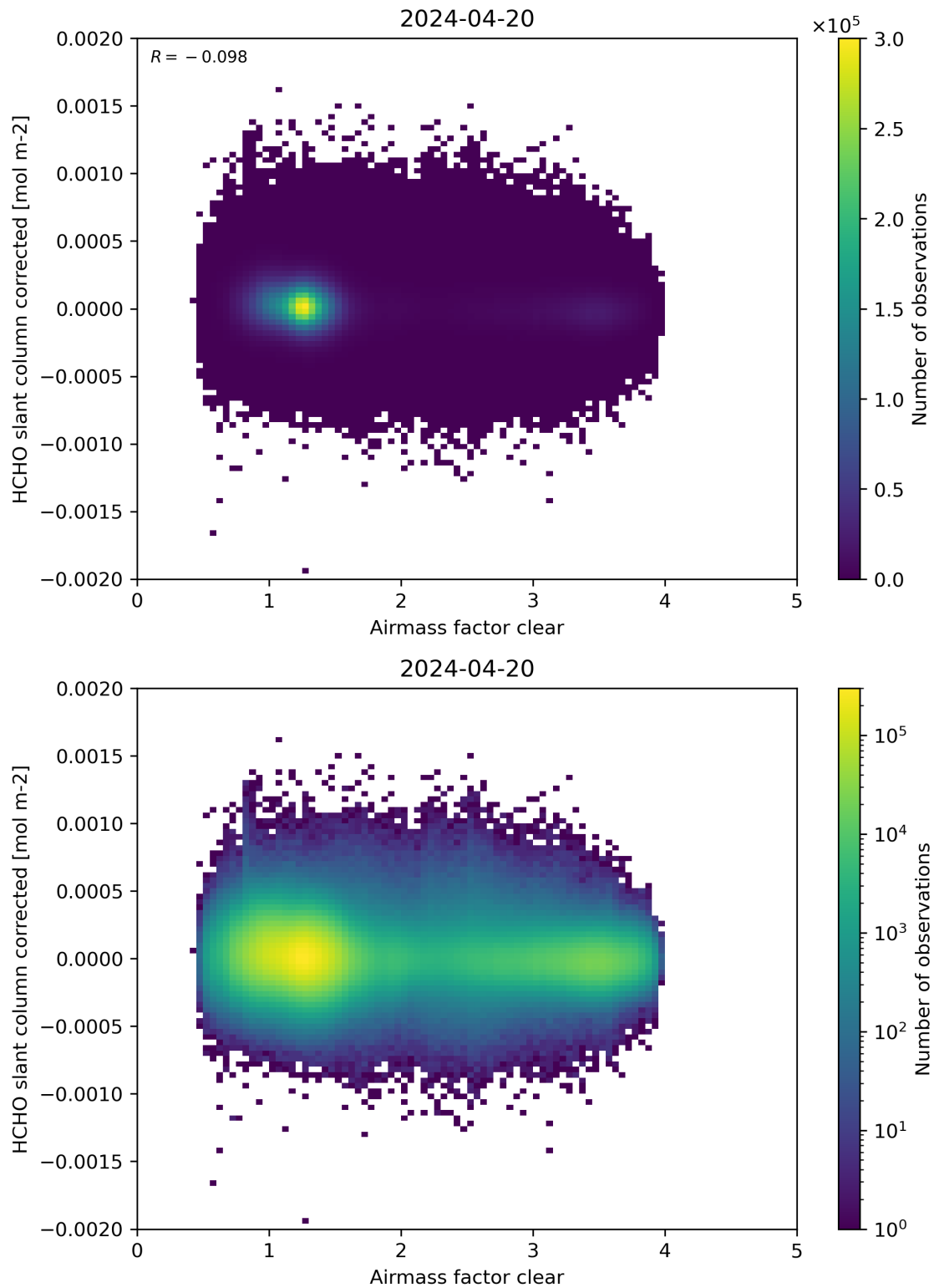
Figure 74: Scatter density plot of “Airmass factor clear” against “HCHO slant column corrected” for 2024-04-19 to 2024-04-21.
