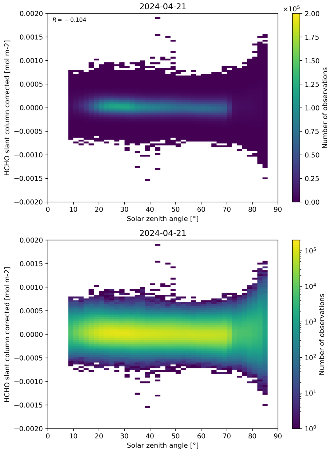
Figure 171: Scatter density plot of “Solar zenith angle” against “HCHO slant column corrected” for 2024-04-21 to 2024-04-22.
