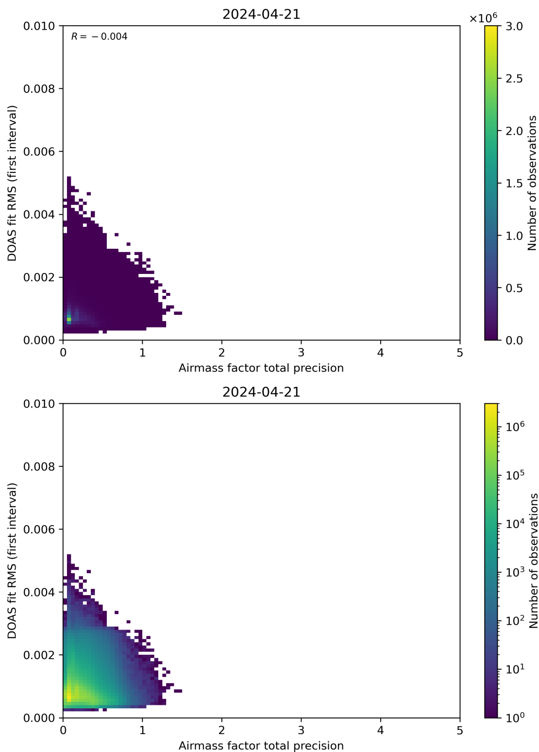
Figure 105: Scatter density plot of “Airmass factor total precision” against “DOAS fit RMS (first interval)” for 2024-04-21 to 2024-04-22.
