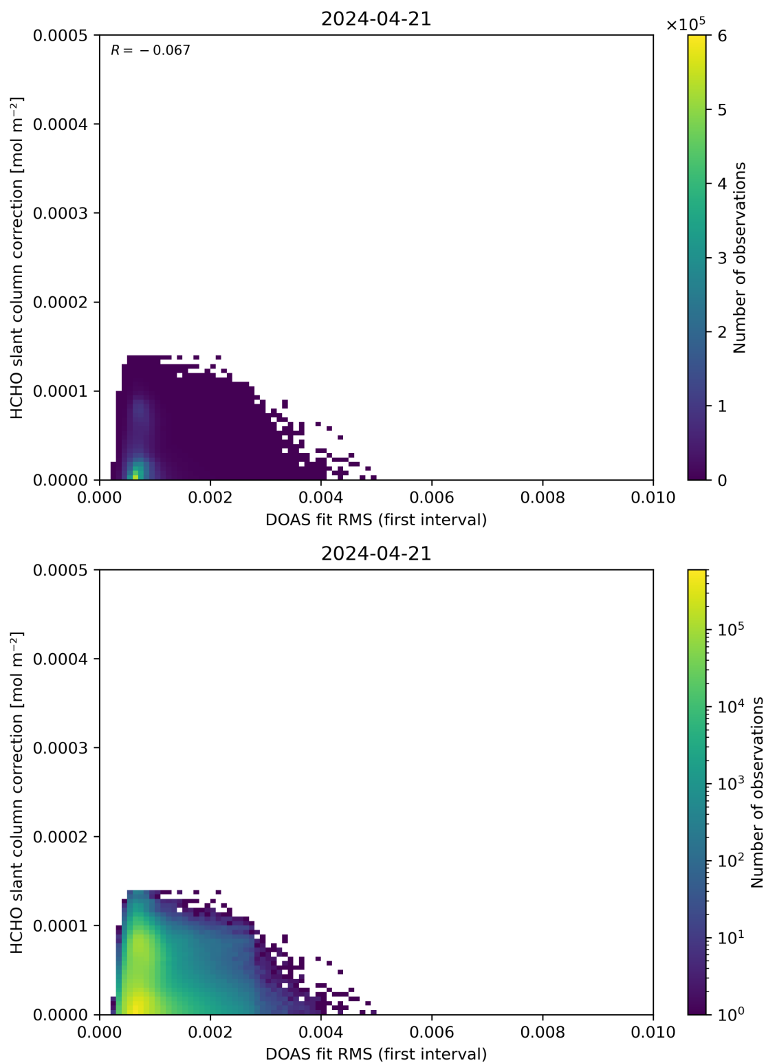
Figure 63: Scatter density plot of “DOAS fit RMS (first interval)” against “HCHO slant column correction” for 2024-04-21 to 2024-04-22.
