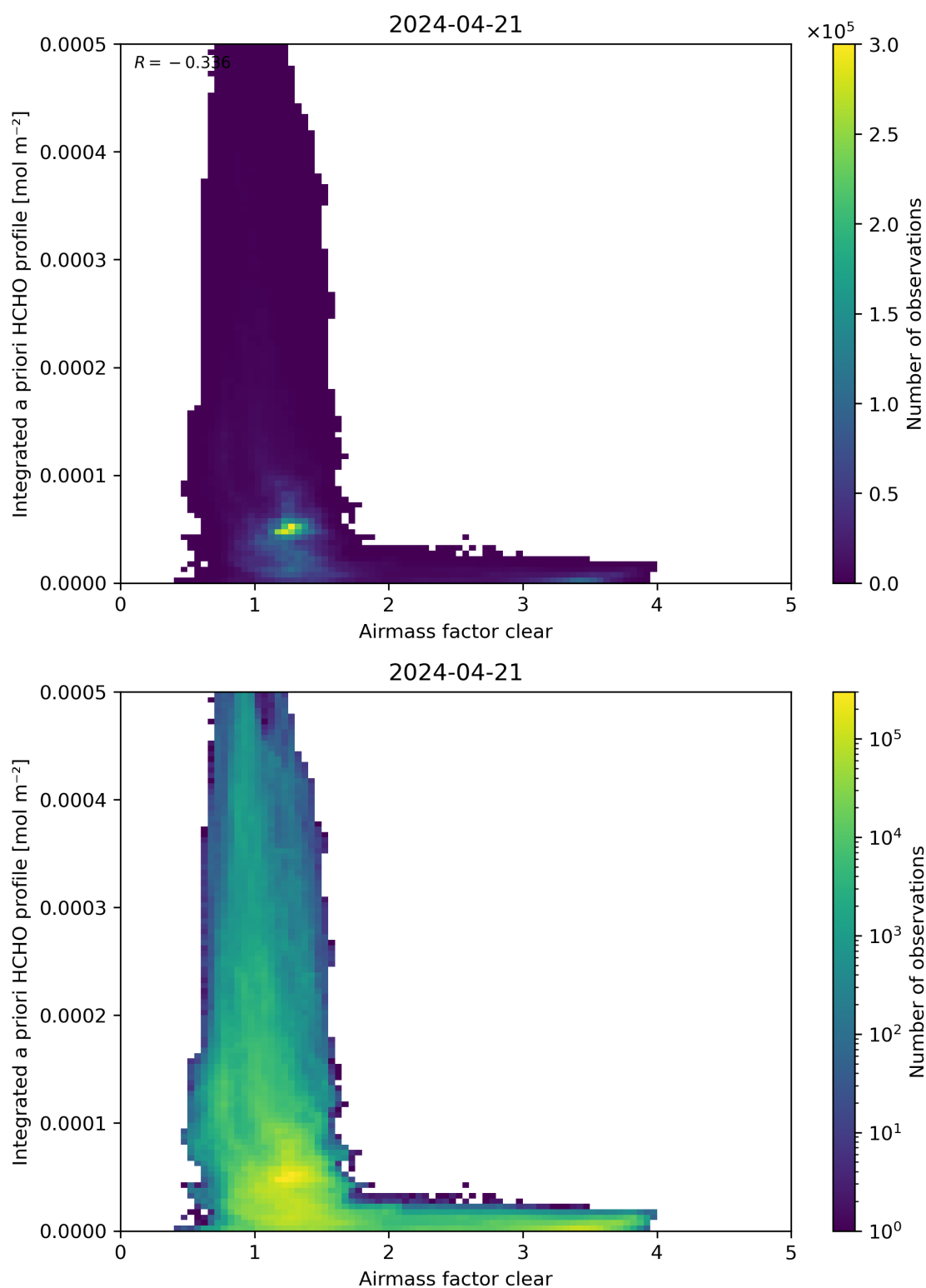
Figure 76: Scatter density plot of “Airmass factor clear” against “Integrated a priori HCHO profile” for 2024-04-21 to 2024-04-22.
