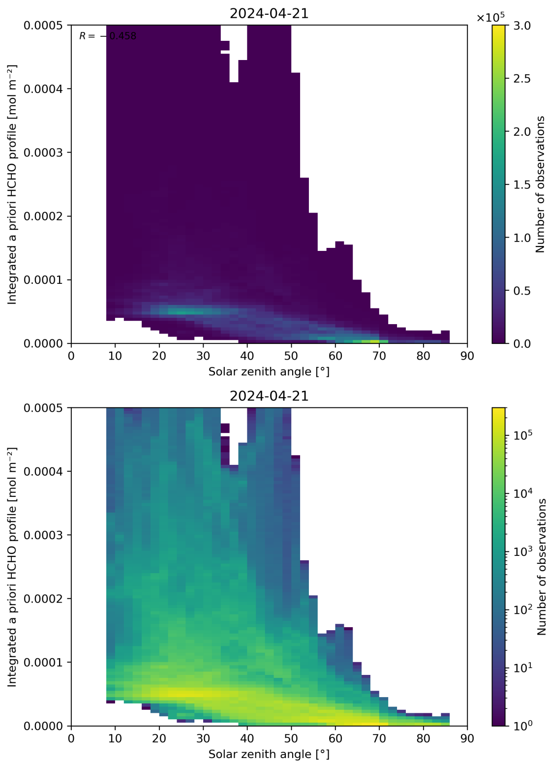
Figure 180: Scatter density plot of “Solar zenith angle” against “Integrated a priori HCHO profile” for 2024-04-21 to 2024-04-22.
