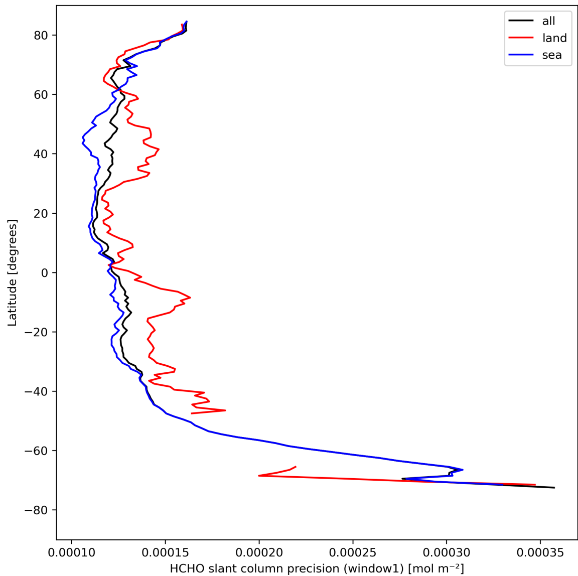
Figure 25: Zonal average of “HCHO slant column precision (window1)” for 2024-04-21 to 2024-04-22.
