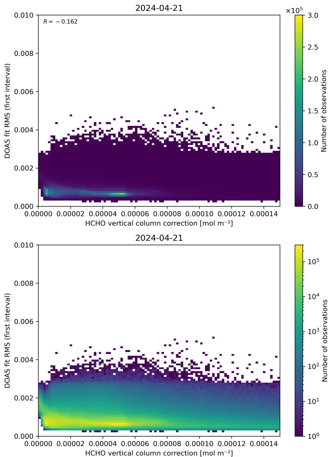
Figure 112: Scatter density plot of “HCHO vertical column correction” against “DOAS fit RMS (first interval)” for 2024-04-21 to 2024-04-22.
