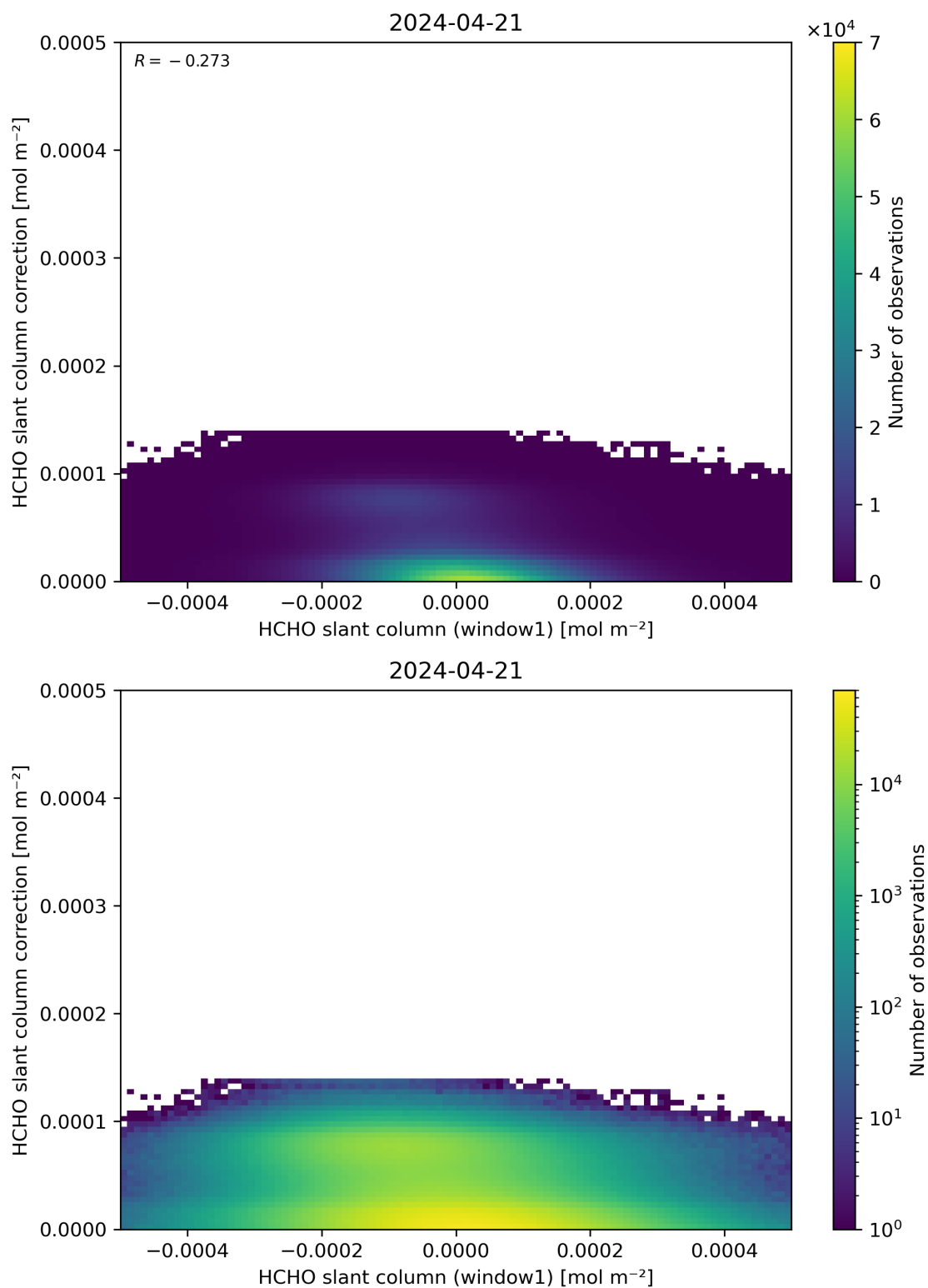
Figure 83: Scatter density plot of “HCHO slant column (window1)” against “HCHO slant column correction” for 2024-04-21 to 2024-04-22.
