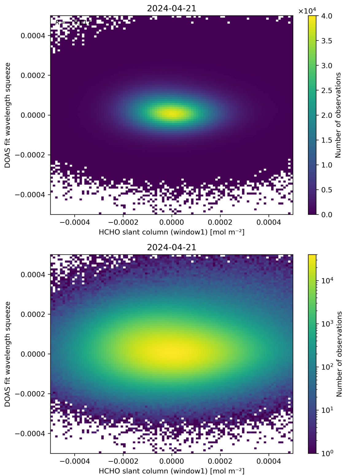
Figure 80: Scatter density plot of “HCHO slant column (window1)” against “DOAS fit wavelength squeeze” for 2024-04-21 to 2024-04-22.
