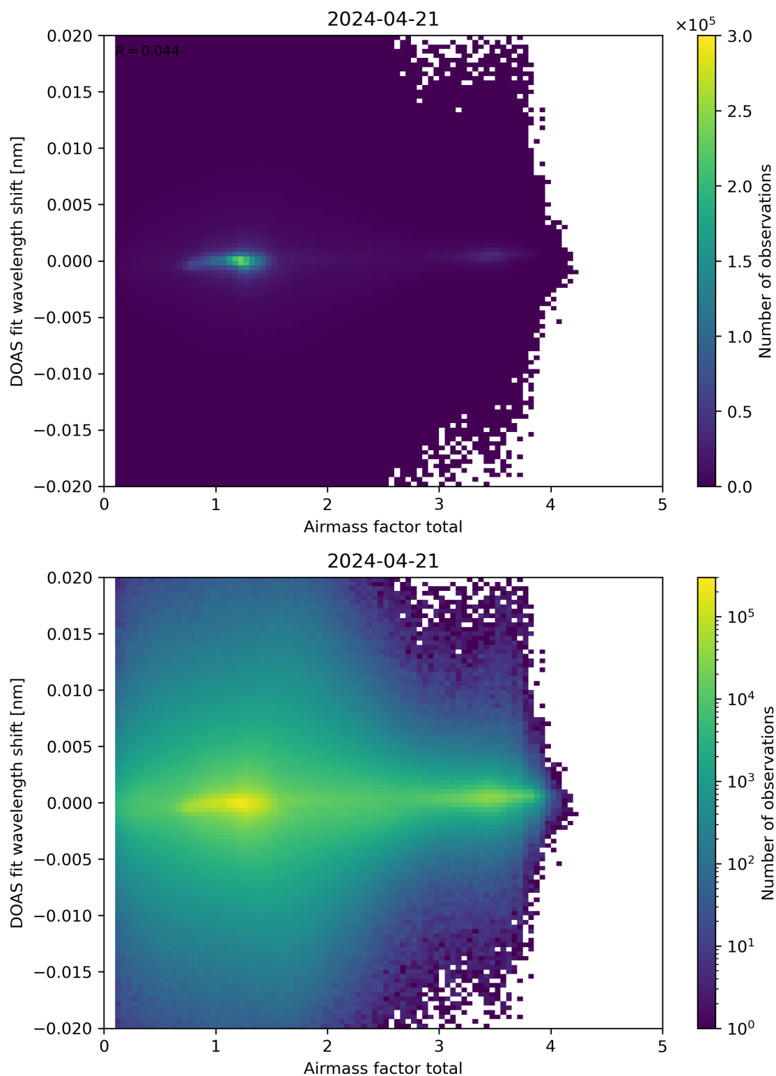
Figure 98: Scatter density plot of “Airmass factor total” against “DOAS fit wavelength shift” for 2024-04-21 to 2024-04-22.
