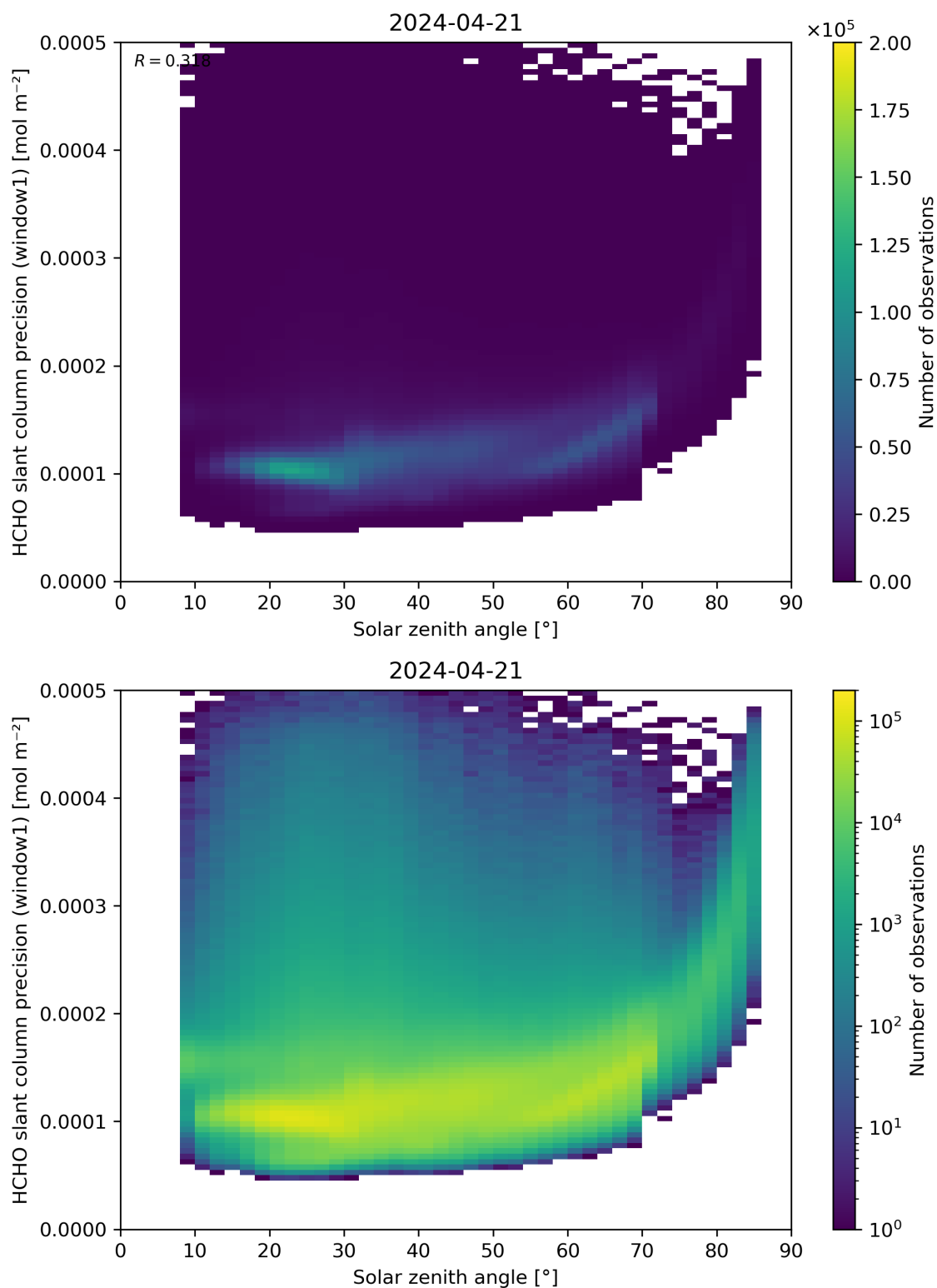
Figure 174: Scatter density plot of “Solar zenith angle” against “HCHO slant column precision (window1)” for 2024-04-21 to 2024-04-22.
