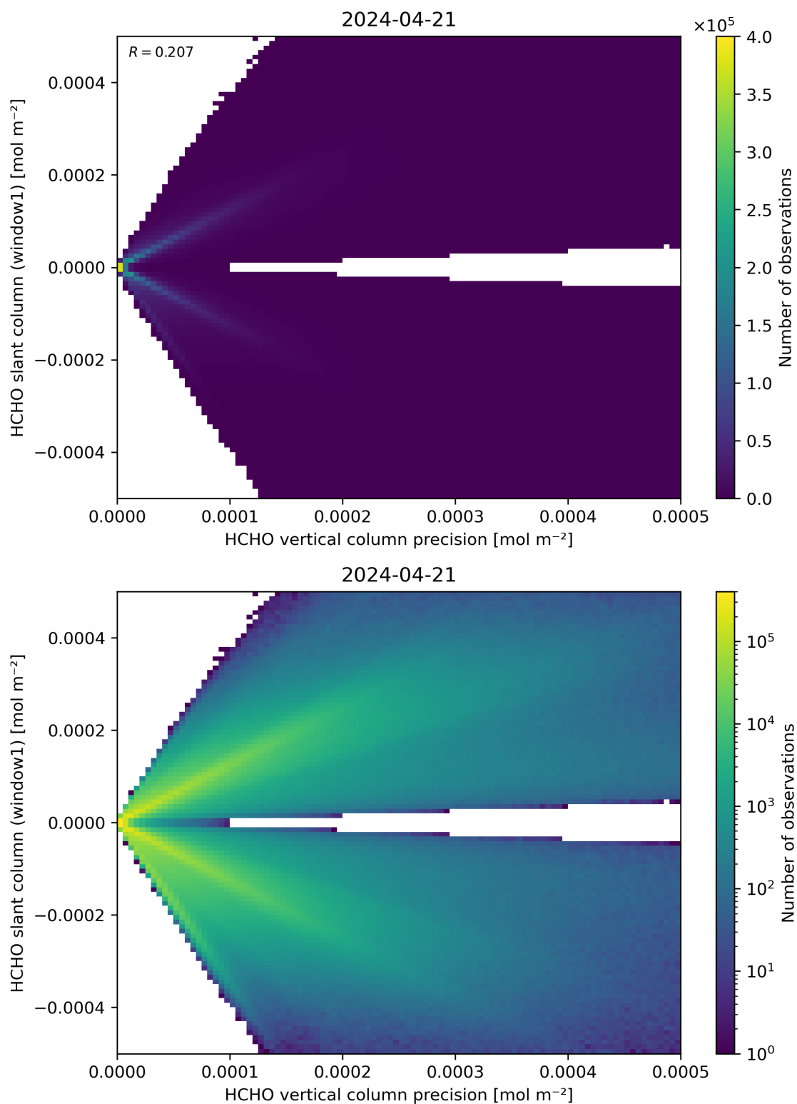
Figure 142: Scatter density plot of “HCHO vertical column precision” against “HCHO slant column (window1)” for 2024-04-21 to 2024-04-22.
