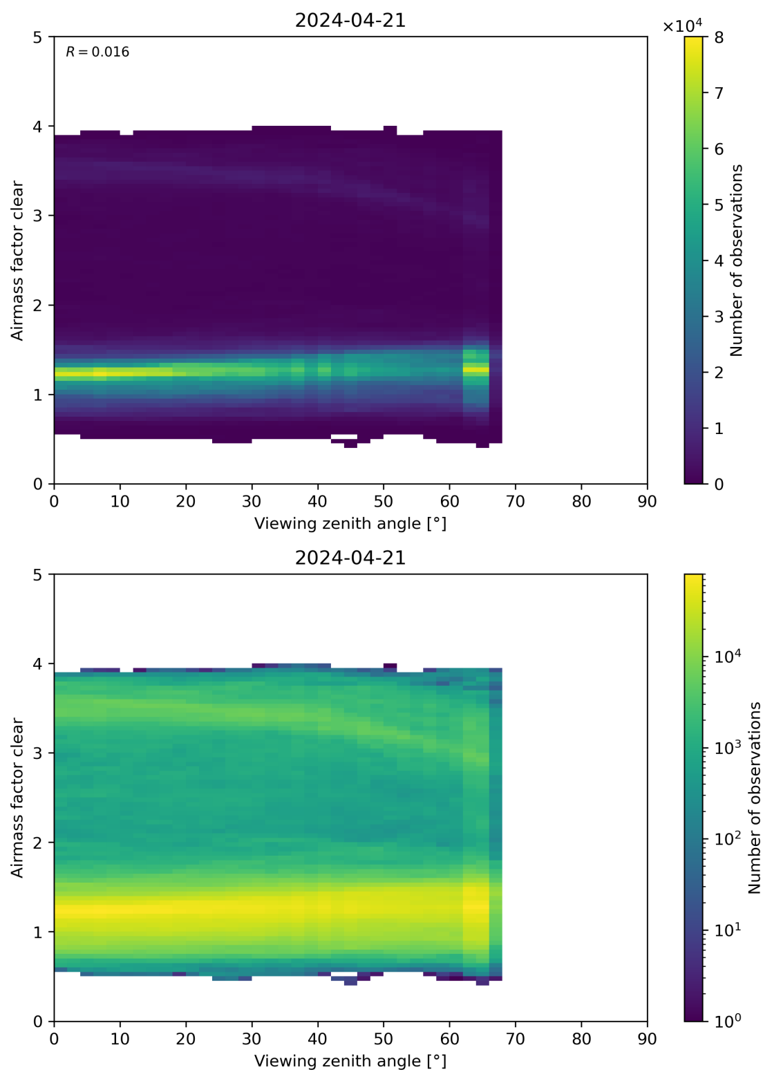
Figure 185: Scatter density plot of “Viewing zenith angle” against “Airmass factor clear” for 2024-04-21 to 2024-04-22.
