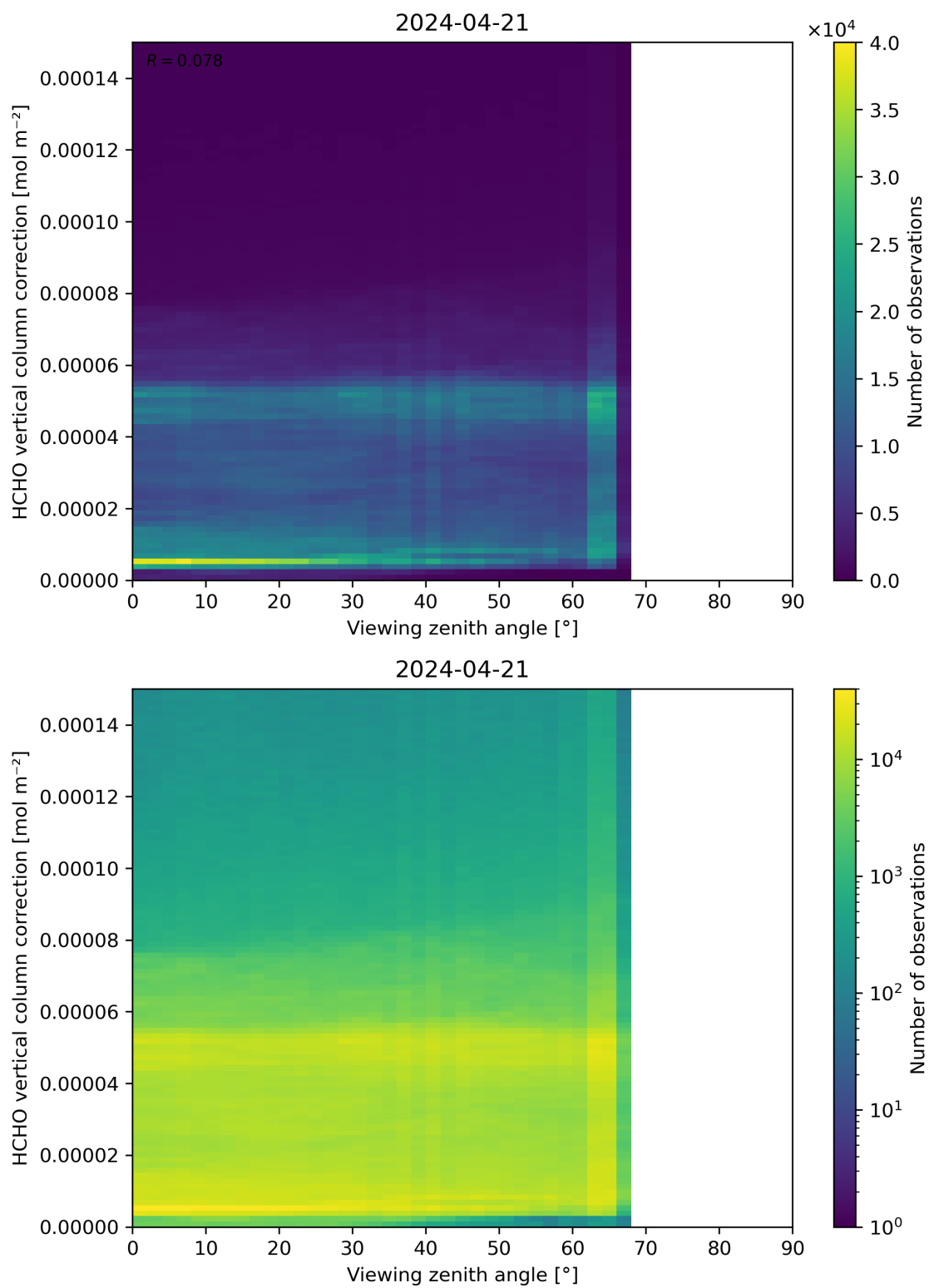
Figure 193: Scatter density plot of “Viewing zenith angle” against “HCHO vertical column correction” for 2024-04-21 to 2024-04-22.
