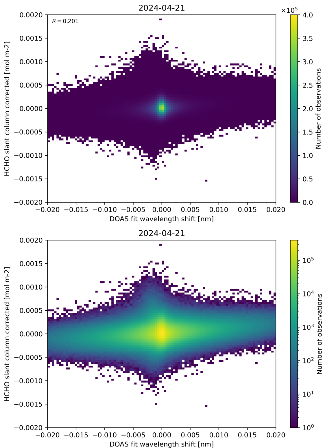
Figure 66: Scatter density plot of “DOAS fit wavelength shift” against “HCHO slant column corrected” for 2024-04-21 to 2024-04-22.
