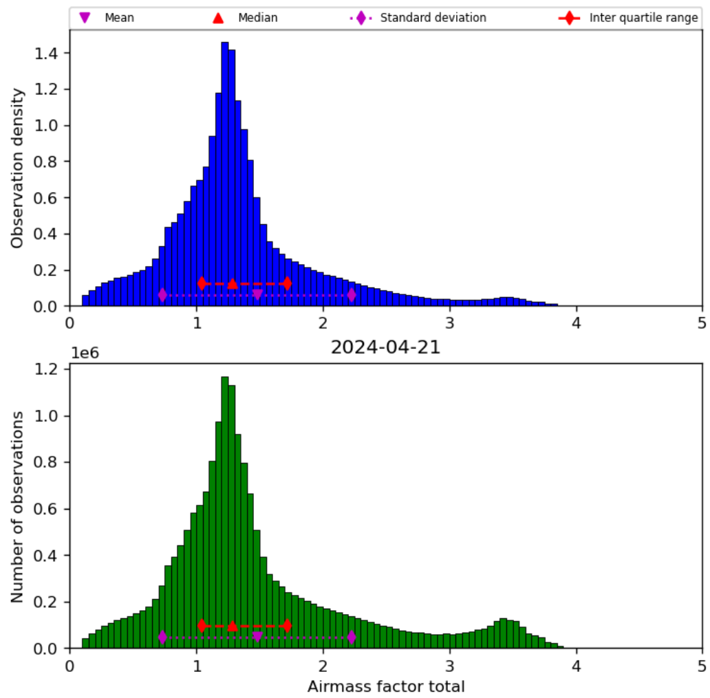
Figure 40: Histogram of “Airmass factor total” for 2024-04-21 to 2024-04-22
