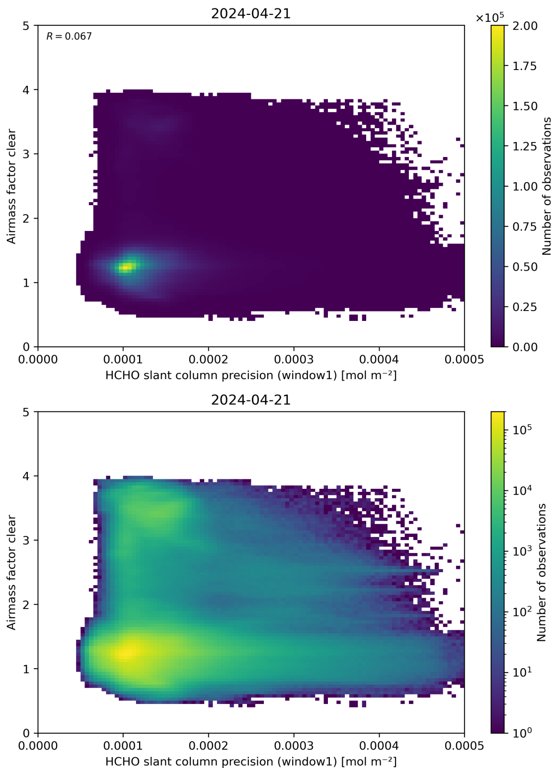
Figure 91: Scatter density plot of “HCHO slant column precision (window1)” against “Airmass factor clear” for 2024-04-21 to 2024-04-22.
