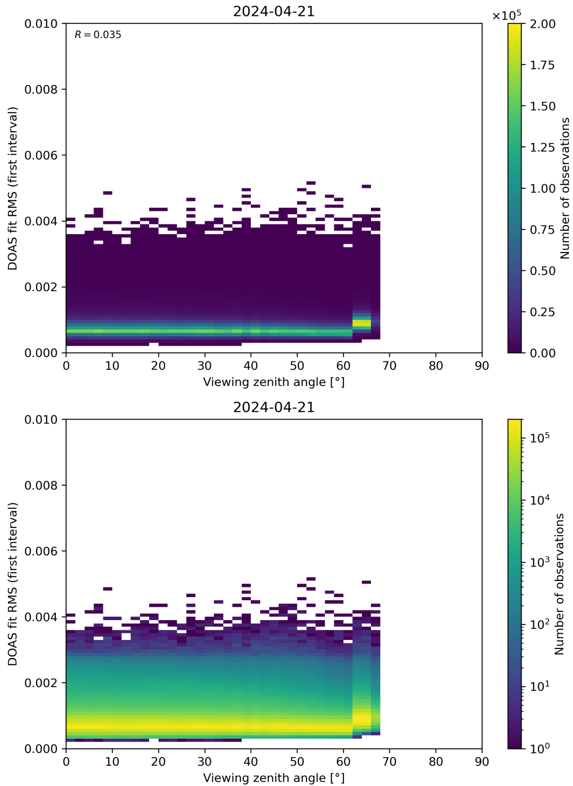
Figure 182: Scatter density plot of “Viewing zenith angle” against “DOAS fit RMS (first interval)” for 2024-04-21 to 2024-04-22.
