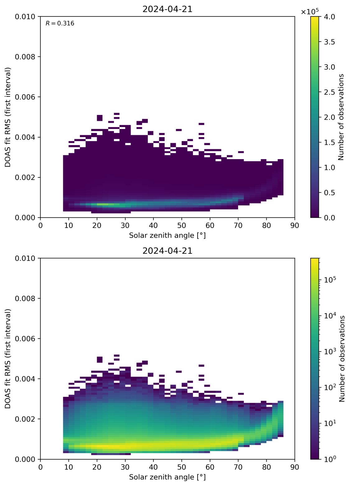
Figure 167: Scatter density plot of “Solar zenith angle” against “DOAS fit RMS (first interval)” for 2024-04-21 to 2024-04-22.
