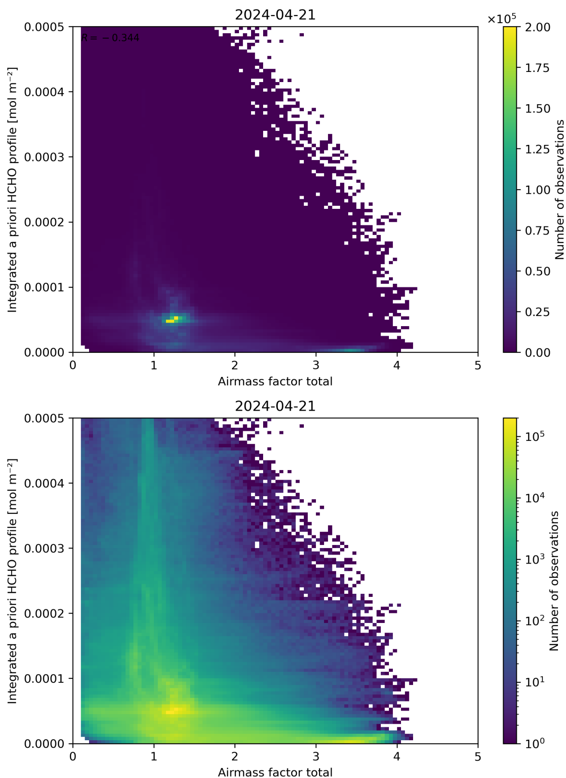
Figure 104: Scatter density plot of “Airmass factor total” against “Integrated a priori HCHO profile” for 2024-04-21 to 2024-04-22.
