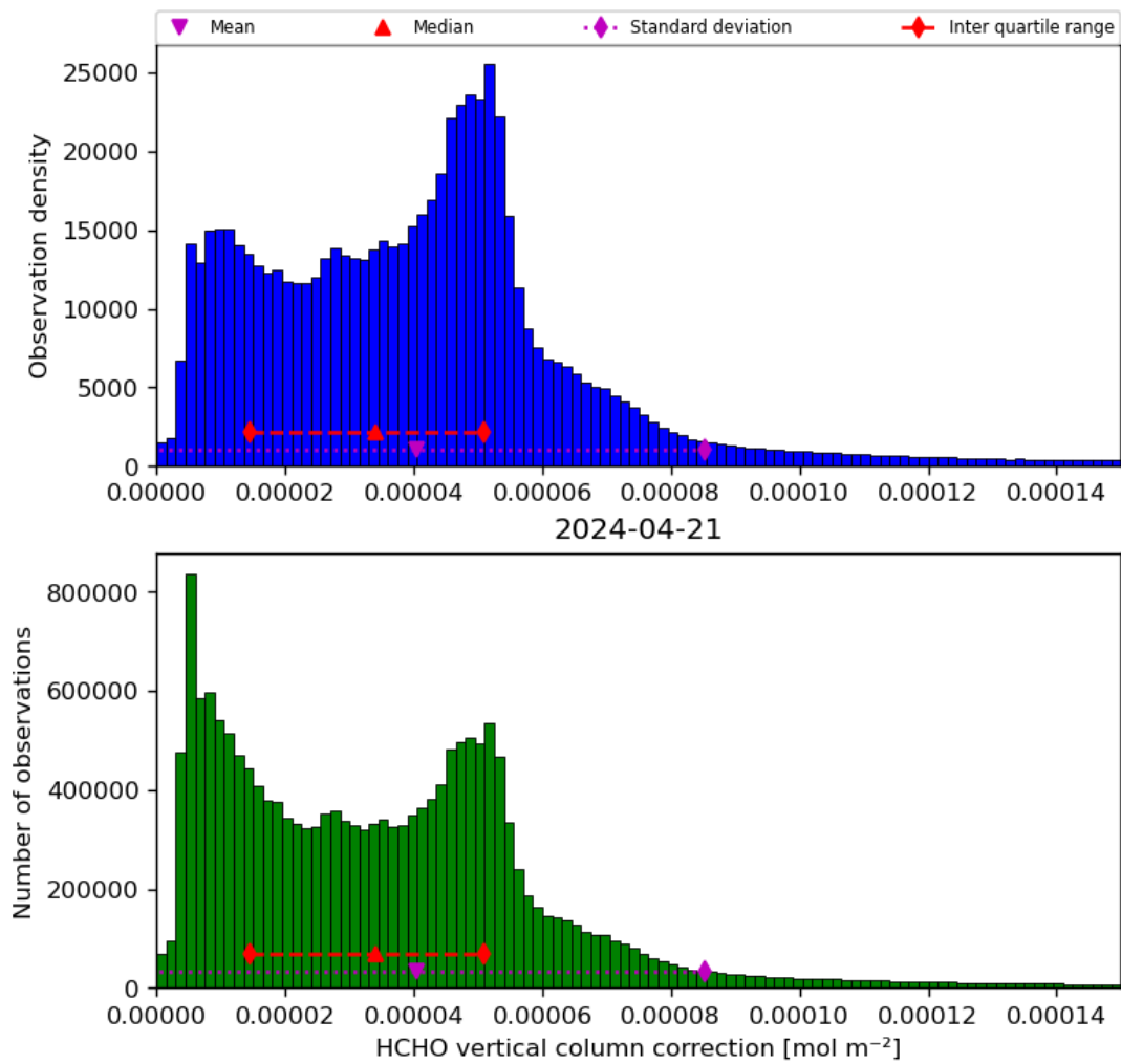
Figure 37: Histogram of “HCHO vertical column correction” for 2024-04-21 to 2024-04-22
