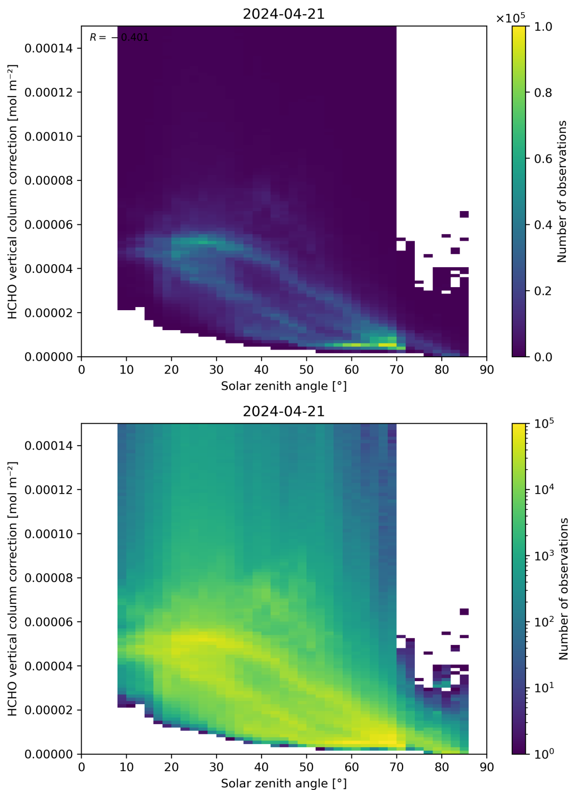
Figure 178: Scatter density plot of “Solar zenith angle” against “HCHO vertical column correction” for 2024-04-21 to 2024-04-22.
