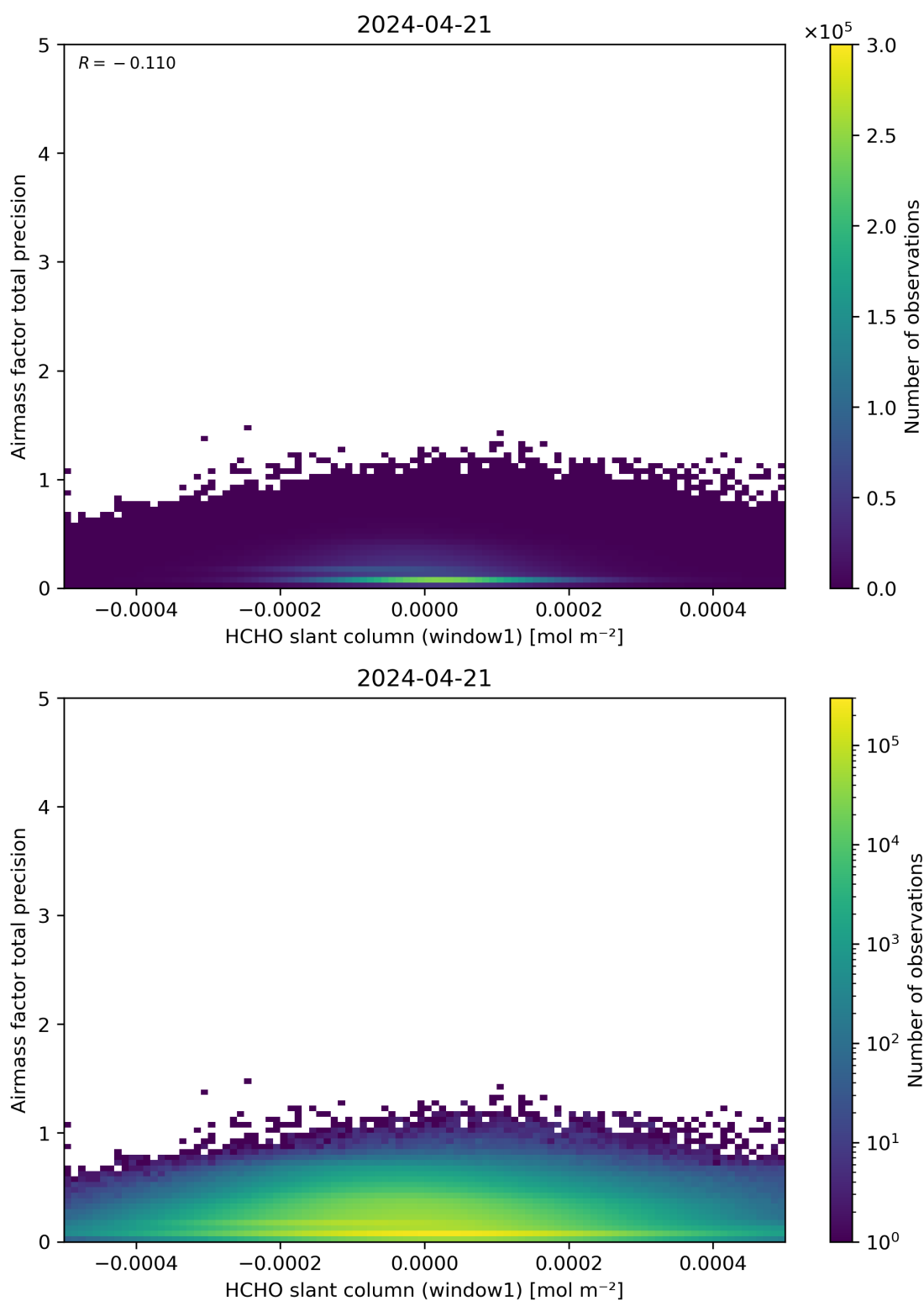
Figure 86: Scatter density plot of “HCHO slant column (window1)” against “Airmass factor total precision” for 2024-04-21 to 2024-04-22.
