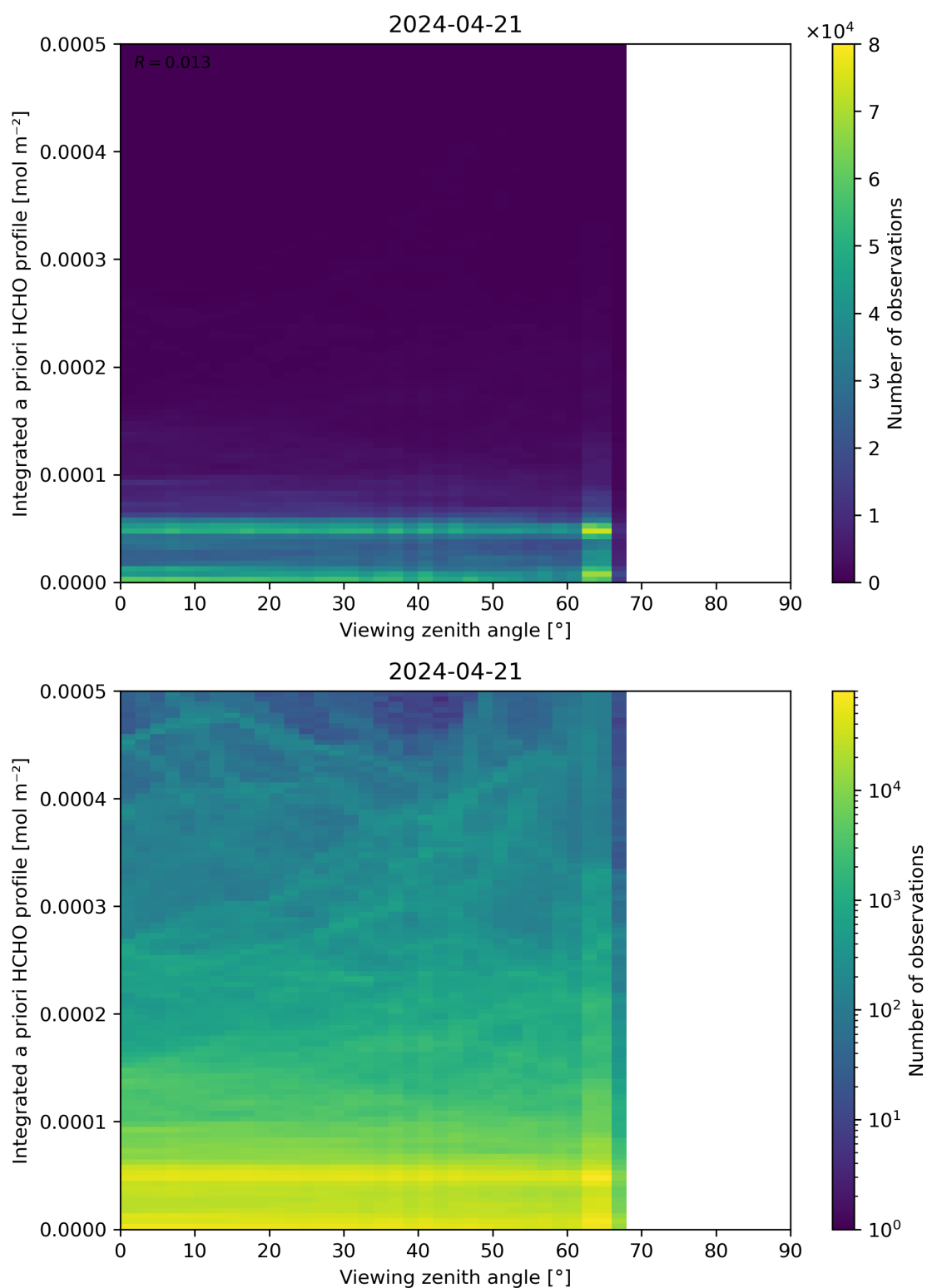
Figure 195: Scatter density plot of “Viewing zenith angle” against “Integrated a priori HCHO profile” for 2024-04-21 to 2024-04-22.
