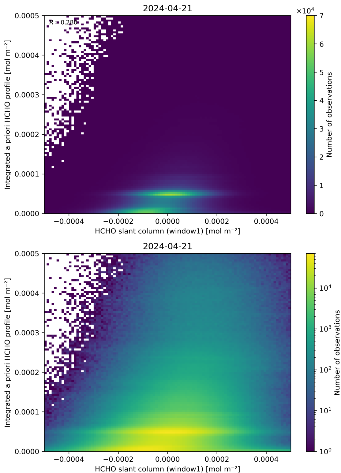
Figure 87: Scatter density plot of “HCHO slant column (window1)” against “Integrated a priori HCHO profile” for 2024-04-21 to 2024-04-22.
