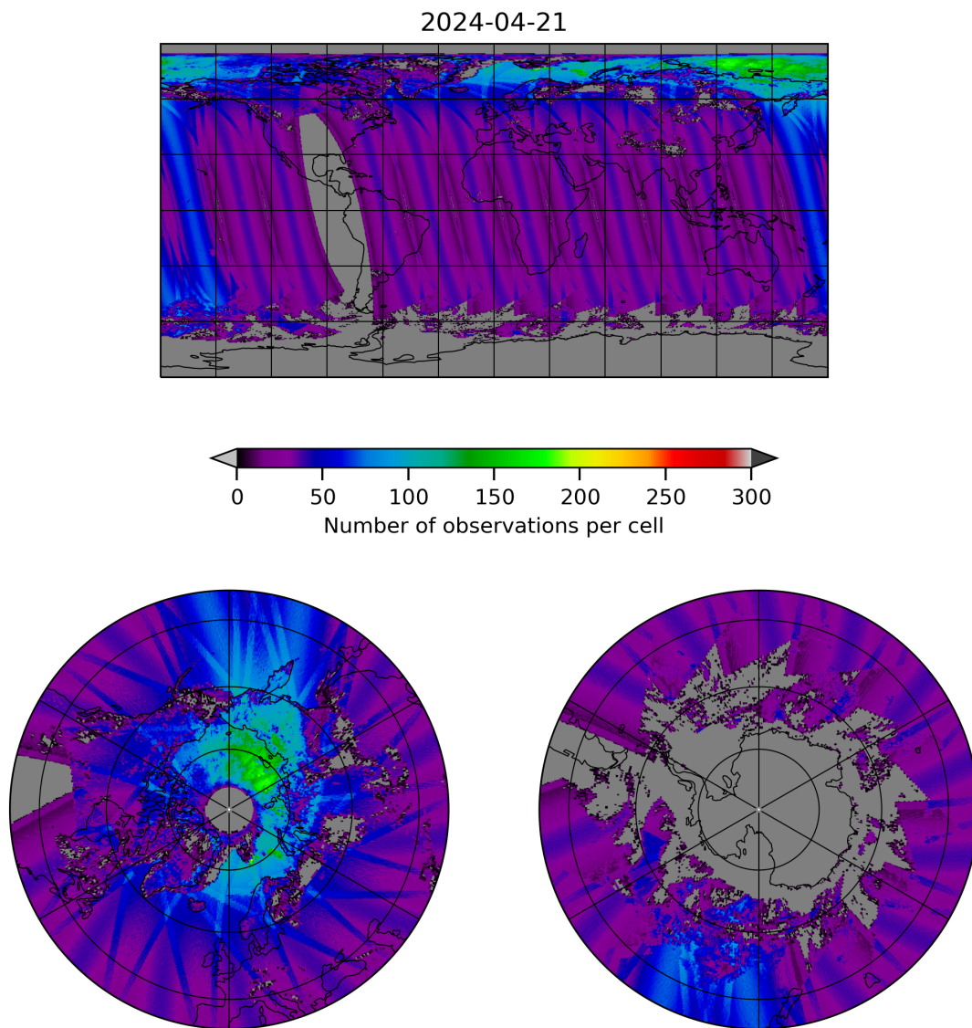
Figure 19: Map of the number of observations for 2024-04-21 to 2024-04-22
