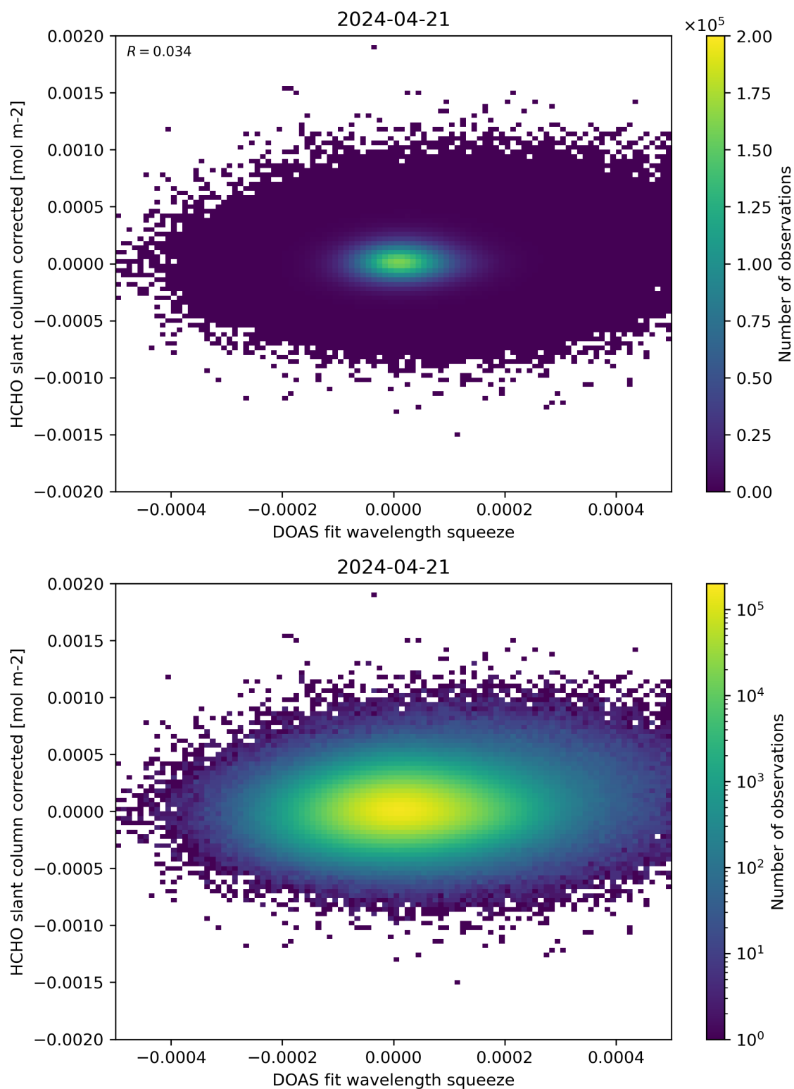
Figure 69: Scatter density plot of “DOAS fit wavelength squeeze” against “HCHO slant column corrected” for 2024-04-21 to 2024-04-22.
