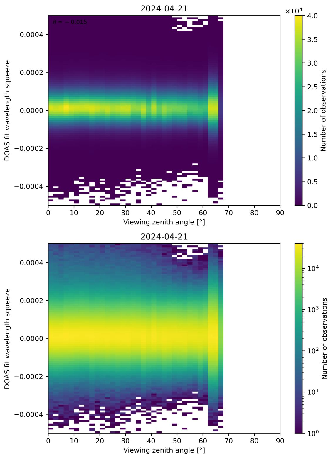
Figure 184: Scatter density plot of “Viewing zenith angle” against “DOAS fit wavelength squeeze” for 2024-04-21 to 2024-04-22.
