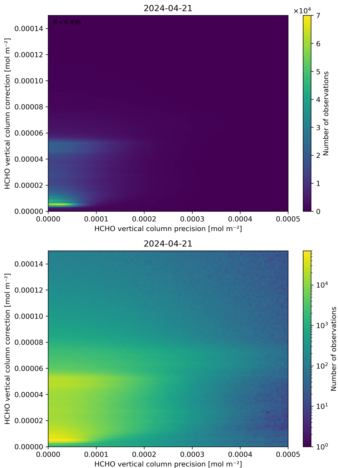
Figure 146: Scatter density plot of “HCHO vertical column precision” against “HCHO vertical column correction” for 2024-04-21 to 2024-04-22.
