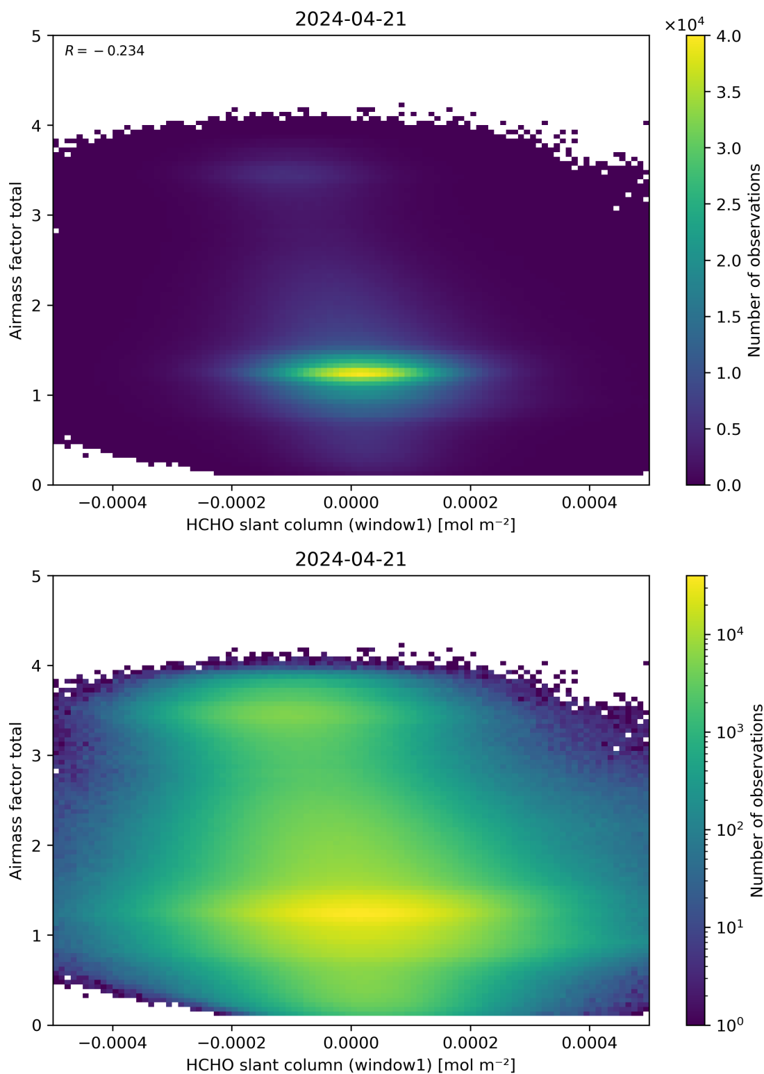
Figure 85: Scatter density plot of “HCHO slant column (window1)” against “Airmass factor total” for 2024-04-21 to 2024-04-22.
