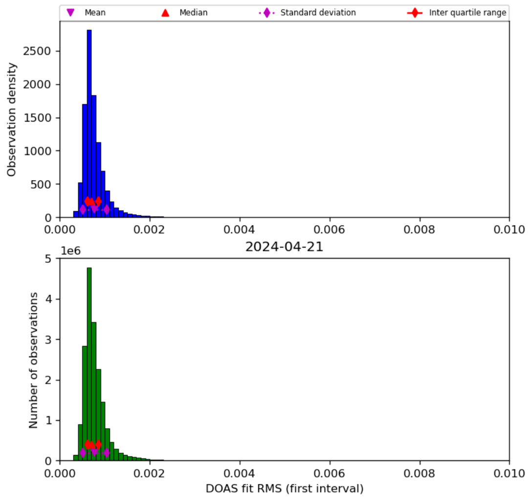
Figure 46: Histogram of “DOAS fit RMS (first interval)” for 2024-04-21 to 2024-04-22
