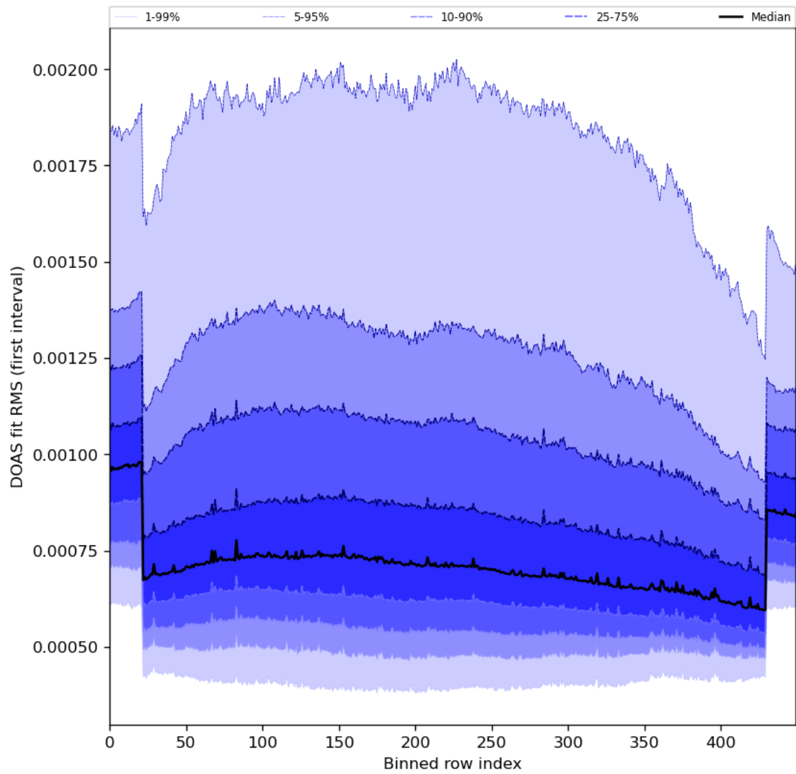
Figure 60: Along track statistics of “DOAS fit RMS (first interval)” for 2024-04-21 to 2024-04-22
