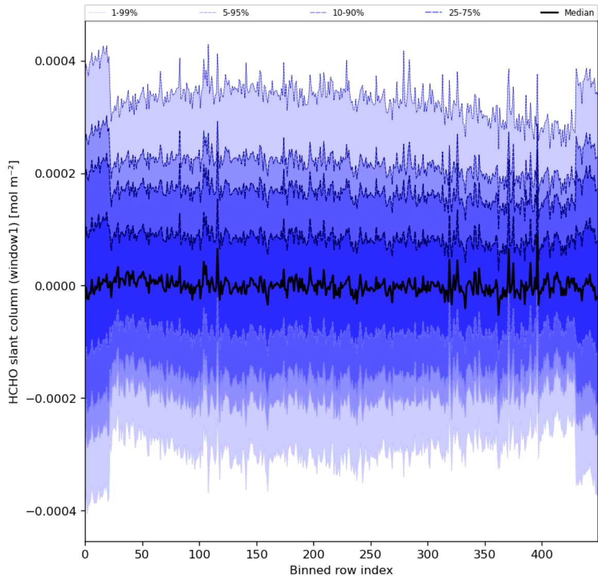
Figure 52: Along track statistics of “HCHO slant column (window1)” for 2024-04-21 to 2024-04-22
