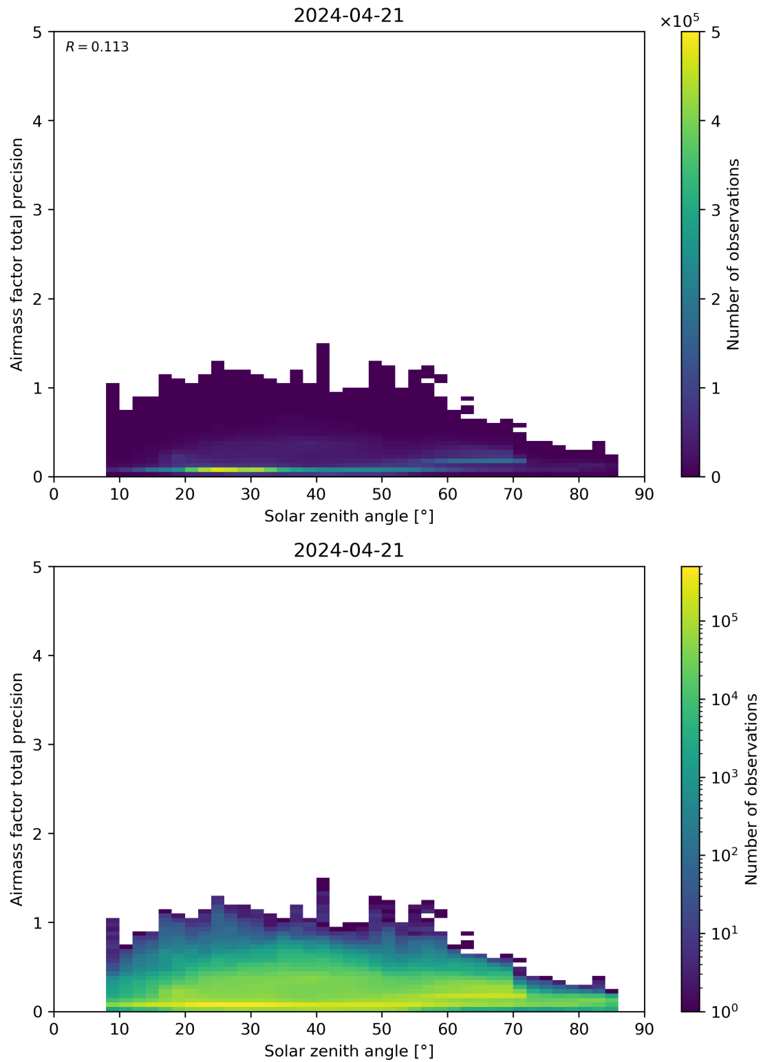
Figure 176: Scatter density plot of “Solar zenith angle” against “Airmass factor total precision” for 2024-04-21 to 2024-04-22.
