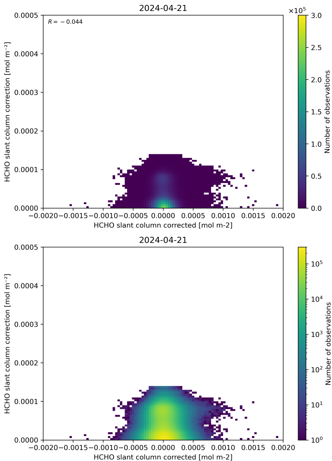
Figure 77: Scatter density plot of “HCHO slant column corrected” against “HCHO slant column correction” for 2024-04-21 to 2024-04-22.
