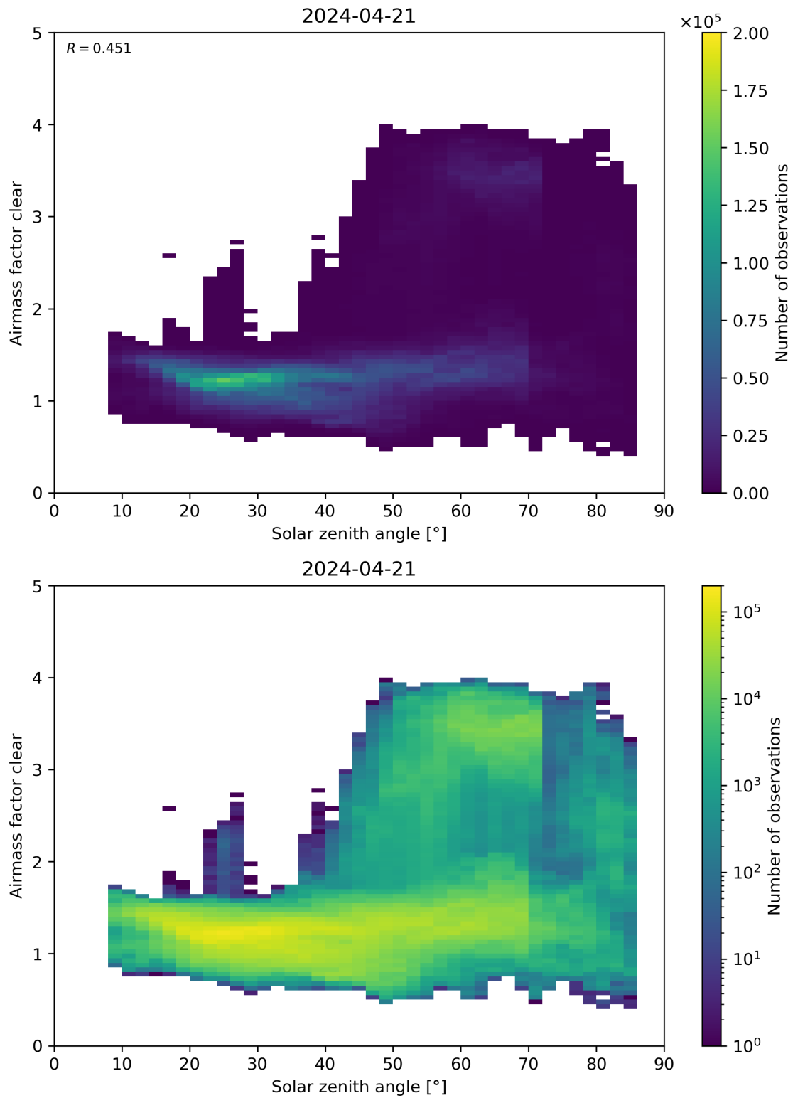
Figure 170: Scatter density plot of “Solar zenith angle” against “Airmass factor clear” for 2024-04-21 to 2024-04-22.
