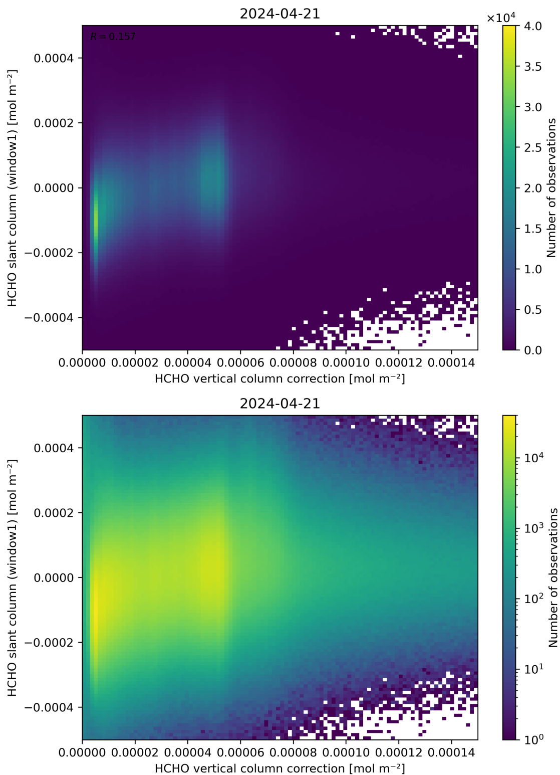
Figure 118: Scatter density plot of “HCHO vertical column correction” against “HCHO slant column (window1)” for 2024-04-21 to 2024-04-22.
