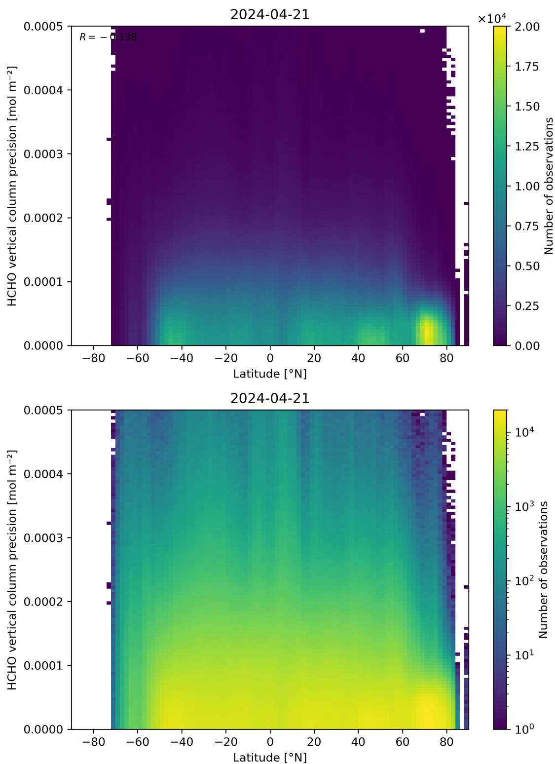
Figure 165: Scatter density plot of “Latitude” against “HCHO vertical column precision” for 2024-04-21 to 2024-04-22.
