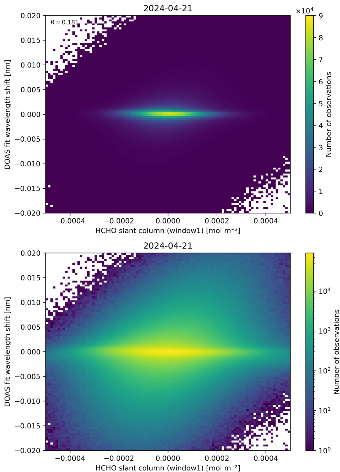
Figure 79: Scatter density plot of “HCHO slant column (window1)” against “DOAS fit wavelength shift” for 2024-04-21 to 2024-04-22.
