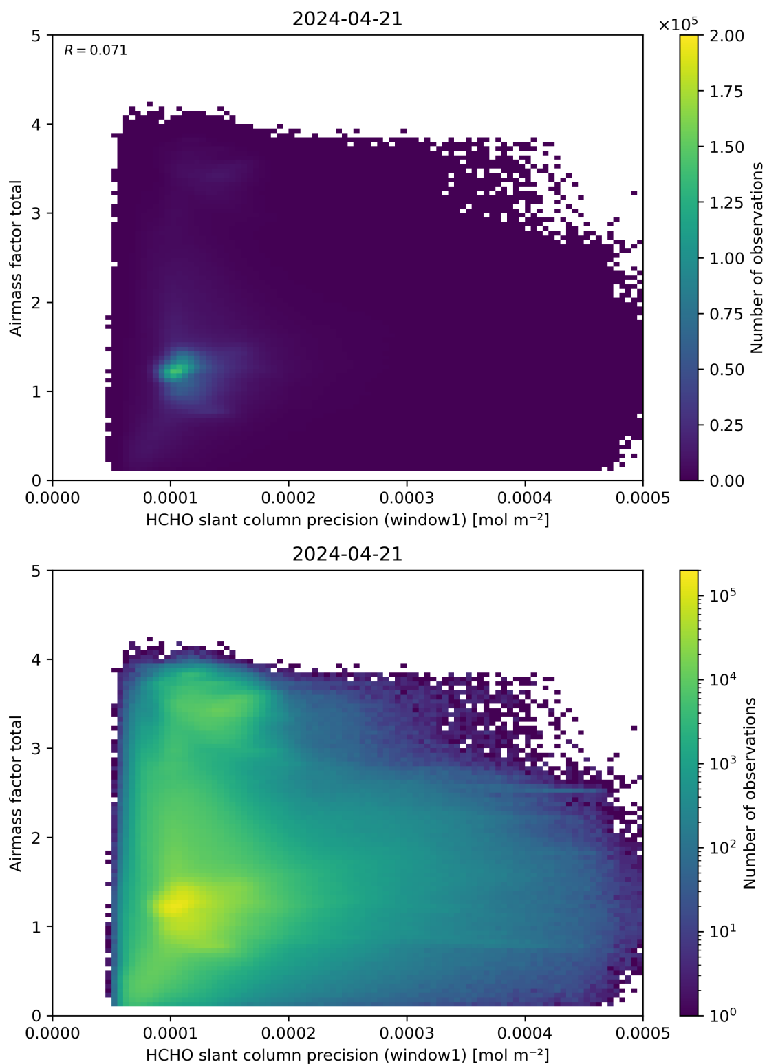
Figure 94: Scatter density plot of “HCHO slant column precision (window1)” against “Airmass factor total” for 2024-04-21 to 2024-04-22.
