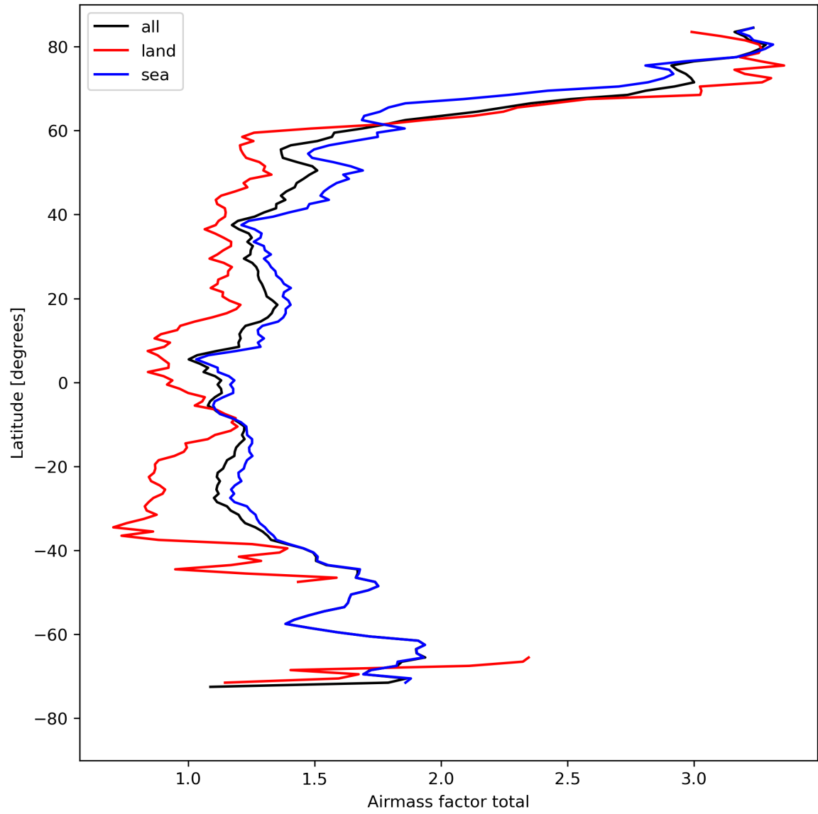
Figure 26: Zonal average of “Airmass factor total” for 2024-04-21 to 2024-04-22.
