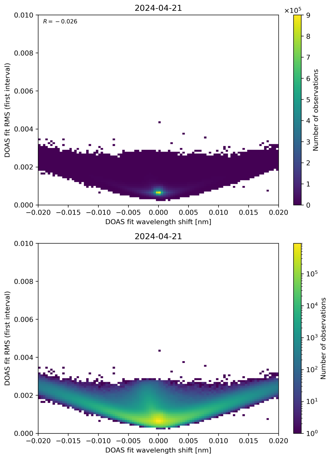
Figure 64: Scatter density plot of “DOAS fit wavelength shift” against “DOAS fit RMS (first interval)” for 2024-04-21 to 2024-04-22.
