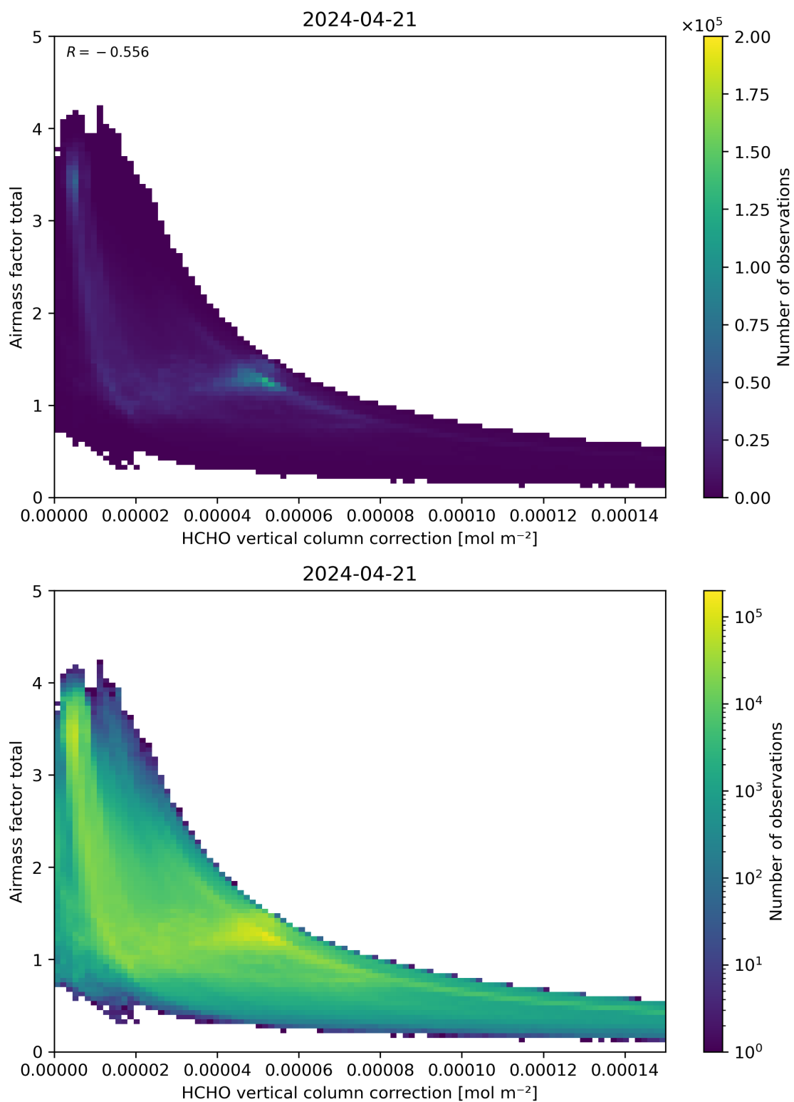
Figure 120: Scatter density plot of “HCHO vertical column correction” against “Airmass factor total” for 2024-04-21 to 2024-04-22.
