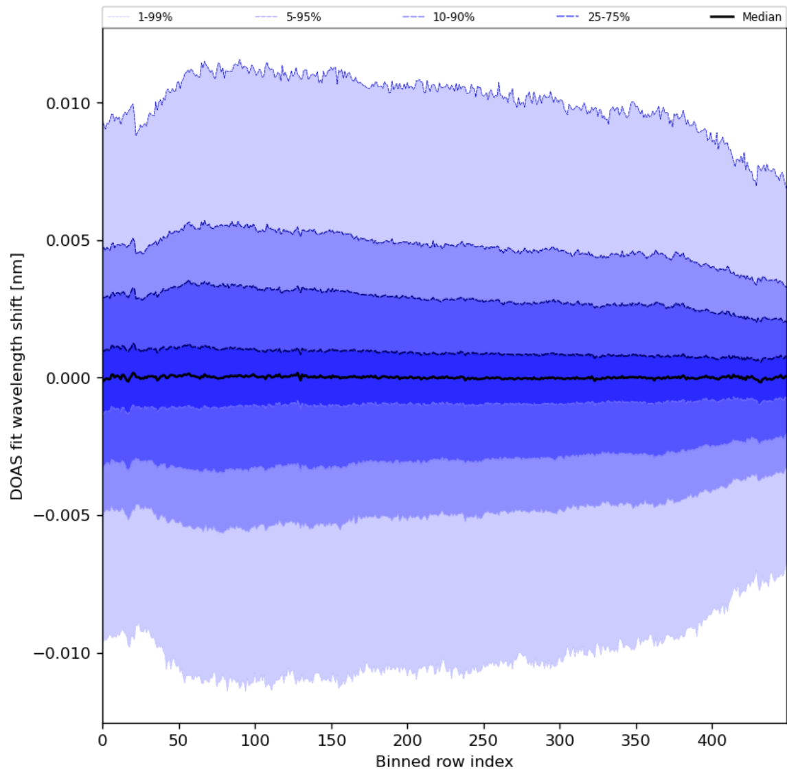
Figure 58: Along track statistics of “DOAS fit wavelength shift” for 2024-04-21 to 2024-04-22
