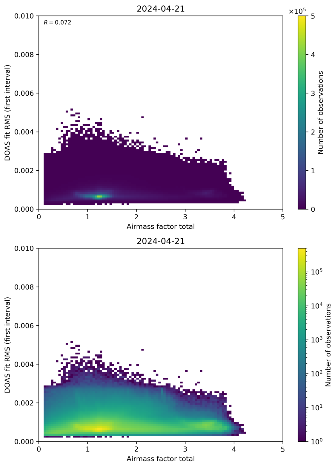
Figure 97: Scatter density plot of “Airmass factor total” against “DOAS fit RMS (first interval)” for 2024-04-21 to 2024-04-22.
