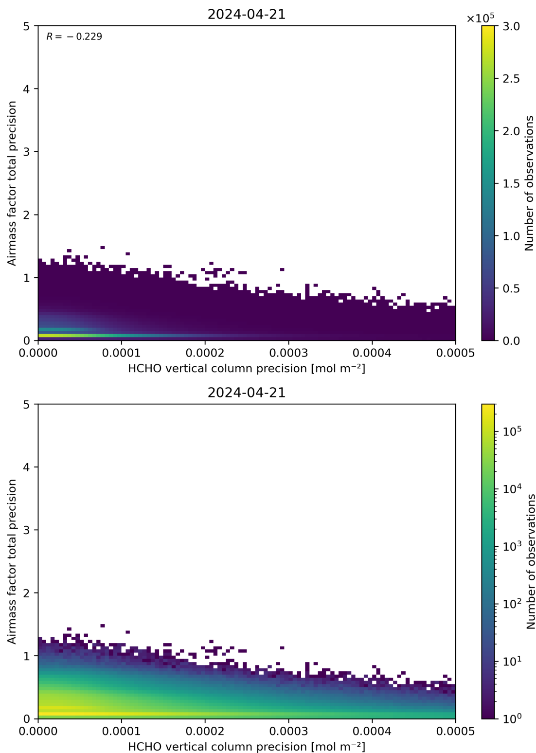
Figure 145: Scatter density plot of “HCHO vertical column precision” against “Airmass factor total precision” for 2024-04-21 to 2024-04-22.
