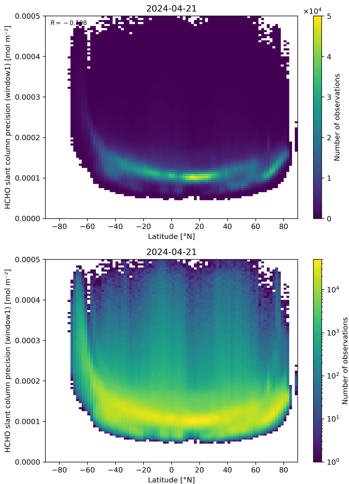
Figure 160: Scatter density plot of “Latitude” against “HCHO slant column precision (window1)” for 2024-04-21 to 2024-04-22.
