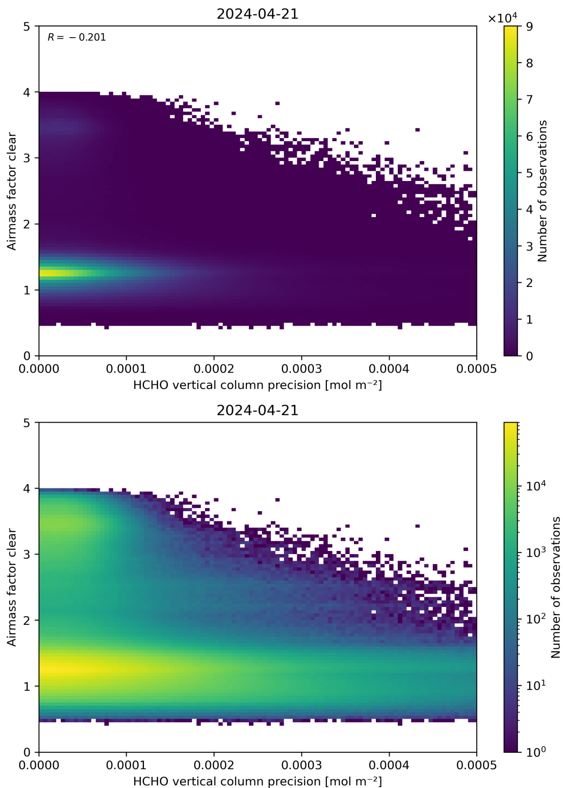
Figure 139: Scatter density plot of “HCHO vertical column precision” against “Airmass factor clear” for 2024-04-21 to 2024-04-22.
