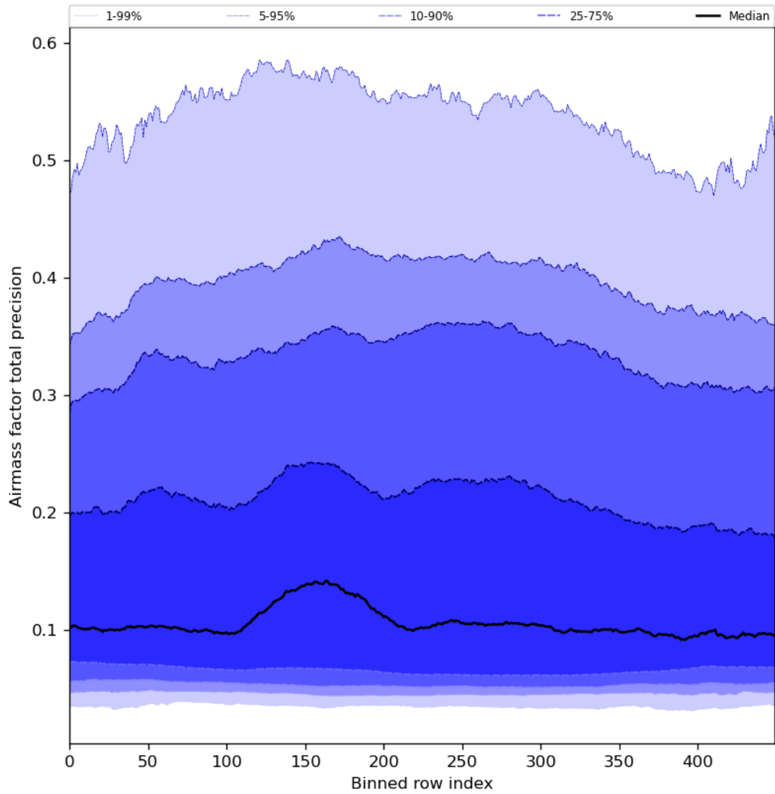
Figure 55: Along track statistics of “Airmass factor total precision” for 2024-04-21 to 2024-04-22
