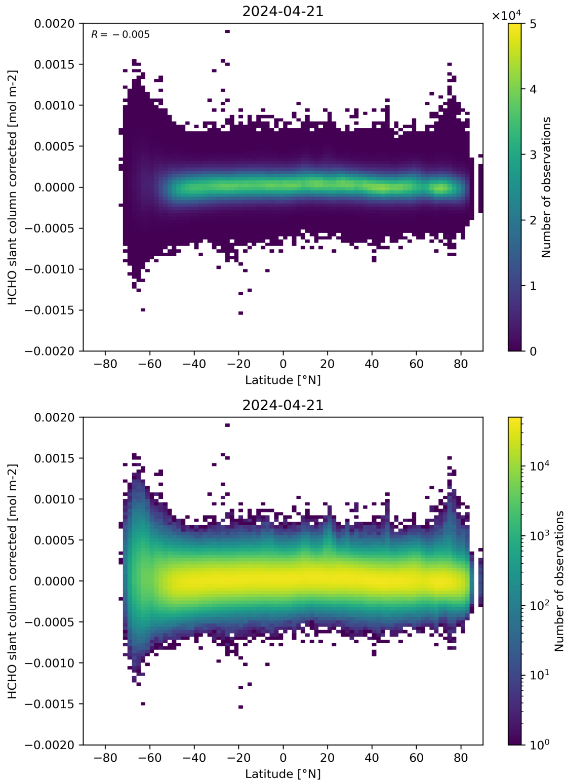
Figure 157: Scatter density plot of “Latitude” against “HCHO slant column corrected” for 2024-04-21 to 2024-04-22.
