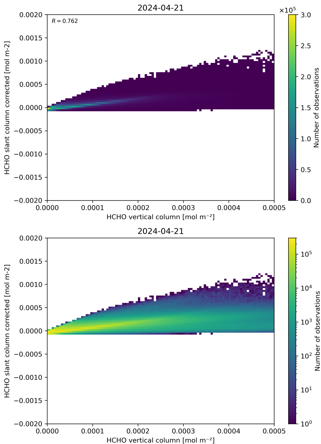
Figure 127: Scatter density plot of “HCHO vertical column” against “HCHO slant column corrected” for 2024-04-21 to 2024-04-22.
