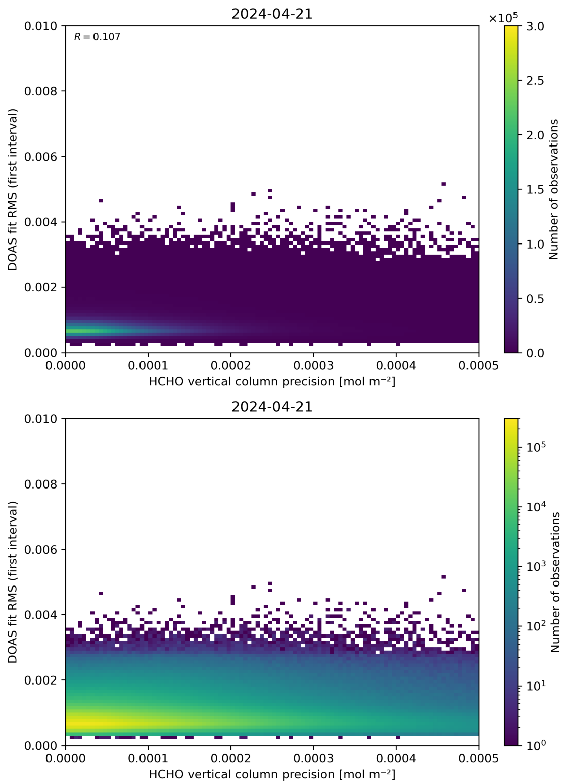
Figure 136: Scatter density plot of “HCHO vertical column precision” against “DOAS fit RMS (first interval)” for 2024-04-21 to 2024-04-22.
