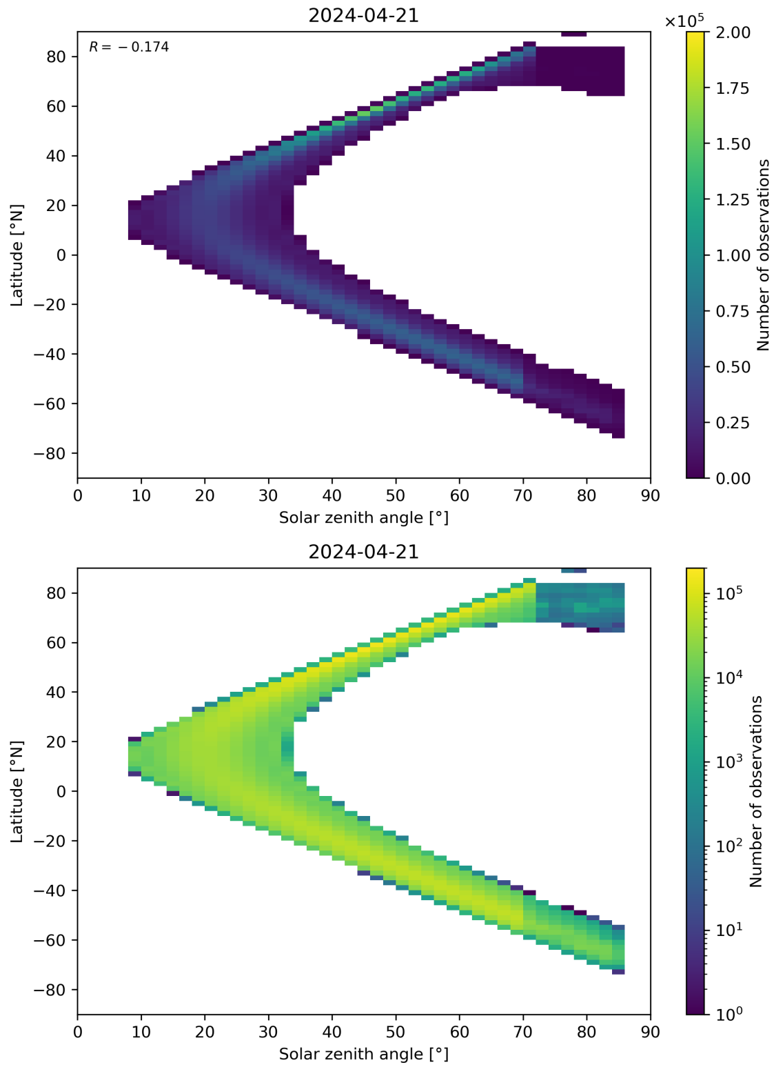
Figure 181: Scatter density plot of “Solar zenith angle” against “Latitude” for 2024-04-21 to 2024-04-22.
