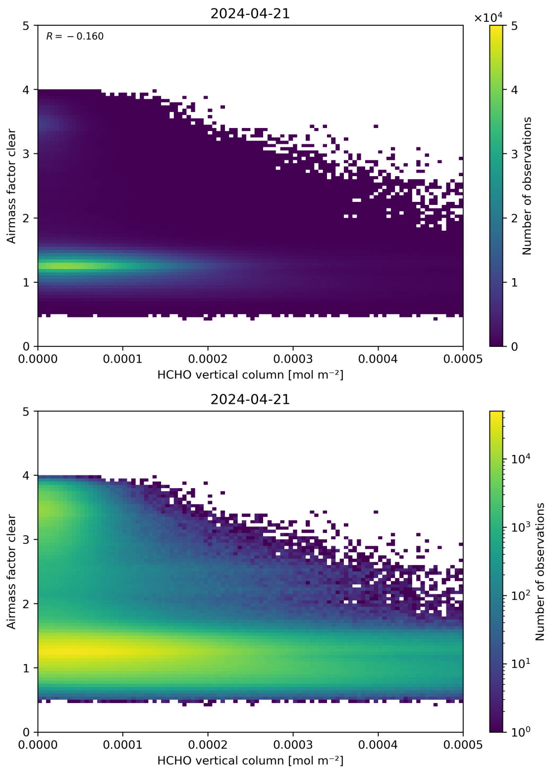
Figure 126: Scatter density plot of “HCHO vertical column” against “Airmass factor clear” for 2024-04-21 to 2024-04-22.
