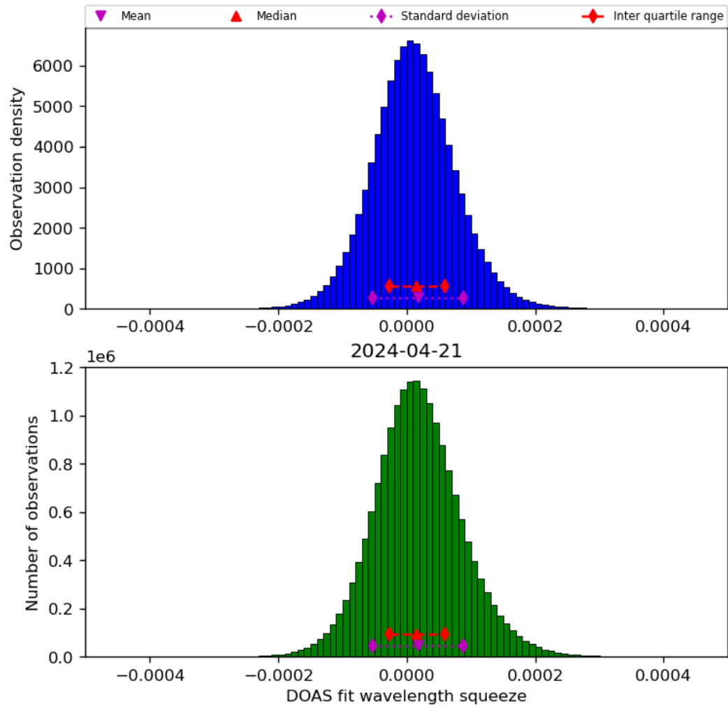
Figure 45: Histogram of “DOAS fit wavelength squeeze” for 2024-04-21 to 2024-04-22
