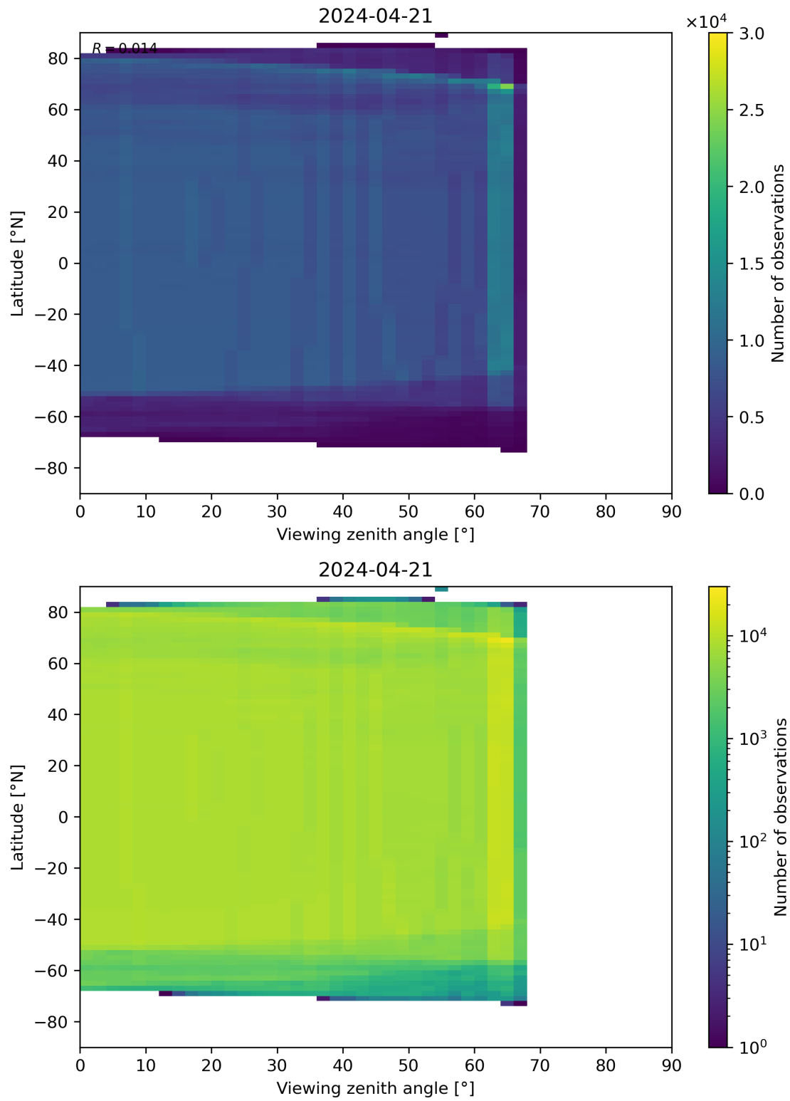
Figure 196: Scatter density plot of “Viewing zenith angle” against “Latitude” for 2024-04-21 to 2024-04-22.
