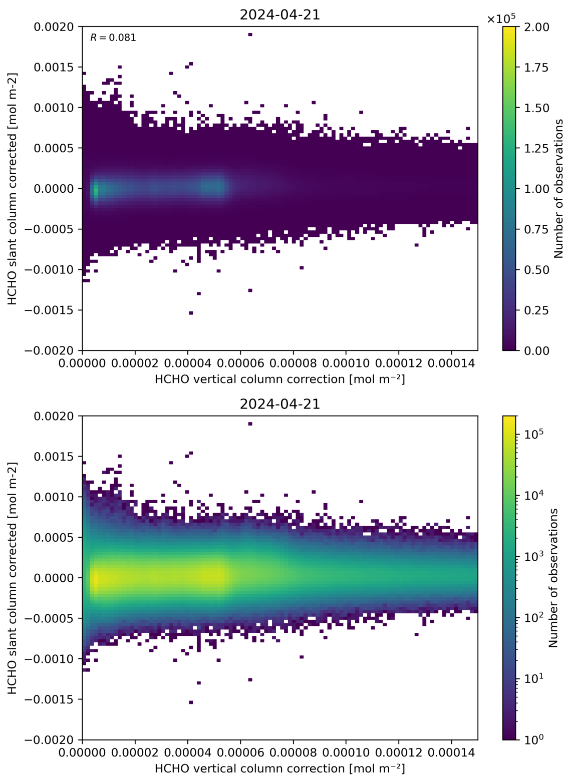
Figure 116: Scatter density plot of “HCHO vertical column correction” against “HCHO slant column corrected” for 2024-04-21 to 2024-04-22.
