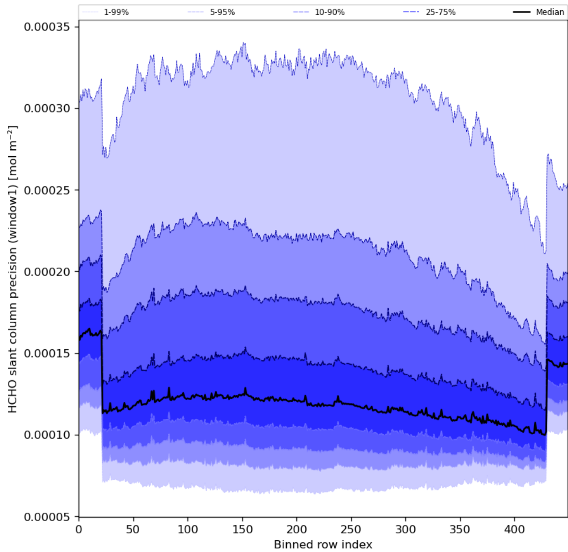
Figure 53: Along track statistics of “HCHO slant column precision (window1)” for 2024-04-21 to 2024-04-22
