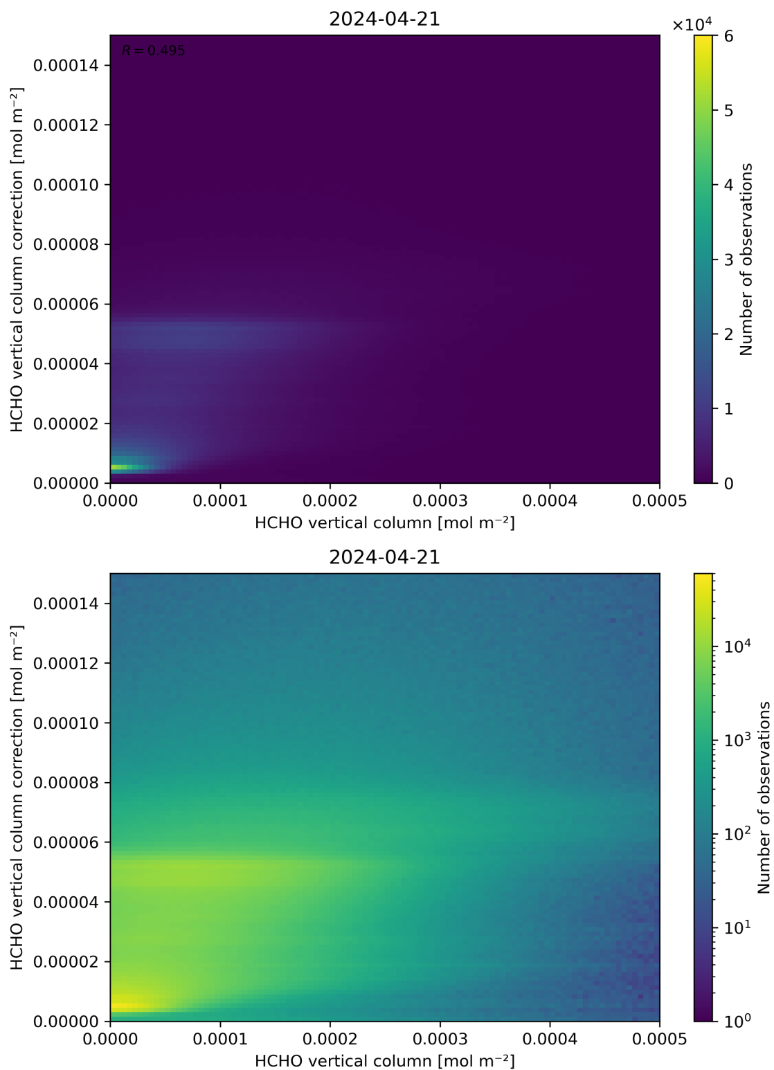
Figure 133: Scatter density plot of “HCHO vertical column” against “HCHO vertical column correction” for 2024-04-21 to 2024-04-22.
