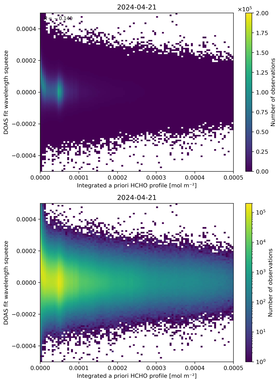
Figure 150: Scatter density plot of “Integrated a priori HCHO profile” against “DOAS fit wavelength squeeze” for 2024-04-21 to 2024-04-22.
