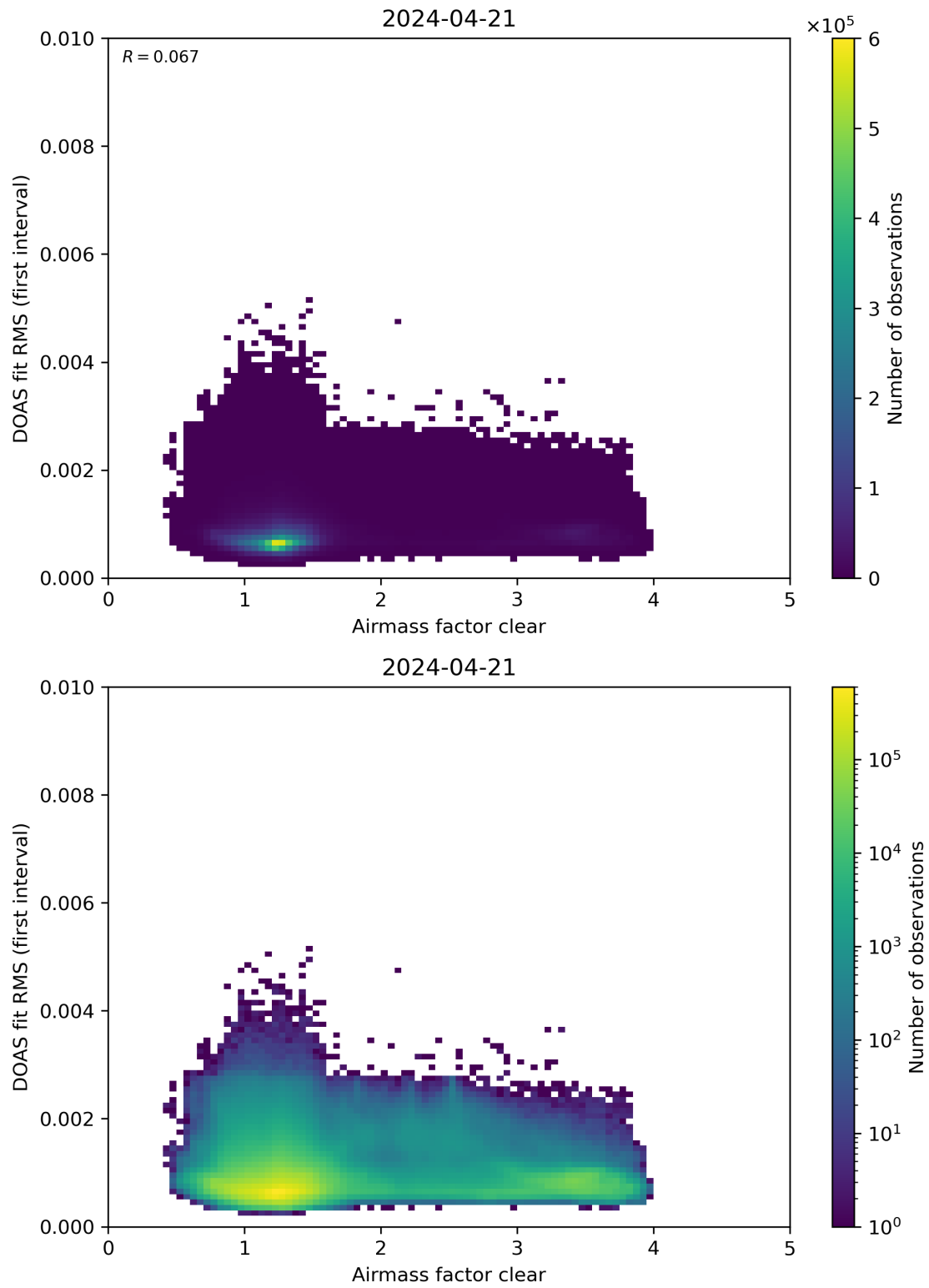
Figure 71: Scatter density plot of “Airmass factor clear” against “DOAS fit RMS (first interval)” for 2024-04-21 to 2024-04-22.
