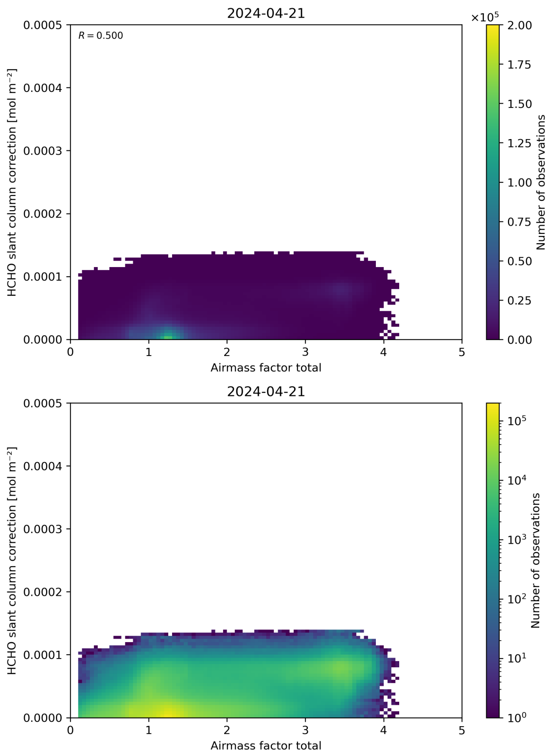
Figure 102: Scatter density plot of “Airmass factor total” against “HCHO slant column correction” for 2024-04-21 to 2024-04-22.
