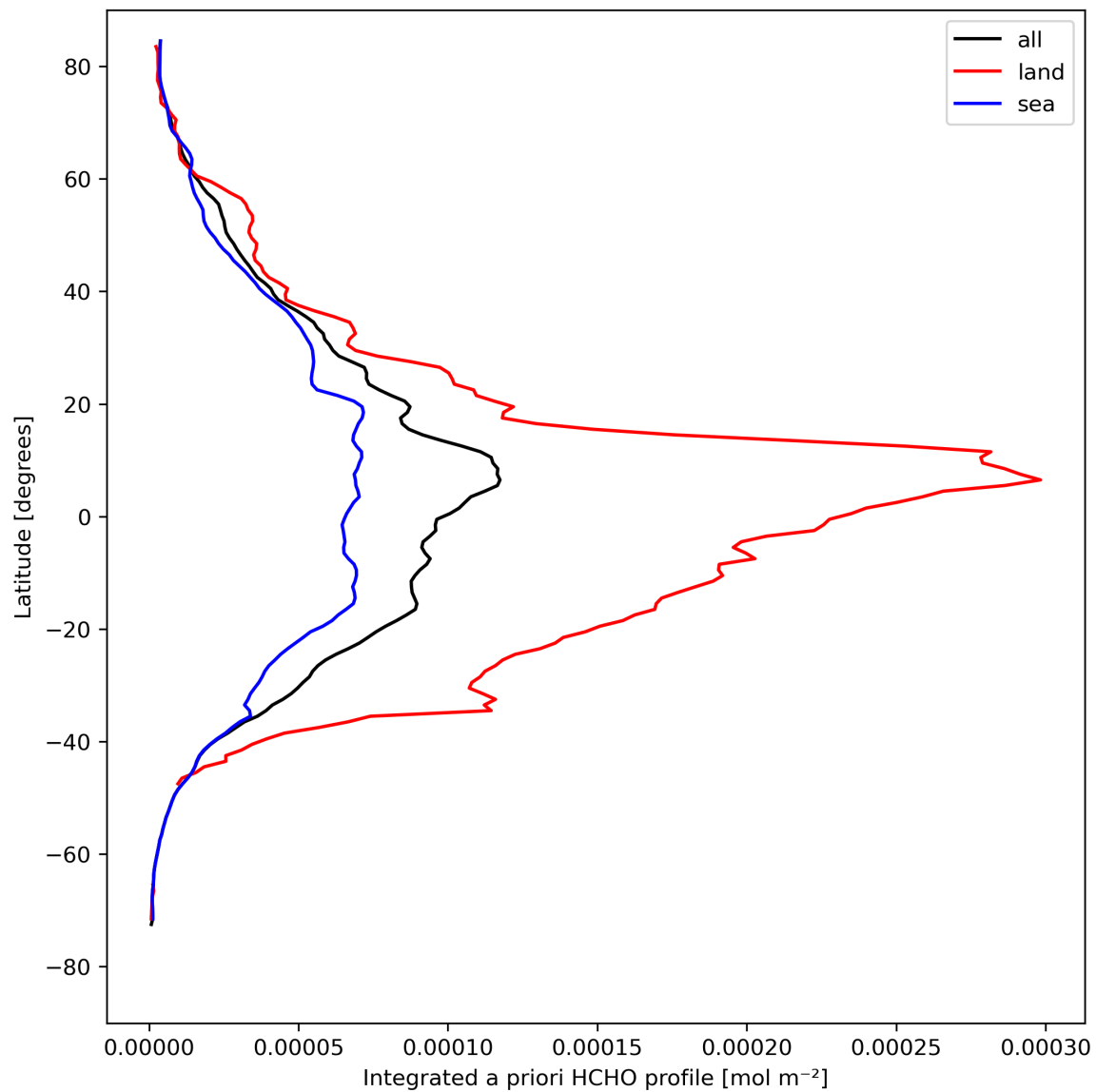
Figure 29: Zonal average of “Integrated a priori HCHO profile” for 2024-04-21 to 2024-04-22.
