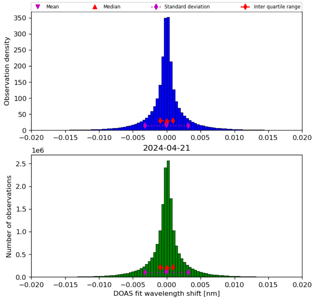
Figure 44: Histogram of “DOAS fit wavelength shift” for 2024-04-21 to 2024-04-22
