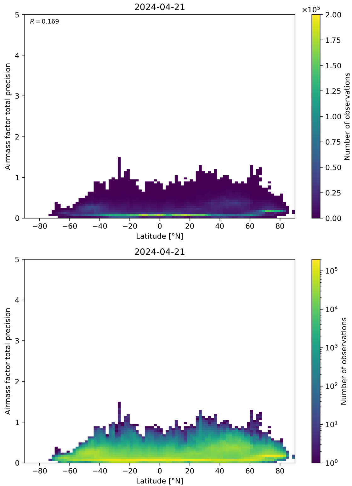
Figure 162: Scatter density plot of “Latitude” against “Airmass factor total precision” for 2024-04-21 to 2024-04-22.
