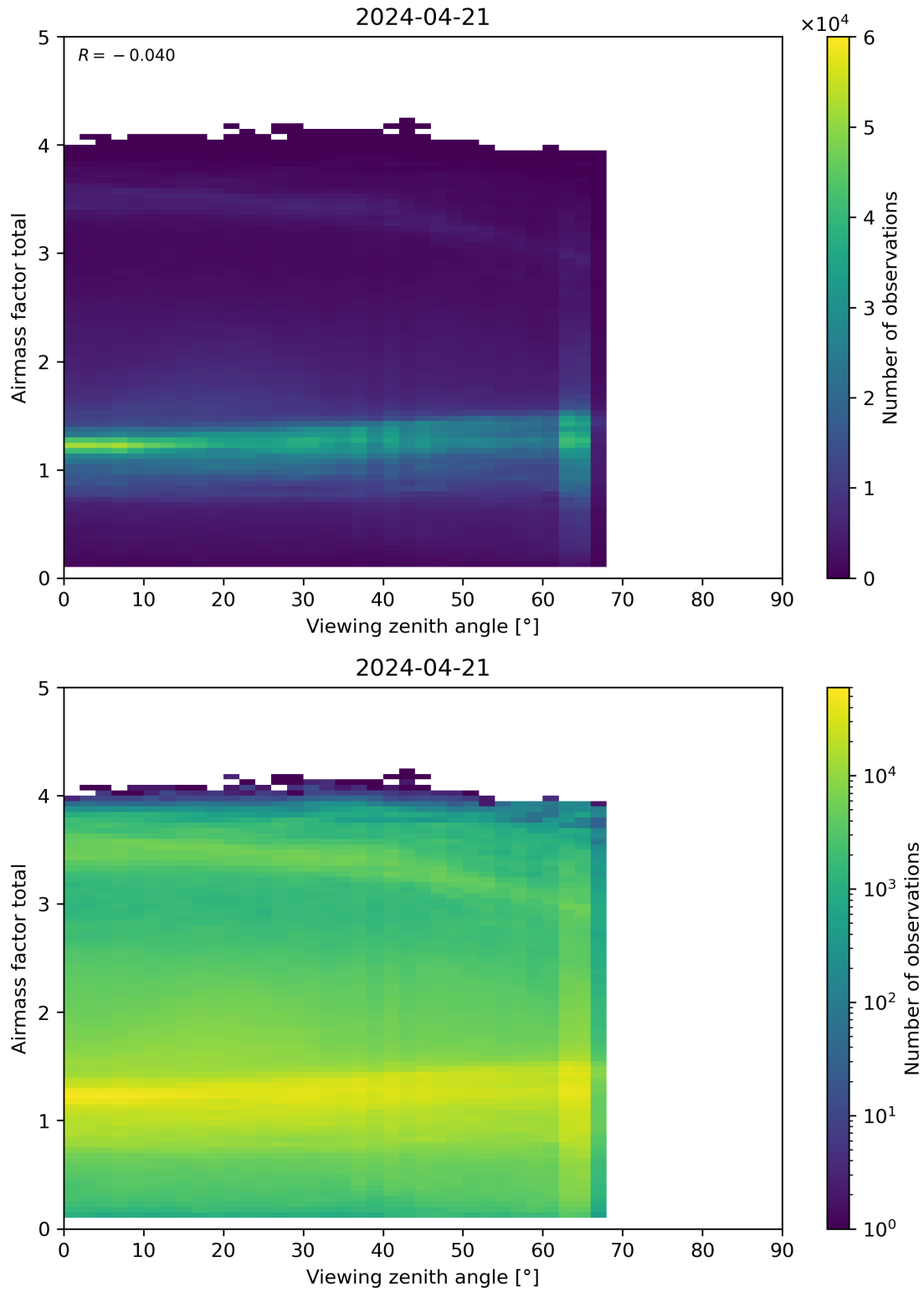
Figure 190: Scatter density plot of “Viewing zenith angle” against “Airmass factor total” for 2024-04-21 to 2024-04-22.
