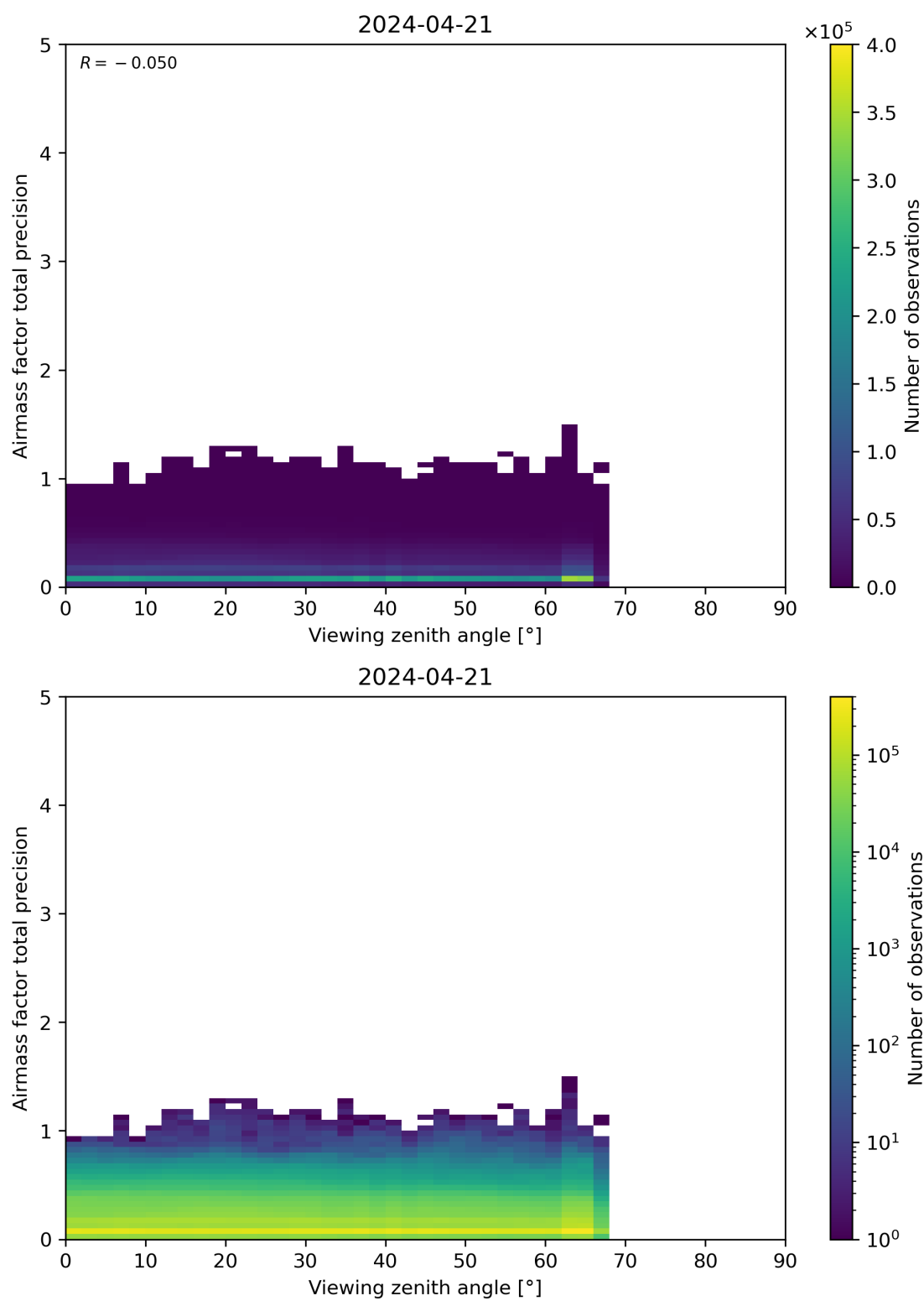
Figure 191: Scatter density plot of “Viewing zenith angle” against “Airmass factor total precision” for 2024-04-21 to 2024-04-22.
