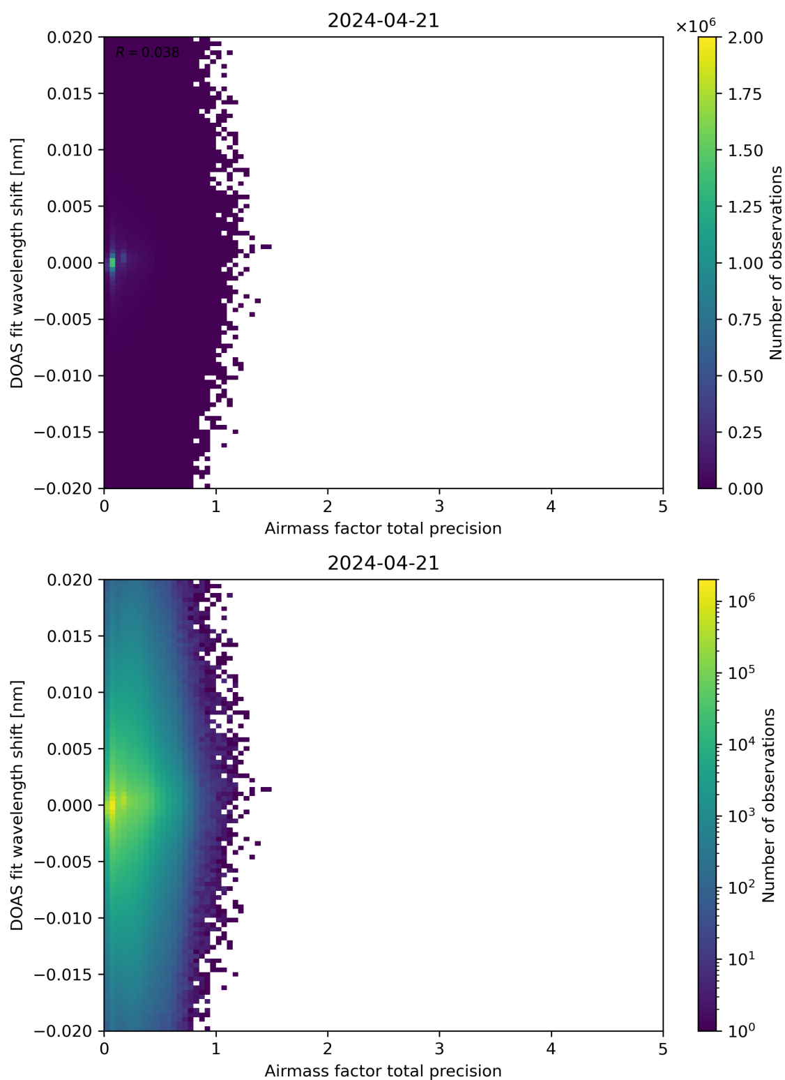
Figure 106: Scatter density plot of “Airmass factor total precision” against “DOAS fit wavelength shift” for 2024-04-21 to 2024-04-22.
