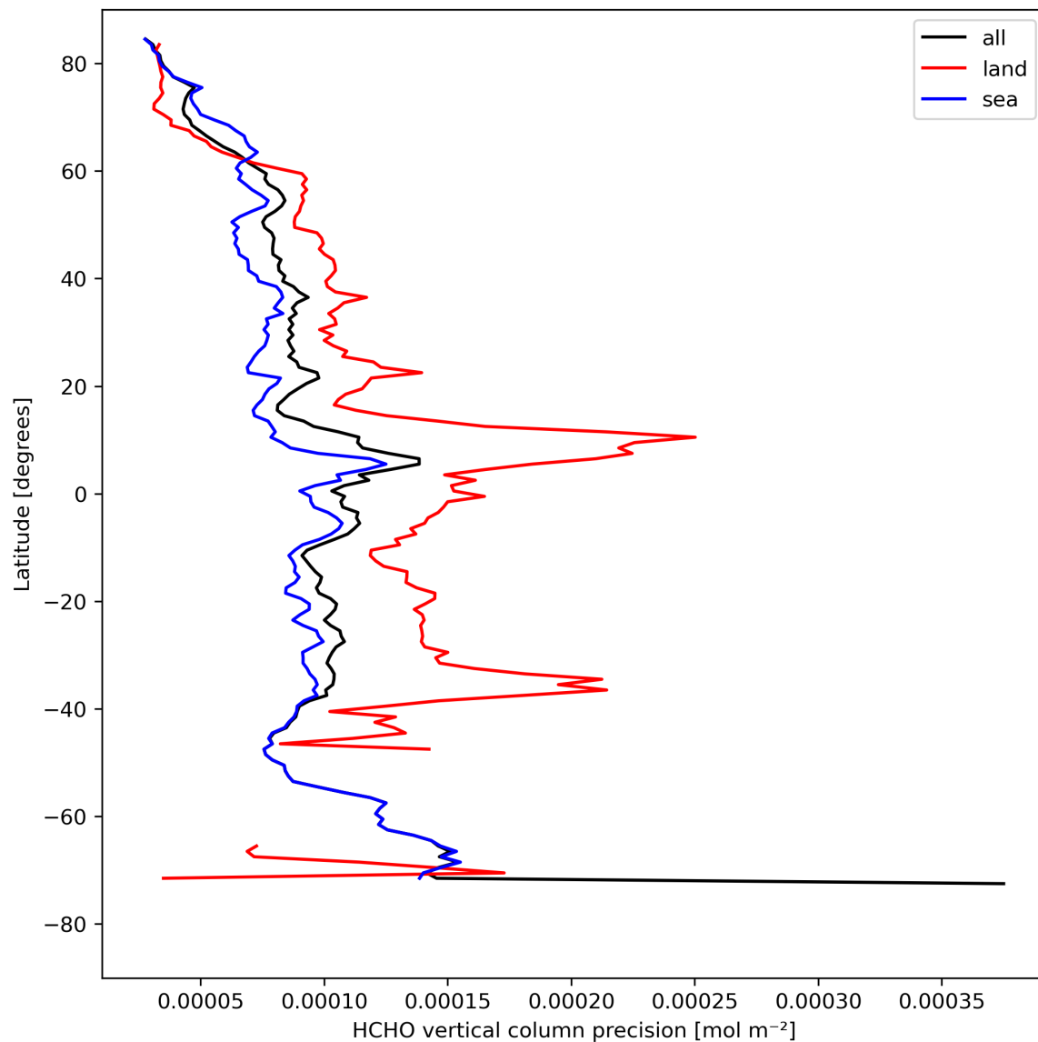
Figure 22: Zonal average of “HCHO vertical column precision” for 2024-04-21 to 2024-04-22.
