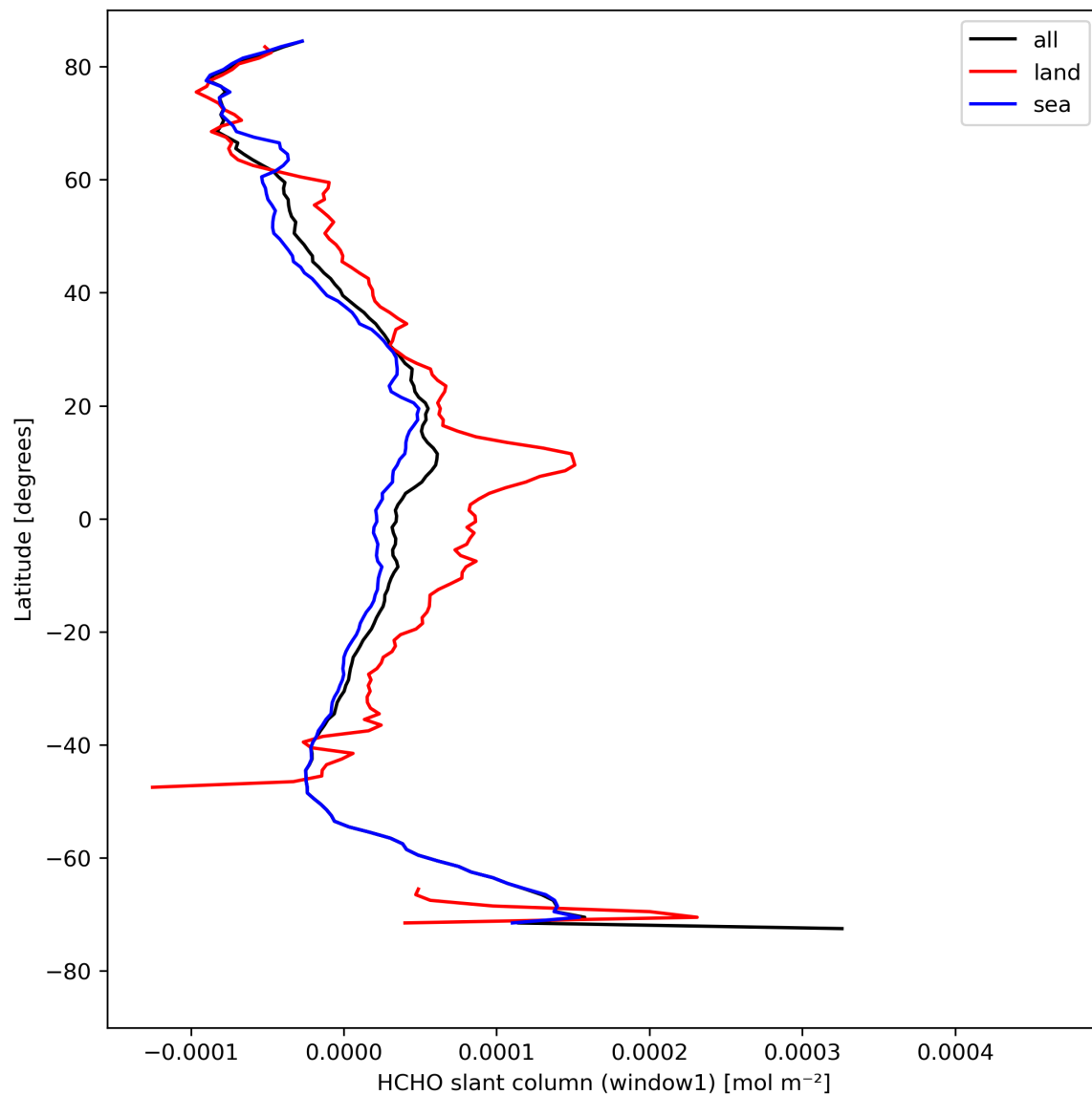
Figure 24: Zonal average of “HCHO slant column (window1)” for 2024-04-21 to 2024-04-22.
