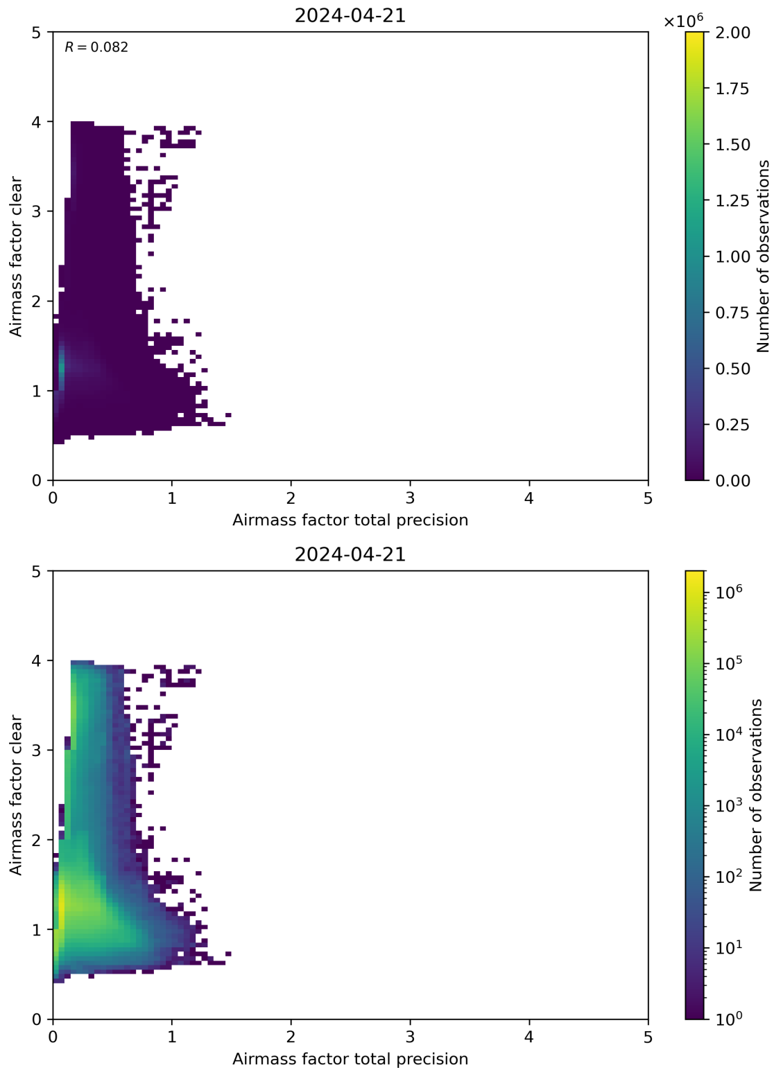
Figure 108: Scatter density plot of “Airmass factor total precision” against “Airmass factor clear” for 2024-04-21 to 2024-04-22.
