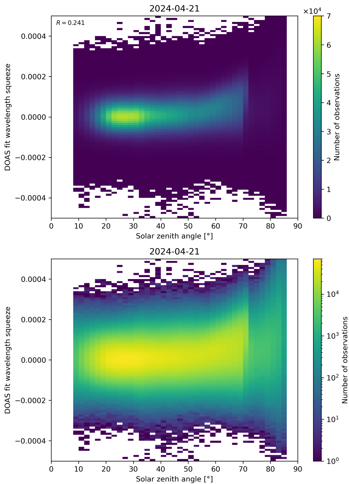
Figure 169: Scatter density plot of “Solar zenith angle” against “DOAS fit wavelength squeeze” for 2024-04-21 to 2024-04-22.
