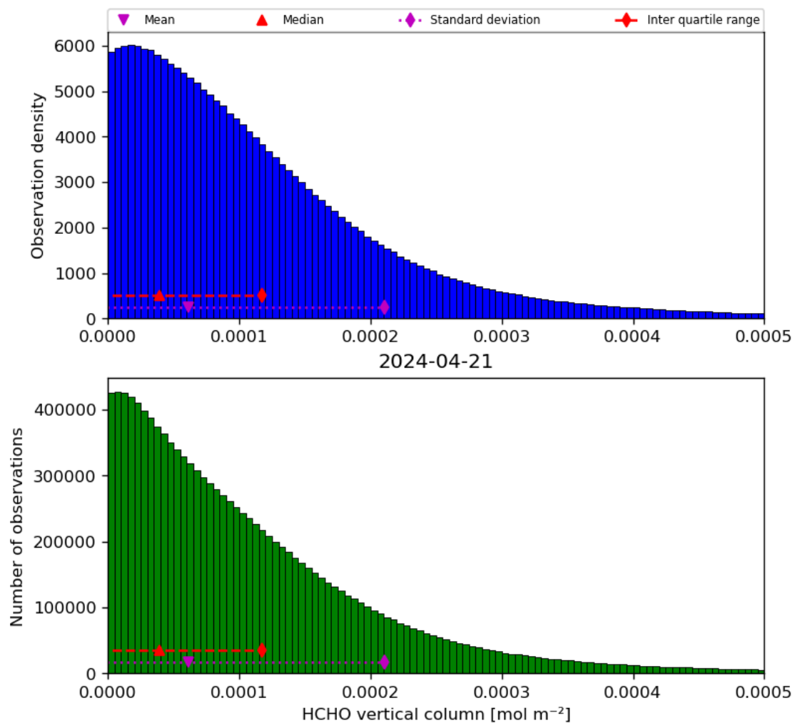
Figure 35: Histogram of “HCHO vertical column” for 2024-04-21 to 2024-04-22
