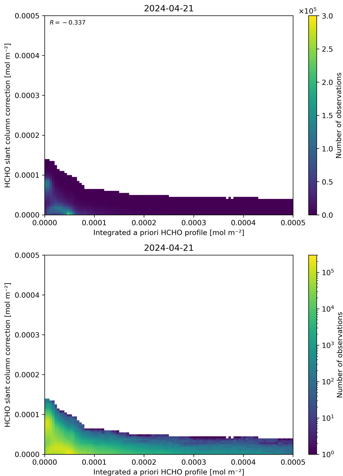
Figure 152: Scatter density plot of “Integrated a priori HCHO profile” against “HCHO slant column correction” for 2024-04-21 to 2024-04-22.
