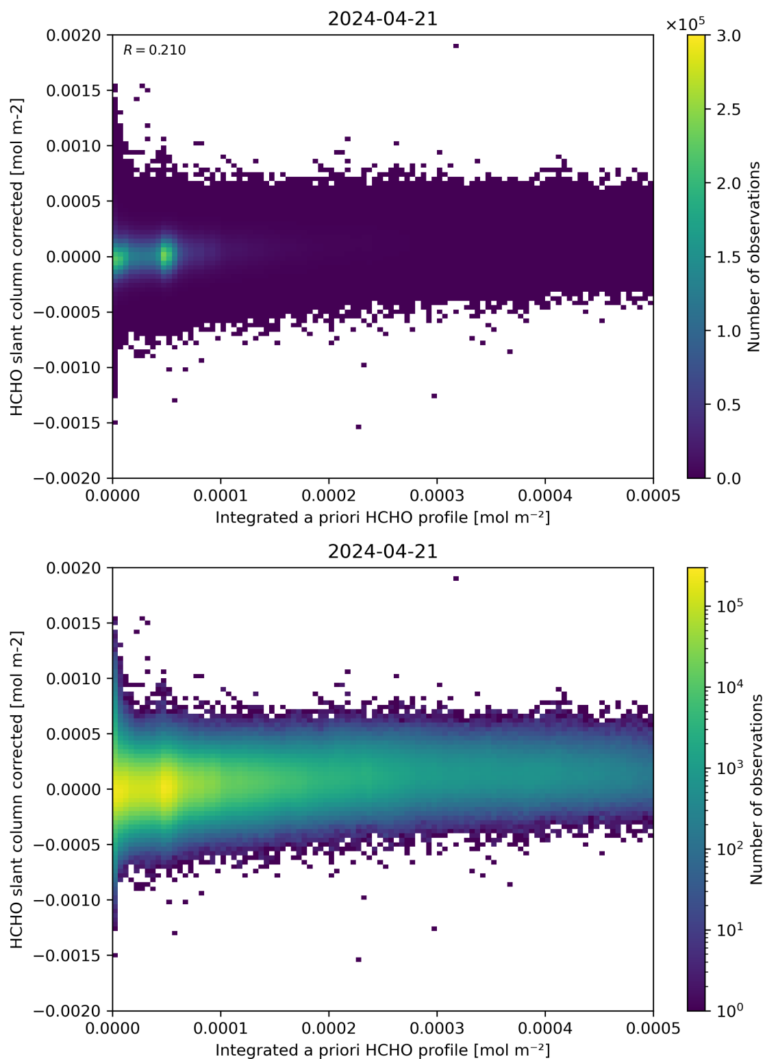
Figure 151: Scatter density plot of “Integrated a priori HCHO profile” against “HCHO slant column corrected” for 2024-04-21 to 2024-04-22.
