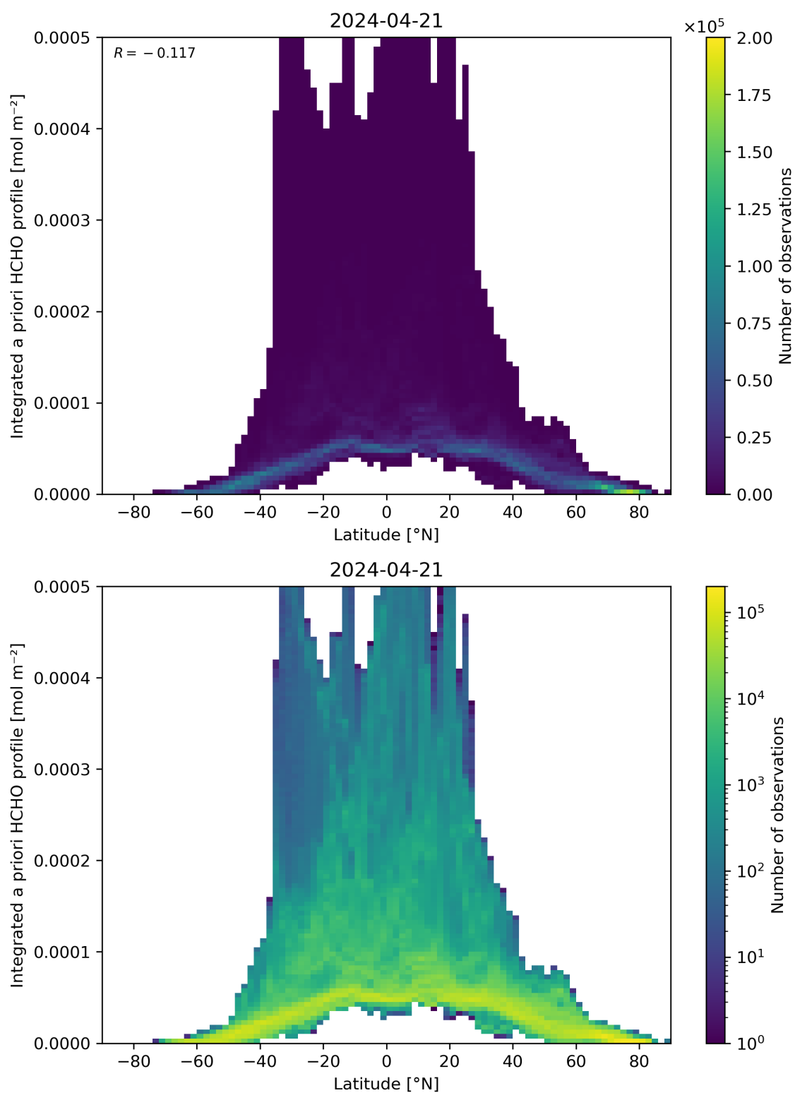
Figure 166: Scatter density plot of “Latitude” against “Integrated a priori HCHO profile” for 2024-04-21 to 2024-04-22.
