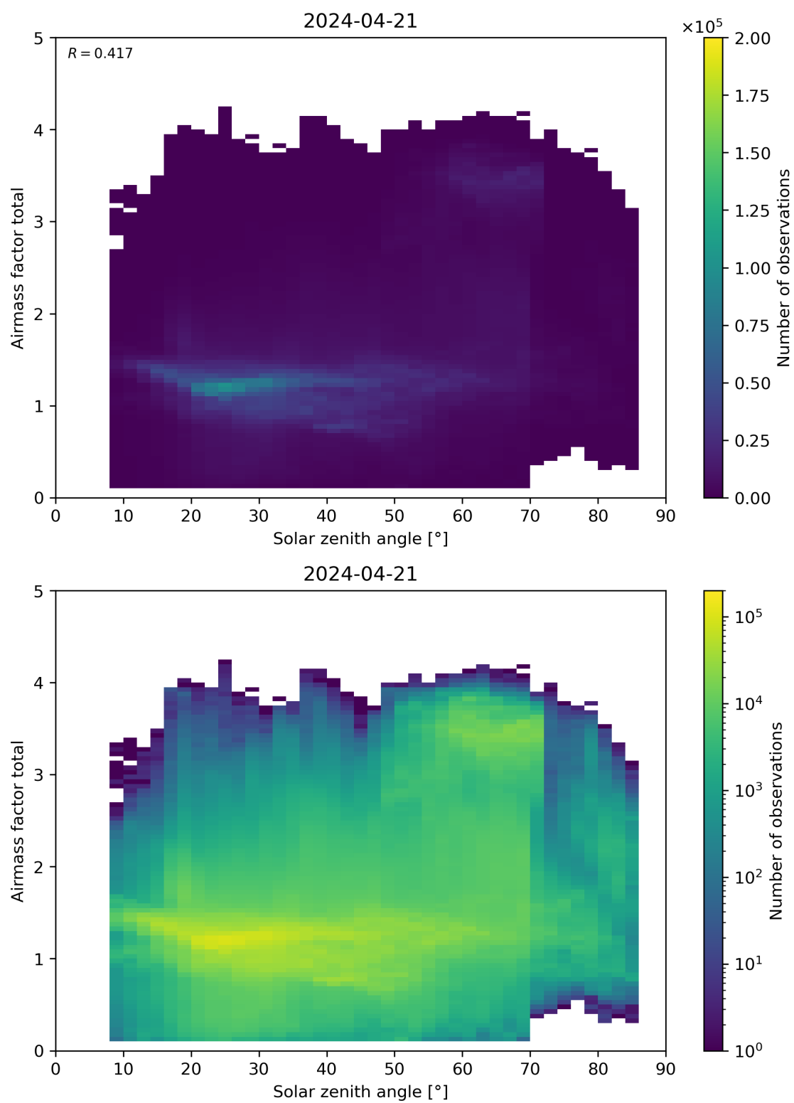
Figure 175: Scatter density plot of “Solar zenith angle” against “Airmass factor total” for 2024-04-21 to 2024-04-22.
