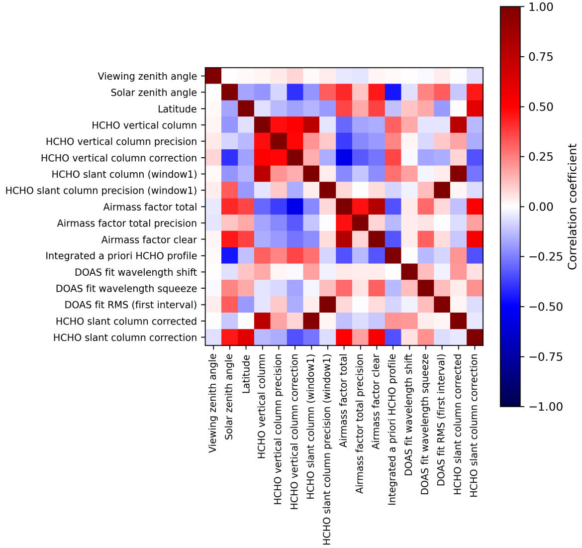
Figure 2: Map of correlation matrix for 2024-04-21 to 2024-04-22.
