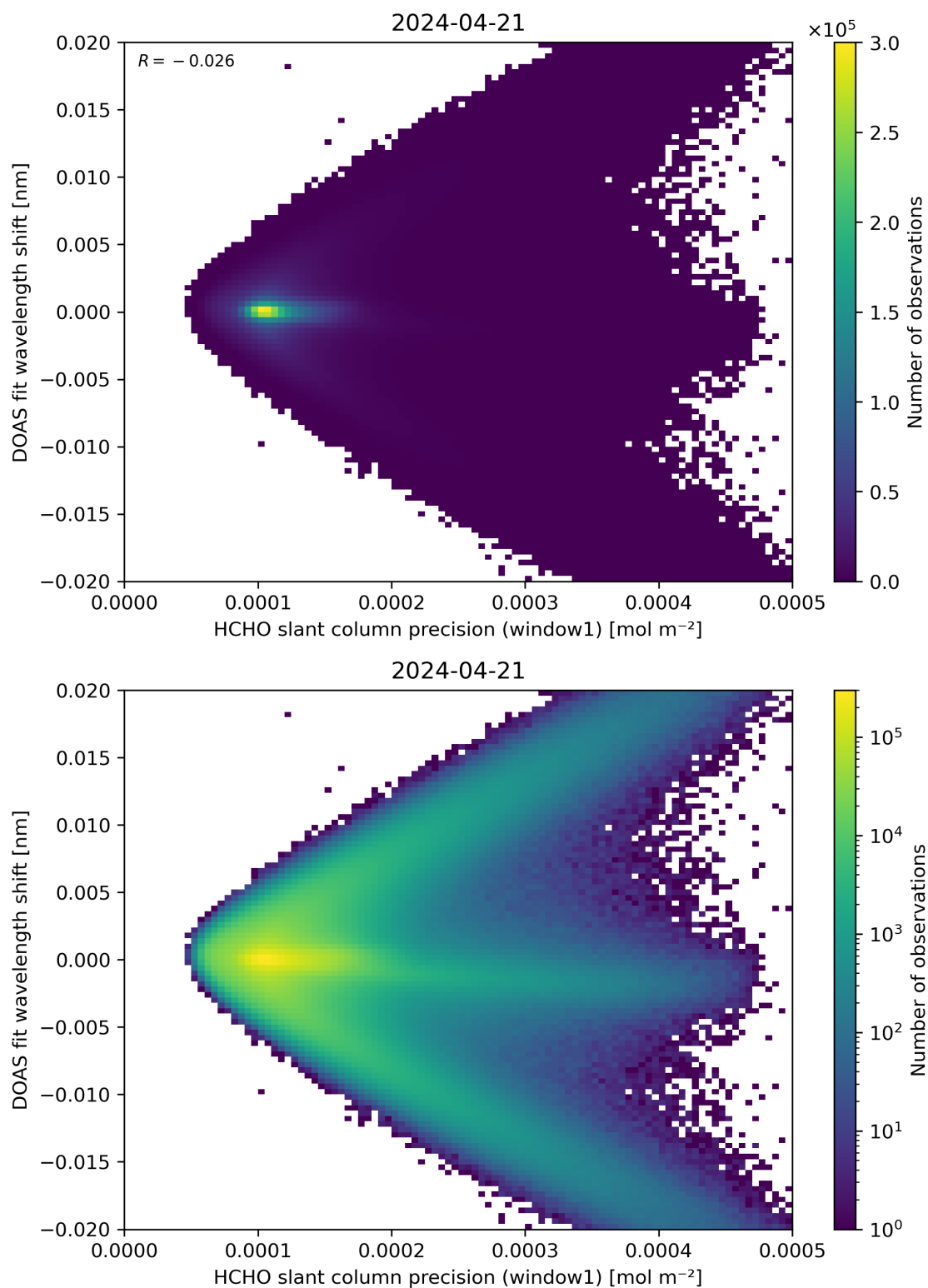
Figure 89: Scatter density plot of “HCHO slant column precision (window1)” against “DOAS fit wavelength shift” for 2024-04-21 to 2024-04-22.
