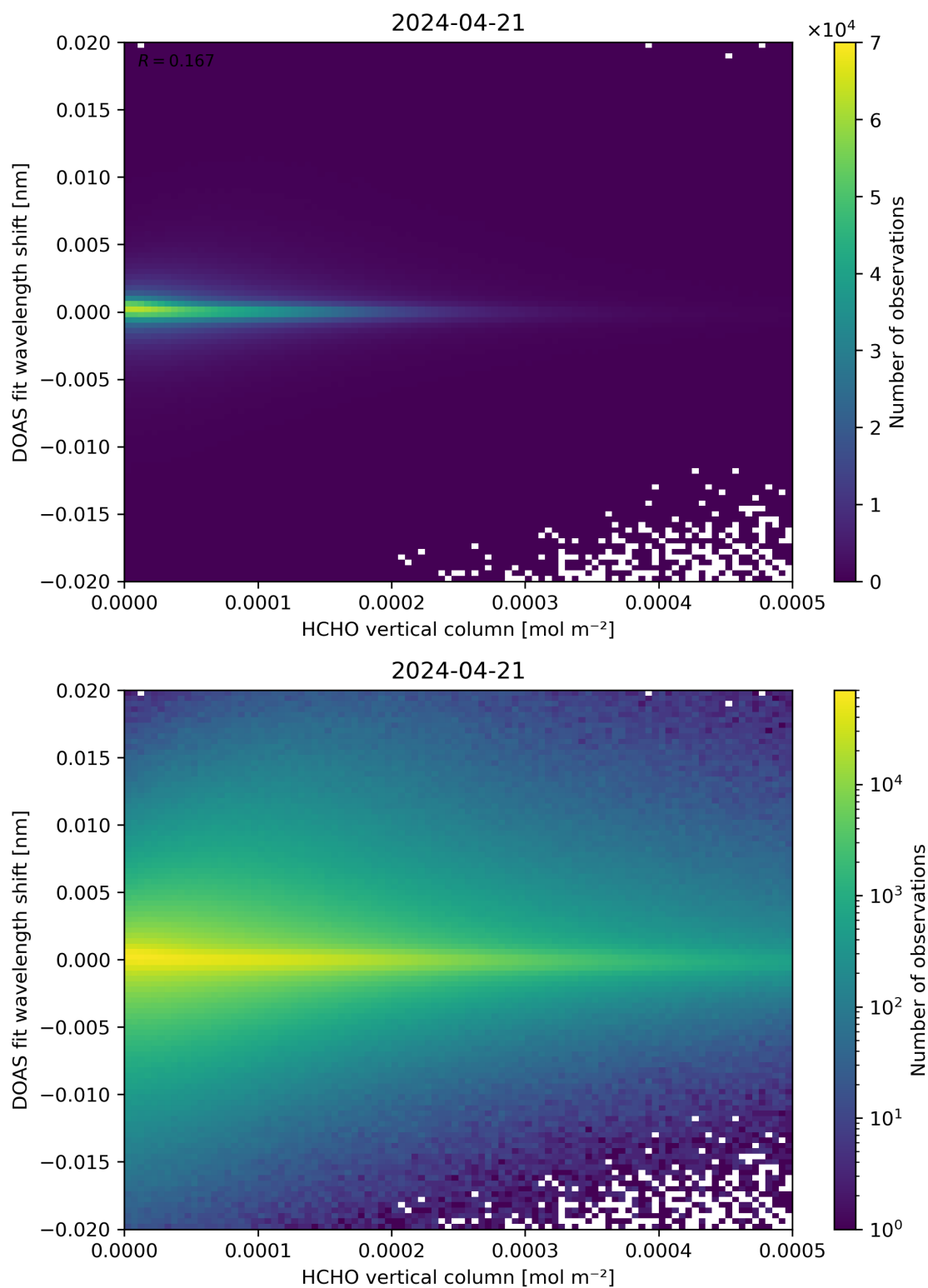
Figure 124: Scatter density plot of “HCHO vertical column” against “DOAS fit wavelength shift” for 2024-04-21 to 2024-04-22.
