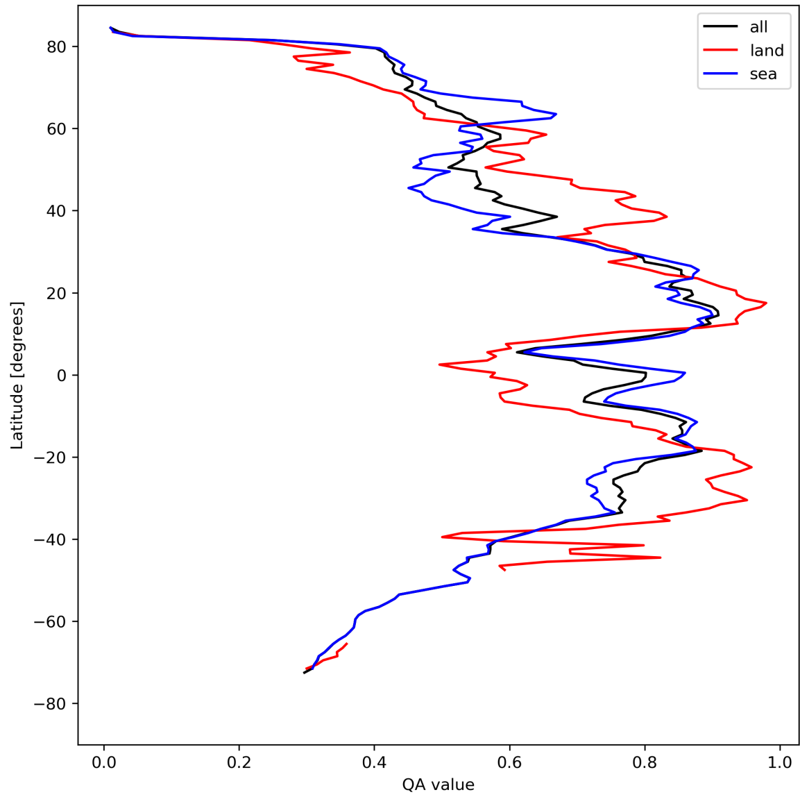
Figure 20: Zonal average of “QA value” for 2024-04-21 to 2024-04-22.
