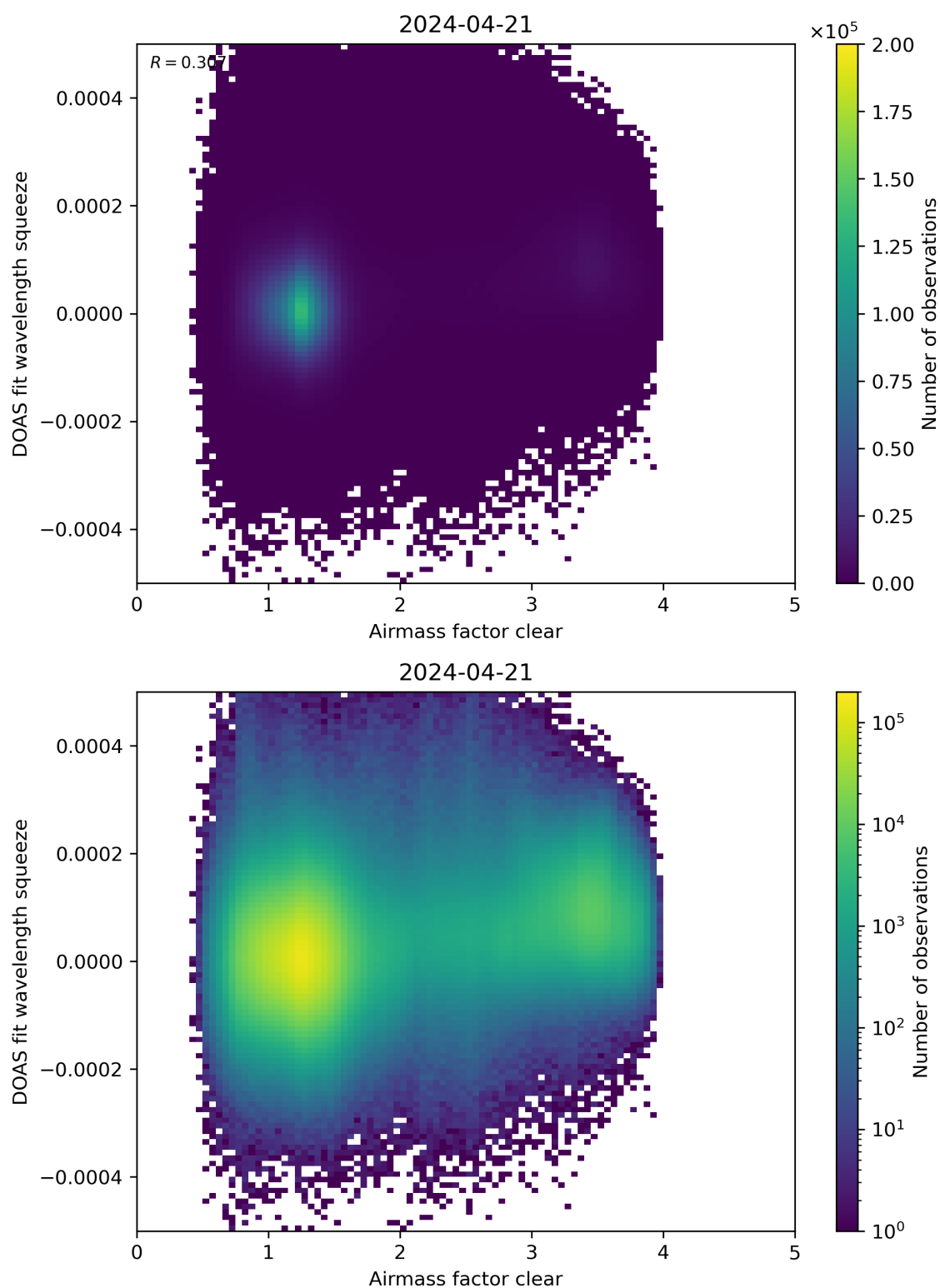
Figure 73: Scatter density plot of “Airmass factor clear” against “DOAS fit wavelength squeeze” for 2024-04-21 to 2024-04-22.
