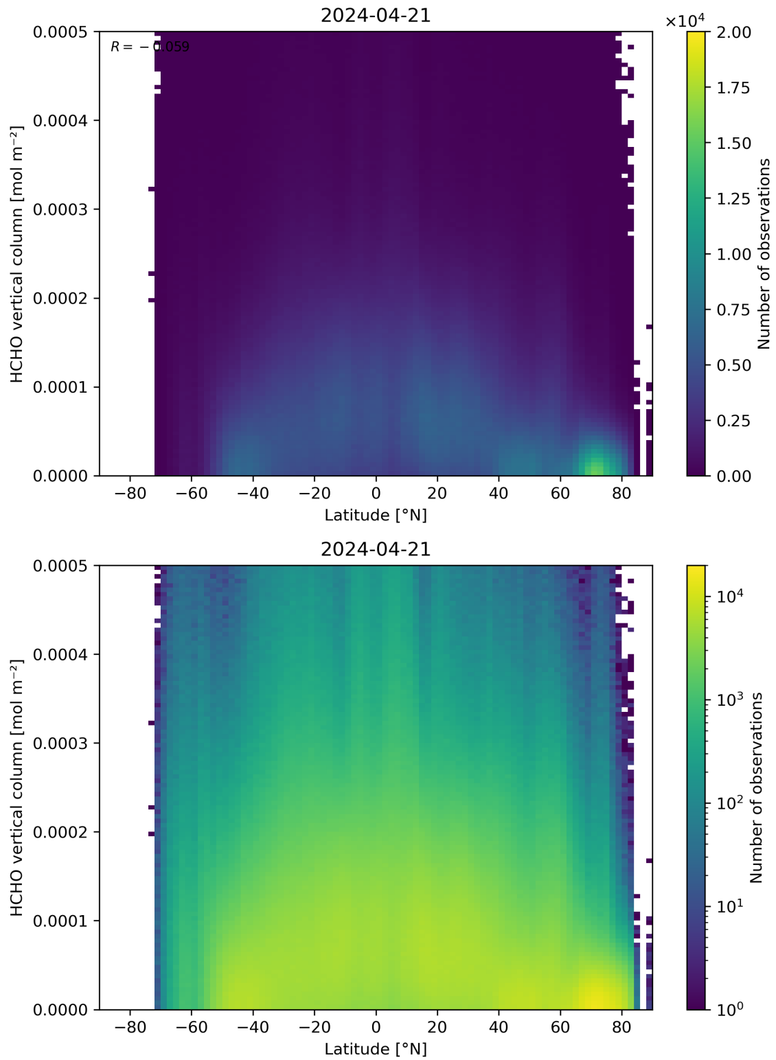
Figure 163: Scatter density plot of “Latitude” against “HCHO vertical column” for 2024-04-21 to 2024-04-22.
