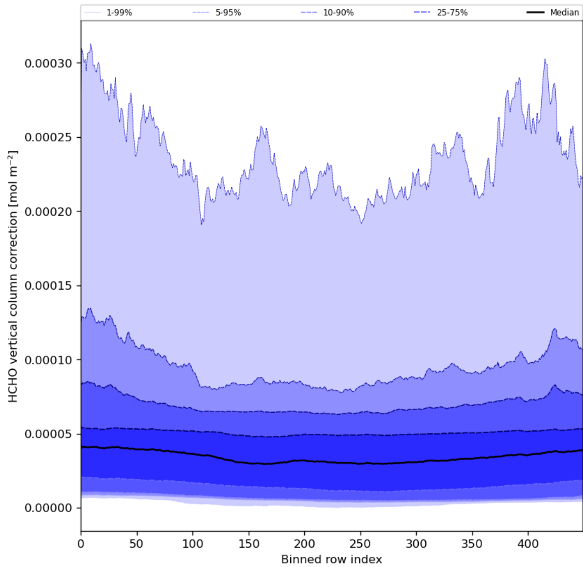
Figure 51: Along track statistics of “HCHO vertical column correction” for 2024-04-21 to 2024-04-22
