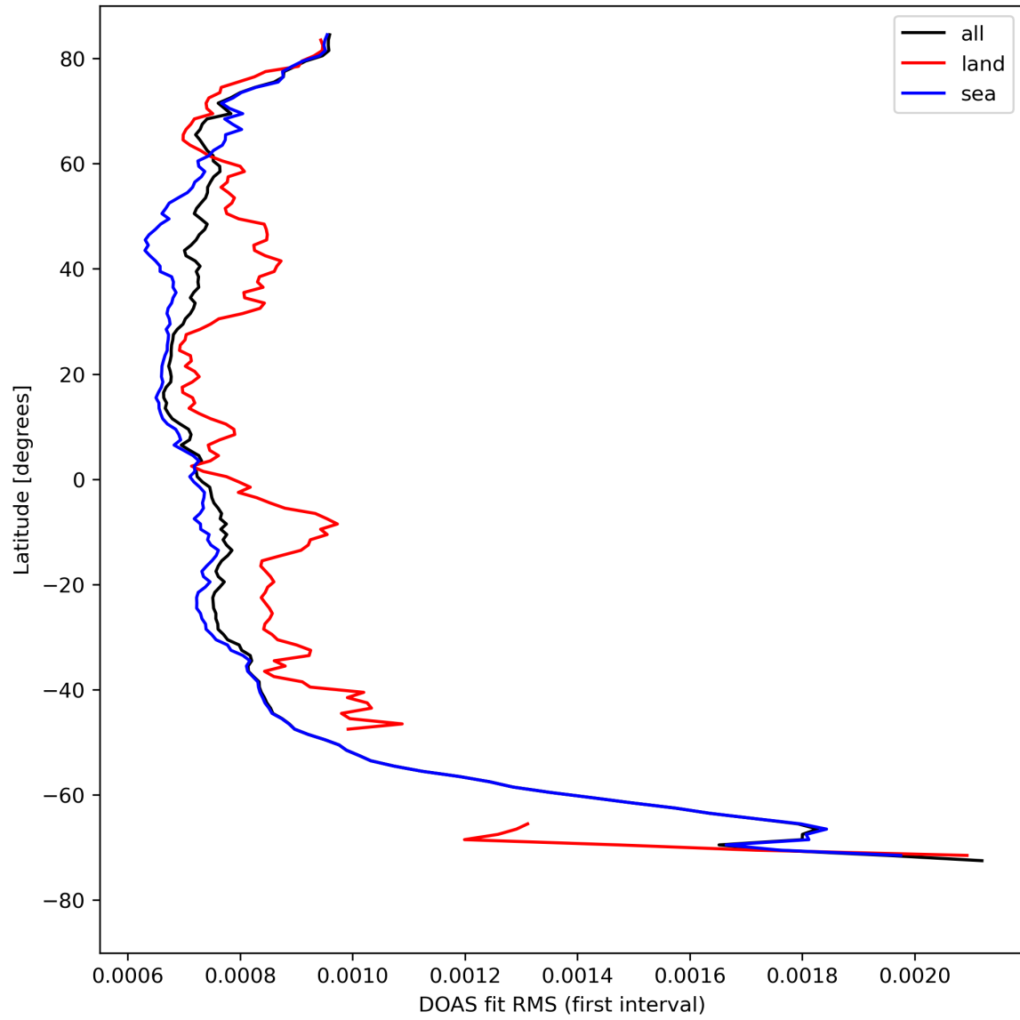
Figure 32: Zonal average of “DOAS fit RMS (first interval)” for 2024-04-21 to 2024-04-22.
