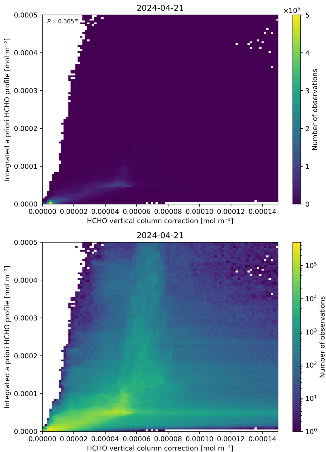
Figure 122: Scatter density plot of “HCHO vertical column correction” against “Integrated a priori HCHO profile” for 2024-04-21 to 2024-04-22.
