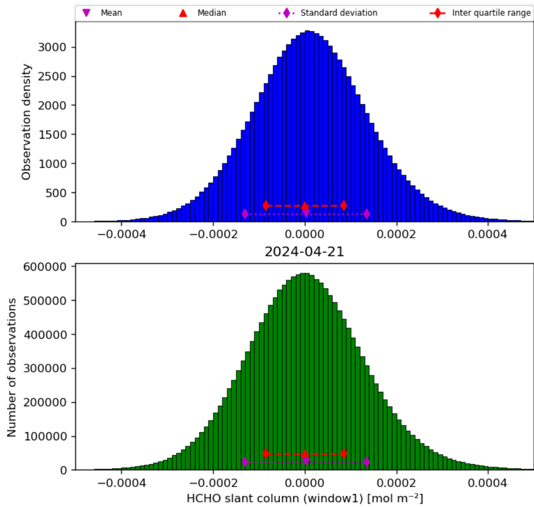
Figure 38: Histogram of “HCHO slant column (window1)” for 2024-04-21 to 2024-04-22
