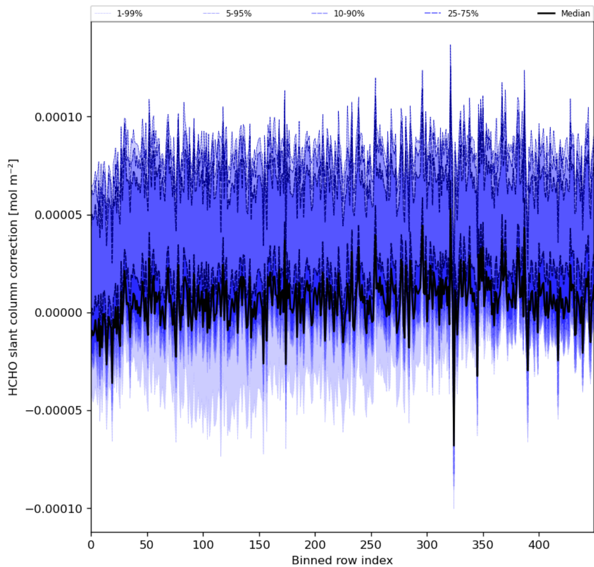
Figure 61: Along track statistics of “HCHO slant column correction” for 2024-04-21 to 2024-04-22
