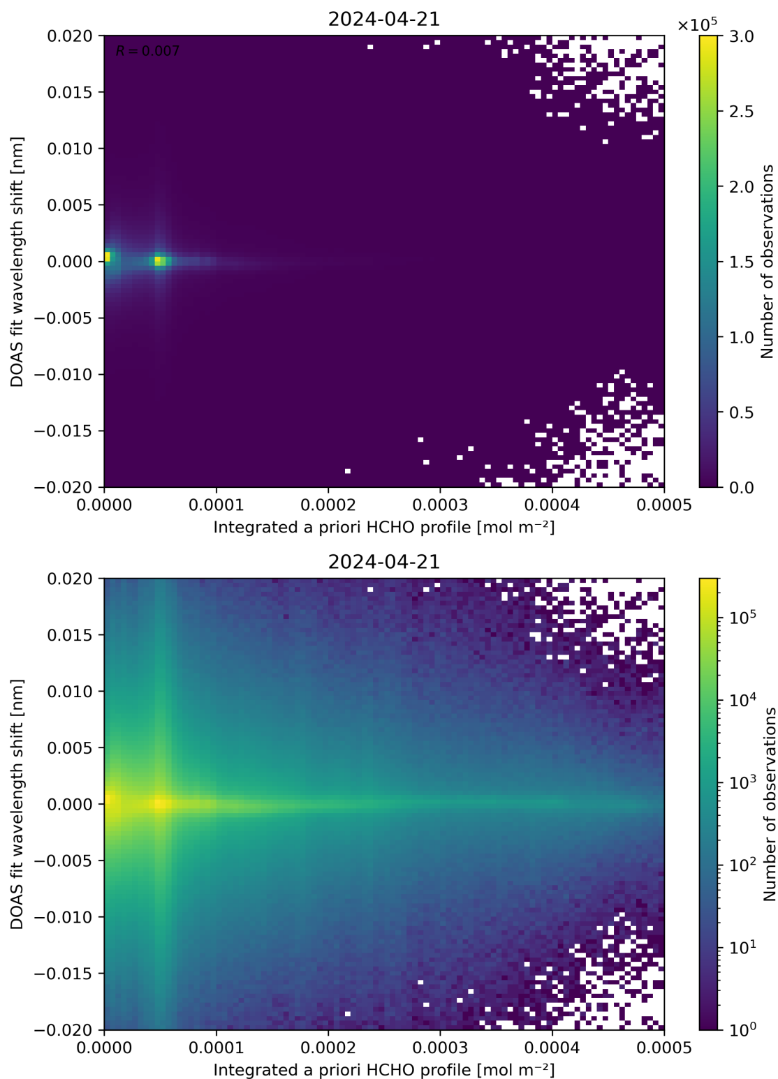
Figure 149: Scatter density plot of “Integrated a priori HCHO profile” against “DOAS fit wavelength shift” for 2024-04-21 to 2024-04-22.
