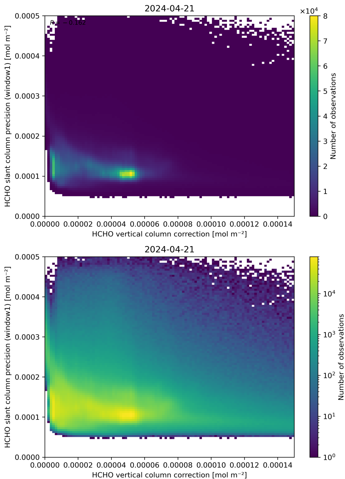
Figure 119: Scatter density plot of “HCHO vertical column correction” against “HCHO slant column precision (window1)” for 2024-04-21 to 2024-04-22.
