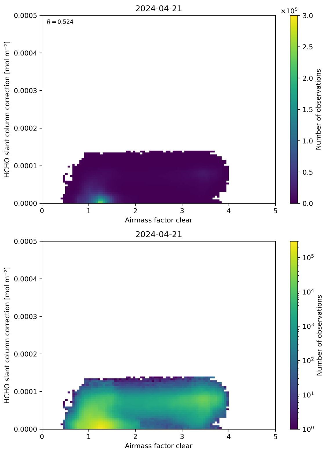
Figure 75: Scatter density plot of “Airmass factor clear” against “HCHO slant column correction” for 2024-04-21 to 2024-04-22.
