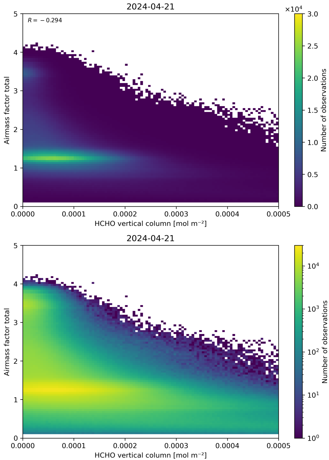
Figure 131: Scatter density plot of “HCHO vertical column” against “Airmass factor total” for 2024-04-21 to 2024-04-22.
