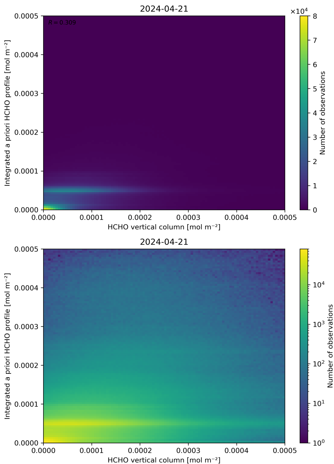
Figure 135: Scatter density plot of “HCHO vertical column” against “Integrated a priori HCHO profile” for 2024-04-21 to 2024-04-22.
