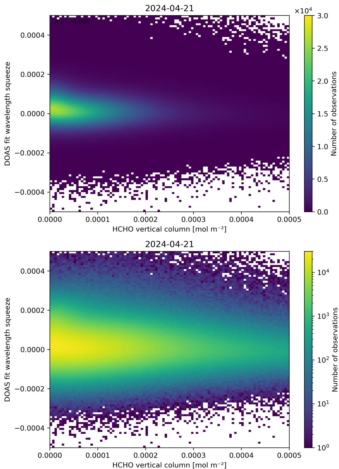
Figure 125: Scatter density plot of “HCHO vertical column” against “DOAS fit wavelength squeeze” for 2024-04-21 to 2024-04-22.
