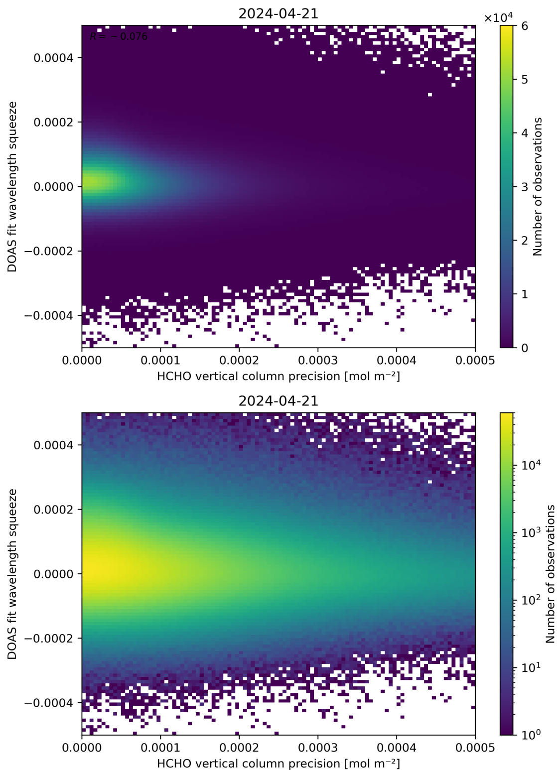
Figure 138: Scatter density plot of “HCHO vertical column precision” against “DOAS fit wavelength squeeze” for 2024-04-21 to 2024-04-22.
