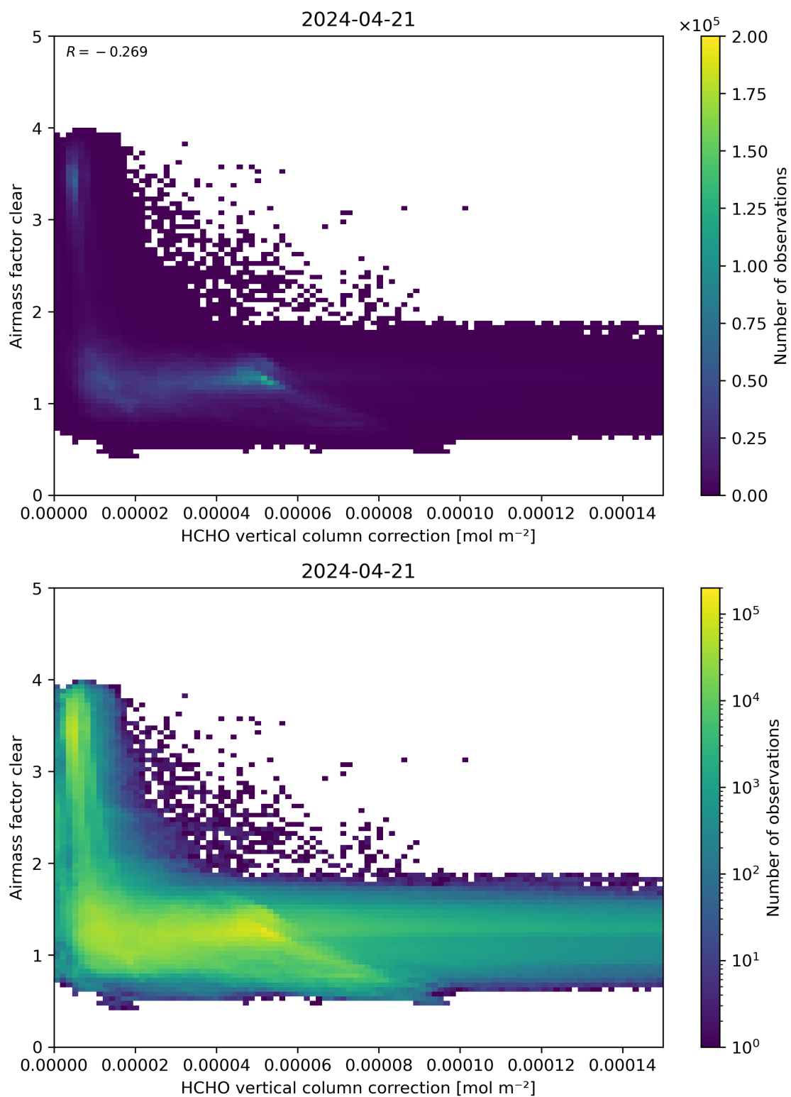
Figure 115: Scatter density plot of “HCHO vertical column correction” against “Airmass factor clear” for 2024-04-21 to 2024-04-22.
