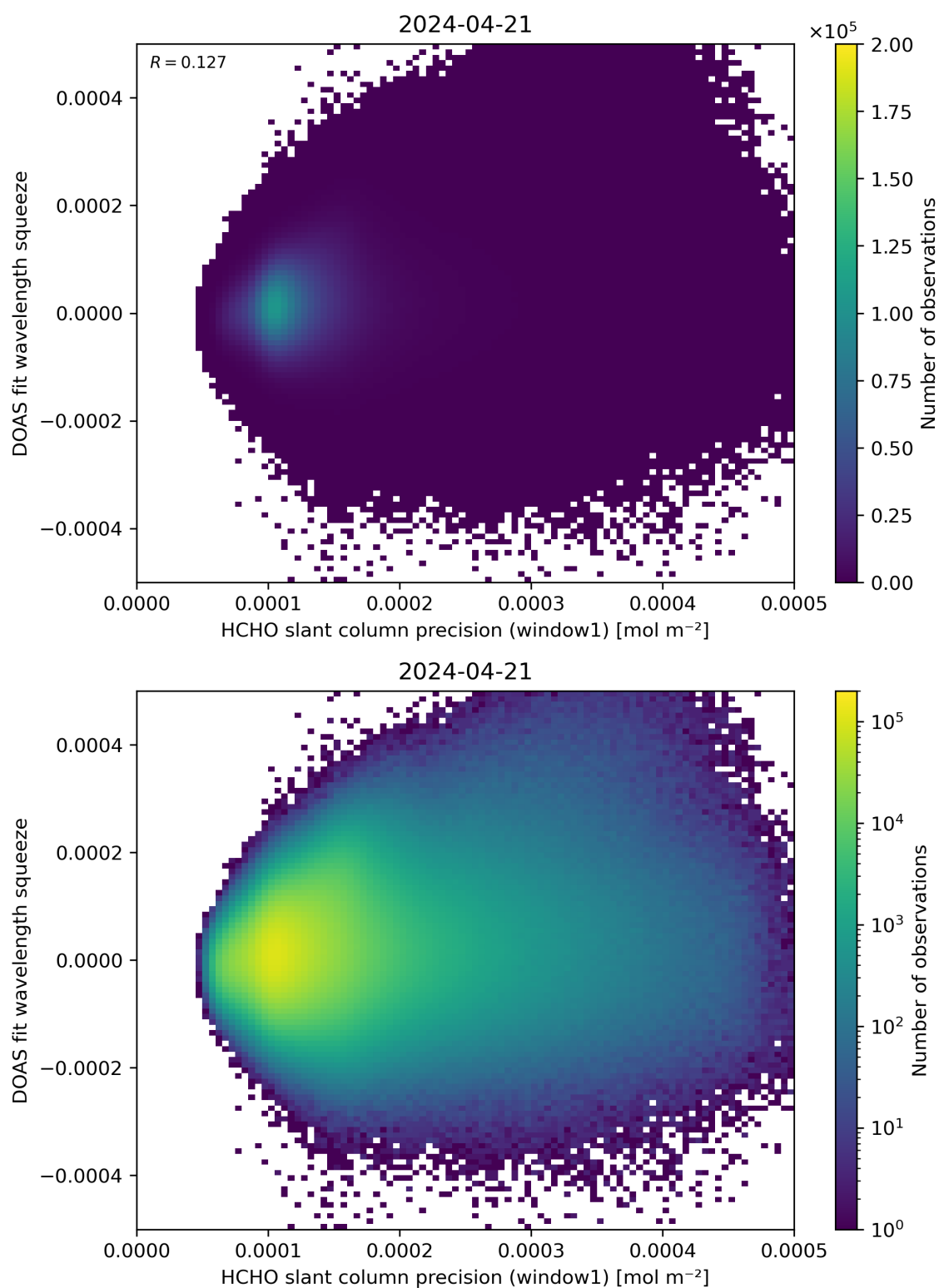
Figure 90: Scatter density plot of “HCHO slant column precision (window1)” against “DOAS fit wavelength squeeze” for 2024-04-21 to 2024-04-22.
