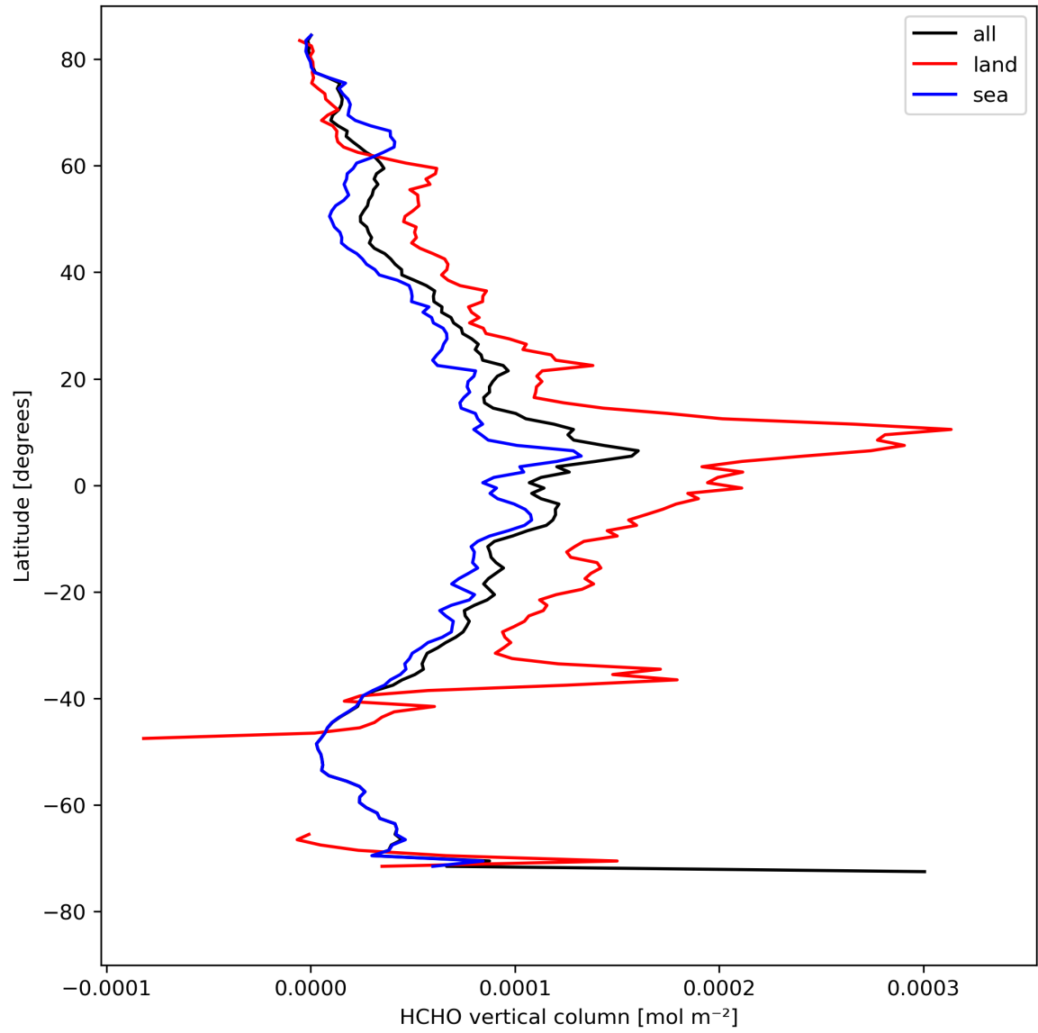
Figure 21: Zonal average of “HCHO vertical column” for 2024-04-21 to 2024-04-22.
