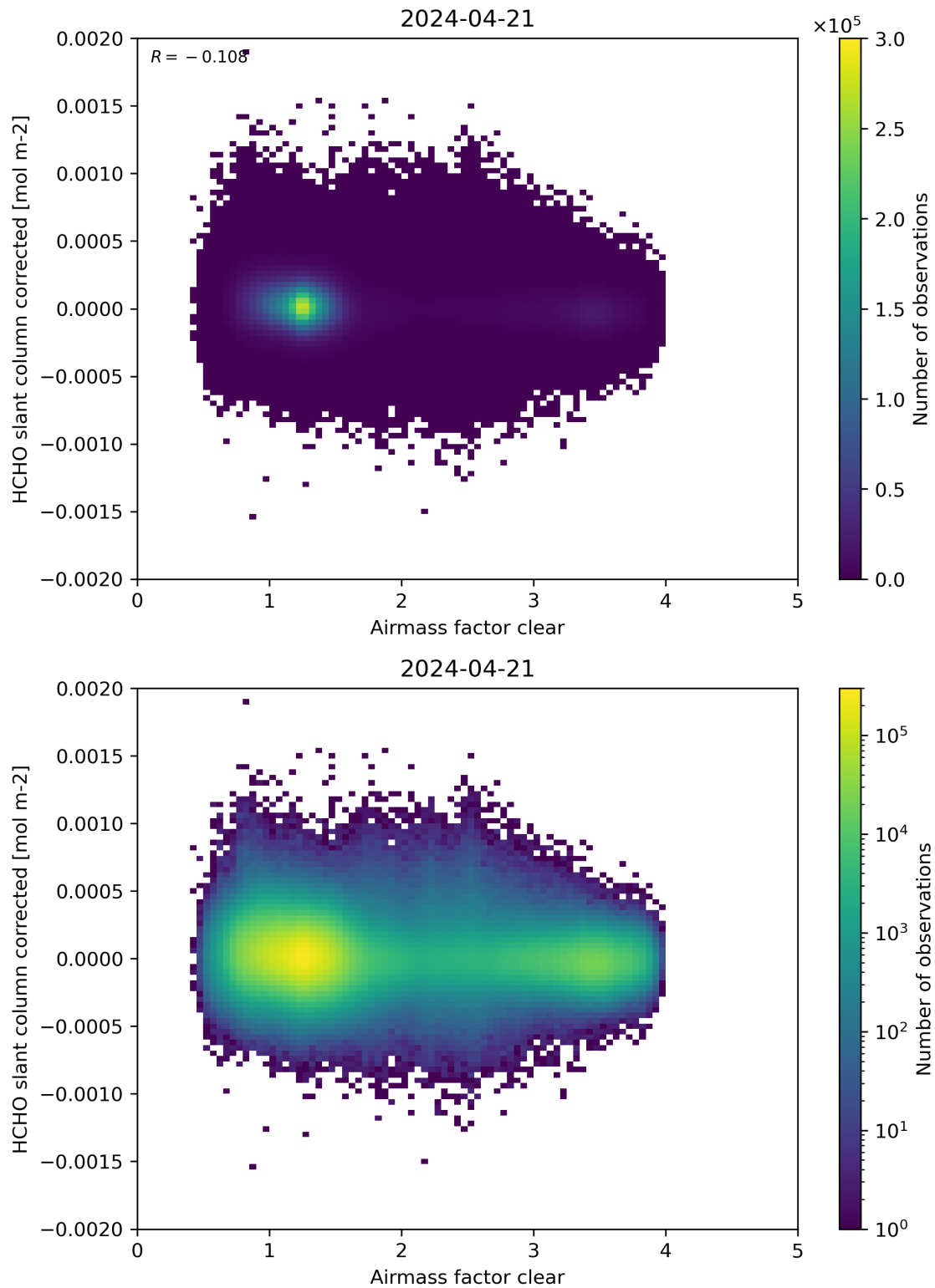
Figure 74: Scatter density plot of “Airmass factor clear” against “HCHO slant column corrected” for 2024-04-21 to 2024-04-22.
