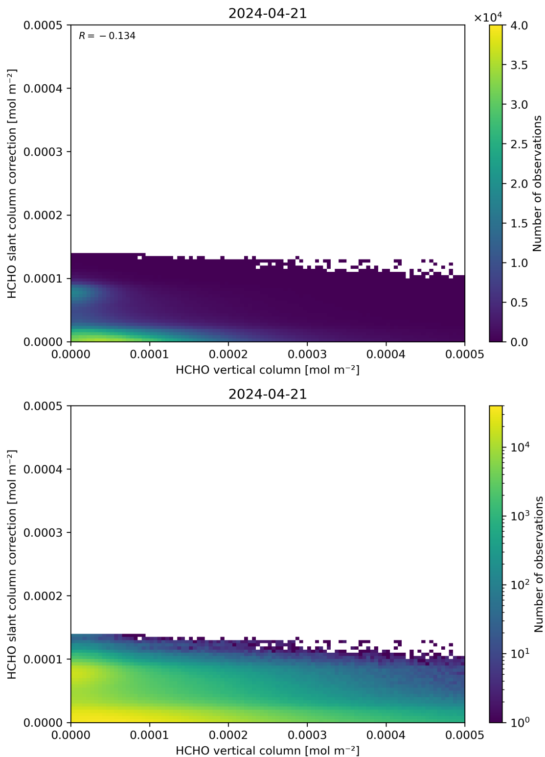
Figure 128: Scatter density plot of “HCHO vertical column” against “HCHO slant column correction” for 2024-04-21 to 2024-04-22.
