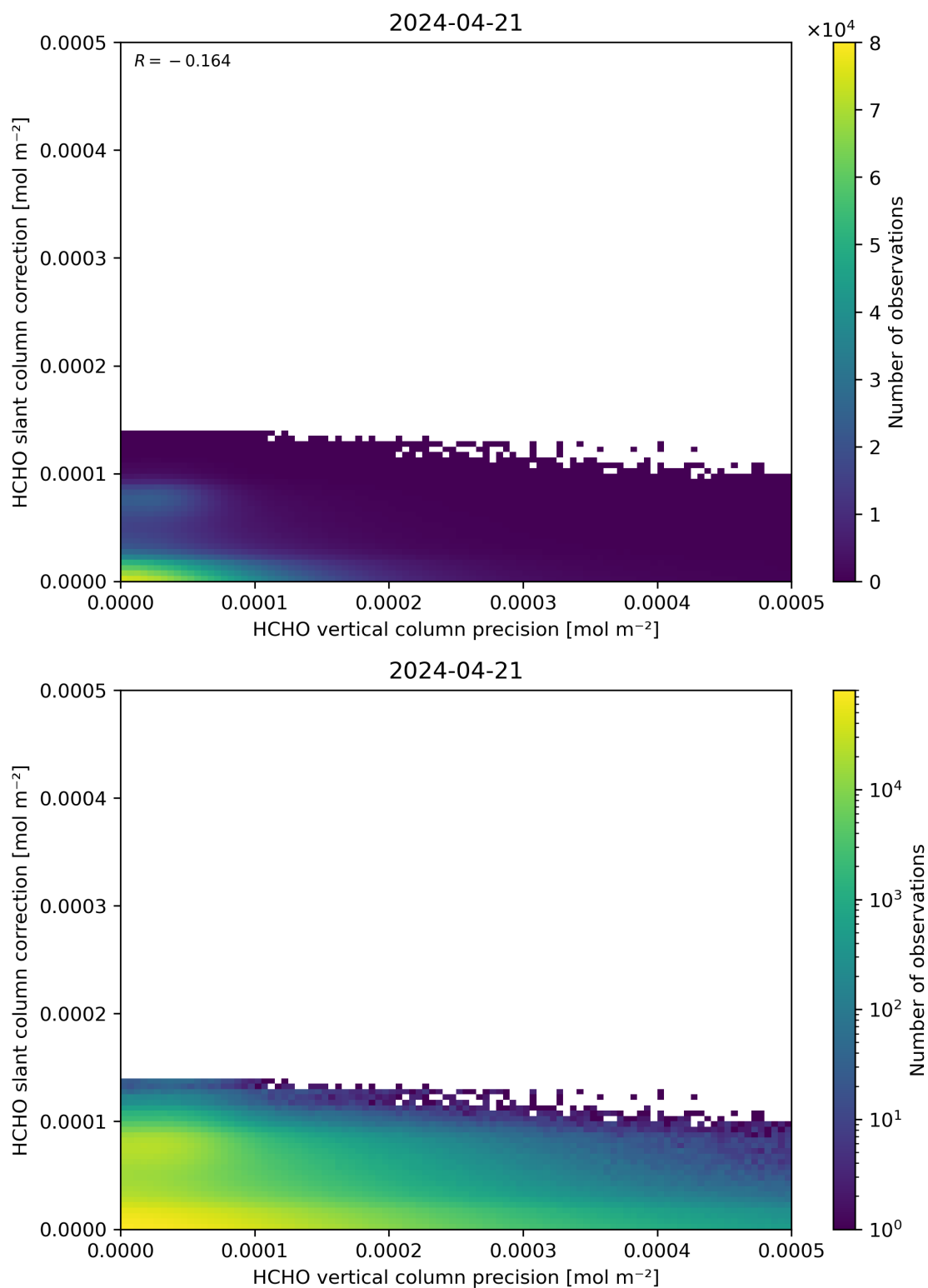
Figure 141: Scatter density plot of “HCHO vertical column precision” against “HCHO slant column correction” for 2024-04-21 to 2024-04-22.
