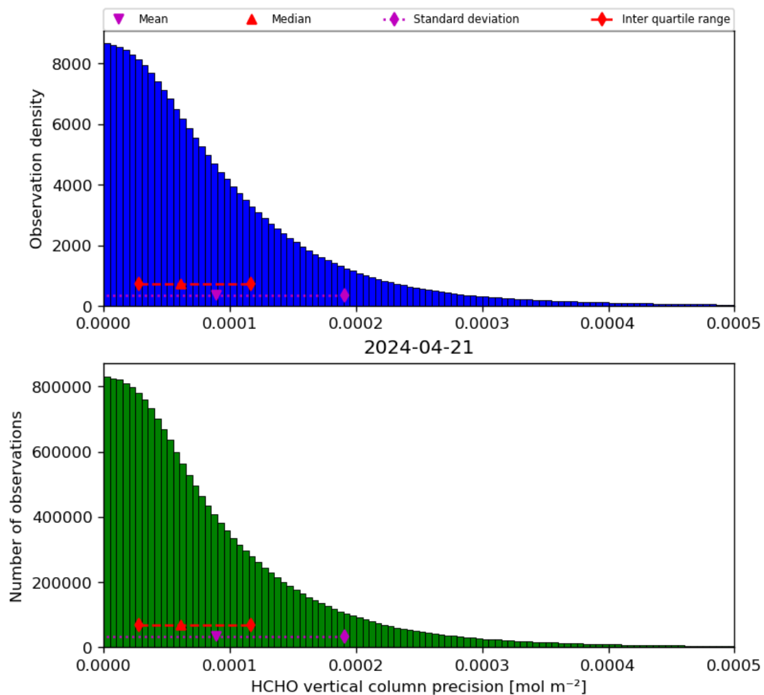
Figure 36: Histogram of “HCHO vertical column precision” for 2024-04-21 to 2024-04-22
