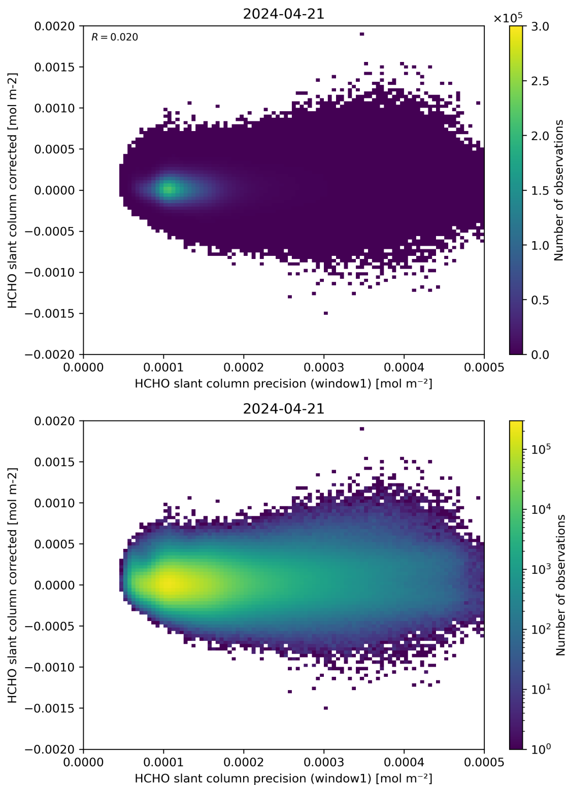
Figure 92: Scatter density plot of “HCHO slant column precision (window1)” against “HCHO slant column corrected” for 2024-04-21 to 2024-04-22.
