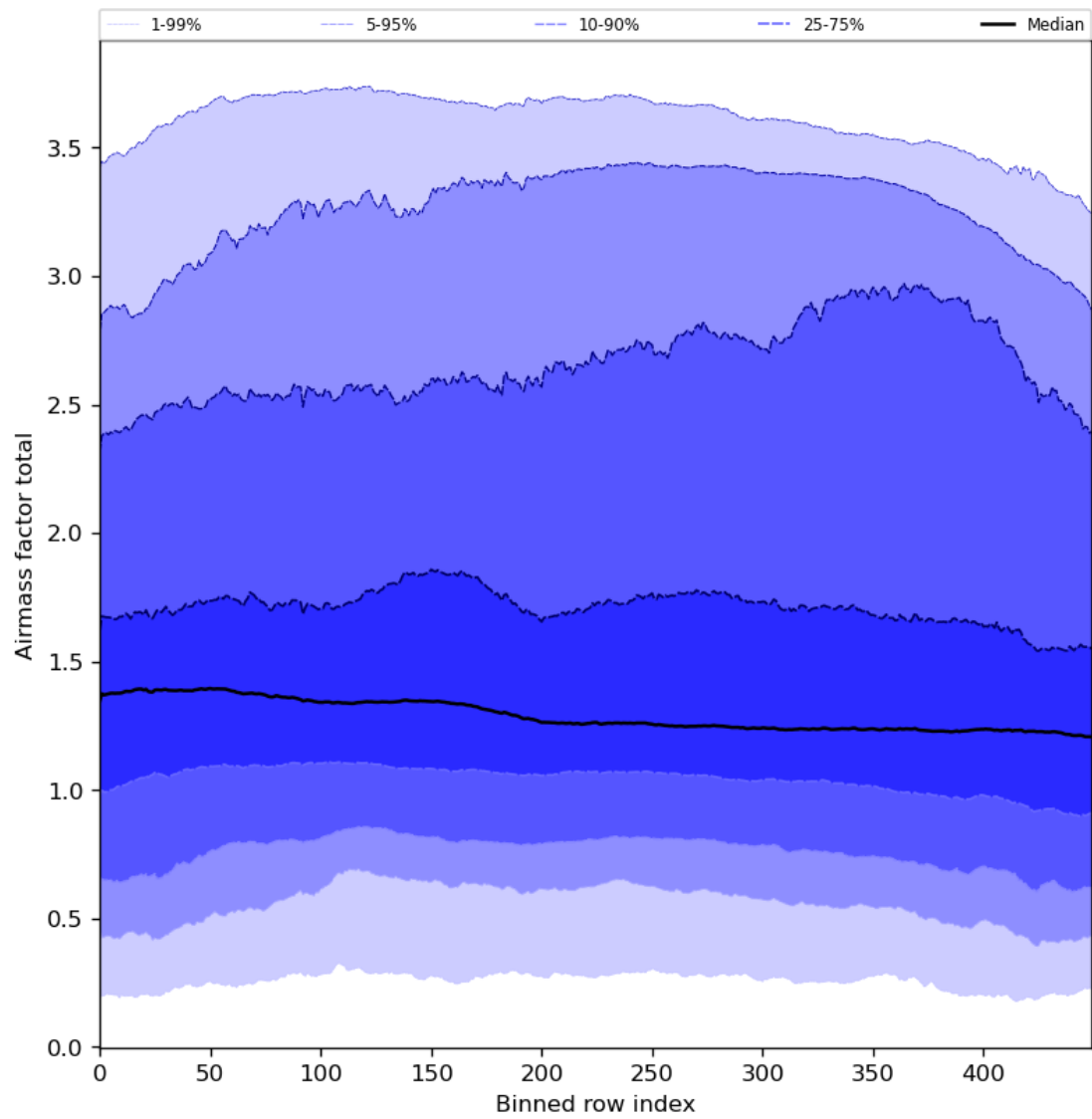
Figure 54: Along track statistics of “Airmass factor total” for 2024-04-21 to 2024-04-22
