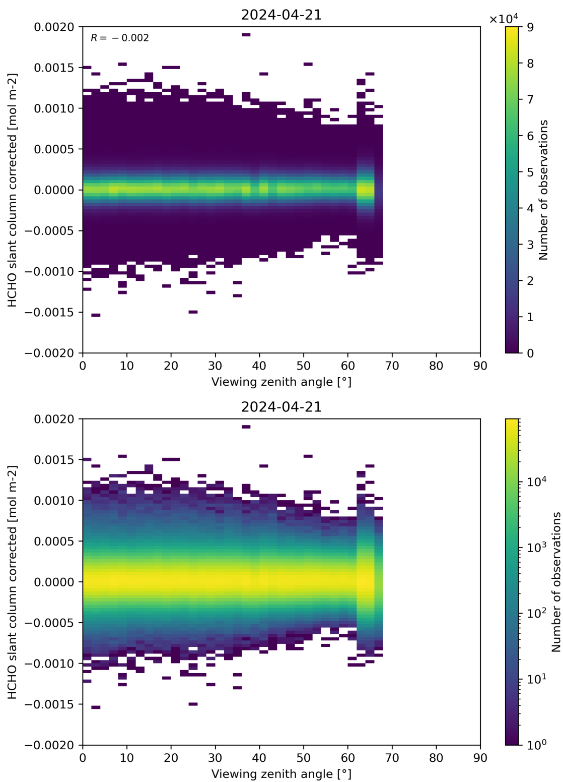
Figure 186: Scatter density plot of “Viewing zenith angle” against “HCHO slant column corrected” for 2024-04-21 to 2024-04-22.
