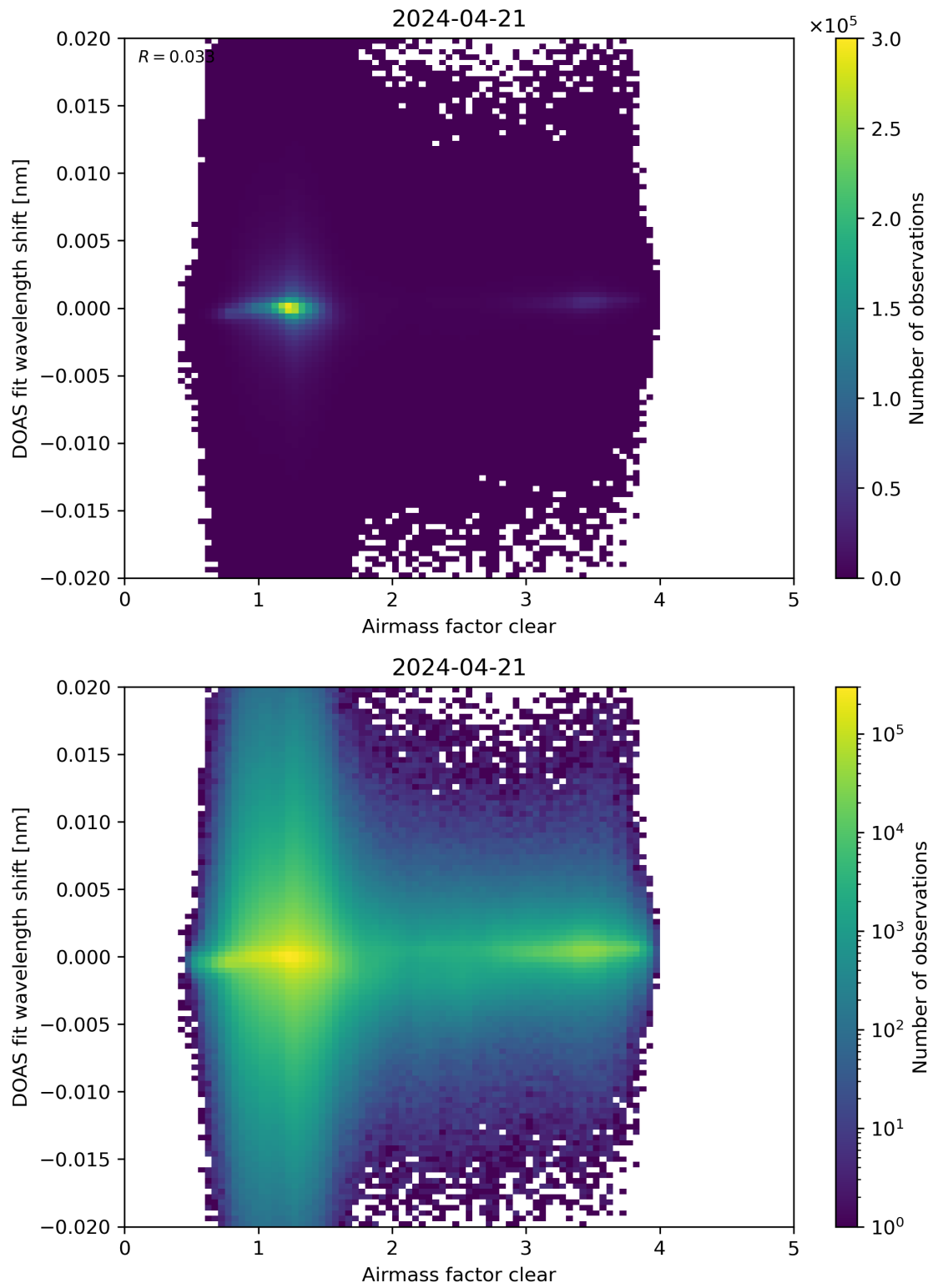
Figure 72: Scatter density plot of “Airmass factor clear” against “DOAS fit wavelength shift” for 2024-04-21 to 2024-04-22.
