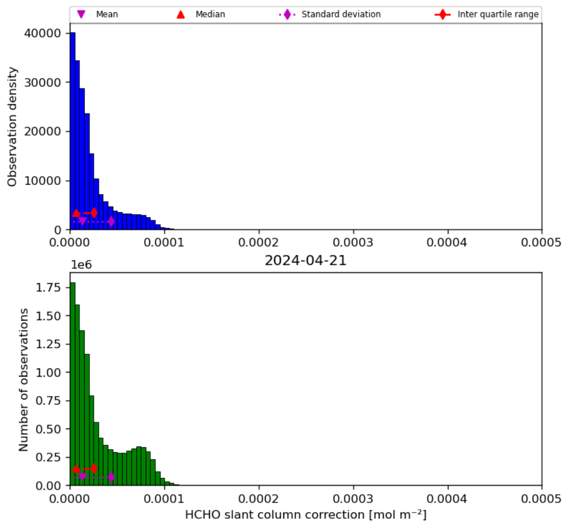
Figure 47: Histogram of “HCHO slant column correction” for 2024-04-21 to 2024-04-22
