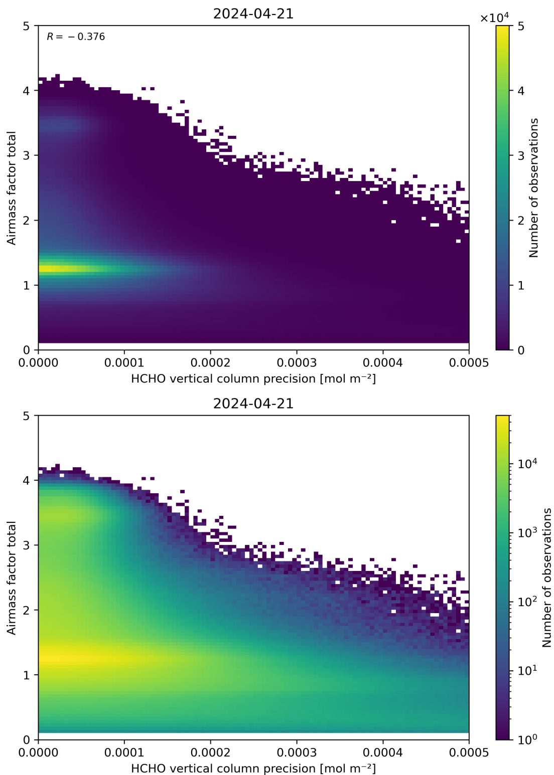
Figure 144: Scatter density plot of “HCHO vertical column precision” against “Airmass factor total” for 2024-04-21 to 2024-04-22.
