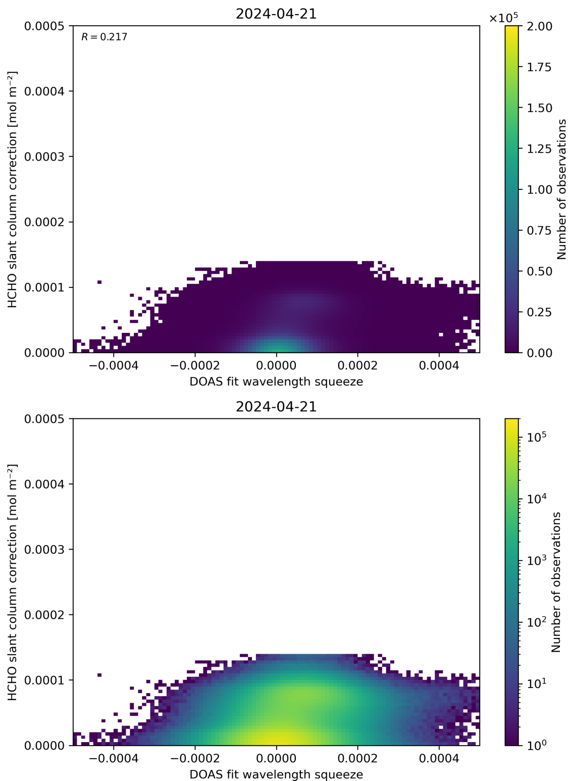
Figure 70: Scatter density plot of “DOAS fit wavelength squeeze” against “HCHO slant column correction” for 2024-04-21 to 2024-04-22.
