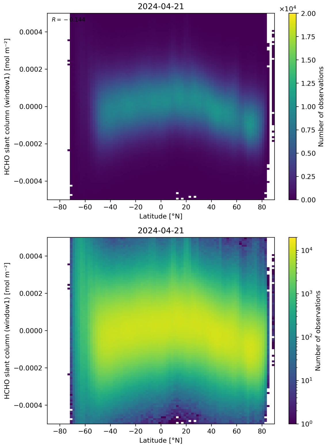
Figure 159: Scatter density plot of “Latitude” against “HCHO slant column (window1)” for 2024-04-21 to 2024-04-22.
