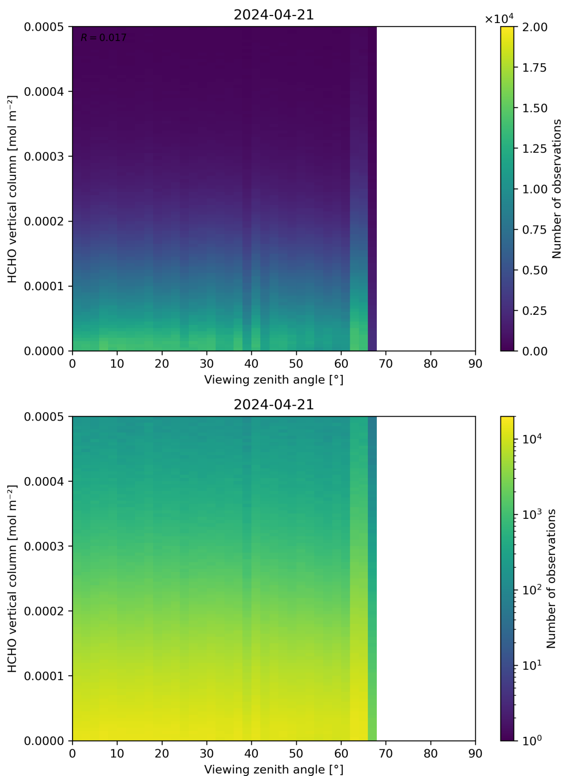
Figure 192: Scatter density plot of “Viewing zenith angle” against “HCHO vertical column” for 2024-04-21 to 2024-04-22.
