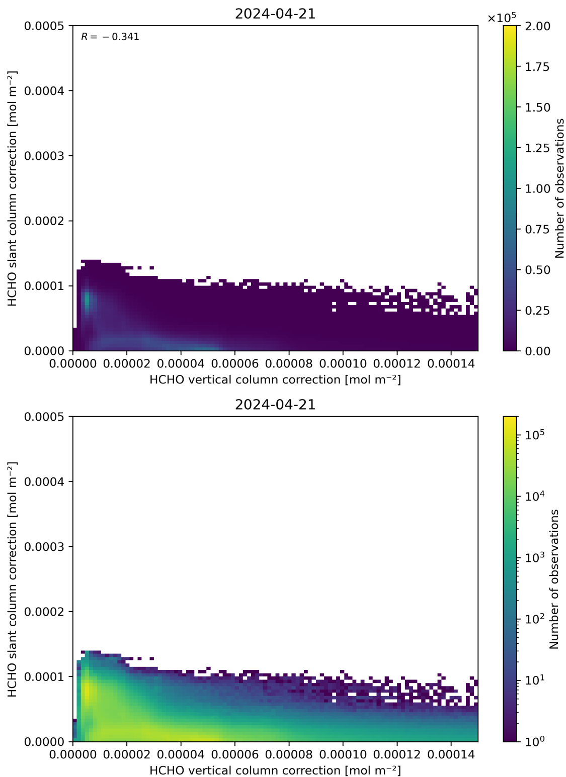
Figure 117: Scatter density plot of “HCHO vertical column correction” against “HCHO slant column correction” for 2024-04-21 to 2024-04-22.
