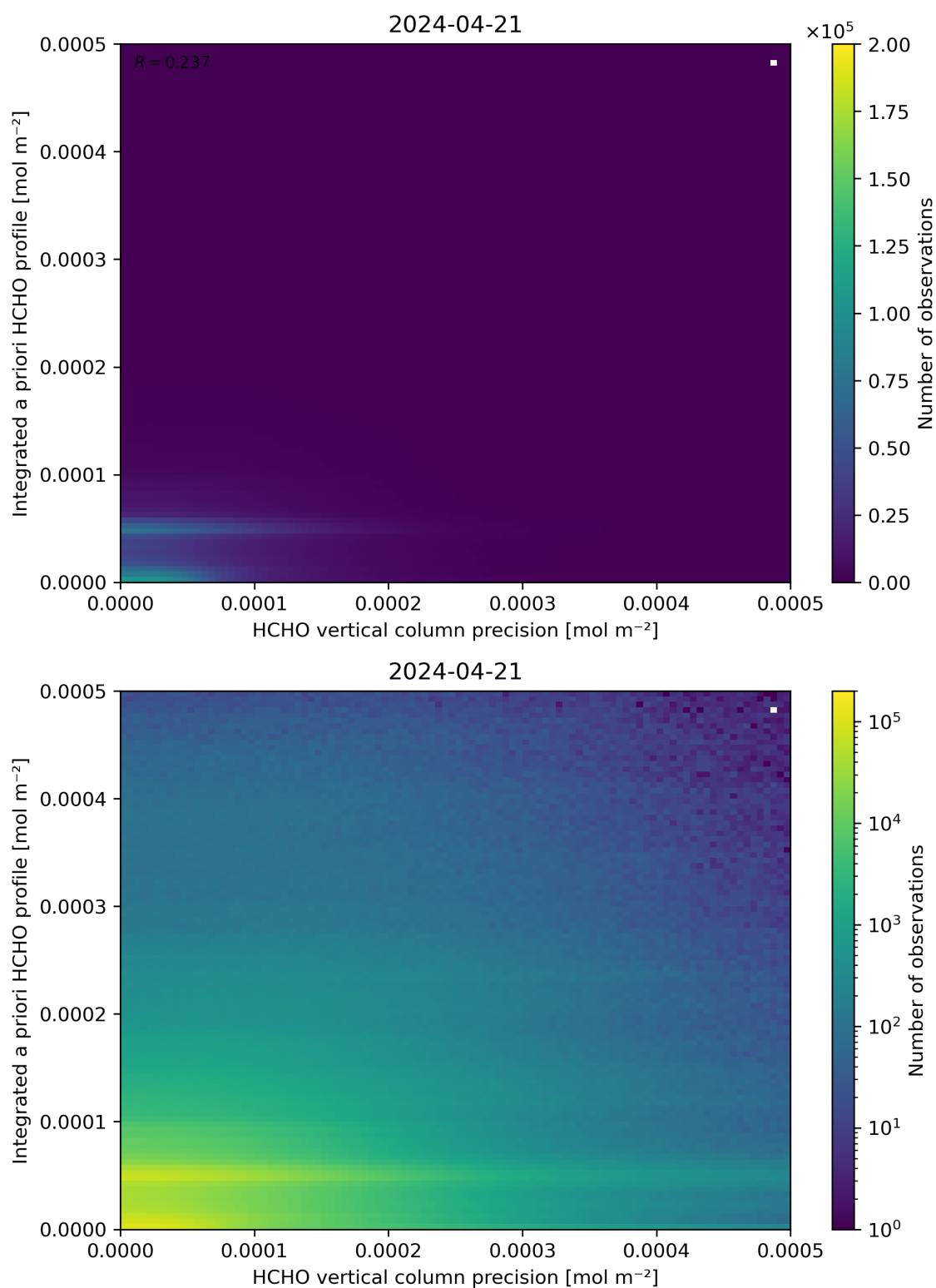
Figure 147: Scatter density plot of “HCHO vertical column precision” against “Integrated a priori HCHO profile” for 2024-04-21 to 2024-04-22.
