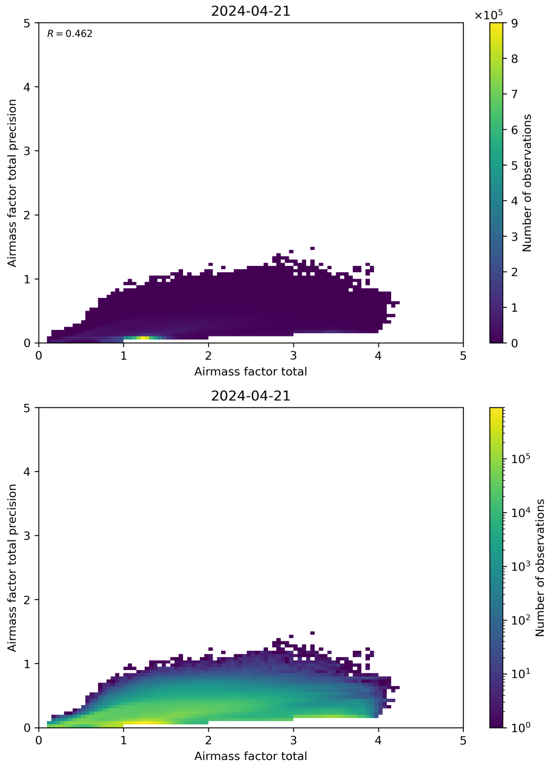
Figure 103: Scatter density plot of “Airmass factor total” against “Airmass factor total precision” for 2024-04-21 to 2024-04-22.
