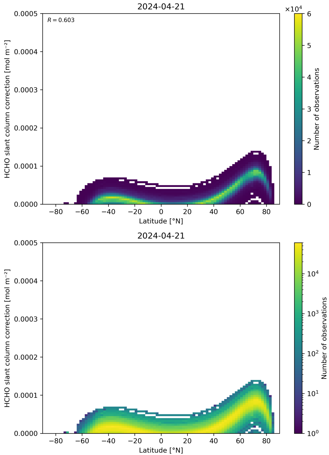
Figure 158: Scatter density plot of “Latitude” against “HCHO slant column correction” for 2024-04-21 to 2024-04-22.
