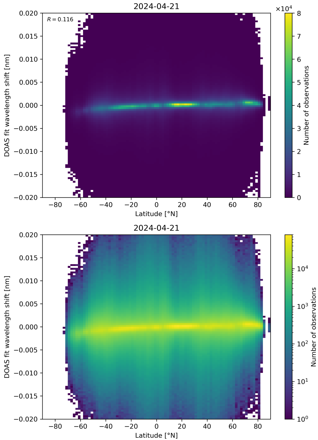
Figure 154: Scatter density plot of “Latitude” against “DOAS fit wavelength shift” for 2024-04-21 to 2024-04-22.
