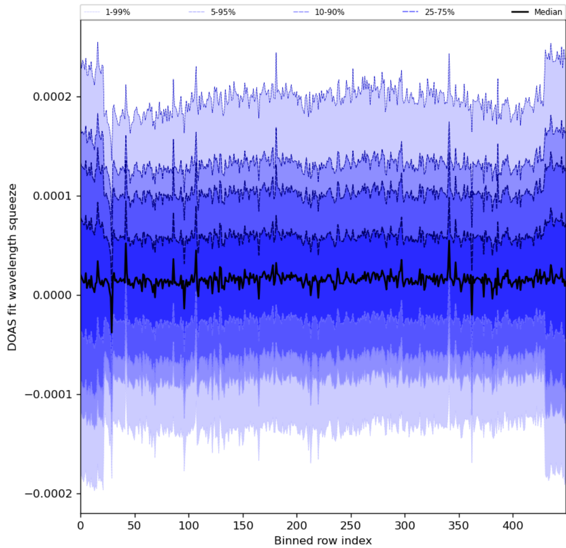
Figure 59: Along track statistics of “DOAS fit wavelength squeeze” for 2024-04-21 to 2024-04-22
