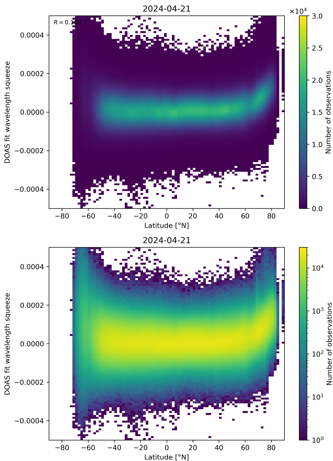
Figure 155: Scatter density plot of “Latitude” against “DOAS fit wavelength squeeze” for 2024-04-21 to 2024-04-22.
