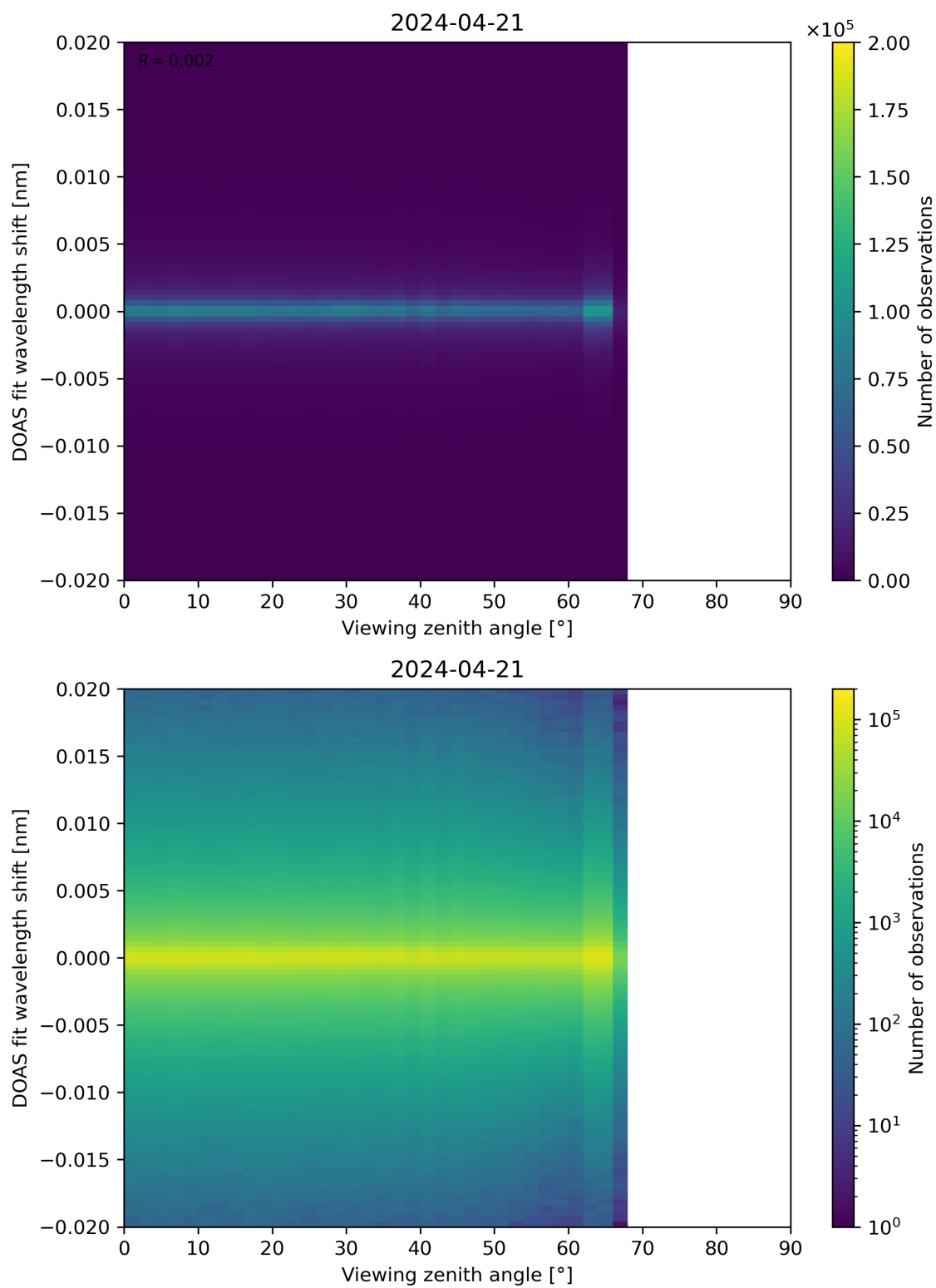
Figure 183: Scatter density plot of “Viewing zenith angle” against “DOAS fit wavelength shift” for 2024-04-21 to 2024-04-22.
