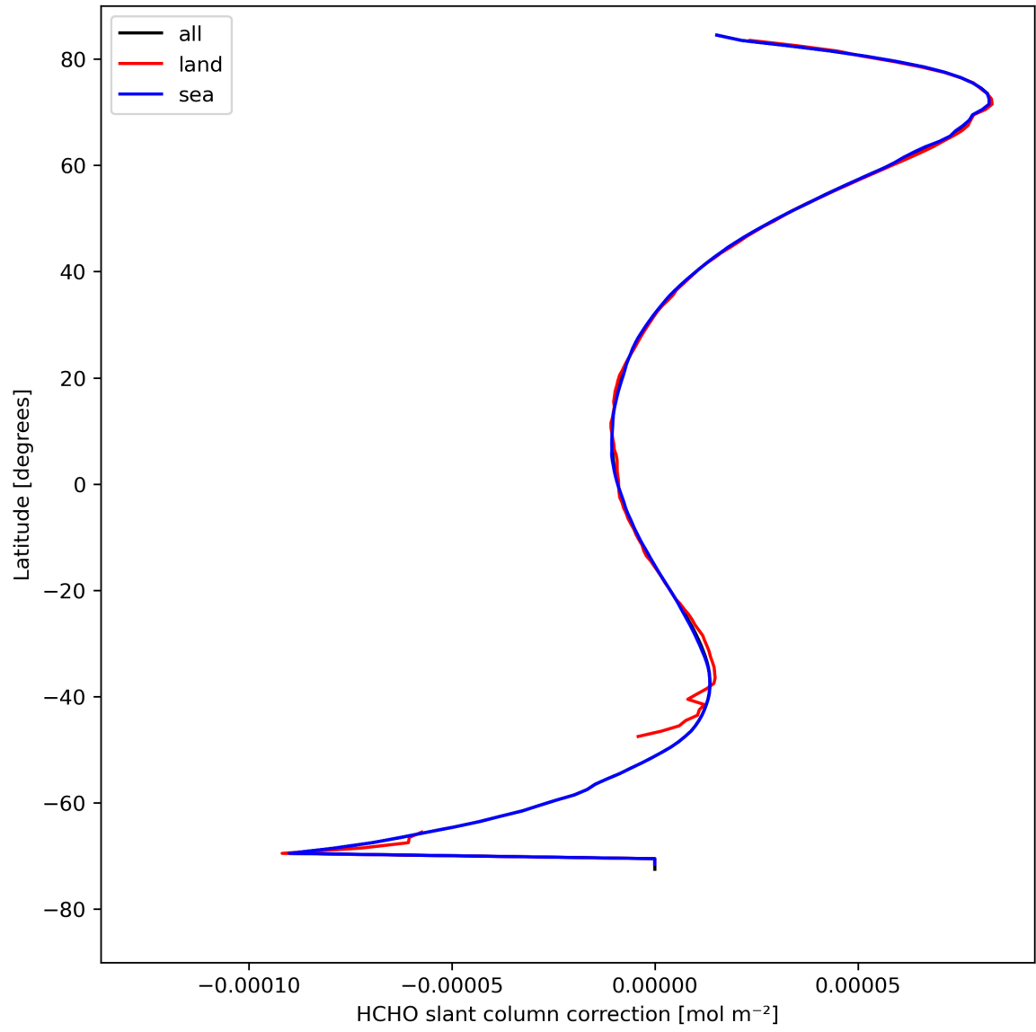
Figure 33: Zonal average of “HCHO slant column correction” for 2024-04-21 to 2024-04-22.
