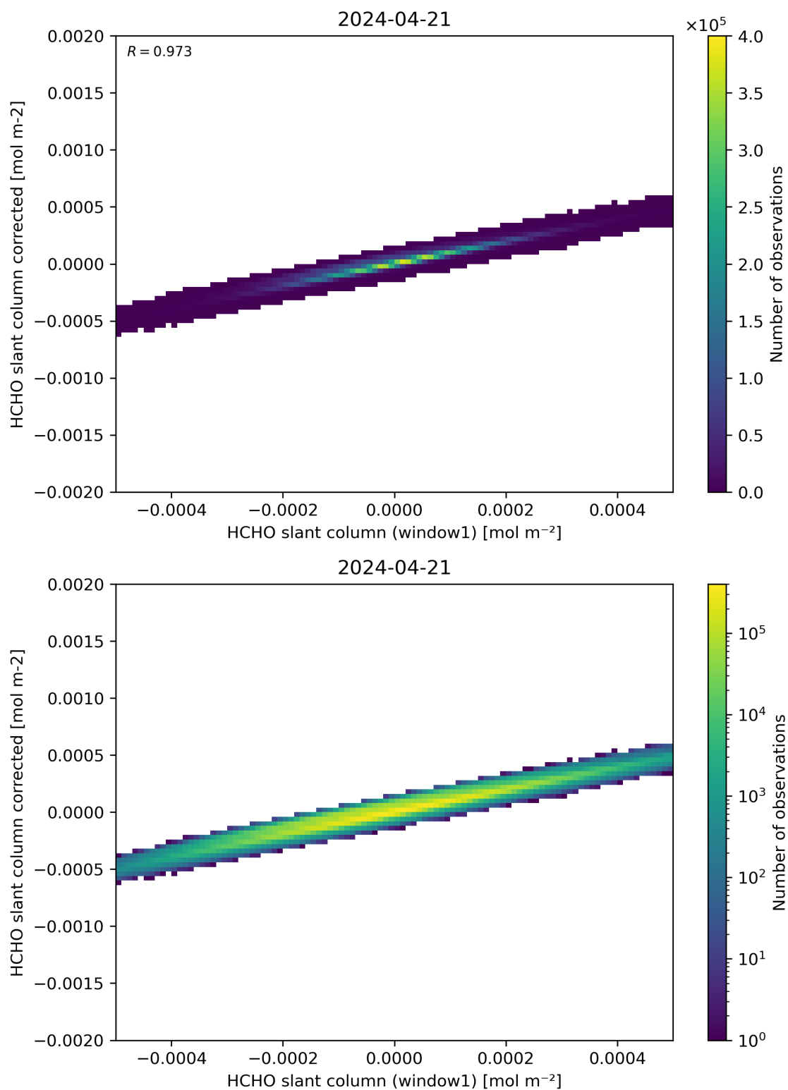
Figure 82: Scatter density plot of “HCHO slant column (window1)” against “HCHO slant column corrected” for 2024-04-21 to 2024-04-22.
