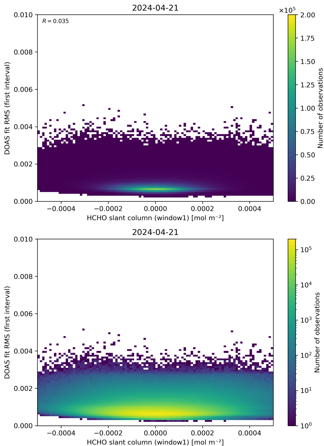
Figure 78: Scatter density plot of “HCHO slant column (window1)” against “DOAS fit RMS (first interval)” for 2024-04-21 to 2024-04-22.
