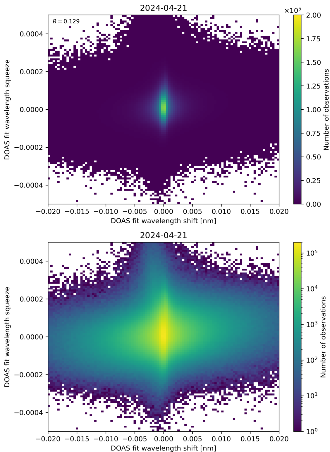
Figure 65: Scatter density plot of “DOAS fit wavelength shift” against “DOAS fit wavelength squeeze” for 2024-04-21 to 2024-04-22.
