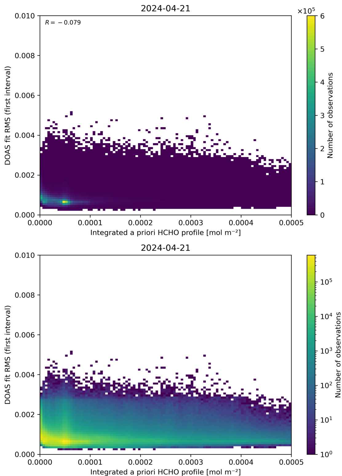
Figure 148: Scatter density plot of “Integrated a priori HCHO profile” against “DOAS fit RMS (first interval)” for 2024-04-21 to 2024-04-22.
