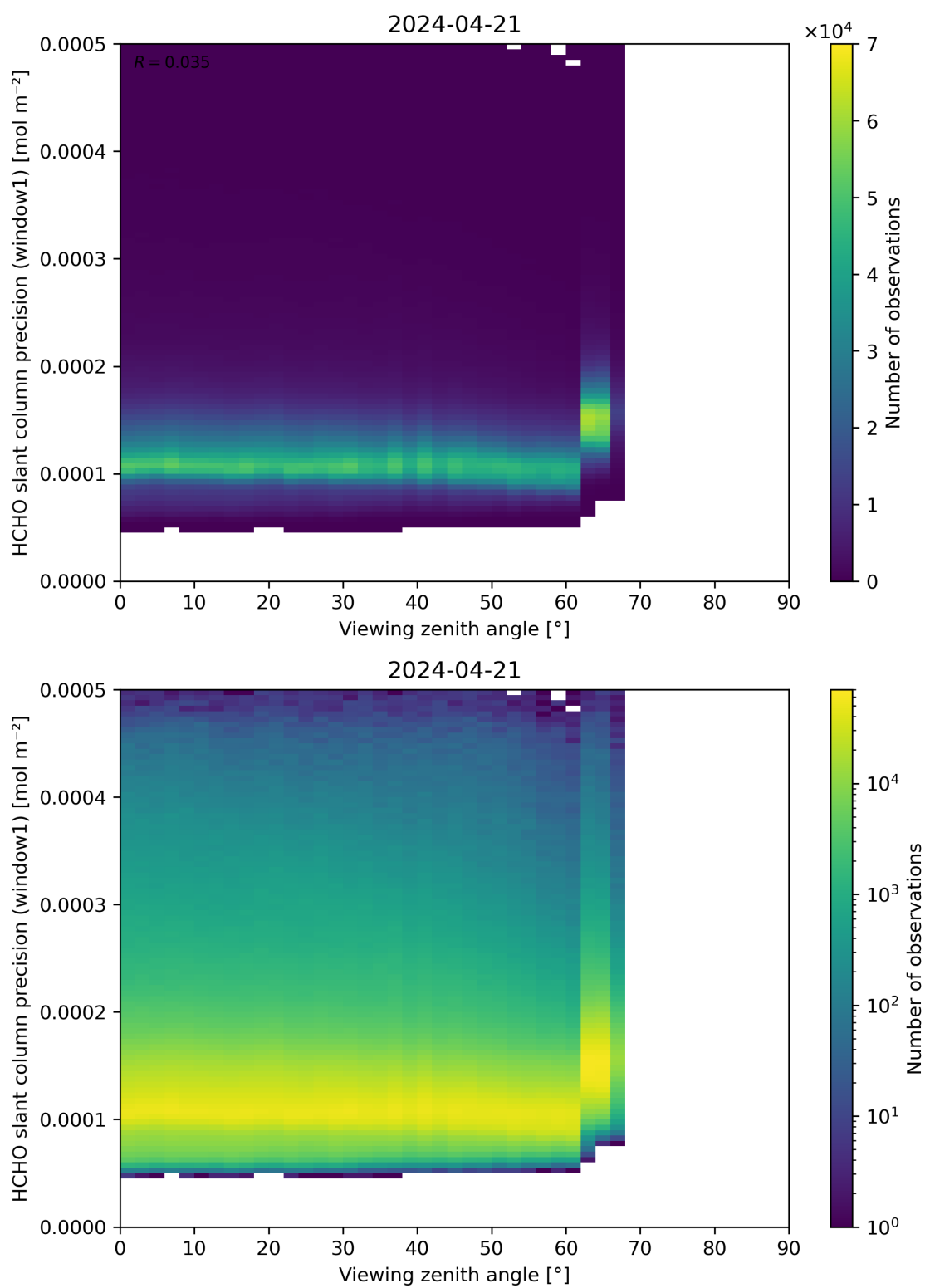
Figure 189: Scatter density plot of “Viewing zenith angle” against “HCHO slant column precision (window1)” for 2024-04-21 to 2024-04-22.
