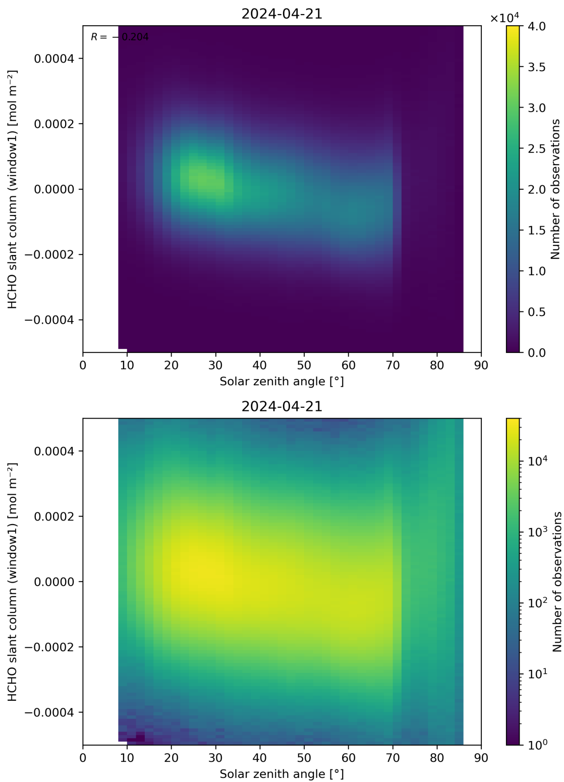
Figure 173: Scatter density plot of “Solar zenith angle” against “HCHO slant column (window1)” for 2024-04-21 to 2024-04-22.
