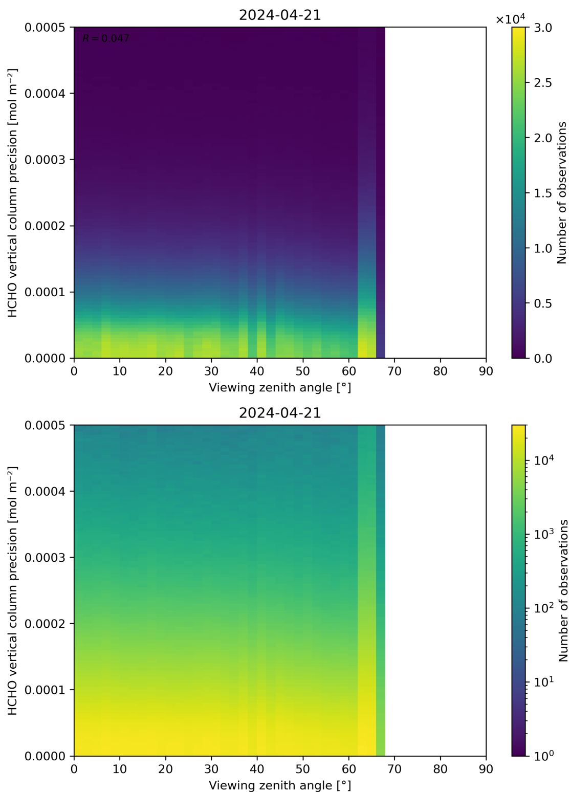
Figure 194: Scatter density plot of “Viewing zenith angle” against “HCHO vertical column precision” for 2024-04-21 to 2024-04-22.
