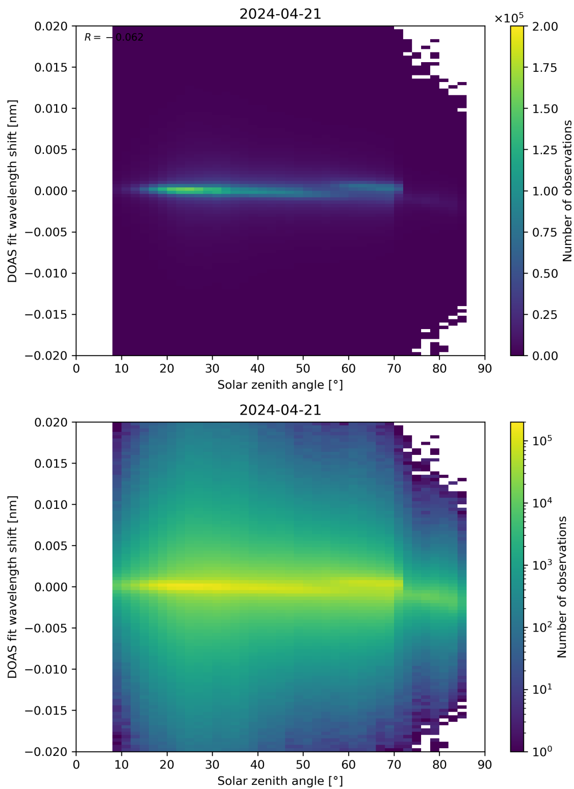
Figure 168: Scatter density plot of “Solar zenith angle” against “DOAS fit wavelength shift” for 2024-04-21 to 2024-04-22.
