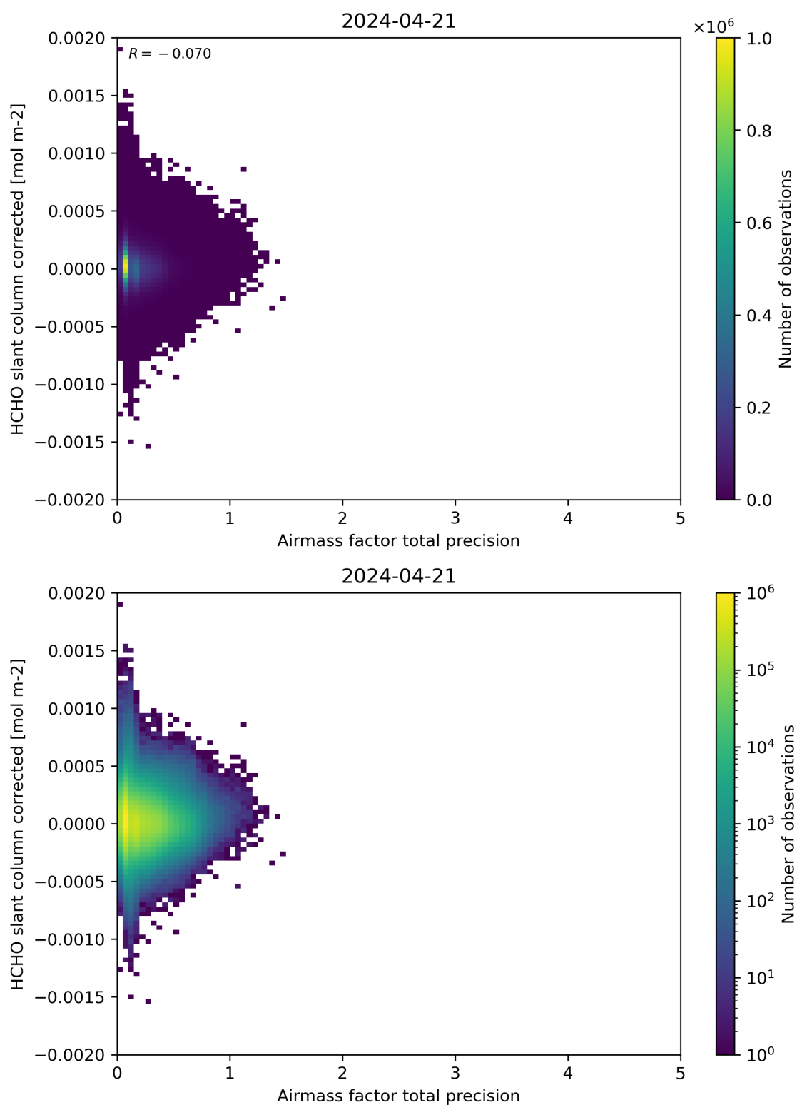
Figure 109: Scatter density plot of “Airmass factor total precision” against “HCHO slant column corrected” for 2024-04-21 to 2024-04-22.
