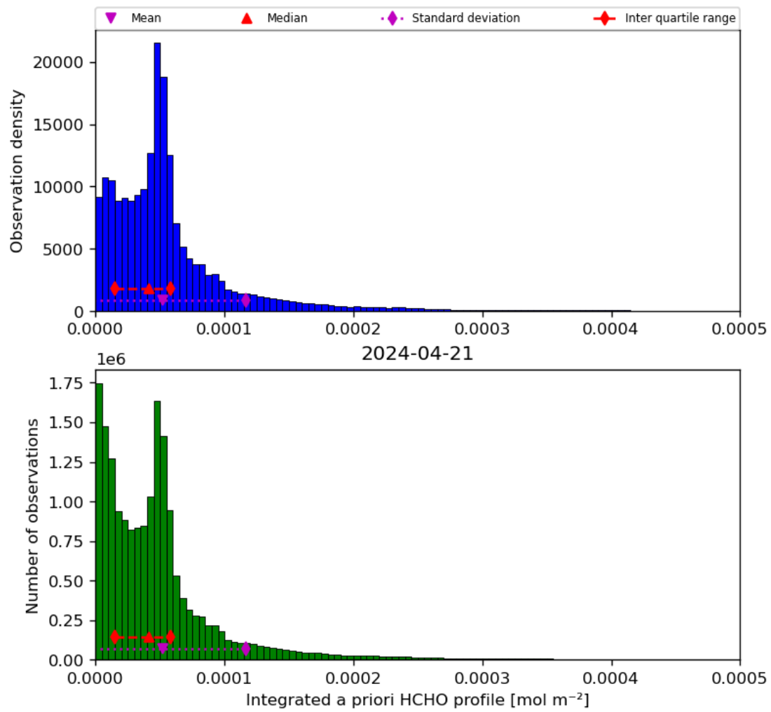
Figure 43: Histogram of “Integrated a priori HCHO profile” for 2024-04-21 to 2024-04-22
