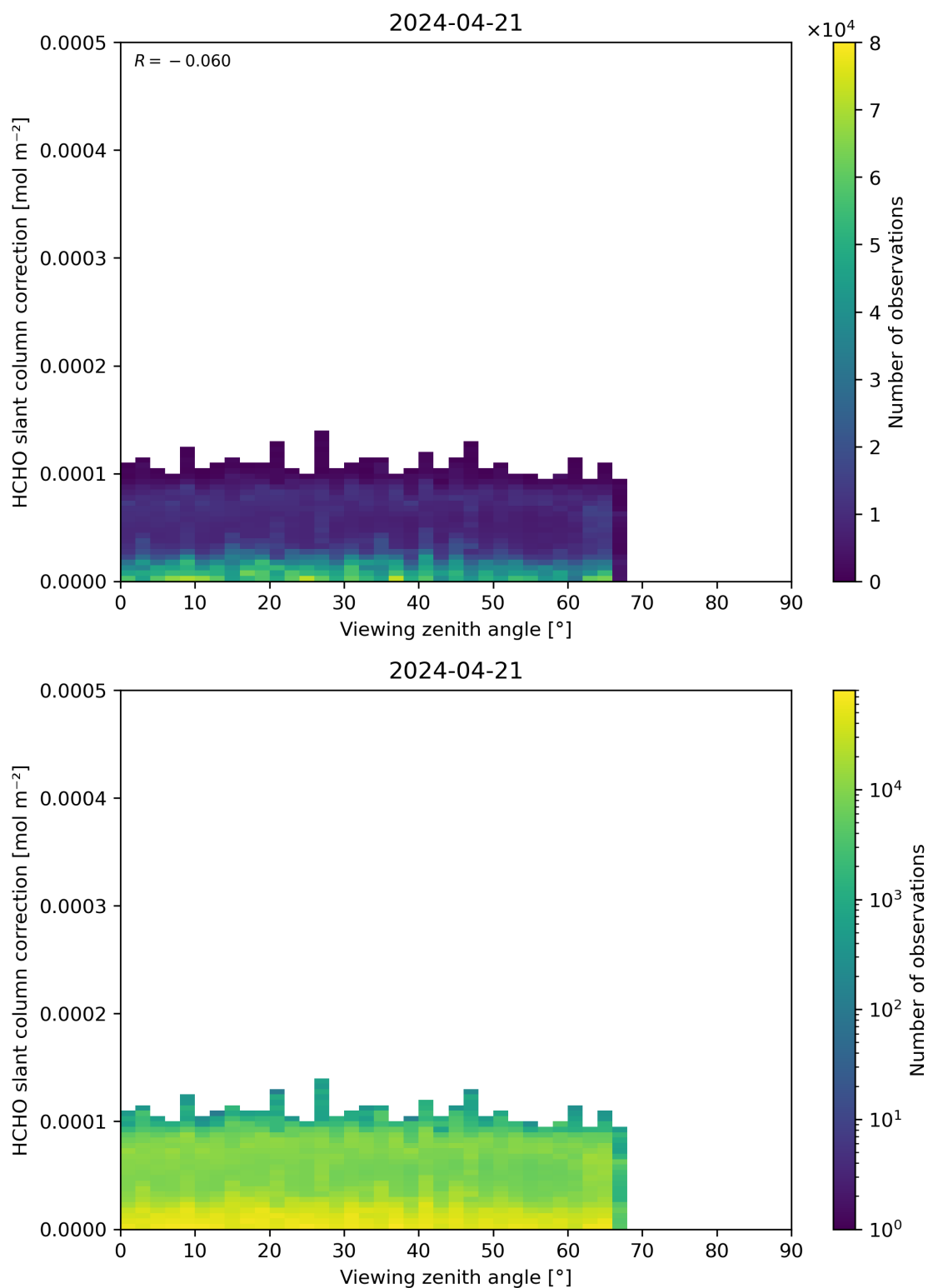
Figure 187: Scatter density plot of “Viewing zenith angle” against “HCHO slant column correction” for 2024-04-21 to 2024-04-22.
