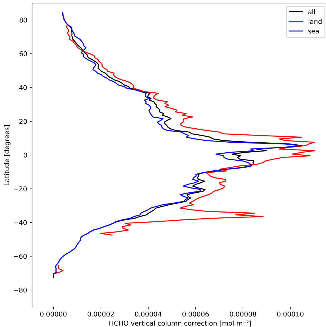
Figure 23: Zonal average of “HCHO vertical column correction” for 2024-04-21 to 2024-04-22.
