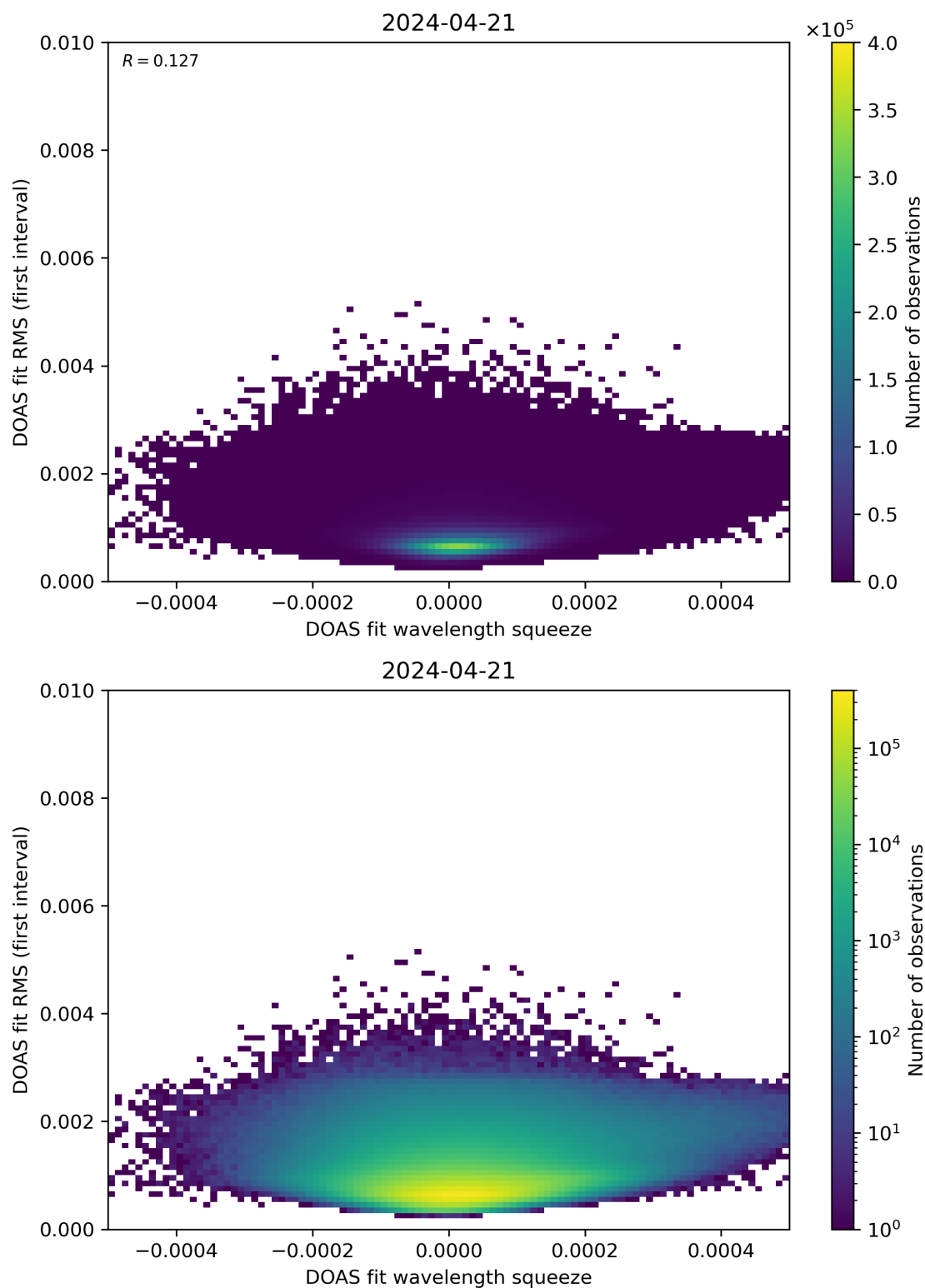
Figure 68: Scatter density plot of “DOAS fit wavelength squeeze” against “DOAS fit RMS (first interval)” for 2024-04-21 to 2024-04-22.
