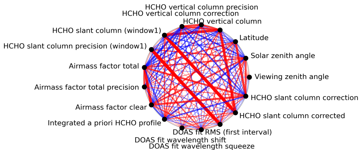
Figure 1: Map of correlation graph for 2024-04-21 to 2024-04-22.
