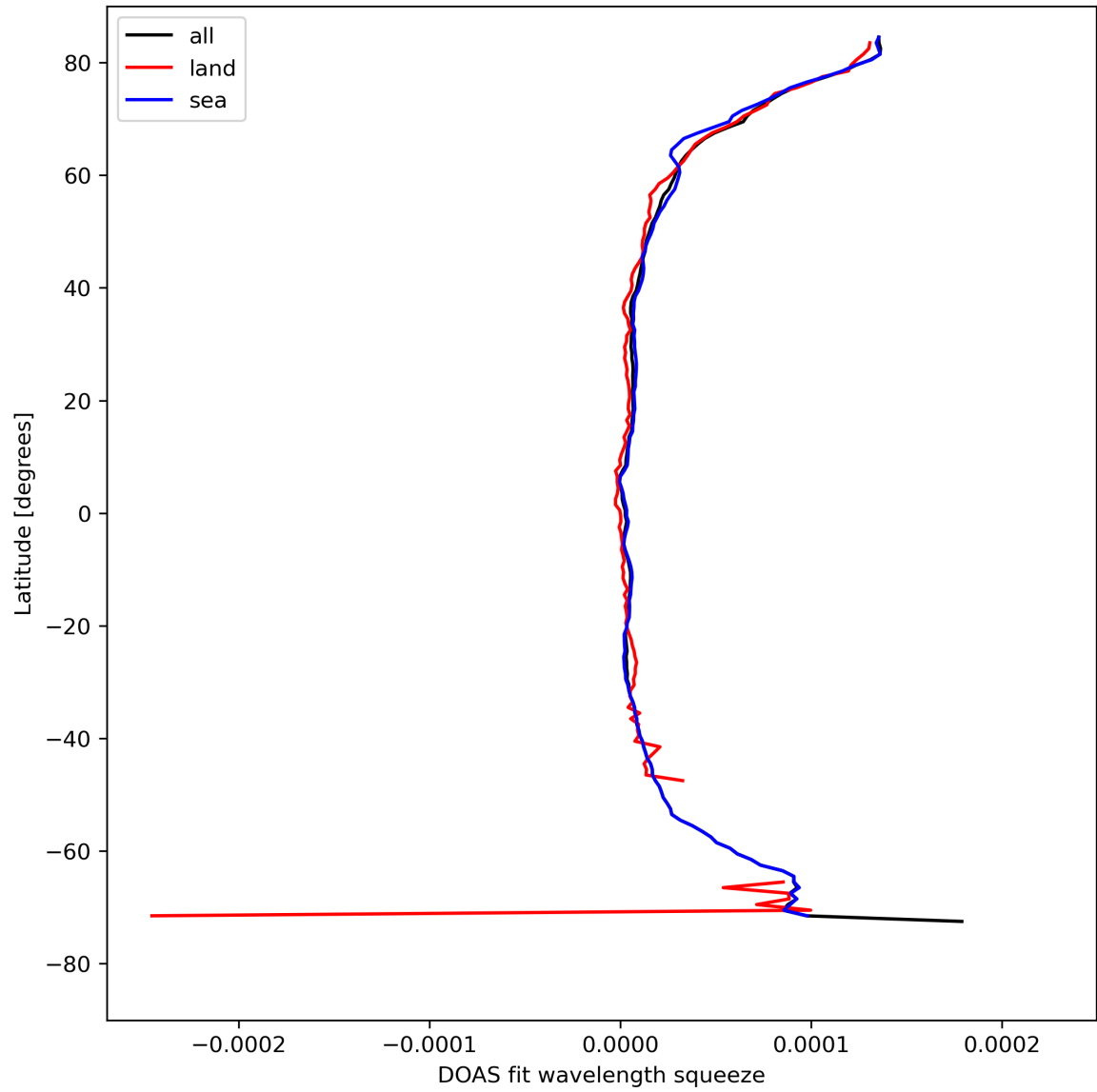
Figure 31: Zonal average of “DOAS fit wavelength squeeze” for 2024-04-21 to 2024-04-22.
