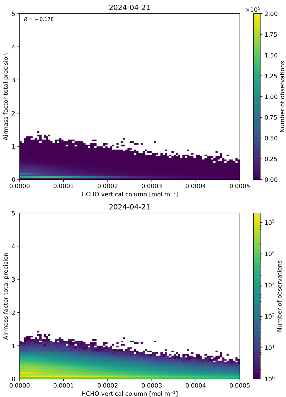
Figure 132: Scatter density plot of “HCHO vertical column” against “Airmass factor total precision” for 2024-04-21 to 2024-04-22.
