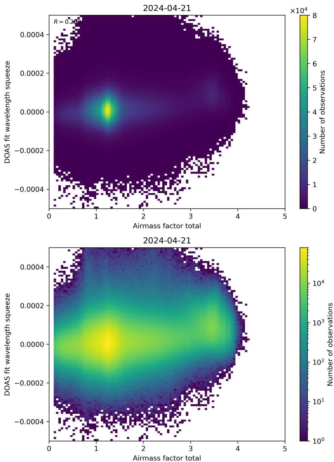
Figure 99: Scatter density plot of “Airmass factor total” against “DOAS fit wavelength squeeze” for 2024-04-21 to 2024-04-22.
