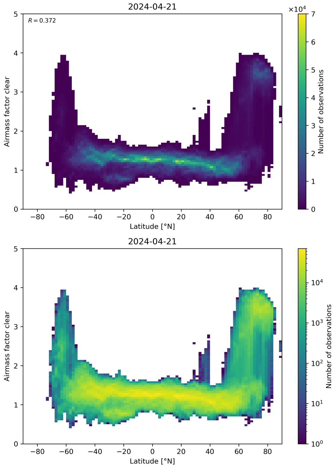
Figure 156: Scatter density plot of “Latitude” against “Airmass factor clear” for 2024-04-21 to 2024-04-22.
