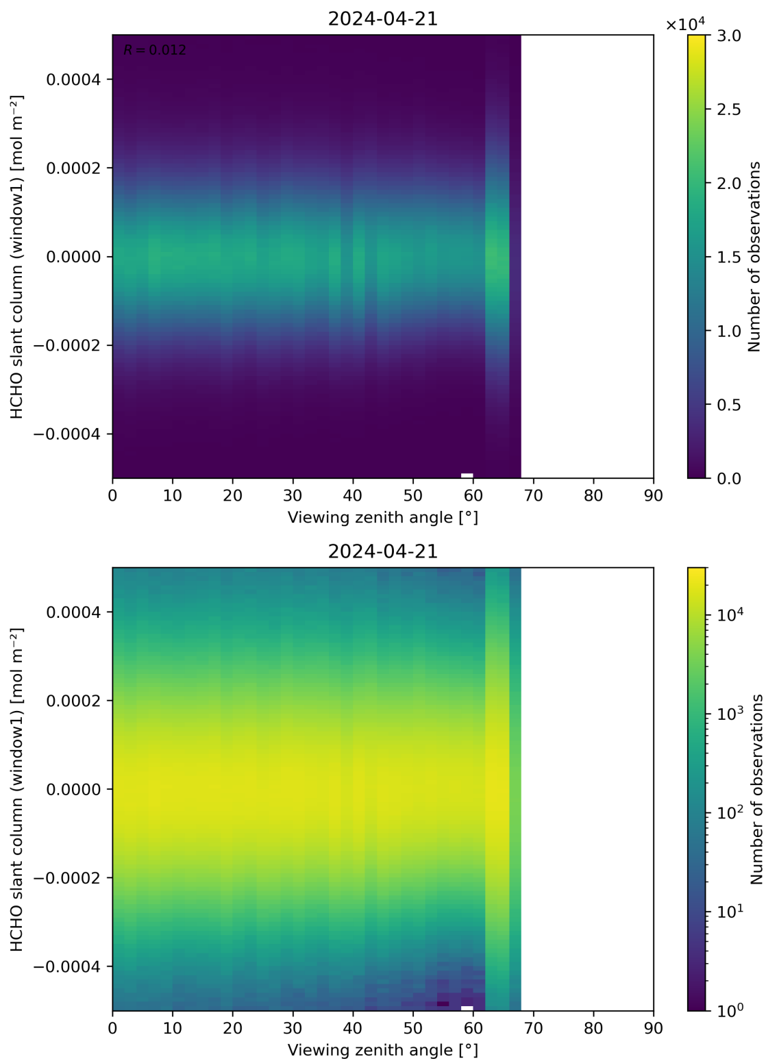
Figure 188: Scatter density plot of “Viewing zenith angle” against “HCHO slant column (window1)” for 2024-04-21 to 2024-04-22.
