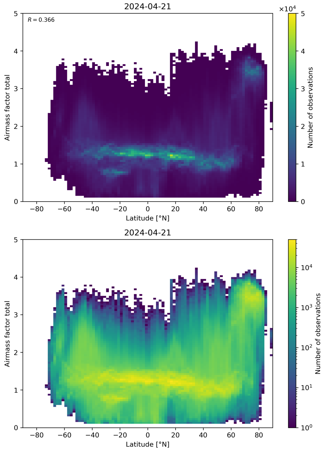
Figure 161: Scatter density plot of “Latitude” against “Airmass factor total” for 2024-04-21 to 2024-04-22.
