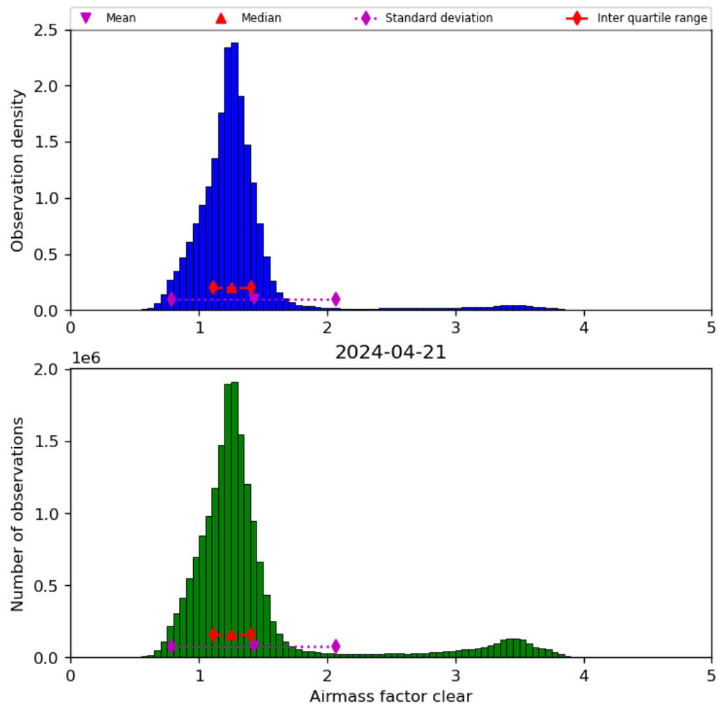
Figure 42: Histogram of “Airmass factor clear” for 2024-04-21 to 2024-04-22
