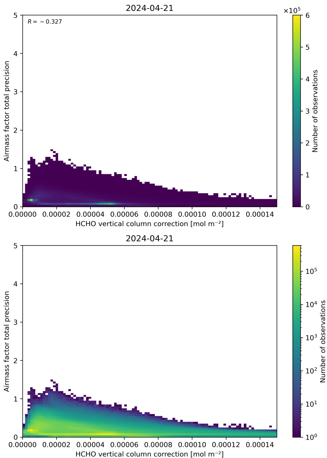
Figure 121: Scatter density plot of “HCHO vertical column correction” against “Airmass factor total precision” for 2024-04-21 to 2024-04-22.
