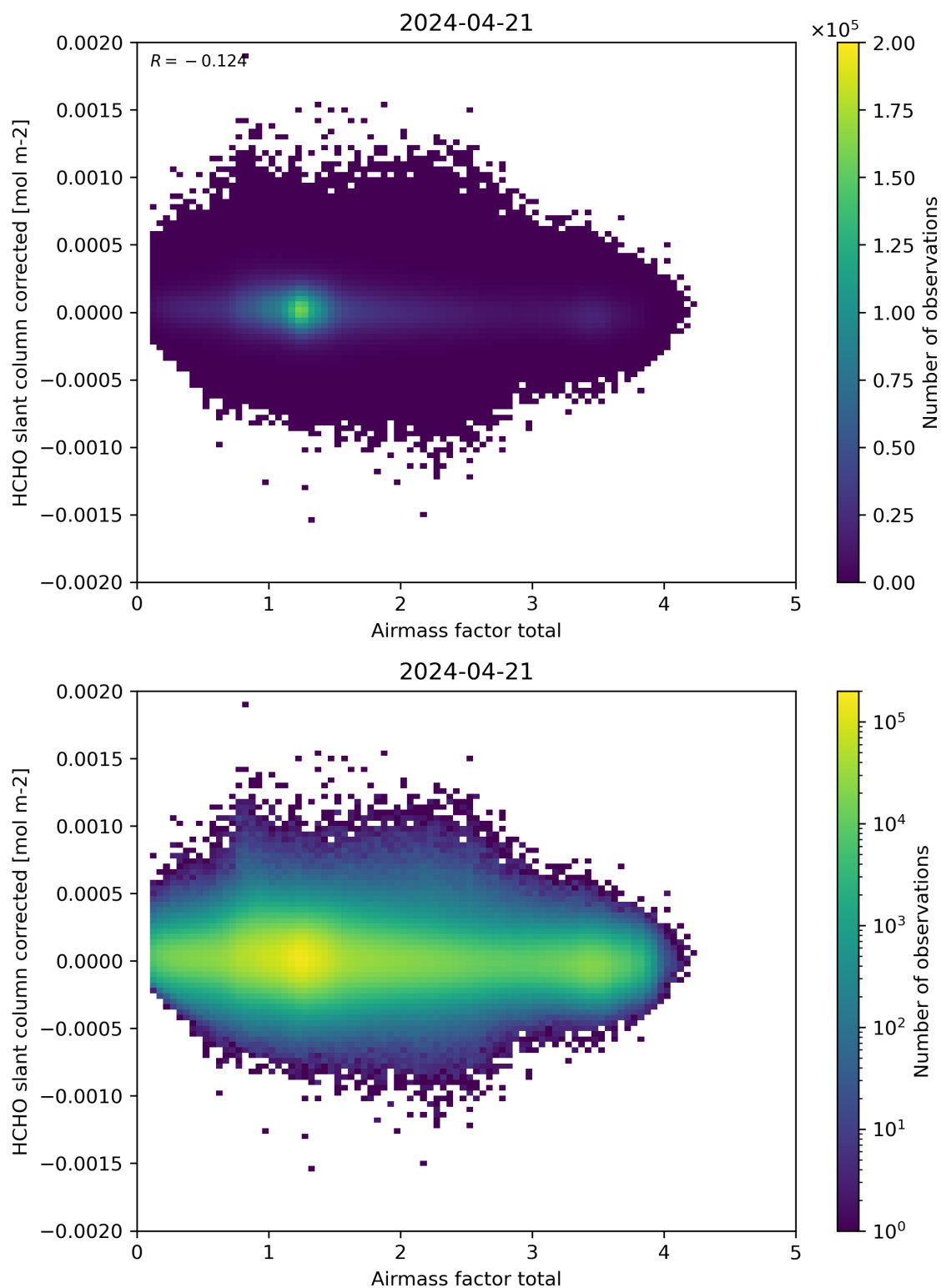
Figure 101: Scatter density plot of “Airmass factor total” against “HCHO slant column corrected” for 2024-04-21 to 2024-04-22.
