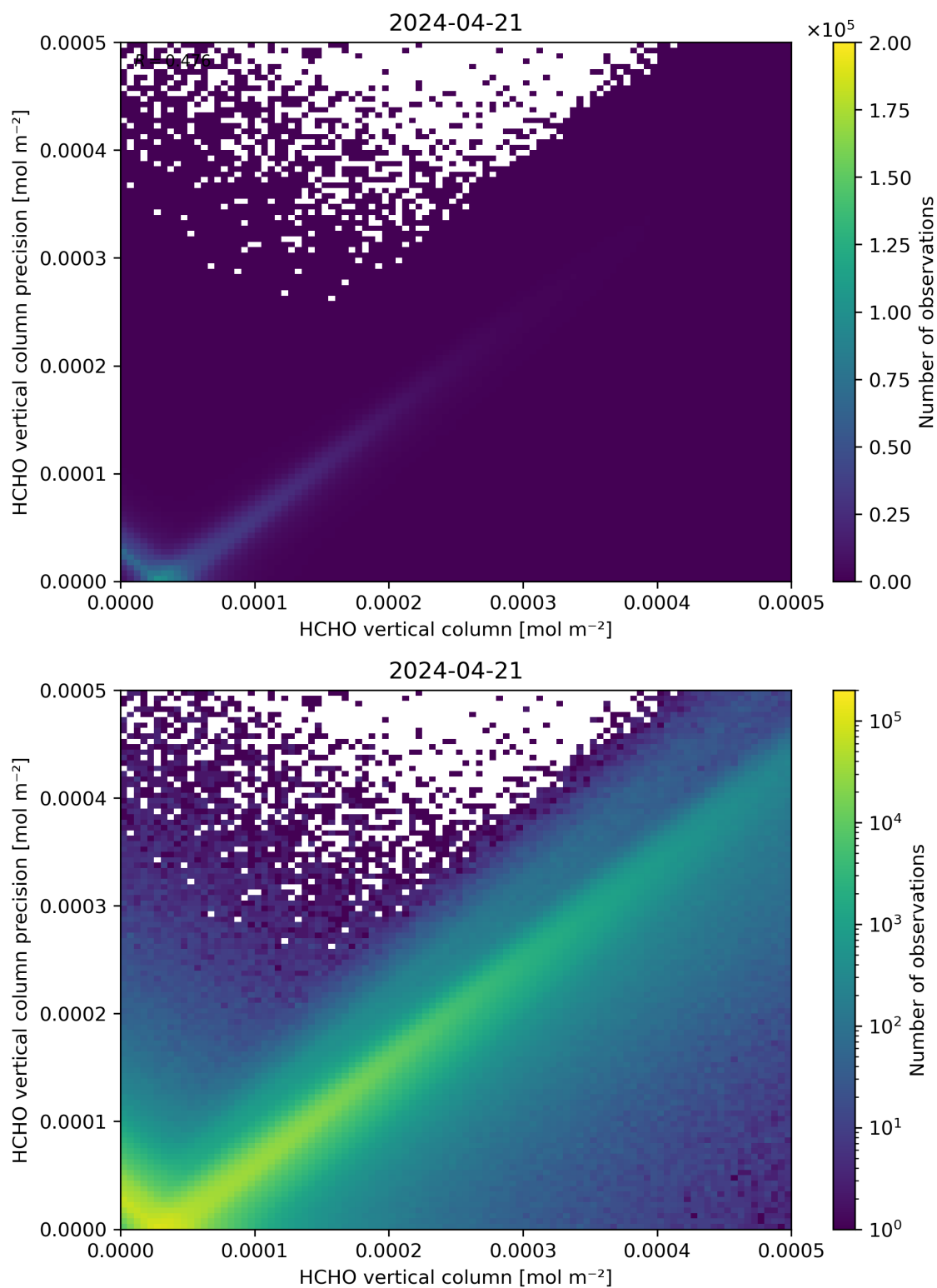
Figure 134: Scatter density plot of “HCHO vertical column” against “HCHO vertical column precision” for 2024-04-21 to 2024-04-22.
