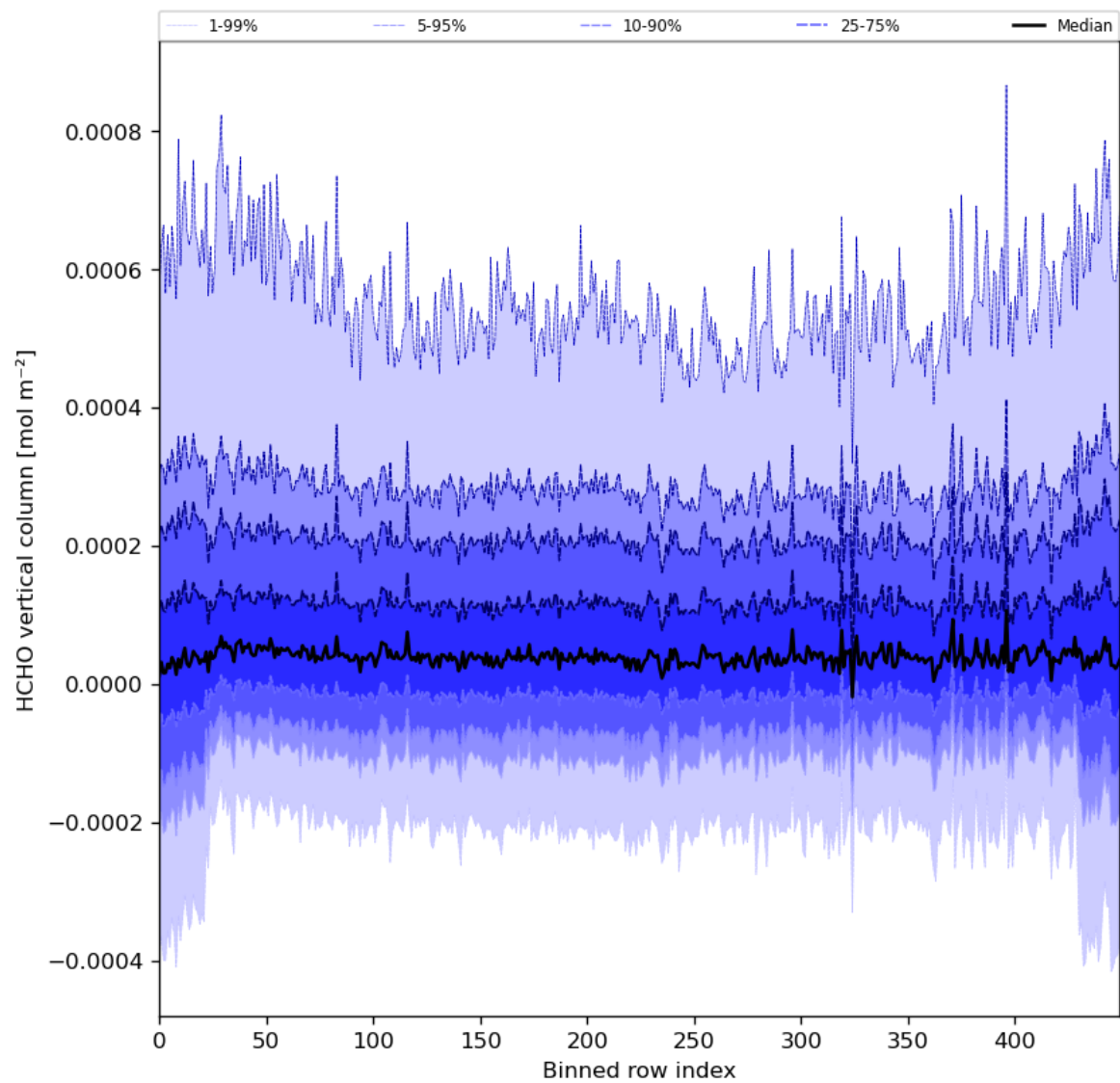
Figure 49: Along track statistics of “HCHO vertical column” for 2024-04-21 to 2024-04-22
