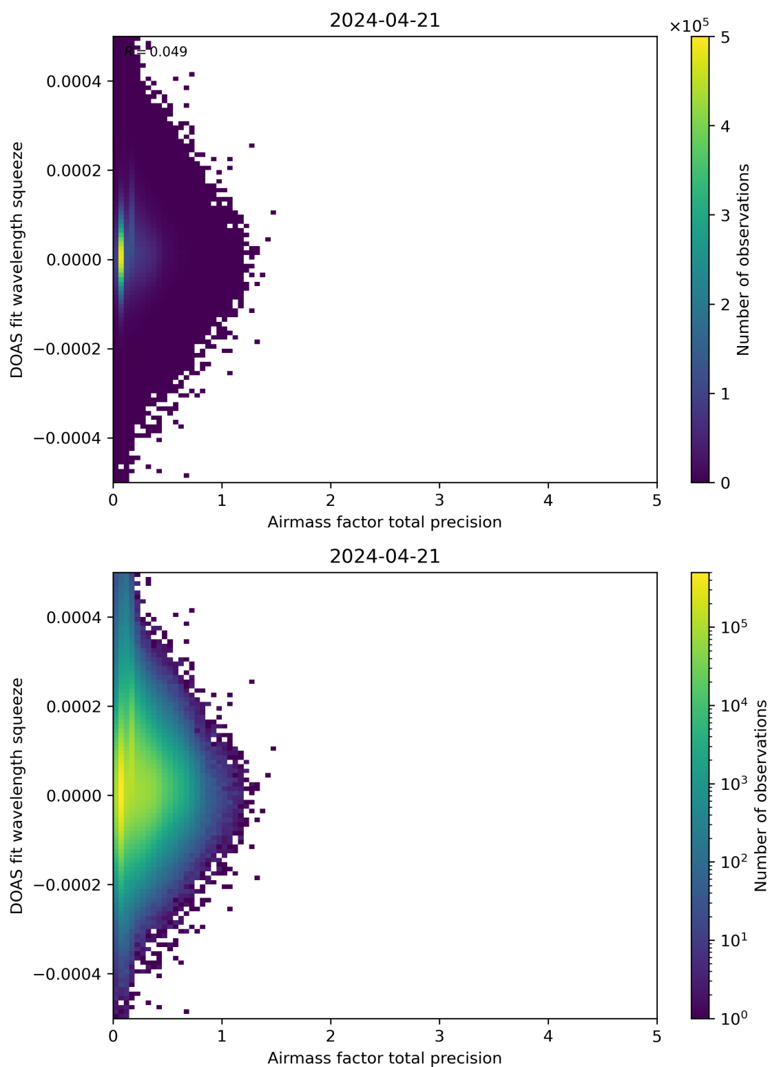
Figure 107: Scatter density plot of “Airmass factor total precision” against “DOAS fit wavelength squeeze” for 2024-04-21 to 2024-04-22.
