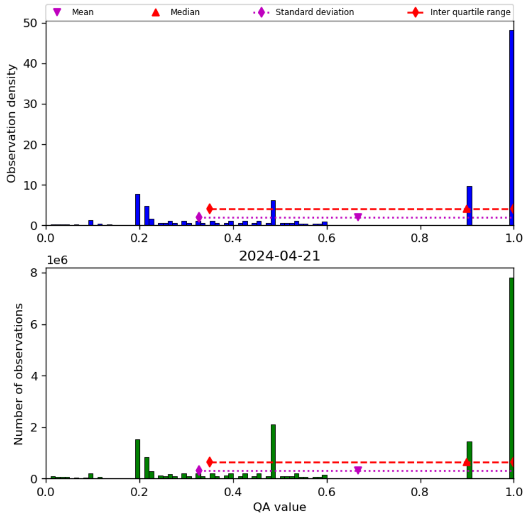
Figure 34: Histogram of “QA value” for 2024-04-21 to 2024-04-22
