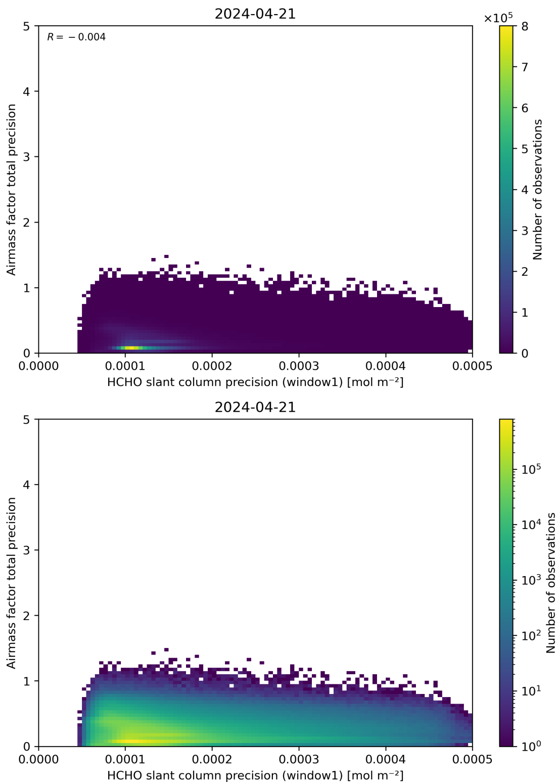
Figure 95: Scatter density plot of “HCHO slant column precision (window1)” against “Airmass factor total precision” for 2024-04-21 to 2024-04-22.
