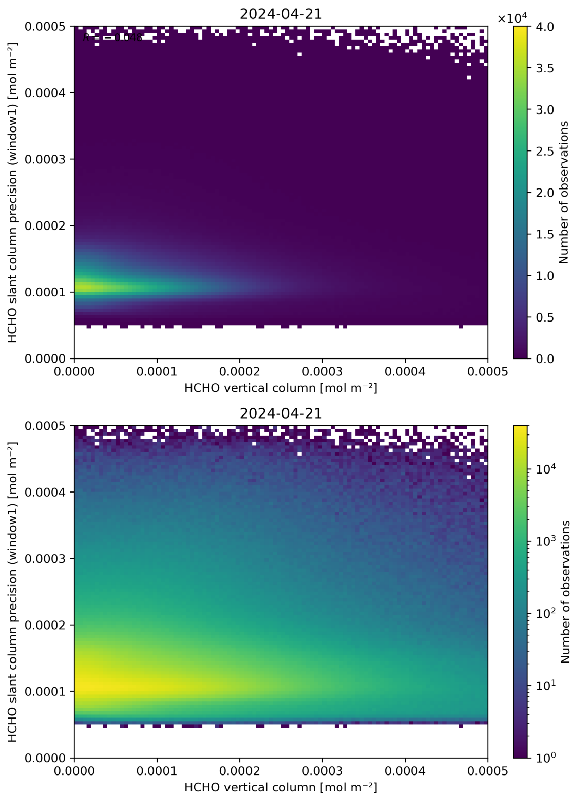
Figure 130: Scatter density plot of “HCHO vertical column” against “HCHO slant column precision (window1)” for 2024-04-21 to 2024-04-22.
