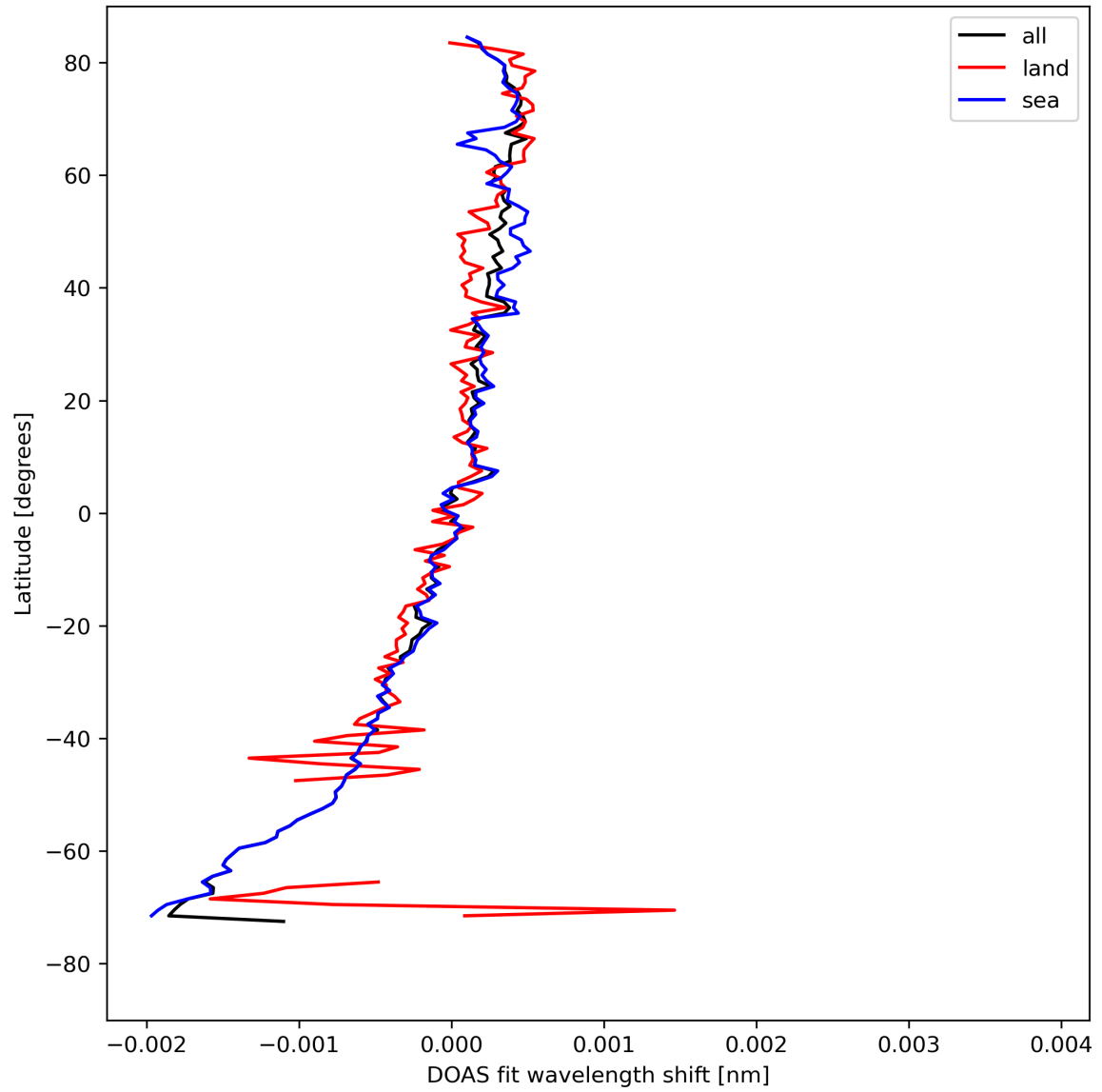
Figure 30: Zonal average of “DOAS fit wavelength shift” for 2024-04-21 to 2024-04-22.
