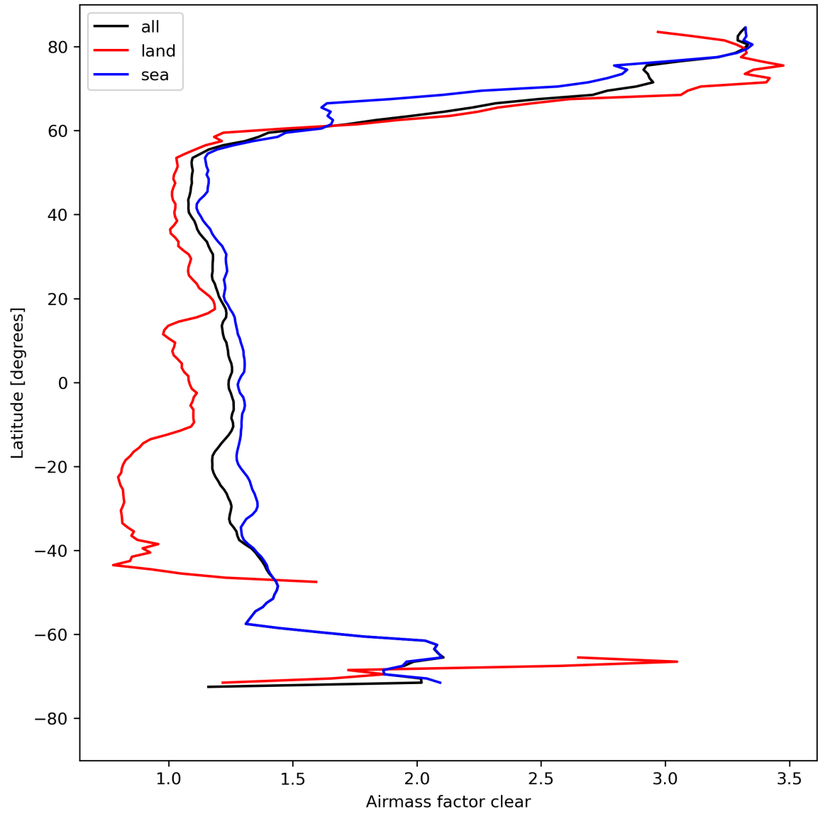
Figure 28: Zonal average of “Airmass factor clear” for 2024-04-21 to 2024-04-22.
