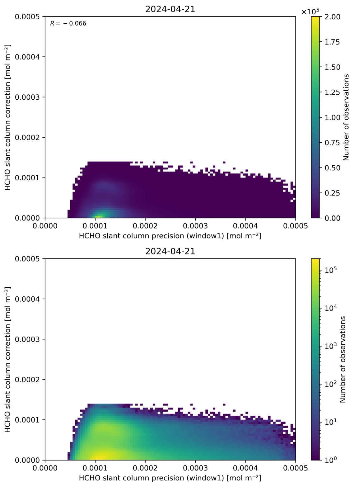
Figure 93: Scatter density plot of “HCHO slant column precision (window1)” against “HCHO slant column correction” for 2024-04-21 to 2024-04-22.
