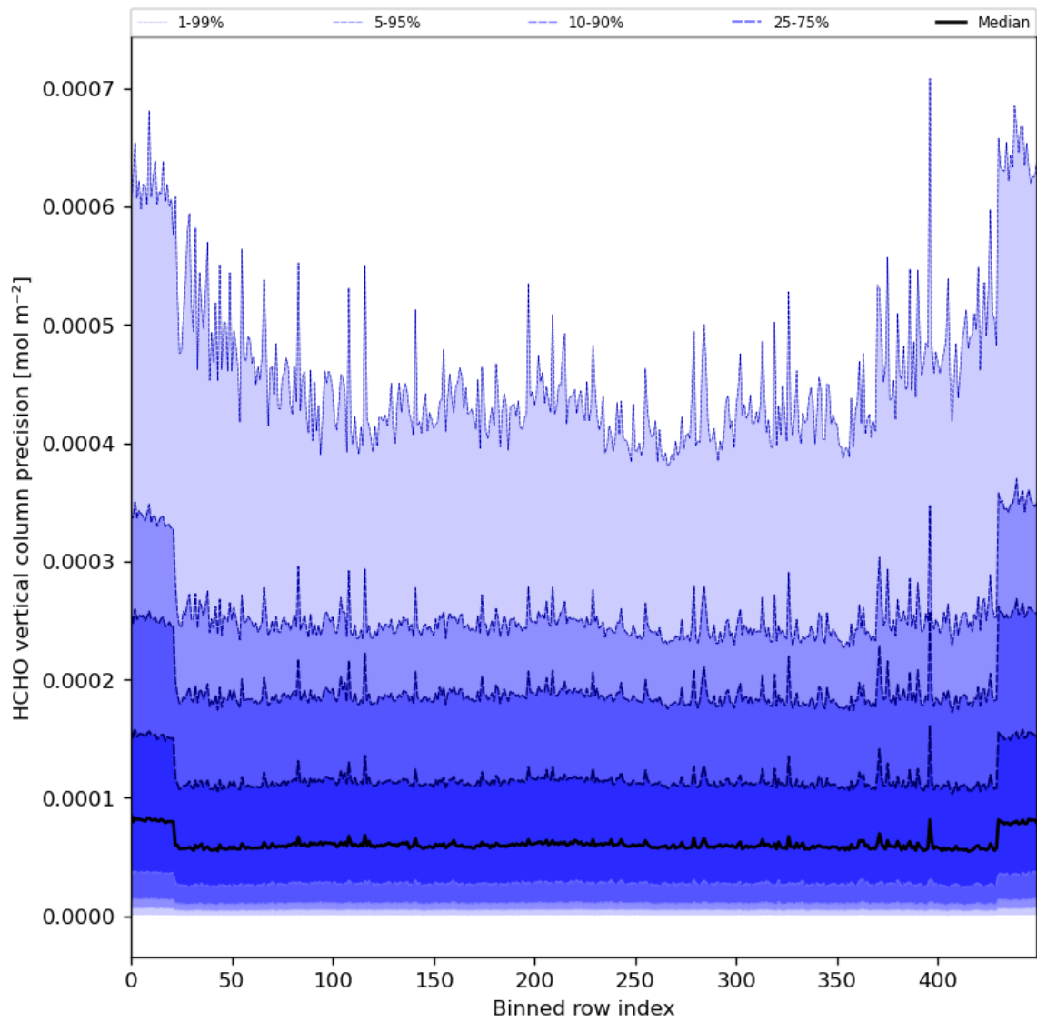
Figure 50: Along track statistics of “HCHO vertical column precision” for 2024-04-21 to 2024-04-22
