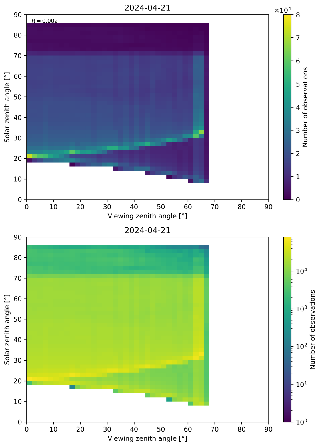
Figure 197: Scatter density plot of “Viewing zenith angle” against “Solar zenith angle” for 2024-04-21 to 2024-04-22.
