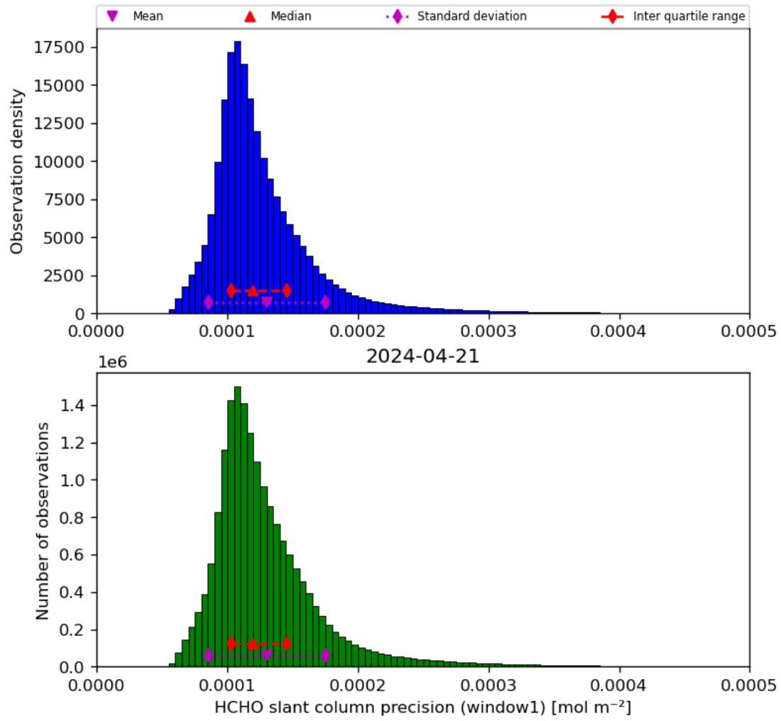
Figure 39: Histogram of “HCHO slant column precision (window1)” for 2024-04-21 to 2024-04-22
