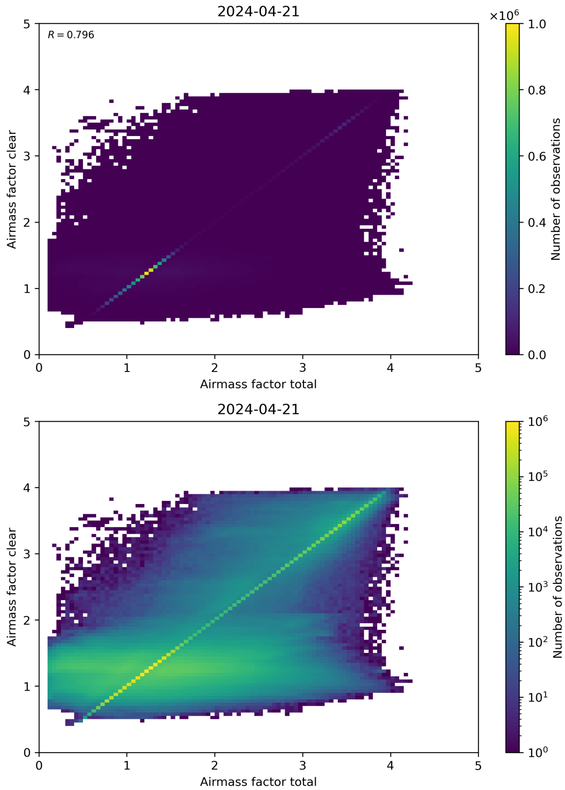
Figure 100: Scatter density plot of “Airmass factor total” against “Airmass factor clear” for 2024-04-21 to 2024-04-22.
