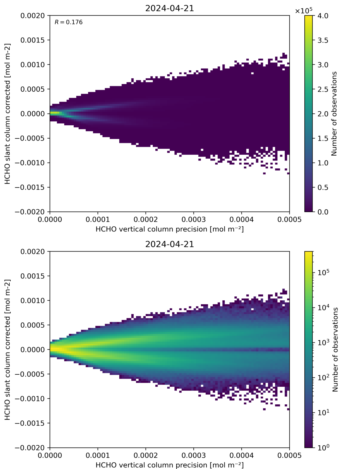
Figure 140: Scatter density plot of “HCHO vertical column precision” against “HCHO slant column corrected” for 2024-04-21 to 2024-04-22.
