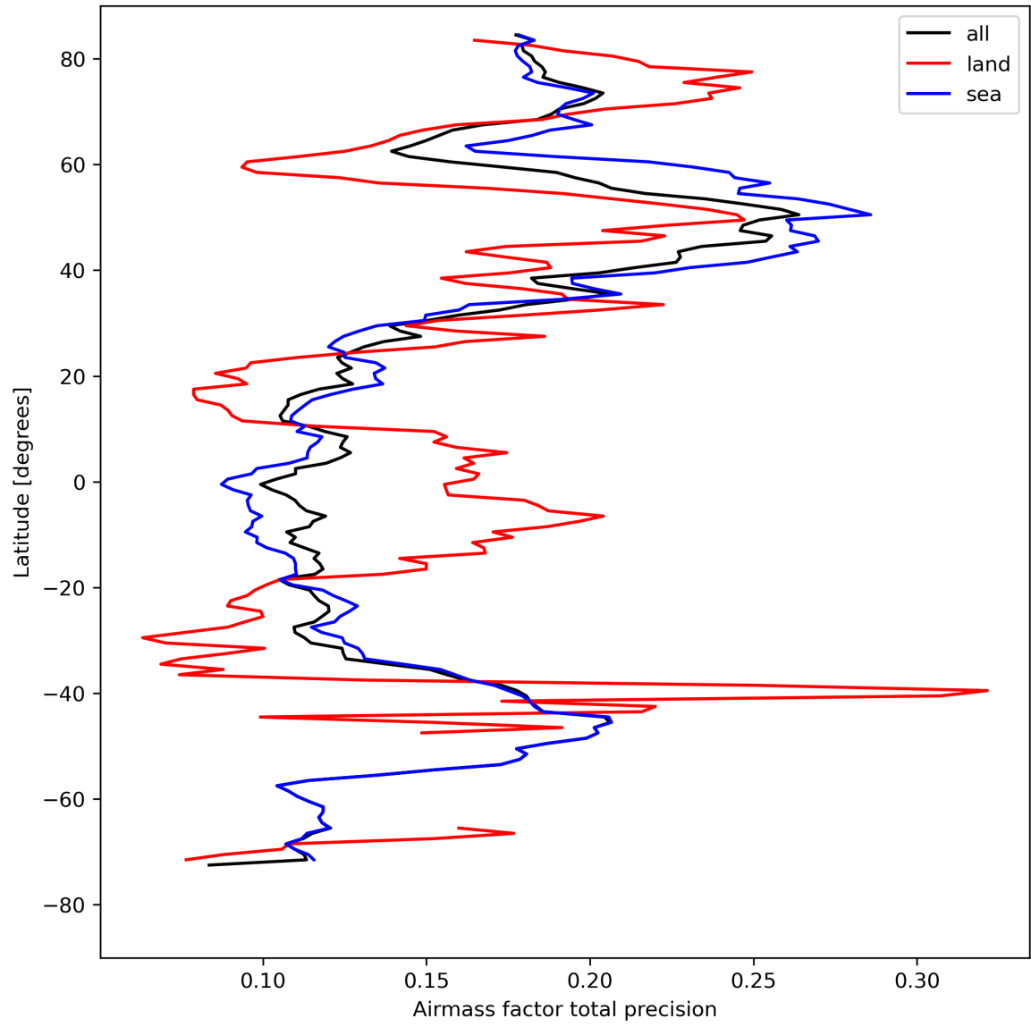
Figure 27: Zonal average of “Airmass factor total precision” for 2024-04-21 to 2024-04-22.
