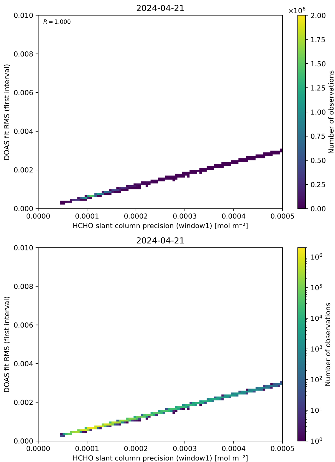
Figure 88: Scatter density plot of “HCHO slant column precision (window1)” against “DOAS fit RMS (first interval)” for 2024-04-21 to 2024-04-22.
