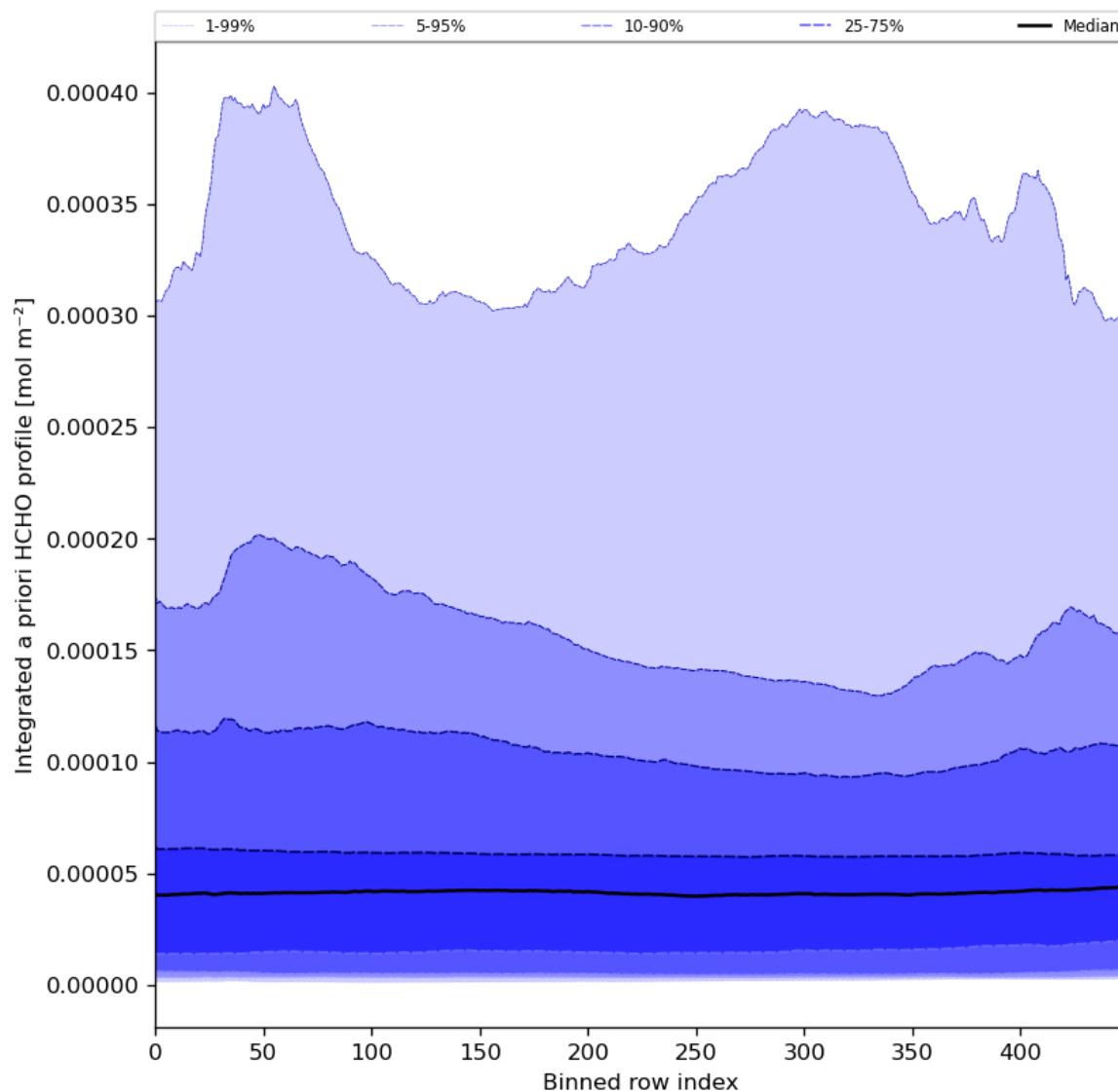
Figure 57: Along track statistics of “Integrated a priori HCHO profile” for 2024-04-21 to 2024-04-22
