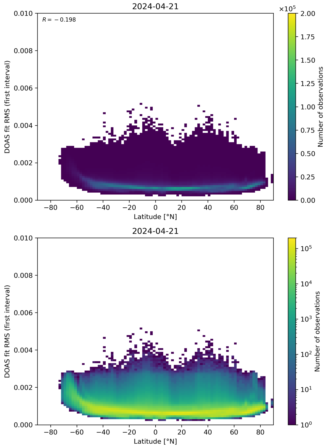
Figure 153: Scatter density plot of “Latitude” against “DOAS fit RMS (first interval)” for 2024-04-21 to 2024-04-22.
