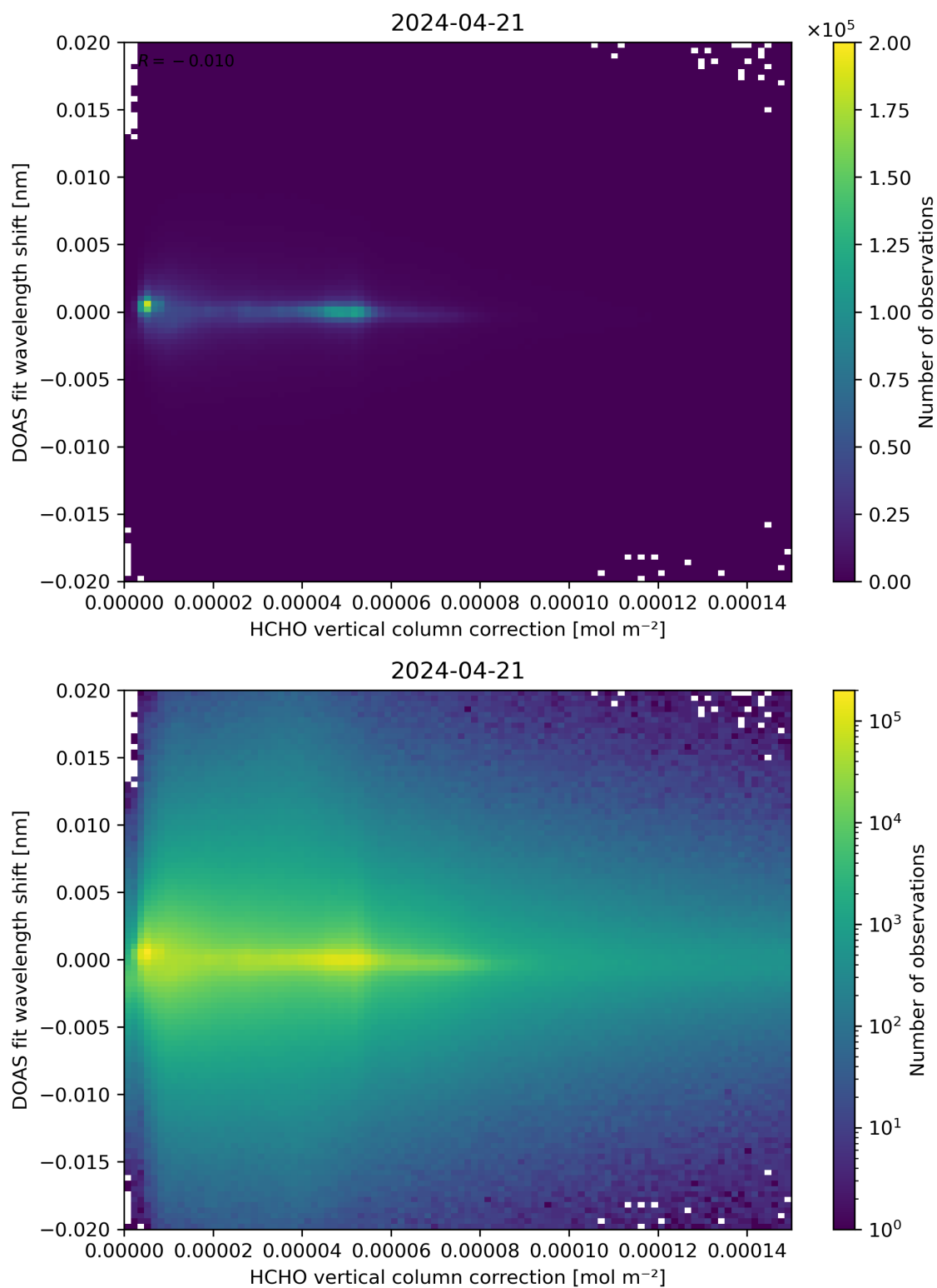
Figure 113: Scatter density plot of “HCHO vertical column correction” against “DOAS fit wavelength shift” for 2024-04-21 to 2024-04-22.
