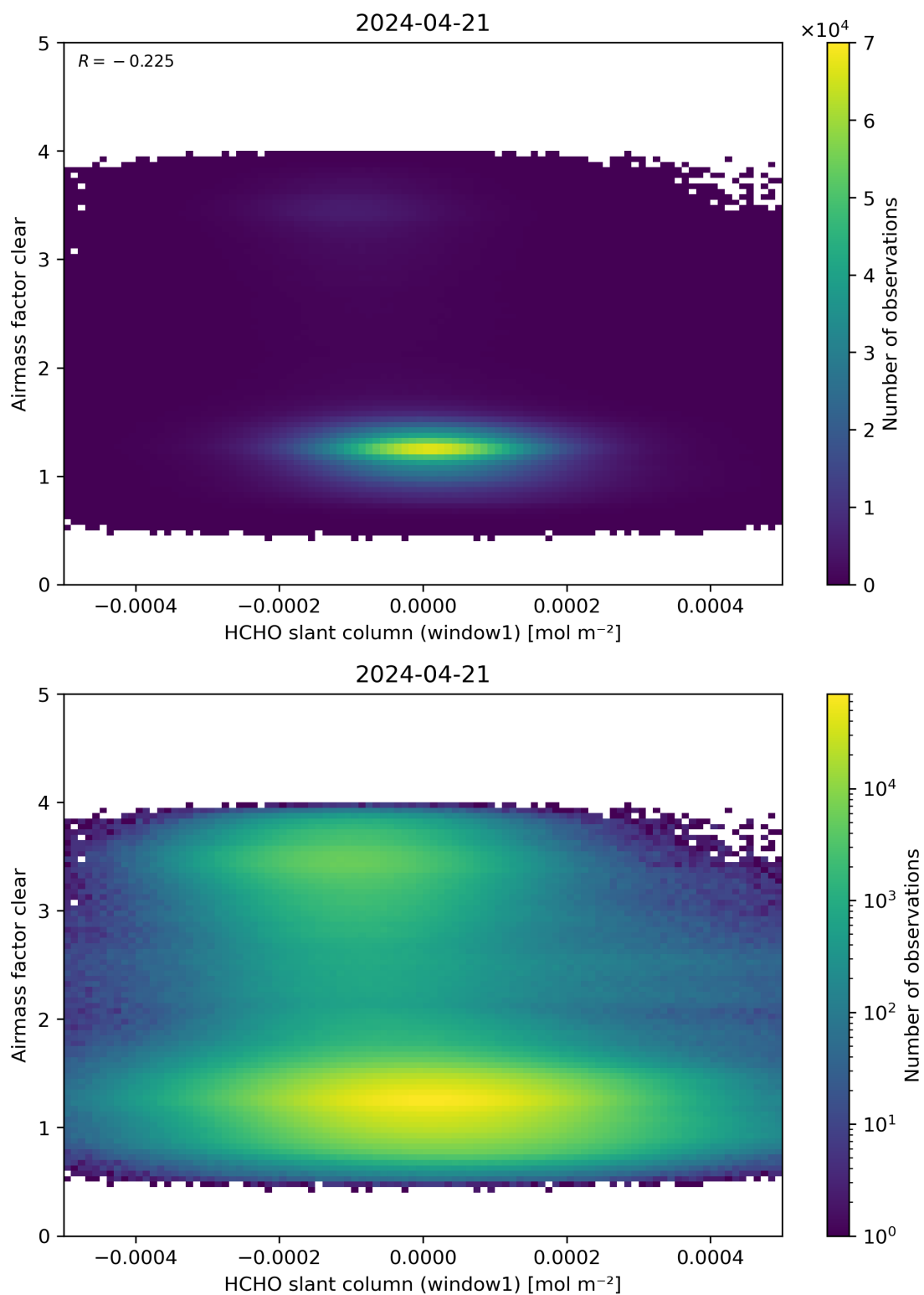
Figure 81: Scatter density plot of “HCHO slant column (window1)” against “Airmass factor clear” for 2024-04-21 to 2024-04-22.
