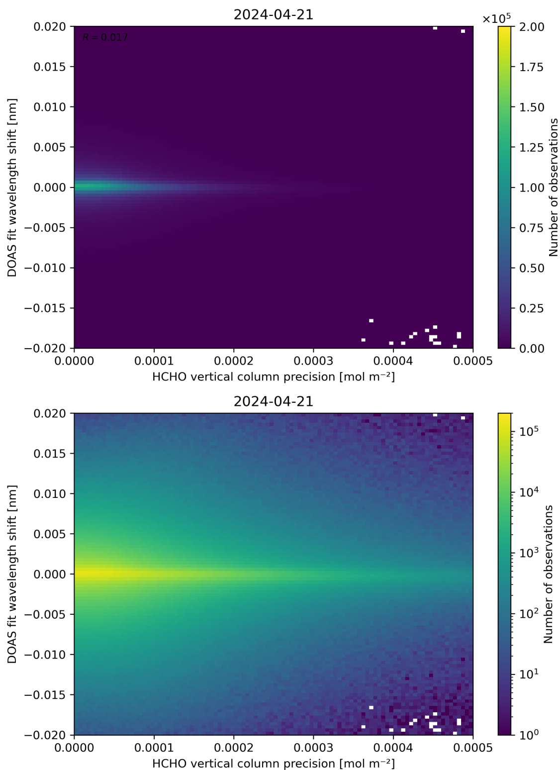
Figure 137: Scatter density plot of “HCHO vertical column precision” against “DOAS fit wavelength shift” for 2024-04-21 to 2024-04-22.
