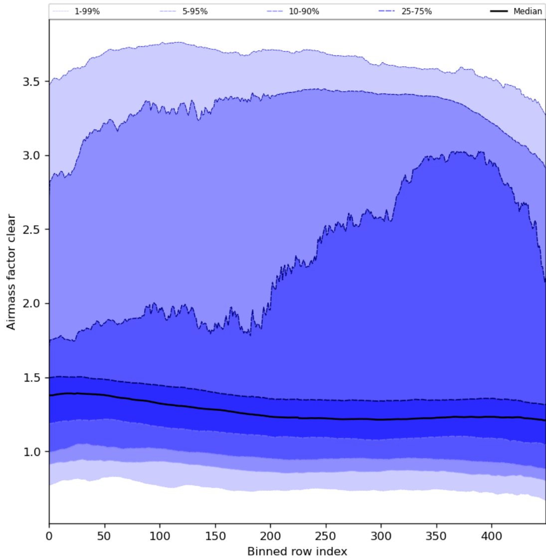
Figure 56: Along track statistics of “Airmass factor clear” for 2024-04-21 to 2024-04-22
