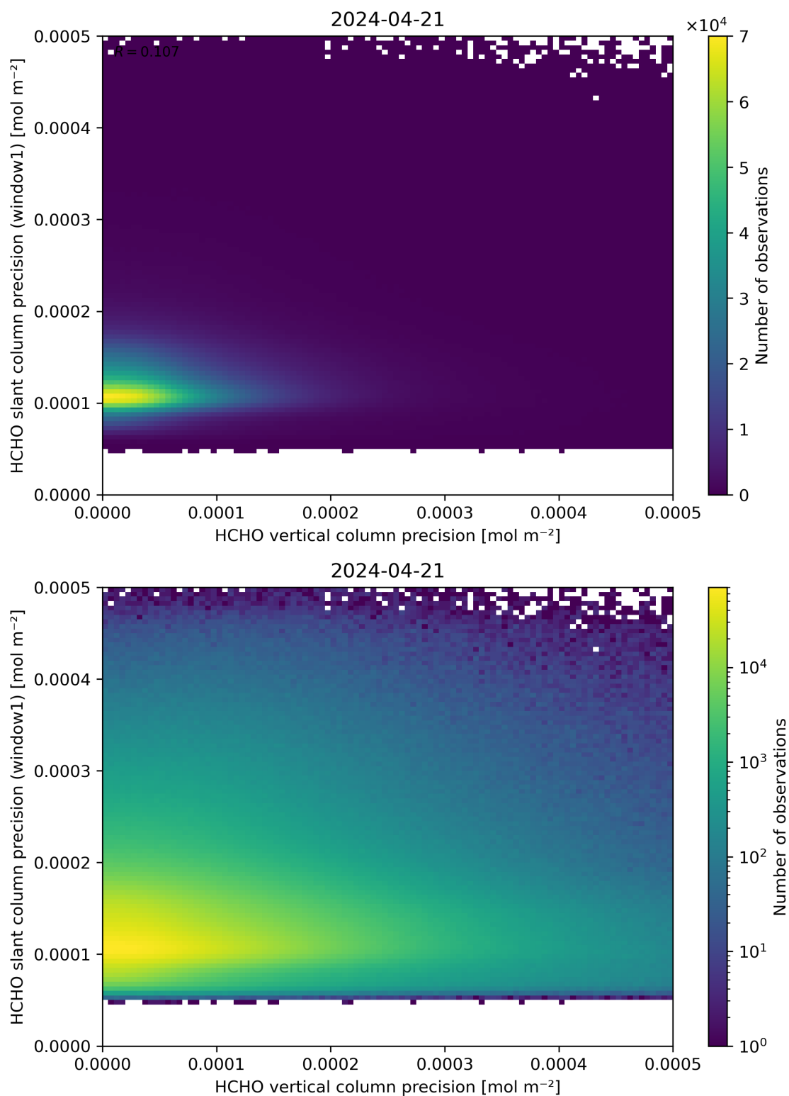
Figure 143: Scatter density plot of “HCHO vertical column precision” against “HCHO slant column precision (window1)” for 2024-04-21 to 2024-04-22.
