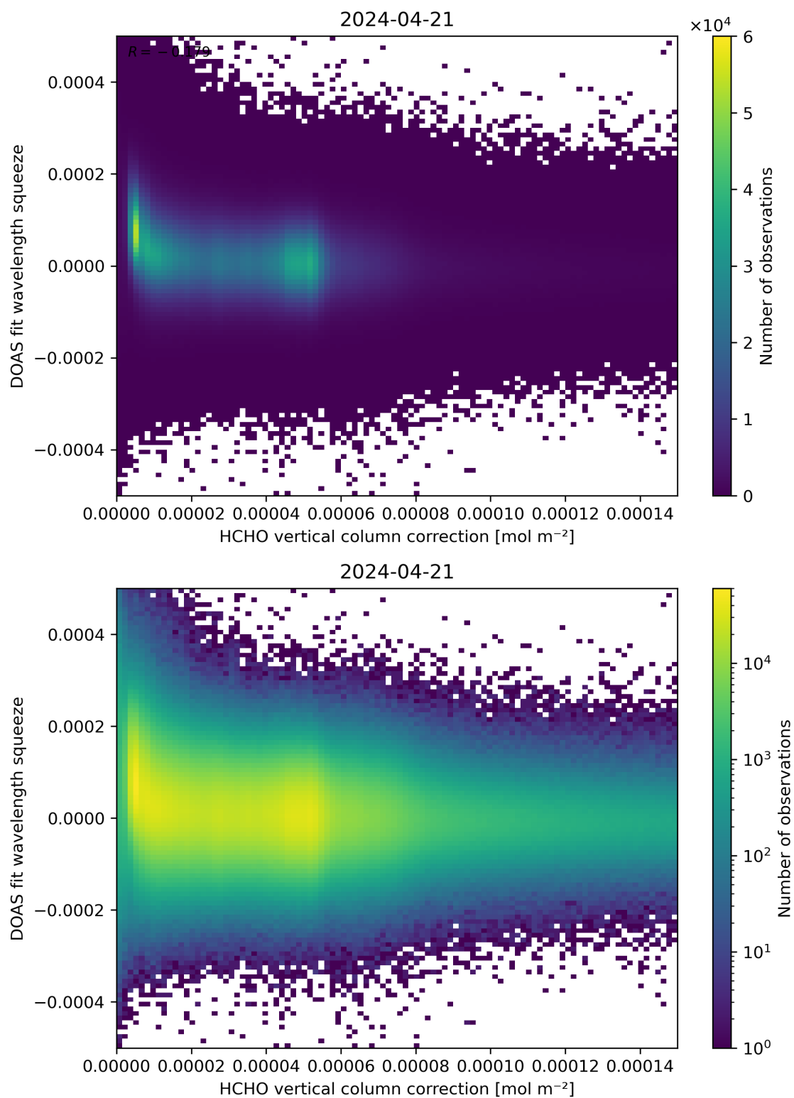
Figure 114: Scatter density plot of “HCHO vertical column correction” against “DOAS fit wavelength squeeze” for 2024-04-21 to 2024-04-22.
