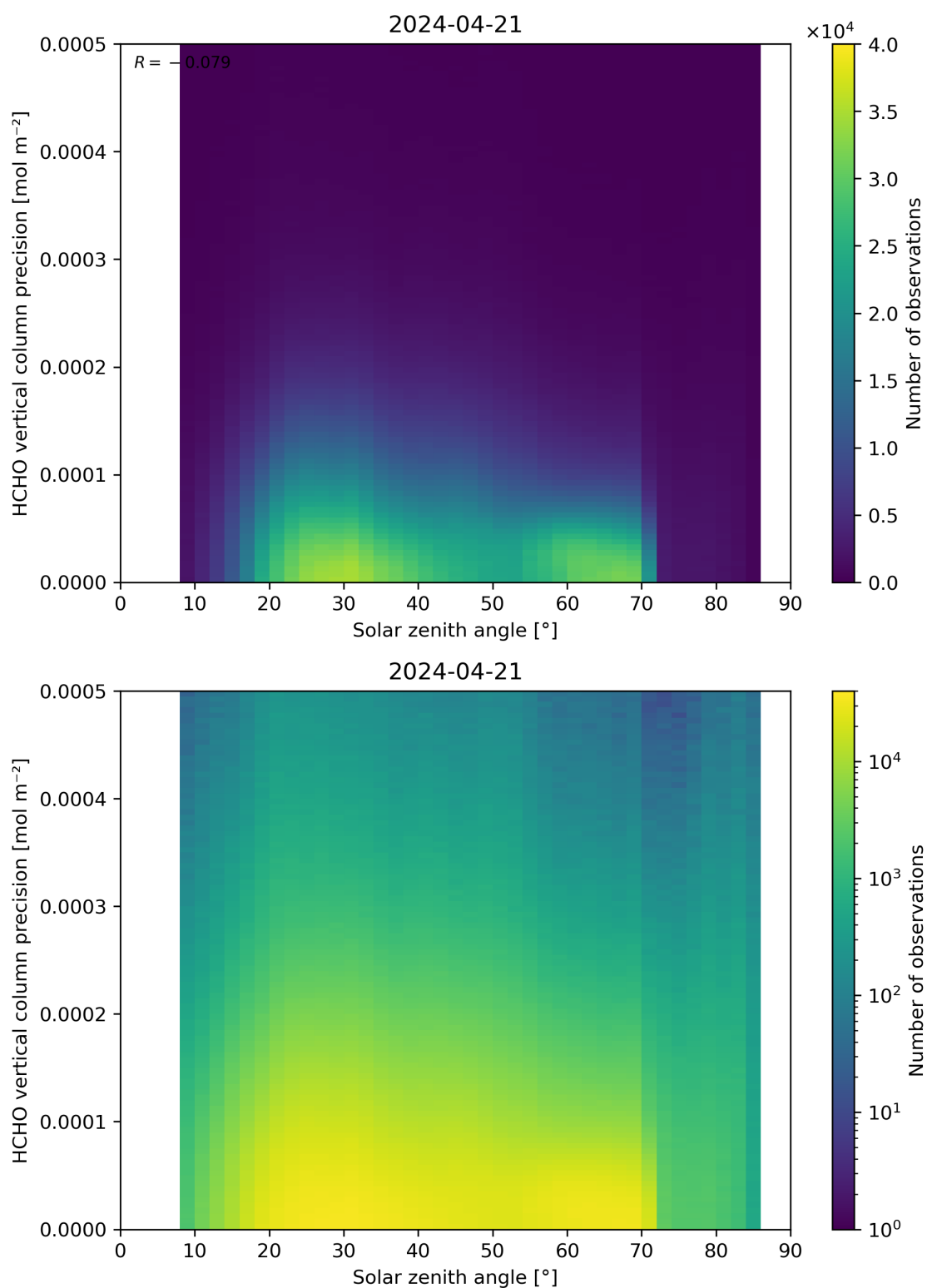
Figure 179: Scatter density plot of “Solar zenith angle” against “HCHO vertical column precision” for 2024-04-21 to 2024-04-22.
