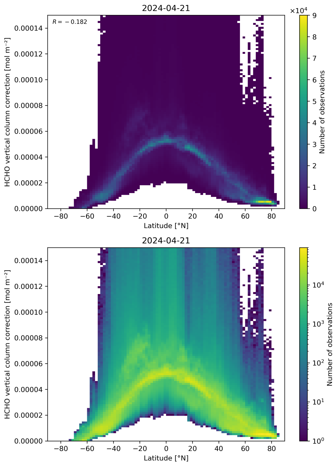
Figure 164: Scatter density plot of “Latitude” against “HCHO vertical column correction” for 2024-04-21 to 2024-04-22.
