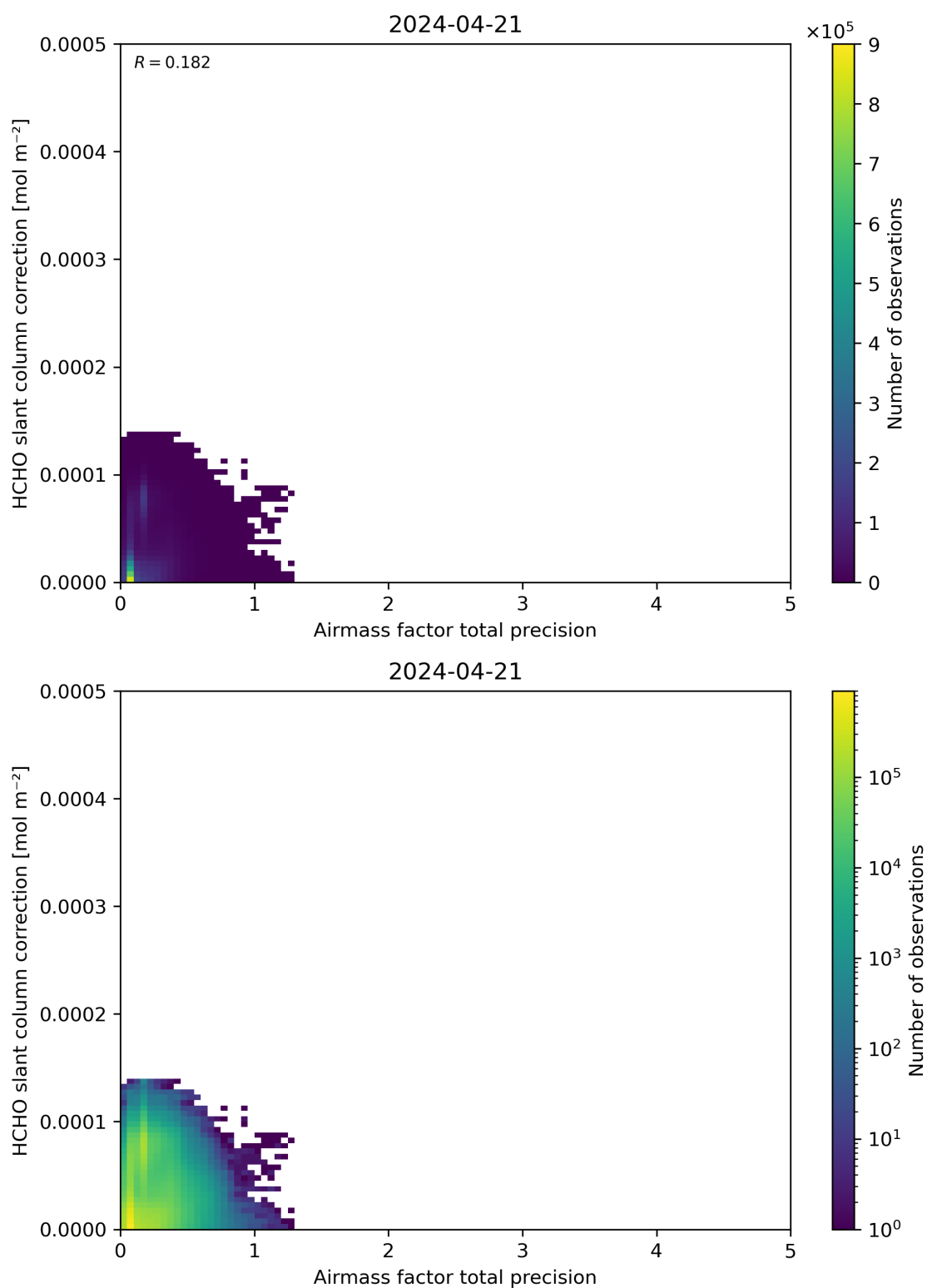
Figure 110: Scatter density plot of “Airmass factor total precision” against “HCHO slant column correction” for 2024-04-21 to 2024-04-22.
