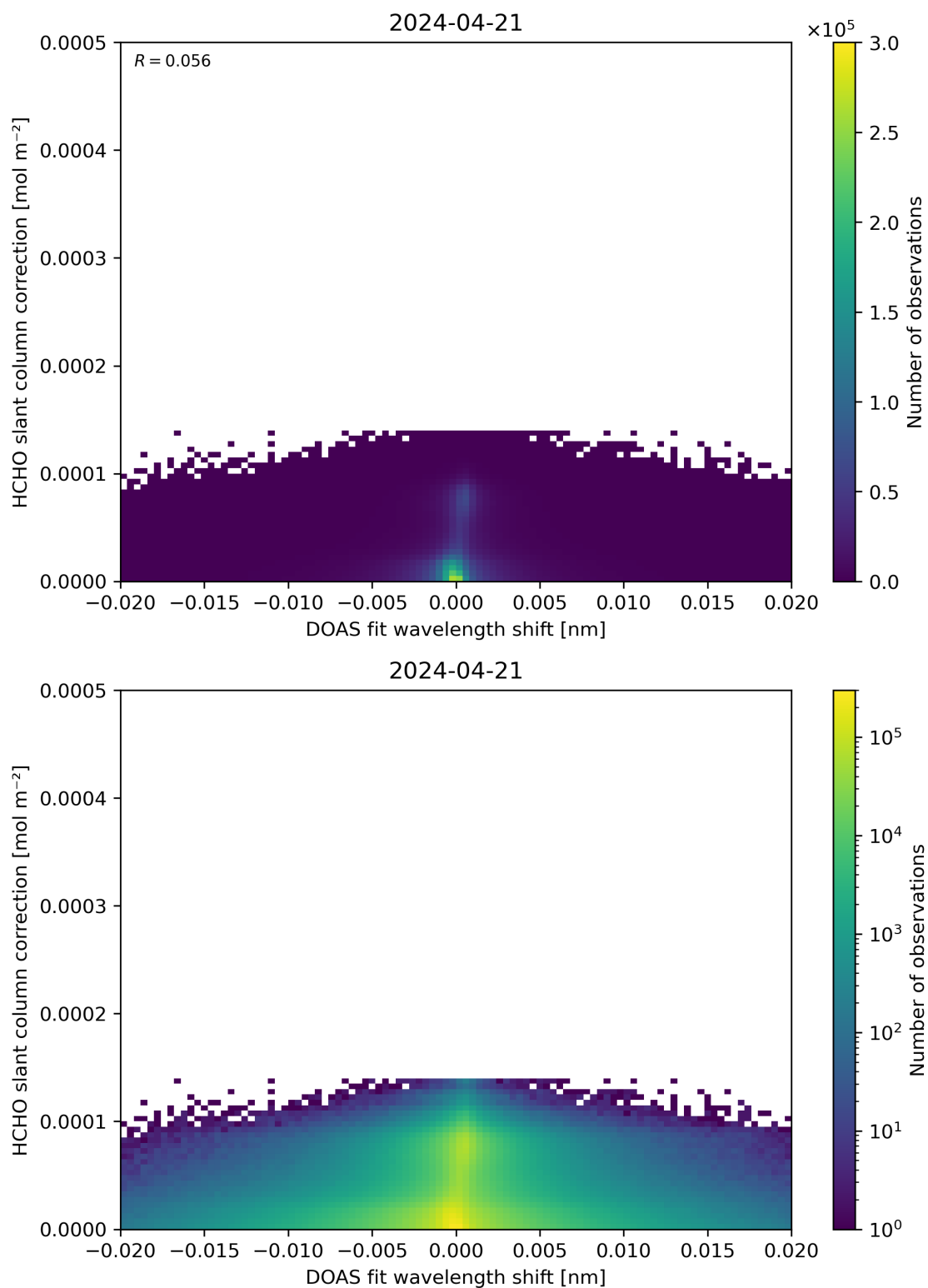
Figure 67: Scatter density plot of “DOAS fit wavelength shift” against “HCHO slant column correction” for 2024-04-21 to 2024-04-22.
