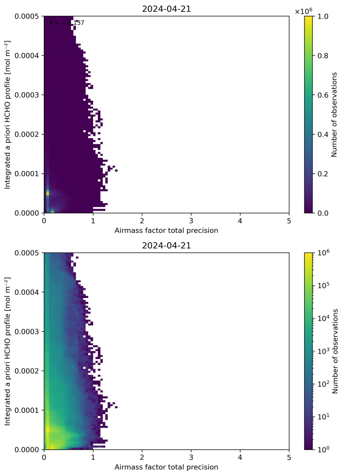
Figure 111: Scatter density plot of “Airmass factor total precision” against “Integrated a priori HCHO profile” for 2024-04-21 to 2024-04-22.
