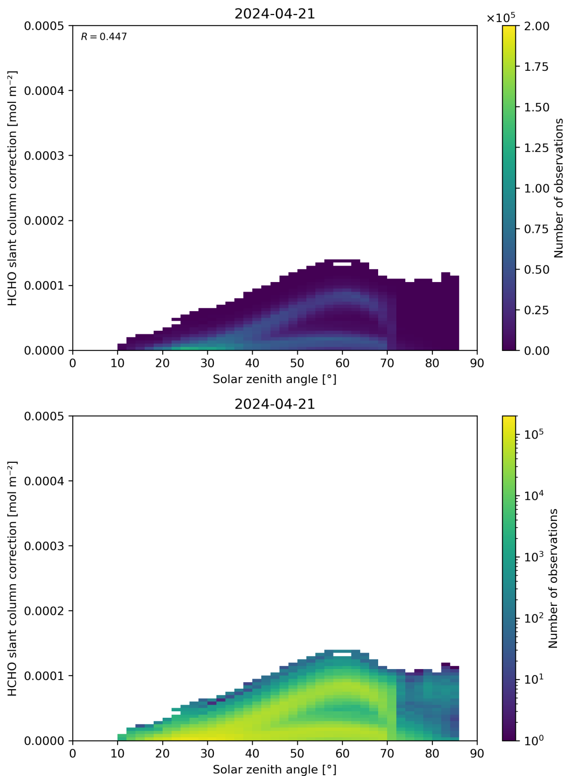
Figure 172: Scatter density plot of “Solar zenith angle” against “HCHO slant column correction” for 2024-04-21 to 2024-04-22.
