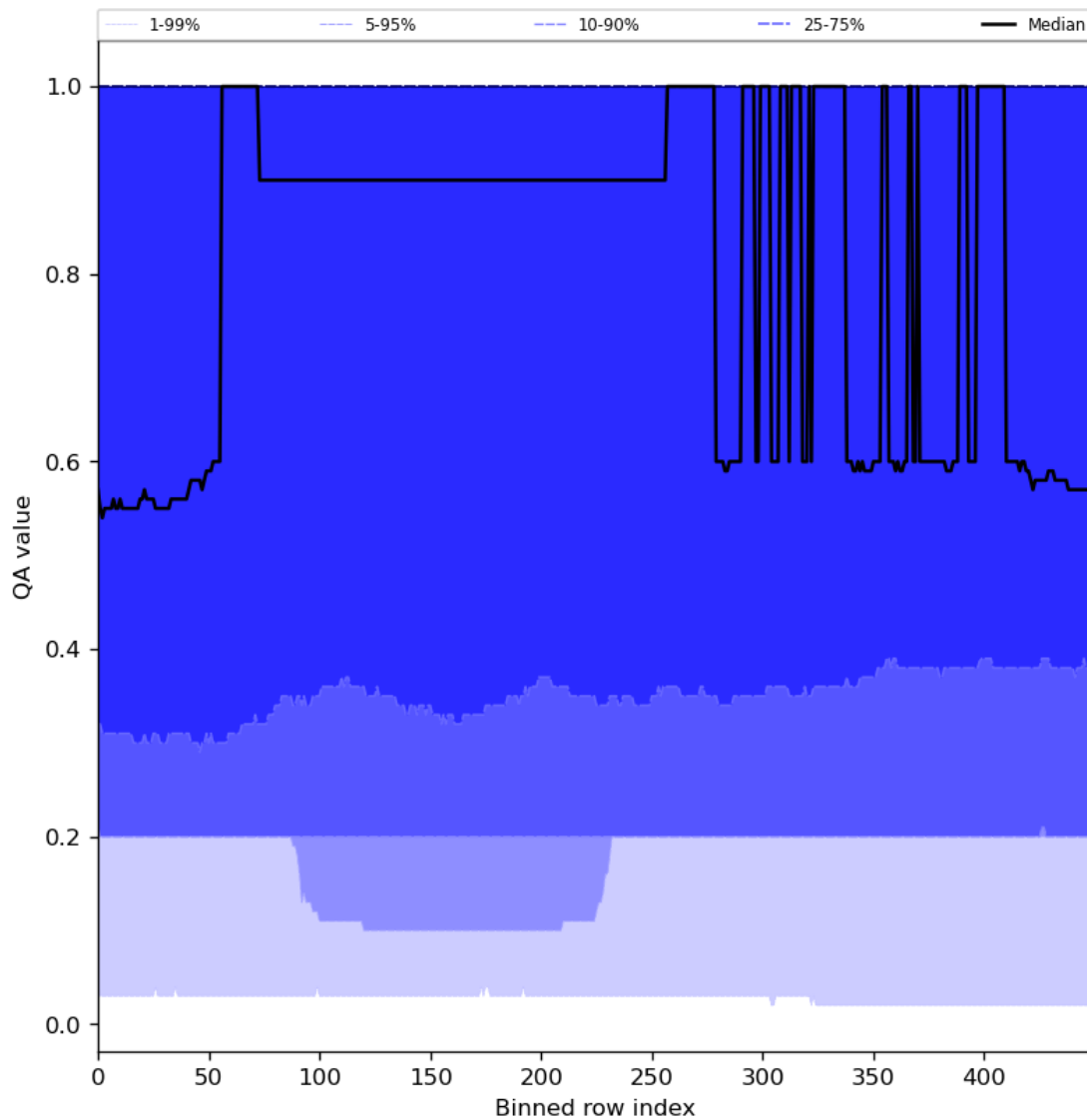
Figure 48: Along track statistics of “QA value” for 2024-04-21 to 2024-04-22
