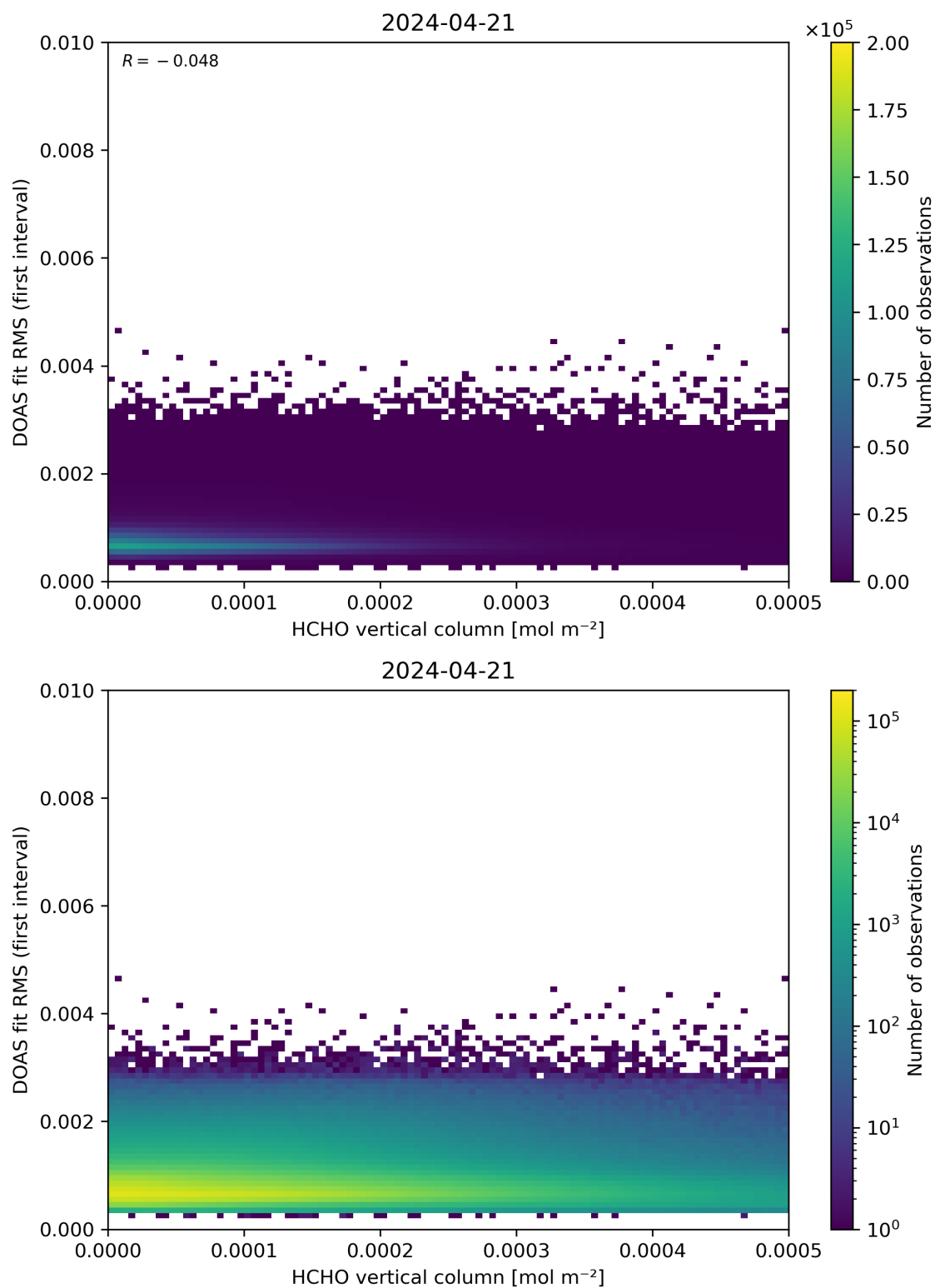
Figure 123: Scatter density plot of “HCHO vertical column” against “DOAS fit RMS (first interval)” for 2024-04-21 to 2024-04-22.
