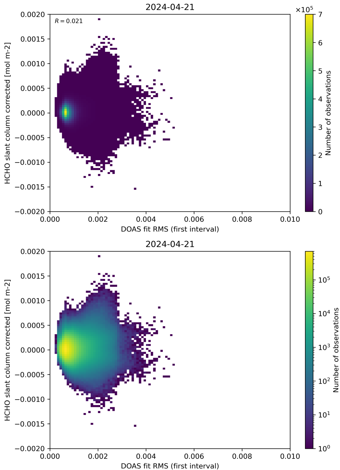
Figure 62: Scatter density plot of “DOAS fit RMS (first interval)” against “HCHO slant column corrected” for 2024-04-21 to 2024-04-22.
