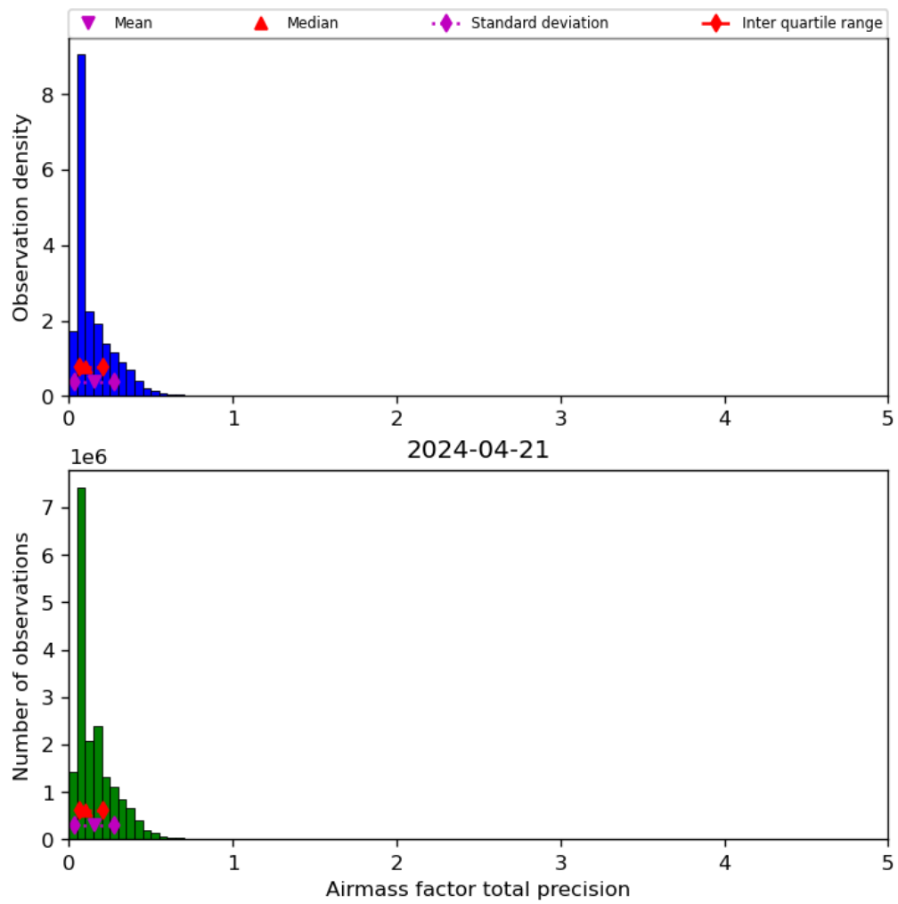
Figure 41: Histogram of “Airmass factor total precision” for 2024-04-21 to 2024-04-22
