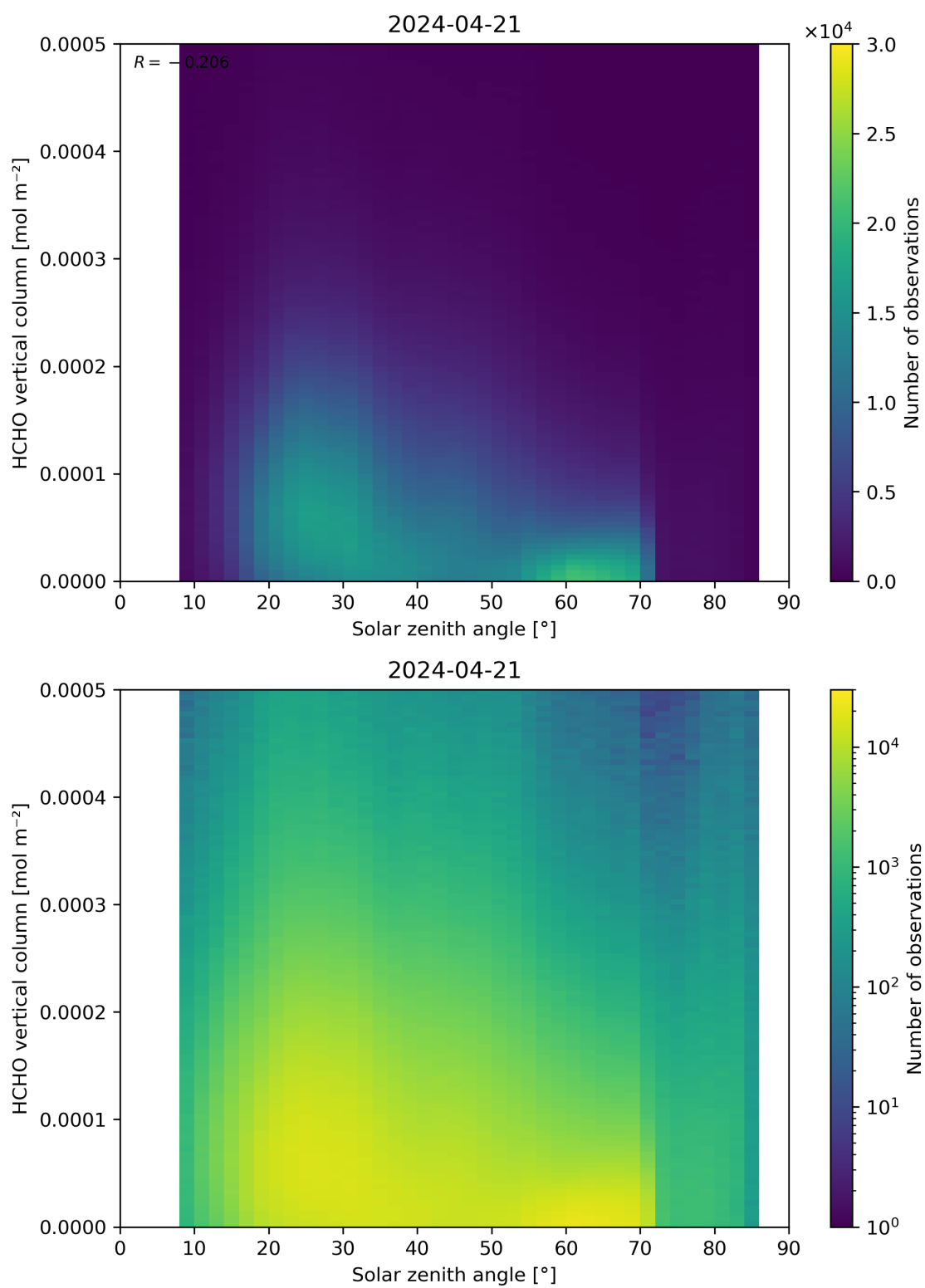
Figure 177: Scatter density plot of “Solar zenith angle” against “HCHO vertical column” for 2024-04-21 to 2024-04-22.
