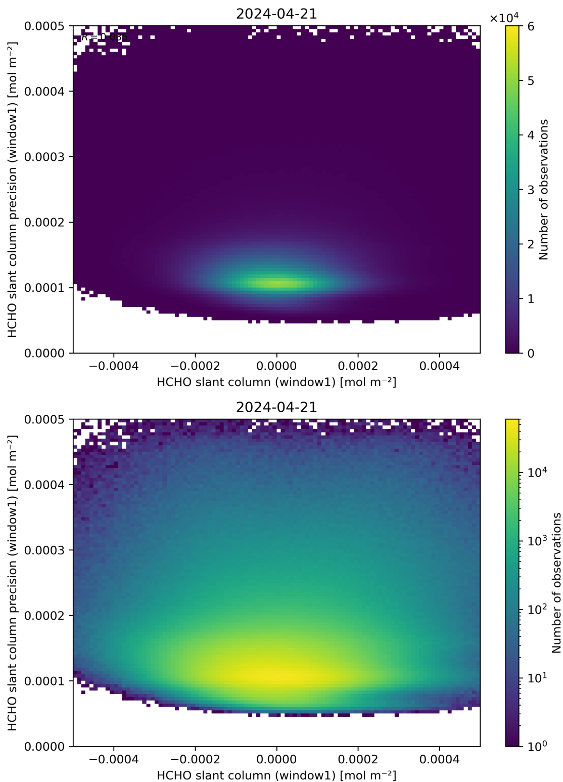
Figure 84: Scatter density plot of “HCHO slant column (window1)” against “HCHO slant column precision (window1)” for 2024-04-21 to 2024-04-22.
