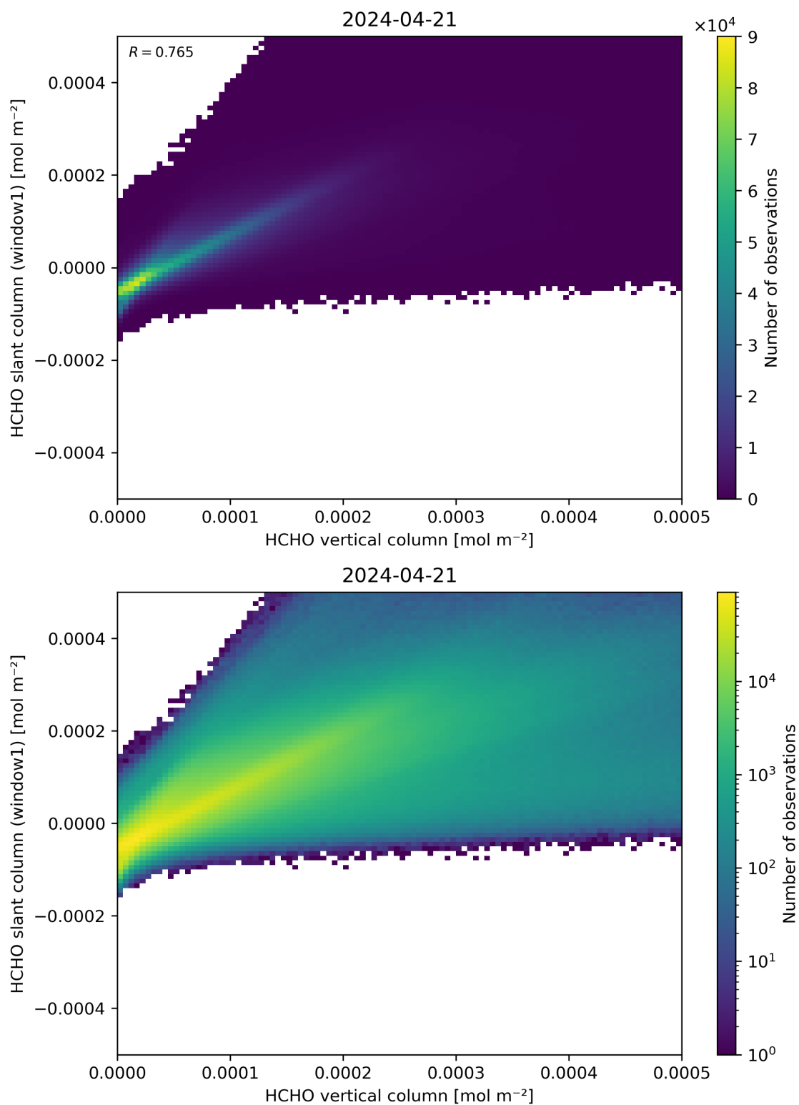
Figure 129: Scatter density plot of “HCHO vertical column” against “HCHO slant column (window1)” for 2024-04-21 to 2024-04-22.
