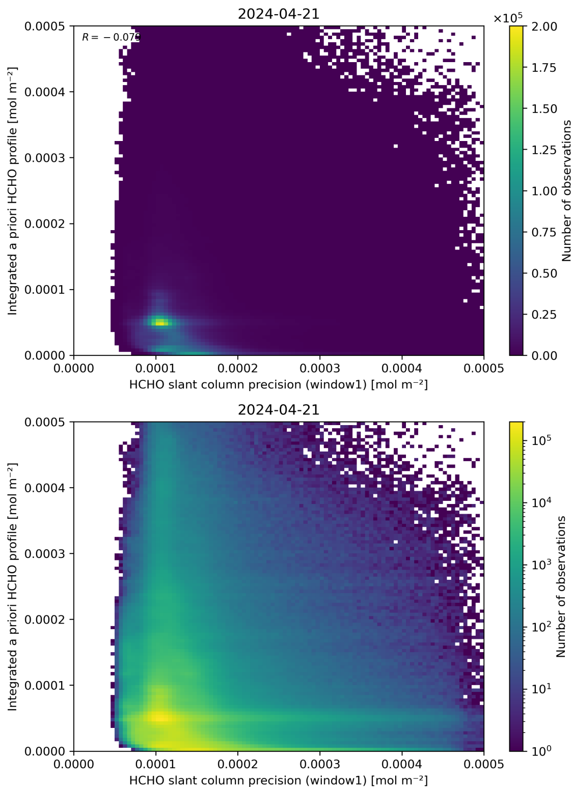
Figure 96: Scatter density plot of “HCHO slant column precision (window1)” against “Integrated a priori HCHO profile” for 2024-04-21 to 2024-04-22.
