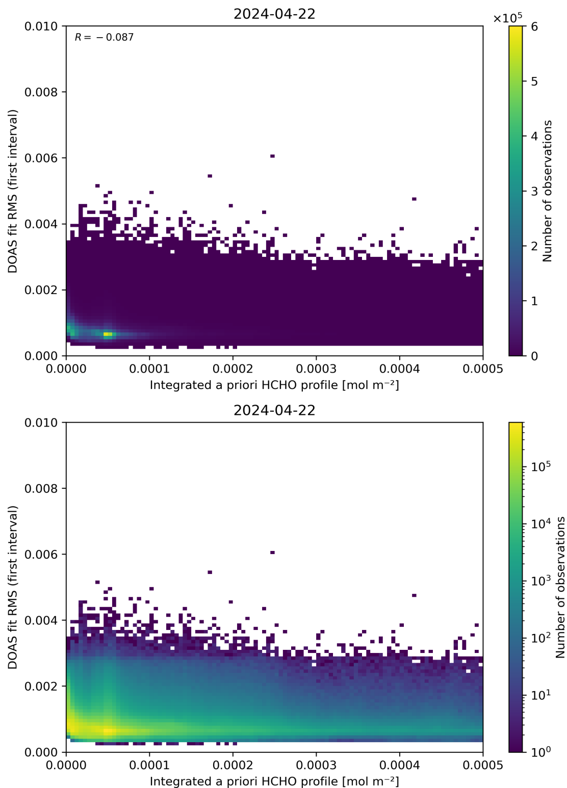
Figure 148: Scatter density plot of “Integrated a priori HCHO profile” against “DOAS fit RMS (first interval)” for 2024-04-21 to 2024-04-23.
