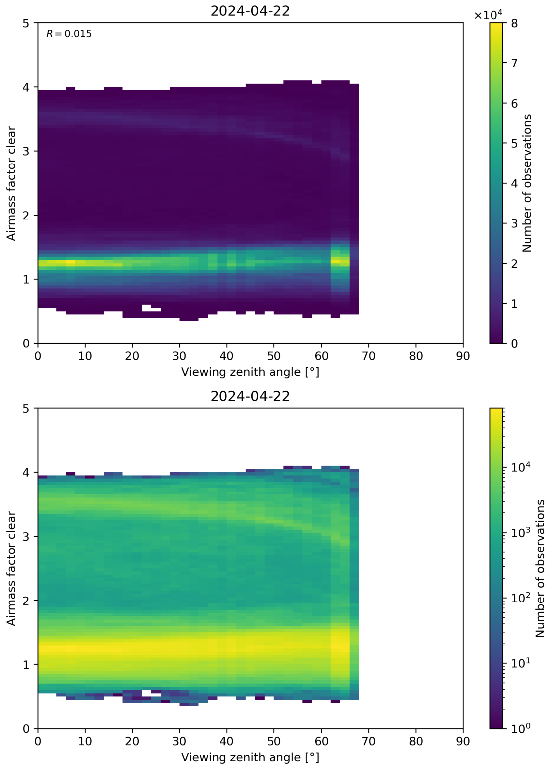
Figure 185: Scatter density plot of “Viewing zenith angle” against “Airmass factor clear” for 2024-04-21 to 2024-04-23.
