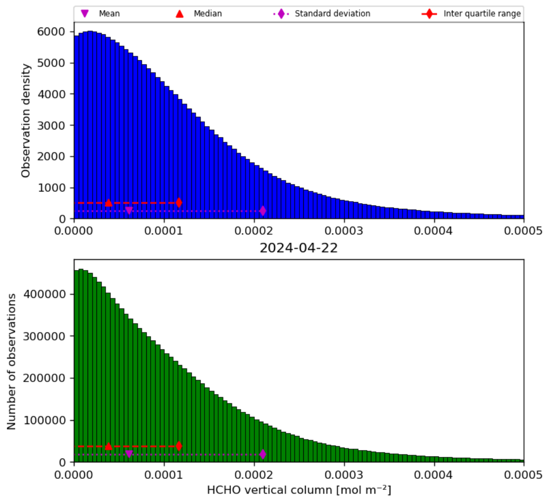
Figure 35: Histogram of “HCHO vertical column” for 2024-04-21 to 2024-04-23
