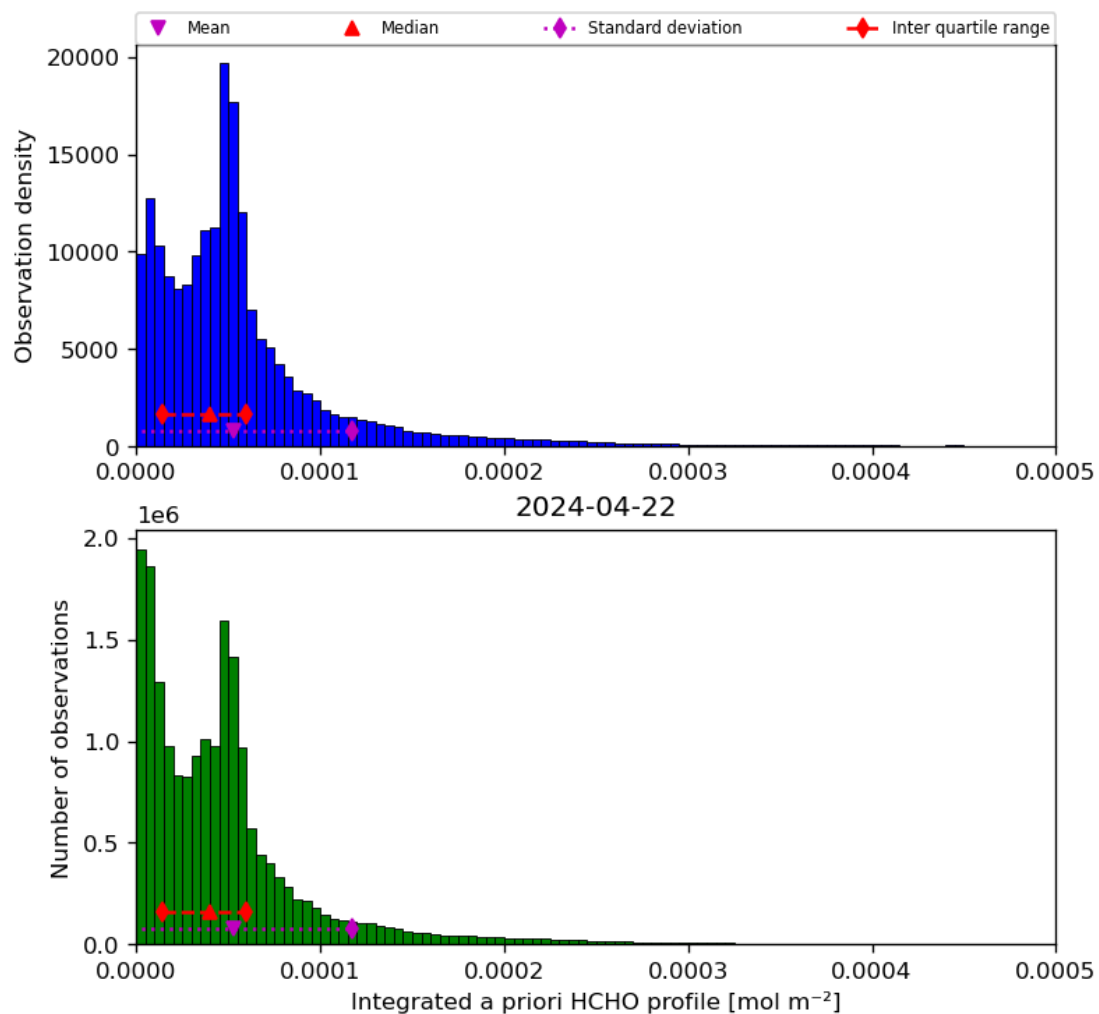
Figure 43: Histogram of “Integrated a priori HCHO profile” for 2024-04-21 to 2024-04-23
