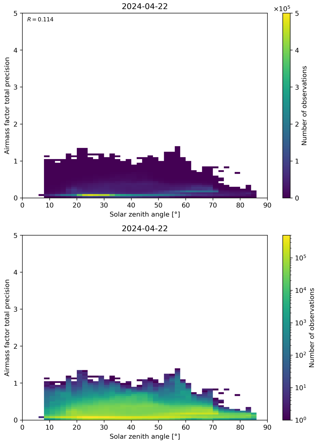
Figure 176: Scatter density plot of “Solar zenith angle” against “Airmass factor total precision” for 2024-04-21 to 2024-04-23.
