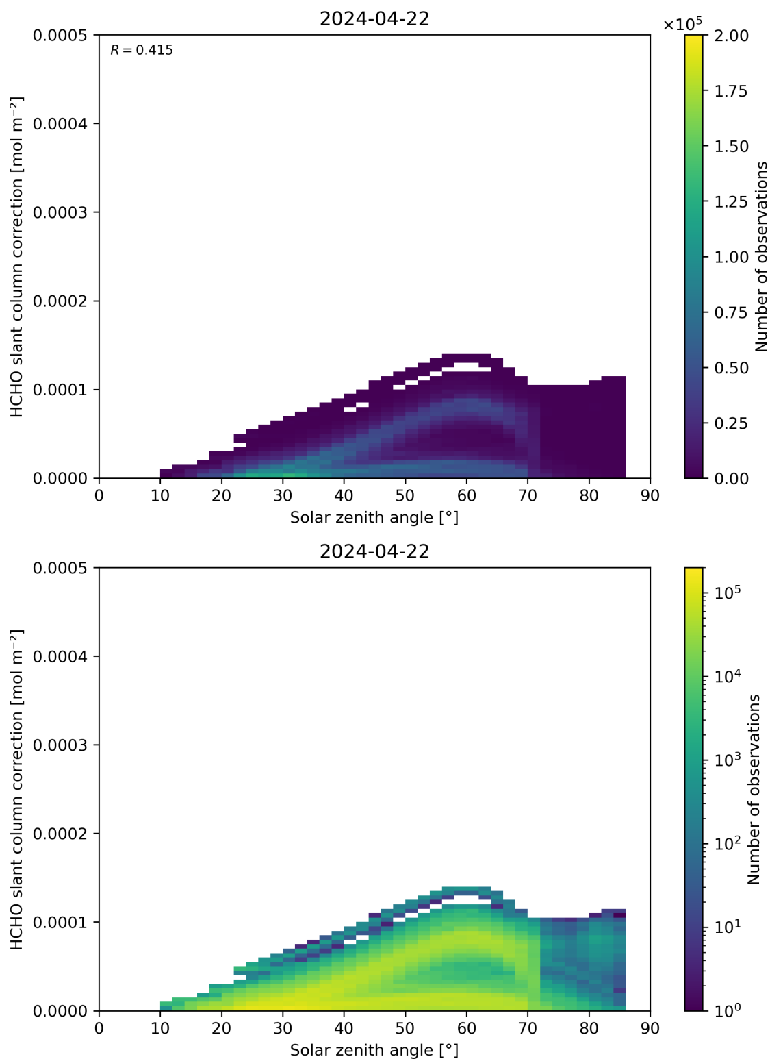
Figure 172: Scatter density plot of “Solar zenith angle” against “HCHO slant column correction” for 2024-04-21 to 2024-04-23.
