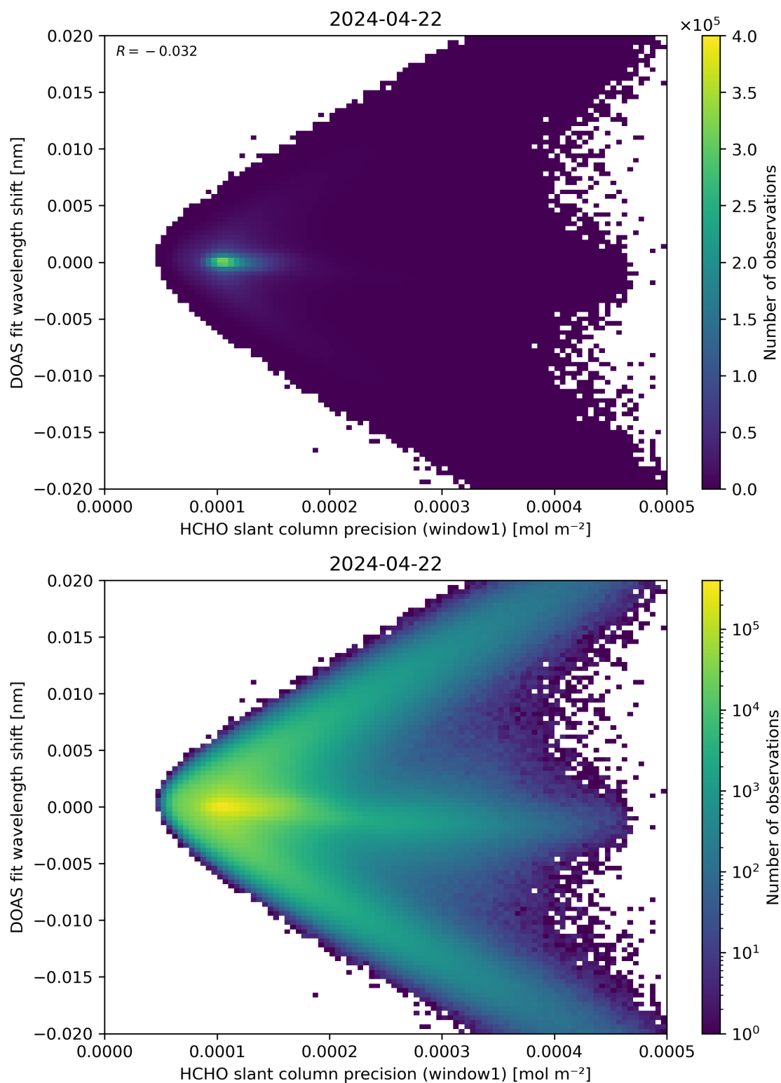
Figure 89: Scatter density plot of “HCHO slant column precision (window1)” against “DOAS fit wavelength shift” for 2024-04-21 to 2024-04-23.
