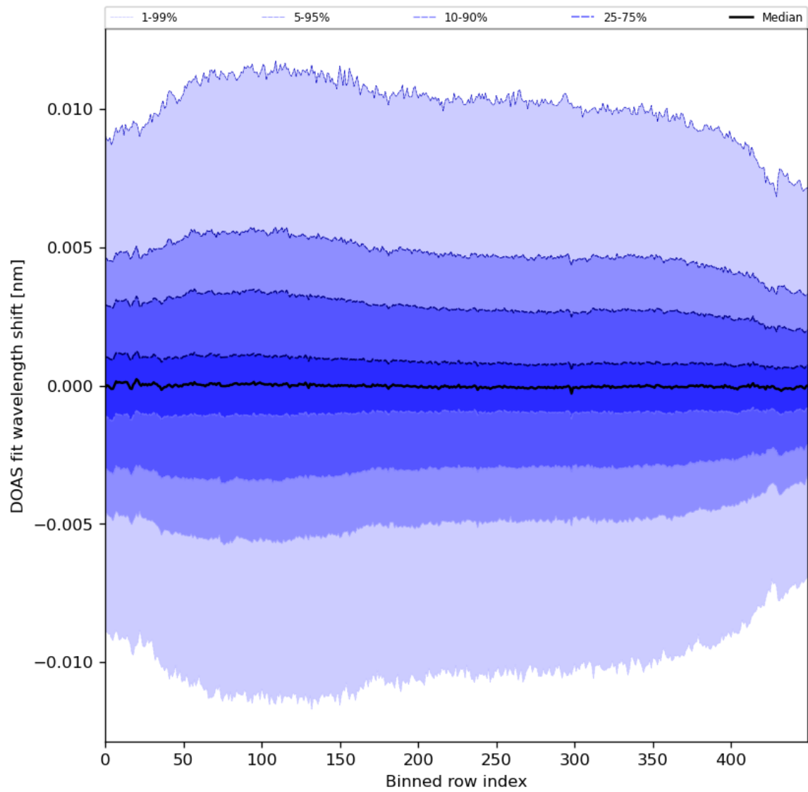
Figure 58: Along track statistics of “DOAS fit wavelength shift” for 2024-04-21 to 2024-04-23
