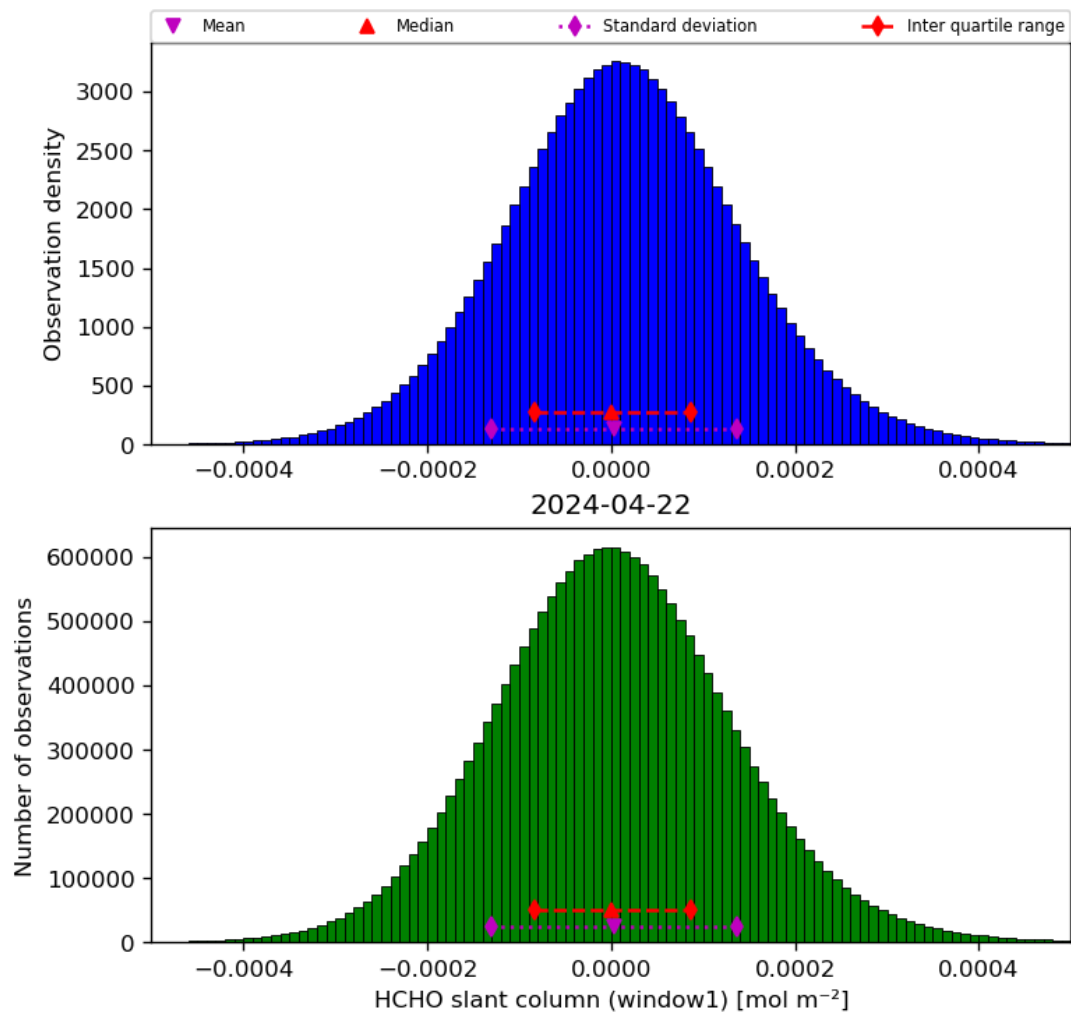
Figure 38: Histogram of “HCHO slant column (window1)” for 2024-04-21 to 2024-04-23
