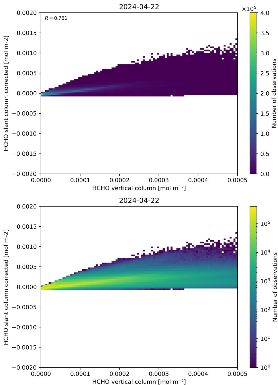
Figure 127: Scatter density plot of “HCHO vertical column” against “HCHO slant column corrected” for 2024-04-21 to 2024-04-23.
