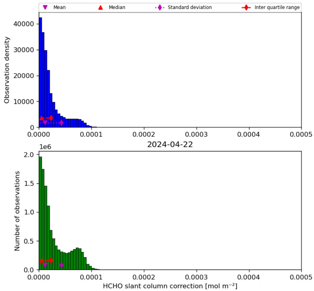
Figure 47: Histogram of “HCHO slant column correction” for 2024-04-21 to 2024-04-23
