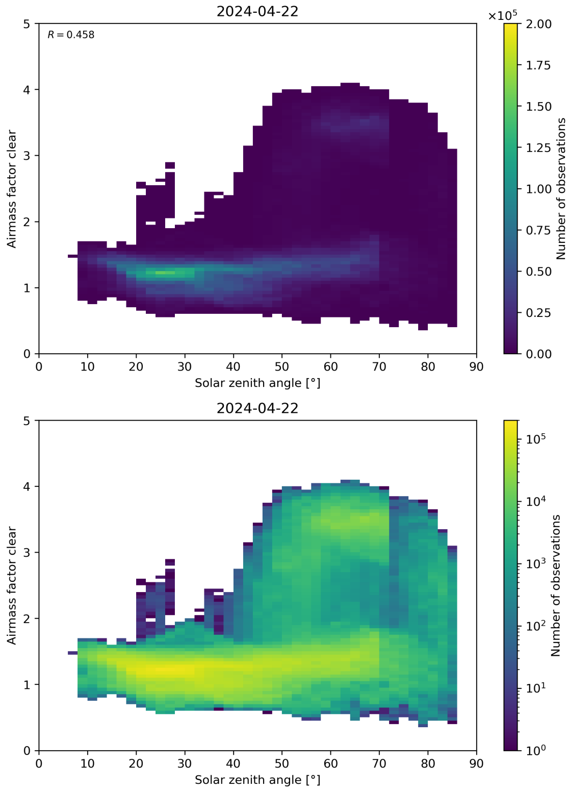
Figure 170: Scatter density plot of “Solar zenith angle” against “Airmass factor clear” for 2024-04-21 to 2024-04-23.
