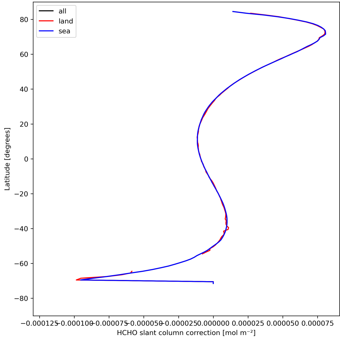
Figure 33: Zonal average of “HCHO slant column correction” for 2024-04-21 to 2024-04-23.
