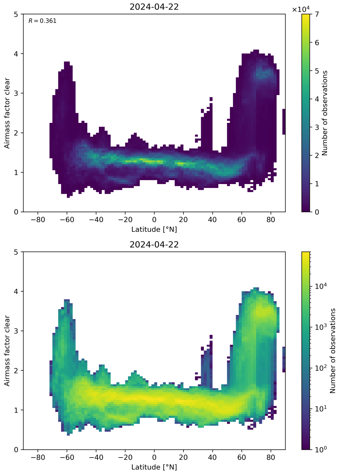
Figure 156: Scatter density plot of “Latitude” against “Airmass factor clear” for 2024-04-21 to 2024-04-23.
