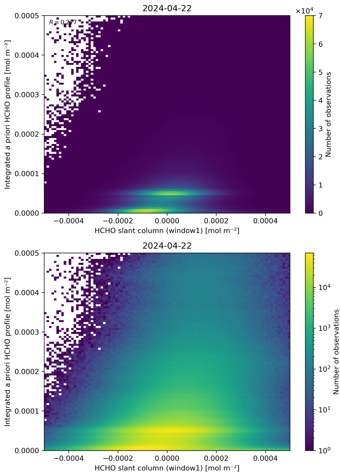
Figure 87: Scatter density plot of “HCHO slant column (window1)” against “Integrated a priori HCHO profile” for 2024-04-21 to 2024-04-23.
