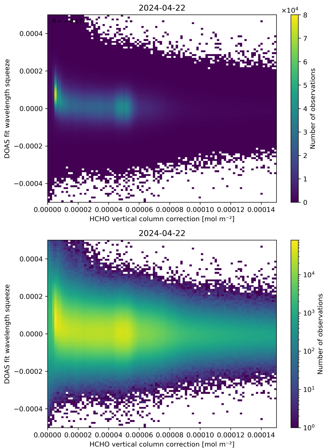
Figure 114: Scatter density plot of “HCHO vertical column correction” against “DOAS fit wavelength squeeze” for 2024-04-21 to 2024-04-23.
