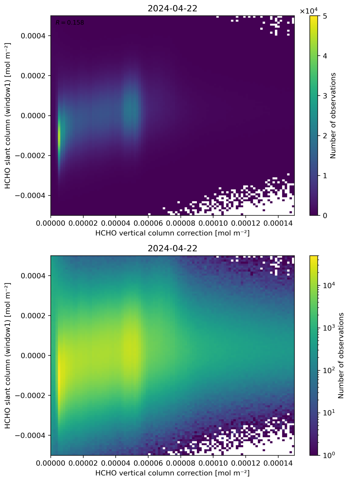
Figure 118: Scatter density plot of “HCHO vertical column correction” against “HCHO slant column (window1)” for 2024-04-21 to 2024-04-23.
