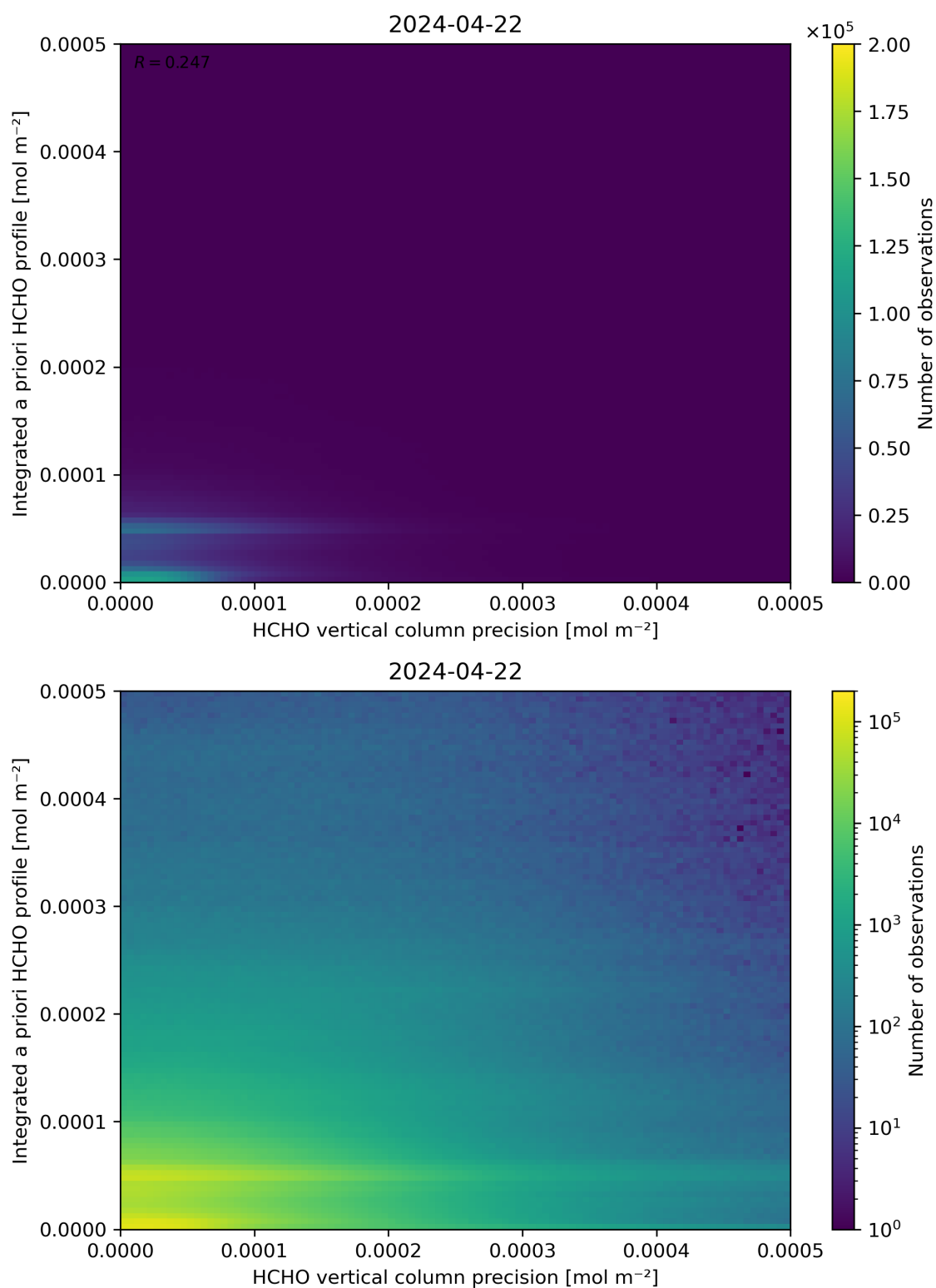
Figure 147: Scatter density plot of “HCHO vertical column precision” against “Integrated a priori HCHO profile” for 2024-04-21 to 2024-04-23.
