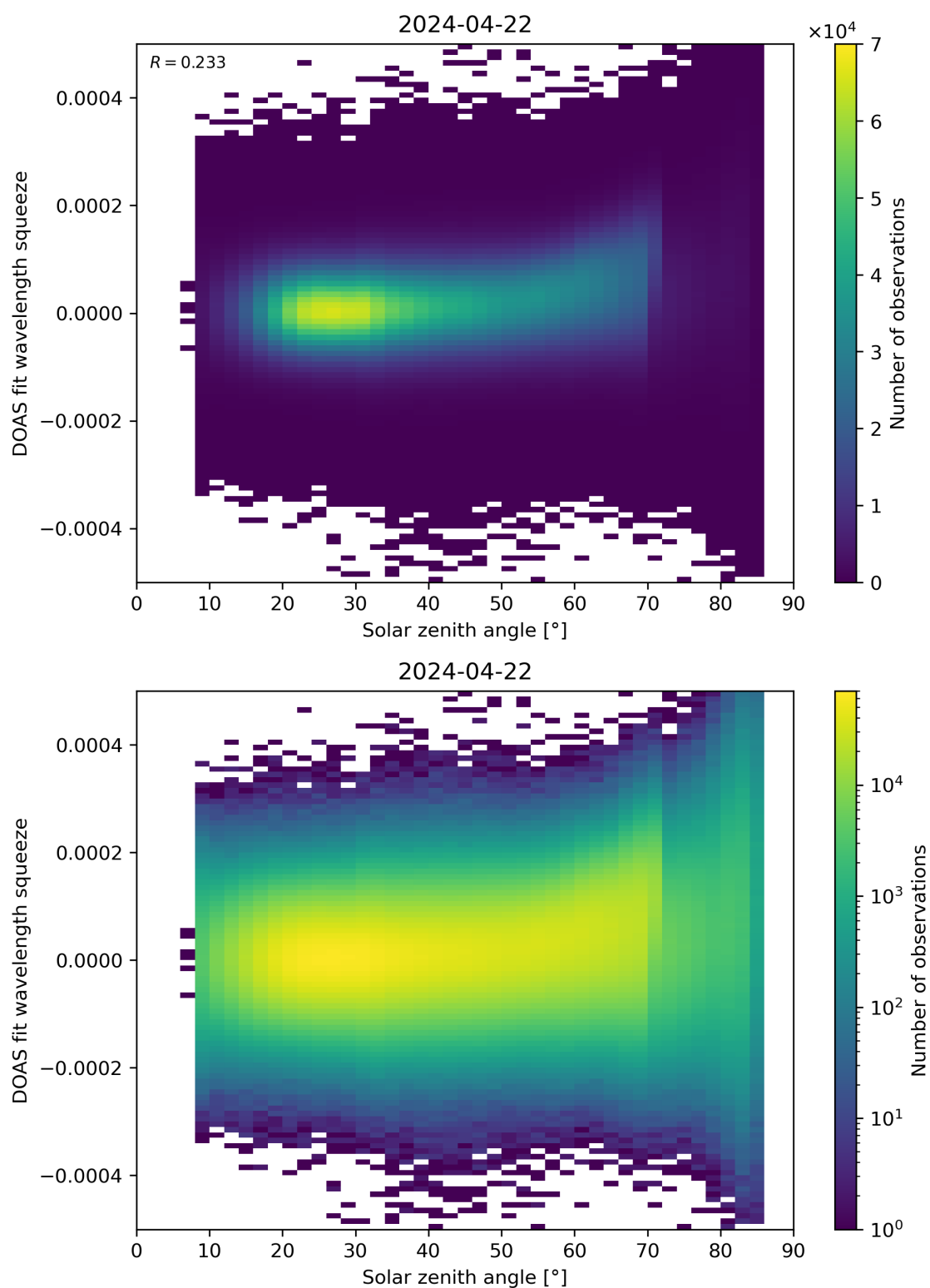
Figure 169: Scatter density plot of “Solar zenith angle” against “DOAS fit wavelength squeeze” for 2024-04-21 to 2024-04-23.
