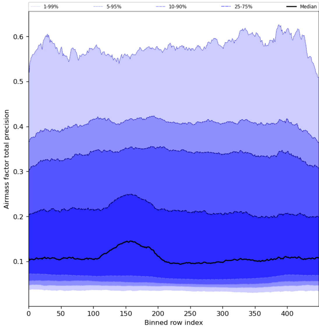
Figure 55: Along track statistics of “Airmass factor total precision” for 2024-04-21 to 2024-04-23
