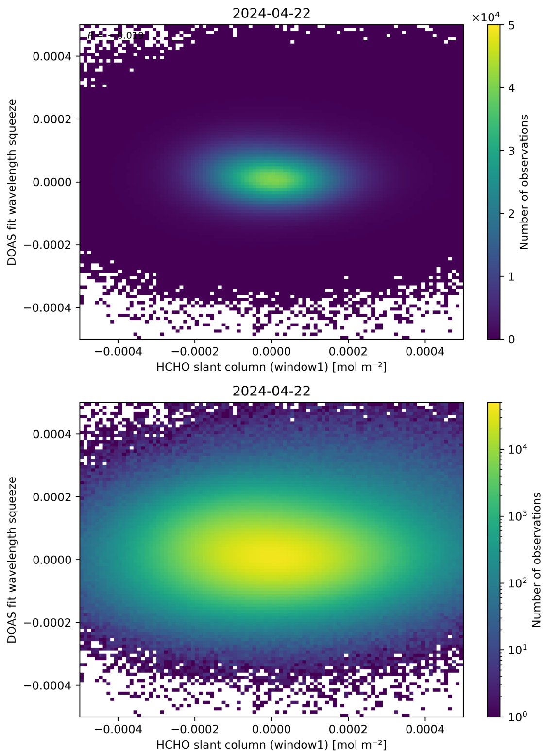
Figure 80: Scatter density plot of “HCHO slant column (window1)” against “DOAS fit wavelength squeeze” for 2024-04-21 to 2024-04-23.
