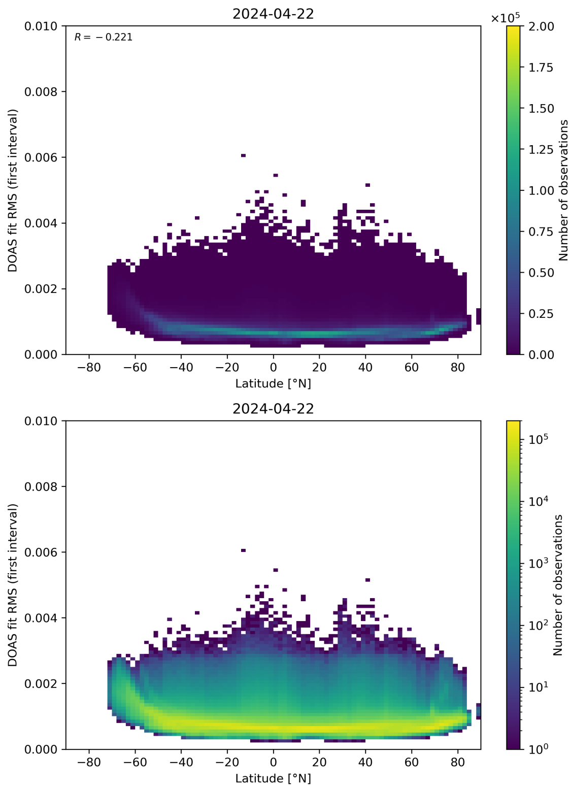
Figure 153: Scatter density plot of “Latitude” against “DOAS fit RMS (first interval)” for 2024-04-21 to 2024-04-23.
