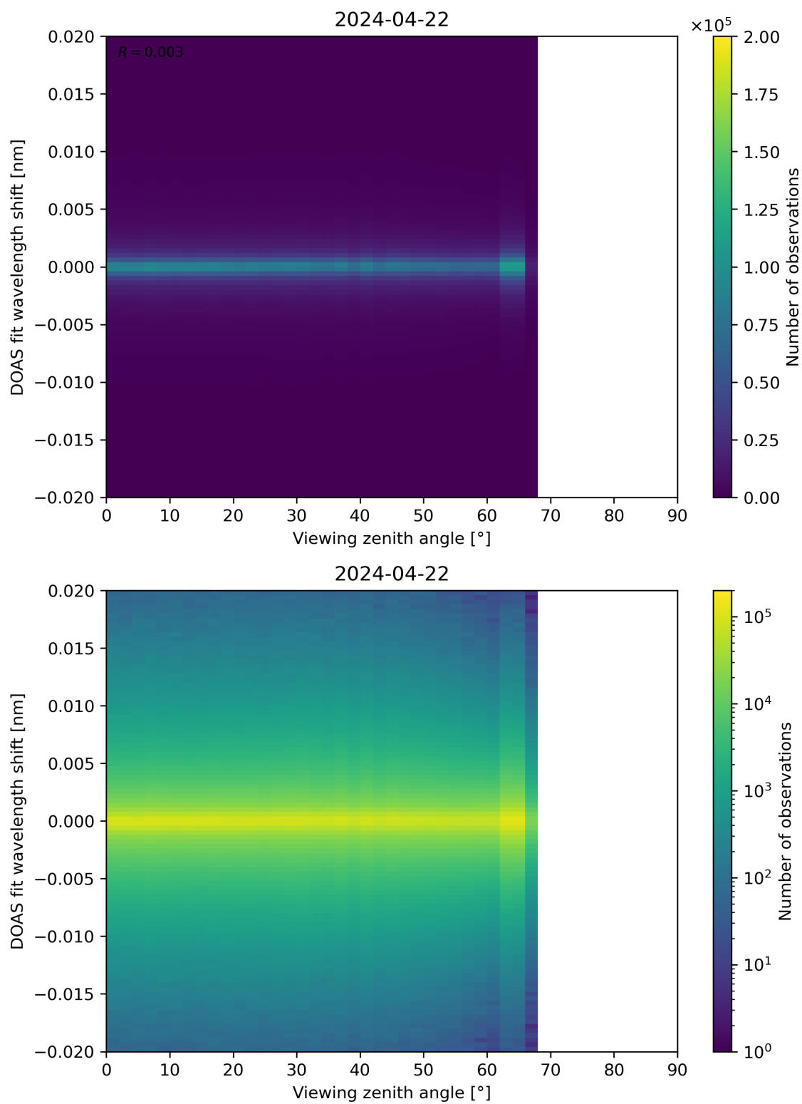
Figure 183: Scatter density plot of “Viewing zenith angle” against “DOAS fit wavelength shift” for 2024-04-21 to 2024-04-23.
