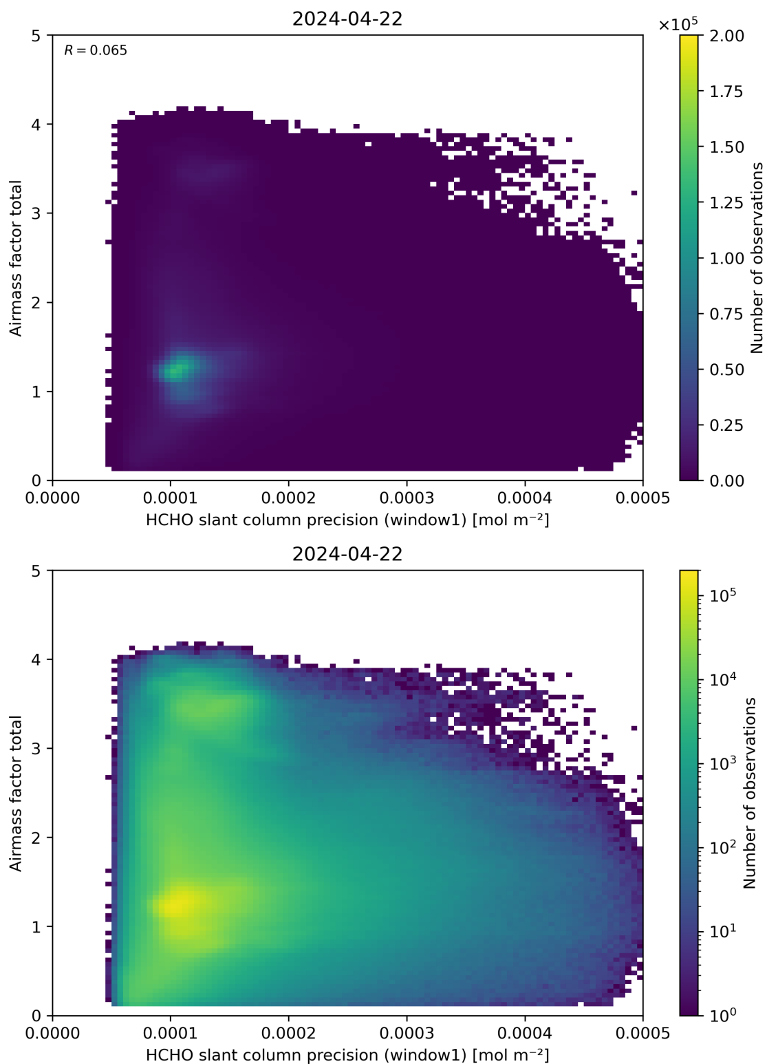
Figure 94: Scatter density plot of “HCHO slant column precision (window1)” against “Airmass factor total” for 2024-04-21 to 2024-04-23.
