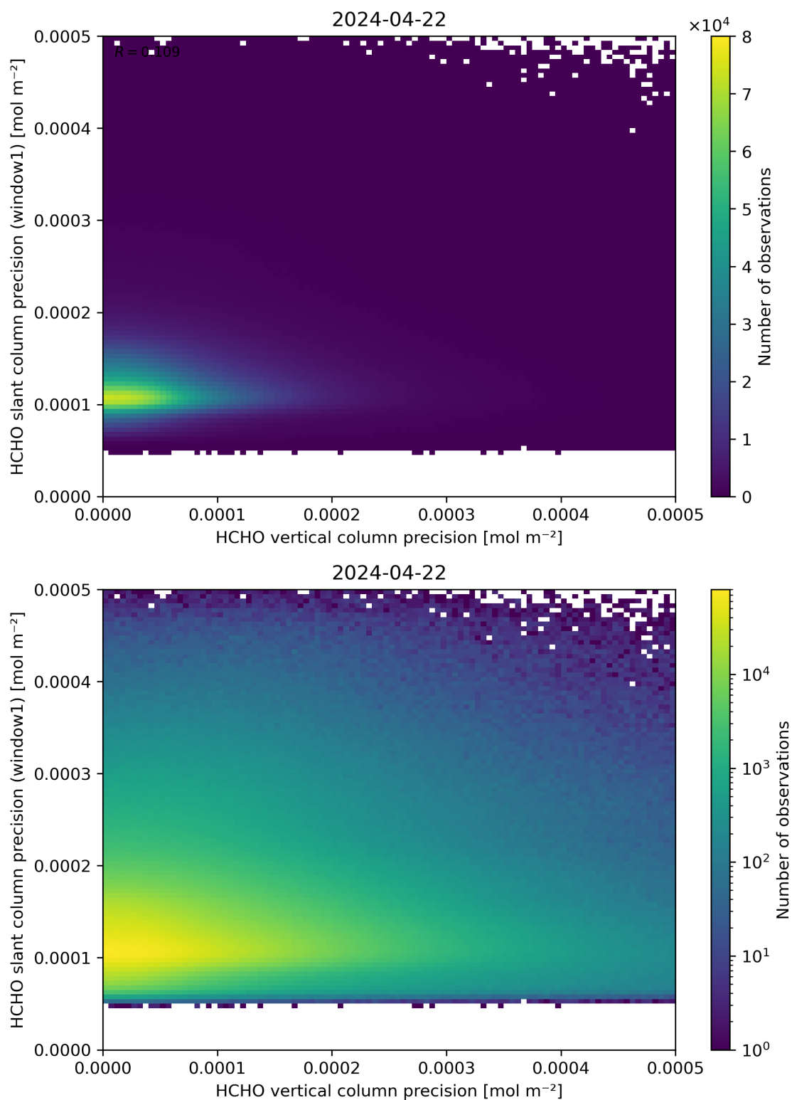
Figure 143: Scatter density plot of “HCHO vertical column precision” against “HCHO slant column precision (window1)” for 2024-04-21 to 2024-04-23.
