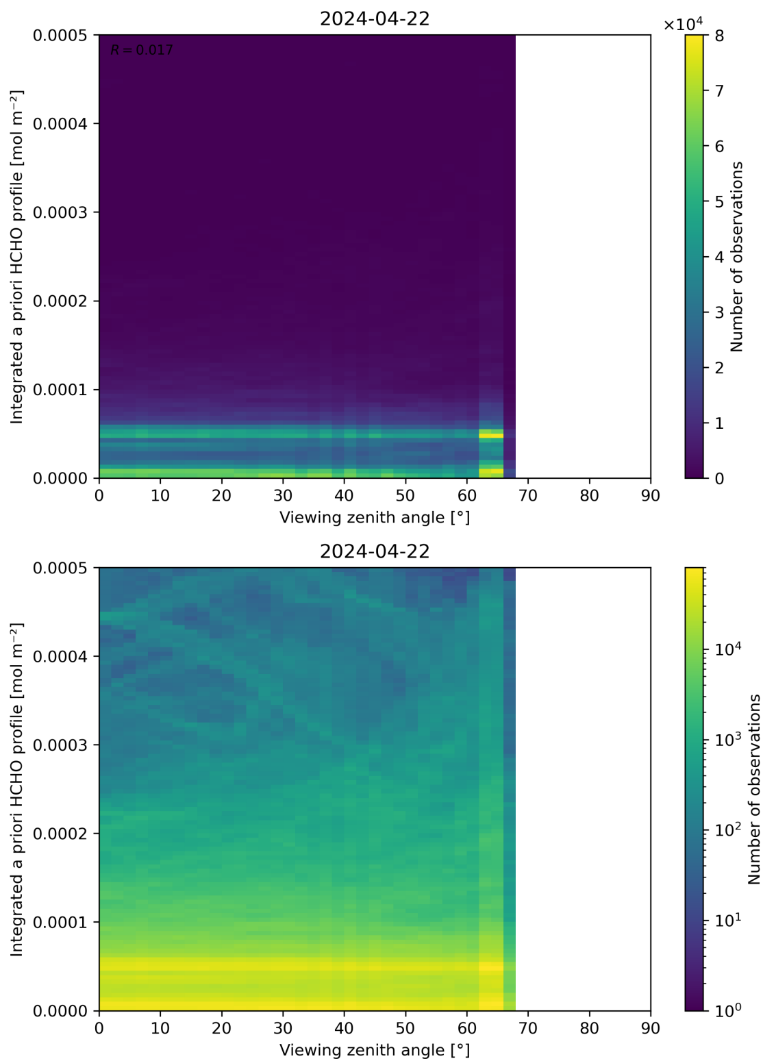
Figure 195: Scatter density plot of “Viewing zenith angle” against “Integrated a priori HCHO profile” for 2024-04-21 to 2024-04-23.
