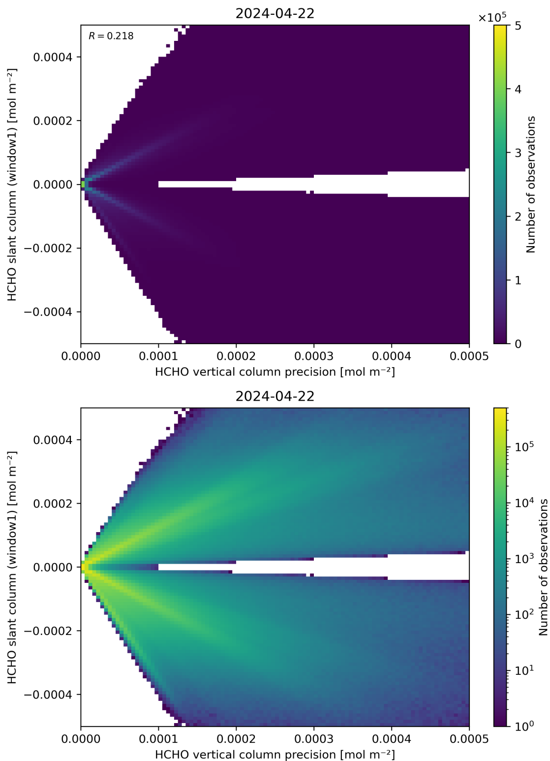
Figure 142: Scatter density plot of “HCHO vertical column precision” against “HCHO slant column (window1)” for 2024-04-21 to 2024-04-23.
