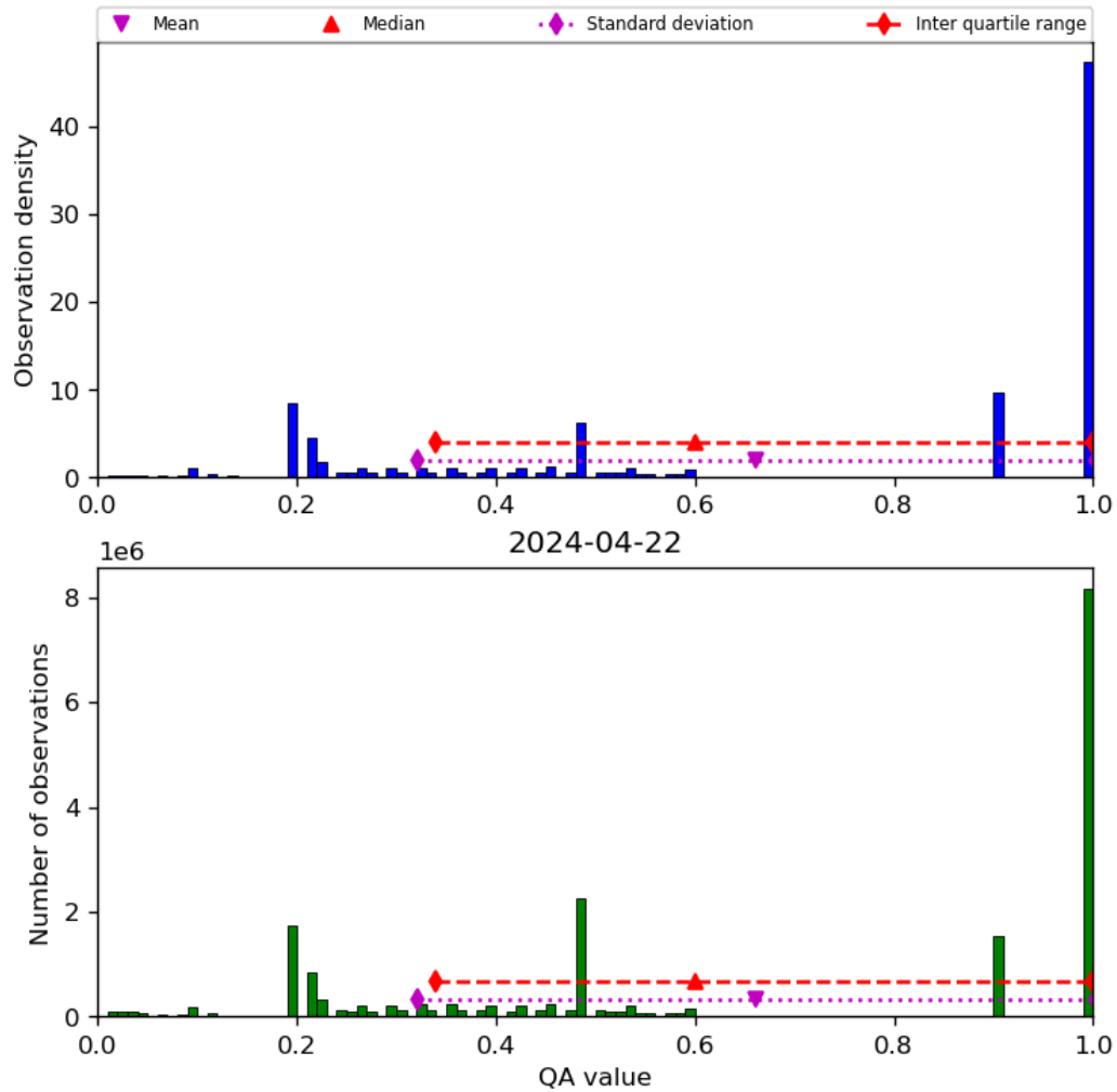
Figure 34: Histogram of “QA value” for 2024-04-21 to 2024-04-23
