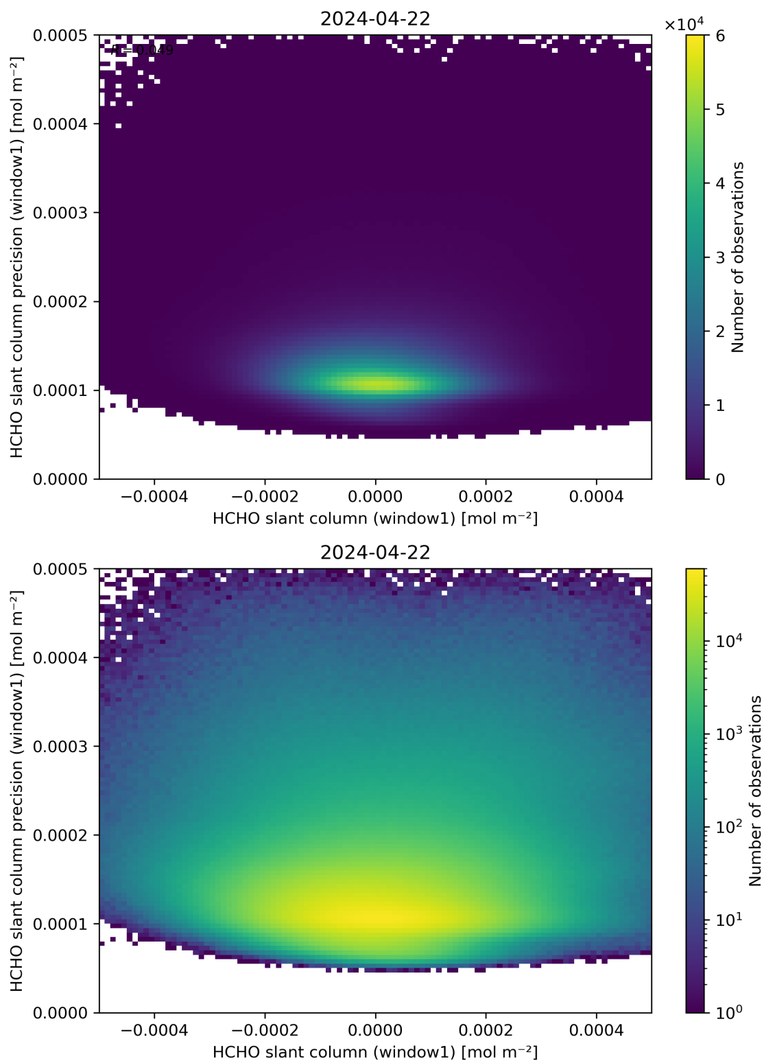
Figure 84: Scatter density plot of “HCHO slant column (window1)” against “HCHO slant column precision (window1)” for 2024-04-21 to 2024-04-23.
