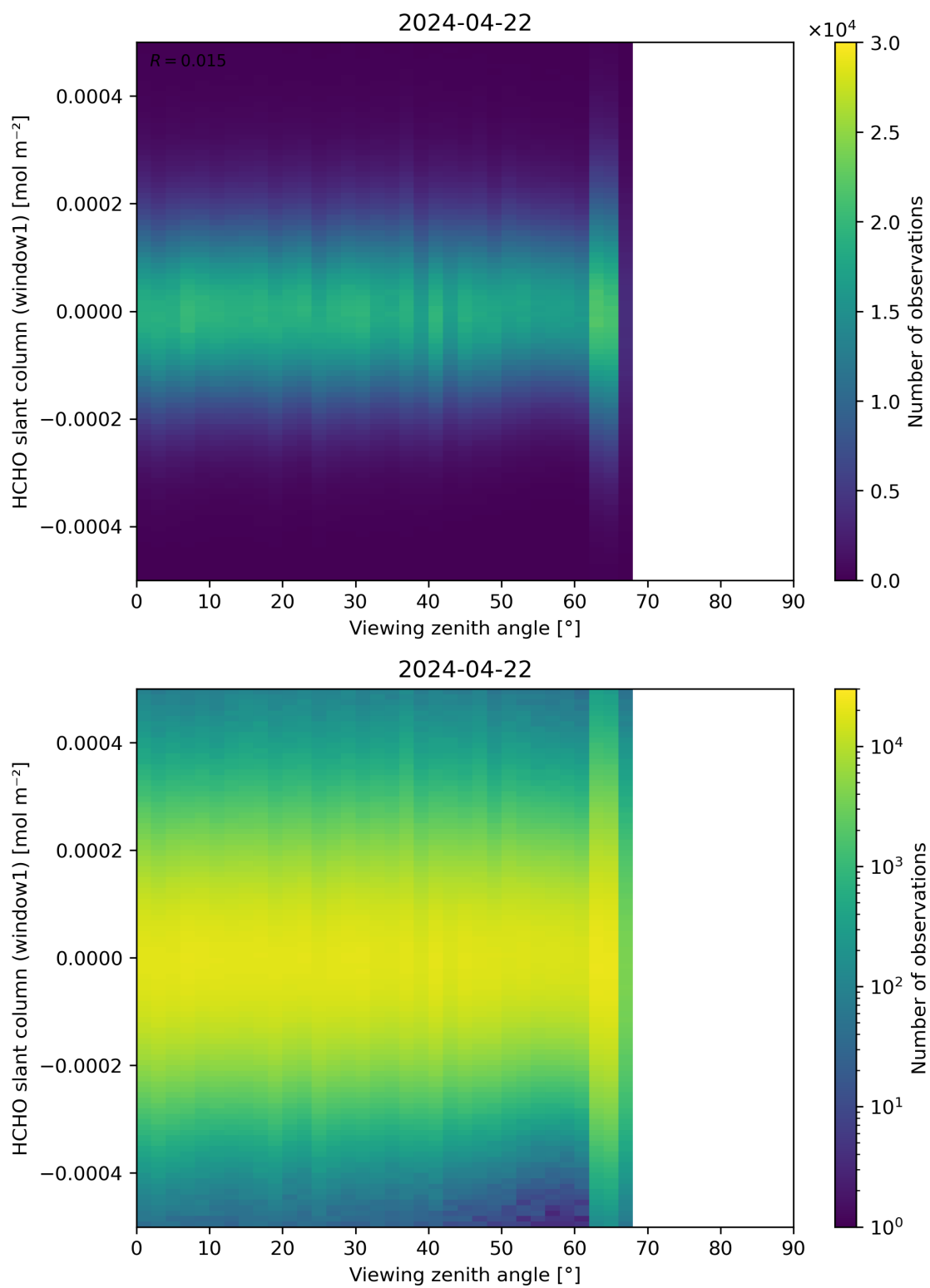
Figure 188: Scatter density plot of “Viewing zenith angle” against “HCHO slant column (window1)” for 2024-04-21 to 2024-04-23.
