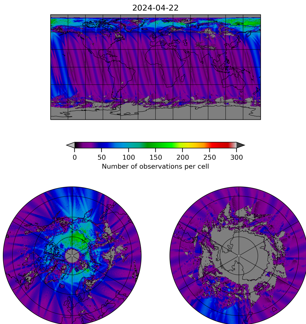
Figure 19: Map of the number of observations for 2024-04-21 to 2024-04-23
