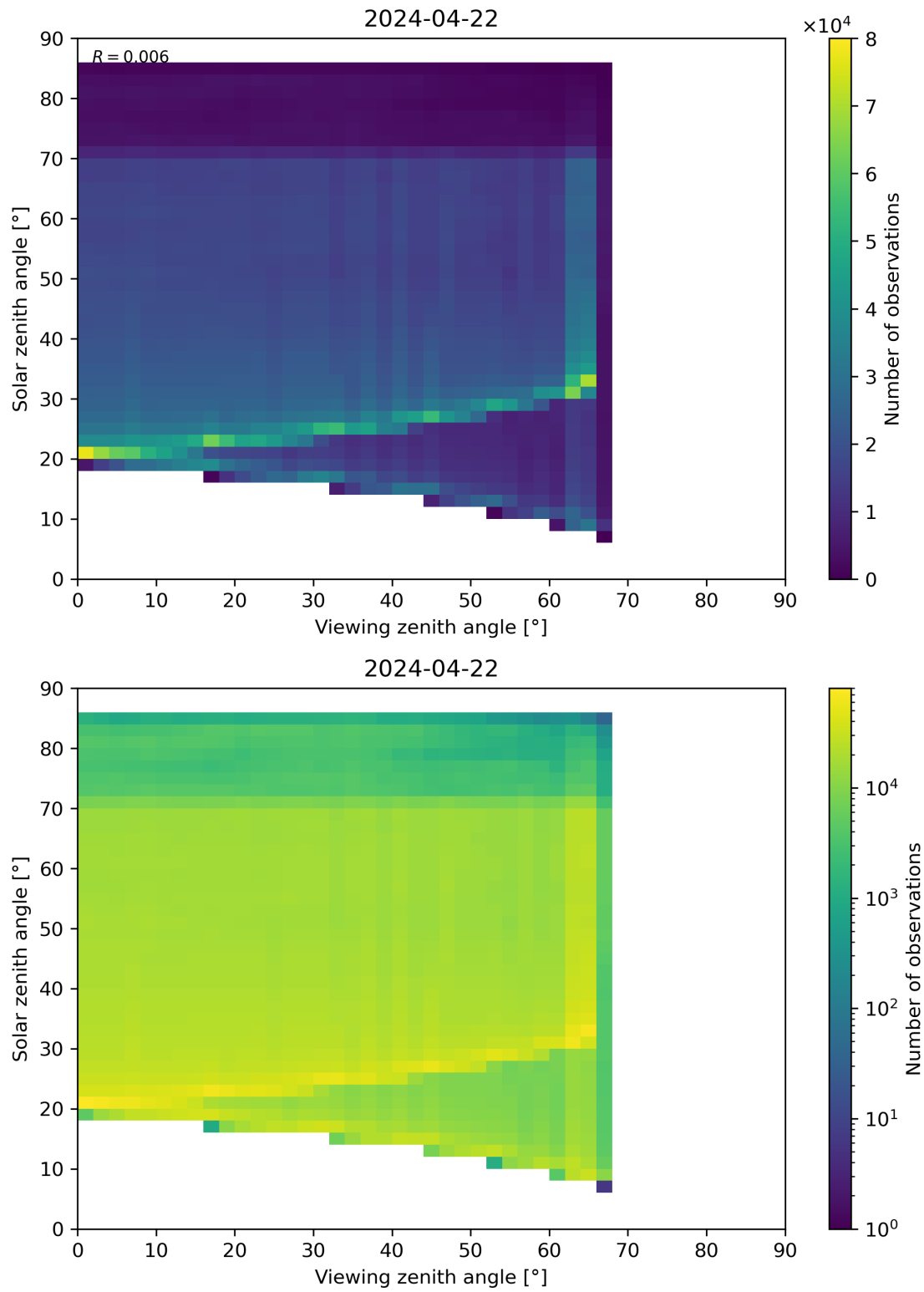
Figure 197: Scatter density plot of “Viewing zenith angle” against “Solar zenith angle” for 2024-04-21 to 2024-04-23.
