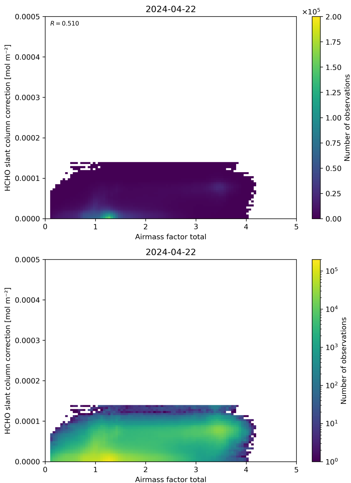
Figure 102: Scatter density plot of “Airmass factor total” against “HCHO slant column correction” for 2024-04-21 to 2024-04-23.
