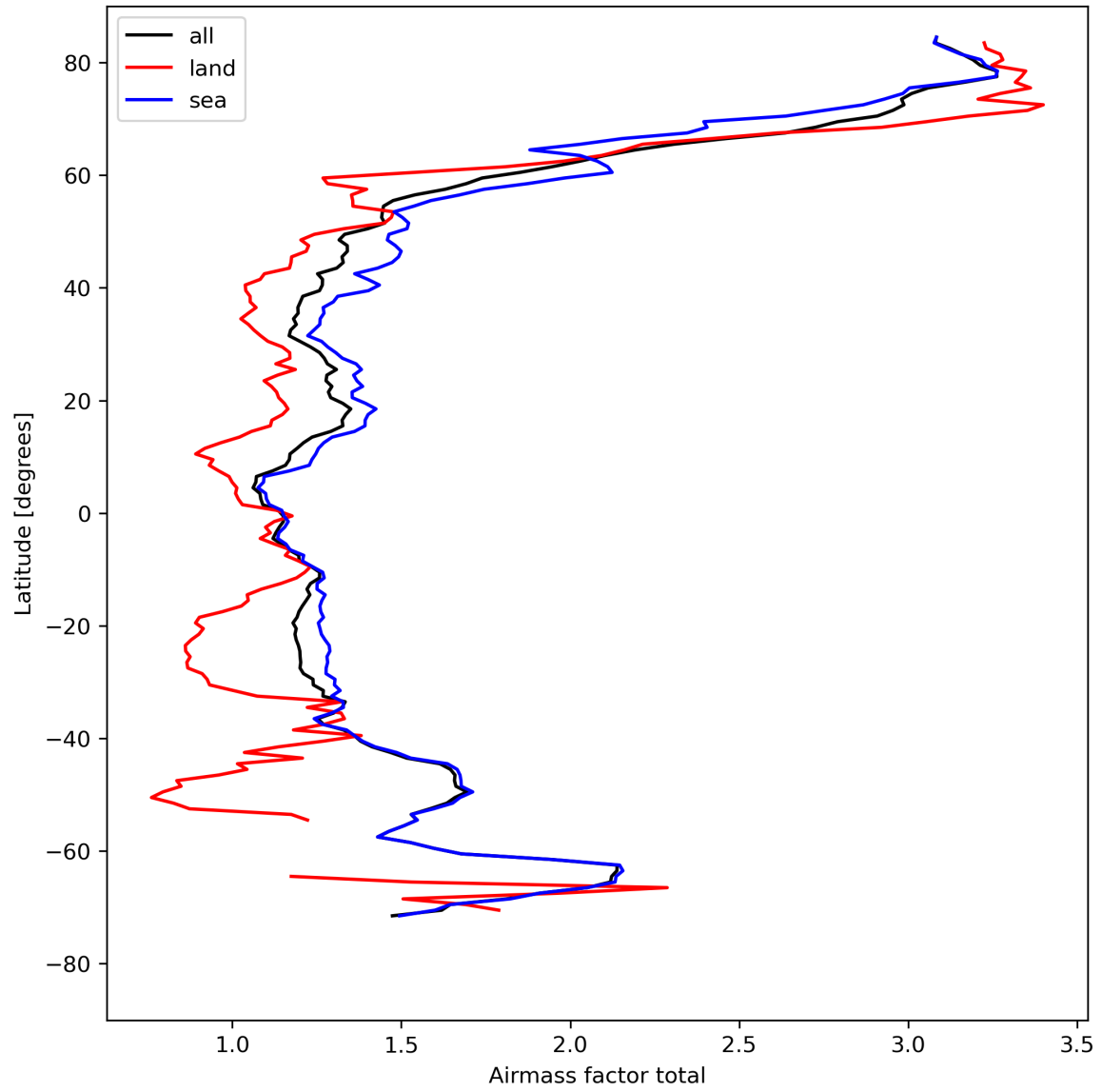
Figure 26: Zonal average of “Airmass factor total” for 2024-04-21 to 2024-04-23.
