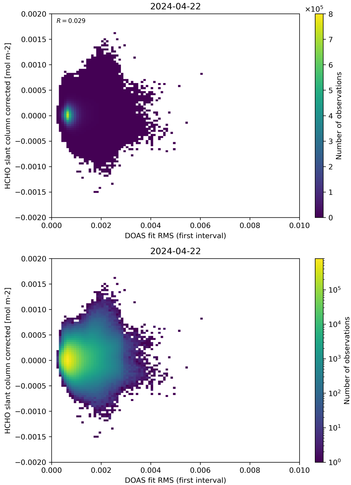
Figure 62: Scatter density plot of “DOAS fit RMS (first interval)” against “HCHO slant column corrected” for 2024-04-21 to 2024-04-23.
