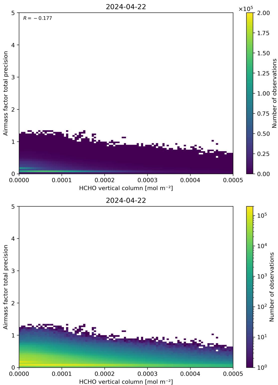
Figure 132: Scatter density plot of “HCHO vertical column” against “Airmass factor total precision” for 2024-04-21 to 2024-04-23.
