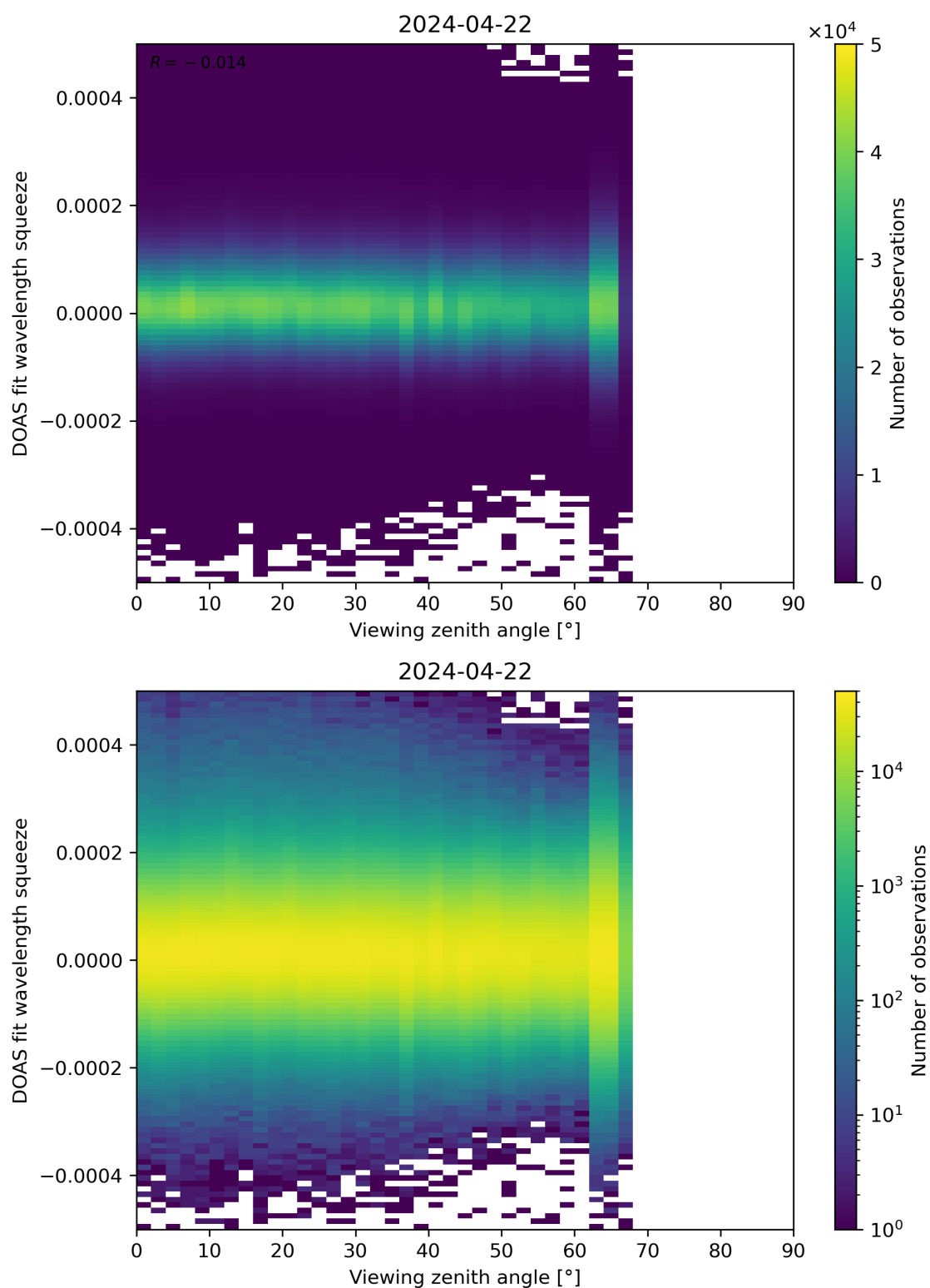
Figure 184: Scatter density plot of “Viewing zenith angle” against “DOAS fit wavelength squeeze” for 2024-04-21 to 2024-04-23.
