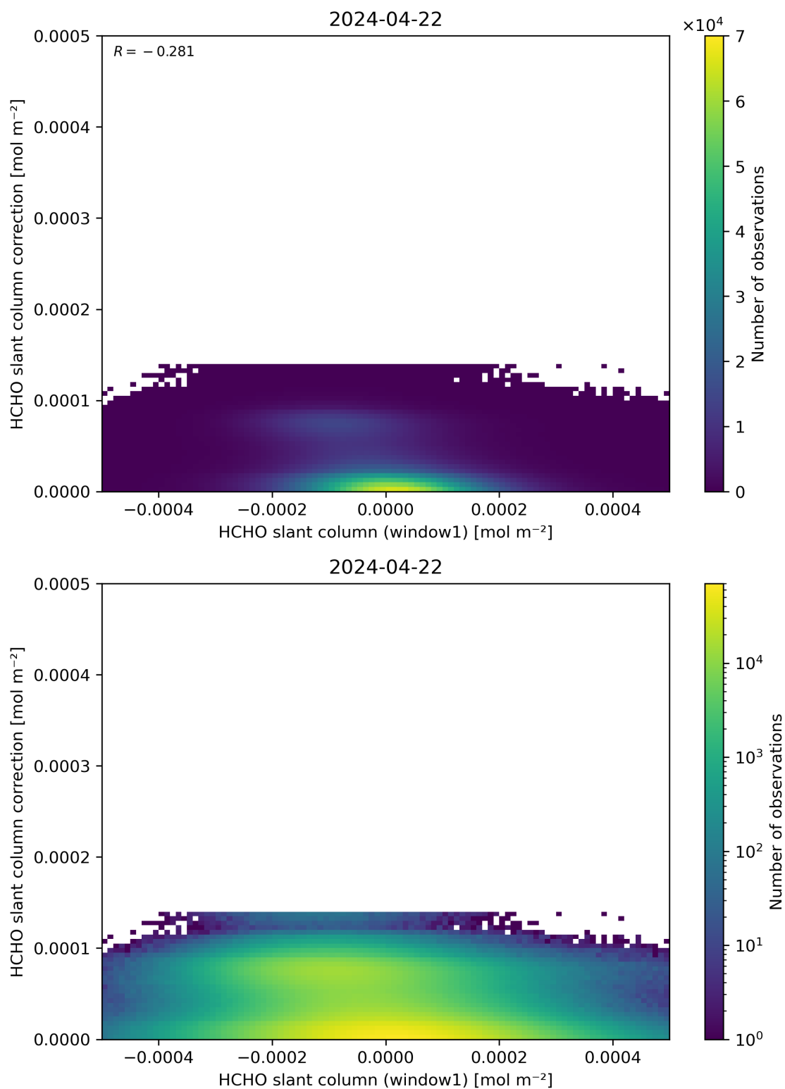
Figure 83: Scatter density plot of “HCHO slant column (window1)” against “HCHO slant column correction” for 2024-04-21 to 2024-04-23.
