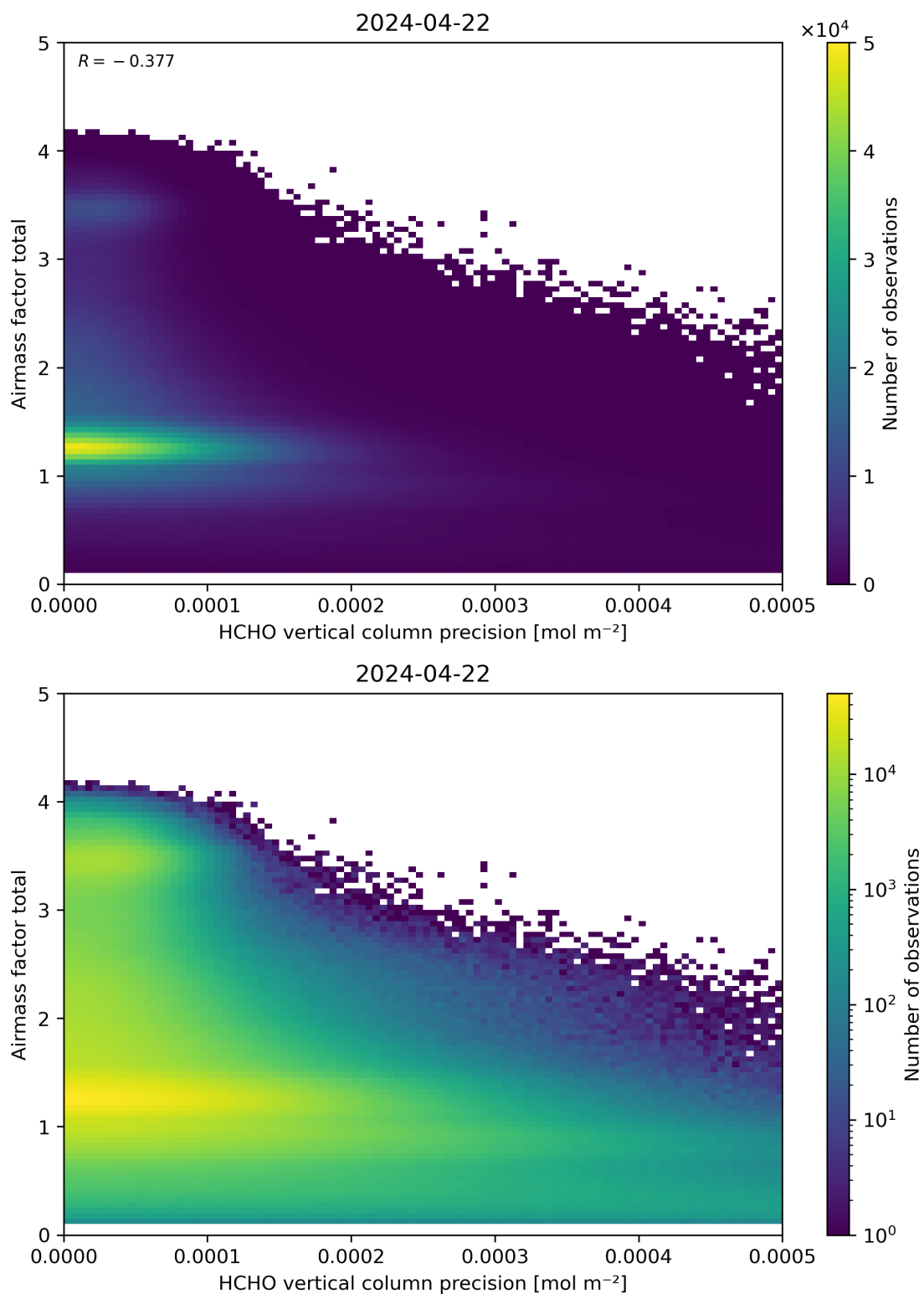
Figure 144: Scatter density plot of “HCHO vertical column precision” against “Airmass factor total” for 2024-04-21 to 2024-04-23.
