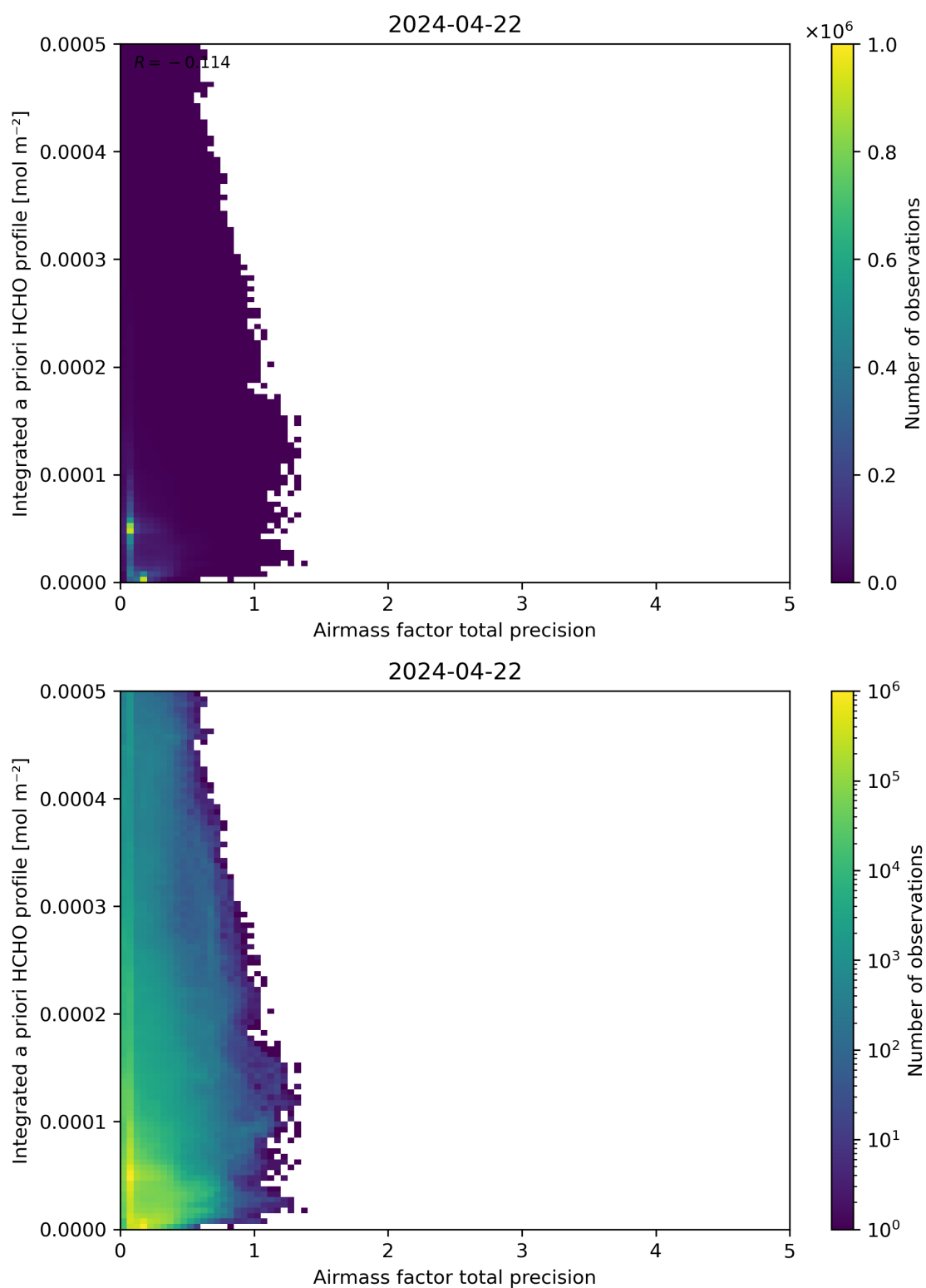
Figure 111: Scatter density plot of “Airmass factor total precision” against “Integrated a priori HCHO profile” for 2024-04-21 to 2024-04-23.
