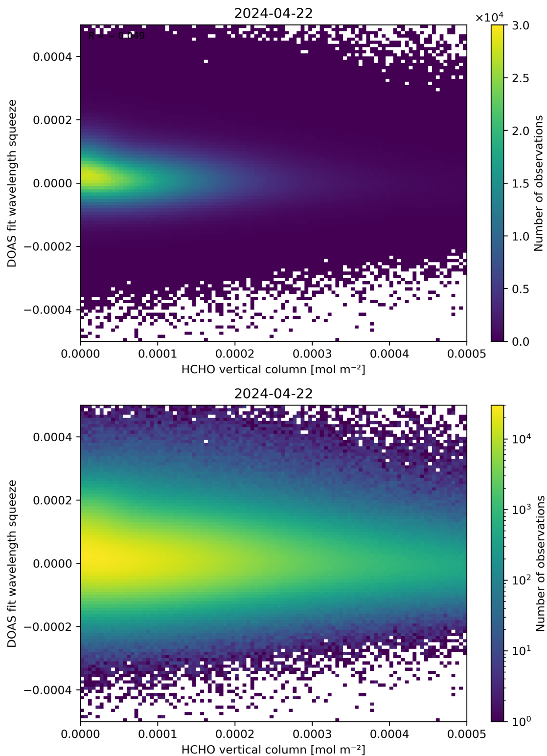
Figure 125: Scatter density plot of “HCHO vertical column” against “DOAS fit wavelength squeeze” for 2024-04-21 to 2024-04-23.
