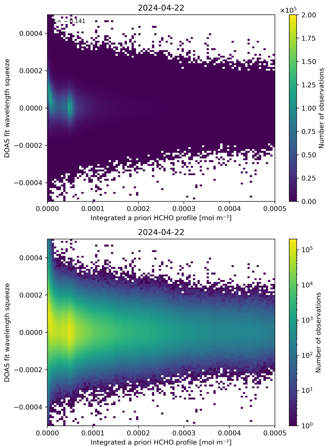
Figure 150: Scatter density plot of “Integrated a priori HCHO profile” against “DOAS fit wavelength squeeze” for 2024-04-21 to 2024-04-23.
