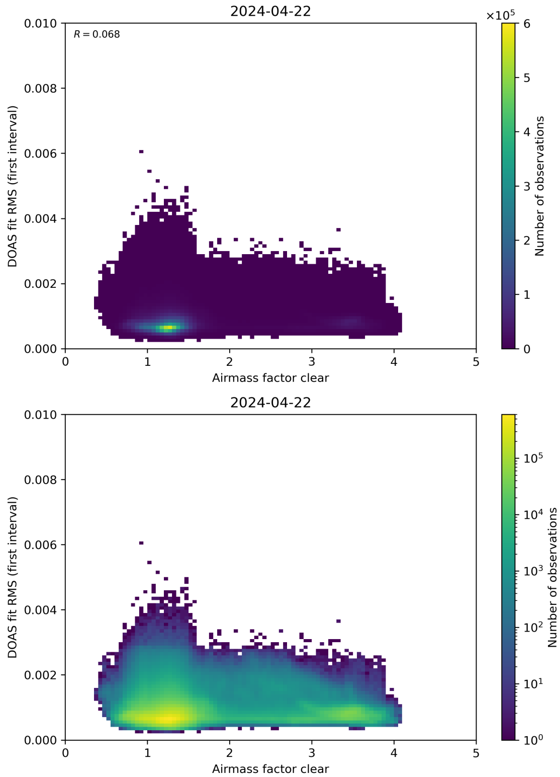
Figure 71: Scatter density plot of “Airmass factor clear” against “DOAS fit RMS (first interval)” for 2024-04-21 to 2024-04-23.
