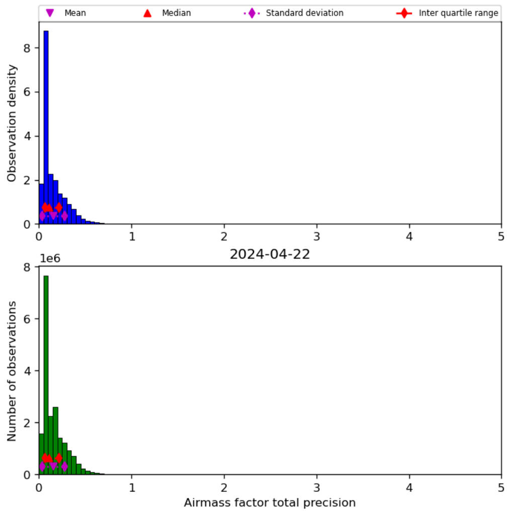
Figure 41: Histogram of “Airmass factor total precision” for 2024-04-21 to 2024-04-23
