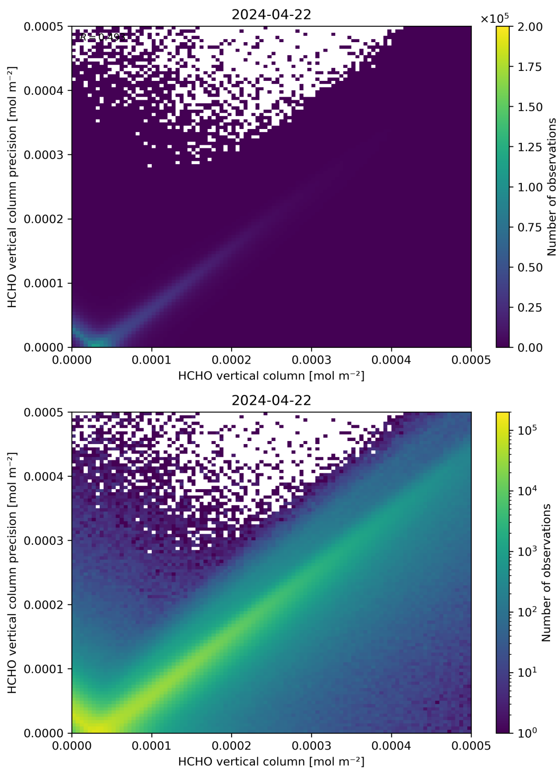
Figure 134: Scatter density plot of “HCHO vertical column” against “HCHO vertical column precision” for 2024-04-21 to 2024-04-23.
