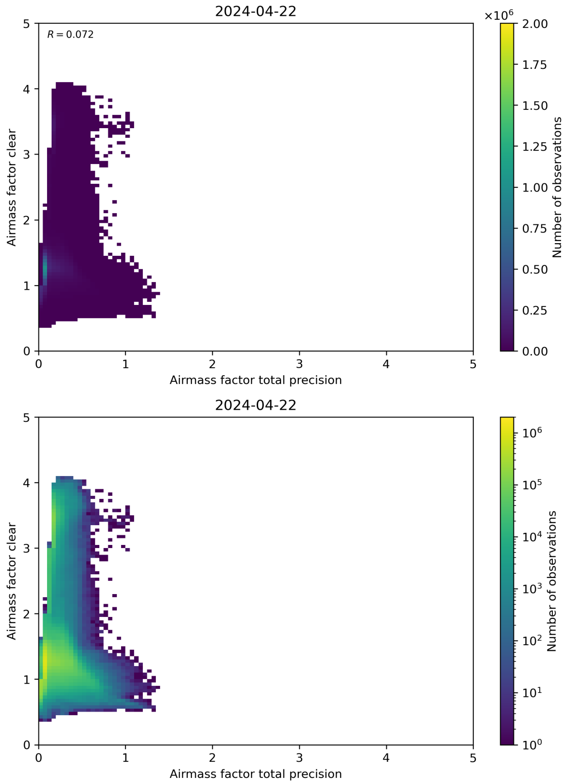
Figure 108: Scatter density plot of “Airmass factor total precision” against “Airmass factor clear” for 2024-04-21 to 2024-04-23.
