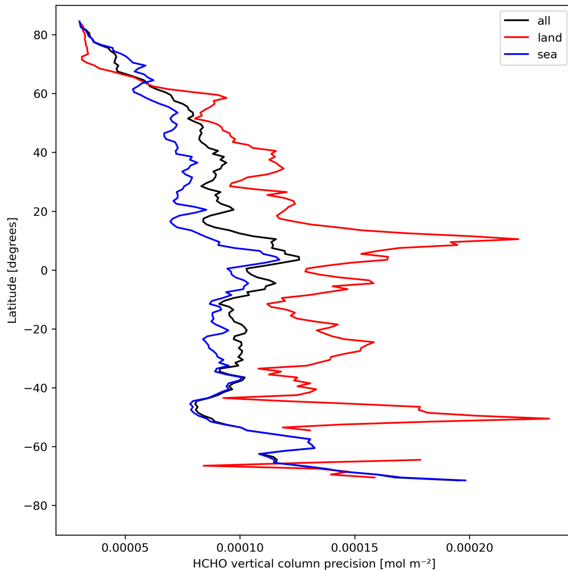
Figure 22: Zonal average of “HCHO vertical column precision” for 2024-04-21 to 2024-04-23.
