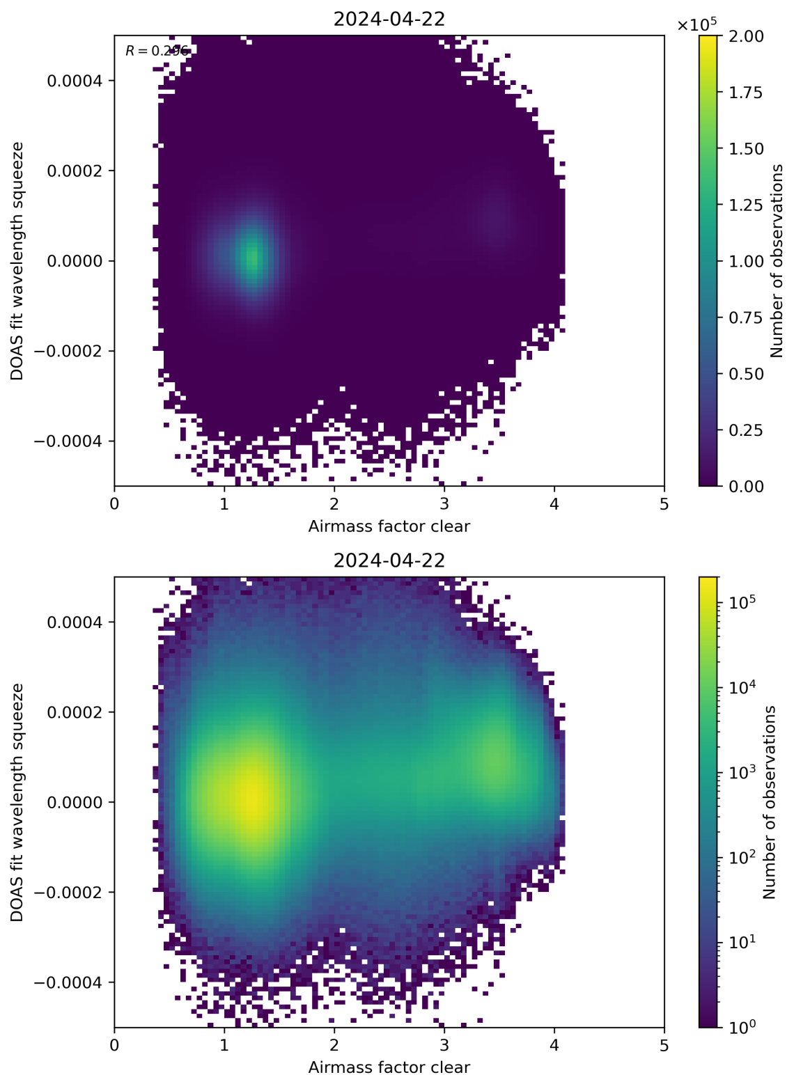
Figure 73: Scatter density plot of “Airmass factor clear” against “DOAS fit wavelength squeeze” for 2024-04-21 to 2024-04-23.
