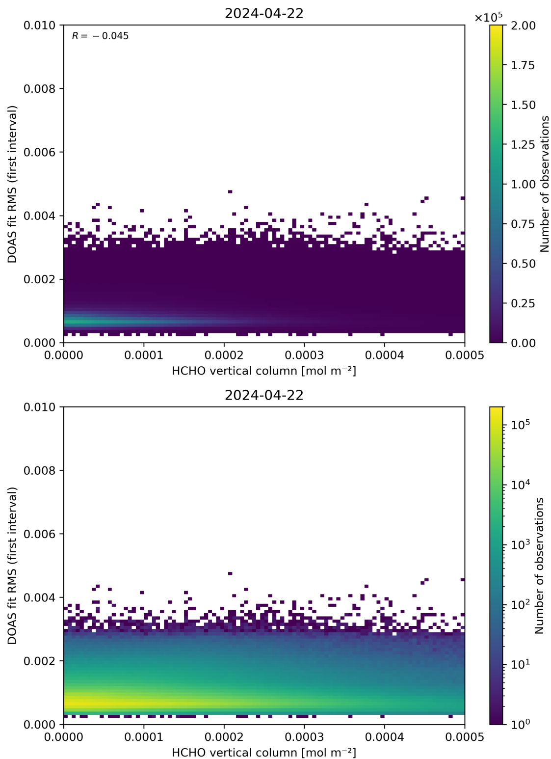
Figure 123: Scatter density plot of “HCHO vertical column” against “DOAS fit RMS (first interval)” for 2024-04-21 to 2024-04-23.
