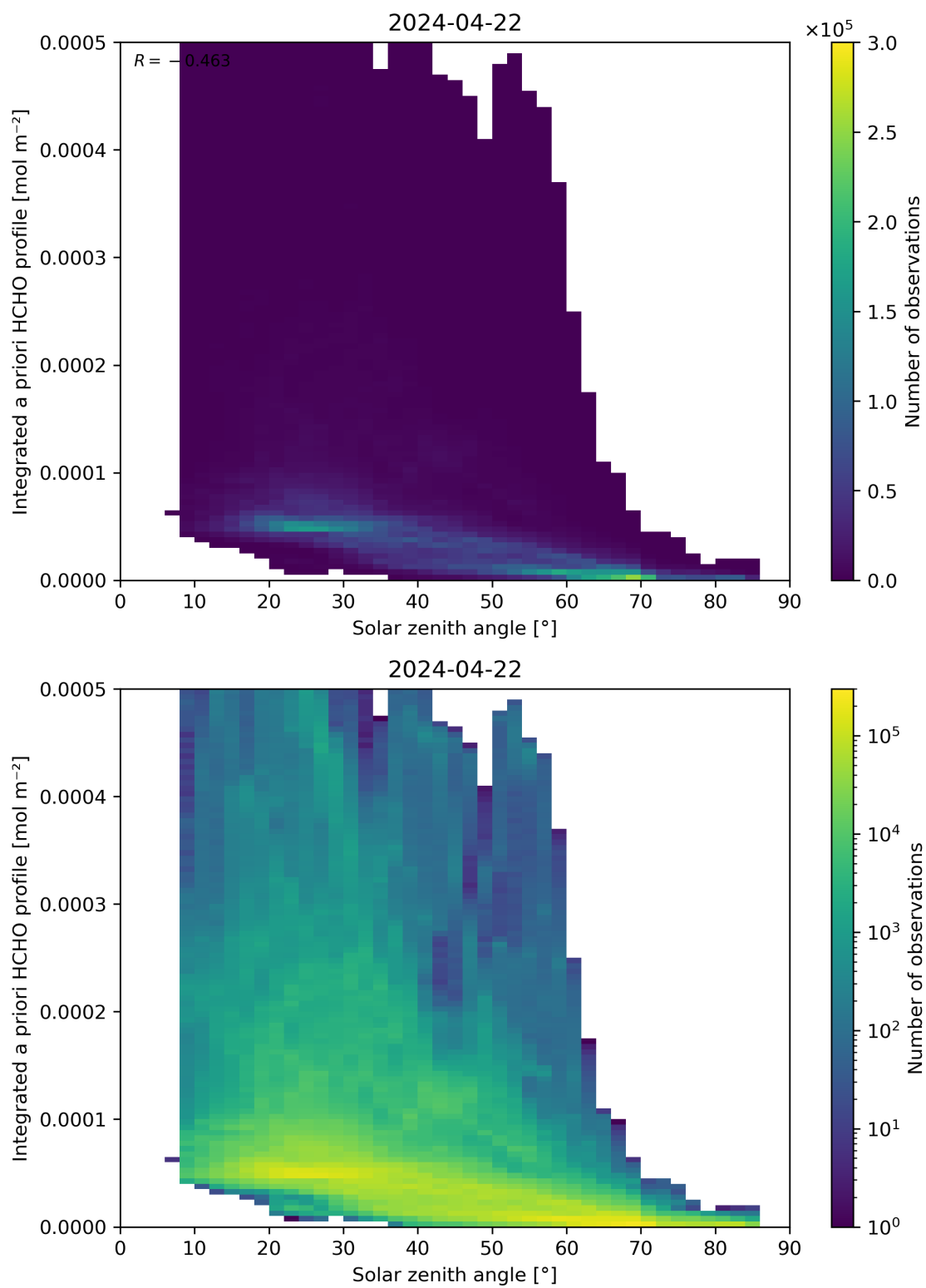
Figure 180: Scatter density plot of “Solar zenith angle” against “Integrated a priori HCHO profile” for 2024-04-21 to 2024-04-23.
