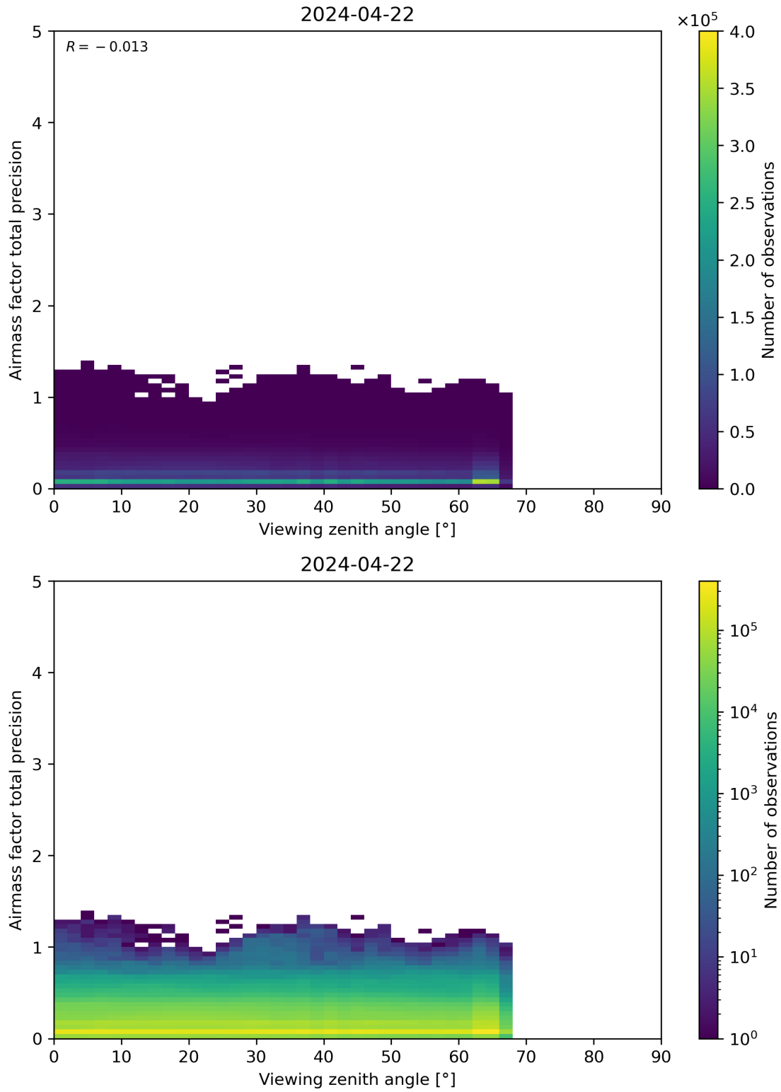
Figure 191: Scatter density plot of “Viewing zenith angle” against “Airmass factor total precision” for 2024-04-21 to 2024-04-23.
