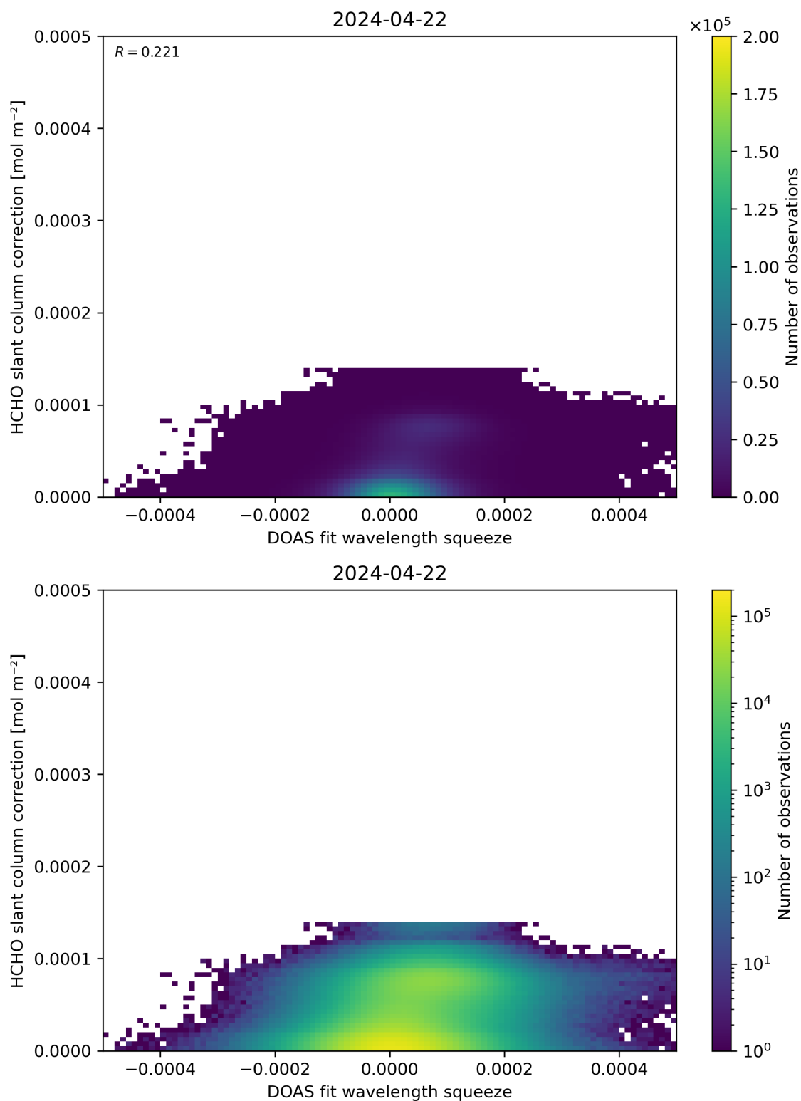
Figure 70: Scatter density plot of “DOAS fit wavelength squeeze” against “HCHO slant column correction” for 2024-04-21 to 2024-04-23.
