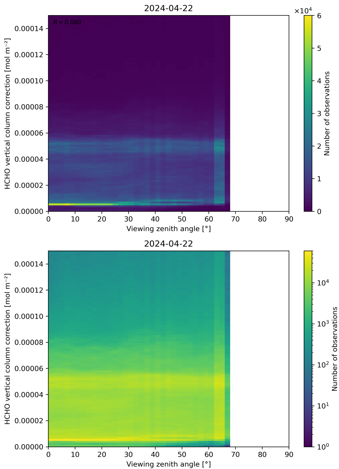
Figure 193: Scatter density plot of “Viewing zenith angle” against “HCHO vertical column correction” for 2024-04-21 to 2024-04-23.
