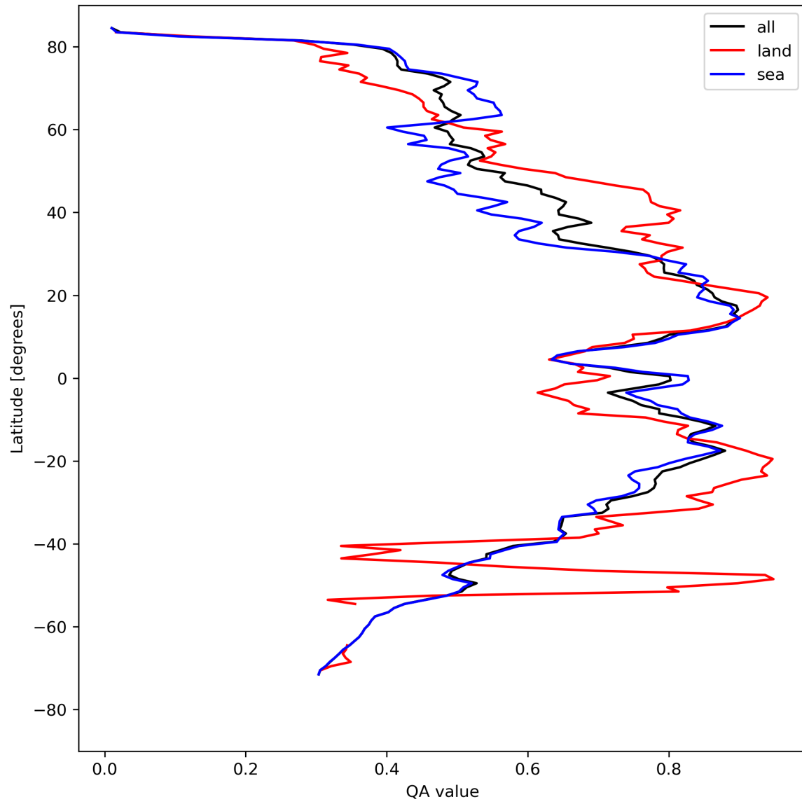
Figure 20: Zonal average of “QA value” for 2024-04-21 to 2024-04-23.
