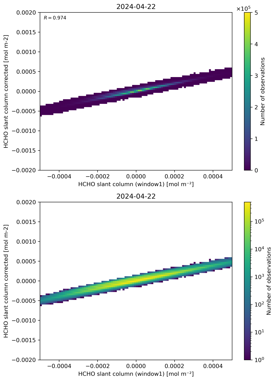
Figure 82: Scatter density plot of “HCHO slant column (window1)” against “HCHO slant column corrected” for 2024-04-21 to 2024-04-23.
