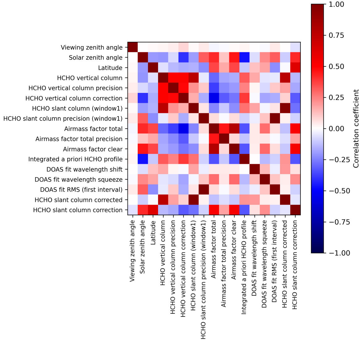
Figure 2: Map of correlation matrix for 2024-04-21 to 2024-04-23.
