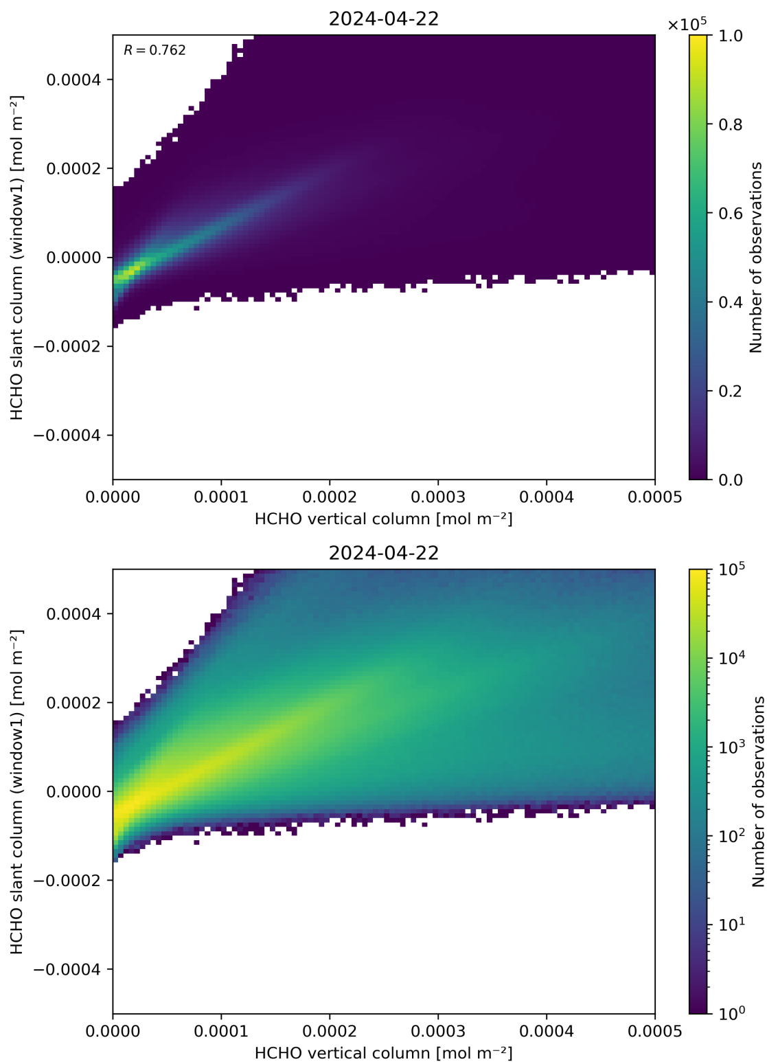
Figure 129: Scatter density plot of “HCHO vertical column” against “HCHO slant column (window1)” for 2024-04-21 to 2024-04-23.
