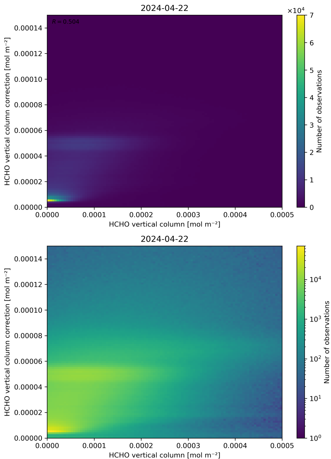
Figure 133: Scatter density plot of “HCHO vertical column” against “HCHO vertical column correction” for 2024-04-21 to 2024-04-23.
