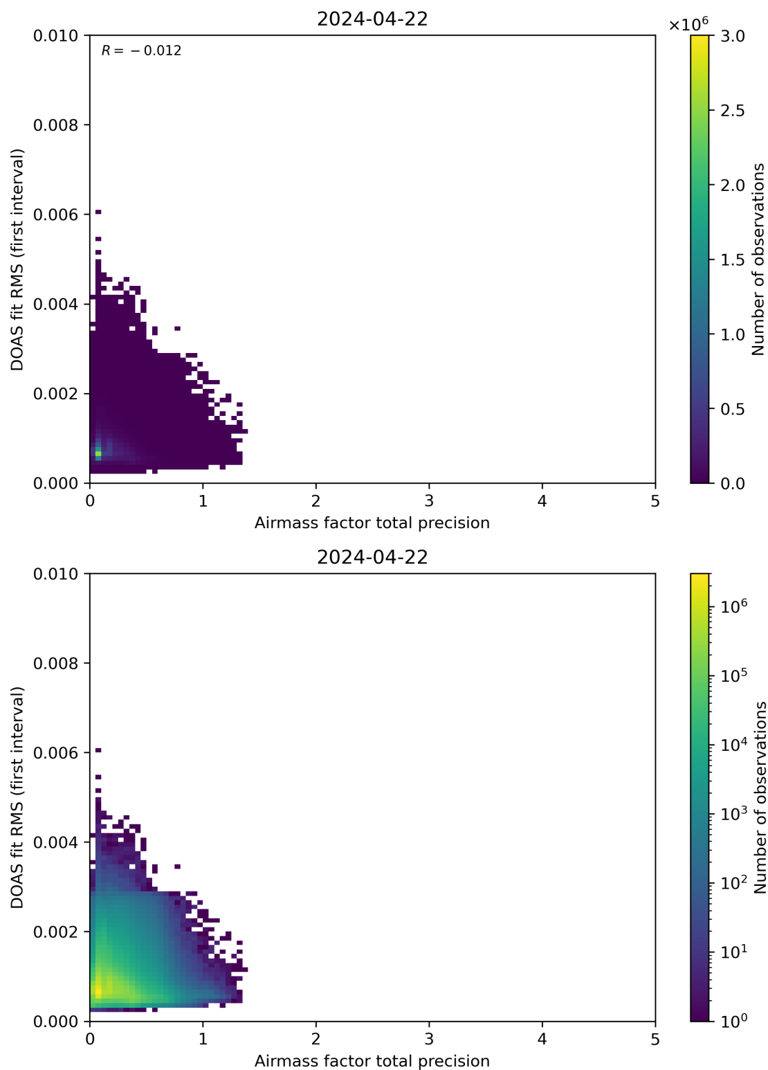
Figure 105: Scatter density plot of “Airmass factor total precision” against “DOAS fit RMS (first interval)” for 2024-04-21 to 2024-04-23.
