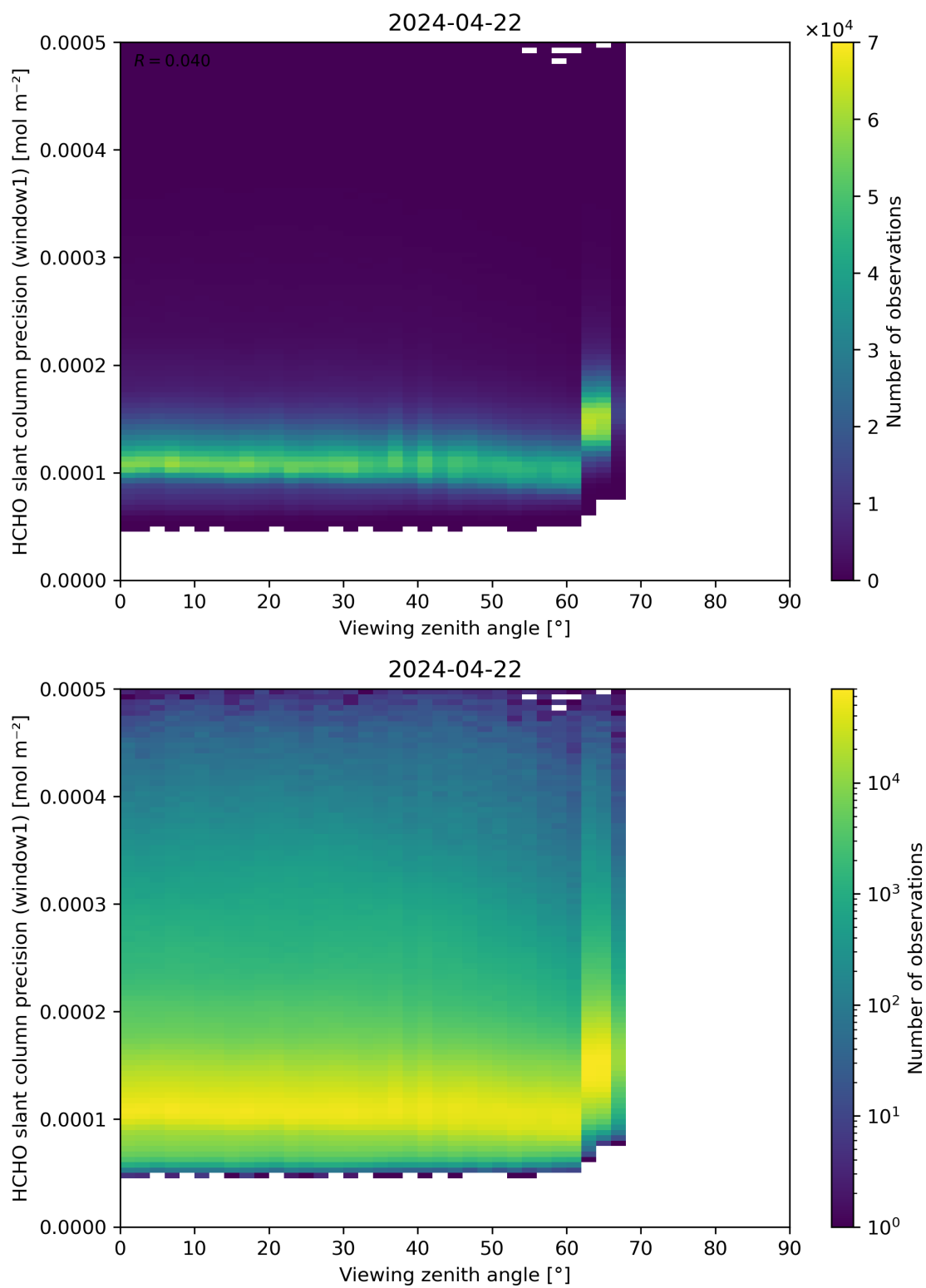
Figure 189: Scatter density plot of “Viewing zenith angle” against “HCHO slant column precision (window1)” for 2024-04-21 to 2024-04-23.
