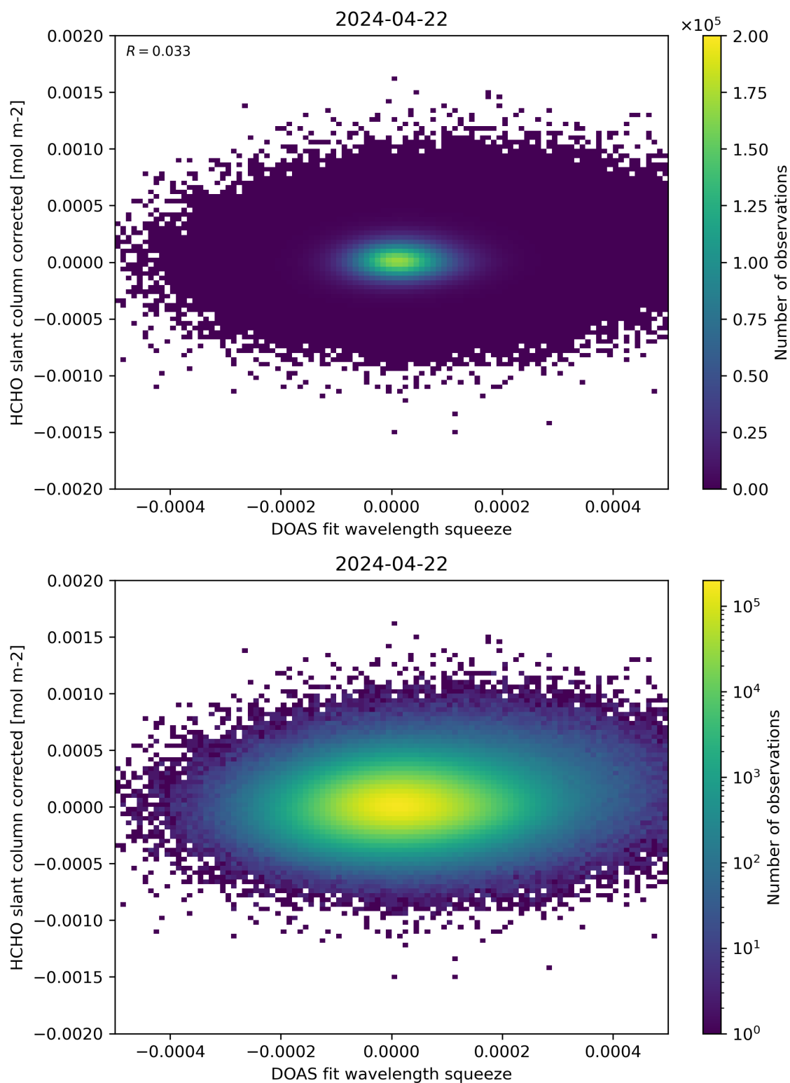
Figure 69: Scatter density plot of “DOAS fit wavelength squeeze” against “HCHO slant column corrected” for 2024-04-21 to 2024-04-23.
