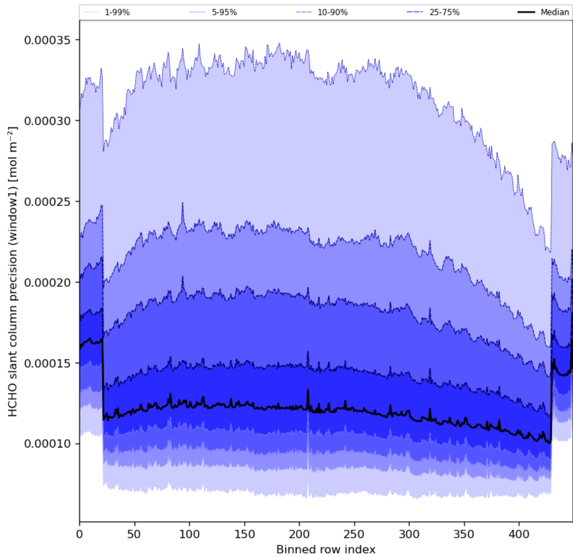
Figure 53: Along track statistics of “HCHO slant column precision (window1)” for 2024-04-23 to 2024-04-25
