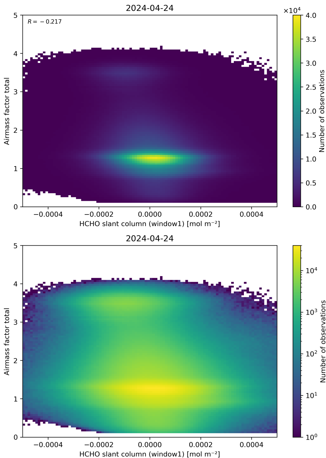
Figure 85: Scatter density plot of “HCHO slant column (window1)” against “Airmass factor total” for 2024-04-23 to 2024-04-25.
