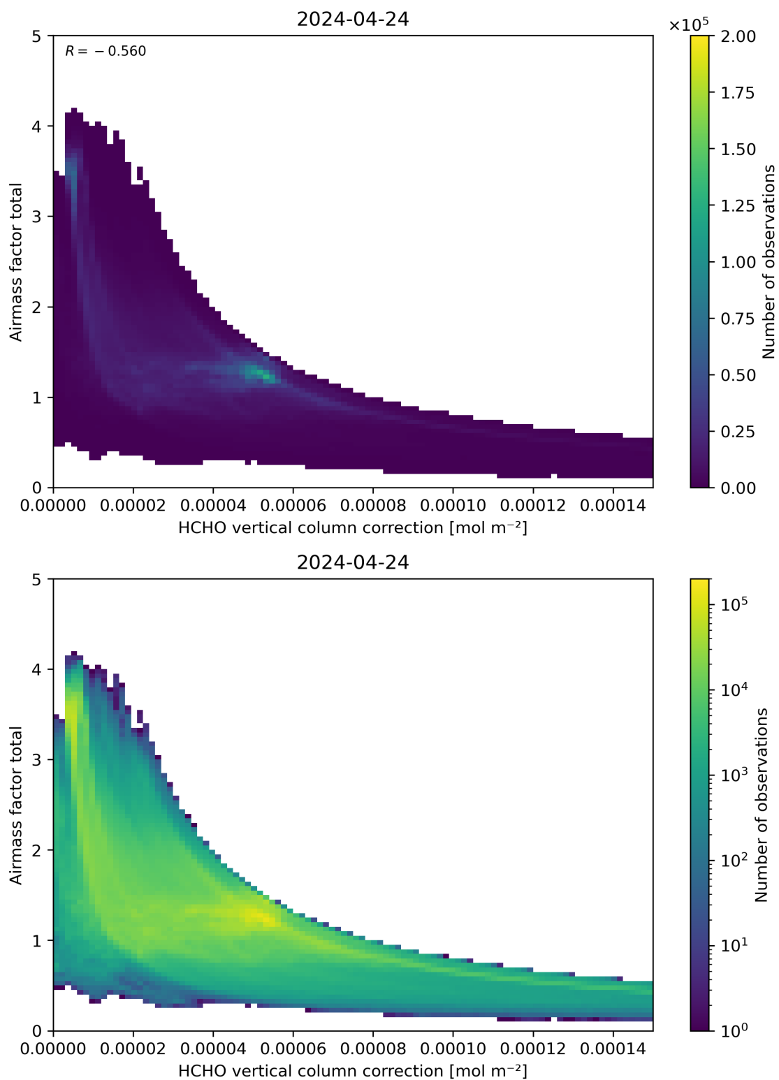
Figure 120: Scatter density plot of “HCHO vertical column correction” against “Airmass factor total” for 2024-04-23 to 2024-04-25.
