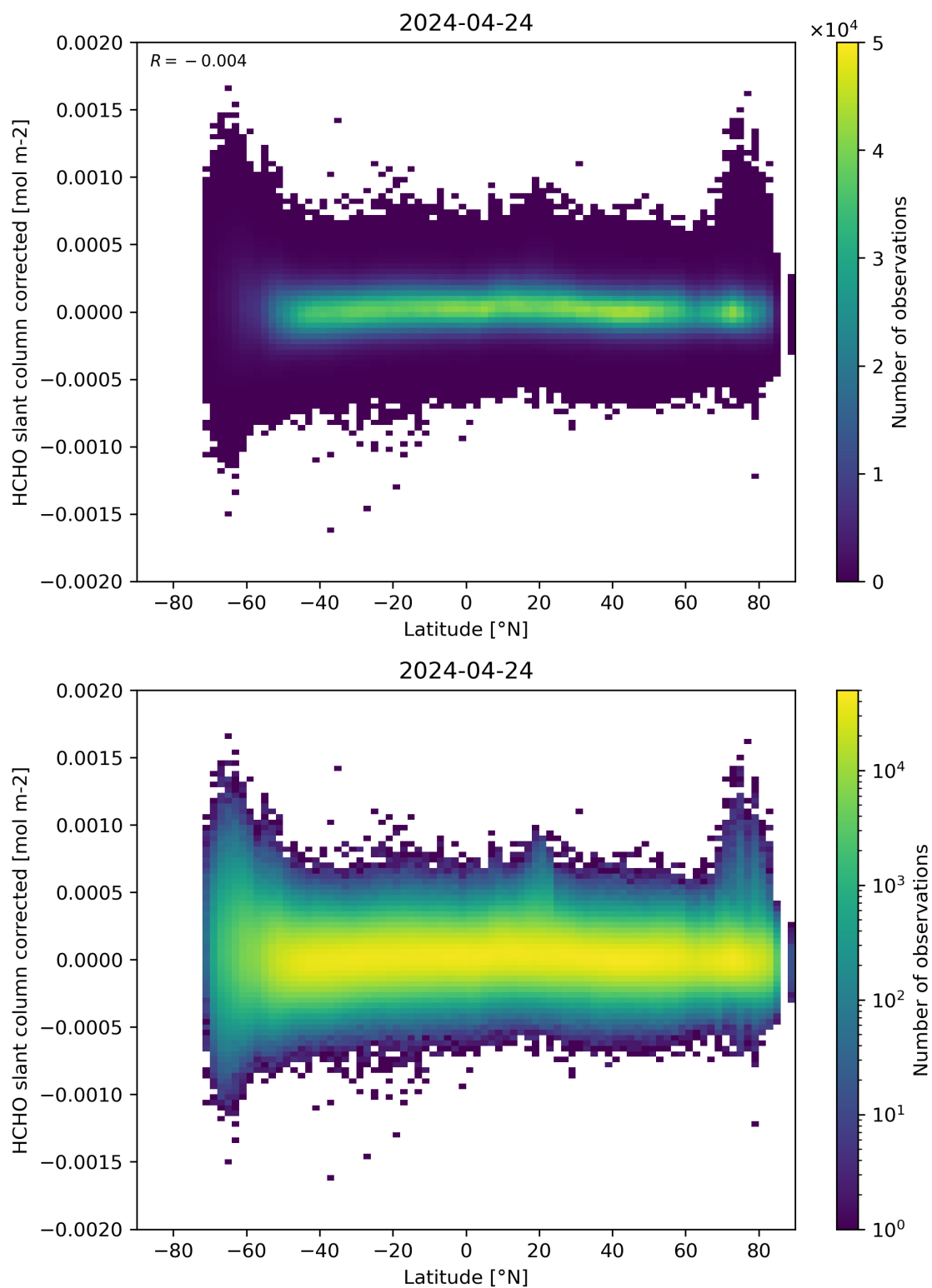
Figure 157: Scatter density plot of “Latitude” against “HCHO slant column corrected” for 2024-04-23 to 2024-04-25.
