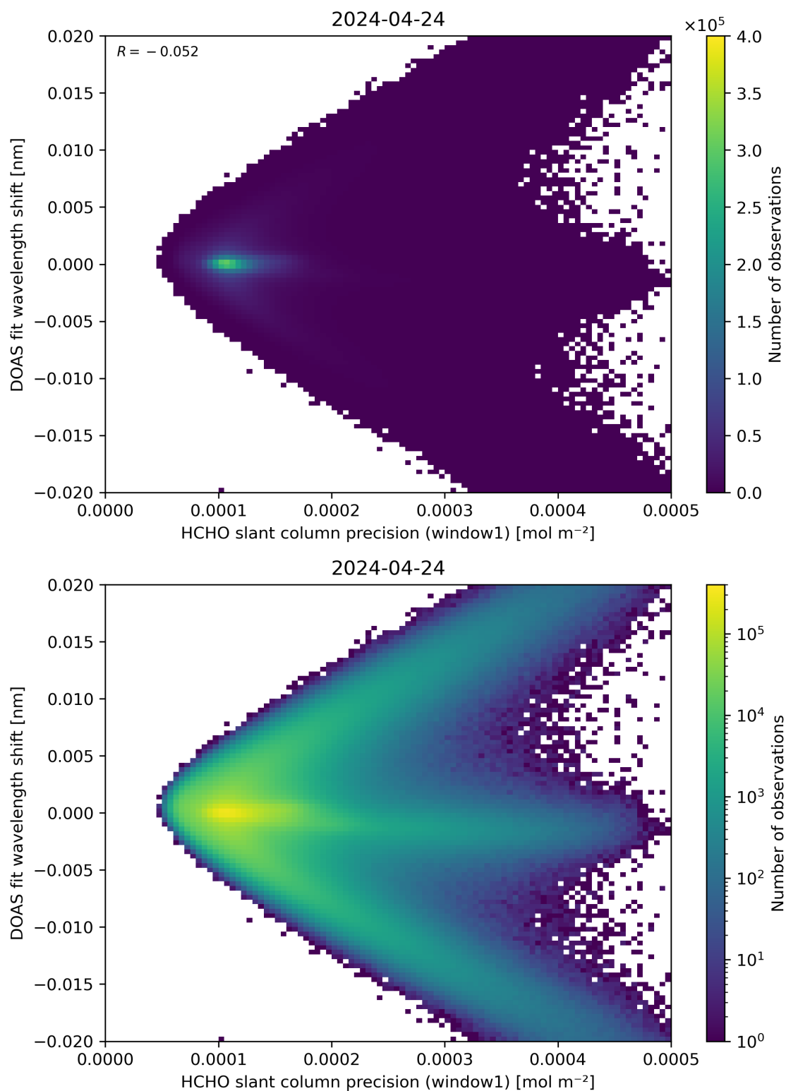
Figure 89: Scatter density plot of “HCHO slant column precision (window1)” against “DOAS fit wavelength shift” for 2024-04-23 to 2024-04-25.
