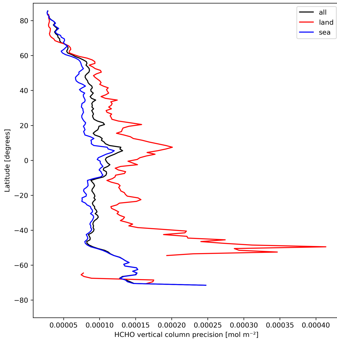
Figure 22: Zonal average of “HCHO vertical column precision” for 2024-04-23 to 2024-04-25.
