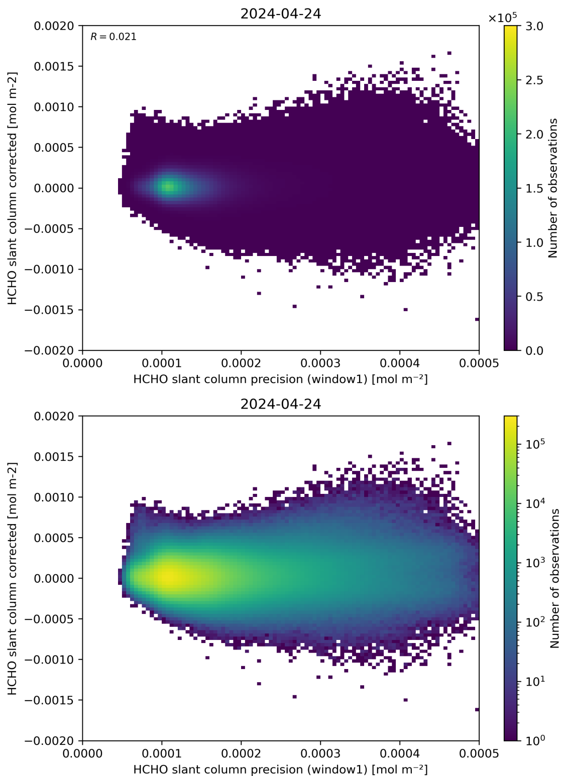
Figure 92: Scatter density plot of “HCHO slant column precision (window1)” against “HCHO slant column corrected” for 2024-04-23 to 2024-04-25.
