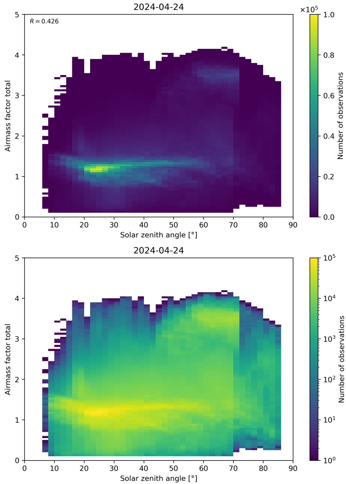
Figure 175: Scatter density plot of “Solar zenith angle” against “Airmass factor total” for 2024-04-23 to 2024-04-25.
