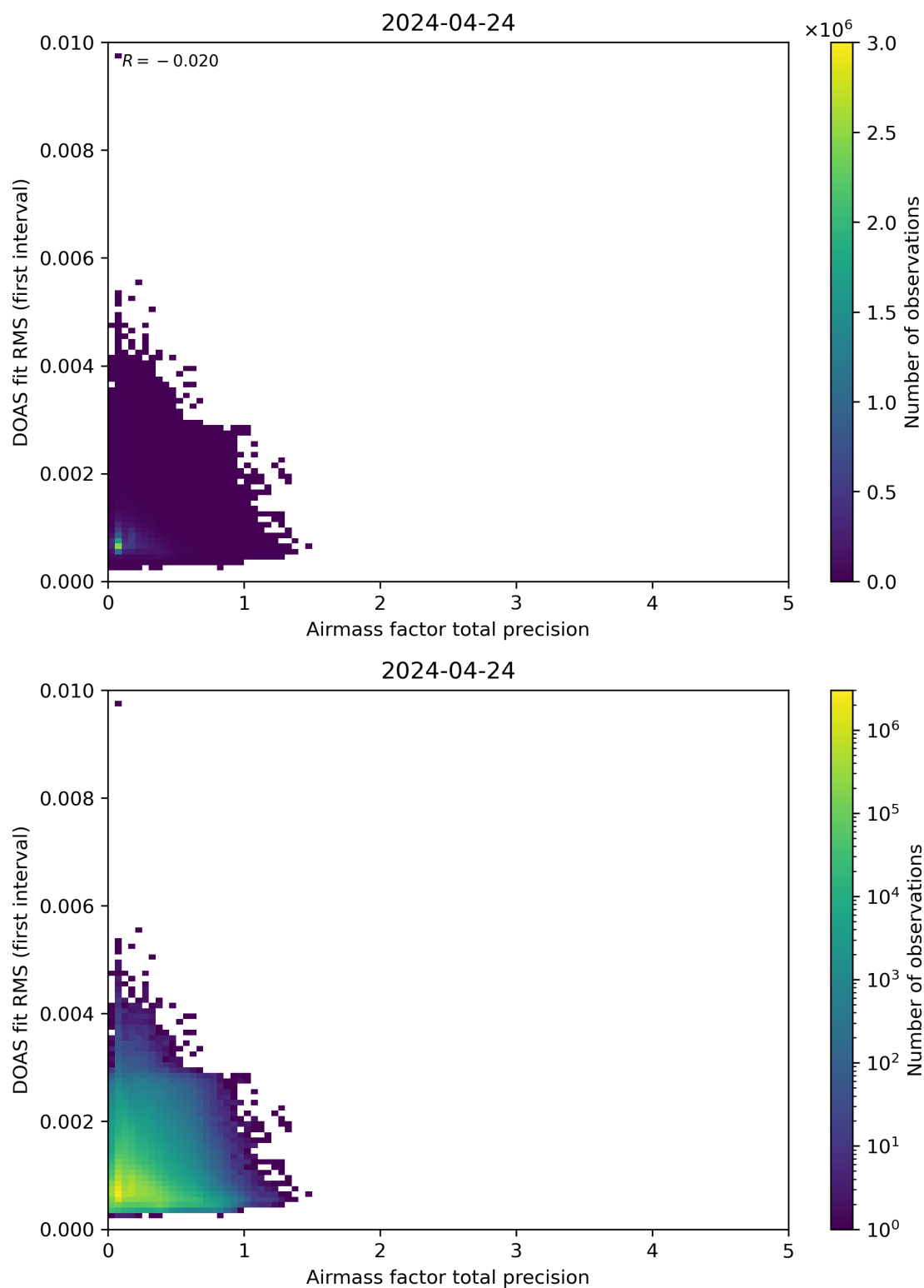
Figure 105: Scatter density plot of “Airmass factor total precision” against “DOAS fit RMS (first interval)” for 2024-04-23 to 2024-04-25.
