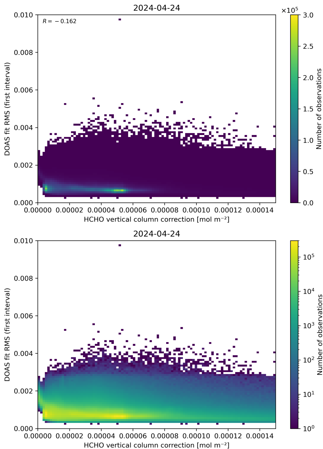
Figure 112: Scatter density plot of “HCHO vertical column correction” against “DOAS fit RMS (first interval)” for 2024-04-23 to 2024-04-25.
