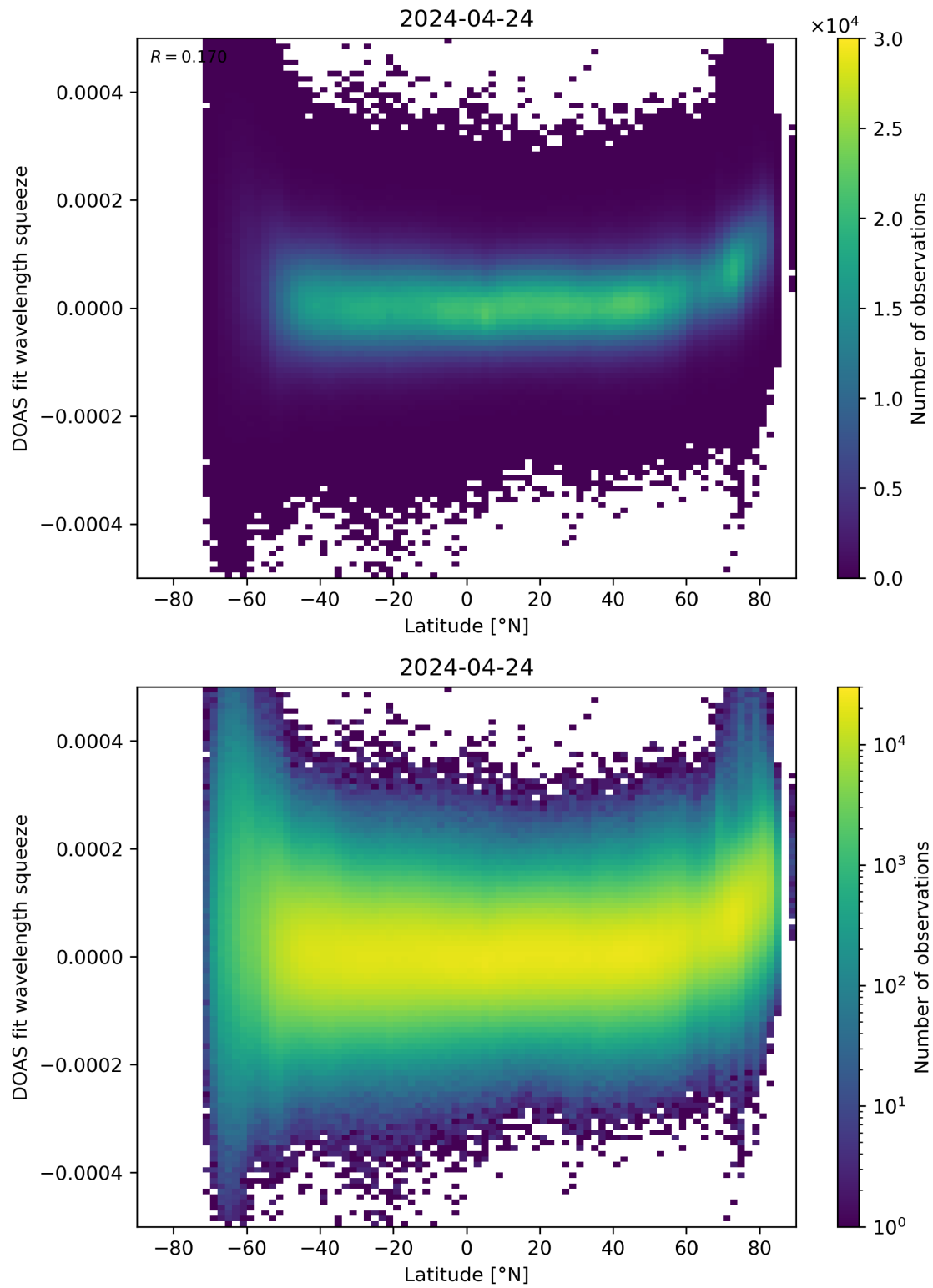
Figure 155: Scatter density plot of “Latitude” against “DOAS fit wavelength squeeze” for 2024-04-23 to 2024-04-25.
