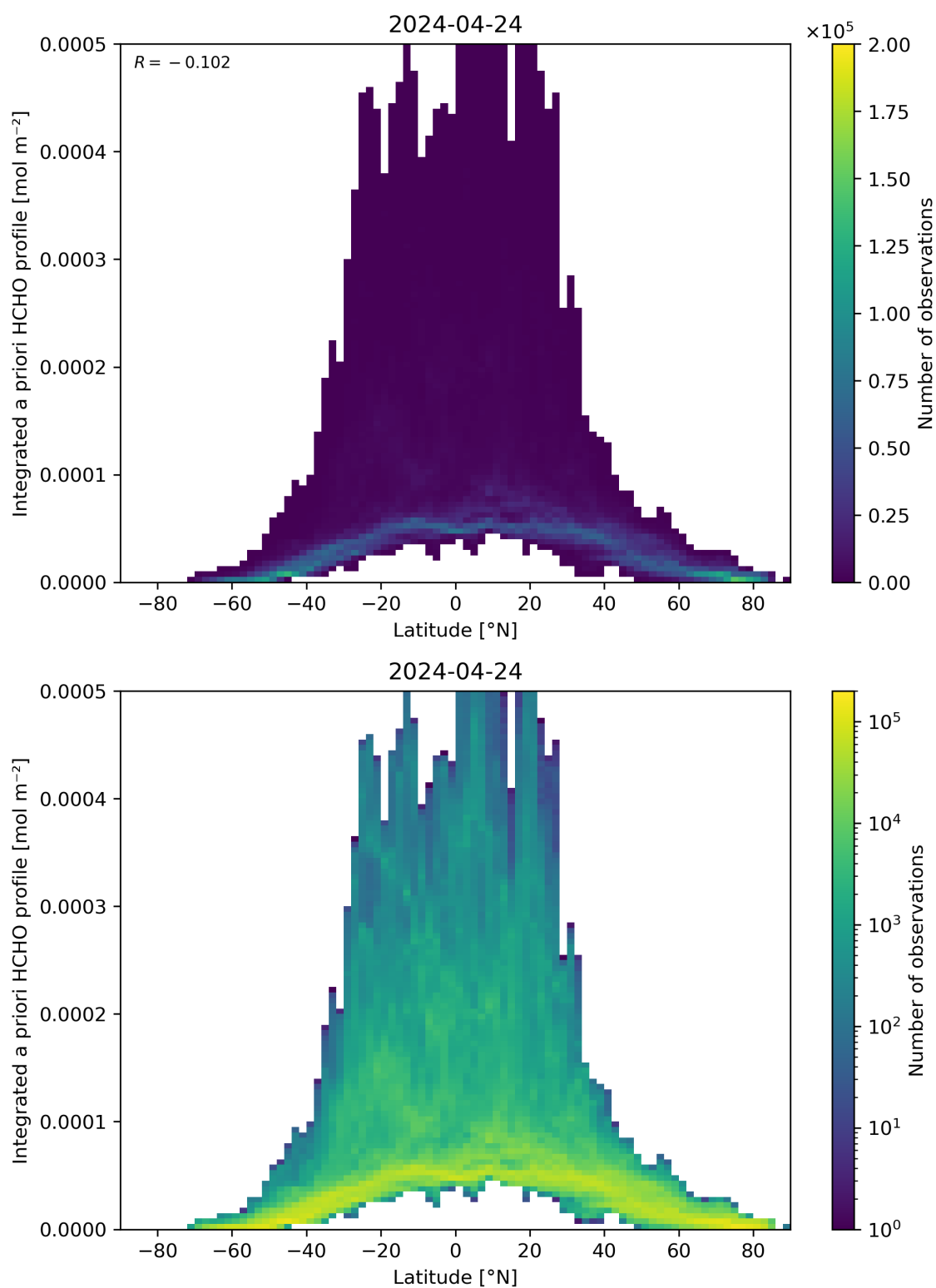
Figure 166: Scatter density plot of “Latitude” against “Integrated a priori HCHO profile” for 2024-04-23 to 2024-04-25.
