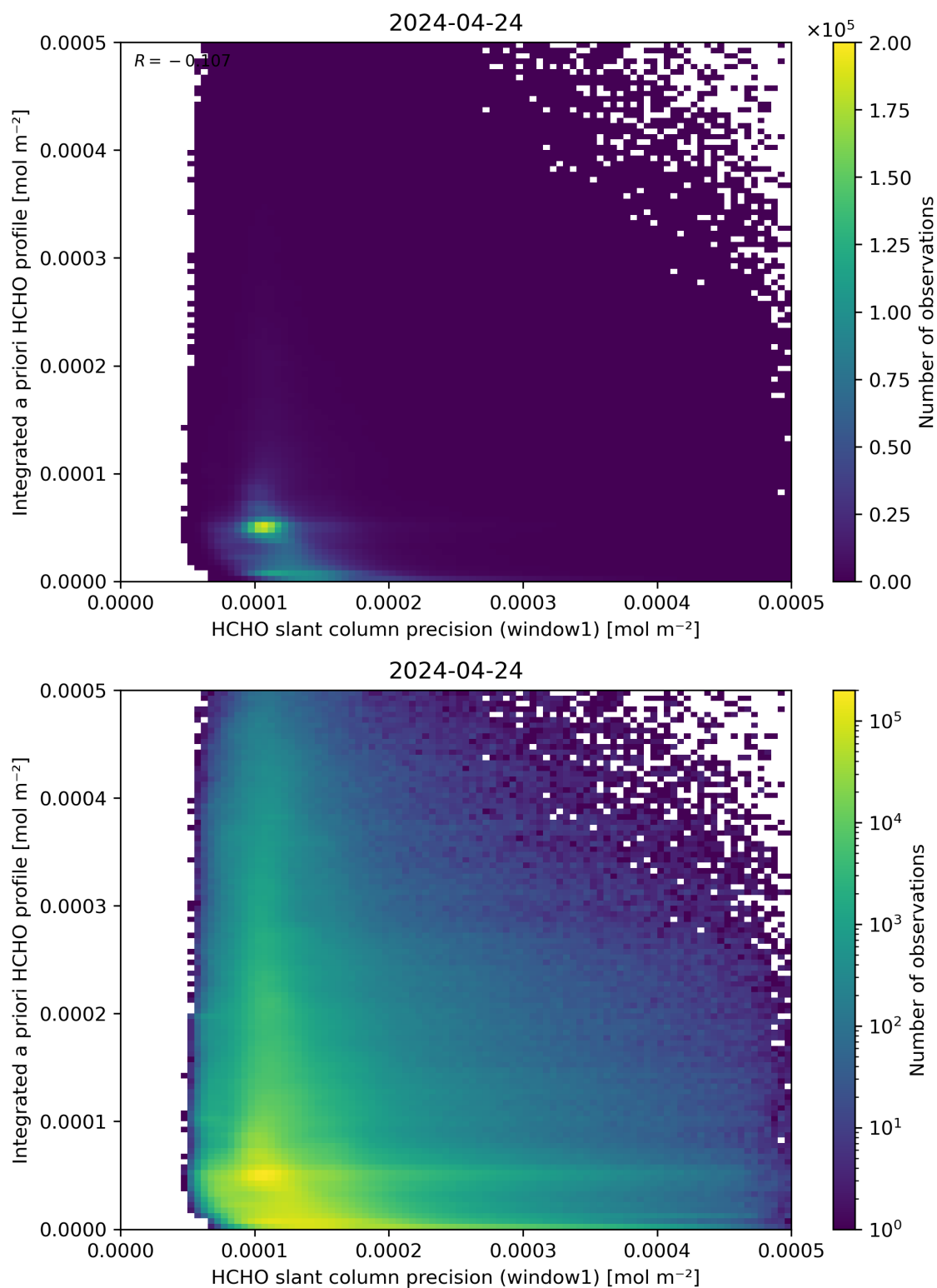
Figure 96: Scatter density plot of “HCHO slant column precision (window1)” against “Integrated a priori HCHO profile” for 2024-04-23 to 2024-04-25.
