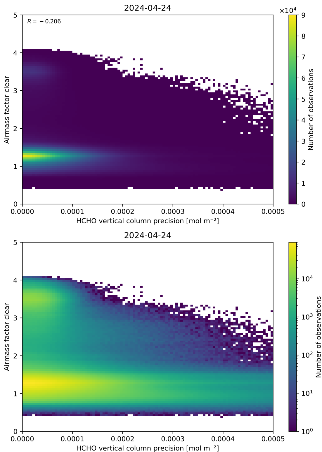
Figure 139: Scatter density plot of “HCHO vertical column precision” against “Airmass factor clear” for 2024-04-23 to 2024-04-25.
