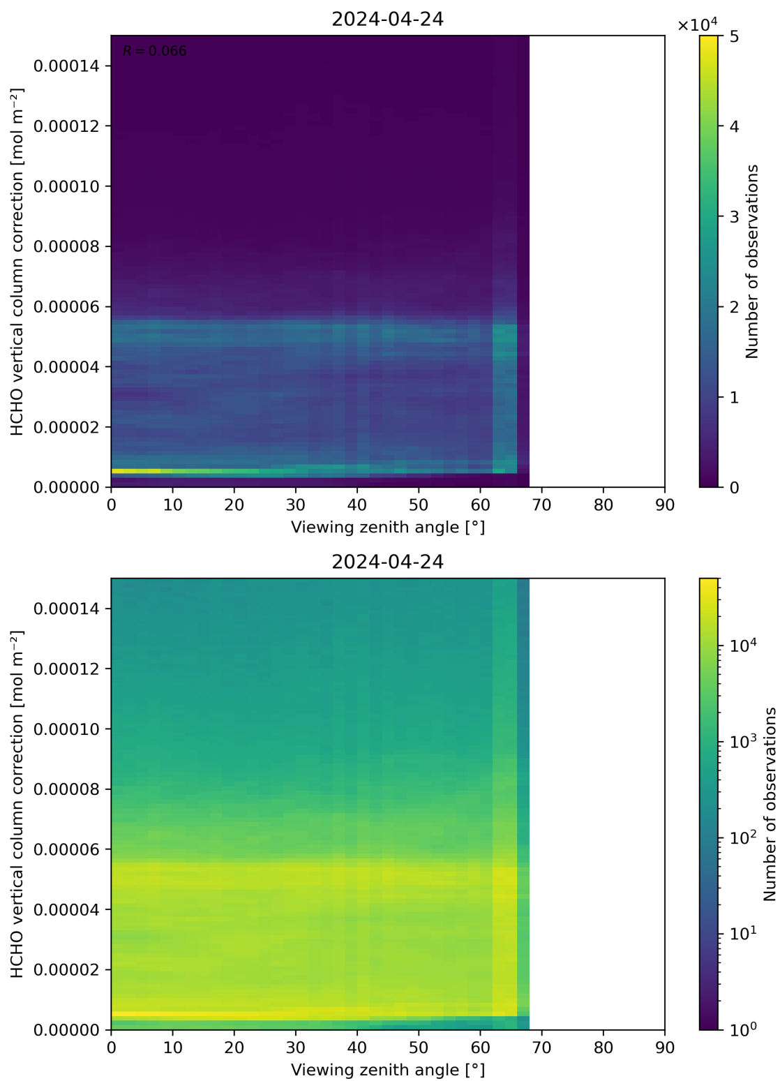
Figure 193: Scatter density plot of “Viewing zenith angle” against “HCHO vertical column correction” for 2024-04-23 to 2024-04-25.
