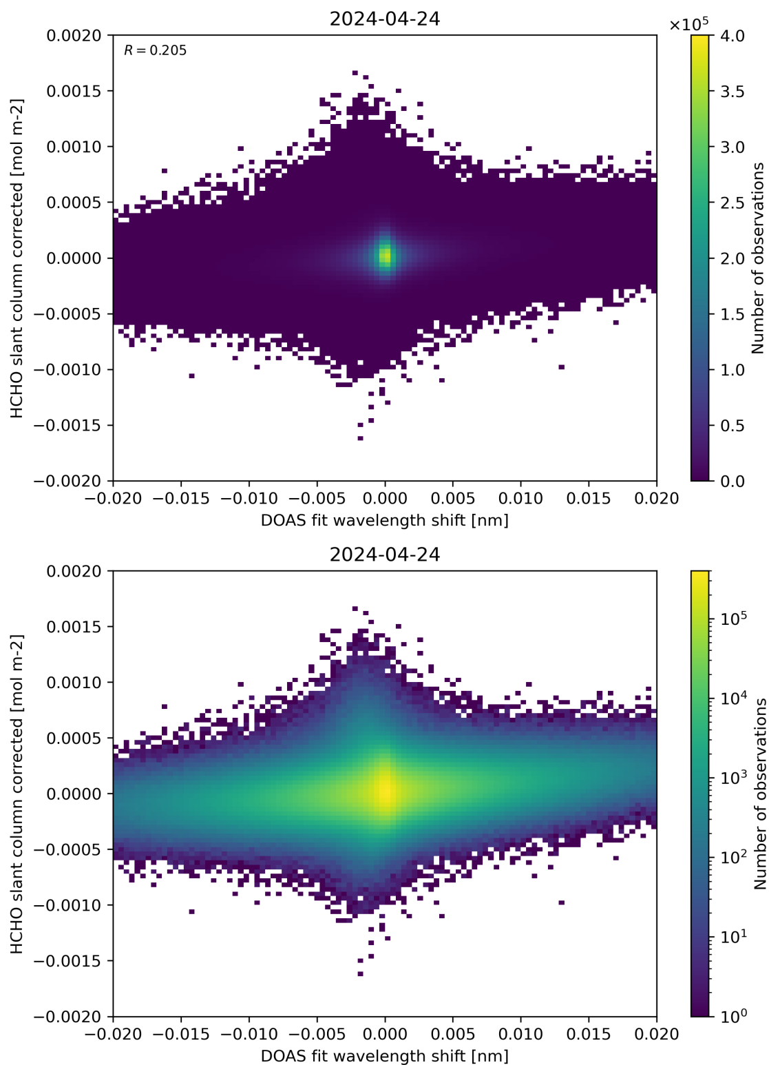
Figure 66: Scatter density plot of “DOAS fit wavelength shift” against “HCHO slant column corrected” for 2024-04-23 to 2024-04-25.
