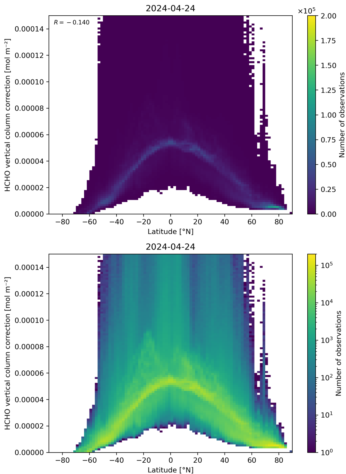
Figure 164: Scatter density plot of “Latitude” against “HCHO vertical column correction” for 2024-04-23 to 2024-04-25.
