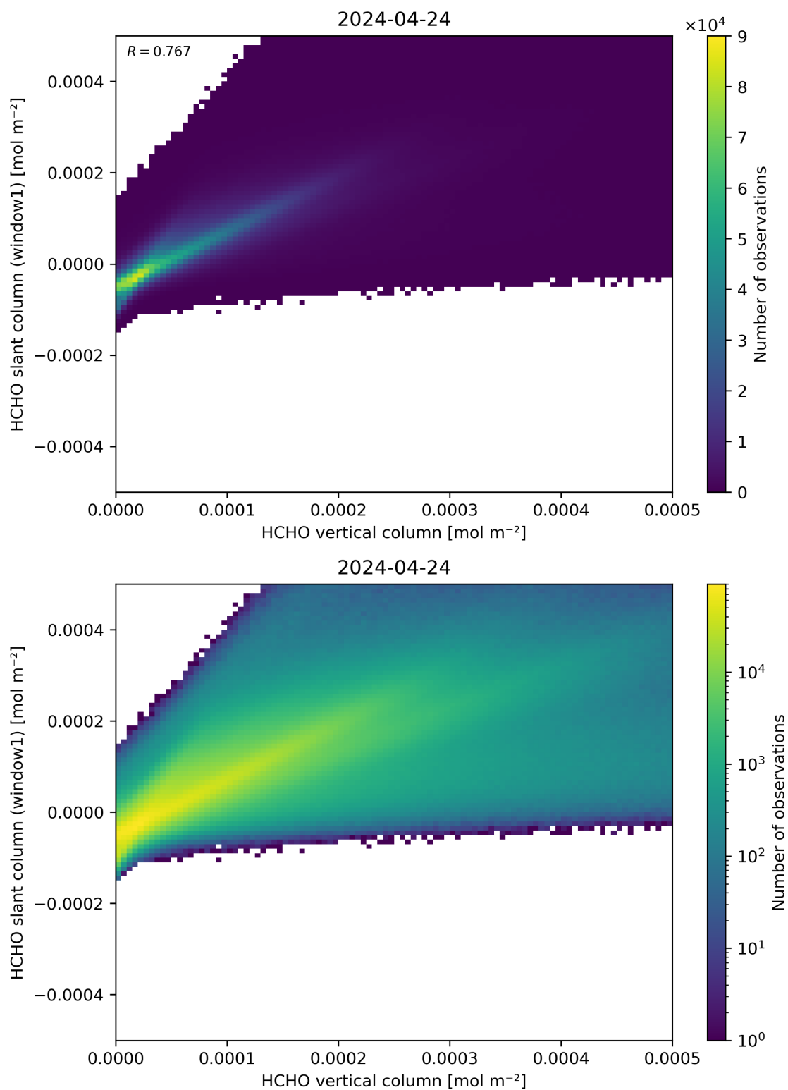
Figure 129: Scatter density plot of “HCHO vertical column” against “HCHO slant column (window1)” for 2024-04-23 to 2024-04-25.
