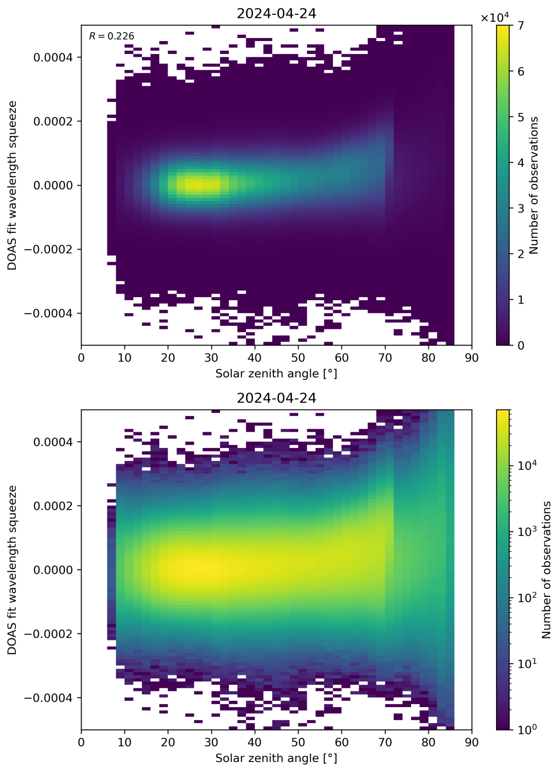
Figure 169: Scatter density plot of “Solar zenith angle” against “DOAS fit wavelength squeeze” for 2024-04-23 to 2024-04-25.
