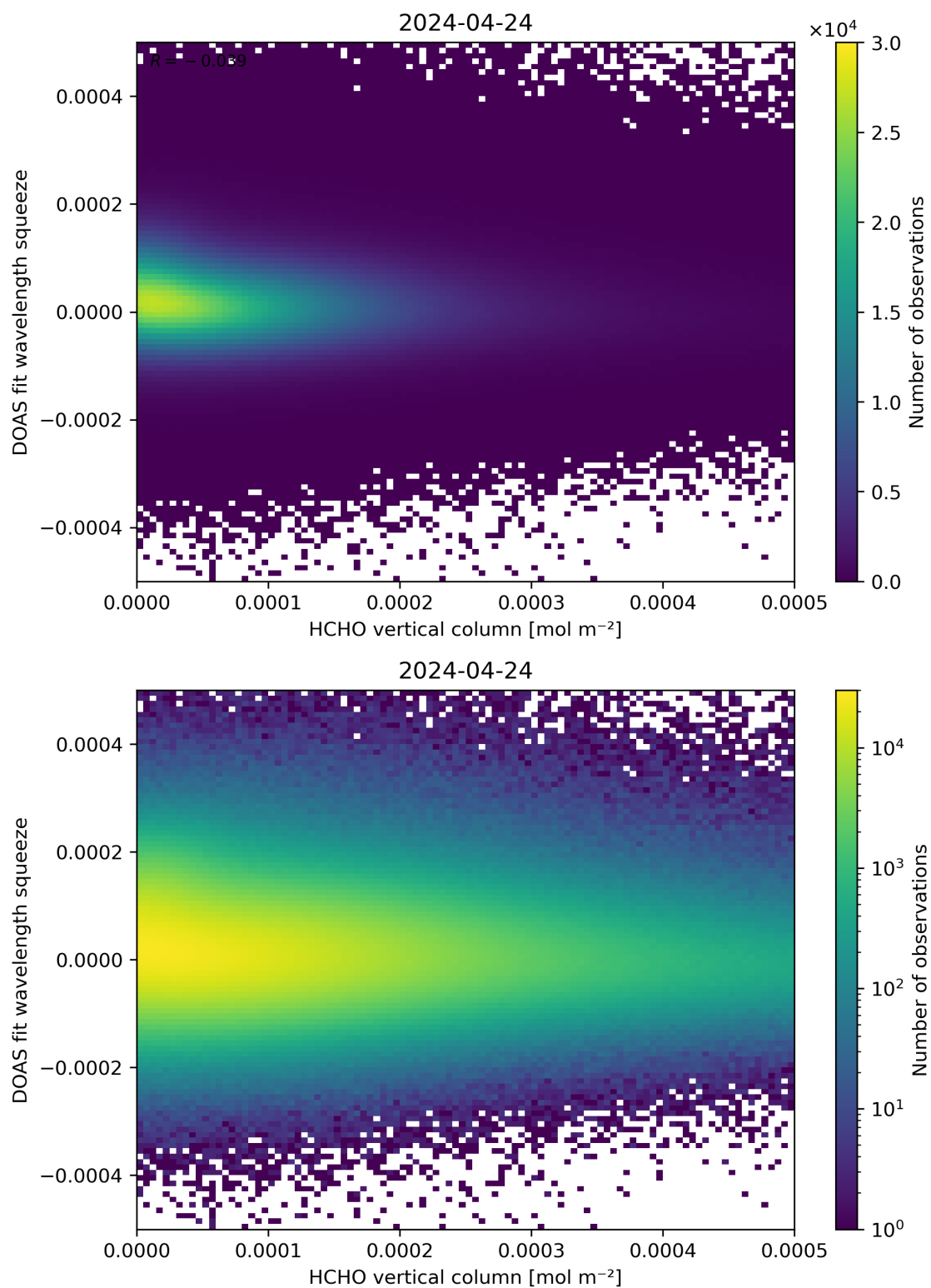
Figure 125: Scatter density plot of “HCHO vertical column” against “DOAS fit wavelength squeeze” for 2024-04-23 to 2024-04-25.
