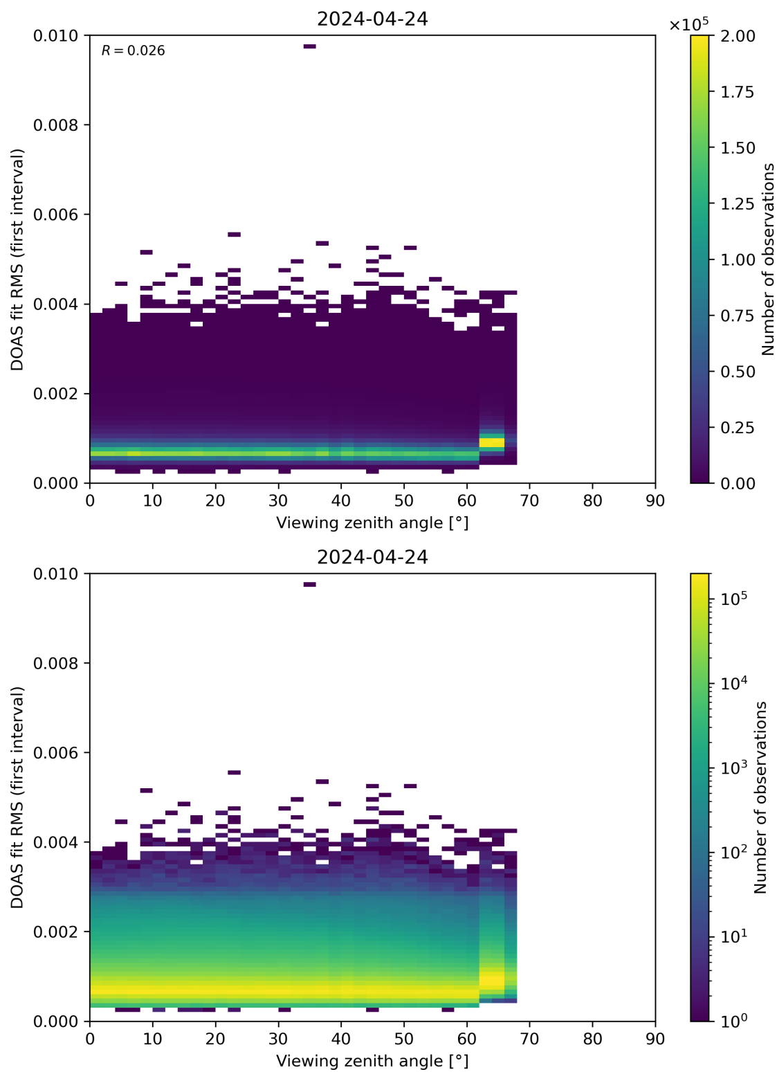
Figure 182: Scatter density plot of “Viewing zenith angle” against “DOAS fit RMS (first interval)” for 2024-04-23 to 2024-04-25.
