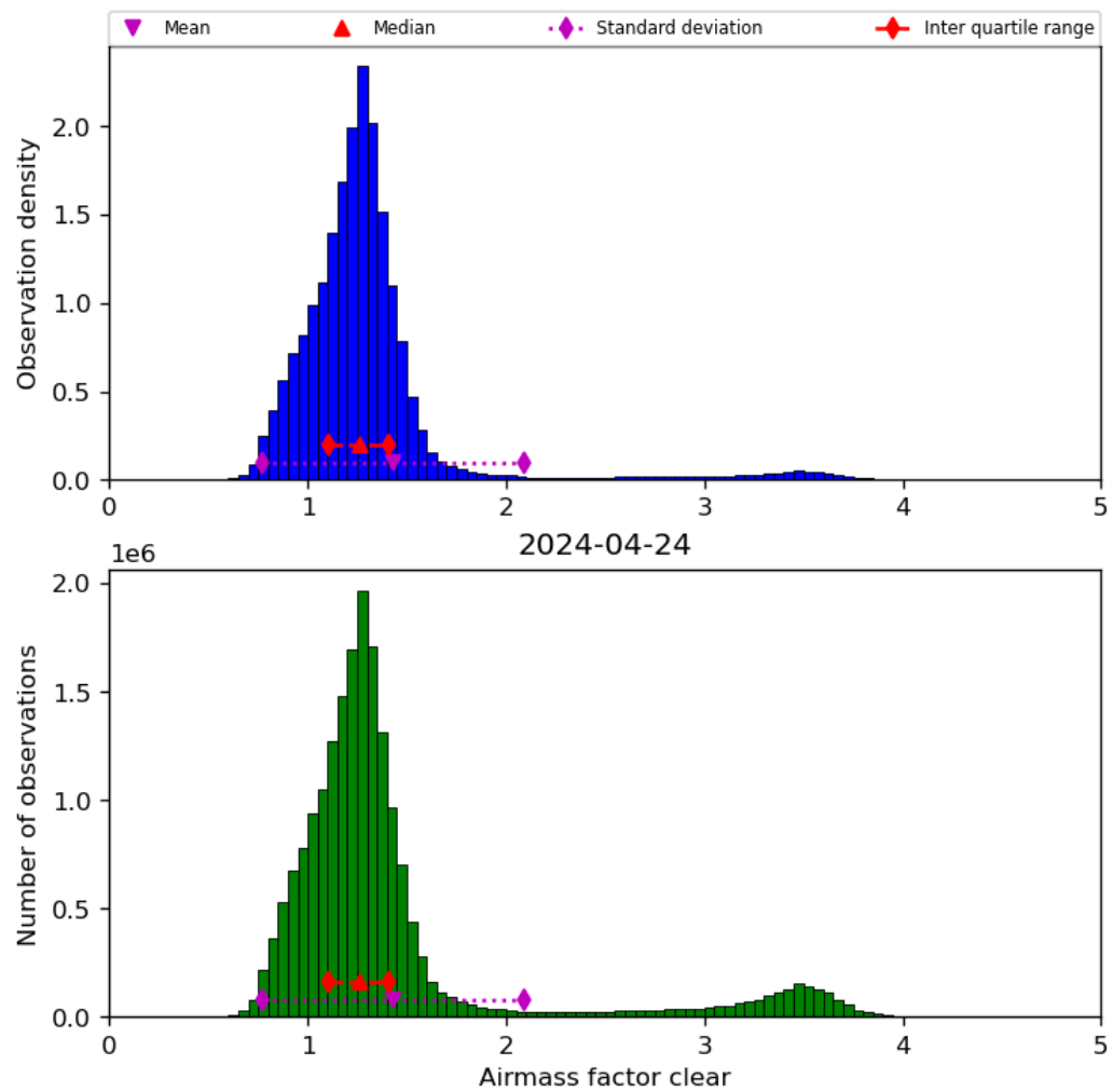
Figure 42: Histogram of “Airmass factor clear” for 2024-04-23 to 2024-04-25
