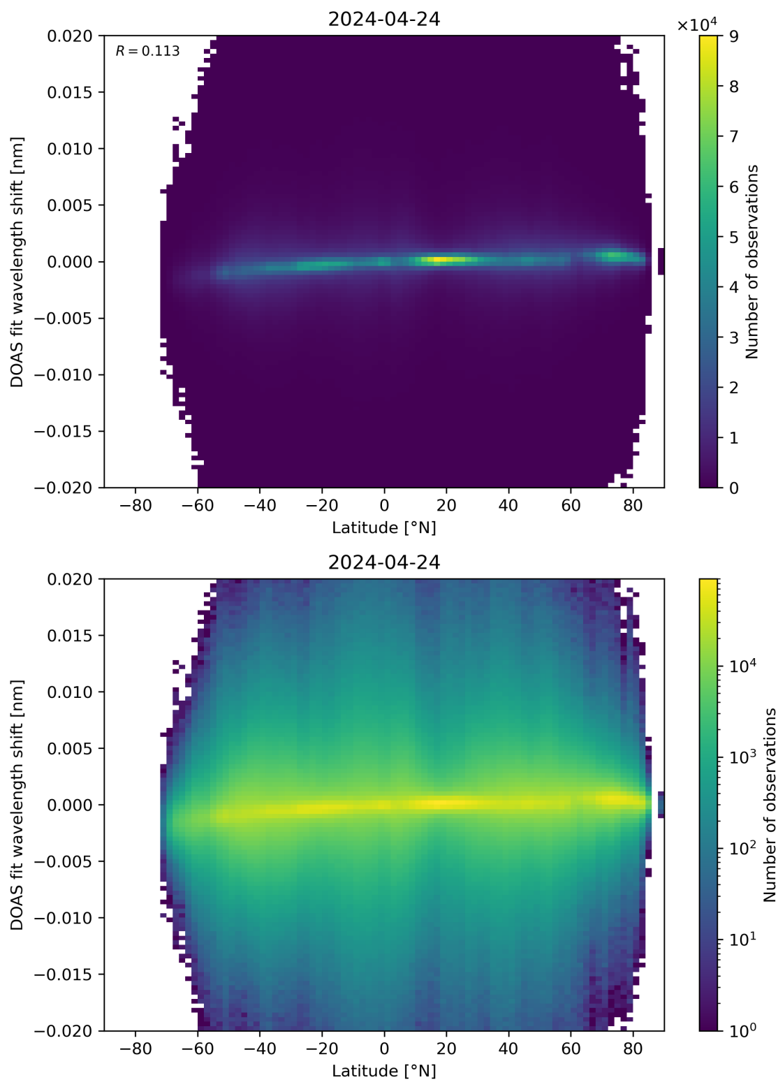
Figure 154: Scatter density plot of “Latitude” against “DOAS fit wavelength shift” for 2024-04-23 to 2024-04-25.
