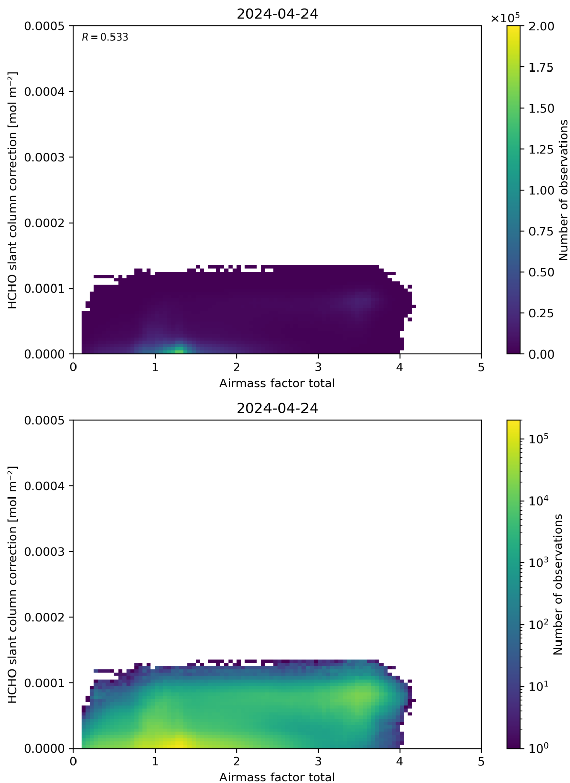
Figure 102: Scatter density plot of “Airmass factor total” against “HCHO slant column correction” for 2024-04-23 to 2024-04-25.
