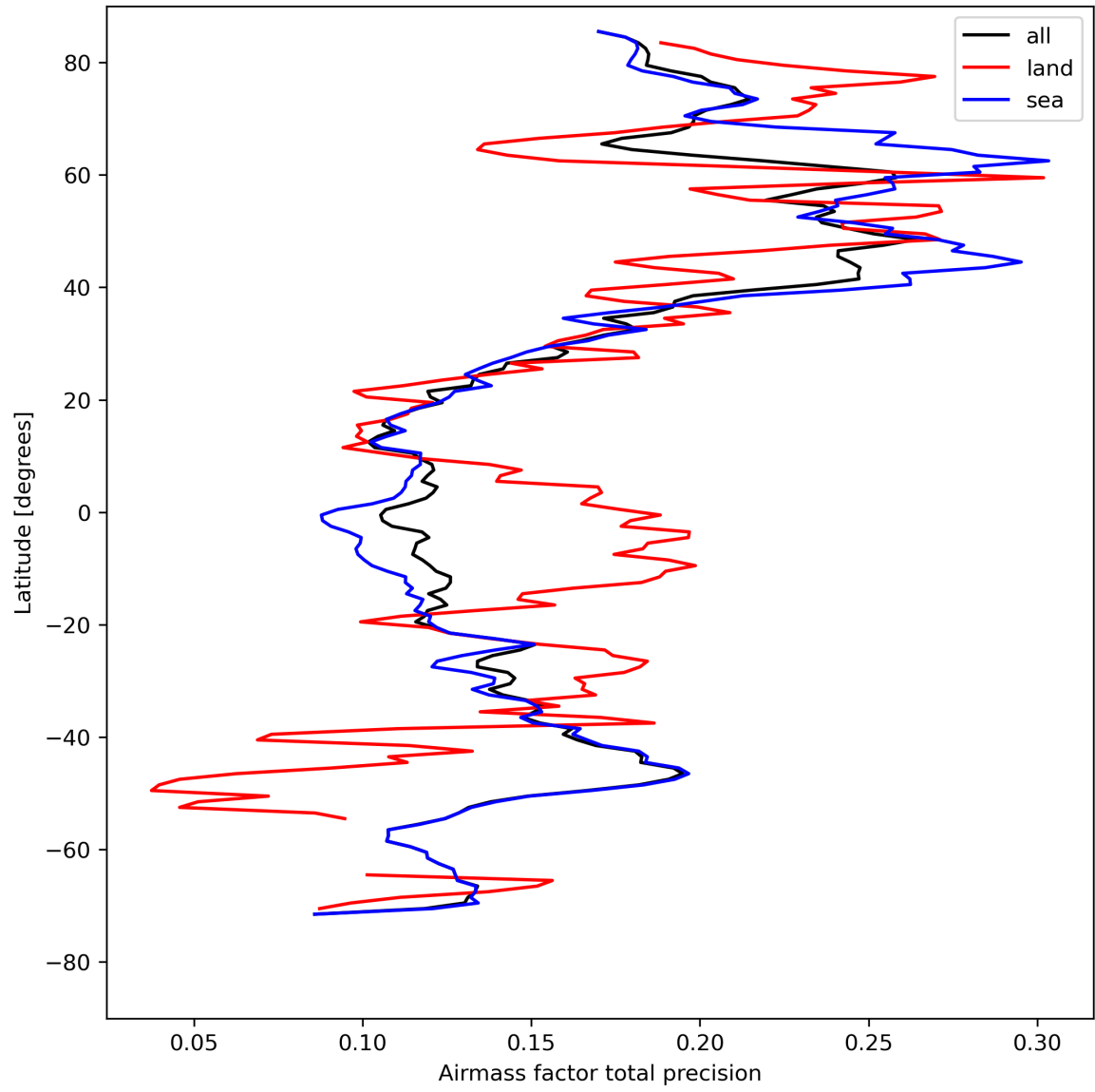
Figure 27: Zonal average of “Airmass factor total precision” for 2024-04-23 to 2024-04-25.
