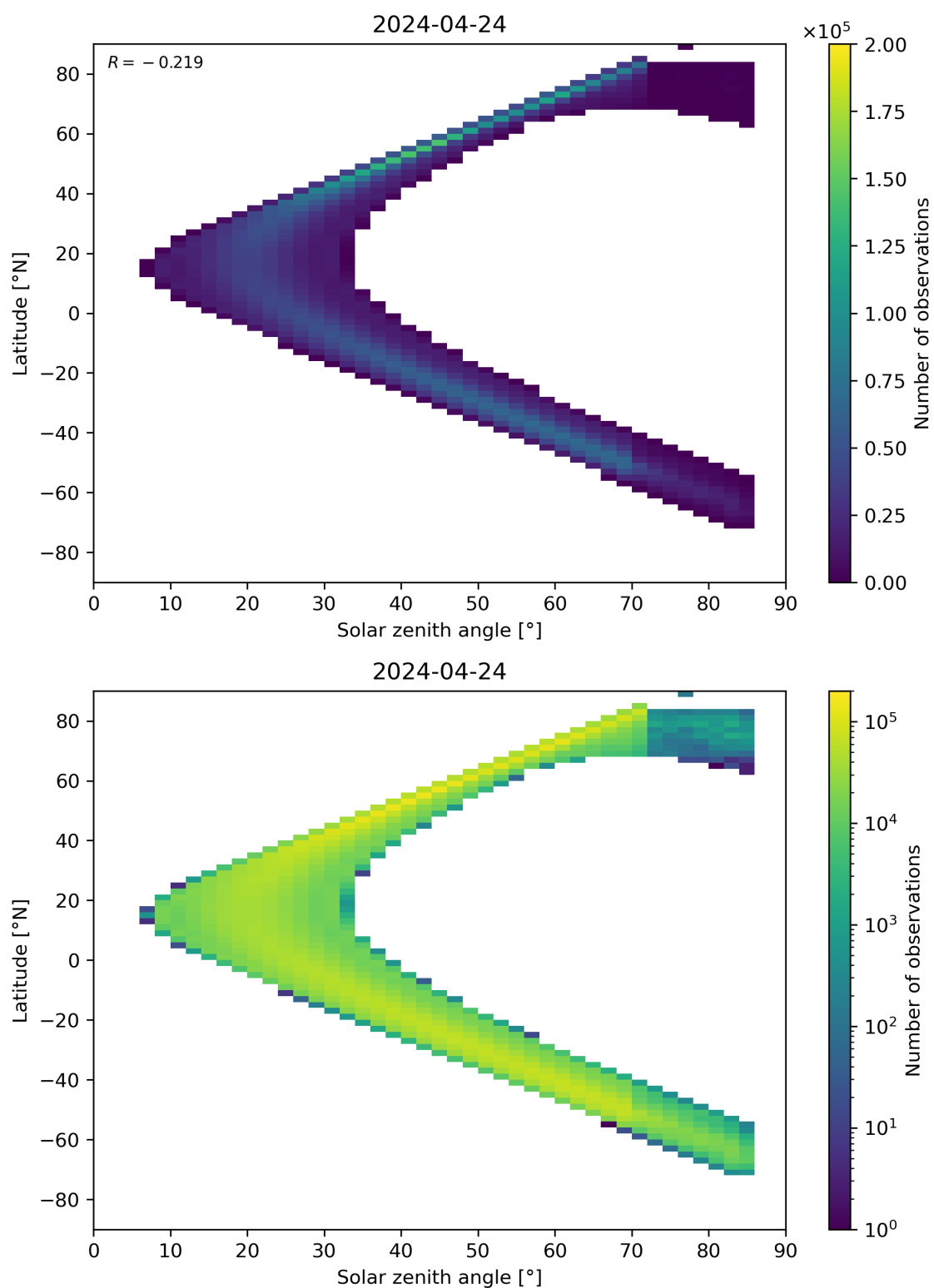
Figure 181: Scatter density plot of “Solar zenith angle” against “Latitude” for 2024-04-23 to 2024-04-25.
