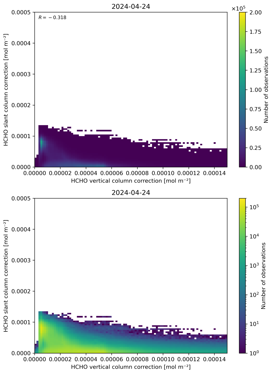
Figure 117: Scatter density plot of “HCHO vertical column correction” against “HCHO slant column correction” for 2024-04-23 to 2024-04-25.
