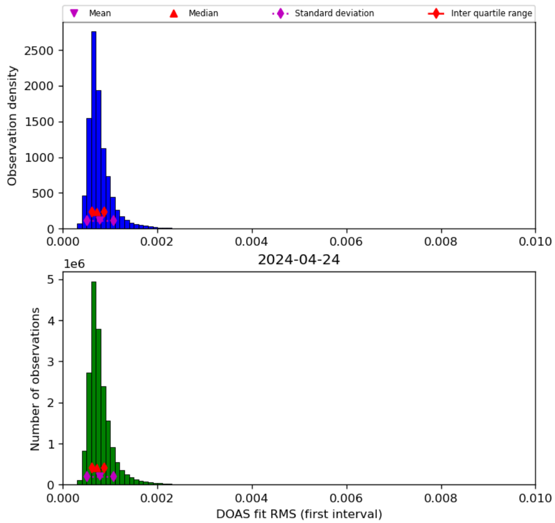
Figure 46: Histogram of “DOAS fit RMS (first interval)” for 2024-04-23 to 2024-04-25
