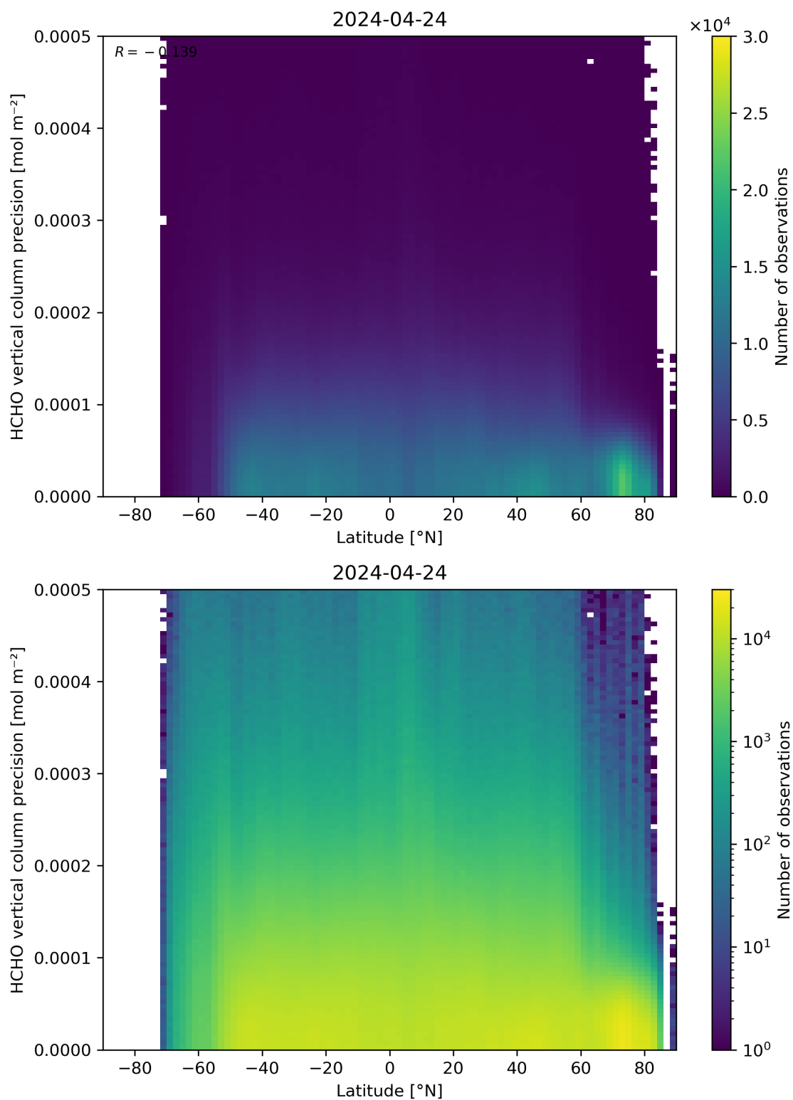
Figure 165: Scatter density plot of “Latitude” against “HCHO vertical column precision” for 2024-04-23 to 2024-04-25.
