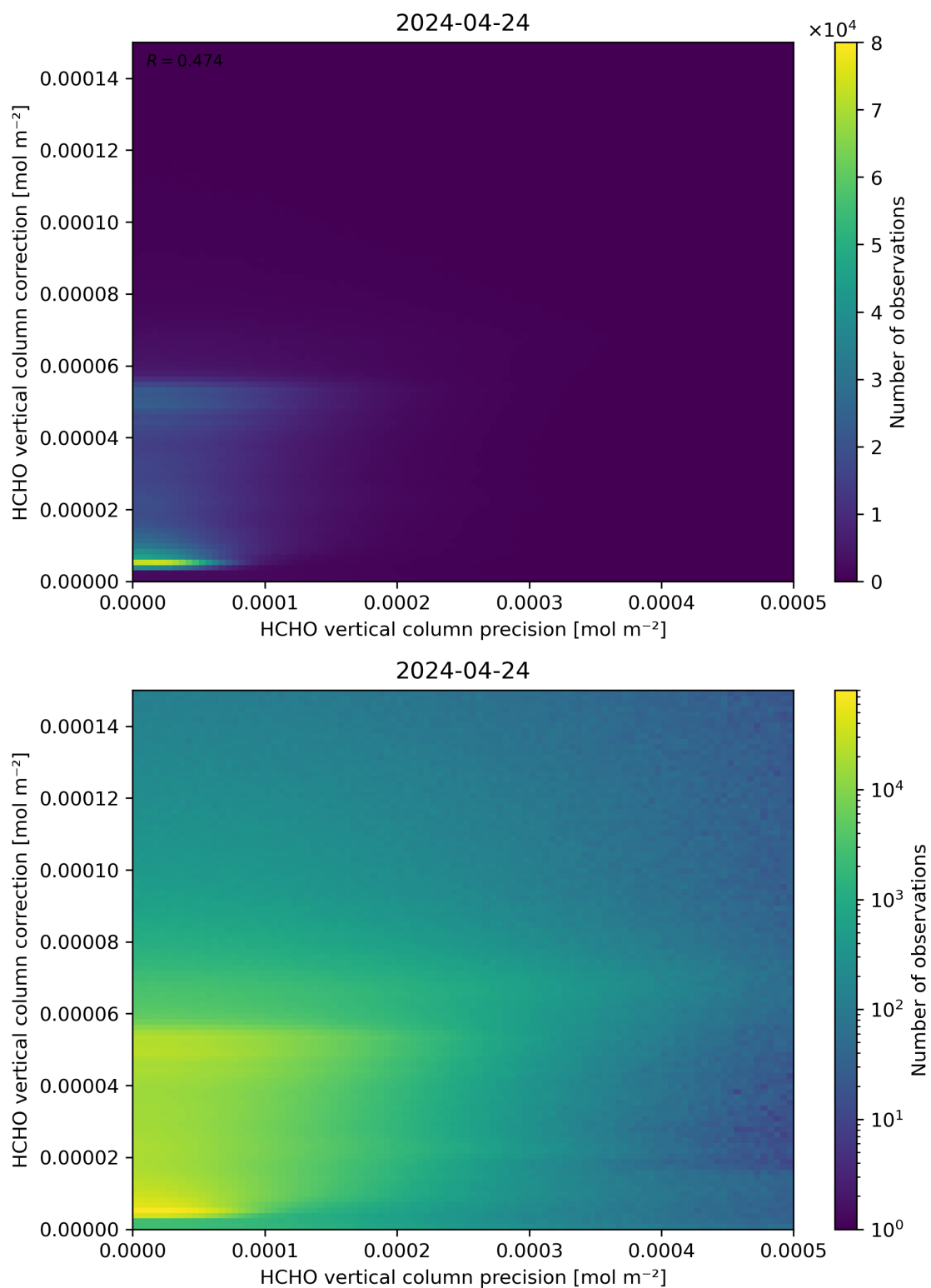
Figure 146: Scatter density plot of “HCHO vertical column precision” against “HCHO vertical column correction” for 2024-04-23 to 2024-04-25.
