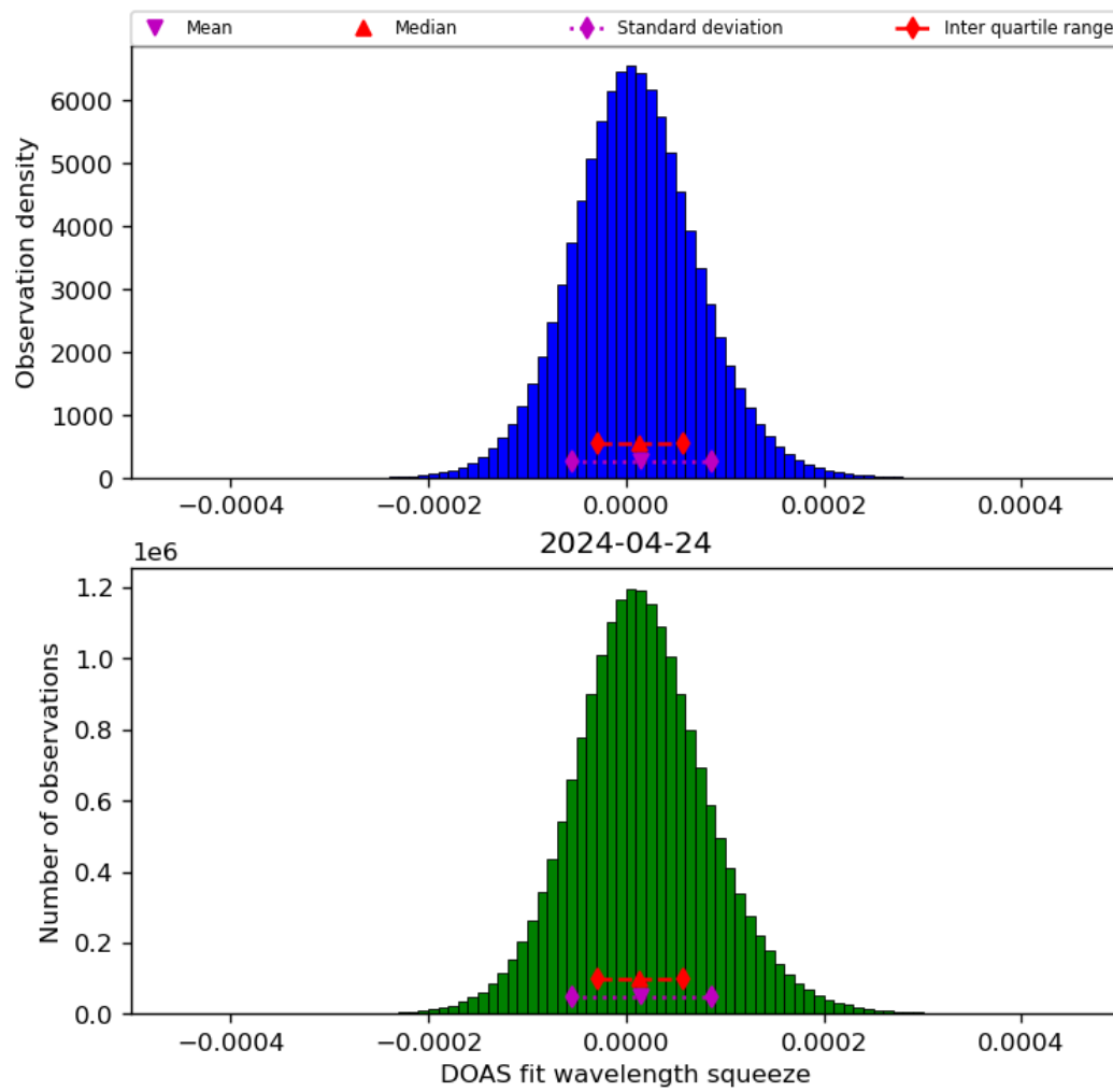
Figure 45: Histogram of “DOAS fit wavelength squeeze” for 2024-04-23 to 2024-04-25
