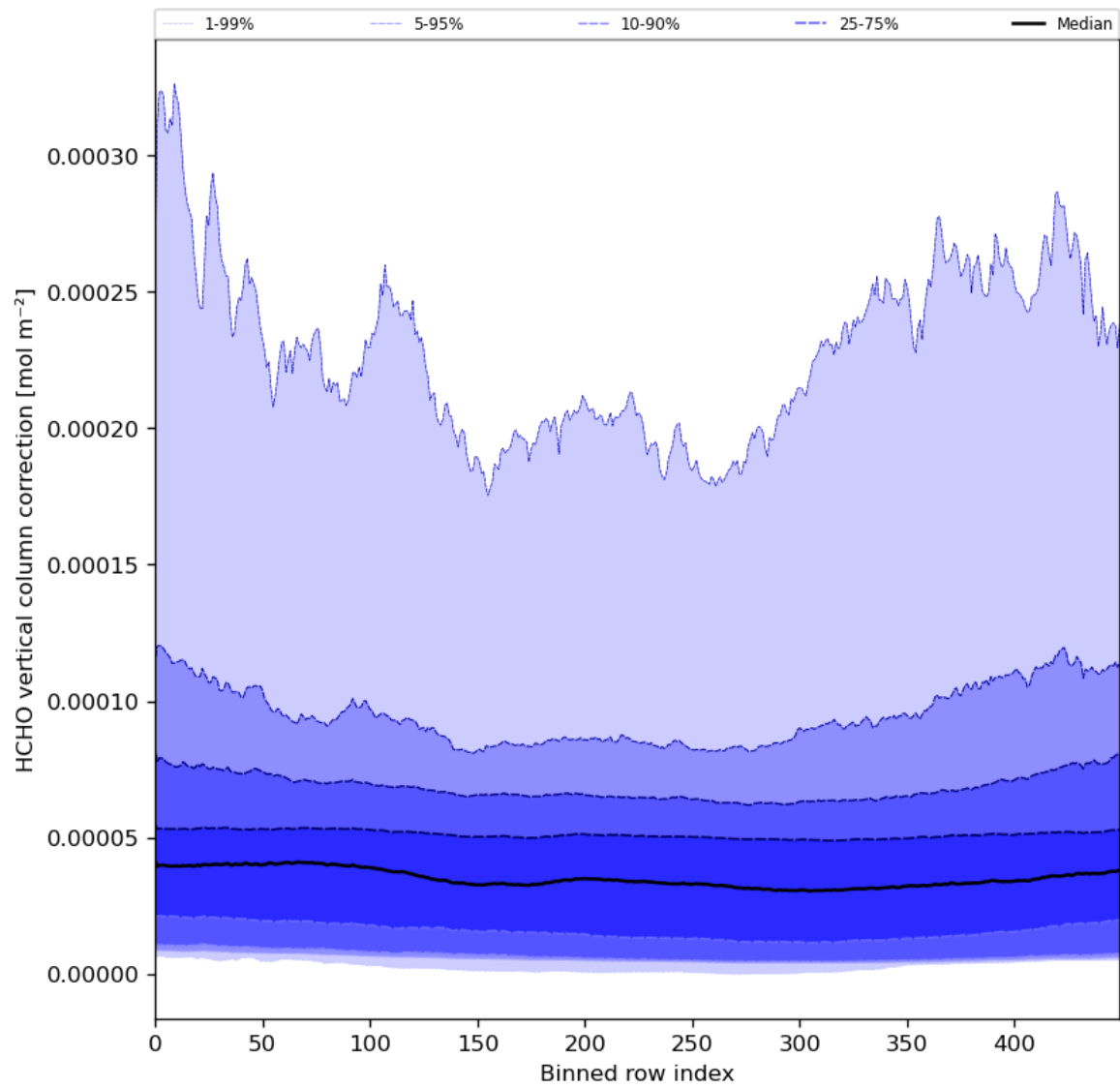
Figure 51: Along track statistics of “HCHO vertical column correction” for 2024-04-23 to 2024-04-25
