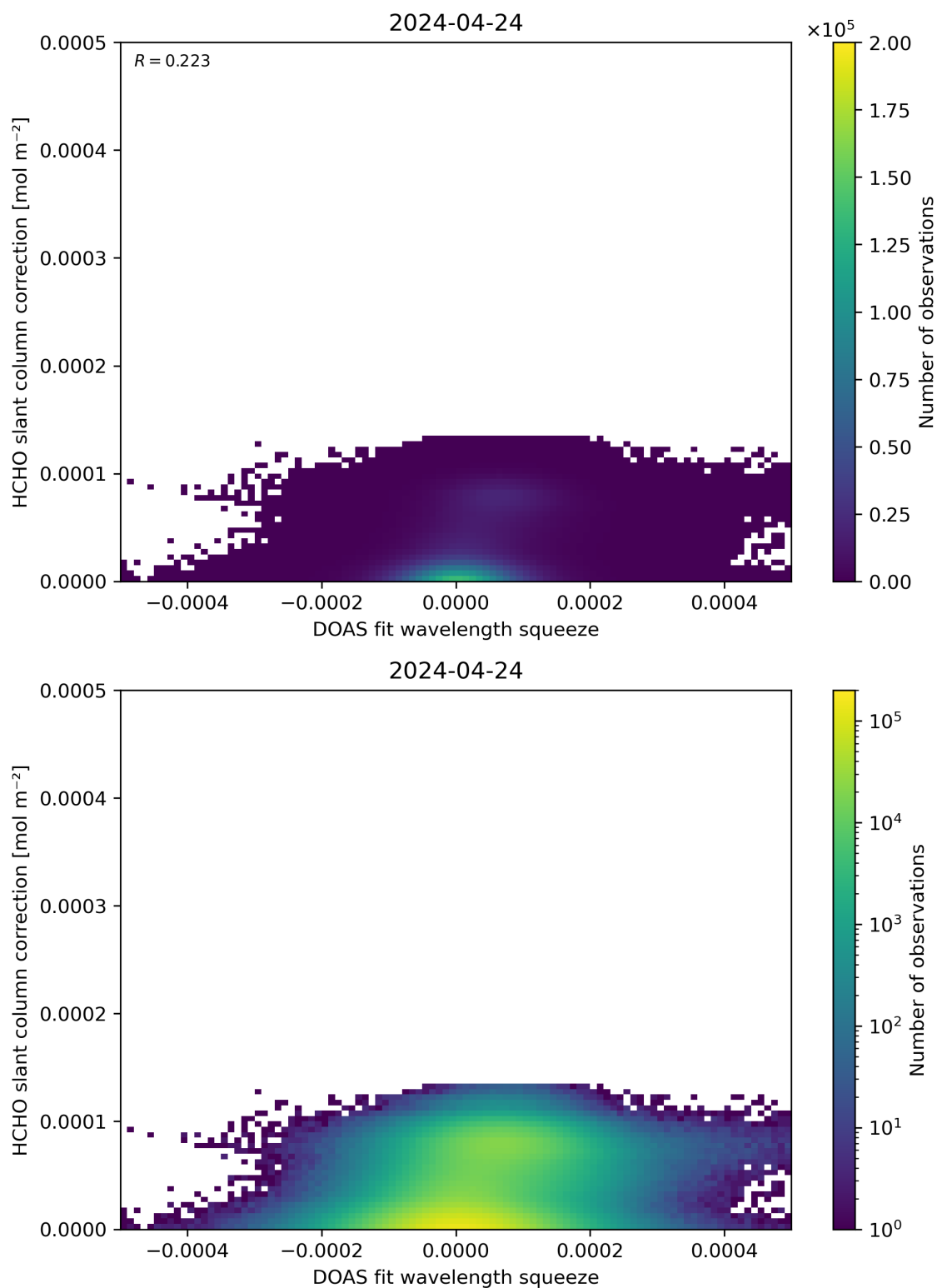
Figure 70: Scatter density plot of “DOAS fit wavelength squeeze” against “HCHO slant column correction” for 2024-04-23 to 2024-04-25.
