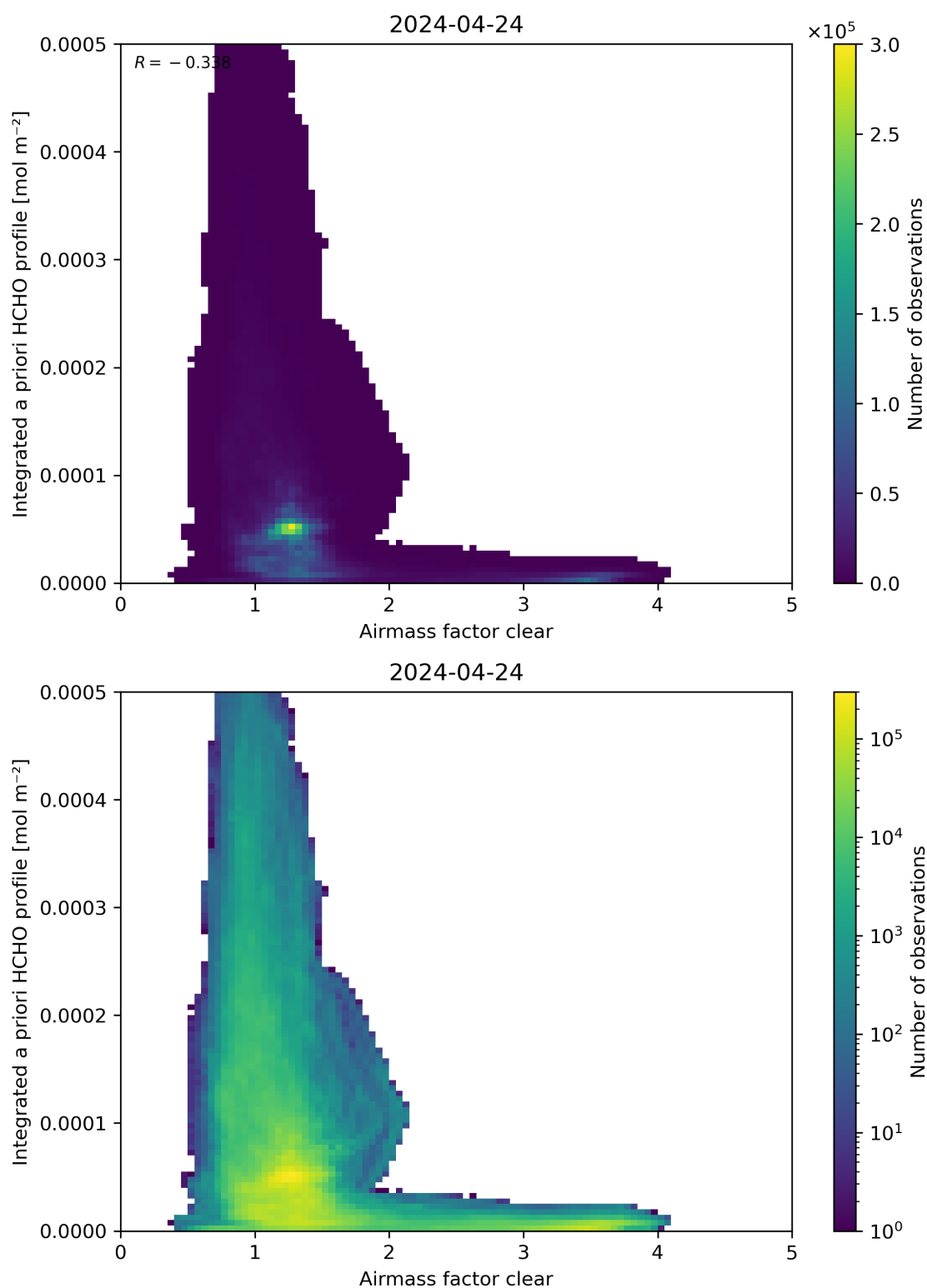
Figure 76: Scatter density plot of “Airmass factor clear” against “Integrated a priori HCHO profile” for 2024-04-23 to 2024-04-25.
