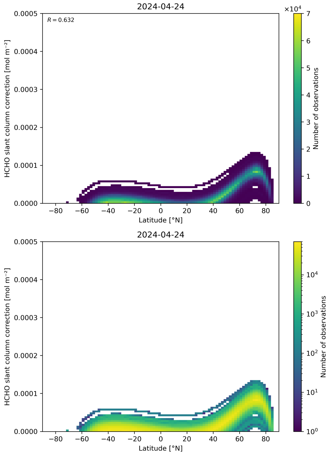
Figure 158: Scatter density plot of “Latitude” against “HCHO slant column correction” for 2024-04-23 to 2024-04-25.
