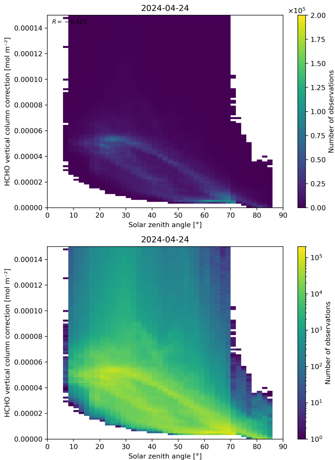
Figure 178: Scatter density plot of “Solar zenith angle” against “HCHO vertical column correction” for 2024-04-23 to 2024-04-25.
