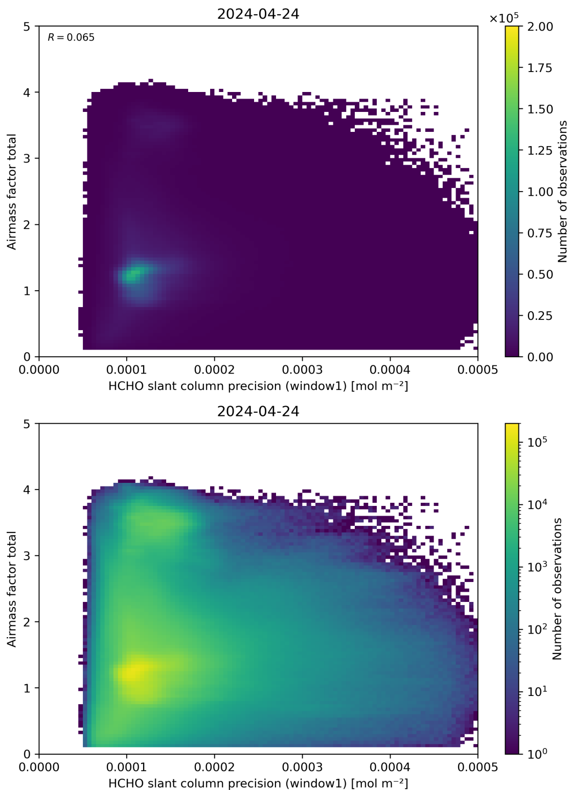
Figure 94: Scatter density plot of “HCHO slant column precision (window1)” against “Airmass factor total” for 2024-04-23 to 2024-04-25.
