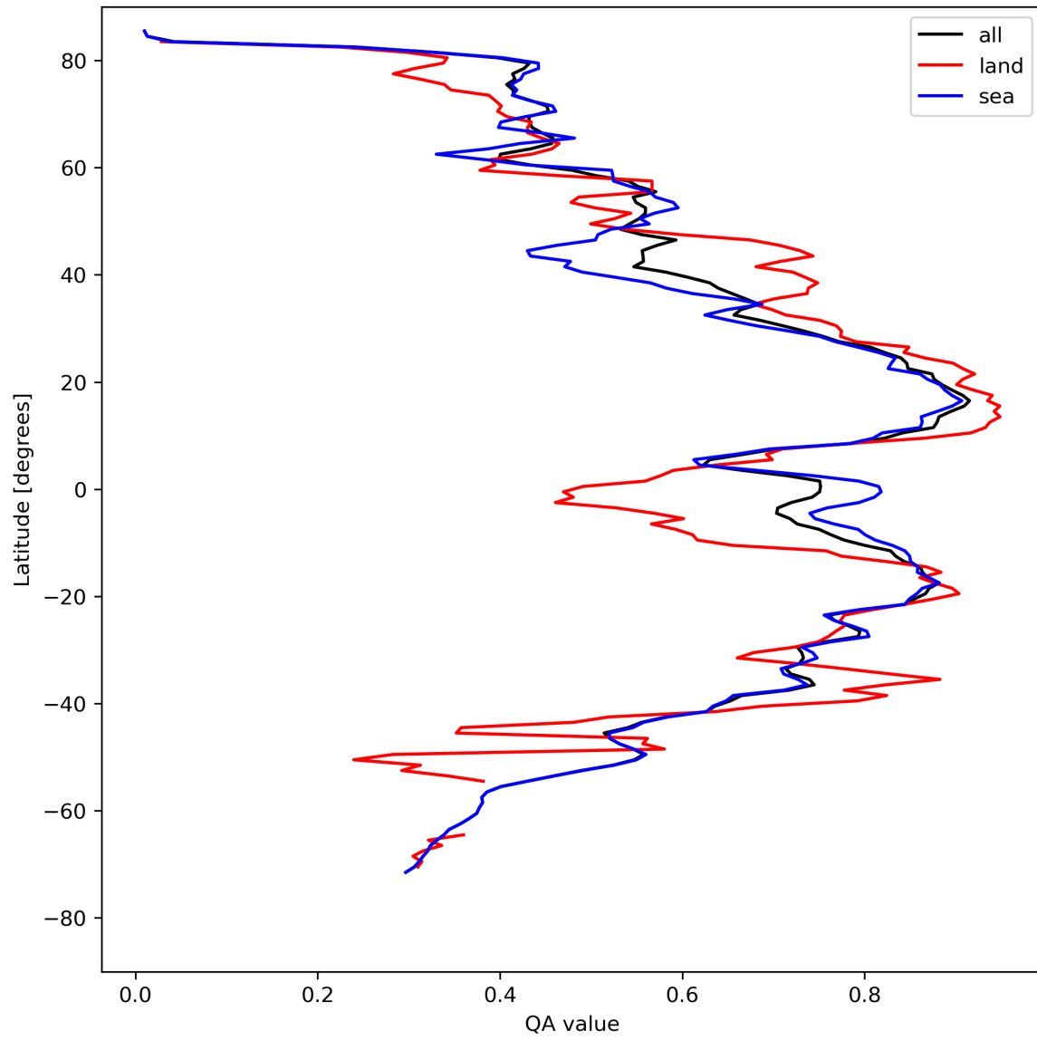
Figure 20: Zonal average of “QA value” for 2024-04-23 to 2024-04-25.
