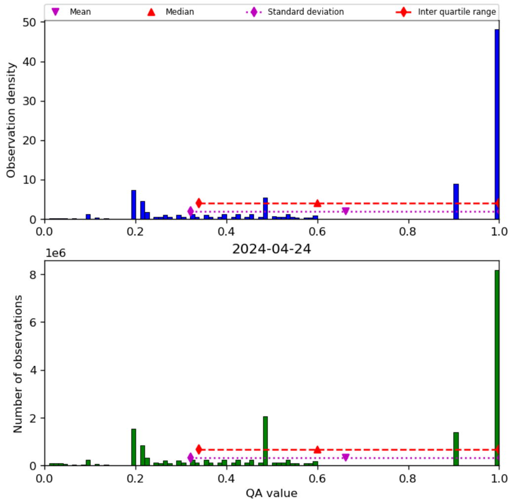
Figure 34: Histogram of “QA value” for 2024-04-23 to 2024-04-25
