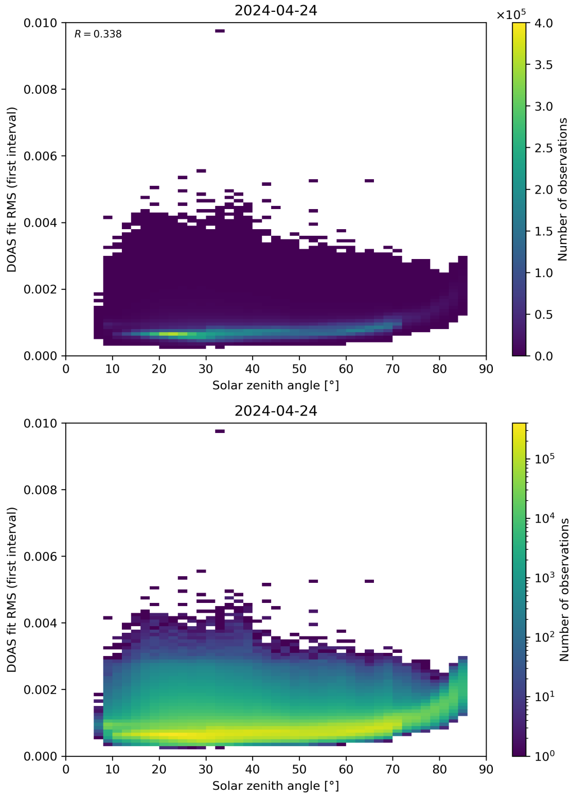
Figure 167: Scatter density plot of “Solar zenith angle” against “DOAS fit RMS (first interval)” for 2024-04-23 to 2024-04-25.
