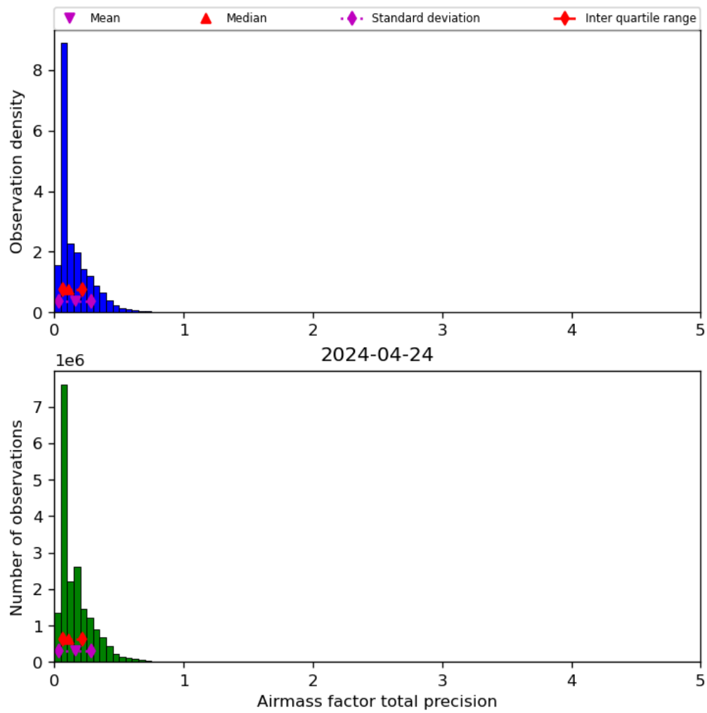
Figure 41: Histogram of "Airmass factor total precision" for 2024-04-23 to 2024-04-25
