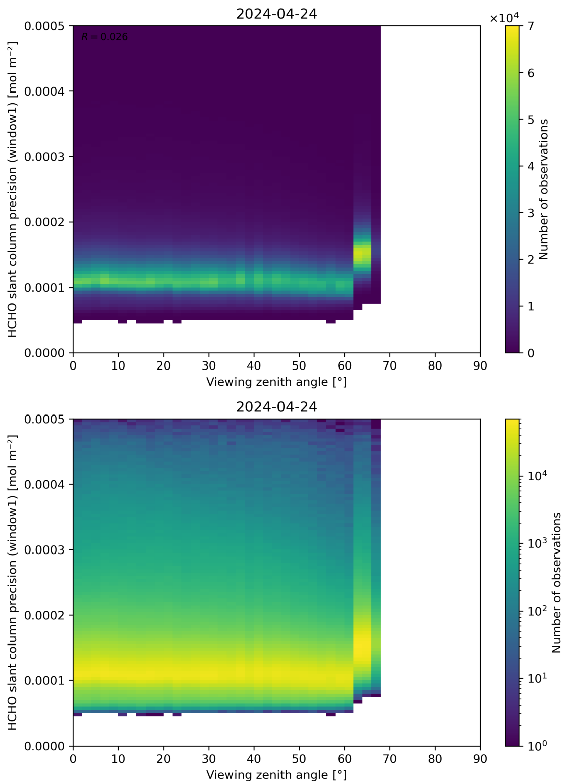
Figure 189: Scatter density plot of “Viewing zenith angle” against “HCHO slant column precision (window1)” for 2024-04-23 to 2024-04-25.
