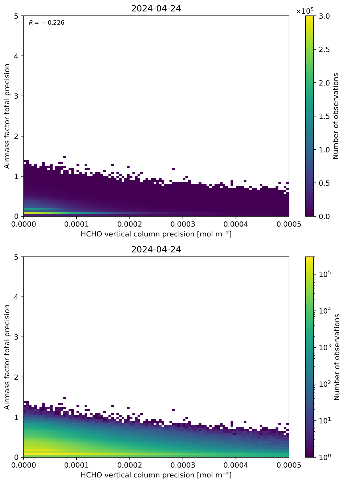
Figure 145: Scatter density plot of “HCHO vertical column precision” against “Airmass factor total precision” for 2024-04-23 to 2024-04-25.
