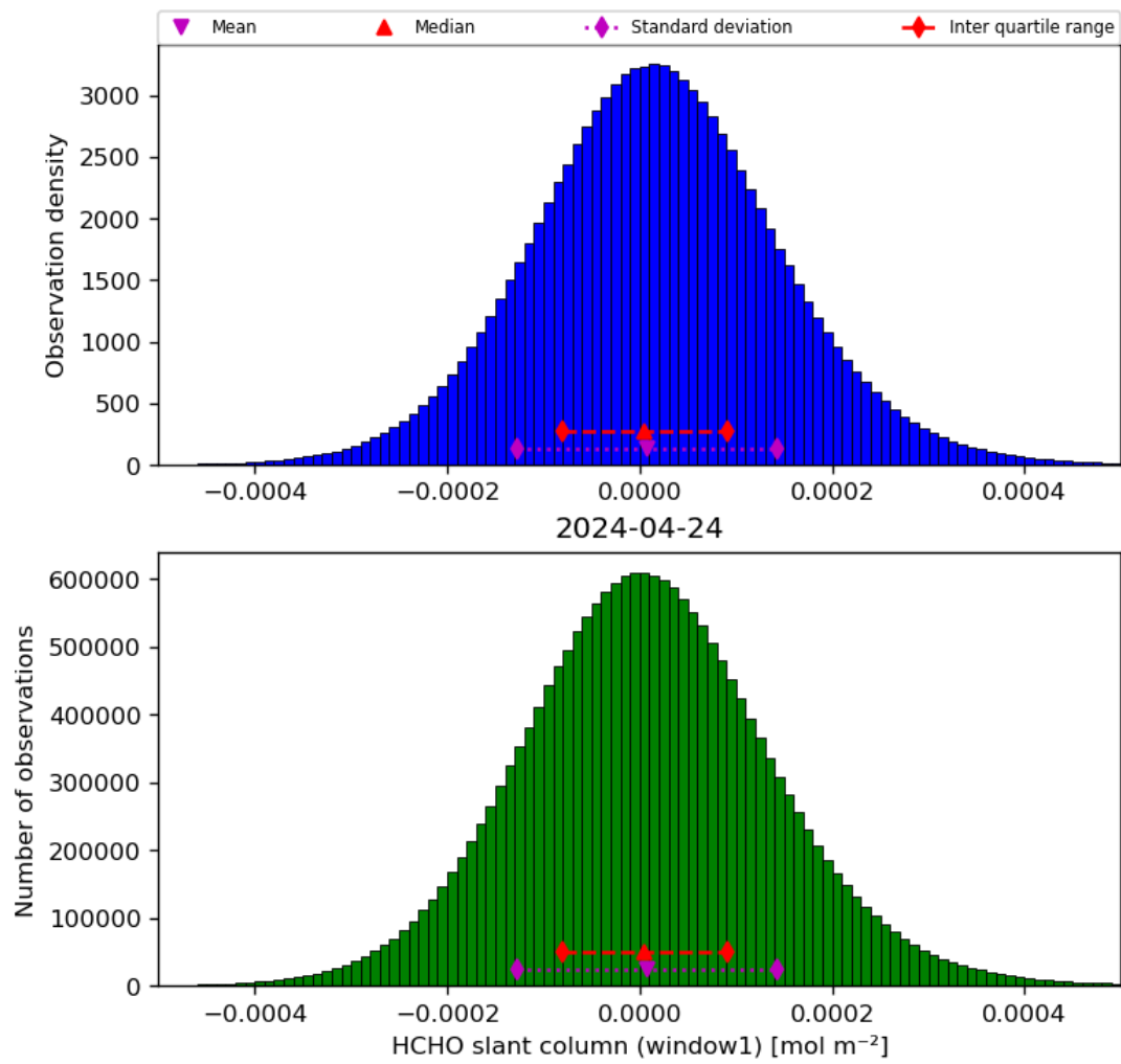
Figure 38: Histogram of “HCHO slant column (window1)” for 2024-04-23 to 2024-04-25
