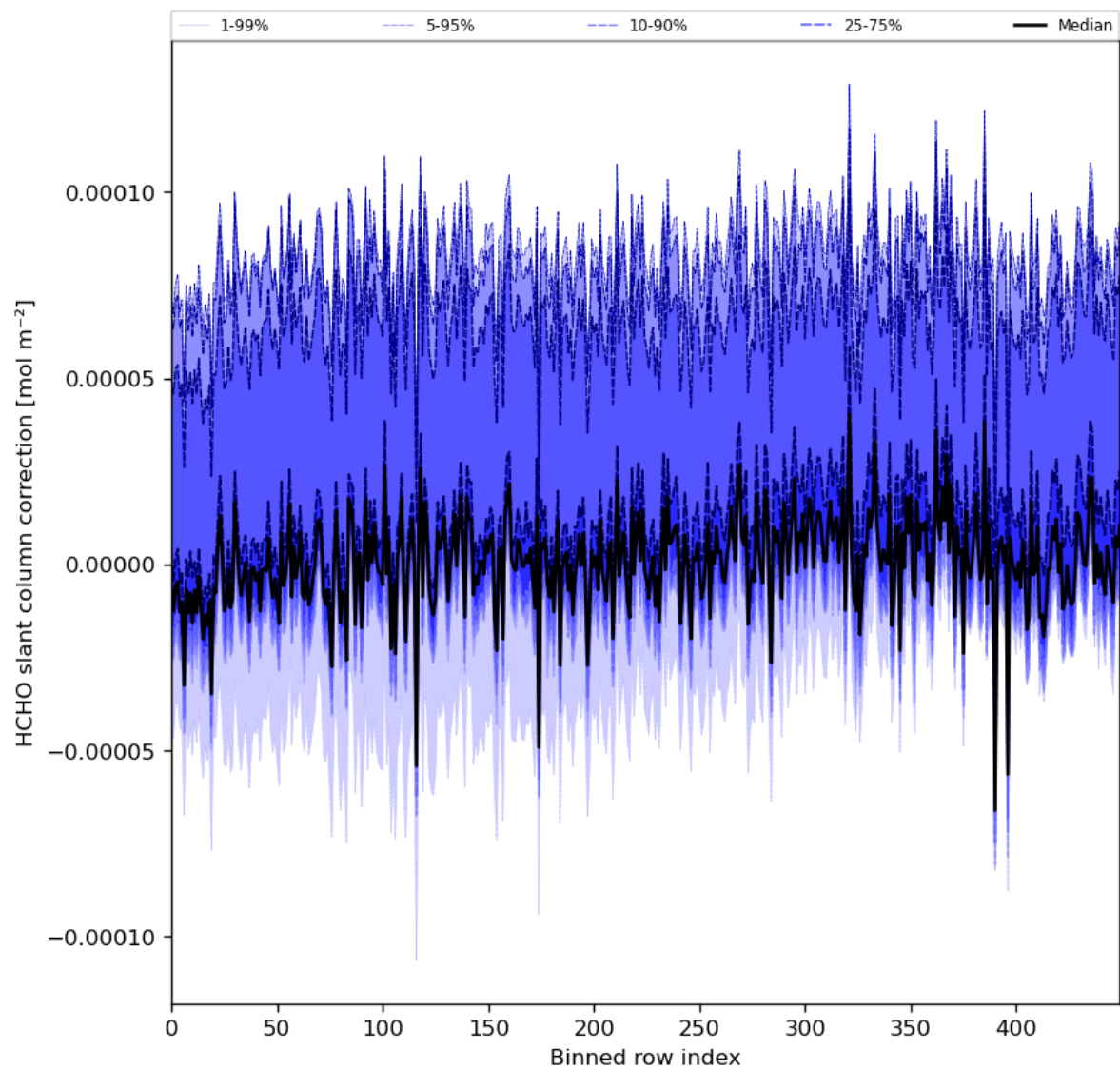
Figure 61: Along track statistics of “HCHO slant column correction” for 2024-04-23 to 2024-04-25
