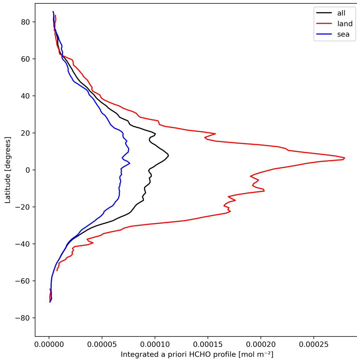
Figure 29: Zonal average of “Integrated a priori HCHO profile” for 2024-04-23 to 2024-04-25.
