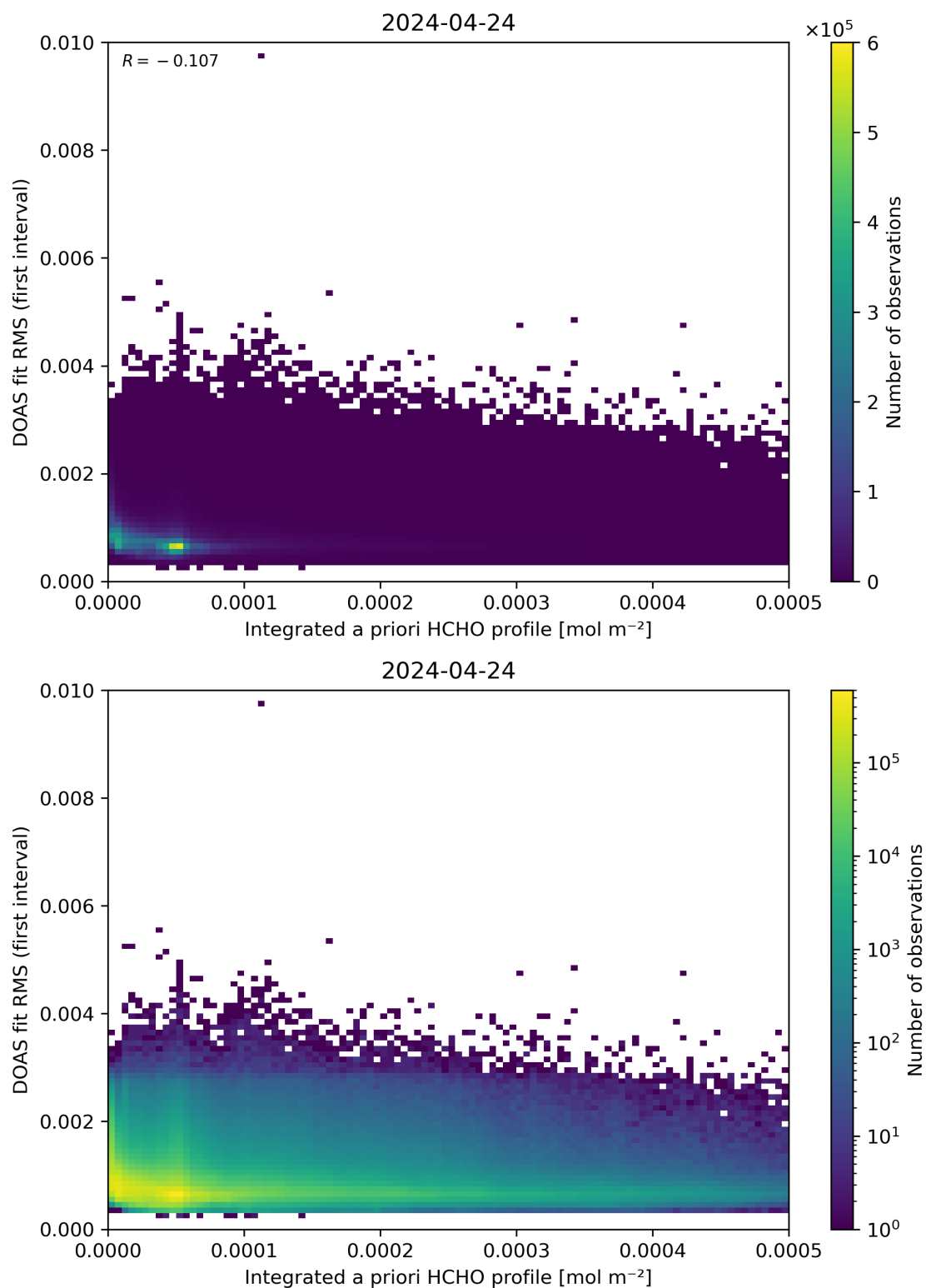
Figure 148: Scatter density plot of “Integrated a priori HCHO profile” against “DOAS fit RMS (first interval)” for 2024-04-23 to 2024-04-25.
