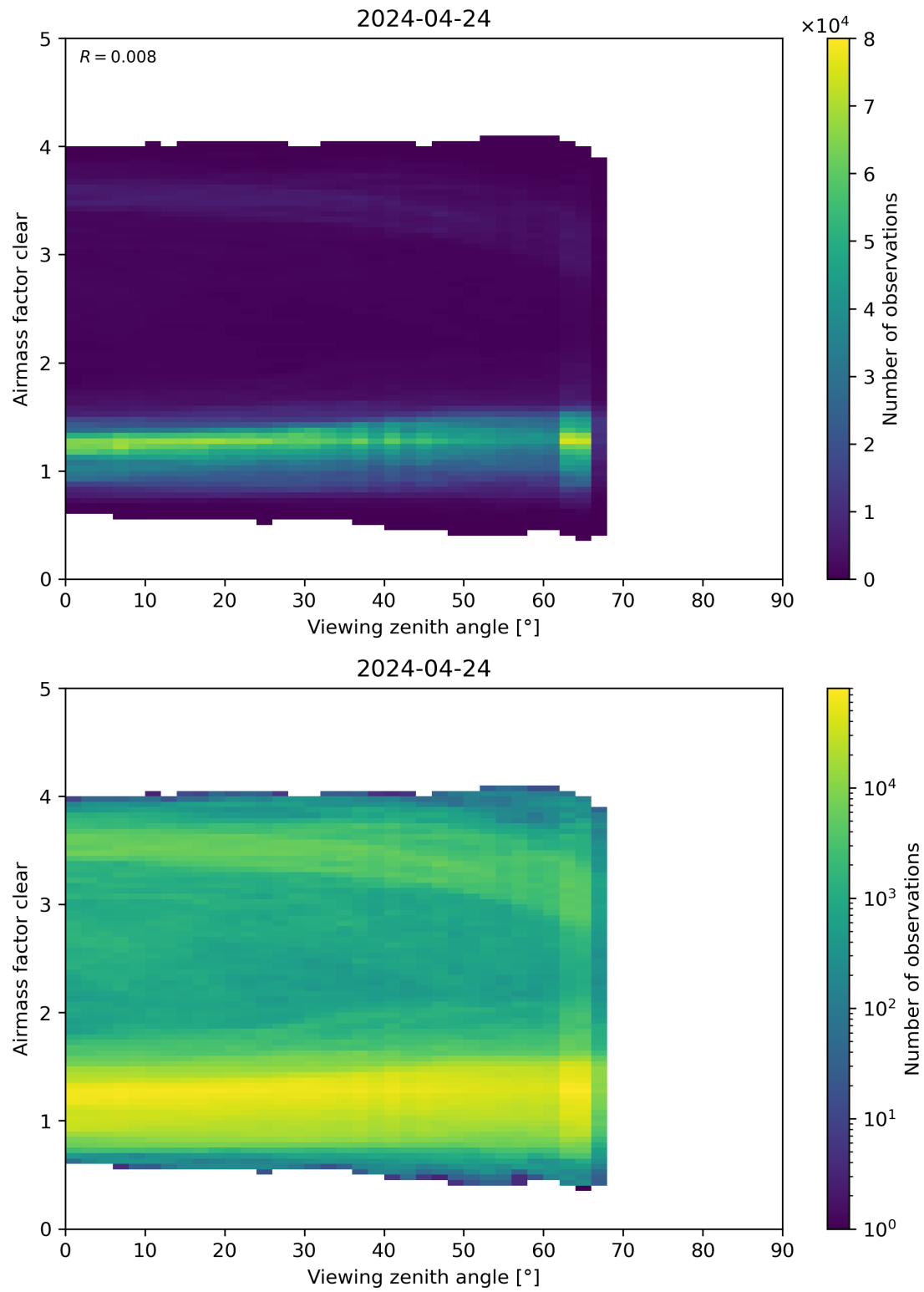
Figure 185: Scatter density plot of “Viewing zenith angle” against “Airmass factor clear” for 2024-04-23 to 2024-04-25.
