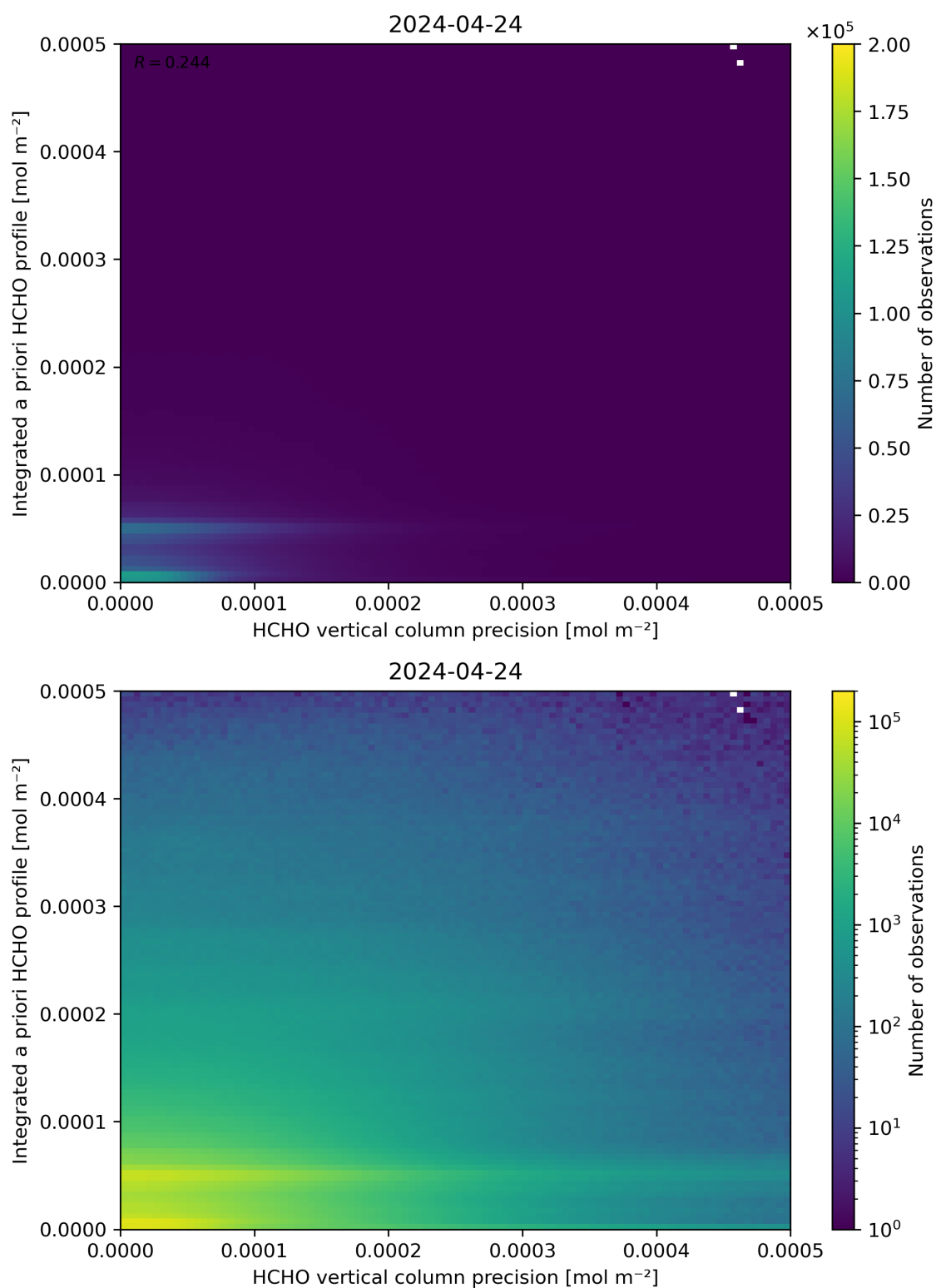
Figure 147: Scatter density plot of “HCHO vertical column precision” against “Integrated a priori HCHO profile” for 2024-04-23 to 2024-04-25.
