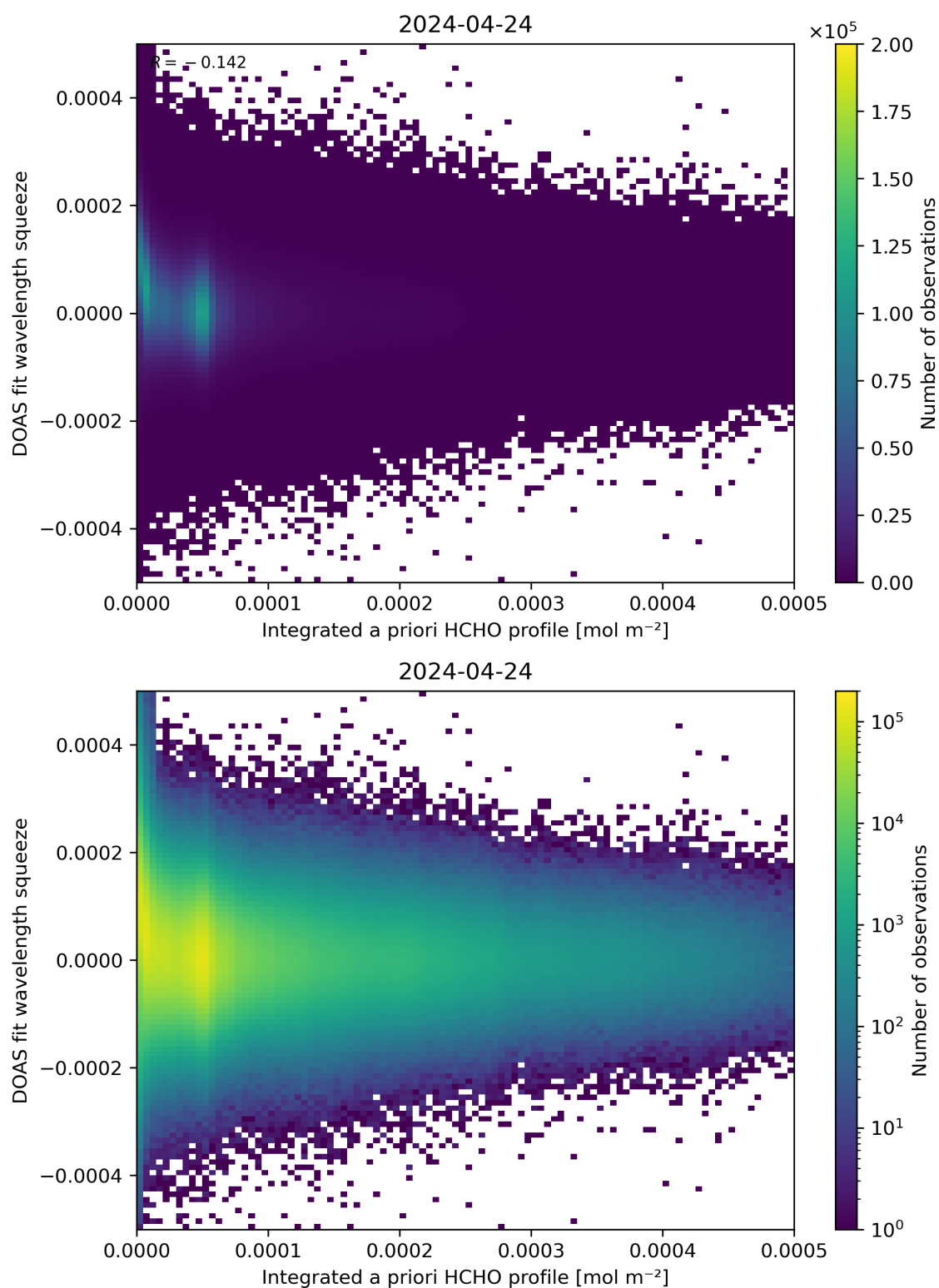
Figure 150: Scatter density plot of “Integrated a priori HCHO profile” against “DOAS fit wavelength squeeze” for 2024-04-23 to 2024-04-25.
