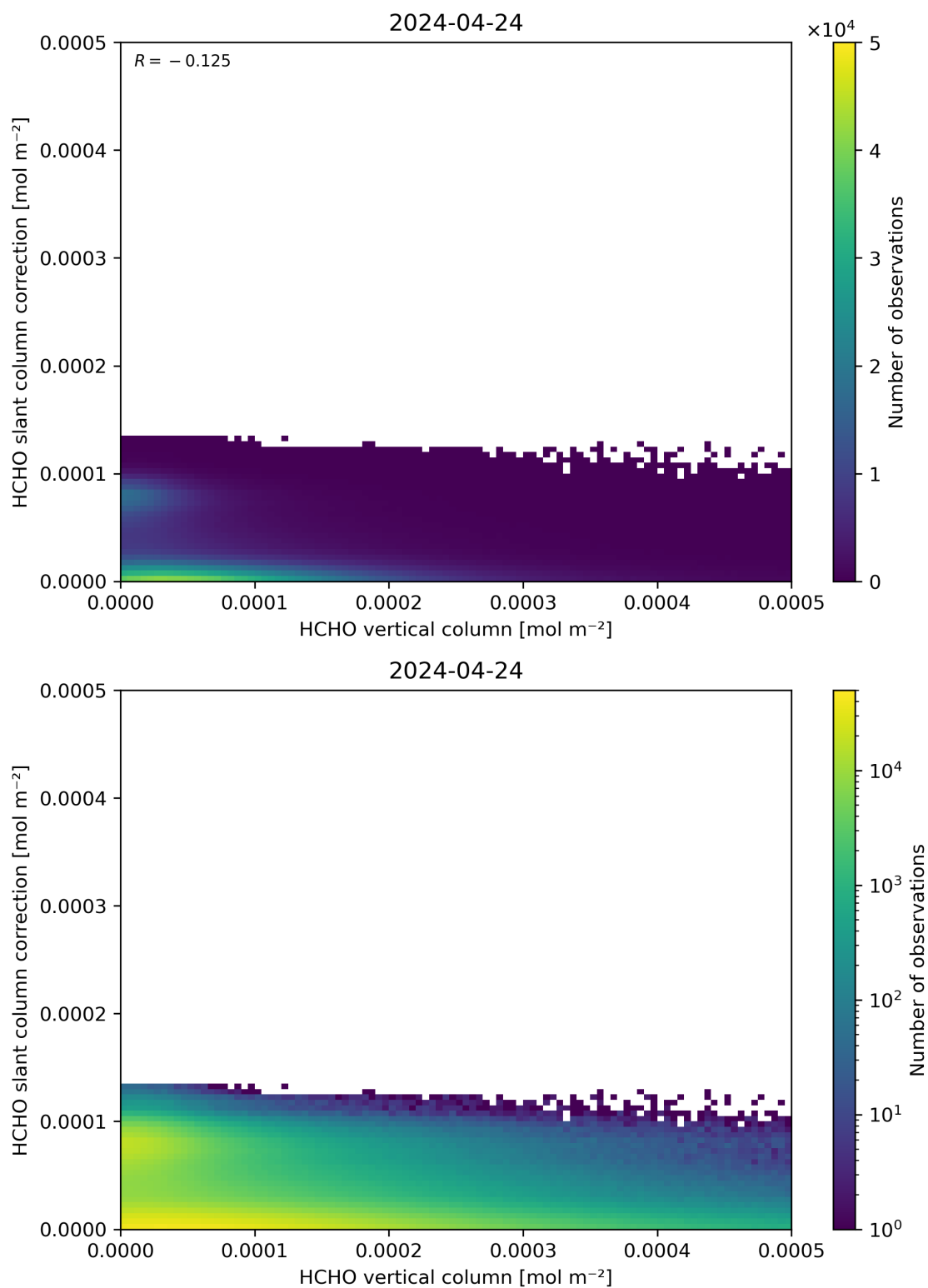
Figure 128: Scatter density plot of “HCHO vertical column” against “HCHO slant column correction” for 2024-04-23 to 2024-04-25.
