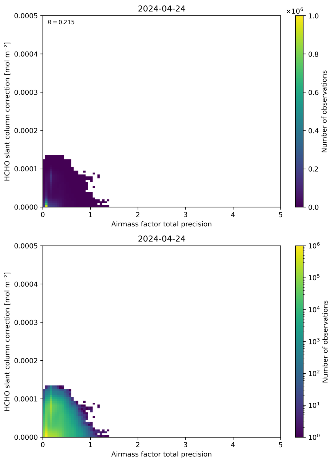
Figure 110: Scatter density plot of “Airmass factor total precision” against “HCHO slant column correction” for 2024-04-23 to 2024-04-25.
