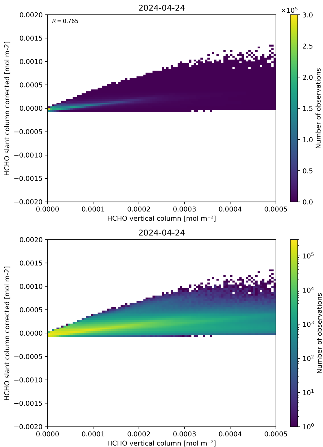
Figure 127: Scatter density plot of “HCHO vertical column” against “HCHO slant column corrected” for 2024-04-23 to 2024-04-25.
