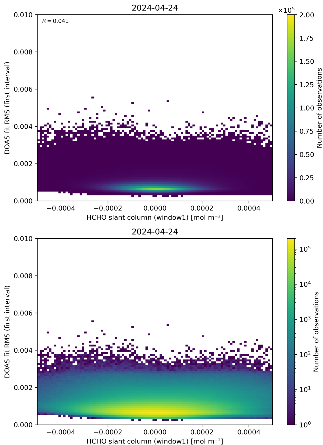
Figure 78: Scatter density plot of “HCHO slant column (window1)” against “DOAS fit RMS (first interval)” for 2024-04-23 to 2024-04-25.
