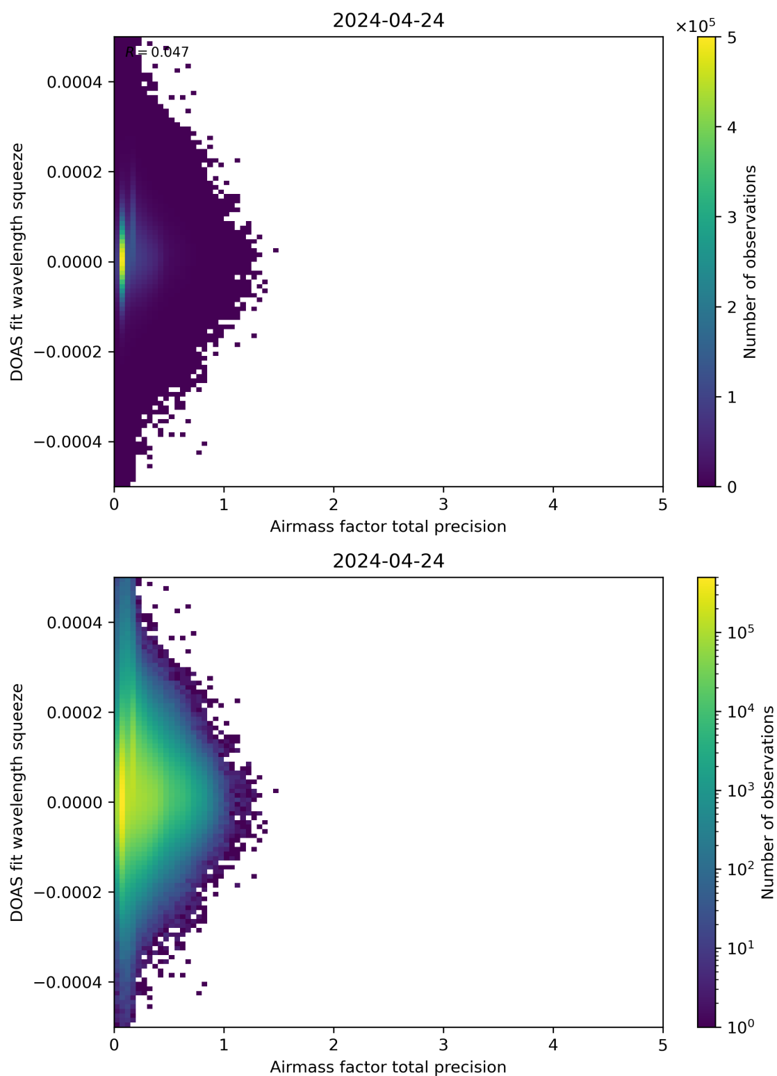
Figure 107: Scatter density plot of “Airmass factor total precision” against “DOAS fit wavelength squeeze” for 2024-04-23 to 2024-04-25.
