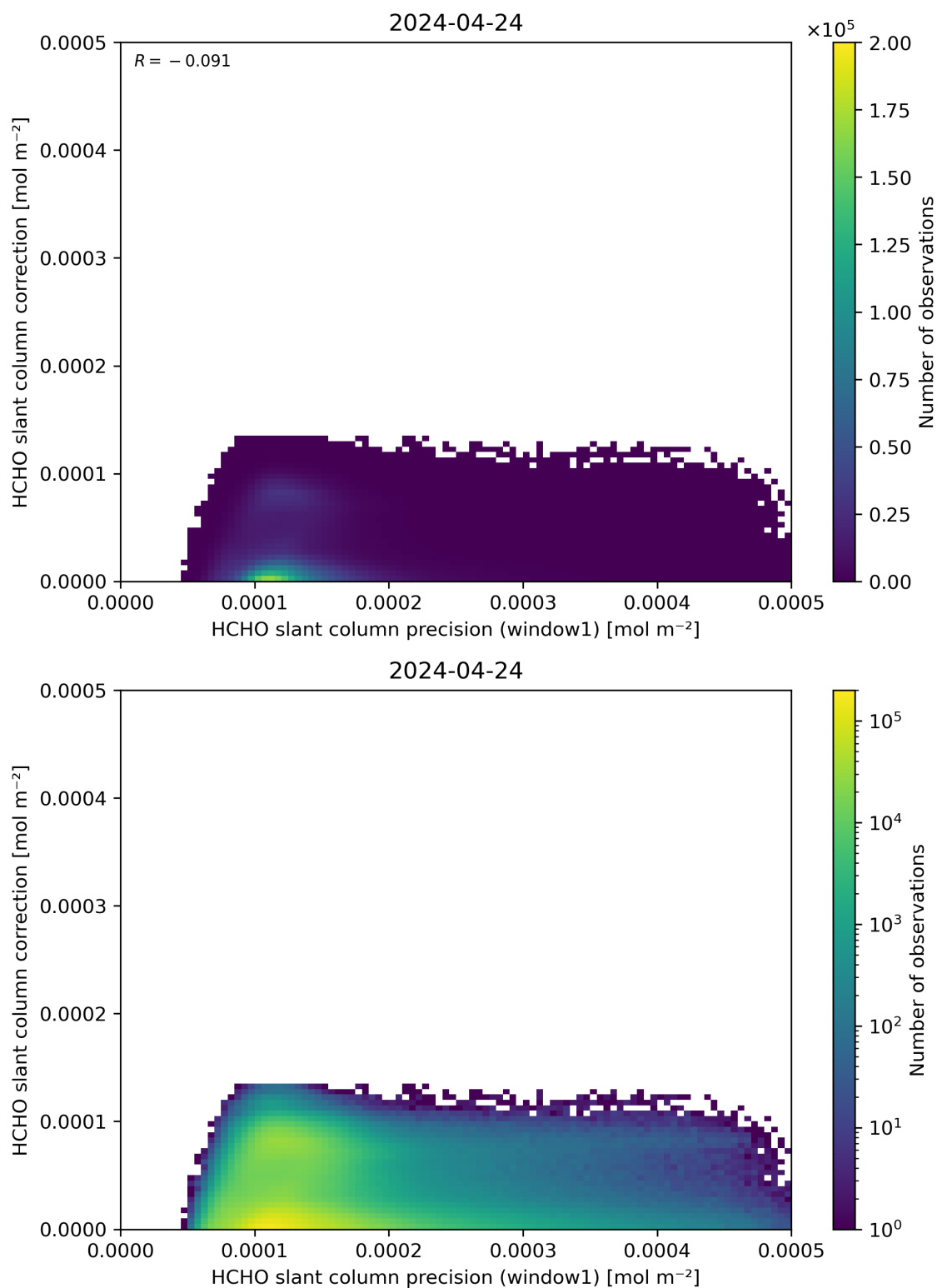
Figure 93: Scatter density plot of “HCHO slant column precision (window1)” against “HCHO slant column correction” for 2024-04-23 to 2024-04-25.
