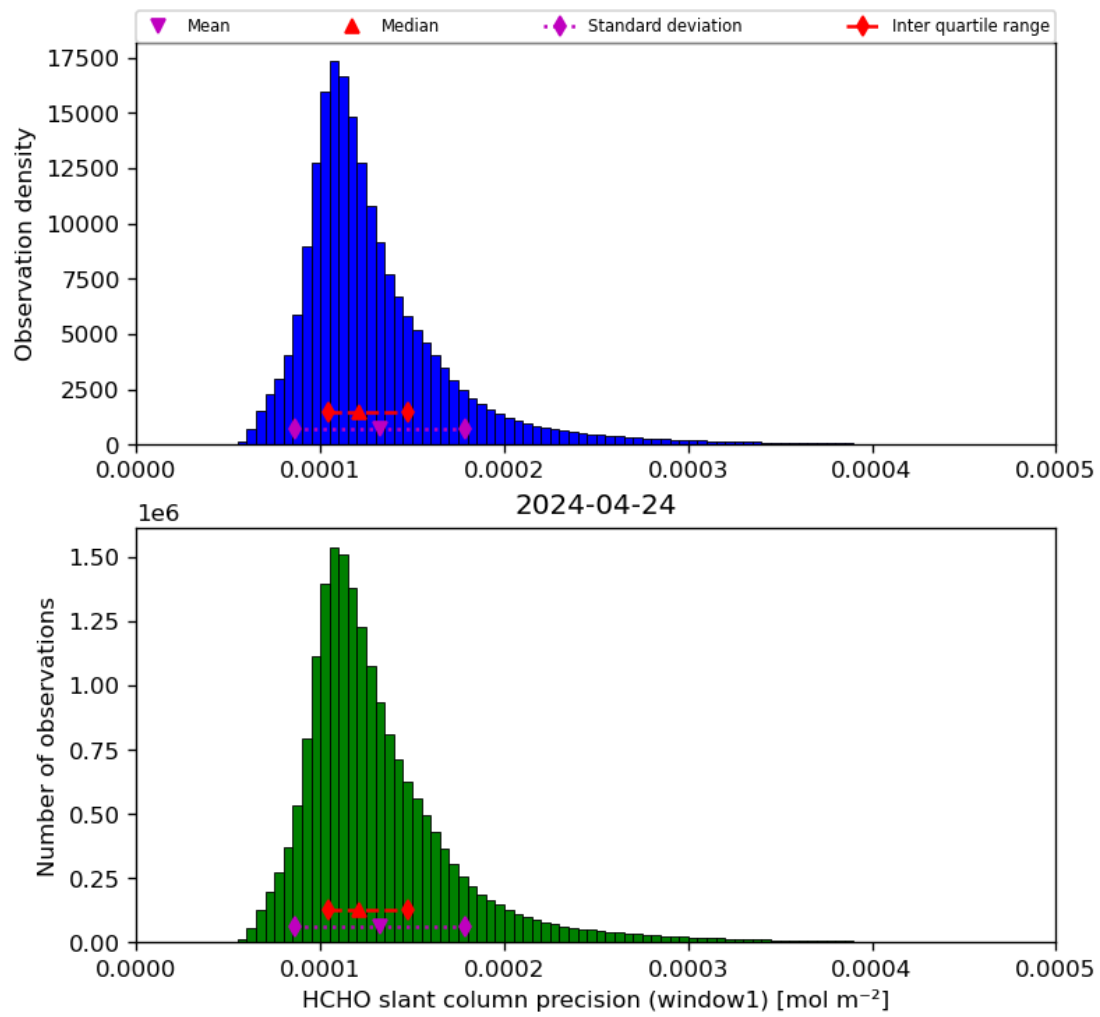
Figure 39: Histogram of “HCHO slant column precision (window1)” for 2024-04-23 to 2024-04-25
