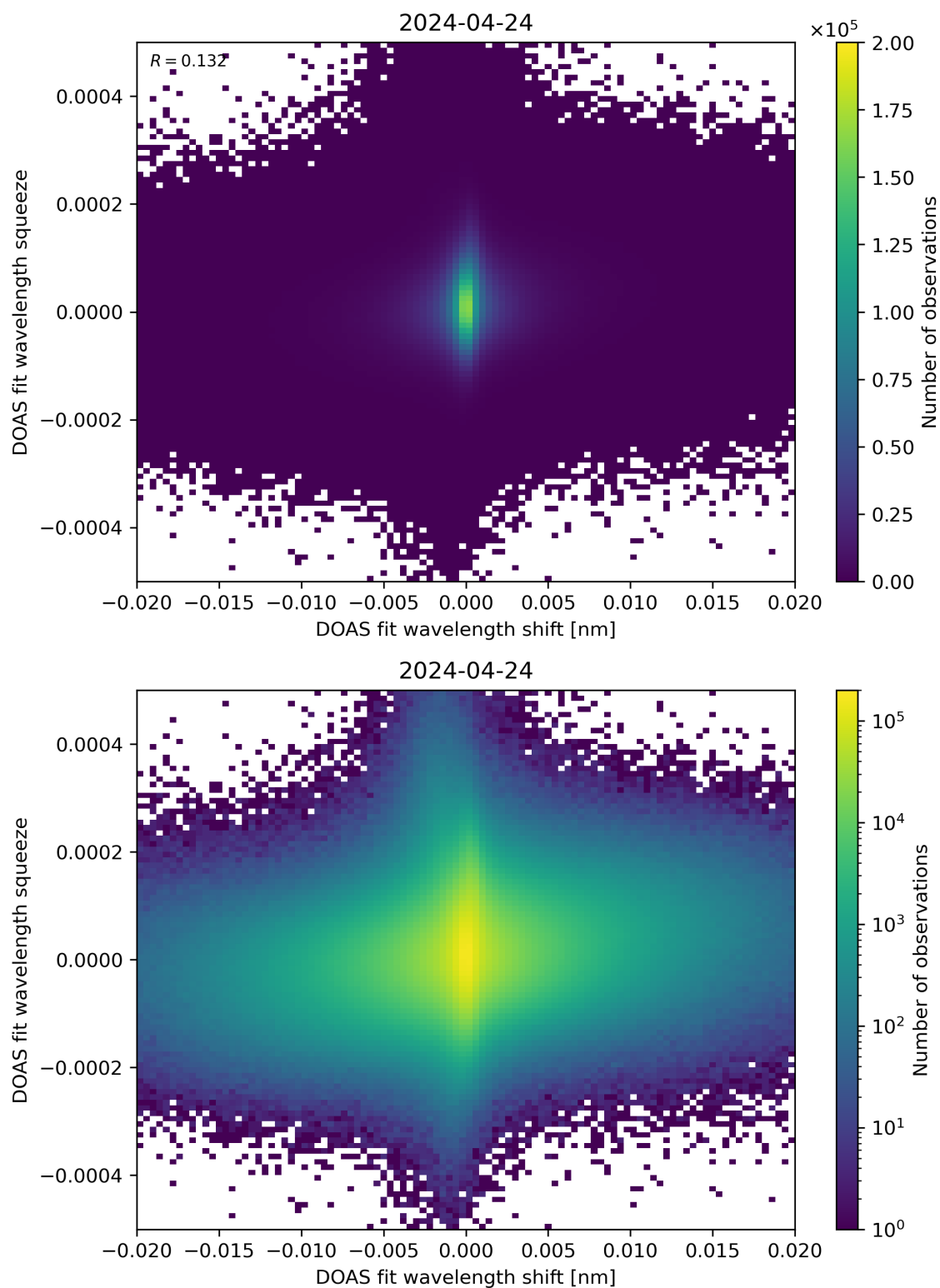
Figure 65: Scatter density plot of “DOAS fit wavelength shift” against “DOAS fit wavelength squeeze” for 2024-04-23 to 2024-04-25.
