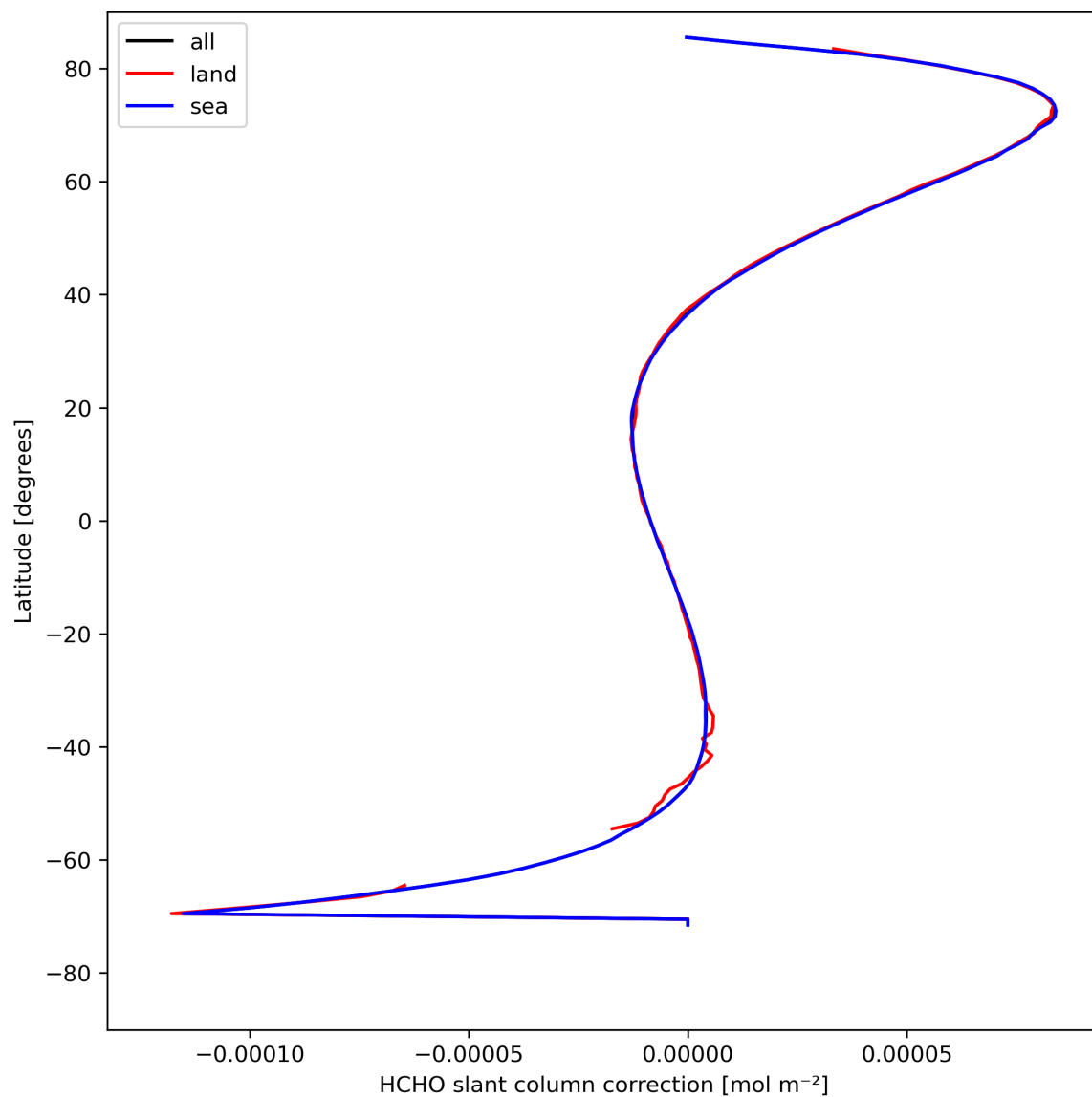
Figure 33: Zonal average of “HCHO slant column correction” for 2024-04-23 to 2024-04-25.
