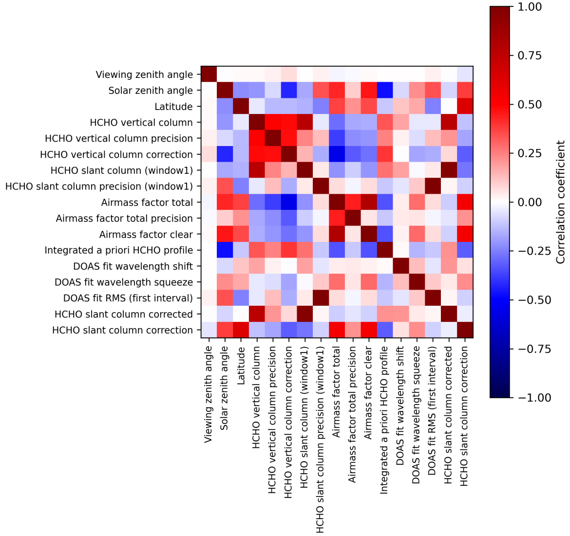
Figure 2: Map of correlation matrix for 2024-04-23 to 2024-04-25.
