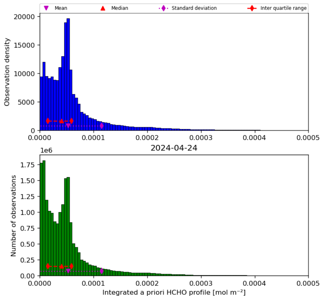
Figure 43: Histogram of “Integrated a priori HCHO profile” for 2024-04-23 to 2024-04-25
