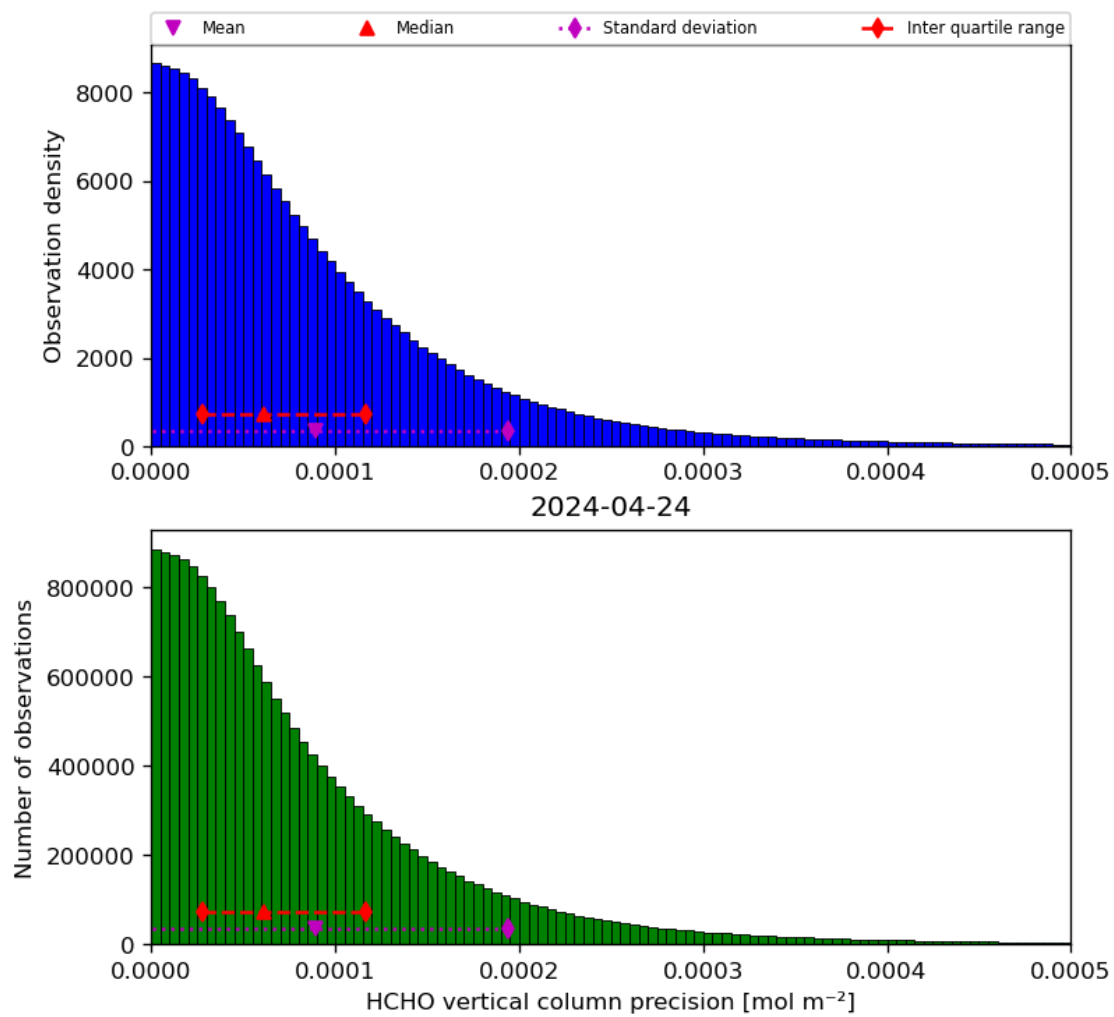
Figure 36: Histogram of “HCHO vertical column precision” for 2024-04-23 to 2024-04-25
