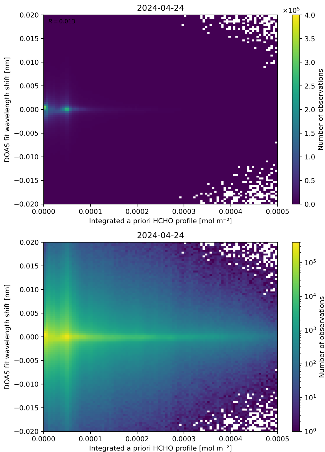
Figure 149: Scatter density plot of “Integrated a priori HCHO profile” against “DOAS fit wavelength shift” for 2024-04-23 to 2024-04-25.
