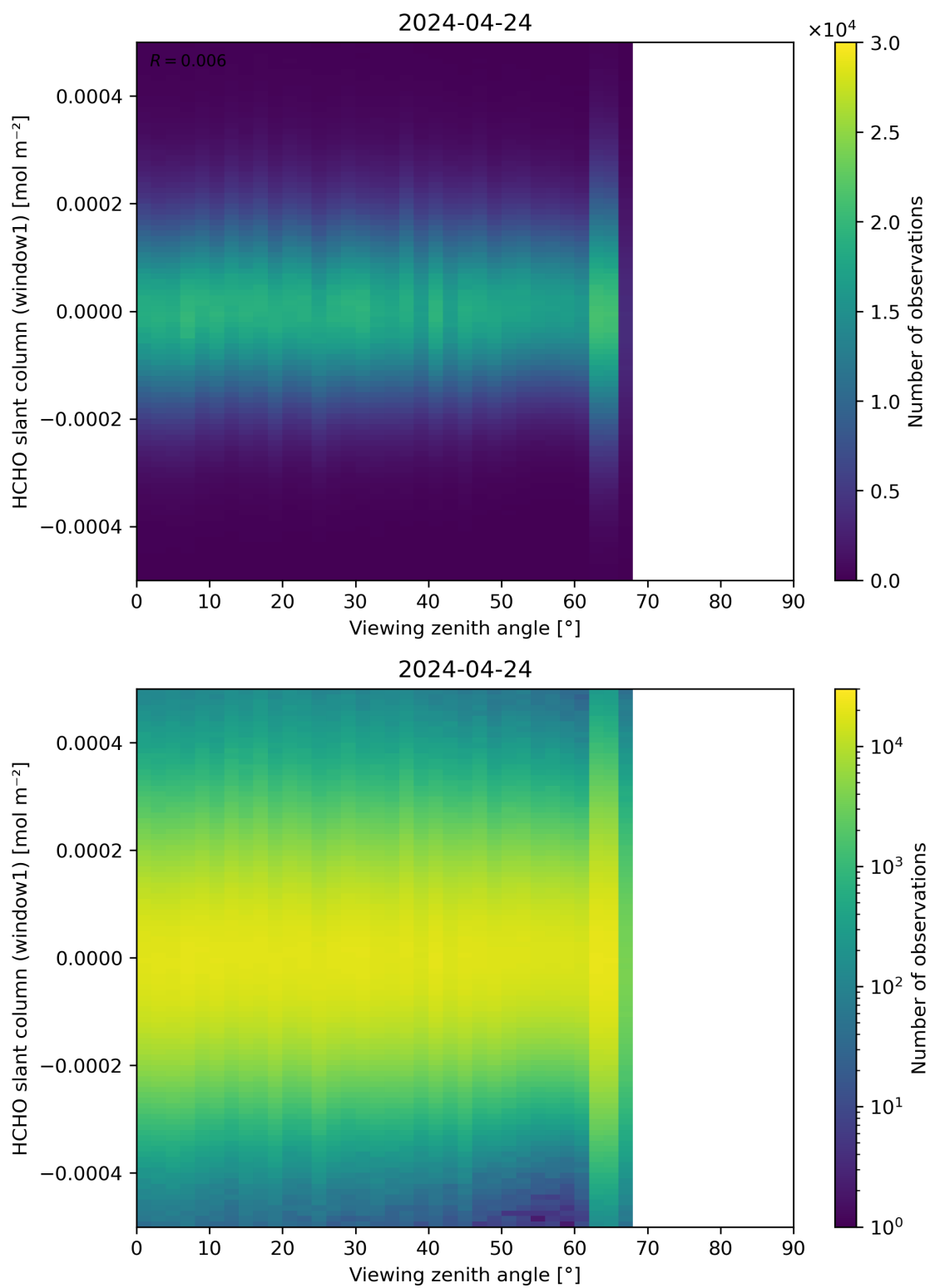
Figure 188: Scatter density plot of “Viewing zenith angle” against “HCHO slant column (window1)” for 2024-04-23 to 2024-04-25.
