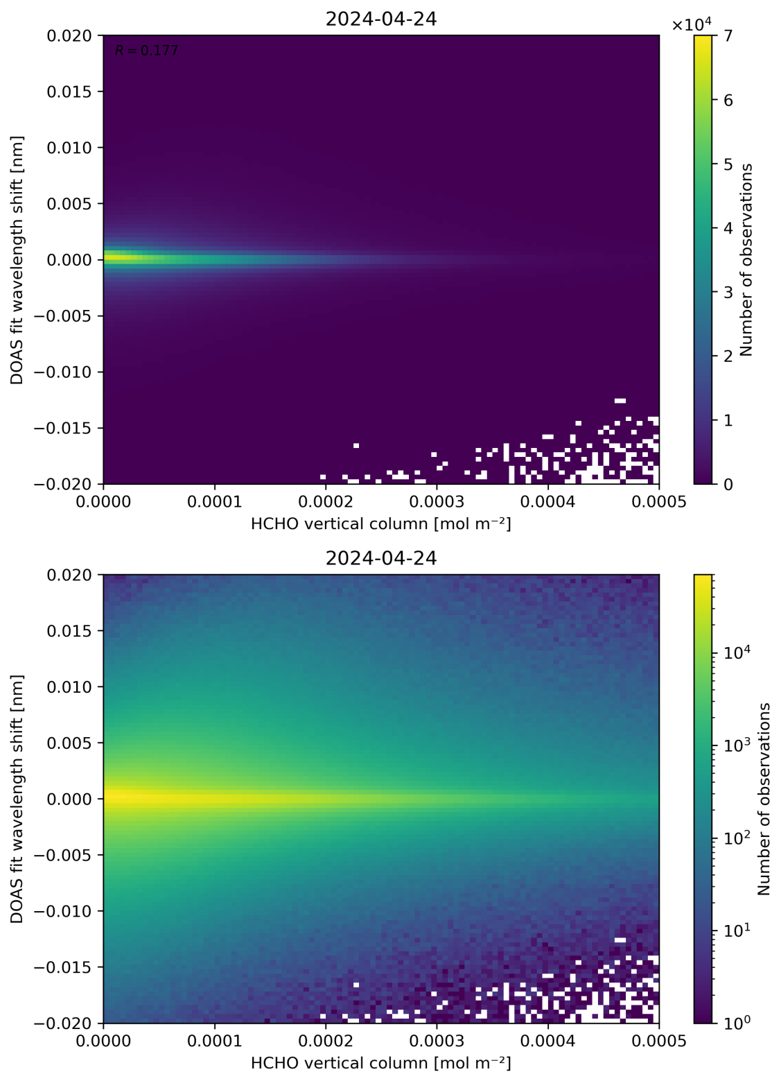
Figure 124: Scatter density plot of “HCHO vertical column” against “DOAS fit wavelength shift” for 2024-04-23 to 2024-04-25.
