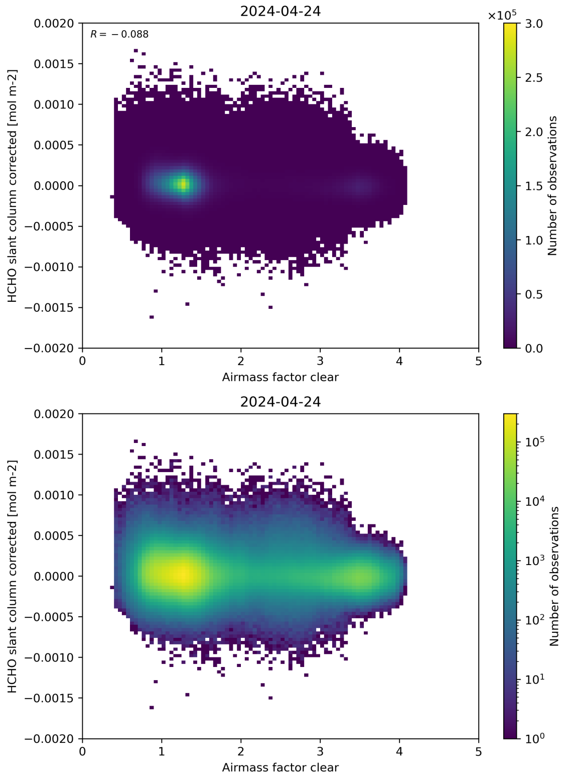
Figure 74: Scatter density plot of “Airmass factor clear” against “HCHO slant column corrected” for 2024-04-23 to 2024-04-25.
