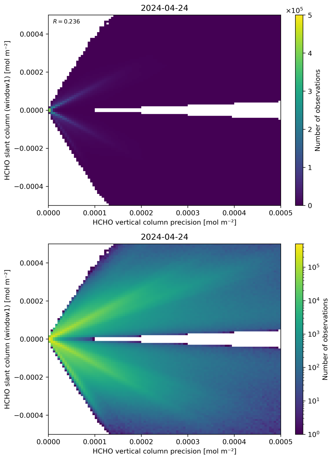
Figure 142: Scatter density plot of “HCHO vertical column precision” against “HCHO slant column (window1)” for 2024-04-23 to 2024-04-25.
