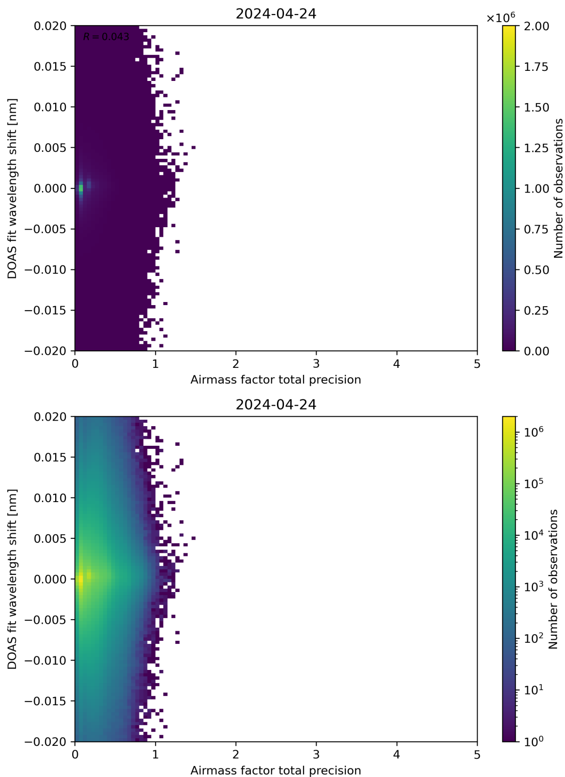
Figure 106: Scatter density plot of “Airmass factor total precision” against “DOAS fit wavelength shift” for 2024-04-23 to 2024-04-25.
