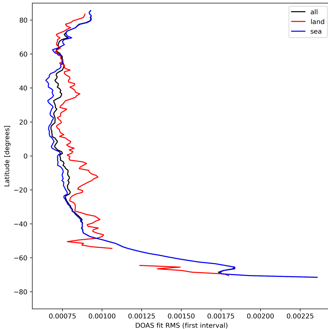
Figure 32: Zonal average of "DOAS fit RMS (first interval)" for 2024-04-23 to 2024-04-25.
