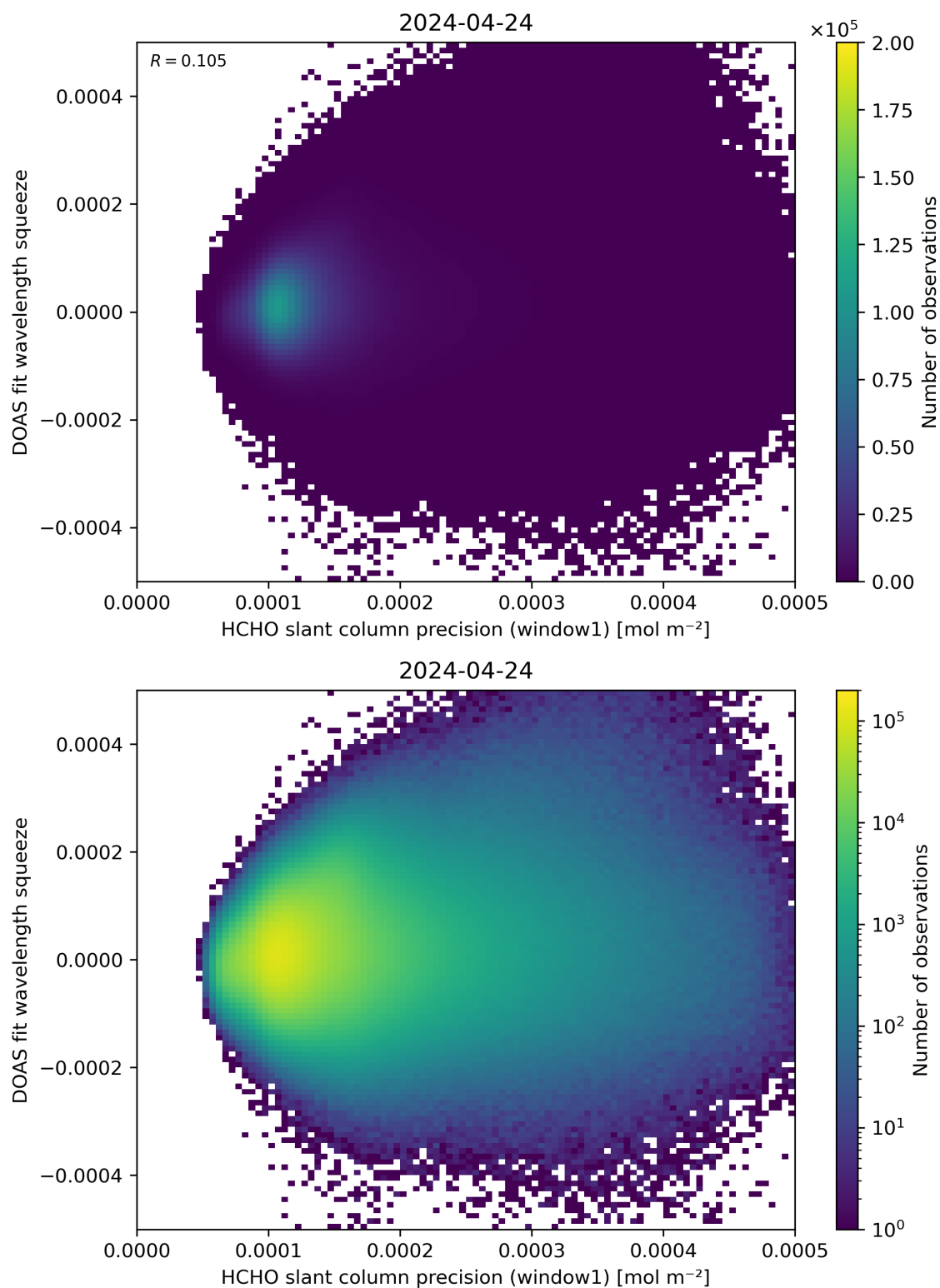
Figure 90: Scatter density plot of “HCHO slant column precision (window1)” against “DOAS fit wavelength squeeze” for 2024-04-23 to 2024-04-25.
