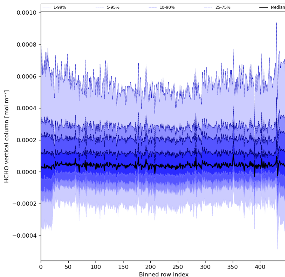
Figure 49: Along track statistics of “HCHO vertical column” for 2024-04-23 to 2024-04-25
