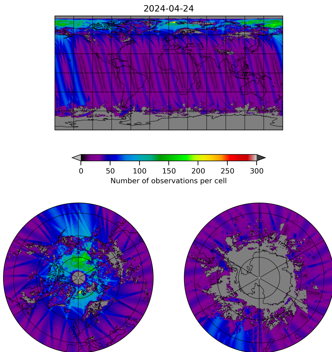
Figure 19: Map of the number of observations for 2024-04-23 to 2024-04-25
