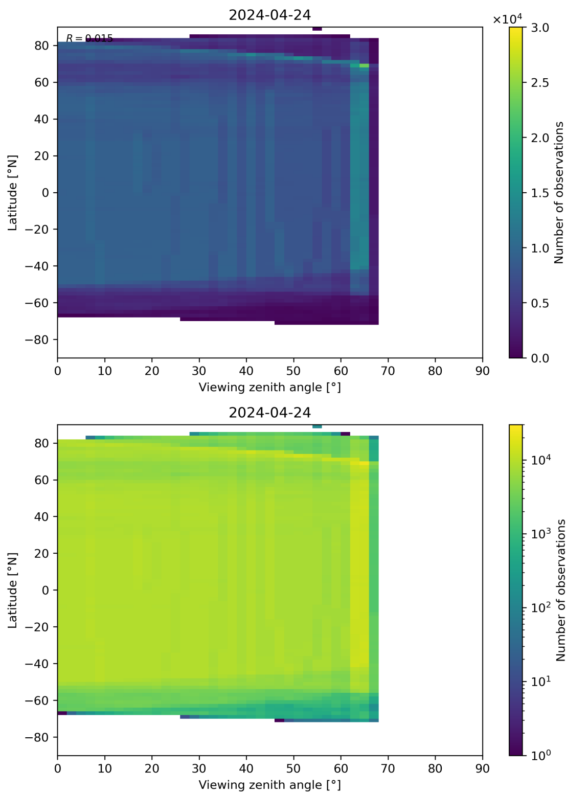
Figure 196: Scatter density plot of “Viewing zenith angle” against “Latitude” for 2024-04-23 to 2024-04-25.
