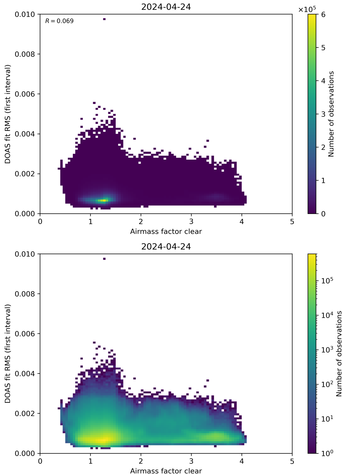
Figure 71: Scatter density plot of “Airmass factor clear” against “DOAS fit RMS (first interval)” for 2024-04-23 to 2024-04-25.
