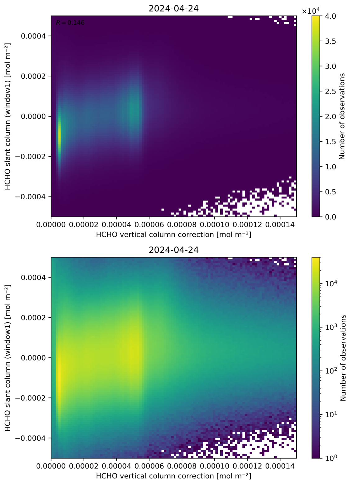
Figure 118: Scatter density plot of “HCHO vertical column correction” against “HCHO slant column (window1)” for 2024-04-23 to 2024-04-25.
