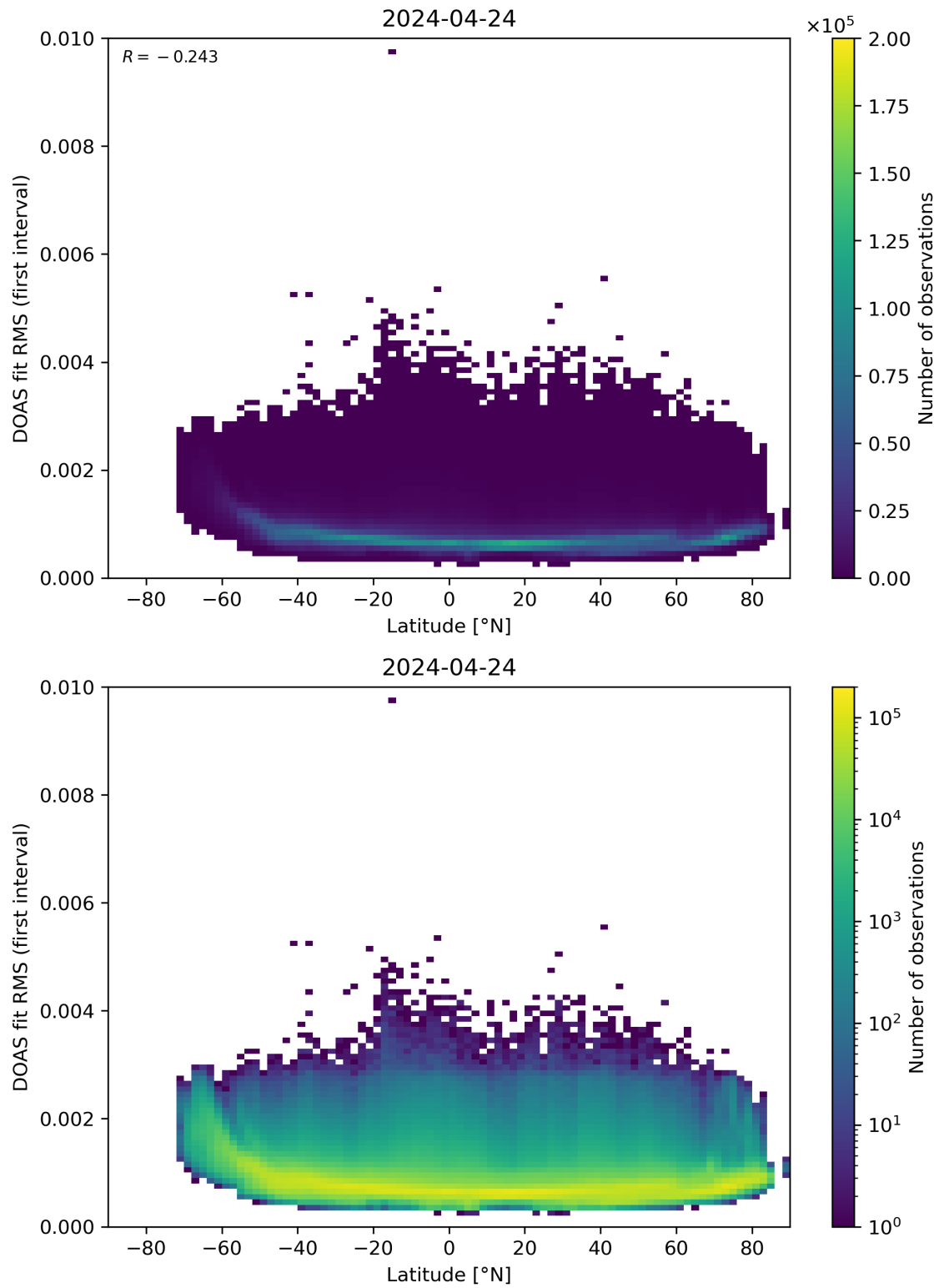
Figure 153: Scatter density plot of “Latitude” against “DOAS fit RMS (first interval)” for 2024-04-23 to 2024-04-25.
