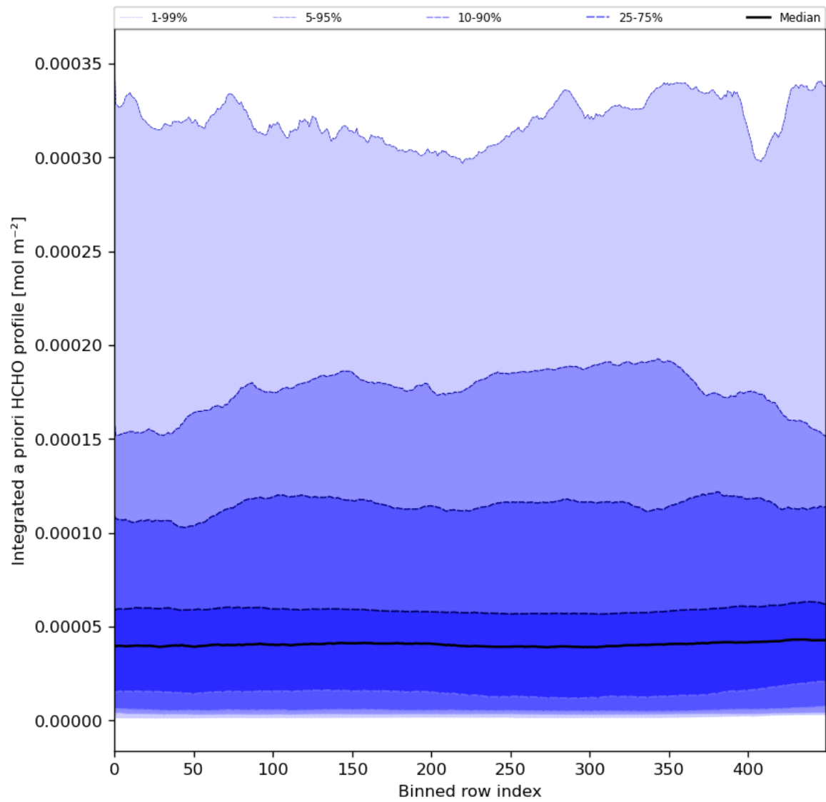
Figure 57: Along track statistics of “Integrated a priori HCHO profile” for 2024-04-23 to 2024-04-25
