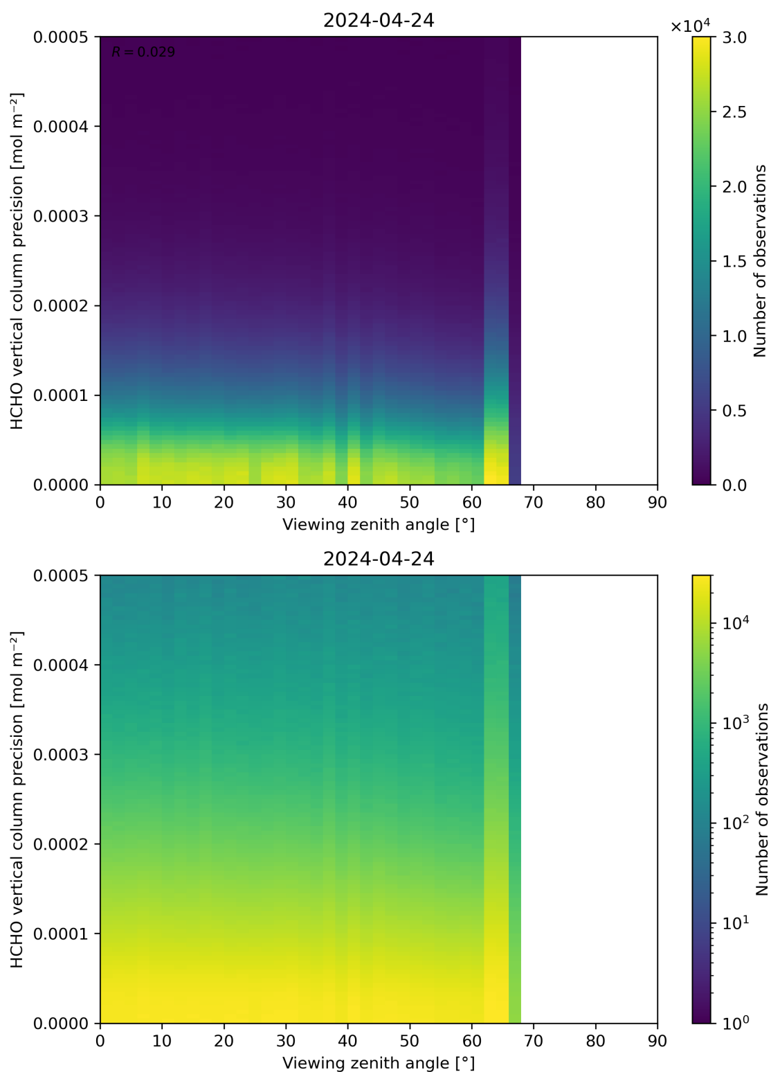
Figure 194: Scatter density plot of “Viewing zenith angle” against “HCHO vertical column precision” for 2024-04-23 to 2024-04-25.
