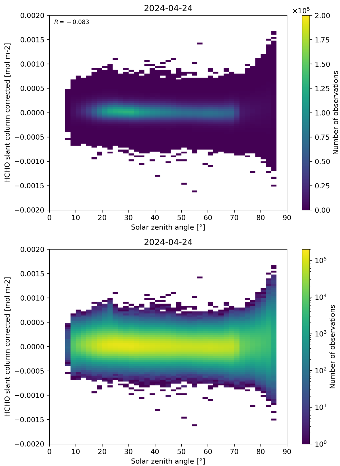
Figure 171: Scatter density plot of “Solar zenith angle” against “HCHO slant column corrected” for 2024-04-23 to 2024-04-25.
