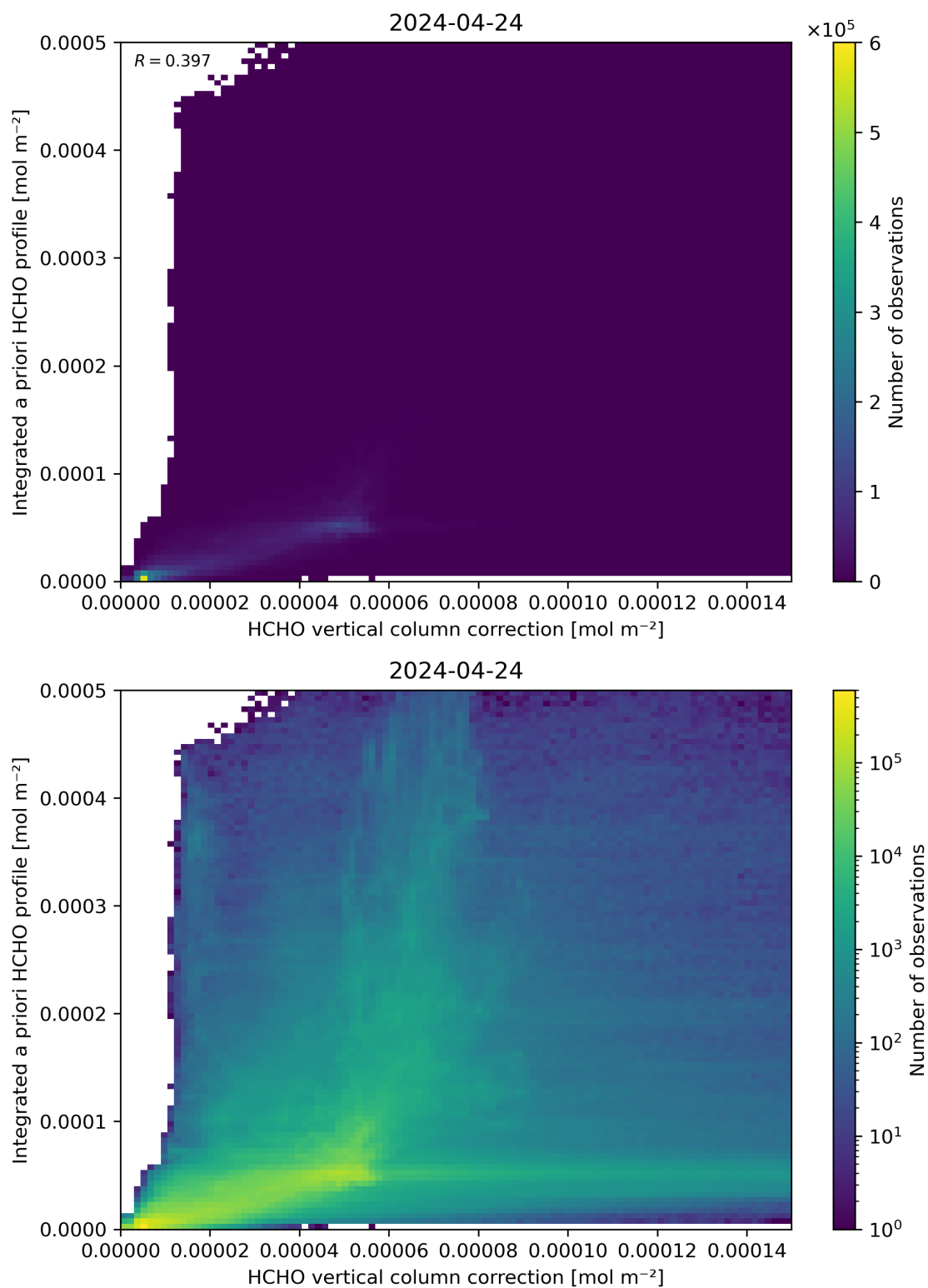
Figure 122: Scatter density plot of “HCHO vertical column correction” against “Integrated a priori HCHO profile” for 2024-04-23 to 2024-04-25.
