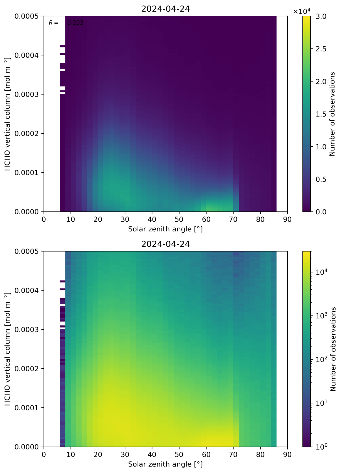
Figure 177: Scatter density plot of “Solar zenith angle” against “HCHO vertical column” for 2024-04-23 to 2024-04-25.
