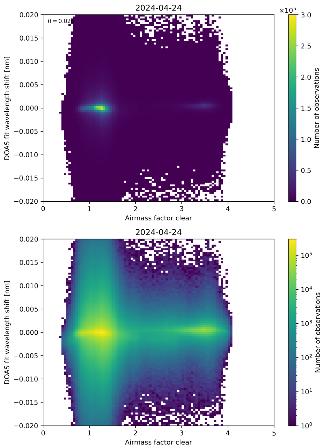
Figure 72: Scatter density plot of “Airmass factor clear” against “DOAS fit wavelength shift” for 2024-04-23 to 2024-04-25.
