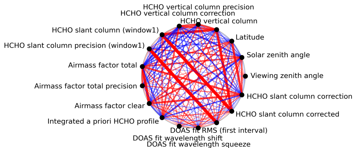
Figure 1: Map of correlation graph for 2024-04-23 to 2024-04-25.
