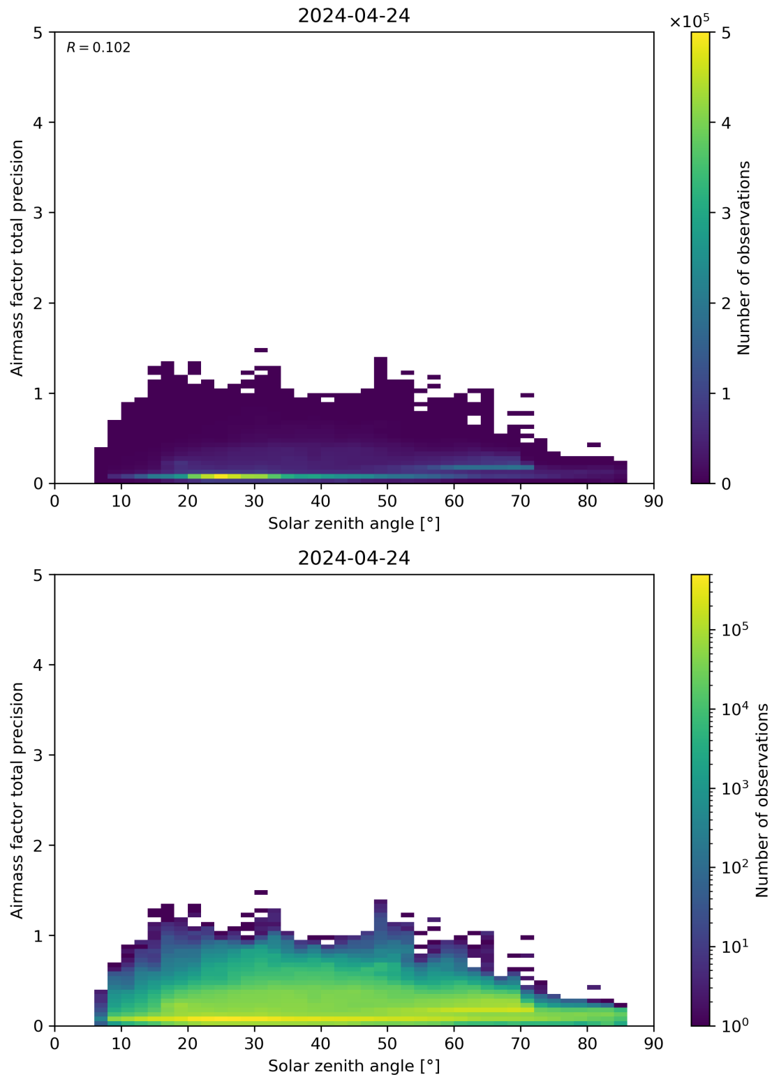
Figure 176: Scatter density plot of “Solar zenith angle” against “Airmass factor total precision” for 2024-04-23 to 2024-04-25.
