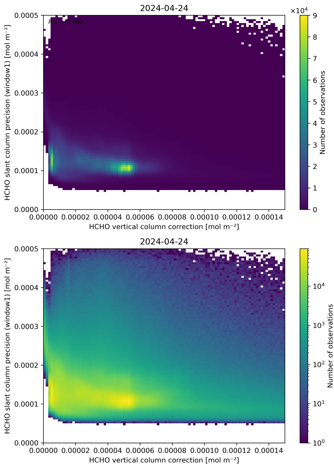
Figure 119: Scatter density plot of “HCHO vertical column correction” against “HCHO slant column precision (window1)” for 2024-04-23 to 2024-04-25.
