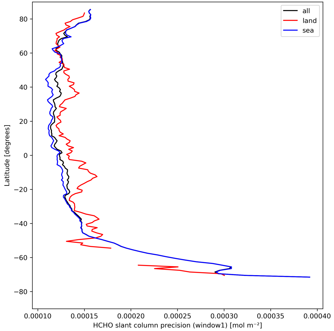
Figure 25: Zonal average of “HCHO slant column precision (window1)” for 2024-04-23 to 2024-04-25.
