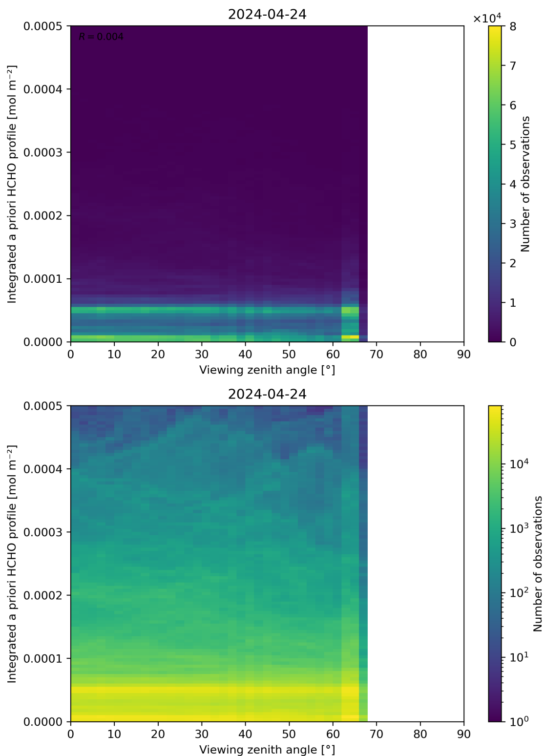
Figure 195: Scatter density plot of “Viewing zenith angle” against “Integrated a priori HCHO profile” for 2024-04-23 to 2024-04-25.
