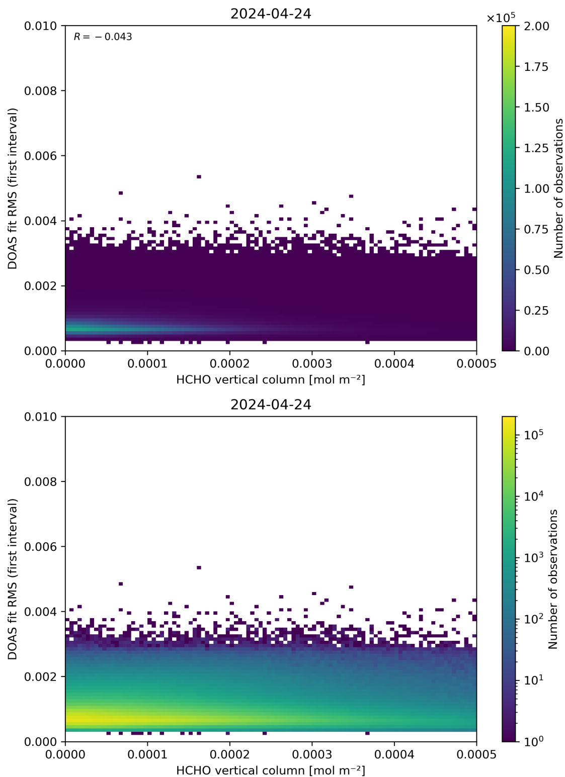
Figure 123: Scatter density plot of “HCHO vertical column” against “DOAS fit RMS (first interval)” for 2024-04-23 to 2024-04-25.
