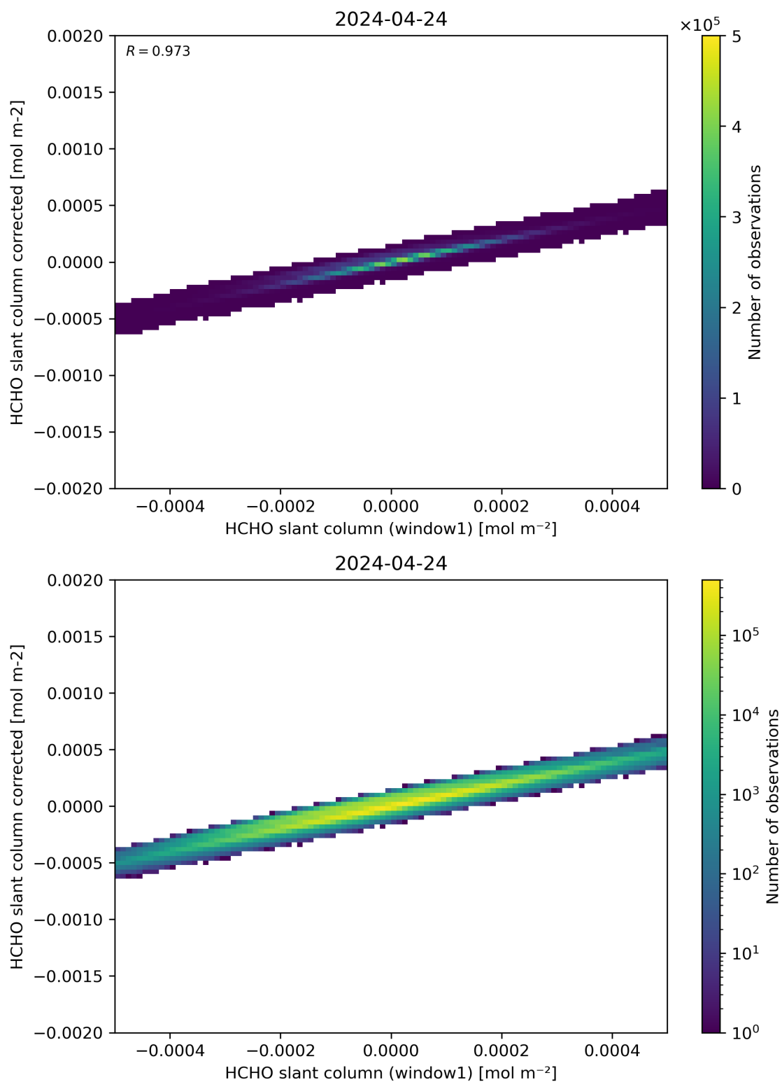
Figure 82: Scatter density plot of “HCHO slant column (window1)” against “HCHO slant column corrected” for 2024-04-23 to 2024-04-25.
