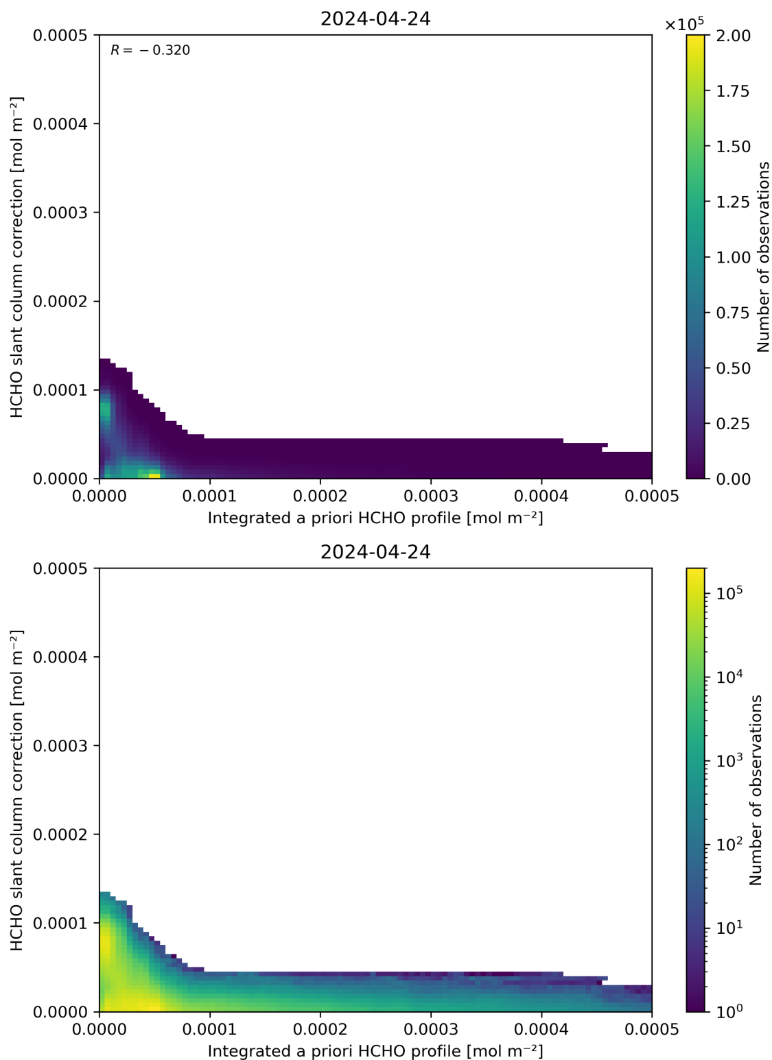
Figure 152: Scatter density plot of “Integrated a priori HCHO profile” against “HCHO slant column correction” for 2024-04-23 to 2024-04-25.
