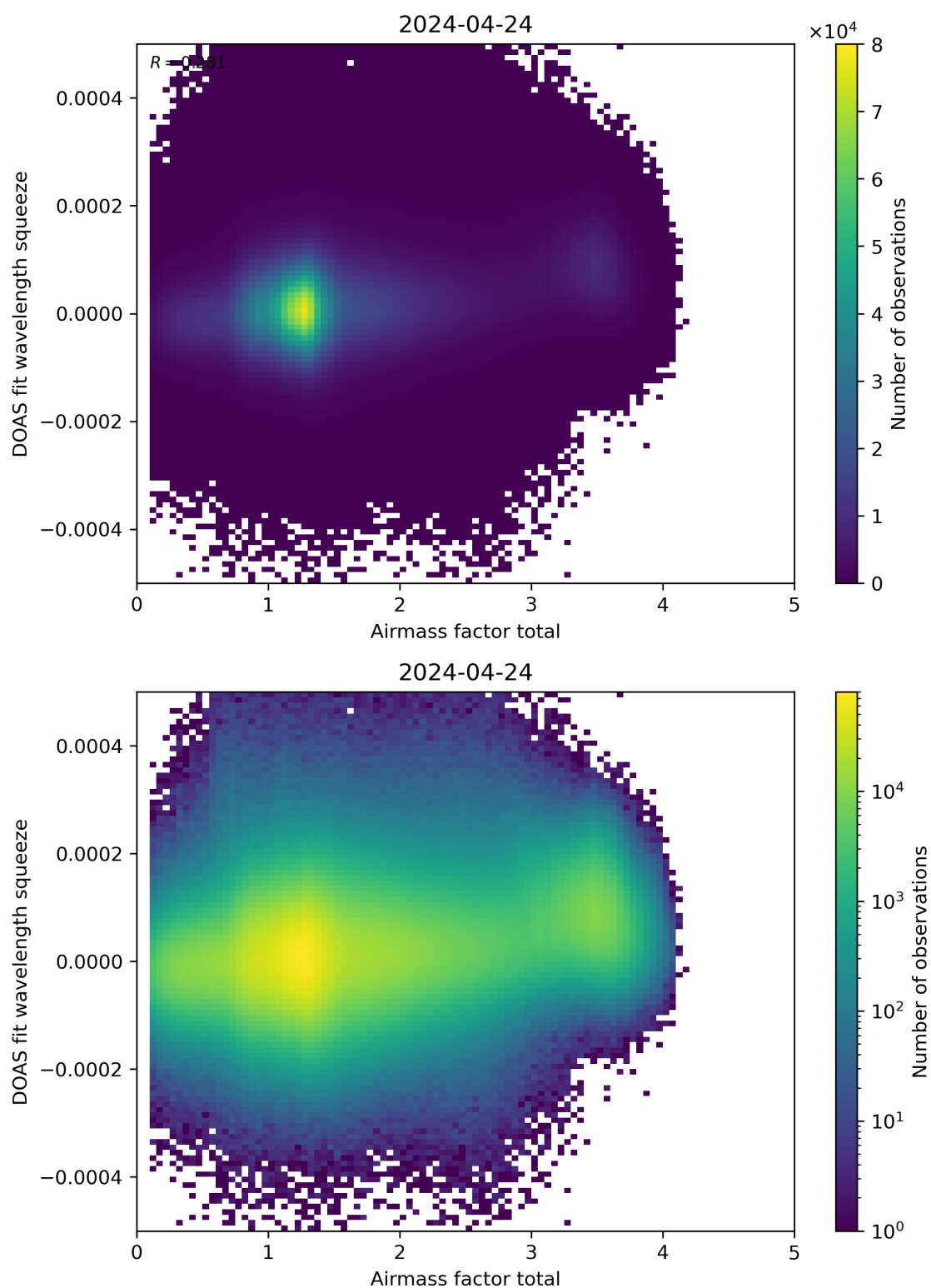
Figure 99: Scatter density plot of “Airmass factor total” against “DOAS fit wavelength squeeze” for 2024-04-23 to 2024-04-25.
