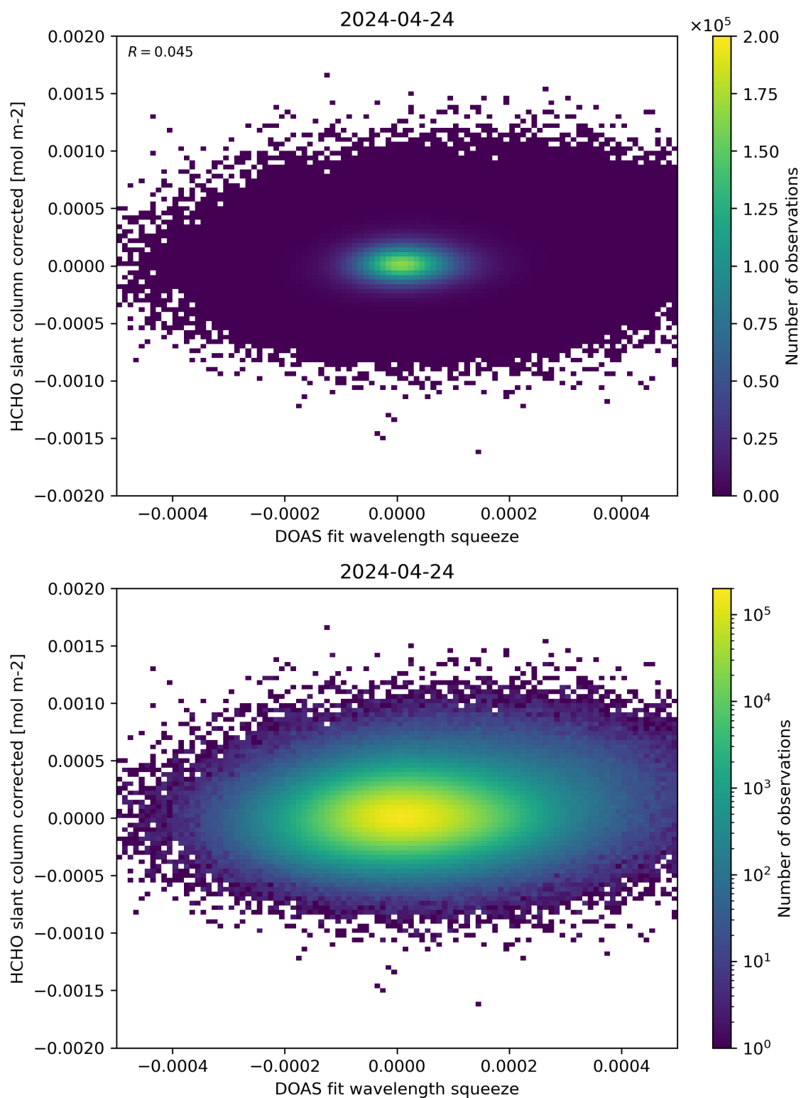
Figure 69: Scatter density plot of “DOAS fit wavelength squeeze” against “HCHO slant column corrected” for 2024-04-23 to 2024-04-25.
