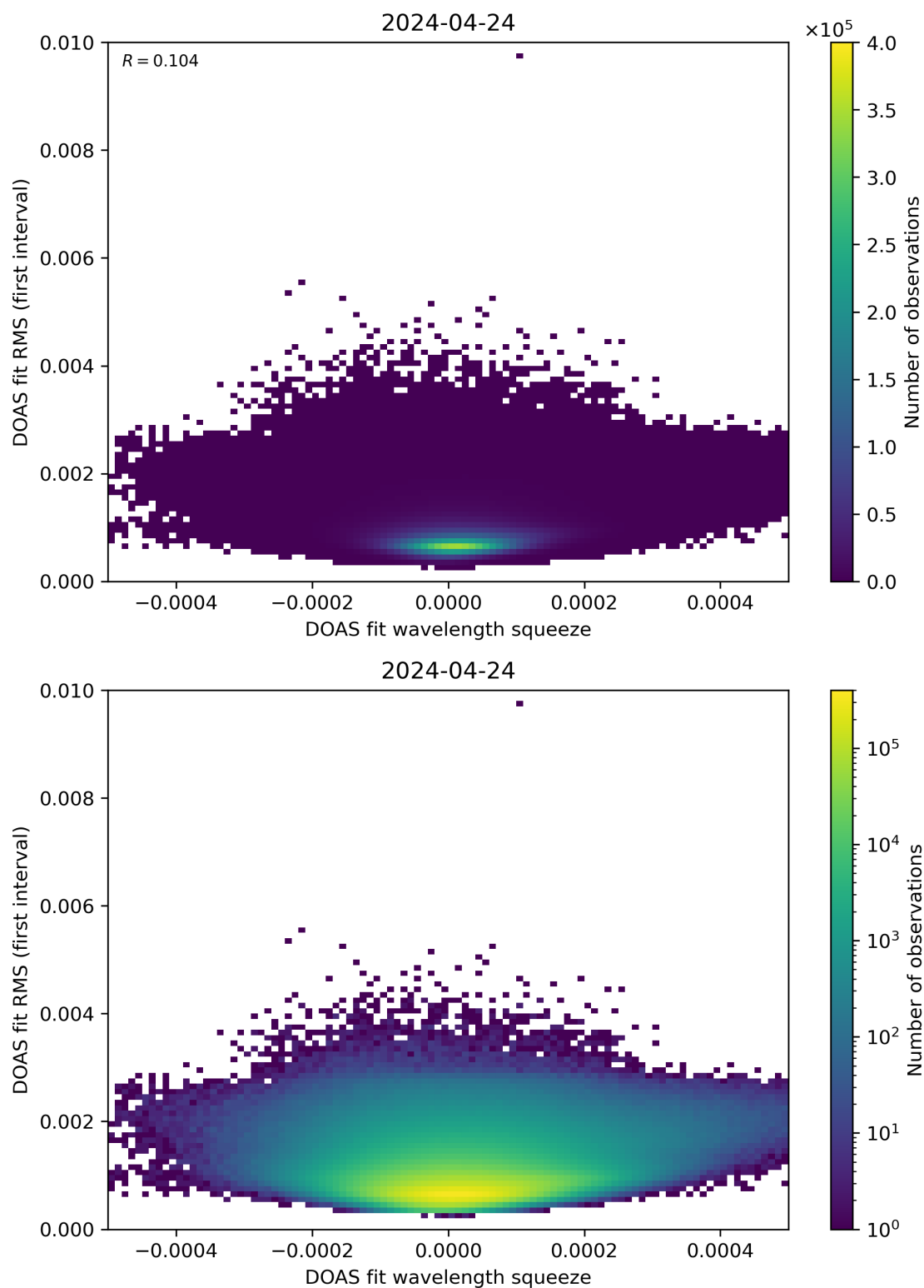
Figure 68: Scatter density plot of “DOAS fit wavelength squeeze” against “DOAS fit RMS (first interval)” for 2024-04-23 to 2024-04-25.
