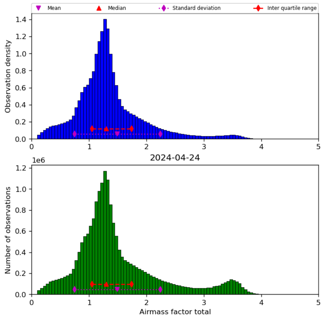
Figure 40: Histogram of “Airmass factor total” for 2024-04-23 to 2024-04-25
