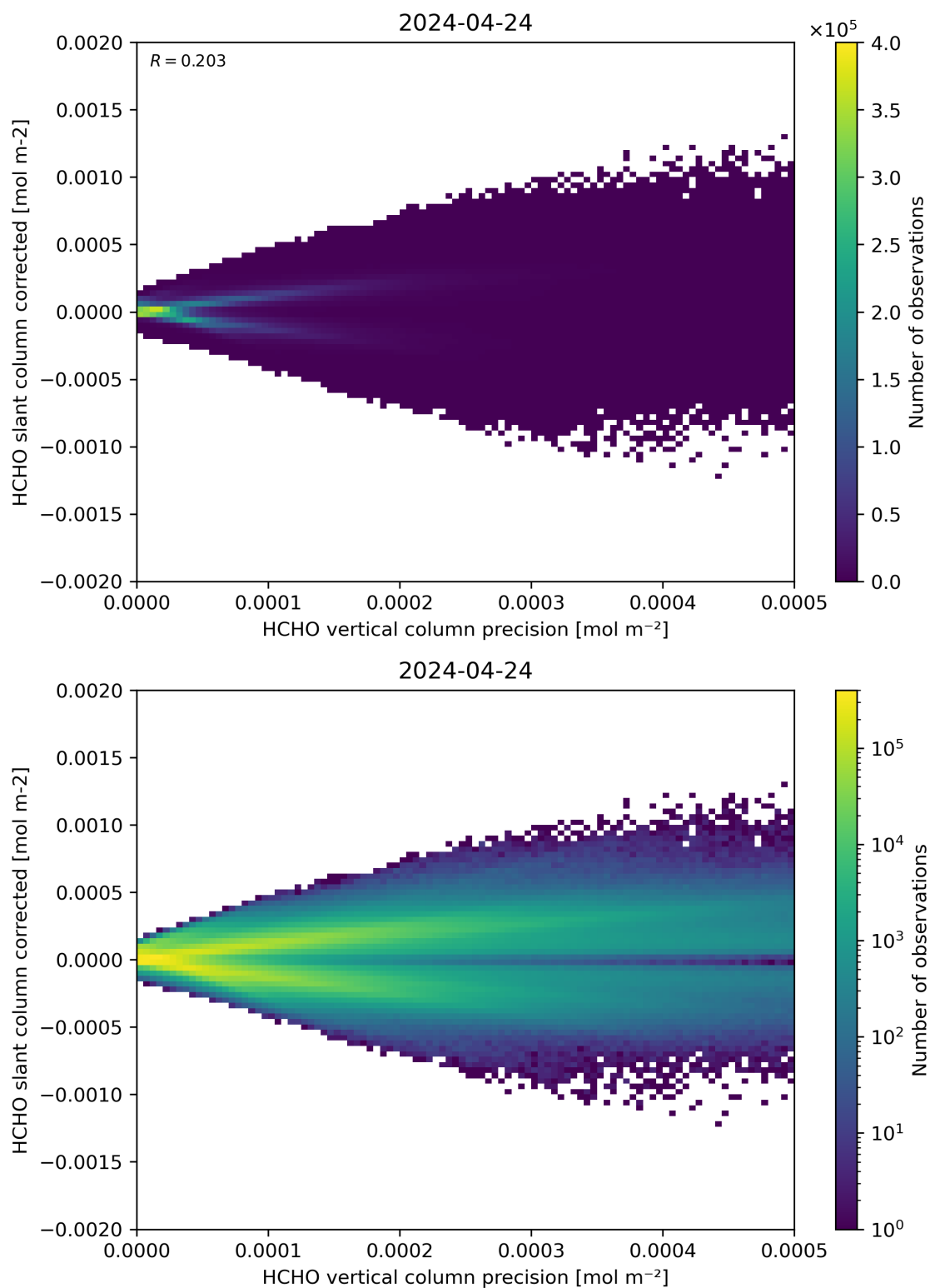
Figure 140: Scatter density plot of “HCHO vertical column precision” against “HCHO slant column corrected” for 2024-04-23 to 2024-04-25.
