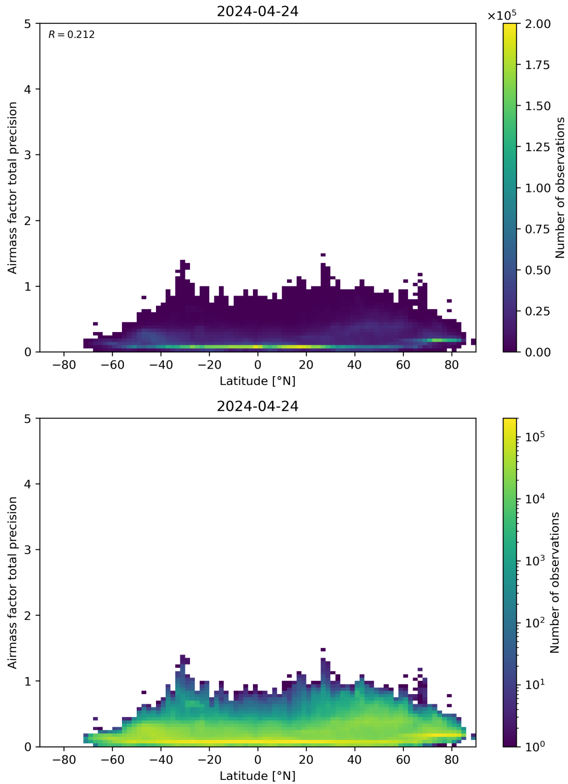
Figure 162: Scatter density plot of “Latitude” against “Airmass factor total precision” for 2024-04-23 to 2024-04-25.
