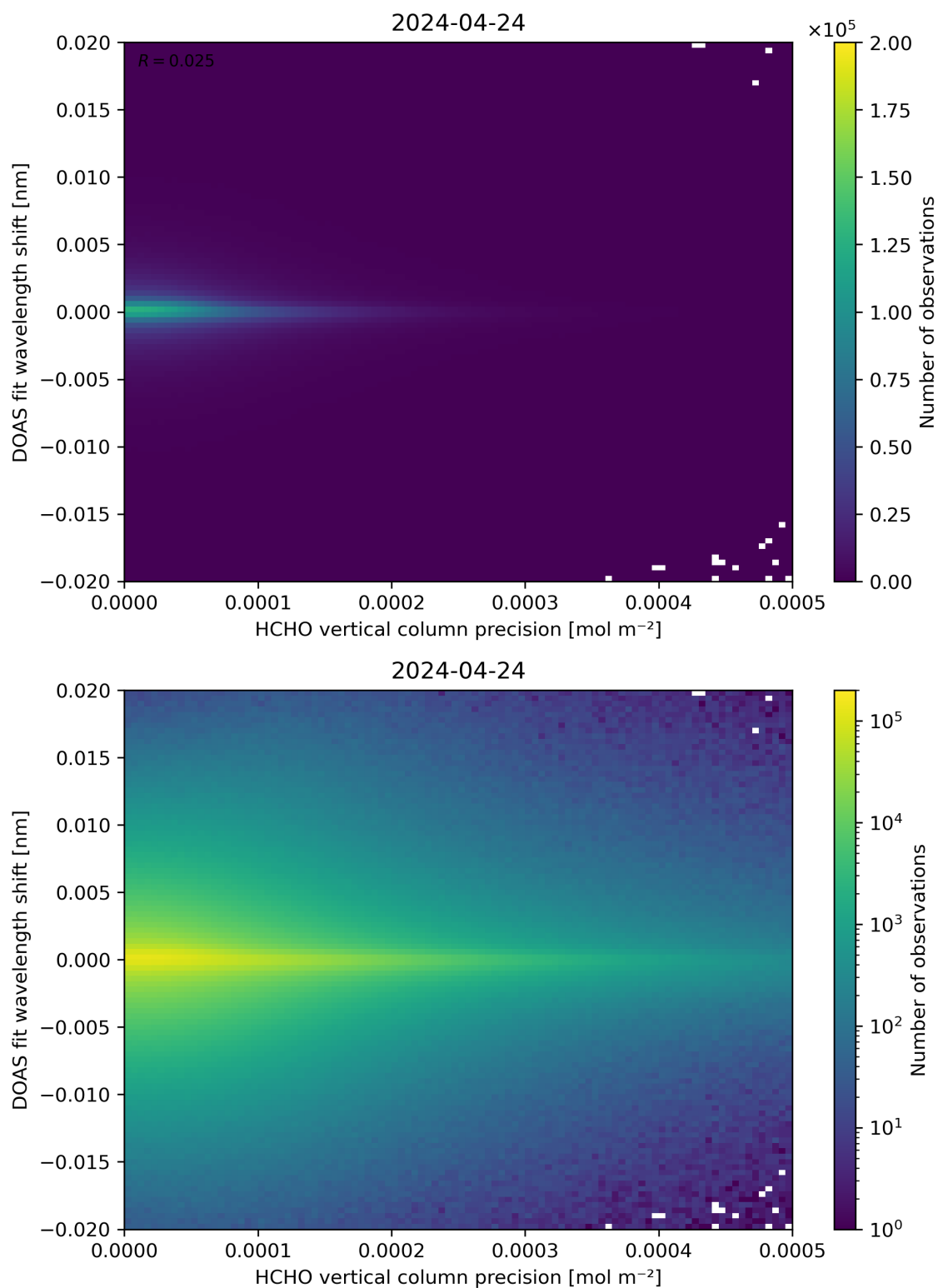
Figure 137: Scatter density plot of “HCHO vertical column precision” against “DOAS fit wavelength shift” for 2024-04-23 to 2024-04-25.
