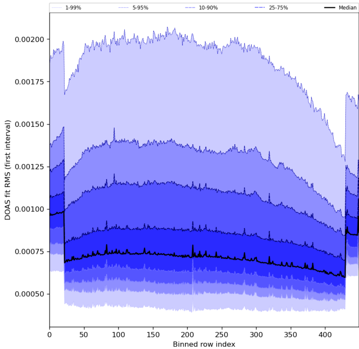
Figure 60: Along track statistics of “DOAS fit RMS (first interval)” for 2024-04-23 to 2024-04-25
