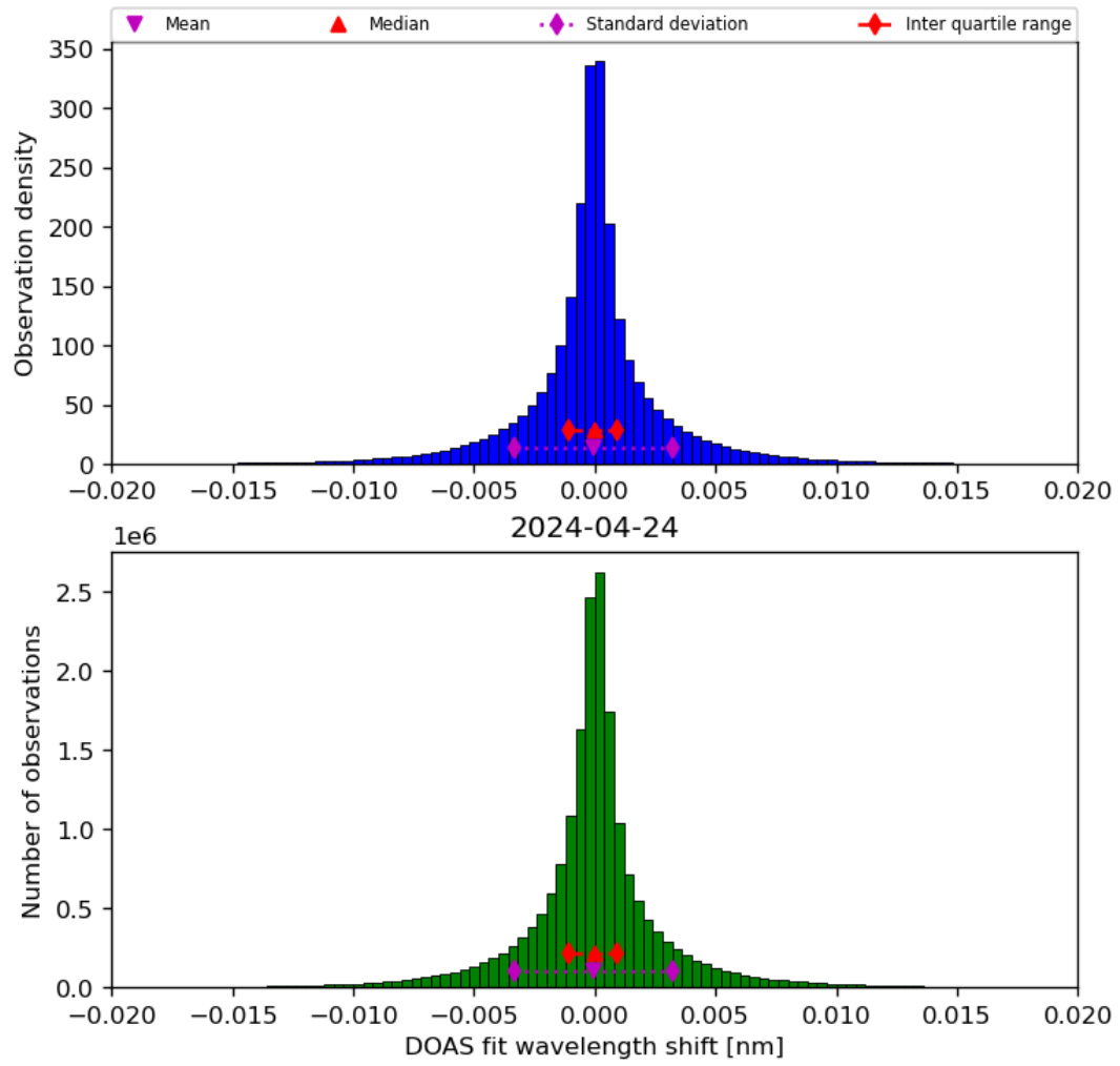
Figure 44: Histogram of “DOAS fit wavelength shift” for 2024-04-23 to 2024-04-25
