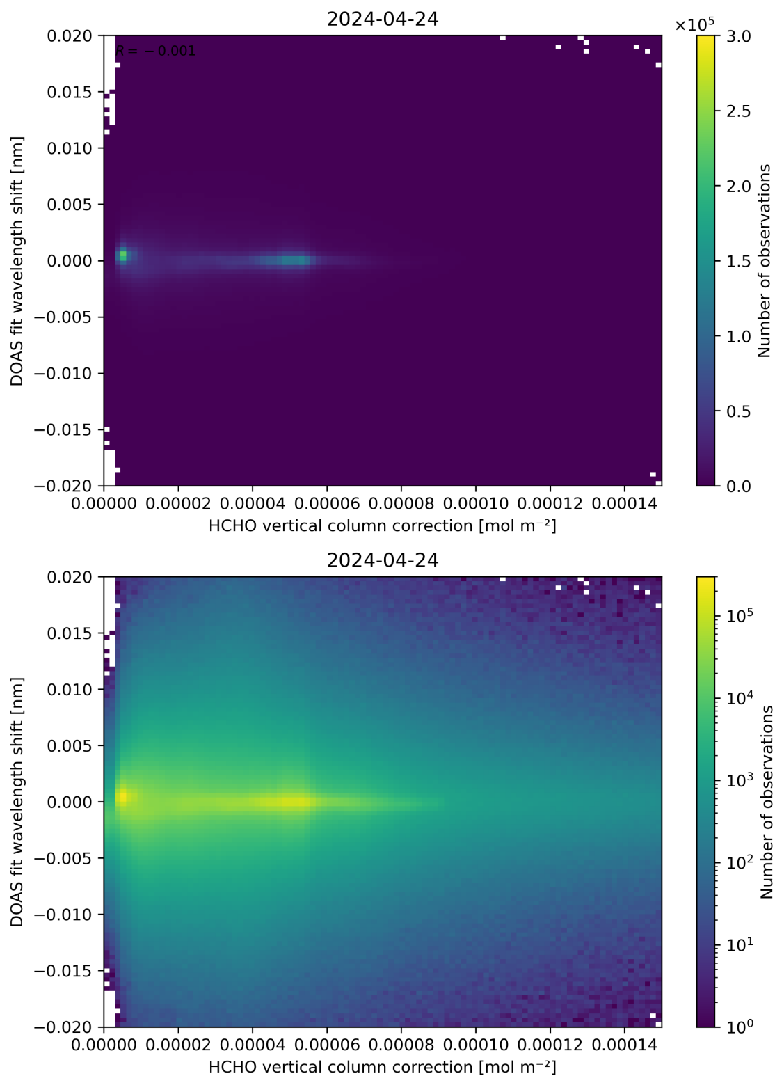
Figure 113: Scatter density plot of “HCHO vertical column correction” against “DOAS fit wavelength shift” for 2024-04-23 to 2024-04-25.
