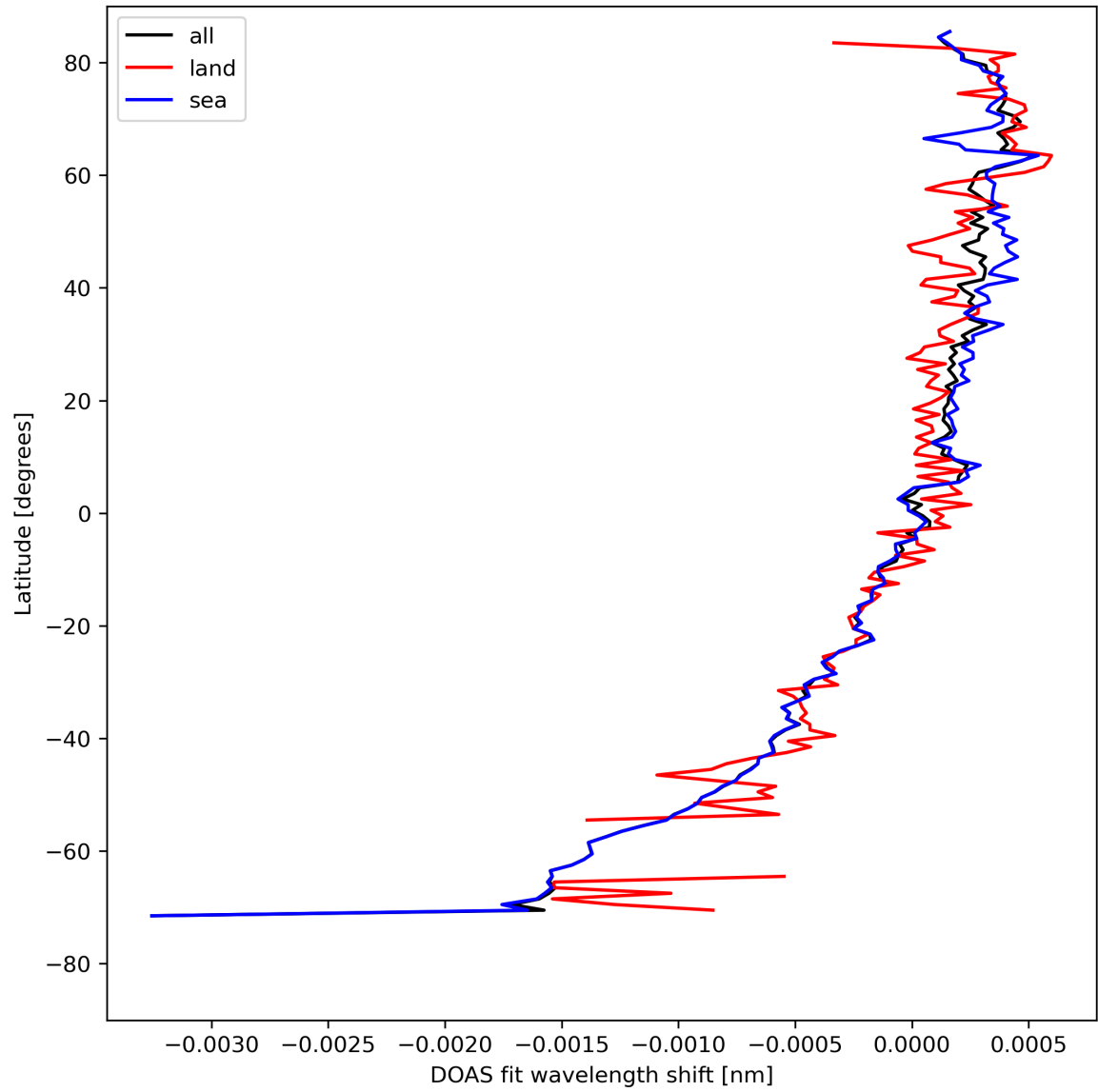
Figure 30: Zonal average of “DOAS fit wavelength shift” for 2024-04-23 to 2024-04-25.
