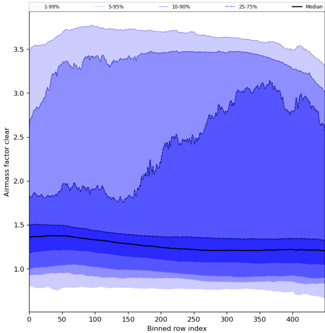
Figure 56: Along track statistics of “Airmass factor clear” for 2024-04-23 to 2024-04-25
