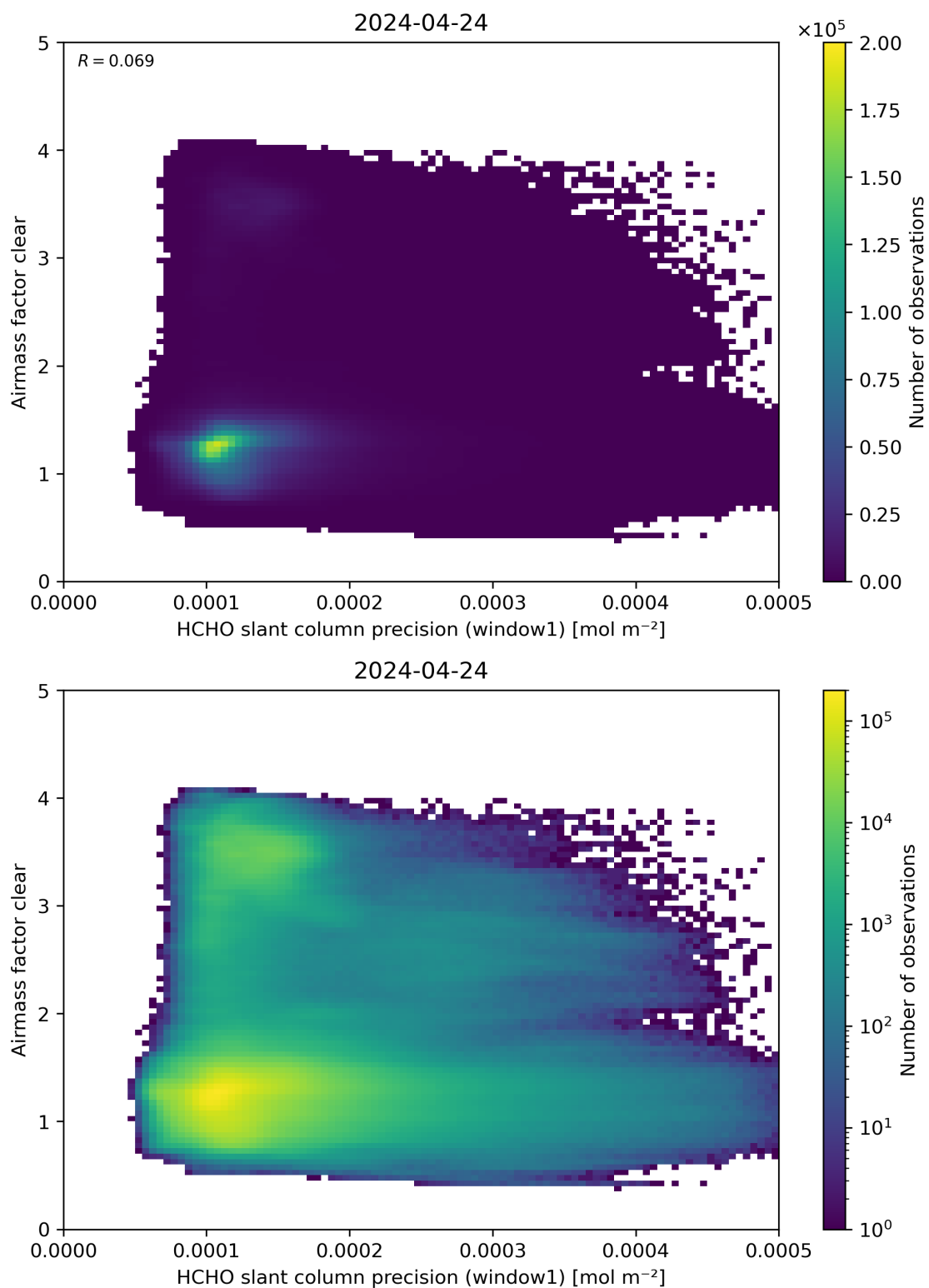
Figure 91: Scatter density plot of “HCHO slant column precision (window1)” against “Airmass factor clear” for 2024-04-23 to 2024-04-25.
