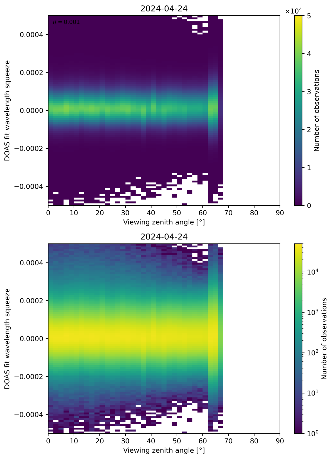
Figure 184: Scatter density plot of “Viewing zenith angle” against “DOAS fit wavelength squeeze” for 2024-04-23 to 2024-04-25.
