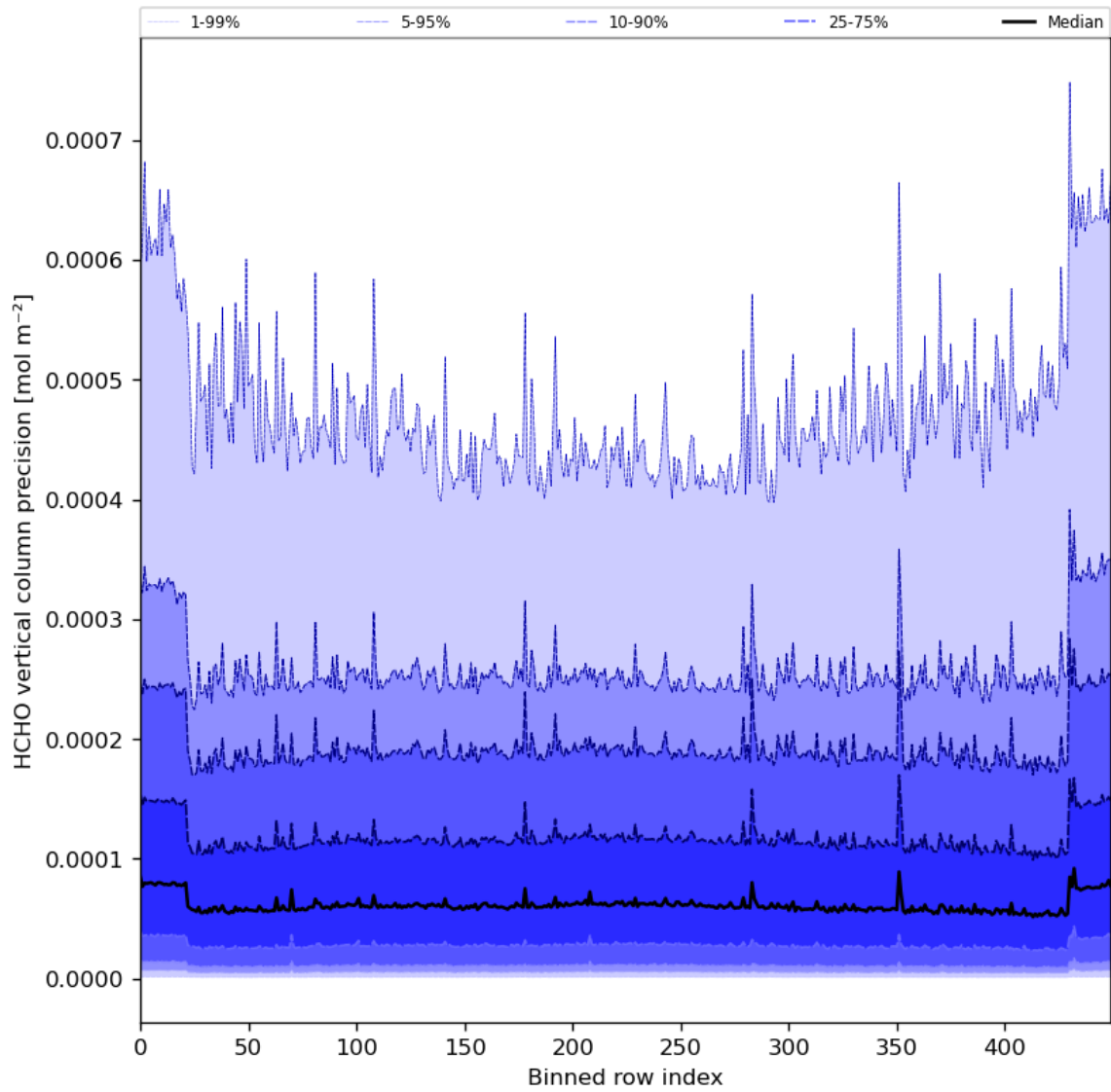
Figure 50: Along track statistics of “HCHO vertical column precision” for 2024-04-23 to 2024-04-25
