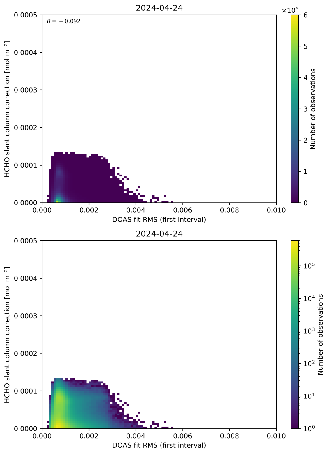
Figure 63: Scatter density plot of “DOAS fit RMS (first interval)” against “HCHO slant column correction” for 2024-04-23 to 2024-04-25.
