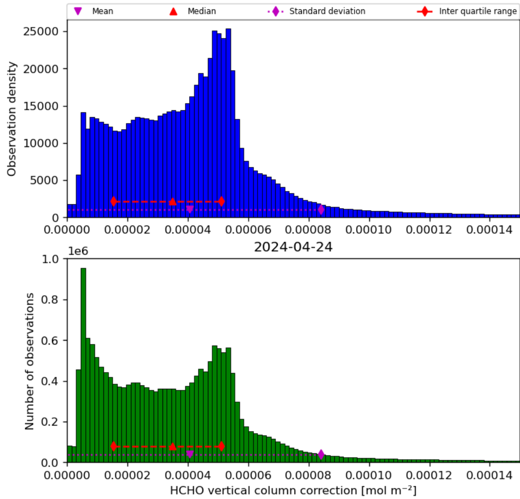
Figure 37: Histogram of “HCHO vertical column correction” for 2024-04-23 to 2024-04-25
