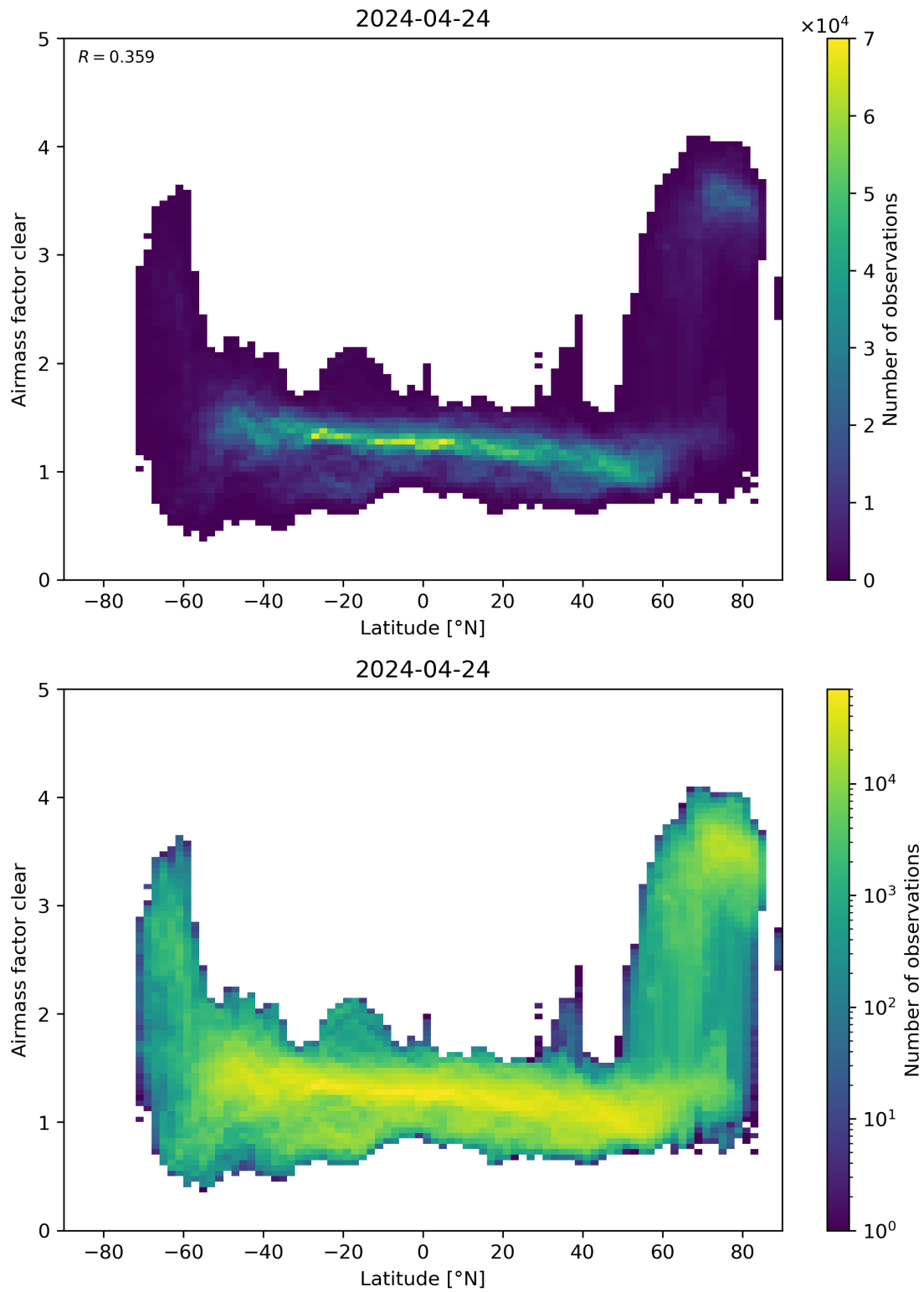
Figure 156: Scatter density plot of “Latitude” against “Airmass factor clear” for 2024-04-23 to 2024-04-25.
