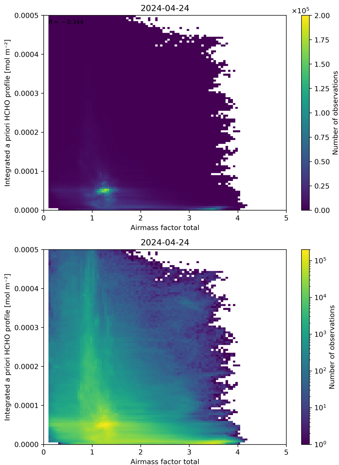
Figure 104: Scatter density plot of “Airmass factor total” against “Integrated a priori HCHO profile” for 2024-04-23 to 2024-04-25.
