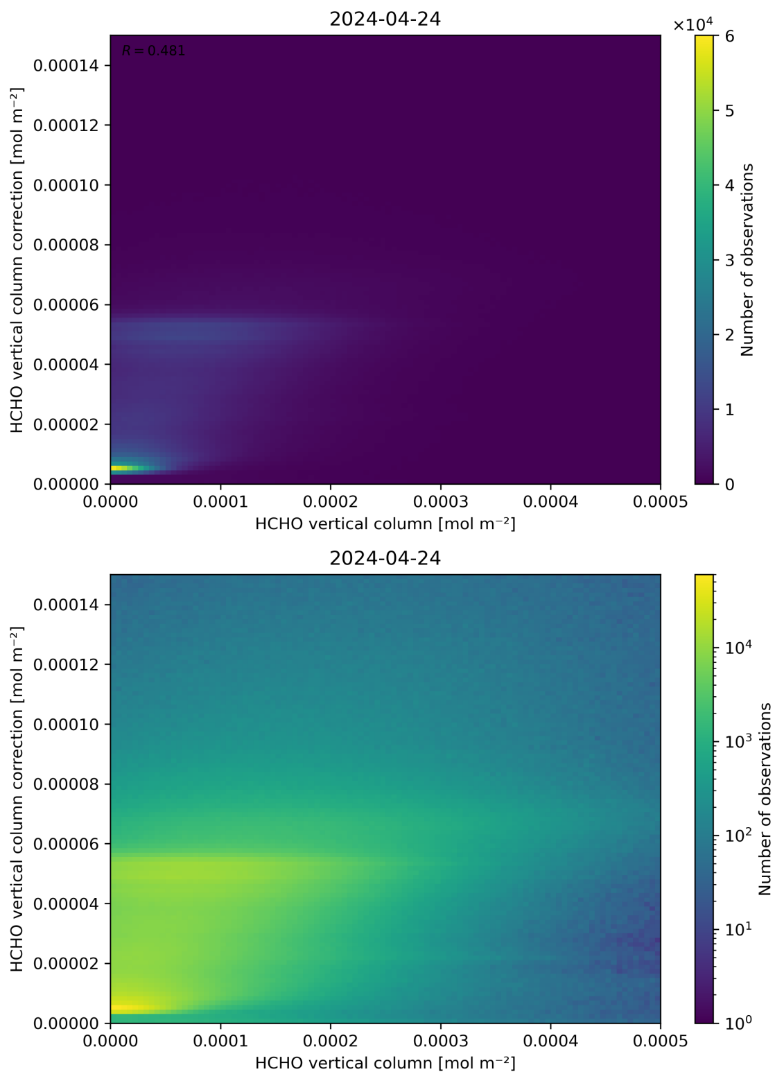
Figure 133: Scatter density plot of “HCHO vertical column” against “HCHO vertical column correction” for 2024-04-23 to 2024-04-25.
