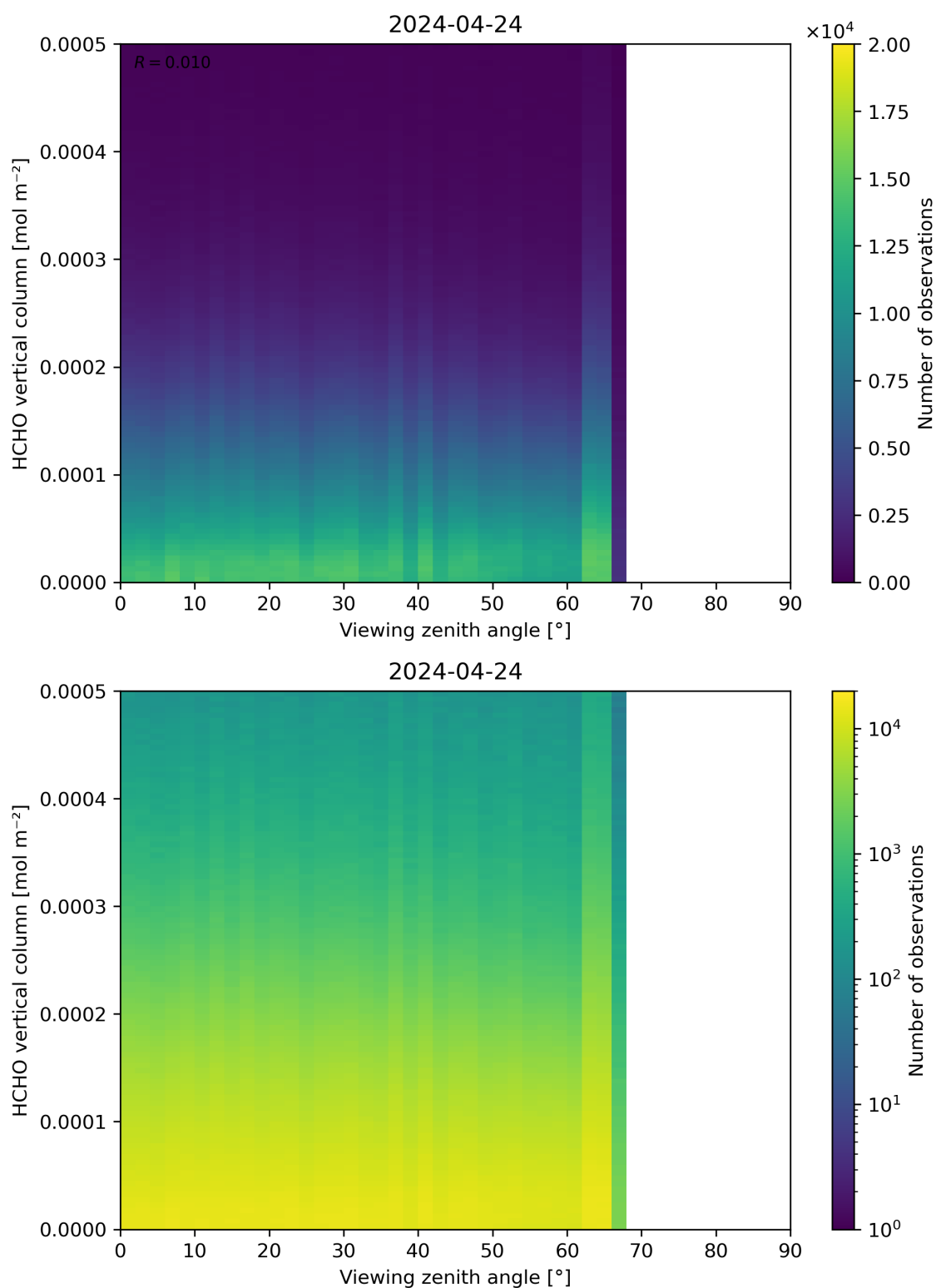
Figure 192: Scatter density plot of “Viewing zenith angle” against “HCHO vertical column” for 2024-04-23 to 2024-04-25.
