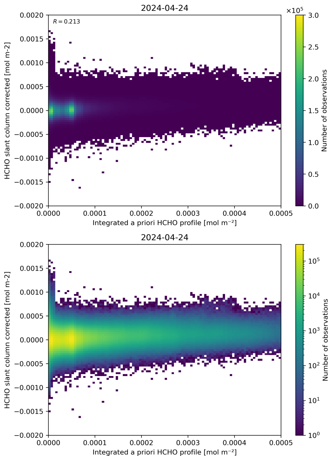
Figure 151: Scatter density plot of “Integrated a priori HCHO profile” against “HCHO slant column corrected” for 2024-04-23 to 2024-04-25.
