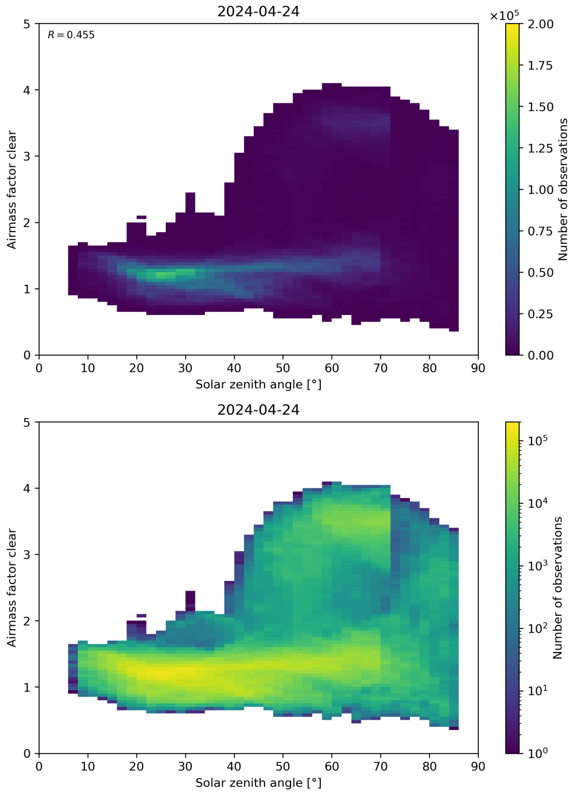
Figure 170: Scatter density plot of “Solar zenith angle” against “Airmass factor clear” for 2024-04-23 to 2024-04-25.
