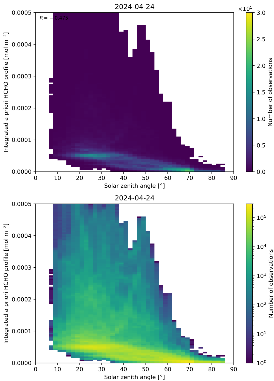
Figure 180: Scatter density plot of “Solar zenith angle” against “Integrated a priori HCHO profile” for 2024-04-23 to 2024-04-25.
