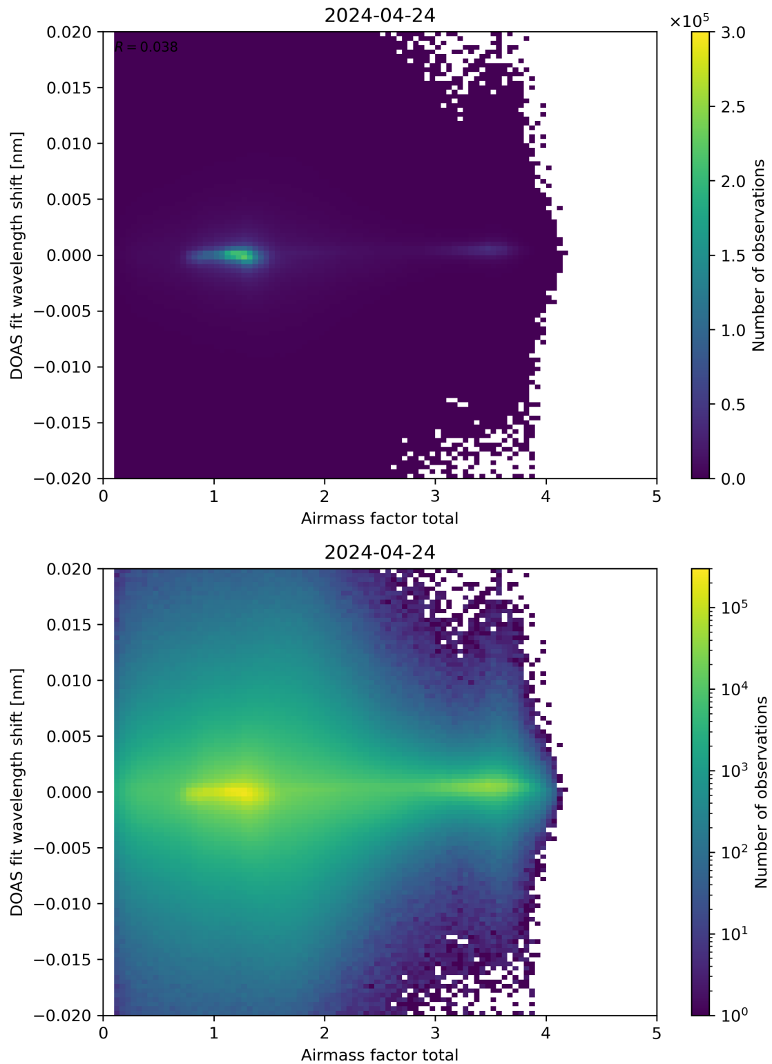
Figure 98: Scatter density plot of “Airmass factor total” against “DOAS fit wavelength shift” for 2024-04-23 to 2024-04-25.
