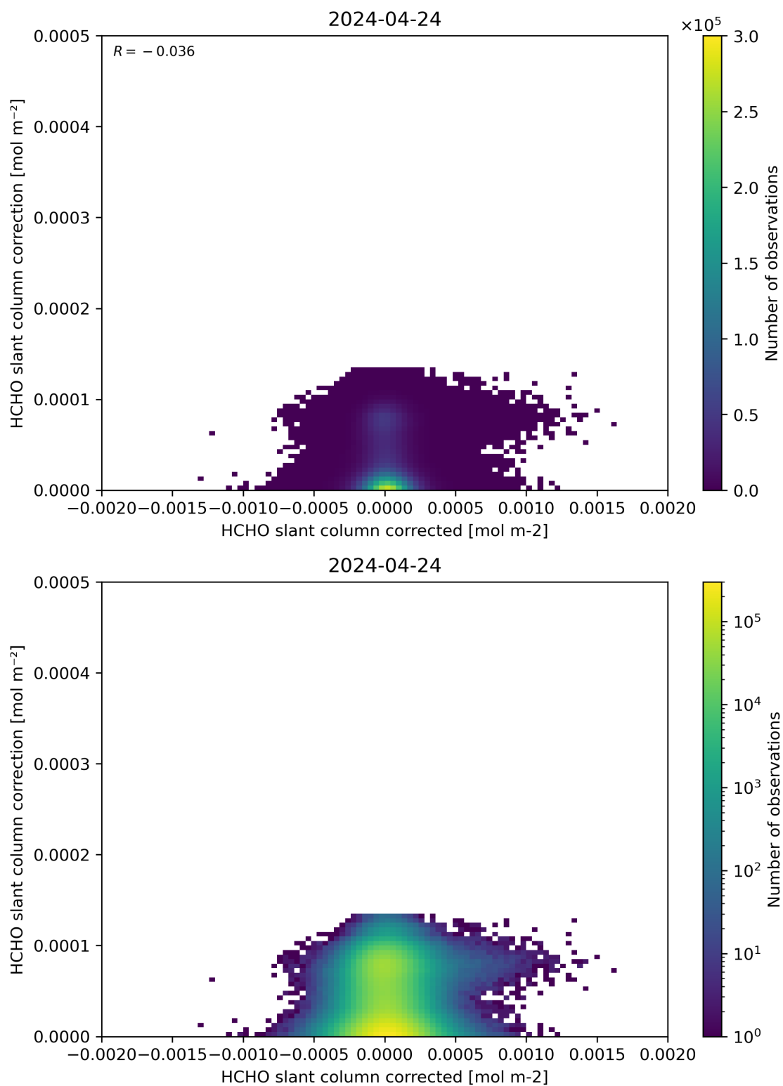
Figure 77: Scatter density plot of “HCHO slant column corrected” against “HCHO slant column correction” for 2024-04-23 to 2024-04-25.
