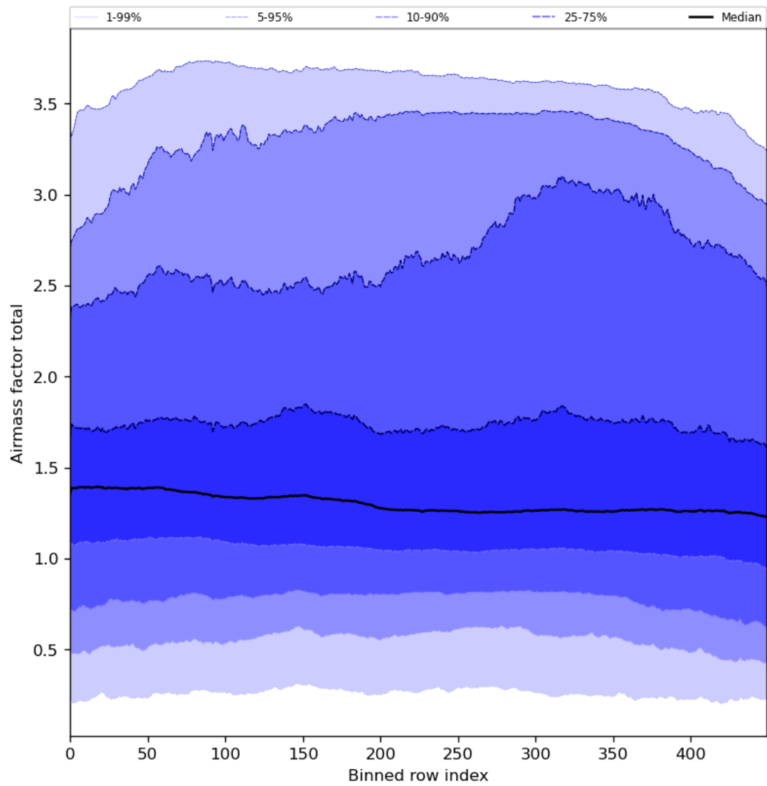
Figure 54: Along track statistics of “Airmass factor total” for 2024-04-23 to 2024-04-25
