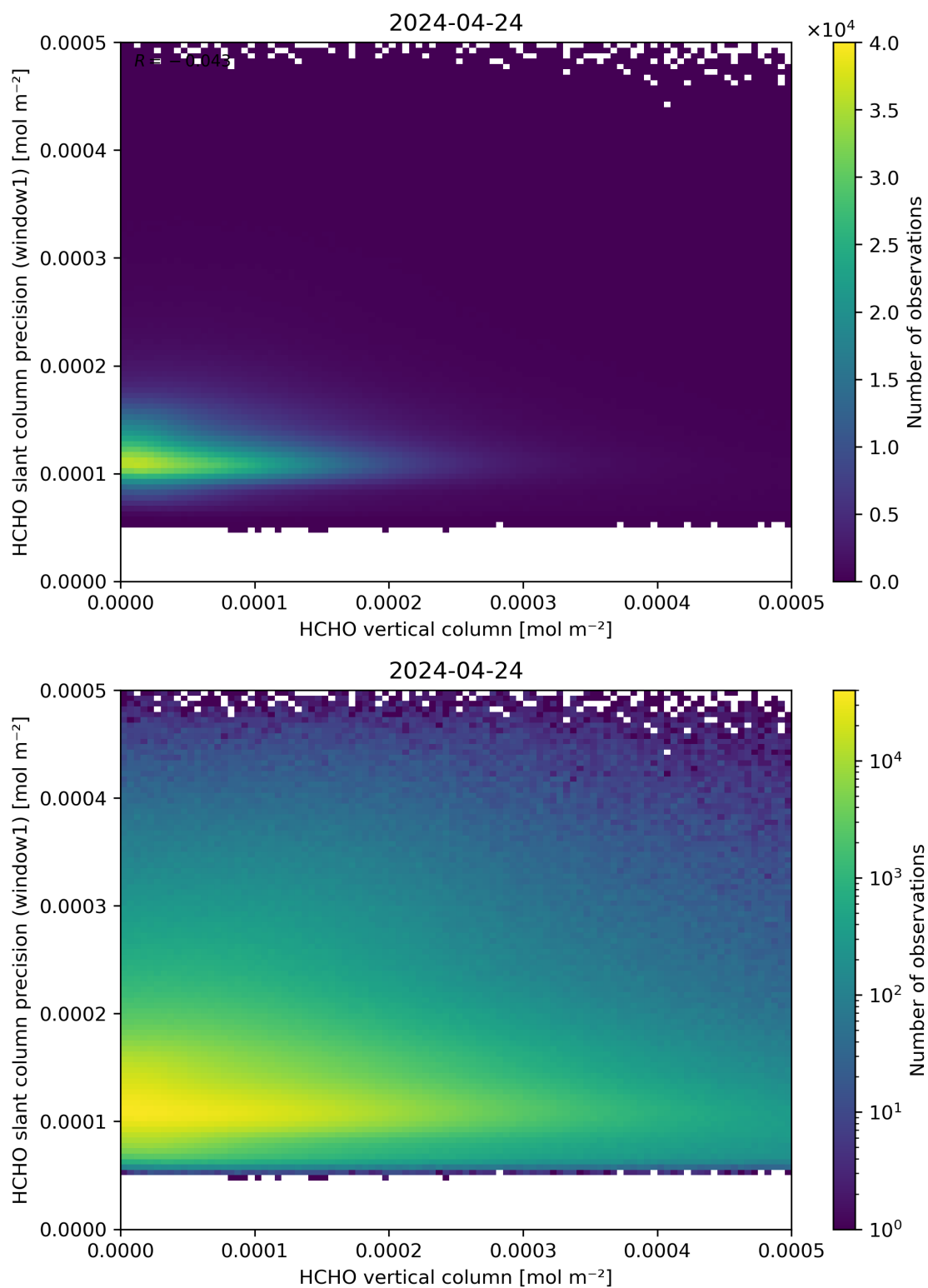
Figure 130: Scatter density plot of “HCHO vertical column” against “HCHO slant column precision (window1)” for 2024-04-23 to 2024-04-25.
