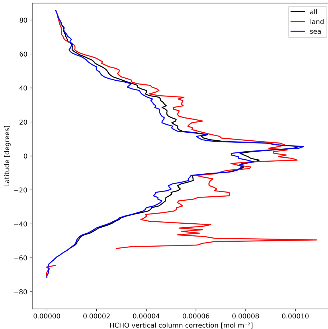
Figure 23: Zonal average of “HCHO vertical column correction” for 2024-04-23 to 2024-04-25.
