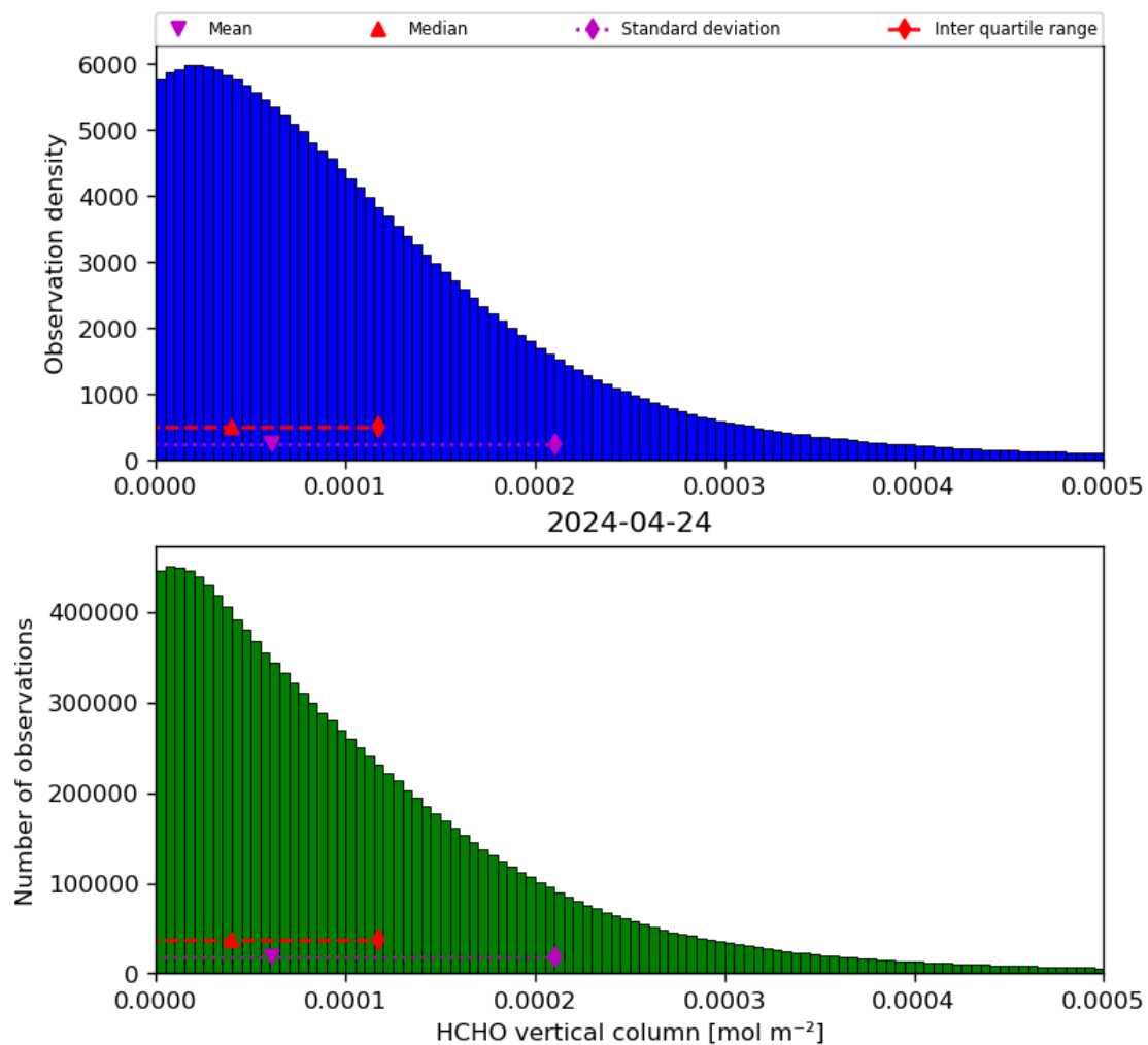
Figure 35: Histogram of “HCHO vertical column” for 2024-04-23 to 2024-04-25
