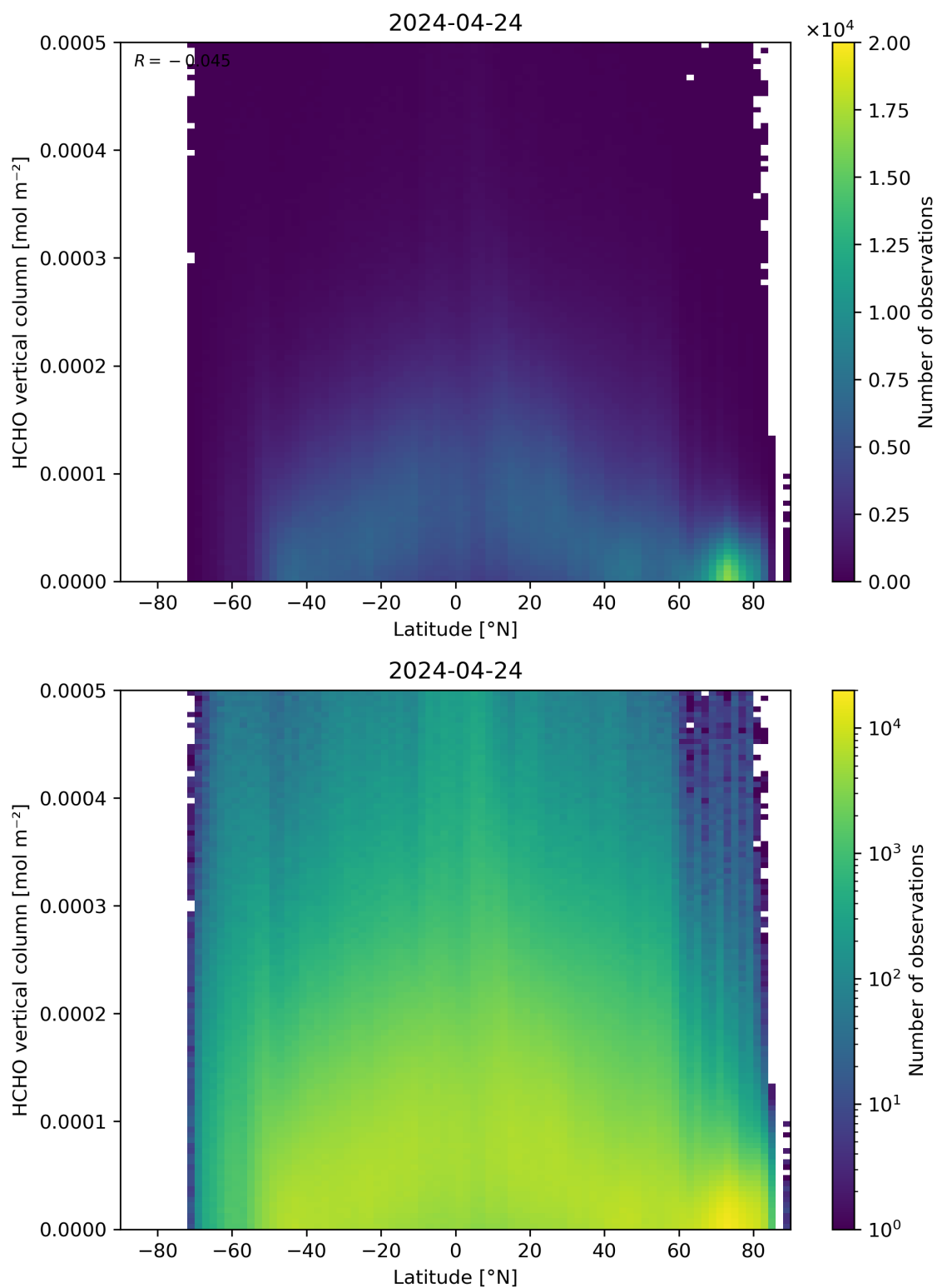
Figure 163: Scatter density plot of “Latitude” against “HCHO vertical column” for 2024-04-23 to 2024-04-25.
