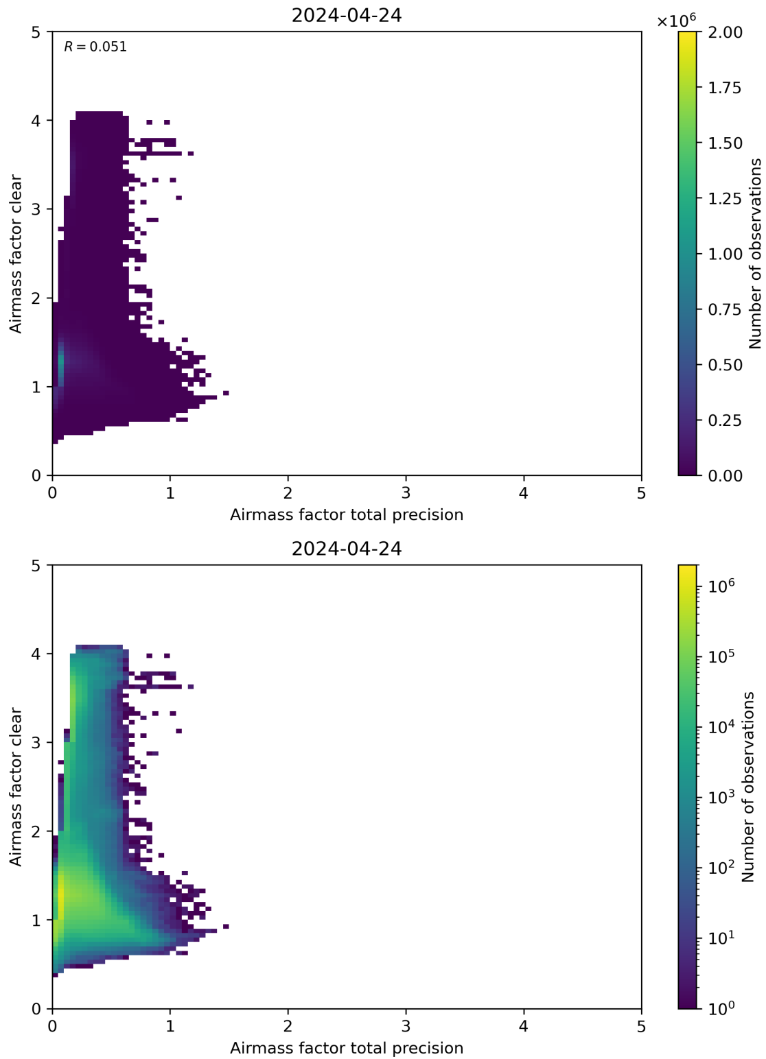
Figure 108: Scatter density plot of “Airmass factor total precision” against “Airmass factor clear” for 2024-04-23 to 2024-04-25.
