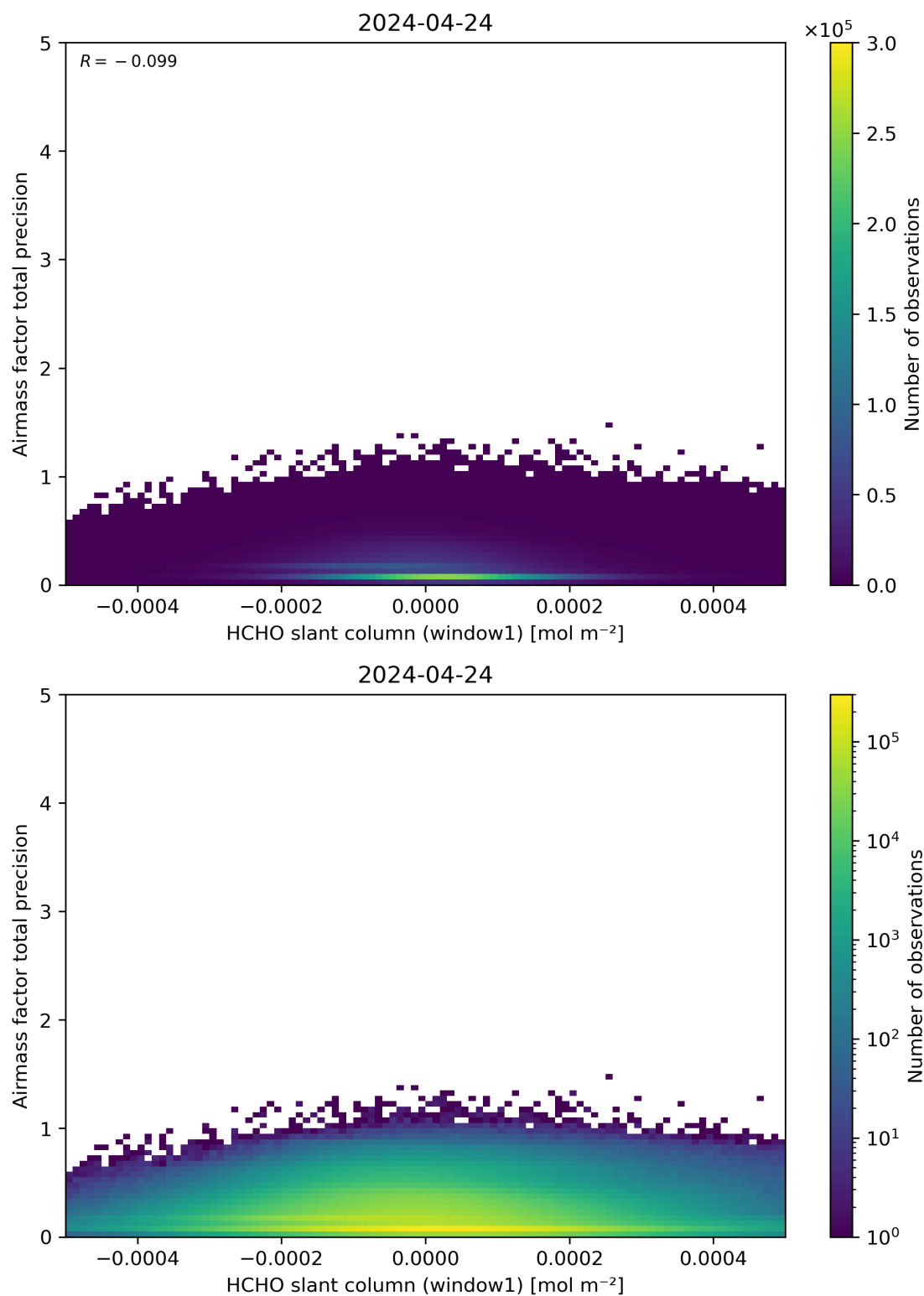
Figure 86: Scatter density plot of “HCHO slant column (window1)” against “Airmass factor total precision” for 2024-04-23 to 2024-04-25.
