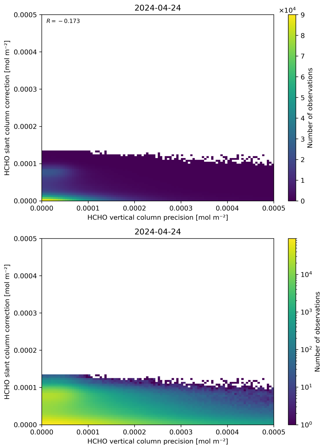
Figure 141: Scatter density plot of “HCHO vertical column precision” against “HCHO slant column correction” for 2024-04-23 to 2024-04-25.
