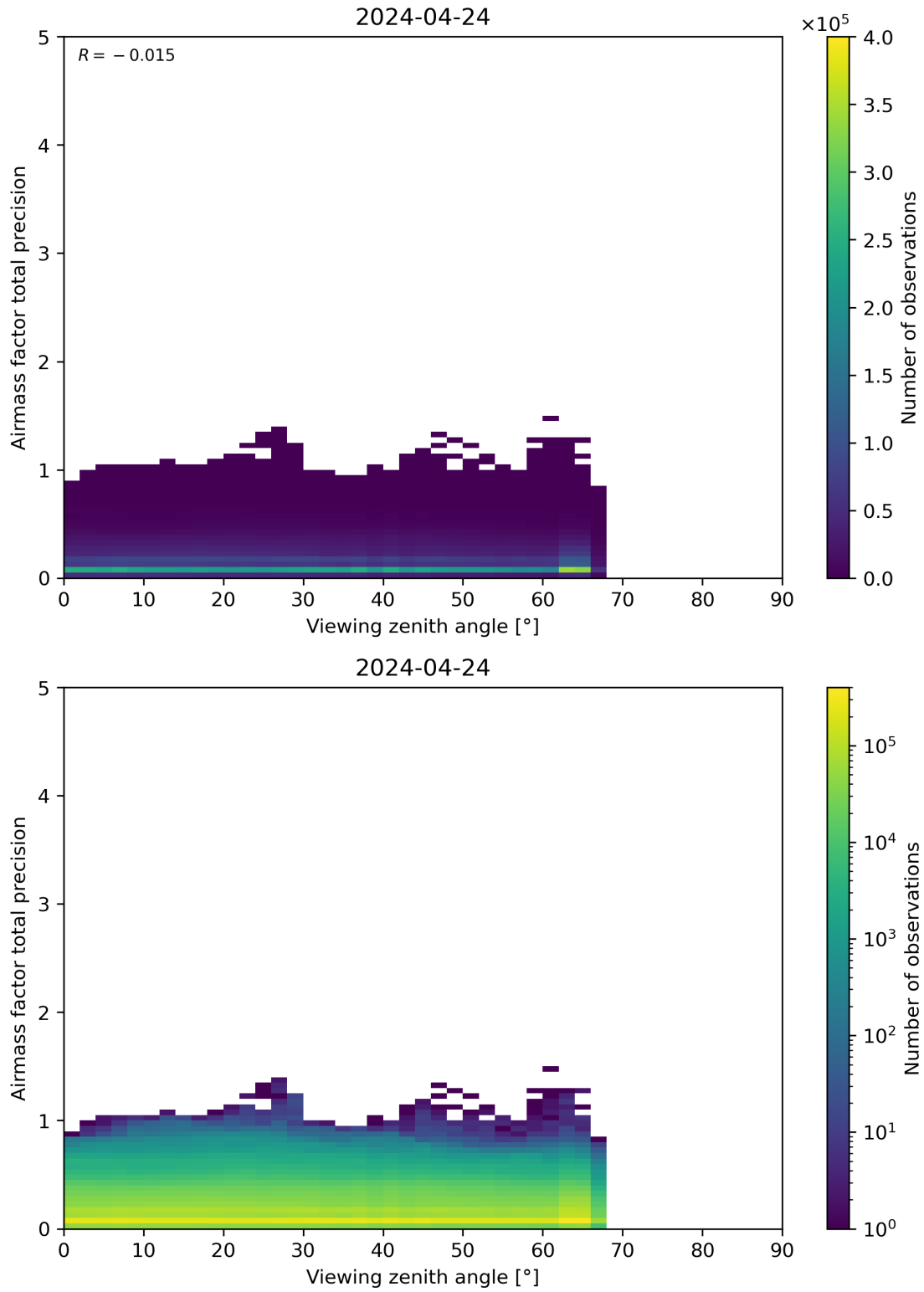
Figure 191: Scatter density plot of “Viewing zenith angle” against “Airmass factor total precision” for 2024-04-23 to 2024-04-25.
