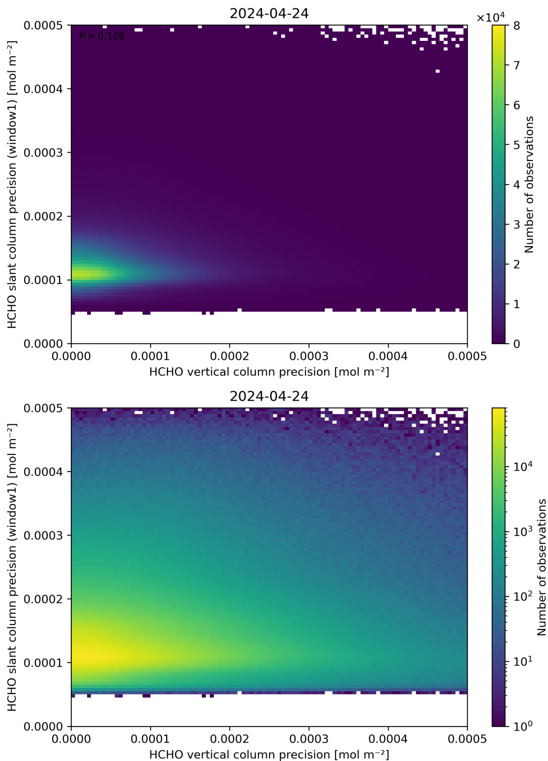
Figure 143: Scatter density plot of “HCHO vertical column precision” against “HCHO slant column precision (window1)” for 2024-04-23 to 2024-04-25.
