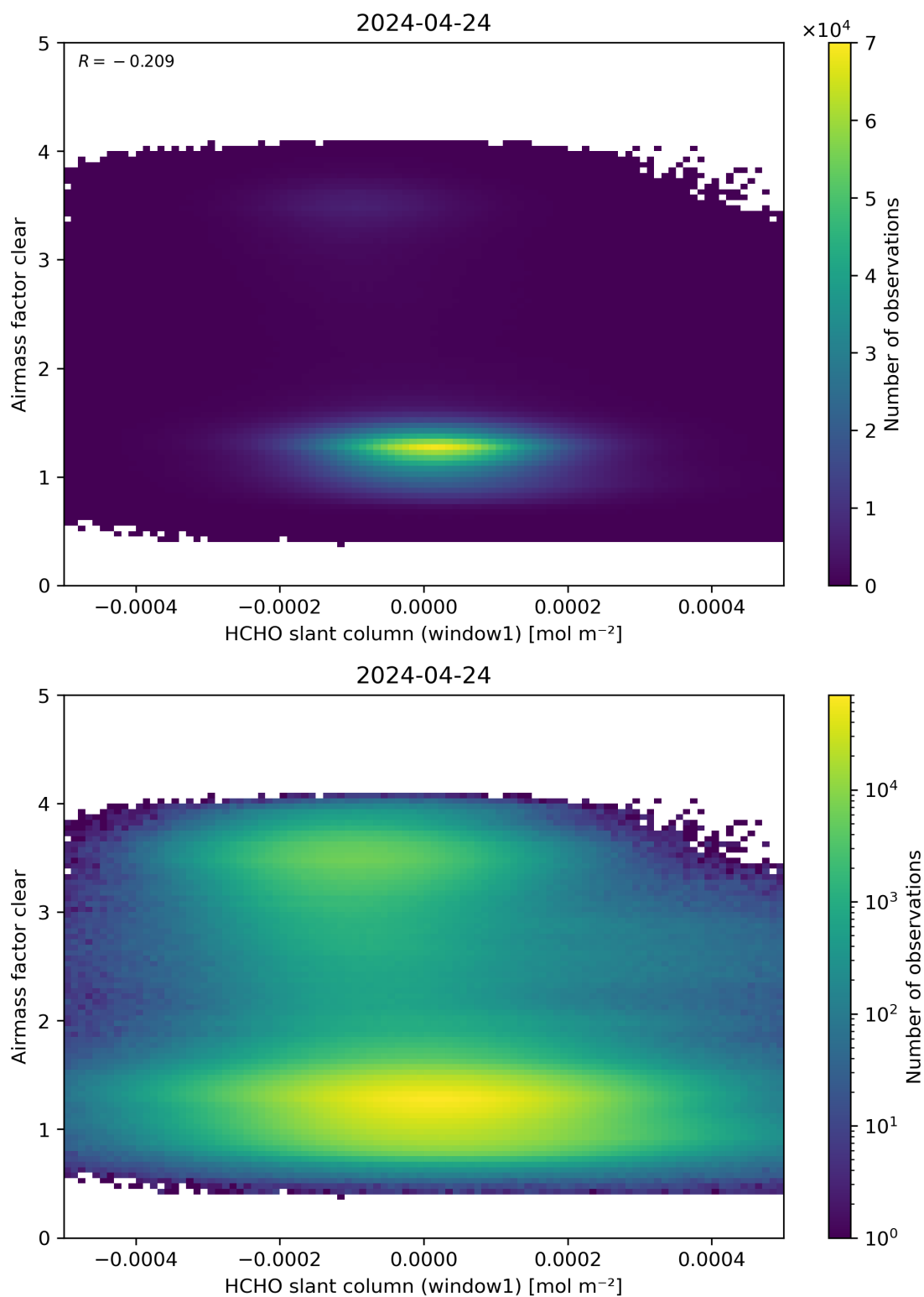
Figure 81: Scatter density plot of “HCHO slant column (window1)” against “Airmass factor clear” for 2024-04-23 to 2024-04-25.
