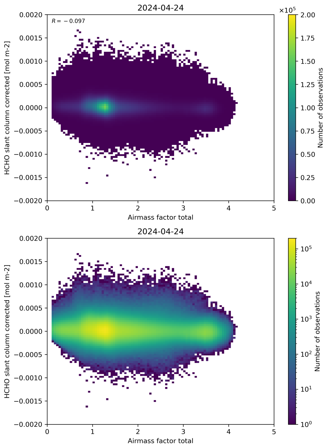
Figure 101: Scatter density plot of “Airmass factor total” against “HCHO slant column corrected” for 2024-04-23 to 2024-04-25.
