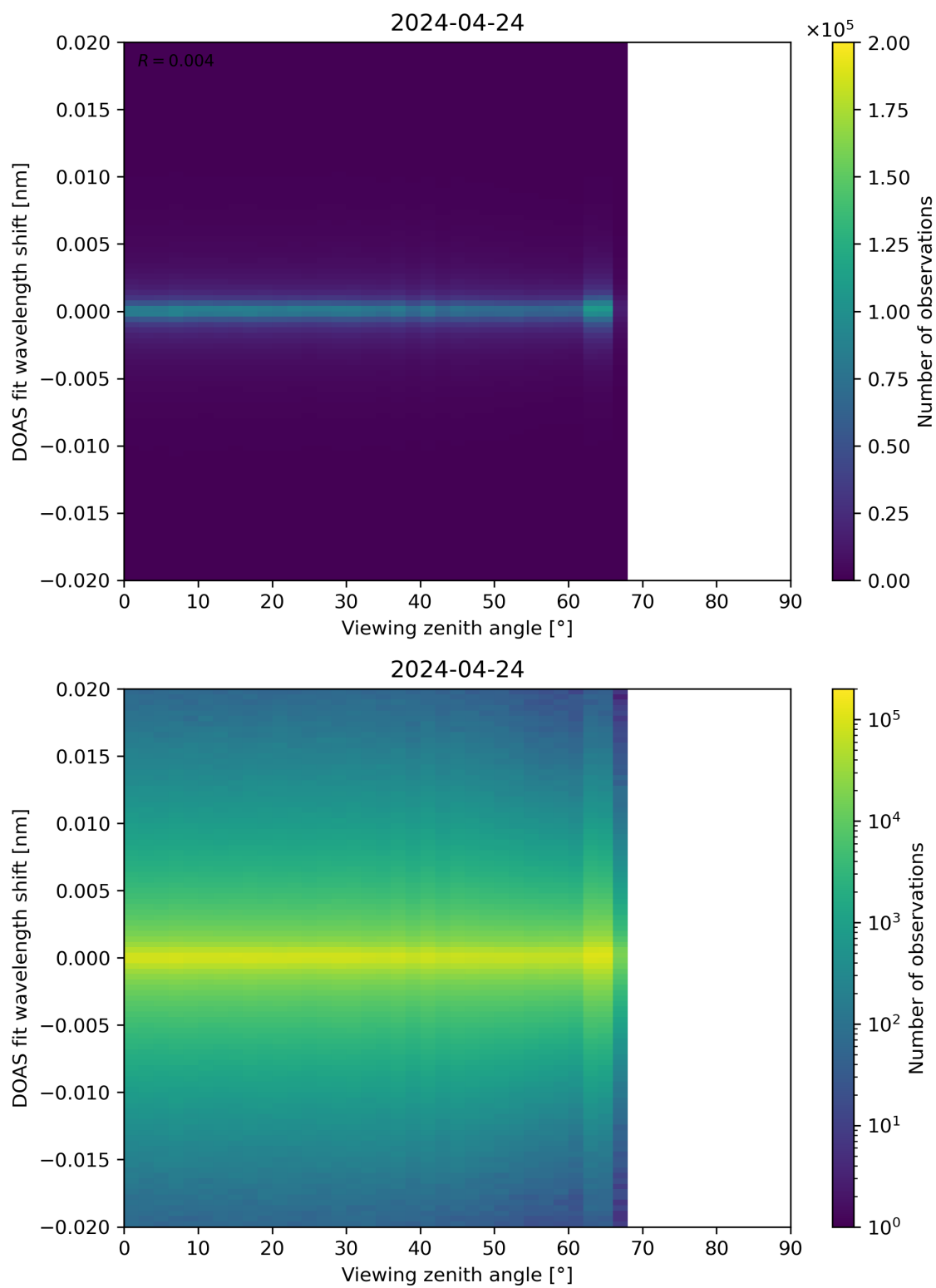
Figure 183: Scatter density plot of “Viewing zenith angle” against “DOAS fit wavelength shift” for 2024-04-23 to 2024-04-25.
