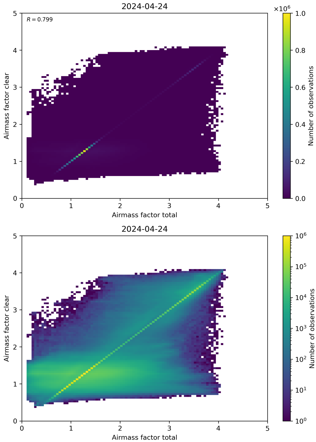
Figure 100: Scatter density plot of “Airmass factor total” against “Airmass factor clear” for 2024-04-23 to 2024-04-25.
