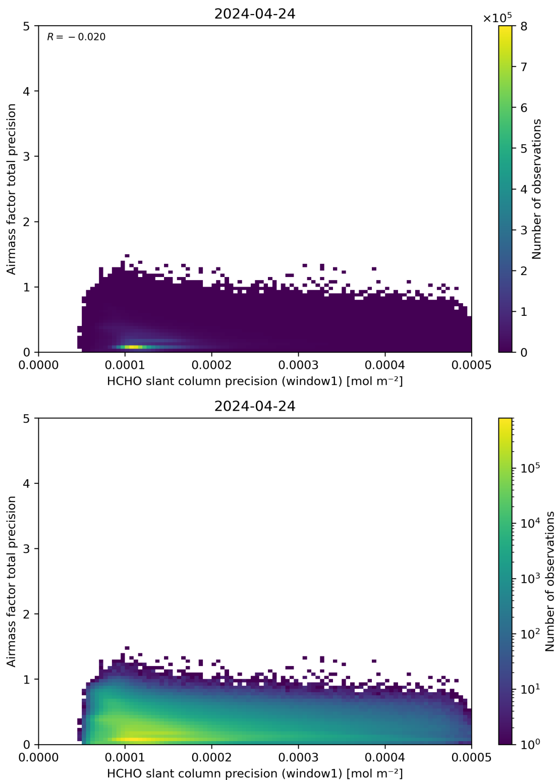
Figure 95: Scatter density plot of “HCHO slant column precision (window1)” against “Airmass factor total precision” for 2024-04-23 to 2024-04-25.
