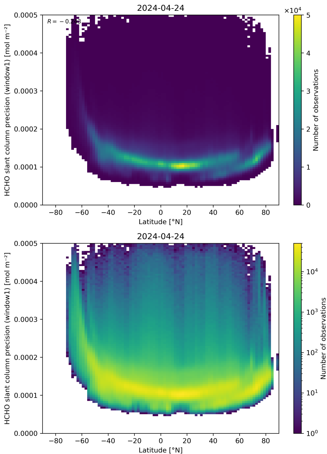
Figure 160: Scatter density plot of “Latitude” against “HCHO slant column precision (window1)” for 2024-04-23 to 2024-04-25.
