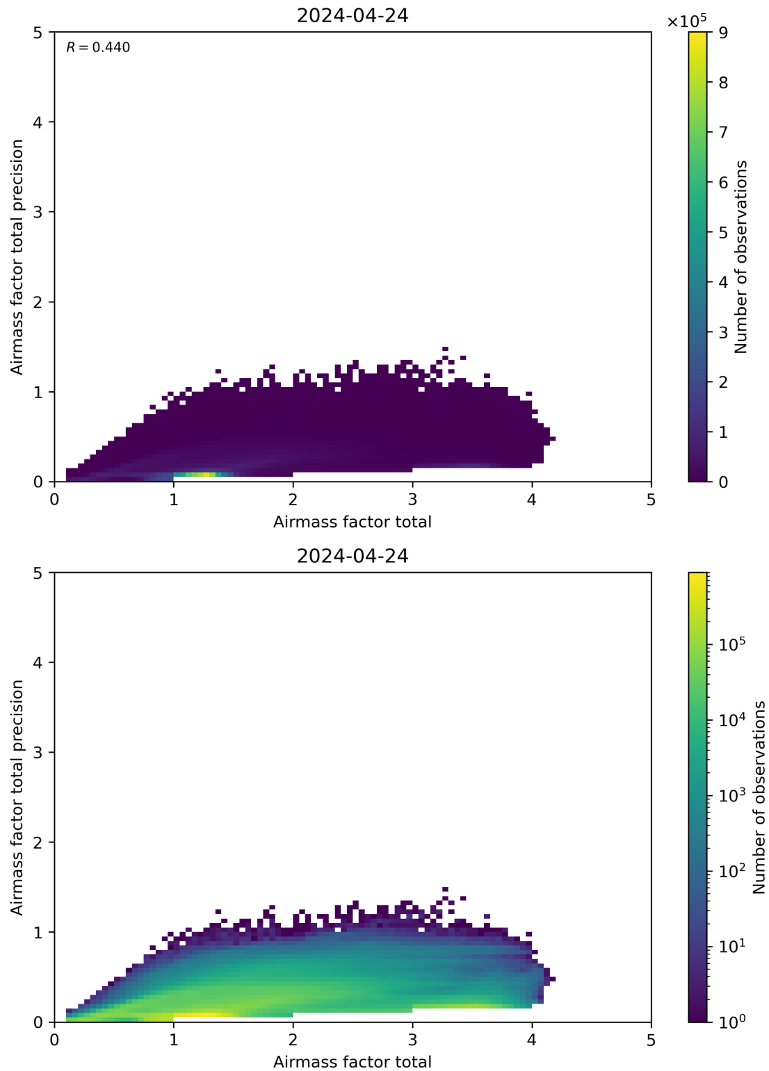
Figure 103: Scatter density plot of “Airmass factor total” against “Airmass factor total precision” for 2024-04-23 to 2024-04-25.
