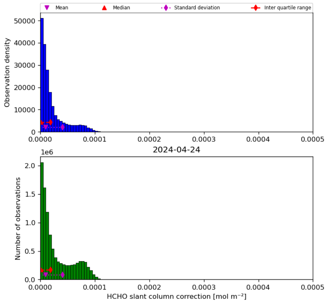
Figure 47: Histogram of “HCHO slant column correction” for 2024-04-23 to 2024-04-25
