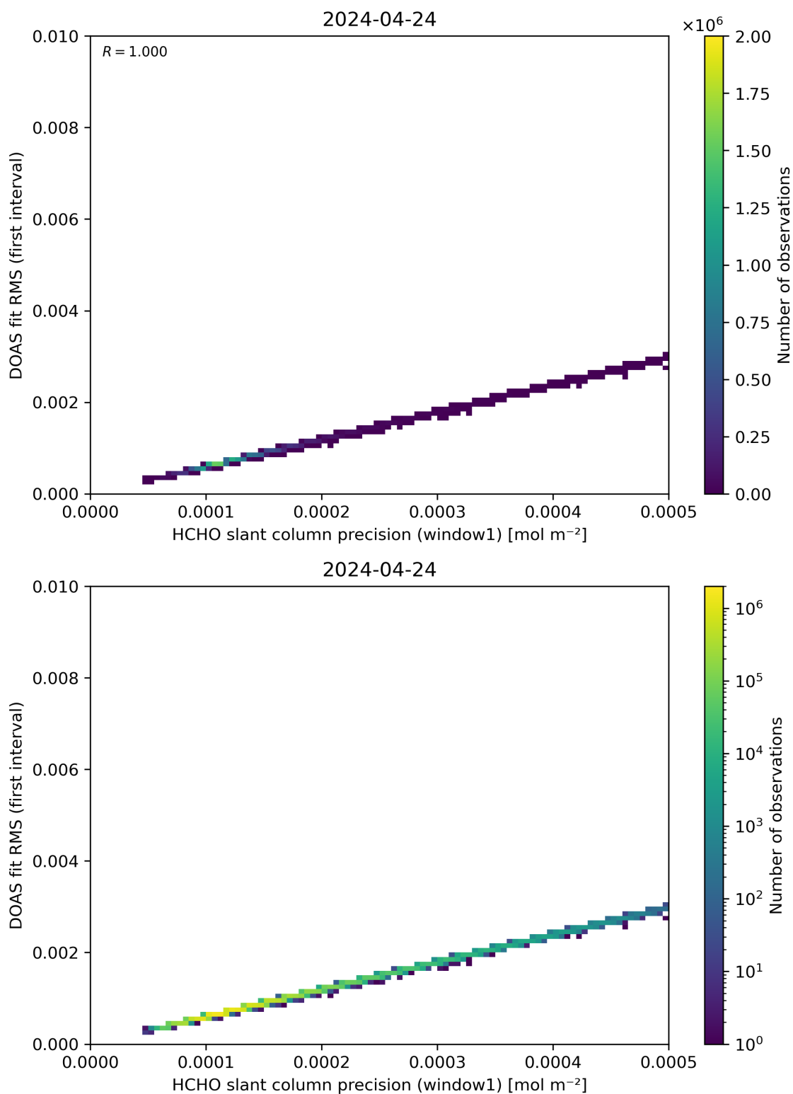
Figure 88: Scatter density plot of “HCHO slant column precision (window1)” against “DOAS fit RMS (first interval)” for 2024-04-23 to 2024-04-25.
