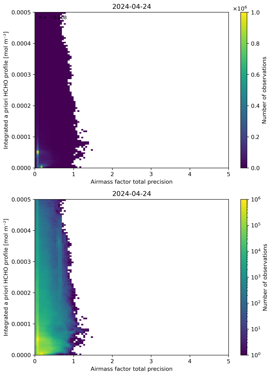
Figure 111: Scatter density plot of “Airmass factor total precision” against “Integrated a priori HCHO profile” for 2024-04-23 to 2024-04-25.
