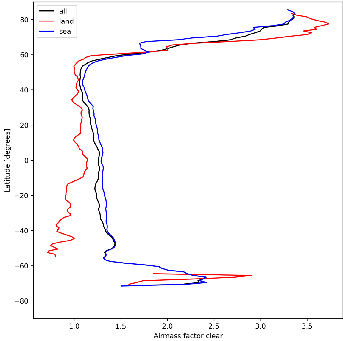
Figure 28: Zonal average of “Airmass factor clear” for 2024-04-23 to 2024-04-25.
