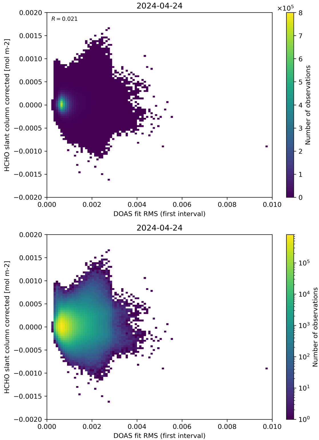
Figure 62: Scatter density plot of “DOAS fit RMS (first interval)” against “HCHO slant column corrected” for 2024-04-23 to 2024-04-25.
