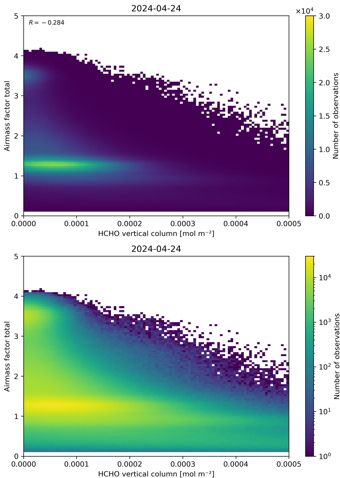
Figure 131: Scatter density plot of “HCHO vertical column” against “Airmass factor total” for 2024-04-23 to 2024-04-25.
