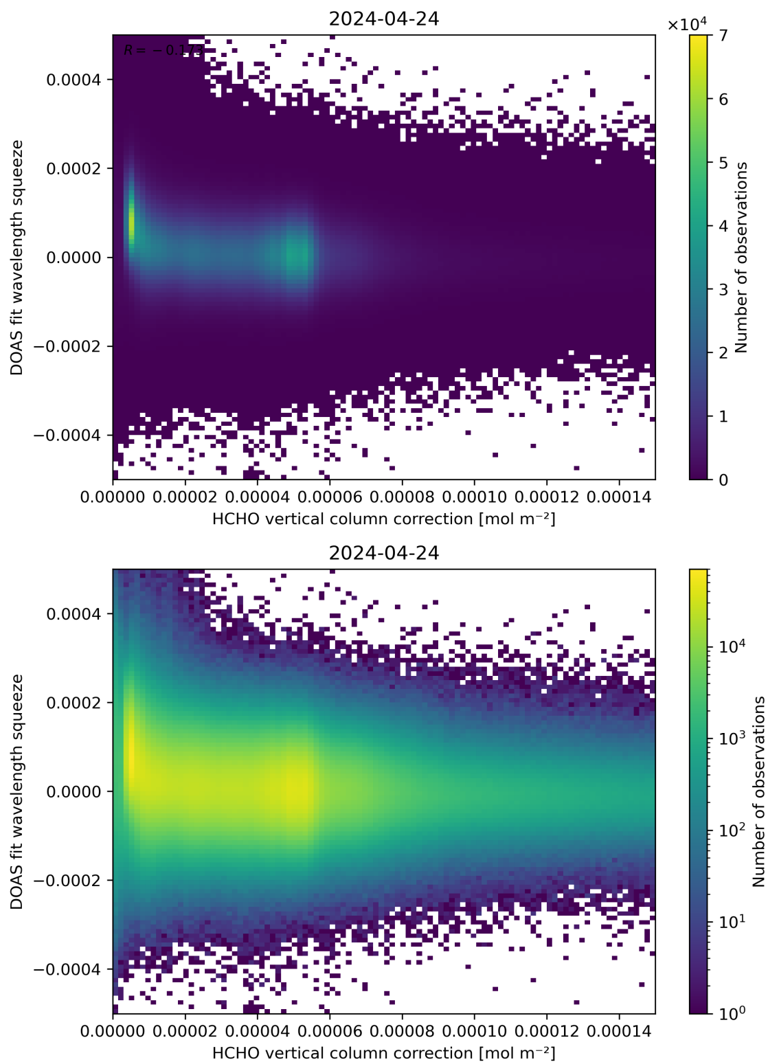
Figure 114: Scatter density plot of “HCHO vertical column correction” against “DOAS fit wavelength squeeze” for 2024-04-23 to 2024-04-25.
