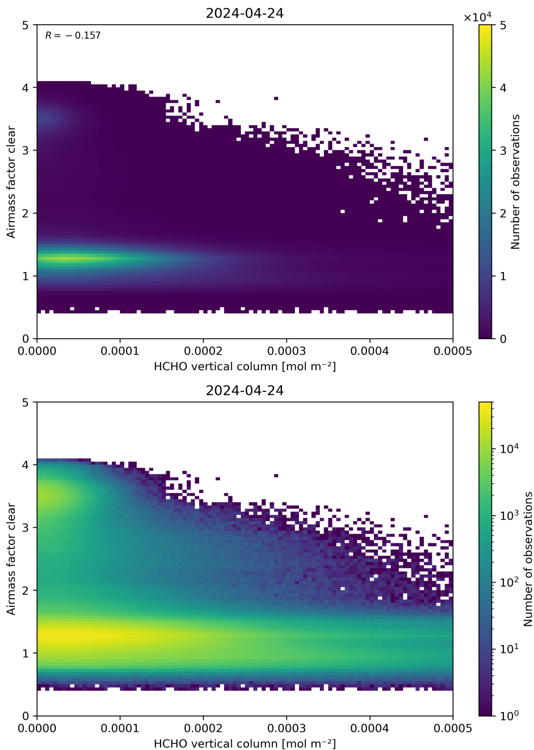
Figure 126: Scatter density plot of “HCHO vertical column” against “Airmass factor clear” for 2024-04-23 to 2024-04-25.
