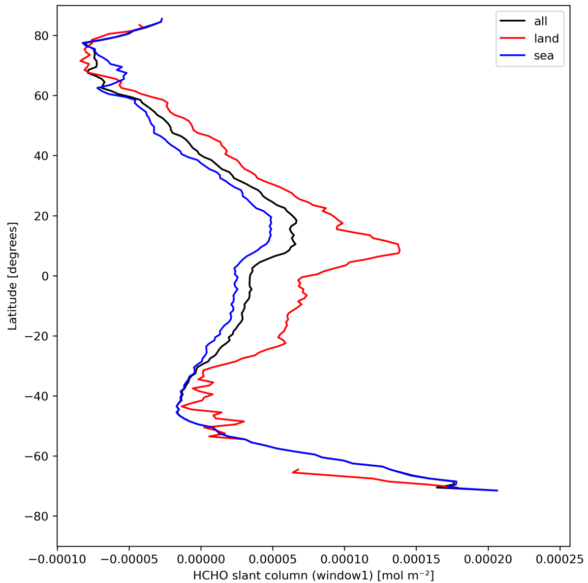
Figure 24: Zonal average of “HCHO slant column (window1)” for 2024-04-23 to 2024-04-25.
