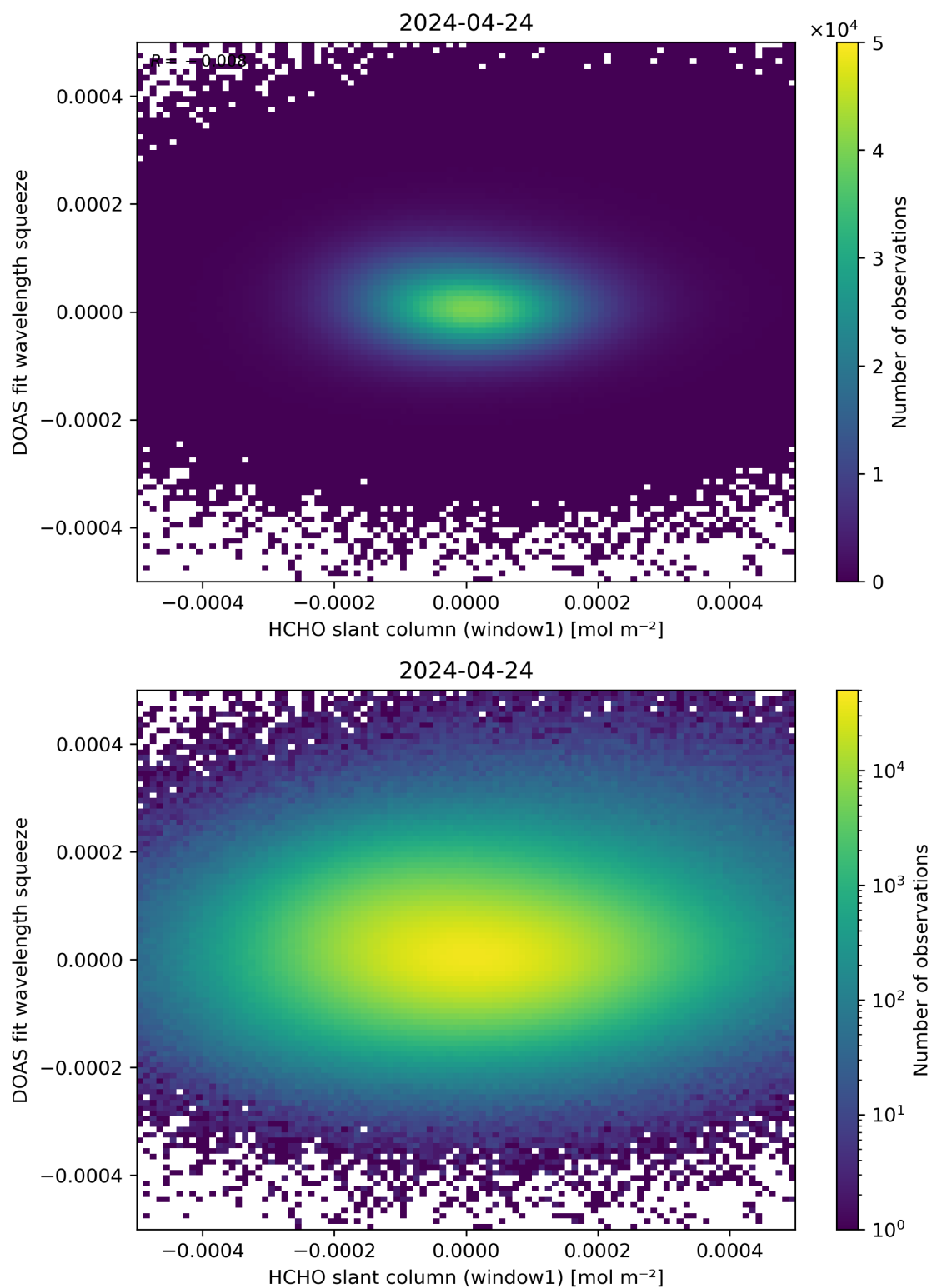
Figure 80: Scatter density plot of “HCHO slant column (window1)” against “DOAS fit wavelength squeeze” for 2024-04-23 to 2024-04-25.
