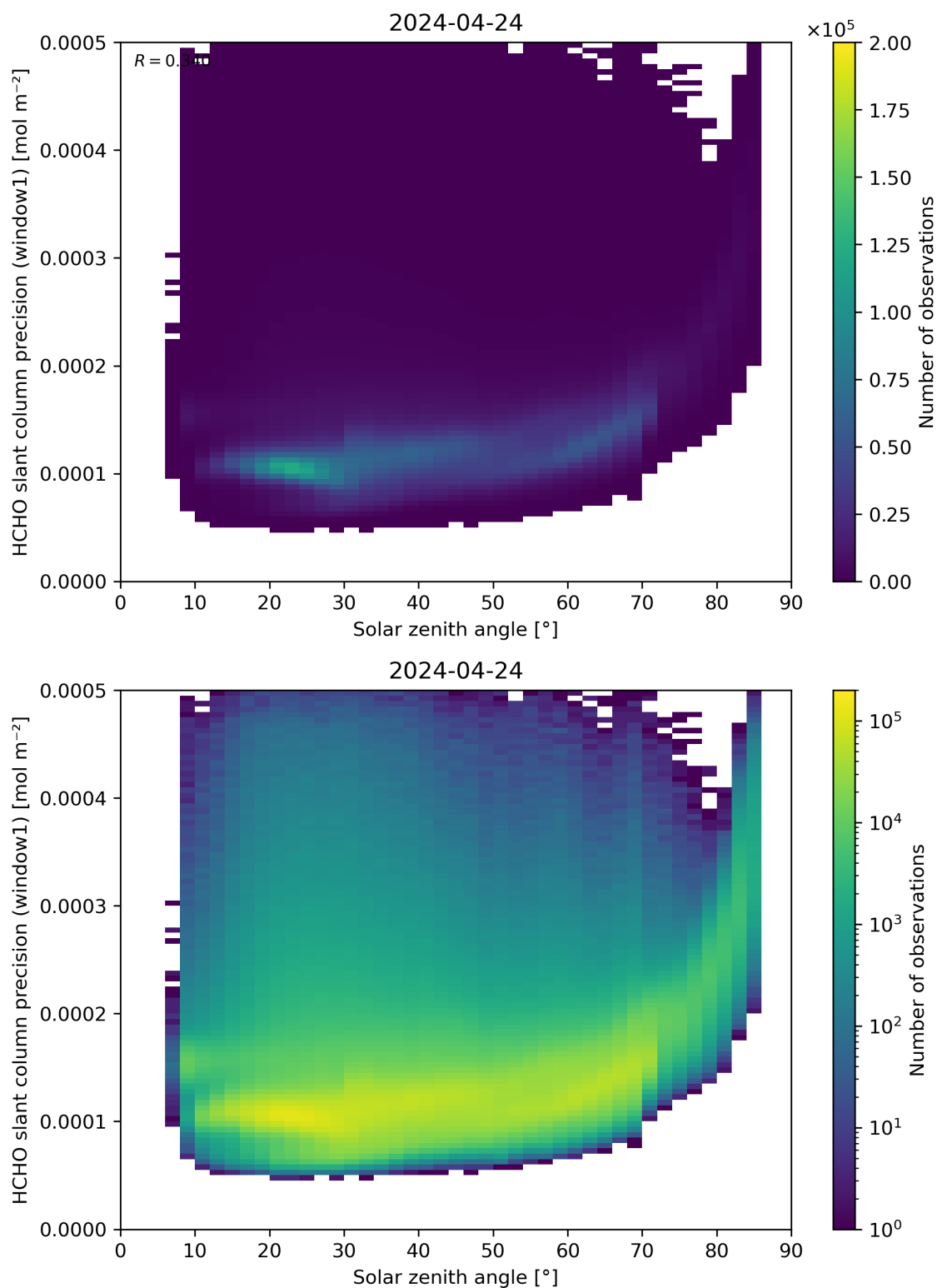
Figure 174: Scatter density plot of “Solar zenith angle” against “HCHO slant column precision (window1)” for 2024-04-23 to 2024-04-25.
