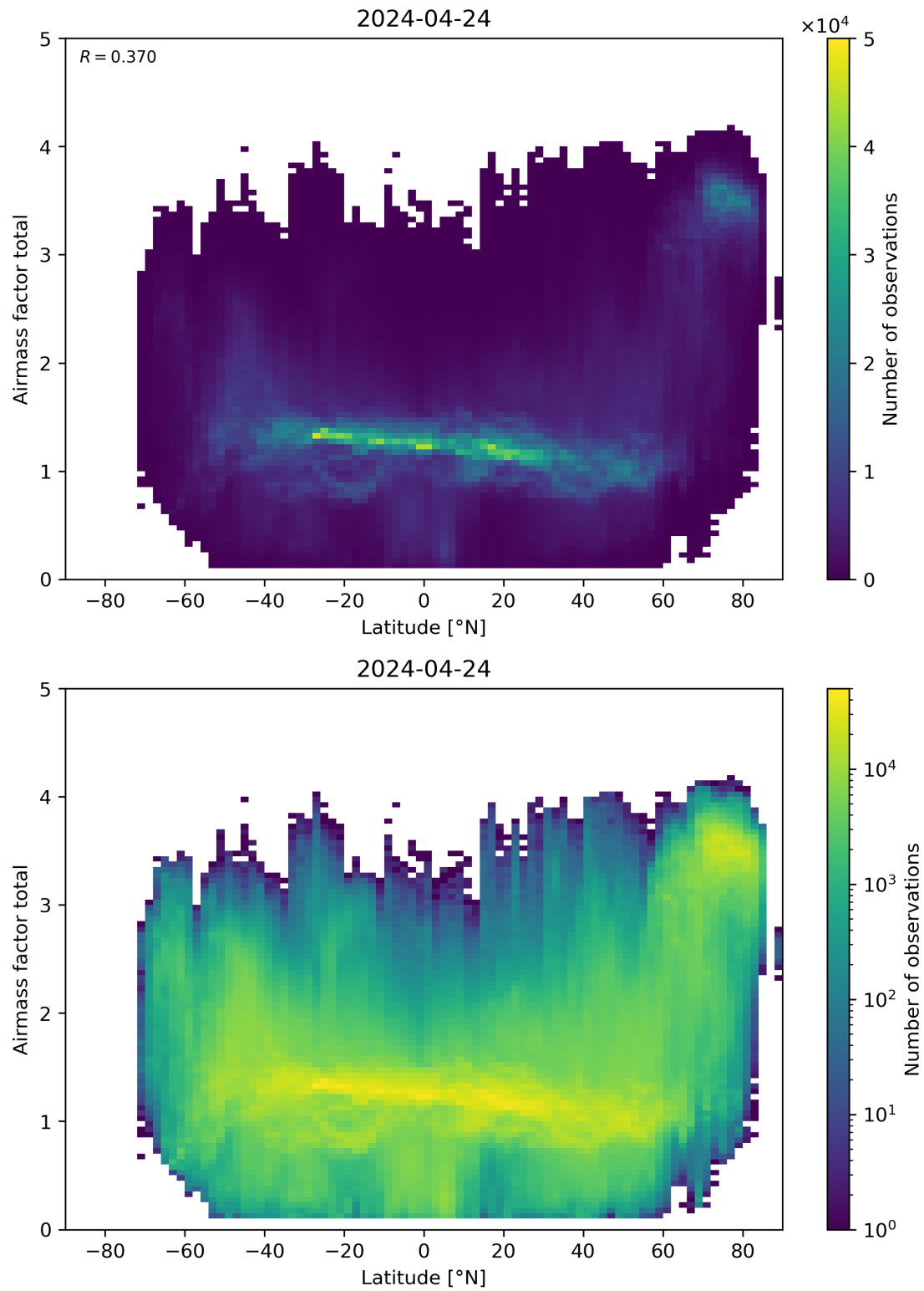
Figure 161: Scatter density plot of “Latitude” against “Airmass factor total” for 2024-04-23 to 2024-04-25.
