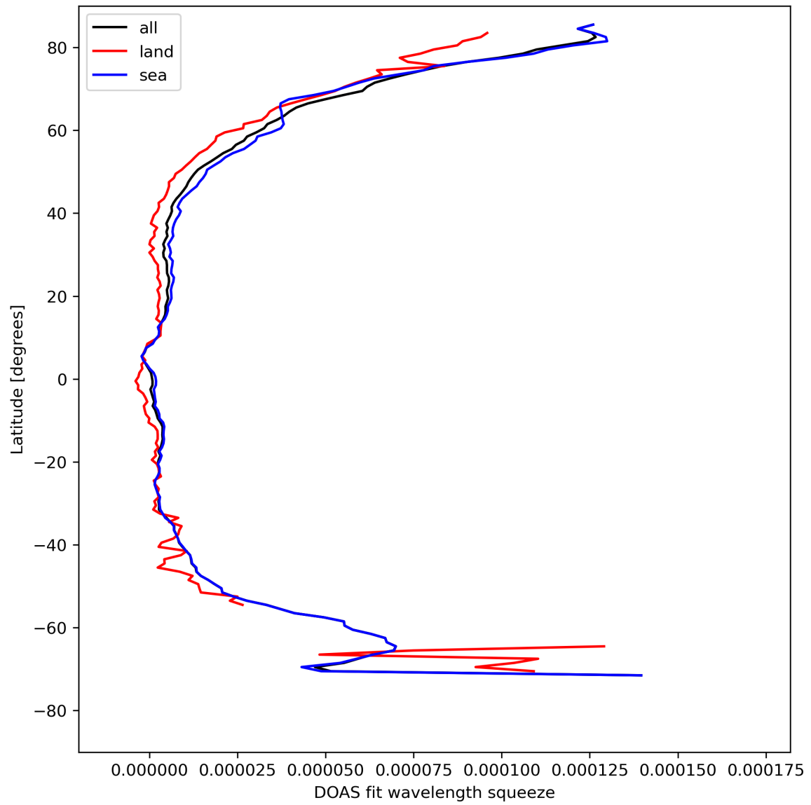
Figure 31: Zonal average of “DOAS fit wavelength squeeze” for 2024-04-23 to 2024-04-25.
