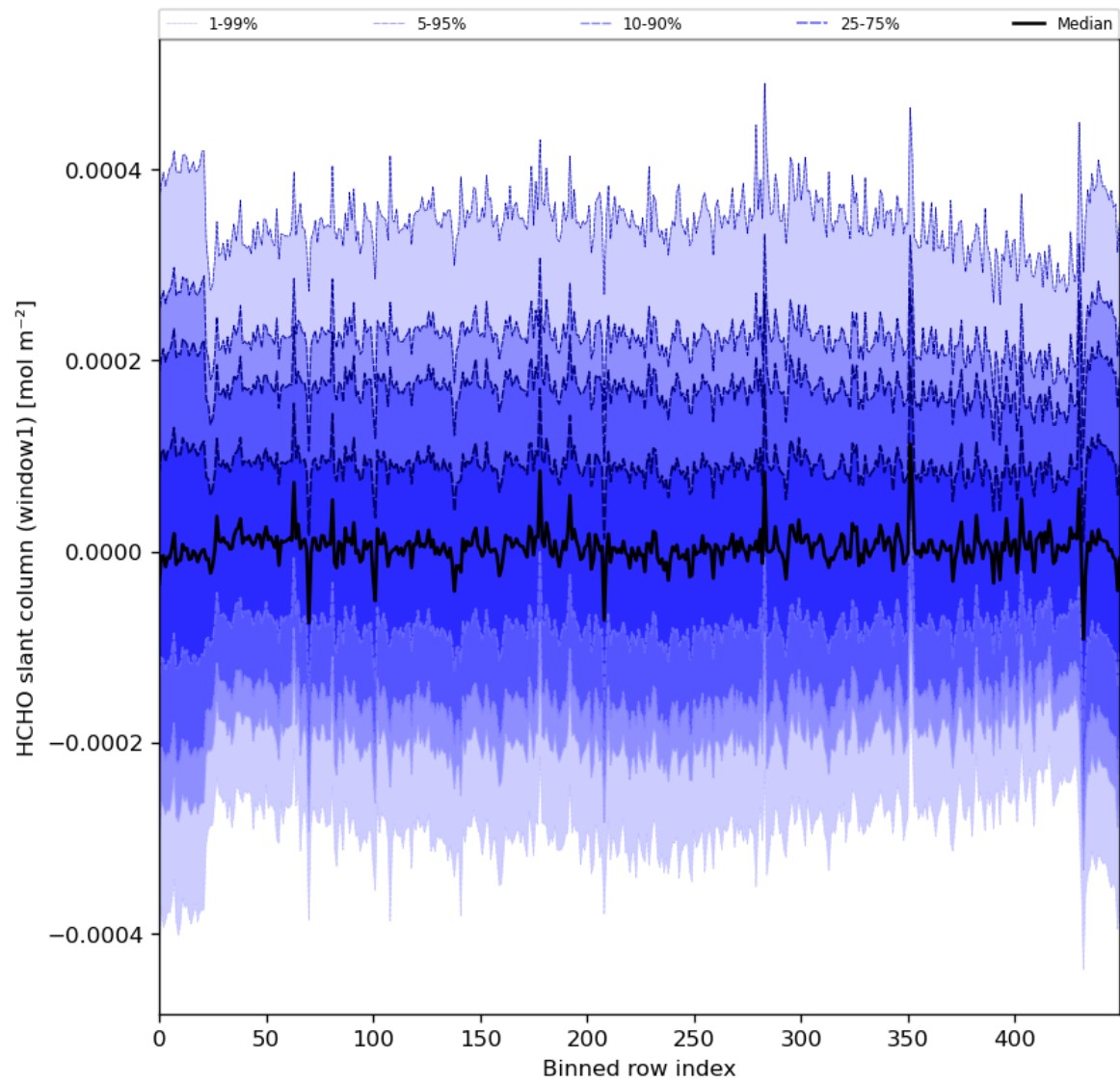
Figure 52: Along track statistics of “HCHO slant column (window1)” for 2024-04-23 to 2024-04-25
