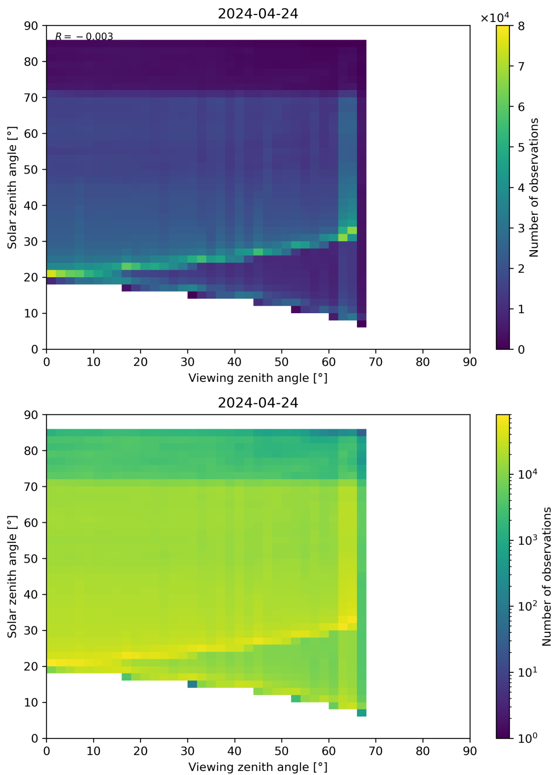
Figure 197: Scatter density plot of “Viewing zenith angle” against “Solar zenith angle” for 2024-04-23 to 2024-04-25.
