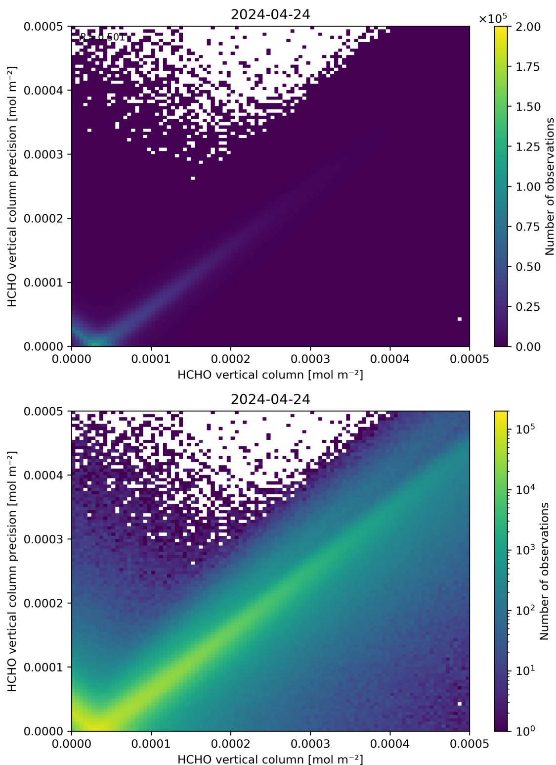
Figure 134: Scatter density plot of “HCHO vertical column” against “HCHO vertical column precision” for 2024-04-23 to 2024-04-25.
