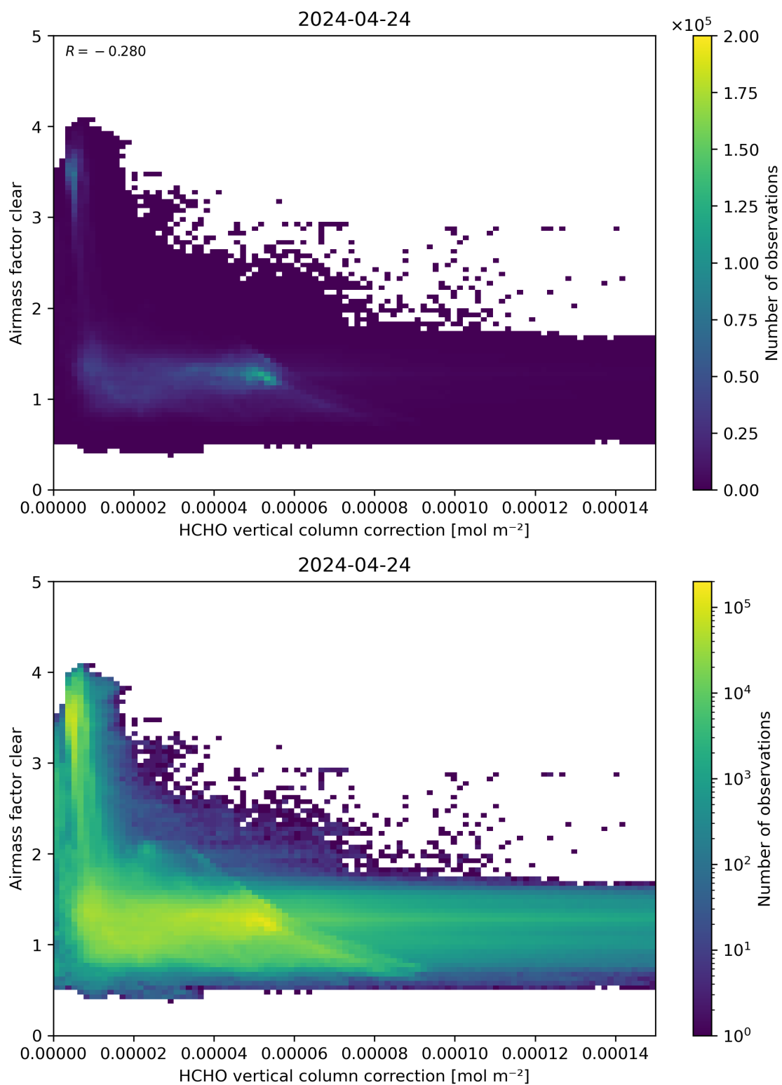
Figure 115: Scatter density plot of “HCHO vertical column correction” against “Airmass factor clear” for 2024-04-23 to 2024-04-25.
