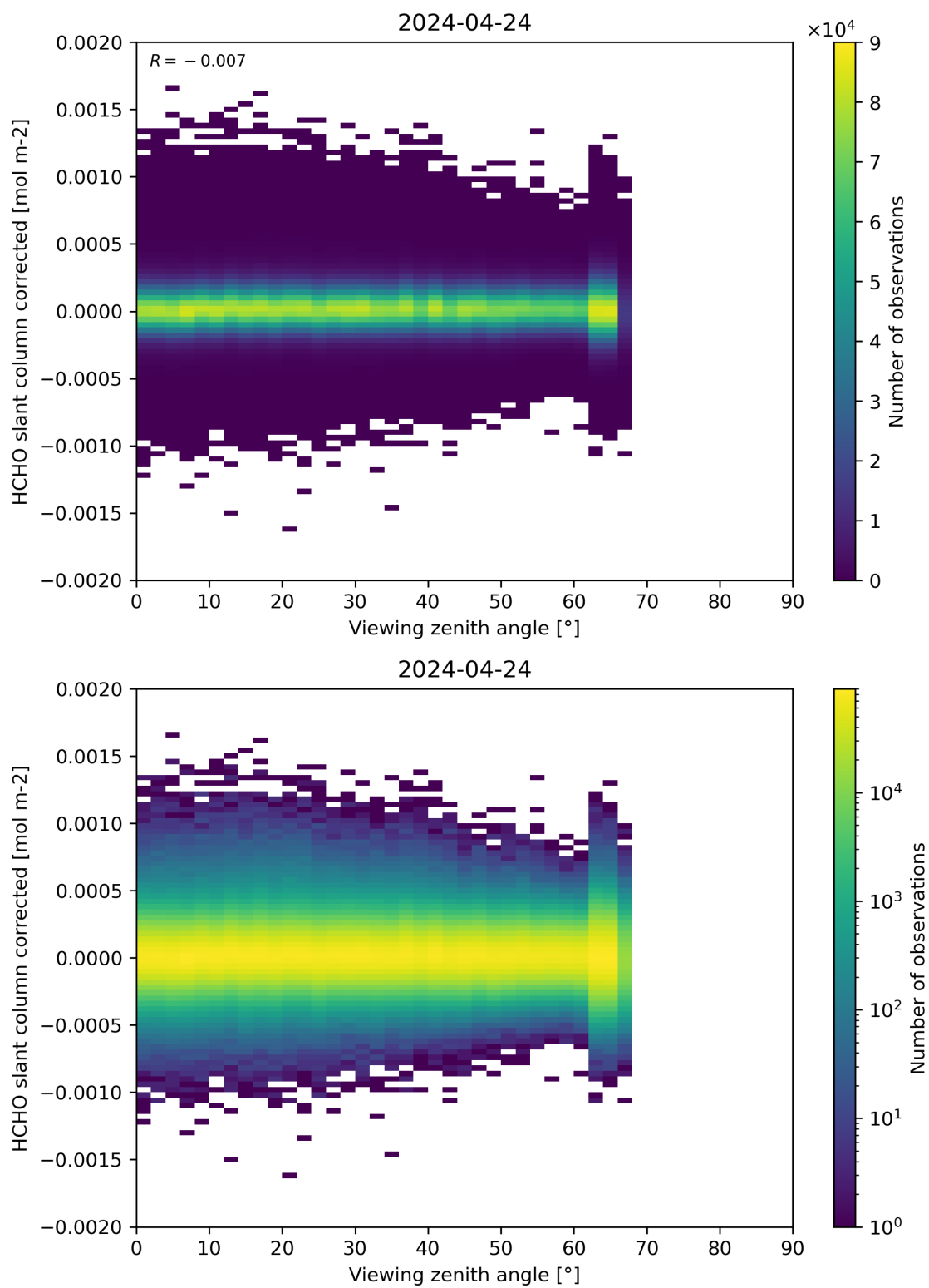
Figure 186: Scatter density plot of “Viewing zenith angle” against “HCHO slant column corrected” for 2024-04-23 to 2024-04-25.
