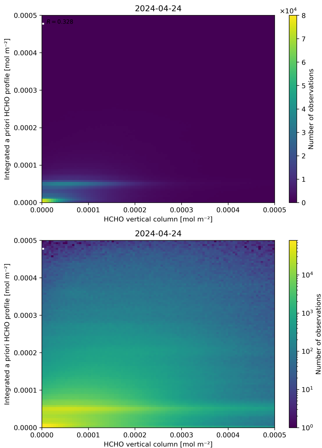
Figure 135: Scatter density plot of “HCHO vertical column” against “Integrated a priori HCHO profile” for 2024-04-23 to 2024-04-25.
