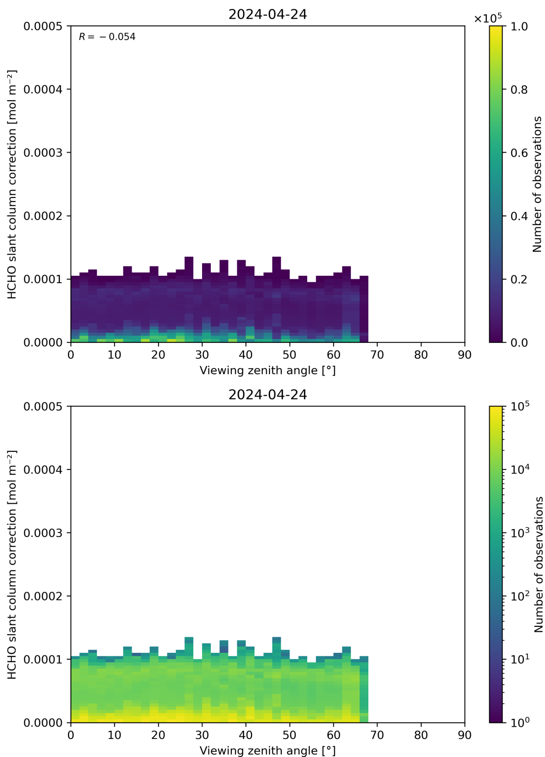
Figure 187: Scatter density plot of “Viewing zenith angle” against “HCHO slant column correction” for 2024-04-23 to 2024-04-25.
