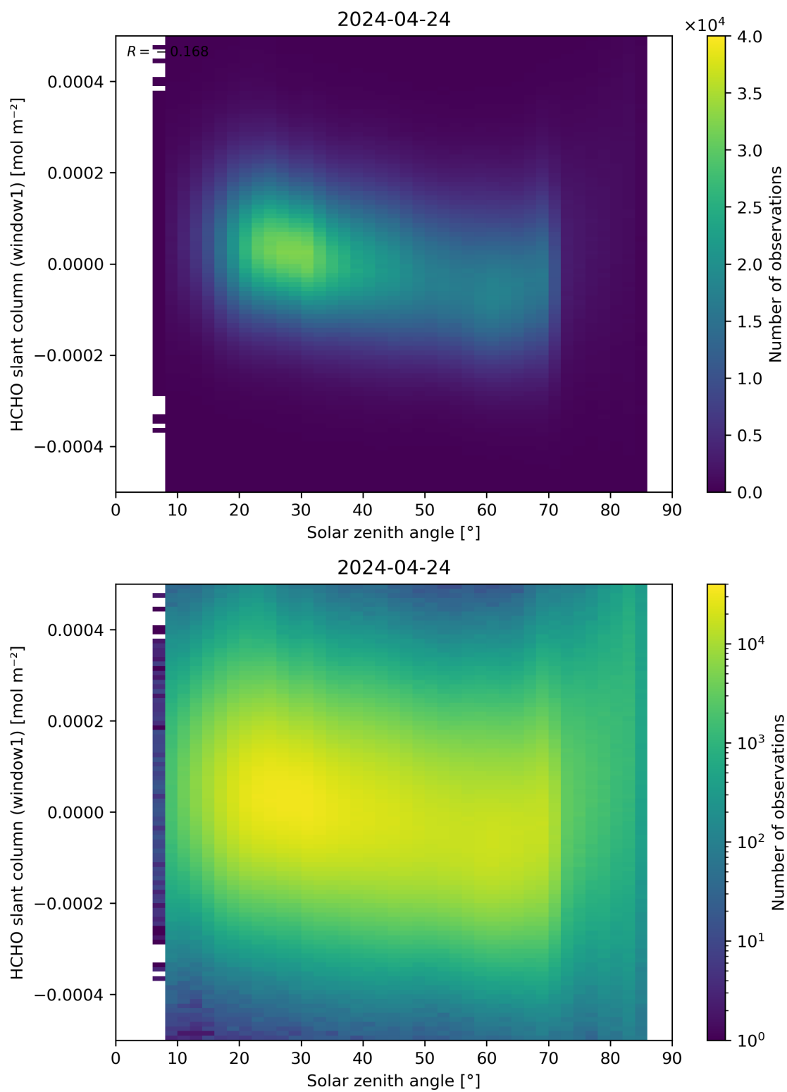
Figure 173: Scatter density plot of “Solar zenith angle” against “HCHO slant column (window1)” for 2024-04-23 to 2024-04-25.
