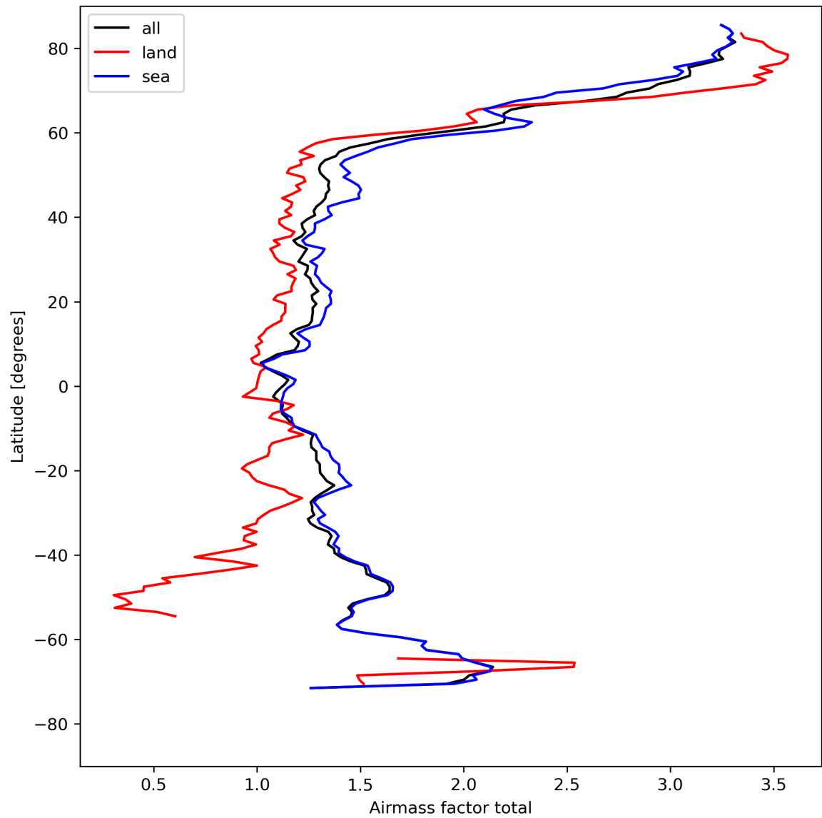
Figure 26: Zonal average of “Airmass factor total” for 2024-04-23 to 2024-04-25.
