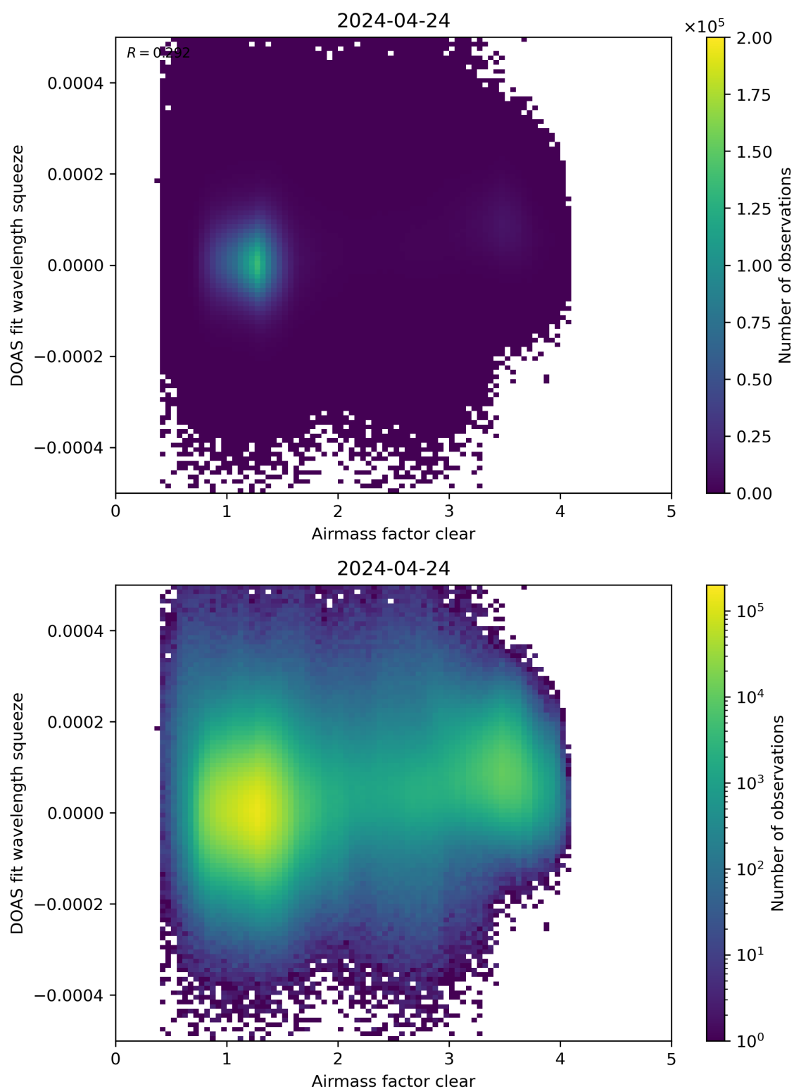
Figure 73: Scatter density plot of “Airmass factor clear” against “DOAS fit wavelength squeeze” for 2024-04-23 to 2024-04-25.
