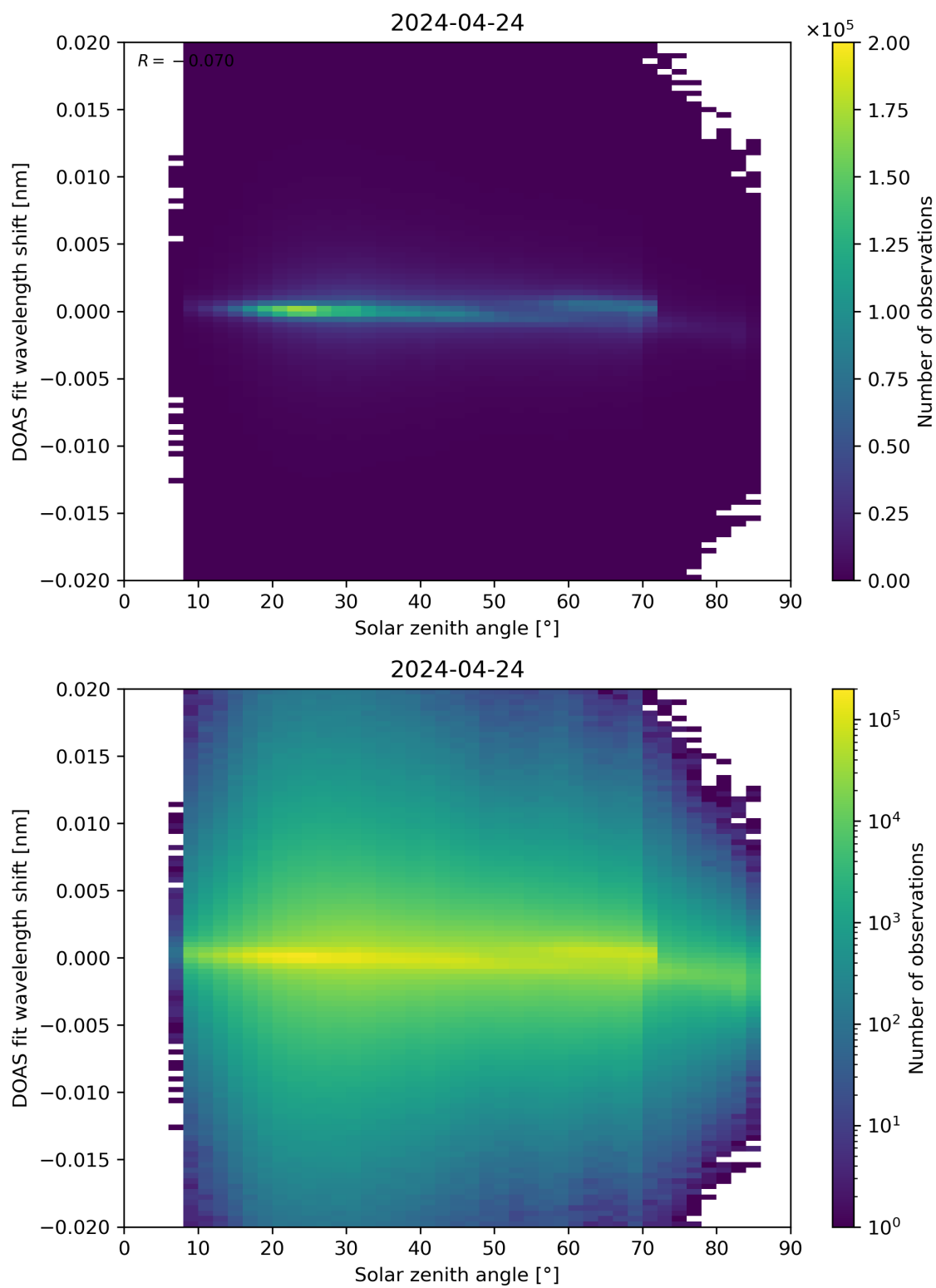
Figure 168: Scatter density plot of “Solar zenith angle” against “DOAS fit wavelength shift” for 2024-04-23 to 2024-04-25.
