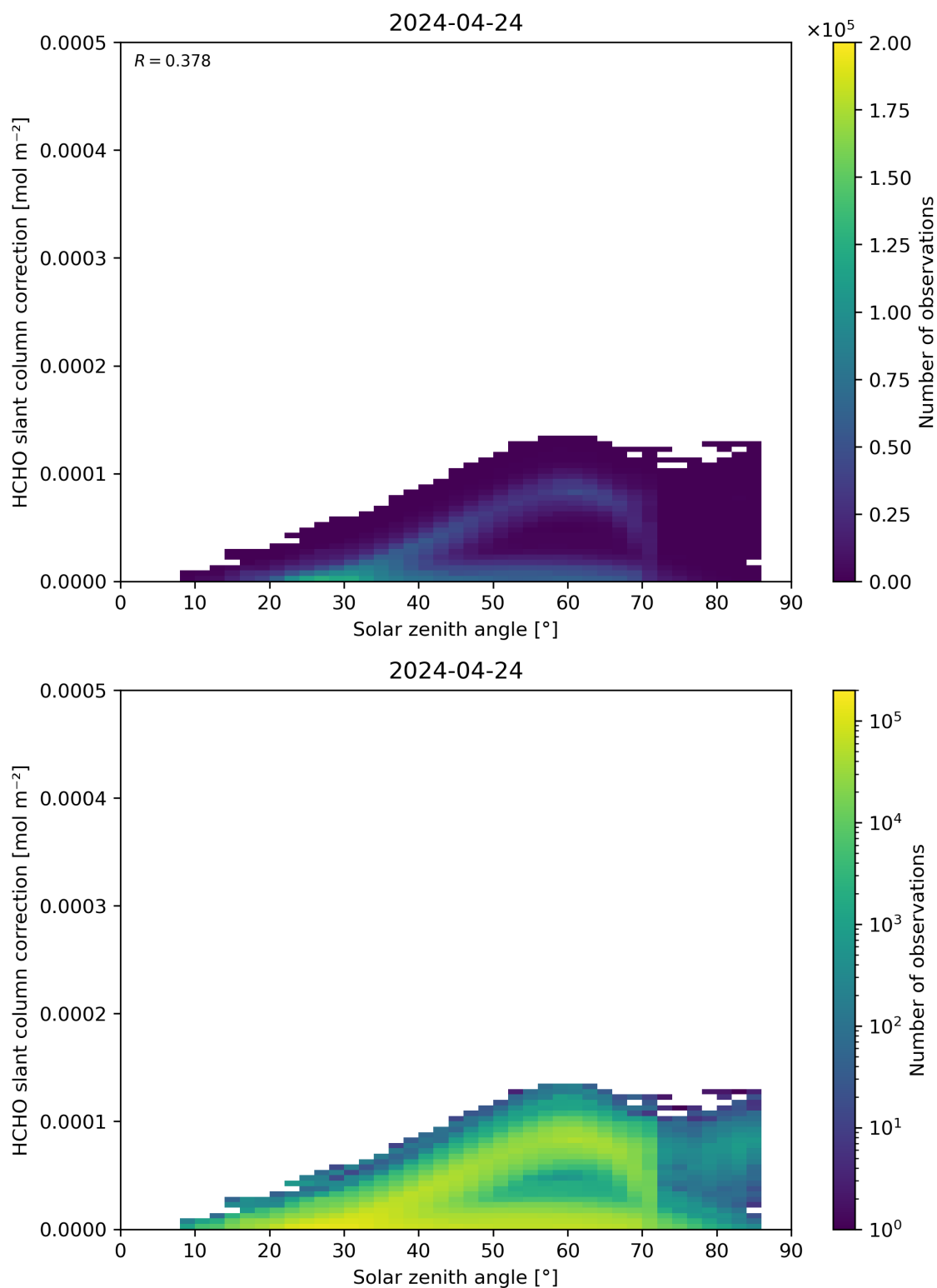
Figure 172: Scatter density plot of “Solar zenith angle” against “HCHO slant column correction” for 2024-04-23 to 2024-04-25.
