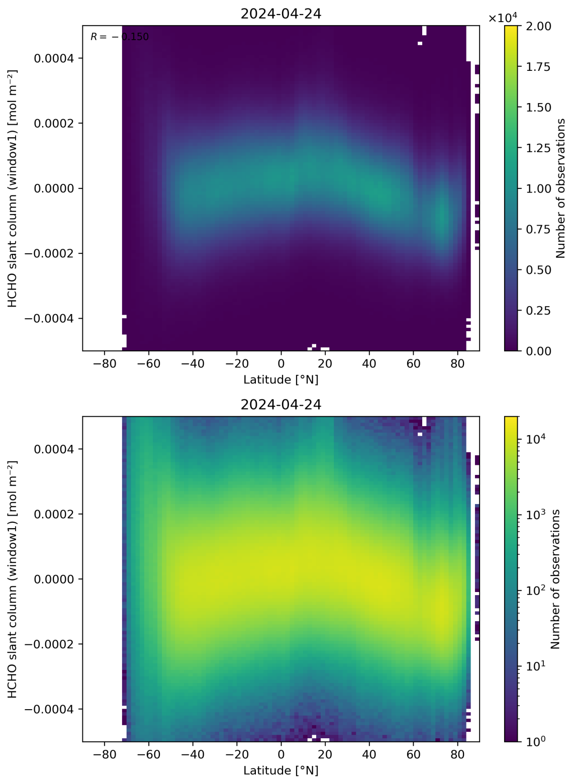
Figure 159: Scatter density plot of “Latitude” against “HCHO slant column (window1)” for 2024-04-23 to 2024-04-25.
