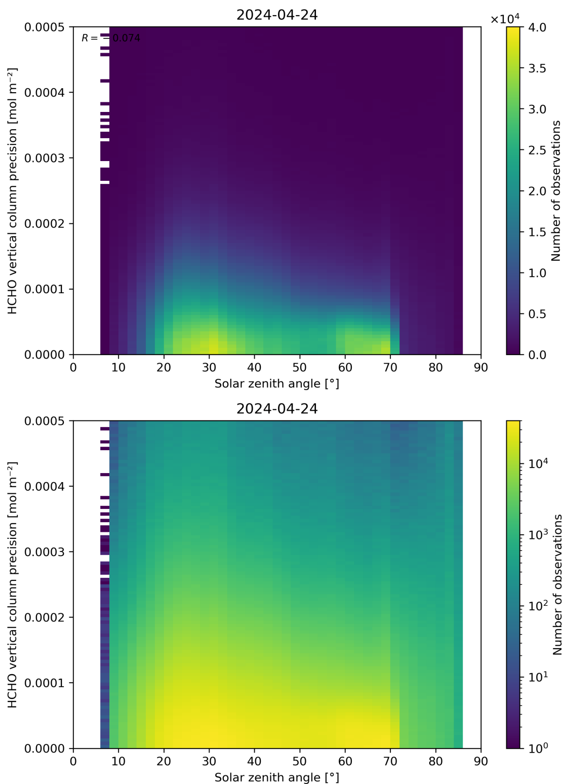
Figure 179: Scatter density plot of “Solar zenith angle” against “HCHO vertical column precision” for 2024-04-23 to 2024-04-25.
