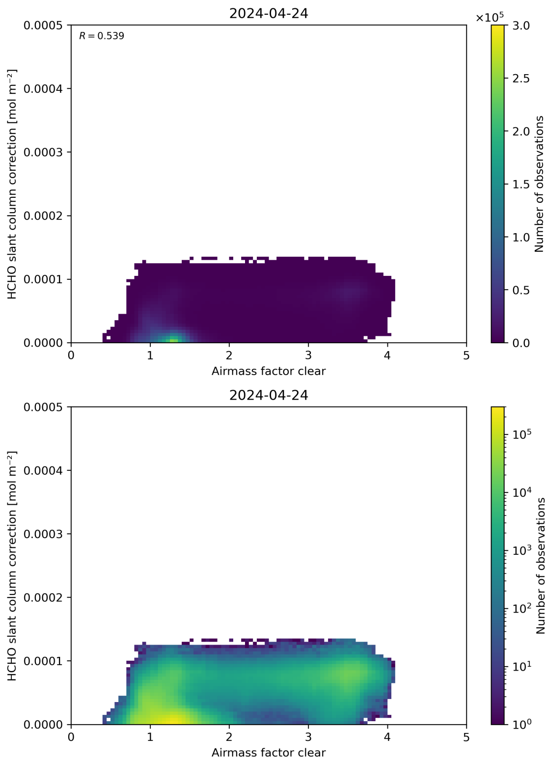
Figure 75: Scatter density plot of “Airmass factor clear” against “HCHO slant column correction” for 2024-04-23 to 2024-04-25.
