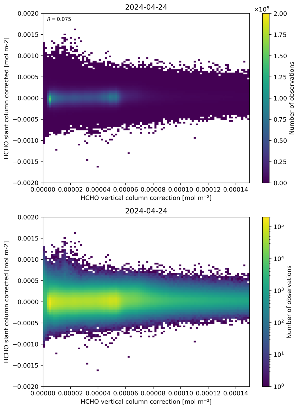
Figure 116: Scatter density plot of “HCHO vertical column correction” against “HCHO slant column corrected” for 2024-04-23 to 2024-04-25.
