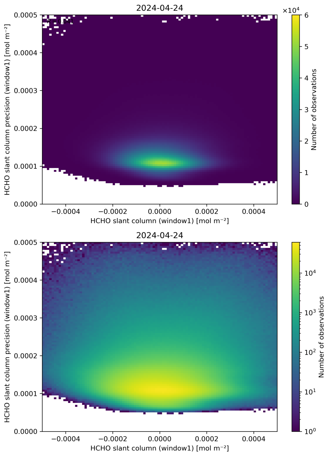
Figure 84: Scatter density plot of “HCHO slant column (window1)” against “HCHO slant column precision (window1)” for 2024-04-23 to 2024-04-25.
