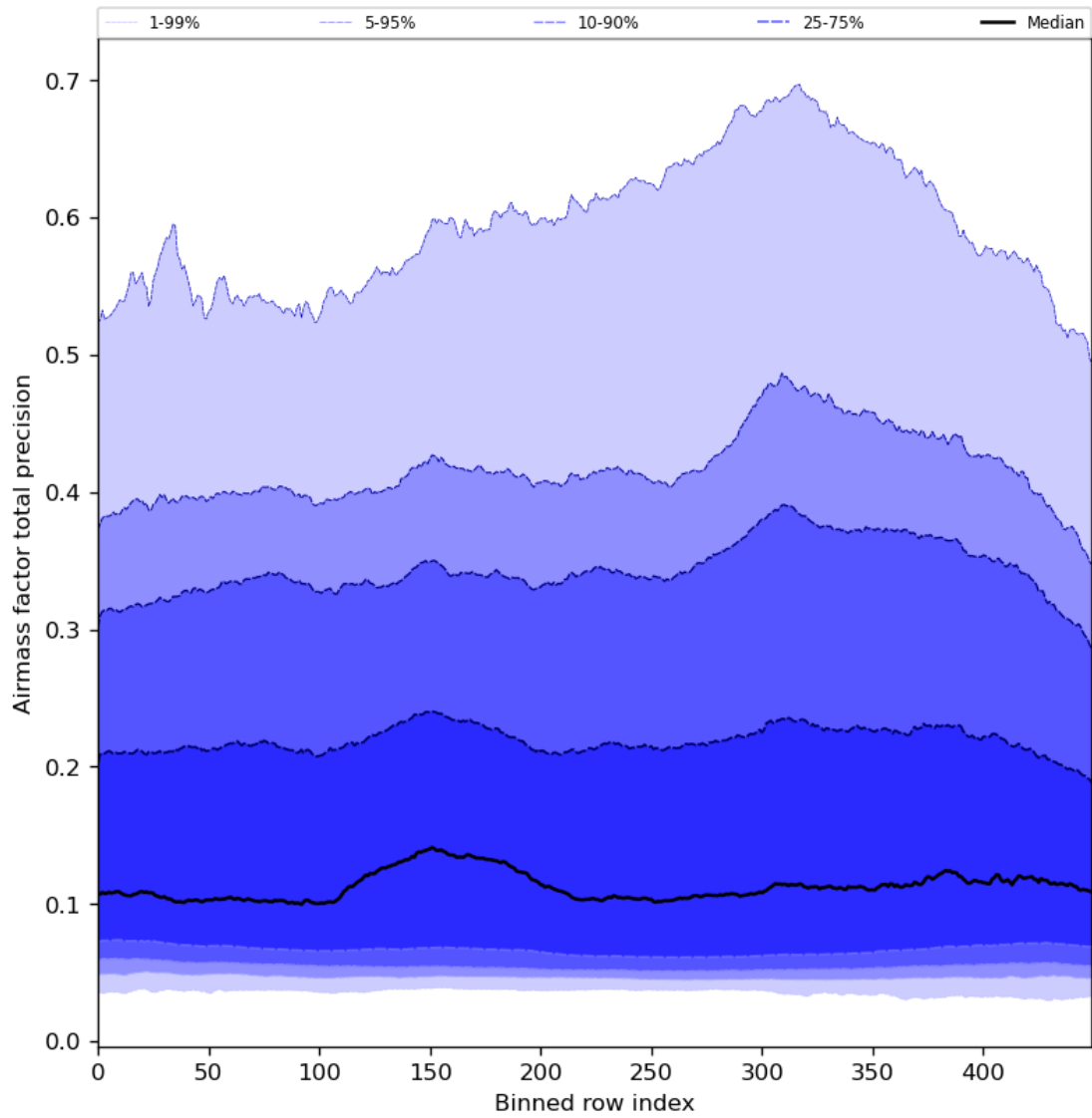
Figure 55: Along track statistics of “Airmass factor total precision” for 2024-04-23 to 2024-04-25
