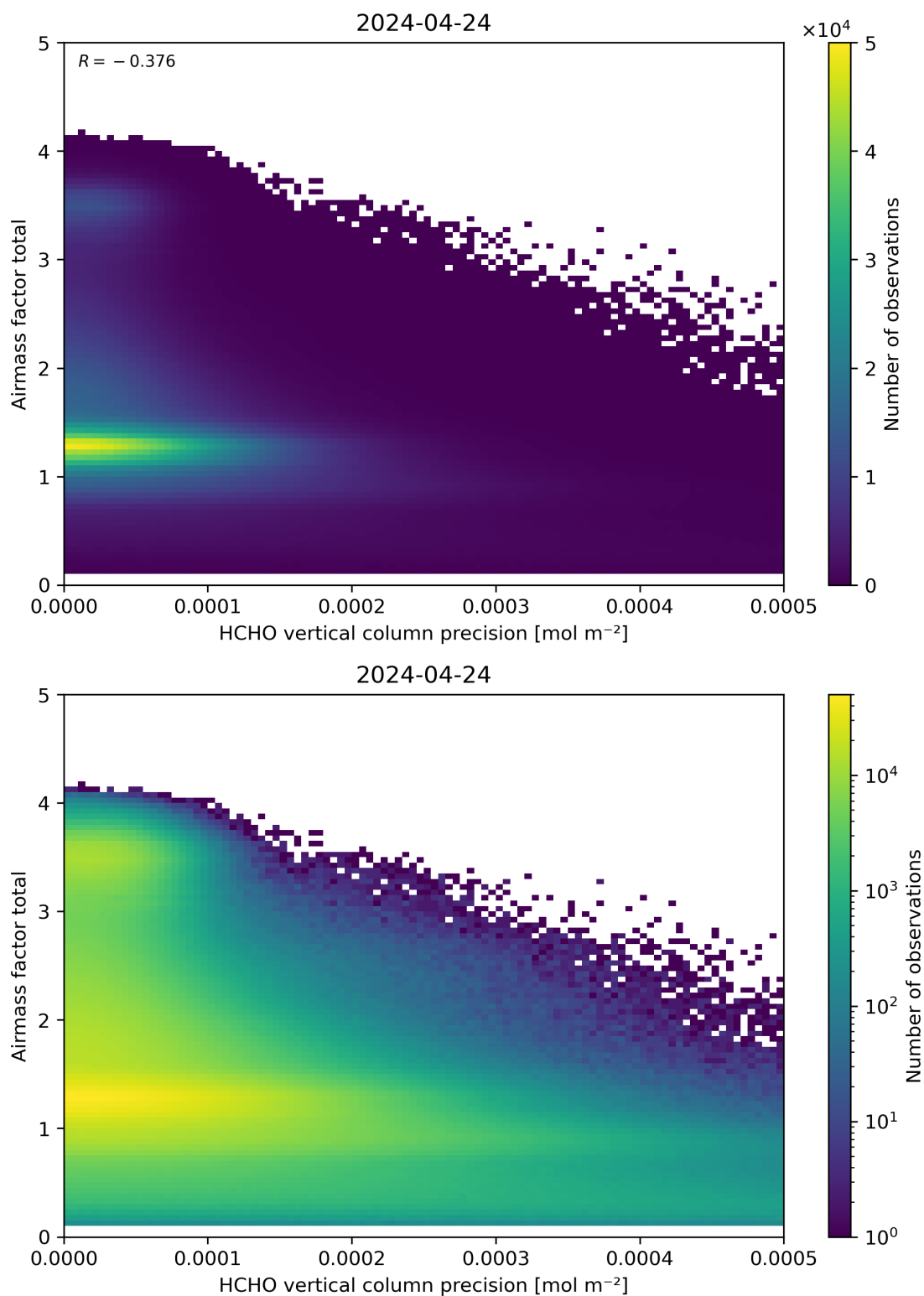
Figure 144: Scatter density plot of “HCHO vertical column precision” against “Airmass factor total” for 2024-04-23 to 2024-04-25.
