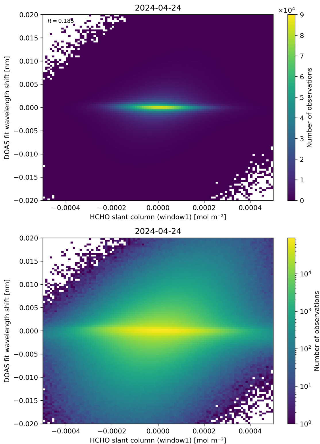
Figure 79: Scatter density plot of “HCHO slant column (window1)” against “DOAS fit wavelength shift” for 2024-04-23 to 2024-04-25.
