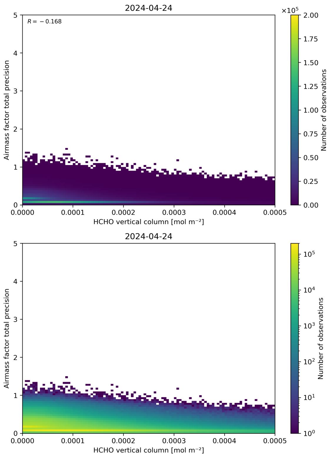
Figure 132: Scatter density plot of “HCHO vertical column” against “Airmass factor total precision” for 2024-04-23 to 2024-04-25.
