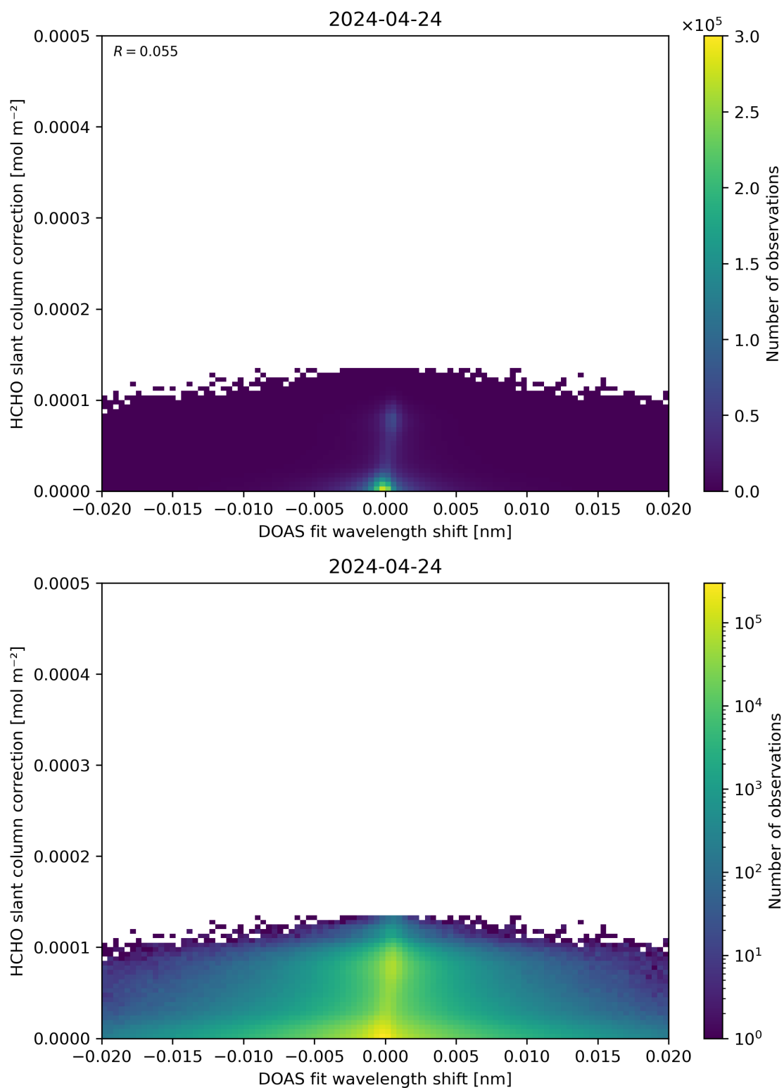
Figure 67: Scatter density plot of “DOAS fit wavelength shift” against “HCHO slant column correction” for 2024-04-23 to 2024-04-25.
