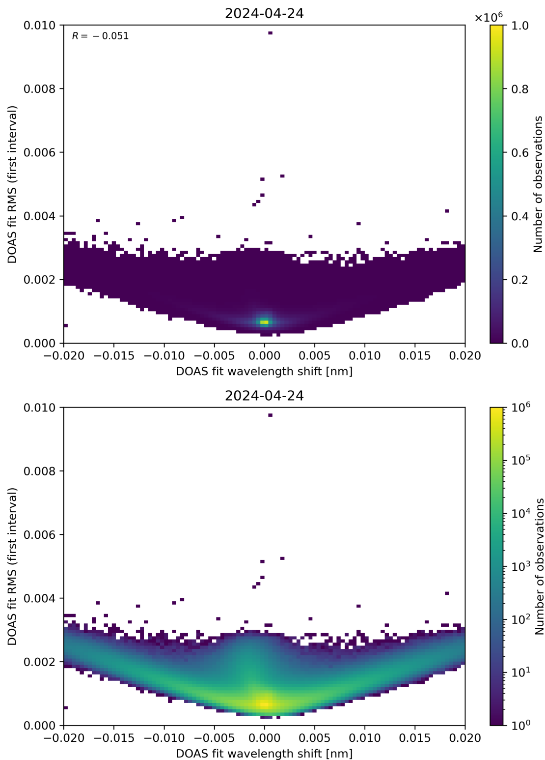
Figure 64: Scatter density plot of “DOAS fit wavelength shift” against “DOAS fit RMS (first interval)” for 2024-04-23 to 2024-04-25.
