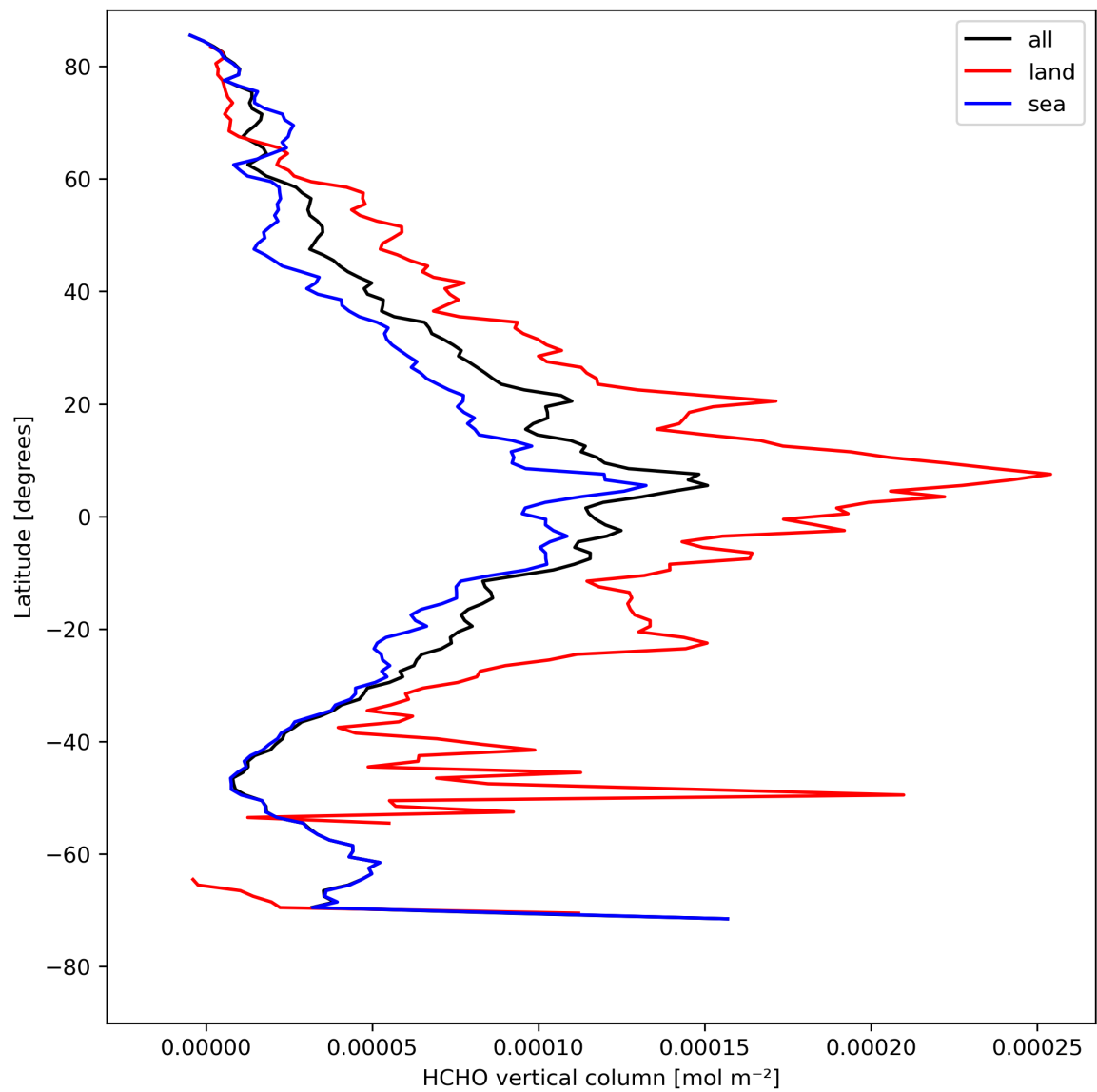
Figure 21: Zonal average of “HCHO vertical column” for 2024-04-23 to 2024-04-25.
