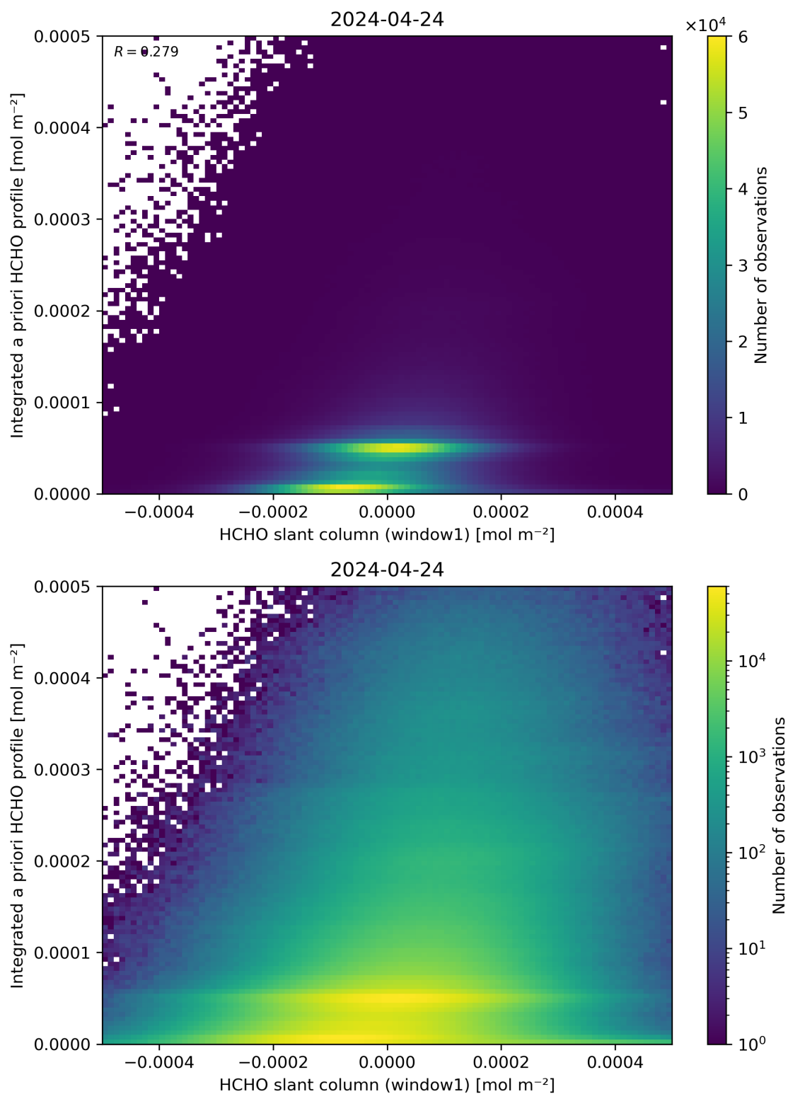
Figure 87: Scatter density plot of “HCHO slant column (window1)” against “Integrated a priori HCHO profile” for 2024-04-23 to 2024-04-25.
