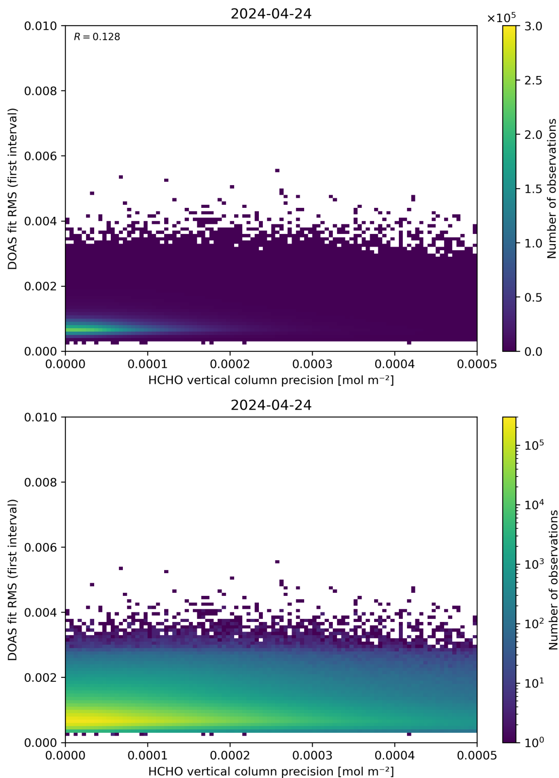
Figure 136: Scatter density plot of “HCHO vertical column precision” against “DOAS fit RMS (first interval)” for 2024-04-23 to 2024-04-25.
