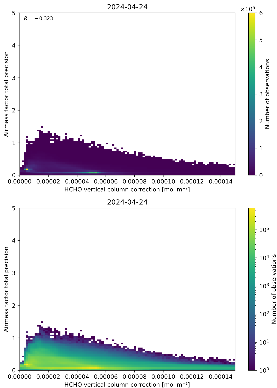
Figure 121: Scatter density plot of “HCHO vertical column correction” against “Airmass factor total precision” for 2024-04-23 to 2024-04-25.
