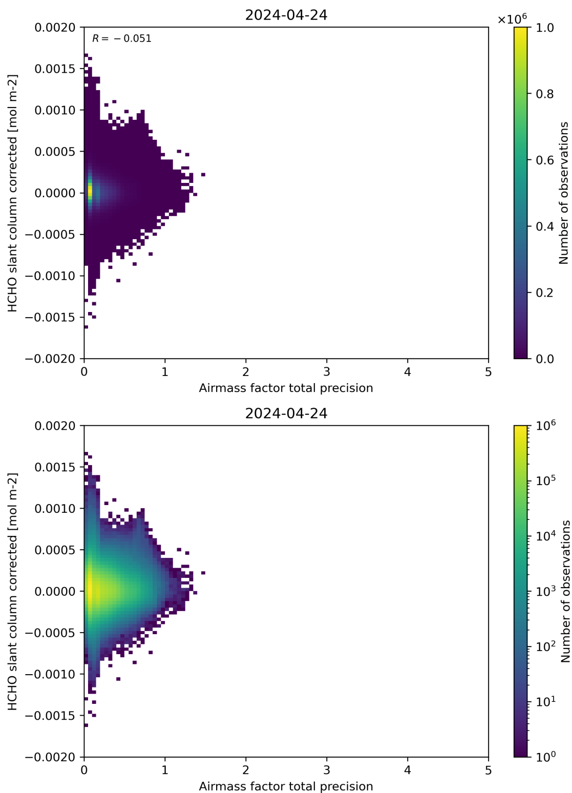
Figure 109: Scatter density plot of “Airmass factor total precision” against “HCHO slant column corrected” for 2024-04-23 to 2024-04-25.
