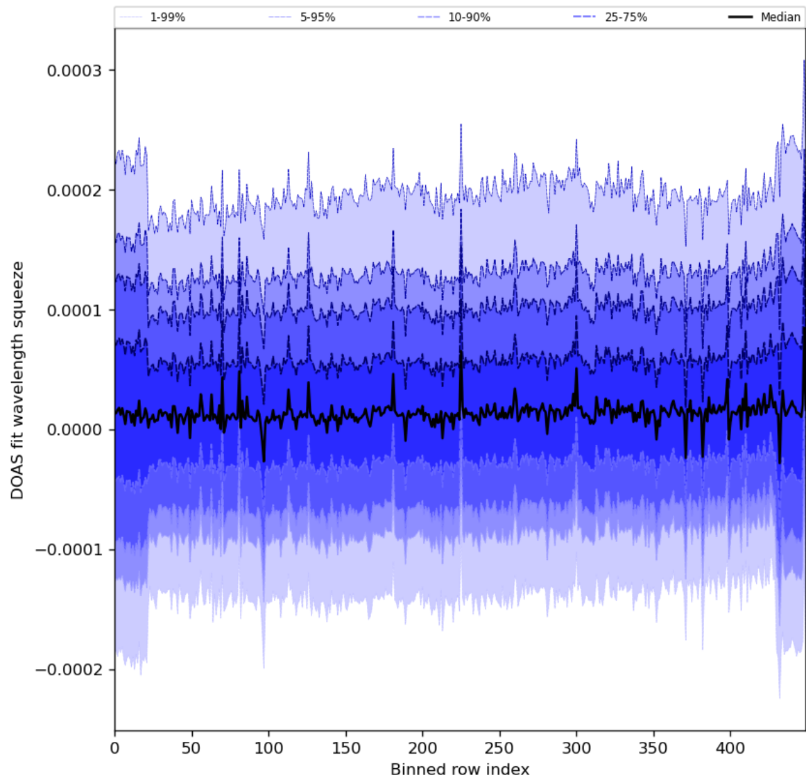
Figure 59: Along track statistics of “DOAS fit wavelength squeeze” for 2024-04-23 to 2024-04-25
