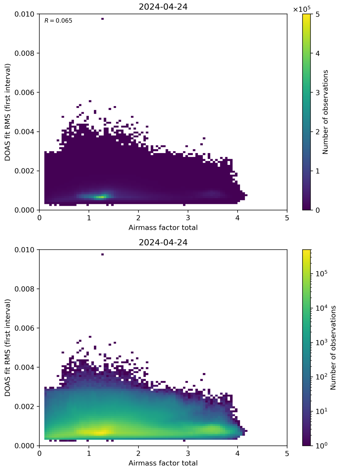
Figure 97: Scatter density plot of “Airmass factor total” against “DOAS fit RMS (first interval)” for 2024-04-23 to 2024-04-25.
