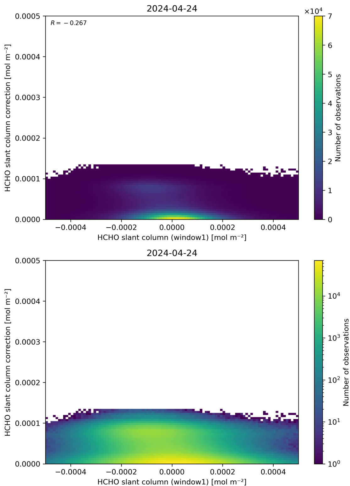
Figure 83: Scatter density plot of “HCHO slant column (window1)” against “HCHO slant column correction” for 2024-04-23 to 2024-04-25.
