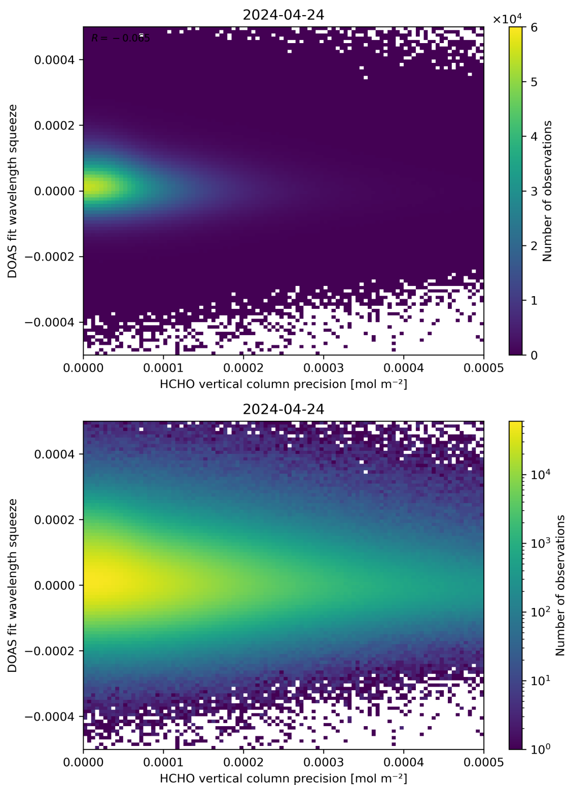
Figure 138: Scatter density plot of “HCHO vertical column precision” against “DOAS fit wavelength squeeze” for 2024-04-23 to 2024-04-25.
