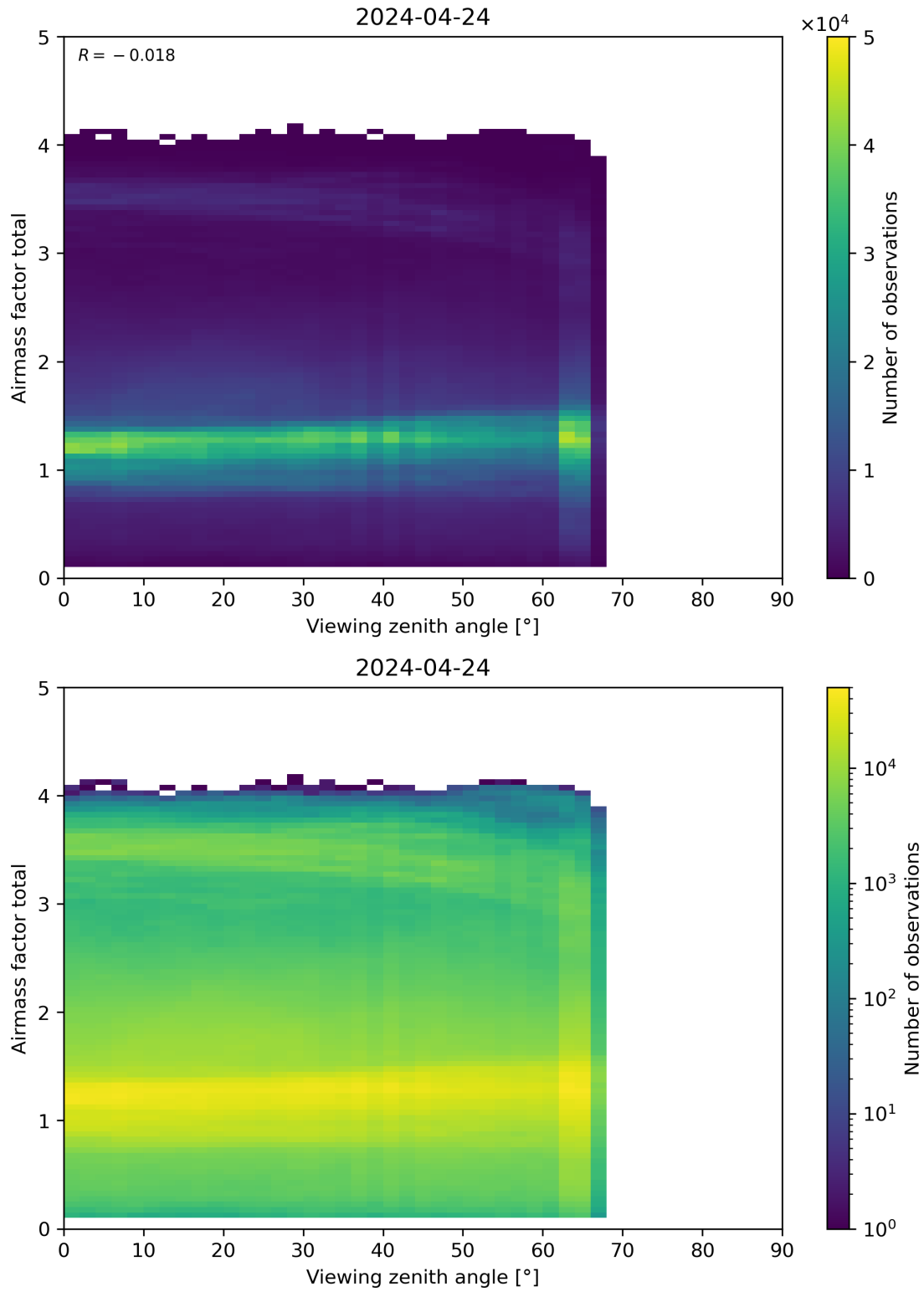
Figure 190: Scatter density plot of “Viewing zenith angle” against “Airmass factor total” for 2024-04-23 to 2024-04-25.
