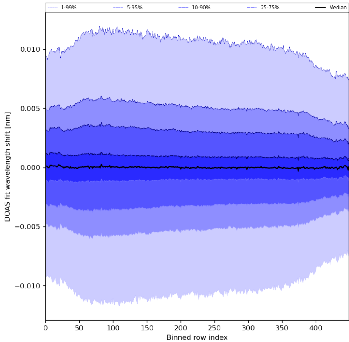
Figure 58: Along track statistics of “DOAS fit wavelength shift” for 2024-04-23 to 2024-04-25
