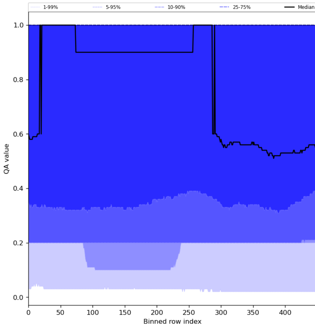
Figure 48: Along track statistics of “QA value” for 2024-04-23 to 2024-04-25
