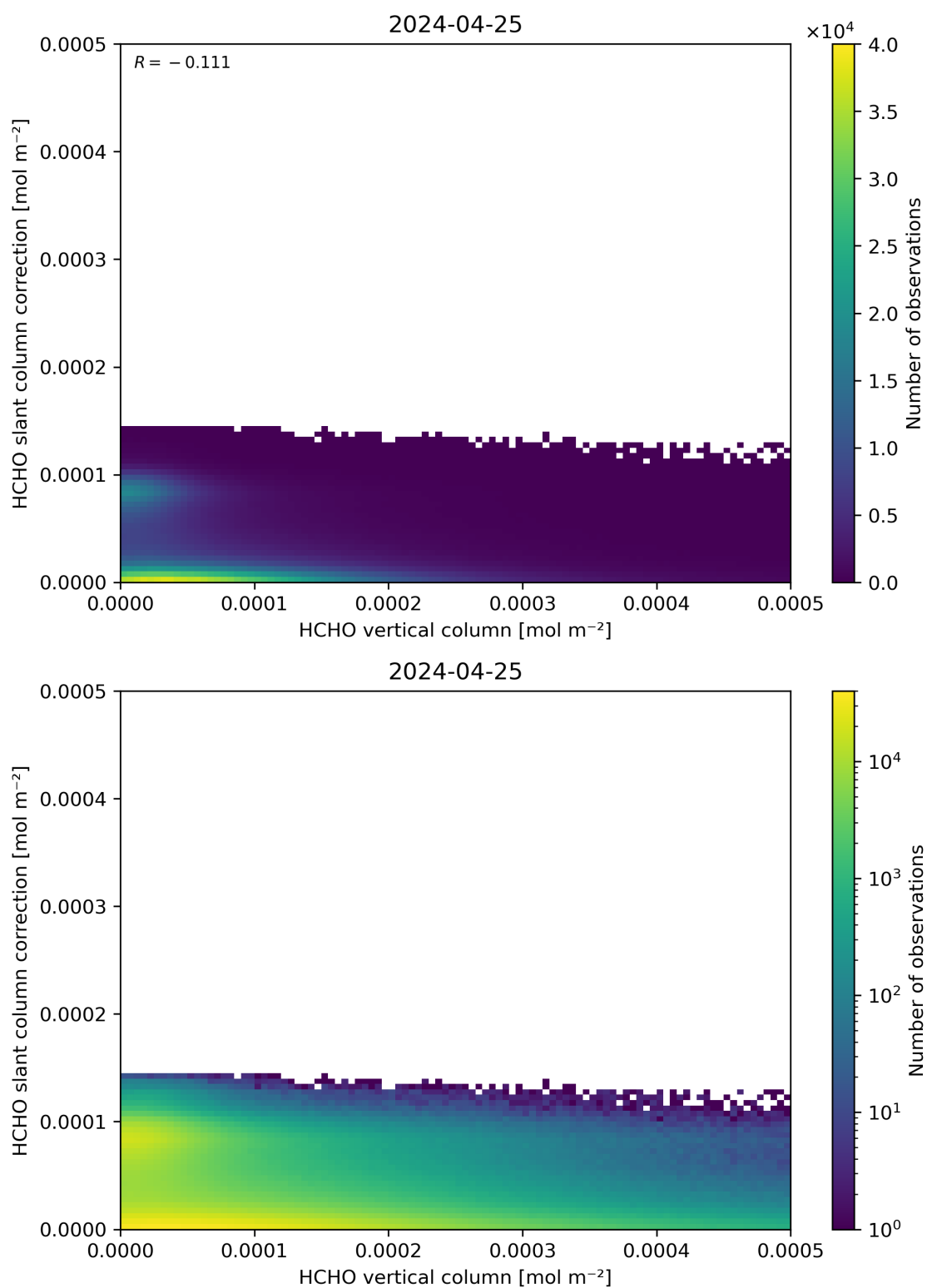
Figure 128: Scatter density plot of “HCHO vertical column” against “HCHO slant column correction” for 2024-04-24 to 2024-04-26.
