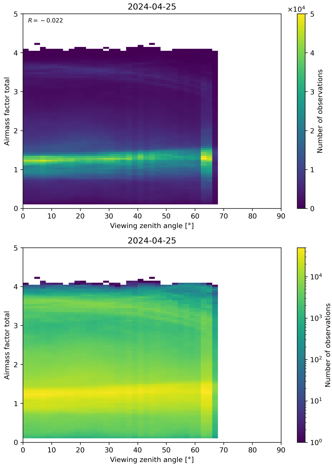
Figure 190: Scatter density plot of “Viewing zenith angle” against “Airmass factor total” for 2024-04-24 to 2024-04-26.
