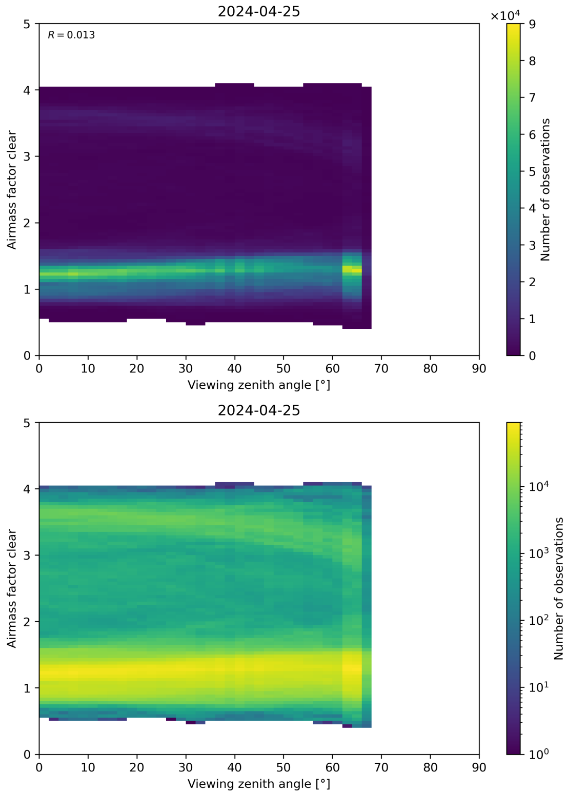
Figure 185: Scatter density plot of “Viewing zenith angle” against “Airmass factor clear” for 2024-04-24 to 2024-04-26.
