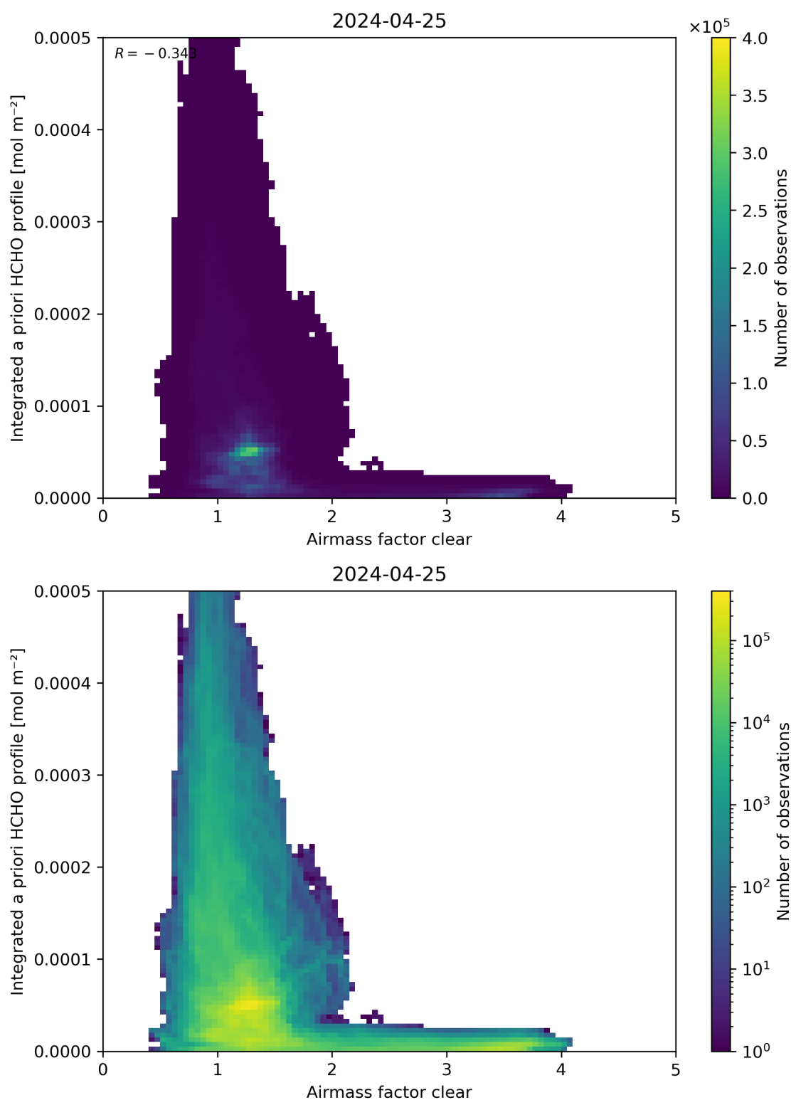
Figure 76: Scatter density plot of “Airmass factor clear” against “Integrated a priori HCHO profile” for 2024-04-24 to 2024-04-26.
