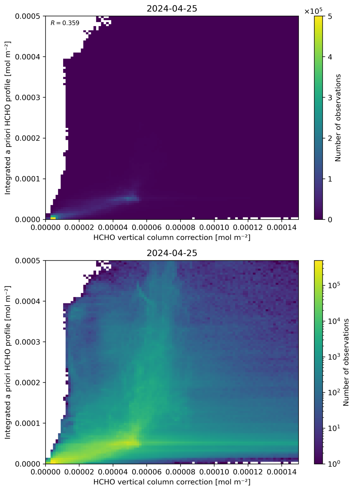
Figure 122: Scatter density plot of “HCHO vertical column correction” against “Integrated a priori HCHO profile” for 2024-04-24 to 2024-04-26.
