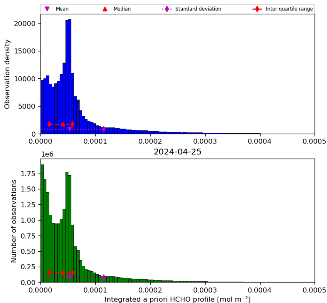
Figure 43: Histogram of “Integrated a priori HCHO profile” for 2024-04-24 to 2024-04-26
