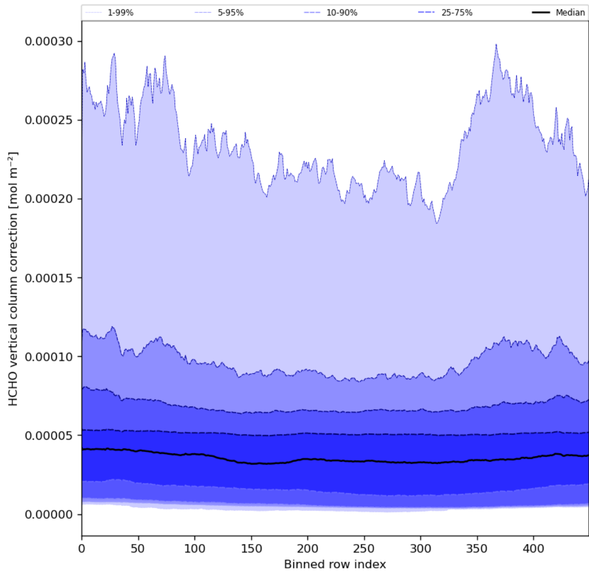
Figure 51: Along track statistics of “HCHO vertical column correction” for 2024-04-24 to 2024-04-26
