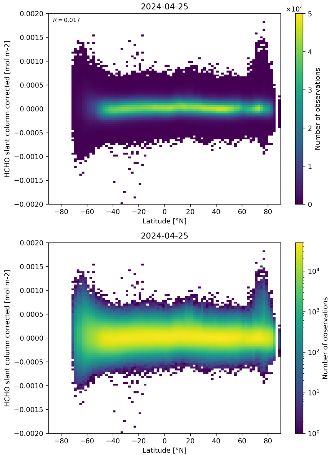
Figure 157: Scatter density plot of “Latitude” against “HCHO slant column corrected” for 2024-04-24 to 2024-04-26.
