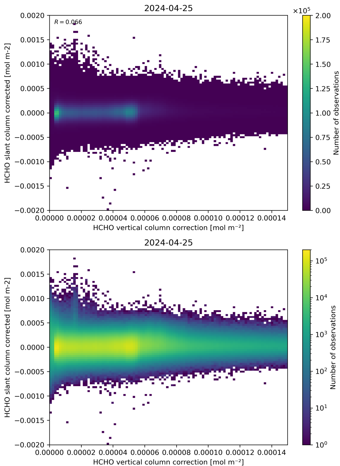
Figure 116: Scatter density plot of “HCHO vertical column correction” against “HCHO slant column corrected” for 2024-04-24 to 2024-04-26.
