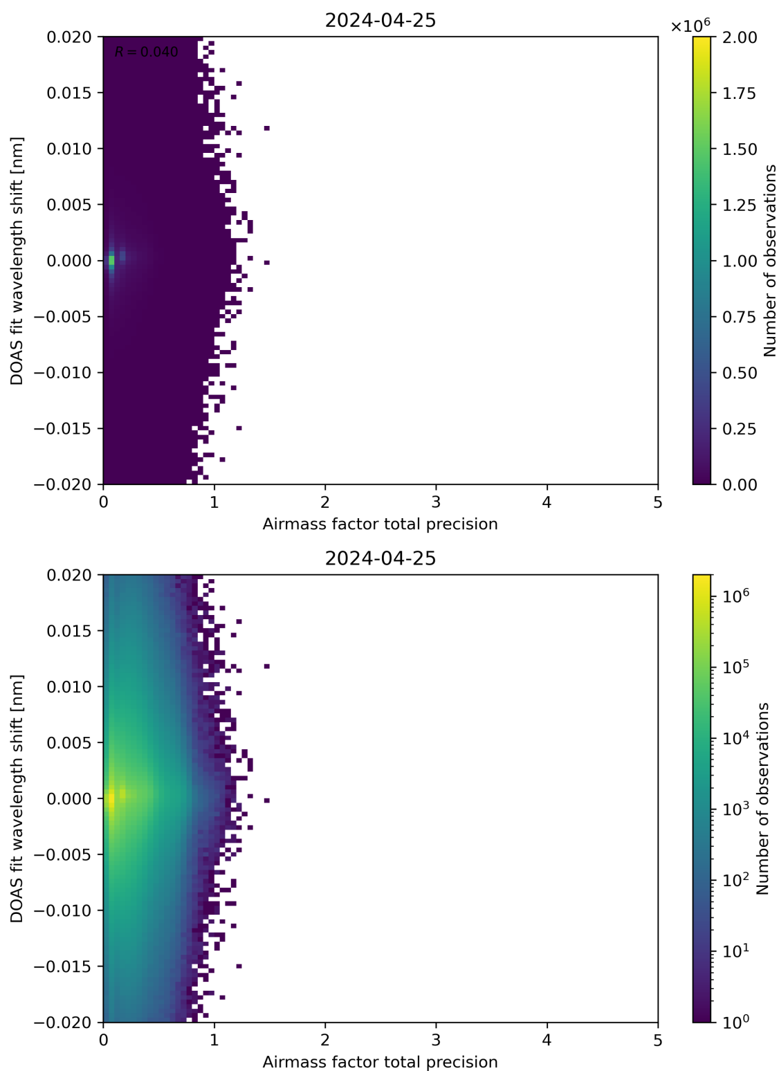
Figure 106: Scatter density plot of “Airmass factor total precision” against “DOAS fit wavelength shift” for 2024-04-24 to 2024-04-26.
