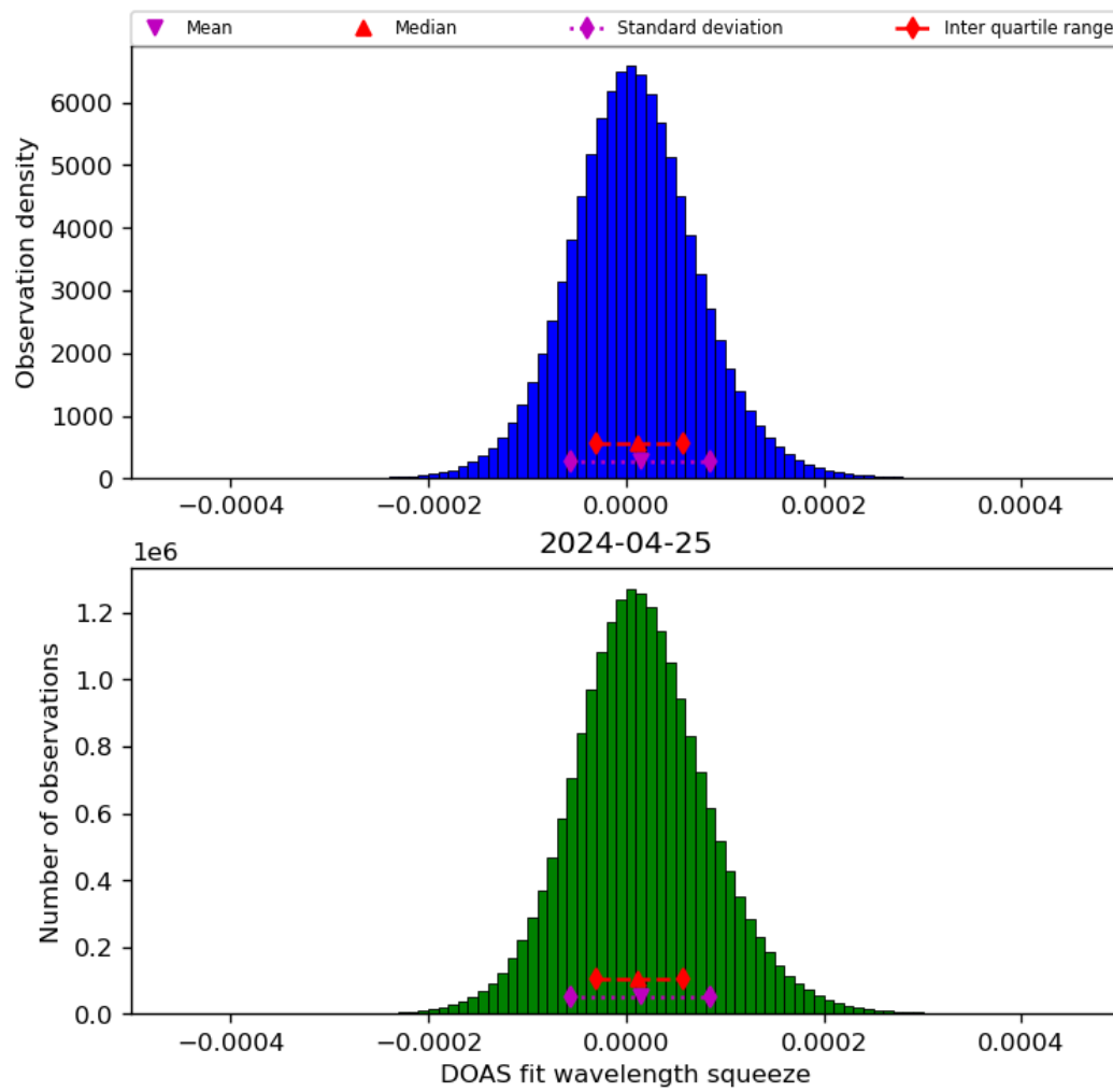
Figure 45: Histogram of “DOAS fit wavelength squeeze” for 2024-04-24 to 2024-04-26
