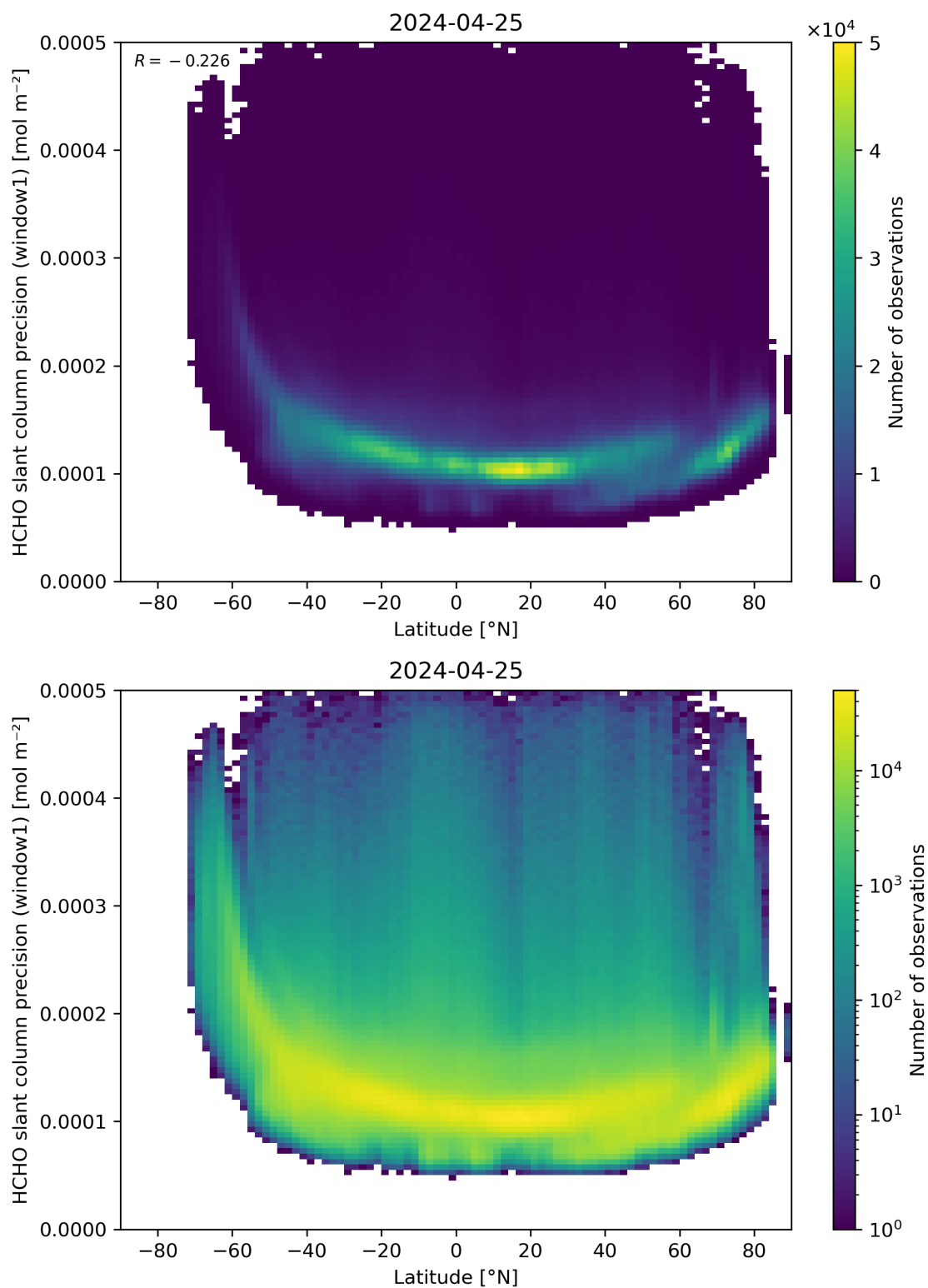
Figure 160: Scatter density plot of “Latitude” against “HCHO slant column precision (window1)” for 2024-04-24 to 2024-04-26.
