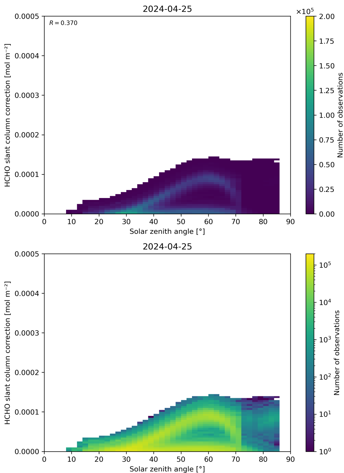
Figure 172: Scatter density plot of “Solar zenith angle” against “HCHO slant column correction” for 2024-04-24 to 2024-04-26.
