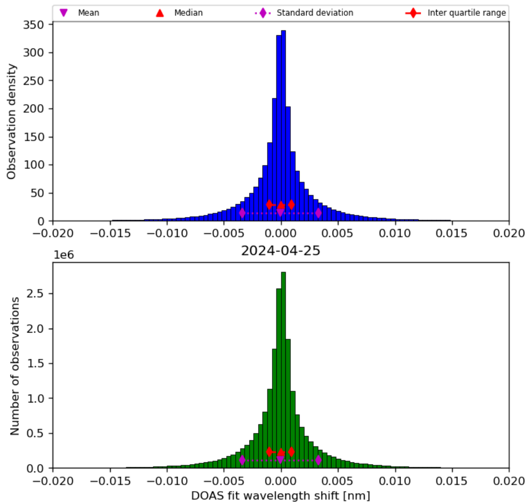
Figure 44: Histogram of “DOAS fit wavelength shift” for 2024-04-24 to 2024-04-26
