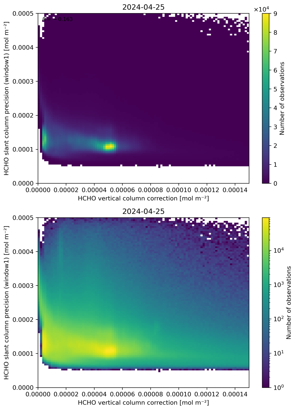
Figure 119: Scatter density plot of “HCHO vertical column correction” against “HCHO slant column precision (window1)” for 2024-04-24 to 2024-04-26.
