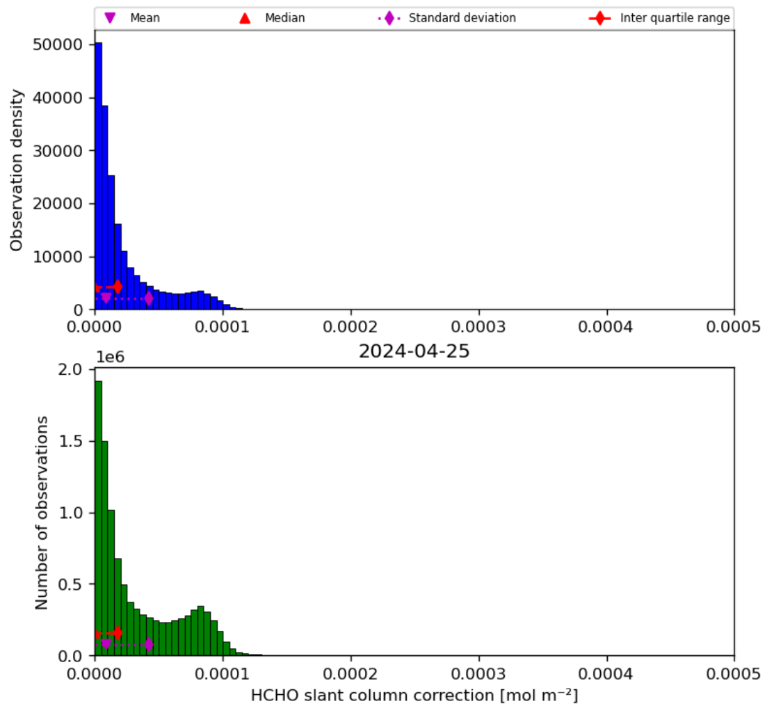
Figure 47: Histogram of “HCHO slant column correction” for 2024-04-24 to 2024-04-26
