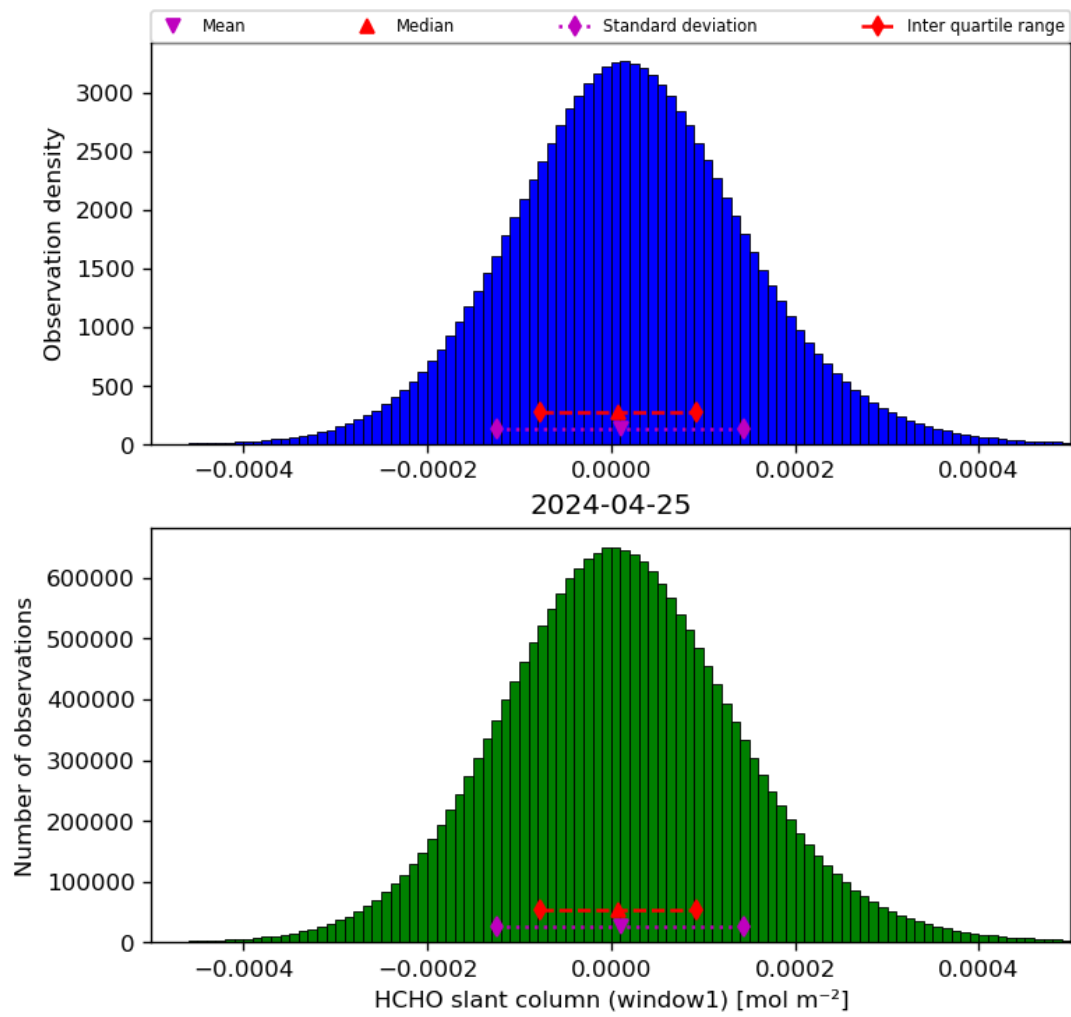
Figure 38: Histogram of “HCHO slant column (window1)” for 2024-04-24 to 2024-04-26
