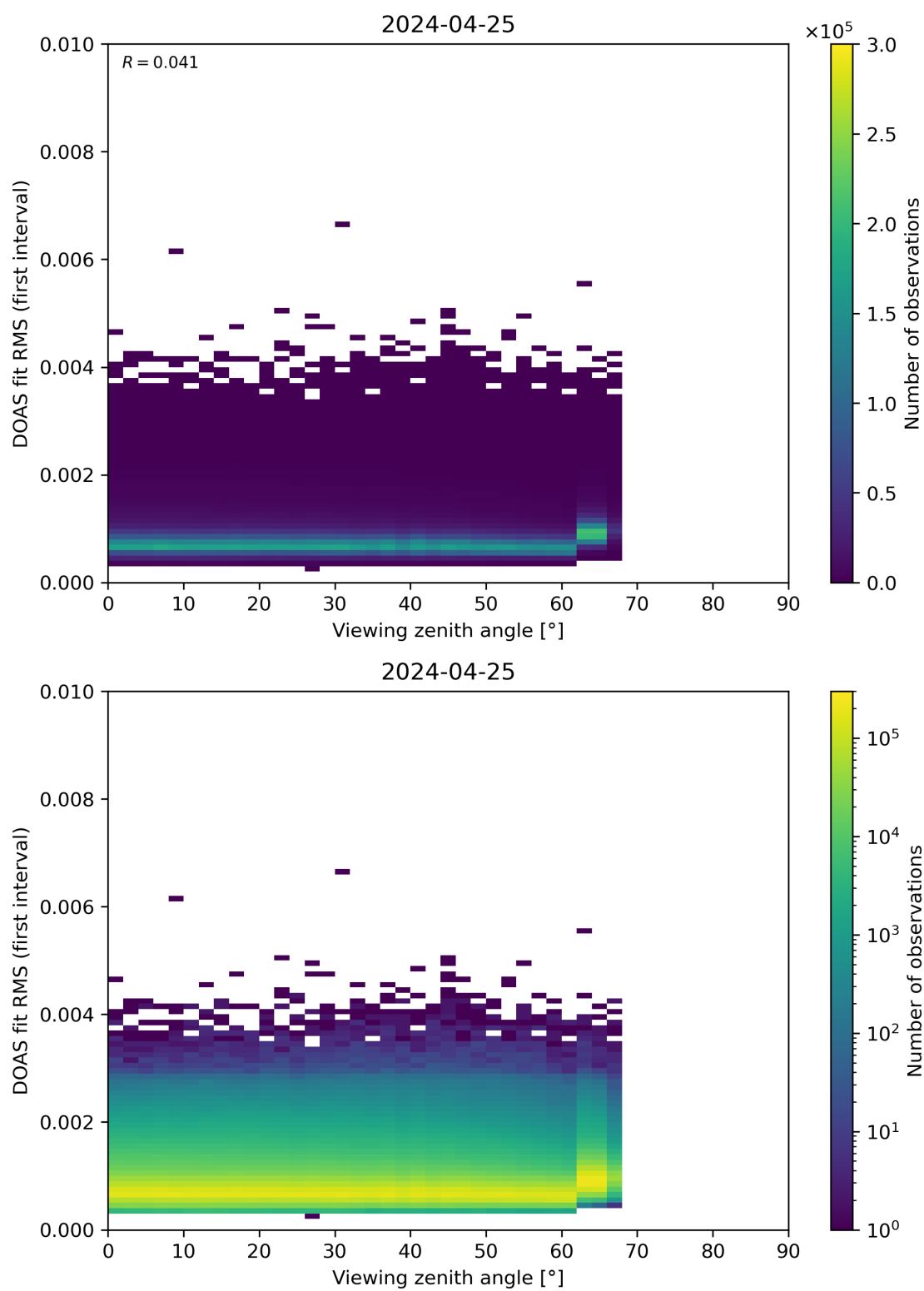
Figure 182: Scatter density plot of “Viewing zenith angle” against “DOAS fit RMS (first interval)” for 2024-04-24 to 2024-04-26.
