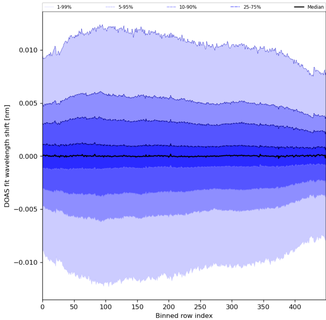
Figure 58: Along track statistics of “DOAS fit wavelength shift” for 2024-04-24 to 2024-04-26
