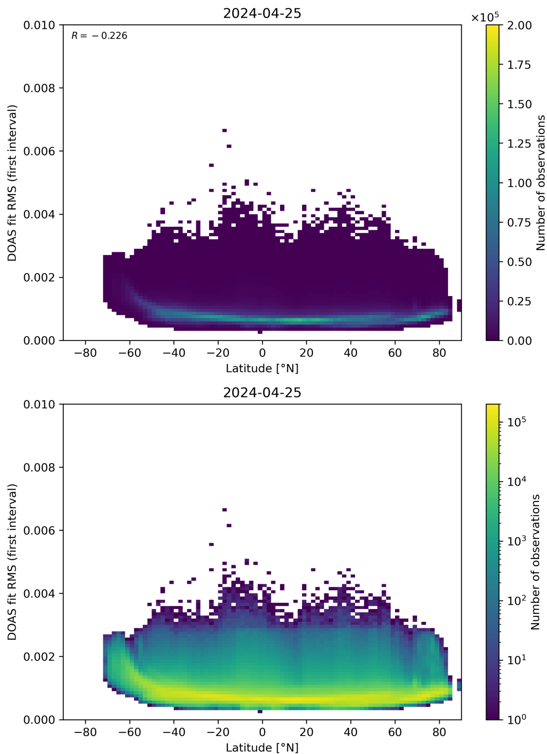
Figure 153: Scatter density plot of “Latitude” against “DOAS fit RMS (first interval)” for 2024-04-24 to 2024-04-26.
