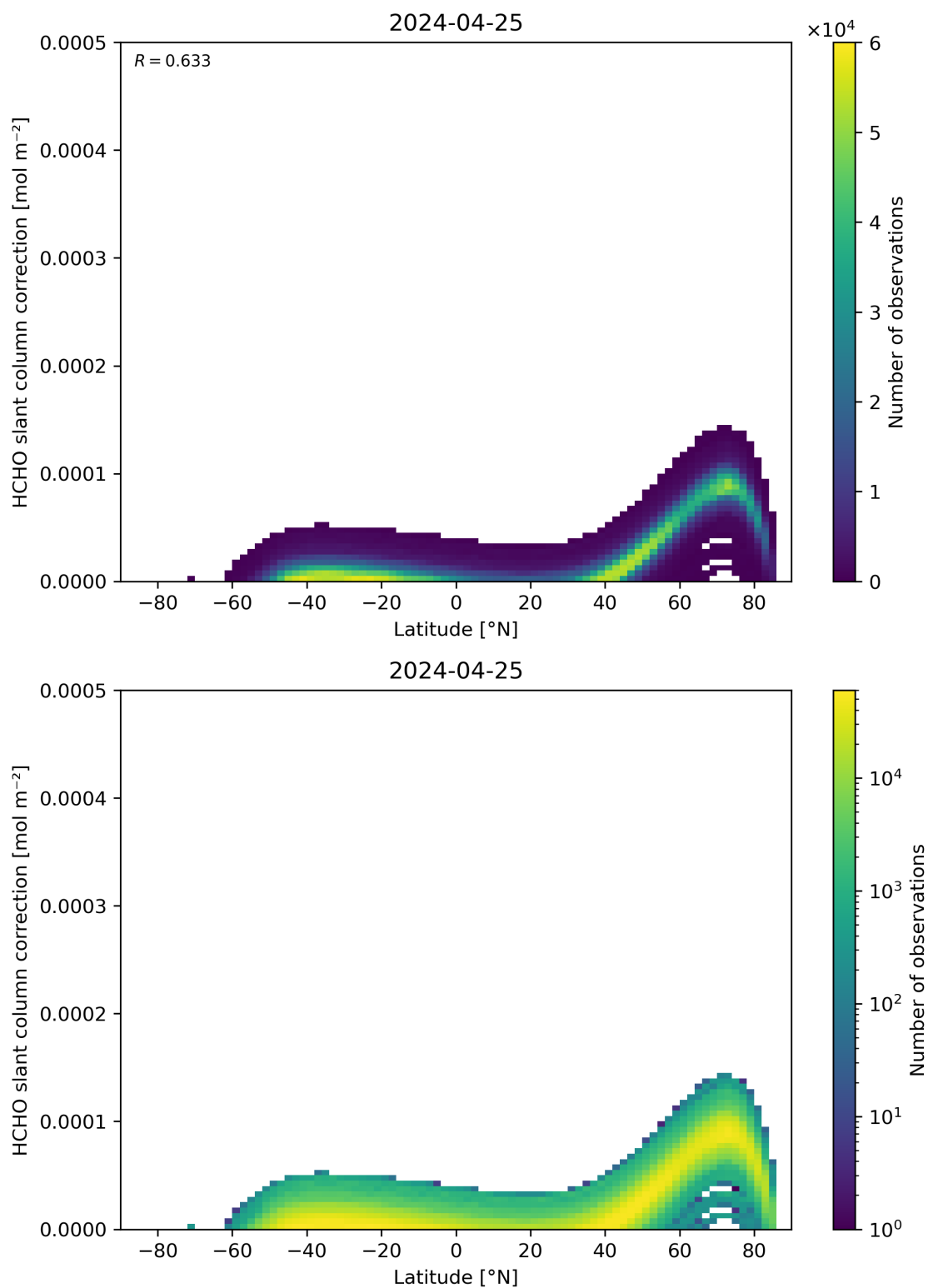
Figure 158: Scatter density plot of “Latitude” against “HCHO slant column correction” for 2024-04-24 to 2024-04-26.
