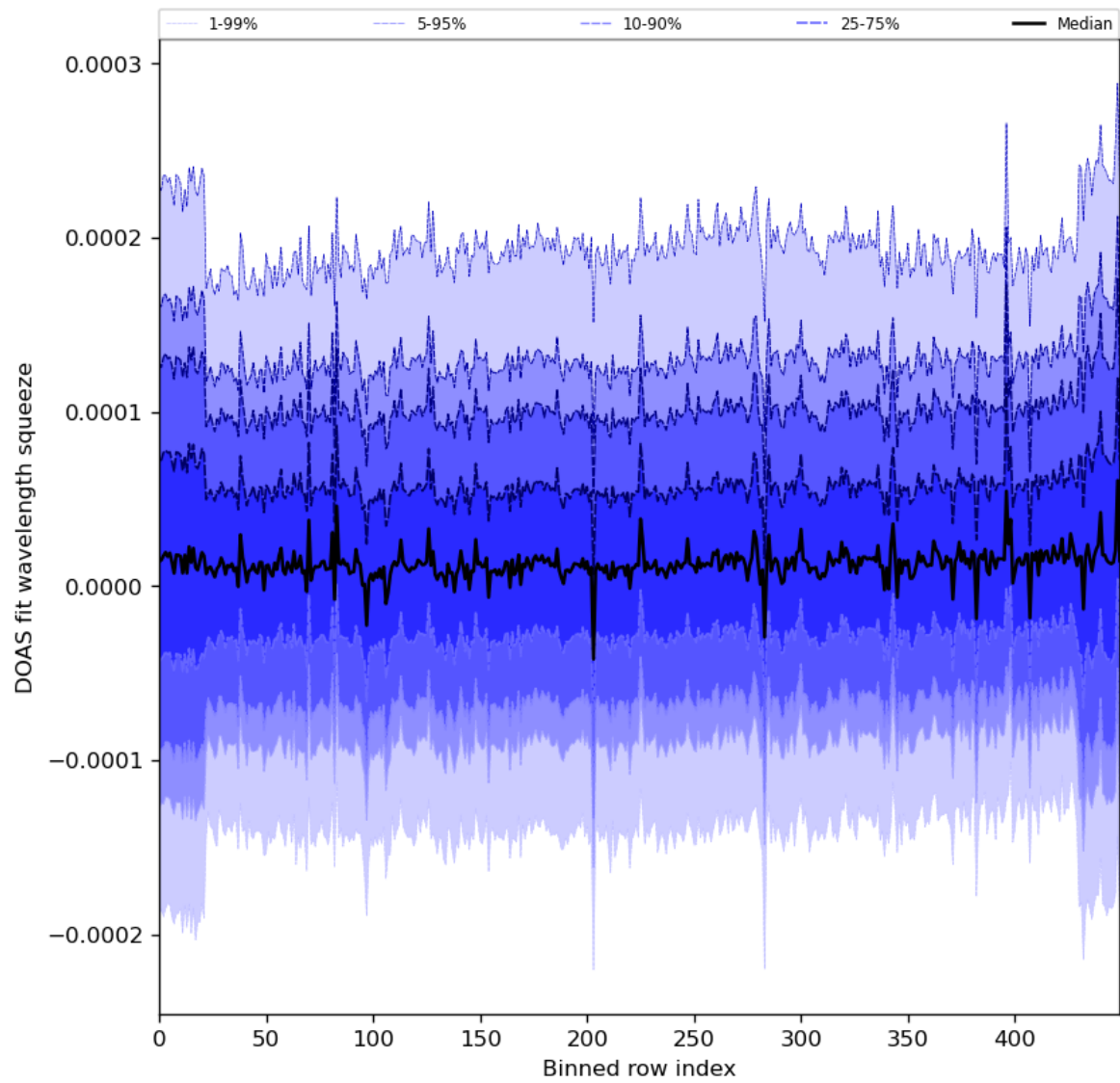
Figure 59: Along track statistics of “DOAS fit wavelength squeeze” for 2024-04-24 to 2024-04-26
