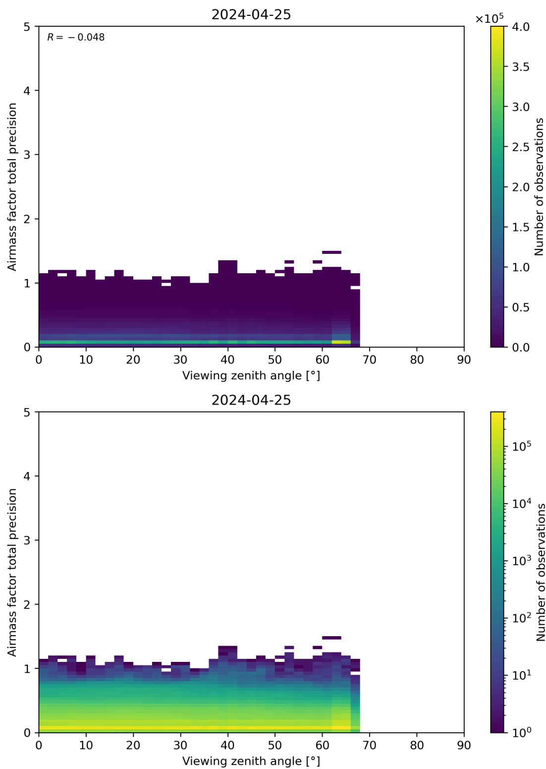
Figure 191: Scatter density plot of “Viewing zenith angle” against “Airmass factor total precision” for 2024-04-24 to 2024-04-26.
