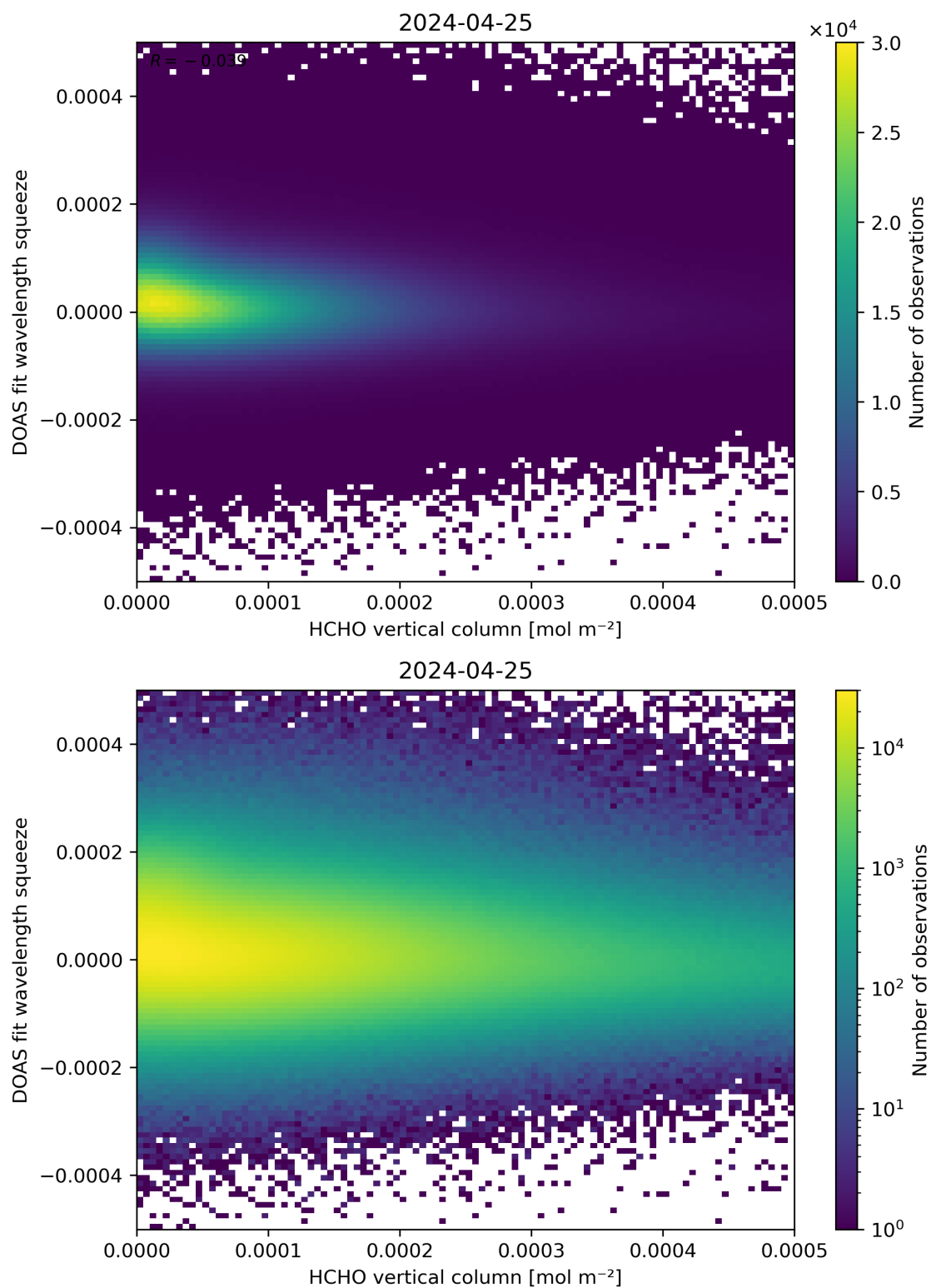
Figure 125: Scatter density plot of “HCHO vertical column” against “DOAS fit wavelength squeeze” for 2024-04-24 to 2024-04-26.
