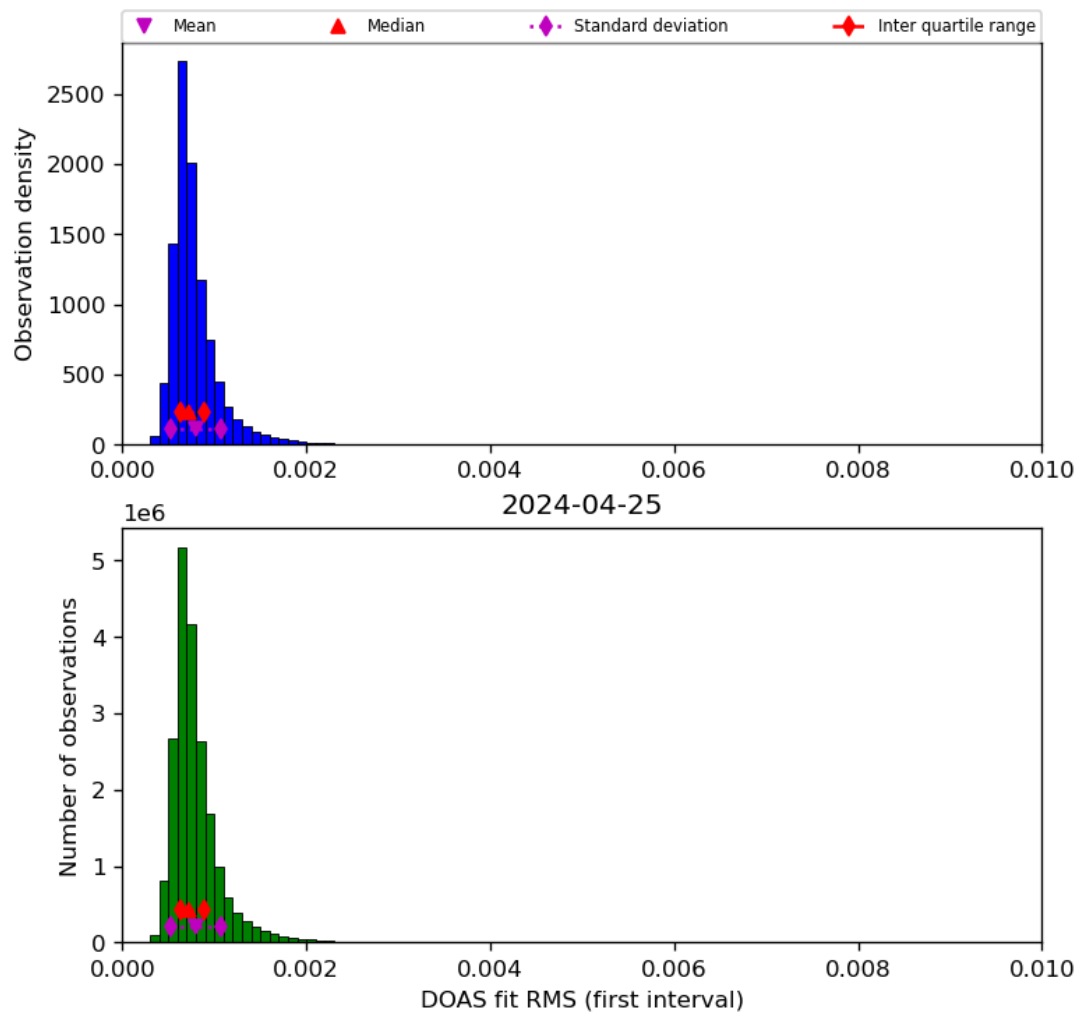
Figure 46: Histogram of “DOAS fit RMS (first interval)” for 2024-04-24 to 2024-04-26
