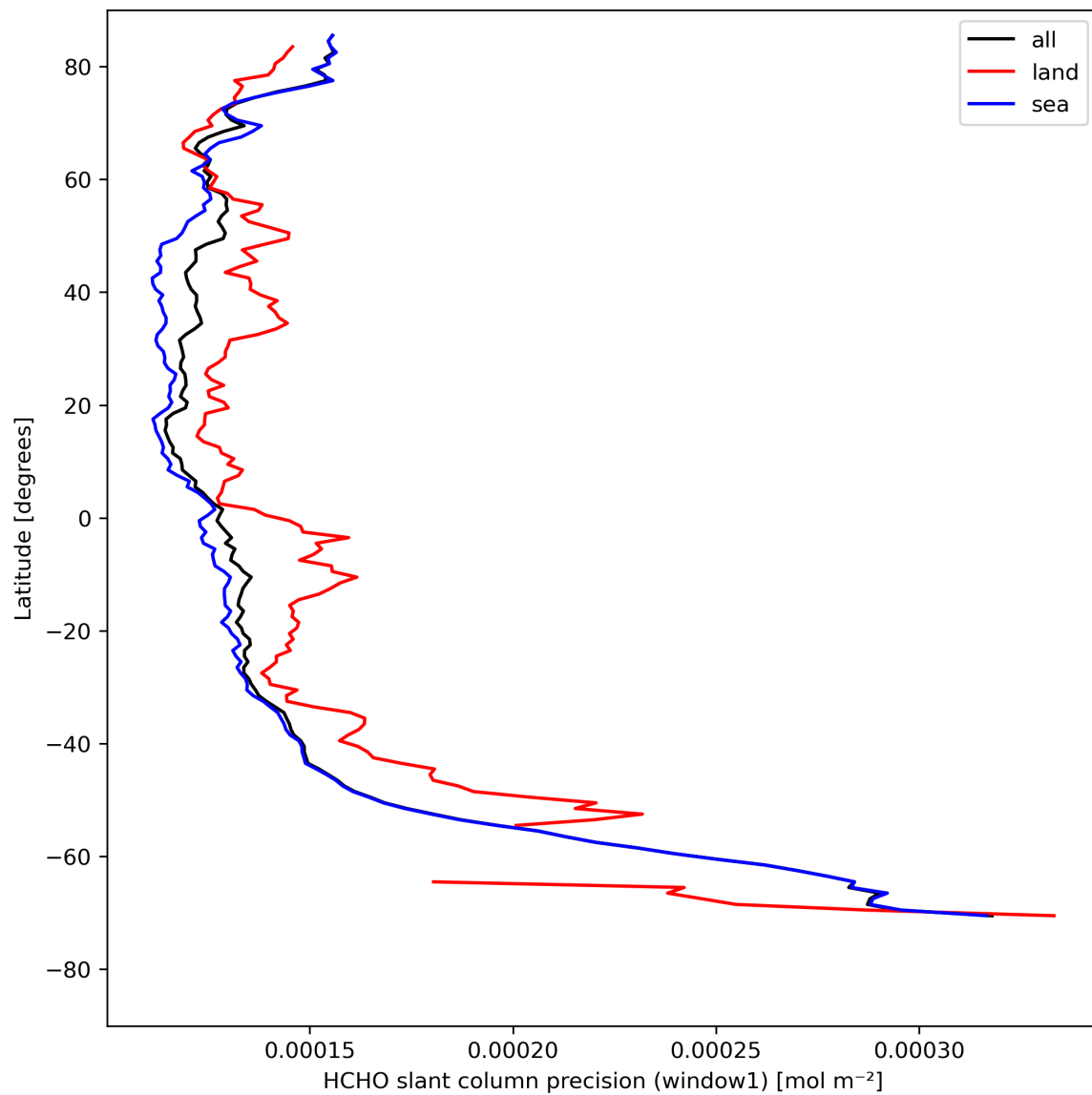
Figure 25: Zonal average of “HCHO slant column precision (window1)” for 2024-04-24 to 2024-04-26.
