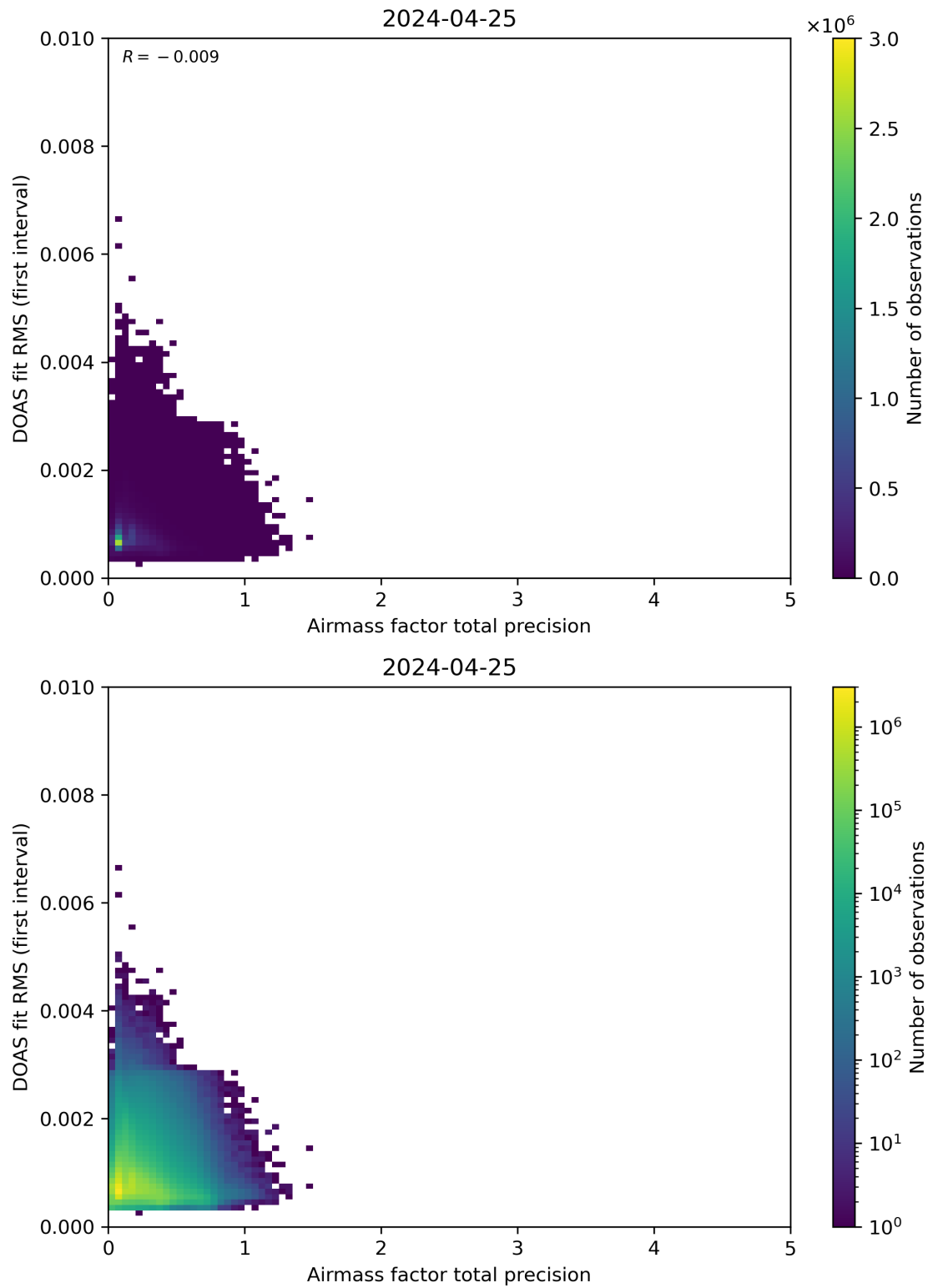
Figure 105: Scatter density plot of “Airmass factor total precision” against “DOAS fit RMS (first interval)” for 2024-04-24 to 2024-04-26.
