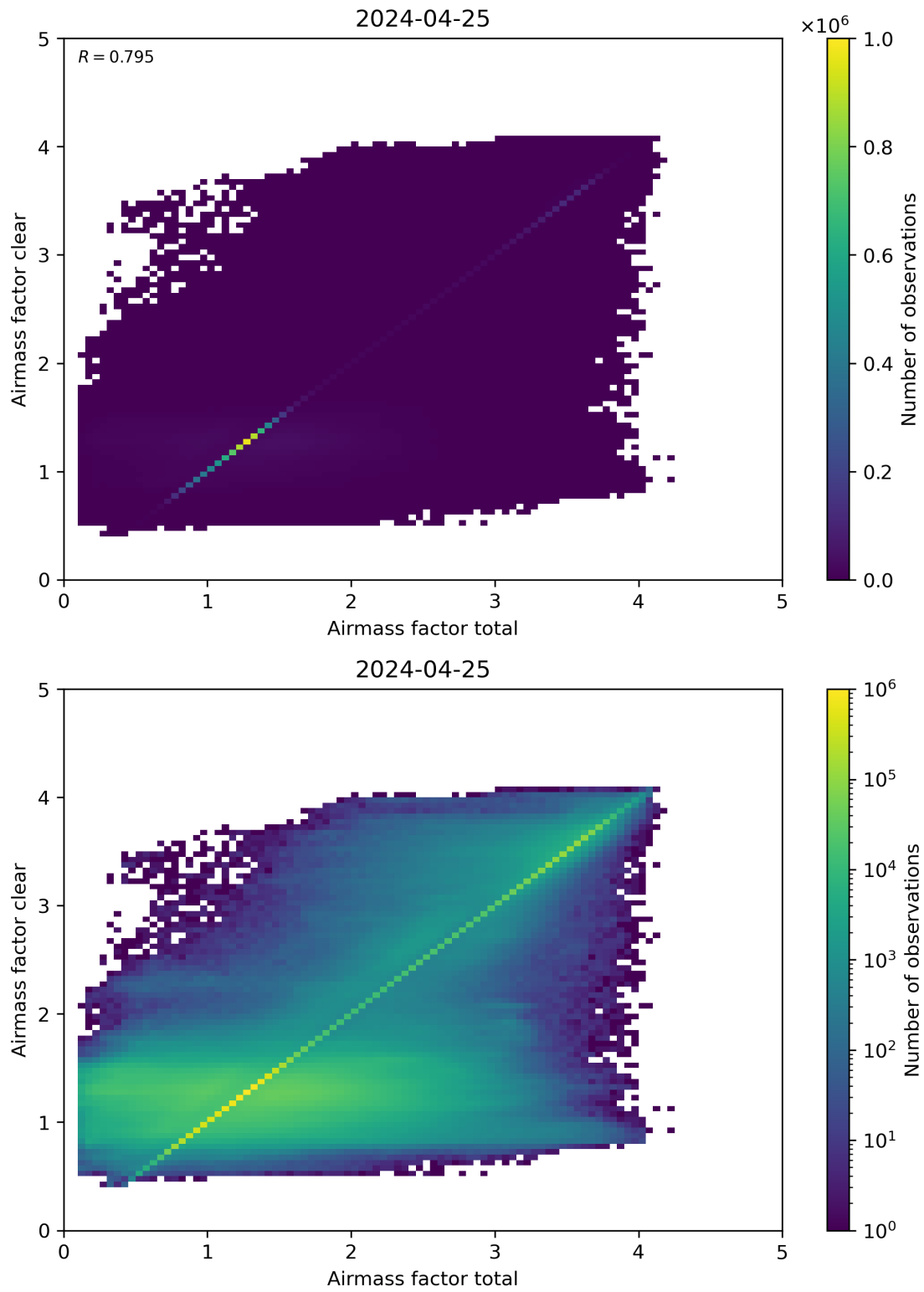
Figure 100: Scatter density plot of “Airmass factor total” against “Airmass factor clear” for 2024-04-24 to 2024-04-26.
