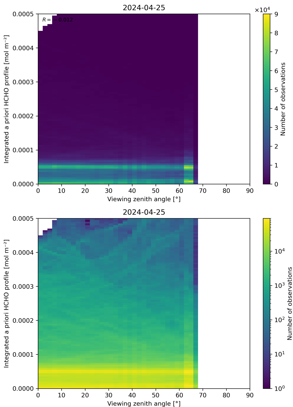
Figure 195: Scatter density plot of “Viewing zenith angle” against “Integrated a priori HCHO profile” for 2024-04-24 to 2024-04-26.
