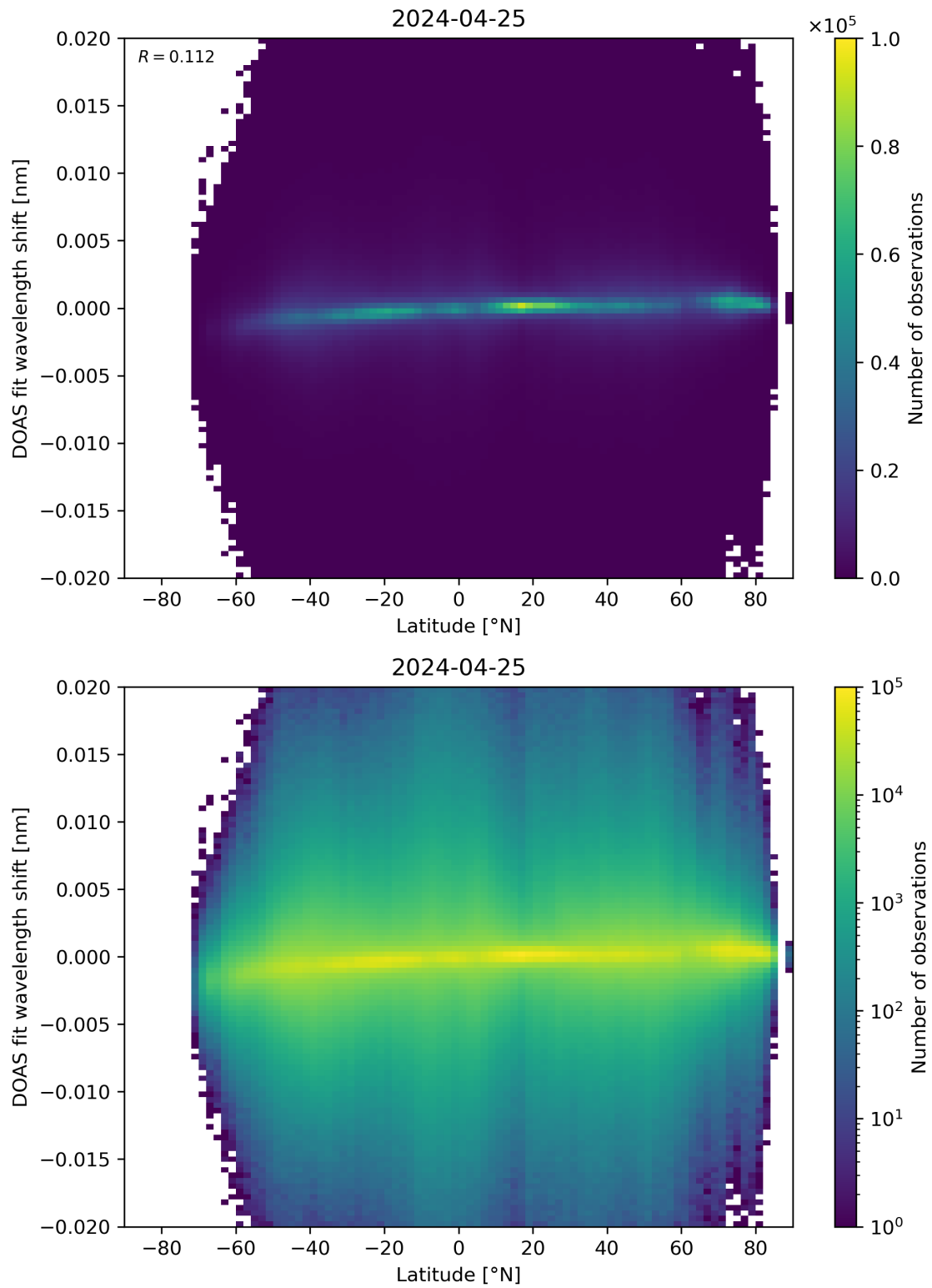
Figure 154: Scatter density plot of “Latitude” against “DOAS fit wavelength shift” for 2024-04-24 to 2024-04-26.
