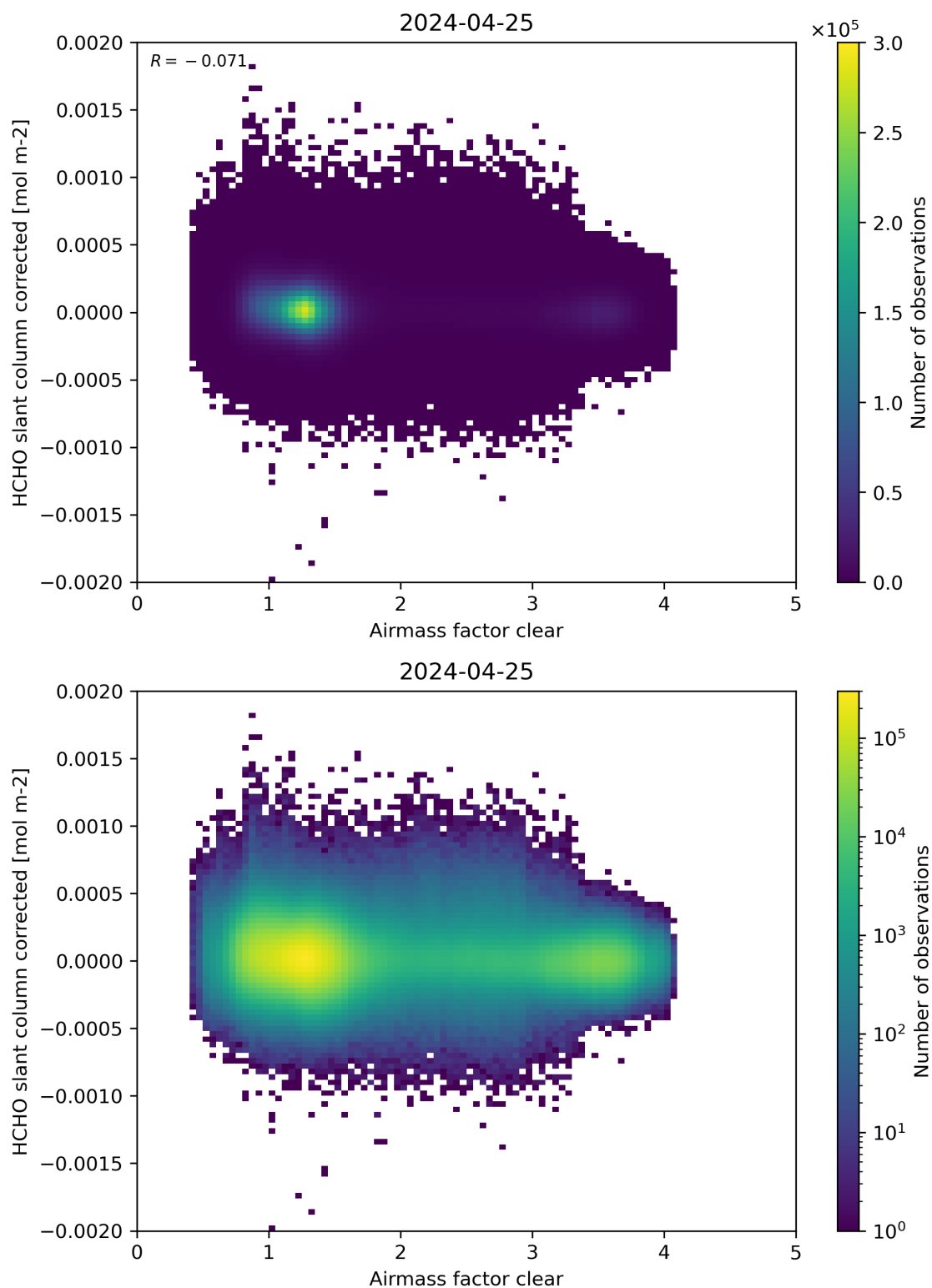
Figure 74: Scatter density plot of “Airmass factor clear” against “HCHO slant column corrected” for 2024-04-24 to 2024-04-26.
