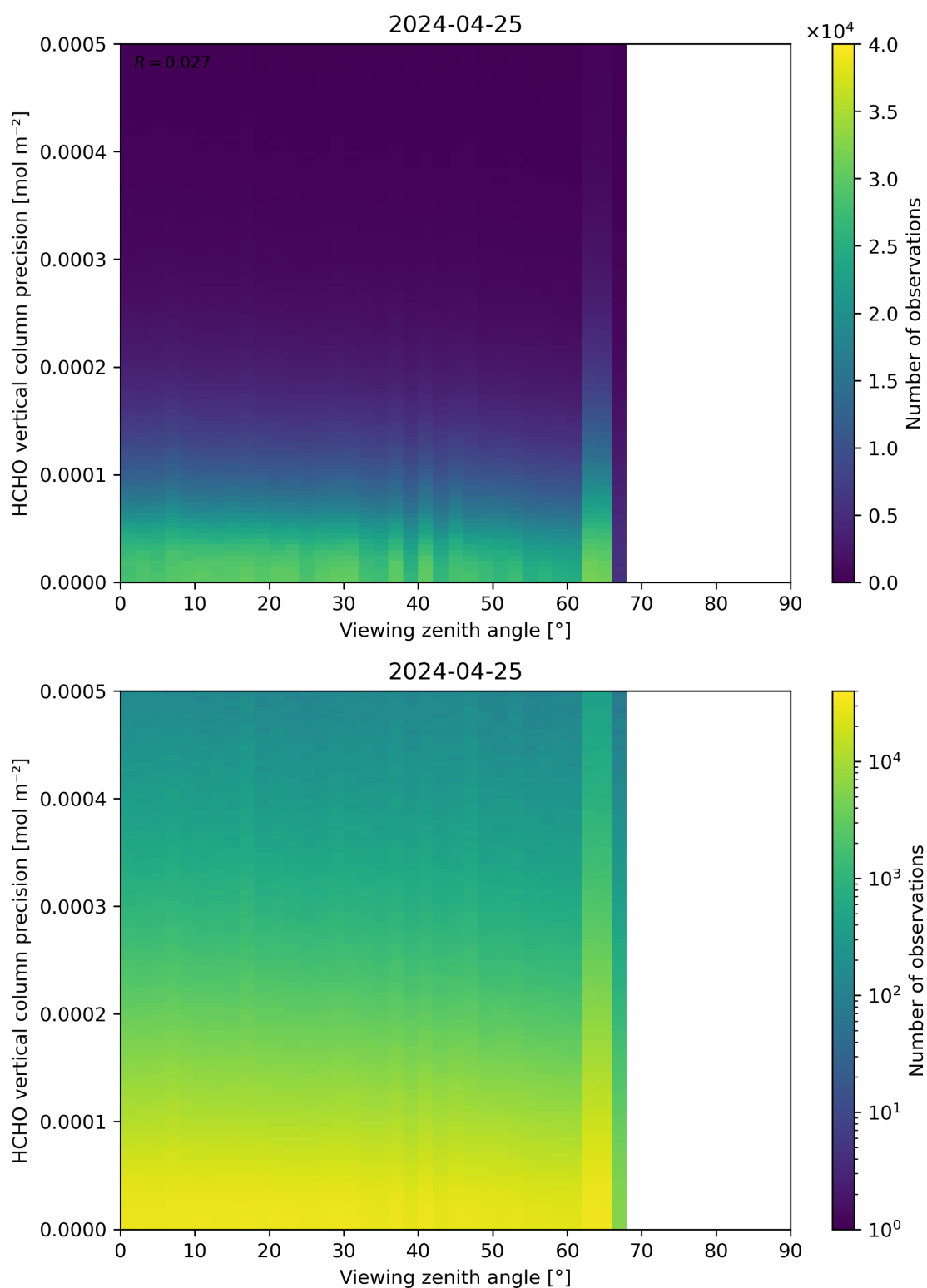
Figure 194: Scatter density plot of “Viewing zenith angle” against “HCHO vertical column precision” for 2024-04-24 to 2024-04-26.
