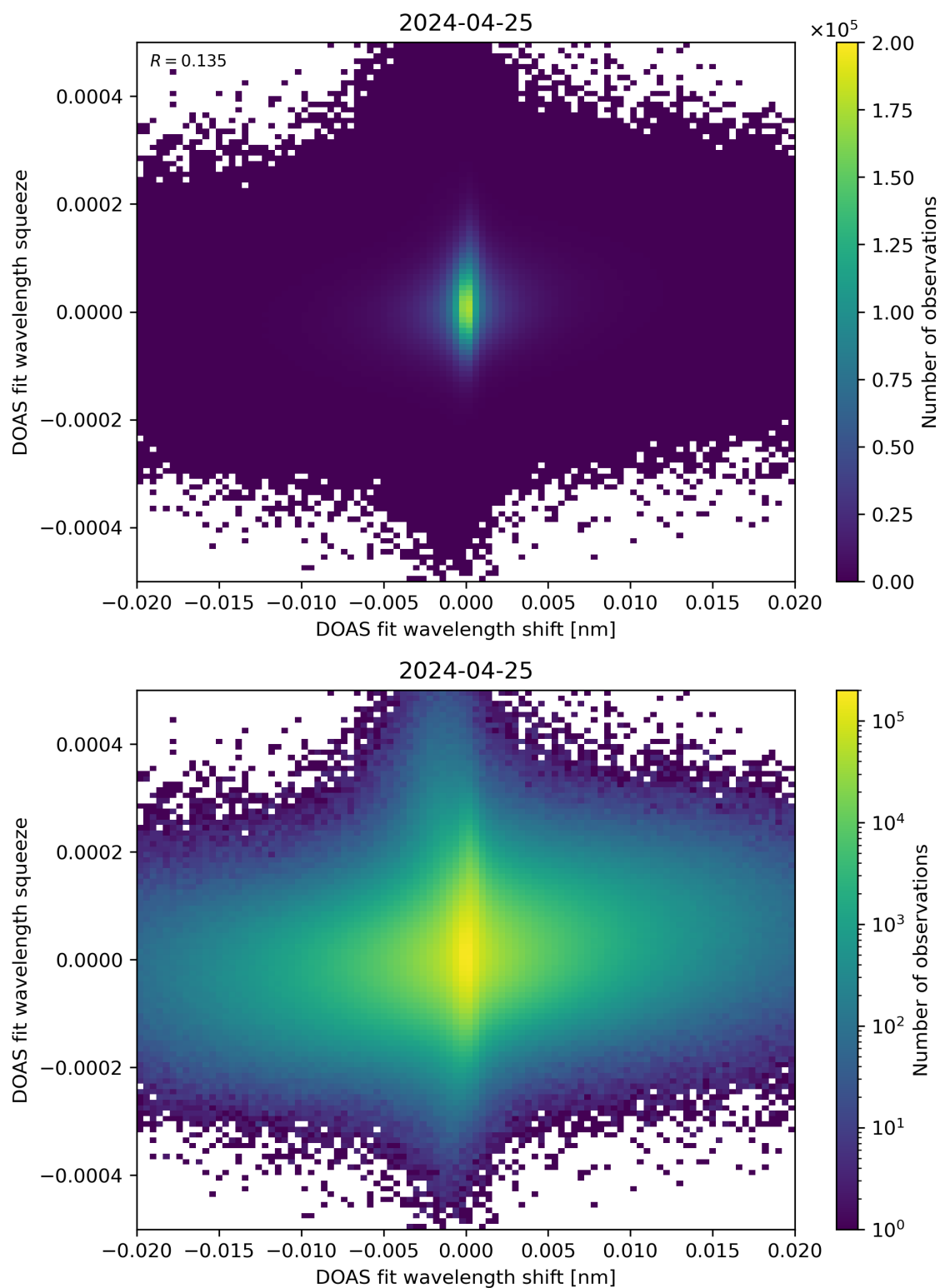
Figure 65: Scatter density plot of “DOAS fit wavelength shift” against “DOAS fit wavelength squeeze” for 2024-04-24 to 2024-04-26.
