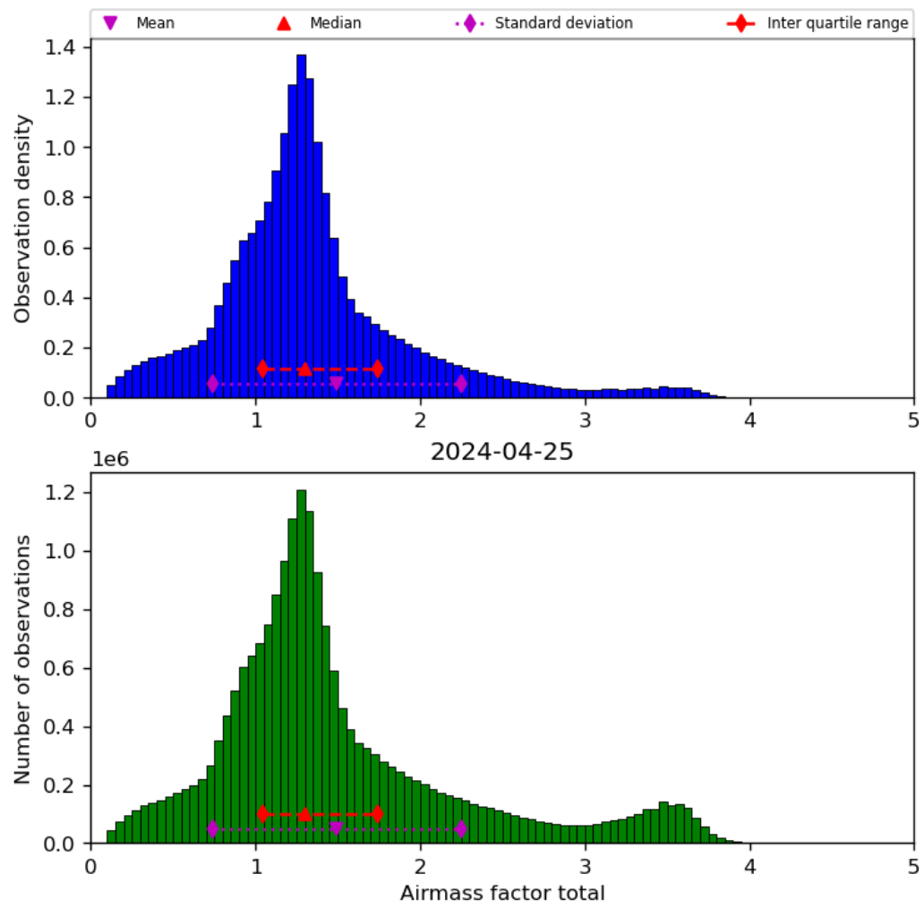
Figure 40: Histogram of “Airmass factor total” for 2024-04-24 to 2024-04-26
