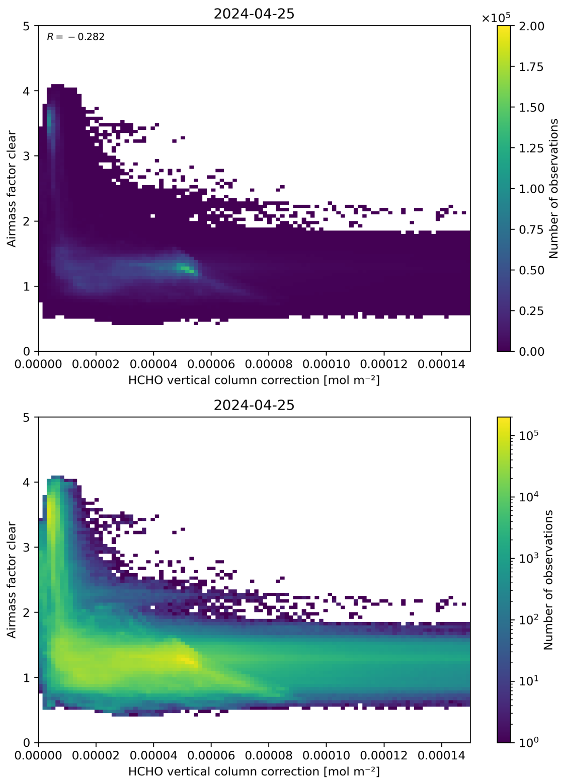
Figure 115: Scatter density plot of “HCHO vertical column correction” against “Airmass factor clear” for 2024-04-24 to 2024-04-26.
