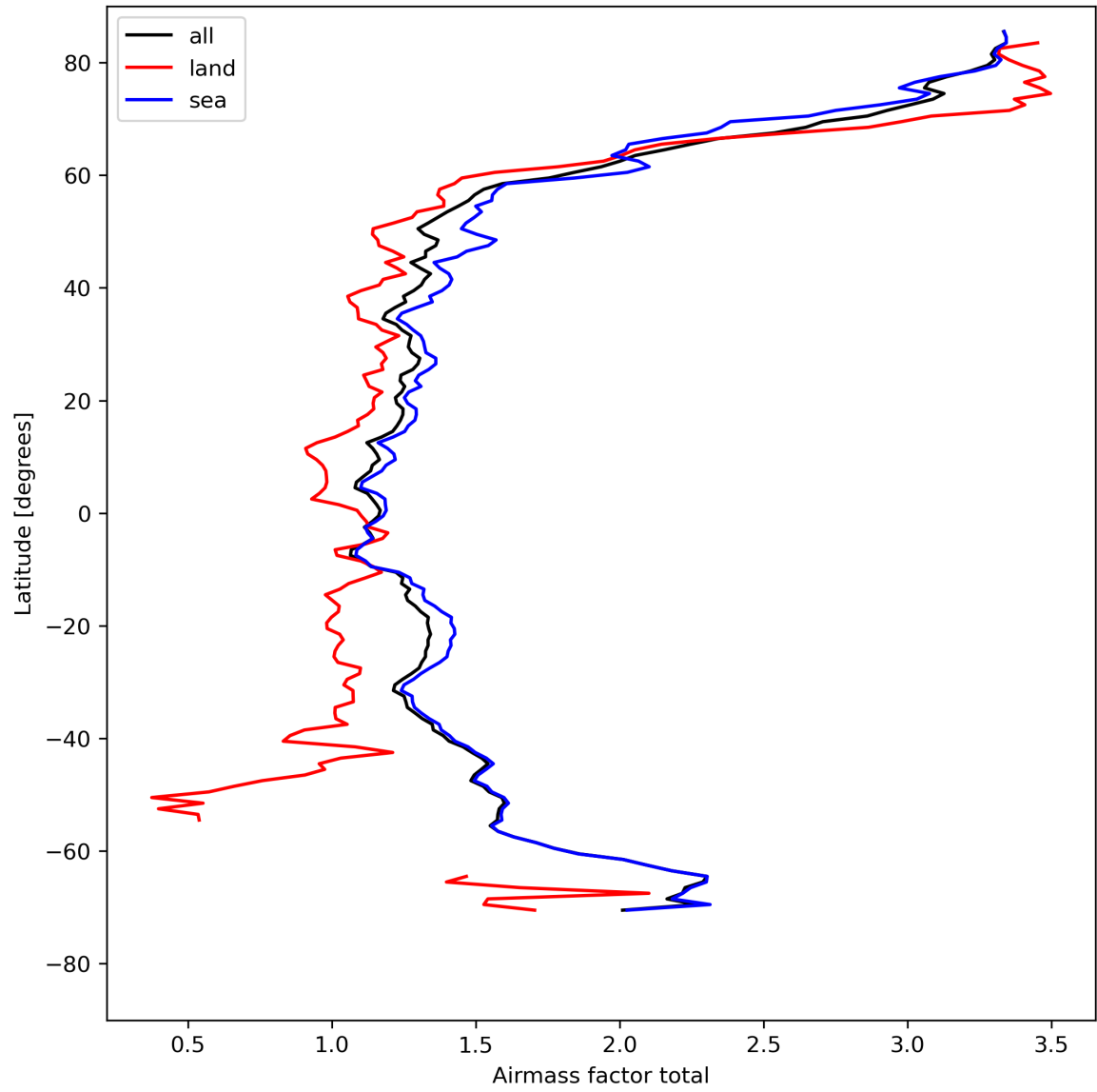
Figure 26: Zonal average of “Airmass factor total” for 2024-04-24 to 2024-04-26.
