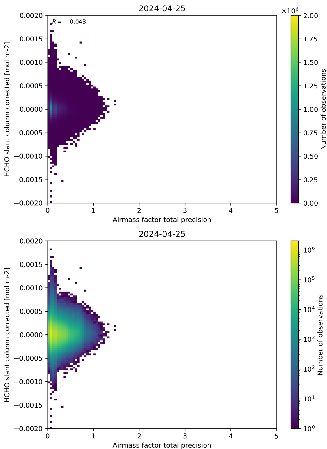
Figure 109: Scatter density plot of “Airmass factor total precision” against “HCHO slant column corrected” for 2024-04-24 to 2024-04-26.
