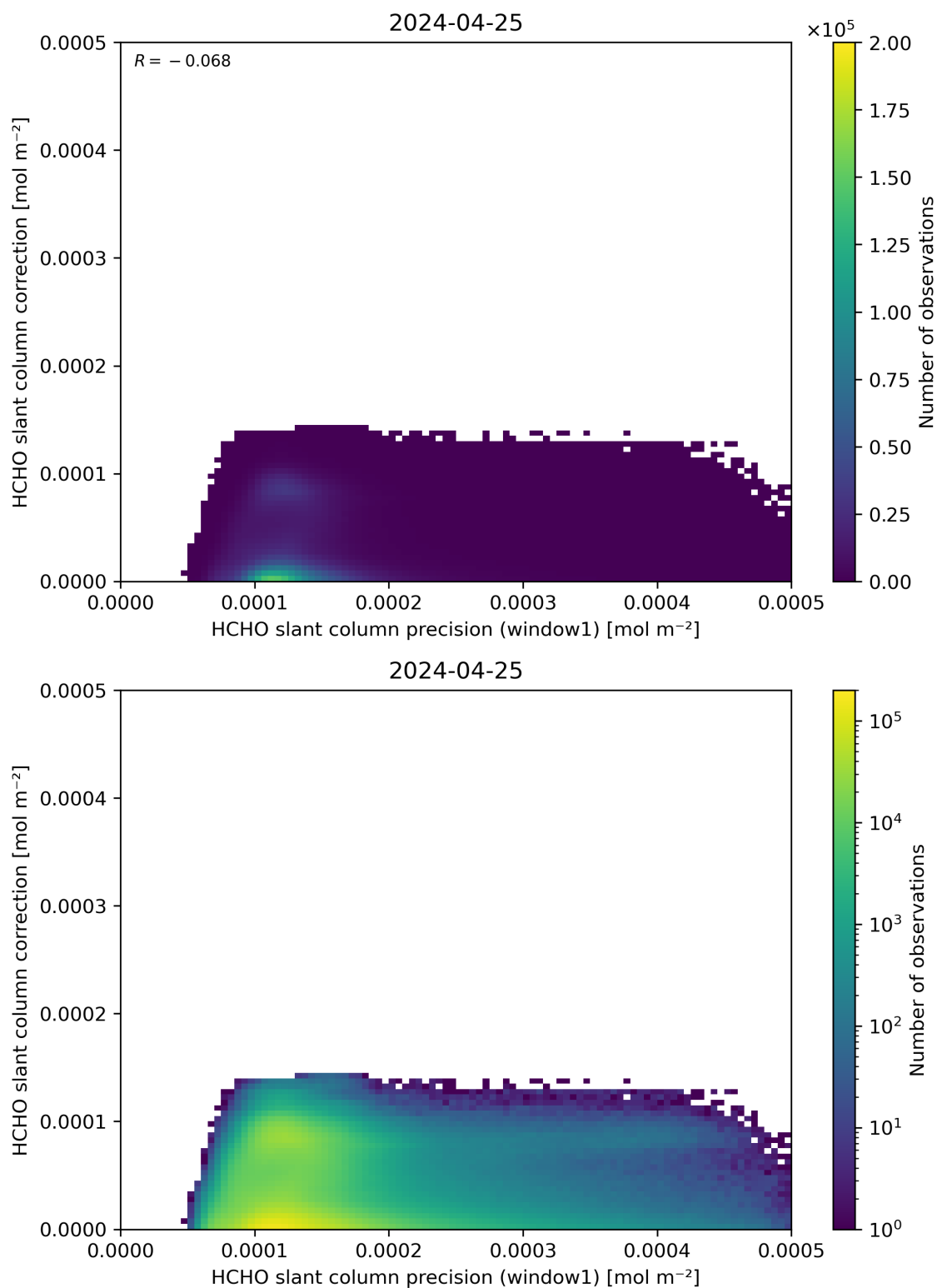
Figure 93: Scatter density plot of “HCHO slant column precision (window1)” against “HCHO slant column correction” for 2024-04-24 to 2024-04-26.
