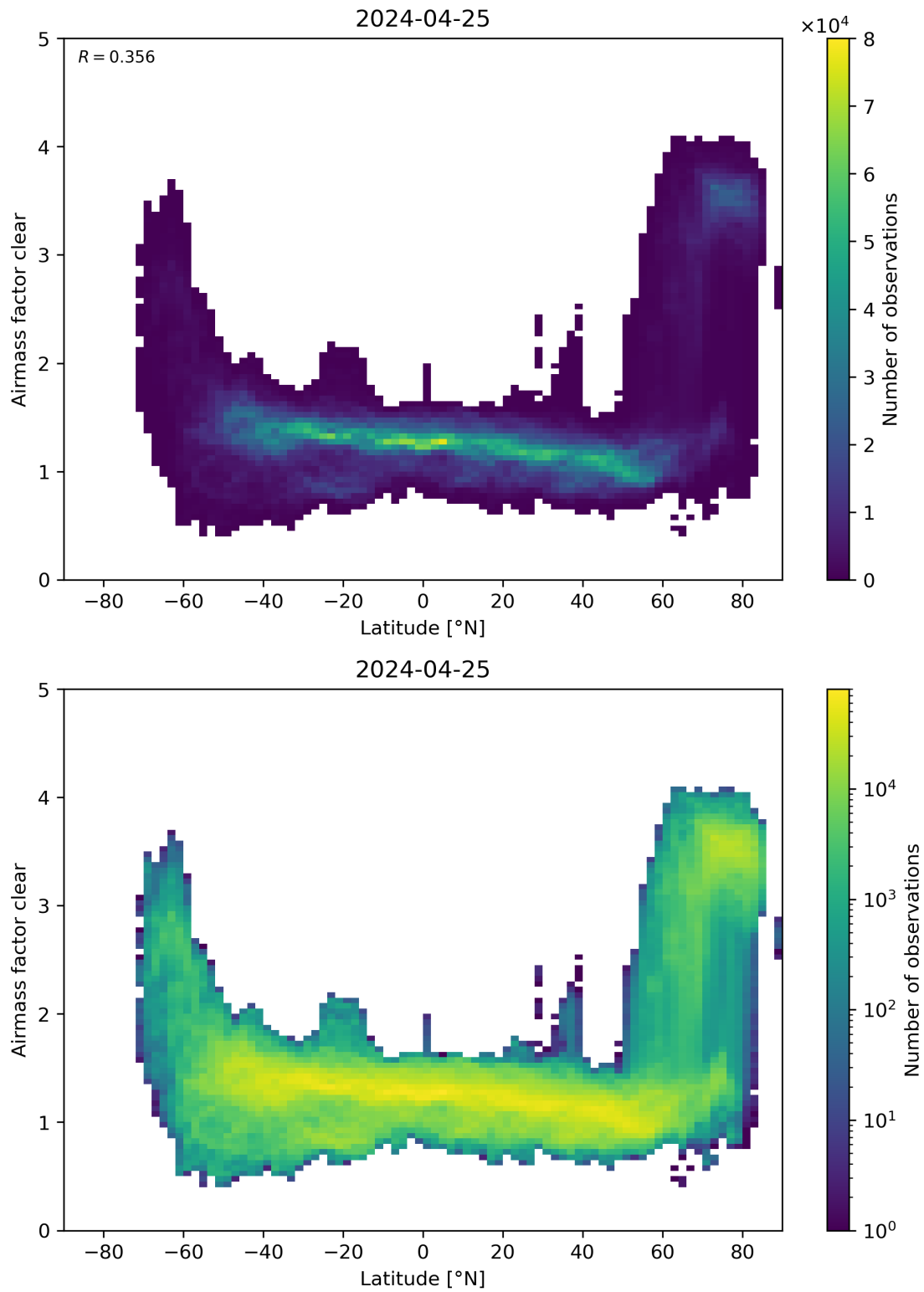
Figure 156: Scatter density plot of “Latitude” against “Airmass factor clear” for 2024-04-24 to 2024-04-26.
