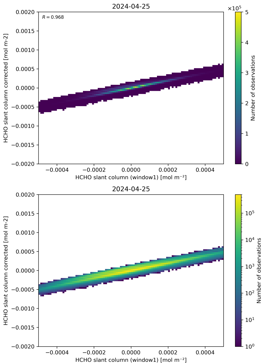
Figure 82: Scatter density plot of “HCHO slant column (window1)” against “HCHO slant column corrected” for 2024-04-24 to 2024-04-26.
