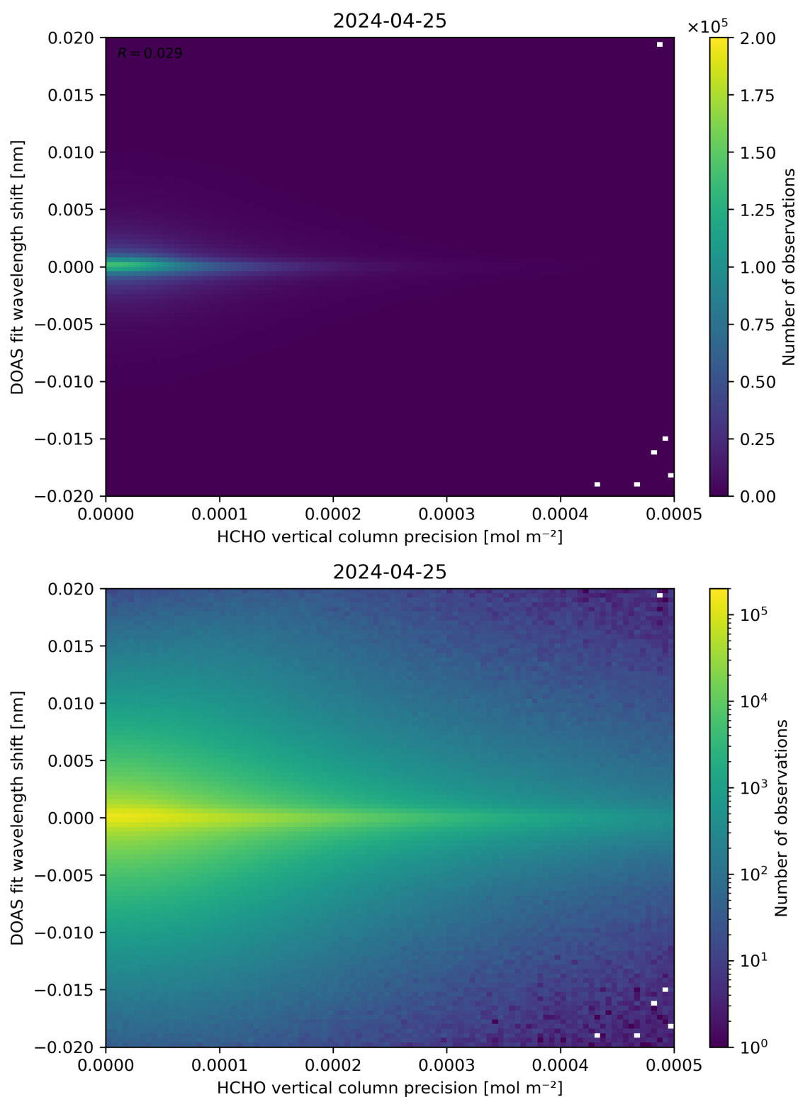
Figure 137: Scatter density plot of “HCHO vertical column precision” against “DOAS fit wavelength shift” for 2024-04-24 to 2024-04-26.
