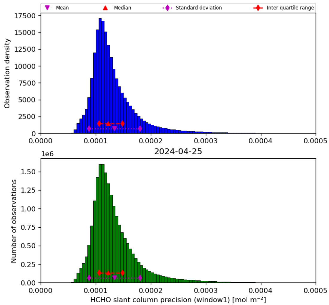
Figure 39: Histogram of “HCHO slant column precision (window1)” for 2024-04-24 to 2024-04-26
