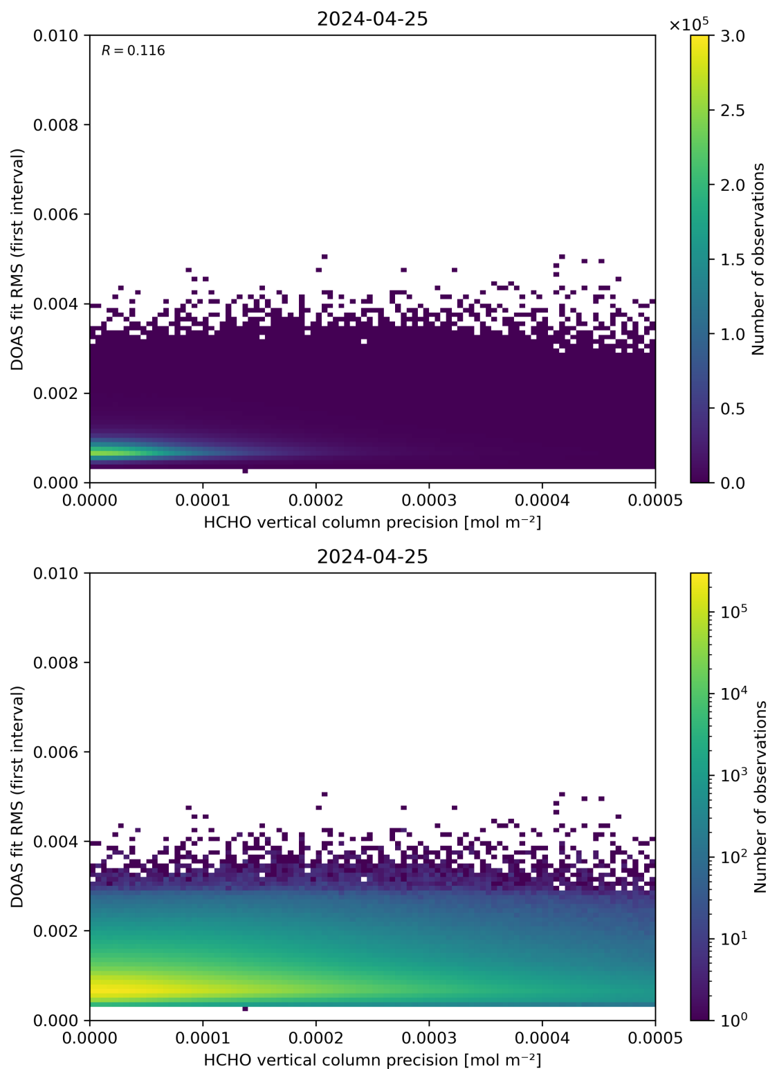
Figure 136: Scatter density plot of “HCHO vertical column precision” against “DOAS fit RMS (first interval)” for 2024-04-24 to 2024-04-26.
