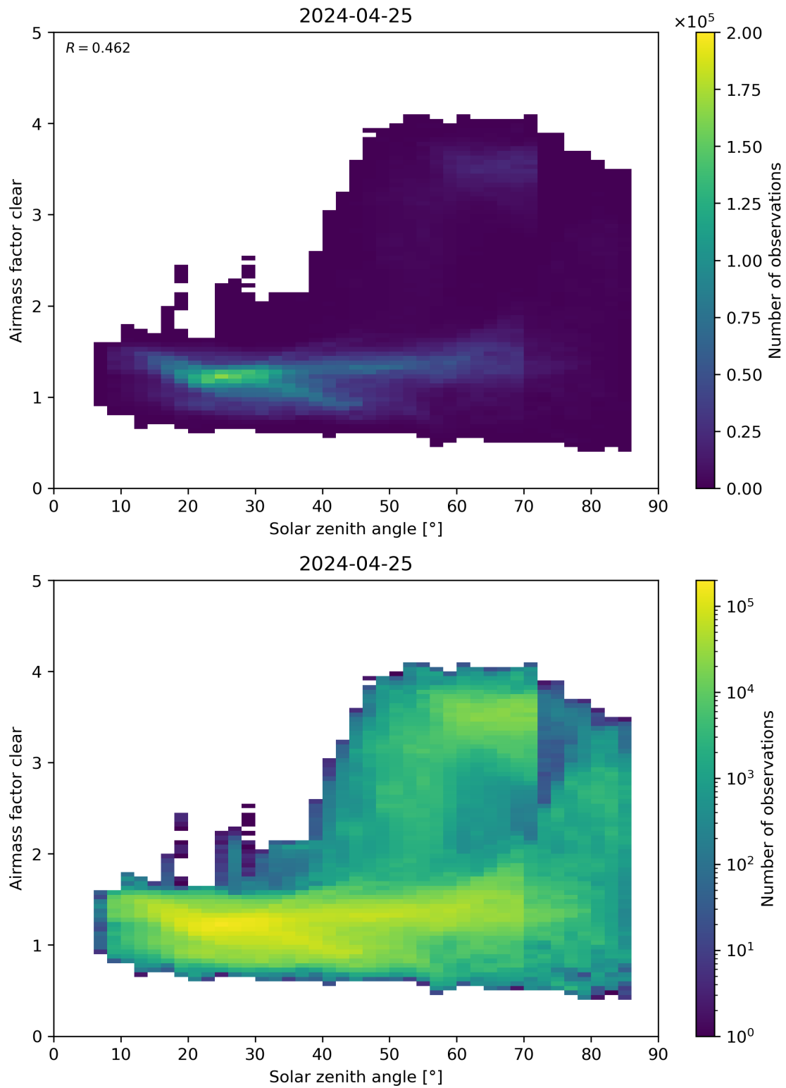
Figure 170: Scatter density plot of “Solar zenith angle” against “Airmass factor clear” for 2024-04-24 to 2024-04-26.
