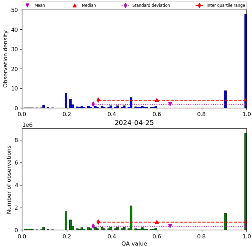
Figure 34: Histogram of “QA value” for 2024-04-24 to 2024-04-26
