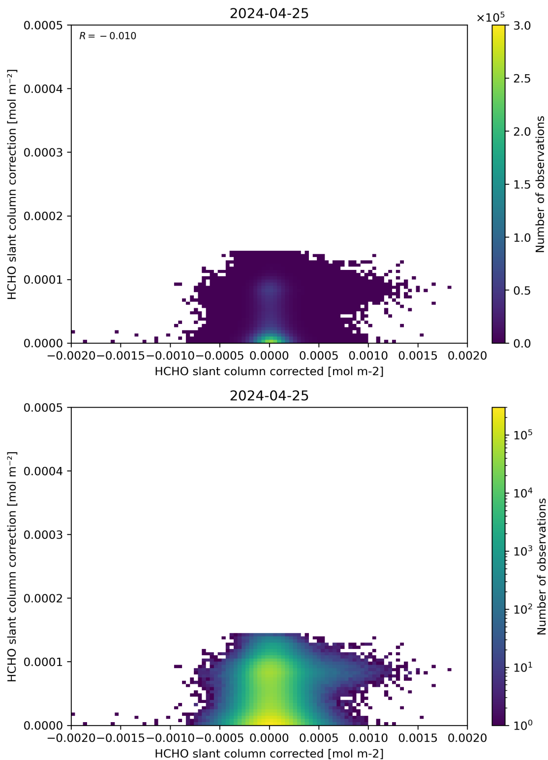
Figure 77: Scatter density plot of “HCHO slant column corrected” against “HCHO slant column correction” for 2024-04-24 to 2024-04-26.
