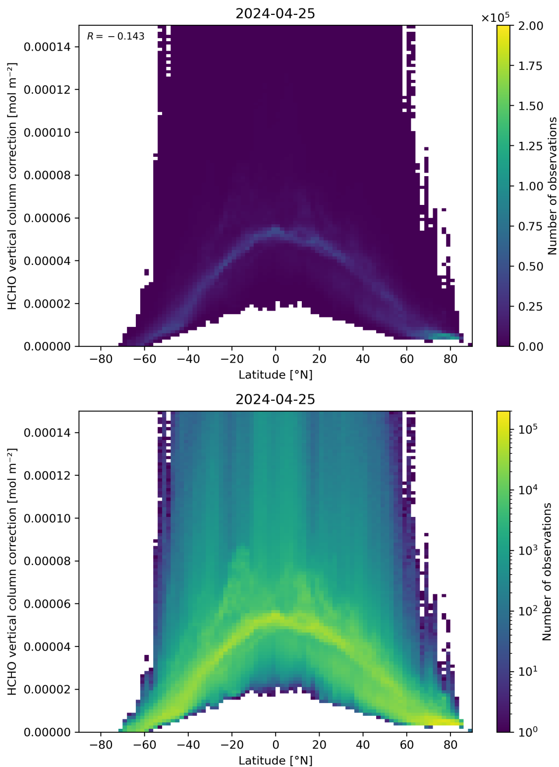
Figure 164: Scatter density plot of “Latitude” against “HCHO vertical column correction” for 2024-04-24 to 2024-04-26.
