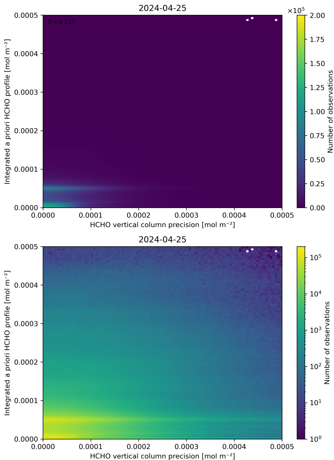
Figure 147: Scatter density plot of “HCHO vertical column precision” against “Integrated a priori HCHO profile” for 2024-04-24 to 2024-04-26.
