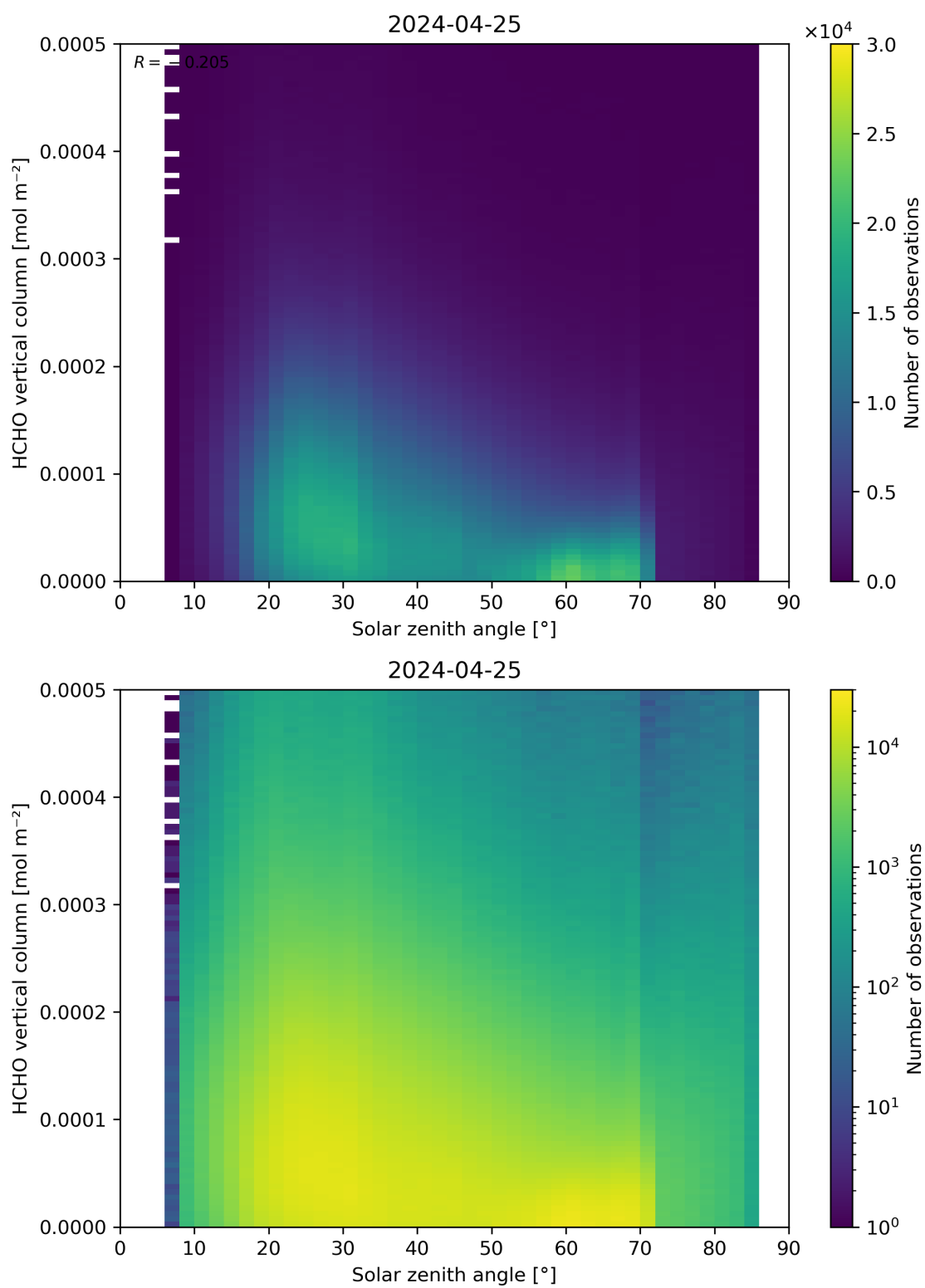
Figure 177: Scatter density plot of “Solar zenith angle” against “HCHO vertical column” for 2024-04-24 to 2024-04-26.
