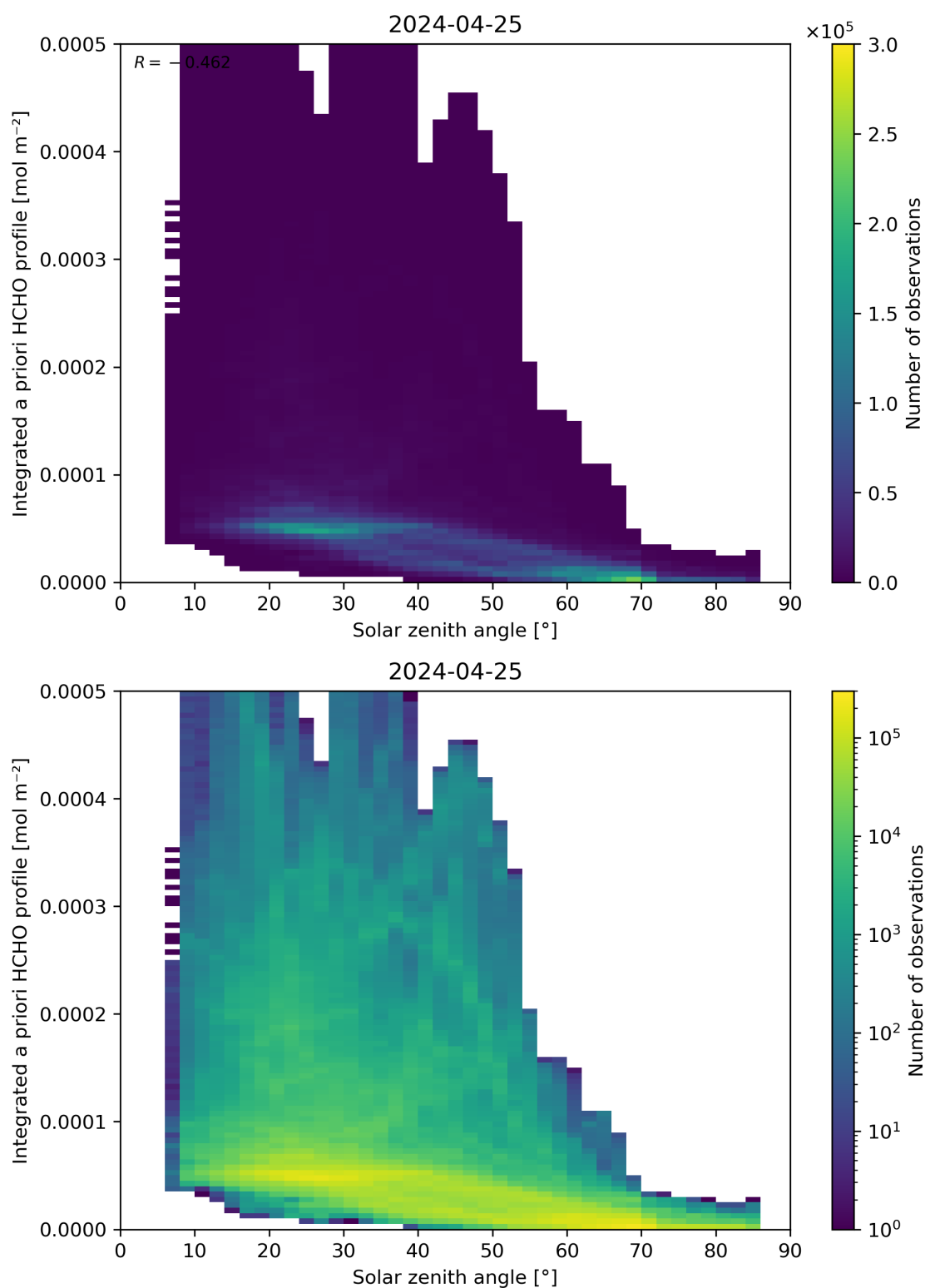
Figure 180: Scatter density plot of “Solar zenith angle” against “Integrated a priori HCHO profile” for 2024-04-24 to 2024-04-26.
