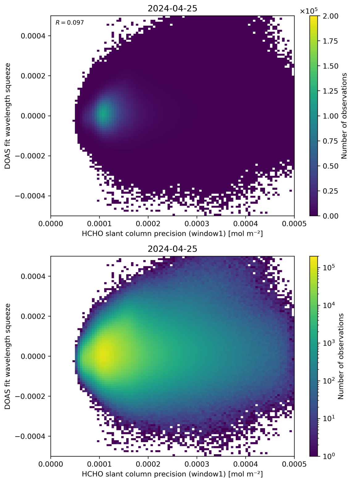
Figure 90: Scatter density plot of “HCHO slant column precision (window1)” against “DOAS fit wavelength squeeze” for 2024-04-24 to 2024-04-26.
