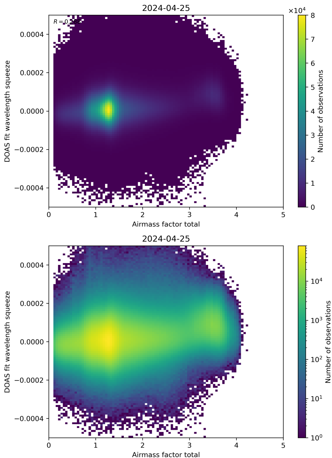
Figure 99: Scatter density plot of “Airmass factor total” against “DOAS fit wavelength squeeze” for 2024-04-24 to 2024-04-26.
