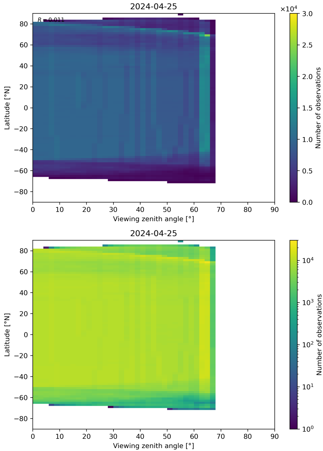
Figure 196: Scatter density plot of “Viewing zenith angle” against “Latitude” for 2024-04-24 to 2024-04-26.
