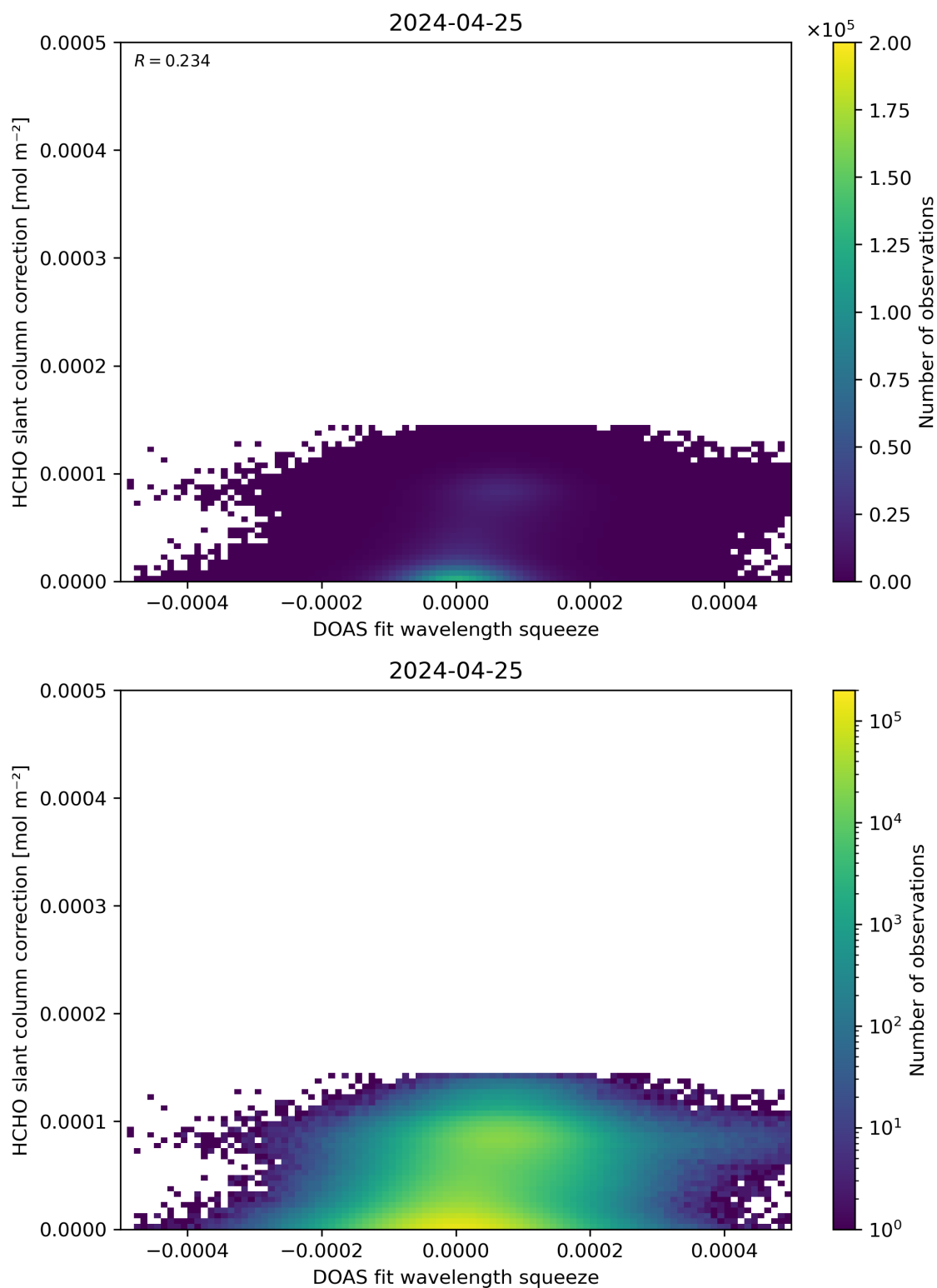
Figure 70: Scatter density plot of “DOAS fit wavelength squeeze” against “HCHO slant column correction” for 2024-04-24 to 2024-04-26.
