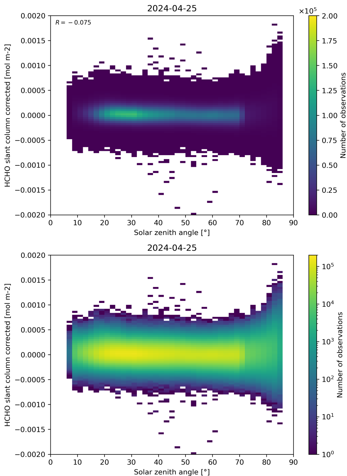
Figure 171: Scatter density plot of “Solar zenith angle” against “HCHO slant column corrected” for 2024-04-24 to 2024-04-26.
