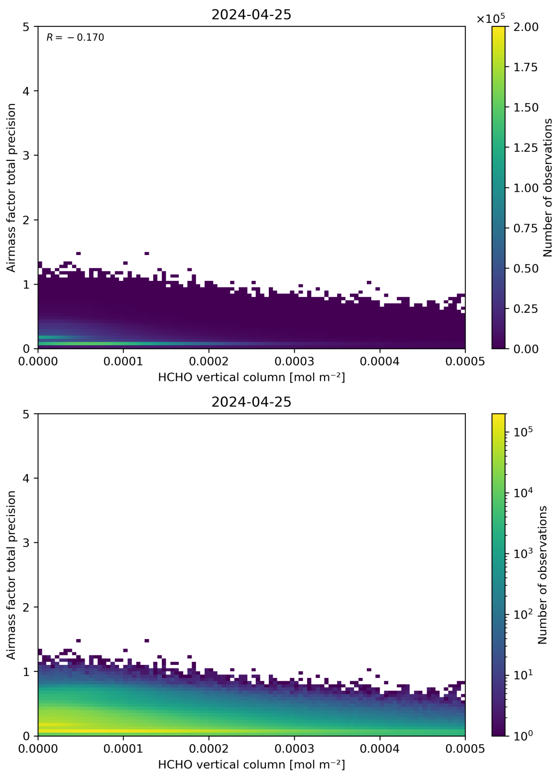
Figure 132: Scatter density plot of “HCHO vertical column” against “Airmass factor total precision” for 2024-04-24 to 2024-04-26.
