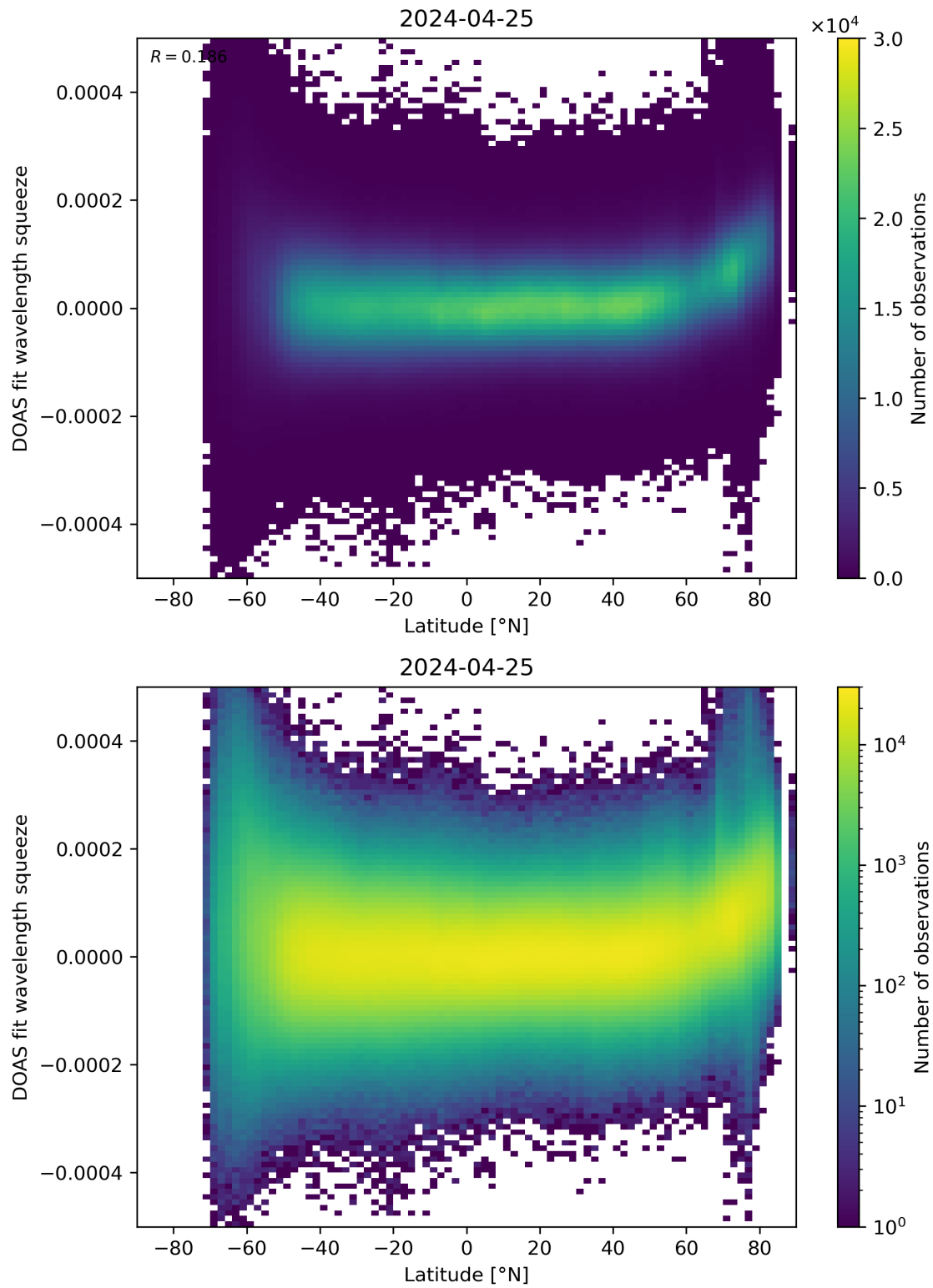
Figure 155: Scatter density plot of “Latitude” against “DOAS fit wavelength squeeze” for 2024-04-24 to 2024-04-26.
