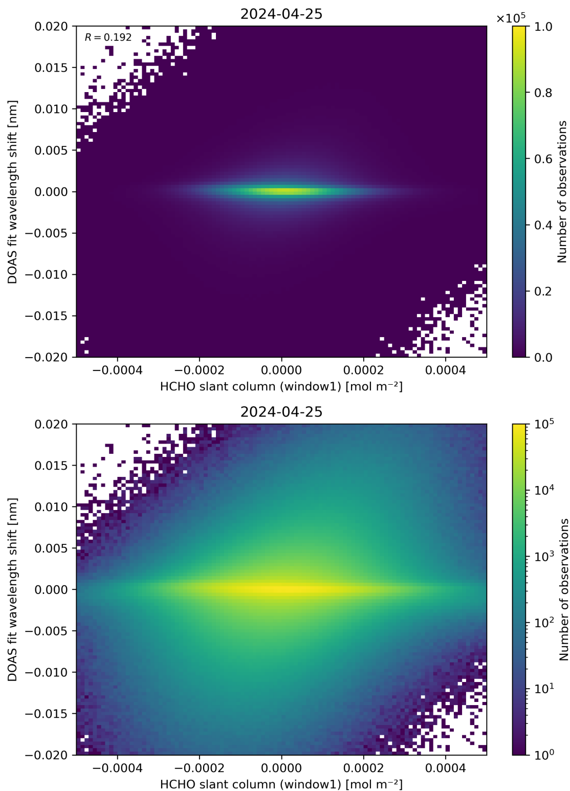
Figure 79: Scatter density plot of “HCHO slant column (window1)” against “DOAS fit wavelength shift” for 2024-04-24 to 2024-04-26.
