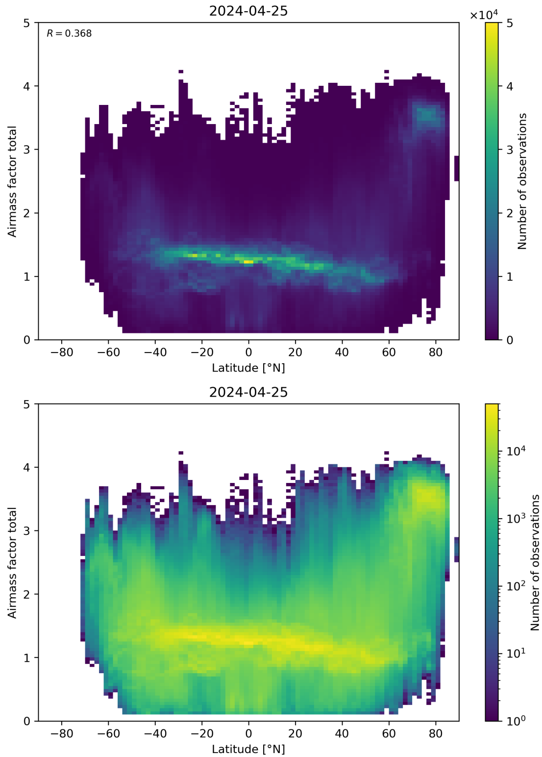
Figure 161: Scatter density plot of “Latitude” against “Airmass factor total” for 2024-04-24 to 2024-04-26.
