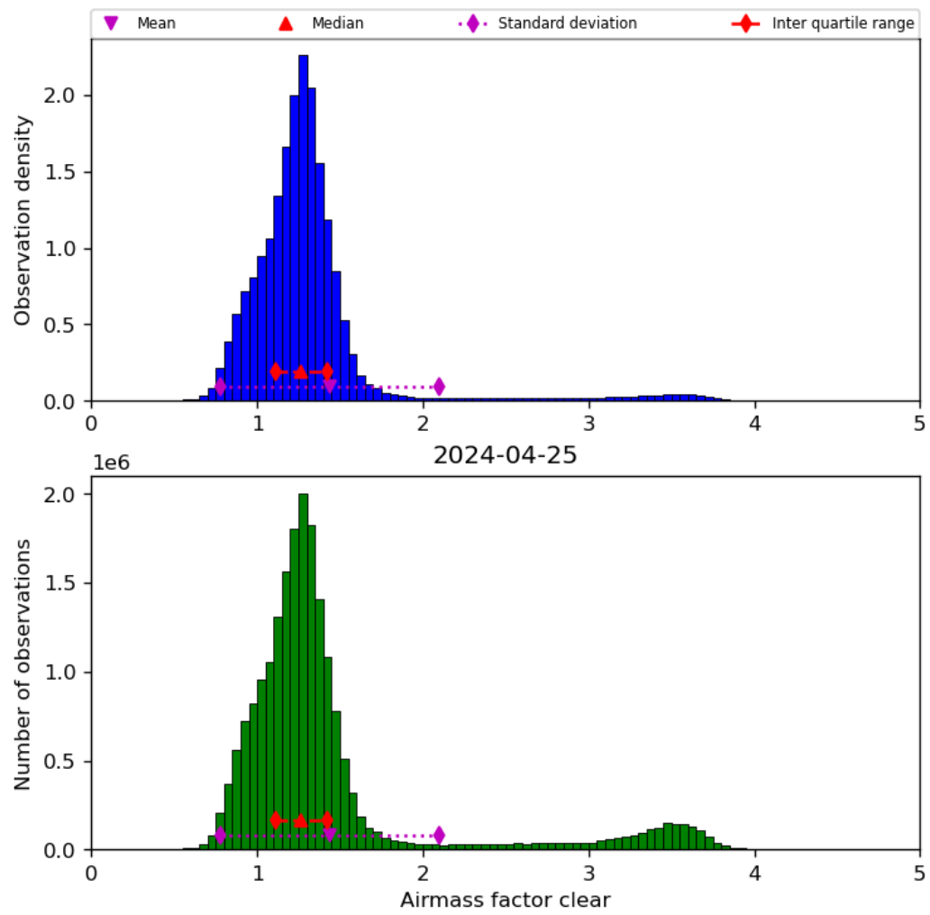
Figure 42: Histogram of “Airmass factor clear” for 2024-04-24 to 2024-04-26
