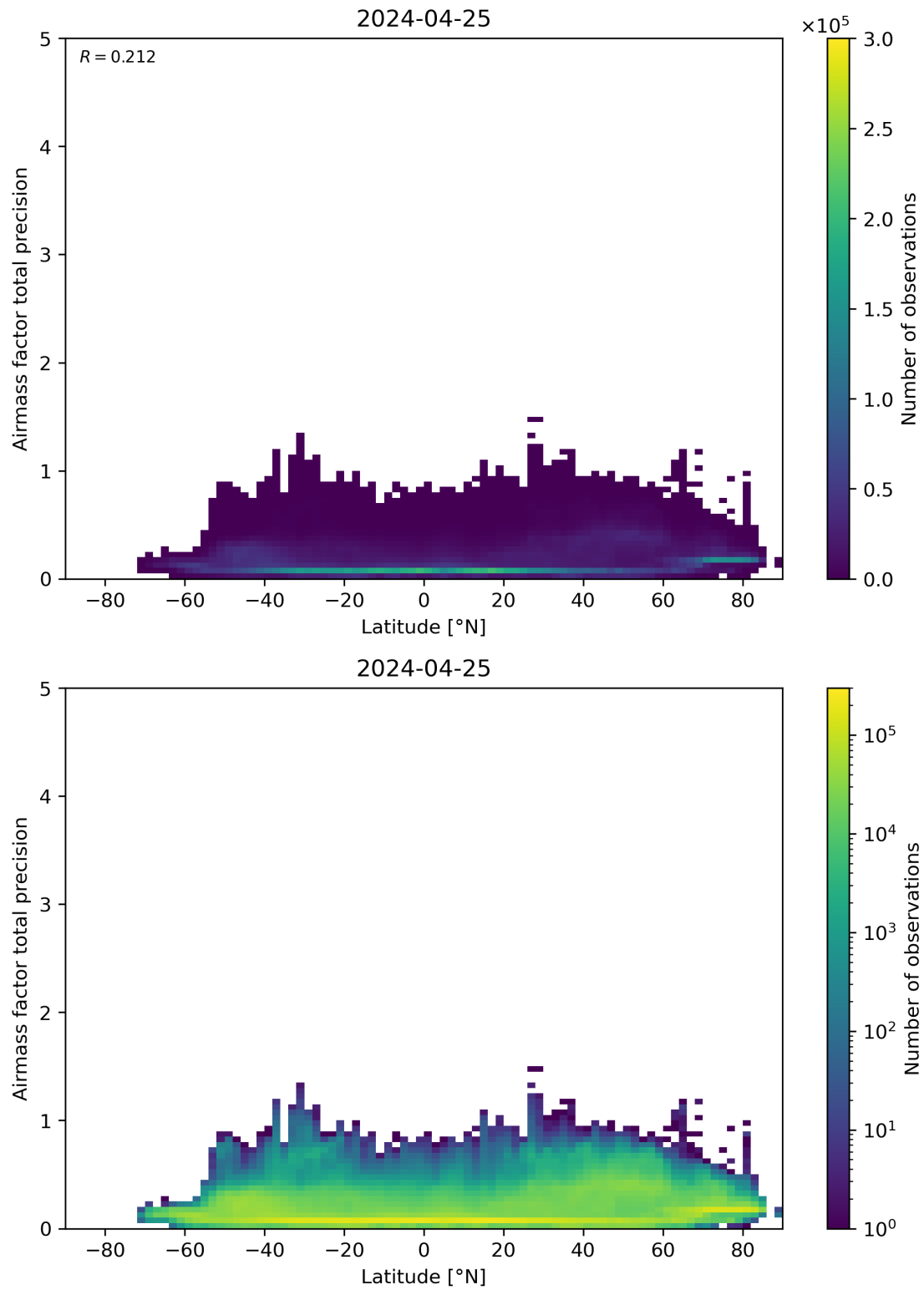
Figure 162: Scatter density plot of “Latitude” against “Airmass factor total precision” for 2024-04-24 to 2024-04-26.
