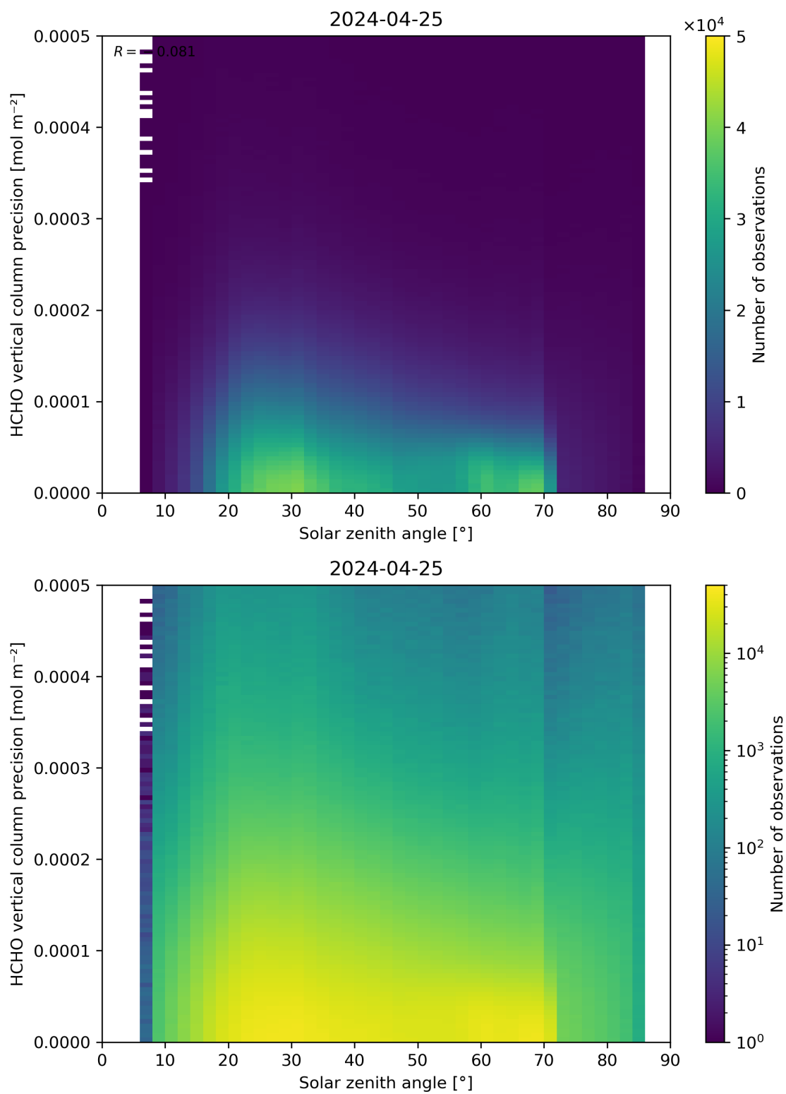
Figure 179: Scatter density plot of “Solar zenith angle” against “HCHO vertical column precision” for 2024-04-24 to 2024-04-26.
