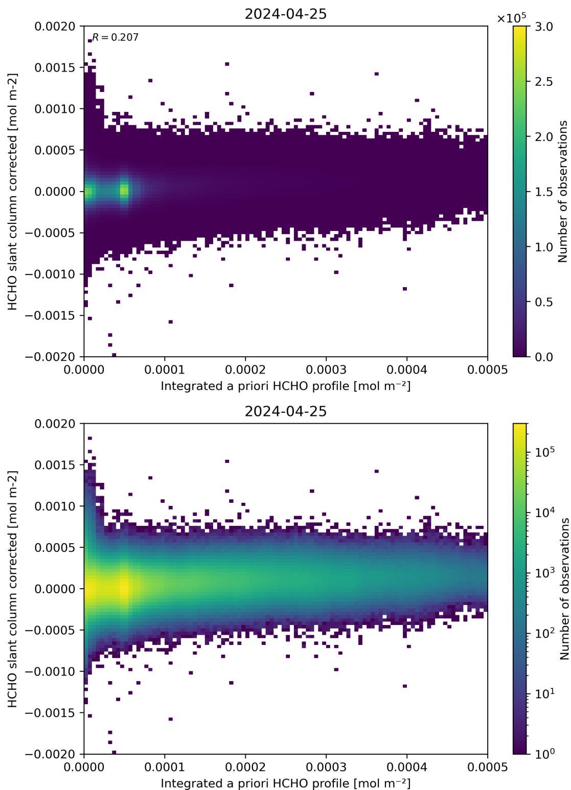
Figure 151: Scatter density plot of “Integrated a priori HCHO profile” against “HCHO slant column corrected” for 2024-04-24 to 2024-04-26.
