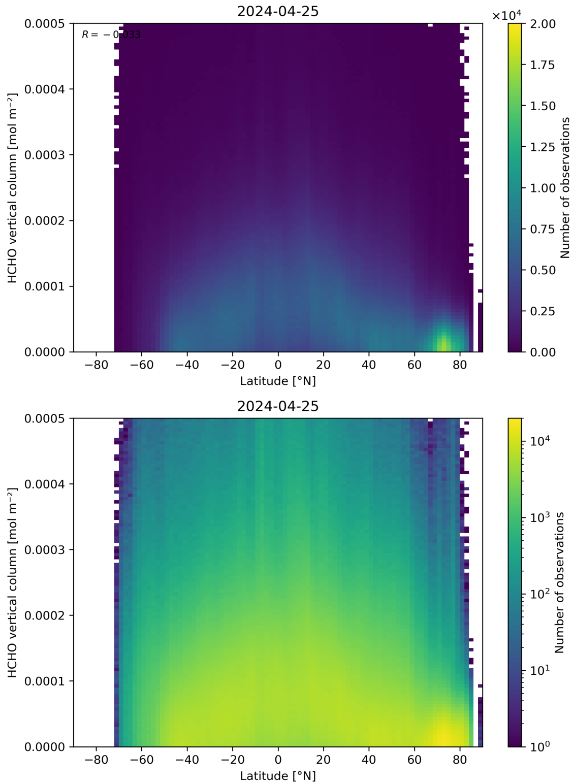
Figure 163: Scatter density plot of “Latitude” against “HCHO vertical column” for 2024-04-24 to 2024-04-26.
