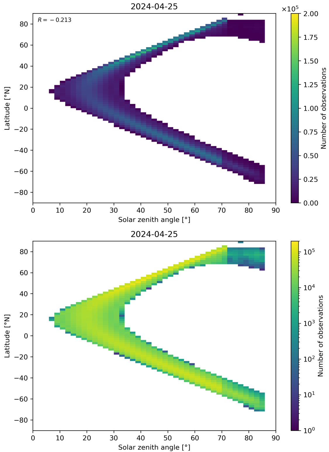
Figure 181: Scatter density plot of “Solar zenith angle” against “Latitude” for 2024-04-24 to 2024-04-26.
