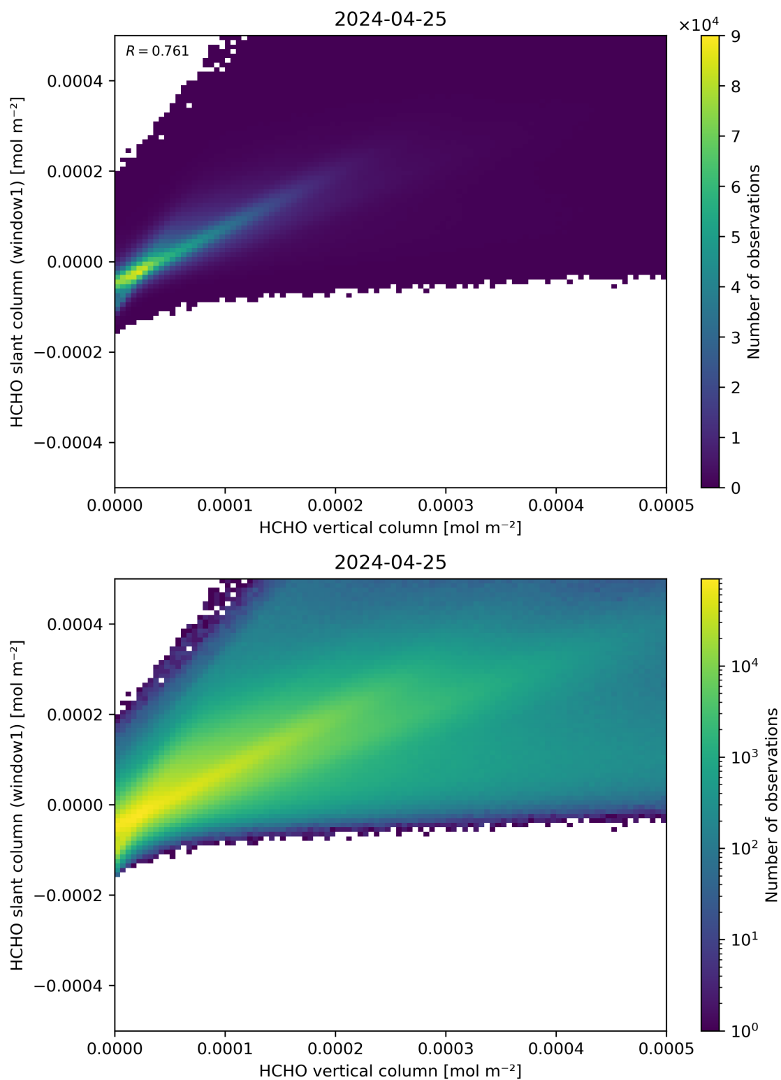
Figure 129: Scatter density plot of “HCHO vertical column” against “HCHO slant column (window1)” for 2024-04-24 to 2024-04-26.
