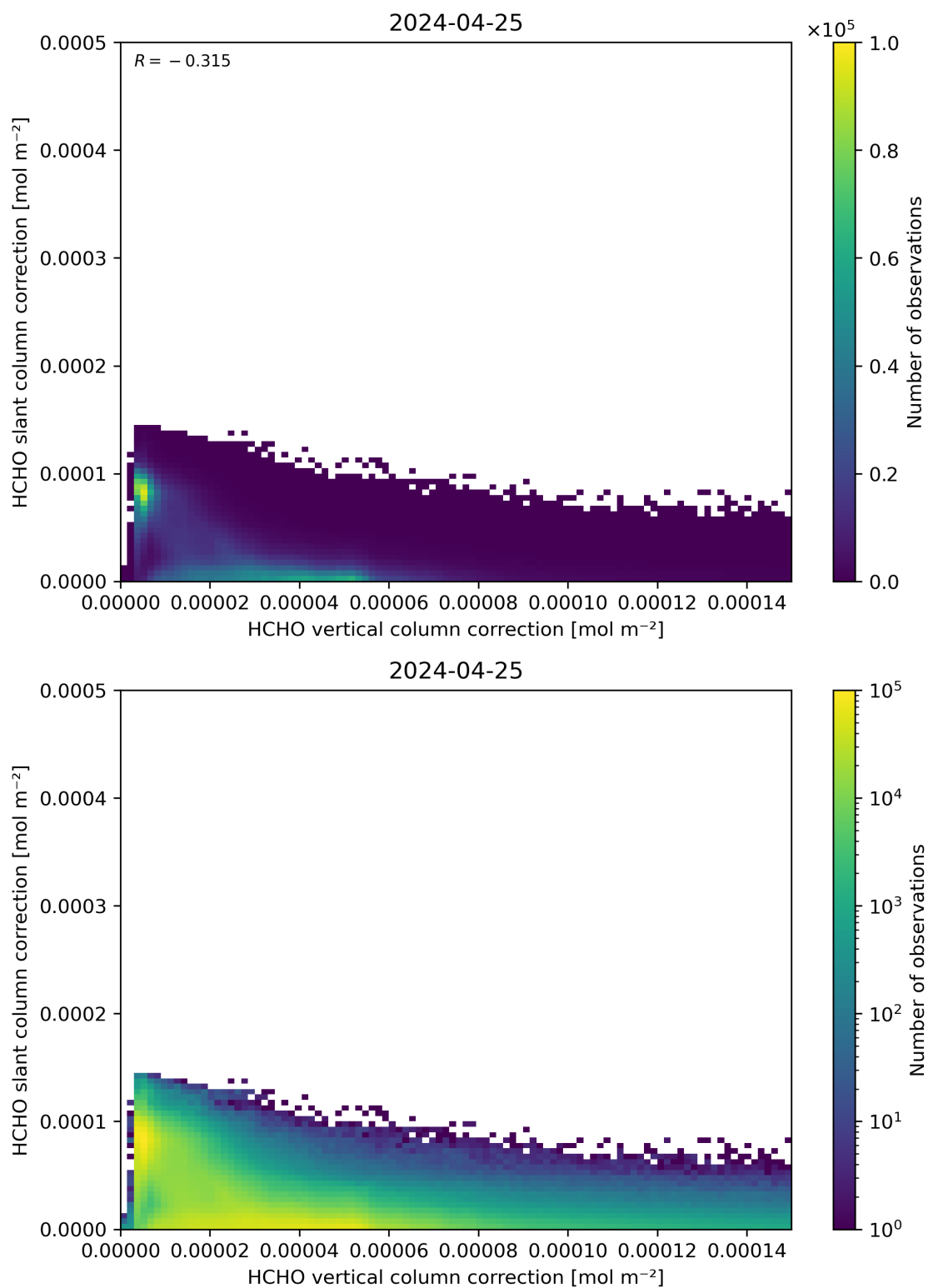
Figure 117: Scatter density plot of “HCHO vertical column correction” against “HCHO slant column correction” for 2024-04-24 to 2024-04-26.
