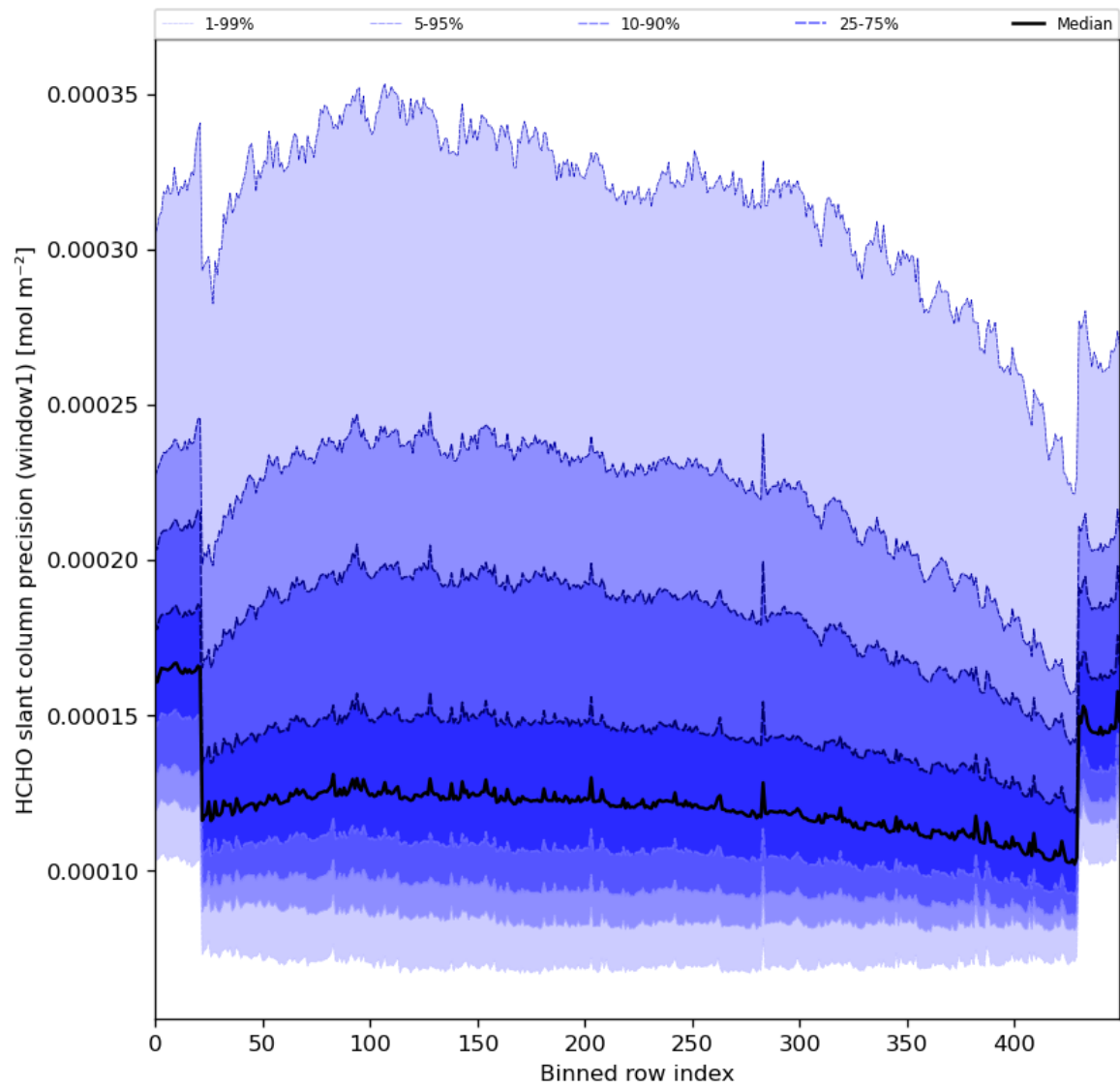
Figure 53: Along track statistics of “HCHO slant column precision (window1)” for 2024-04-24 to 2024-04-26
