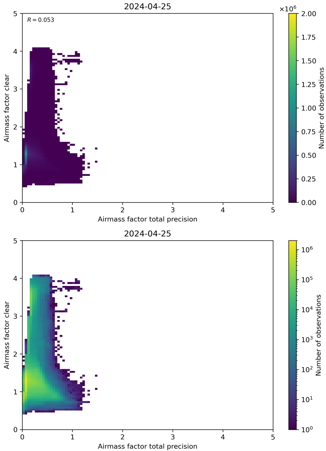
Figure 108: Scatter density plot of “Airmass factor total precision” against “Airmass factor clear” for 2024-04-24 to 2024-04-26.
