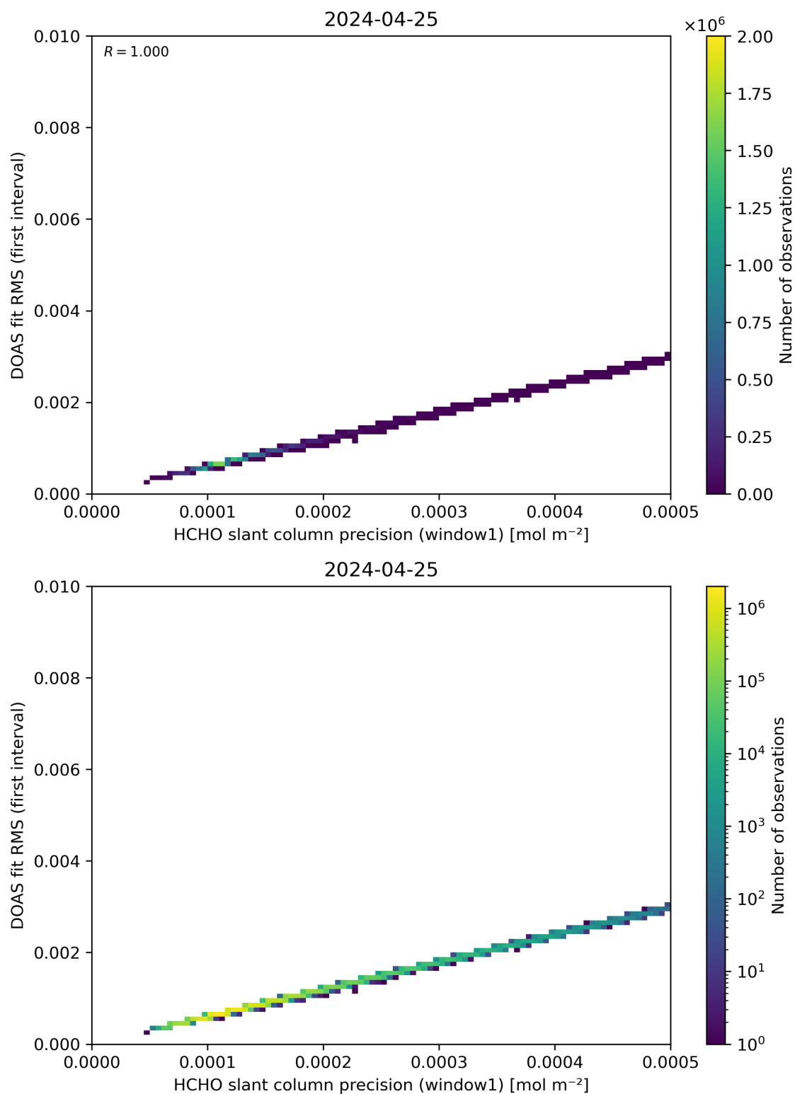
Figure 88: Scatter density plot of “HCHO slant column precision (window1)” against “DOAS fit RMS (first interval)” for 2024-04-24 to 2024-04-26.
