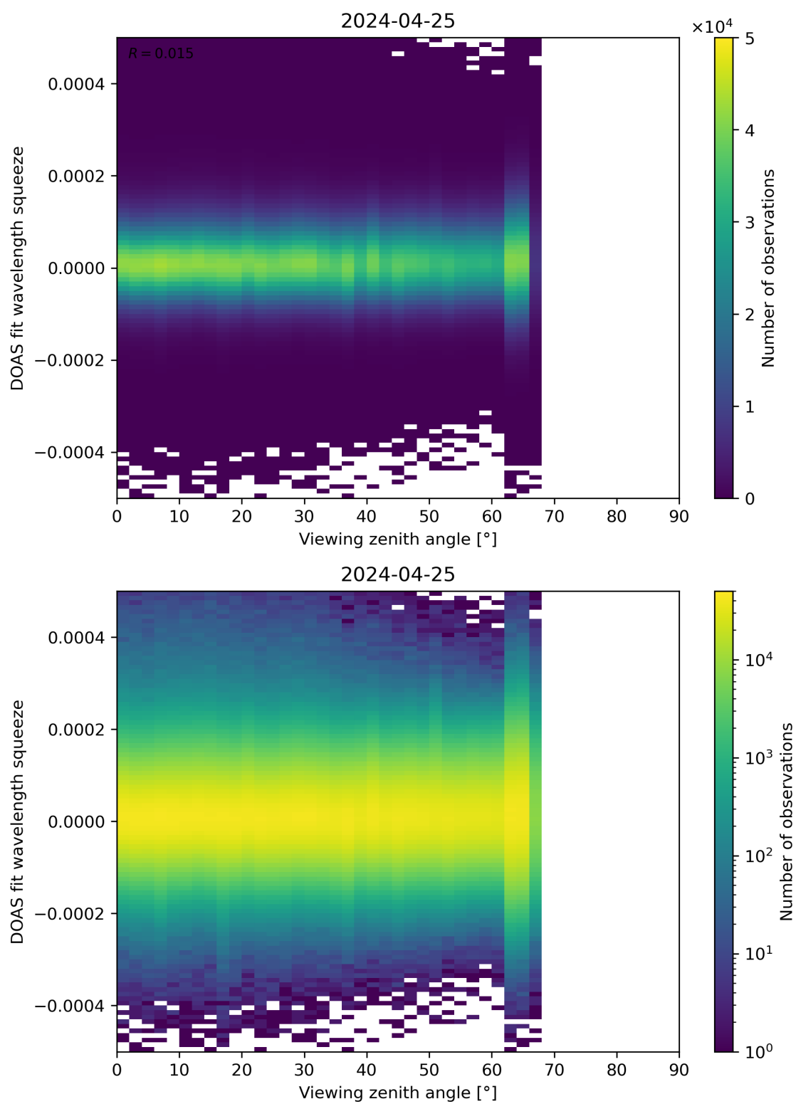
Figure 184: Scatter density plot of “Viewing zenith angle” against “DOAS fit wavelength squeeze” for 2024-04-24 to 2024-04-26.
