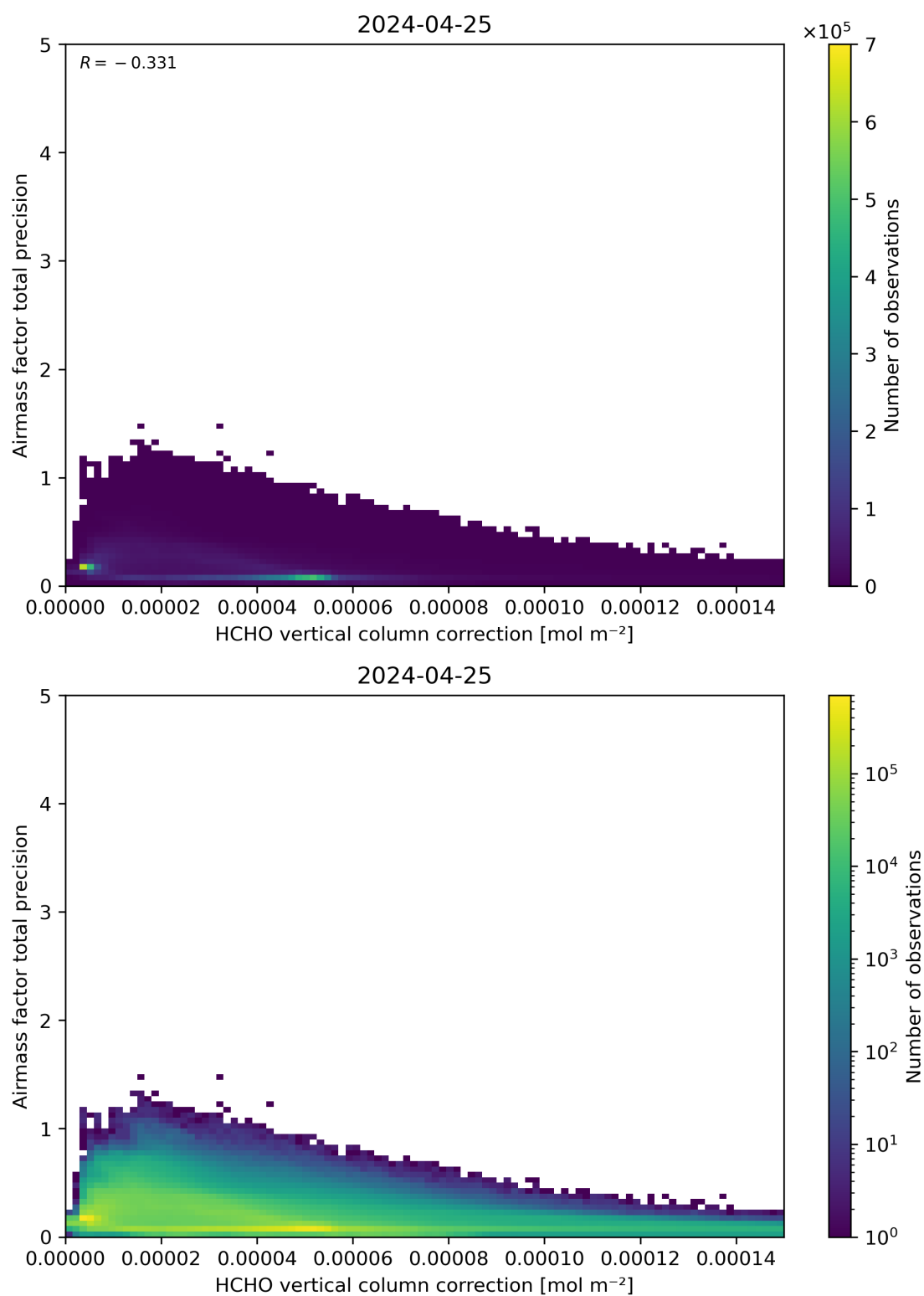
Figure 121: Scatter density plot of “HCHO vertical column correction” against “Airmass factor total precision” for 2024-04-24 to 2024-04-26.
