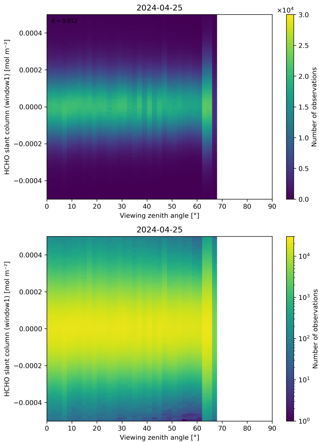
Figure 188: Scatter density plot of “Viewing zenith angle” against “HCHO slant column (window1)” for 2024-04-24 to 2024-04-26.
