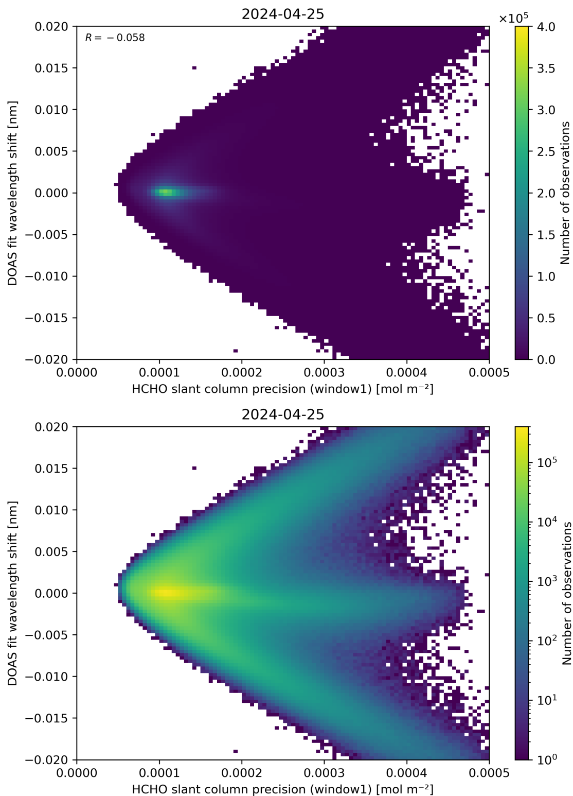
Figure 89: Scatter density plot of “HCHO slant column precision (window1)” against “DOAS fit wavelength shift” for 2024-04-24 to 2024-04-26.
