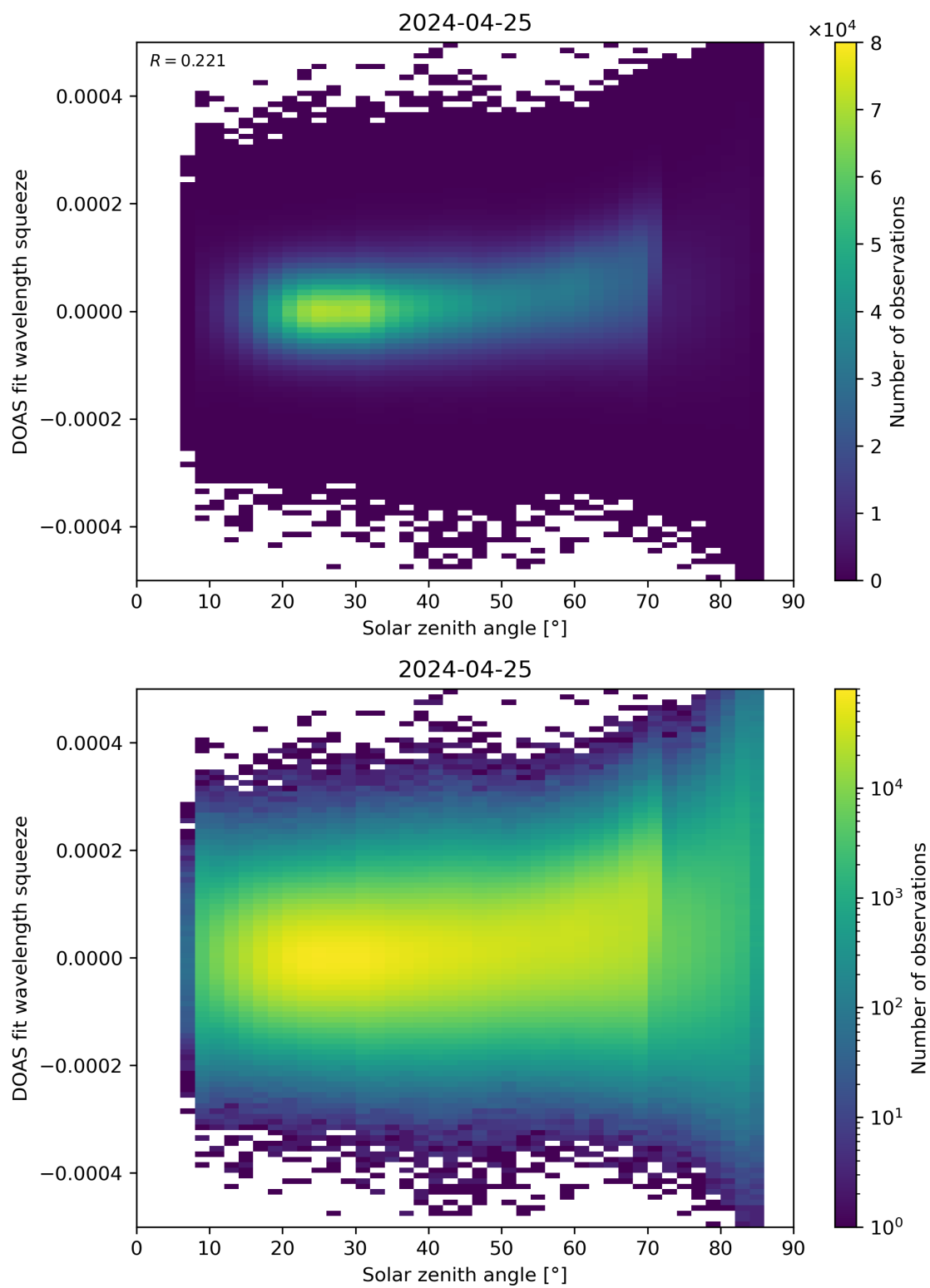
Figure 169: Scatter density plot of “Solar zenith angle” against “DOAS fit wavelength squeeze” for 2024-04-24 to 2024-04-26.
