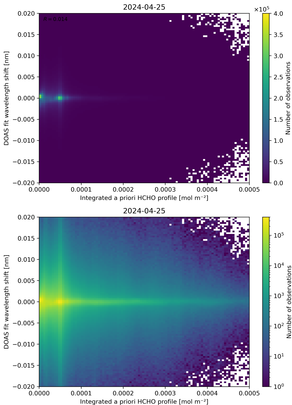
Figure 149: Scatter density plot of “Integrated a priori HCHO profile” against “DOAS fit wavelength shift” for 2024-04-24 to 2024-04-26.
