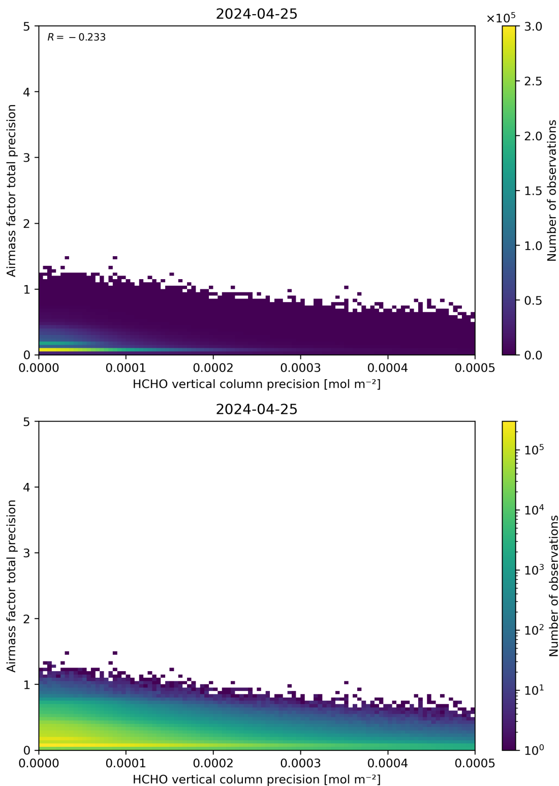
Figure 145: Scatter density plot of “HCHO vertical column precision” against “Airmass factor total precision” for 2024-04-24 to 2024-04-26.
