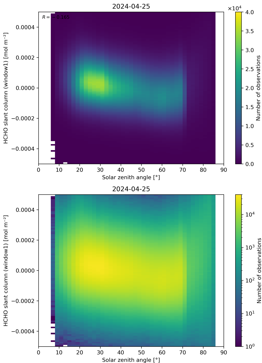
Figure 173: Scatter density plot of “Solar zenith angle” against “HCHO slant column (window1)” for 2024-04-24 to 2024-04-26.
