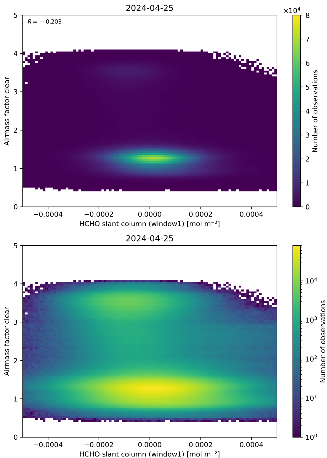
Figure 81: Scatter density plot of “HCHO slant column (window1)” against “Airmass factor clear” for 2024-04-24 to 2024-04-26.
