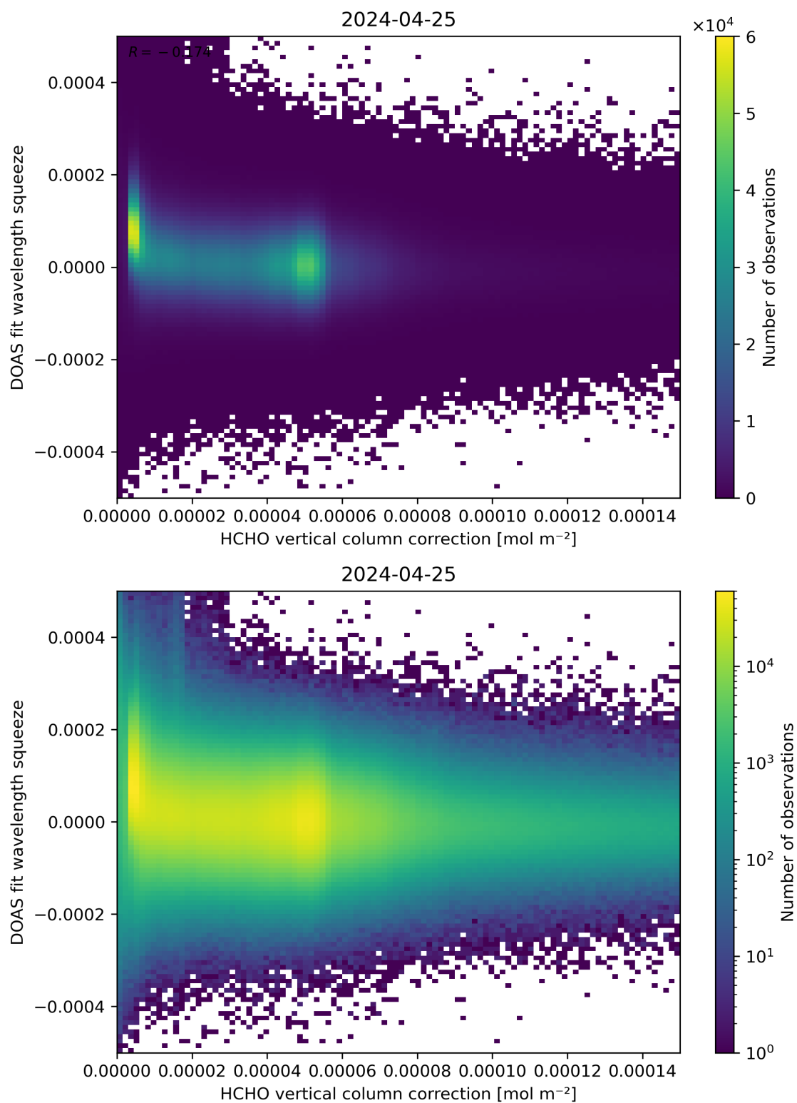
Figure 114: Scatter density plot of “HCHO vertical column correction” against “DOAS fit wavelength squeeze” for 2024-04-24 to 2024-04-26.
