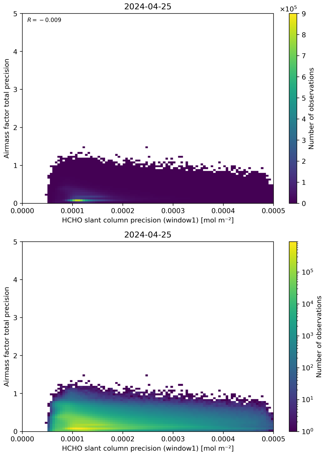
Figure 95: Scatter density plot of “HCHO slant column precision (window1)” against “Airmass factor total precision” for 2024-04-24 to 2024-04-26.
