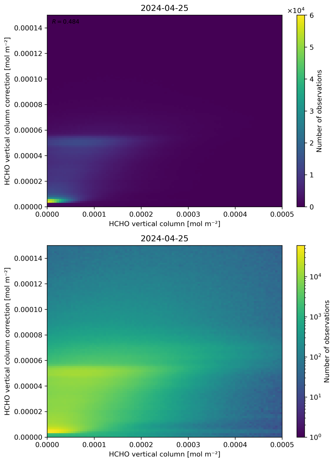
Figure 133: Scatter density plot of “HCHO vertical column” against “HCHO vertical column correction” for 2024-04-24 to 2024-04-26.
