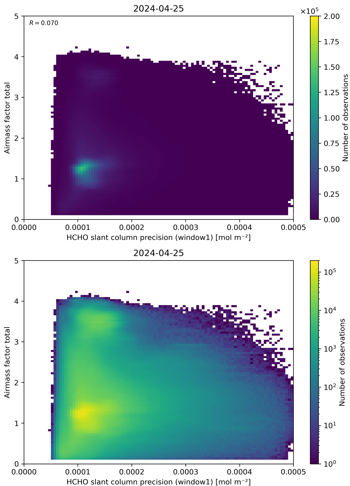
Figure 94: Scatter density plot of “HCHO slant column precision (window1)” against “Airmass factor total” for 2024-04-24 to 2024-04-26.
