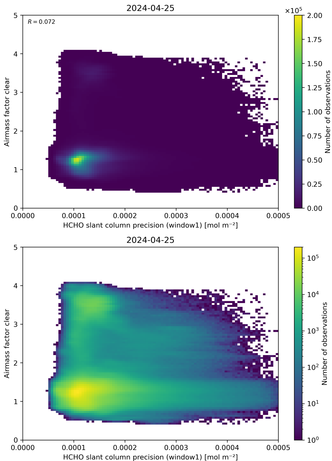
Figure 91: Scatter density plot of “HCHO slant column precision (window1)” against “Airmass factor clear” for 2024-04-24 to 2024-04-26.
