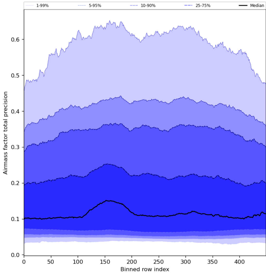
Figure 55: Along track statistics of “Airmass factor total precision” for 2024-04-24 to 2024-04-26
