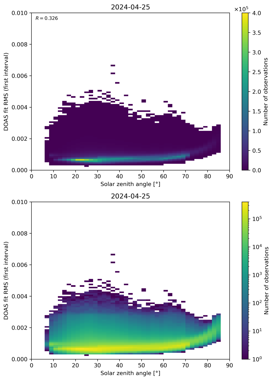
Figure 167: Scatter density plot of “Solar zenith angle” against “DOAS fit RMS (first interval)” for 2024-04-24 to 2024-04-26.
