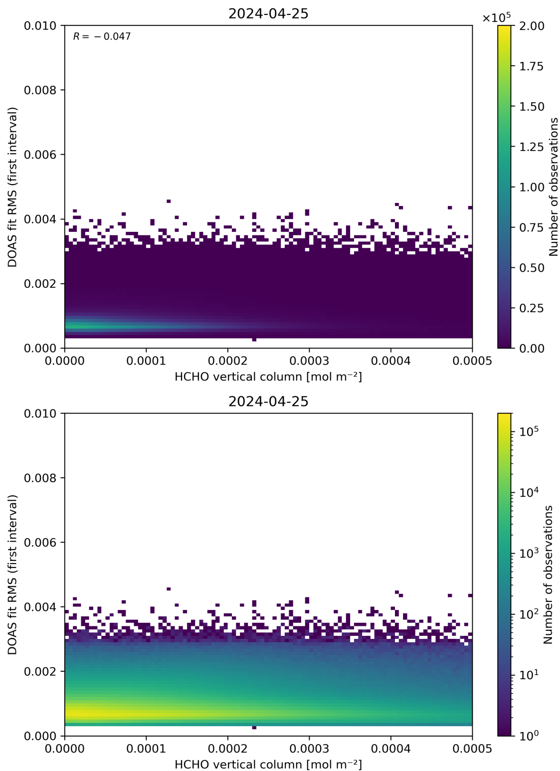
Figure 123: Scatter density plot of “HCHO vertical column” against “DOAS fit RMS (first interval)” for 2024-04-24 to 2024-04-26.
