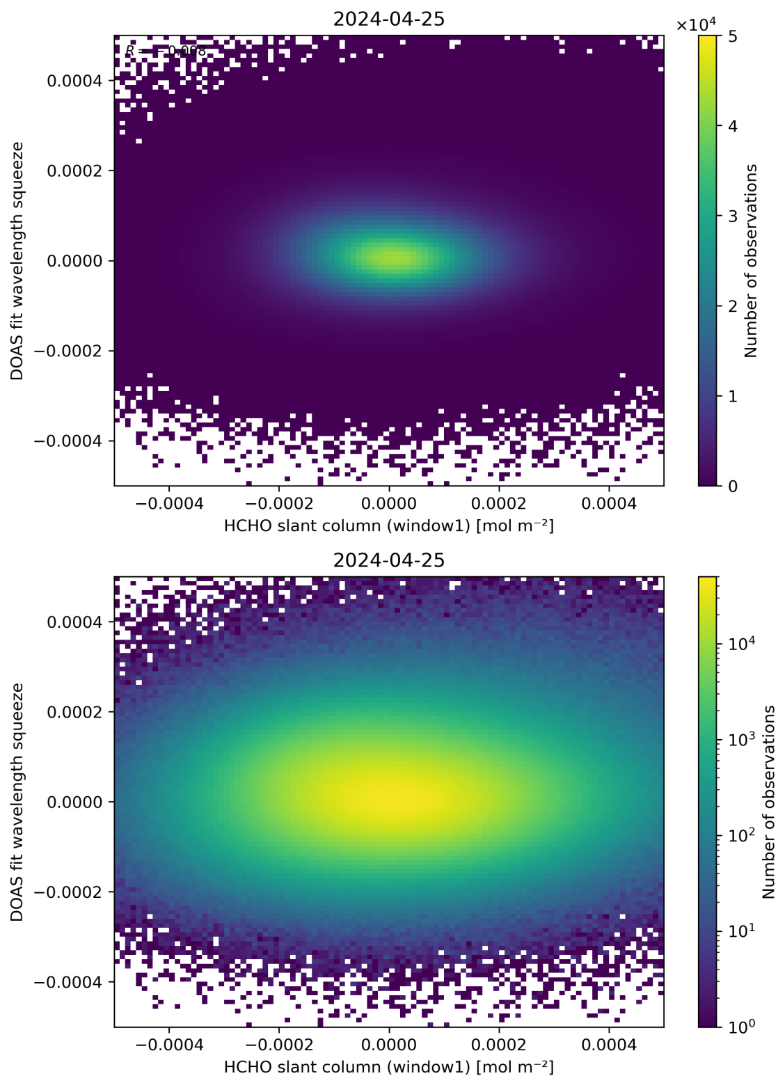
Figure 80: Scatter density plot of “HCHO slant column (window1)” against “DOAS fit wavelength squeeze” for 2024-04-24 to 2024-04-26.
