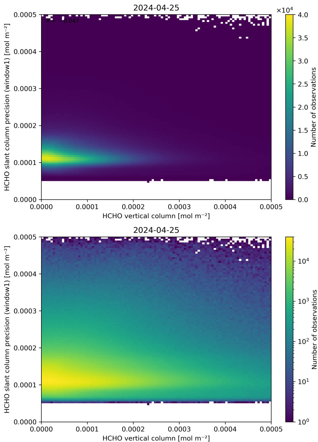
Figure 130: Scatter density plot of “HCHO vertical column” against “HCHO slant column precision (window1)” for 2024-04-24 to 2024-04-26.
