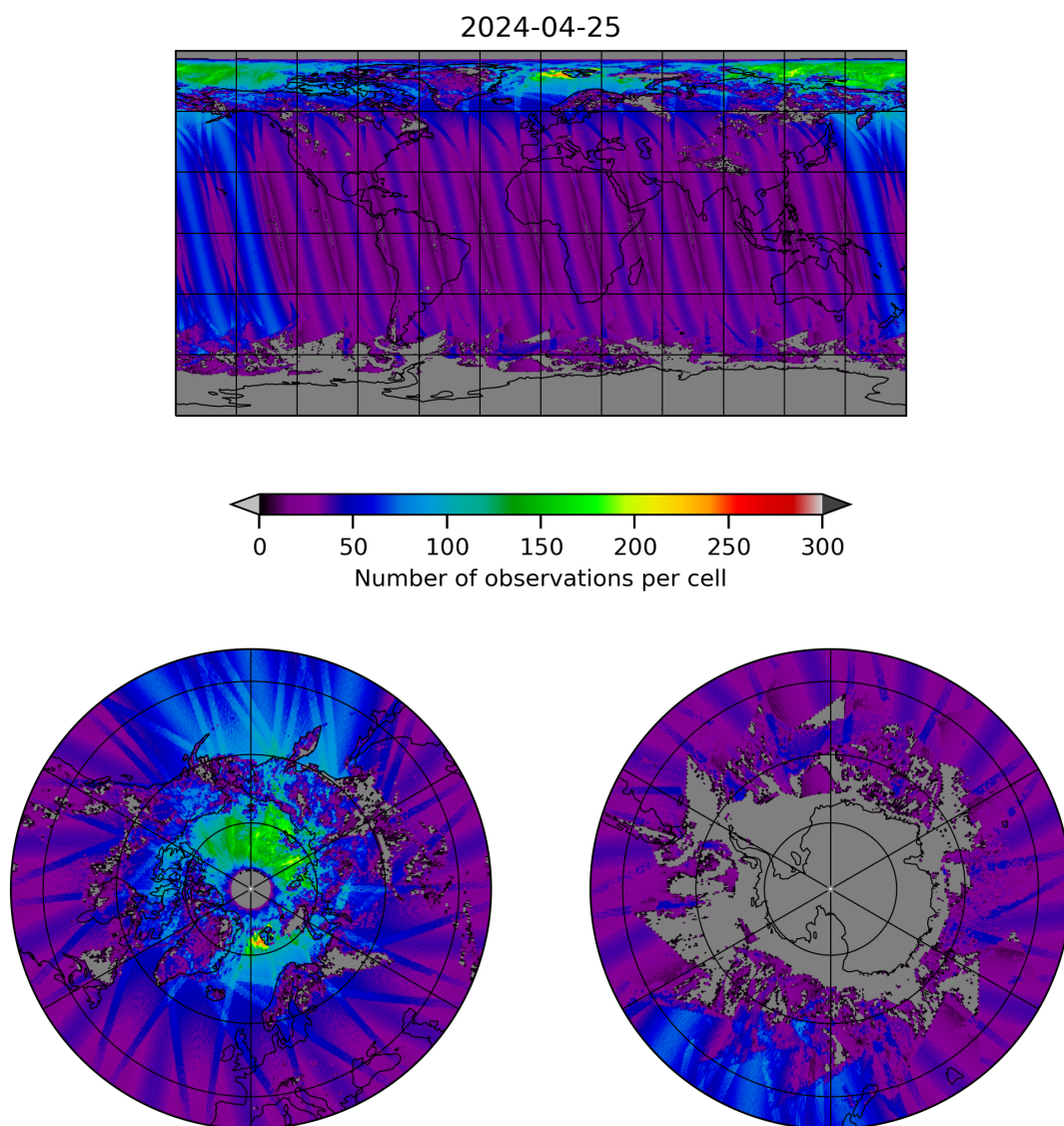
Figure 19: Map of the number of observations for 2024-04-24 to 2024-04-26
