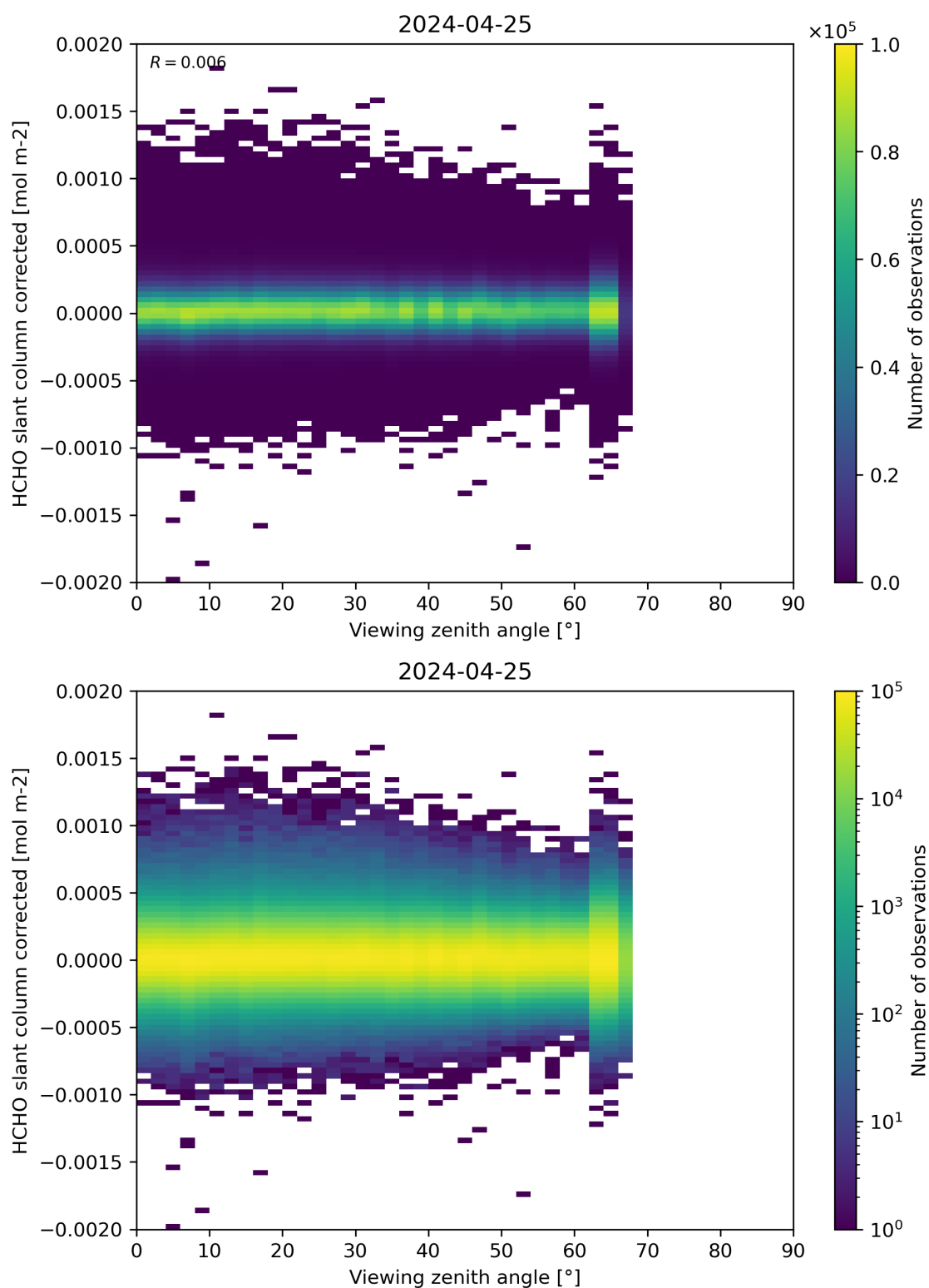
Figure 186: Scatter density plot of “Viewing zenith angle” against “HCHO slant column corrected” for 2024-04-24 to 2024-04-26.
