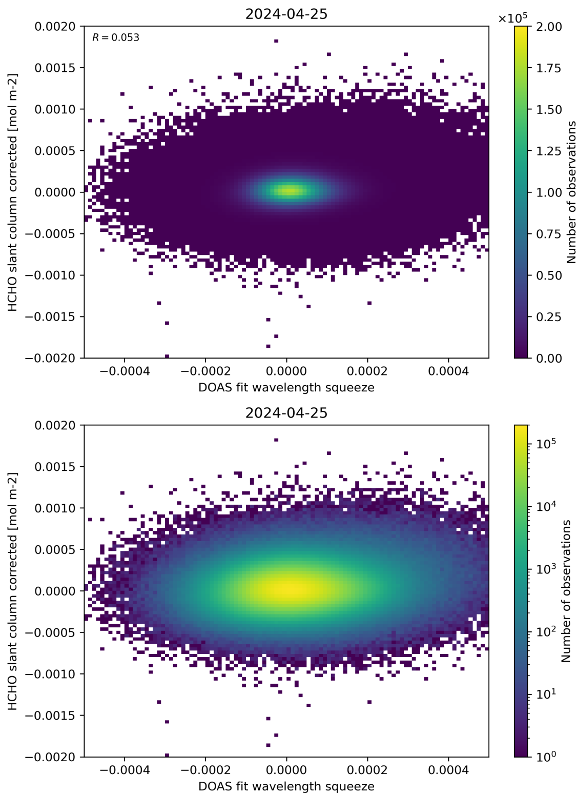
Figure 69: Scatter density plot of “DOAS fit wavelength squeeze” against “HCHO slant column corrected” for 2024-04-24 to 2024-04-26.
