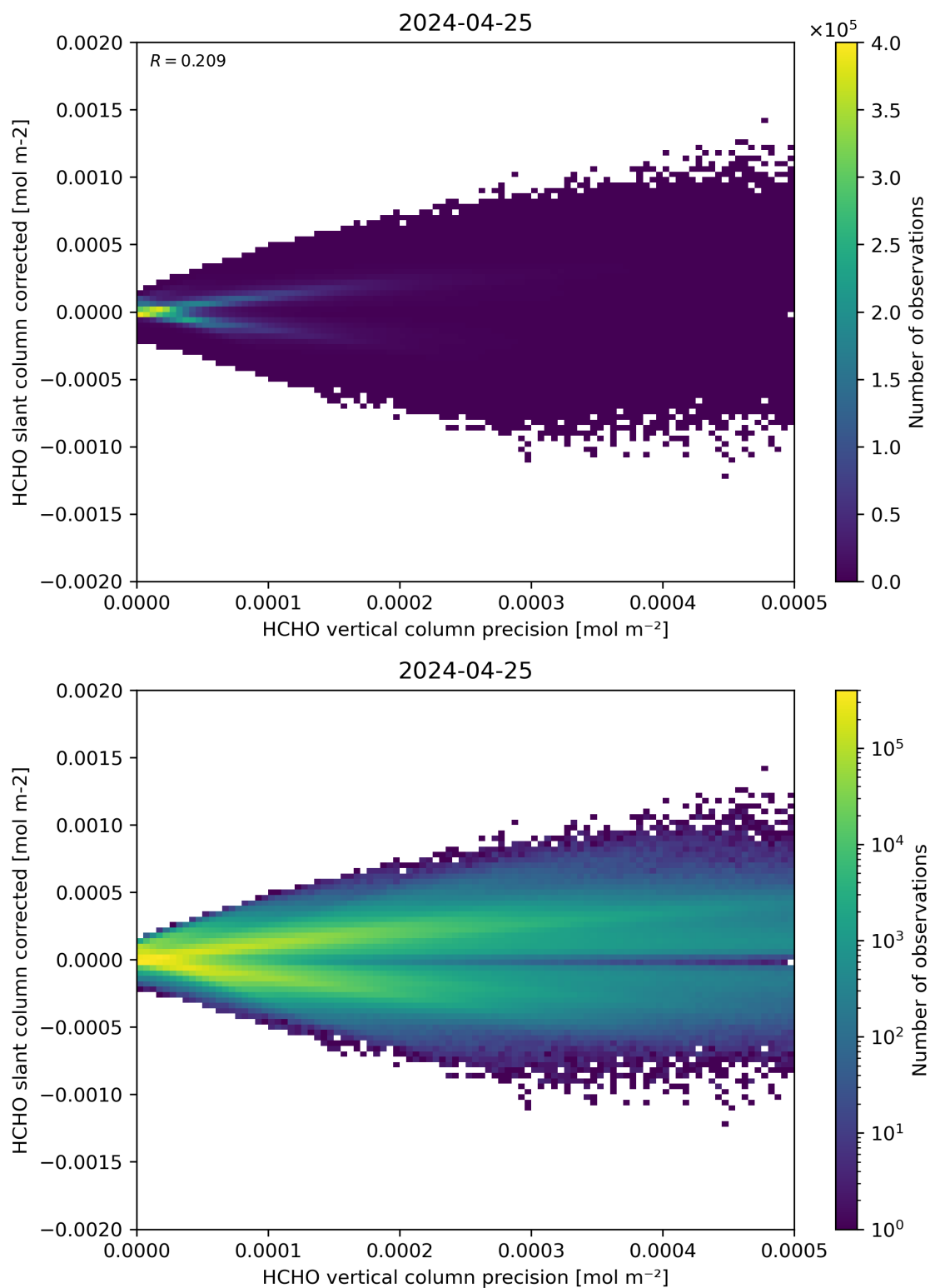
Figure 140: Scatter density plot of “HCHO vertical column precision” against “HCHO slant column corrected” for 2024-04-24 to 2024-04-26.
