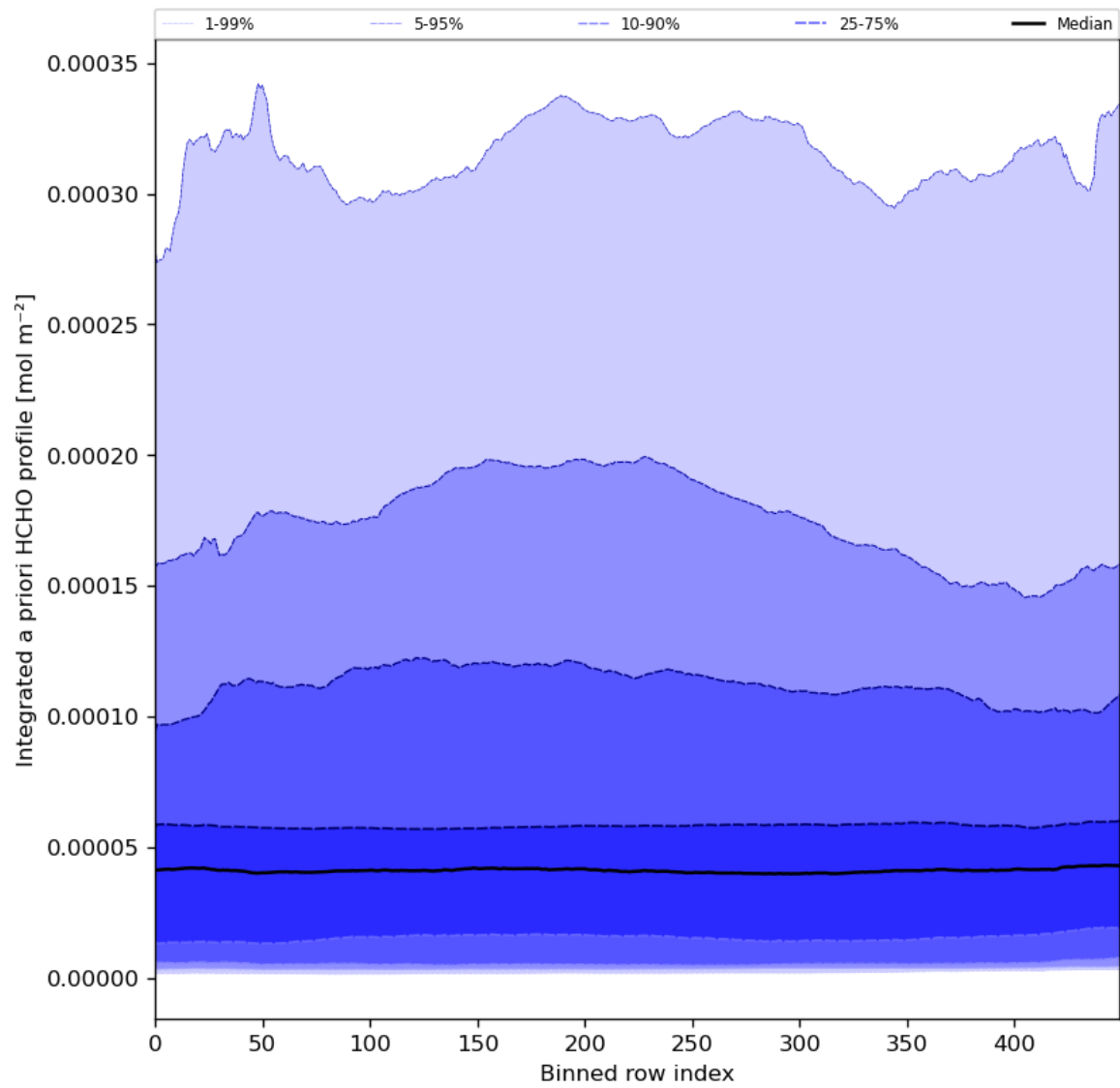
Figure 57: Along track statistics of “Integrated a priori HCHO profile” for 2024-04-24 to 2024-04-26
