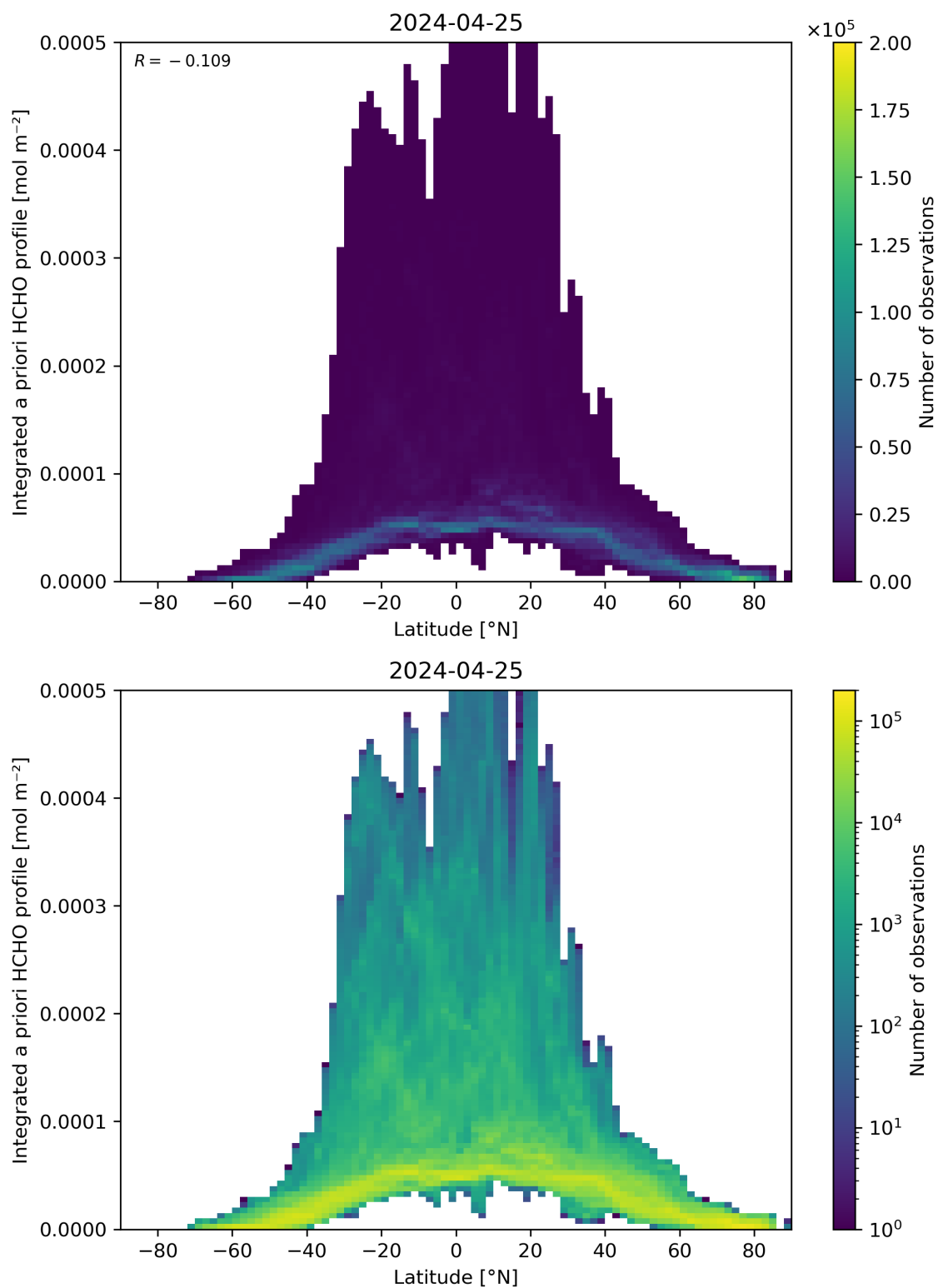
Figure 166: Scatter density plot of “Latitude” against “Integrated a priori HCHO profile” for 2024-04-24 to 2024-04-26.
