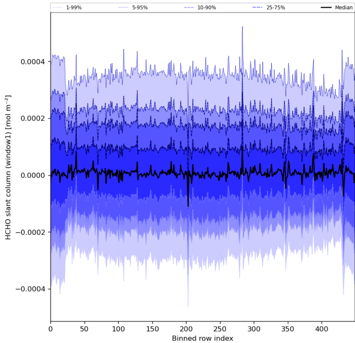
Figure 52: Along track statistics of “HCHO slant column (window1)” for 2024-04-24 to 2024-04-26
