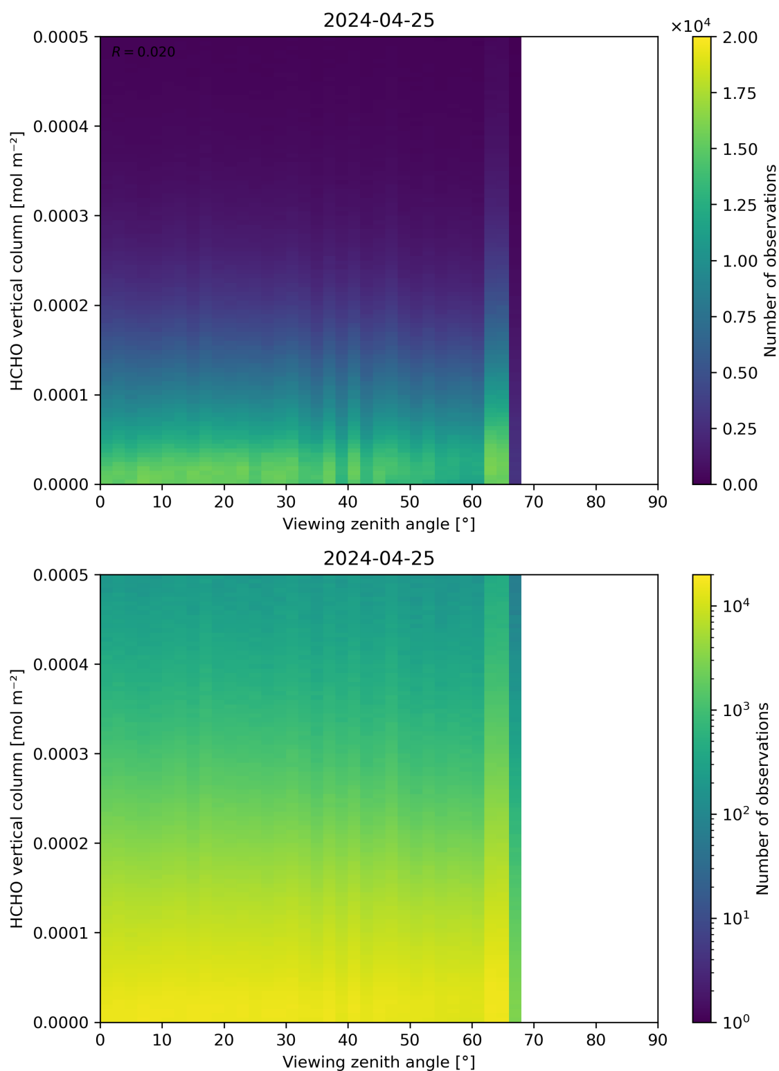
Figure 192: Scatter density plot of “Viewing zenith angle” against “HCHO vertical column” for 2024-04-24 to 2024-04-26.
