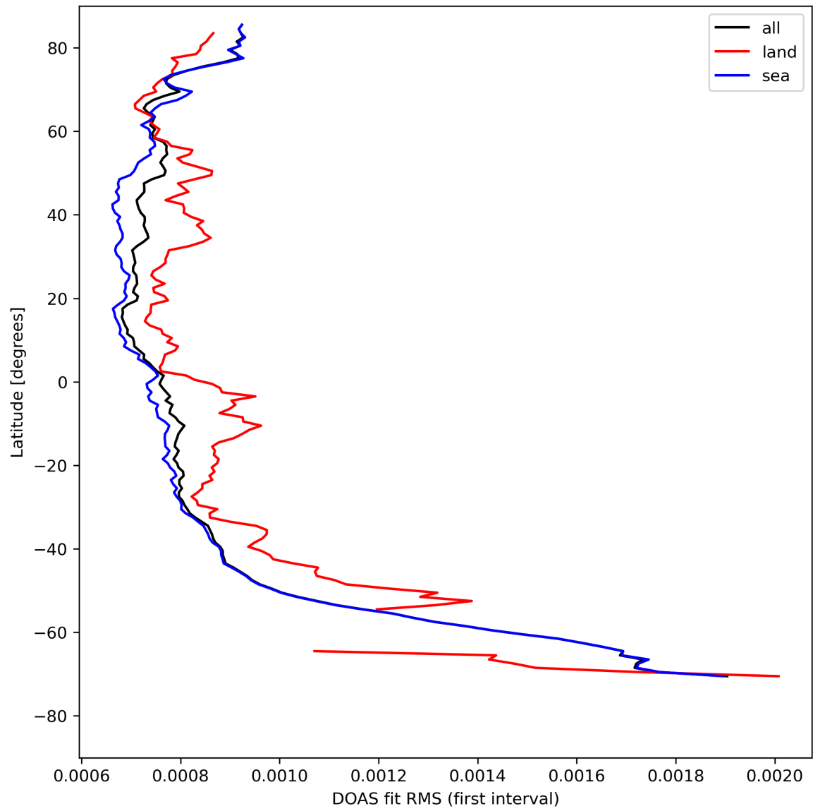
Figure 32: Zonal average of “DOAS fit RMS (first interval)” for 2024-04-24 to 2024-04-26.
