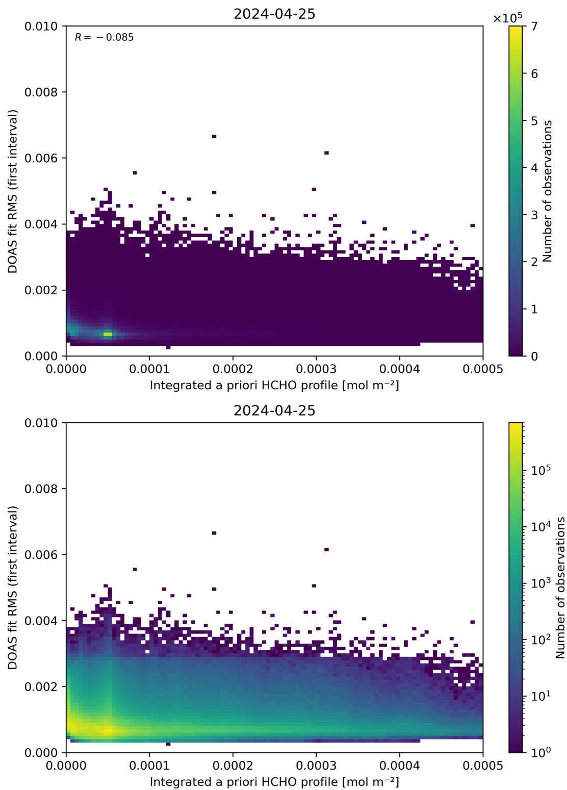
Figure 148: Scatter density plot of “Integrated a priori HCHO profile” against “DOAS fit RMS (first interval)” for 2024-04-24 to 2024-04-26.
