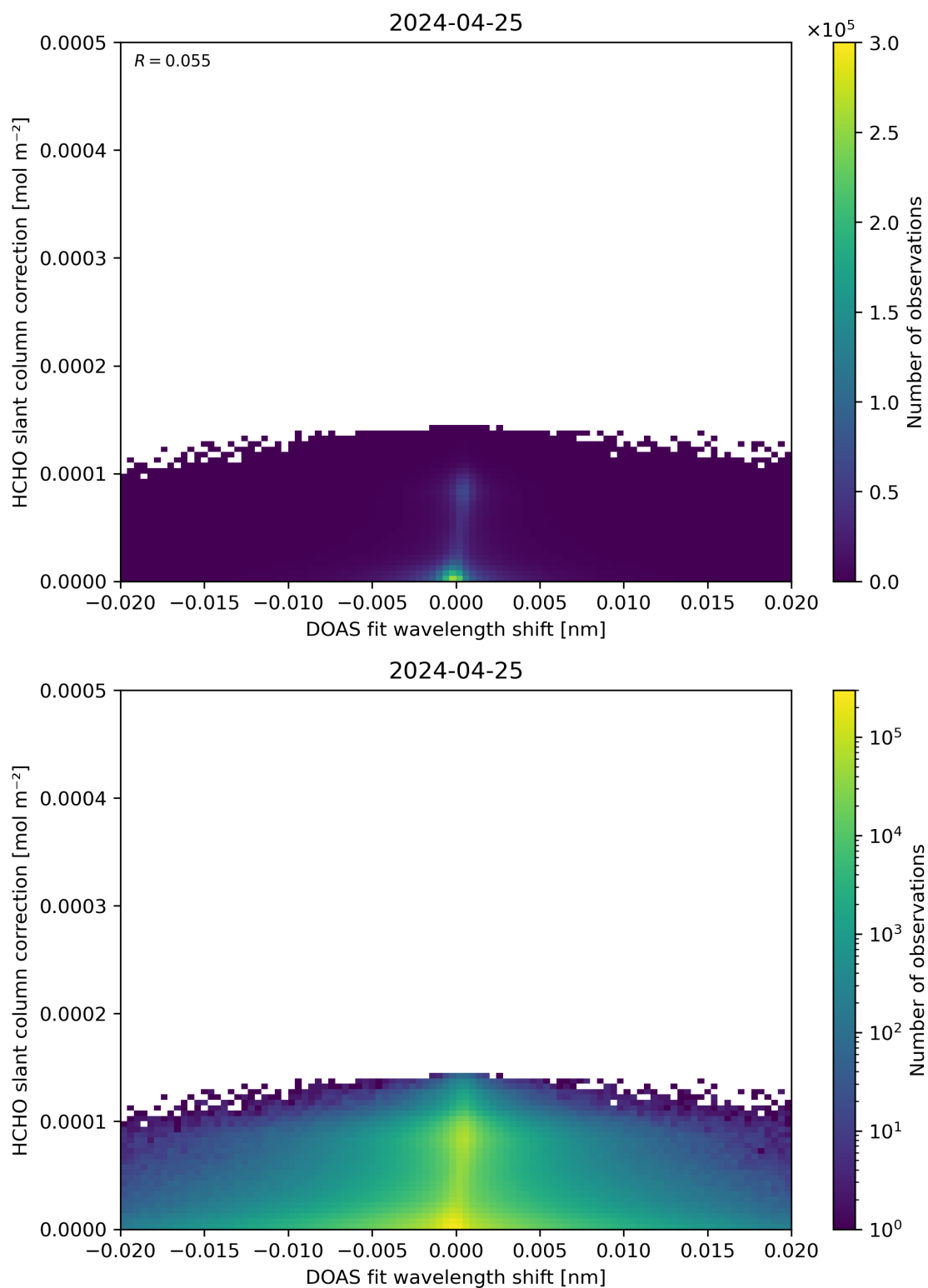
Figure 67: Scatter density plot of “DOAS fit wavelength shift” against “HCHO slant column correction” for 2024-04-24 to 2024-04-26.
