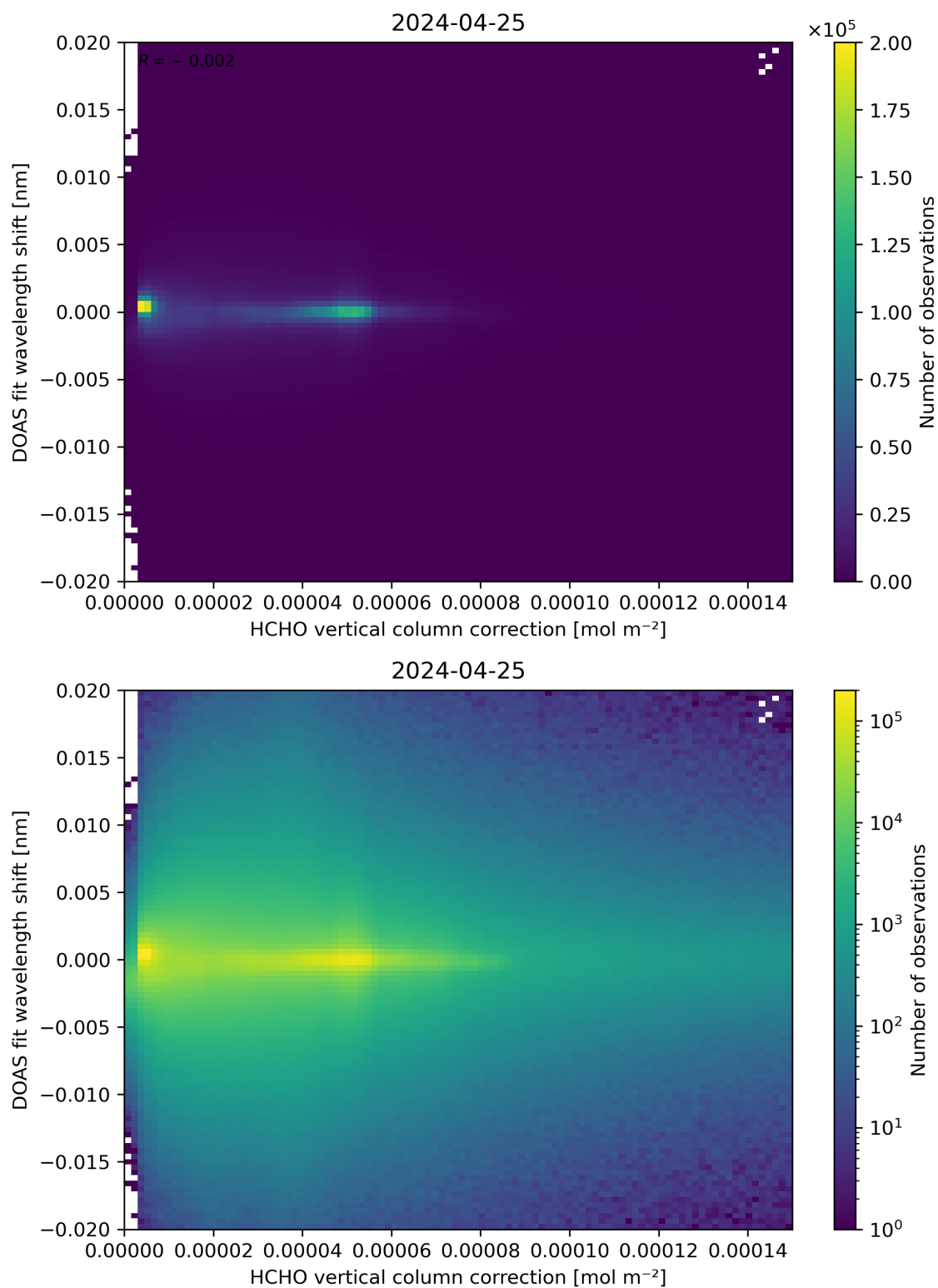
Figure 113: Scatter density plot of “HCHO vertical column correction” against “DOAS fit wavelength shift” for 2024-04-24 to 2024-04-26.
