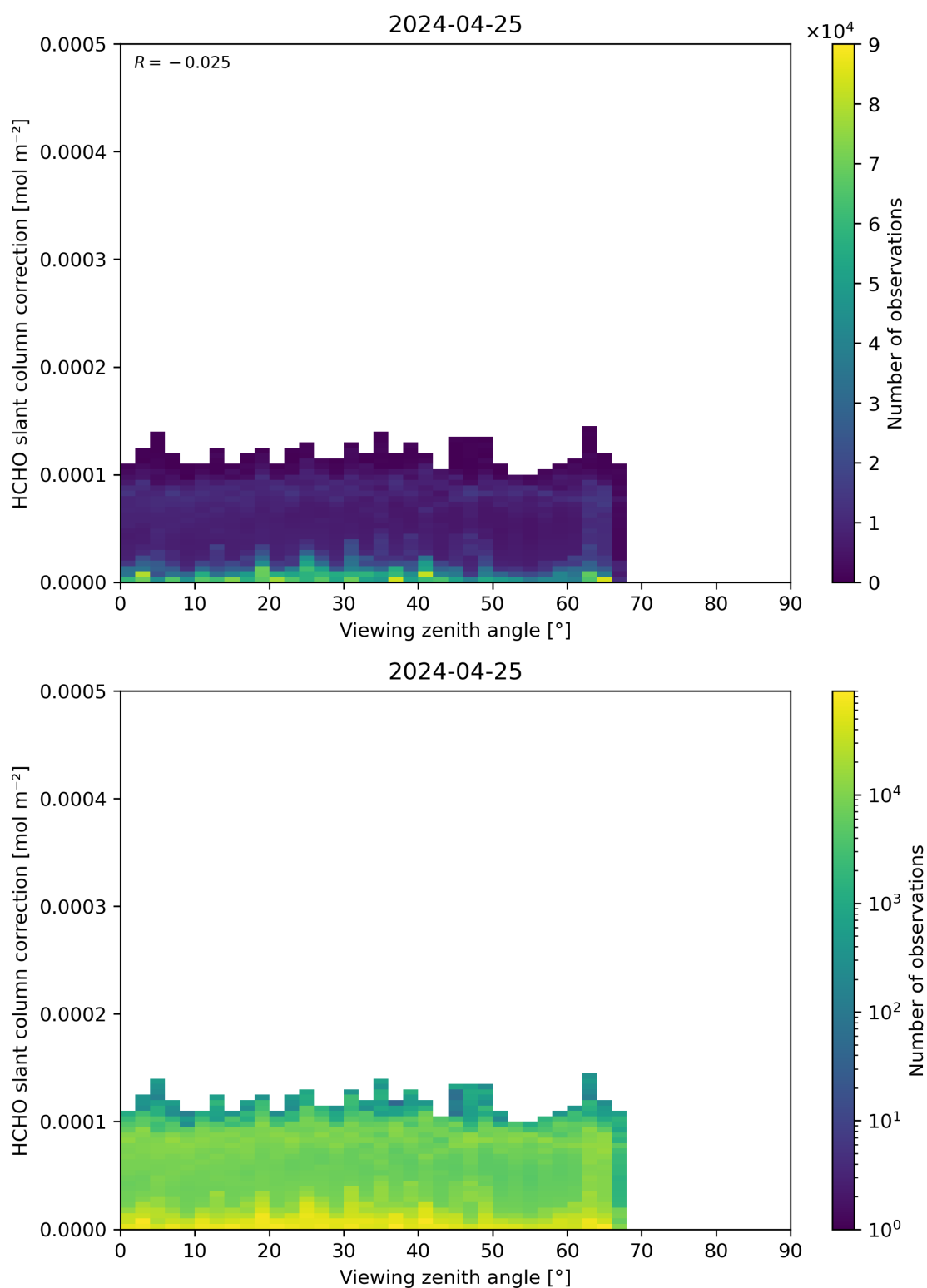
Figure 187: Scatter density plot of “Viewing zenith angle” against “HCHO slant column correction” for 2024-04-24 to 2024-04-26.
