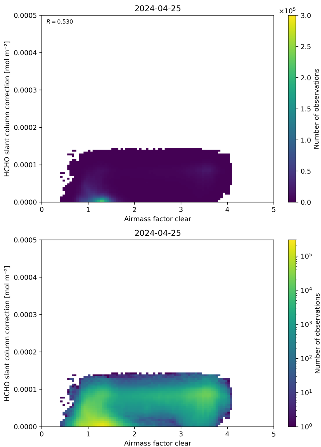
Figure 75: Scatter density plot of “Airmass factor clear” against “HCHO slant column correction” for 2024-04-24 to 2024-04-26.
