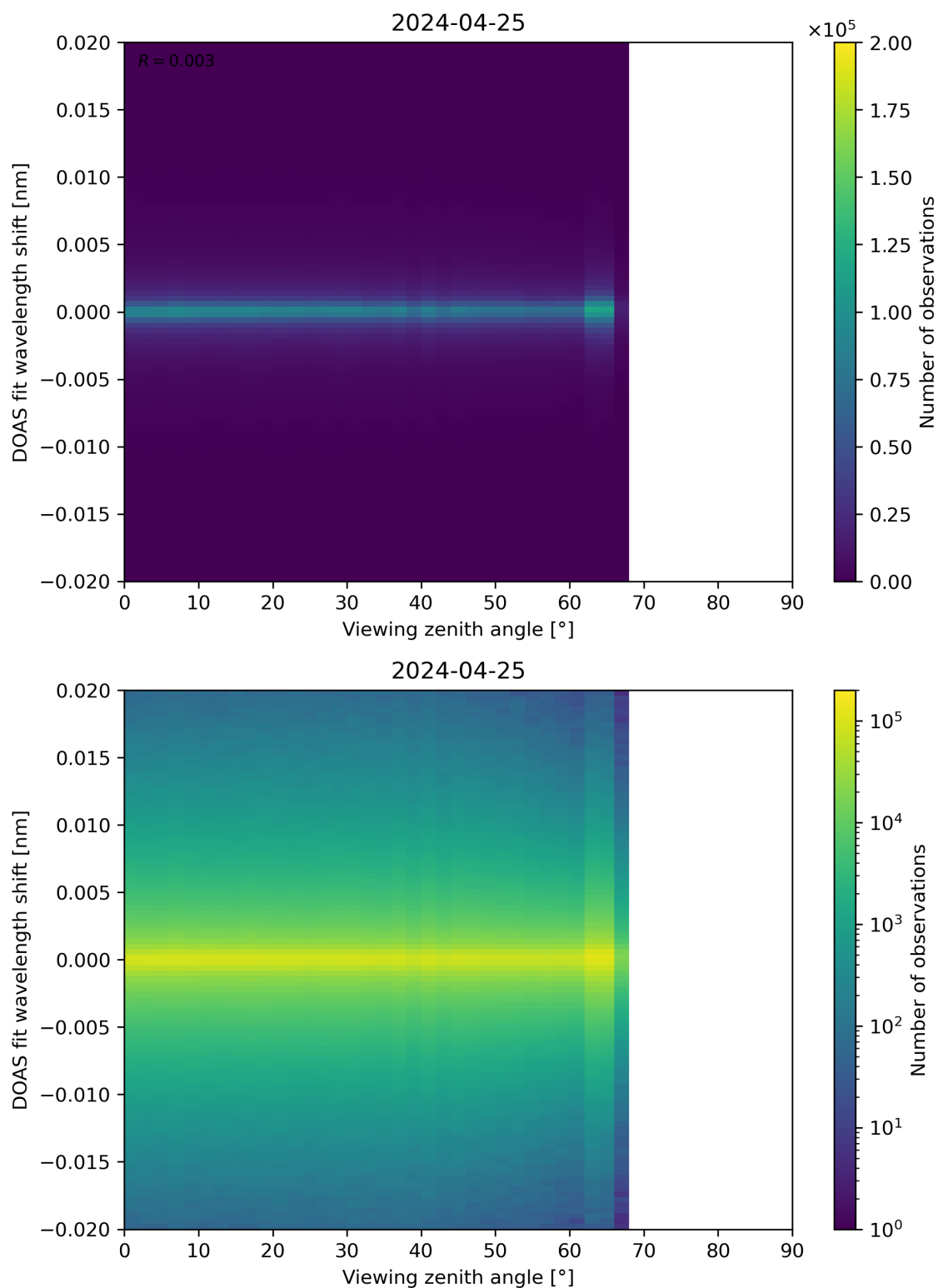
Figure 183: Scatter density plot of “Viewing zenith angle” against “DOAS fit wavelength shift” for 2024-04-24 to 2024-04-26.
