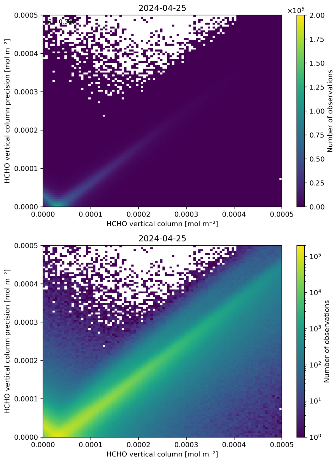
Figure 134: Scatter density plot of “HCHO vertical column” against “HCHO vertical column precision” for 2024-04-24 to 2024-04-26.
