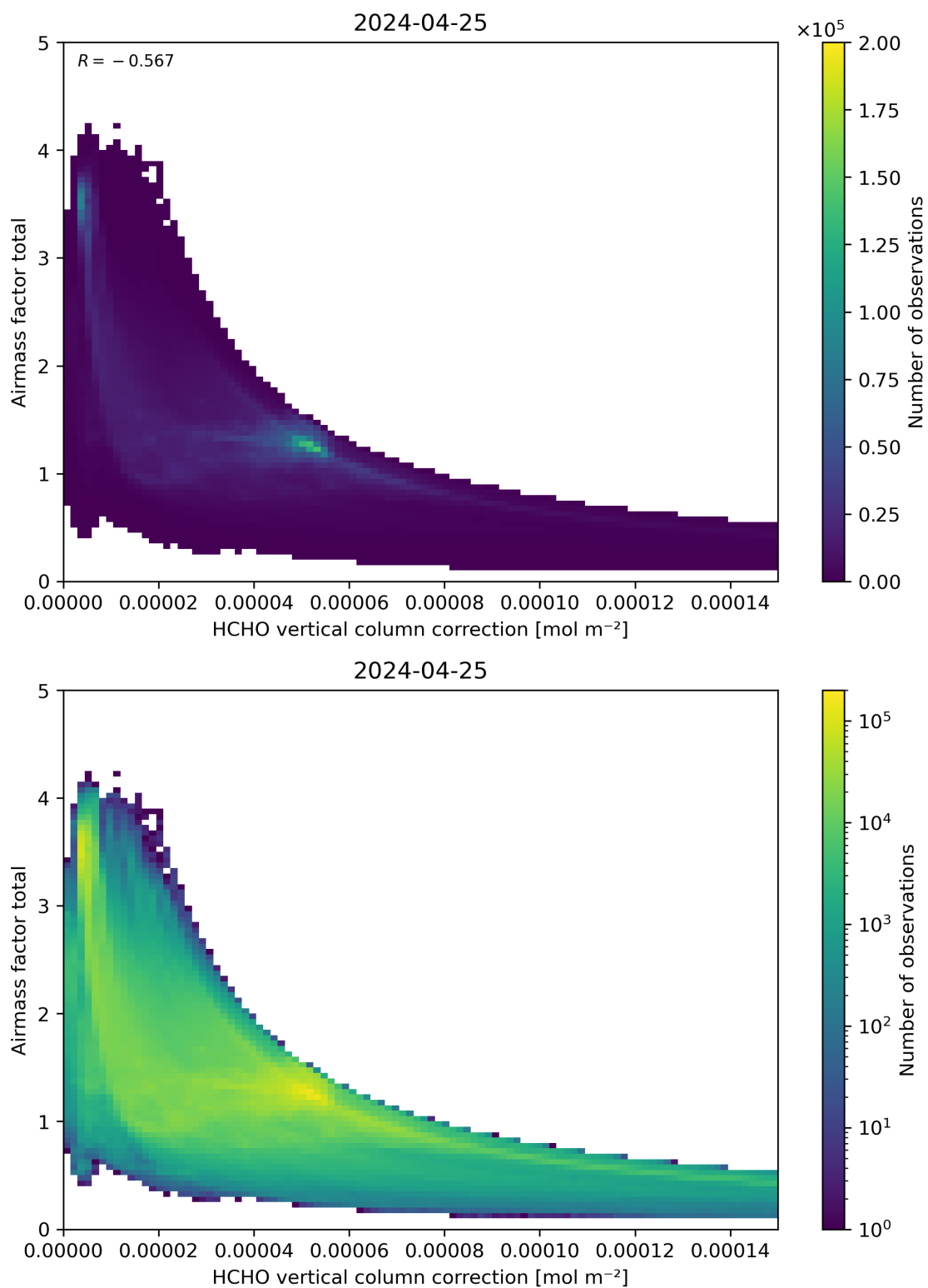
Figure 120: Scatter density plot of “HCHO vertical column correction” against “Airmass factor total” for 2024-04-24 to 2024-04-26.
