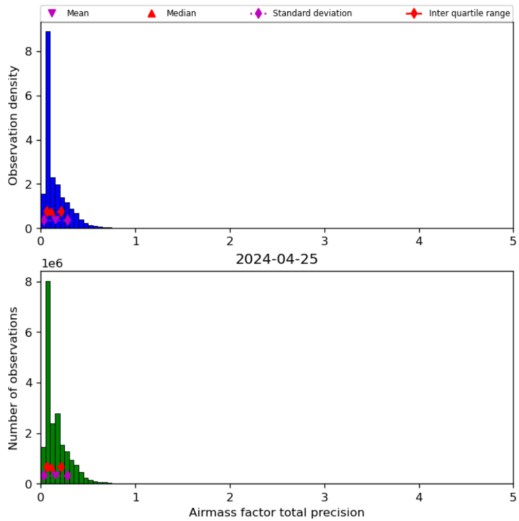
Figure 41: Histogram of “Airmass factor total precision” for 2024-04-24 to 2024-04-26
