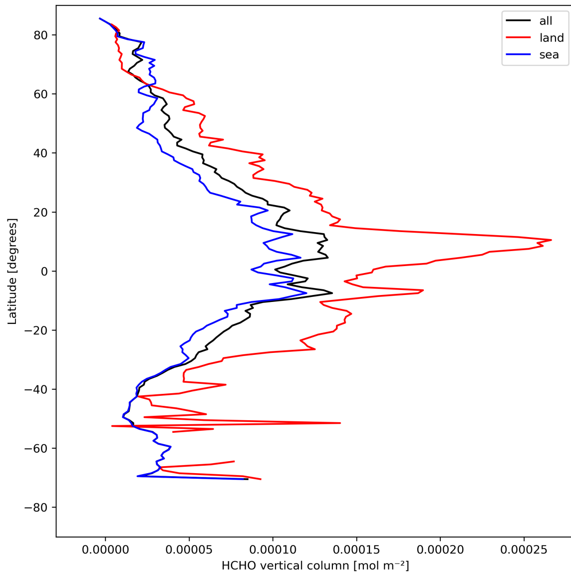
Figure 21: Zonal average of “HCHO vertical column” for 2024-04-24 to 2024-04-26.
