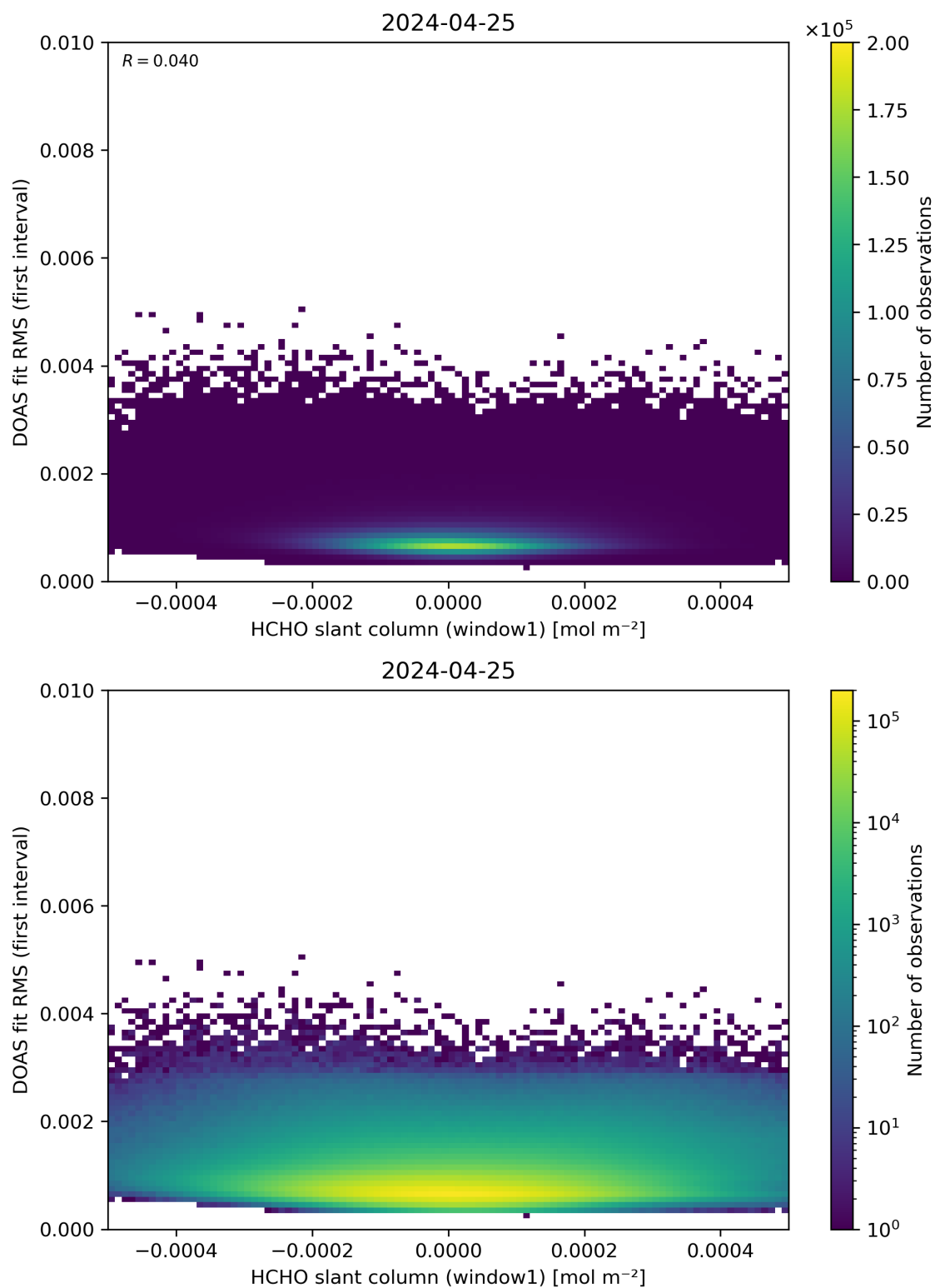
Figure 78: Scatter density plot of “HCHO slant column (window1)” against “DOAS fit RMS (first interval)” for 2024-04-24 to 2024-04-26.
