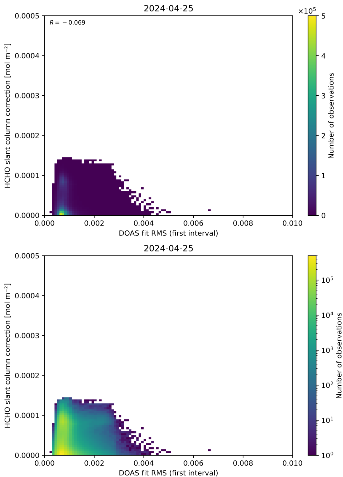
Figure 63: Scatter density plot of “DOAS fit RMS (first interval)” against “HCHO slant column correction” for 2024-04-24 to 2024-04-26.
