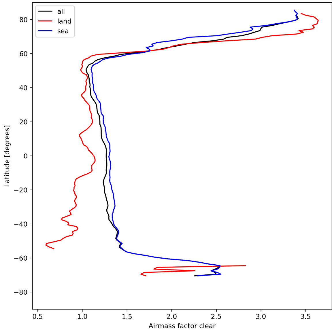
Figure 28: Zonal average of “Airmass factor clear” for 2024-04-24 to 2024-04-26.
