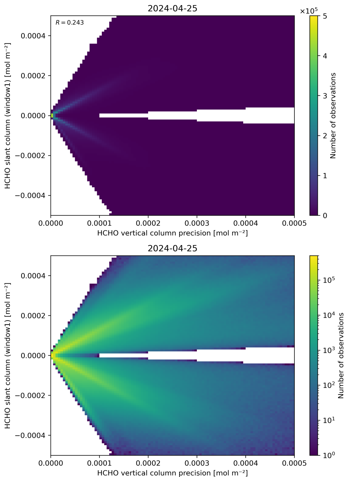
Figure 142: Scatter density plot of “HCHO vertical column precision” against “HCHO slant column (window1)” for 2024-04-24 to 2024-04-26.
