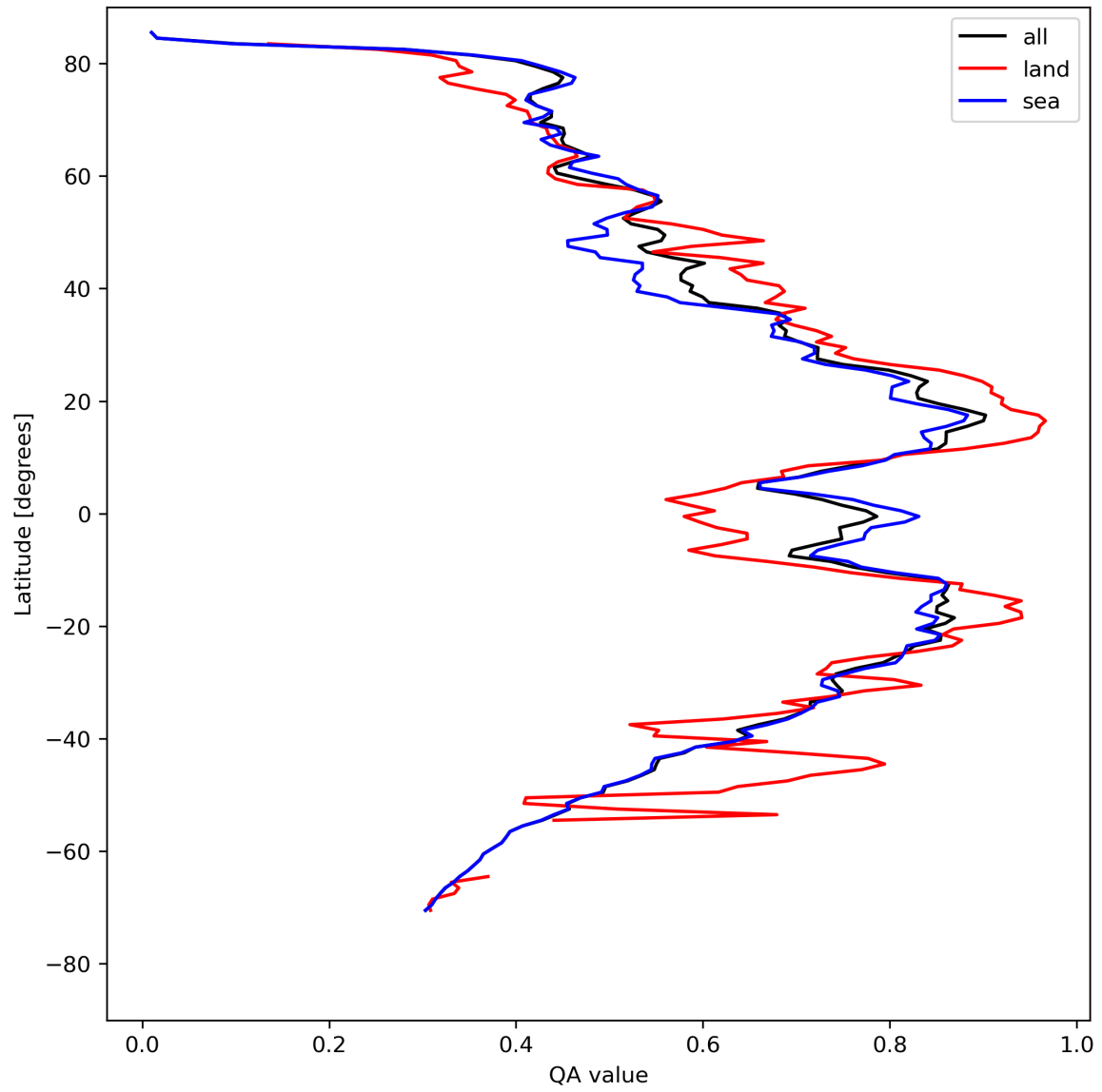
Figure 20: Zonal average of “QA value” for 2024-04-24 to 2024-04-26.
