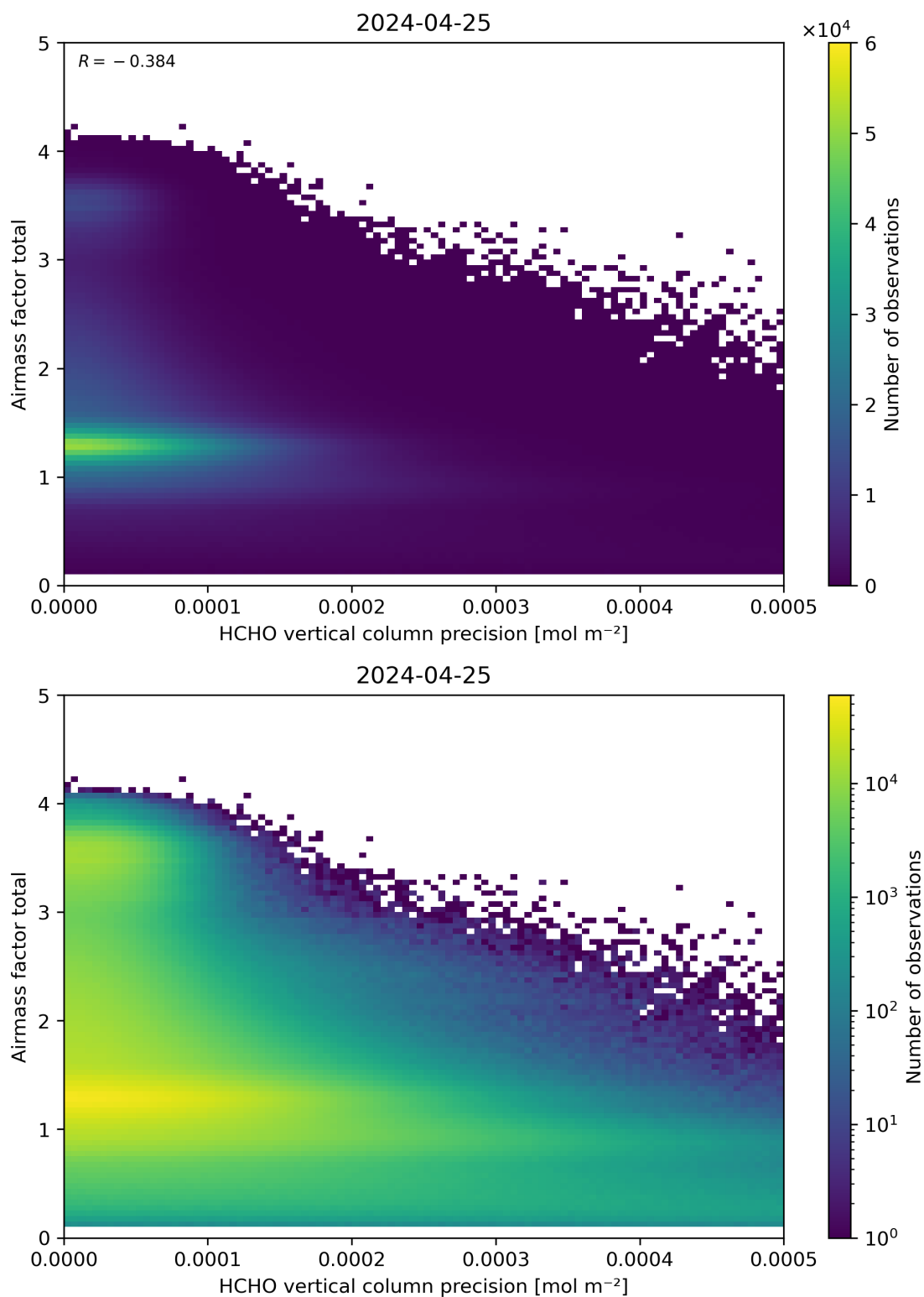
Figure 144: Scatter density plot of “HCHO vertical column precision” against “Airmass factor total” for 2024-04-24 to 2024-04-26.
