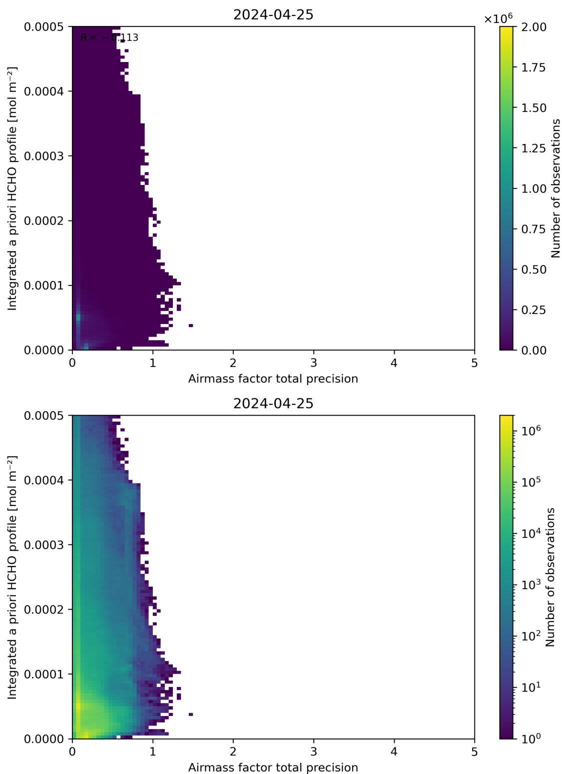
Figure 111: Scatter density plot of “Airmass factor total precision” against “Integrated a priori HCHO profile” for 2024-04-24 to 2024-04-26.
