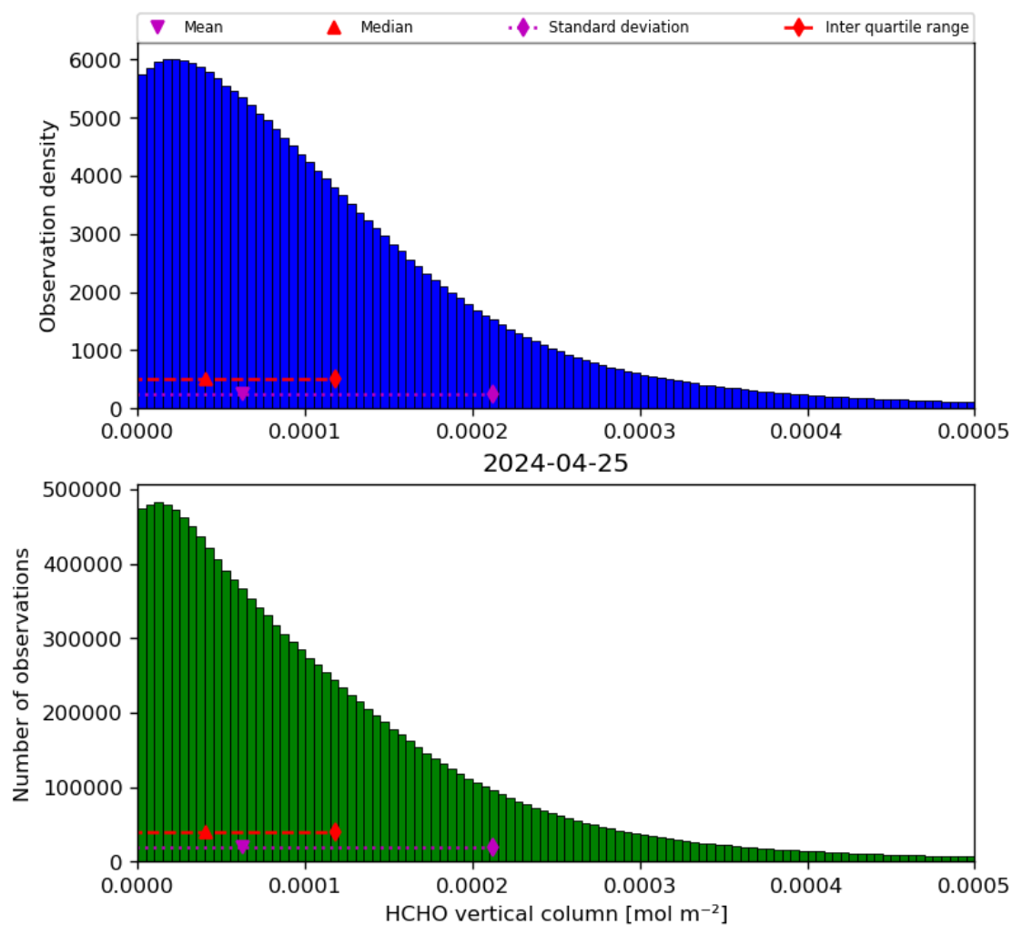
Figure 35: Histogram of “HCHO vertical column” for 2024-04-24 to 2024-04-26
