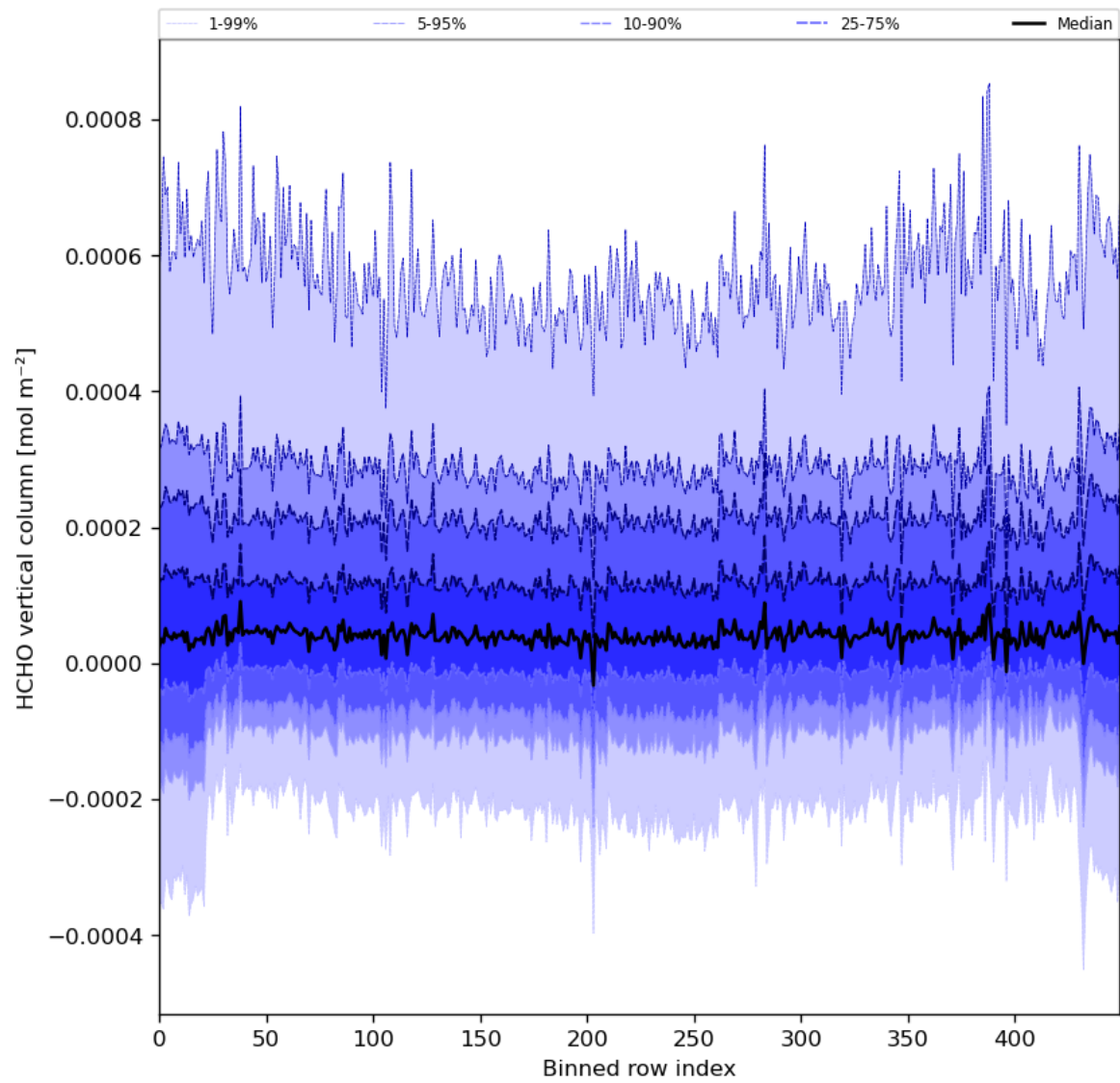
Figure 49: Along track statistics of “HCHO vertical column” for 2024-04-24 to 2024-04-26
