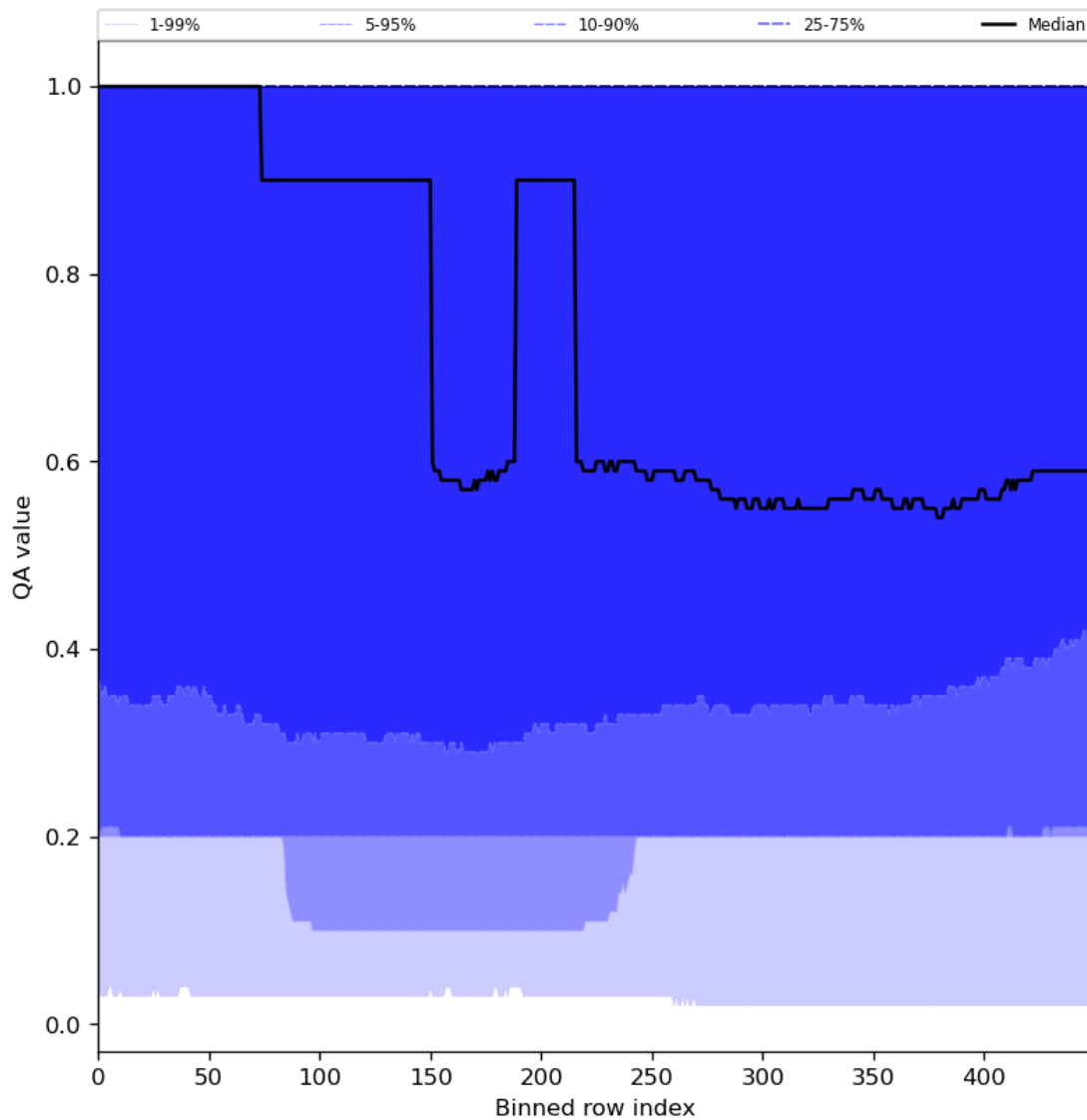
Figure 48: Along track statistics of “QA value” for 2024-04-24 to 2024-04-26
