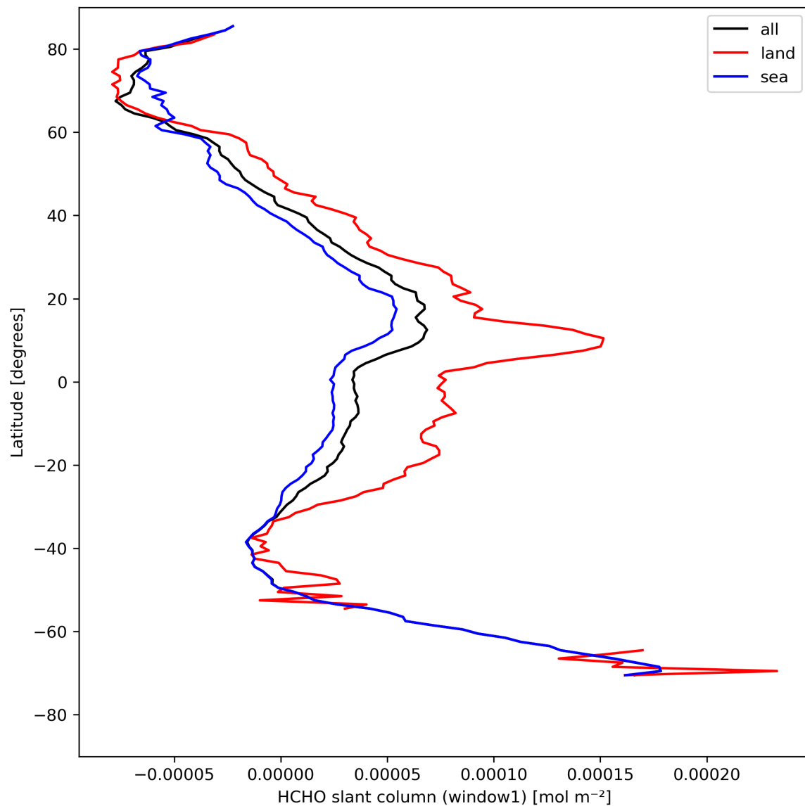
Figure 24: Zonal average of “HCHO slant column (window1)” for 2024-04-24 to 2024-04-26.
