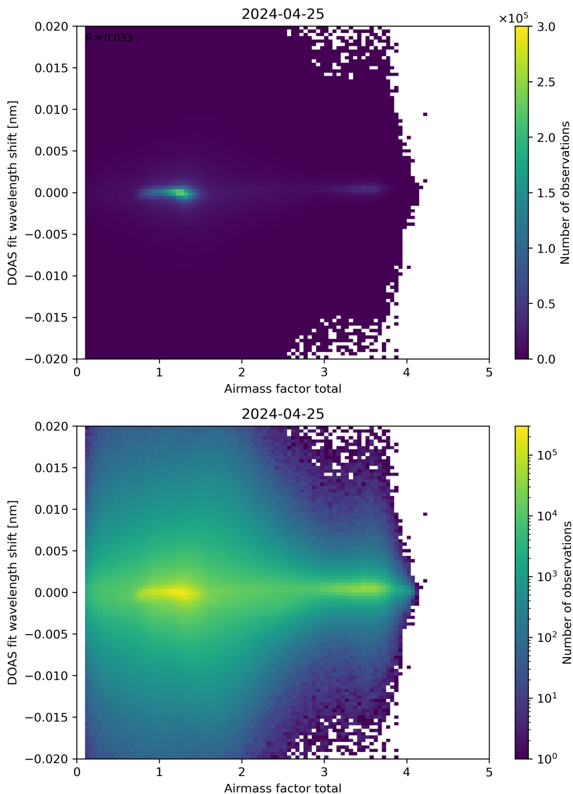
Figure 98: Scatter density plot of “Airmass factor total” against “DOAS fit wavelength shift” for 2024-04-24 to 2024-04-26.
