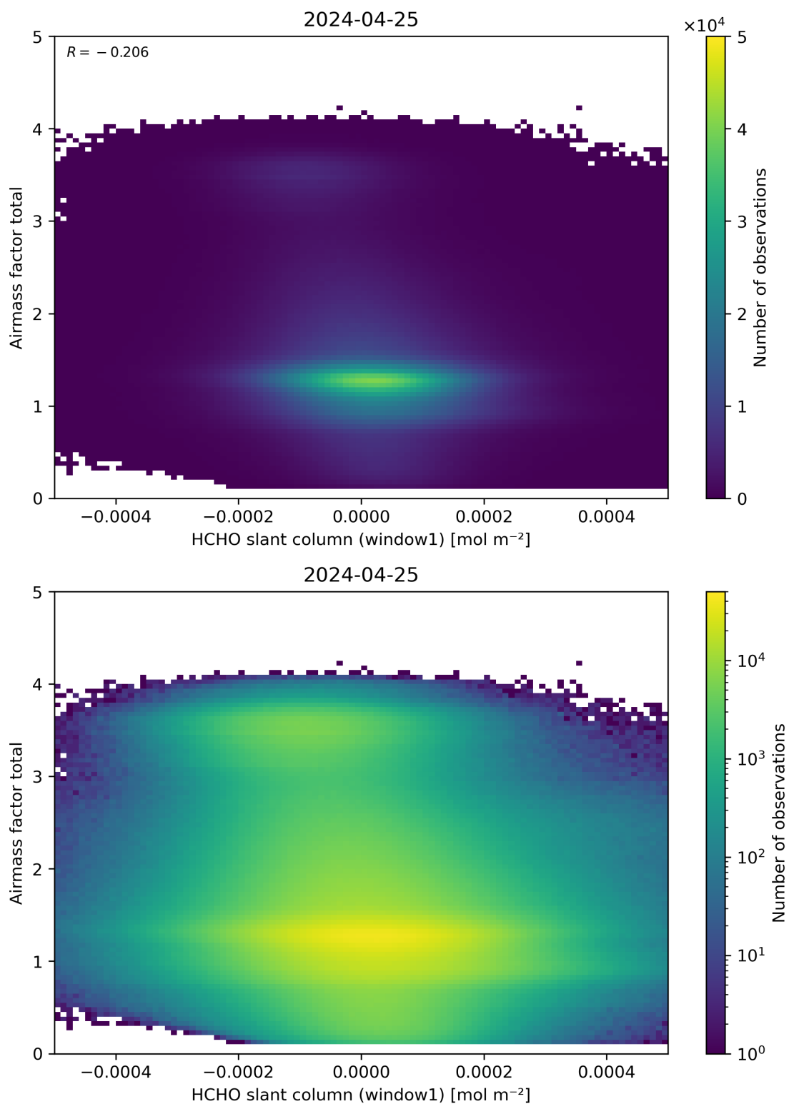
Figure 85: Scatter density plot of “HCHO slant column (window1)” against “Airmass factor total” for 2024-04-24 to 2024-04-26.
