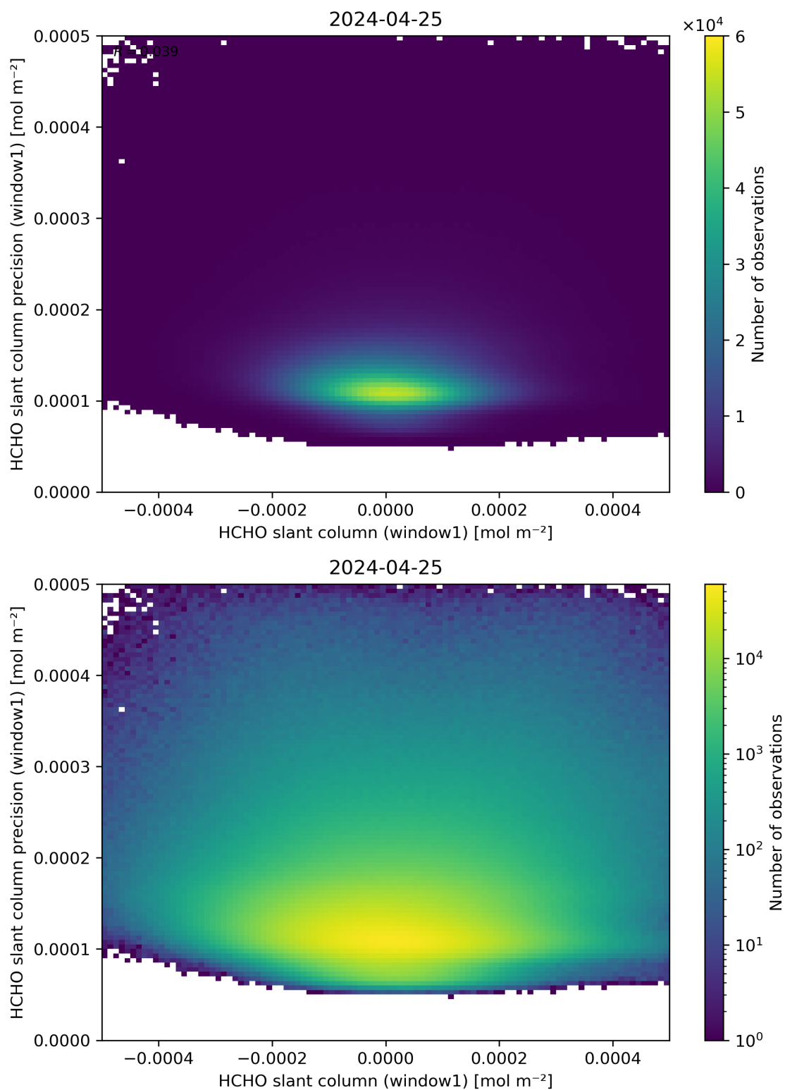
Figure 84: Scatter density plot of “HCHO slant column (window1)” against “HCHO slant column precision (window1)” for 2024-04-24 to 2024-04-26.
