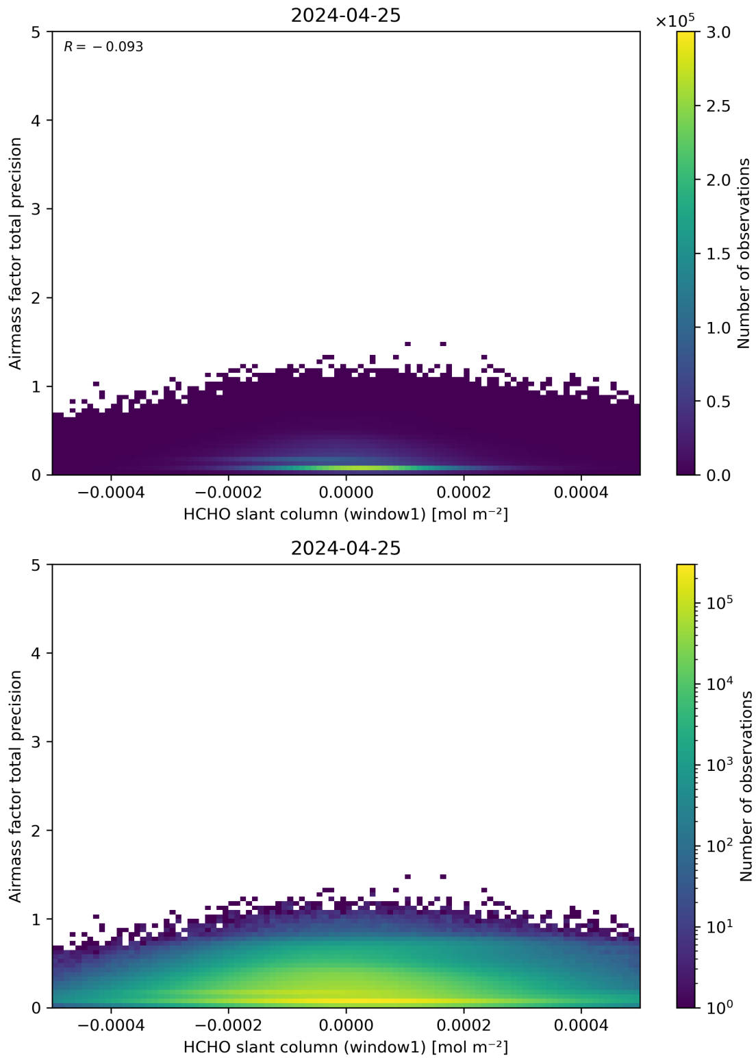
Figure 86: Scatter density plot of “HCHO slant column (window1)” against “Airmass factor total precision” for 2024-04-24 to 2024-04-26.
