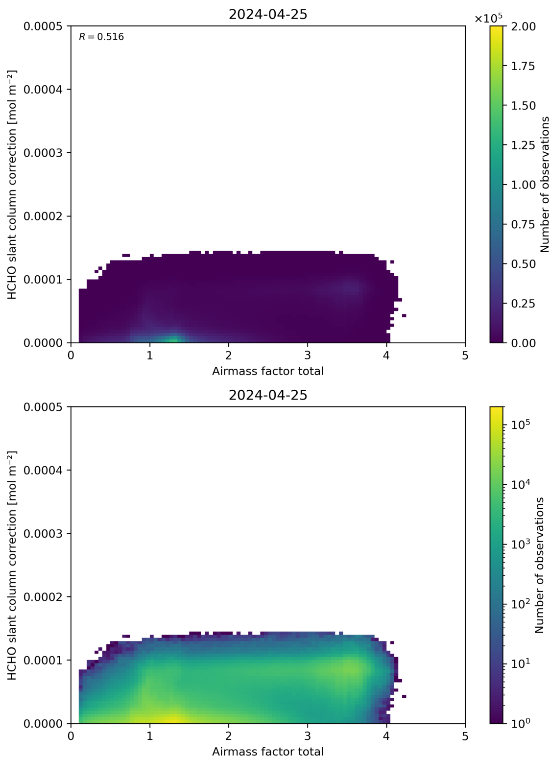
Figure 102: Scatter density plot of “Airmass factor total” against “HCHO slant column correction” for 2024-04-24 to 2024-04-26.
