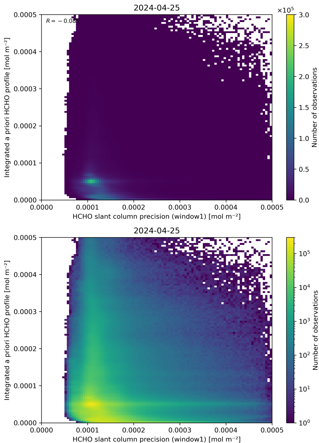
Figure 96: Scatter density plot of “HCHO slant column precision (window1)” against “Integrated a priori HCHO profile” for 2024-04-24 to 2024-04-26.
