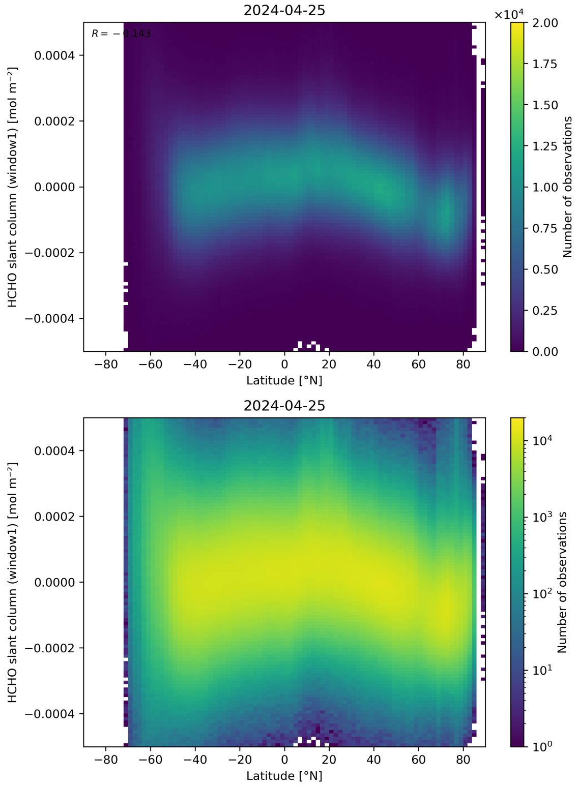
Figure 159: Scatter density plot of “Latitude” against “HCHO slant column (window1)” for 2024-04-24 to 2024-04-26.
