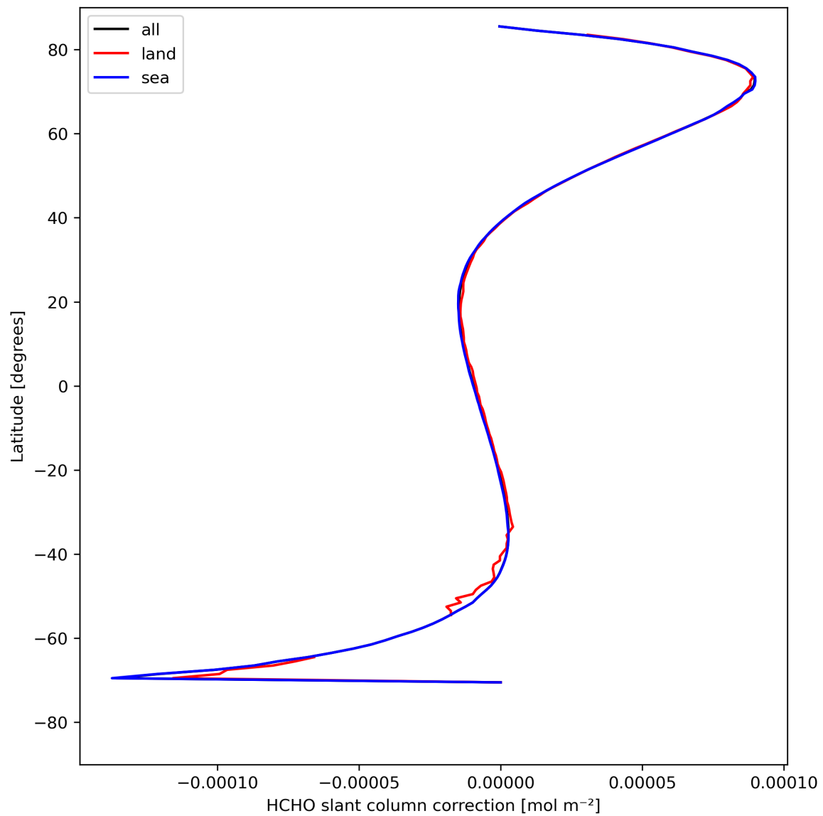
Figure 33: Zonal average of “HCHO slant column correction” for 2024-04-24 to 2024-04-26.
