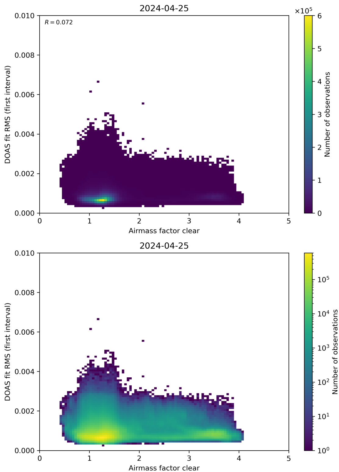
Figure 71: Scatter density plot of “Airmass factor clear” against “DOAS fit RMS (first interval)” for 2024-04-24 to 2024-04-26.
