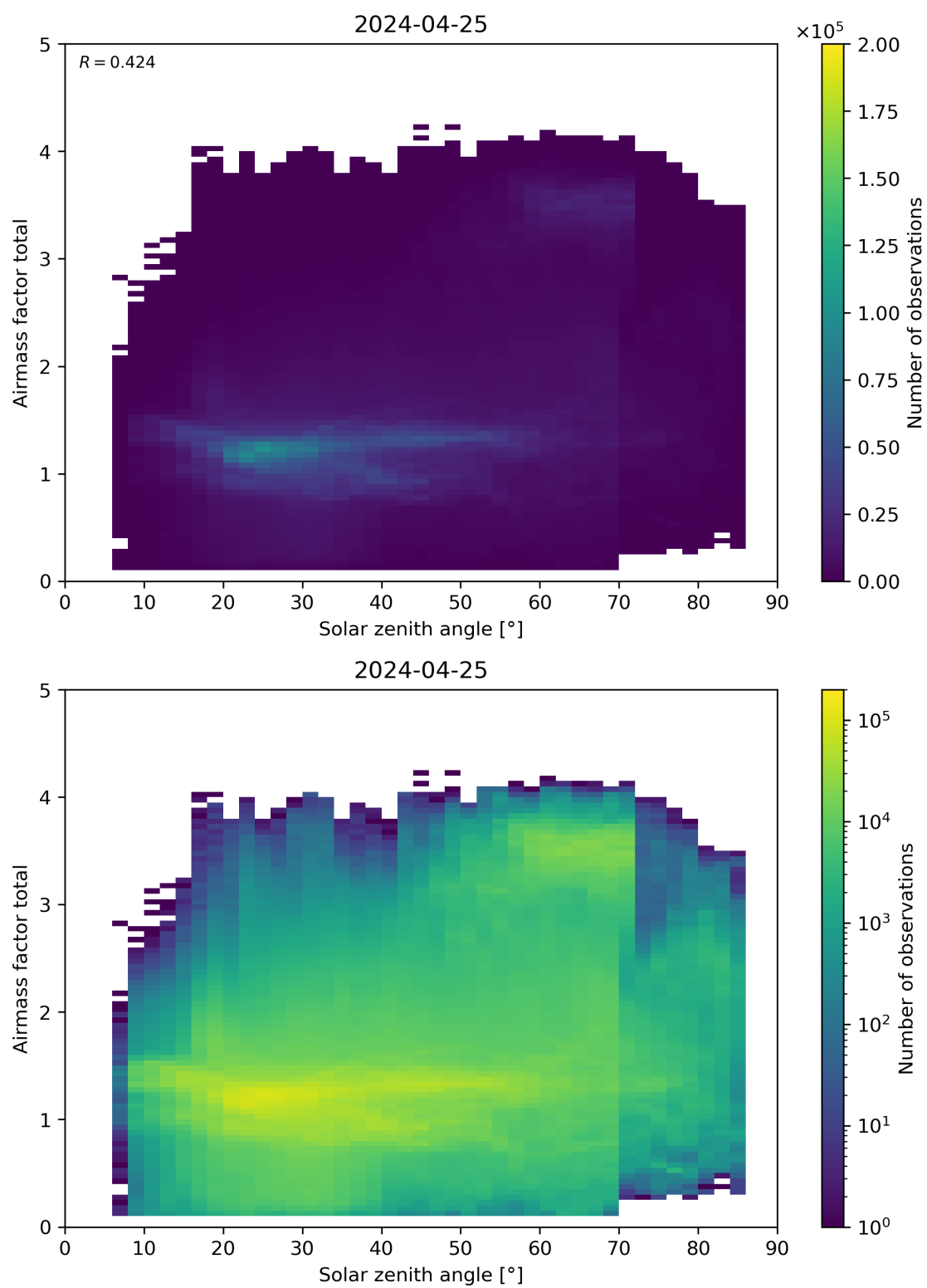
Figure 175: Scatter density plot of “Solar zenith angle” against “Airmass factor total” for 2024-04-24 to 2024-04-26.
