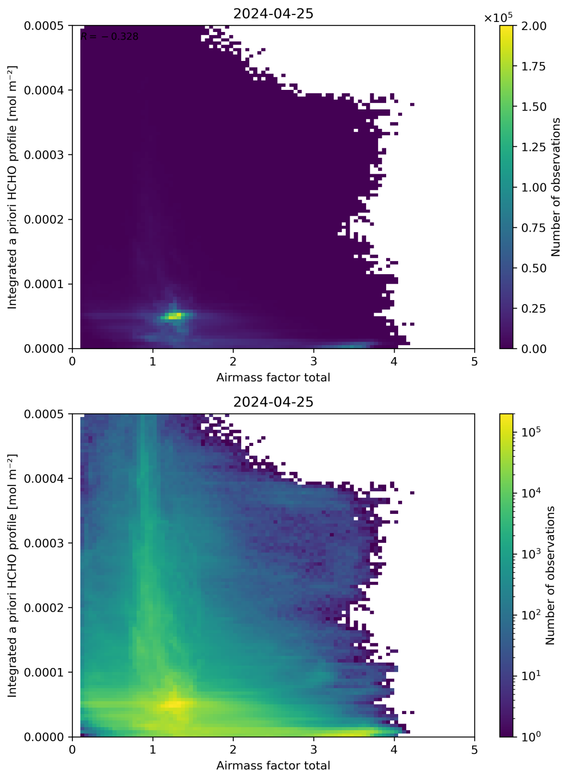
Figure 104: Scatter density plot of “Airmass factor total” against “Integrated a priori HCHO profile” for 2024-04-24 to 2024-04-26.
