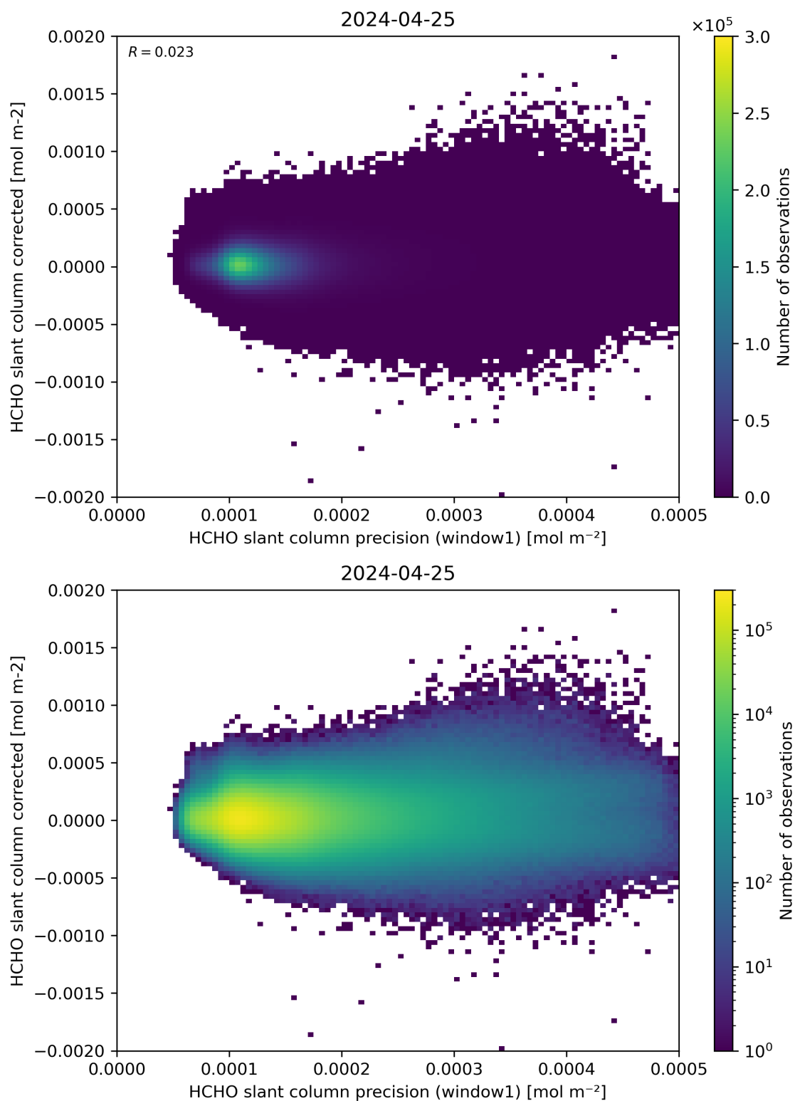
Figure 92: Scatter density plot of “HCHO slant column precision (window1)” against “HCHO slant column corrected” for 2024-04-24 to 2024-04-26.
