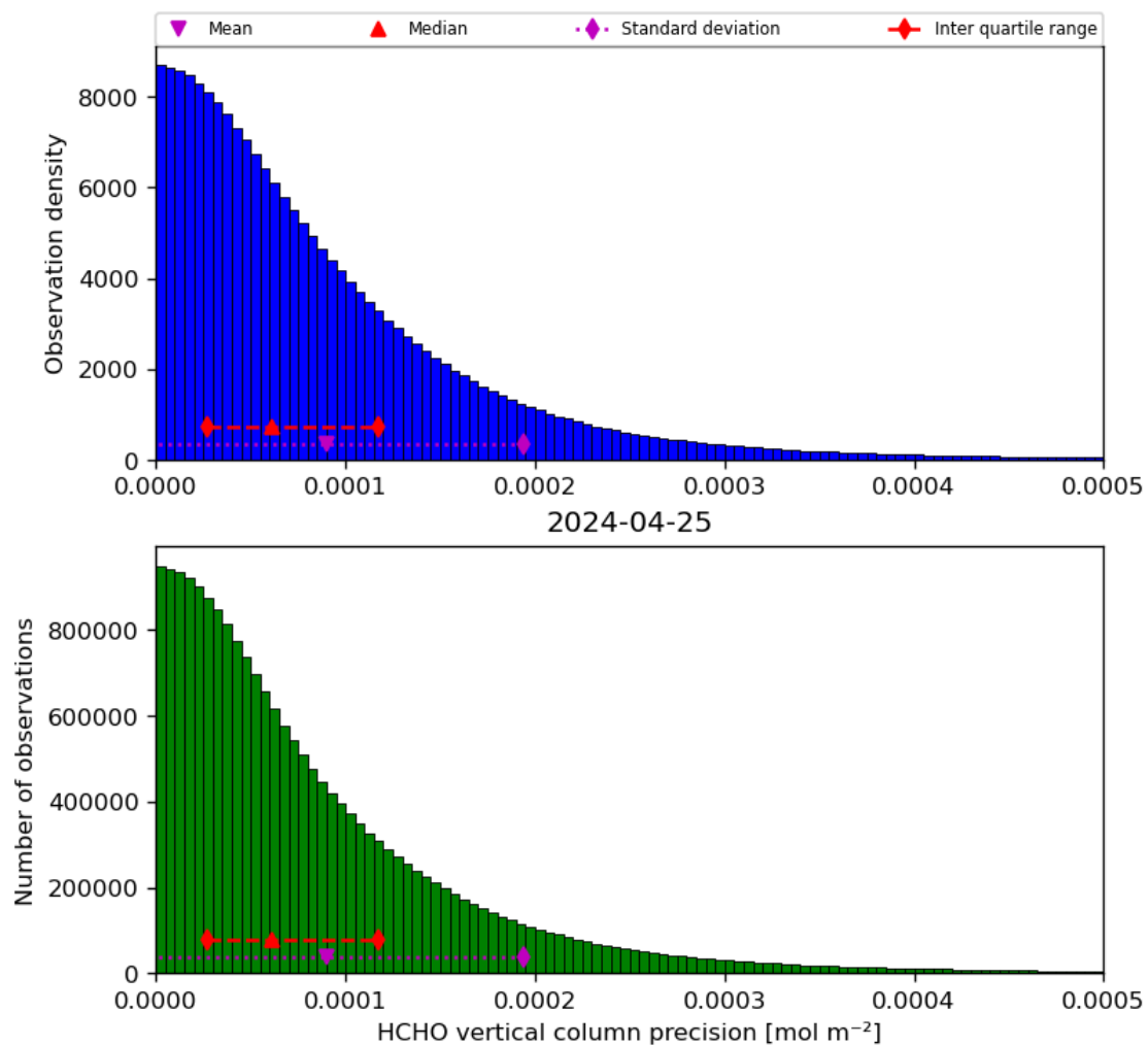
Figure 36: Histogram of "HCHO vertical column precision" for 2024-04-24 to 2024-04-26
