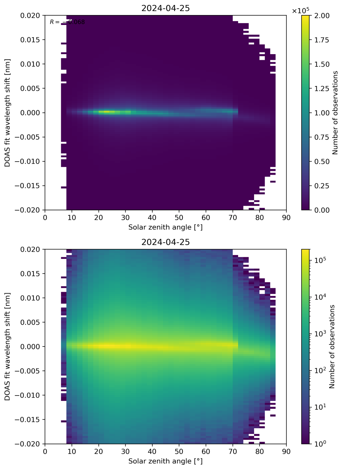
Figure 168: Scatter density plot of “Solar zenith angle” against “DOAS fit wavelength shift” for 2024-04-24 to 2024-04-26.
