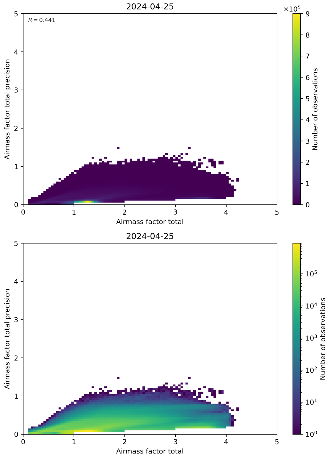
Figure 103: Scatter density plot of “Airmass factor total” against “Airmass factor total precision” for 2024-04-24 to 2024-04-26.
