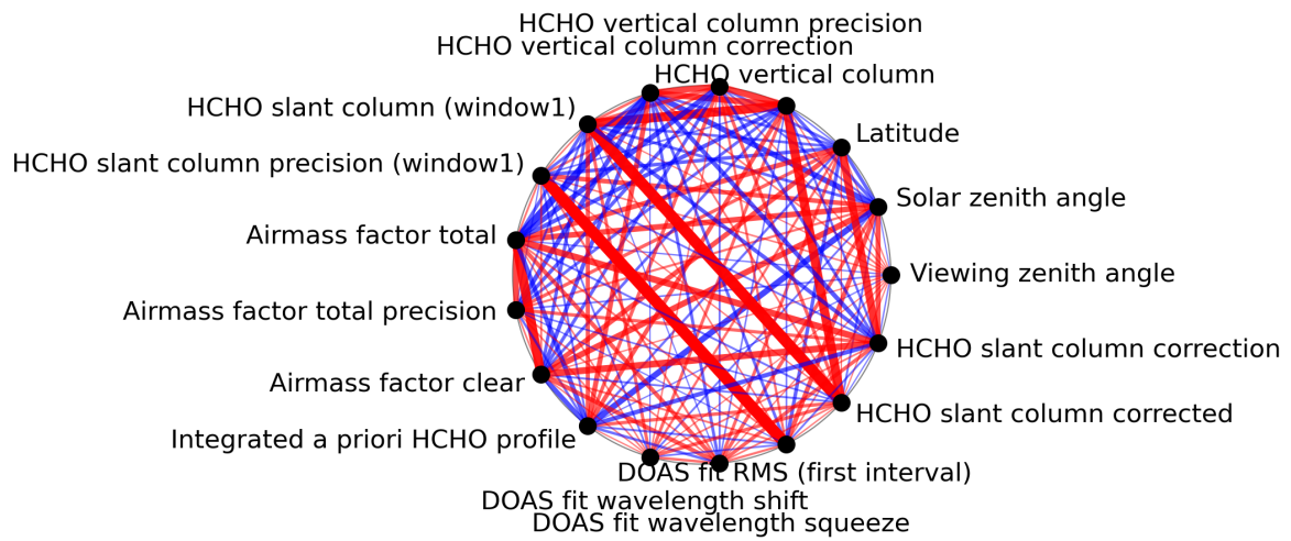
Figure 1: Map of correlation graph for 2024-04-24 to 2024-04-26.
