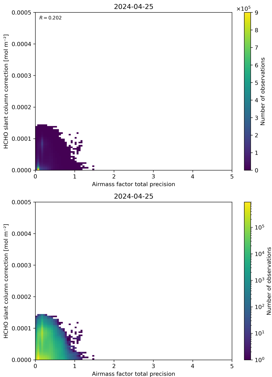
Figure 110: Scatter density plot of “Airmass factor total precision” against “HCHO slant column correction” for 2024-04-24 to 2024-04-26.
