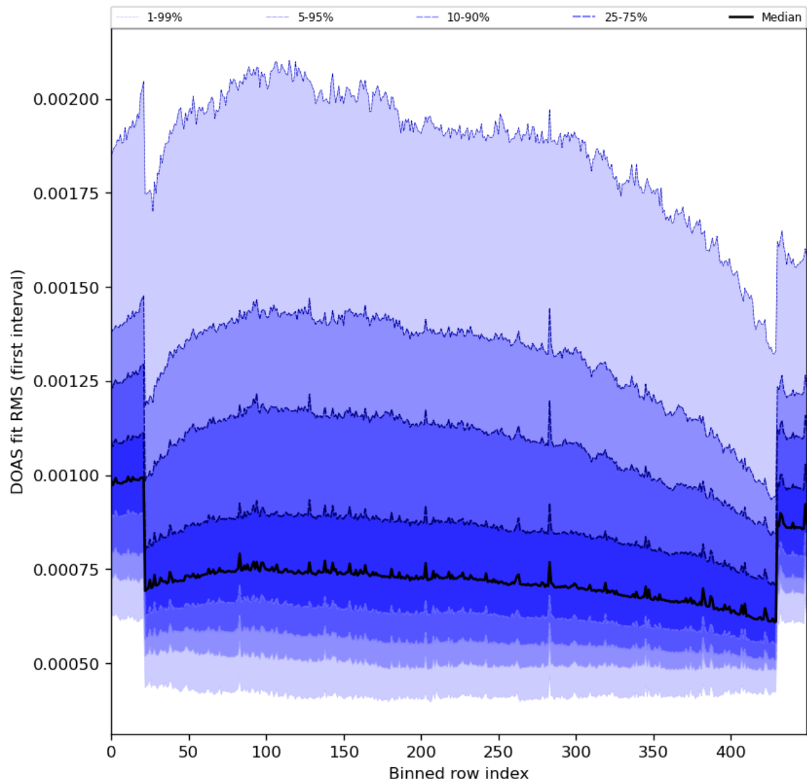
Figure 60: Along track statistics of “DOAS fit RMS (first interval)” for 2024-04-24 to 2024-04-26
