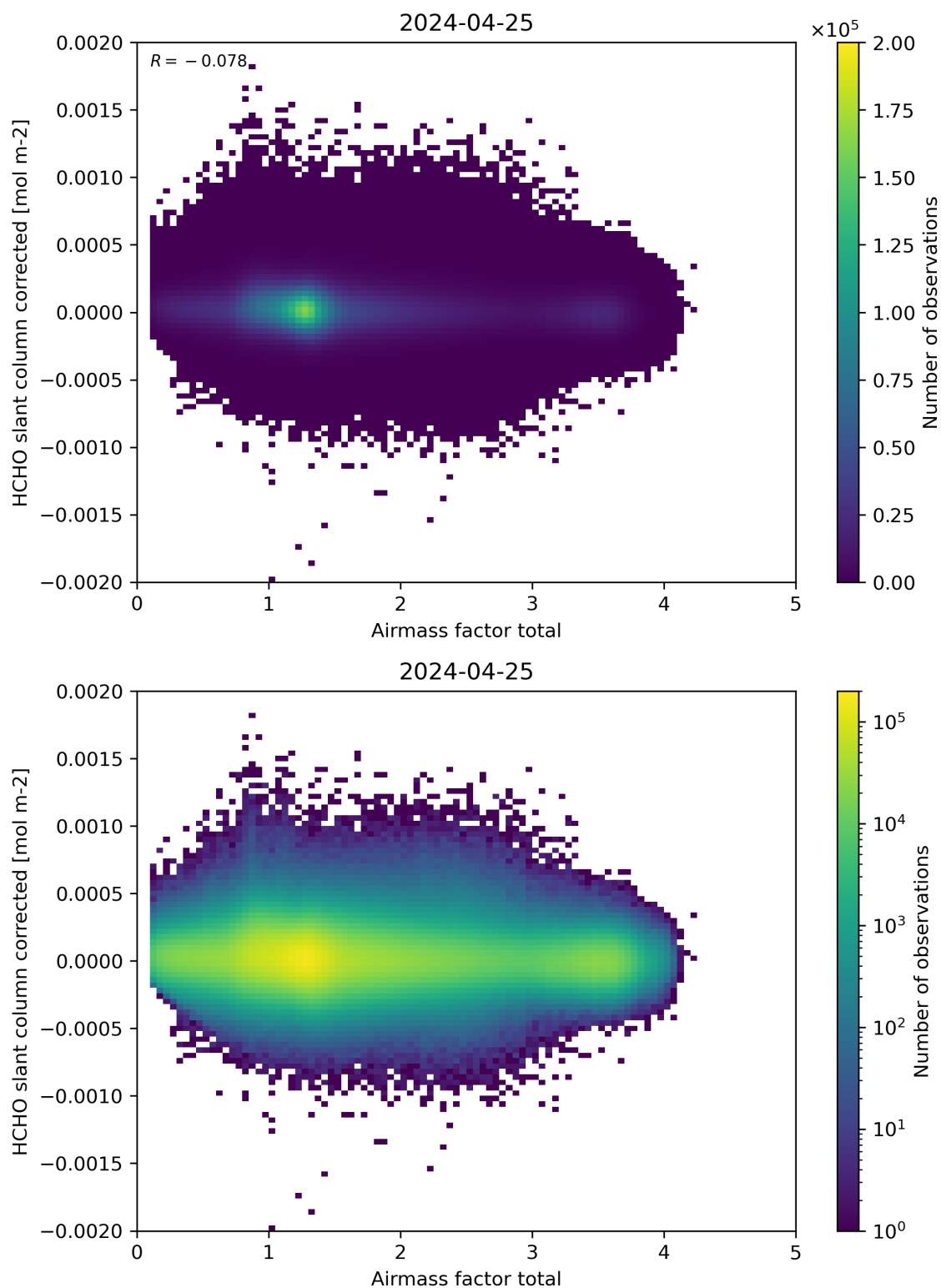
Figure 101: Scatter density plot of “Airmass factor total” against “HCHO slant column corrected” for 2024-04-24 to 2024-04-26.
