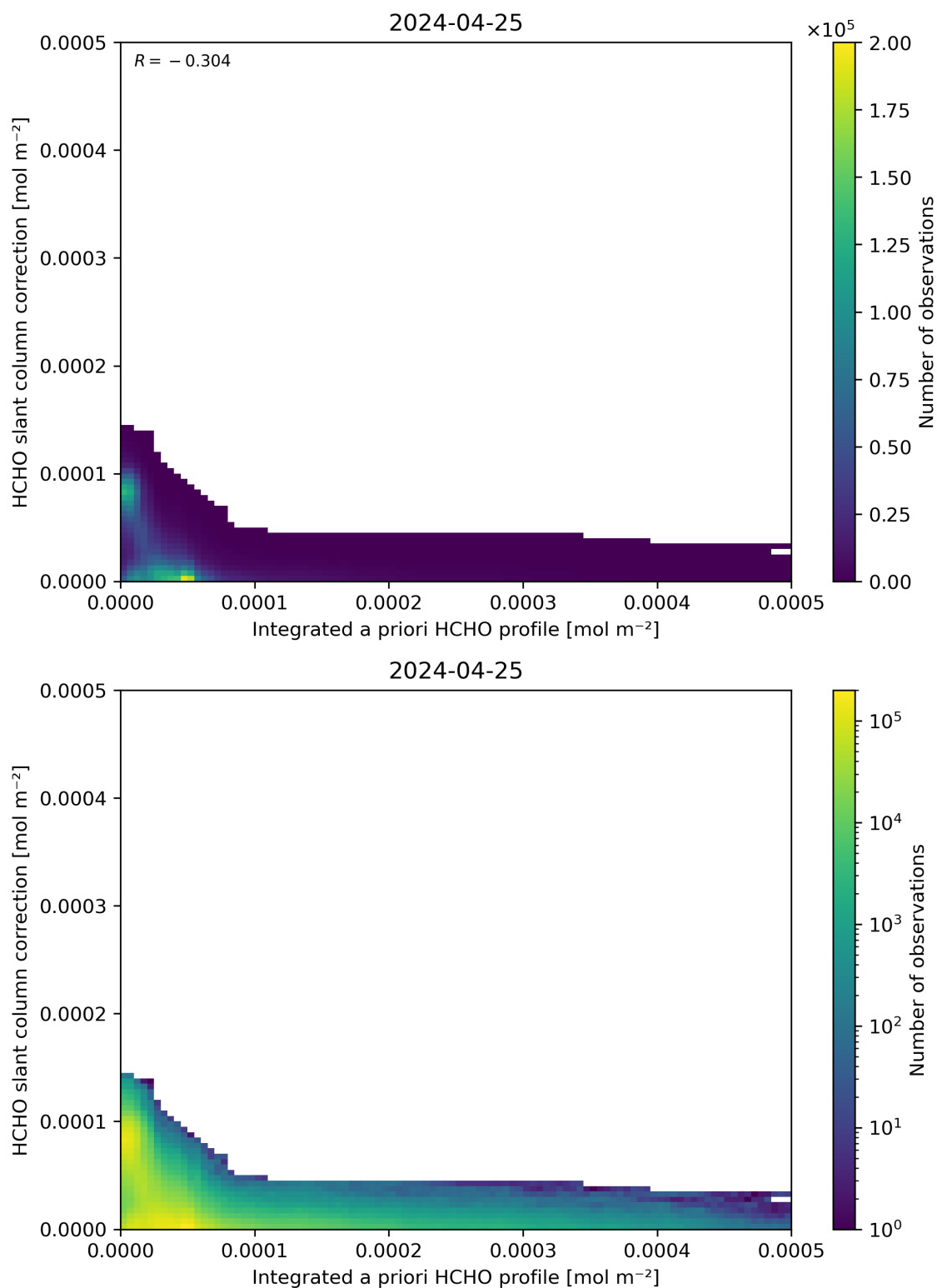
Figure 152: Scatter density plot of “Integrated a priori HCHO profile” against “HCHO slant column correction” for 2024-04-24 to 2024-04-26.
