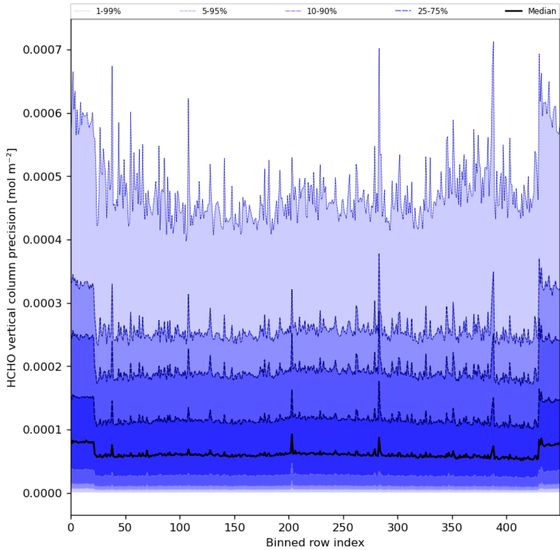
Figure 50: Along track statistics of “HCHO vertical column precision” for 2024-04-24 to 2024-04-26
