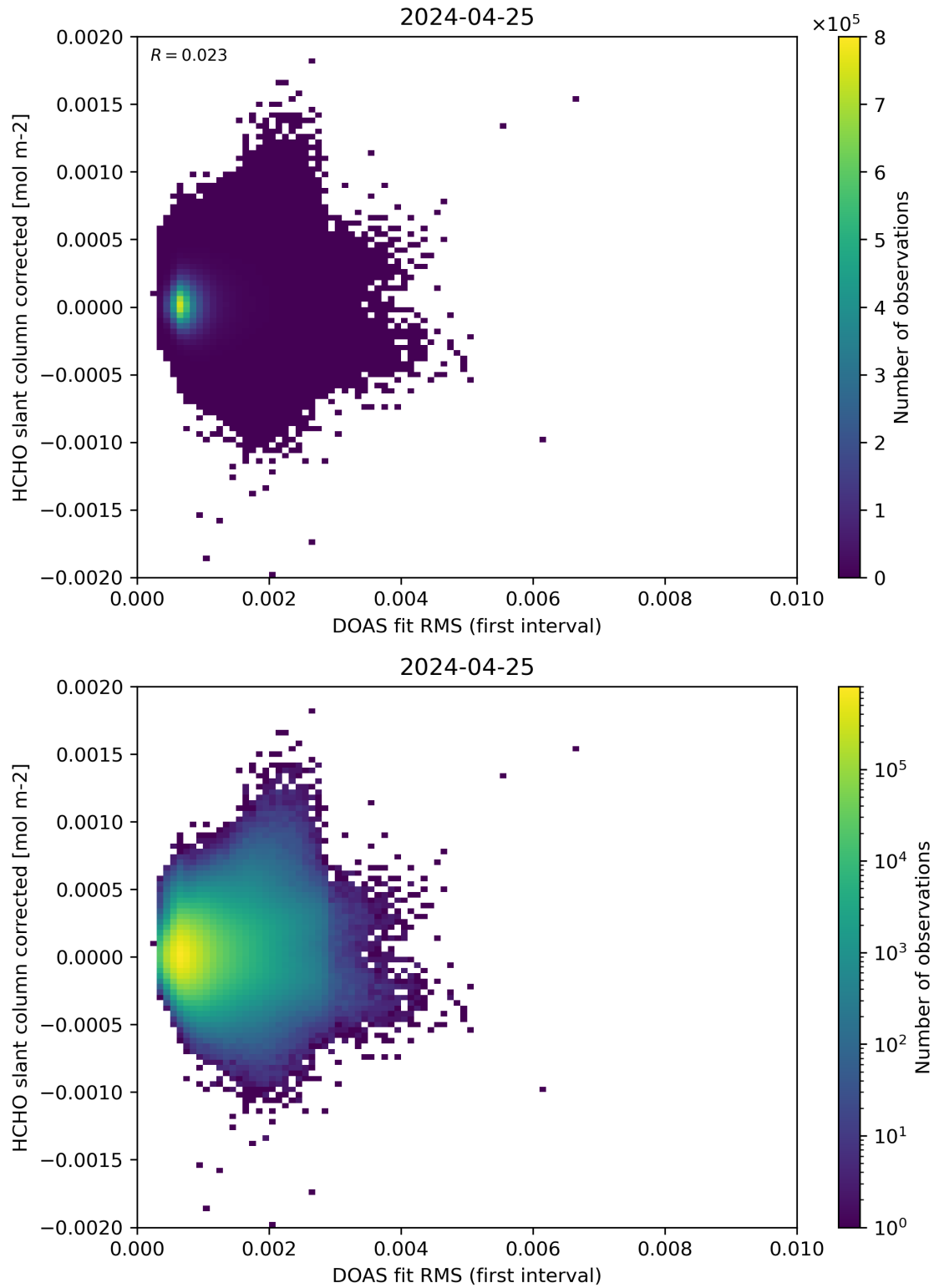
Figure 62: Scatter density plot of “DOAS fit RMS (first interval)” against “HCHO slant column corrected” for 2024-04-24 to 2024-04-26.
