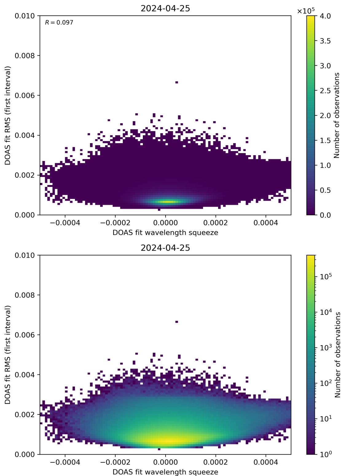
Figure 68: Scatter density plot of “DOAS fit wavelength squeeze” against “DOAS fit RMS (first interval)” for 2024-04-24 to 2024-04-26.
