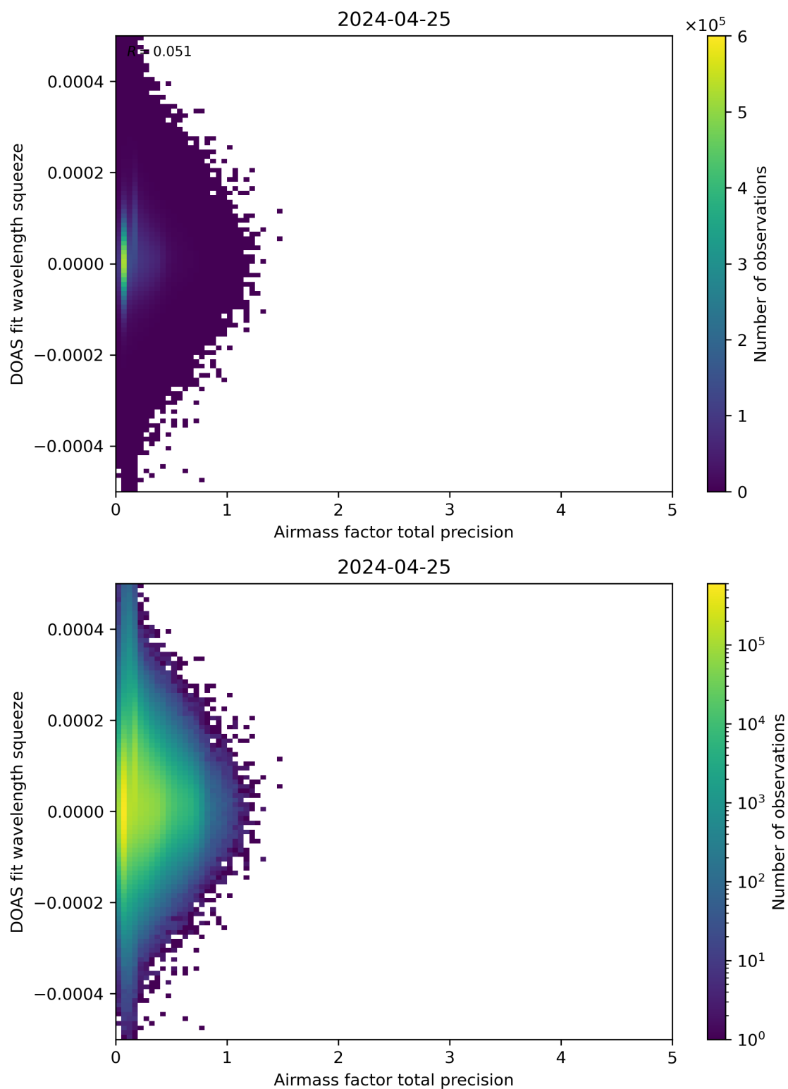
Figure 107: Scatter density plot of “Airmass factor total precision” against “DOAS fit wavelength squeeze” for 2024-04-24 to 2024-04-26.
