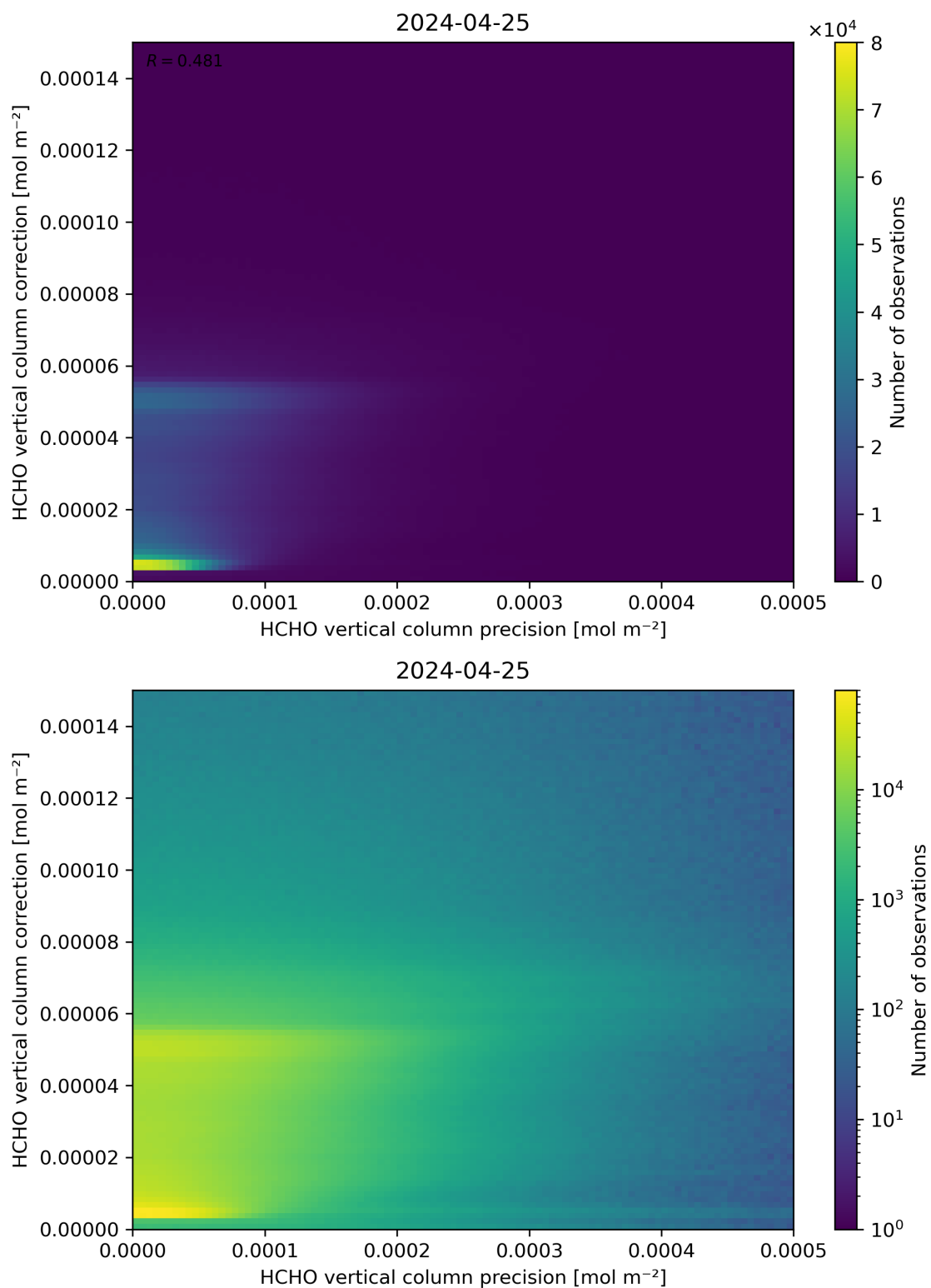
Figure 146: Scatter density plot of “HCHO vertical column precision” against “HCHO vertical column correction” for 2024-04-24 to 2024-04-26.
