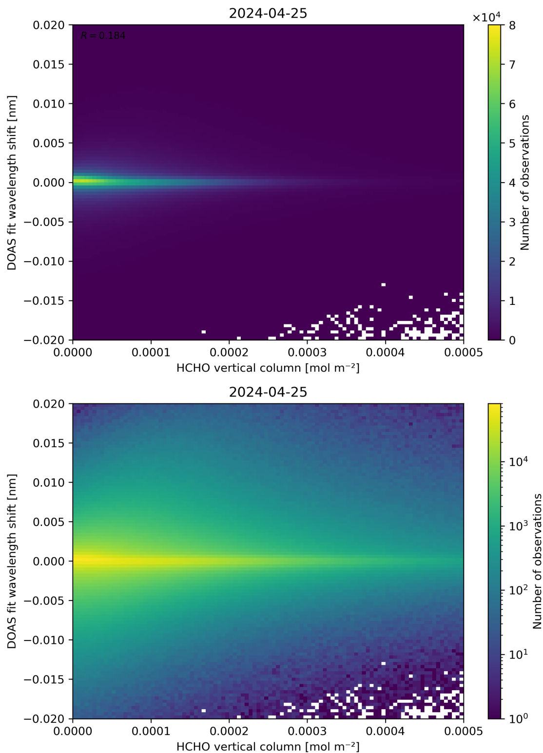
Figure 124: Scatter density plot of “HCHO vertical column” against “DOAS fit wavelength shift” for 2024-04-24 to 2024-04-26.
