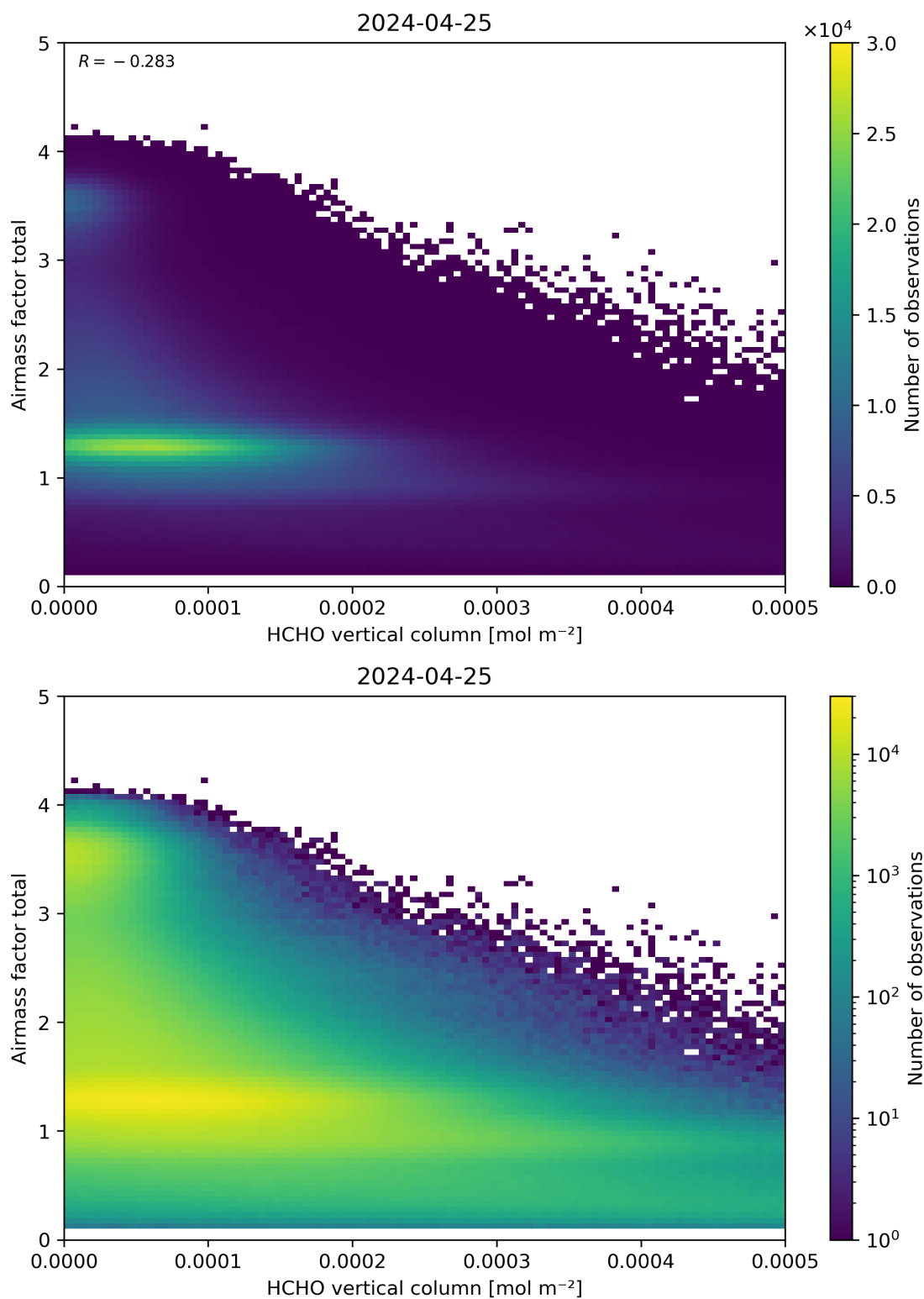
Figure 131: Scatter density plot of “HCHO vertical column” against “Airmass factor total” for 2024-04-24 to 2024-04-26.
