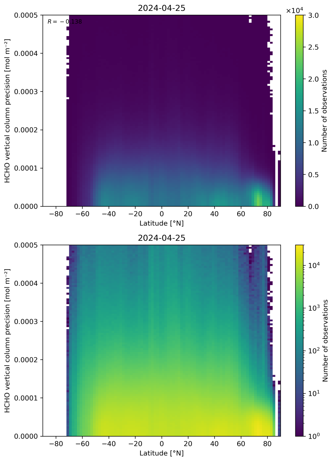
Figure 165: Scatter density plot of “Latitude” against “HCHO vertical column precision” for 2024-04-24 to 2024-04-26.
