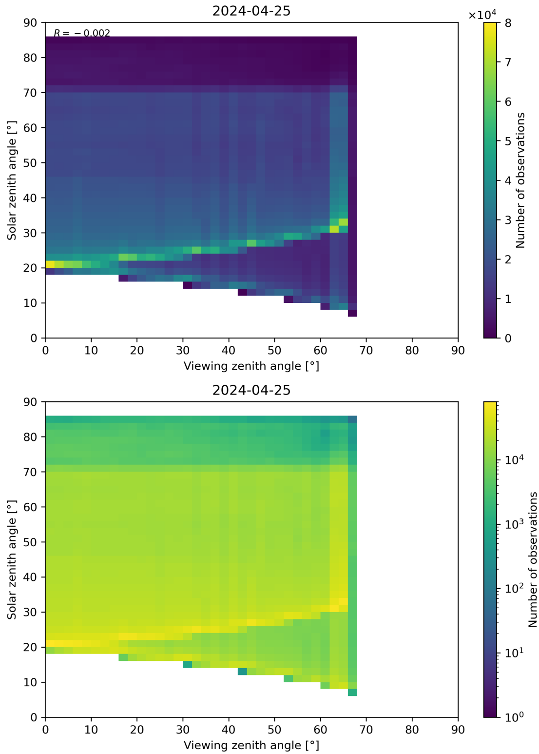
Figure 197: Scatter density plot of “Viewing zenith angle” against “Solar zenith angle” for 2024-04-24 to 2024-04-26.
