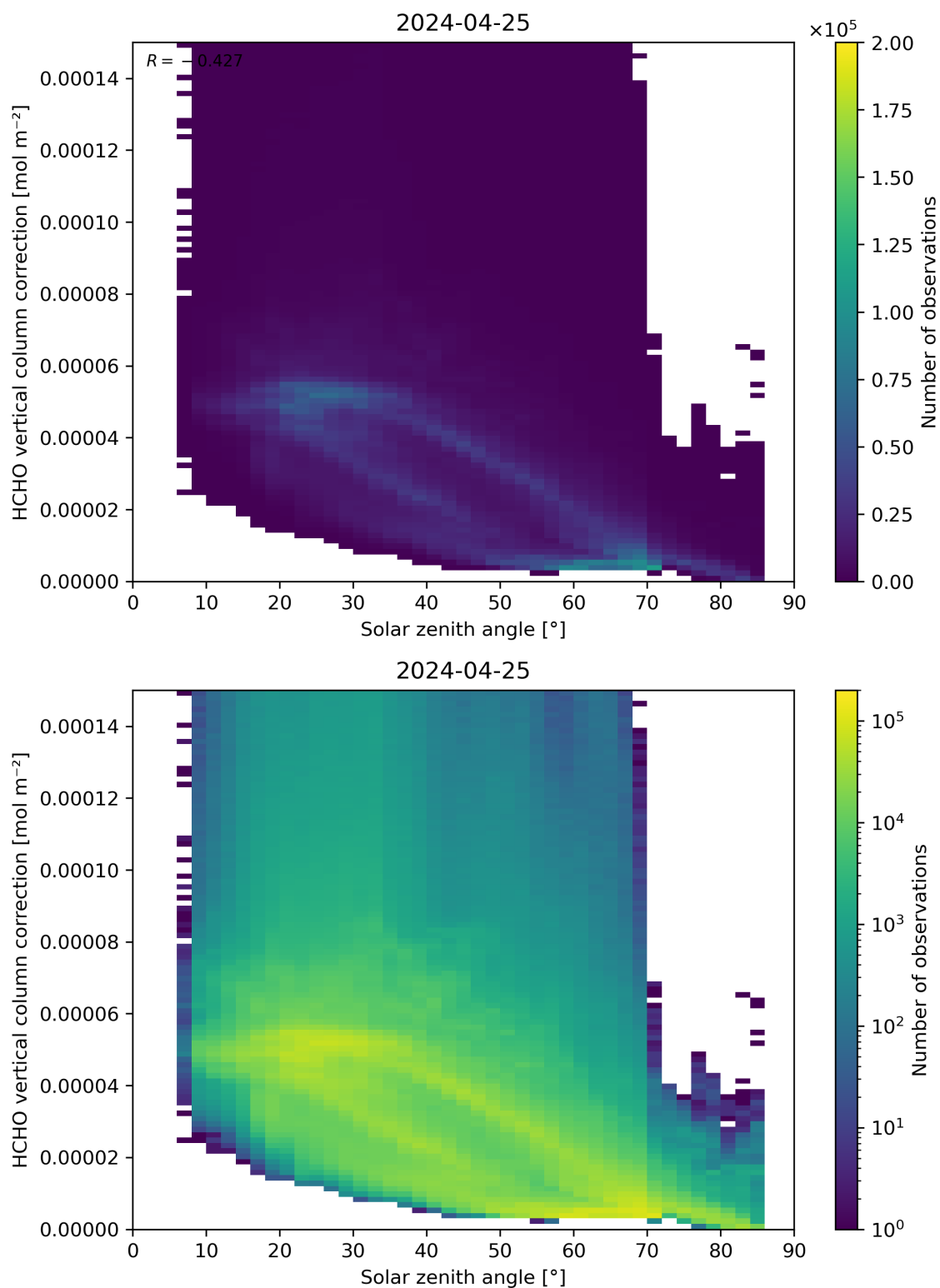
Figure 178: Scatter density plot of “Solar zenith angle” against “HCHO vertical column correction” for 2024-04-24 to 2024-04-26.
