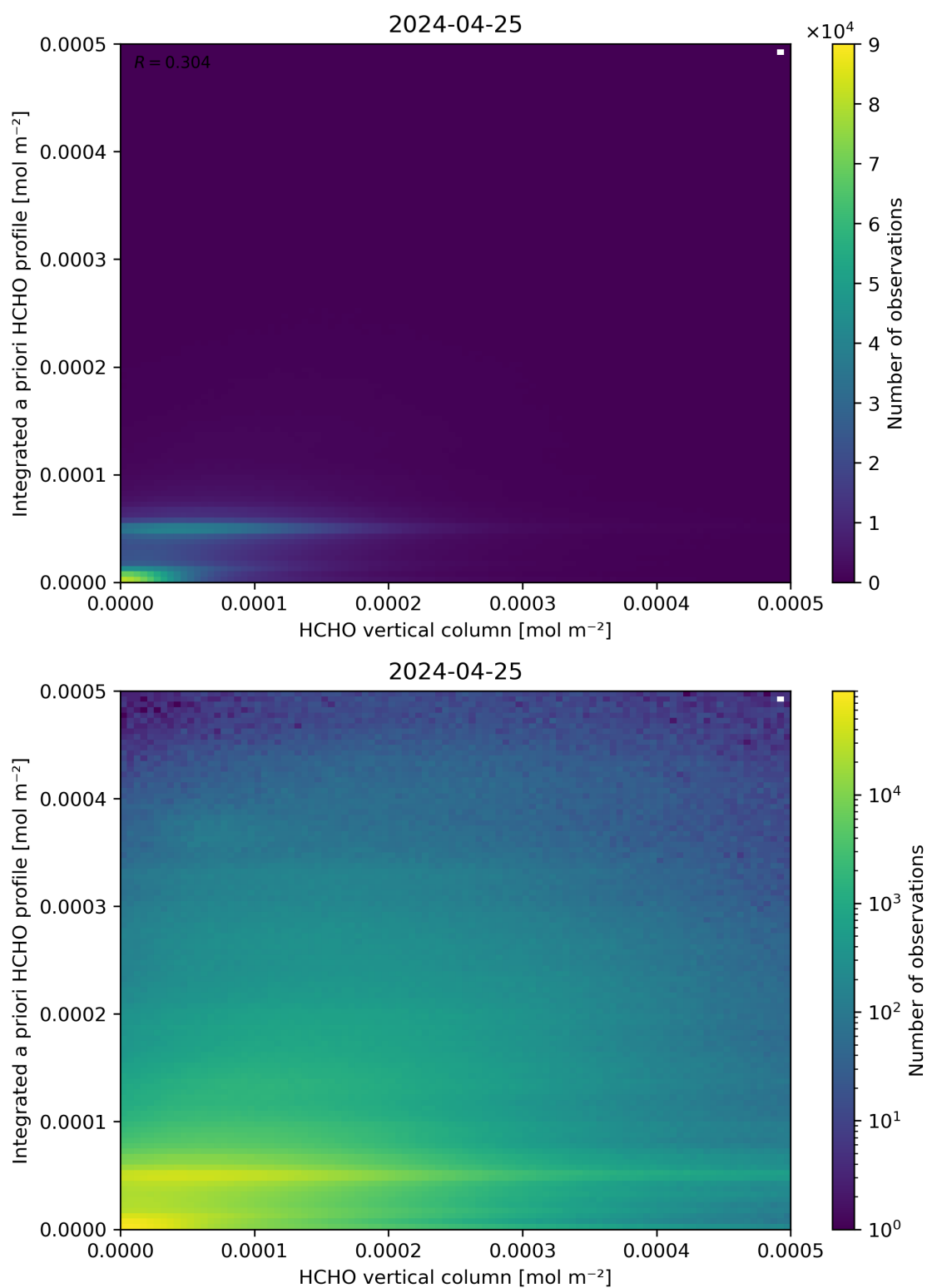
Figure 135: Scatter density plot of “HCHO vertical column” against “Integrated a priori HCHO profile” for 2024-04-24 to 2024-04-26.
