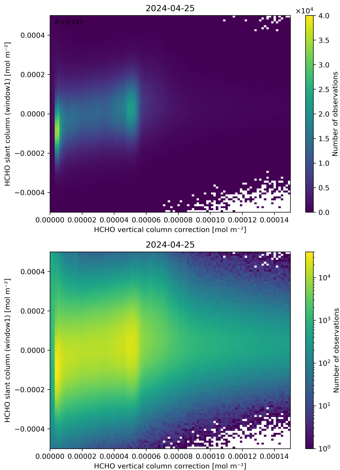
Figure 118: Scatter density plot of “HCHO vertical column correction” against “HCHO slant column (window1)” for 2024-04-24 to 2024-04-26.
