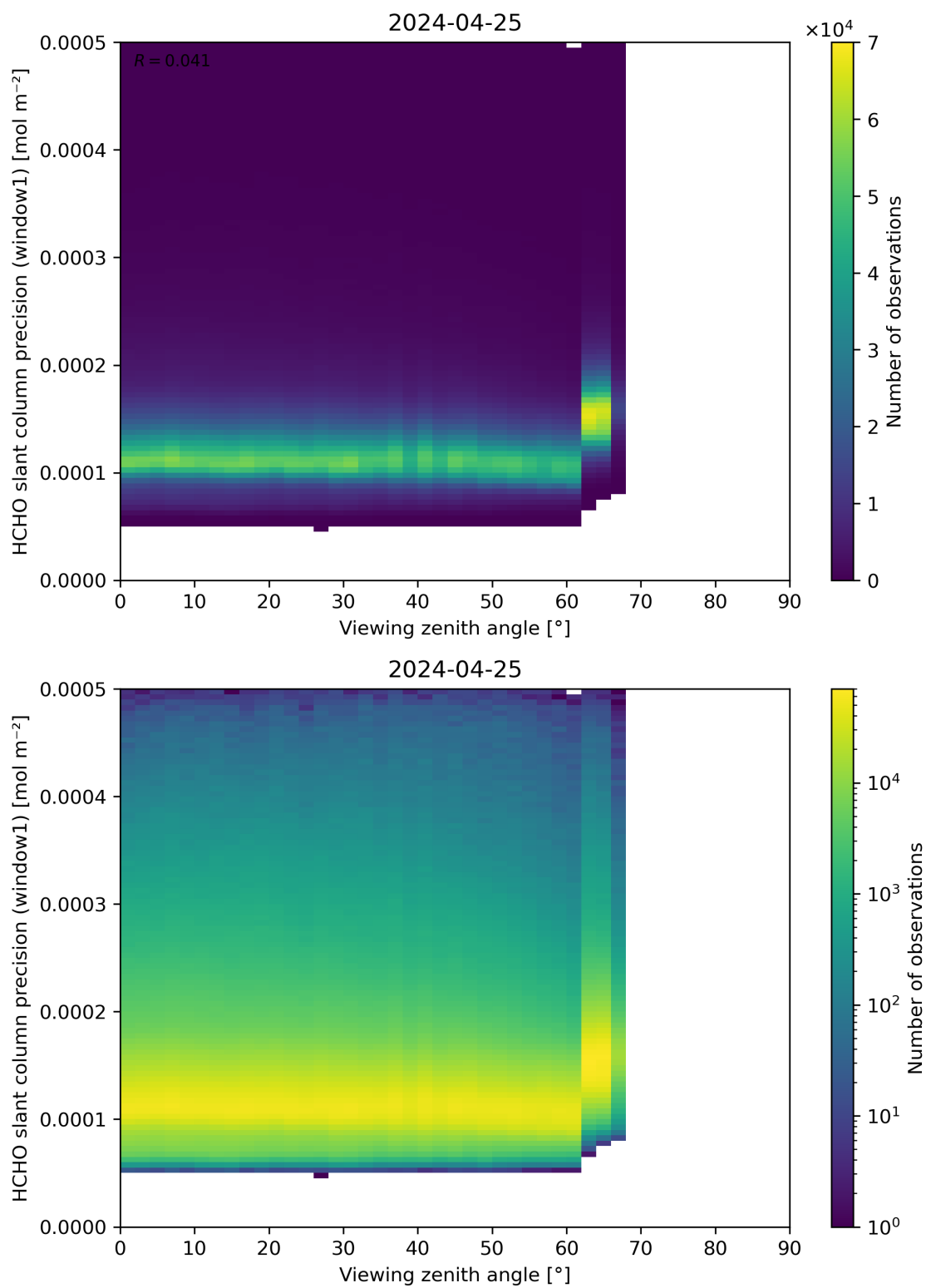
Figure 189: Scatter density plot of “Viewing zenith angle” against “HCHO slant column precision (window1)” for 2024-04-24 to 2024-04-26.
