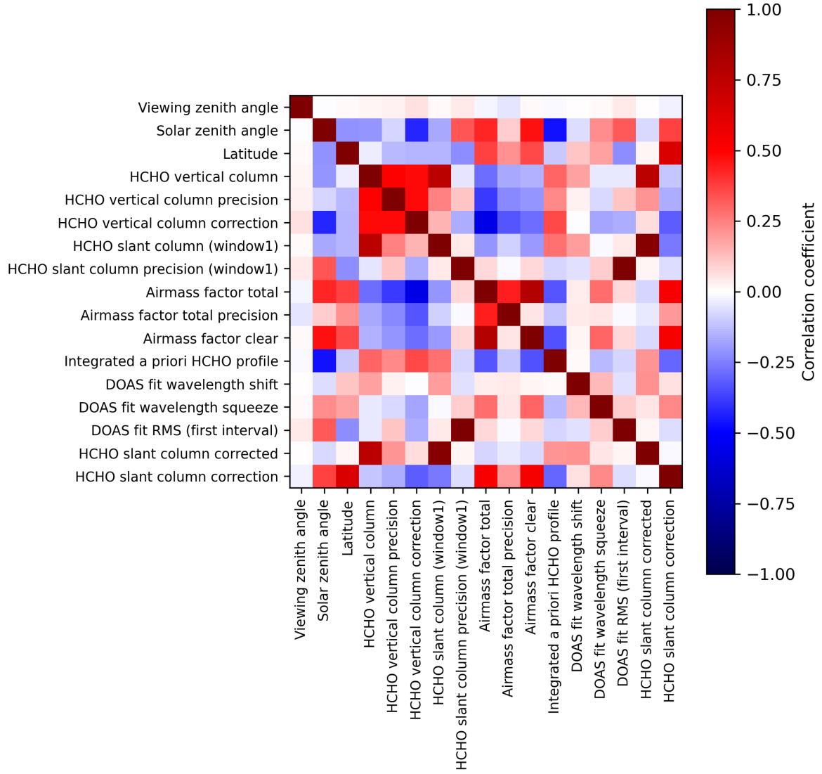
Figure 2: Map of correlation matrix for 2024-04-24 to 2024-04-26.
