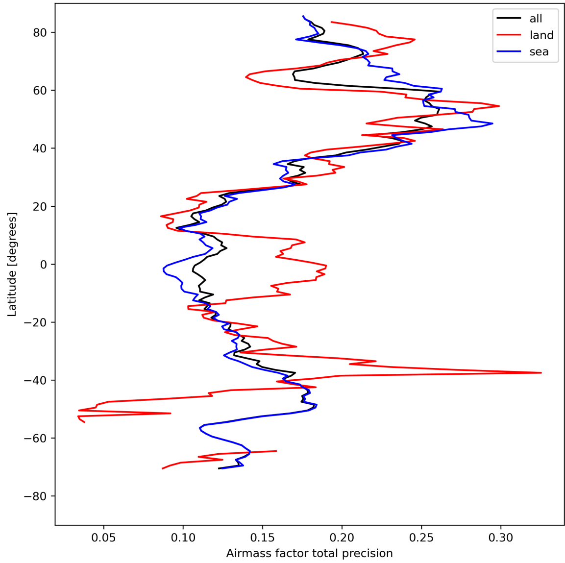
Figure 27: Zonal average of “Airmass factor total precision” for 2024-04-24 to 2024-04-26.
