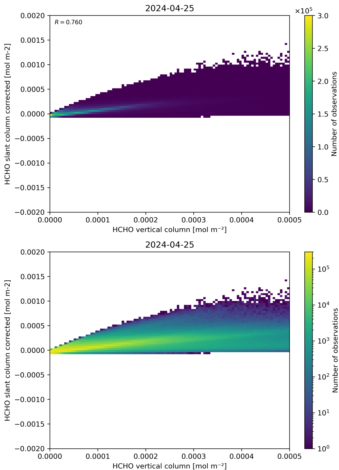
Figure 127: Scatter density plot of “HCHO vertical column” against “HCHO slant column corrected” for 2024-04-24 to 2024-04-26.
