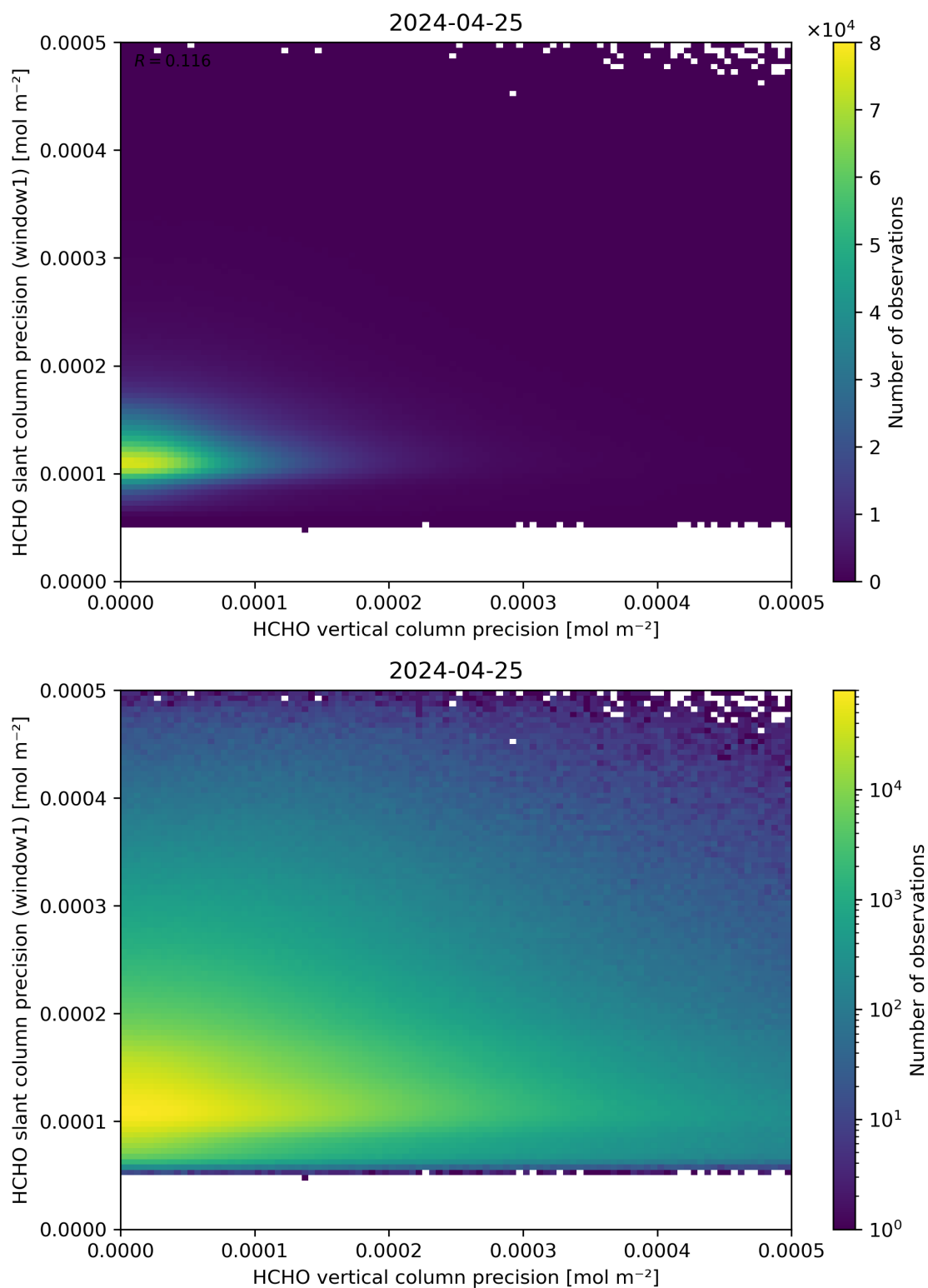
Figure 143: Scatter density plot of “HCHO vertical column precision” against “HCHO slant column precision (window1)” for 2024-04-24 to 2024-04-26.
