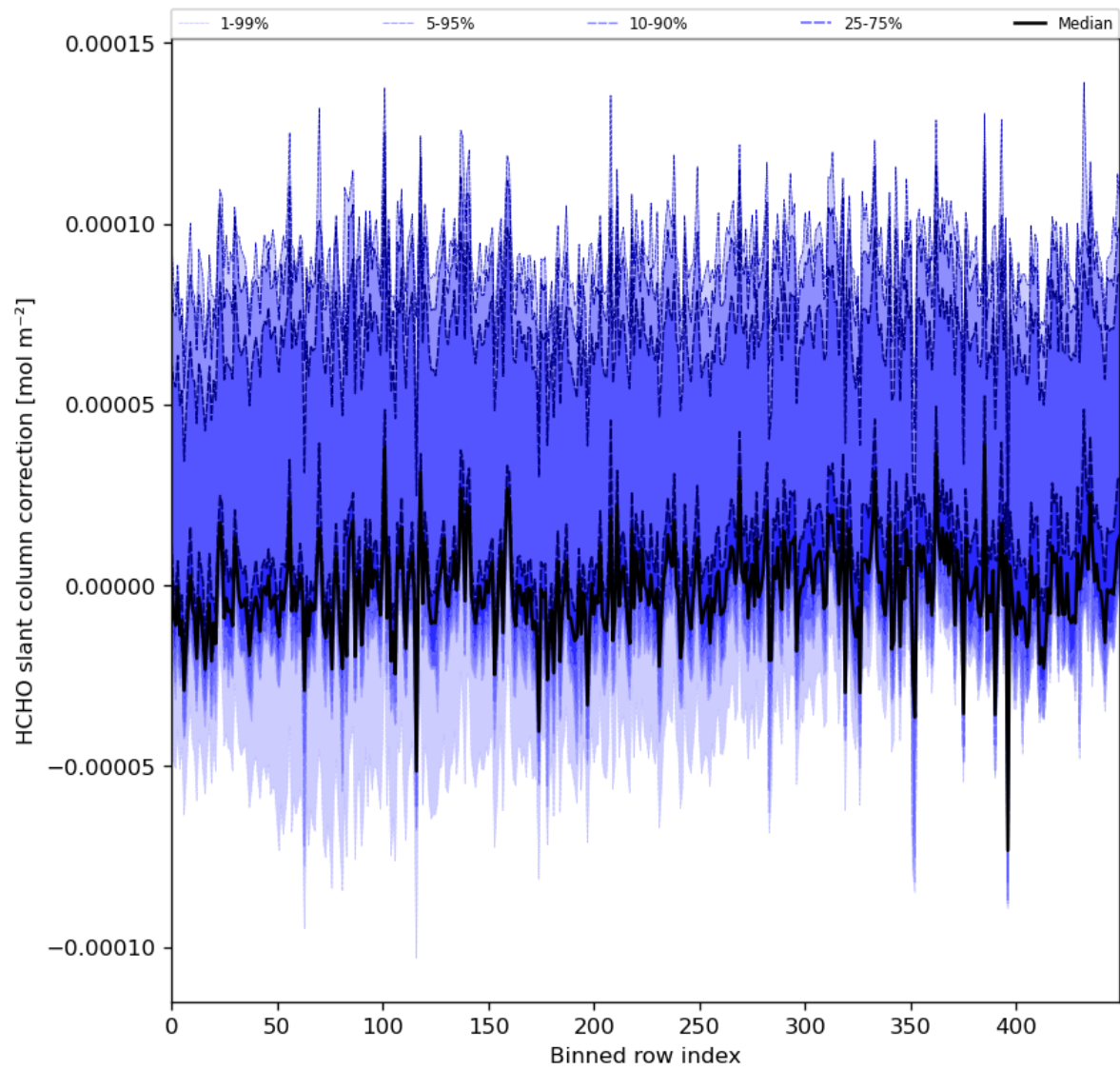
Figure 61: Along track statistics of “HCHO slant column correction” for 2024-04-24 to 2024-04-26
