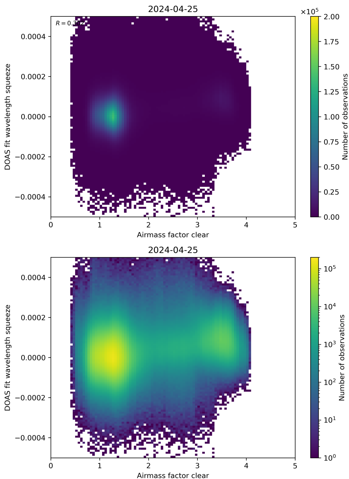
Figure 73: Scatter density plot of “Airmass factor clear” against “DOAS fit wavelength squeeze” for 2024-04-24 to 2024-04-26.
