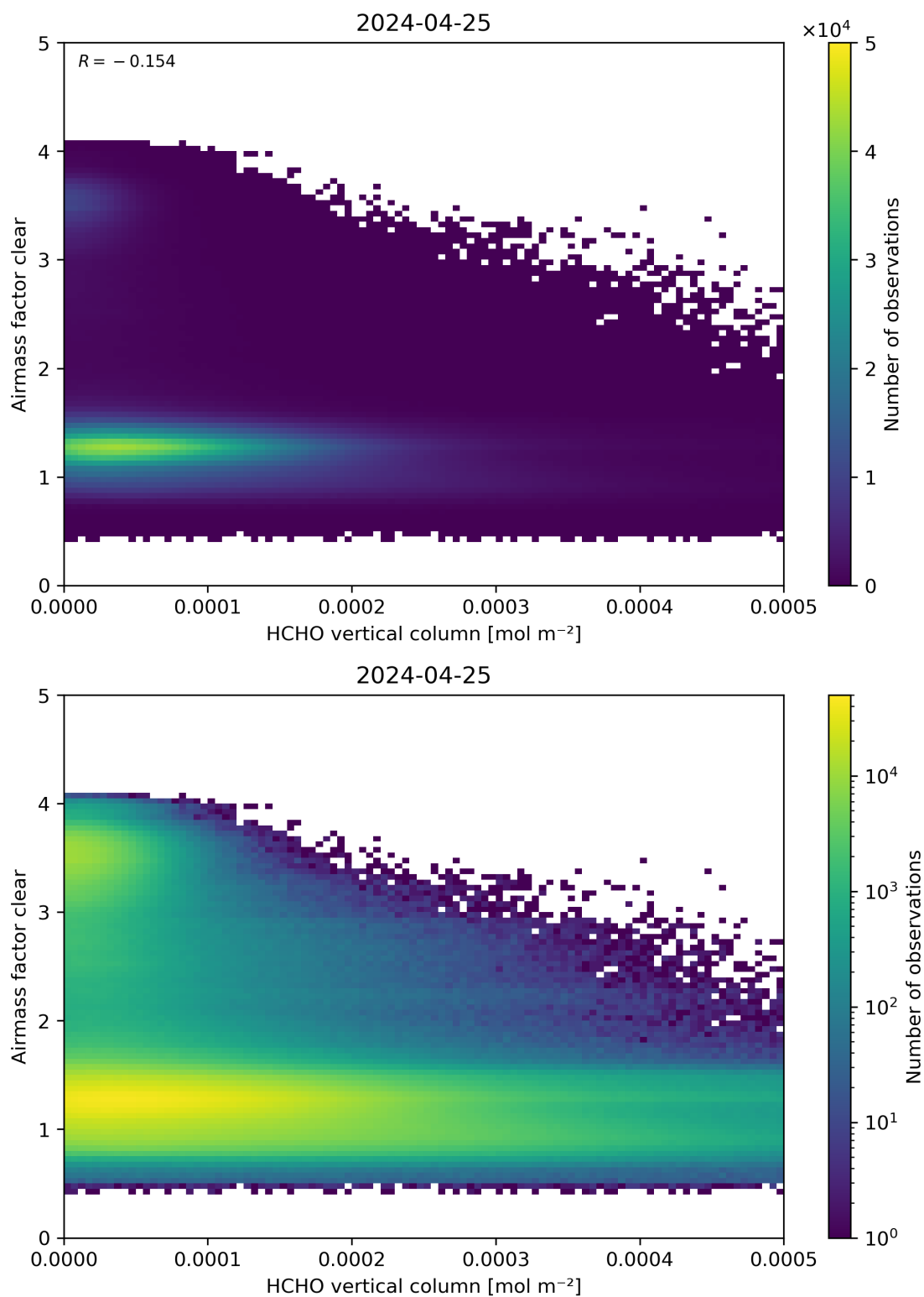
Figure 126: Scatter density plot of “HCHO vertical column” against “Airmass factor clear” for 2024-04-24 to 2024-04-26.
