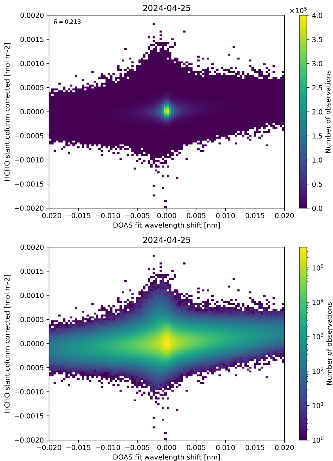
Figure 66: Scatter density plot of “DOAS fit wavelength shift” against “HCHO slant column corrected” for 2024-04-24 to 2024-04-26.
