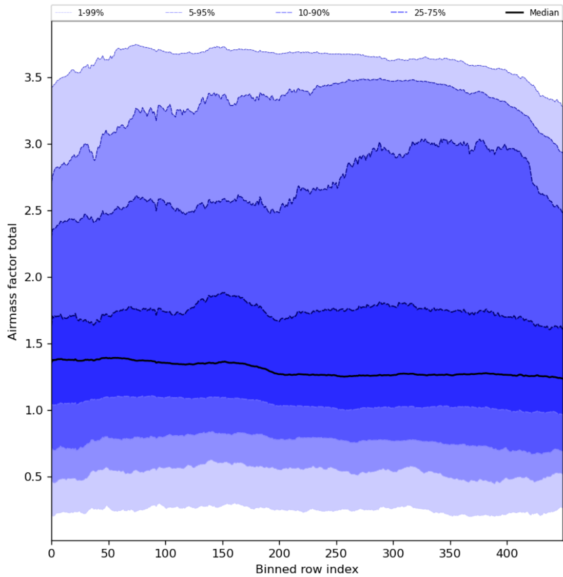
Figure 54: Along track statistics of “Airmass factor total” for 2024-04-24 to 2024-04-26
