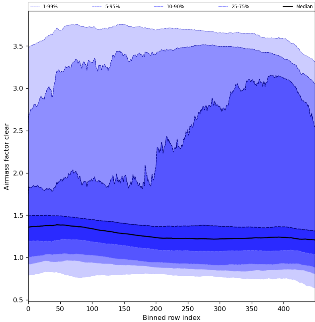
Figure 56: Along track statistics of “Airmass factor clear” for 2024-04-24 to 2024-04-26
