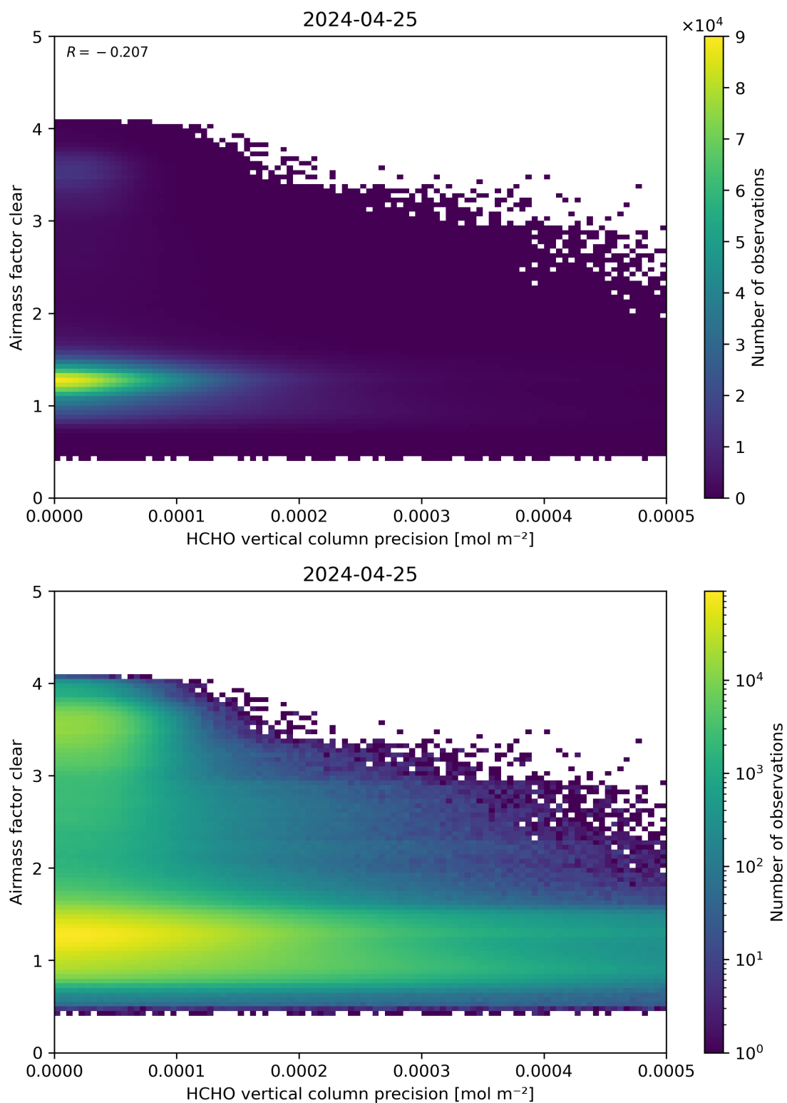
Figure 139: Scatter density plot of “HCHO vertical column precision” against “Airmass factor clear” for 2024-04-24 to 2024-04-26.
