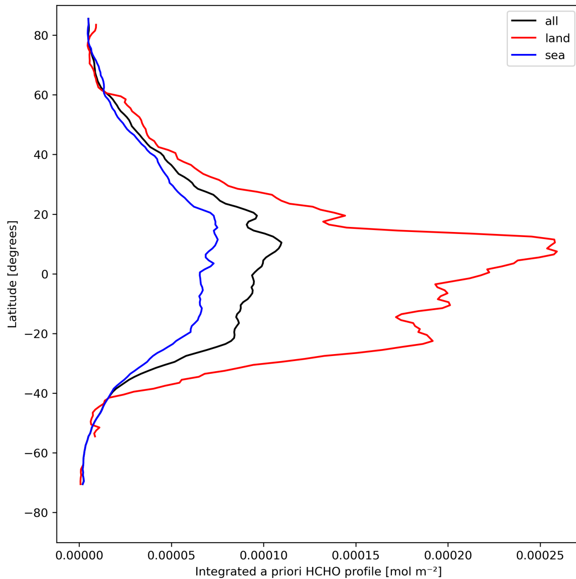
Figure 29: Zonal average of “Integrated a priori HCHO profile” for 2024-04-24 to 2024-04-26.
