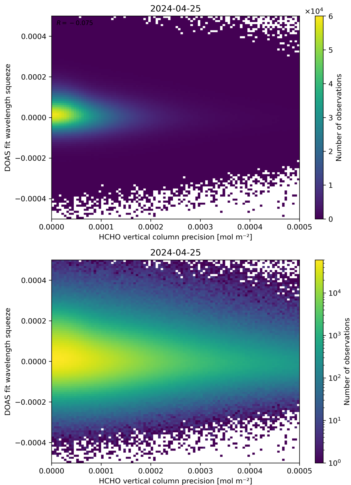
Figure 138: Scatter density plot of “HCHO vertical column precision” against “DOAS fit wavelength squeeze” for 2024-04-24 to 2024-04-26.
