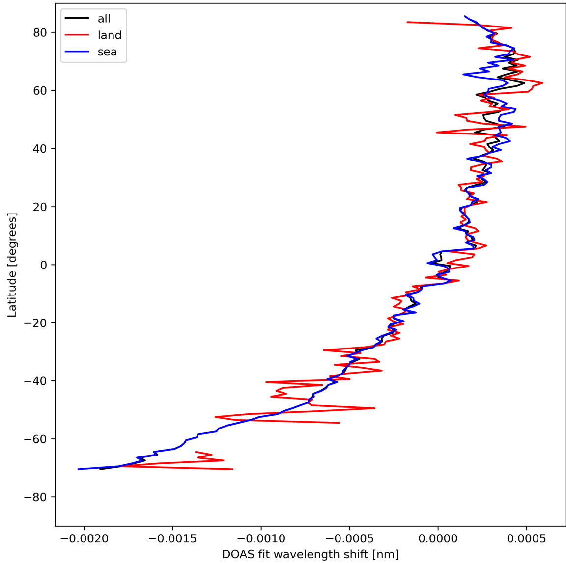
Figure 30: Zonal average of “DOAS fit wavelength shift” for 2024-04-24 to 2024-04-26.
