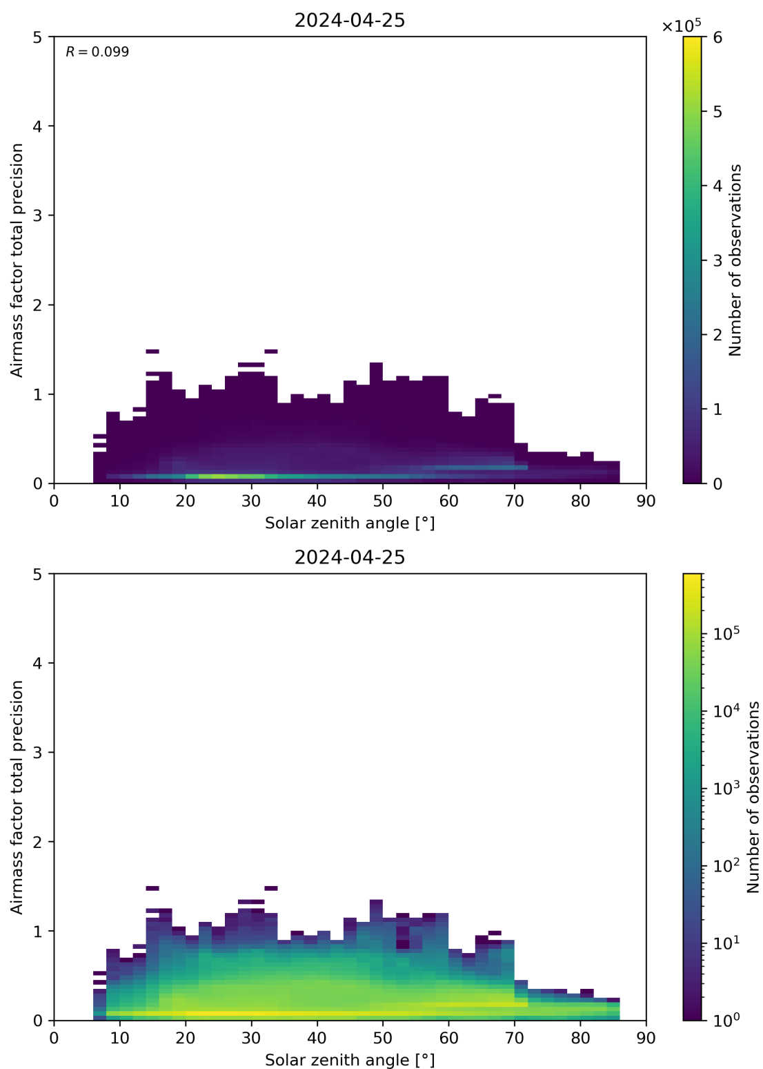
Figure 176: Scatter density plot of “Solar zenith angle” against “Airmass factor total precision” for 2024-04-24 to 2024-04-26.
