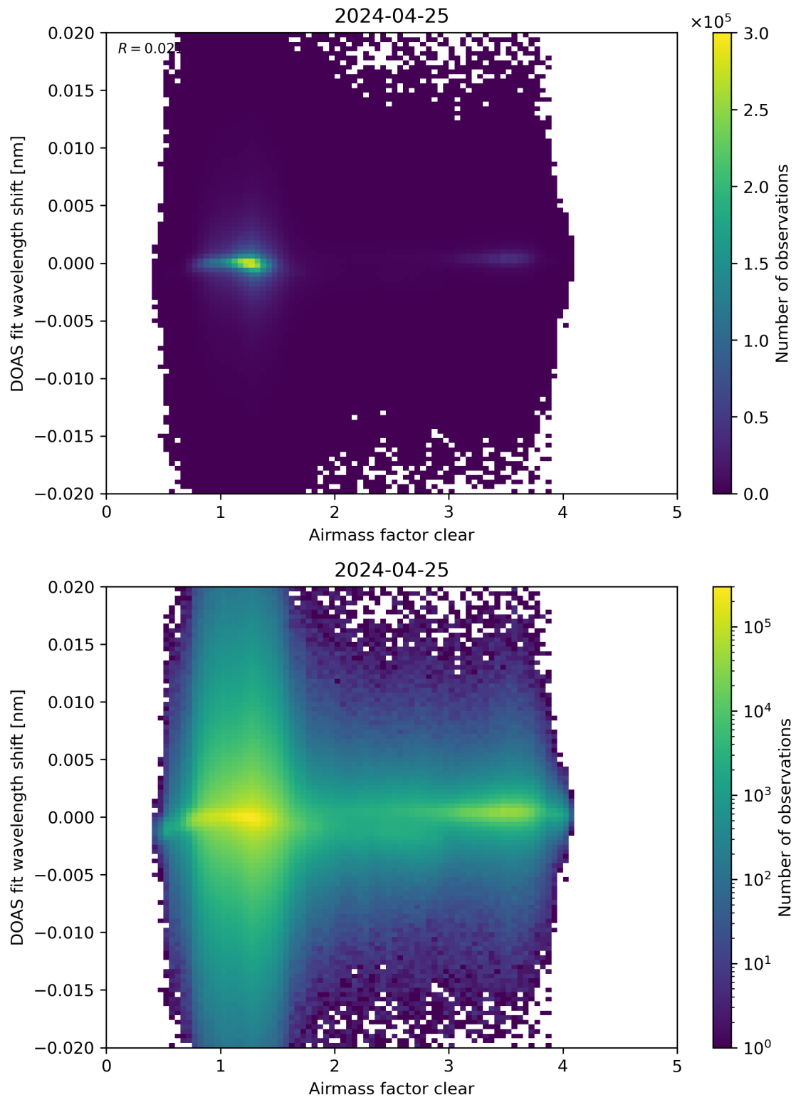
Figure 72: Scatter density plot of “Airmass factor clear” against “DOAS fit wavelength shift” for 2024-04-24 to 2024-04-26.
