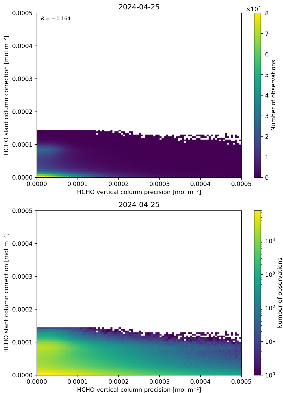
Figure 141: Scatter density plot of “HCHO vertical column precision” against “HCHO slant column correction” for 2024-04-24 to 2024-04-26.
