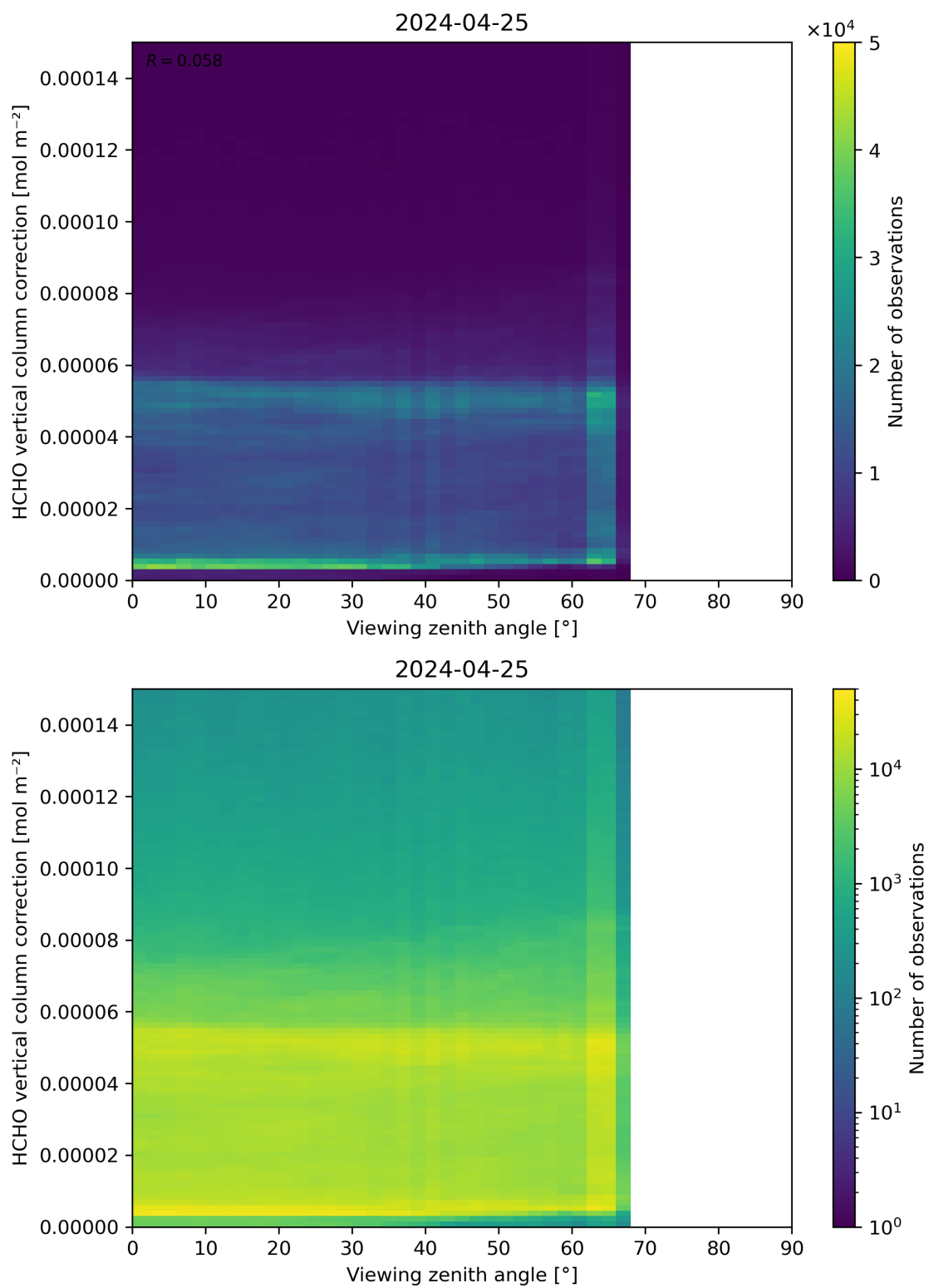
Figure 193: Scatter density plot of “Viewing zenith angle” against “HCHO vertical column correction” for 2024-04-24 to 2024-04-26.
