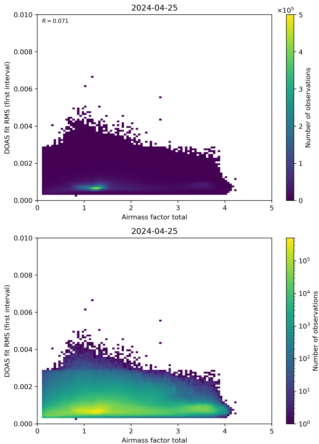
Figure 97: Scatter density plot of “Airmass factor total” against “DOAS fit RMS (first interval)” for 2024-04-24 to 2024-04-26.
