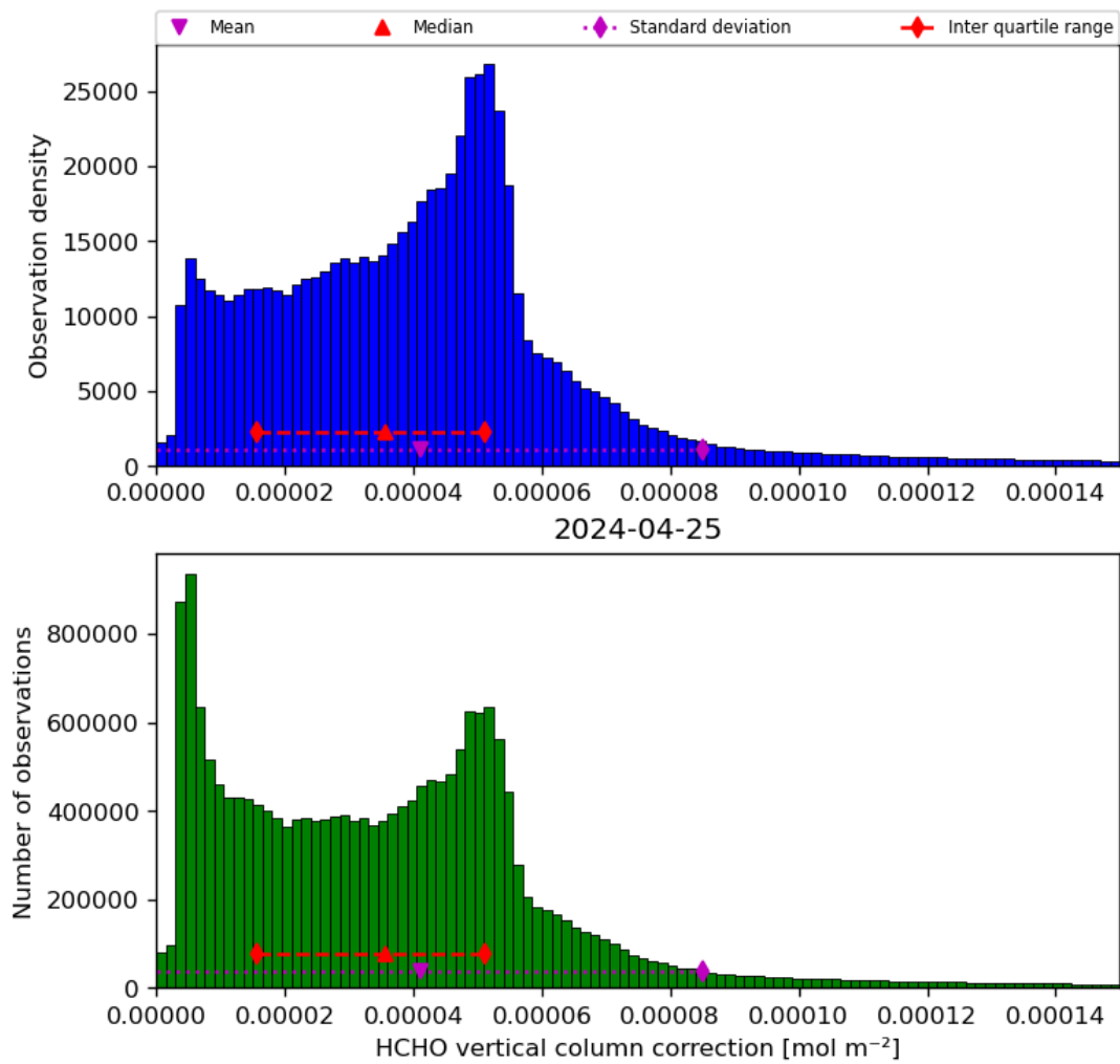
Figure 37: Histogram of “HCHO vertical column correction” for 2024-04-24 to 2024-04-26
