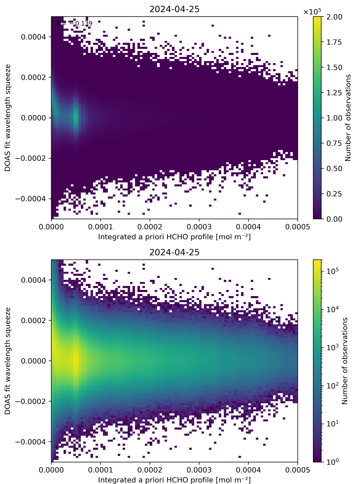
Figure 150: Scatter density plot of “Integrated a priori HCHO profile” against “DOAS fit wavelength squeeze” for 2024-04-24 to 2024-04-26.
