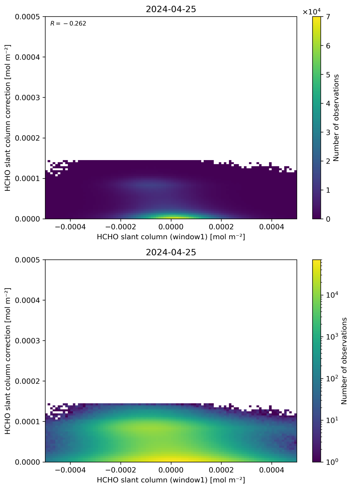
Figure 83: Scatter density plot of “HCHO slant column (window1)” against “HCHO slant column correction” for 2024-04-24 to 2024-04-26.
