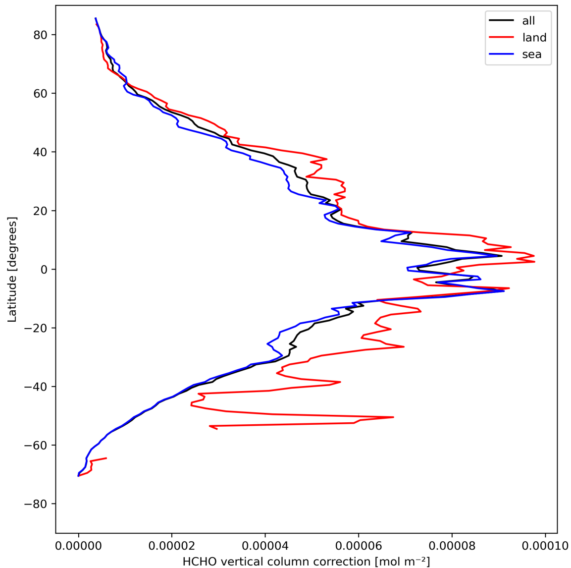
Figure 23: Zonal average of “HCHO vertical column correction” for 2024-04-24 to 2024-04-26.
