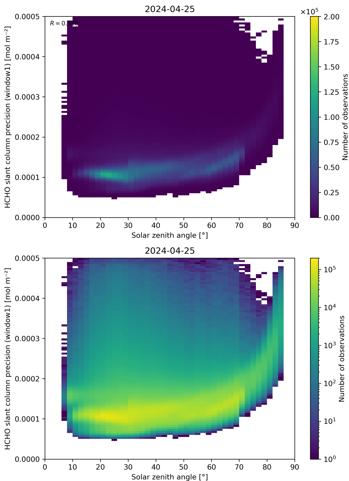
Figure 174: Scatter density plot of “Solar zenith angle” against “HCHO slant column precision (window1)” for 2024-04-24 to 2024-04-26.
