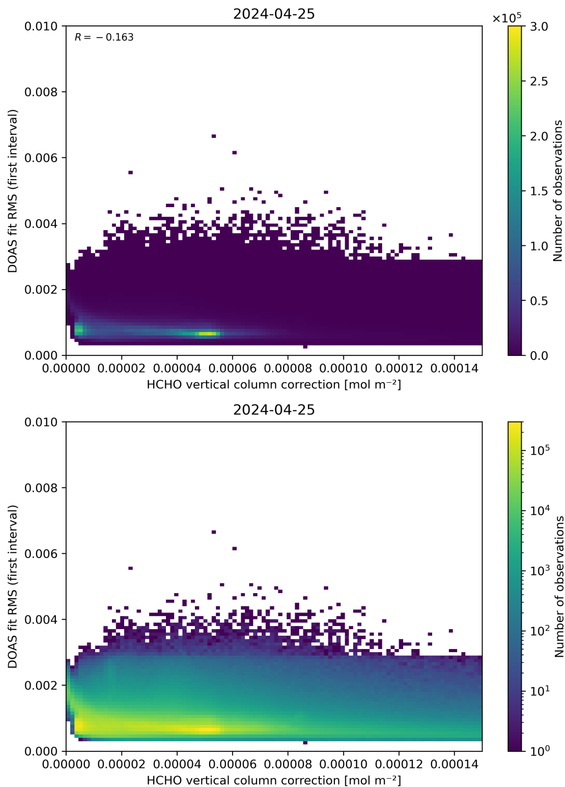
Figure 112: Scatter density plot of “HCHO vertical column correction” against “DOAS fit RMS (first interval)” for 2024-04-24 to 2024-04-26.
