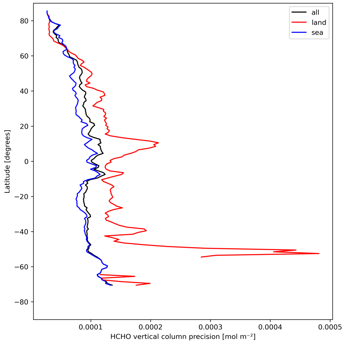
Figure 22: Zonal average of “HCHO vertical column precision” for 2024-04-24 to 2024-04-26.
