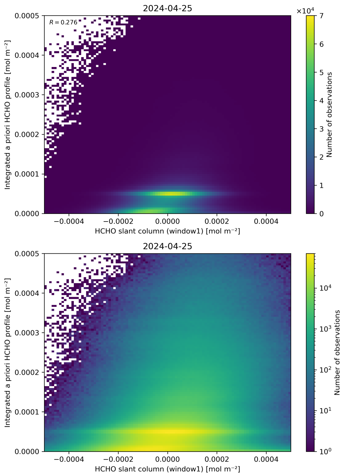
Figure 87: Scatter density plot of “HCHO slant column (window1)” against “Integrated a priori HCHO profile” for 2024-04-24 to 2024-04-26.
