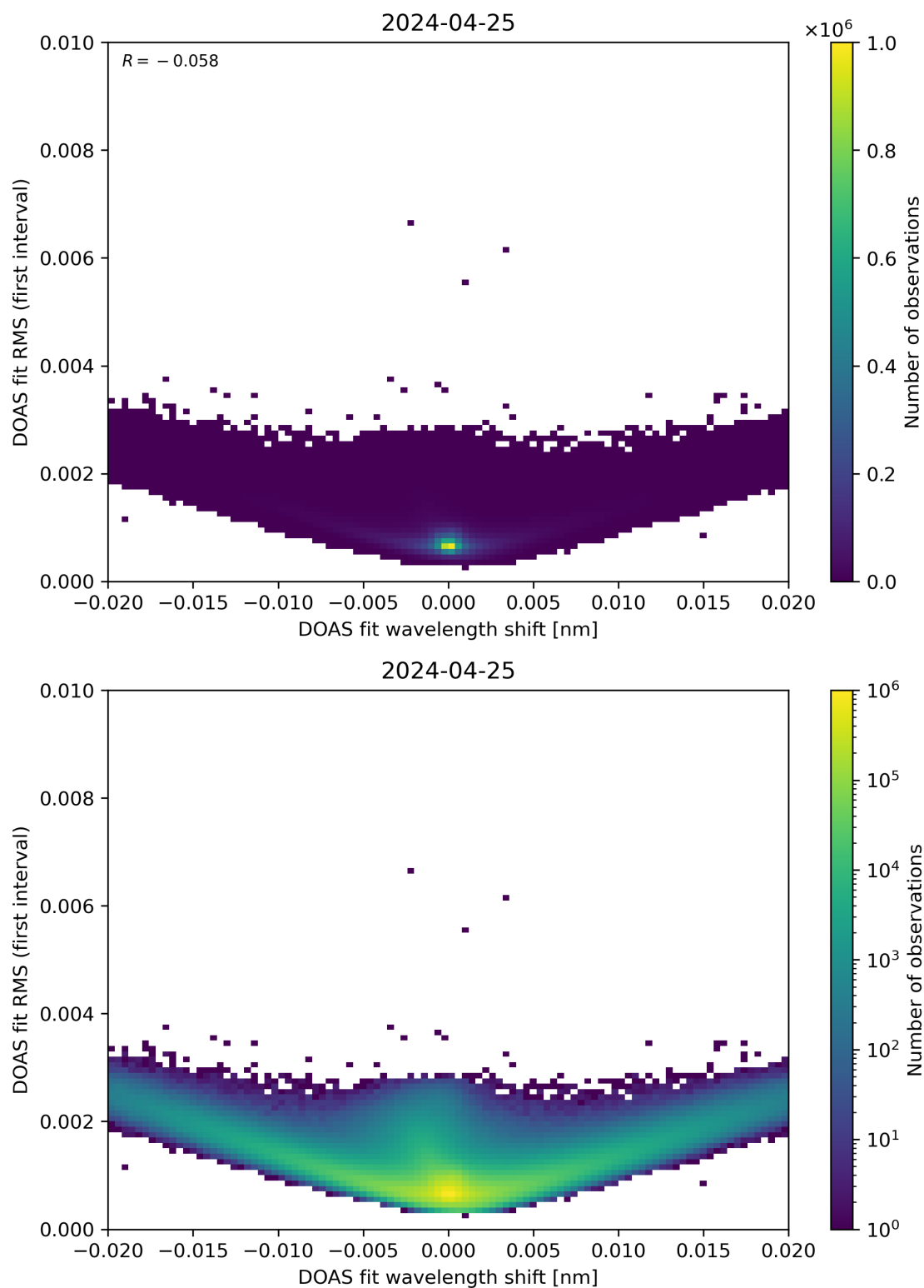
Figure 64: Scatter density plot of “DOAS fit wavelength shift” against “DOAS fit RMS (first interval)” for 2024-04-24 to 2024-04-26.
