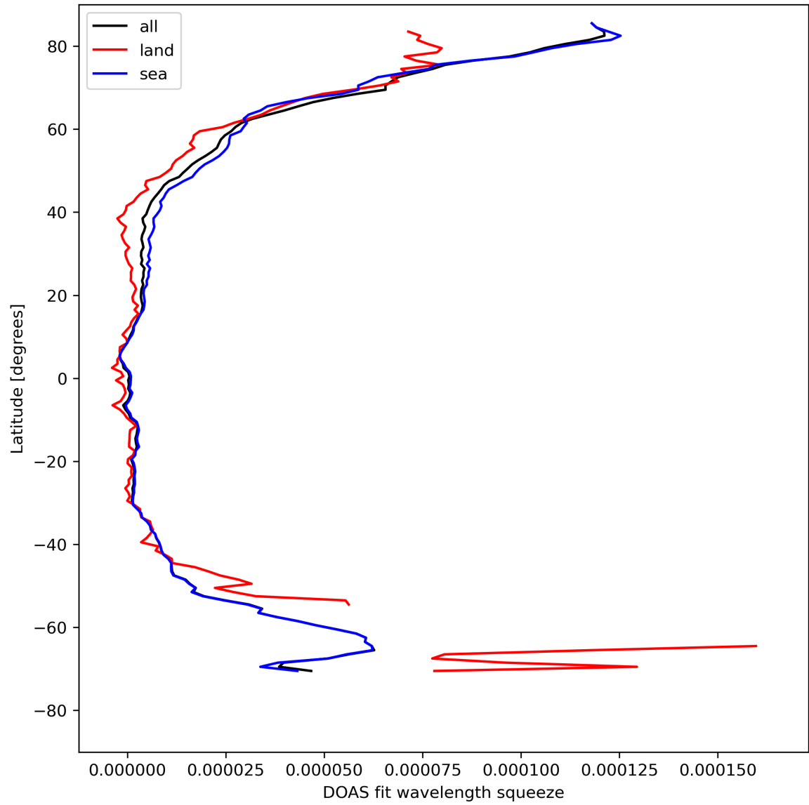
Figure 31: Zonal average of “DOAS fit wavelength squeeze” for 2024-04-24 to 2024-04-26.
