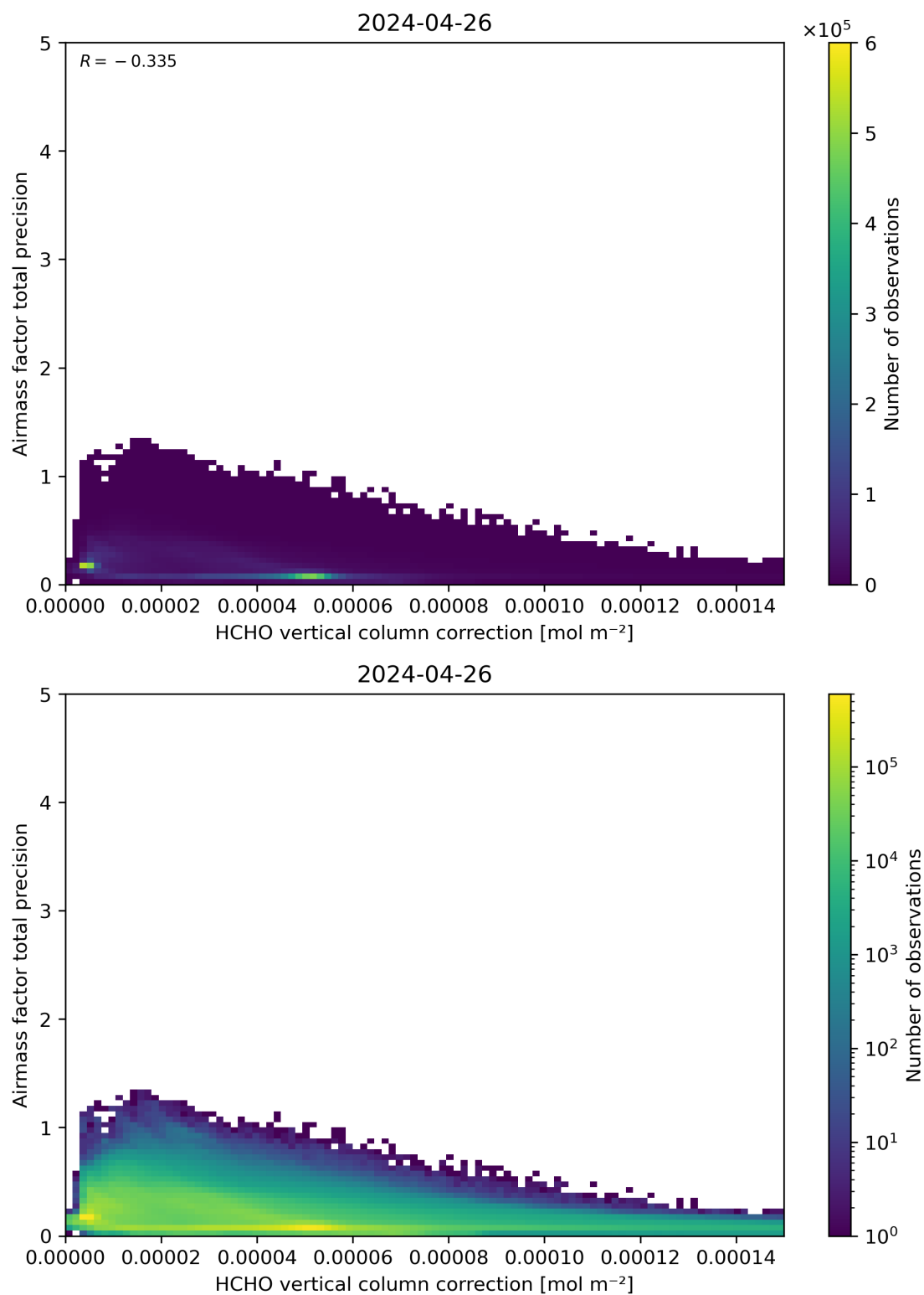
Figure 121: Scatter density plot of “HCHO vertical column correction” against “Airmass factor total precision” for 2024-04-26 to 2024-04-27.
