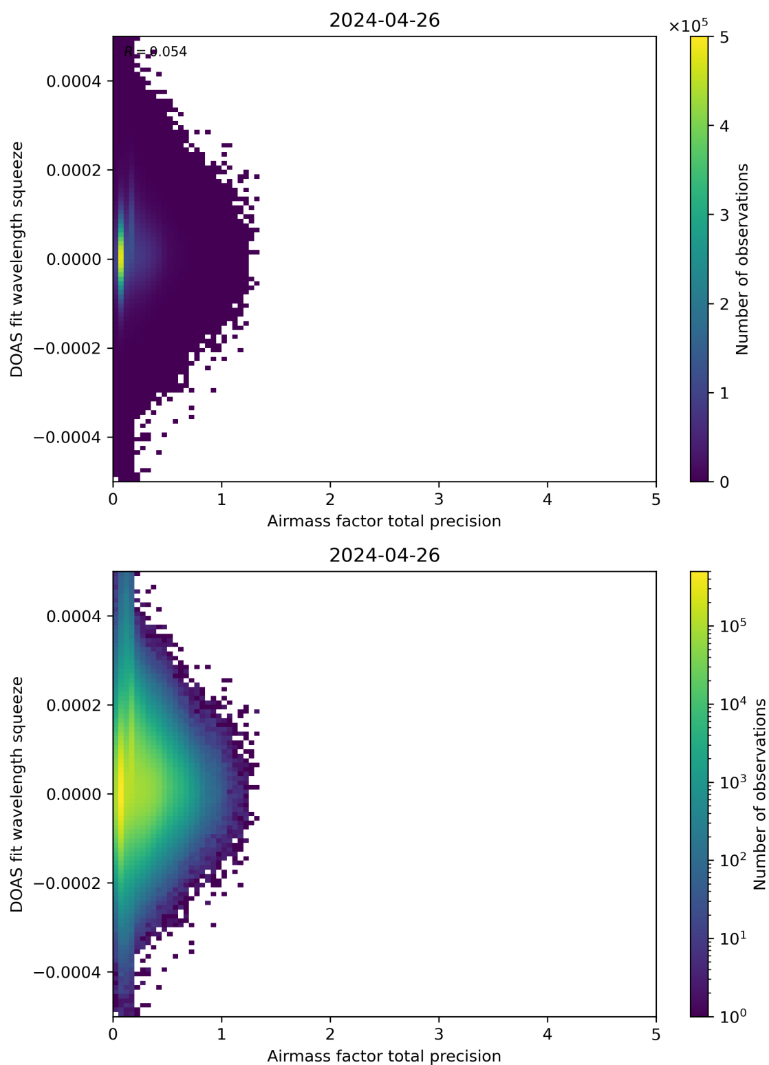
Figure 107: Scatter density plot of “Airmass factor total precision” against “DOAS fit wavelength squeeze” for 2024-04-26 to 2024-04-27.
