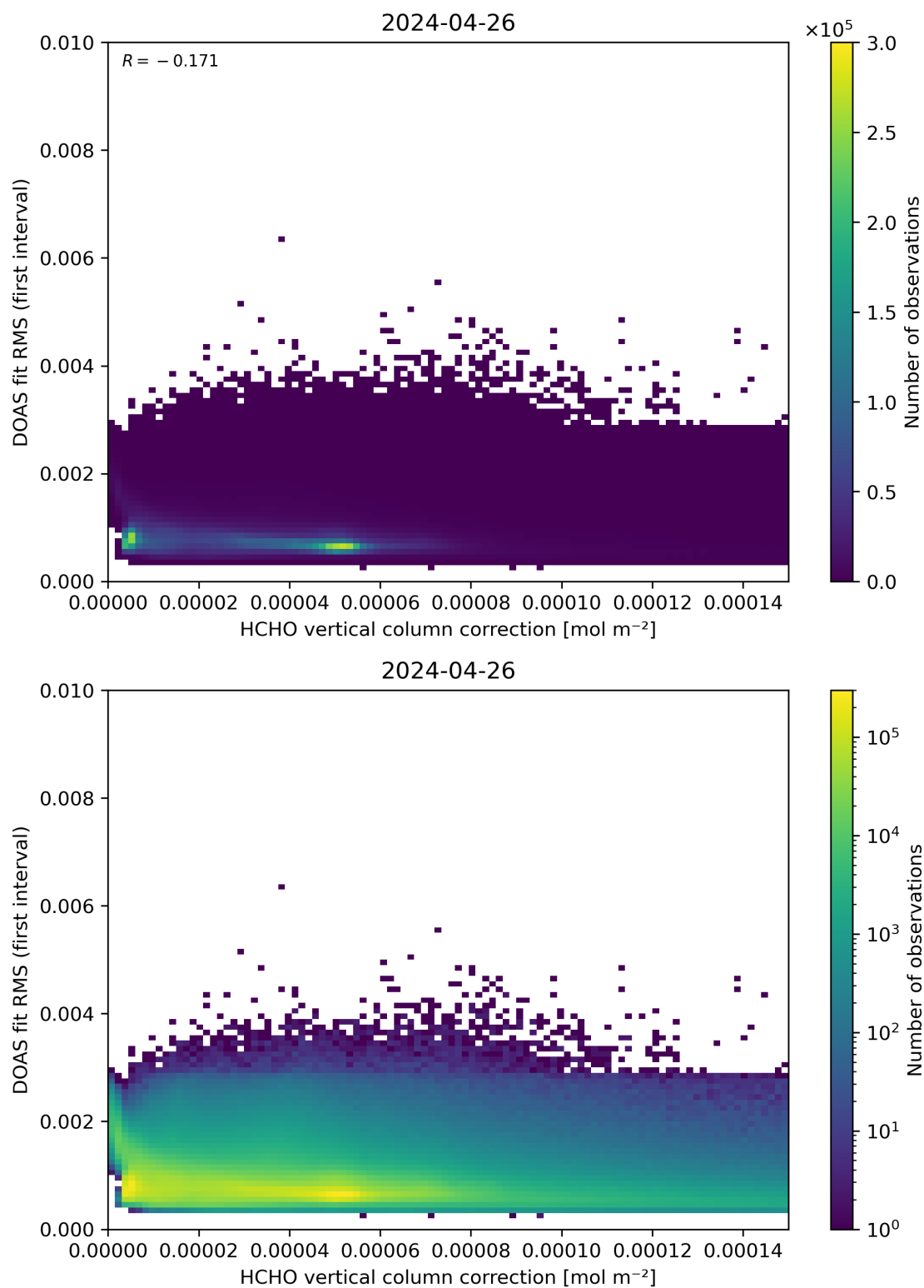
Figure 112: Scatter density plot of “HCHO vertical column correction” against “DOAS fit RMS (first interval)” for 2024-04-26 to 2024-04-27.
