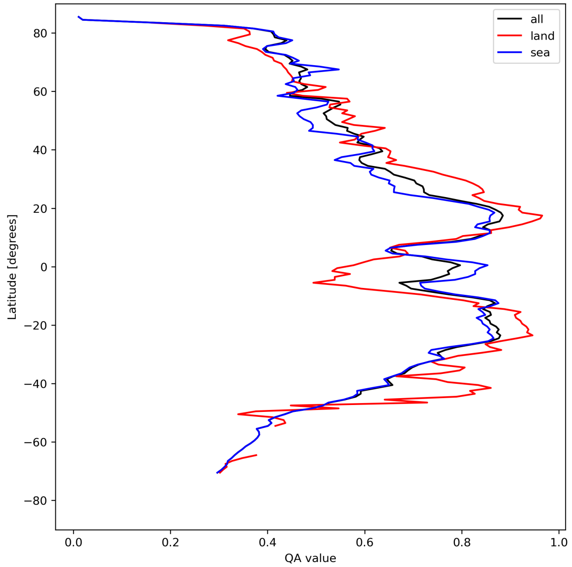
Figure 20: Zonal average of “QA value” for 2024-04-26 to 2024-04-27.
