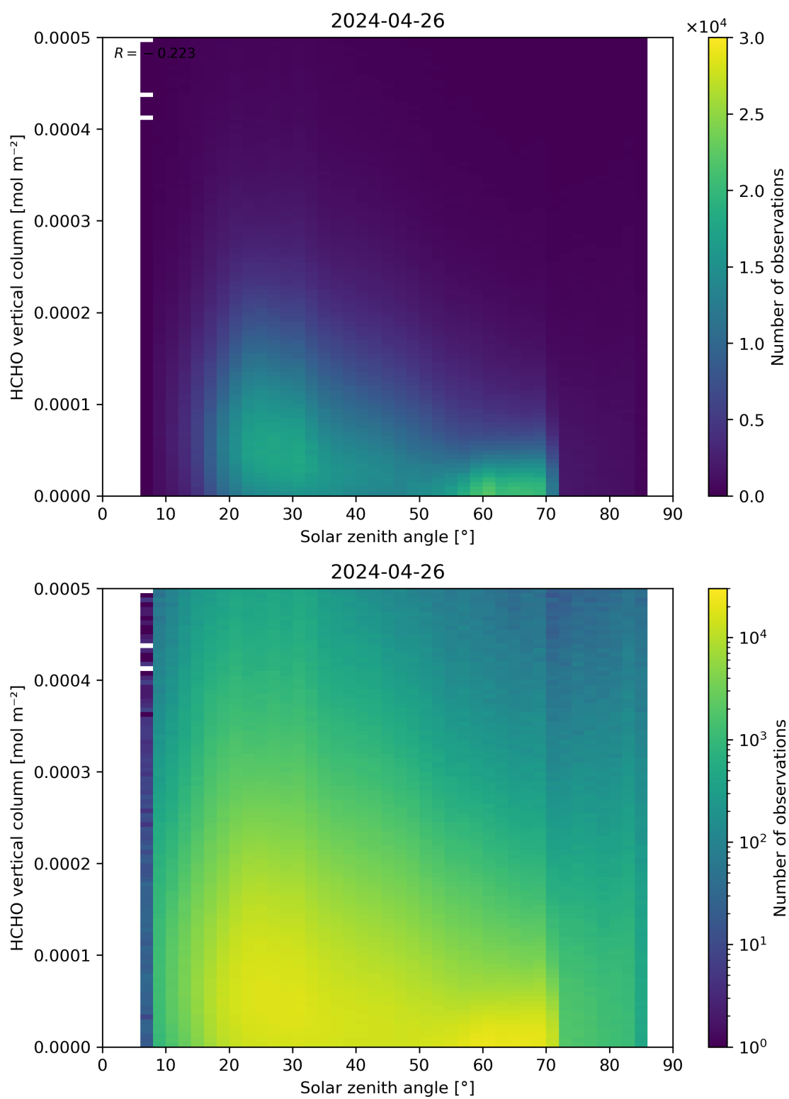
Figure 177: Scatter density plot of “Solar zenith angle” against “HCHO vertical column” for 2024-04-26 to 2024-04-27.
