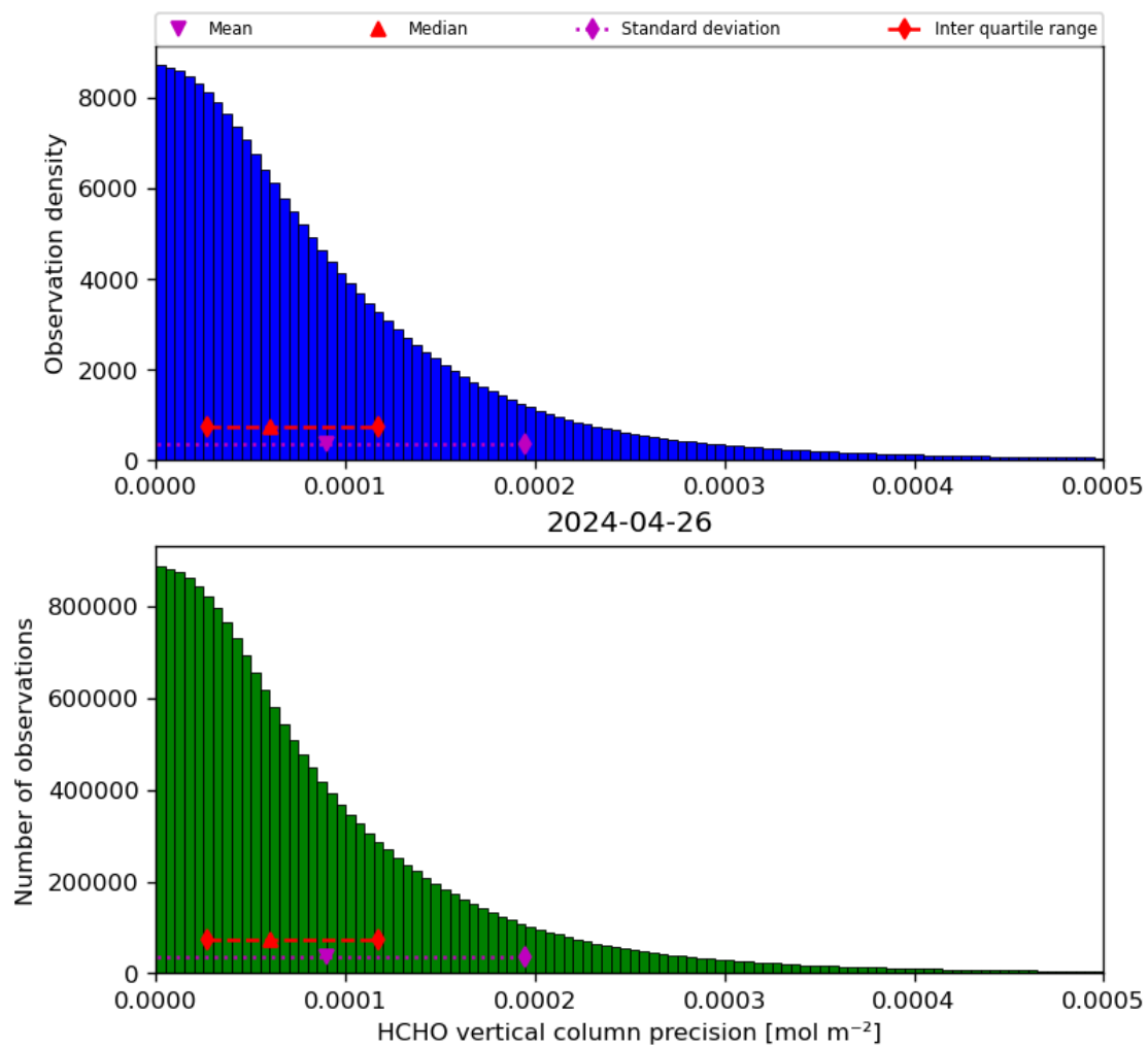
Figure 36: Histogram of “HCHO vertical column precision” for 2024-04-26 to 2024-04-27
