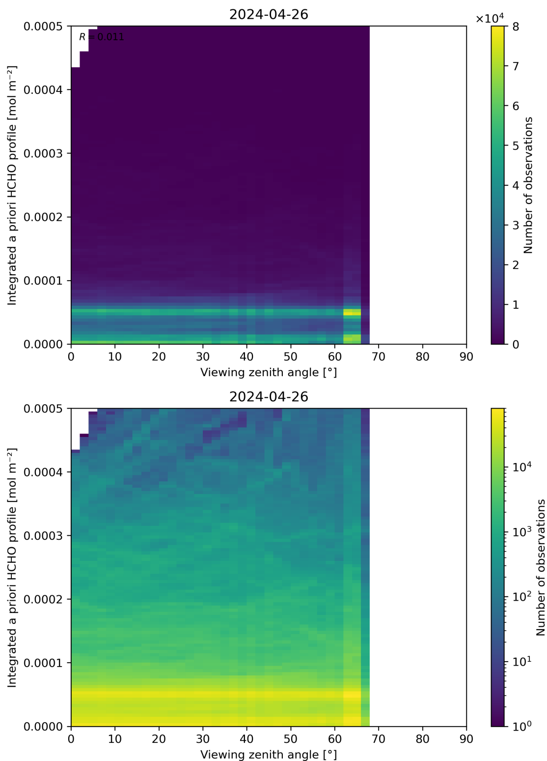
Figure 195: Scatter density plot of “Viewing zenith angle” against “Integrated a priori HCHO profile” for 2024-04-26 to 2024-04-27.
