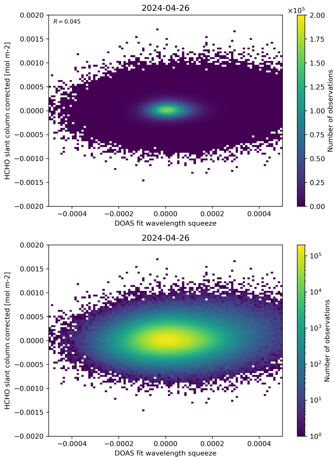
Figure 69: Scatter density plot of “DOAS fit wavelength squeeze” against “HCHO slant column corrected” for 2024-04-26 to 2024-04-27.
