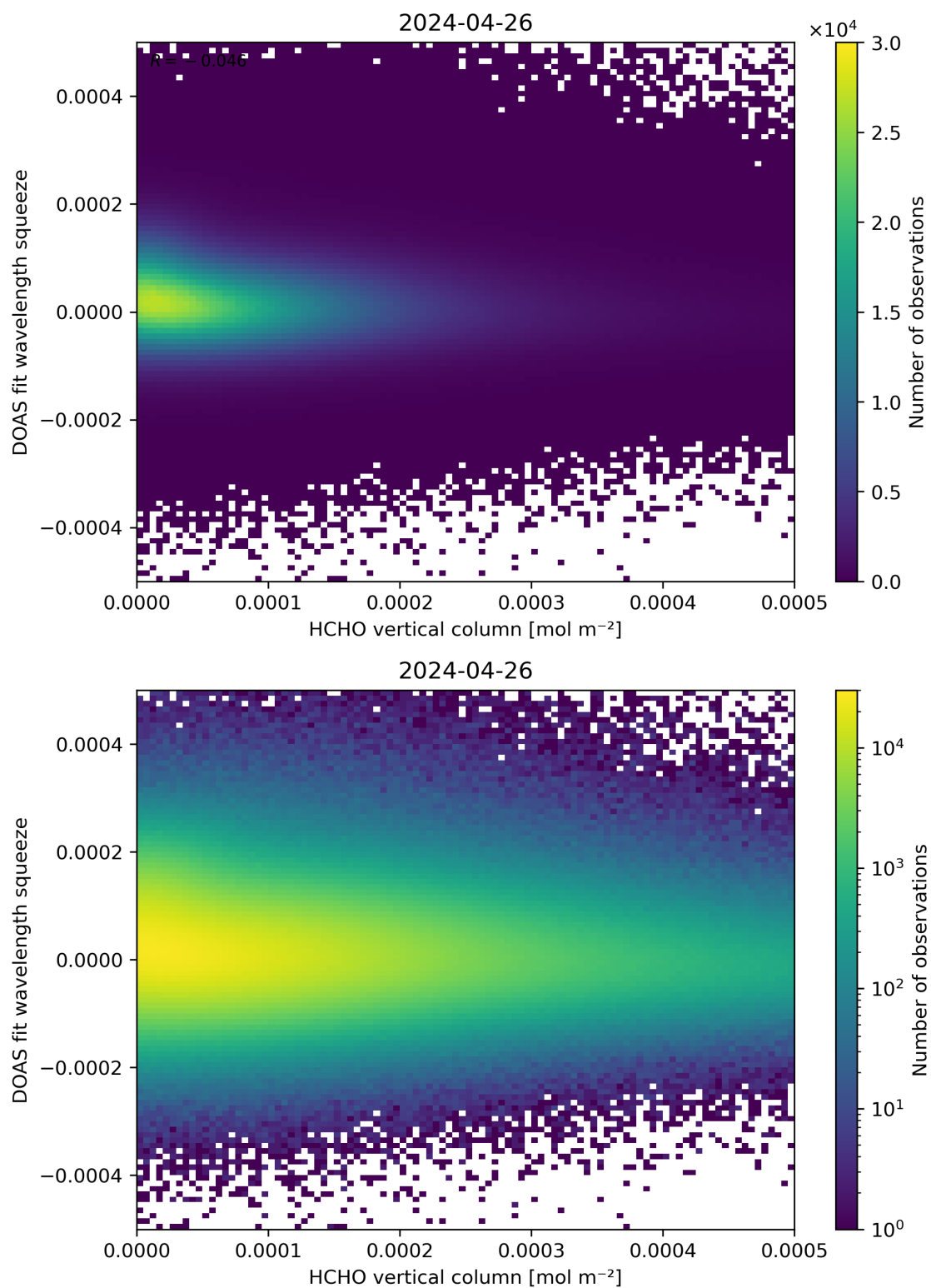
Figure 125: Scatter density plot of “HCHO vertical column” against “DOAS fit wavelength squeeze” for 2024-04-26 to 2024-04-27.
