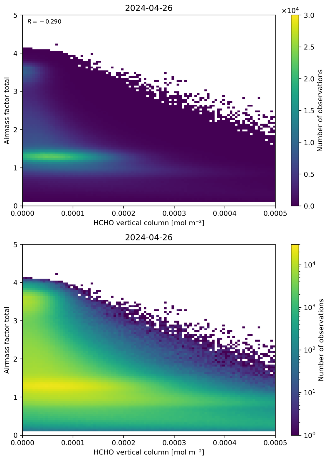
Figure 131: Scatter density plot of “HCHO vertical column” against “Airmass factor total” for 2024-04-26 to 2024-04-27.
