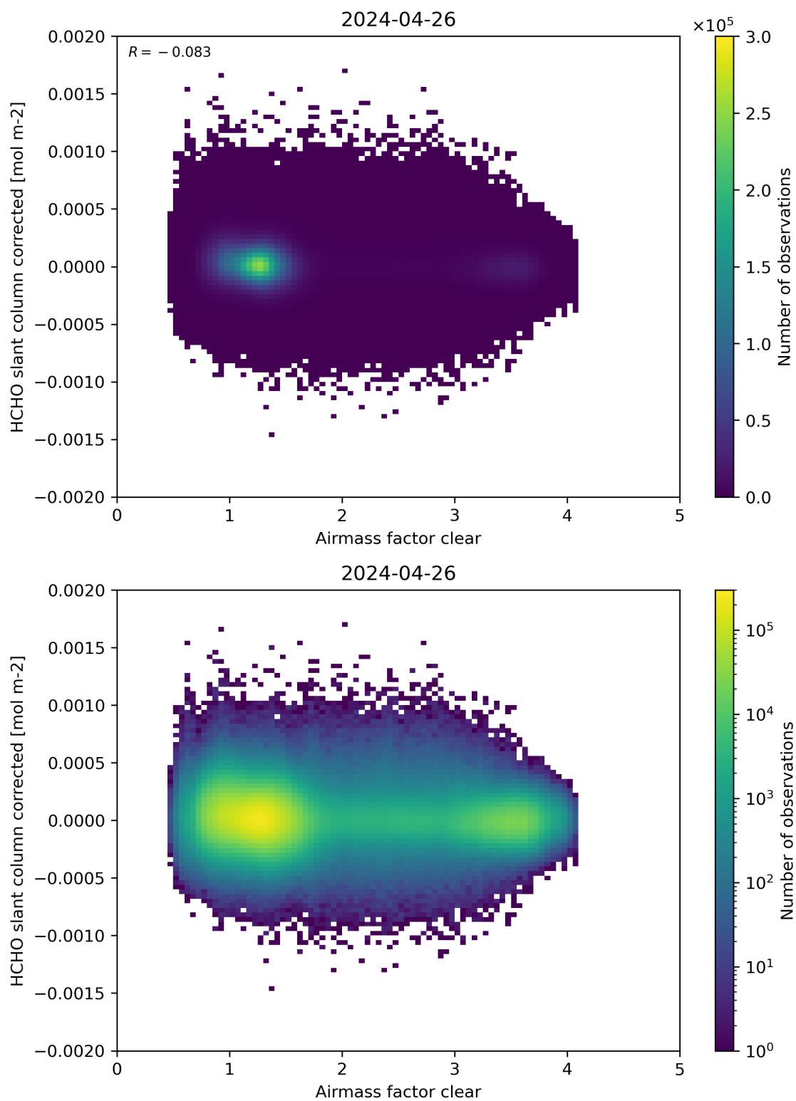
Figure 74: Scatter density plot of “Airmass factor clear” against “HCHO slant column corrected” for 2024-04-26 to 2024-04-27.
