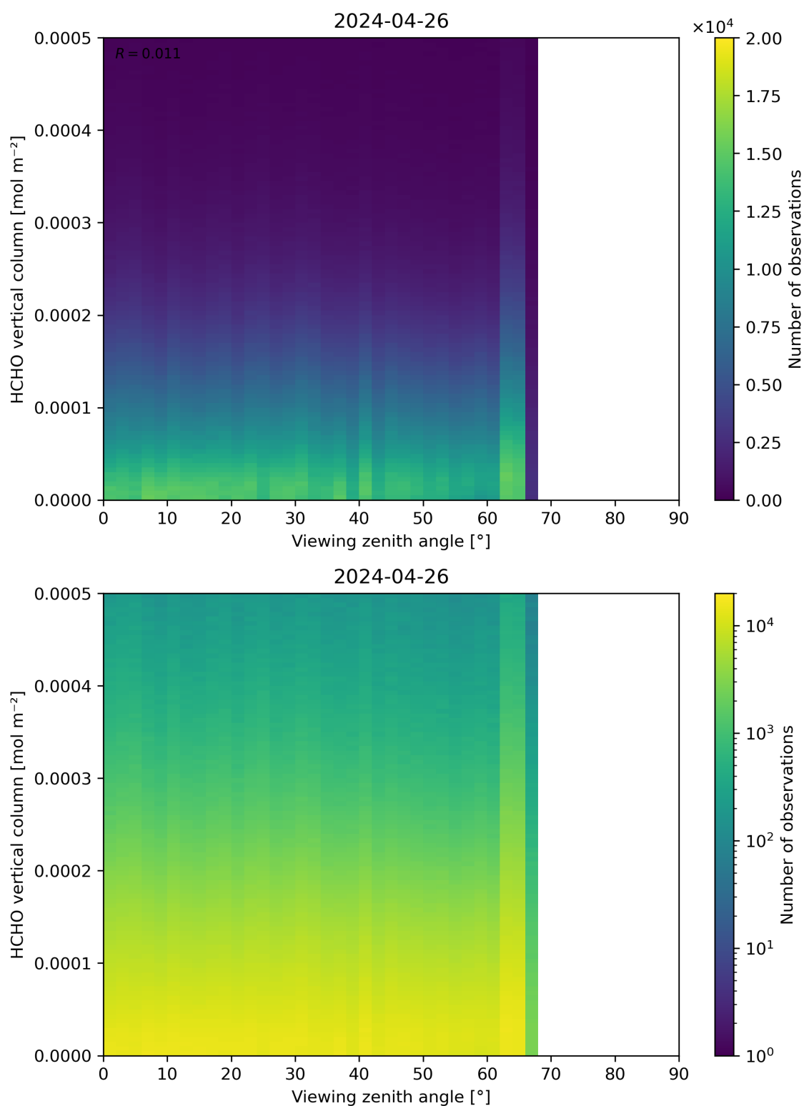
Figure 192: Scatter density plot of “Viewing zenith angle” against “HCHO vertical column” for 2024-04-26 to 2024-04-27.
