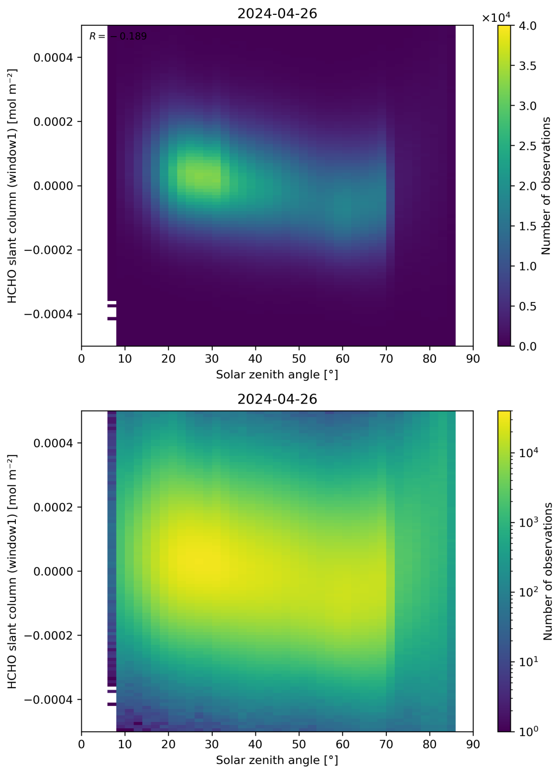
Figure 173: Scatter density plot of “Solar zenith angle” against “HCHO slant column (window1)” for 2024-04-26 to 2024-04-27.
