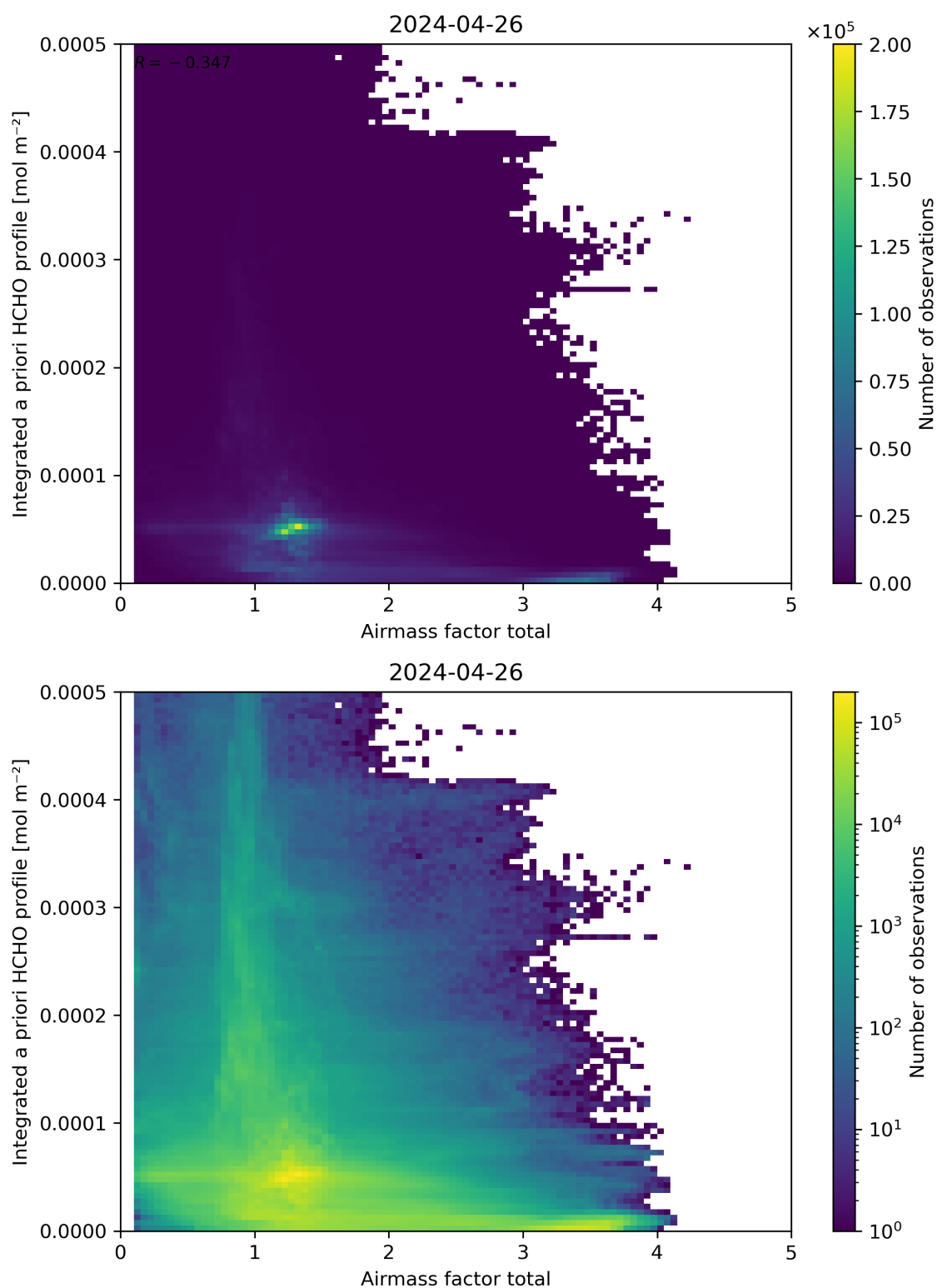
Figure 104: Scatter density plot of “Airmass factor total” against “Integrated a priori HCHO profile” for 2024-04-26 to 2024-04-27.
