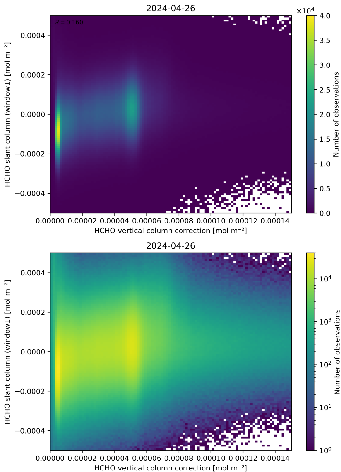
Figure 118: Scatter density plot of “HCHO vertical column correction” against “HCHO slant column (window1)” for 2024-04-26 to 2024-04-27.
