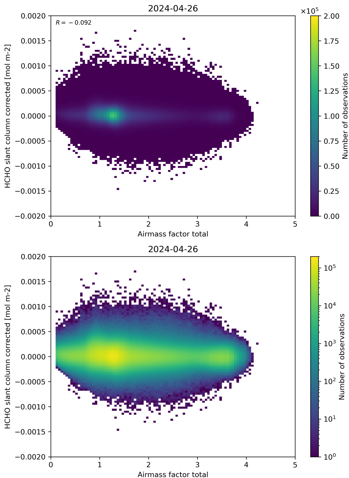
Figure 101: Scatter density plot of “Airmass factor total” against “HCHO slant column corrected” for 2024-04-26 to 2024-04-27.
