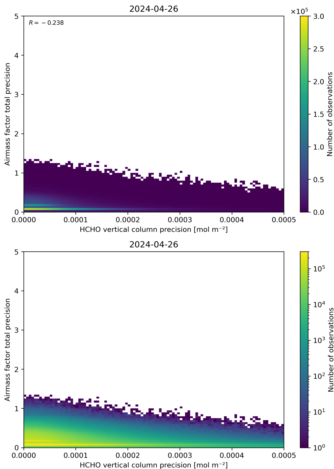
Figure 145: Scatter density plot of “HCHO vertical column precision” against “Airmass factor total precision” for 2024-04-26 to 2024-04-27.
