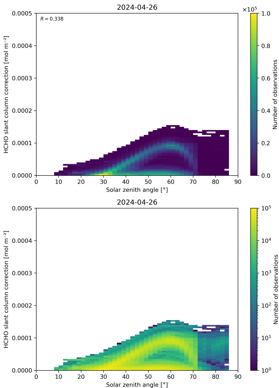
Figure 172: Scatter density plot of “Solar zenith angle” against “HCHO slant column correction” for 2024-04-26 to 2024-04-27.
