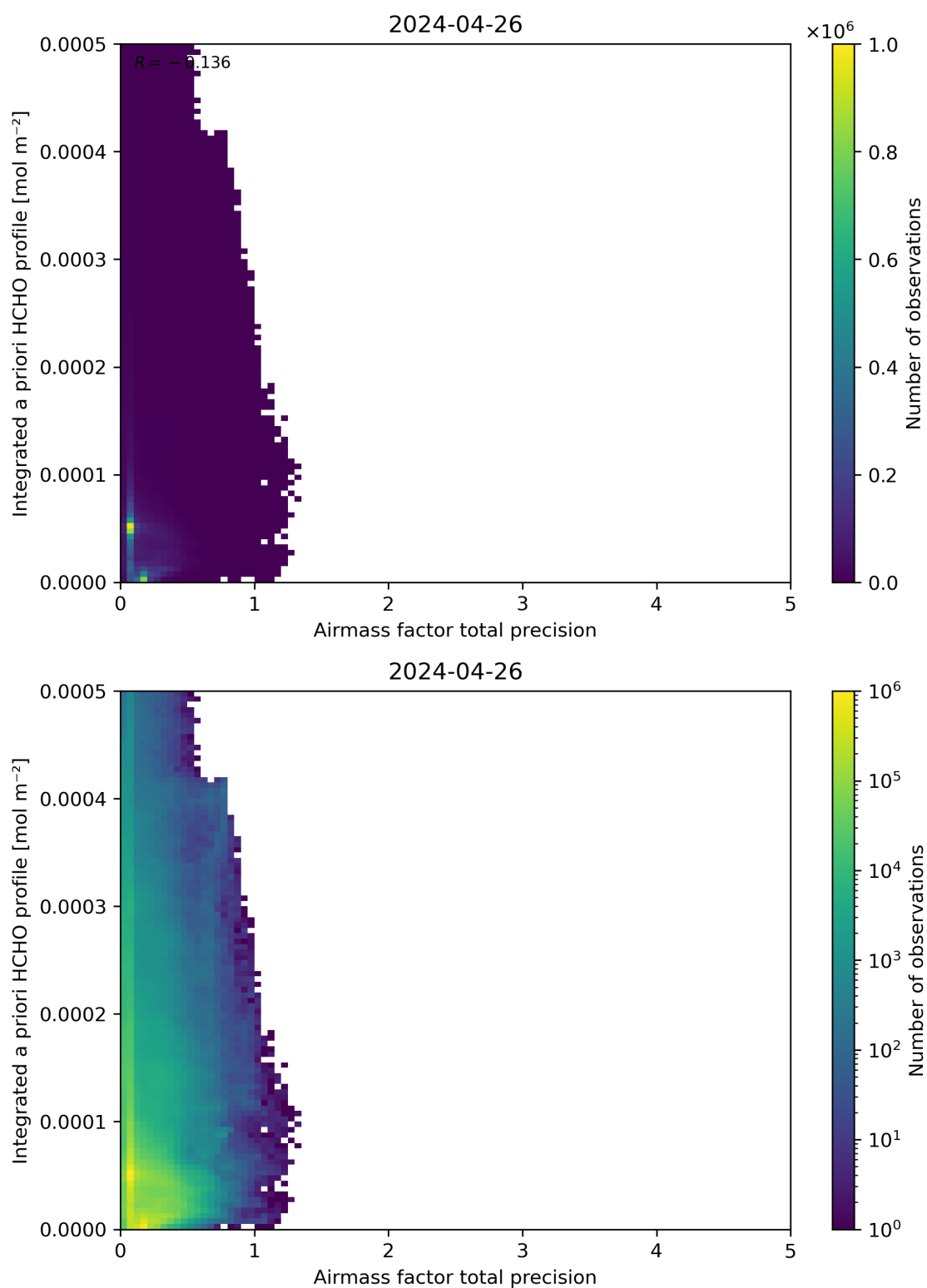
Figure 111: Scatter density plot of “Airmass factor total precision” against “Integrated a priori HCHO profile” for 2024-04-26 to 2024-04-27.
