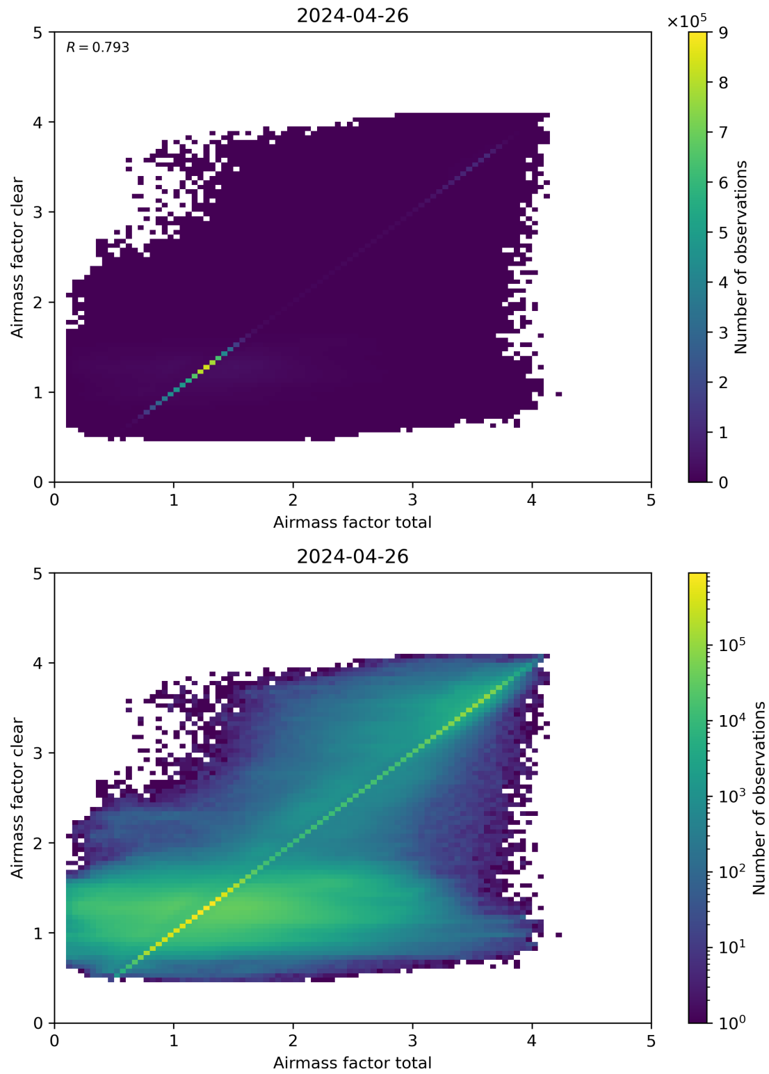
Figure 100: Scatter density plot of “Airmass factor total” against “Airmass factor clear” for 2024-04-26 to 2024-04-27.
