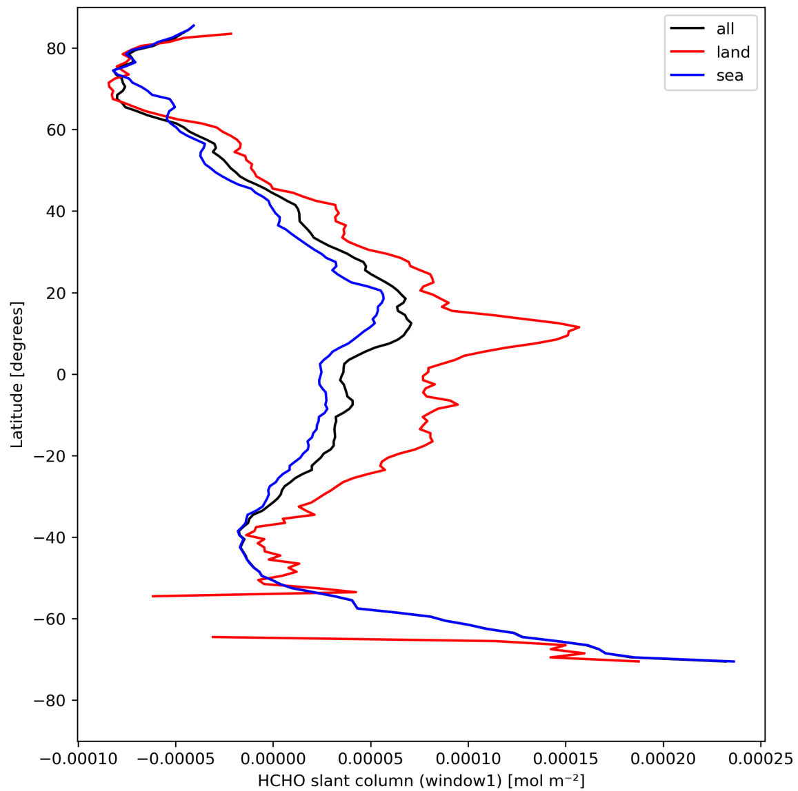
Figure 24: Zonal average of “HCHO slant column (window1)” for 2024-04-26 to 2024-04-27.
