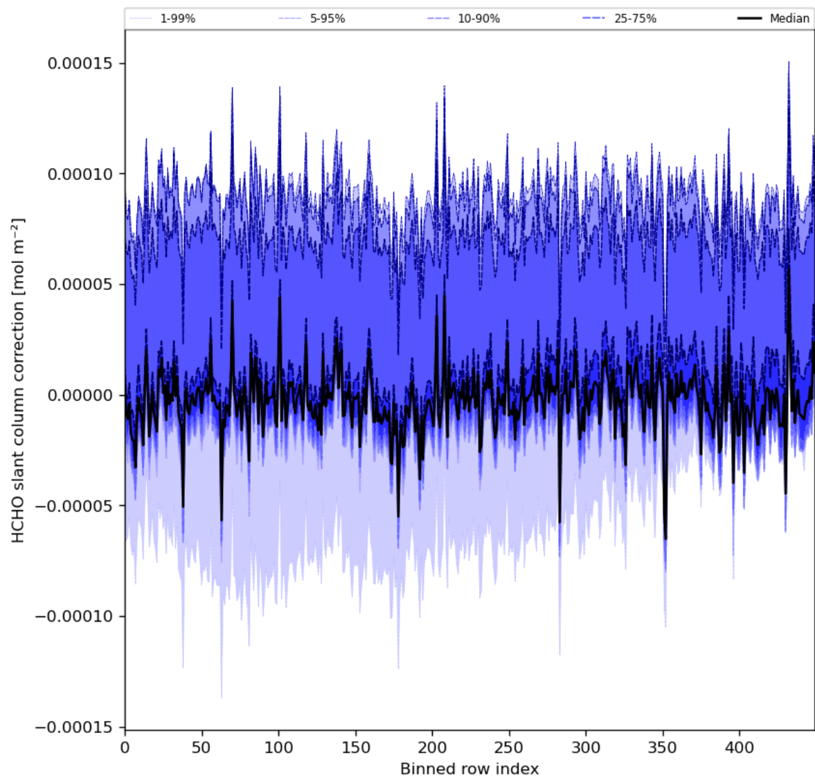
Figure 61: Along track statistics of “HCHO slant column correction” for 2024-04-26 to 2024-04-27
