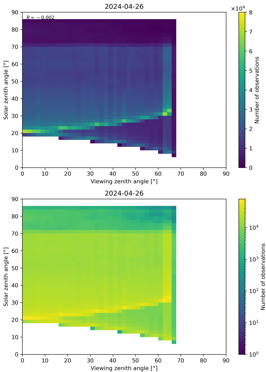
Figure 197: Scatter density plot of “Viewing zenith angle” against “Solar zenith angle” for 2024-04-26 to 2024-04-27.
