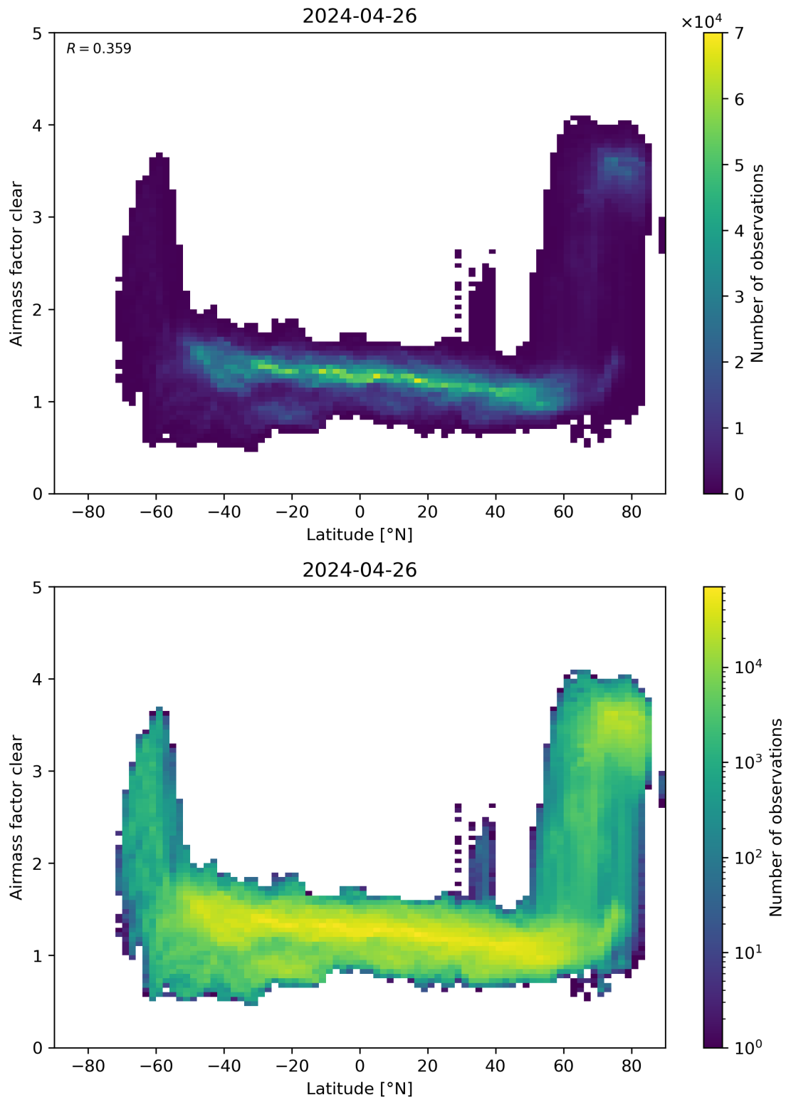
Figure 156: Scatter density plot of “Latitude” against “Airmass factor clear” for 2024-04-26 to 2024-04-27.
