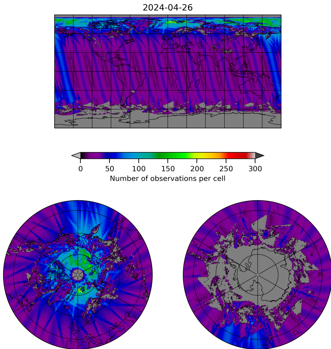
Figure 19: Map of the number of observations for 2024-04-26 to 2024-04-27
