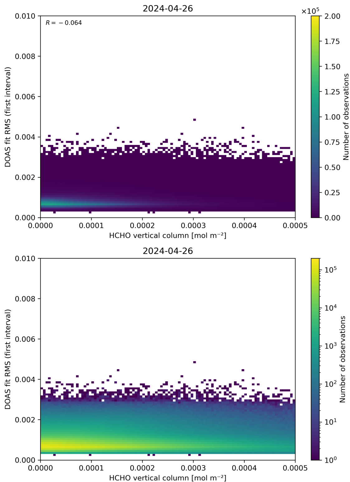
Figure 123: Scatter density plot of “HCHO vertical column” against “DOAS fit RMS (first interval)” for 2024-04-26 to 2024-04-27.
