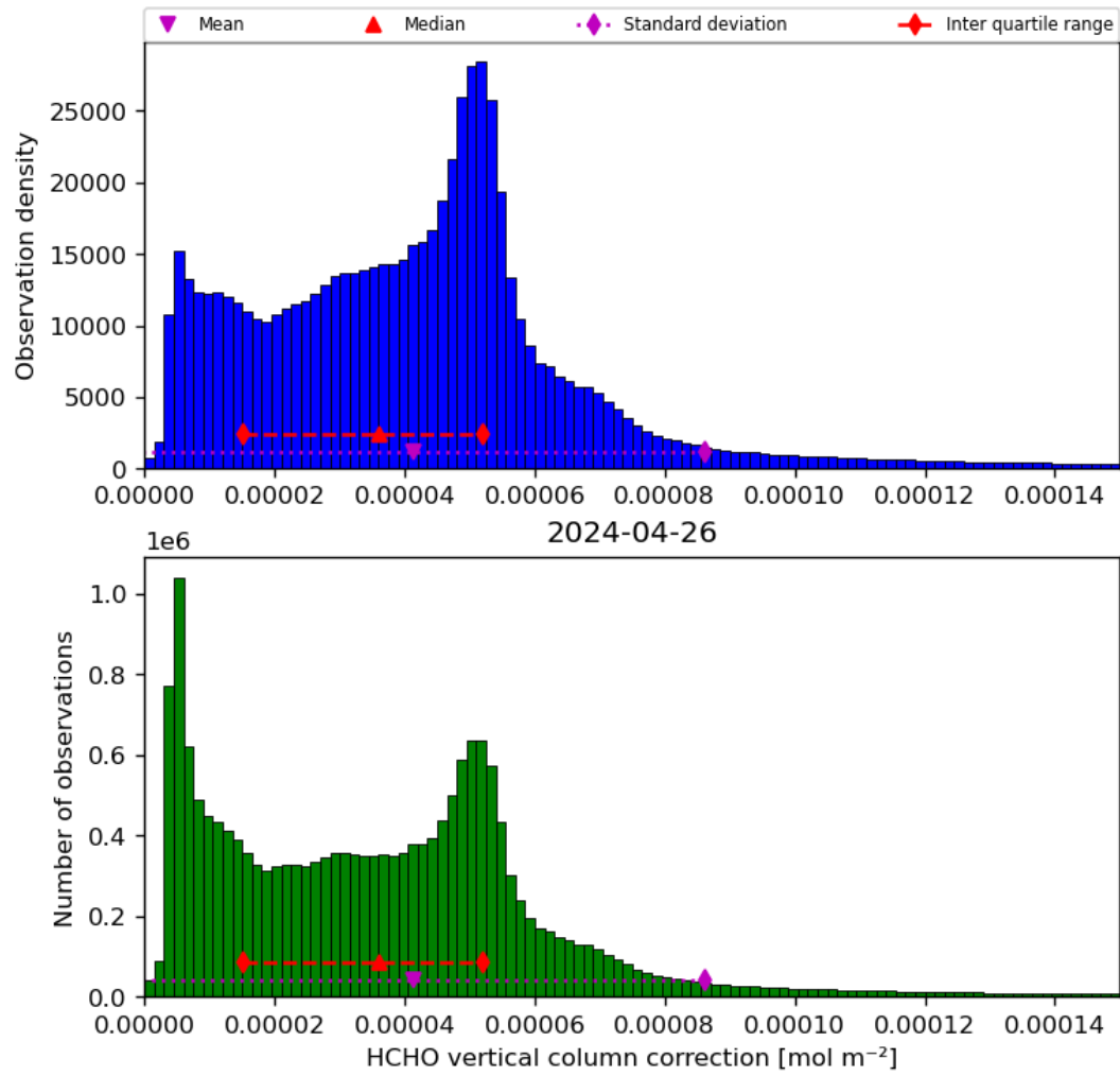
Figure 37: Histogram of “HCHO vertical column correction” for 2024-04-26 to 2024-04-27
