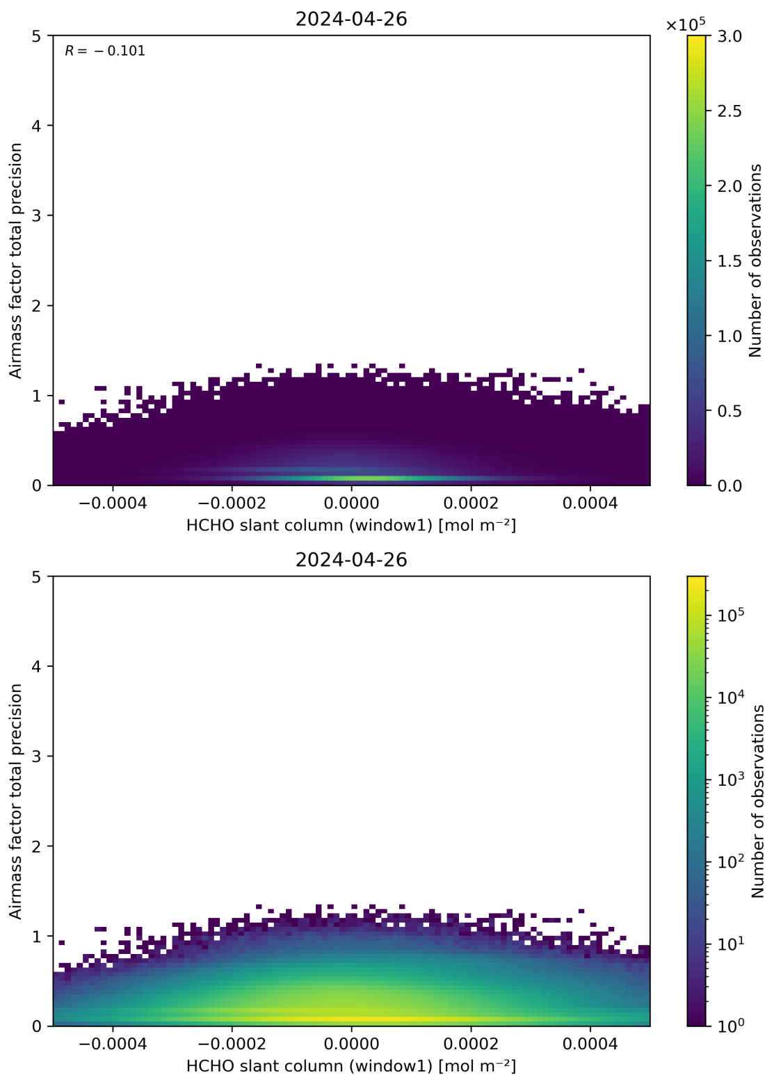
Figure 86: Scatter density plot of “HCHO slant column (window1)” against “Airmass factor total precision” for 2024-04-26 to 2024-04-27.
