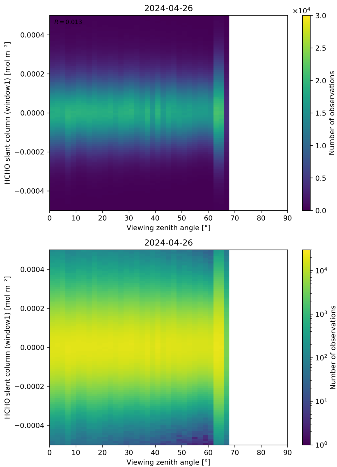
Figure 188: Scatter density plot of “Viewing zenith angle” against “HCHO slant column (window1)” for 2024-04-26 to 2024-04-27.
