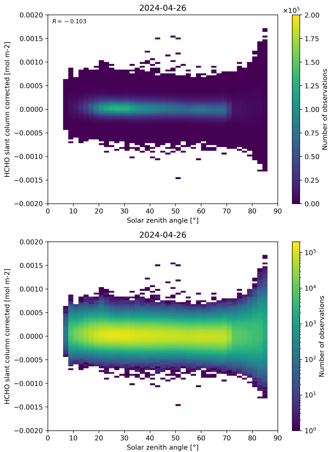
Figure 171: Scatter density plot of “Solar zenith angle” against “HCHO slant column corrected” for 2024-04-26 to 2024-04-27.
