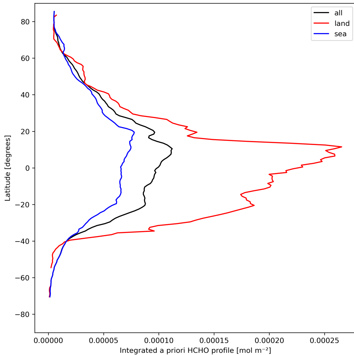
Figure 29: Zonal average of “Integrated a priori HCHO profile” for 2024-04-26 to 2024-04-27.
