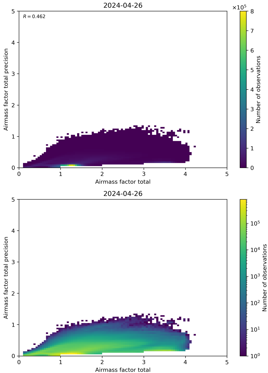
Figure 103: Scatter density plot of “Airmass factor total” against “Airmass factor total precision” for 2024-04-26 to 2024-04-27.
