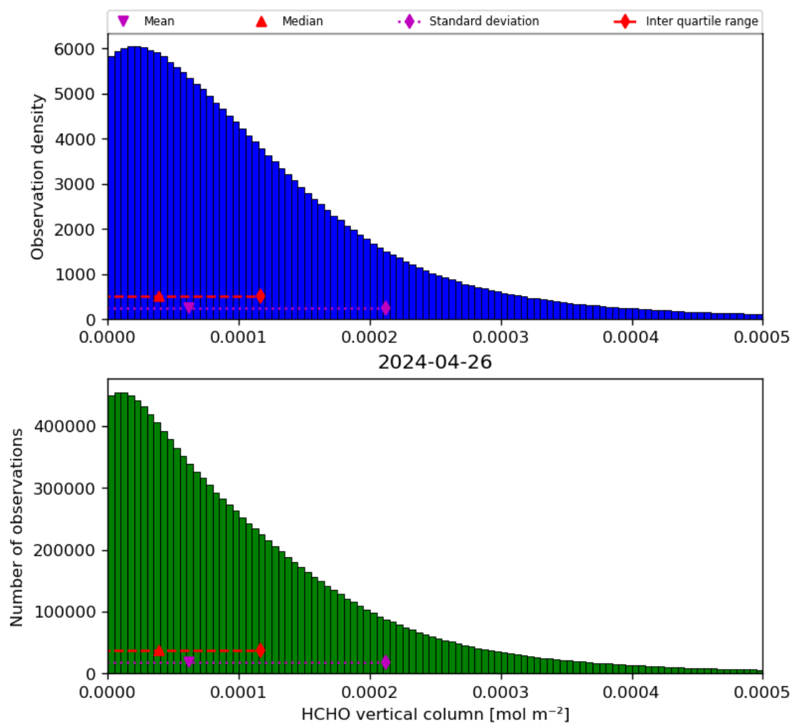
Figure 35: Histogram of “HCHO vertical column” for 2024-04-26 to 2024-04-27
