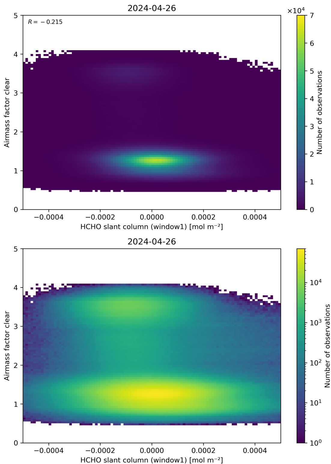
Figure 81: Scatter density plot of “HCHO slant column (window1)” against “Airmass factor clear” for 2024-04-26 to 2024-04-27.
