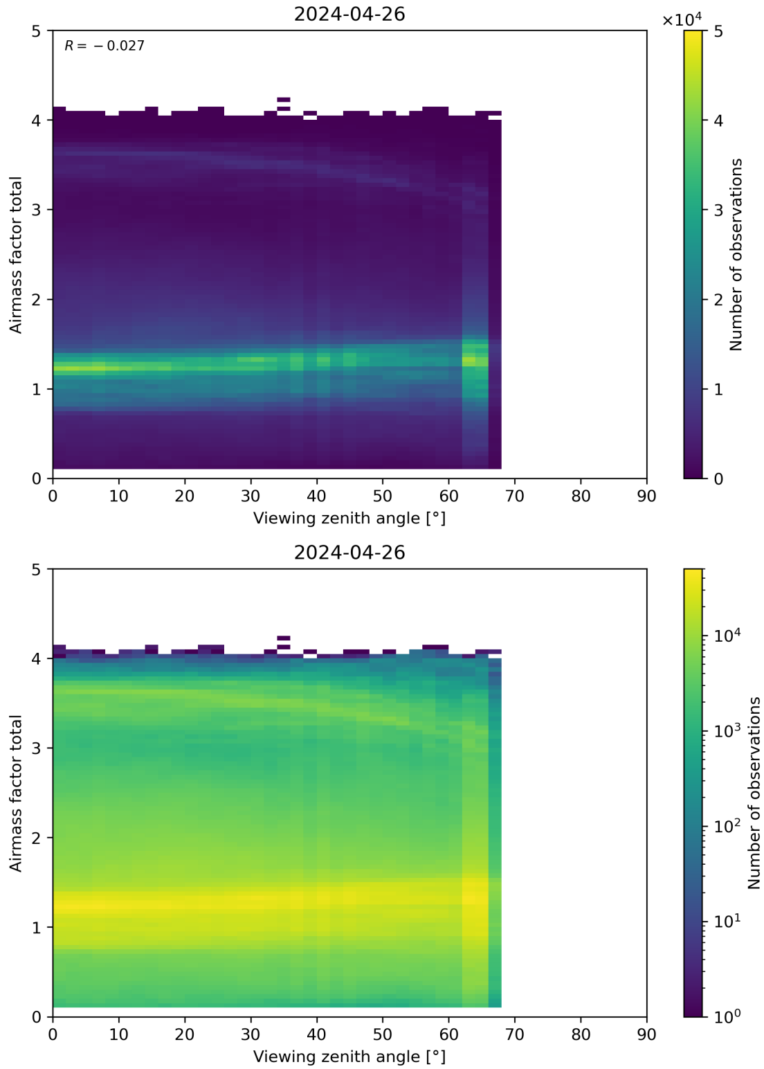
Figure 190: Scatter density plot of “Viewing zenith angle” against “Airmass factor total” for 2024-04-26 to 2024-04-27.
