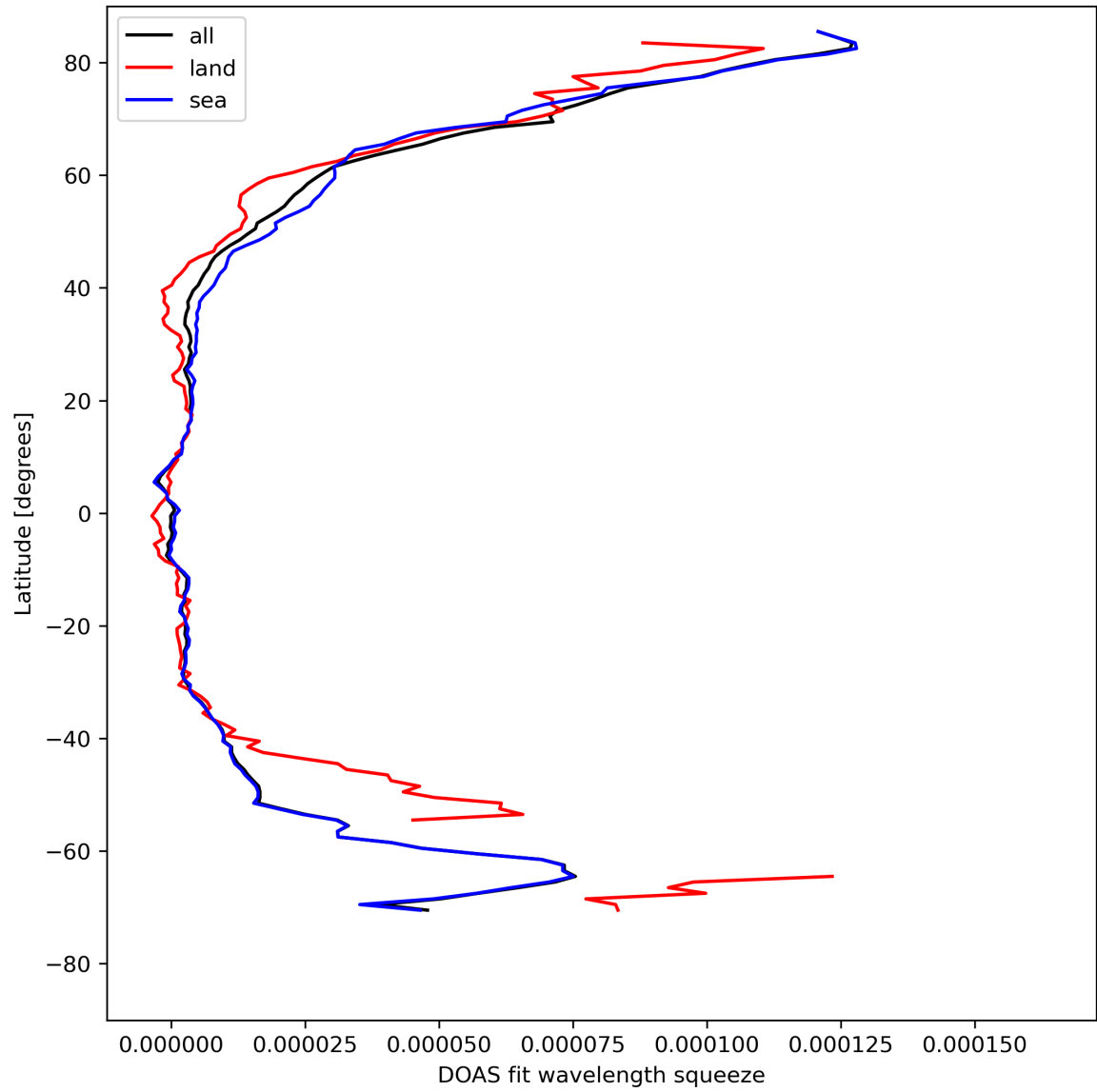
Figure 31: Zonal average of “DOAS fit wavelength squeeze” for 2024-04-26 to 2024-04-27.
