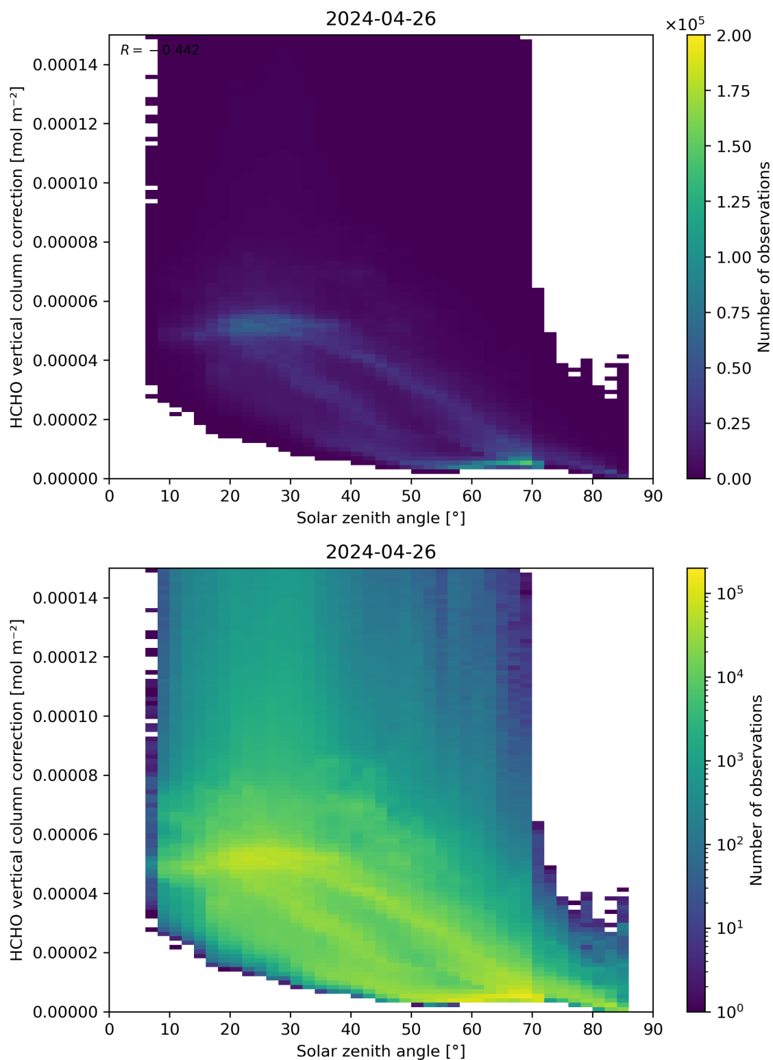
Figure 178: Scatter density plot of “Solar zenith angle” against “HCHO vertical column correction” for 2024-04-26 to 2024-04-27.
