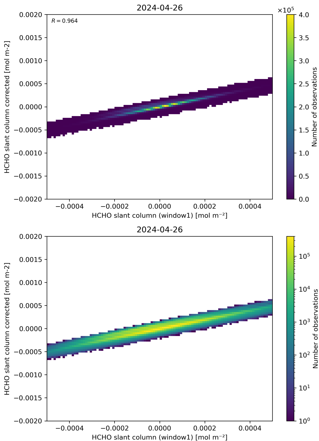
Figure 82: Scatter density plot of “HCHO slant column (window1)” against “HCHO slant column corrected” for 2024-04-26 to 2024-04-27.
