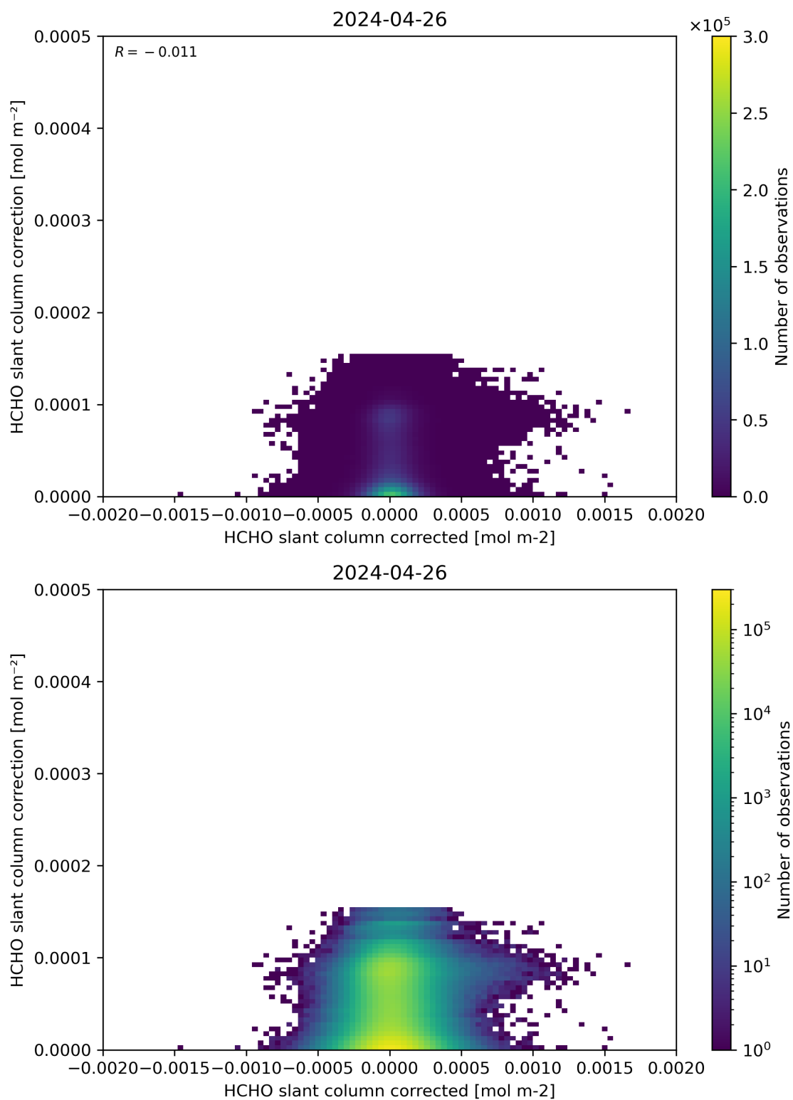
Figure 77: Scatter density plot of “HCHO slant column corrected” against “HCHO slant column correction” for 2024-04-26 to 2024-04-27.
