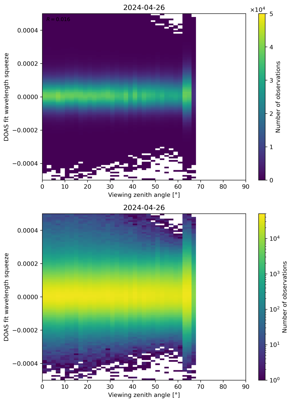
Figure 184: Scatter density plot of “Viewing zenith angle” against “DOAS fit wavelength squeeze” for 2024-04-26 to 2024-04-27.
