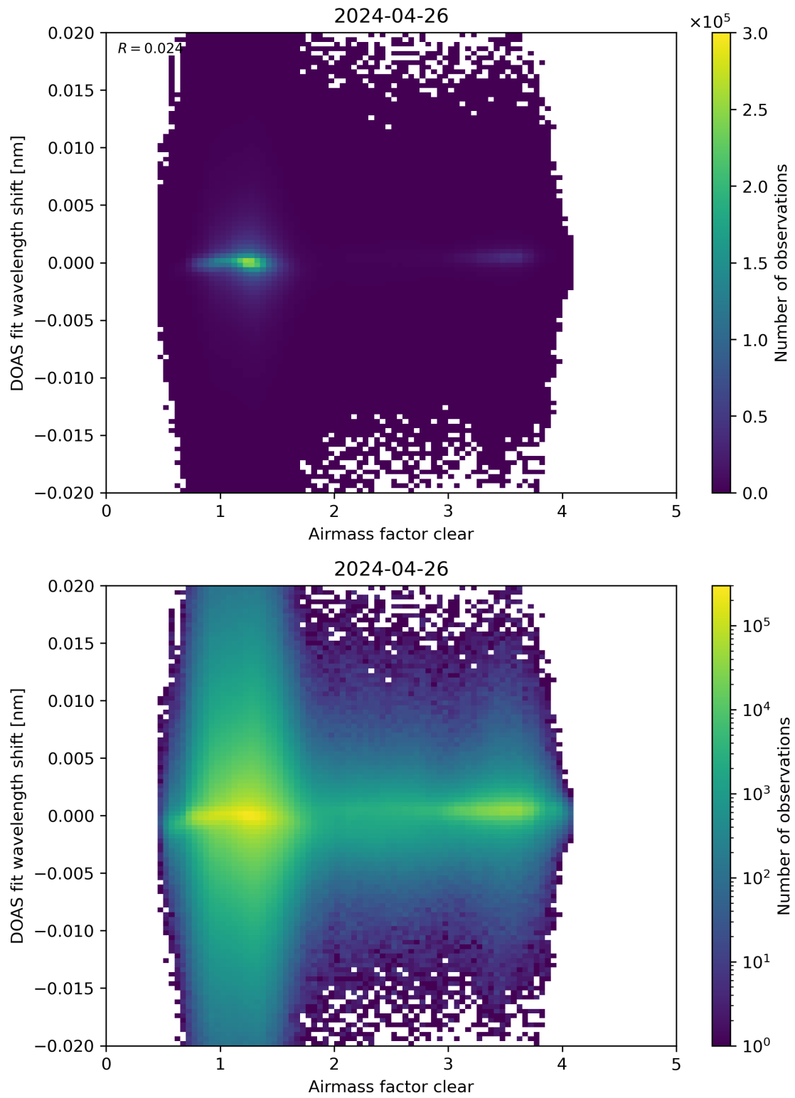
Figure 72: Scatter density plot of “Airmass factor clear” against “DOAS fit wavelength shift” for 2024-04-26 to 2024-04-27.
