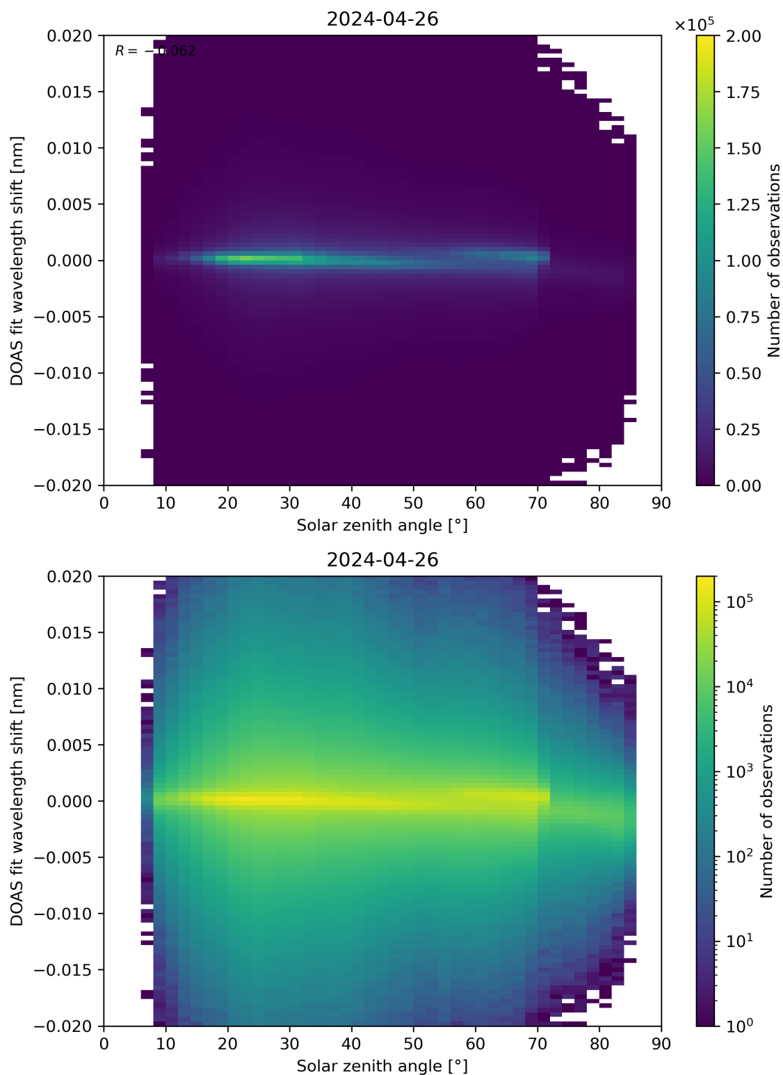
Figure 168: Scatter density plot of “Solar zenith angle” against “DOAS fit wavelength shift” for 2024-04-26 to 2024-04-27.
