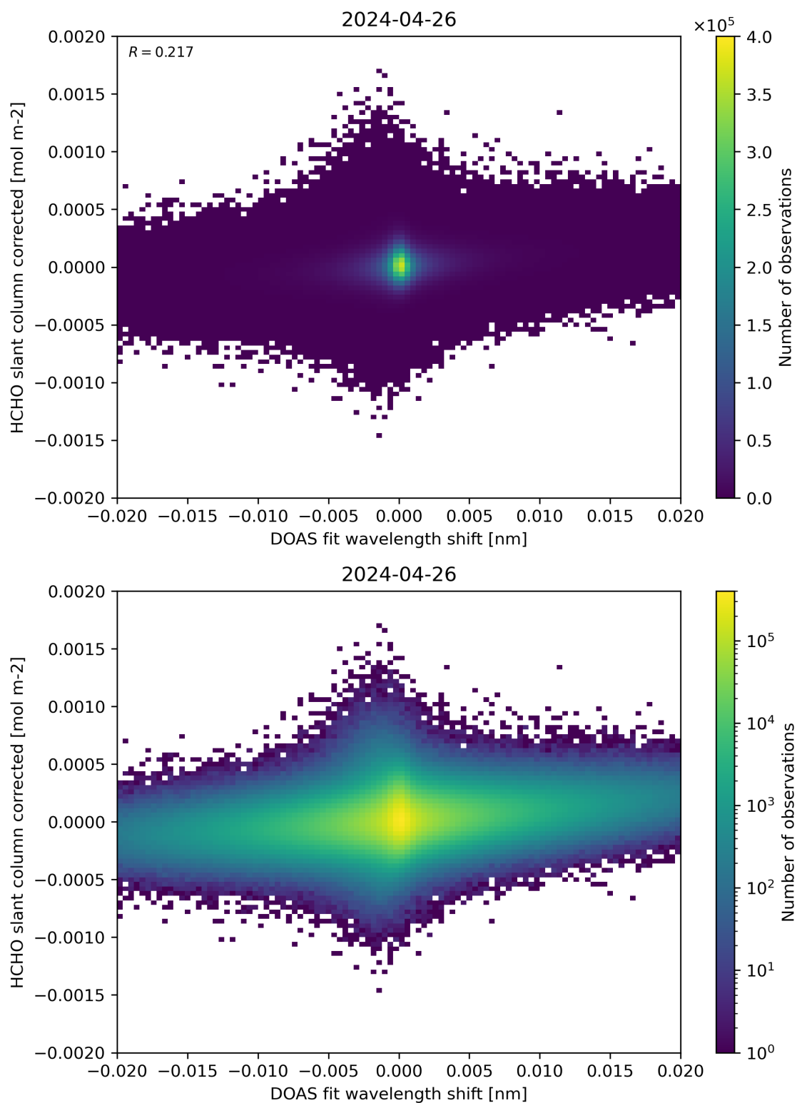
Figure 66: Scatter density plot of “DOAS fit wavelength shift” against “HCHO slant column corrected” for 2024-04-26 to 2024-04-27.
