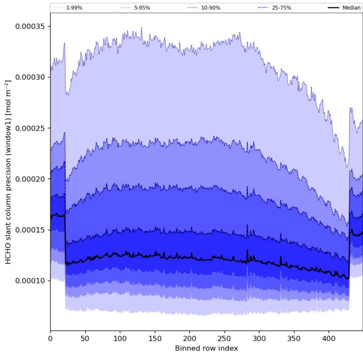
Figure 53: Along track statistics of “HCHO slant column precision (window1)” for 2024-04-26 to 2024-04-27
