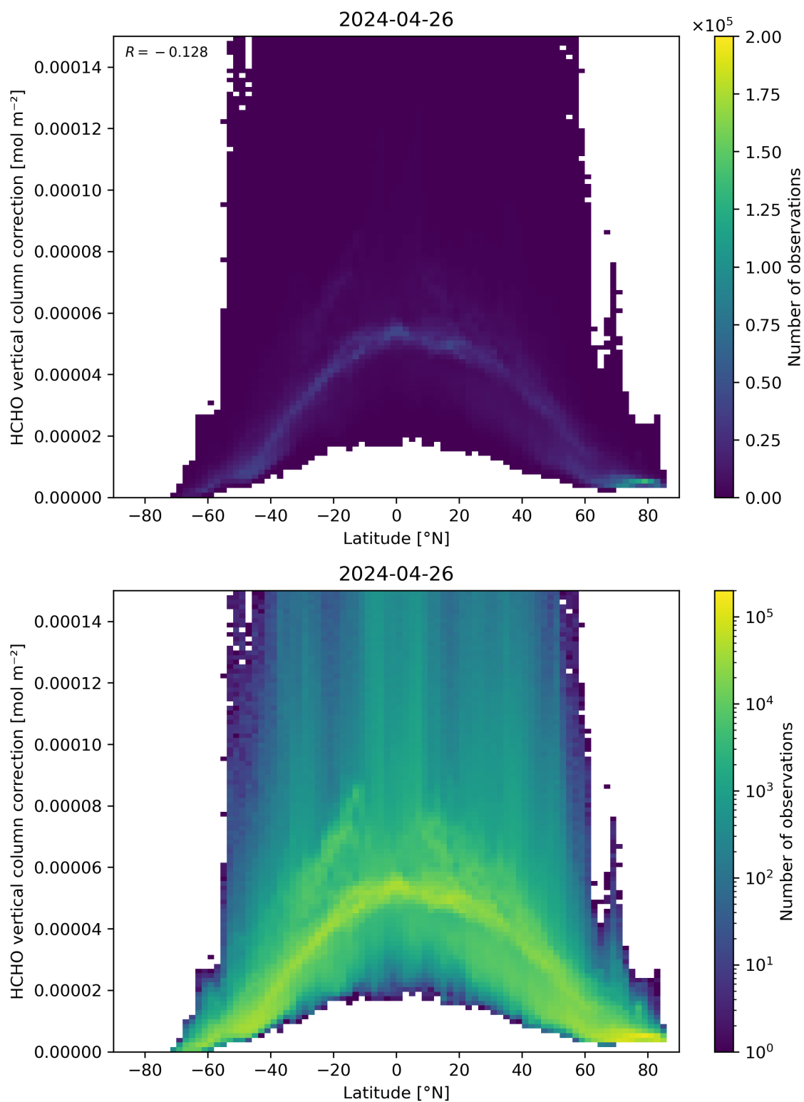
Figure 164: Scatter density plot of “Latitude” against “HCHO vertical column correction” for 2024-04-26 to 2024-04-27.
