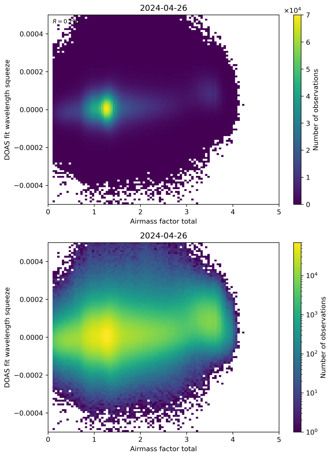
Figure 99: Scatter density plot of “Airmass factor total” against “DOAS fit wavelength squeeze” for 2024-04-26 to 2024-04-27.
