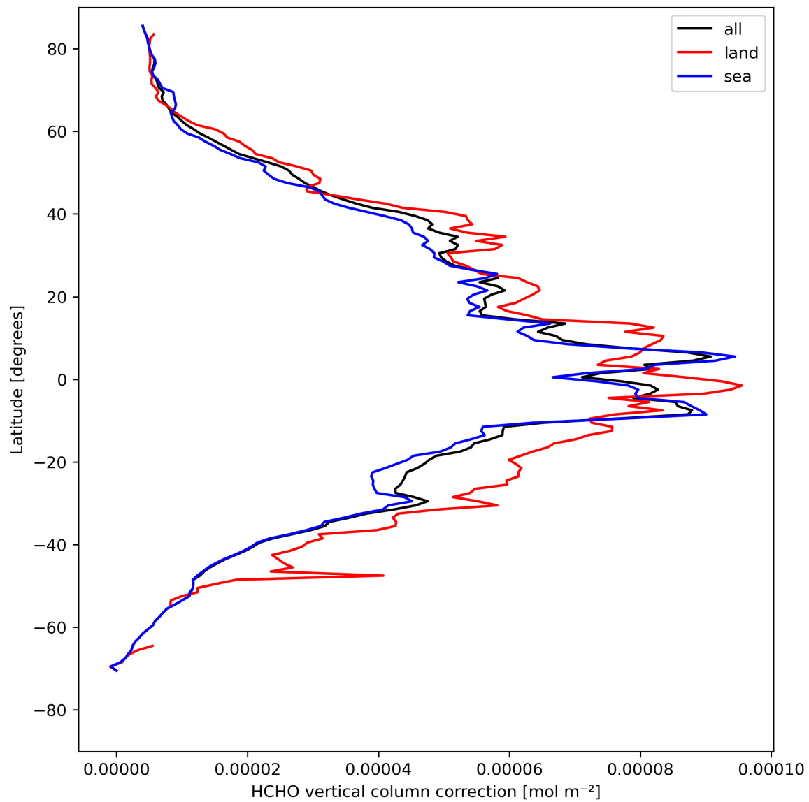
Figure 23: Zonal average of “HCHO vertical column correction” for 2024-04-26 to 2024-04-27.
