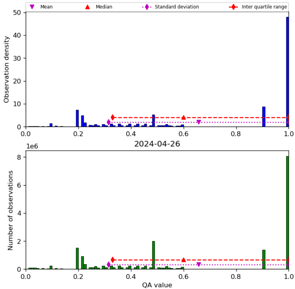
Figure 34: Histogram of “QA value” for 2024-04-26 to 2024-04-27
