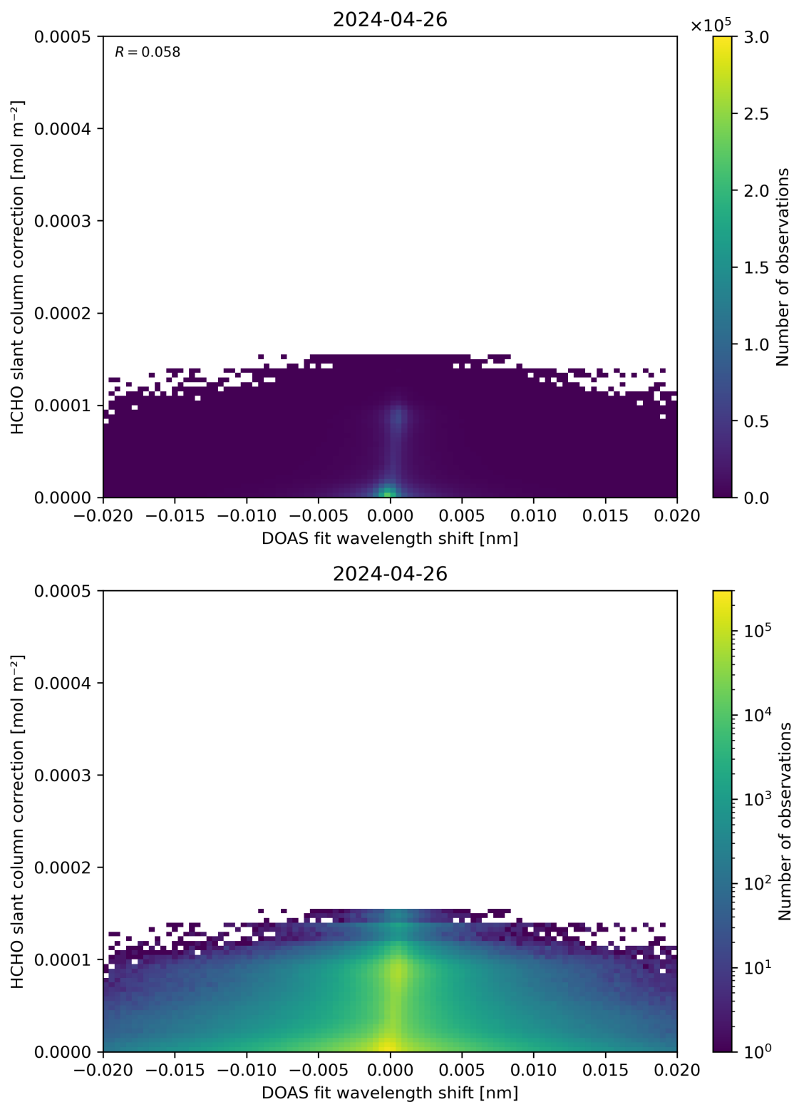
Figure 67: Scatter density plot of “DOAS fit wavelength shift” against “HCHO slant column correction” for 2024-04-26 to 2024-04-27.
