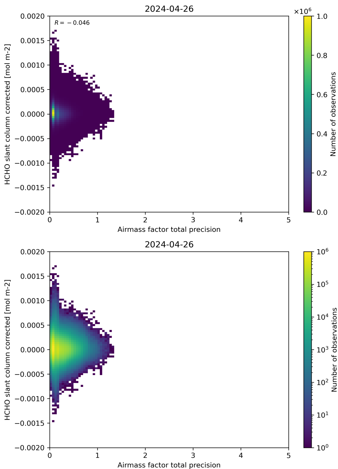
Figure 109: Scatter density plot of “Airmass factor total precision” against “HCHO slant column corrected” for 2024-04-26 to 2024-04-27.
