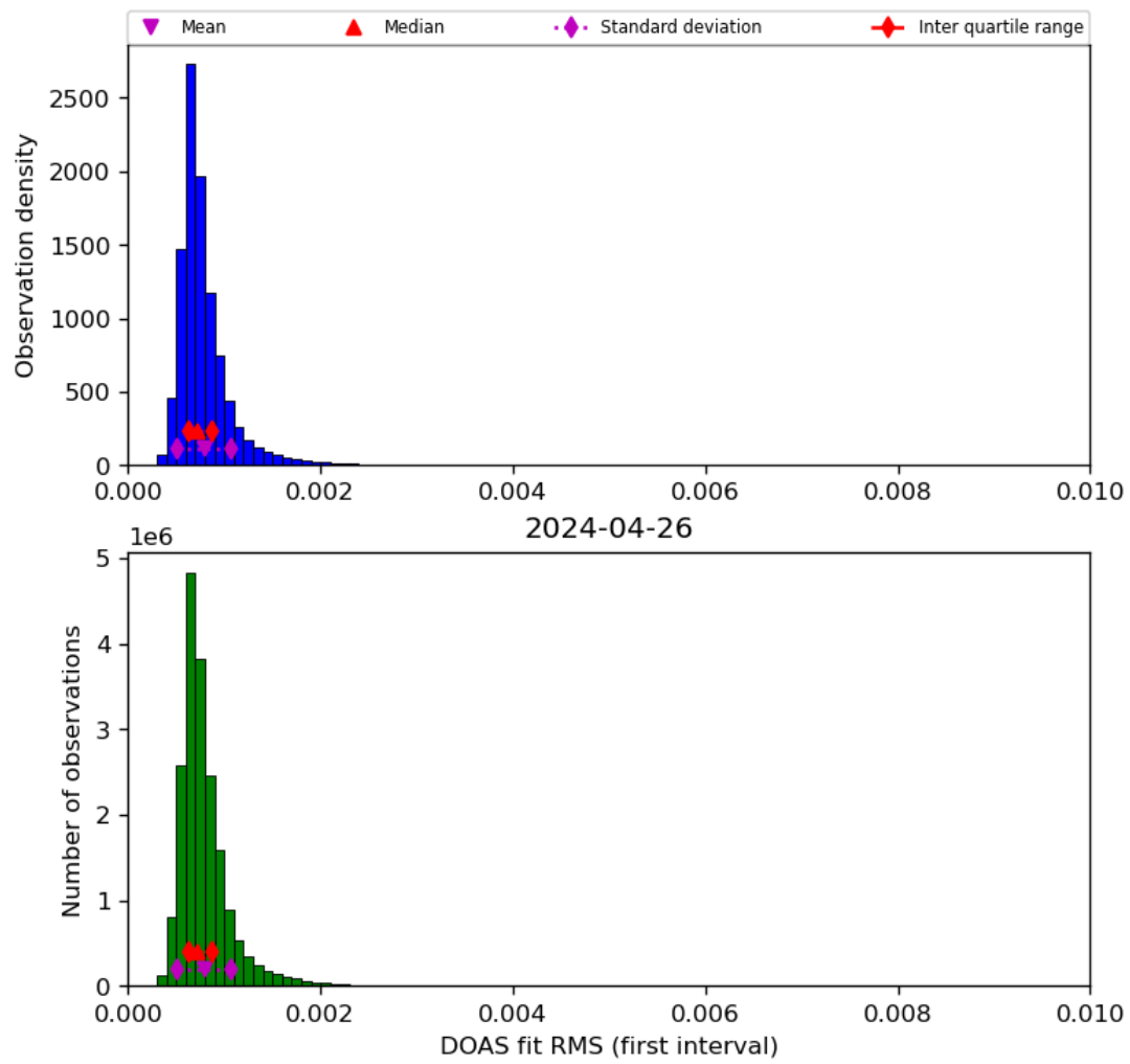
Figure 46: Histogram of “DOAS fit RMS (first interval)” for 2024-04-26 to 2024-04-27
