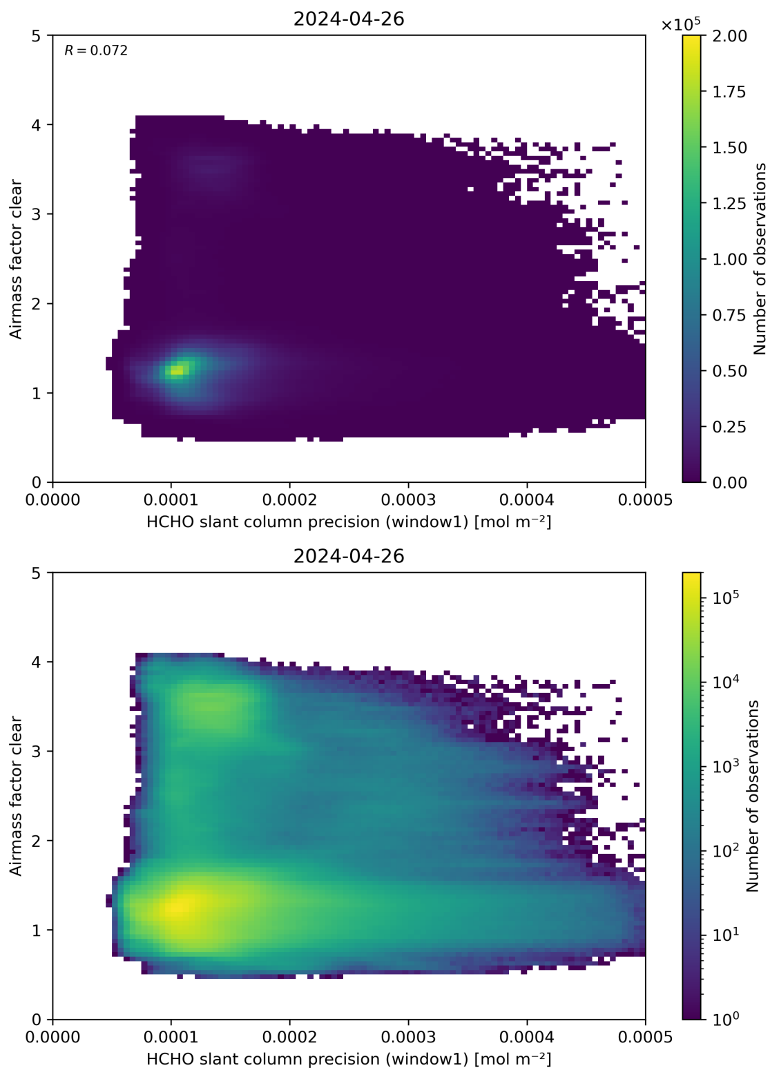
Figure 91: Scatter density plot of “HCHO slant column precision (window1)” against “Airmass factor clear” for 2024-04-26 to 2024-04-27.
