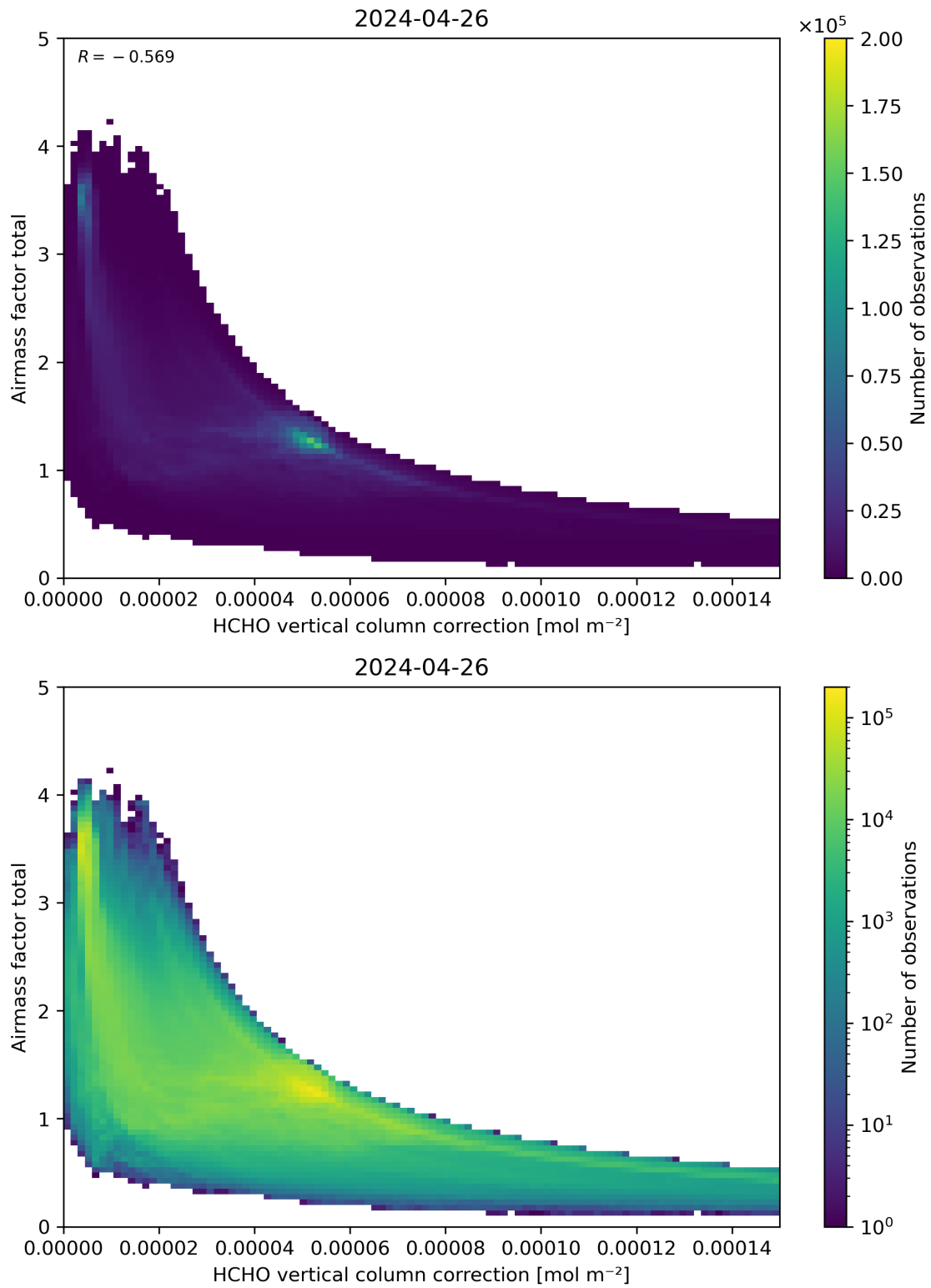
Figure 120: Scatter density plot of “HCHO vertical column correction” against “Airmass factor total” for 2024-04-26 to 2024-04-27.
