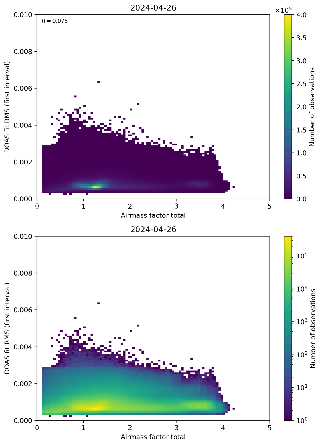
Figure 97: Scatter density plot of “Airmass factor total” against “DOAS fit RMS (first interval)” for 2024-04-26 to 2024-04-27.
