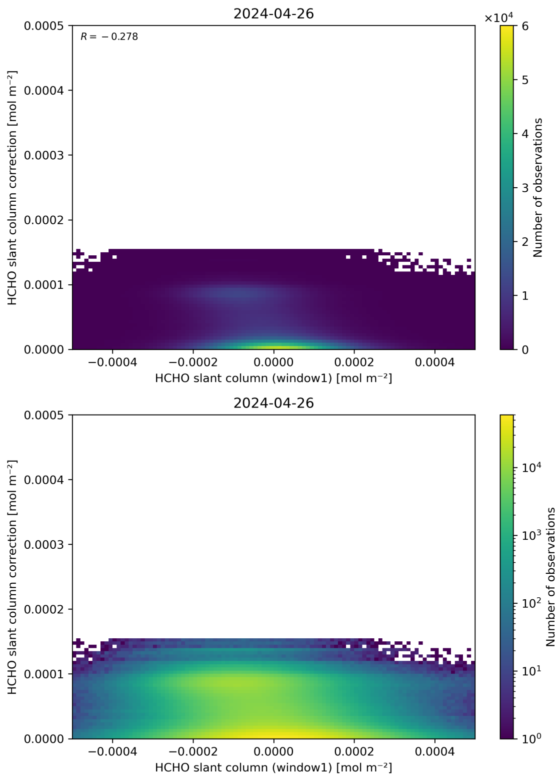
Figure 83: Scatter density plot of “HCHO slant column (window1)” against “HCHO slant column correction” for 2024-04-26 to 2024-04-27.
