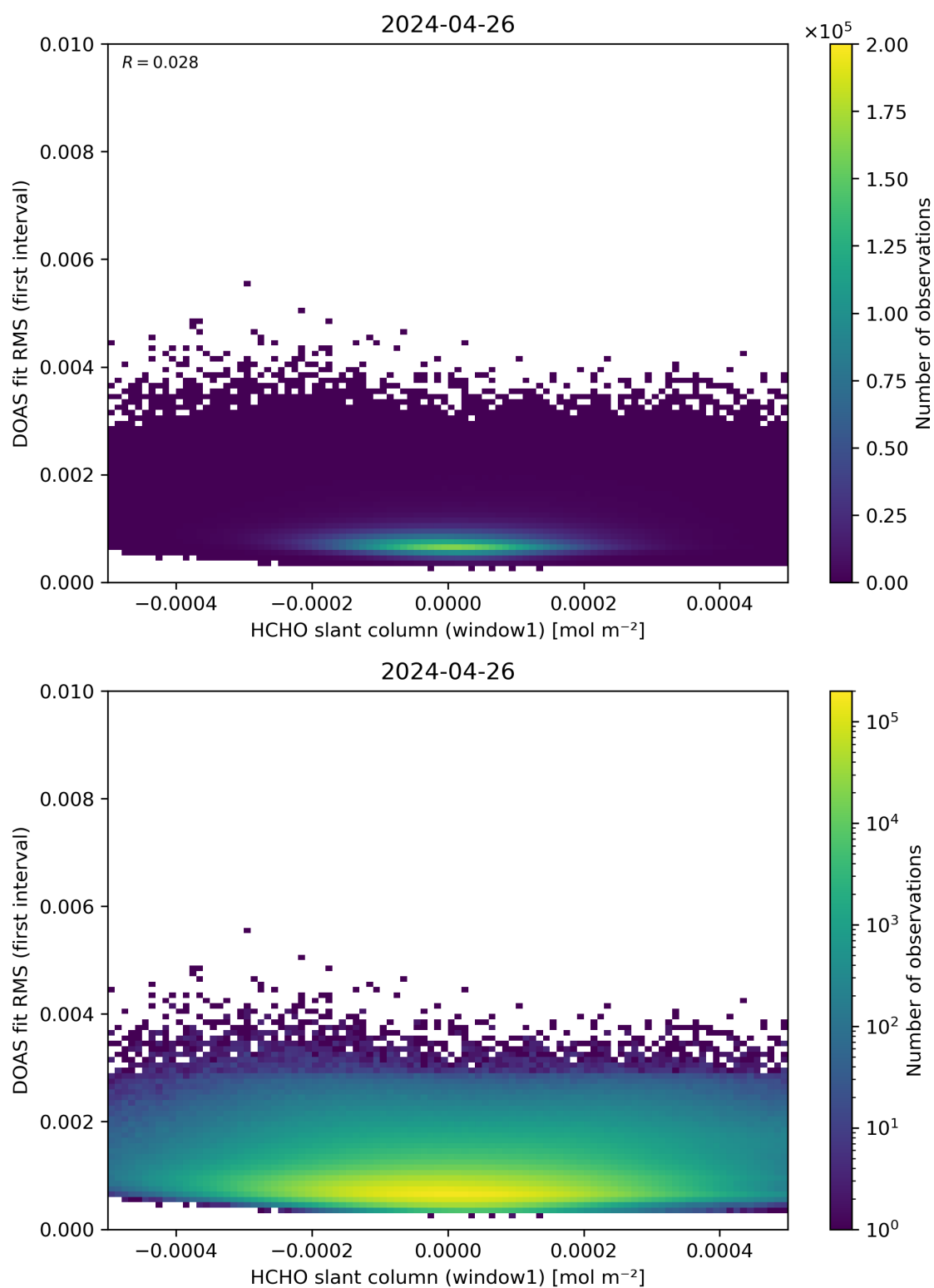
Figure 78: Scatter density plot of “HCHO slant column (window1)” against “DOAS fit RMS (first interval)” for 2024-04-26 to 2024-04-27.
