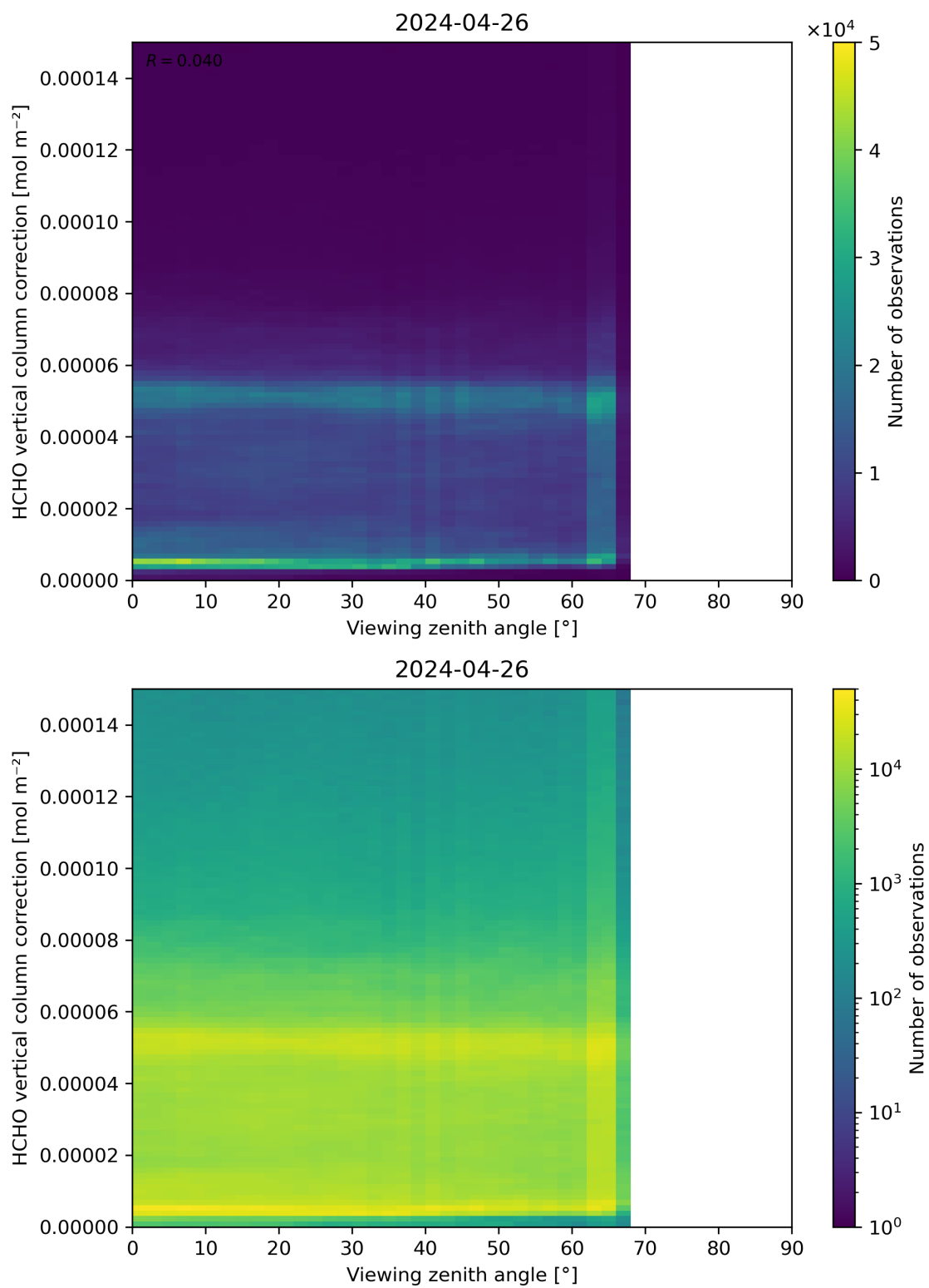
Figure 193: Scatter density plot of “Viewing zenith angle” against “HCHO vertical column correction” for 2024-04-26 to 2024-04-27.
