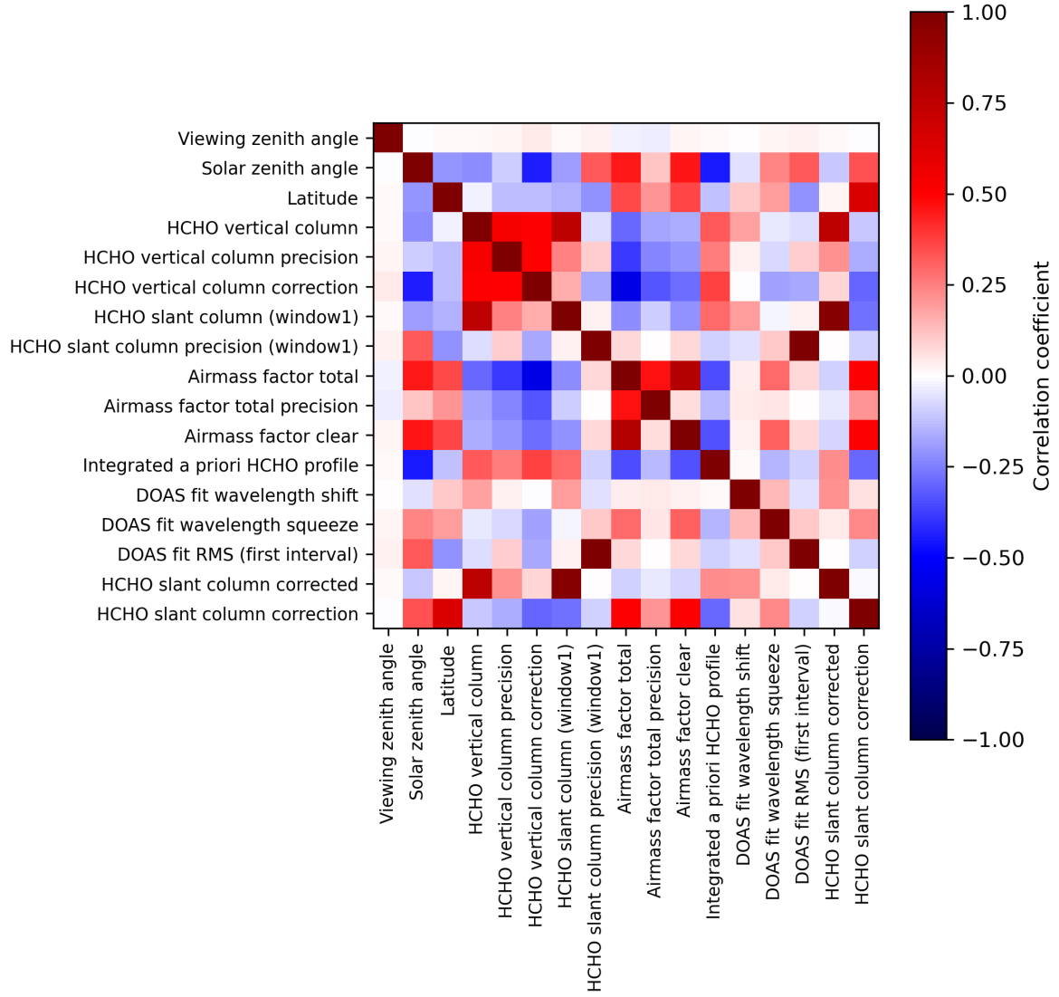
Figure 2: Map of correlation matrix for 2024-04-26 to 2024-04-27.
