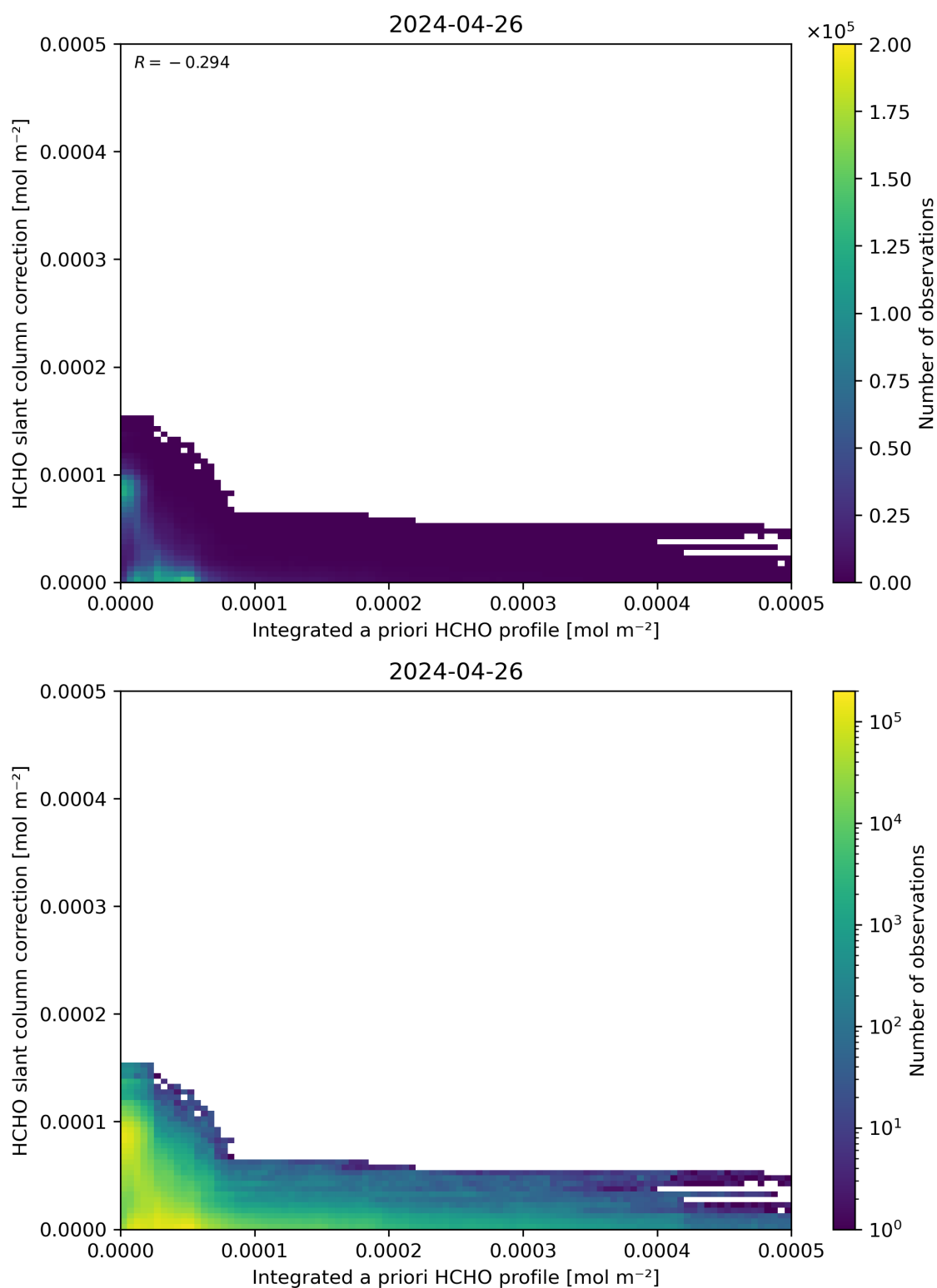
Figure 152: Scatter density plot of “Integrated a priori HCHO profile” against “HCHO slant column correction” for 2024-04-26 to 2024-04-27.
