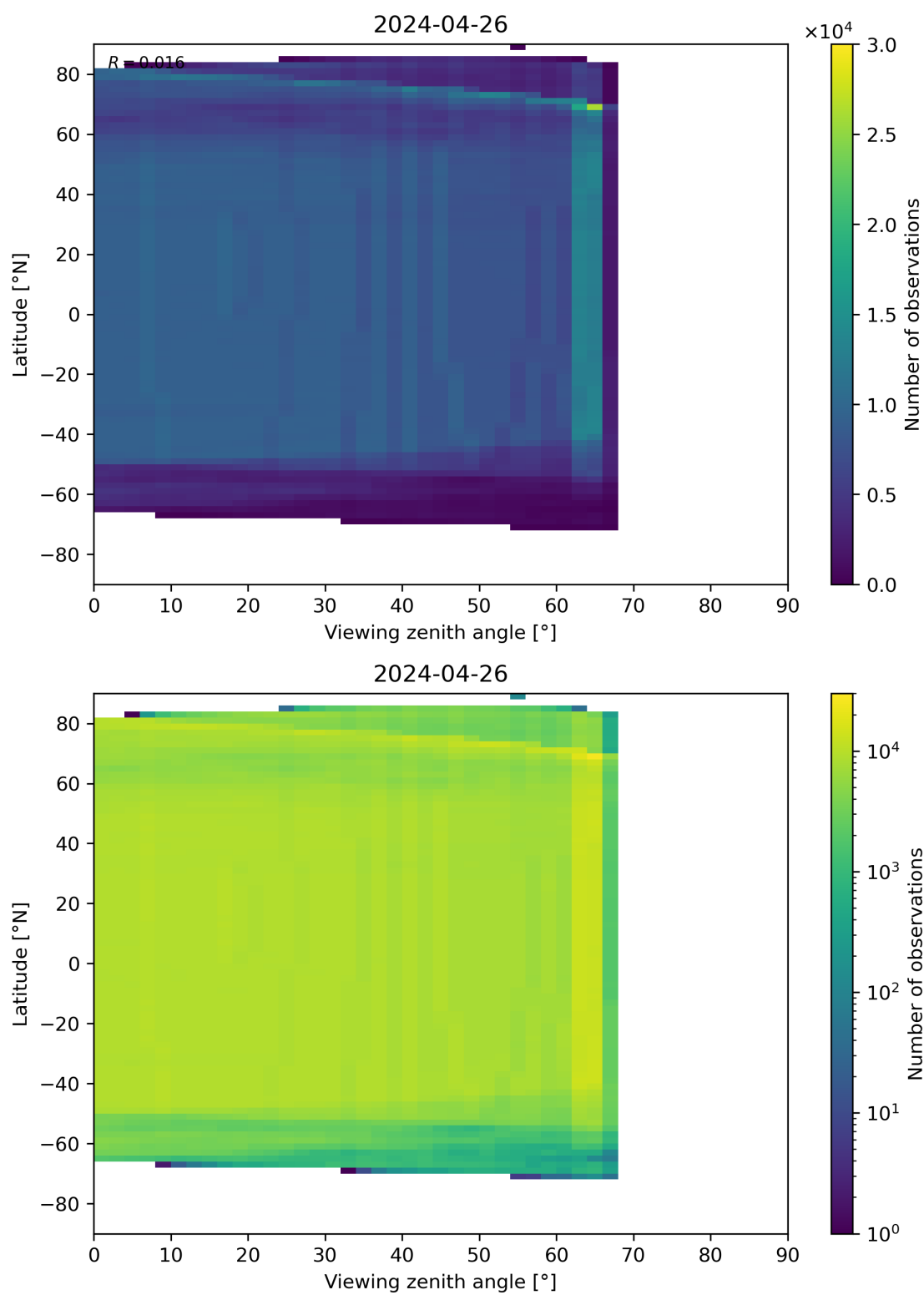
Figure 196: Scatter density plot of “Viewing zenith angle” against “Latitude” for 2024-04-26 to 2024-04-27.
