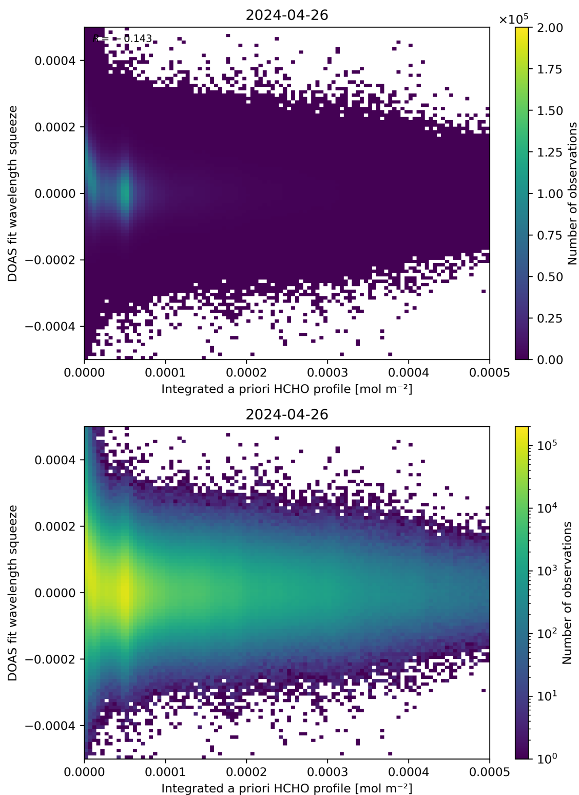
Figure 150: Scatter density plot of “Integrated a priori HCHO profile” against “DOAS fit wavelength squeeze” for 2024-04-26 to 2024-04-27.
