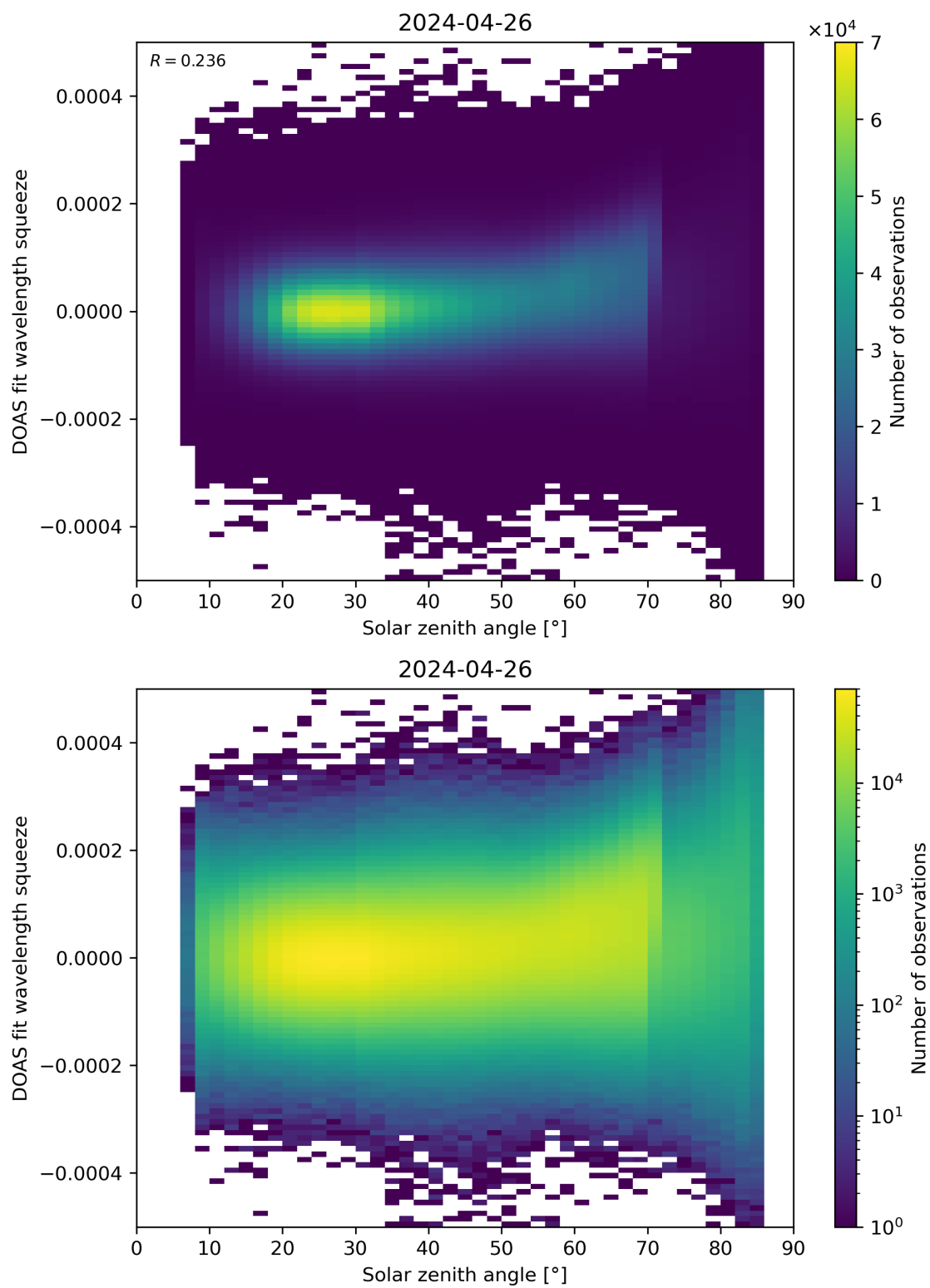
Figure 169: Scatter density plot of “Solar zenith angle” against “DOAS fit wavelength squeeze” for 2024-04-26 to 2024-04-27.
