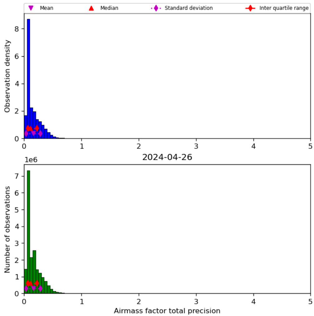
Figure 41: Histogram of “Airmass factor total precision” for 2024-04-26 to 2024-04-27
