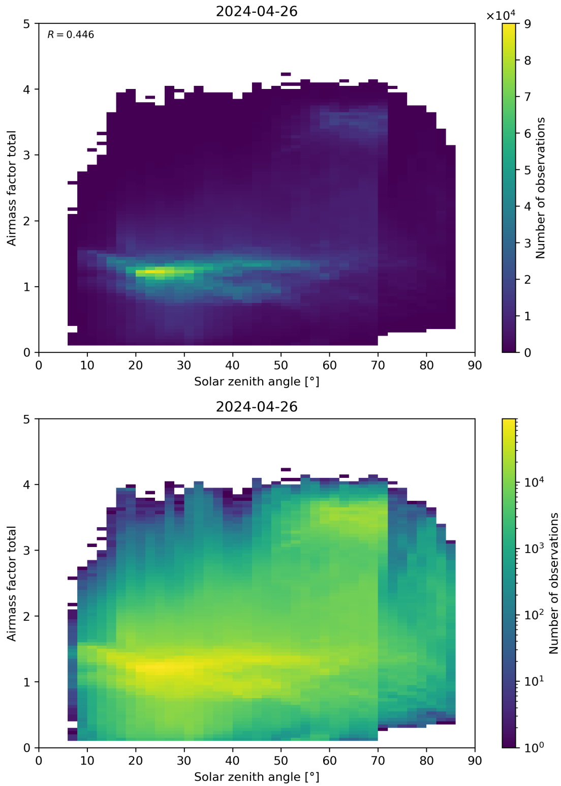
Figure 175: Scatter density plot of “Solar zenith angle” against “Airmass factor total” for 2024-04-26 to 2024-04-27.
