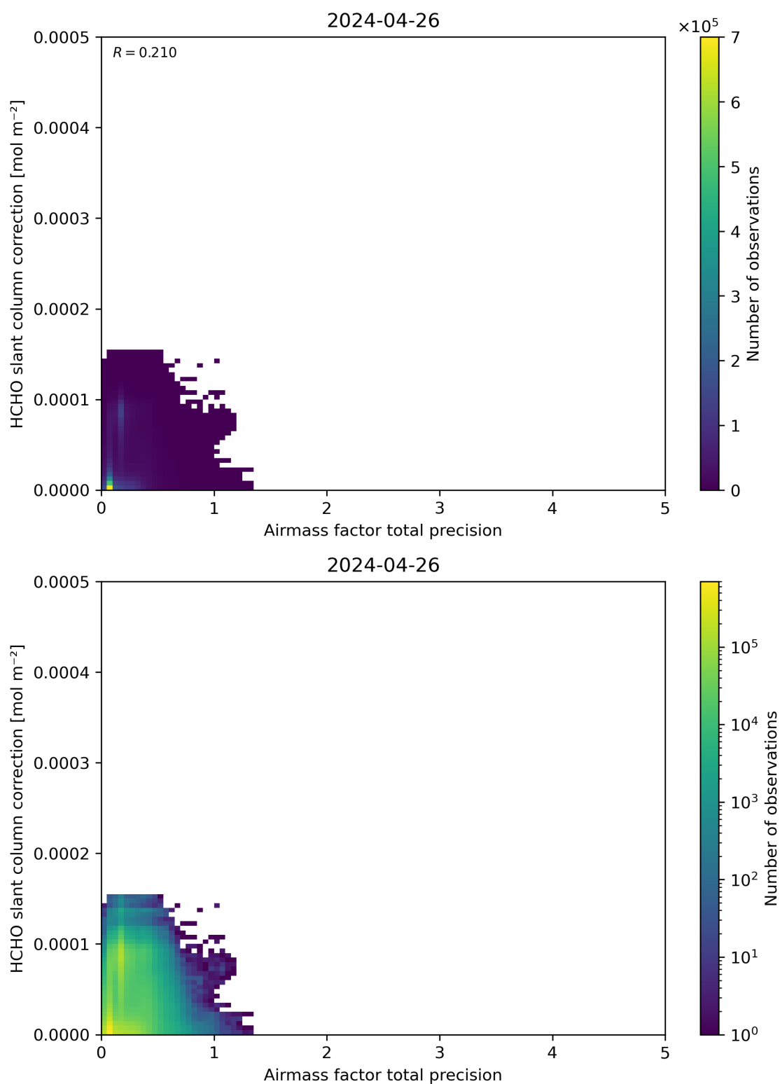
Figure 110: Scatter density plot of “Airmass factor total precision” against “HCHO slant column correction” for 2024-04-26 to 2024-04-27.
