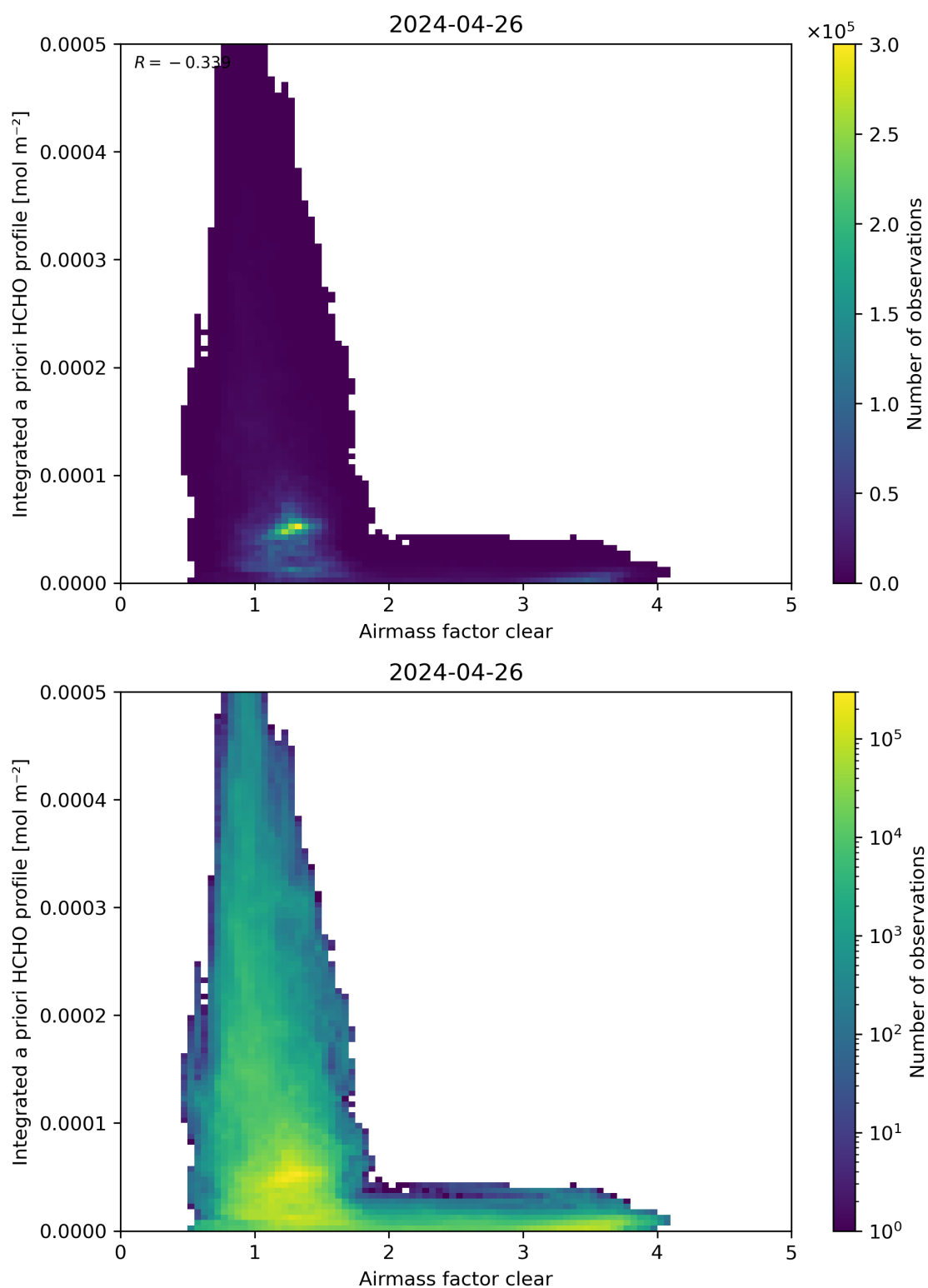
Figure 76: Scatter density plot of “Airmass factor clear” against “Integrated a priori HCHO profile” for 2024-04-26 to 2024-04-27.
