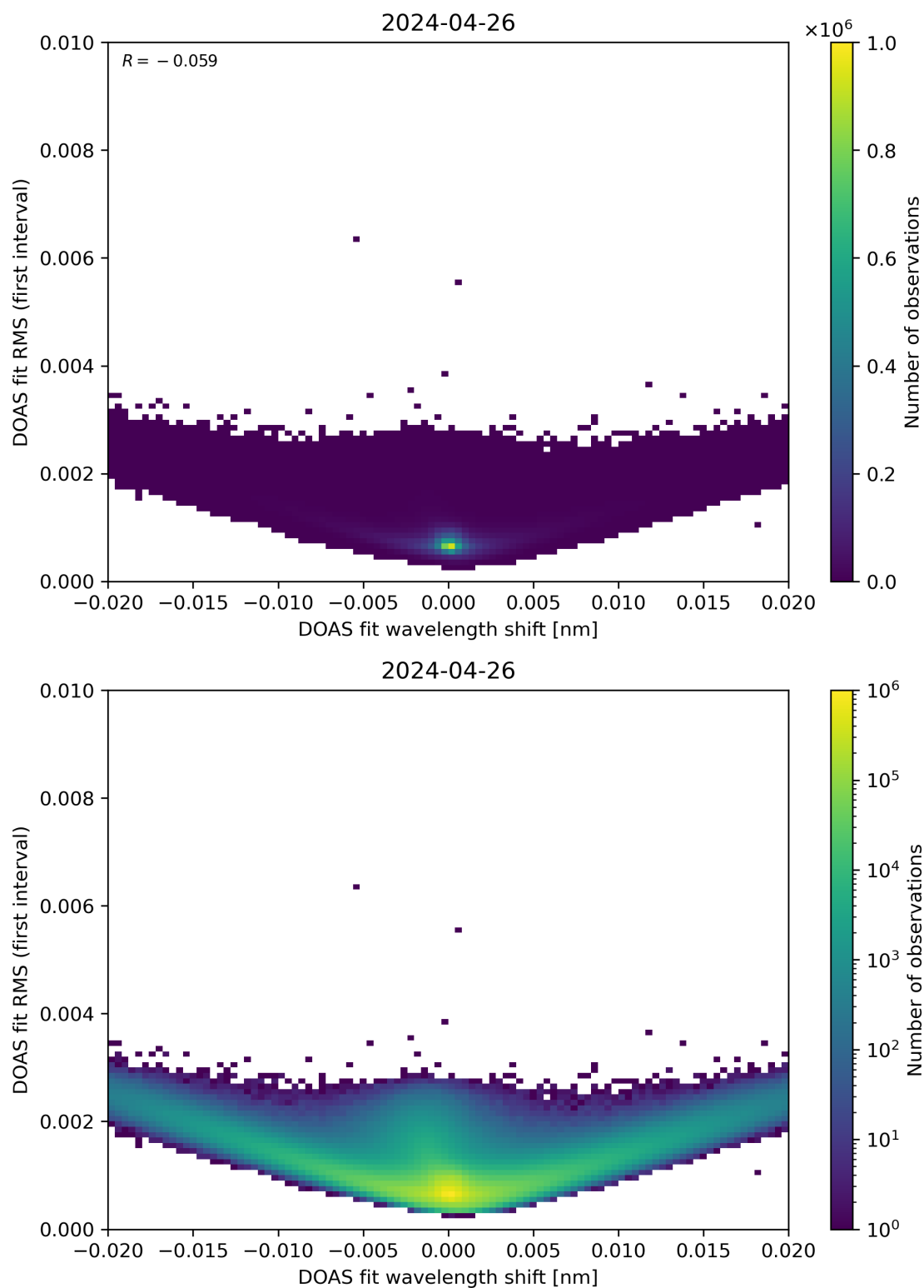
Figure 64: Scatter density plot of “DOAS fit wavelength shift” against “DOAS fit RMS (first interval)” for 2024-04-26 to 2024-04-27.
