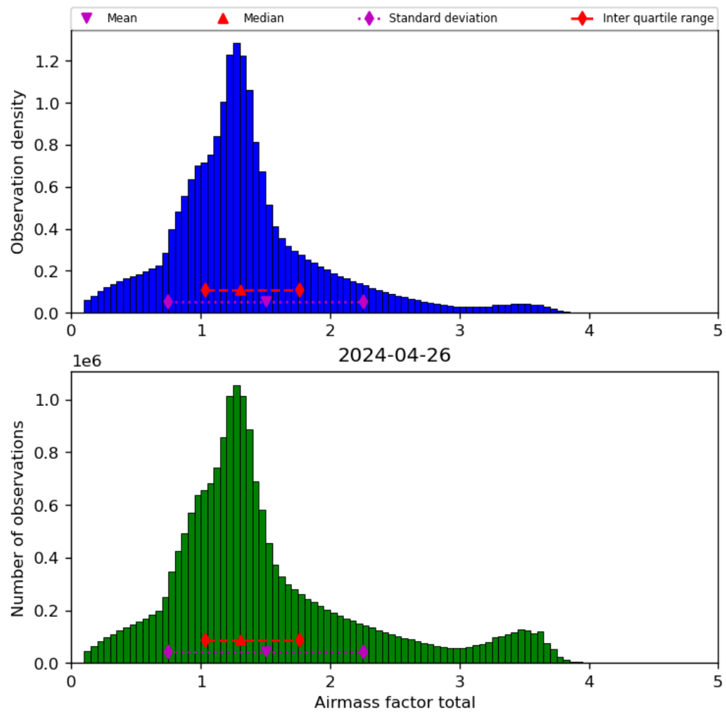
Figure 40: Histogram of “Airmass factor total” for 2024-04-26 to 2024-04-27
