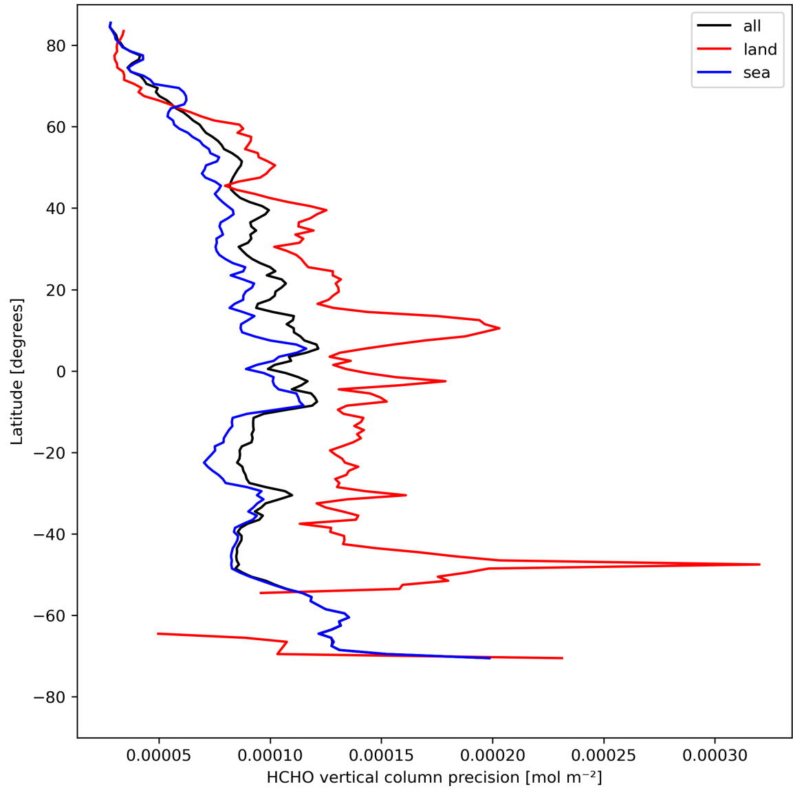
Figure 22: Zonal average of “HCHO vertical column precision” for 2024-04-26 to 2024-04-27.
