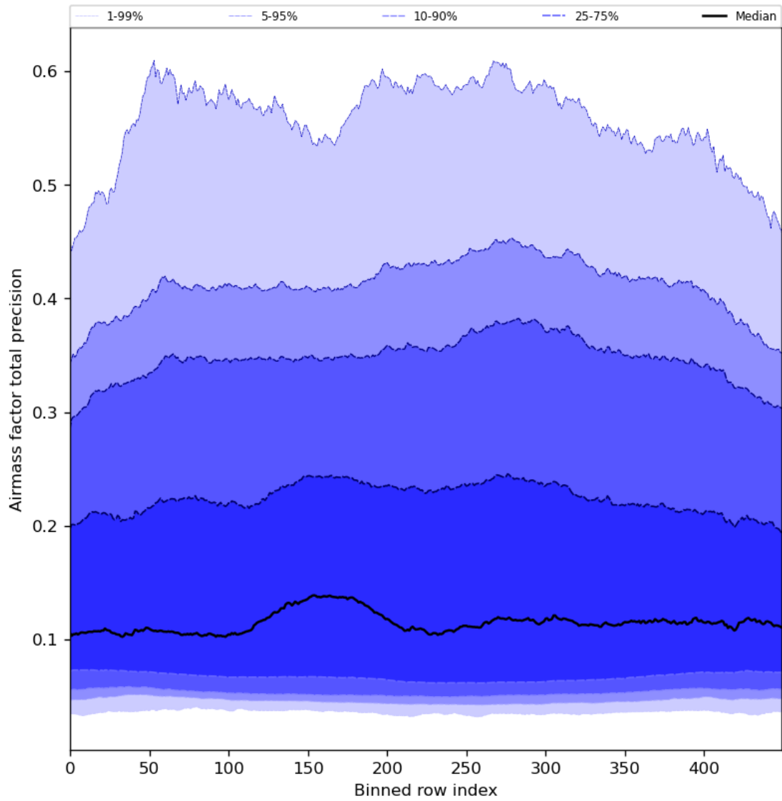
Figure 55: Along track statistics of “Airmass factor total precision” for 2024-04-26 to 2024-04-27
