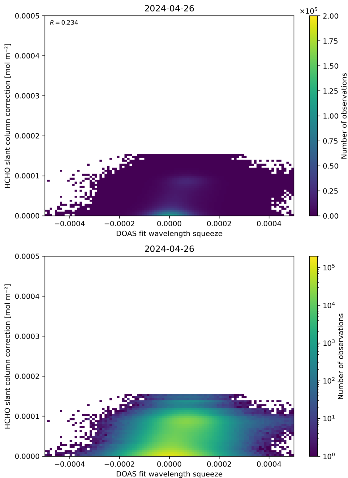
Figure 70: Scatter density plot of “DOAS fit wavelength squeeze” against “HCHO slant column correction” for 2024-04-26 to 2024-04-27.
