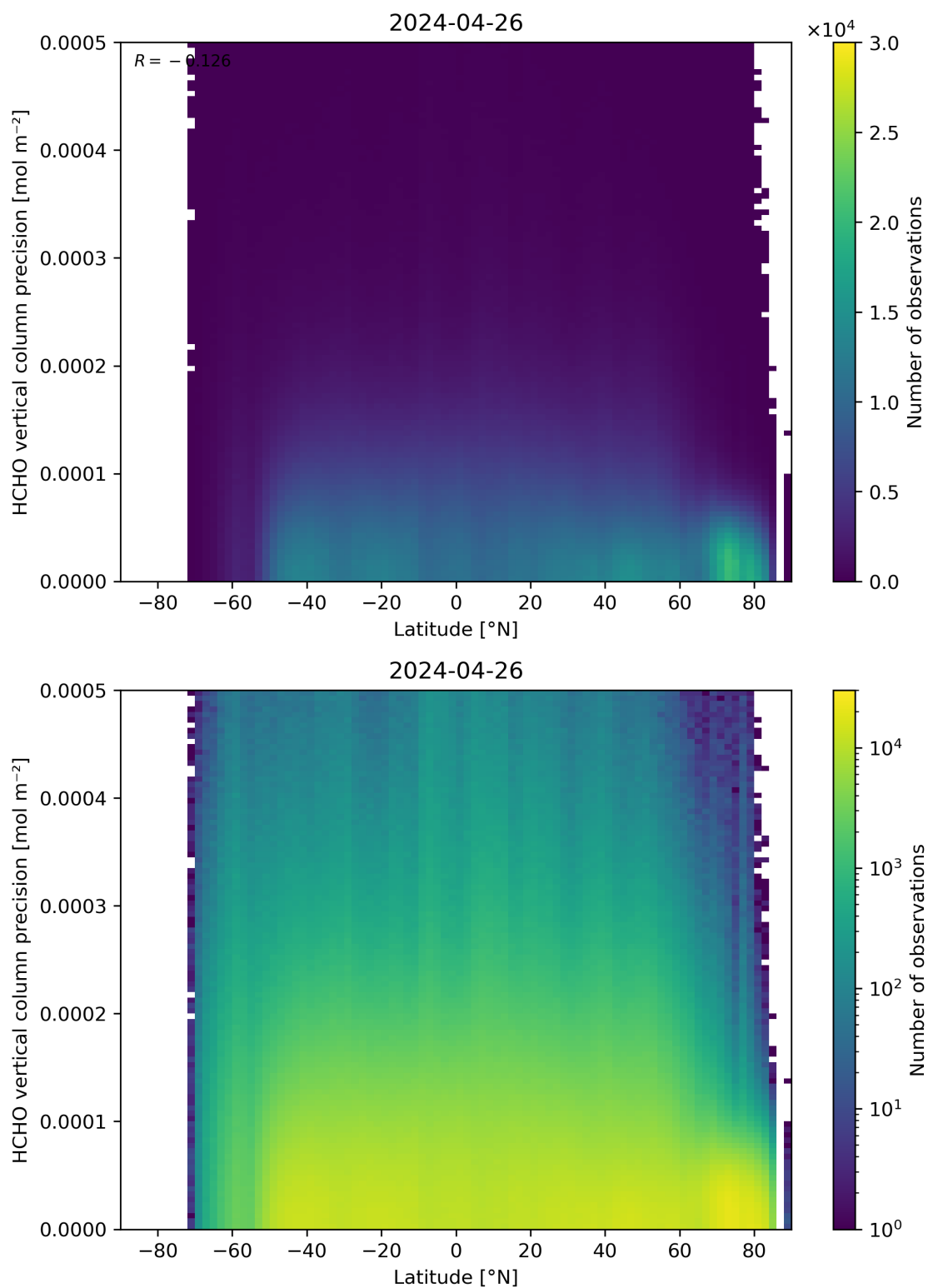
Figure 165: Scatter density plot of “Latitude” against “HCHO vertical column precision” for 2024-04-26 to 2024-04-27.
