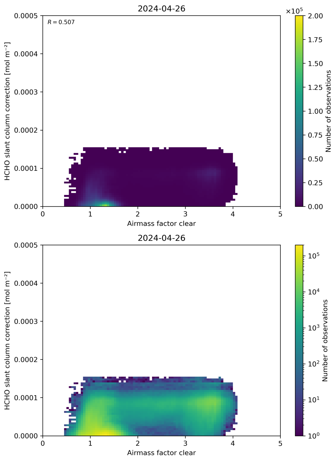
Figure 75: Scatter density plot of “Airmass factor clear” against “HCHO slant column correction” for 2024-04-26 to 2024-04-27.
