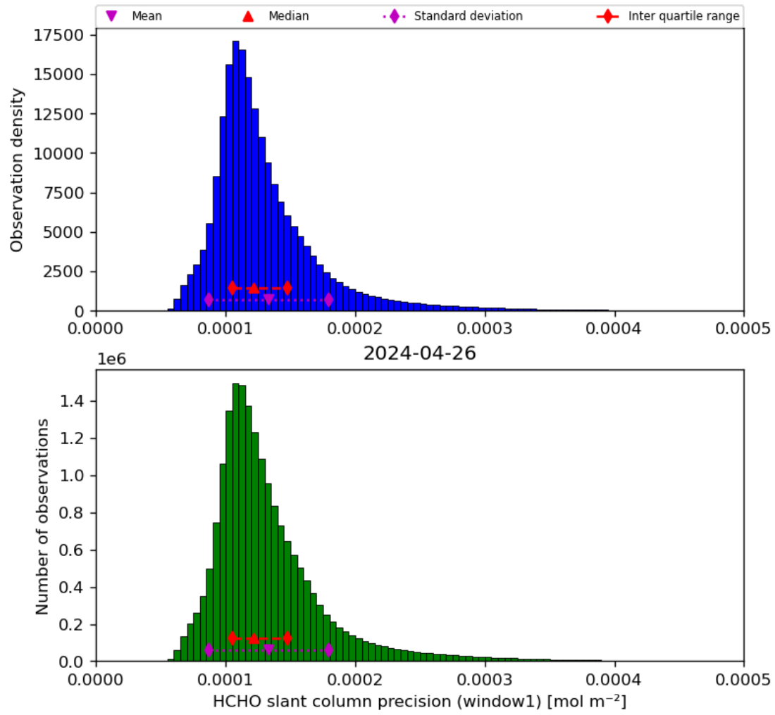
Figure 39: Histogram of “HCHO slant column precision (window1)” for 2024-04-26 to 2024-04-27
