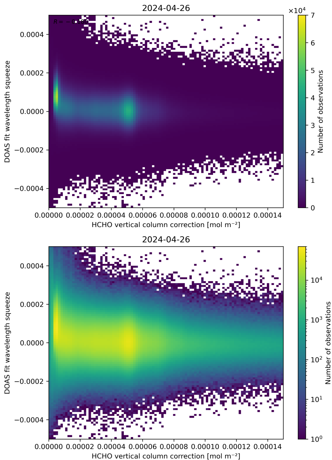
Figure 114: Scatter density plot of “HCHO vertical column correction” against “DOAS fit wavelength squeeze” for 2024-04-26 to 2024-04-27.
