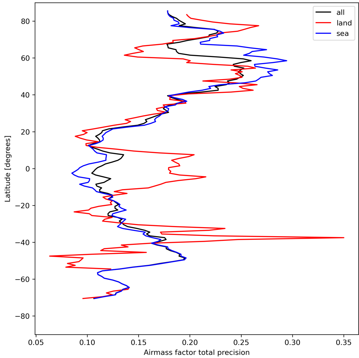
Figure 27: Zonal average of “Airmass factor total precision” for 2024-04-26 to 2024-04-27.
