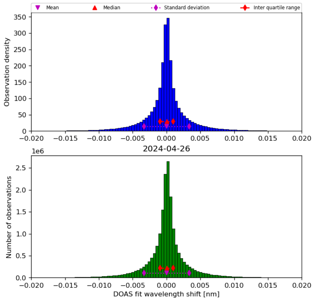
Figure 44: Histogram of “DOAS fit wavelength shift” for 2024-04-26 to 2024-04-27
