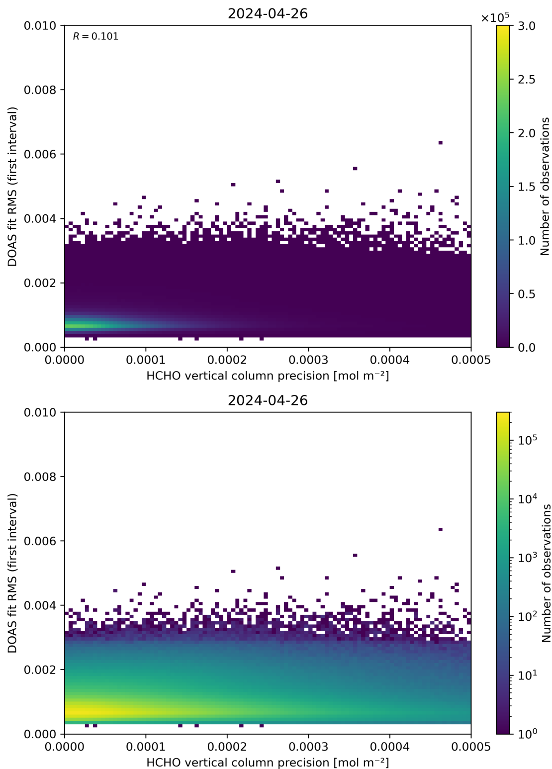
Figure 136: Scatter density plot of “HCHO vertical column precision” against “DOAS fit RMS (first interval)” for 2024-04-26 to 2024-04-27.
