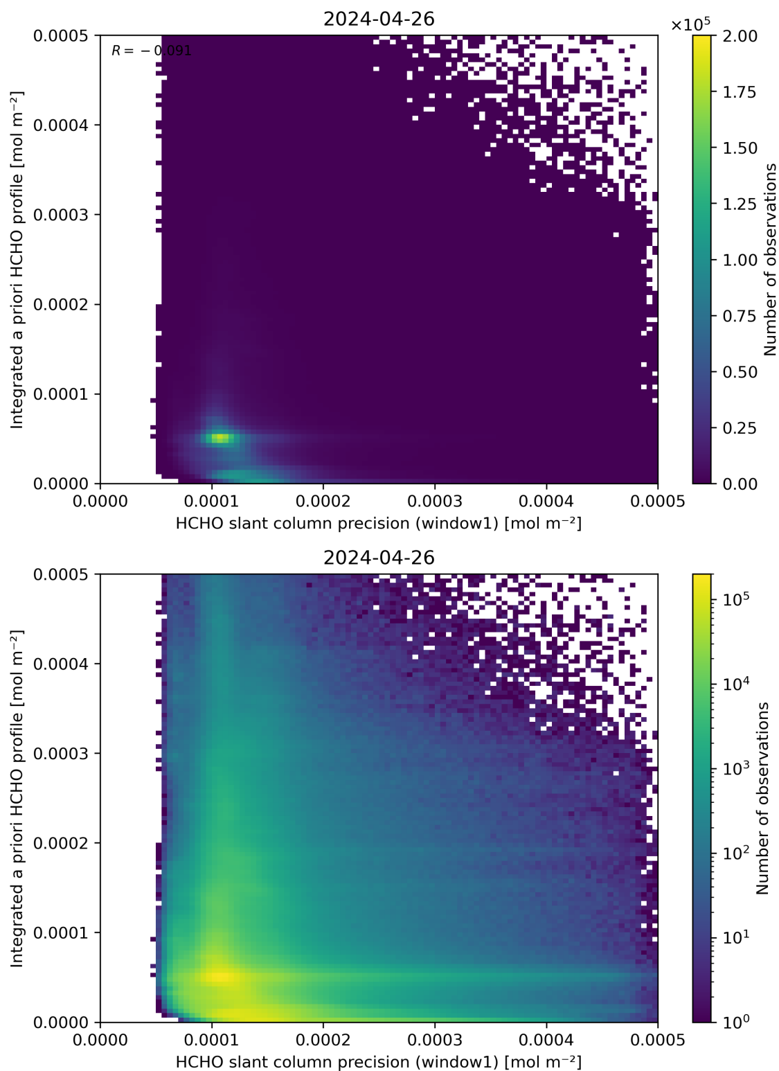
Figure 96: Scatter density plot of “HCHO slant column precision (window1)” against “Integrated a priori HCHO profile” for 2024-04-26 to 2024-04-27.
