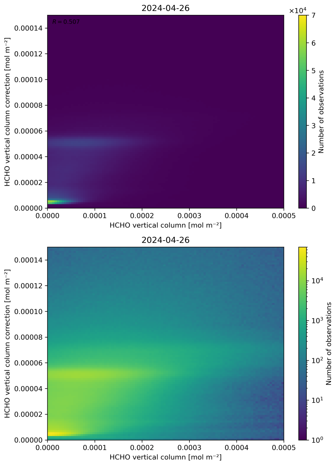
Figure 133: Scatter density plot of “HCHO vertical column” against “HCHO vertical column correction” for 2024-04-26 to 2024-04-27.
