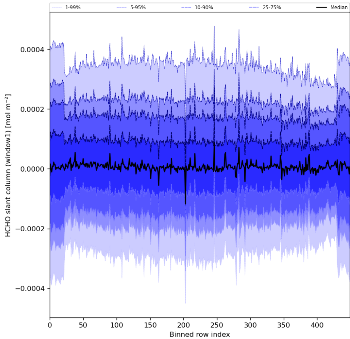
Figure 52: Along track statistics of “HCHO slant column (window1)” for 2024-04-26 to 2024-04-27
