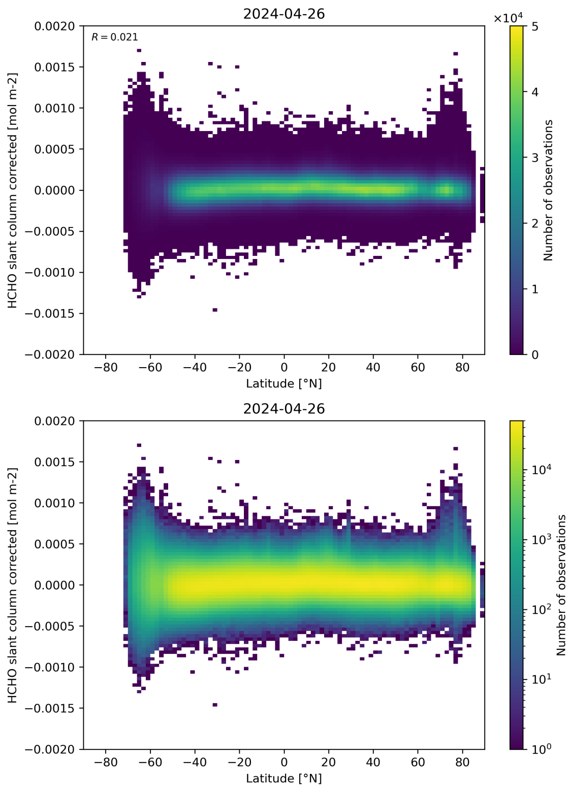
Figure 157: Scatter density plot of “Latitude” against “HCHO slant column corrected” for 2024-04-26 to 2024-04-27.
