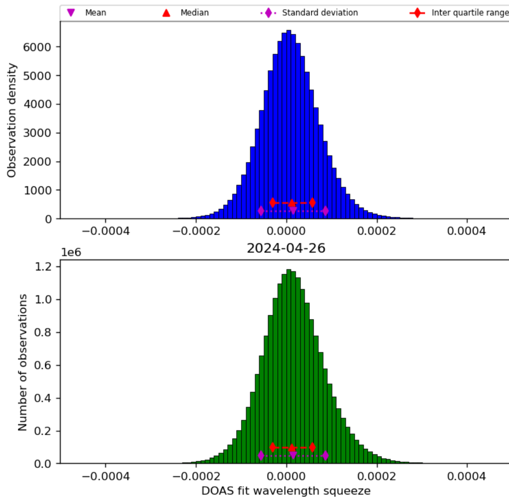
Figure 45: Histogram of “DOAS fit wavelength squeeze” for 2024-04-26 to 2024-04-27
