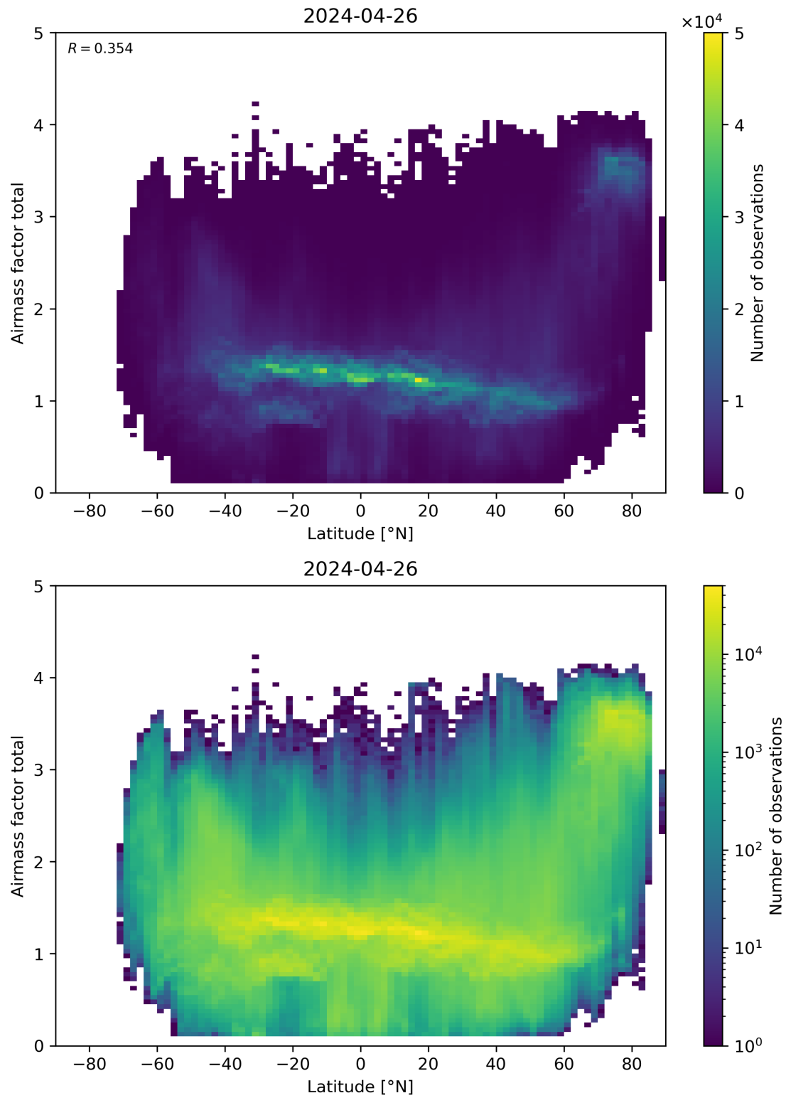
Figure 161: Scatter density plot of “Latitude” against “Airmass factor total” for 2024-04-26 to 2024-04-27.
