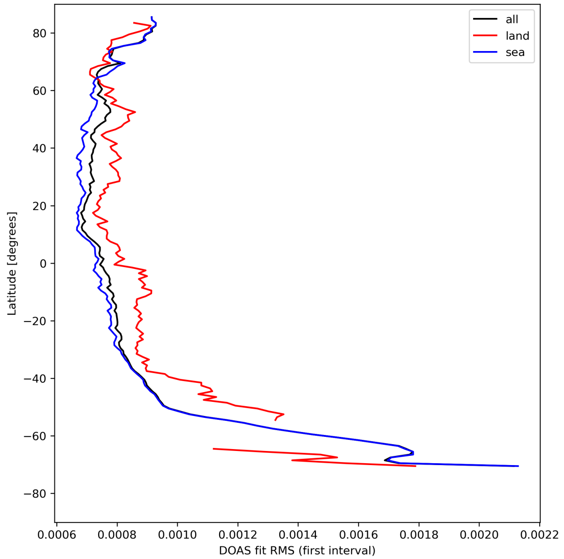
Figure 32: Zonal average of “DOAS fit RMS (first interval)” for 2024-04-26 to 2024-04-27.
