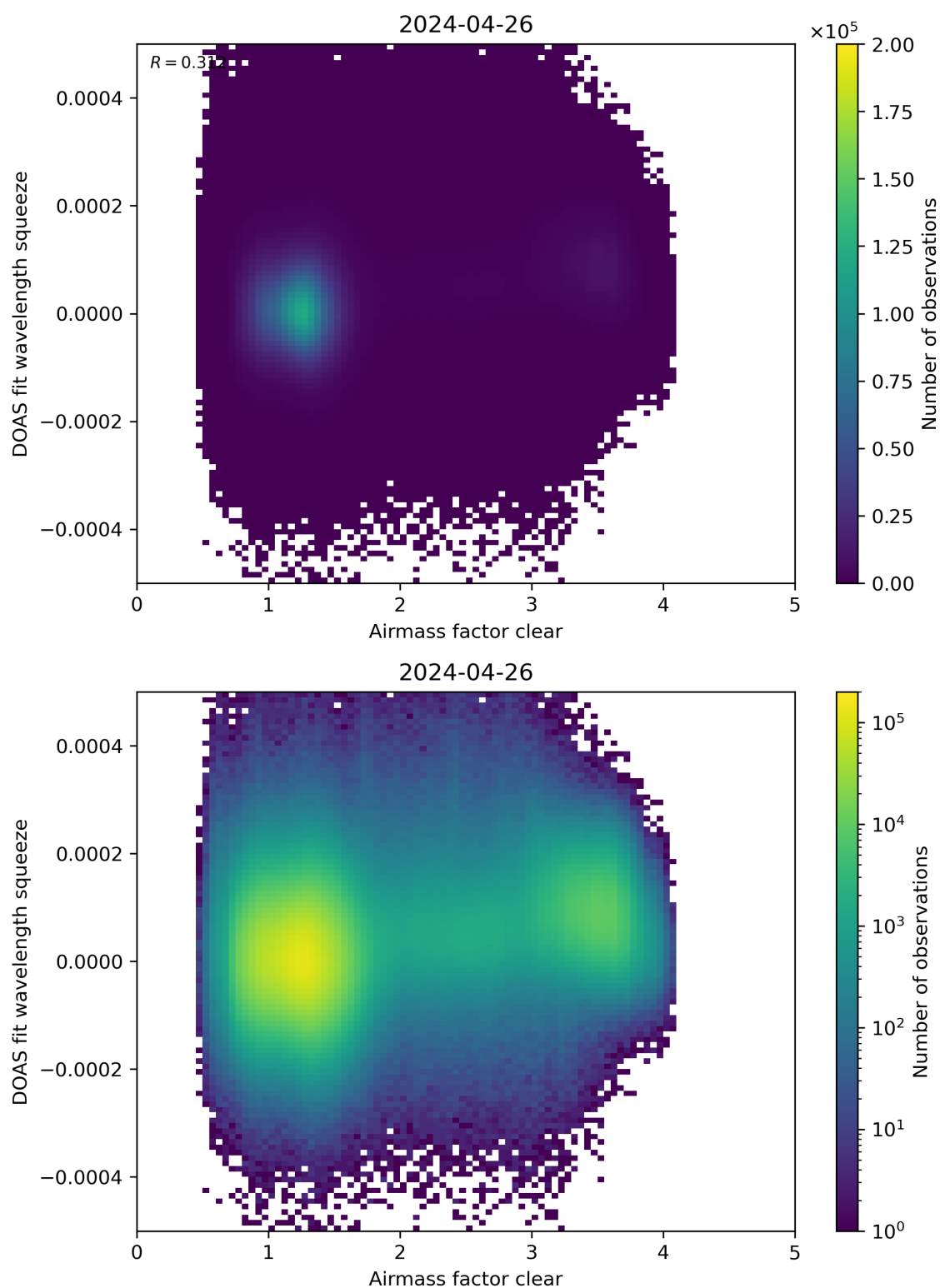
Figure 73: Scatter density plot of “Airmass factor clear” against “DOAS fit wavelength squeeze” for 2024-04-26 to 2024-04-27.
