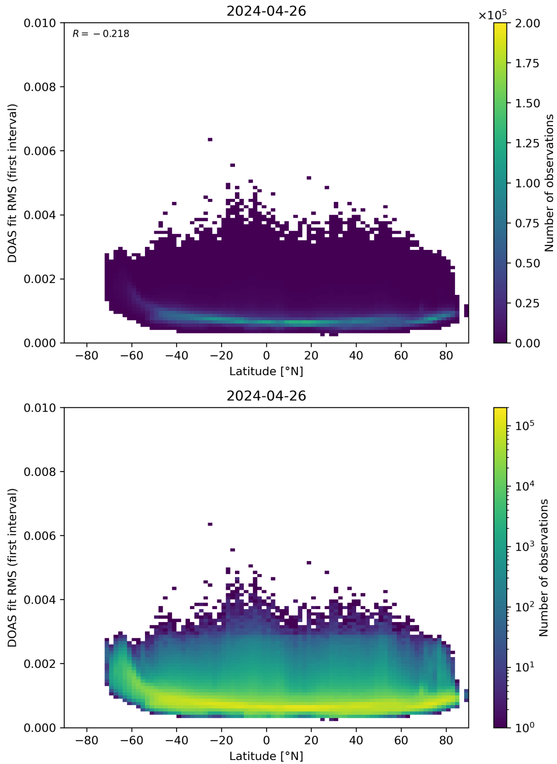
Figure 153: Scatter density plot of “Latitude” against “DOAS fit RMS (first interval)” for 2024-04-26 to 2024-04-27.
