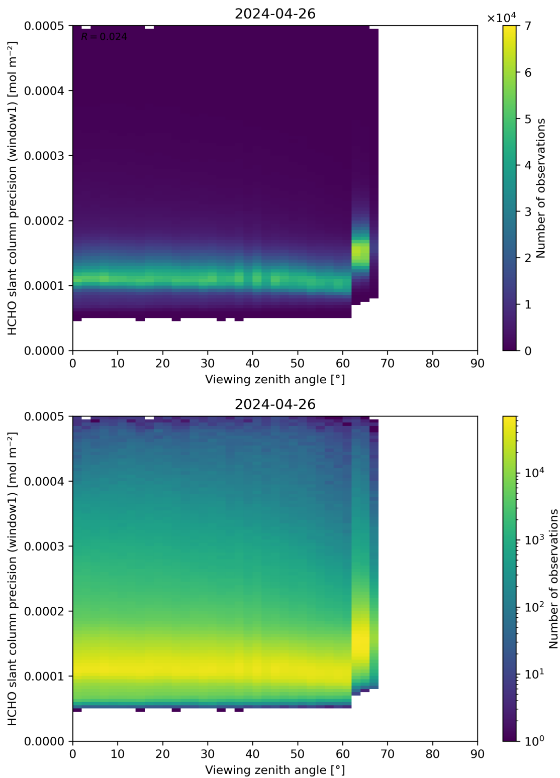
Figure 189: Scatter density plot of “Viewing zenith angle” against “HCHO slant column precision (window1)” for 2024-04-26 to 2024-04-27.
