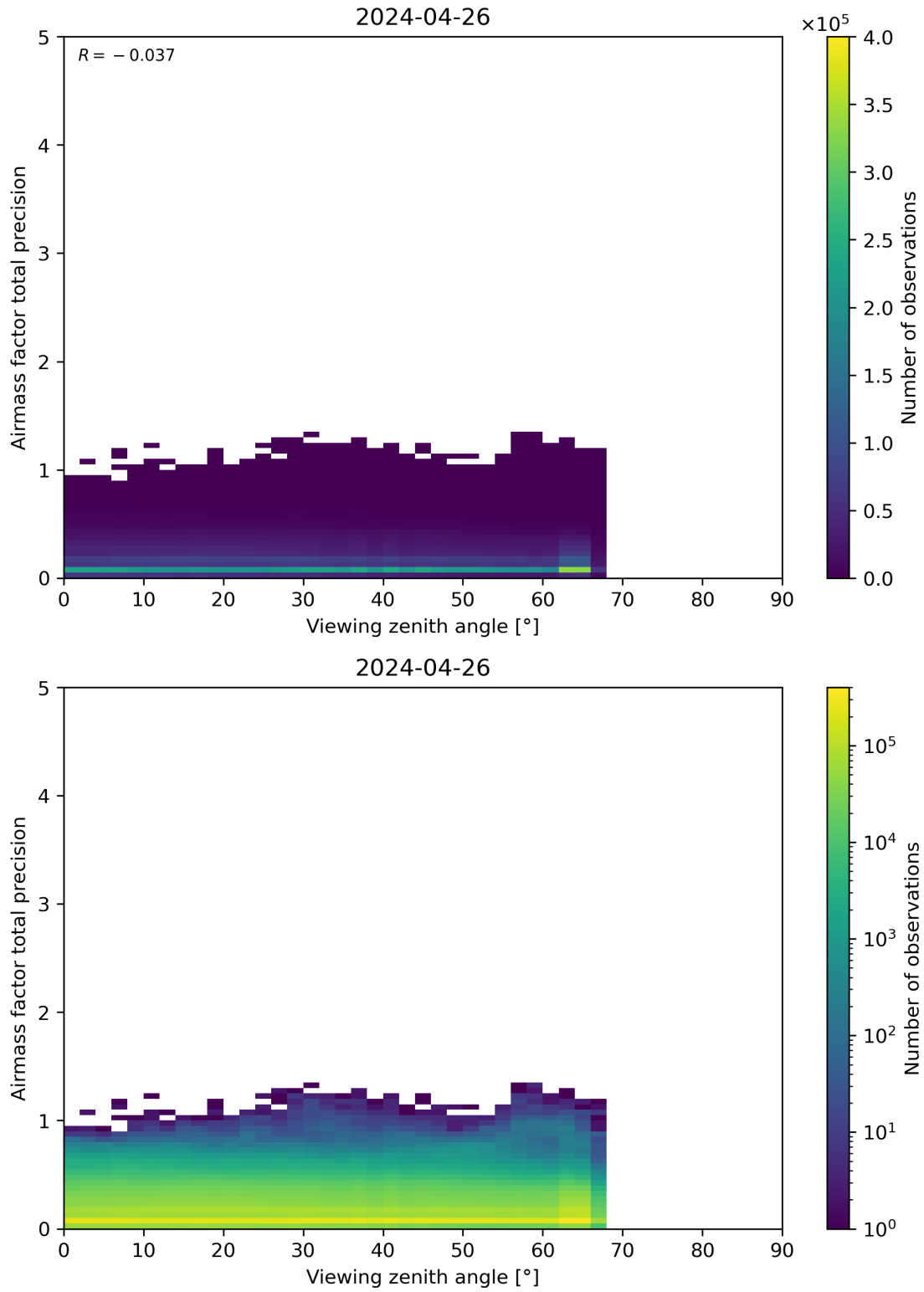
Figure 191: Scatter density plot of “Viewing zenith angle” against “Airmass factor total precision” for 2024-04-26 to 2024-04-27.
