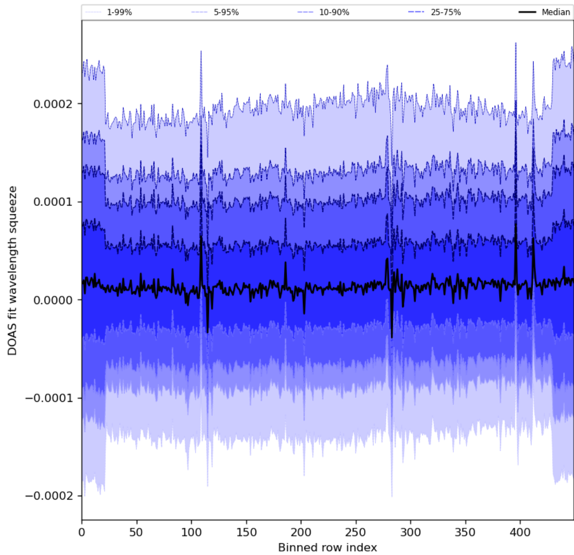
Figure 59: Along track statistics of “DOAS fit wavelength squeeze” for 2024-04-26 to 2024-04-27
