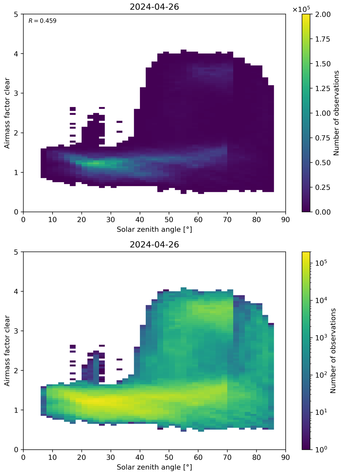
Figure 170: Scatter density plot of “Solar zenith angle” against “Airmass factor clear” for 2024-04-26 to 2024-04-27.
