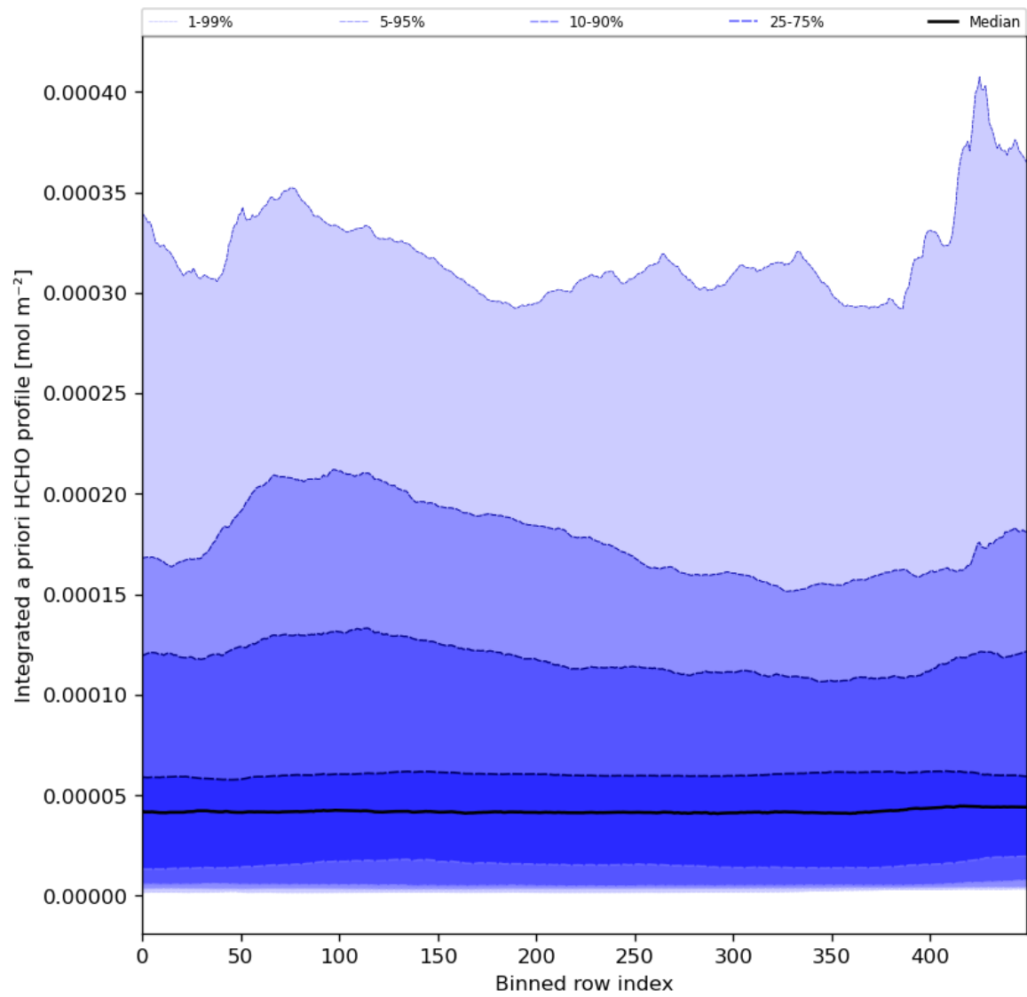
Figure 57: Along track statistics of “Integrated a priori HCHO profile” for 2024-04-26 to 2024-04-27
