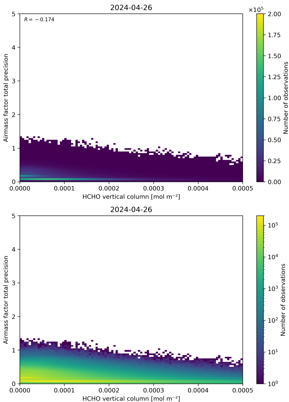
Figure 132: Scatter density plot of “HCHO vertical column” against “Airmass factor total precision” for 2024-04-26 to 2024-04-27.
