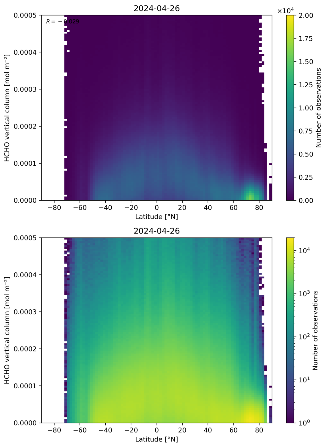
Figure 163: Scatter density plot of “Latitude” against “HCHO vertical column” for 2024-04-26 to 2024-04-27.
