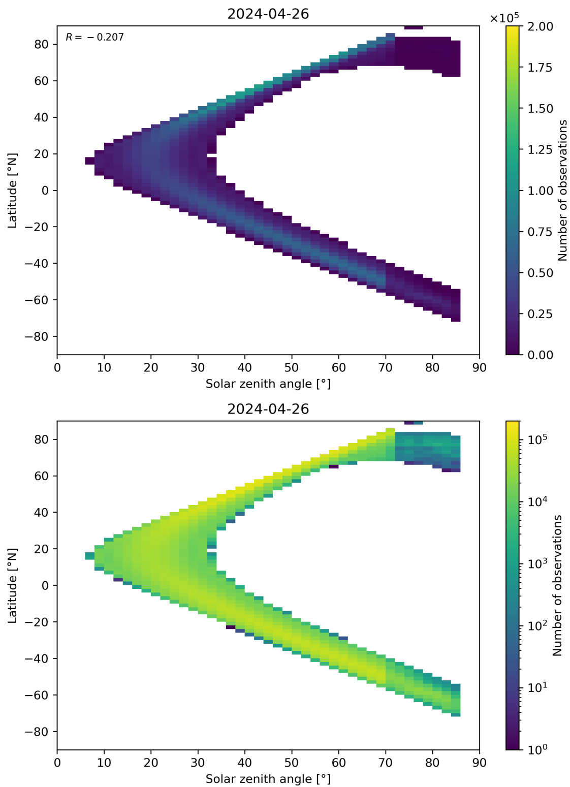
Figure 181: Scatter density plot of “Solar zenith angle” against “Latitude” for 2024-04-26 to 2024-04-27.
