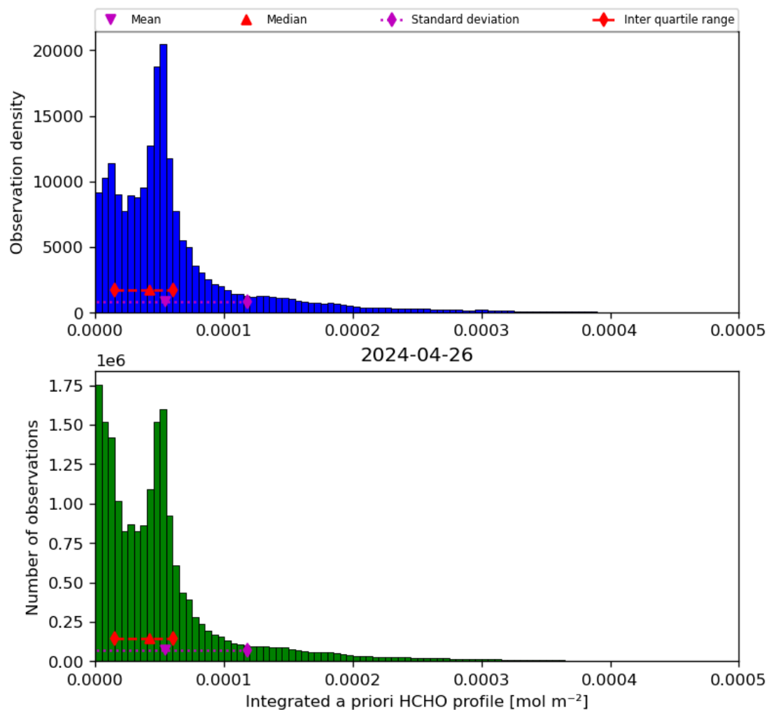
Figure 43: Histogram of “Integrated a priori HCHO profile” for 2024-04-26 to 2024-04-27
