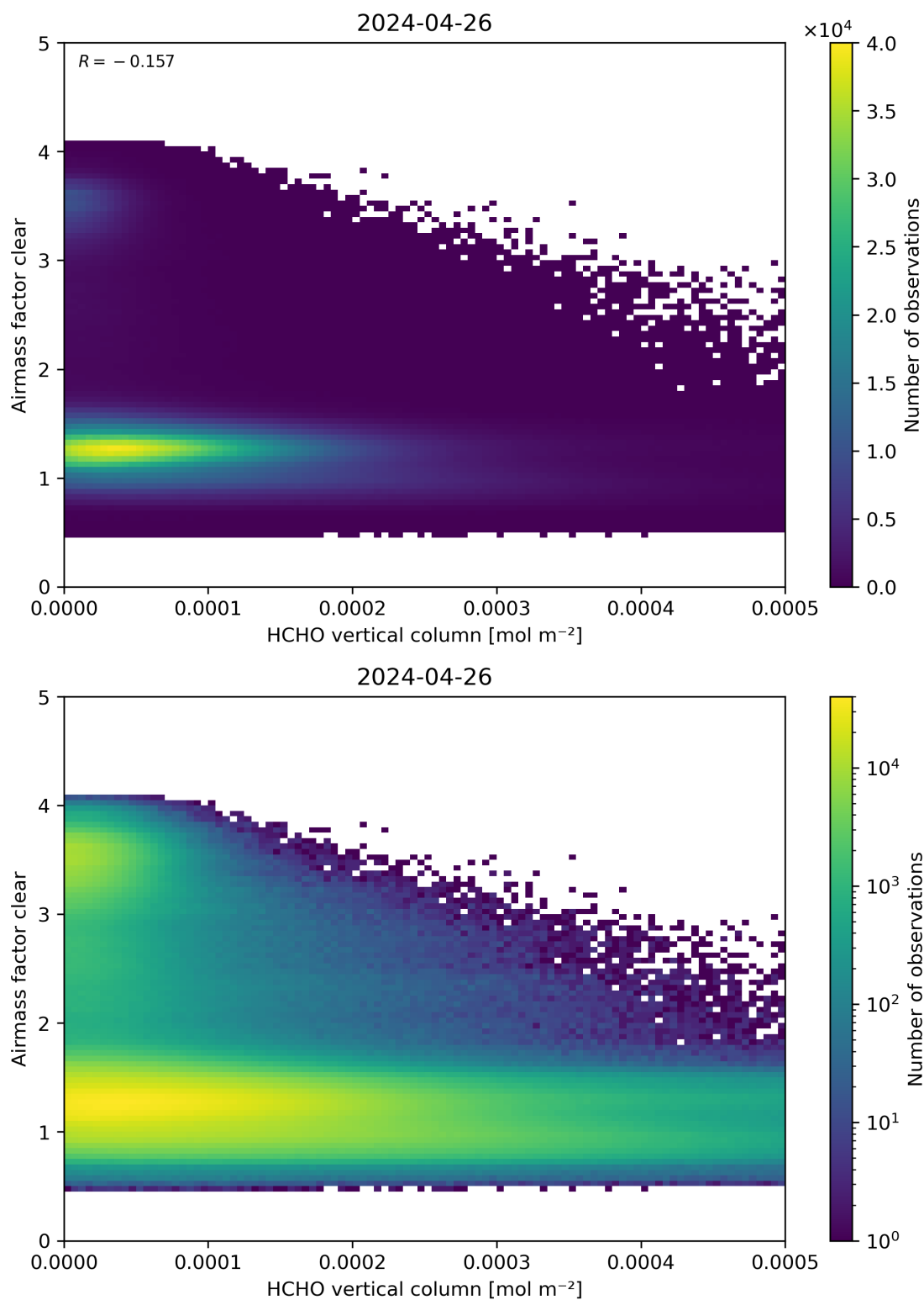
Figure 126: Scatter density plot of “HCHO vertical column” against “Airmass factor clear” for 2024-04-26 to 2024-04-27.
