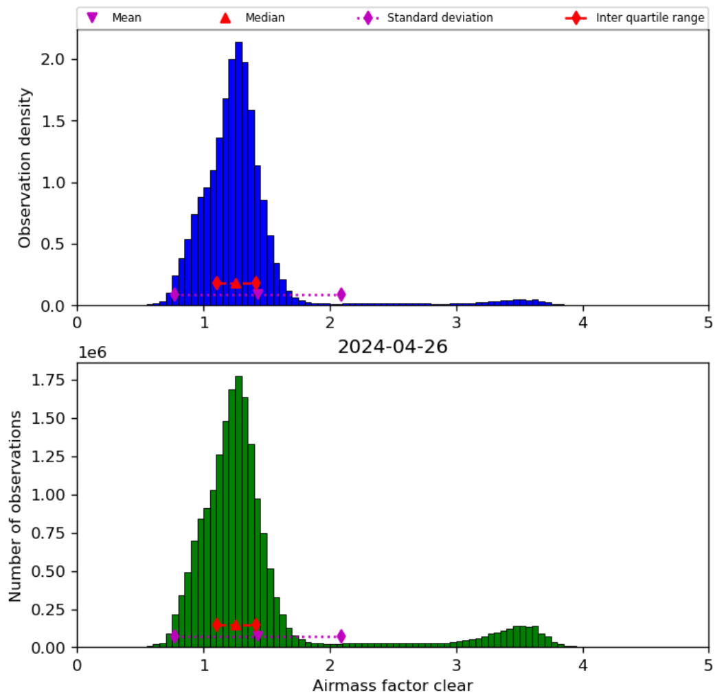
Figure 42: Histogram of “Airmass factor clear” for 2024-04-26 to 2024-04-27
