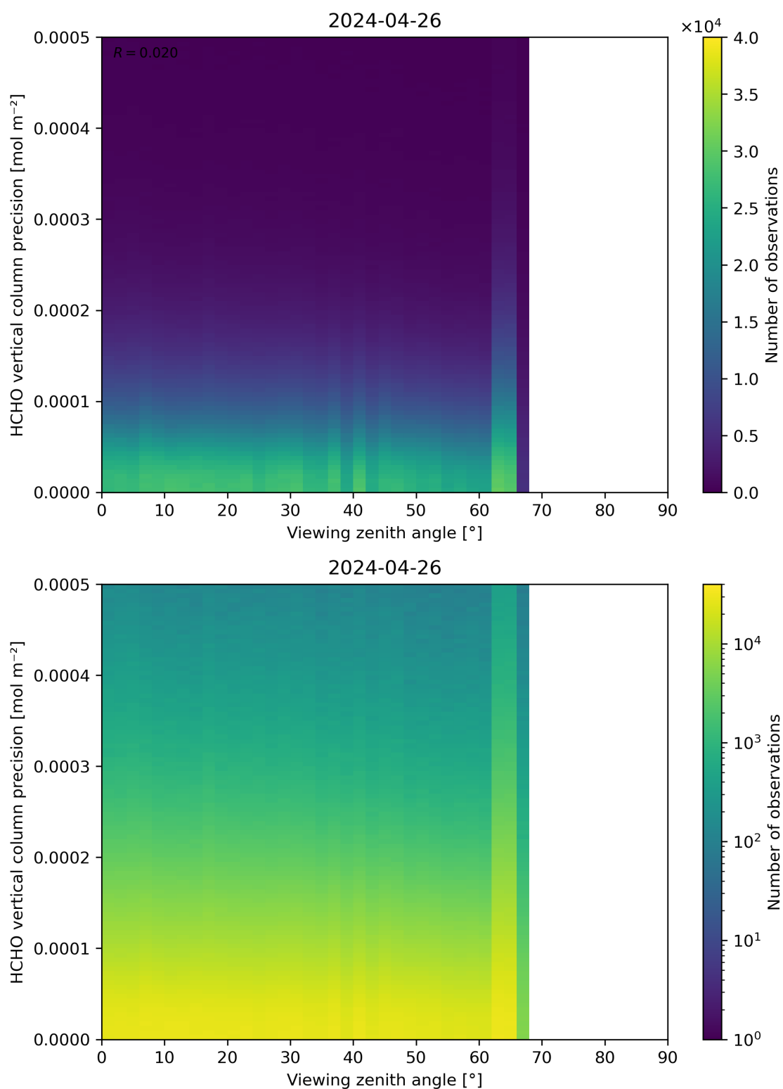
Figure 194: Scatter density plot of “Viewing zenith angle” against “HCHO vertical column precision” for 2024-04-26 to 2024-04-27.
