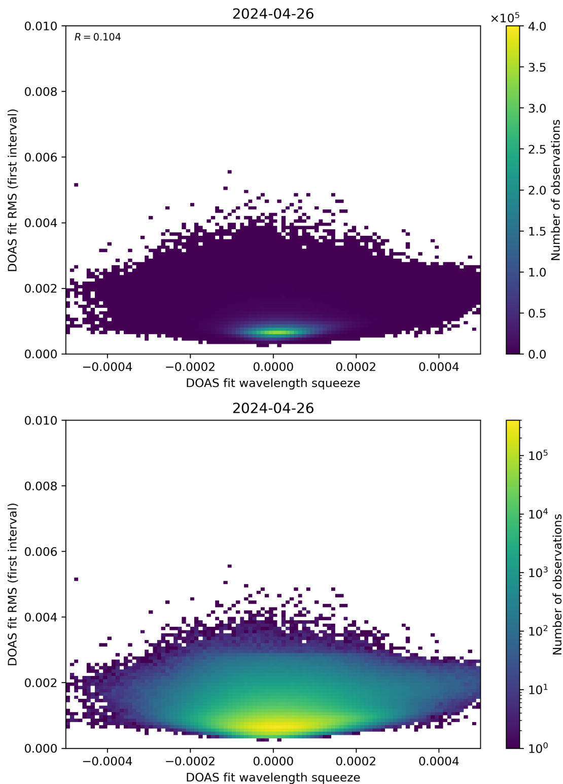
Figure 68: Scatter density plot of “DOAS fit wavelength squeeze” against “DOAS fit RMS (first interval)” for 2024-04-26 to 2024-04-27.
