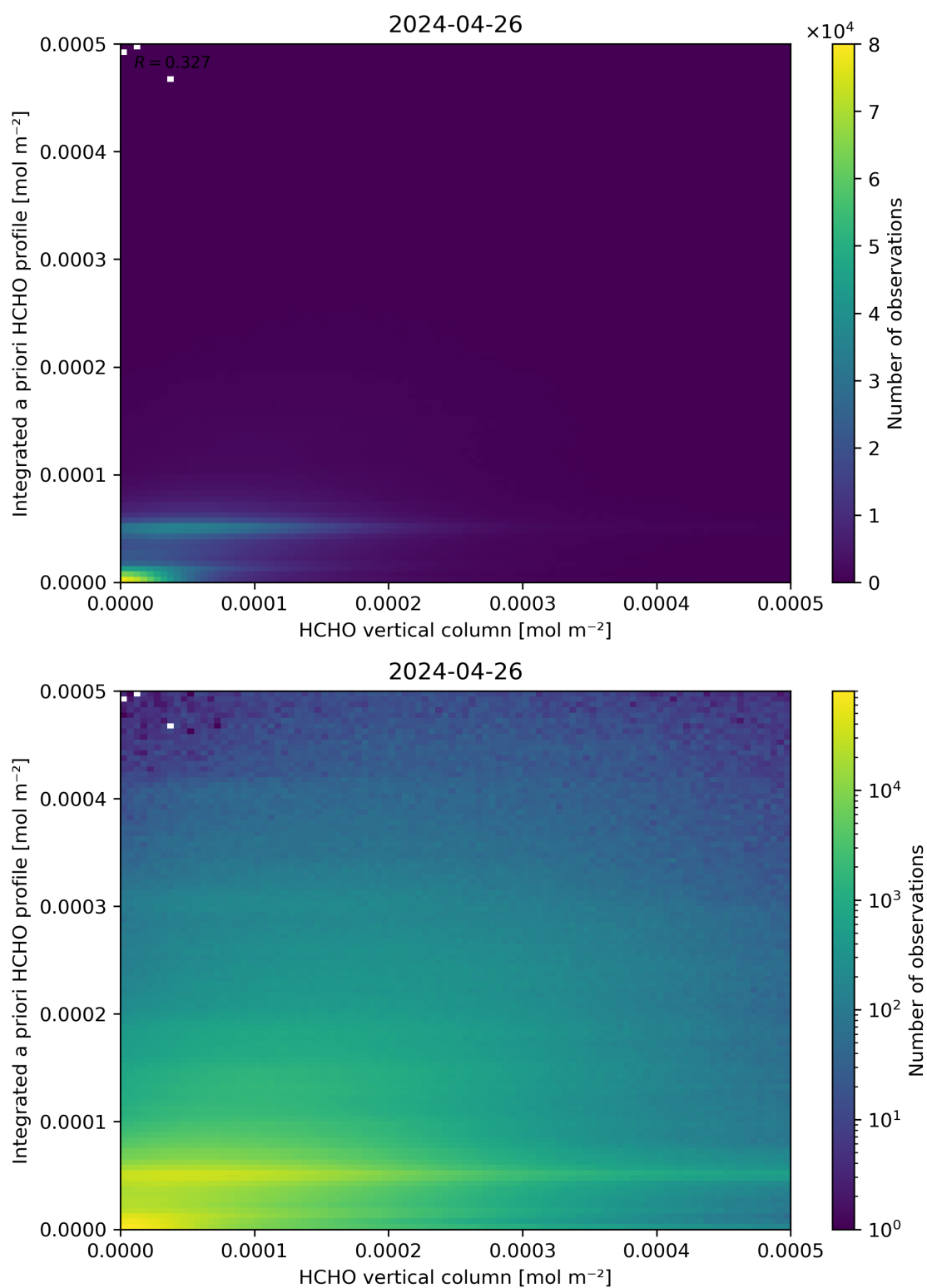
Figure 135: Scatter density plot of “HCHO vertical column” against “Integrated a priori HCHO profile” for 2024-04-26 to 2024-04-27.
