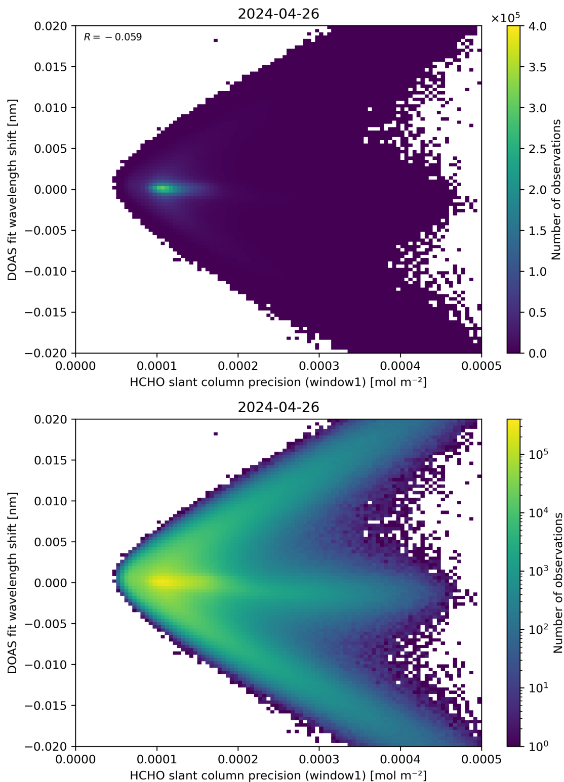
Figure 89: Scatter density plot of “HCHO slant column precision (window1)” against “DOAS fit wavelength shift” for 2024-04-26 to 2024-04-27.
