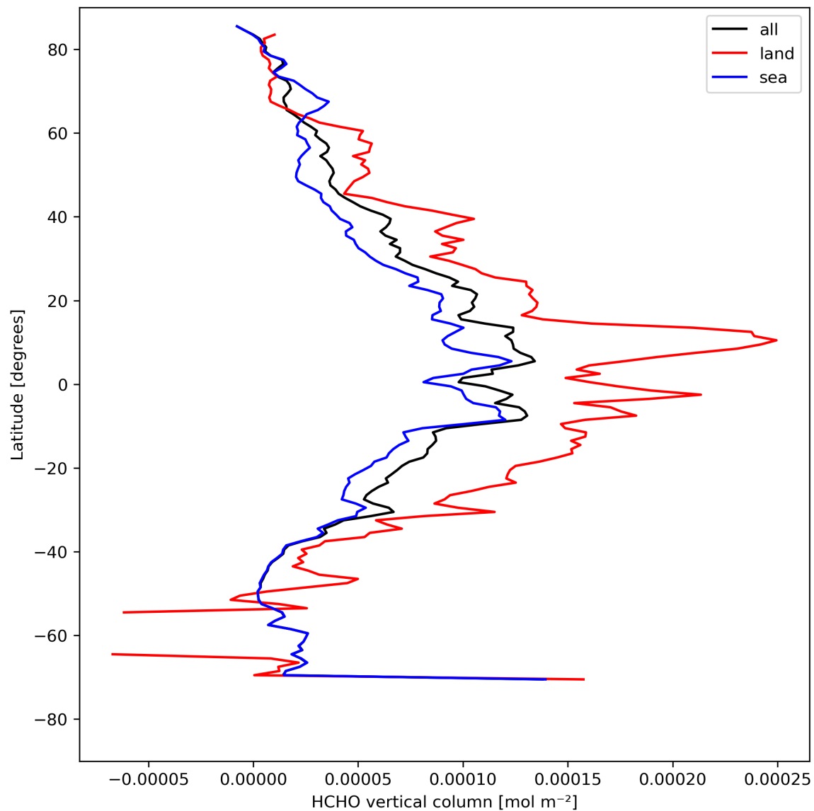
Figure 21: Zonal average of “HCHO vertical column” for 2024-04-26 to 2024-04-27.
