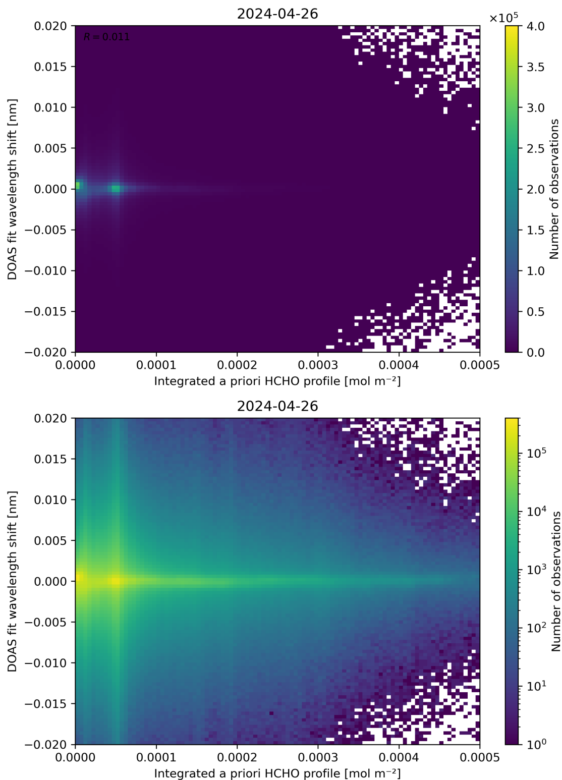
Figure 149: Scatter density plot of “Integrated a priori HCHO profile” against “DOAS fit wavelength shift” for 2024-04-26 to 2024-04-27.
