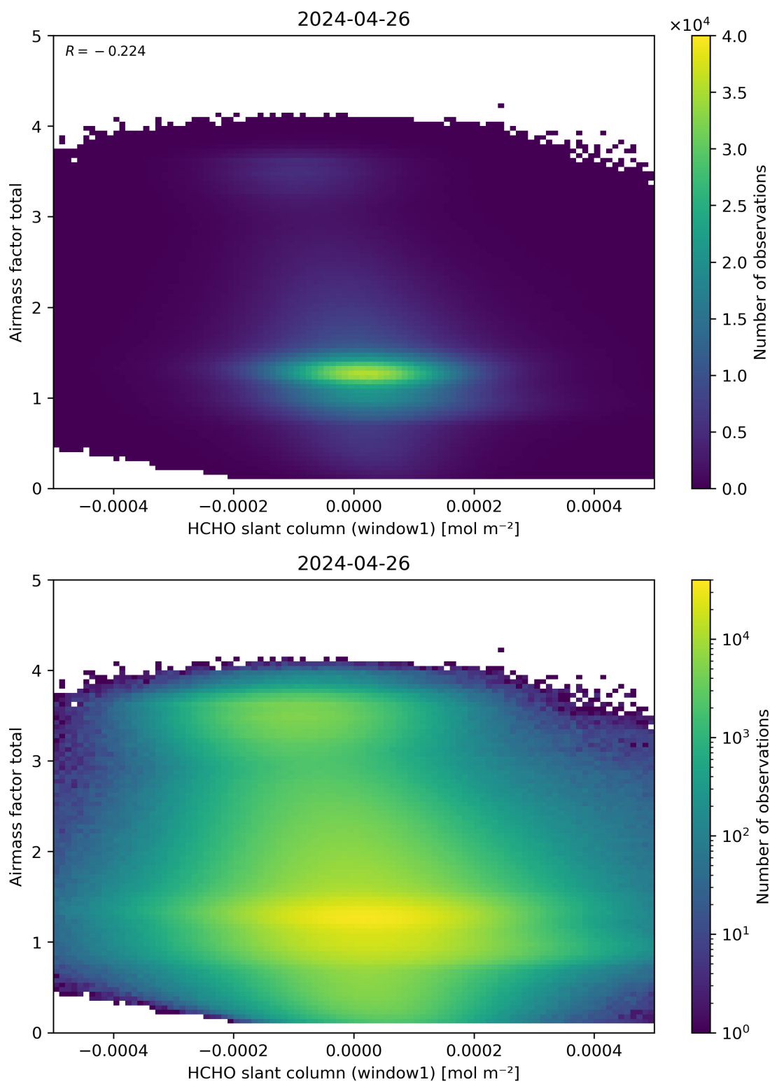
Figure 85: Scatter density plot of “HCHO slant column (window1)” against “Airmass factor total” for 2024-04-26 to 2024-04-27.
