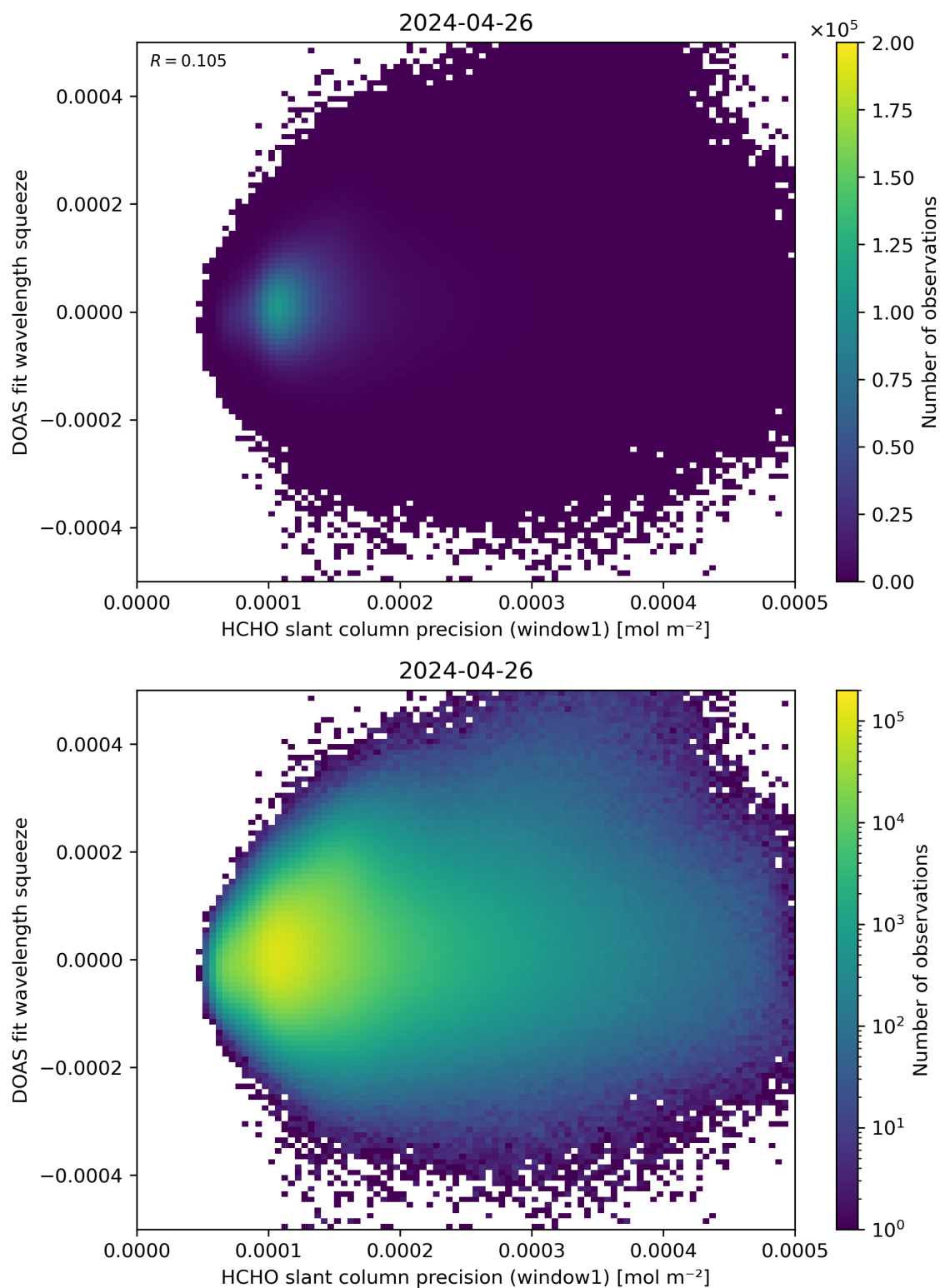
Figure 90: Scatter density plot of “HCHO slant column precision (window1)” against “DOAS fit wavelength squeeze” for 2024-04-26 to 2024-04-27.
