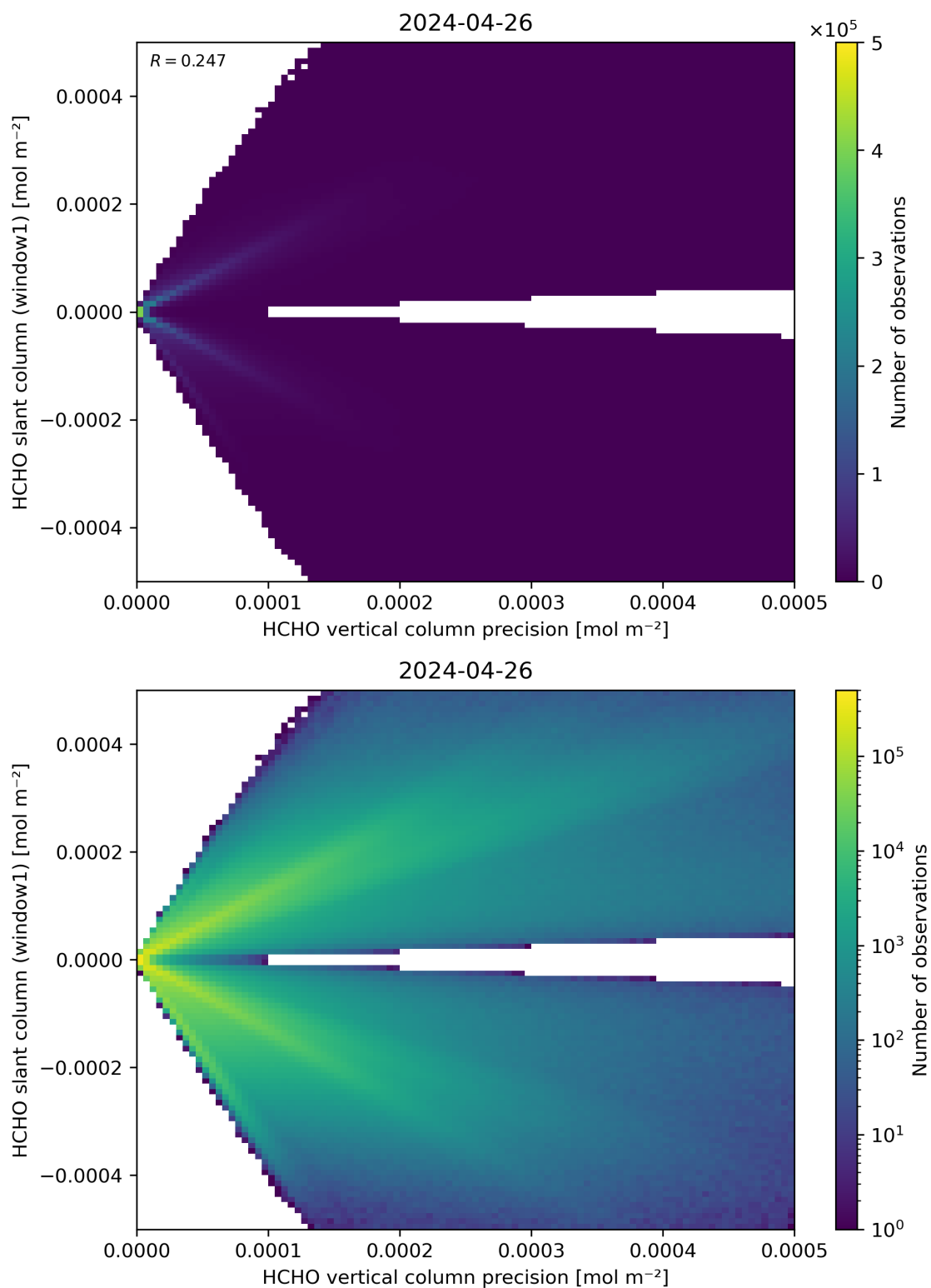
Figure 142: Scatter density plot of “HCHO vertical column precision” against “HCHO slant column (window1)” for 2024-04-26 to 2024-04-27.
