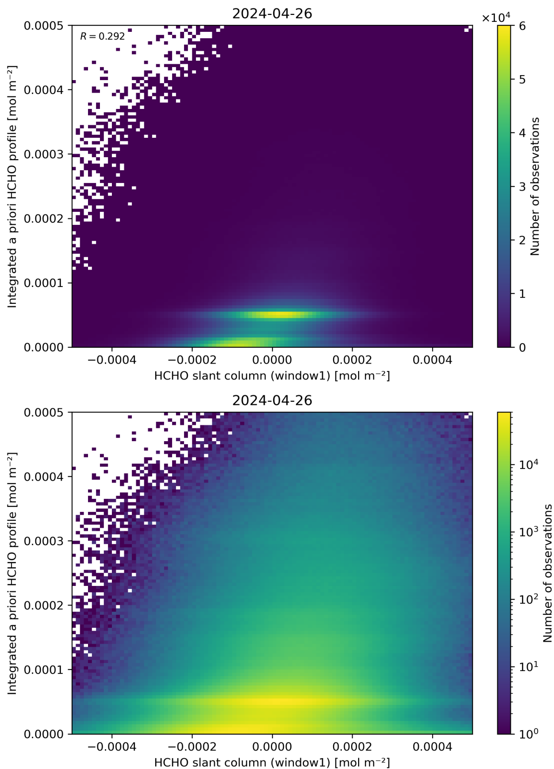
Figure 87: Scatter density plot of “HCHO slant column (window1)” against “Integrated a priori HCHO profile” for 2024-04-26 to 2024-04-27.
