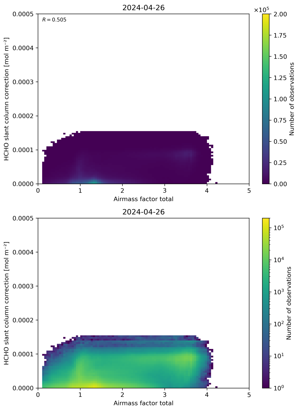
Figure 102: Scatter density plot of “Airmass factor total” against “HCHO slant column correction” for 2024-04-26 to 2024-04-27.
