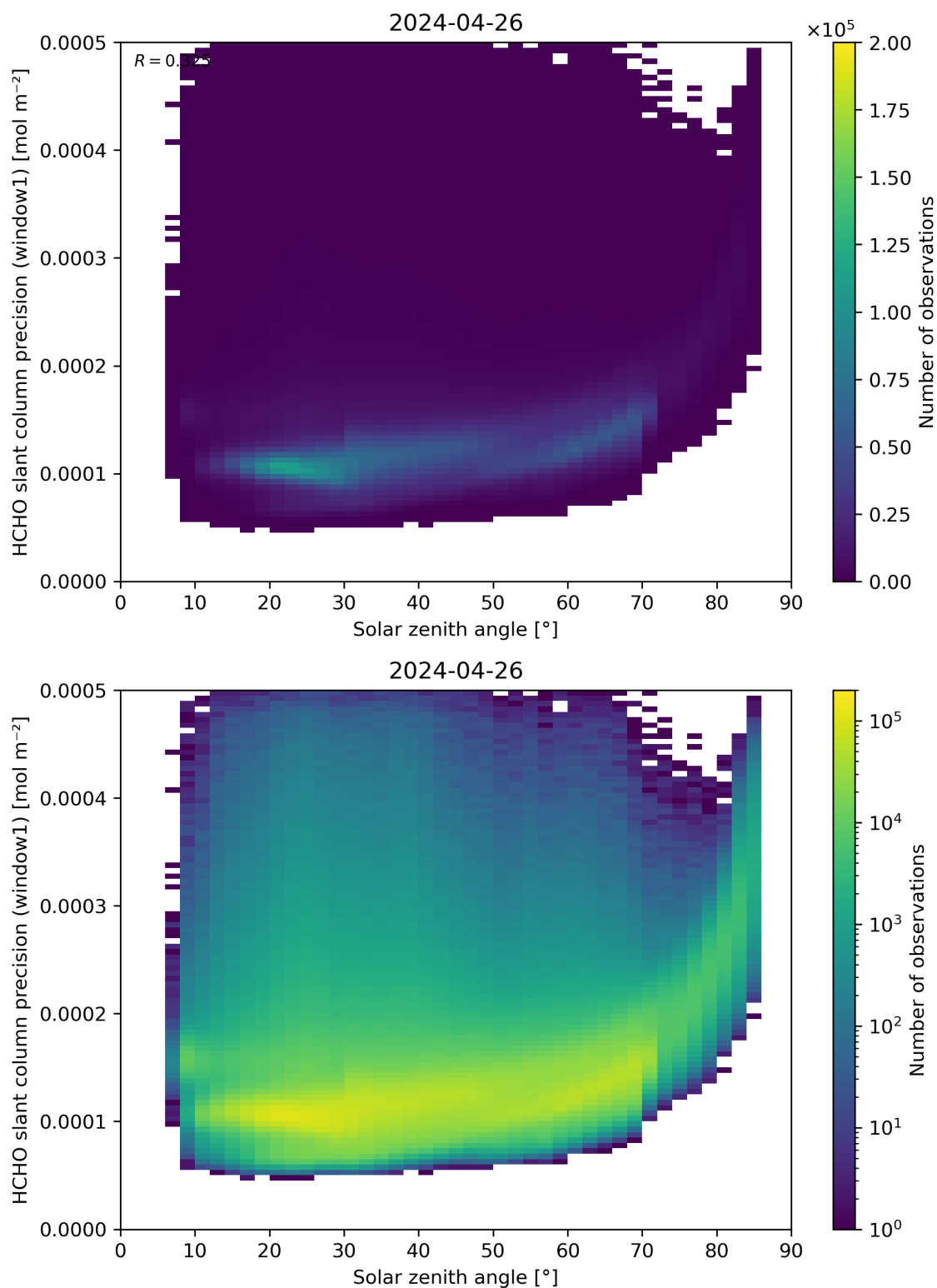
Figure 174: Scatter density plot of “Solar zenith angle” against “HCHO slant column precision (window1)” for 2024-04-26 to 2024-04-27.
