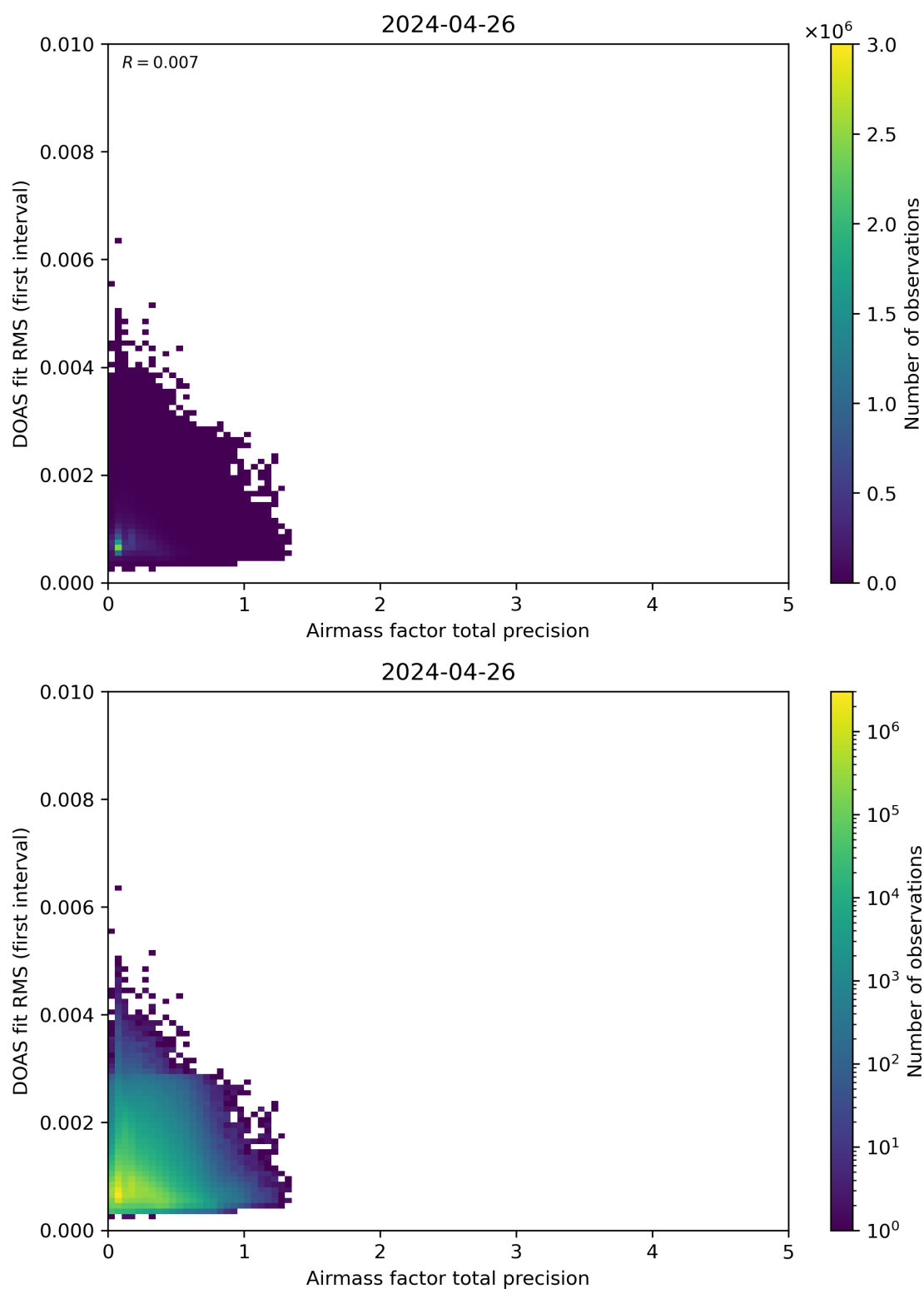
Figure 105: Scatter density plot of “Airmass factor total precision” against “DOAS fit RMS (first interval)” for 2024-04-26 to 2024-04-27.
