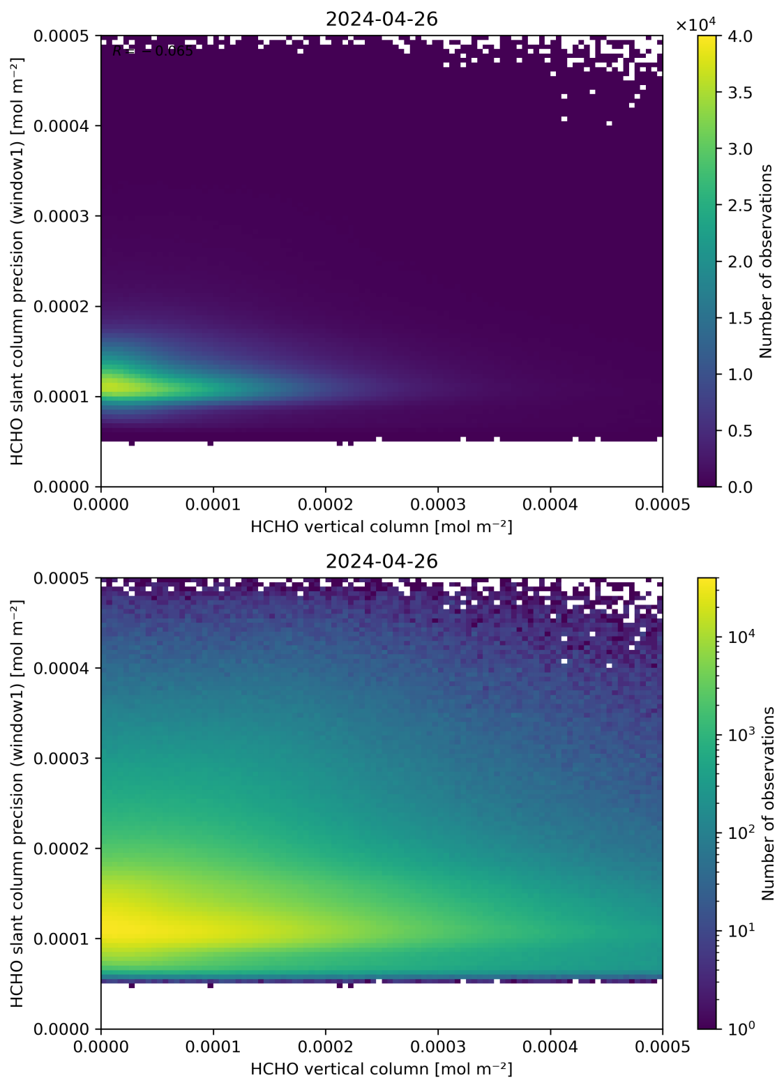
Figure 130: Scatter density plot of “HCHO vertical column” against “HCHO slant column precision (window1)” for 2024-04-26 to 2024-04-27.
