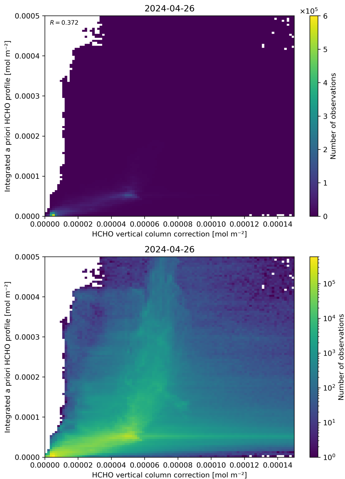
Figure 122: Scatter density plot of “HCHO vertical column correction” against “Integrated a priori HCHO profile” for 2024-04-26 to 2024-04-27.
