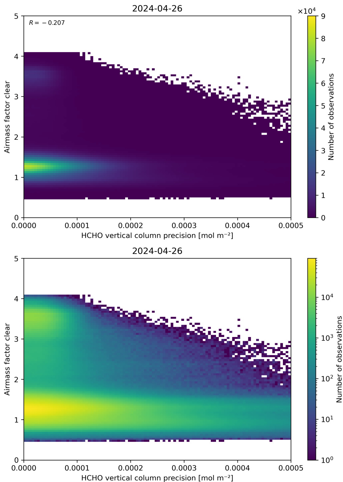
Figure 139: Scatter density plot of “HCHO vertical column precision” against “Airmass factor clear” for 2024-04-26 to 2024-04-27.
