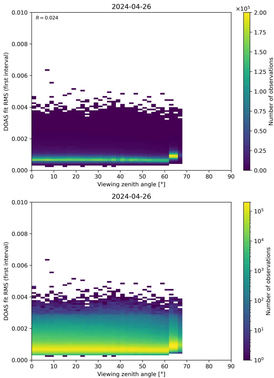
Figure 182: Scatter density plot of “Viewing zenith angle” against “DOAS fit RMS (first interval)” for 2024-04-26 to 2024-04-27.
