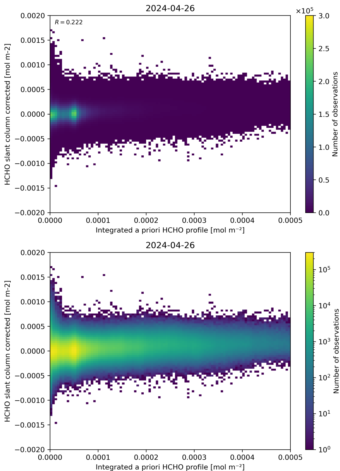
Figure 151: Scatter density plot of “Integrated a priori HCHO profile” against “HCHO slant column corrected” for 2024-04-26 to 2024-04-27.
