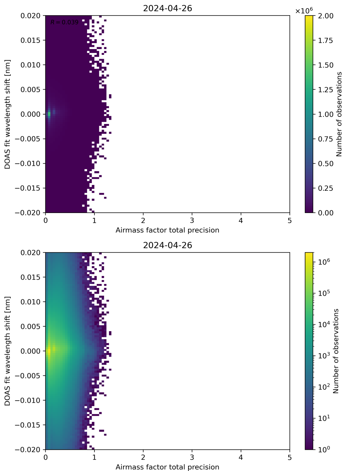
Figure 106: Scatter density plot of “Airmass factor total precision” against “DOAS fit wavelength shift” for 2024-04-26 to 2024-04-27.
