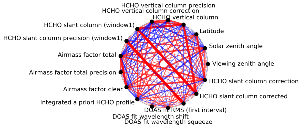
Figure 1: Map of correlation graph for 2024-04-26 to 2024-04-27.
