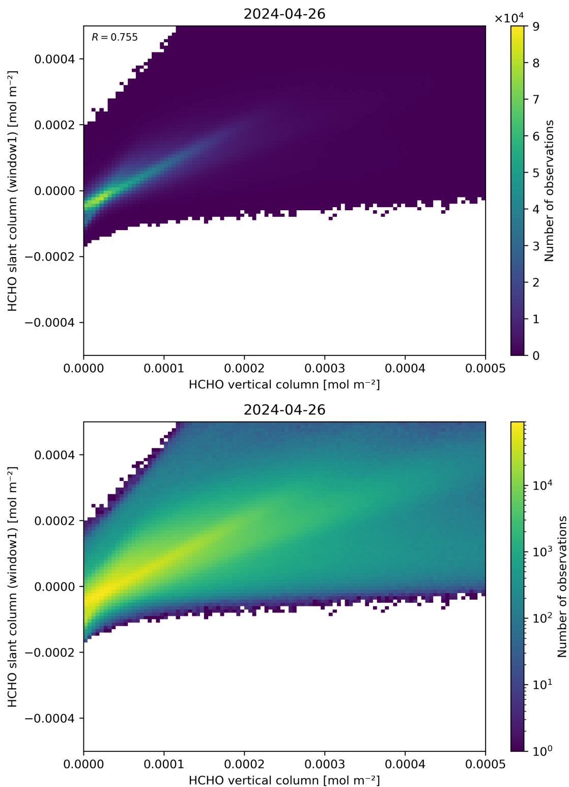
Figure 129: Scatter density plot of “HCHO vertical column” against “HCHO slant column (window1)” for 2024-04-26 to 2024-04-27.
