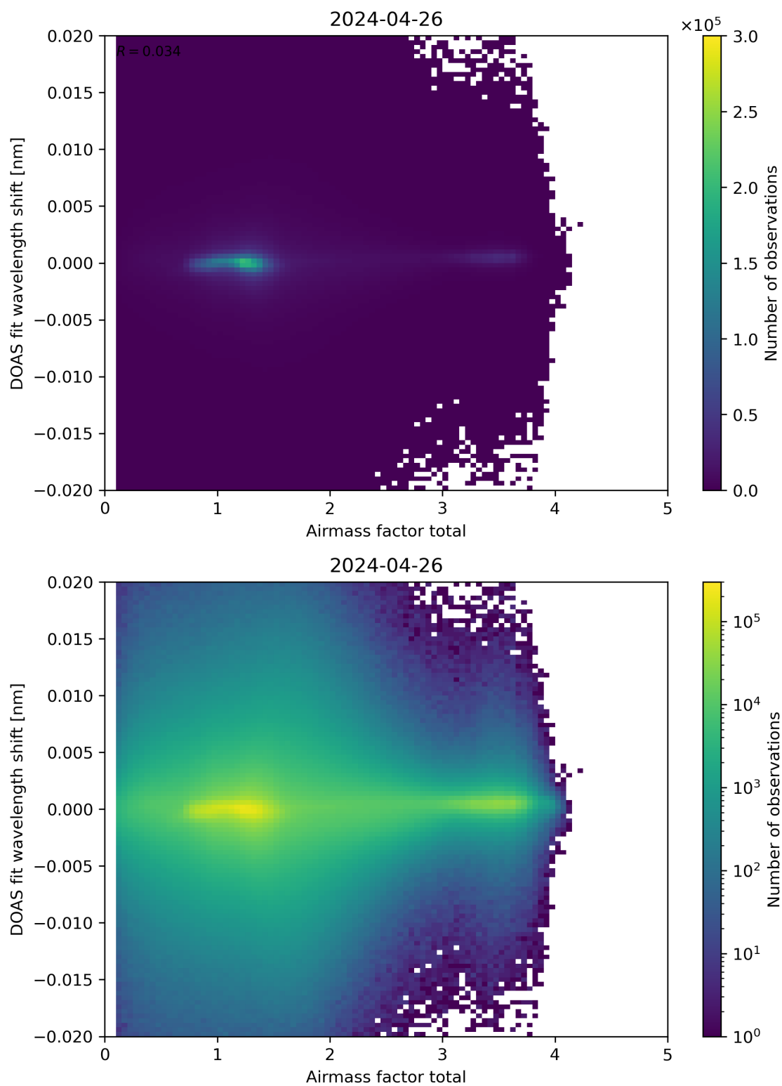
Figure 98: Scatter density plot of “Airmass factor total” against “DOAS fit wavelength shift” for 2024-04-26 to 2024-04-27.
