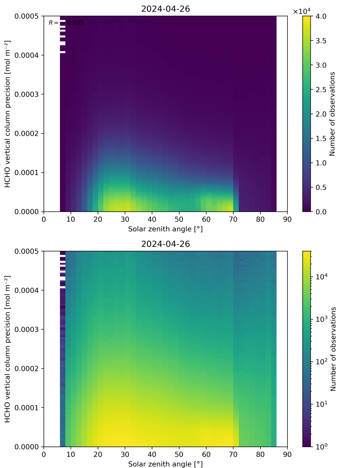
Figure 179: Scatter density plot of “Solar zenith angle” against “HCHO vertical column precision” for 2024-04-26 to 2024-04-27.
