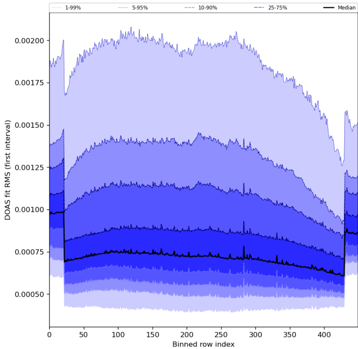
Figure 60: Along track statistics of “DOAS fit RMS (first interval)” for 2024-04-26 to 2024-04-27
