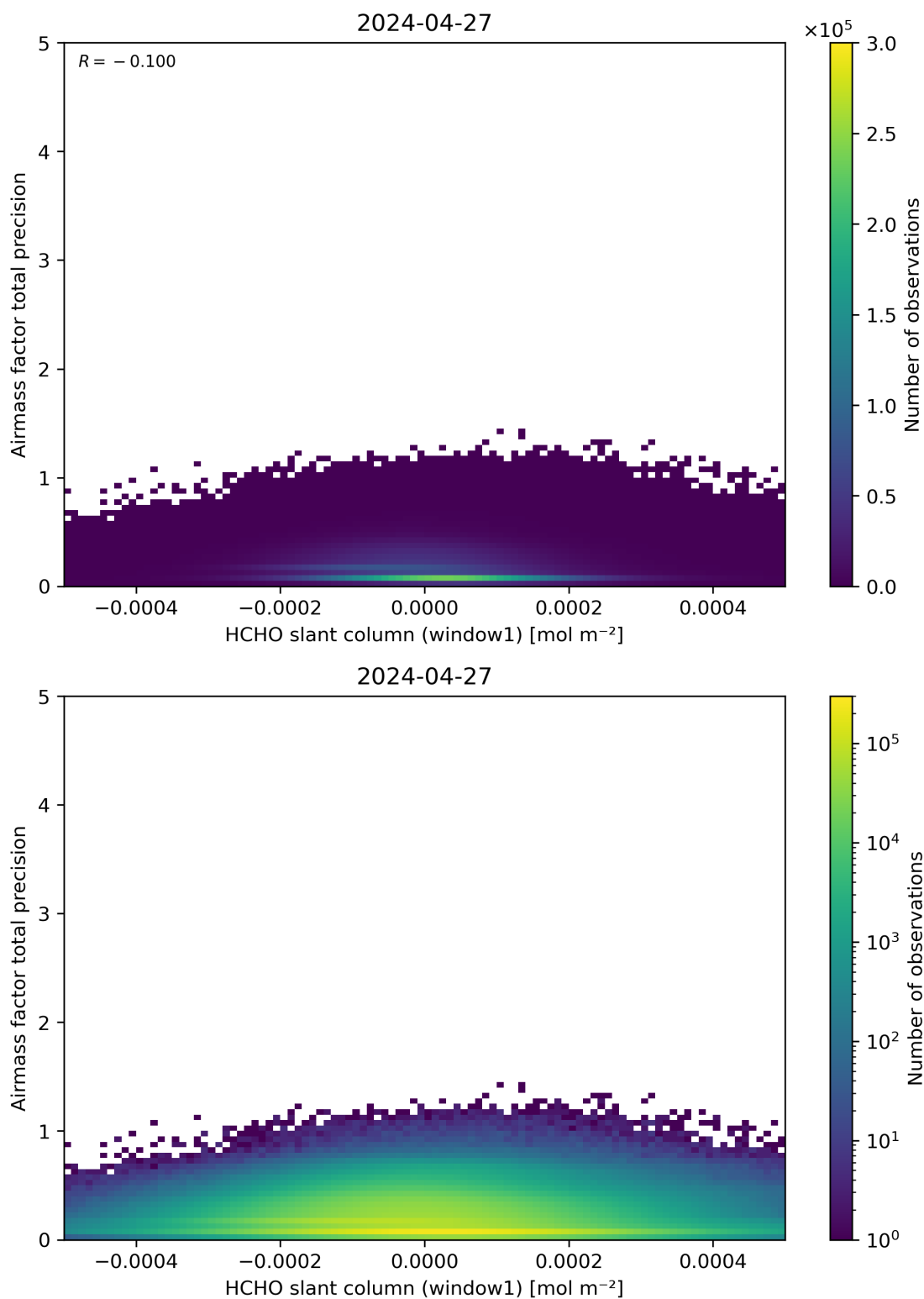
Figure 86: Scatter density plot of “HCHO slant column (window1)” against “Airmass factor total precision” for 2024-04-26 to 2024-04-28.
