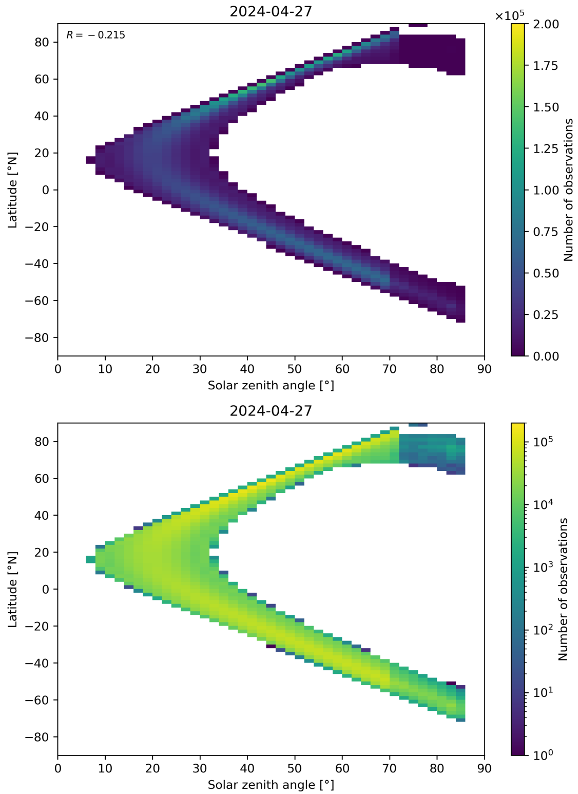
Figure 181: Scatter density plot of “Solar zenith angle” against “Latitude” for 2024-04-26 to 2024-04-28.
