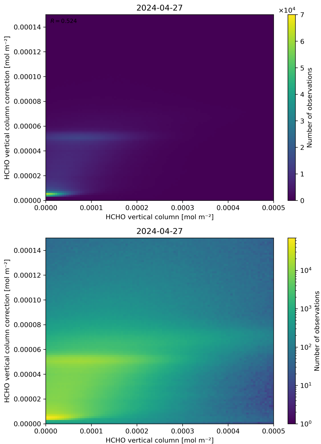
Figure 133: Scatter density plot of “HCHO vertical column” against “HCHO vertical column correction” for 2024-04-26 to 2024-04-28.
