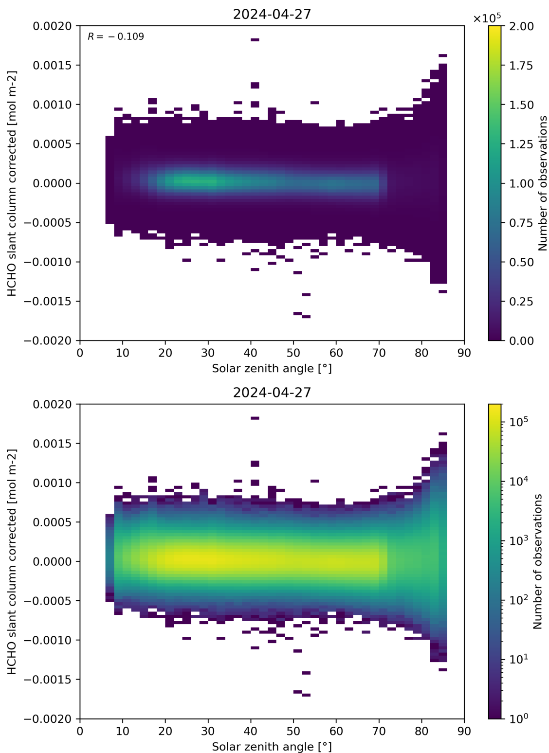
Figure 171: Scatter density plot of “Solar zenith angle” against “HCHO slant column corrected” for 2024-04-26 to 2024-04-28.
