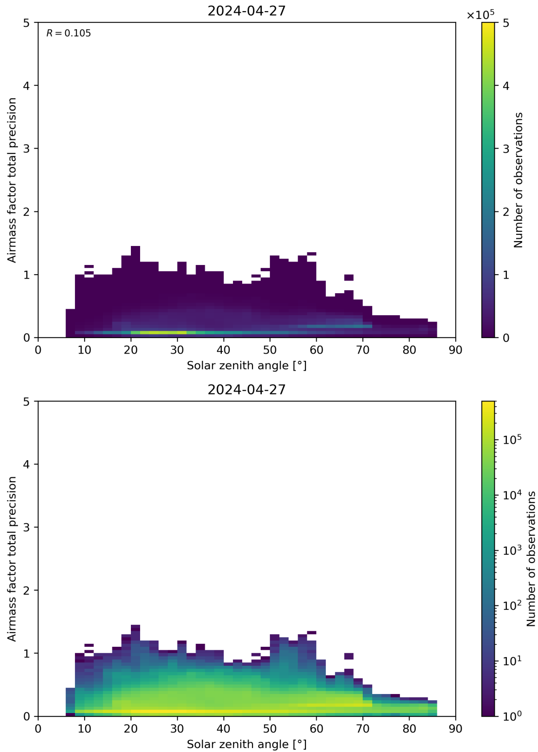
Figure 176: Scatter density plot of “Solar zenith angle” against “Airmass factor total precision” for 2024-04-26 to 2024-04-28.
