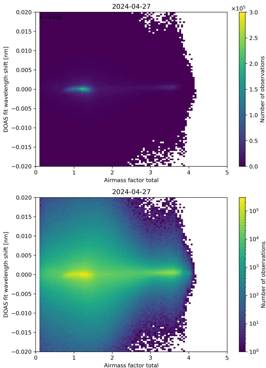
Figure 98: Scatter density plot of “Airmass factor total” against “DOAS fit wavelength shift” for 2024-04-26 to 2024-04-28.
