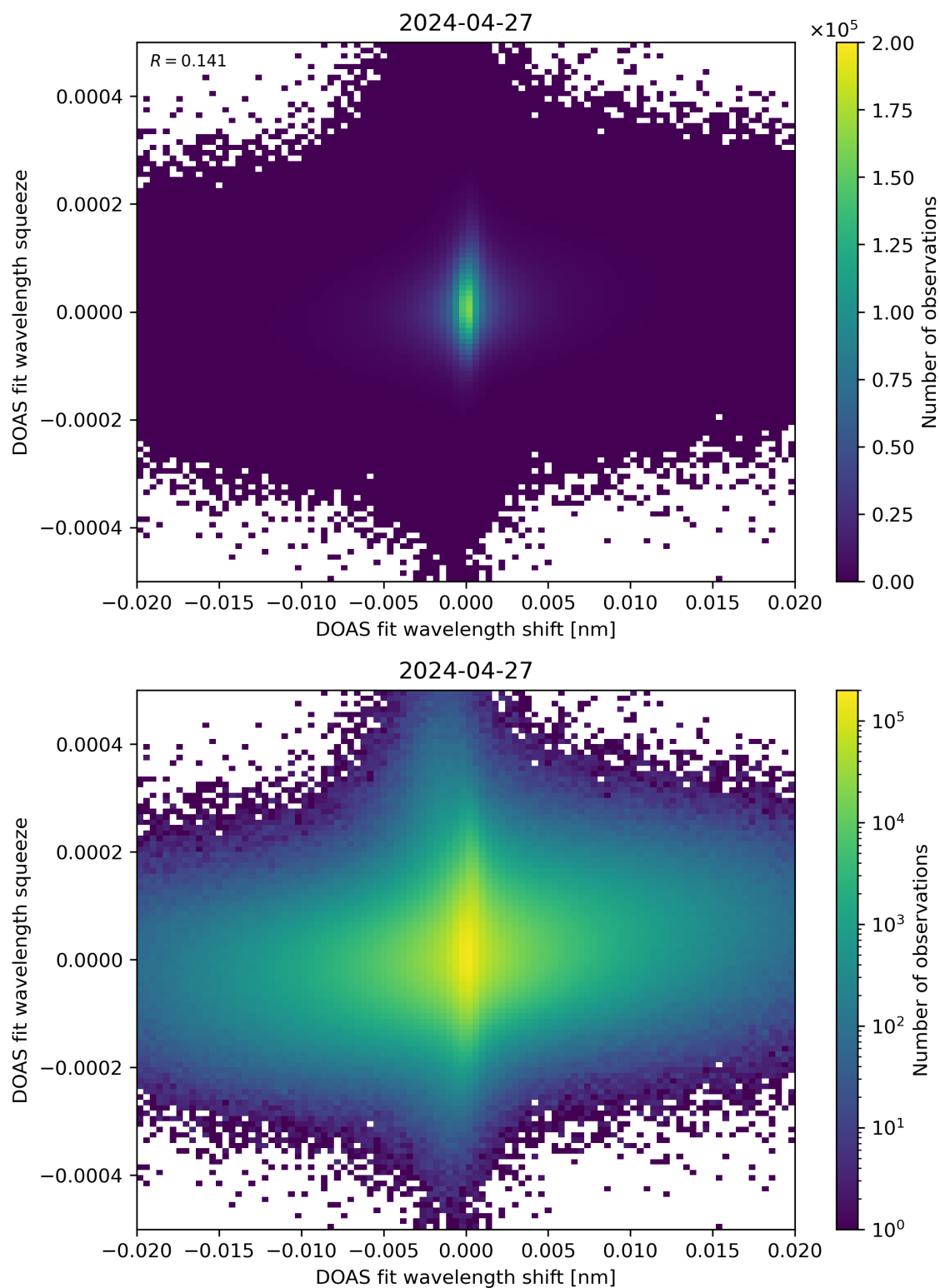
Figure 65: Scatter density plot of “DOAS fit wavelength shift” against “DOAS fit wavelength squeeze” for 2024-04-26 to 2024-04-28.
