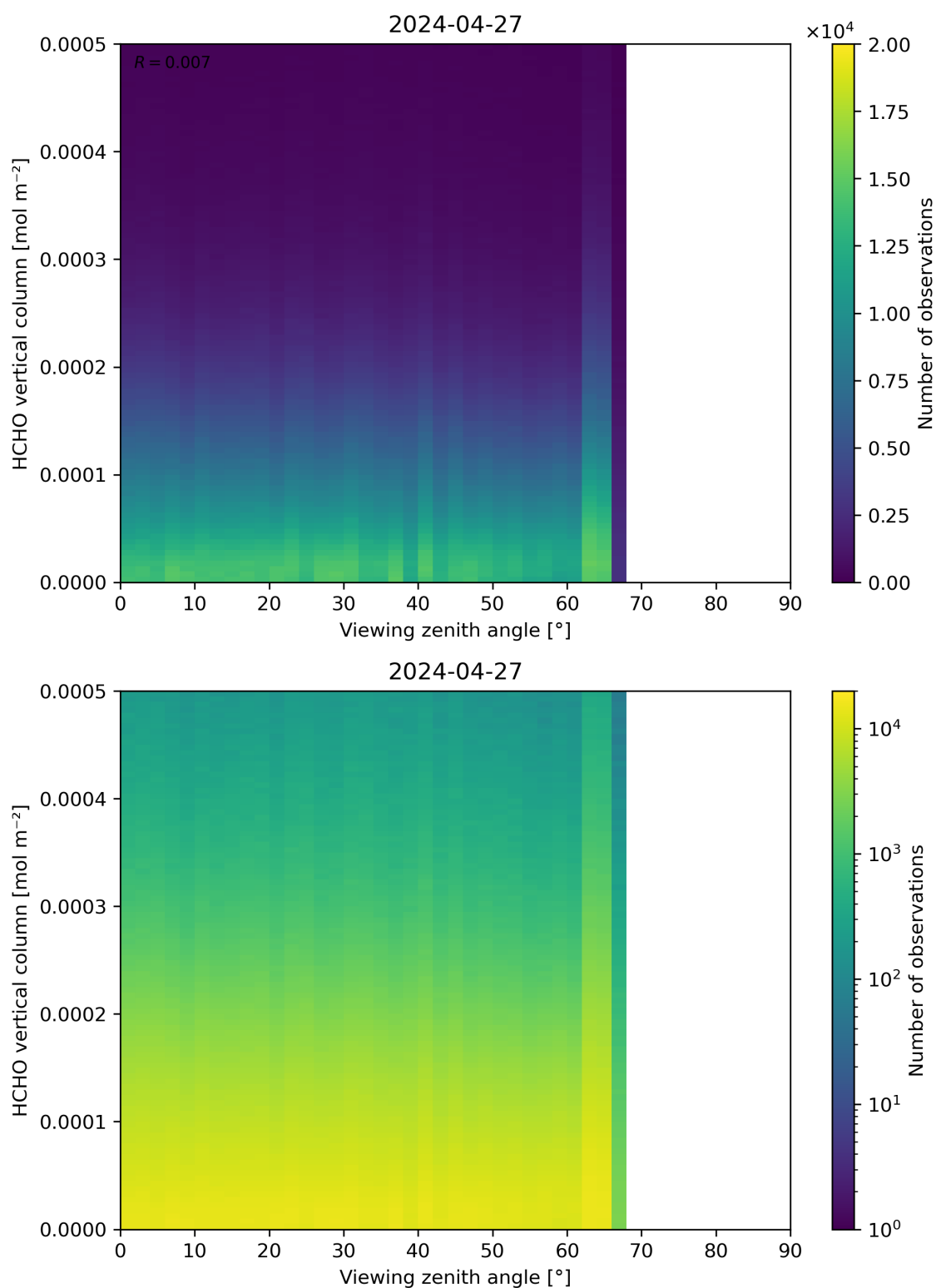
Figure 192: Scatter density plot of “Viewing zenith angle” against “HCHO vertical column” for 2024-04-26 to 2024-04-28.
