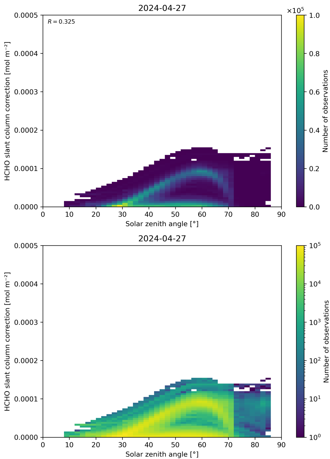
Figure 172: Scatter density plot of “Solar zenith angle” against “HCHO slant column correction” for 2024-04-26 to 2024-04-28.
