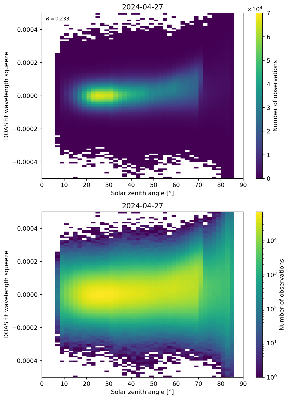
Figure 169: Scatter density plot of “Solar zenith angle” against “DOAS fit wavelength squeeze” for 2024-04-26 to 2024-04-28.
