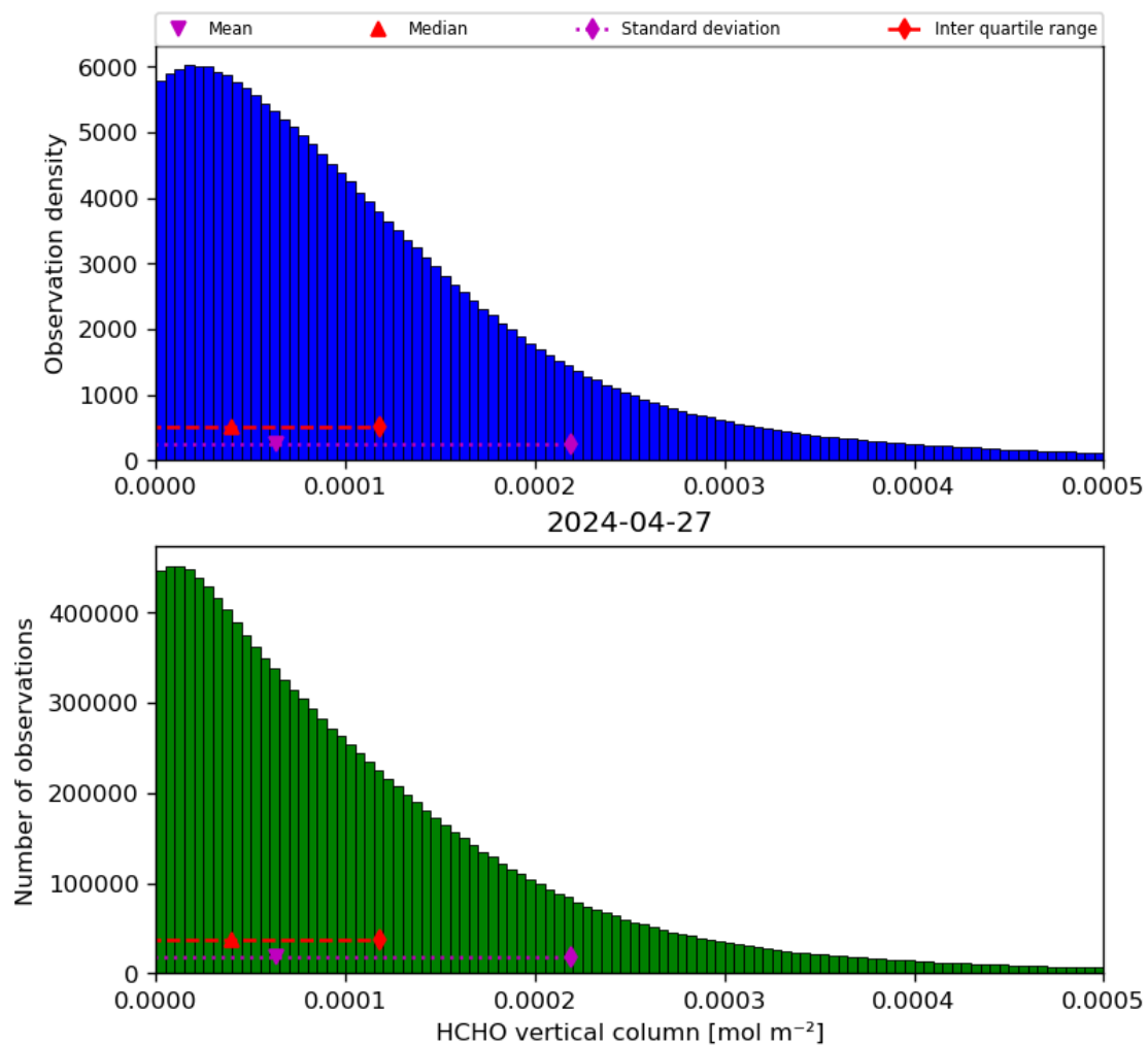
Figure 35: Histogram of “HCHO vertical column” for 2024-04-26 to 2024-04-28
