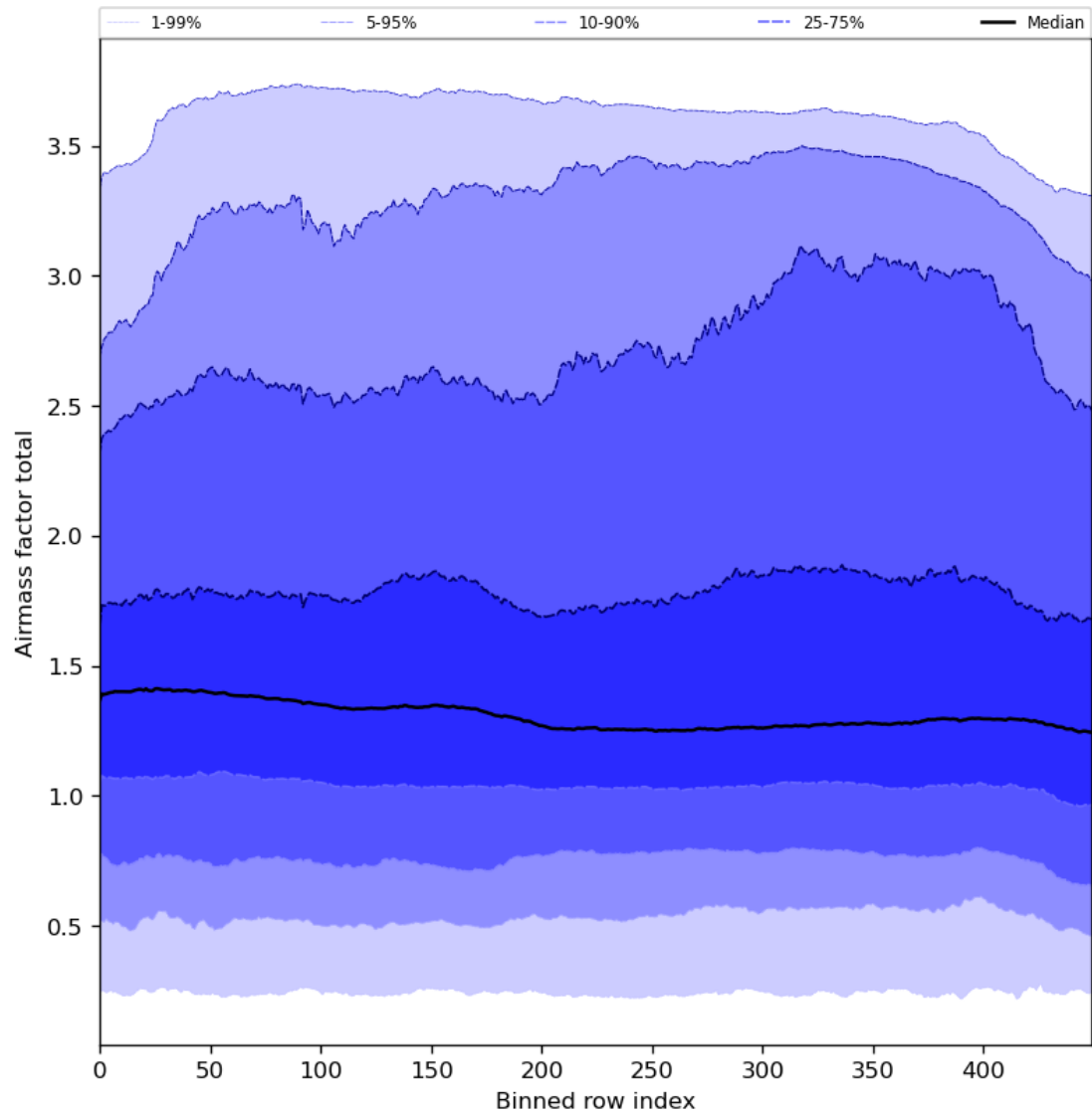
Figure 54: Along track statistics of “Airmass factor total” for 2024-04-26 to 2024-04-28
