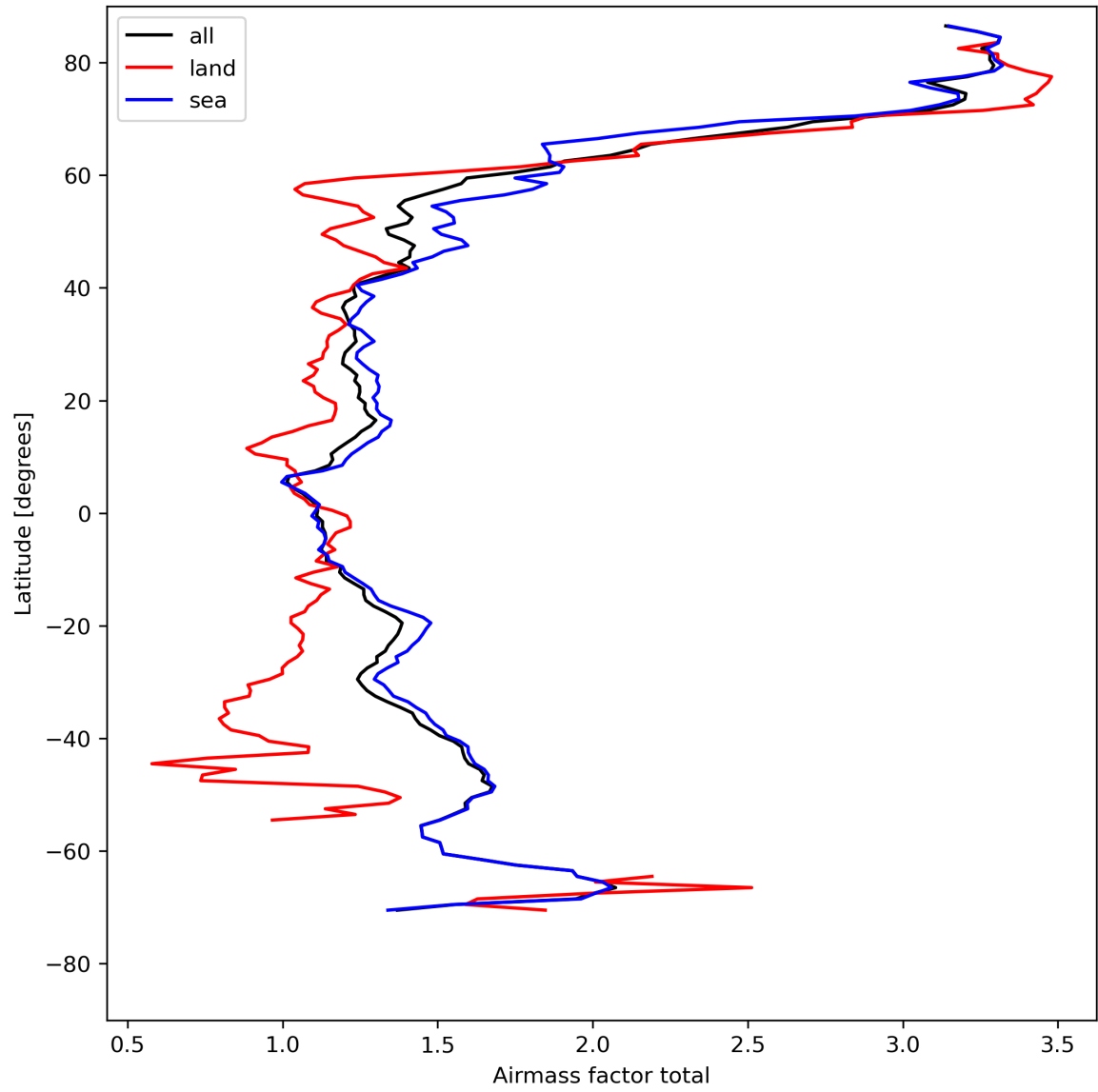
Figure 26: Zonal average of “Airmass factor total” for 2024-04-26 to 2024-04-28.
