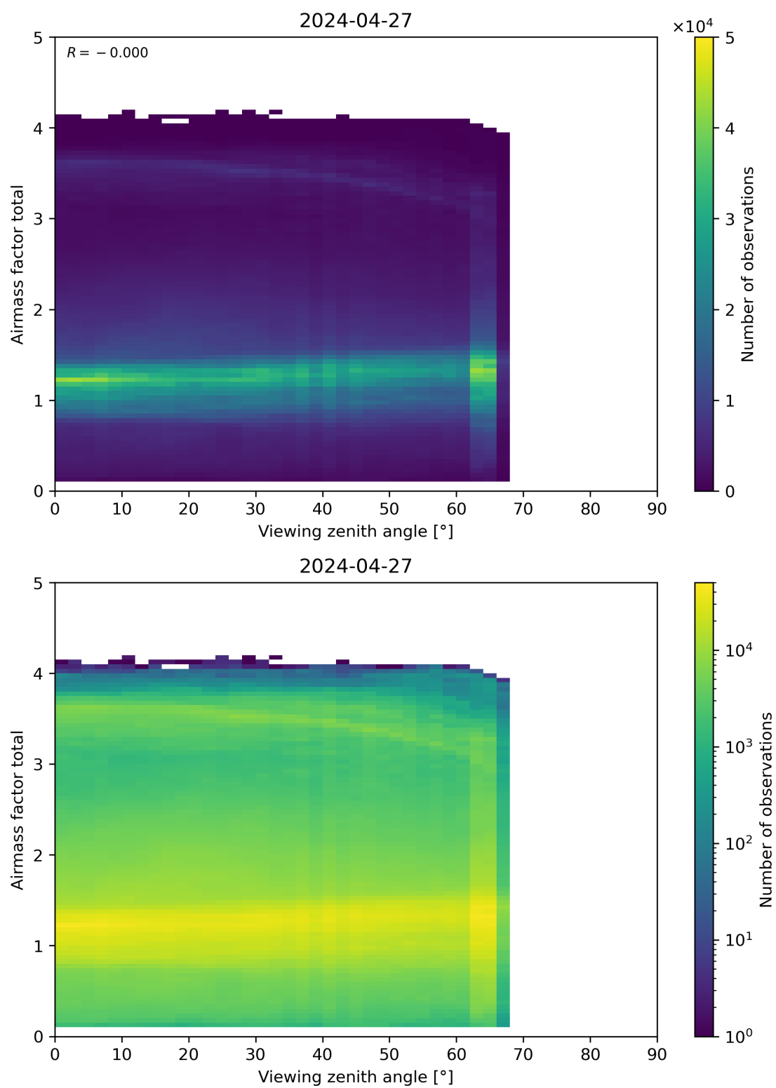
Figure 190: Scatter density plot of “Viewing zenith angle” against “Airmass factor total” for 2024-04-26 to 2024-04-28.
