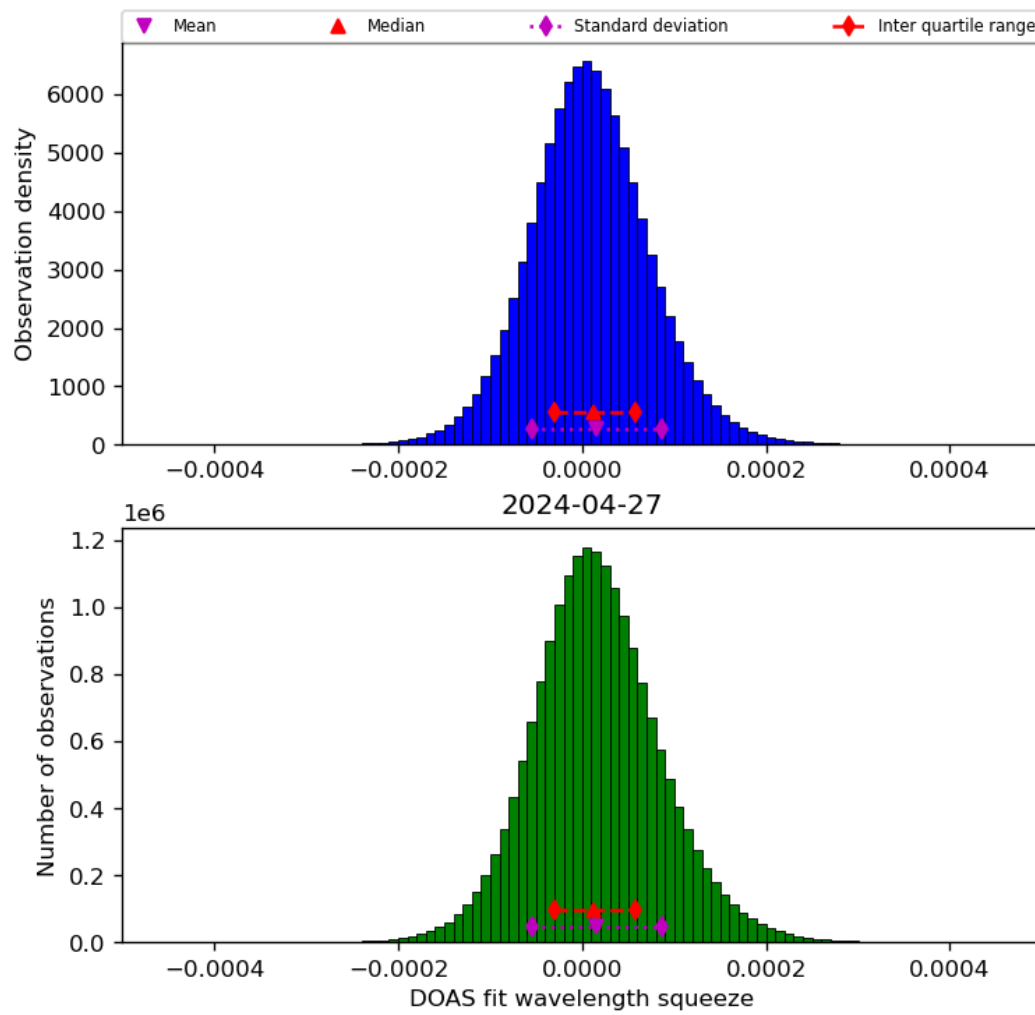
Figure 45: Histogram of “DOAS fit wavelength squeeze” for 2024-04-26 to 2024-04-28
