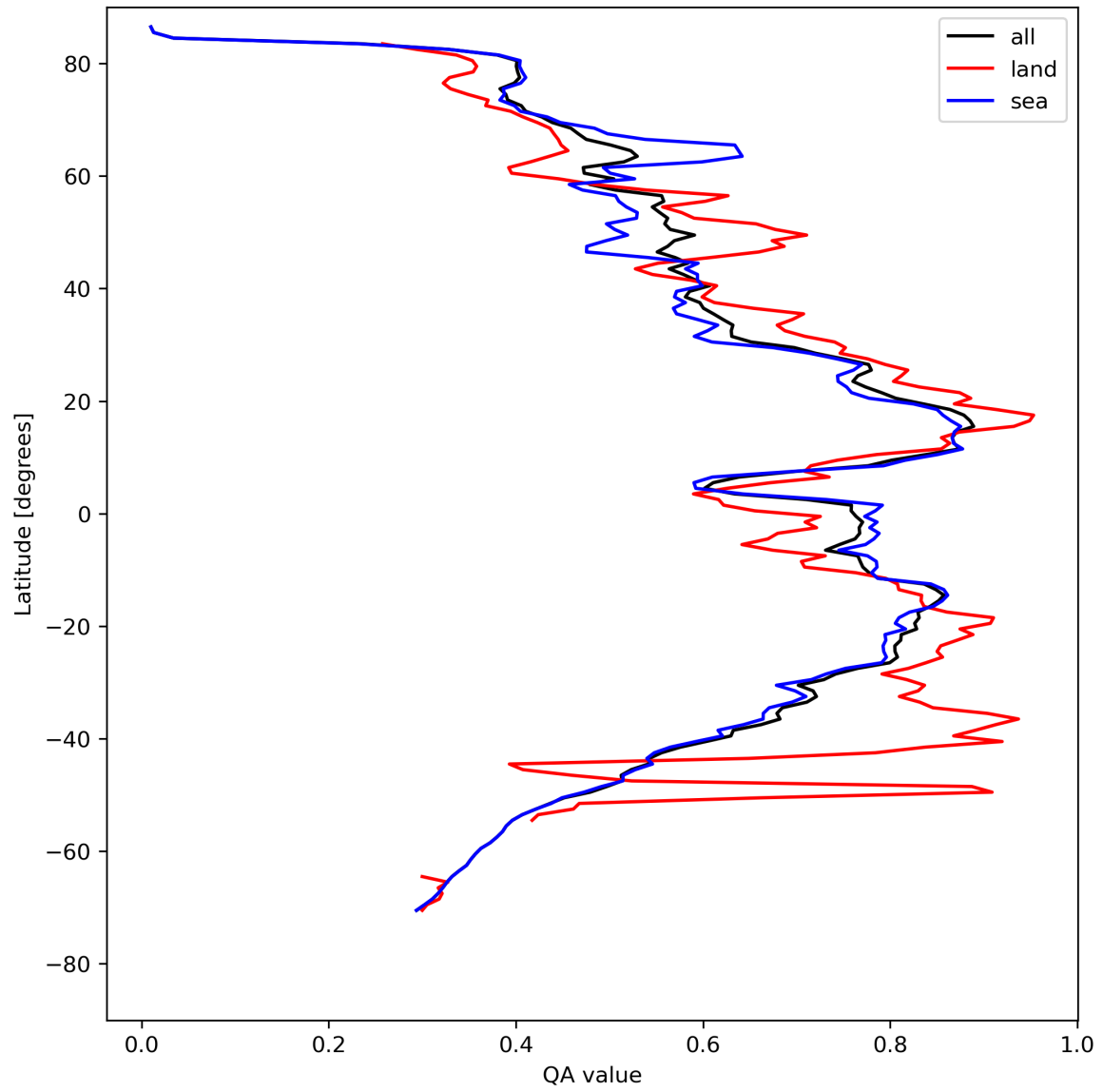
Figure 20: Zonal average of “QA value” for 2024-04-26 to 2024-04-28.
