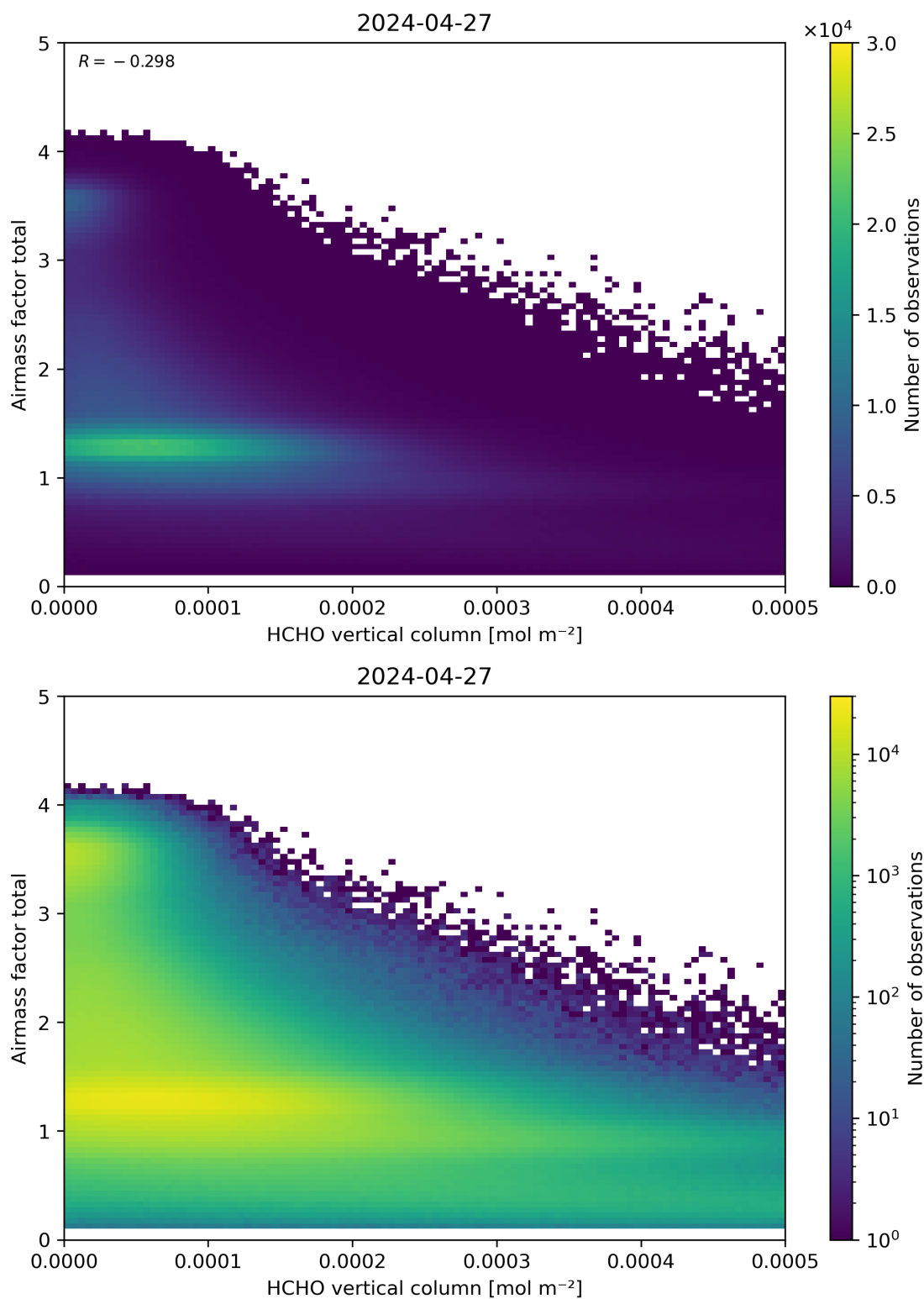
Figure 131: Scatter density plot of “HCHO vertical column” against “Airmass factor total” for 2024-04-26 to 2024-04-28.
