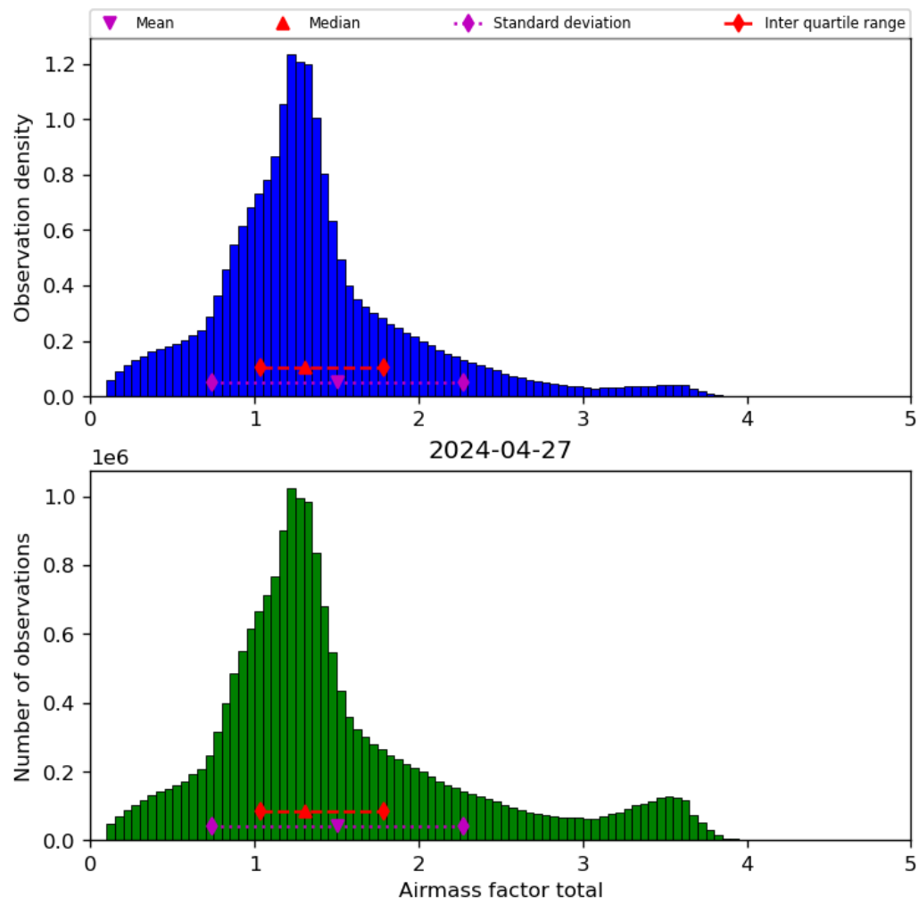
Figure 40: Histogram of “Airmass factor total” for 2024-04-26 to 2024-04-28
