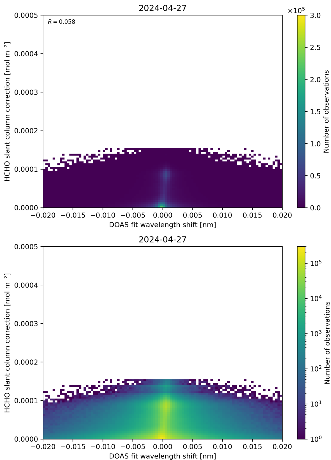
Figure 67: Scatter density plot of “DOAS fit wavelength shift” against “HCHO slant column correction” for 2024-04-26 to 2024-04-28.
