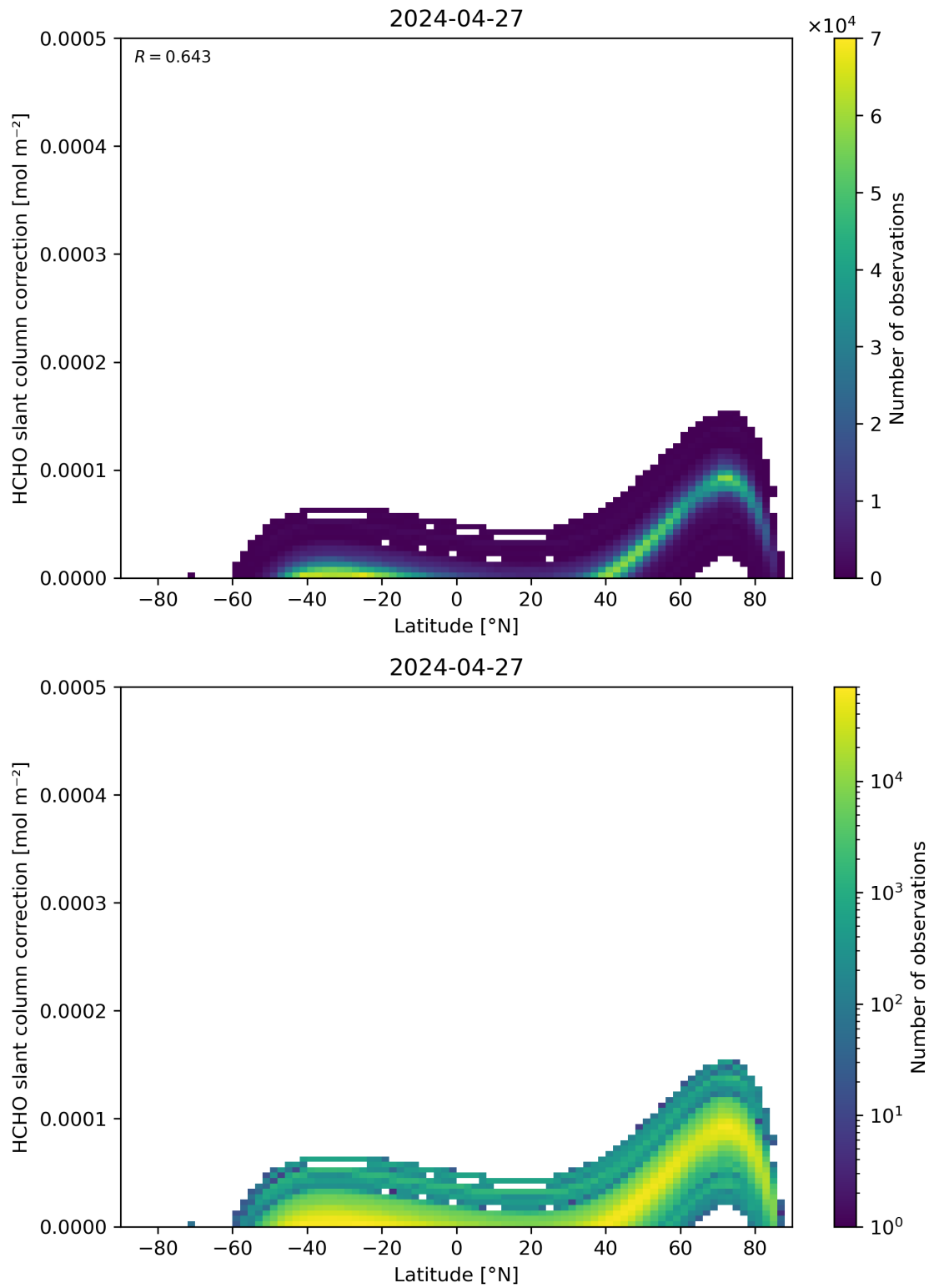
Figure 158: Scatter density plot of “Latitude” against “HCHO slant column correction” for 2024-04-26 to 2024-04-28.
