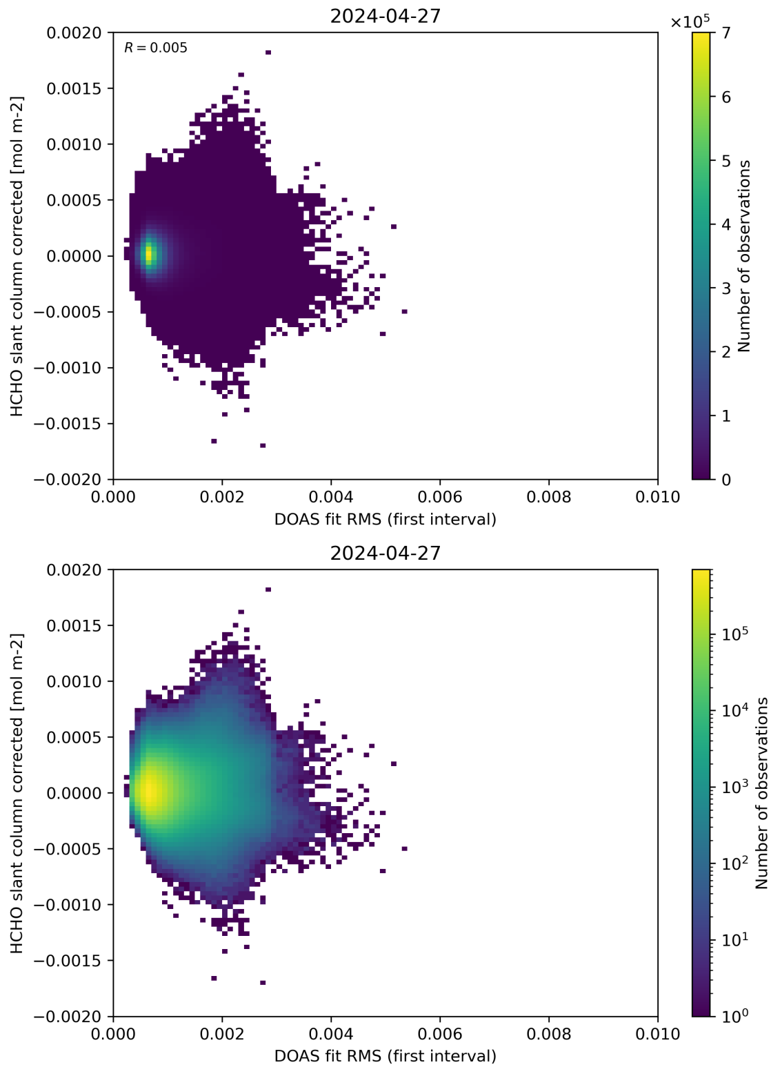
Figure 62: Scatter density plot of “DOAS fit RMS (first interval)” against “HCHO slant column corrected” for 2024-04-26 to 2024-04-28.
