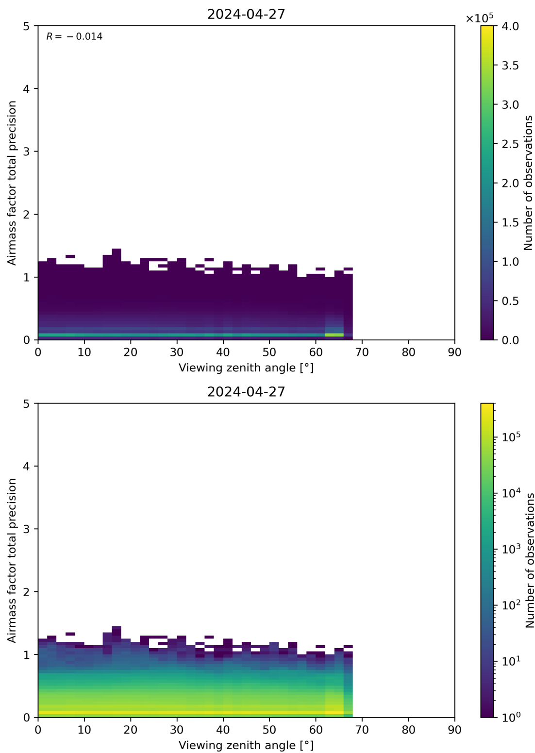
Figure 191: Scatter density plot of “Viewing zenith angle” against “Airmass factor total precision” for 2024-04-26 to 2024-04-28.
