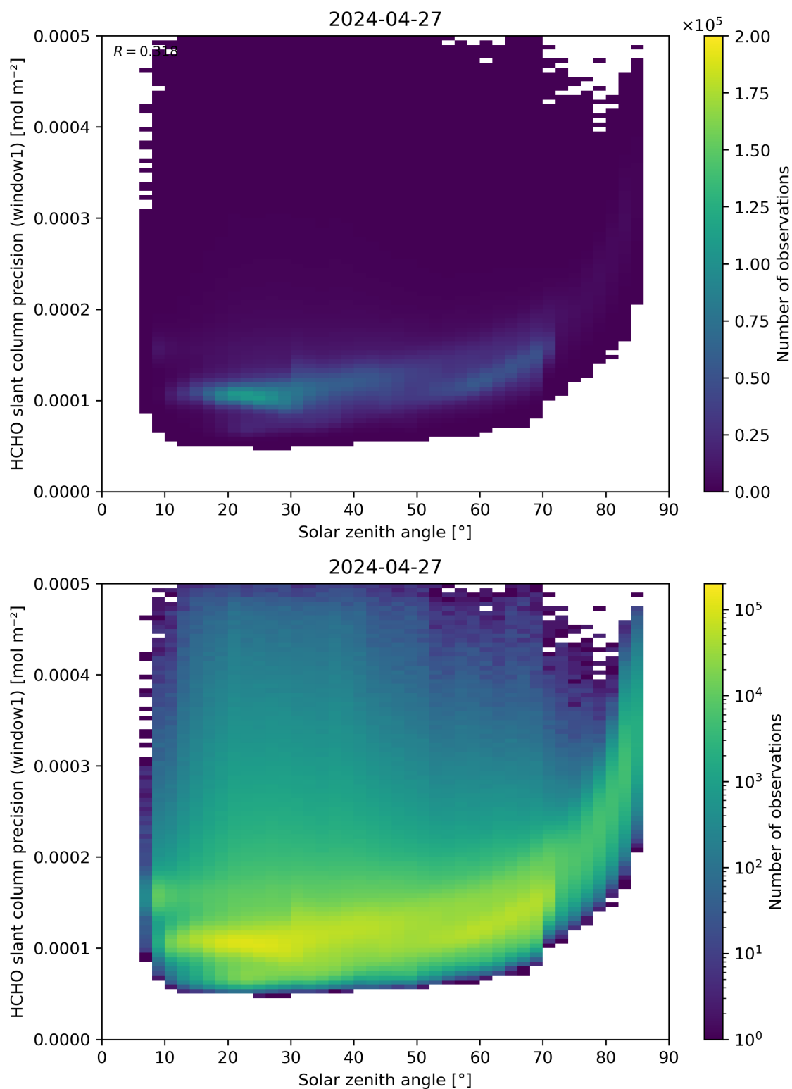
Figure 174: Scatter density plot of “Solar zenith angle” against “HCHO slant column precision (window1)” for 2024-04-26 to 2024-04-28.
