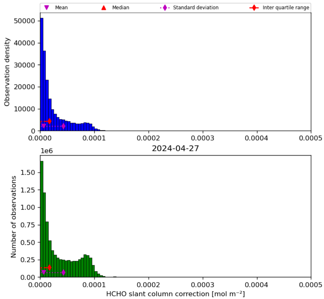
Figure 47: Histogram of “HCHO slant column correction” for 2024-04-26 to 2024-04-28
