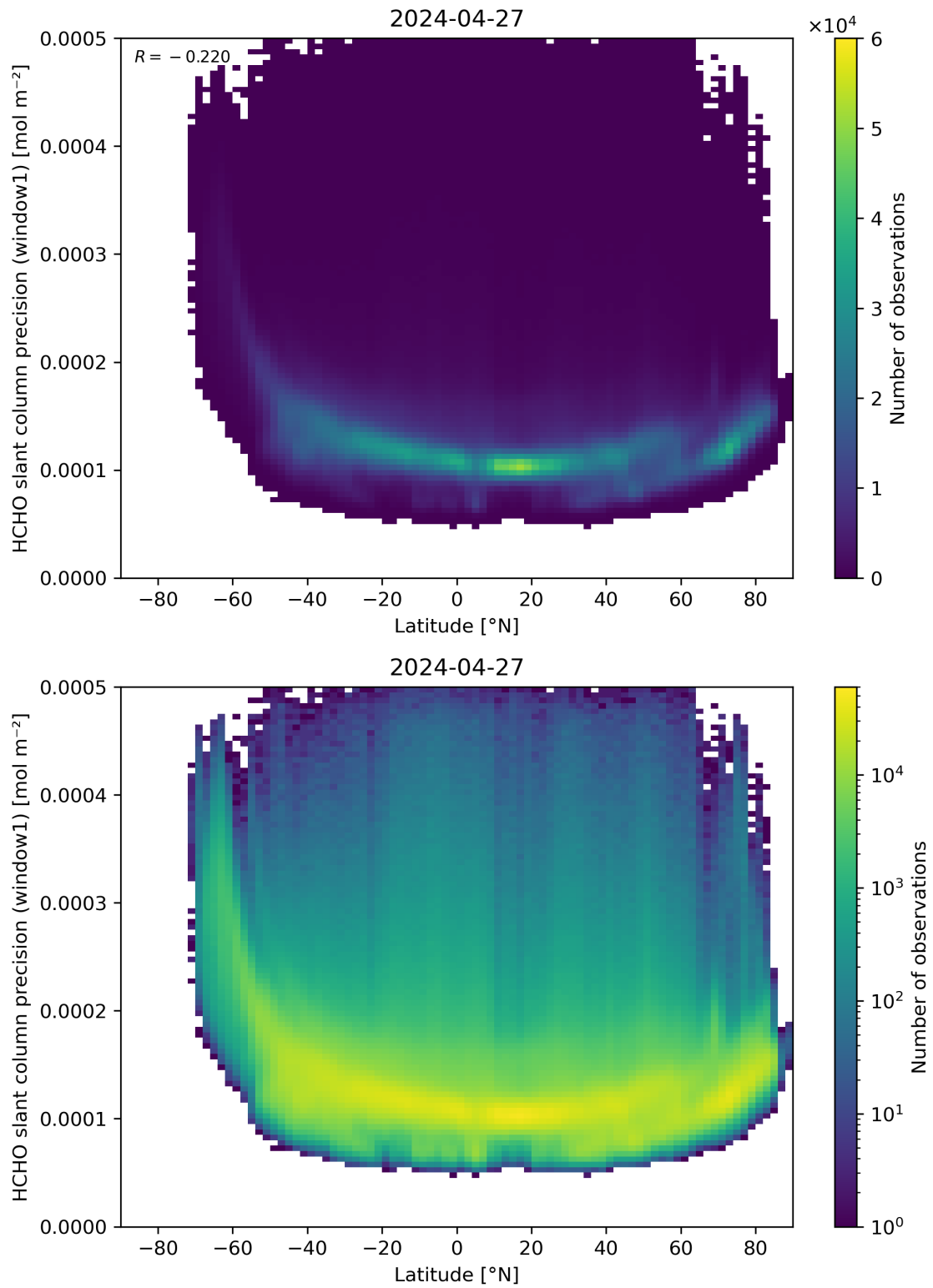
Figure 160: Scatter density plot of “Latitude” against “HCHO slant column precision (window1)” for 2024-04-26 to 2024-04-28.
