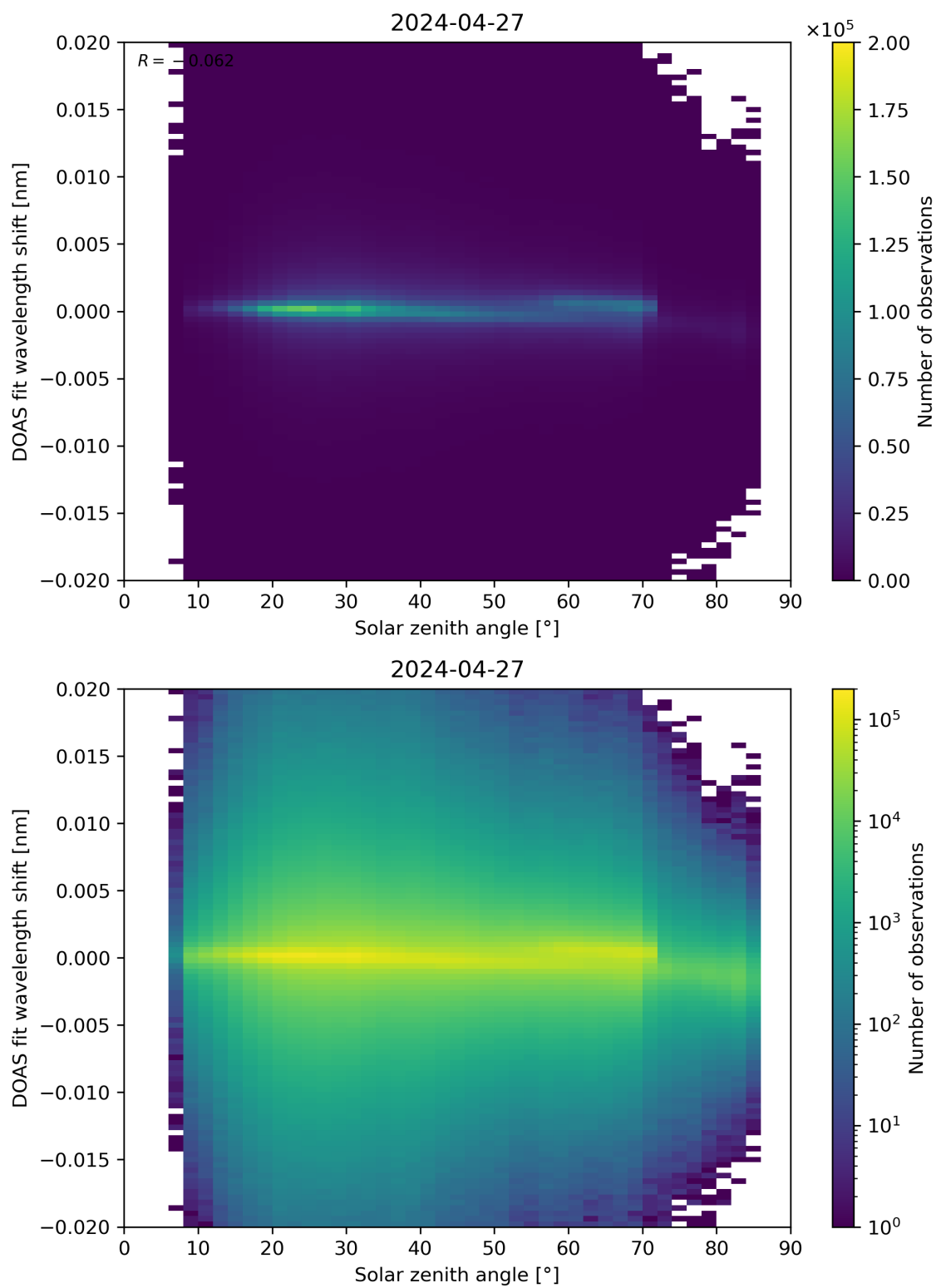
Figure 168: Scatter density plot of “Solar zenith angle” against “DOAS fit wavelength shift” for 2024-04-26 to 2024-04-28.
