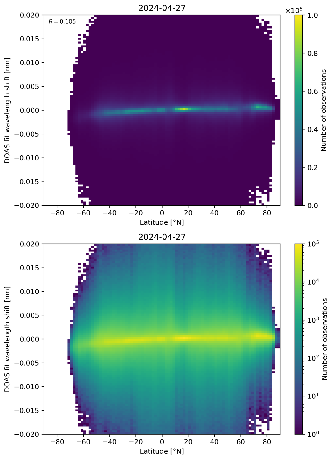
Figure 154: Scatter density plot of “Latitude” against “DOAS fit wavelength shift” for 2024-04-26 to 2024-04-28.
