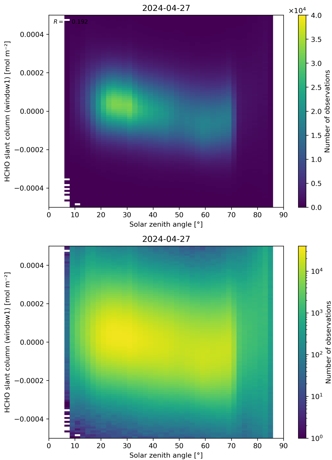
Figure 173: Scatter density plot of “Solar zenith angle” against “HCHO slant column (window1)” for 2024-04-26 to 2024-04-28.
