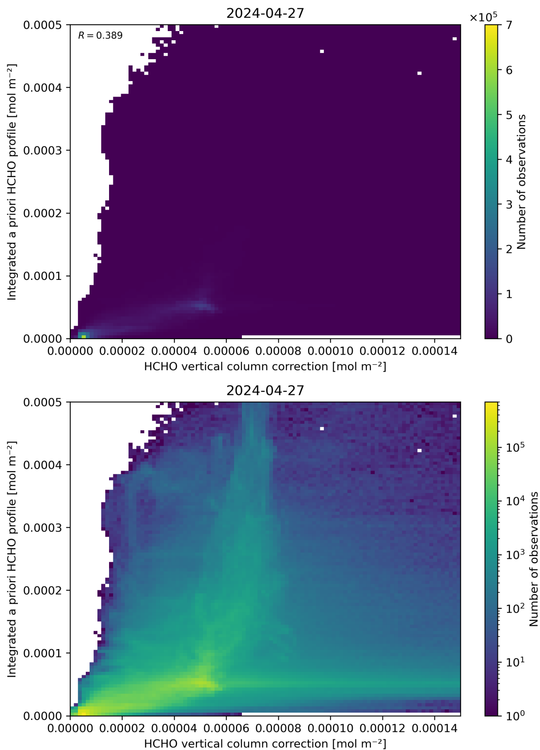
Figure 122: Scatter density plot of “HCHO vertical column correction” against “Integrated a priori HCHO profile” for 2024-04-26 to 2024-04-28.
