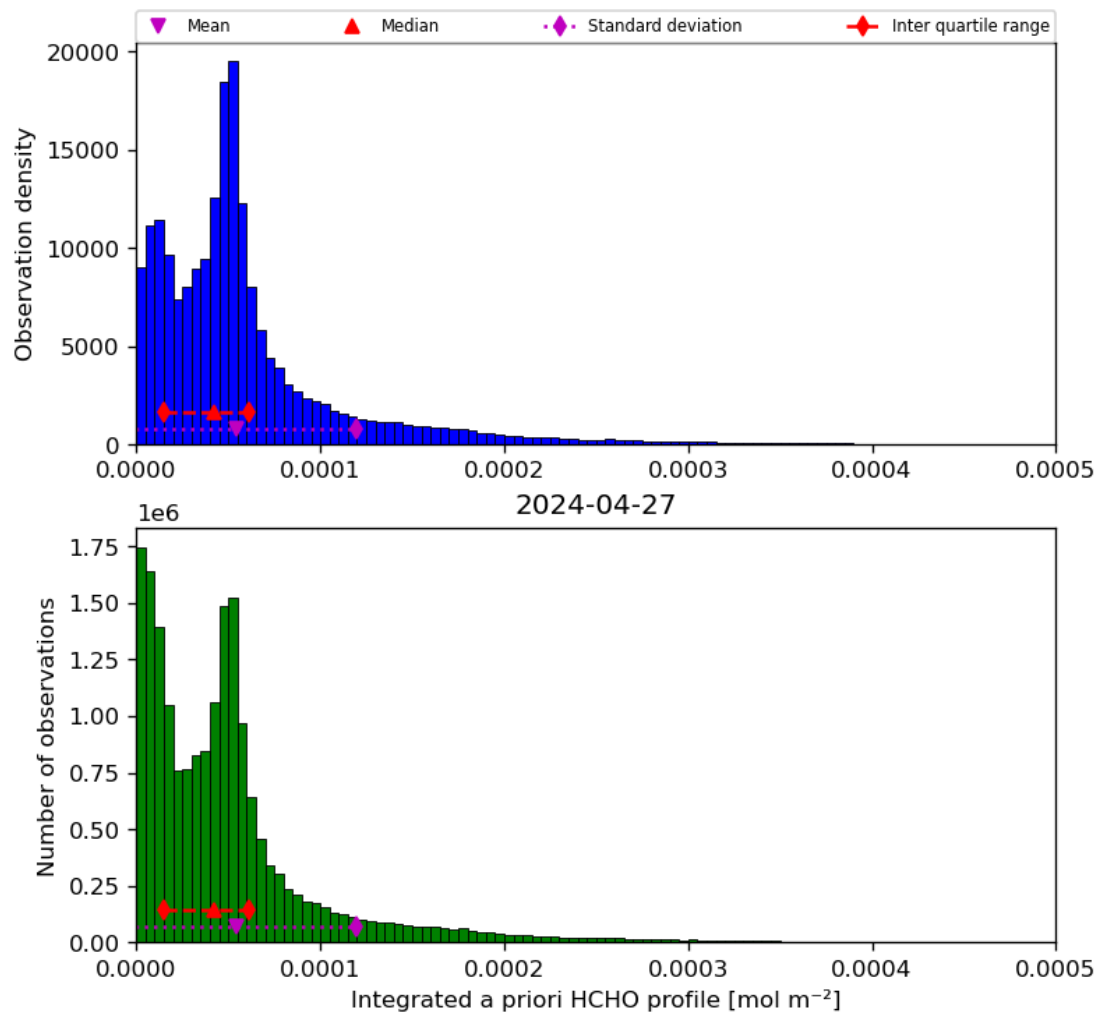
Figure 43: Histogram of “Integrated a priori HCHO profile” for 2024-04-26 to 2024-04-28
