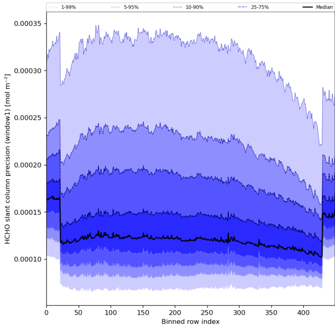
Figure 53: Along track statistics of “HCHO slant column precision (window1)” for 2024-04-26 to 2024-04-28
