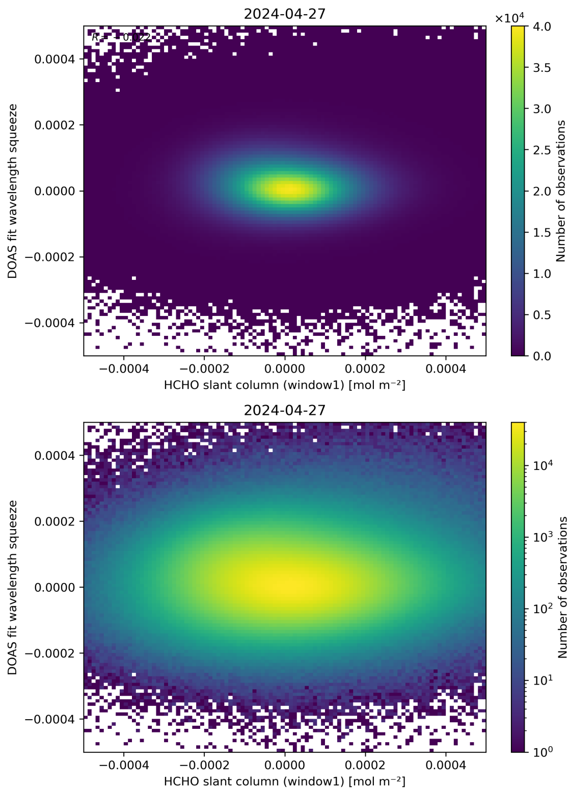
Figure 80: Scatter density plot of “HCHO slant column (window1)” against “DOAS fit wavelength squeeze” for 2024-04-26 to 2024-04-28.
