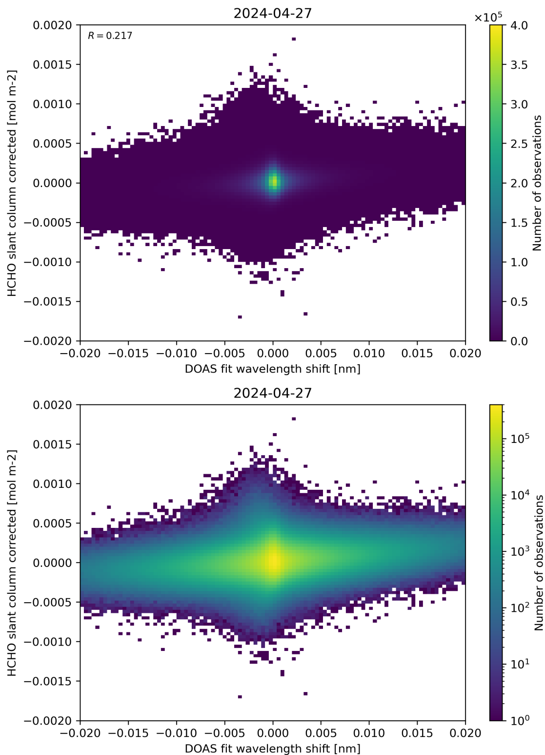
Figure 66: Scatter density plot of “DOAS fit wavelength shift” against “HCHO slant column corrected” for 2024-04-26 to 2024-04-28.
