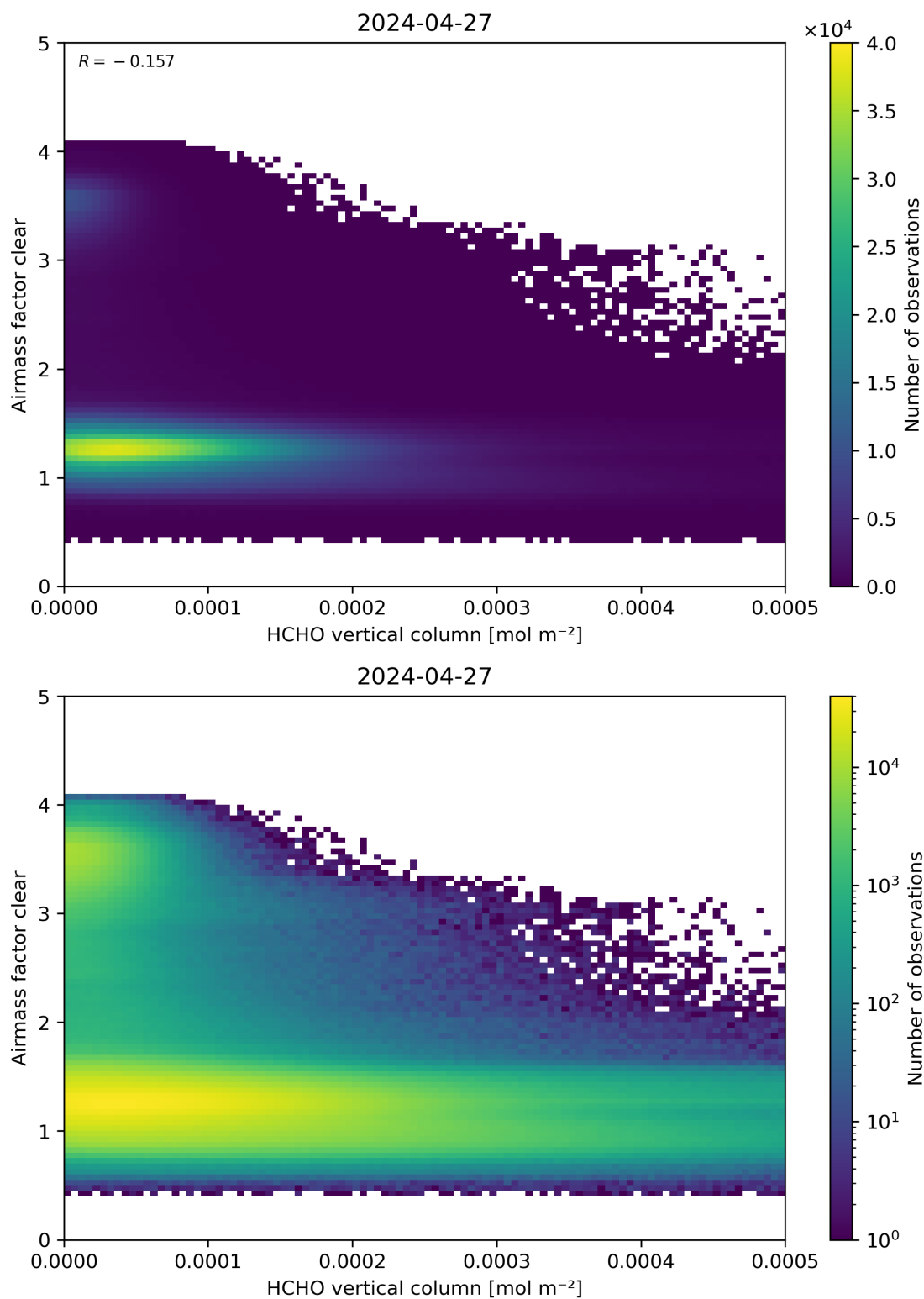
Figure 126: Scatter density plot of “HCHO vertical column” against “Airmass factor clear” for 2024-04-26 to 2024-04-28.
