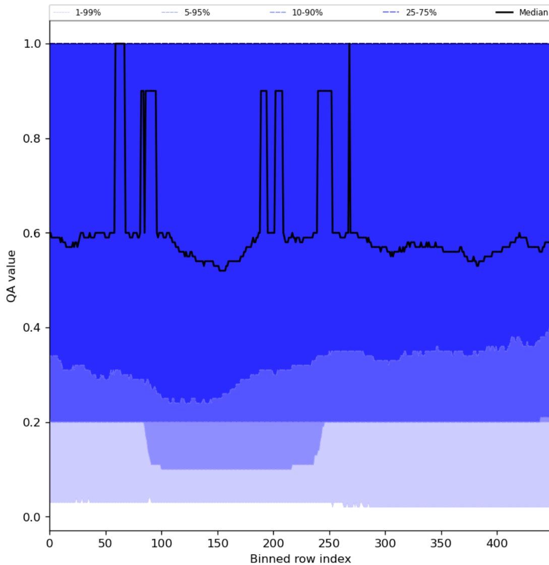
Figure 48: Along track statistics of “QA value” for 2024-04-26 to 2024-04-28
