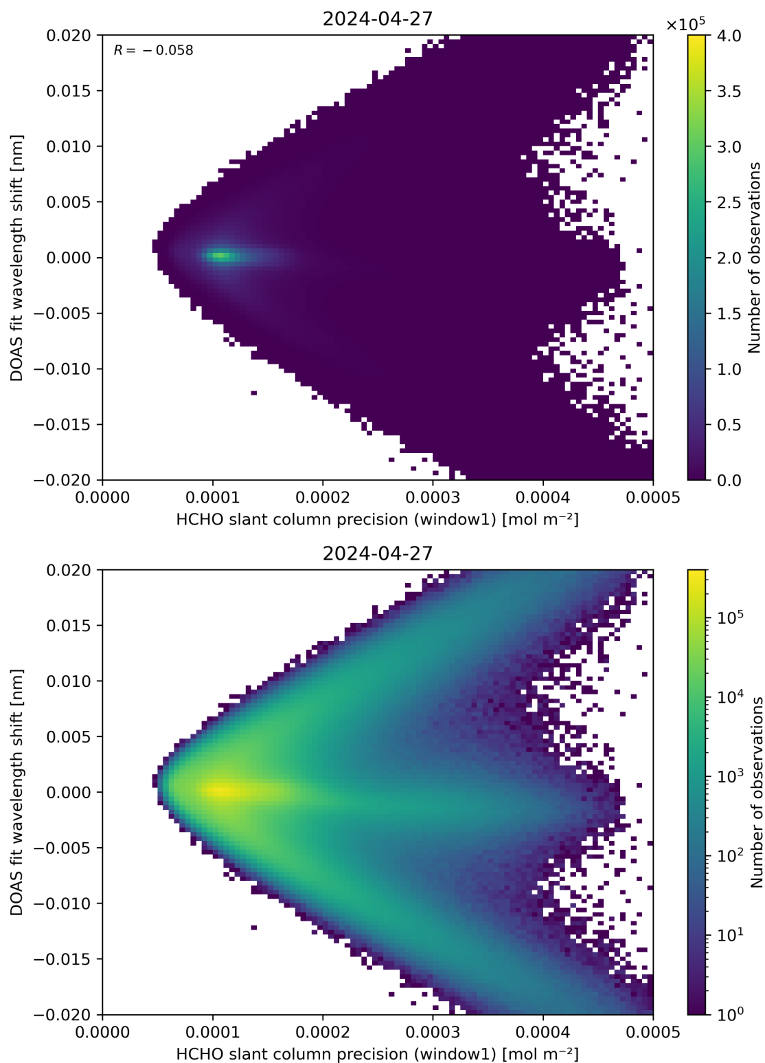
Figure 89: Scatter density plot of “HCHO slant column precision (window1)” against “DOAS fit wavelength shift” for 2024-04-26 to 2024-04-28.
