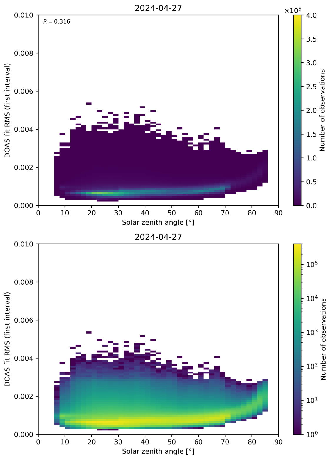
Figure 167: Scatter density plot of “Solar zenith angle” against “DOAS fit RMS (first interval)” for 2024-04-26 to 2024-04-28.
