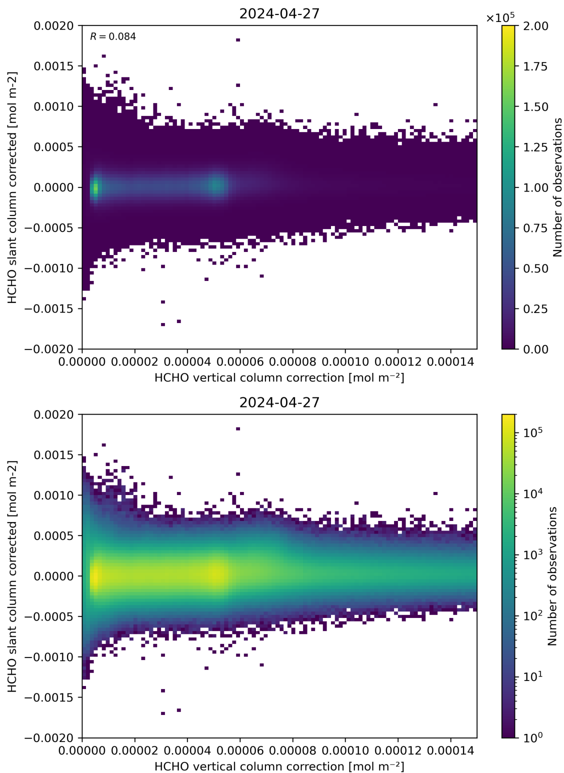
Figure 116: Scatter density plot of “HCHO vertical column correction” against “HCHO slant column corrected” for 2024-04-26 to 2024-04-28.
