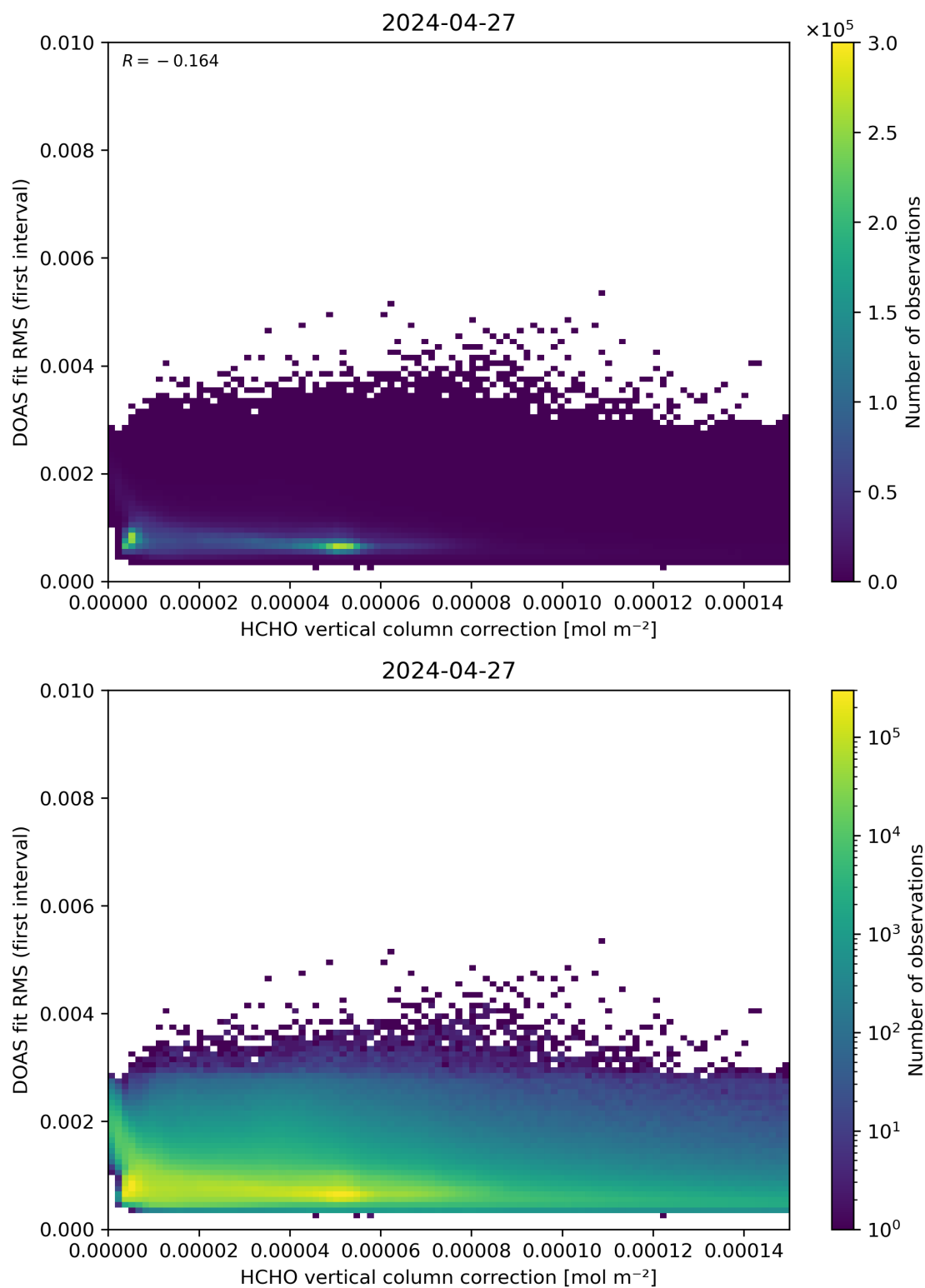
Figure 112: Scatter density plot of “HCHO vertical column correction” against “DOAS fit RMS (first interval)” for 2024-04-26 to 2024-04-28.
