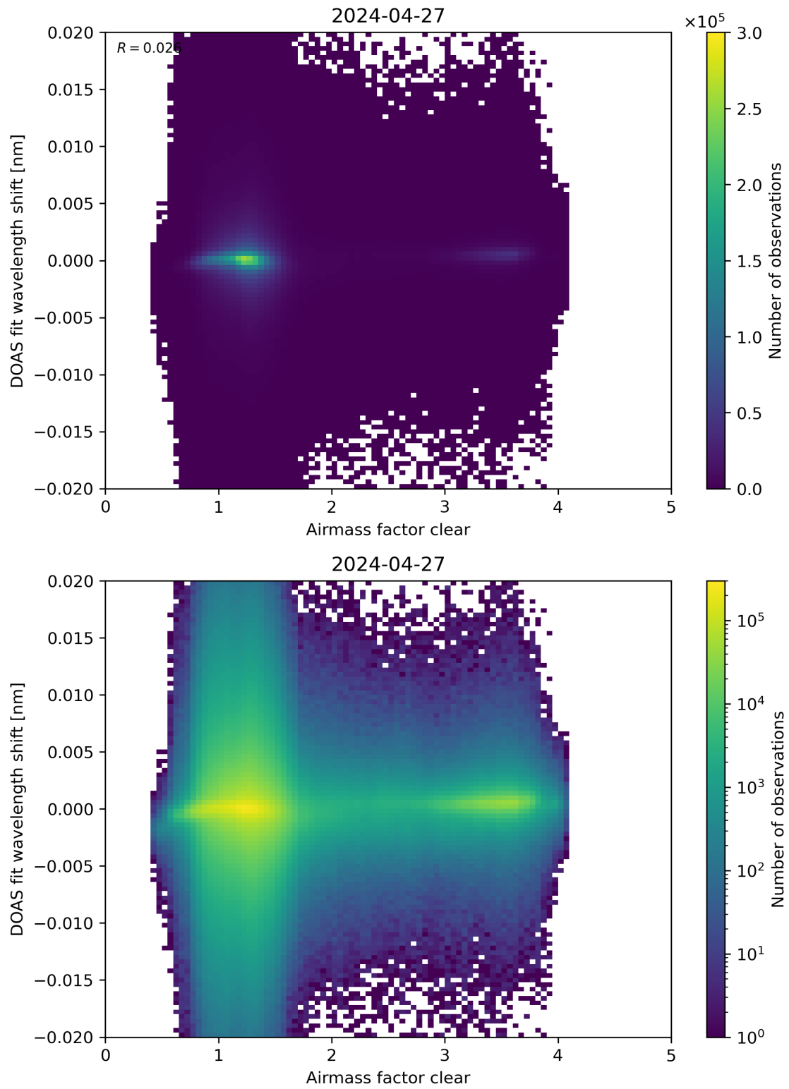
Figure 72: Scatter density plot of “Airmass factor clear” against “DOAS fit wavelength shift” for 2024-04-26 to 2024-04-28.
