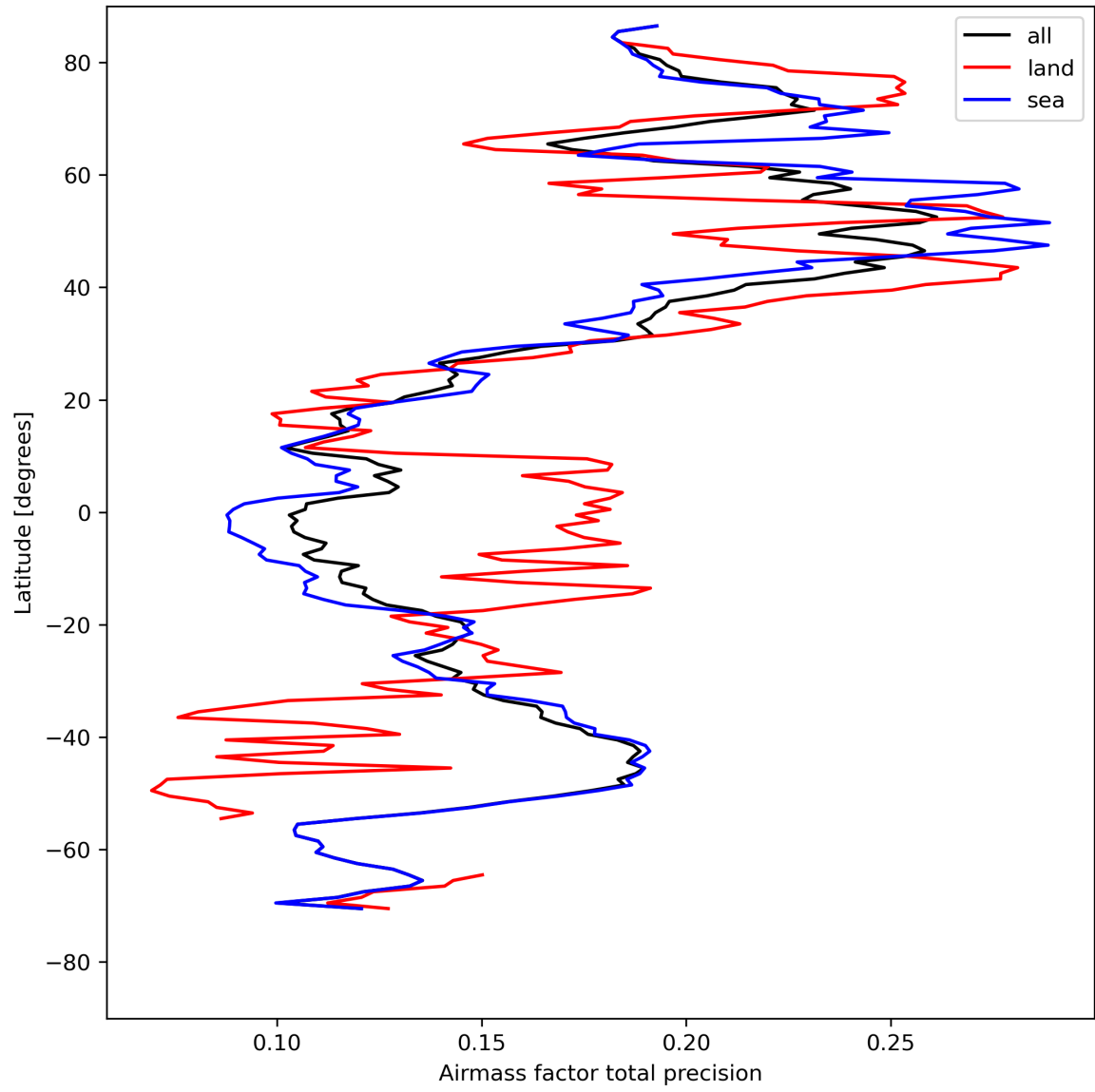
Figure 27: Zonal average of “Airmass factor total precision” for 2024-04-26 to 2024-04-28.
