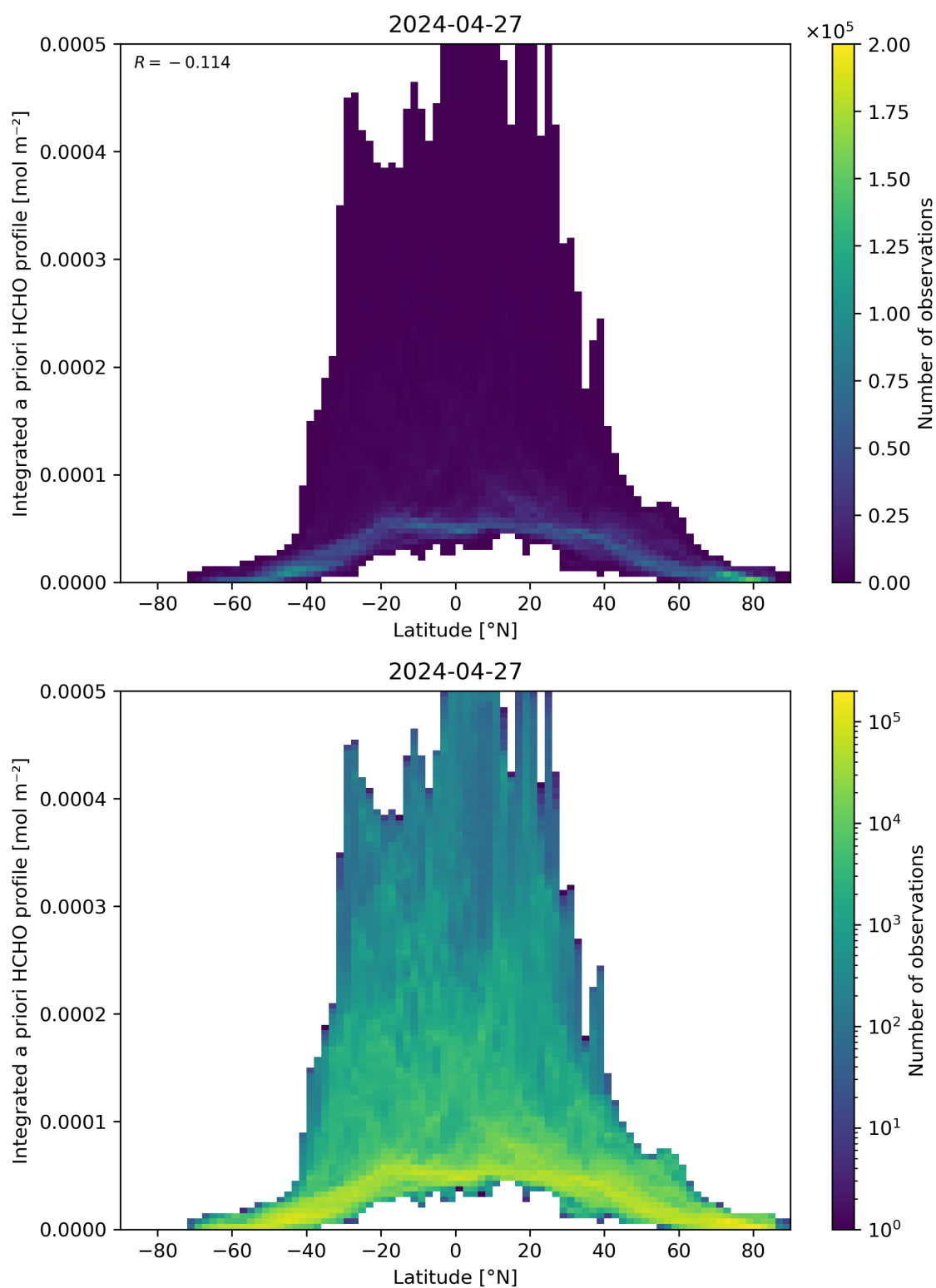
Figure 166: Scatter density plot of “Latitude” against “Integrated a priori HCHO profile” for 2024-04-26 to 2024-04-28.
