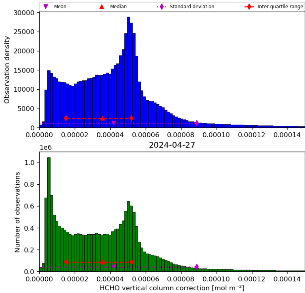
Figure 37: Histogram of “HCHO vertical column correction” for 2024-04-26 to 2024-04-28
