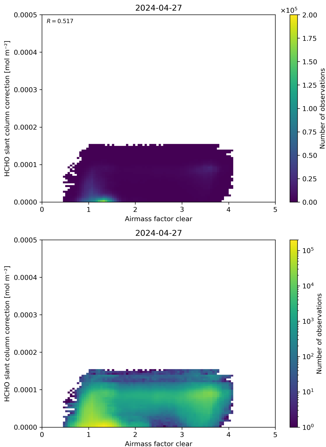
Figure 75: Scatter density plot of “Airmass factor clear” against “HCHO slant column correction” for 2024-04-26 to 2024-04-28.
