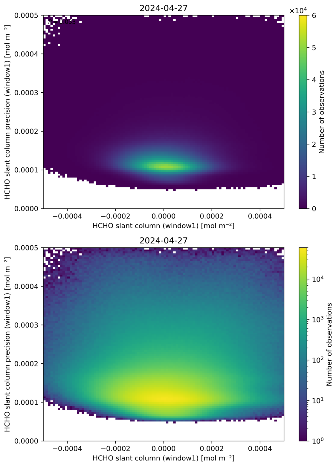
Figure 84: Scatter density plot of “HCHO slant column (window1)” against “HCHO slant column precision (window1)” for 2024-04-26 to 2024-04-28.
