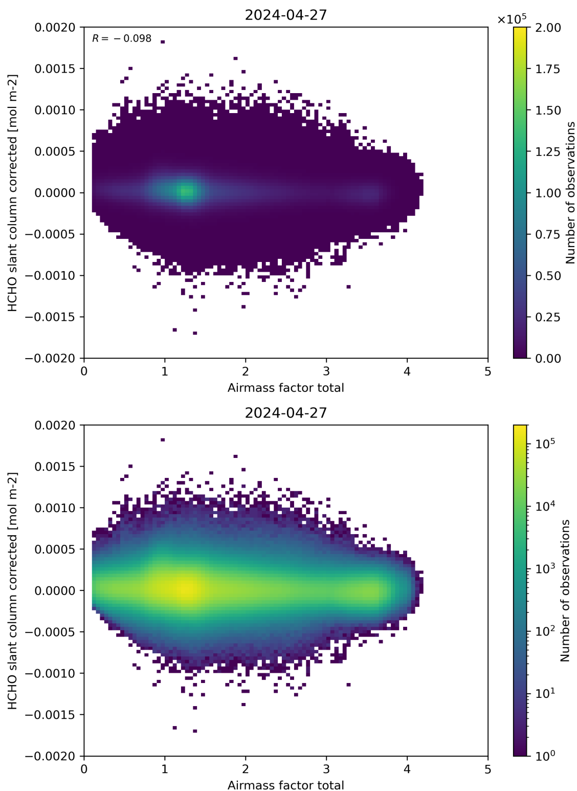
Figure 101: Scatter density plot of “Airmass factor total” against “HCHO slant column corrected” for 2024-04-26 to 2024-04-28.
