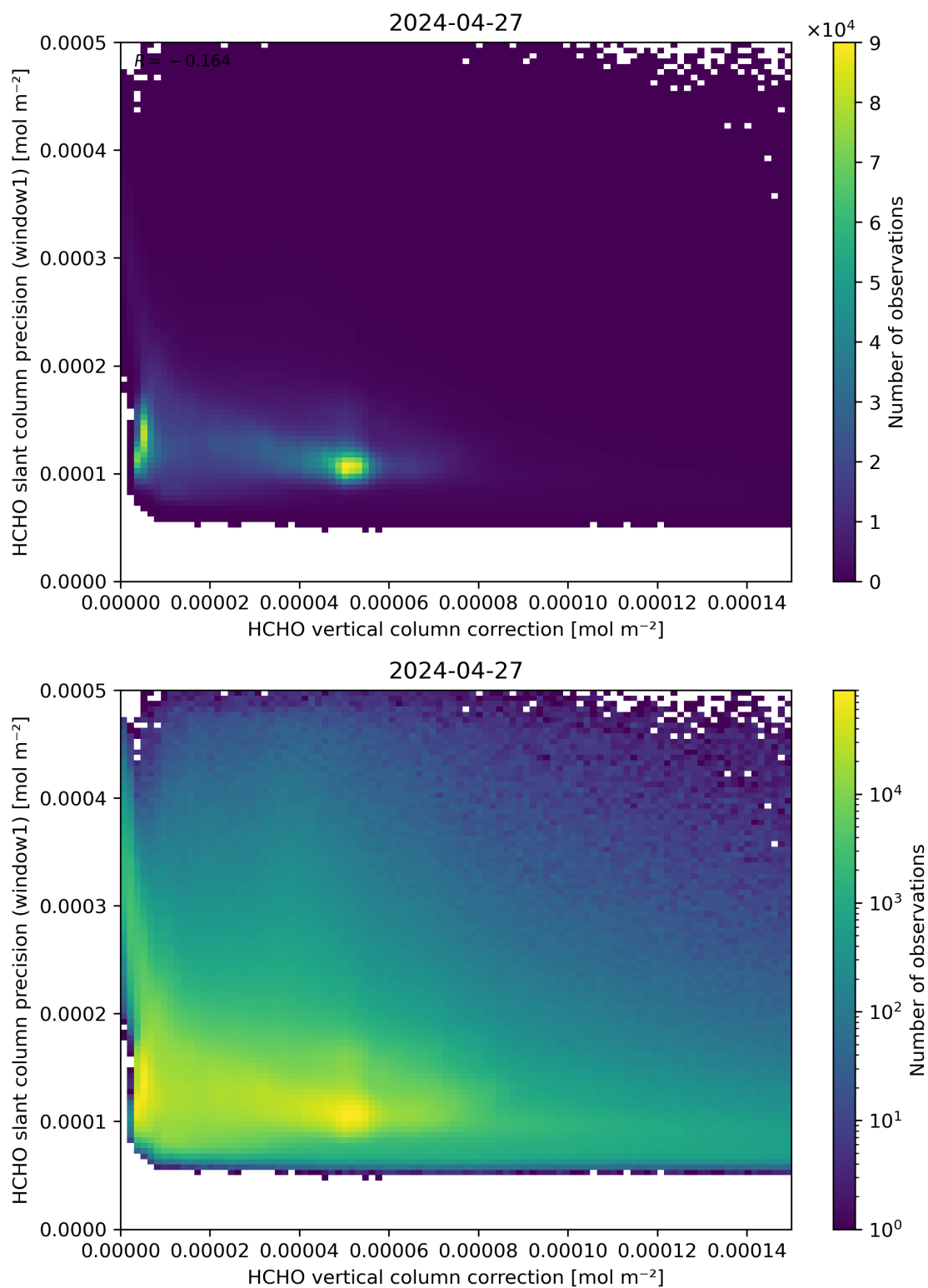
Figure 119: Scatter density plot of “HCHO vertical column correction” against “HCHO slant column precision (window1)” for 2024-04-26 to 2024-04-28.
