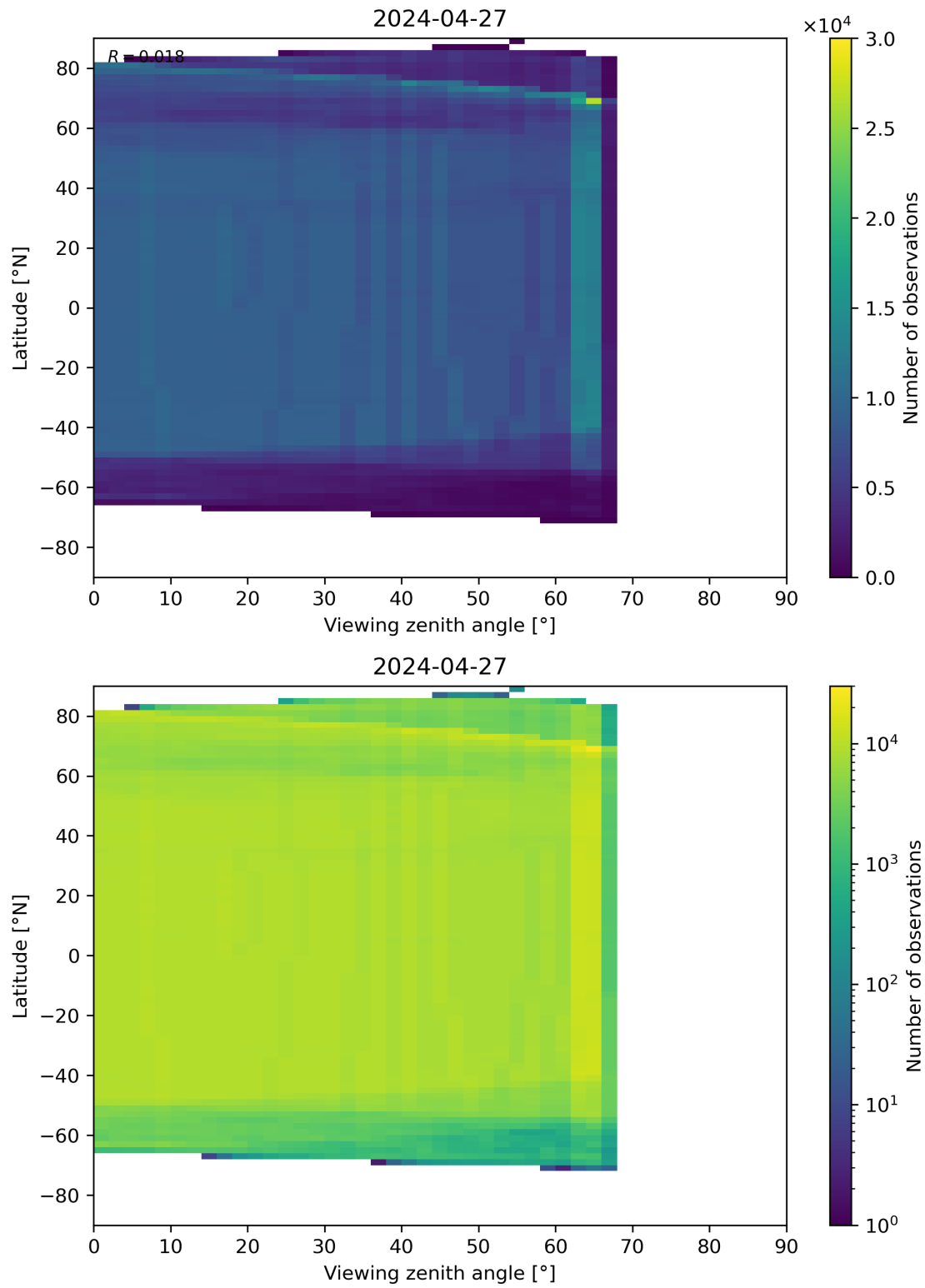
Figure 196: Scatter density plot of “Viewing zenith angle” against “Latitude” for 2024-04-26 to 2024-04-28.
