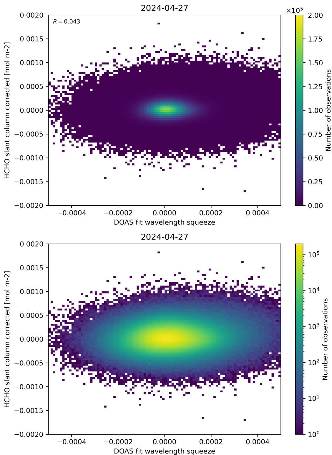
Figure 69: Scatter density plot of “DOAS fit wavelength squeeze” against “HCHO slant column corrected” for 2024-04-26 to 2024-04-28.
