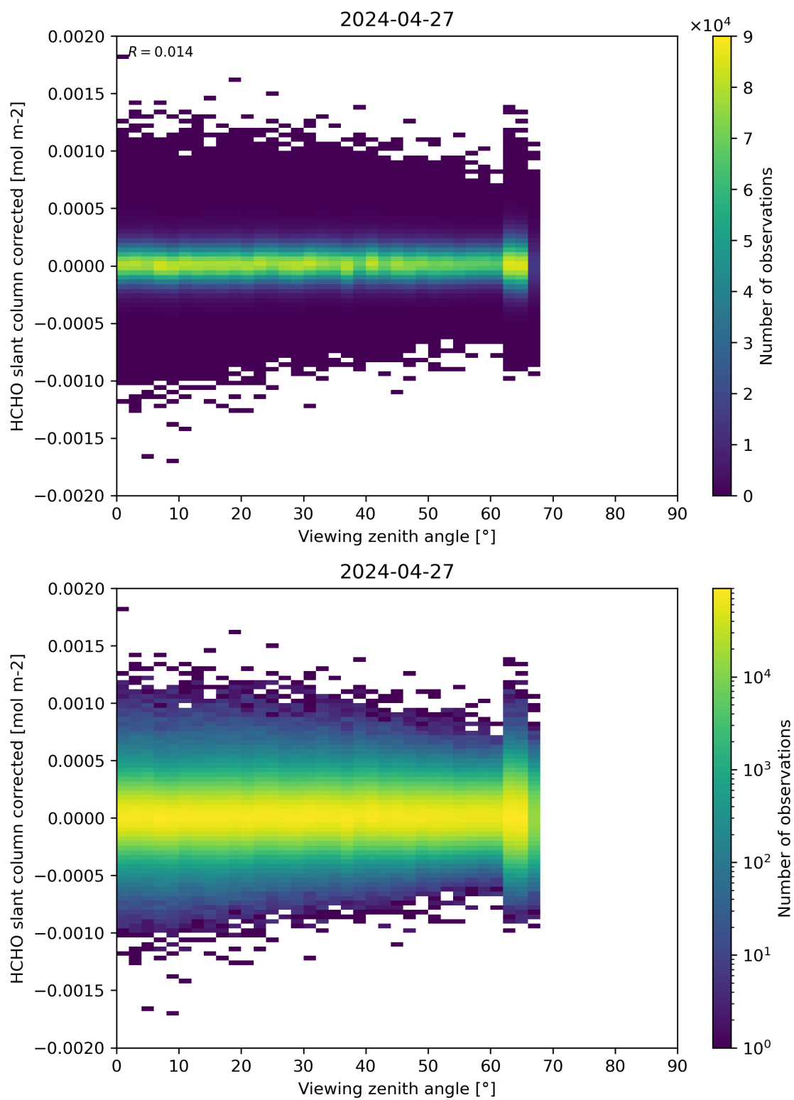
Figure 186: Scatter density plot of “Viewing zenith angle” against “HCHO slant column corrected” for 2024-04-26 to 2024-04-28.
