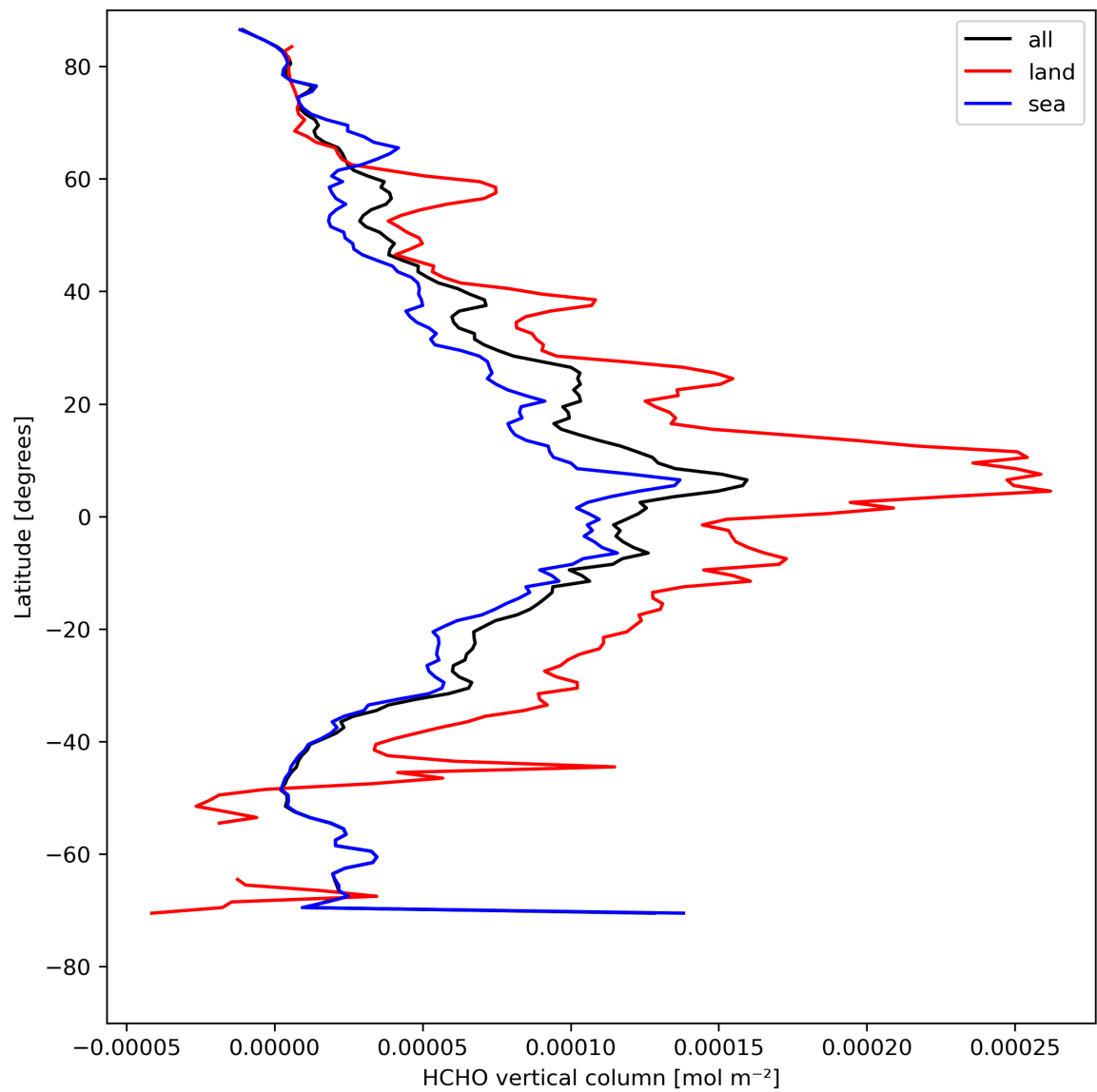
Figure 21: Zonal average of “HCHO vertical column” for 2024-04-26 to 2024-04-28.
