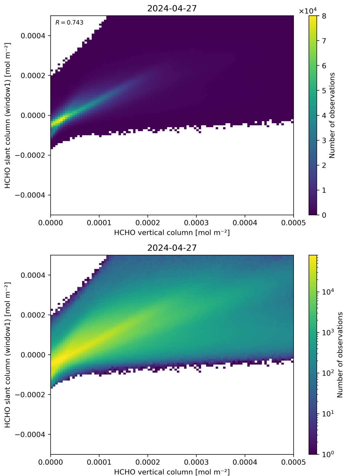
Figure 129: Scatter density plot of “HCHO vertical column” against “HCHO slant column (window1)” for 2024-04-26 to 2024-04-28.
