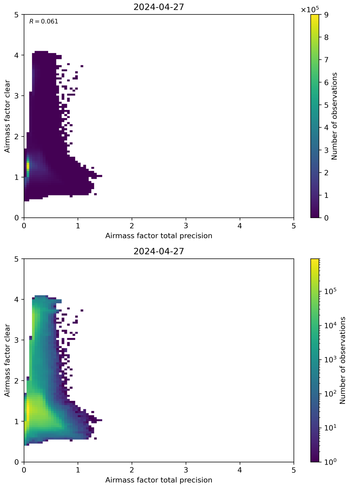
Figure 108: Scatter density plot of “Airmass factor total precision” against “Airmass factor clear” for 2024-04-26 to 2024-04-28.
