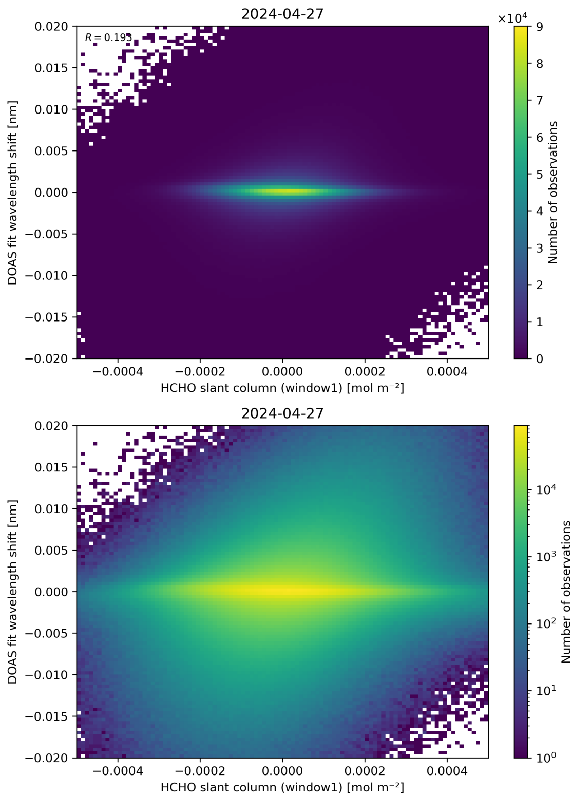
Figure 79: Scatter density plot of “HCHO slant column (window1)” against “DOAS fit wavelength shift” for 2024-04-26 to 2024-04-28.
