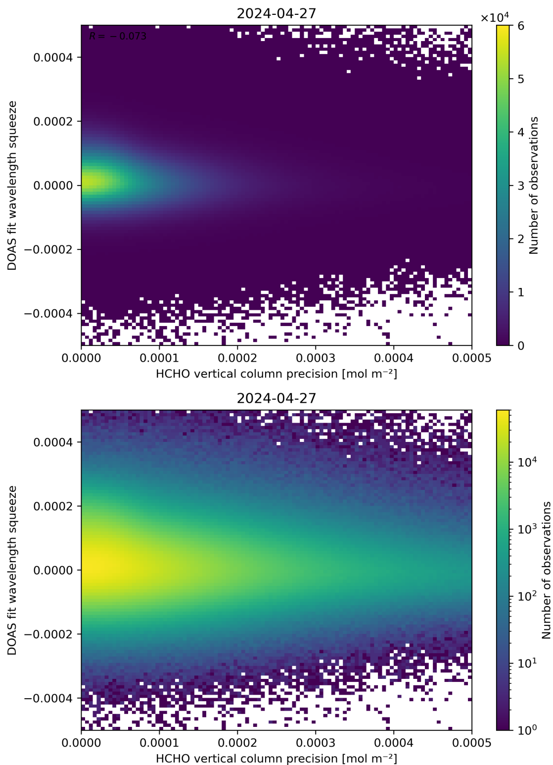
Figure 138: Scatter density plot of “HCHO vertical column precision” against “DOAS fit wavelength squeeze” for 2024-04-26 to 2024-04-28.
