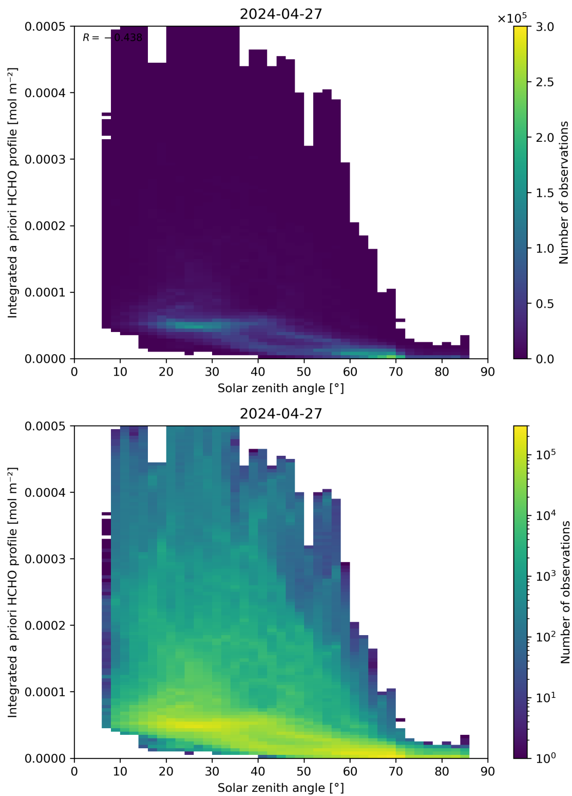
Figure 180: Scatter density plot of “Solar zenith angle” against “Integrated a priori HCHO profile” for 2024-04-26 to 2024-04-28.
