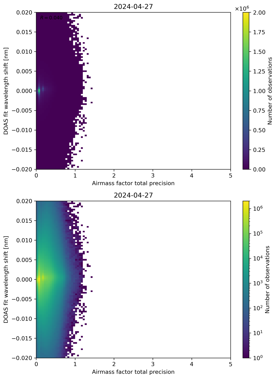
Figure 106: Scatter density plot of “Airmass factor total precision” against “DOAS fit wavelength shift” for 2024-04-26 to 2024-04-28.
