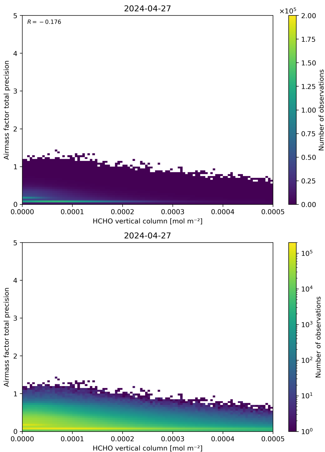
Figure 132: Scatter density plot of “HCHO vertical column” against “Airmass factor total precision” for 2024-04-26 to 2024-04-28.
