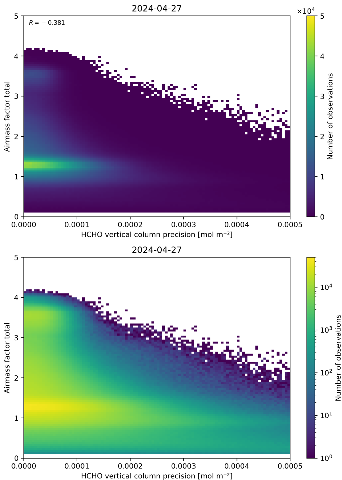
Figure 144: Scatter density plot of “HCHO vertical column precision” against “Airmass factor total” for 2024-04-26 to 2024-04-28.
