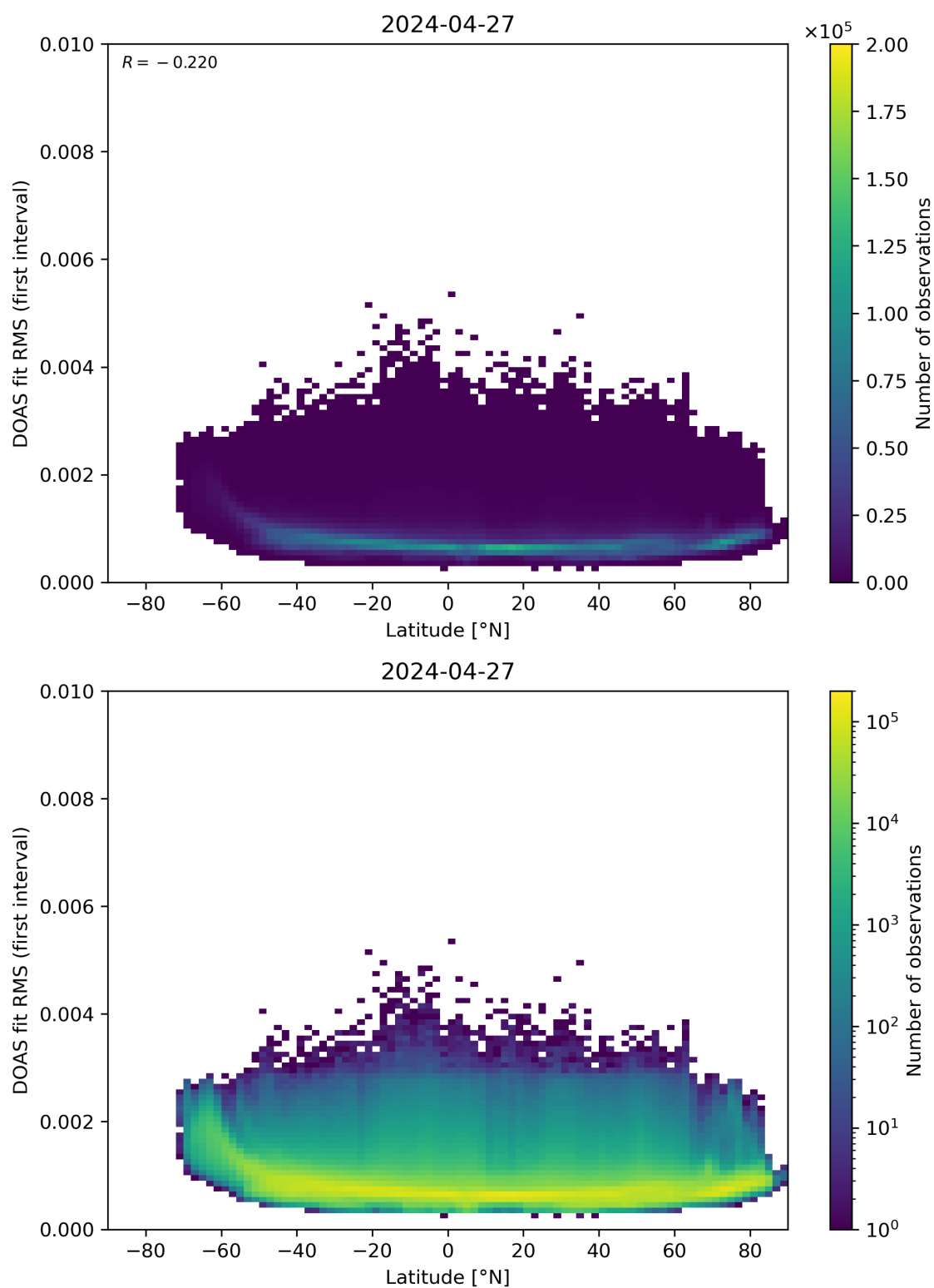
Figure 153: Scatter density plot of “Latitude” against “DOAS fit RMS (first interval)” for 2024-04-26 to 2024-04-28.
