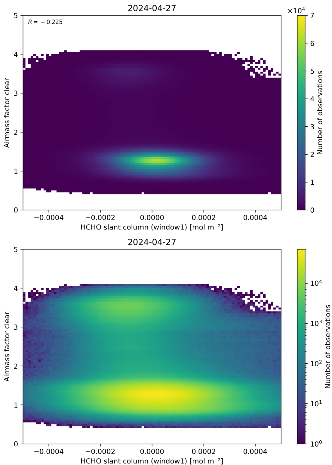
Figure 81: Scatter density plot of “HCHO slant column (window1)” against “Airmass factor clear” for 2024-04-26 to 2024-04-28.
