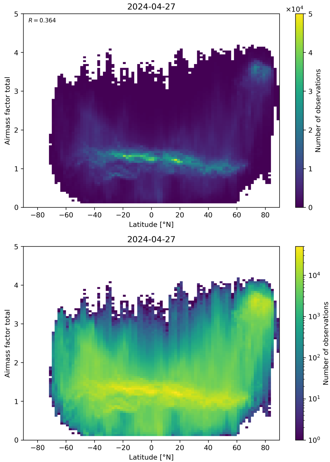
Figure 161: Scatter density plot of “Latitude” against “Airmass factor total” for 2024-04-26 to 2024-04-28.
