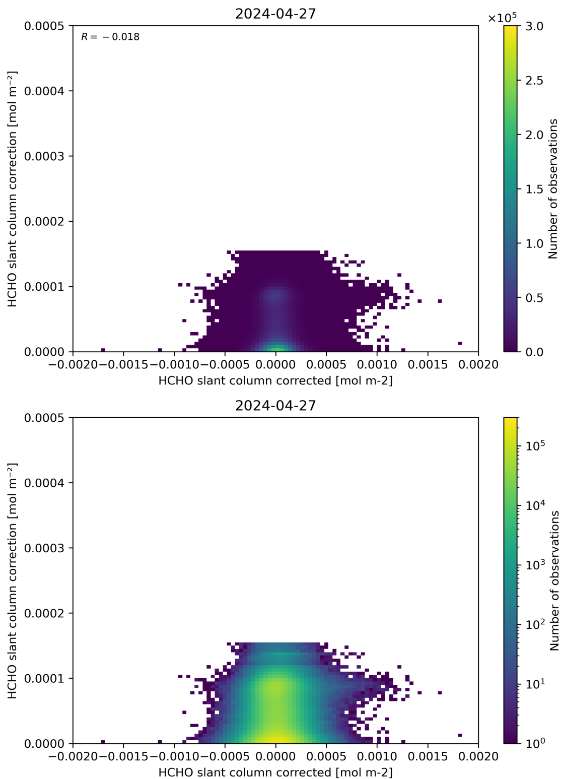
Figure 77: Scatter density plot of “HCHO slant column corrected” against “HCHO slant column correction” for 2024-04-26 to 2024-04-28.
