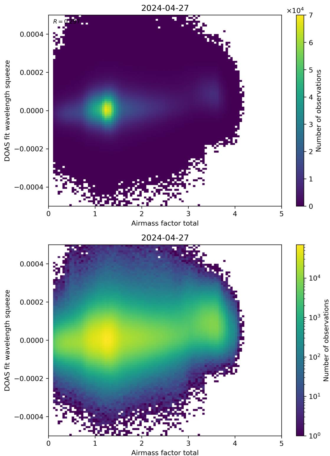
Figure 99: Scatter density plot of “Airmass factor total” against “DOAS fit wavelength squeeze” for 2024-04-26 to 2024-04-28.
