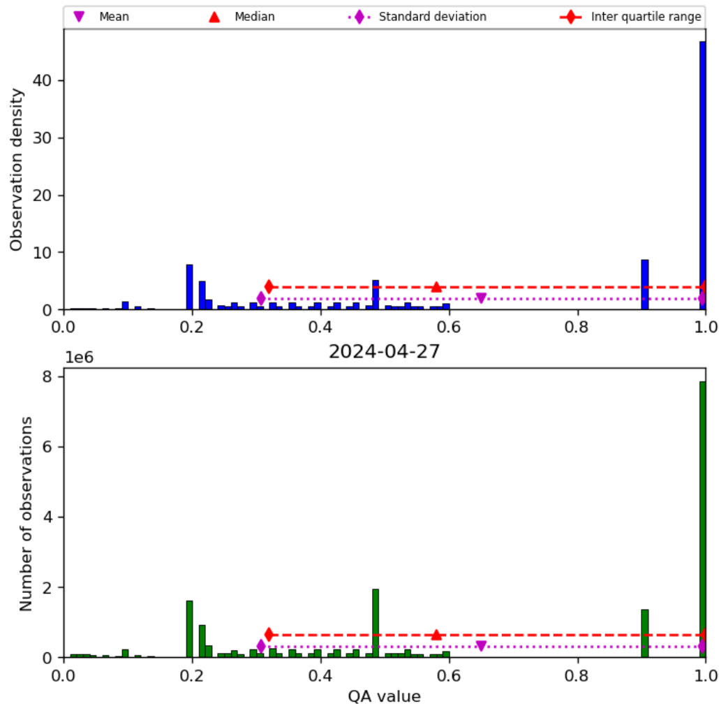
Figure 34: Histogram of “QA value” for 2024-04-26 to 2024-04-28
