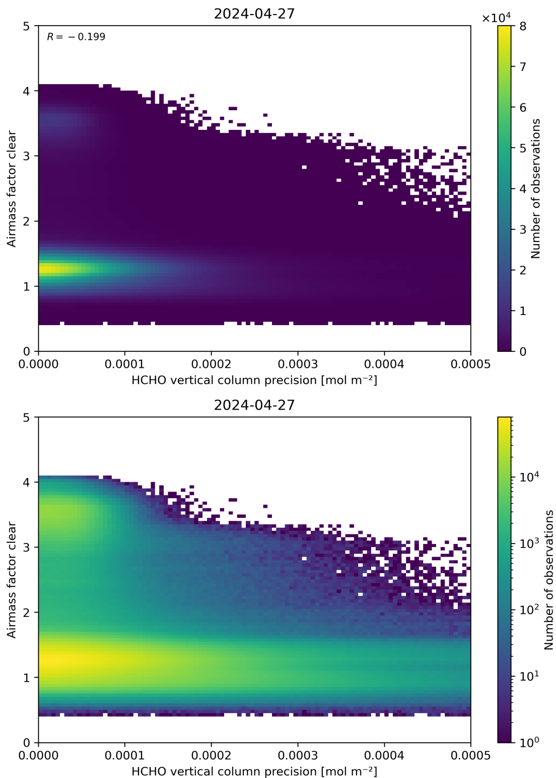
Figure 139: Scatter density plot of “HCHO vertical column precision” against “Airmass factor clear” for 2024-04-26 to 2024-04-28.
