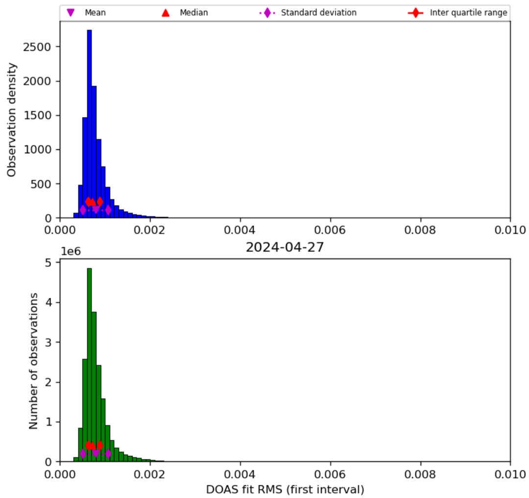
Figure 46: Histogram of “DOAS fit RMS (first interval)” for 2024-04-26 to 2024-04-28
