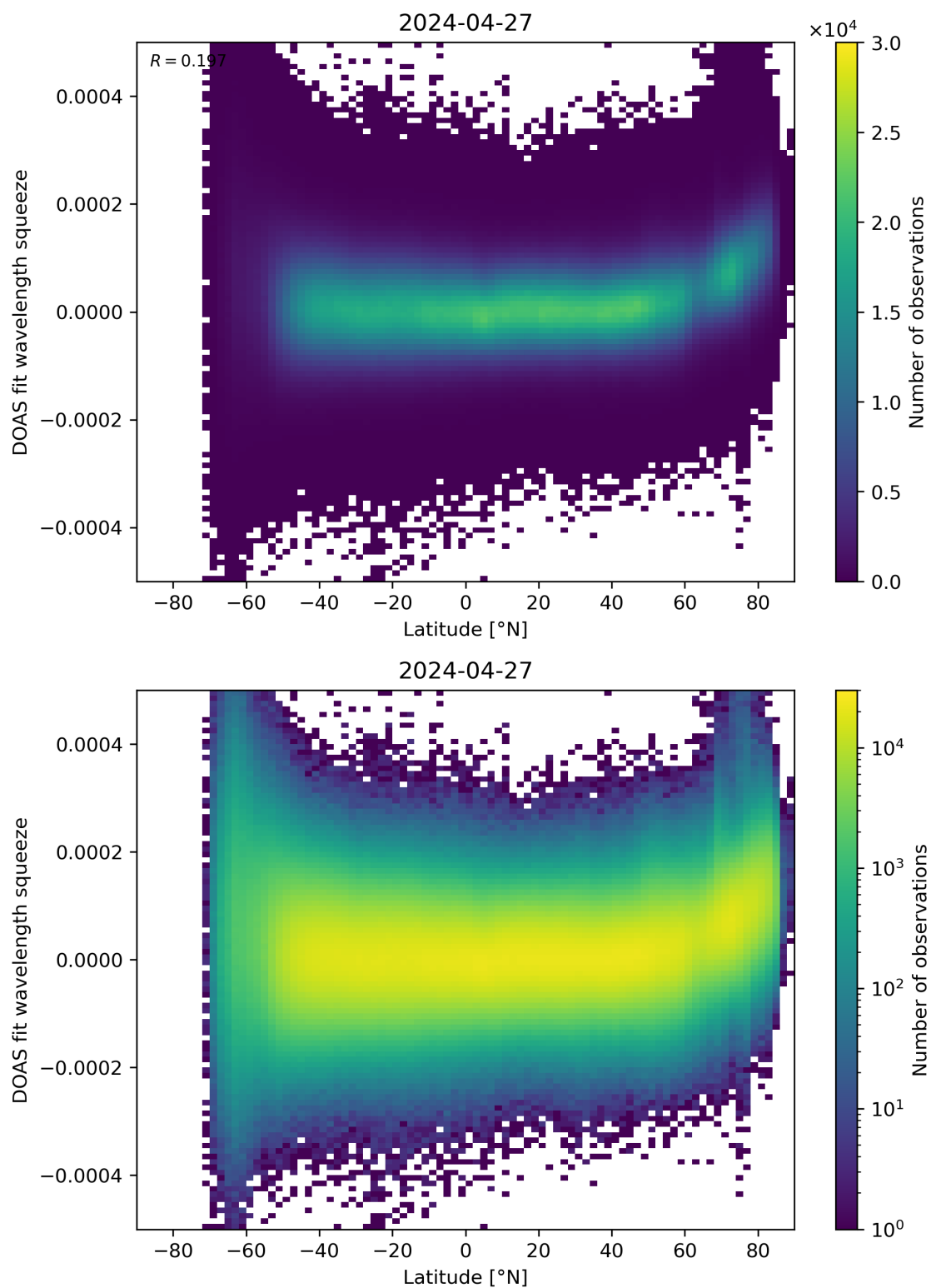
Figure 155: Scatter density plot of “Latitude” against “DOAS fit wavelength squeeze” for 2024-04-26 to 2024-04-28.
