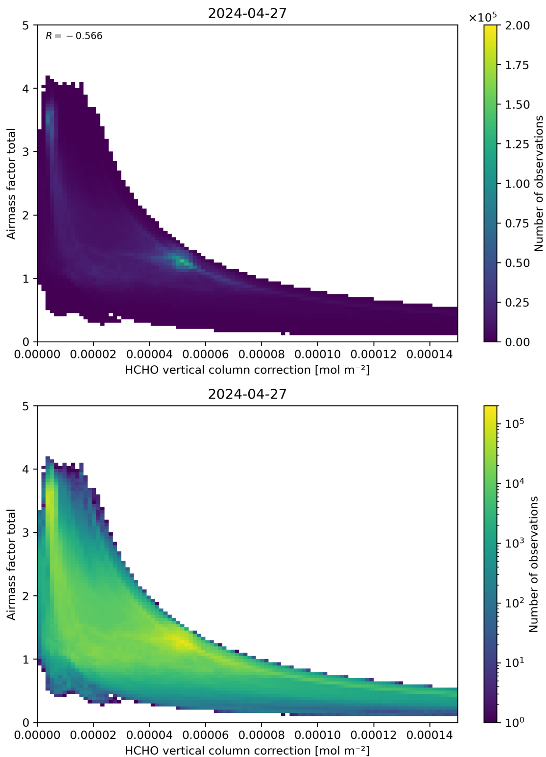
Figure 120: Scatter density plot of “HCHO vertical column correction” against “Airmass factor total” for 2024-04-26 to 2024-04-28.
