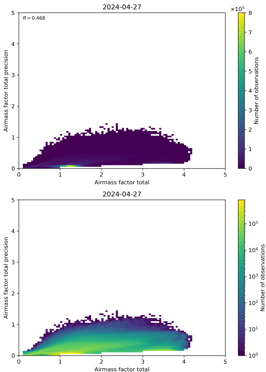
Figure 103: Scatter density plot of “Airmass factor total” against “Airmass factor total precision” for 2024-04-26 to 2024-04-28.
