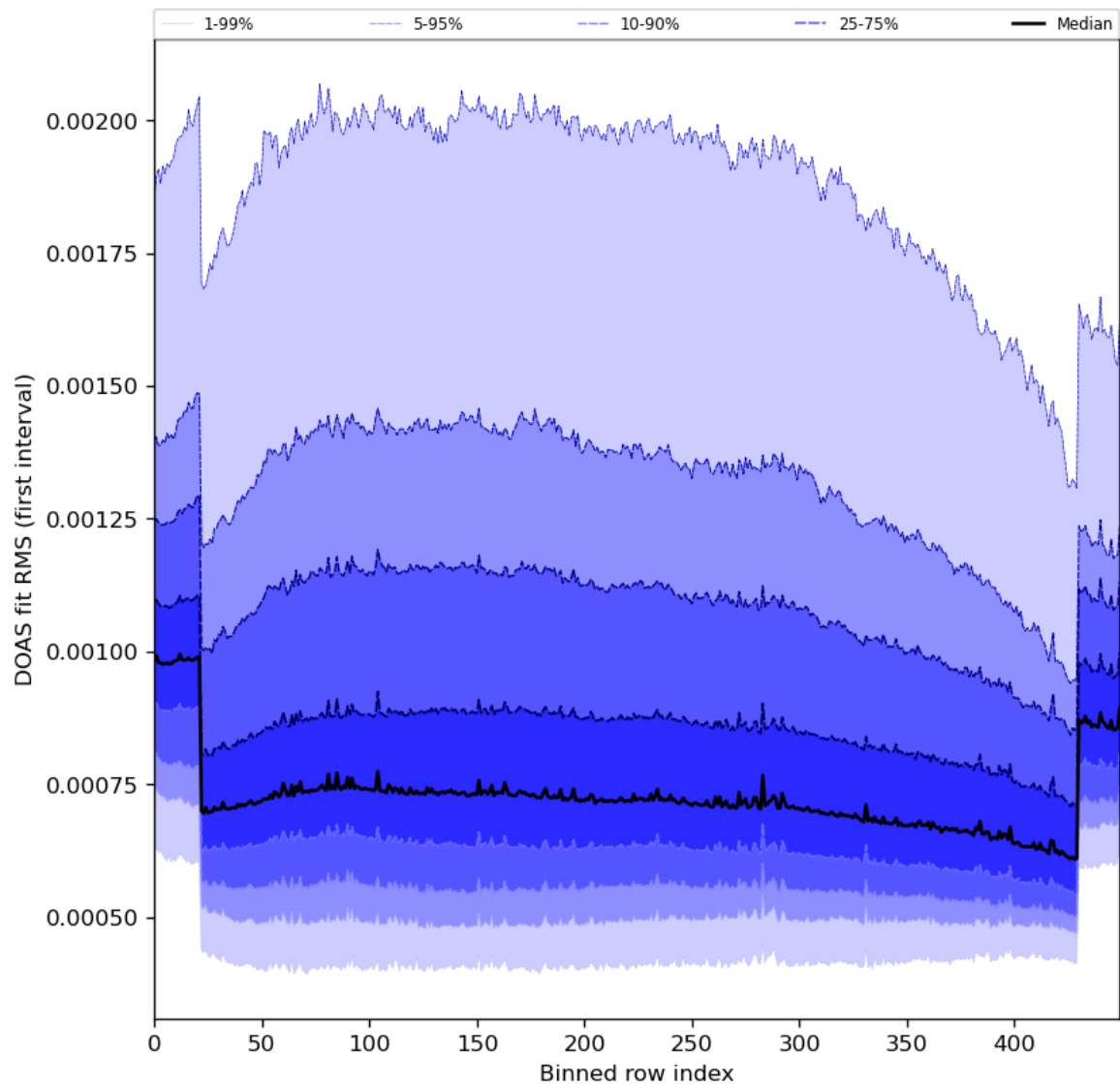
Figure 60: Along track statistics of “DOAS fit RMS (first interval)” for 2024-04-26 to 2024-04-28
