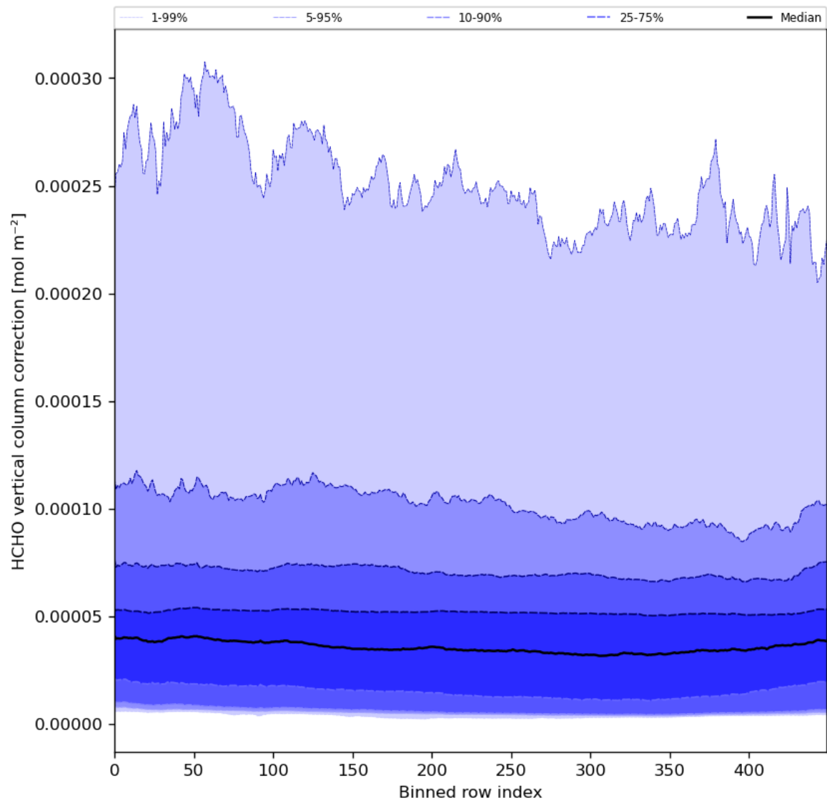
Figure 51: Along track statistics of “HCHO vertical column correction” for 2024-04-26 to 2024-04-28
