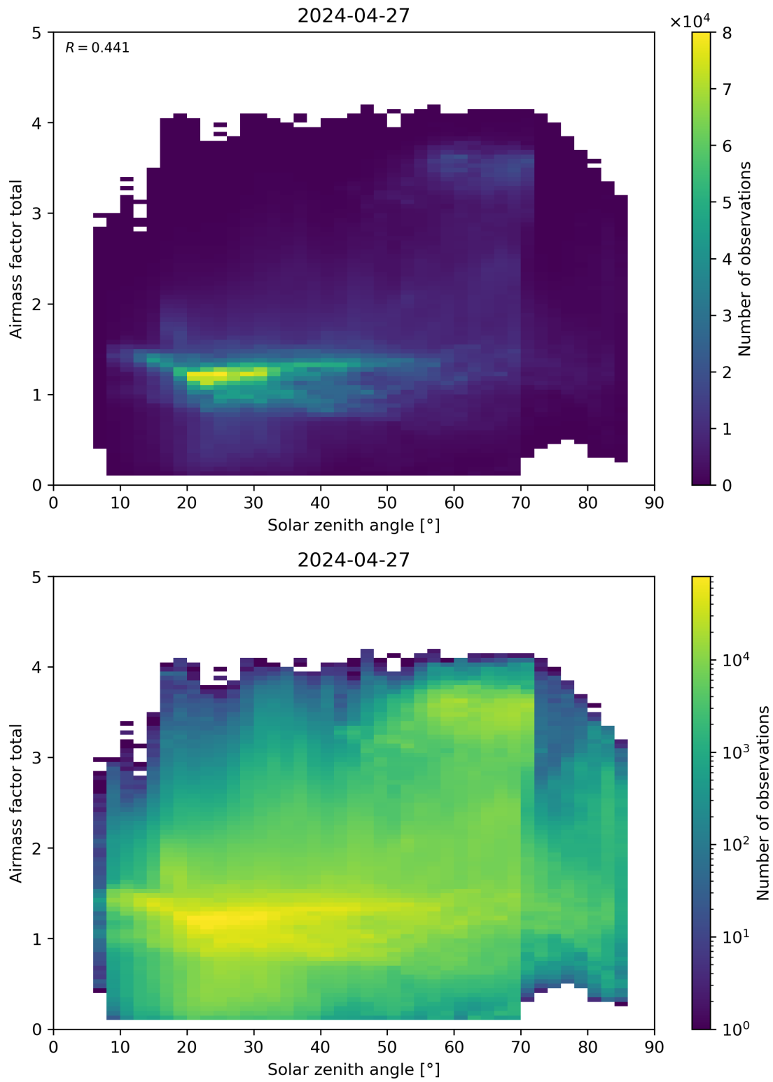
Figure 175: Scatter density plot of “Solar zenith angle” against “Airmass factor total” for 2024-04-26 to 2024-04-28.
