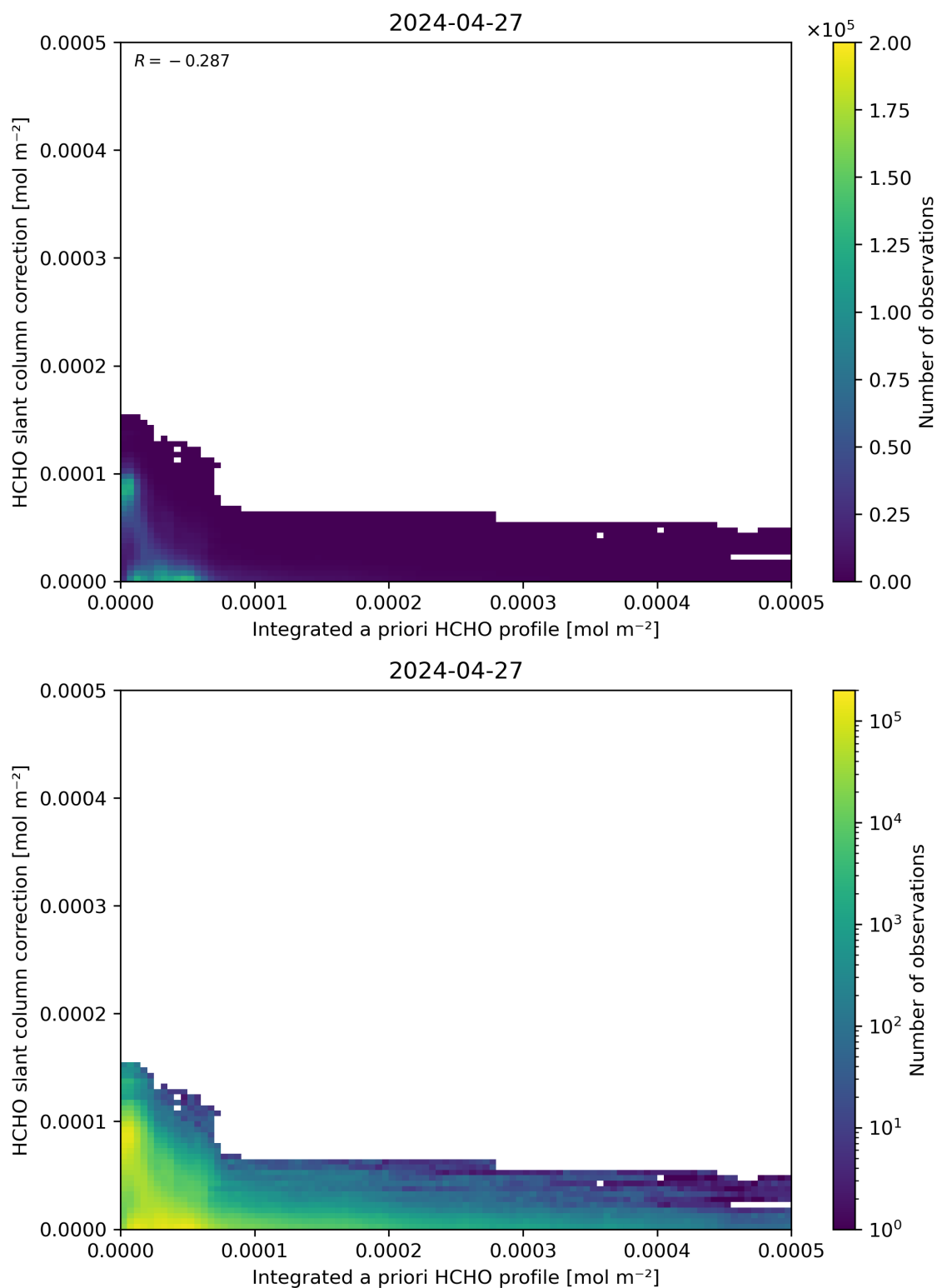
Figure 152: Scatter density plot of “Integrated a priori HCHO profile” against “HCHO slant column correction” for 2024-04-26 to 2024-04-28.
