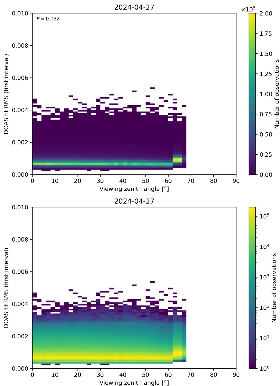
Figure 182: Scatter density plot of “Viewing zenith angle” against “DOAS fit RMS (first interval)” for 2024-04-26 to 2024-04-28.
