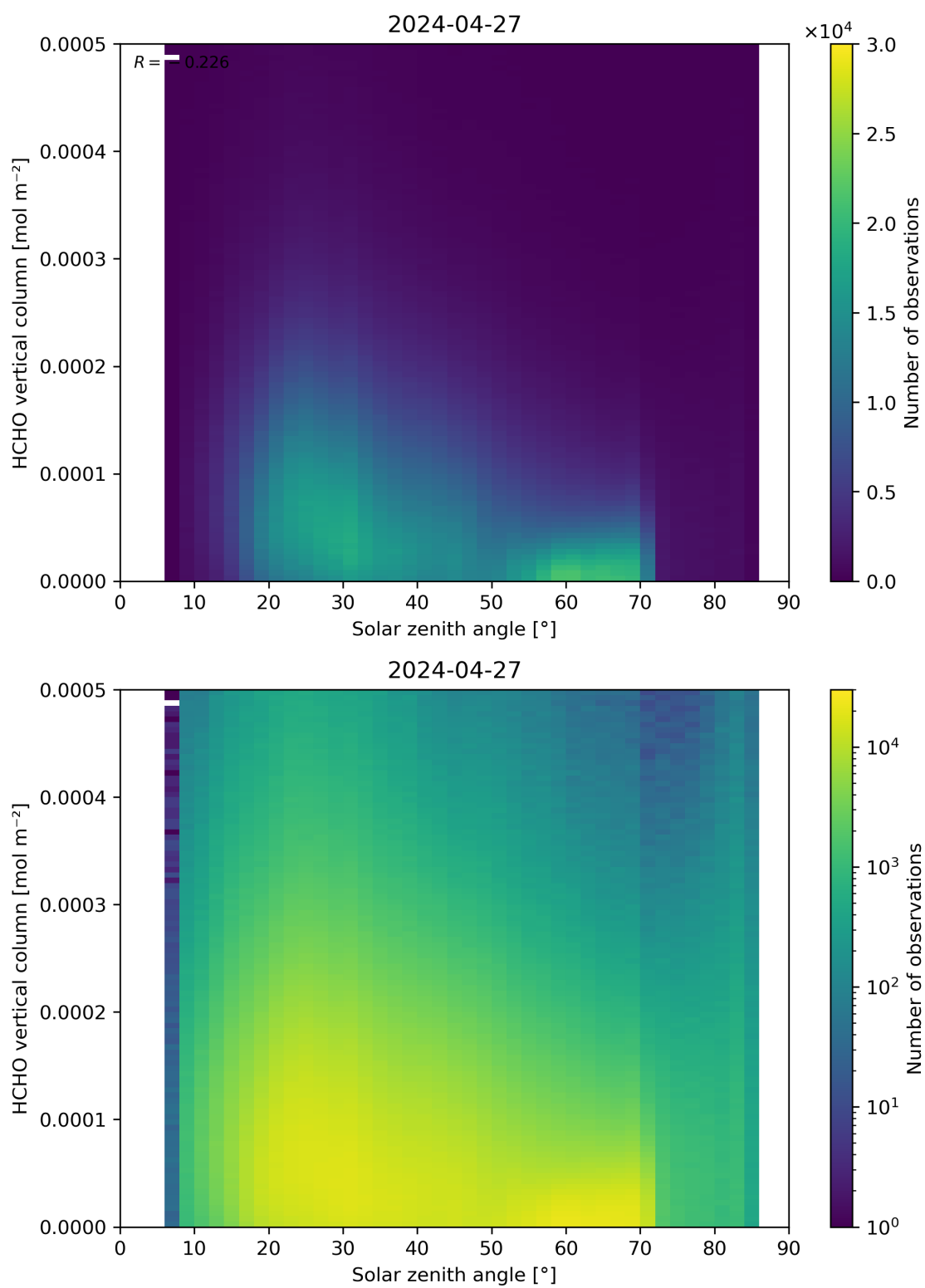
Figure 177: Scatter density plot of “Solar zenith angle” against “HCHO vertical column” for 2024-04-26 to 2024-04-28.
