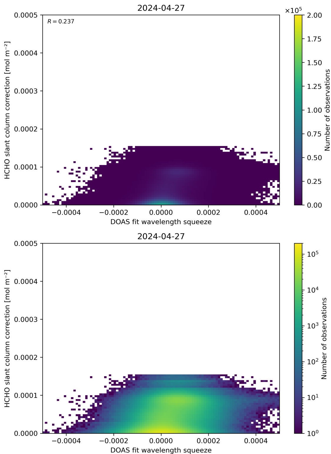
Figure 70: Scatter density plot of “DOAS fit wavelength squeeze” against “HCHO slant column correction” for 2024-04-26 to 2024-04-28.
