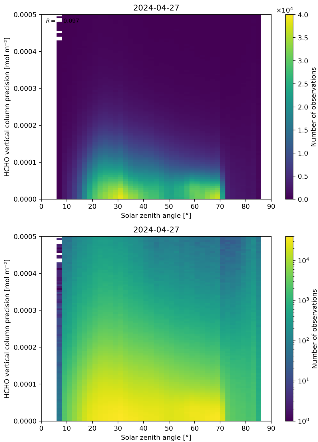
Figure 179: Scatter density plot of “Solar zenith angle” against “HCHO vertical column precision” for 2024-04-26 to 2024-04-28.
