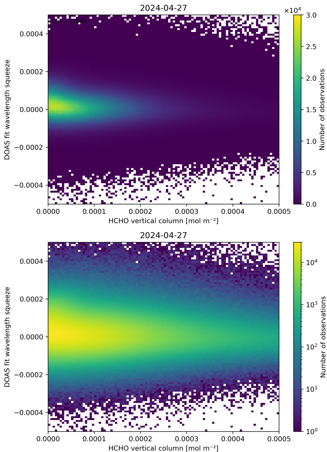
Figure 125: Scatter density plot of “HCHO vertical column” against “DOAS fit wavelength squeeze” for 2024-04-26 to 2024-04-28.
