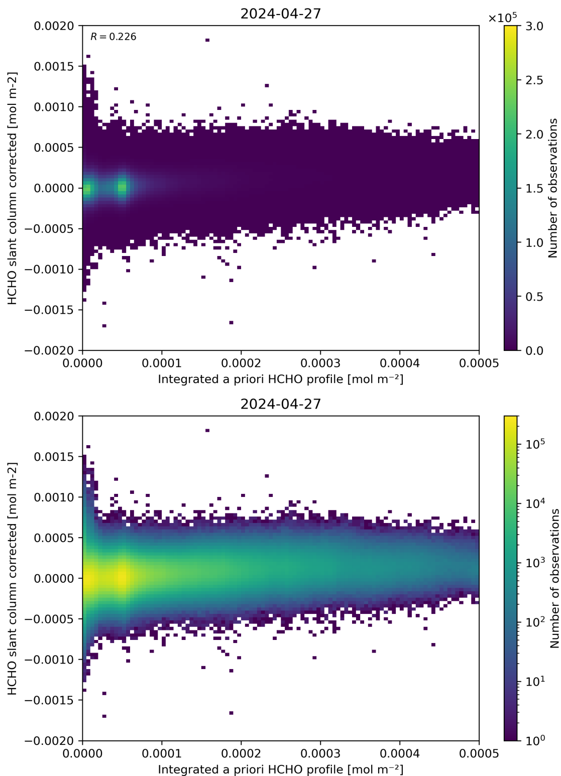
Figure 151: Scatter density plot of “Integrated a priori HCHO profile” against “HCHO slant column corrected” for 2024-04-26 to 2024-04-28.
