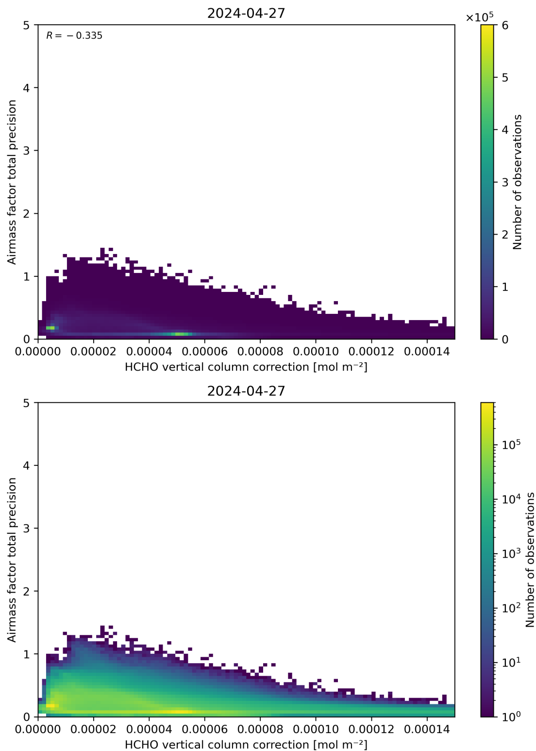
Figure 121: Scatter density plot of “HCHO vertical column correction” against “Airmass factor total precision” for 2024-04-26 to 2024-04-28.
