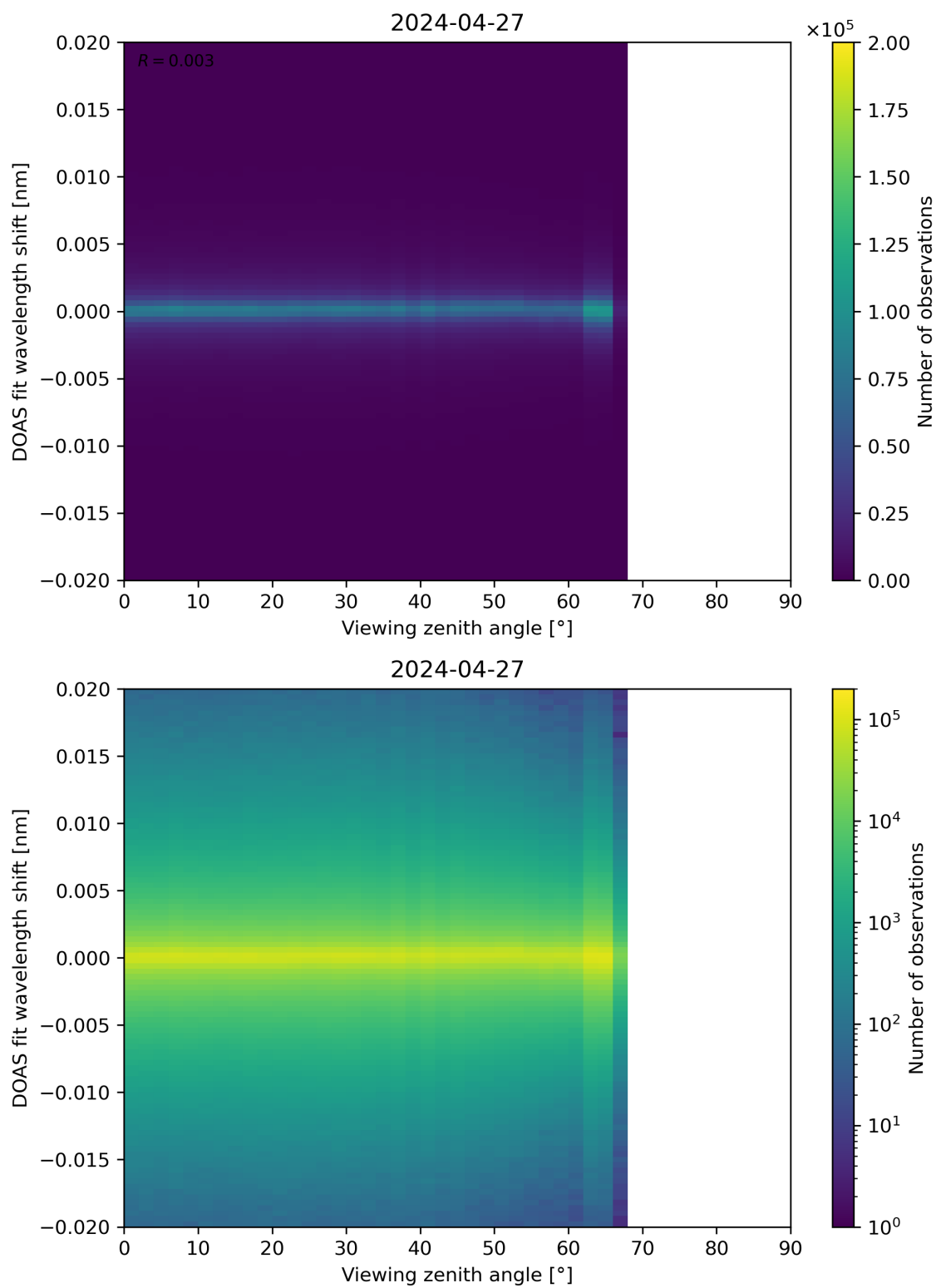
Figure 183: Scatter density plot of “Viewing zenith angle” against “DOAS fit wavelength shift” for 2024-04-26 to 2024-04-28.
