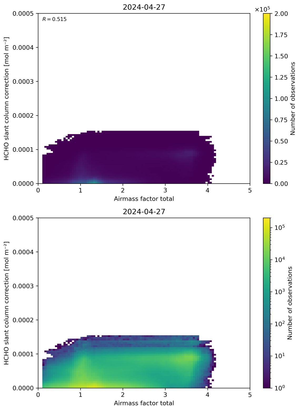
Figure 102: Scatter density plot of “Airmass factor total” against “HCHO slant column correction” for 2024-04-26 to 2024-04-28.
