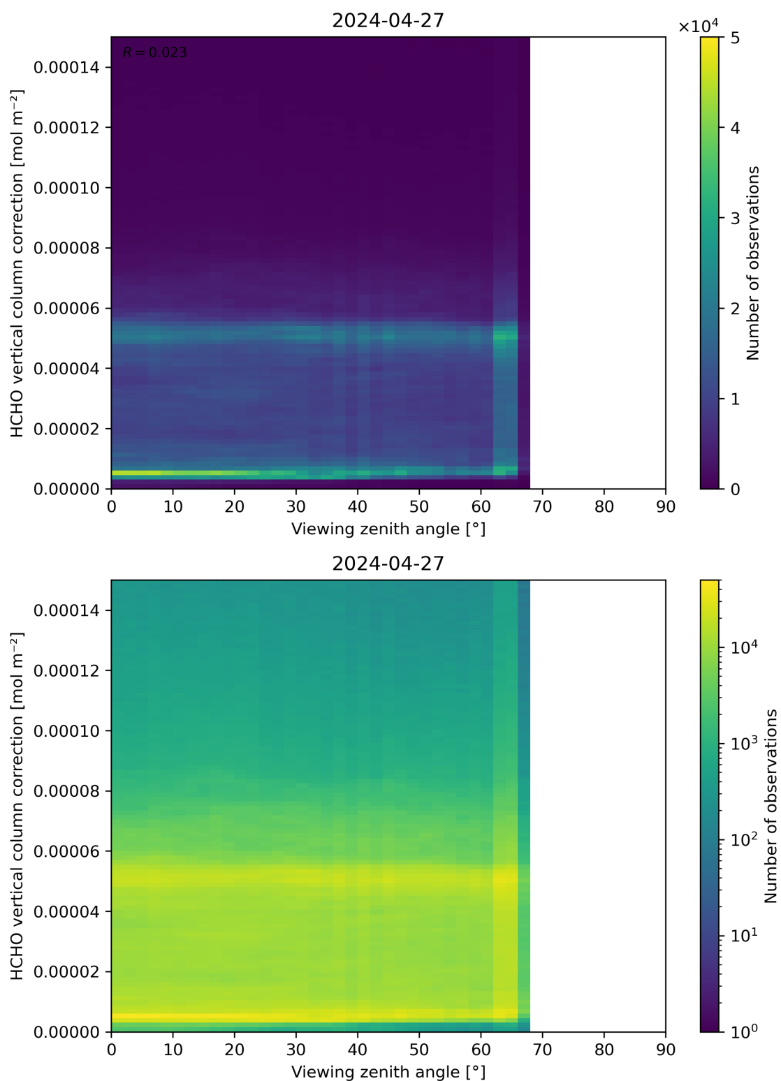
Figure 193: Scatter density plot of “Viewing zenith angle” against “HCHO vertical column correction” for 2024-04-26 to 2024-04-28.
