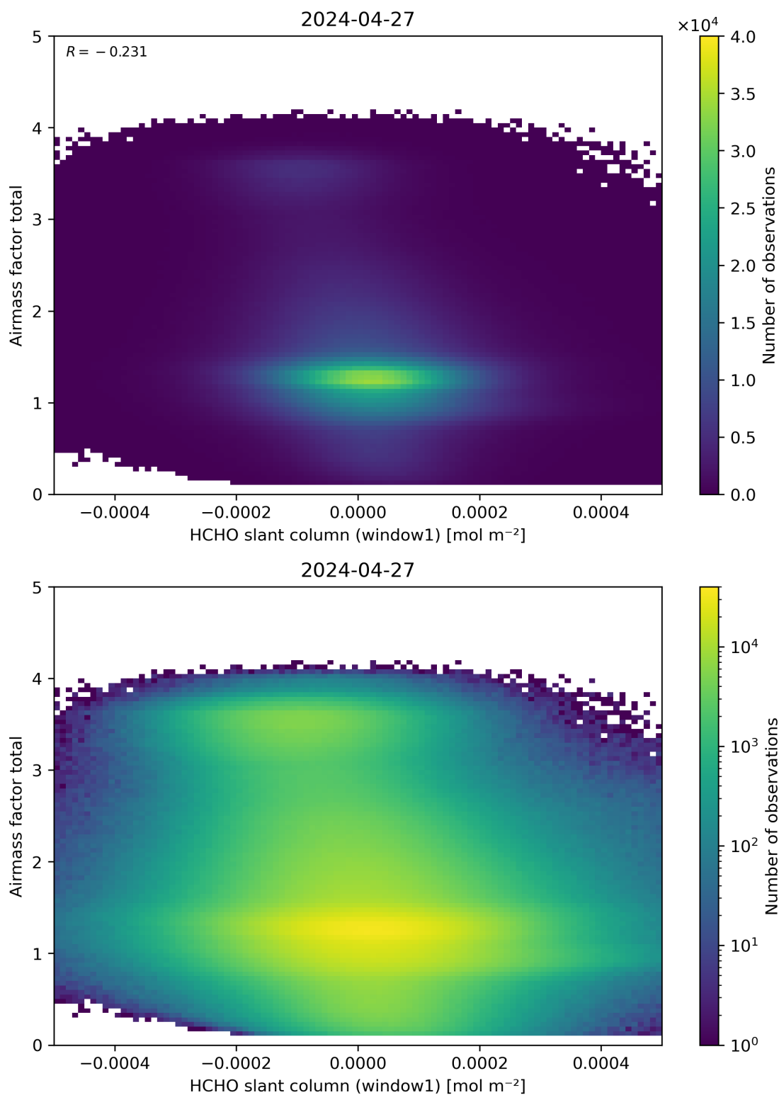
Figure 85: Scatter density plot of “HCHO slant column (window1)” against “Airmass factor total” for 2024-04-26 to 2024-04-28.
