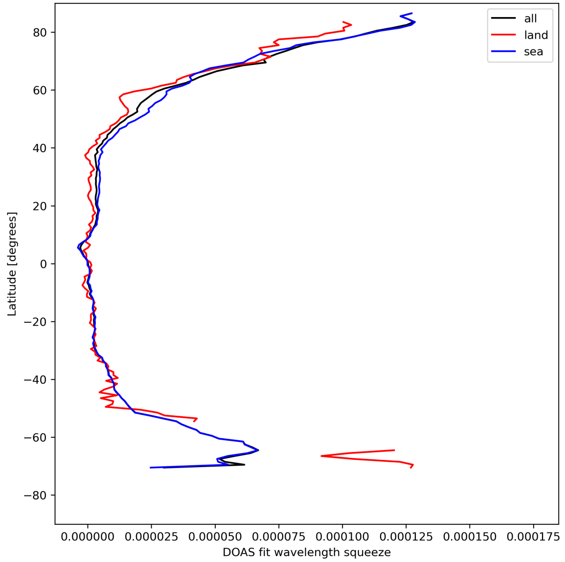
Figure 31: Zonal average of “DOAS fit wavelength squeeze” for 2024-04-26 to 2024-04-28.
