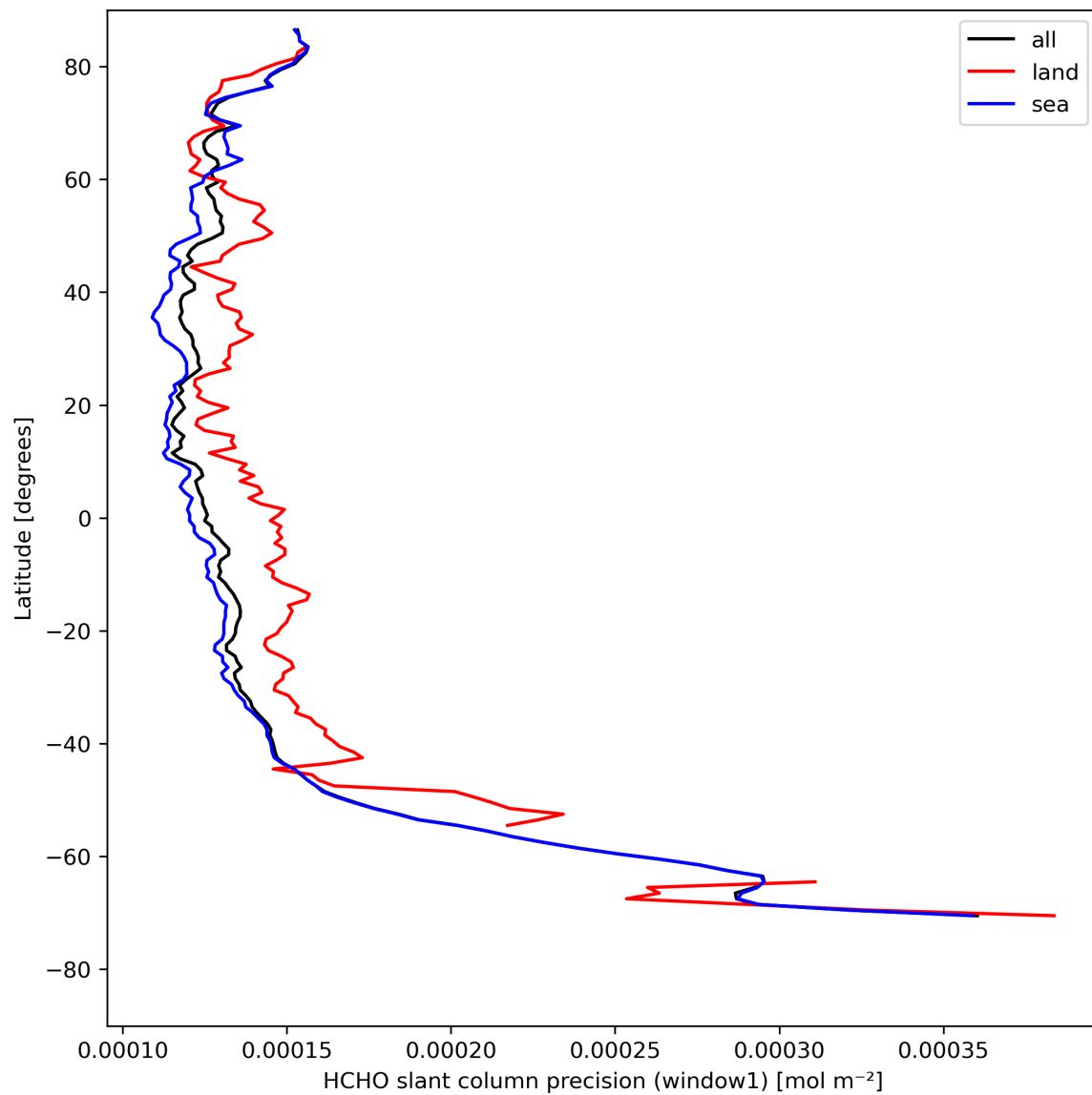
Figure 25: Zonal average of “HCHO slant column precision (window1)” for 2024-04-26 to 2024-04-28.
