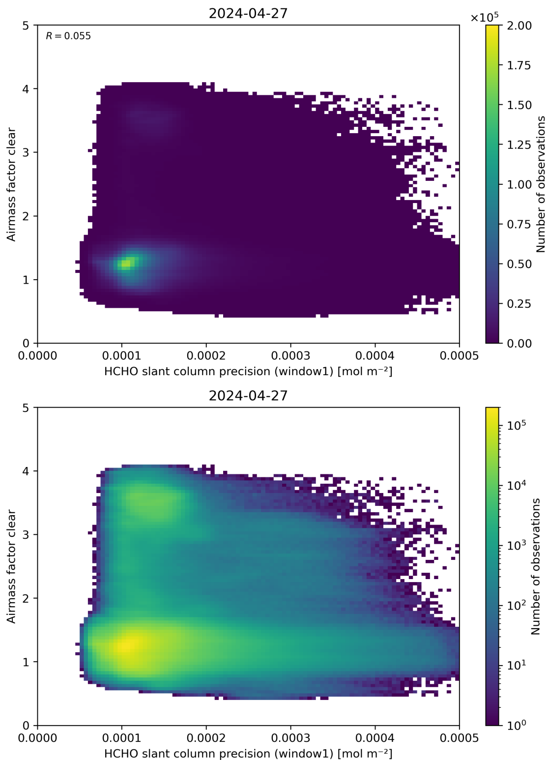
Figure 91: Scatter density plot of “HCHO slant column precision (window1)” against “Airmass factor clear” for 2024-04-26 to 2024-04-28.
