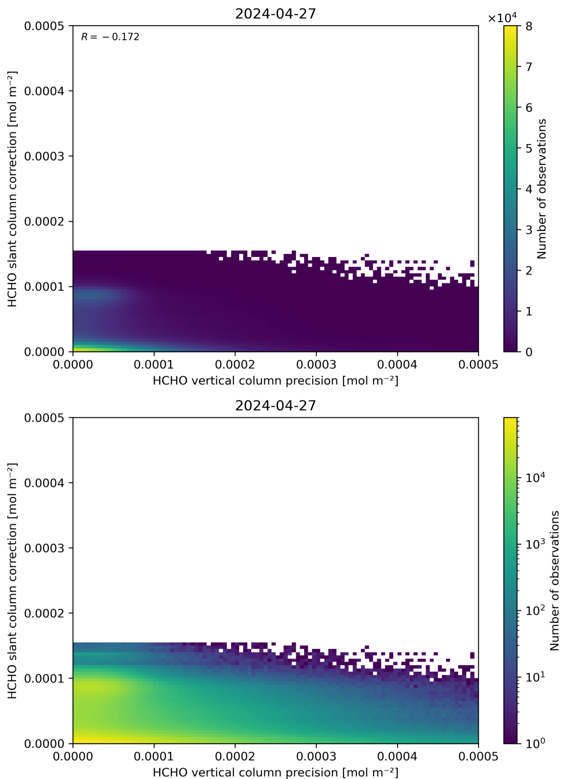
Figure 141: Scatter density plot of “HCHO vertical column precision” against “HCHO slant column correction” for 2024-04-26 to 2024-04-28.
