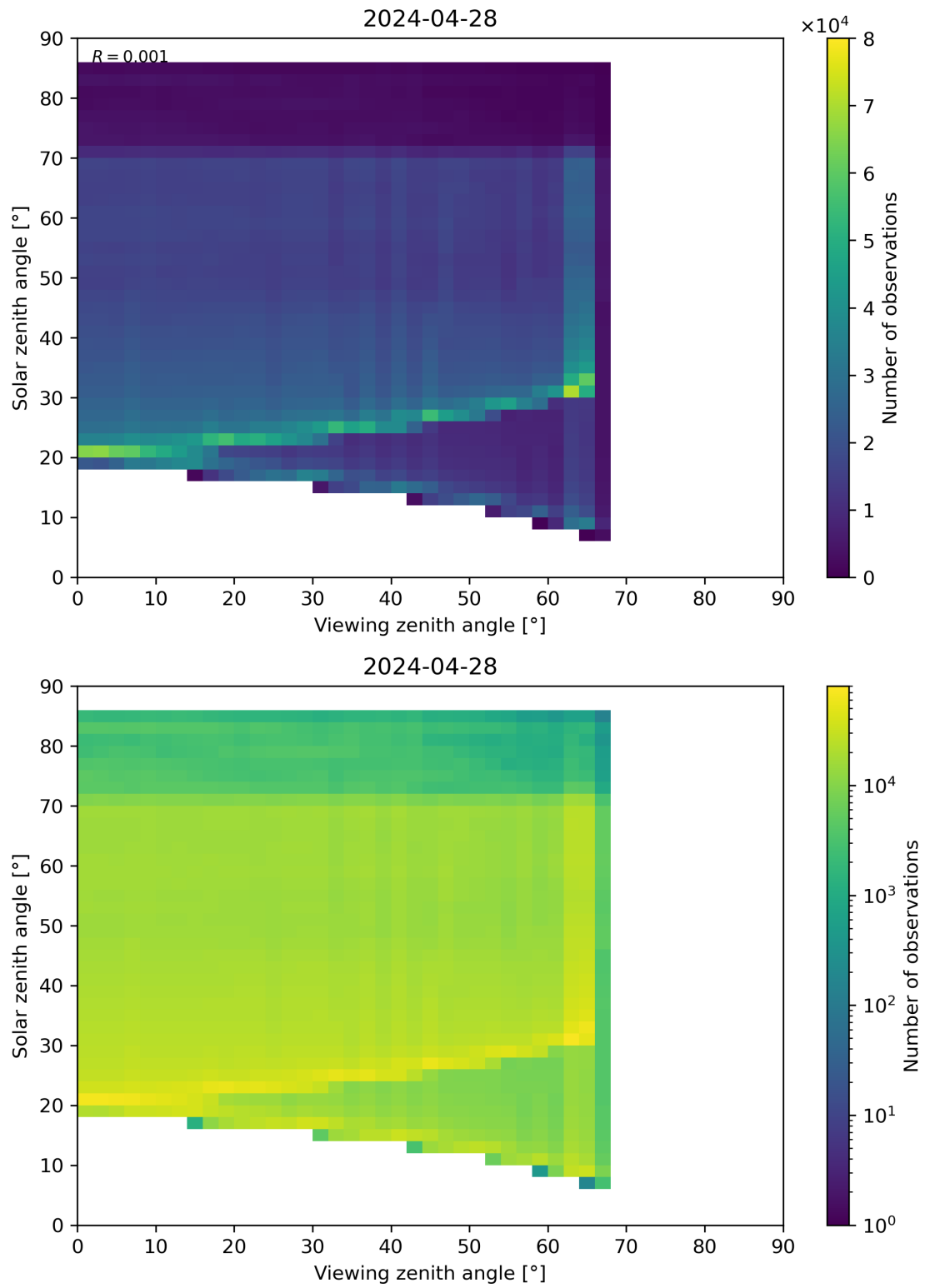
Figure 197: Scatter density plot of “Viewing zenith angle” against “Solar zenith angle” for 2024-04-27 to 2024-04-29.
