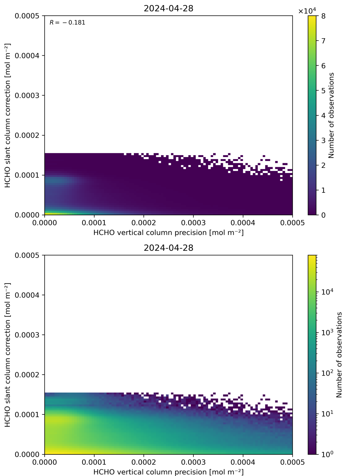
Figure 141: Scatter density plot of “HCHO vertical column precision” against “HCHO slant column correction” for 2024-04-27 to 2024-04-29.
