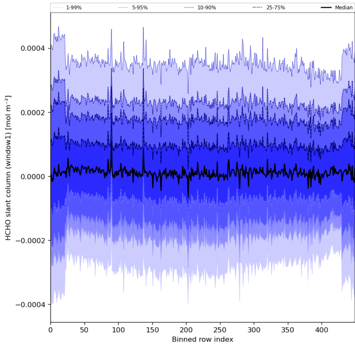
Figure 52: Along track statistics of “HCHO slant column (window1)” for 2024-04-27 to 2024-04-29
