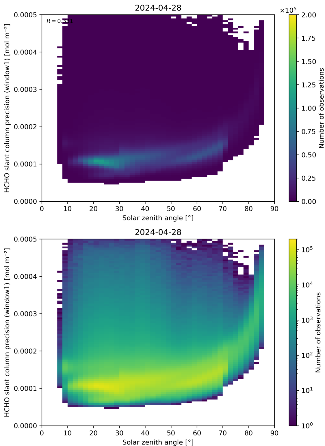
Figure 174: Scatter density plot of “Solar zenith angle” against “HCHO slant column precision (window1)” for 2024-04-27 to 2024-04-29.
