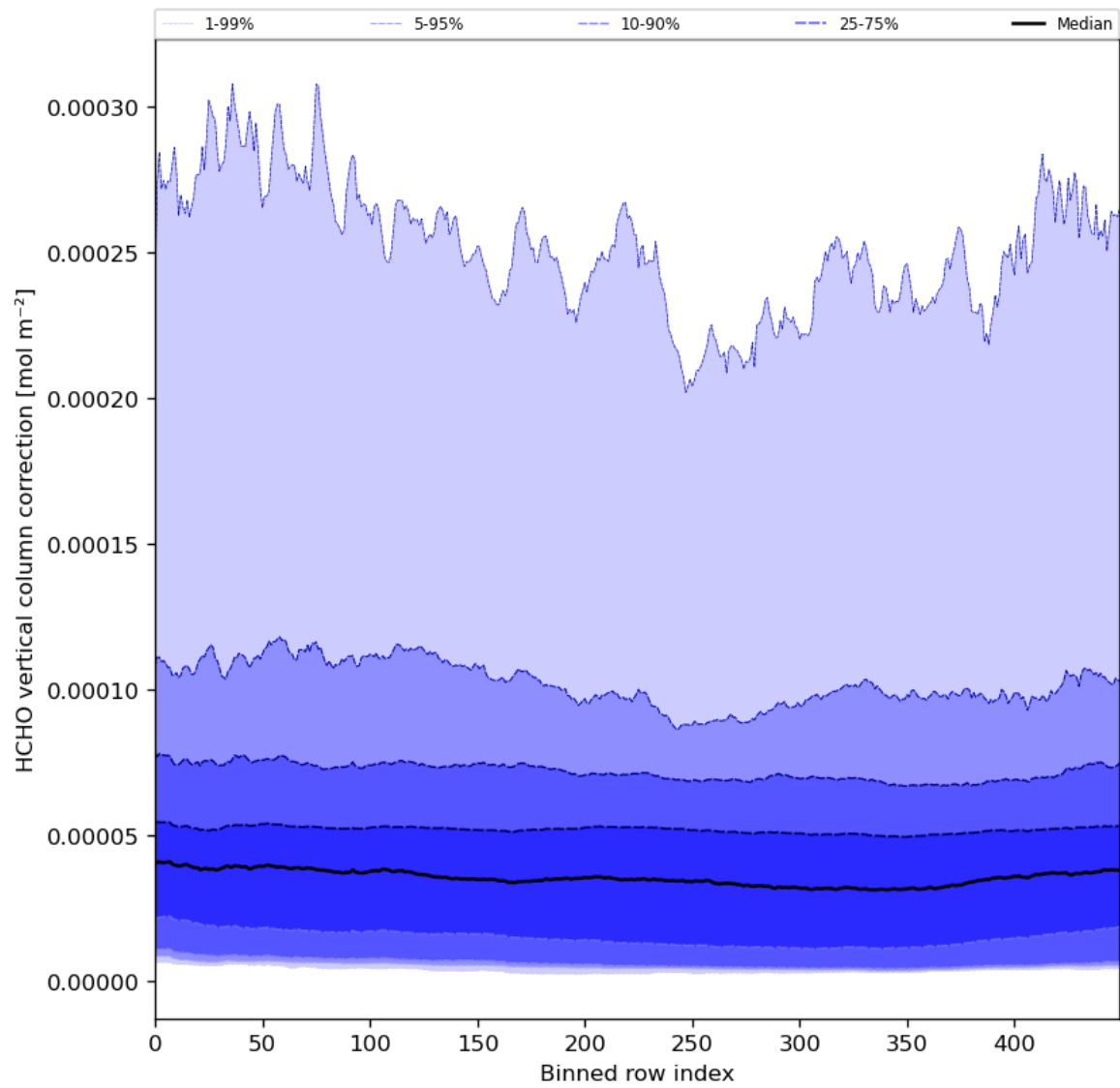
Figure 51: Along track statistics of “HCHO vertical column correction” for 2024-04-27 to 2024-04-29
