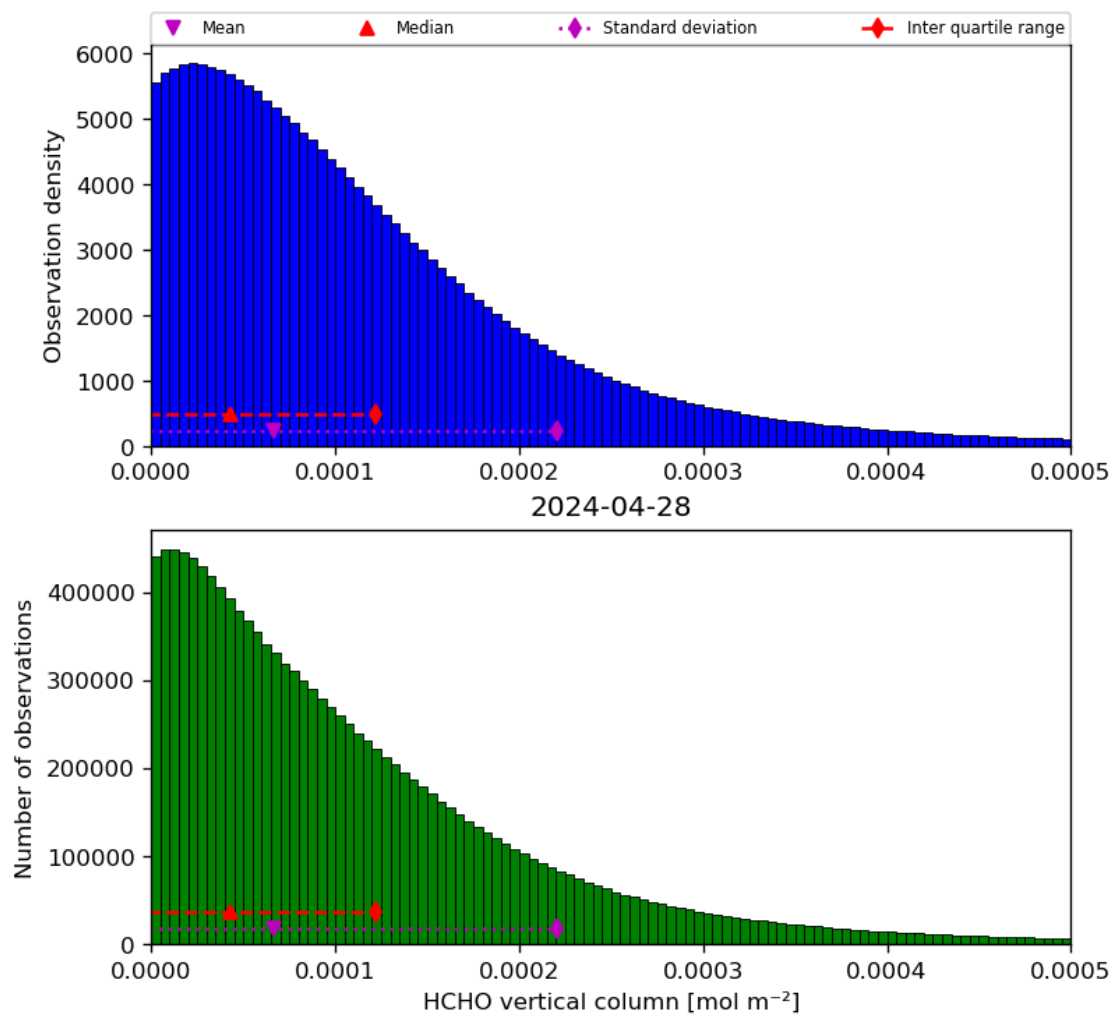
Figure 35: Histogram of “HCHO vertical column” for 2024-04-27 to 2024-04-29
