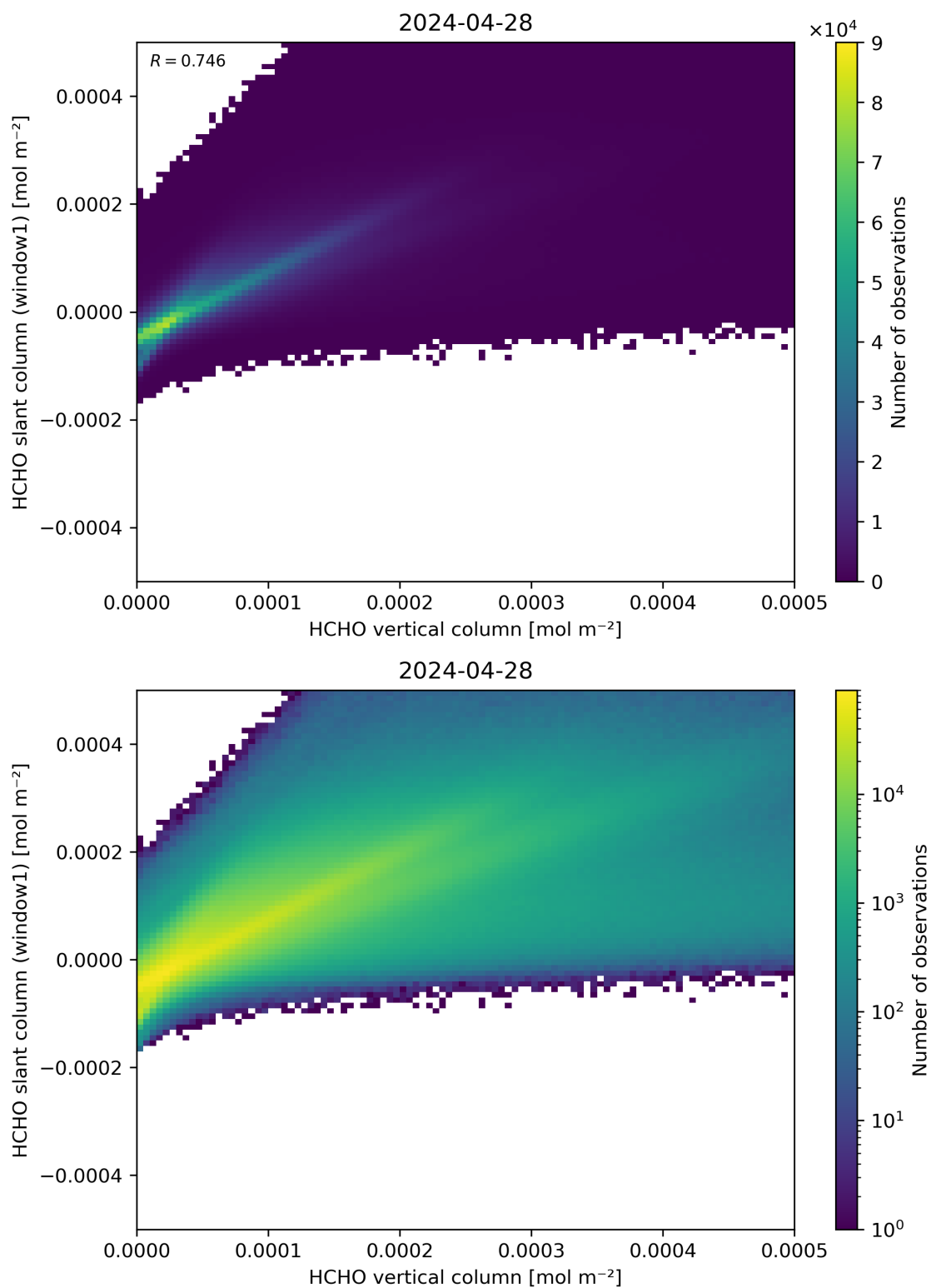
Figure 129: Scatter density plot of “HCHO vertical column” against “HCHO slant column (window1)” for 2024-04-27 to 2024-04-29.
