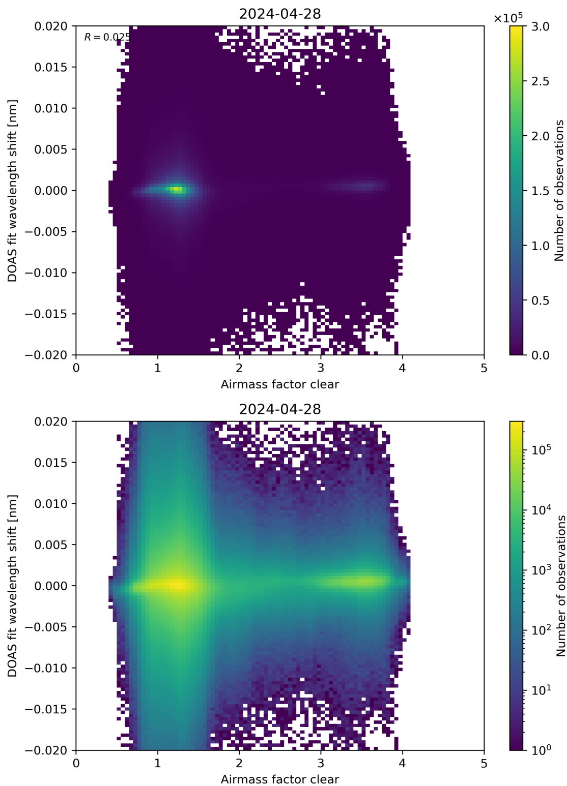
Figure 72: Scatter density plot of “Airmass factor clear” against “DOAS fit wavelength shift” for 2024-04-27 to 2024-04-29.
