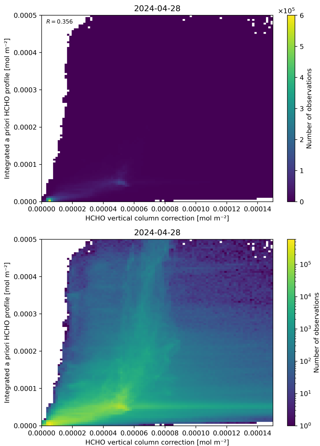
Figure 122: Scatter density plot of “HCHO vertical column correction” against “Integrated a priori HCHO profile” for 2024-04-27 to 2024-04-29.
