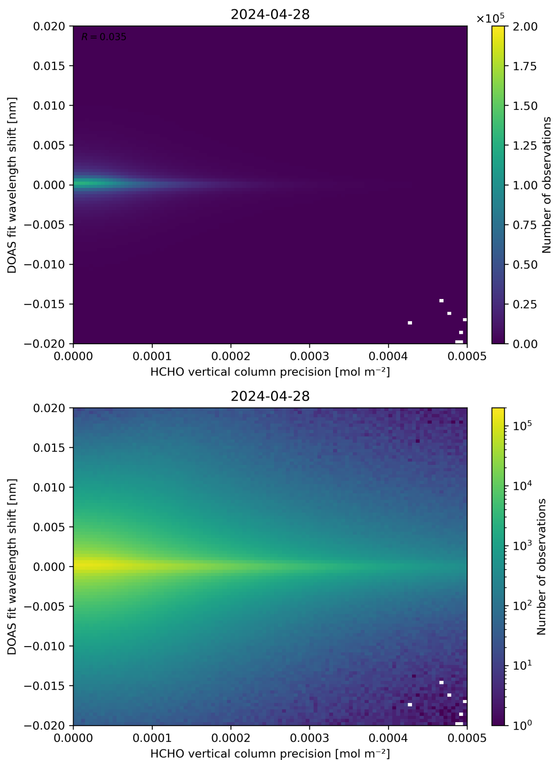
Figure 137: Scatter density plot of “HCHO vertical column precision” against “DOAS fit wavelength shift” for 2024-04-27 to 2024-04-29.
