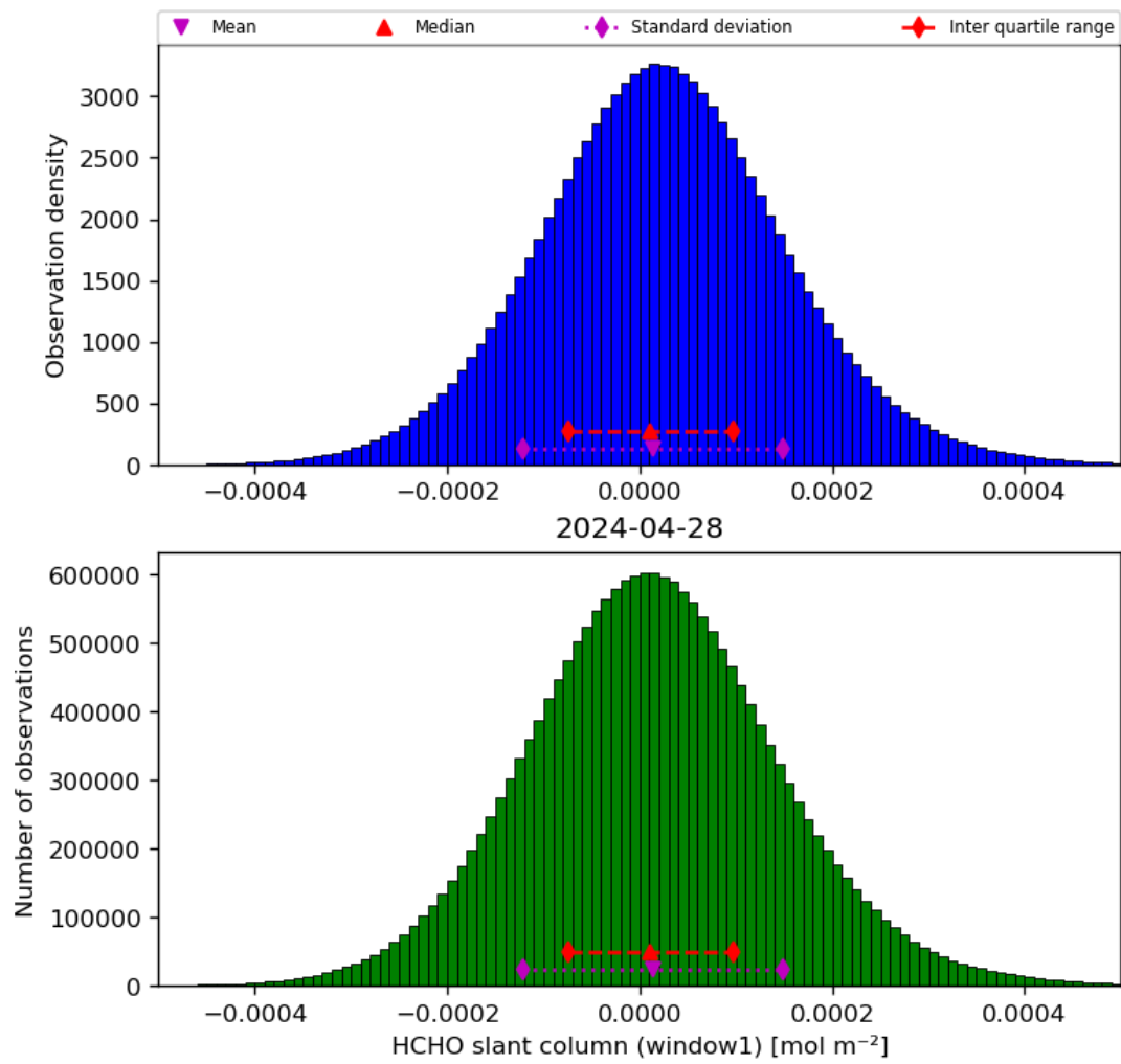
Figure 38: Histogram of “HCHO slant column (window1)” for 2024-04-27 to 2024-04-29
