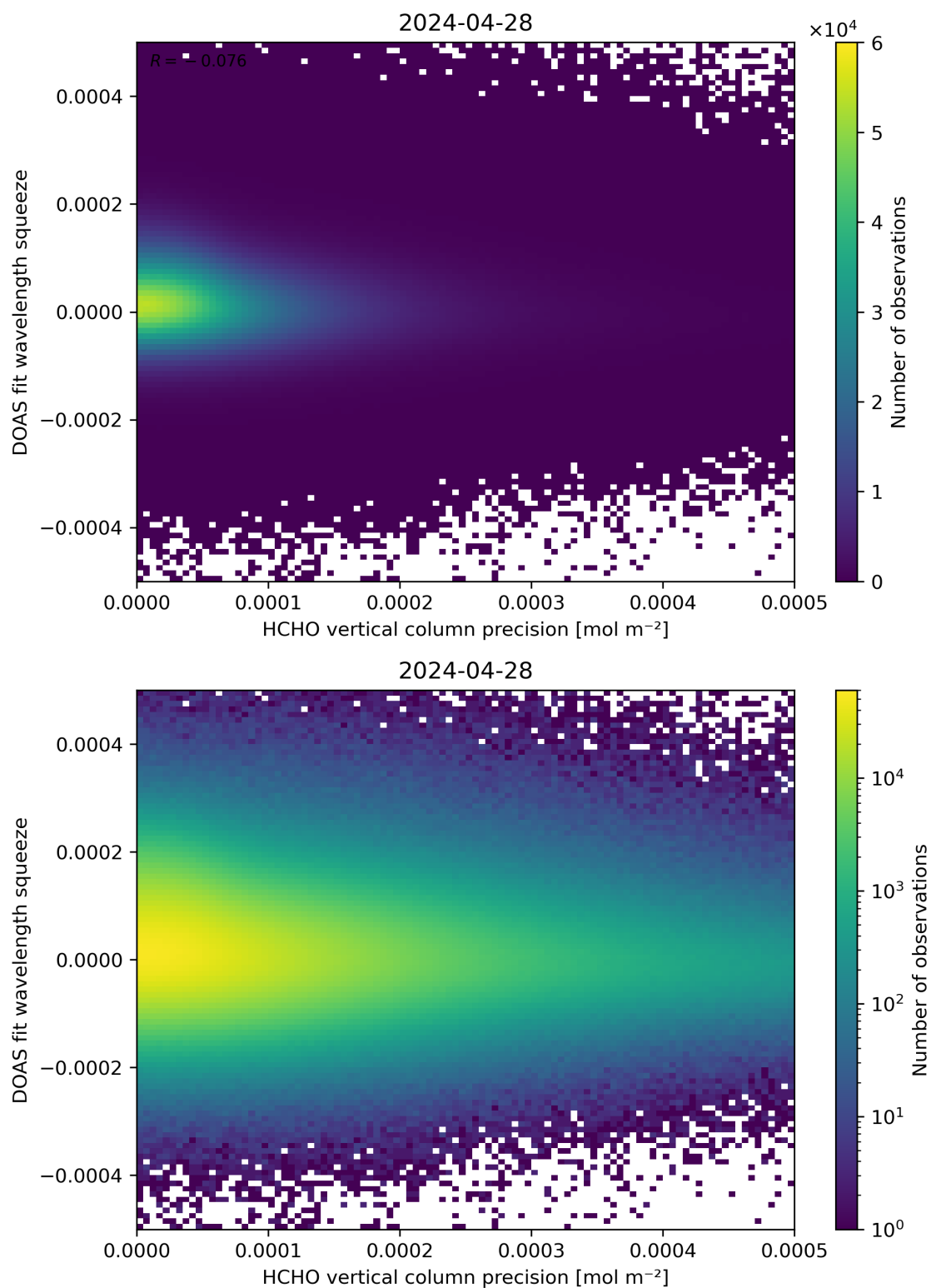
Figure 138: Scatter density plot of “HCHO vertical column precision” against “DOAS fit wavelength squeeze” for 2024-04-27 to 2024-04-29.
