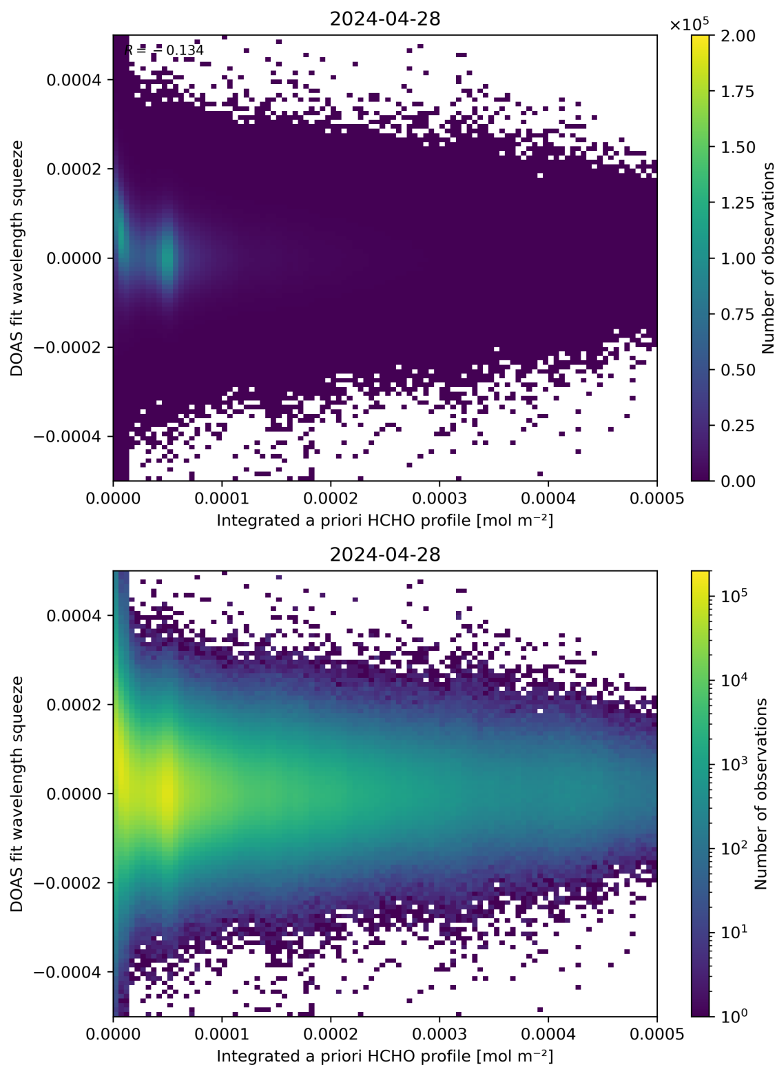
Figure 150: Scatter density plot of “Integrated a priori HCHO profile” against “DOAS fit wavelength squeeze” for 2024-04-27 to 2024-04-29.
