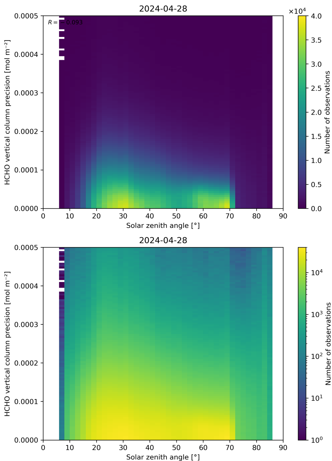
Figure 179: Scatter density plot of “Solar zenith angle” against “HCHO vertical column precision” for 2024-04-27 to 2024-04-29.
