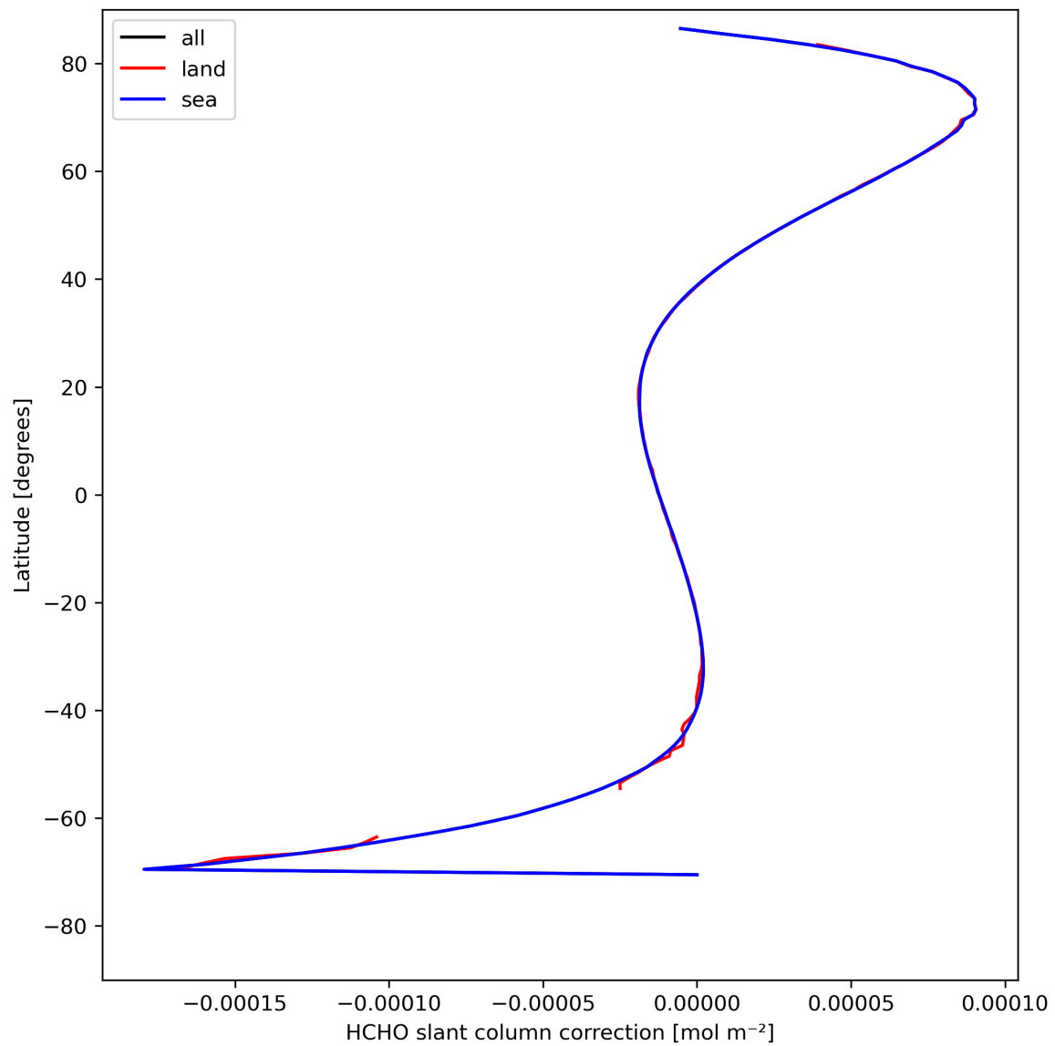
Figure 33: Zonal average of “HCHO slant column correction” for 2024-04-27 to 2024-04-29.
