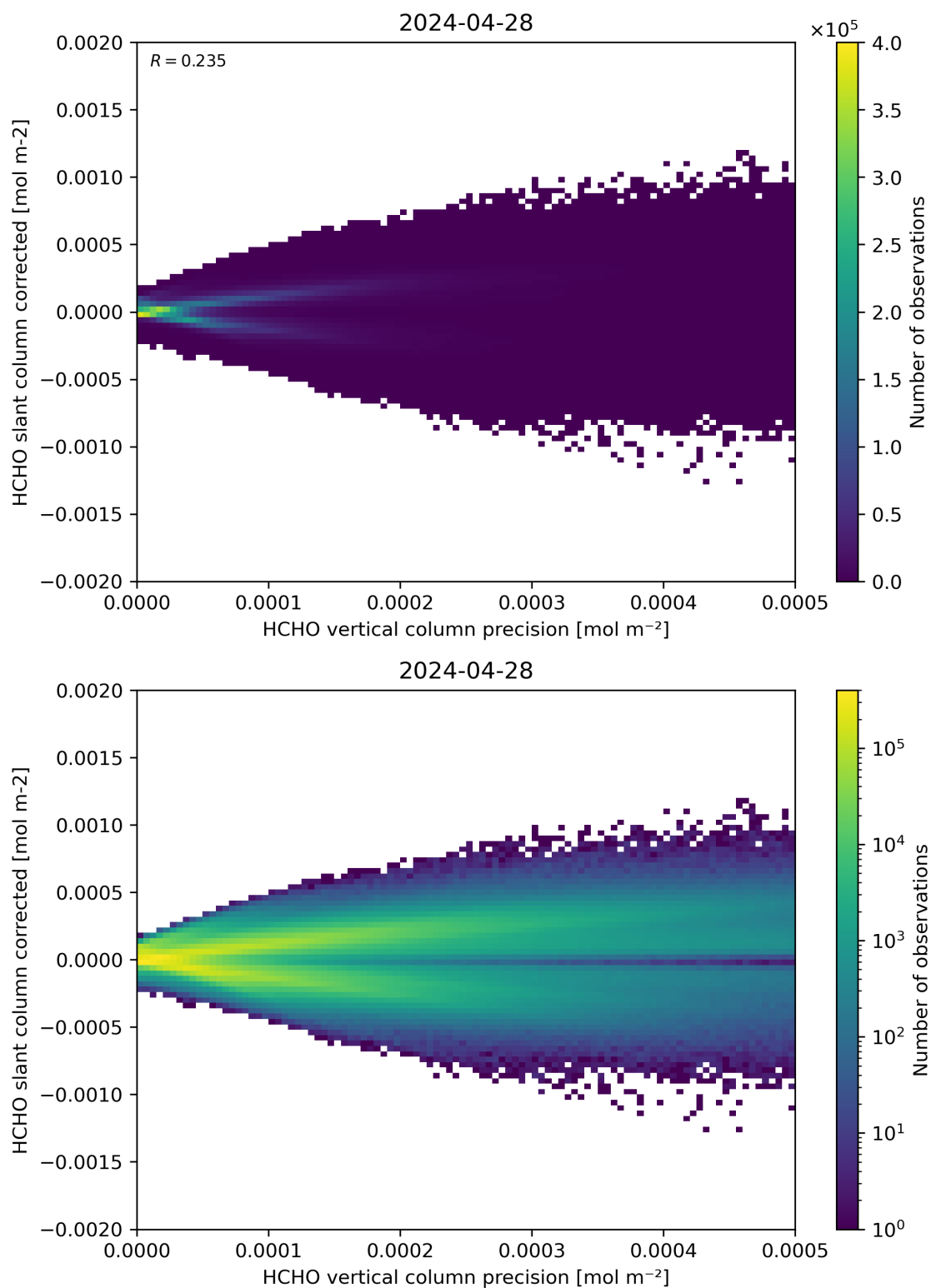
Figure 140: Scatter density plot of “HCHO vertical column precision” against “HCHO slant column corrected” for 2024-04-27 to 2024-04-29.
