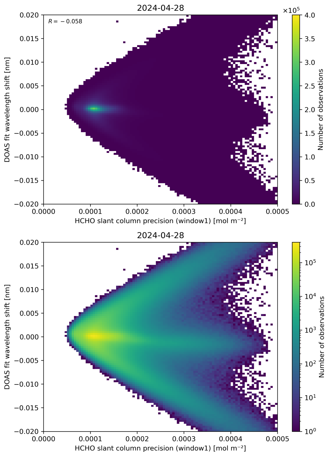
Figure 89: Scatter density plot of “HCHO slant column precision (window1)” against “DOAS fit wavelength shift” for 2024-04-27 to 2024-04-29.
