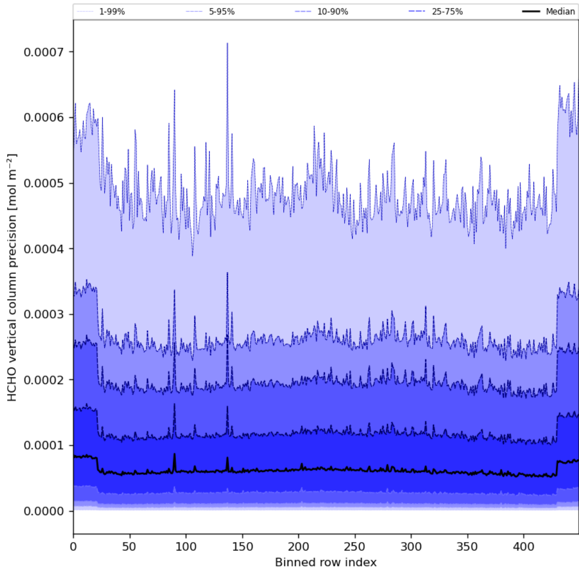
Figure 50: Along track statistics of “HCHO vertical column precision” for 2024-04-27 to 2024-04-29
