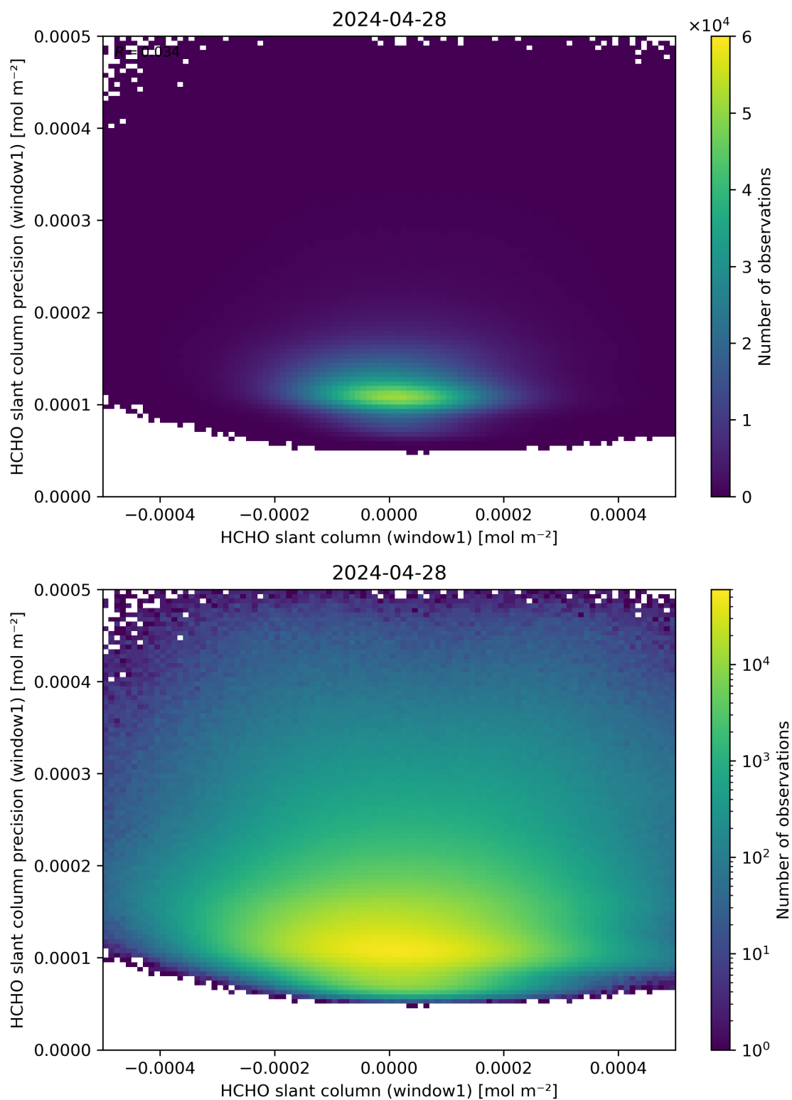
Figure 84: Scatter density plot of “HCHO slant column (window1)” against “HCHO slant column precision (window1)” for 2024-04-27 to 2024-04-29.
