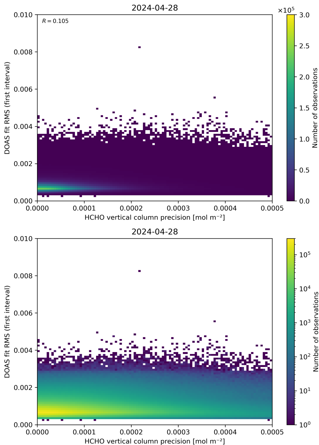
Figure 136: Scatter density plot of “HCHO vertical column precision” against “DOAS fit RMS (first interval)” for 2024-04-27 to 2024-04-29.
