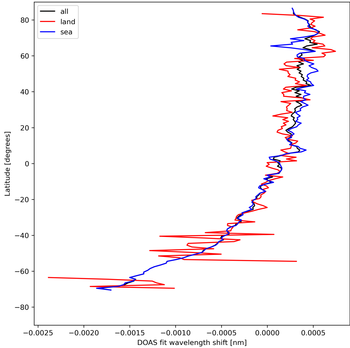
Figure 30: Zonal average of “DOAS fit wavelength shift” for 2024-04-27 to 2024-04-29.
