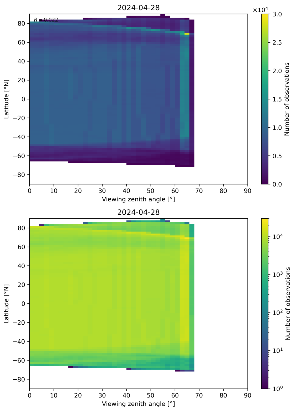
Figure 196: Scatter density plot of “Viewing zenith angle” against “Latitude” for 2024-04-27 to 2024-04-29.
