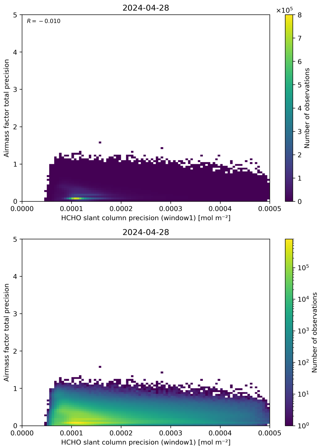
Figure 95: Scatter density plot of “HCHO slant column precision (window1)” against “Airmass factor total precision” for 2024-04-27 to 2024-04-29.
