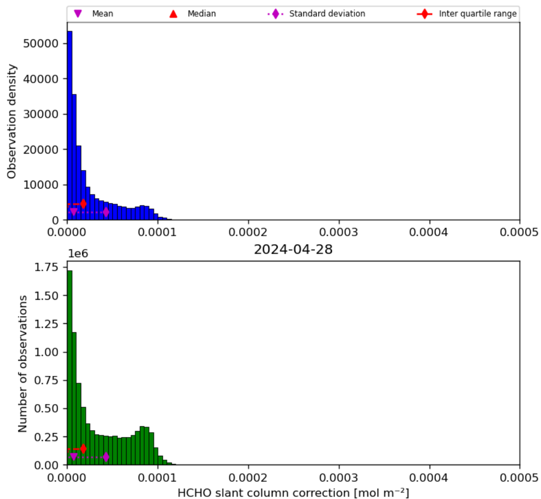
Figure 47: Histogram of “HCHO slant column correction” for 2024-04-27 to 2024-04-29
