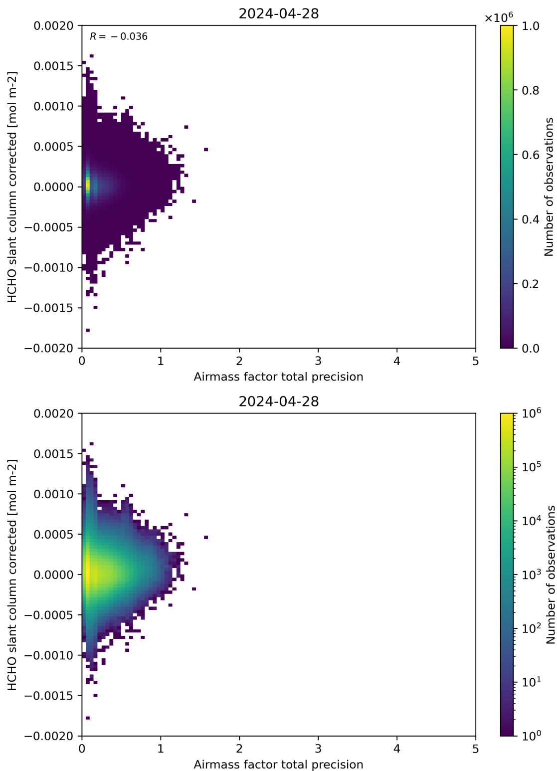
Figure 109: Scatter density plot of “Airmass factor total precision” against “HCHO slant column corrected” for 2024-04-27 to 2024-04-29.
