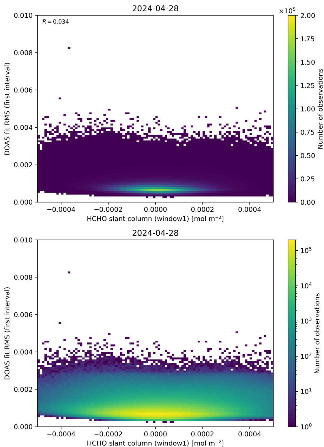
Figure 78: Scatter density plot of “HCHO slant column (window1)” against “DOAS fit RMS (first interval)” for 2024-04-27 to 2024-04-29.
