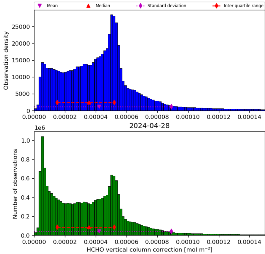
Figure 37: Histogram of “HCHO vertical column correction” for 2024-04-27 to 2024-04-29
