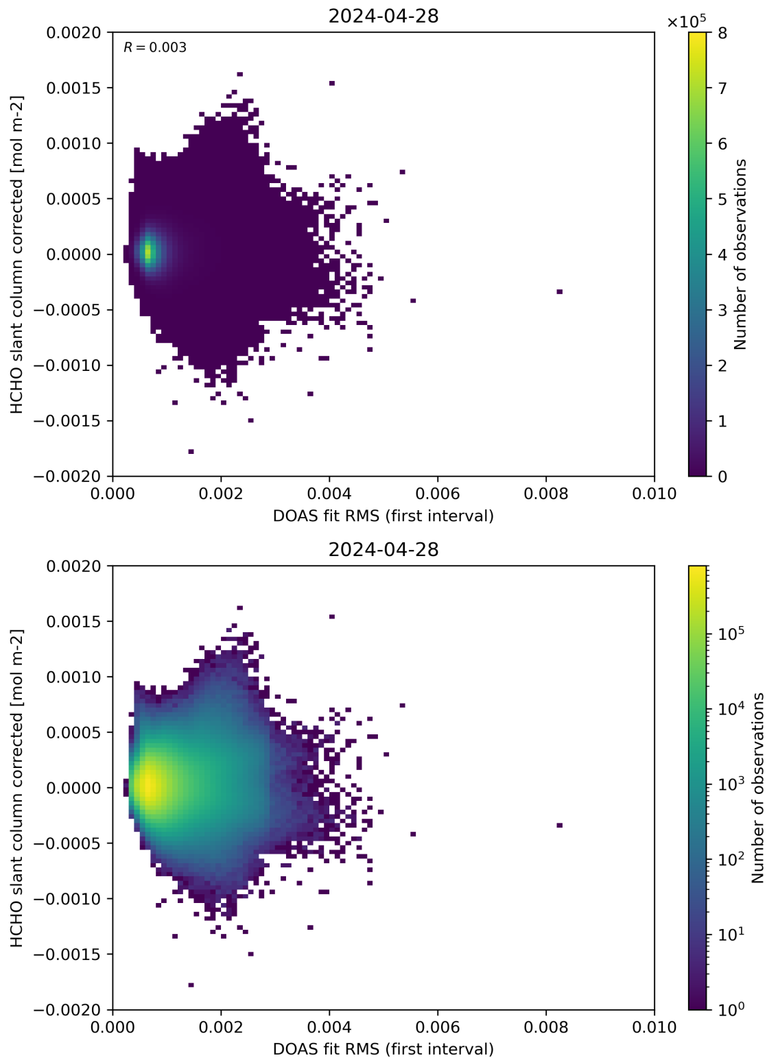
Figure 62: Scatter density plot of “DOAS fit RMS (first interval)” against “HCHO slant column corrected” for 2024-04-27 to 2024-04-29.
