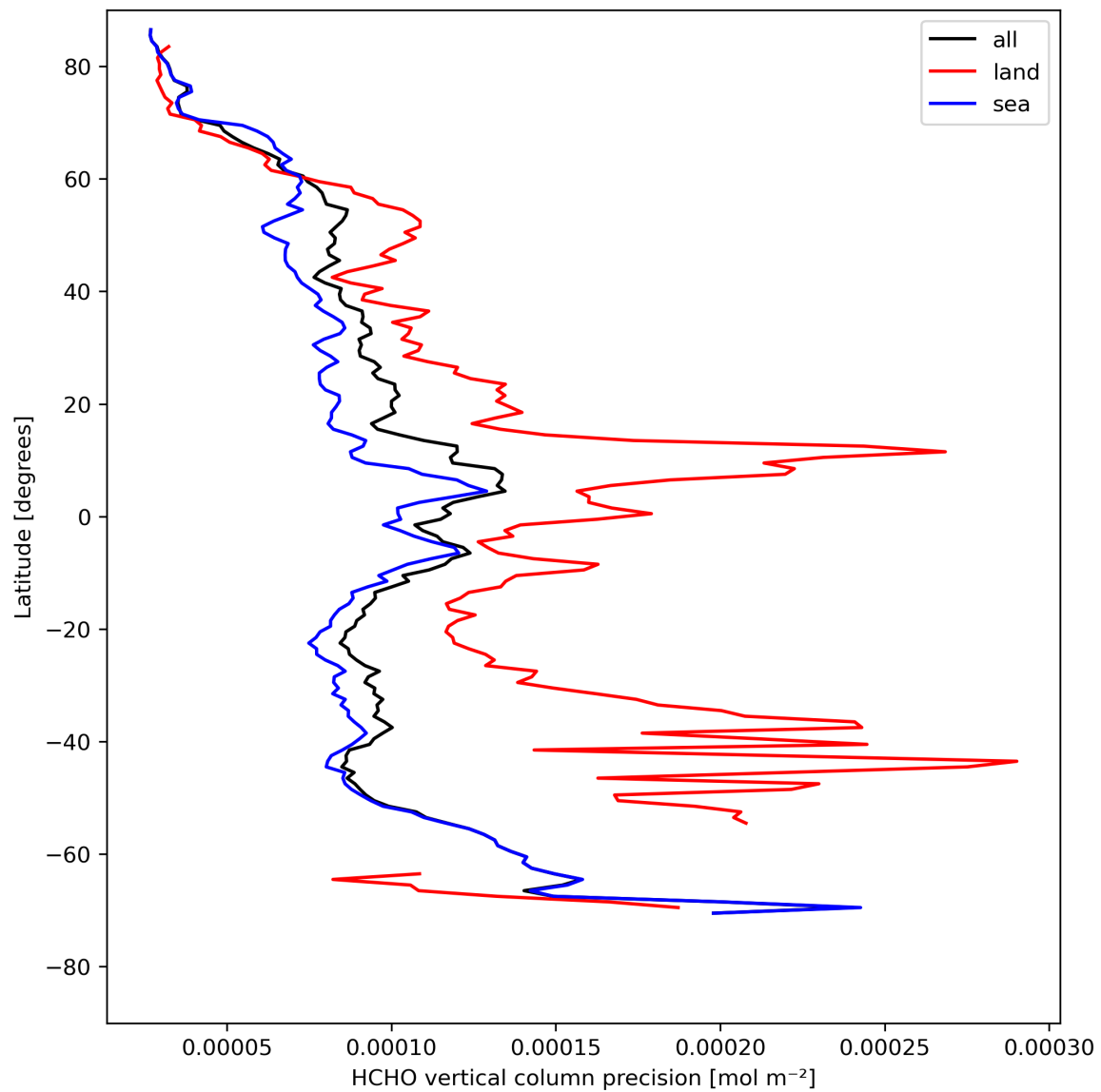
Figure 22: Zonal average of “HCHO vertical column precision” for 2024-04-27 to 2024-04-29.
