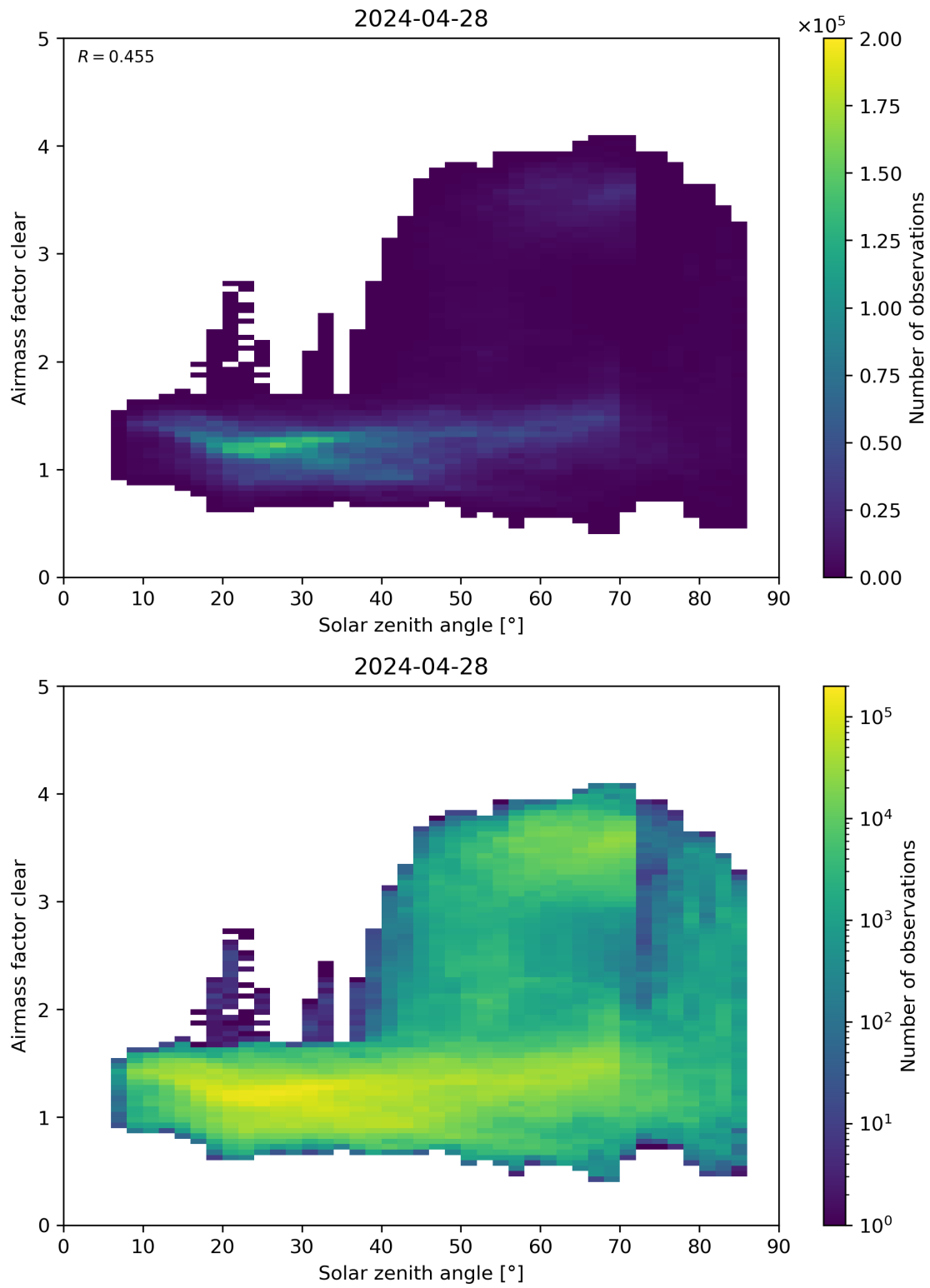
Figure 170: Scatter density plot of “Solar zenith angle” against “Airmass factor clear” for 2024-04-27 to 2024-04-29.
