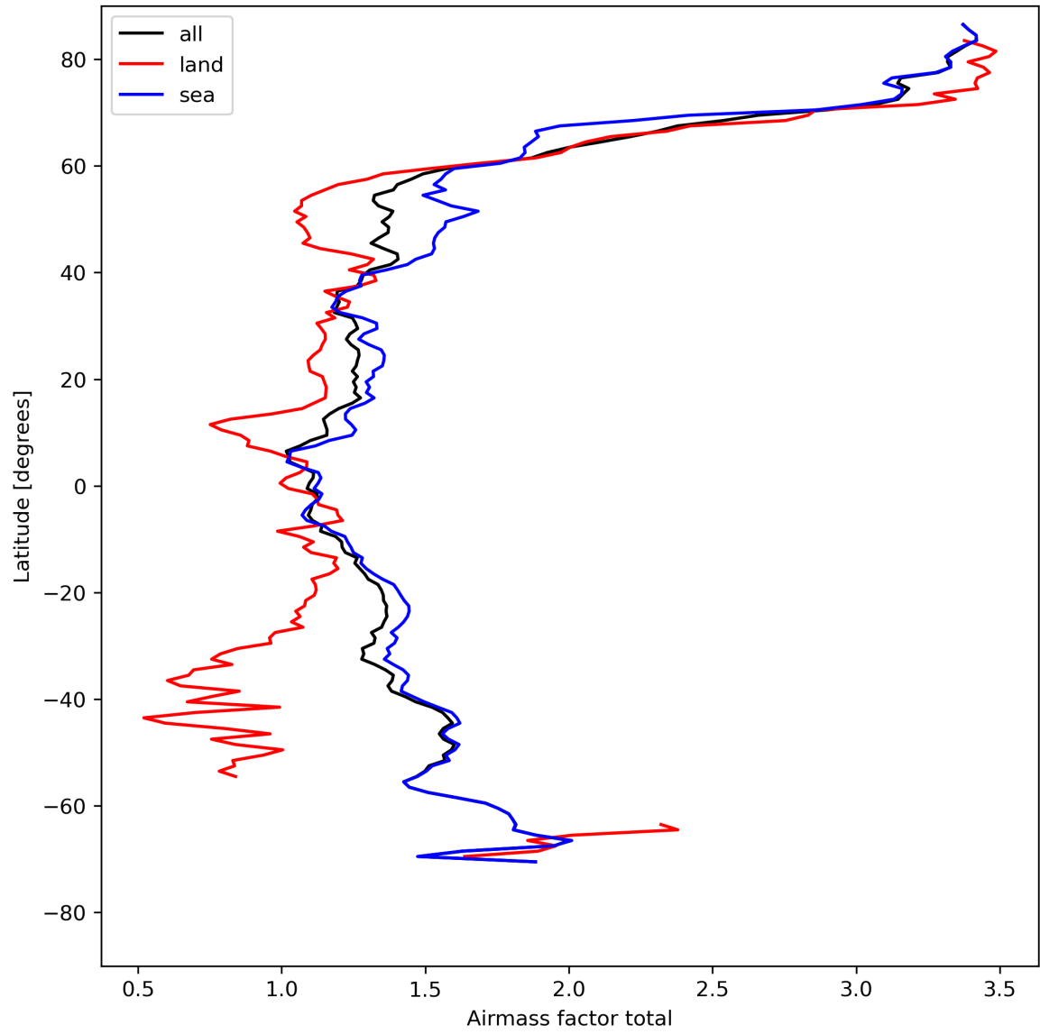
Figure 26: Zonal average of “Airmass factor total” for 2024-04-27 to 2024-04-29.
