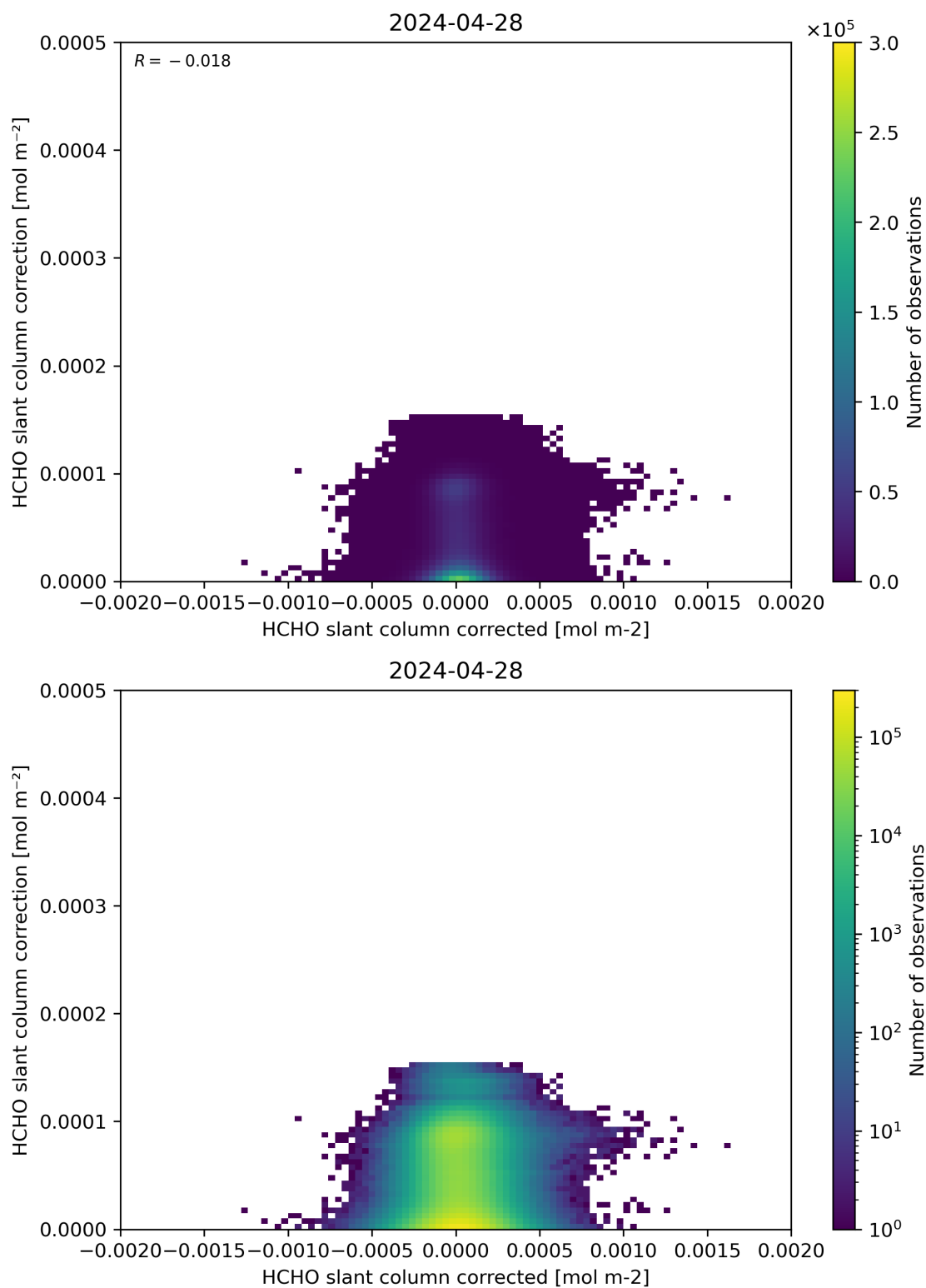
Figure 77: Scatter density plot of “HCHO slant column corrected” against “HCHO slant column correction” for 2024-04-27 to 2024-04-29.
