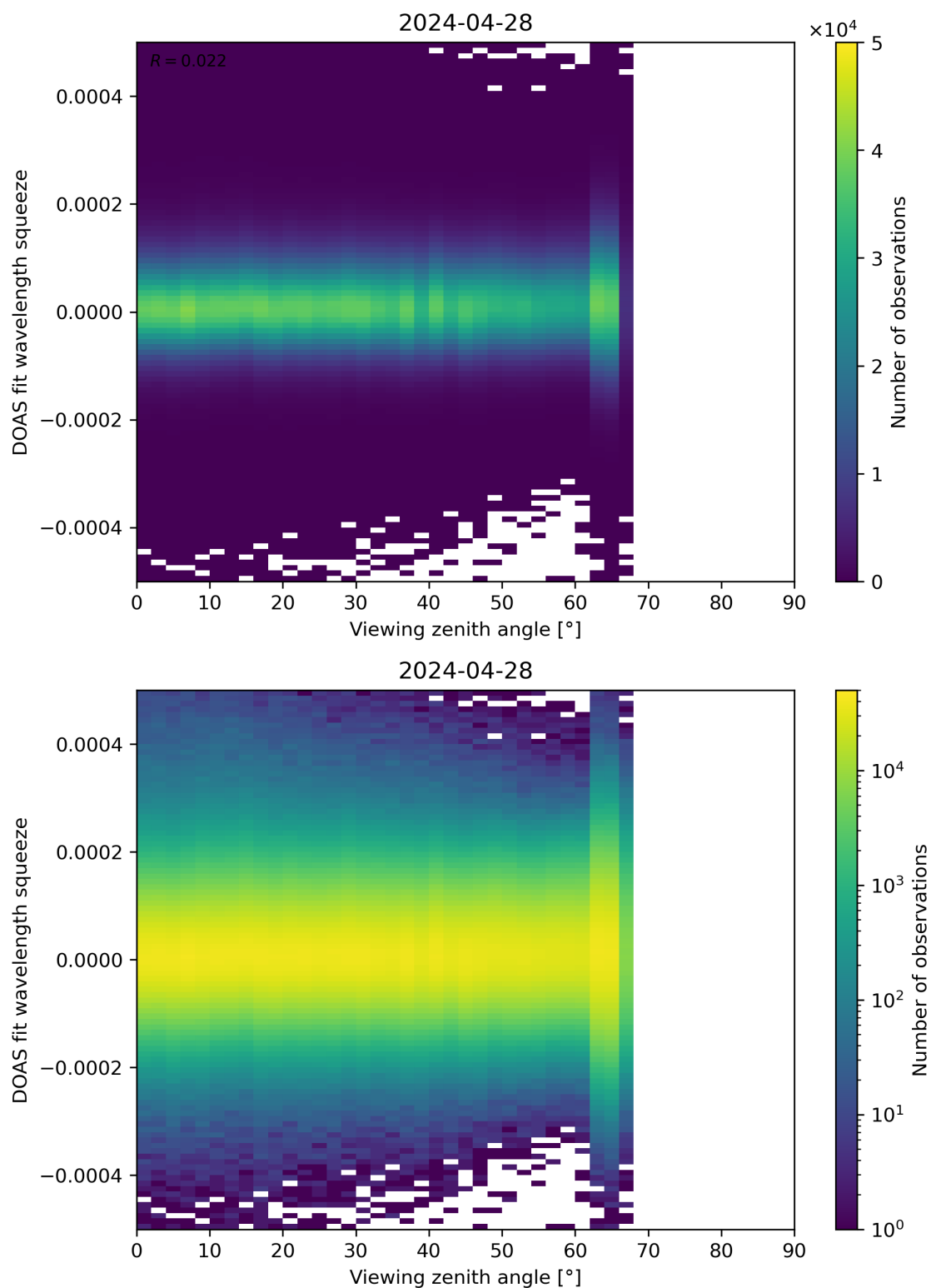
Figure 184: Scatter density plot of “Viewing zenith angle” against “DOAS fit wavelength squeeze” for 2024-04-27 to 2024-04-29.
