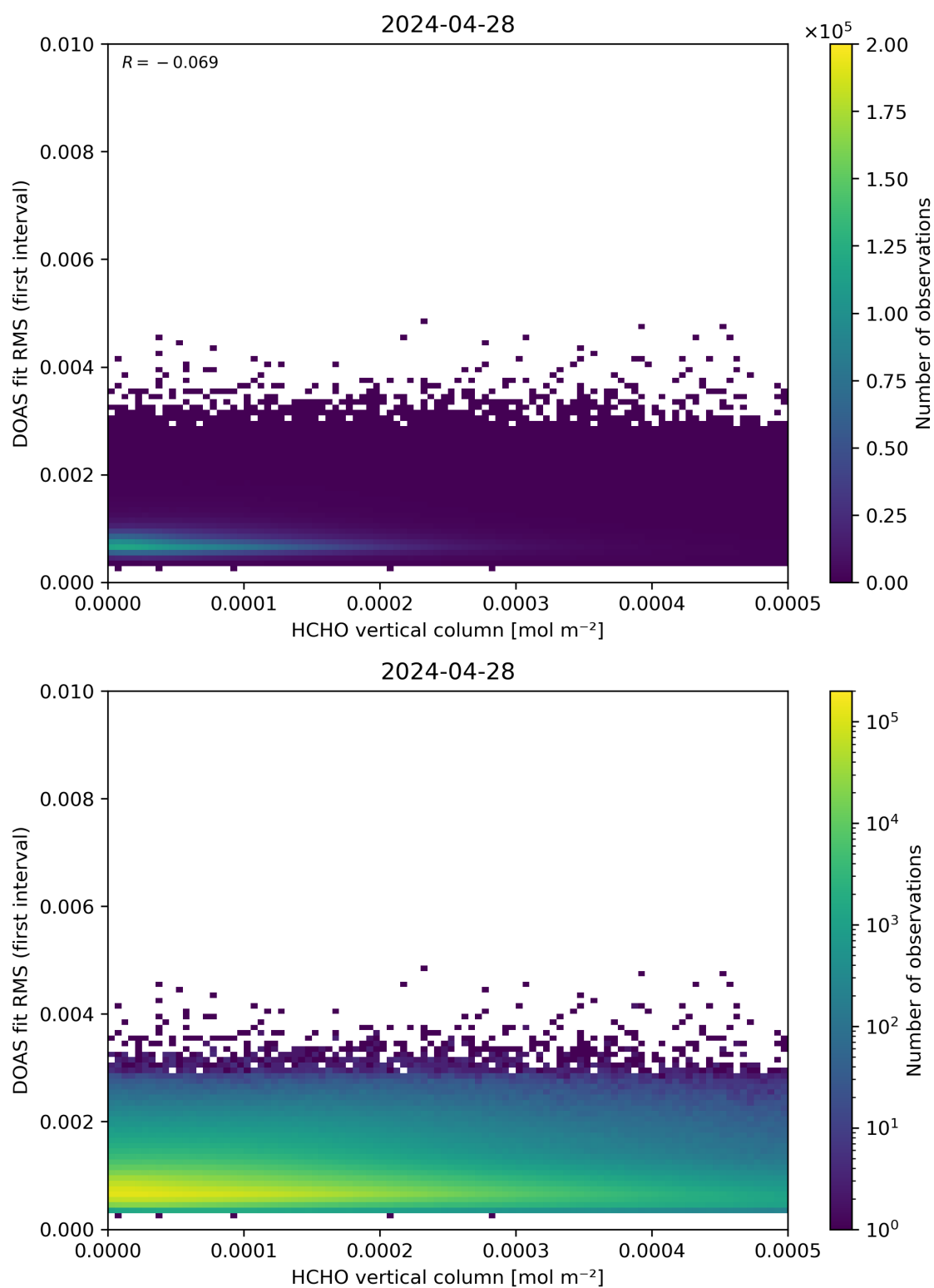
Figure 123: Scatter density plot of “HCHO vertical column” against “DOAS fit RMS (first interval)” for 2024-04-27 to 2024-04-29.
