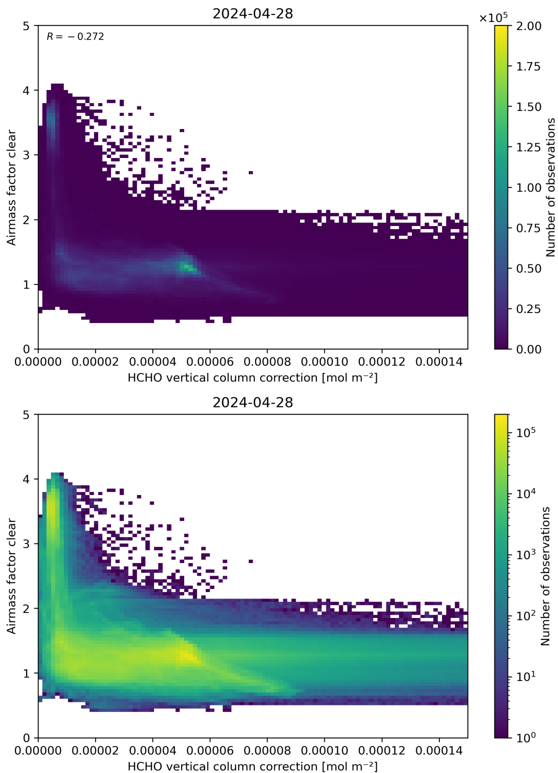
Figure 115: Scatter density plot of “HCHO vertical column correction” against “Airmass factor clear” for 2024-04-27 to 2024-04-29.
