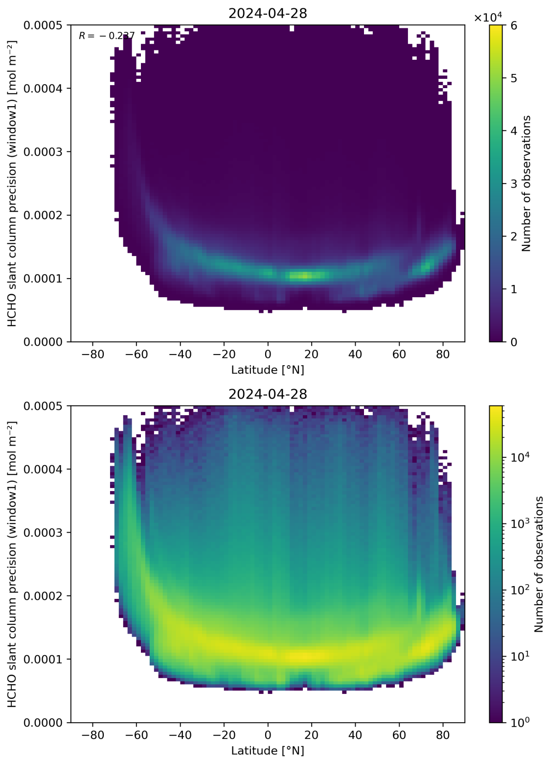
Figure 160: Scatter density plot of “Latitude” against “HCHO slant column precision (window1)” for 2024-04-27 to 2024-04-29.
