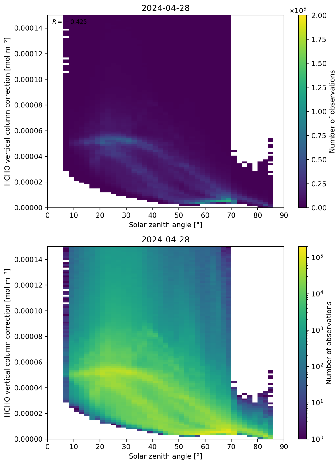
Figure 178: Scatter density plot of “Solar zenith angle” against “HCHO vertical column correction” for 2024-04-27 to 2024-04-29.
