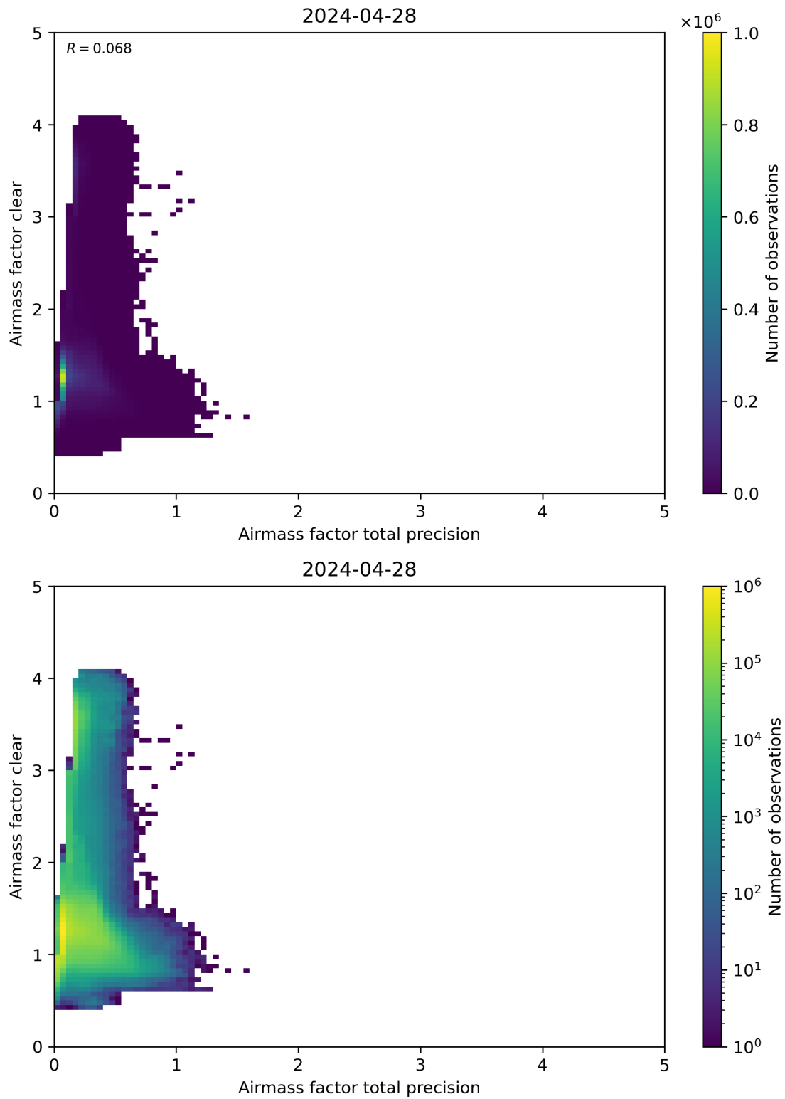
Figure 108: Scatter density plot of “Airmass factor total precision” against “Airmass factor clear” for 2024-04-27 to 2024-04-29.
