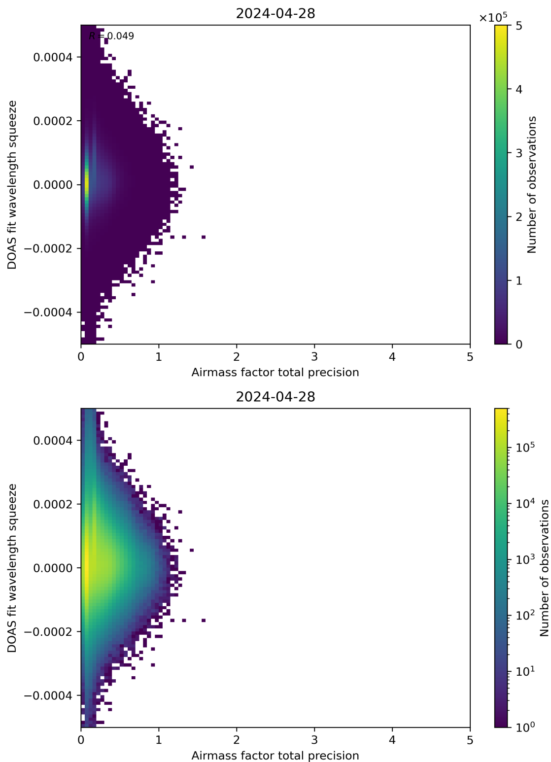
Figure 107: Scatter density plot of “Airmass factor total precision” against “DOAS fit wavelength squeeze” for 2024-04-27 to 2024-04-29.
