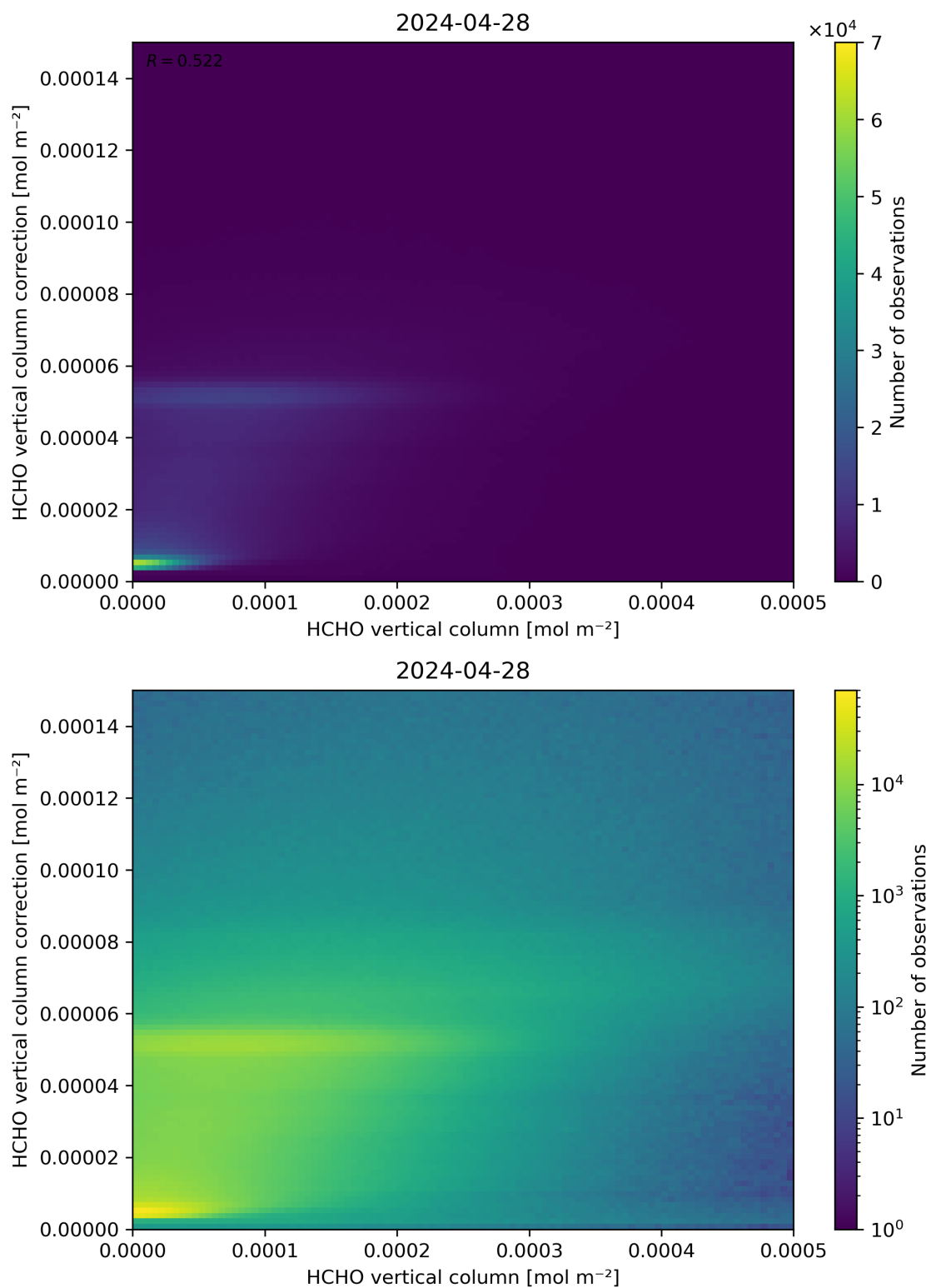
Figure 133: Scatter density plot of “HCHO vertical column” against “HCHO vertical column correction” for 2024-04-27 to 2024-04-29.
