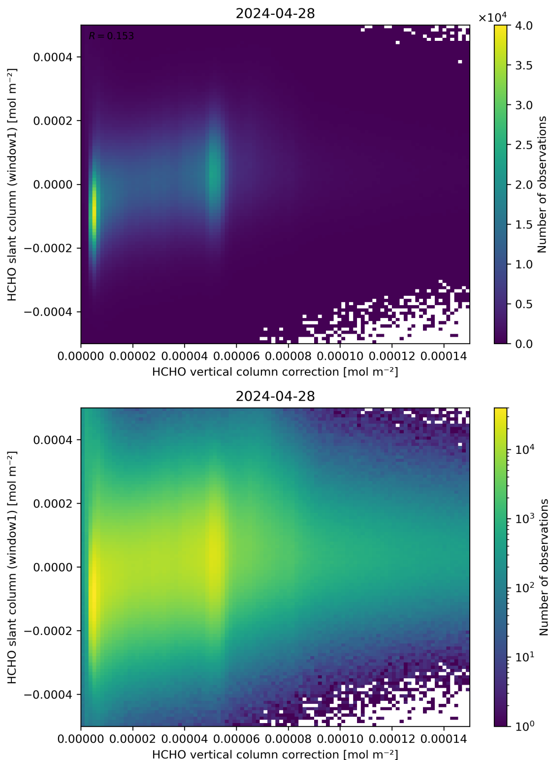
Figure 118: Scatter density plot of “HCHO vertical column correction” against “HCHO slant column (window1)” for 2024-04-27 to 2024-04-29.
