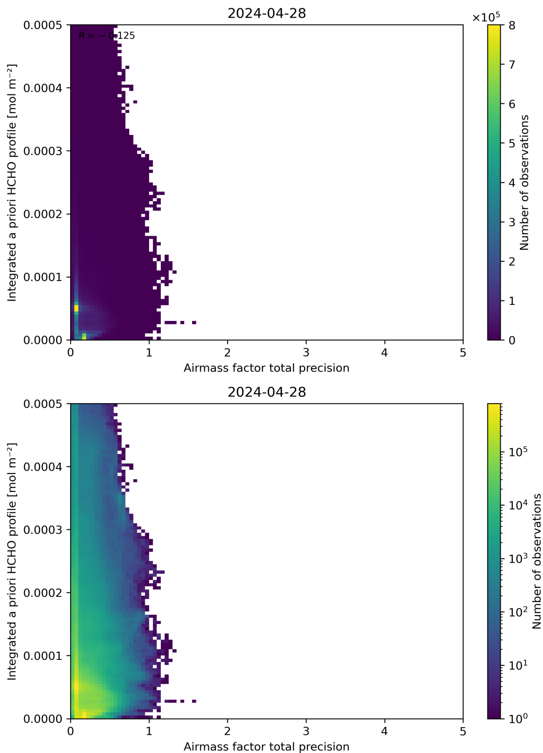
Figure 111: Scatter density plot of “Airmass factor total precision” against “Integrated a priori HCHO profile” for 2024-04-27 to 2024-04-29.
