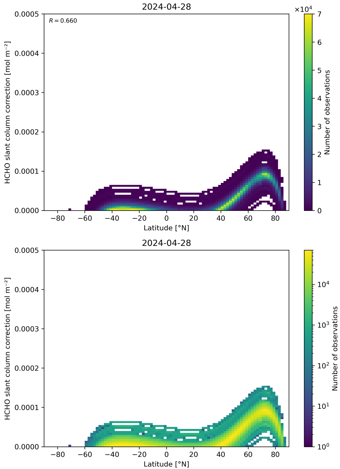
Figure 158: Scatter density plot of “Latitude” against “HCHO slant column correction” for 2024-04-27 to 2024-04-29.
