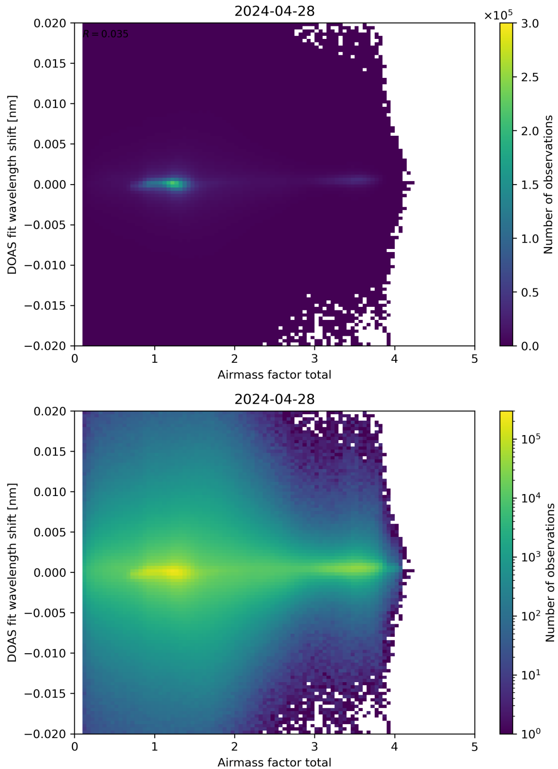
Figure 98: Scatter density plot of “Airmass factor total” against “DOAS fit wavelength shift” for 2024-04-27 to 2024-04-29.
