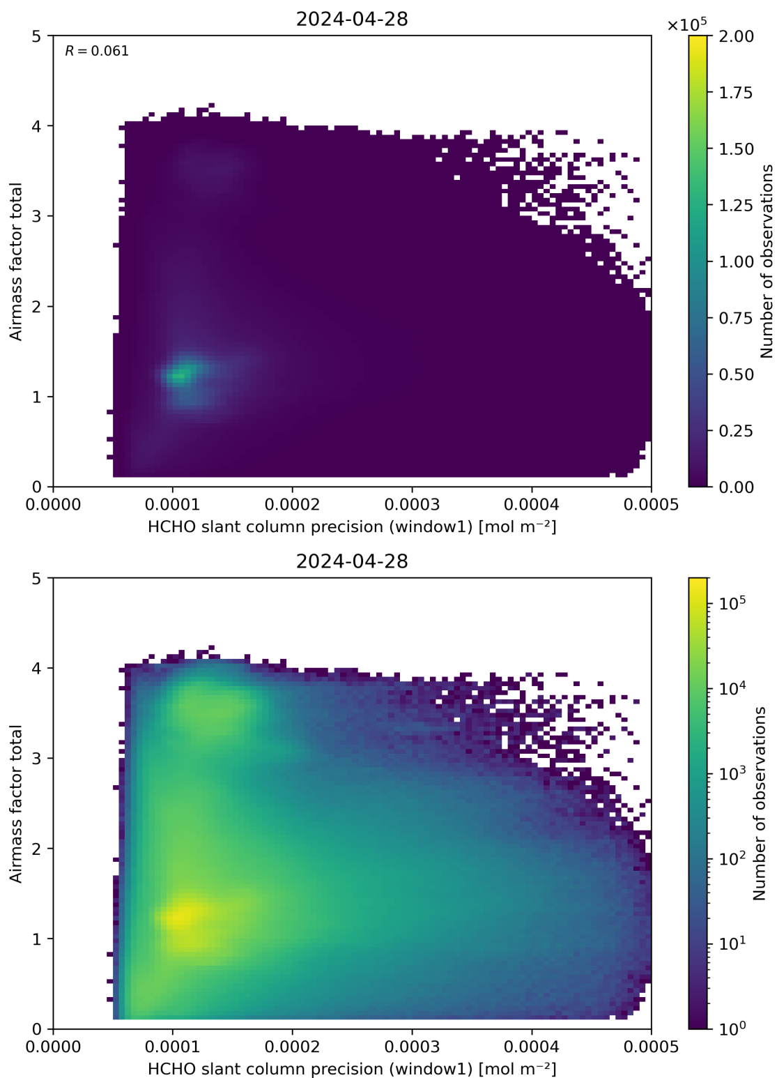
Figure 94: Scatter density plot of “HCHO slant column precision (window1)” against “Airmass factor total” for 2024-04-27 to 2024-04-29.
