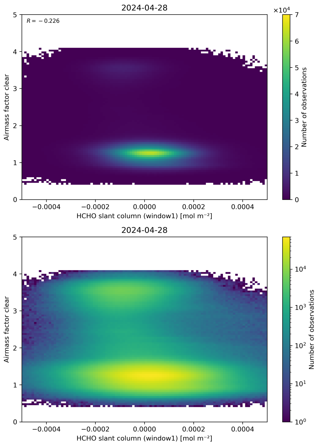
Figure 81: Scatter density plot of “HCHO slant column (window1)” against “Airmass factor clear” for 2024-04-27 to 2024-04-29.
