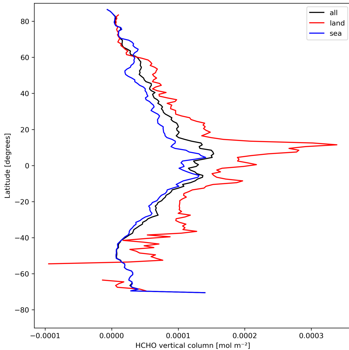
Figure 21: Zonal average of “HCHO vertical column” for 2024-04-27 to 2024-04-29.
