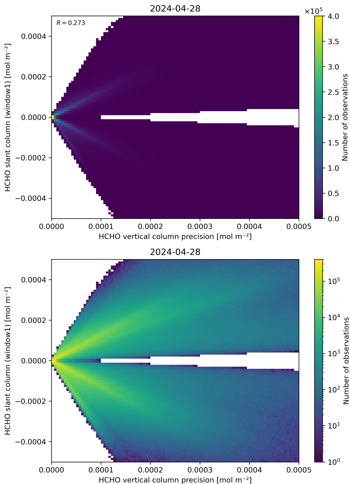
Figure 142: Scatter density plot of “HCHO vertical column precision” against “HCHO slant column (window1)” for 2024-04-27 to 2024-04-29.
