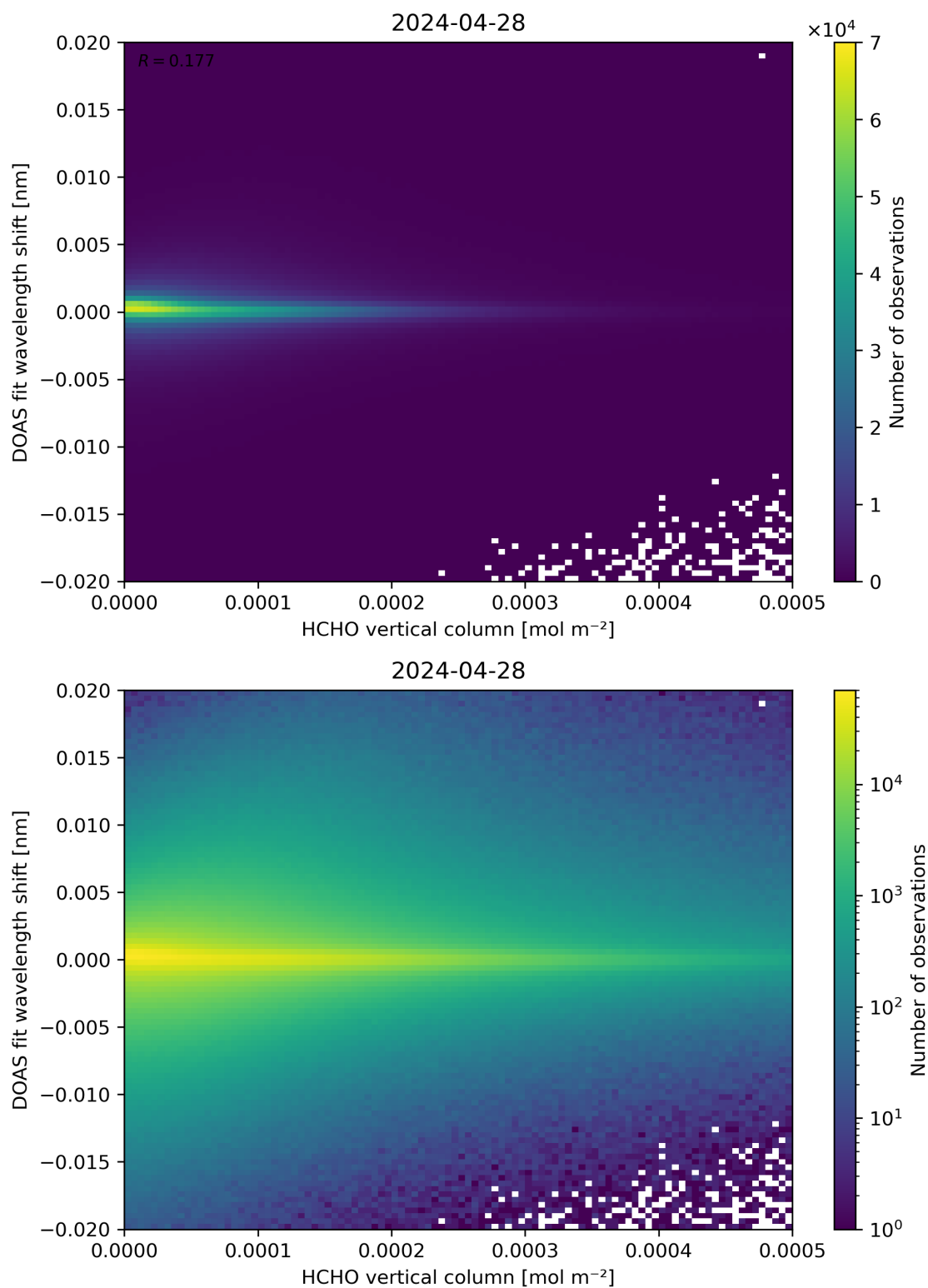
Figure 124: Scatter density plot of “HCHO vertical column” against “DOAS fit wavelength shift” for 2024-04-27 to 2024-04-29.
