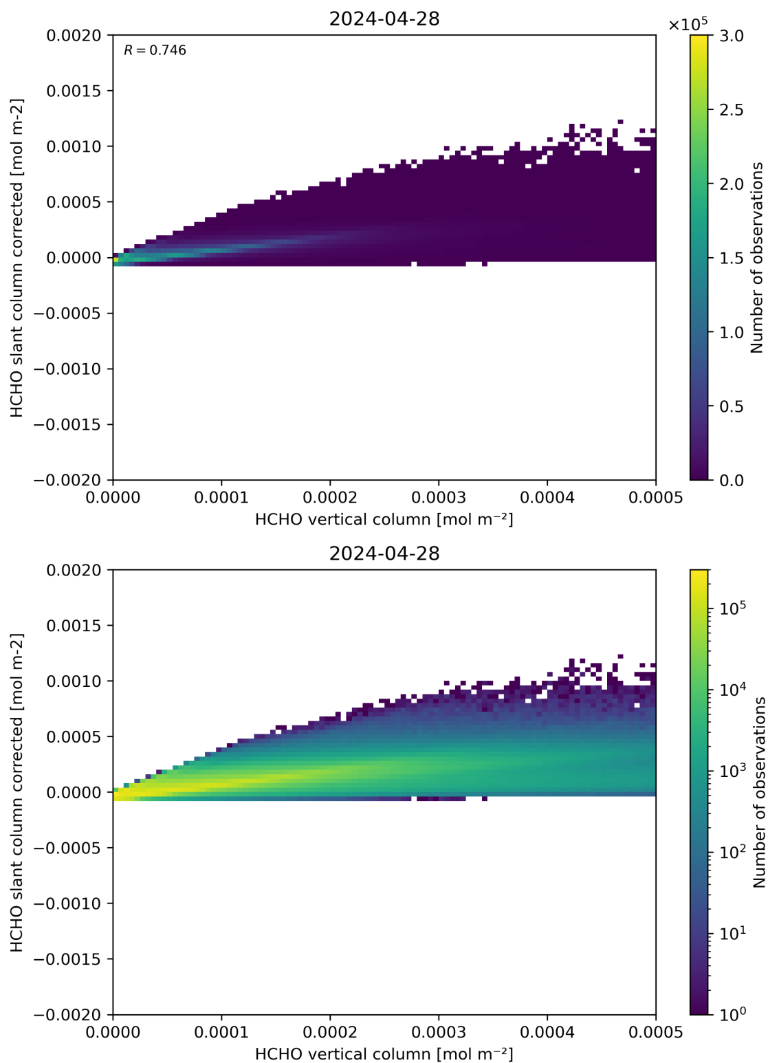
Figure 127: Scatter density plot of “HCHO vertical column” against “HCHO slant column corrected” for 2024-04-27 to 2024-04-29.
