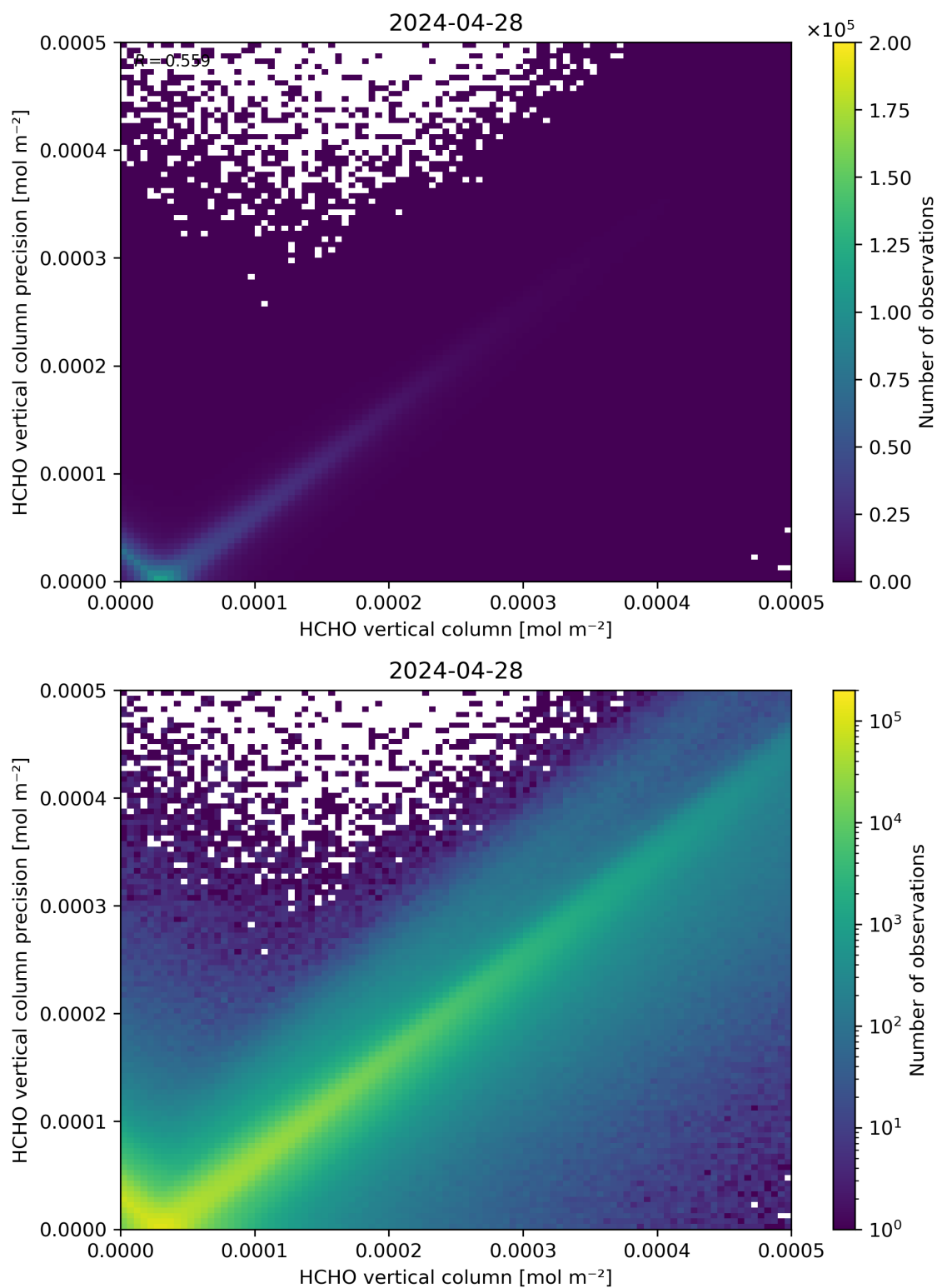
Figure 134: Scatter density plot of “HCHO vertical column” against “HCHO vertical column precision” for 2024-04-27 to 2024-04-29.
