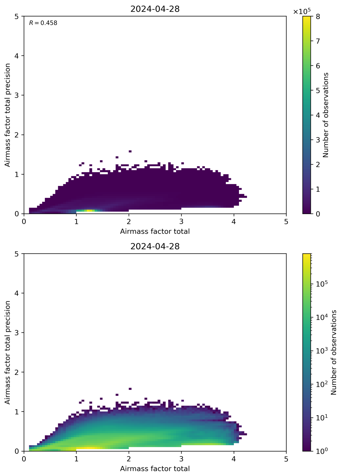
Figure 103: Scatter density plot of “Airmass factor total” against “Airmass factor total precision” for 2024-04-27 to 2024-04-29.
