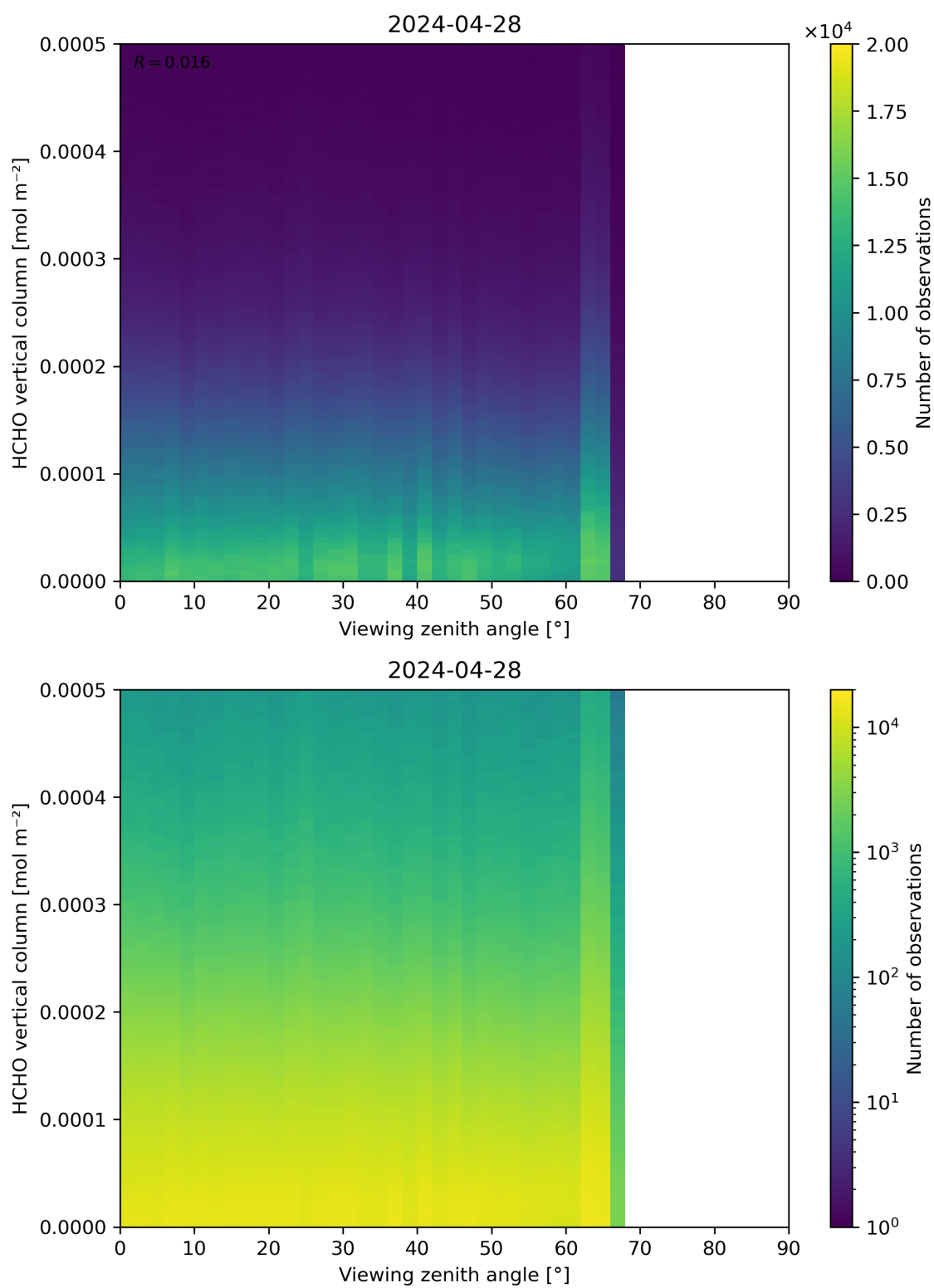
Figure 192: Scatter density plot of “Viewing zenith angle” against “HCHO vertical column” for 2024-04-27 to 2024-04-29.
