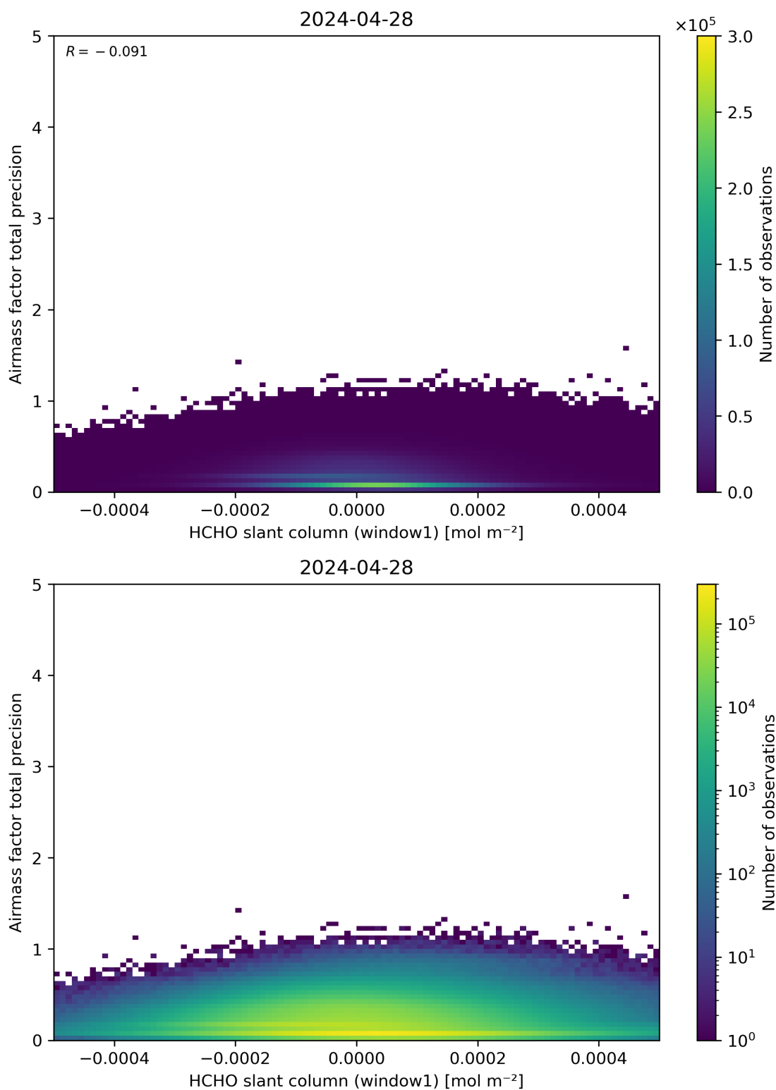
Figure 86: Scatter density plot of “HCHO slant column (window1)” against “Airmass factor total precision” for 2024-04-27 to 2024-04-29.
