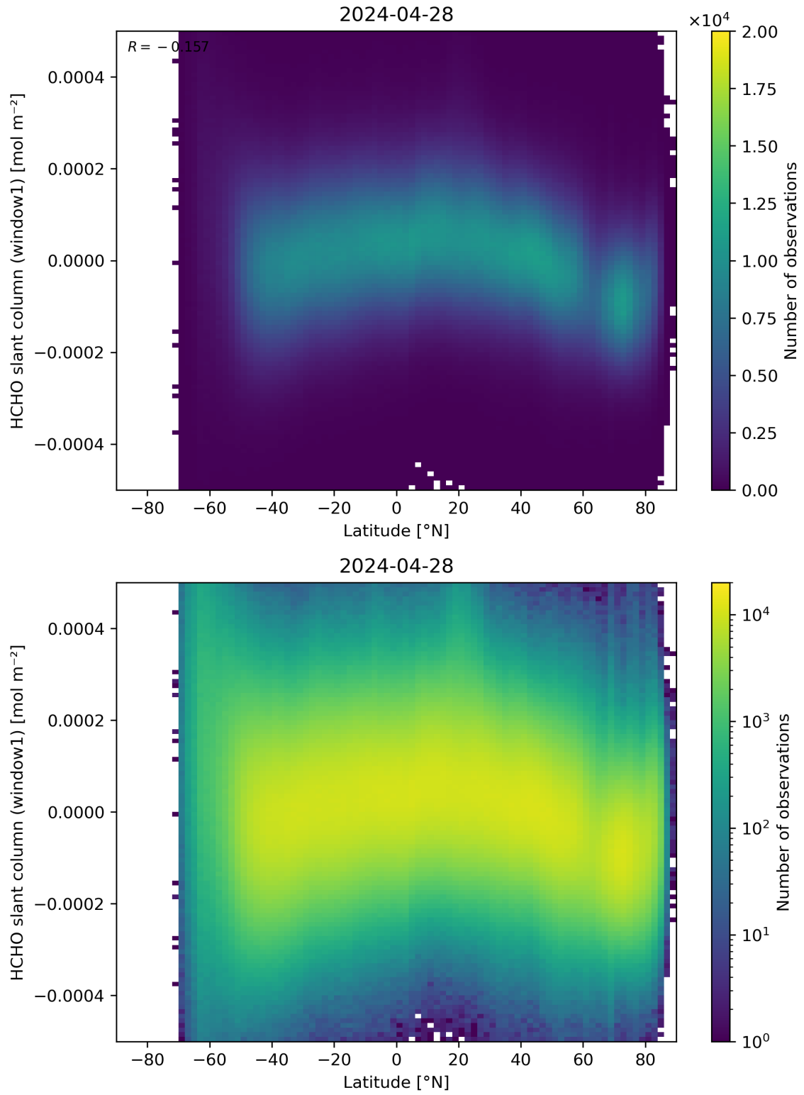
Figure 159: Scatter density plot of “Latitude” against “HCHO slant column (window1)” for 2024-04-27 to 2024-04-29.
