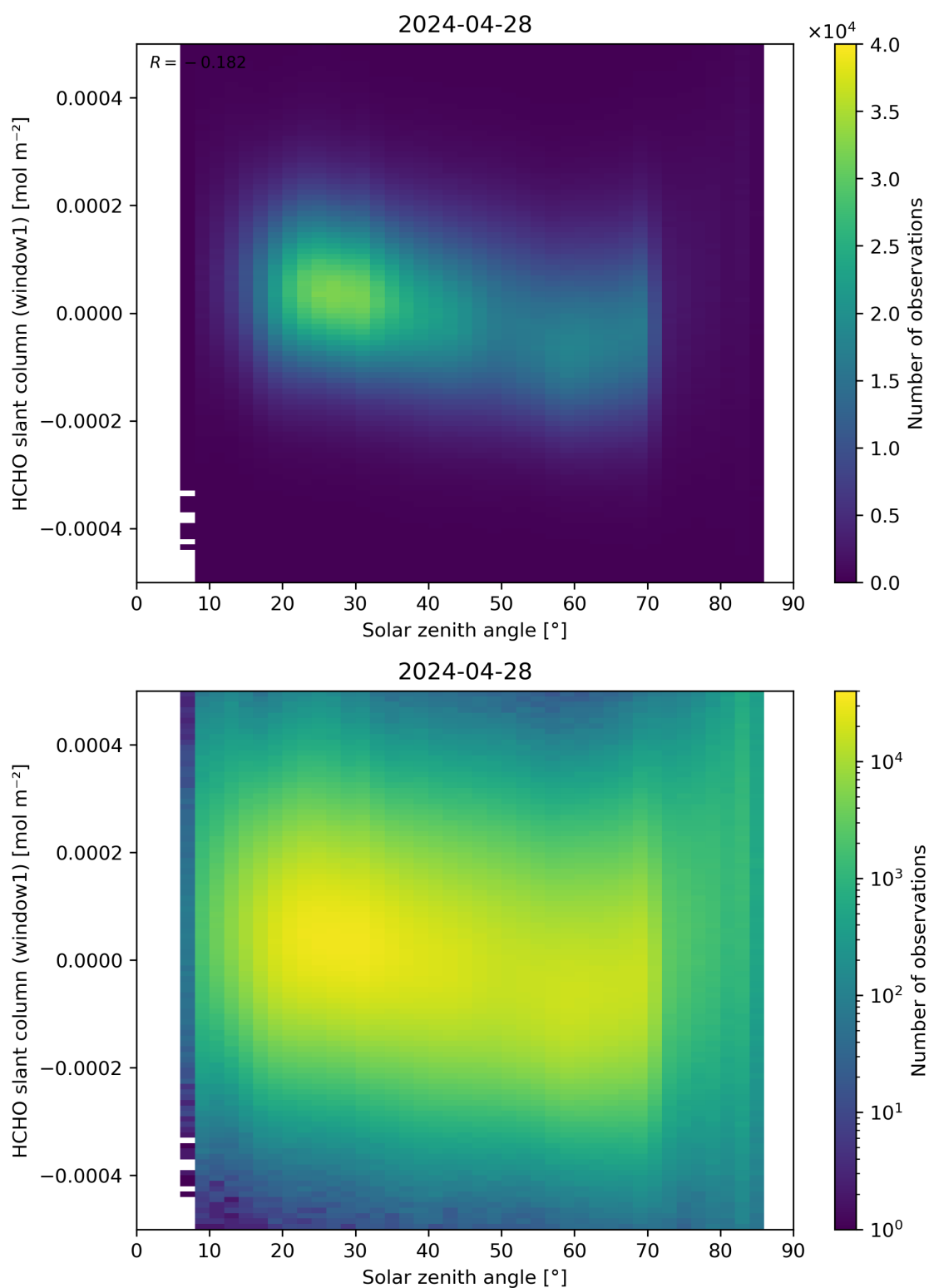
Figure 173: Scatter density plot of “Solar zenith angle” against “HCHO slant column (window1)” for 2024-04-27 to 2024-04-29.
