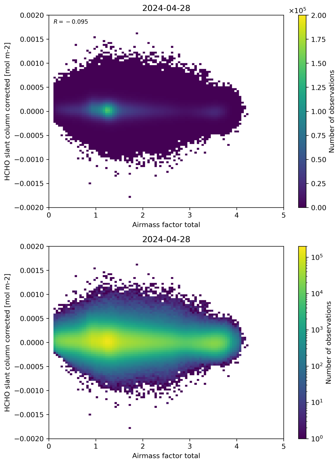
Figure 101: Scatter density plot of “Airmass factor total” against “HCHO slant column corrected” for 2024-04-27 to 2024-04-29.
