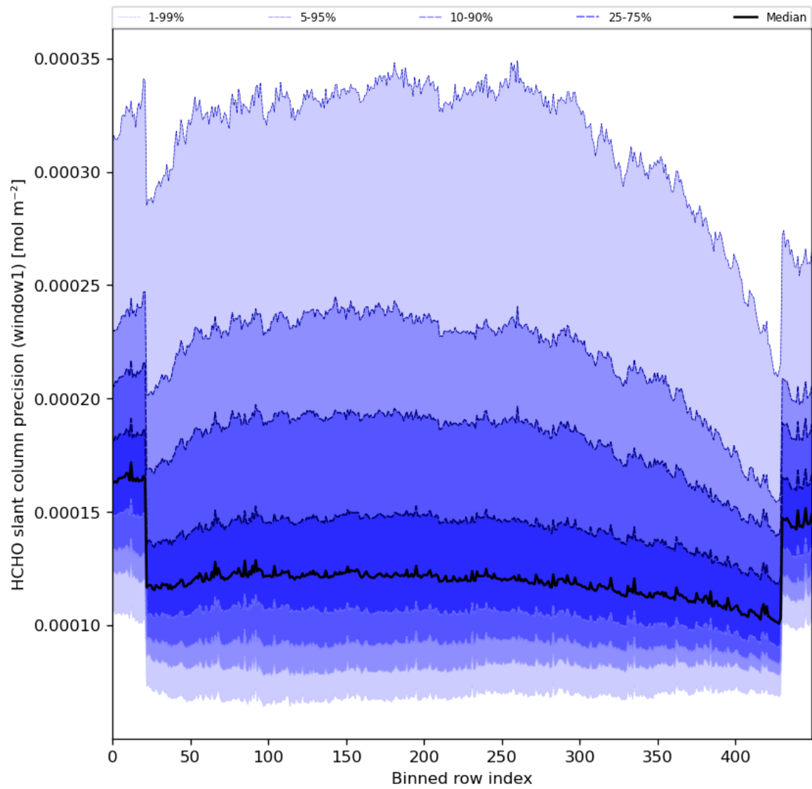
Figure 53: Along track statistics of “HCHO slant column precision (window1)” for 2024-04-27 to 2024-04-29
