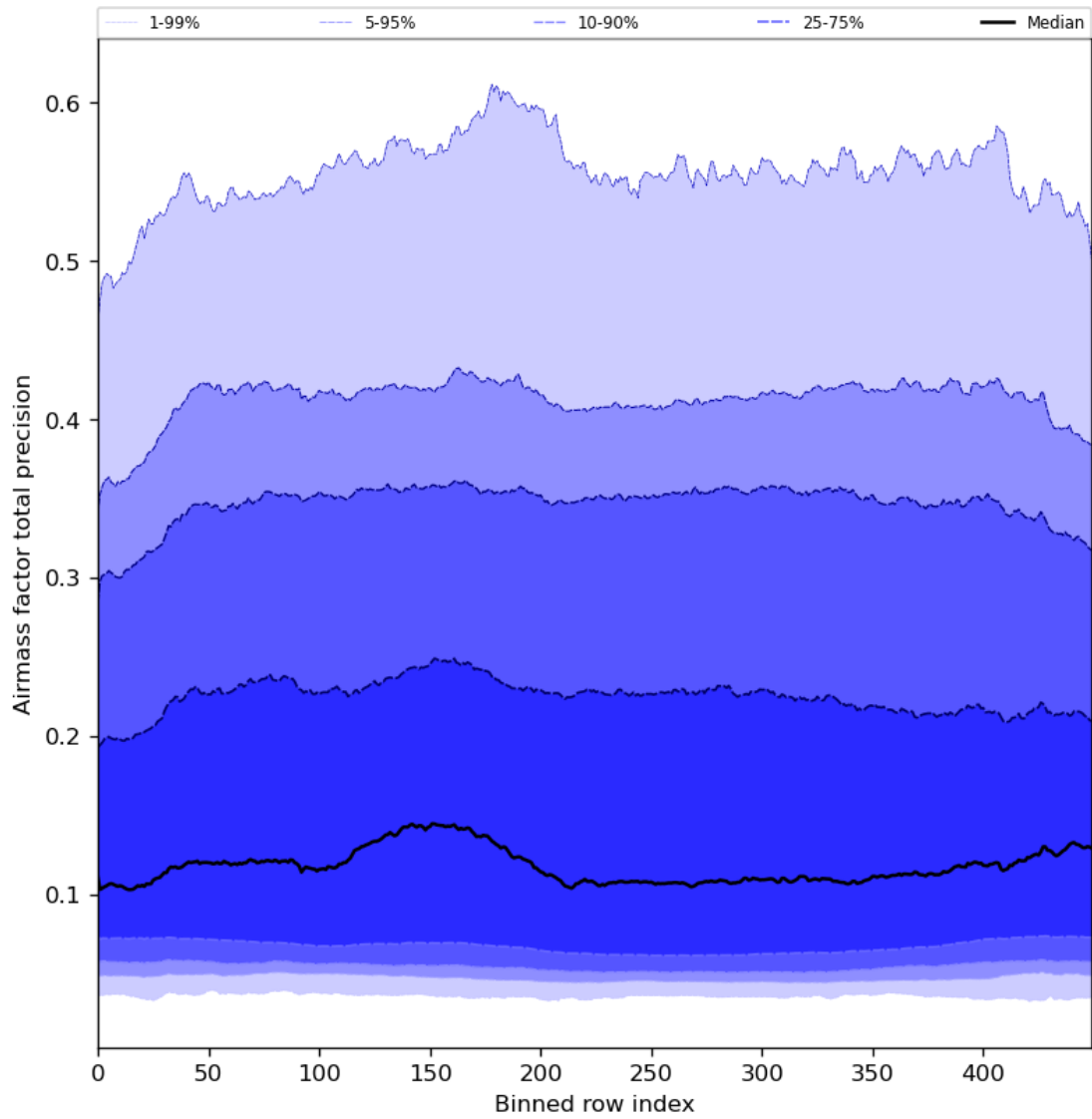
Figure 55: Along track statistics of “Airmass factor total precision” for 2024-04-27 to 2024-04-29
