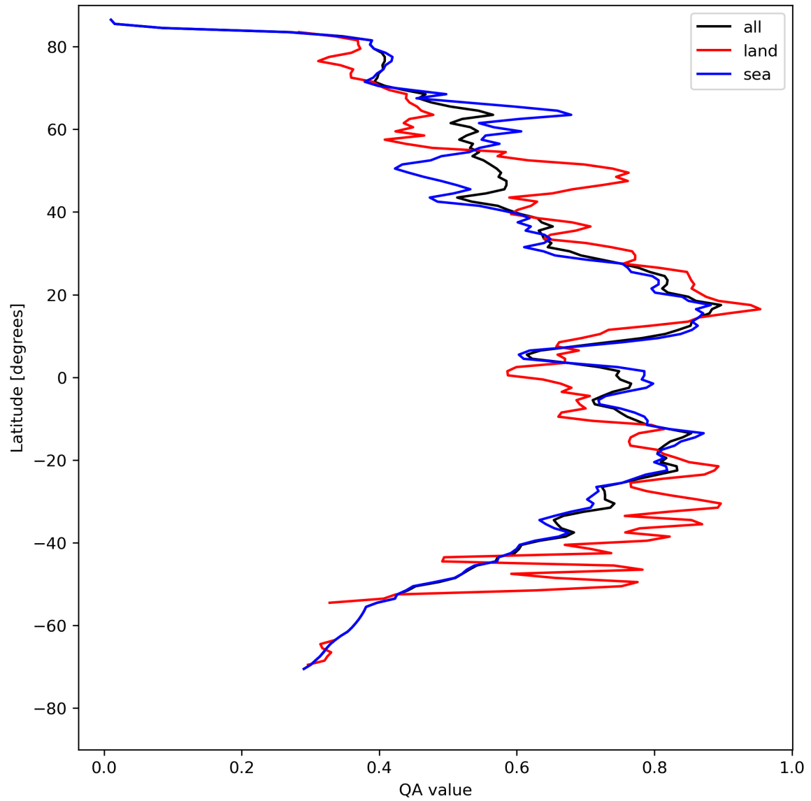
Figure 20: Zonal average of “QA value” for 2024-04-27 to 2024-04-29.
