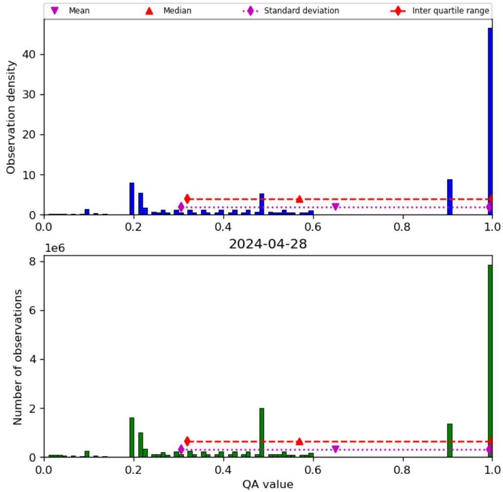
Figure 34: Histogram of “QA value” for 2024-04-27 to 2024-04-29
