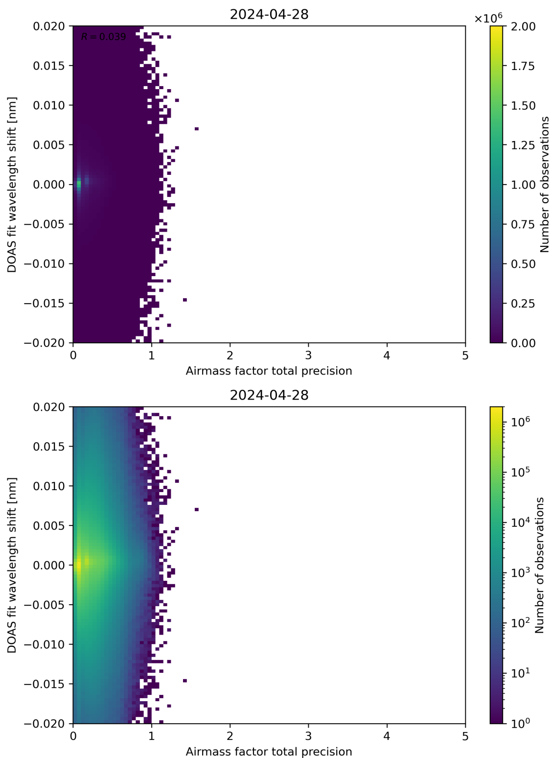
Figure 106: Scatter density plot of “Airmass factor total precision” against “DOAS fit wavelength shift” for 2024-04-27 to 2024-04-29.
