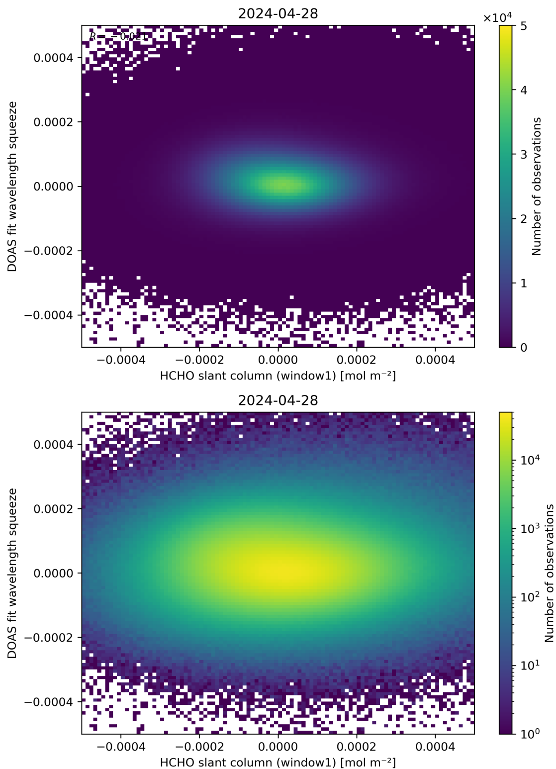
Figure 80: Scatter density plot of “HCHO slant column (window1)” against “DOAS fit wavelength squeeze” for 2024-04-27 to 2024-04-29.
