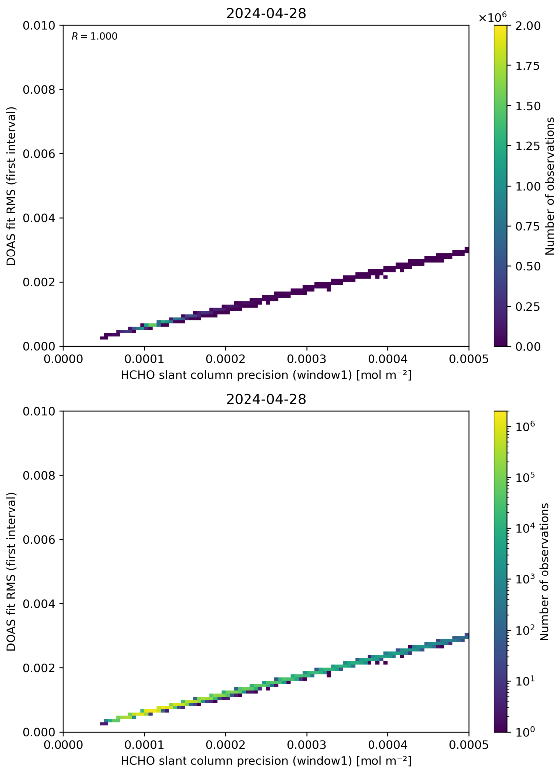
Figure 88: Scatter density plot of “HCHO slant column precision (window1)” against “DOAS fit RMS (first interval)” for 2024-04-27 to 2024-04-29.
