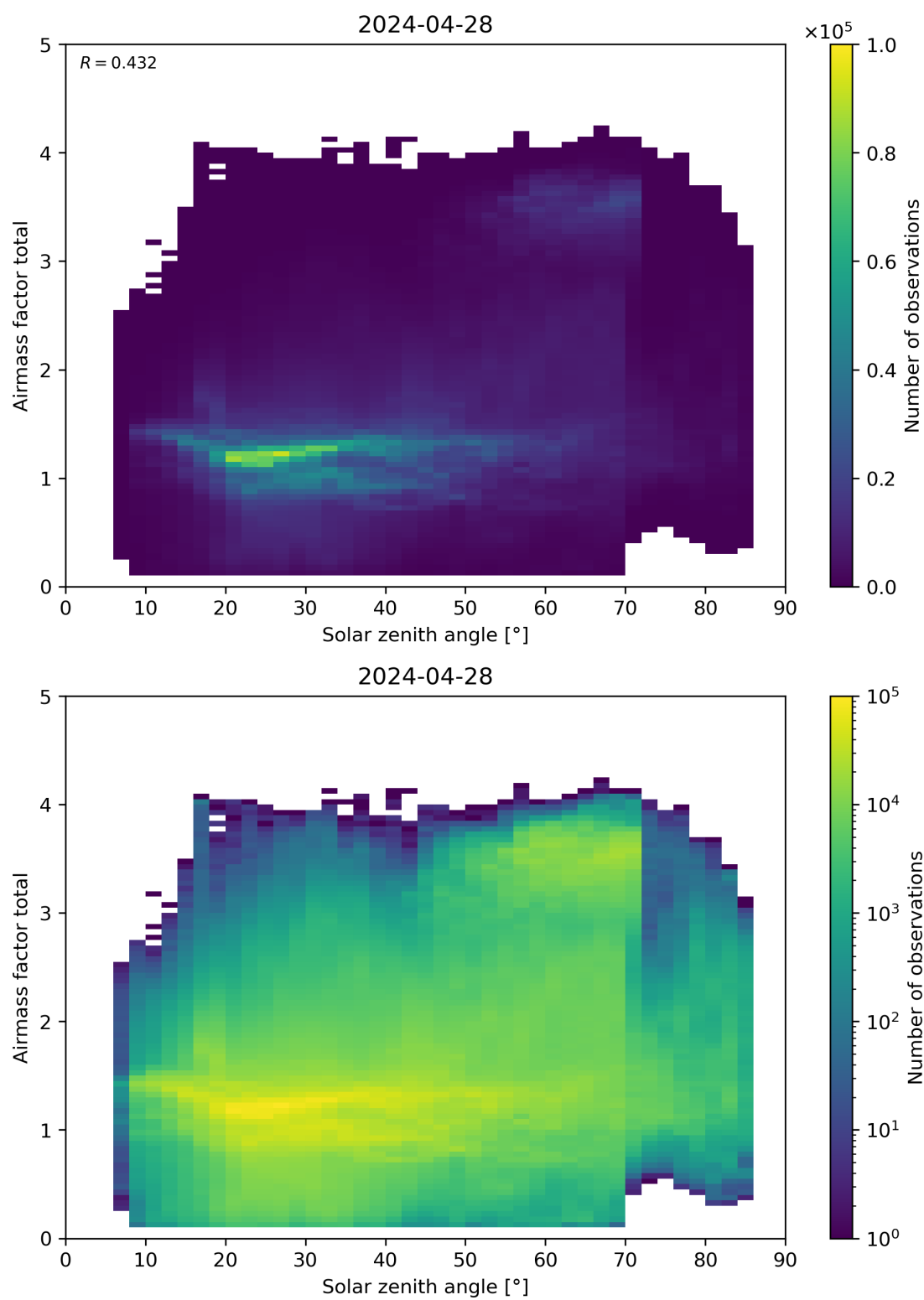
Figure 175: Scatter density plot of “Solar zenith angle” against “Airmass factor total” for 2024-04-27 to 2024-04-29.
