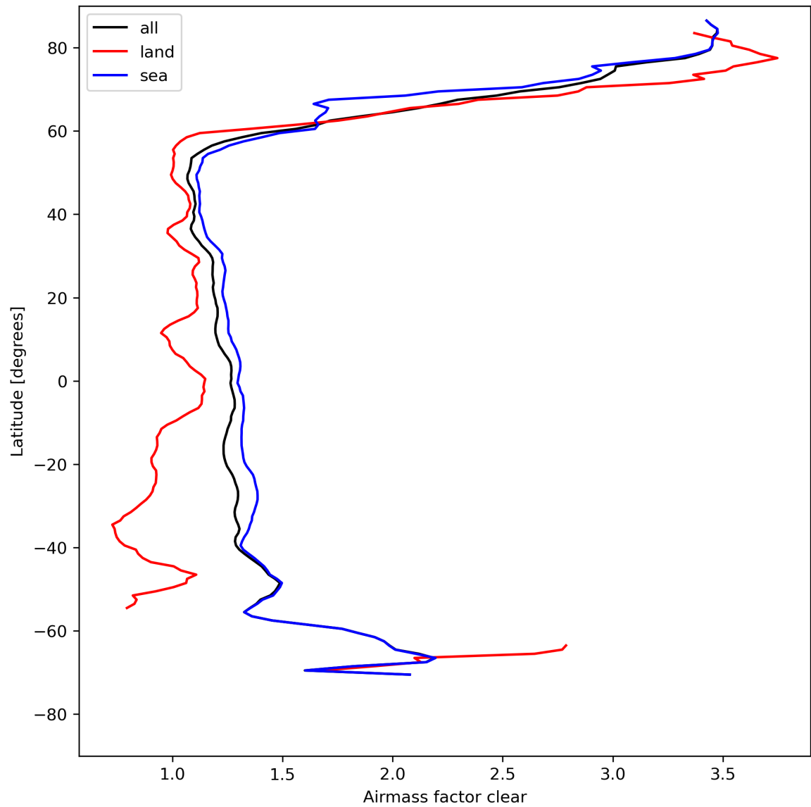
Figure 28: Zonal average of “Airmass factor clear” for 2024-04-27 to 2024-04-29.
