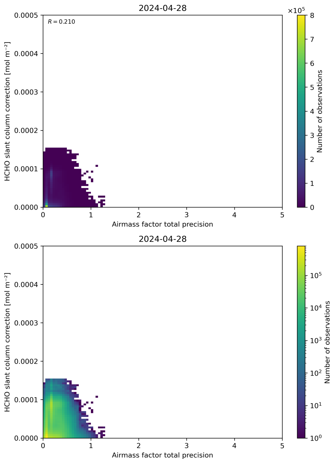
Figure 110: Scatter density plot of “Airmass factor total precision” against “HCHO slant column correction” for 2024-04-27 to 2024-04-29.
