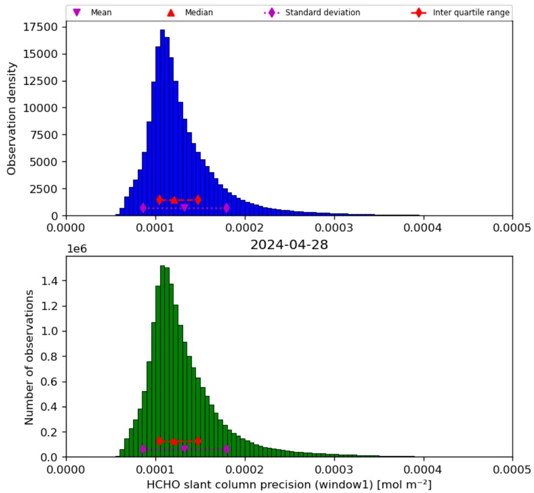
Figure 39: Histogram of “HCHO slant column precision (window1)” for 2024-04-27 to 2024-04-29
