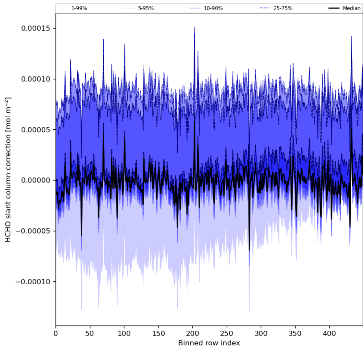
Figure 61: Along track statistics of “HCHO slant column correction” for 2024-04-27 to 2024-04-29
