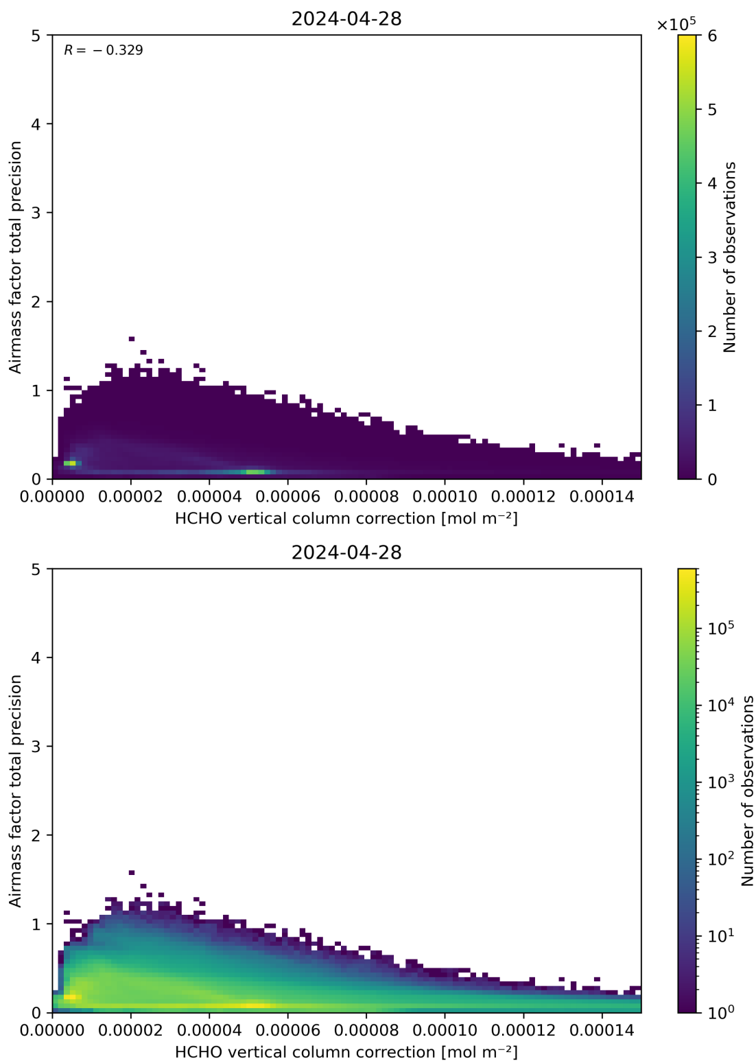
Figure 121: Scatter density plot of “HCHO vertical column correction” against “Airmass factor total precision” for 2024-04-27 to 2024-04-29.
