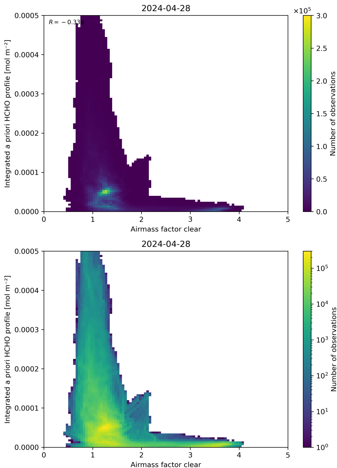
Figure 76: Scatter density plot of “Airmass factor clear” against “Integrated a priori HCHO profile” for 2024-04-27 to 2024-04-29.
