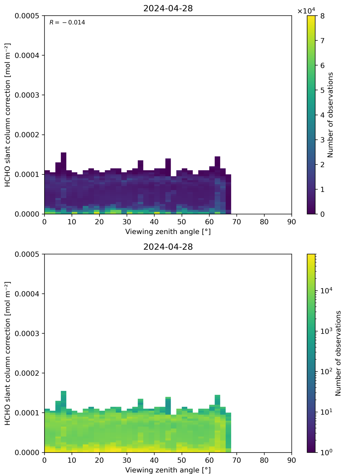
Figure 187: Scatter density plot of “Viewing zenith angle” against “HCHO slant column correction” for 2024-04-27 to 2024-04-29.
