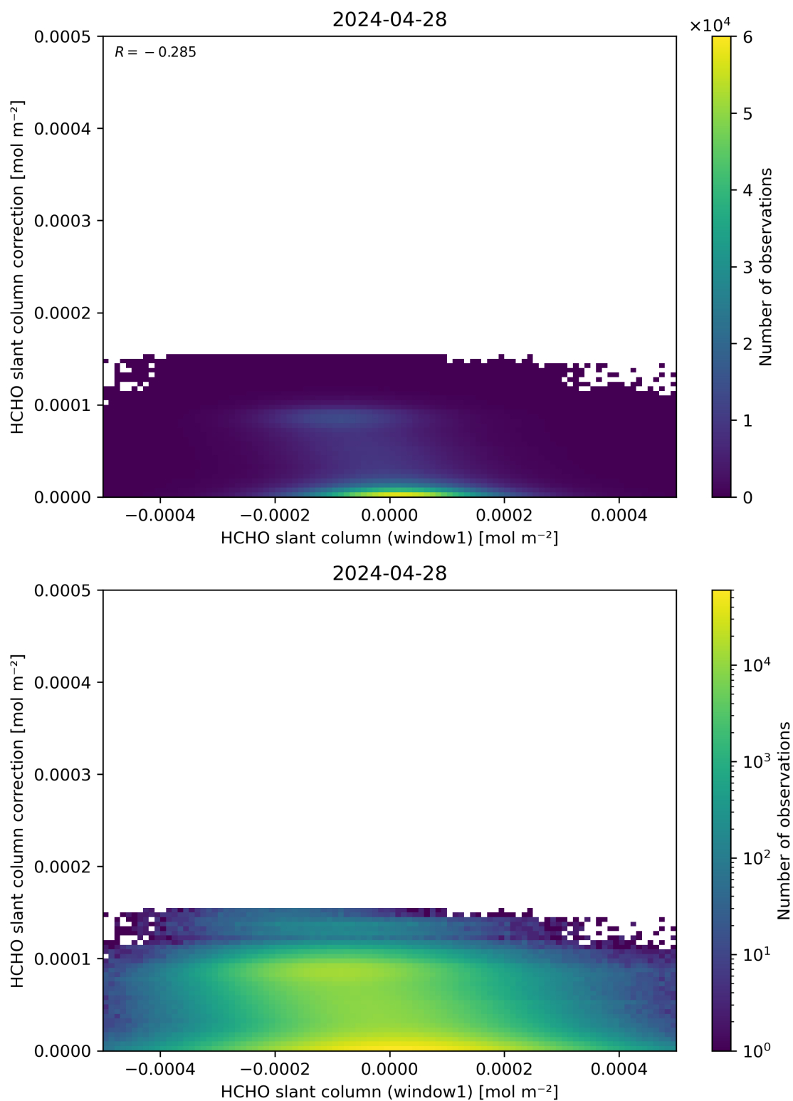
Figure 83: Scatter density plot of “HCHO slant column (window1)” against “HCHO slant column correction” for 2024-04-27 to 2024-04-29.
