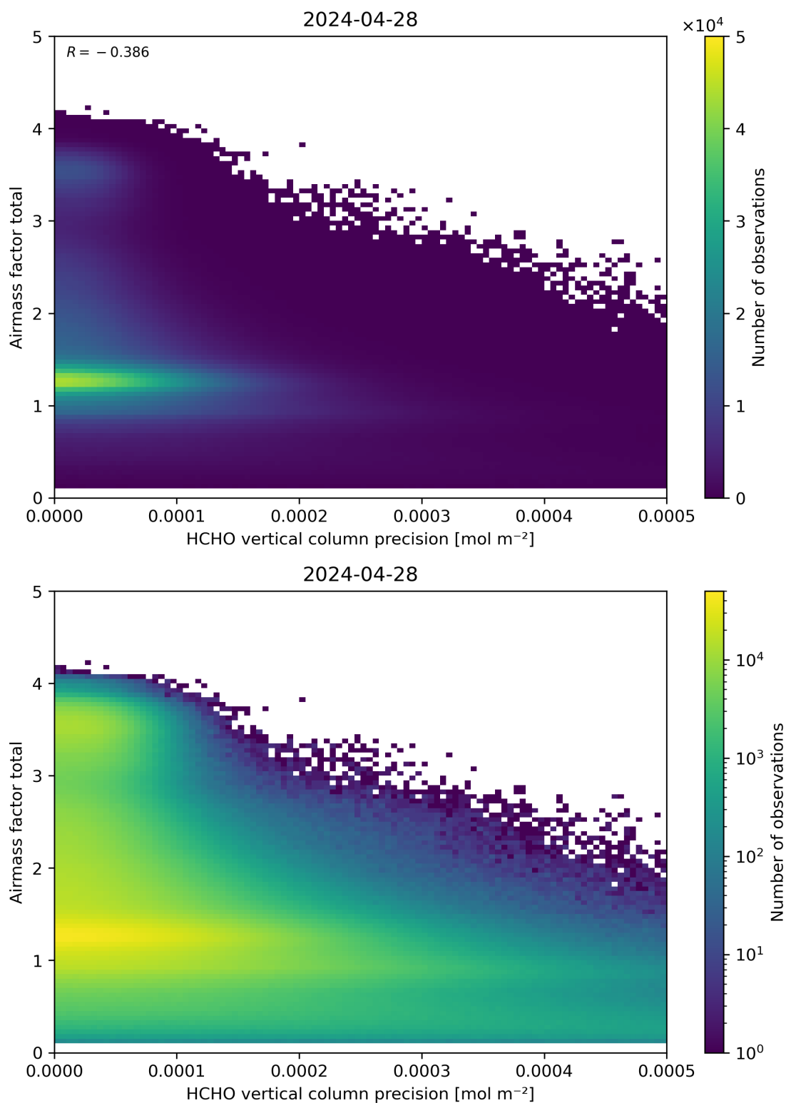
Figure 144: Scatter density plot of “HCHO vertical column precision” against “Airmass factor total” for 2024-04-27 to 2024-04-29.
