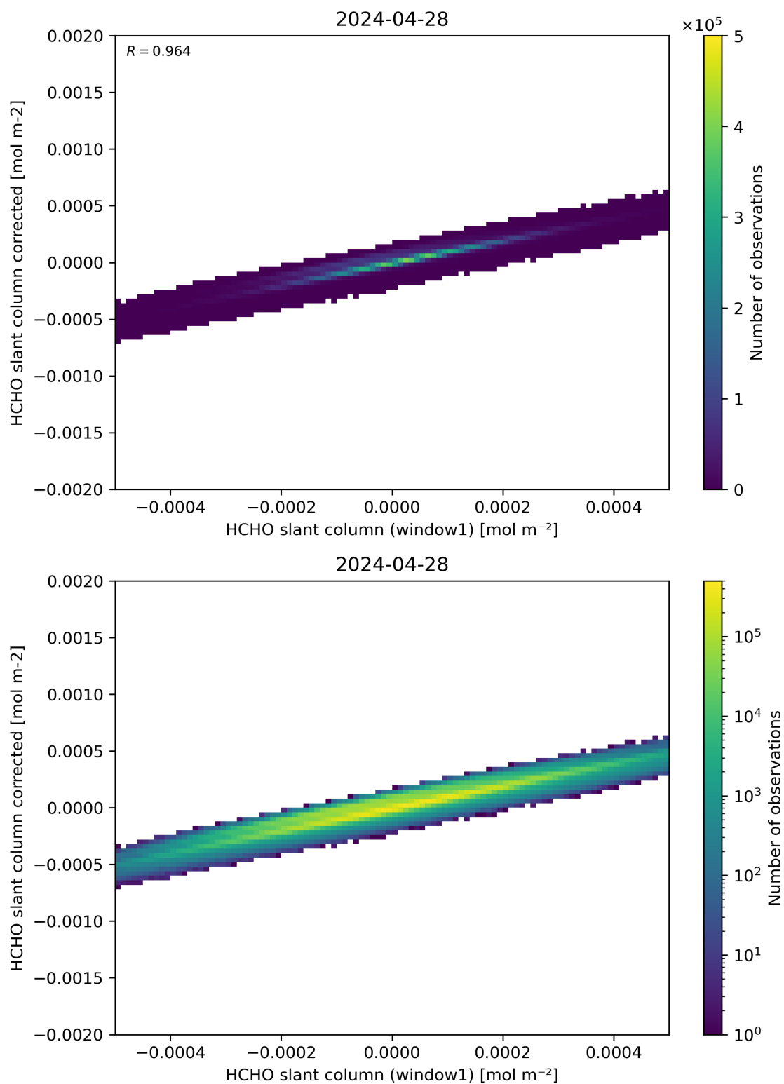
Figure 82: Scatter density plot of “HCHO slant column (window1)” against “HCHO slant column corrected” for 2024-04-27 to 2024-04-29.
