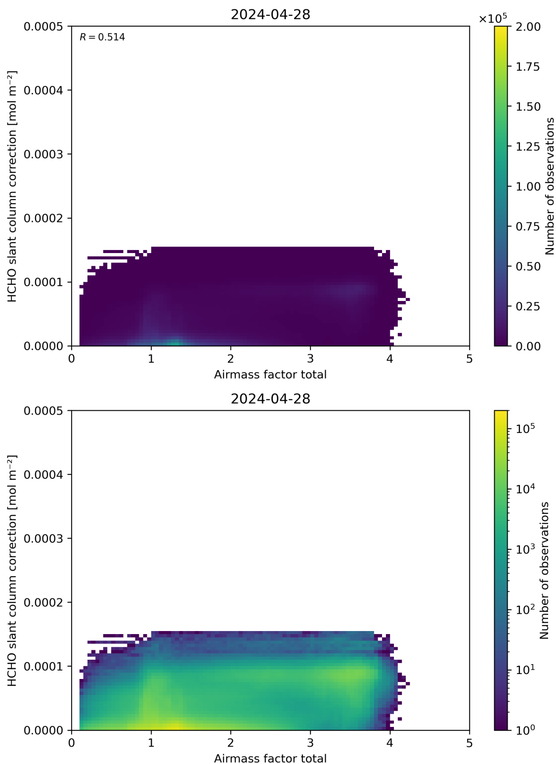
Figure 102: Scatter density plot of “Airmass factor total” against “HCHO slant column correction” for 2024-04-27 to 2024-04-29.
