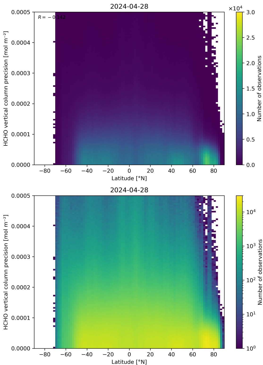
Figure 165: Scatter density plot of “Latitude” against “HCHO vertical column precision” for 2024-04-27 to 2024-04-29.
