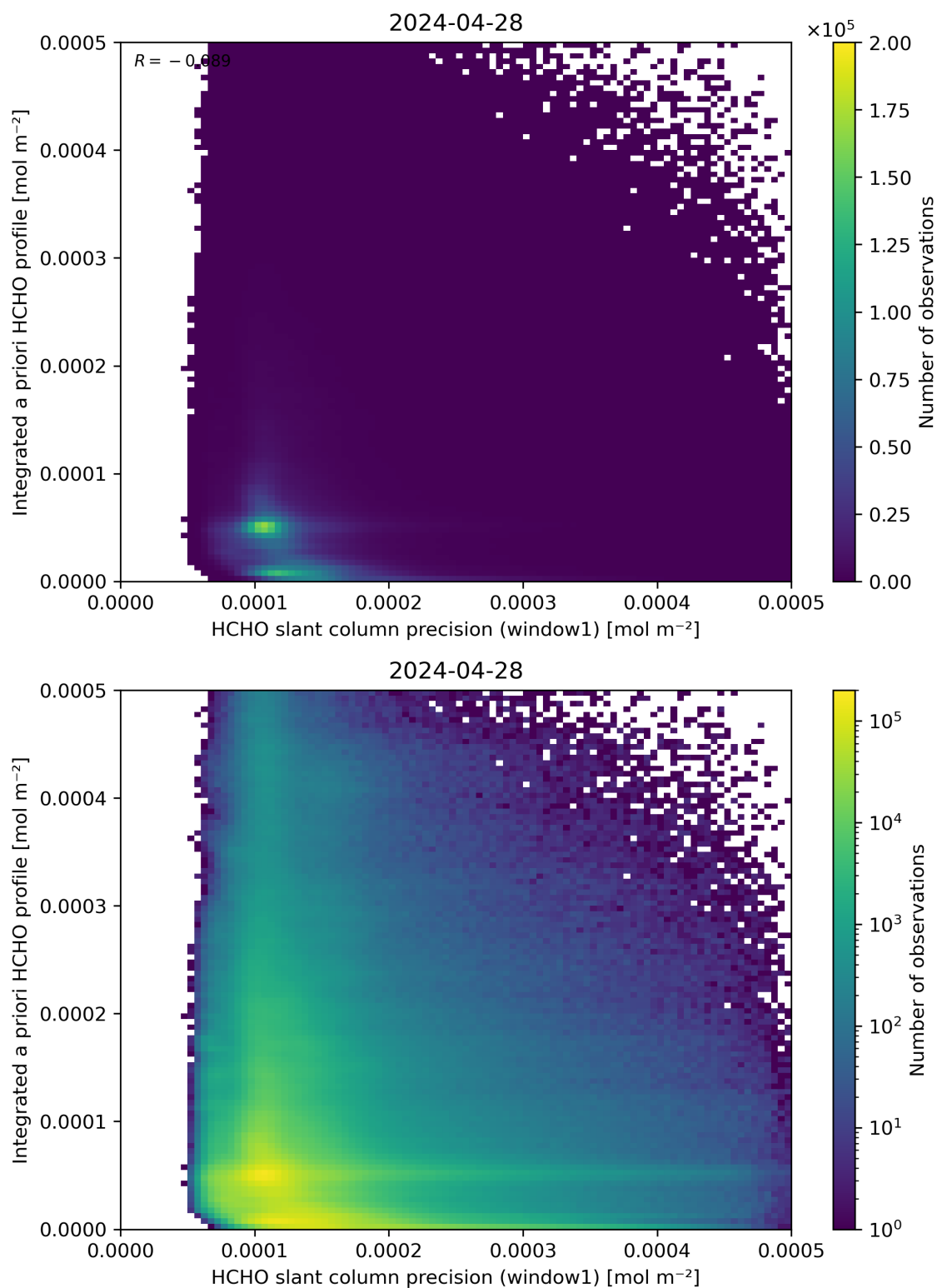
Figure 96: Scatter density plot of “HCHO slant column precision (window1)” against “Integrated a priori HCHO profile” for 2024-04-27 to 2024-04-29.
