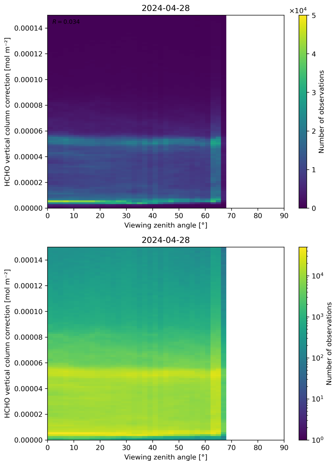
Figure 193: Scatter density plot of “Viewing zenith angle” against “HCHO vertical column correction” for 2024-04-27 to 2024-04-29.
