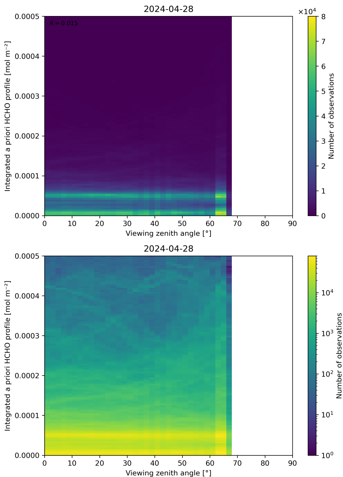
Figure 195: Scatter density plot of “Viewing zenith angle” against “Integrated a priori HCHO profile” for 2024-04-27 to 2024-04-29.
