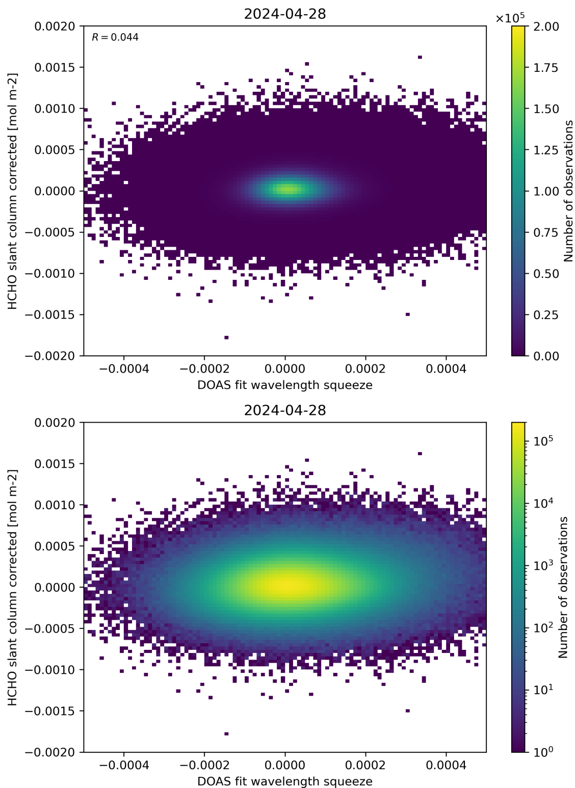
Figure 69: Scatter density plot of “DOAS fit wavelength squeeze” against “HCHO slant column corrected” for 2024-04-27 to 2024-04-29.
