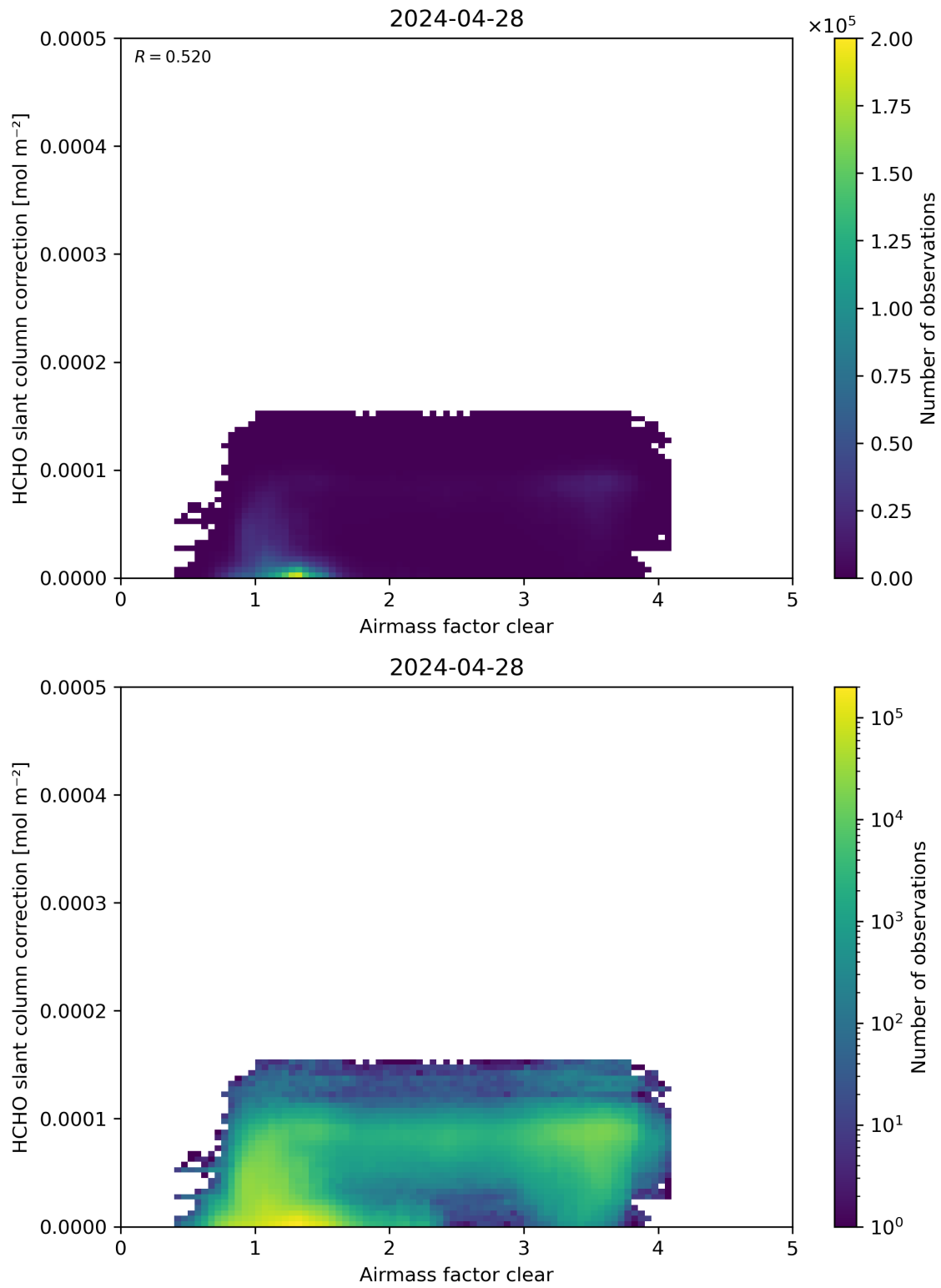
Figure 75: Scatter density plot of “Airmass factor clear” against “HCHO slant column correction” for 2024-04-27 to 2024-04-29.
