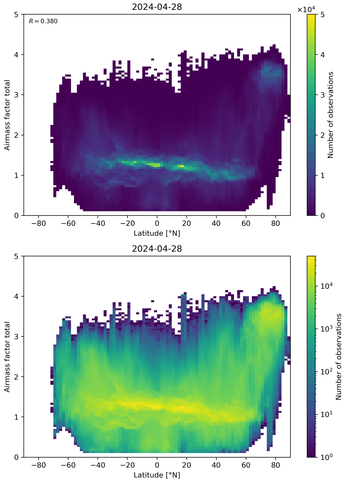
Figure 161: Scatter density plot of “Latitude” against “Airmass factor total” for 2024-04-27 to 2024-04-29.
