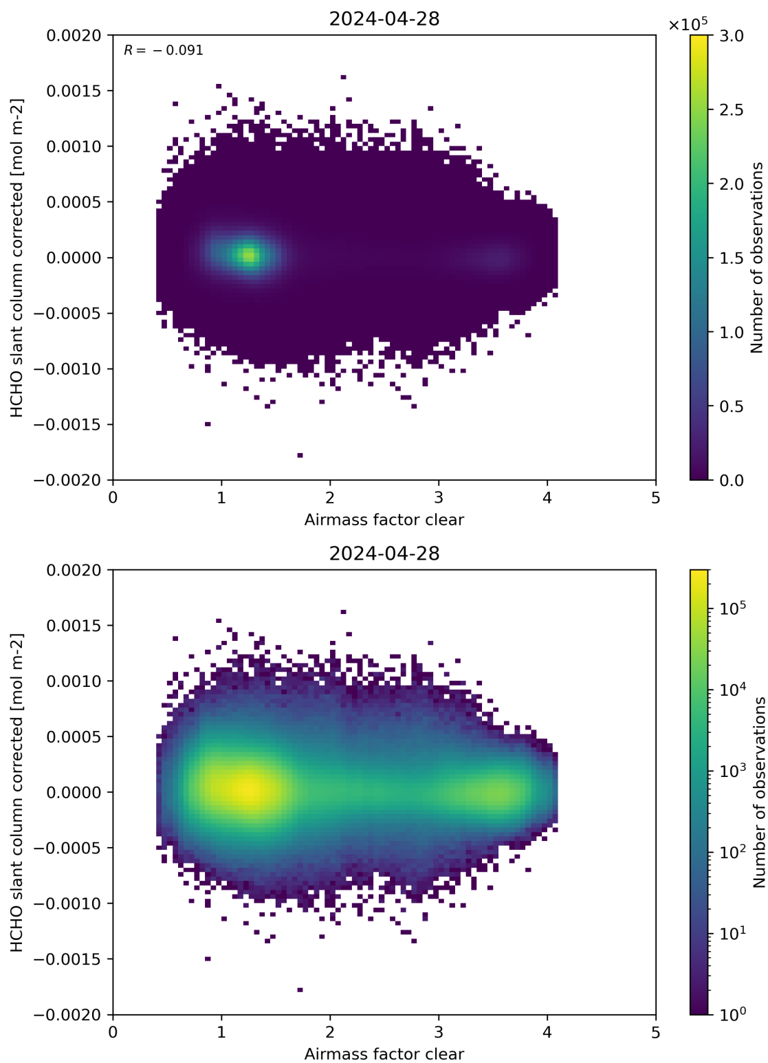
Figure 74: Scatter density plot of “Airmass factor clear” against “HCHO slant column corrected” for 2024-04-27 to 2024-04-29.
