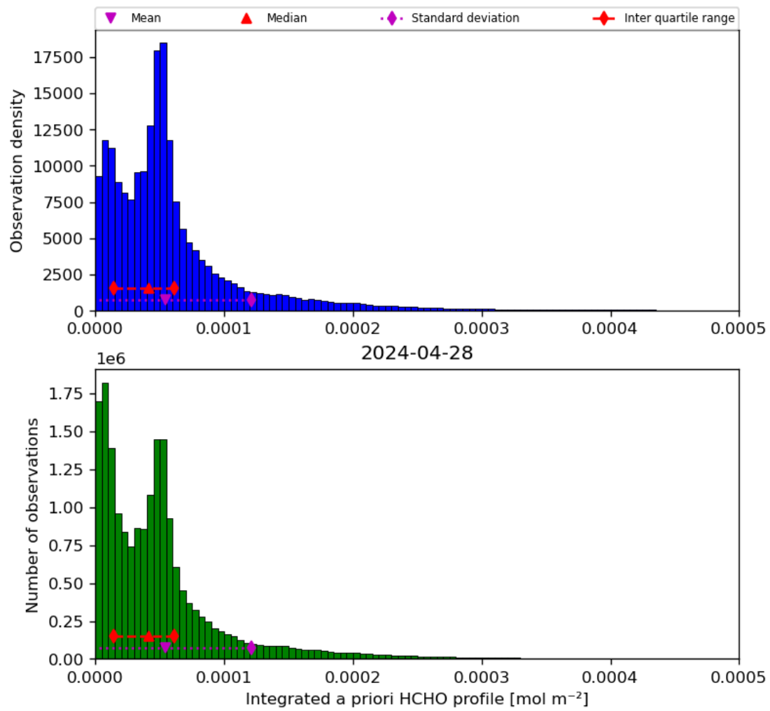
Figure 43: Histogram of “Integrated a priori HCHO profile” for 2024-04-27 to 2024-04-29
