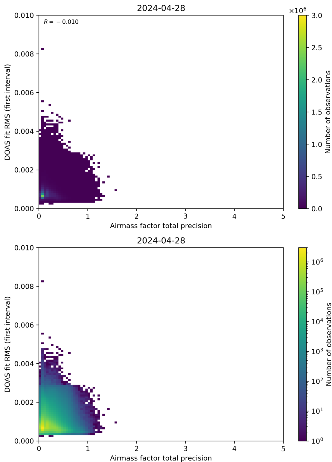
Figure 105: Scatter density plot of “Airmass factor total precision” against “DOAS fit RMS (first interval)” for 2024-04-27 to 2024-04-29.
