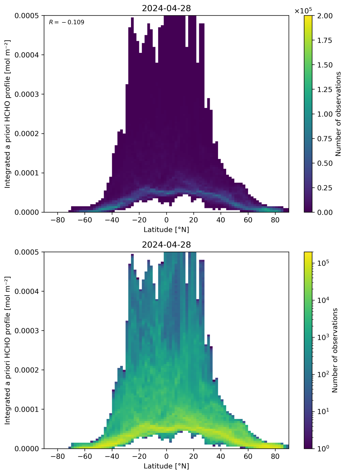
Figure 166: Scatter density plot of “Latitude” against “Integrated a priori HCHO profile” for 2024-04-27 to 2024-04-29.
