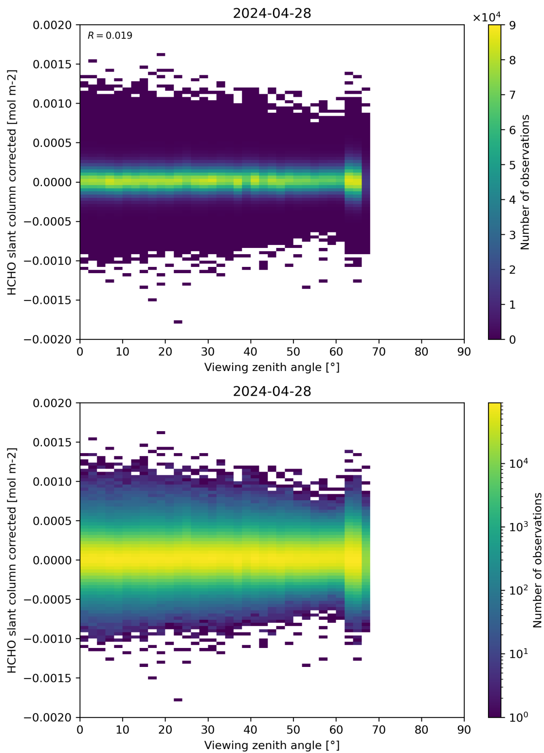
Figure 186: Scatter density plot of “Viewing zenith angle” against “HCHO slant column corrected” for 2024-04-27 to 2024-04-29.
