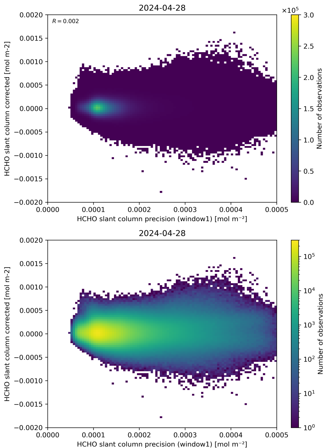
Figure 92: Scatter density plot of “HCHO slant column precision (window1)” against “HCHO slant column corrected” for 2024-04-27 to 2024-04-29.
