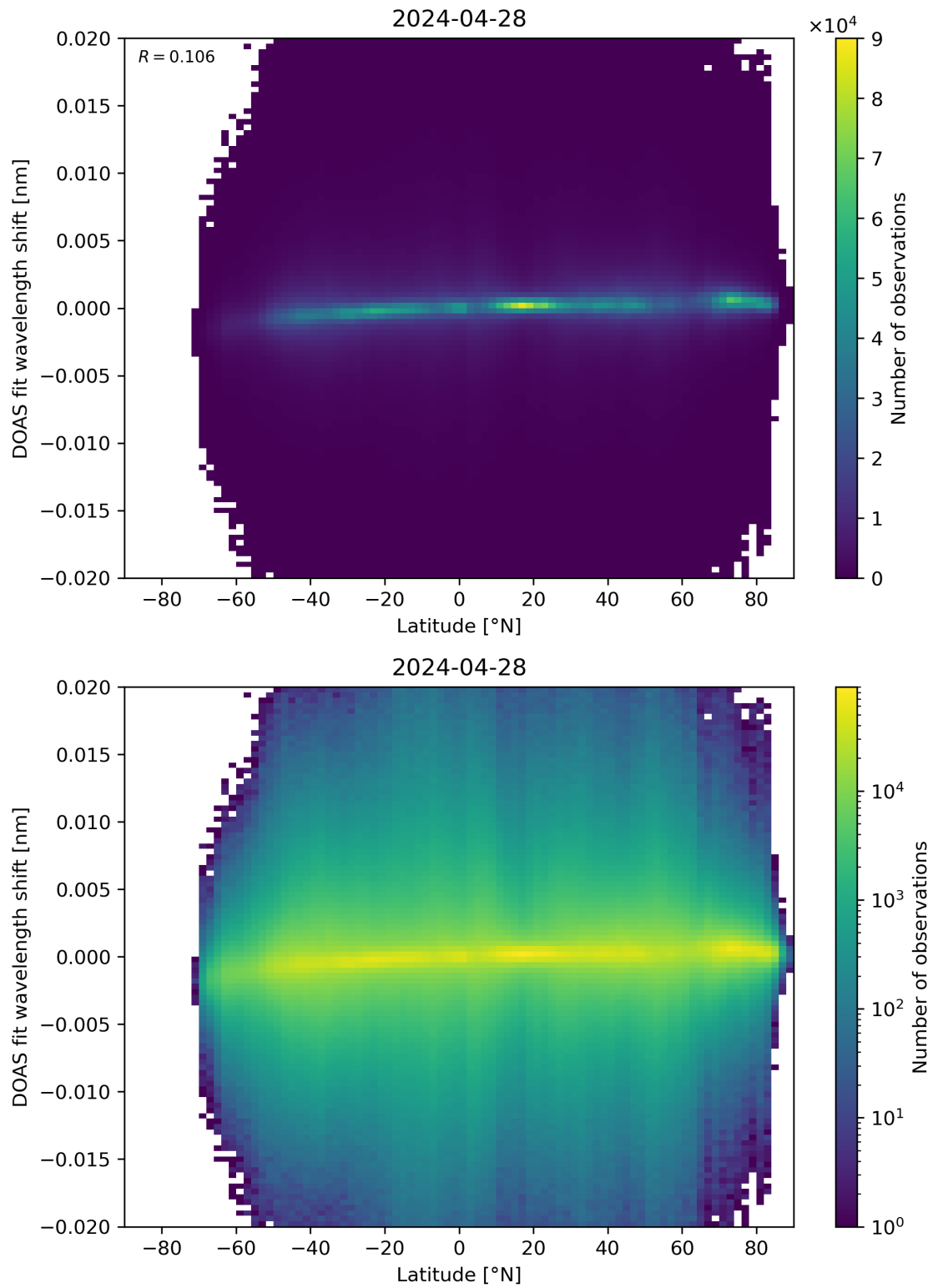
Figure 154: Scatter density plot of “Latitude” against “DOAS fit wavelength shift” for 2024-04-27 to 2024-04-29.
