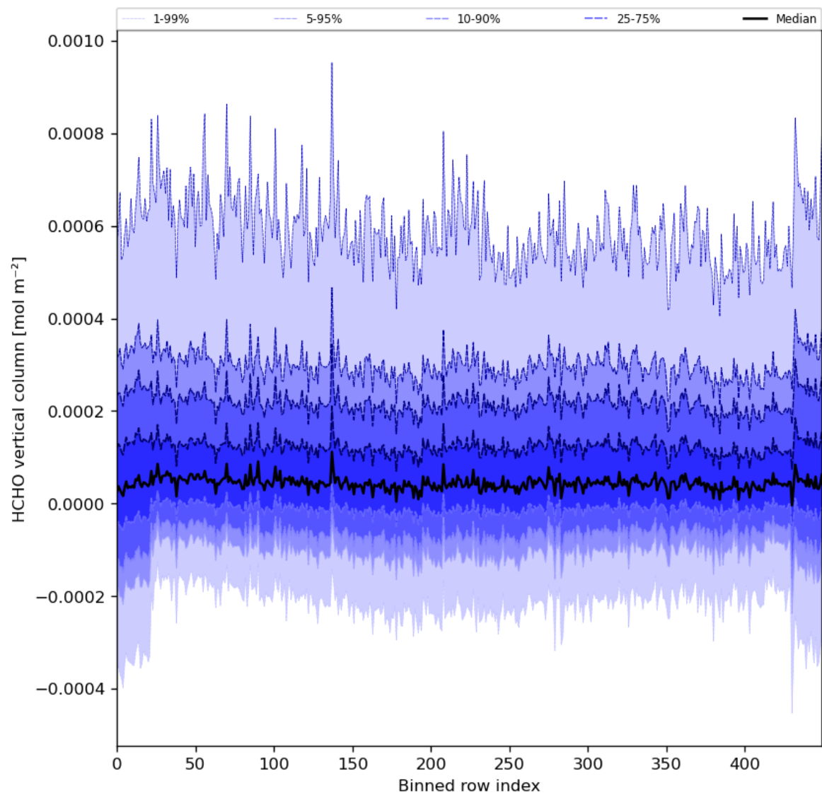
Figure 49: Along track statistics of “HCHO vertical column” for 2024-04-27 to 2024-04-29
