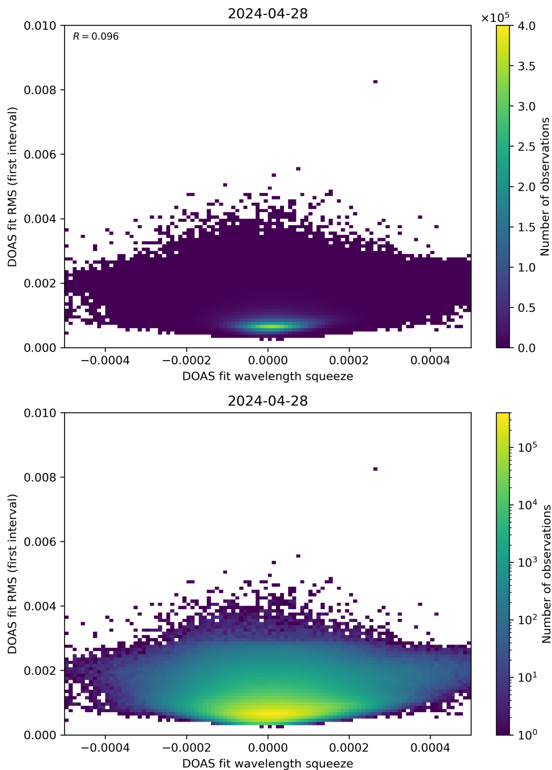
Figure 68: Scatter density plot of “DOAS fit wavelength squeeze” against “DOAS fit RMS (first interval)” for 2024-04-27 to 2024-04-29.
