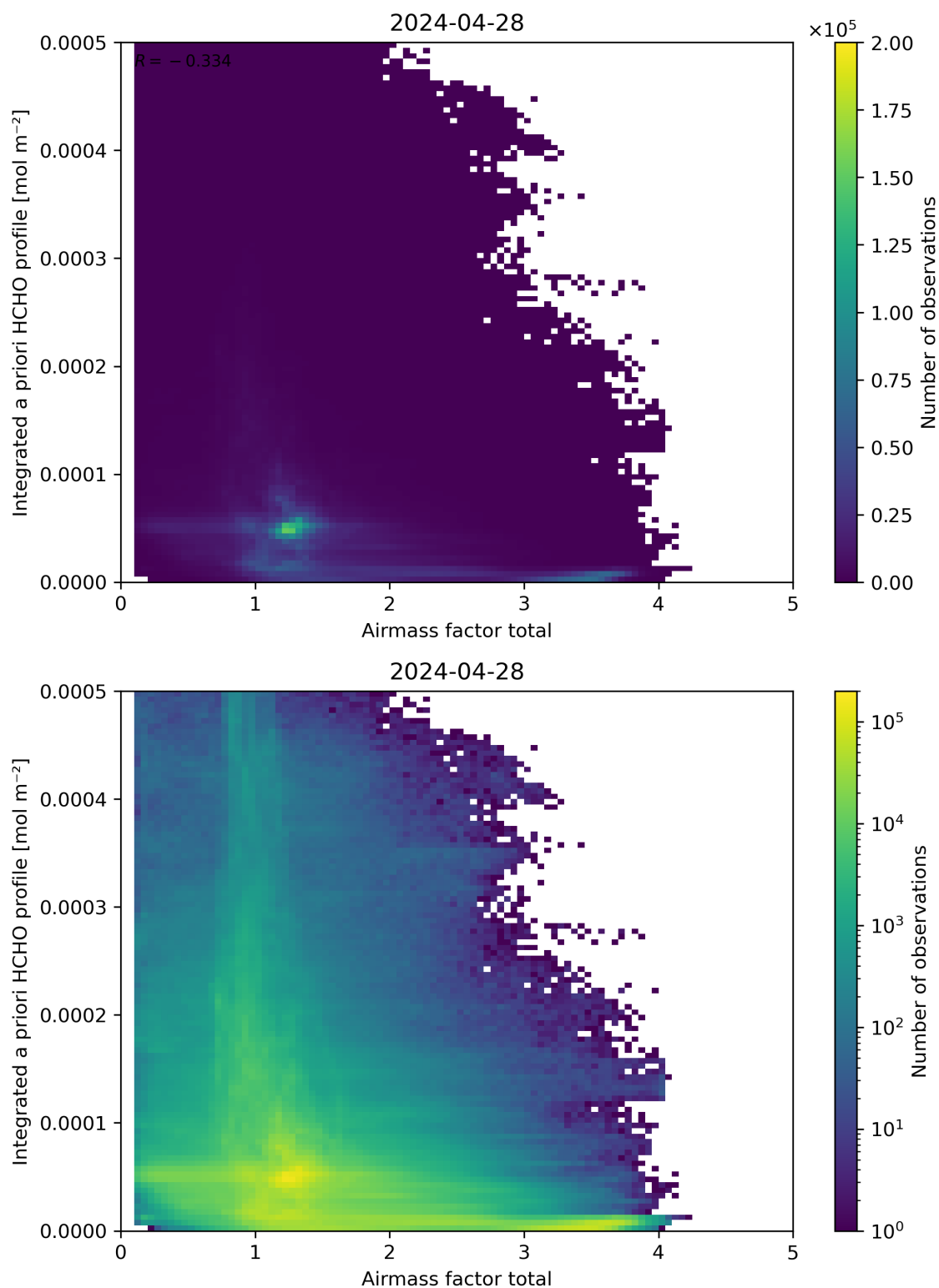
Figure 104: Scatter density plot of “Airmass factor total” against “Integrated a priori HCHO profile” for 2024-04-27 to 2024-04-29.
