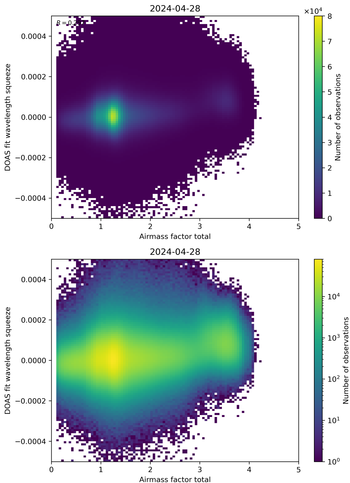
Figure 99: Scatter density plot of “Airmass factor total” against “DOAS fit wavelength squeeze” for 2024-04-27 to 2024-04-29.
