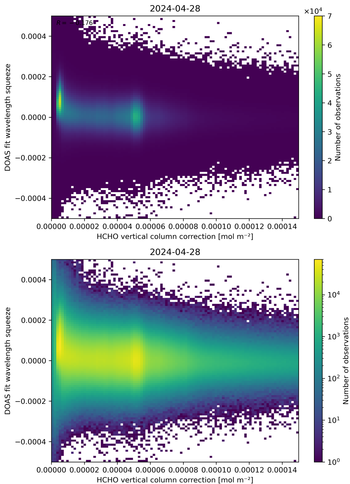
Figure 114: Scatter density plot of “HCHO vertical column correction” against “DOAS fit wavelength squeeze” for 2024-04-27 to 2024-04-29.
