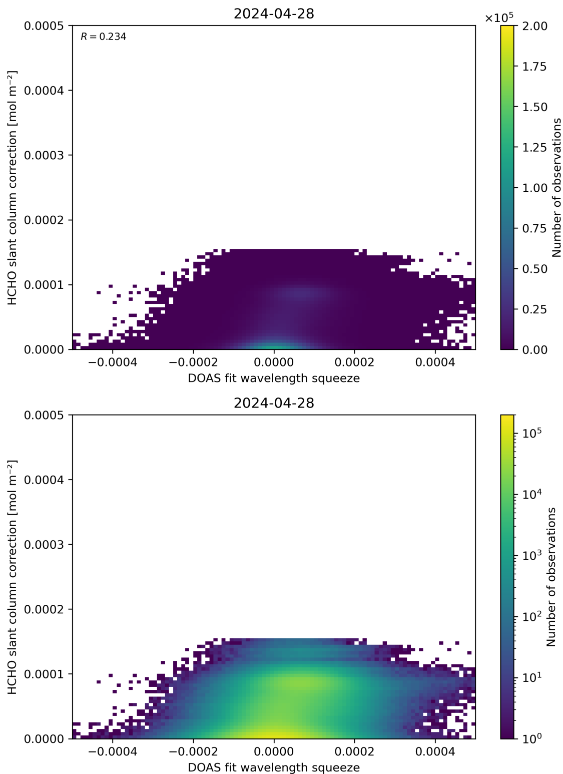
Figure 70: Scatter density plot of “DOAS fit wavelength squeeze” against “HCHO slant column correction” for 2024-04-27 to 2024-04-29.
