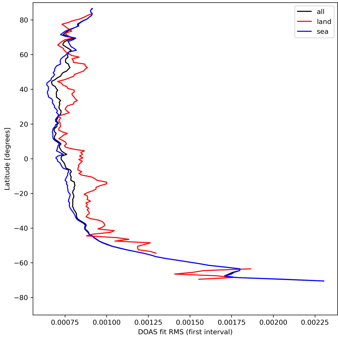
Figure 32: Zonal average of “DOAS fit RMS (first interval)” for 2024-04-27 to 2024-04-29.
