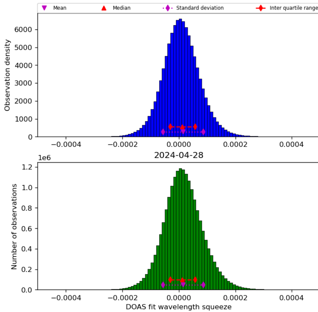
Figure 45: Histogram of “DOAS fit wavelength squeeze” for 2024-04-27 to 2024-04-29
