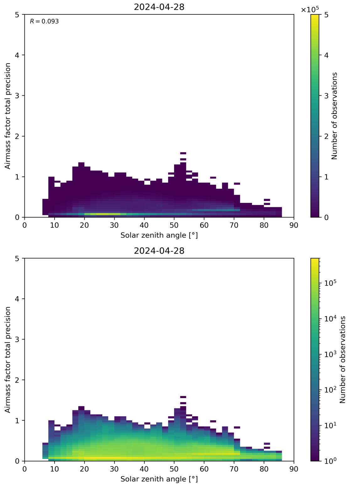
Figure 176: Scatter density plot of “Solar zenith angle” against “Airmass factor total precision” for 2024-04-27 to 2024-04-29.
