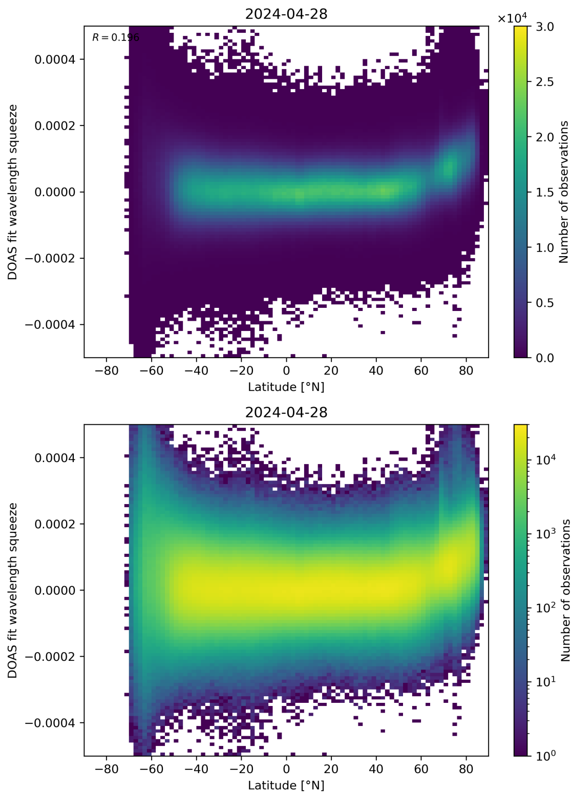
Figure 155: Scatter density plot of “Latitude” against “DOAS fit wavelength squeeze” for 2024-04-27 to 2024-04-29.
