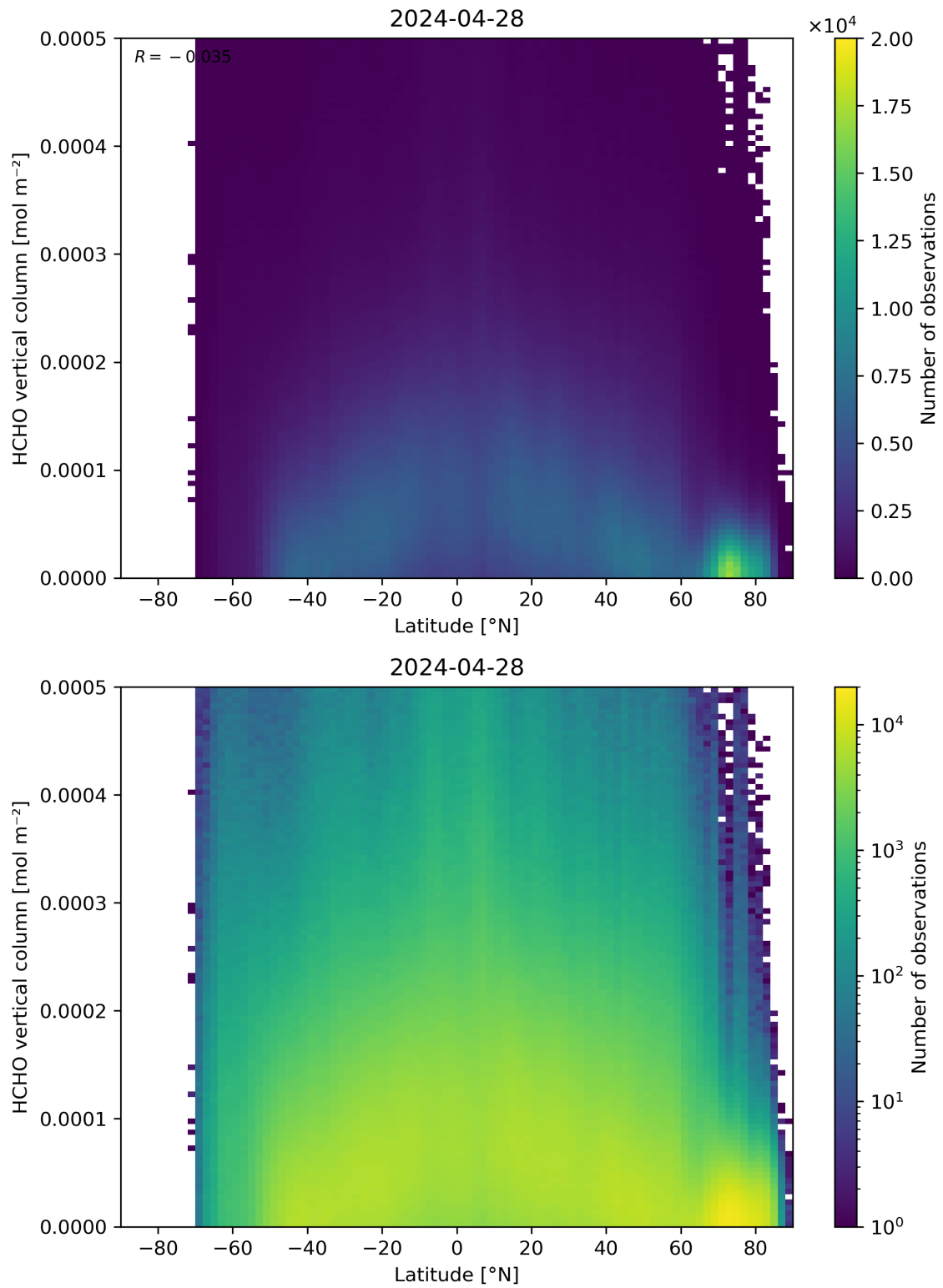
Figure 163: Scatter density plot of “Latitude” against “HCHO vertical column” for 2024-04-27 to 2024-04-29.
