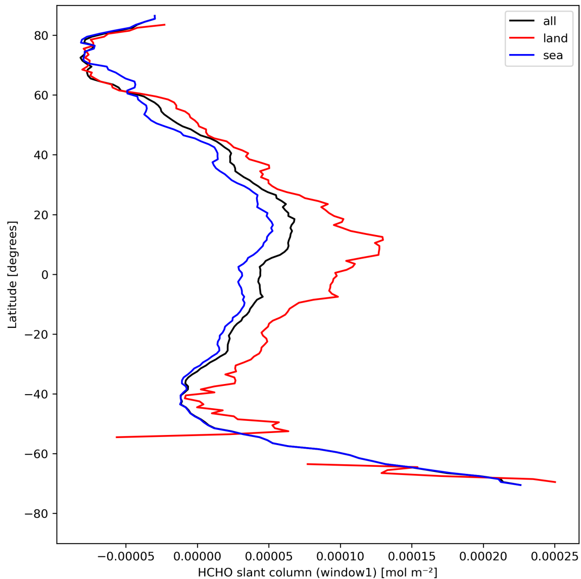
Figure 24: Zonal average of “HCHO slant column (window1)” for 2024-04-27 to 2024-04-29.
