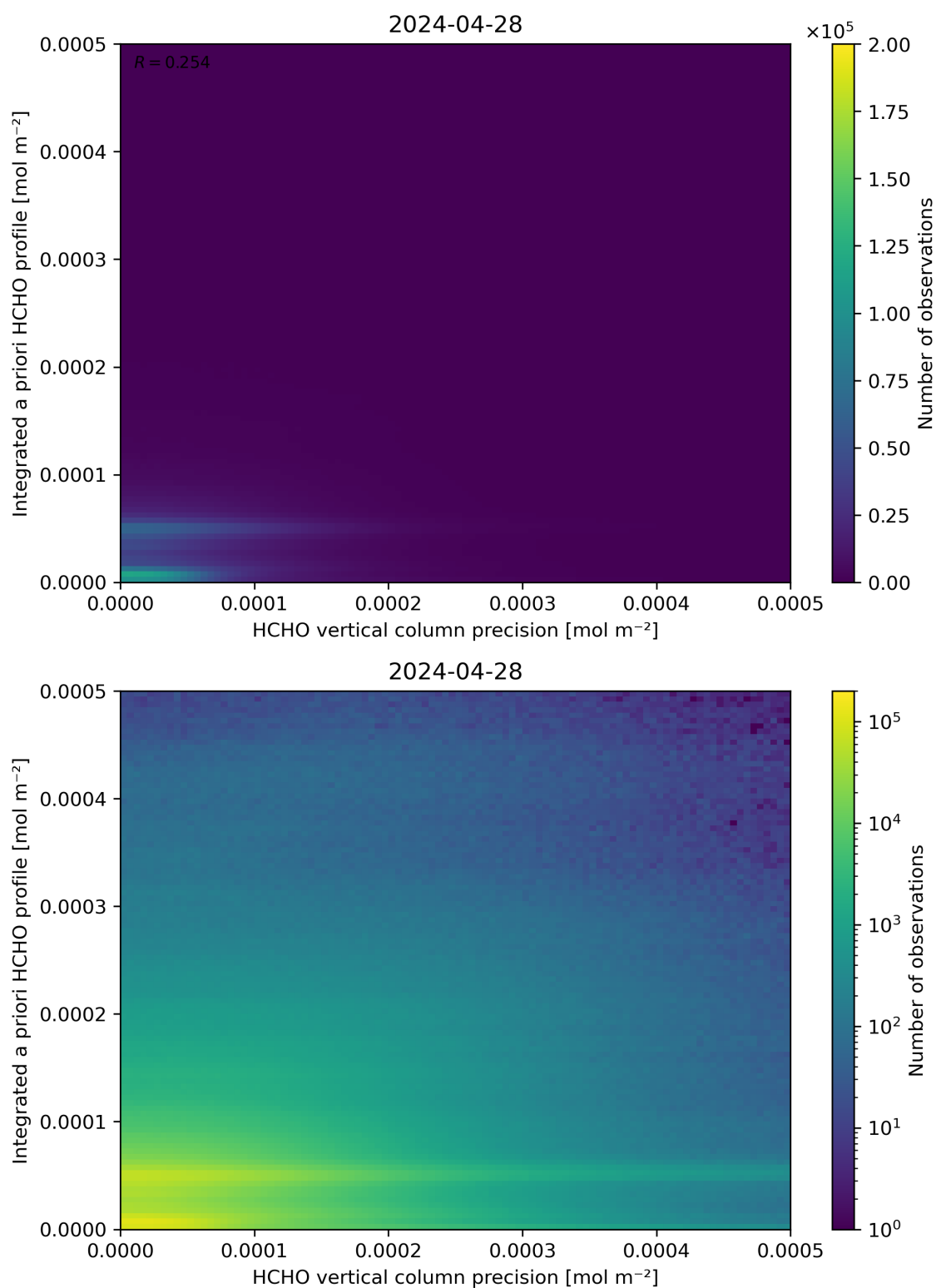
Figure 147: Scatter density plot of “HCHO vertical column precision” against “Integrated a priori HCHO profile” for 2024-04-27 to 2024-04-29.
