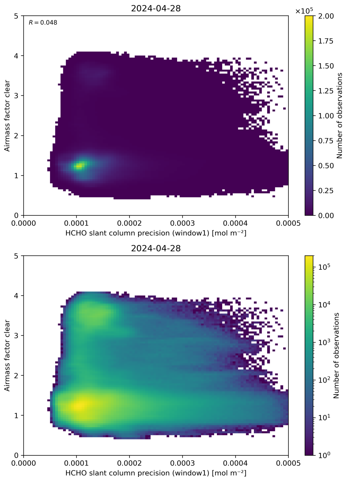
Figure 91: Scatter density plot of “HCHO slant column precision (window1)” against “Airmass factor clear” for 2024-04-27 to 2024-04-29.
