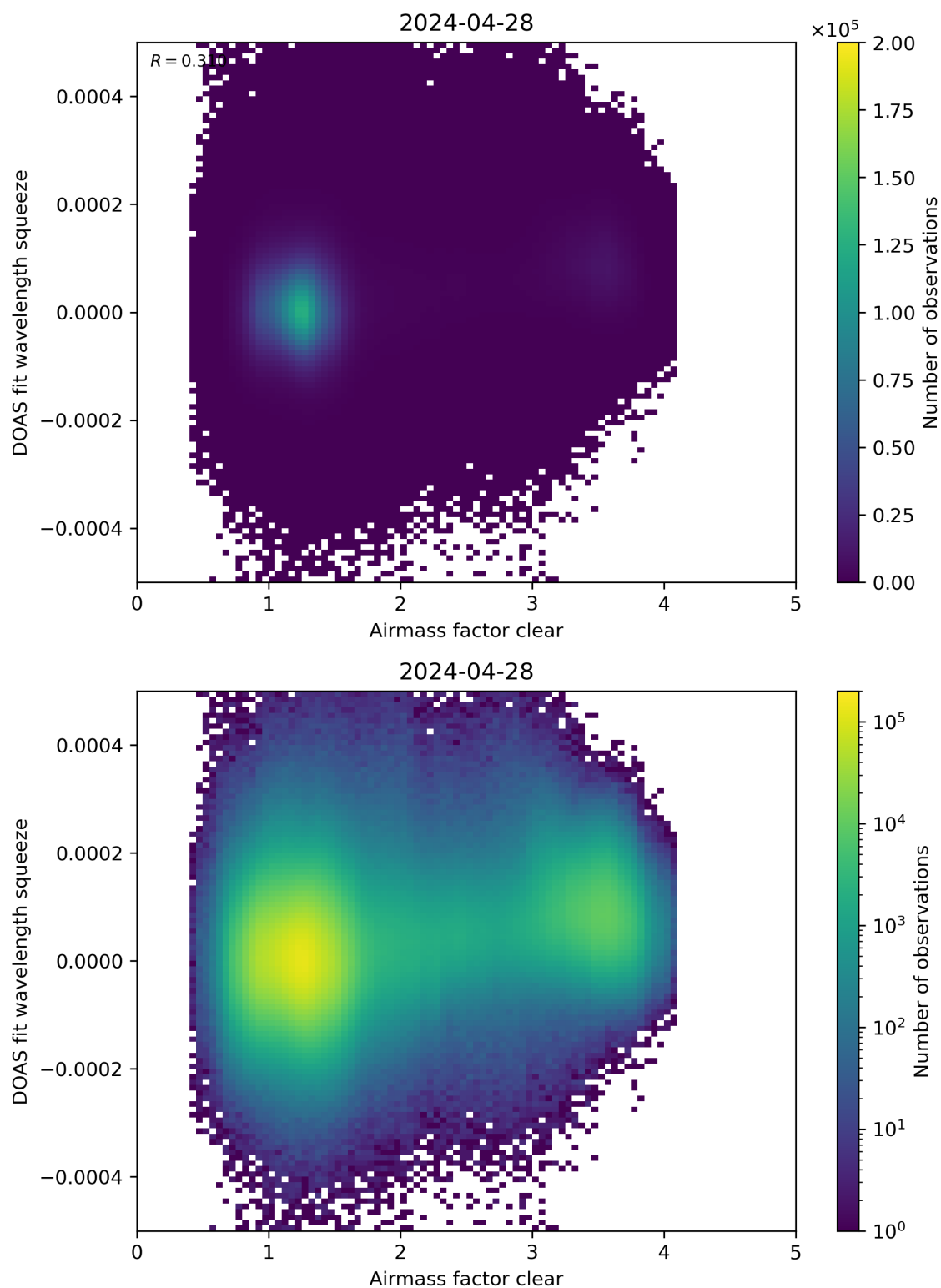
Figure 73: Scatter density plot of “Airmass factor clear” against “DOAS fit wavelength squeeze” for 2024-04-27 to 2024-04-29.
