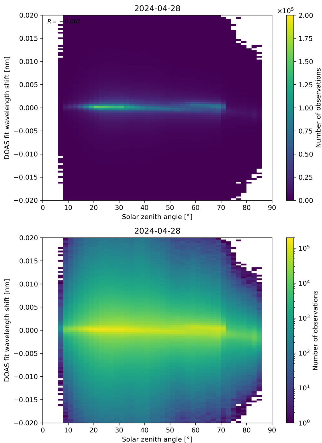
Figure 168: Scatter density plot of “Solar zenith angle” against “DOAS fit wavelength shift” for 2024-04-27 to 2024-04-29.
