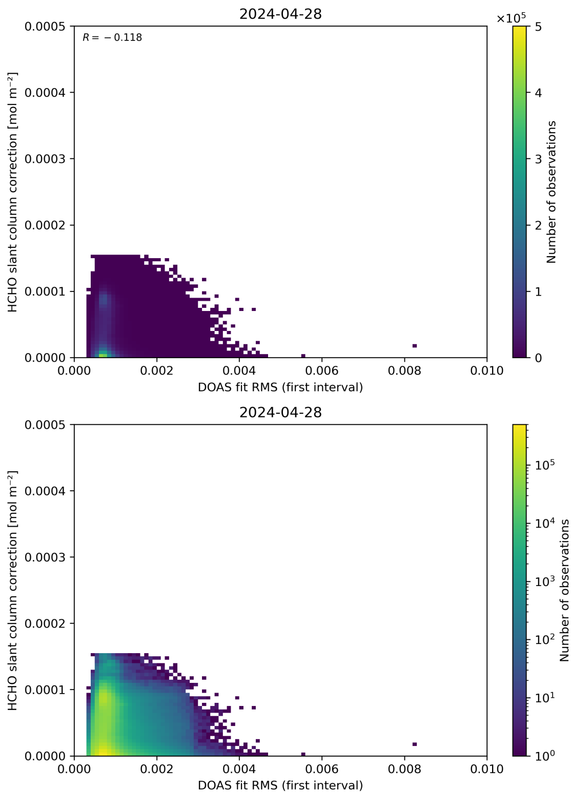
Figure 63: Scatter density plot of “DOAS fit RMS (first interval)” against “HCHO slant column correction” for 2024-04-27 to 2024-04-29.
