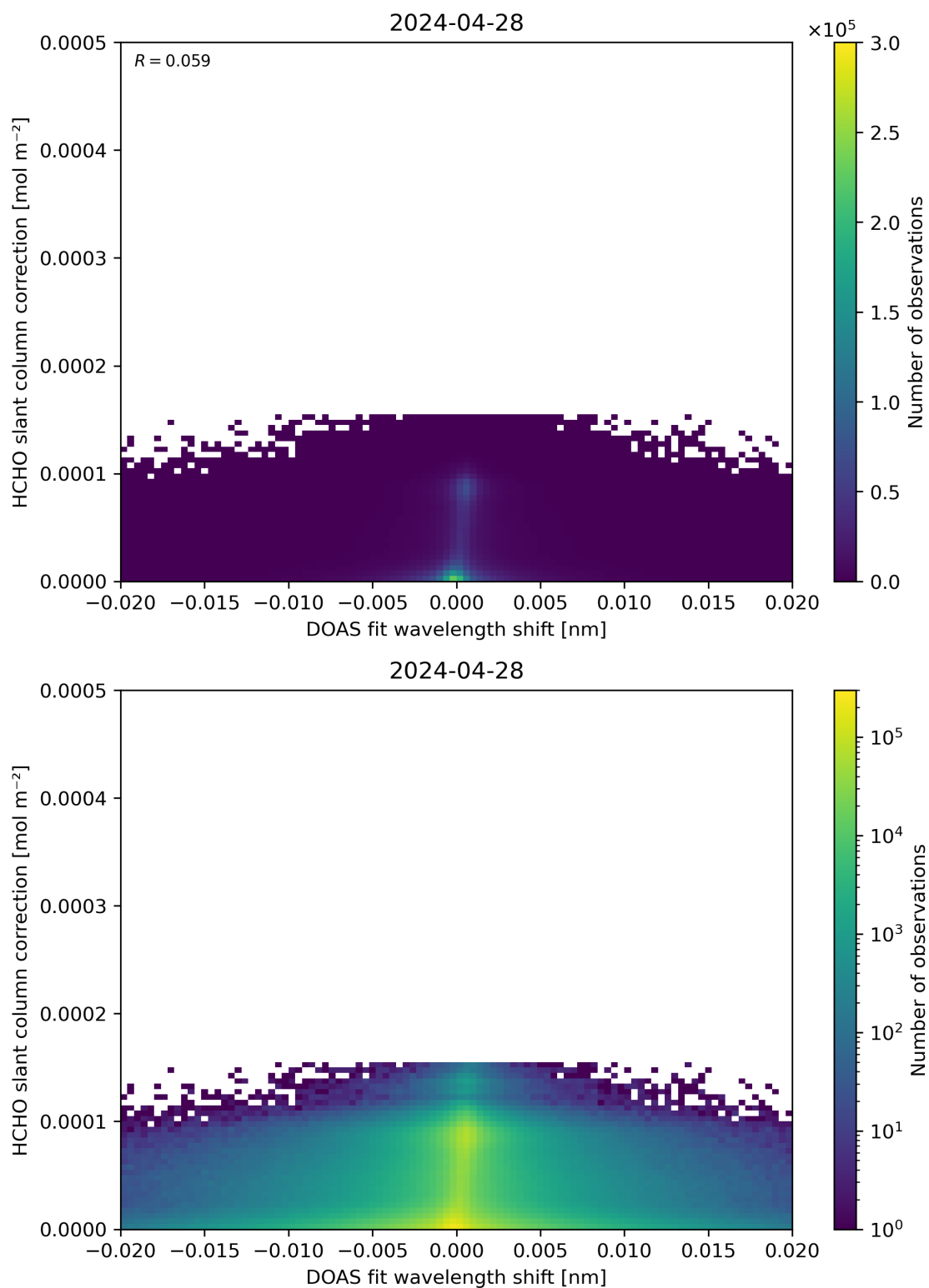
Figure 67: Scatter density plot of “DOAS fit wavelength shift” against “HCHO slant column correction” for 2024-04-27 to 2024-04-29.
