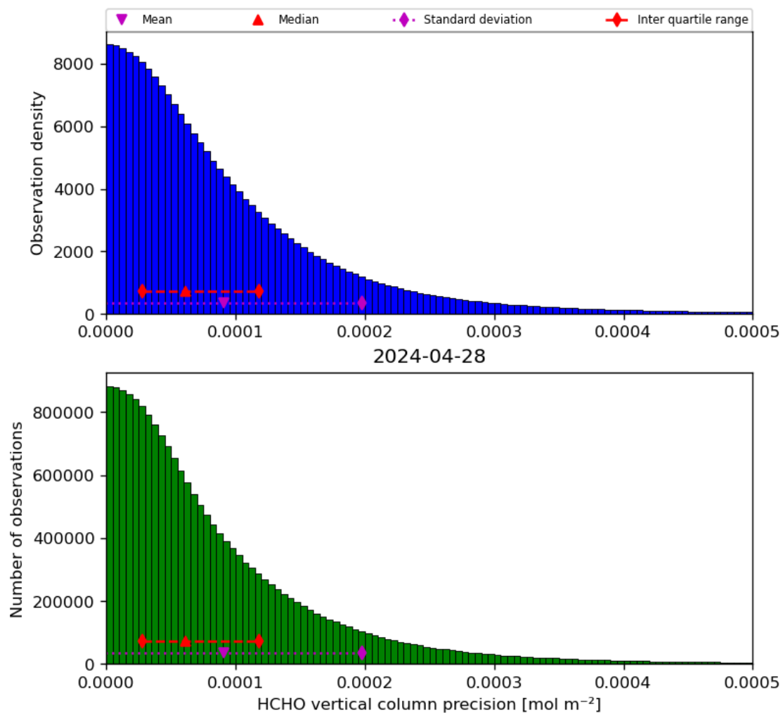
Figure 36: Histogram of “HCHO vertical column precision” for 2024-04-27 to 2024-04-29
