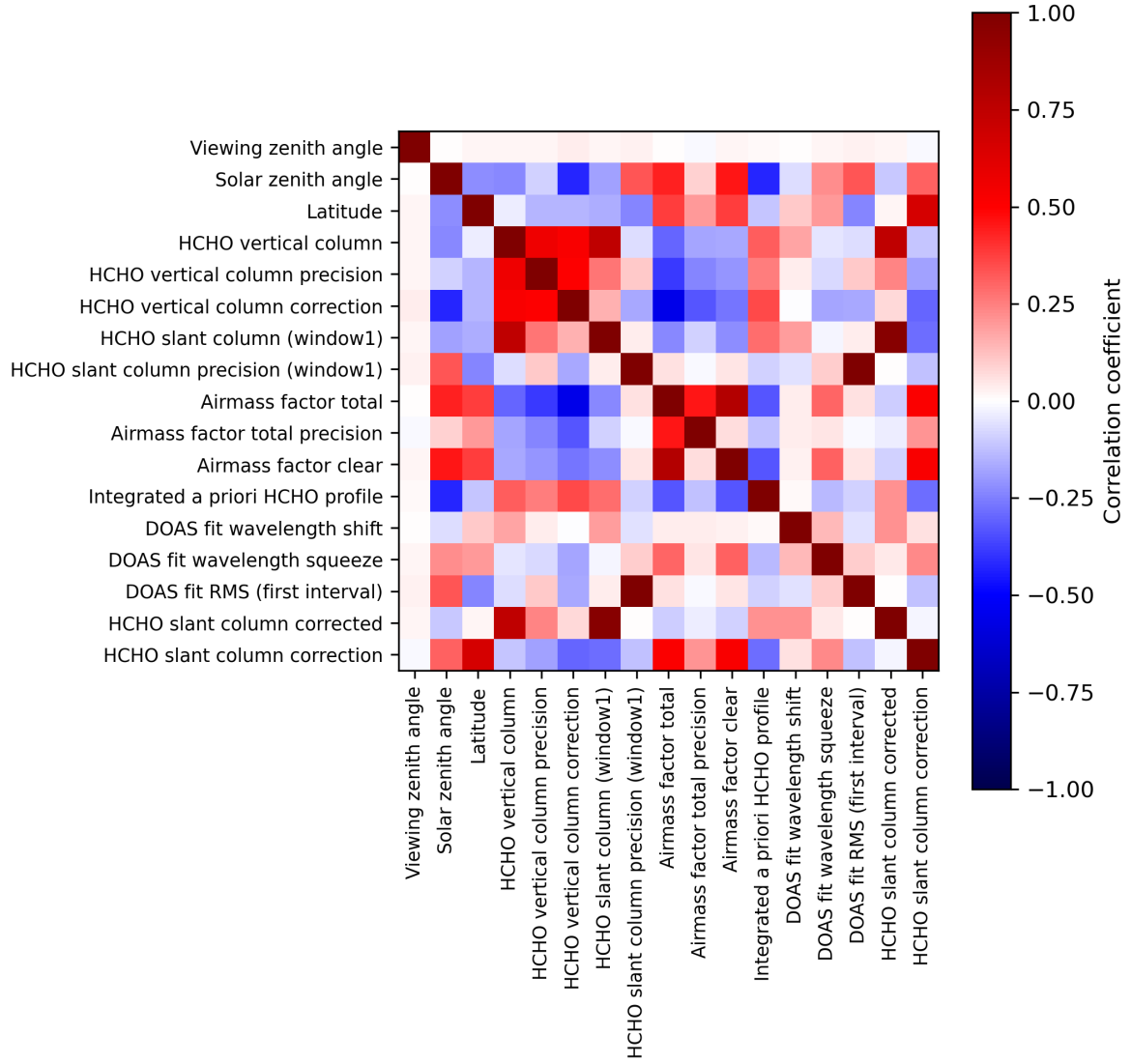
Figure 2: Map of correlation matrix for 2024-04-27 to 2024-04-29.
