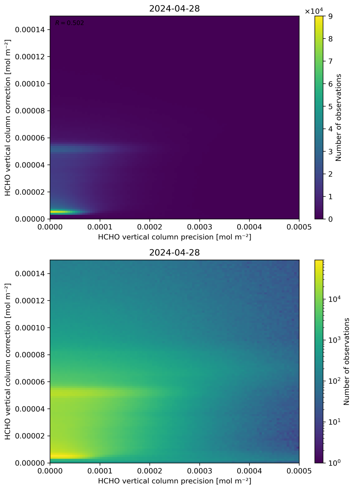
Figure 146: Scatter density plot of “HCHO vertical column precision” against “HCHO vertical column correction” for 2024-04-27 to 2024-04-29.
