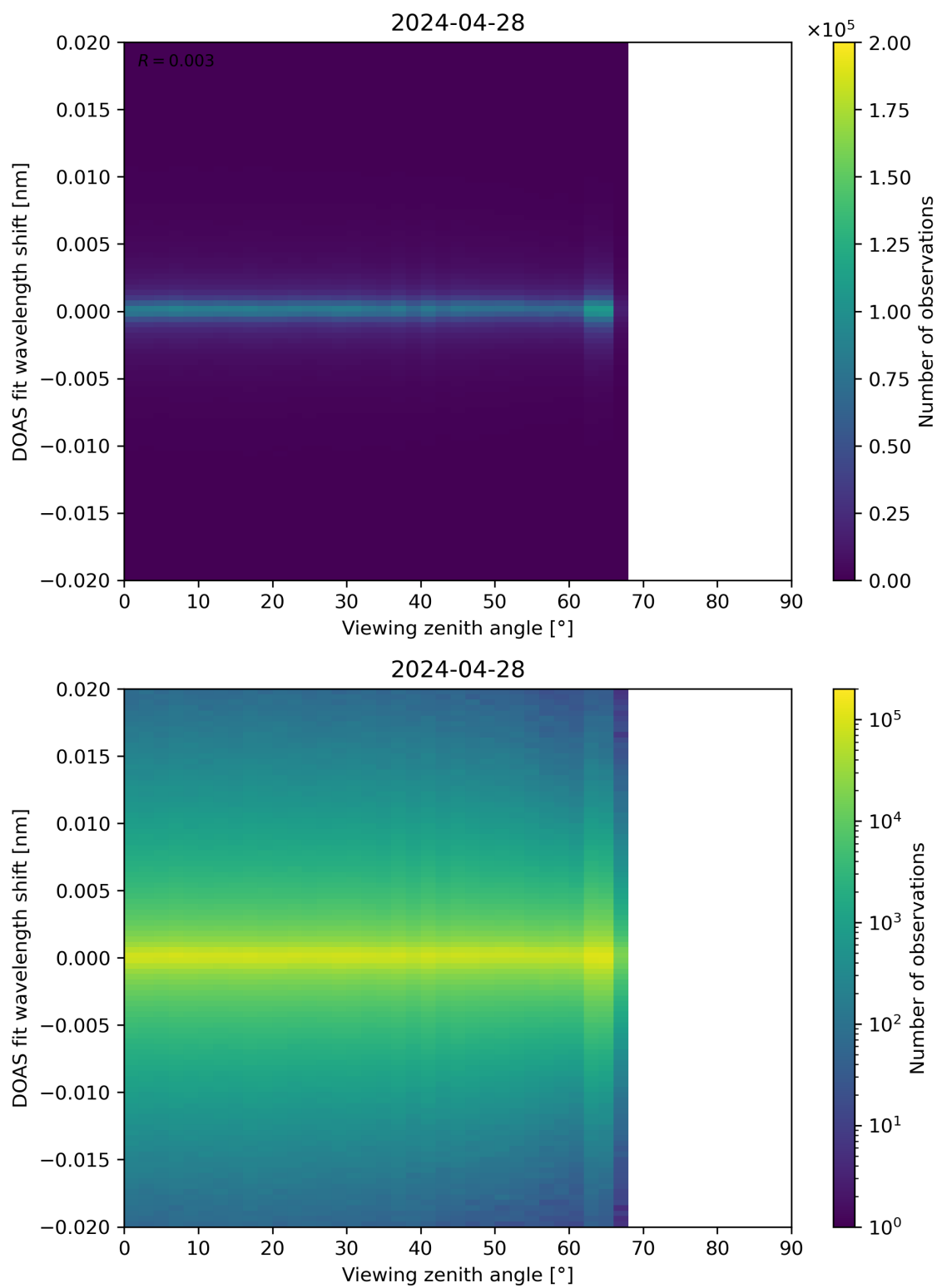
Figure 183: Scatter density plot of “Viewing zenith angle” against “DOAS fit wavelength shift” for 2024-04-27 to 2024-04-29.
