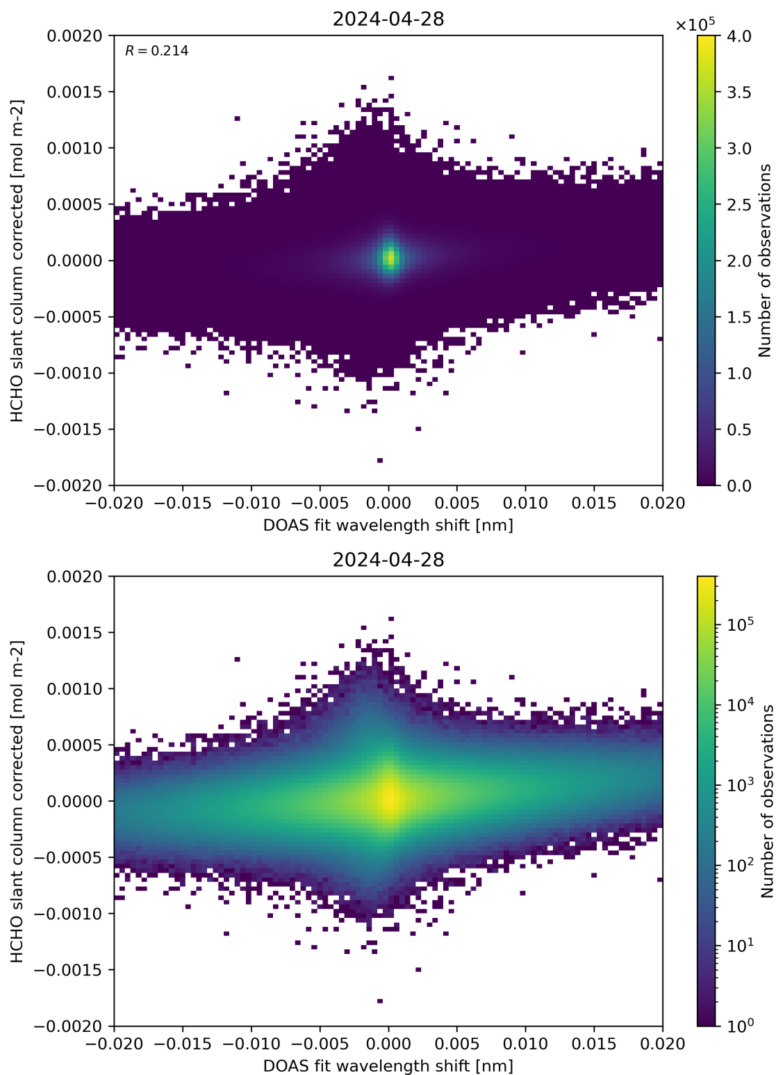
Figure 66: Scatter density plot of “DOAS fit wavelength shift” against “HCHO slant column corrected” for 2024-04-27 to 2024-04-29.
