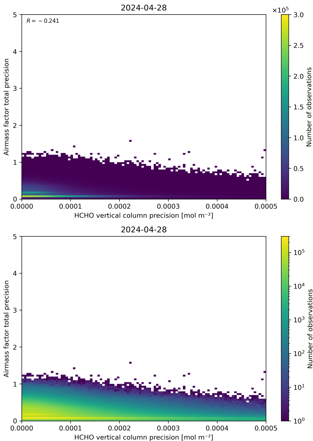
Figure 145: Scatter density plot of “HCHO vertical column precision” against “Airmass factor total precision” for 2024-04-27 to 2024-04-29.
