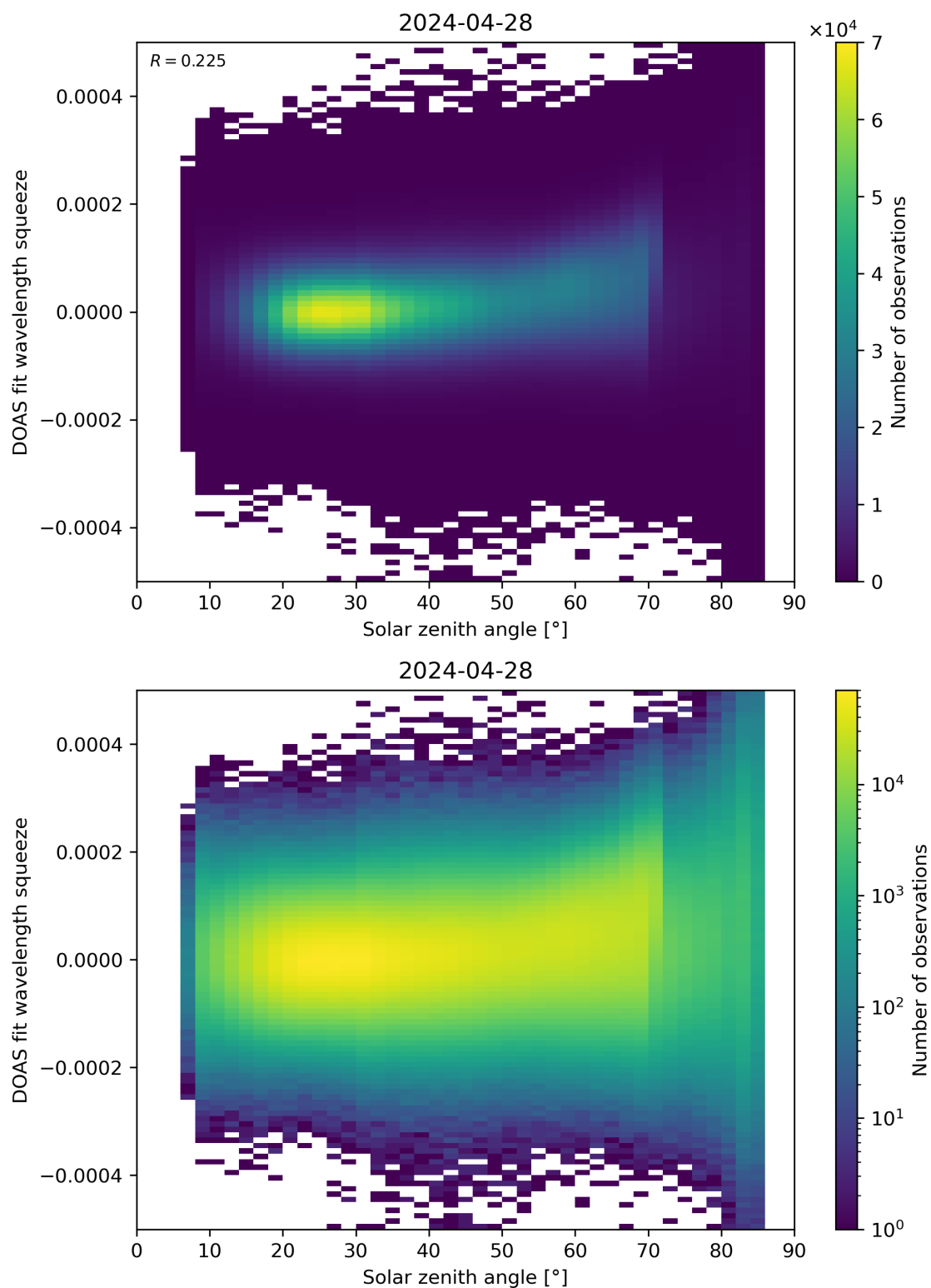
Figure 169: Scatter density plot of “Solar zenith angle” against “DOAS fit wavelength squeeze” for 2024-04-27 to 2024-04-29.
