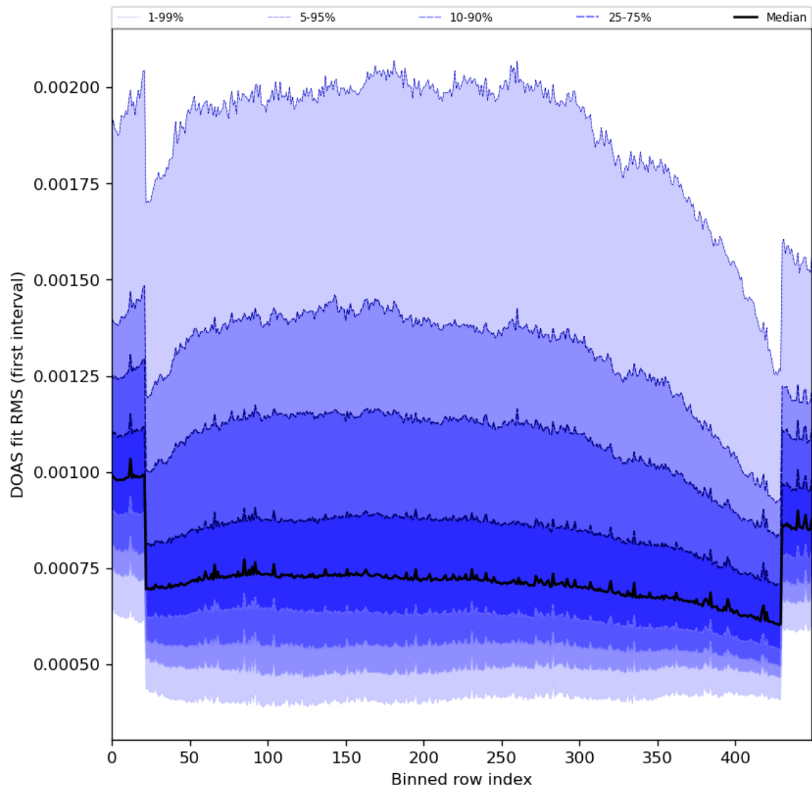
Figure 60: Along track statistics of “DOAS fit RMS (first interval)” for 2024-04-27 to 2024-04-29
