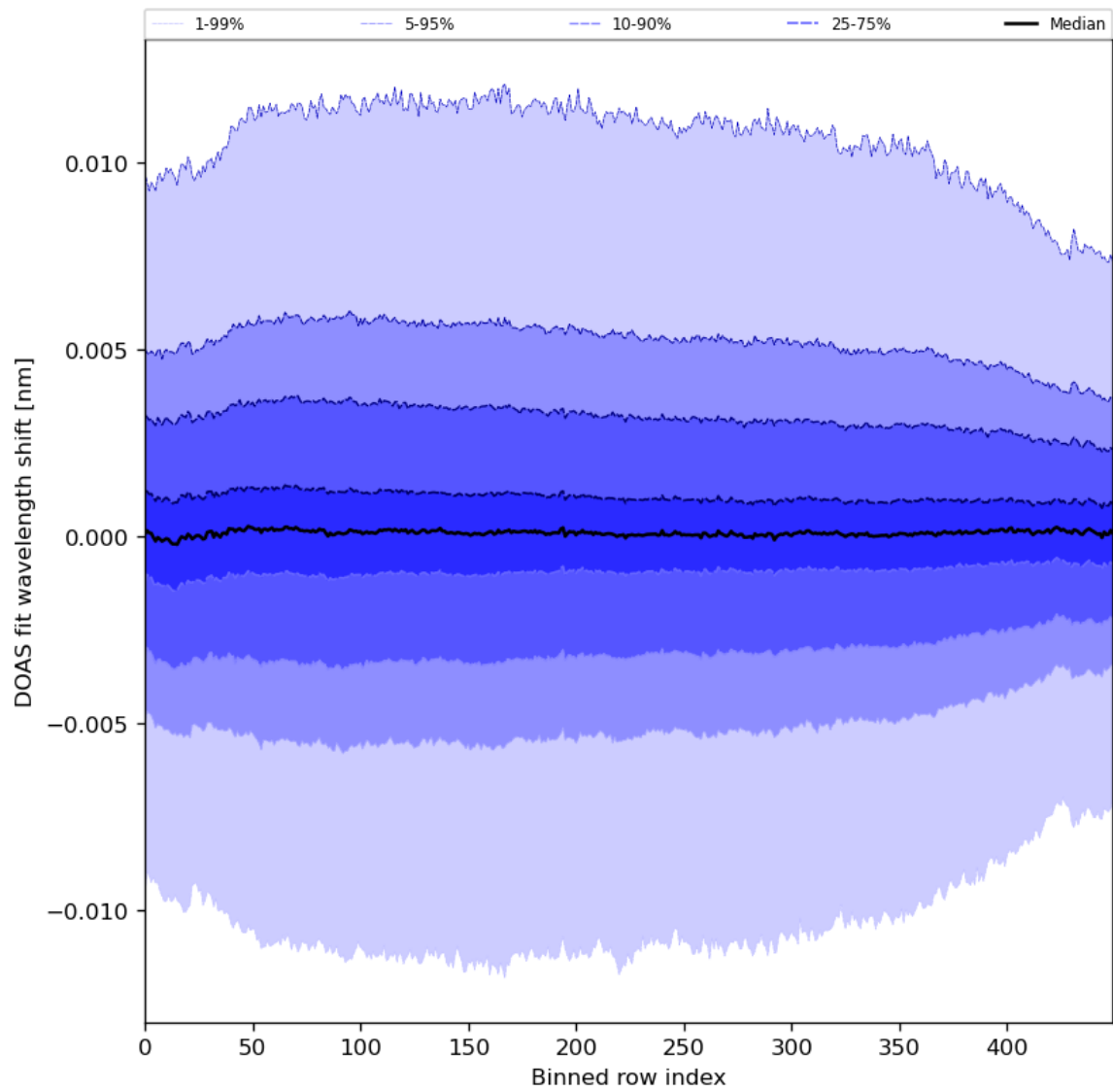
Figure 58: Along track statistics of “DOAS fit wavelength shift” for 2024-04-27 to 2024-04-29
