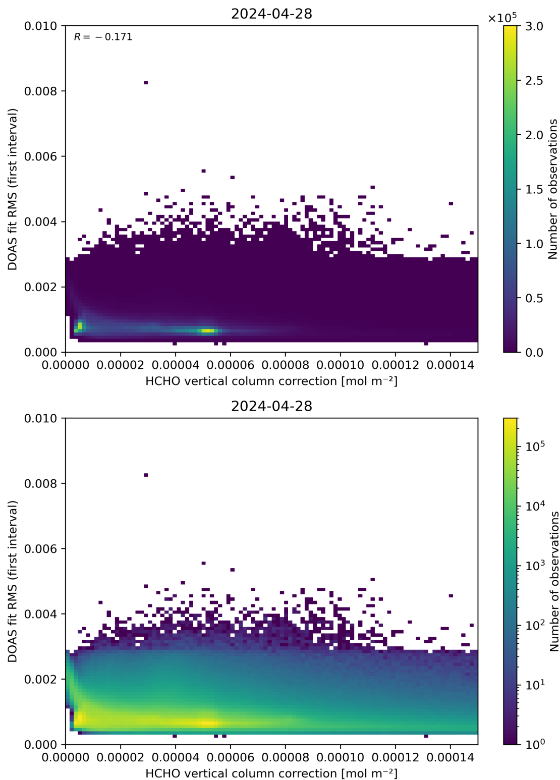
Figure 112: Scatter density plot of “HCHO vertical column correction” against “DOAS fit RMS (first interval)” for 2024-04-27 to 2024-04-29.
