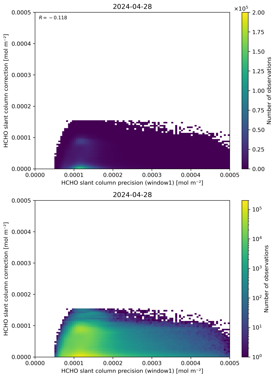
Figure 93: Scatter density plot of “HCHO slant column precision (window1)” against “HCHO slant column correction” for 2024-04-27 to 2024-04-29.
