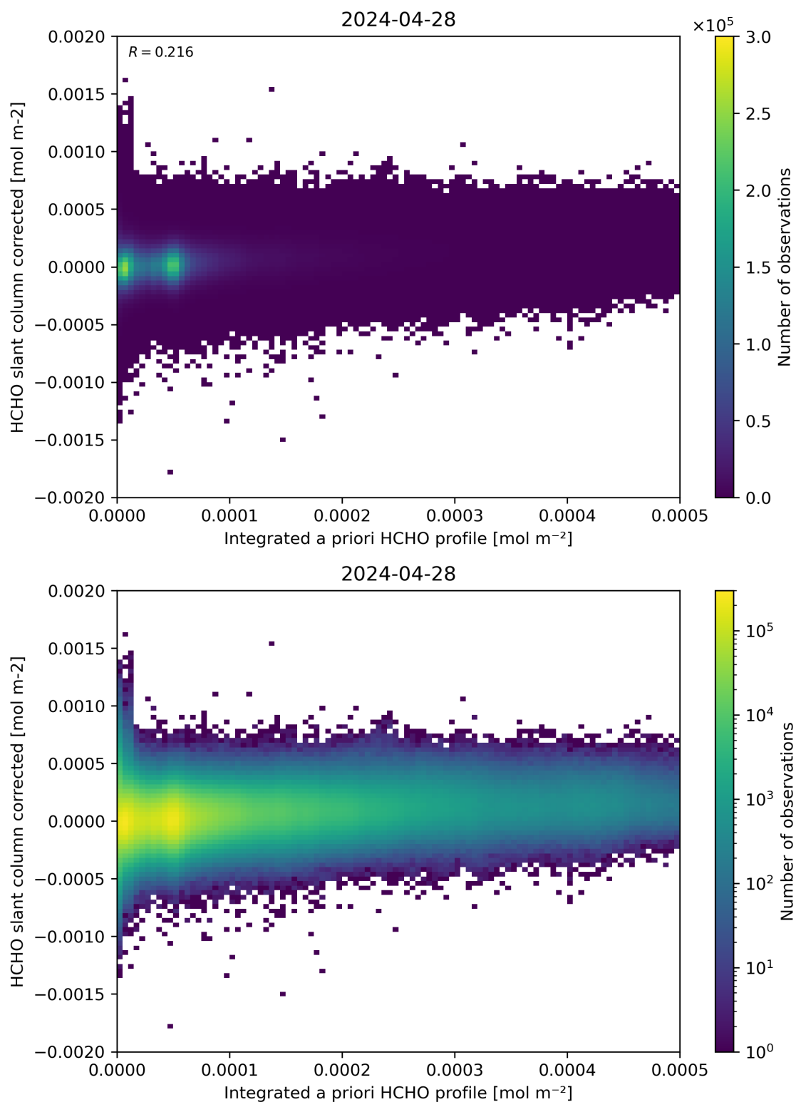
Figure 151: Scatter density plot of “Integrated a priori HCHO profile” against “HCHO slant column corrected” for 2024-04-27 to 2024-04-29.
