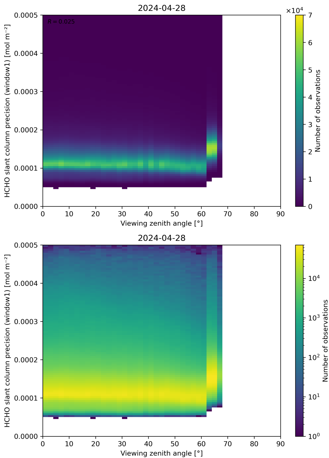
Figure 189: Scatter density plot of “Viewing zenith angle” against “HCHO slant column precision (window1)” for 2024-04-27 to 2024-04-29.
