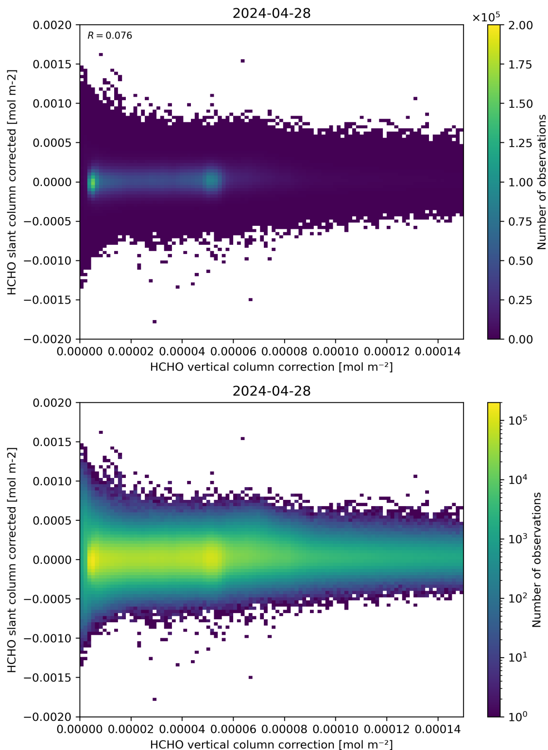
Figure 116: Scatter density plot of “HCHO vertical column correction” against “HCHO slant column corrected” for 2024-04-27 to 2024-04-29.
