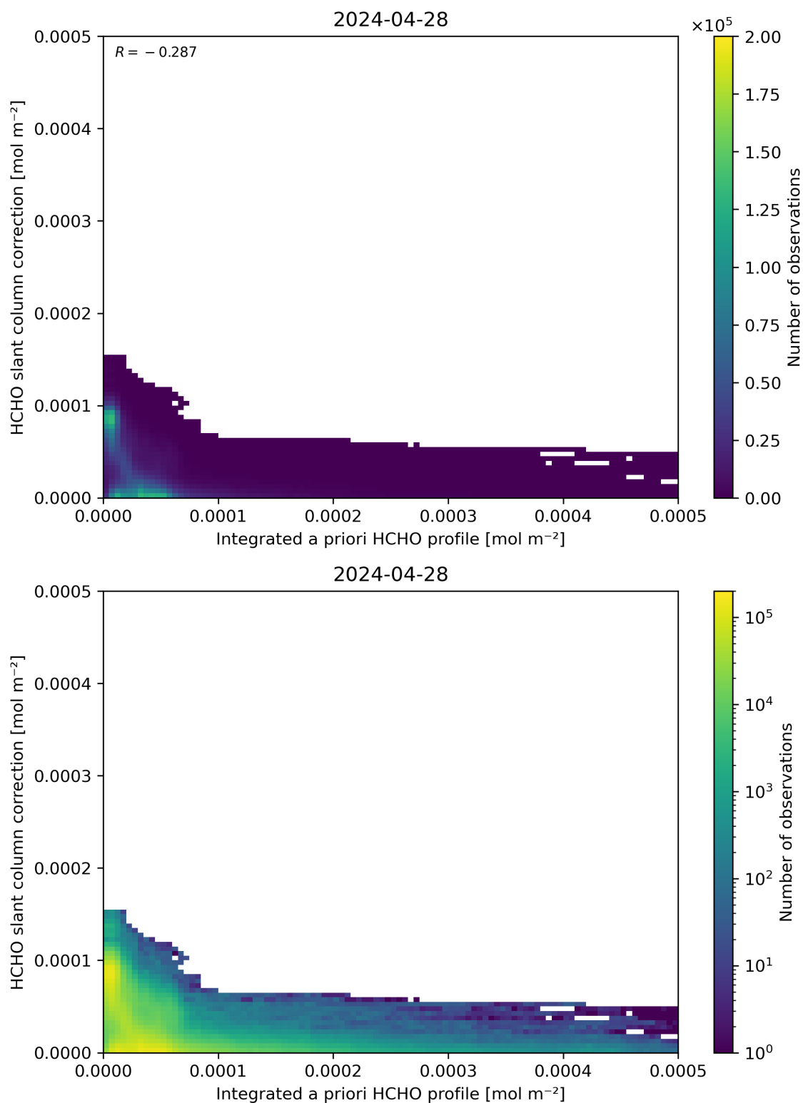
Figure 152: Scatter density plot of “Integrated a priori HCHO profile” against “HCHO slant column correction” for 2024-04-27 to 2024-04-29.
