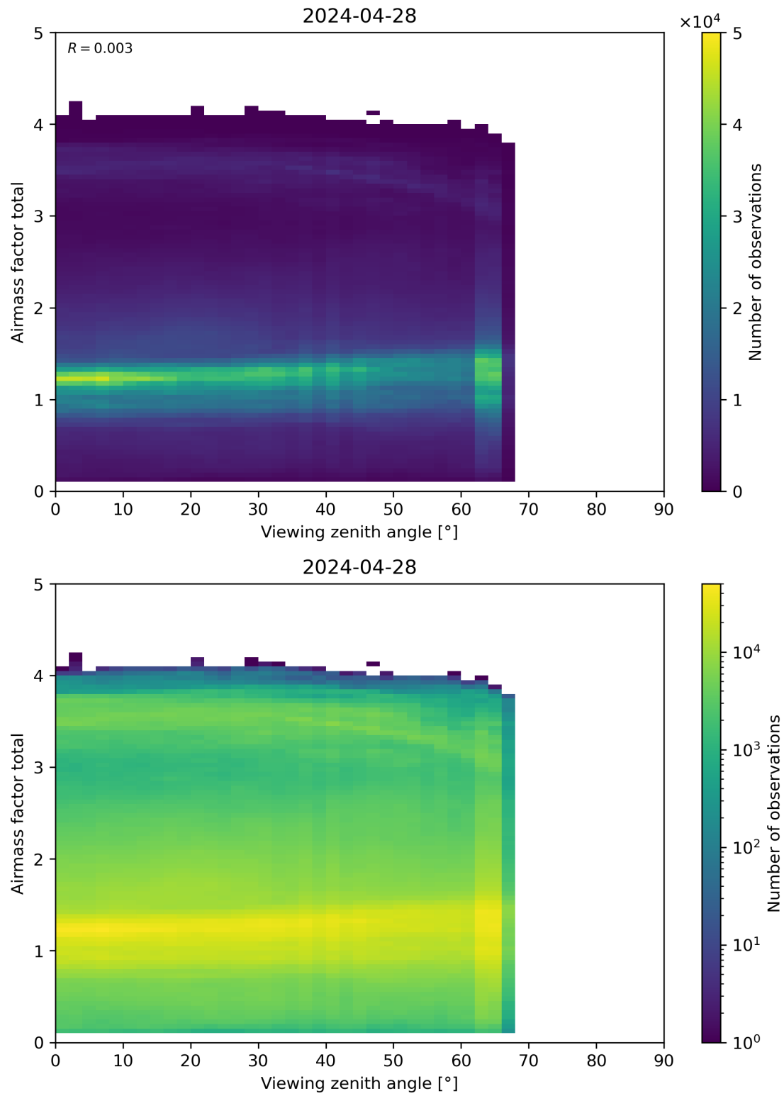
Figure 190: Scatter density plot of “Viewing zenith angle” against “Airmass factor total” for 2024-04-27 to 2024-04-29.
