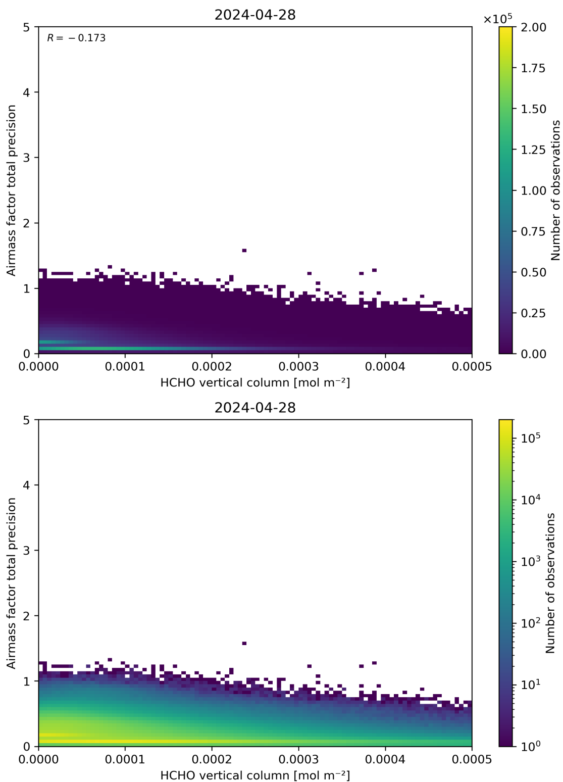
Figure 132: Scatter density plot of “HCHO vertical column” against “Airmass factor total precision” for 2024-04-27 to 2024-04-29.
