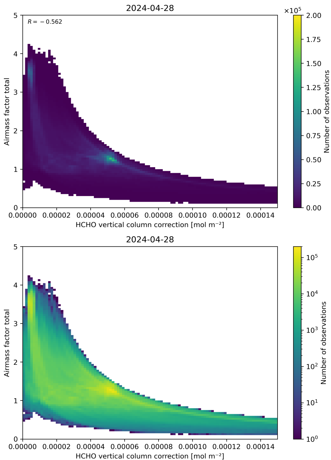
Figure 120: Scatter density plot of “HCHO vertical column correction” against “Airmass factor total” for 2024-04-27 to 2024-04-29.
