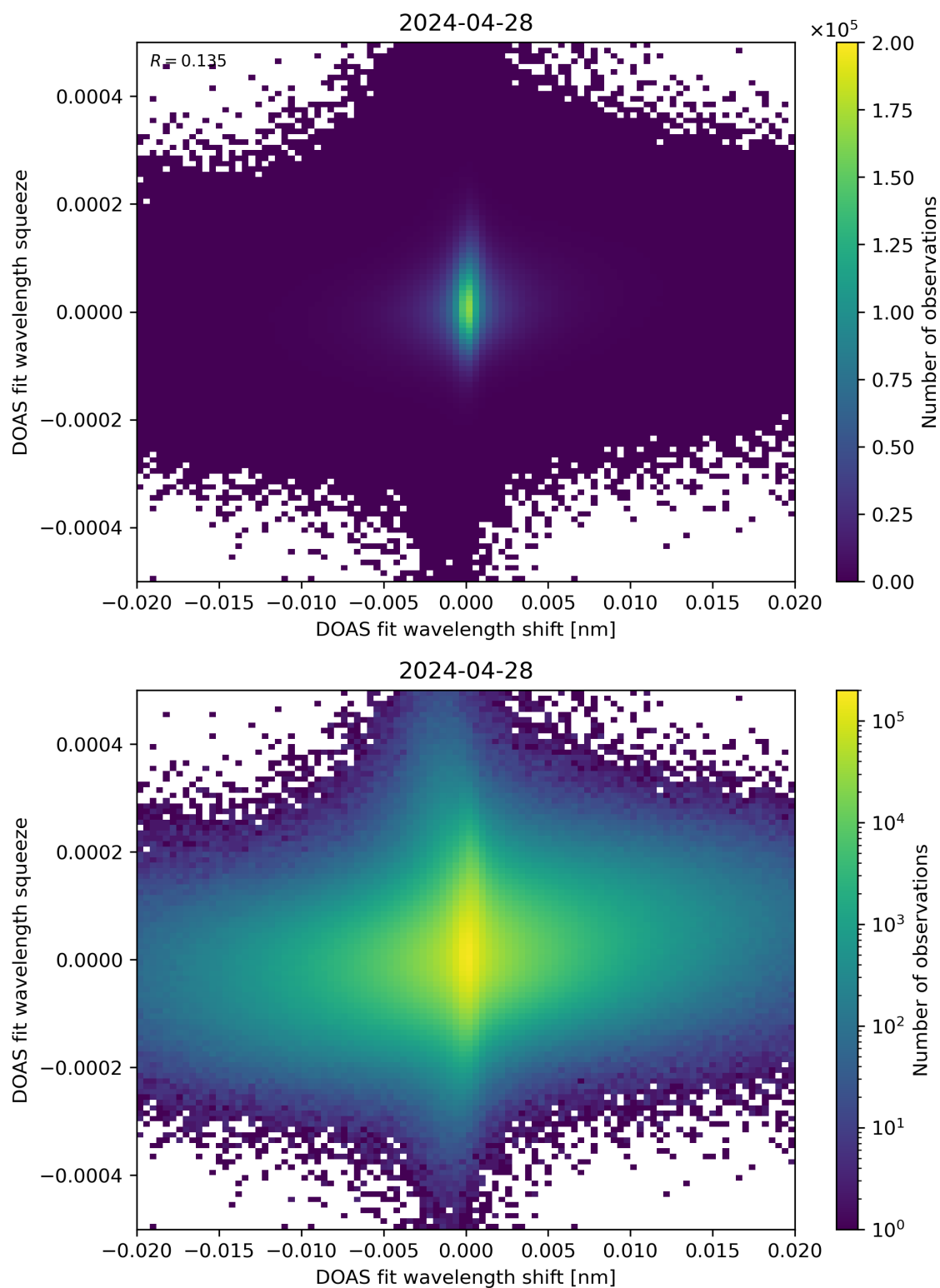
Figure 65: Scatter density plot of “DOAS fit wavelength shift” against “DOAS fit wavelength squeeze” for 2024-04-27 to 2024-04-29.
