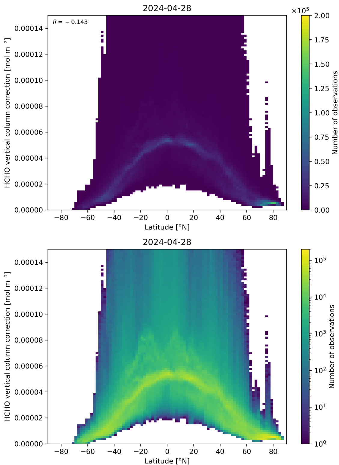
Figure 164: Scatter density plot of “Latitude” against “HCHO vertical column correction” for 2024-04-27 to 2024-04-29.
