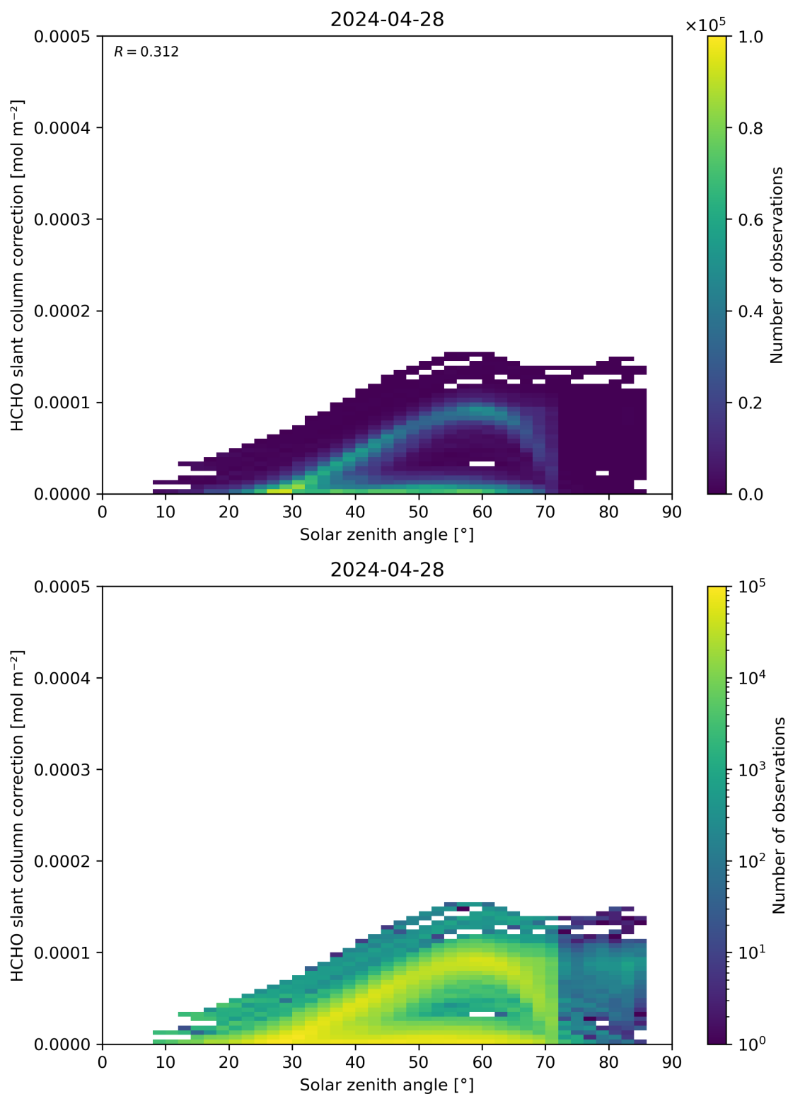
Figure 172: Scatter density plot of “Solar zenith angle” against “HCHO slant column correction” for 2024-04-27 to 2024-04-29.
