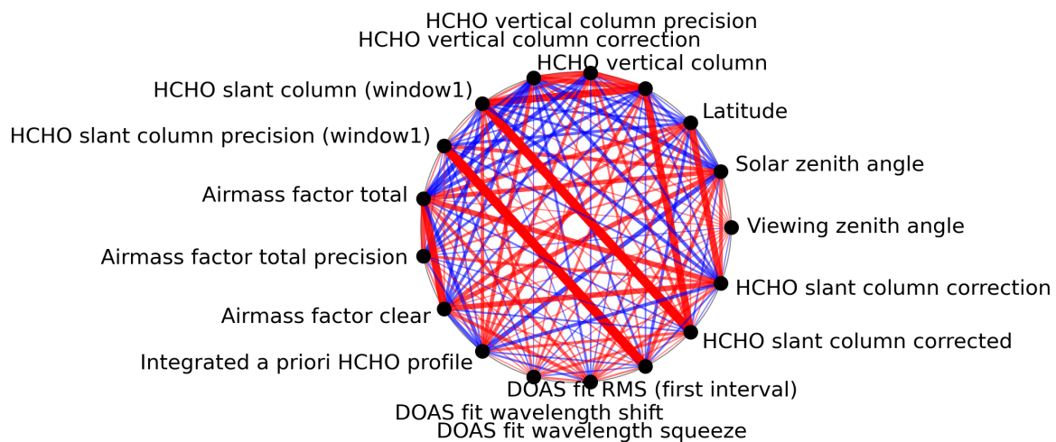
Figure 1: Map of correlation graph for 2024-04-27 to 2024-04-29.
