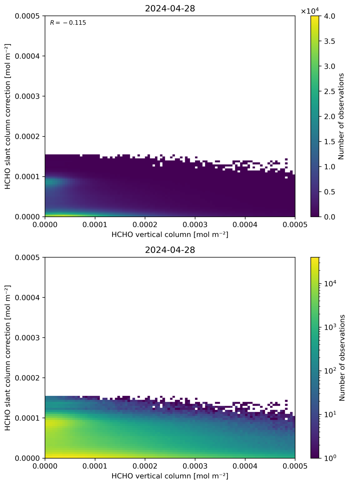
Figure 128: Scatter density plot of “HCHO vertical column” against “HCHO slant column correction” for 2024-04-27 to 2024-04-29.
