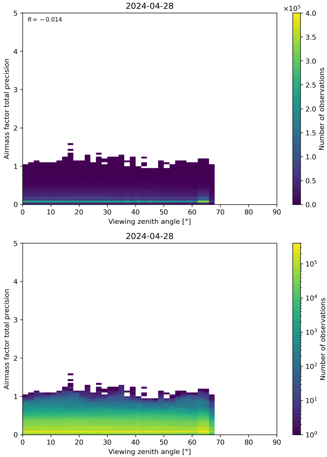
Figure 191: Scatter density plot of “Viewing zenith angle” against “Airmass factor total precision” for 2024-04-27 to 2024-04-29.
