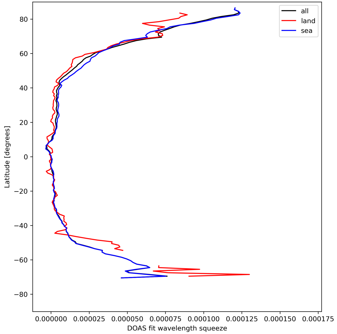
Figure 31: Zonal average of “DOAS fit wavelength squeeze” for 2024-04-27 to 2024-04-29.
