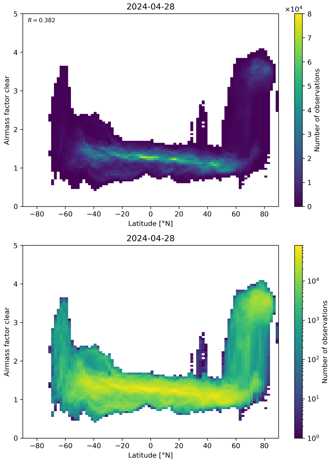
Figure 156: Scatter density plot of “Latitude” against “Airmass factor clear” for 2024-04-27 to 2024-04-29.
