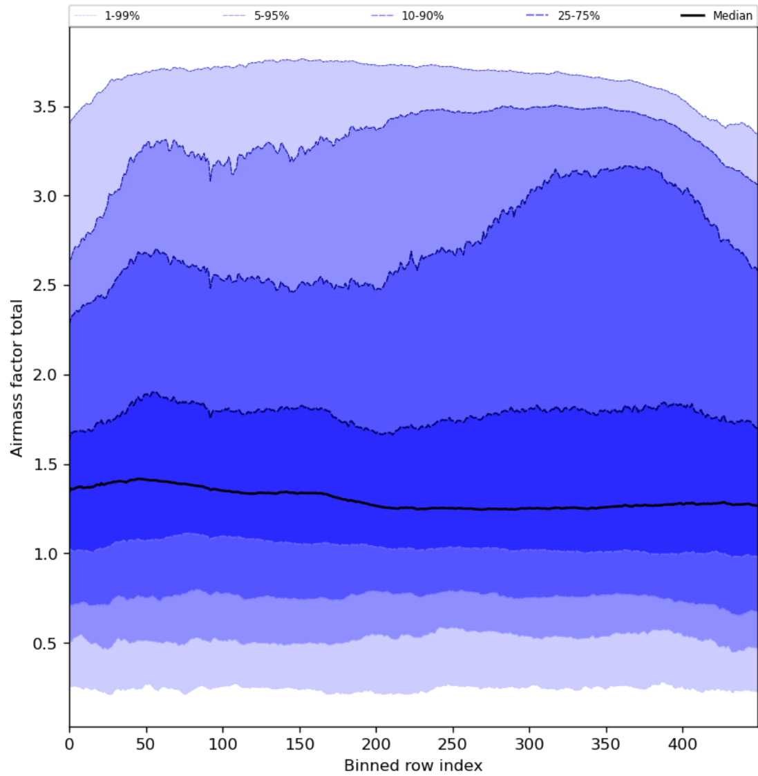
Figure 54: Along track statistics of “Airmass factor total” for 2024-04-27 to 2024-04-29
