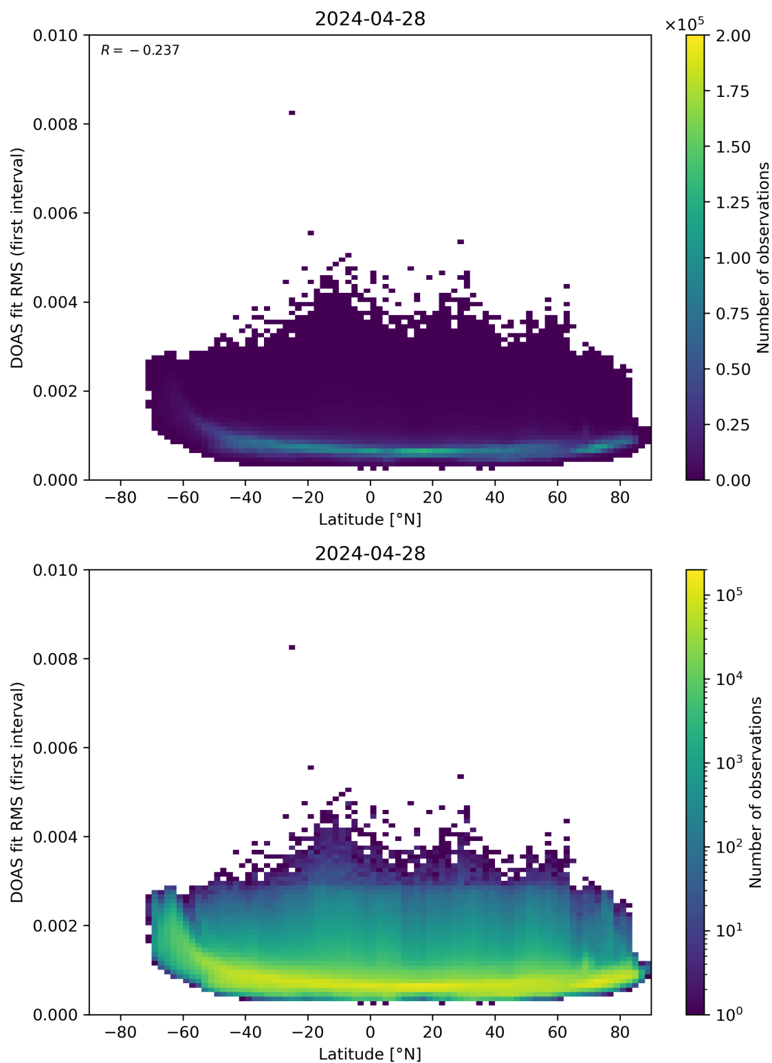
Figure 153: Scatter density plot of “Latitude” against “DOAS fit RMS (first interval)” for 2024-04-27 to 2024-04-29.
