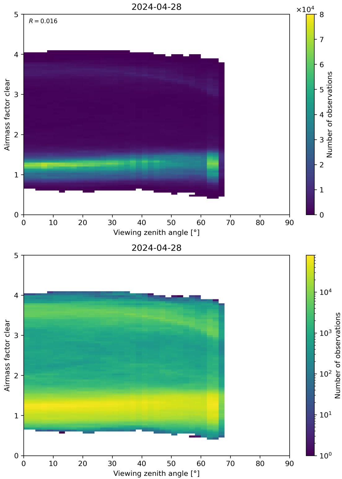
Figure 185: Scatter density plot of “Viewing zenith angle” against “Airmass factor clear” for 2024-04-27 to 2024-04-29.
