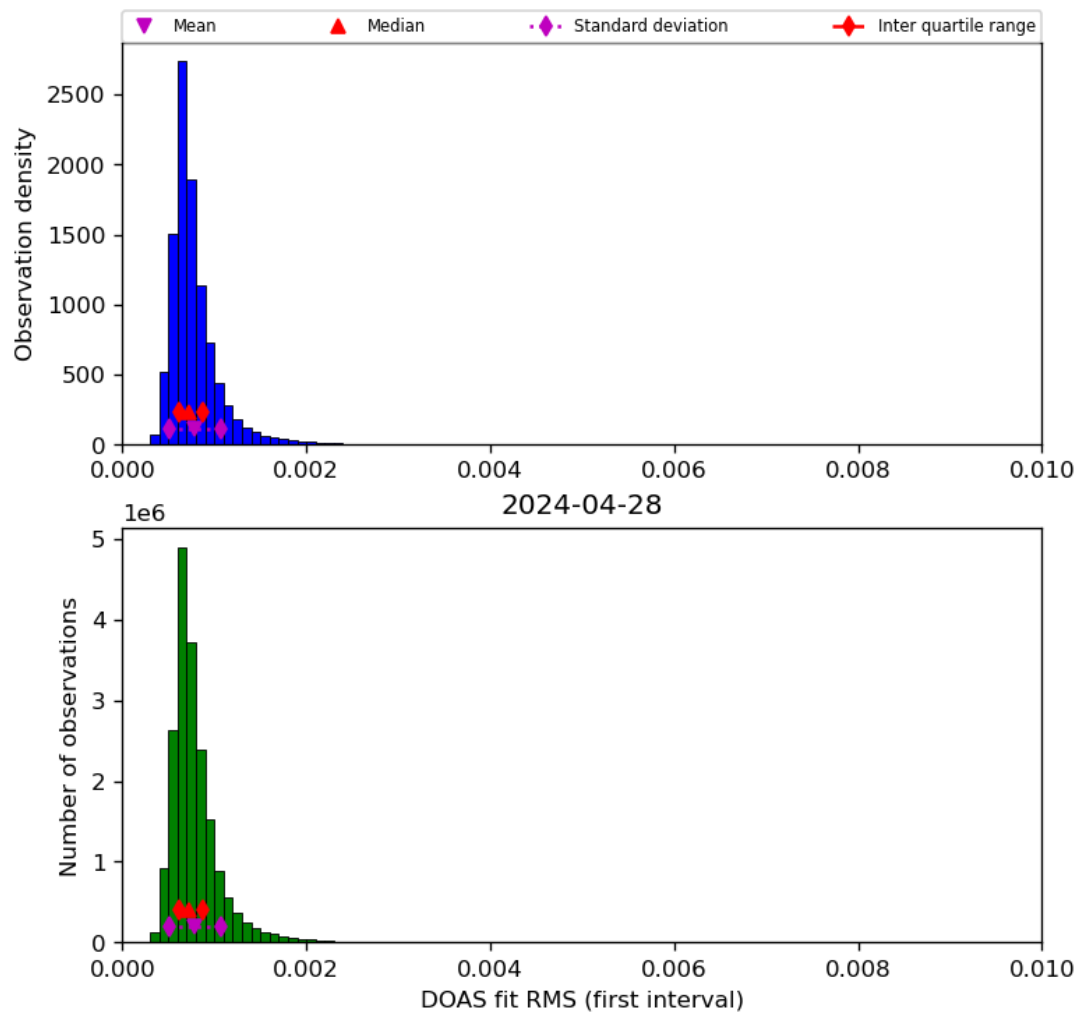
Figure 46: Histogram of “DOAS fit RMS (first interval)” for 2024-04-27 to 2024-04-29
