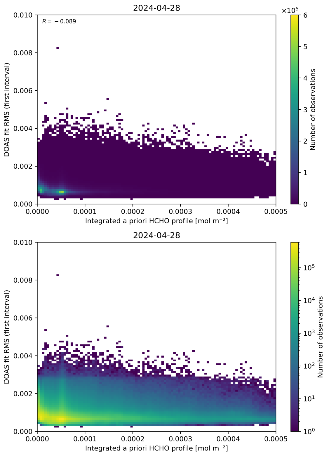
Figure 148: Scatter density plot of “Integrated a priori HCHO profile” against “DOAS fit RMS (first interval)” for 2024-04-27 to 2024-04-29.
