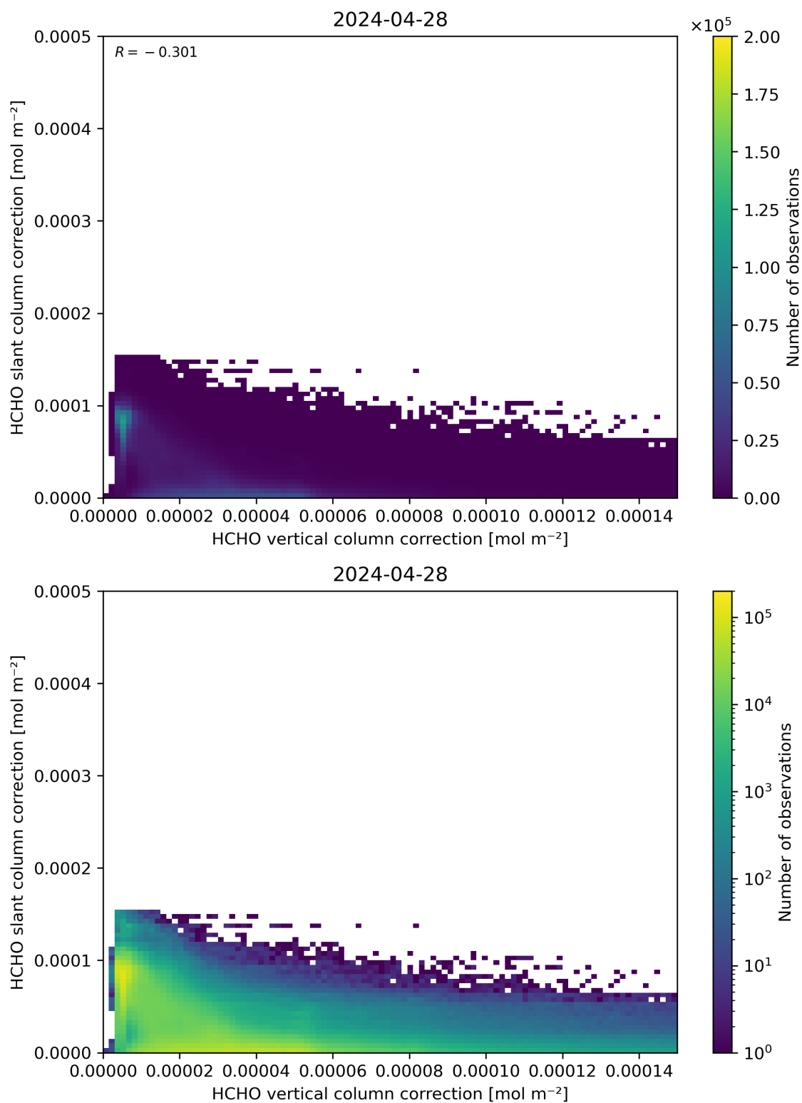
Figure 117: Scatter density plot of “HCHO vertical column correction” against “HCHO slant column correction” for 2024-04-27 to 2024-04-29.
