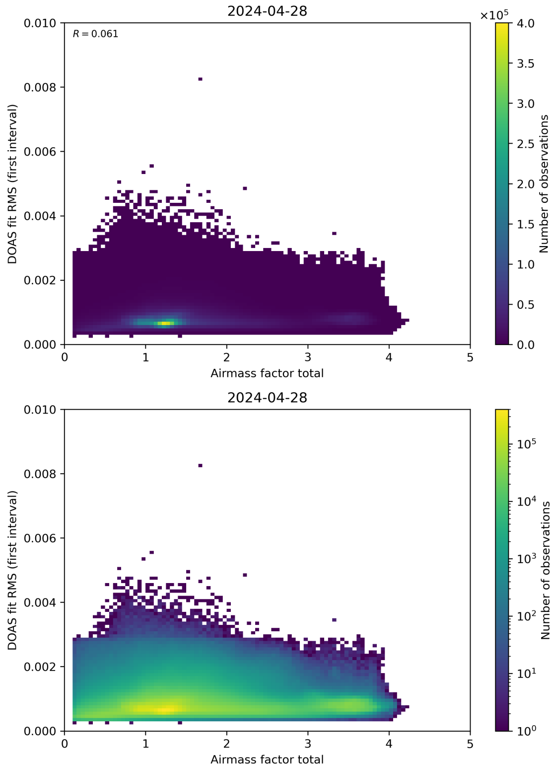
Figure 97: Scatter density plot of “Airmass factor total” against “DOAS fit RMS (first interval)” for 2024-04-27 to 2024-04-29.
