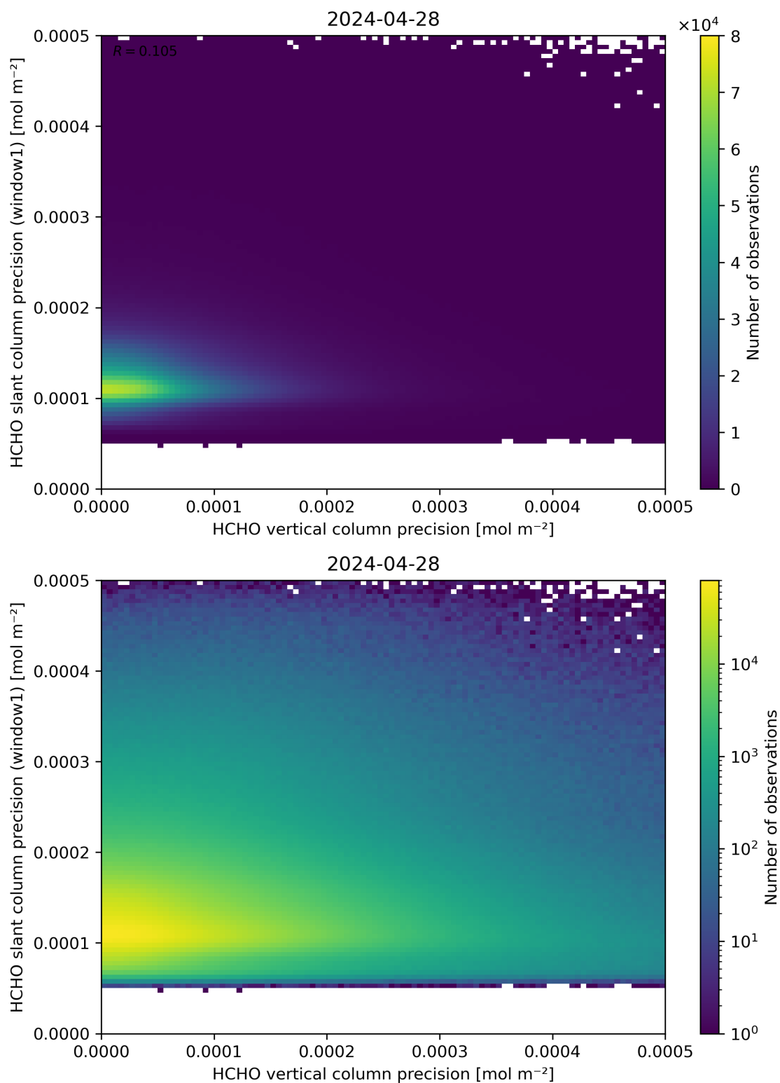
Figure 143: Scatter density plot of “HCHO vertical column precision” against “HCHO slant column precision (window1)” for 2024-04-27 to 2024-04-29.
