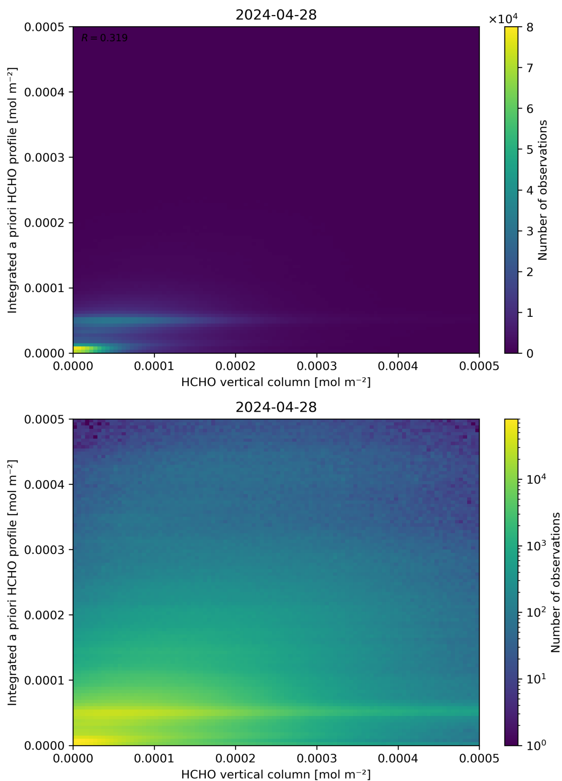
Figure 135: Scatter density plot of “HCHO vertical column” against “Integrated a priori HCHO profile” for 2024-04-27 to 2024-04-29.
