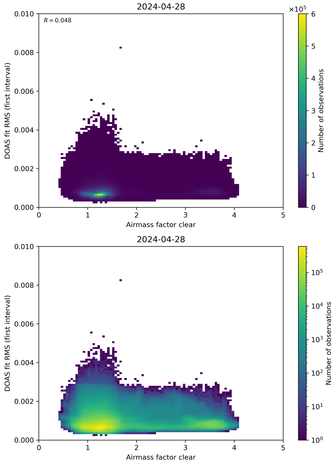
Figure 71: Scatter density plot of “Airmass factor clear” against “DOAS fit RMS (first interval)” for 2024-04-27 to 2024-04-29.
