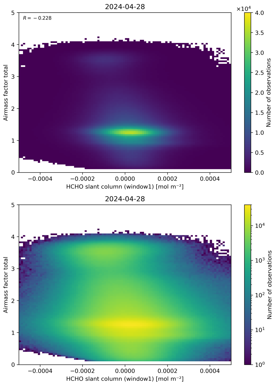
Figure 85: Scatter density plot of “HCHO slant column (window1)” against “Airmass factor total” for 2024-04-27 to 2024-04-29.
