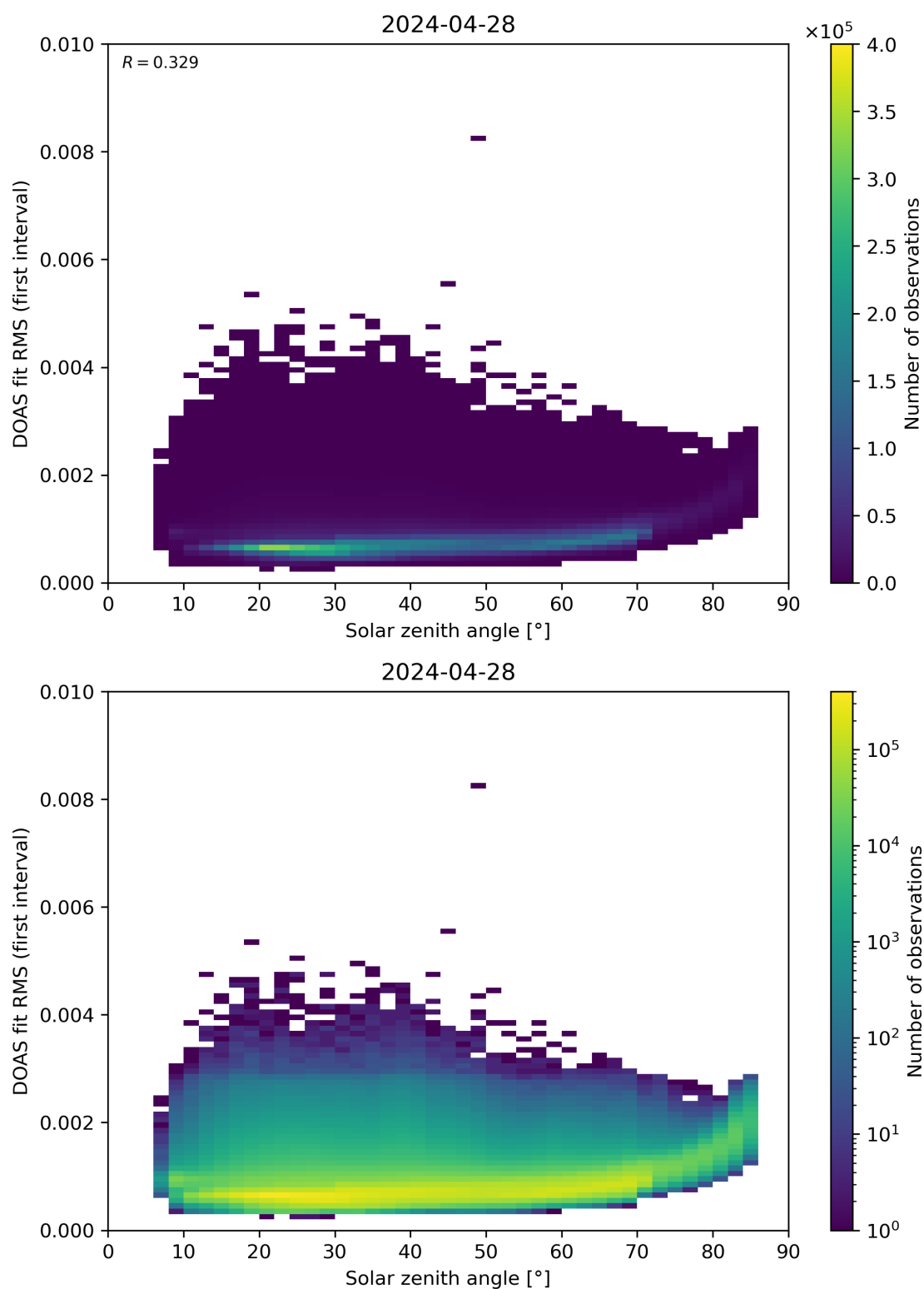
Figure 167: Scatter density plot of “Solar zenith angle” against “DOAS fit RMS (first interval)” for 2024-04-27 to 2024-04-29.
