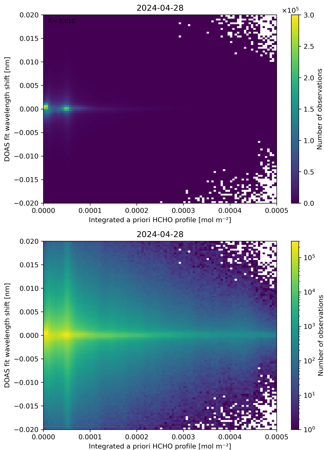
Figure 149: Scatter density plot of “Integrated a priori HCHO profile” against “DOAS fit wavelength shift” for 2024-04-27 to 2024-04-29.
