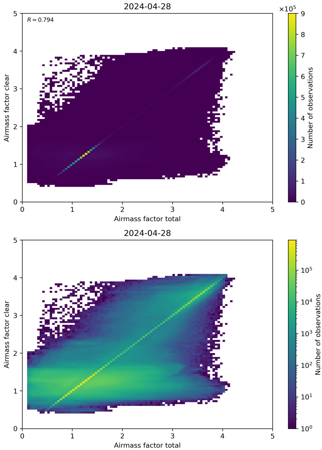
Figure 100: Scatter density plot of “Airmass factor total” against “Airmass factor clear” for 2024-04-27 to 2024-04-29.
