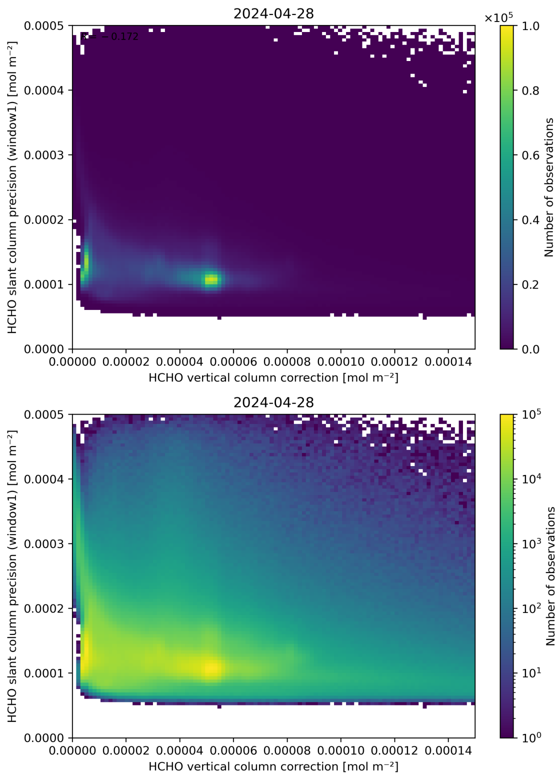
Figure 119: Scatter density plot of “HCHO vertical column correction” against “HCHO slant column precision (window1)” for 2024-04-27 to 2024-04-29.
