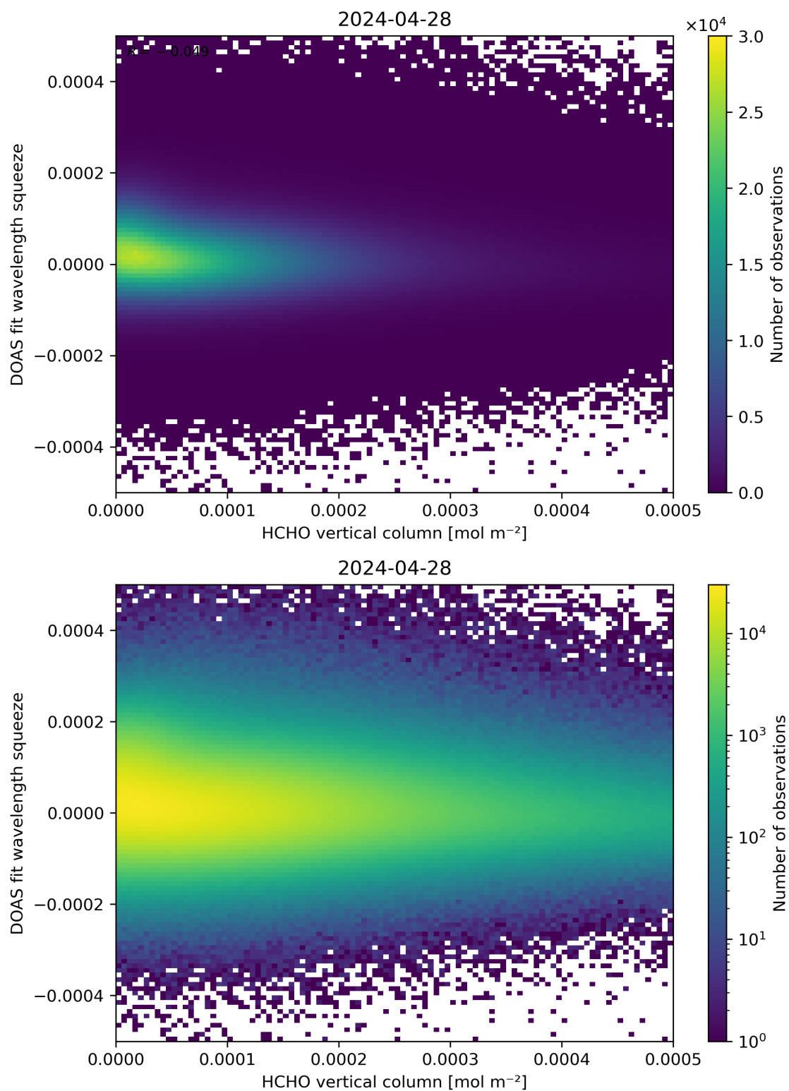
Figure 125: Scatter density plot of “HCHO vertical column” against “DOAS fit wavelength squeeze” for 2024-04-27 to 2024-04-29.
