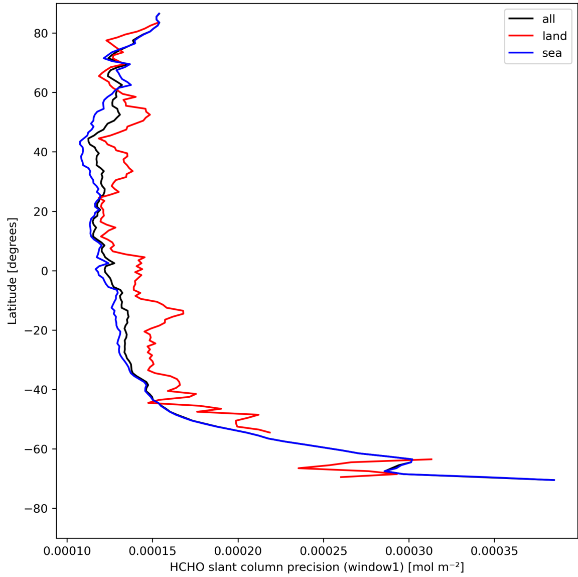
Figure 25: Zonal average of "HCHO slant column precision (window1)" for 2024-04-27 to 2024-04-29.
