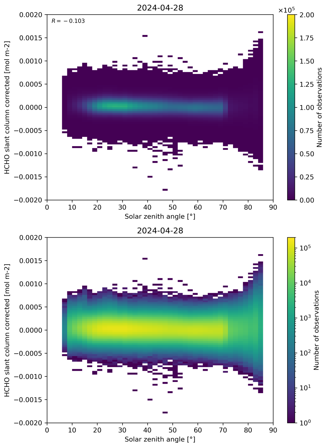
Figure 171: Scatter density plot of “Solar zenith angle” against “HCHO slant column corrected” for 2024-04-27 to 2024-04-29.
