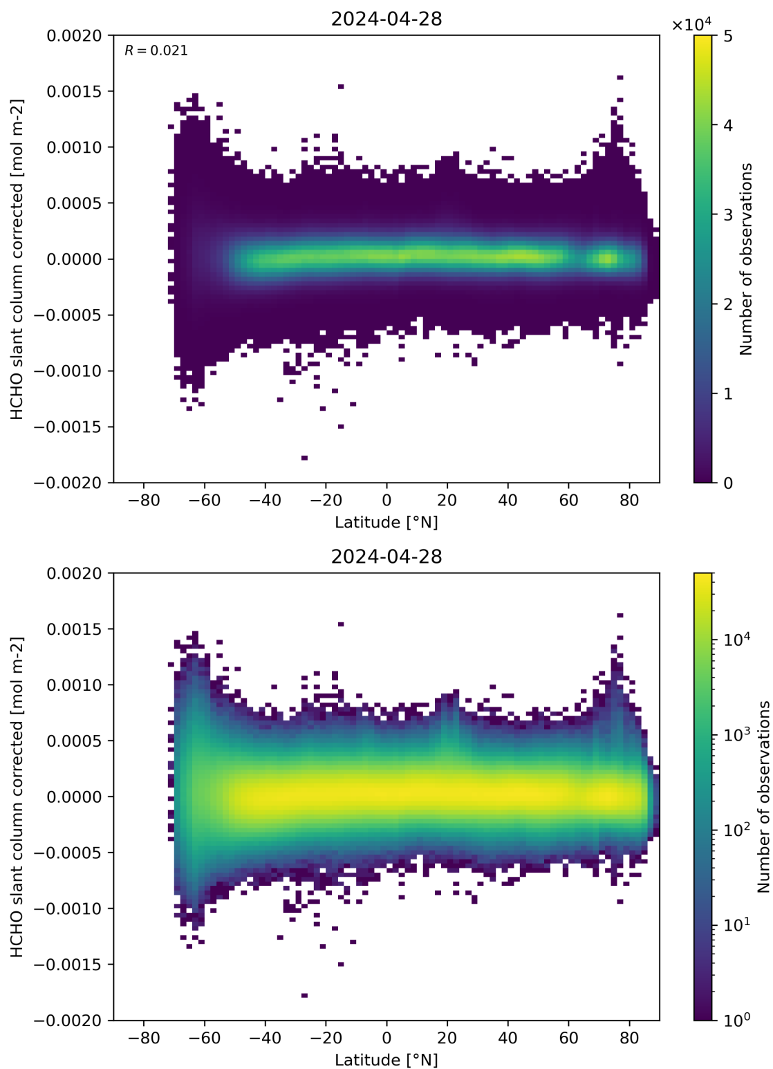
Figure 157: Scatter density plot of “Latitude” against “HCHO slant column corrected” for 2024-04-27 to 2024-04-29.
