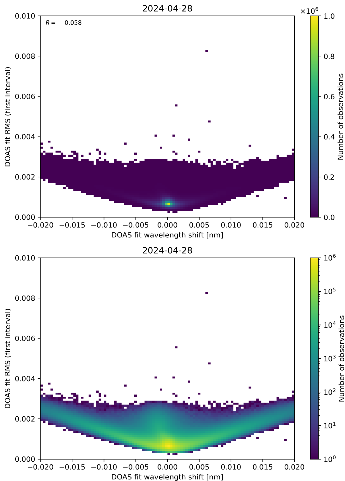
Figure 64: Scatter density plot of “DOAS fit wavelength shift” against “DOAS fit RMS (first interval)” for 2024-04-27 to 2024-04-29.
