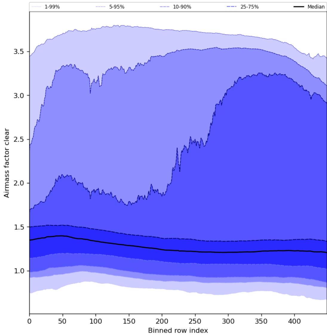
Figure 56: Along track statistics of “Airmass factor clear” for 2024-04-27 to 2024-04-29
