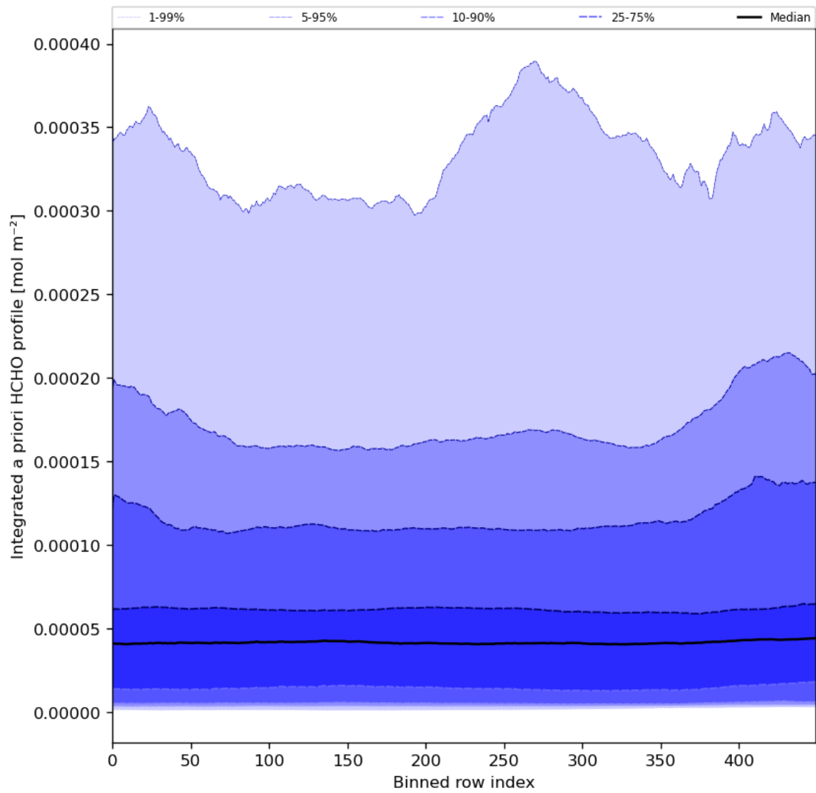
Figure 57: Along track statistics of “Integrated a priori HCHO profile” for 2024-04-27 to 2024-04-29
