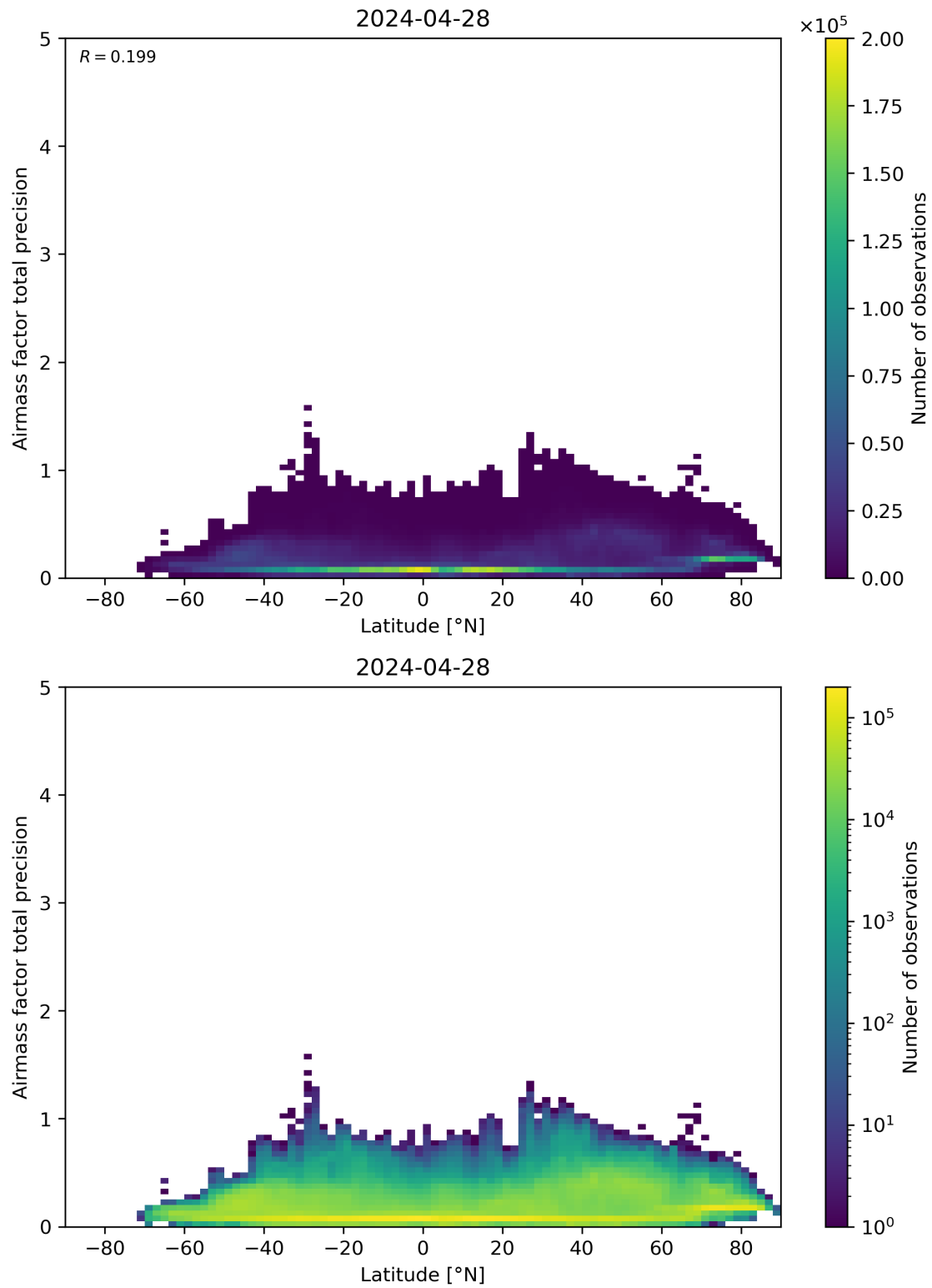
Figure 162: Scatter density plot of “Latitude” against “Airmass factor total precision” for 2024-04-27 to 2024-04-29.
