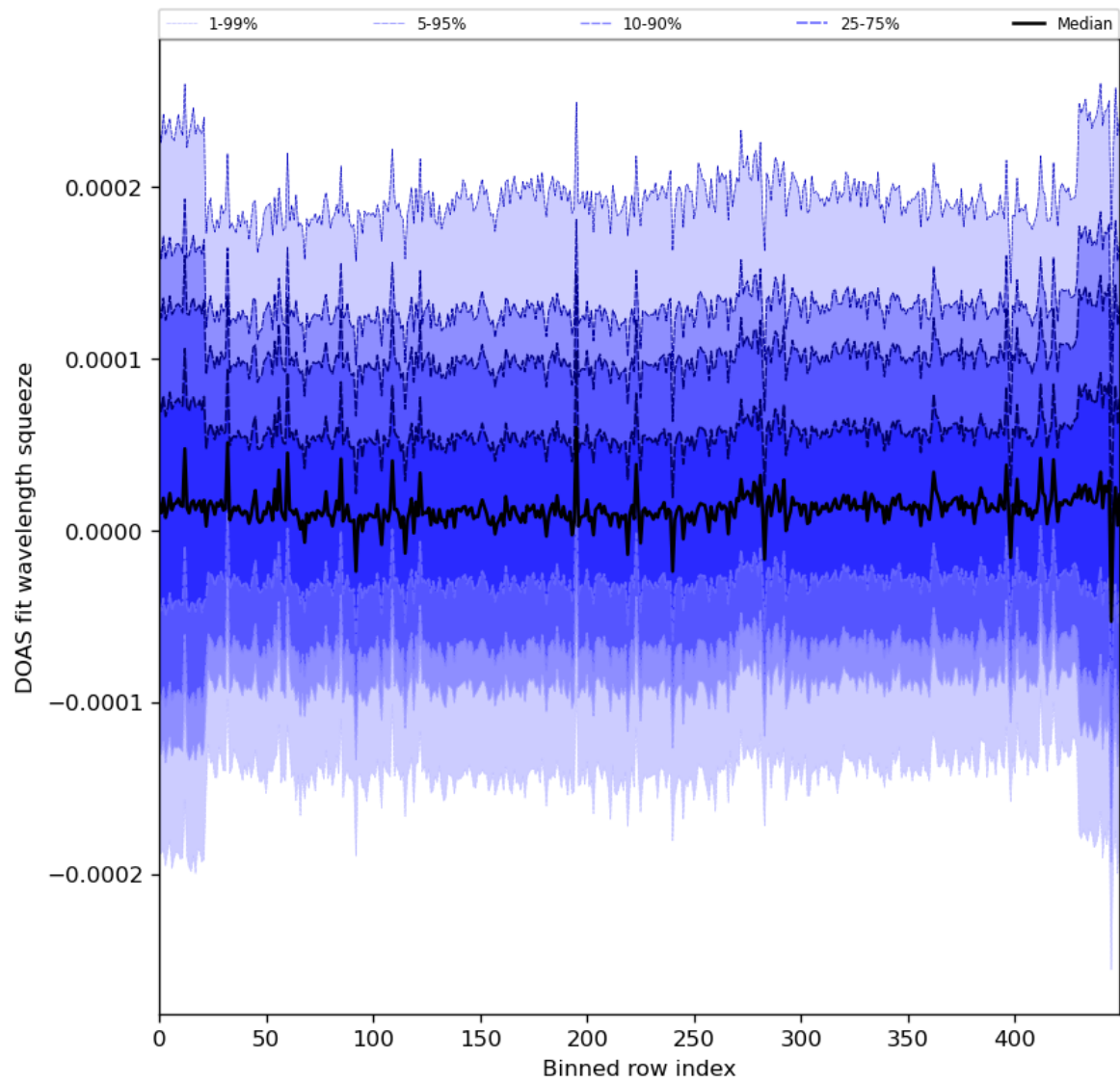
Figure 59: Along track statistics of “DOAS fit wavelength squeeze” for 2024-04-27 to 2024-04-29
