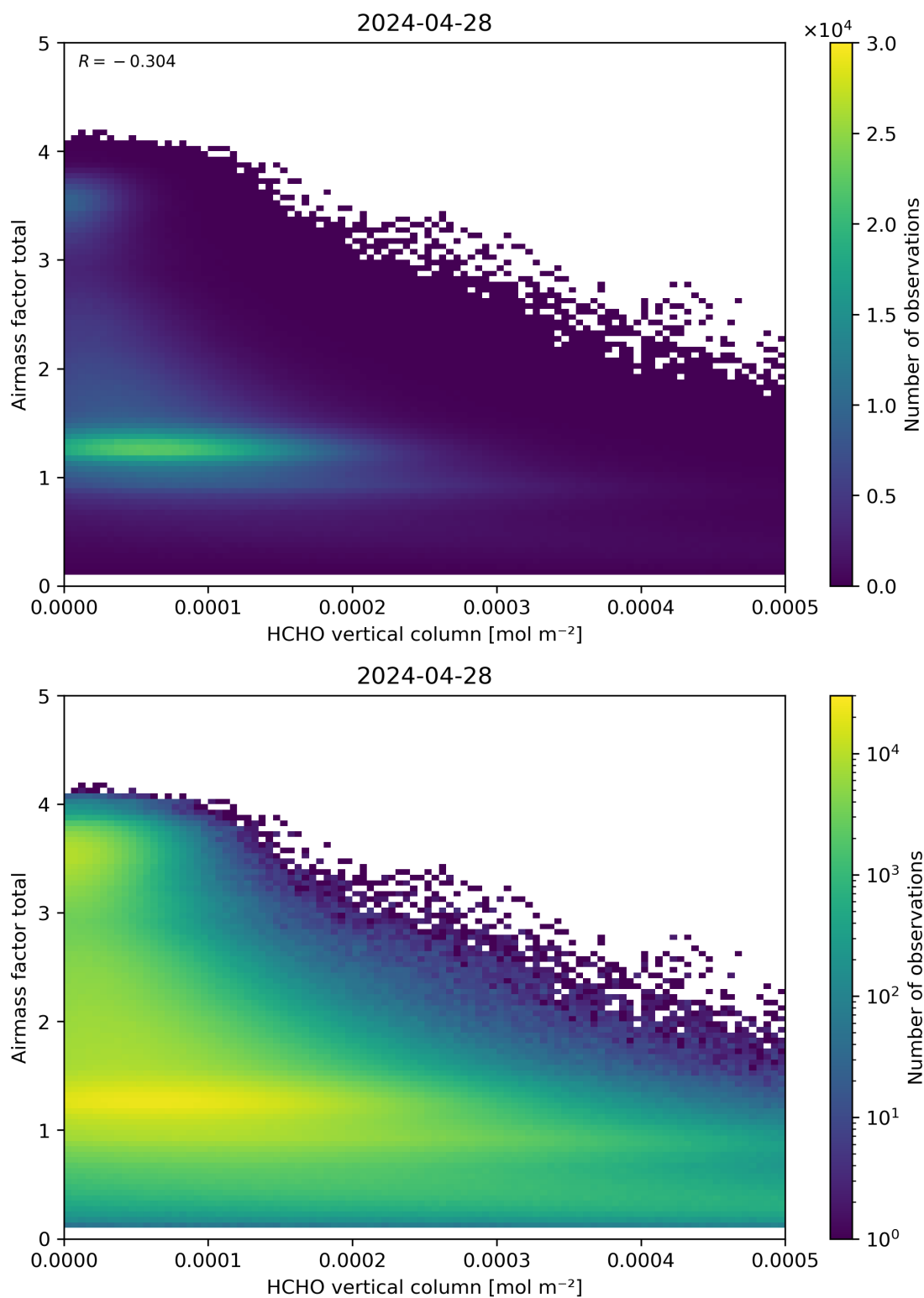
Figure 131: Scatter density plot of “HCHO vertical column” against “Airmass factor total” for 2024-04-27 to 2024-04-29.
