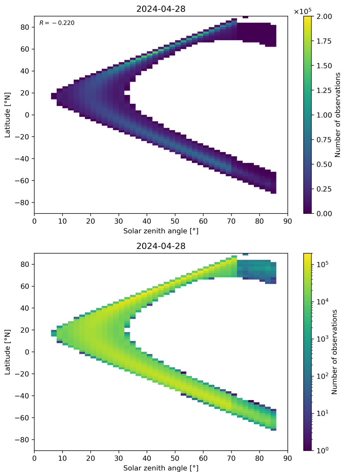
Figure 181: Scatter density plot of “Solar zenith angle” against “Latitude” for 2024-04-27 to 2024-04-29.
