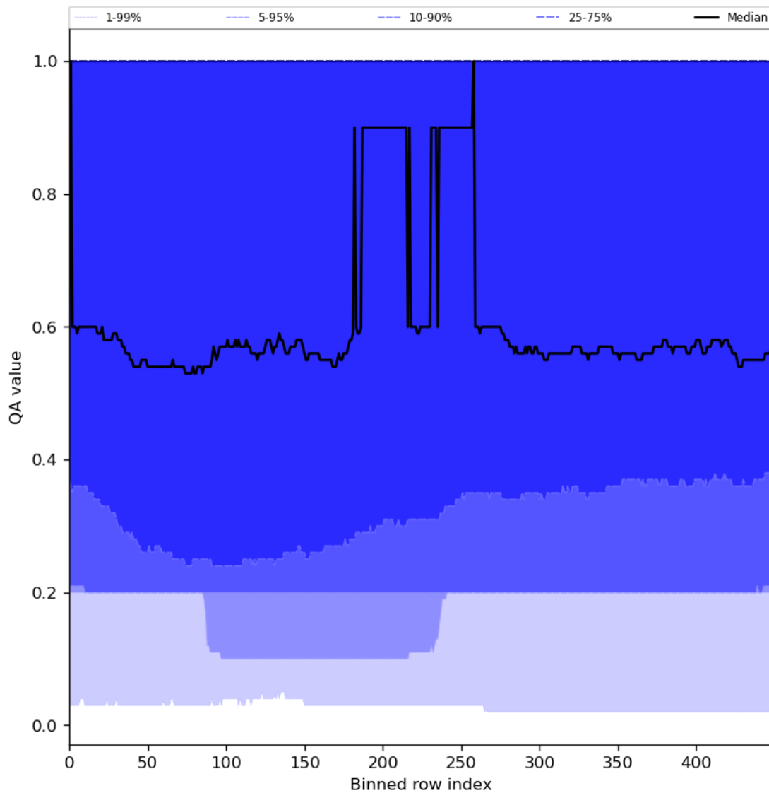
Figure 48: Along track statistics of “QA value” for 2024-04-27 to 2024-04-29
