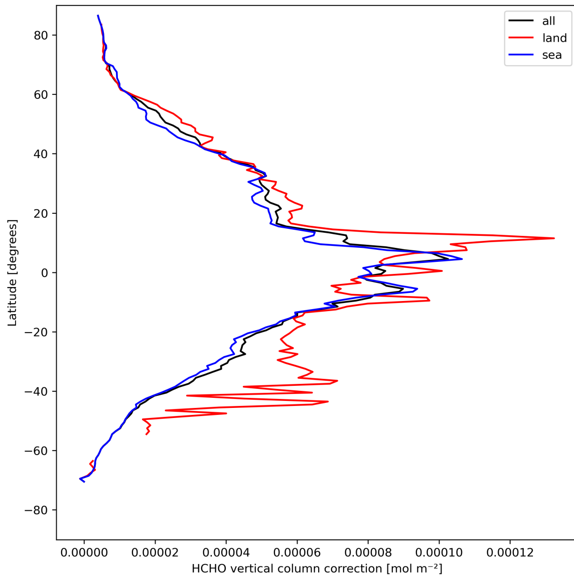
Figure 23: Zonal average of “HCHO vertical column correction” for 2024-04-27 to 2024-04-29.
