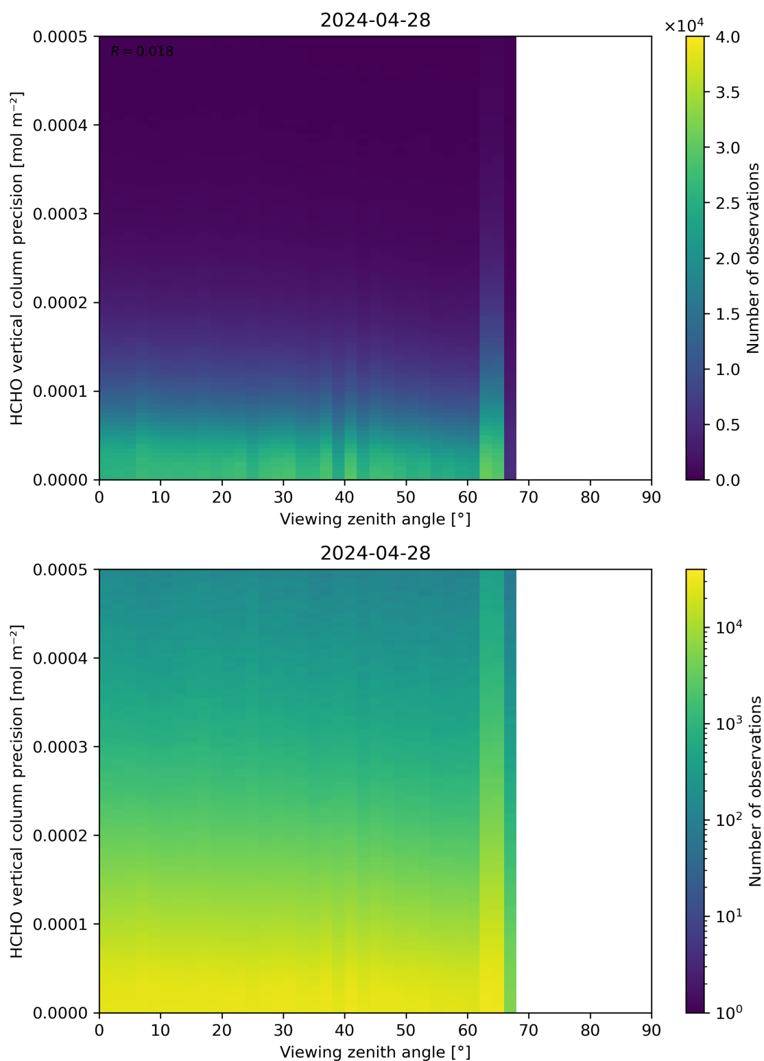
Figure 194: Scatter density plot of “Viewing zenith angle” against “HCHO vertical column precision” for 2024-04-27 to 2024-04-29.
