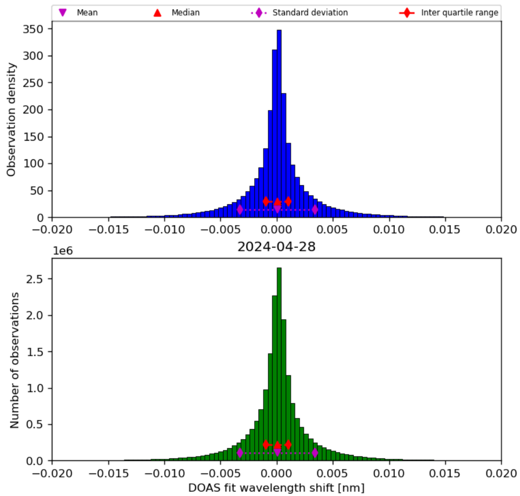
Figure 44: Histogram of “DOAS fit wavelength shift” for 2024-04-27 to 2024-04-29
