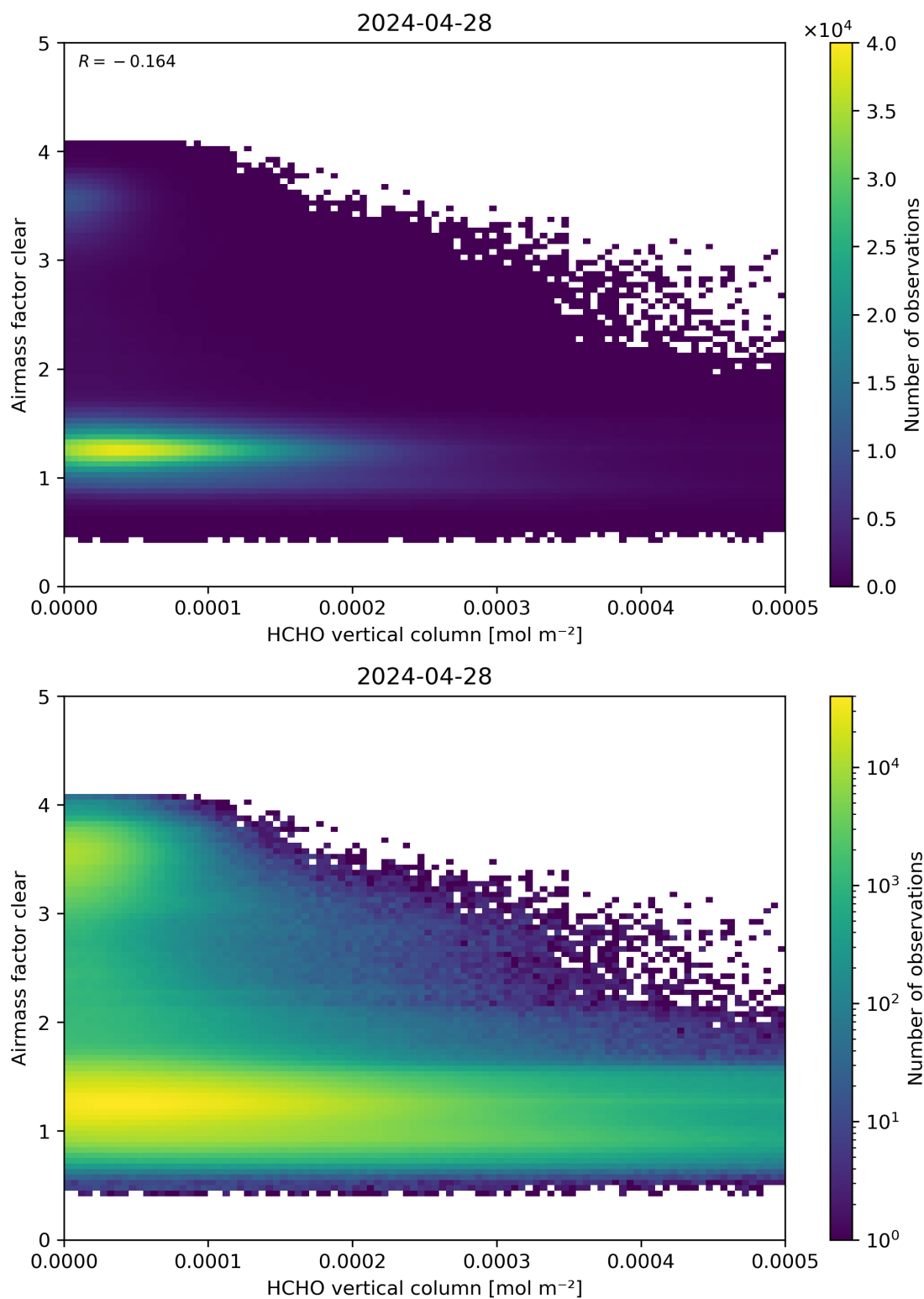
Figure 126: Scatter density plot of “HCHO vertical column” against “Airmass factor clear” for 2024-04-27 to 2024-04-29.
