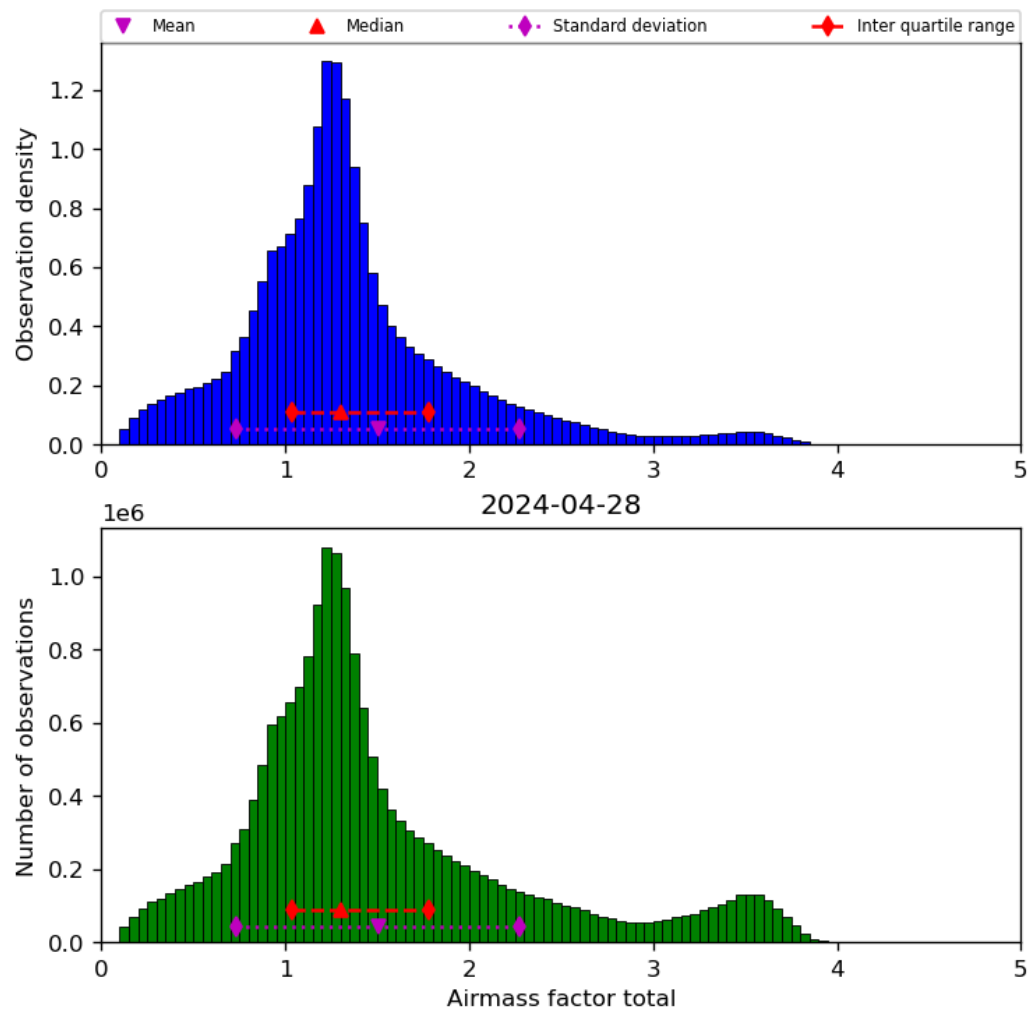
Figure 40: Histogram of “Airmass factor total” for 2024-04-27 to 2024-04-29
