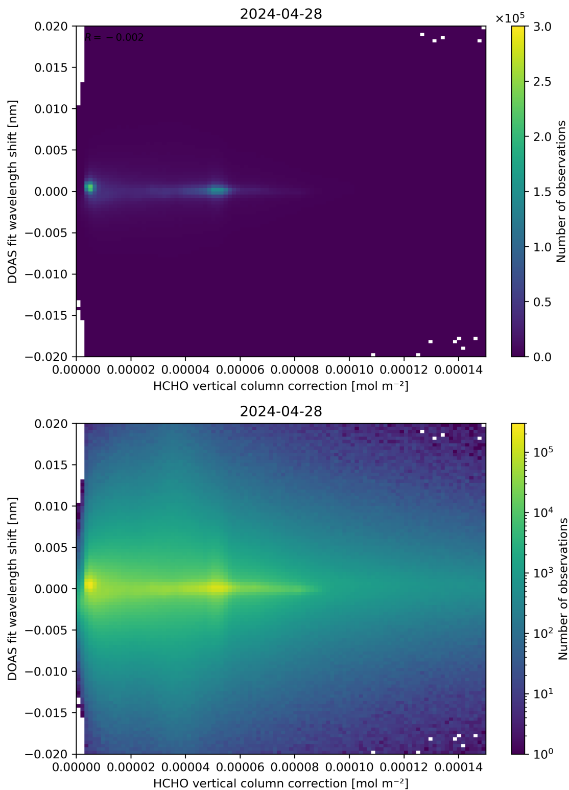
Figure 113: Scatter density plot of “HCHO vertical column correction” against “DOAS fit wavelength shift” for 2024-04-27 to 2024-04-29.
