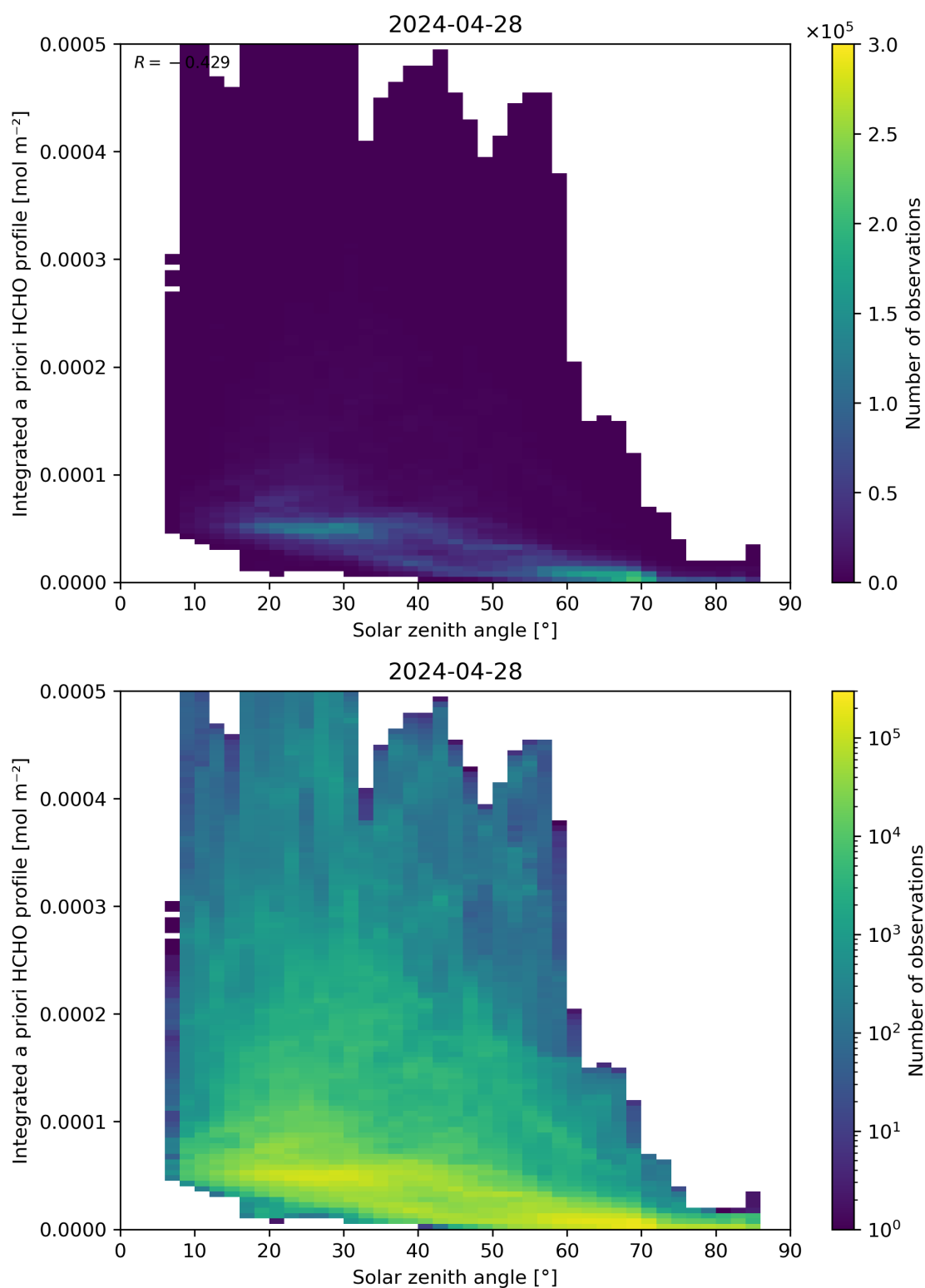
Figure 180: Scatter density plot of “Solar zenith angle” against “Integrated a priori HCHO profile” for 2024-04-27 to 2024-04-29.
