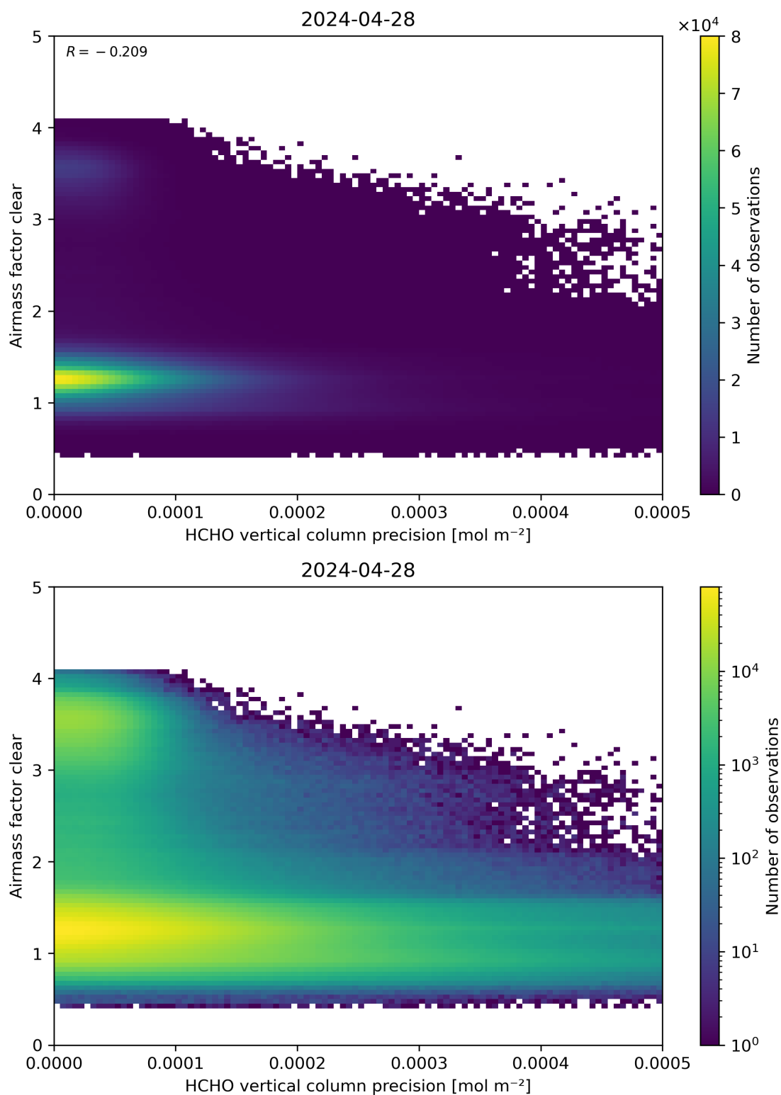
Figure 139: Scatter density plot of “HCHO vertical column precision” against “Airmass factor clear” for 2024-04-27 to 2024-04-29.
