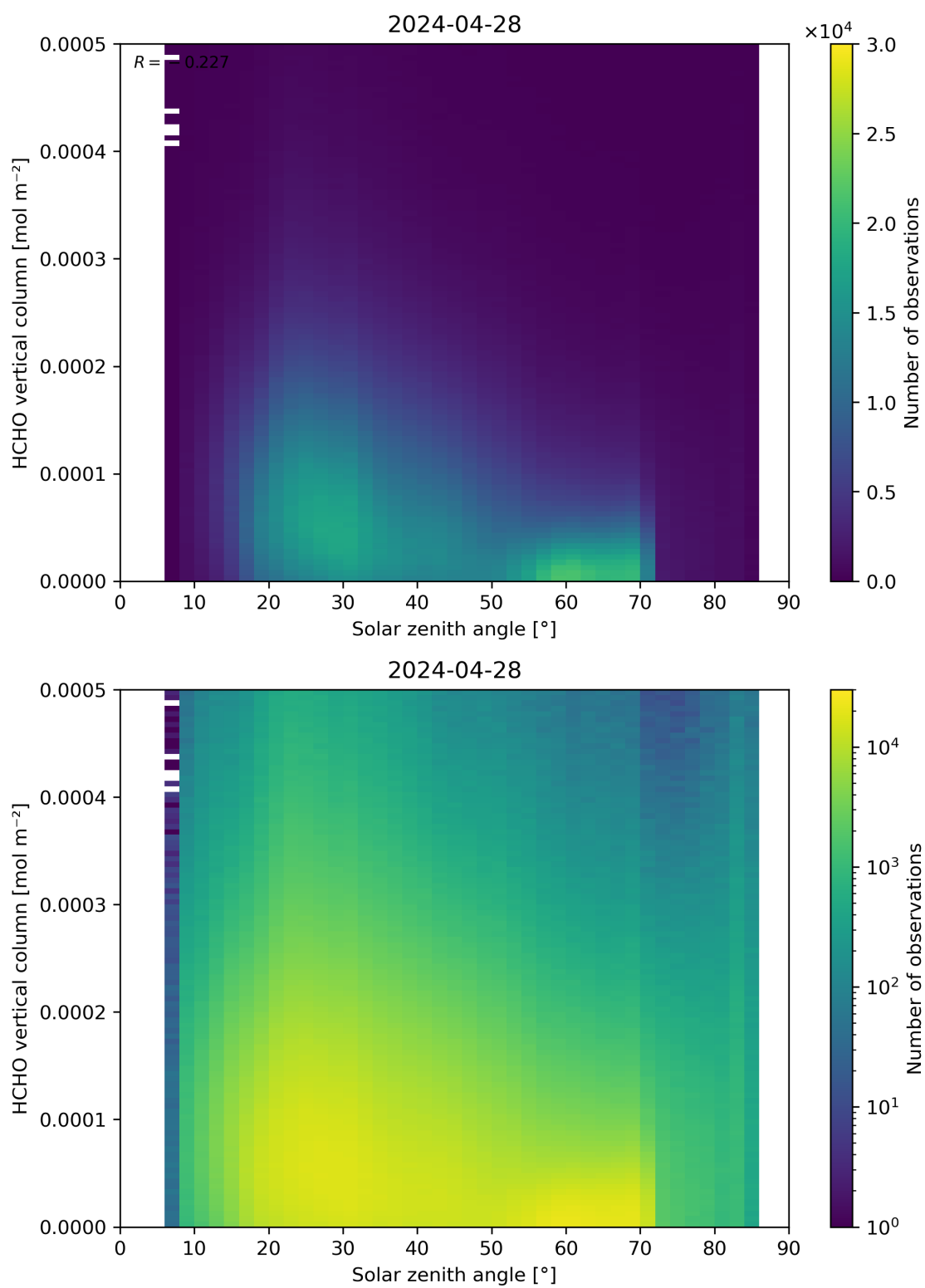
Figure 177: Scatter density plot of “Solar zenith angle” against “HCHO vertical column” for 2024-04-27 to 2024-04-29.
