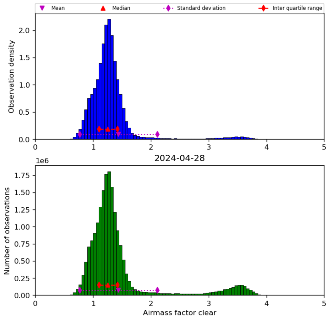
Figure 42: Histogram of “Airmass factor clear” for 2024-04-27 to 2024-04-29
