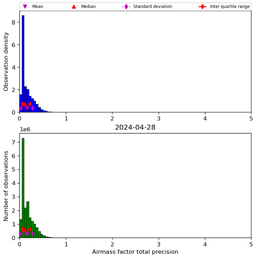
Figure 41: Histogram of “Airmass factor total precision” for 2024-04-27 to 2024-04-29
