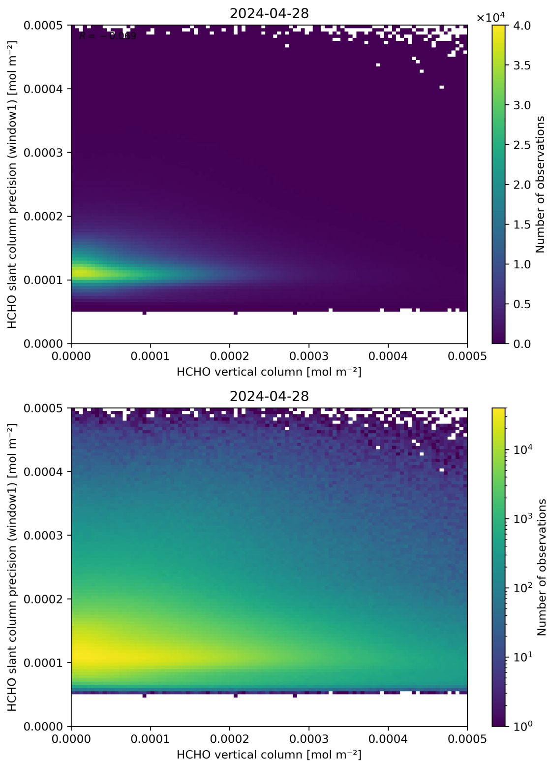
Figure 130: Scatter density plot of “HCHO vertical column” against “HCHO slant column precision (window1)” for 2024-04-27 to 2024-04-29.
