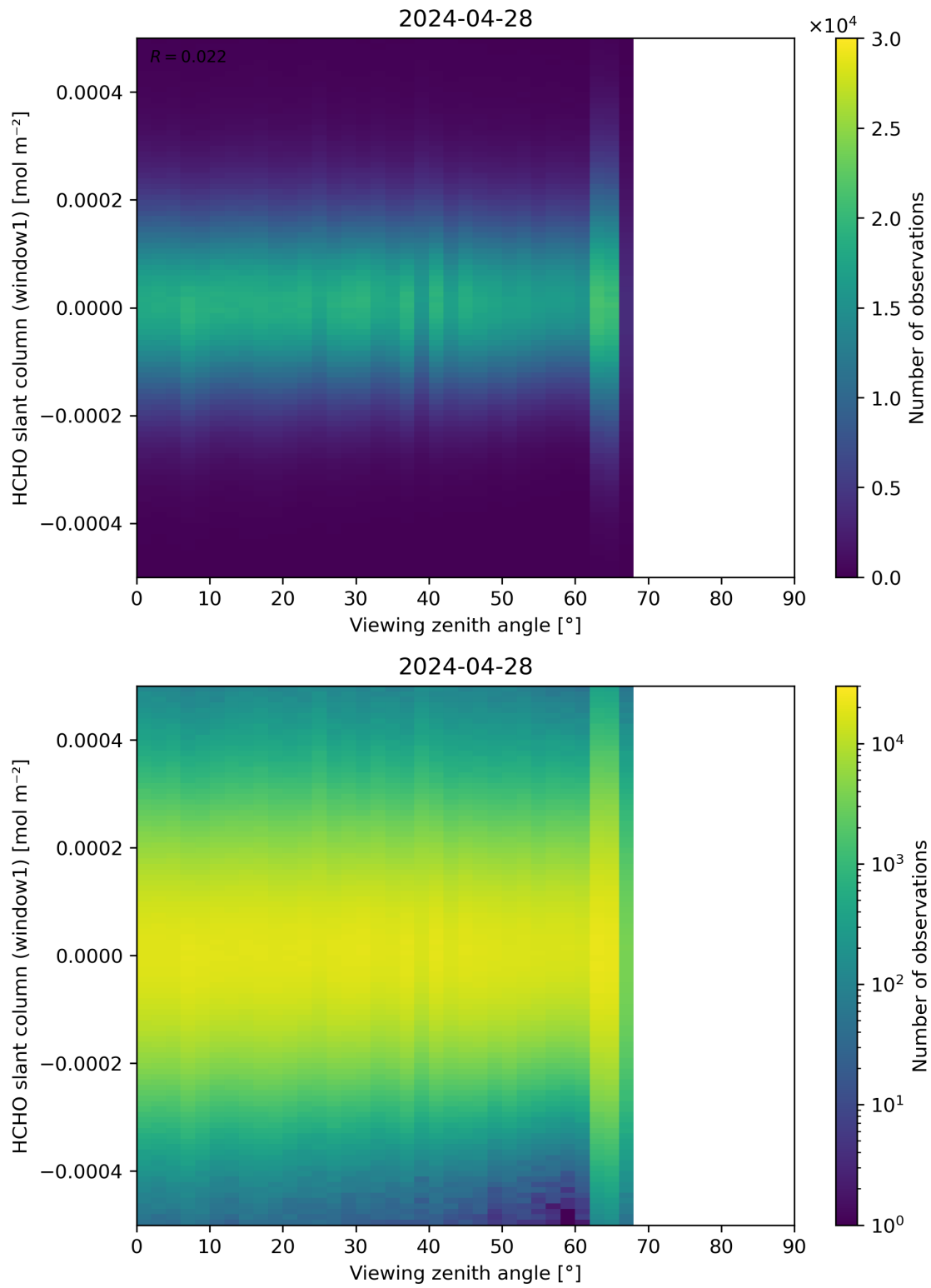
Figure 188: Scatter density plot of “Viewing zenith angle” against “HCHO slant column (window1)” for 2024-04-27 to 2024-04-29.
