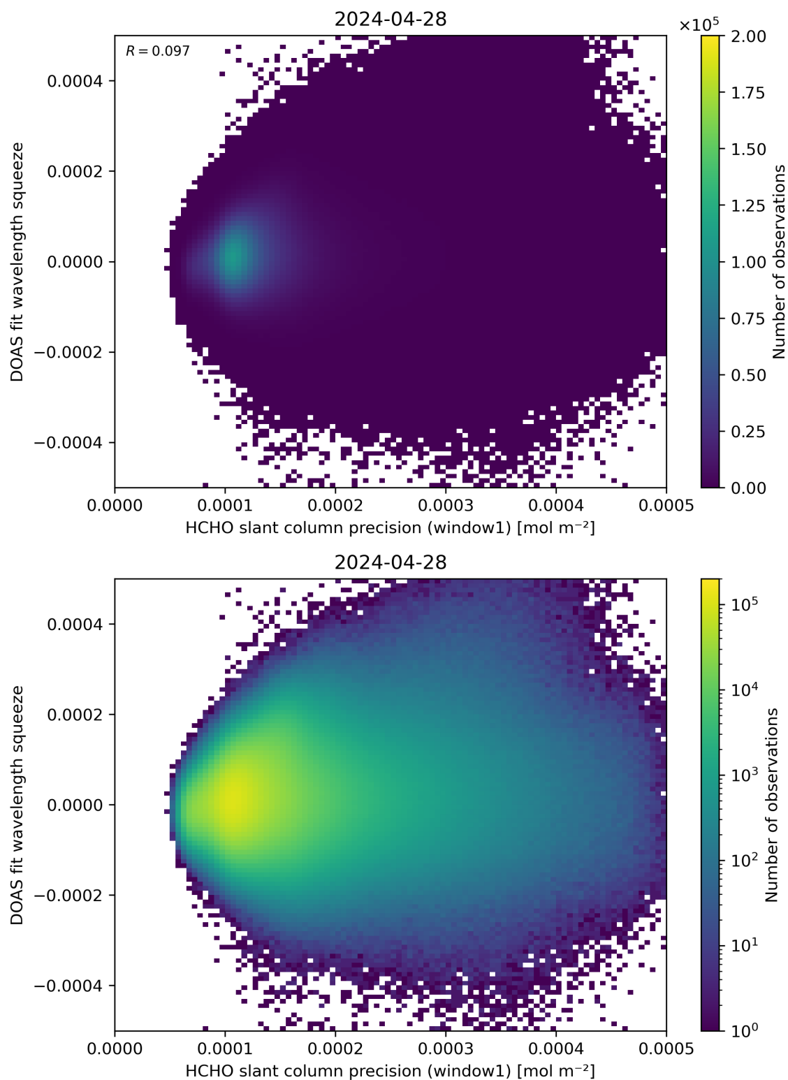
Figure 90: Scatter density plot of “HCHO slant column precision (window1)” against “DOAS fit wavelength squeeze” for 2024-04-27 to 2024-04-29.
