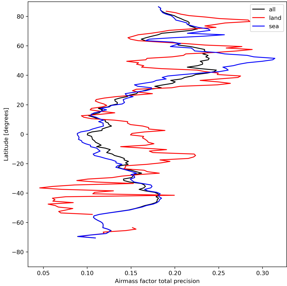
Figure 27: Zonal average of “Airmass factor total precision” for 2024-04-27 to 2024-04-29.
