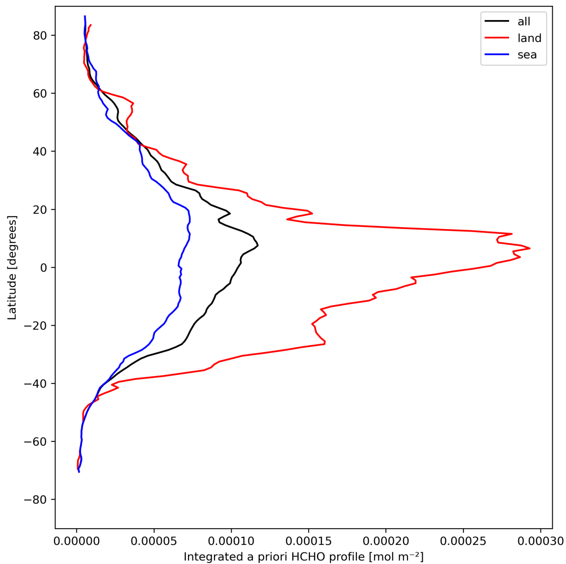
Figure 29: Zonal average of “Integrated a priori HCHO profile” for 2024-04-27 to 2024-04-29.
