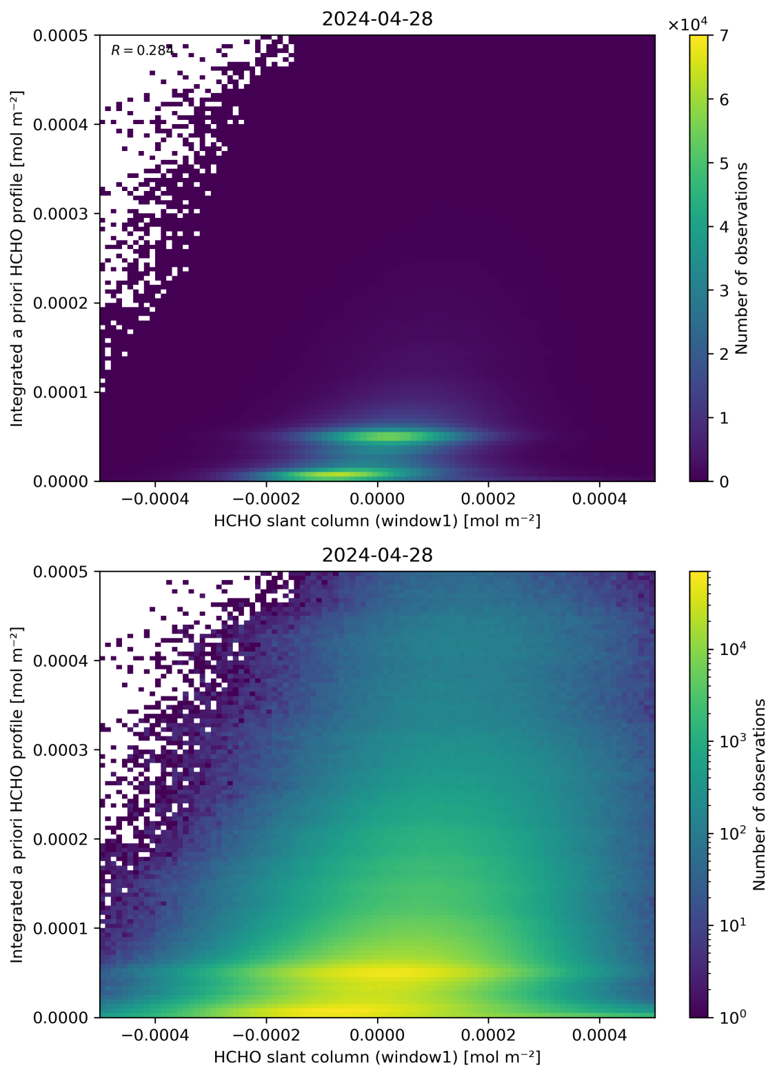
Figure 87: Scatter density plot of “HCHO slant column (window1)” against “Integrated a priori HCHO profile” for 2024-04-27 to 2024-04-29.
