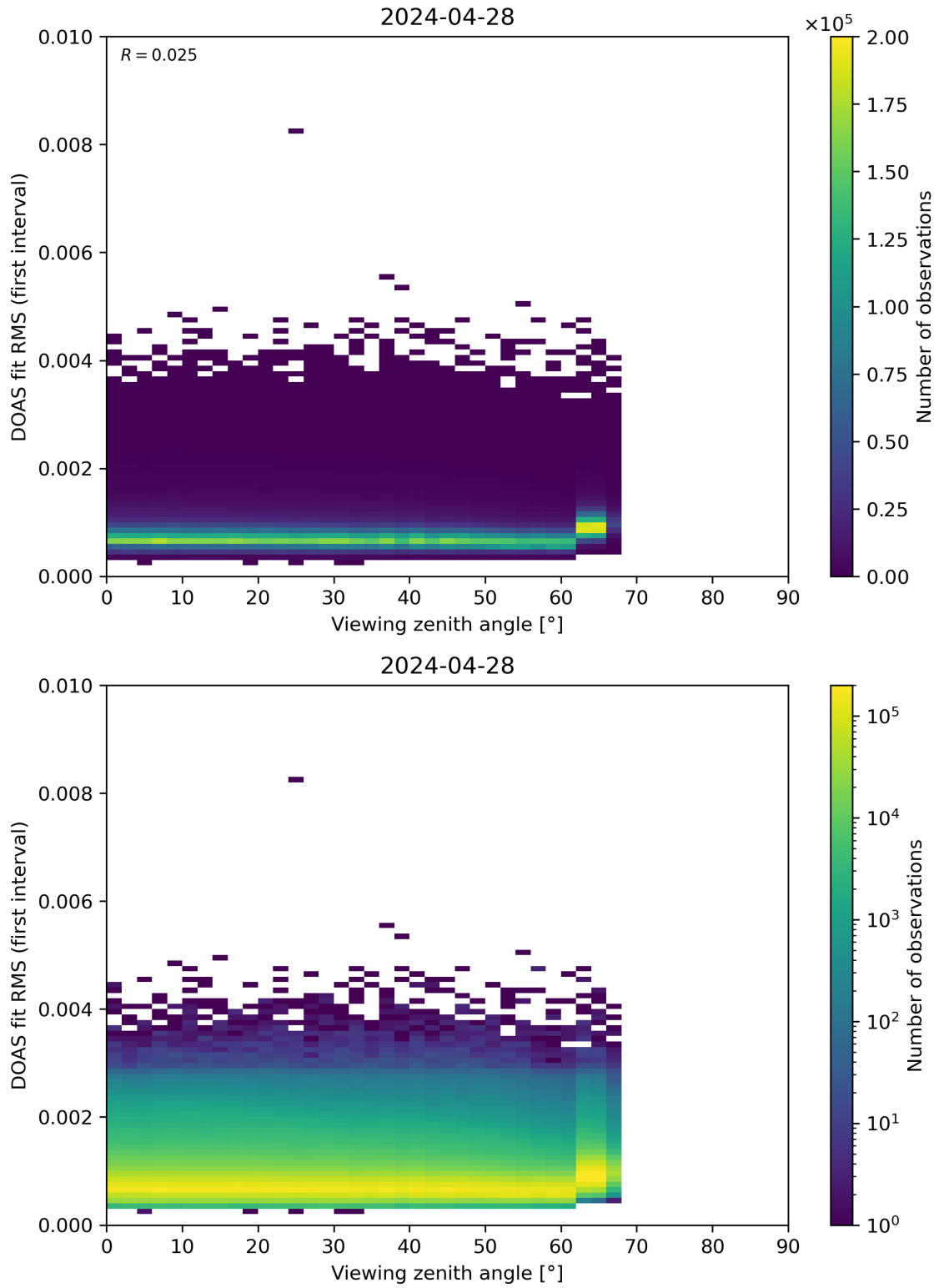
Figure 182: Scatter density plot of “Viewing zenith angle” against “DOAS fit RMS (first interval)” for 2024-04-27 to 2024-04-29.
