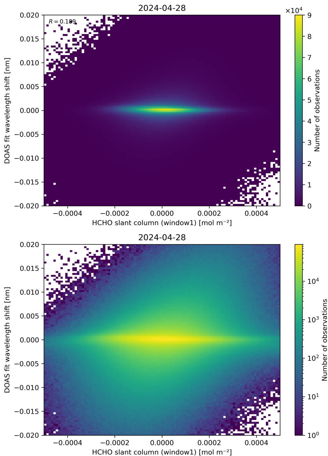
Figure 79: Scatter density plot of “HCHO slant column (window1)” against “DOAS fit wavelength shift” for 2024-04-27 to 2024-04-29.
