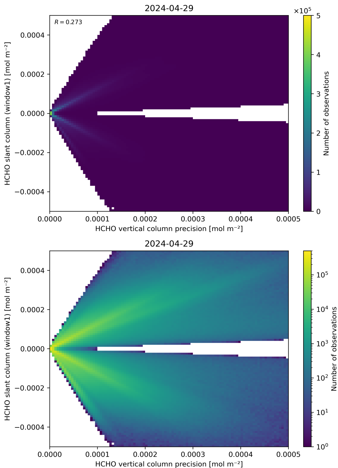
Figure 142: Scatter density plot of “HCHO vertical column precision” against “HCHO slant column (window1)” for 2024-04-28 to 2024-04-30.
