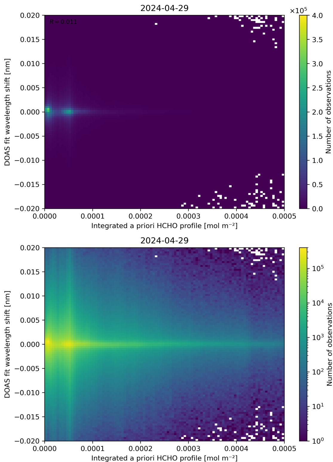
Figure 149: Scatter density plot of “Integrated a priori HCHO profile” against “DOAS fit wavelength shift” for 2024-04-28 to 2024-04-30.
