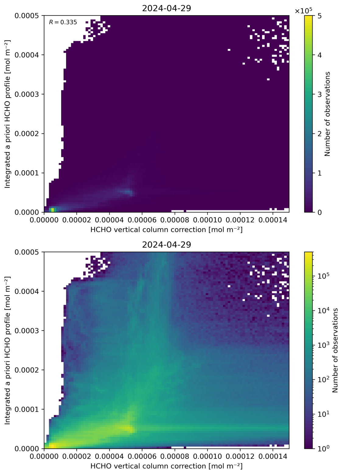
Figure 122: Scatter density plot of “HCHO vertical column correction” against “Integrated a priori HCHO profile” for 2024-04-28 to 2024-04-30.
