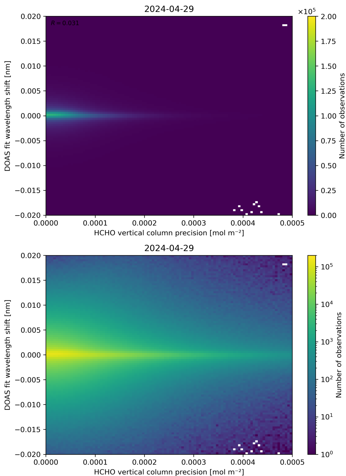
Figure 137: Scatter density plot of “HCHO vertical column precision” against “DOAS fit wavelength shift” for 2024-04-28 to 2024-04-30.
