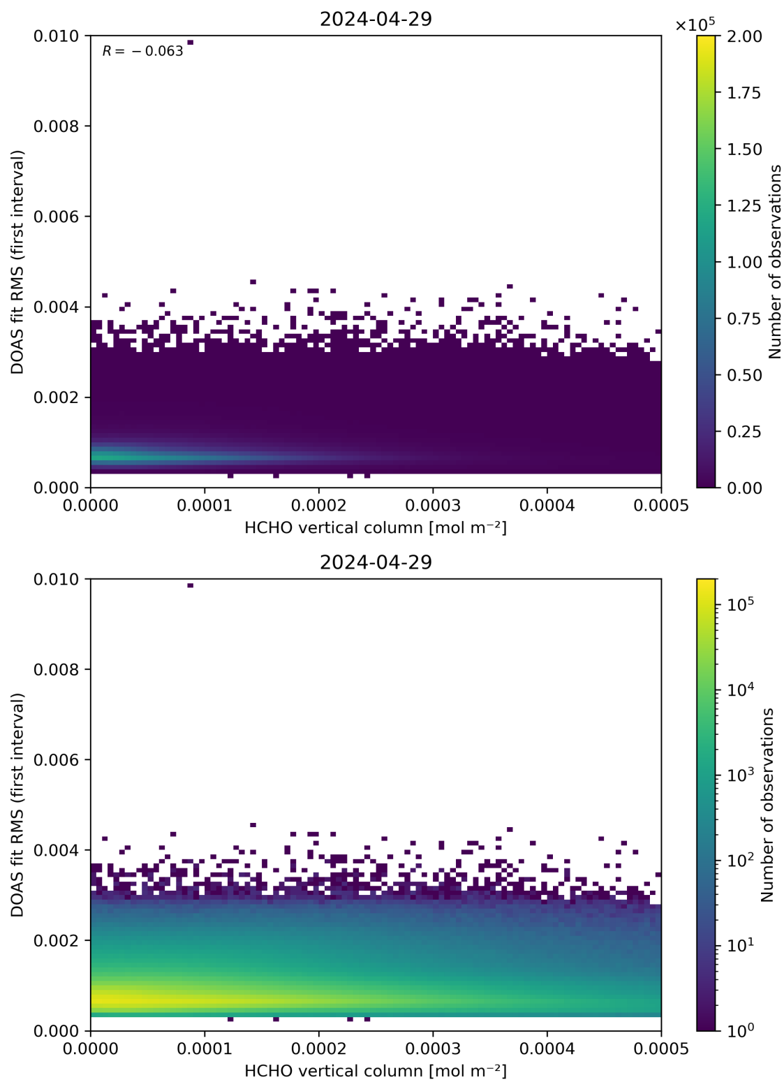
Figure 123: Scatter density plot of “HCHO vertical column” against “DOAS fit RMS (first interval)” for 2024-04-28 to 2024-04-30.
