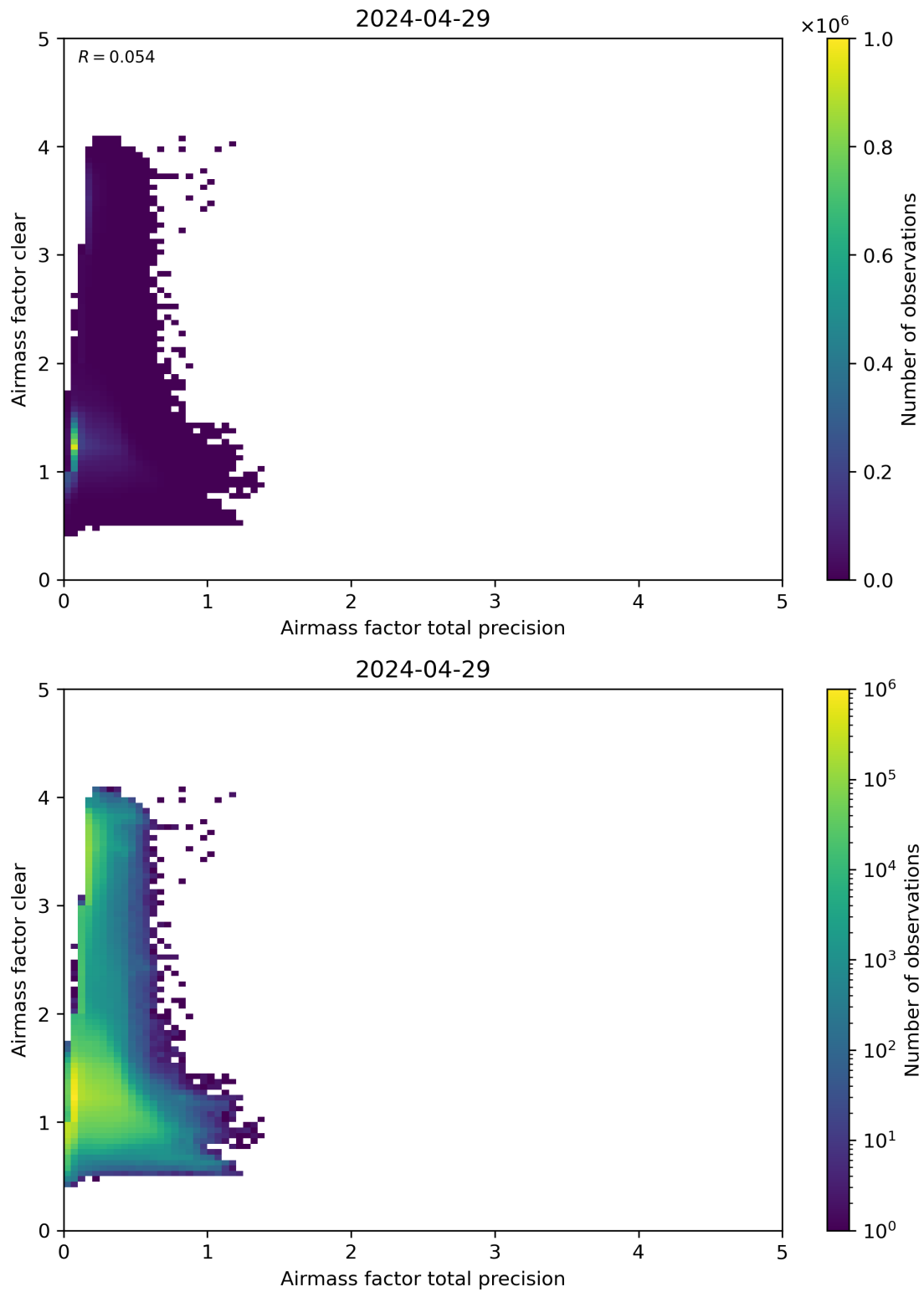
Figure 108: Scatter density plot of “Airmass factor total precision” against “Airmass factor clear” for 2024-04-28 to 2024-04-30.
