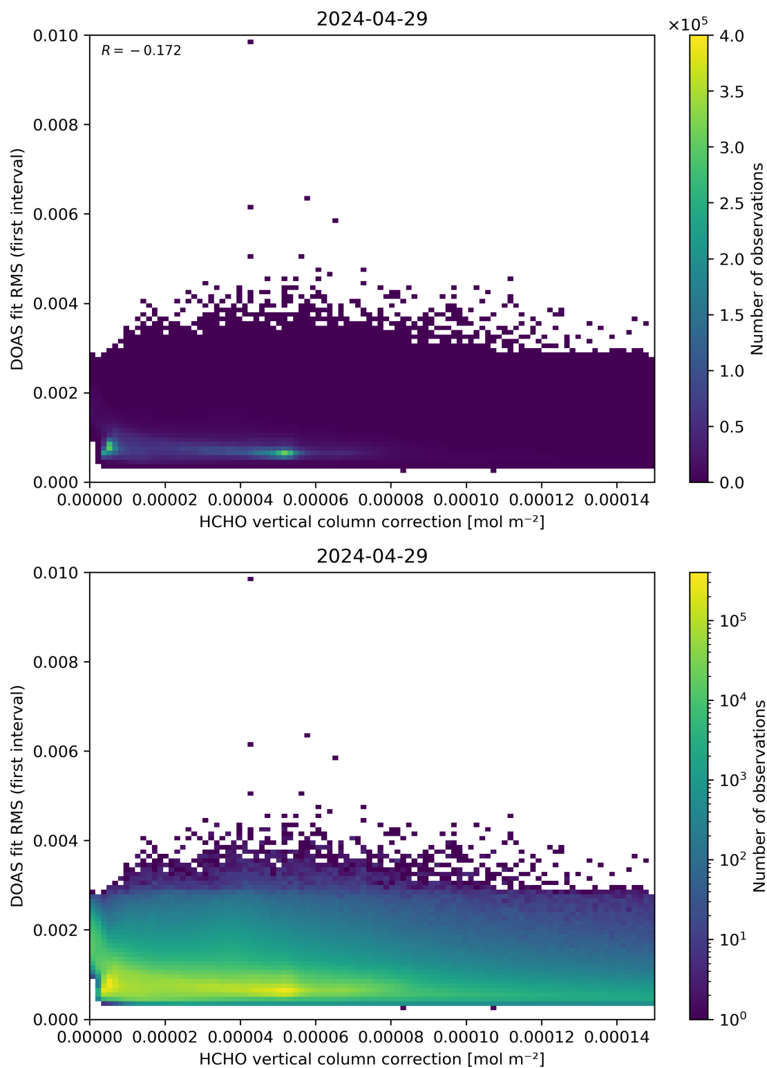
Figure 112: Scatter density plot of “HCHO vertical column correction” against “DOAS fit RMS (first interval)” for 2024-04-28 to 2024-04-30.
