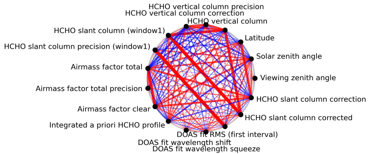
Figure 1: Map of correlation graph for 2024-04-28 to 2024-04-30.
