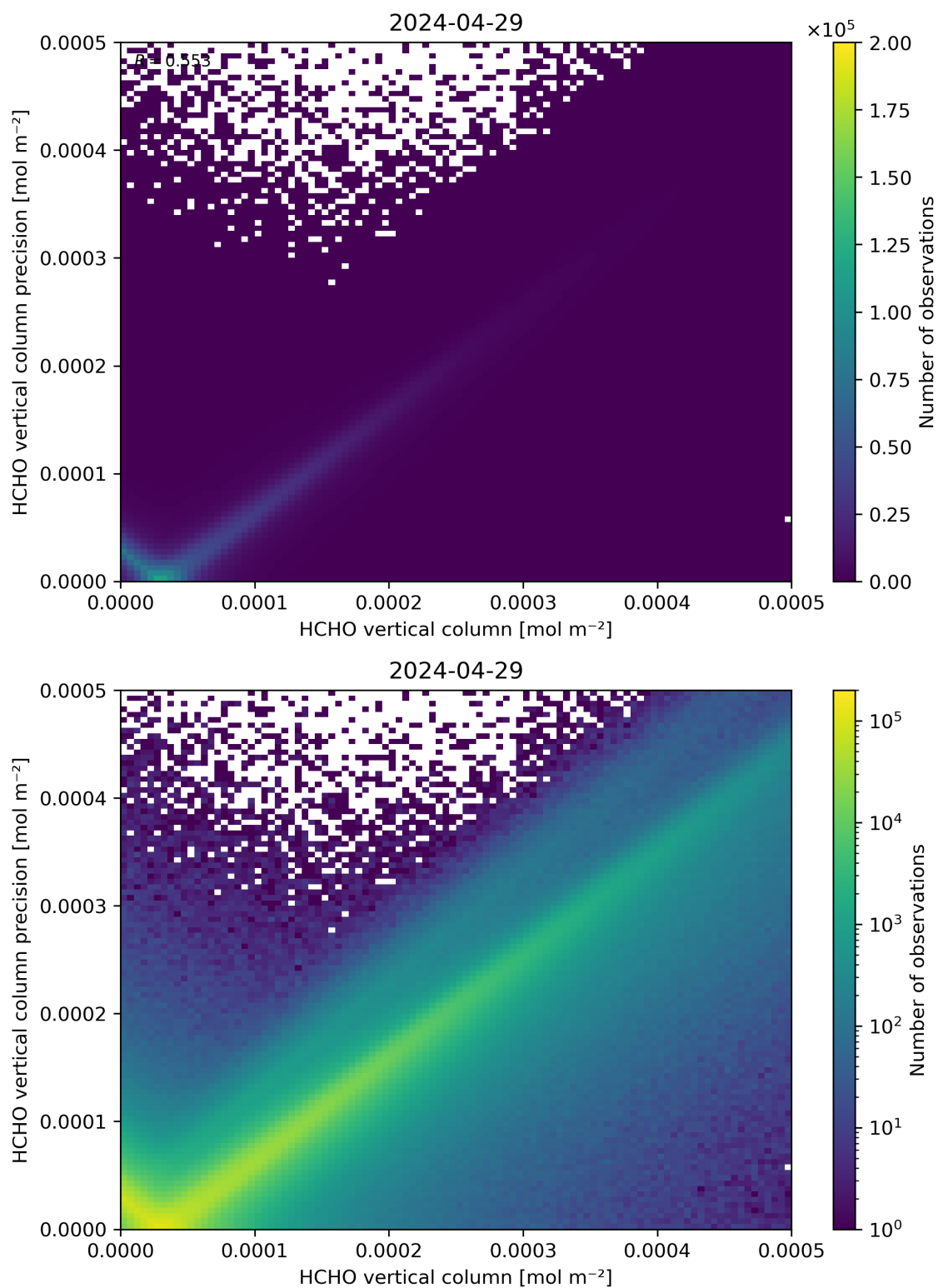
Figure 134: Scatter density plot of “HCHO vertical column” against “HCHO vertical column precision” for 2024-04-28 to 2024-04-30.
