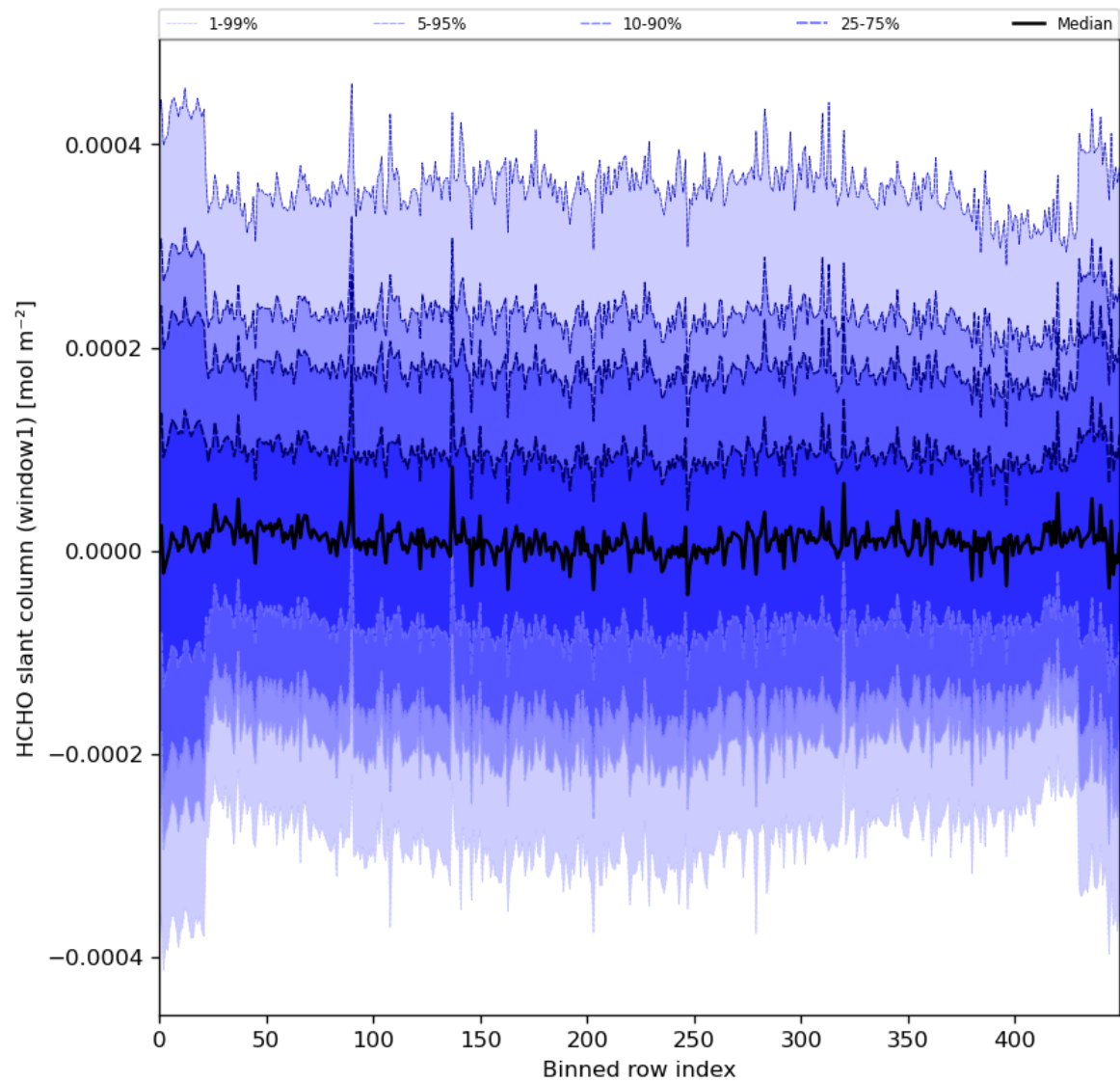
Figure 52: Along track statistics of “HCHO slant column (window1)” for 2024-04-28 to 2024-04-30
