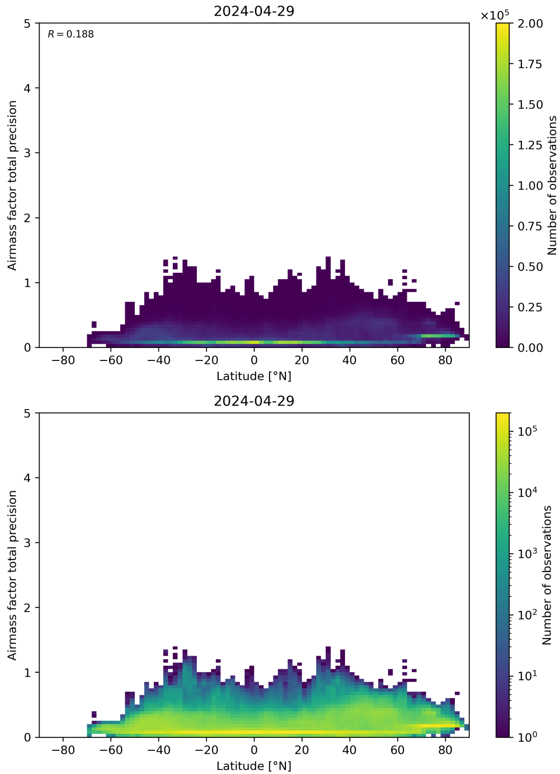
Figure 162: Scatter density plot of “Latitude” against “Airmass factor total precision” for 2024-04-28 to 2024-04-30.
