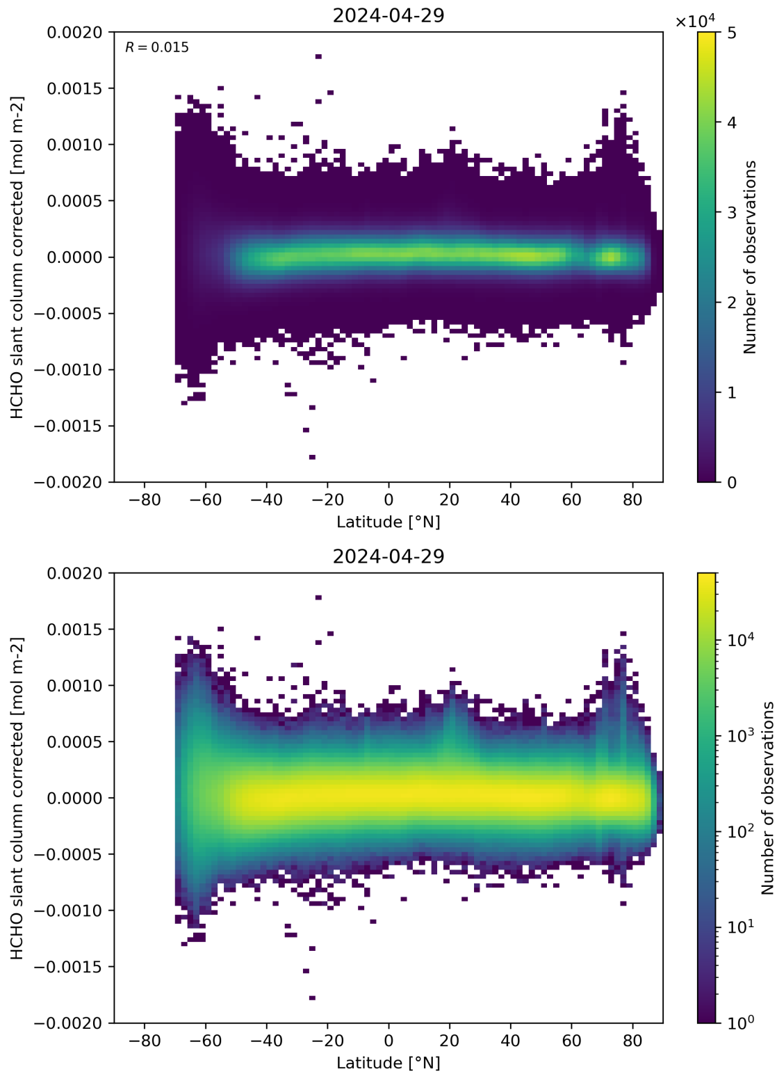
Figure 157: Scatter density plot of “Latitude” against “HCHO slant column corrected” for 2024-04-28 to 2024-04-30.
