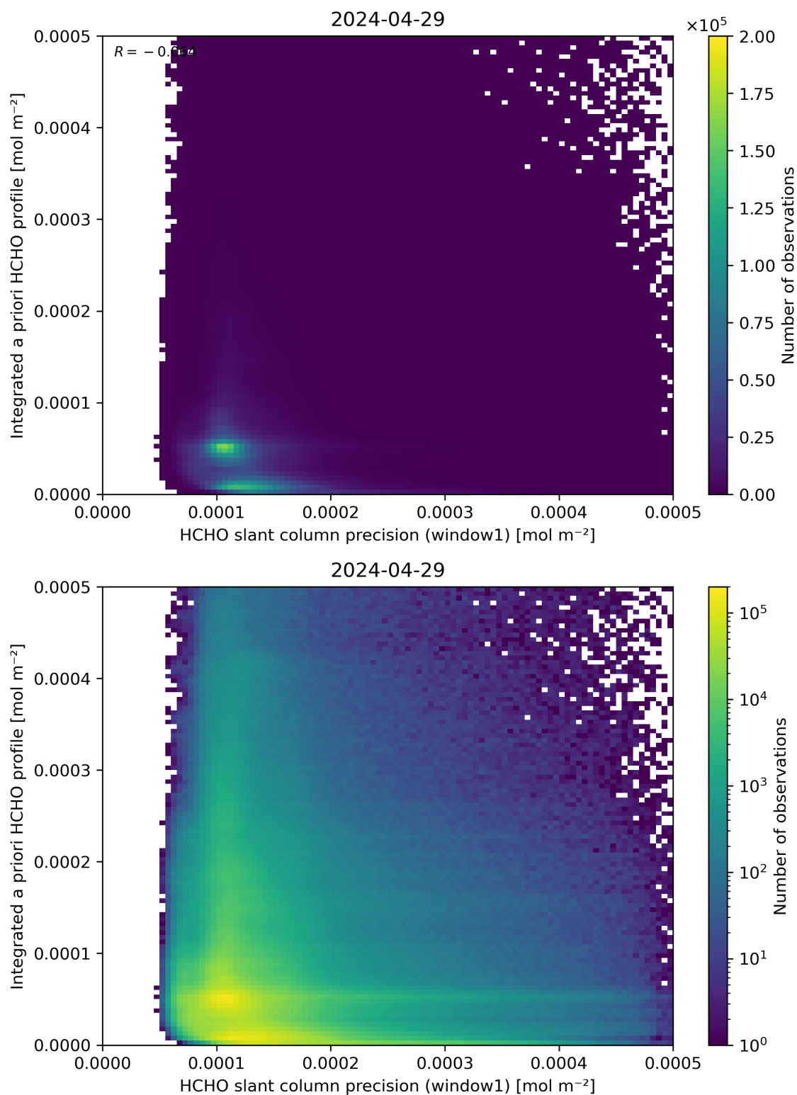
Figure 96: Scatter density plot of “HCHO slant column precision (window1)” against “Integrated a priori HCHO profile” for 2024-04-28 to 2024-04-30.
