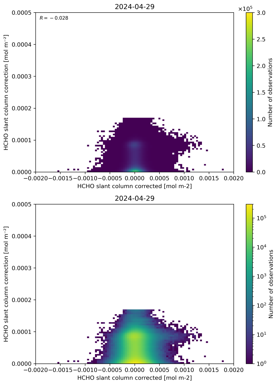
Figure 77: Scatter density plot of “HCHO slant column corrected” against “HCHO slant column correction” for 2024-04-28 to 2024-04-30.
