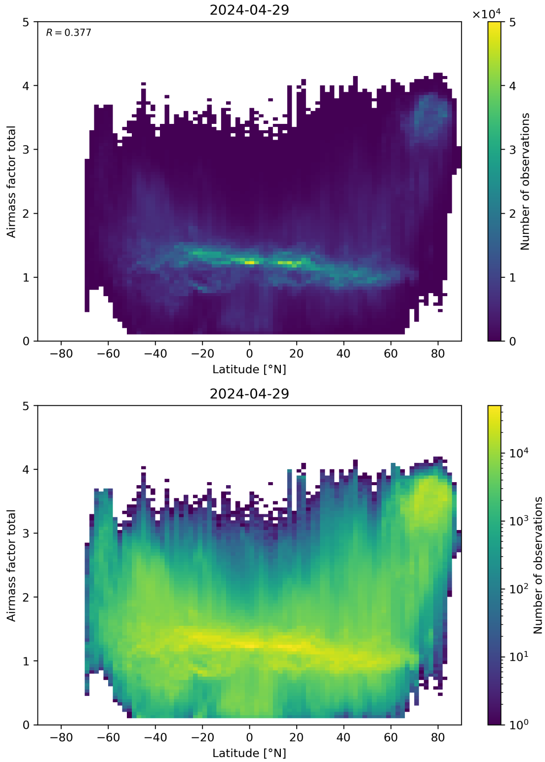
Figure 161: Scatter density plot of “Latitude” against “Airmass factor total” for 2024-04-28 to 2024-04-30.
