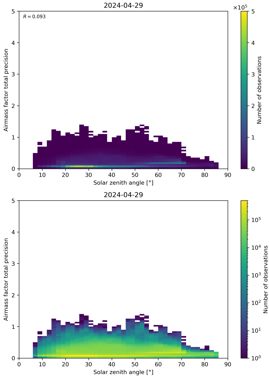
Figure 176: Scatter density plot of “Solar zenith angle” against “Airmass factor total precision” for 2024-04-28 to 2024-04-30.
