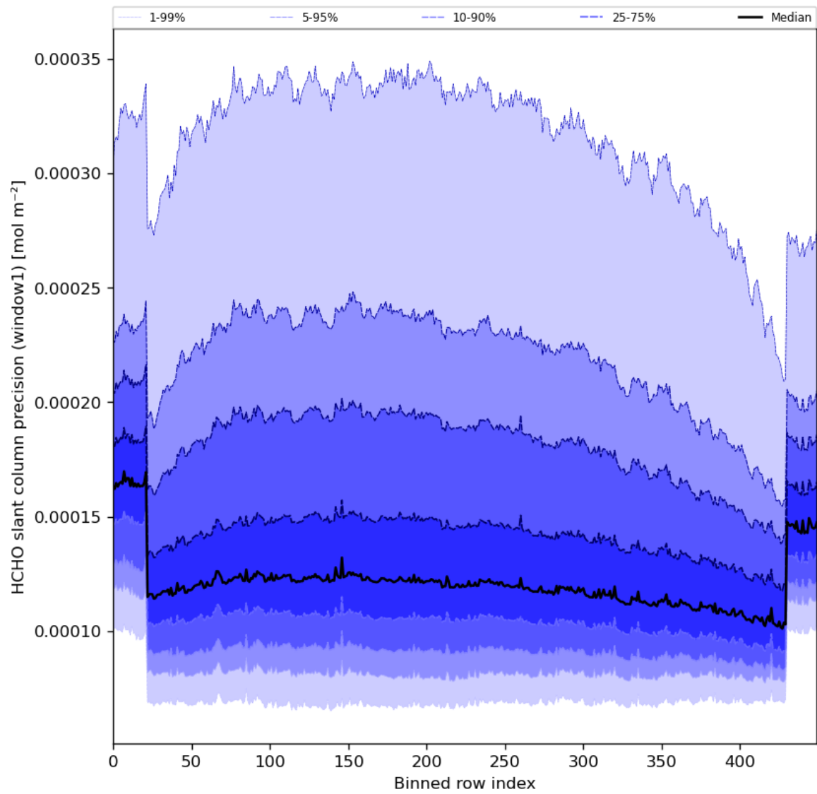
Figure 53: Along track statistics of “HCHO slant column precision (window1)” for 2024-04-28 to 2024-04-30
