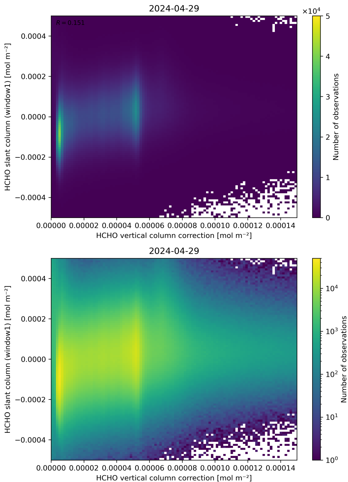
Figure 118: Scatter density plot of “HCHO vertical column correction” against “HCHO slant column (window1)” for 2024-04-28 to 2024-04-30.
