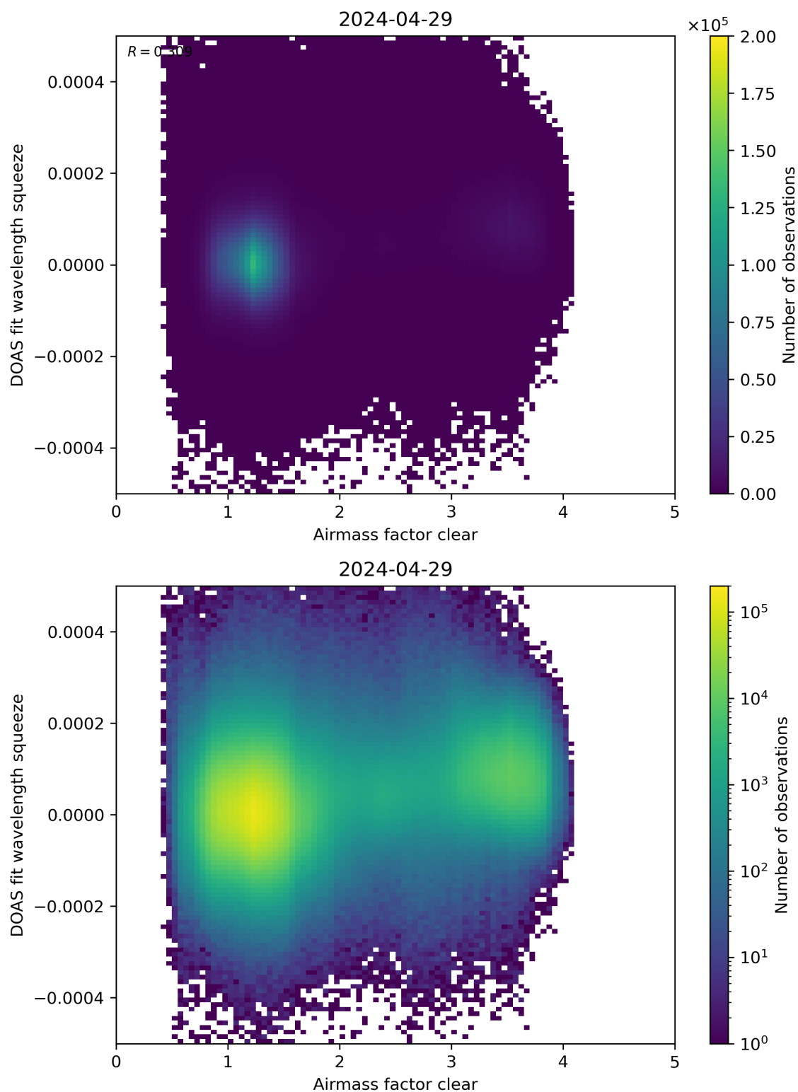
Figure 73: Scatter density plot of “Airmass factor clear” against “DOAS fit wavelength squeeze” for 2024-04-28 to 2024-04-30.
