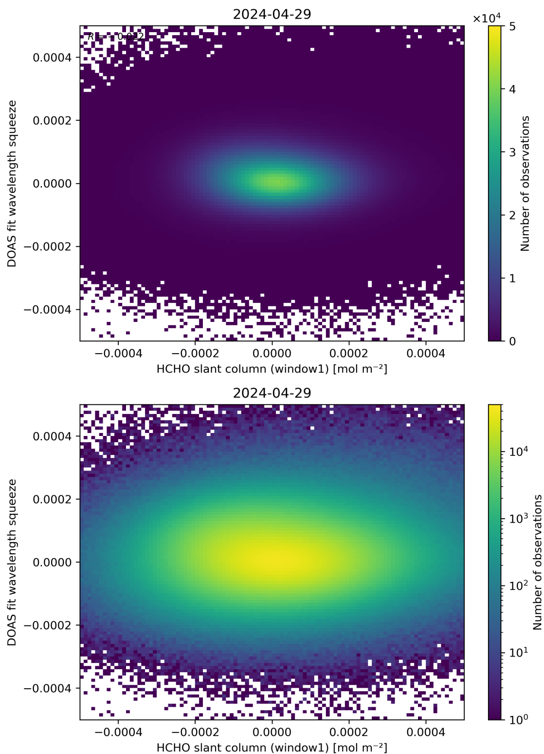
Figure 80: Scatter density plot of “HCHO slant column (window1)” against “DOAS fit wavelength squeeze” for 2024-04-28 to 2024-04-30.
