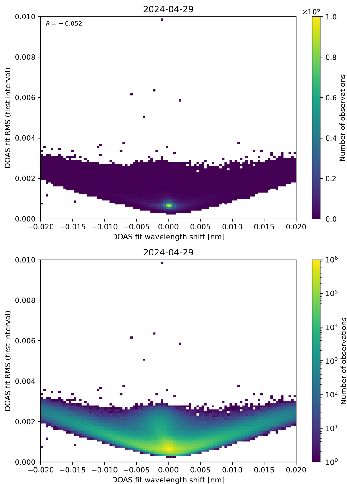
Figure 64: Scatter density plot of “DOAS fit wavelength shift” against “DOAS fit RMS (first interval)” for 2024-04-28 to 2024-04-30.
