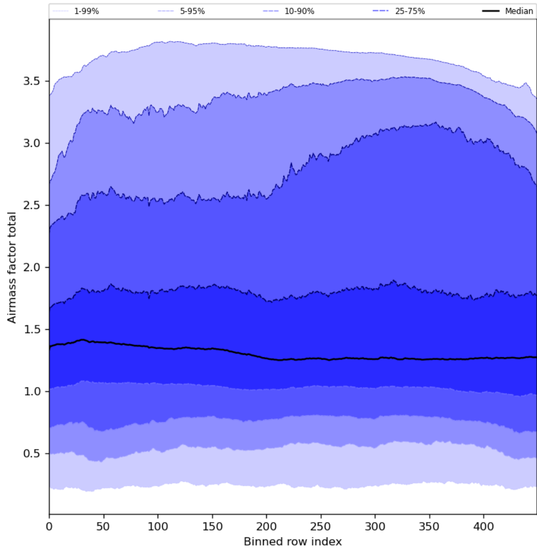
Figure 54: Along track statistics of “Airmass factor total” for 2024-04-28 to 2024-04-30
