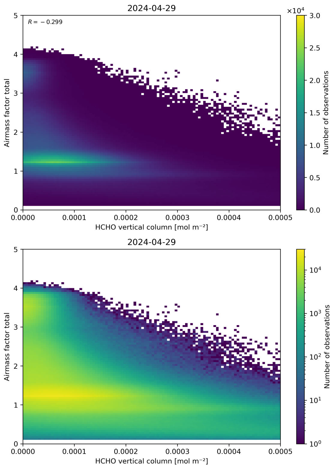
Figure 131: Scatter density plot of “HCHO vertical column” against “Airmass factor total” for 2024-04-28 to 2024-04-30.
