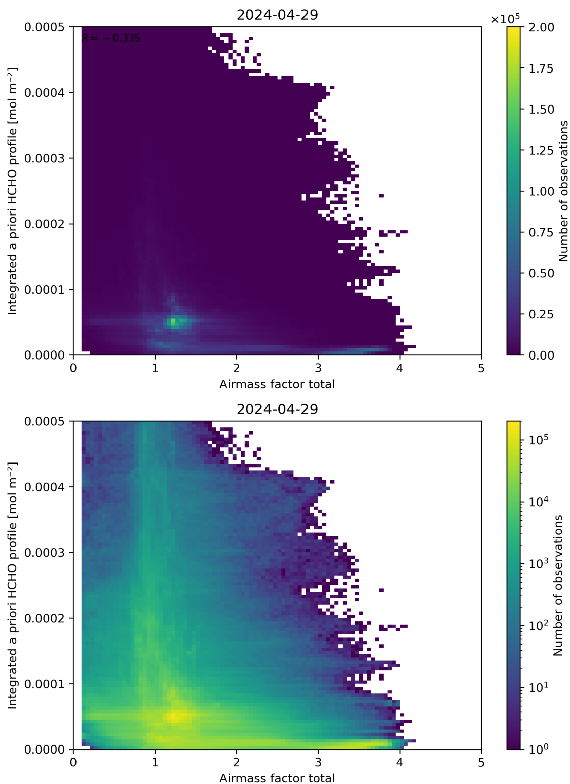
Figure 104: Scatter density plot of “Air mass factor total” against “Integrated a priori HCHO profile” for 2024-04-28 to 2024-04-30.
