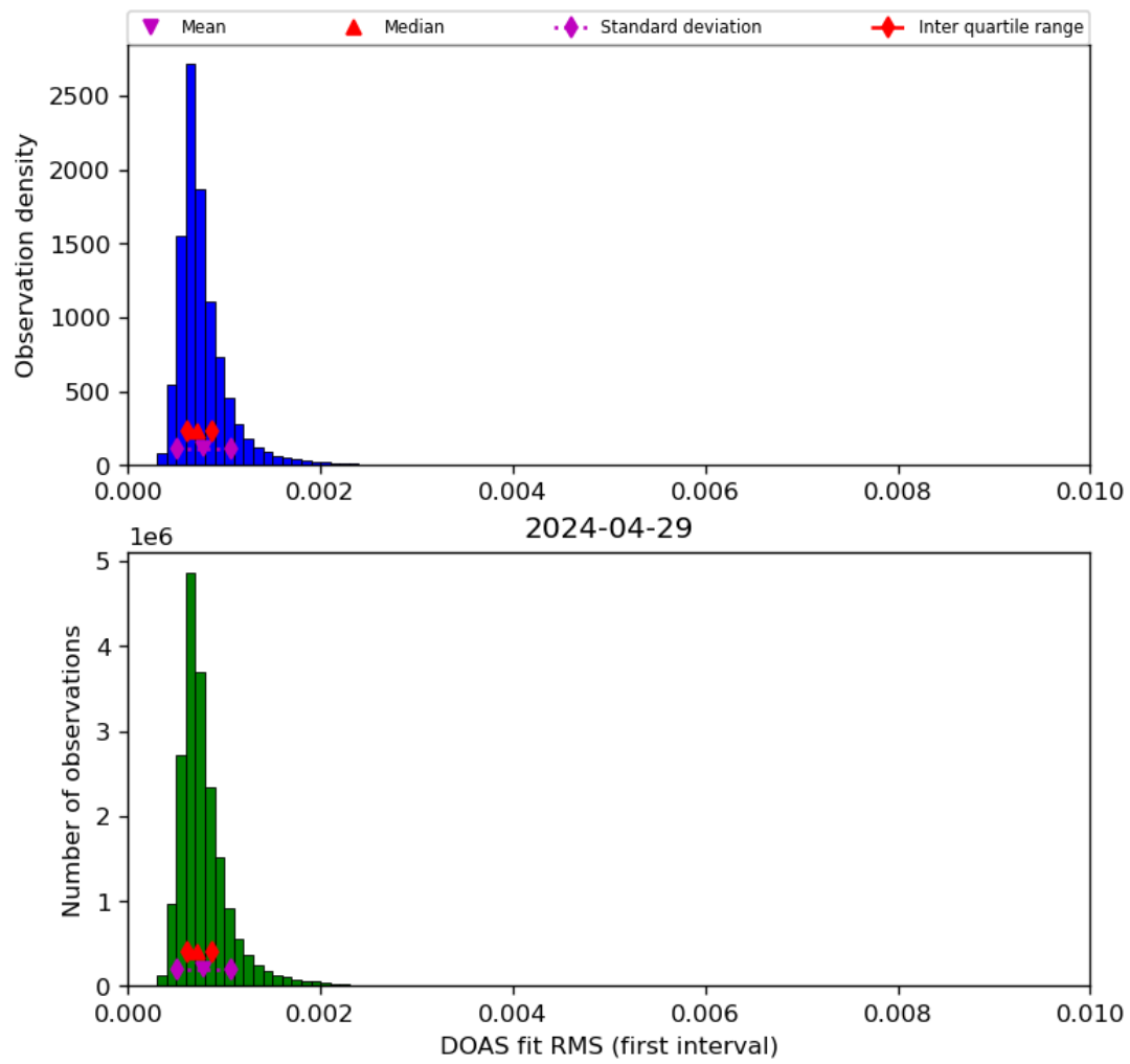
Figure 46: Histogram of “DOAS fit RMS (first interval)” for 2024-04-28 to 2024-04-30
