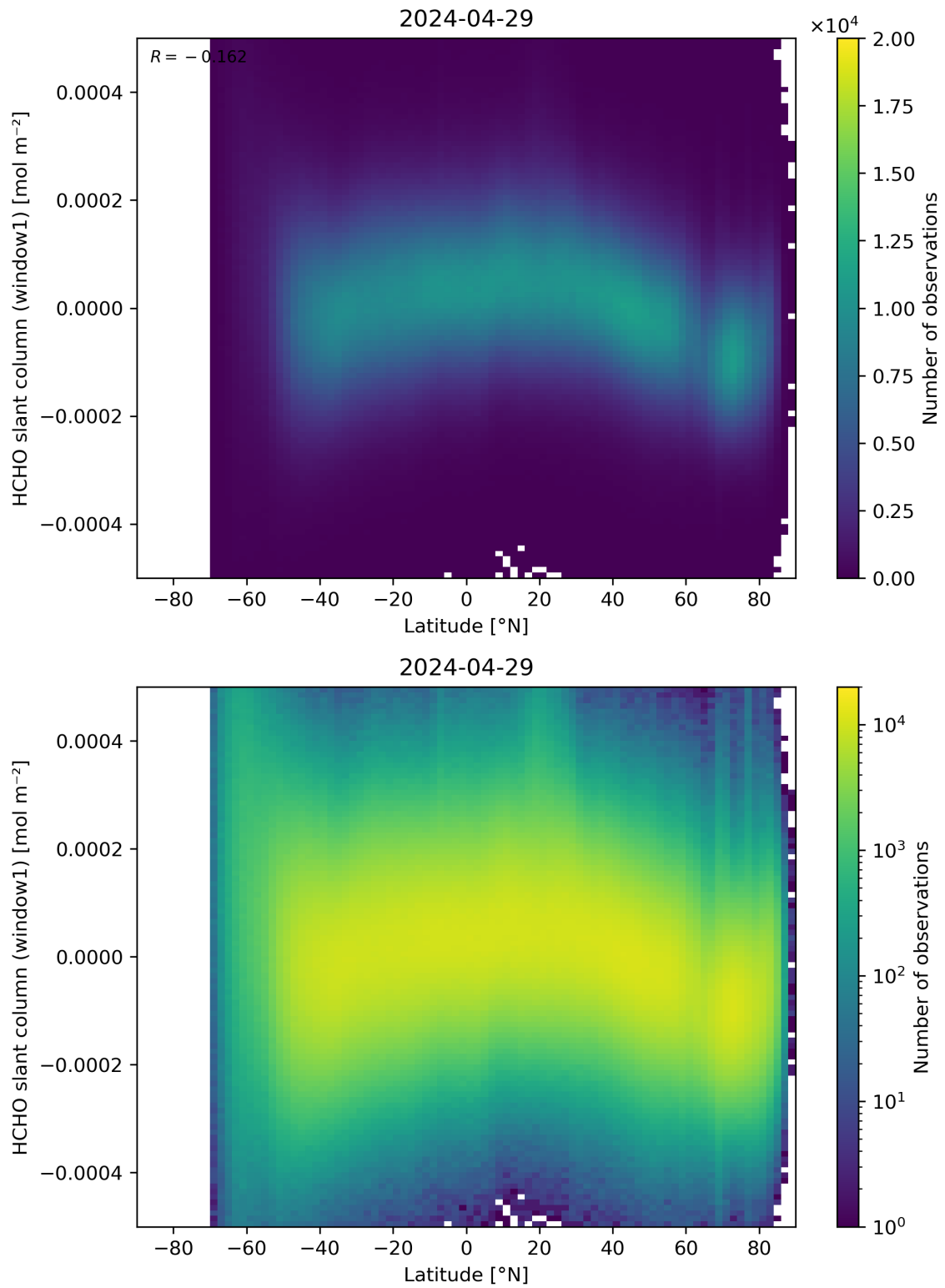
Figure 159: Scatter density plot of “Latitude” against “HCHO slant column (window1)” for 2024-04-28 to 2024-04-30.
