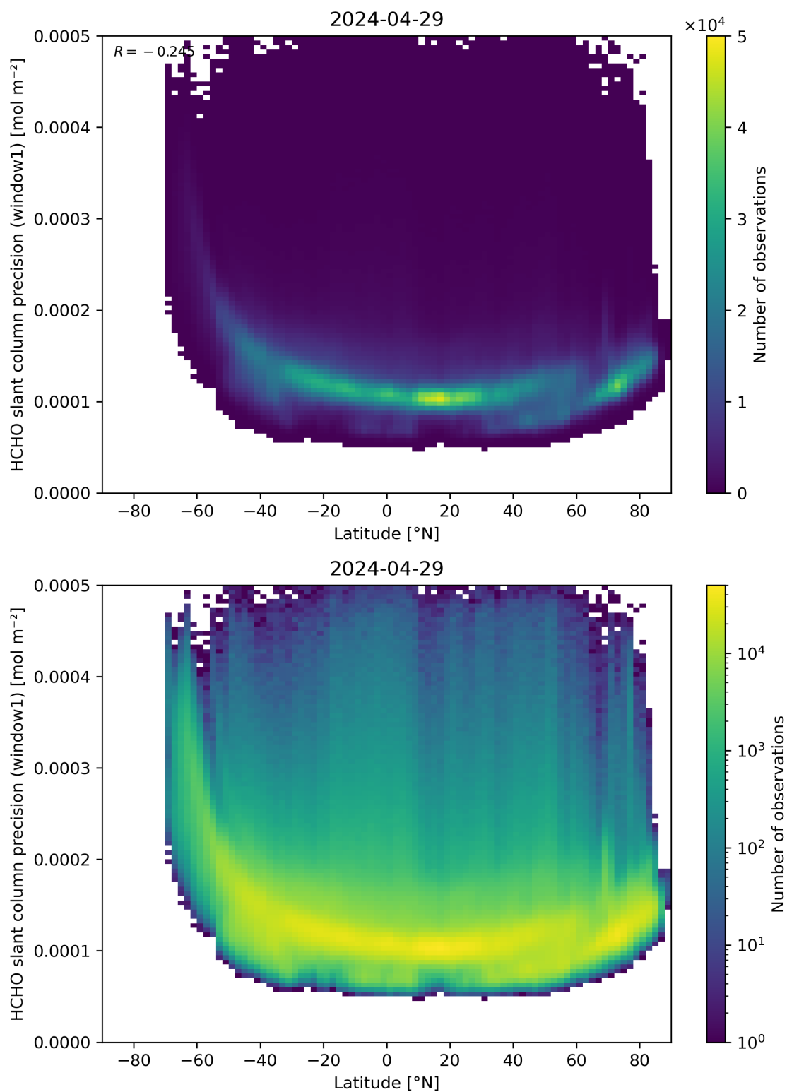
Figure 160: Scatter density plot of “Latitude” against “HCHO slant column precision (window1)” for 2024-04-28 to 2024-04-30.
