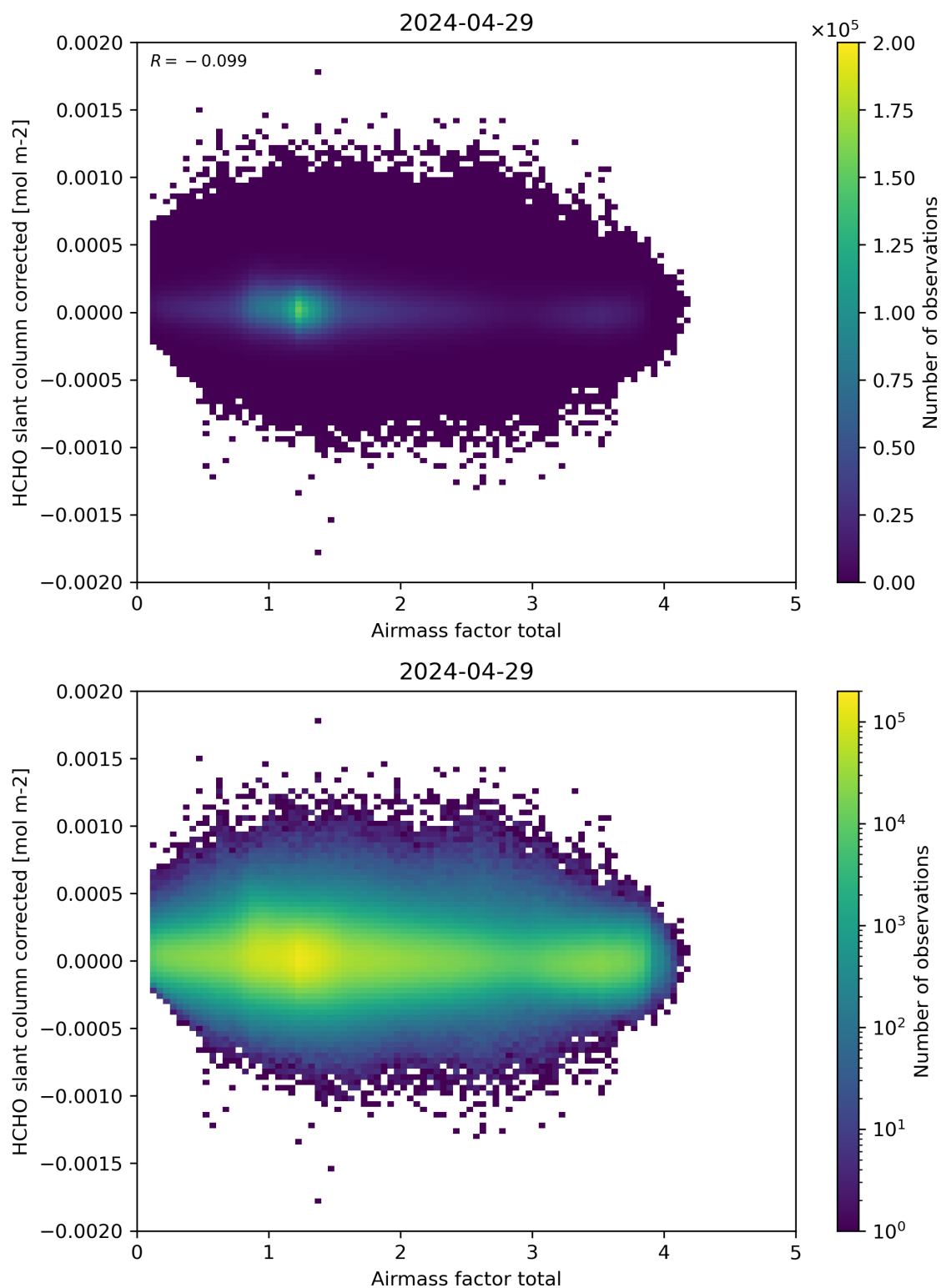
Figure 101: Scatter density plot of “Airmass factor total” against “HCHO slant column corrected” for 2024-04-28 to 2024-04-30.
