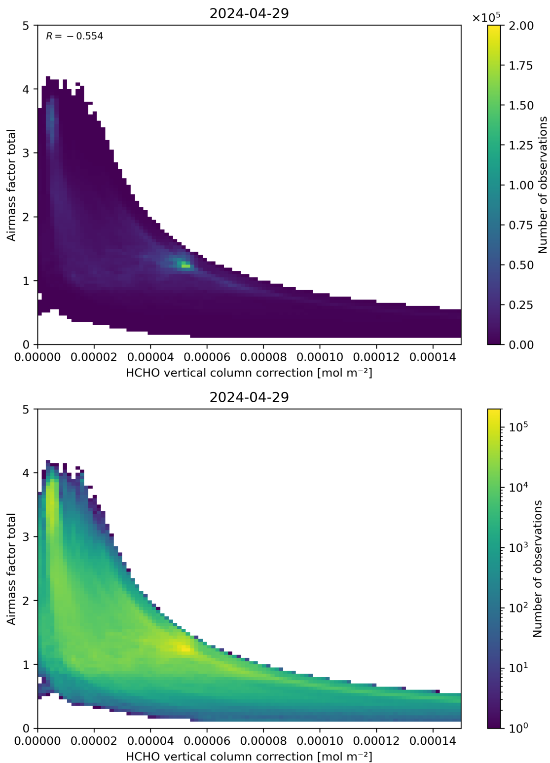
Figure 120: Scatter density plot of “HCHO vertical column correction” against “Airmass factor total” for 2024-04-28 to 2024-04-30.
