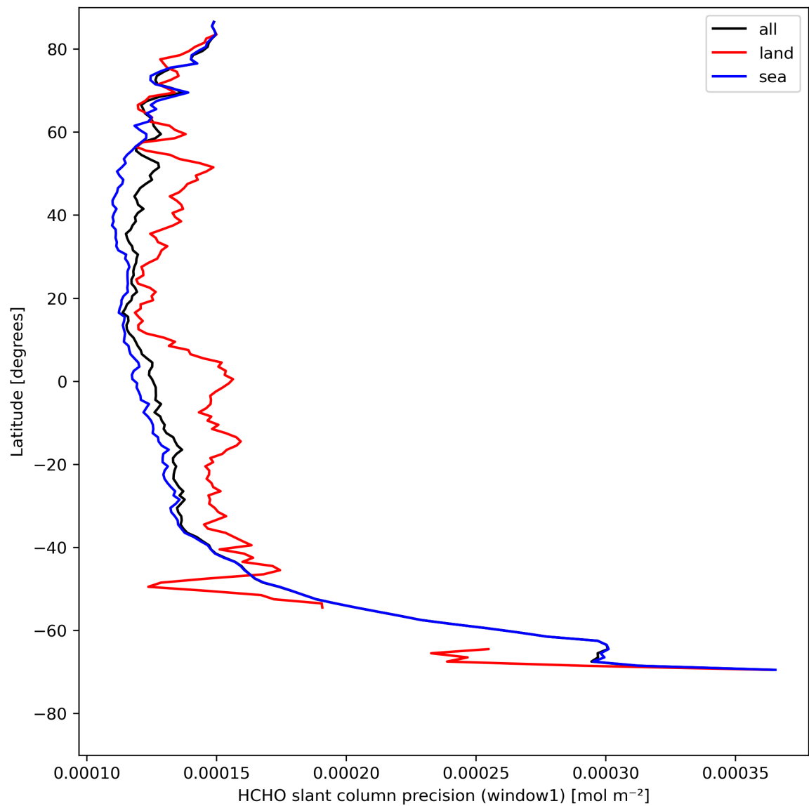
Figure 25: Zonal average of “HCHO slant column precision (window1)” for 2024-04-28 to 2024-04-30.
