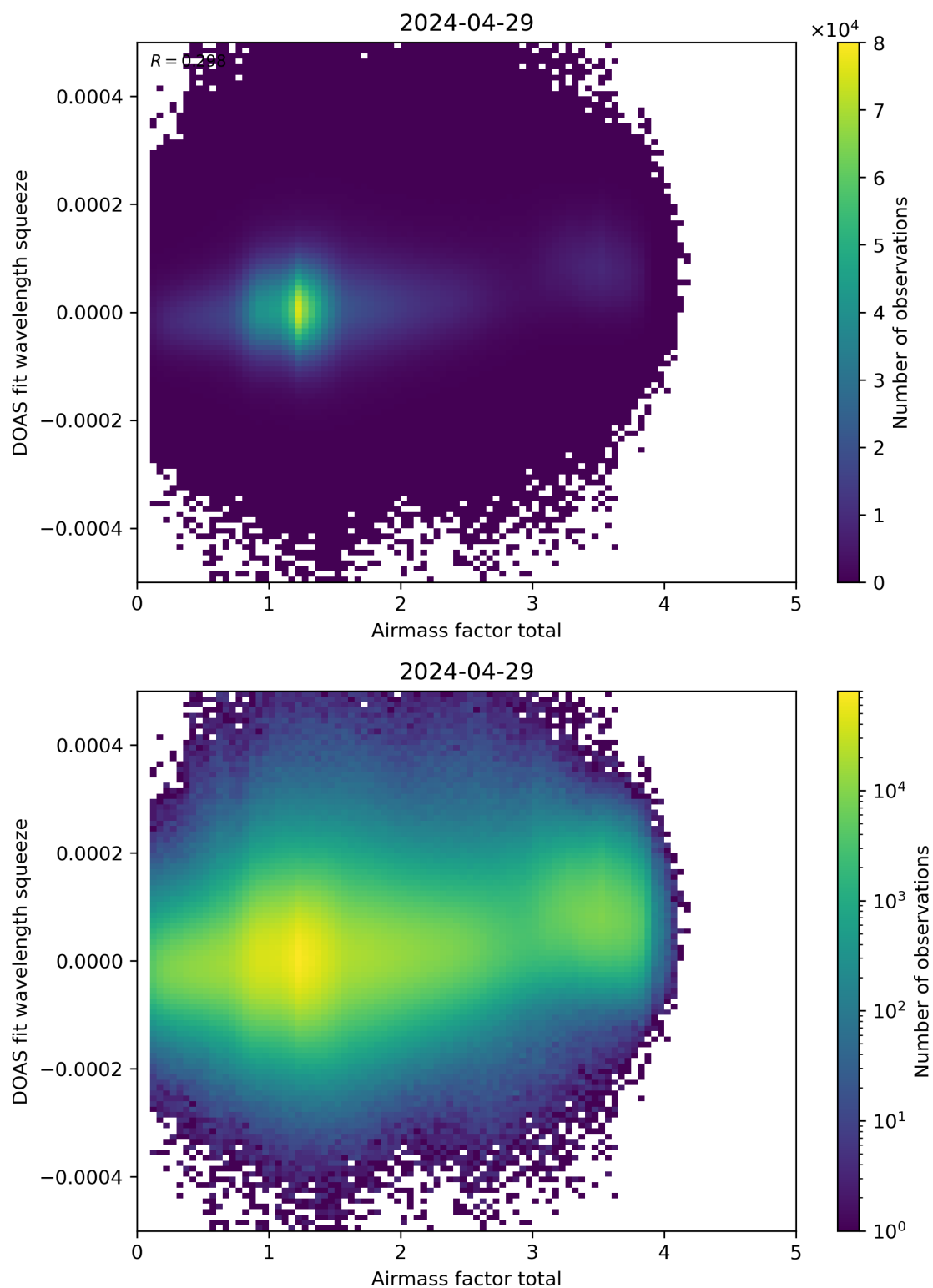
Figure 99: Scatter density plot of “Airmass factor total” against “DOAS fit wavelength squeeze” for 2024-04-28 to 2024-04-30.
