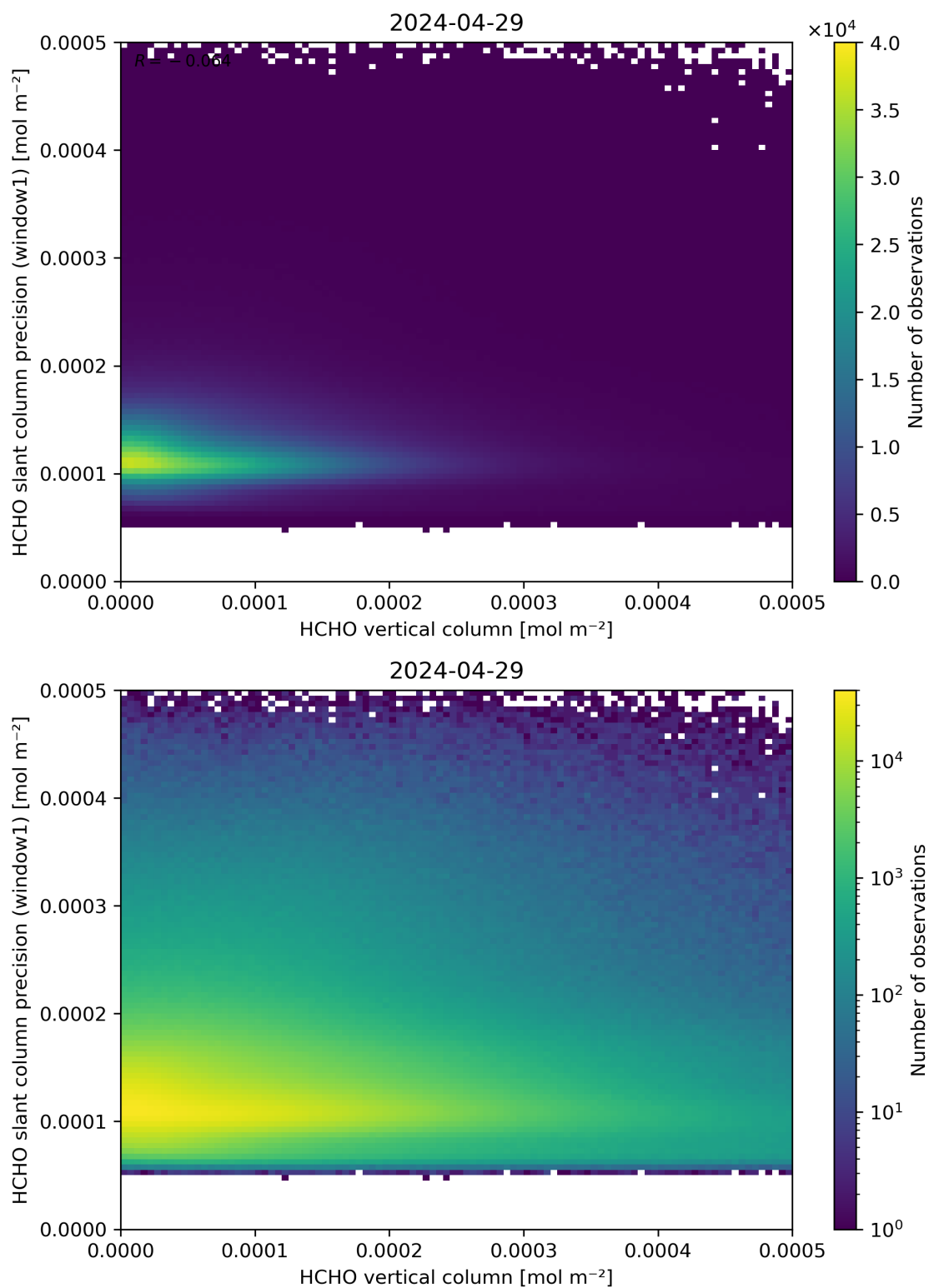
Figure 130: Scatter density plot of “HCHO vertical column” against “HCHO slant column precision (window1)” for 2024-04-28 to 2024-04-30.
