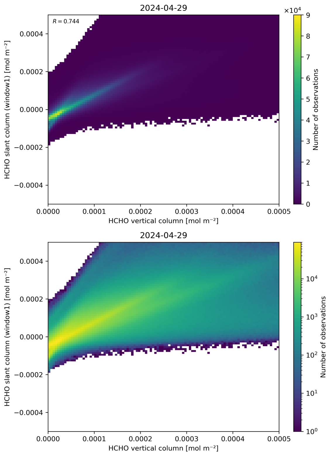
Figure 129: Scatter density plot of “HCHO vertical column” against “HCHO slant column (window1)” for 2024-04-28 to 2024-04-30.
