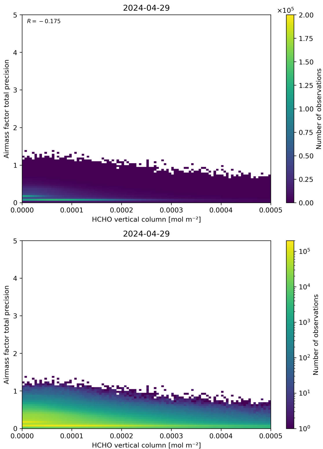
Figure 132: Scatter density plot of “HCHO vertical column” against “Airmass factor total precision” for 2024-04-28 to 2024-04-30.
