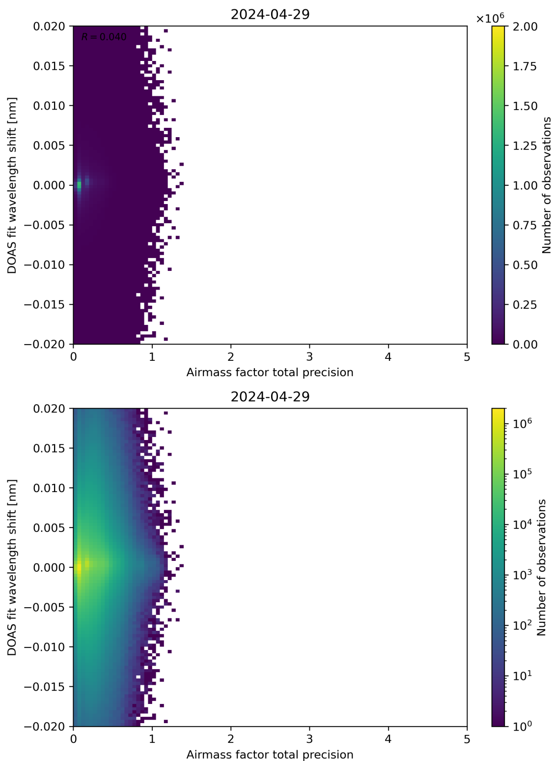
Figure 106: Scatter density plot of “Airmass factor total precision” against “DOAS fit wavelength shift” for 2024-04-28 to 2024-04-30.
