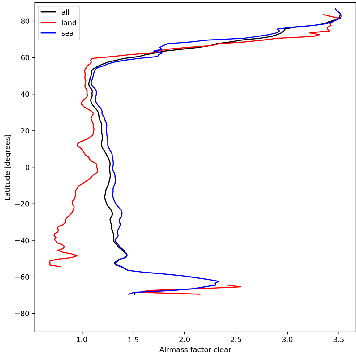
Figure 28: Zonal average of “Airmass factor clear” for 2024-04-28 to 2024-04-30.
