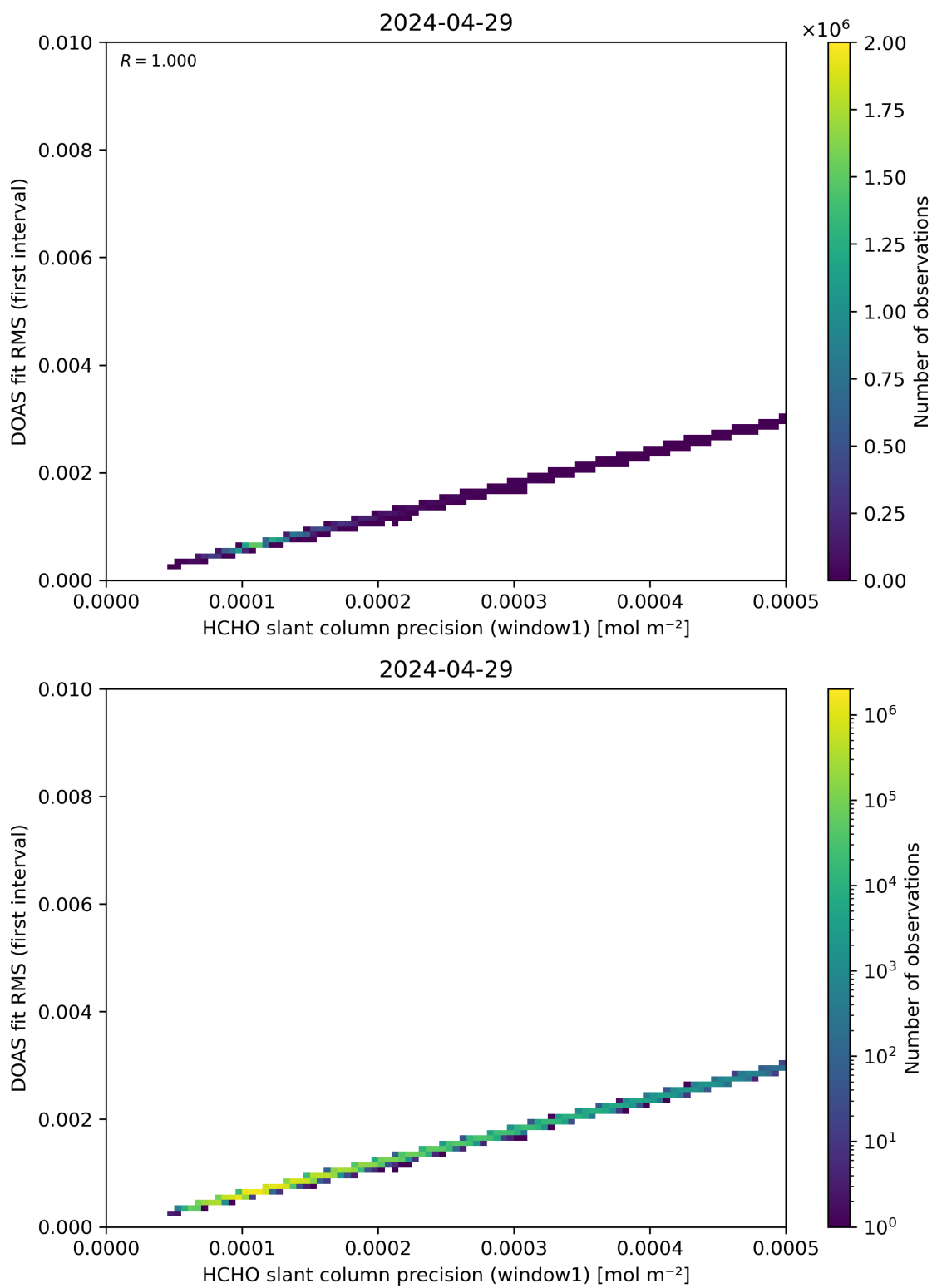
Figure 88: Scatter density plot of “HCHO slant column precision (window1)” against “DOAS fit RMS (first interval)” for 2024-04-28 to 2024-04-30.
