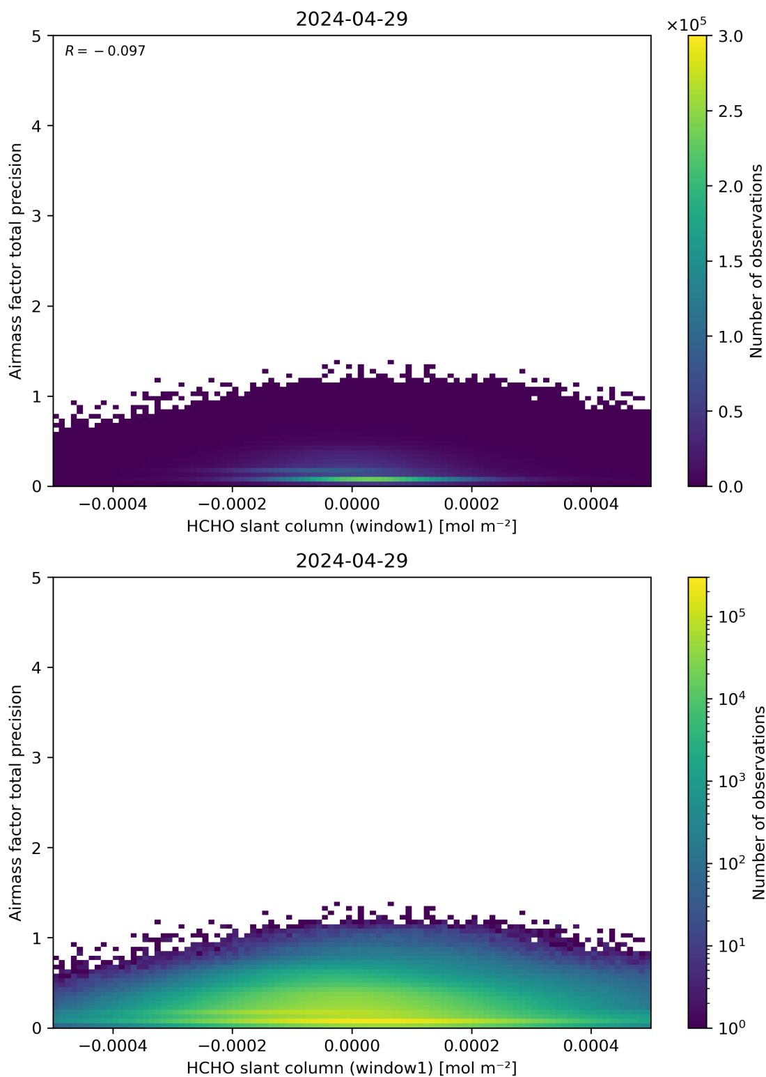
Figure 86: Scatter density plot of “HCHO slant column (window1)” against “Airmass factor total precision” for 2024-04-28 to 2024-04-30.
