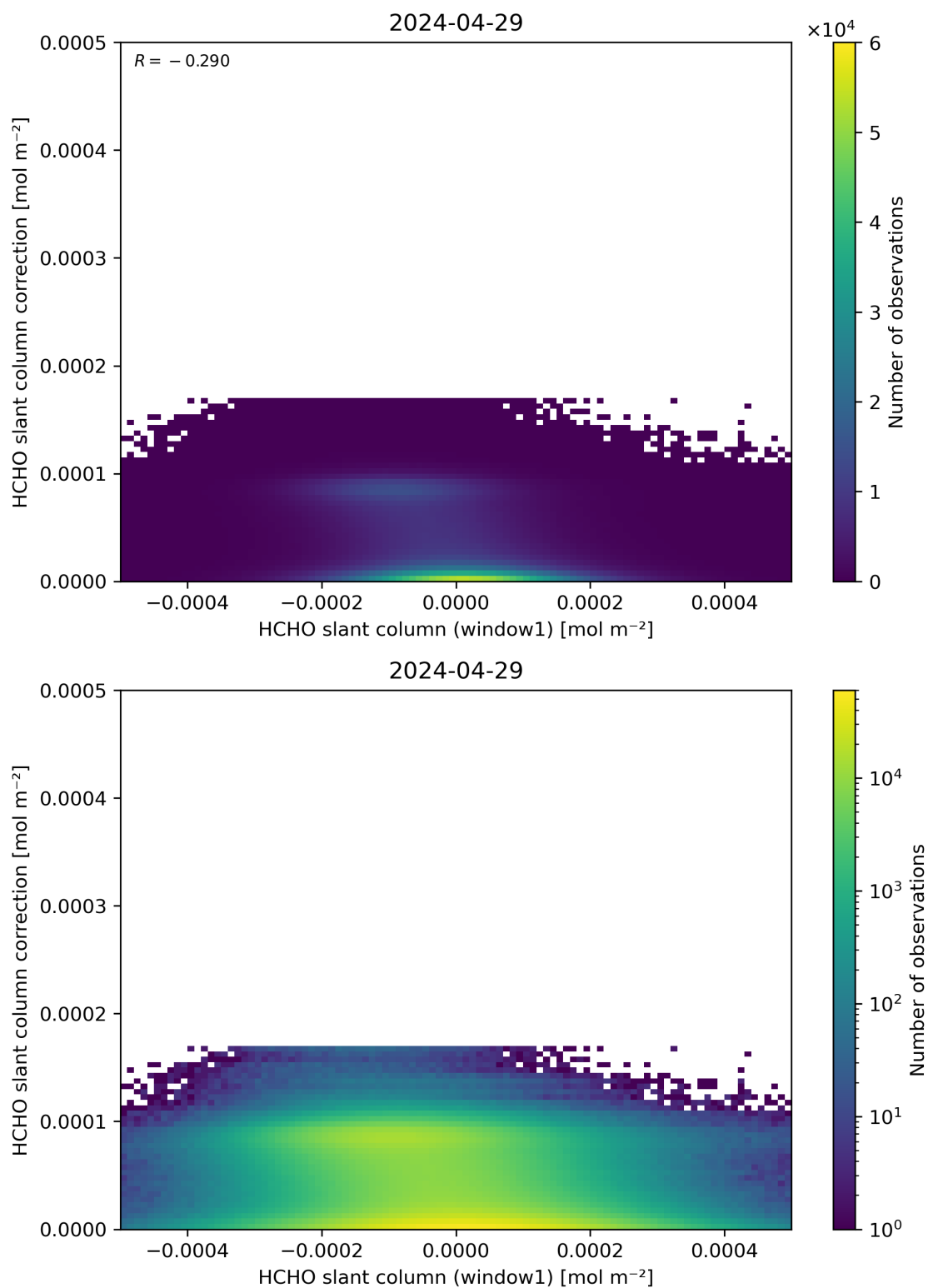
Figure 83: Scatter density plot of “HCHO slant column (window1)” against “HCHO slant column correction” for 2024-04-28 to 2024-04-30.
