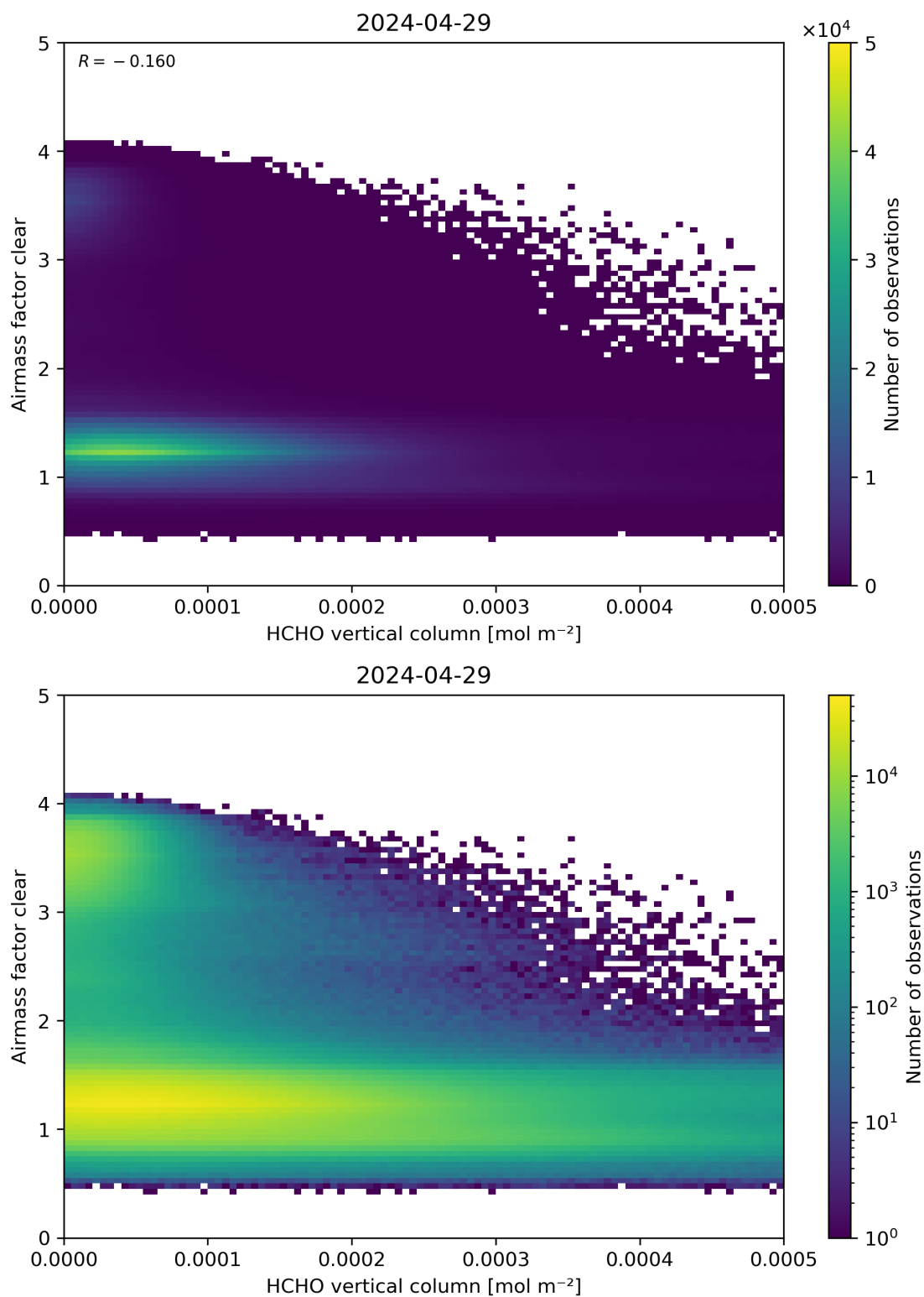
Figure 126: Scatter density plot of “HCHO vertical column” against “Airmass factor clear” for 2024-04-28 to 2024-04-30.
