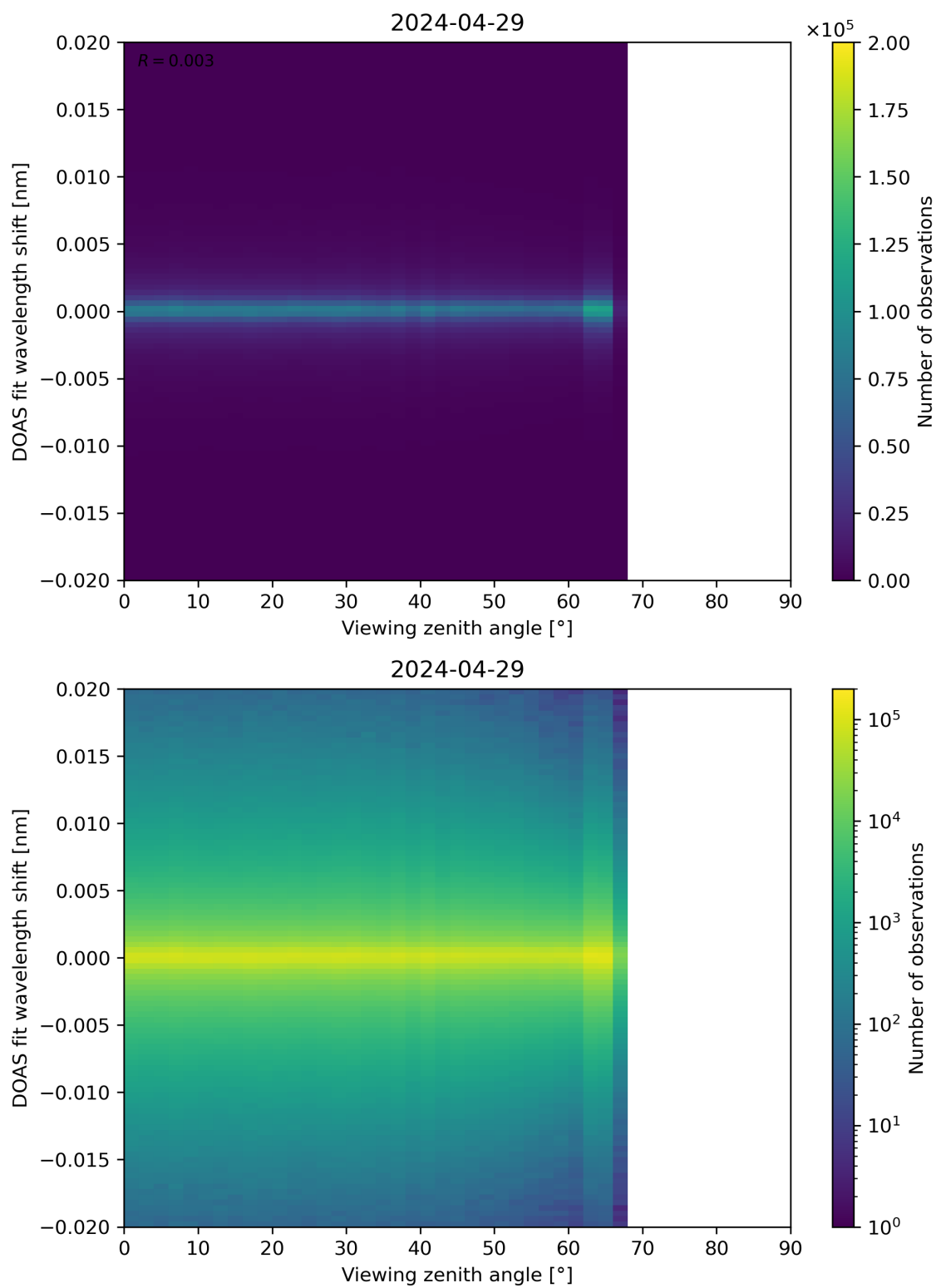
Figure 183: Scatter density plot of “Viewing zenith angle” against “DOAS fit wavelength shift” for 2024-04-28 to 2024-04-30.
