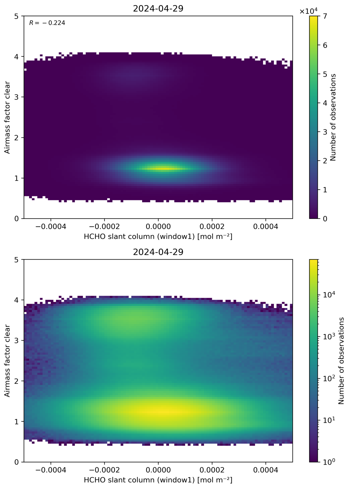
Figure 81: Scatter density plot of “HCHO slant column (window1)” against “Airmass factor clear” for 2024-04-28 to 2024-04-30.
