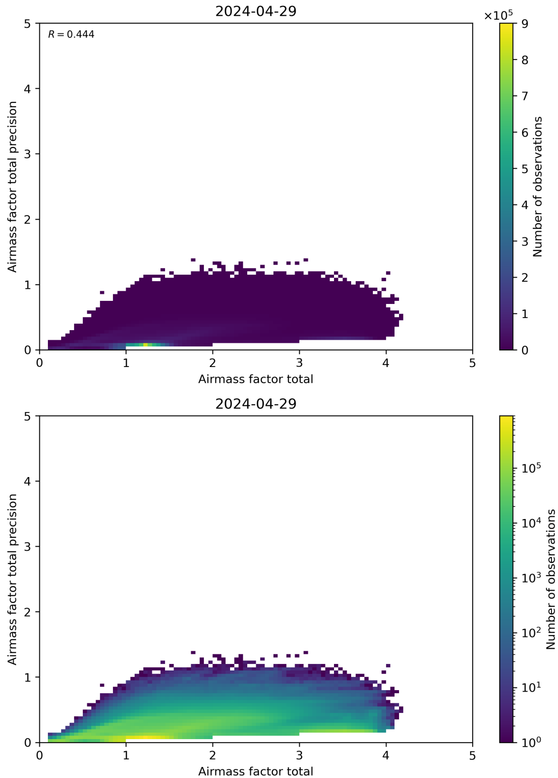
Figure 103: Scatter density plot of “Airmass factor total” against “Airmass factor total precision” for 2024-04-28 to 2024-04-30.
