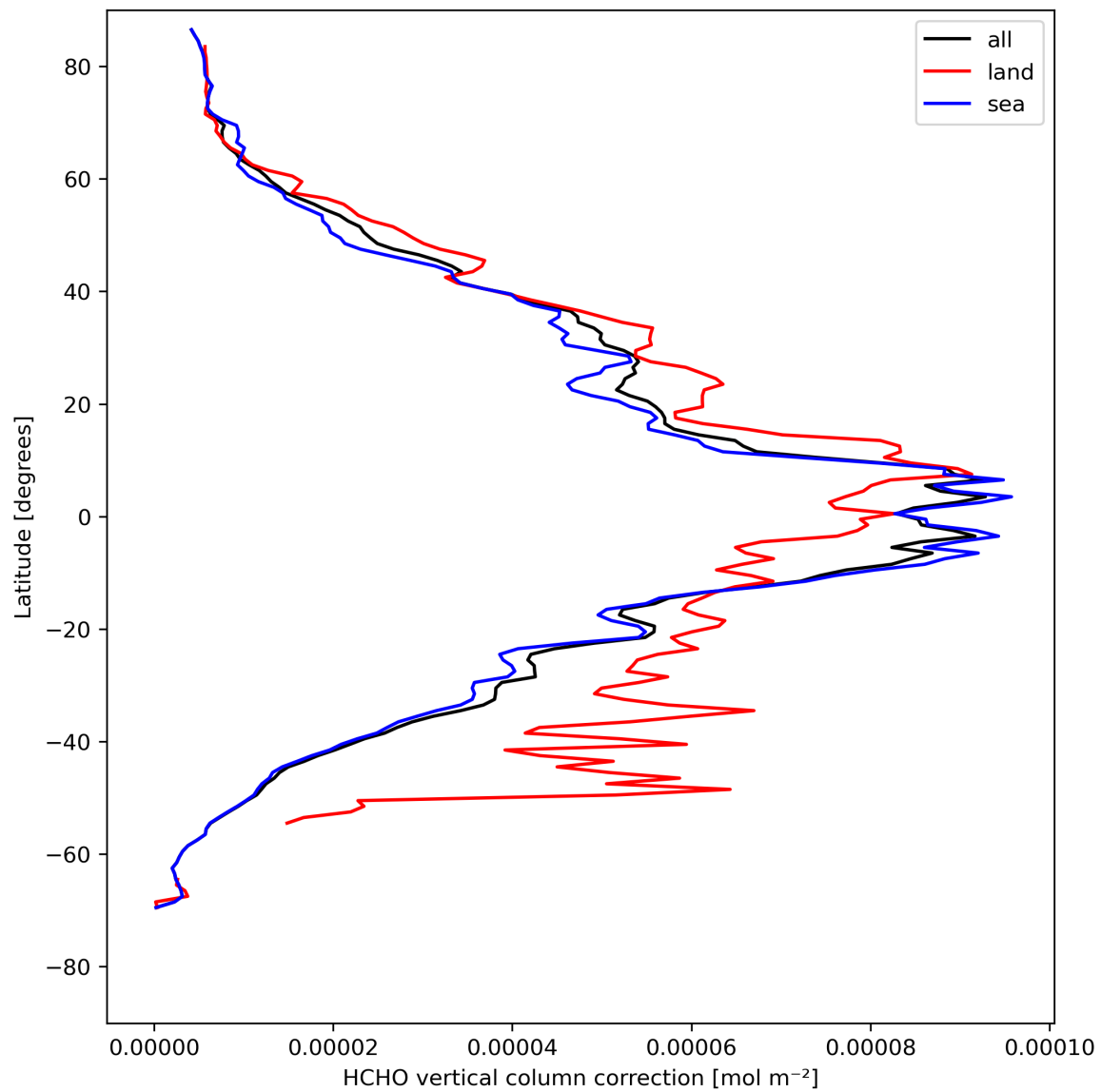
Figure 23: Zonal average of “HCHO vertical column correction” for 2024-04-28 to 2024-04-30.
