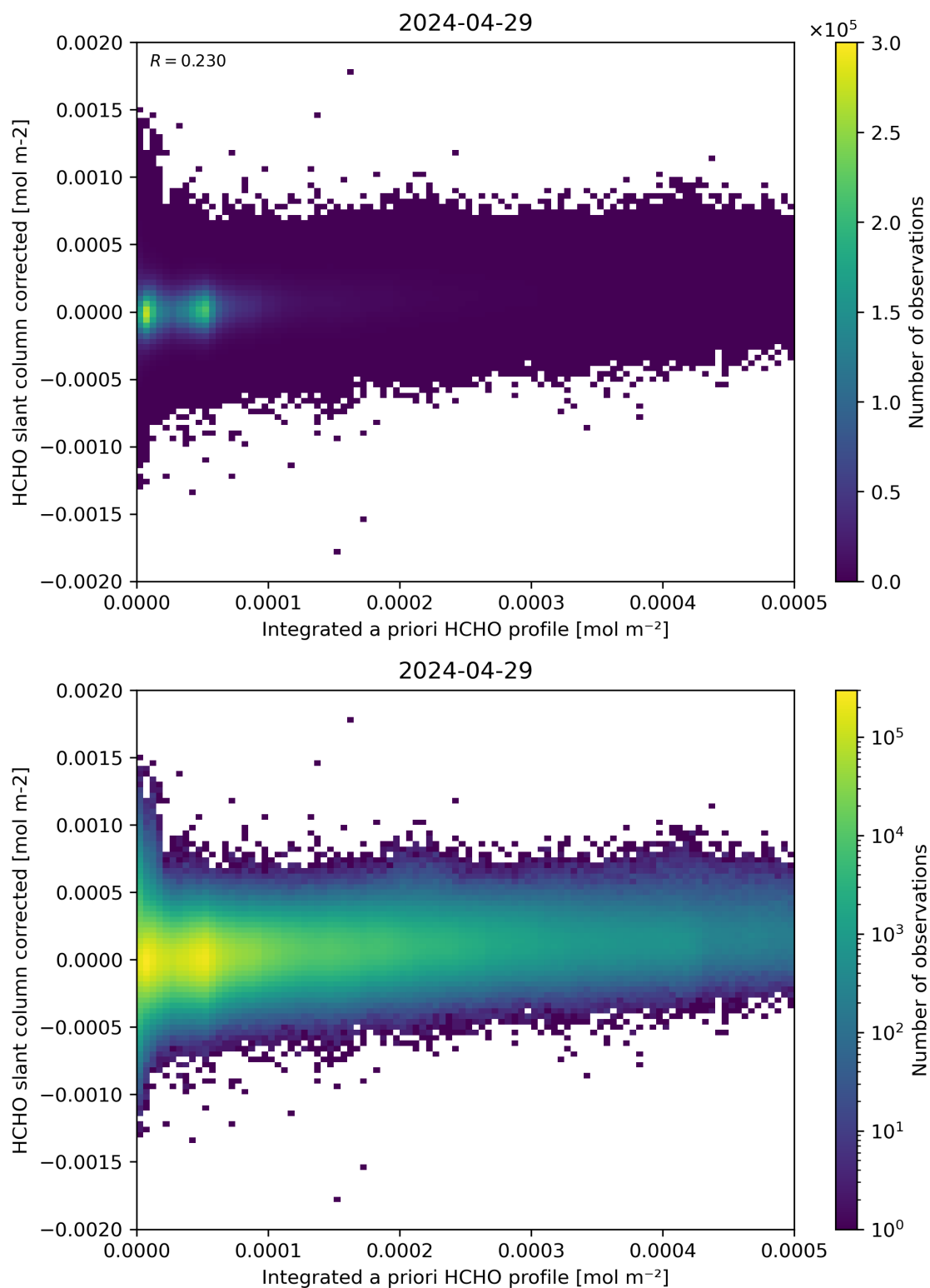
Figure 151: Scatter density plot of “Integrated a priori HCHO profile” against “HCHO slant column corrected” for 2024-04-28 to 2024-04-30.
