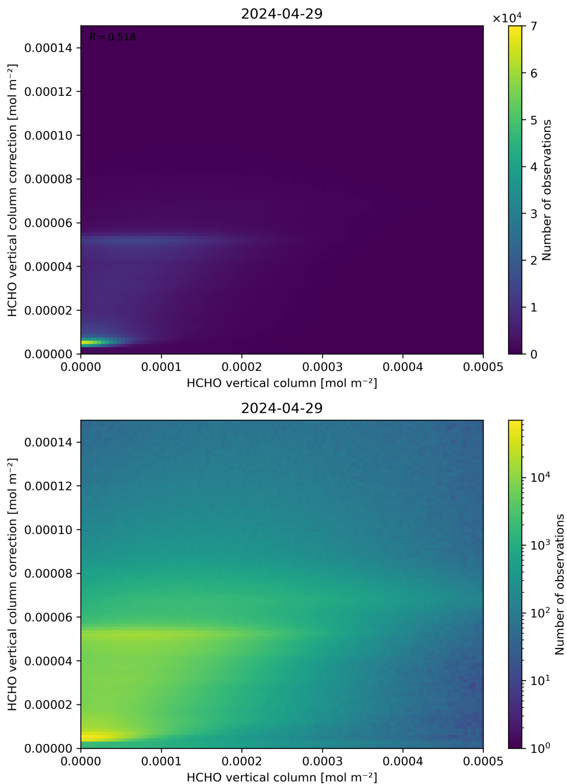
Figure 133: Scatter density plot of “HCHO vertical column” against “HCHO vertical column correction” for 2024-04-28 to 2024-04-30.
