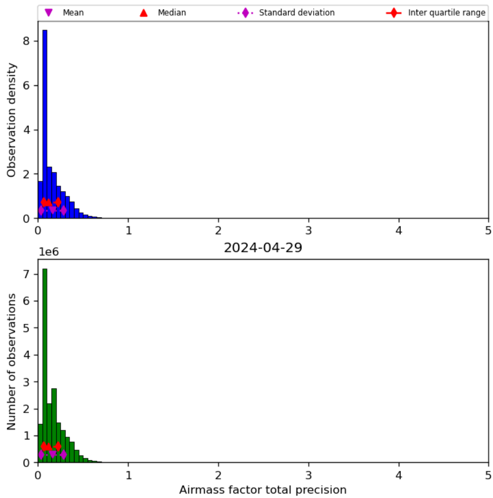
Figure 41: Histogram of “Airmass factor total precision” for 2024-04-28 to 2024-04-30
