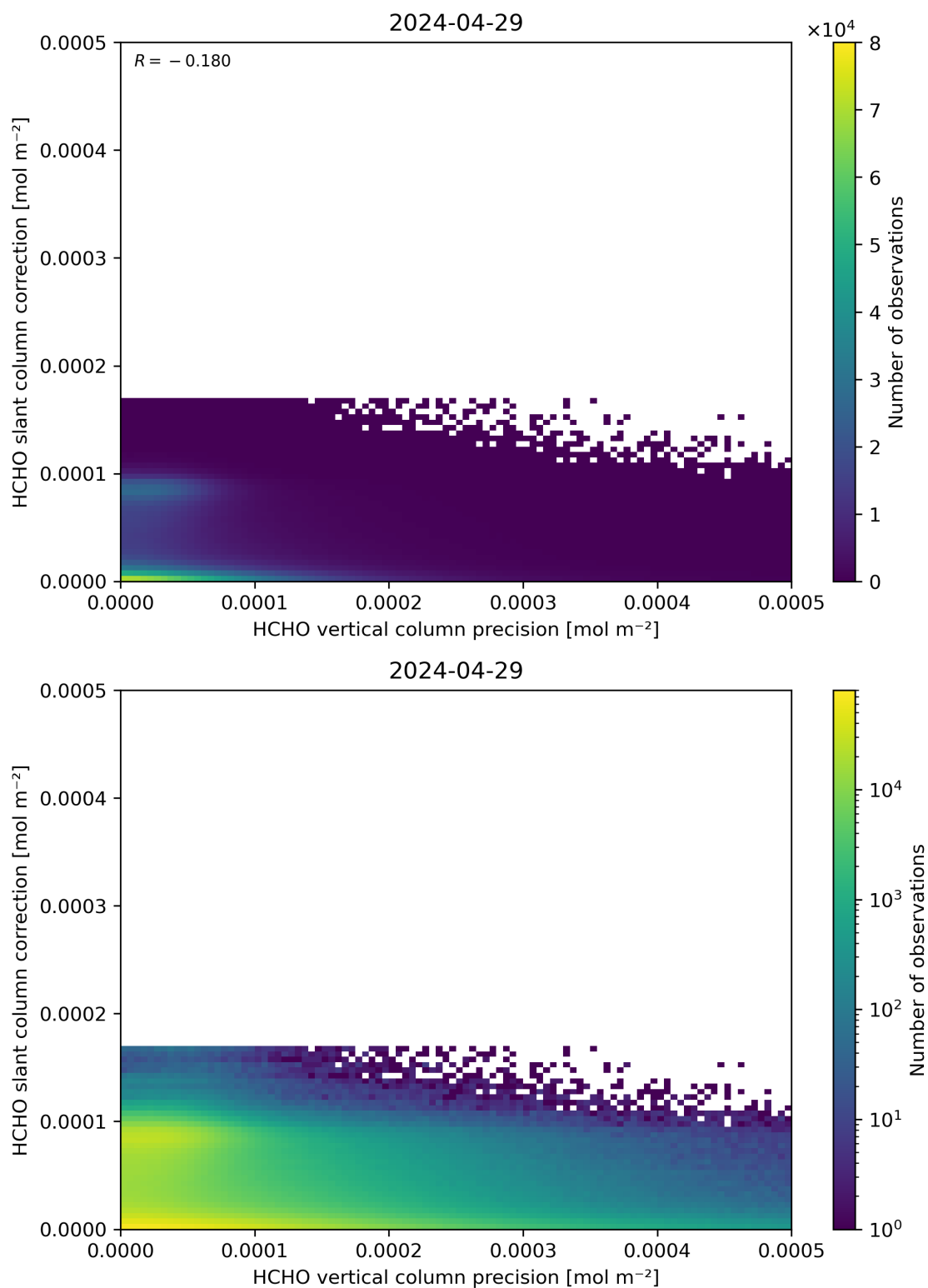
Figure 141: Scatter density plot of “HCHO vertical column precision” against “HCHO slant column correction” for 2024-04-28 to 2024-04-30.
