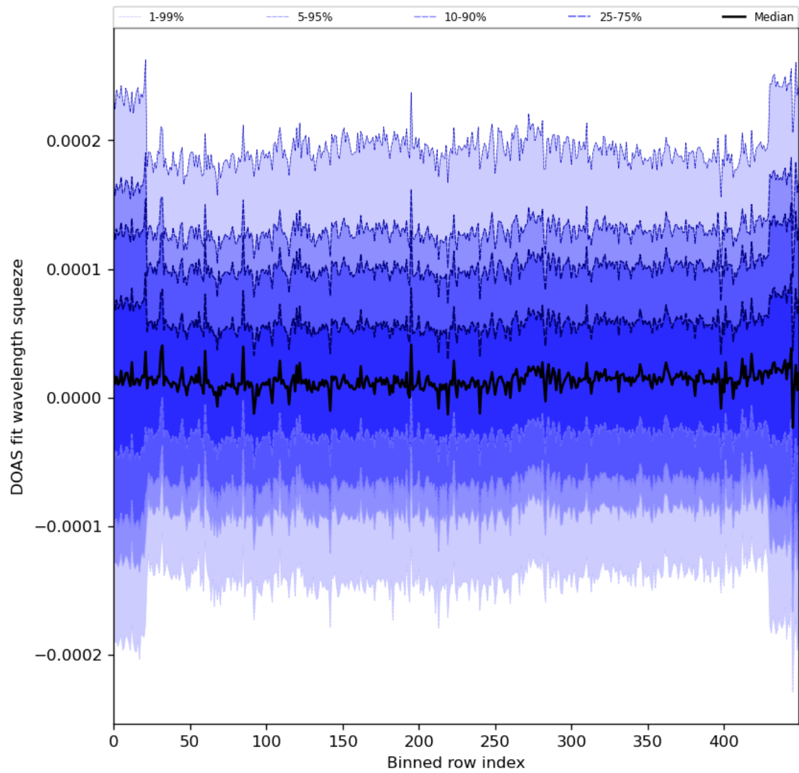
Figure 59: Along track statistics of “DOAS fit wavelength squeeze” for 2024-04-28 to 2024-04-30
