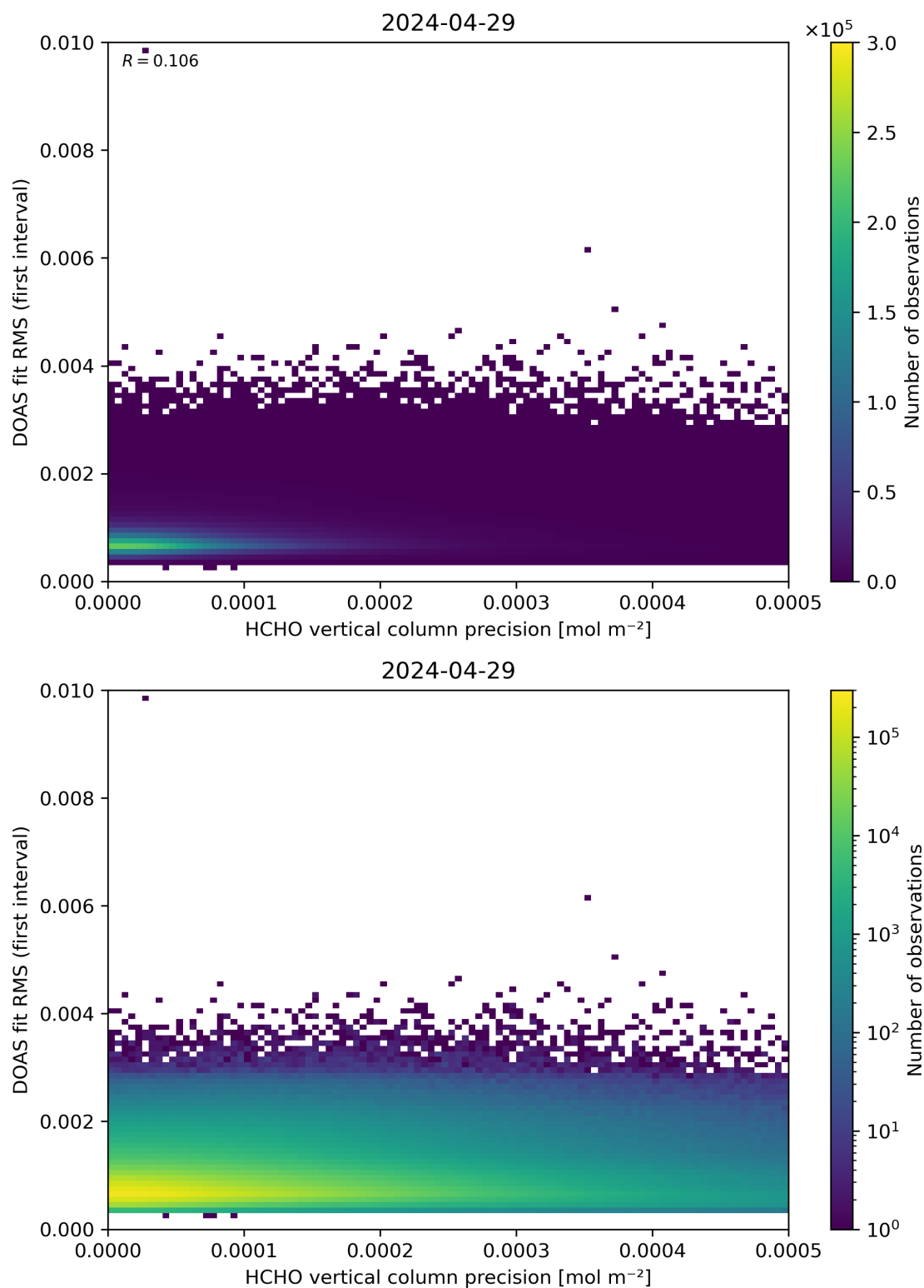
Figure 136: Scatter density plot of “HCHO vertical column precision” against “DOAS fit RMS (first interval)” for 2024-04-28 to 2024-04-30.
