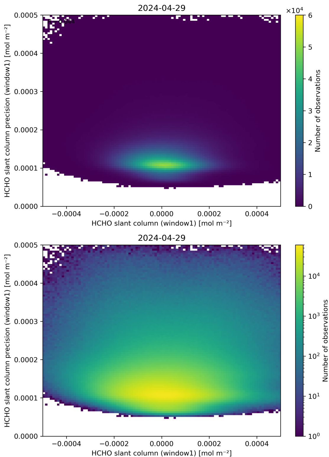
Figure 84: Scatter density plot of “HCHO slant column (window1)” against “HCHO slant column precision (window1)” for 2024-04-28 to 2024-04-30.
