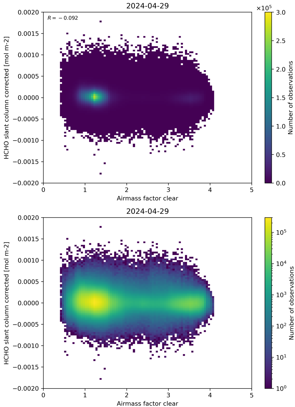
Figure 74: Scatter density plot of “Airmass factor clear” against “HCHO slant column corrected” for 2024-04-28 to 2024-04-30.
