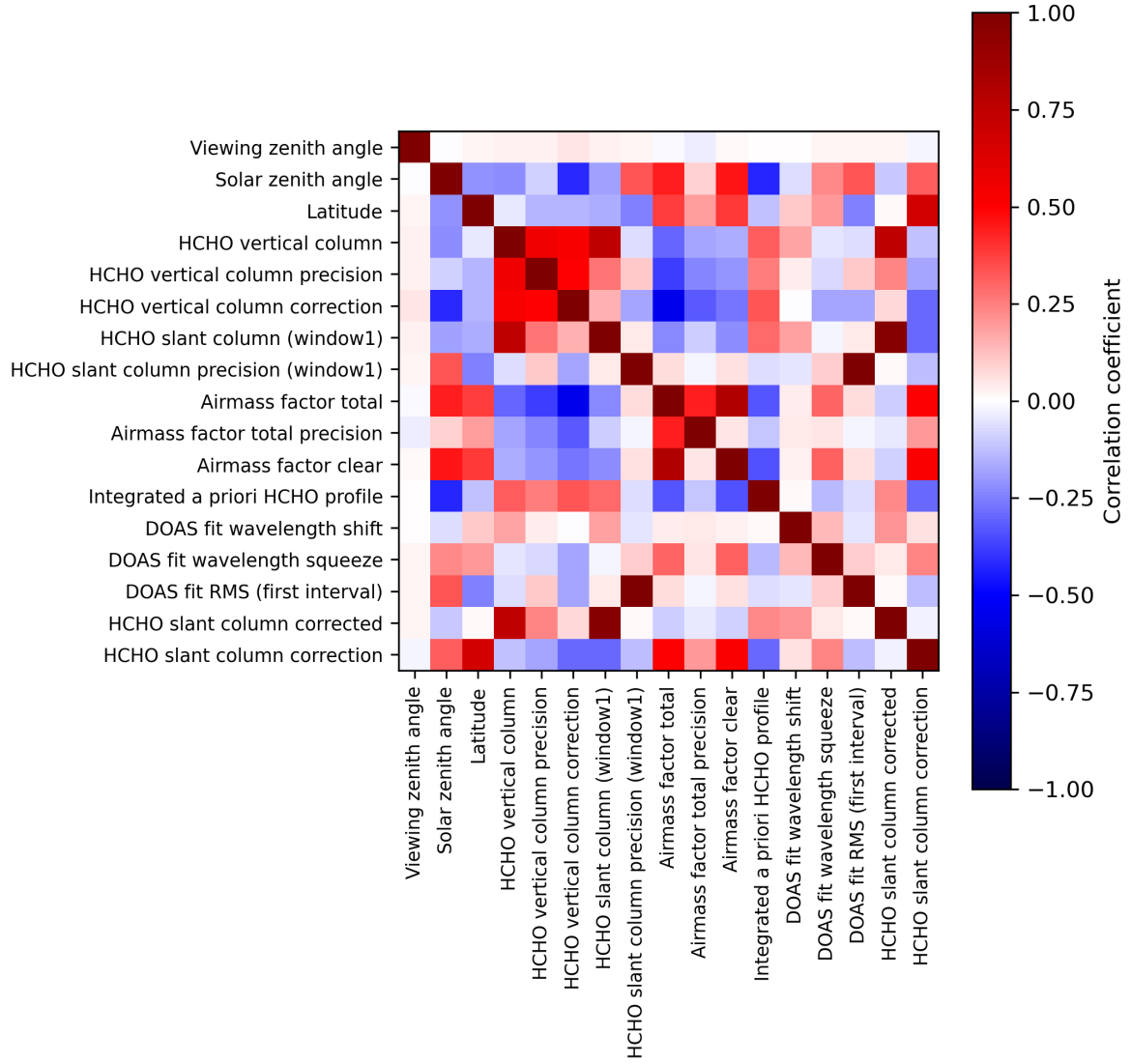
Figure 2: Map of correlation matrix for 2024-04-28 to 2024-04-30.
