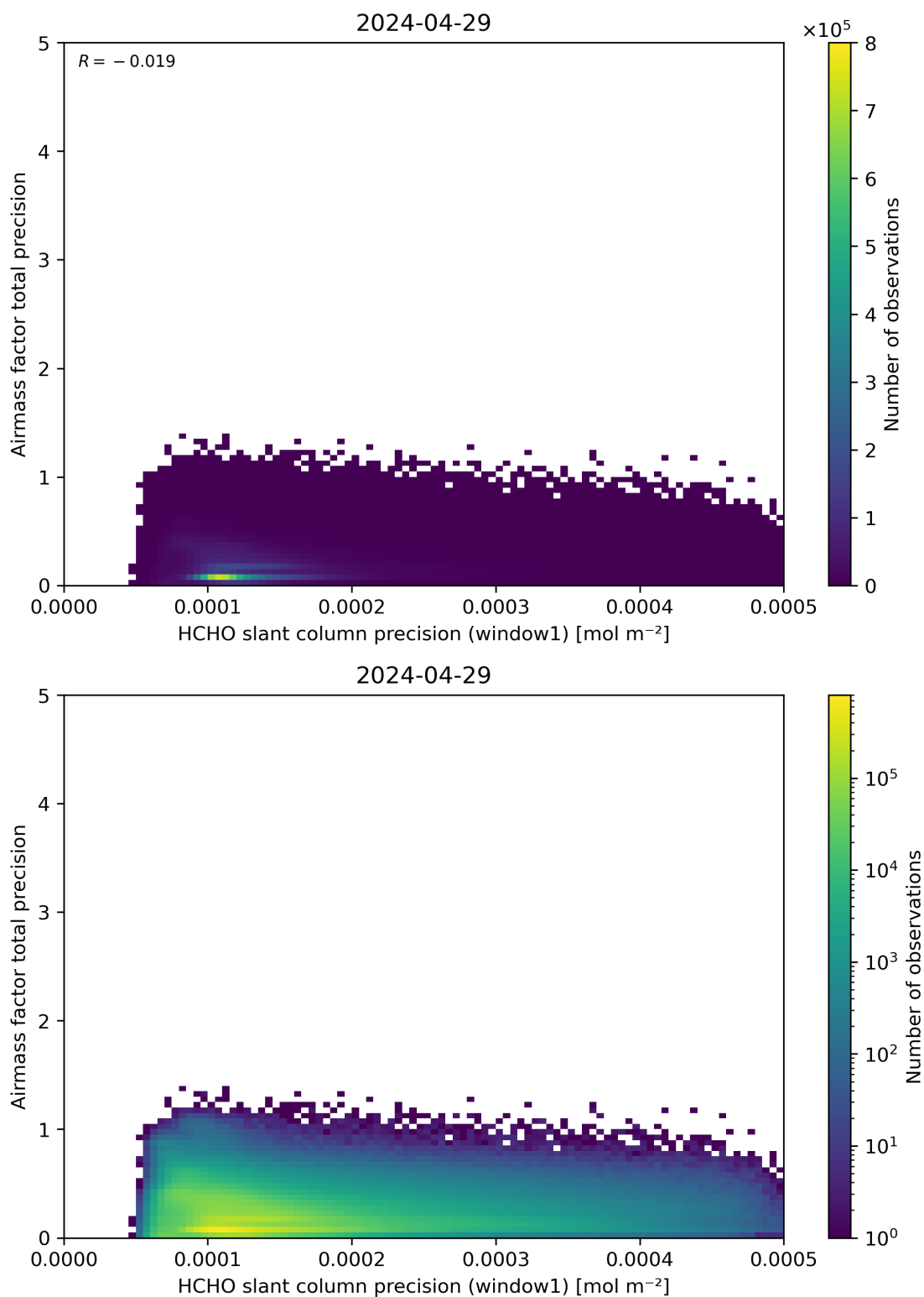
Figure 95: Scatter density plot of “HCHO slant column precision (window1)” against “Airmass factor total precision” for 2024-04-28 to 2024-04-30.
