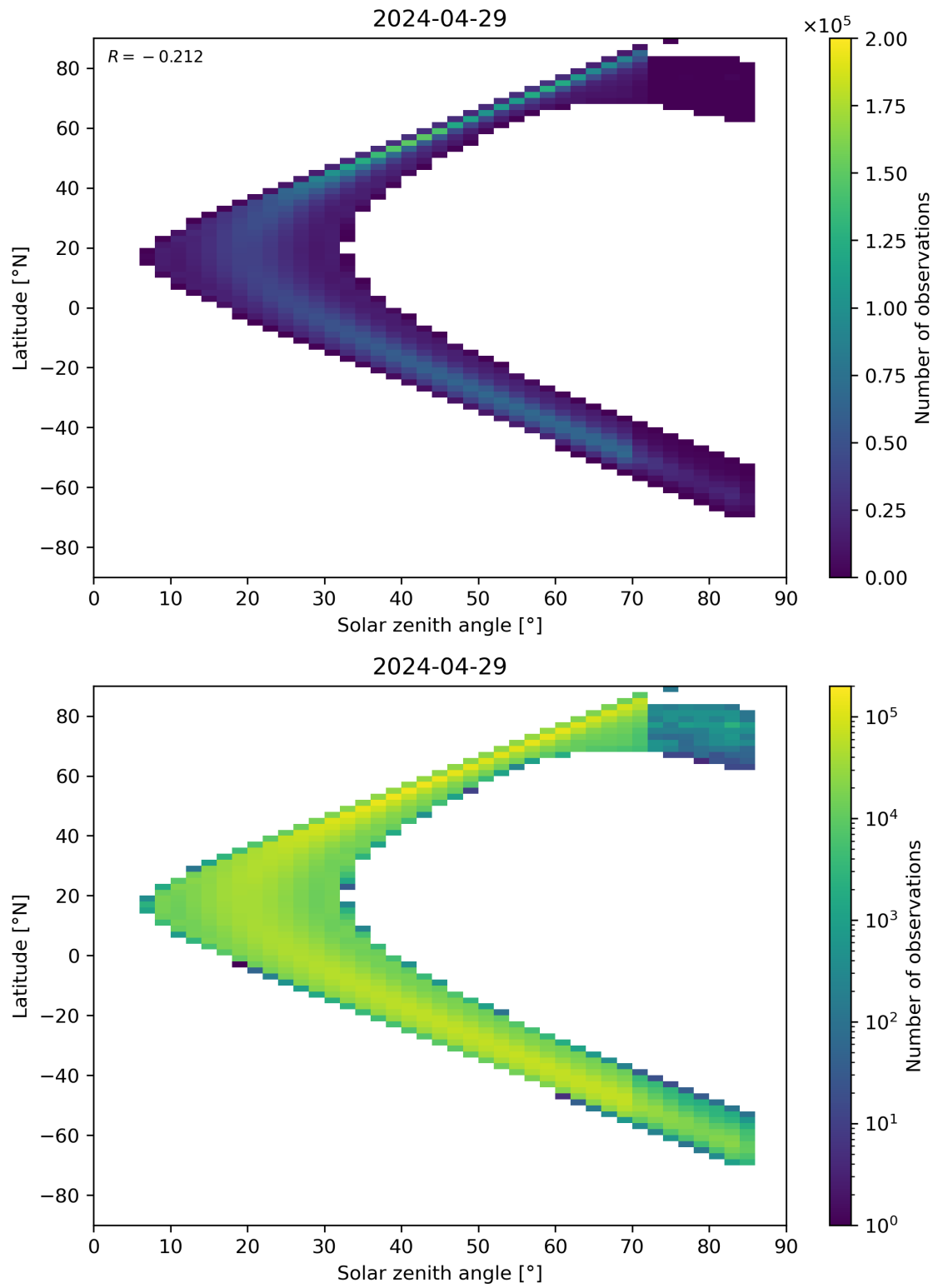
Figure 181: Scatter density plot of “Solar zenith angle” against “Latitude” for 2024-04-28 to 2024-04-30.
