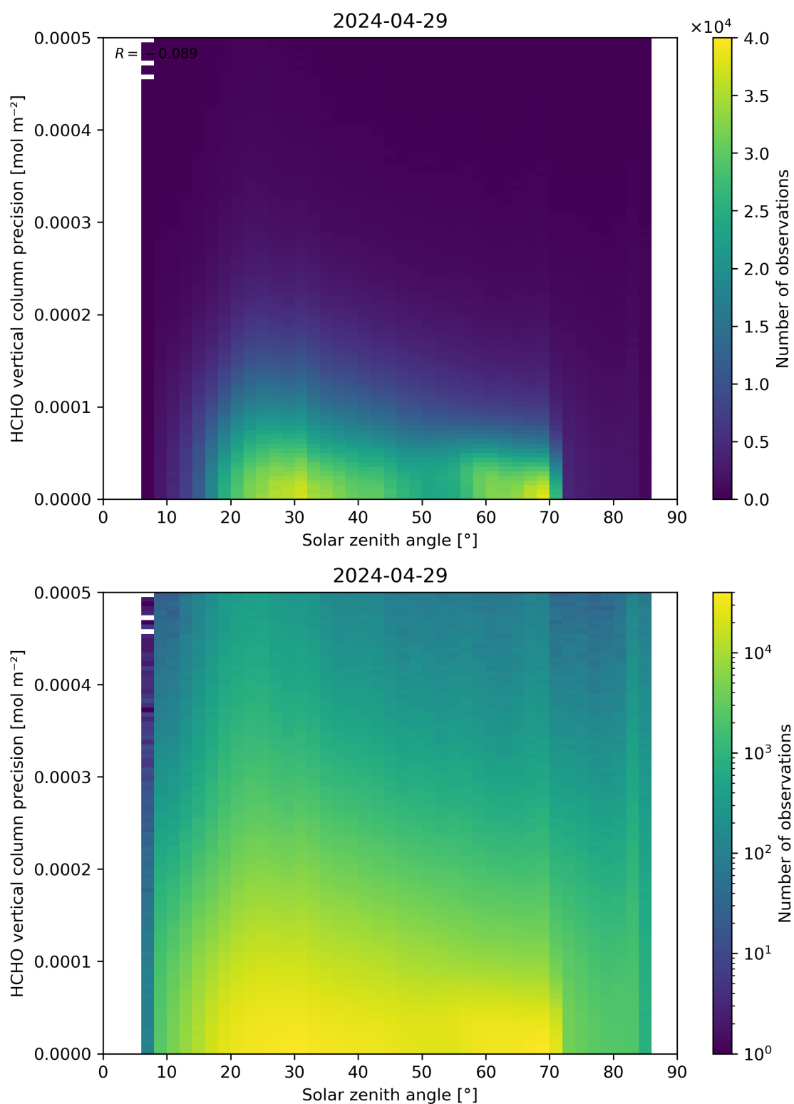
Figure 179: Scatter density plot of “Solar zenith angle” against “HCHO vertical column precision” for 2024-04-28 to 2024-04-30.
