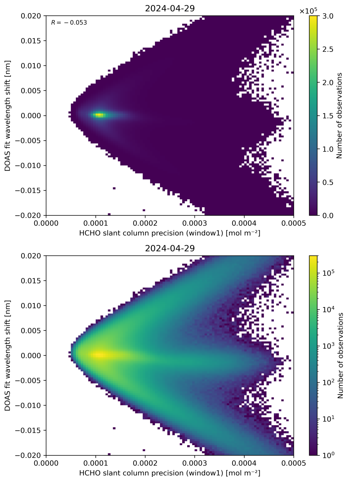
Figure 89: Scatter density plot of “HCHO slant column precision (window1)” against “DOAS fit wavelength shift” for 2024-04-28 to 2024-04-30.
