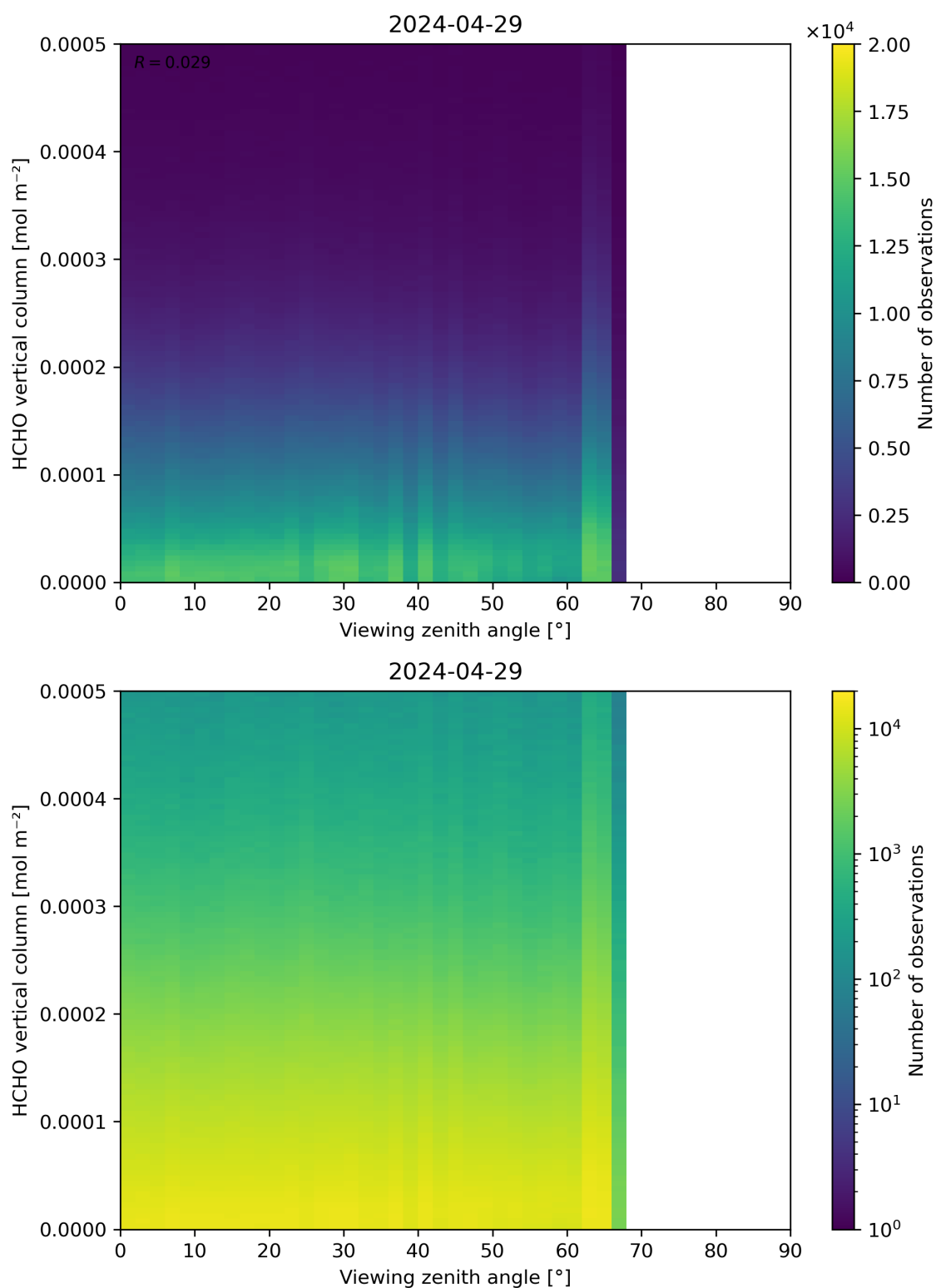
Figure 192: Scatter density plot of “Viewing zenith angle” against “HCHO vertical column” for 2024-04-28 to 2024-04-30.
