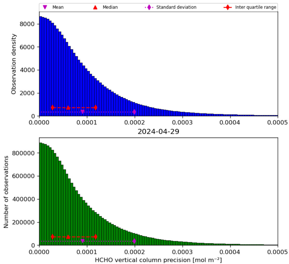
Figure 36: Histogram of “HCHO vertical column precision” for 2024-04-28 to 2024-04-30
