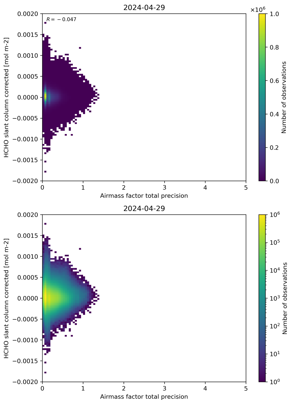
Figure 109: Scatter density plot of “Airmass factor total precision” against “HCHO slant column corrected” for 2024-04-28 to 2024-04-30.
