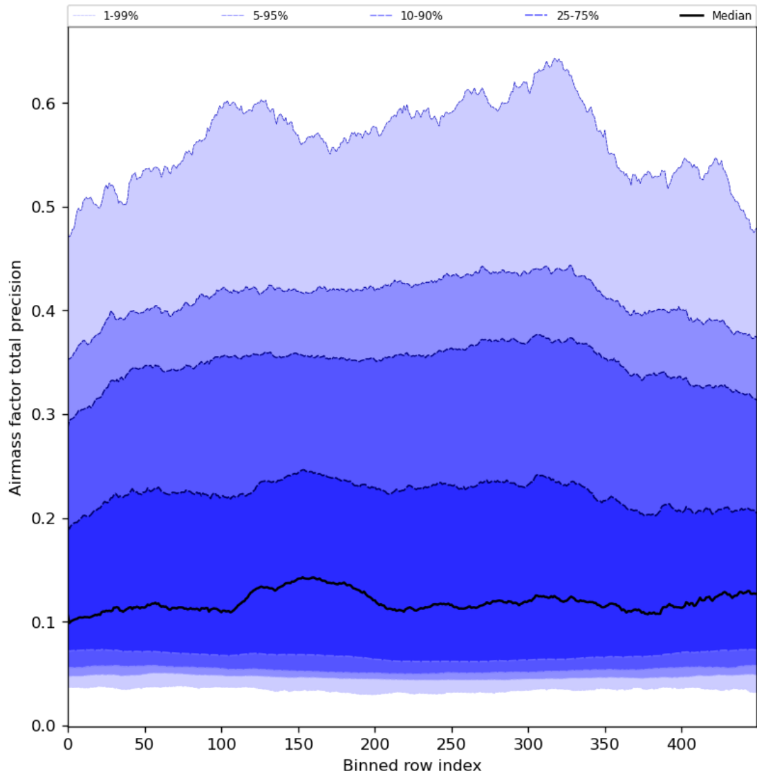
Figure 55: Along track statistics of “Airmass factor total precision” for 2024-04-28 to 2024-04-30
