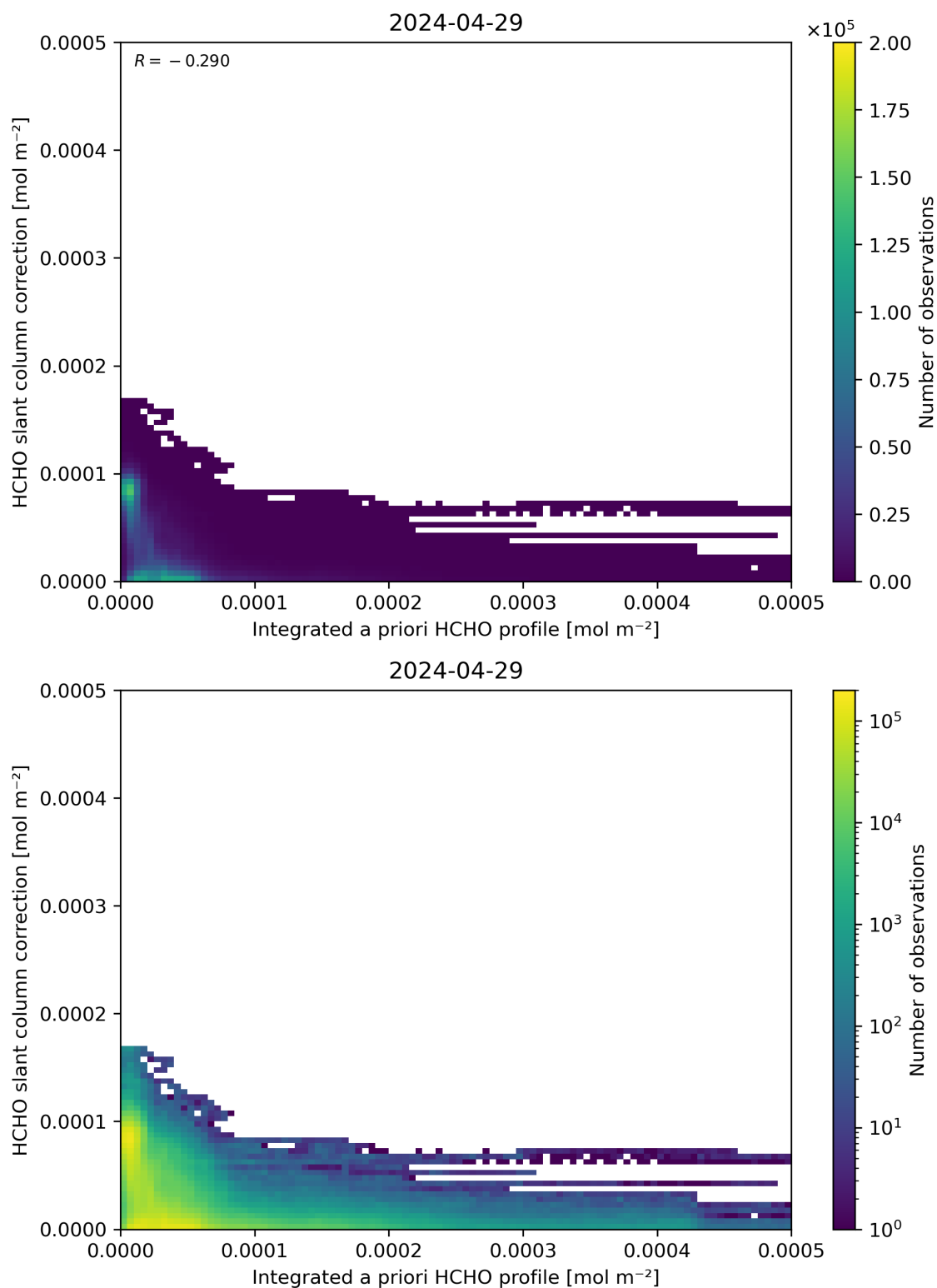
Figure 152: Scatter density plot of “Integrated a priori HCHO profile” against “HCHO slant column correction” for 2024-04-28 to 2024-04-30.
