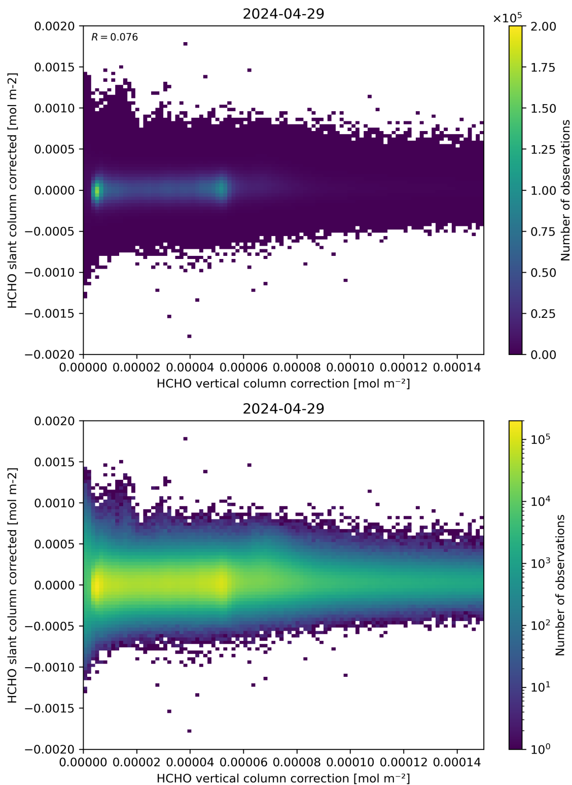
Figure 116: Scatter density plot of “HCHO vertical column correction” against “HCHO slant column corrected” for 2024-04-28 to 2024-04-30.
