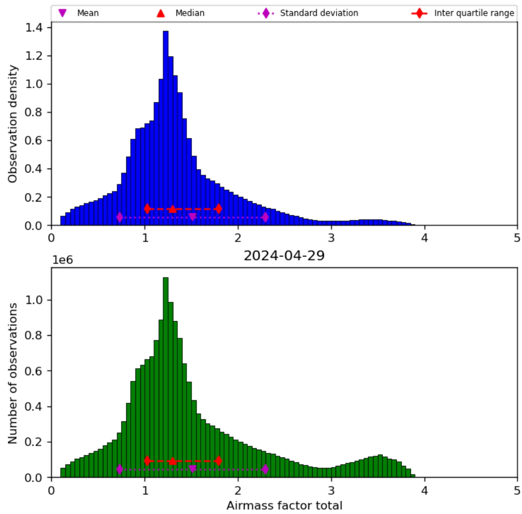
Figure 40: Histogram of “Airmass factor total” for 2024-04-28 to 2024-04-30
