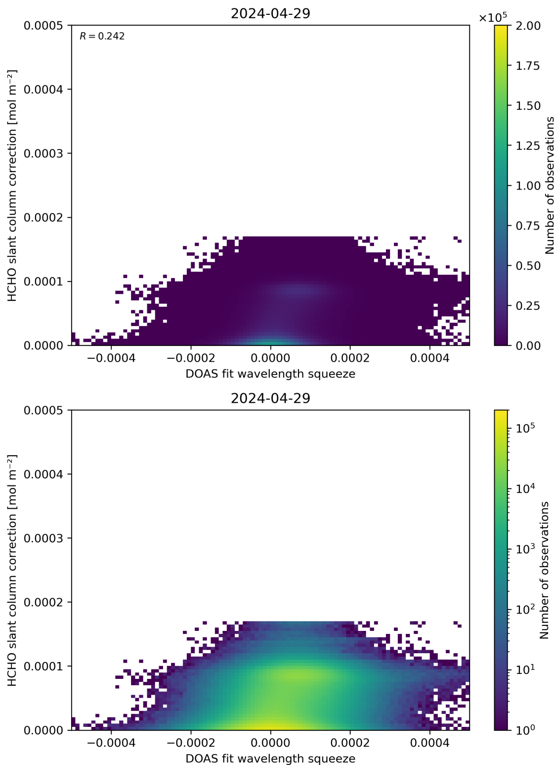
Figure 70: Scatter density plot of “DOAS fit wavelength squeeze” against “HCHO slant column correction” for 2024-04-28 to 2024-04-30.
