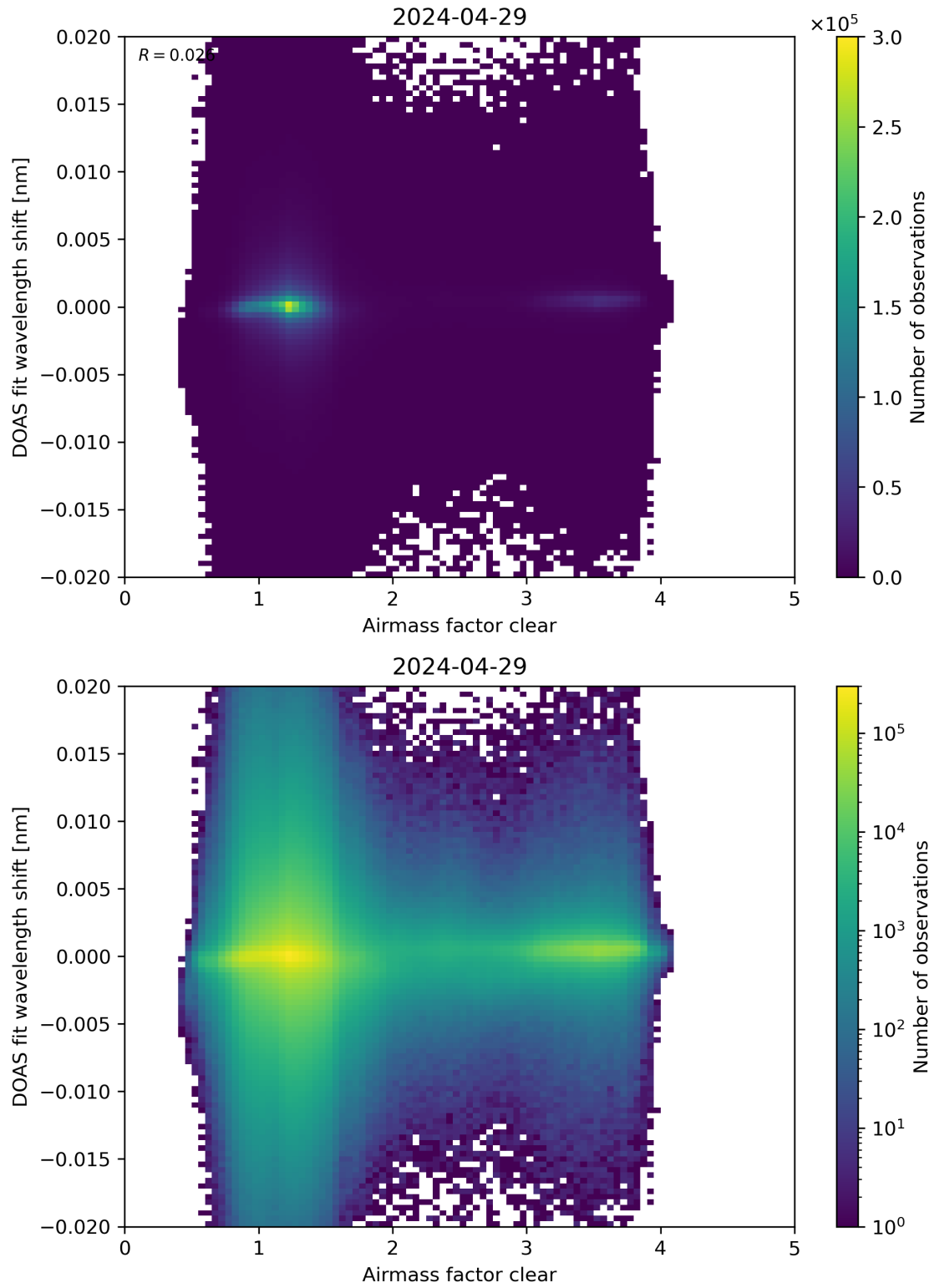
Figure 72: Scatter density plot of “Airmass factor clear” against “DOAS fit wavelength shift” for 2024-04-28 to 2024-04-30.
