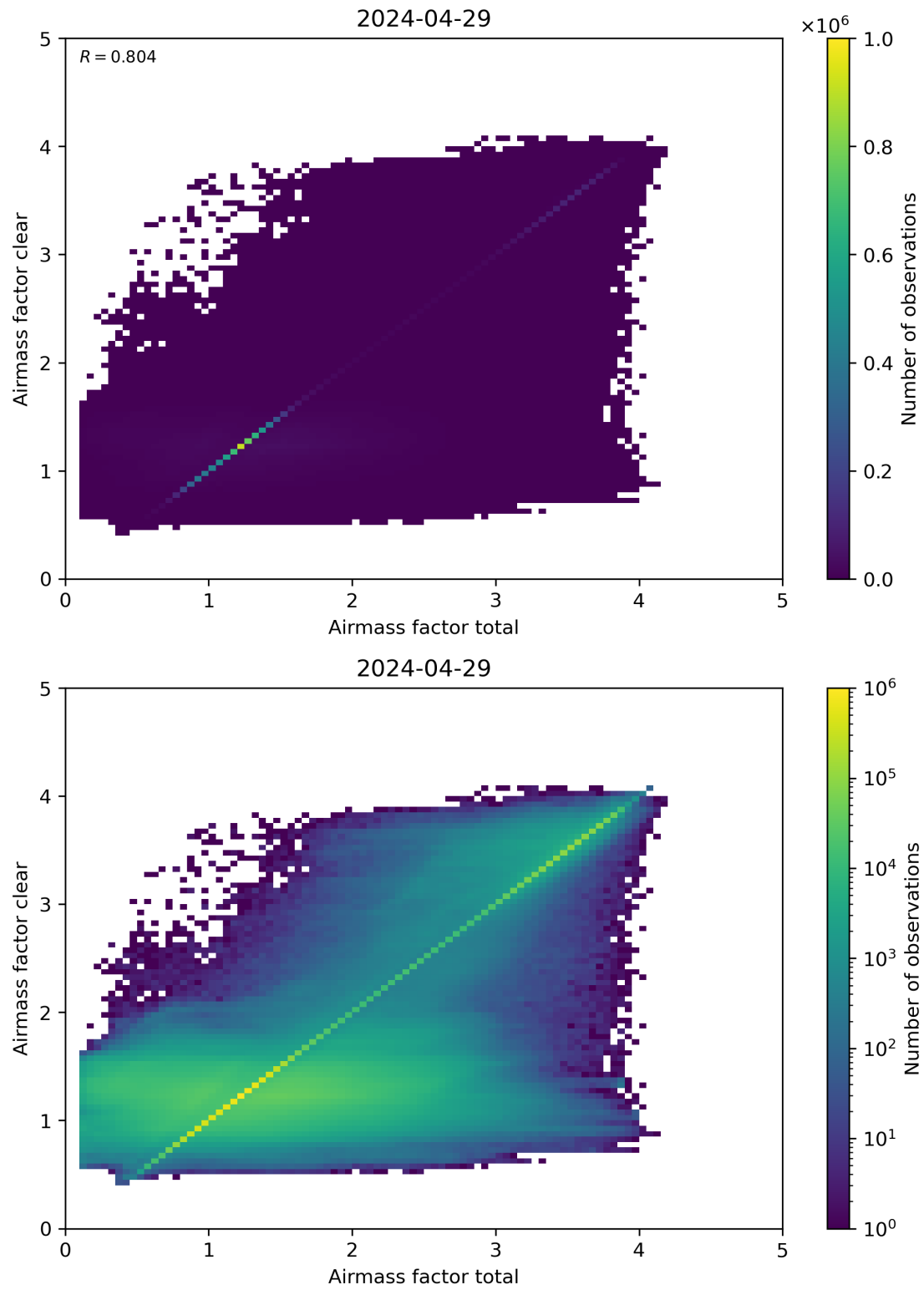
Figure 100: Scatter density plot of “Airmass factor total” against “Airmass factor clear” for 2024-04-28 to 2024-04-30.
