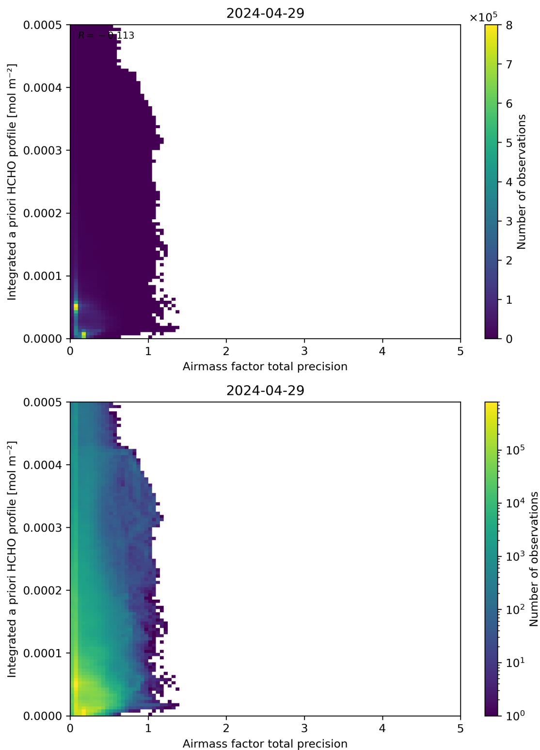
Figure 111: Scatter density plot of “Airmass factor total precision” against “Integrated a priori HCHO profile” for 2024-04-28 to 2024-04-30.
