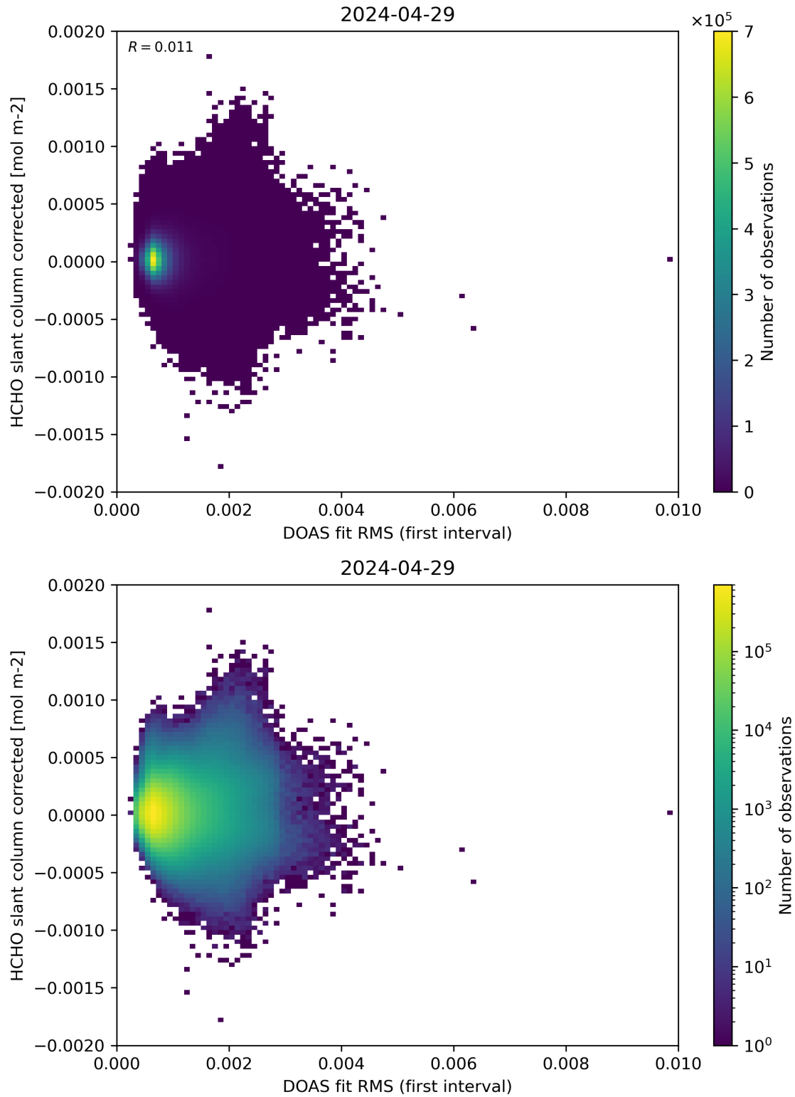
Figure 62: Scatter density plot of “DOAS fit RMS (first interval)” against “HCHO slant column corrected” for 2024-04-28 to 2024-04-30.
