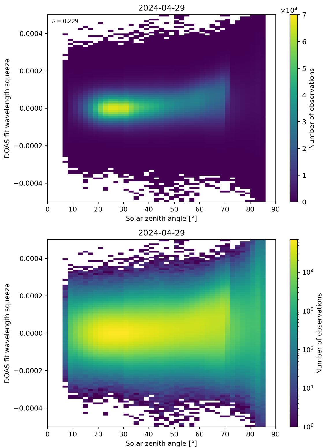
Figure 169: Scatter density plot of “Solar zenith angle” against “DOAS fit wavelength squeeze” for 2024-04-28 to 2024-04-30.
