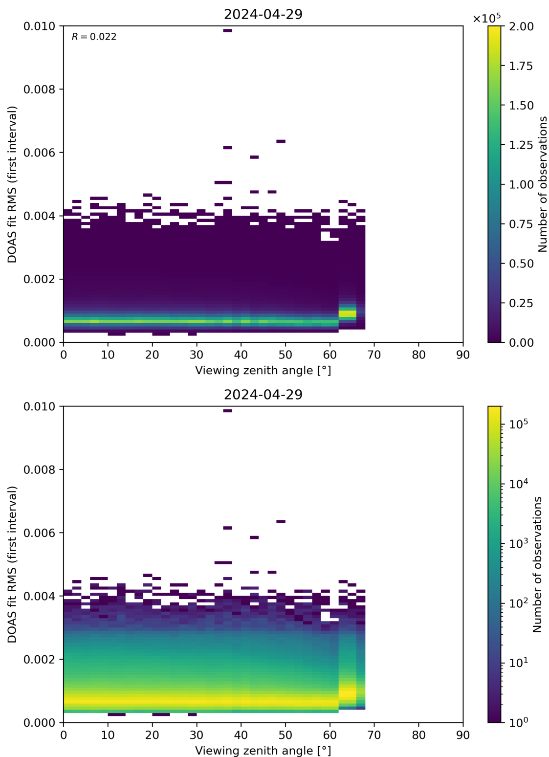
Figure 182: Scatter density plot of “Viewing zenith angle” against “DOAS fit RMS (first interval)” for 2024-04-28 to 2024-04-30.
