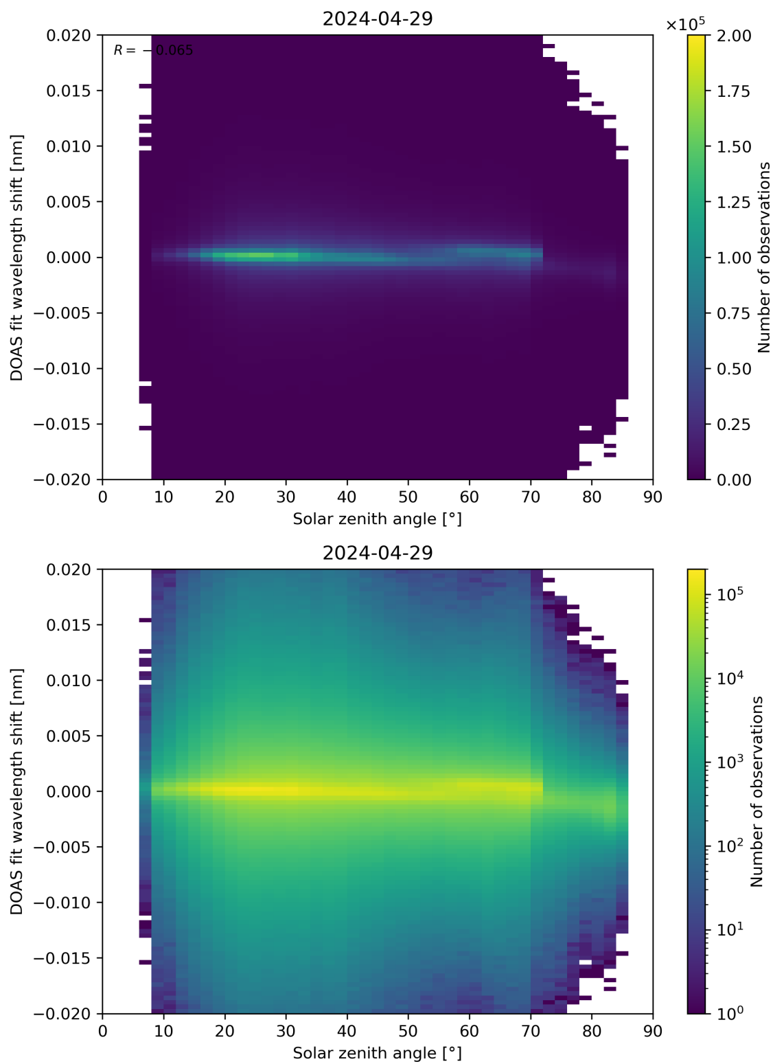
Figure 168: Scatter density plot of “Solar zenith angle” against “DOAS fit wavelength shift” for 2024-04-28 to 2024-04-30.
