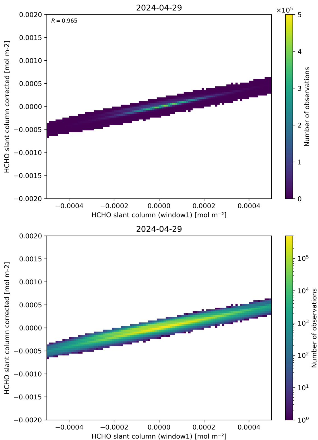
Figure 82: Scatter density plot of “HCHO slant column (window1)” against “HCHO slant column corrected” for 2024-04-28 to 2024-04-30.
