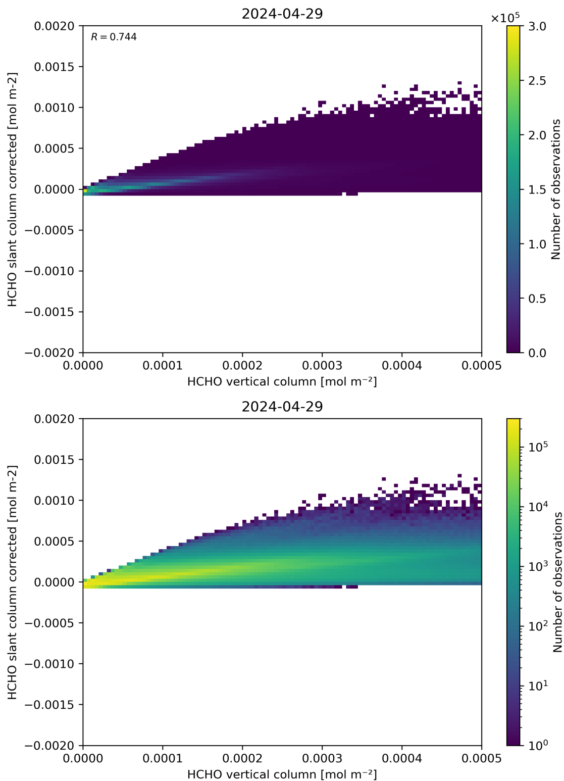
Figure 127: Scatter density plot of “HCHO vertical column” against “HCHO slant column corrected” for 2024-04-28 to 2024-04-30.
