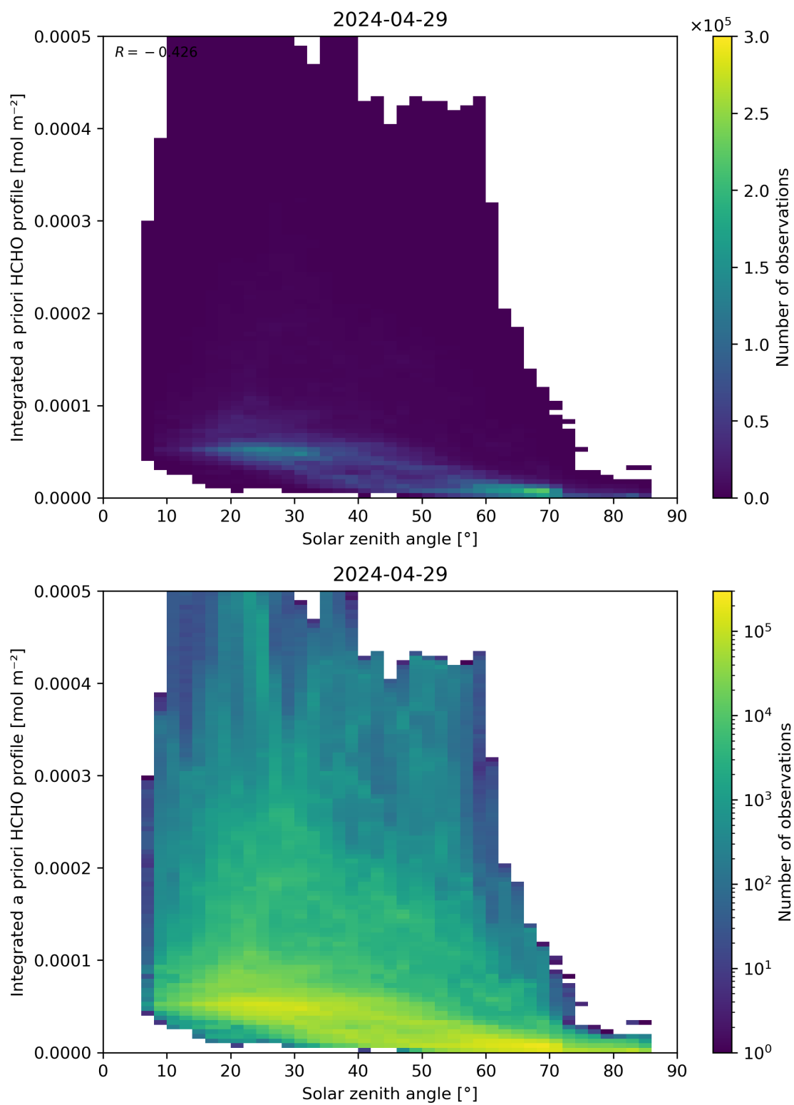
Figure 180: Scatter density plot of “Solar zenith angle” against “Integrated a priori HCHO profile” for 2024-04-28 to 2024-04-30.
