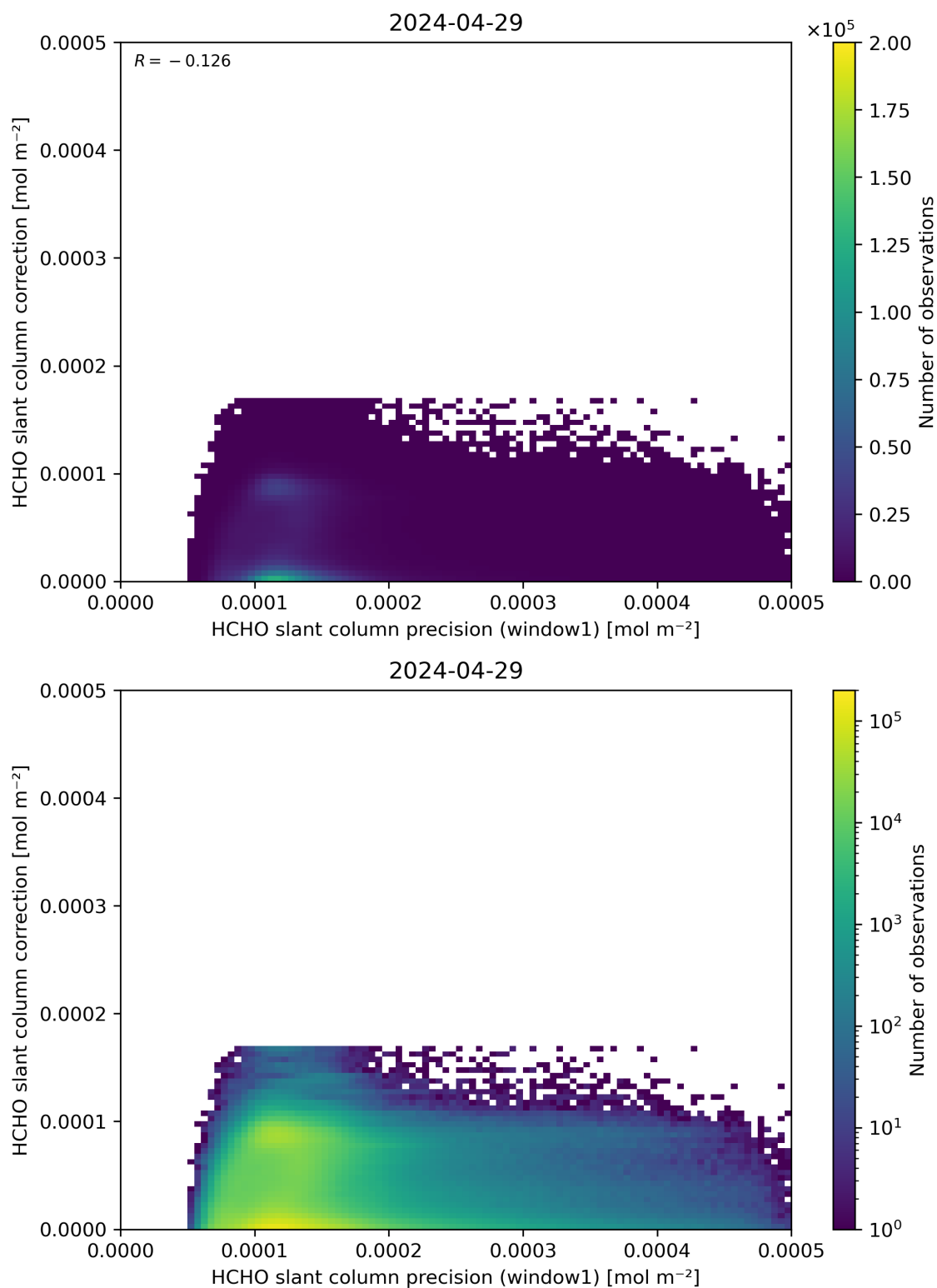
Figure 93: Scatter density plot of “HCHO slant column precision (window1)” against “HCHO slant column correction” for 2024-04-28 to 2024-04-30.
