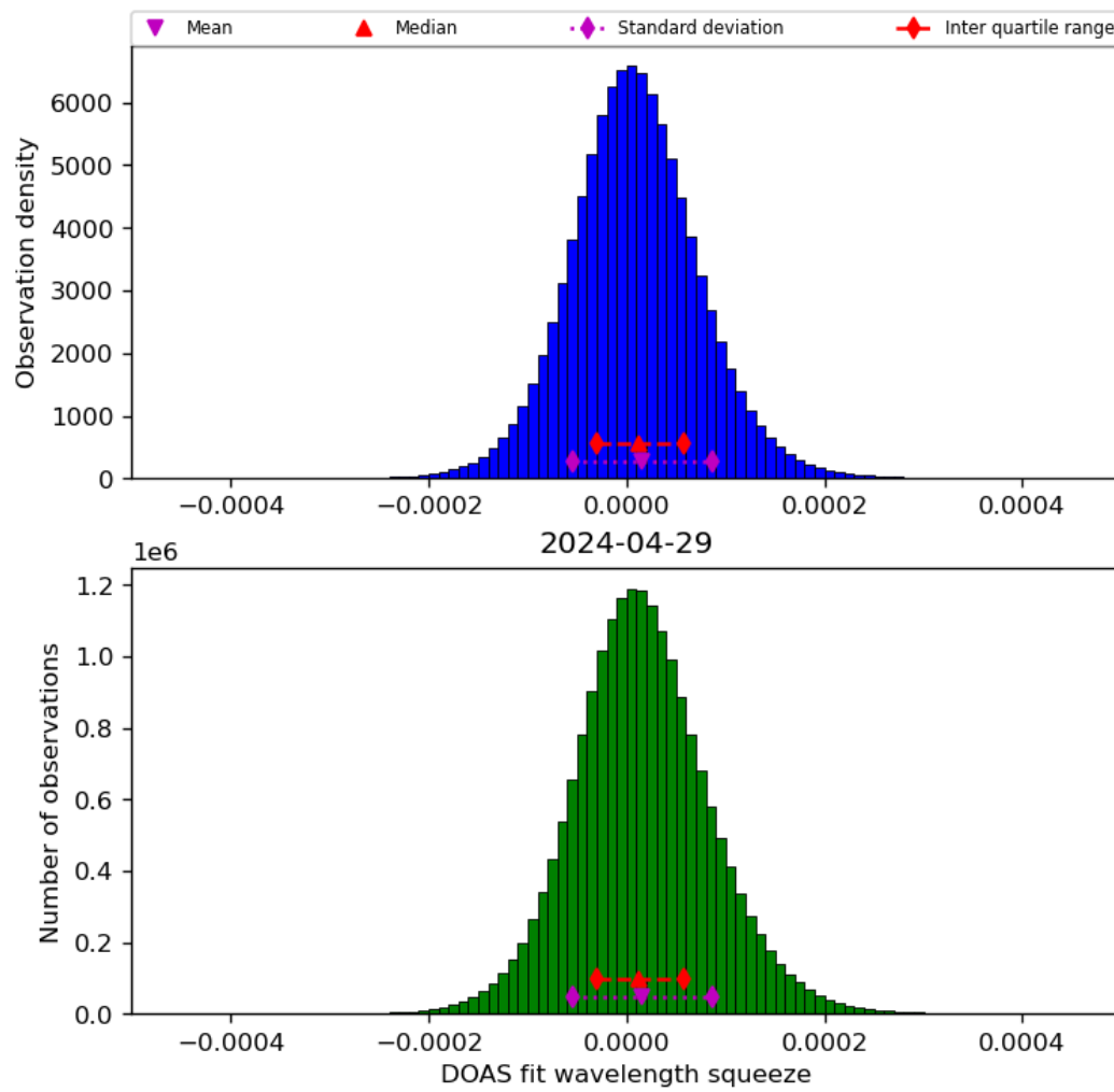
Figure 45: Histogram of “DOAS fit wavelength squeeze” for 2024-04-28 to 2024-04-30
