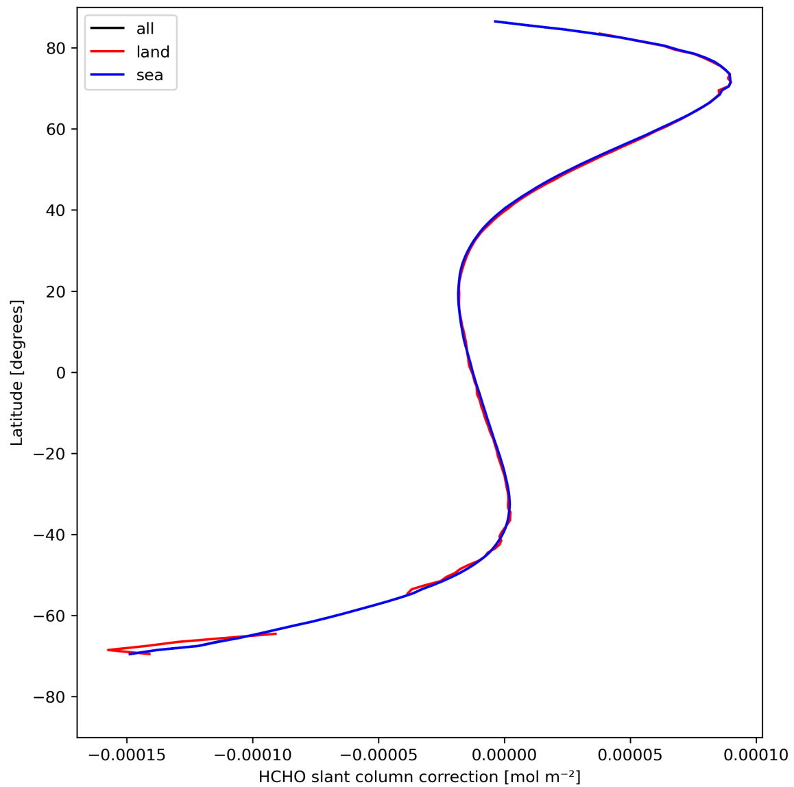
Figure 33: Zonal average of “HCHO slant column correction” for 2024-04-28 to 2024-04-30.
