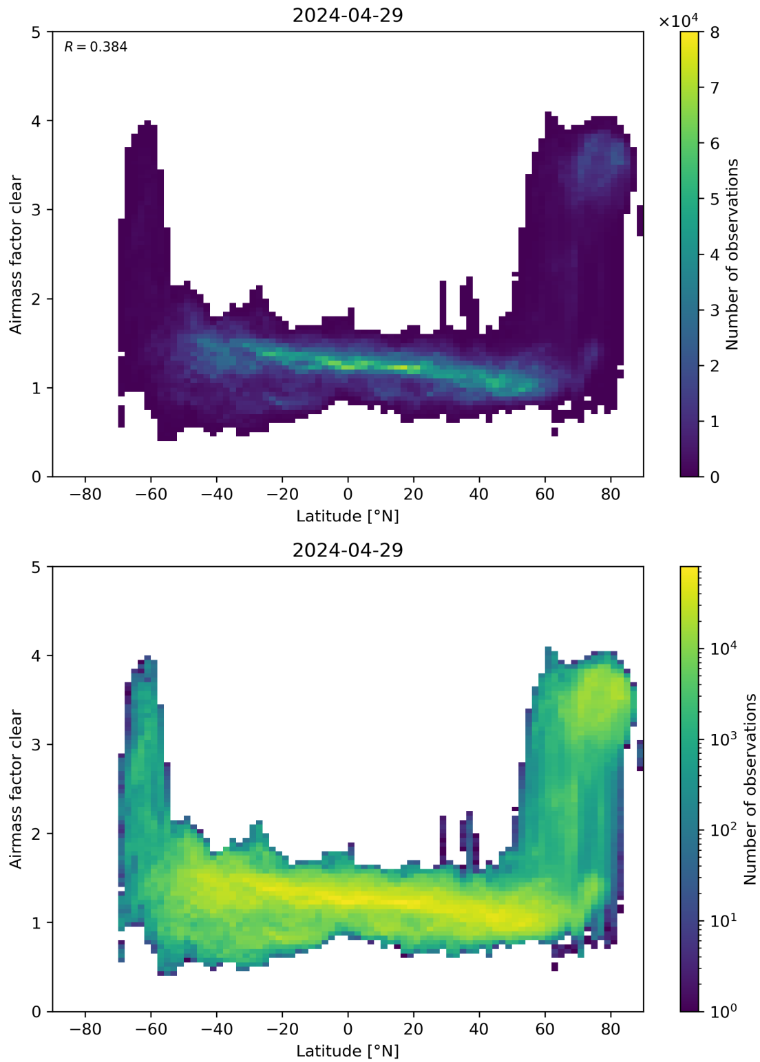
Figure 156: Scatter density plot of “Latitude” against “Airmass factor clear” for 2024-04-28 to 2024-04-30.
