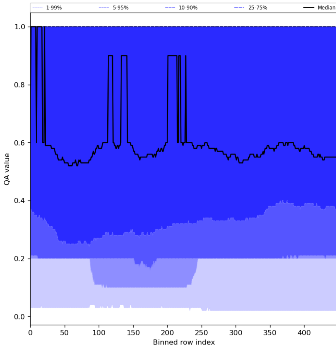
Figure 48: Along track statistics of “QA value” for 2024-04-28 to 2024-04-30
