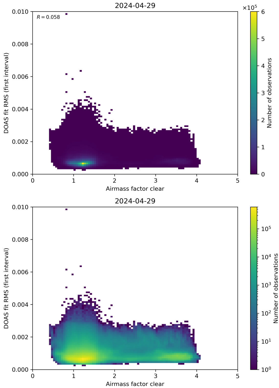
Figure 71: Scatter density plot of “Airmass factor clear” against “DOAS fit RMS (first interval)” for 2024-04-28 to 2024-04-30.
