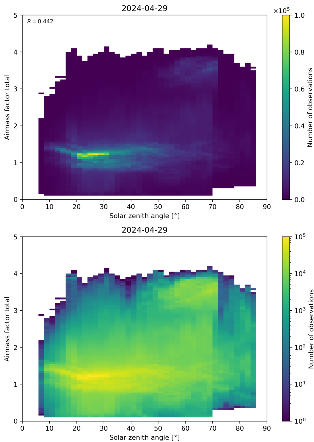
Figure 175: Scatter density plot of “Solar zenith angle” against “Airmass factor total” for 2024-04-28 to 2024-04-30.
