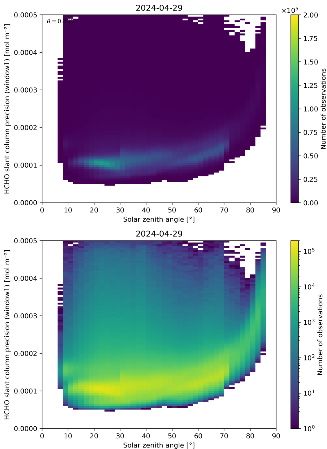
Figure 174: Scatter density plot of “Solar zenith angle” against “HCHO slant column precision (window1)” for 2024-04-28 to 2024-04-30.
