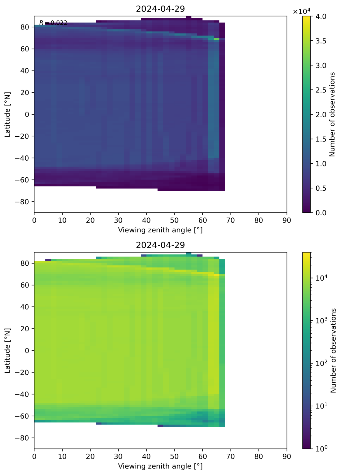
Figure 196: Scatter density plot of “Viewing zenith angle” against “Latitude” for 2024-04-28 to 2024-04-30.
