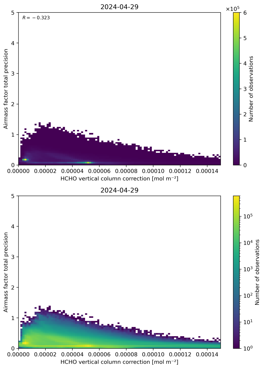
Figure 121: Scatter density plot of “HCHO vertical column correction” against “Airmass factor total precision” for 2024-04-28 to 2024-04-30.
