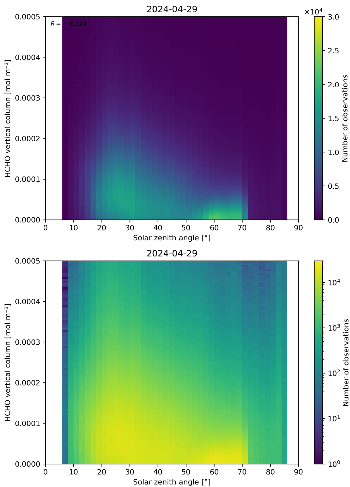
Figure 177: Scatter density plot of “Solar zenith angle” against “HCHO vertical column” for 2024-04-28 to 2024-04-30.
