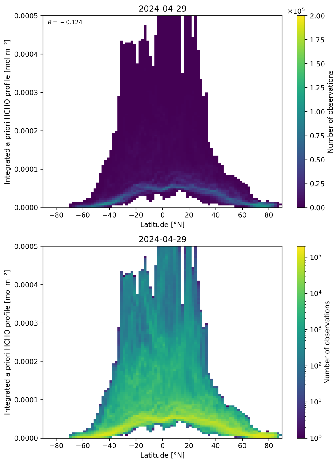
Figure 166: Scatter density plot of “Latitude” against “Integrated a priori HCHO profile” for 2024-04-28 to 2024-04-30.
