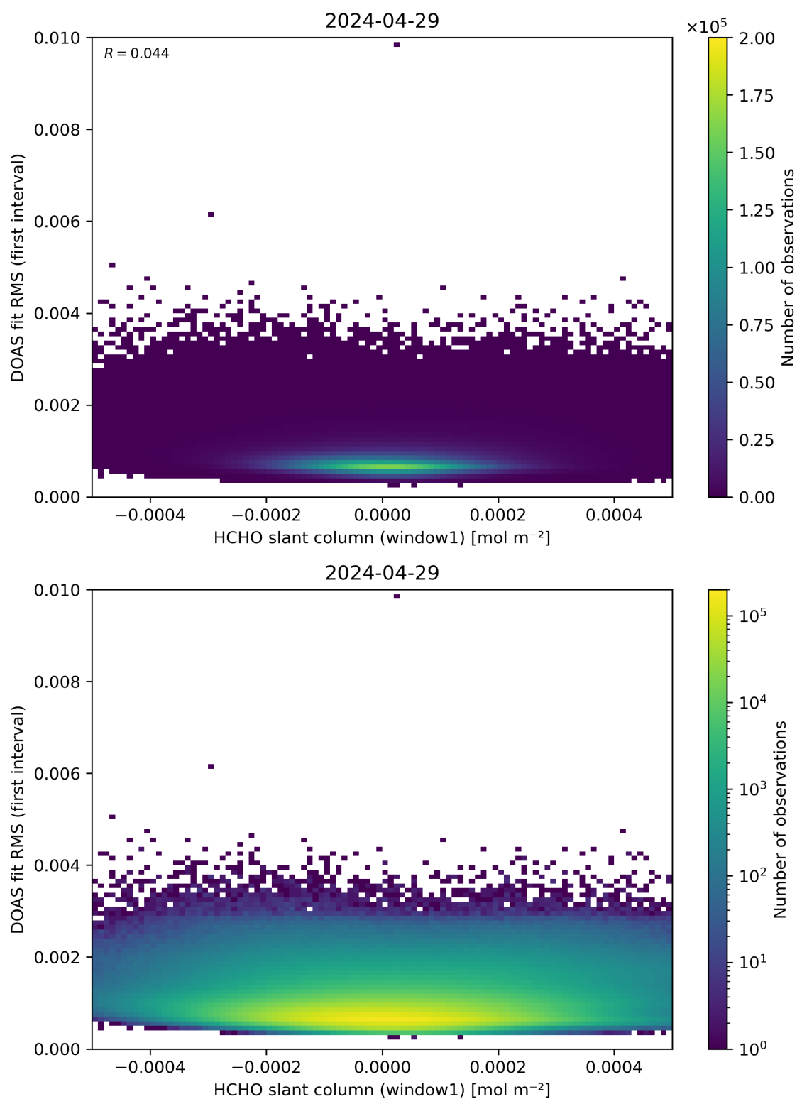
Figure 78: Scatter density plot of “HCHO slant column (window1)” against “DOAS fit RMS (first interval)” for 2024-04-28 to 2024-04-30.
