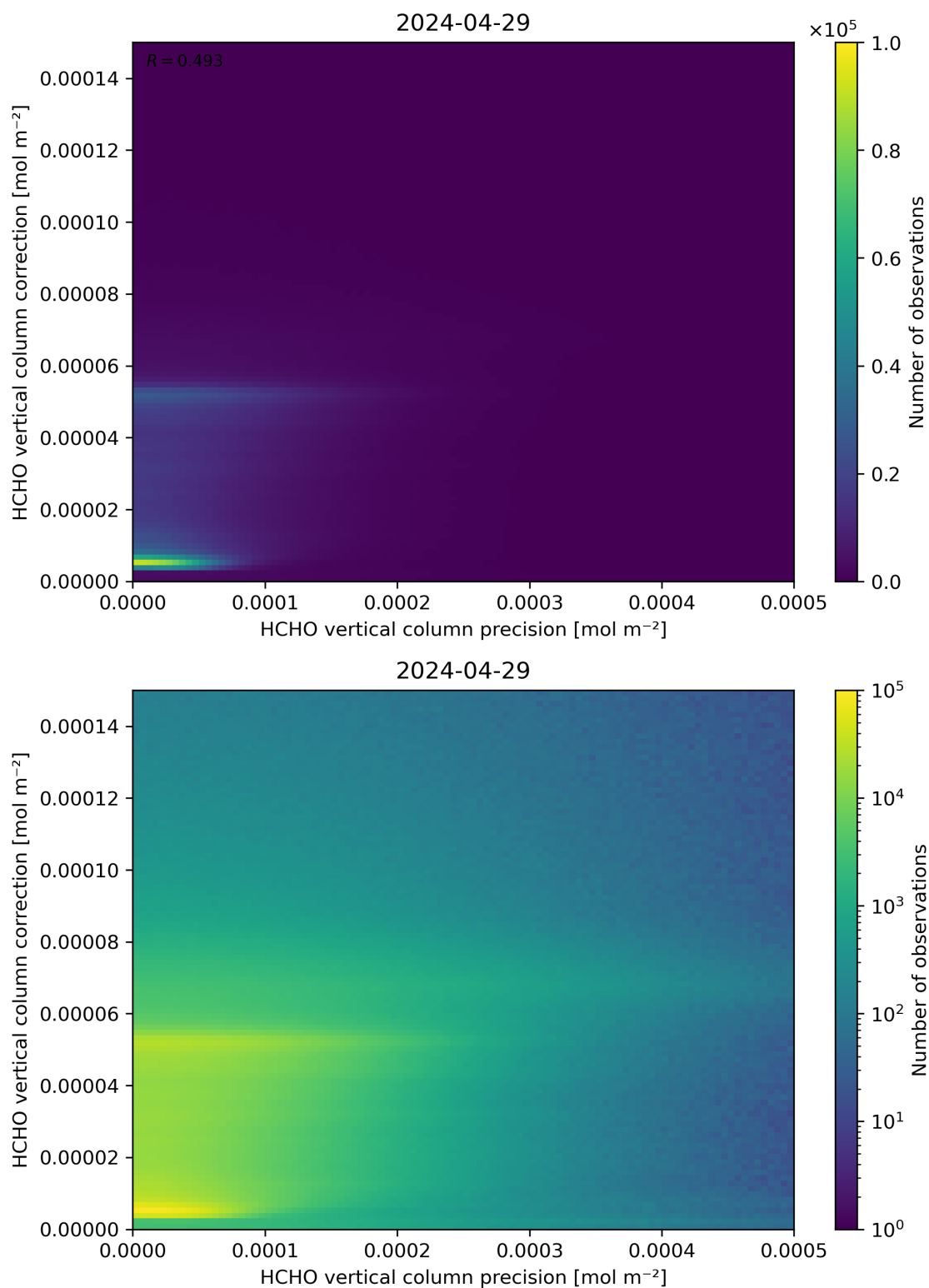
Figure 146: Scatter density plot of “HCHO vertical column precision” against “HCHO vertical column correction” for 2024-04-28 to 2024-04-30.
