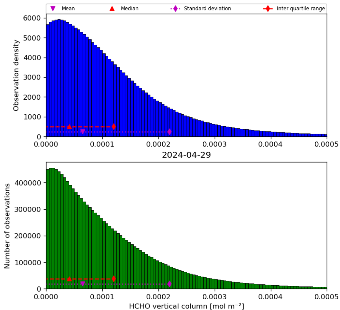
Figure 35: Histogram of “HCHO vertical column” for 2024-04-28 to 2024-04-30
