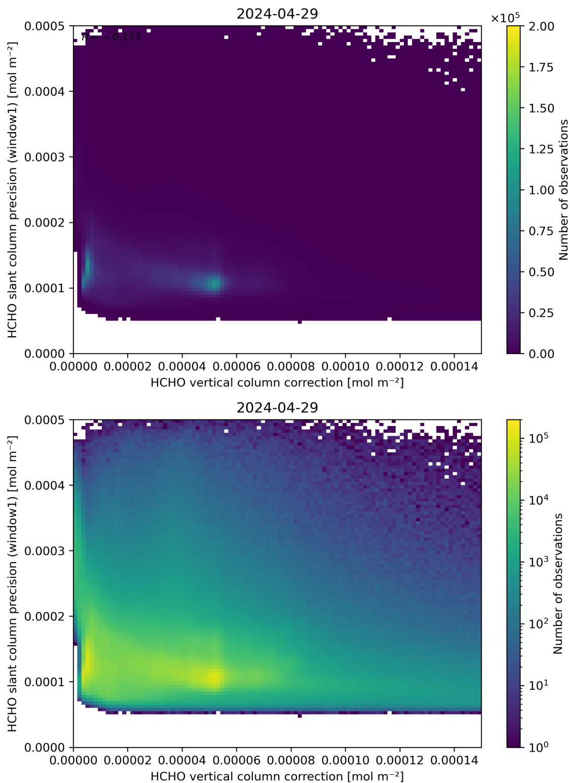
Figure 119: Scatter density plot of “HCHO vertical column correction” against “HCHO slant column precision (window1)” for 2024-04-28 to 2024-04-30.
