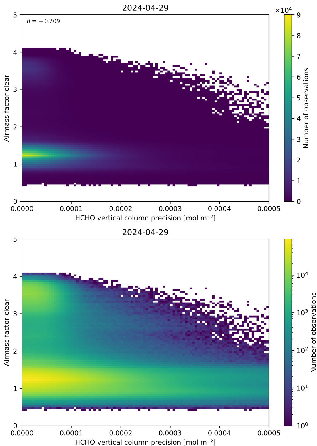
Figure 139: Scatter density plot of “HCHO vertical column precision” against “Airmass factor clear” for 2024-04-28 to 2024-04-30.
