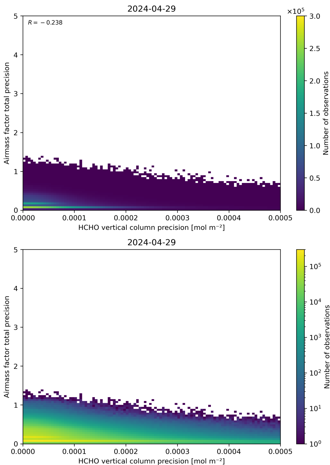
Figure 145: Scatter density plot of “HCHO vertical column precision” against “Airmass factor total precision” for 2024-04-28 to 2024-04-30.
