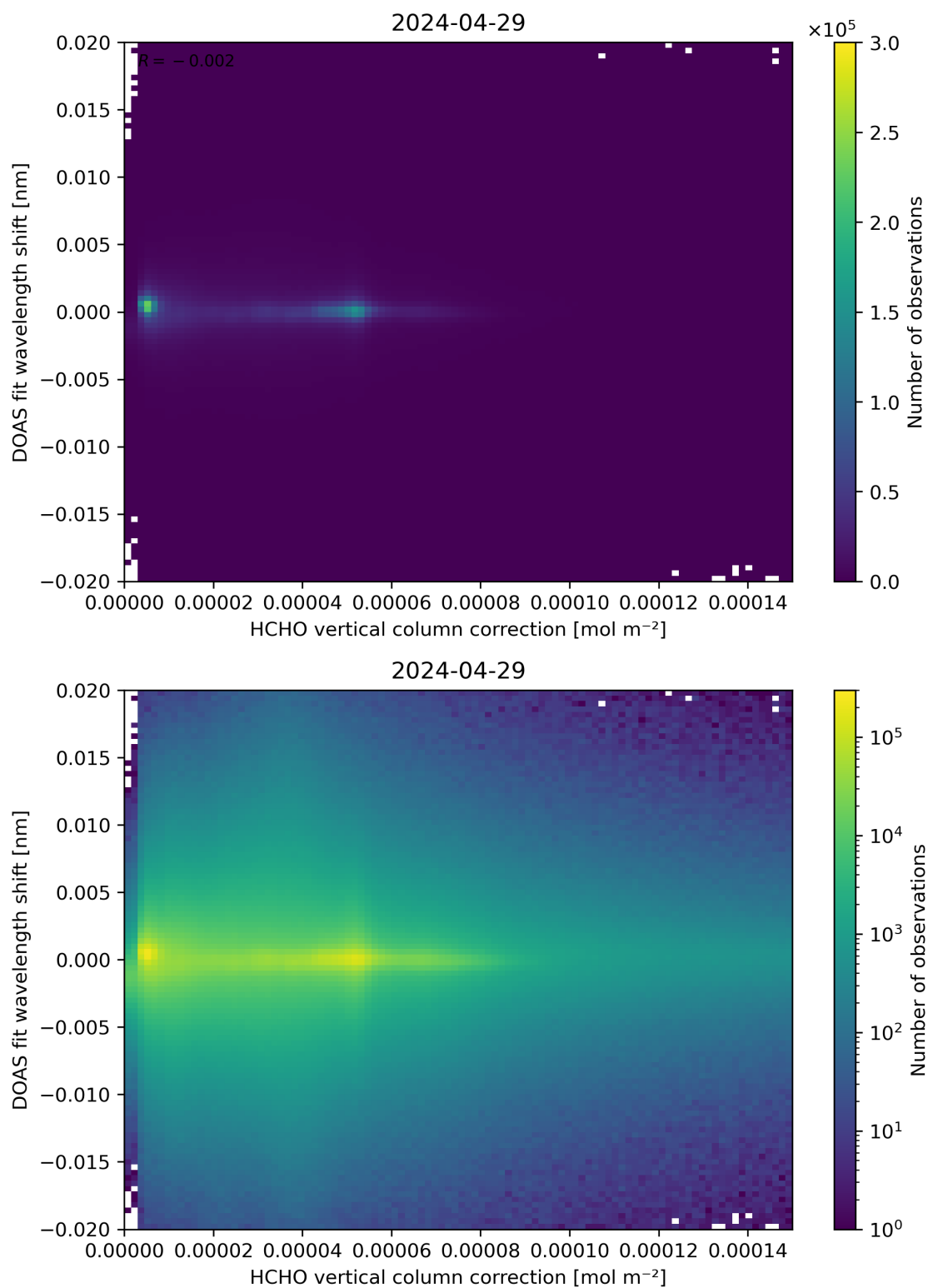
Figure 113: Scatter density plot of “HCHO vertical column correction” against “DOAS fit wavelength shift” for 2024-04-28 to 2024-04-30.
