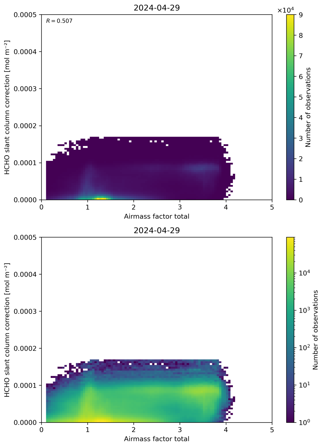
Figure 102: Scatter density plot of “Airmass factor total” against “HCHO slant column correction” for 2024-04-28 to 2024-04-30.
