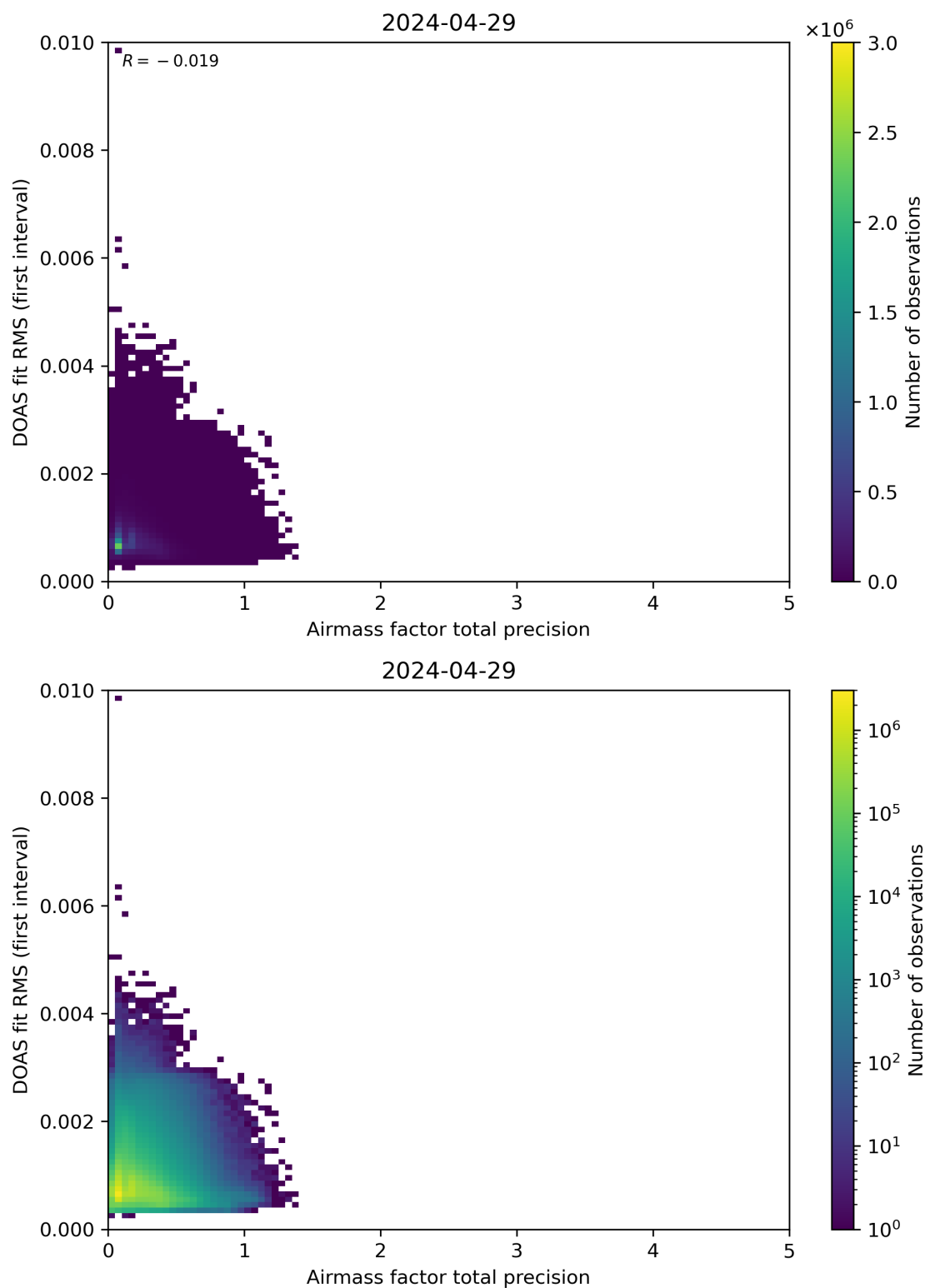
Figure 105: Scatter density plot of “Airmass factor total precision” against “DOAS fit RMS (first interval)” for 2024-04-28 to 2024-04-30.
