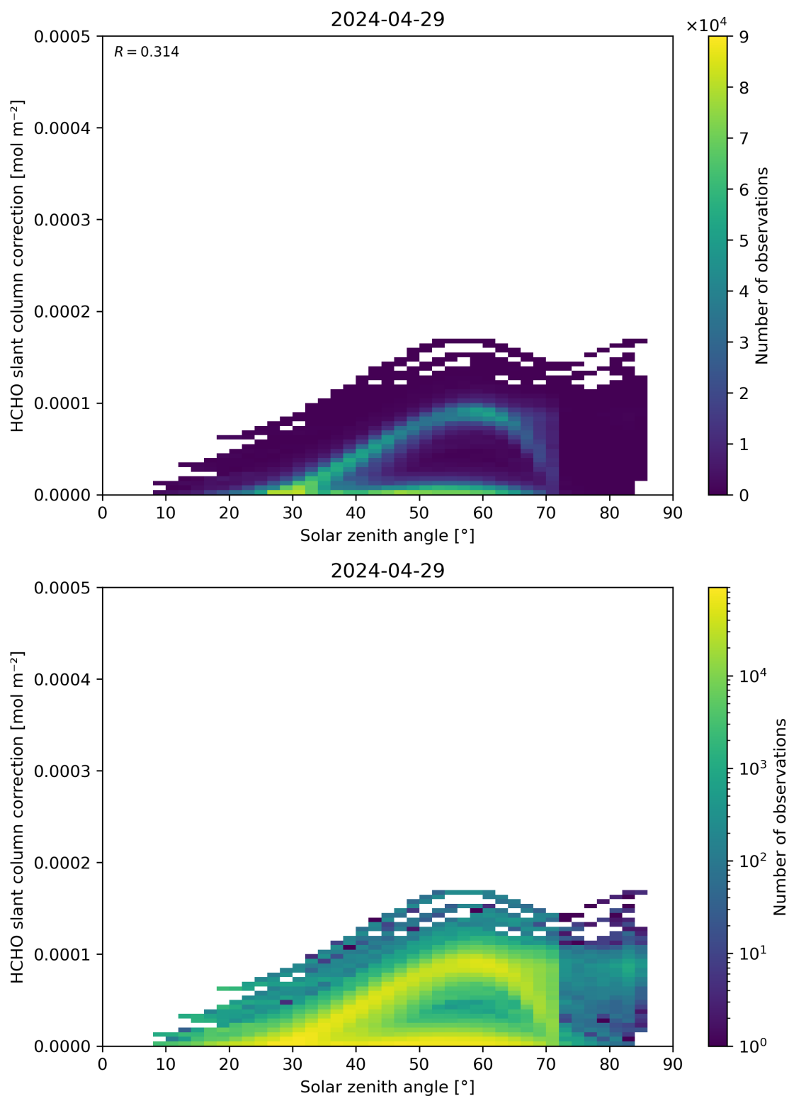
Figure 172: Scatter density plot of “Solar zenith angle” against “HCHO slant column correction” for 2024-04-28 to 2024-04-30.
