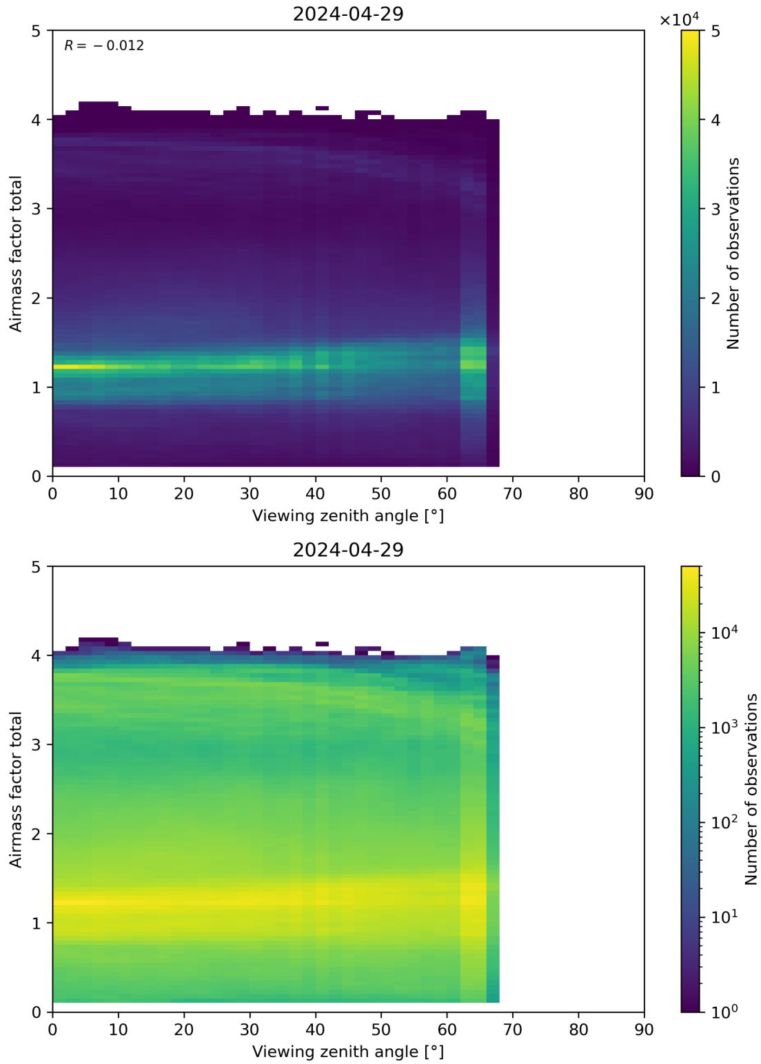
Figure 190: Scatter density plot of “Viewing zenith angle” against “Airmass factor total” for 2024-04-28 to 2024-04-30.
