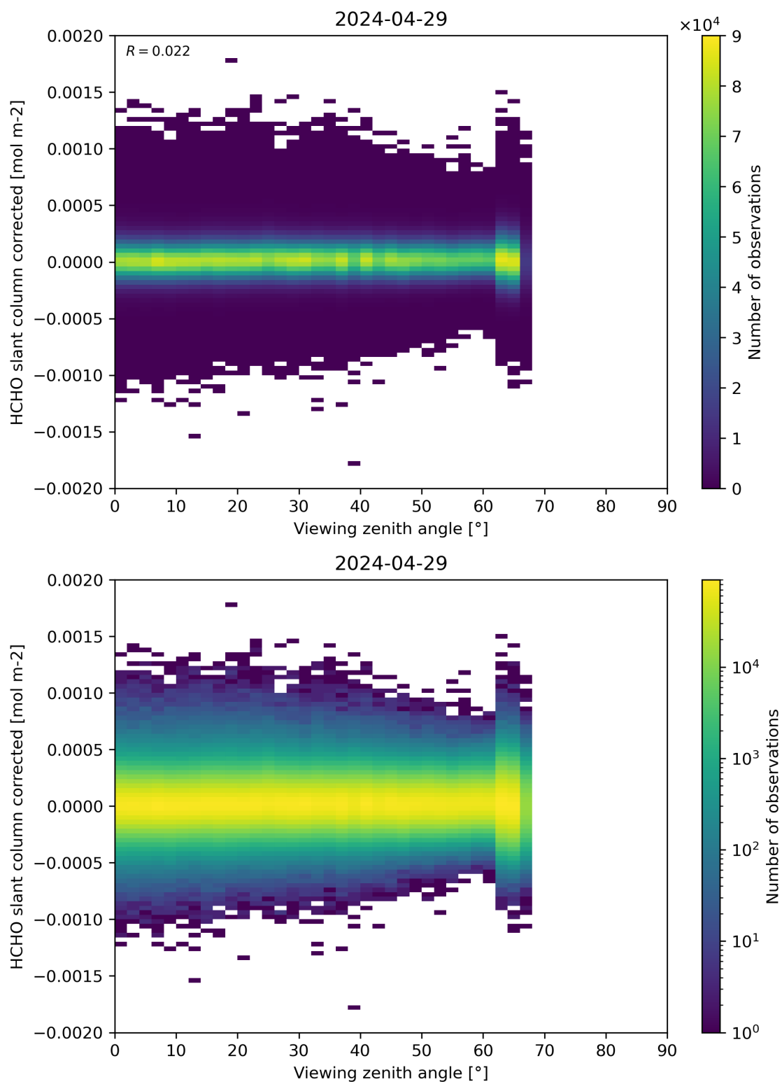
Figure 186: Scatter density plot of “Viewing zenith angle” against “HCHO slant column corrected” for 2024-04-28 to 2024-04-30.
