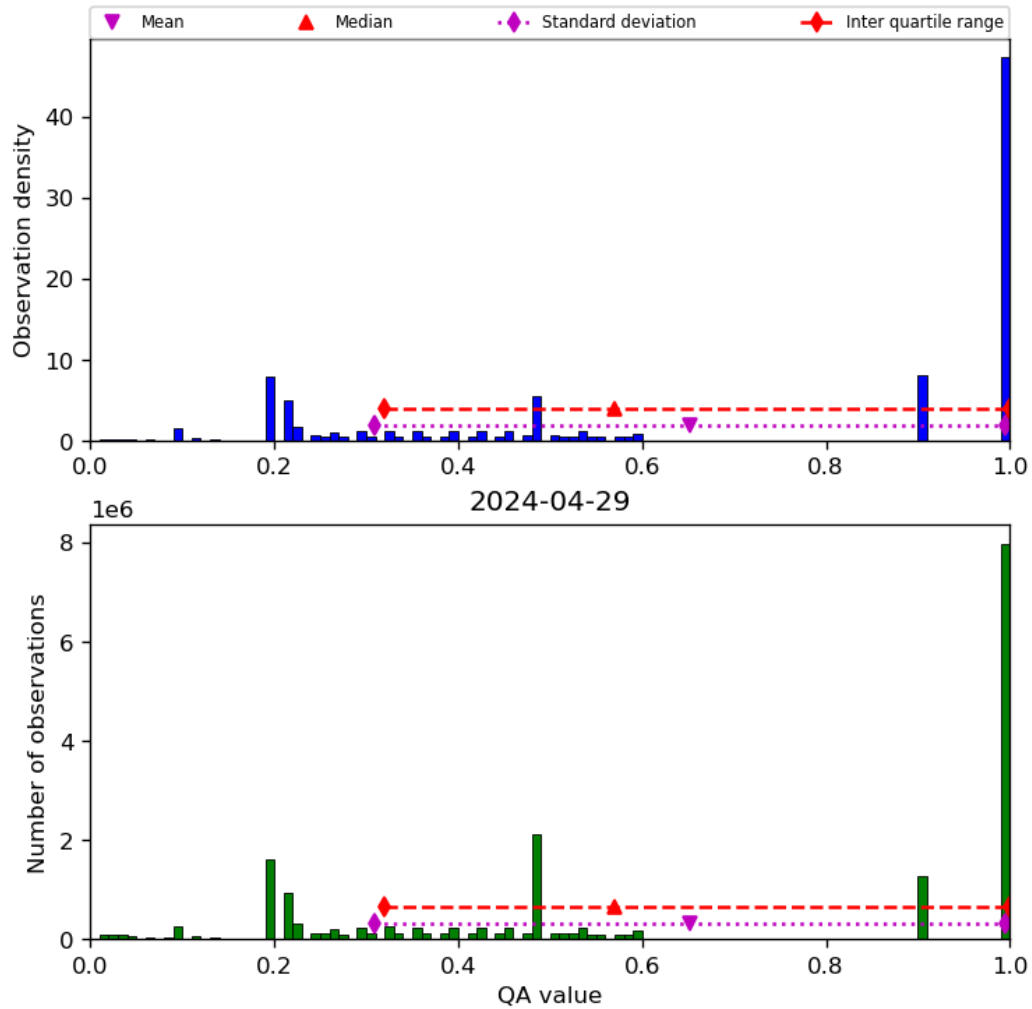
Figure 34: Histogram of “QA value” for 2024-04-28 to 2024-04-30
