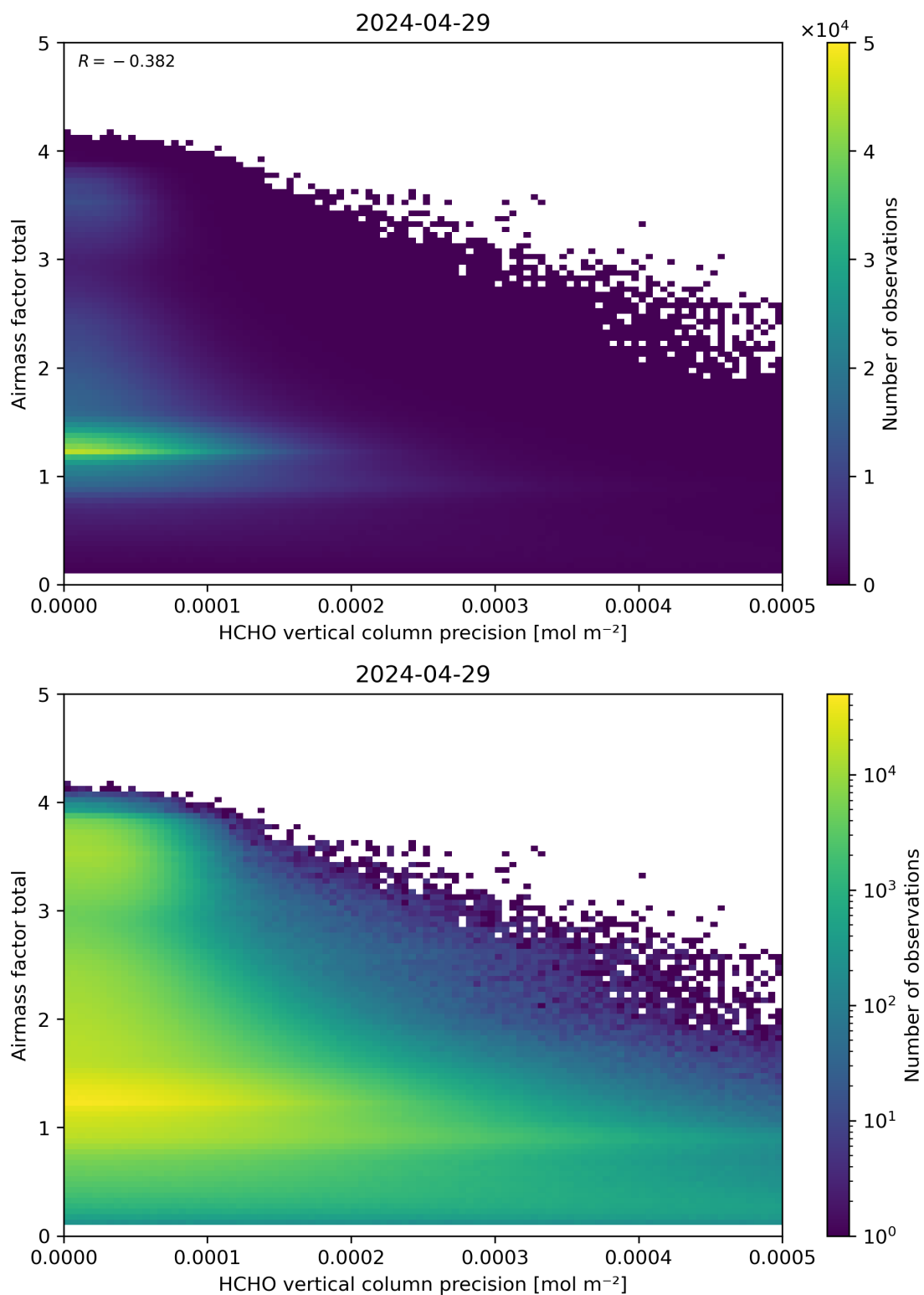
Figure 144: Scatter density plot of “HCHO vertical column precision” against “Airmass factor total” for 2024-04-28 to 2024-04-30.
