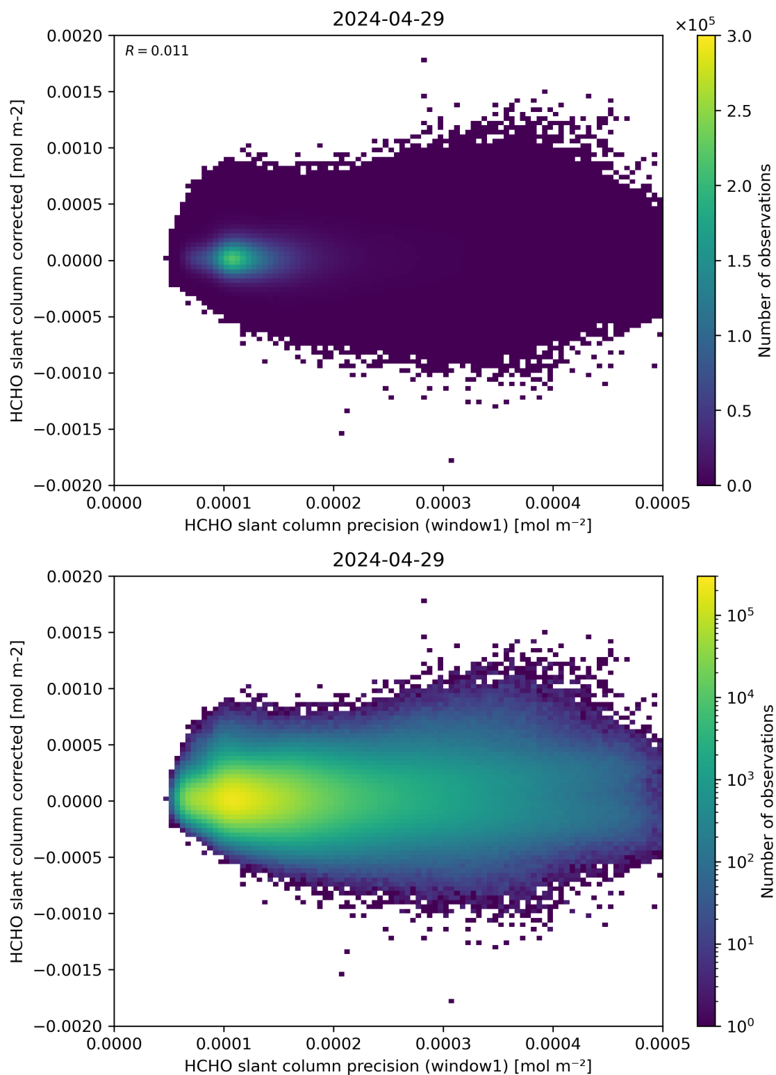
Figure 92: Scatter density plot of “HCHO slant column precision (window1)” against “HCHO slant column corrected” for 2024-04-28 to 2024-04-30.
