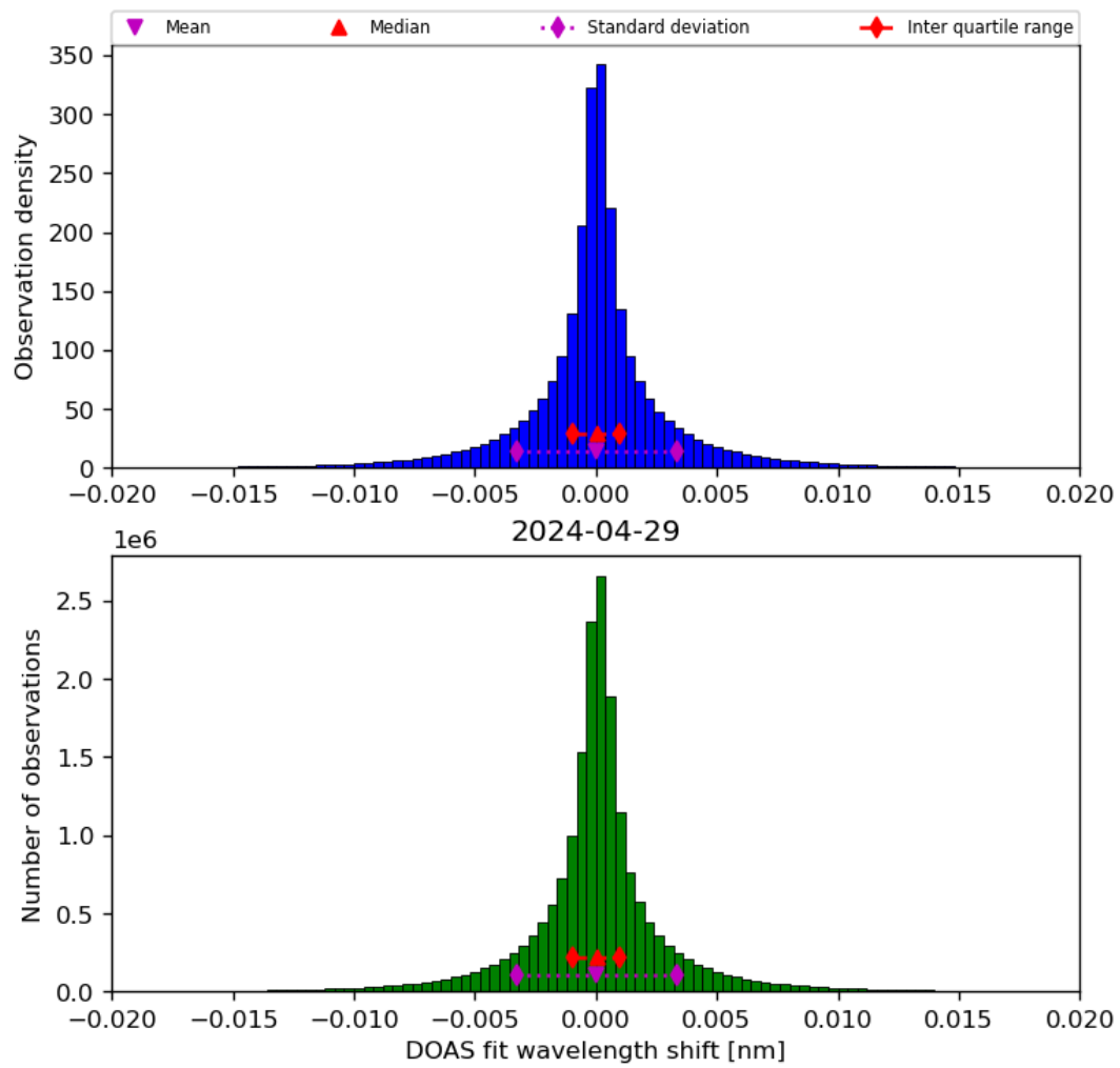
Figure 44: Histogram of “DOAS fit wavelength shift” for 2024-04-28 to 2024-04-30
