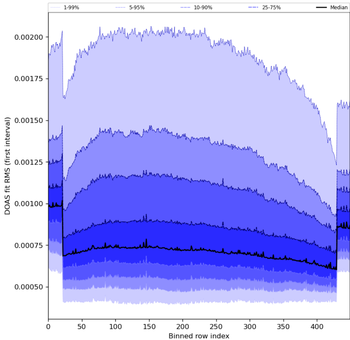
Figure 60: Along track statistics of “DOAS fit RMS (first interval)” for 2024-04-28 to 2024-04-30
