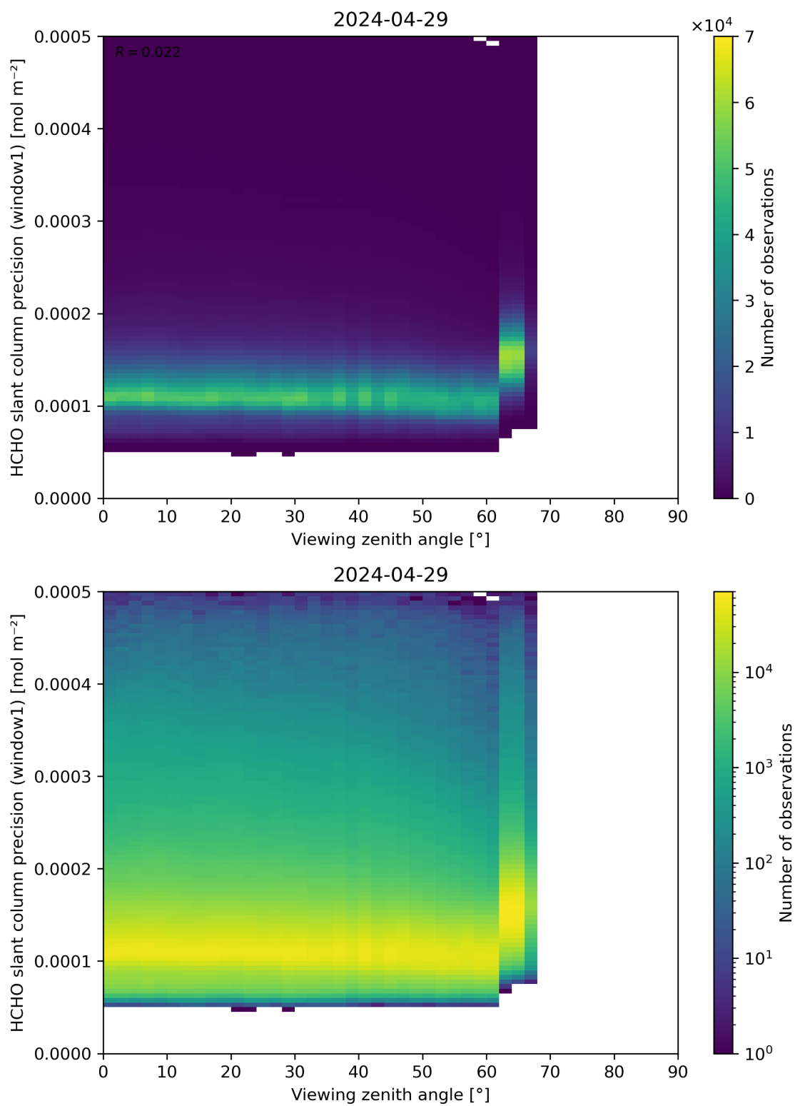
Figure 189: Scatter density plot of “Viewing zenith angle” against “HCHO slant column precision (window1)” for 2024-04-28 to 2024-04-30.
