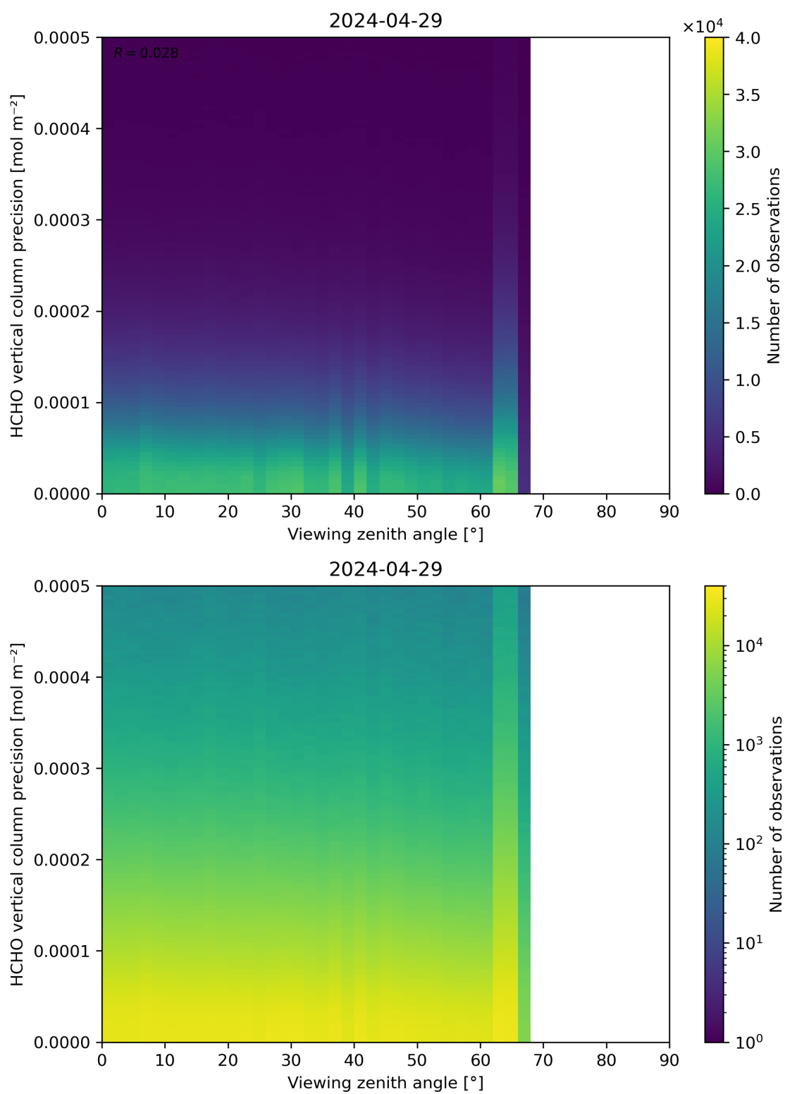
Figure 194: Scatter density plot of “Viewing zenith angle” against “HCHO vertical column precision” for 2024-04-28 to 2024-04-30.
