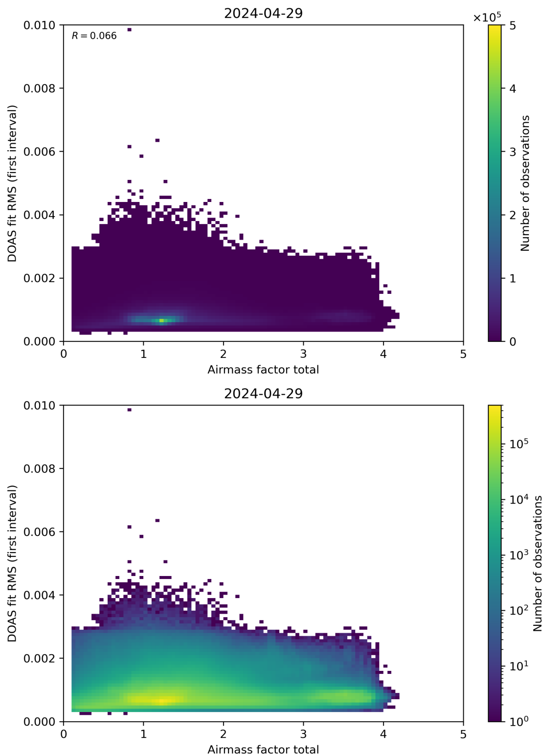
Figure 97: Scatter density plot of “Airmass factor total” against “DOAS fit RMS (first interval)” for 2024-04-28 to 2024-04-30.
