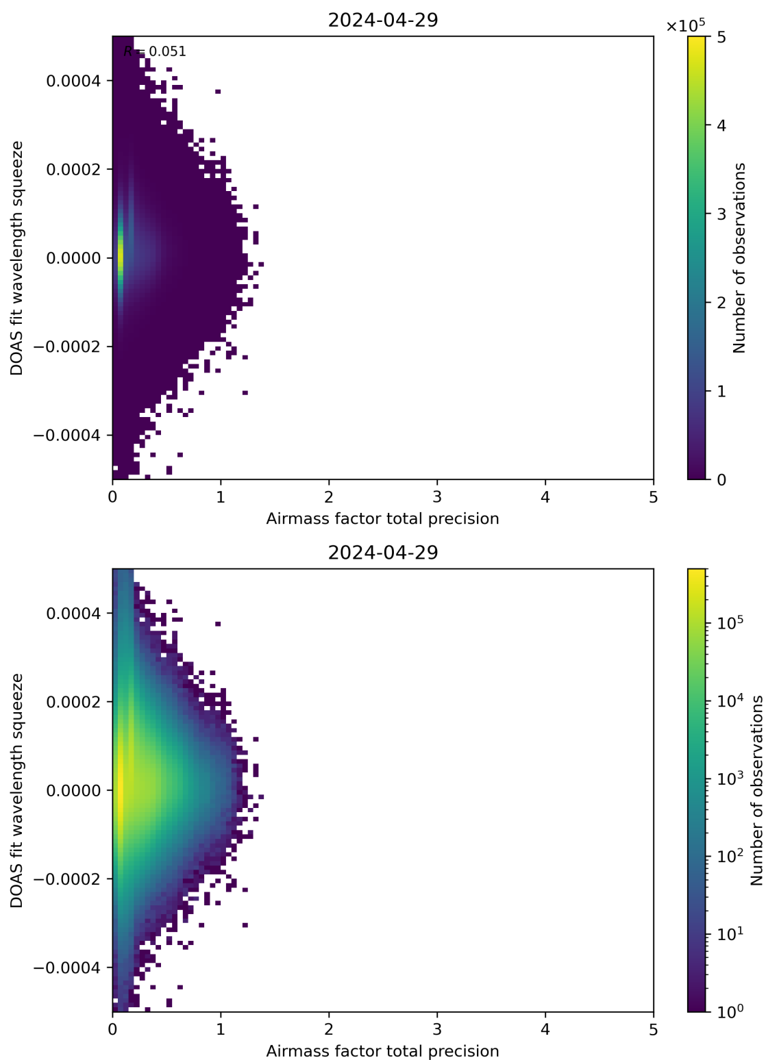
Figure 107: Scatter density plot of “Airmass factor total precision” against “DOAS fit wavelength squeeze” for 2024-04-28 to 2024-04-30.
