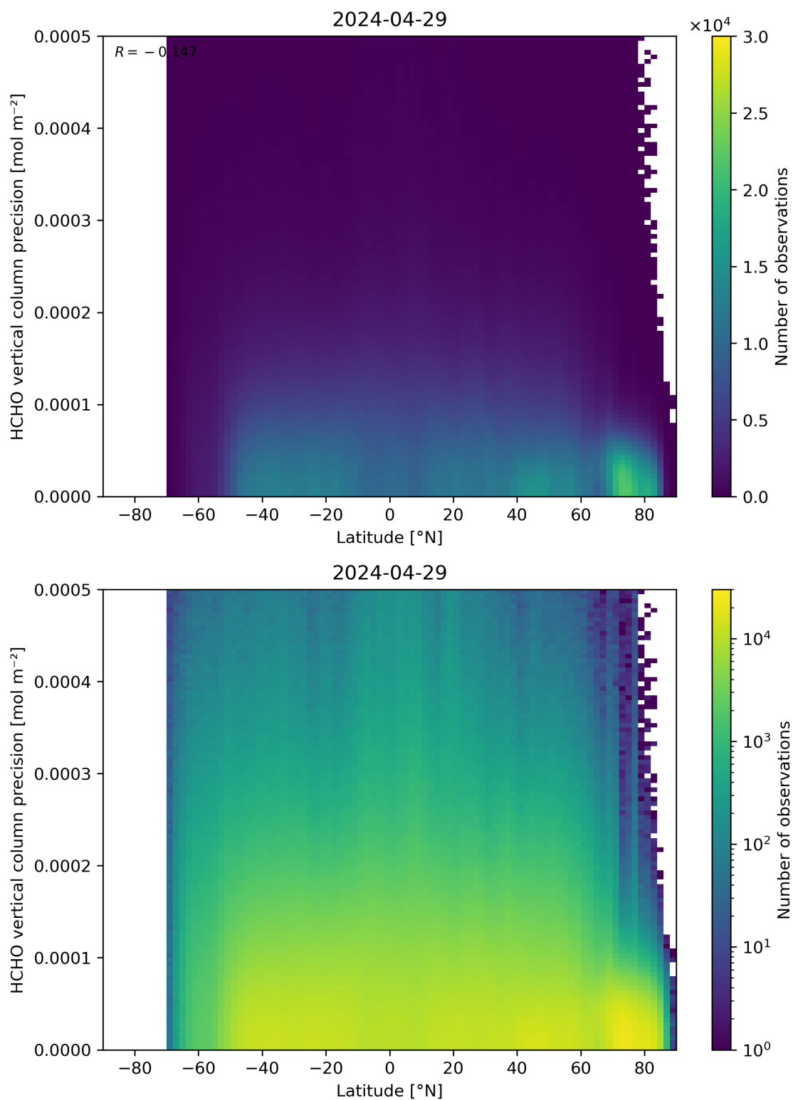
Figure 165: Scatter density plot of “Latitude” against “HCHO vertical column precision” for 2024-04-28 to 2024-04-30.
