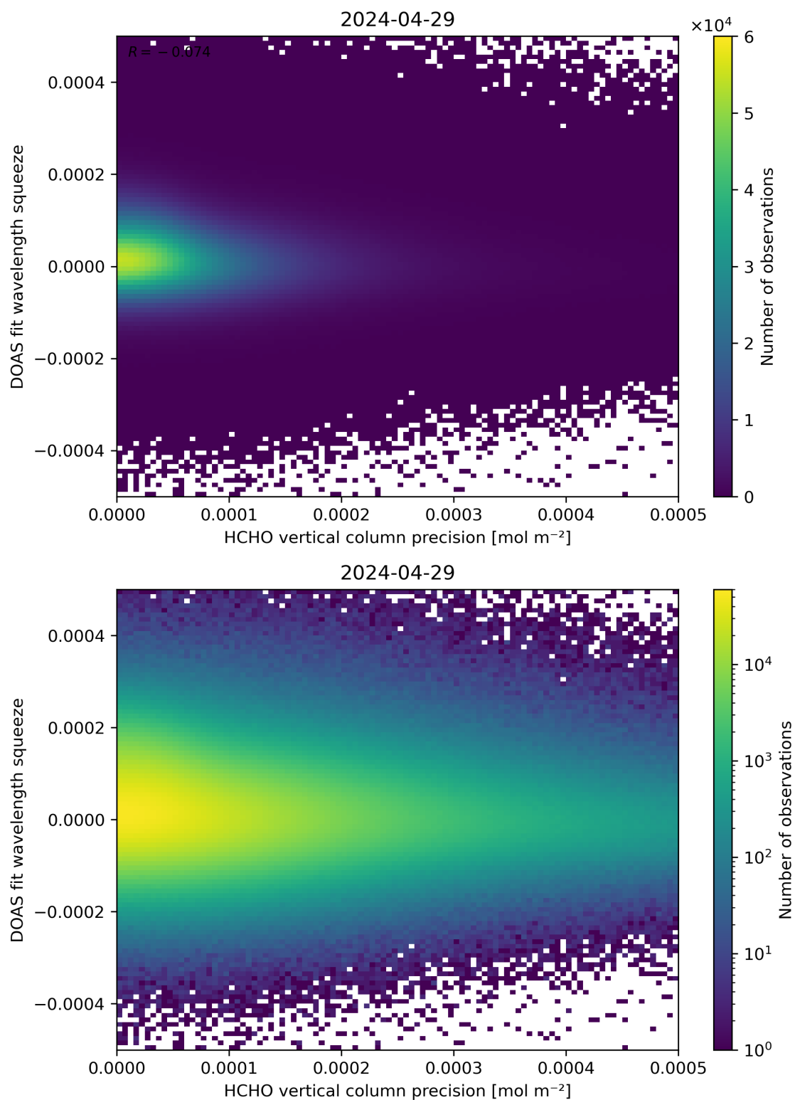
Figure 138: Scatter density plot of “HCHO vertical column precision” against “DOAS fit wavelength squeeze” for 2024-04-28 to 2024-04-30.
