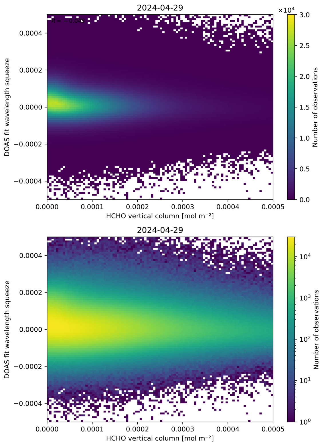
Figure 125: Scatter density plot of “HCHO vertical column” against “DOAS fit wavelength squeeze” for 2024-04-28 to 2024-04-30.
