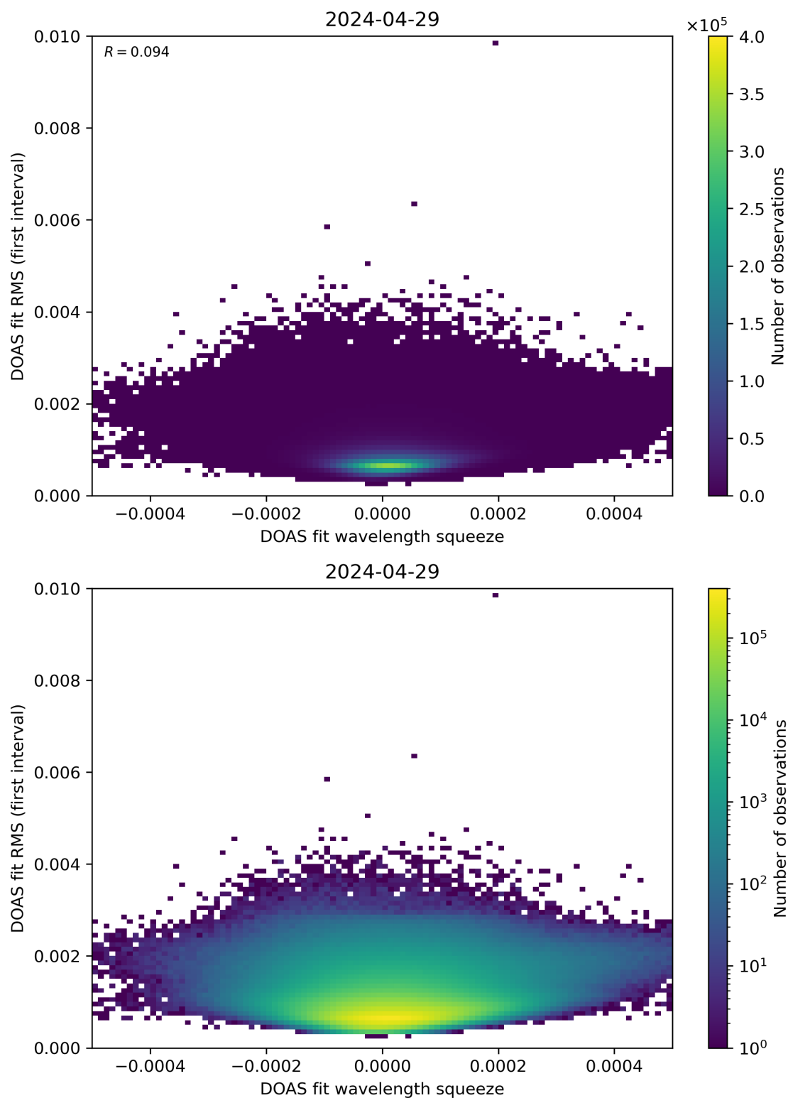
Figure 68: Scatter density plot of “DOAS fit wavelength squeeze” against “DOAS fit RMS (first interval)” for 2024-04-28 to 2024-04-30.
