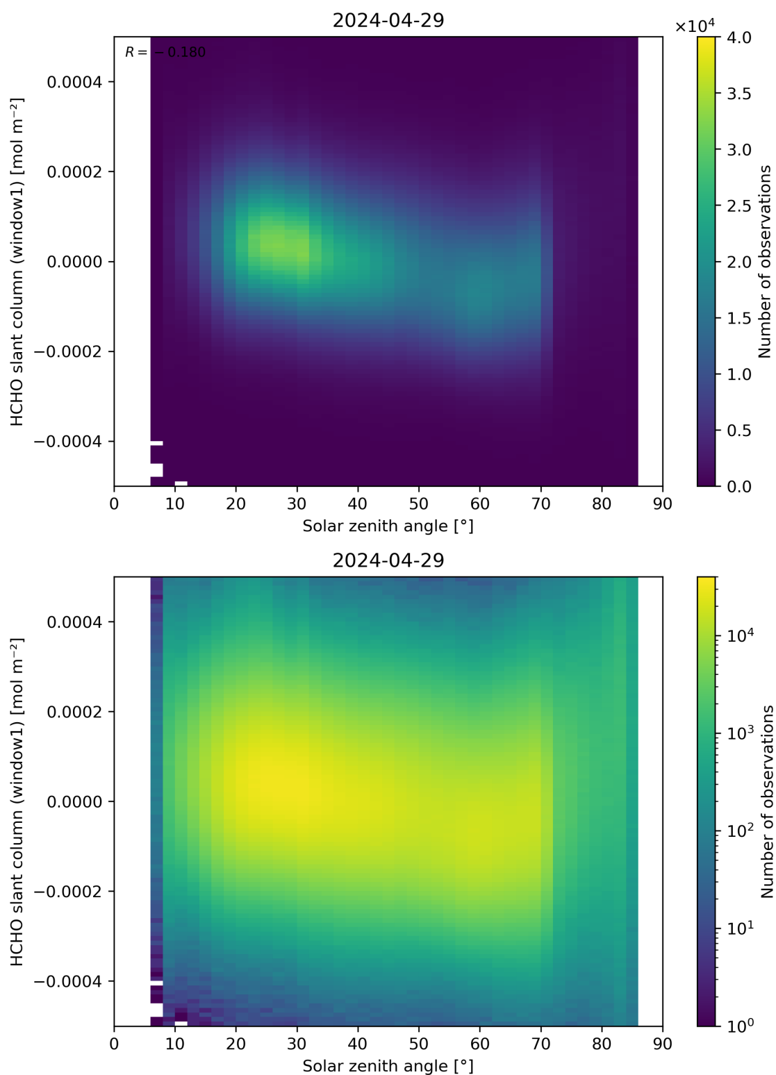
Figure 173: Scatter density plot of “Solar zenith angle” against “HCHO slant column (window1)” for 2024-04-28 to 2024-04-30.
