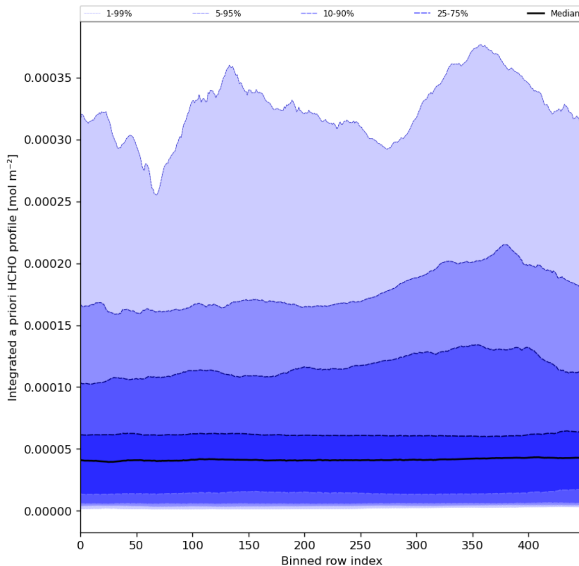
Figure 57: Along track statistics of “Integrated a priori HCHO profile” for 2024-04-28 to 2024-04-30
