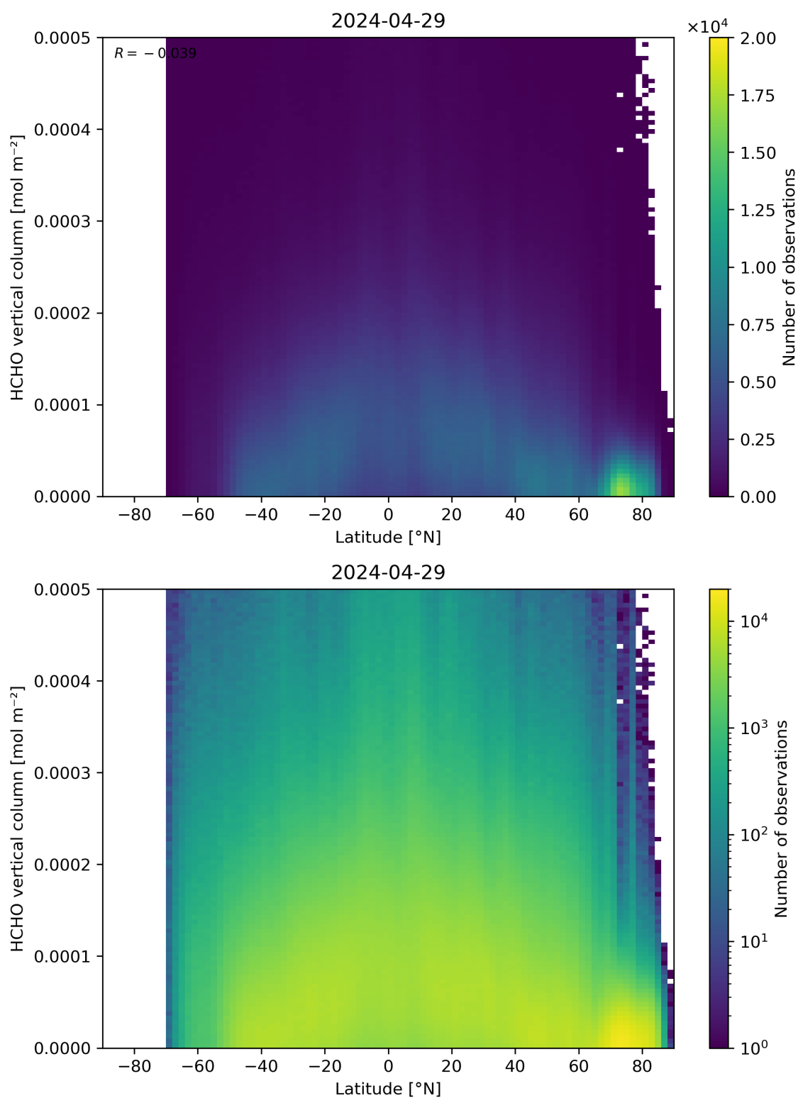
Figure 163: Scatter density plot of “Latitude” against “HCHO vertical column” for 2024-04-28 to 2024-04-30.
