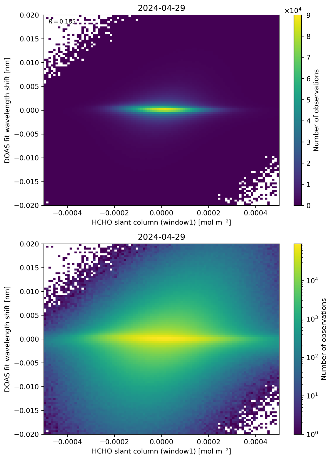
Figure 79: Scatter density plot of “HCHO slant column (window1)” against “DOAS fit wavelength shift” for 2024-04-28 to 2024-04-30.
