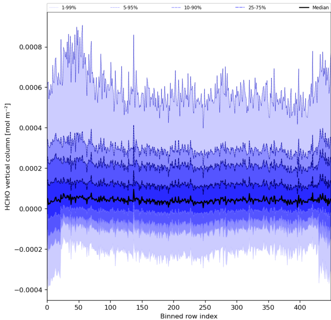
Figure 49: Along track statistics of “HCHO vertical column” for 2024-04-28 to 2024-04-30
