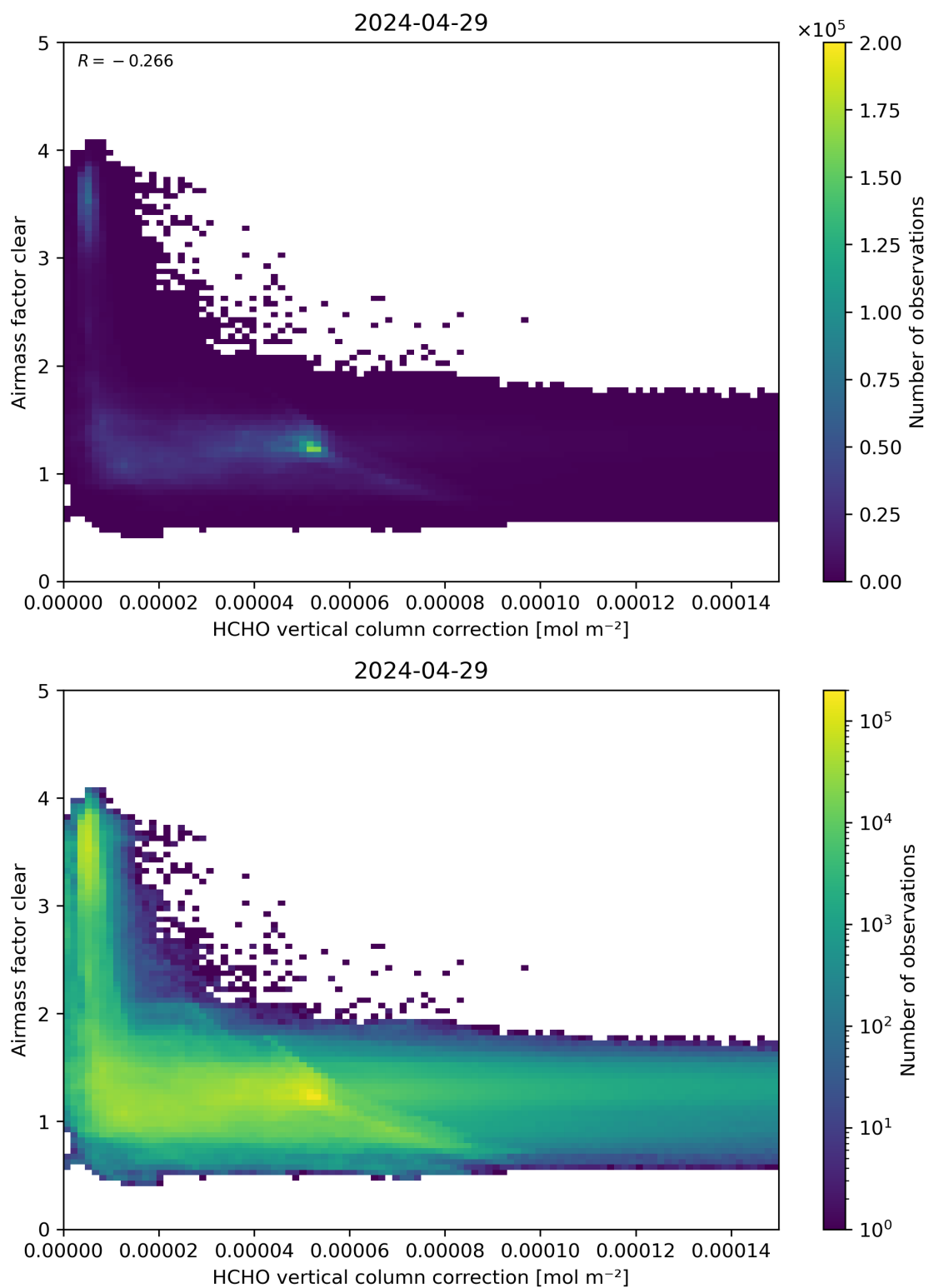
Figure 115: Scatter density plot of “HCHO vertical column correction” against “Airmass factor clear” for 2024-04-28 to 2024-04-30.
