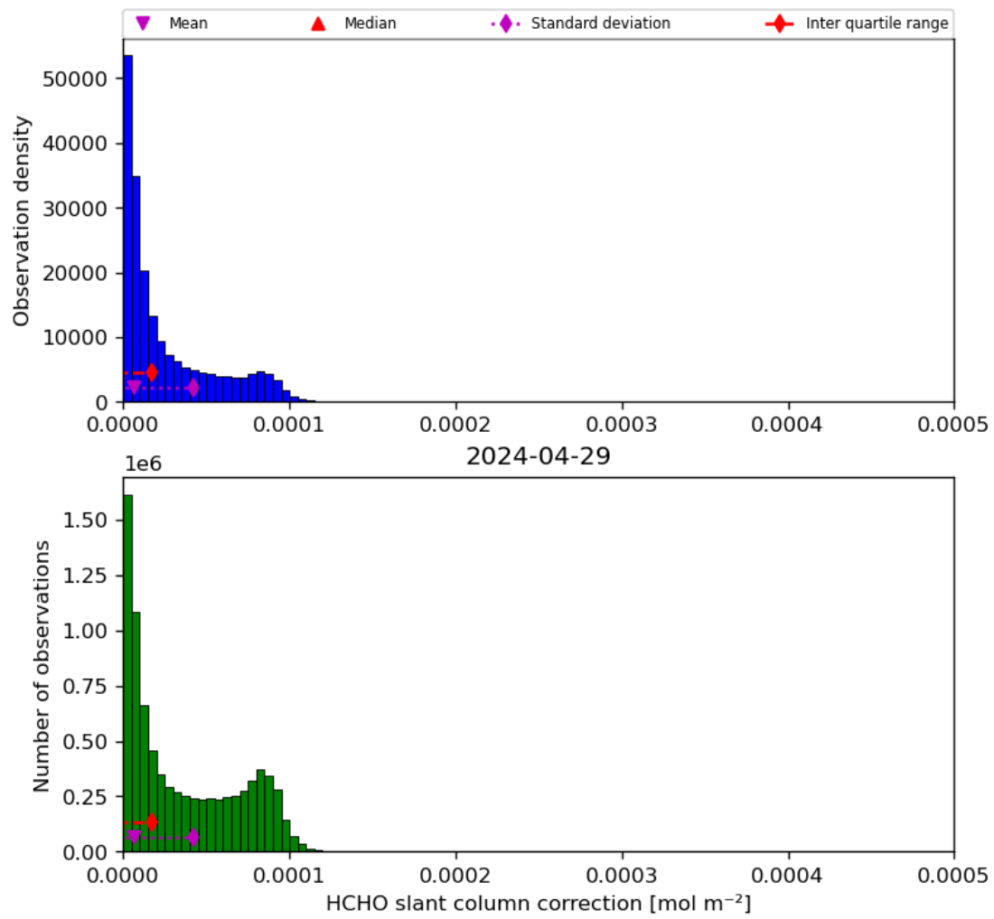
Figure 47: Histogram of “HCHO slant column correction” for 2024-04-28 to 2024-04-30
