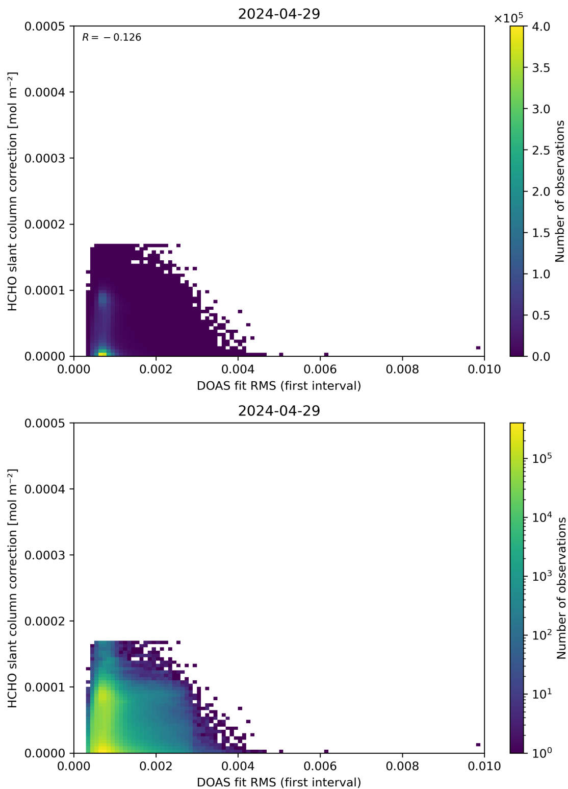
Figure 63: Scatter density plot of “DOAS fit RMS (first interval)” against “HCHO slant column correction” for 2024-04-28 to 2024-04-30.
