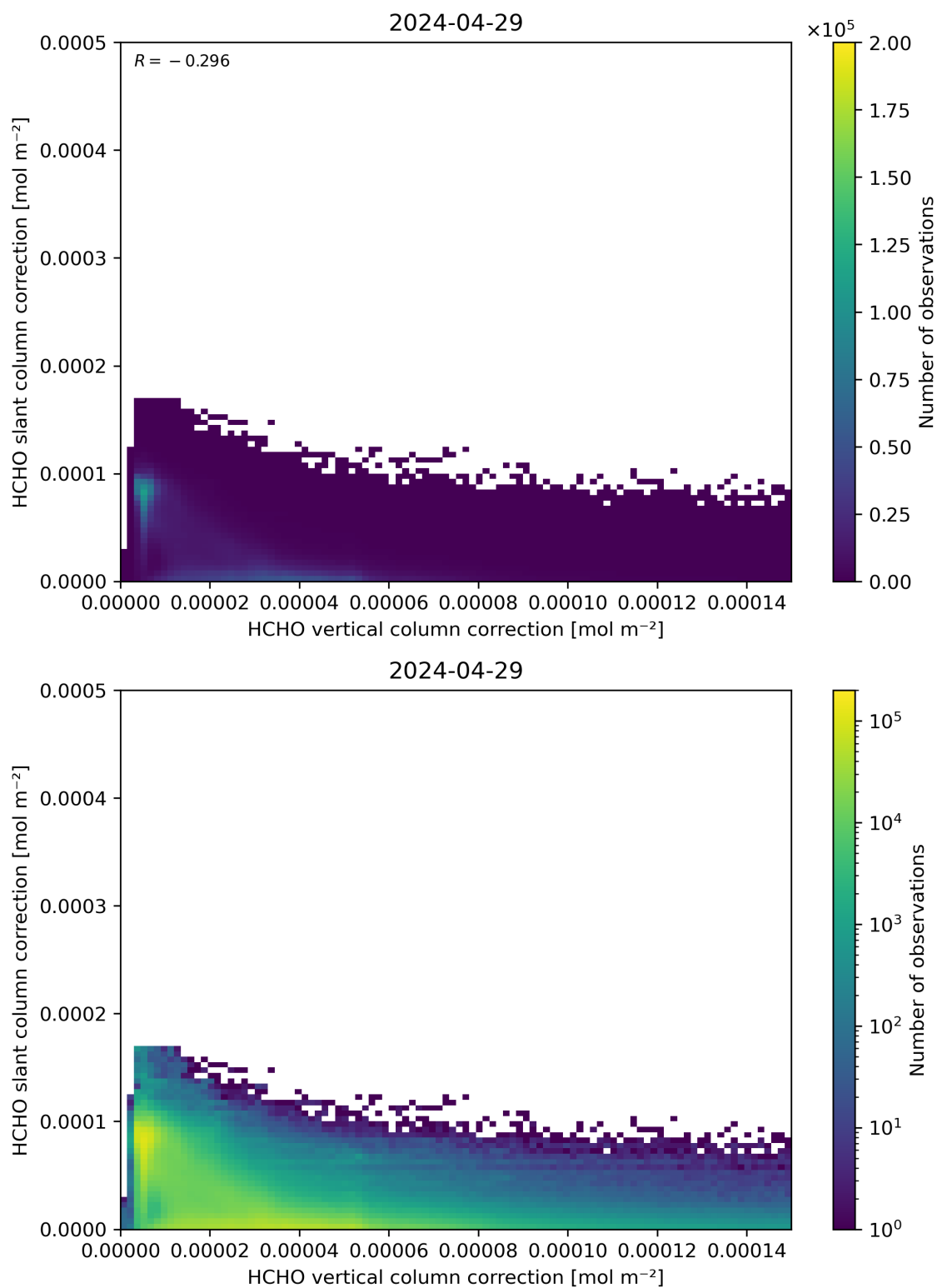
Figure 117: Scatter density plot of “HCHO vertical column correction” against “HCHO slant column correction” for 2024-04-28 to 2024-04-30.
