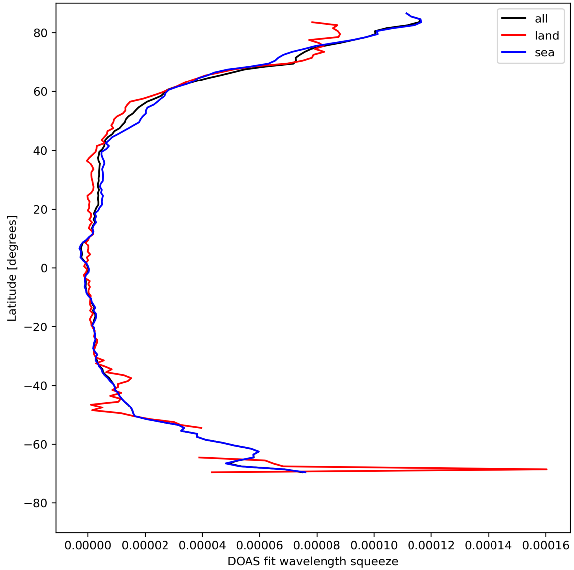
Figure 31: Zonal average of “DOAS fit wavelength squeeze” for 2024-04-28 to 2024-04-30.
