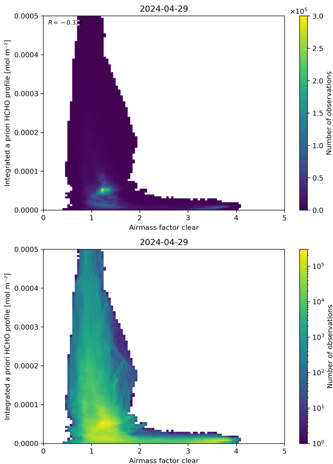
Figure 76: Scatter density plot of “Airmass factor clear” against “Integrated a priori HCHO profile” for 2024-04-28 to 2024-04-30.
