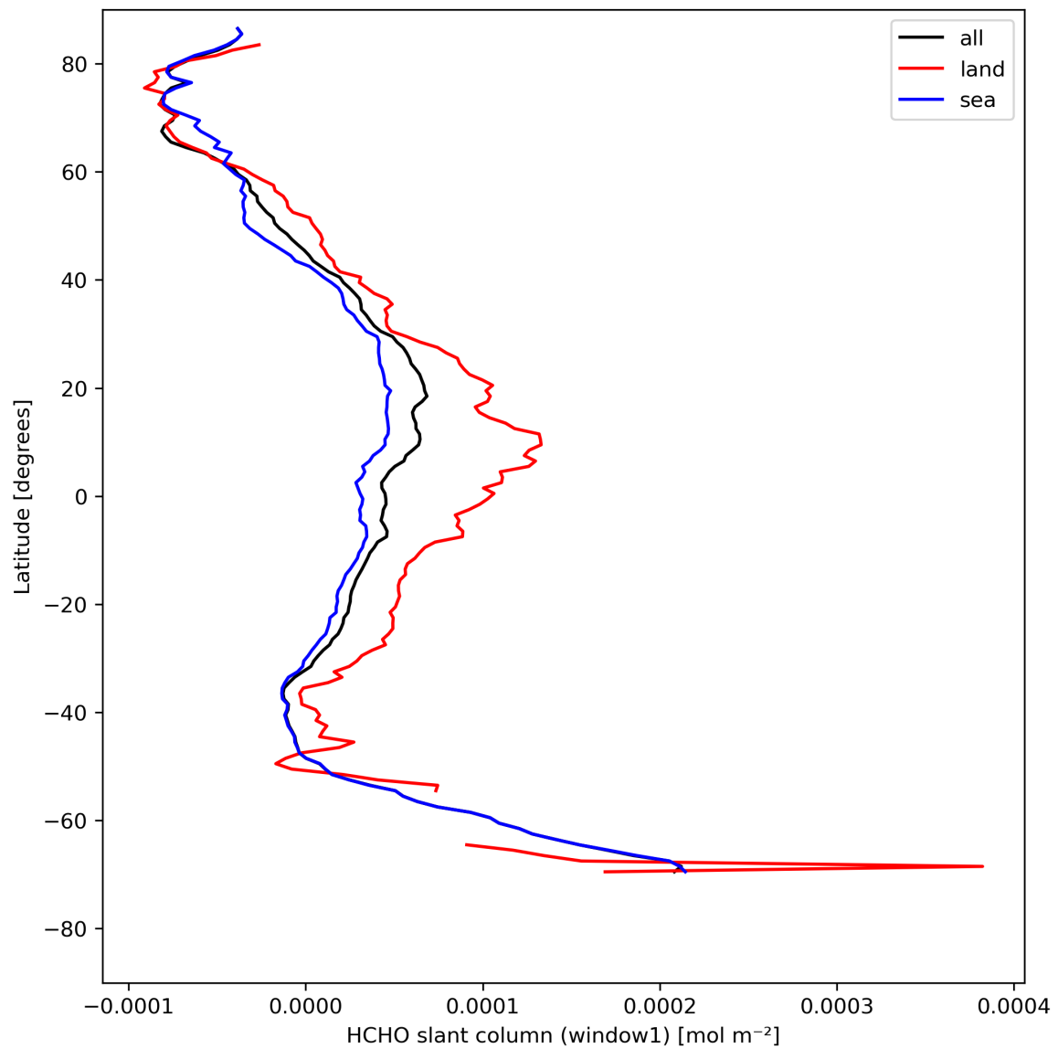
Figure 24: Zonal average of “HCHO slant column (window1)” for 2024-04-28 to 2024-04-30.
