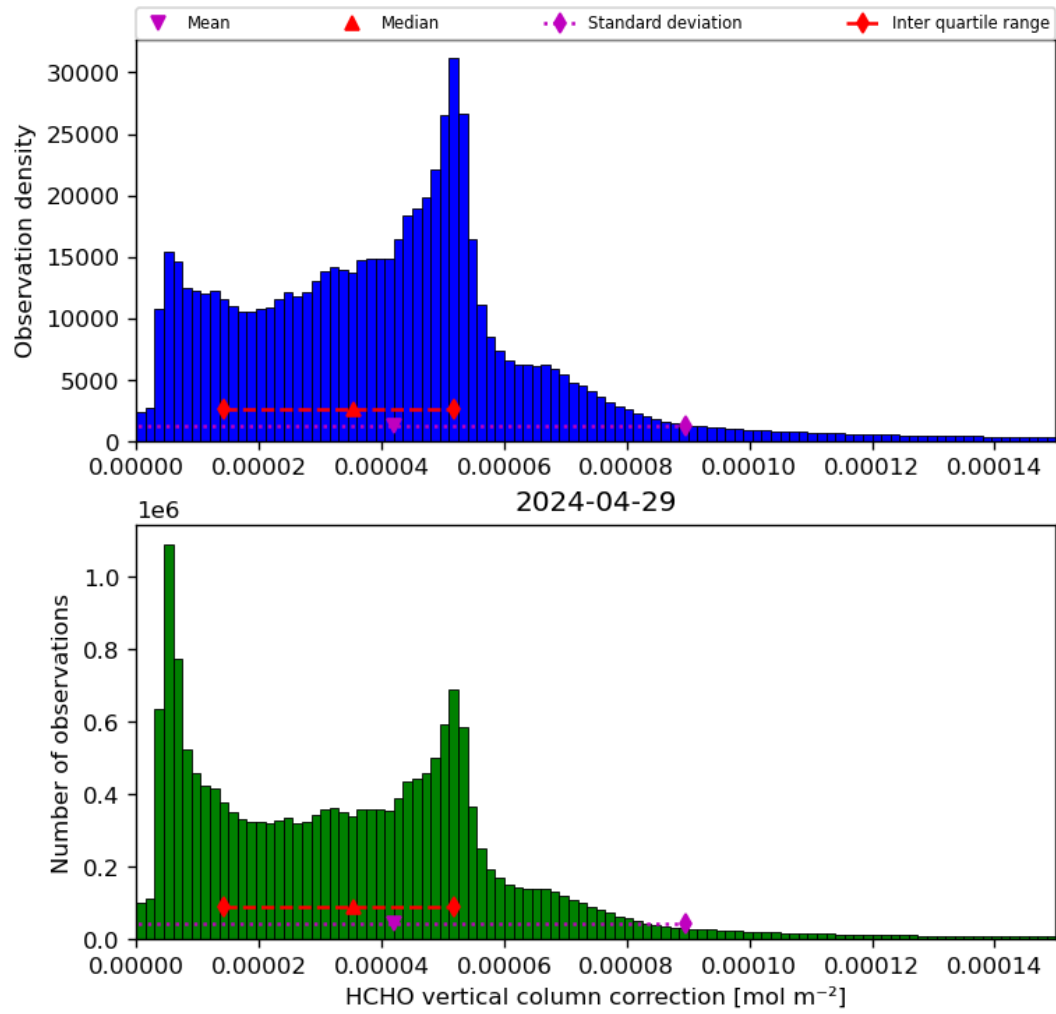
Figure 37: Histogram of “HCHO vertical column correction” for 2024-04-28 to 2024-04-30
