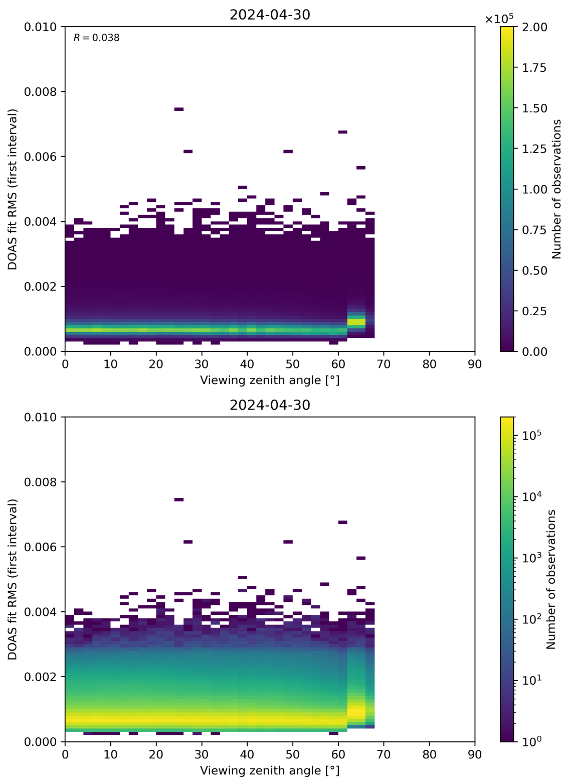
Figure 182: Scatter density plot of “Viewing zenith angle” against “DOAS fit RMS (first interval)” for 2024-04-29 to 2024-05-01.
