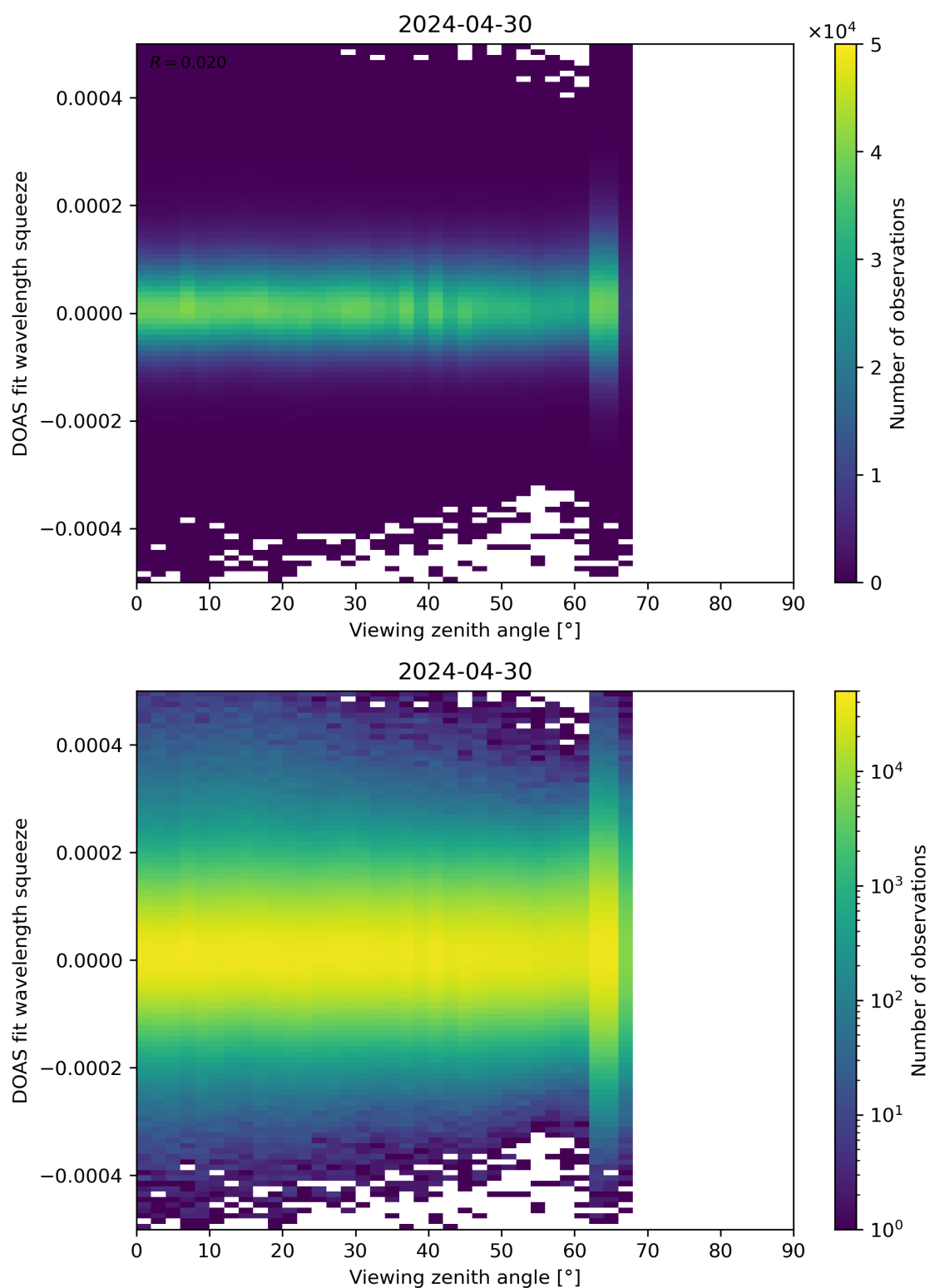
Figure 184: Scatter density plot of “Viewing zenith angle” against “DOAS fit wavelength squeeze” for 2024-04-29 to 2024-05-01.
