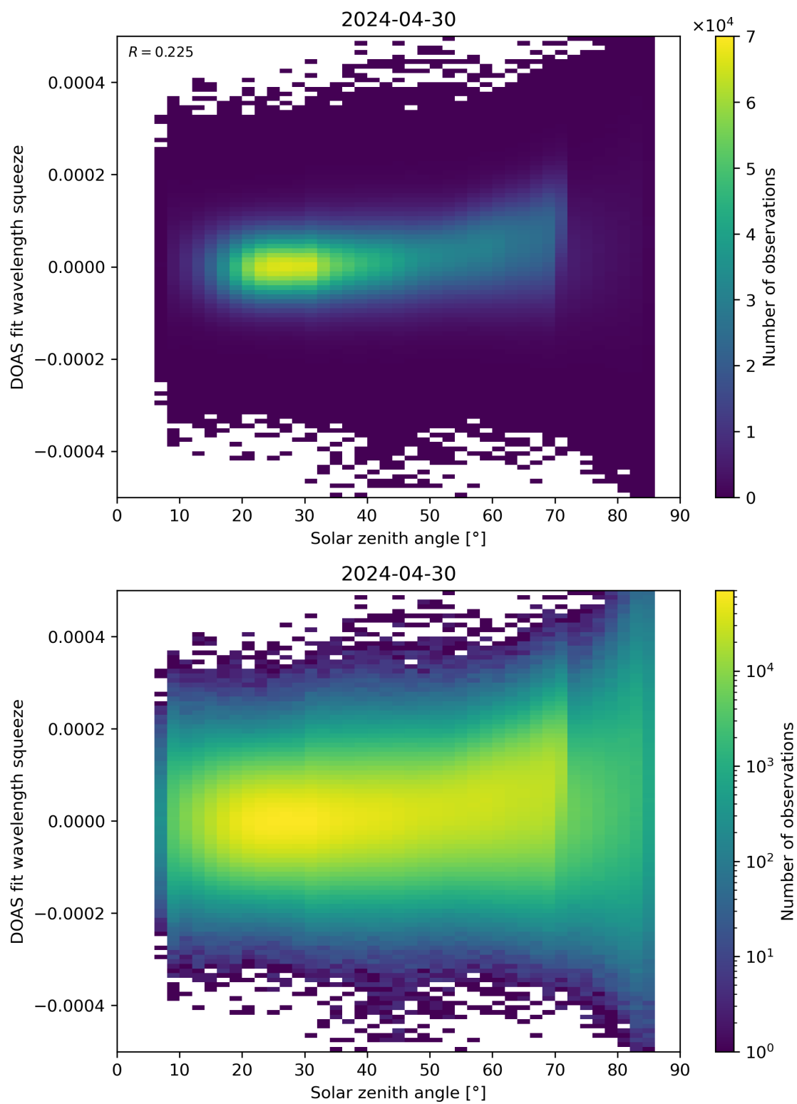
Figure 169: Scatter density plot of “Solar zenith angle” against “DOAS fit wavelength squeeze” for 2024-04-29 to 2024-05-01.
