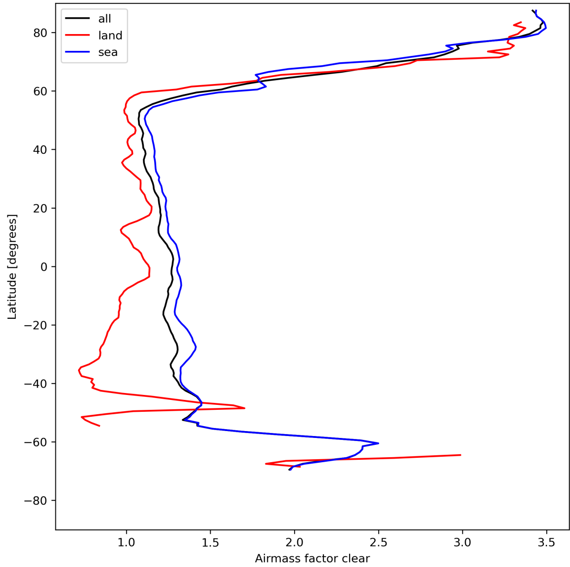
Figure 28: Zonal average of “Airmass factor clear” for 2024-04-29 to 2024-05-01.
