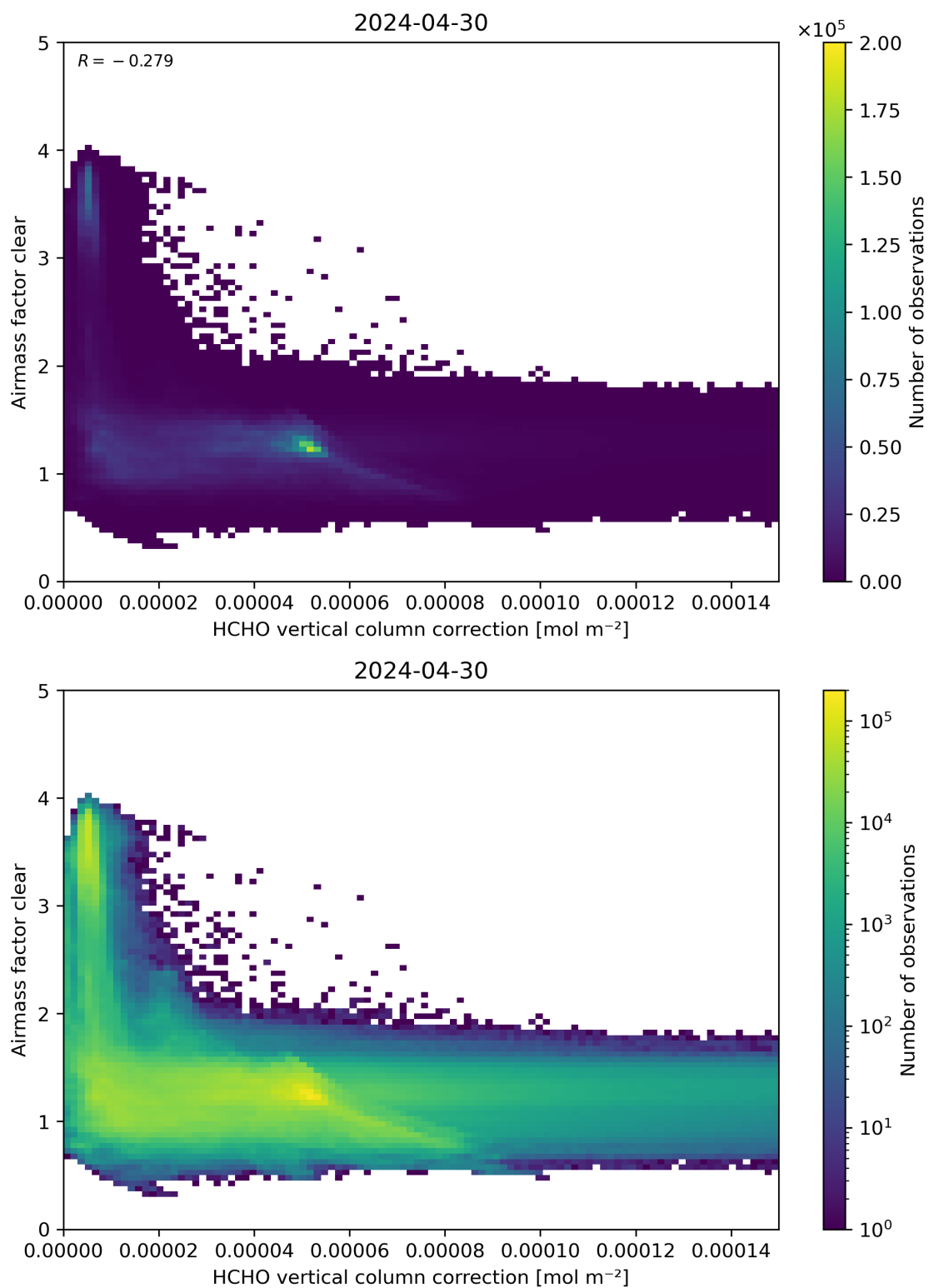
Figure 115: Scatter density plot of “HCHO vertical column correction” against “Airmass factor clear” for 2024-04-29 to 2024-05-01.
