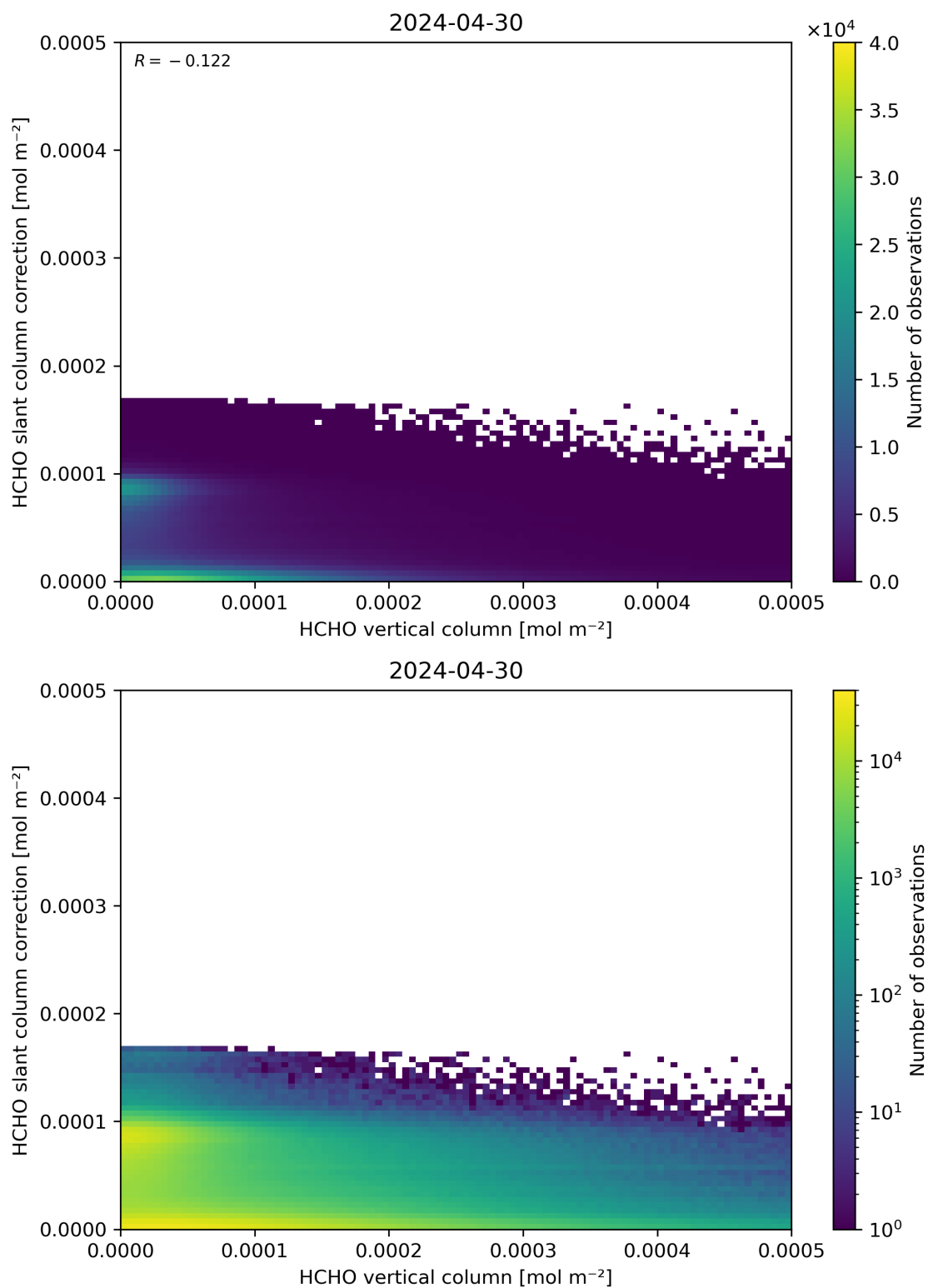
Figure 128: Scatter density plot of “HCHO vertical column” against “HCHO slant column correction” for 2024-04-29 to 2024-05-01.
