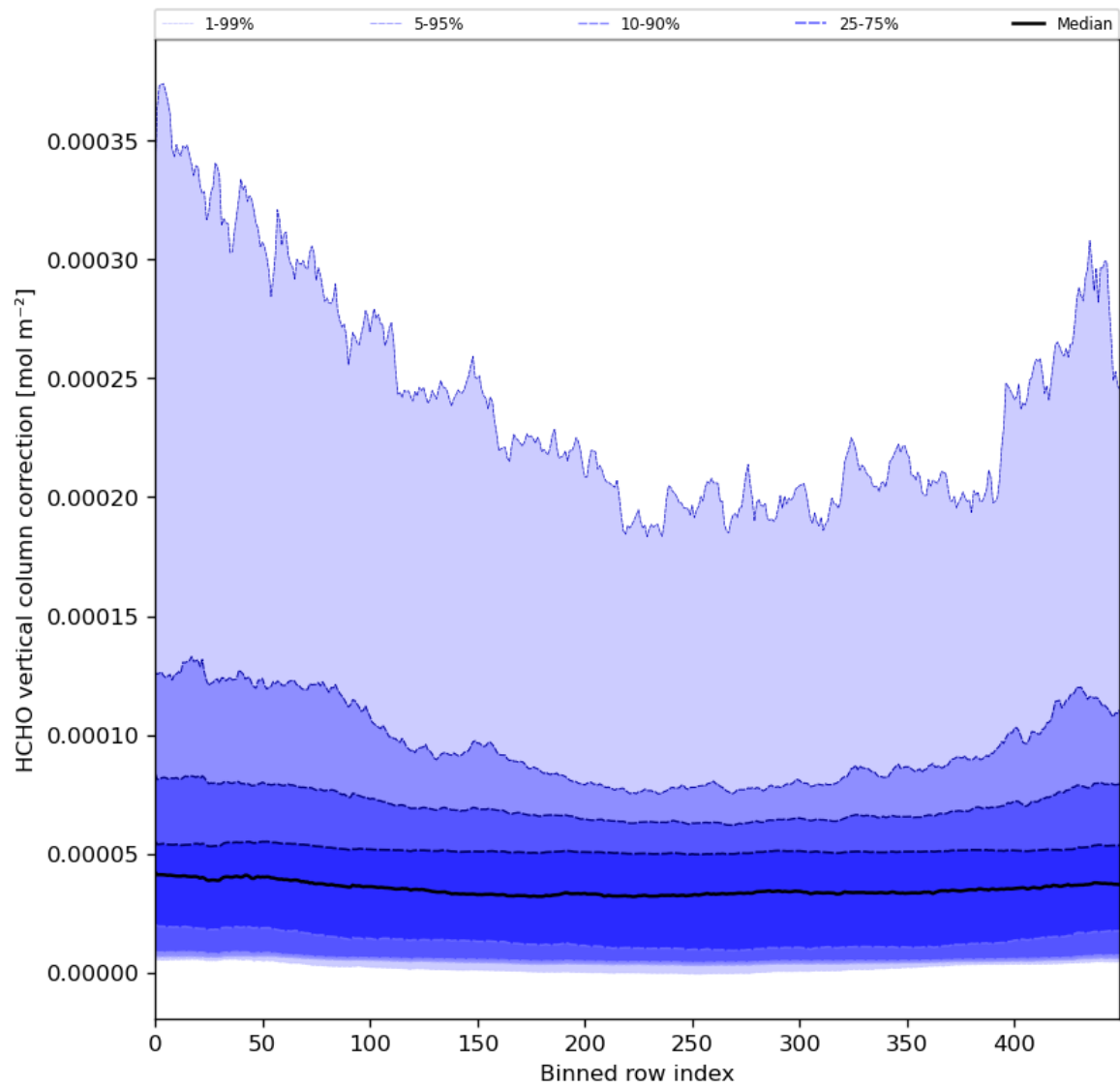
Figure 51: Along track statistics of “HCHO vertical column correction” for 2024-04-29 to 2024-05-01
