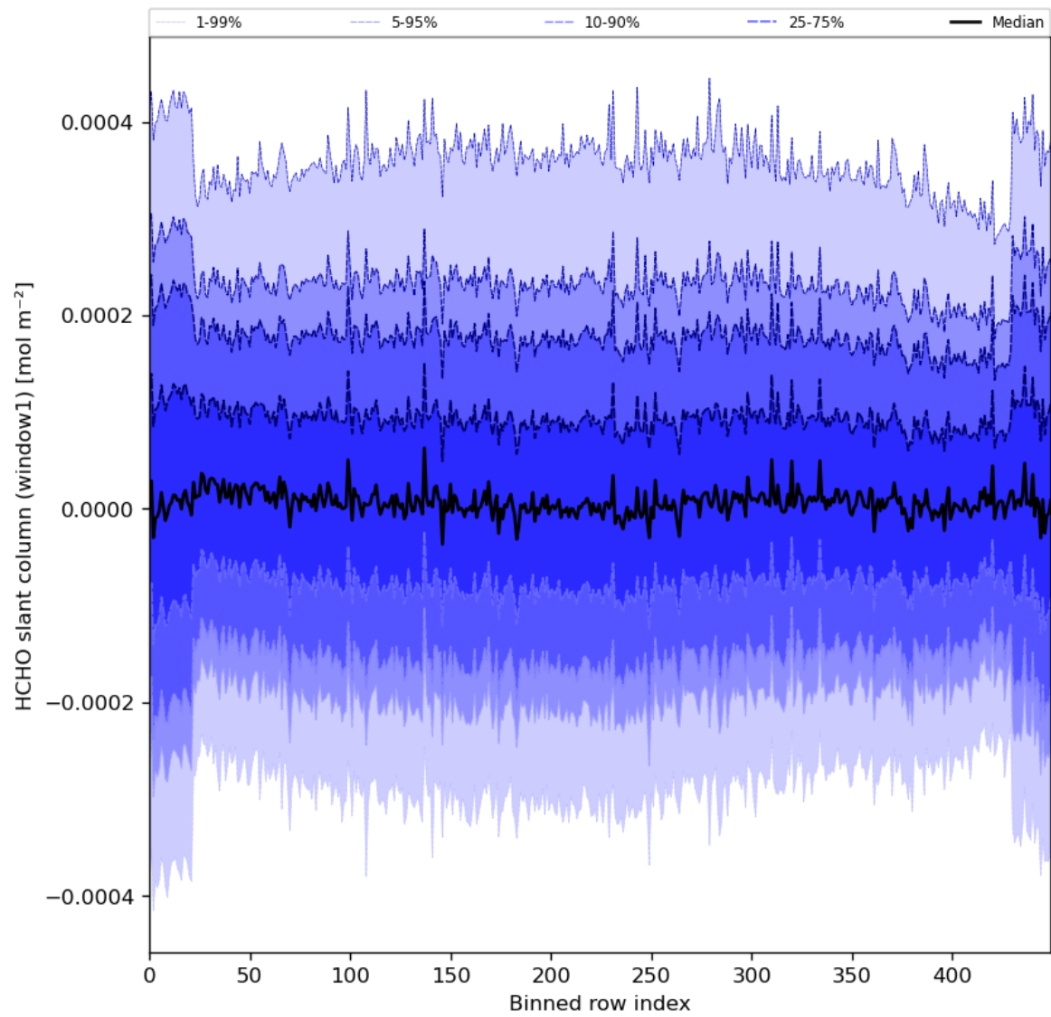
Figure 52: Along track statistics of “HCHO slant column (window1)” for 2024-04-29 to 2024-05-01
