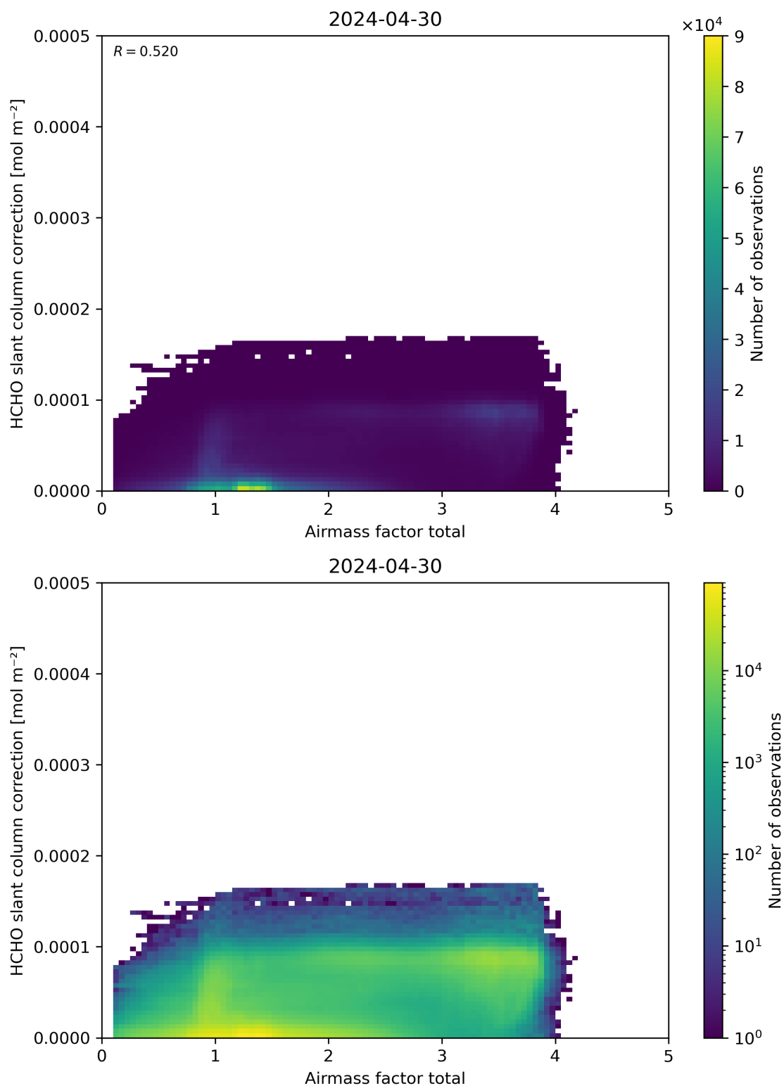
Figure 102: Scatter density plot of “Airmass factor total” against “HCHO slant column correction” for 2024-04-29 to 2024-05-01.
