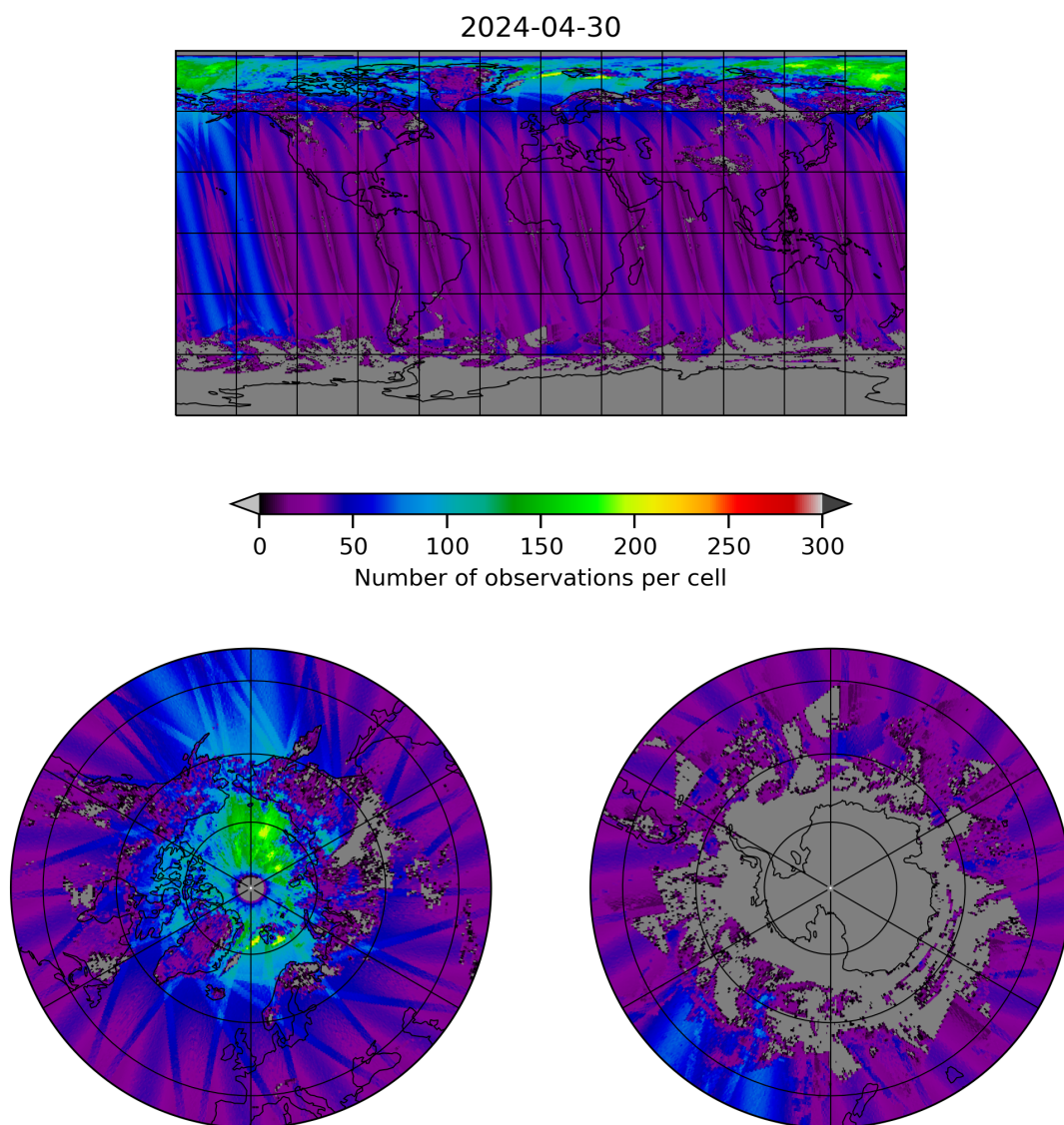
Figure 19: Map of the number of observations for 2024-04-29 to 2024-05-01
