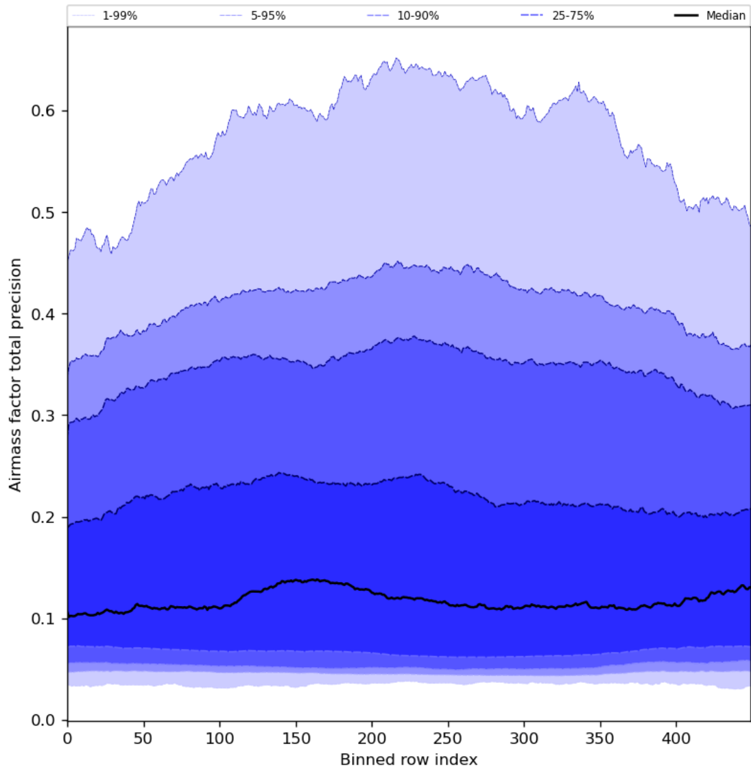
Figure 55: Along track statistics of “Airmass factor total precision” for 2024-04-29 to 2024-05-01
