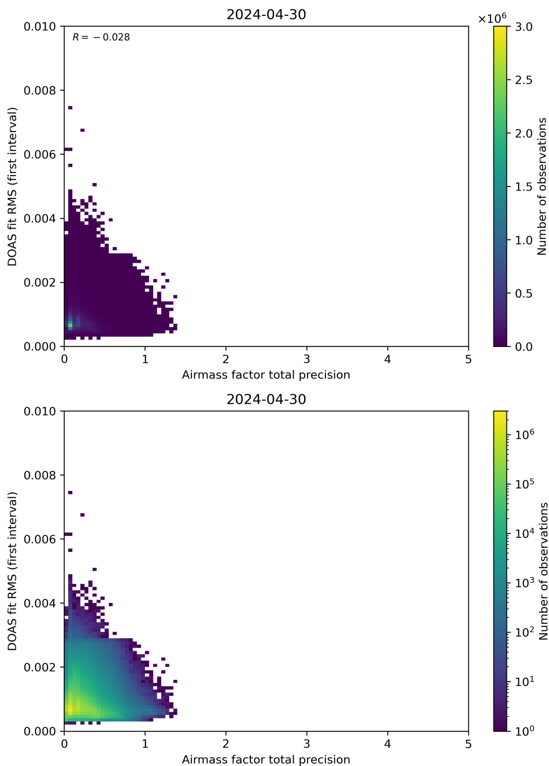
Figure 105: Scatter density plot of “Airmass factor total precision” against “DOAS fit RMS (first interval)” for 2024-04-29 to 2024-05-01.
