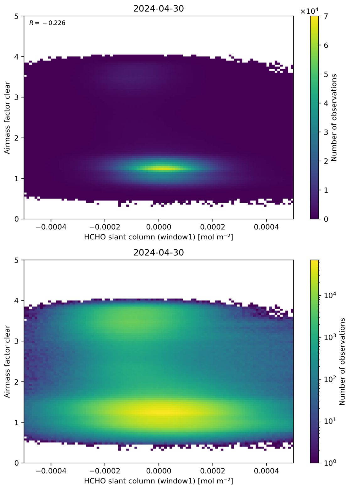
Figure 81: Scatter density plot of “HCHO slant column (window1)” against “Airmass factor clear” for 2024-04-29 to 2024-05-01.
