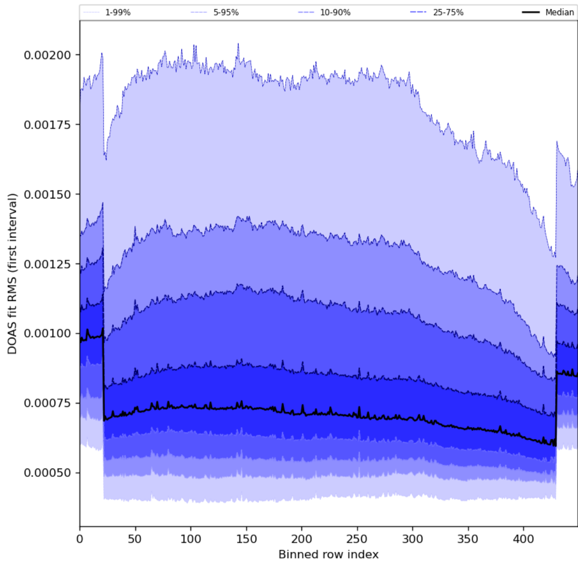
Figure 60: Along track statistics of “DOAS fit RMS (first interval)” for 2024-04-29 to 2024-05-01
