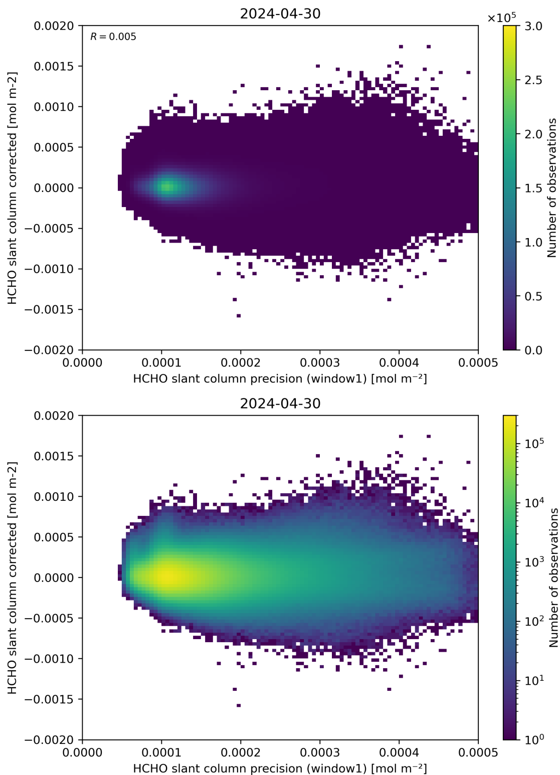
Figure 92: Scatter density plot of “HCHO slant column precision (window1)” against “HCHO slant column corrected” for 2024-04-29 to 2024-05-01.
