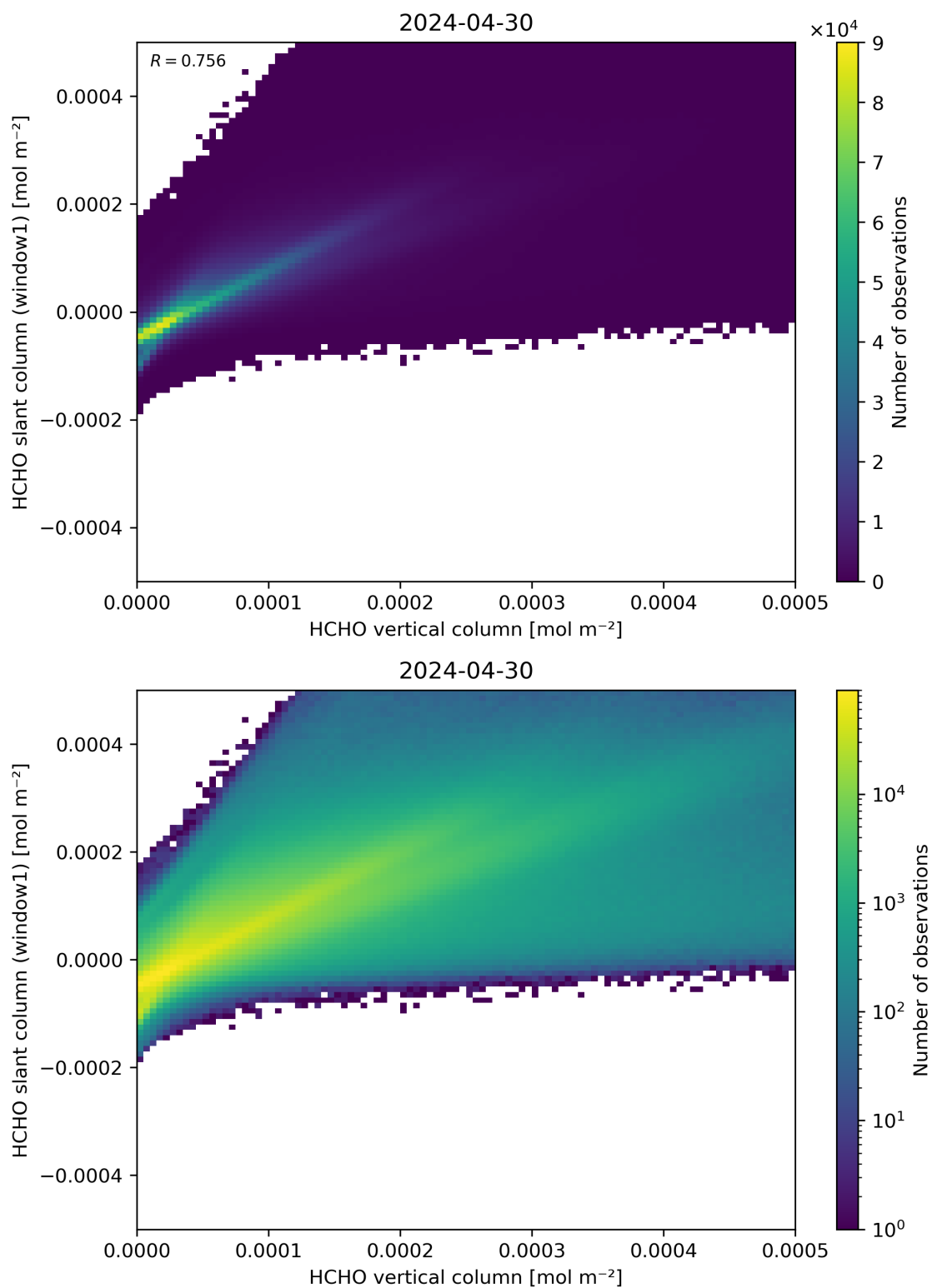
Figure 129: Scatter density plot of “HCHO vertical column” against “HCHO slant column (window1)” for 2024-04-29 to 2024-05-01.
