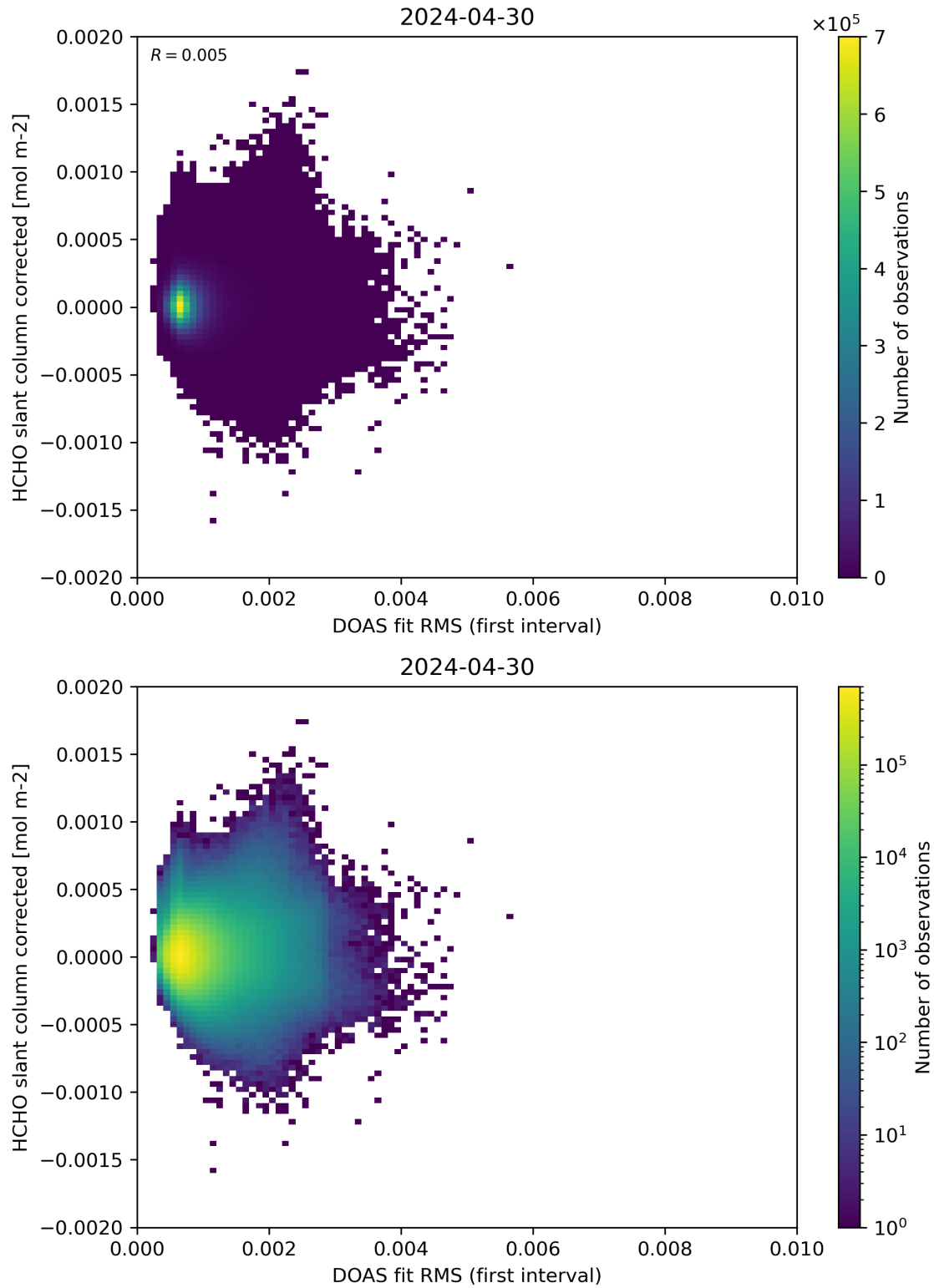
Figure 62: Scatter density plot of “DOAS fit RMS (first interval)” against “HCHO slant column corrected” for 2024-04-29 to 2024-05-01.
