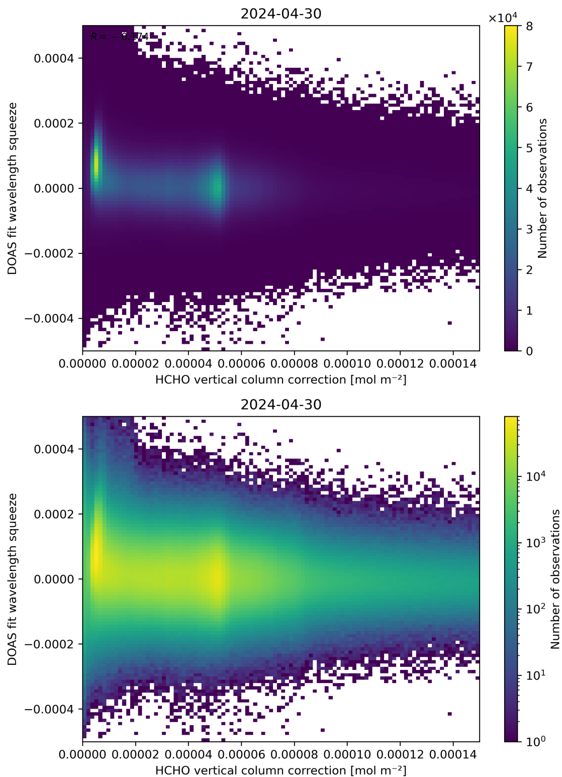
Figure 114: Scatter density plot of “HCHO vertical column correction” against “DOAS fit wavelength squeeze” for 2024-04-29 to 2024-05-01.
