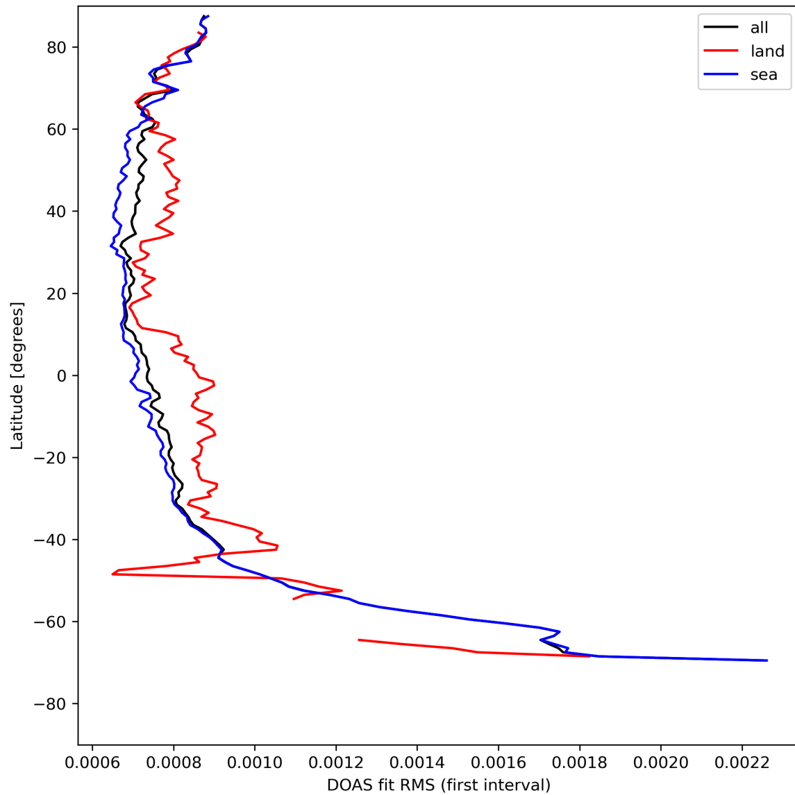
Figure 32: Zonal average of “DOAS fit RMS (first interval)” for 2024-04-29 to 2024-05-01.
