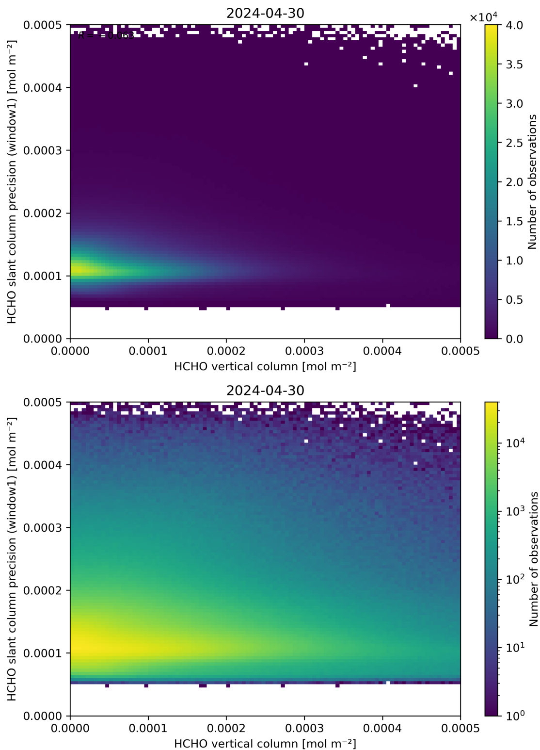
Figure 130: Scatter density plot of “HCHO vertical column” against “HCHO slant column precision (window1)” for 2024-04-29 to 2024-05-01.
