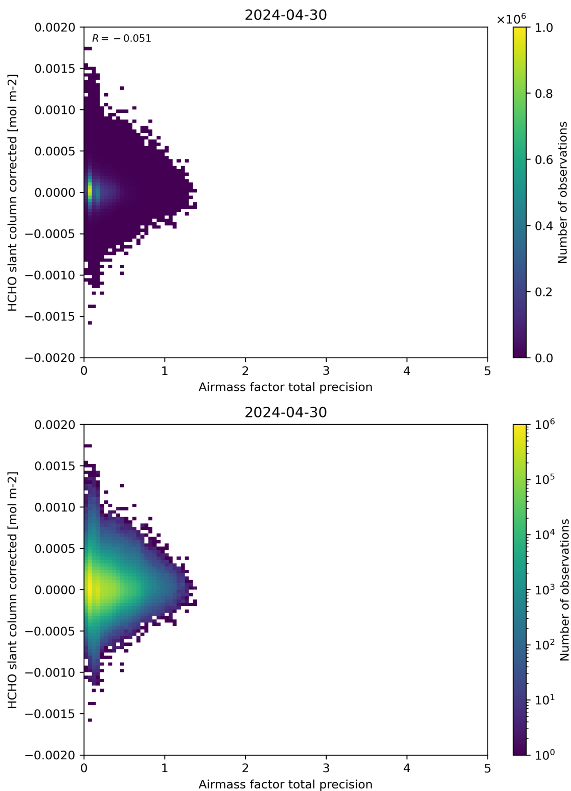
Figure 109: Scatter density plot of “Airmass factor total precision” against “HCHO slant column corrected” for 2024-04-29 to 2024-05-01.
