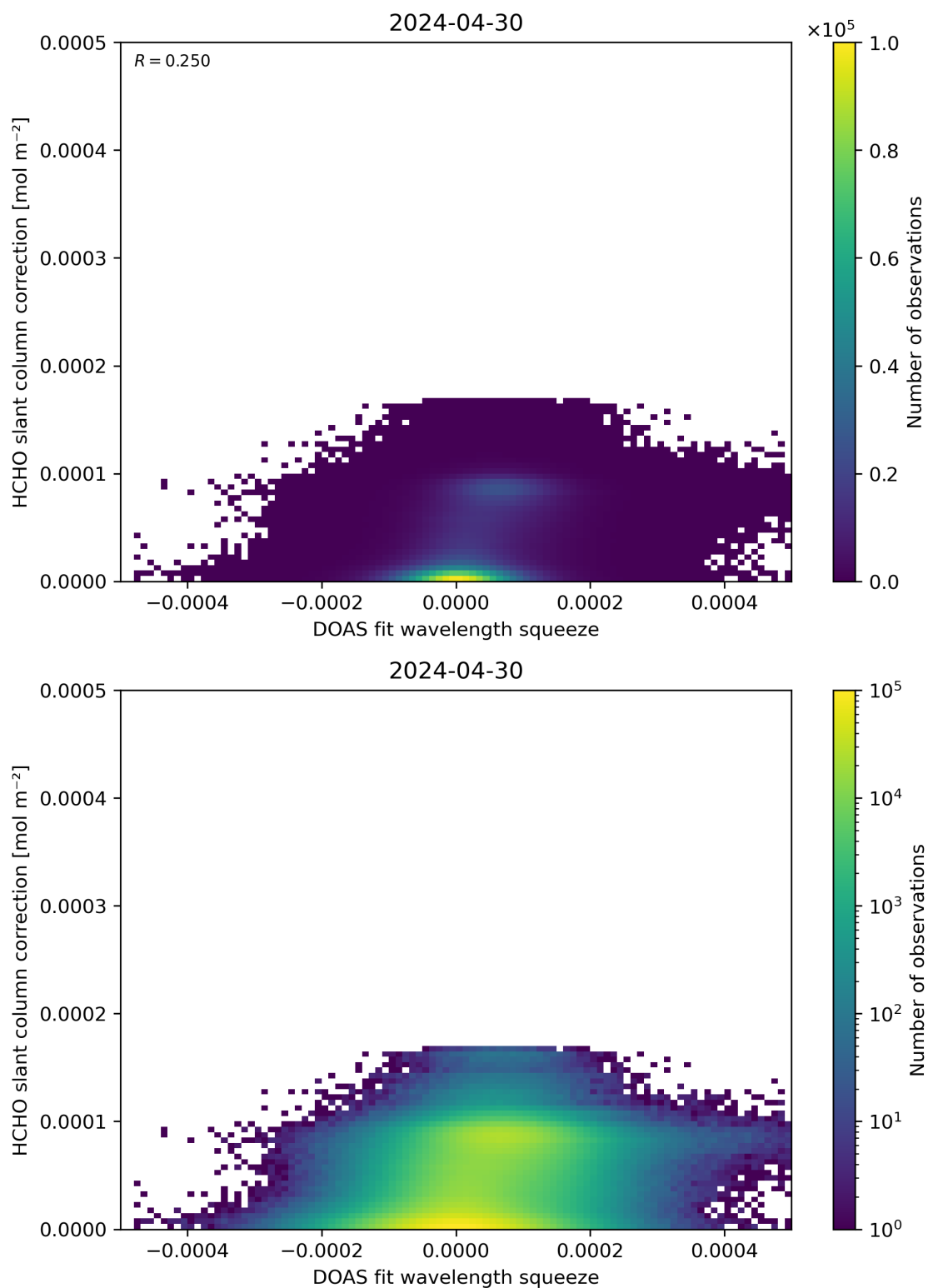
Figure 70: Scatter density plot of “DOAS fit wavelength squeeze” against “HCHO slant column correction” for 2024-04-29 to 2024-05-01.
