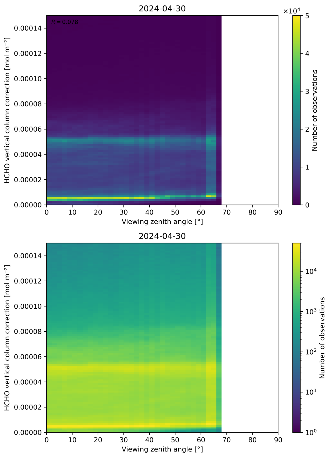
Figure 193: Scatter density plot of “Viewing zenith angle” against “HCHO vertical column correction” for 2024-04-29 to 2024-05-01.
