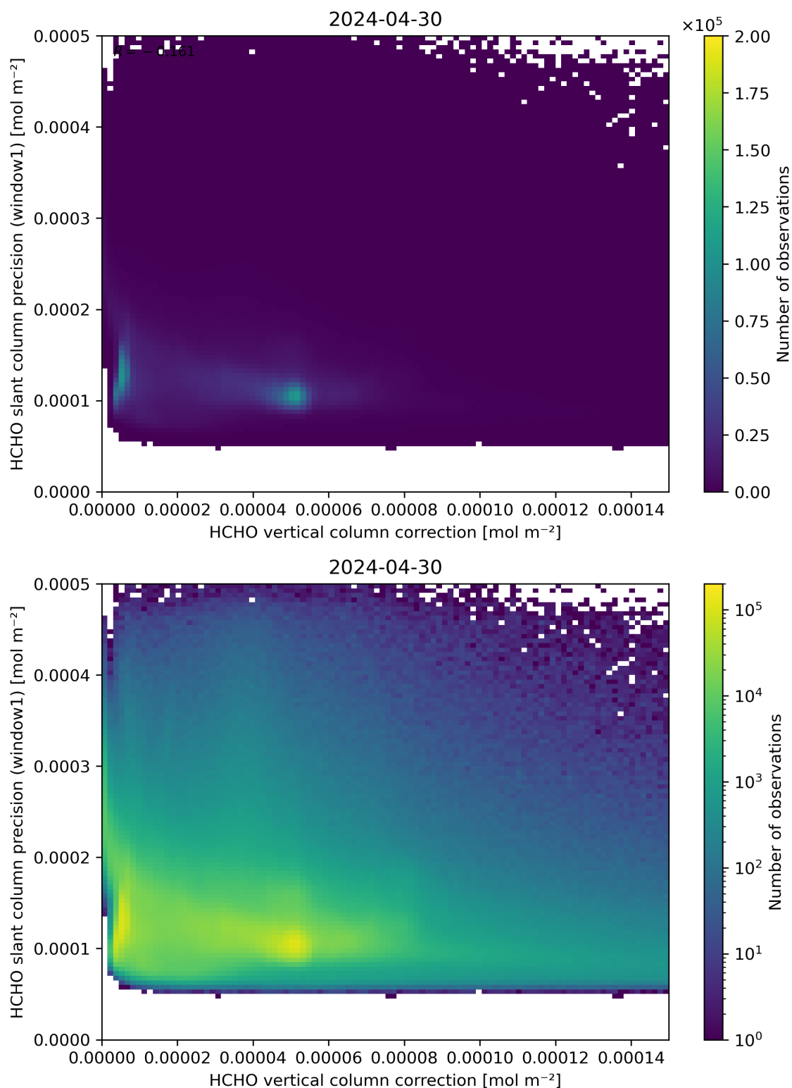
Figure 119: Scatter density plot of “HCHO vertical column correction” against “HCHO slant column precision (window1)” for 2024-04-29 to 2024-05-01.
