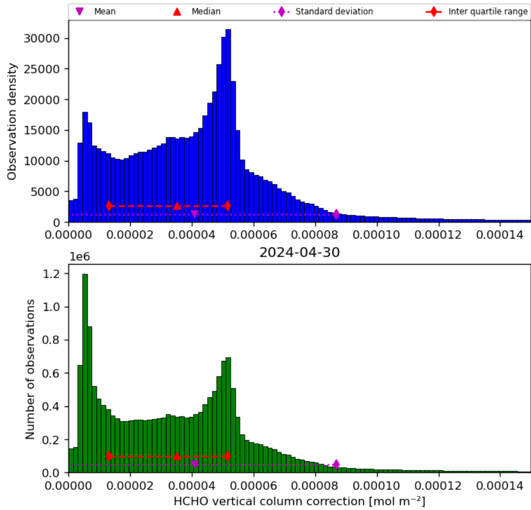
Figure 37: Histogram of “HCHO vertical column correction” for 2024-04-29 to 2024-05-01
