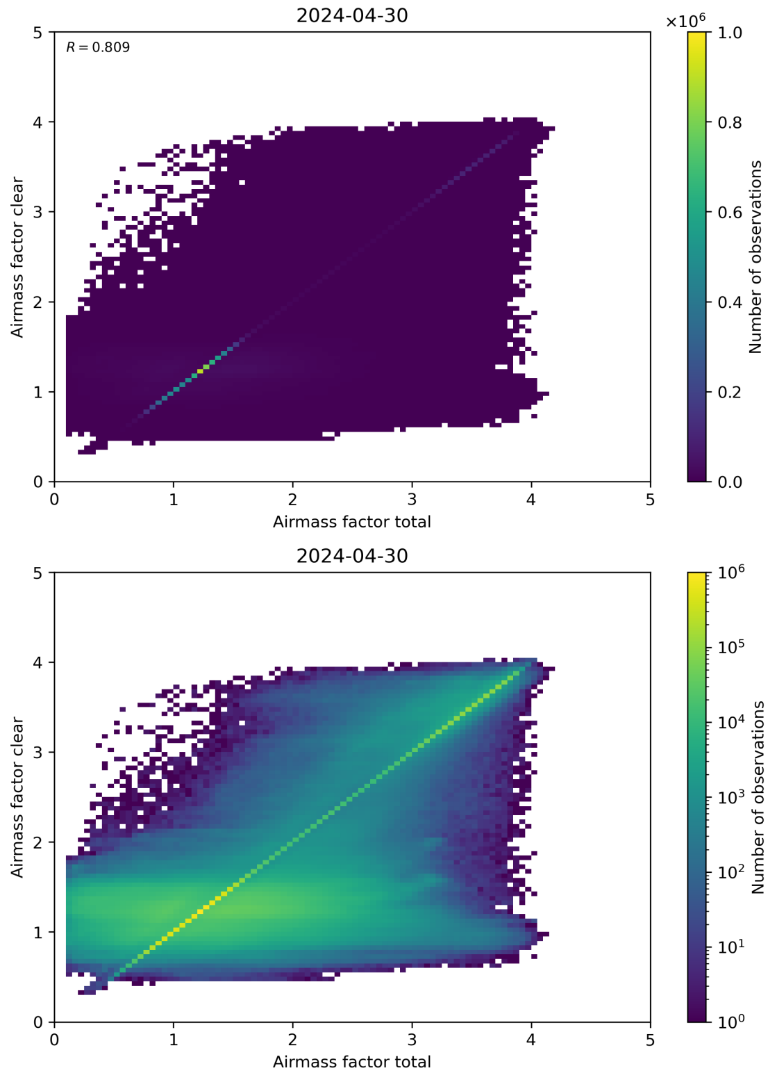
Figure 100: Scatter density plot of “Airmass factor total” against “Airmass factor clear” for 2024-04-29 to 2024-05-01.
