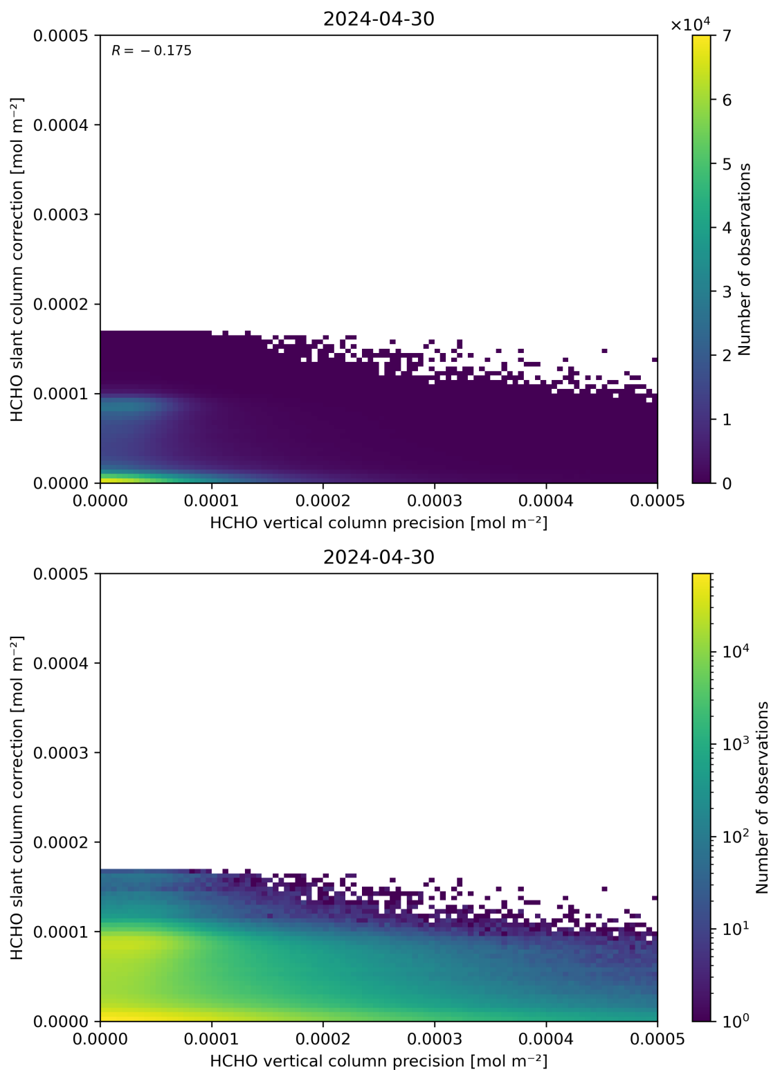
Figure 141: Scatter density plot of “HCHO vertical column precision” against “HCHO slant column correction” for 2024-04-29 to 2024-05-01.
