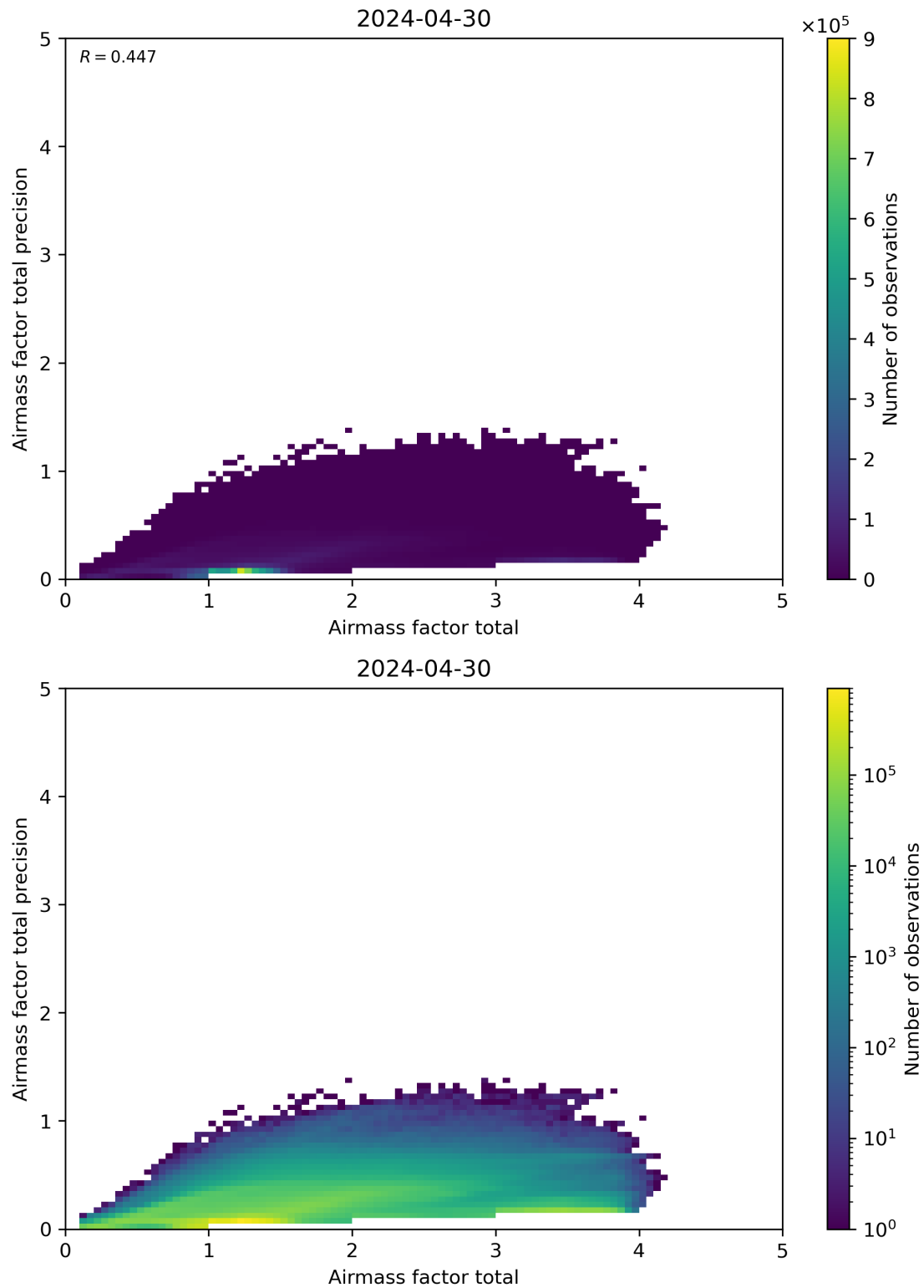
Figure 103: Scatter density plot of “Airmass factor total” against “Airmass factor total precision” for 2024-04-29 to 2024-05-01.
