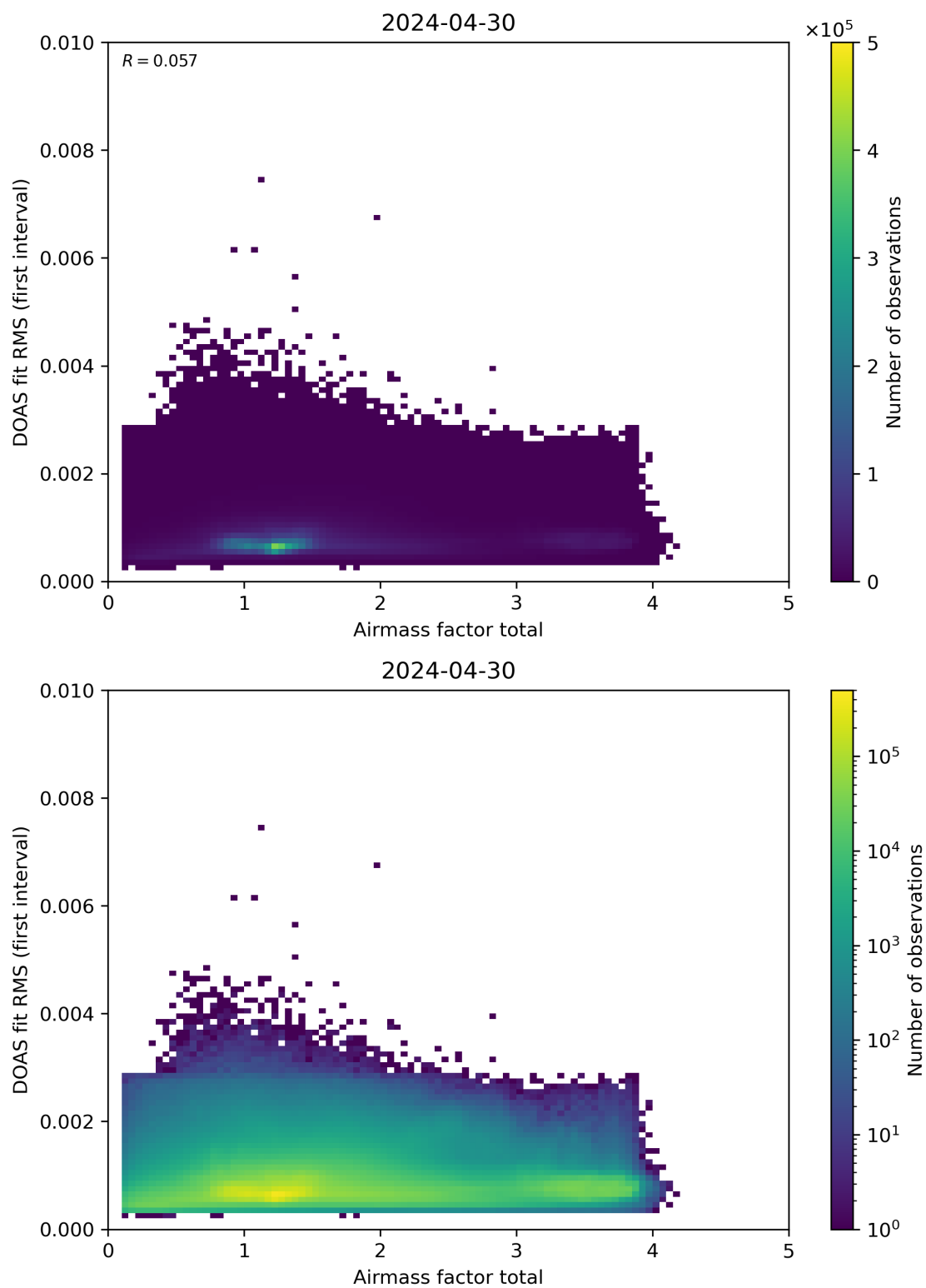
Figure 97: Scatter density plot of “Airmass factor total” against “DOAS fit RMS (first interval)” for 2024-04-29 to 2024-05-01.
