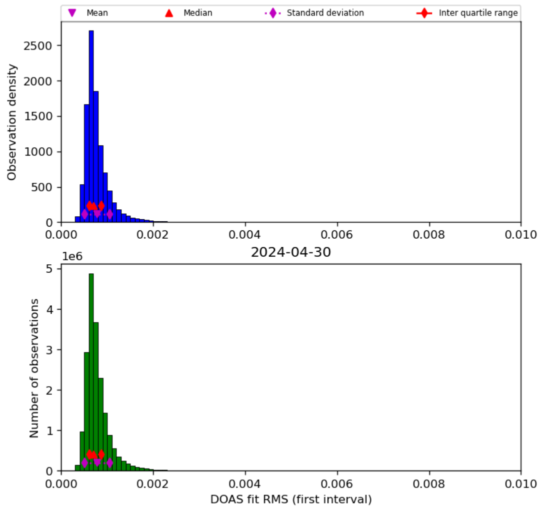
Figure 46: Histogram of “DOAS fit RMS (first interval)” for 2024-04-29 to 2024-05-01
