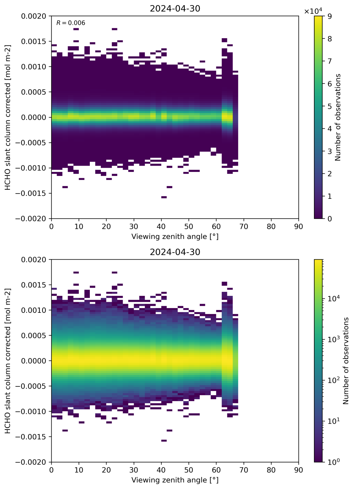
Figure 186: Scatter density plot of “Viewing zenith angle” against “HCHO slant column corrected” for 2024-04-29 to 2024-05-01.
