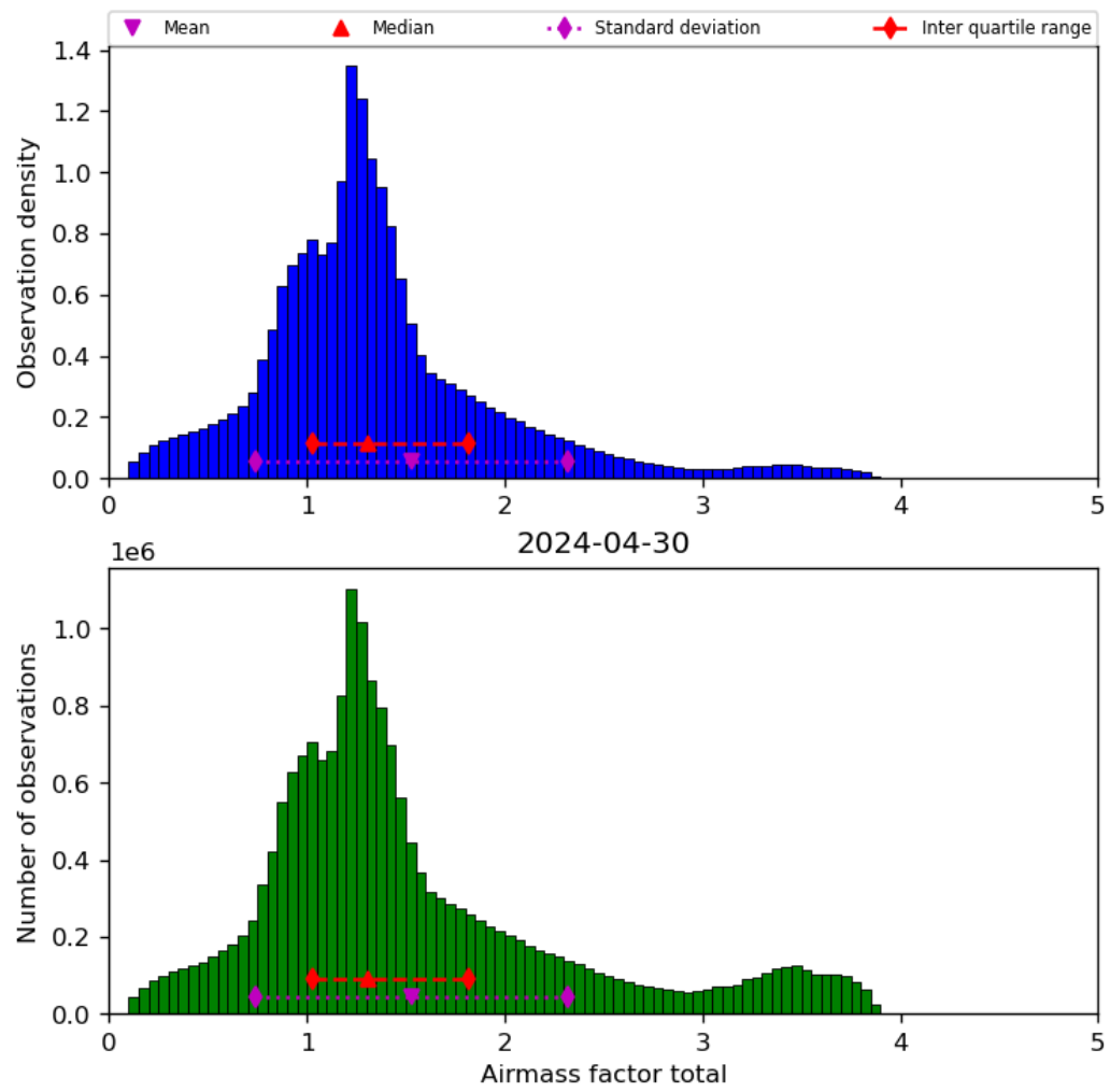
Figure 40: Histogram of “Airmass factor total” for 2024-04-29 to 2024-05-01
