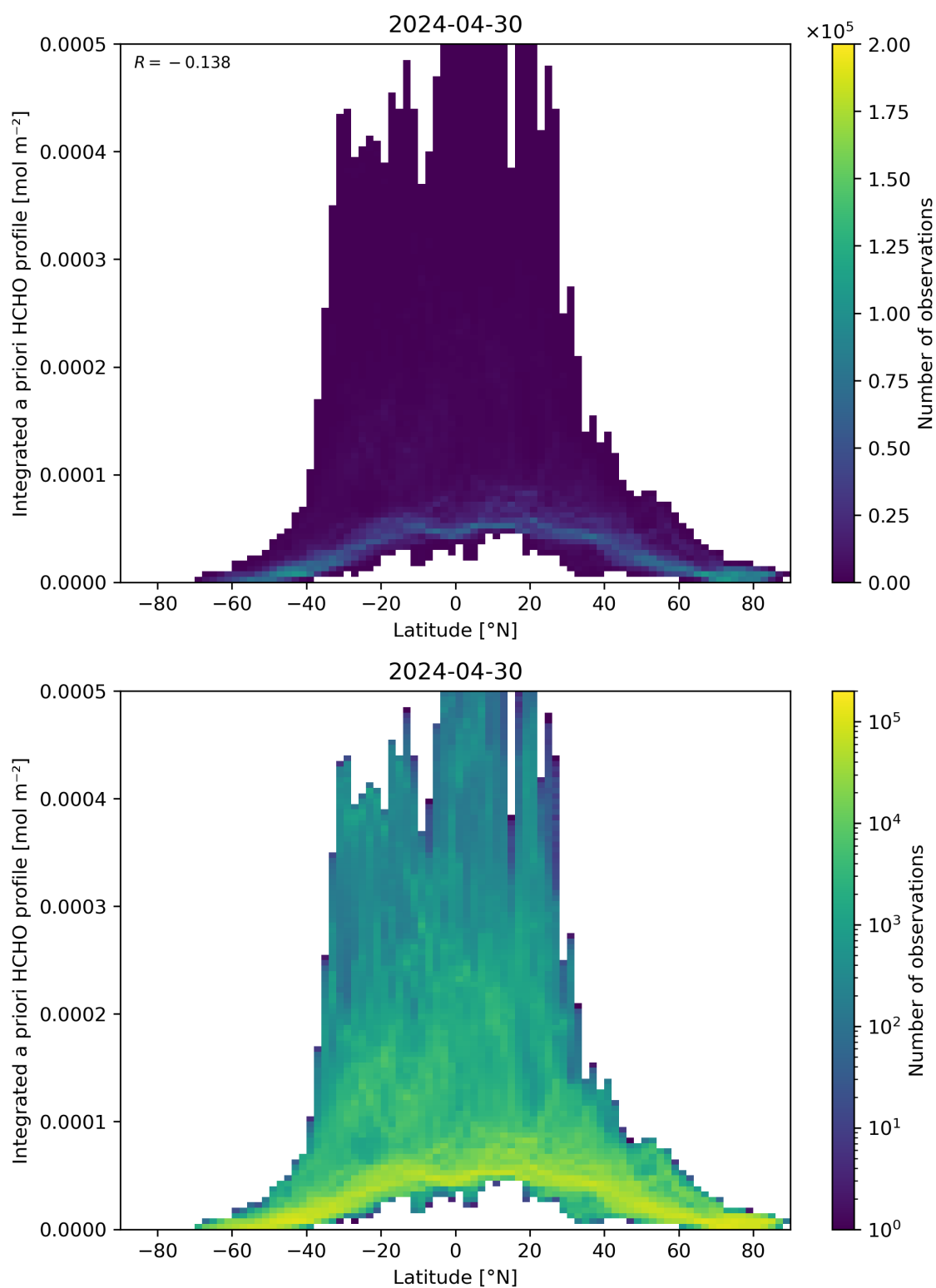
Figure 166: Scatter density plot of “Latitude” against “Integrated a priori HCHO profile” for 2024-04-29 to 2024-05-01.
