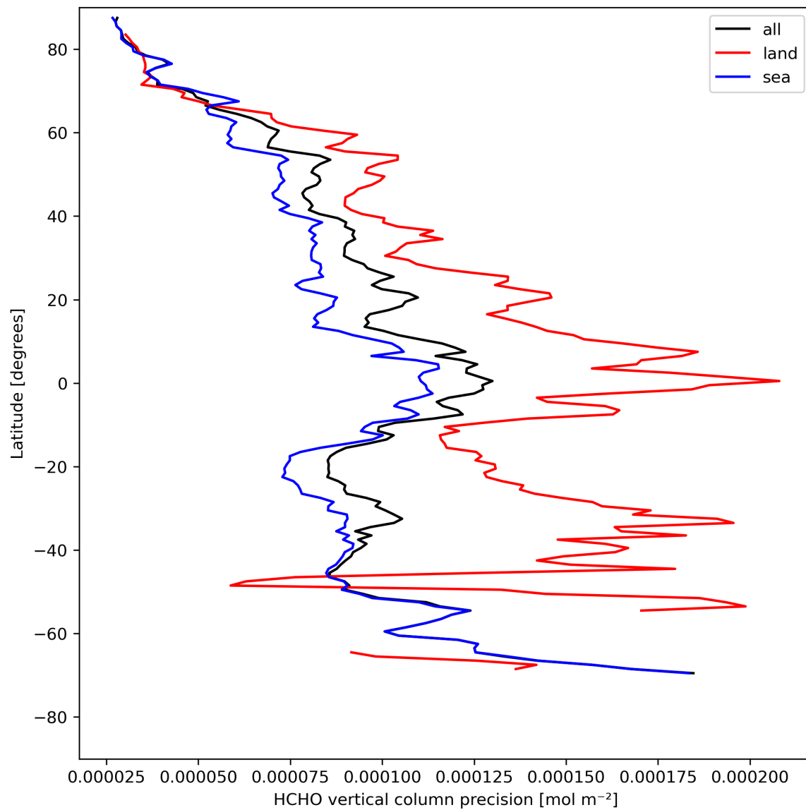
Figure 22: Zonal average of “HCHO vertical column precision” for 2024-04-29 to 2024-05-01.
