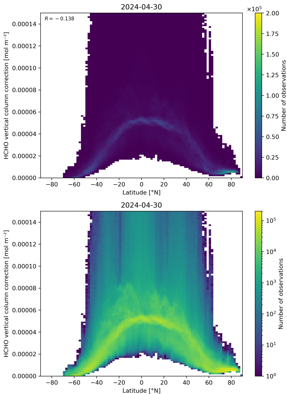
Figure 164: Scatter density plot of “Latitude” against “HCHO vertical column correction” for 2024-04-29 to 2024-05-01.
