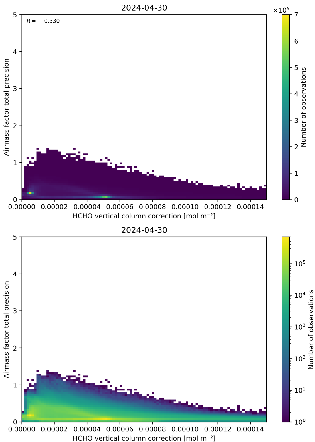
Figure 121: Scatter density plot of “HCHO vertical column correction” against “Airmass factor total precision” for 2024-04-29 to 2024-05-01.
