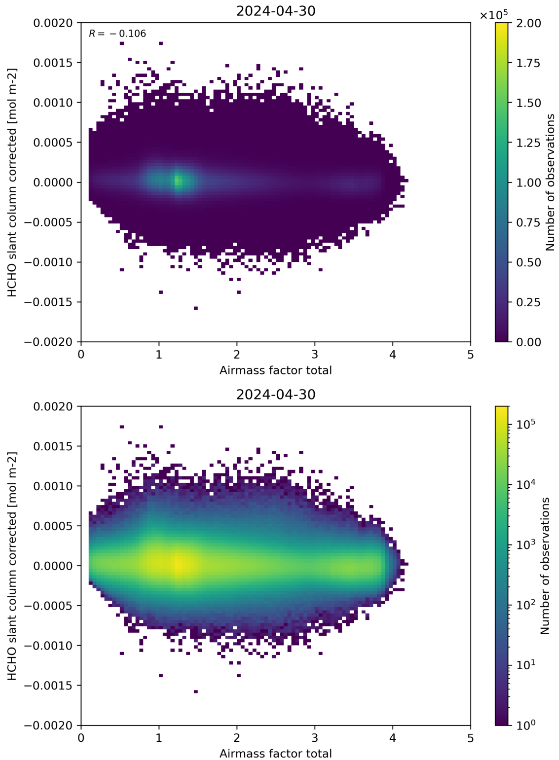
Figure 101: Scatter density plot of “Airmass factor total” against “HCHO slant column corrected” for 2024-04-29 to 2024-05-01.
