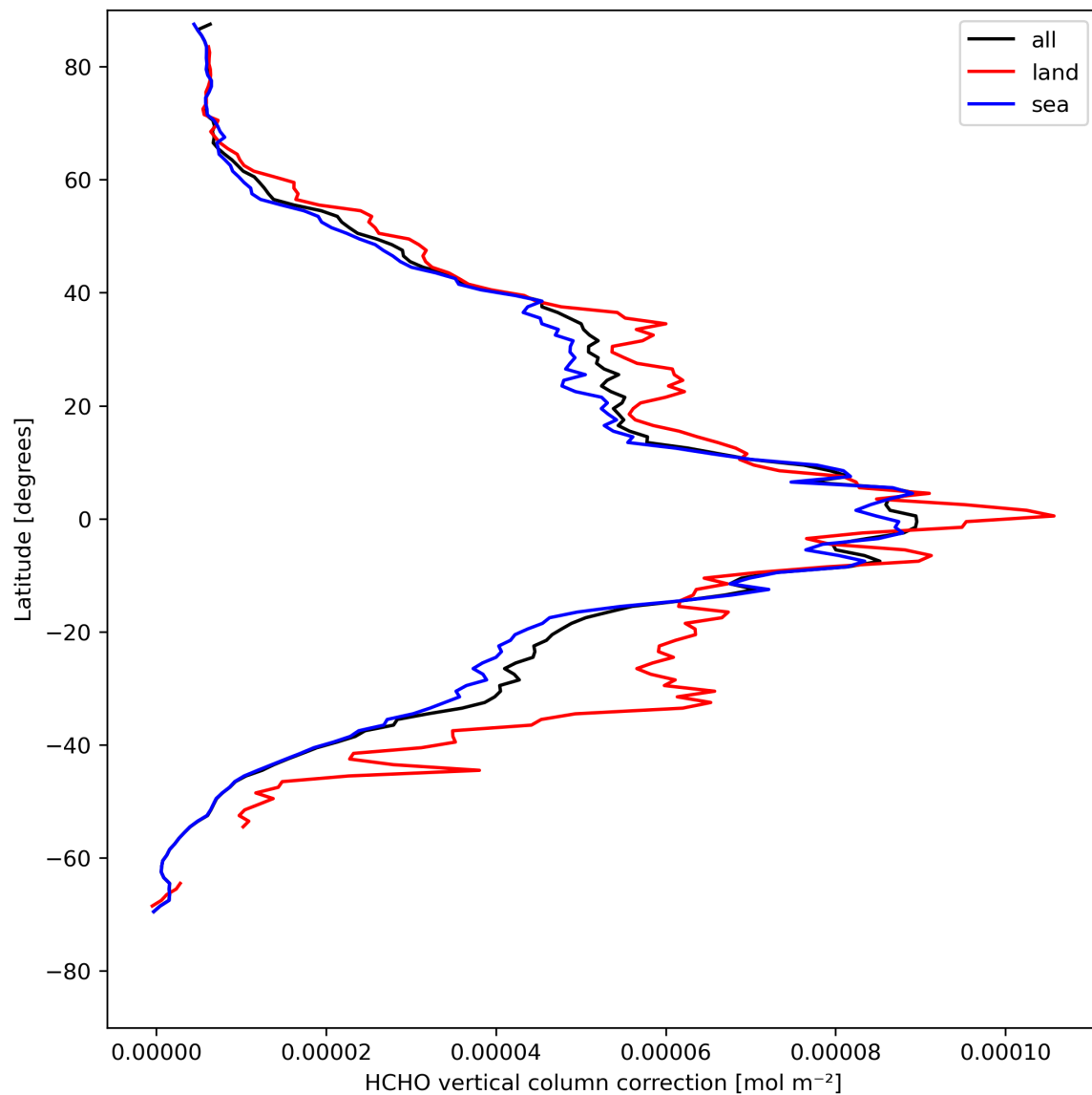
Figure 23: Zonal average of “HCHO vertical column correction” for 2024-04-29 to 2024-05-01.
