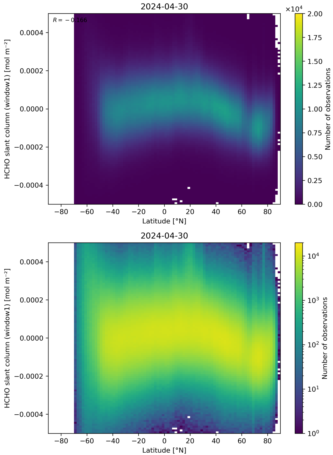
Figure 159: Scatter density plot of “Latitude” against “HCHO slant column (window1)” for 2024-04-29 to 2024-05-01.
