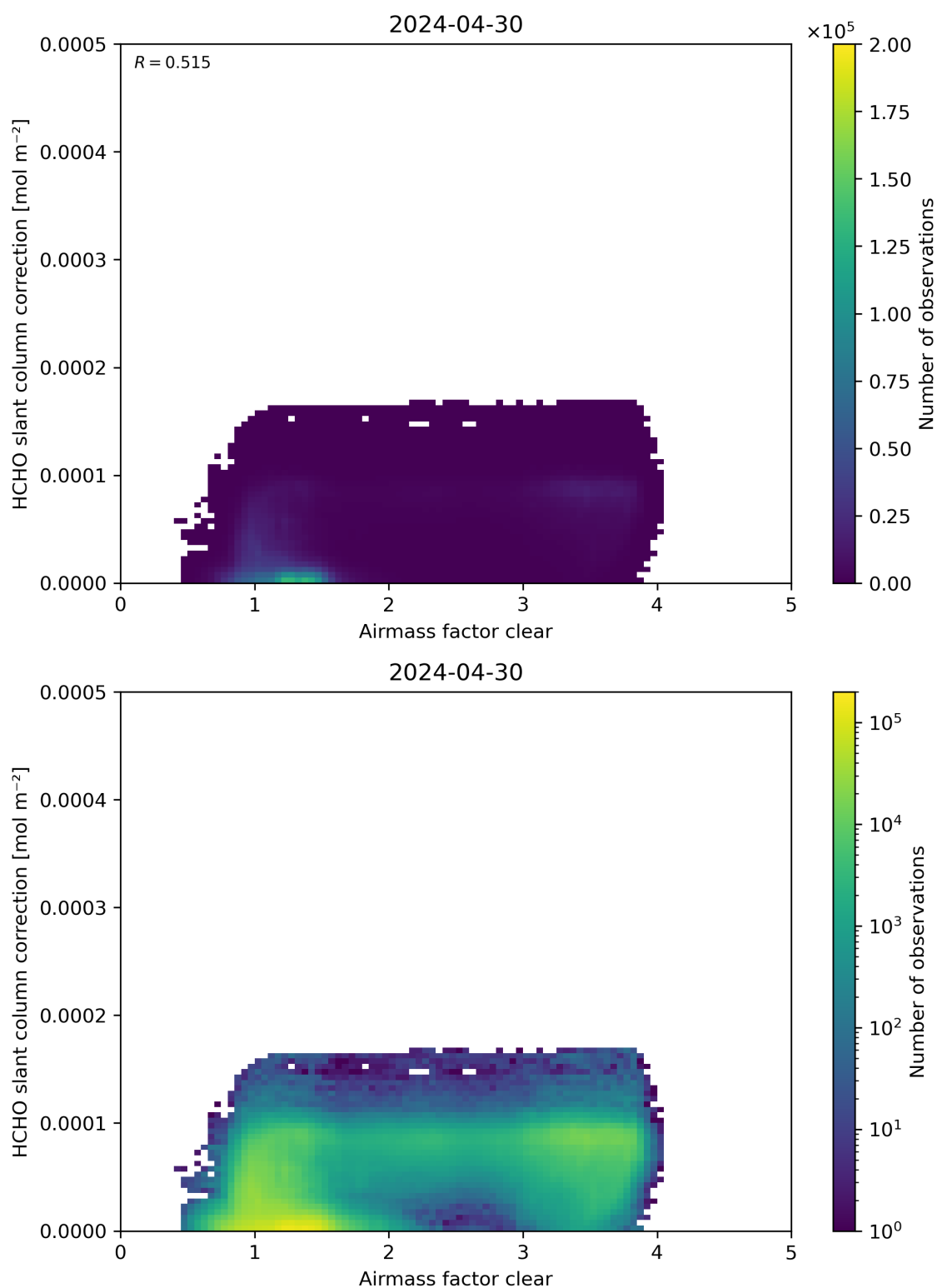
Figure 75: Scatter density plot of “Airmass factor clear” against “HCHO slant column correction” for 2024-04-29 to 2024-05-01.
