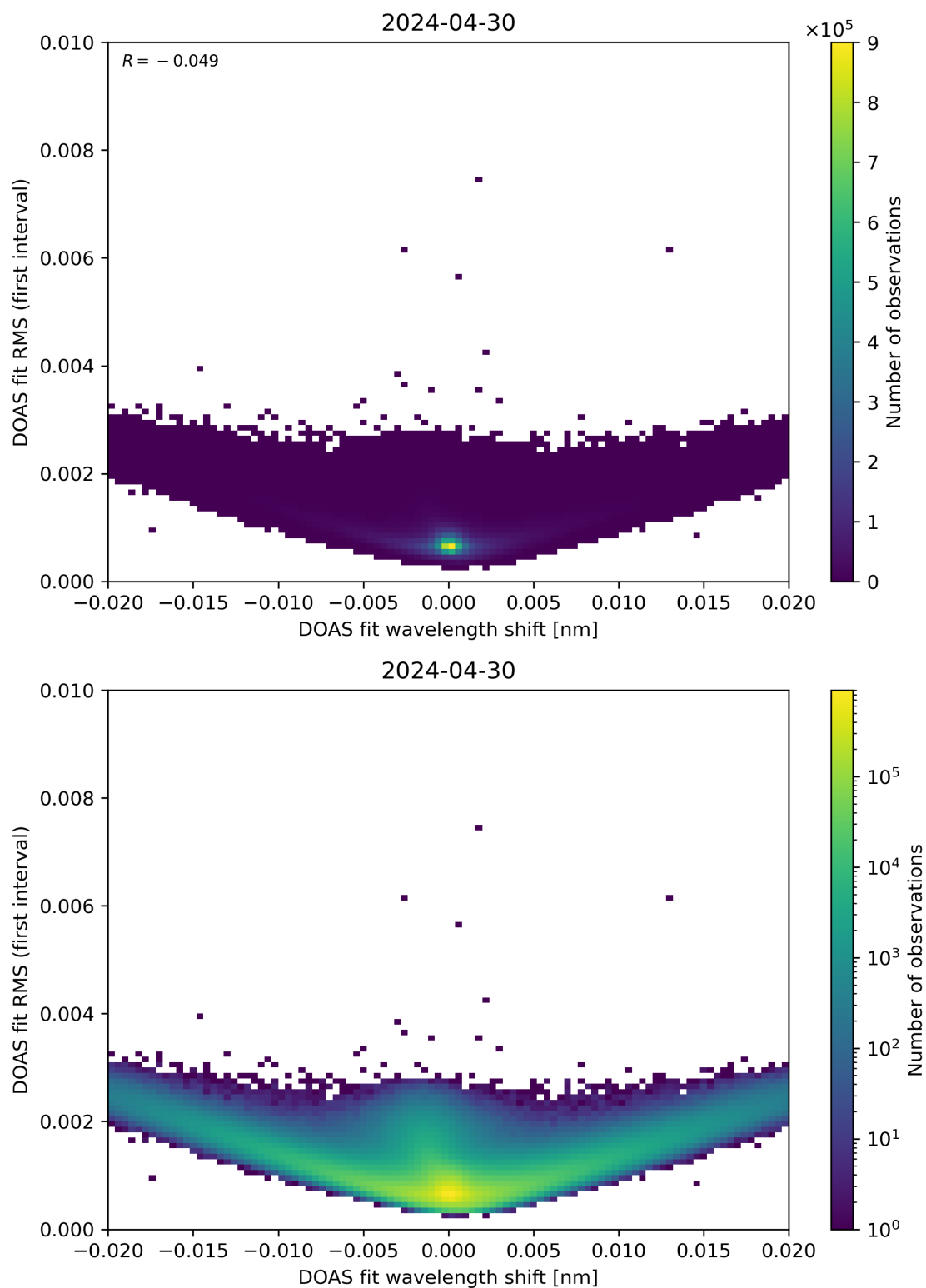
Figure 64: Scatter density plot of “DOAS fit wavelength shift” against “DOAS fit RMS (first interval)” for 2024-04-29 to 2024-05-01.
