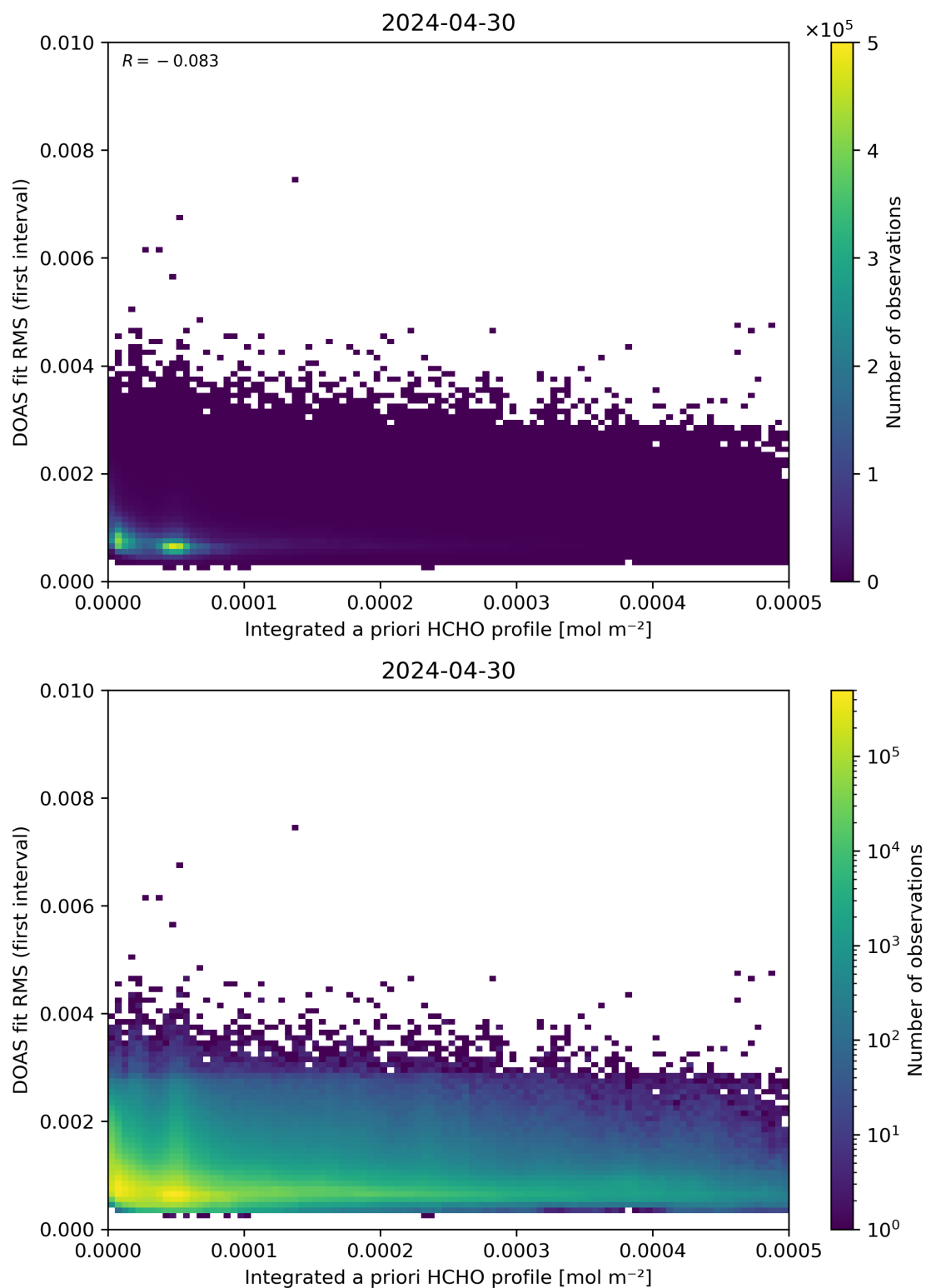
Figure 148: Scatter density plot of “Integrated a priori HCHO profile” against “DOAS fit RMS (first interval)” for 2024-04-29 to 2024-05-01.
