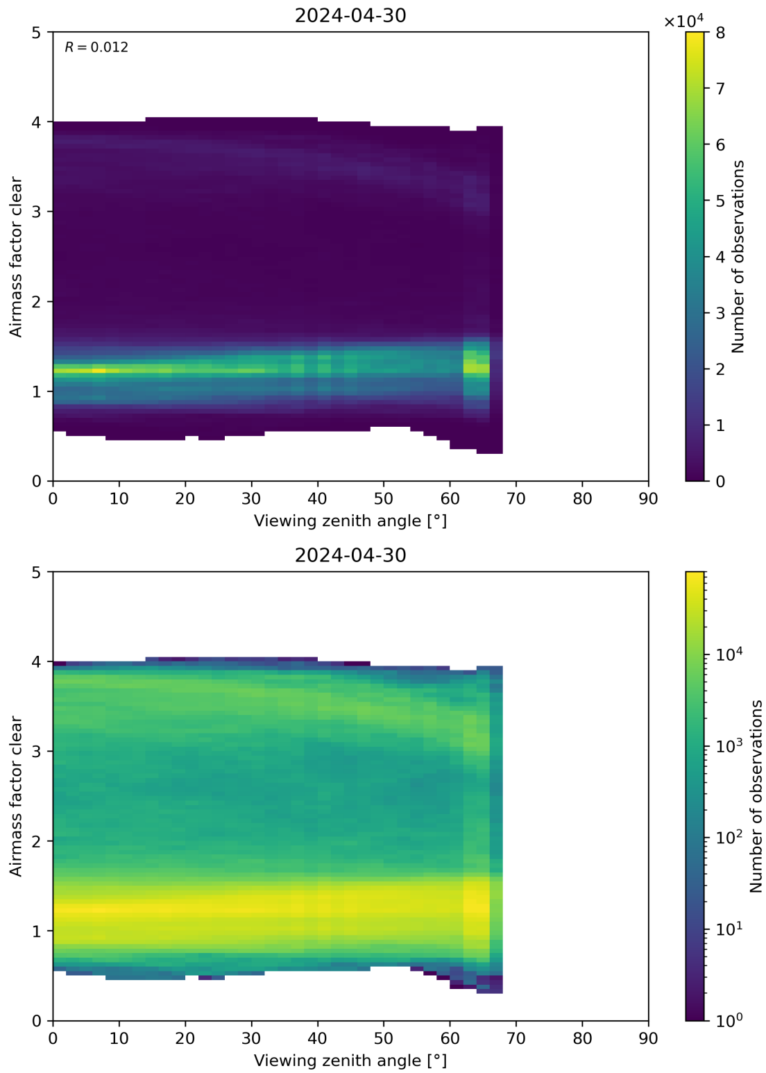
Figure 185: Scatter density plot of “Viewing zenith angle” against “Airmass factor clear” for 2024-04-29 to 2024-05-01.
