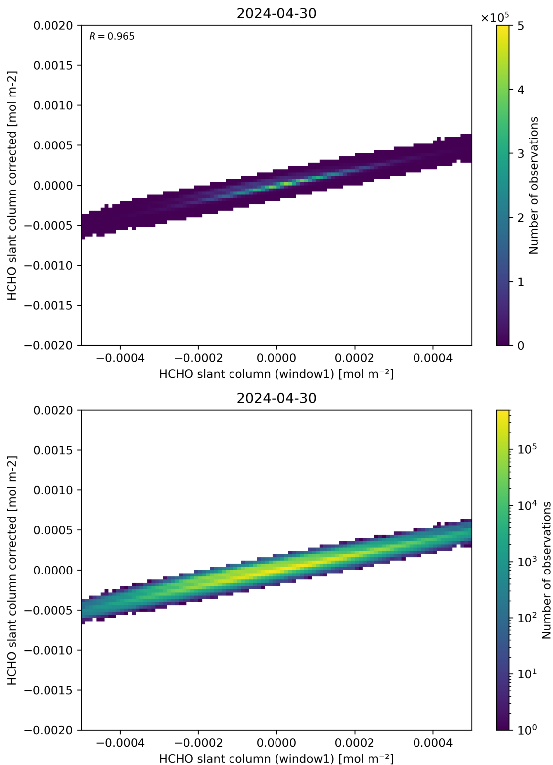
Figure 82: Scatter density plot of “HCHO slant column (window1)” against “HCHO slant column corrected” for 2024-04-29 to 2024-05-01.
