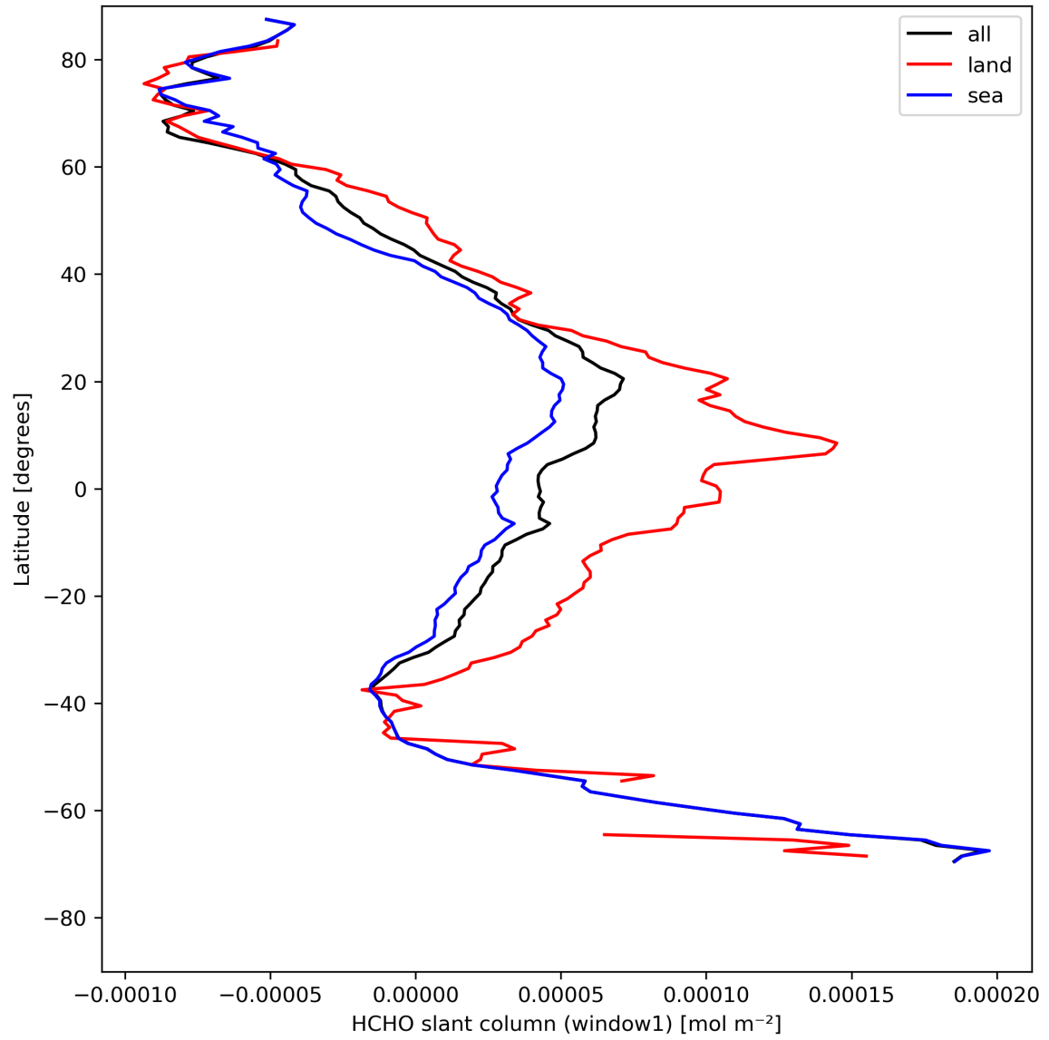
Figure 24: Zonal average of “HCHO slant column (window1)” for 2024-04-29 to 2024-05-01.
