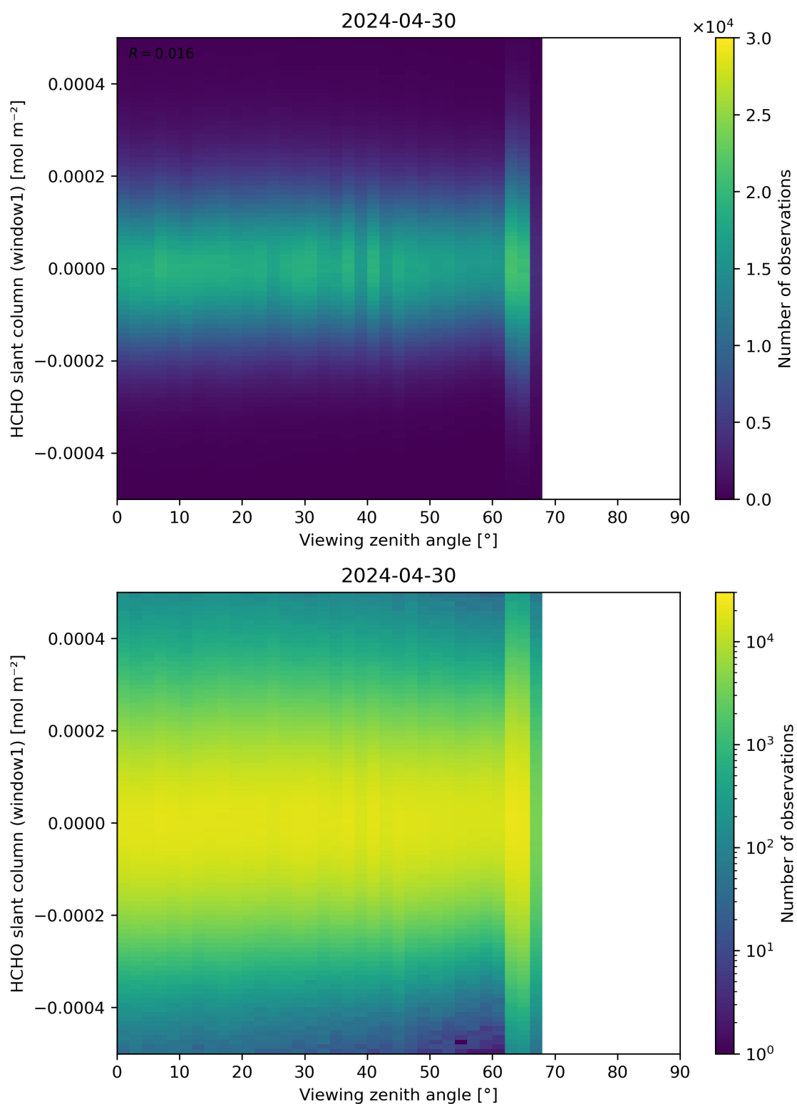
Figure 188: Scatter density plot of “Viewing zenith angle” against “HCHO slant column (window1)” for 2024-04-29 to 2024-05-01.
