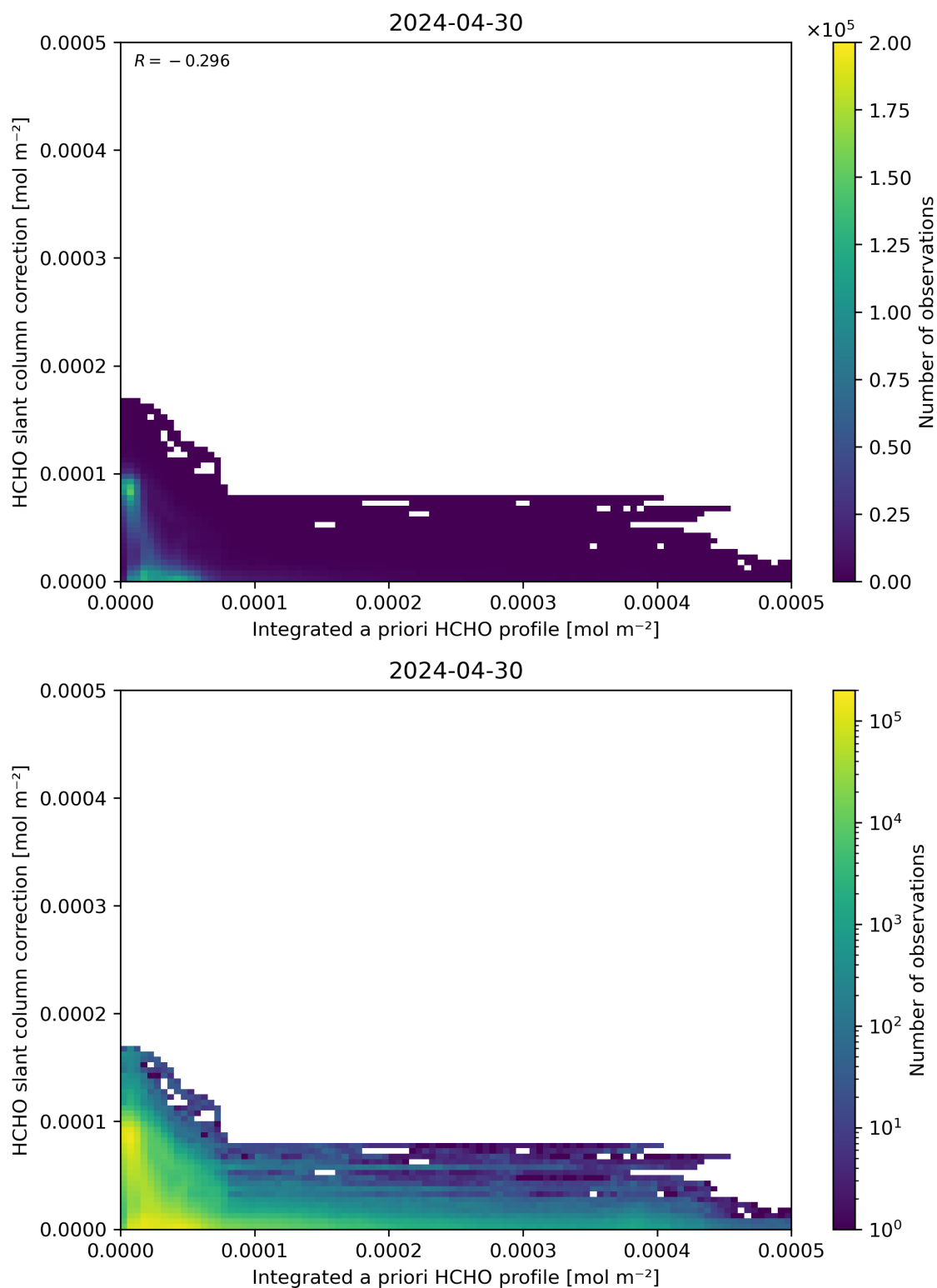
Figure 152: Scatter density plot of “Integrated a priori HCHO profile” against “HCHO slant column correction” for 2024-04-29 to 2024-05-01.
