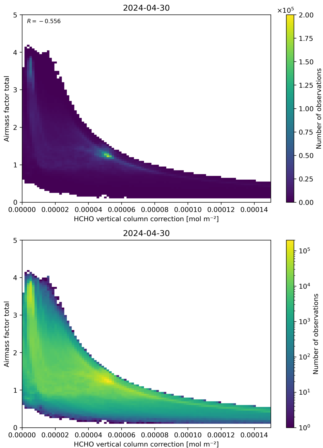
Figure 120: Scatter density plot of “HCHO vertical column correction” against “Airmass factor total” for 2024-04-29 to 2024-05-01.
