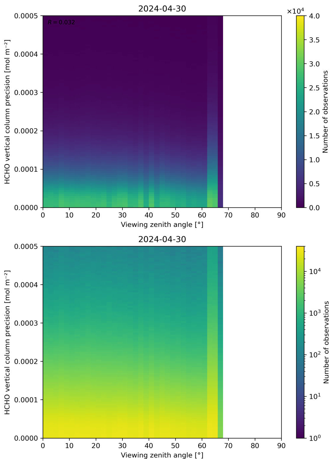
Figure 194: Scatter density plot of “Viewing zenith angle” against “HCHO vertical column precision” for 2024-04-29 to 2024-05-01.
