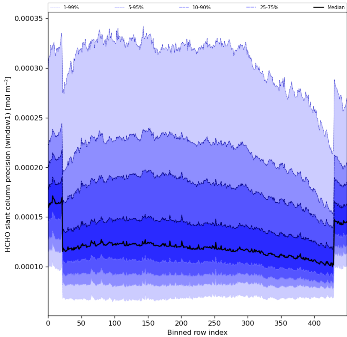
Figure 53: Along track statistics of “HCHO slant column precision (window1)” for 2024-04-29 to 2024-05-01
