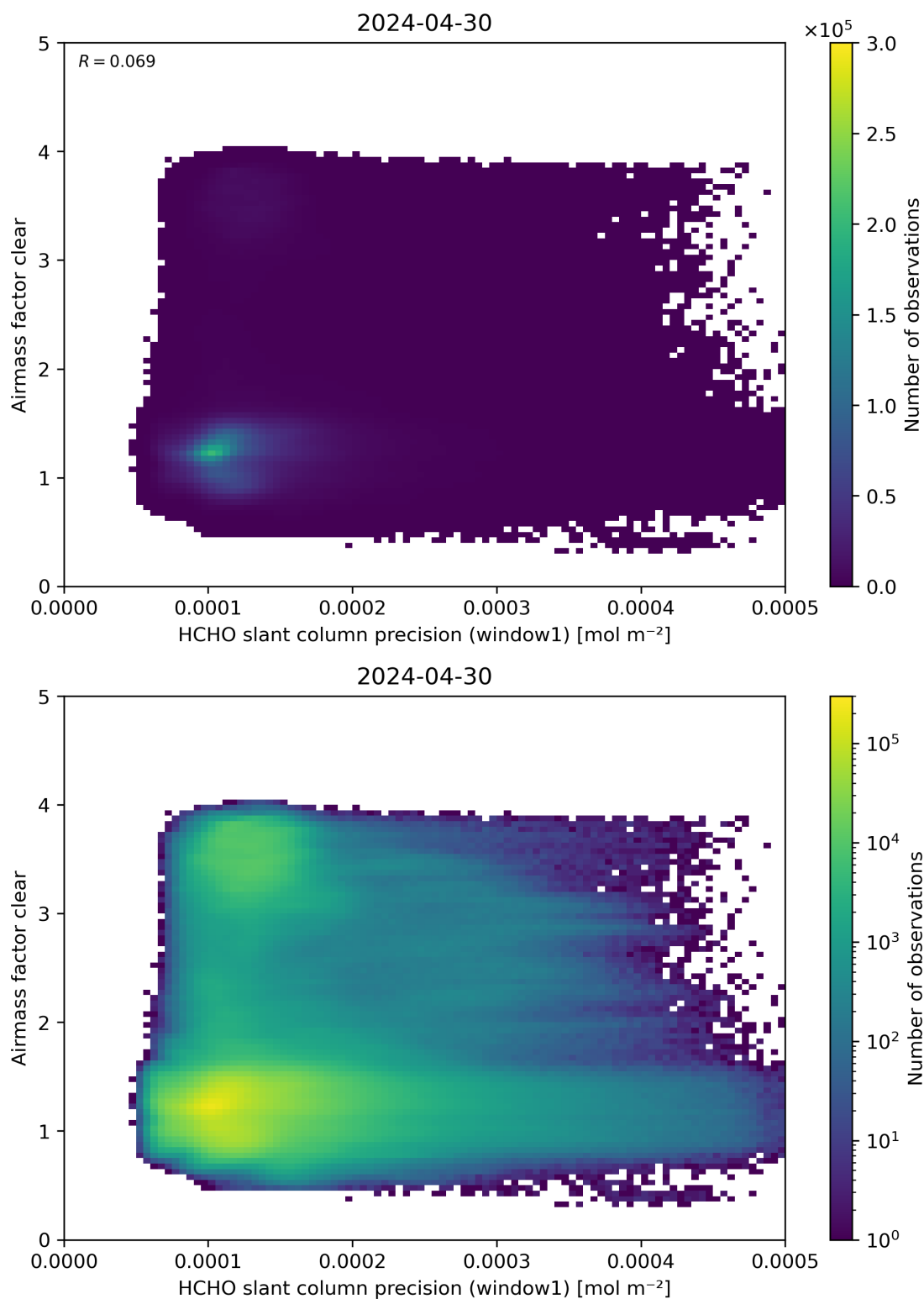
Figure 91: Scatter density plot of “HCHO slant column precision (window1)” against “Airmass factor clear” for 2024-04-29 to 2024-05-01.
