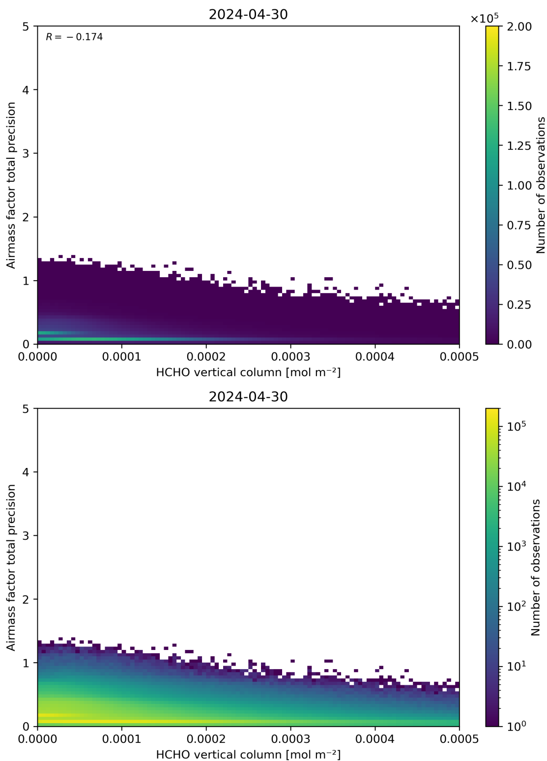
Figure 132: Scatter density plot of “HCHO vertical column” against “Airmass factor total precision” for 2024-04-29 to 2024-05-01.
