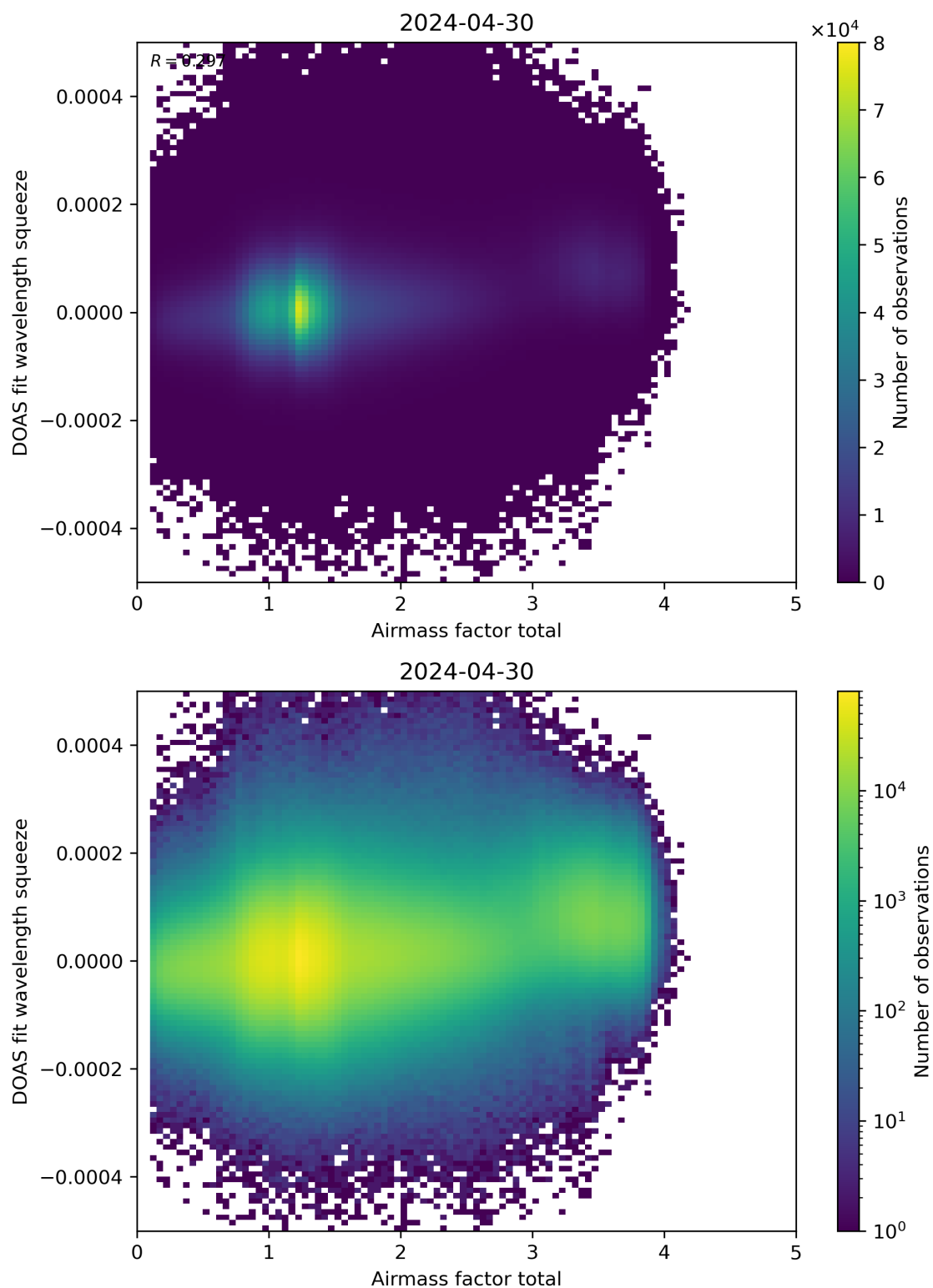
Figure 99: Scatter density plot of “Airmass factor total” against “DOAS fit wavelength squeeze” for 2024-04-29 to 2024-05-01.
