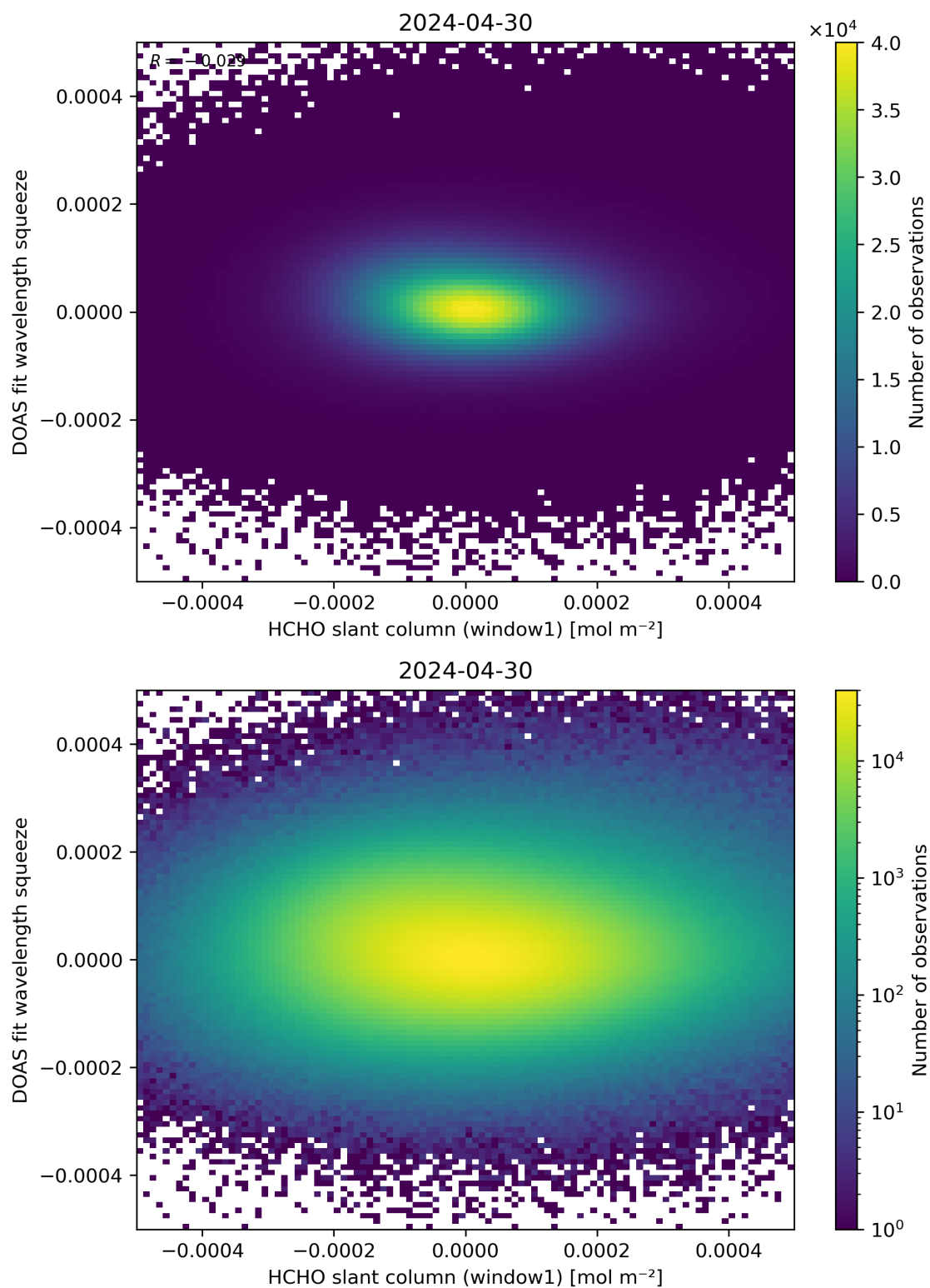
Figure 80: Scatter density plot of “HCHO slant column (window1)” against “DOAS fit wavelength squeeze” for 2024-04-29 to 2024-05-01.
