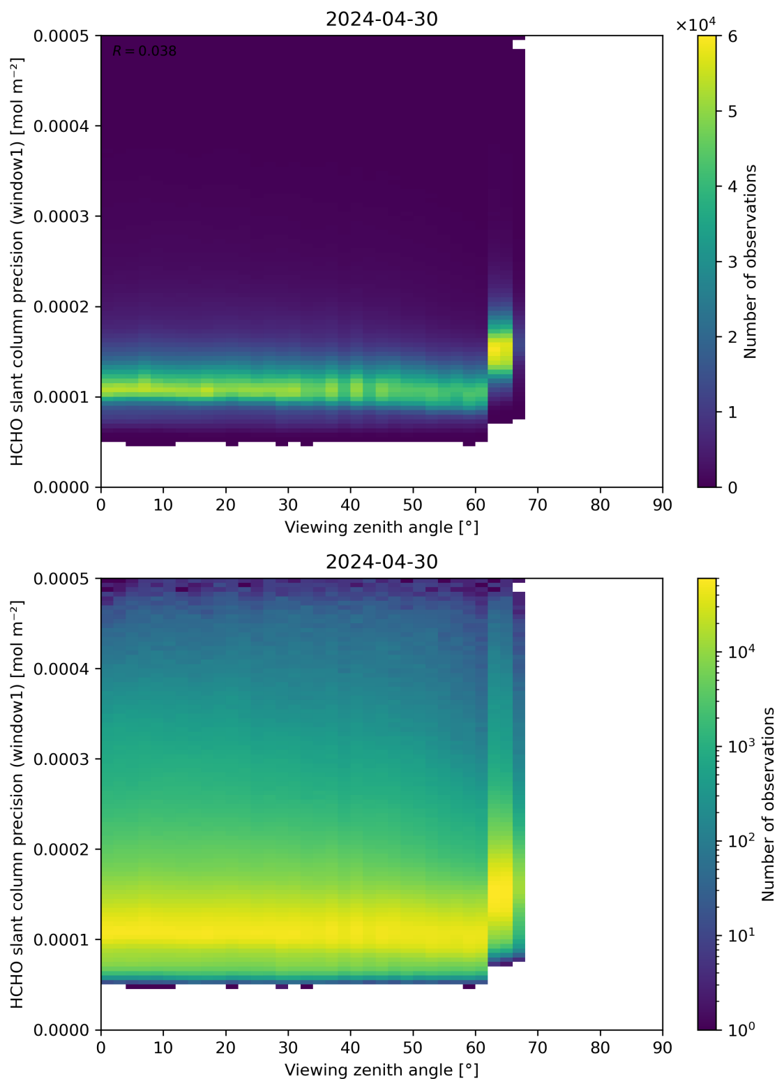
Figure 189: Scatter density plot of “Viewing zenith angle” against “HCHO slant column precision (window1)” for 2024-04-29 to 2024-05-01.
