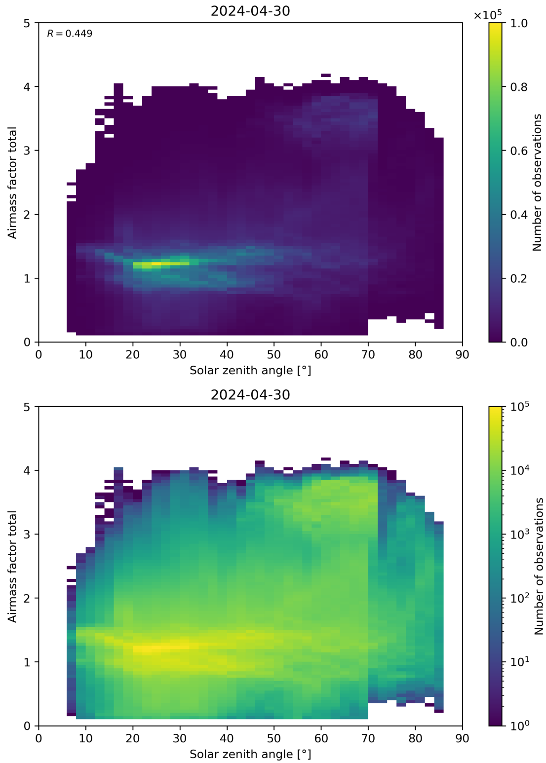
Figure 175: Scatter density plot of “Solar zenith angle” against “Airmass factor total” for 2024-04-29 to 2024-05-01.
