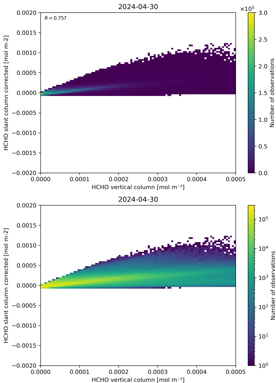
Figure 127: Scatter density plot of “HCHO vertical column” against “HCHO slant column corrected” for 2024-04-29 to 2024-05-01.
