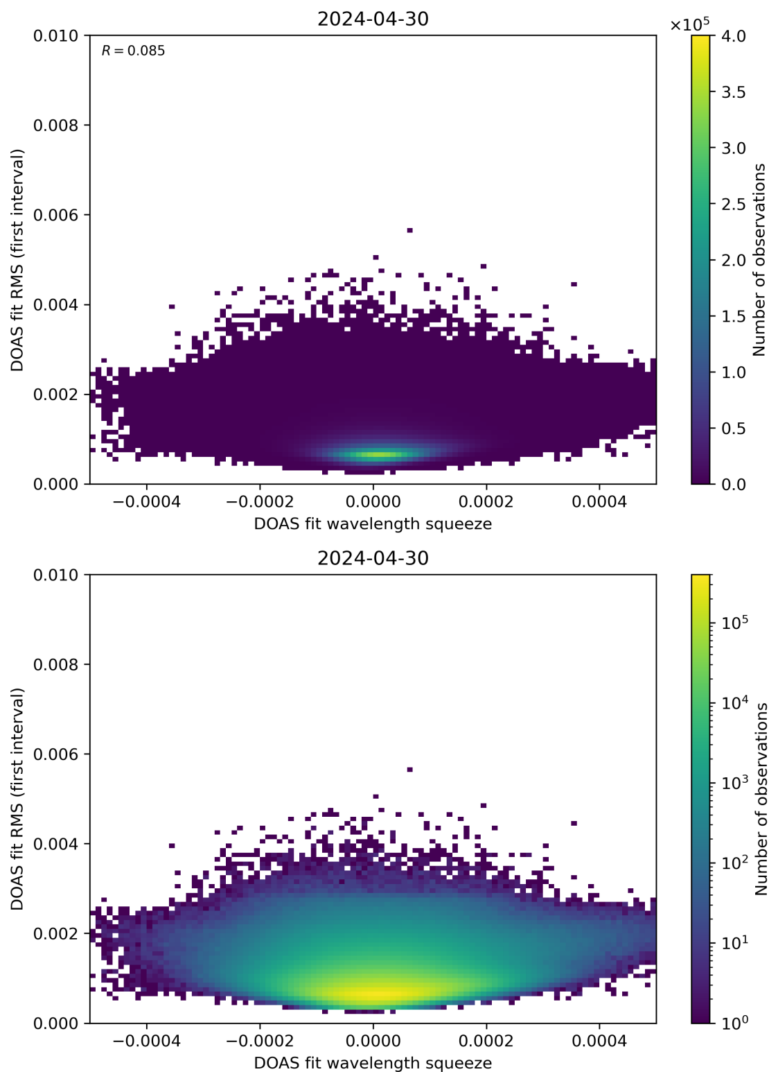
Figure 68: Scatter density plot of “DOAS fit wavelength squeeze” against “DOAS fit RMS (first interval)” for 2024-04-29 to 2024-05-01.
