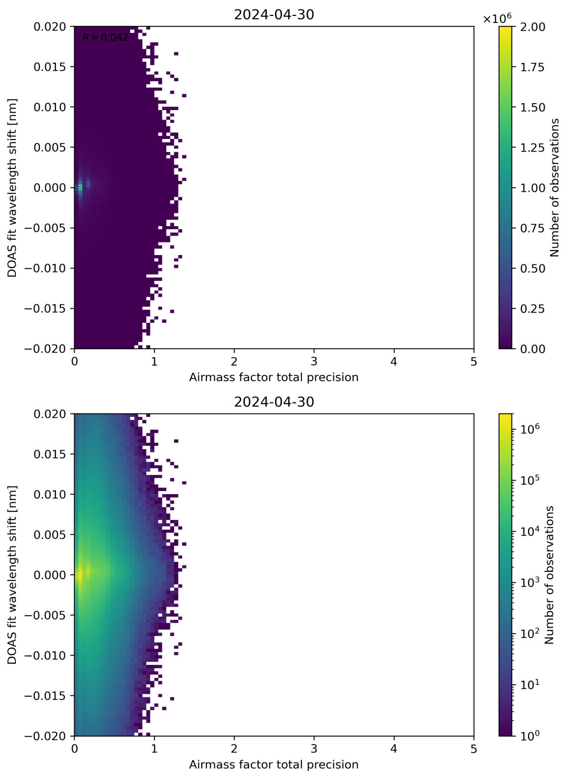
Figure 106: Scatter density plot of “Airmass factor total precision” against “DOAS fit wavelength shift” for 2024-04-29 to 2024-05-01.
