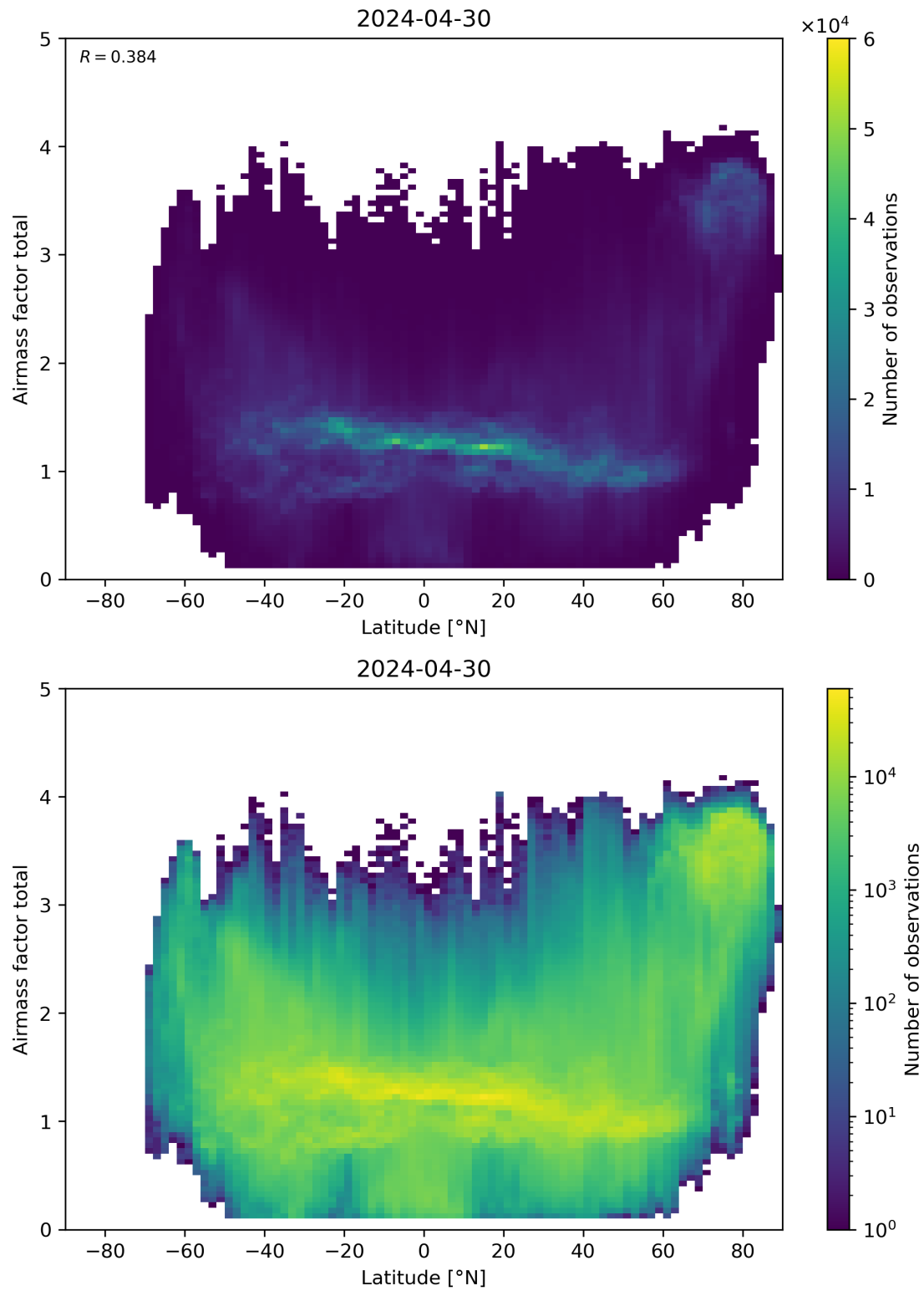
Figure 161: Scatter density plot of “Latitude” against “Airmass factor total” for 2024-04-29 to 2024-05-01.
