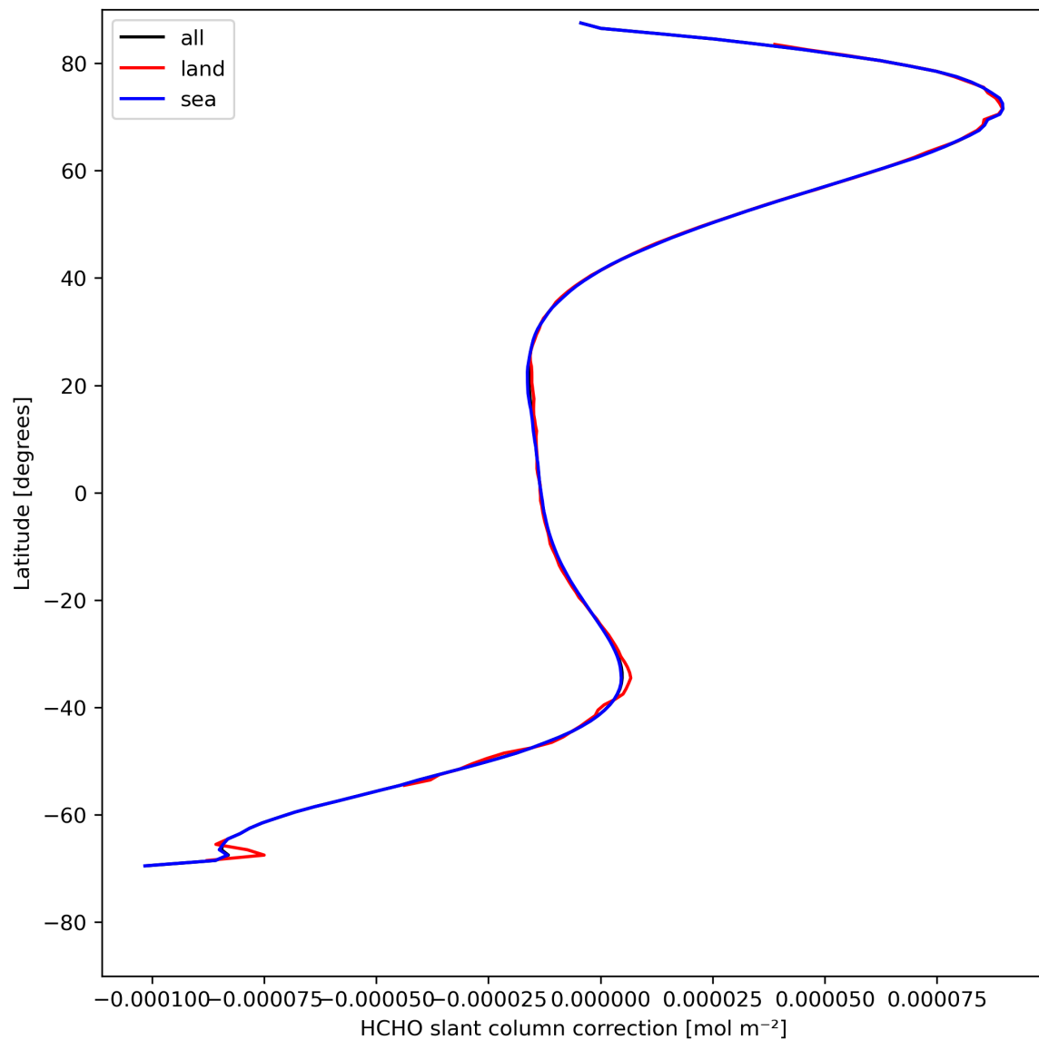
Figure 33: Zonal average of “HCHO slant column correction” for 2024-04-29 to 2024-05-01.
