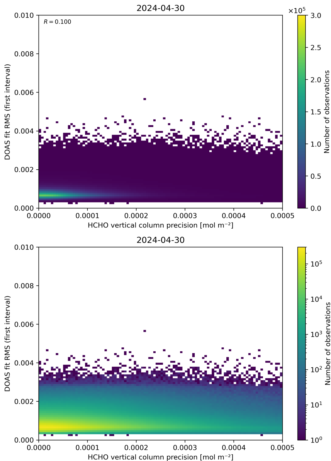
Figure 136: Scatter density plot of “HCHO vertical column precision” against “DOAS fit RMS (first interval)” for 2024-04-29 to 2024-05-01.
