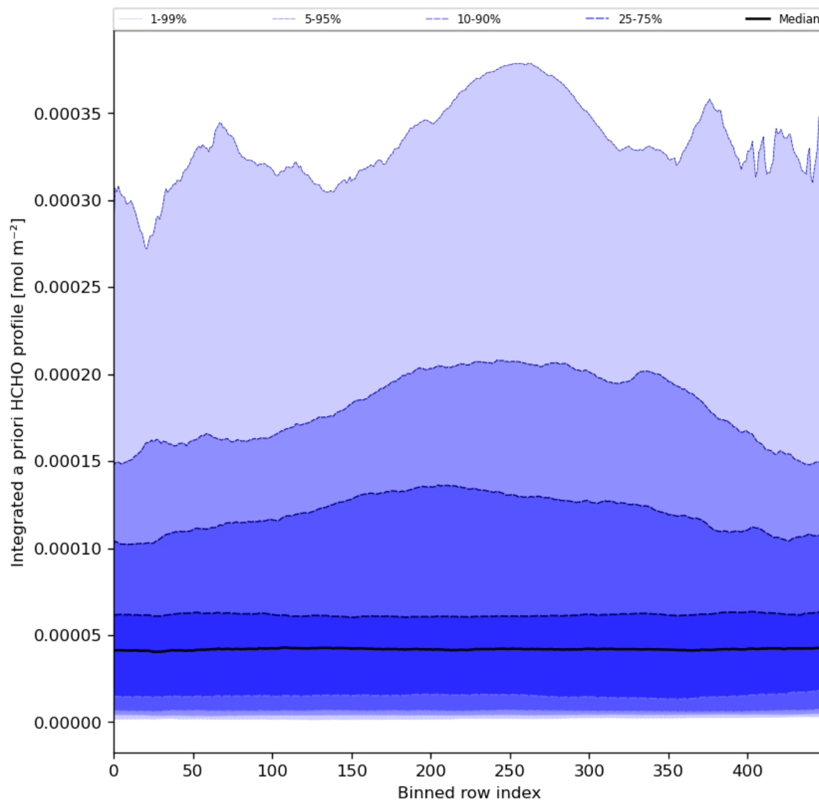
Figure 57: Along track statistics of “Integrated a priori HCHO profile” for 2024-04-29 to 2024-05-01
