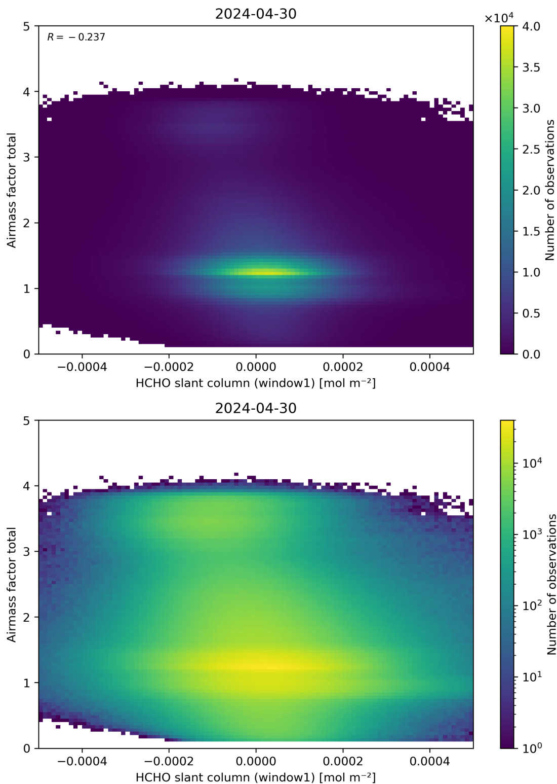
Figure 85: Scatter density plot of “HCHO slant column (window1)” against “Airmass factor total” for 2024-04-29 to 2024-05-01.
