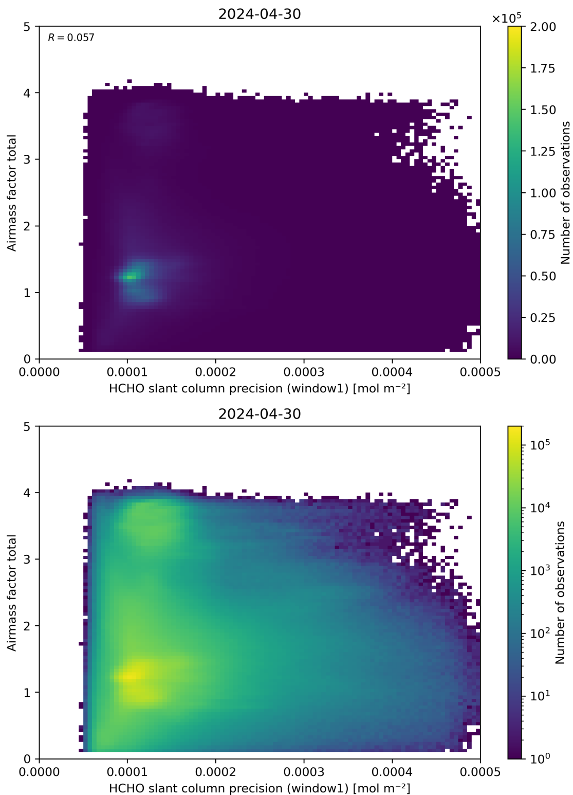
Figure 94: Scatter density plot of “HCHO slant column precision (window1)” against “Airmass factor total” for 2024-04-29 to 2024-05-01.
