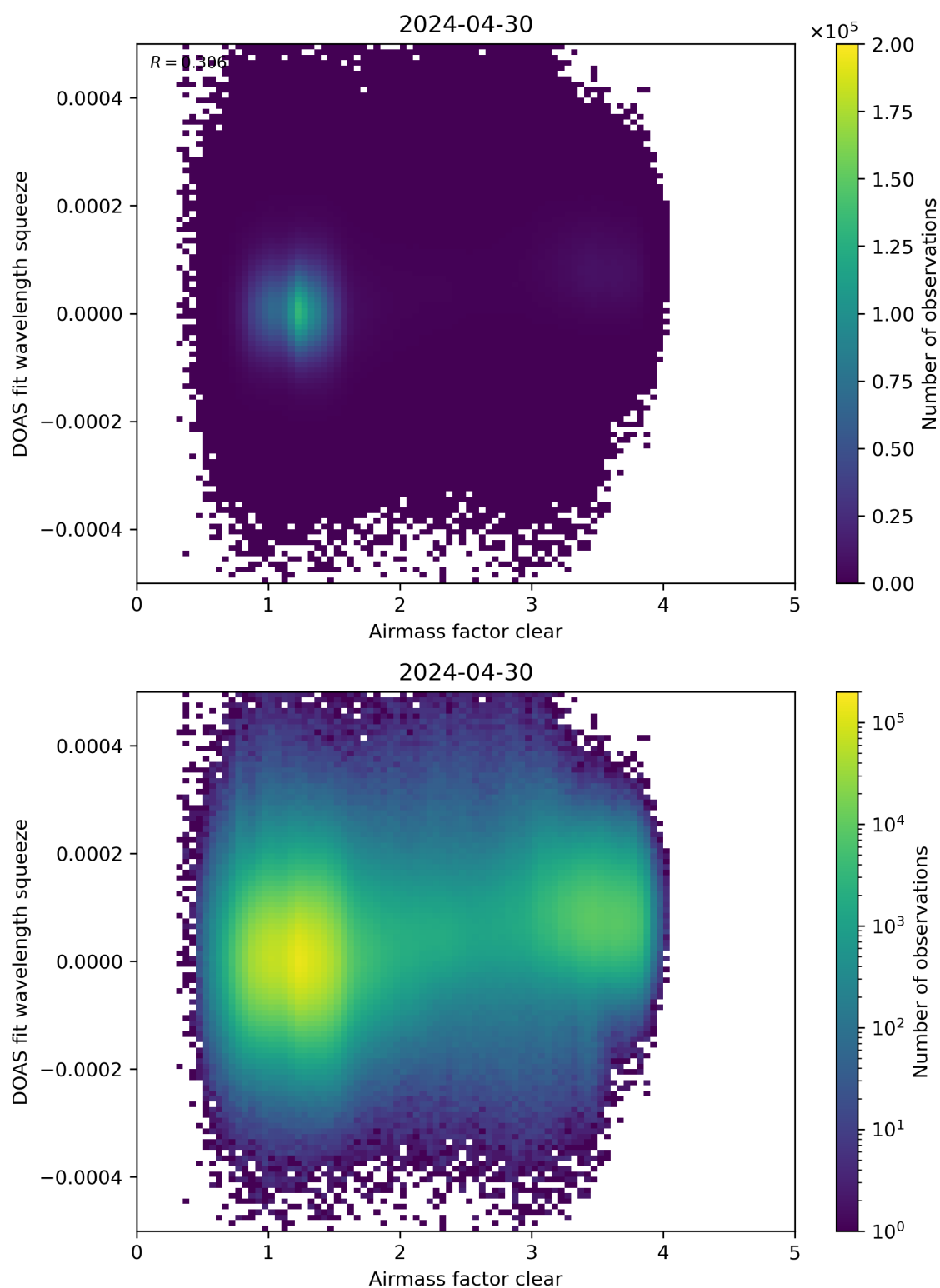
Figure 73: Scatter density plot of “Airmass factor clear” against “DOAS fit wavelength squeeze” for 2024-04-29 to 2024-05-01.
