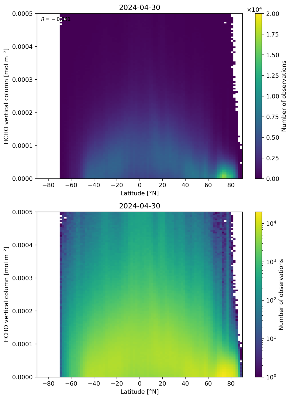
Figure 163: Scatter density plot of “Latitude” against “HCHO vertical column” for 2024-04-29 to 2024-05-01.
