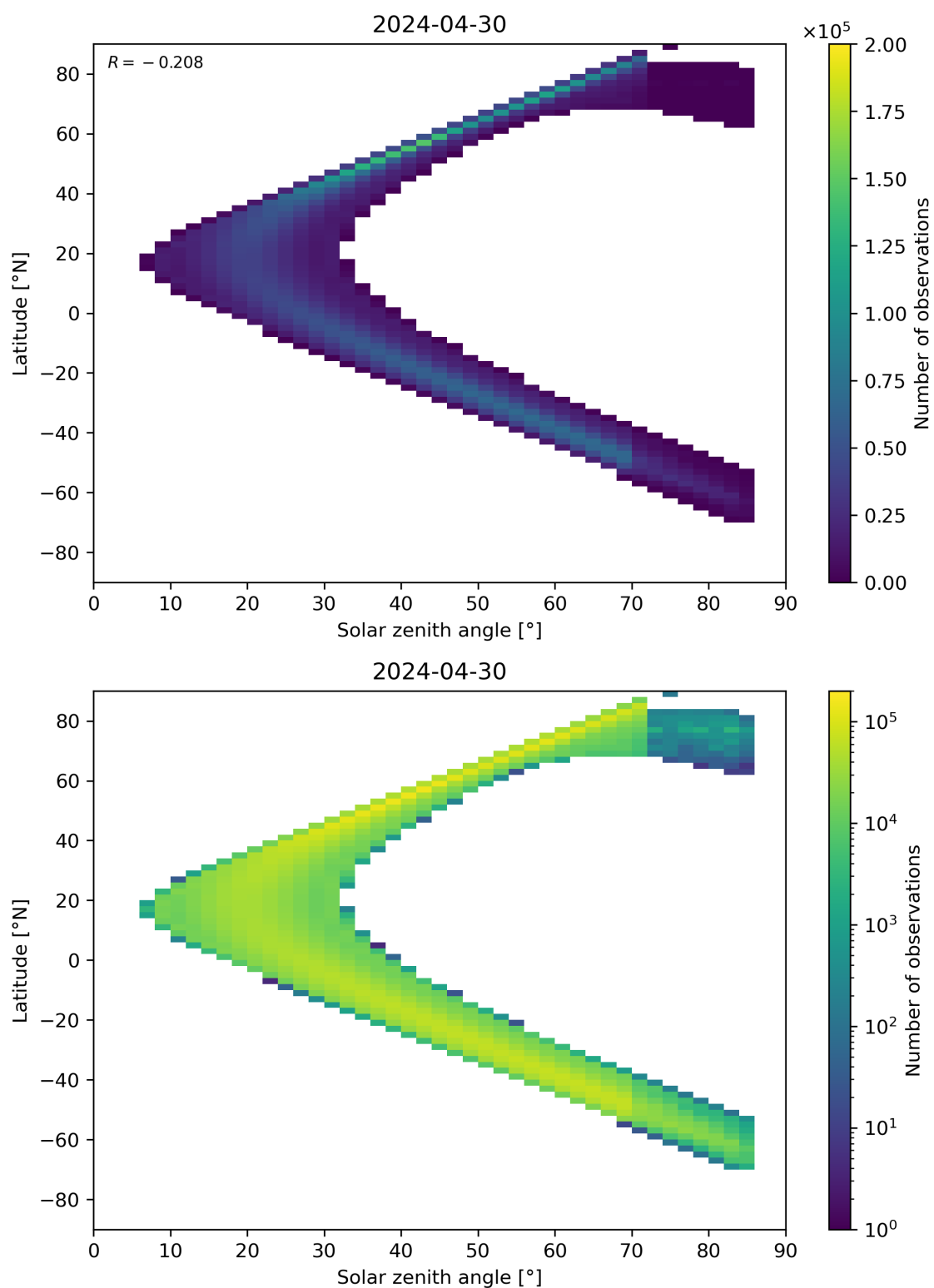
Figure 181: Scatter density plot of “Solar zenith angle” against “Latitude” for 2024-04-29 to 2024-05-01.
