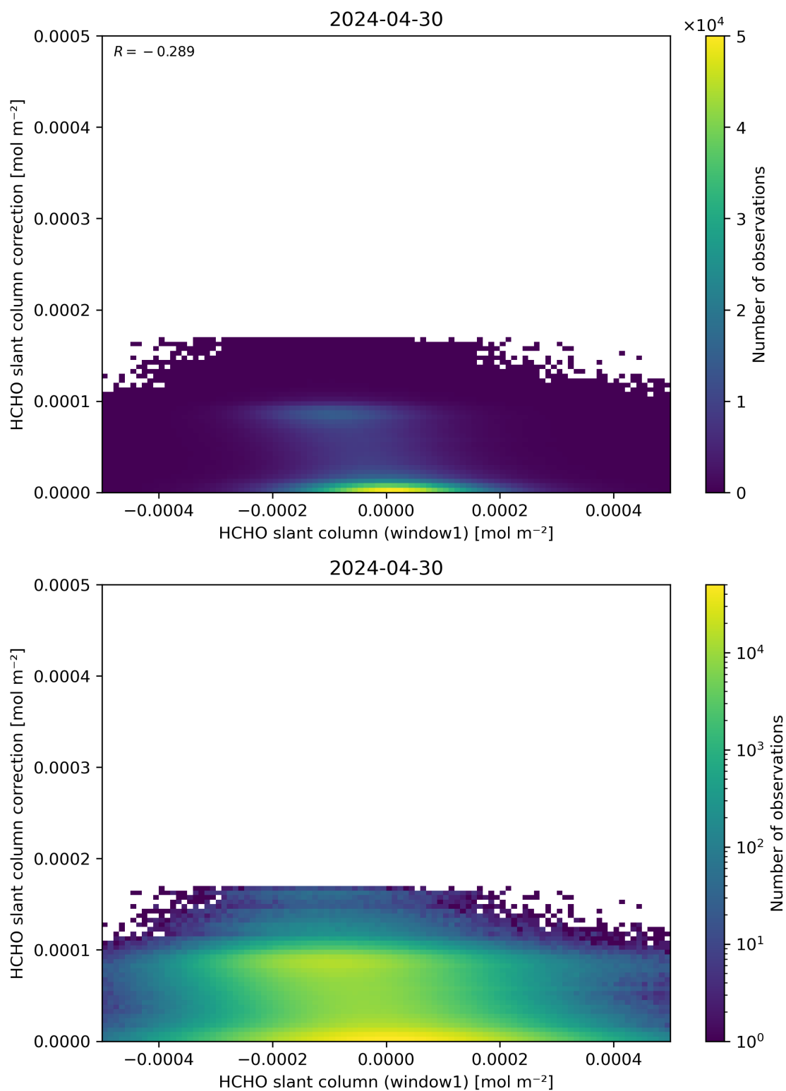
Figure 83: Scatter density plot of “HCHO slant column (window1)” against “HCHO slant column correction” for 2024-04-29 to 2024-05-01.
