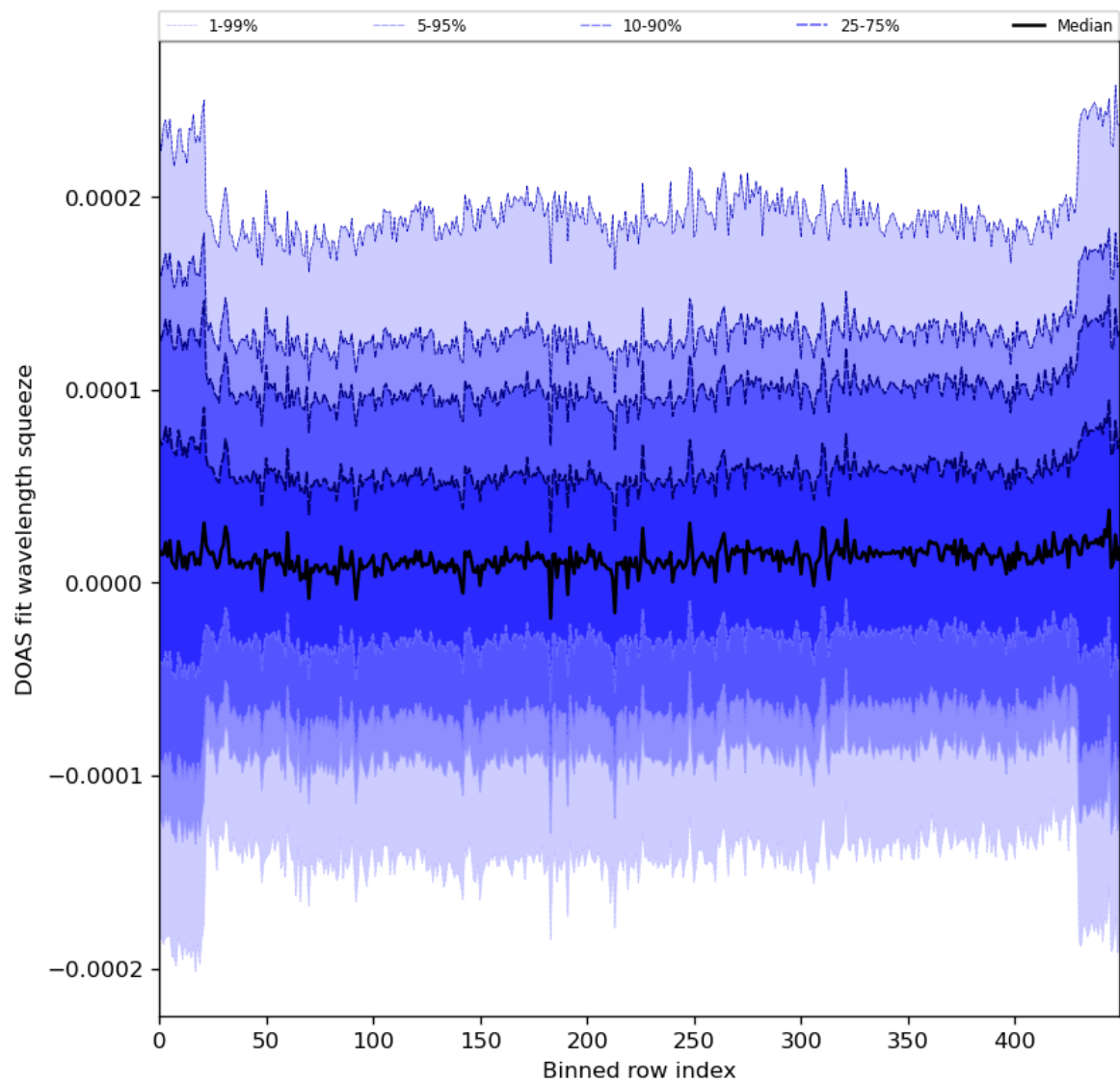
Figure 59: Along track statistics of “DOAS fit wavelength squeeze” for 2024-04-29 to 2024-05-01
