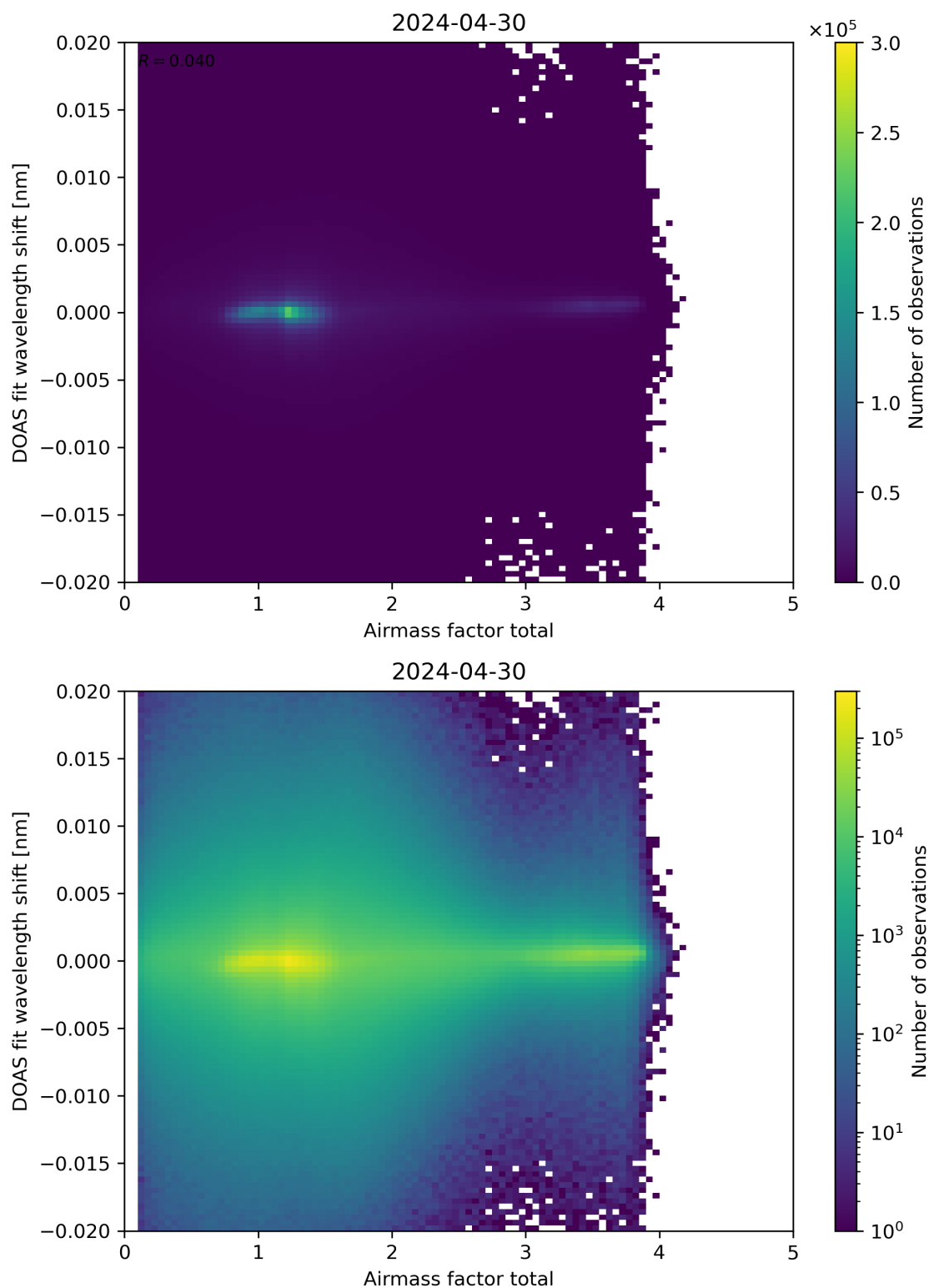
Figure 98: Scatter density plot of “Airmass factor total” against “DOAS fit wavelength shift” for 2024-04-29 to 2024-05-01.
