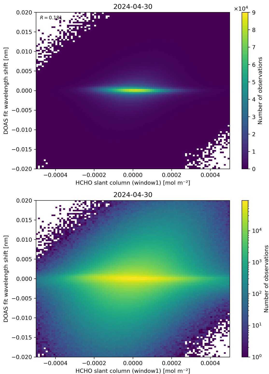
Figure 79: Scatter density plot of “HCHO slant column (window1)” against “DOAS fit wavelength shift” for 2024-04-29 to 2024-05-01.
