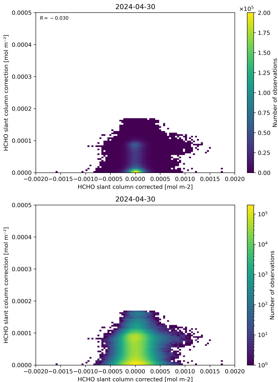
Figure 77: Scatter density plot of “HCHO slant column corrected” against “HCHO slant column correction” for 2024-04-29 to 2024-05-01.
