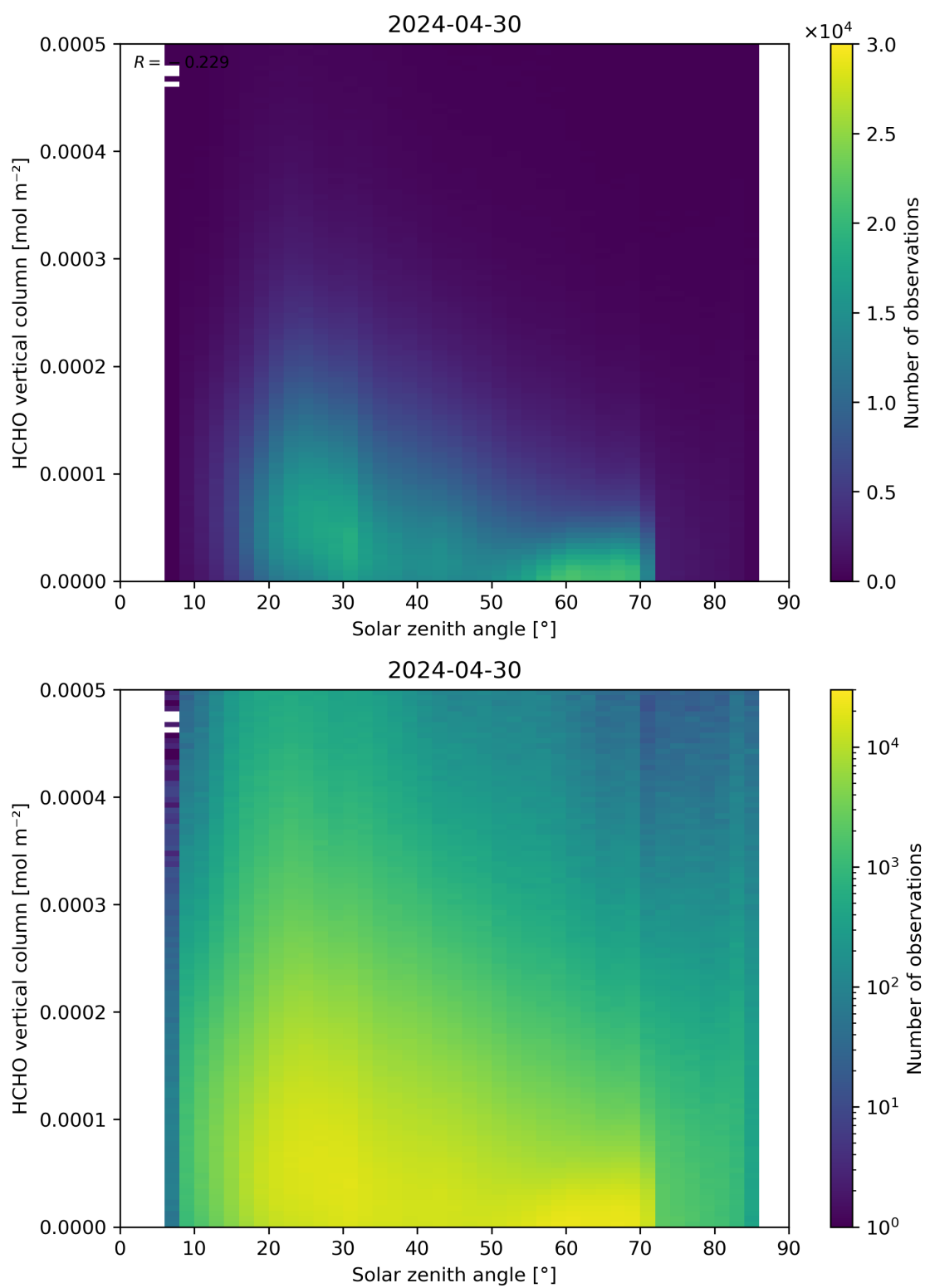
Figure 177: Scatter density plot of “Solar zenith angle” against “HCHO vertical column” for 2024-04-29 to 2024-05-01.
