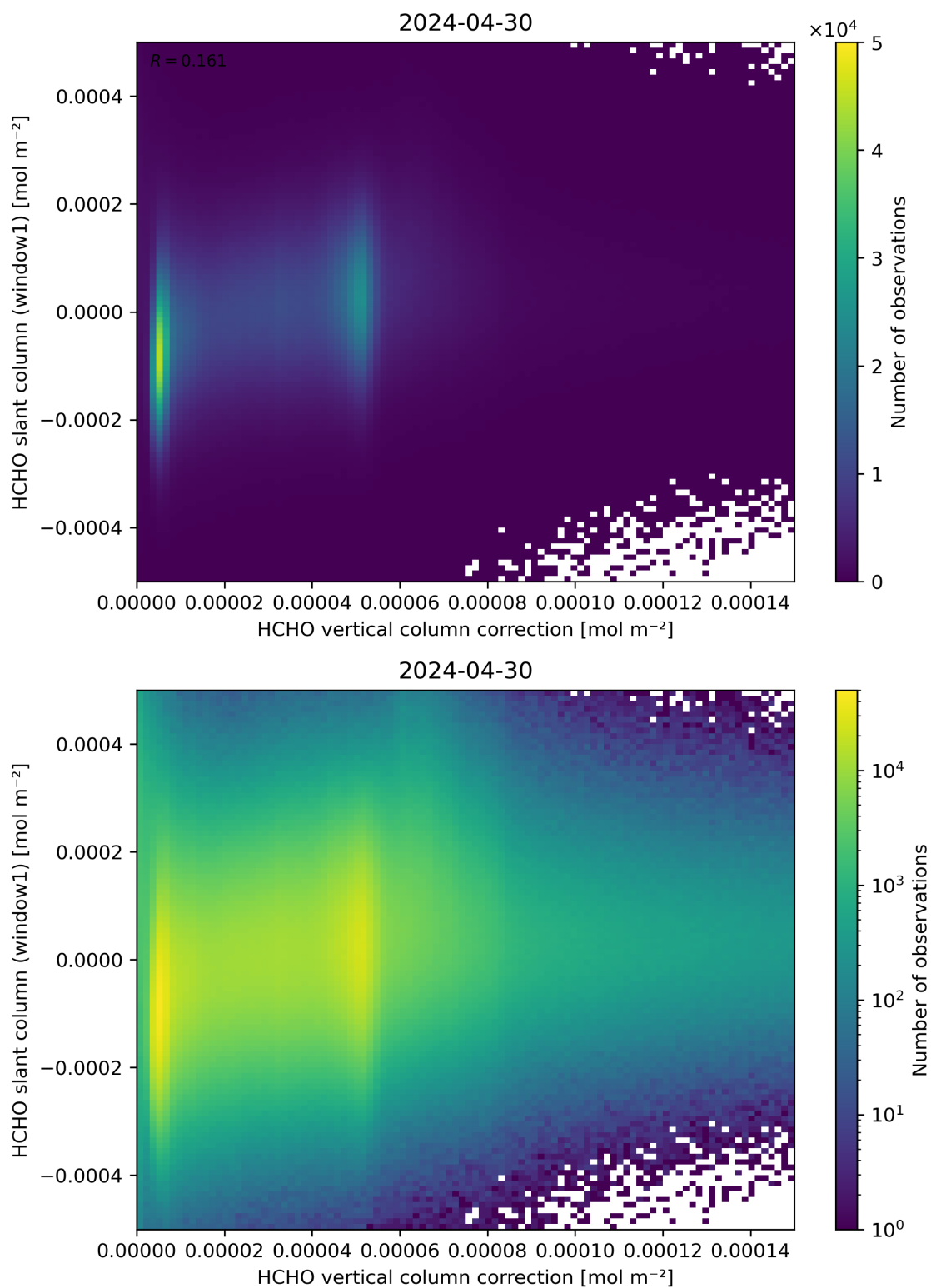
Figure 118: Scatter density plot of “HCHO vertical column correction” against “HCHO slant column (window1)” for 2024-04-29 to 2024-05-01.
