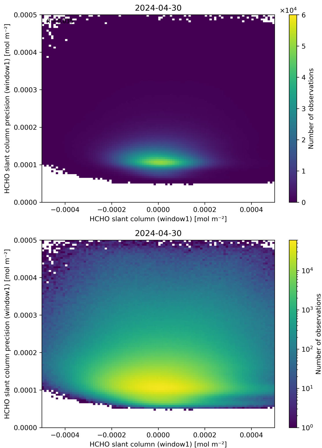
Figure 84: Scatter density plot of “HCHO slant column (window1)” against “HCHO slant column precision (window1)” for 2024-04-29 to 2024-05-01.
