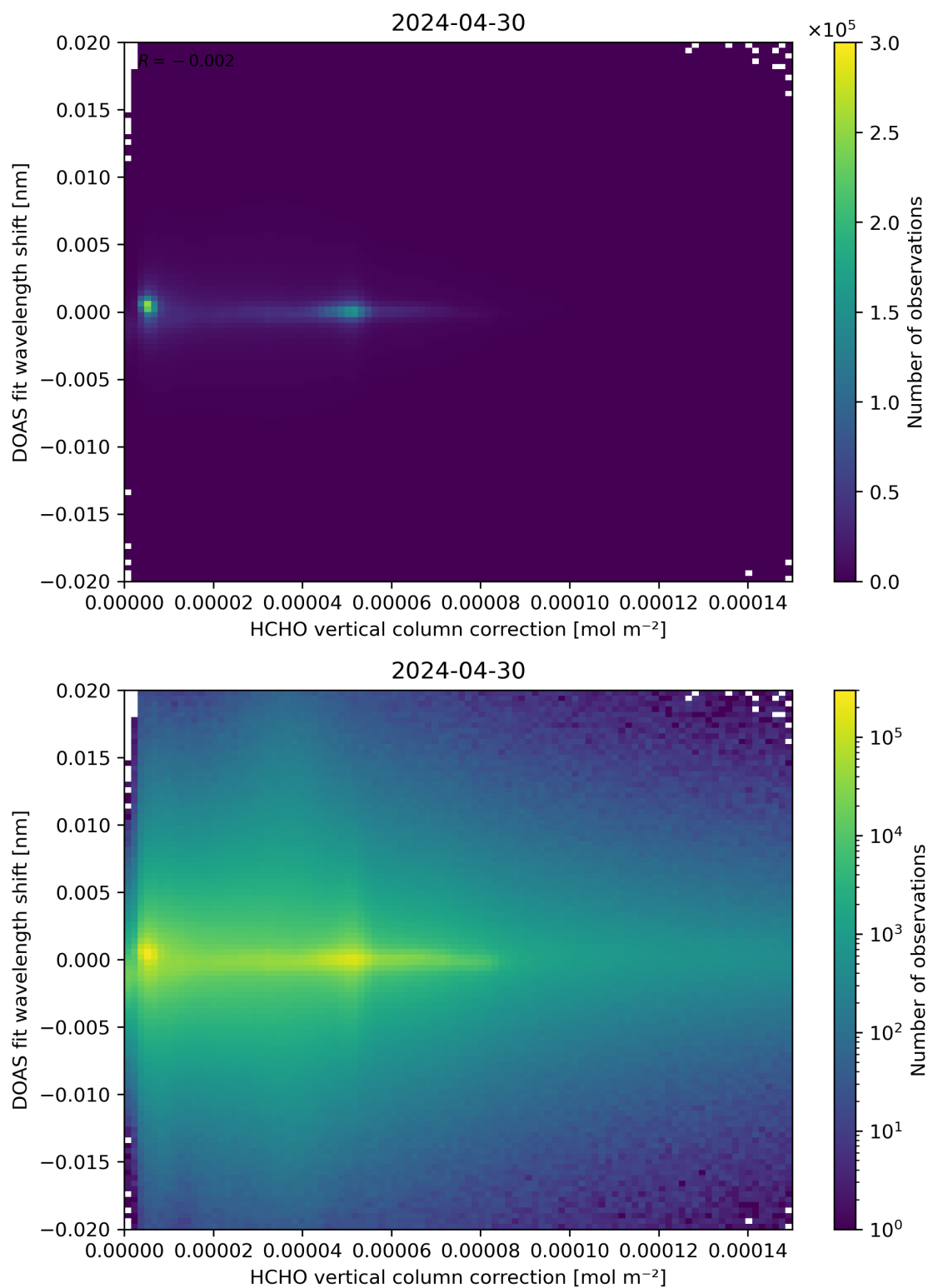
Figure 113: Scatter density plot of “HCHO vertical column correction” against “DOAS fit wavelength shift” for 2024-04-29 to 2024-05-01.
