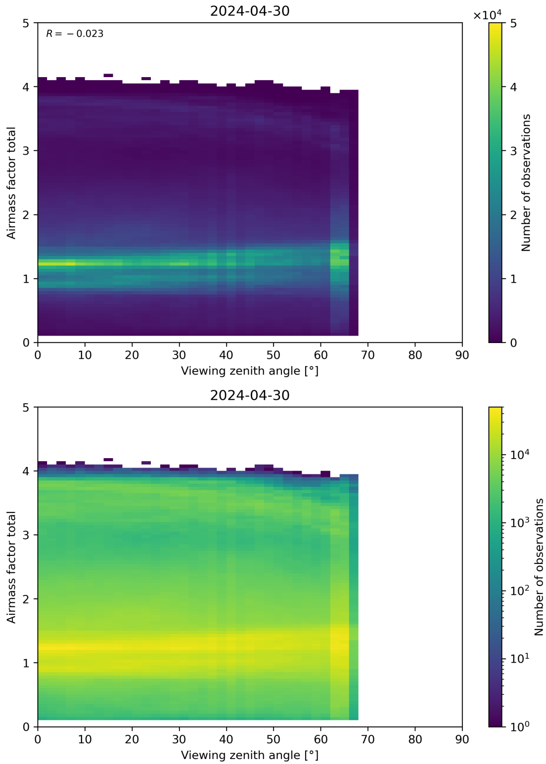
Figure 190: Scatter density plot of “Viewing zenith angle” against “Airmass factor total” for 2024-04-29 to 2024-05-01.
