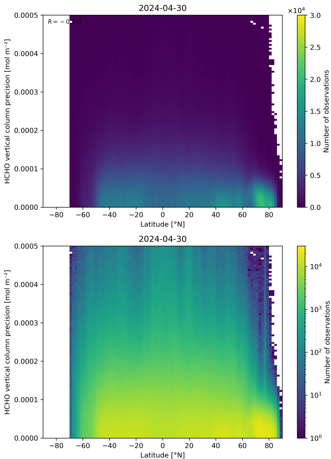
Figure 165: Scatter density plot of “Latitude” against “HCHO vertical column precision” for 2024-04-29 to 2024-05-01.
