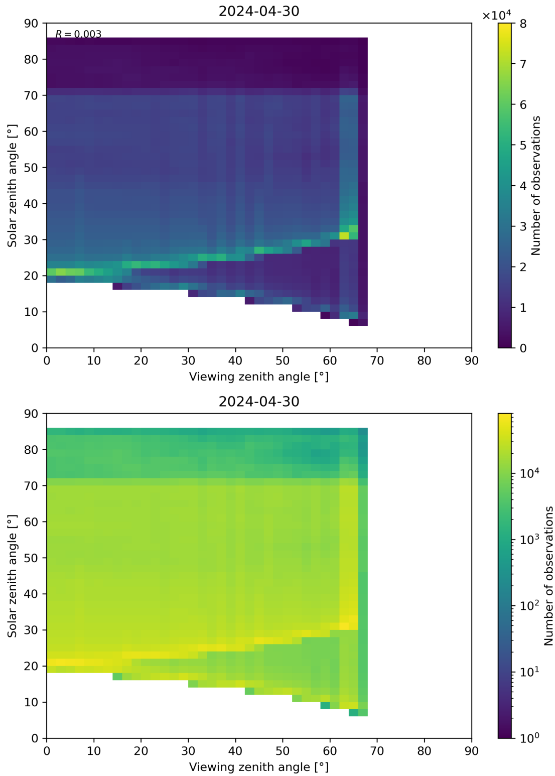
Figure 197: Scatter density plot of “Viewing zenith angle” against “Solar zenith angle” for 2024-04-29 to 2024-05-01.
