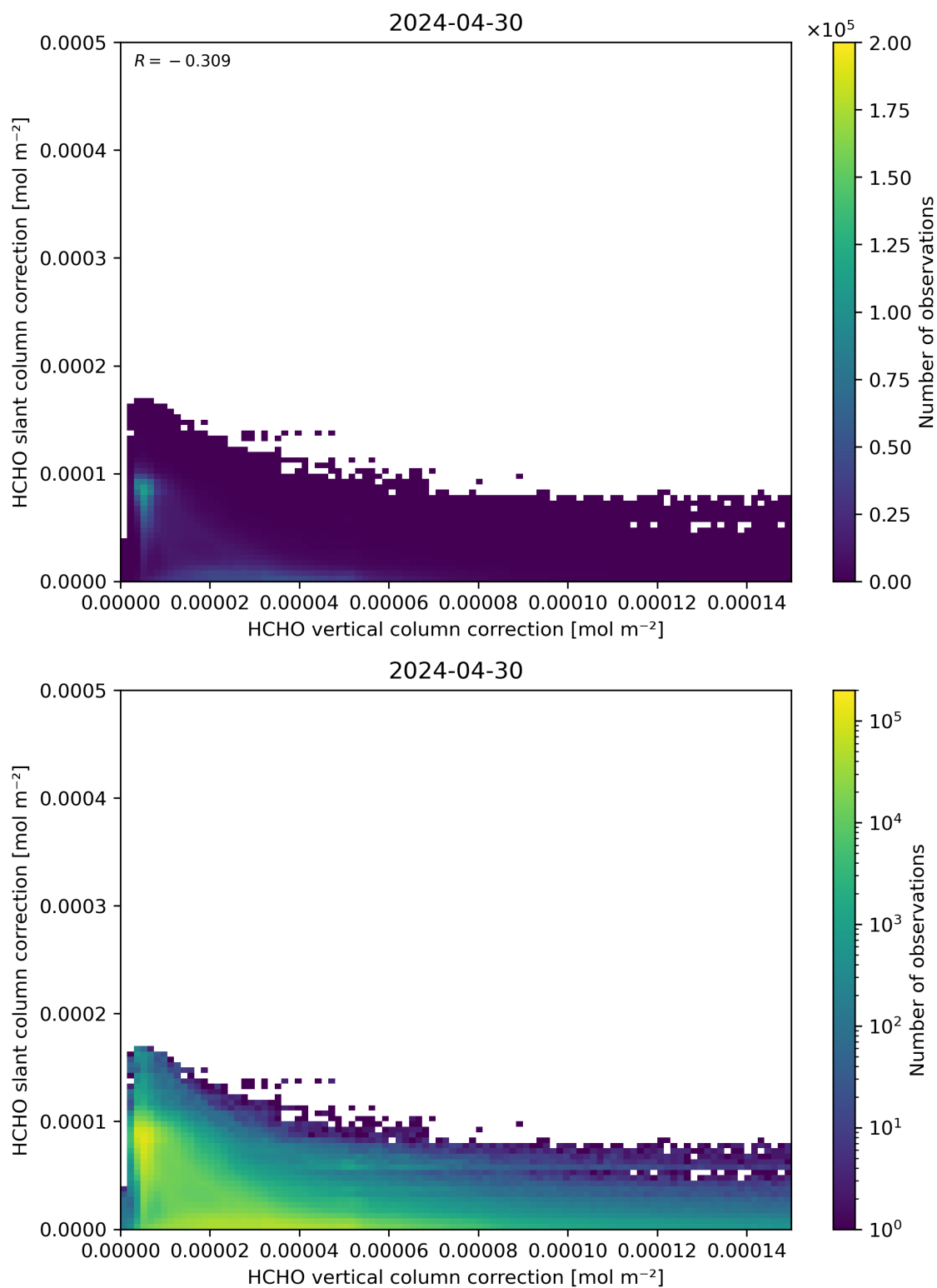
Figure 117: Scatter density plot of “HCHO vertical column correction” against “HCHO slant column correction” for 2024-04-29 to 2024-05-01.
