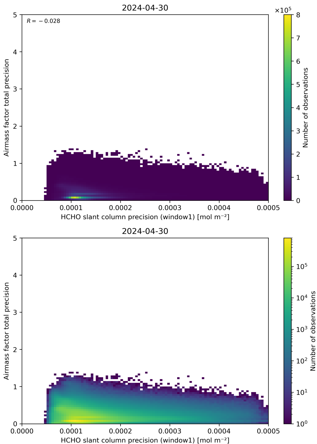
Figure 95: Scatter density plot of “HCHO slant column precision (window1)” against “Airmass factor total precision” for 2024-04-29 to 2024-05-01.
