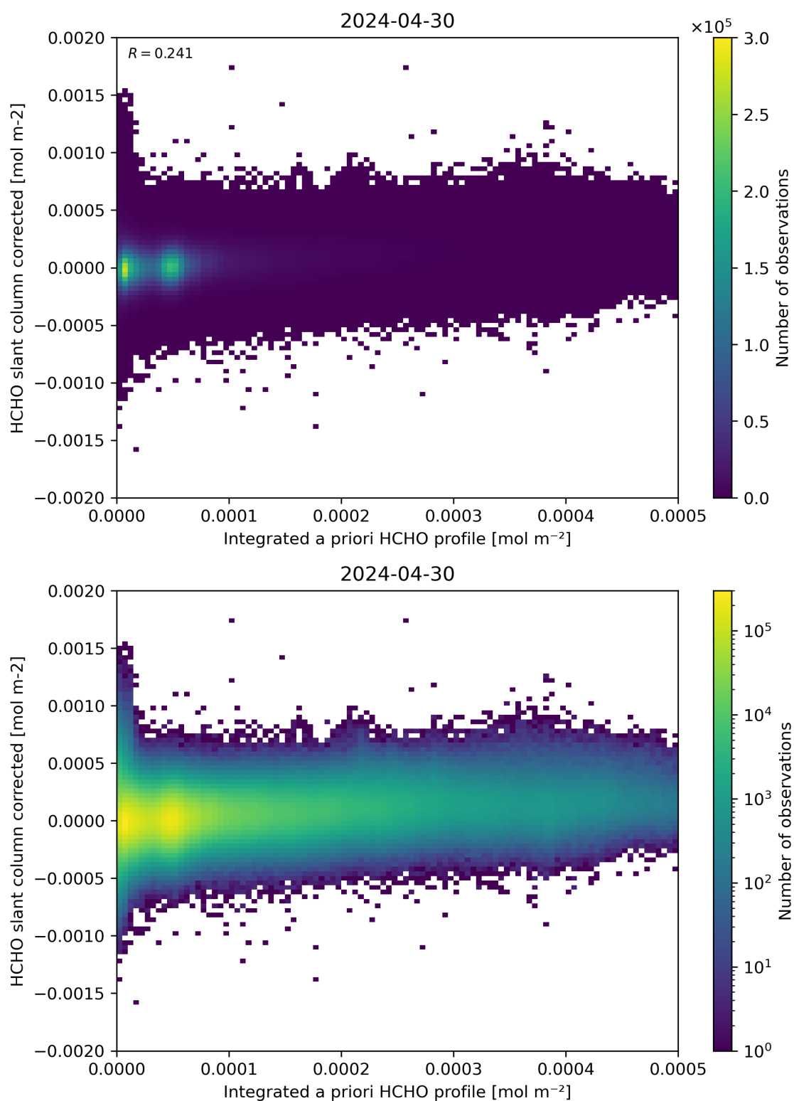
Figure 151: Scatter density plot of “Integrated a priori HCHO profile” against “HCHO slant column corrected” for 2024-04-29 to 2024-05-01.
