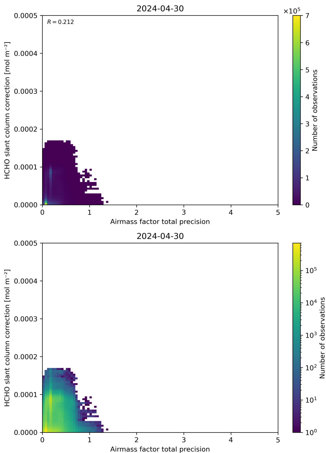
Figure 110: Scatter density plot of “Airmass factor total precision” against “HCHO slant column correction” for 2024-04-29 to 2024-05-01.
