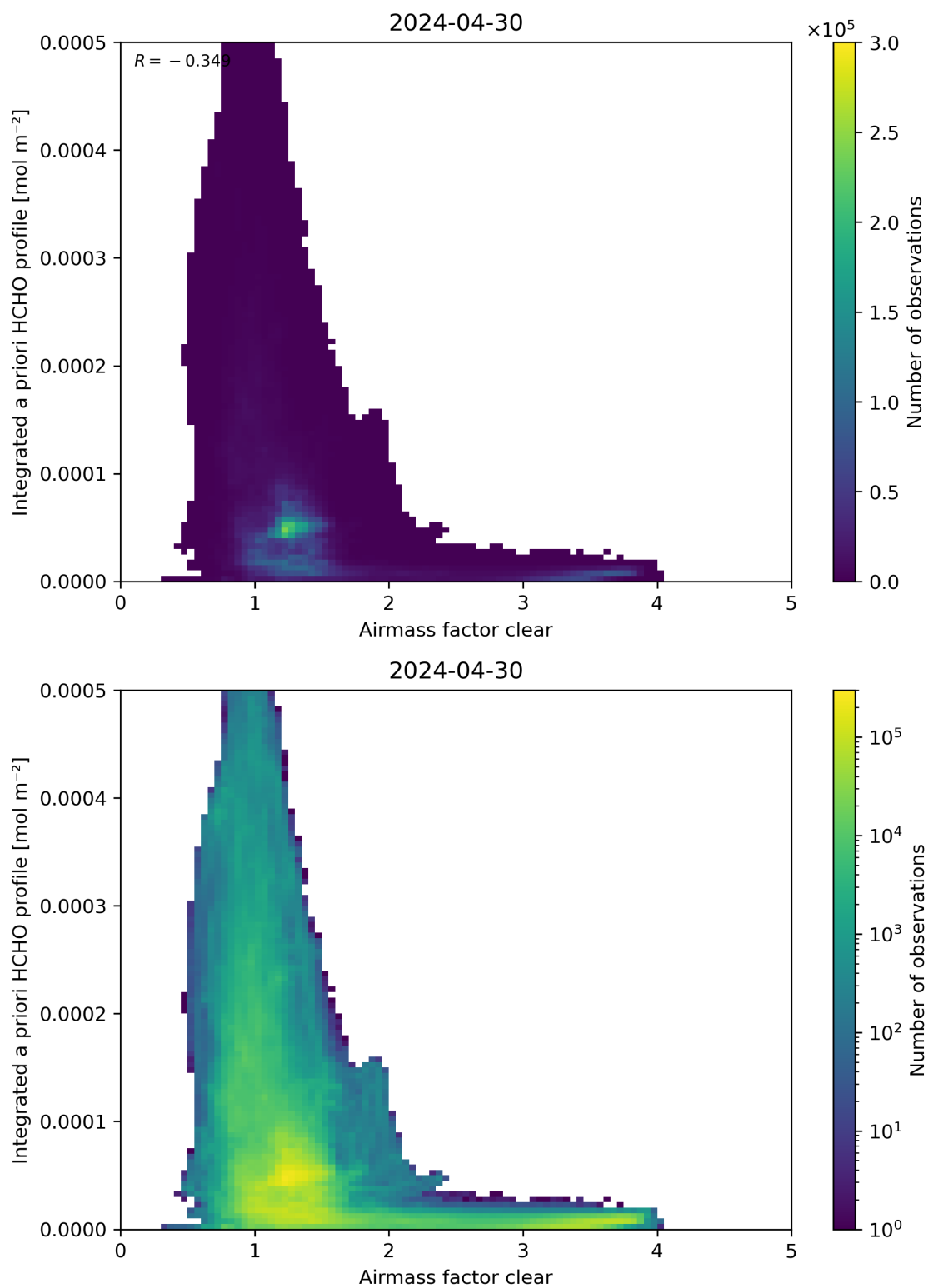
Figure 76: Scatter density plot of “Airmass factor clear” against “Integrated a priori HCHO profile” for 2024-04-29 to 2024-05-01.
