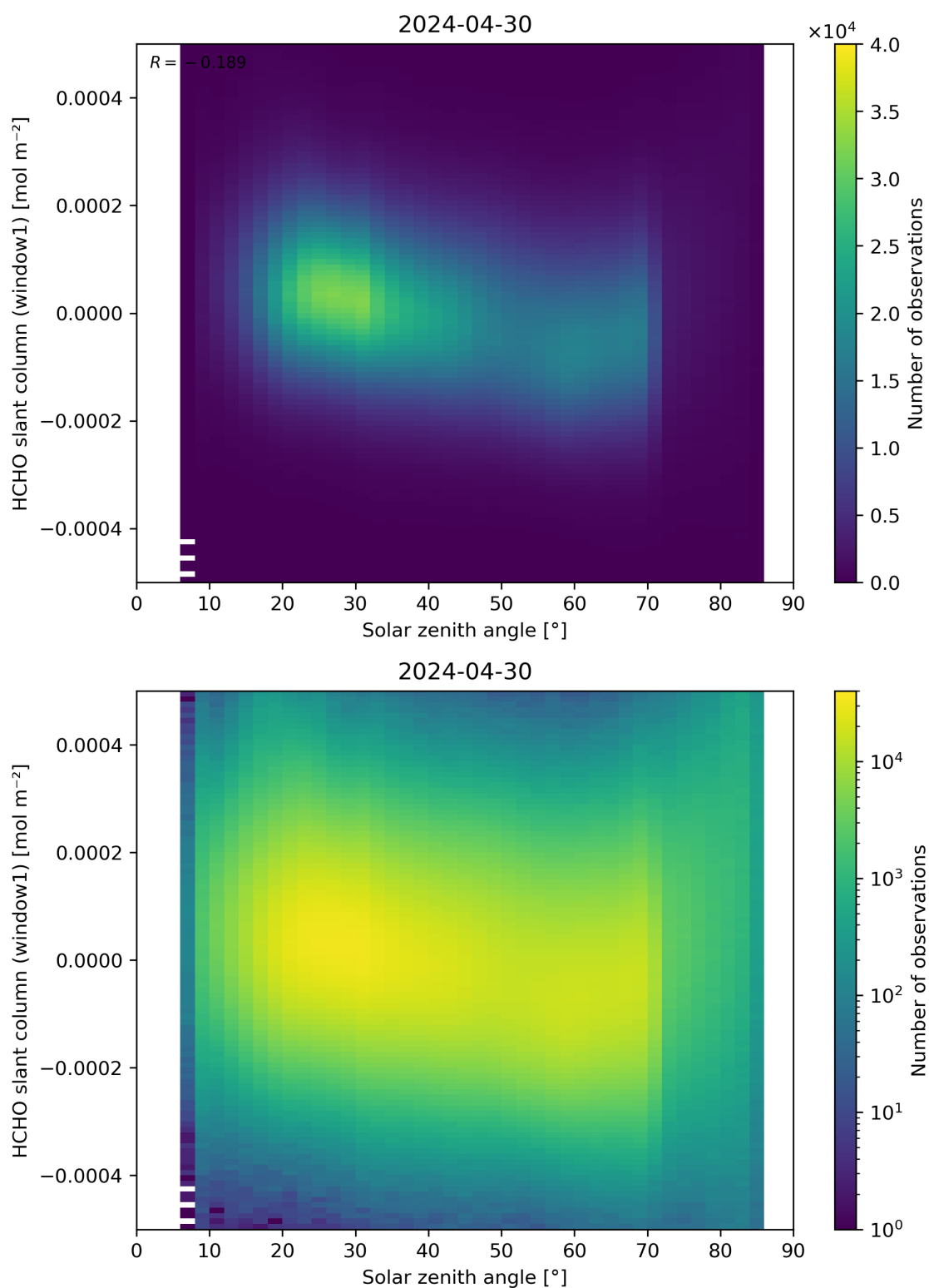
Figure 173: Scatter density plot of “Solar zenith angle” against “HCHO slant column (window1)” for 2024-04-29 to 2024-05-01.
