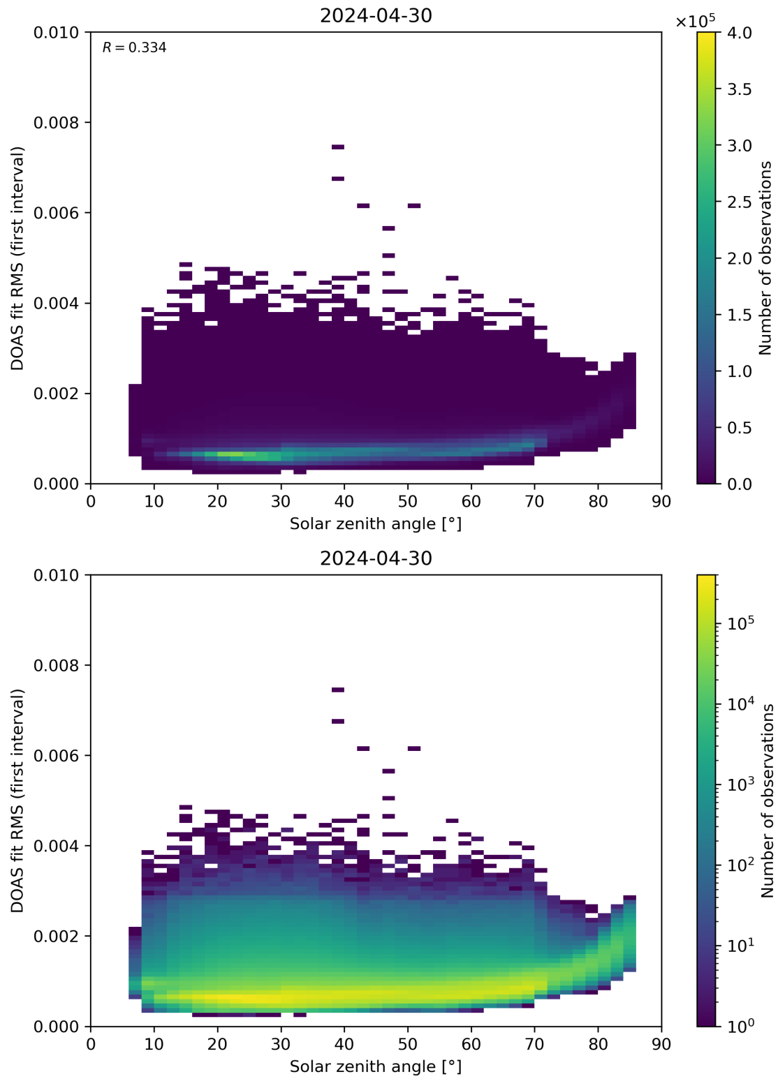
Figure 167: Scatter density plot of “Solar zenith angle” against “DOAS fit RMS (first interval)” for 2024-04-29 to 2024-05-01.
