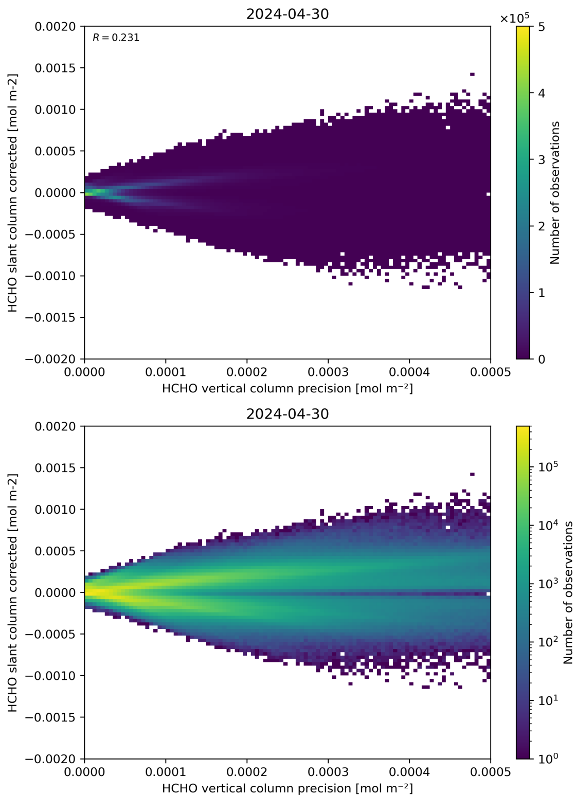
Figure 140: Scatter density plot of “HCHO vertical column precision” against “HCHO slant column corrected” for 2024-04-29 to 2024-05-01.
