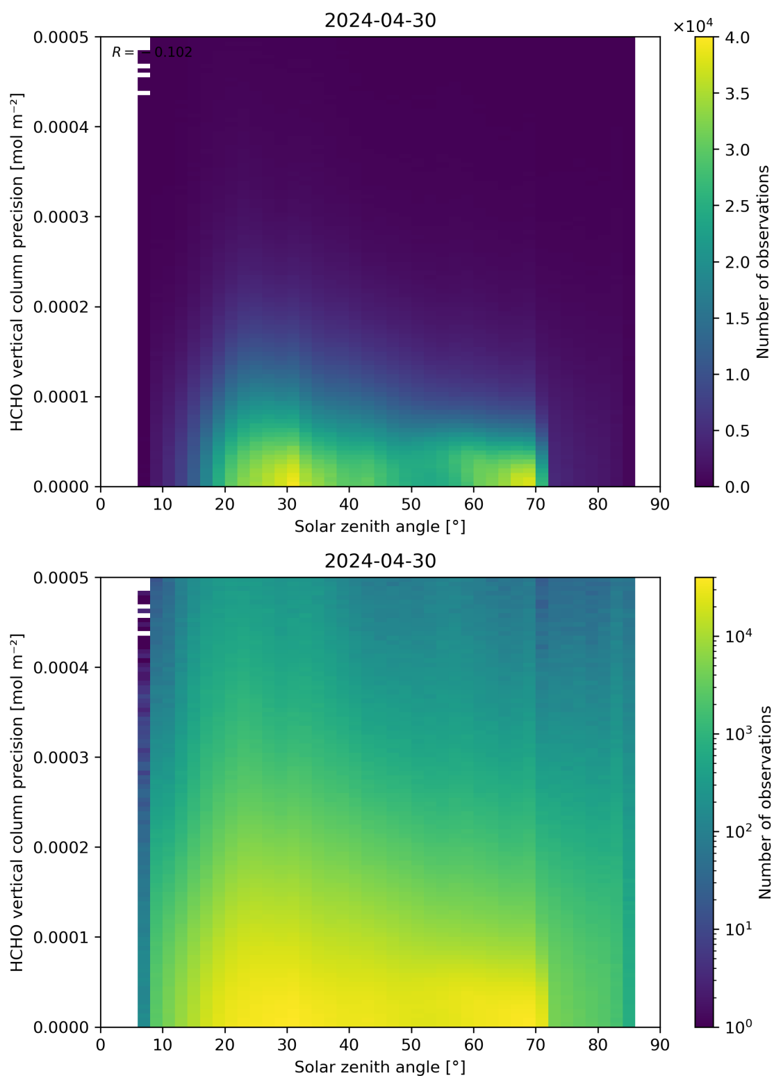
Figure 179: Scatter density plot of “Solar zenith angle” against “HCHO vertical column precision” for 2024-04-29 to 2024-05-01.
