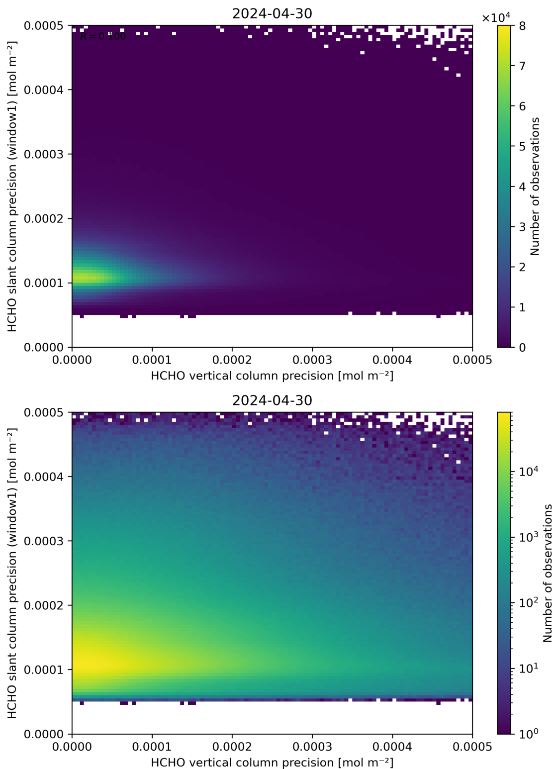
Figure 143: Scatter density plot of “HCHO vertical column precision” against “HCHO slant column precision (window1)” for 2024-04-29 to 2024-05-01.
