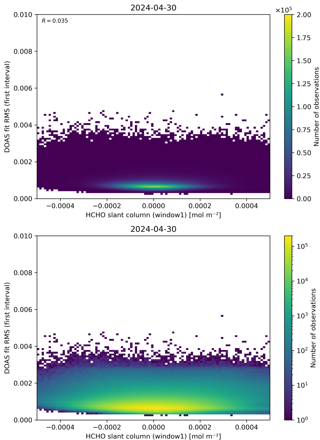
Figure 78: Scatter density plot of “HCHO slant column (window1)” against “DOAS fit RMS (first interval)” for 2024-04-29 to 2024-05-01.
