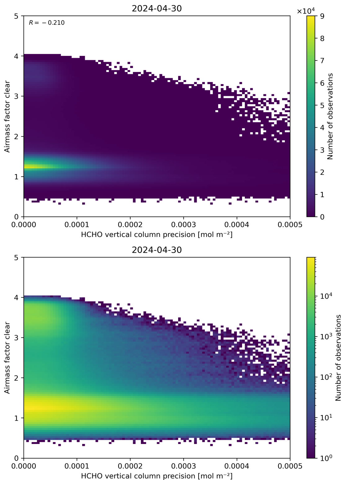
Figure 139: Scatter density plot of “HCHO vertical column precision” against “Airmass factor clear” for 2024-04-29 to 2024-05-01.
