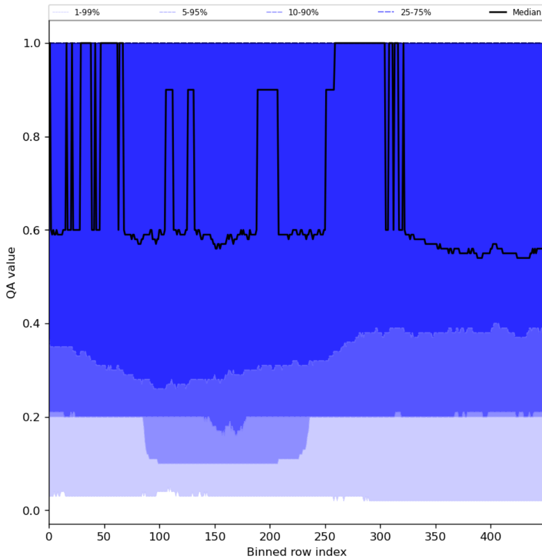
Figure 48: Along track statistics of “QA value” for 2024-04-29 to 2024-05-01
