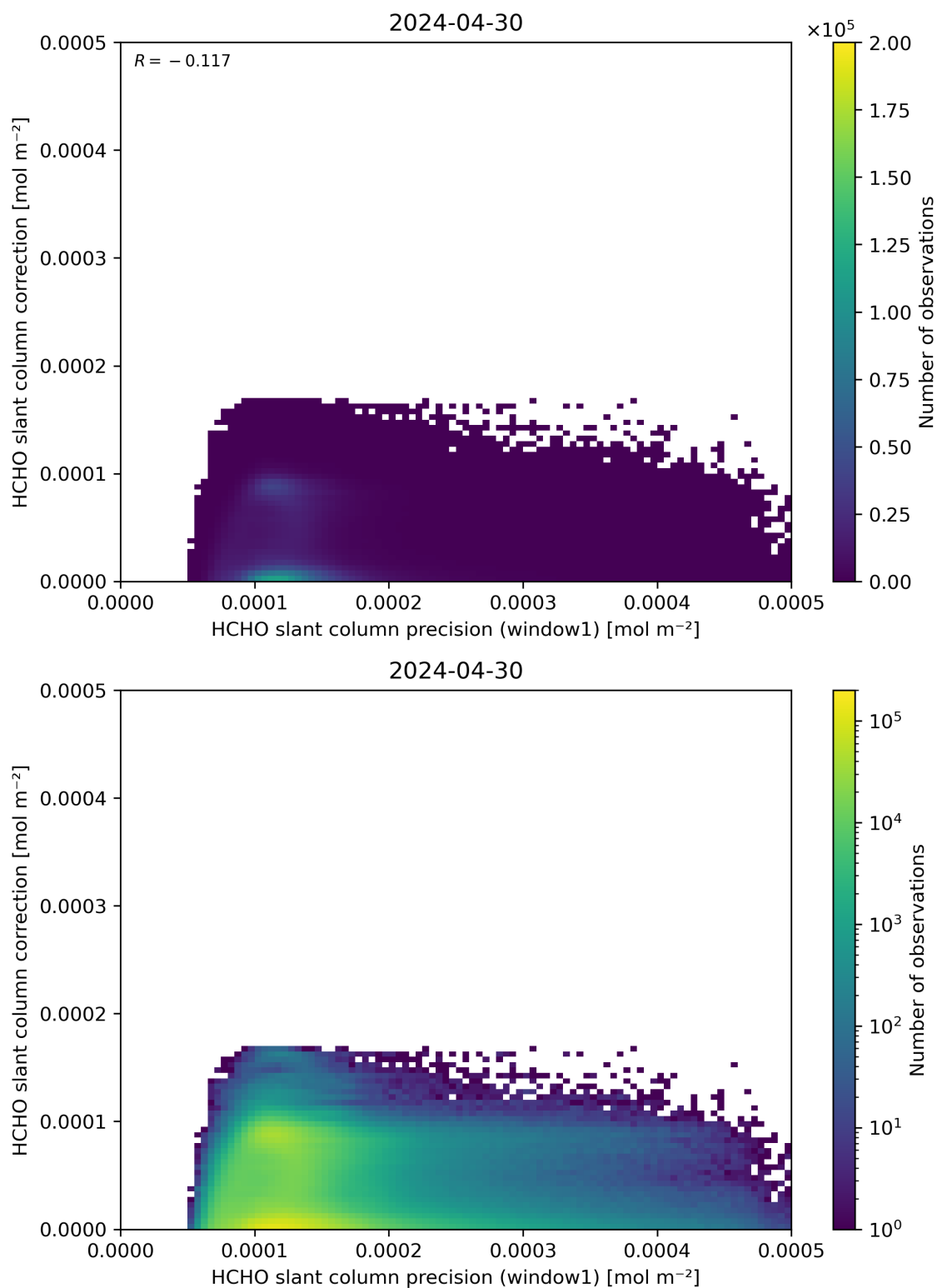
Figure 93: Scatter density plot of “HCHO slant column precision (window1)” against “HCHO slant column correction” for 2024-04-29 to 2024-05-01.
