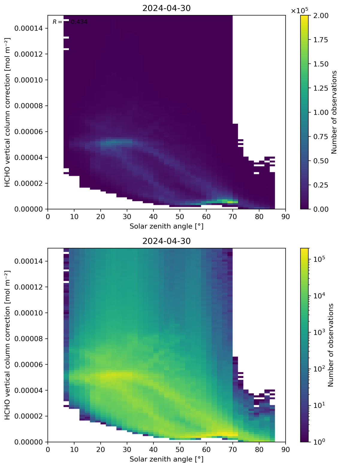
Figure 178: Scatter density plot of “Solar zenith angle” against “HCHO vertical column correction” for 2024-04-29 to 2024-05-01.
