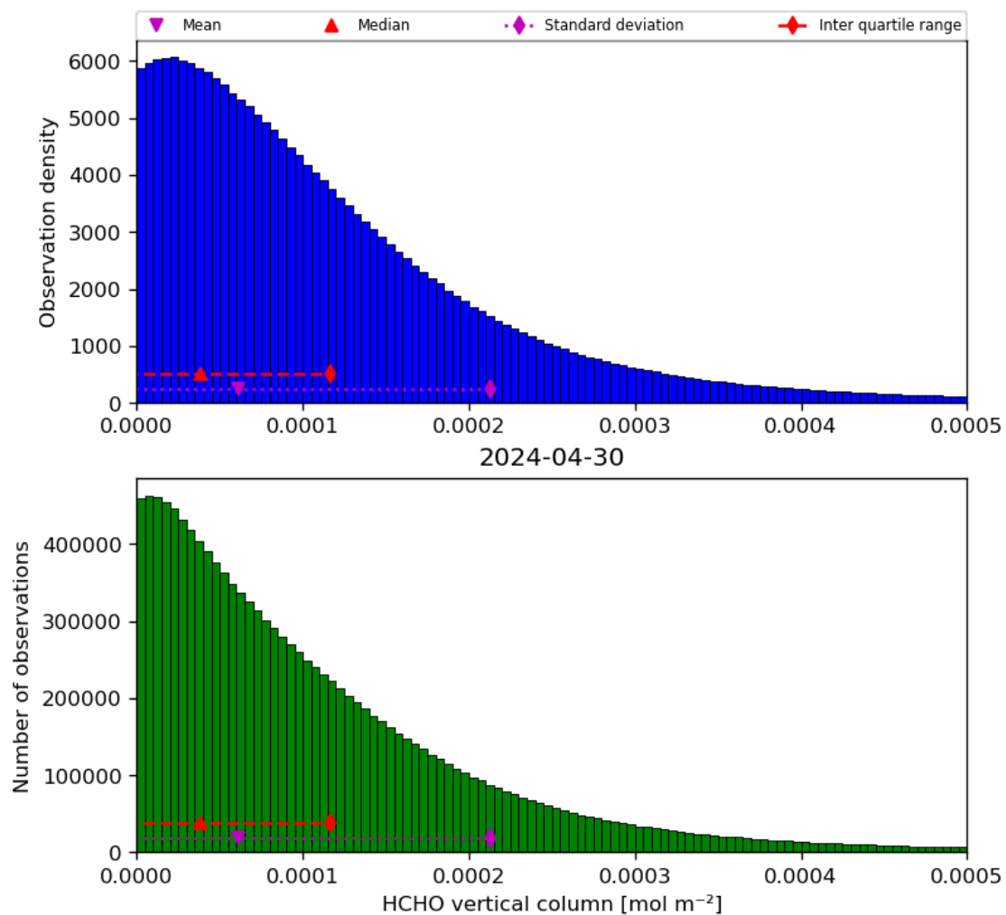
Figure 35: Histogram of “HCHO vertical column” for 2024-04-29 to 2024-05-01
