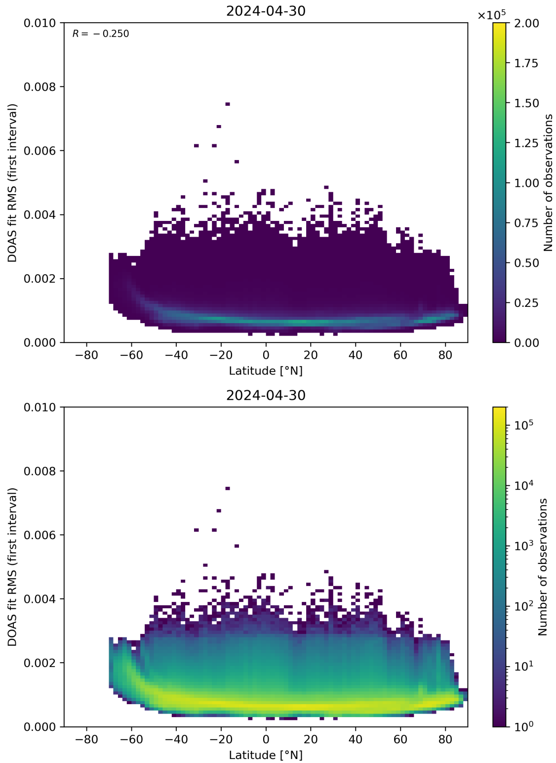
Figure 153: Scatter density plot of “Latitude” against “DOAS fit RMS (first interval)” for 2024-04-29 to 2024-05-01.
