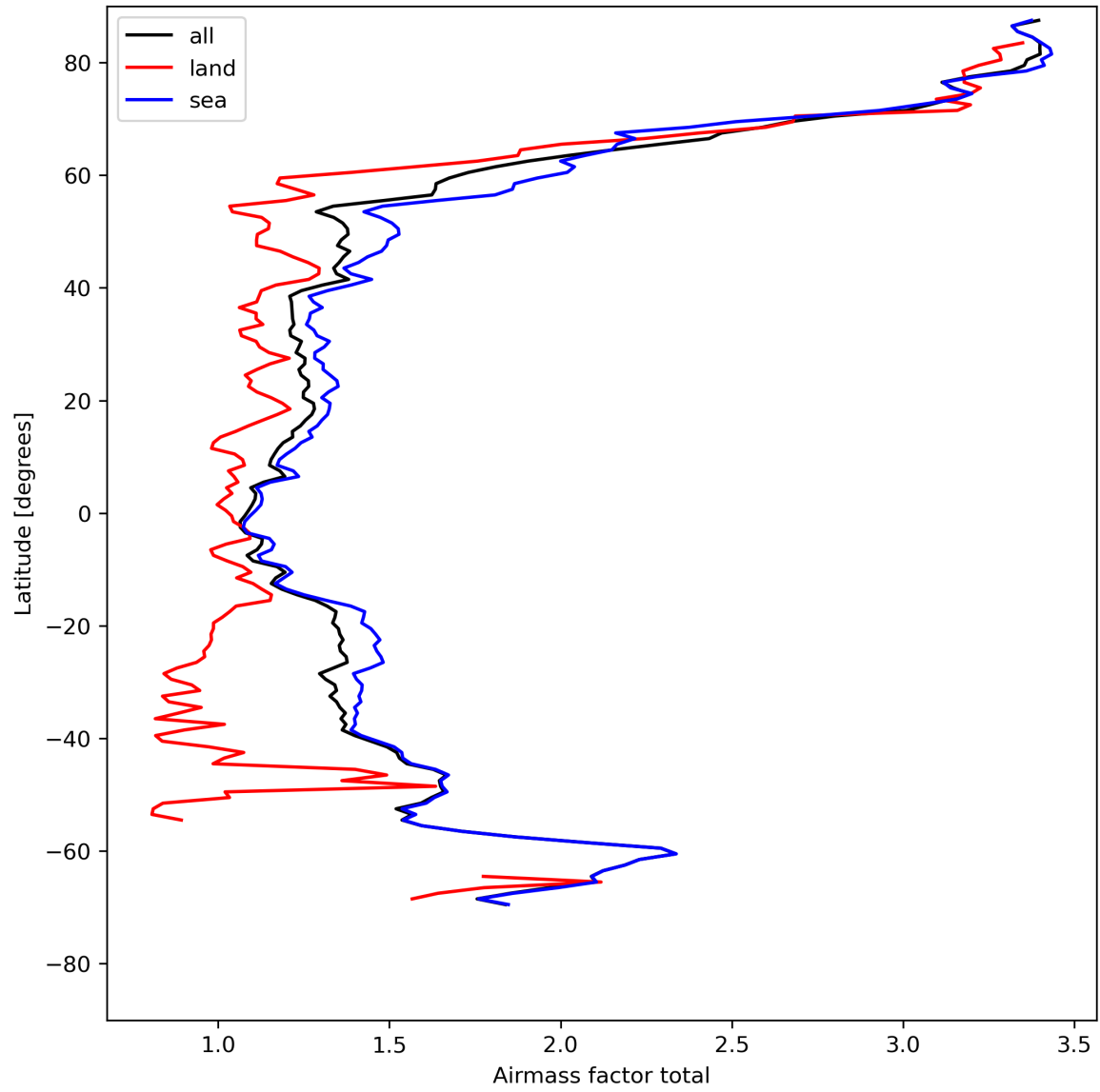
Figure 26: Zonal average of “Airmass factor total” for 2024-04-29 to 2024-05-01.
