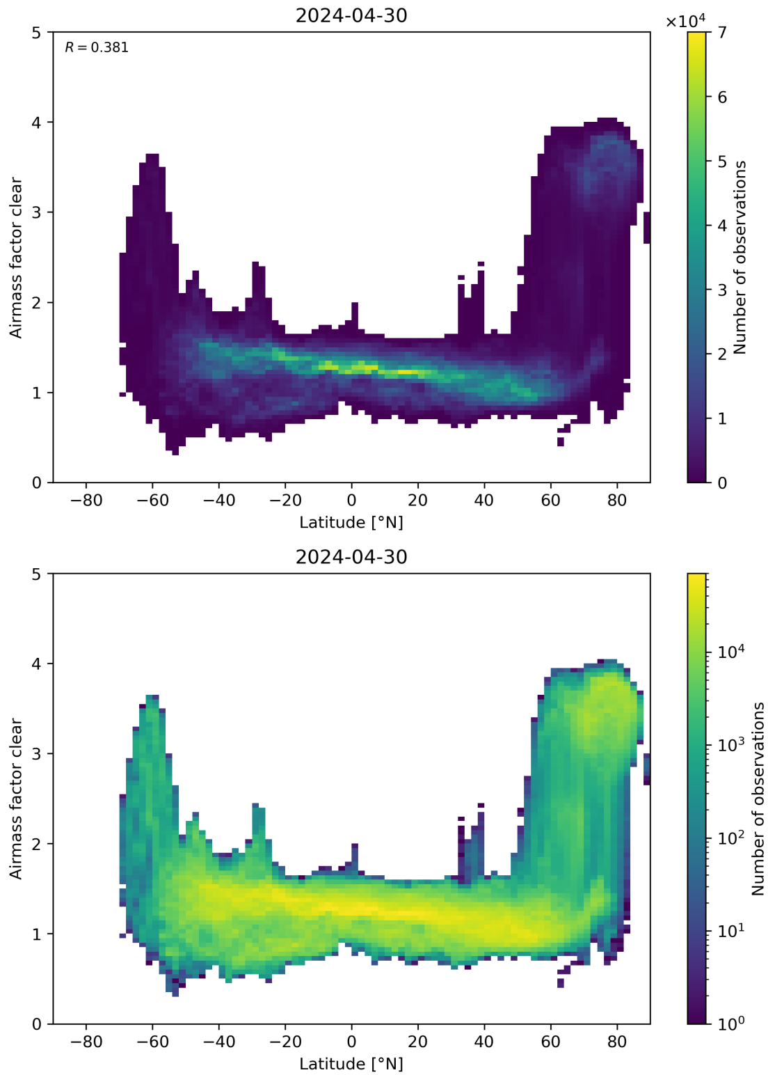
Figure 156: Scatter density plot of “Latitude” against “Airmass factor clear” for 2024-04-29 to 2024-05-01.
