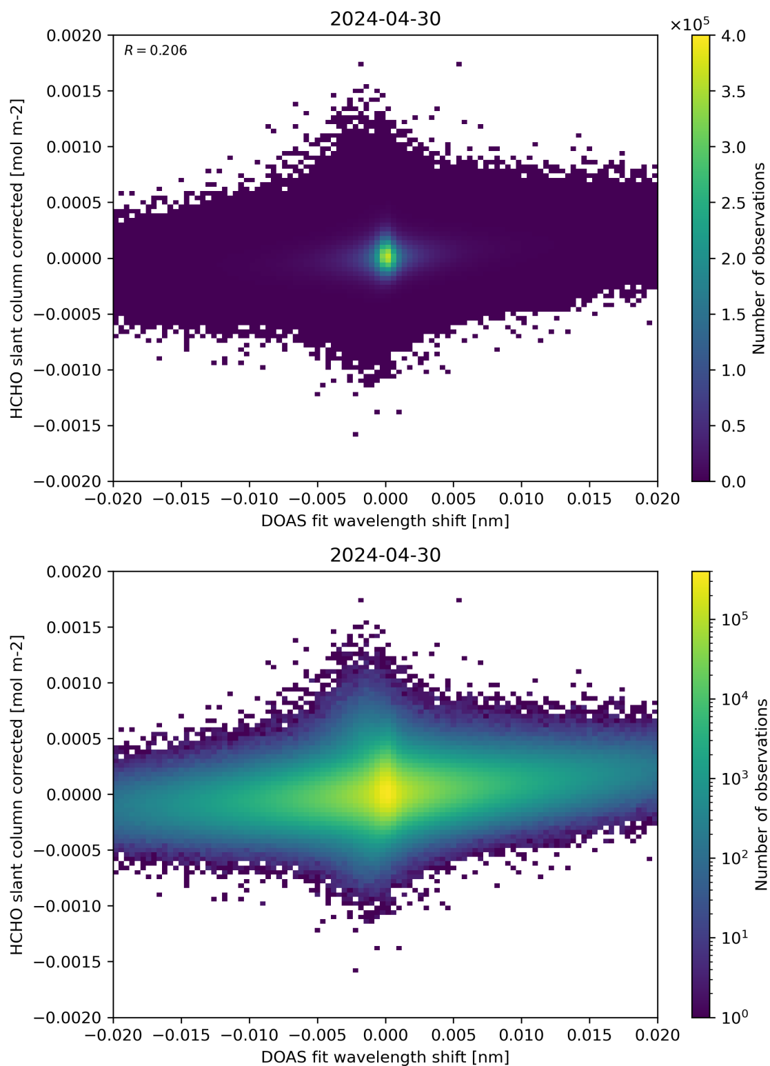
Figure 66: Scatter density plot of “DOAS fit wavelength shift” against “HCHO slant column corrected” for 2024-04-29 to 2024-05-01.
