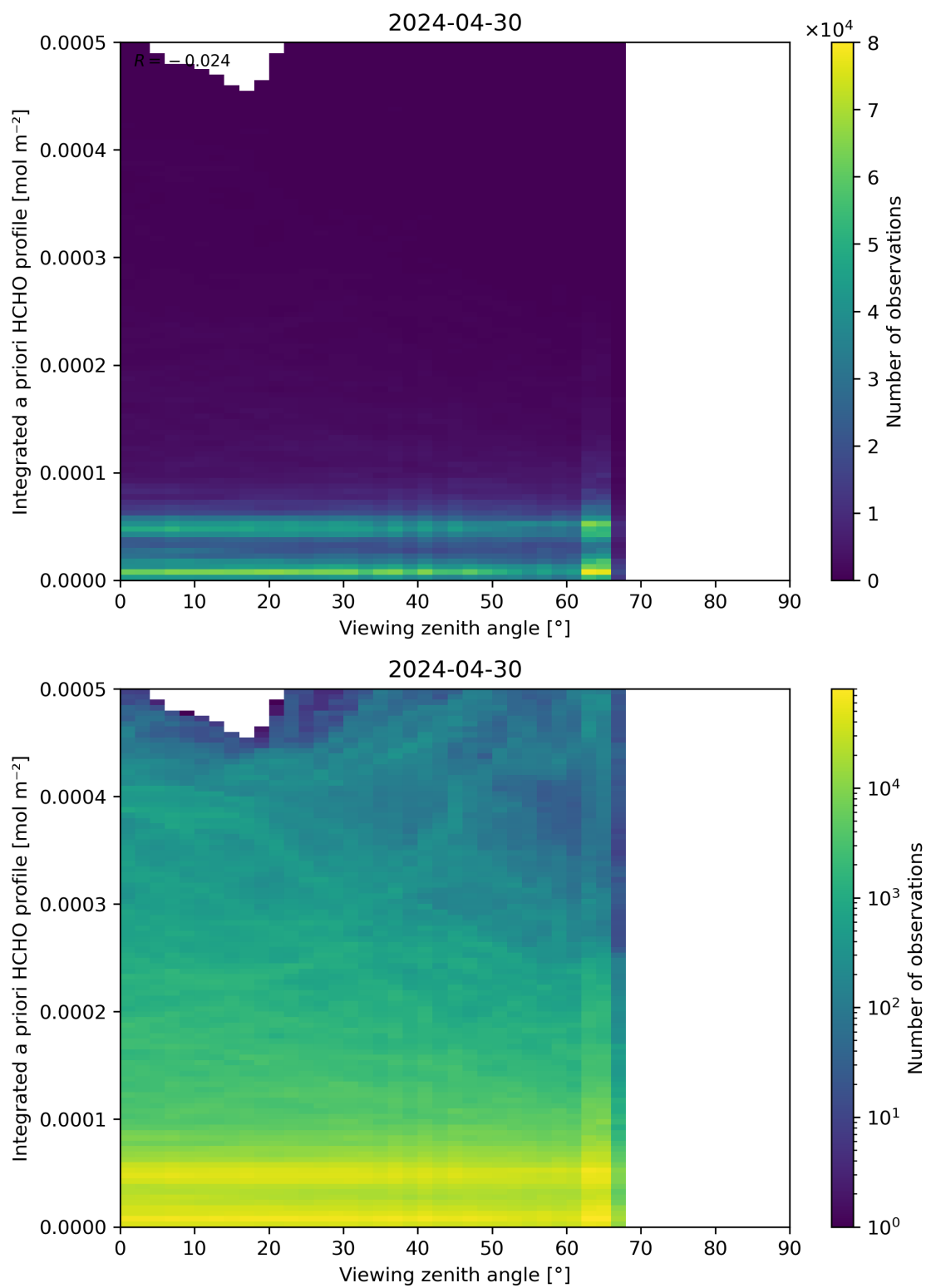
Figure 195: Scatter density plot of “Viewing zenith angle” against “Integrated a priori HCHO profile” for 2024-04-29 to 2024-05-01.
