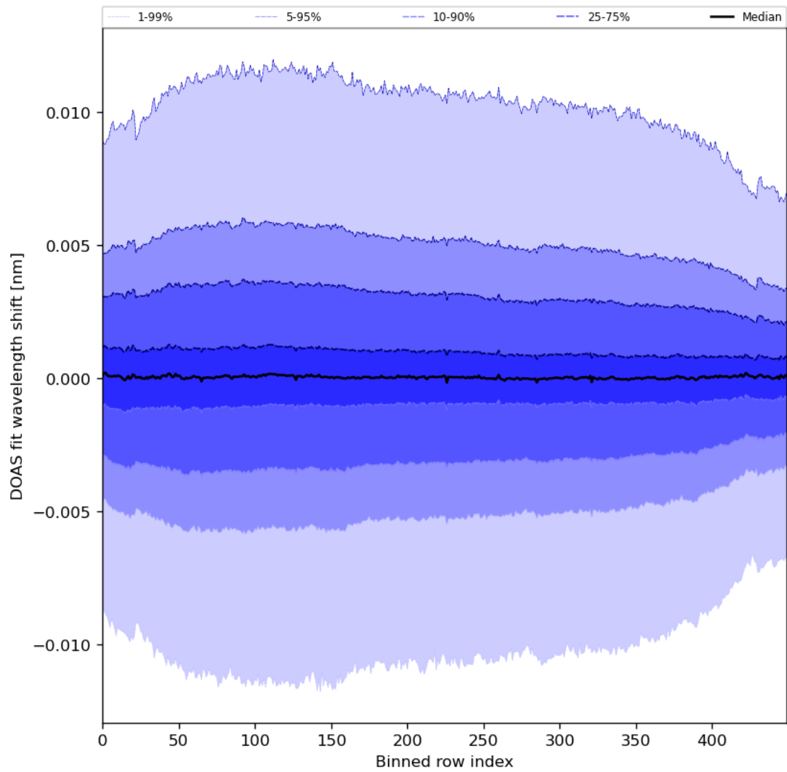
Figure 58: Along track statistics of “DOAS fit wavelength shift” for 2024-04-29 to 2024-05-01
