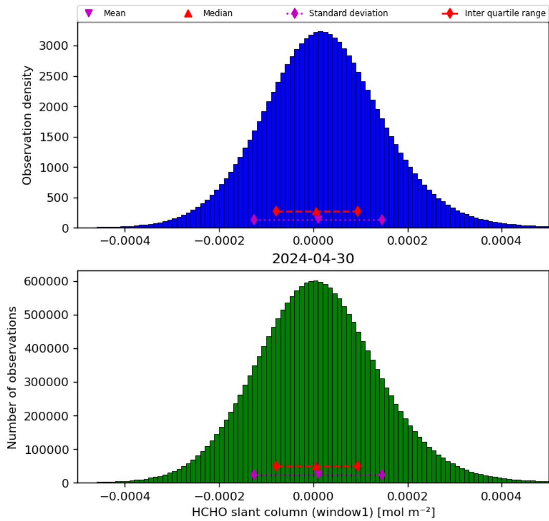
Figure 38: Histogram of “HCHO slant column (window1)” for 2024-04-29 to 2024-05-01
