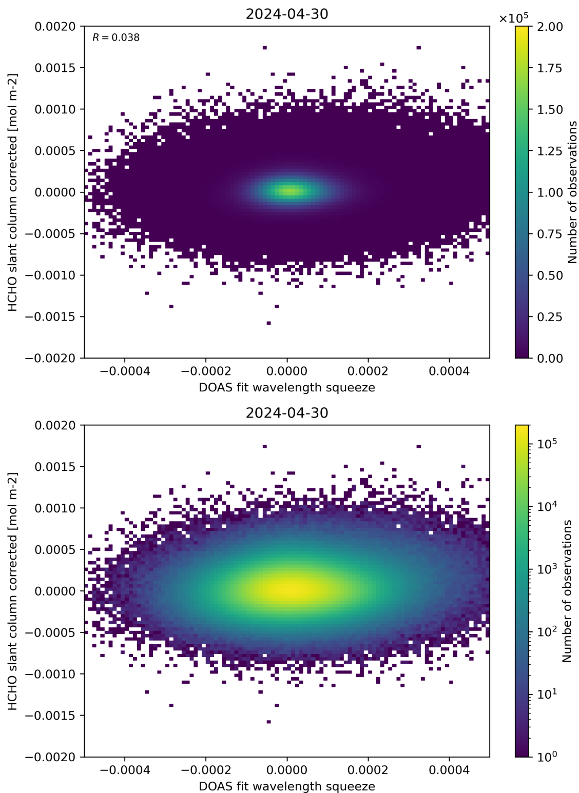
Figure 69: Scatter density plot of “DOAS fit wavelength squeeze” against “HCHO slant column corrected” for 2024-04-29 to 2024-05-01.
