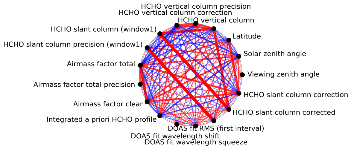
Figure 1: Map of correlation graph for 2024-04-29 to 2024-05-01.
