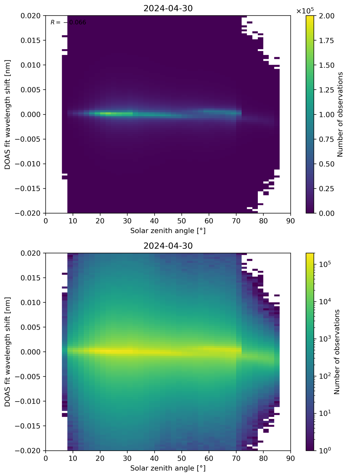
Figure 168: Scatter density plot of “Solar zenith angle” against “DOAS fit wavelength shift” for 2024-04-29 to 2024-05-01.
