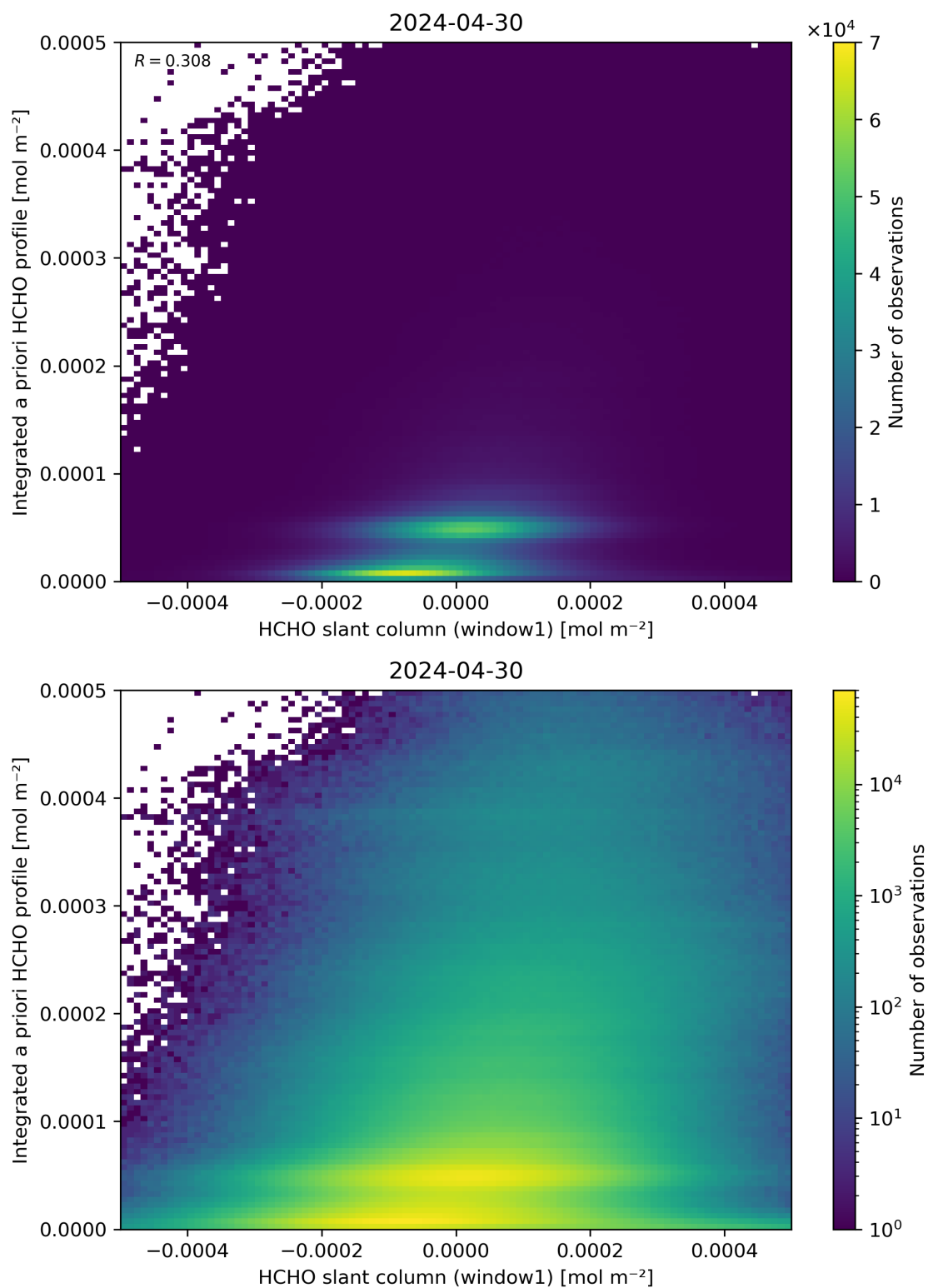
Figure 87: Scatter density plot of “HCHO slant column (window1)” against “Integrated a priori HCHO profile” for 2024-04-29 to 2024-05-01.
