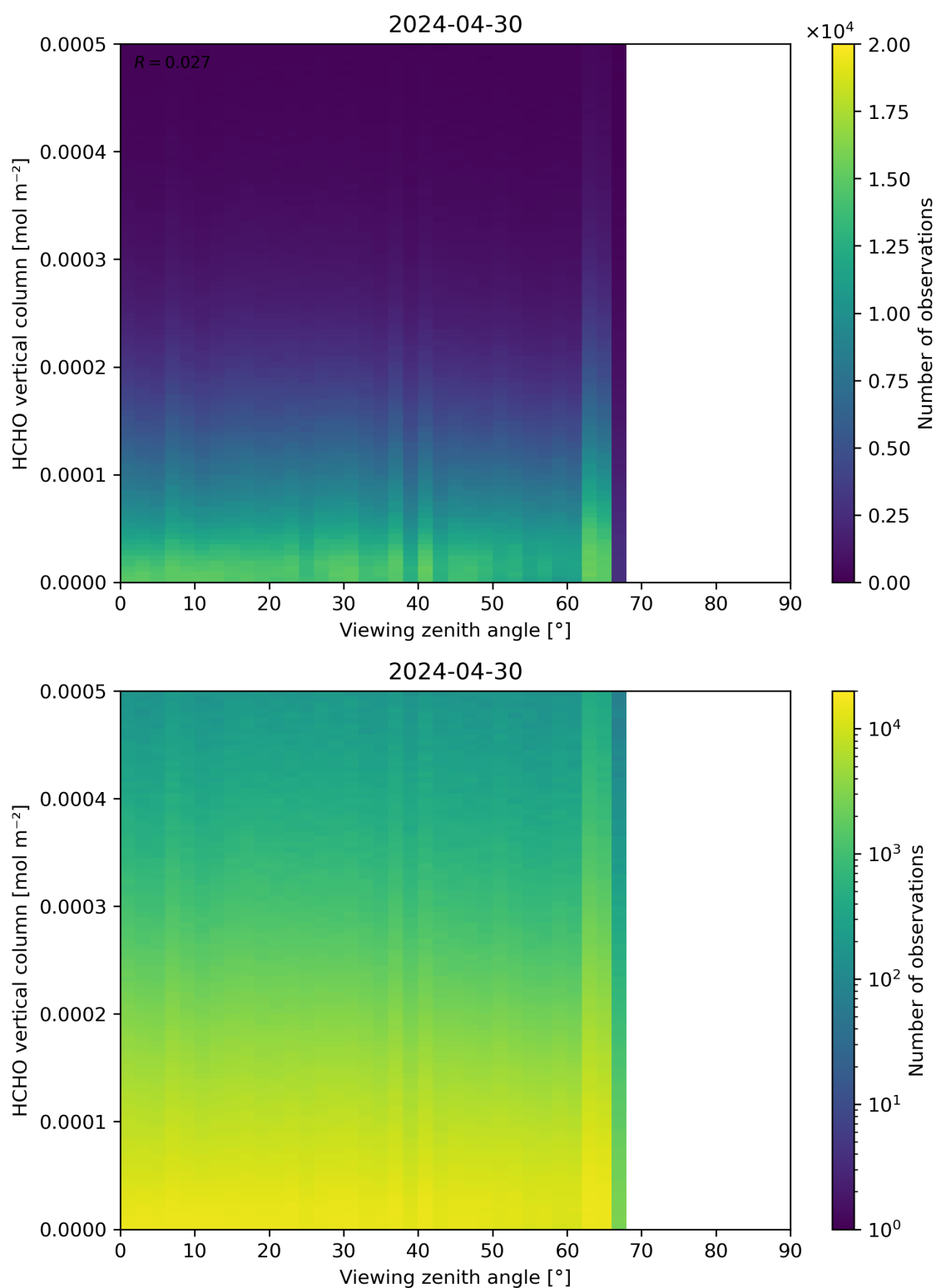
Figure 192: Scatter density plot of “Viewing zenith angle” against “HCHO vertical column” for 2024-04-29 to 2024-05-01.
