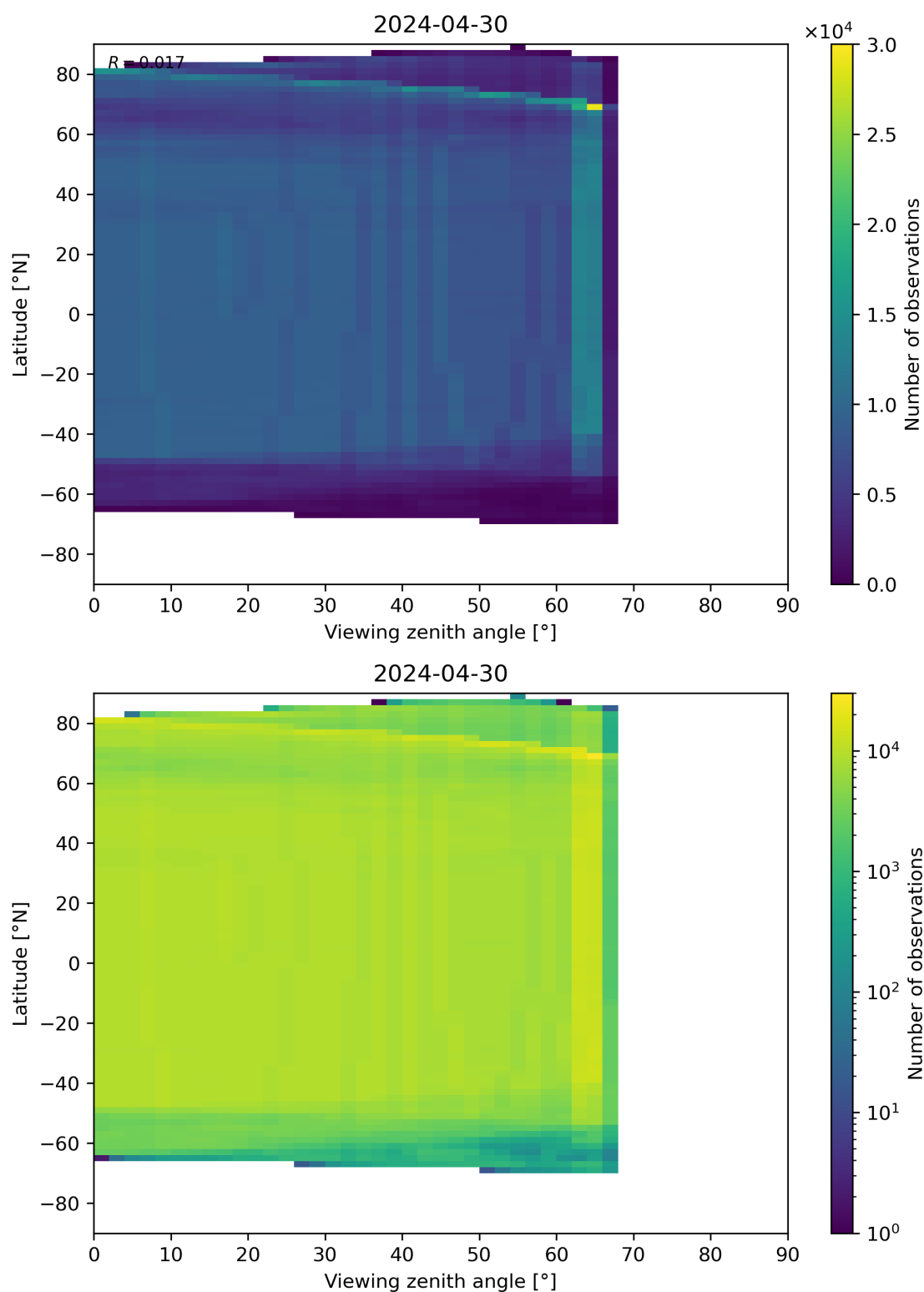
Figure 196: Scatter density plot of “Viewing zenith angle” against “Latitude” for 2024-04-29 to 2024-05-01.
