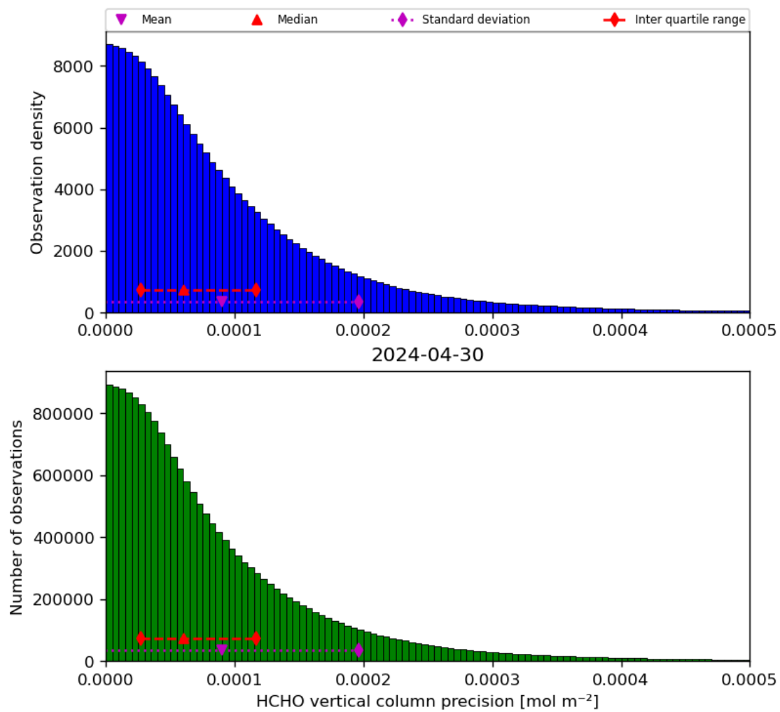
Figure 36: Histogram of “HCHO vertical column precision” for 2024-04-29 to 2024-05-01
