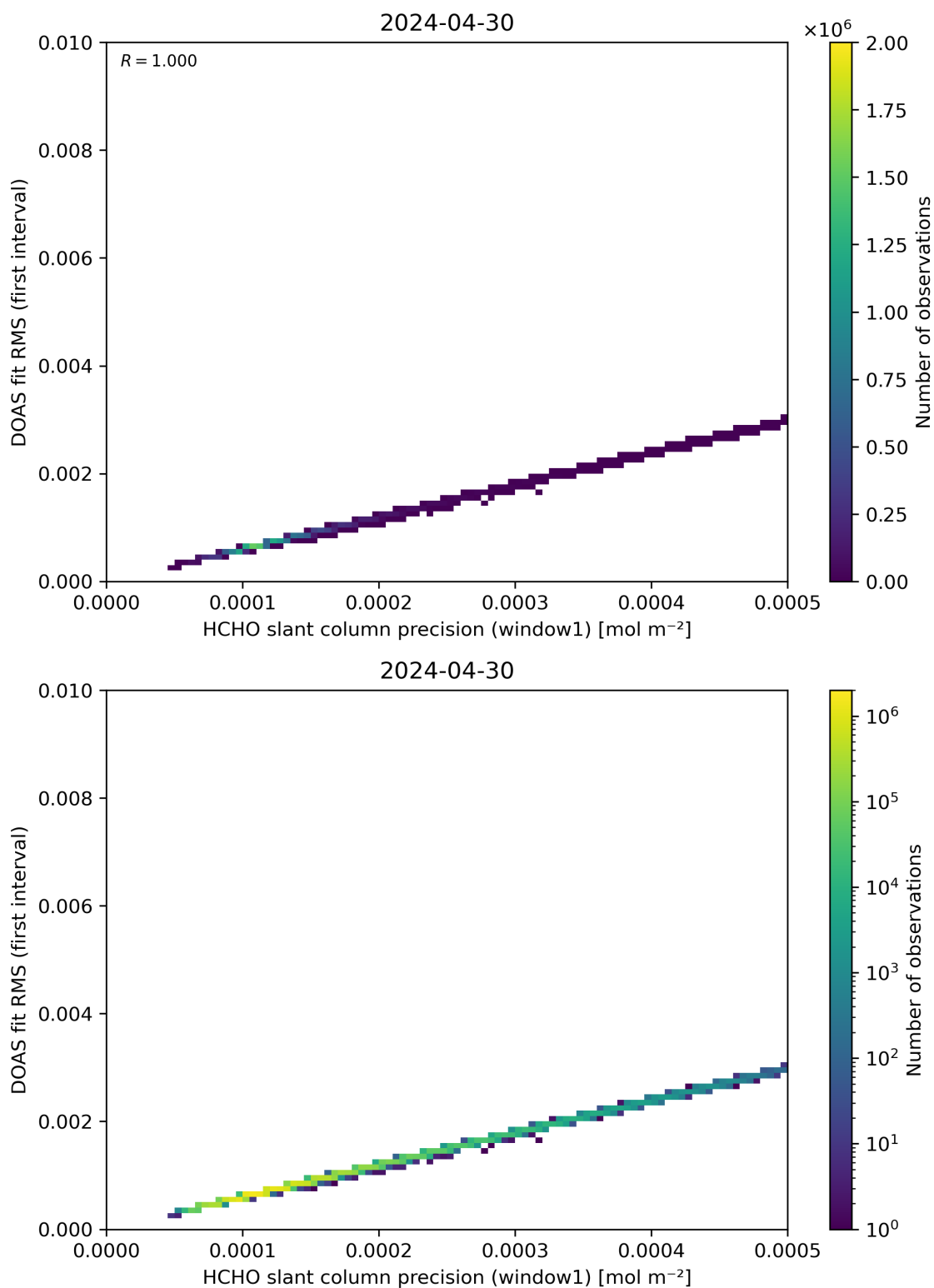
Figure 88: Scatter density plot of “HCHO slant column precision (window1)” against “DOAS fit RMS (first interval)” for 2024-04-29 to 2024-05-01.
