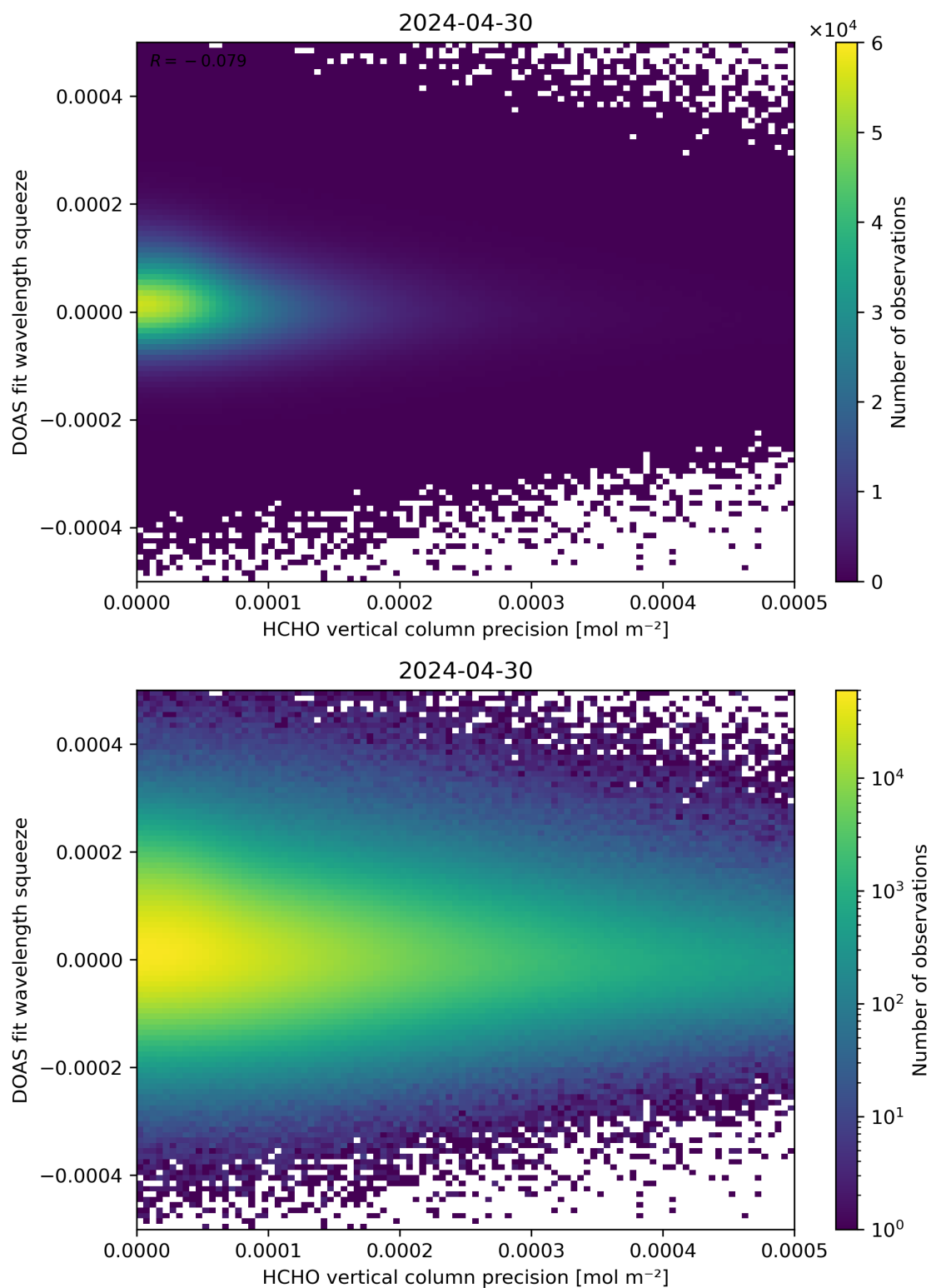
Figure 138: Scatter density plot of “HCHO vertical column precision” against “DOAS fit wavelength squeeze” for 2024-04-29 to 2024-05-01.
