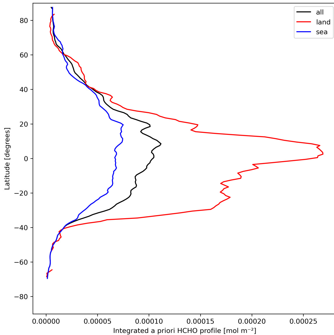
Figure 29: Zonal average of “Integrated a priori HCHO profile” for 2024-04-29 to 2024-05-01.
