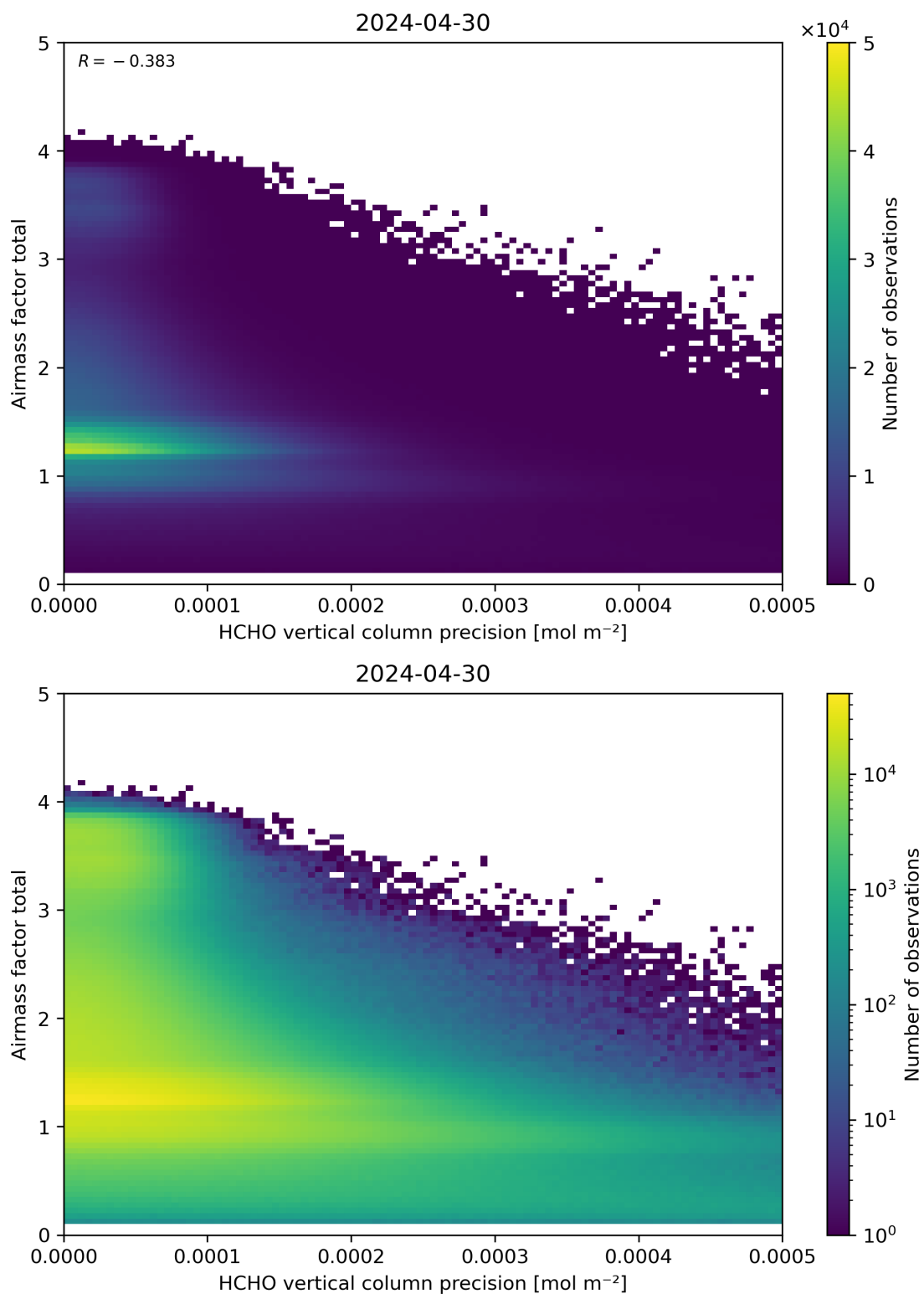
Figure 144: Scatter density plot of “HCHO vertical column precision” against “Airmass factor total” for 2024-04-29 to 2024-05-01.
