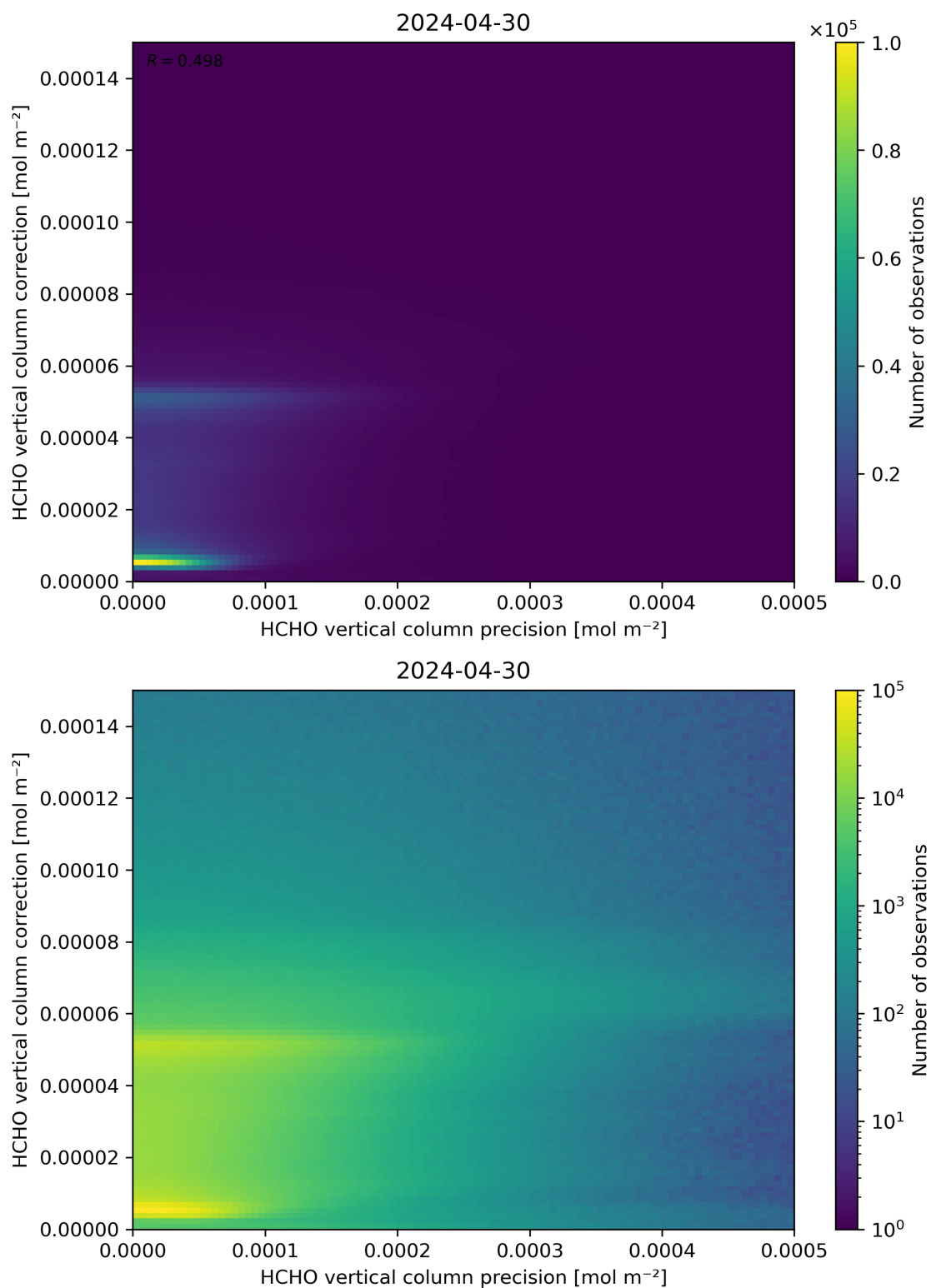
Figure 146: Scatter density plot of “HCHO vertical column precision” against “HCHO vertical column correction” for 2024-04-29 to 2024-05-01.
