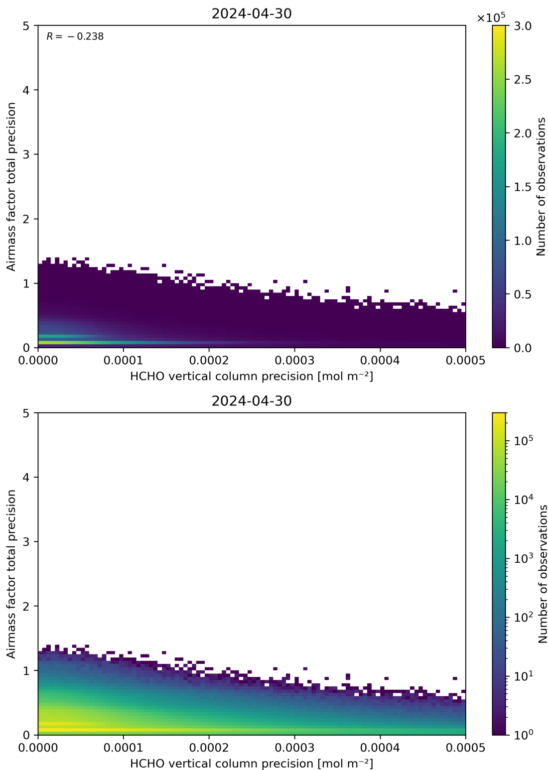
Figure 145: Scatter density plot of “HCHO vertical column precision” against “Airmass factor total precision” for 2024-04-29 to 2024-05-01.
