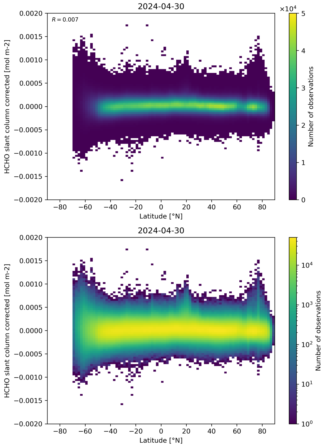
Figure 157: Scatter density plot of “Latitude” against “HCHO slant column corrected” for 2024-04-29 to 2024-05-01.
