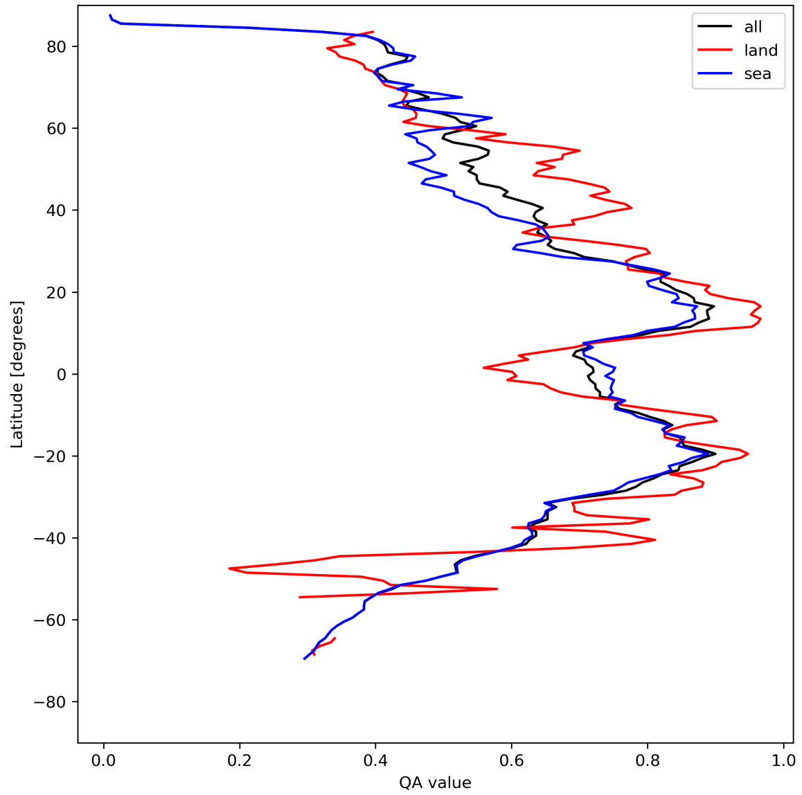
Figure 20: Zonal average of “QA value” for 2024-04-29 to 2024-05-01.
