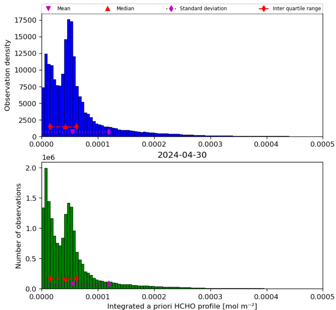
Figure 43: Histogram of “Integrated a priori HCHO profile” for 2024-04-29 to 2024-05-01
