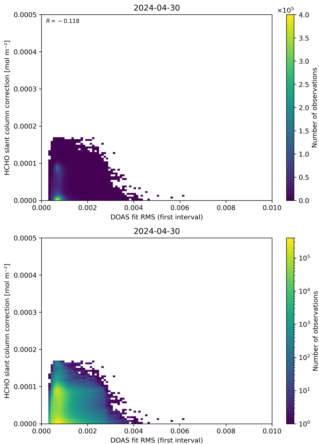
Figure 63: Scatter density plot of “DOAS fit RMS (first interval)” against “HCHO slant column correction” for 2024-04-29 to 2024-05-01.
