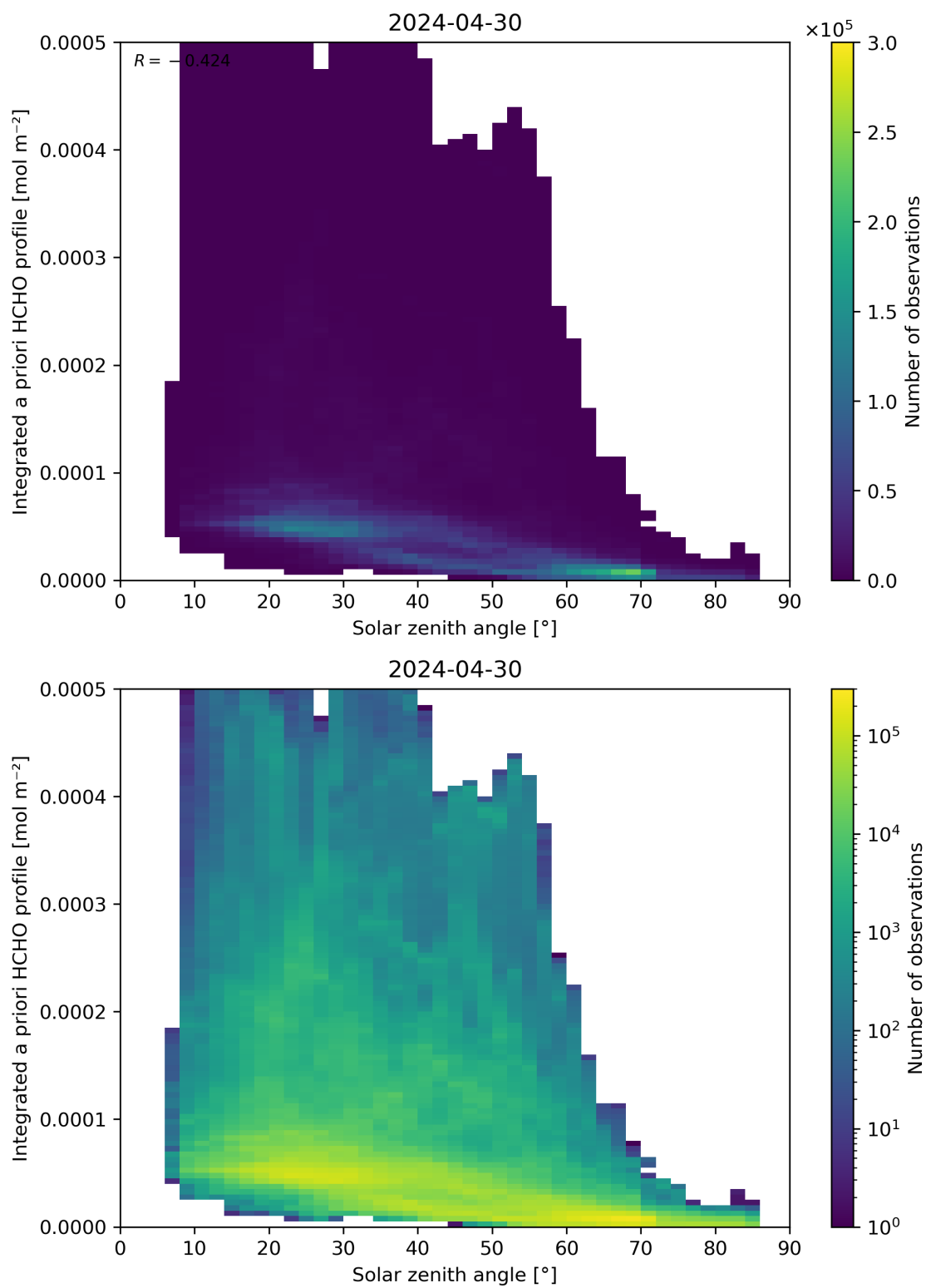
Figure 180: Scatter density plot of “Solar zenith angle” against “Integrated a priori HCHO profile” for 2024-04-29 to 2024-05-01.
