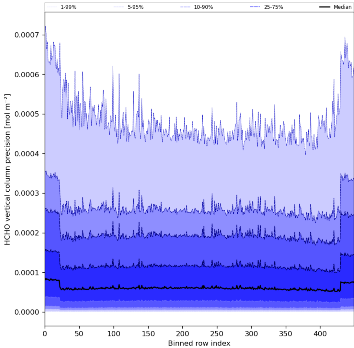
Figure 50: Along track statistics of "HCHO vertical column precision" for 2024-04-29 to 2024-05-01
