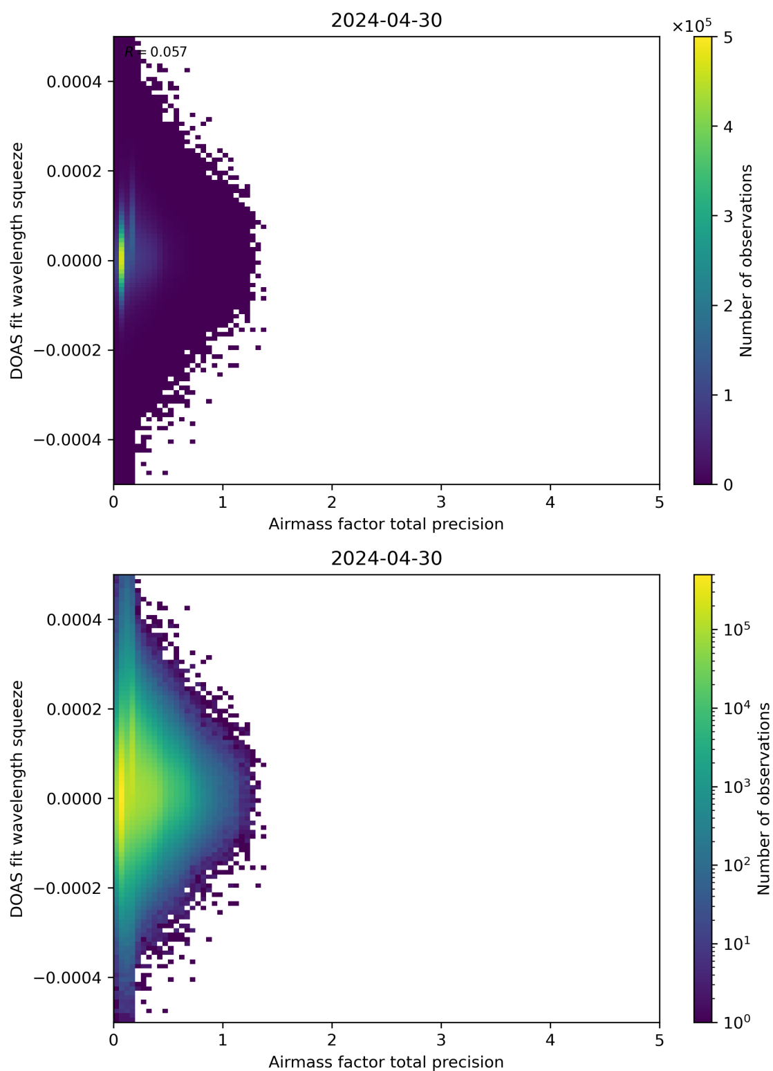
Figure 107: Scatter density plot of “Airmass factor total precision” against “DOAS fit wavelength squeeze” for 2024-04-29 to 2024-05-01.
