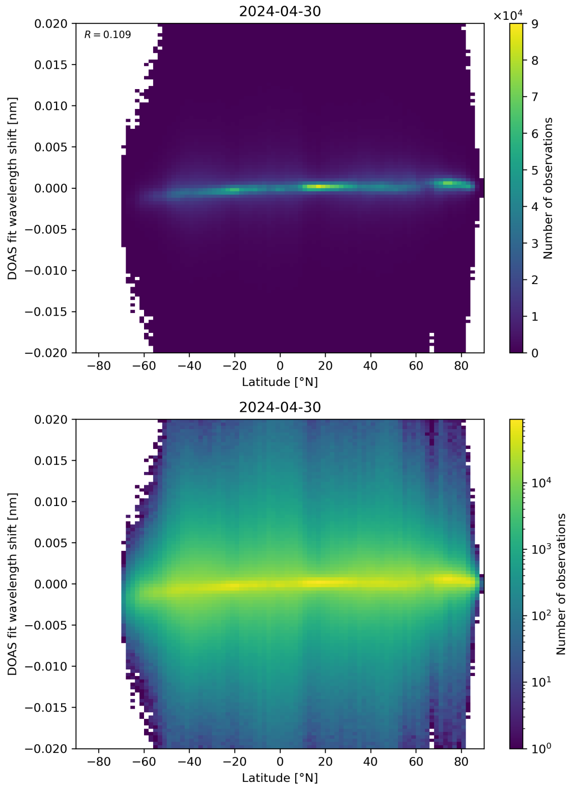
Figure 154: Scatter density plot of “Latitude” against “DOAS fit wavelength shift” for 2024-04-29 to 2024-05-01.
