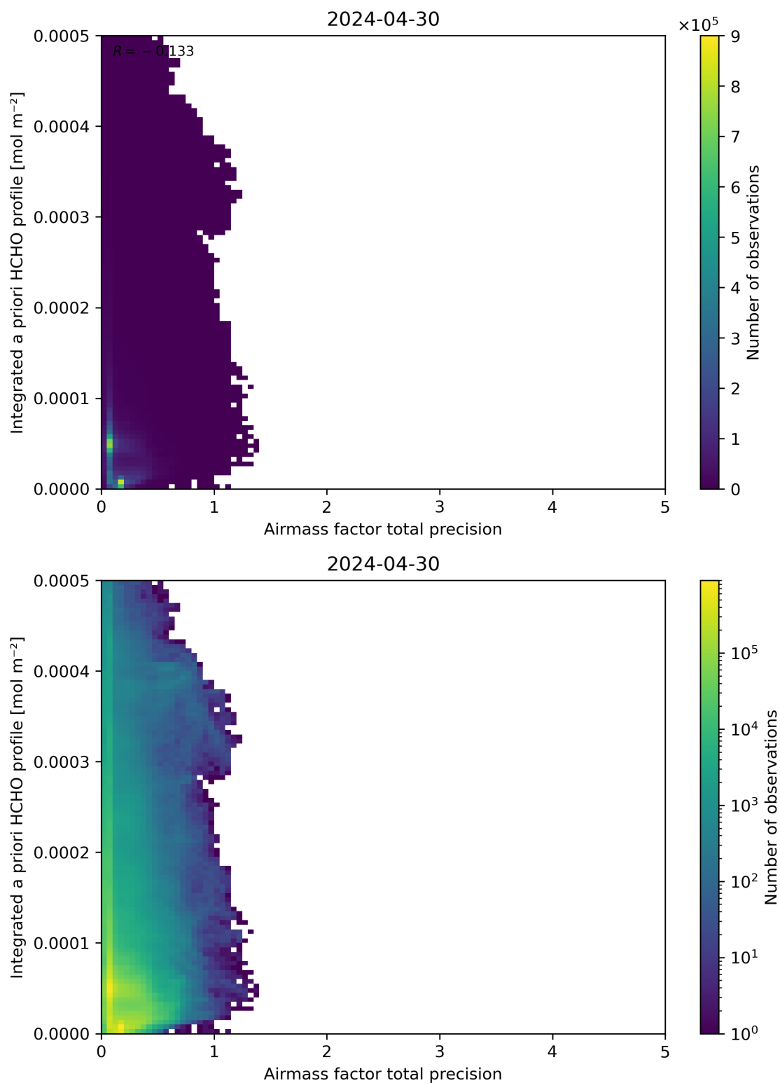
Figure 111: Scatter density plot of “Airmass factor total precision” against “Integrated a priori HCHO profile” for 2024-04-29 to 2024-05-01.
