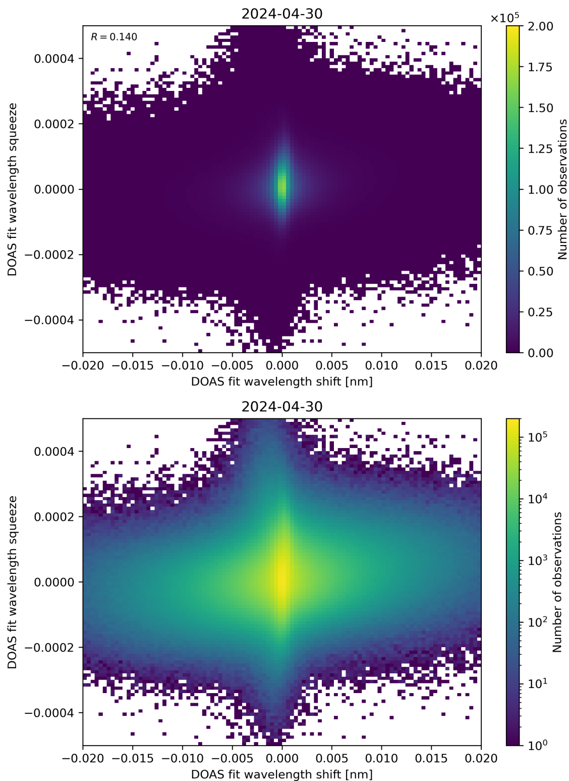
Figure 65: Scatter density plot of “DOAS fit wavelength shift” against “DOAS fit wavelength squeeze” for 2024-04-29 to 2024-05-01.
