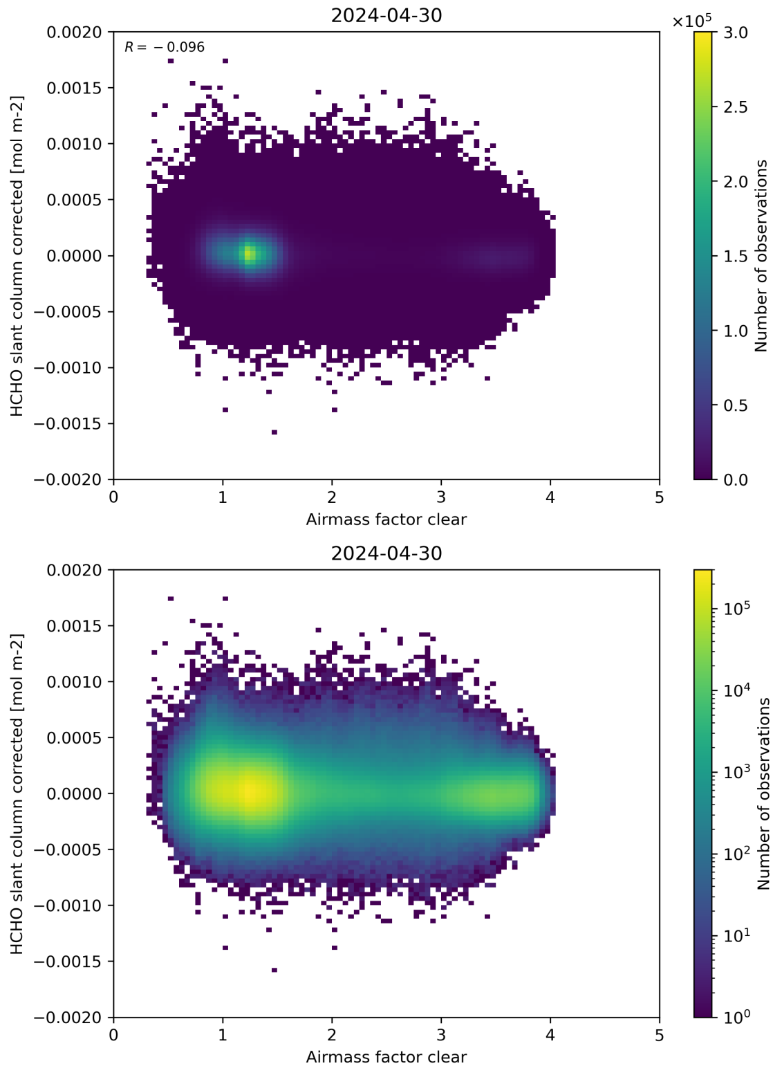
Figure 74: Scatter density plot of “Airmass factor clear” against “HCHO slant column corrected” for 2024-04-29 to 2024-05-01.
