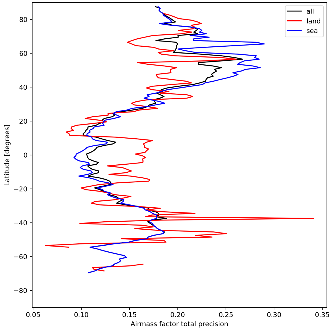
Figure 27: Zonal average of “Airmass factor total precision” for 2024-04-29 to 2024-05-01.
