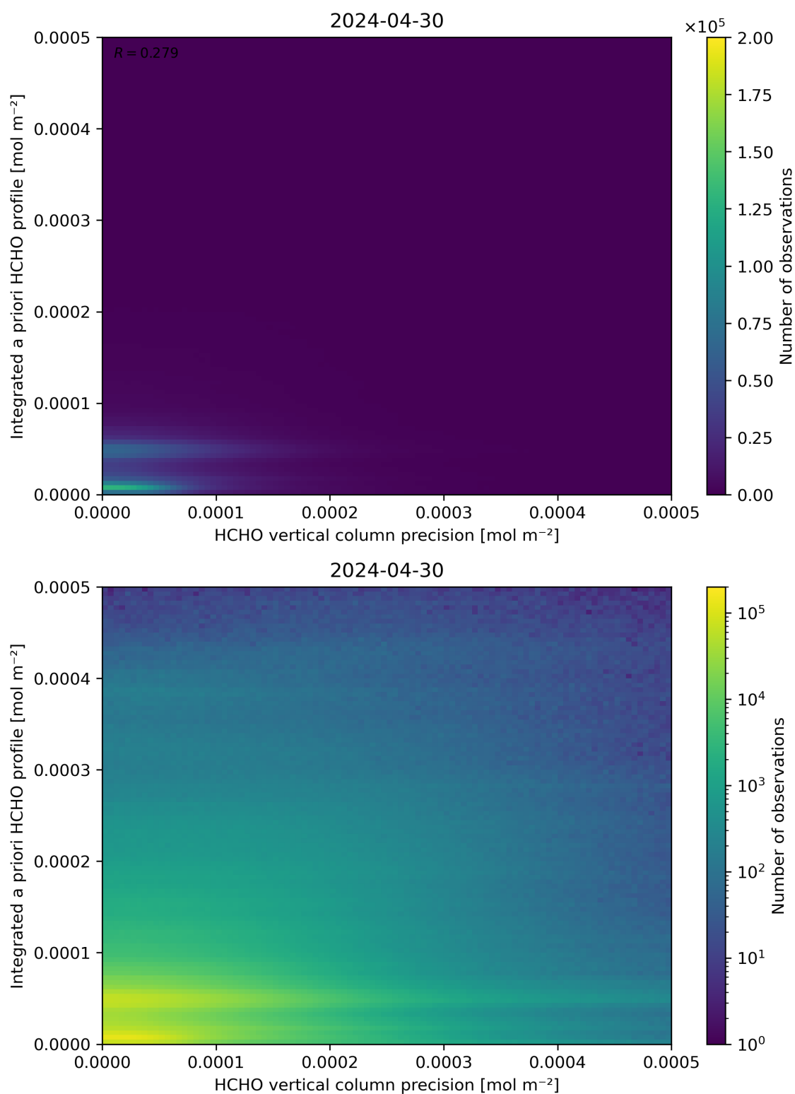
Figure 147: Scatter density plot of “HCHO vertical column precision” against “Integrated a priori HCHO profile” for 2024-04-29 to 2024-05-01.
