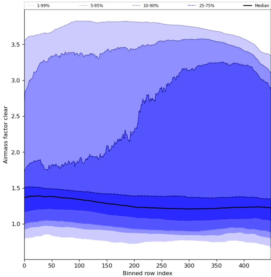
Figure 56: Along track statistics of “Airmass factor clear” for 2024-04-29 to 2024-05-01
