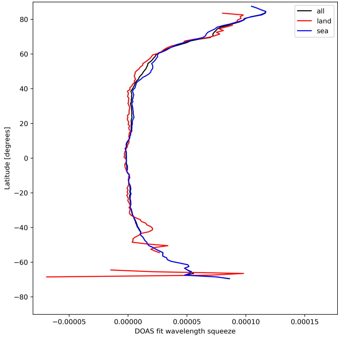
Figure 31: Zonal average of “DOAS fit wavelength squeeze” for 2024-04-29 to 2024-05-01.
