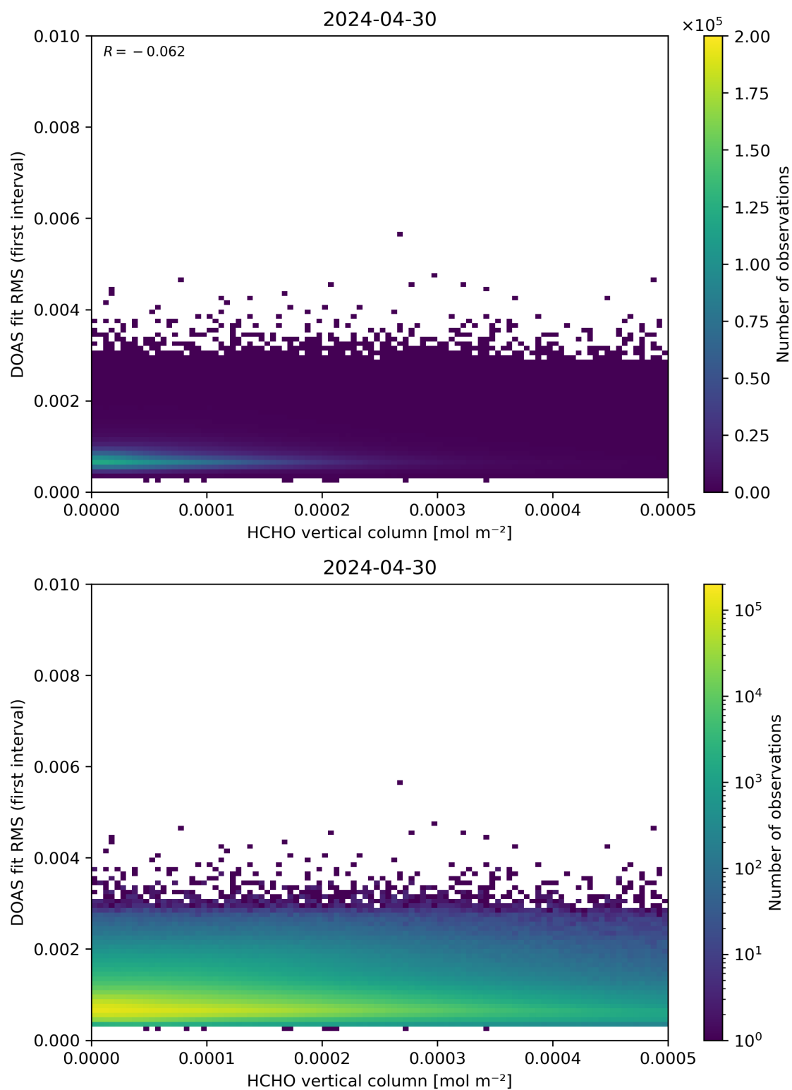
Figure 123: Scatter density plot of “HCHO vertical column” against “DOAS fit RMS (first interval)” for 2024-04-29 to 2024-05-01.
