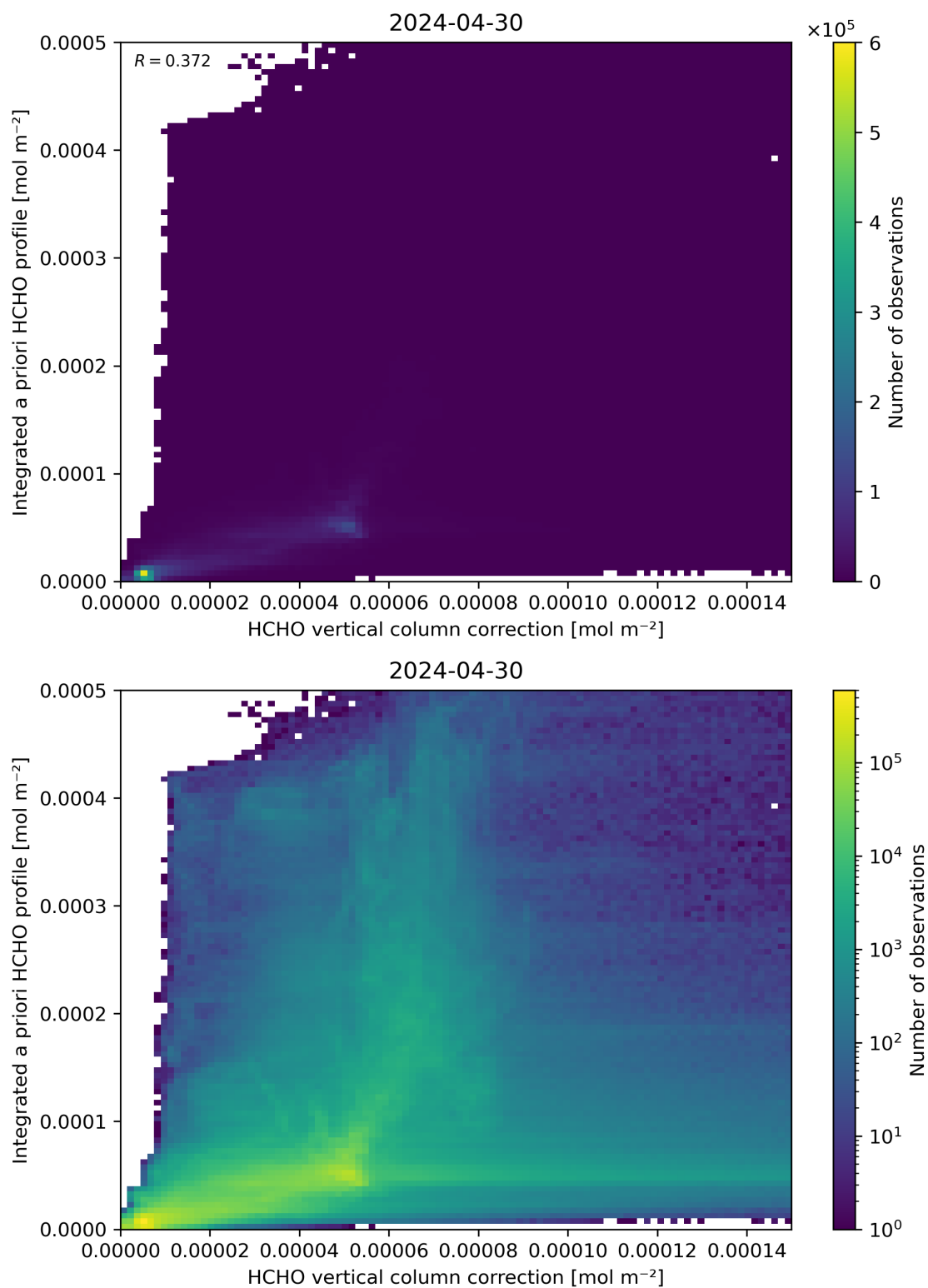
Figure 122: Scatter density plot of “HCHO vertical column correction” against “Integrated a priori HCHO profile” for 2024-04-29 to 2024-05-01.
