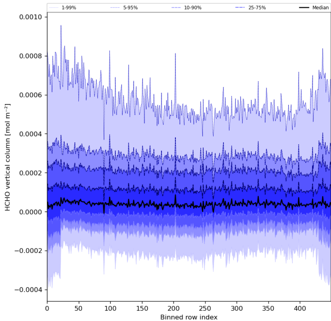
Figure 49: Along track statistics of “HCHO vertical column” for 2024-04-29 to 2024-05-01
