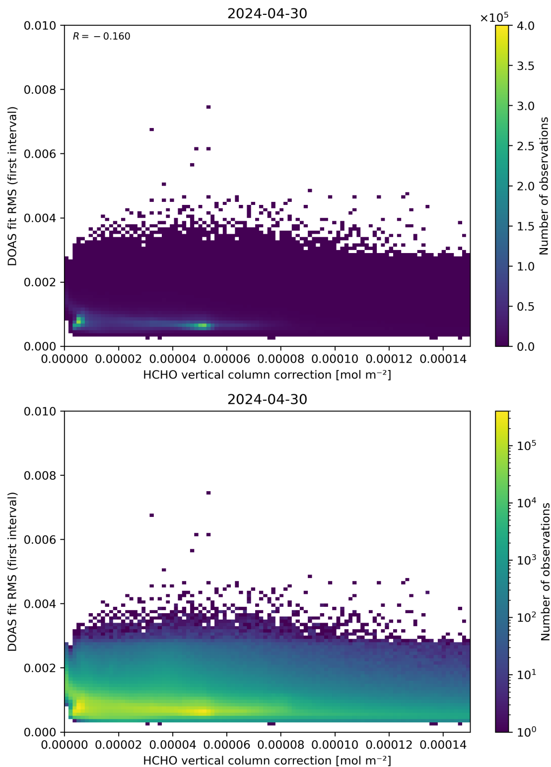
Figure 112: Scatter density plot of “HCHO vertical column correction” against “DOAS fit RMS (first interval)” for 2024-04-29 to 2024-05-01.
