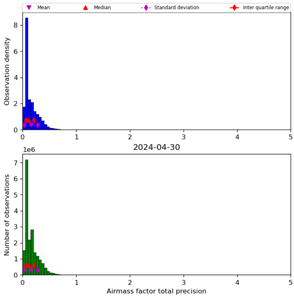
Figure 41: Histogram of “Airmass factor total precision” for 2024-04-29 to 2024-05-01
