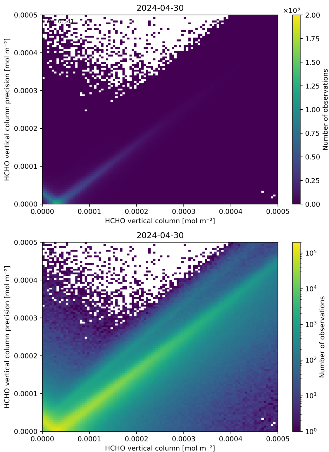
Figure 134: Scatter density plot of “HCHO vertical column” against “HCHO vertical column precision” for 2024-04-29 to 2024-05-01.
