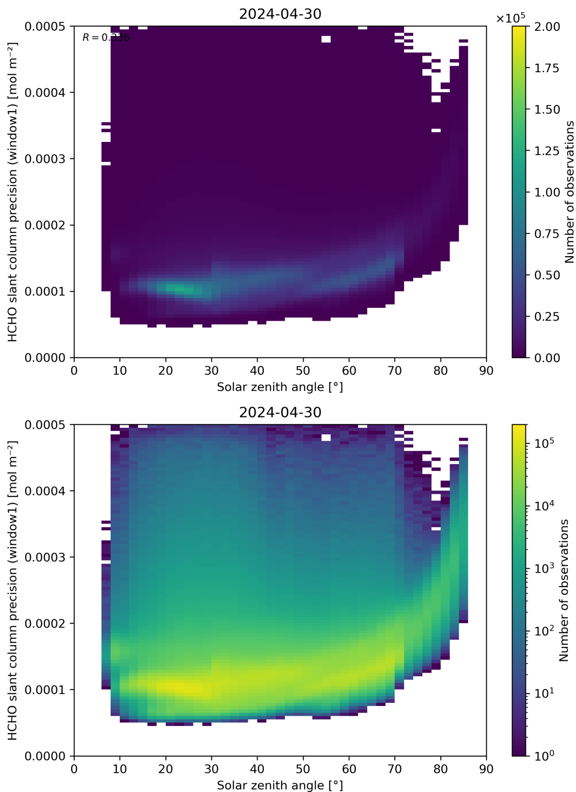
Figure 174: Scatter density plot of “Solar zenith angle” against “HCHO slant column precision (window1)” for 2024-04-29 to 2024-05-01.
