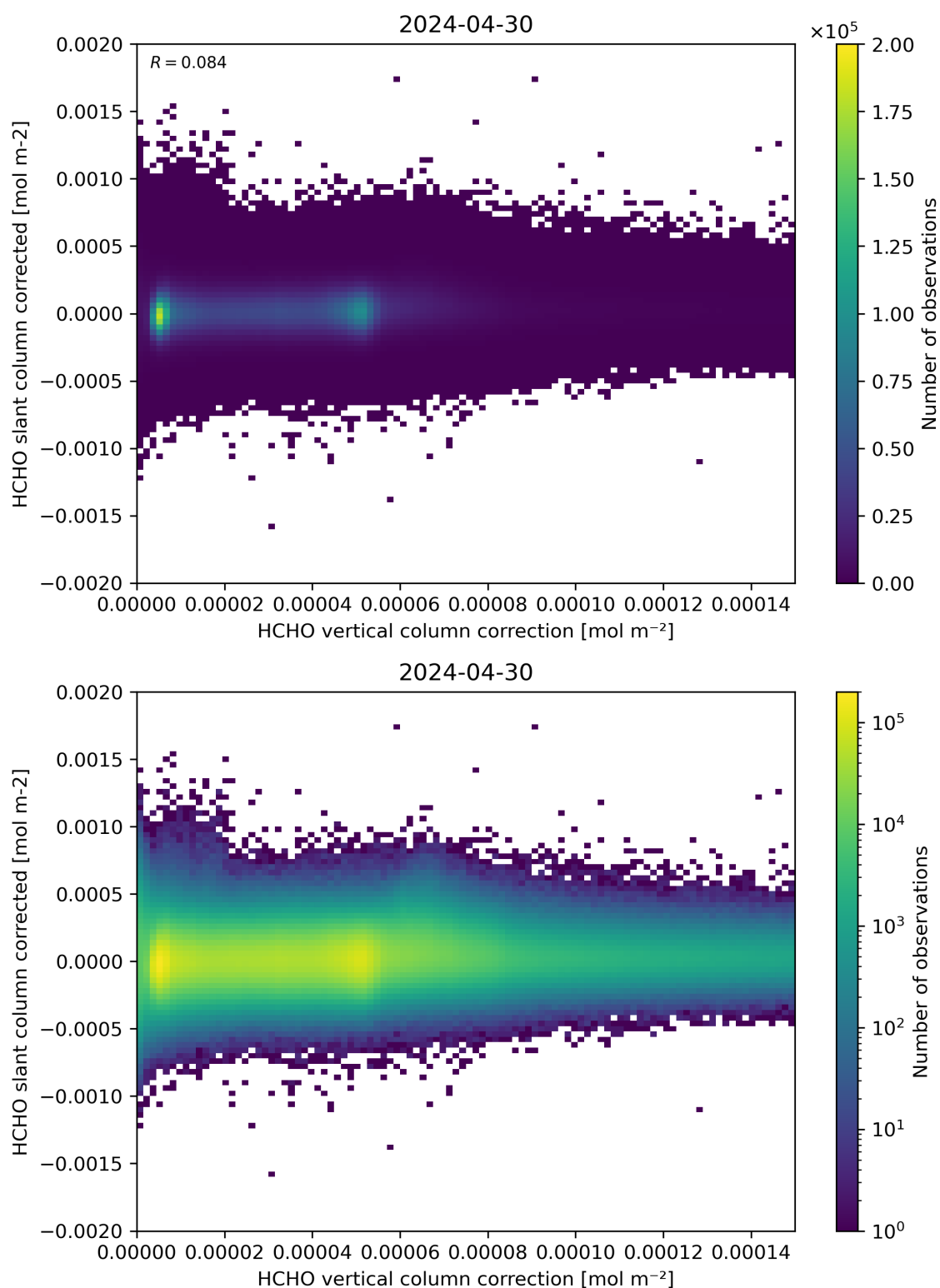
Figure 116: Scatter density plot of “HCHO vertical column correction” against “HCHO slant column corrected” for 2024-04-29 to 2024-05-01.
