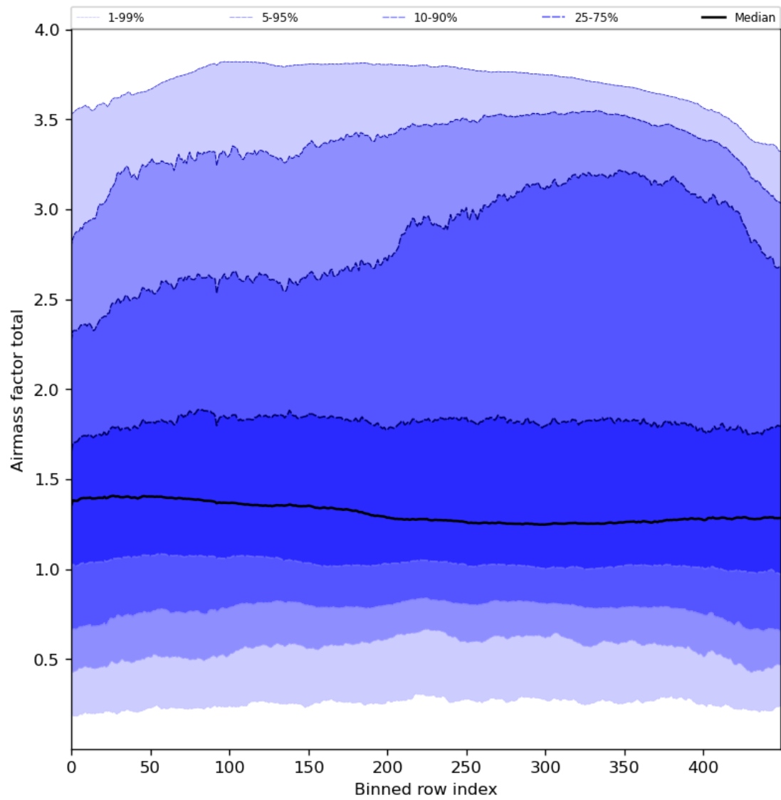
Figure 54: Along track statistics of “Airmass factor total” for 2024-04-29 to 2024-05-01
