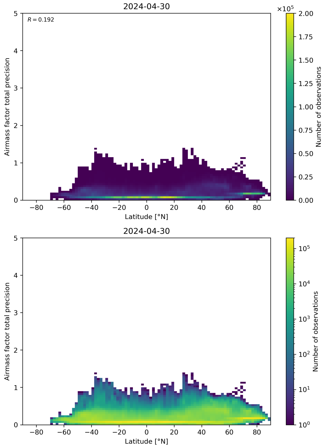
Figure 162: Scatter density plot of “Latitude” against “Airmass factor total precision” for 2024-04-29 to 2024-05-01.
