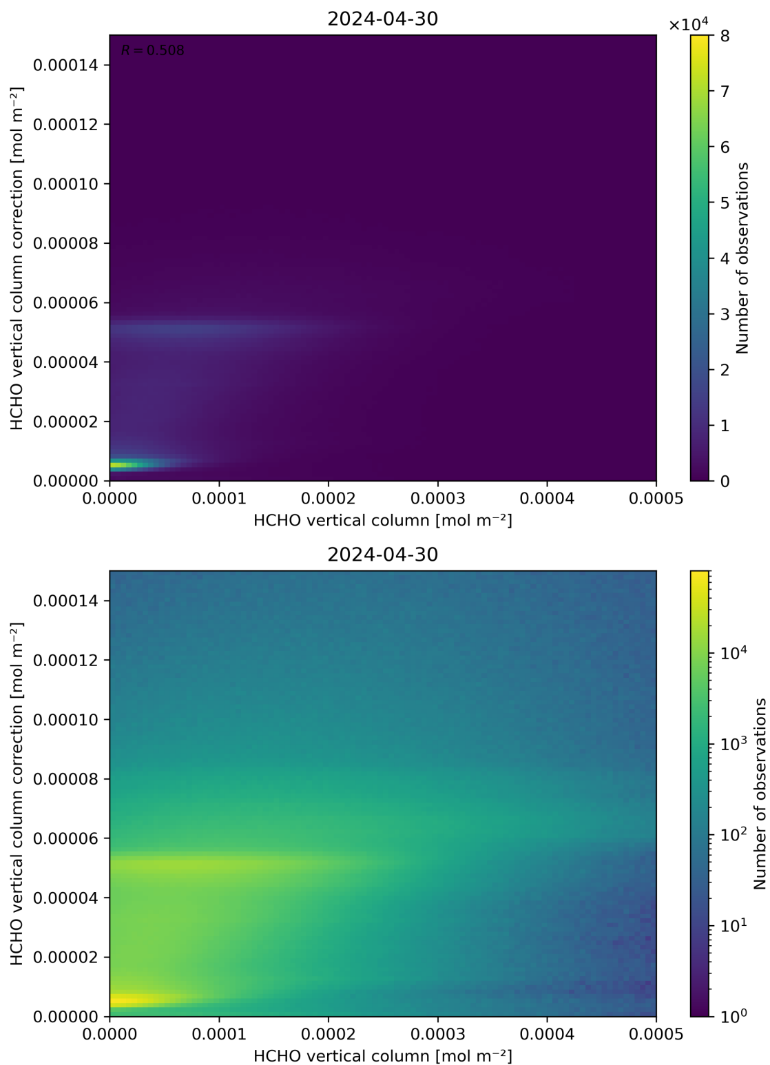
Figure 133: Scatter density plot of “HCHO vertical column” against “HCHO vertical column correction” for 2024-04-29 to 2024-05-01.
