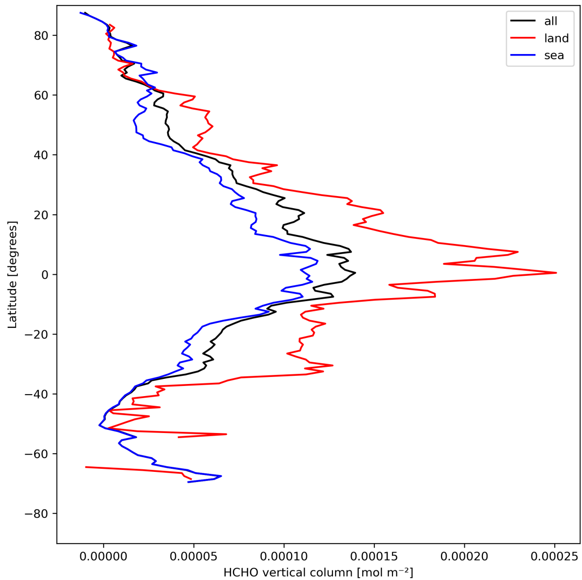
Figure 21: Zonal average of “HCHO vertical column” for 2024-04-29 to 2024-05-01.
