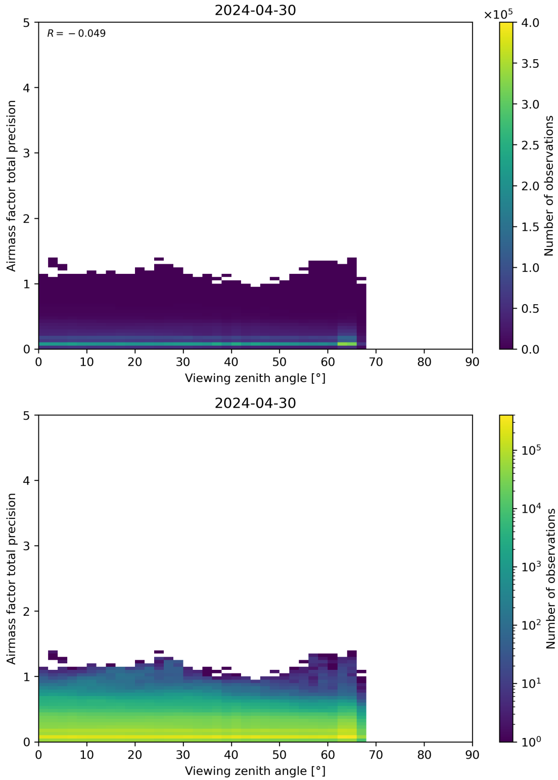
Figure 191: Scatter density plot of “Viewing zenith angle” against “Airmass factor total precision” for 2024-04-29 to 2024-05-01.
