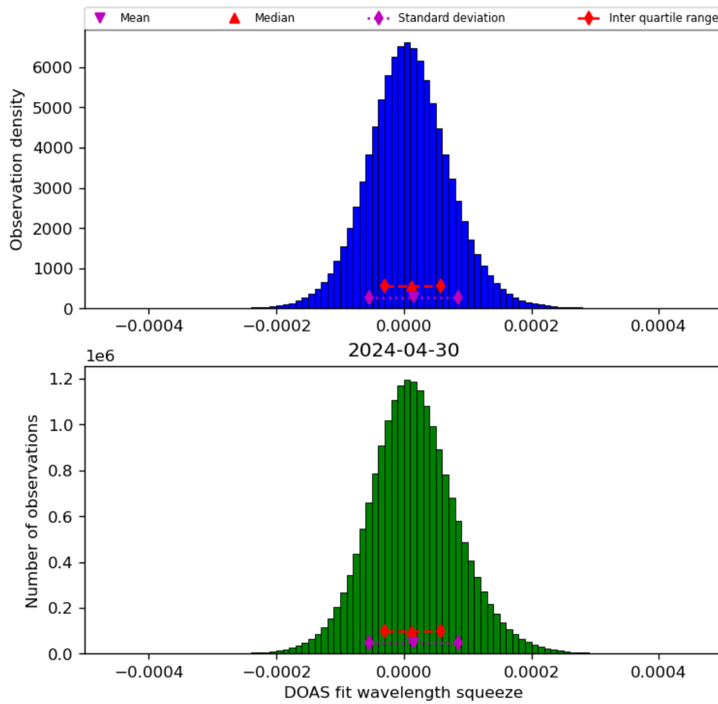
Figure 45: Histogram of “DOAS fit wavelength squeeze” for 2024-04-29 to 2024-05-01
