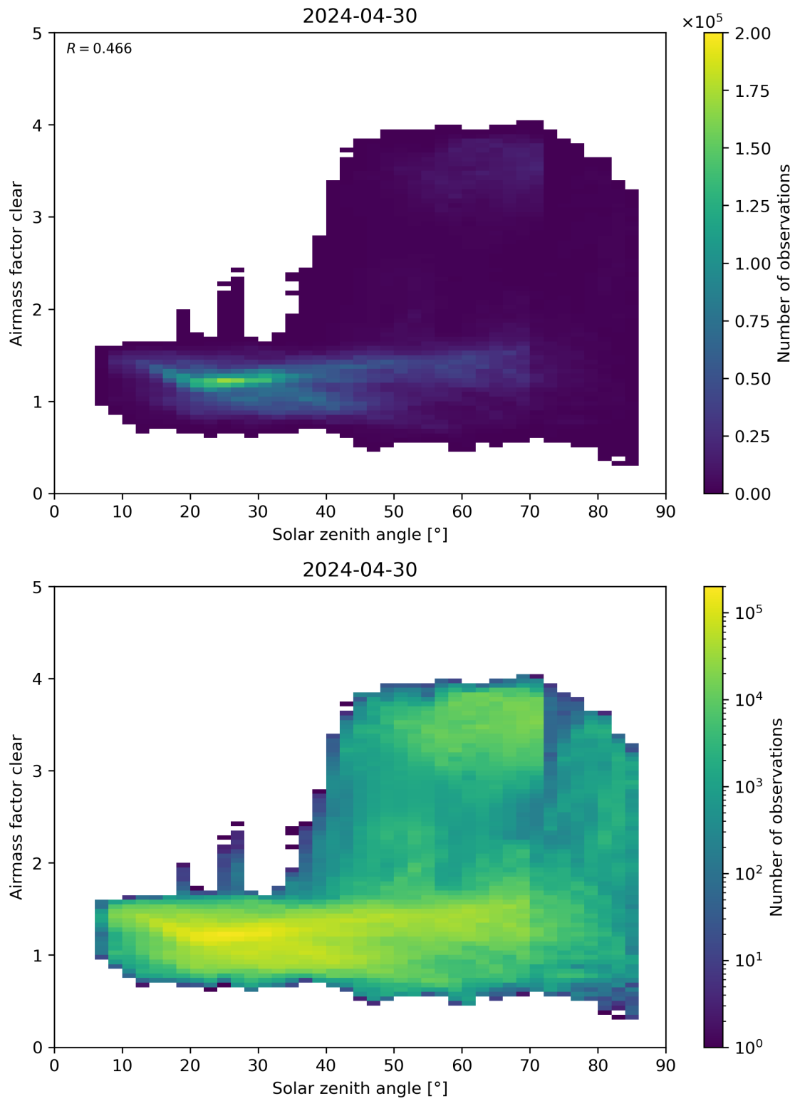
Figure 170: Scatter density plot of “Solar zenith angle” against “Airmass factor clear” for 2024-04-29 to 2024-05-01.
