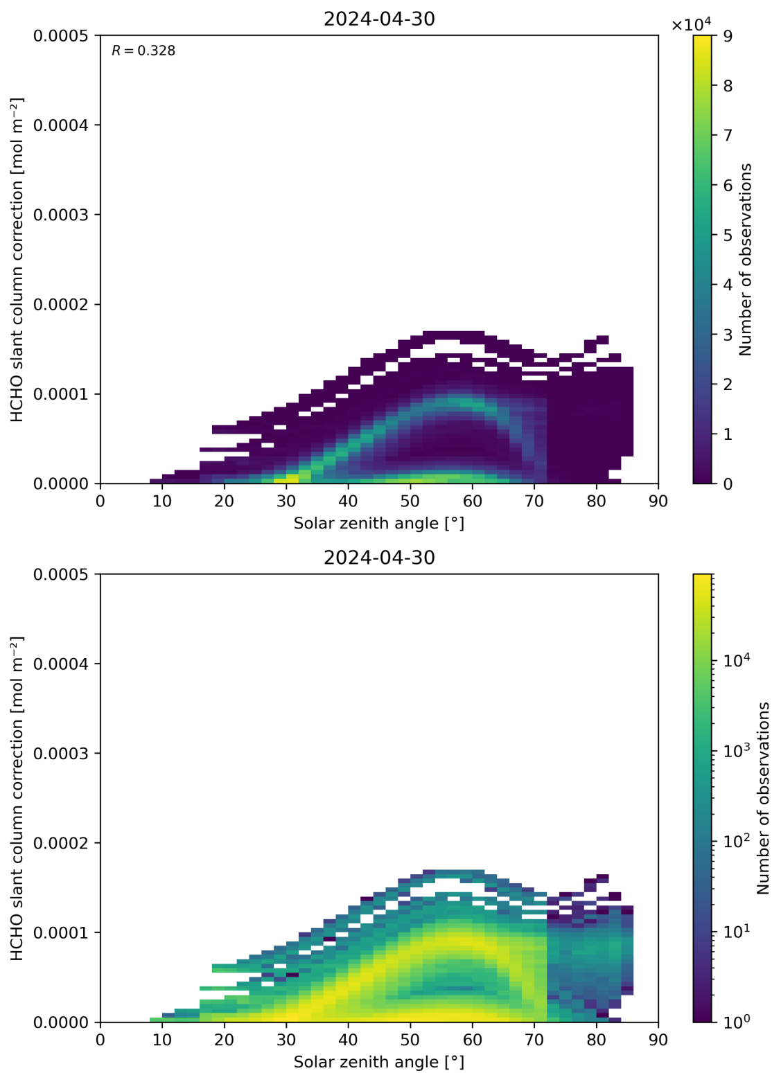
Figure 172: Scatter density plot of “Solar zenith angle” against “HCHO slant column correction” for 2024-04-29 to 2024-05-01.
