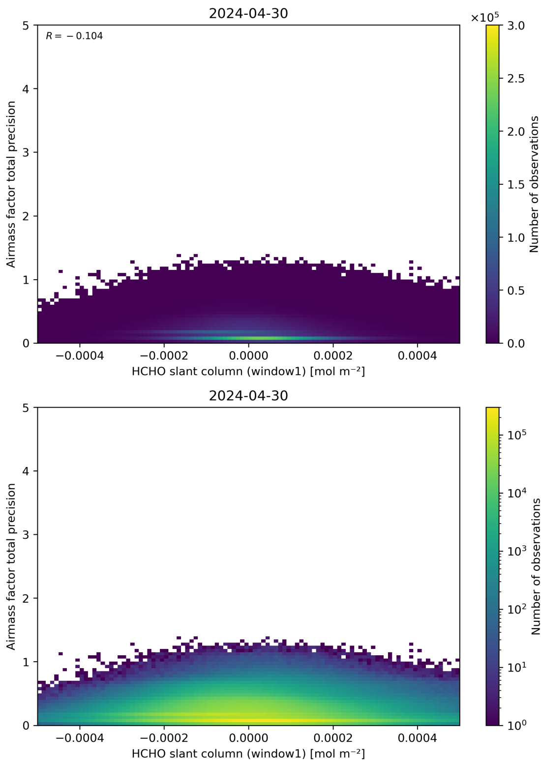
Figure 86: Scatter density plot of “HCHO slant column (window1)” against “Airmass factor total precision” for 2024-04-29 to 2024-05-01.
