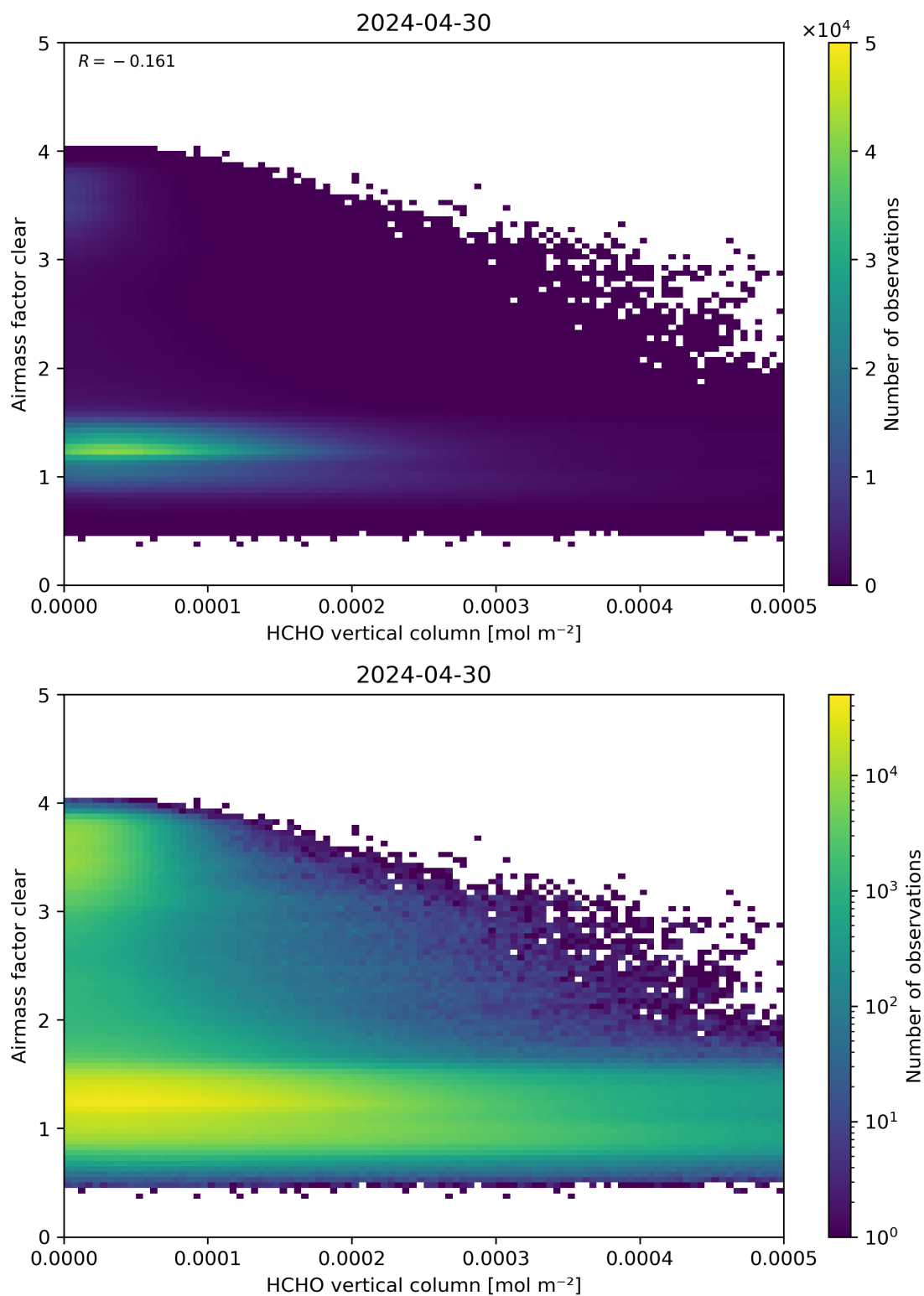
Figure 126: Scatter density plot of “HCHO vertical column” against “Airmass factor clear” for 2024-04-29 to 2024-05-01.
