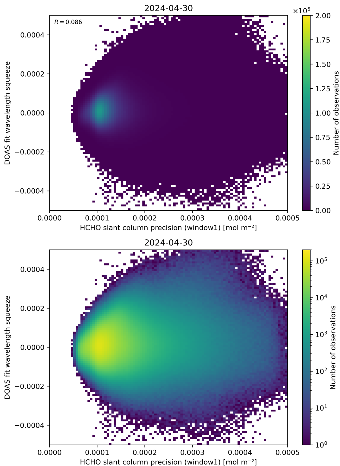
Figure 90: Scatter density plot of “HCHO slant column precision (window1)” against “DOAS fit wavelength squeeze” for 2024-04-29 to 2024-05-01.
