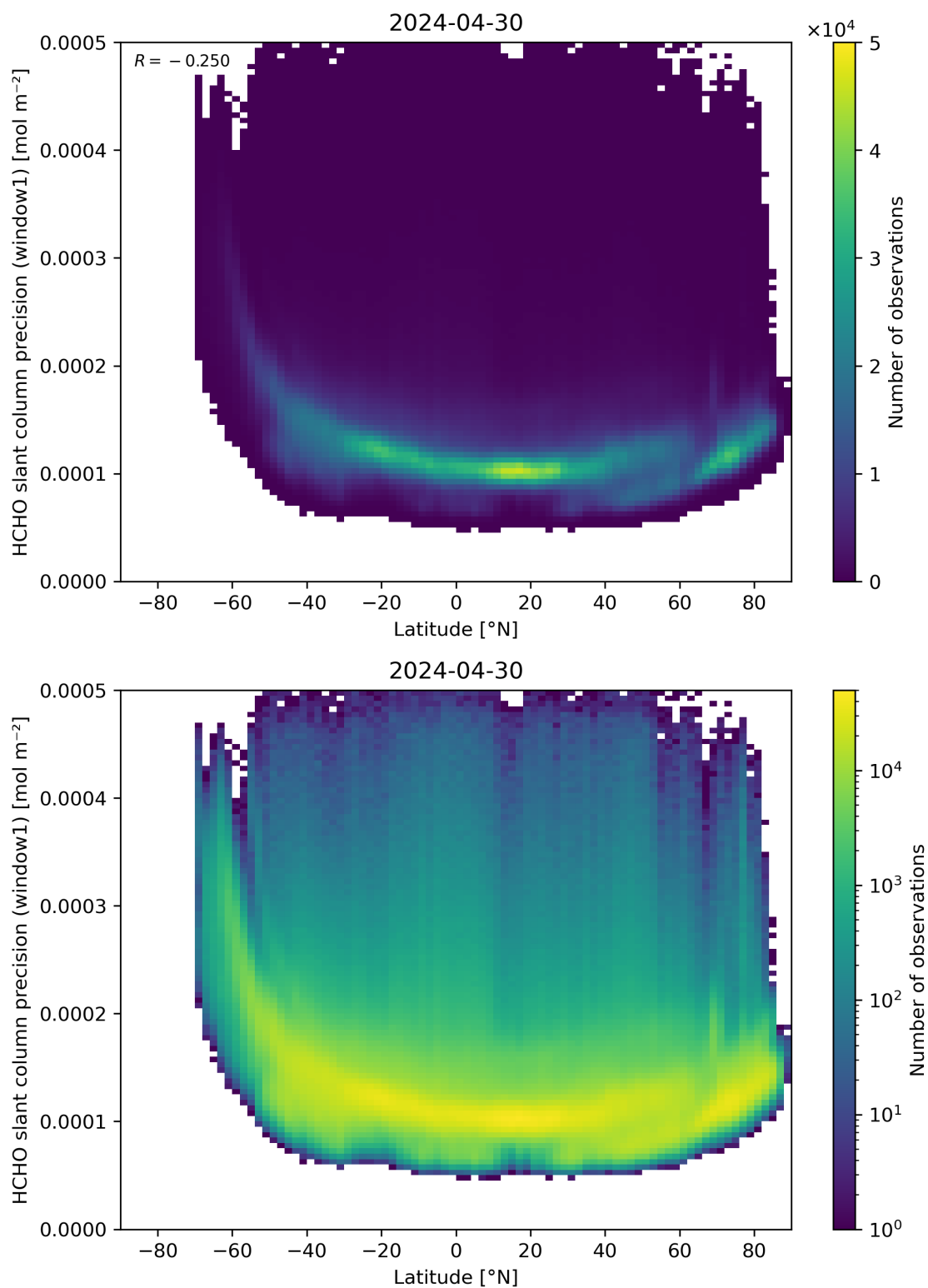
Figure 160: Scatter density plot of “Latitude” against “HCHO slant column precision (window1)” for 2024-04-29 to 2024-05-01.
