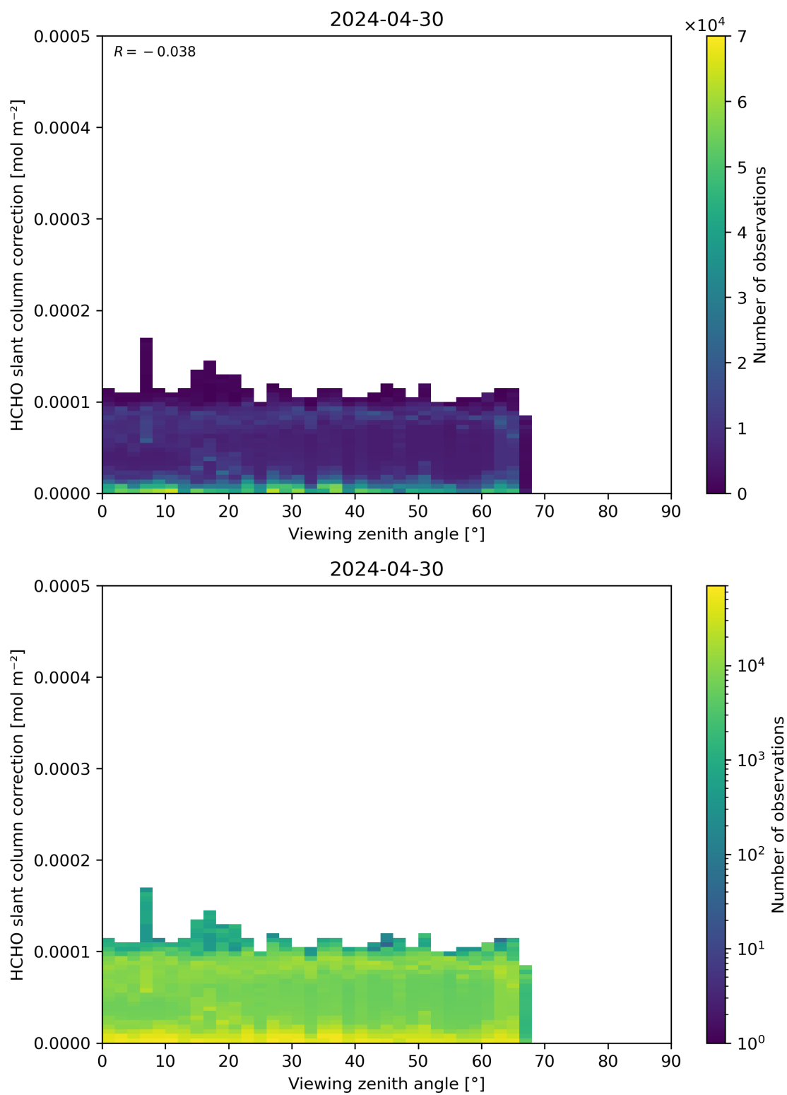
Figure 187: Scatter density plot of “Viewing zenith angle” against “HCHO slant column correction” for 2024-04-29 to 2024-05-01.
