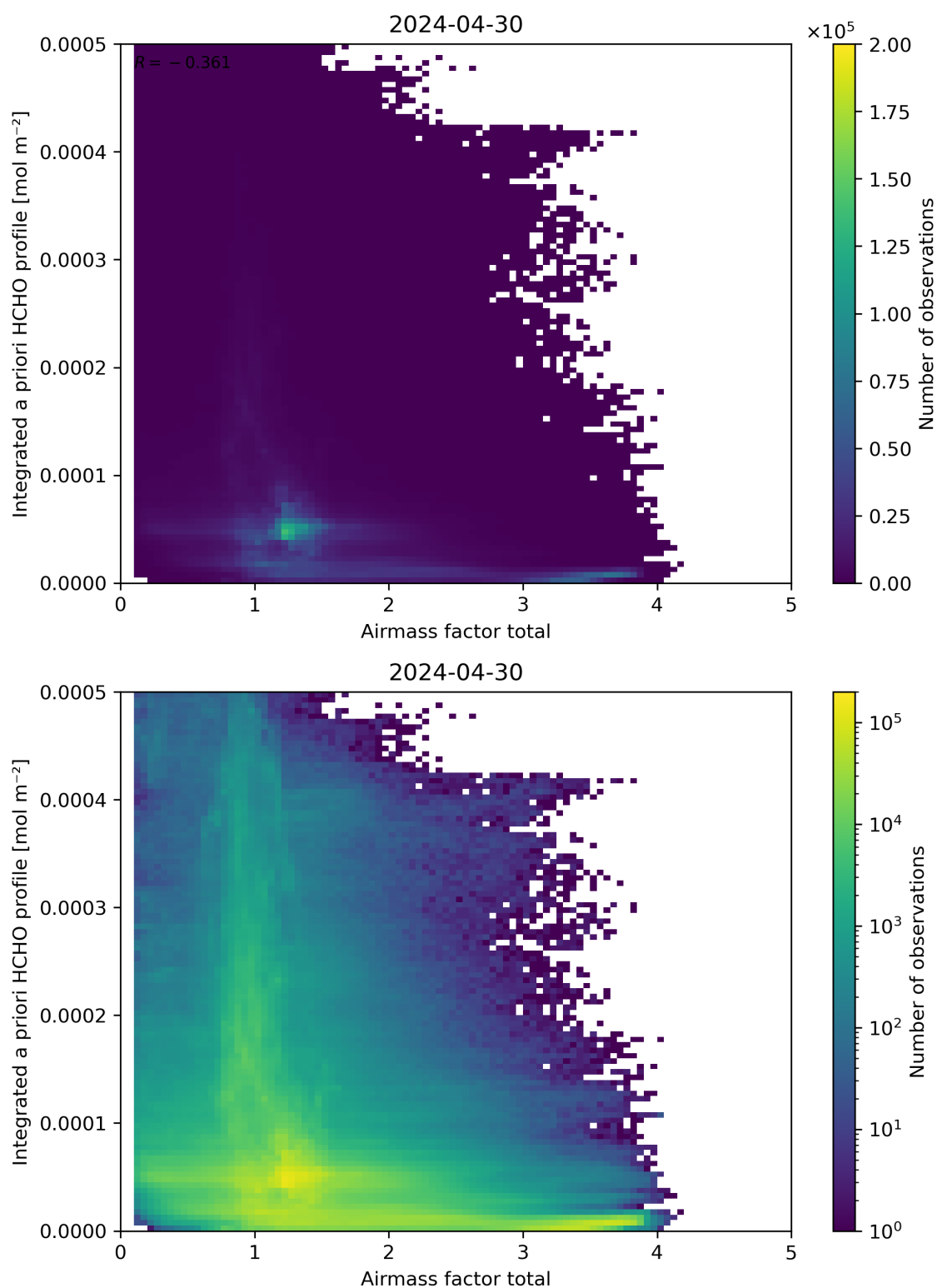
Figure 104: Scatter density plot of “Airmass factor total” against “Integrated a priori HCHO profile” for 2024-04-29 to 2024-05-01.
