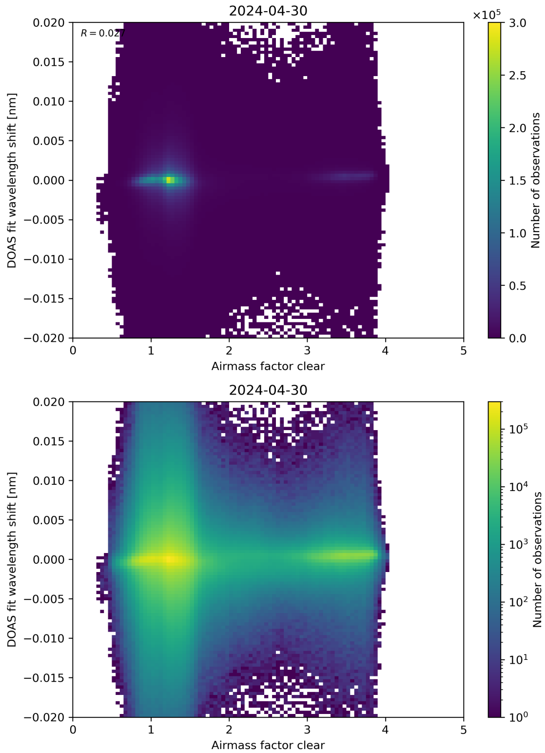
Figure 72: Scatter density plot of “Airmass factor clear” against “DOAS fit wavelength shift” for 2024-04-29 to 2024-05-01.
