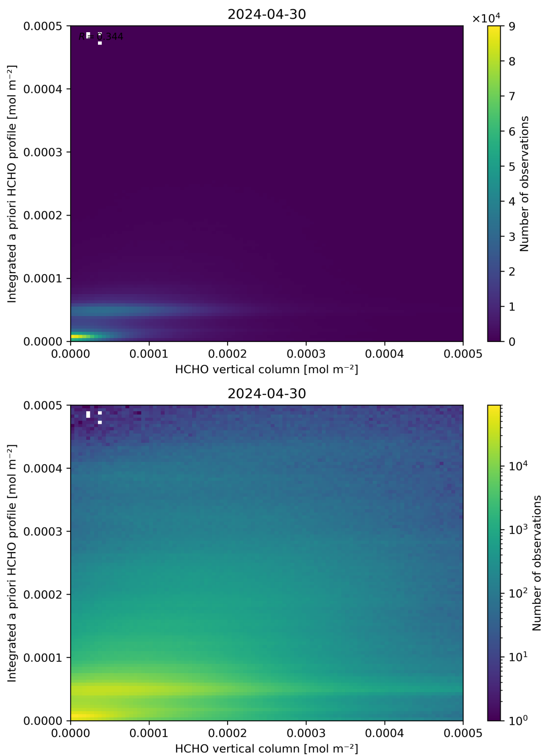
Figure 135: Scatter density plot of “HCHO vertical column” against “Integrated a priori HCHO profile” for 2024-04-29 to 2024-05-01.
