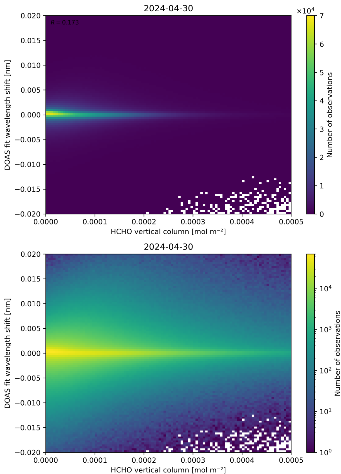
Figure 124: Scatter density plot of “HCHO vertical column” against “DOAS fit wavelength shift” for 2024-04-29 to 2024-05-01.
