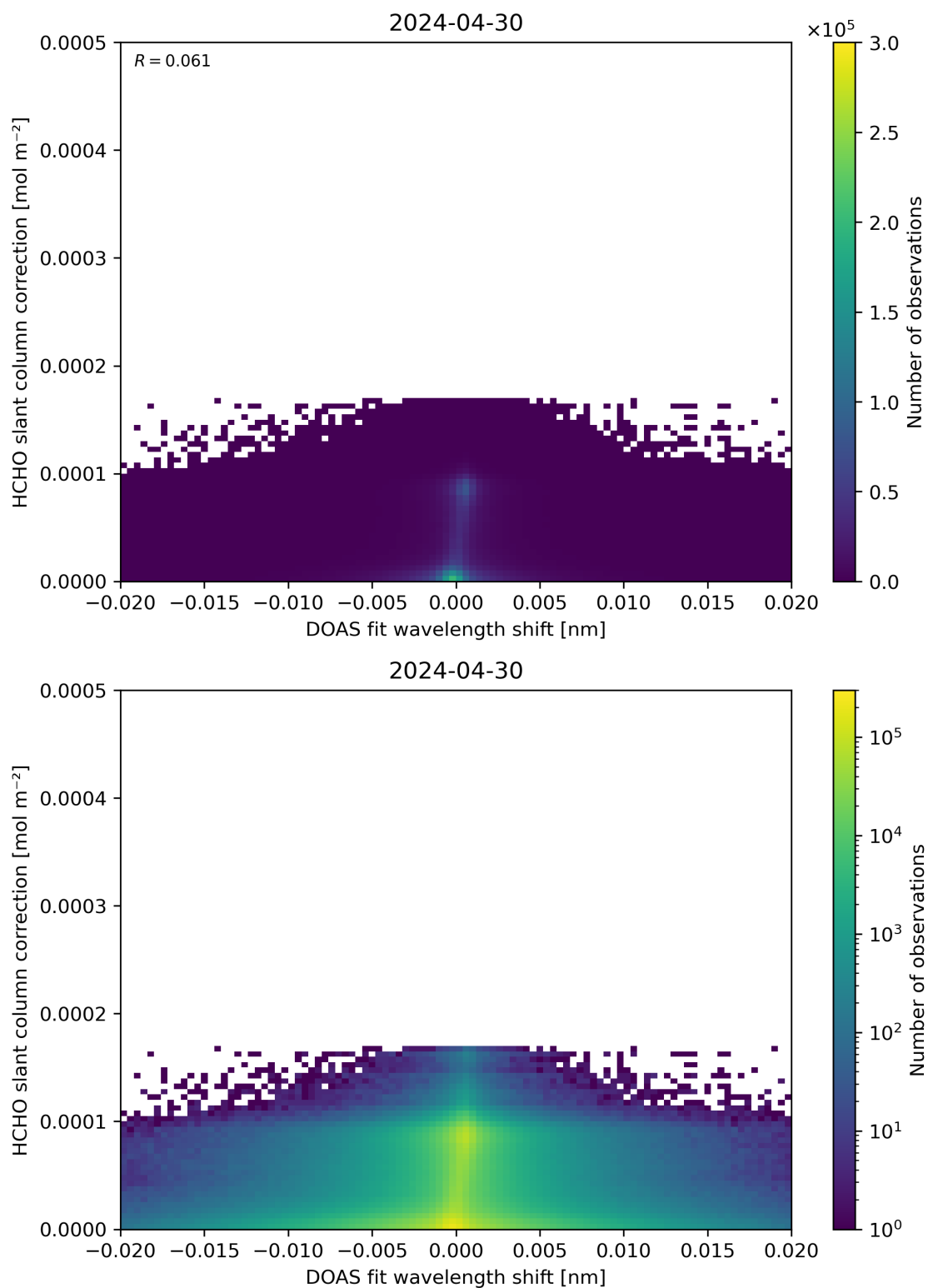
Figure 67: Scatter density plot of “DOAS fit wavelength shift” against “HCHO slant column correction” for 2024-04-29 to 2024-05-01.
