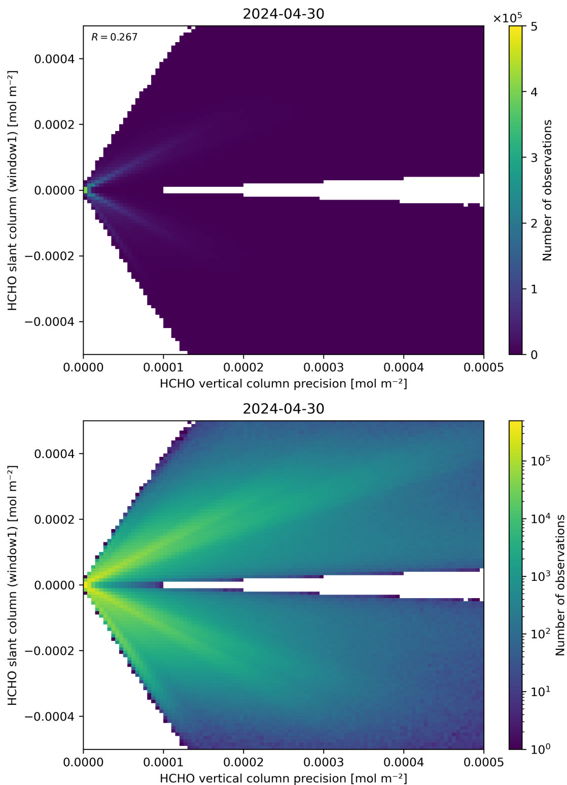
Figure 142: Scatter density plot of “HCHO vertical column precision” against “HCHO slant column (window1)” for 2024-04-29 to 2024-05-01.
