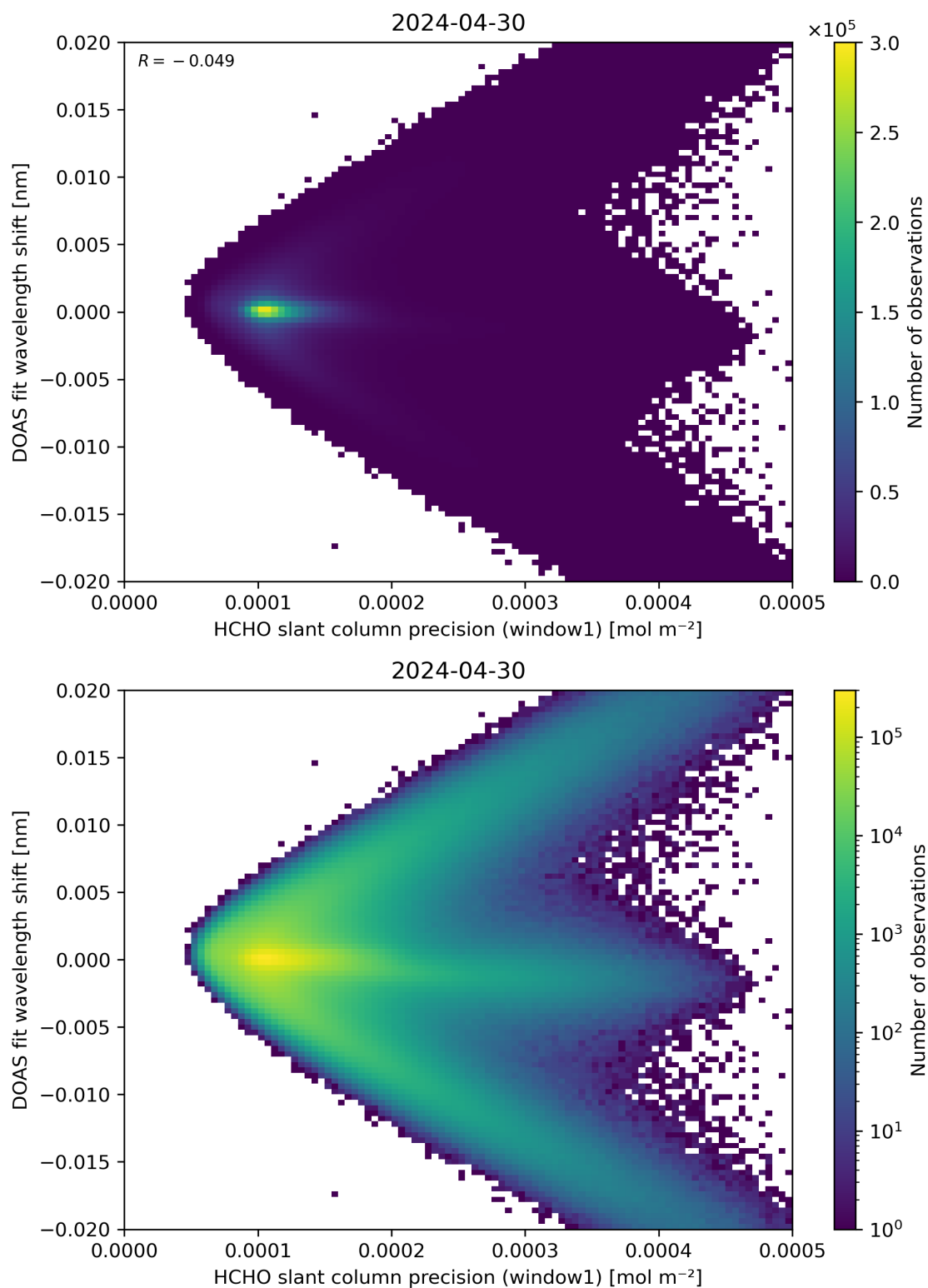
Figure 89: Scatter density plot of “HCHO slant column precision (window1)” against “DOAS fit wavelength shift” for 2024-04-29 to 2024-05-01.
