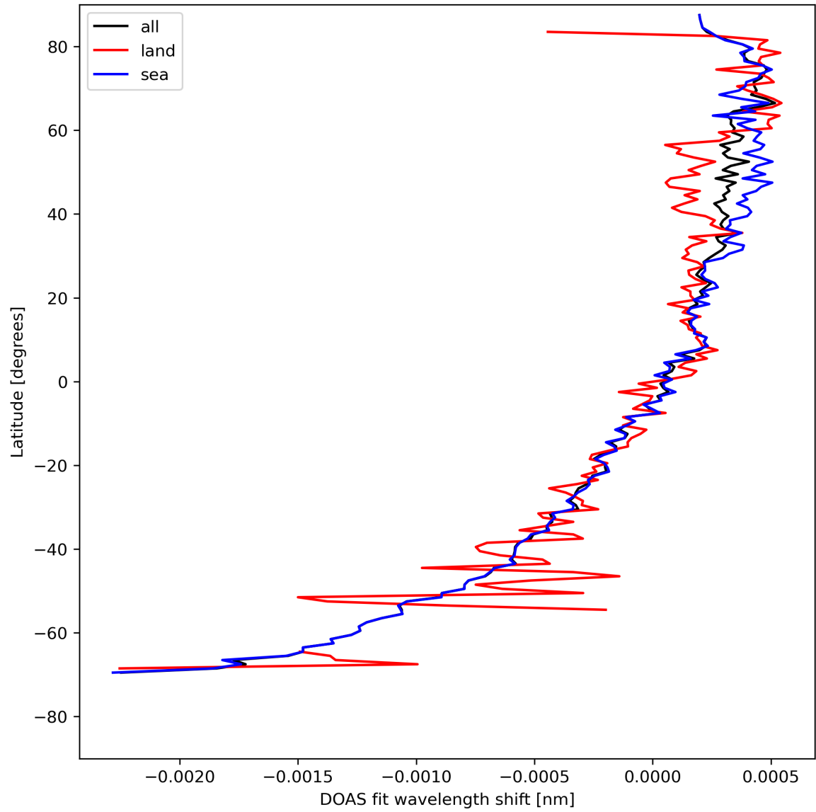
Figure 30: Zonal average of "DOAS fit wavelength shift" for 2024-04-29 to 2024-05-01.
