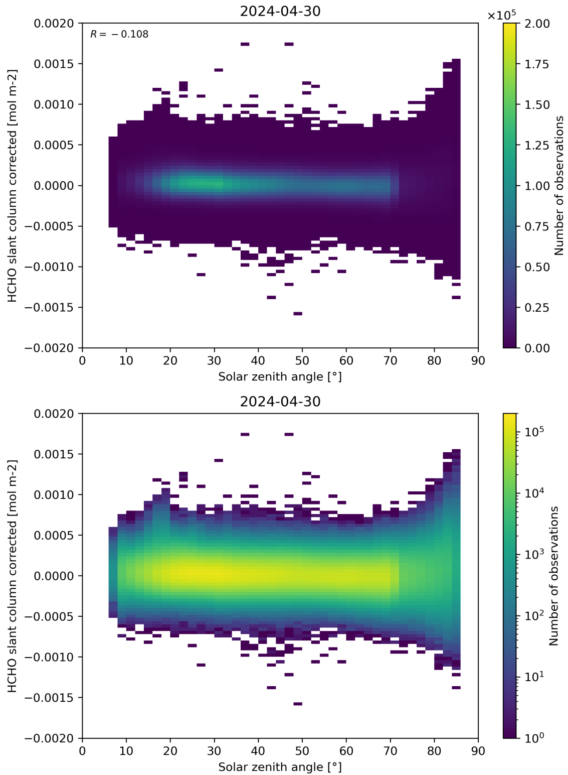
Figure 171: Scatter density plot of “Solar zenith angle” against “HCHO slant column corrected” for 2024-04-29 to 2024-05-01.
