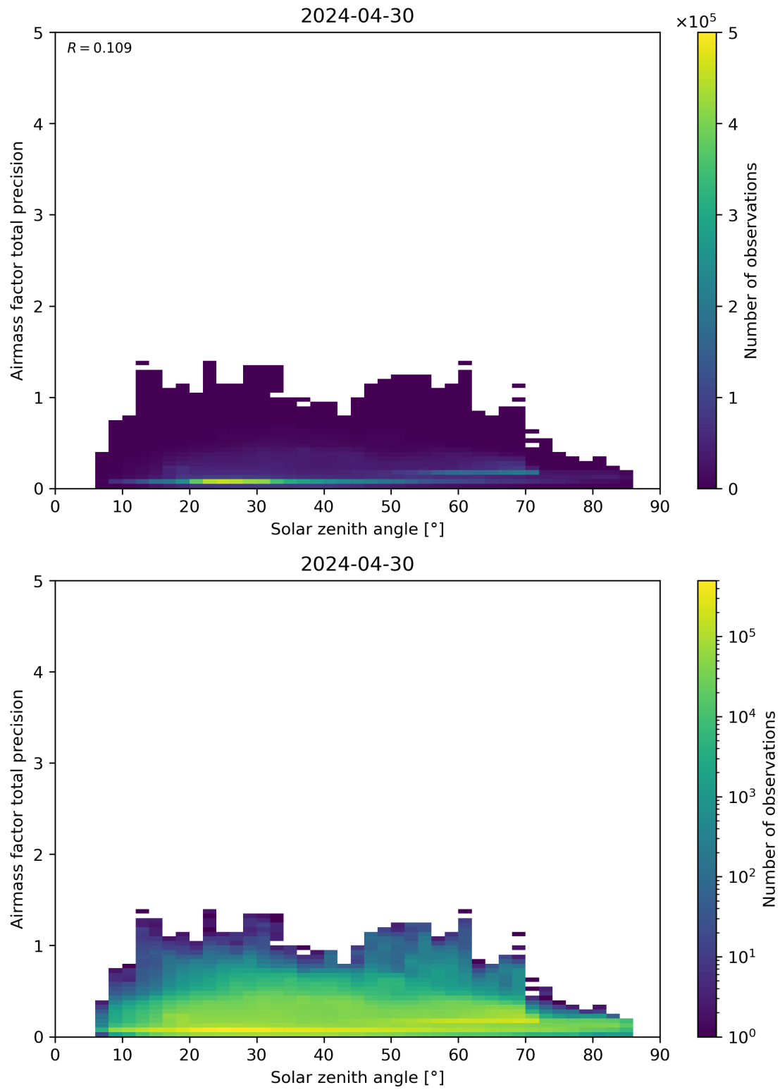
Figure 176: Scatter density plot of “Solar zenith angle” against “Airmass factor total precision” for 2024-04-29 to 2024-05-01.
