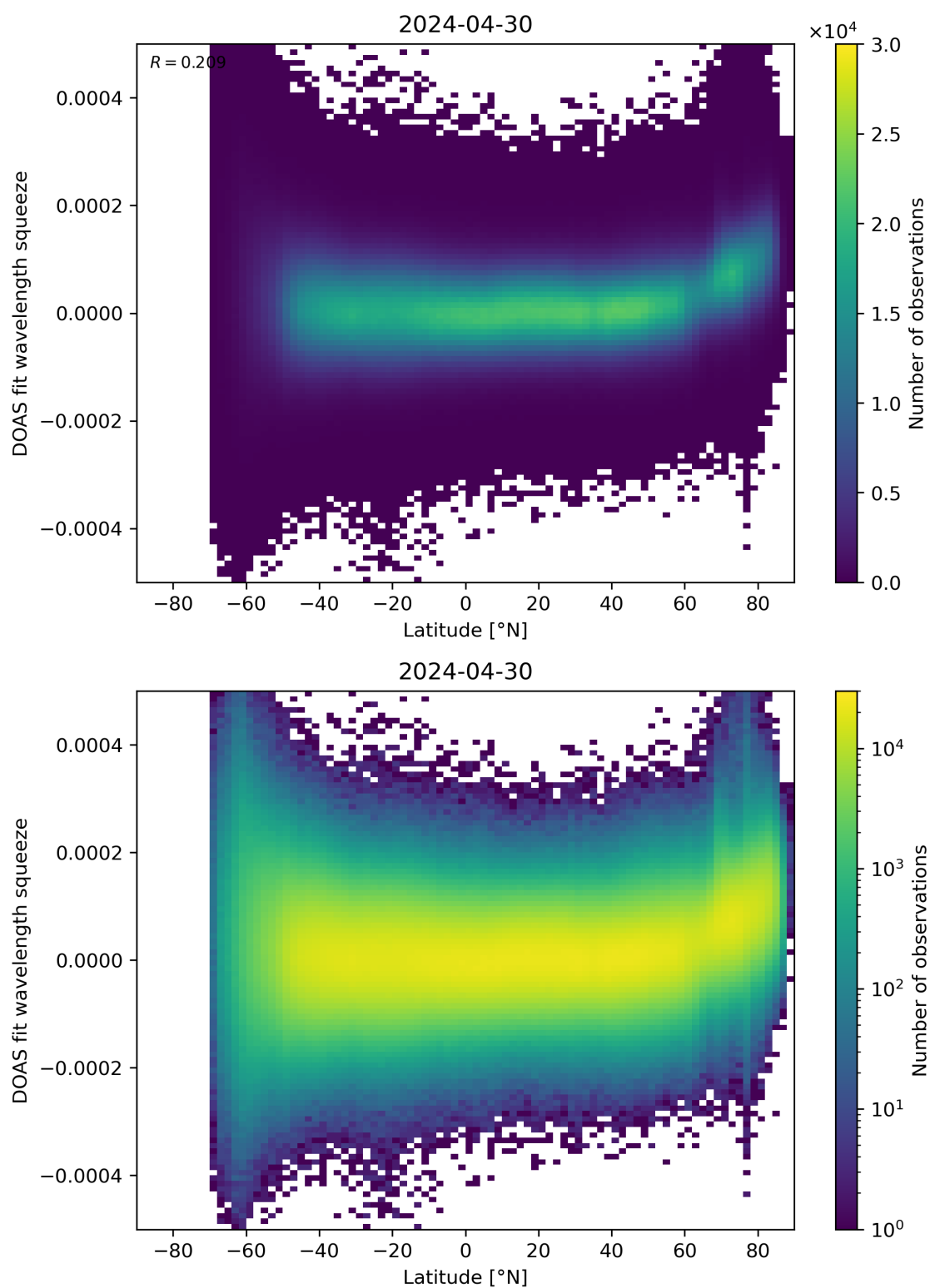
Figure 155: Scatter density plot of “Latitude” against “DOAS fit wavelength squeeze” for 2024-04-29 to 2024-05-01.
