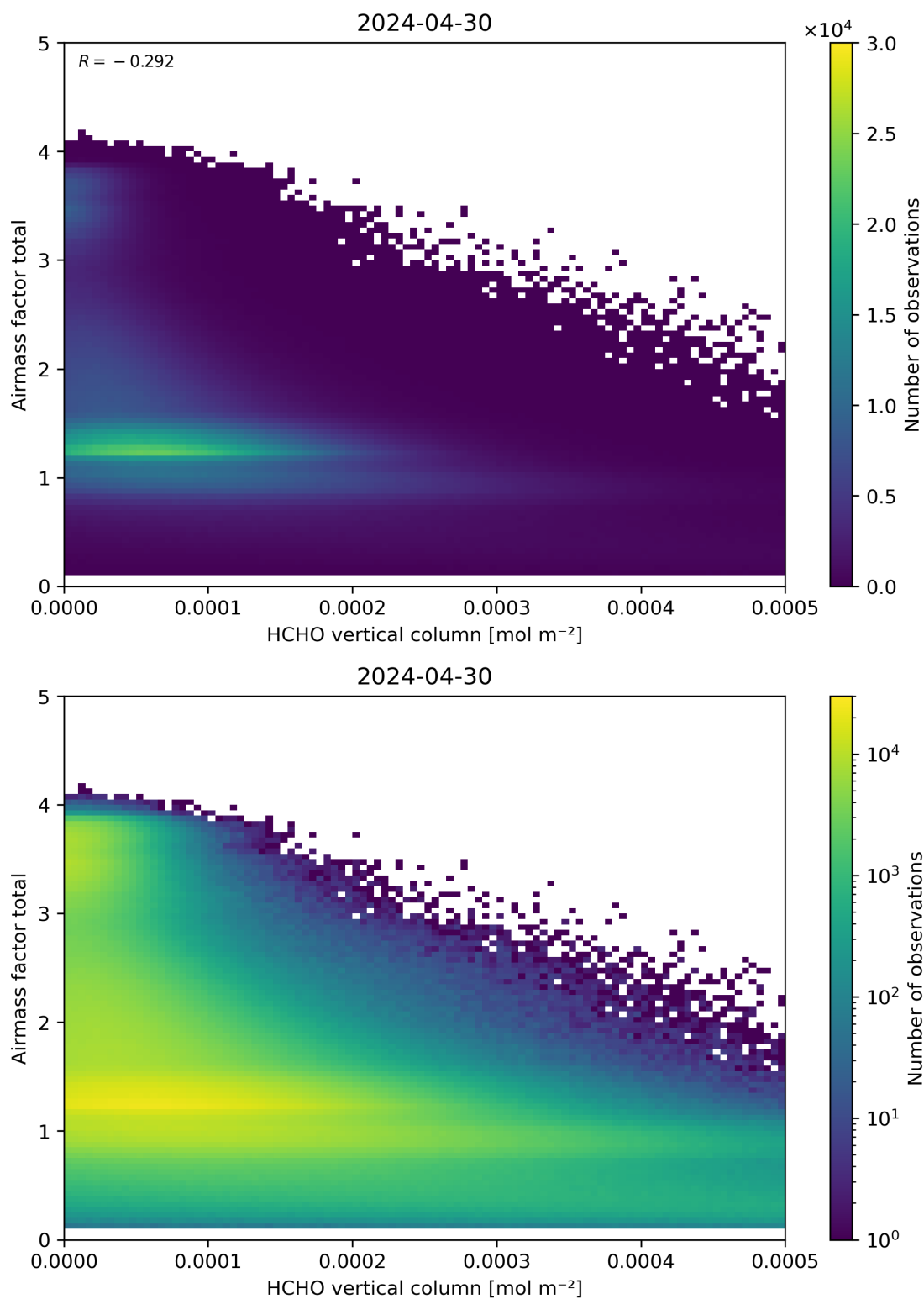
Figure 131: Scatter density plot of “HCHO vertical column” against “Airmass factor total” for 2024-04-29 to 2024-05-01.
