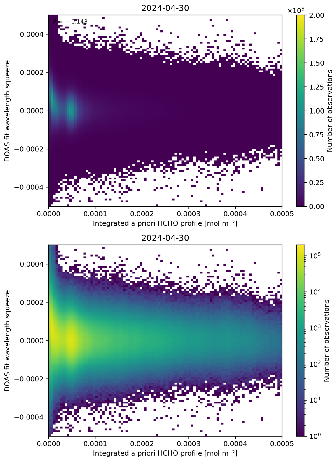
Figure 150: Scatter density plot of “Integrated a priori HCHO profile” against “DOAS fit wavelength squeeze” for 2024-04-29 to 2024-05-01.
