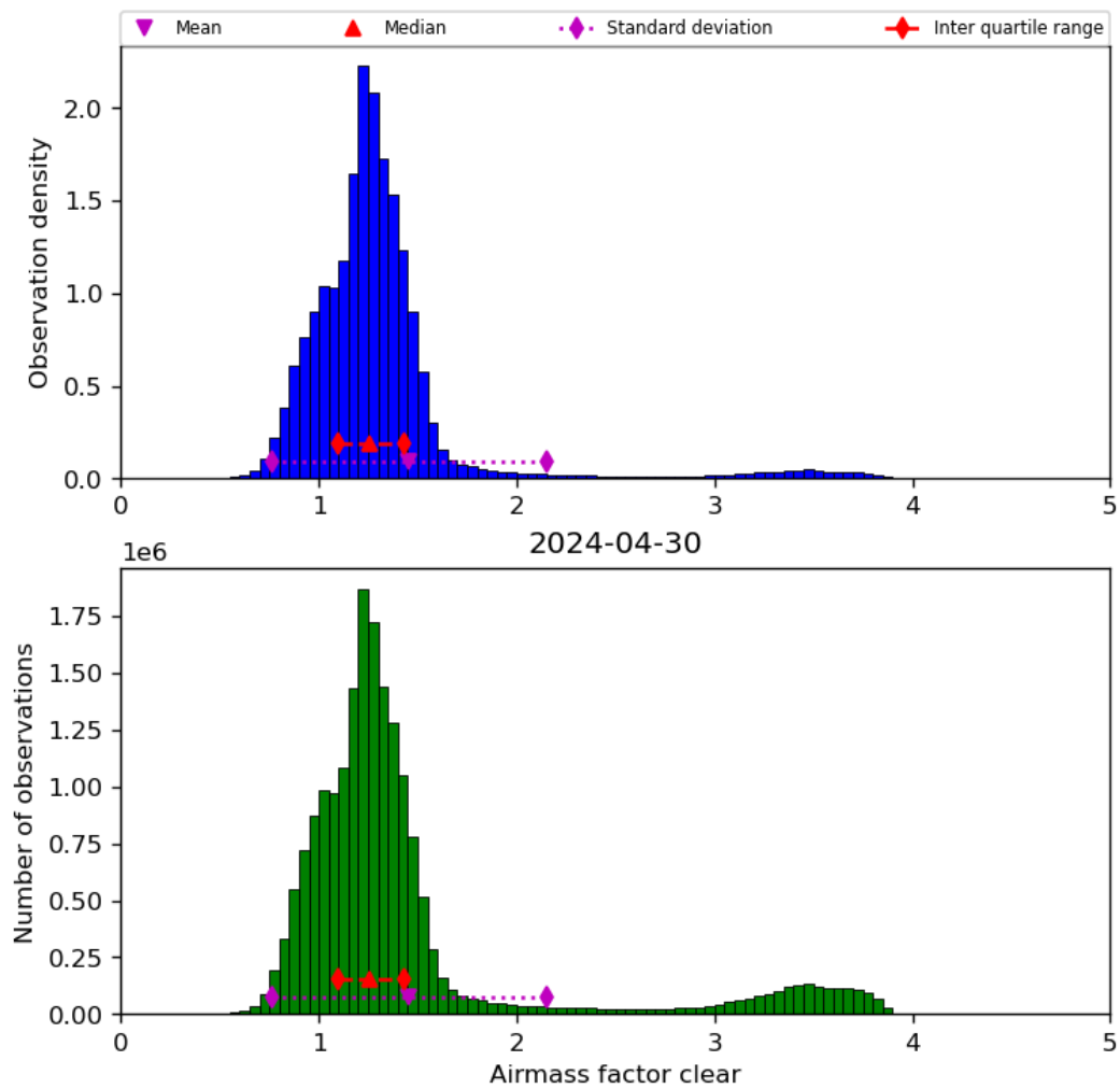
Figure 42: Histogram of “Airmass factor clear” for 2024-04-29 to 2024-05-01
