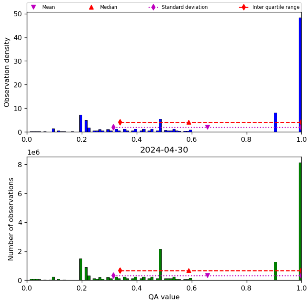
Figure 34: Histogram of “QA value” for 2024-04-29 to 2024-05-01
