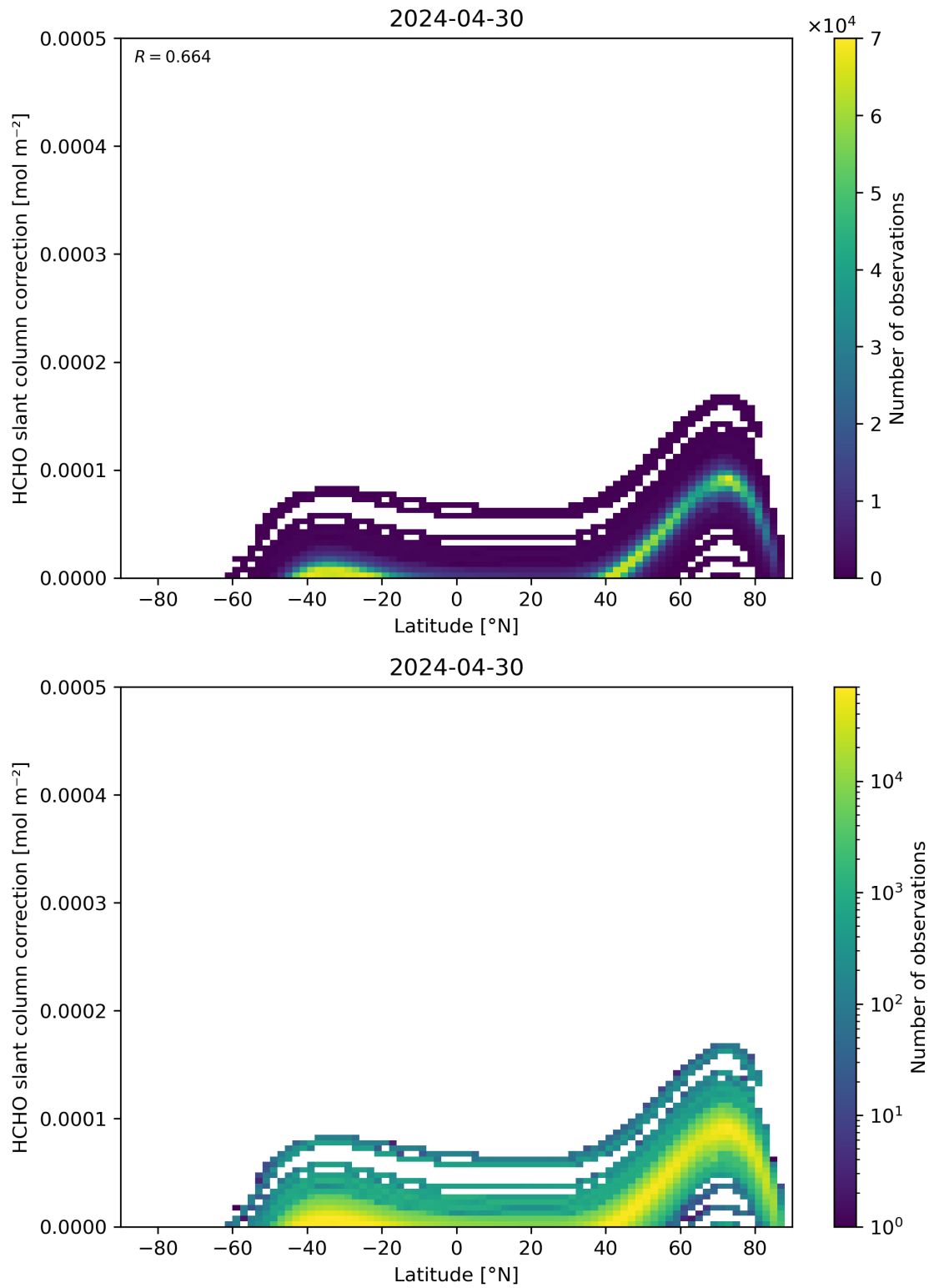
Figure 158: Scatter density plot of “Latitude” against “HCHO slant column correction” for 2024-04-29 to 2024-05-01.
