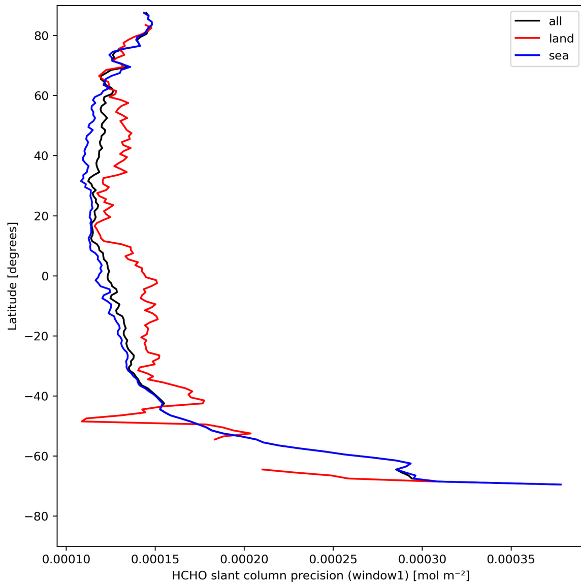
Figure 25: Zonal average of “HCHO slant column precision (window1)” for 2024-04-29 to 2024-05-01.
