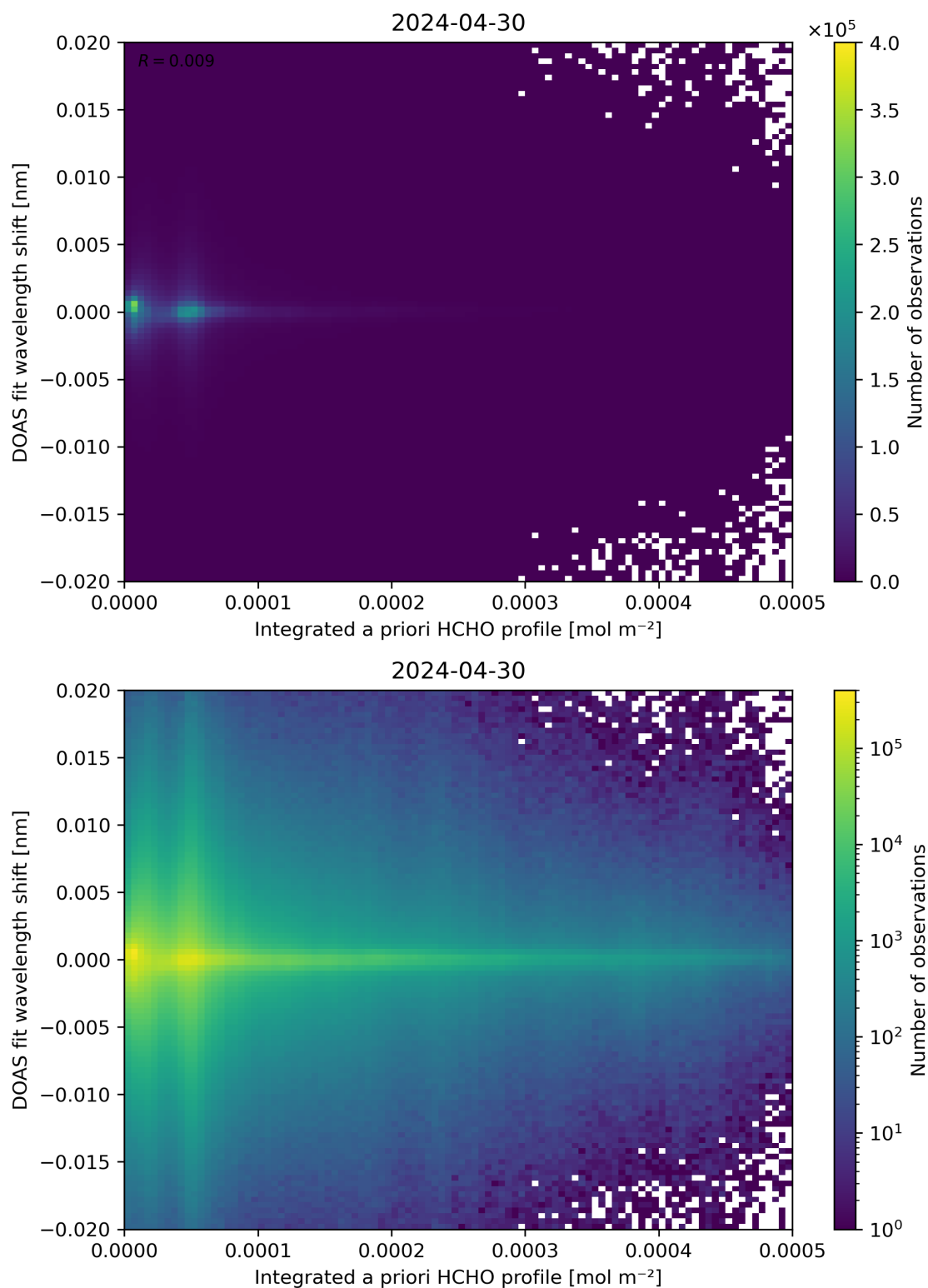
Figure 149: Scatter density plot of “Integrated a priori HCHO profile” against “DOAS fit wavelength shift” for 2024-04-29 to 2024-05-01.
