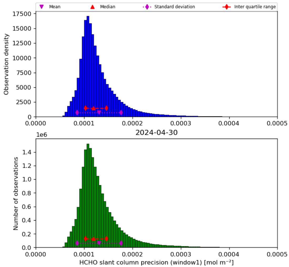
Figure 39: Histogram of “HCHO slant column precision (window1)” for 2024-04-29 to 2024-05-01
