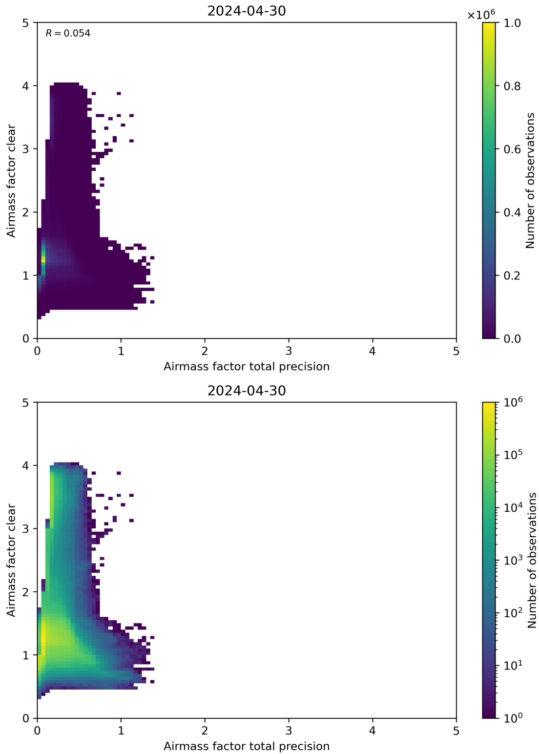
Figure 108: Scatter density plot of “Airmass factor total precision” against “Airmass factor clear” for 2024-04-29 to 2024-05-01.
