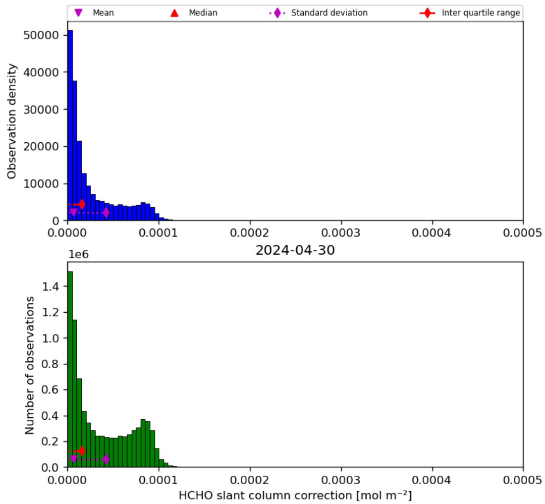
Figure 47: Histogram of “HCHO slant column correction” for 2024-04-29 to 2024-05-01
