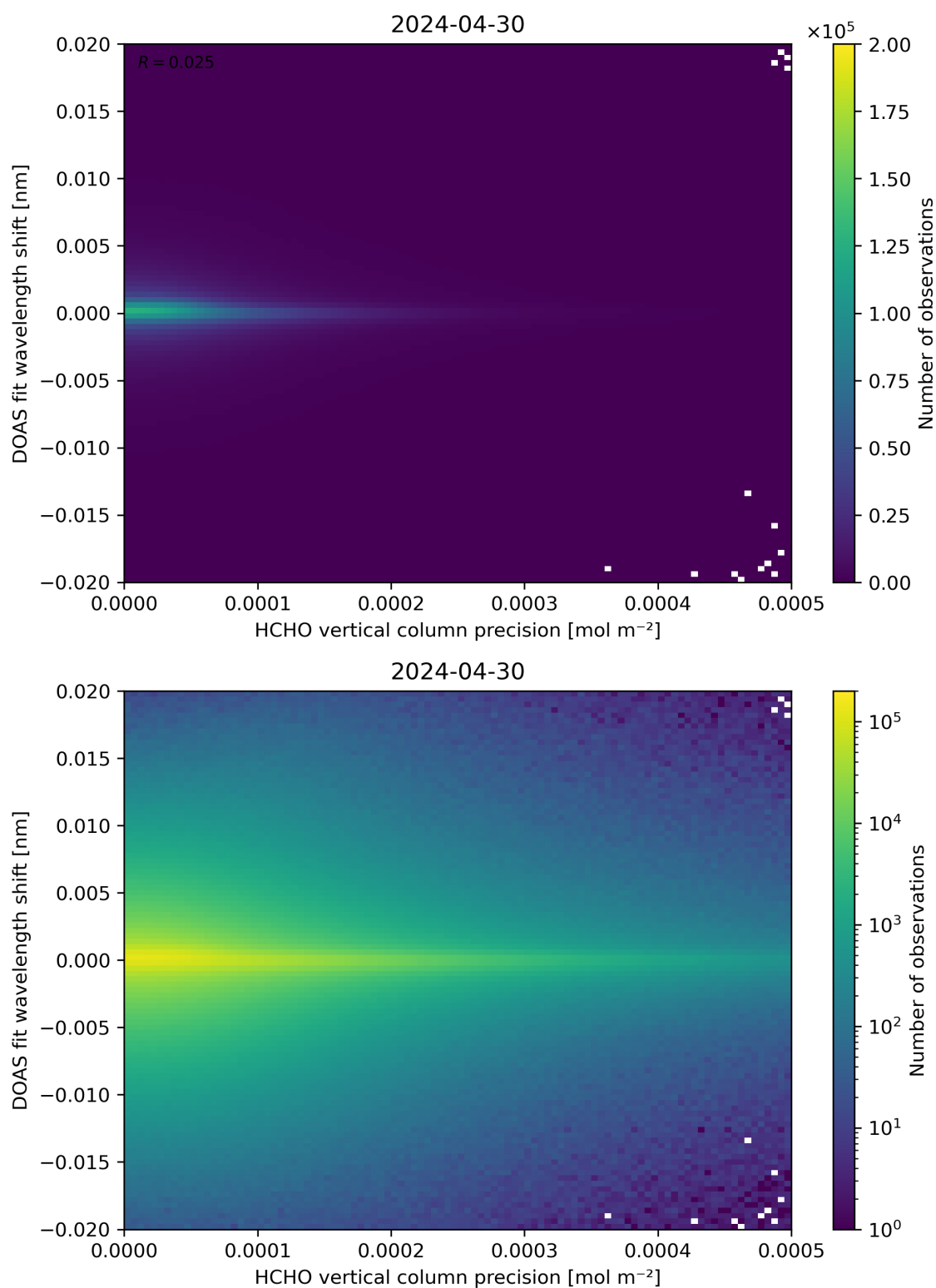
Figure 137: Scatter density plot of “HCHO vertical column precision” against “DOAS fit wavelength shift” for 2024-04-29 to 2024-05-01.
