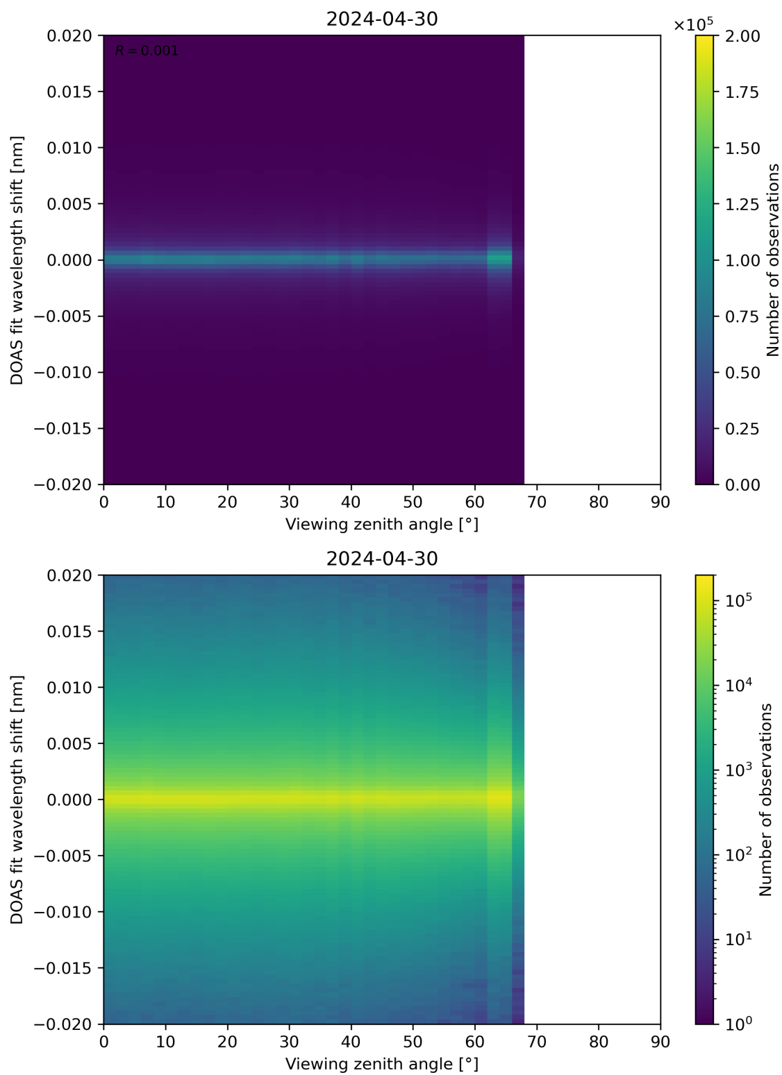
Figure 183: Scatter density plot of “Viewing zenith angle” against “DOAS fit wavelength shift” for 2024-04-29 to 2024-05-01.
