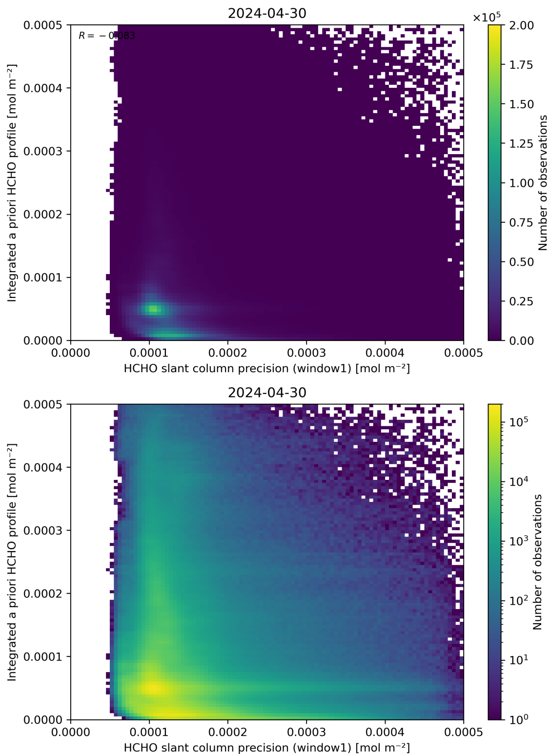
Figure 96: Scatter density plot of “HCHO slant column precision (window1)” against “Integrated a priori HCHO profile” for 2024-04-29 to 2024-05-01.
