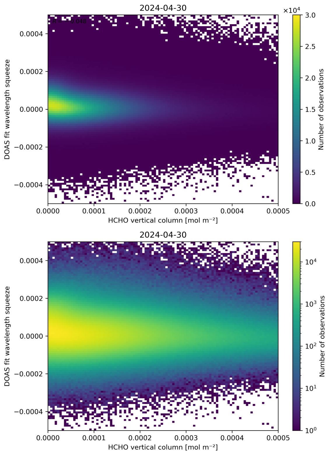
Figure 125: Scatter density plot of “HCHO vertical column” against “DOAS fit wavelength squeeze” for 2024-04-29 to 2024-05-01.
