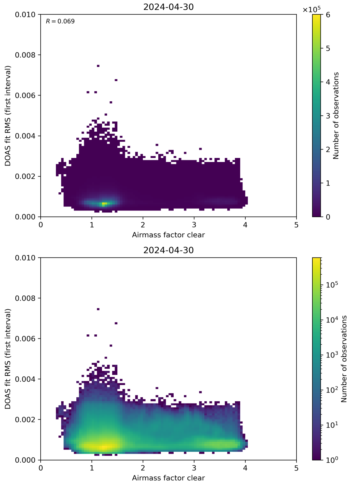
Figure 71: Scatter density plot of “Airmass factor clear” against “DOAS fit RMS (first interval)” for 2024-04-29 to 2024-05-01.
