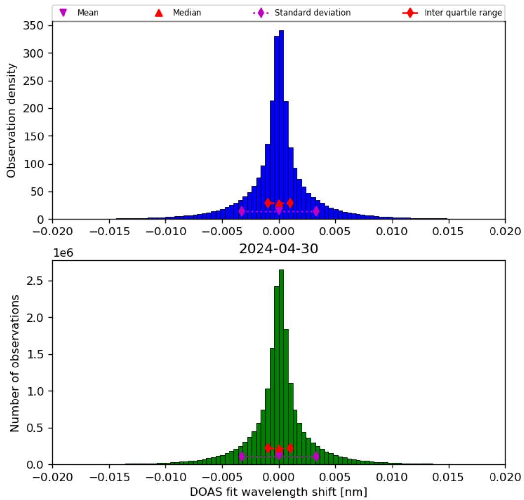
Figure 44: Histogram of “DOAS fit wavelength shift” for 2024-04-29 to 2024-05-01
