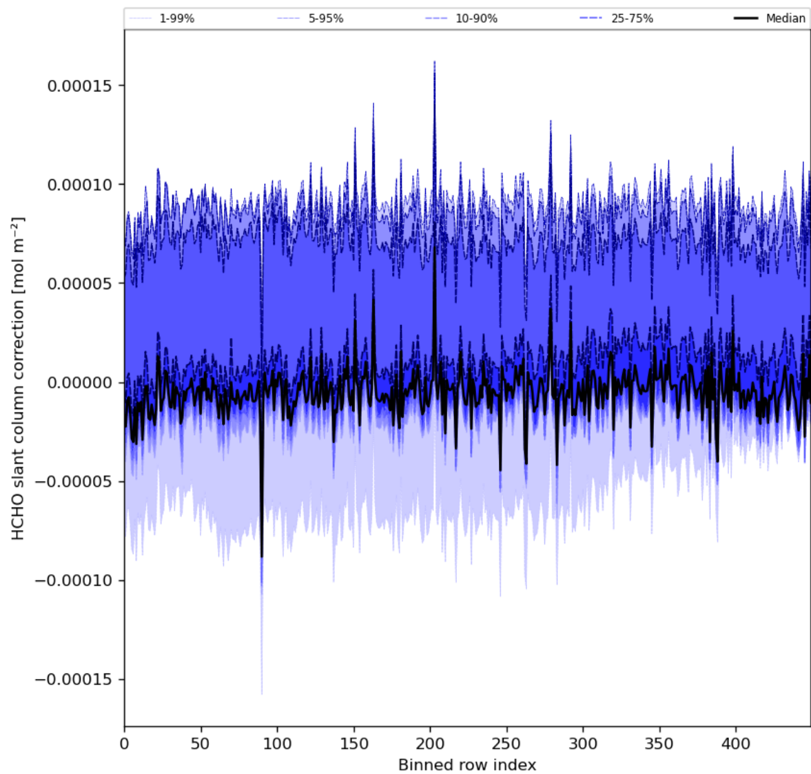
Figure 61: Along track statistics of “HCHO slant column correction” for 2024-04-29 to 2024-05-01
