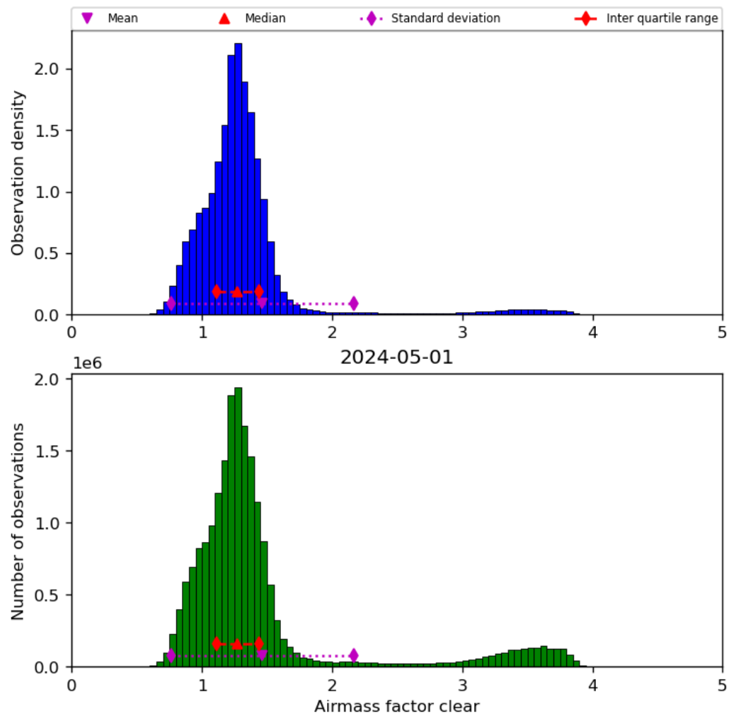
Figure 42: Histogram of “Airmass factor clear” for 2024-04-30 to 2024-05-02
