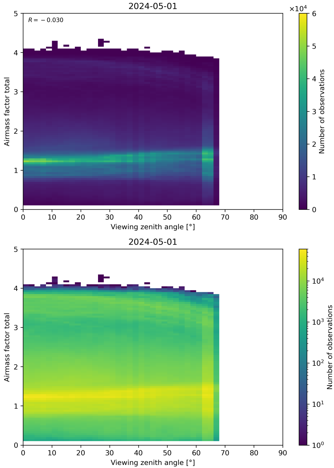
Figure 190: Scatter density plot of “Viewing zenith angle” against “Airmass factor total” for 2024-04-30 to 2024-05-02.
