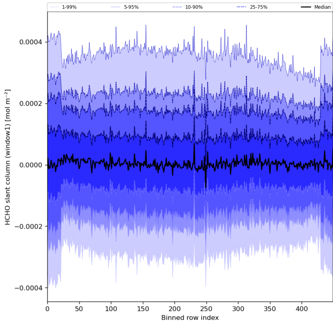
Figure 52: Along track statistics of “HCHO slant column (window1)” for 2024-04-30 to 2024-05-02
