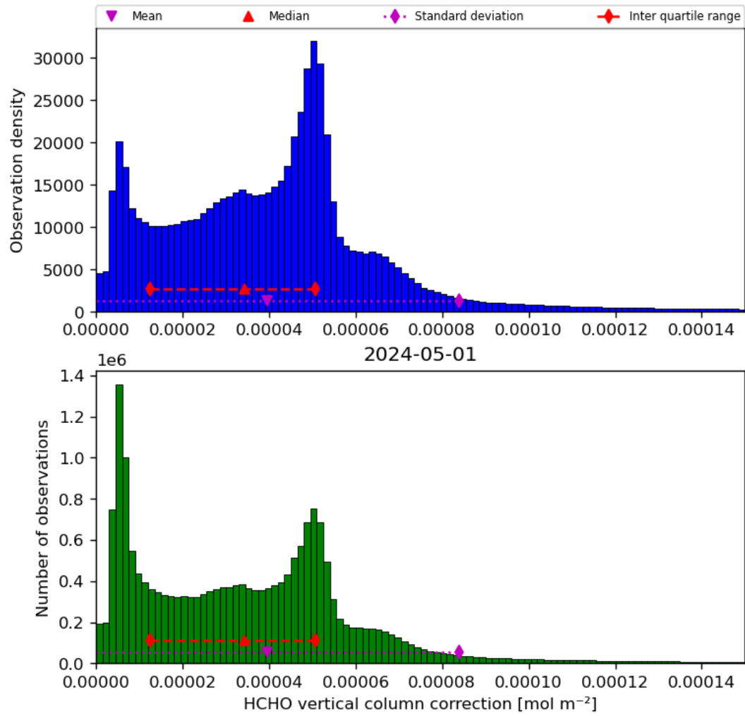
Figure 37: Histogram of “HCHO vertical column correction” for 2024-04-30 to 2024-05-02
