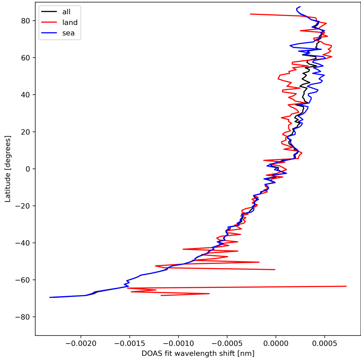
Figure 30: Zonal average of “DOAS fit wavelength shift” for 2024-04-30 to 2024-05-02.
