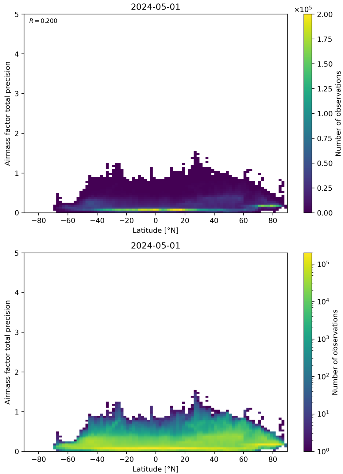
Figure 162: Scatter density plot of “Latitude” against “Airmass factor total precision” for 2024-04-30 to 2024-05-02.
