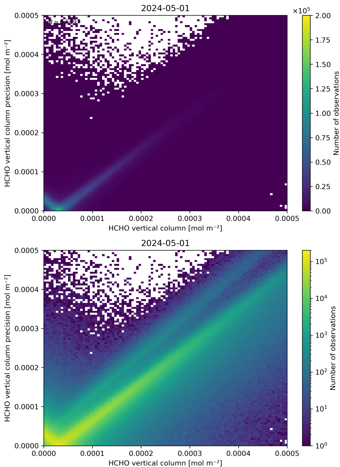
Figure 134: Scatter density plot of “HCHO vertical column” against “HCHO vertical column precision” for 2024-04-30 to 2024-05-02.
