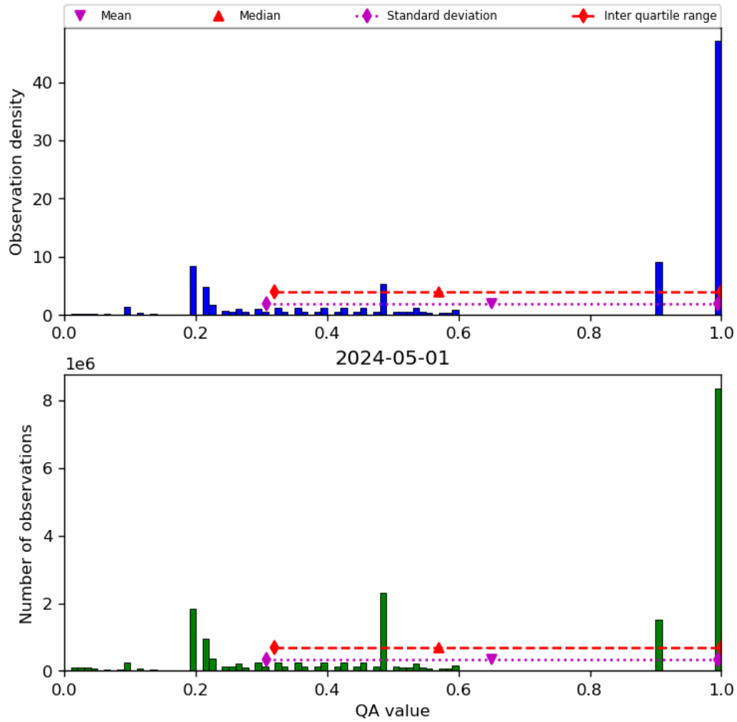
Figure 34: Histogram of “QA value” for 2024-04-30 to 2024-05-02
