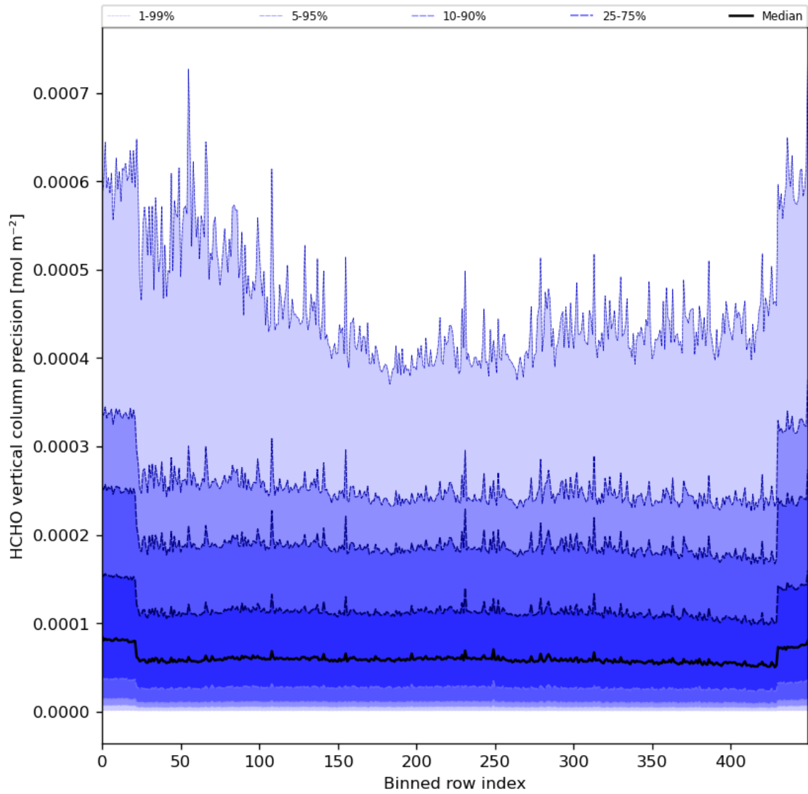
Figure 50: Along track statistics of “HCHO vertical column precision” for 2024-04-30 to 2024-05-02
