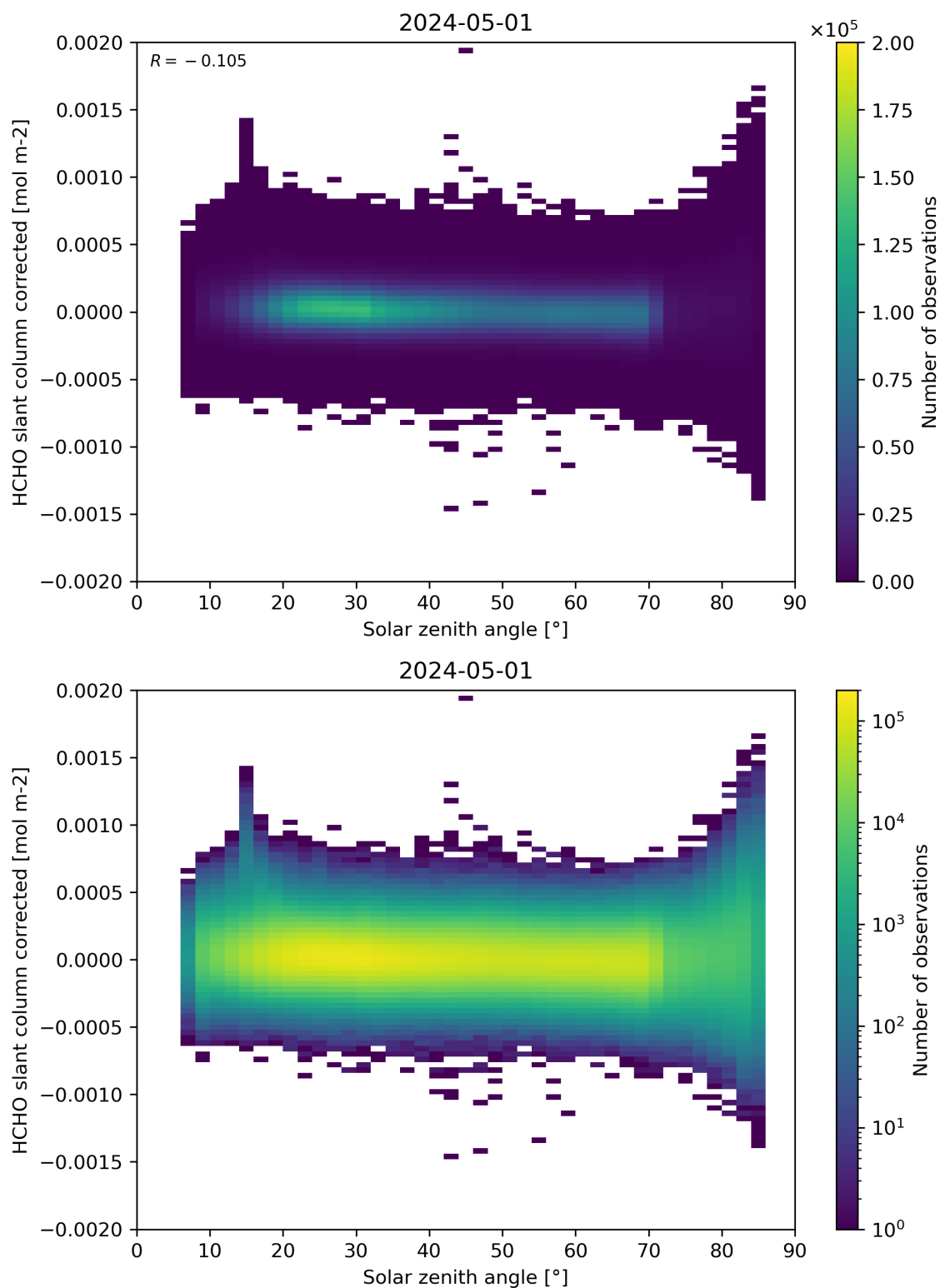
Figure 171: Scatter density plot of “Solar zenith angle” against “HCHO slant column corrected” for 2024-04-30 to 2024-05-02.
