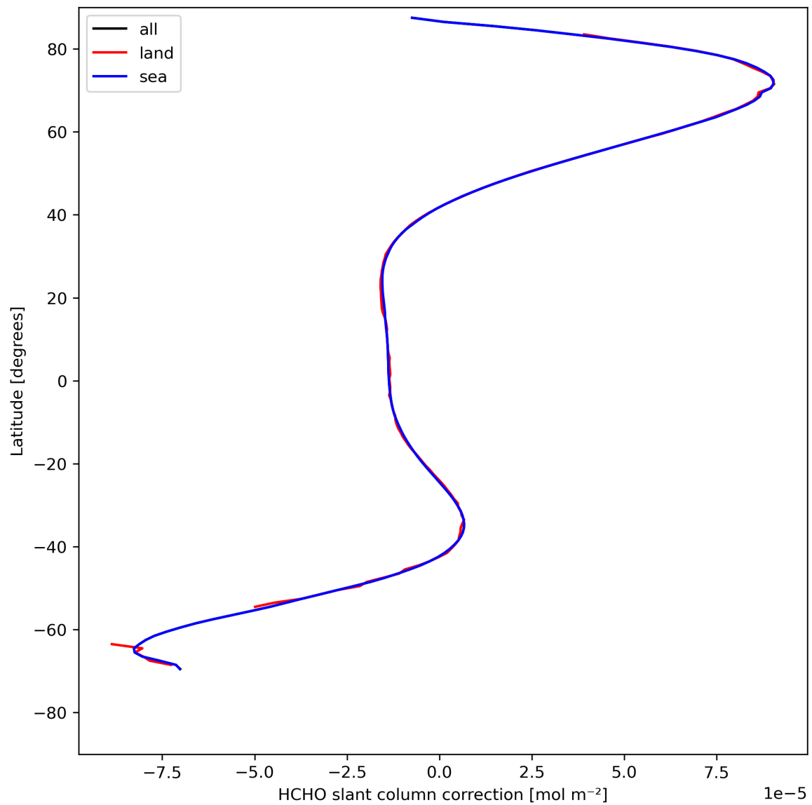
Figure 33: Zonal average of “HCHO slant column correction” for 2024-04-30 to 2024-05-02.
