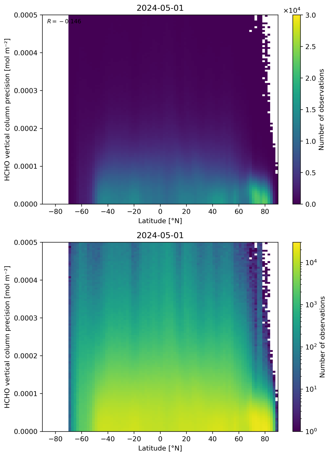
Figure 165: Scatter density plot of “Latitude” against “HCHO vertical column precision” for 2024-04-30 to 2024-05-02.
