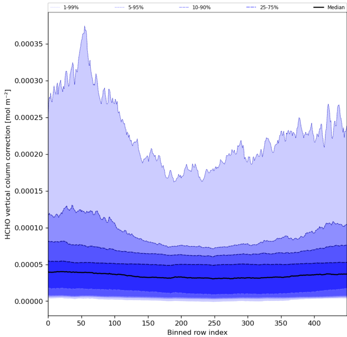
Figure 51: Along track statistics of “HCHO vertical column correction” for 2024-04-30 to 2024-05-02
