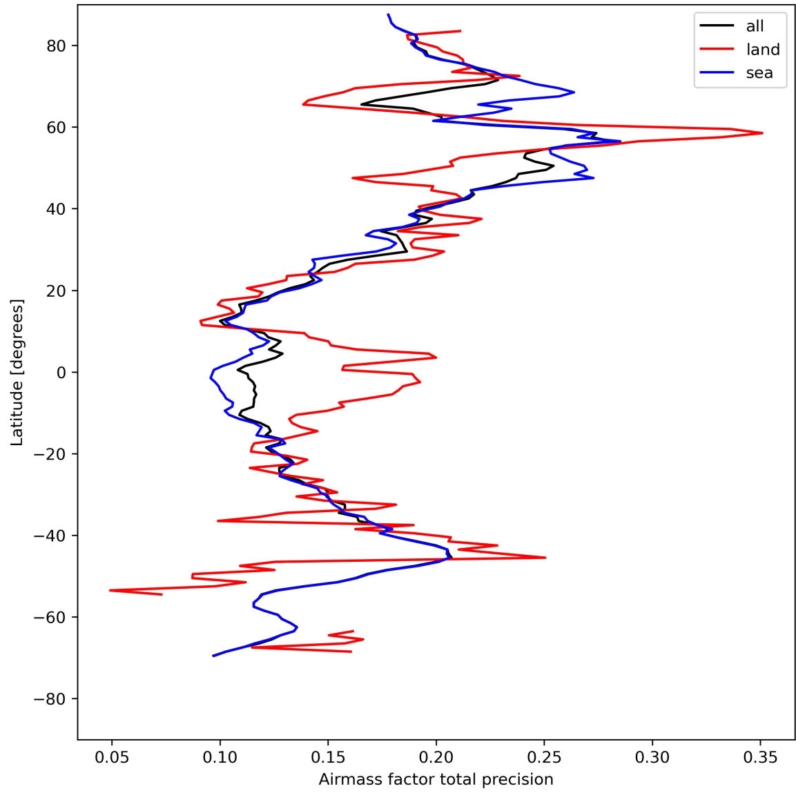
Figure 27: Zonal average of “Airmass factor total precision” for 2024-04-30 to 2024-05-02.
