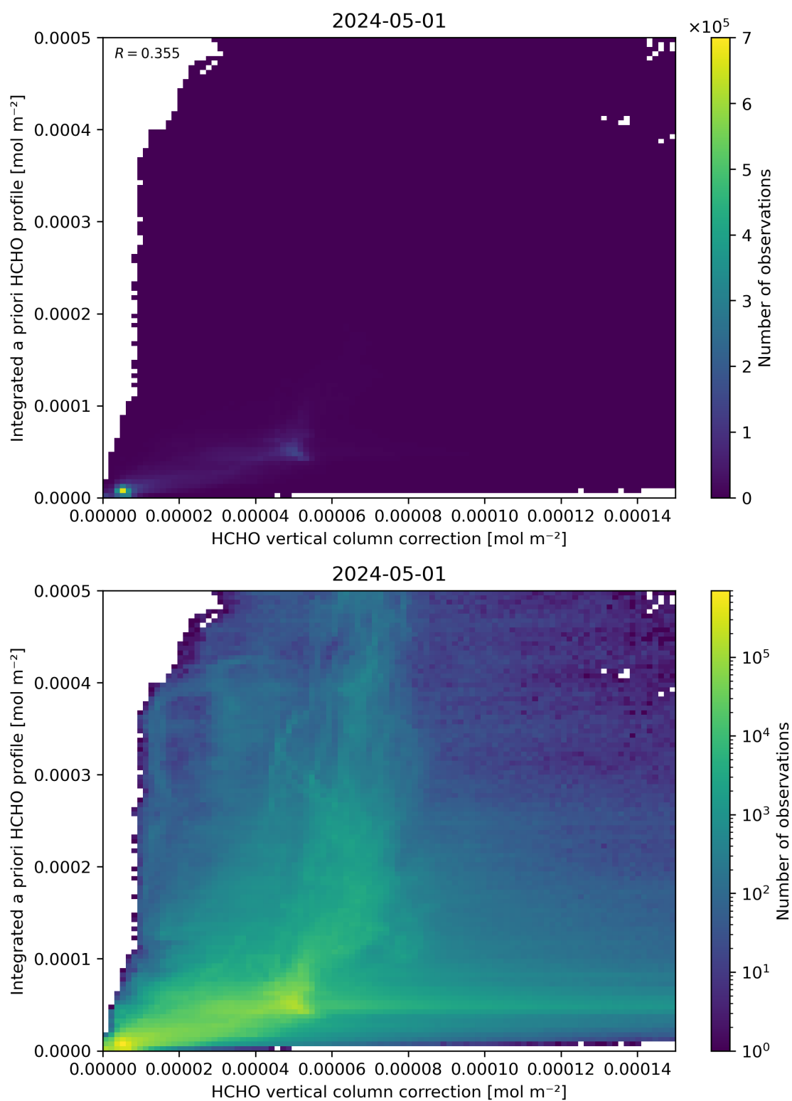
Figure 122: Scatter density plot of “HCHO vertical column correction” against “Integrated a priori HCHO profile” for 2024-04-30 to 2024-05-02.
