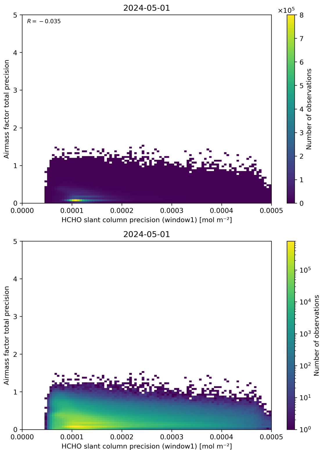
Figure 95: Scatter density plot of “HCHO slant column precision (window1)” against “Airmass factor total precision” for 2024-04-30 to 2024-05-02.
