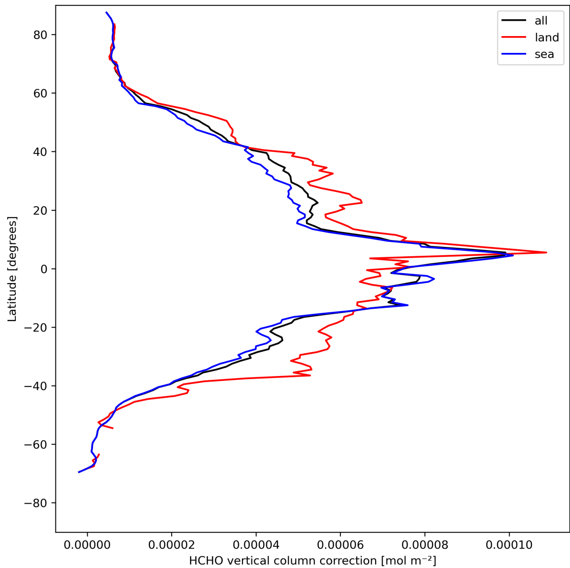
Figure 23: Zonal average of “HCHO vertical column correction” for 2024-04-30 to 2024-05-02.
