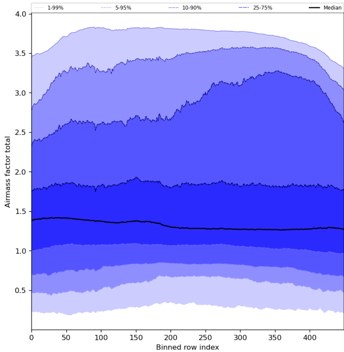
Figure 54: Along track statistics of “Airmass factor total” for 2024-04-30 to 2024-05-02
