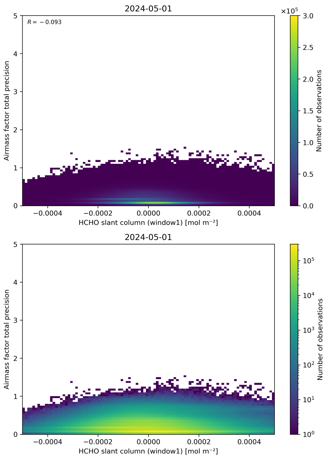
Figure 86: Scatter density plot of “HCHO slant column (window1)” against “Airmass factor total precision” for 2024-04-30 to 2024-05-02.
