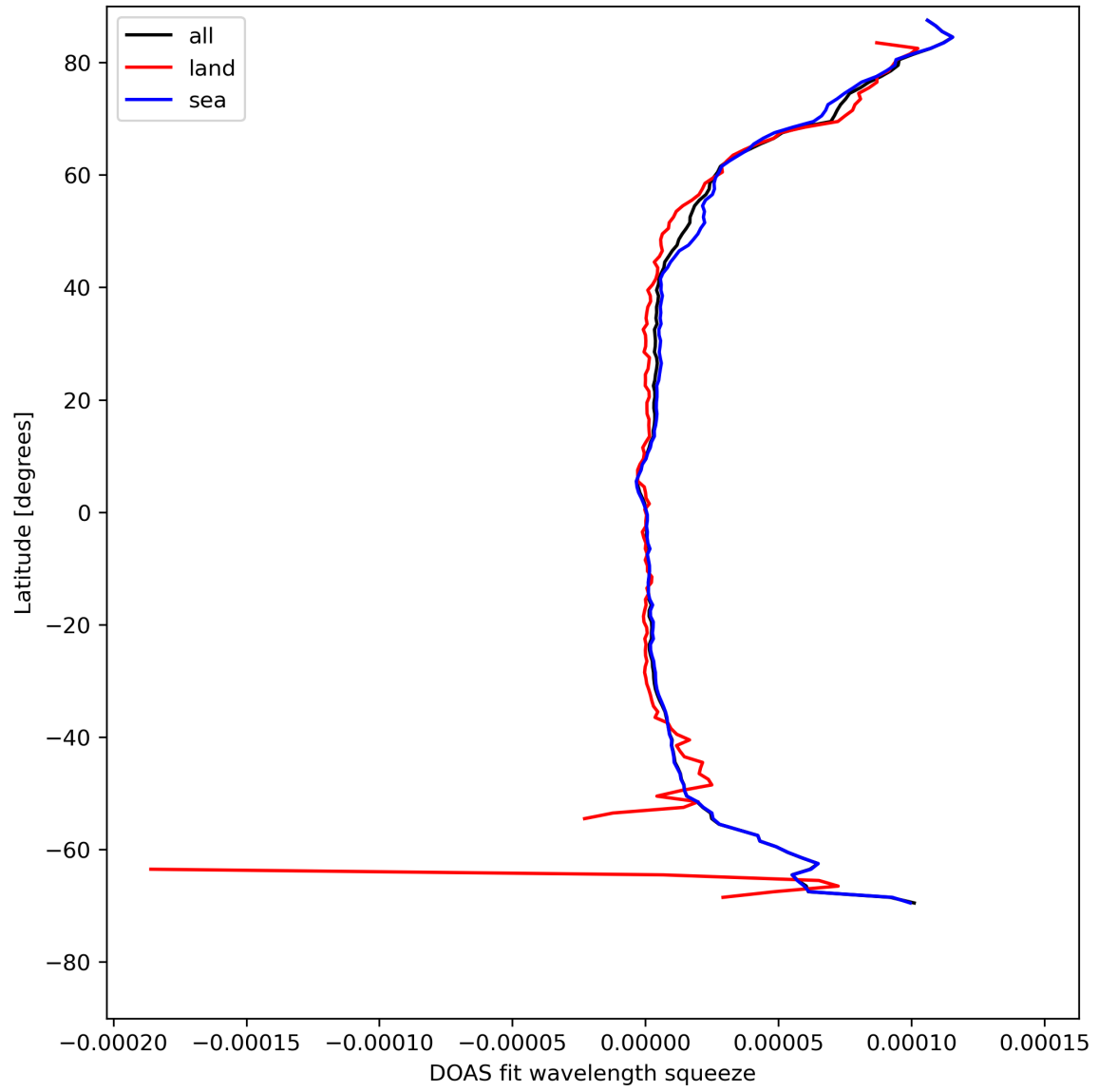
Figure 31: Zonal average of “DOAS fit wavelength squeeze” for 2024-04-30 to 2024-05-02.
