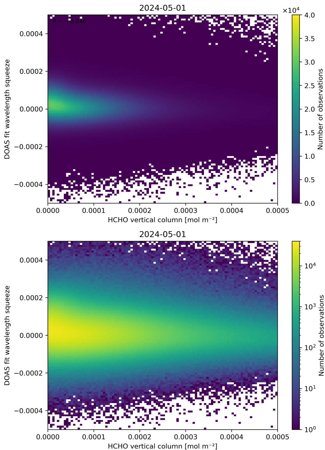
Figure 125: Scatter density plot of “HCHO vertical column” against “DOAS fit wavelength squeeze” for 2024-04-30 to 2024-05-02.
