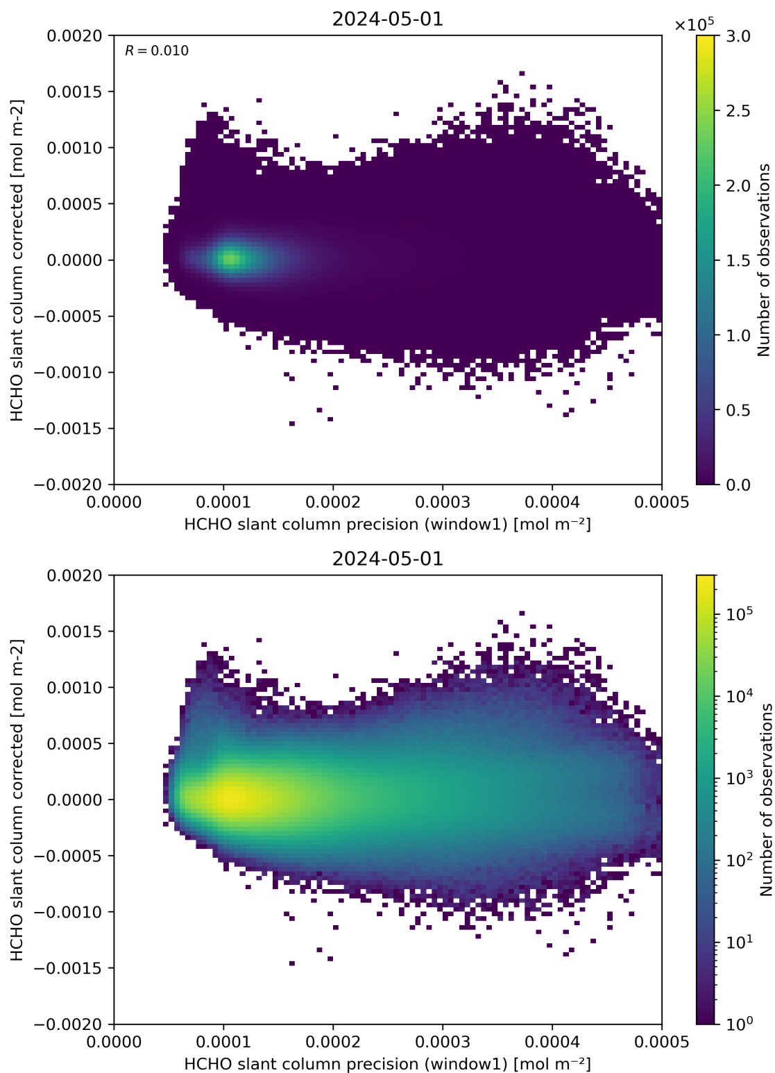
Figure 92: Scatter density plot of “HCHO slant column precision (window1)” against “HCHO slant column corrected” for 2024-04-30 to 2024-05-02.
