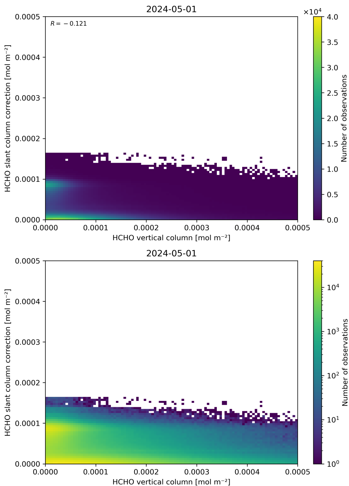
Figure 128: Scatter density plot of “HCHO vertical column” against “HCHO slant column correction” for 2024-04-30 to 2024-05-02.
