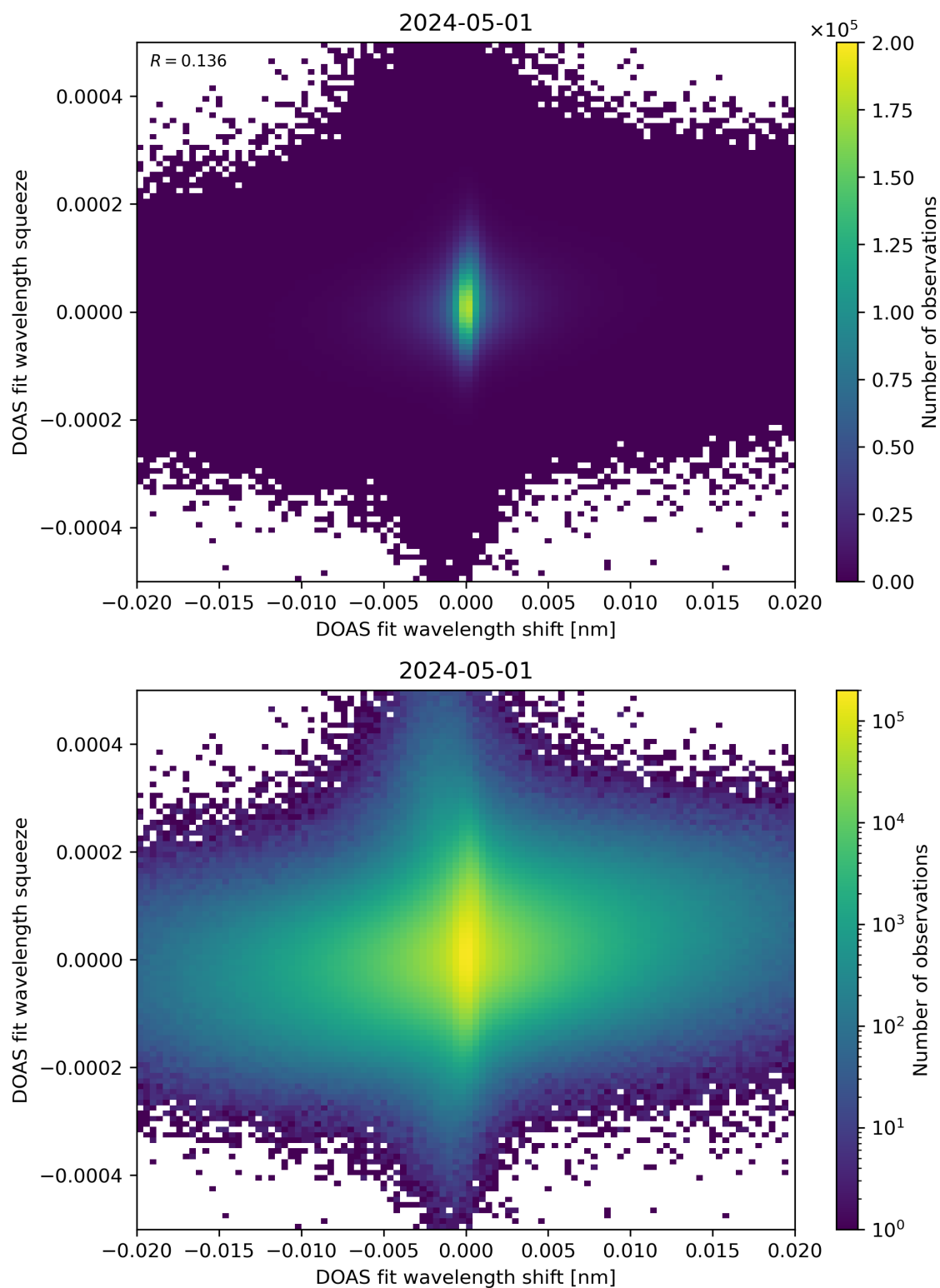
Figure 65: Scatter density plot of “DOAS fit wavelength shift” against “DOAS fit wavelength squeeze” for 2024-04-30 to 2024-05-02.
