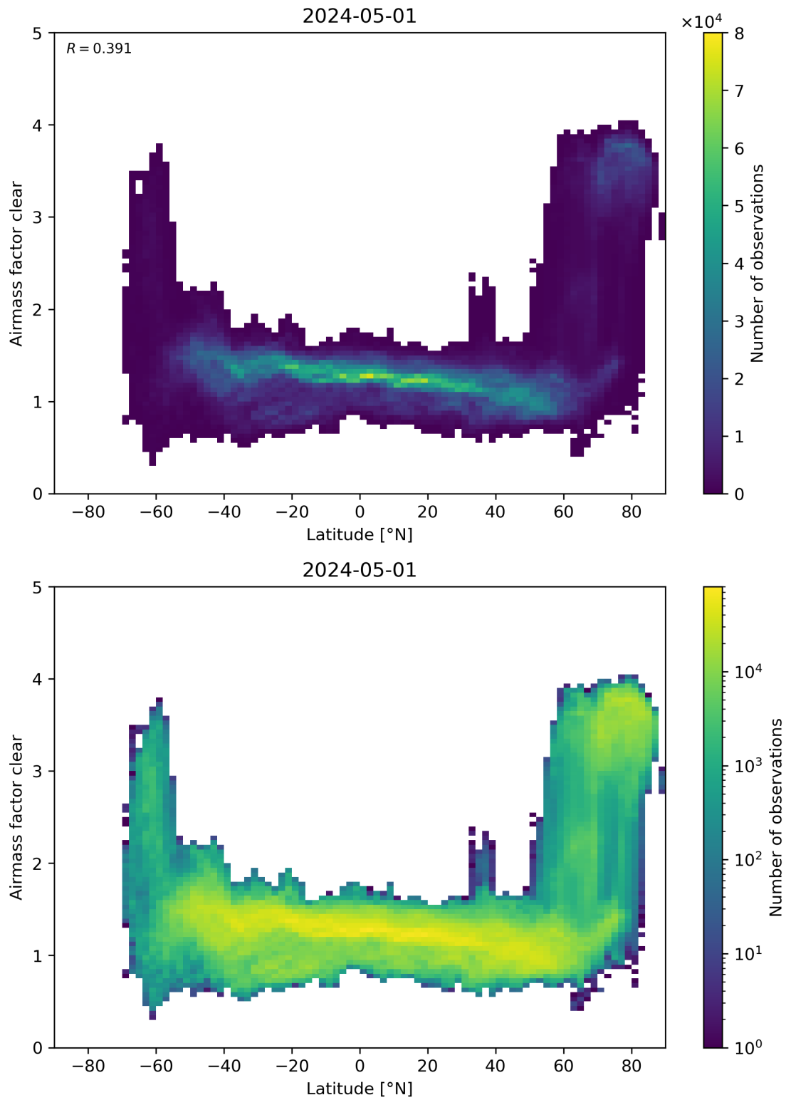
Figure 156: Scatter density plot of “Latitude” against “Airmass factor clear” for 2024-04-30 to 2024-05-02.
