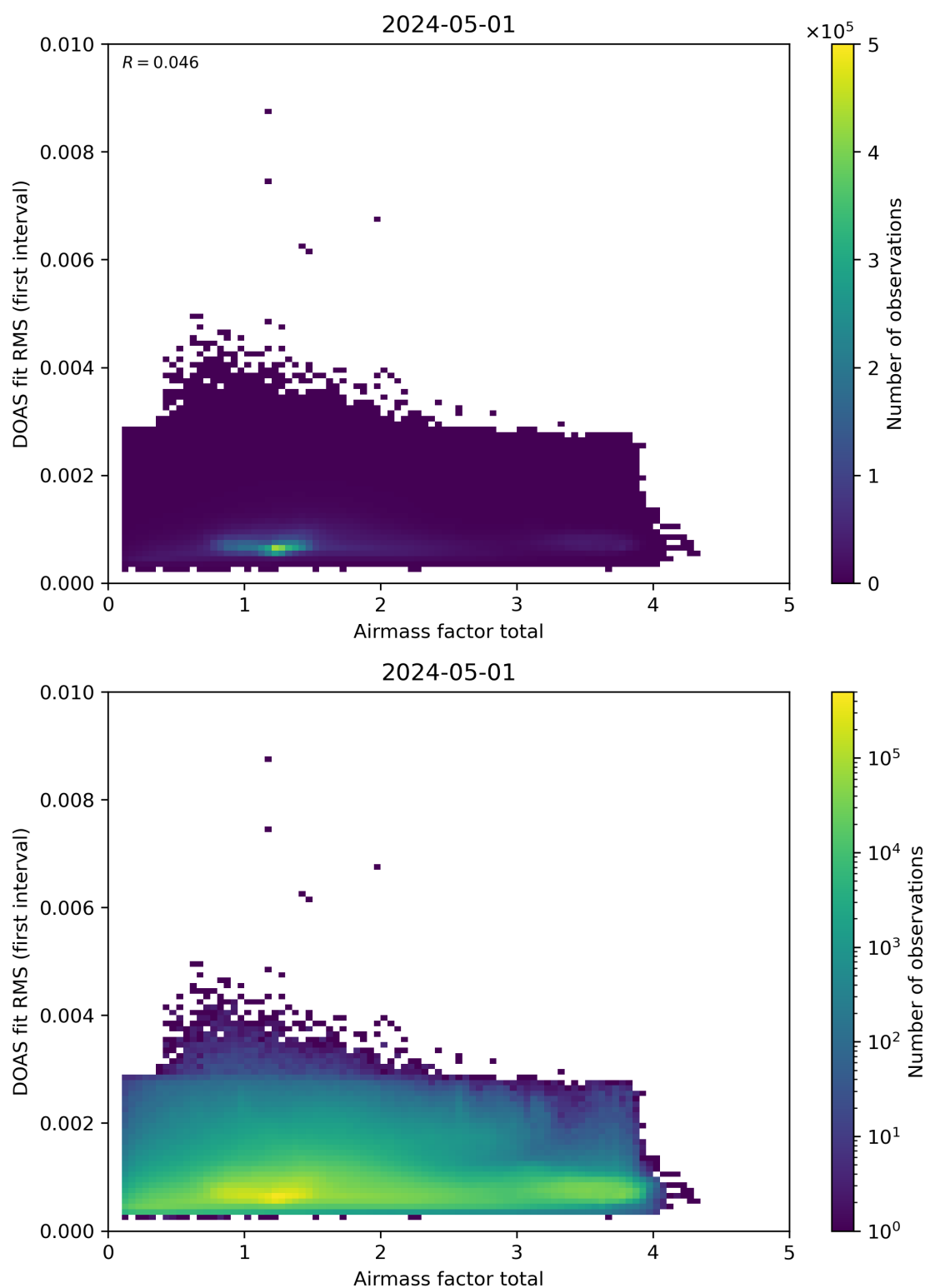
Figure 97: Scatter density plot of “Airmass factor total” against “DOAS fit RMS (first interval)” for 2024-04-30 to 2024-05-02.
