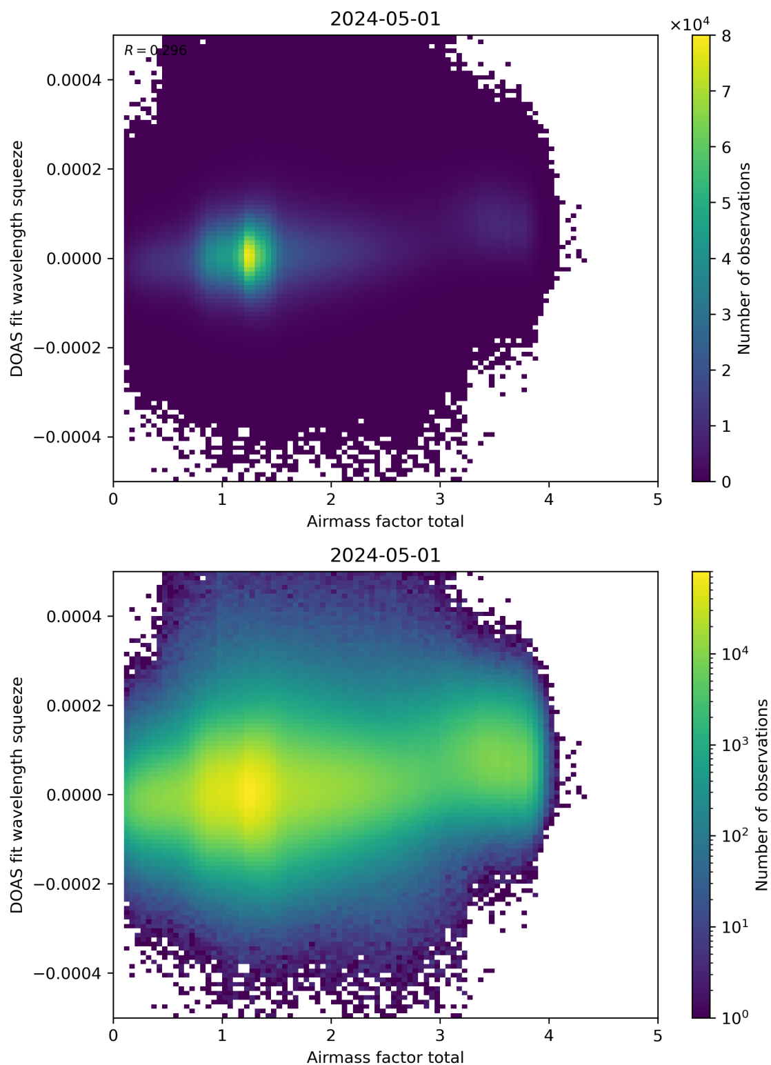
Figure 99: Scatter density plot of “Airmass factor total” against “DOAS fit wavelength squeeze” for 2024-04-30 to 2024-05-02.
