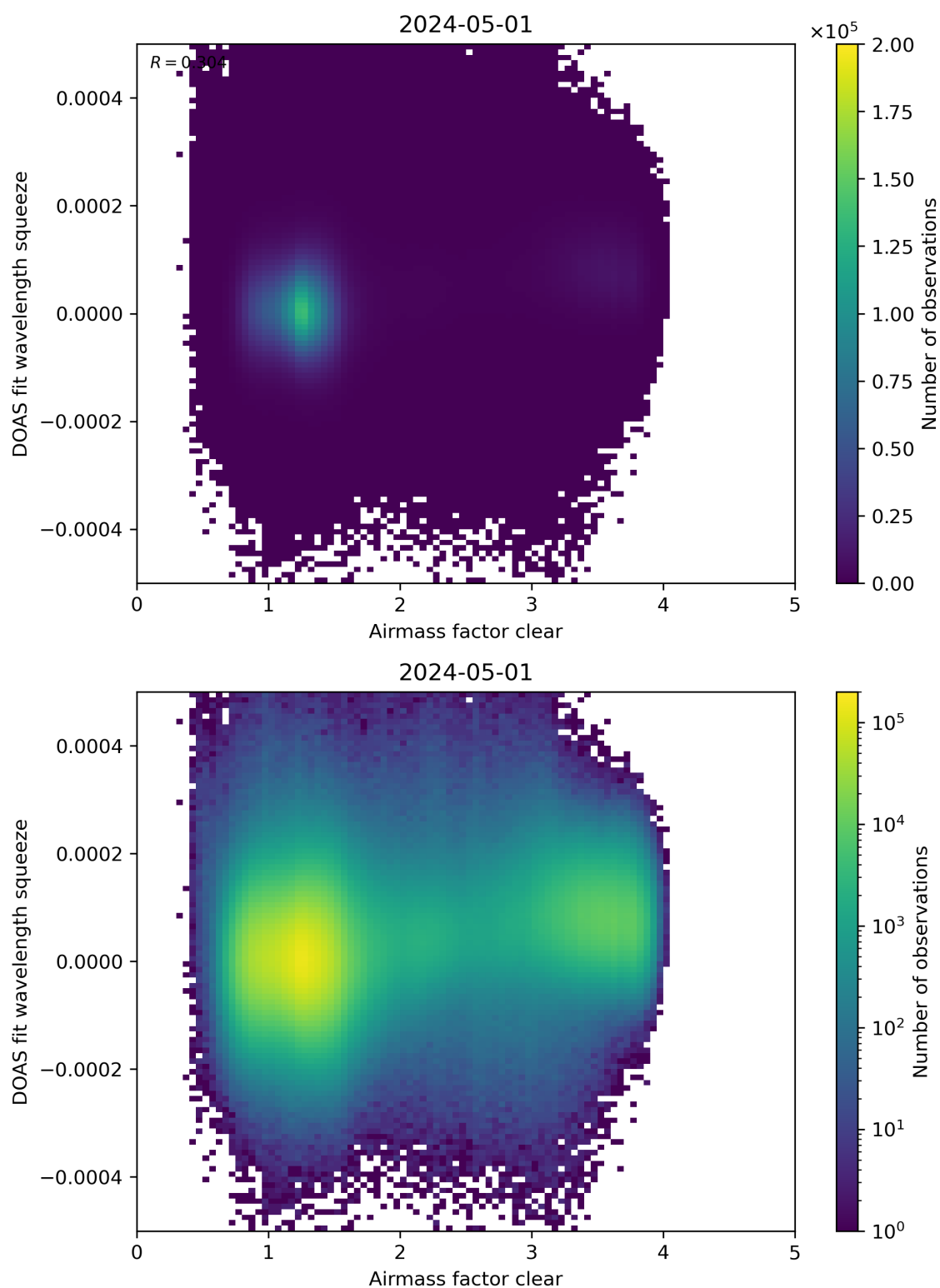
Figure 73: Scatter density plot of “Airmass factor clear” against “DOAS fit wavelength squeeze” for 2024-04-30 to 2024-05-02.
