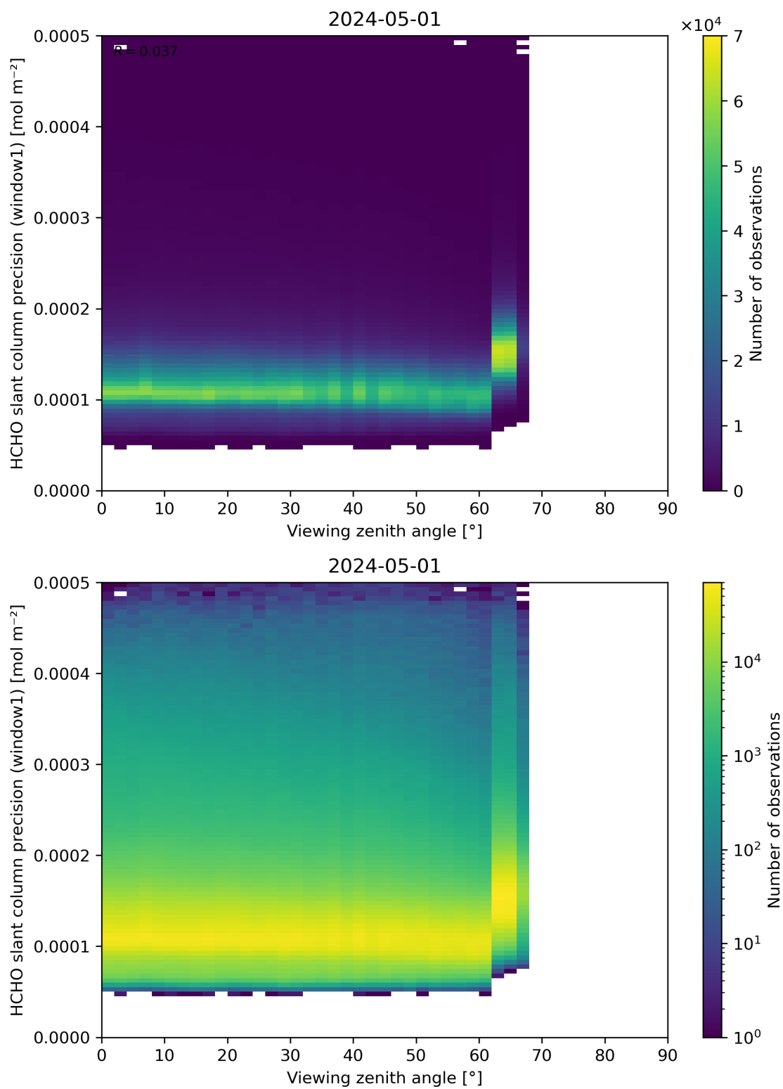
Figure 189: Scatter density plot of “Viewing zenith angle” against “HCHO slant column precision (window1)” for 2024-04-30 to 2024-05-02.
