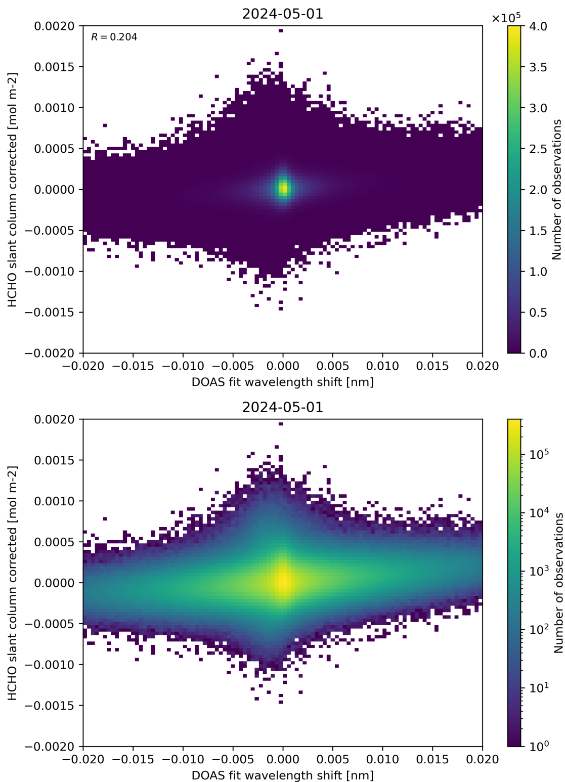
Figure 66: Scatter density plot of “DOAS fit wavelength shift” against “HCHO slant column corrected” for 2024-04-30 to 2024-05-02.
