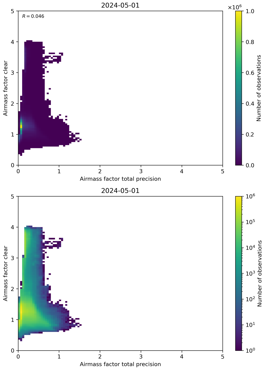
Figure 108: Scatter density plot of “Airmass factor total precision” against “Airmass factor clear” for 2024-04-30 to 2024-05-02.
