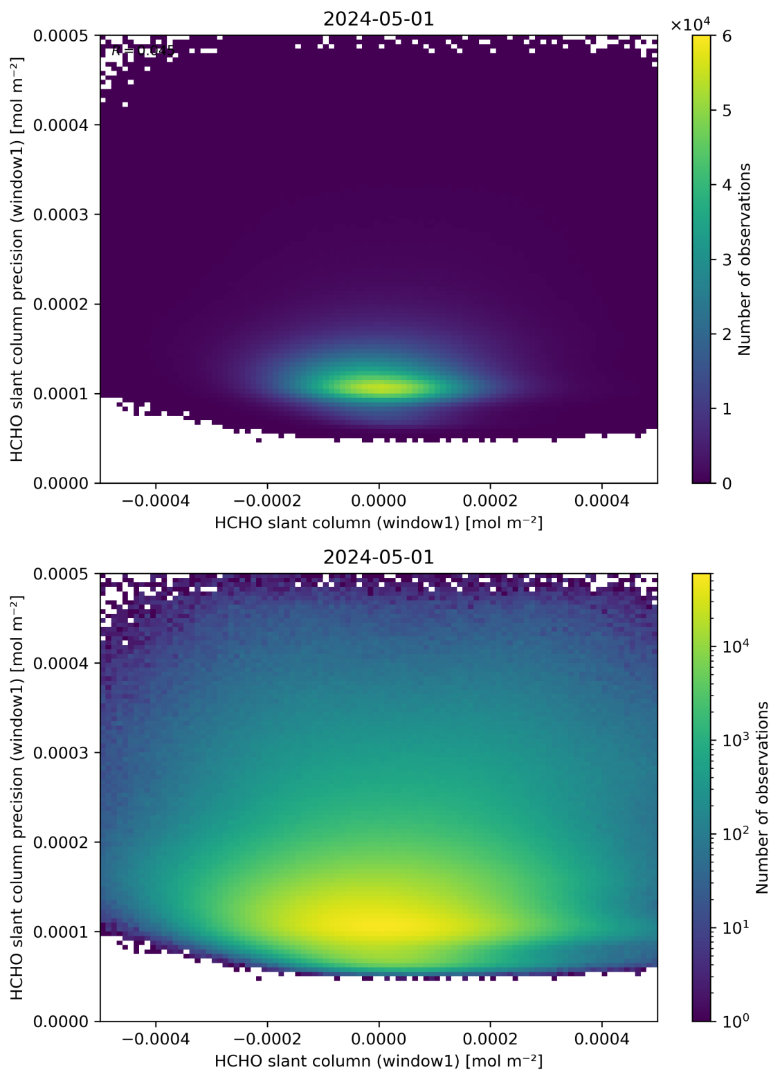
Figure 84: Scatter density plot of “HCHO slant column (window1)” against “HCHO slant column precision (window1)” for 2024-04-30 to 2024-05-02.
