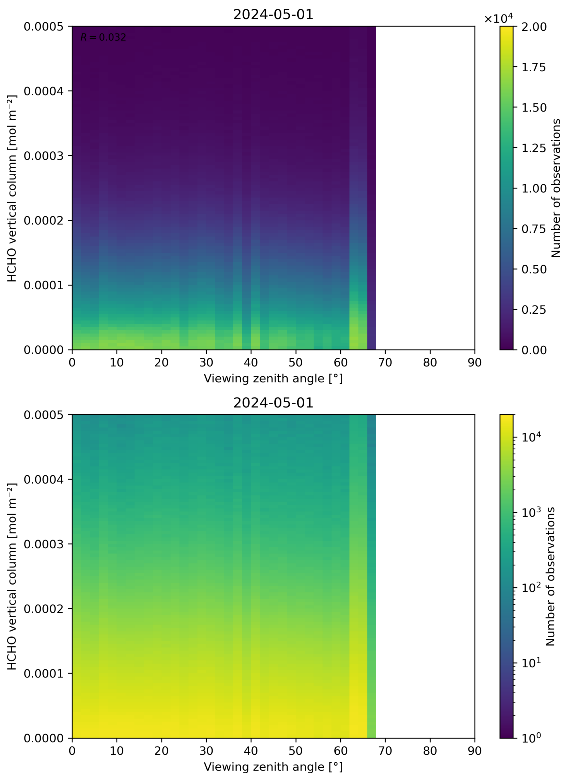
Figure 192: Scatter density plot of “Viewing zenith angle” against “HCHO vertical column” for 2024-04-30 to 2024-05-02.
