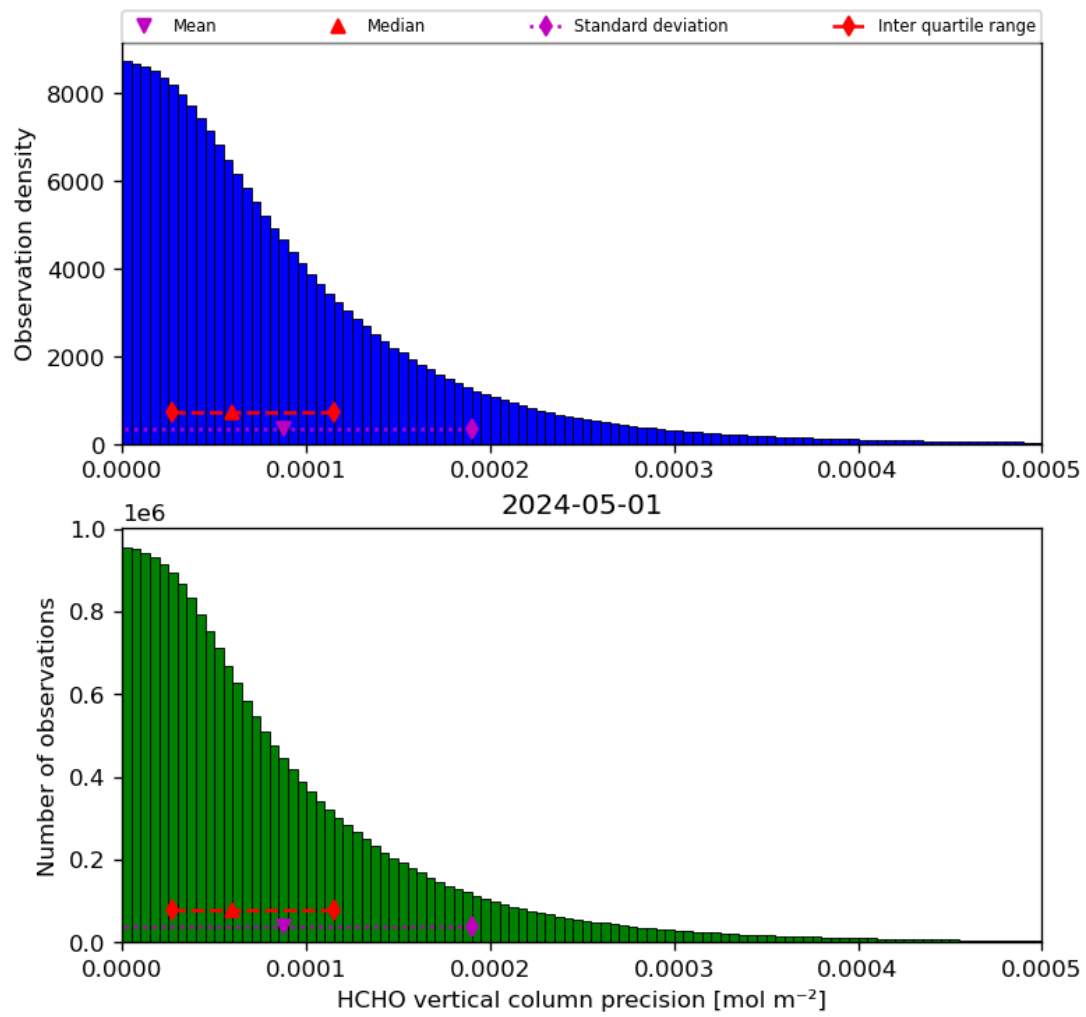
Figure 36: Histogram of “HCHO vertical column precision” for 2024-04-30 to 2024-05-02
