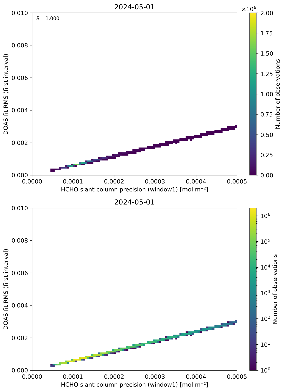
Figure 88: Scatter density plot of “HCHO slant column precision (window1)” against “DOAS fit RMS (first interval)” for 2024-04-30 to 2024-05-02.
