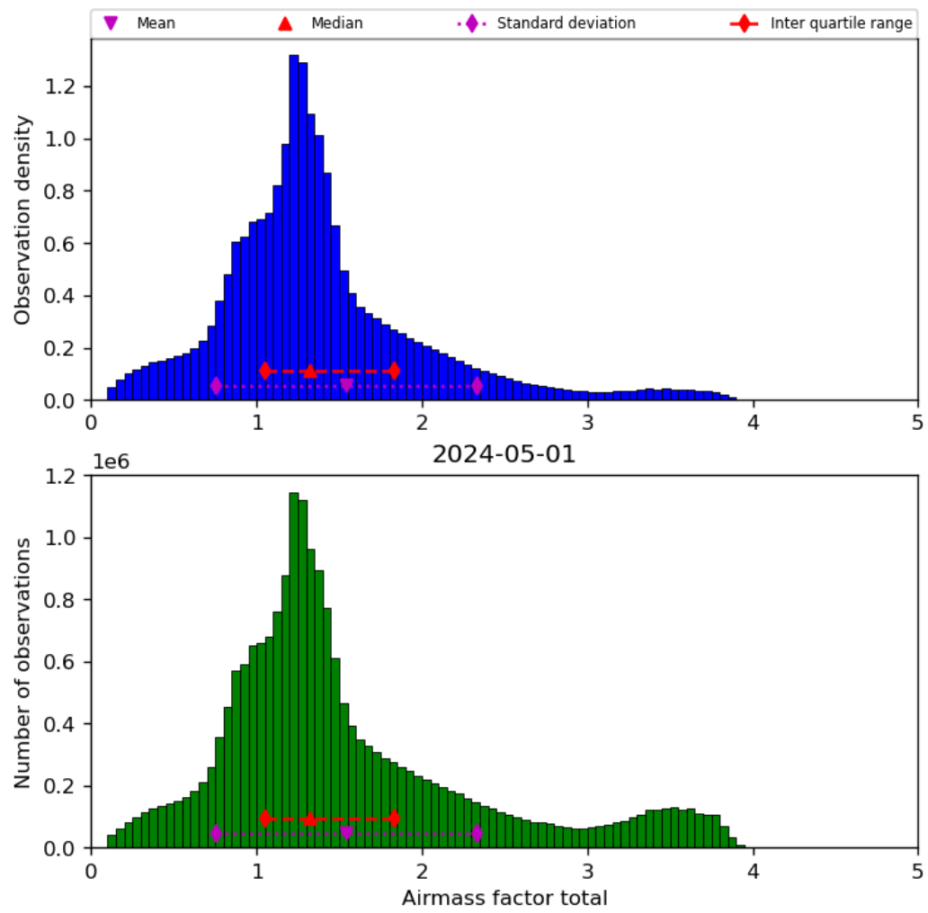
Figure 40: Histogram of “Airmass factor total” for 2024-04-30 to 2024-05-02
