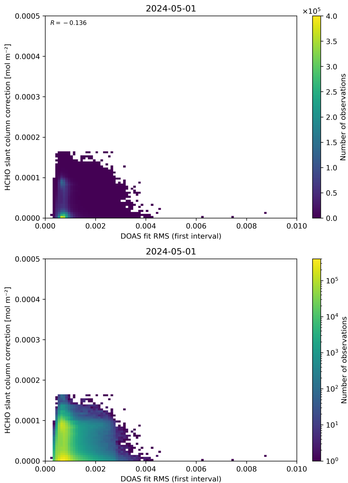
Figure 63: Scatter density plot of “DOAS fit RMS (first interval)” against “HCHO slant column correction” for 2024-04-30 to 2024-05-02.
