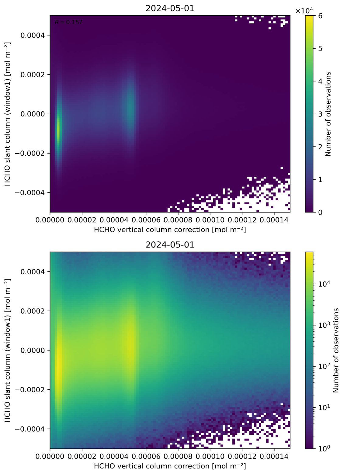
Figure 118: Scatter density plot of “HCHO vertical column correction” against “HCHO slant column (window1)” for 2024-04-30 to 2024-05-02.
