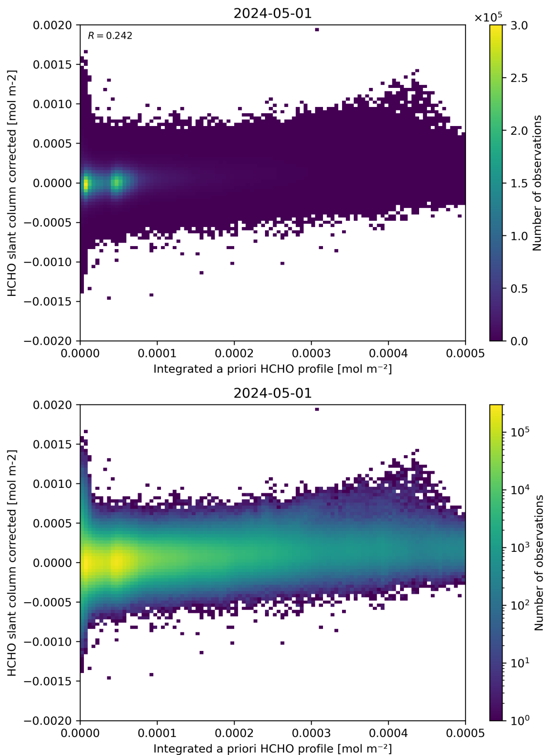
Figure 151: Scatter density plot of “Integrated a priori HCHO profile” against “HCHO slant column corrected” for 2024-04-30 to 2024-05-02.
