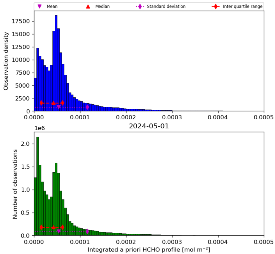
Figure 43: Histogram of “Integrated a priori HCHO profile” for 2024-04-30 to 2024-05-02
