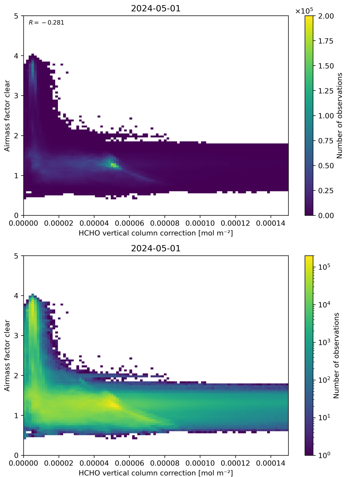
Figure 115: Scatter density plot of “HCHO vertical column correction” against “Airmass factor clear” for 2024-04-30 to 2024-05-02.
