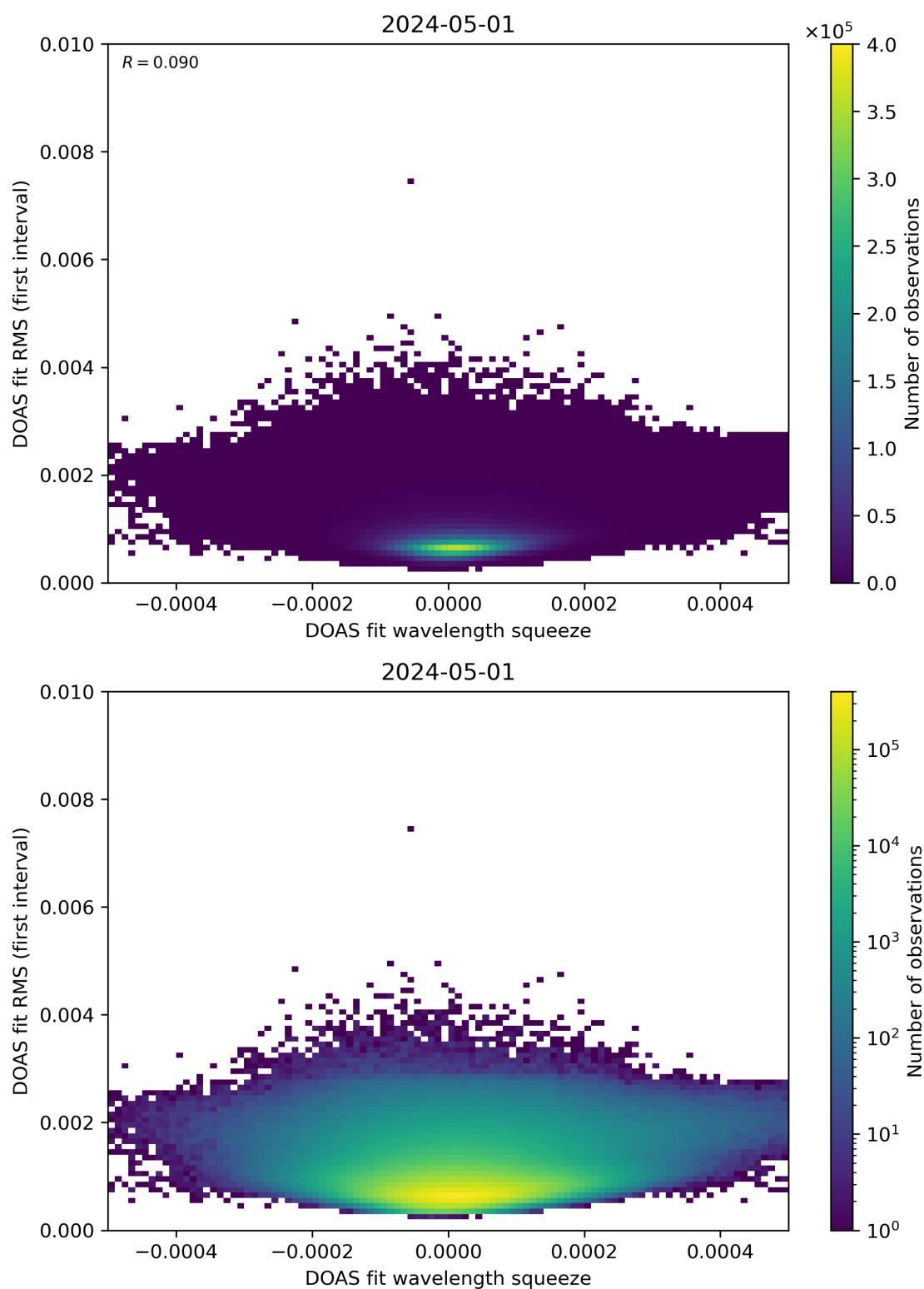
Figure 68: Scatter density plot of “DOAS fit wavelength squeeze” against “DOAS fit RMS (first interval)” for 2024-04-30 to 2024-05-02.
