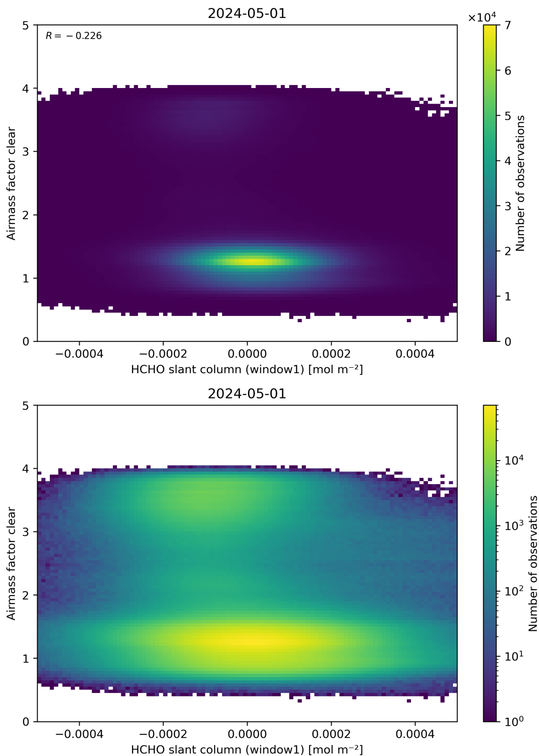
Figure 81: Scatter density plot of “HCHO slant column (window1)” against “Airmass factor clear” for 2024-04-30 to 2024-05-02.
