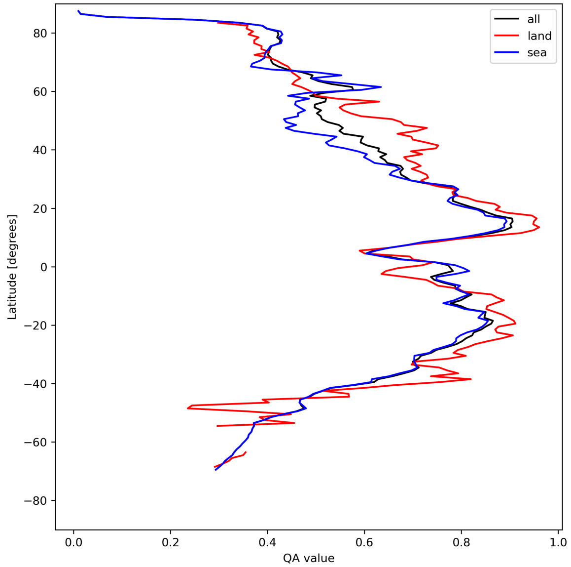
Figure 20: Zonal average of “QA value” for 2024-04-30 to 2024-05-02.
