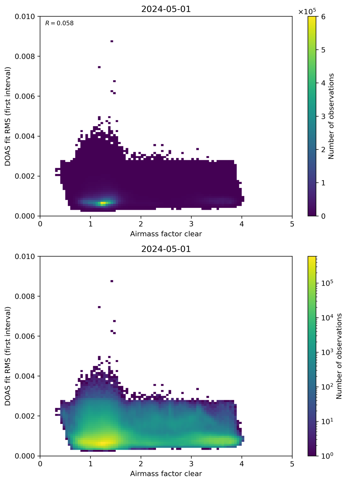
Figure 71: Scatter density plot of “Airmass factor clear” against “DOAS fit RMS (first interval)” for 2024-04-30 to 2024-05-02.
