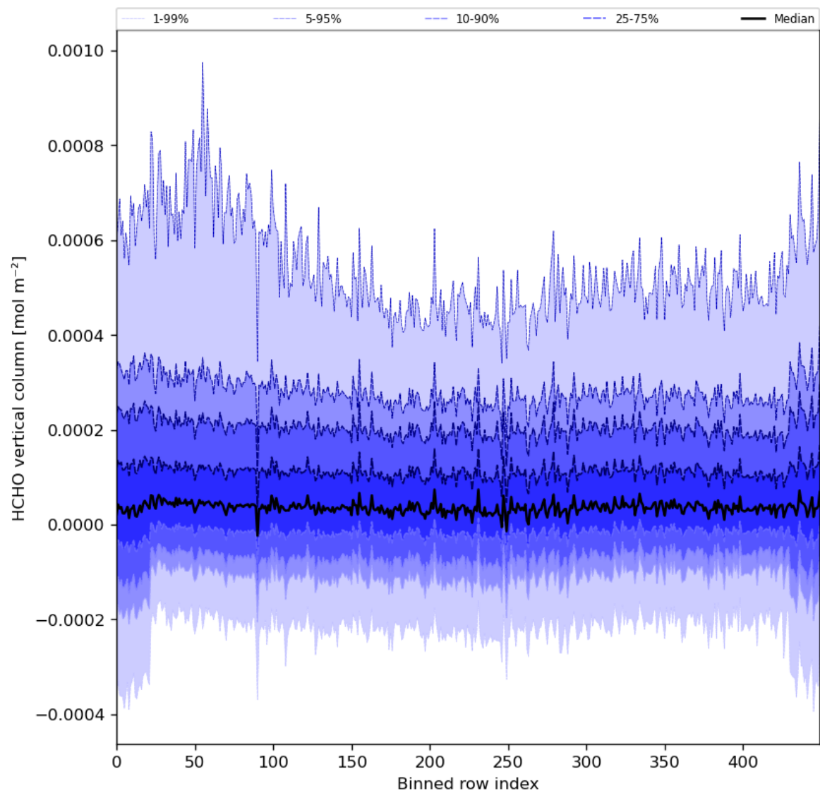
Figure 49: Along track statistics of “HCHO vertical column” for 2024-04-30 to 2024-05-02
