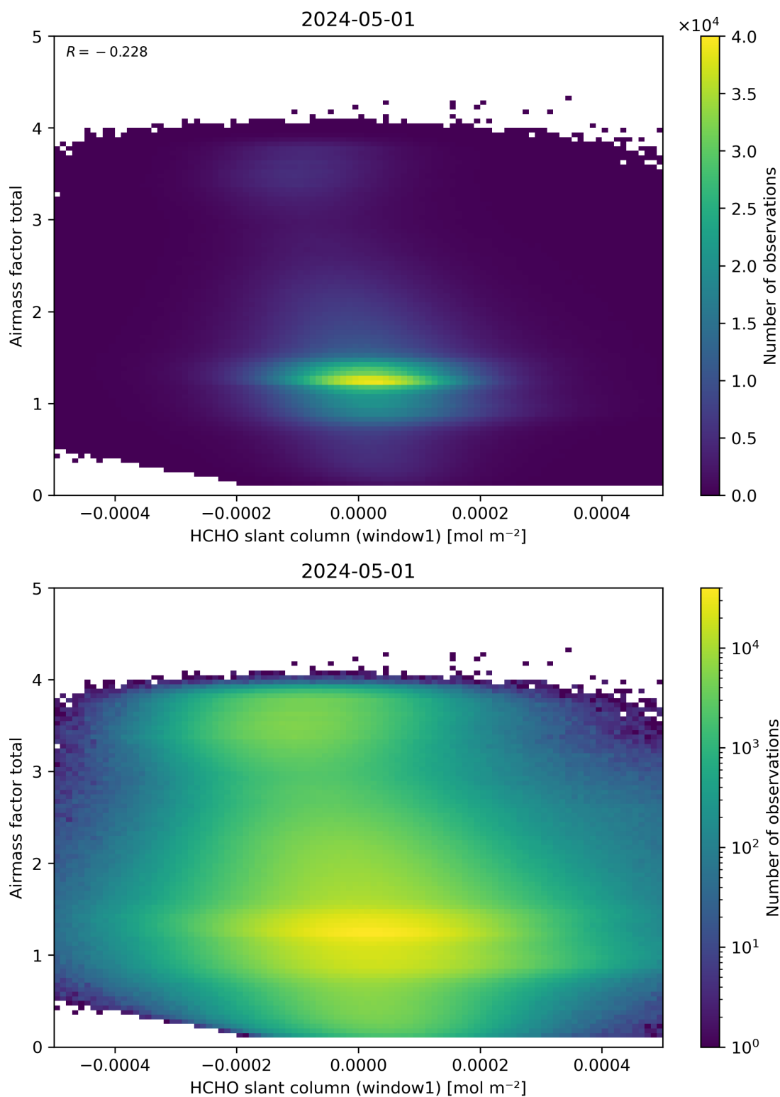
Figure 85: Scatter density plot of “HCHO slant column (window1)” against “Airmass factor total” for 2024-04-30 to 2024-05-02.
