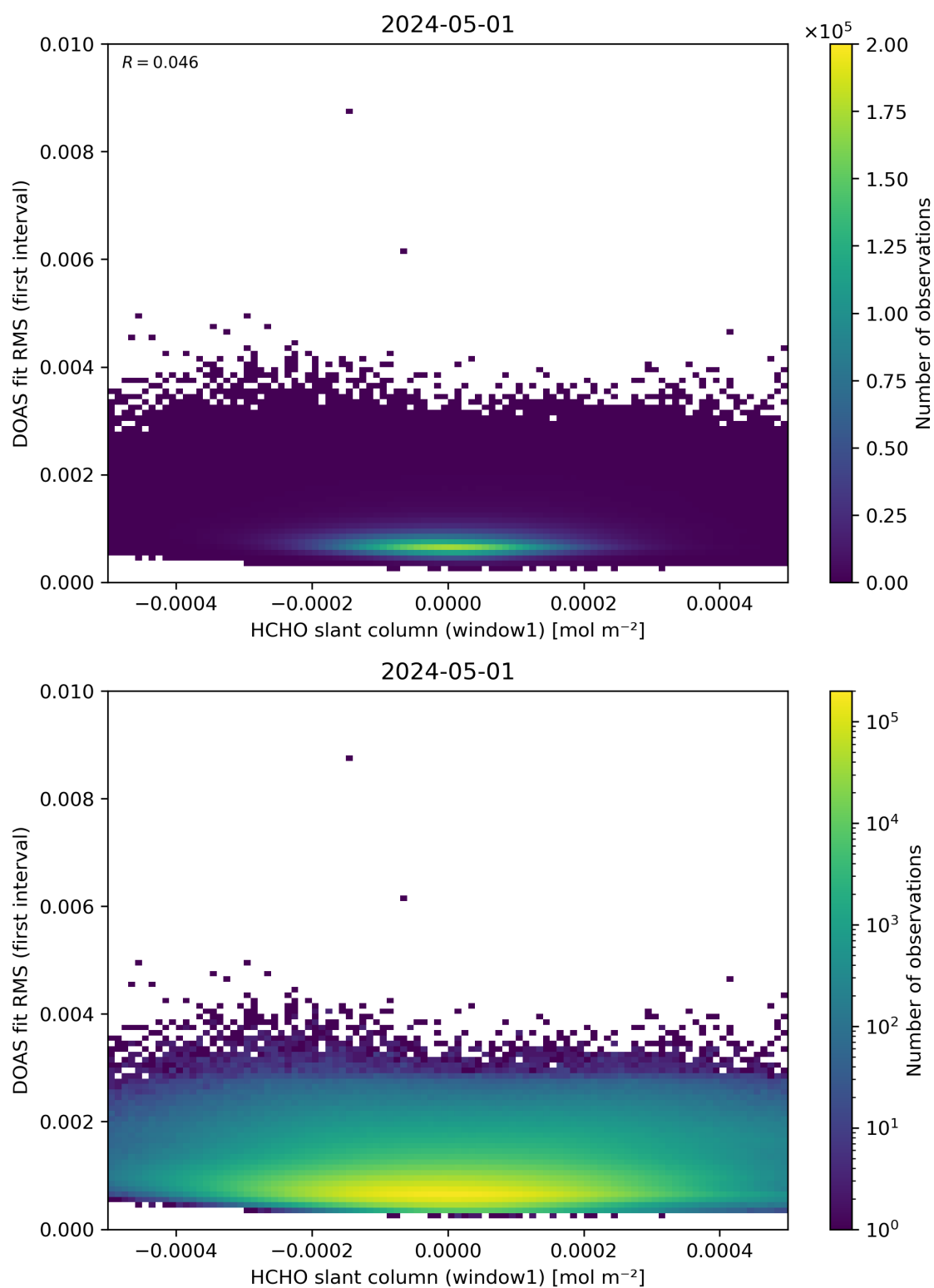
Figure 78: Scatter density plot of “HCHO slant column (window1)” against “DOAS fit RMS (first interval)” for 2024-04-30 to 2024-05-02.
