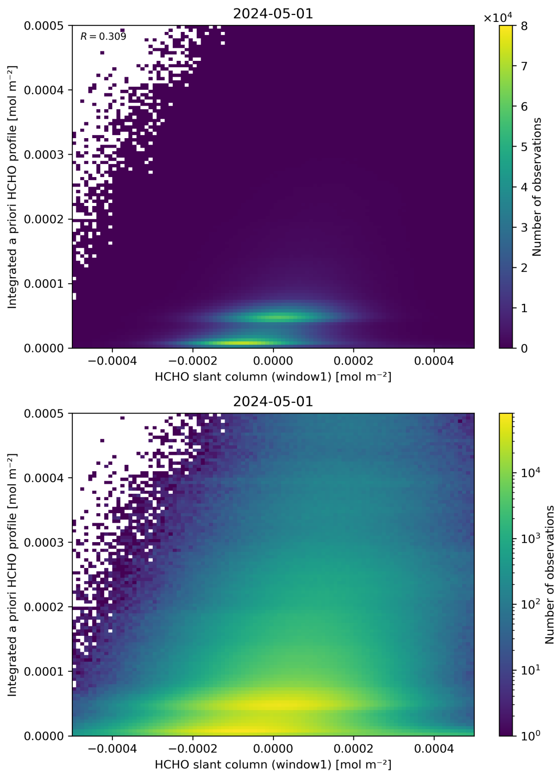
Figure 87: Scatter density plot of “HCHO slant column (window1)” against “Integrated a priori HCHO profile” for 2024-04-30 to 2024-05-02.
