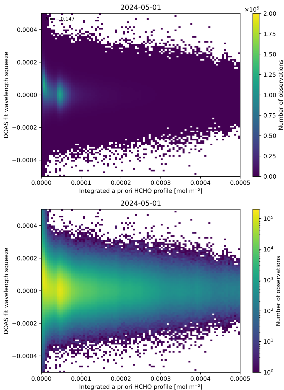
Figure 150: Scatter density plot of “Integrated a priori HCHO profile” against “DOAS fit wavelength squeeze” for 2024-04-30 to 2024-05-02.
