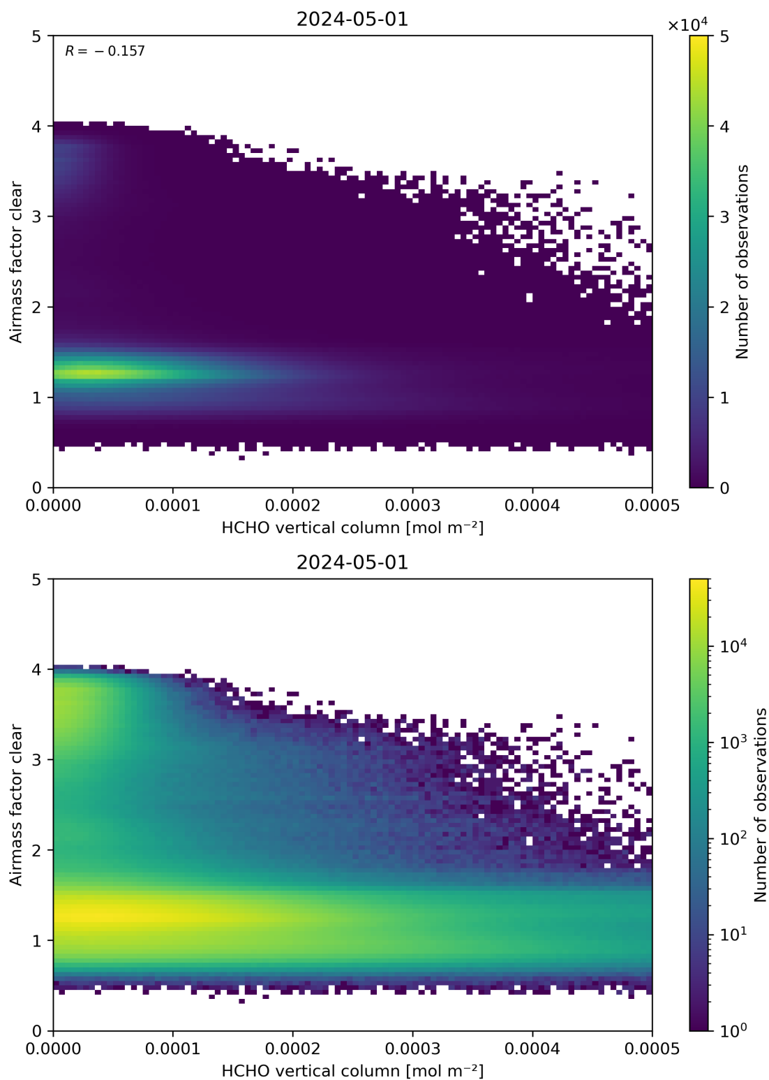
Figure 126: Scatter density plot of “HCHO vertical column” against “Airmass factor clear” for 2024-04-30 to 2024-05-02.
