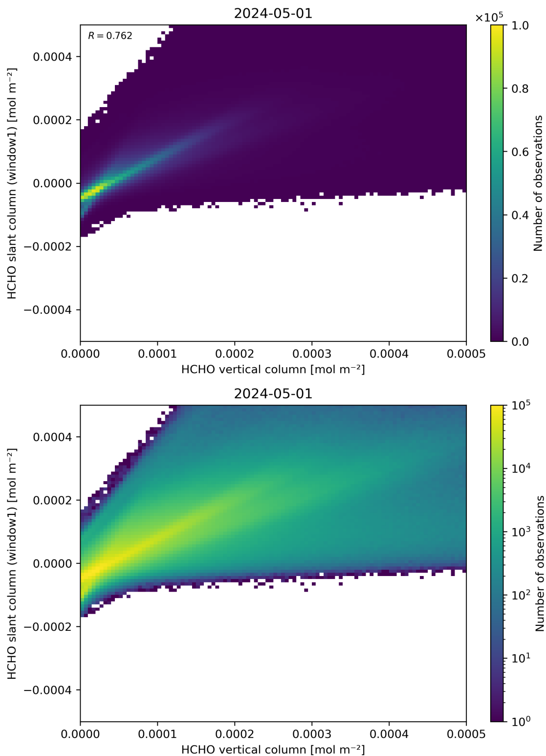
Figure 129: Scatter density plot of “HCHO vertical column” against “HCHO slant column (window1)” for 2024-04-30 to 2024-05-02.
