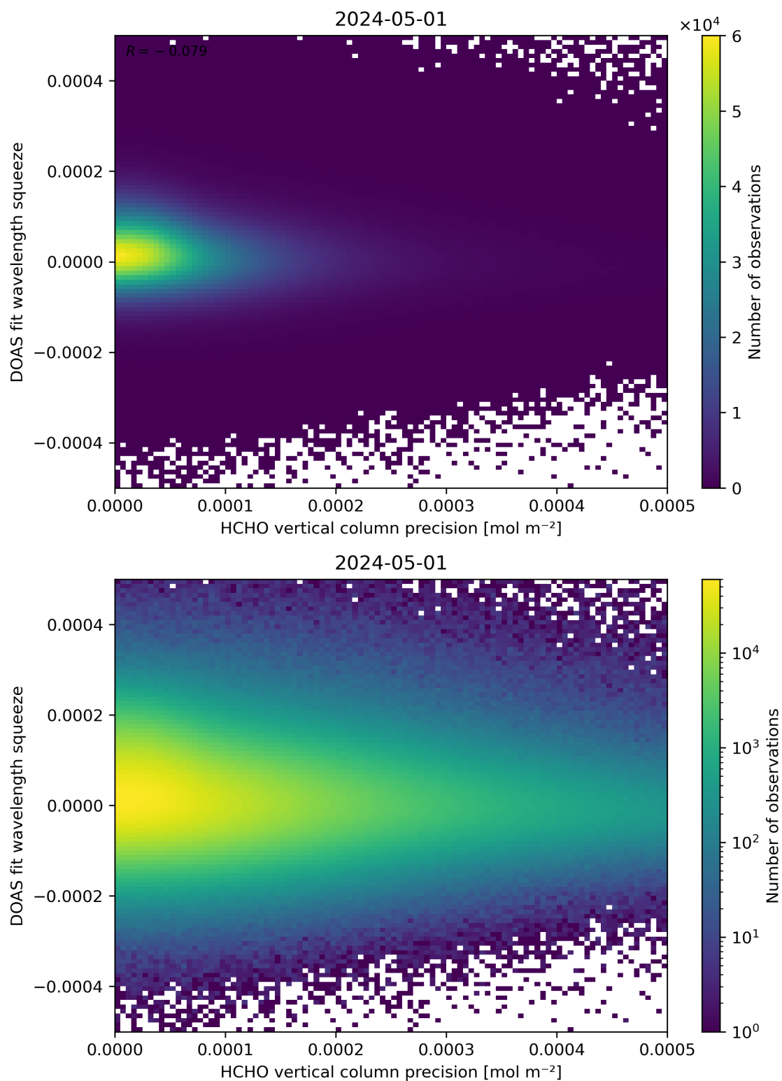
Figure 138: Scatter density plot of “HCHO vertical column precision” against “DOAS fit wavelength squeeze” for 2024-04-30 to 2024-05-02.
