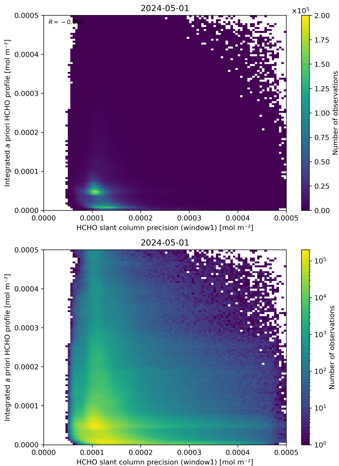
Figure 96: Scatter density plot of “HCHO slant column precision (window1)” against “Integrated a priori HCHO profile” for 2024-04-30 to 2024-05-02.
