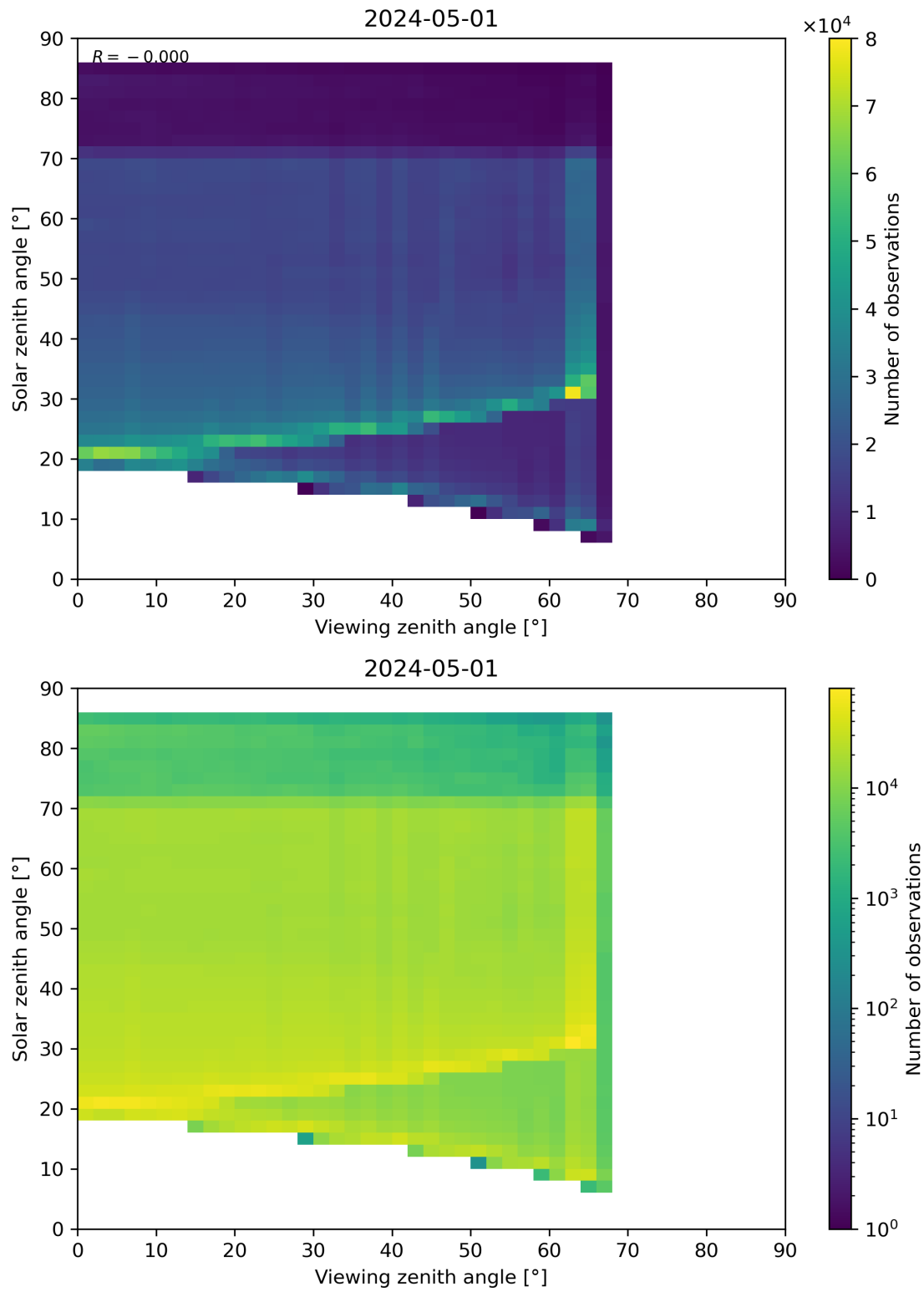
Figure 197: Scatter density plot of “Viewing zenith angle” against “Solar zenith angle” for 2024-04-30 to 2024-05-02.
