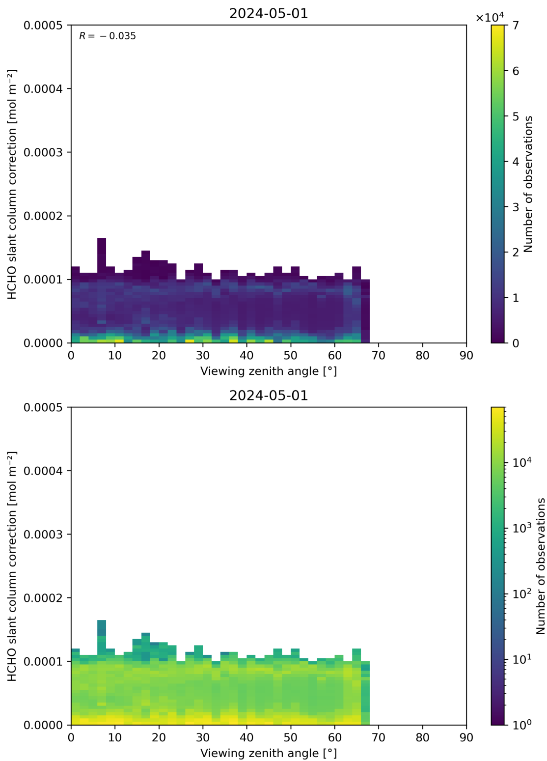
Figure 187: Scatter density plot of “Viewing zenith angle” against “HCHO slant column correction” for 2024-04-30 to 2024-05-02.
