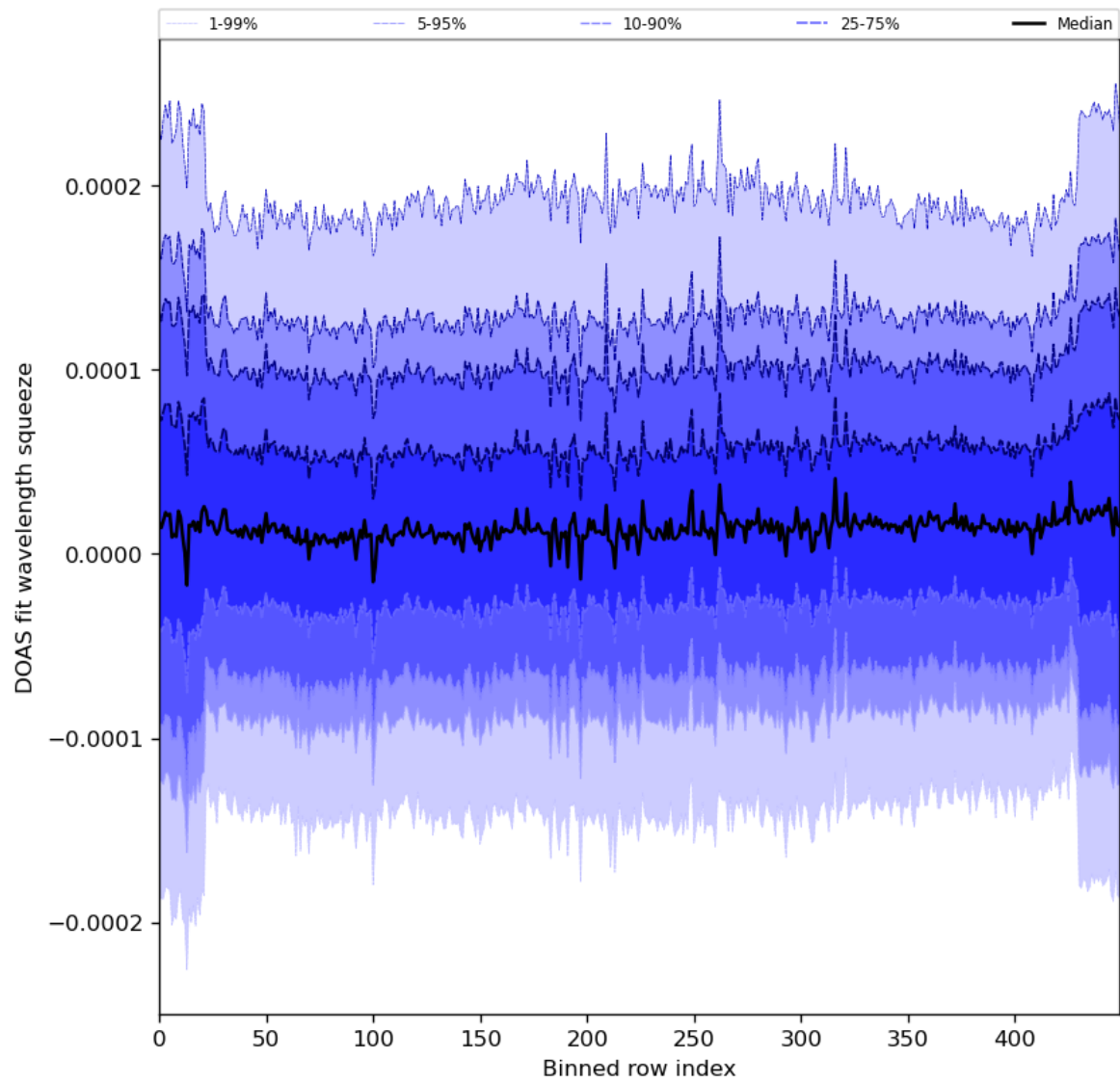
Figure 59: Along track statistics of “DOAS fit wavelength squeeze” for 2024-04-30 to 2024-05-02
