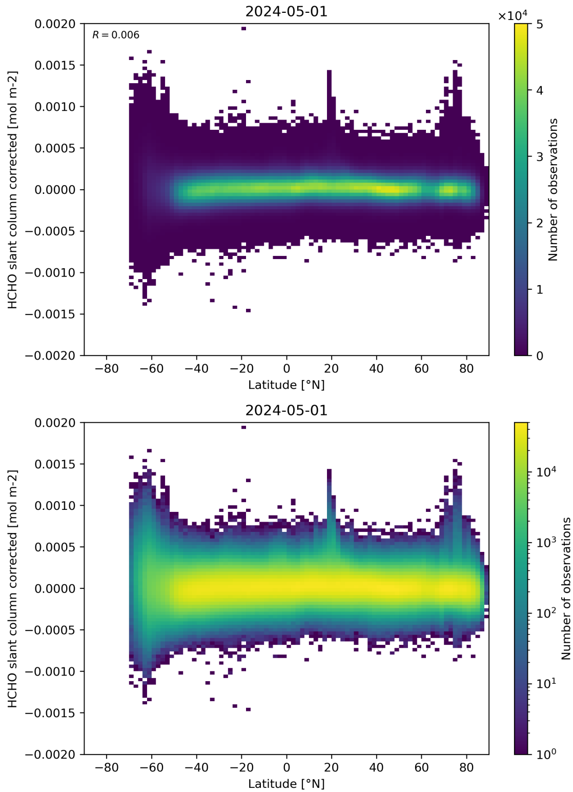
Figure 157: Scatter density plot of “Latitude” against “HCHO slant column corrected” for 2024-04-30 to 2024-05-02.
