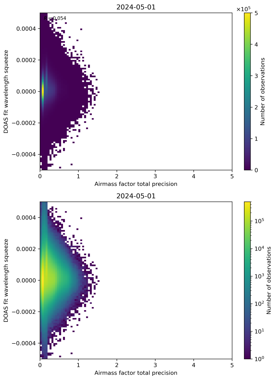
Figure 107: Scatter density plot of “Airmass factor total precision” against “DOAS fit wavelength squeeze” for 2024-04-30 to 2024-05-02.
