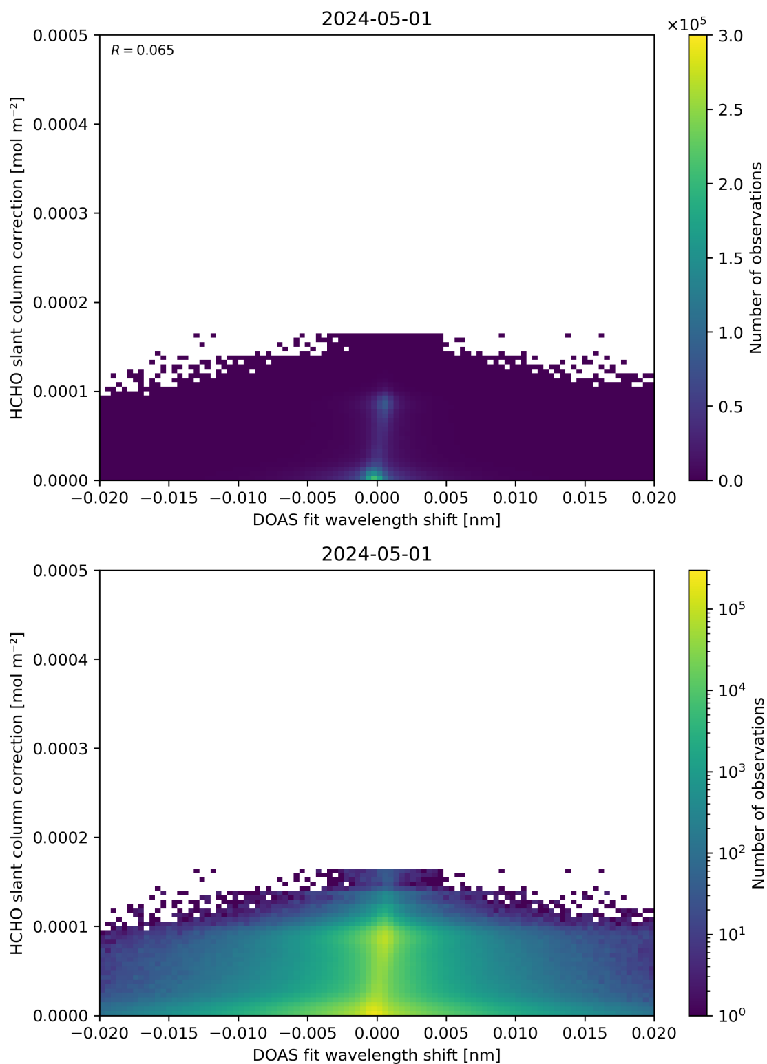
Figure 67: Scatter density plot of “DOAS fit wavelength shift” against “HCHO slant column correction” for 2024-04-30 to 2024-05-02.
