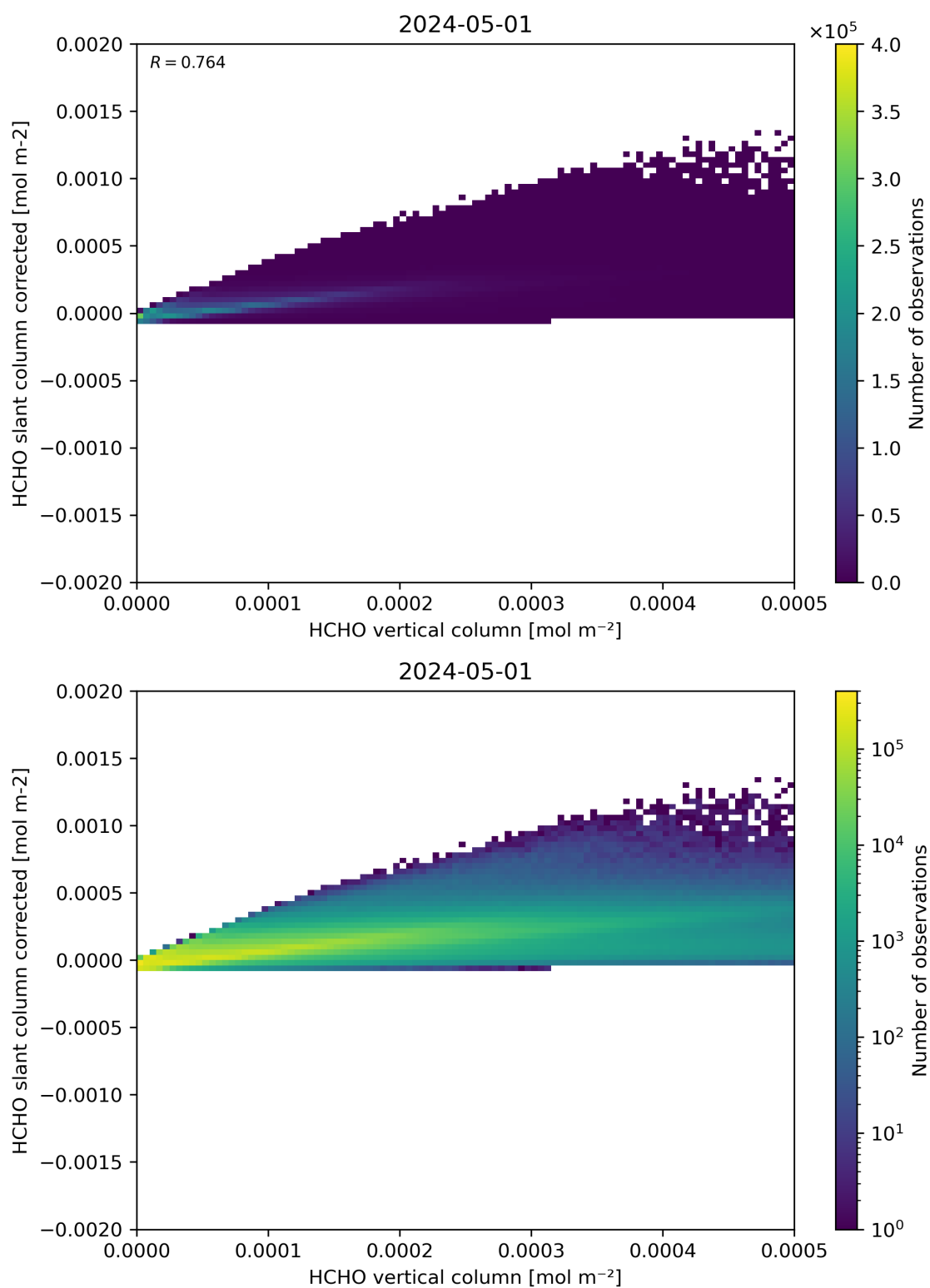
Figure 127: Scatter density plot of “HCHO vertical column” against “HCHO slant column corrected” for 2024-04-30 to 2024-05-02.
