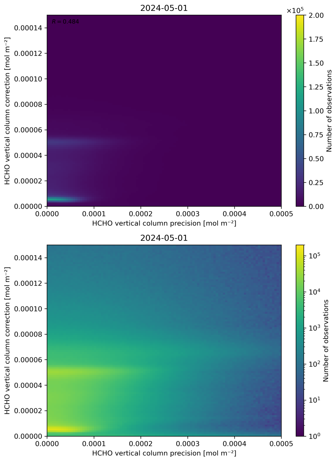
Figure 146: Scatter density plot of “HCHO vertical column precision” against “HCHO vertical column correction” for 2024-04-30 to 2024-05-02.
