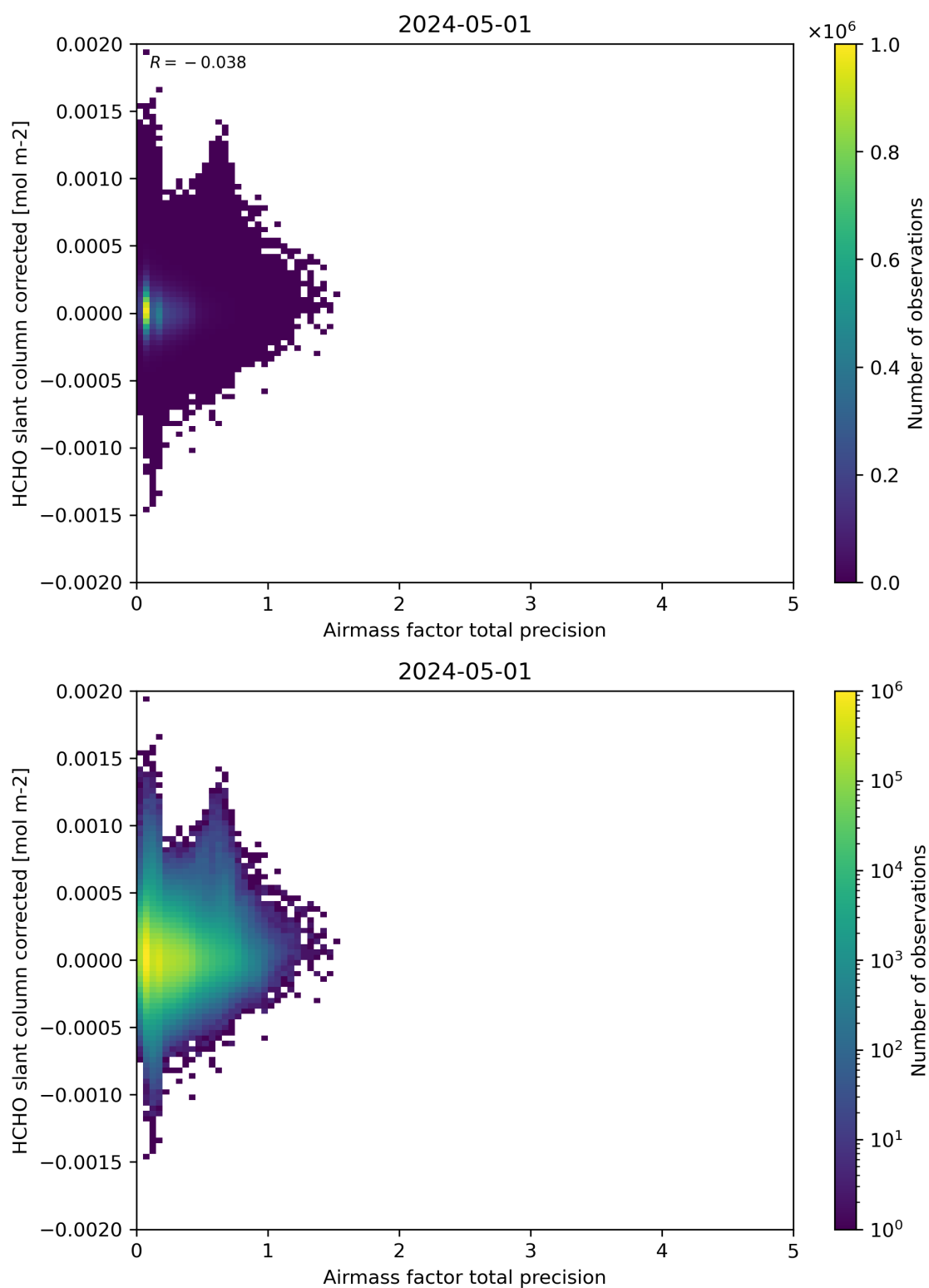
Figure 109: Scatter density plot of “Airmass factor total precision” against “HCHO slant column corrected” for 2024-04-30 to 2024-05-02.
