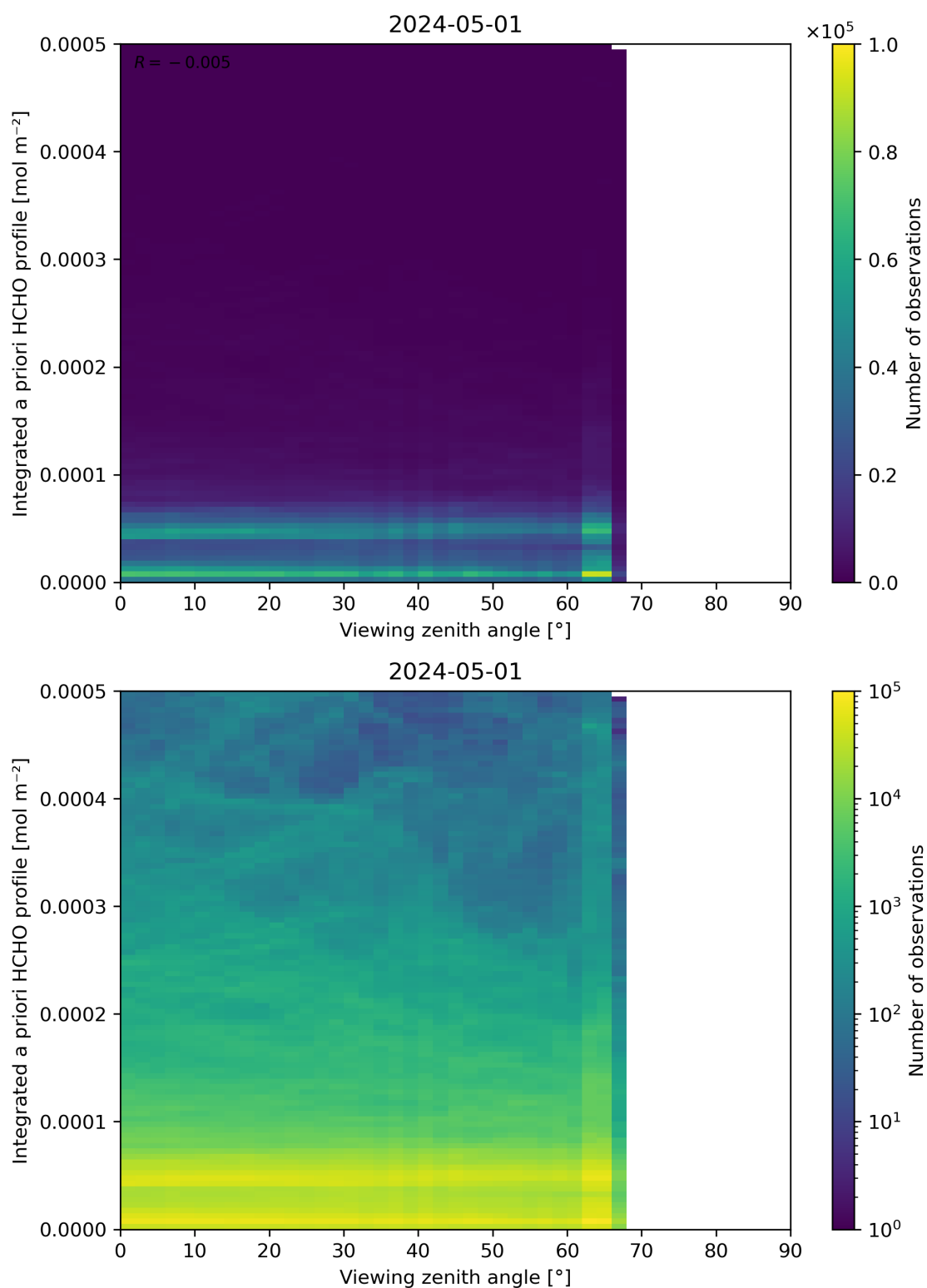
Figure 195: Scatter density plot of “Viewing zenith angle” against “Integrated a priori HCHO profile” for 2024-04-30 to 2024-05-02.
