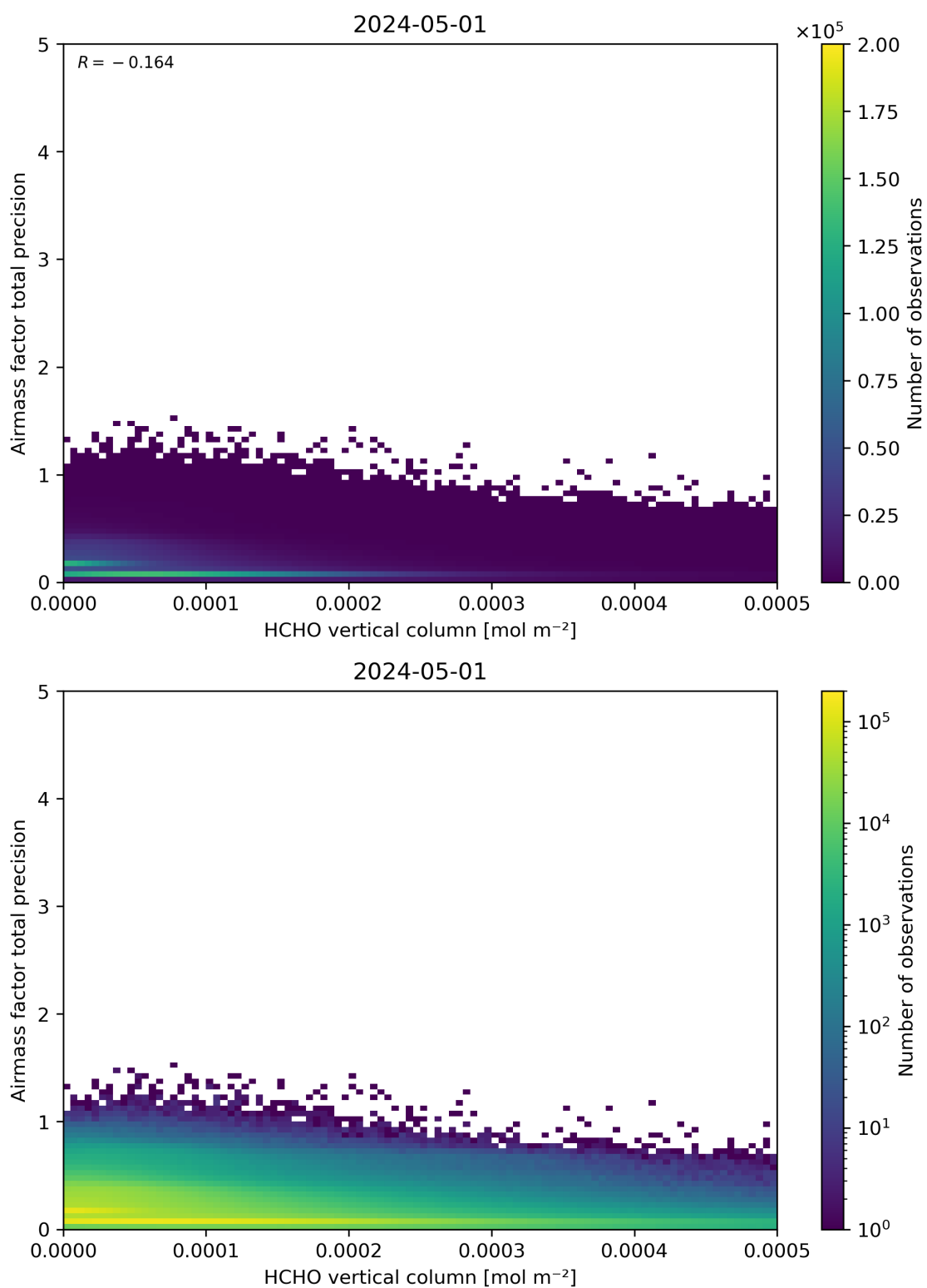
Figure 132: Scatter density plot of “HCHO vertical column” against “Airmass factor total precision” for 2024-04-30 to 2024-05-02.
