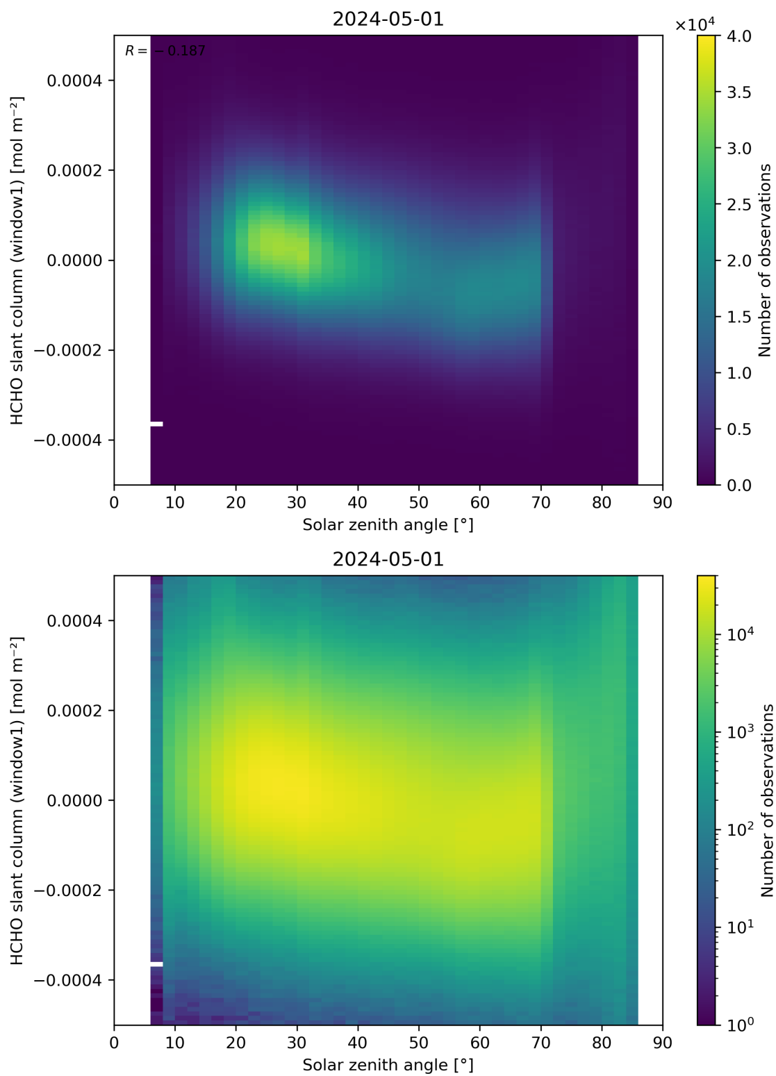
Figure 173: Scatter density plot of “Solar zenith angle” against “HCHO slant column (window1)” for 2024-04-30 to 2024-05-02.
