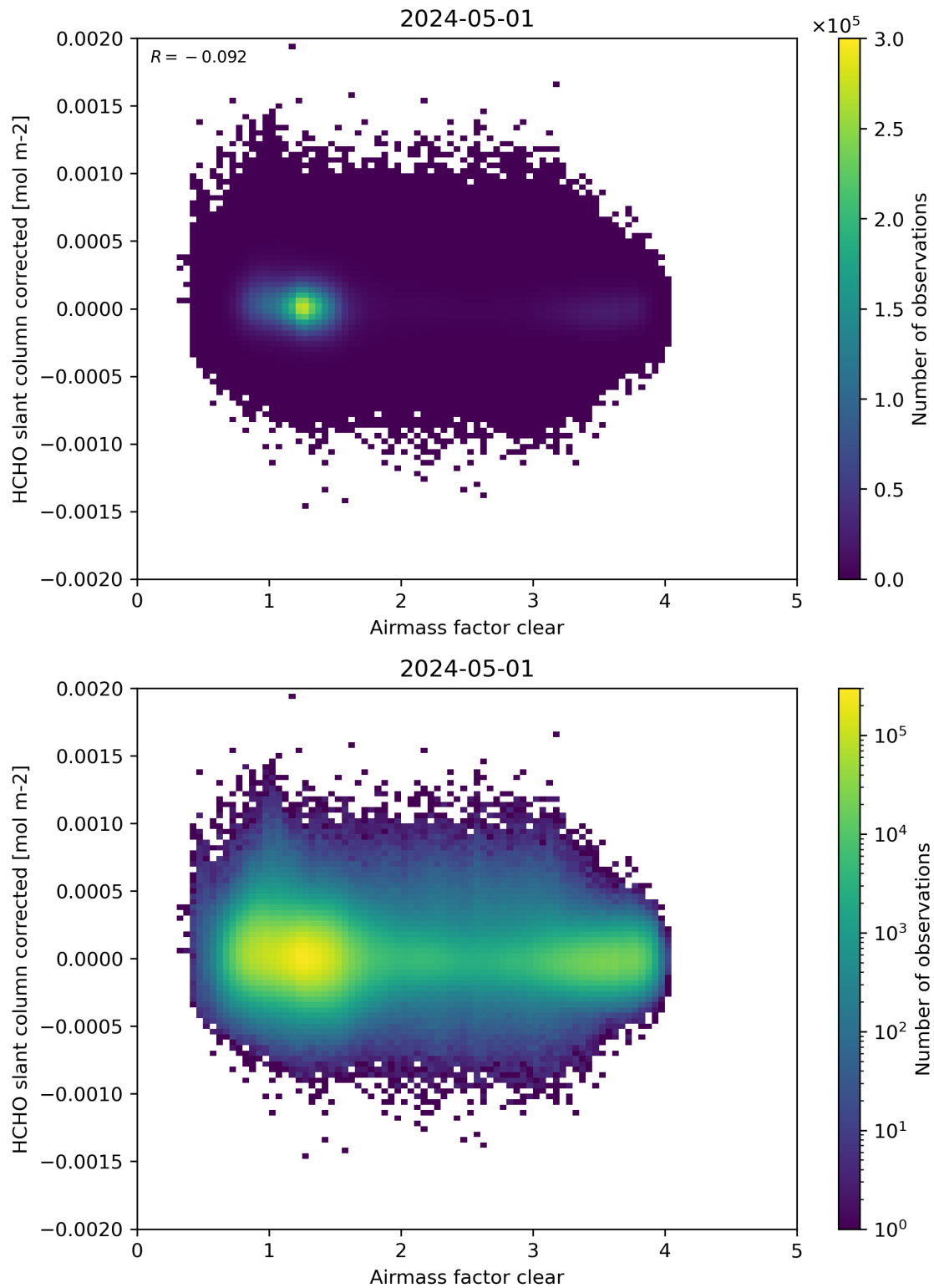
Figure 74: Scatter density plot of “Airmass factor clear” against “HCHO slant column corrected” for 2024-04-30 to 2024-05-02.
