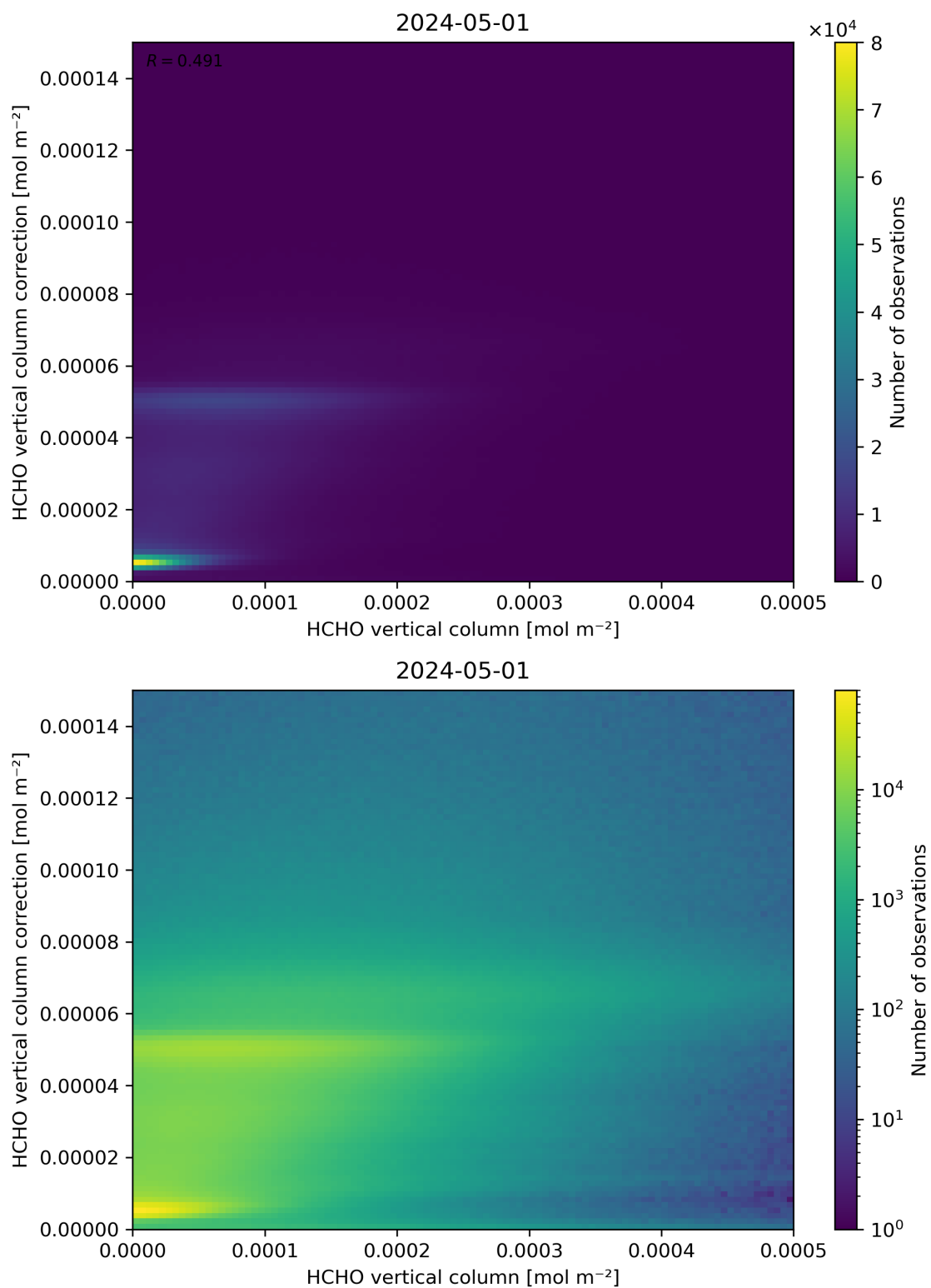
Figure 133: Scatter density plot of “HCHO vertical column” against “HCHO vertical column correction” for 2024-04-30 to 2024-05-02.
