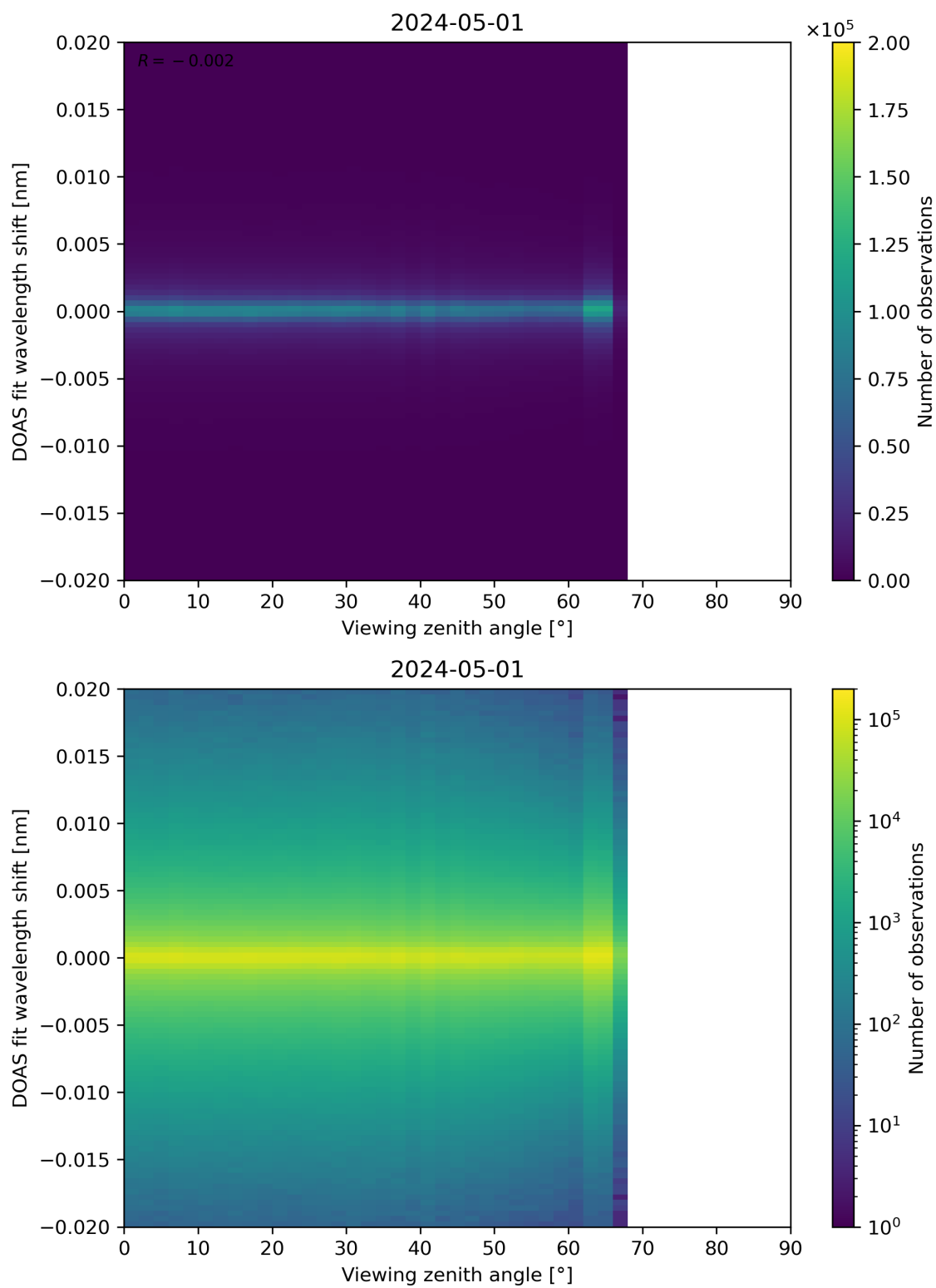
Figure 183: Scatter density plot of “Viewing zenith angle” against “DOAS fit wavelength shift” for 2024-04-30 to 2024-05-02.
