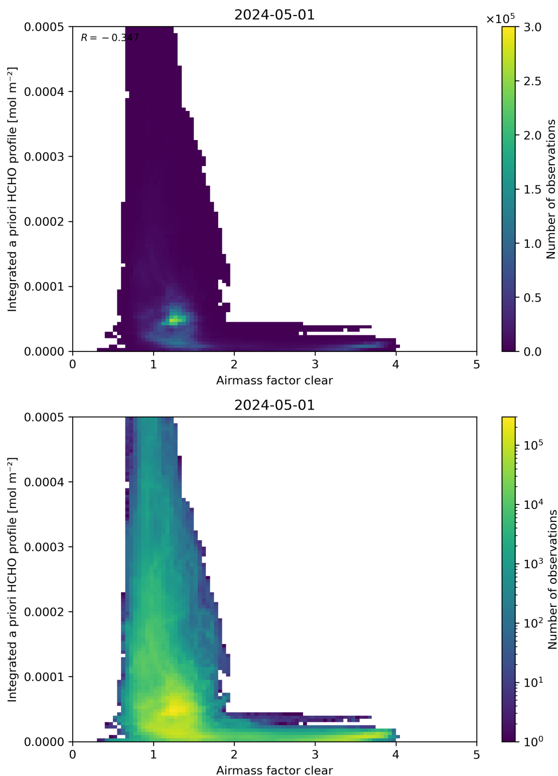
Figure 76: Scatter density plot of “Airmass factor clear” against “Integrated a priori HCHO profile” for 2024-04-30 to 2024-05-02.
