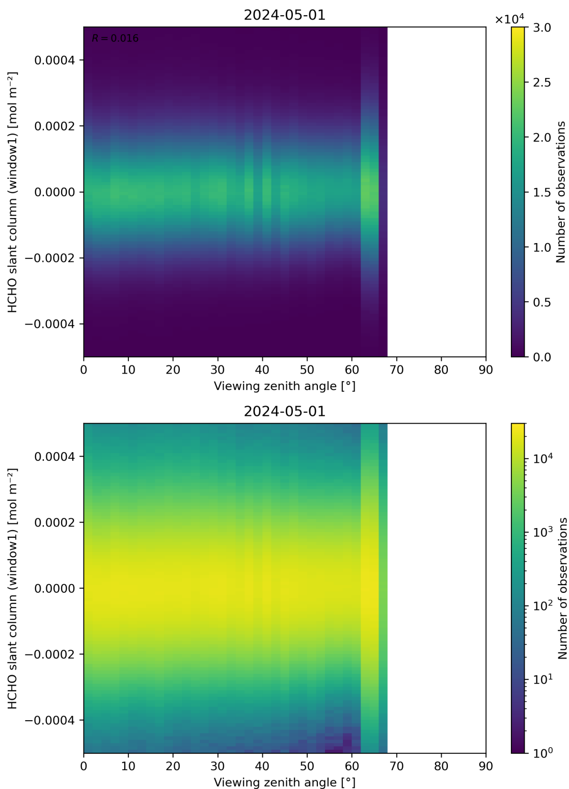
Figure 188: Scatter density plot of “Viewing zenith angle” against “HCHO slant column (window1)” for 2024-04-30 to 2024-05-02.
