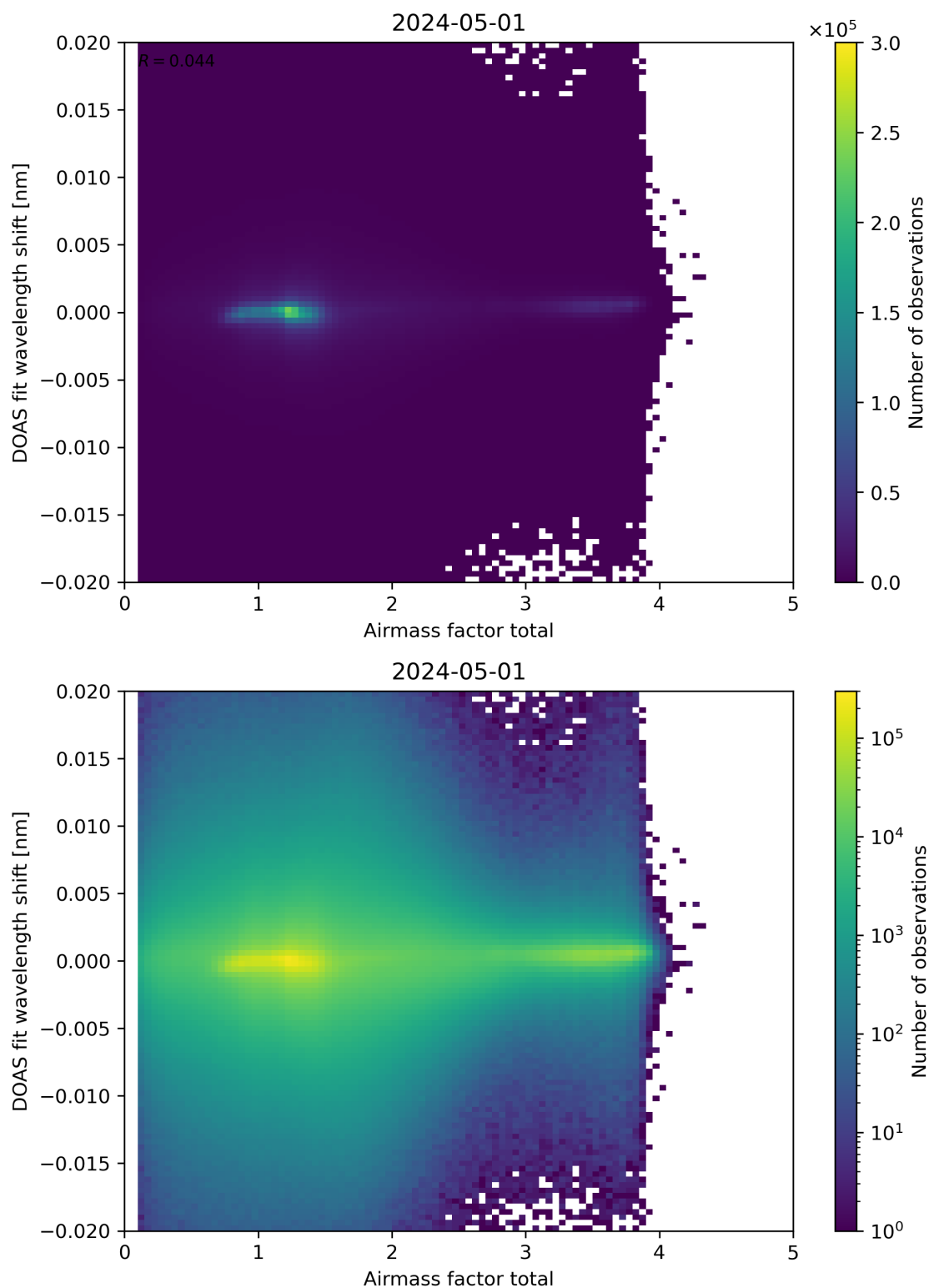
Figure 98: Scatter density plot of “Airmass factor total” against “DOAS fit wavelength shift” for 2024-04-30 to 2024-05-02.
