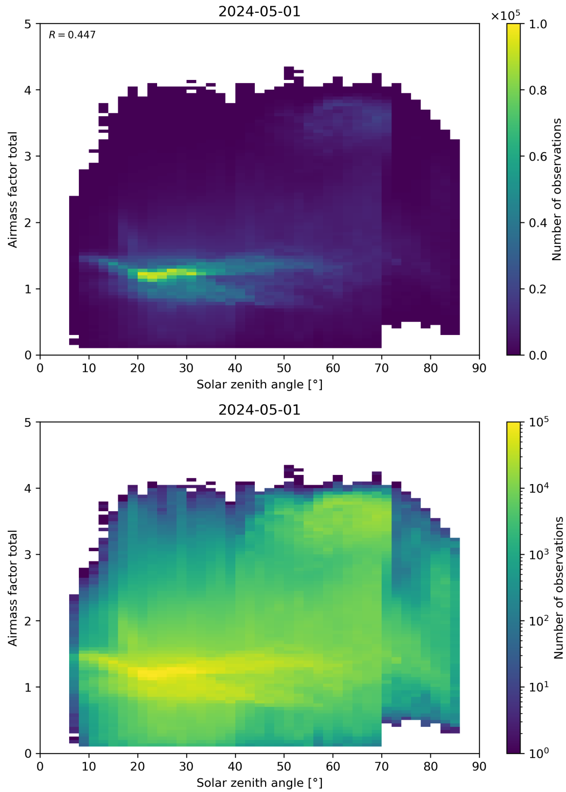
Figure 175: Scatter density plot of “Solar zenith angle” against “Airmass factor total” for 2024-04-30 to 2024-05-02.
