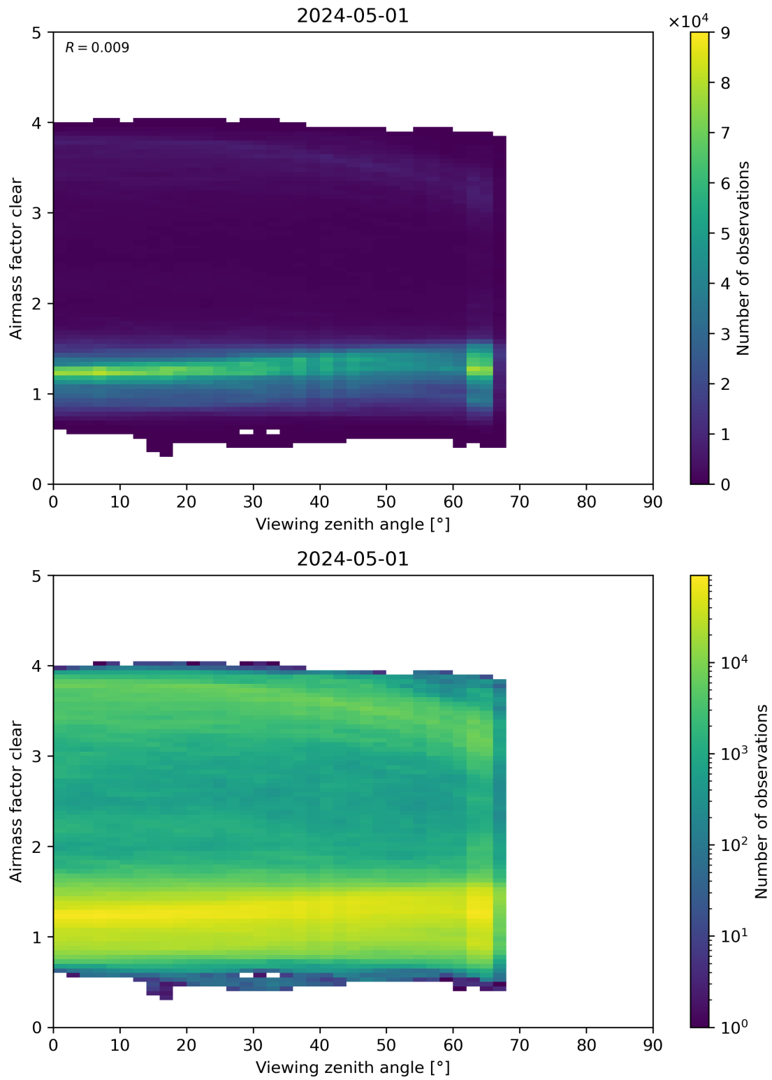
Figure 185: Scatter density plot of “Viewing zenith angle” against “Airmass factor clear” for 2024-04-30 to 2024-05-02.
