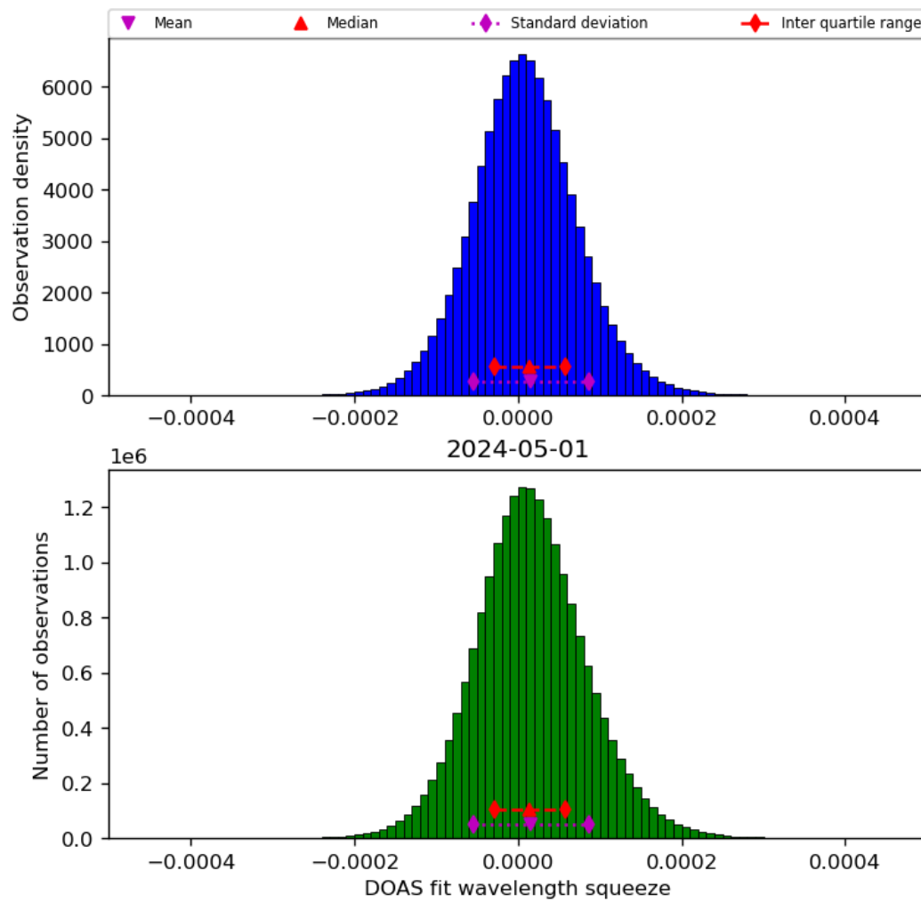
Figure 45: Histogram of “DOAS fit wavelength squeeze” for 2024-04-30 to 2024-05-02
