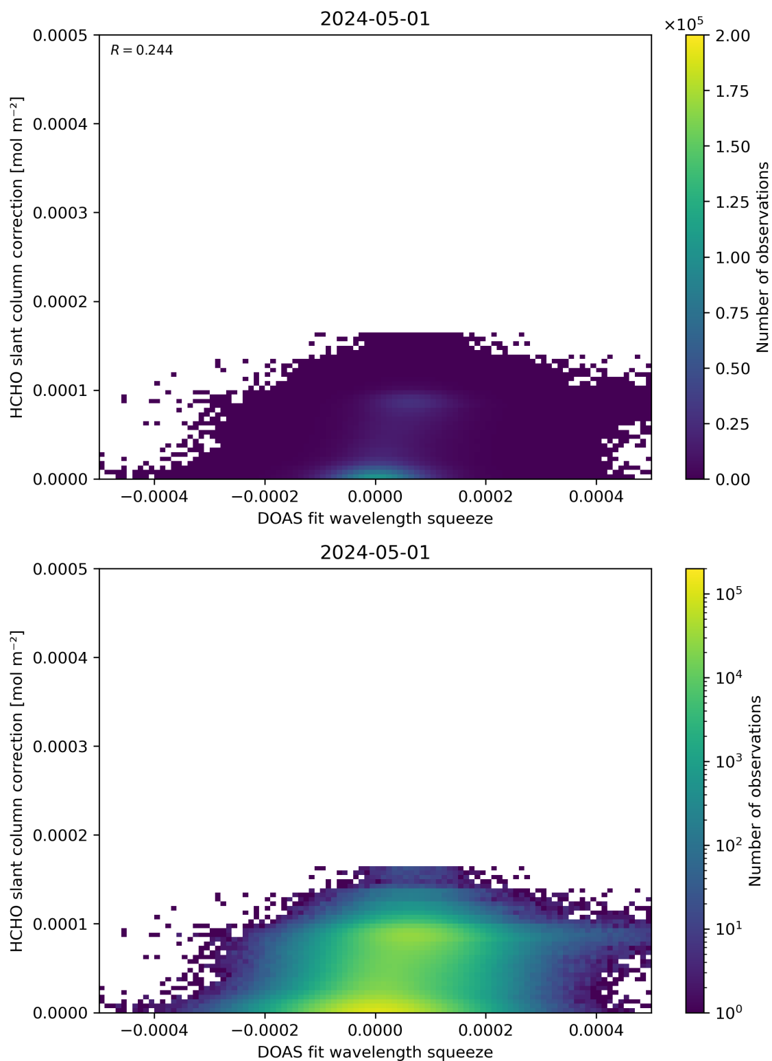
Figure 70: Scatter density plot of “DOAS fit wavelength squeeze” against “HCHO slant column correction” for 2024-04-30 to 2024-05-02.
