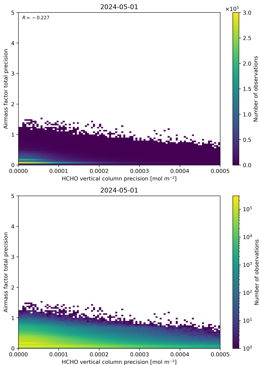
Figure 145: Scatter density plot of “HCHO vertical column precision” against “Airmass factor total precision” for 2024-04-30 to 2024-05-02.
