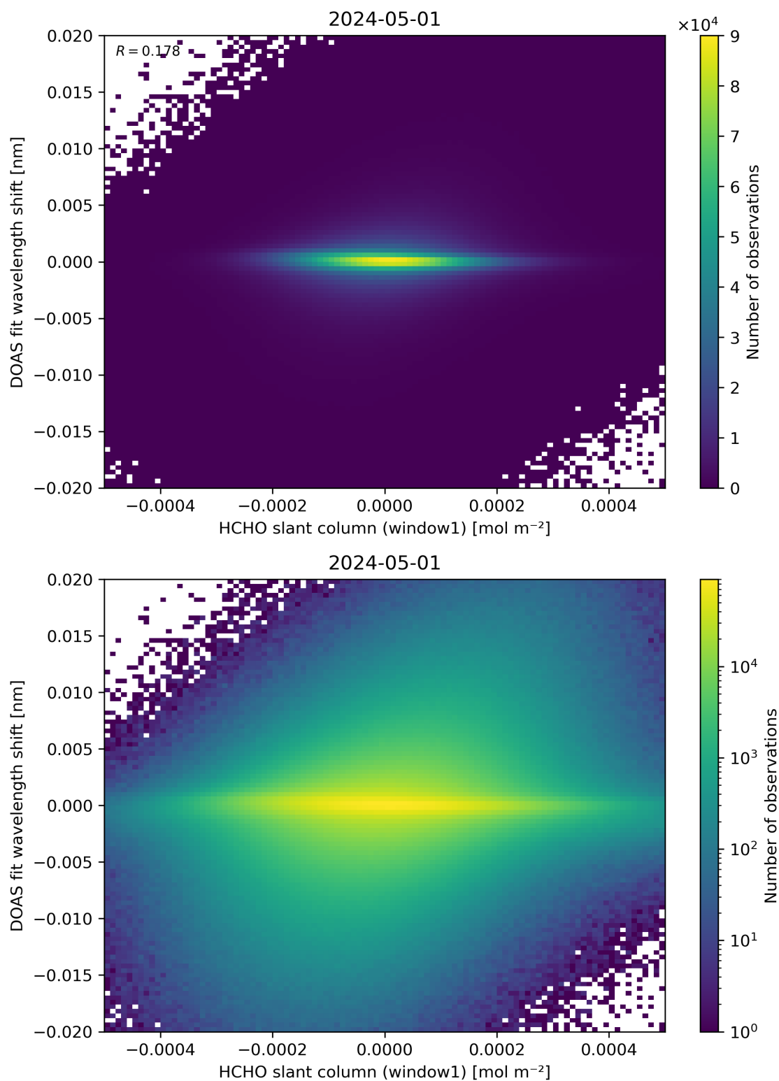
Figure 79: Scatter density plot of “HCHO slant column (window1)” against “DOAS fit wavelength shift” for 2024-04-30 to 2024-05-02.
