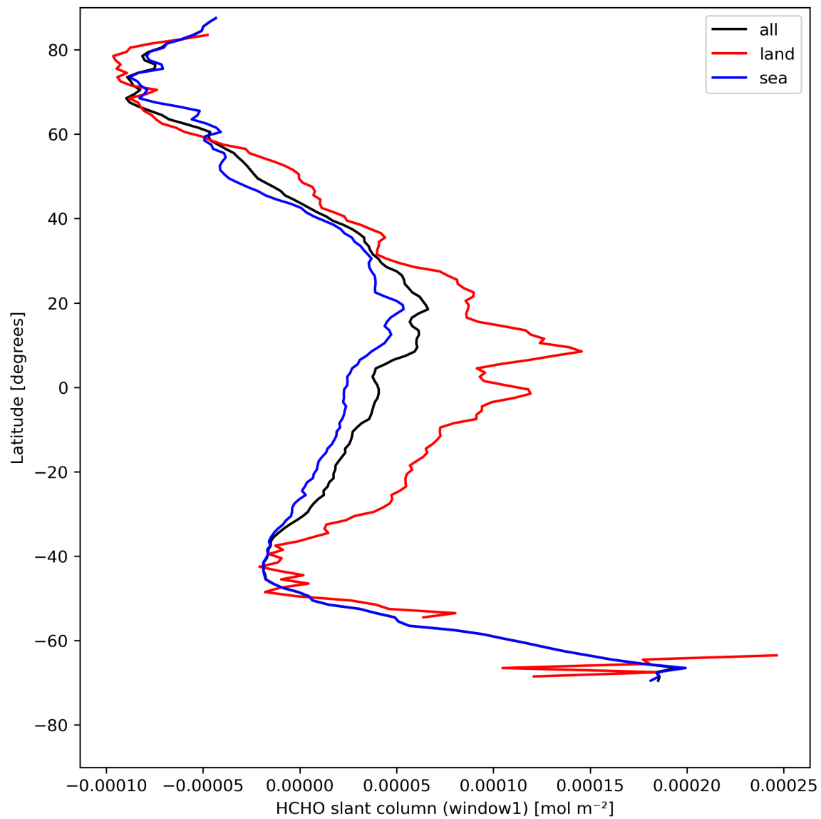
Figure 24: Zonal average of “HCHO slant column (window1)” for 2024-04-30 to 2024-05-02.
