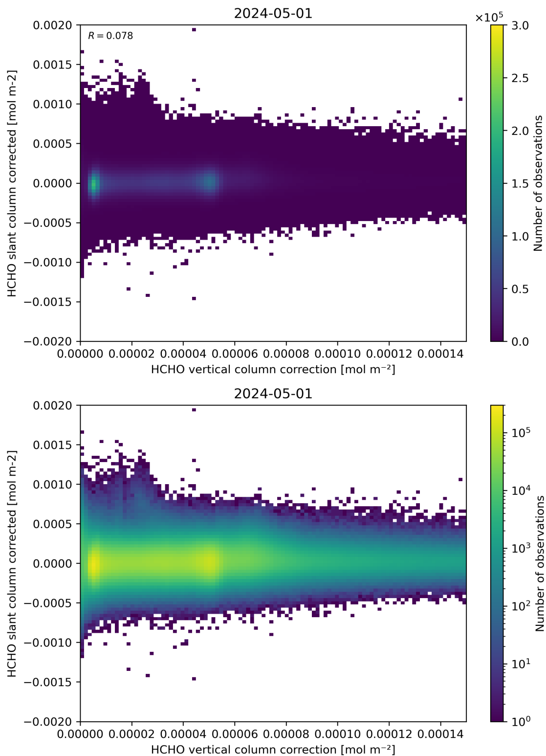
Figure 116: Scatter density plot of “HCHO vertical column correction” against “HCHO slant column corrected” for 2024-04-30 to 2024-05-02.
