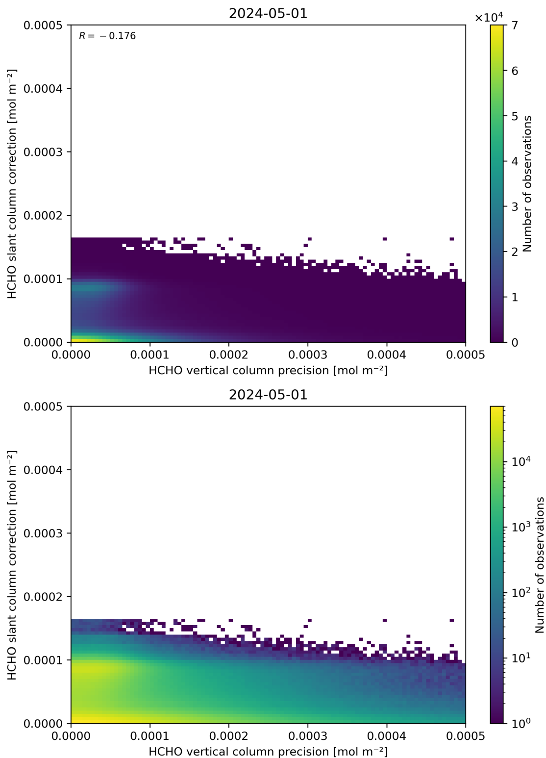
Figure 141: Scatter density plot of “HCHO vertical column precision” against “HCHO slant column correction” for 2024-04-30 to 2024-05-02.
