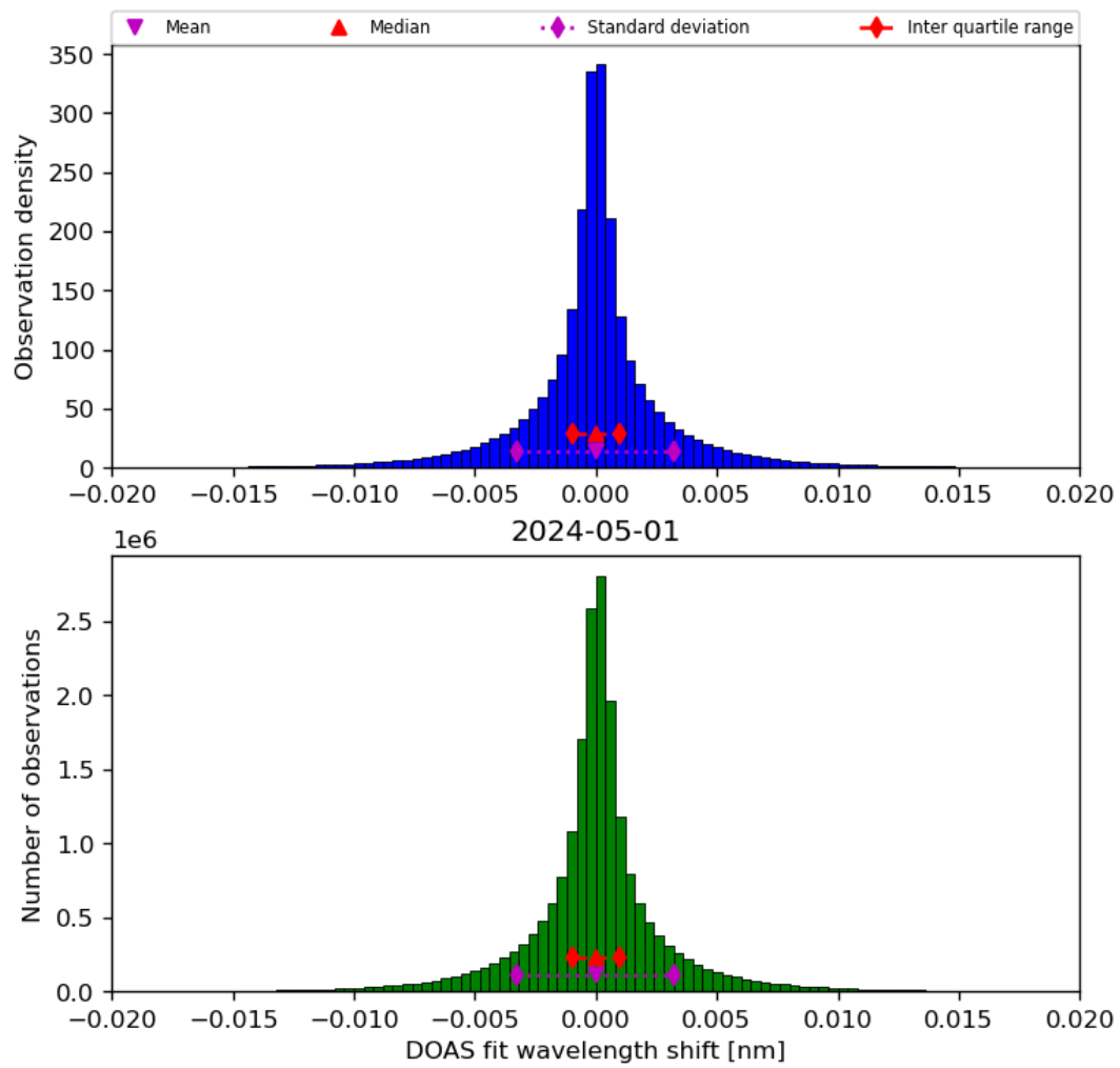
Figure 44: Histogram of “DOAS fit wavelength shift” for 2024-04-30 to 2024-05-02
