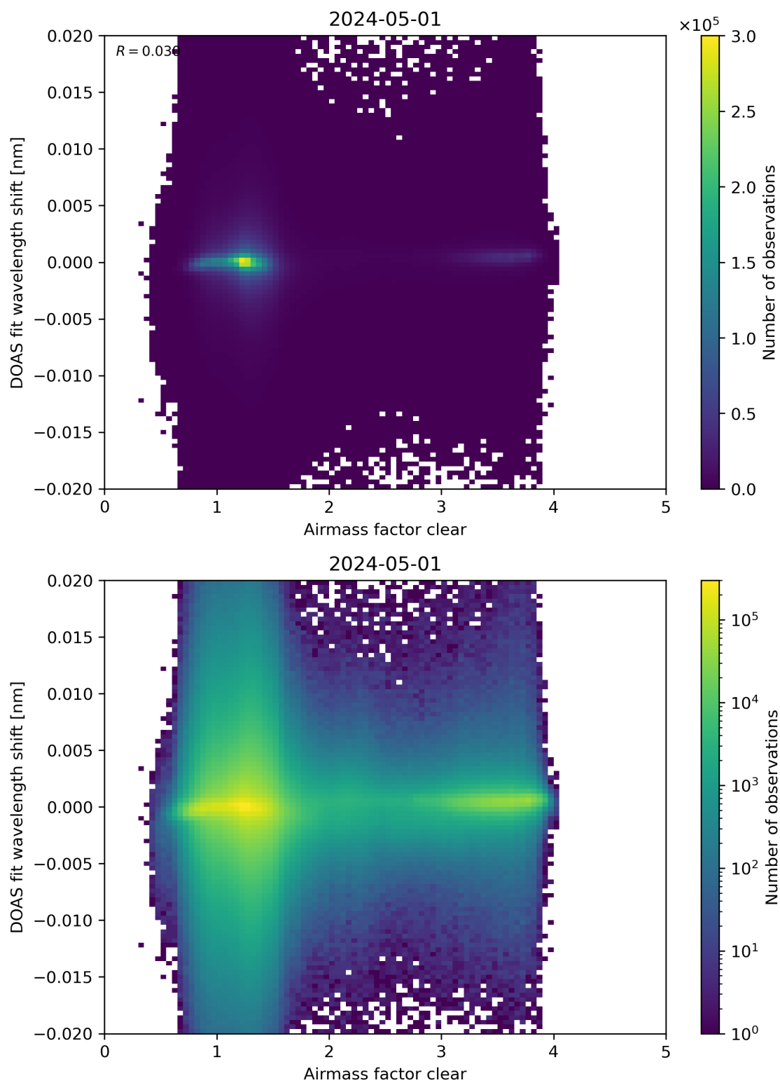
Figure 72: Scatter density plot of “Airmass factor clear” against “DOAS fit wavelength shift” for 2024-04-30 to 2024-05-02.
