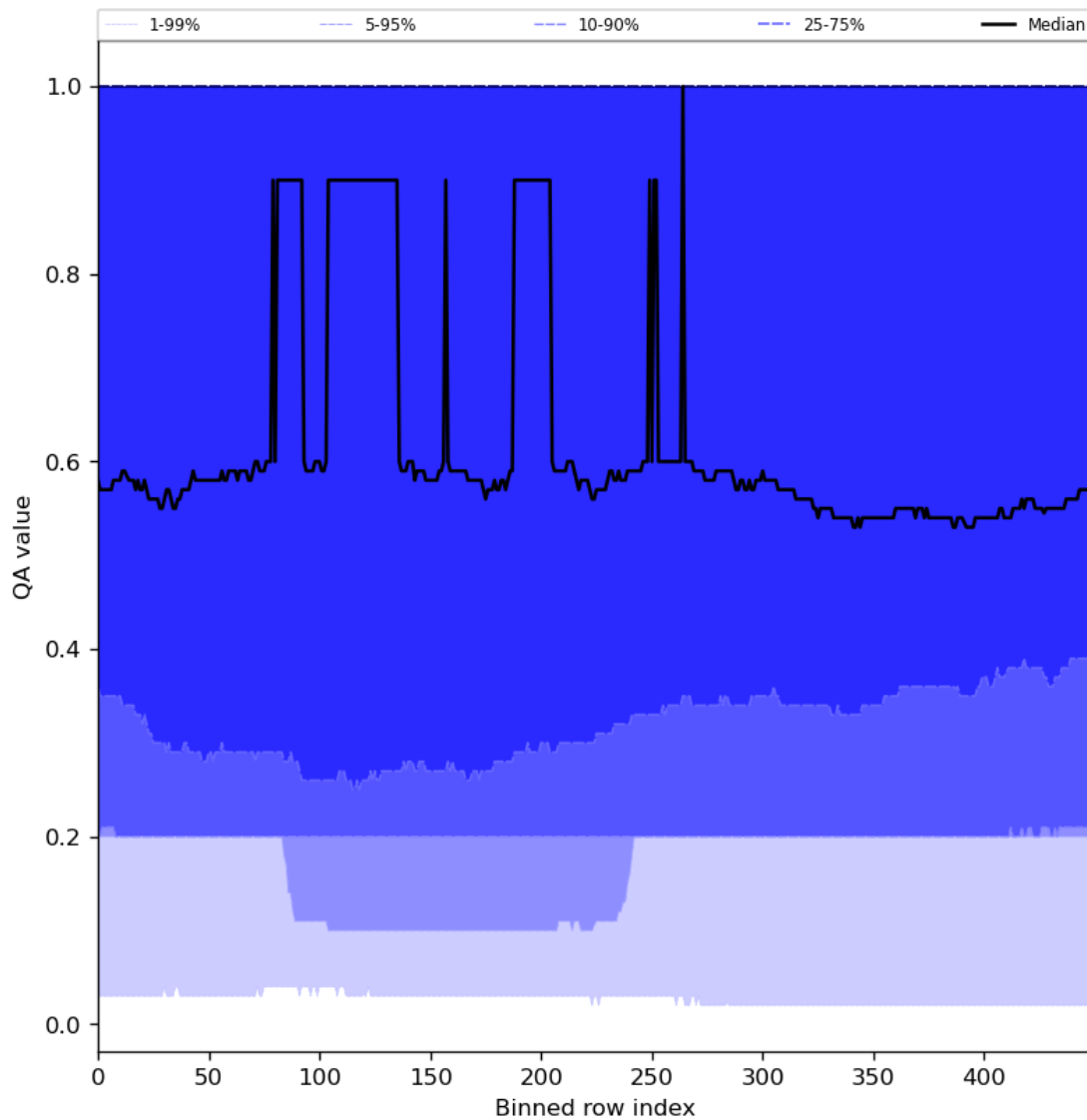
Figure 48: Along track statistics of “QA value” for 2024-04-30 to 2024-05-02
