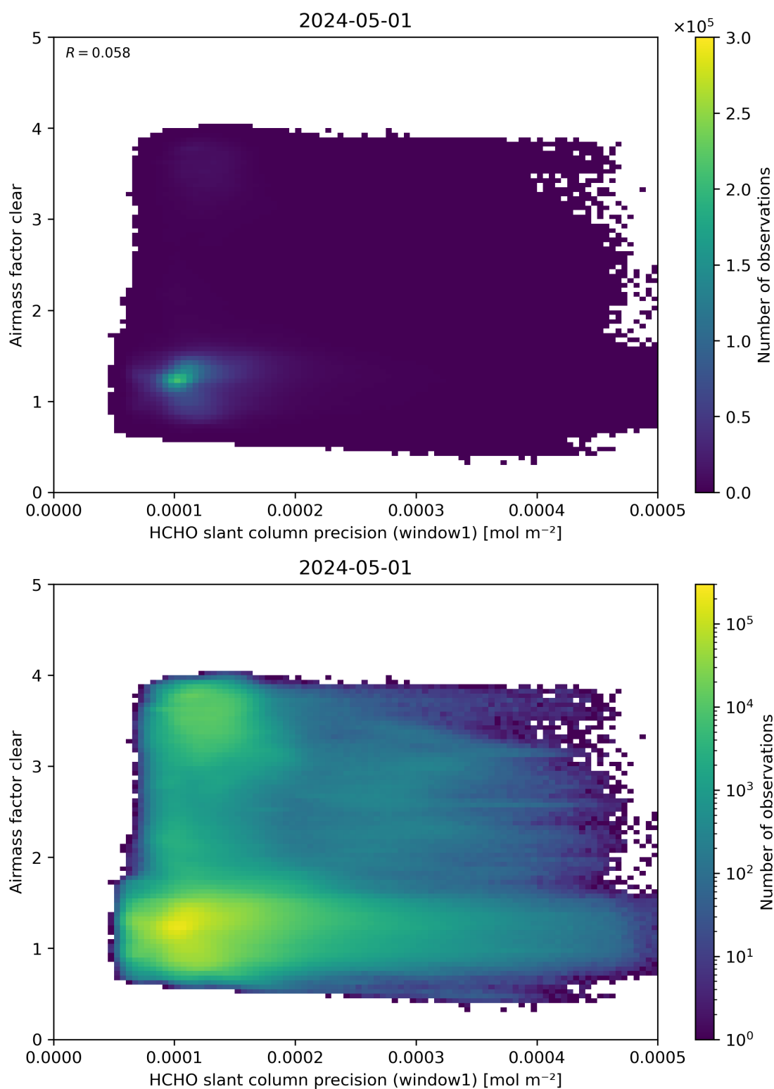
Figure 91: Scatter density plot of “HCHO slant column precision (window1)” against “Airmass factor clear” for 2024-04-30 to 2024-05-02.
