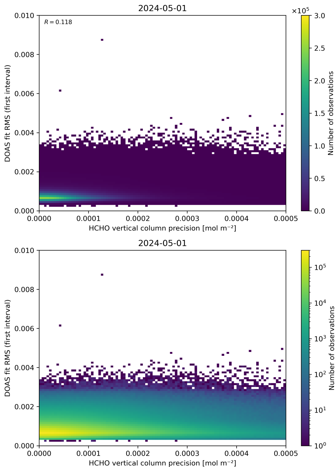
Figure 136: Scatter density plot of “HCHO vertical column precision” against “DOAS fit RMS (first interval)” for 2024-04-30 to 2024-05-02.
