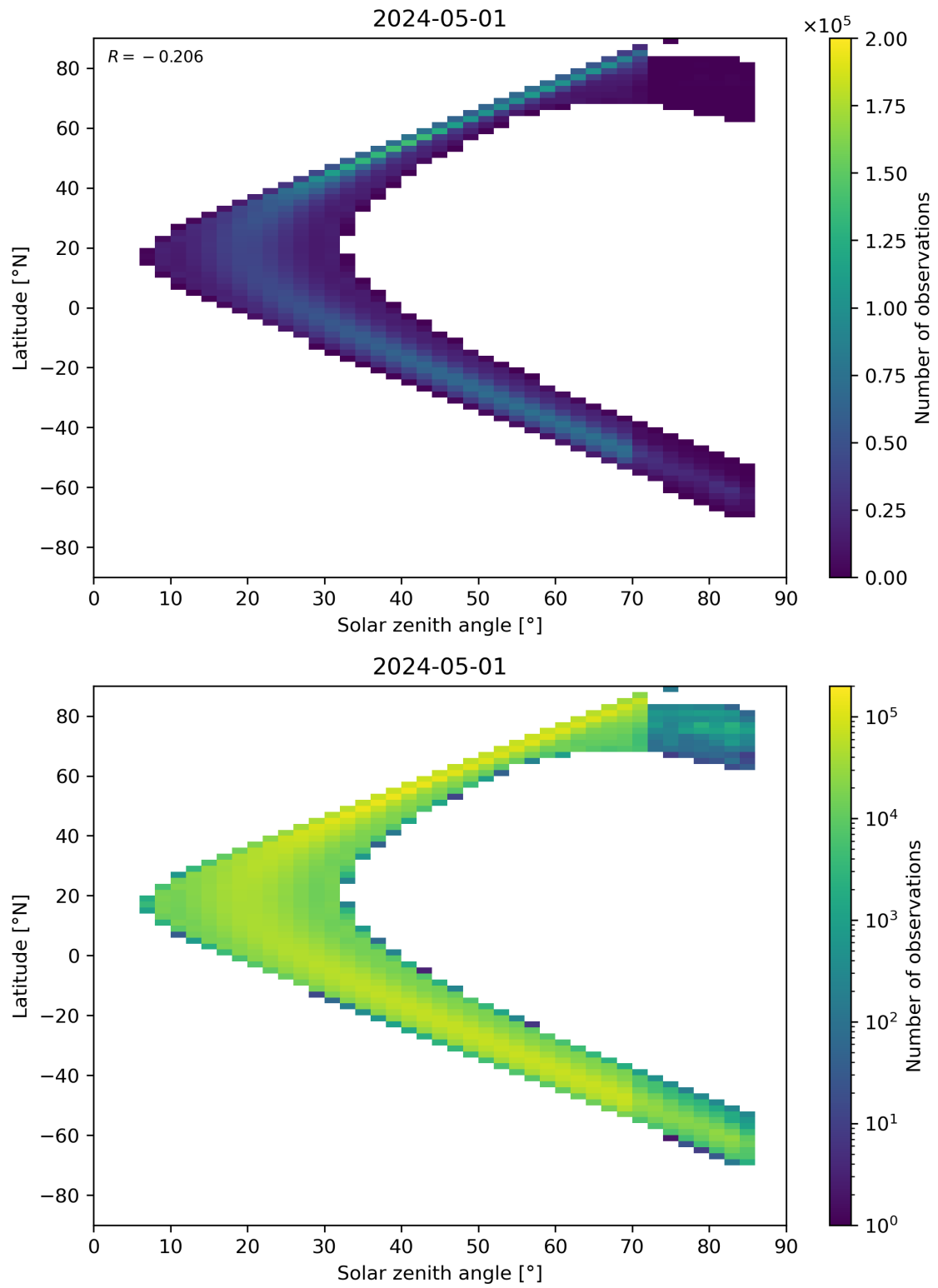
Figure 181: Scatter density plot of “Solar zenith angle” against “Latitude” for 2024-04-30 to 2024-05-02.
