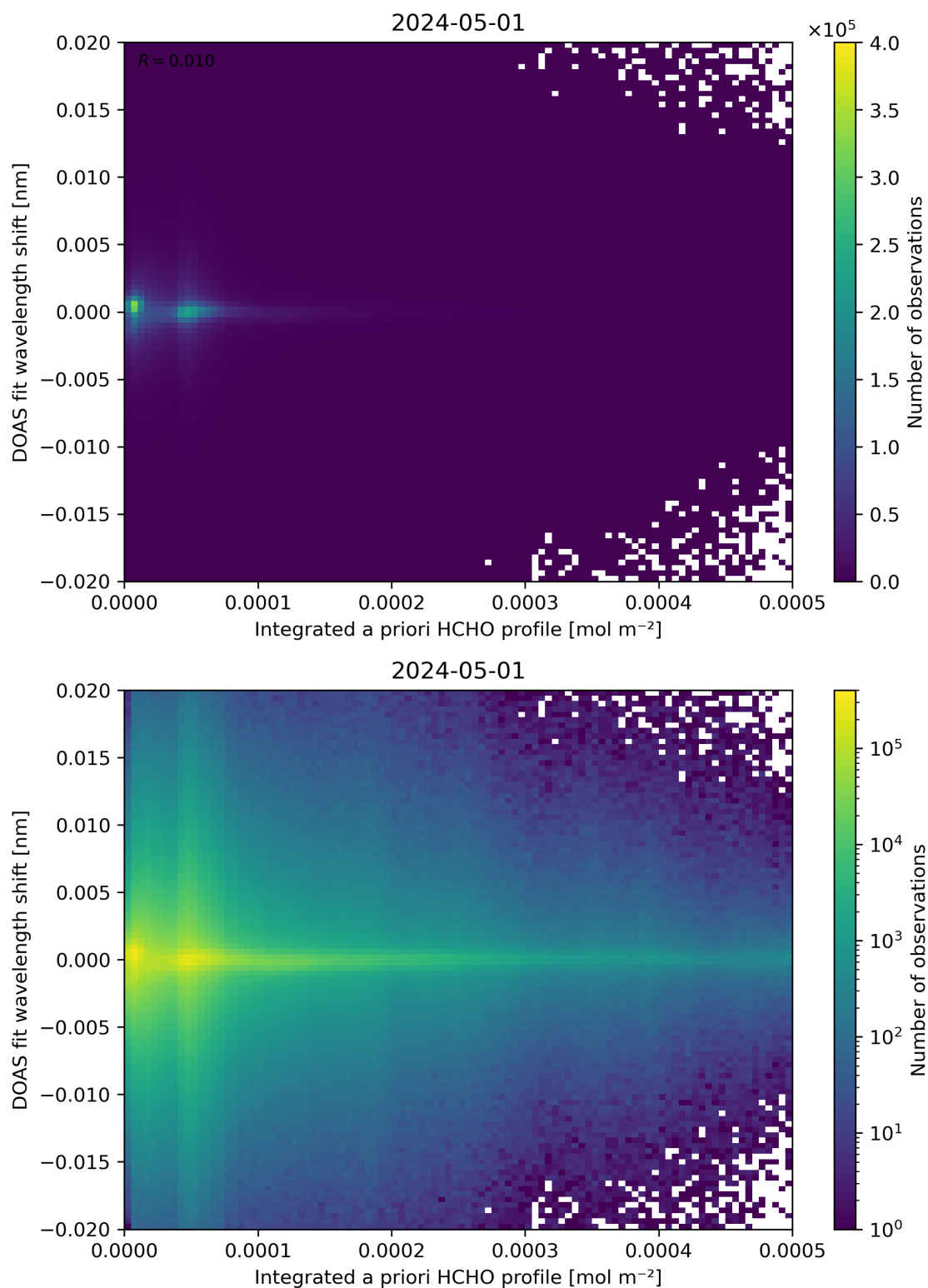
Figure 149: Scatter density plot of “Integrated a priori HCHO profile” against “DOAS fit wavelength shift” for 2024-04-30 to 2024-05-02.
