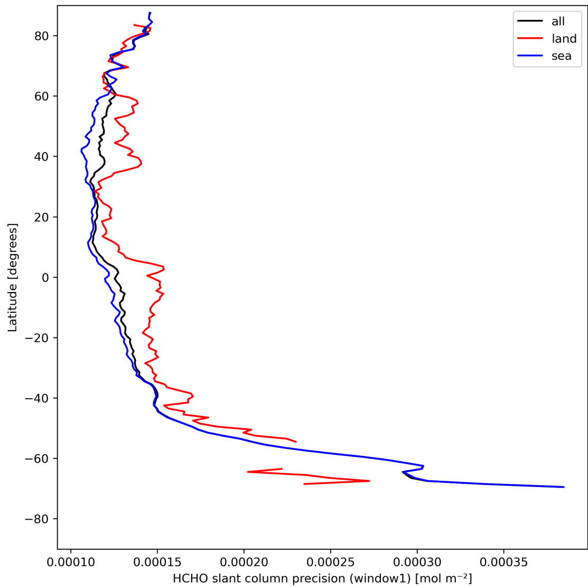
Figure 25: Zonal average of “HCHO slant column precision (window1)” for 2024-04-30 to 2024-05-02.
