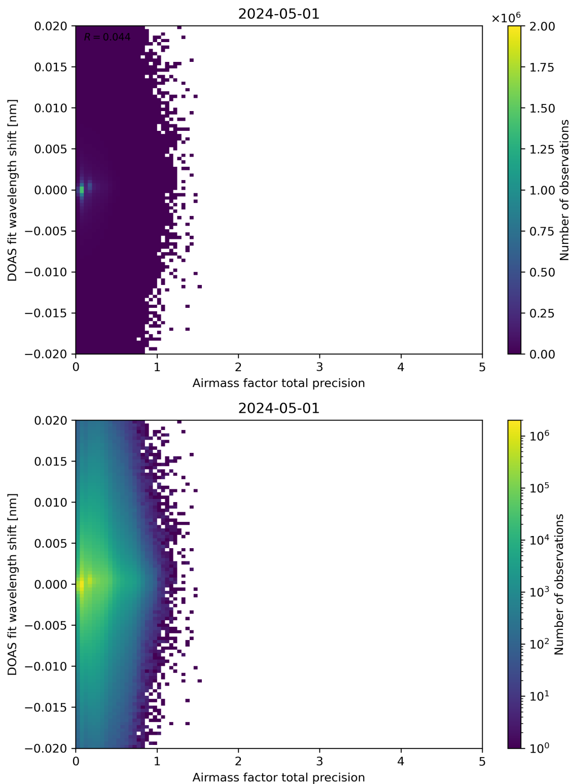
Figure 106: Scatter density plot of “Airmass factor total precision” against “DOAS fit wavelength shift” for 2024-04-30 to 2024-05-02.
