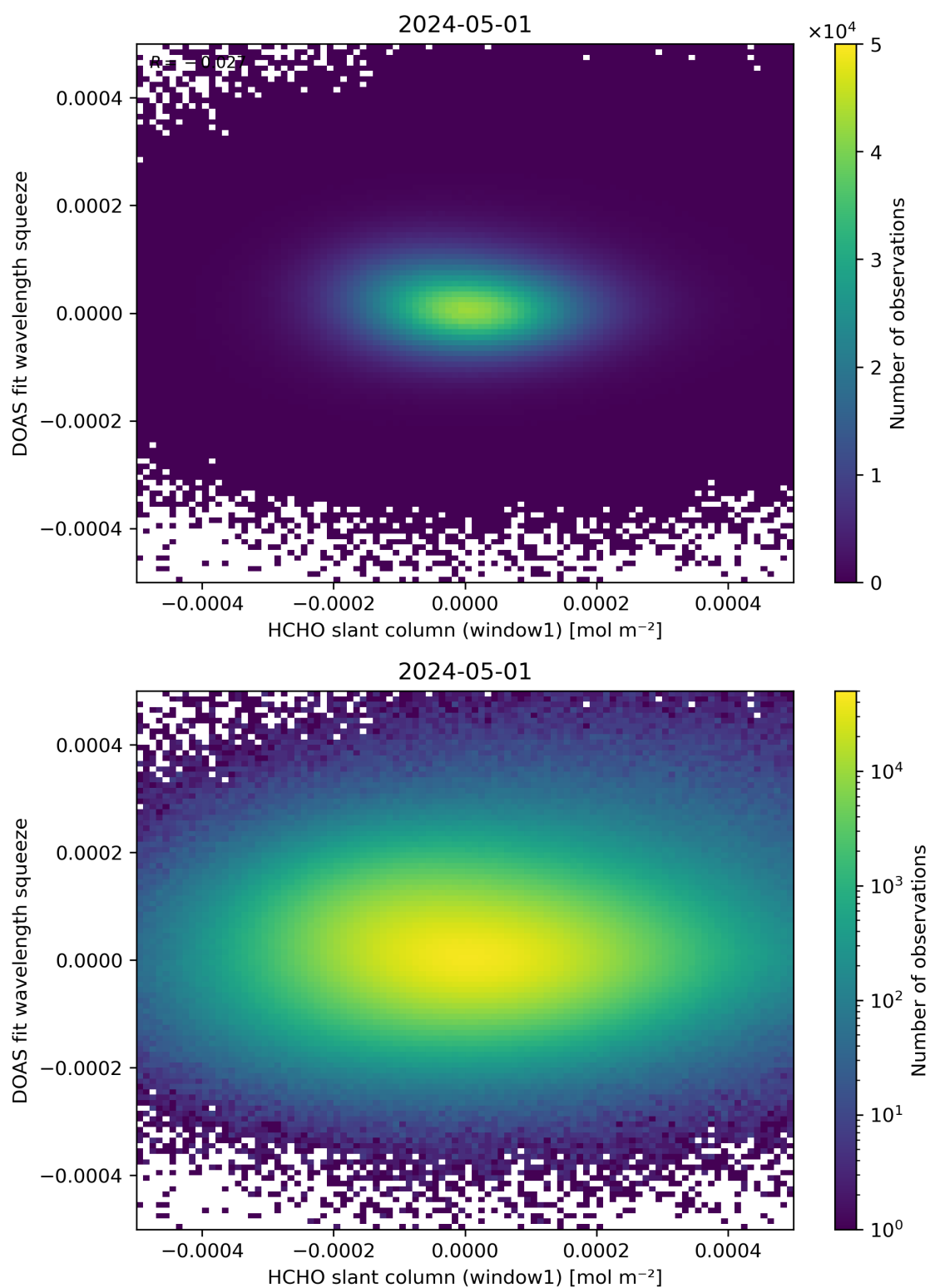
Figure 80: Scatter density plot of “HCHO slant column (window1)” against “DOAS fit wavelength squeeze” for 2024-04-30 to 2024-05-02.
