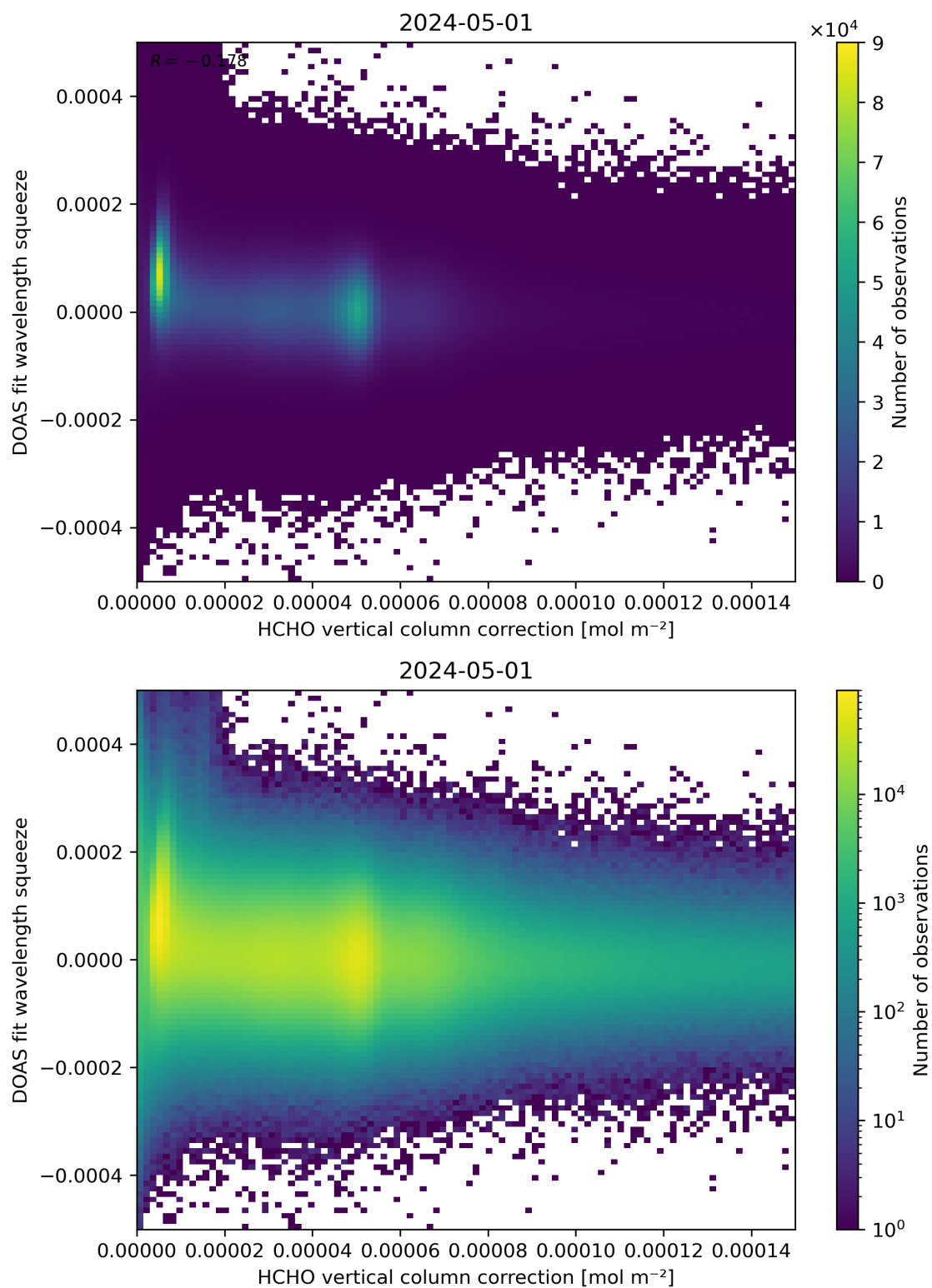
Figure 114: Scatter density plot of “HCHO vertical column correction” against “DOAS fit wavelength squeeze” for 2024-04-30 to 2024-05-02.
