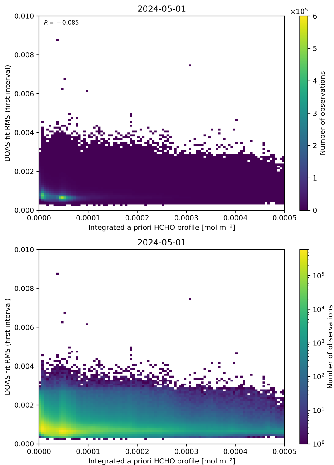
Figure 148: Scatter density plot of “Integrated a priori HCHO profile” against “DOAS fit RMS (first interval)” for 2024-04-30 to 2024-05-02.
