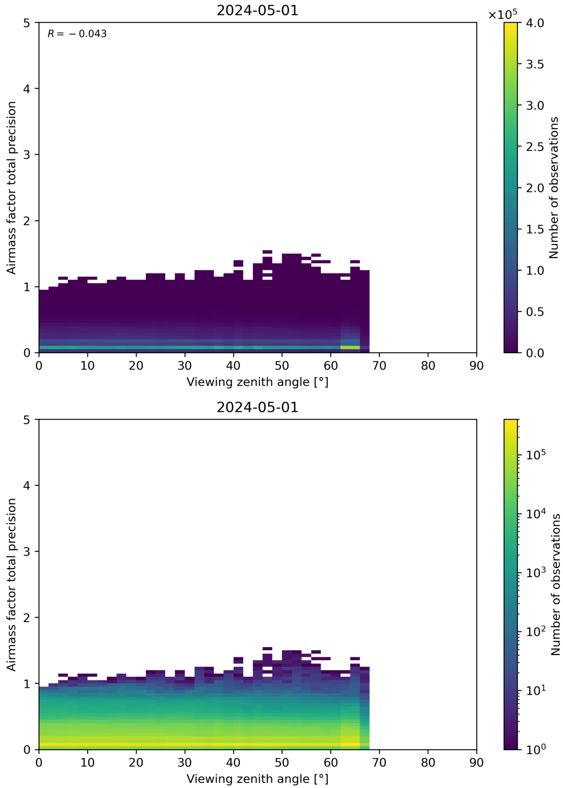
Figure 191: Scatter density plot of “Viewing zenith angle” against “Airmass factor total precision” for 2024-04-30 to 2024-05-02.
