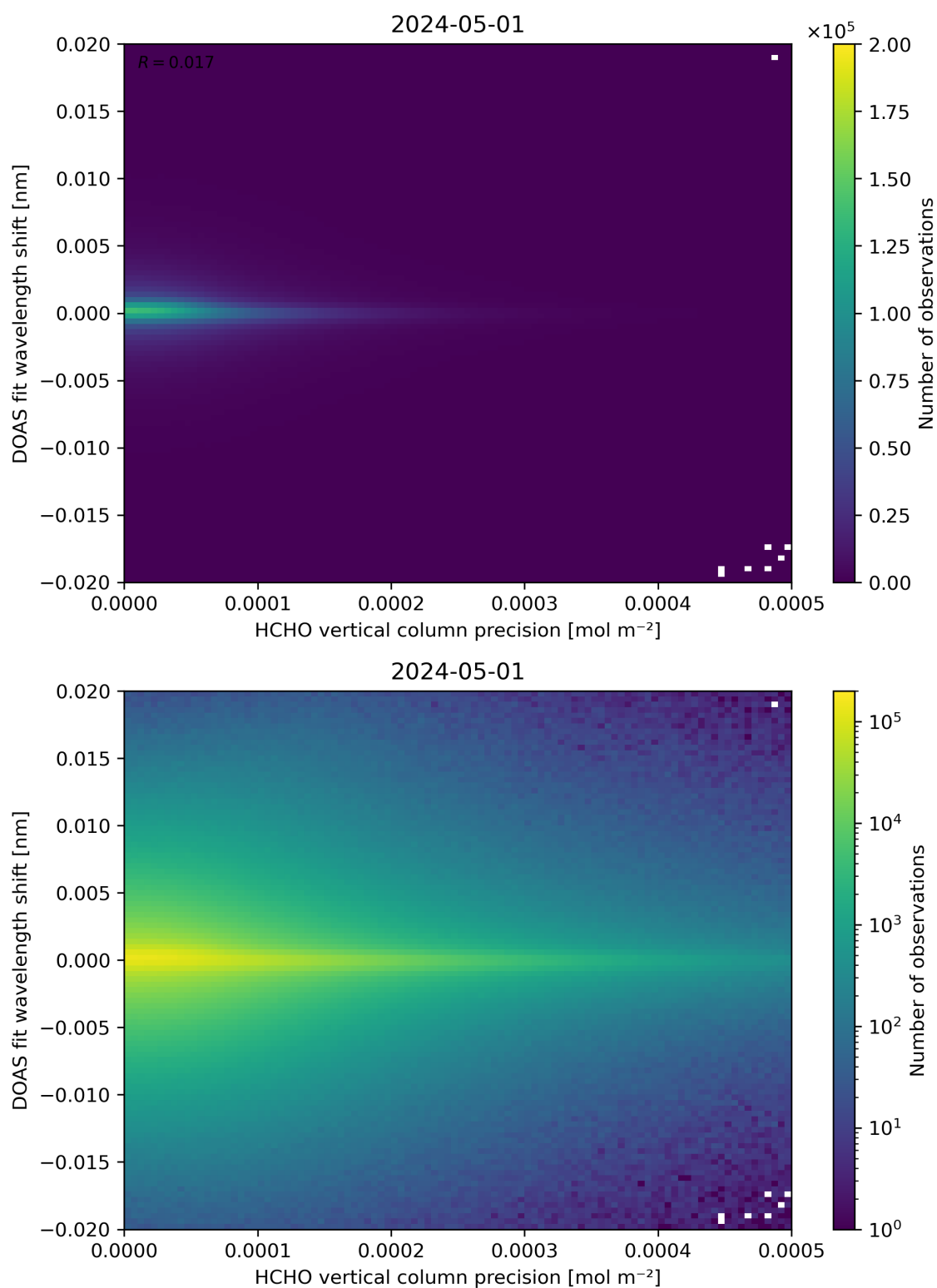
Figure 137: Scatter density plot of “HCHO vertical column precision” against “DOAS fit wavelength shift” for 2024-04-30 to 2024-05-02.
