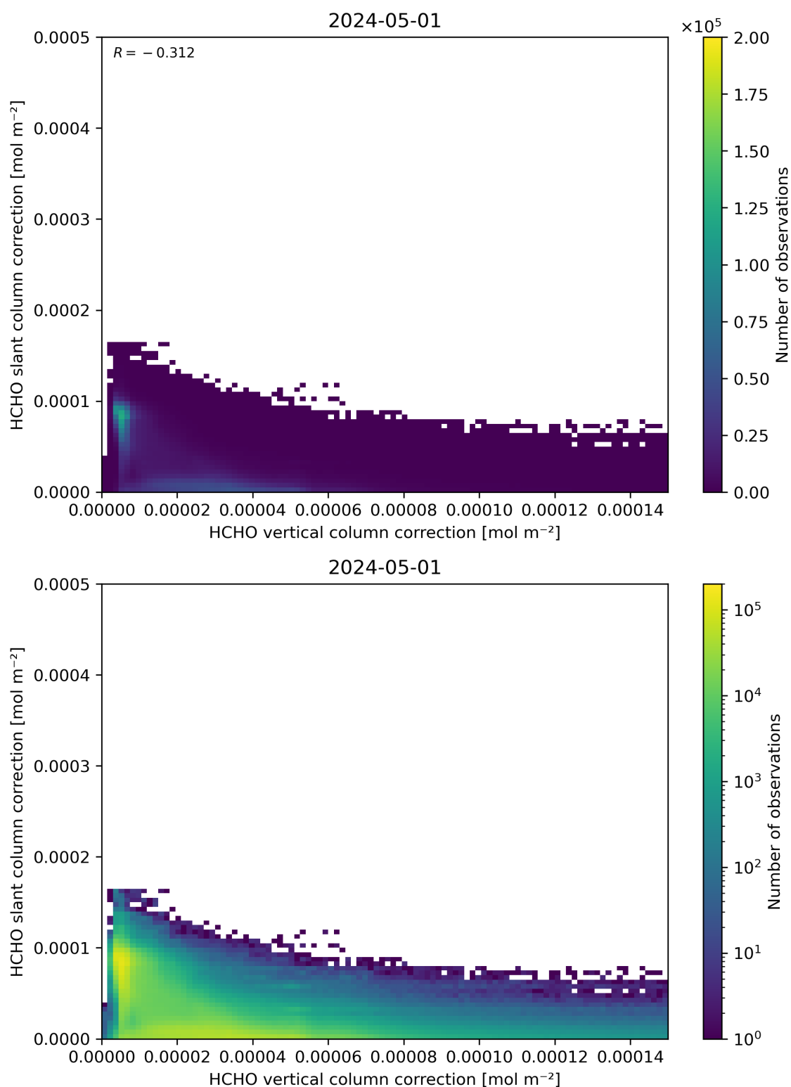
Figure 117: Scatter density plot of “HCHO vertical column correction” against “HCHO slant column correction” for 2024-04-30 to 2024-05-02.
