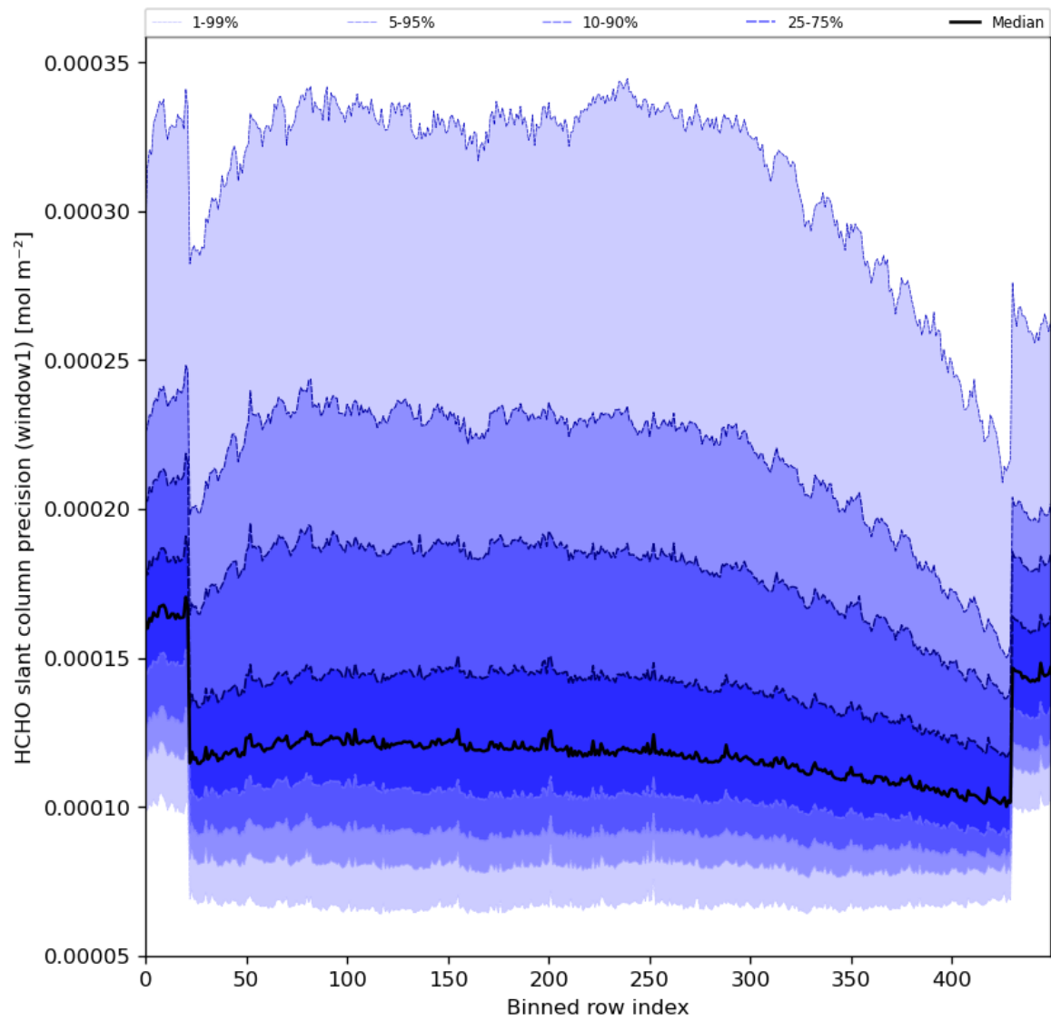
Figure 53: Along track statistics of “HCHO slant column precision (window1)” for 2024-04-30 to 2024-05-02
