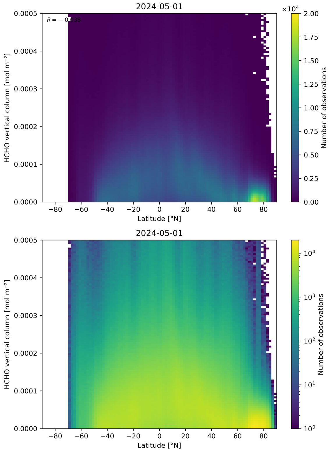
Figure 163: Scatter density plot of “Latitude” against “HCHO vertical column” for 2024-04-30 to 2024-05-02.
