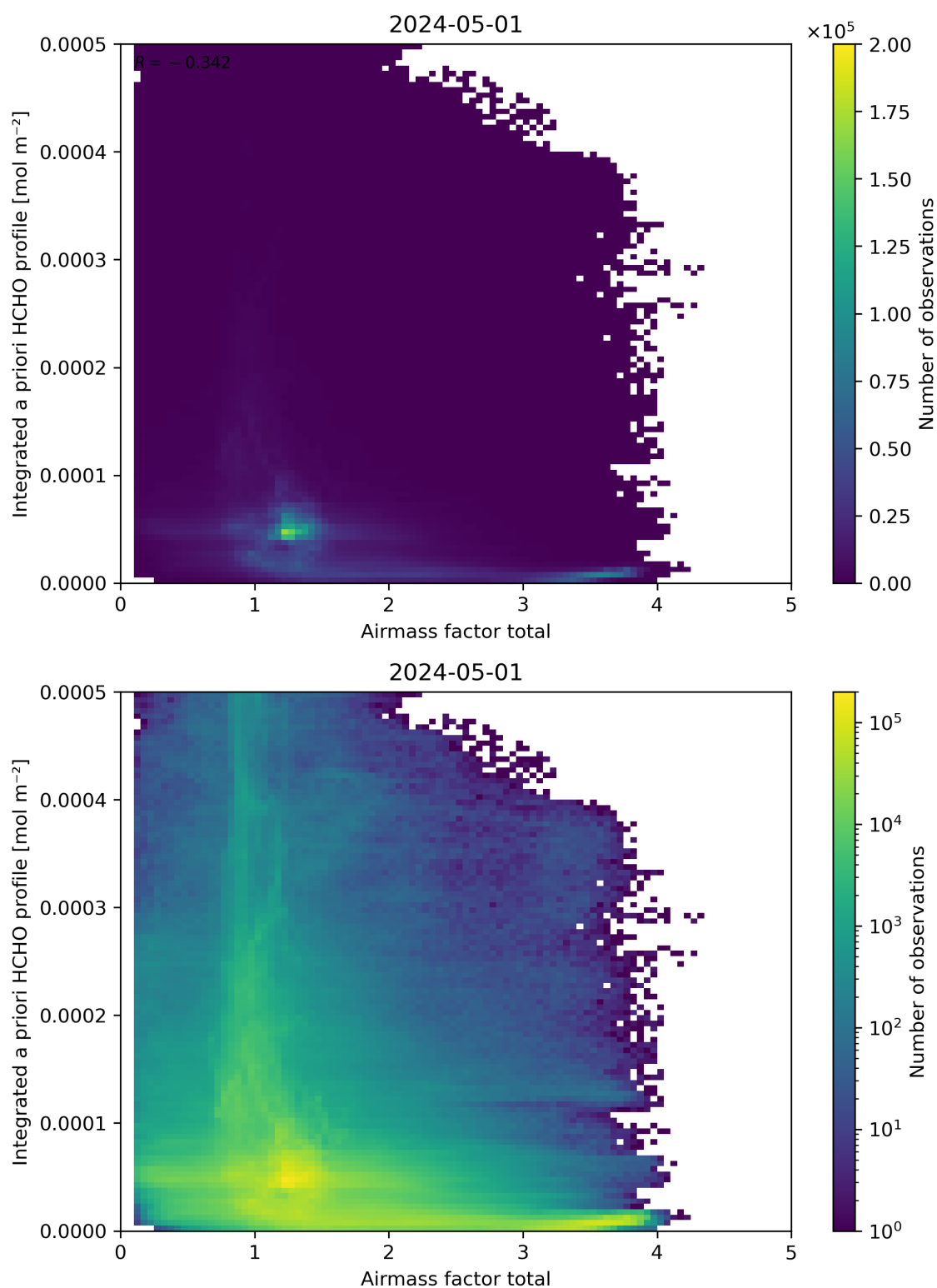
Figure 104: Scatter density plot of “Airmass factor total” against “Integrated a priori HCHO profile” for 2024-04-30 to 2024-05-02.
