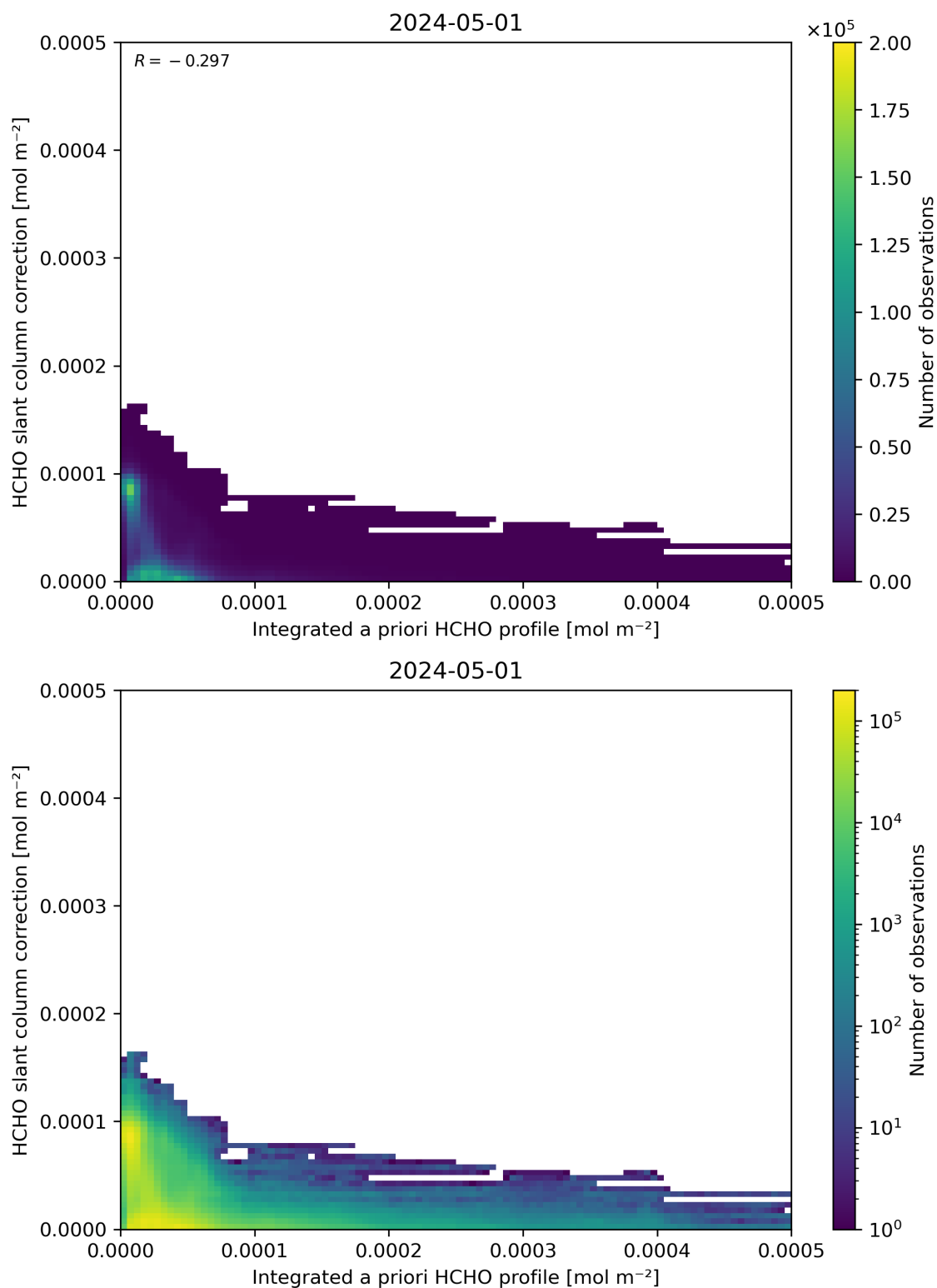
Figure 152: Scatter density plot of “Integrated a priori HCHO profile” against “HCHO slant column correction” for 2024-04-30 to 2024-05-02.
