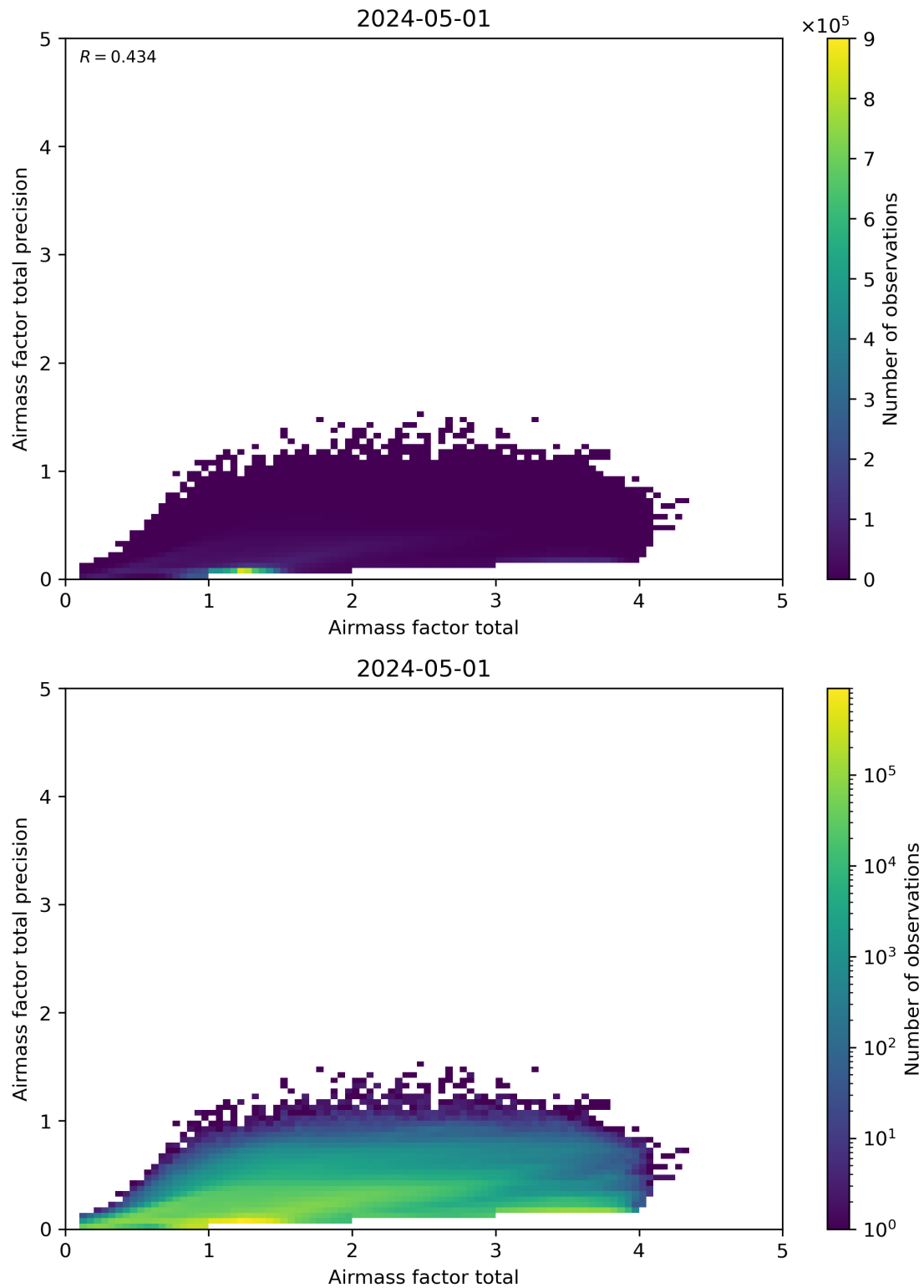
Figure 103: Scatter density plot of “Airmass factor total” against “Airmass factor total precision” for 2024-04-30 to 2024-05-02.
