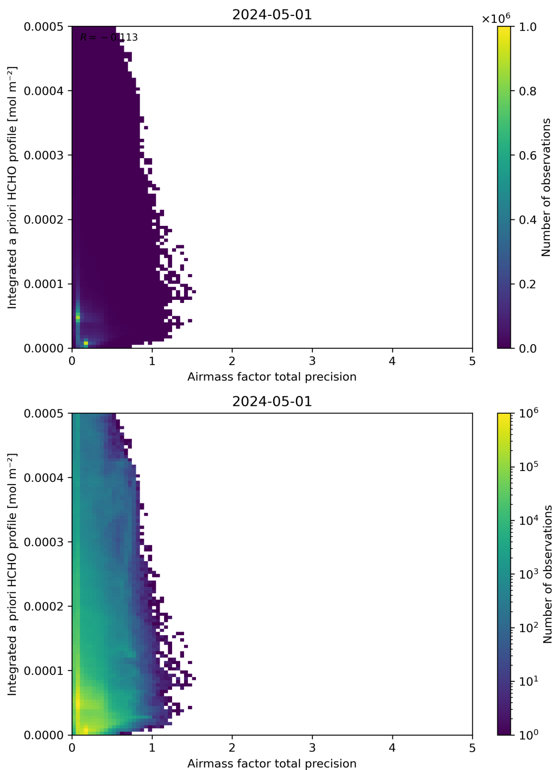
Figure 111: Scatter density plot of “Airmass factor total precision” against “Integrated a priori HCHO profile” for 2024-04-30 to 2024-05-02.
