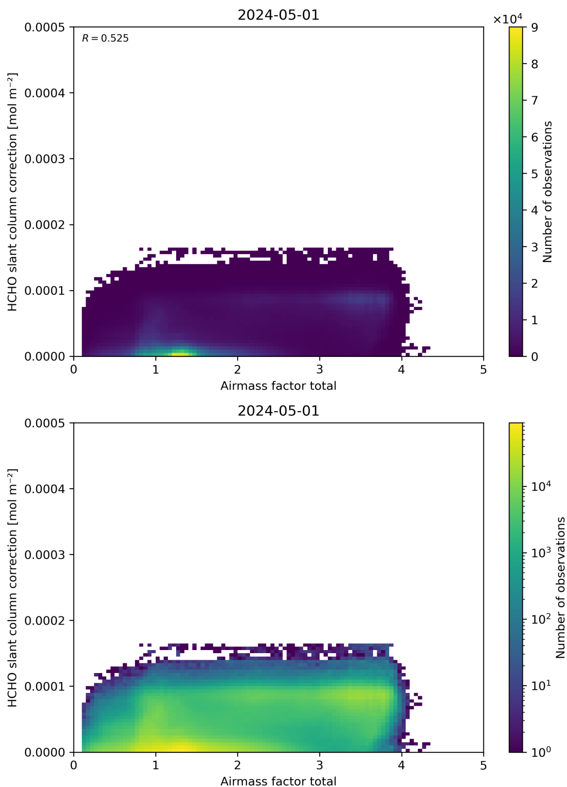
Figure 102: Scatter density plot of “Airmass factor total” against “HCHO slant column correction” for 2024-04-30 to 2024-05-02.
