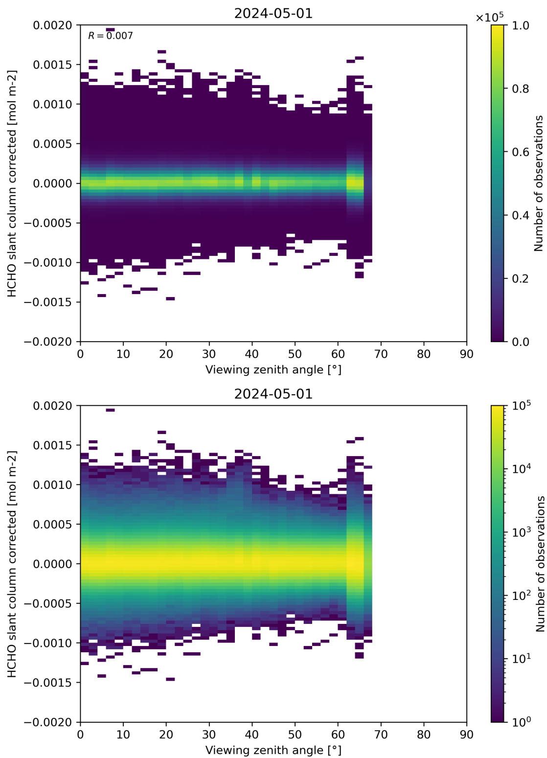
Figure 186: Scatter density plot of “Viewing zenith angle” against “HCHO slant column corrected” for 2024-04-30 to 2024-05-02.
