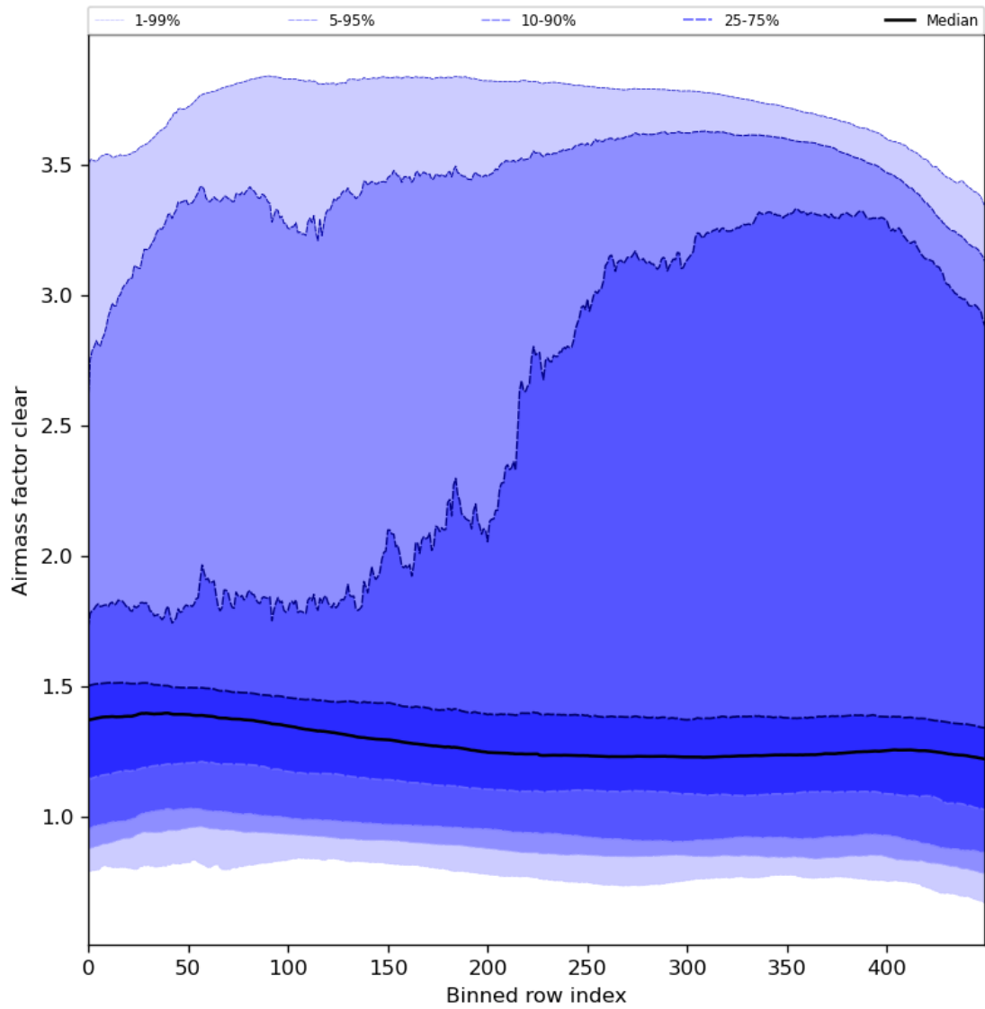
Figure 56: Along track statistics of “Airmass factor clear” for 2024-04-30 to 2024-05-02
