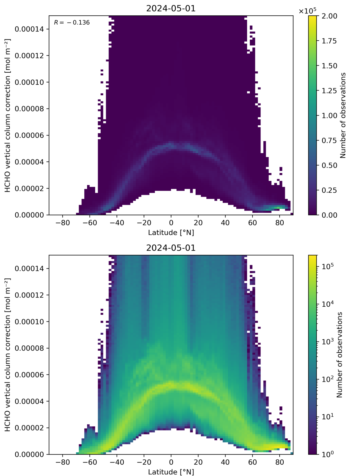
Figure 164: Scatter density plot of “Latitude” against “HCHO vertical column correction” for 2024-04-30 to 2024-05-02.
