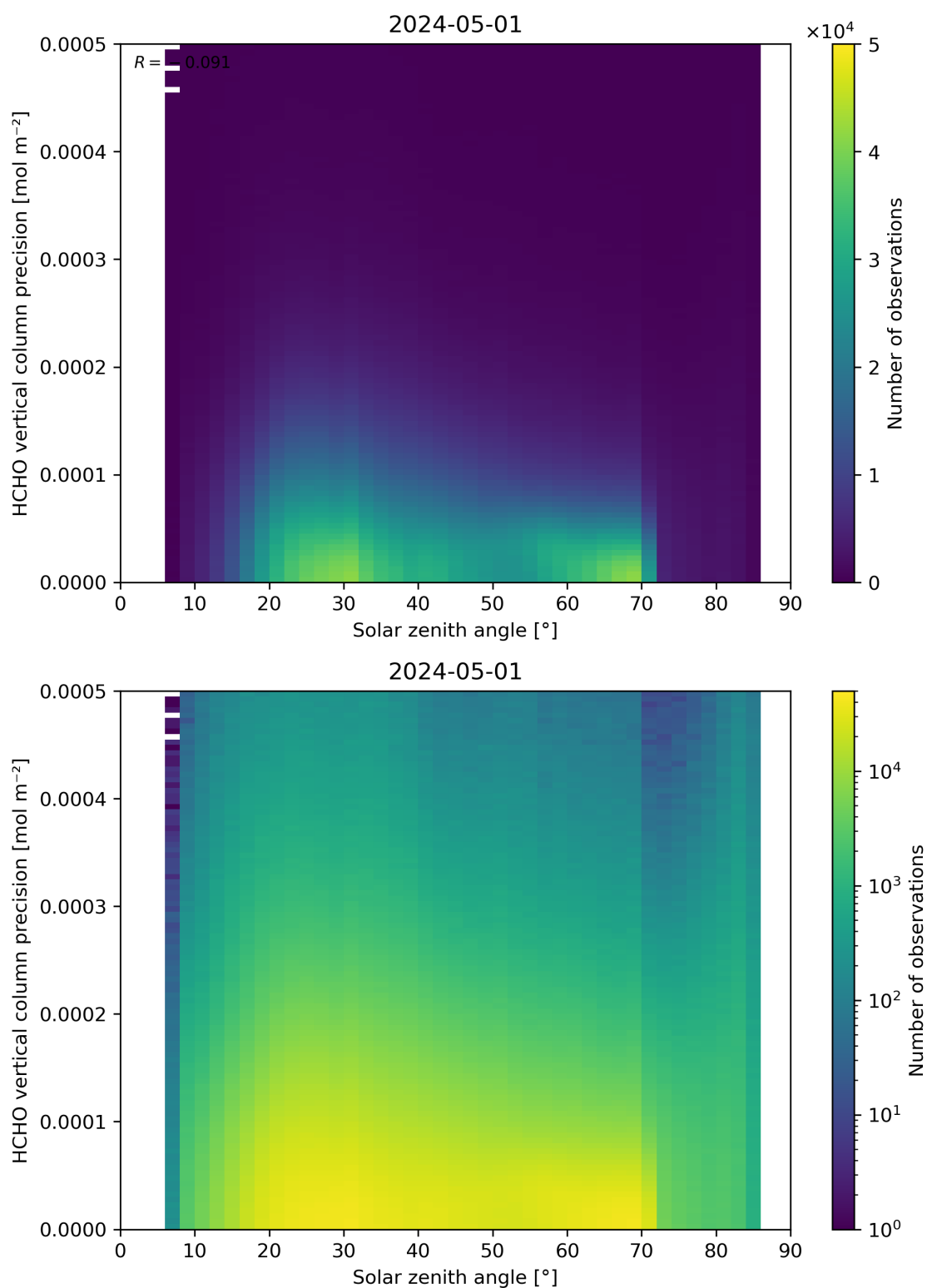
Figure 179: Scatter density plot of “Solar zenith angle” against “HCHO vertical column precision” for 2024-04-30 to 2024-05-02.
