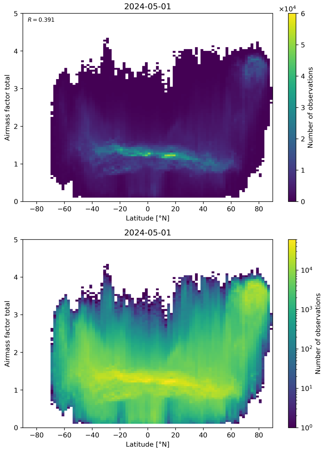
Figure 161: Scatter density plot of “Latitude” against “Airmass factor total” for 2024-04-30 to 2024-05-02.
