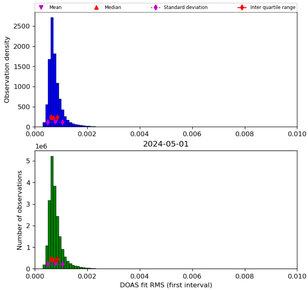
Figure 46: Histogram of “DOAS fit RMS (first interval)” for 2024-04-30 to 2024-05-02
