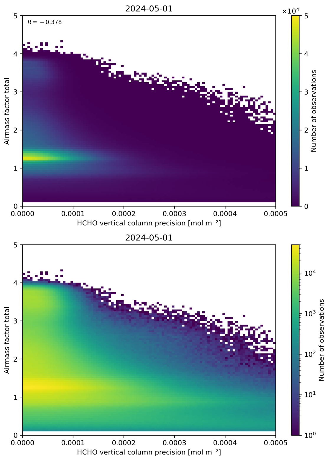
Figure 144: Scatter density plot of “HCHO vertical column precision” against “Airmass factor total” for 2024-04-30 to 2024-05-02.
