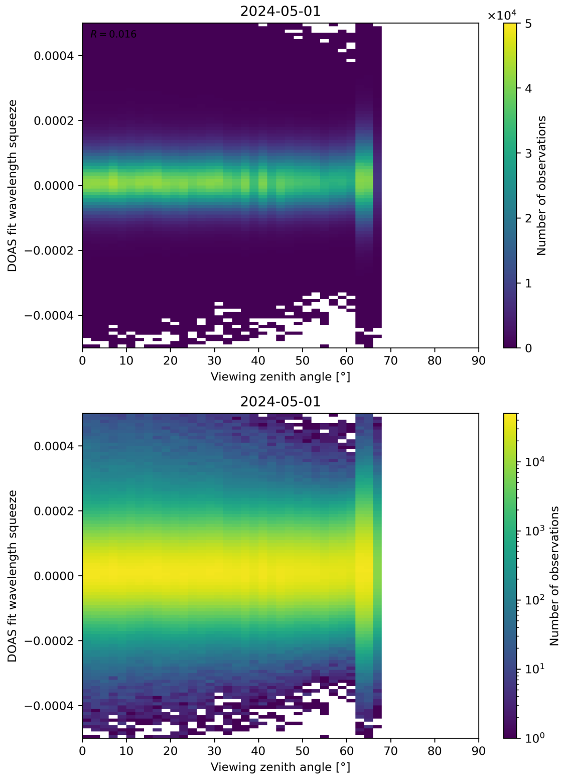
Figure 184: Scatter density plot of “Viewing zenith angle” against “DOAS fit wavelength squeeze” for 2024-04-30 to 2024-05-02.
