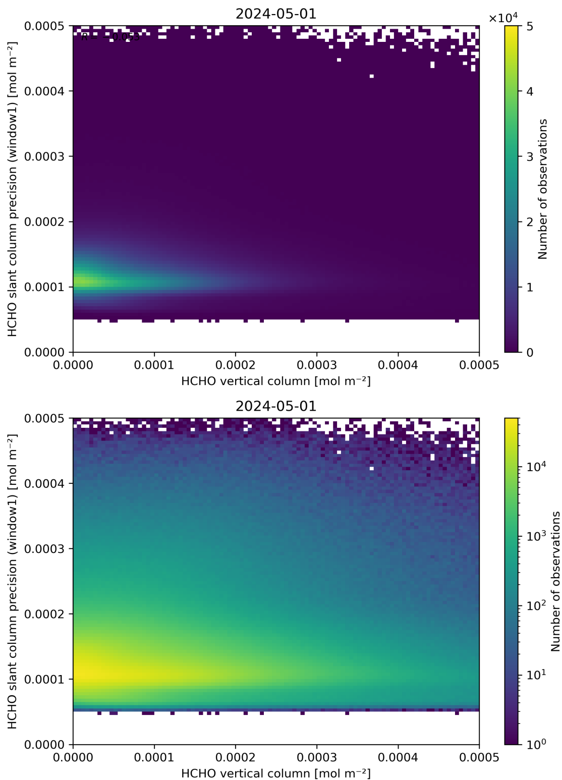
Figure 130: Scatter density plot of “HCHO vertical column” against “HCHO slant column precision (window1)” for 2024-04-30 to 2024-05-02.
