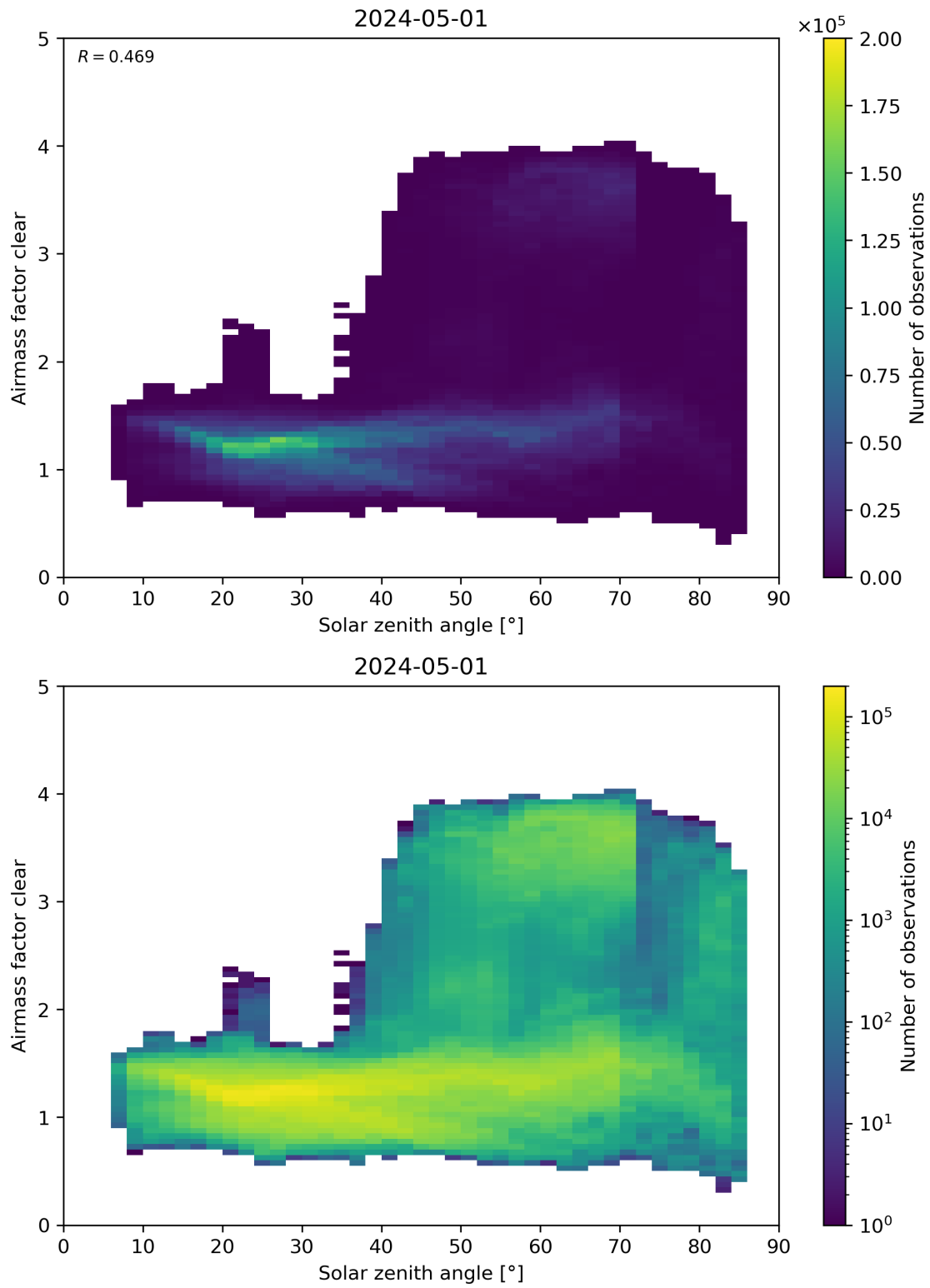
Figure 170: Scatter density plot of “Solar zenith angle” against “Airmass factor clear” for 2024-04-30 to 2024-05-02.
