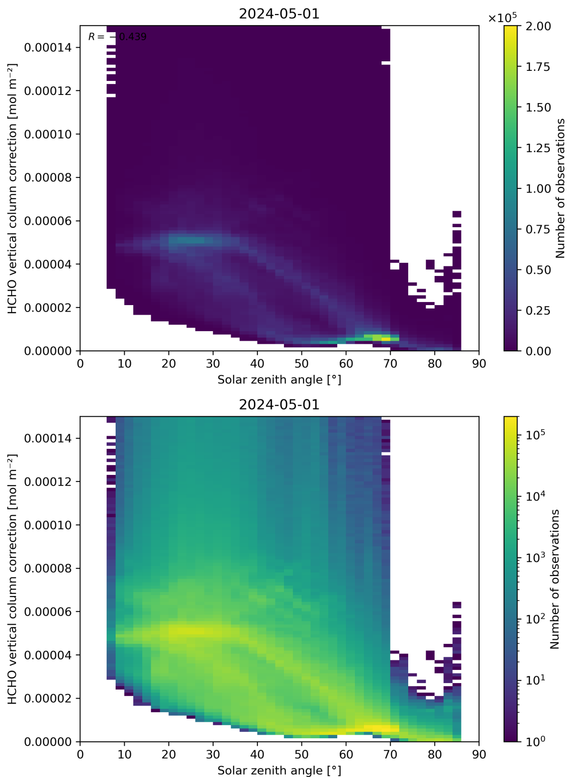
Figure 178: Scatter density plot of “Solar zenith angle” against “HCHO vertical column correction” for 2024-04-30 to 2024-05-02.
