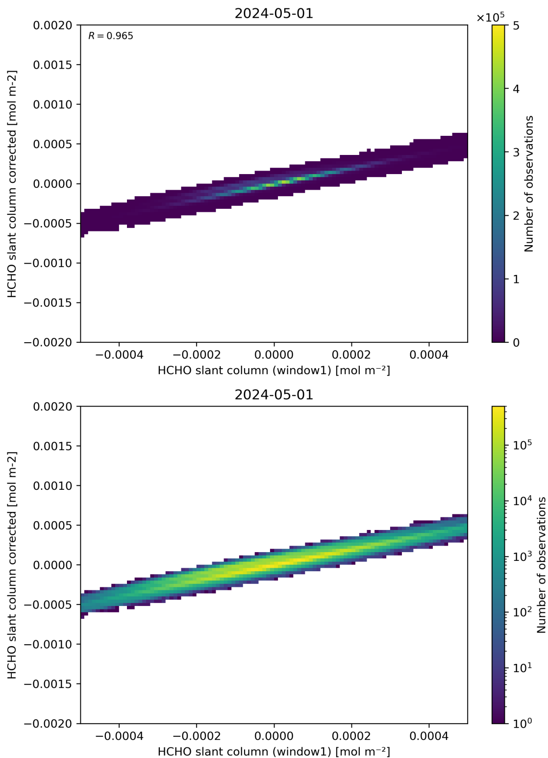
Figure 82: Scatter density plot of “HCHO slant column (window1)” against “HCHO slant column corrected” for 2024-04-30 to 2024-05-02.
