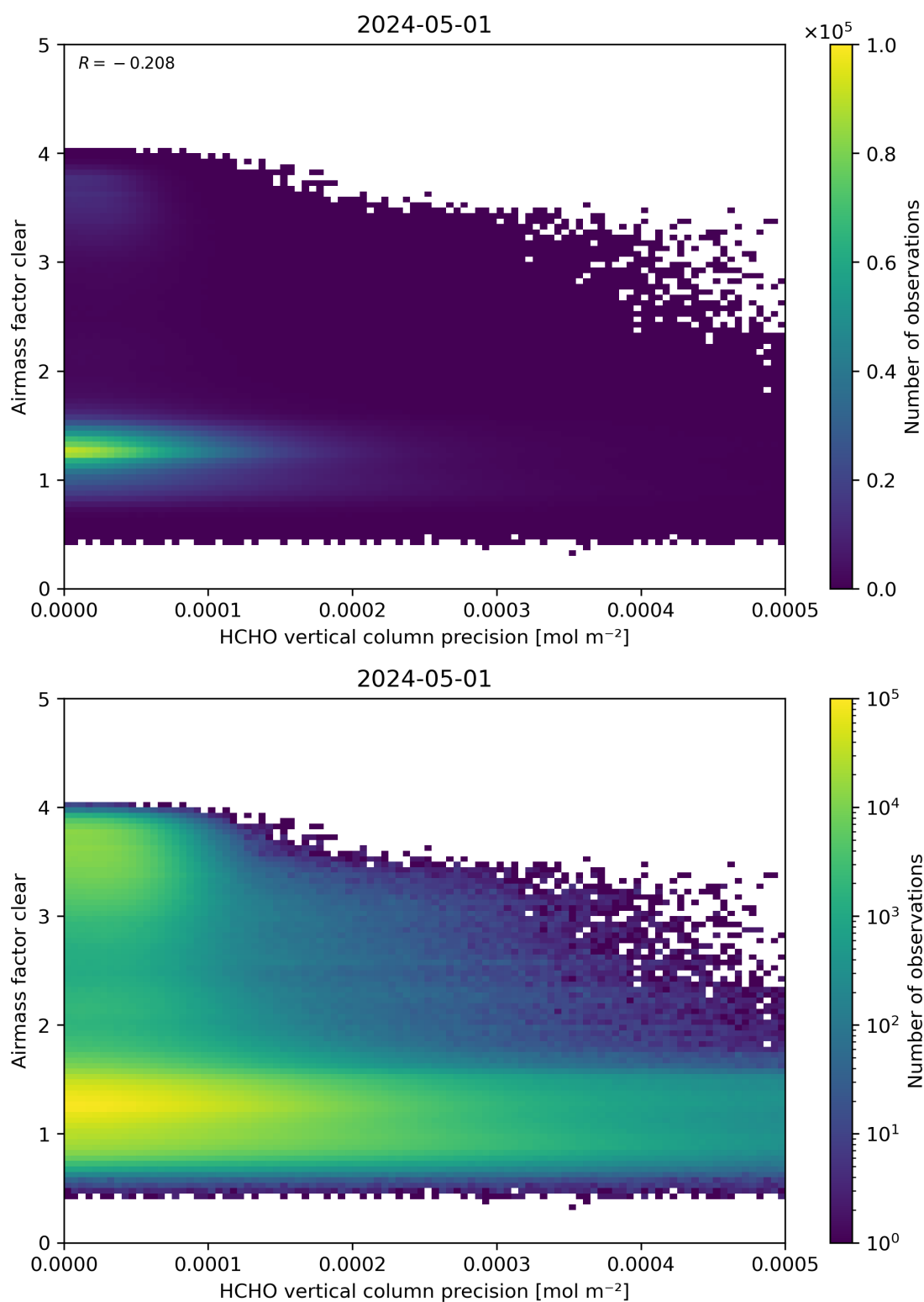
Figure 139: Scatter density plot of “HCHO vertical column precision” against “Airmass factor clear” for 2024-04-30 to 2024-05-02.
