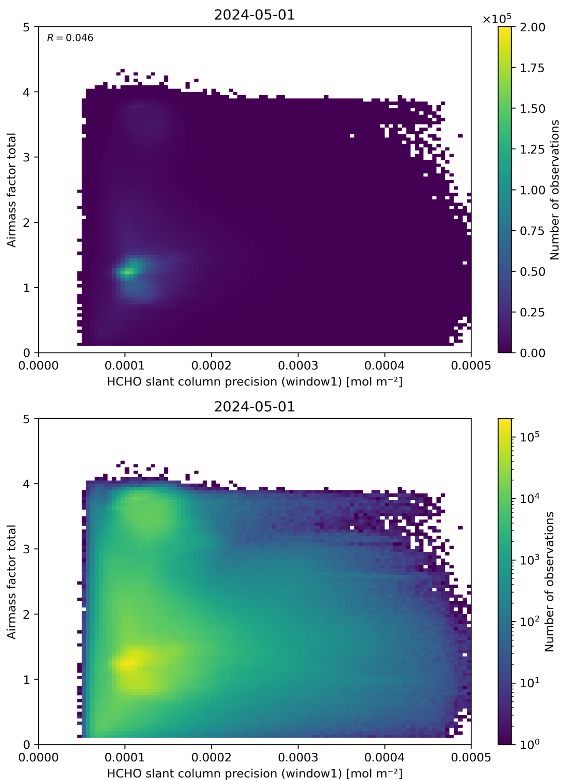
Figure 94: Scatter density plot of “HCHO slant column precision (window1)” against “Airmass factor total” for 2024-04-30 to 2024-05-02.
