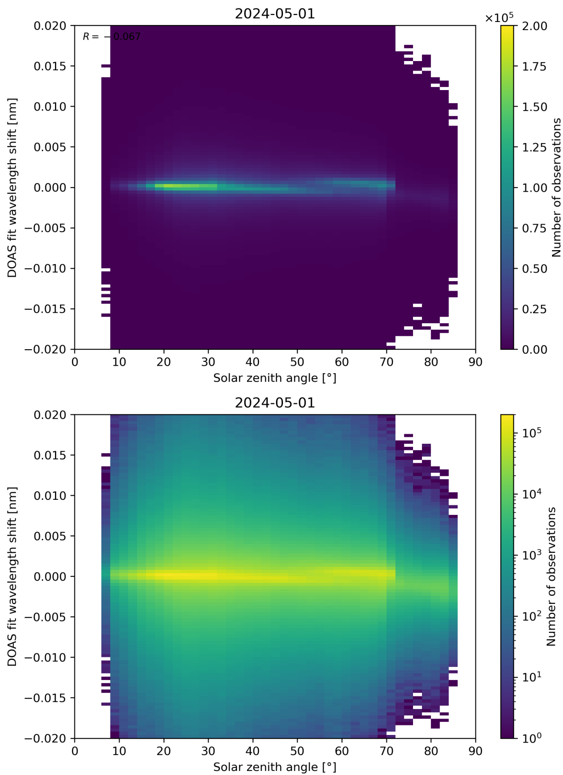
Figure 168: Scatter density plot of “Solar zenith angle” against “DOAS fit wavelength shift” for 2024-04-30 to 2024-05-02.
