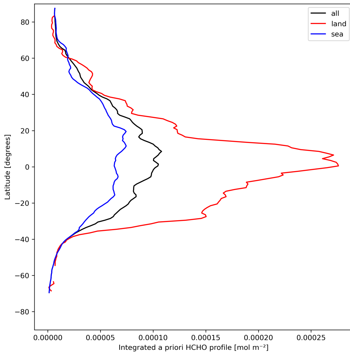
Figure 29: Zonal average of “Integrated a priori HCHO profile” for 2024-04-30 to 2024-05-02.
