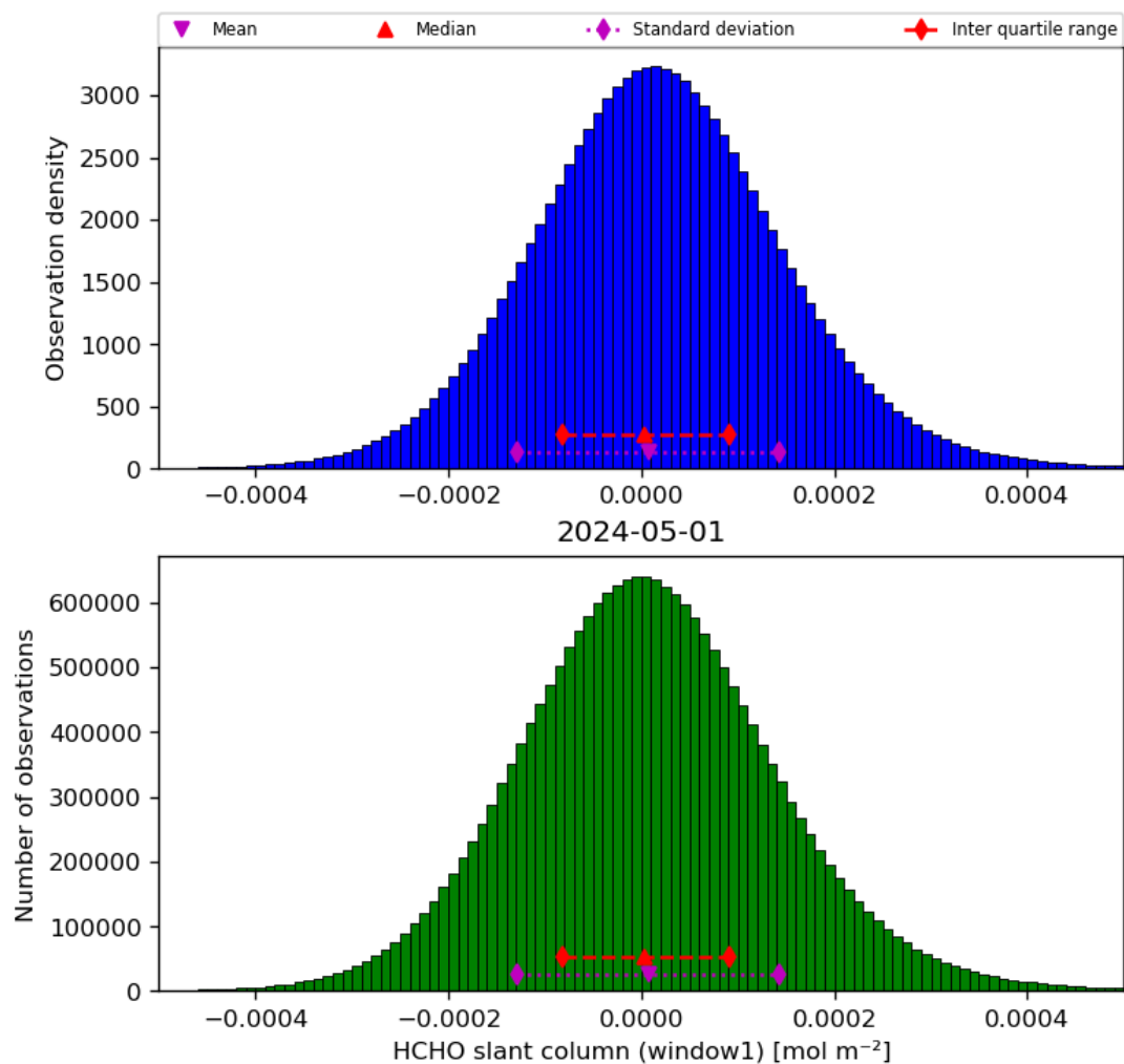
Figure 38: Histogram of “HCHO slant column (window1)” for 2024-04-30 to 2024-05-02
