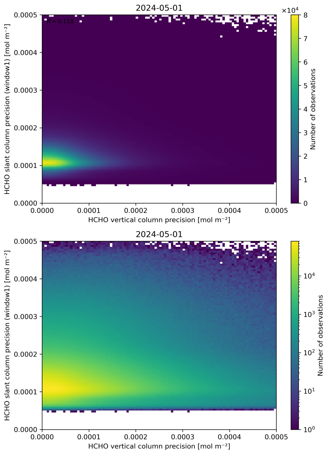
Figure 143: Scatter density plot of “HCHO vertical column precision” against “HCHO slant column precision (window1)” for 2024-04-30 to 2024-05-02.
