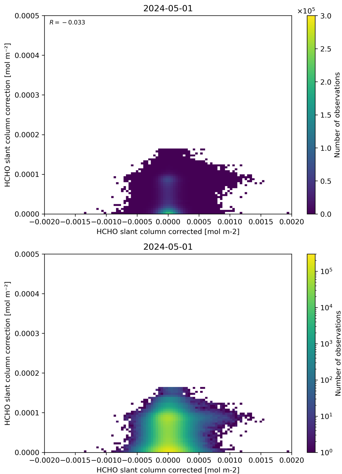
Figure 77: Scatter density plot of “HCHO slant column corrected” against “HCHO slant column correction” for 2024-04-30 to 2024-05-02.
