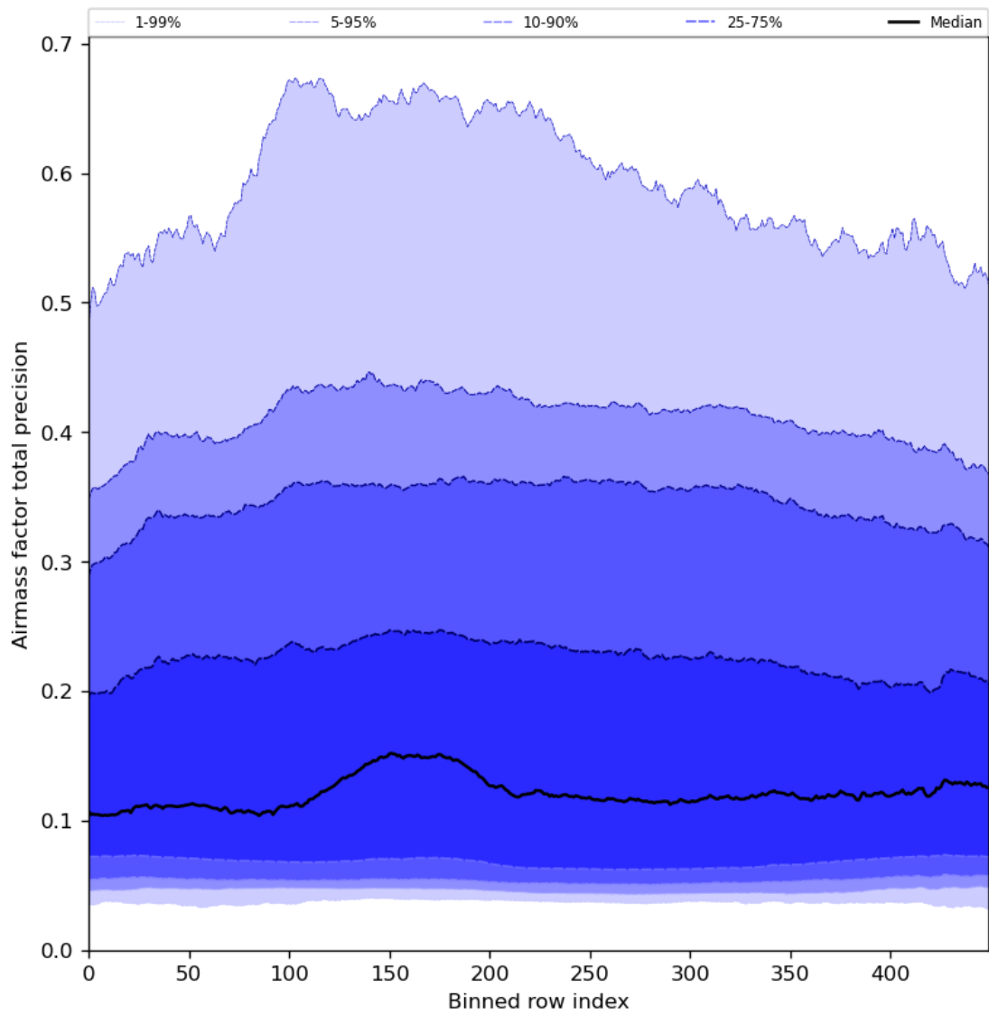
Figure 55: Along track statistics of “Airmass factor total precision” for 2024-04-30 to 2024-05-02
