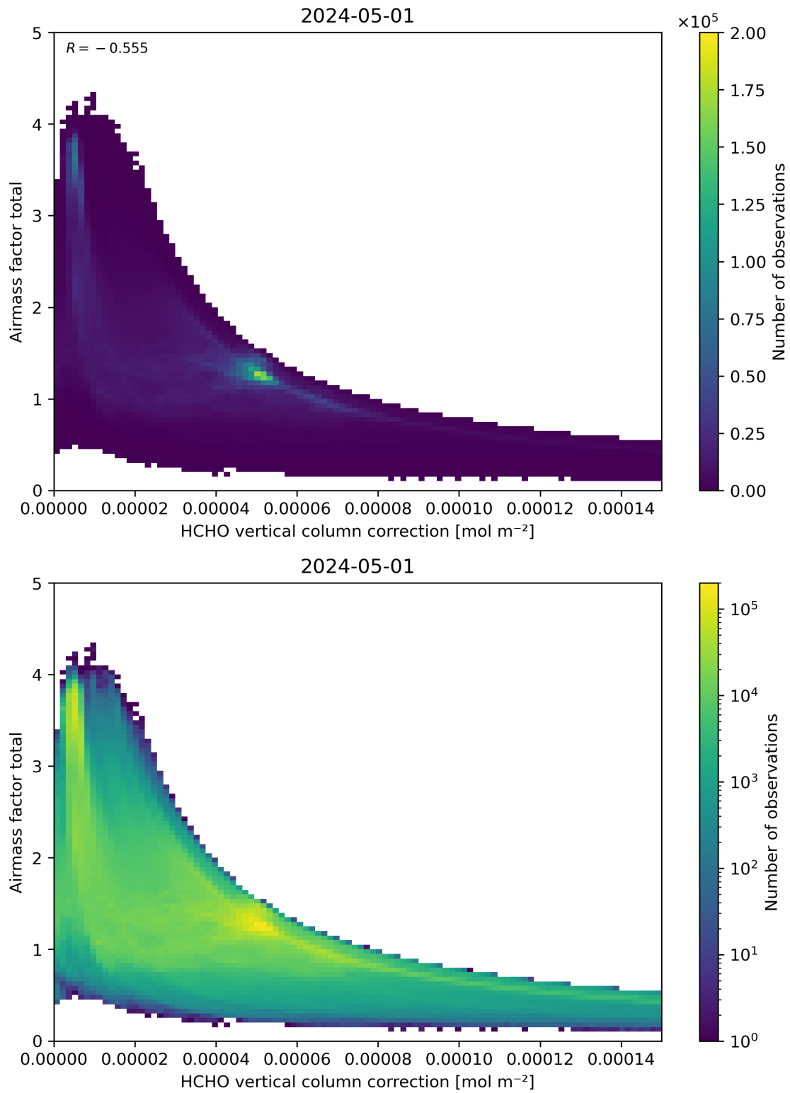
Figure 120: Scatter density plot of “HCHO vertical column correction” against “Airmass factor total” for 2024-04-30 to 2024-05-02.
