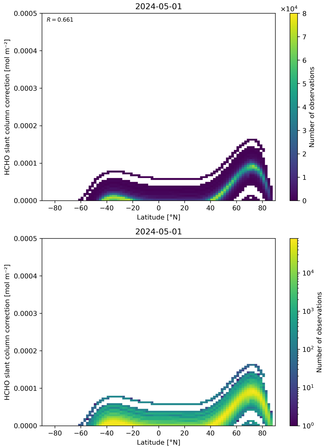
Figure 158: Scatter density plot of “Latitude” against “HCHO slant column correction” for 2024-04-30 to 2024-05-02.
