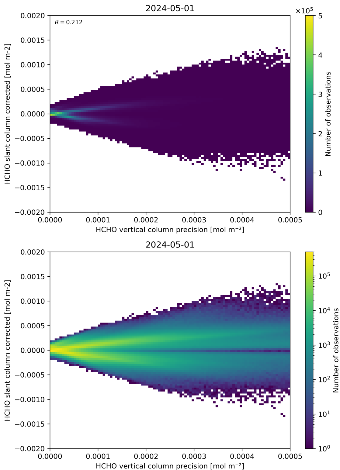
Figure 140: Scatter density plot of “HCHO vertical column precision” against “HCHO slant column corrected” for 2024-04-30 to 2024-05-02.
