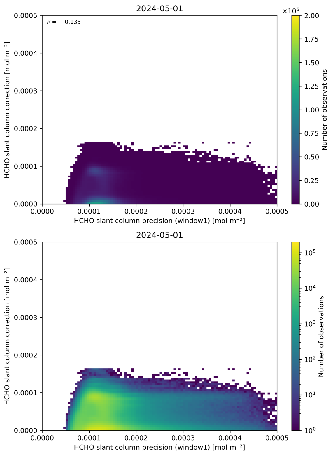
Figure 93: Scatter density plot of “HCHO slant column precision (window1)” against “HCHO slant column correction” for 2024-04-30 to 2024-05-02.
