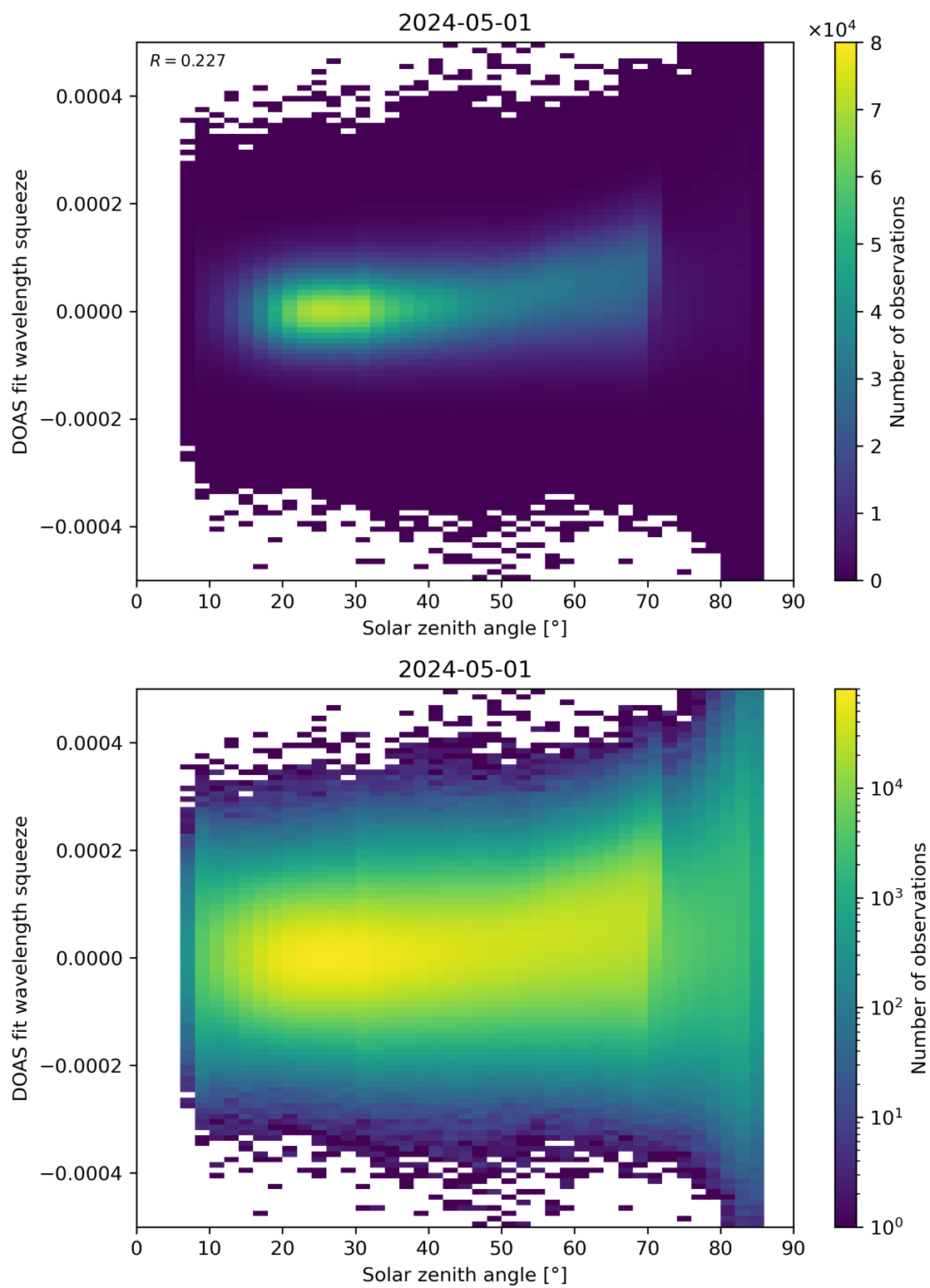
Figure 169: Scatter density plot of “Solar zenith angle” against “DOAS fit wavelength squeeze” for 2024-04-30 to 2024-05-02.
