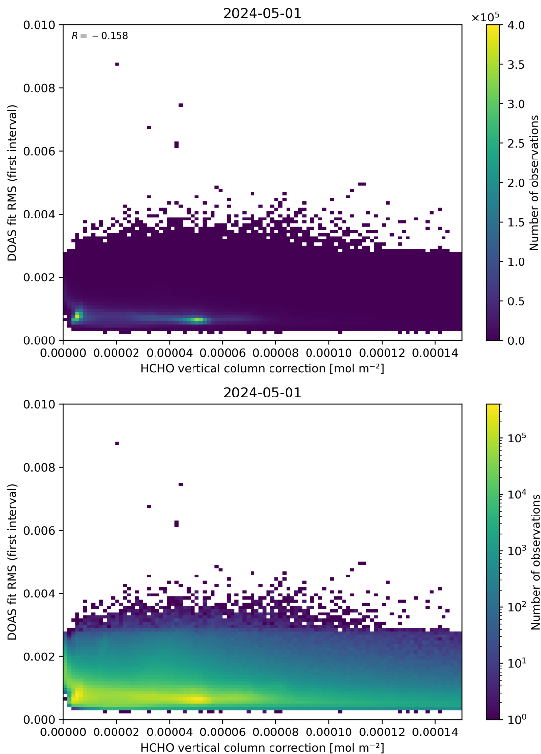
Figure 112: Scatter density plot of “HCHO vertical column correction” against “DOAS fit RMS (first interval)” for 2024-04-30 to 2024-05-02.
