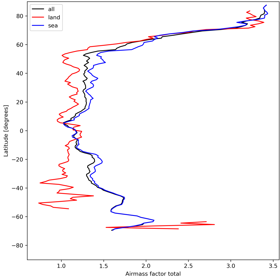
Figure 26: Zonal average of “Airmass factor total” for 2024-04-30 to 2024-05-02.
