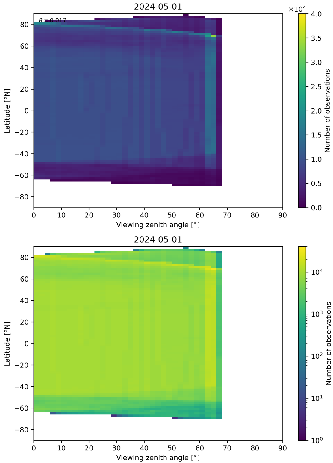
Figure 196: Scatter density plot of “Viewing zenith angle” against “Latitude” for 2024-04-30 to 2024-05-02.
