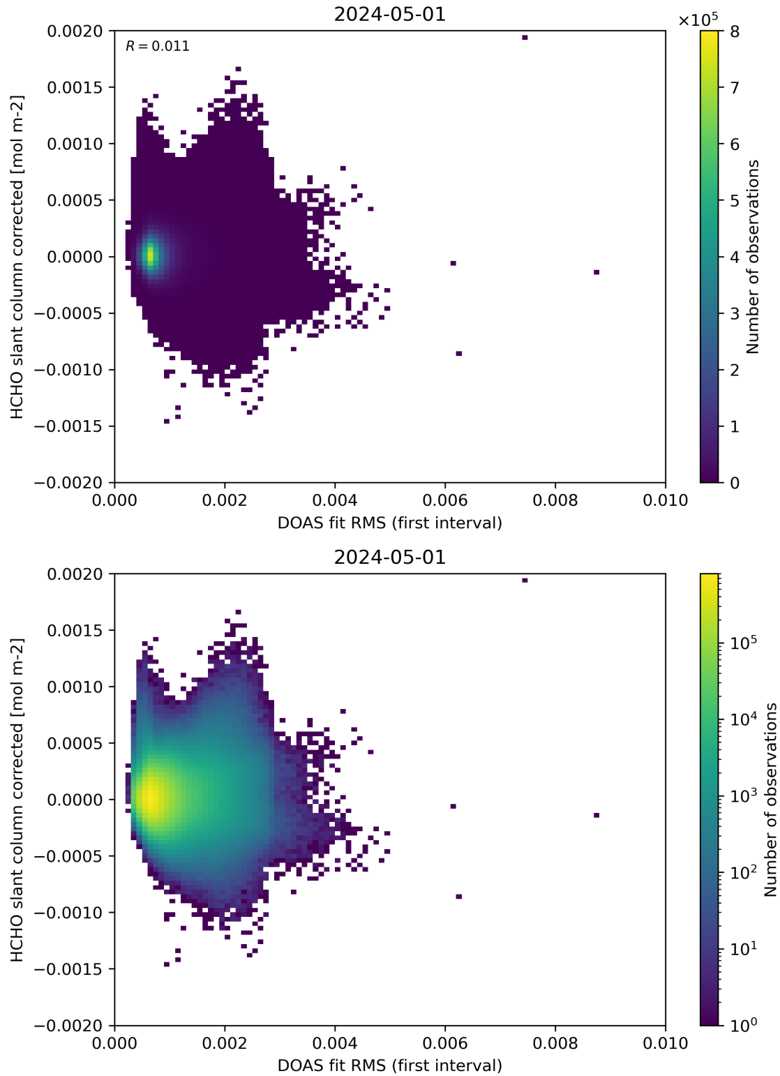
Figure 62: Scatter density plot of “DOAS fit RMS (first interval)” against “HCHO slant column corrected” for 2024-04-30 to 2024-05-02.
