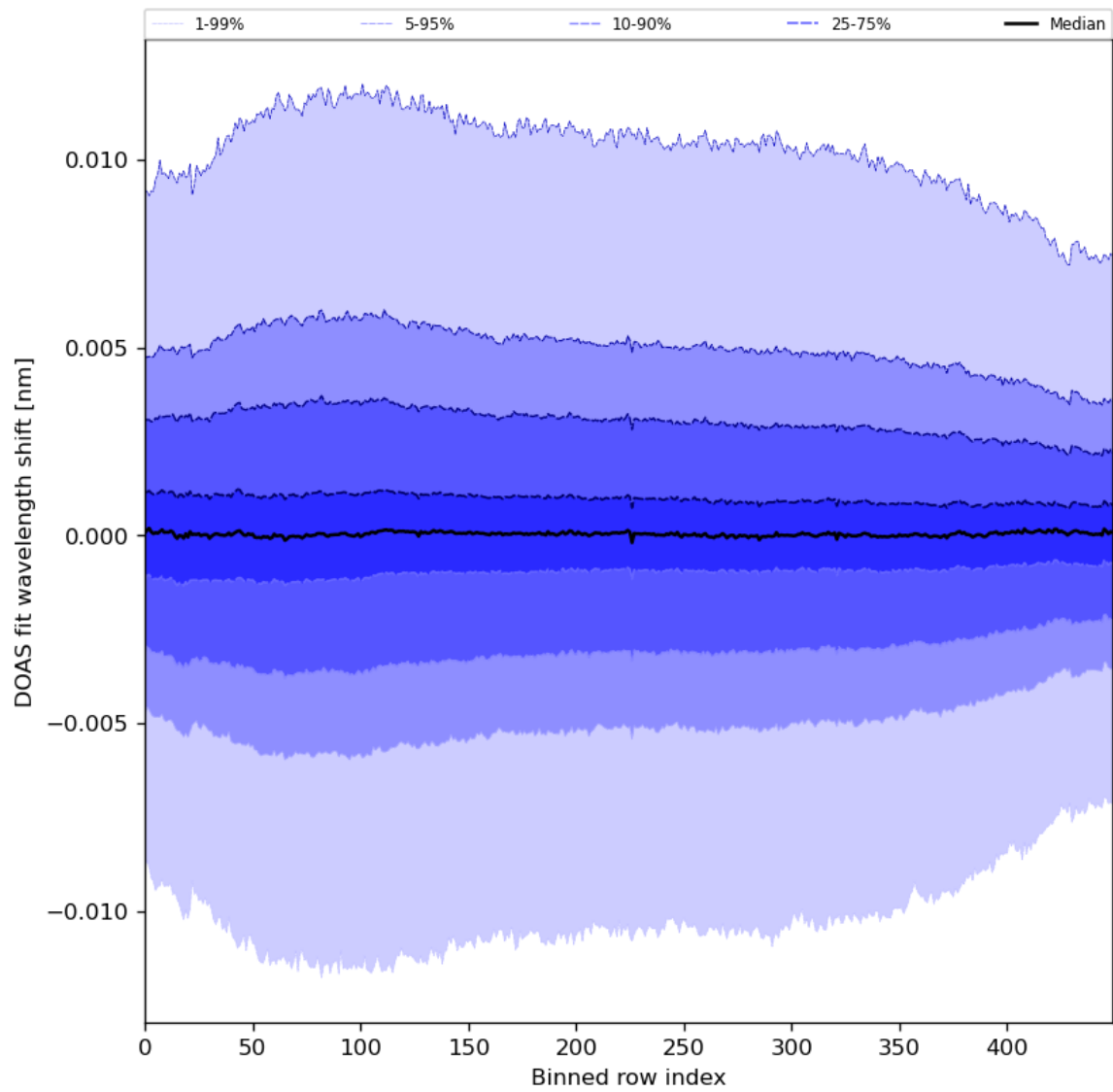
Figure 58: Along track statistics of “DOAS fit wavelength shift” for 2024-04-30 to 2024-05-02
