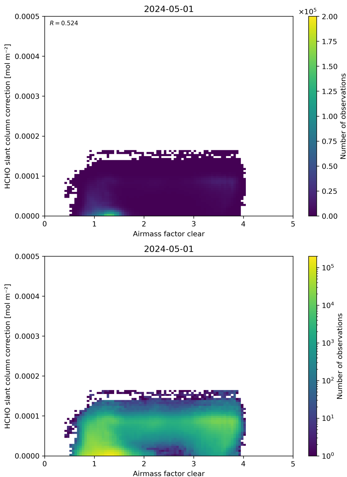
Figure 75: Scatter density plot of “Airmass factor clear” against “HCHO slant column correction” for 2024-04-30 to 2024-05-02.
