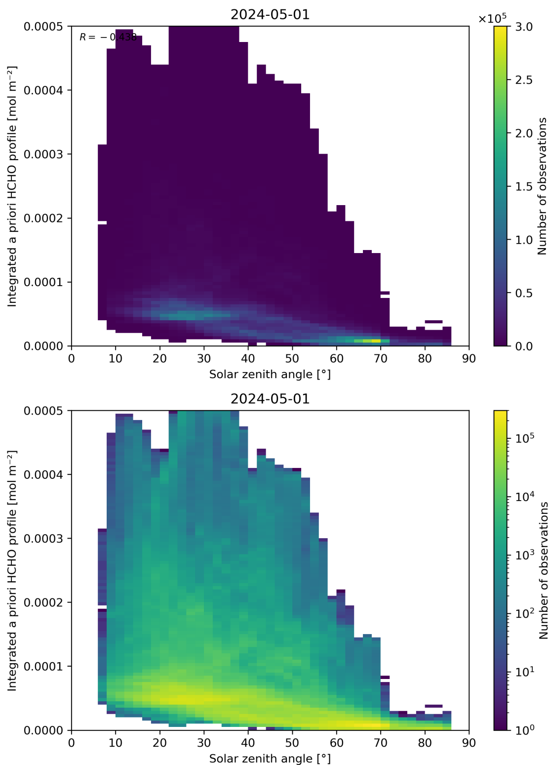
Figure 180: Scatter density plot of “Solar zenith angle” against “Integrated a priori HCHO profile” for 2024-04-30 to 2024-05-02.
