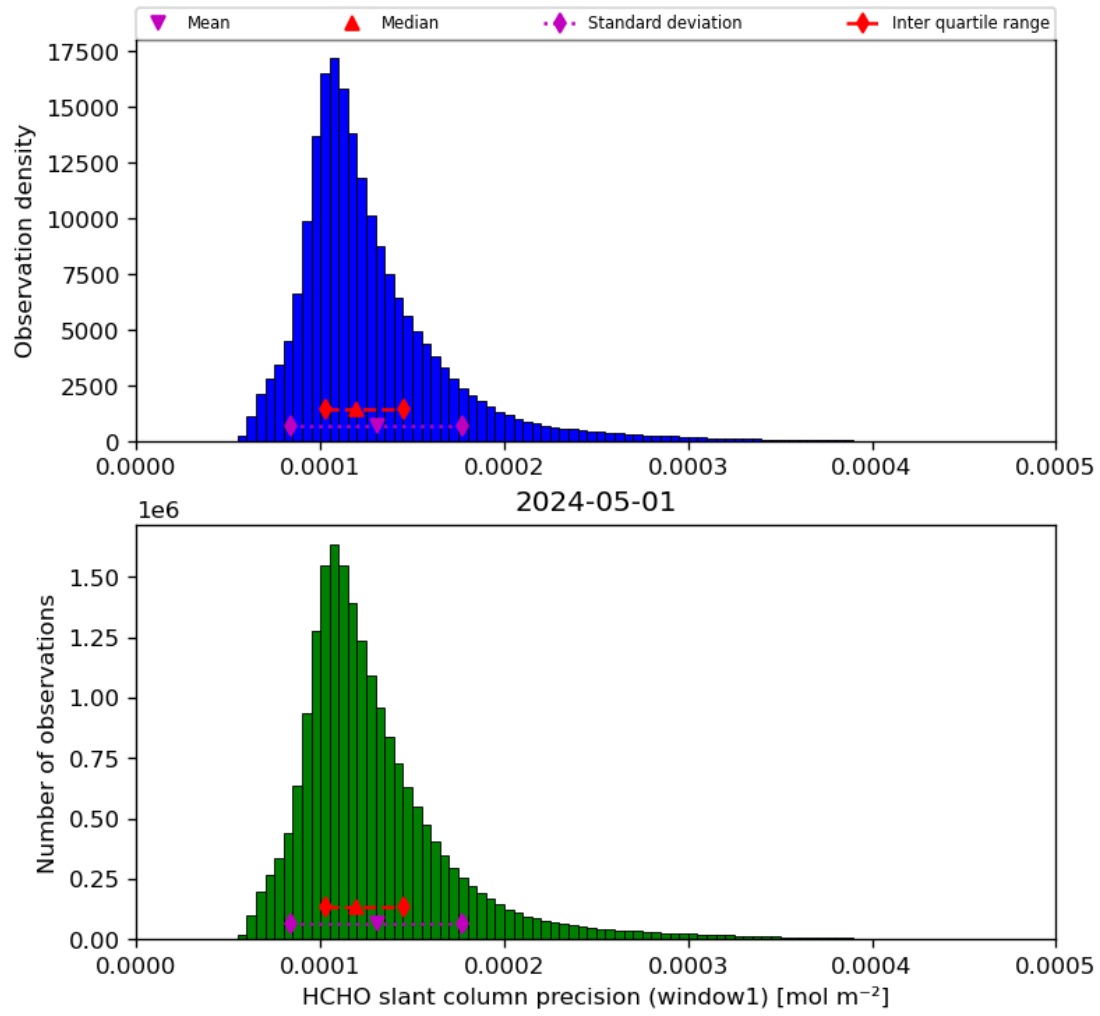
Figure 39: Histogram of “HCHO slant column precision (window1)” for 2024-04-30 to 2024-05-02
