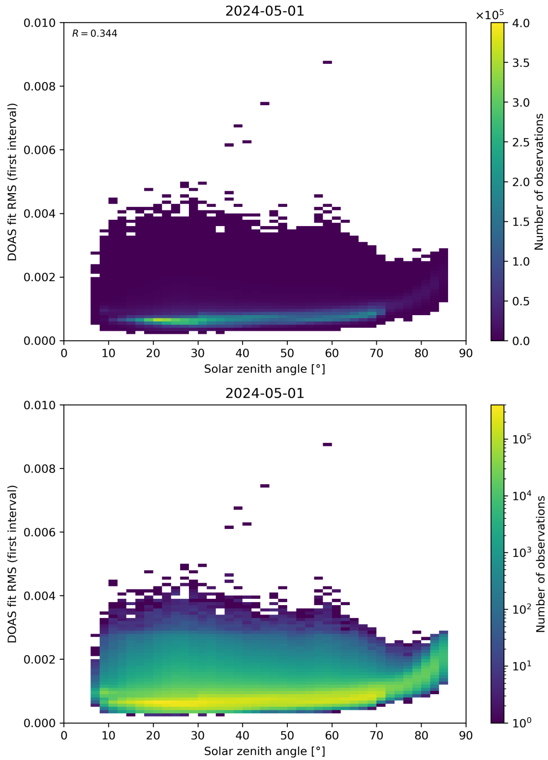
Figure 167: Scatter density plot of “Solar zenith angle” against “DOAS fit RMS (first interval)” for 2024-04-30 to 2024-05-02.
