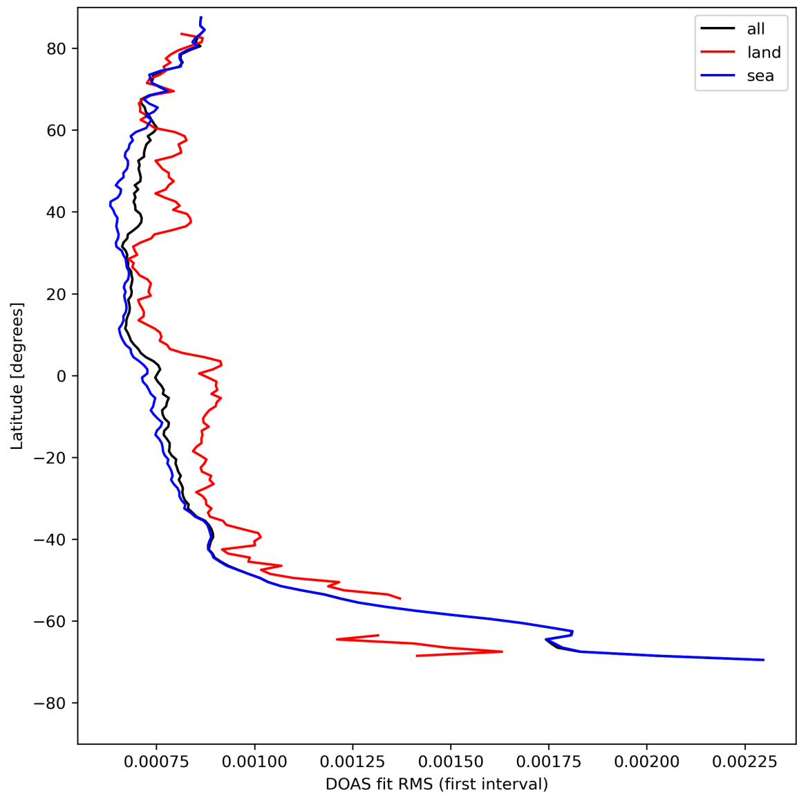
Figure 32: Zonal average of “DOAS fit RMS (first interval)” for 2024-04-30 to 2024-05-02.
