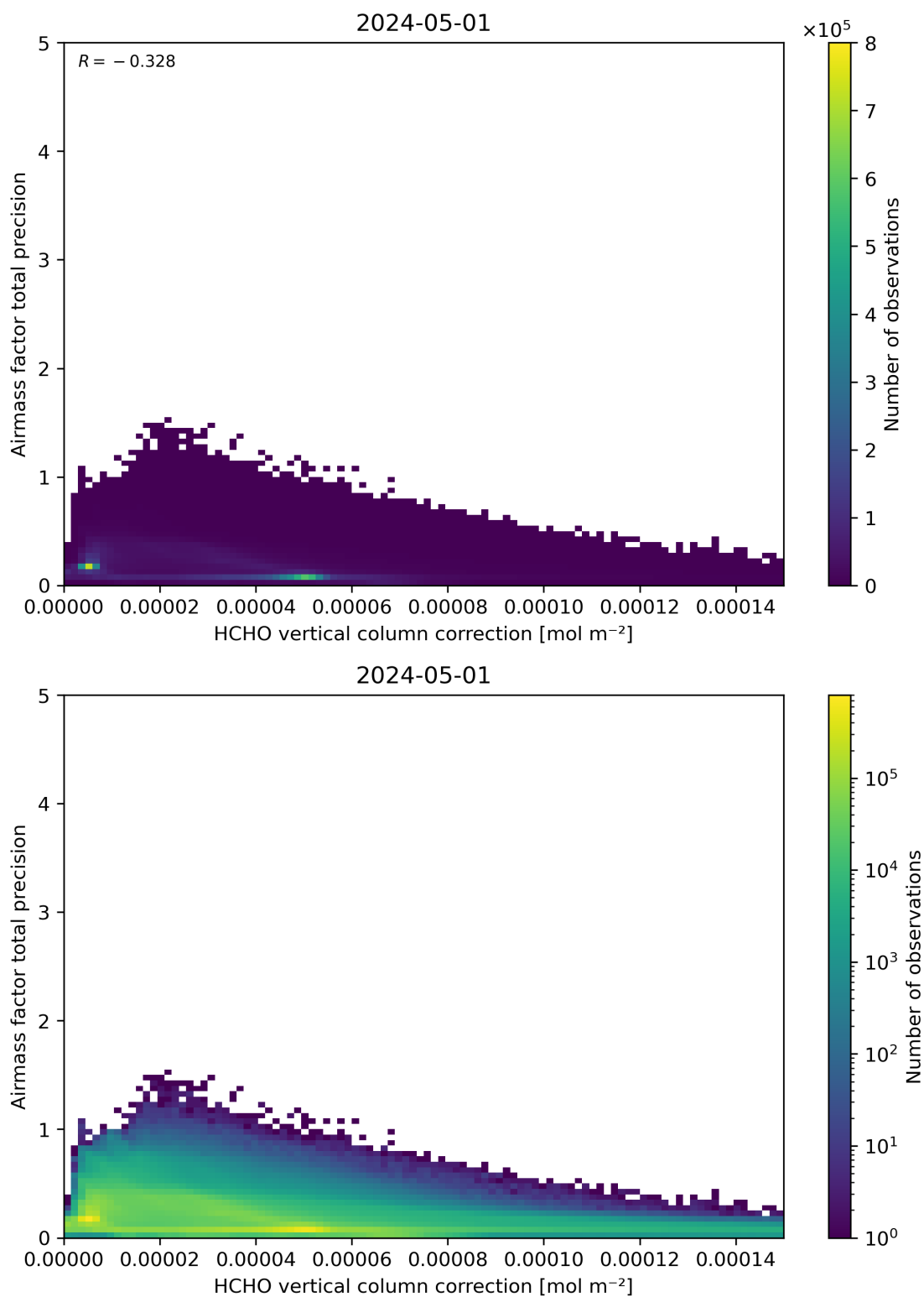
Figure 121: Scatter density plot of “HCHO vertical column correction” against “Airmass factor total precision” for 2024-04-30 to 2024-05-02.
