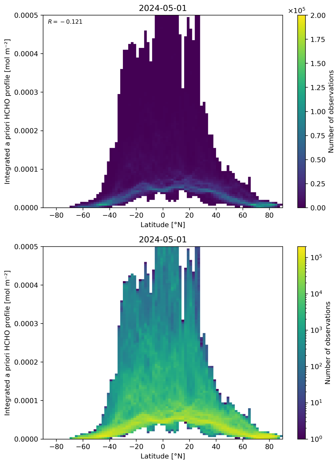
Figure 166: Scatter density plot of “Latitude” against “Integrated a priori HCHO profile” for 2024-04-30 to 2024-05-02.
