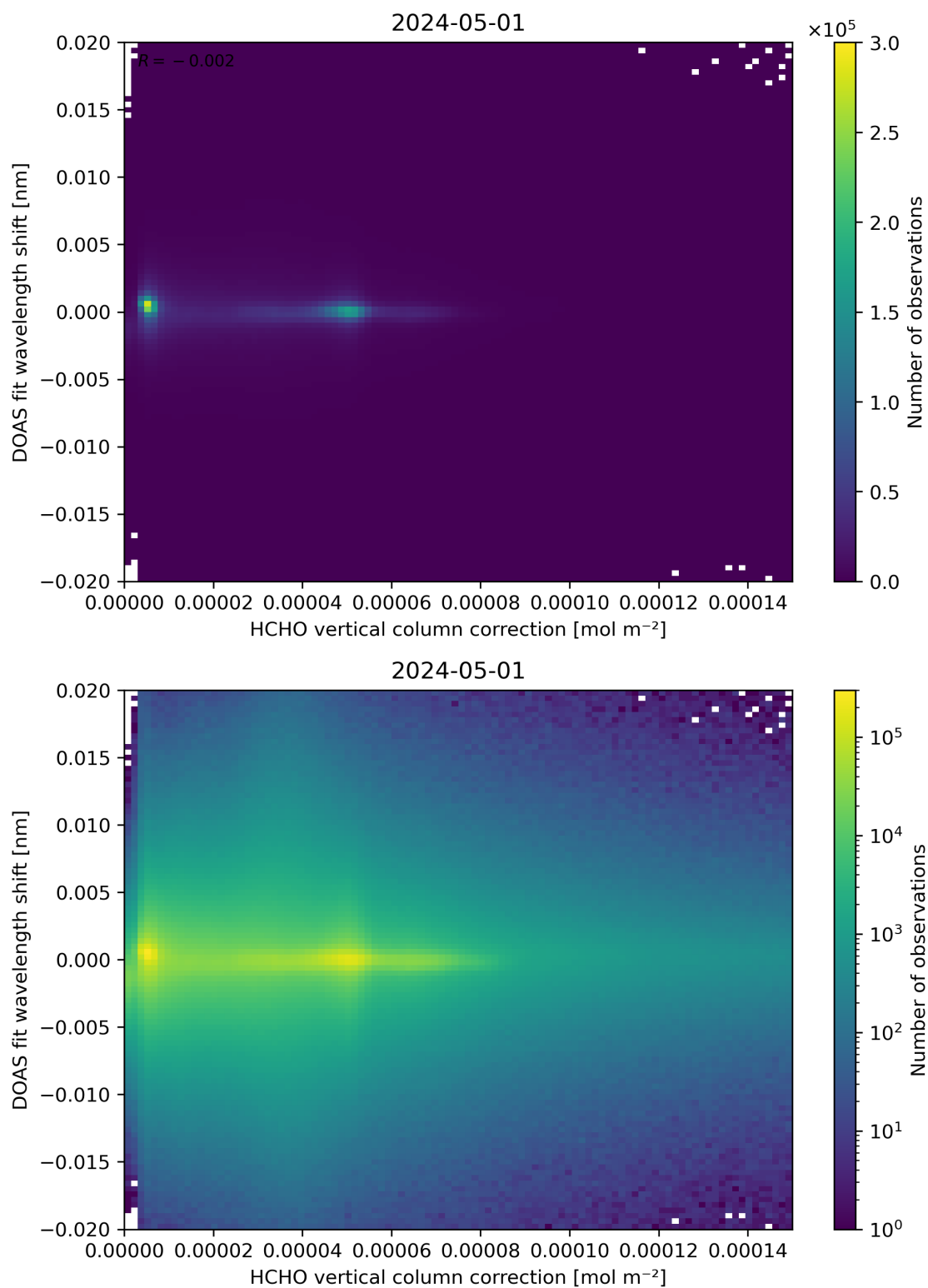
Figure 113: Scatter density plot of “HCHO vertical column correction” against “DOAS fit wavelength shift” for 2024-04-30 to 2024-05-02.
