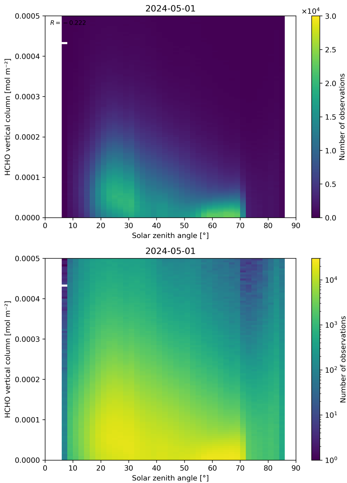
Figure 177: Scatter density plot of “Solar zenith angle” against “HCHO vertical column” for 2024-04-30 to 2024-05-02.
