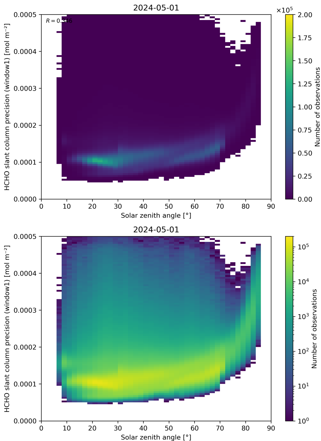
Figure 174: Scatter density plot of “Solar zenith angle” against “HCHO slant column precision (window1)” for 2024-04-30 to 2024-05-02.
