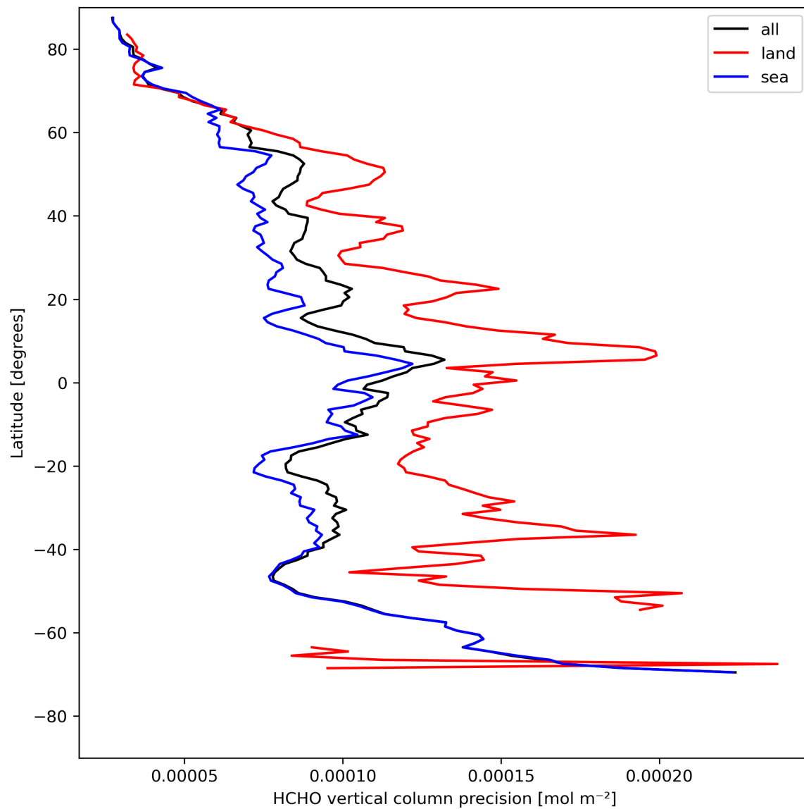
Figure 22: Zonal average of “HCHO vertical column precision” for 2024-04-30 to 2024-05-02.
