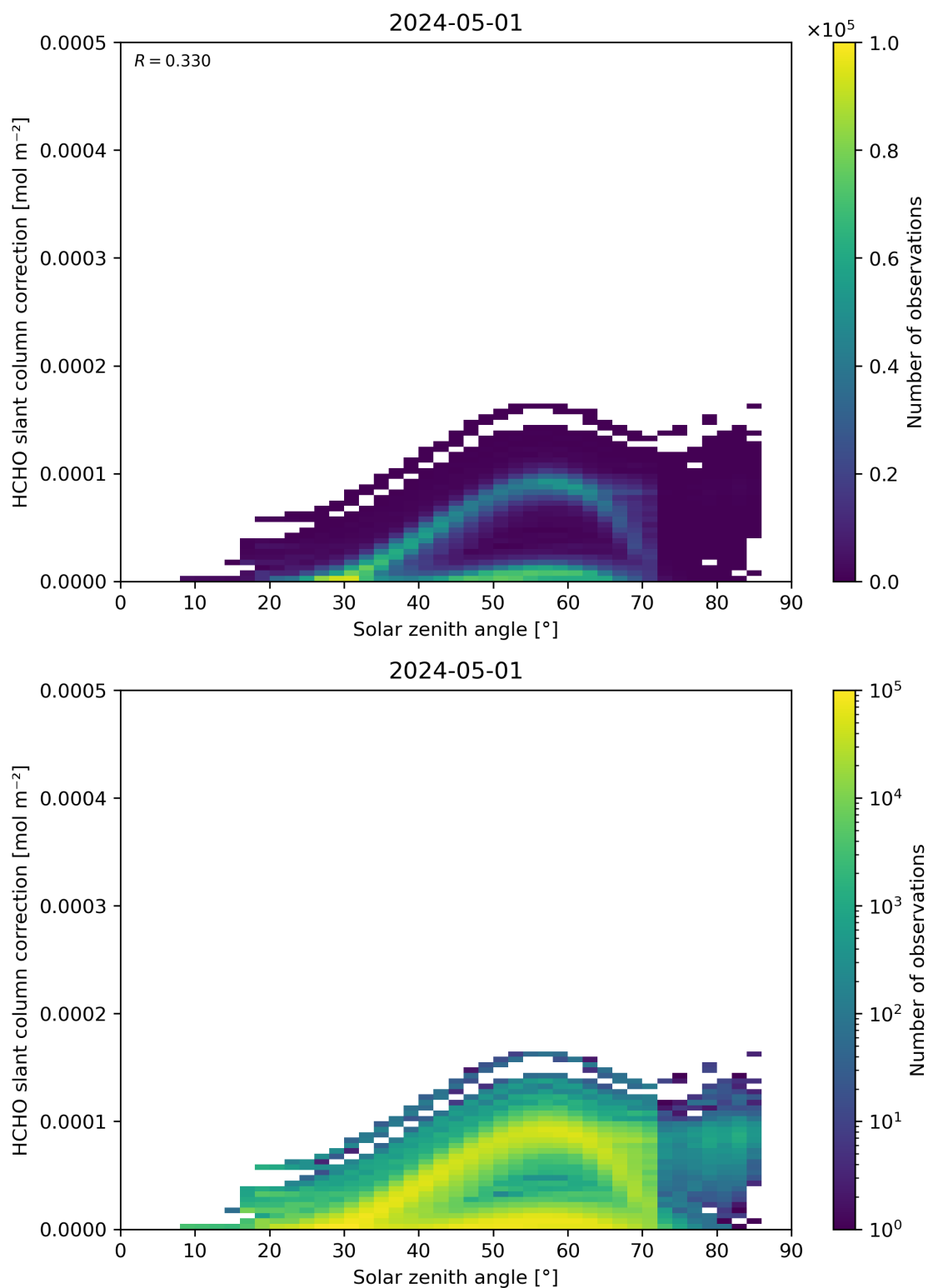
Figure 172: Scatter density plot of “Solar zenith angle” against “HCHO slant column correction” for 2024-04-30 to 2024-05-02.
