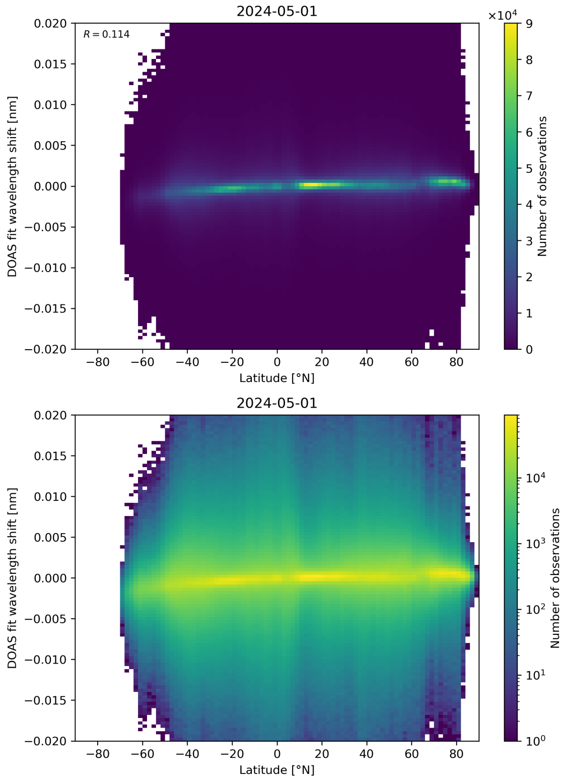
Figure 154: Scatter density plot of “Latitude” against “DOAS fit wavelength shift” for 2024-04-30 to 2024-05-02.
