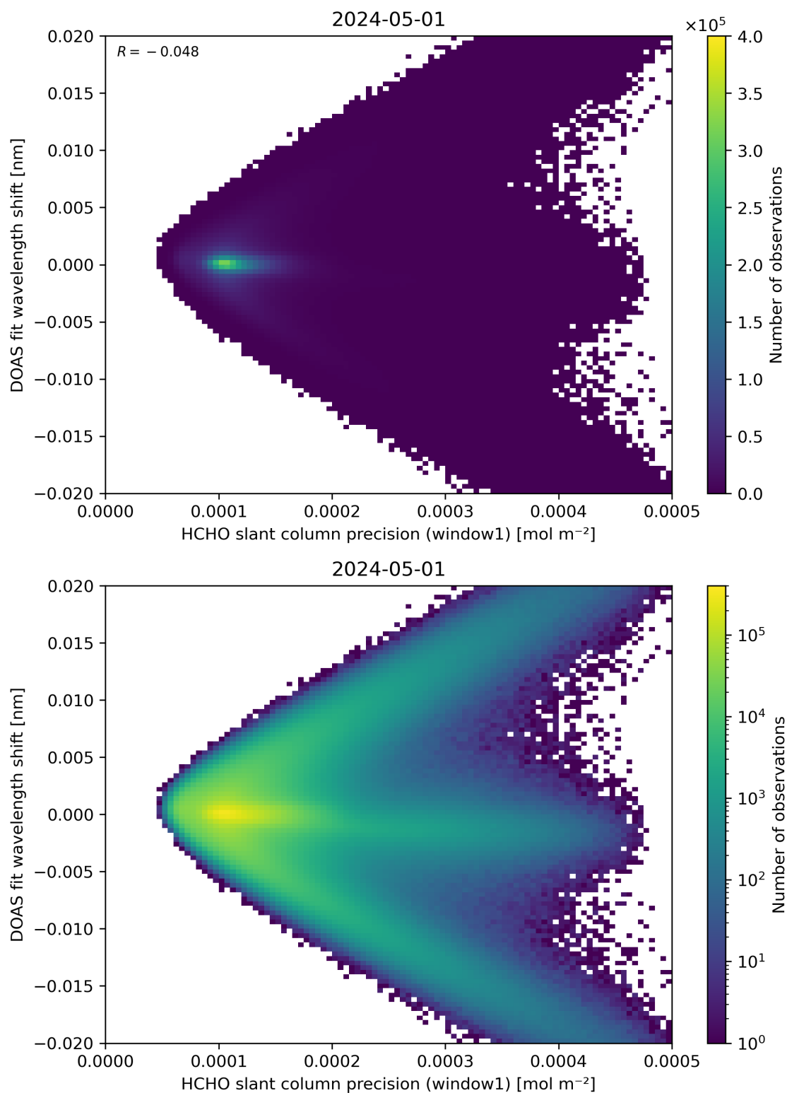
Figure 89: Scatter density plot of “HCHO slant column precision (window1)” against “DOAS fit wavelength shift” for 2024-04-30 to 2024-05-02.
