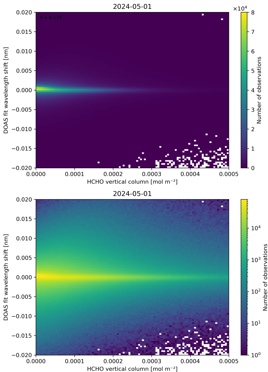
Figure 124: Scatter density plot of “HCHO vertical column” against “DOAS fit wavelength shift” for 2024-04-30 to 2024-05-02.
