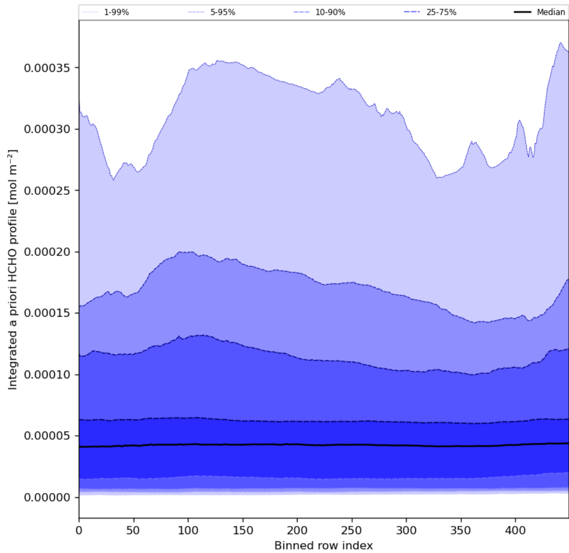
Figure 57: Along track statistics of "Integrated a priori HCHO profile" for 2024-04-30 to 2024-05-02
