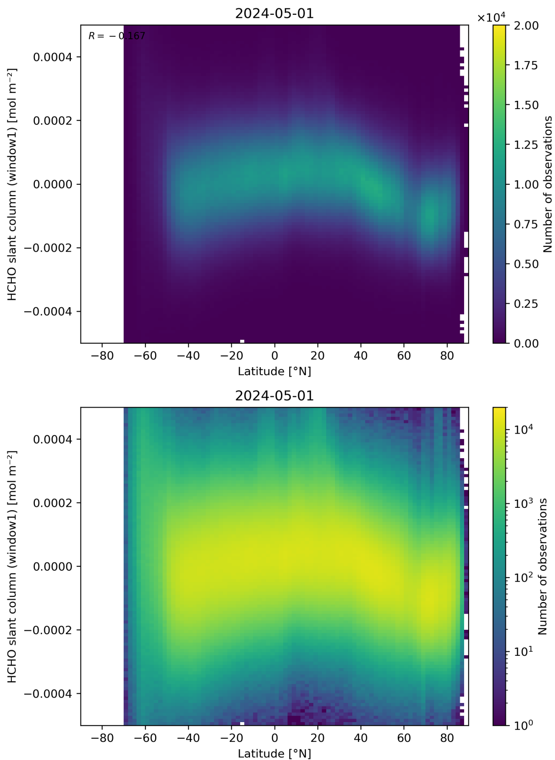
Figure 159: Scatter density plot of “Latitude” against “HCHO slant column (window1)” for 2024-04-30 to 2024-05-02.
