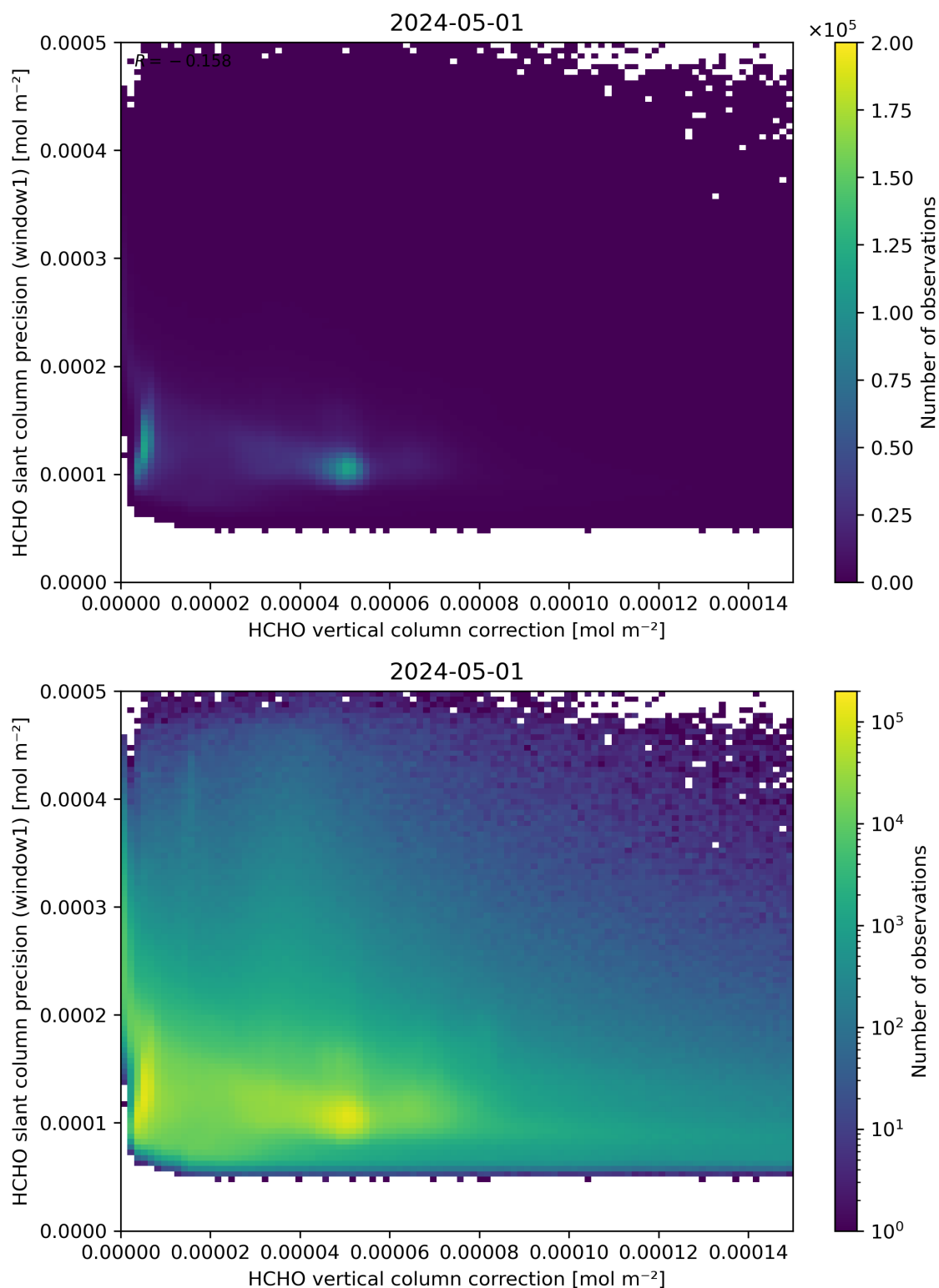
Figure 119: Scatter density plot of “HCHO vertical column correction” against “HCHO slant column precision (window1)” for 2024-04-30 to 2024-05-02.
