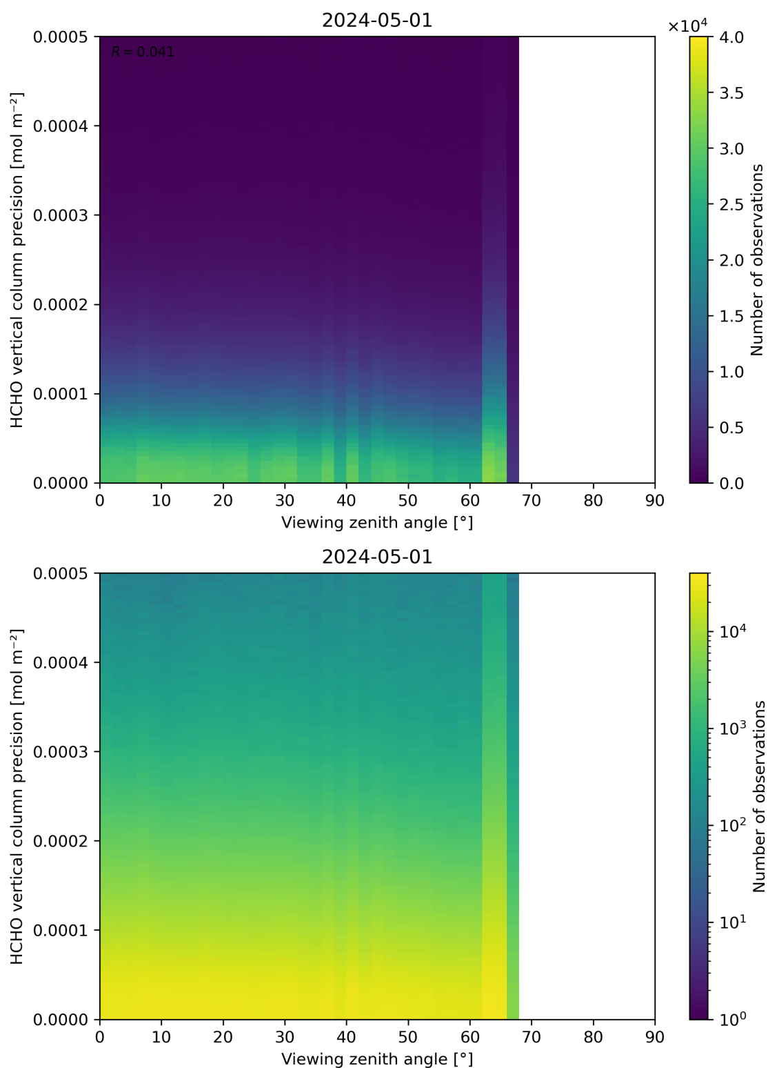
Figure 194: Scatter density plot of “Viewing zenith angle” against “HCHO vertical column precision” for 2024-04-30 to 2024-05-02.
