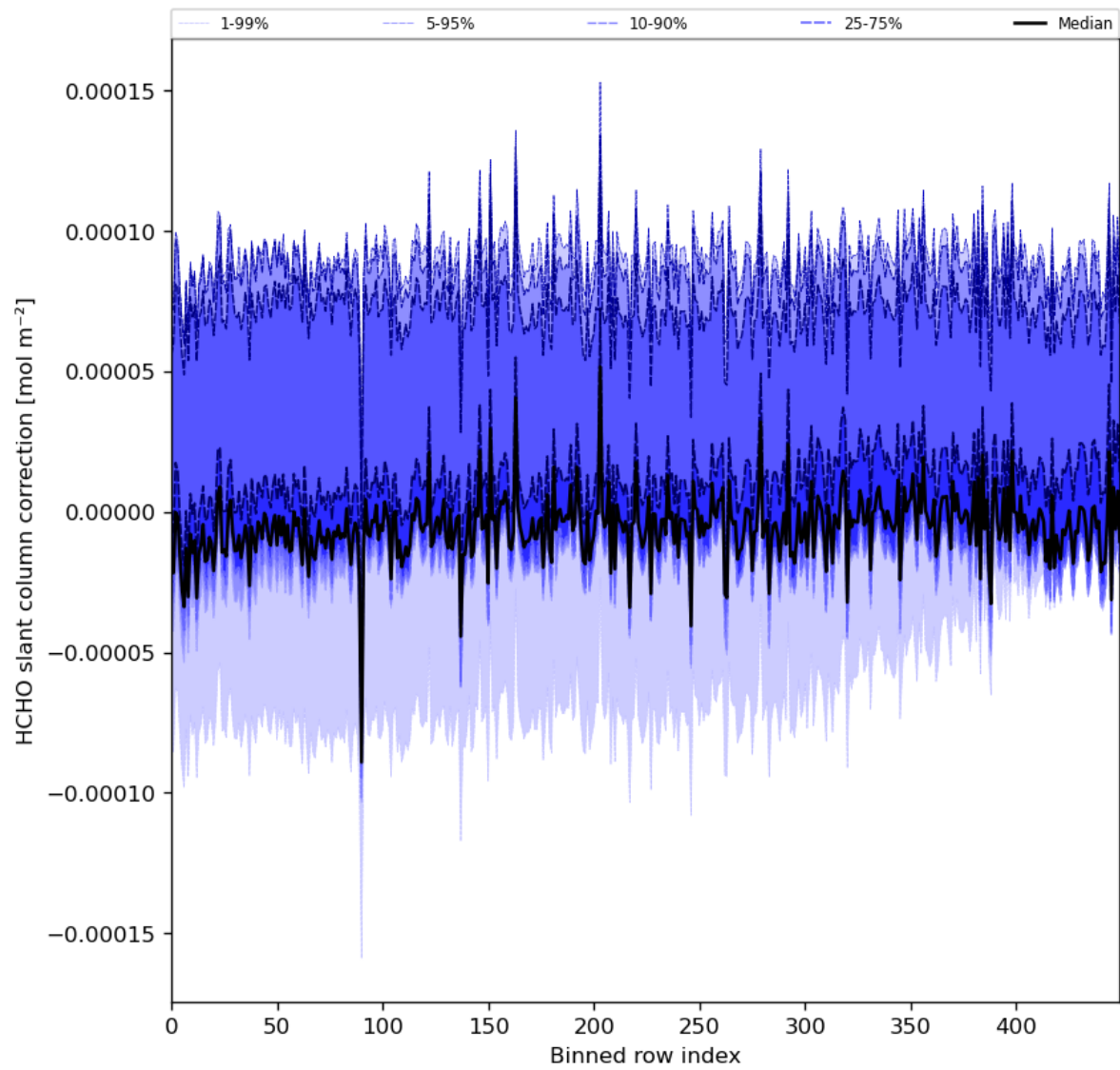
Figure 61: Along track statistics of “HCHO slant column correction” for 2024-04-30 to 2024-05-02
