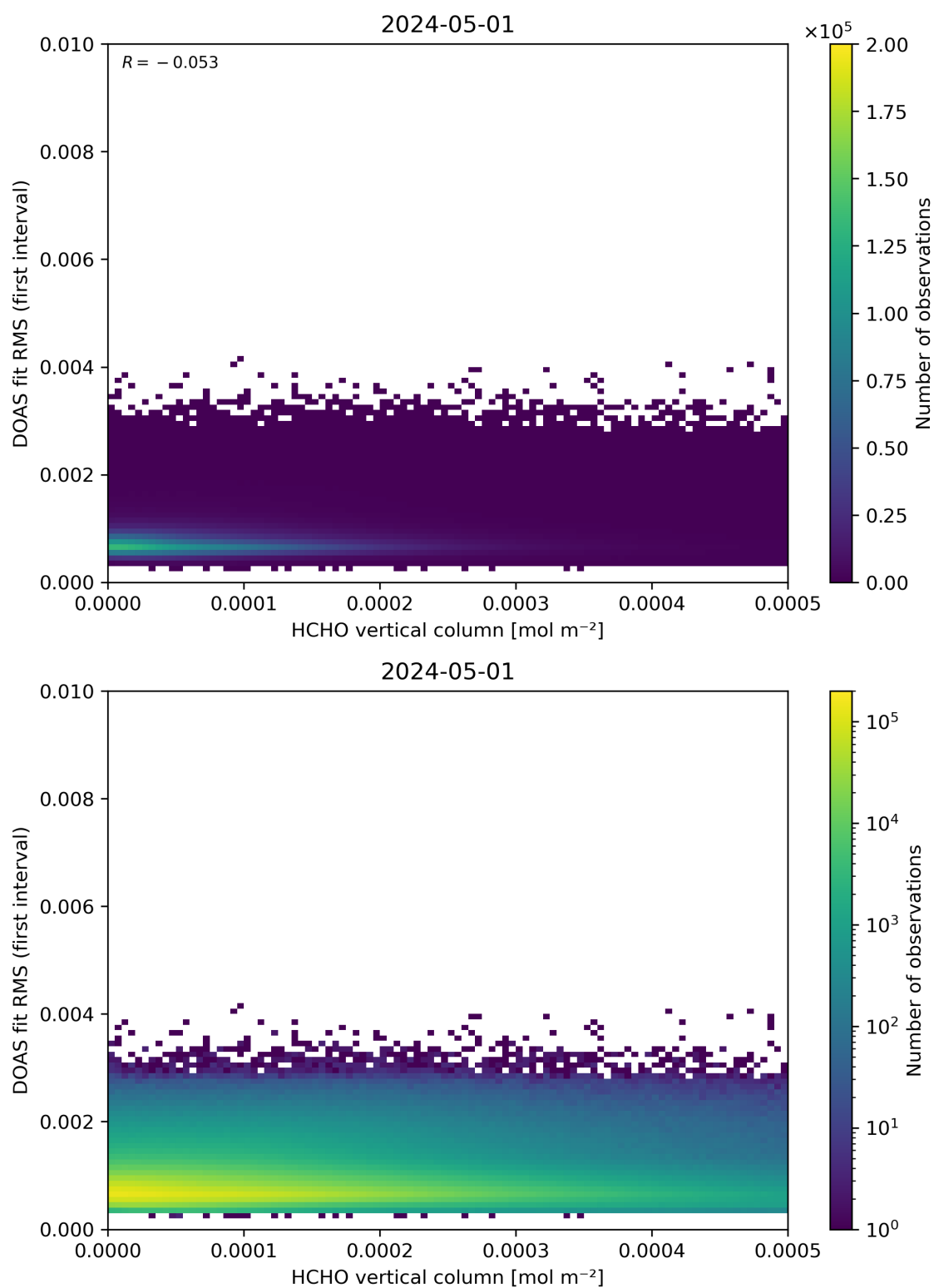
Figure 123: Scatter density plot of “HCHO vertical column” against “DOAS fit RMS (first interval)” for 2024-04-30 to 2024-05-02.
