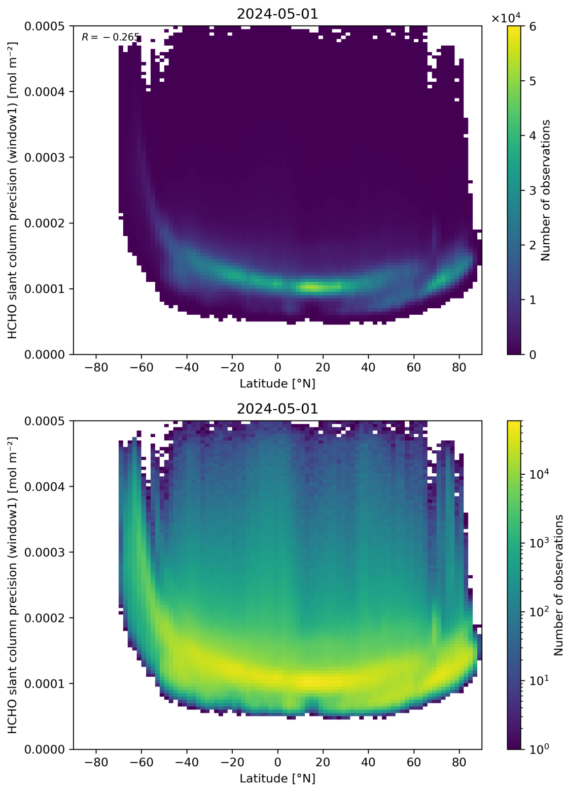
Figure 160: Scatter density plot of “Latitude” against “HCHO slant column precision (window1)” for 2024-04-30 to 2024-05-02.
