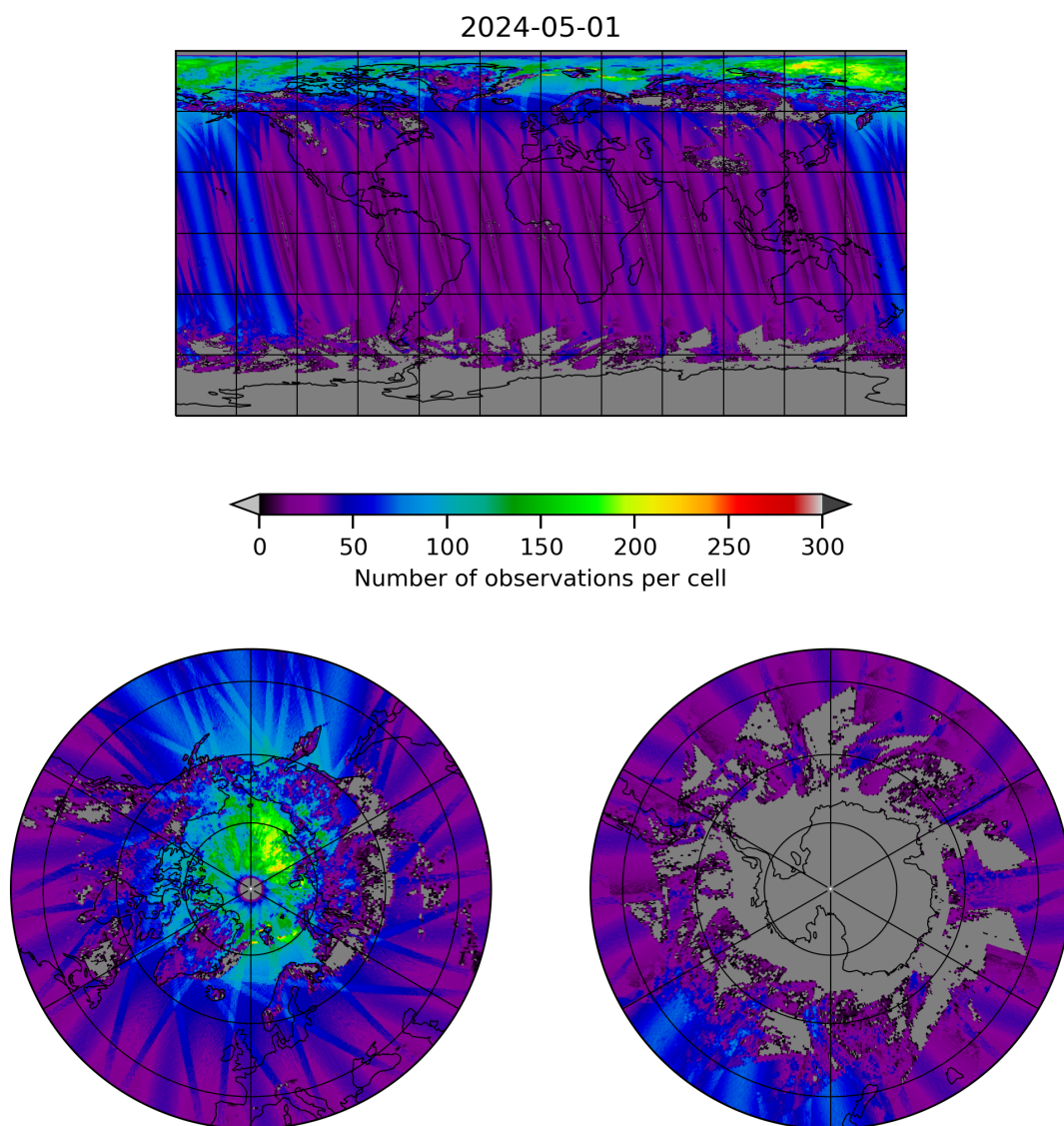
Figure 19: Map of the number of observations for 2024-04-30 to 2024-05-02
