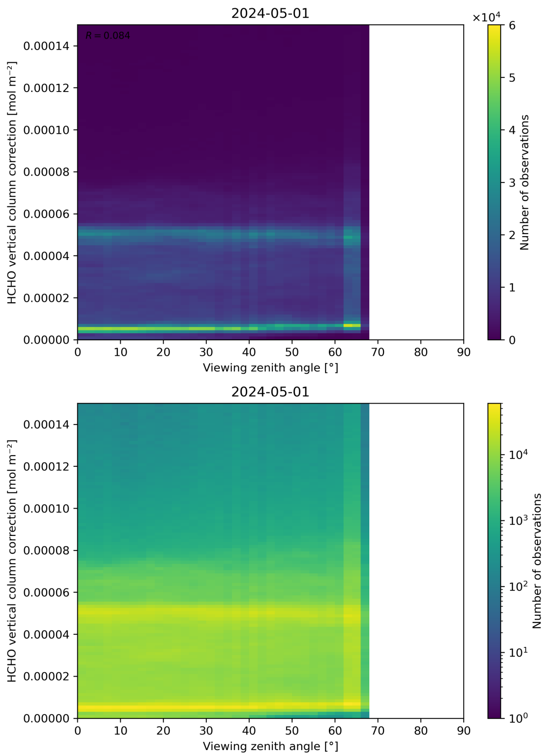
Figure 193: Scatter density plot of “Viewing zenith angle” against “HCHO vertical column correction” for 2024-04-30 to 2024-05-02.
