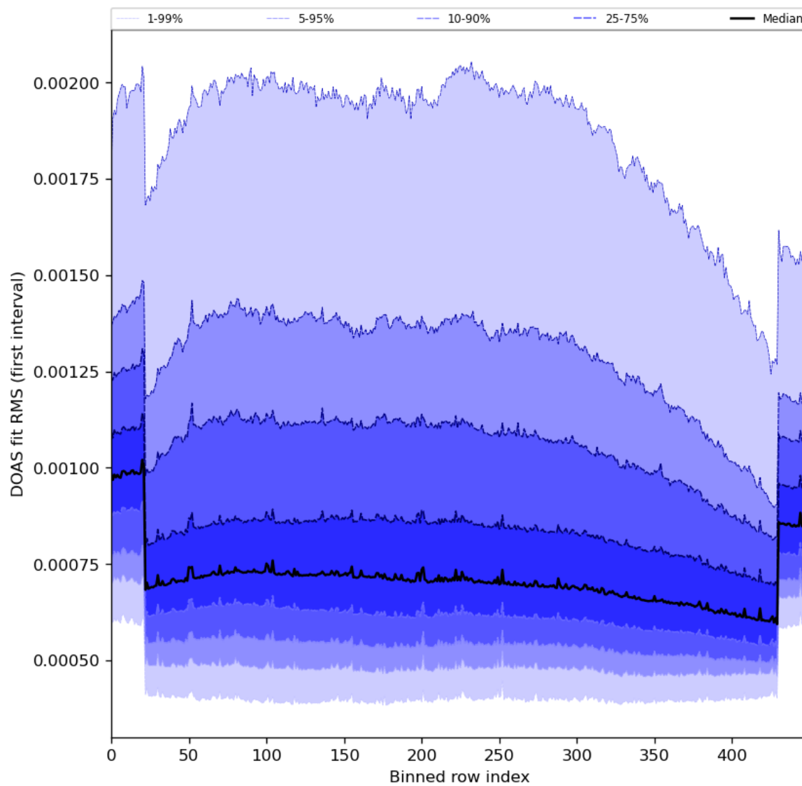
Figure 60: Along track statistics of “DOAS fit RMS (first interval)” for 2024-04-30 to 2024-05-02
