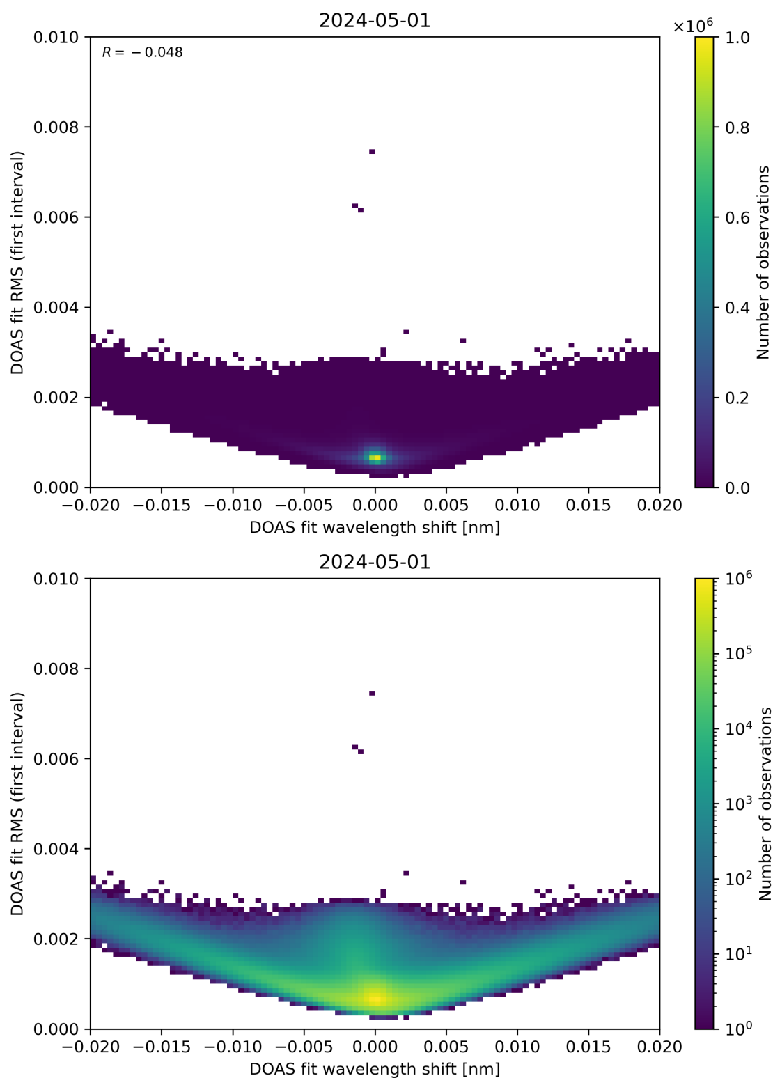
Figure 64: Scatter density plot of “DOAS fit wavelength shift” against “DOAS fit RMS (first interval)” for 2024-04-30 to 2024-05-02.
