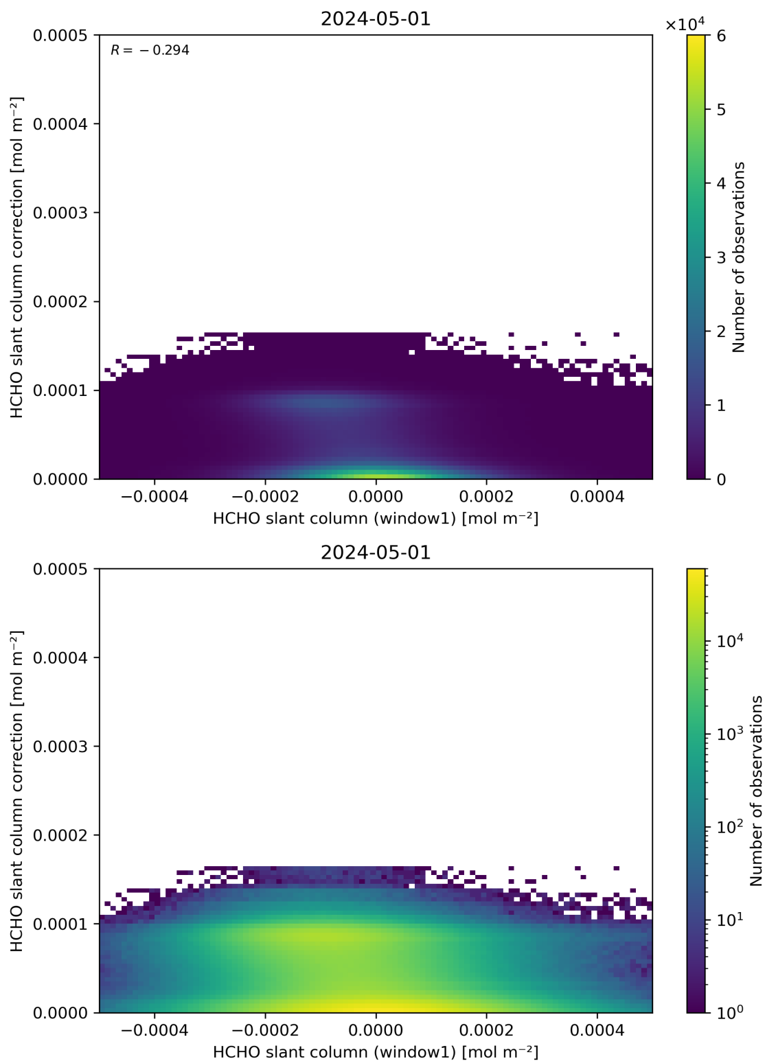
Figure 83: Scatter density plot of “HCHO slant column (window1)” against “HCHO slant column correction” for 2024-04-30 to 2024-05-02.
