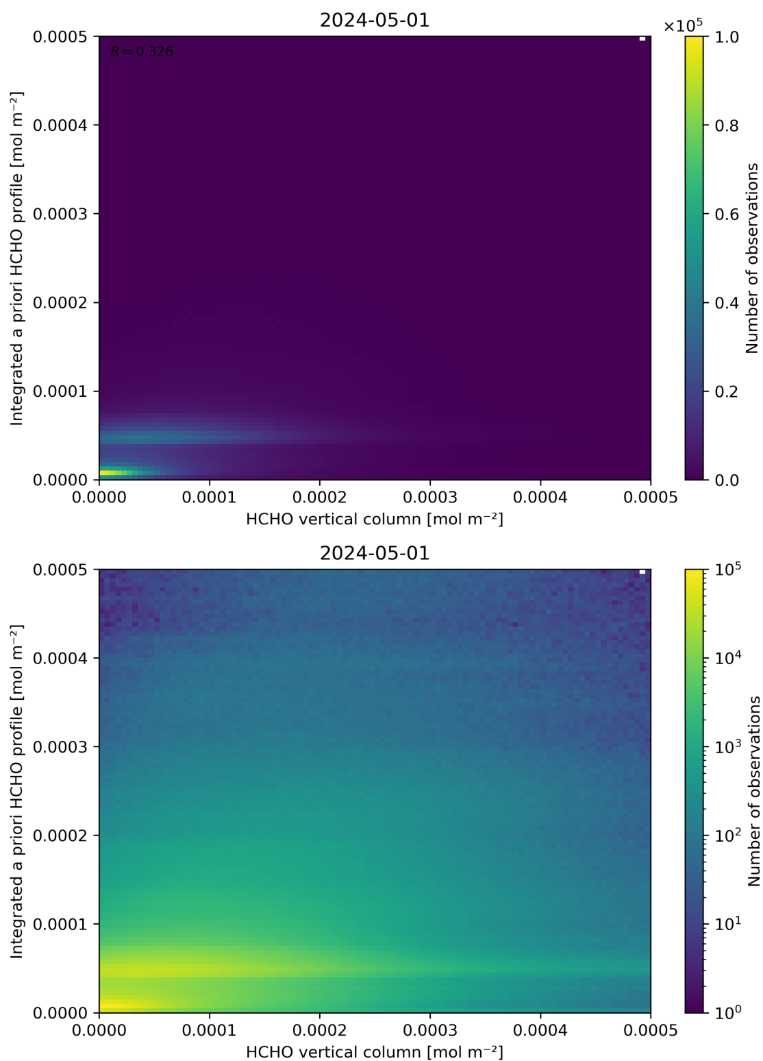
Figure 135: Scatter density plot of “HCHO vertical column” against “Integrated a priori HCHO profile” for 2024-04-30 to 2024-05-02.
