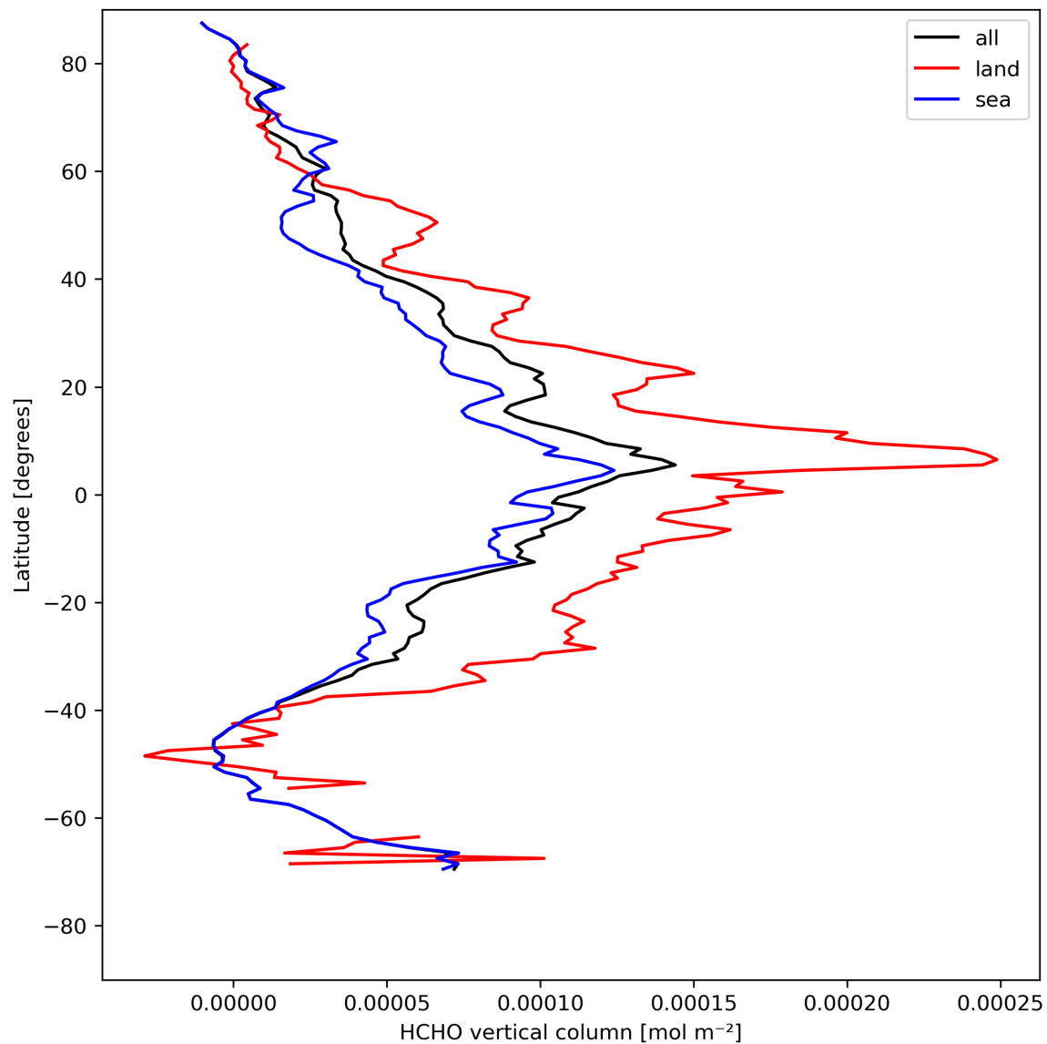
Figure 21: Zonal average of “HCHO vertical column” for 2024-04-30 to 2024-05-02.
