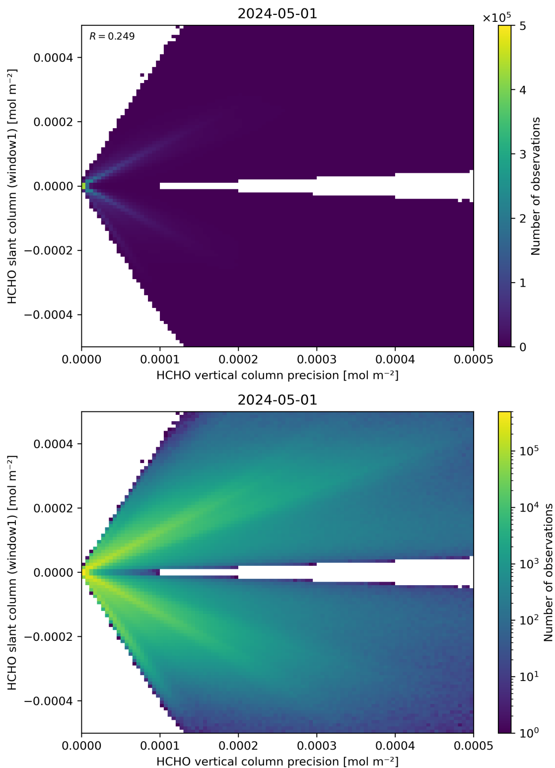
Figure 142: Scatter density plot of “HCHO vertical column precision” against “HCHO slant column (window1)” for 2024-04-30 to 2024-05-02.
