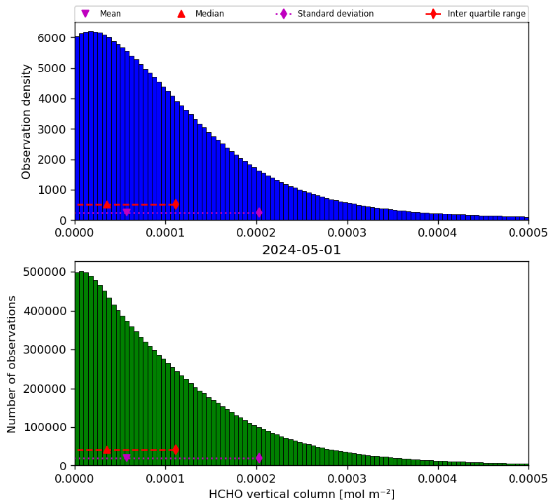
Figure 35: Histogram of “HCHO vertical column” for 2024-04-30 to 2024-05-02
