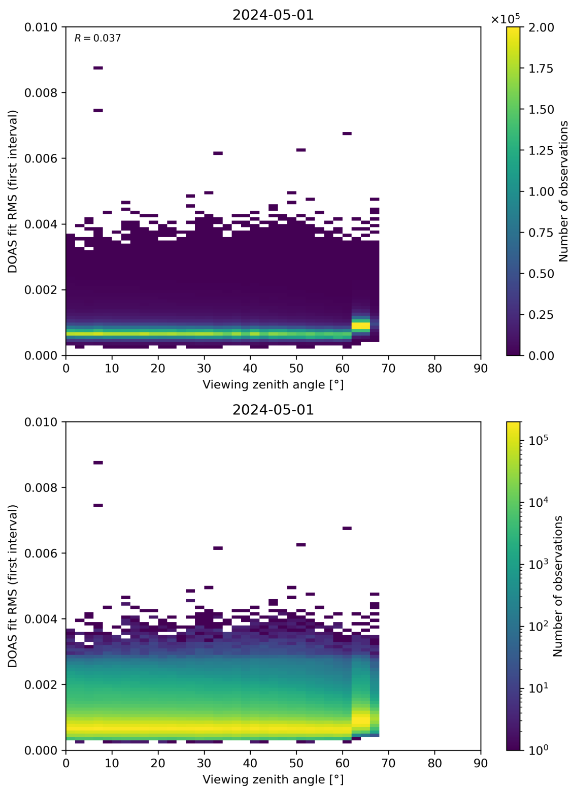
Figure 182: Scatter density plot of “Viewing zenith angle” against “DOAS fit RMS (first interval)” for 2024-04-30 to 2024-05-02.
