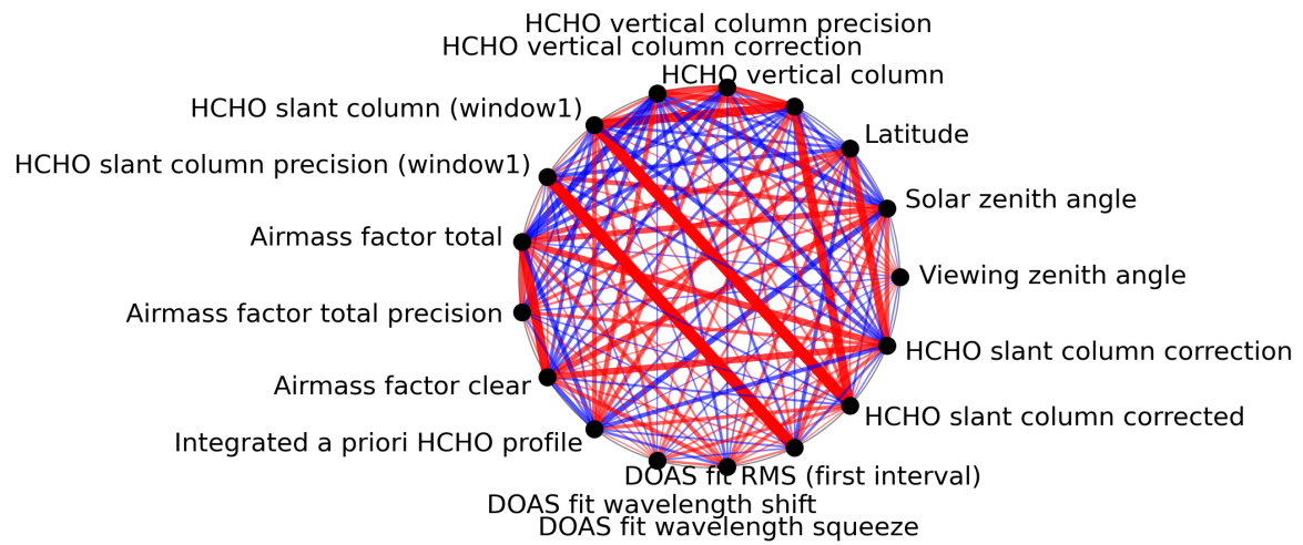
Figure 1: Map of correlation graph for 2024-04-30 to 2024-05-02.
