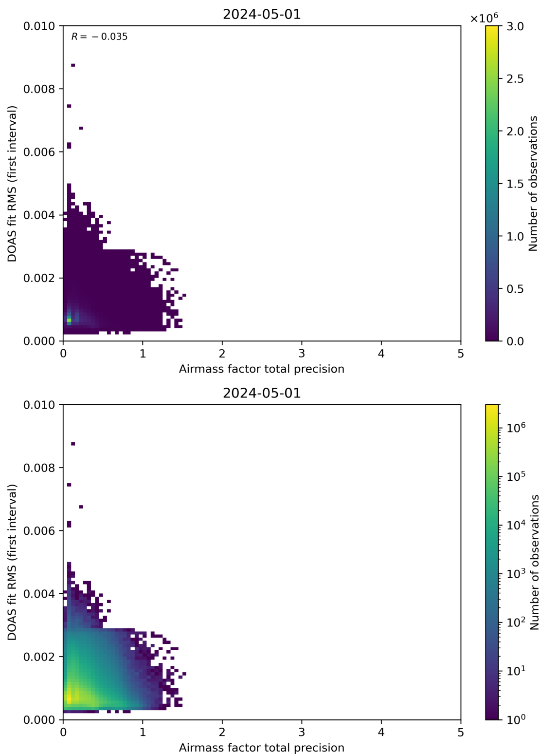
Figure 105: Scatter density plot of “Airmass factor total precision” against “DOAS fit RMS (first interval)” for 2024-04-30 to 2024-05-02.
