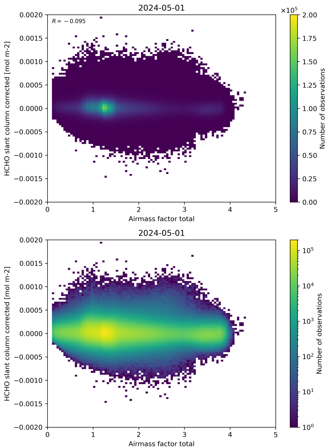
Figure 101: Scatter density plot of “Airmass factor total” against “HCHO slant column corrected” for 2024-04-30 to 2024-05-02.
