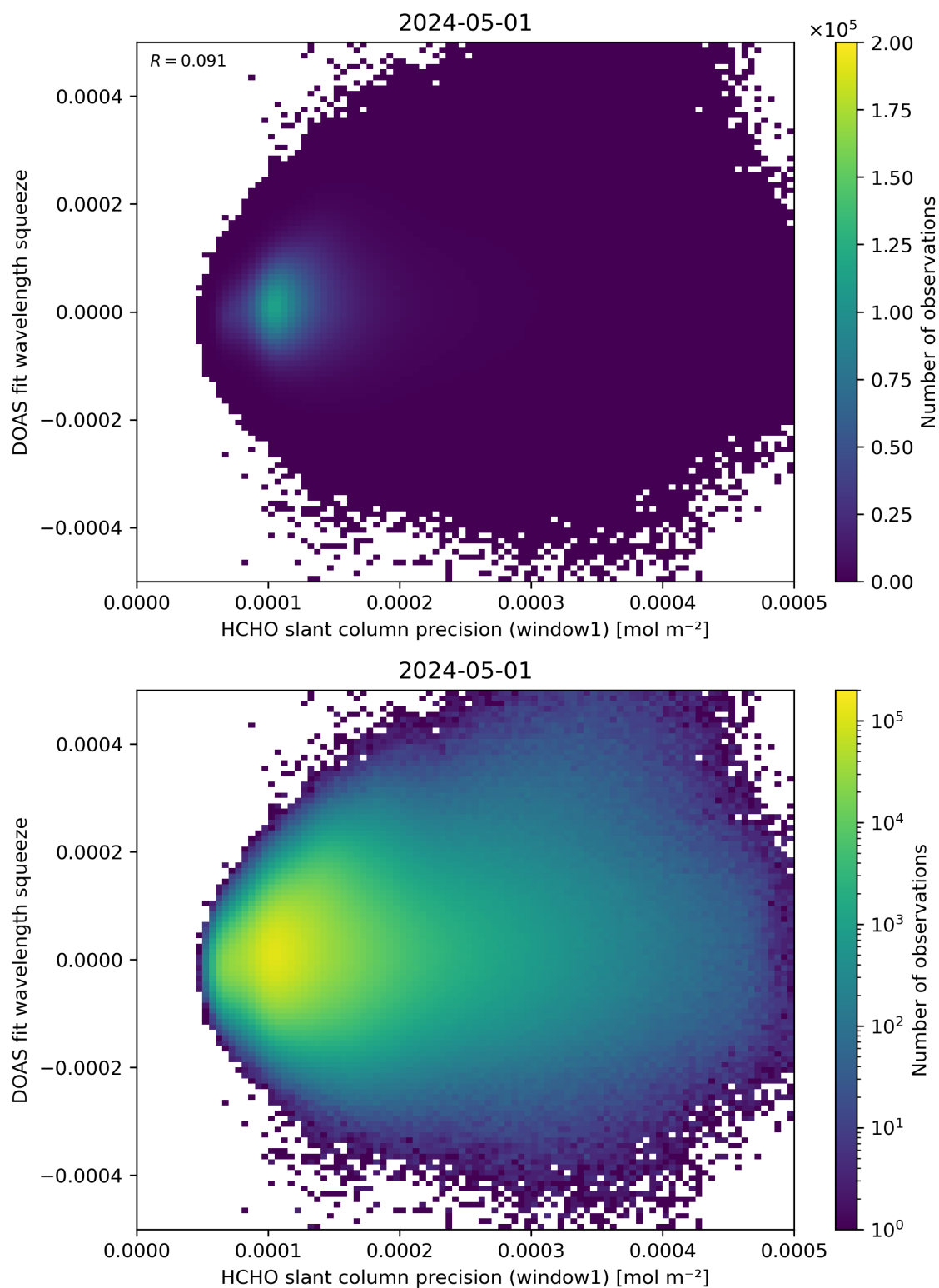
Figure 90: Scatter density plot of “HCHO slant column precision (window1)” against “DOAS fit wavelength squeeze” for 2024-04-30 to 2024-05-02.
