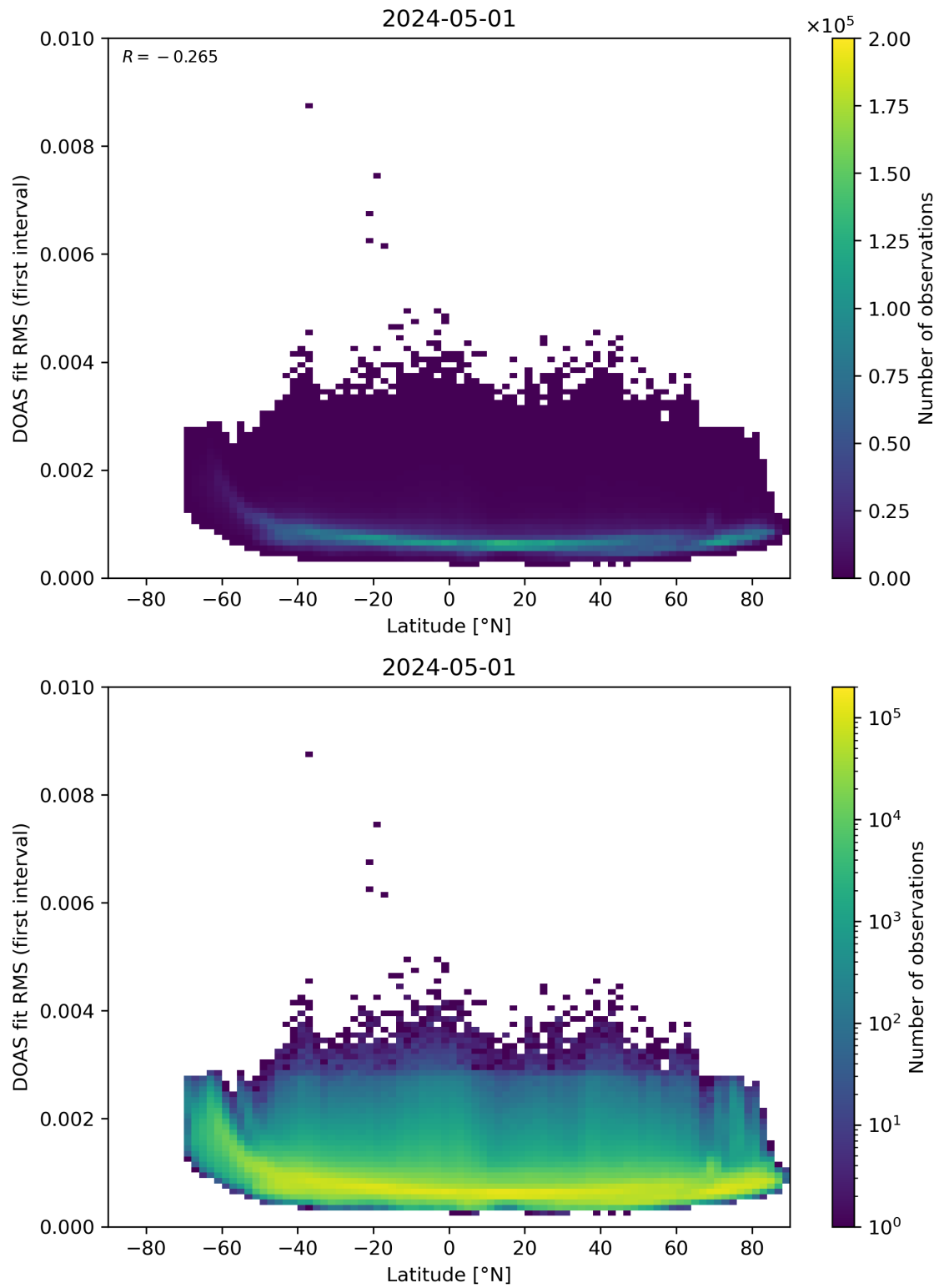
Figure 153: Scatter density plot of “Latitude” against “DOAS fit RMS (first interval)” for 2024-04-30 to 2024-05-02.
