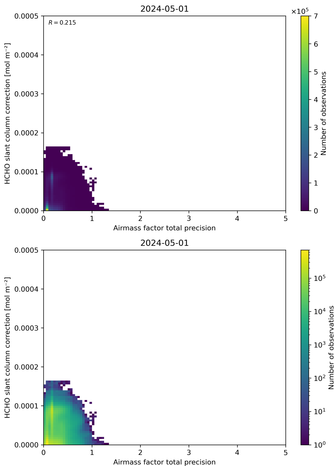
Figure 110: Scatter density plot of “Airmass factor total precision” against “HCHO slant column correction” for 2024-04-30 to 2024-05-02.
