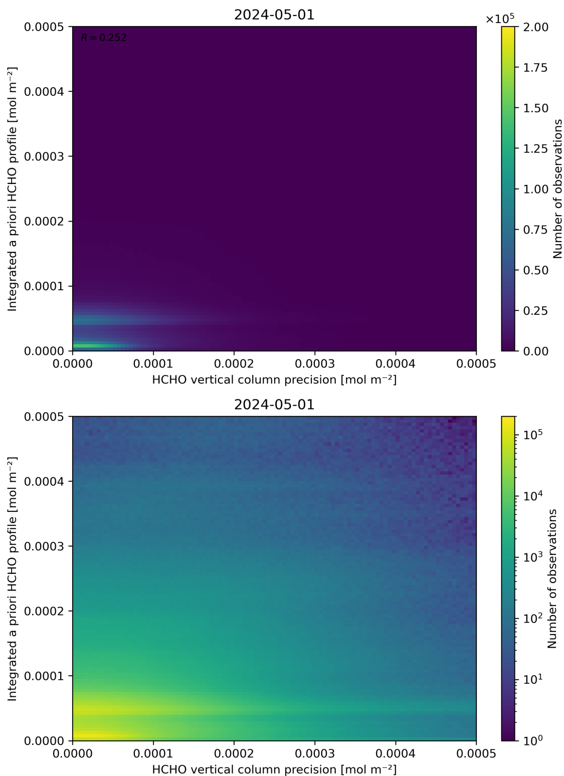
Figure 147: Scatter density plot of “HCHO vertical column precision” against “Integrated a priori HCHO profile” for 2024-04-30 to 2024-05-02.
