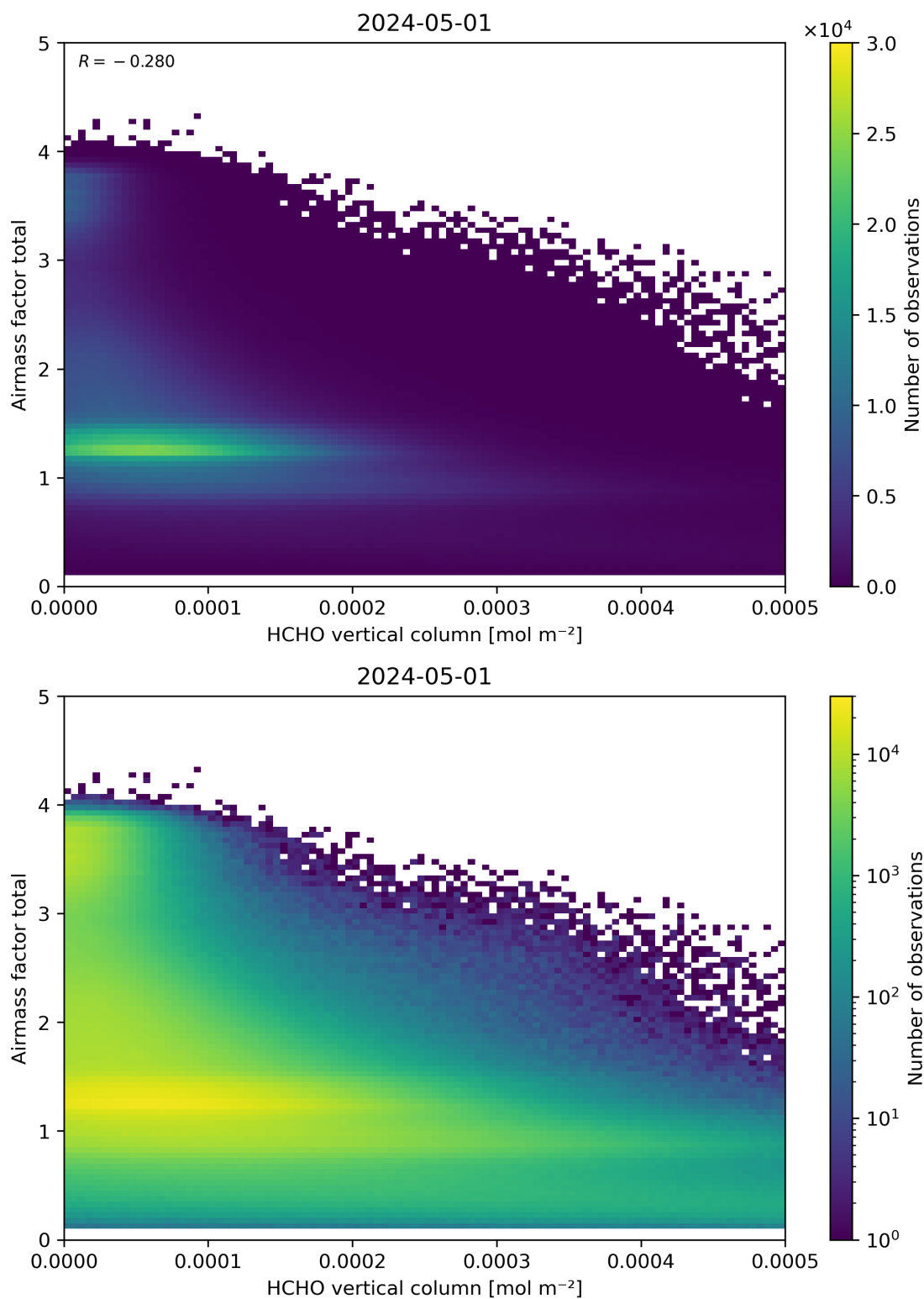
Figure 131: Scatter density plot of “HCHO vertical column” against “Airmass factor total” for 2024-04-30 to 2024-05-02.
