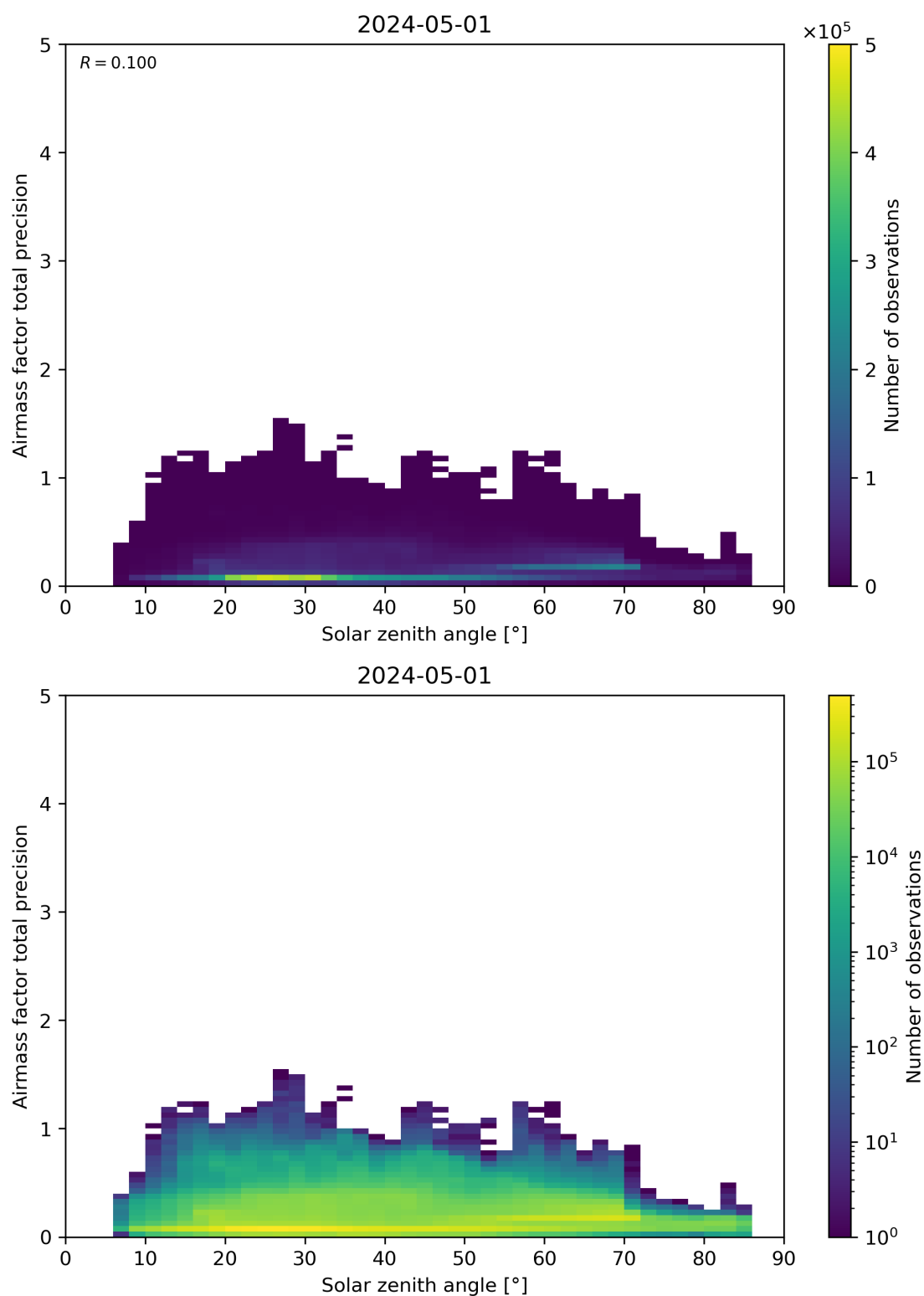
Figure 176: Scatter density plot of “Solar zenith angle” against “Airmass factor total precision” for 2024-04-30 to 2024-05-02.
