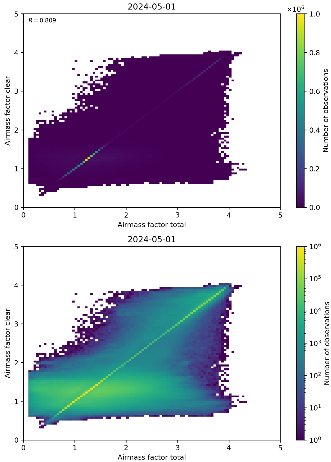
Figure 100: Scatter density plot of “Airmass factor total” against “Airmass factor clear” for 2024-04-30 to 2024-05-02.
