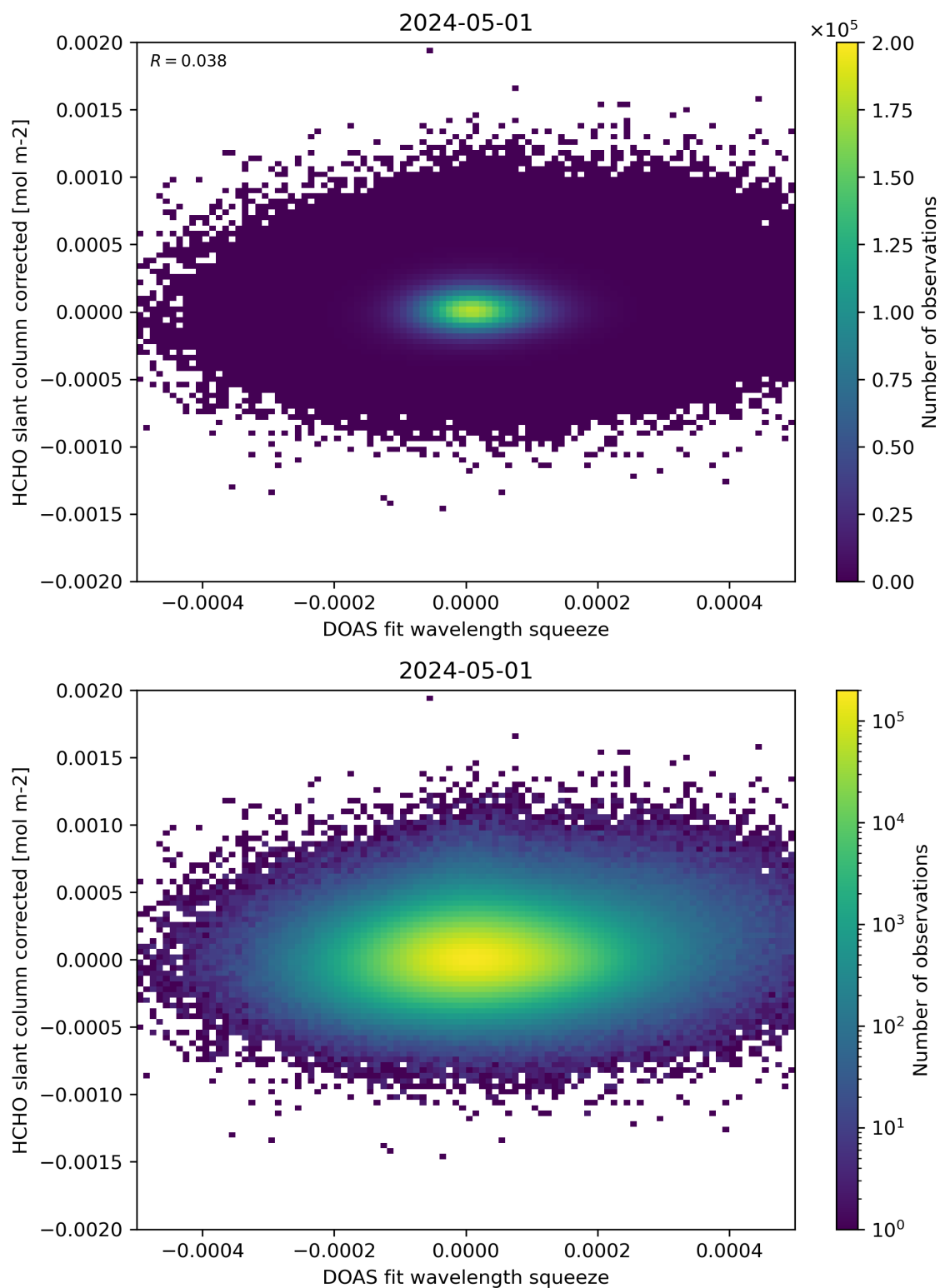
Figure 69: Scatter density plot of “DOAS fit wavelength squeeze” against “HCHO slant column corrected” for 2024-04-30 to 2024-05-02.
