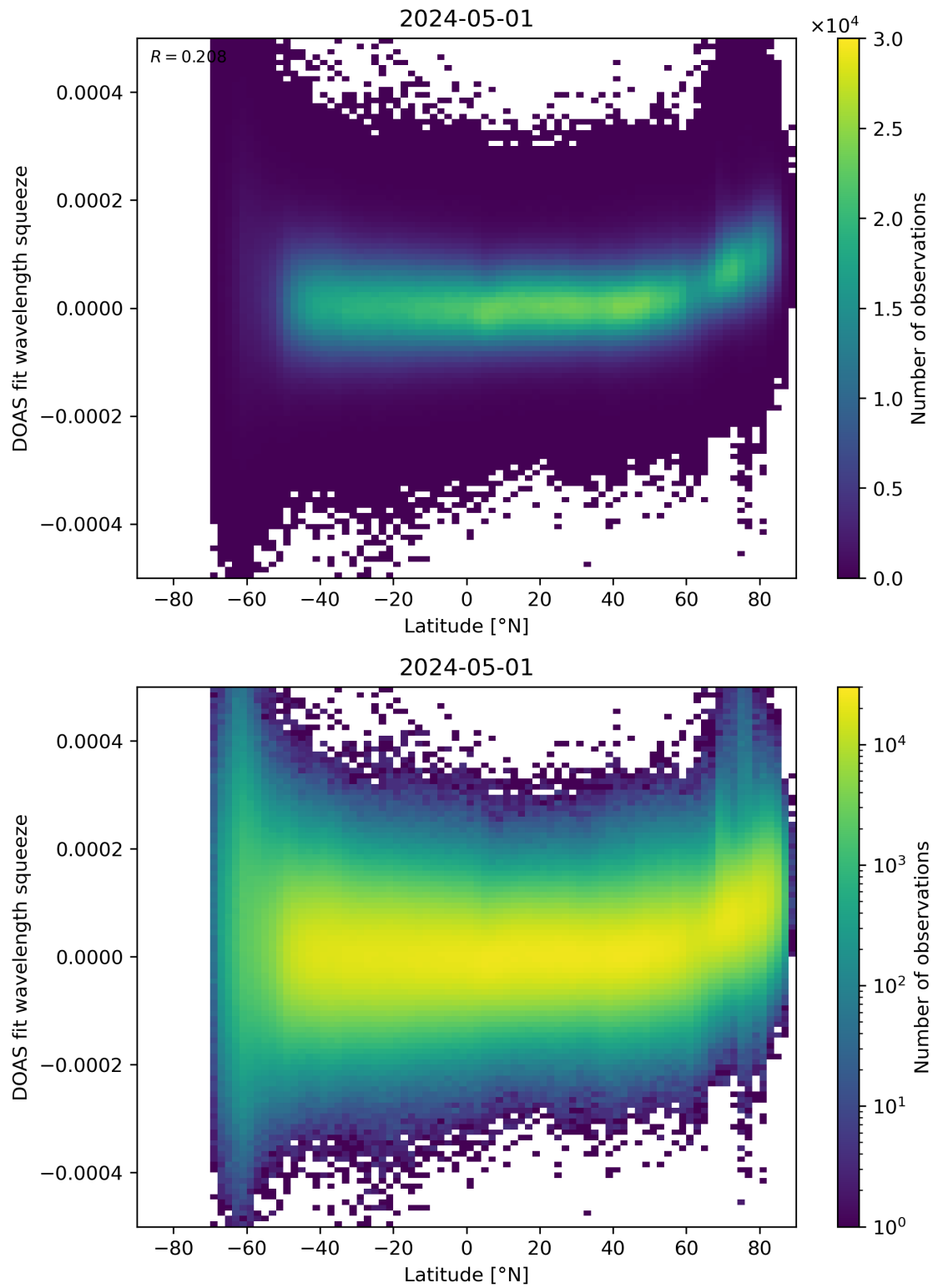
Figure 155: Scatter density plot of “Latitude” against “DOAS fit wavelength squeeze” for 2024-04-30 to 2024-05-02.
