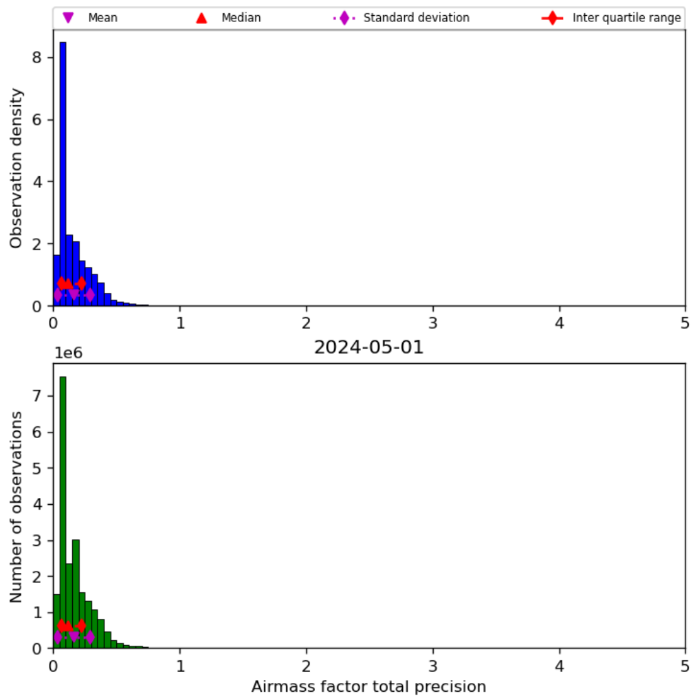
Figure 41: Histogram of “Airmass factor total precision” for 2024-04-30 to 2024-05-02
