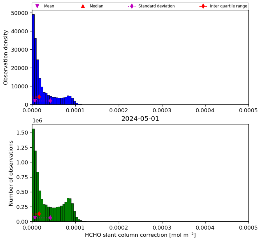
Figure 47: Histogram of “HCHO slant column correction” for 2024-04-30 to 2024-05-02
