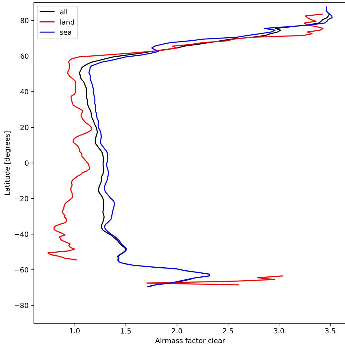
Figure 28: Zonal average of “Airmass factor clear” for 2024-04-30 to 2024-05-02.
