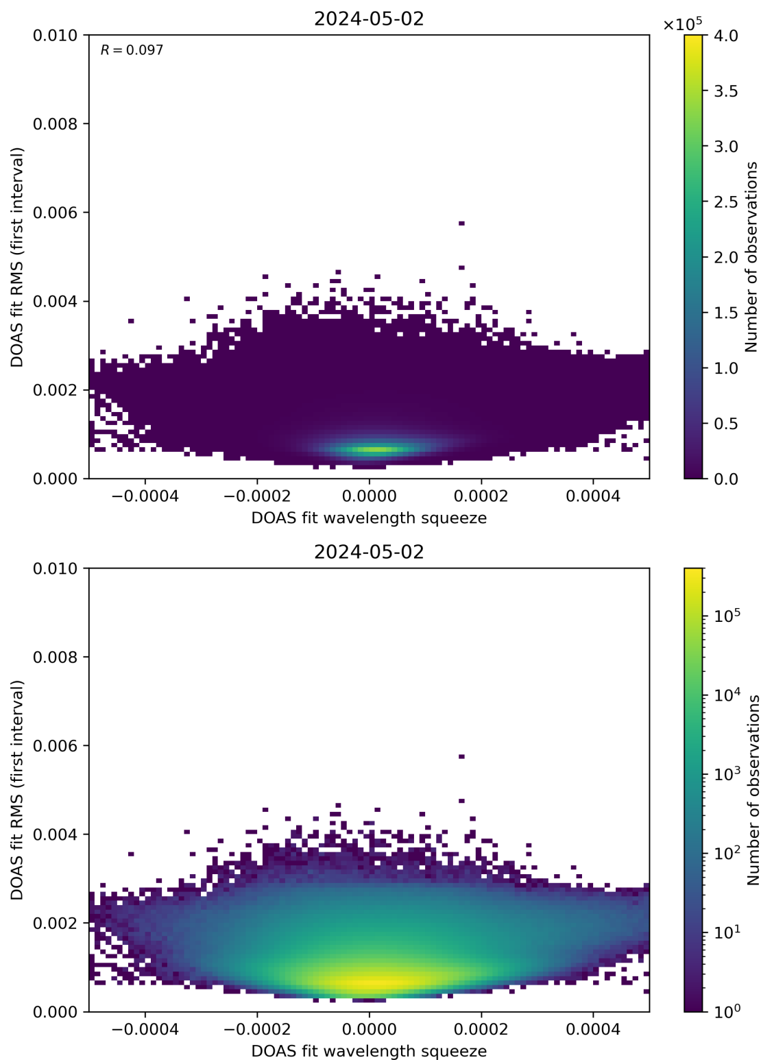
Figure 68: Scatter density plot of “DOAS fit wavelength squeeze” against “DOAS fit RMS (first interval)” for 2024-05-02 to 2024-05-03.
