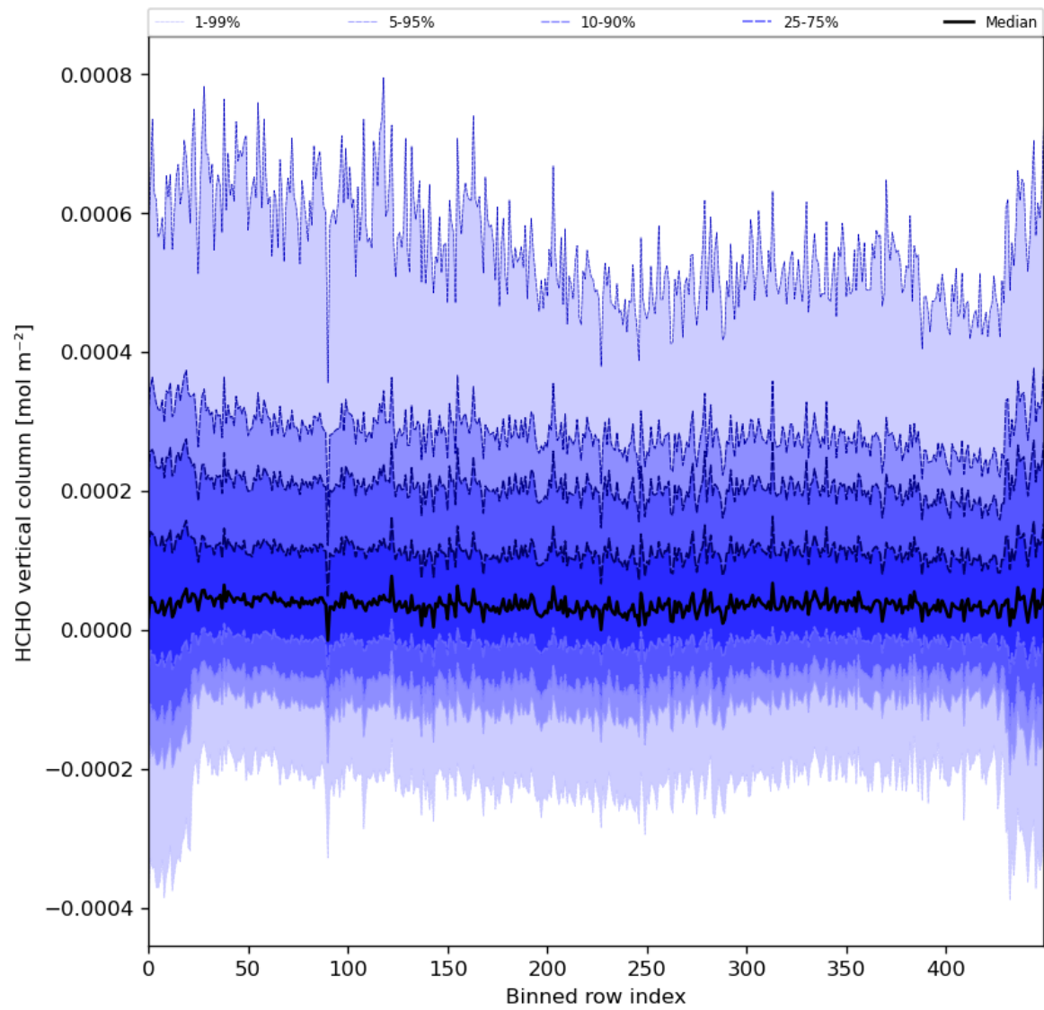
Figure 49: Along track statistics of “HCHO vertical column” for 2024-05-02 to 2024-05-03
