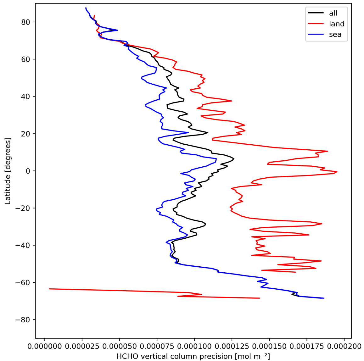
Figure 22: Zonal average of “HCHO vertical column precision” for 2024-05-02 to 2024-05-03.
