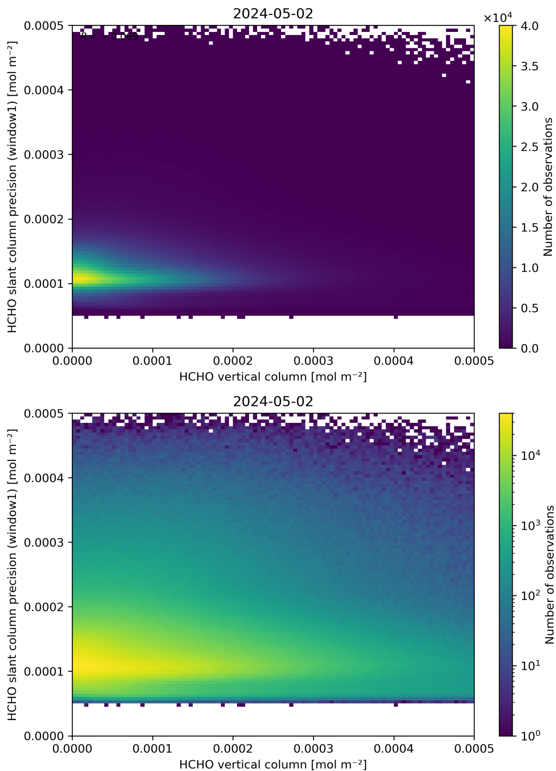
Figure 130: Scatter density plot of “HCHO vertical column” against “HCHO slant column precision (window1)” for 2024-05-02 to 2024-05-03.
