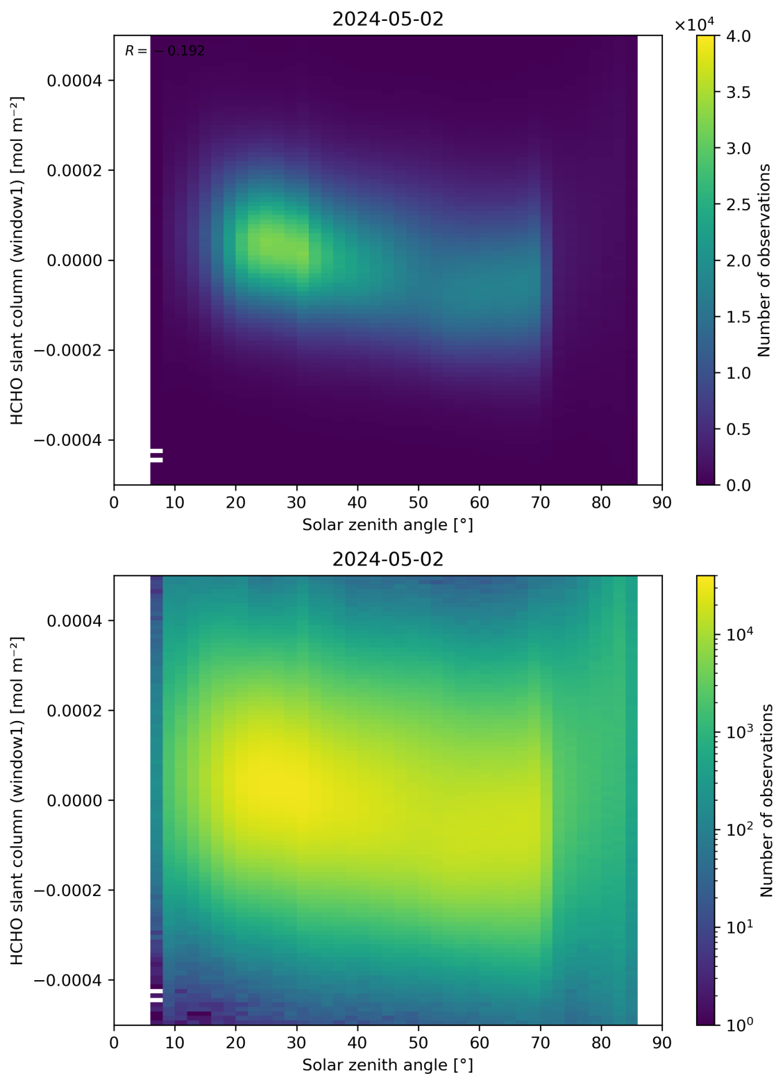
Figure 173: Scatter density plot of “Solar zenith angle” against “HCHO slant column (window1)” for 2024-05-02 to 2024-05-03.
