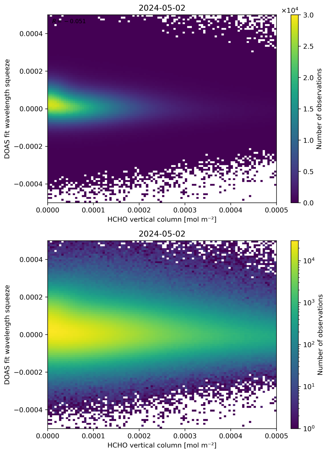
Figure 125: Scatter density plot of “HCHO vertical column” against “DOAS fit wavelength squeeze” for 2024-05-02 to 2024-05-03.
