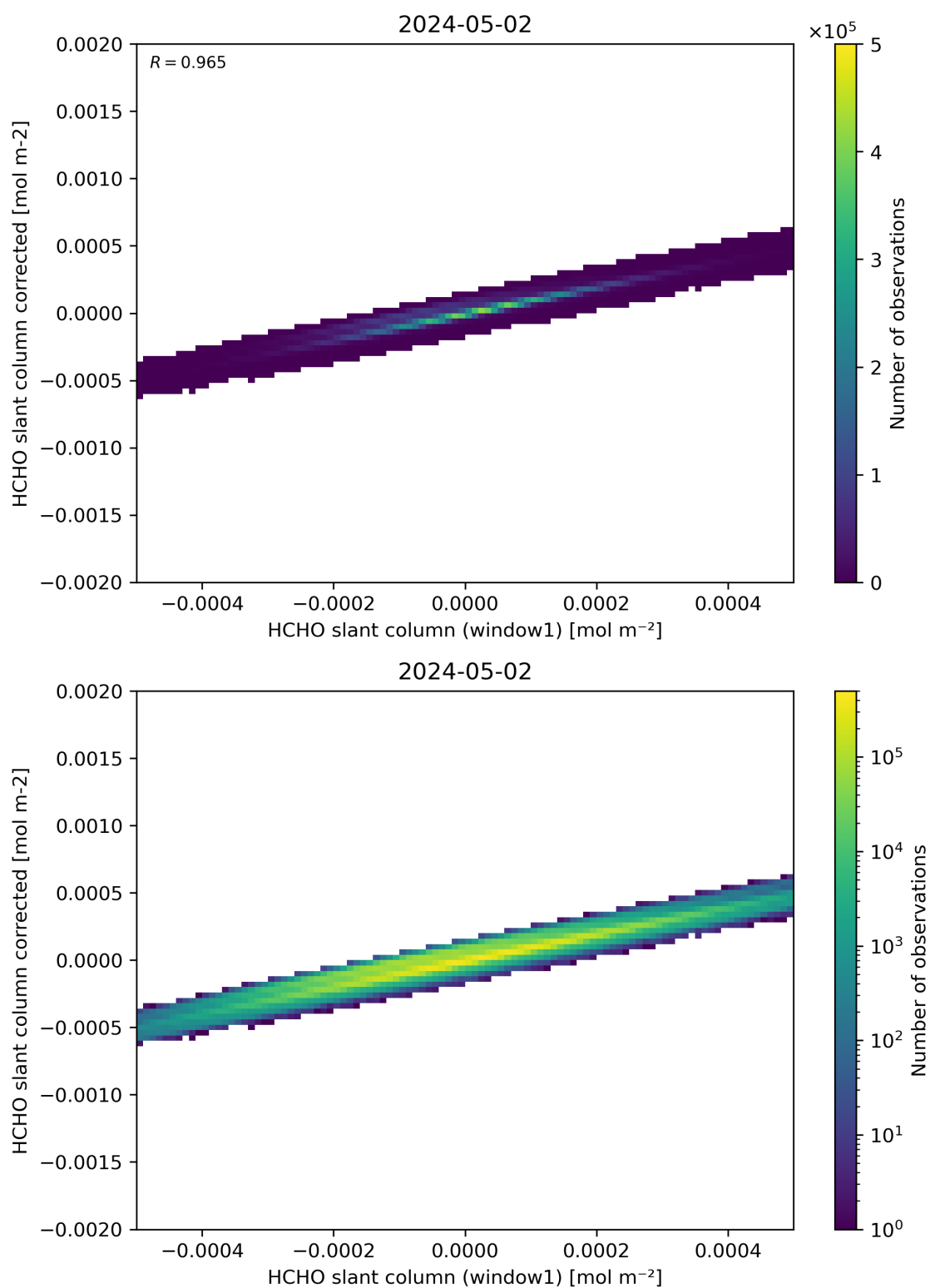
Figure 82: Scatter density plot of “HCHO slant column (window1)” against “HCHO slant column corrected” for 2024-05-02 to 2024-05-03.
