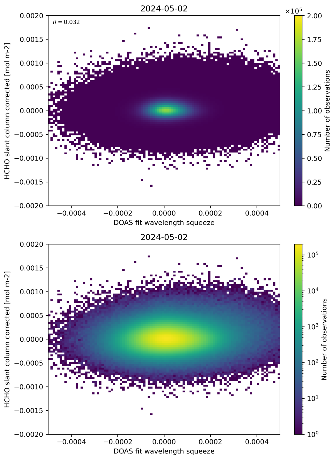
Figure 69: Scatter density plot of “DOAS fit wavelength squeeze” against “HCHO slant column corrected” for 2024-05-02 to 2024-05-03.
