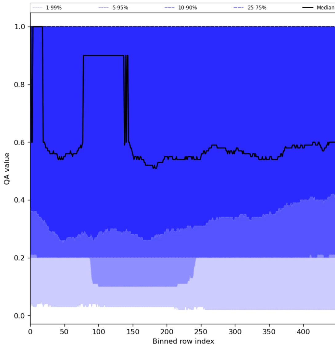
Figure 48: Along track statistics of “QA value” for 2024-05-02 to 2024-05-03
