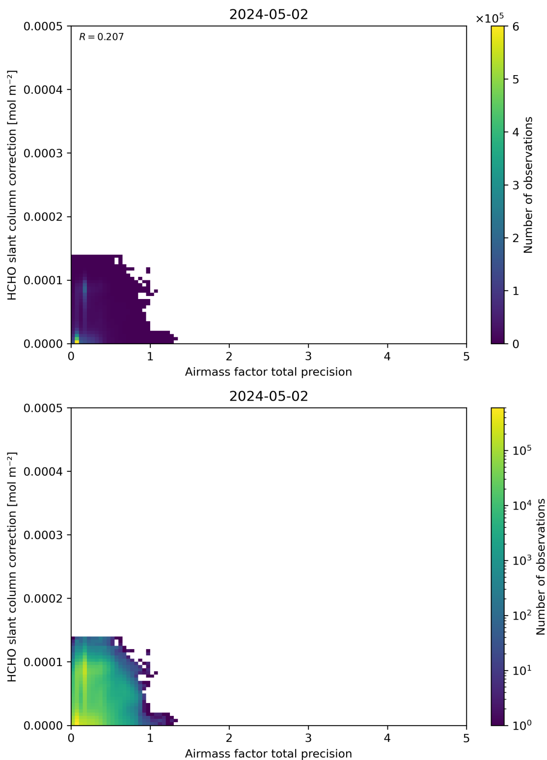
Figure 110: Scatter density plot of “Airmass factor total precision” against “HCHO slant column correction” for 2024-05-02 to 2024-05-03.
