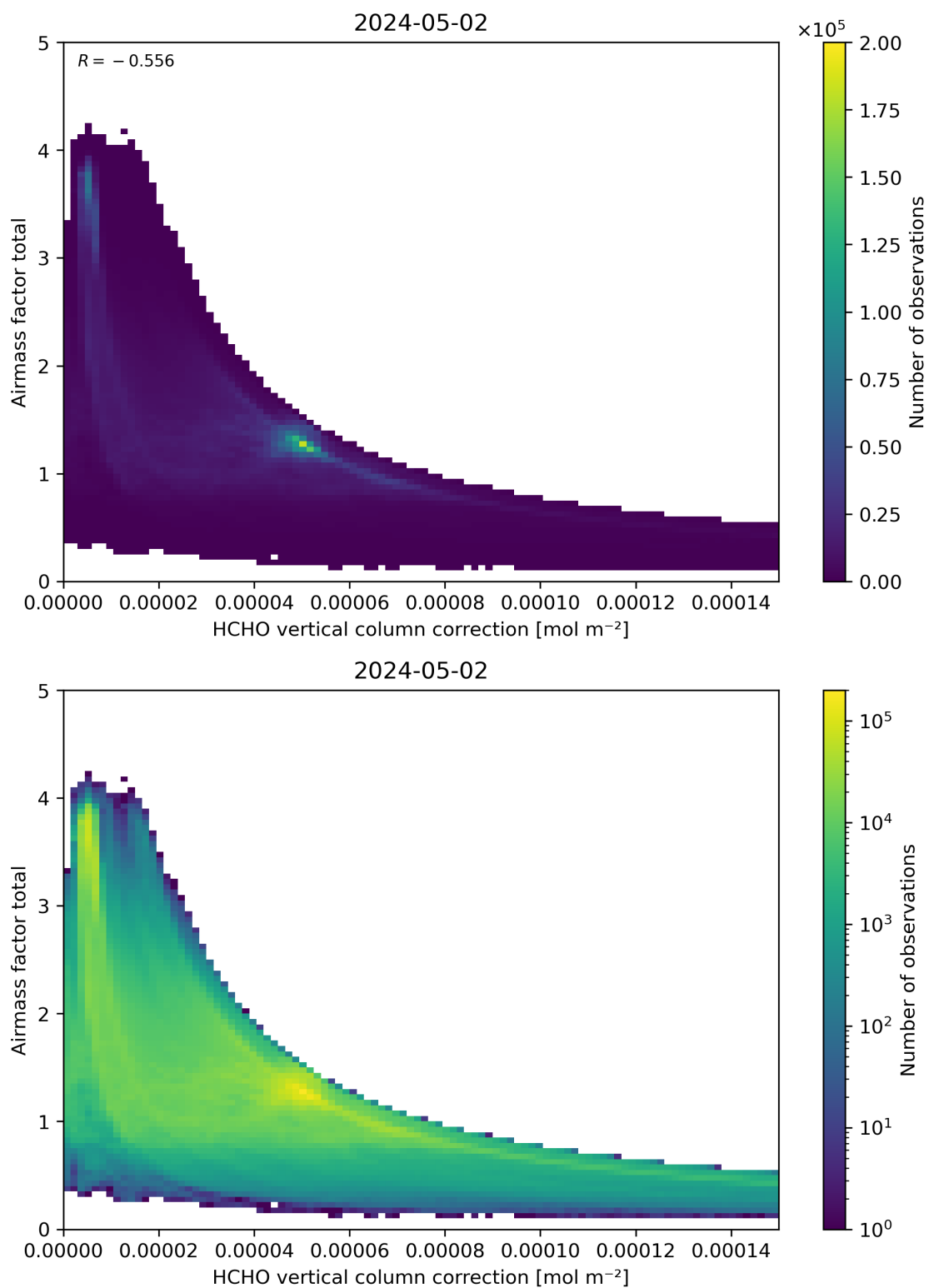
Figure 120: Scatter density plot of “HCHO vertical column correction” against “Airmass factor total” for 2024-05-02 to 2024-05-03.
