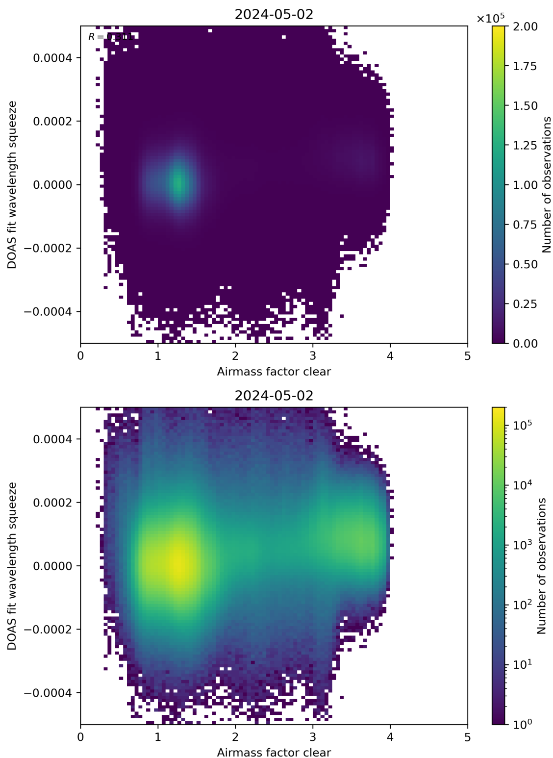
Figure 73: Scatter density plot of “Airmass factor clear” against “DOAS fit wavelength squeeze” for 2024-05-02 to 2024-05-03.
