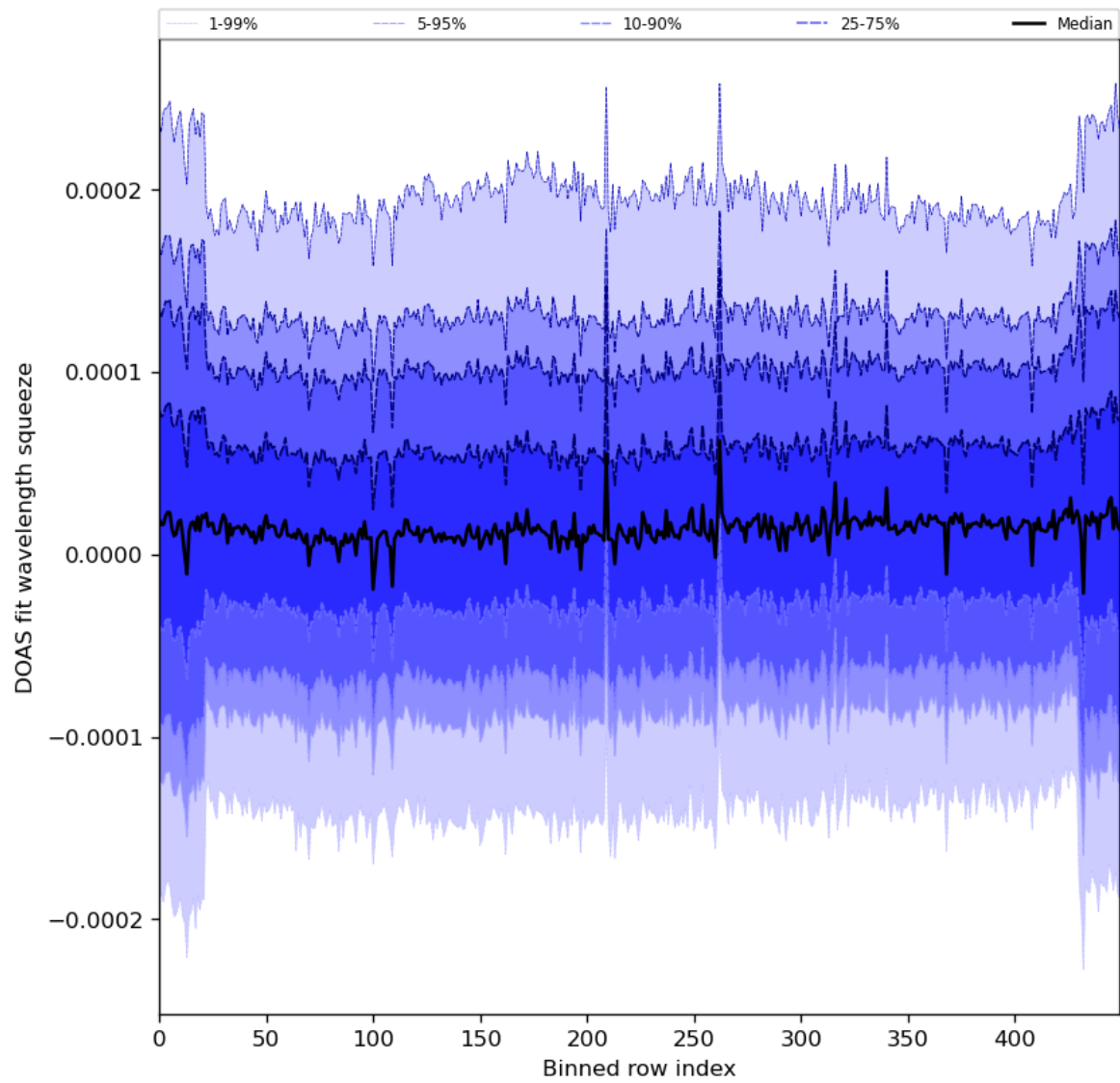
Figure 59: Along track statistics of “DOAS fit wavelength squeeze” for 2024-05-02 to 2024-05-03
