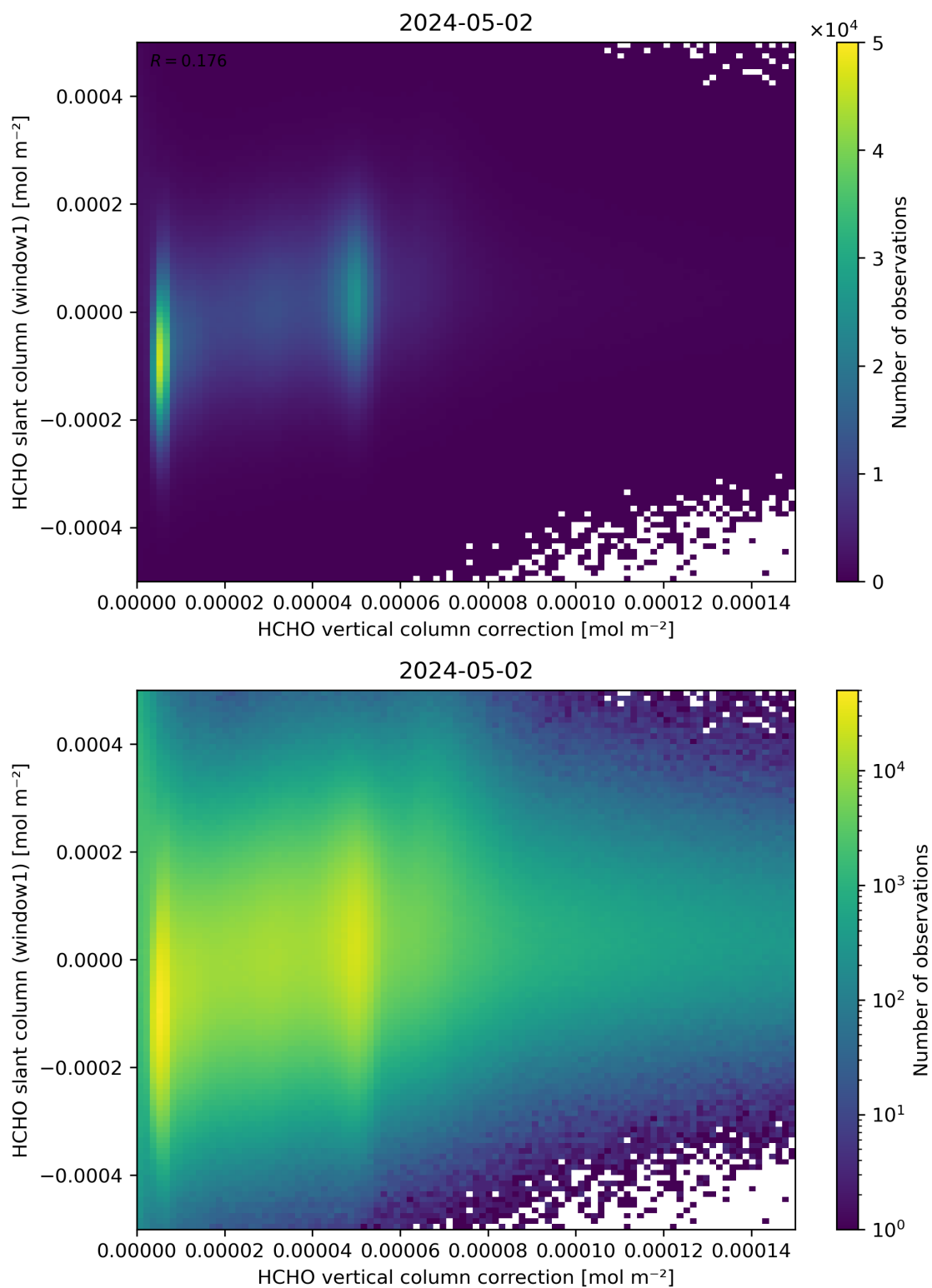
Figure 118: Scatter density plot of “HCHO vertical column correction” against “HCHO slant column (window1)” for 2024-05-02 to 2024-05-03.
