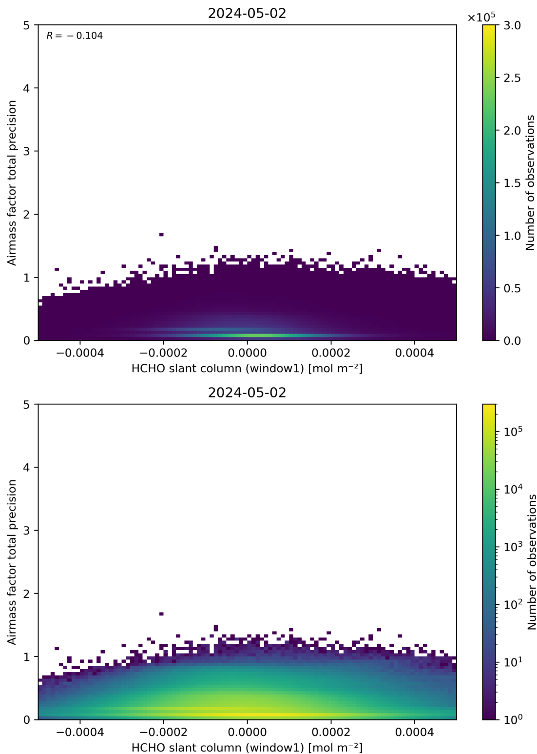
Figure 86: Scatter density plot of “HCHO slant column (window1)” against “Airmass factor total precision” for 2024-05-02 to 2024-05-03.
