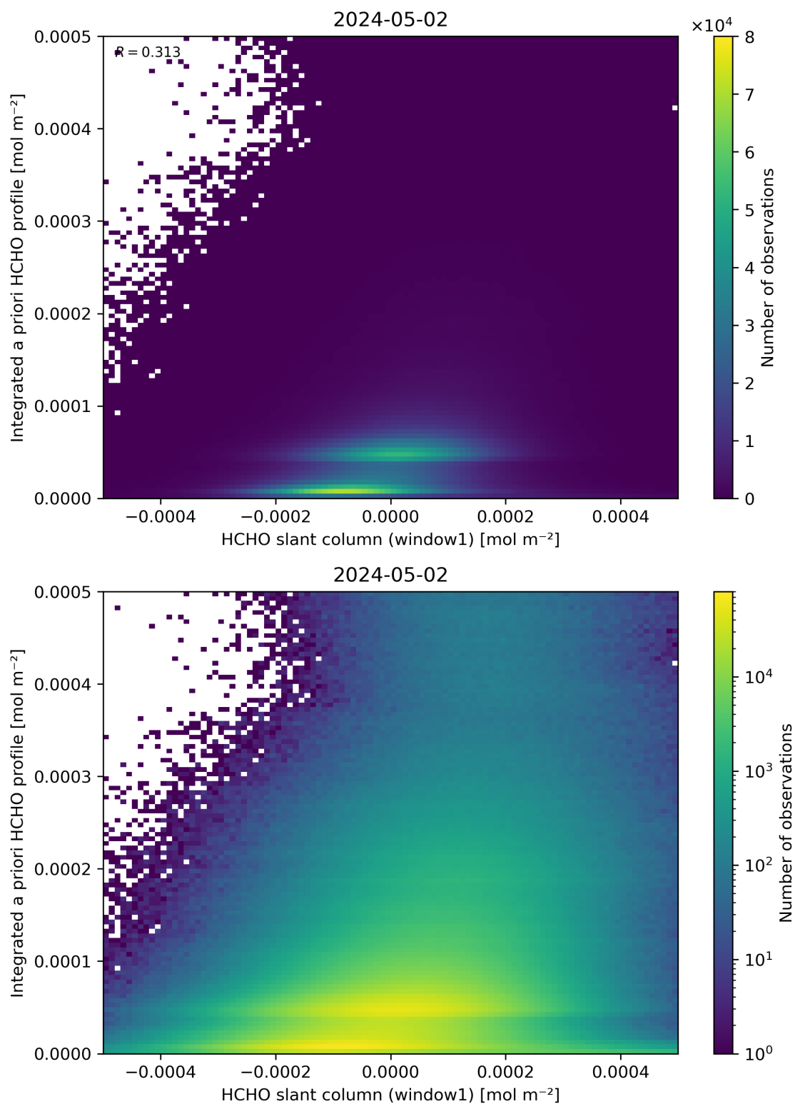
Figure 87: Scatter density plot of “HCHO slant column (window1)” against “Integrated a priori HCHO profile” for 2024-05-02 to 2024-05-03.
