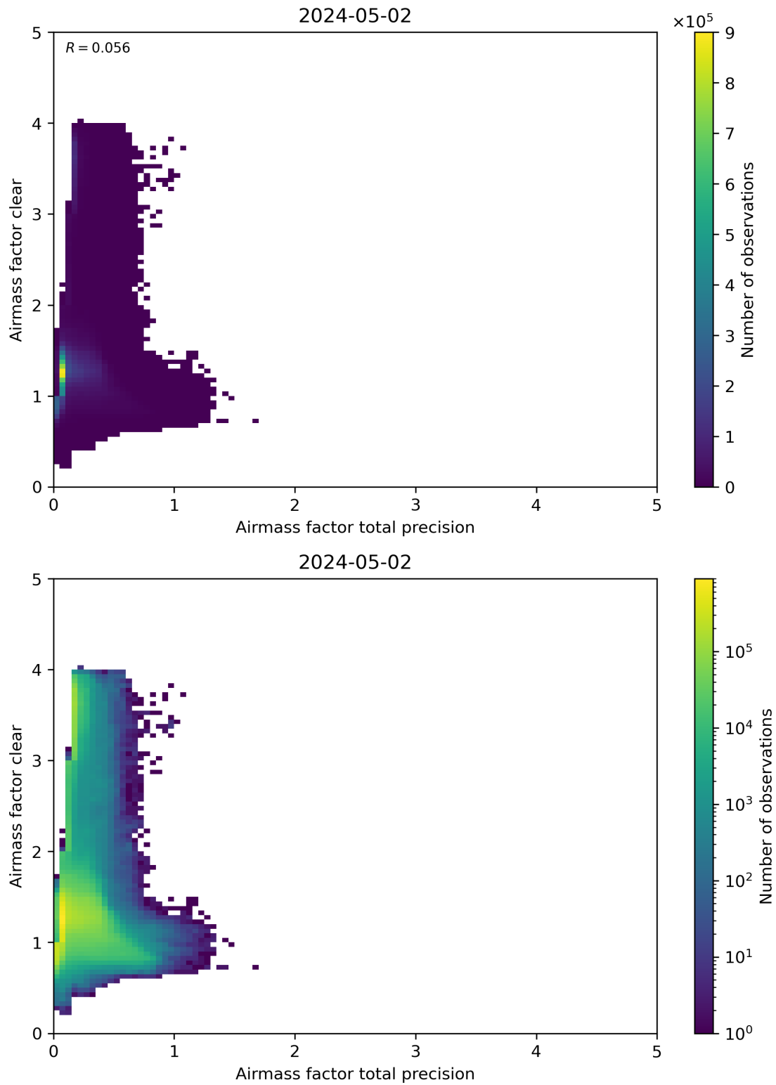
Figure 108: Scatter density plot of “Airmass factor total precision” against “Airmass factor clear” for 2024-05-02 to 2024-05-03.
