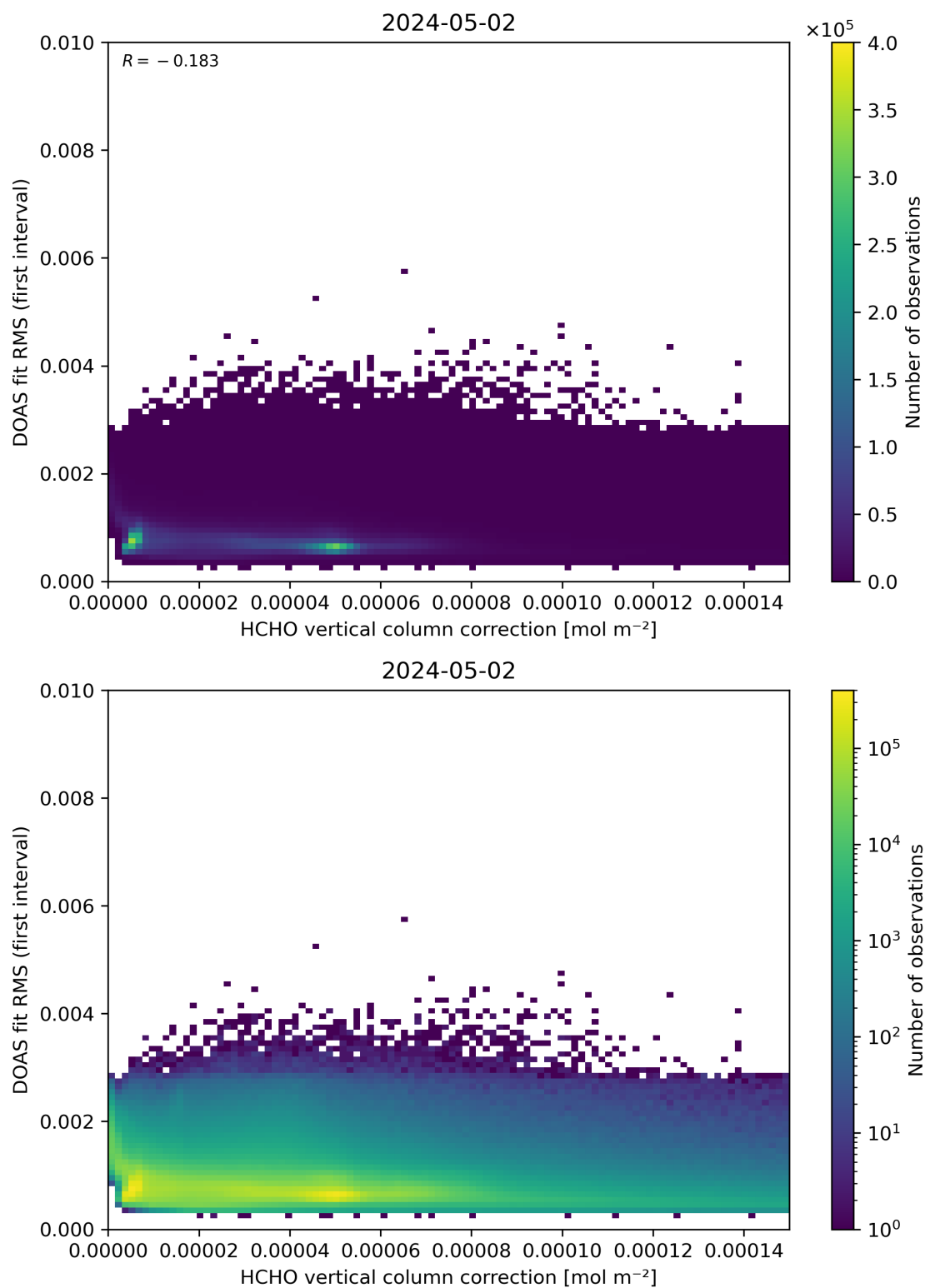
Figure 112: Scatter density plot of “HCHO vertical column correction” against “DOAS fit RMS (first interval)” for 2024-05-02 to 2024-05-03.
