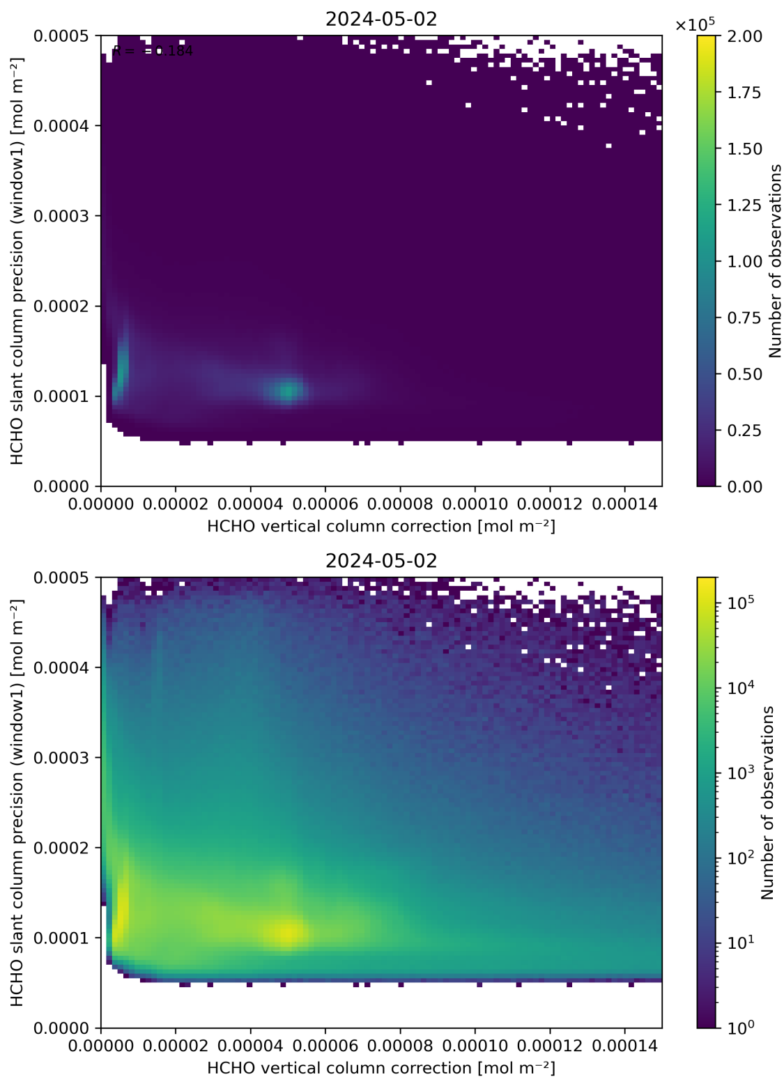
Figure 119: Scatter density plot of “HCHO vertical column correction” against “HCHO slant column precision (window1)” for 2024-05-02 to 2024-05-03.
