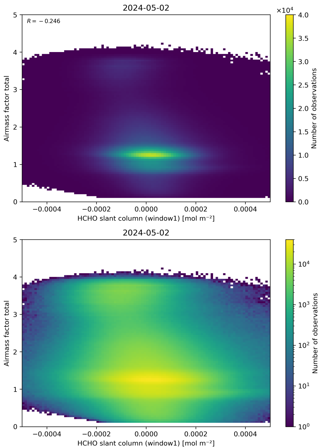
Figure 85: Scatter density plot of “HCHO slant column (window1)” against “Airmass factor total” for 2024-05-02 to 2024-05-03.
