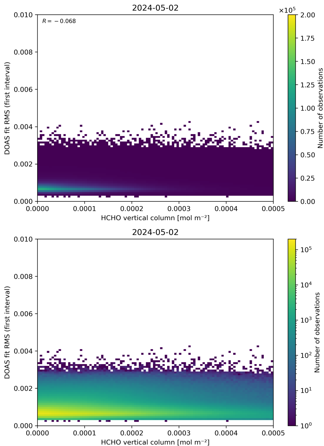
Figure 123: Scatter density plot of “HCHO vertical column” against “DOAS fit RMS (first interval)” for 2024-05-02 to 2024-05-03.
