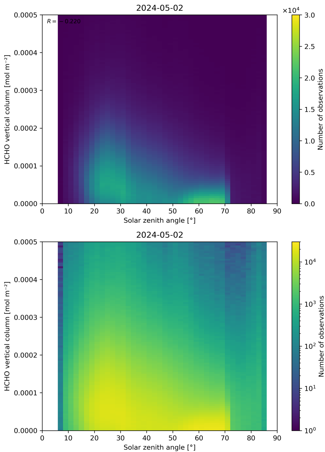
Figure 177: Scatter density plot of “Solar zenith angle” against “HCHO vertical column” for 2024-05-02 to 2024-05-03.
