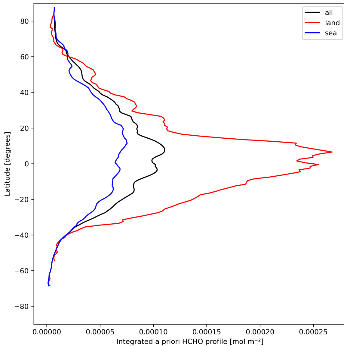
Figure 29: Zonal average of “Integrated a priori HCHO profile” for 2024-05-02 to 2024-05-03.
