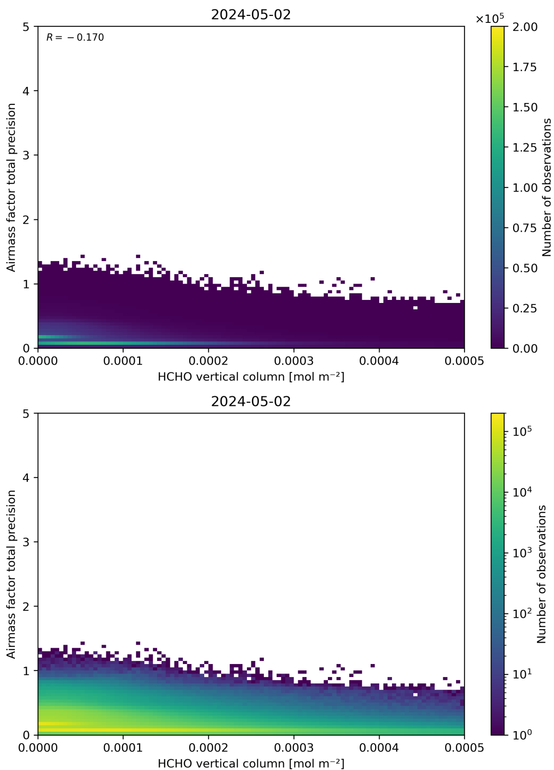
Figure 132: Scatter density plot of “HCHO vertical column” against “Airmass factor total precision” for 2024-05-02 to 2024-05-03.
