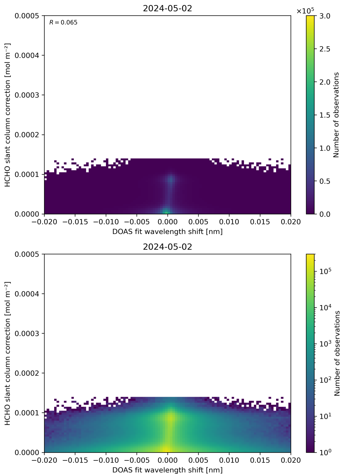
Figure 67: Scatter density plot of “DOAS fit wavelength shift” against “HCHO slant column correction” for 2024-05-02 to 2024-05-03.
