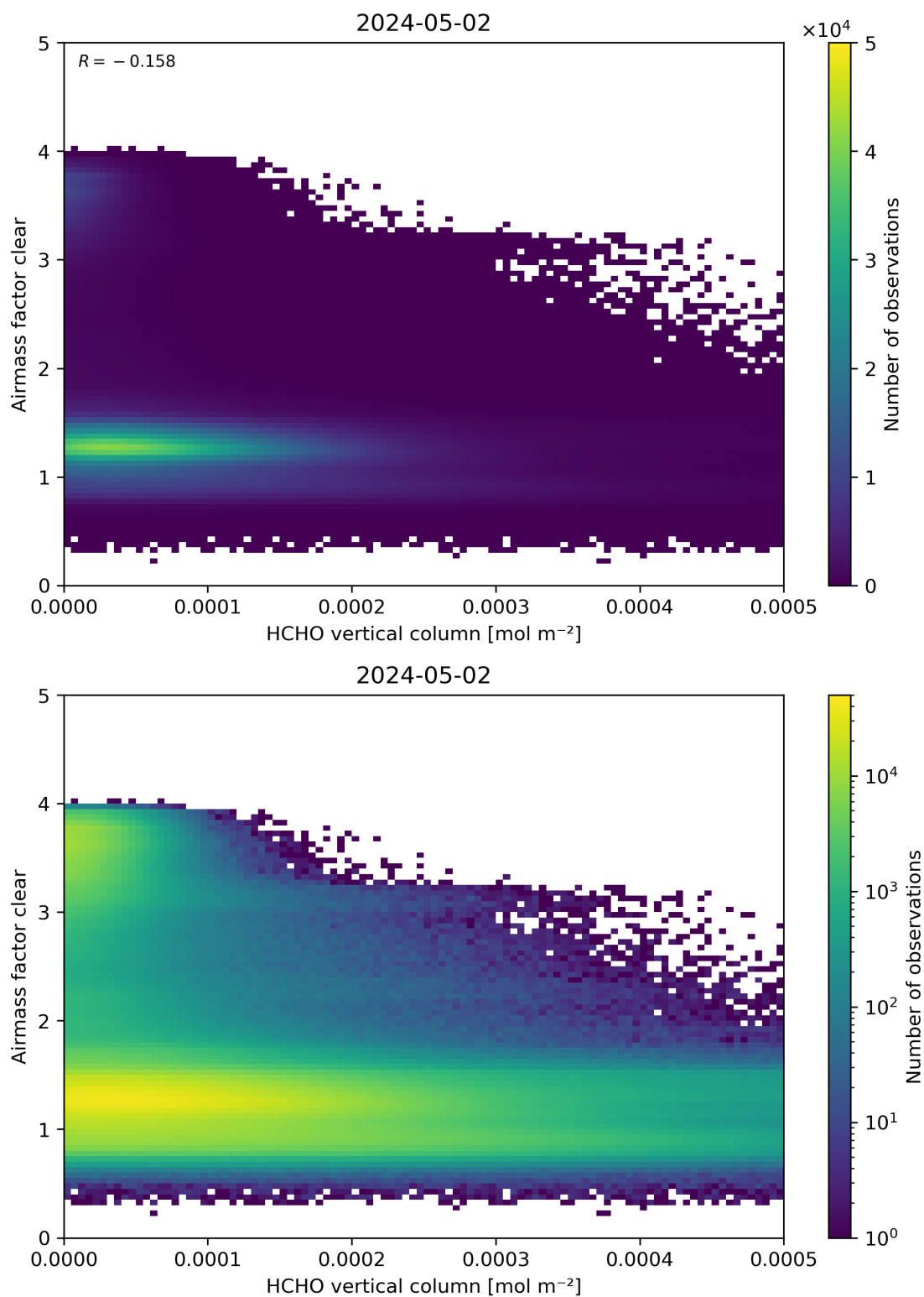
Figure 126: Scatter density plot of “HCHO vertical column” against “Airmass factor clear” for 2024-05-02 to 2024-05-03.
