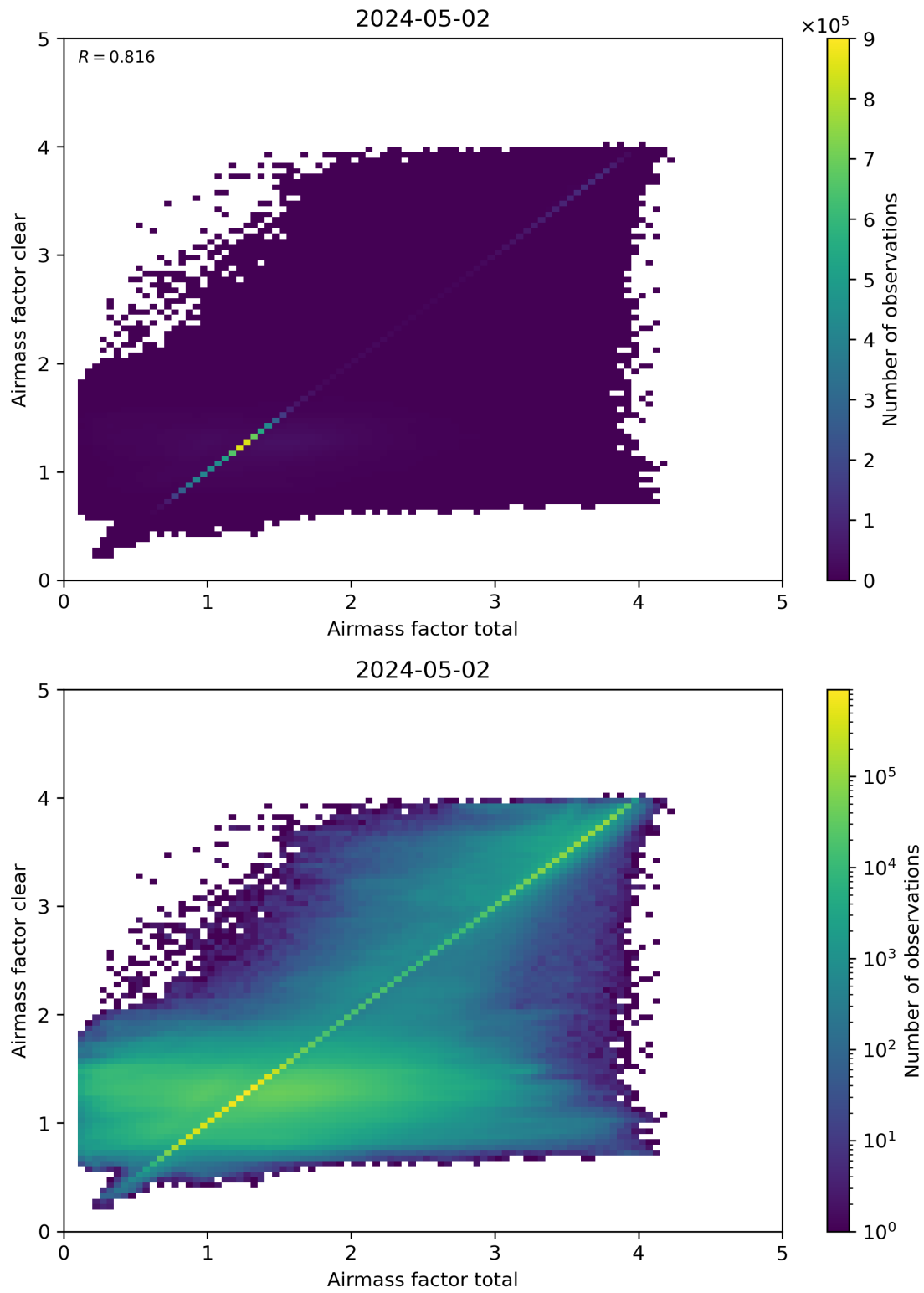
Figure 100: Scatter density plot of “Airmass factor total” against “Airmass factor clear” for 2024-05-02 to 2024-05-03.
