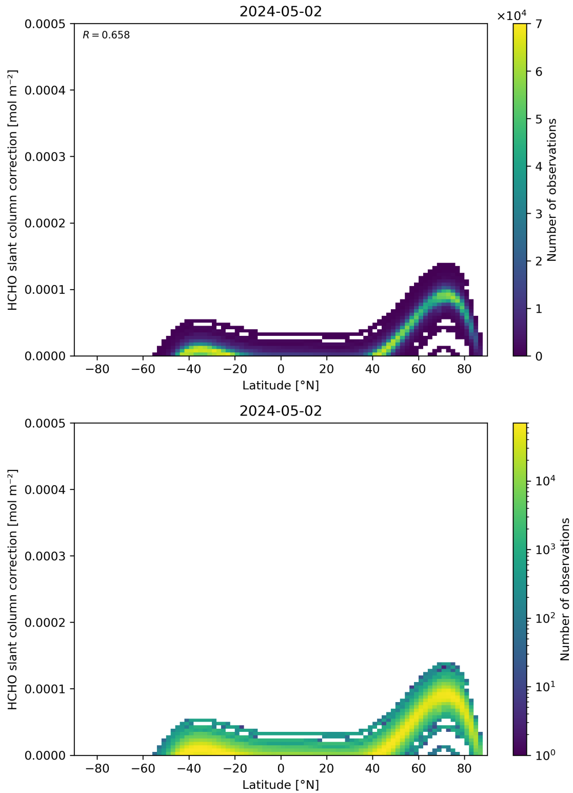
Figure 158: Scatter density plot of “Latitude” against “HCHO slant column correction” for 2024-05-02 to 2024-05-03.
