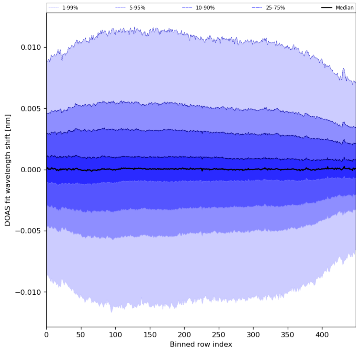
Figure 58: Along track statistics of “DOAS fit wavelength shift” for 2024-05-02 to 2024-05-03
