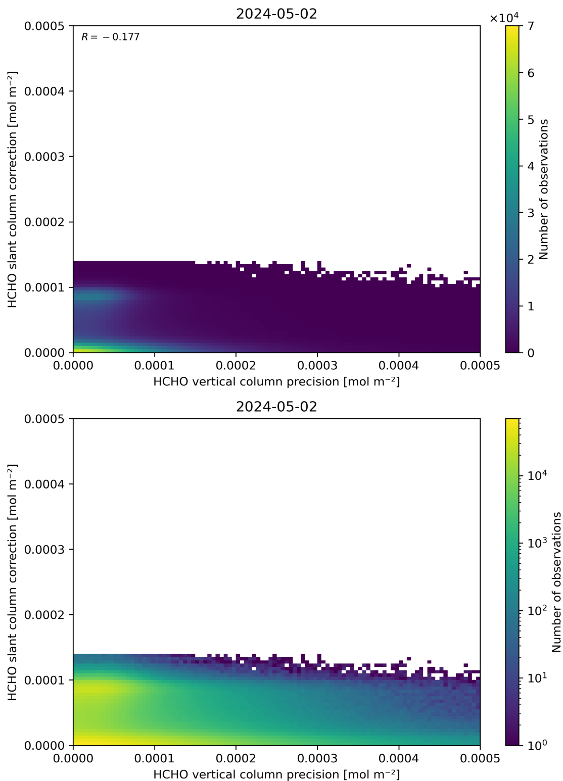
Figure 141: Scatter density plot of “HCHO vertical column precision” against “HCHO slant column correction” for 2024-05-02 to 2024-05-03.
