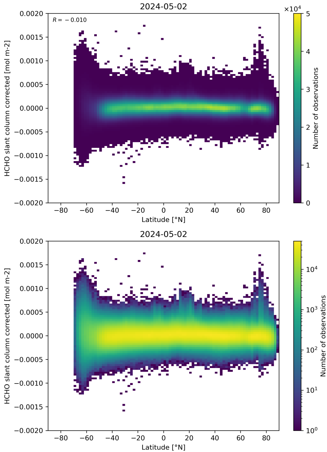
Figure 157: Scatter density plot of “Latitude” against “HCHO slant column corrected” for 2024-05-02 to 2024-05-03.
