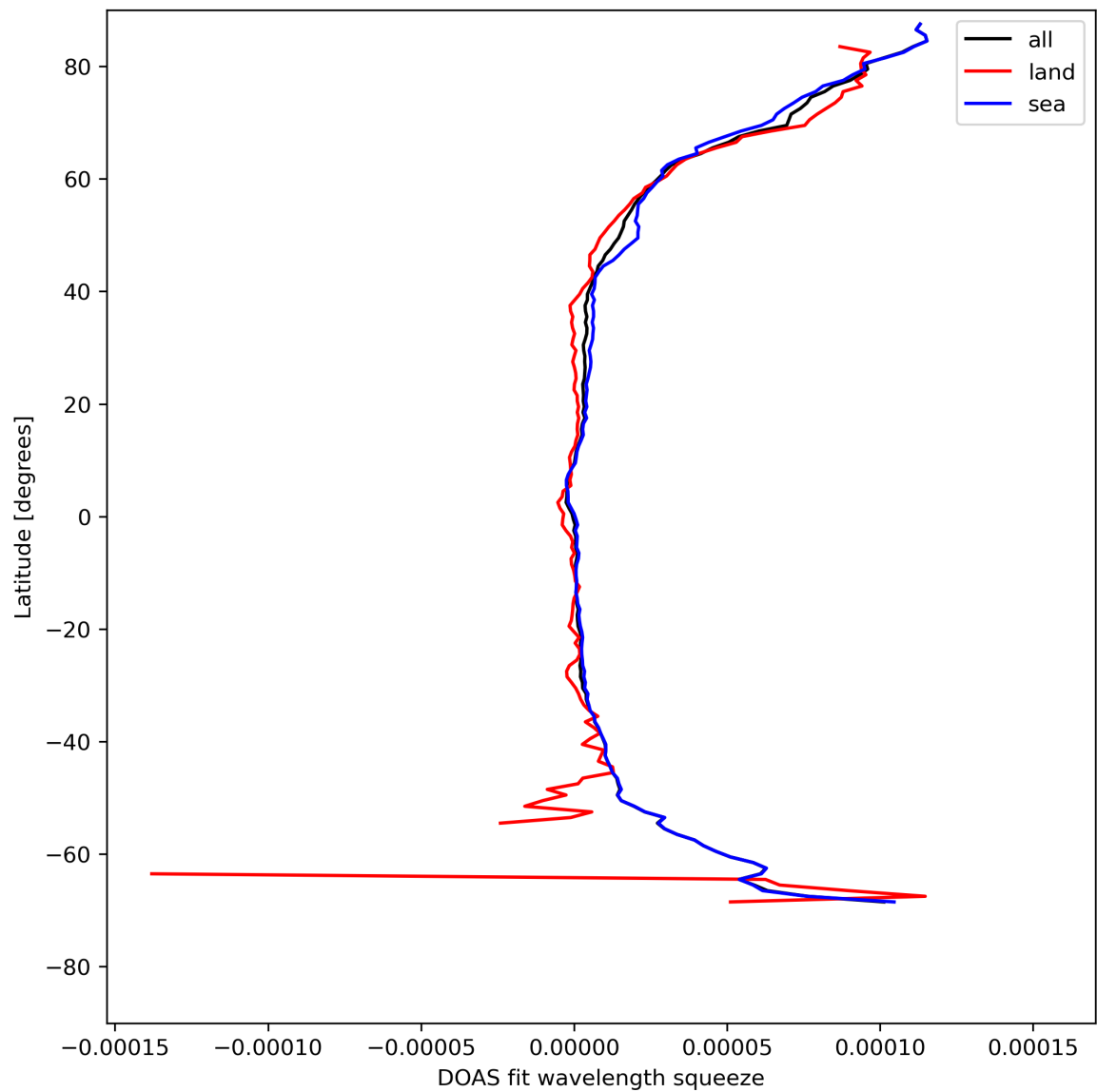
Figure 31: Zonal average of “DOAS fit wavelength squeeze” for 2024-05-02 to 2024-05-03.
