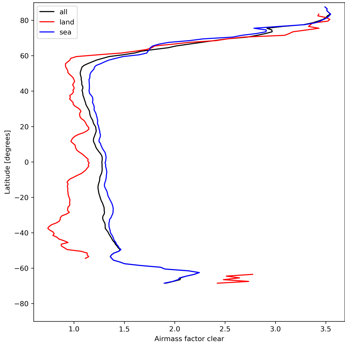
Figure 28: Zonal average of “Airmass factor clear” for 2024-05-02 to 2024-05-03.
