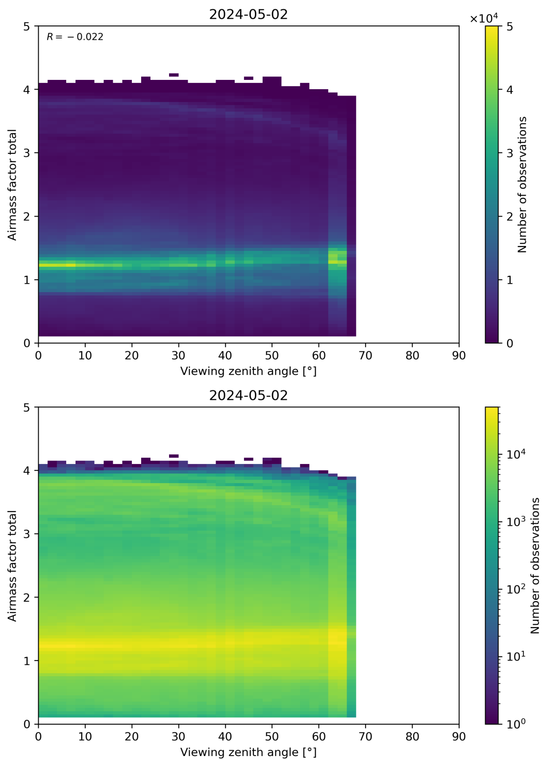
Figure 190: Scatter density plot of “Viewing zenith angle” against “Airmass factor total” for 2024-05-02 to 2024-05-03.
