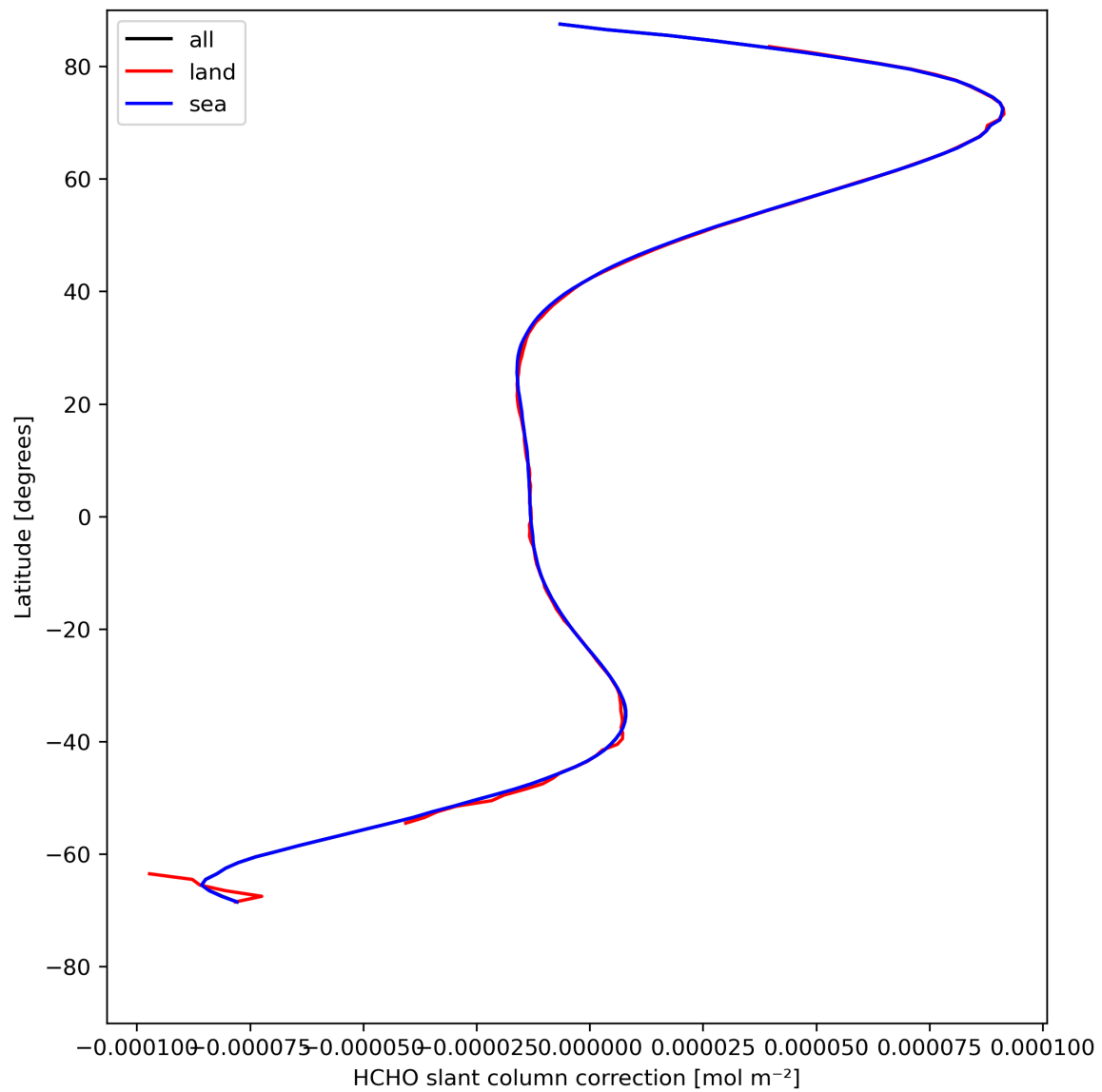
Figure 33: Zonal average of “HCHO slant column correction” for 2024-05-02 to 2024-05-03.
