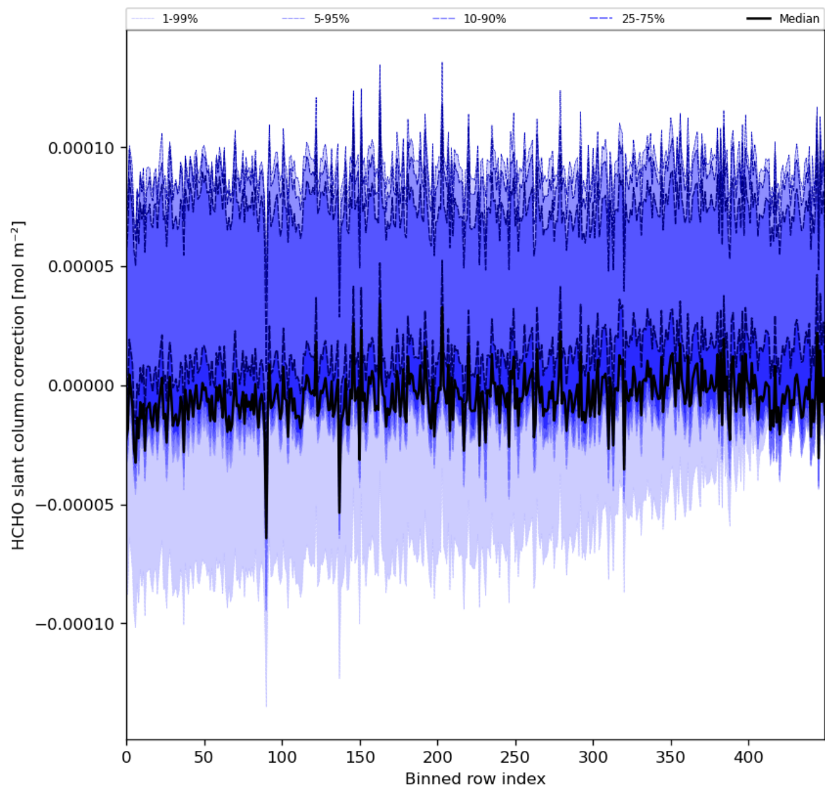
Figure 61: Along track statistics of “HCHO slant column correction” for 2024-05-02 to 2024-05-03
