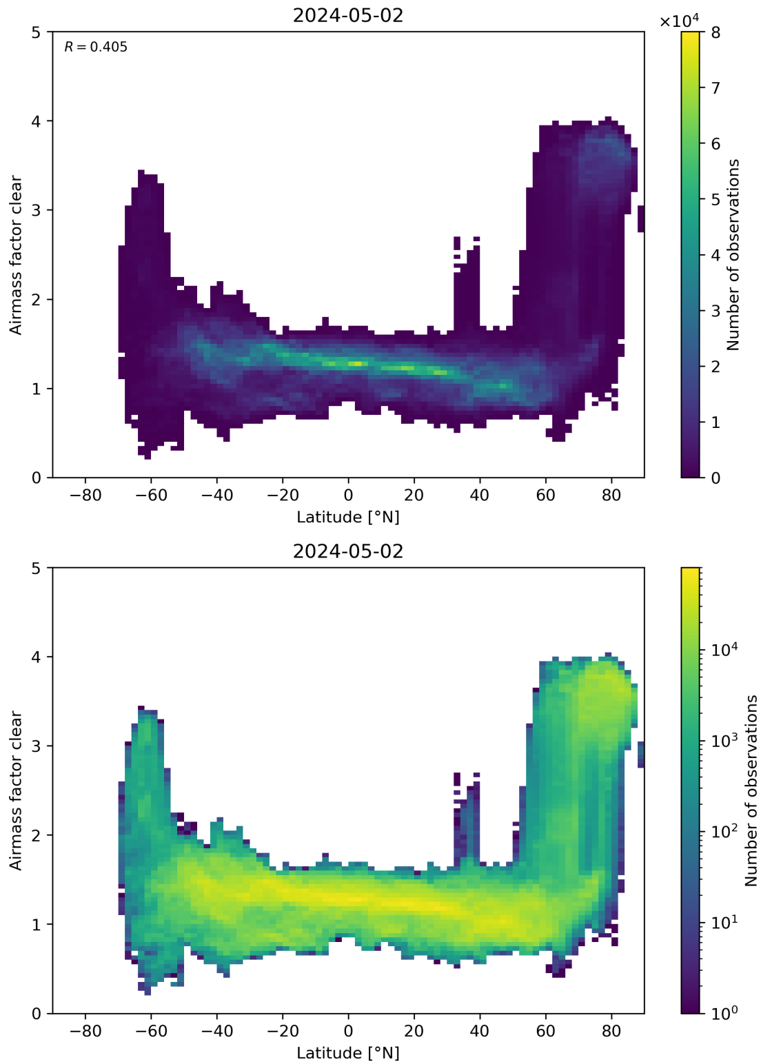
Figure 156: Scatter density plot of “Latitude” against “Airmass factor clear” for 2024-05-02 to 2024-05-03.
