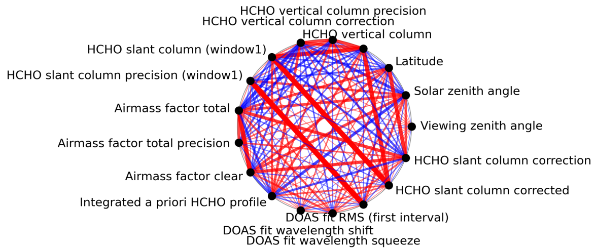
Figure 1: Map of correlation graph for 2024-05-02 to 2024-05-03.
