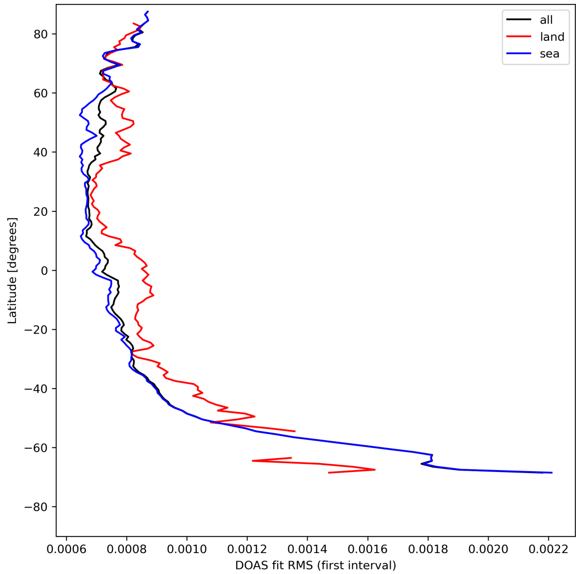
Figure 32: Zonal average of “DOAS fit RMS (first interval)” for 2024-05-02 to 2024-05-03.
