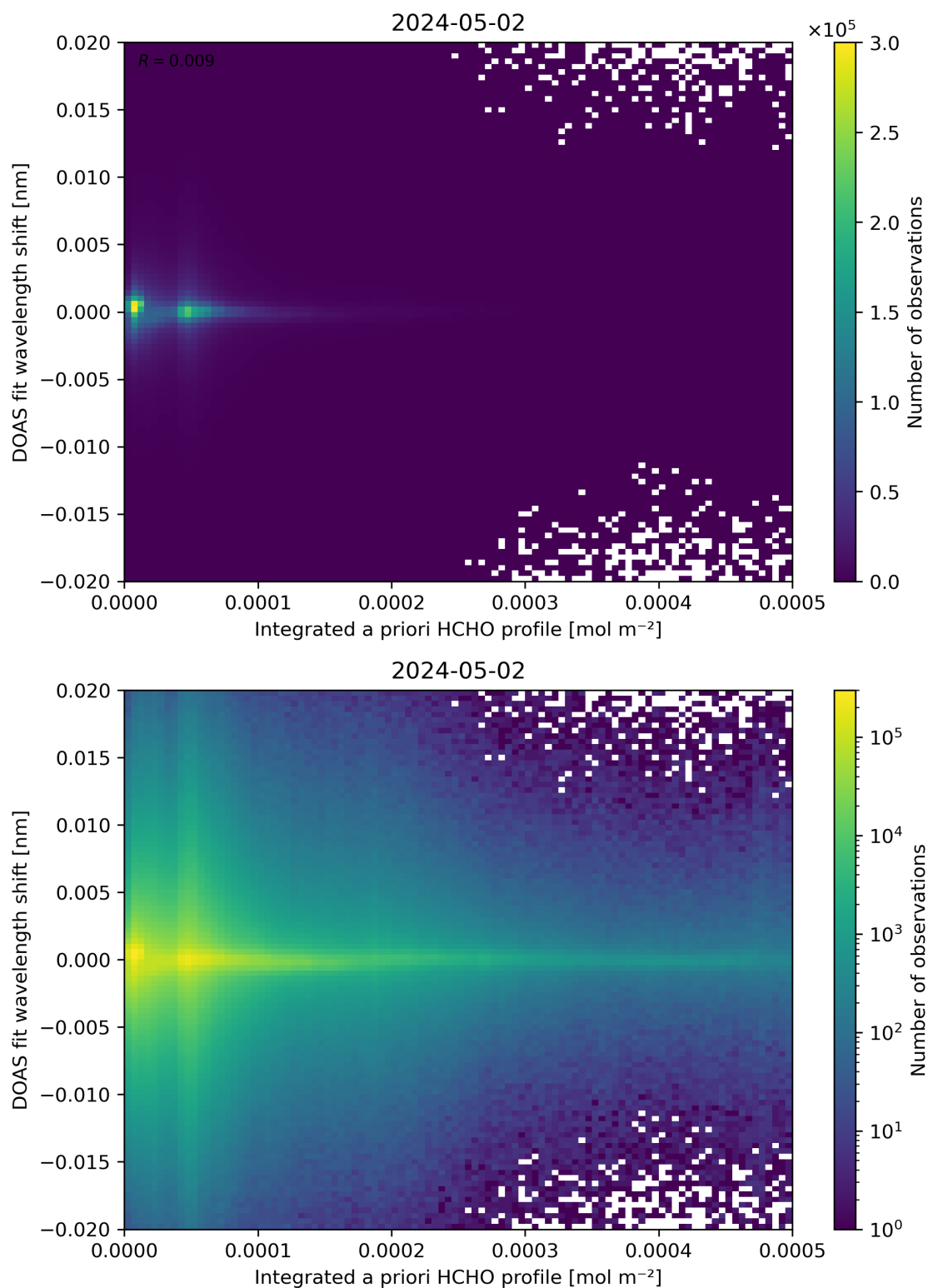
Figure 149: Scatter density plot of “Integrated a priori HCHO profile” against “DOAS fit wavelength shift” for 2024-05-02 to 2024-05-03.
