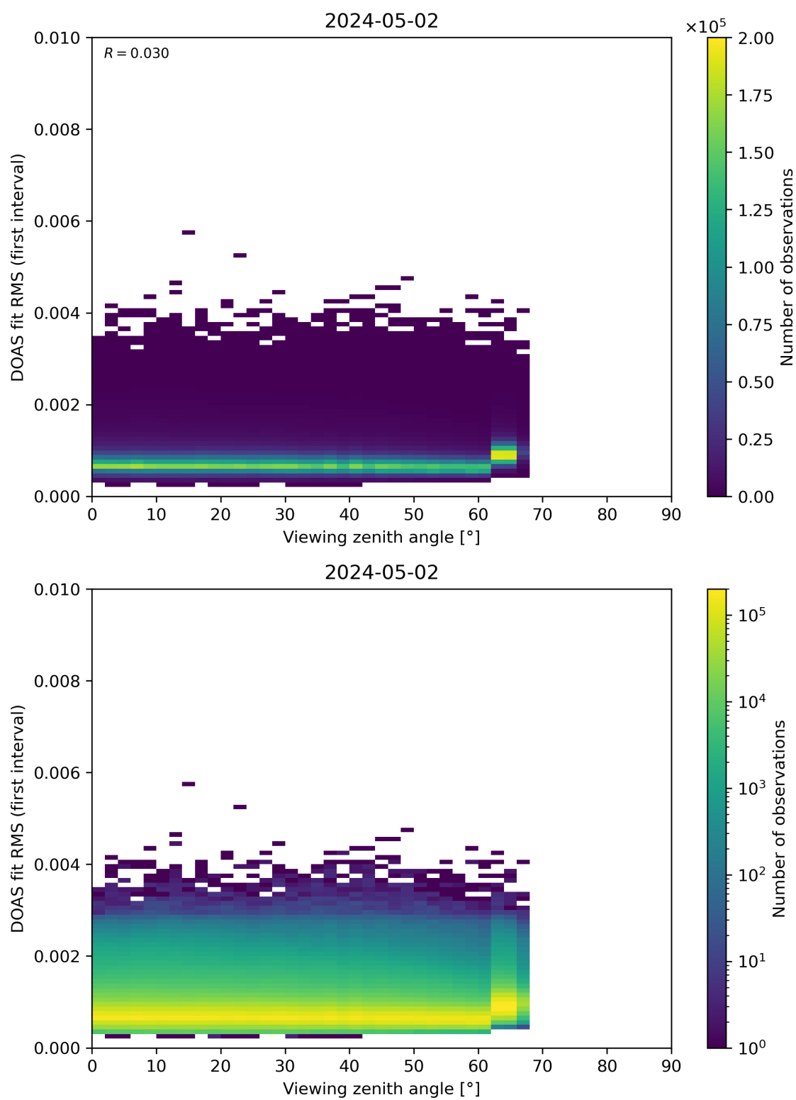
Figure 182: Scatter density plot of “Viewing zenith angle” against “DOAS fit RMS (first interval)” for 2024-05-02 to 2024-05-03.
