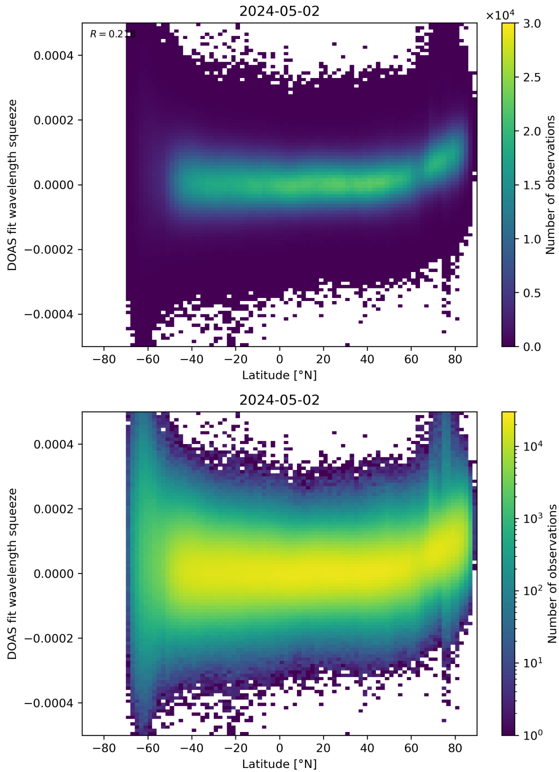
Figure 155: Scatter density plot of “Latitude” against “DOAS fit wavelength squeeze” for 2024-05-02 to 2024-05-03.
