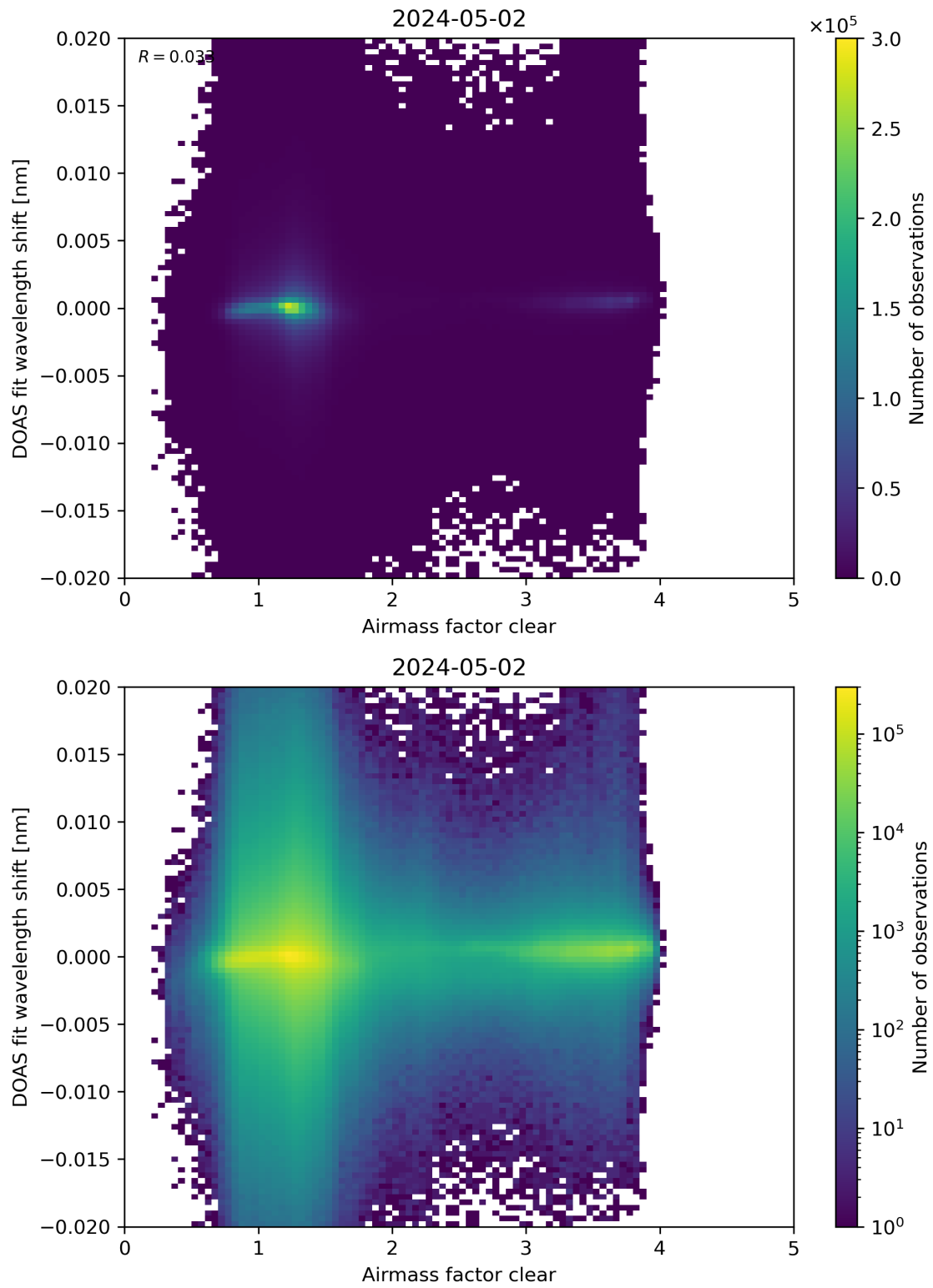
Figure 72: Scatter density plot of “Airmass factor clear” against “DOAS fit wavelength shift” for 2024-05-02 to 2024-05-03.
