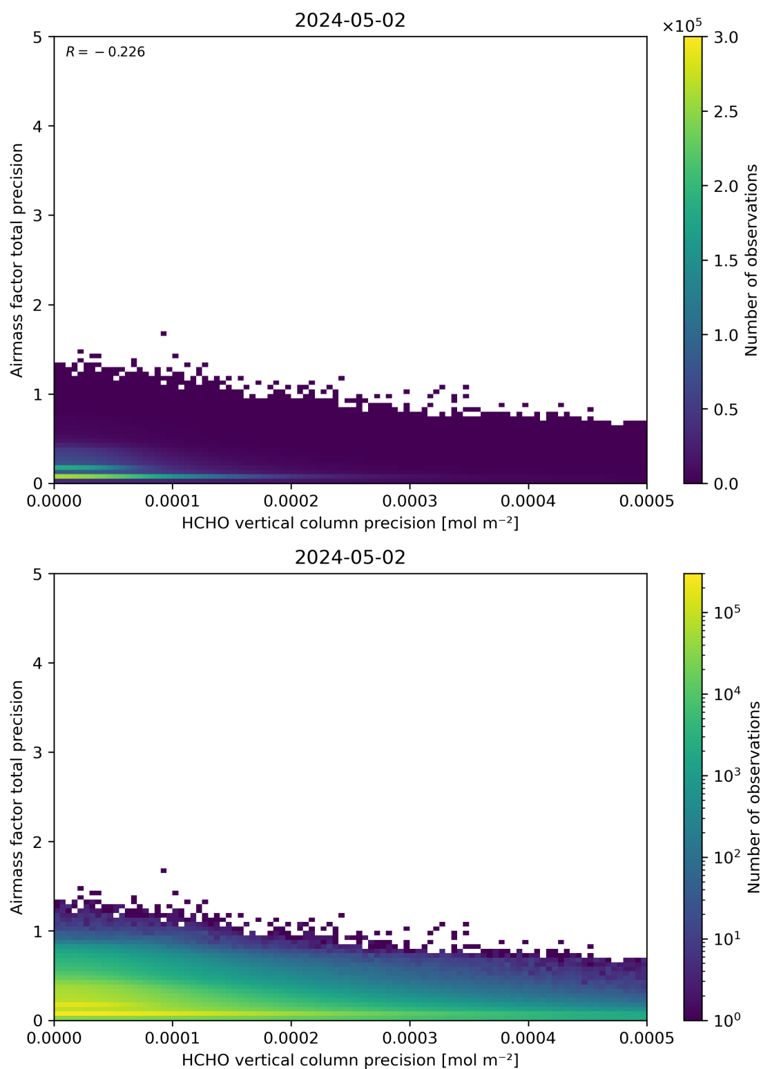
Figure 145: Scatter density plot of “HCHO vertical column precision” against “Airmass factor total precision” for 2024-05-02 to 2024-05-03.
