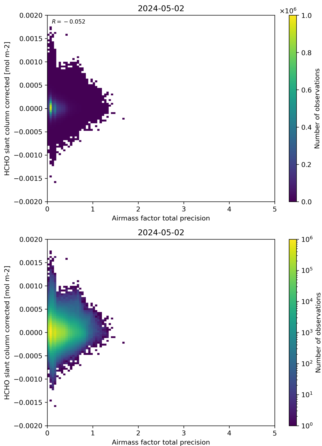
Figure 109: Scatter density plot of “Air mass factor total precision” against “HCHO slant column corrected” for 2024-05-02 to 2024-05-03.
