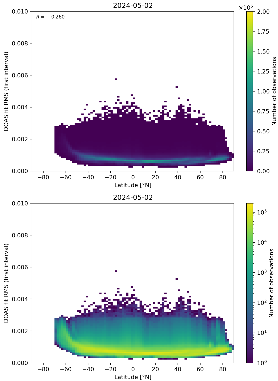
Figure 153: Scatter density plot of “Latitude” against “DOAS fit RMS (first interval)” for 2024-05-02 to 2024-05-03.
