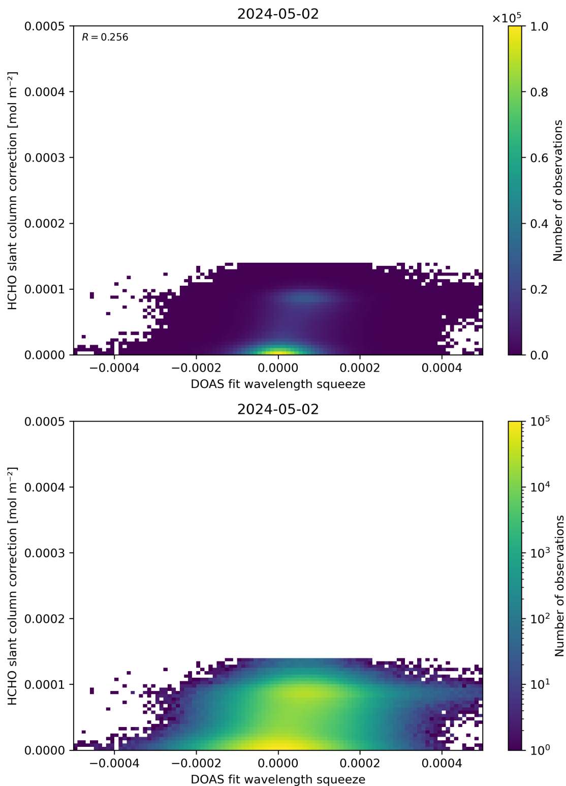
Figure 70: Scatter density plot of “DOAS fit wavelength squeeze” against “HCHO slant column correction” for 2024-05-02 to 2024-05-03.
