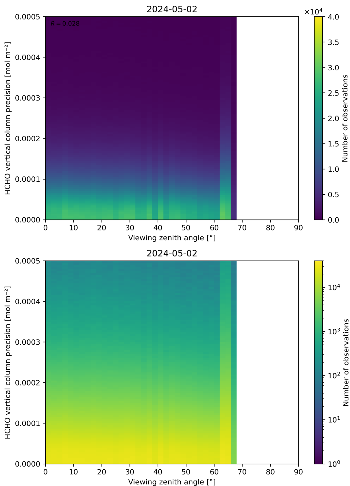
Figure 194: Scatter density plot of “Viewing zenith angle” against “HCHO vertical column precision” for 2024-05-02 to 2024-05-03.
