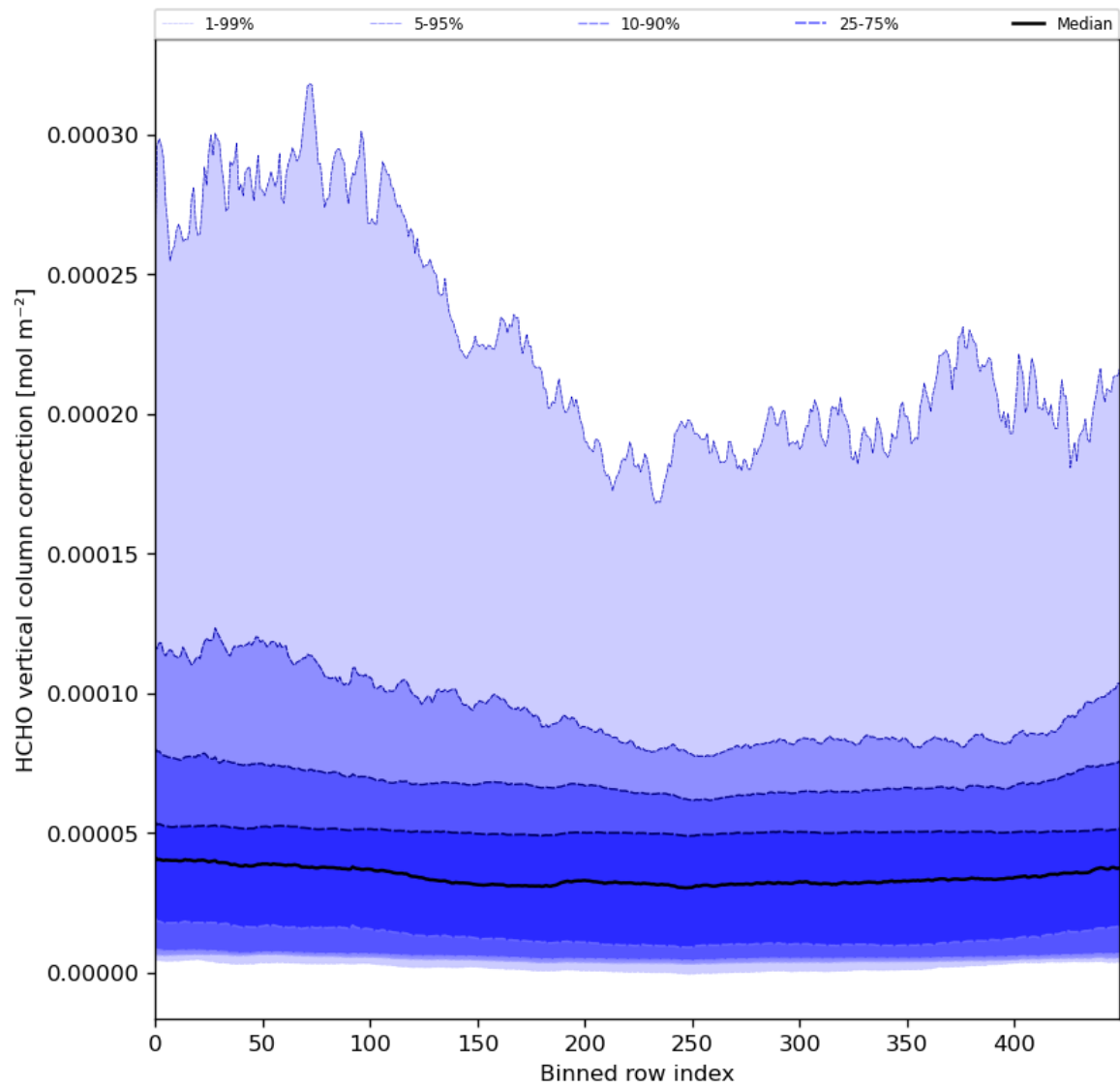
Figure 51: Along track statistics of “HCHO vertical column correction” for 2024-05-02 to 2024-05-03
