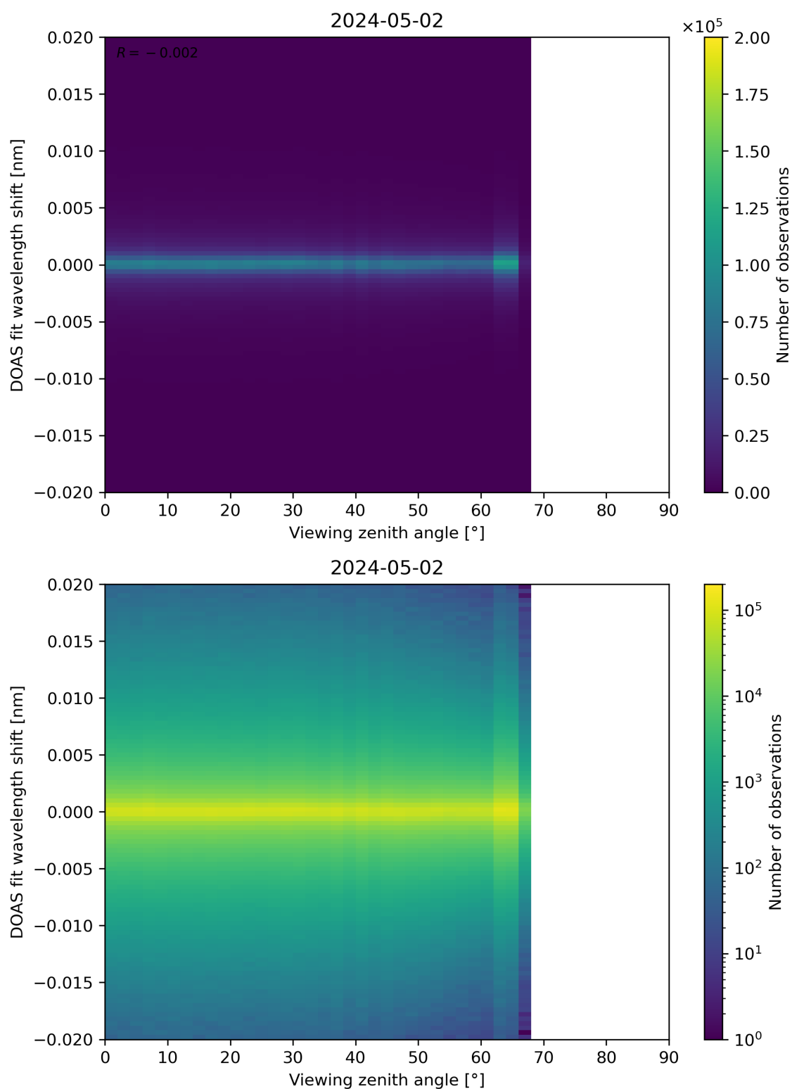
Figure 183: Scatter density plot of “Viewing zenith angle” against “DOAS fit wavelength shift” for 2024-05-02 to 2024-05-03.
