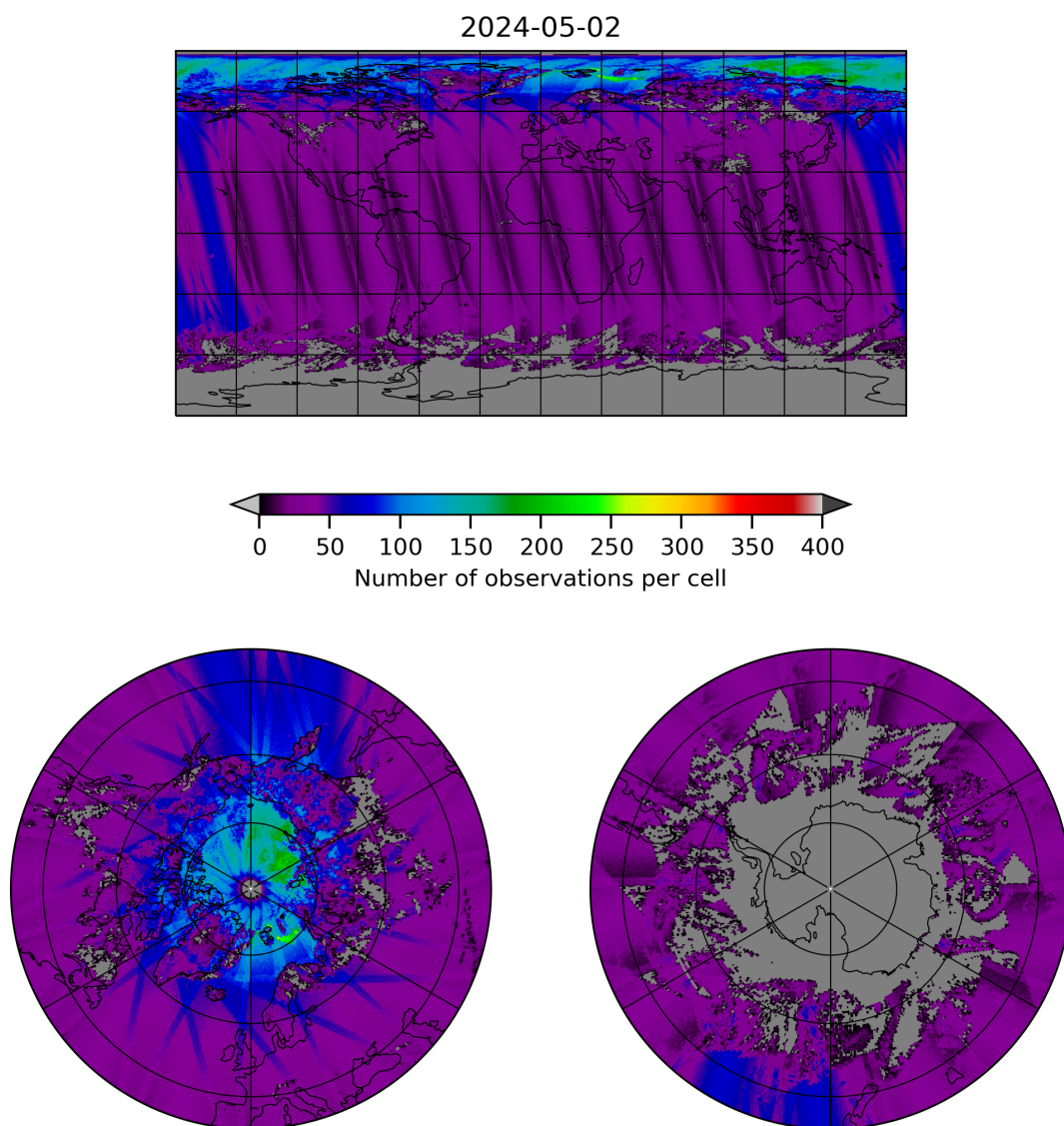
Figure 19: Map of the number of observations for 2024-05-02 to 2024-05-03
