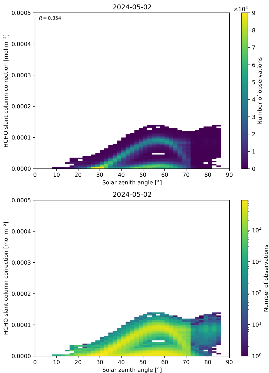
Figure 172: Scatter density plot of “Solar zenith angle” against “HCHO slant column correction” for 2024-05-02 to 2024-05-03.
