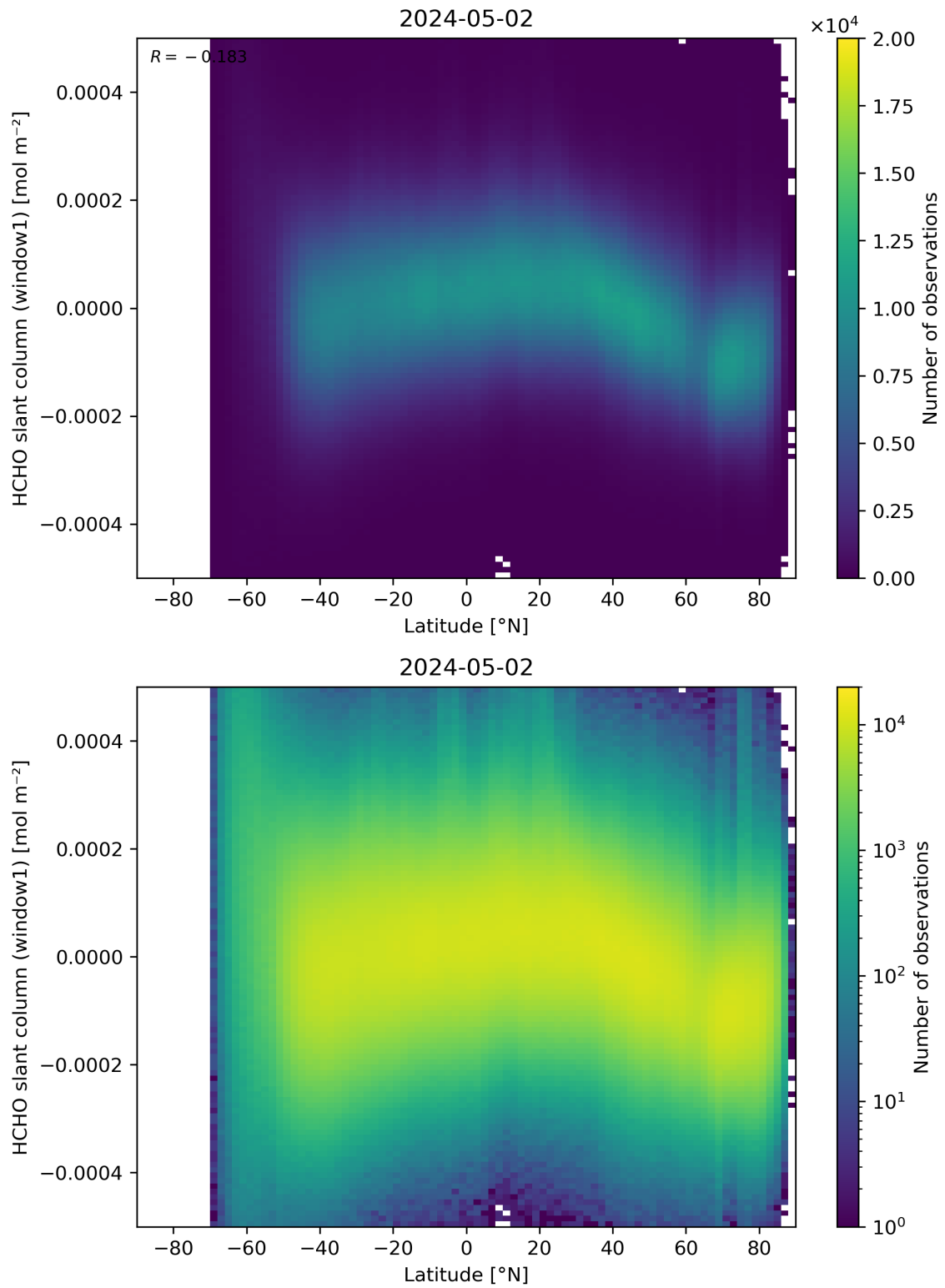
Figure 159: Scatter density plot of “Latitude” against “HCHO slant column (window1)” for 2024-05-02 to 2024-05-03.
