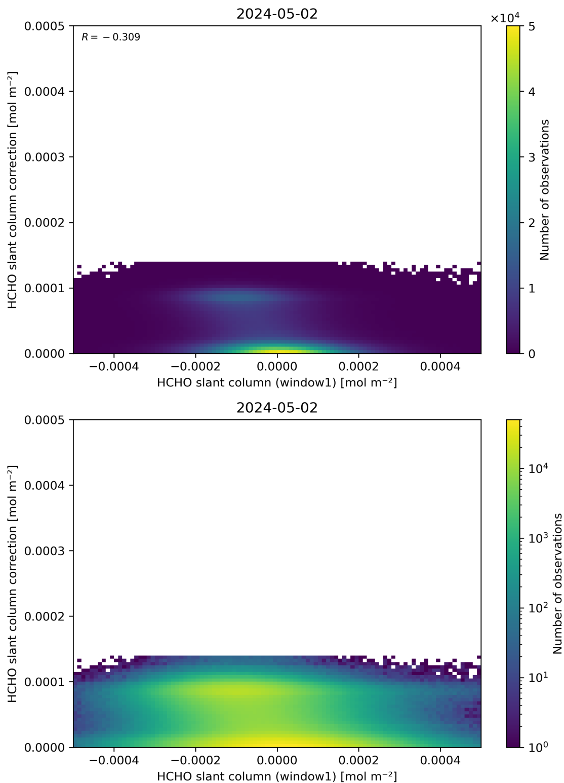
Figure 83: Scatter density plot of “HCHO slant column (window1)” against “HCHO slant column correction” for 2024-05-02 to 2024-05-03.
