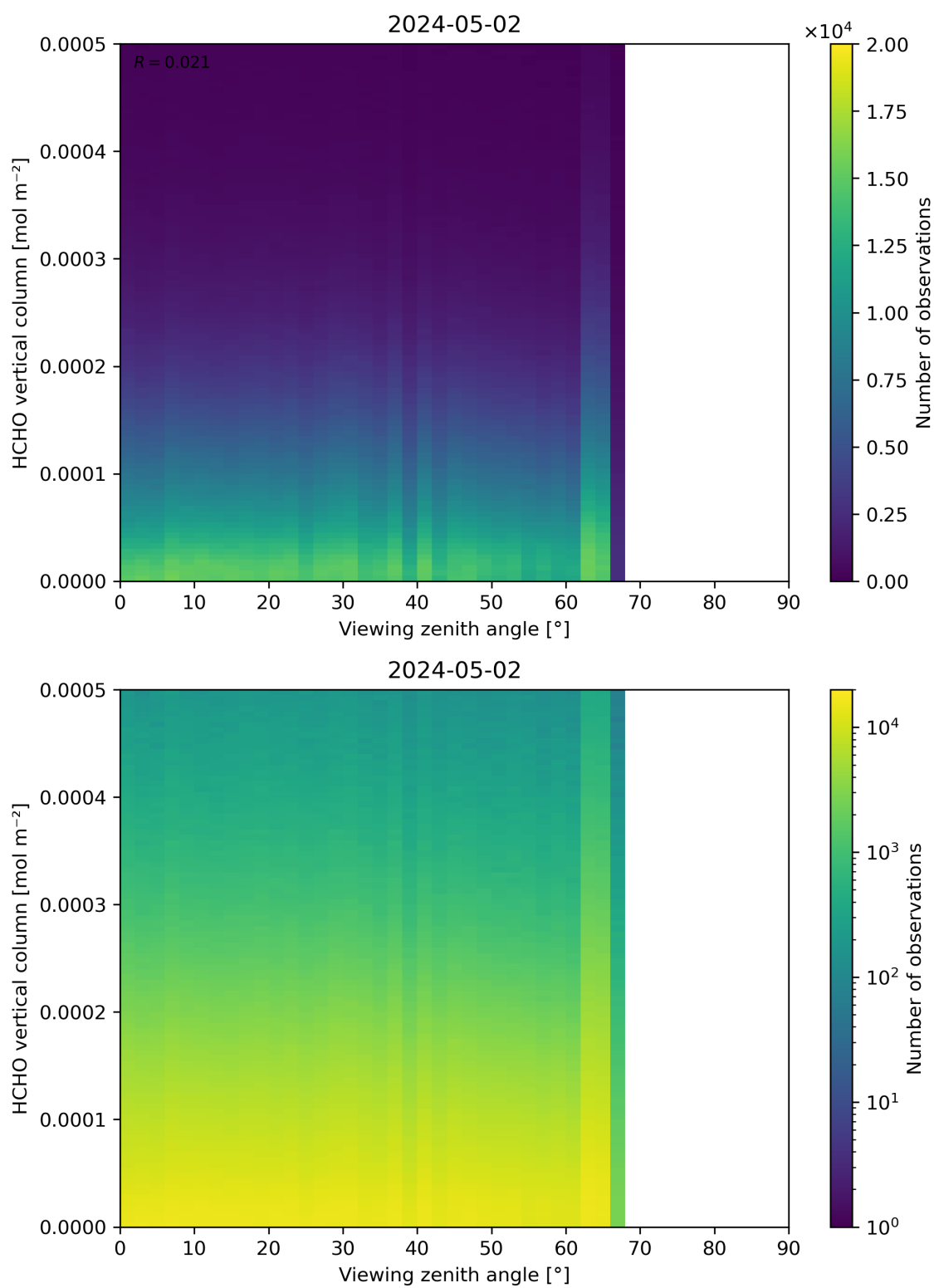
Figure 192: Scatter density plot of “Viewing zenith angle” against “HCHO vertical column” for 2024-05-02 to 2024-05-03.
