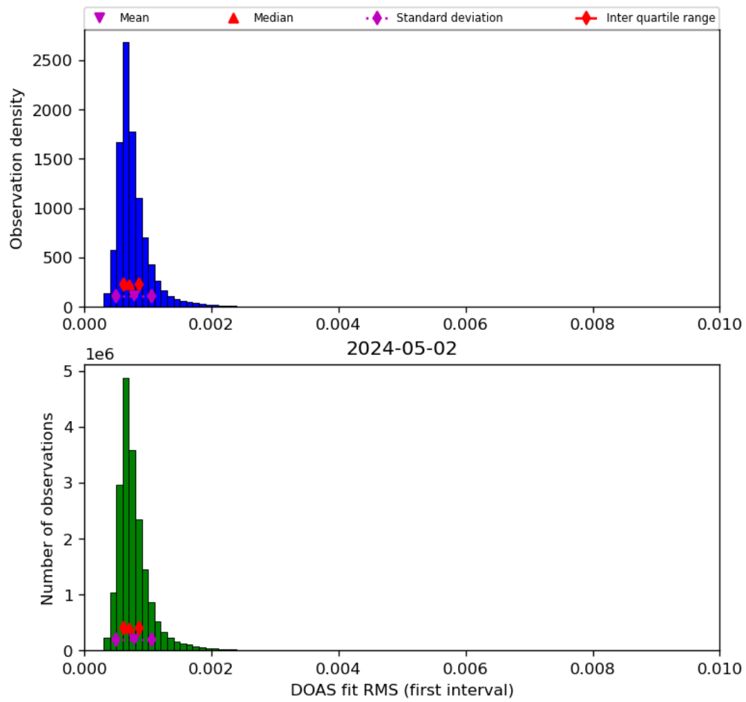
Figure 46: Histogram of “DOAS fit RMS (first interval)” for 2024-05-02 to 2024-05-03
