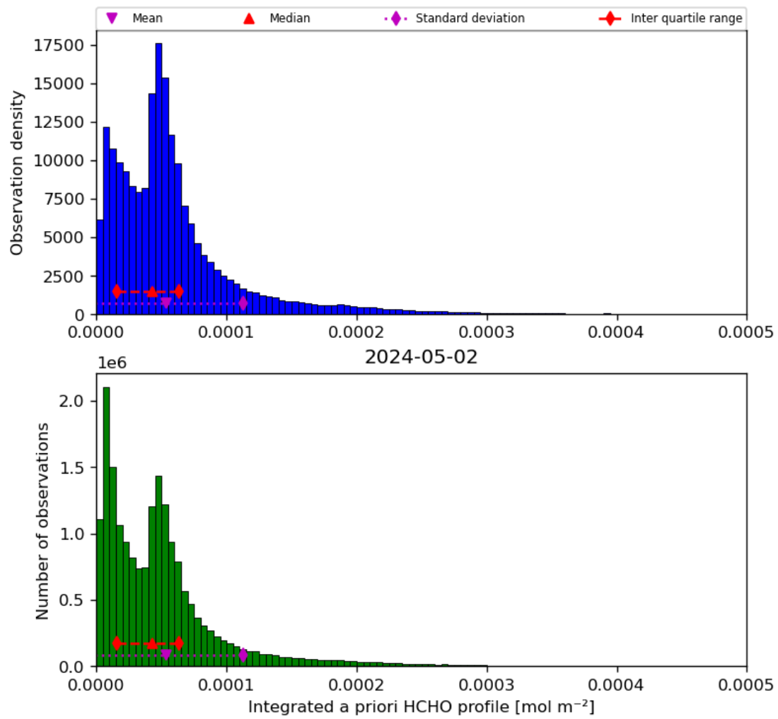
Figure 43: Histogram of “Integrated a priori HCHO profile” for 2024-05-02 to 2024-05-03
