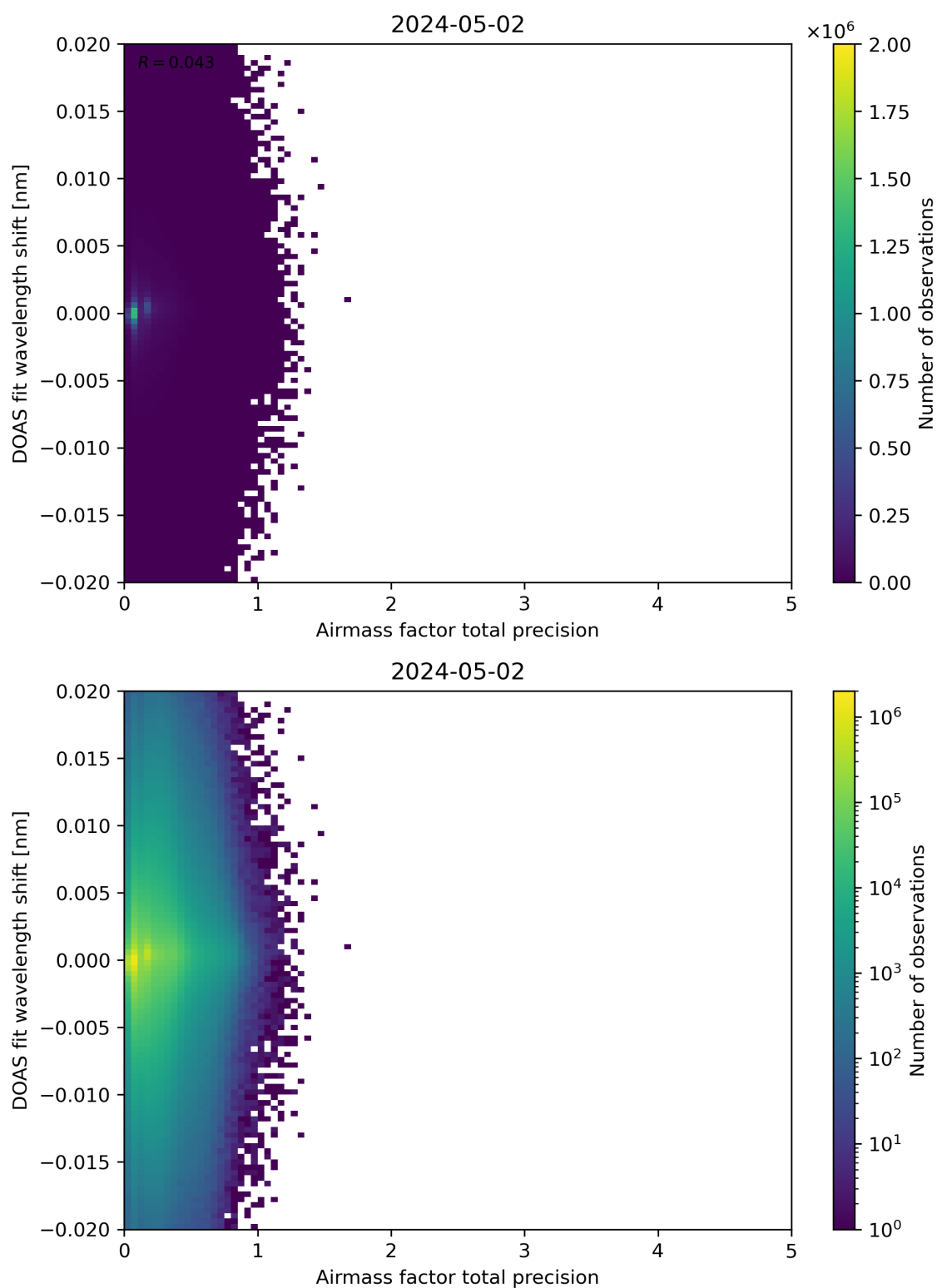
Figure 106: Scatter density plot of “Airmass factor total precision” against “DOAS fit wavelength shift” for 2024-05-02 to 2024-05-03.
