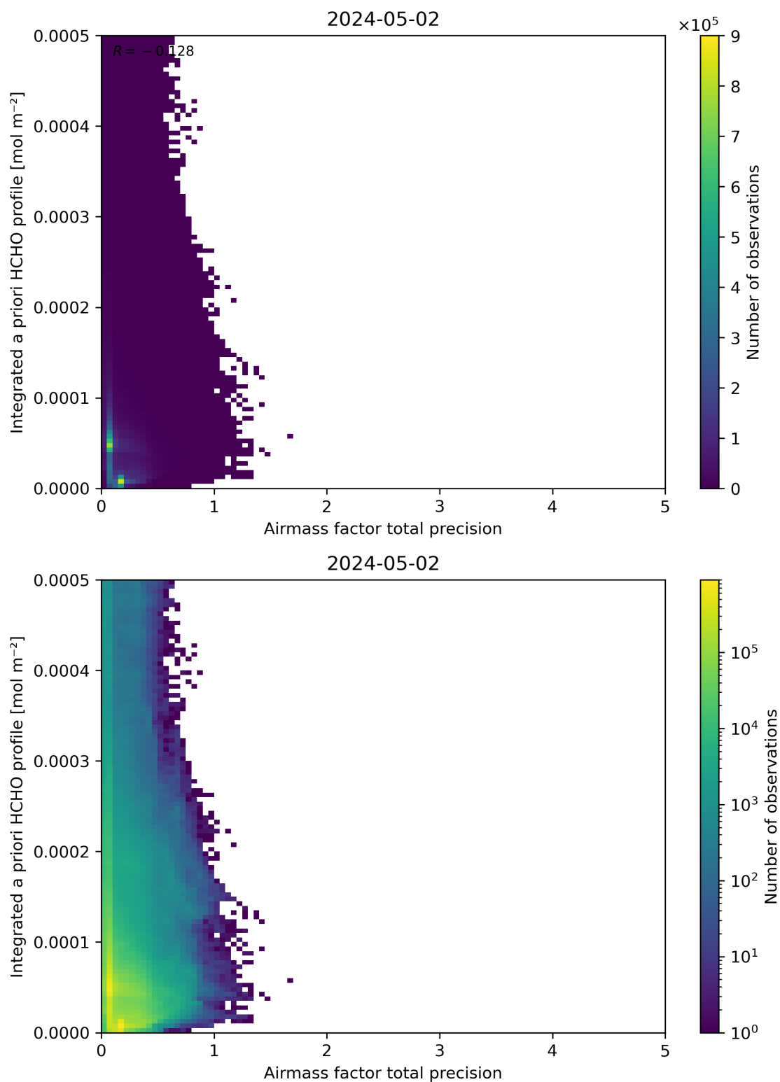
Figure 111: Scatter density plot of “Airmass factor total precision” against “Integrated a priori HCHO profile” for 2024-05-02 to 2024-05-03.
