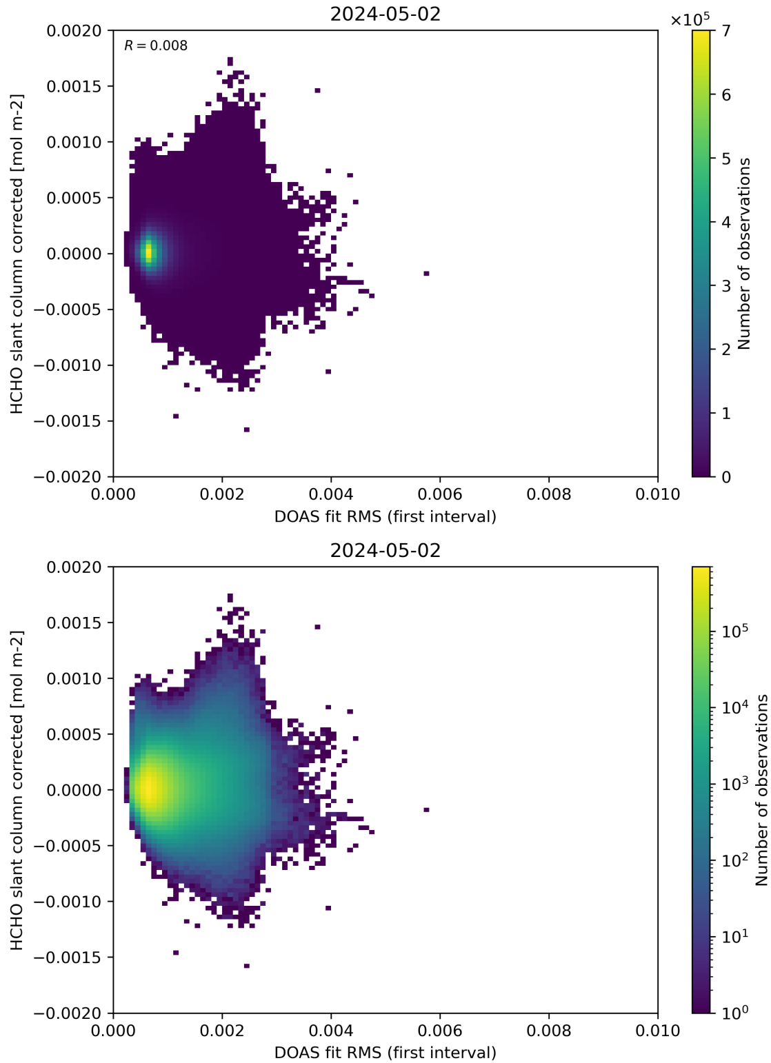
Figure 62: Scatter density plot of “DOAS fit RMS (first interval)” against “HCHO slant column corrected” for 2024-05-02 to 2024-05-03.
