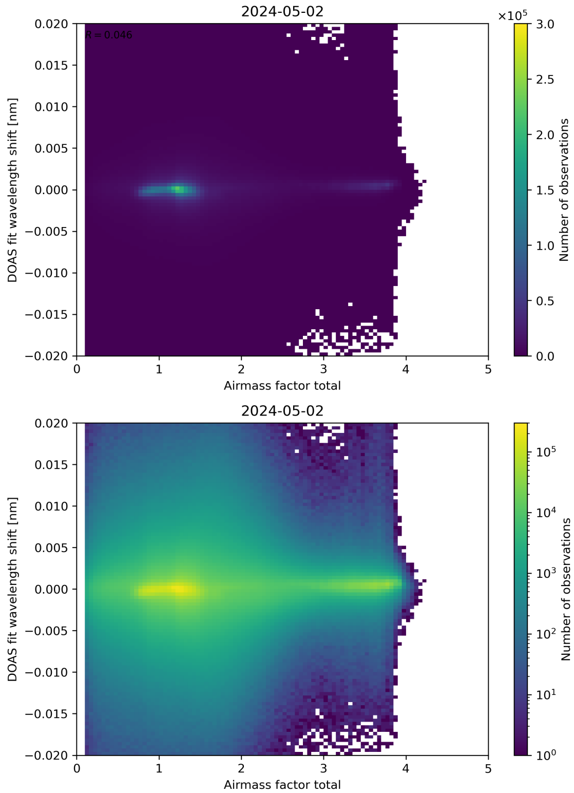
Figure 98: Scatter density plot of “Airmass factor total” against “DOAS fit wavelength shift” for 2024-05-02 to 2024-05-03.
