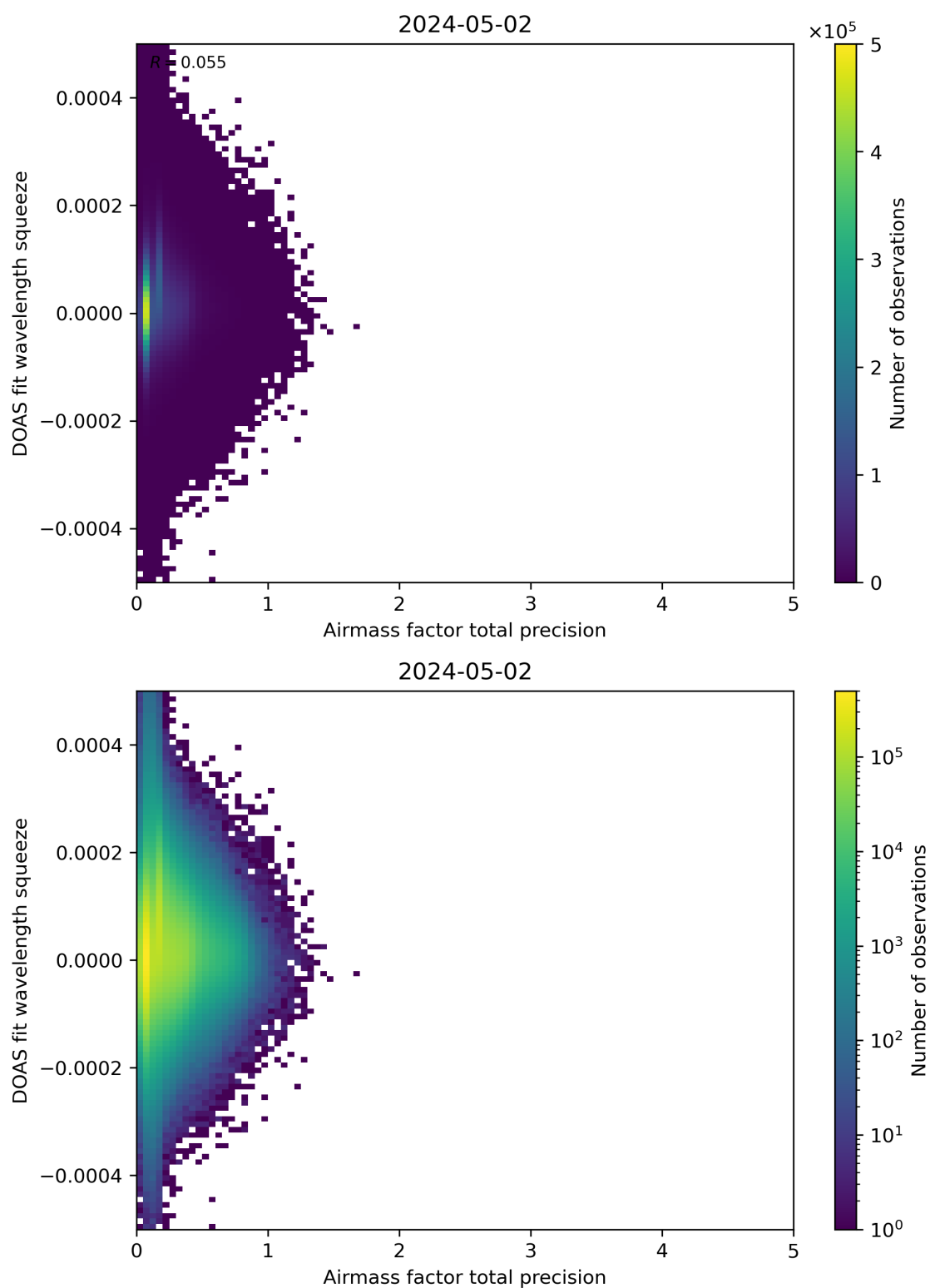
Figure 107: Scatter density plot of “Airmass factor total precision” against “DOAS fit wavelength squeeze” for 2024-05-02 to 2024-05-03.
