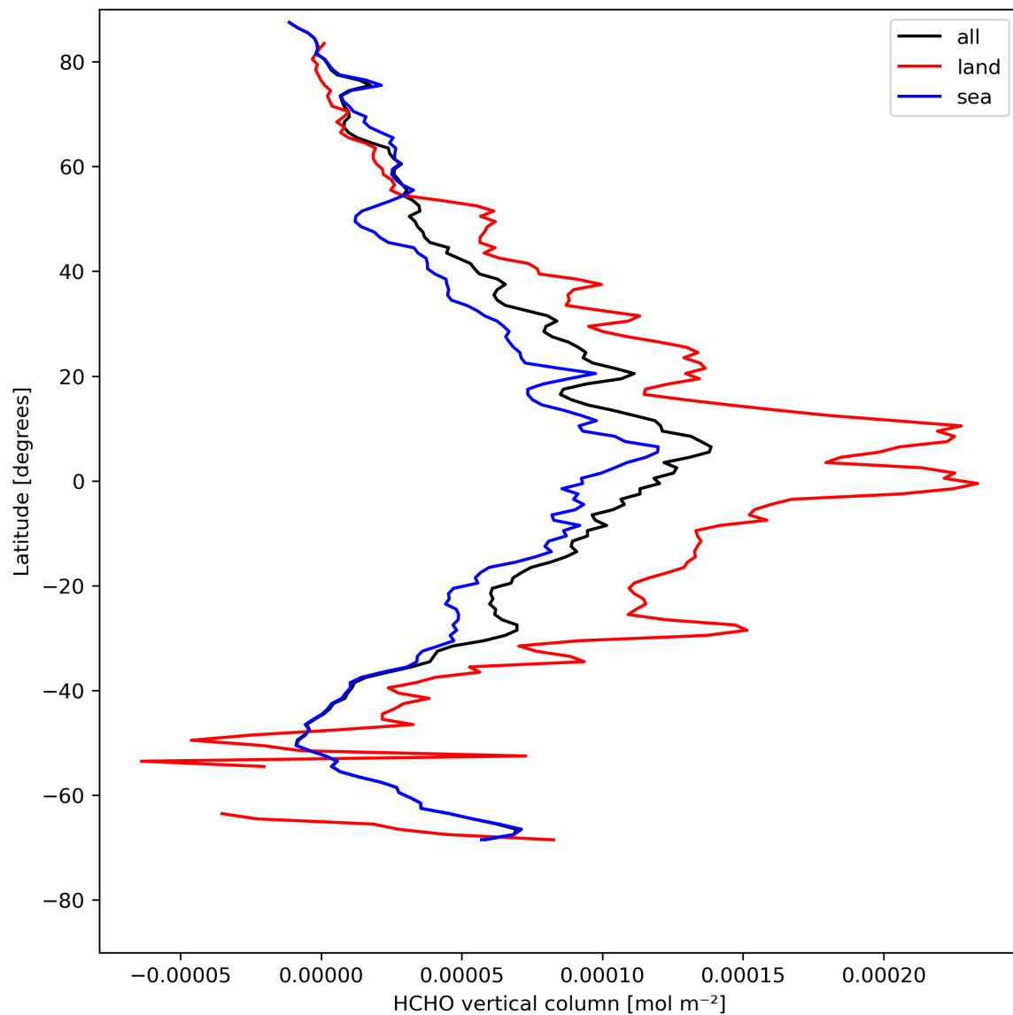
Figure 21: Zonal average of “HCHO vertical column” for 2024-05-02 to 2024-05-03.
