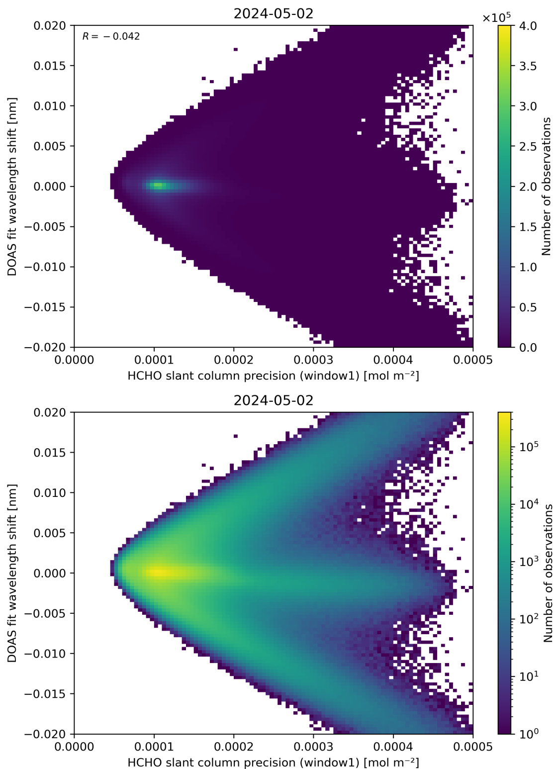
Figure 89: Scatter density plot of “HCHO slant column precision (window1)” against “DOAS fit wavelength shift” for 2024-05-02 to 2024-05-03.
