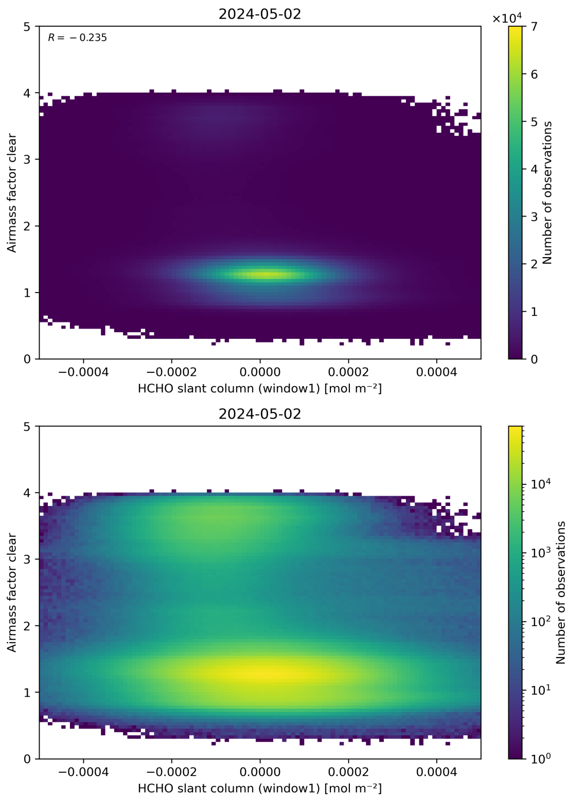
Figure 81: Scatter density plot of “HCHO slant column (window1)” against “Airmass factor clear” for 2024-05-02 to 2024-05-03.
