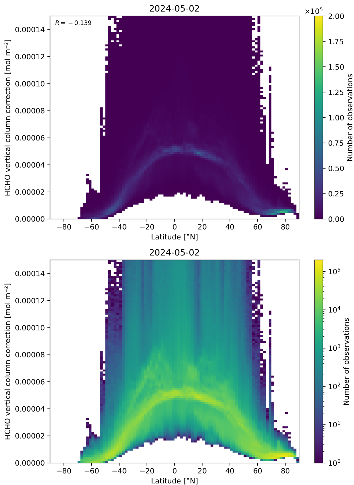
Figure 164: Scatter density plot of “Latitude” against “HCHO vertical column correction” for 2024-05-02 to 2024-05-03.
