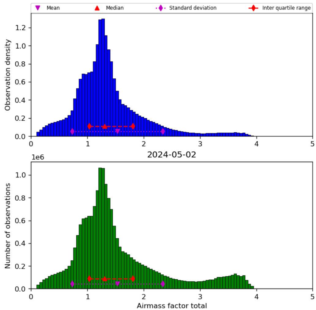
Figure 40: Histogram of “Airmass factor total” for 2024-05-02 to 2024-05-03
