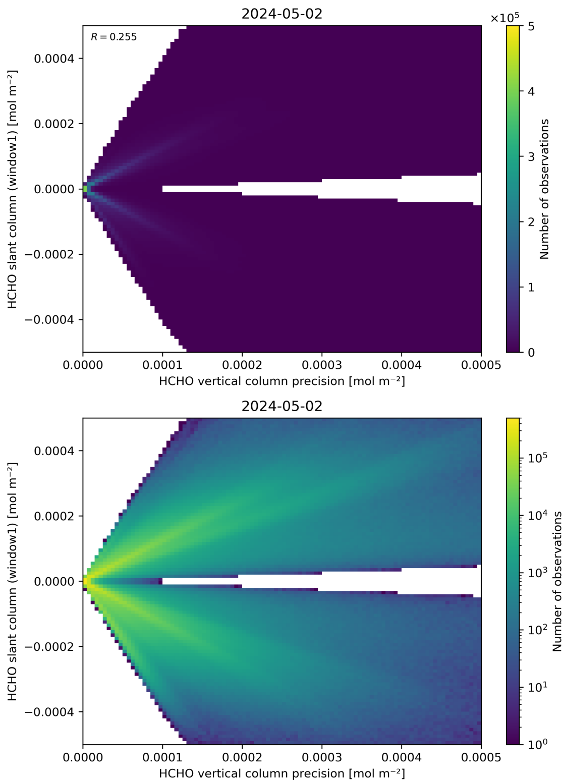
Figure 142: Scatter density plot of “HCHO vertical column precision” against “HCHO slant column (window1)” for 2024-05-02 to 2024-05-03.
