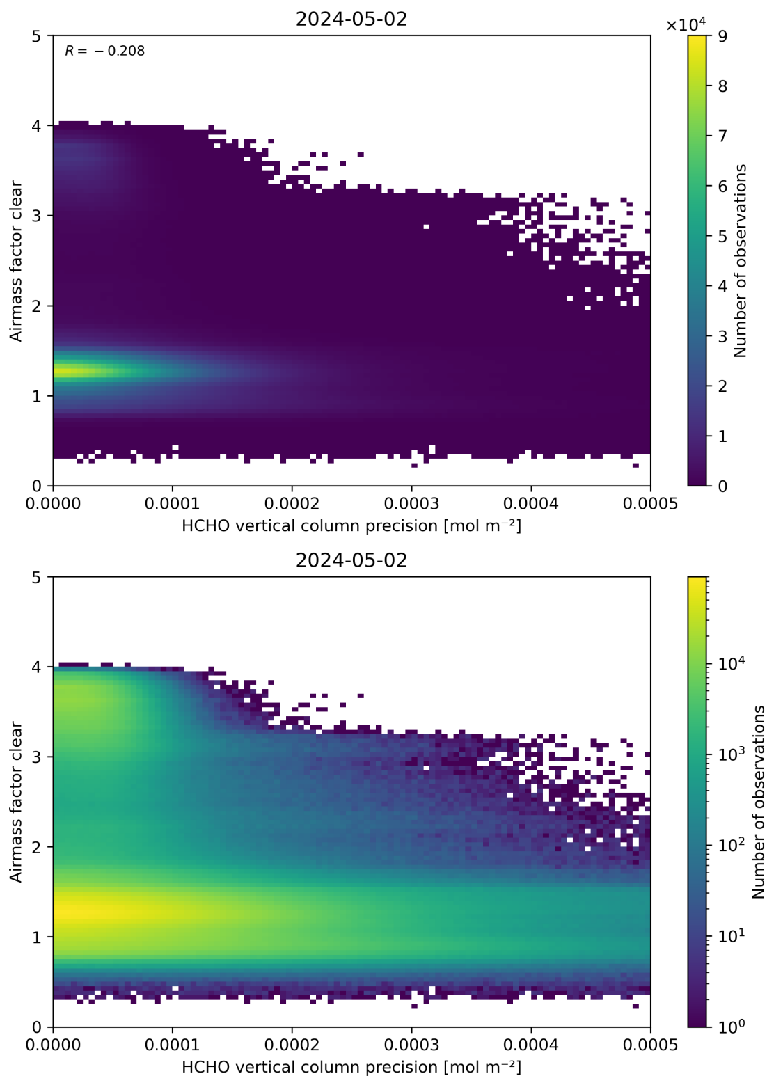
Figure 139: Scatter density plot of “HCHO vertical column precision” against “Airmass factor clear” for 2024-05-02 to 2024-05-03.
