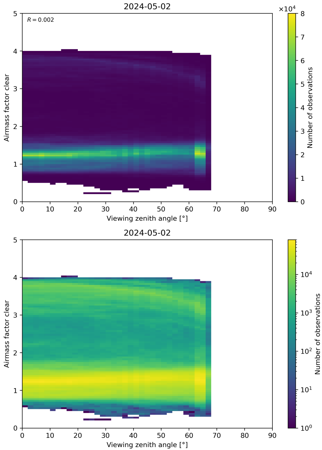
Figure 185: Scatter density plot of “Viewing zenith angle” against “Airmass factor clear” for 2024-05-02 to 2024-05-03.
