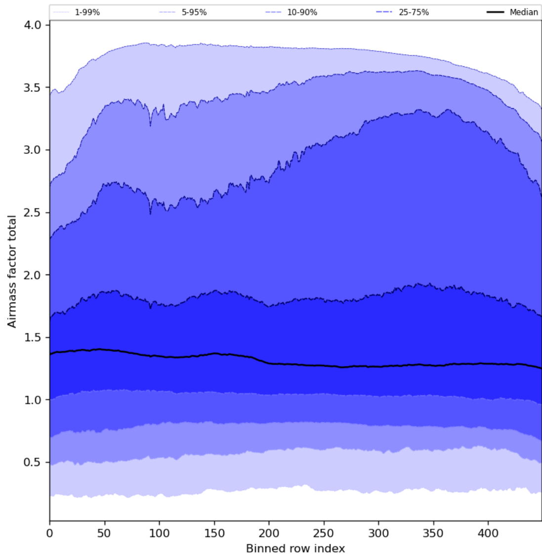
Figure 54: Along track statistics of “Airmass factor total” for 2024-05-02 to 2024-05-03
