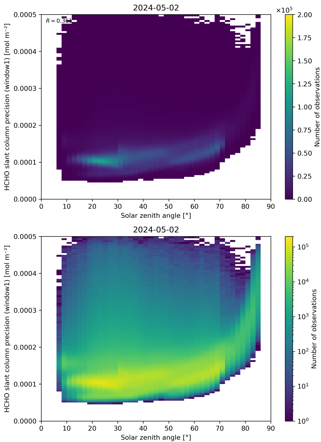
Figure 174: Scatter density plot of “Solar zenith angle” against “HCHO slant column precision (window1)” for 2024-05-02 to 2024-05-03.
