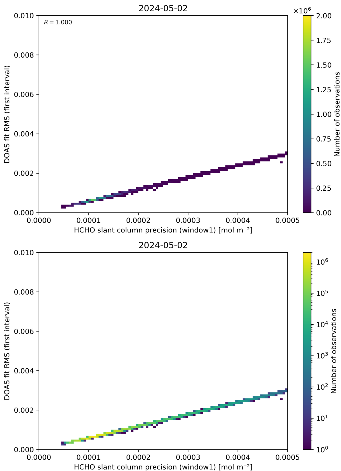
Figure 88: Scatter density plot of “HCHO slant column precision (window1)” against “DOAS fit RMS (first interval)” for 2024-05-02 to 2024-05-03.
