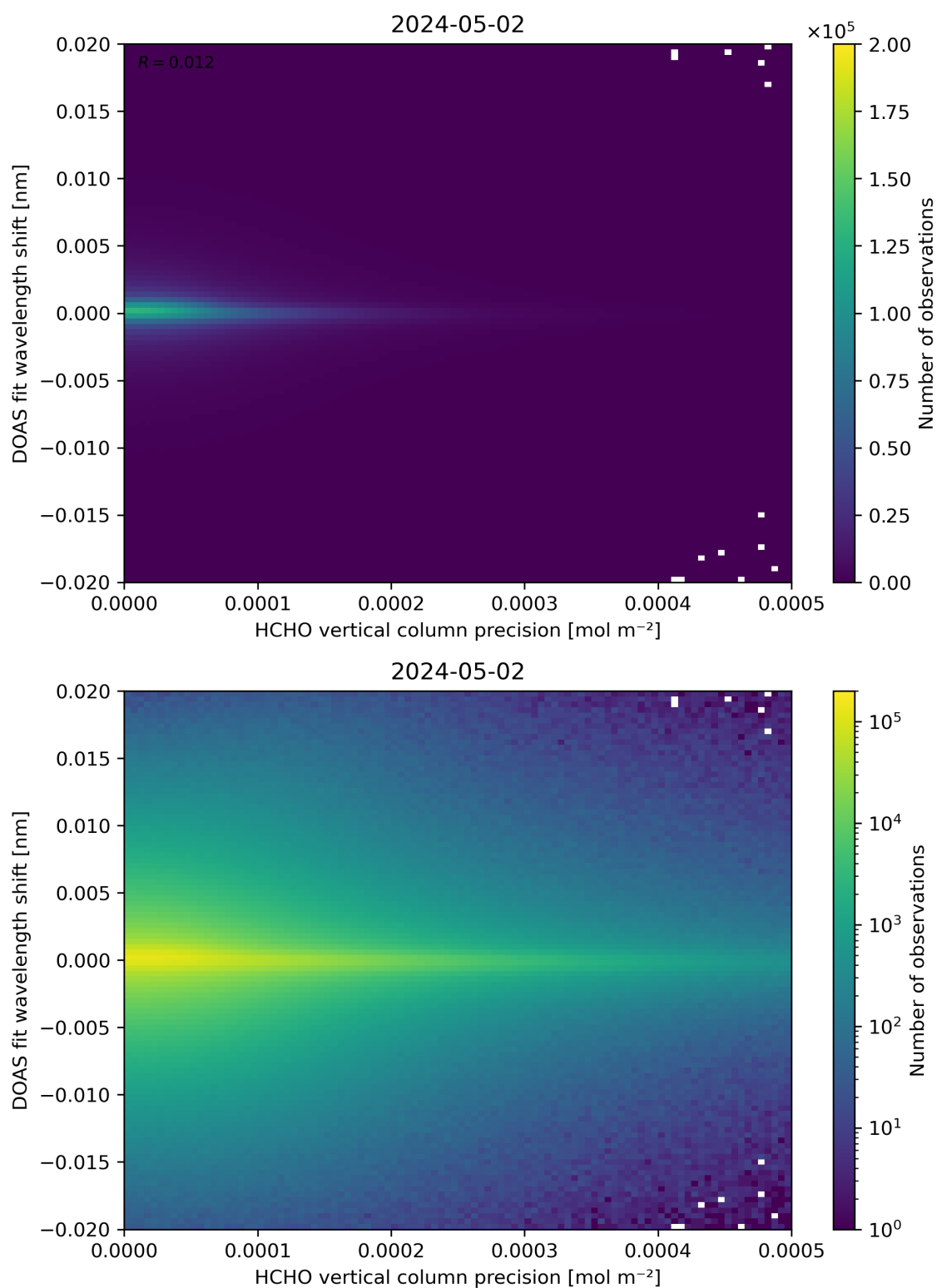
Figure 137: Scatter density plot of “HCHO vertical column precision” against “DOAS fit wavelength shift” for 2024-05-02 to 2024-05-03.
