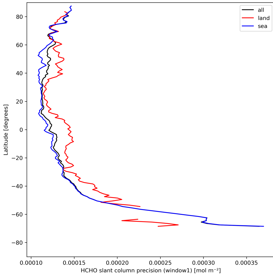
Figure 25: Zonal average of “HCHO slant column precision (window1)” for 2024-05-02 to 2024-05-03.
