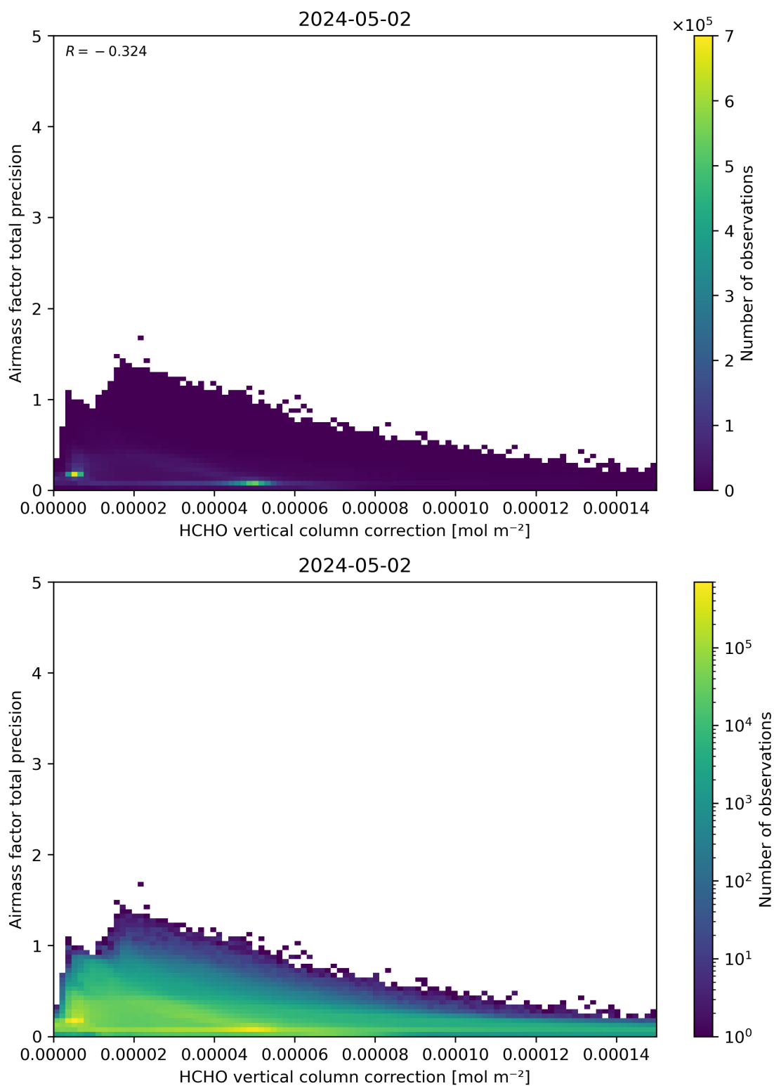
Figure 121: Scatter density plot of “HCHO vertical column correction” against “Airmass factor total precision” for 2024-05-02 to 2024-05-03.
