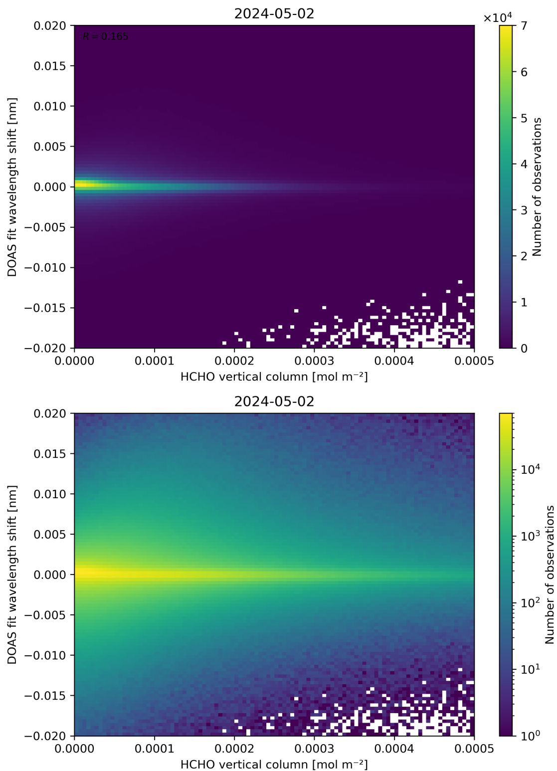
Figure 124: Scatter density plot of “HCHO vertical column” against “DOAS fit wavelength shift” for 2024-05-02 to 2024-05-03.
