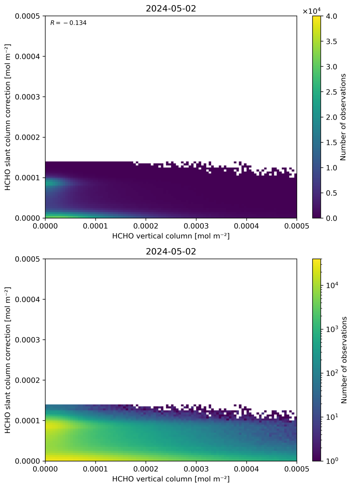
Figure 128: Scatter density plot of “HCHO vertical column” against “HCHO slant column correction” for 2024-05-02 to 2024-05-03.
