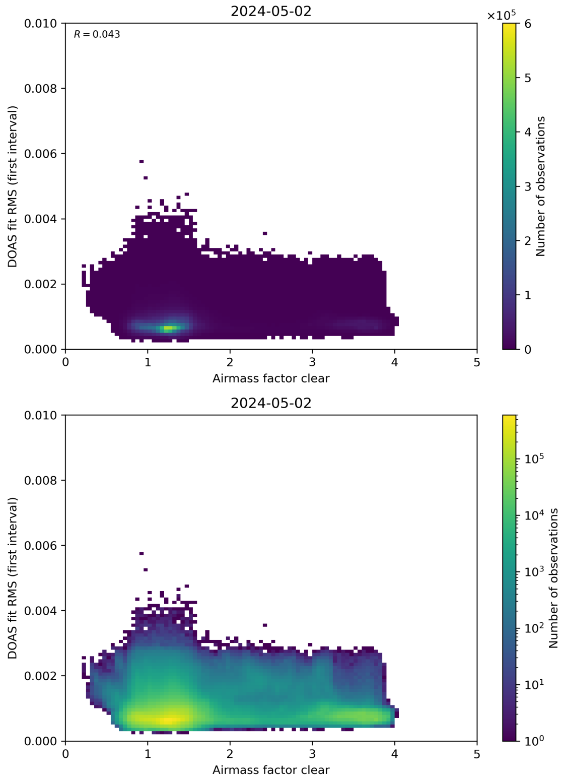
Figure 71: Scatter density plot of “Airmass factor clear” against “DOAS fit RMS (first interval)” for 2024-05-02 to 2024-05-03.
