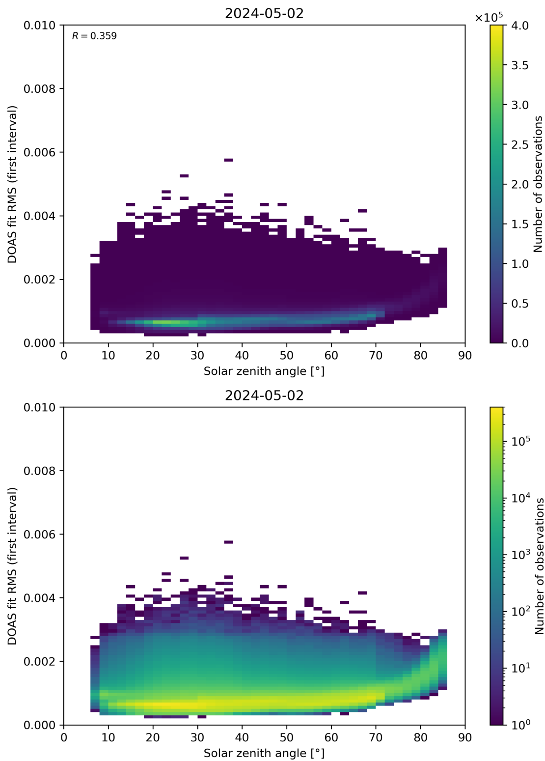
Figure 167: Scatter density plot of “Solar zenith angle” against “DOAS fit RMS (first interval)” for 2024-05-02 to 2024-05-03.
