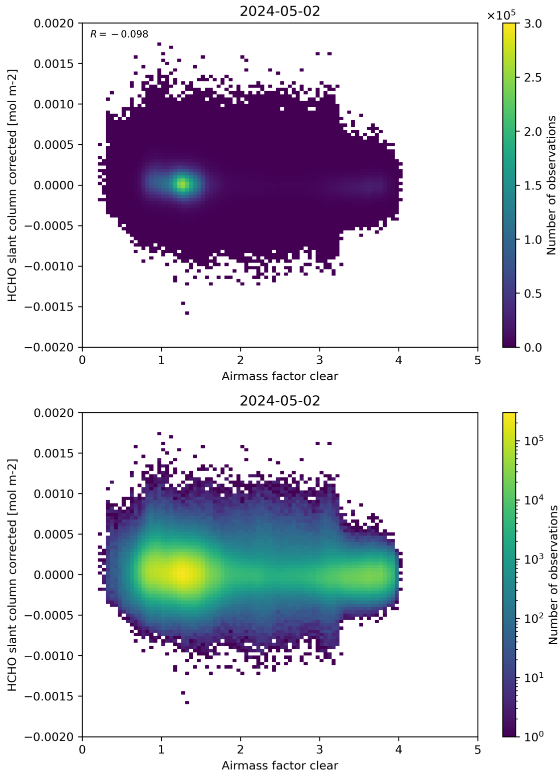
Figure 74: Scatter density plot of “Airmass factor clear” against “HCHO slant column corrected” for 2024-05-02 to 2024-05-03.
