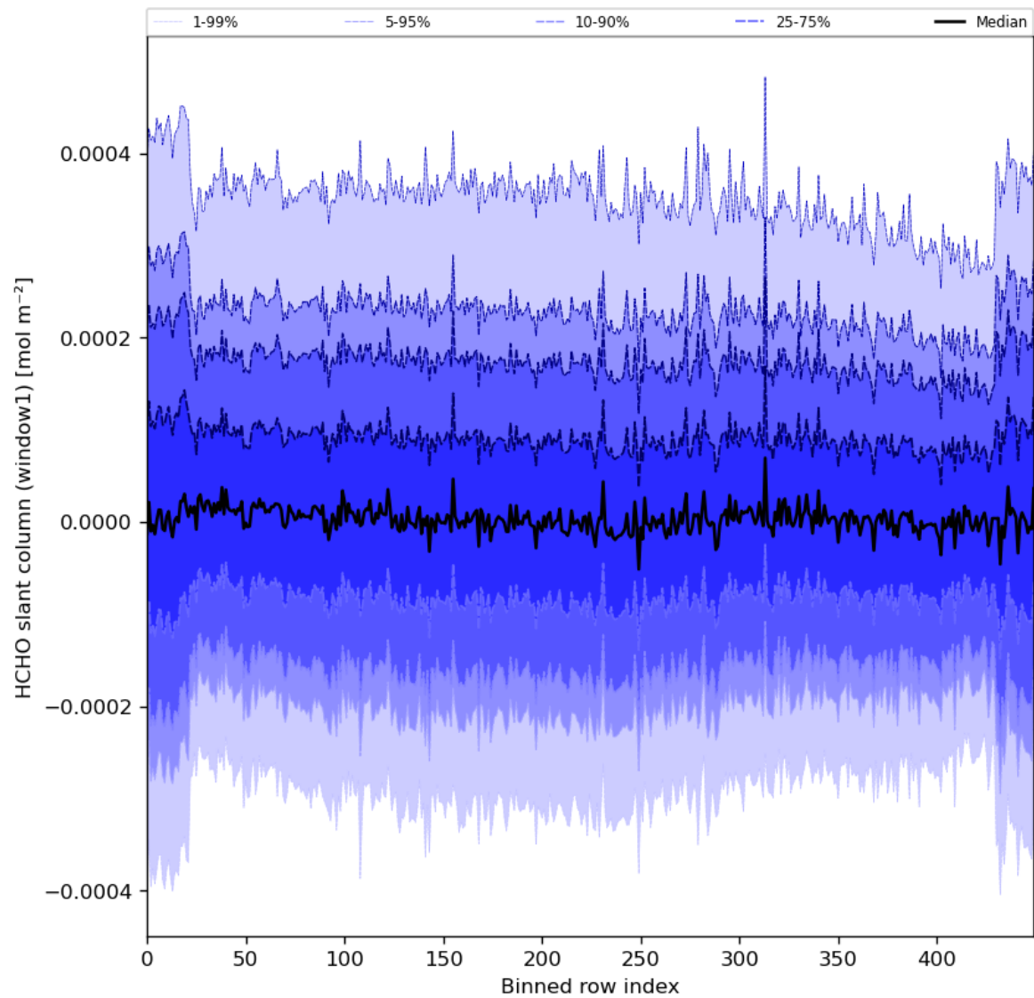
Figure 52: Along track statistics of “HCHO slant column (window1)” for 2024-05-02 to 2024-05-03
