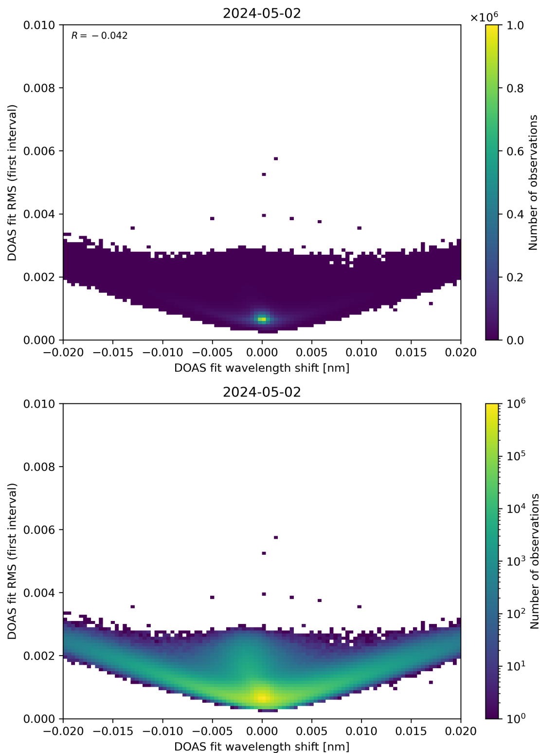
Figure 64: Scatter density plot of “DOAS fit wavelength shift” against “DOAS fit RMS (first interval)” for 2024-05-02 to 2024-05-03.
