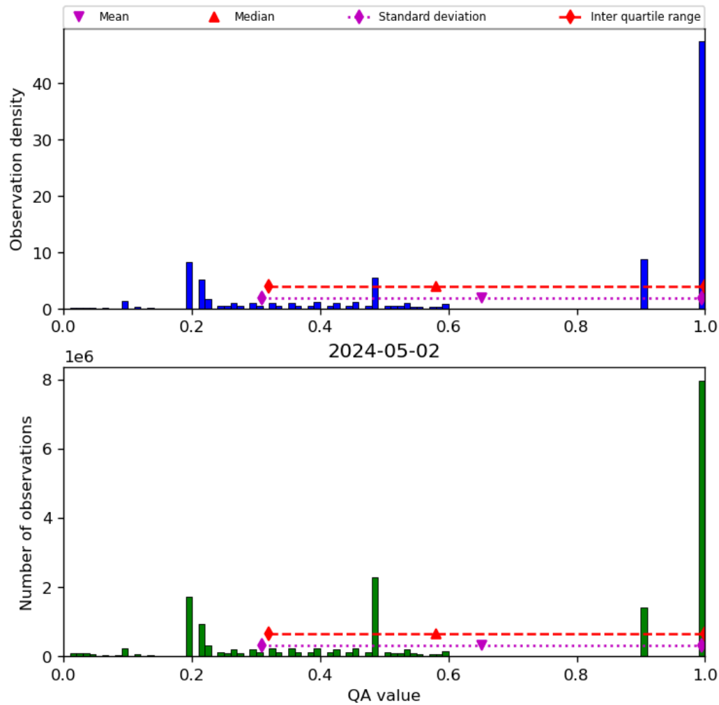
Figure 34: Histogram of “QA value” for 2024-05-02 to 2024-05-03
