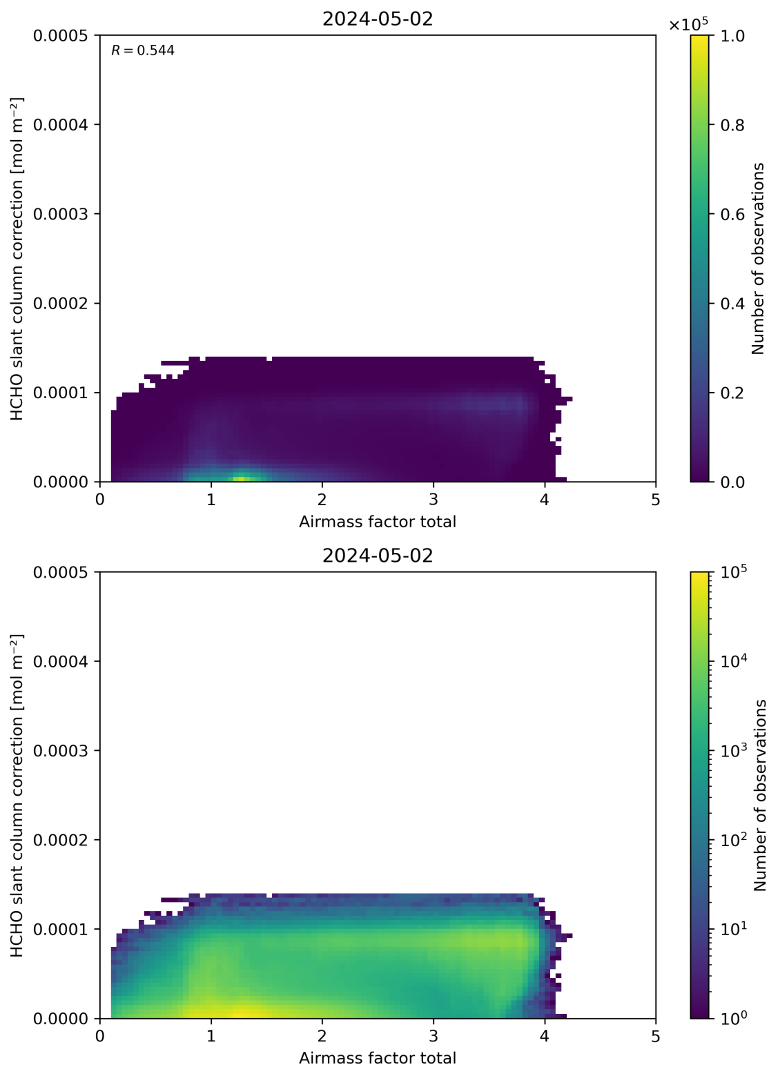
Figure 102: Scatter density plot of “Airmass factor total” against “HCHO slant column correction” for 2024-05-02 to 2024-05-03.
