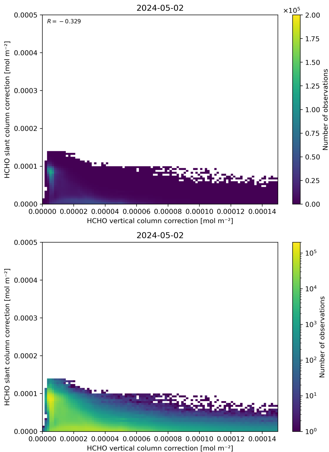
Figure 117: Scatter density plot of “HCHO vertical column correction” against “HCHO slant column correction” for 2024-05-02 to 2024-05-03.
