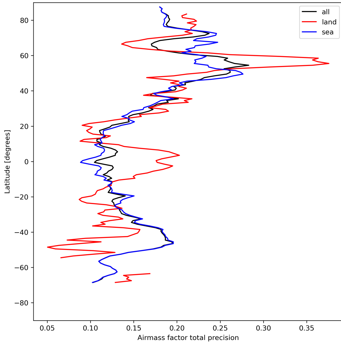
Figure 27: Zonal average of “Airmass factor total precision” for 2024-05-02 to 2024-05-03.
