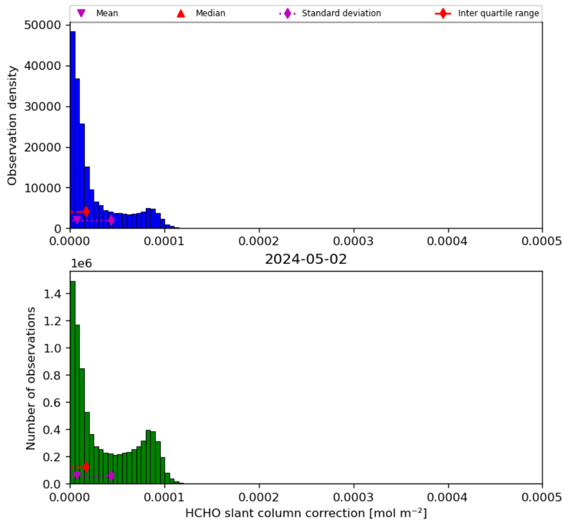
Figure 47: Histogram of “HCHO slant column correction” for 2024-05-02 to 2024-05-03
