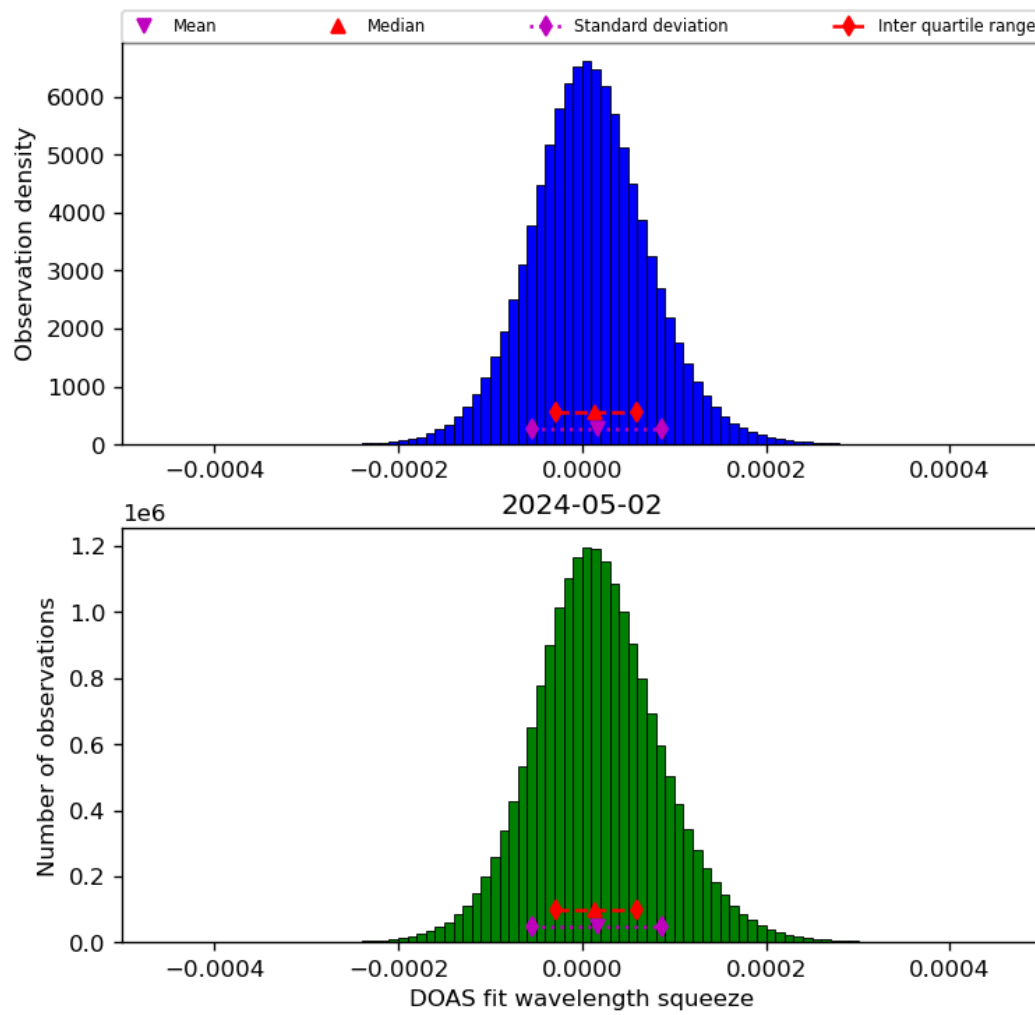
Figure 45: Histogram of “DOAS fit wavelength squeeze” for 2024-05-02 to 2024-05-03
