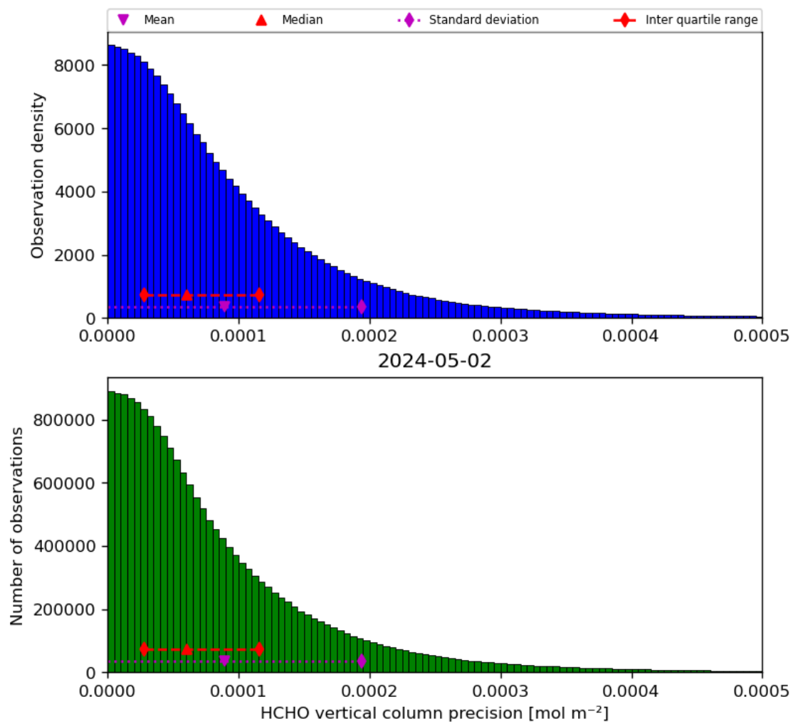
Figure 36: Histogram of “HCHO vertical column precision” for 2024-05-02 to 2024-05-03
