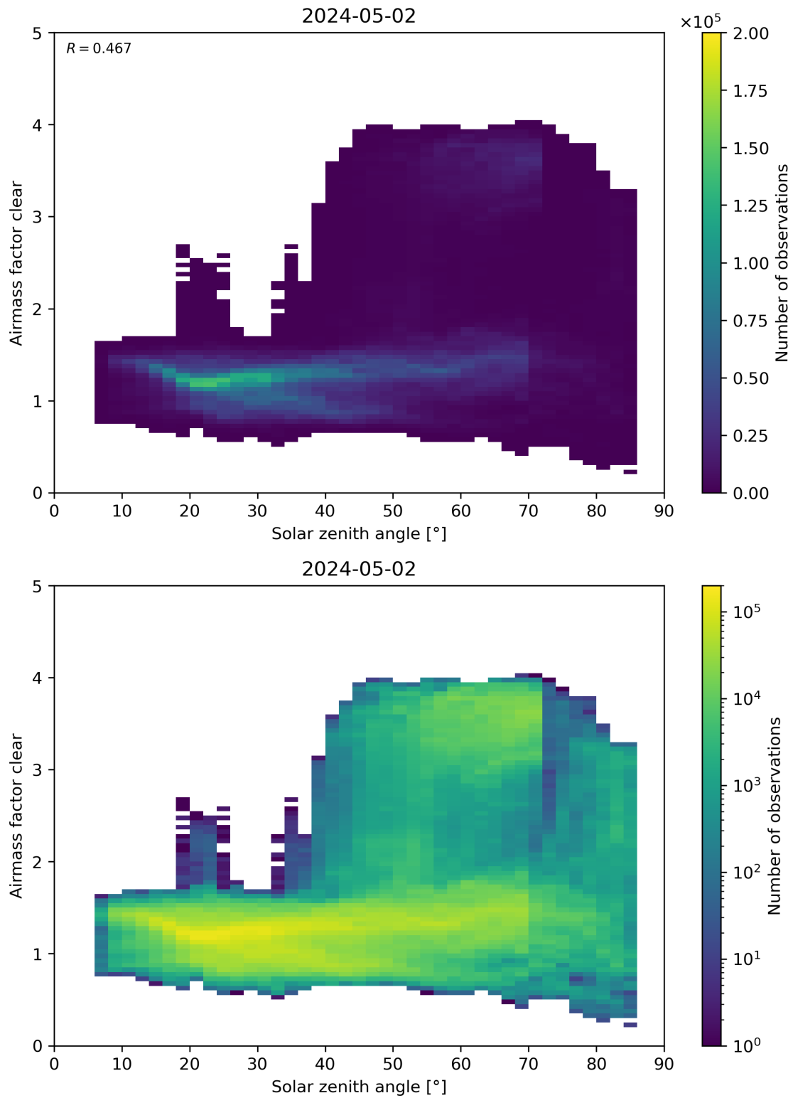
Figure 170: Scatter density plot of “Solar zenith angle” against “Airmass factor clear” for 2024-05-02 to 2024-05-03.
