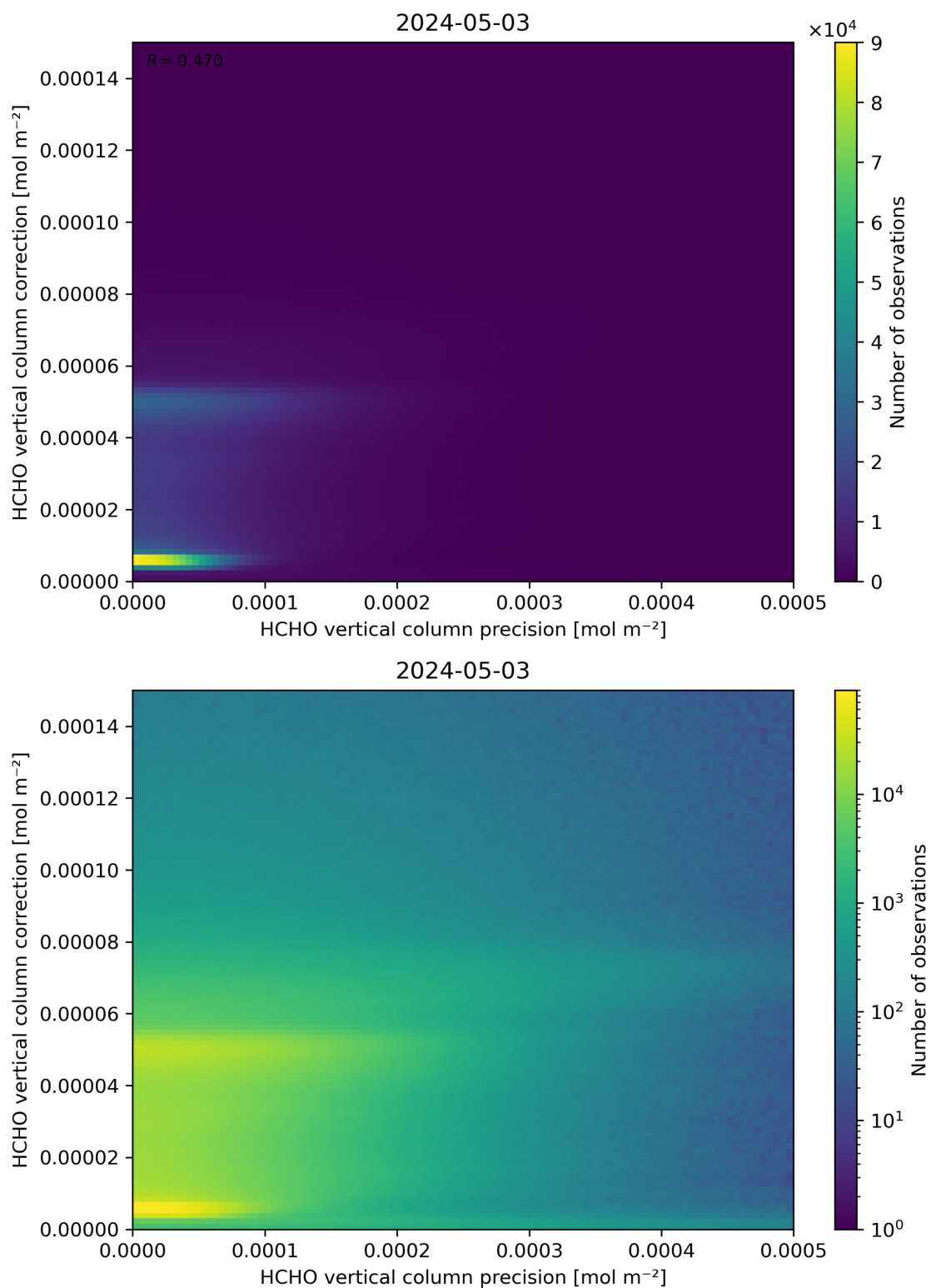
Figure 146: Scatter density plot of “HCHO vertical column precision” against “HCHO vertical column correction” for 2024-05-02 to 2024-05-04.
