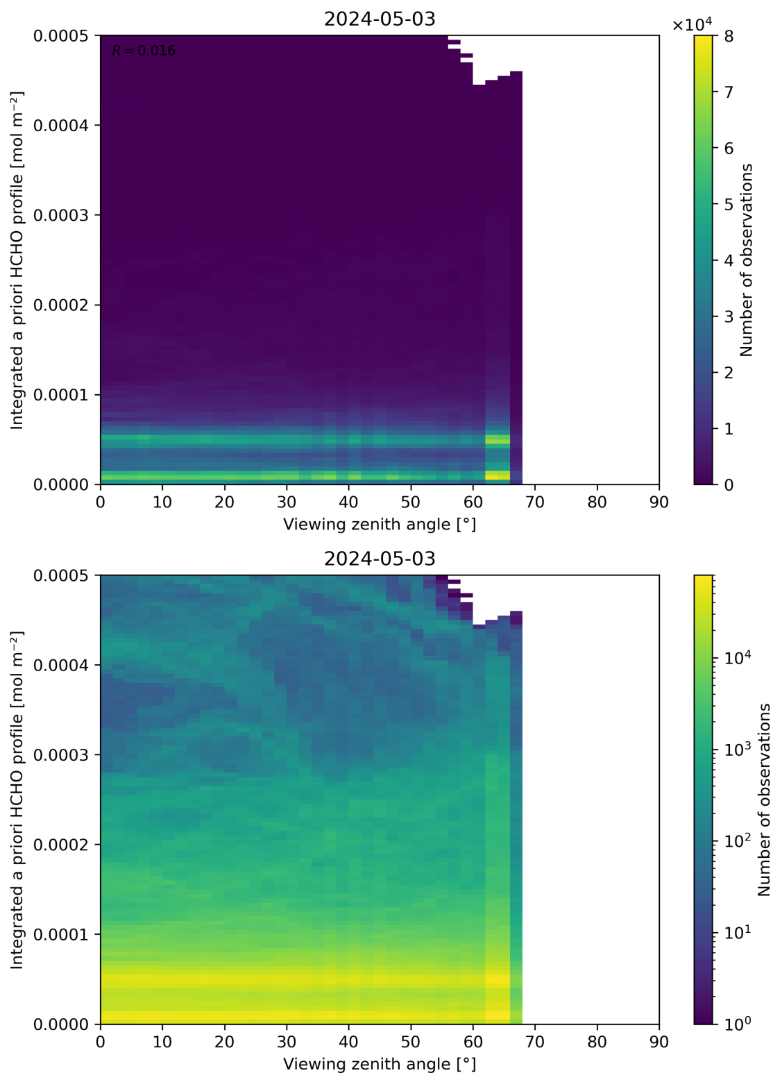
Figure 195: Scatter density plot of “Viewing zenith angle” against “Integrated a priori HCHO profile” for 2024-05-02 to 2024-05-04.
