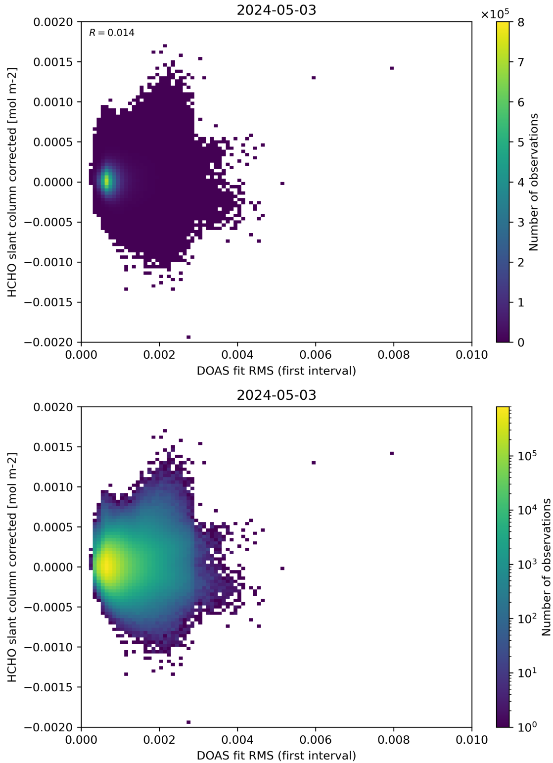
Figure 62: Scatter density plot of “DOAS fit RMS (first interval)” against “HCHO slant column corrected” for 2024-05-02 to 2024-05-04.
