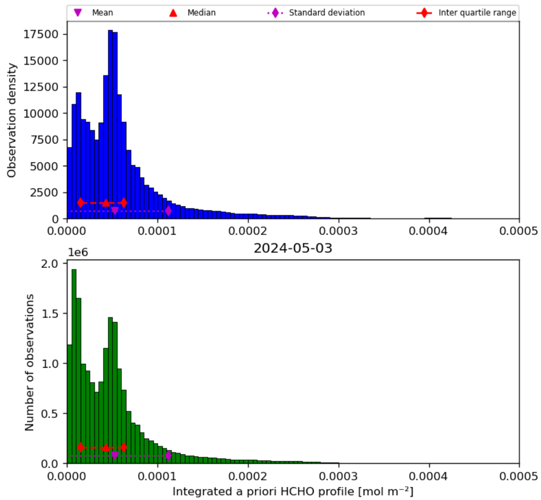
Figure 43: Histogram of “Integrated a priori HCHO profile” for 2024-05-02 to 2024-05-04
