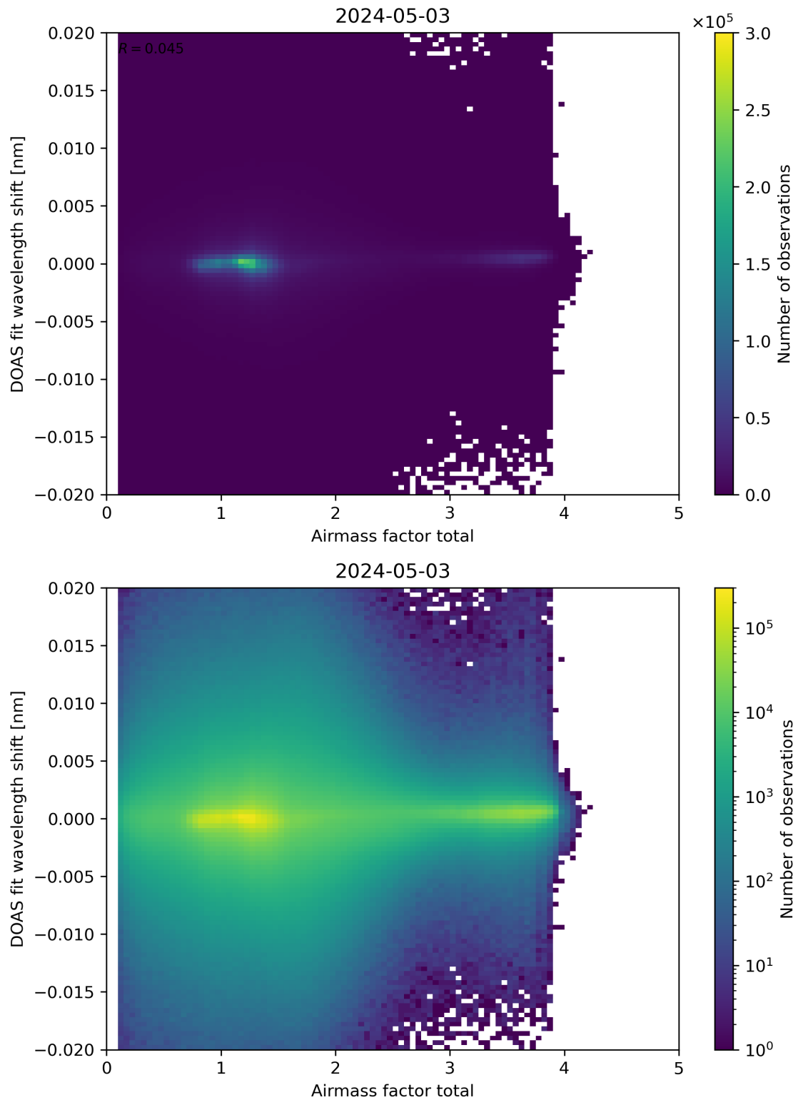
Figure 98: Scatter density plot of “Airmass factor total” against “DOAS fit wavelength shift” for 2024-05-02 to 2024-05-04.
