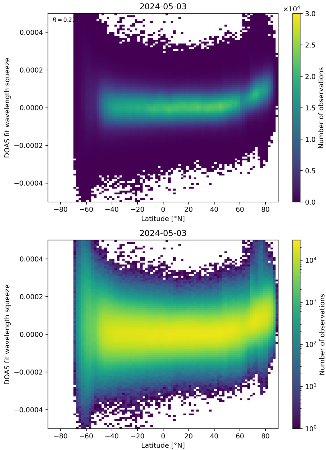
Figure 155: Scatter density plot of “Latitude” against “DOAS fit wavelength squeeze” for 2024-05-02 to 2024-05-04.
