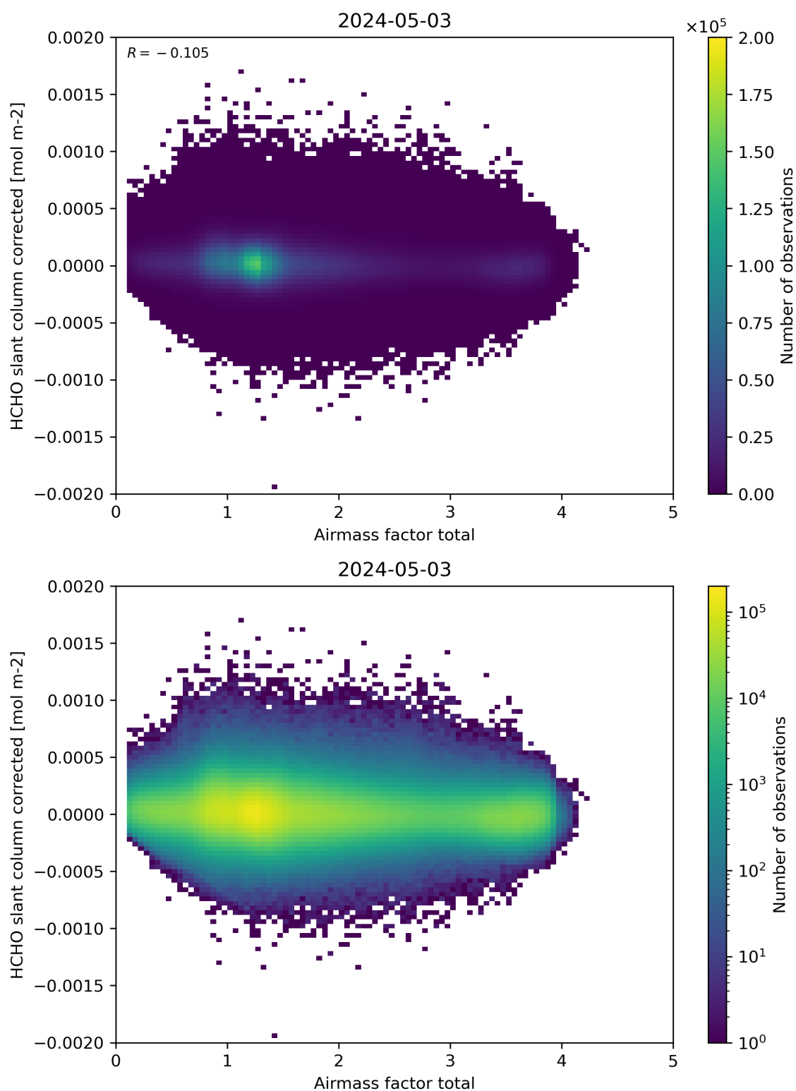
Figure 101: Scatter density plot of “Airmass factor total” against “HCHO slant column corrected” for 2024-05-02 to 2024-05-04.
