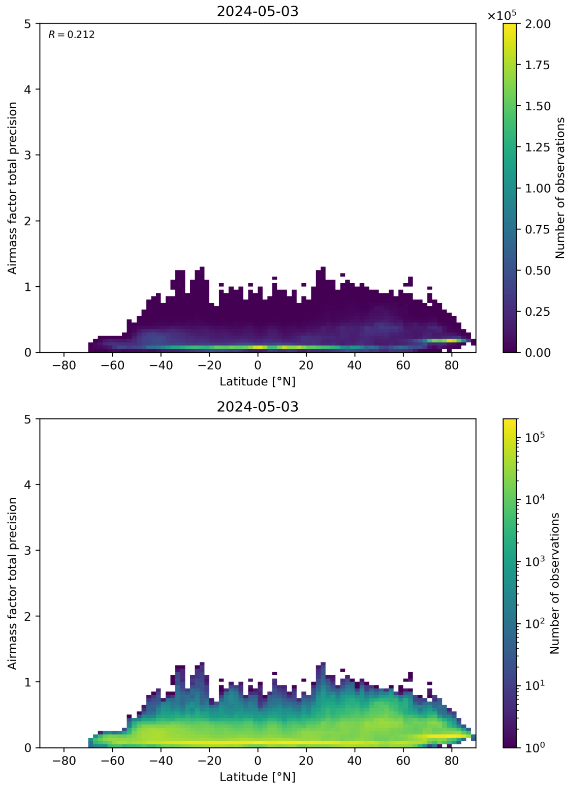
Figure 162: Scatter density plot of “Latitude” against “Airmass factor total precision” for 2024-05-02 to 2024-05-04.
