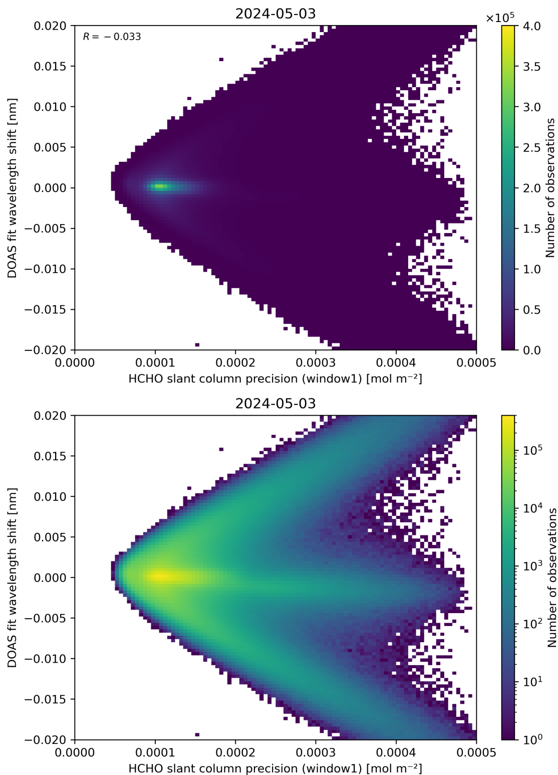
Figure 89: Scatter density plot of “HCHO slant column precision (window1)” against “DOAS fit wavelength shift” for 2024-05-02 to 2024-05-04.
