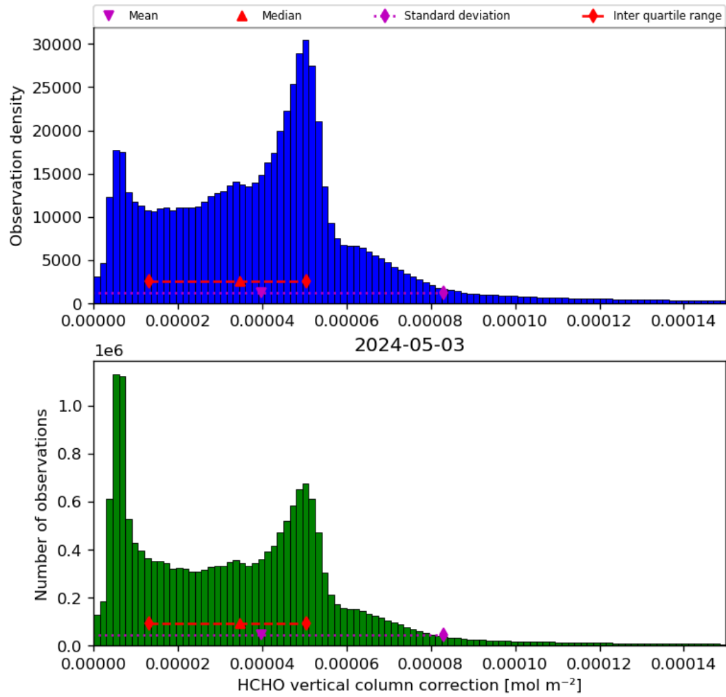
Figure 37: Histogram of “HCHO vertical column correction” for 2024-05-02 to 2024-05-04
