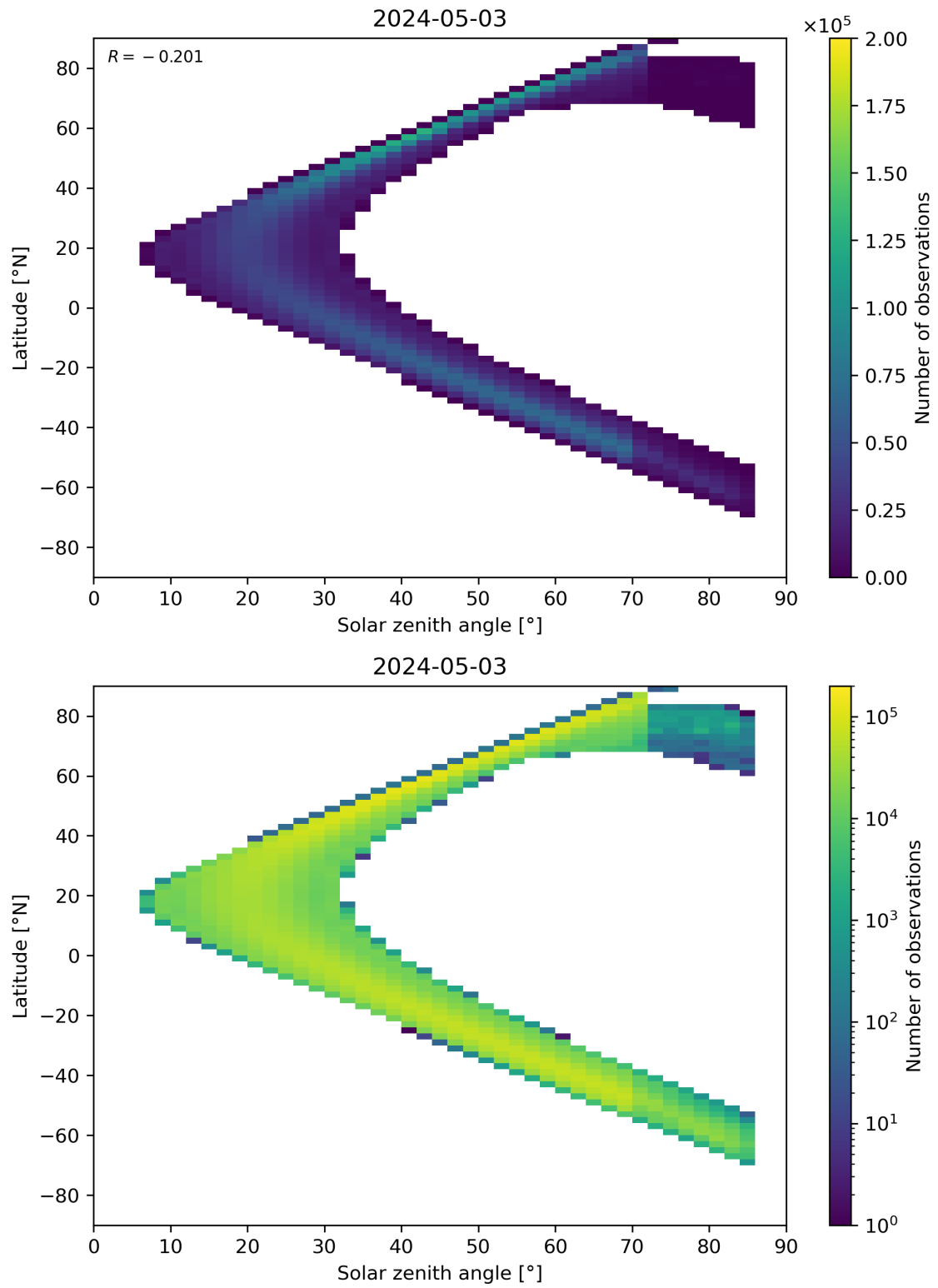
Figure 181: Scatter density plot of “Solar zenith angle” against “Latitude” for 2024-05-02 to 2024-05-04.
