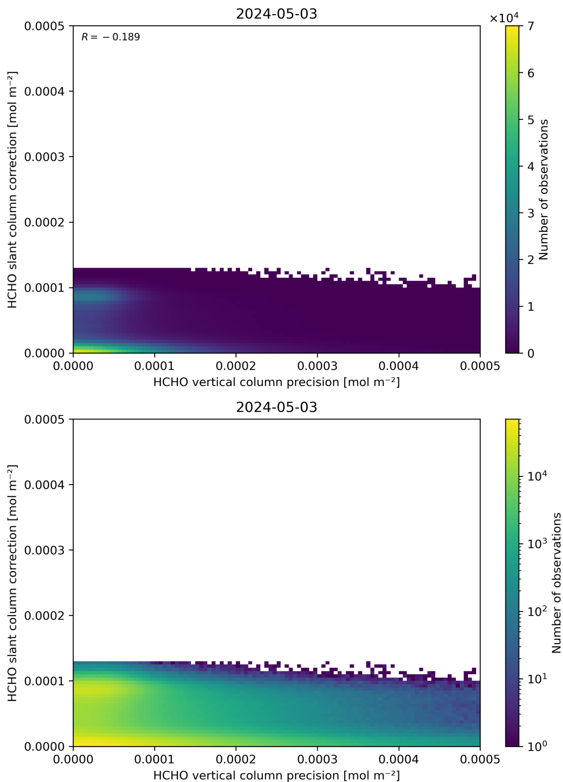
Figure 141: Scatter density plot of “HCHO vertical column precision” against “HCHO slant column correction” for 2024-05-02 to 2024-05-04.
