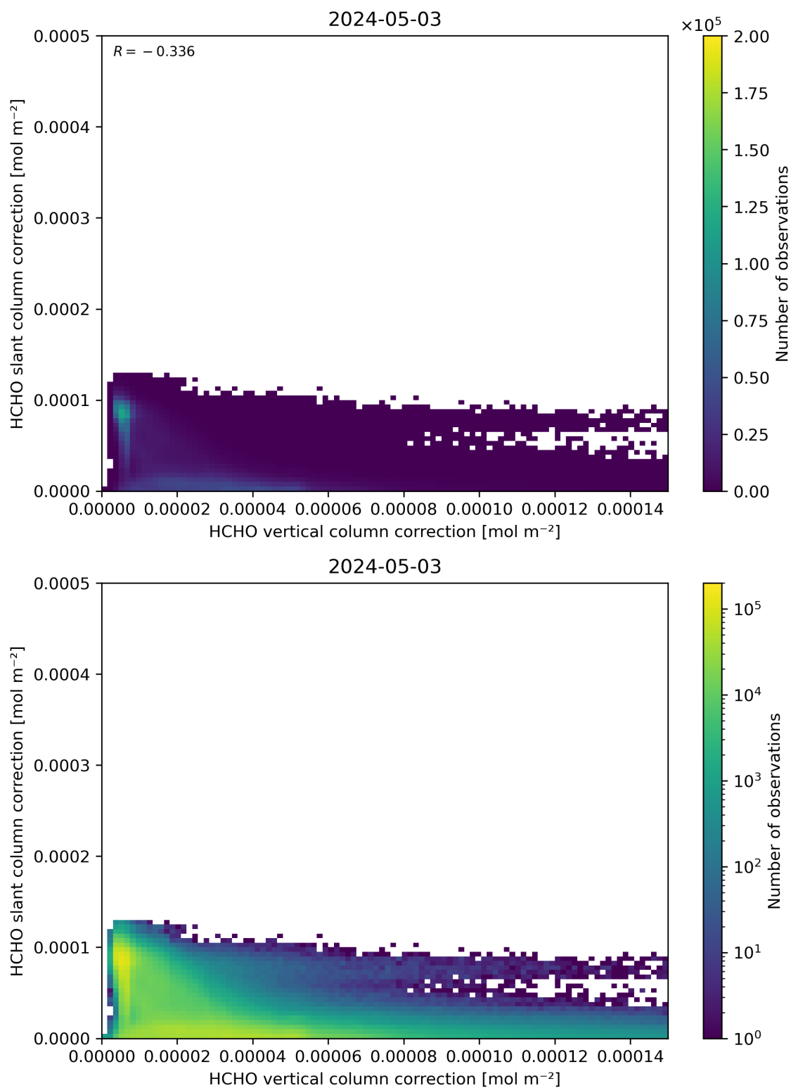
Figure 117: Scatter density plot of “HCHO vertical column correction” against “HCHO slant column correction” for 2024-05-02 to 2024-05-04.
