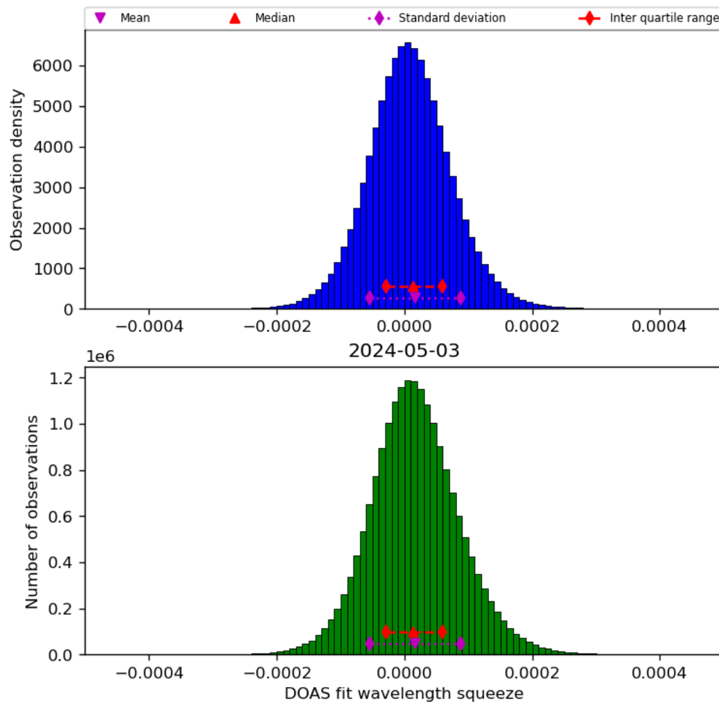
Figure 45: Histogram of “DOAS fit wavelength squeeze” for 2024-05-02 to 2024-05-04
