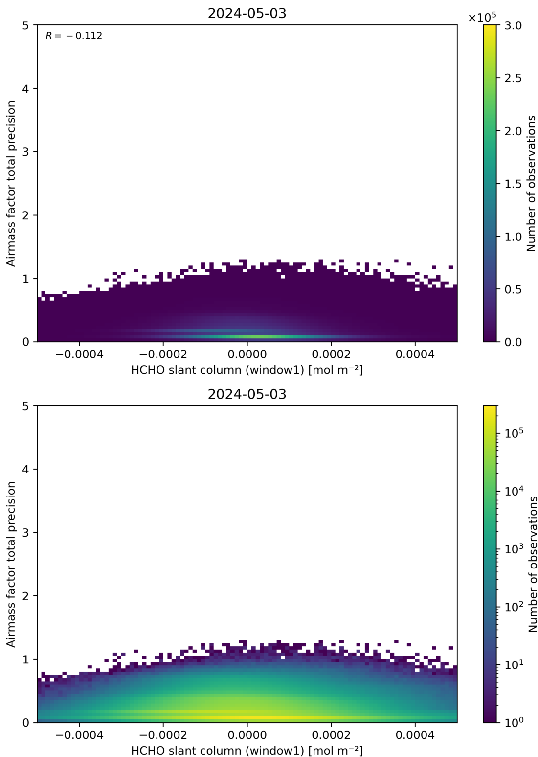
Figure 86: Scatter density plot of “HCHO slant column (window1)” against “Airmass factor total precision” for 2024-05-02 to 2024-05-04.
