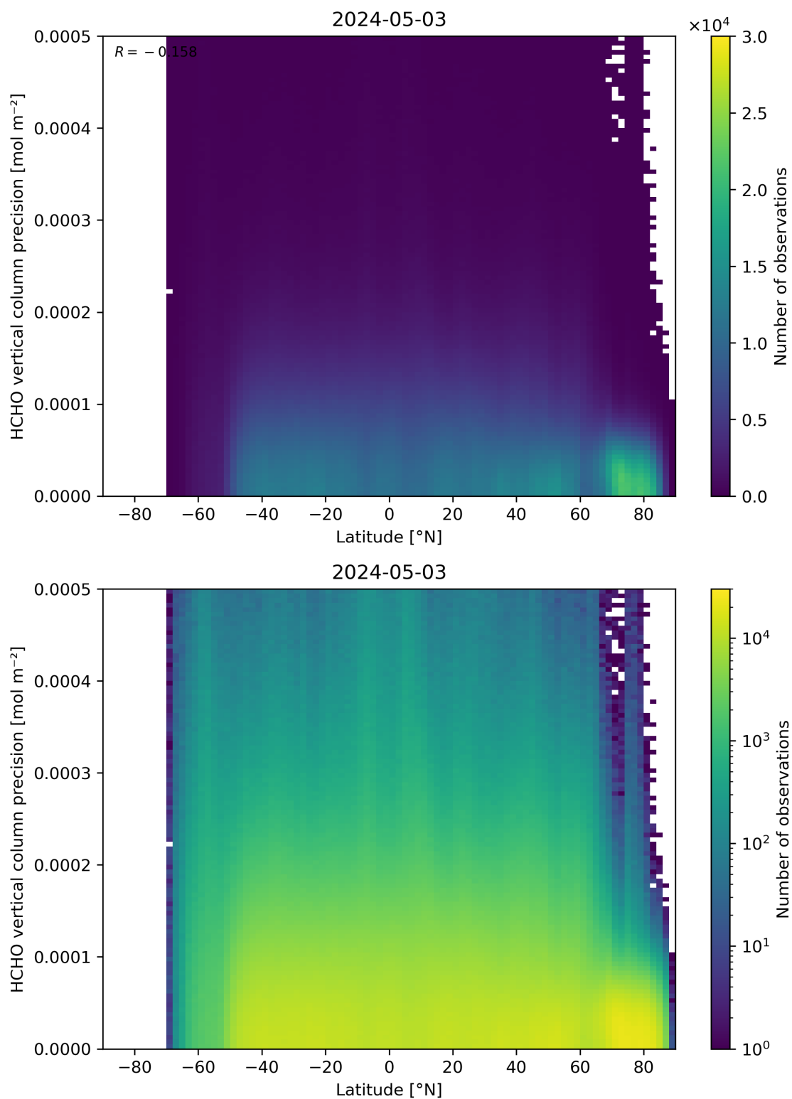
Figure 165: Scatter density plot of “Latitude” against “HCHO vertical column precision” for 2024-05-02 to 2024-05-04.
