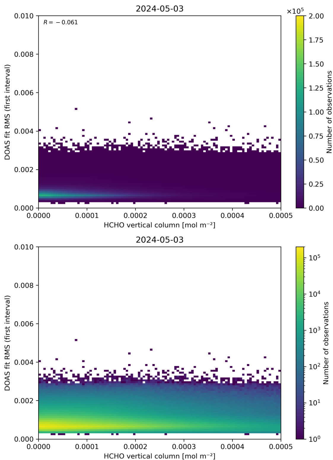
Figure 123: Scatter density plot of “HCHO vertical column” against “DOAS fit RMS (first interval)” for 2024-05-02 to 2024-05-04.
