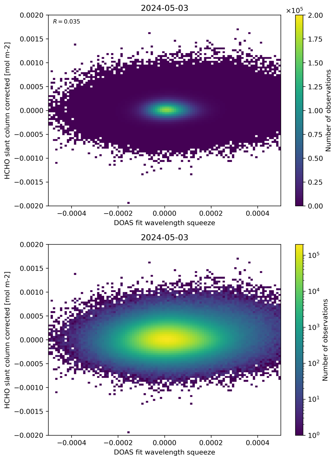
Figure 69: Scatter density plot of “DOAS fit wavelength squeeze” against “HCHO slant column corrected” for 2024-05-02 to 2024-05-04.
