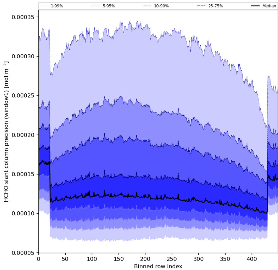
Figure 53: Along track statistics of “HCHO slant column precision (window1)” for 2024-05-02 to 2024-05-04
