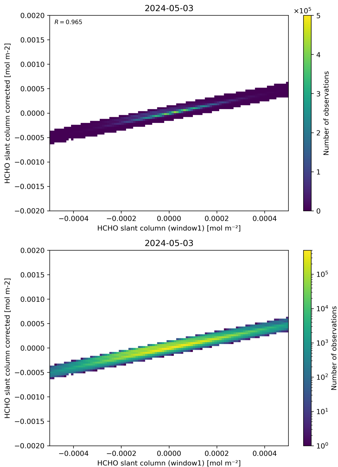
Figure 82: Scatter density plot of “HCHO slant column (window1)” against “HCHO slant column corrected” for 2024-05-02 to 2024-05-04.
