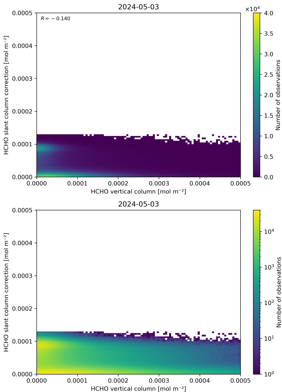
Figure 128: Scatter density plot of “HCHO vertical column” against “HCHO slant column correction” for 2024-05-02 to 2024-05-04.
