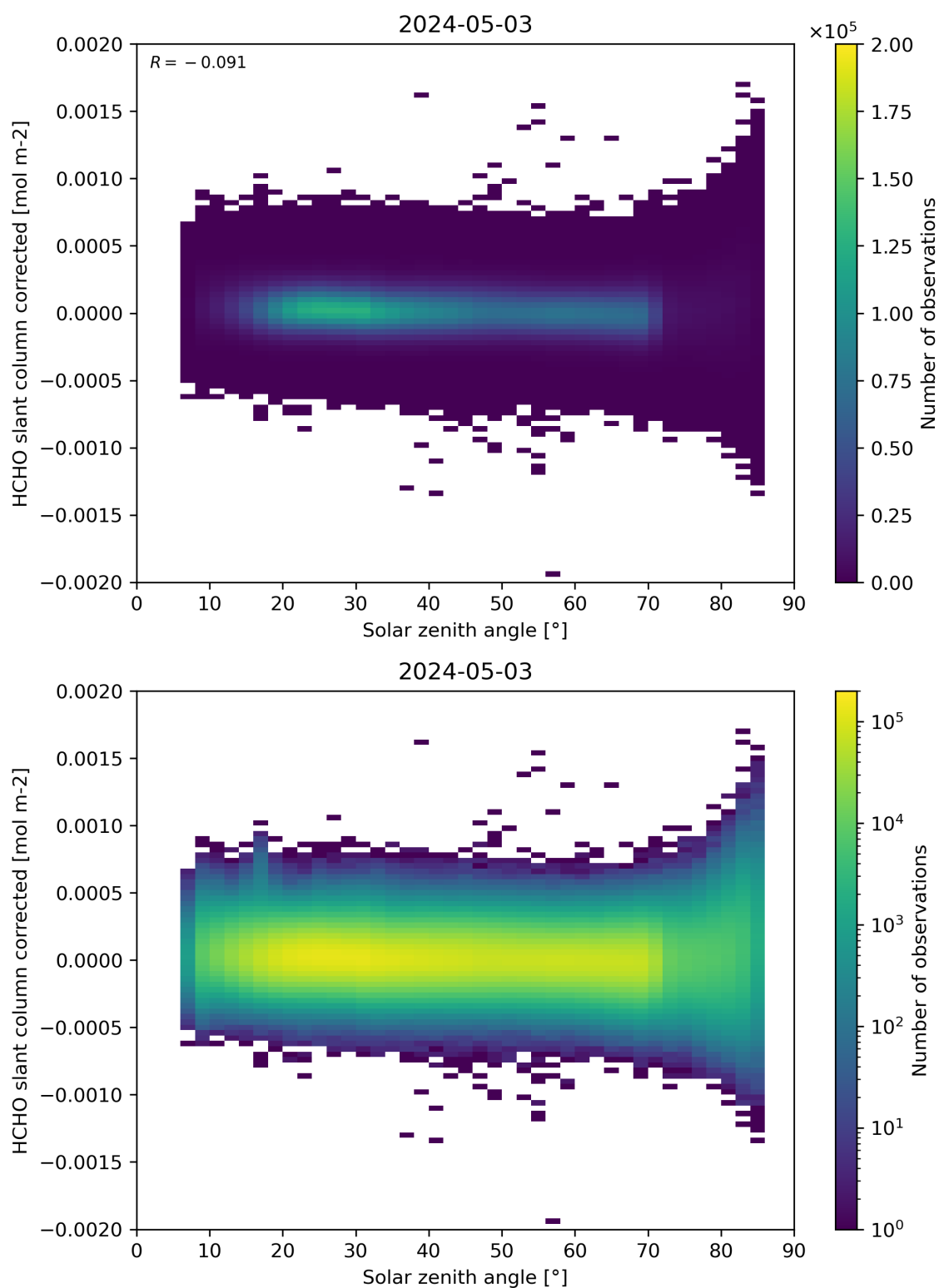
Figure 171: Scatter density plot of “Solar zenith angle” against “HCHO slant column corrected” for 2024-05-02 to 2024-05-04.
