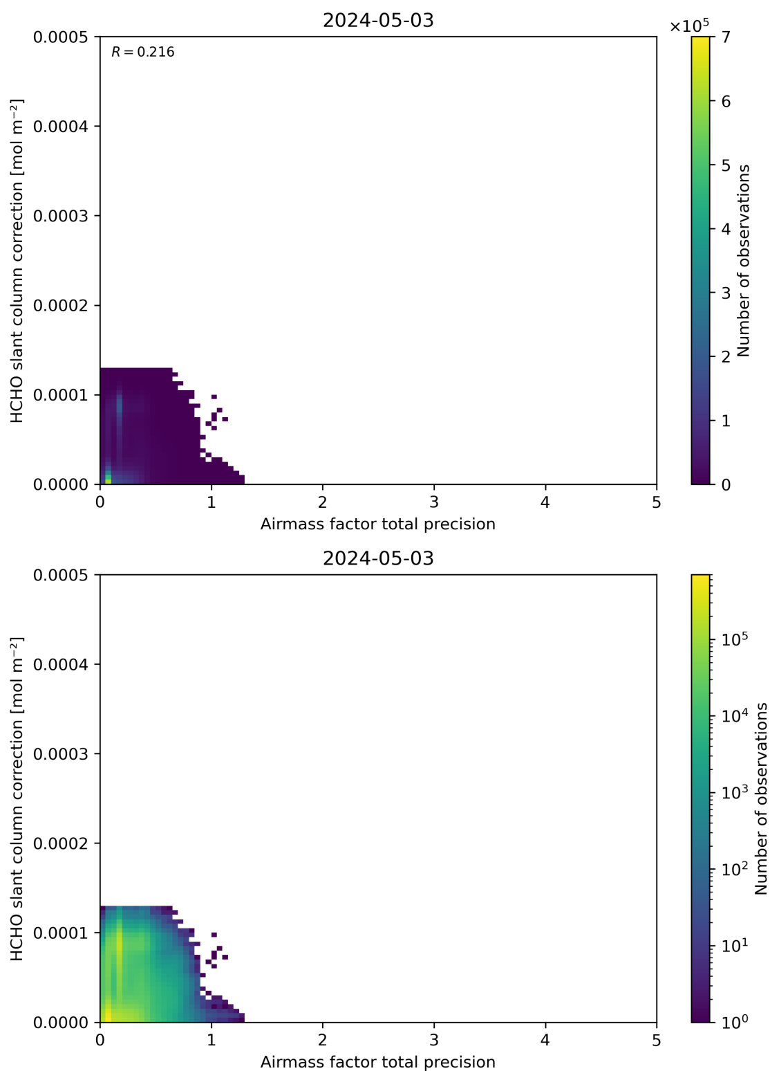
Figure 110: Scatter density plot of “Airmass factor total precision” against “HCHO slant column correction” for 2024-05-02 to 2024-05-04.
