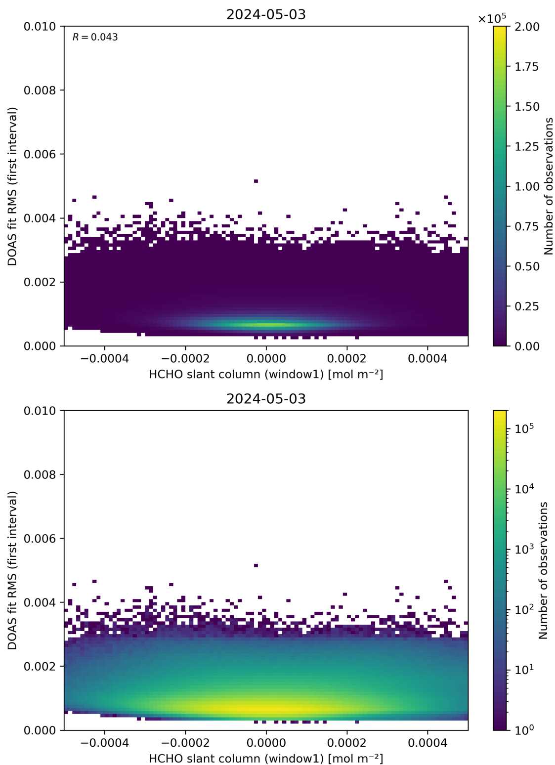
Figure 78: Scatter density plot of “HCHO slant column (window1)” against “DOAS fit RMS (first interval)” for 2024-05-02 to 2024-05-04.
