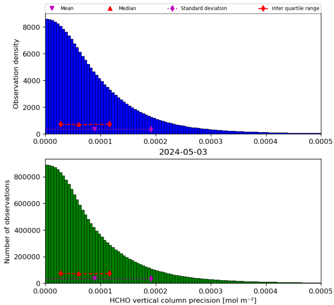
Figure 36: Histogram of “HCHO vertical column precision” for 2024-05-02 to 2024-05-04
