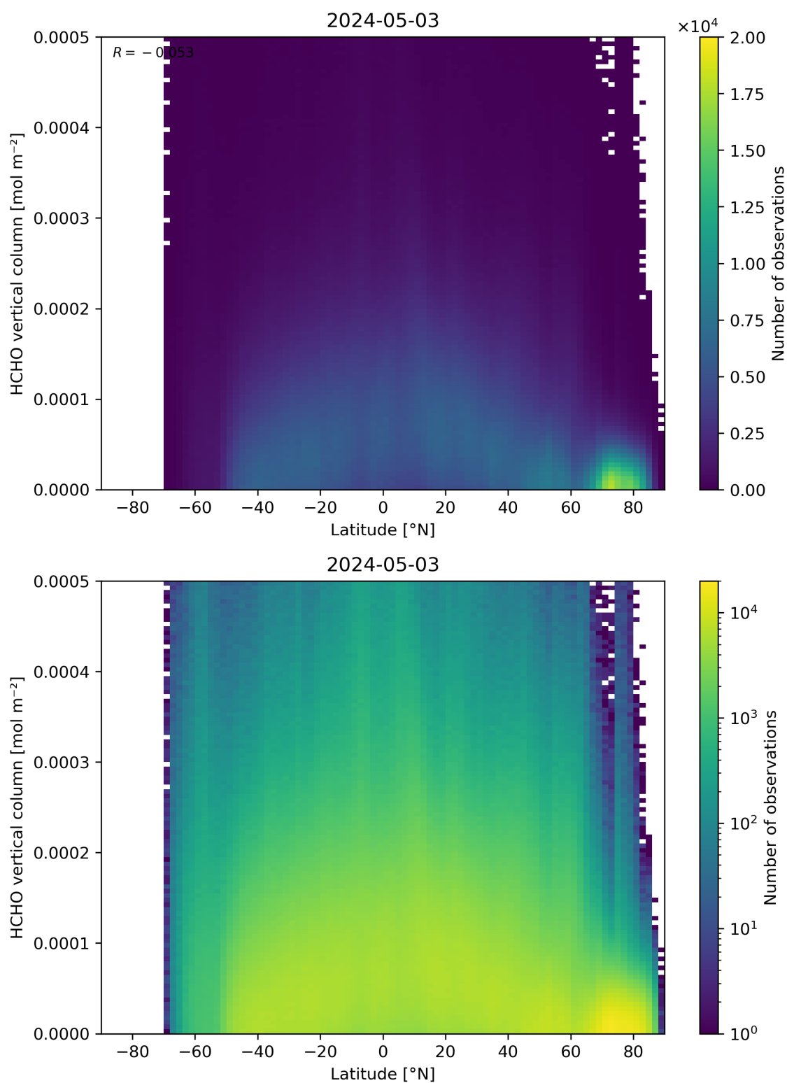
Figure 163: Scatter density plot of “Latitude” against “HCHO vertical column” for 2024-05-02 to 2024-05-04.
