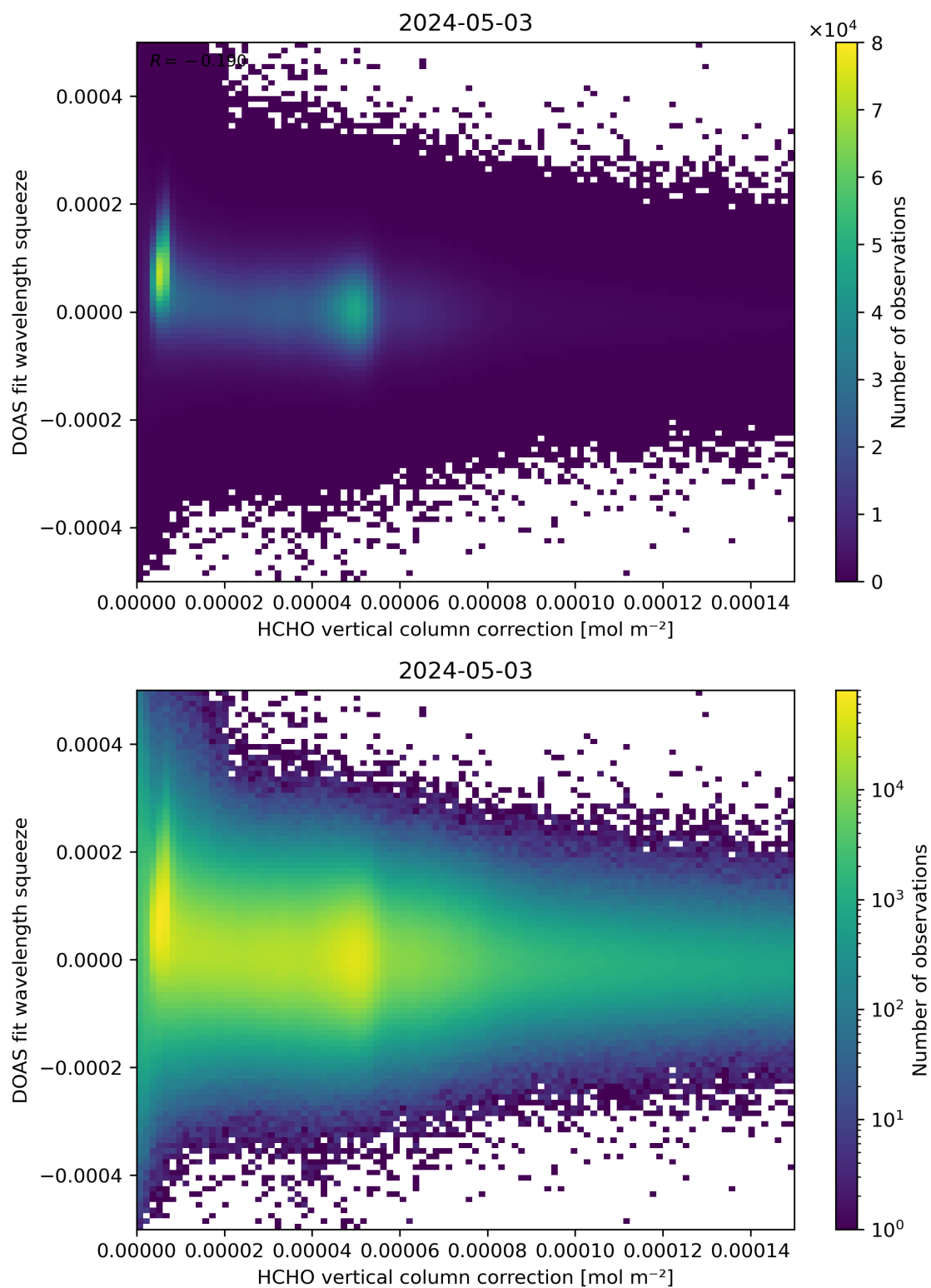
Figure 114: Scatter density plot of “HCHO vertical column correction” against “DOAS fit wavelength squeeze” for 2024-05-02 to 2024-05-04.
