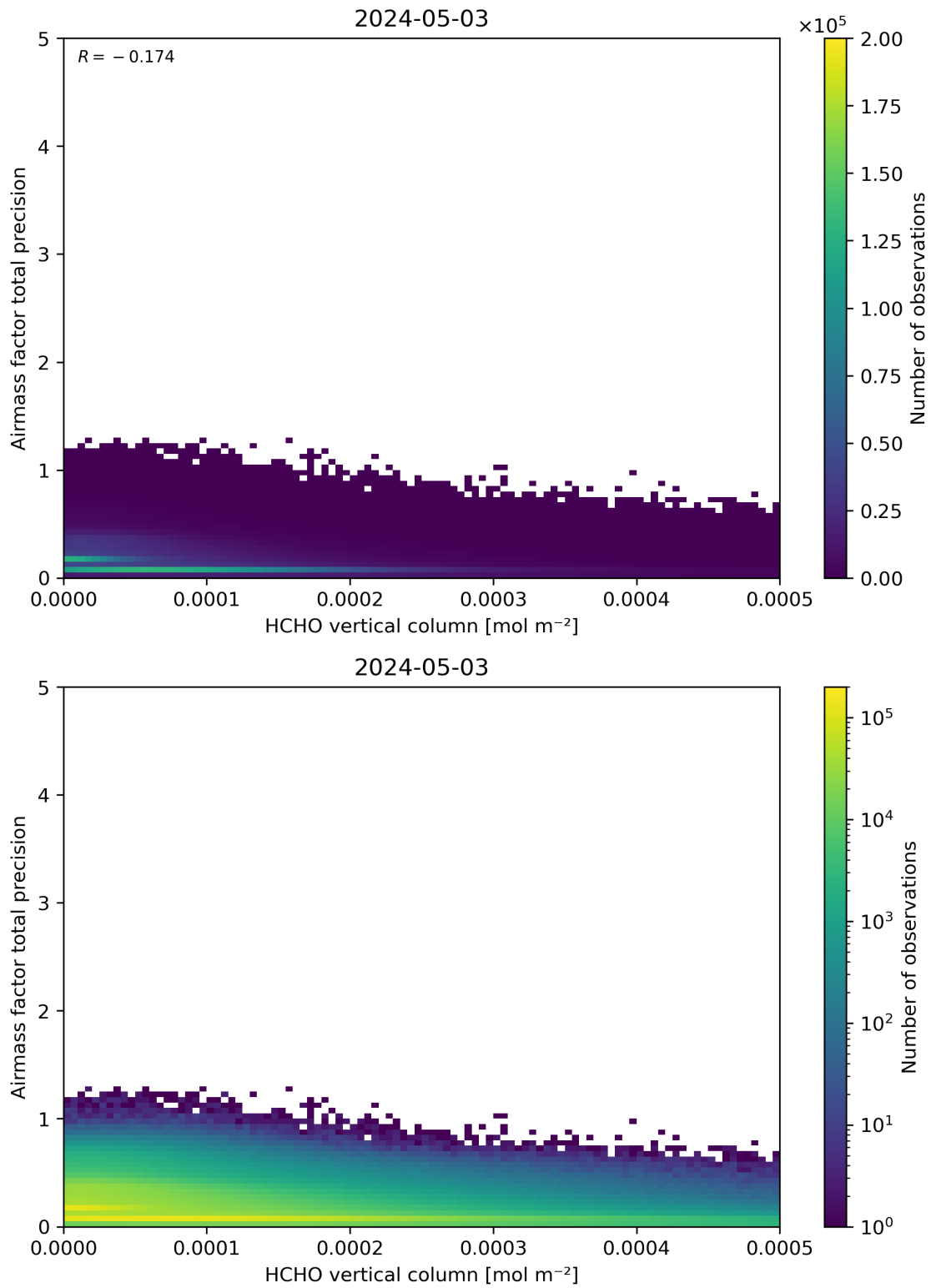
Figure 132: Scatter density plot of “HCHO vertical column” against “Airmass factor total precision” for 2024-05-02 to 2024-05-04.
