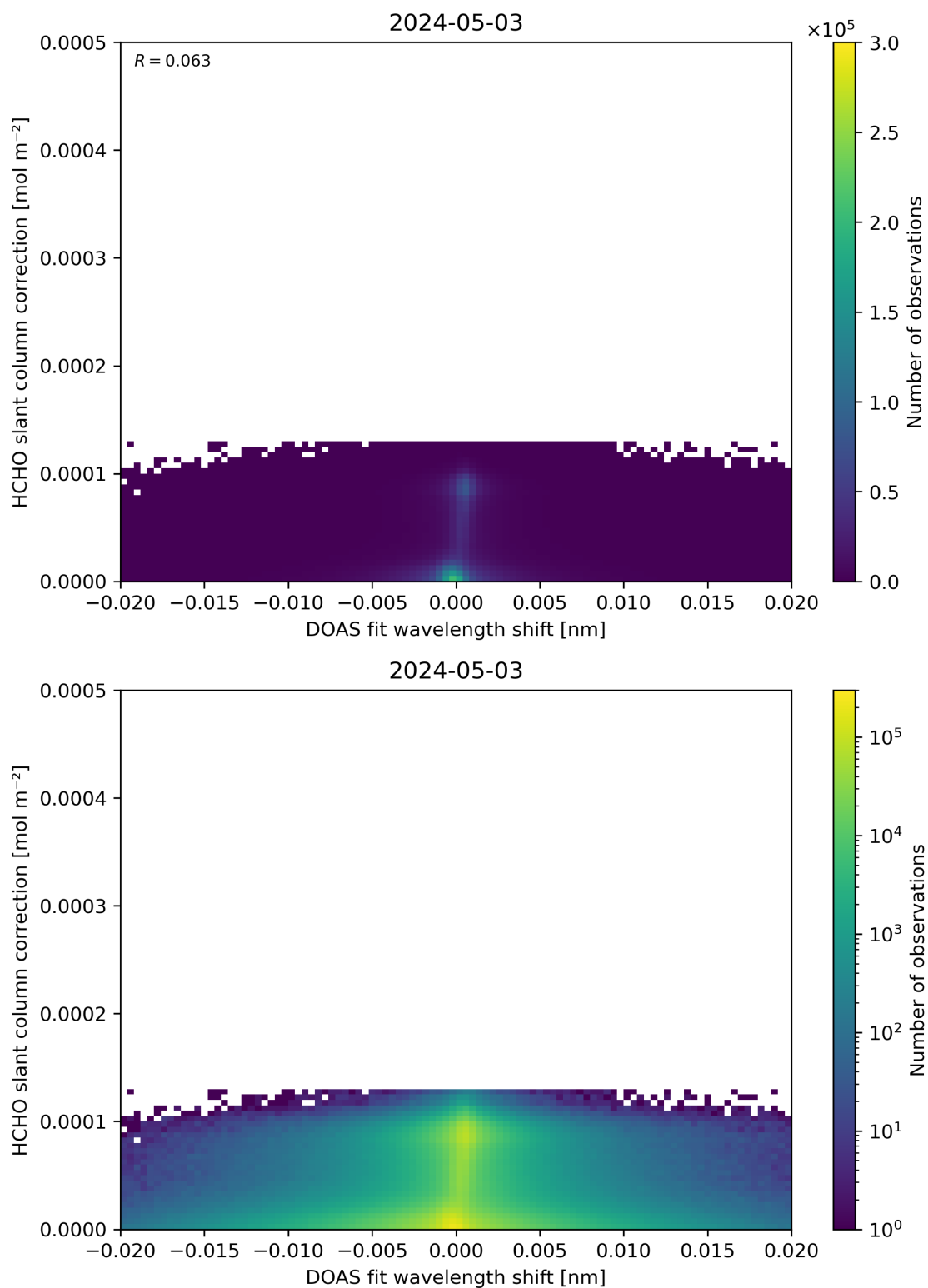
Figure 67: Scatter density plot of “DOAS fit wavelength shift” against “HCHO slant column correction” for 2024-05-02 to 2024-05-04.
