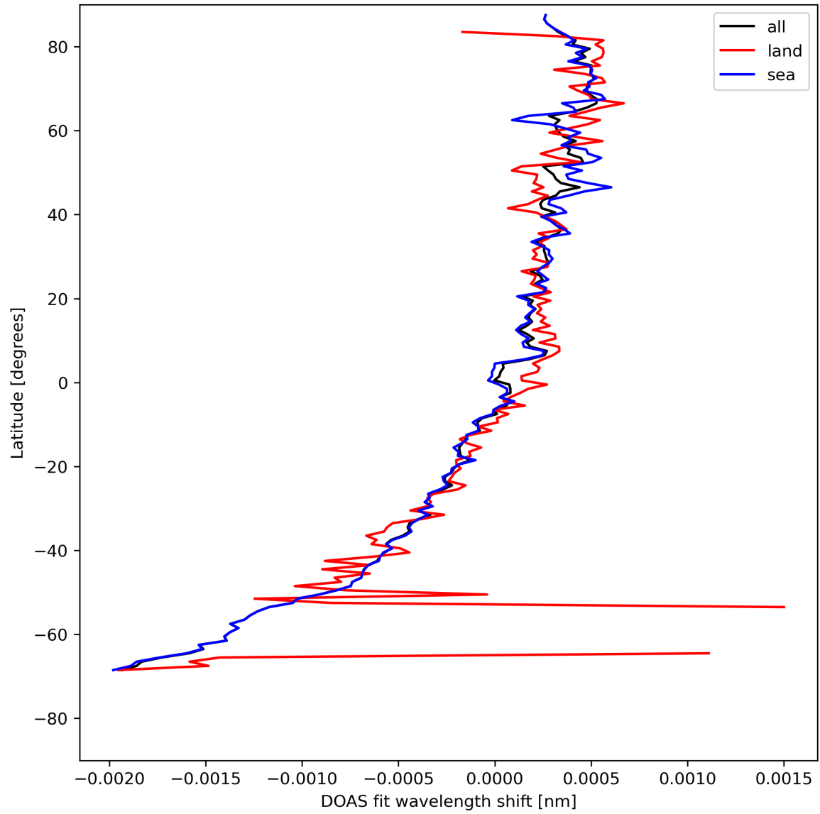
Figure 30: Zonal average of “DOAS fit wavelength shift” for 2024-05-02 to 2024-05-04.
