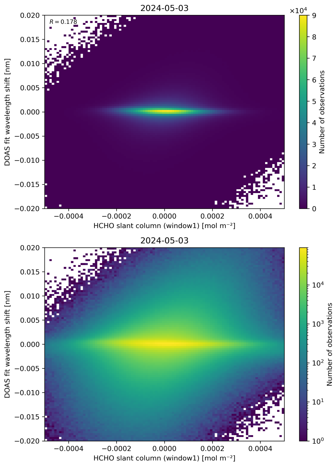
Figure 79: Scatter density plot of “HCHO slant column (window1)” against “DOAS fit wavelength shift” for 2024-05-02 to 2024-05-04.
