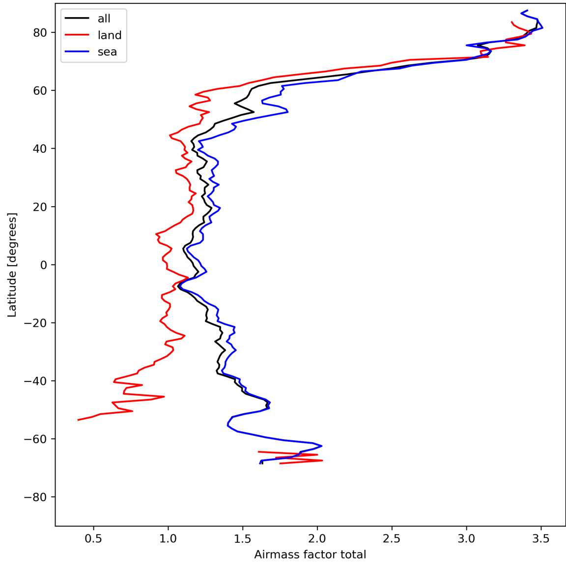
Figure 26: Zonal average of “Airmass factor total” for 2024-05-02 to 2024-05-04.
