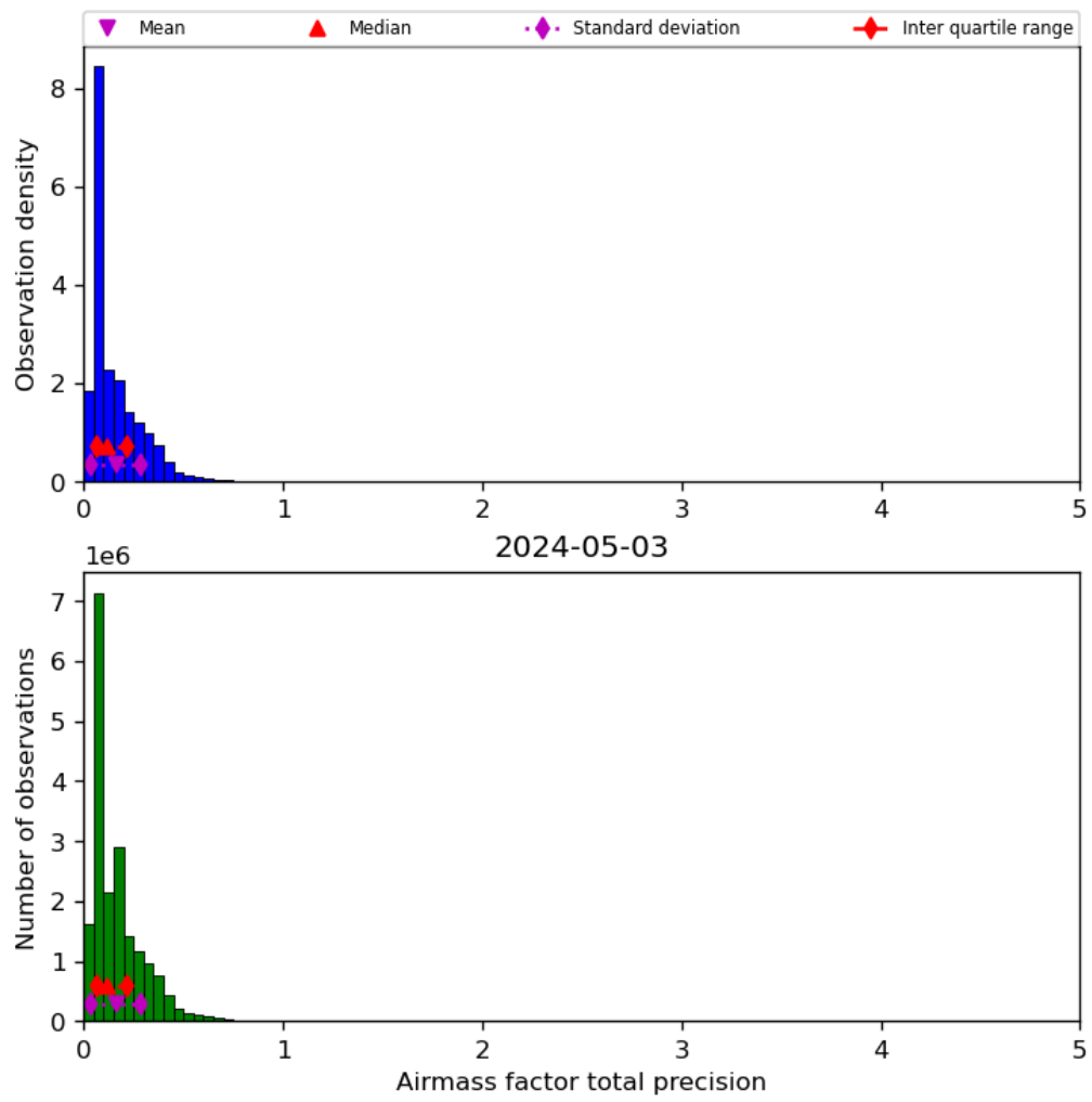
Figure 41: Histogram of “Airmass factor total precision” for 2024-05-02 to 2024-05-04
