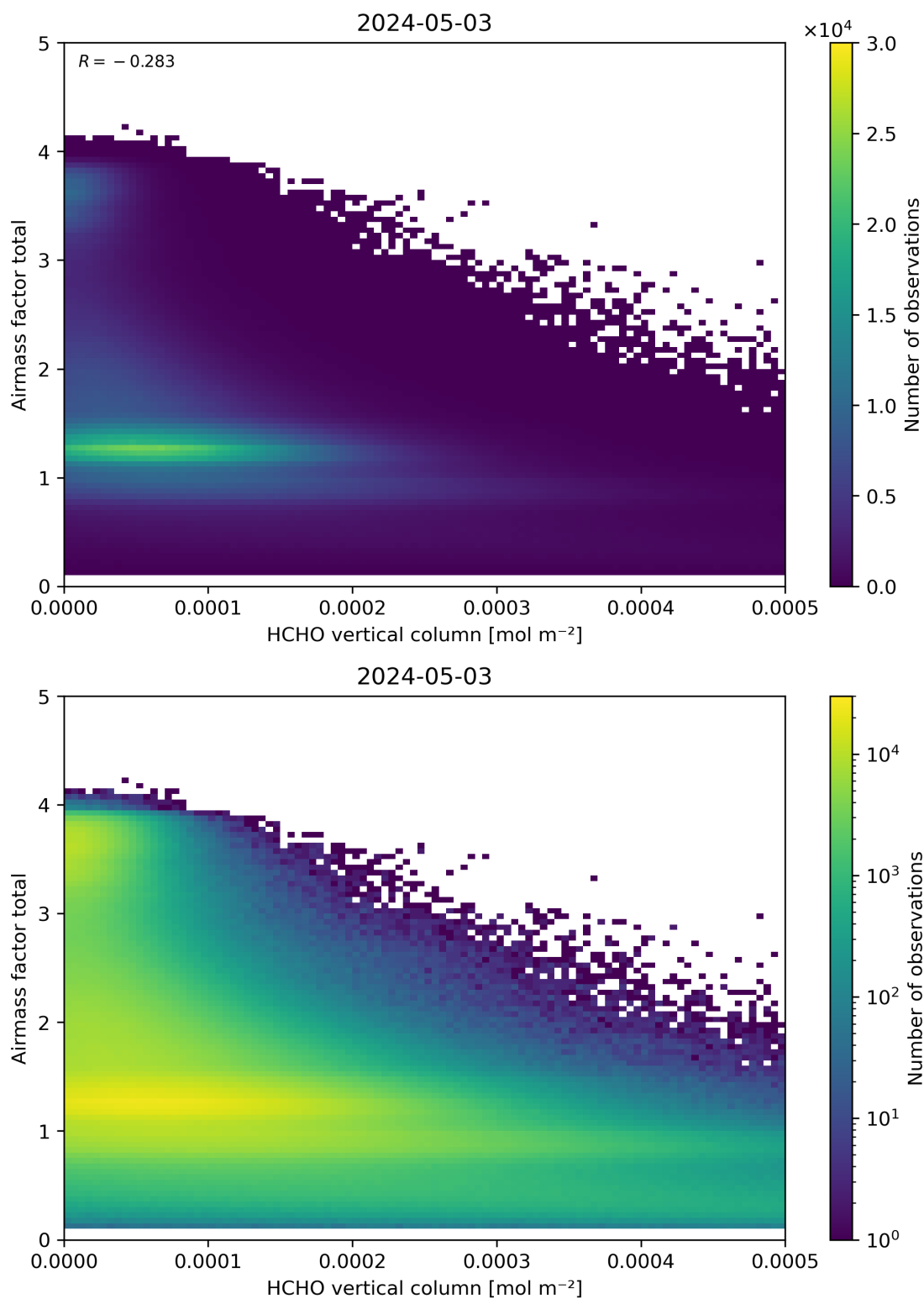
Figure 131: Scatter density plot of “HCHO vertical column” against “Airmass factor total” for 2024-05-02 to 2024-05-04.
