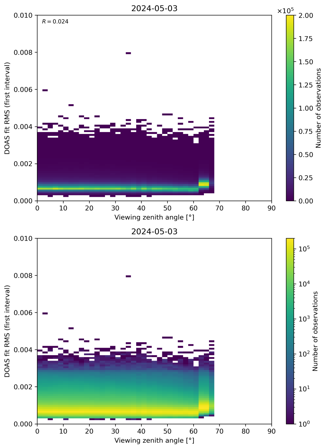
Figure 182: Scatter density plot of “Viewing zenith angle” against “DOAS fit RMS (first interval)” for 2024-05-02 to 2024-05-04.
