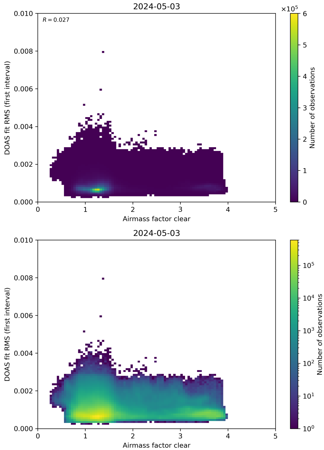
Figure 71: Scatter density plot of “Airmass factor clear” against “DOAS fit RMS (first interval)” for 2024-05-02 to 2024-05-04.
