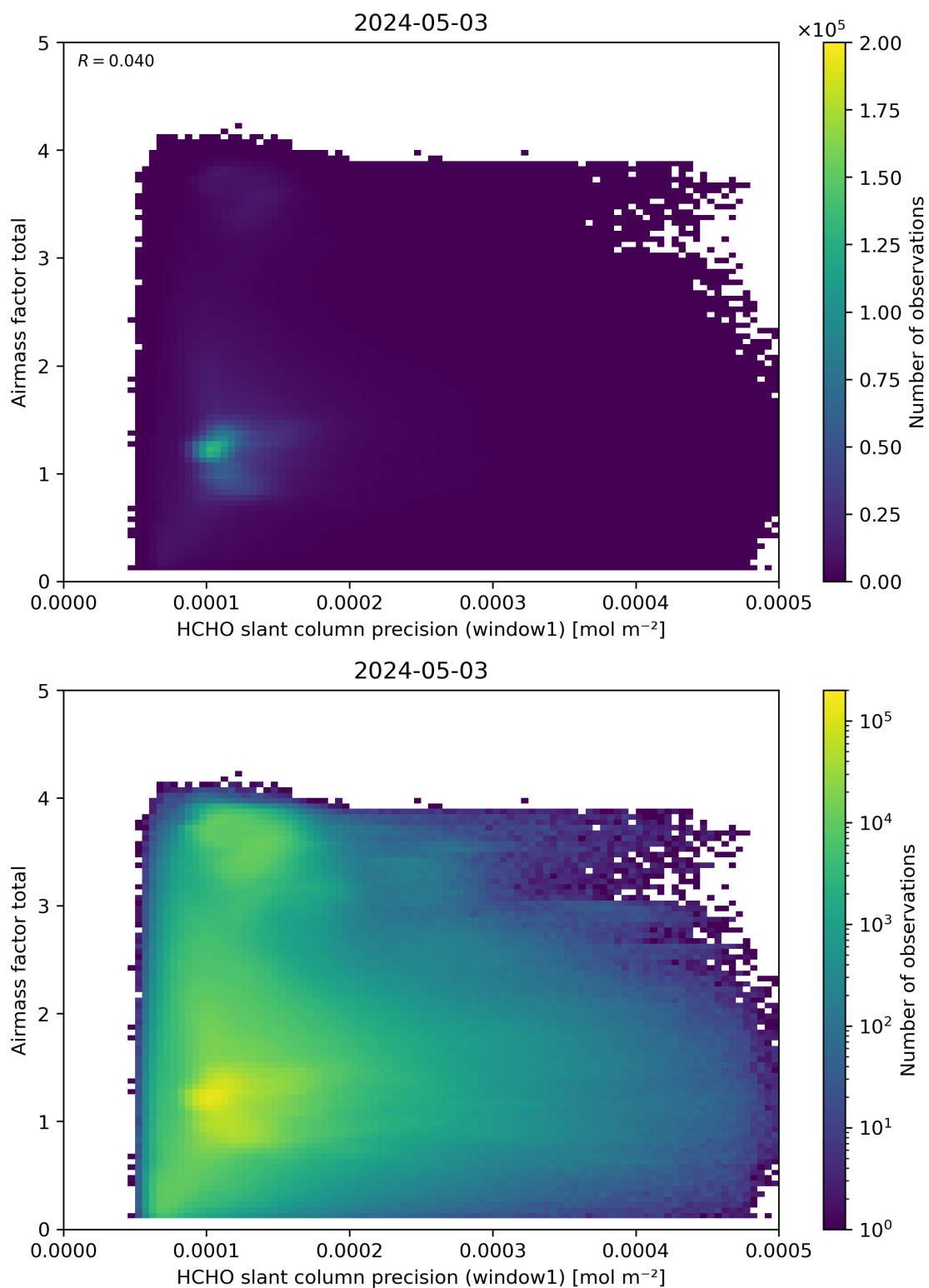
Figure 94: Scatter density plot of “HCHO slant column precision (window1)” against “Airmass factor total” for 2024-05-02 to 2024-05-04.
