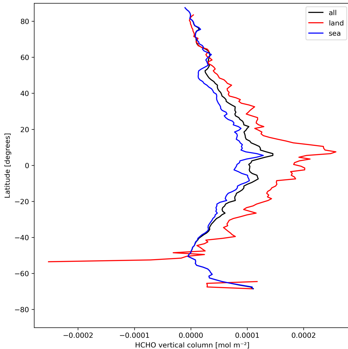
Figure 21: Zonal average of “HCHO vertical column” for 2024-05-02 to 2024-05-04.
