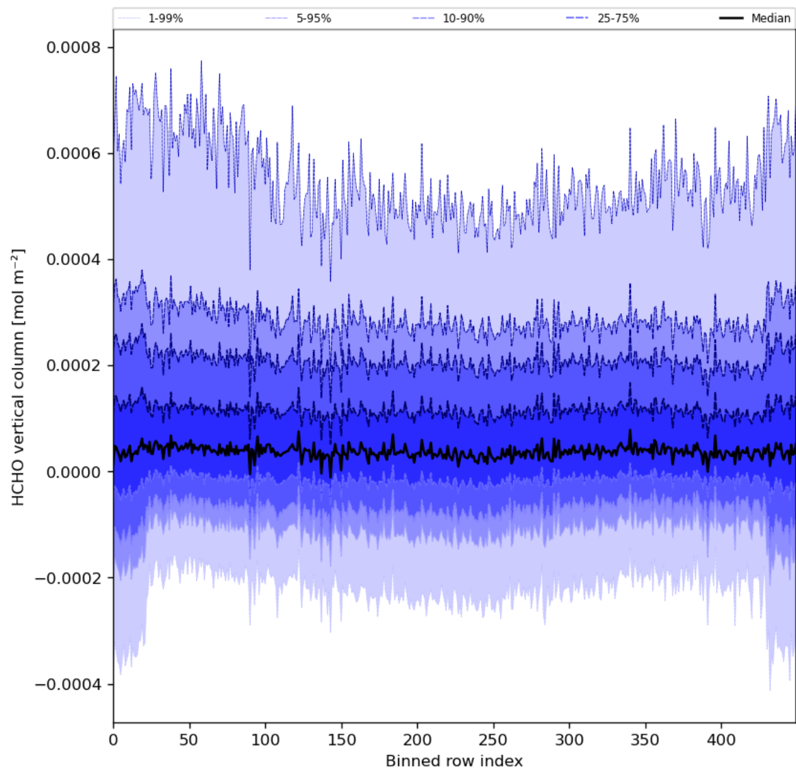
Figure 49: Along track statistics of “HCHO vertical column” for 2024-05-02 to 2024-05-04
