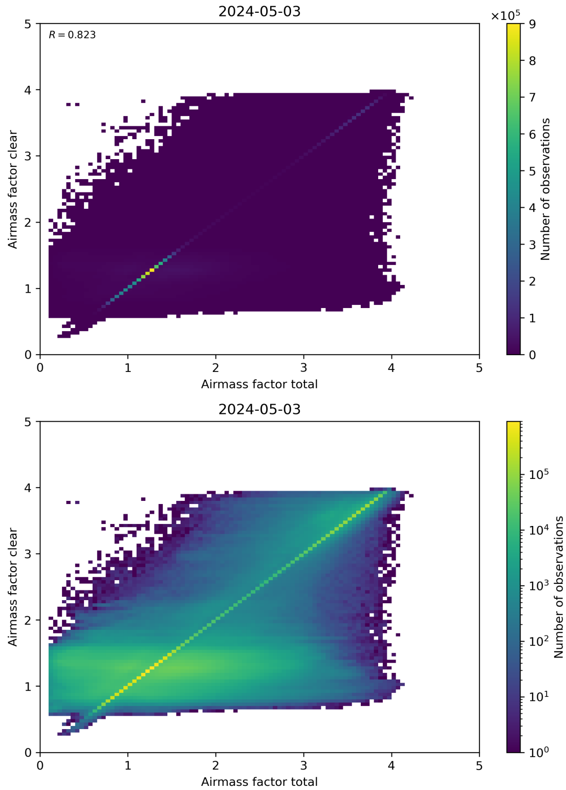
Figure 100: Scatter density plot of “Airmass factor total” against “Airmass factor clear” for 2024-05-02 to 2024-05-04.
