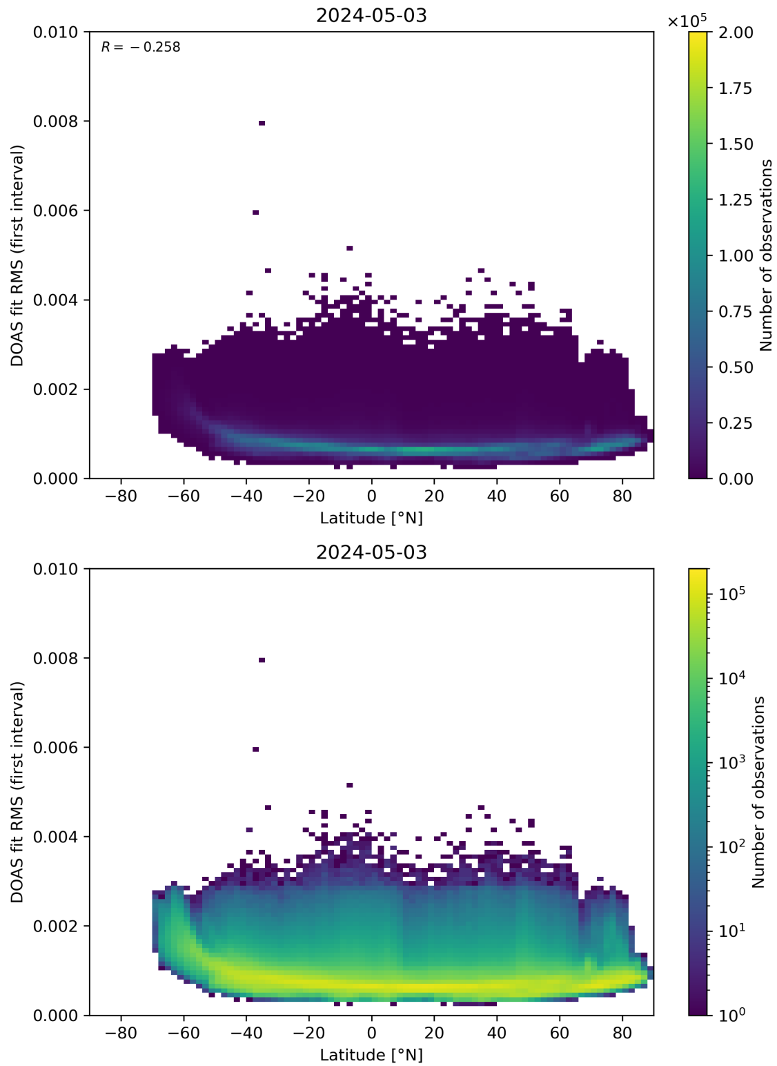
Figure 153: Scatter density plot of “Latitude” against “DOAS fit RMS (first interval)” for 2024-05-02 to 2024-05-04.
