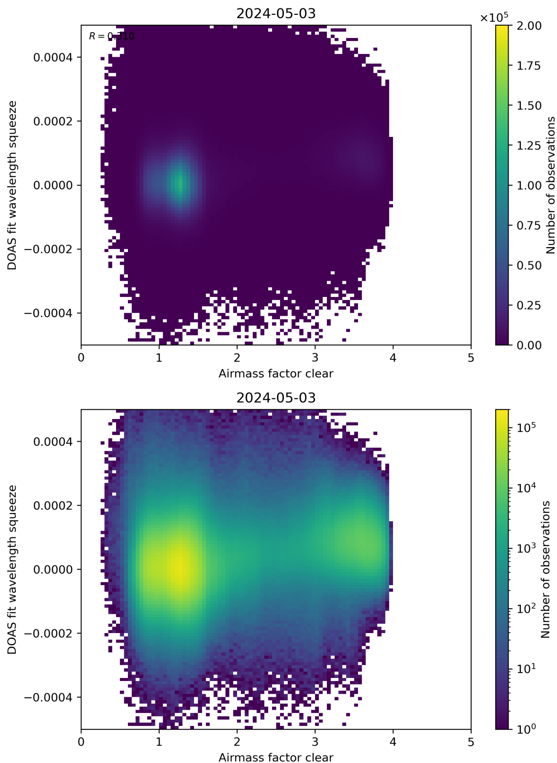
Figure 73: Scatter density plot of “Airmass factor clear” against “DOAS fit wavelength squeeze” for 2024-05-02 to 2024-05-04.
