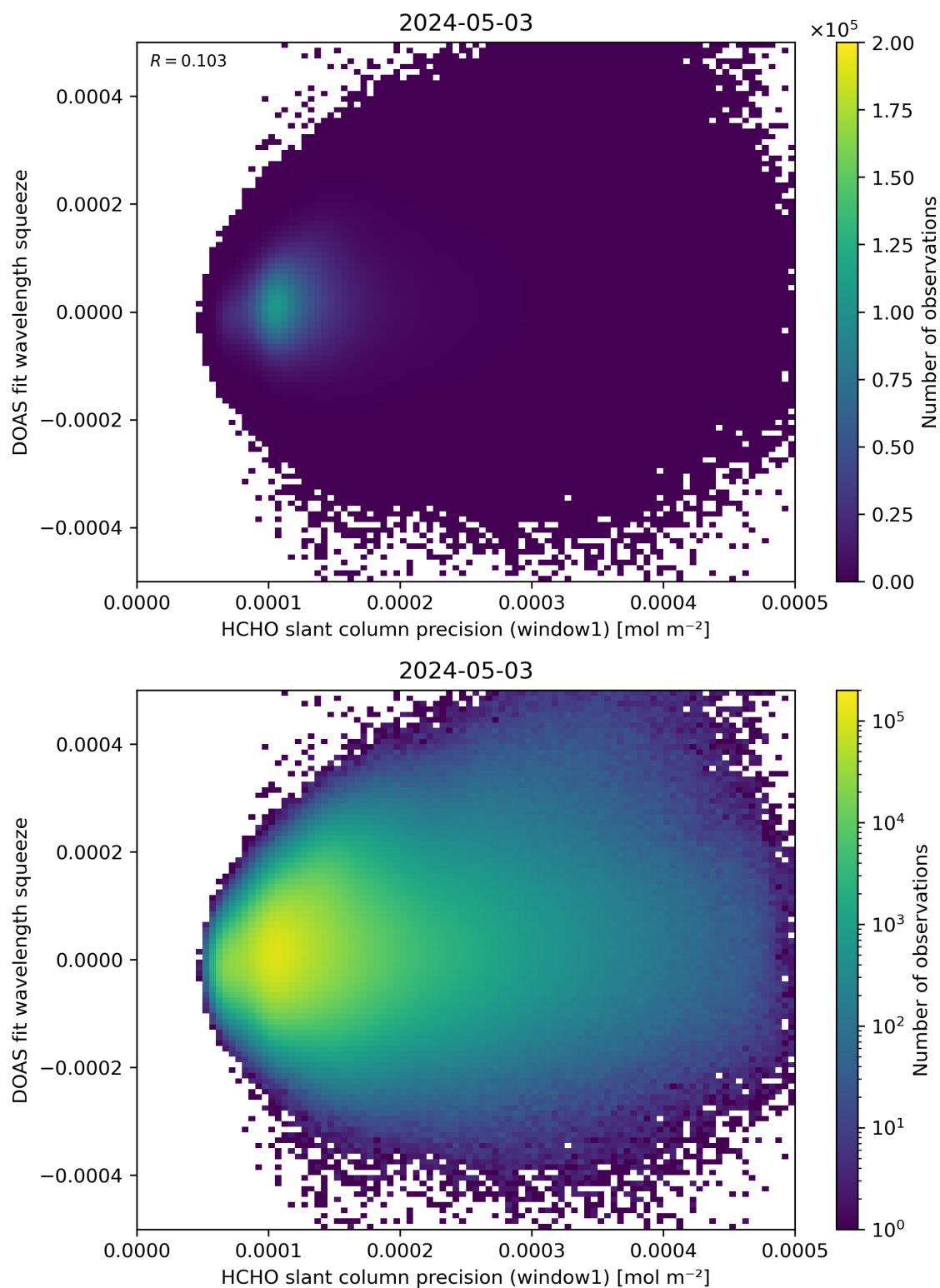
Figure 90: Scatter density plot of “HCHO slant column precision (window1)” against “DOAS fit wavelength squeeze” for 2024-05-02 to 2024-05-04.
