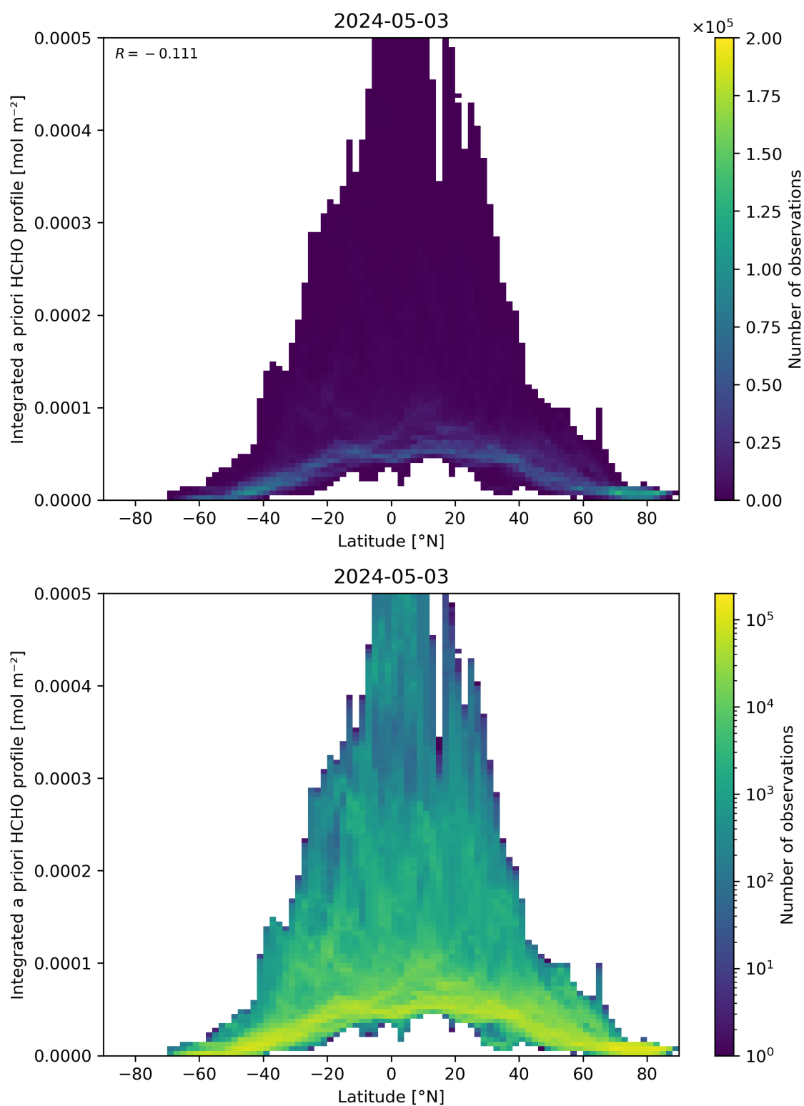
Figure 166: Scatter density plot of “Latitude” against “Integrated a priori HCHO profile” for 2024-05-02 to 2024-05-04.
