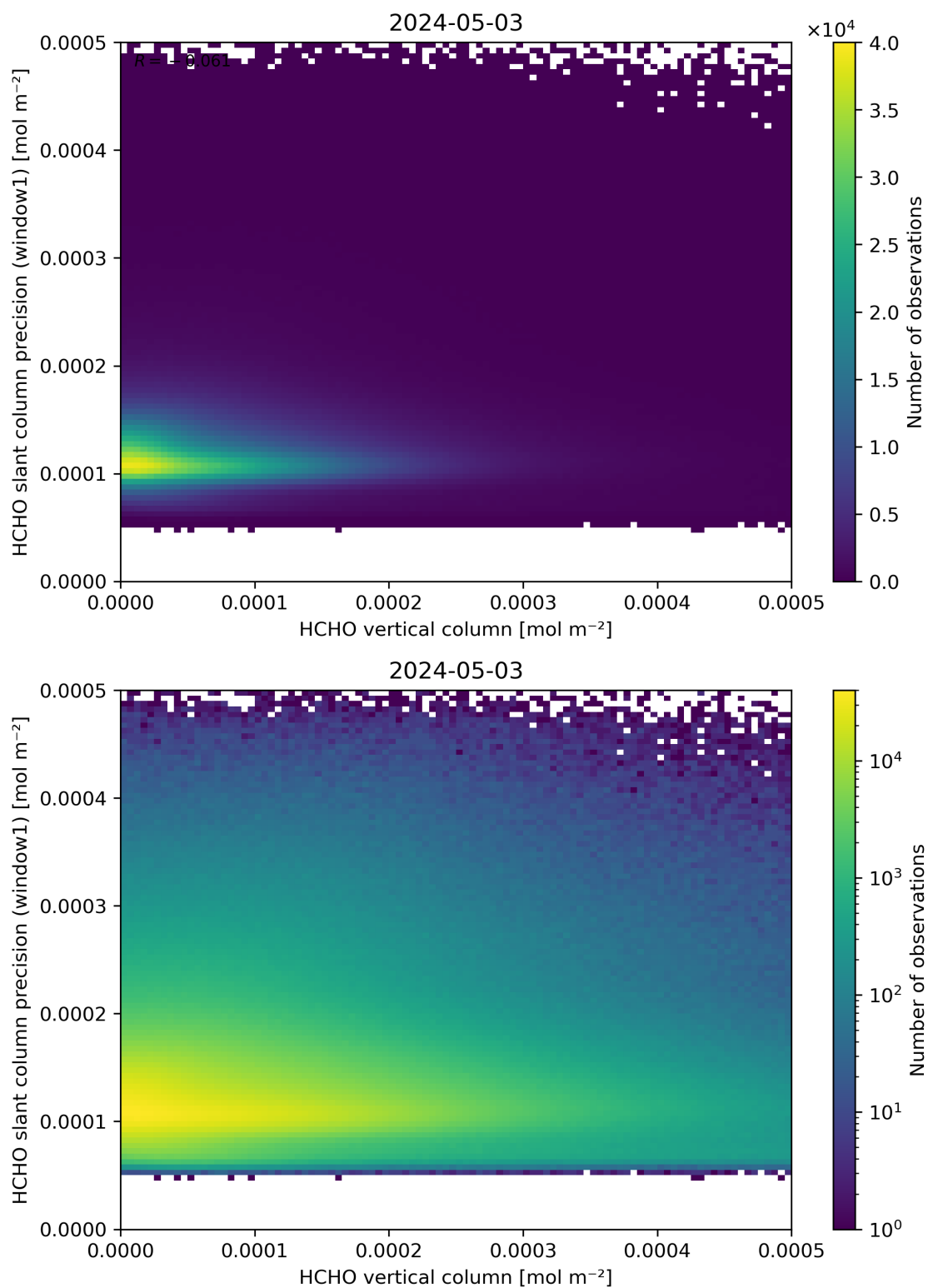
Figure 130: Scatter density plot of “HCHO vertical column” against “HCHO slant column precision (window1)” for 2024-05-02 to 2024-05-04.
