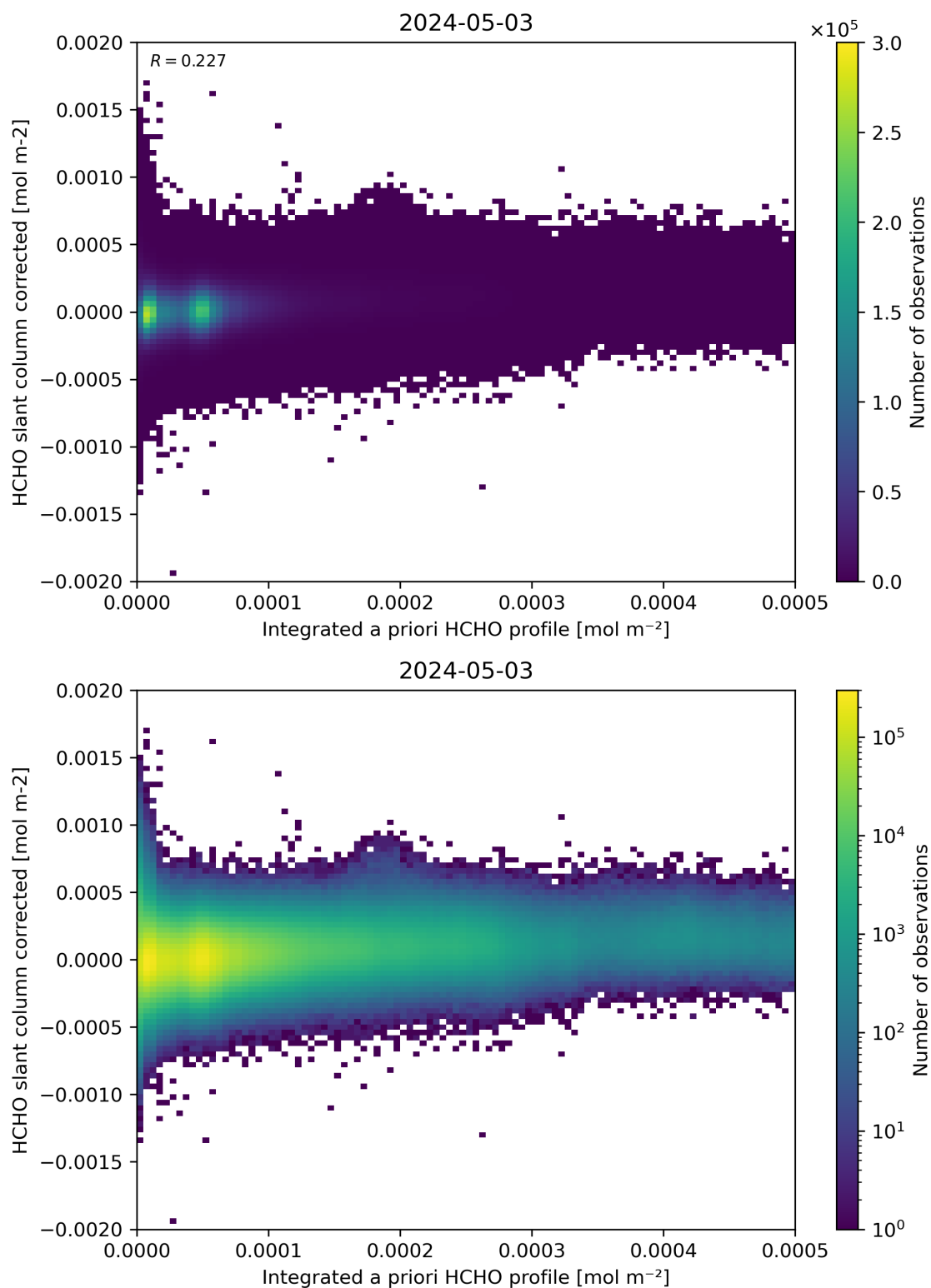
Figure 151: Scatter density plot of “Integrated a priori HCHO profile” against “HCHO slant column corrected” for 2024-05-02 to 2024-05-04.
