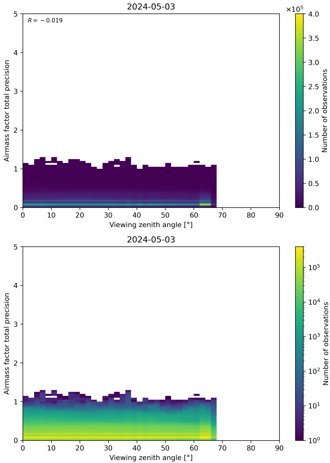
Figure 191: Scatter density plot of “Viewing zenith angle” against “Airmass factor total precision” for 2024-05-02 to 2024-05-04.
