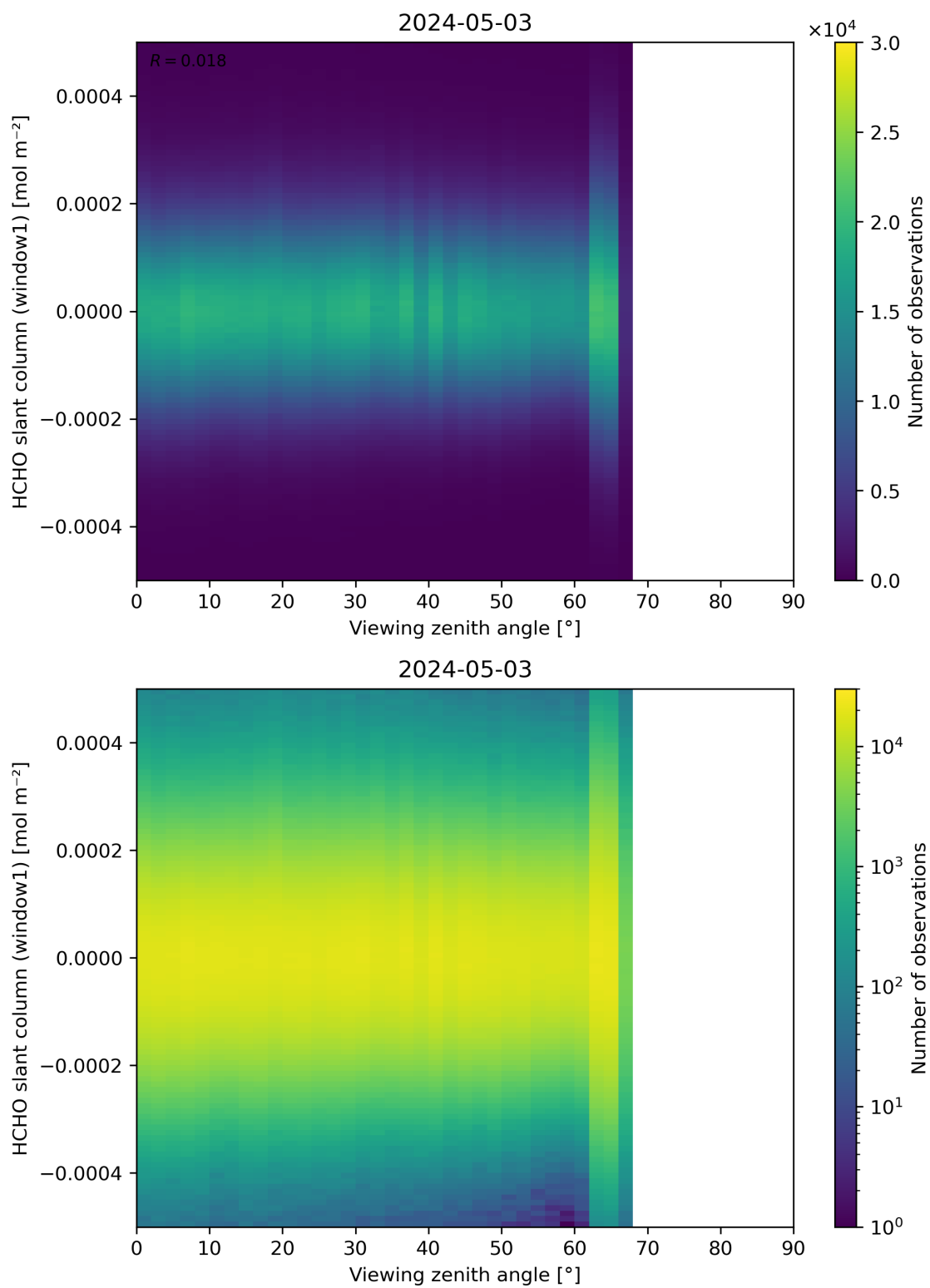
Figure 188: Scatter density plot of “Viewing zenith angle” against “HCHO slant column (window1)” for 2024-05-02 to 2024-05-04.
