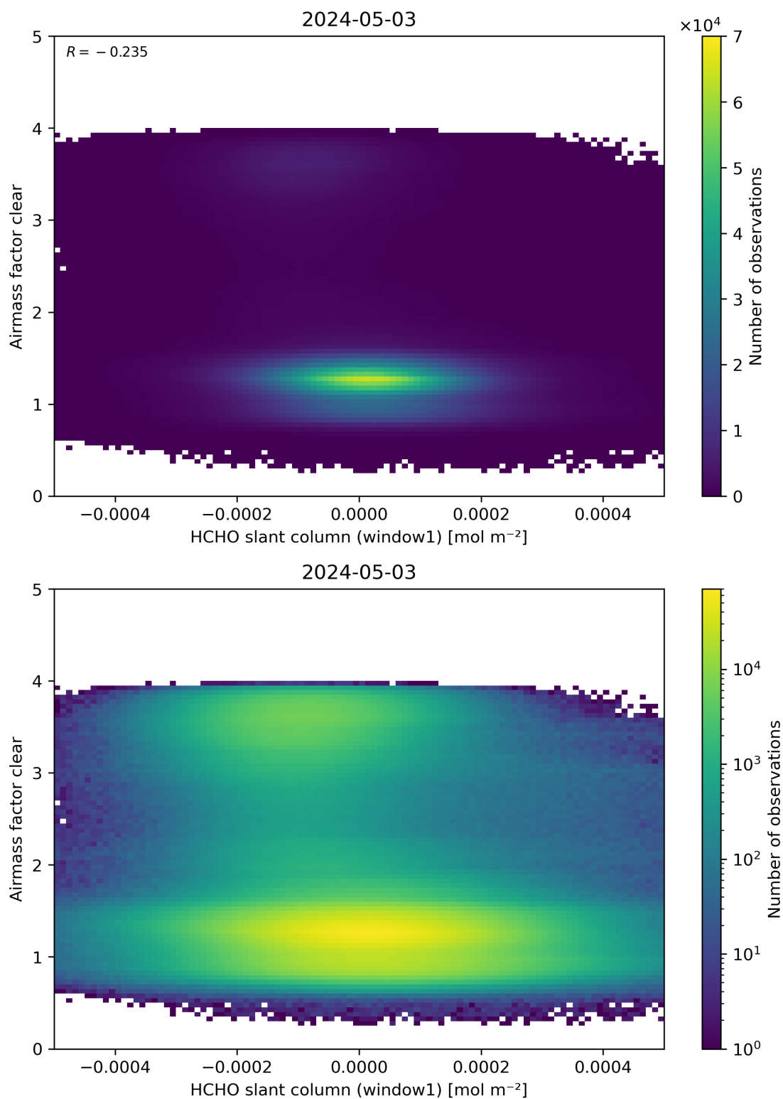
Figure 81: Scatter density plot of “HCHO slant column (window1)” against “Airmass factor clear” for 2024-05-02 to 2024-05-04.
