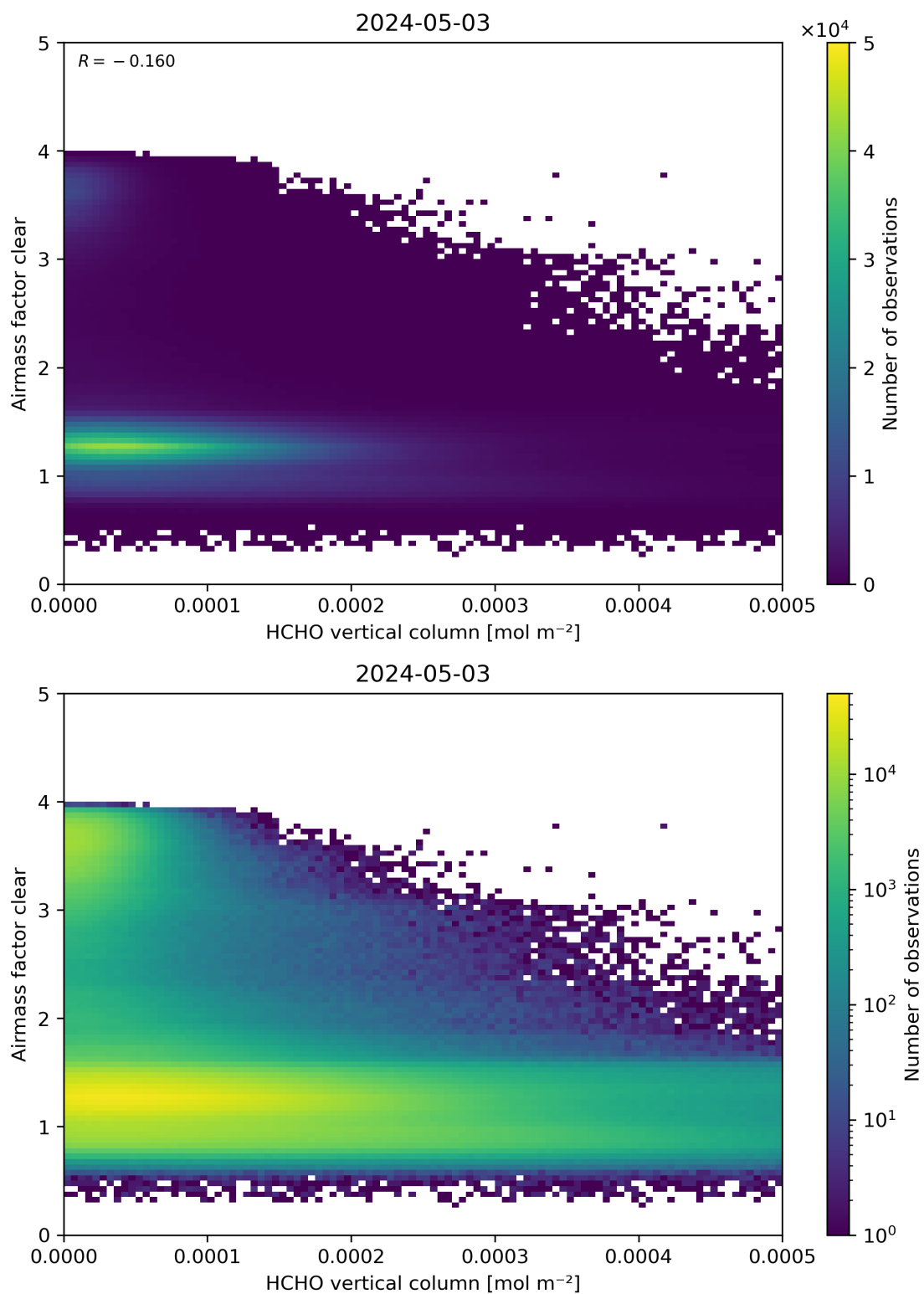
Figure 126: Scatter density plot of “HCHO vertical column” against “Airmass factor clear” for 2024-05-02 to 2024-05-04.
