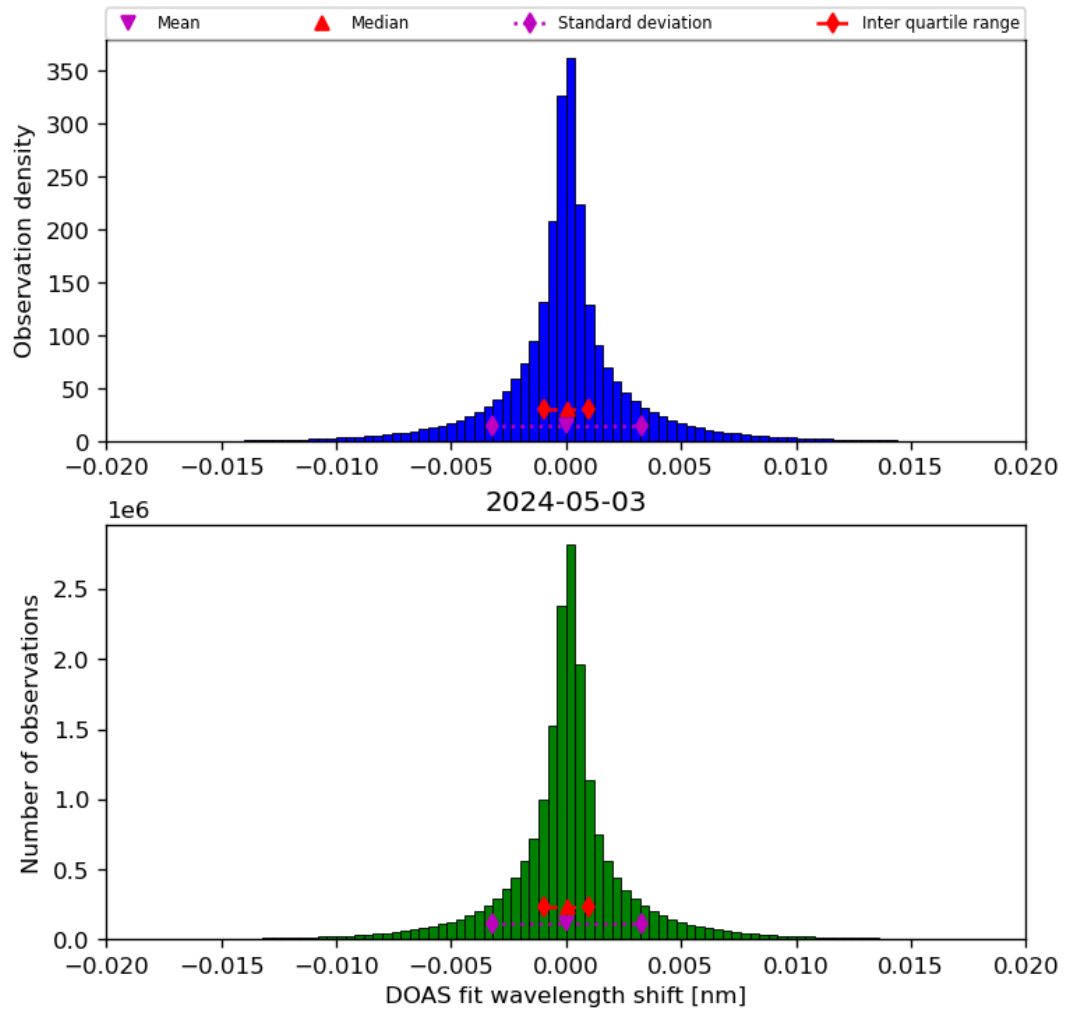
Figure 44: Histogram of “DOAS fit wavelength shift” for 2024-05-02 to 2024-05-04
