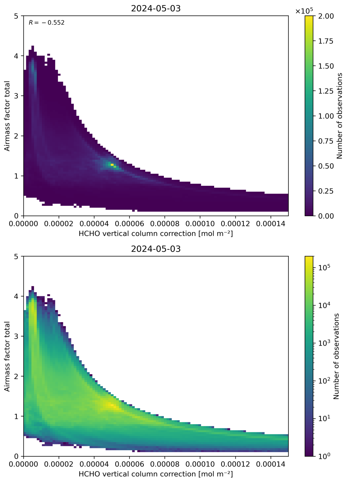
Figure 120: Scatter density plot of “HCHO vertical column correction” against “Airmass factor total” for 2024-05-02 to 2024-05-04.
