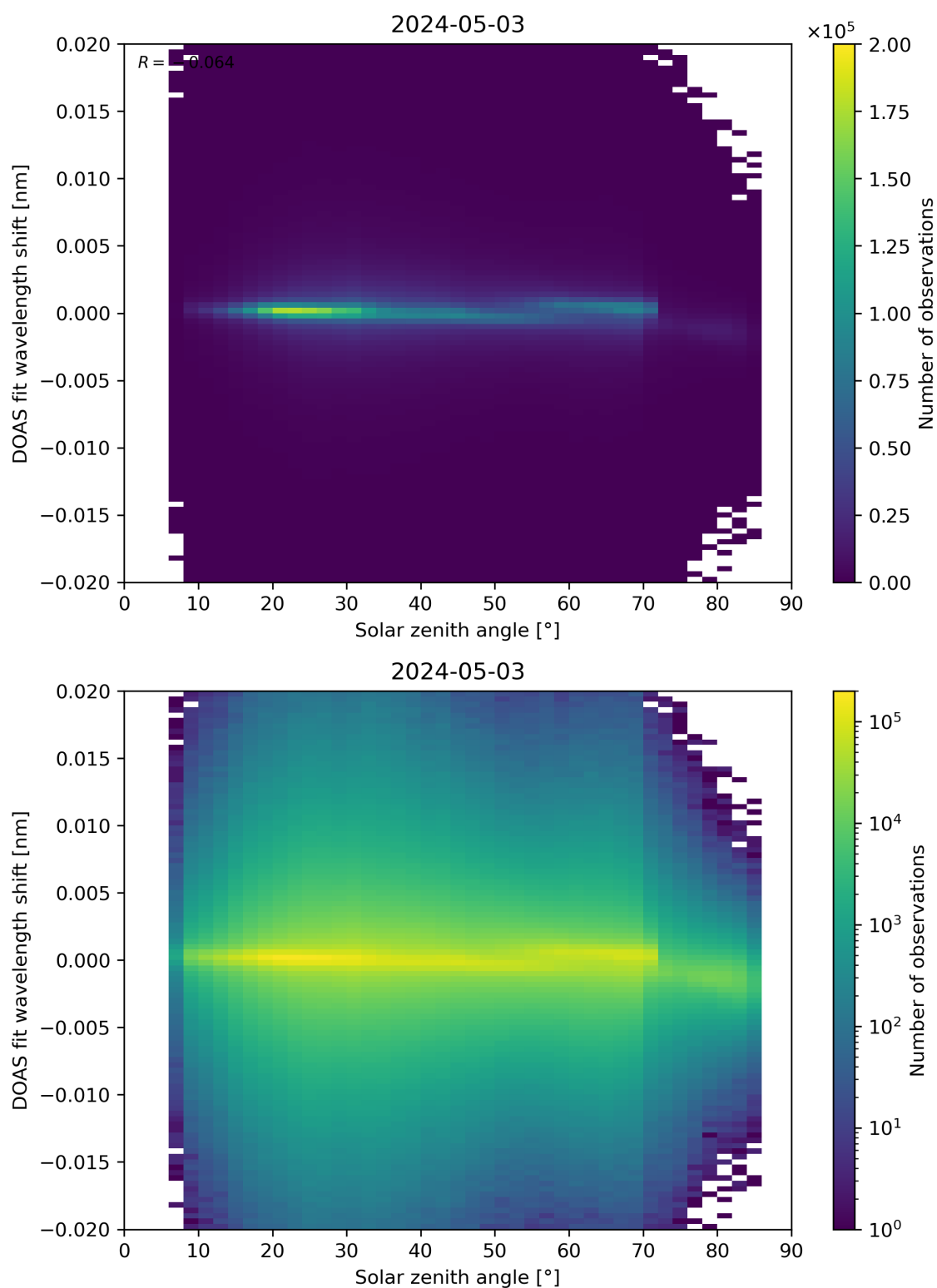
Figure 168: Scatter density plot of “Solar zenith angle” against “DOAS fit wavelength shift” for 2024-05-02 to 2024-05-04.
