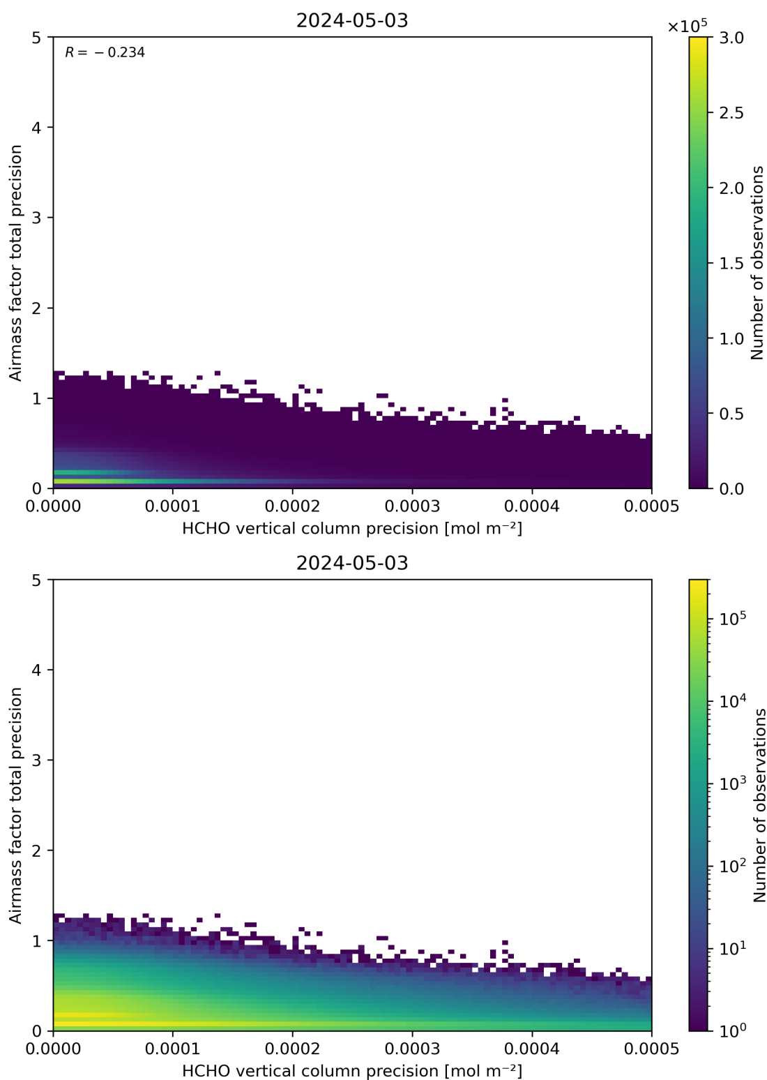
Figure 145: Scatter density plot of “HCHO vertical column precision” against “Airmass factor total precision” for 2024-05-02 to 2024-05-04.
