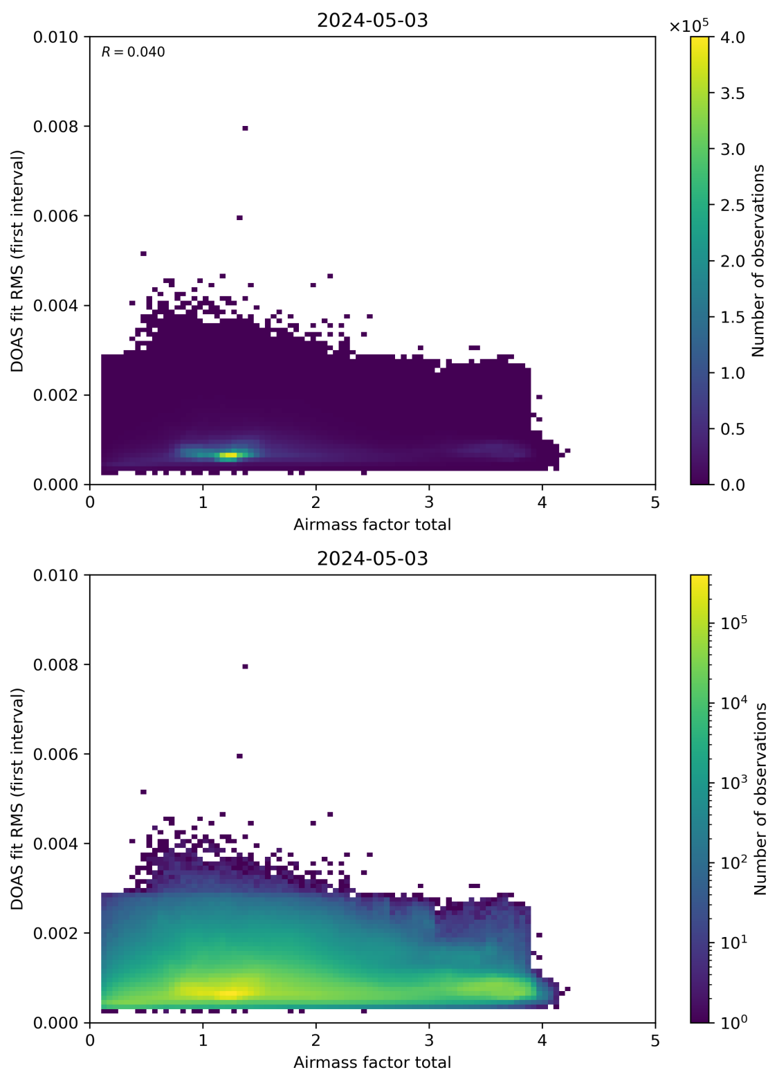
Figure 97: Scatter density plot of “Airmass factor total” against “DOAS fit RMS (first interval)” for 2024-05-02 to 2024-05-04.
