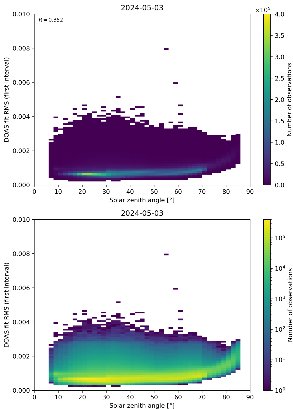
Figure 167: Scatter density plot of “Solar zenith angle” against “DOAS fit RMS (first interval)” for 2024-05-02 to 2024-05-04.
