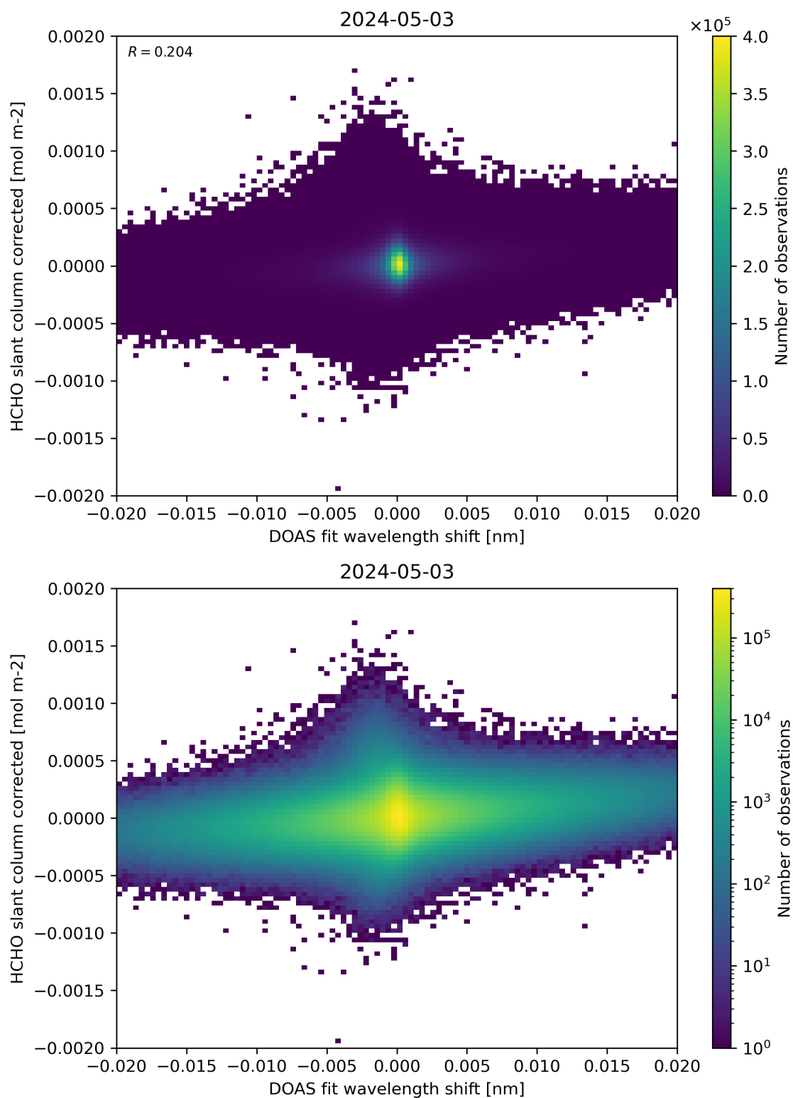
Figure 66: Scatter density plot of “DOAS fit wavelength shift” against “HCHO slant column corrected” for 2024-05-02 to 2024-05-04.
