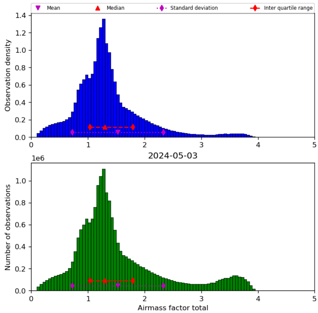
Figure 40: Histogram of “Airmass factor total” for 2024-05-02 to 2024-05-04
