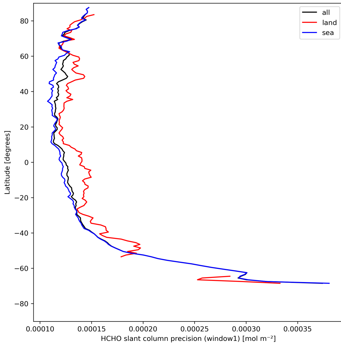
Figure 25: Zonal average of “HCHO slant column precision (window1)” for 2024-05-02 to 2024-05-04.
