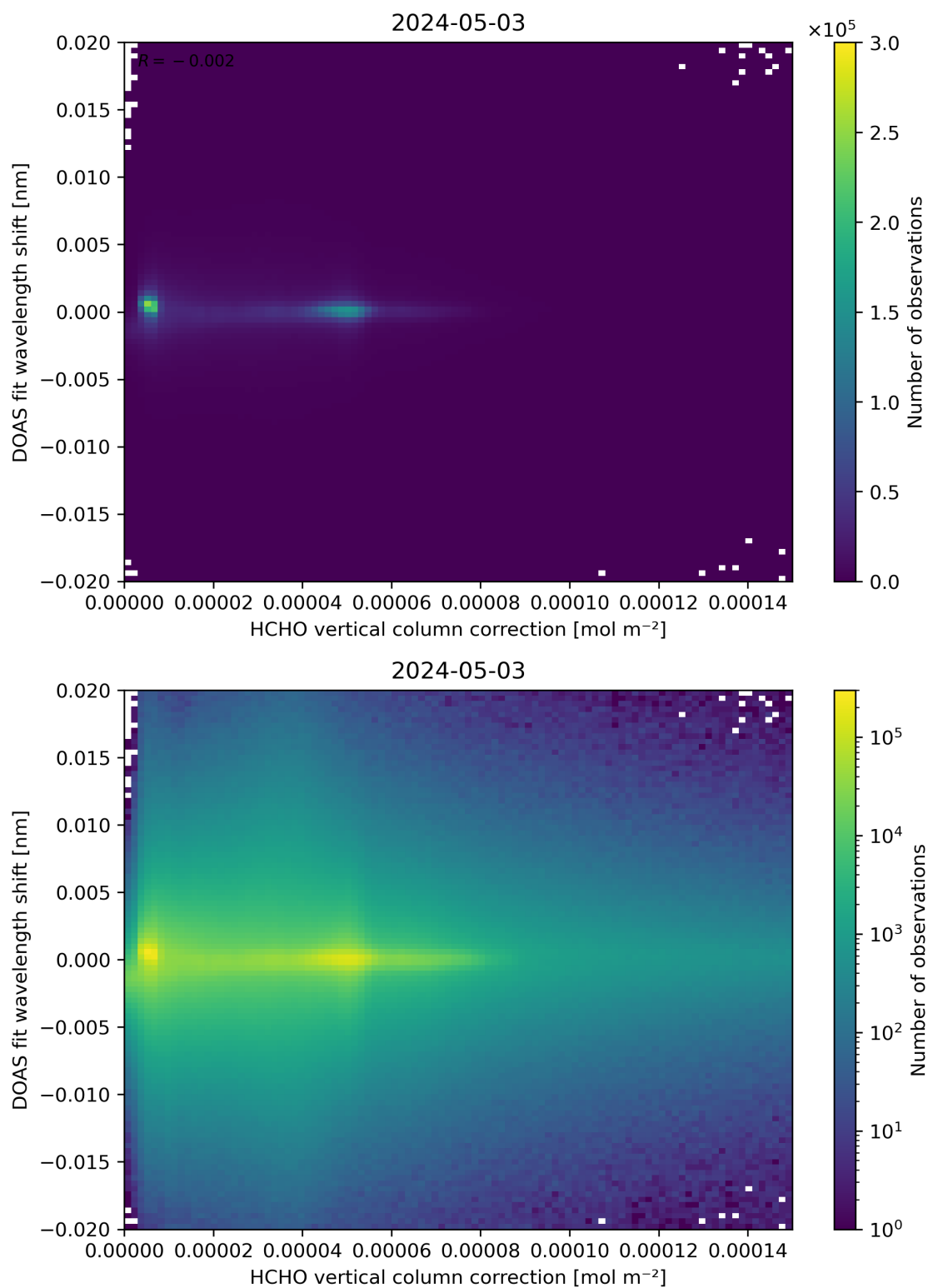
Figure 113: Scatter density plot of “HCHO vertical column correction” against “DOAS fit wavelength shift” for 2024-05-02 to 2024-05-04.
