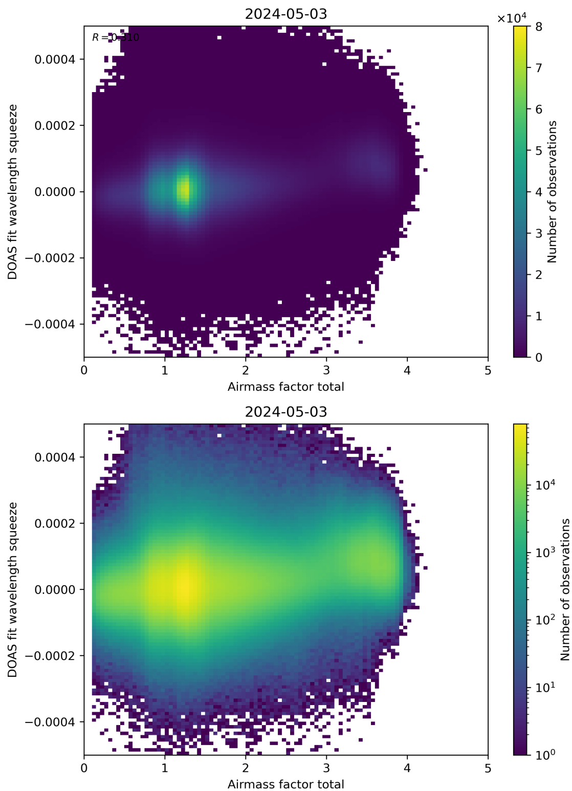
Figure 99: Scatter density plot of “Airmass factor total” against “DOAS fit wavelength squeeze” for 2024-05-02 to 2024-05-04.
