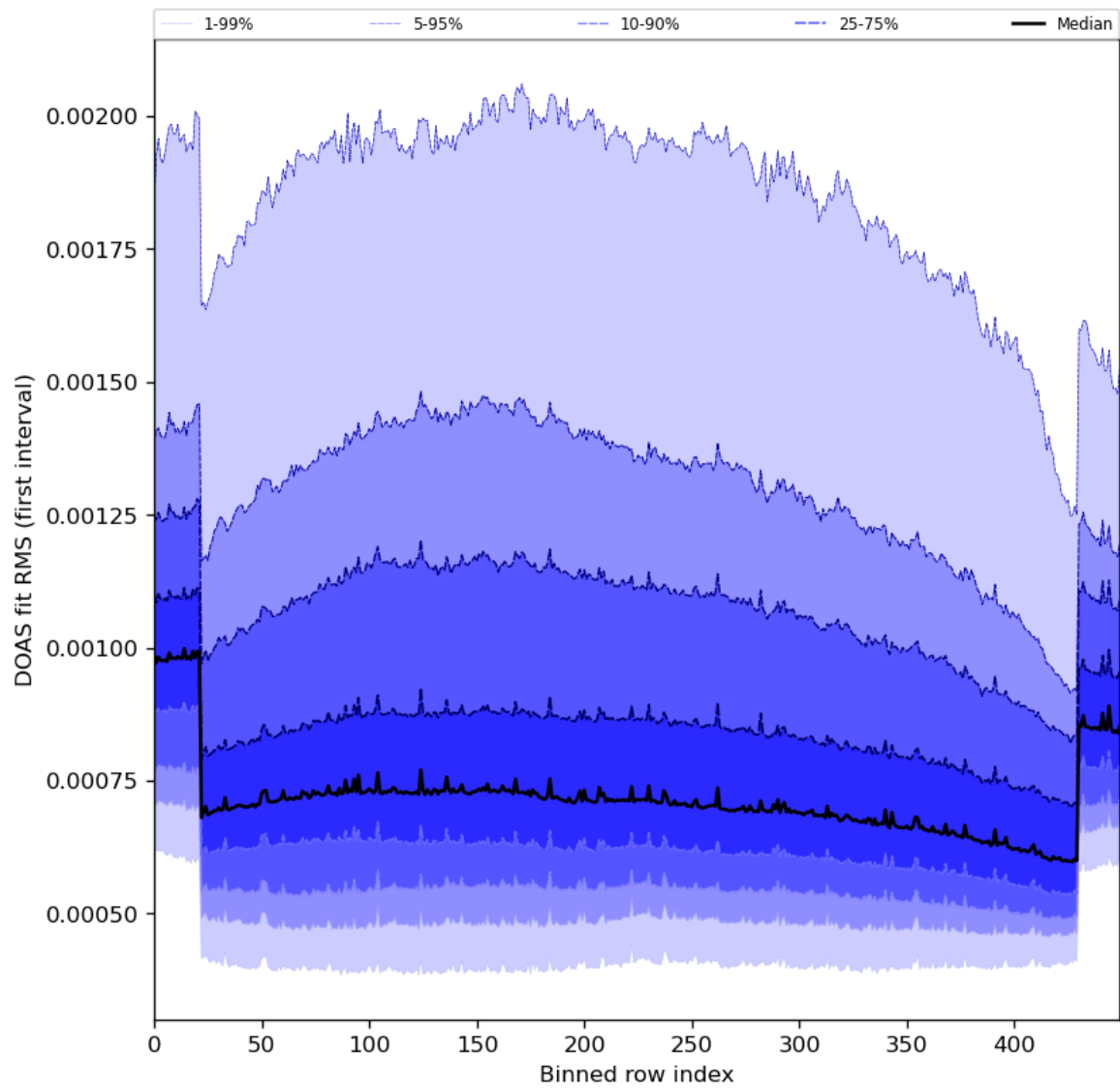
Figure 60: Along track statistics of “DOAS fit RMS (first interval)” for 2024-05-02 to 2024-05-04
