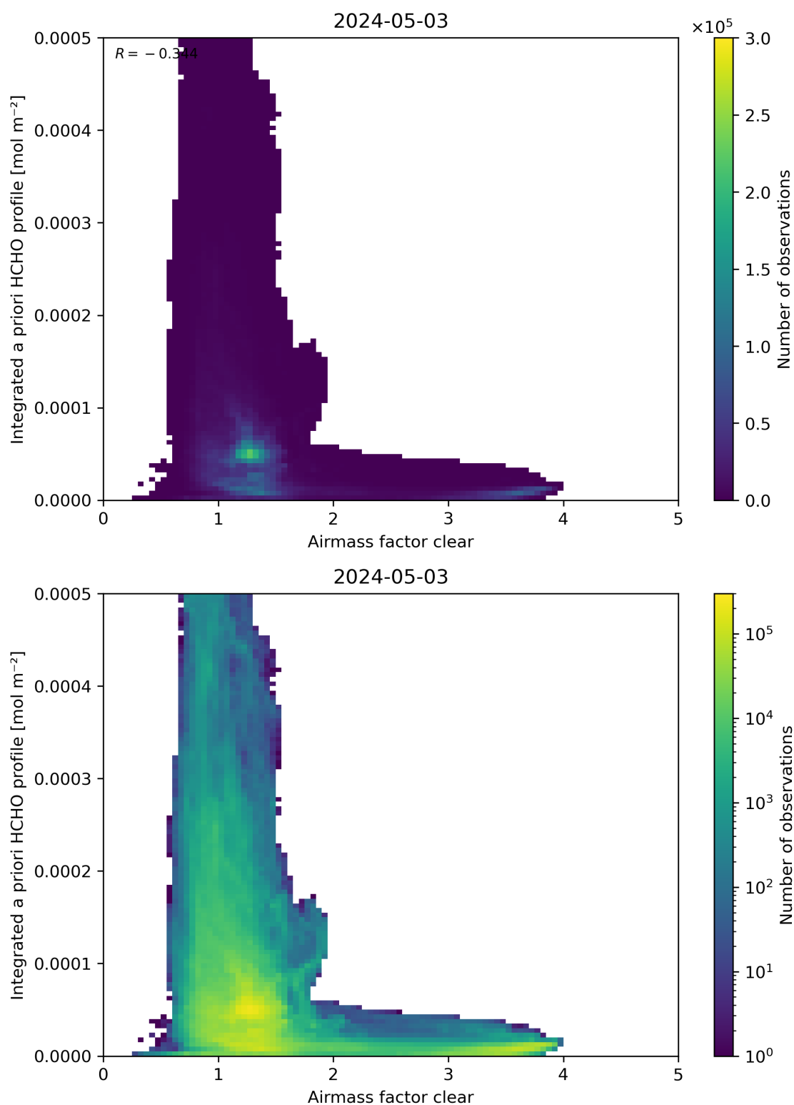
Figure 76: Scatter density plot of “Airmass factor clear” against “Integrated a priori HCHO profile” for 2024-05-02 to 2024-05-04.
