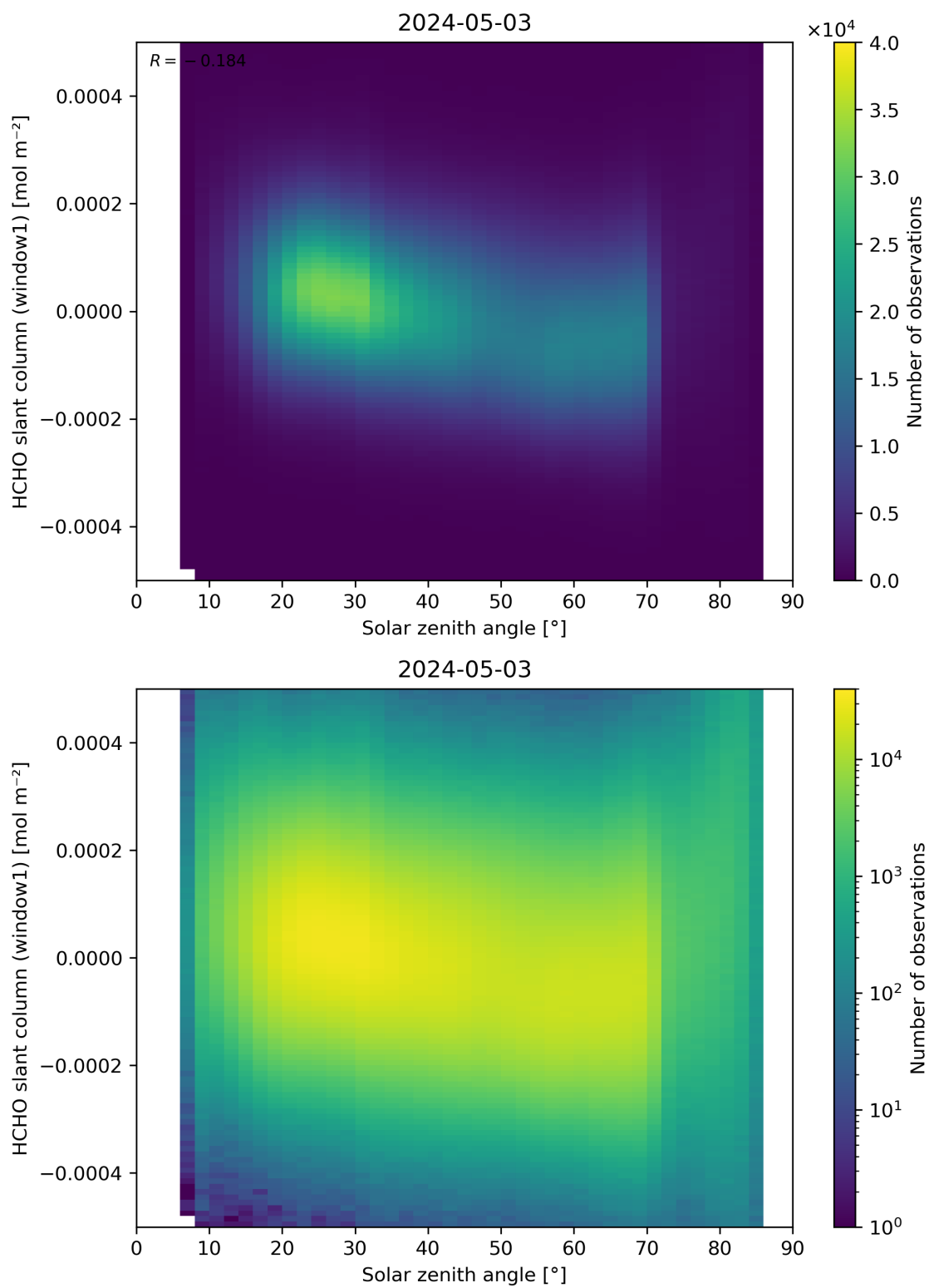
Figure 173: Scatter density plot of “Solar zenith angle” against “HCHO slant column (window1)” for 2024-05-02 to 2024-05-04.
