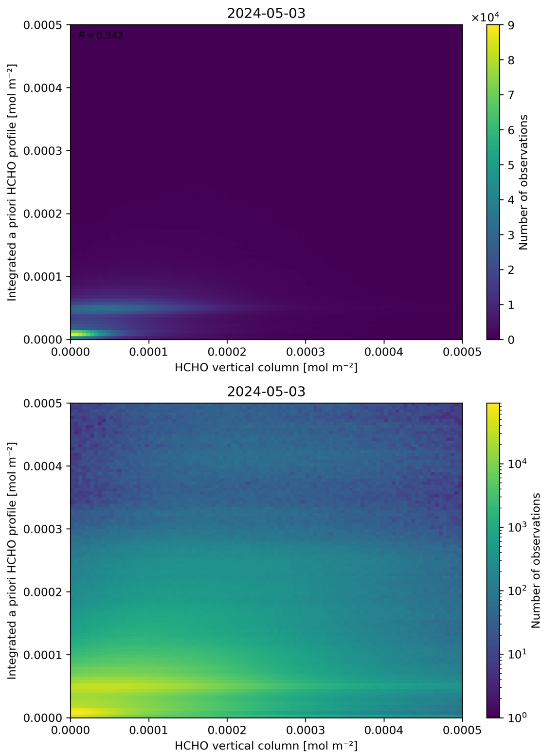
Figure 135: Scatter density plot of “HCHO vertical column” against “Integrated a priori HCHO profile” for 2024-05-02 to 2024-05-04.
