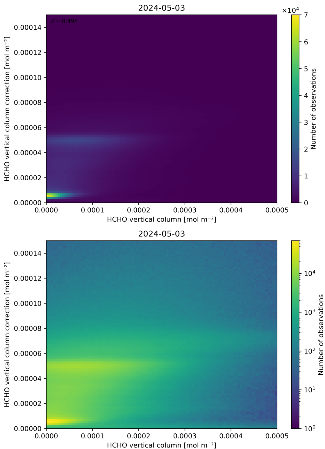
Figure 133: Scatter density plot of “HCHO vertical column” against “HCHO vertical column correction” for 2024-05-02 to 2024-05-04.
