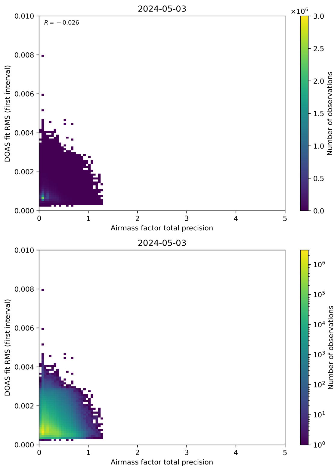
Figure 105: Scatter density plot of “Airmass factor total precision” against “DOAS fit RMS (first interval)” for 2024-05-02 to 2024-05-04.
