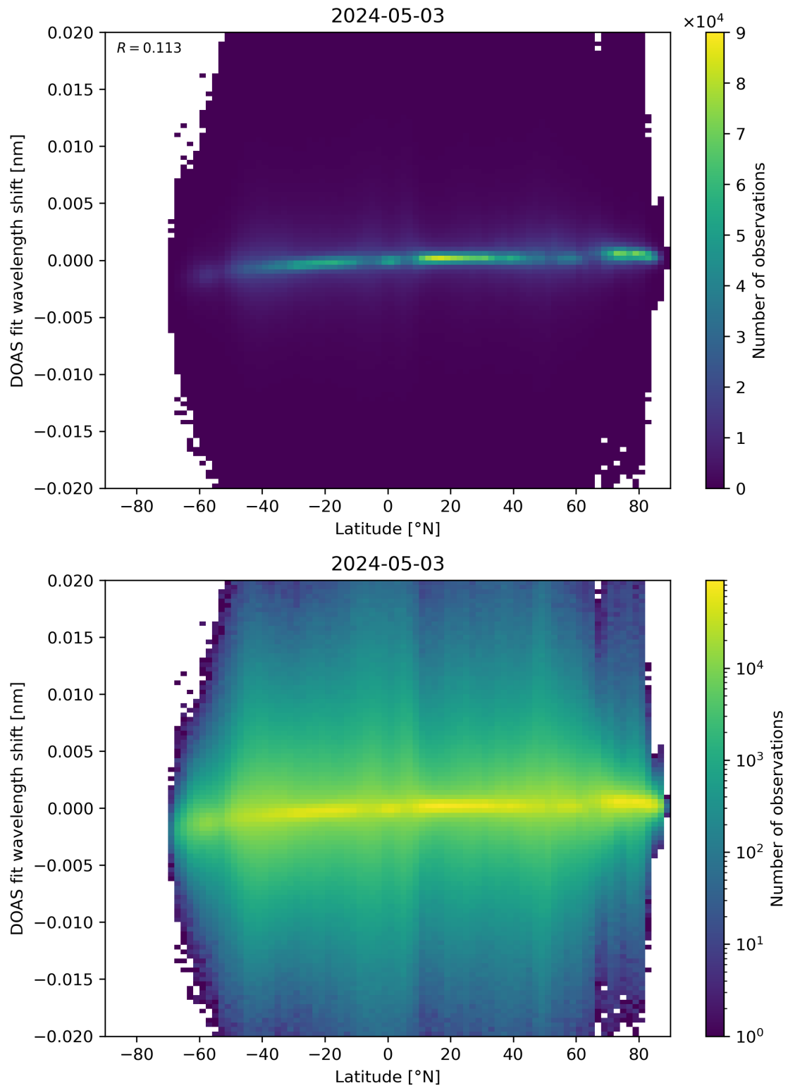
Figure 154: Scatter density plot of “Latitude” against “DOAS fit wavelength shift” for 2024-05-02 to 2024-05-04.
