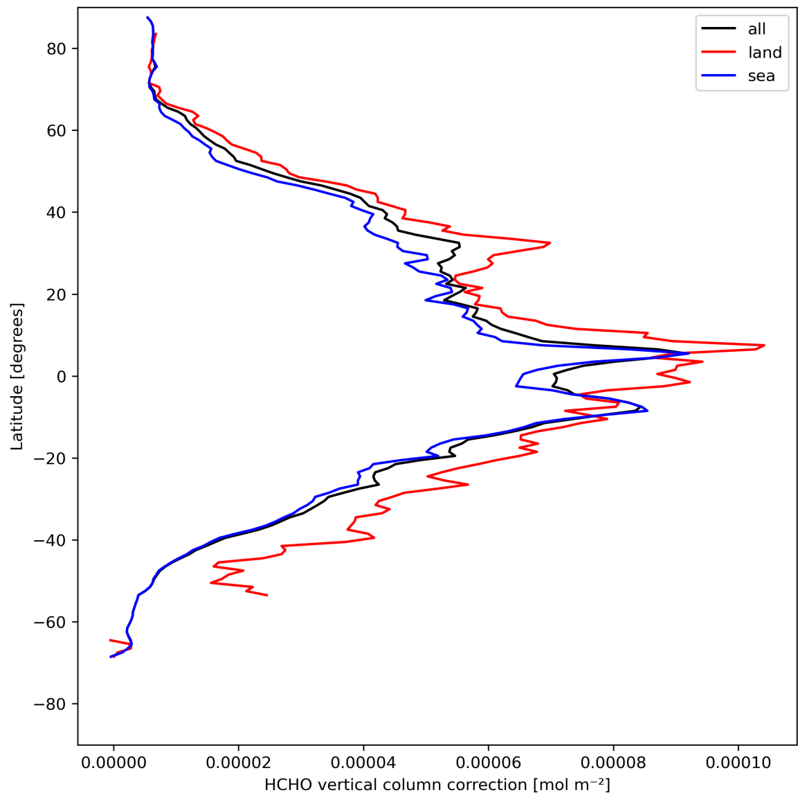
Figure 23: Zonal average of “HCHO vertical column correction” for 2024-05-02 to 2024-05-04.
