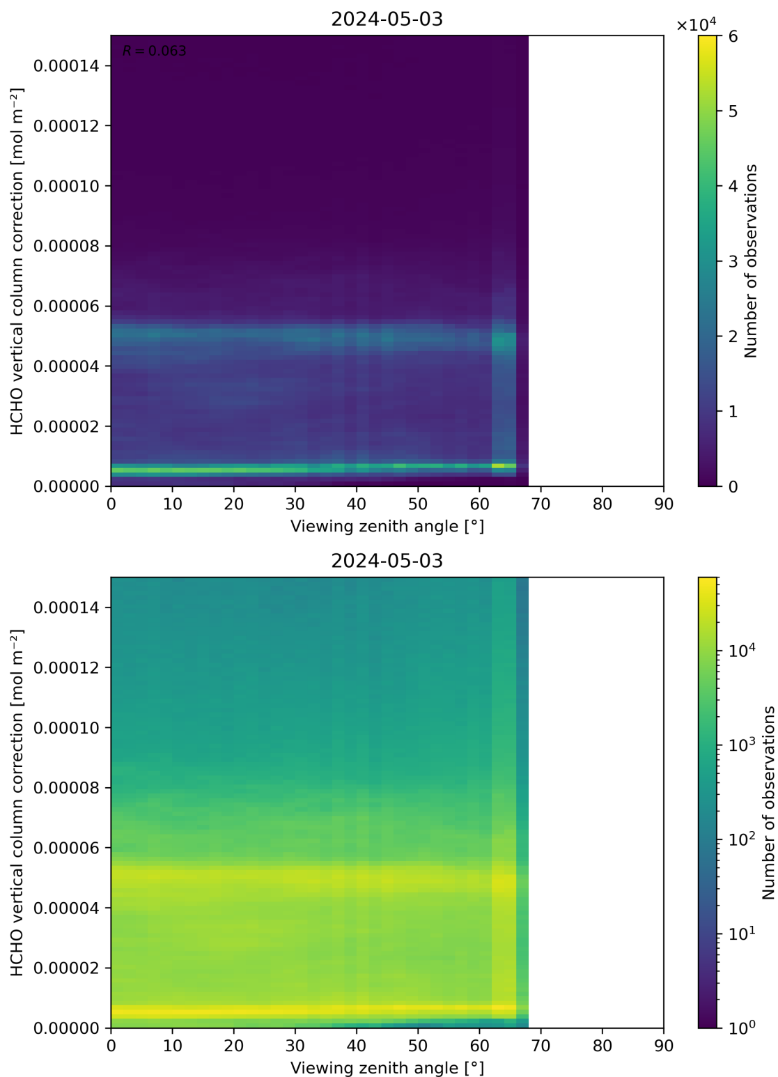
Figure 193: Scatter density plot of “Viewing zenith angle” against “HCHO vertical column correction” for 2024-05-02 to 2024-05-04.
