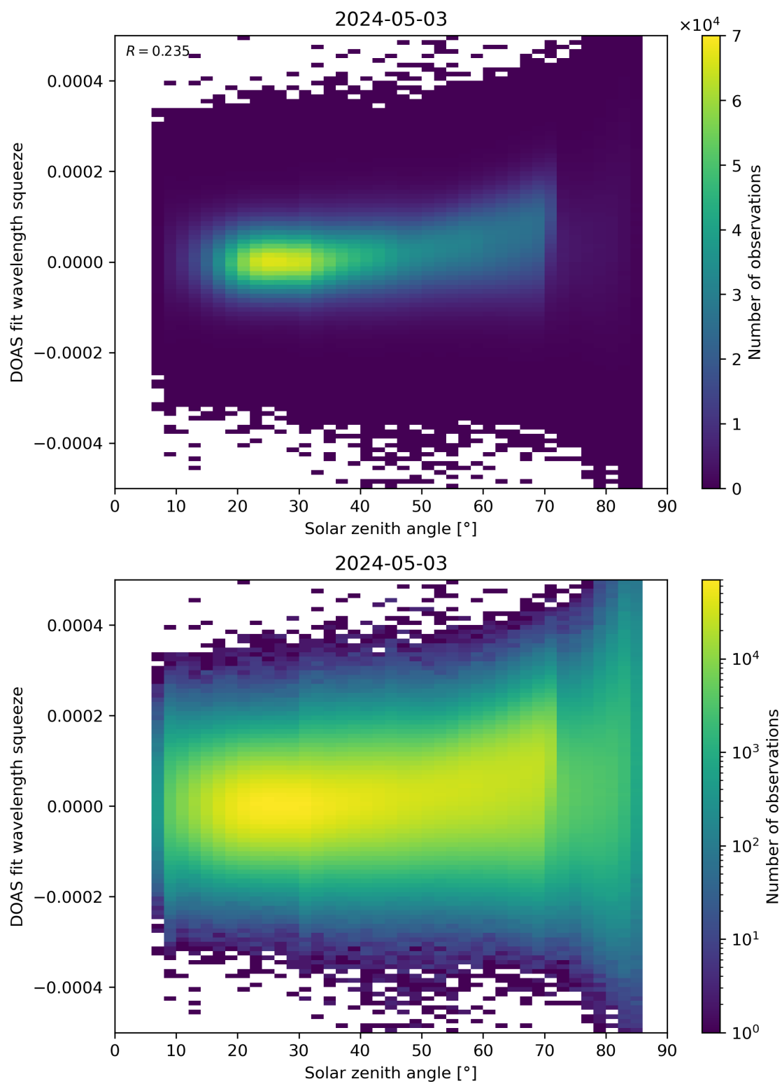
Figure 169: Scatter density plot of “Solar zenith angle” against “DOAS fit wavelength squeeze” for 2024-05-02 to 2024-05-04.
