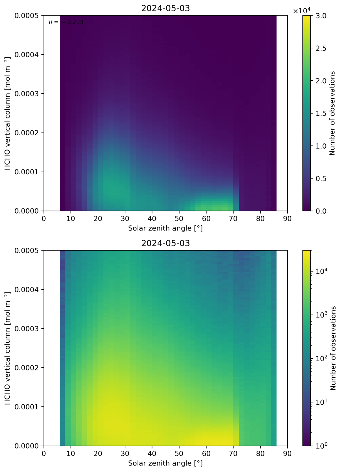
Figure 177: Scatter density plot of “Solar zenith angle” against “HCHO vertical column” for 2024-05-02 to 2024-05-04.
