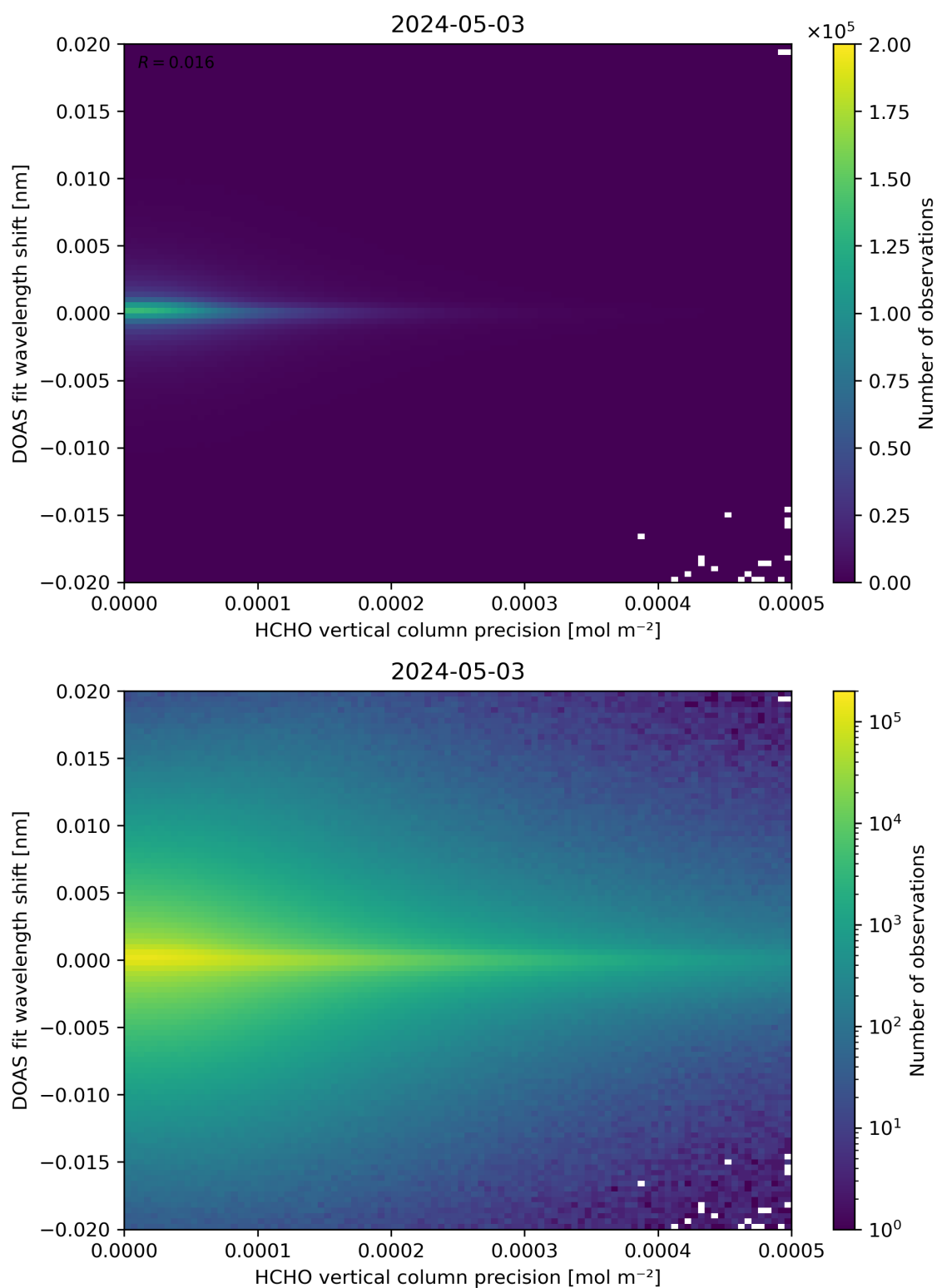
Figure 137: Scatter density plot of “HCHO vertical column precision” against “DOAS fit wavelength shift” for 2024-05-02 to 2024-05-04.
