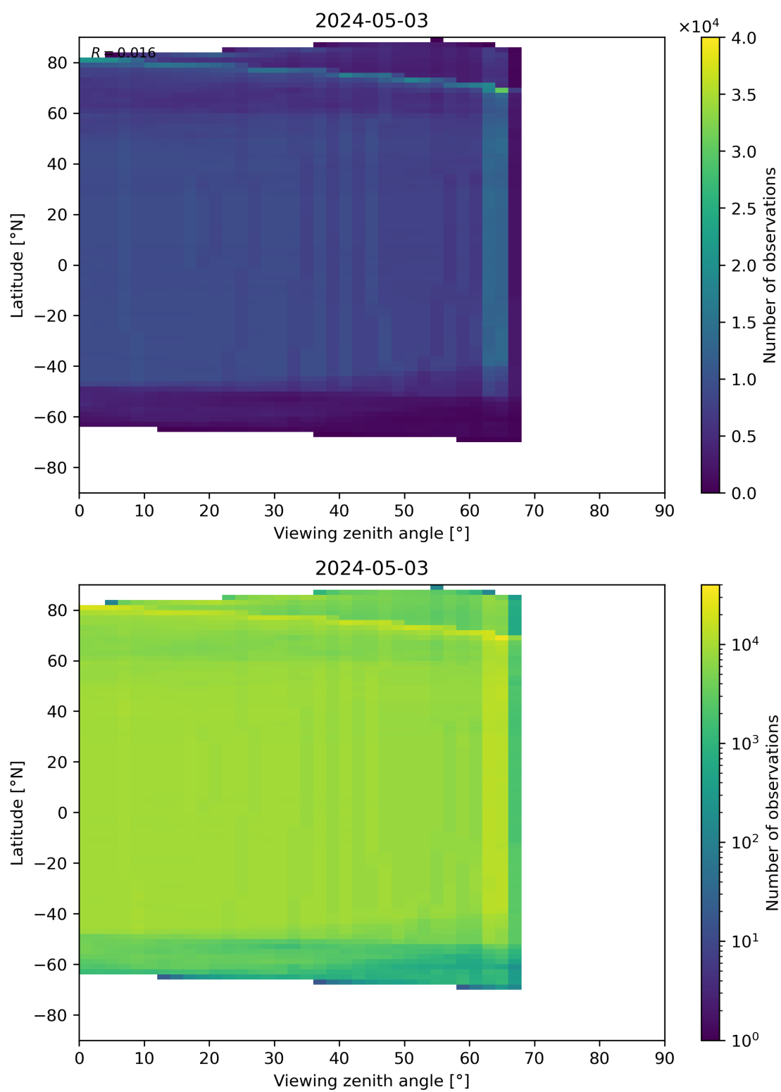
Figure 196: Scatter density plot of “Viewing zenith angle” against “Latitude” for 2024-05-02 to 2024-05-04.
