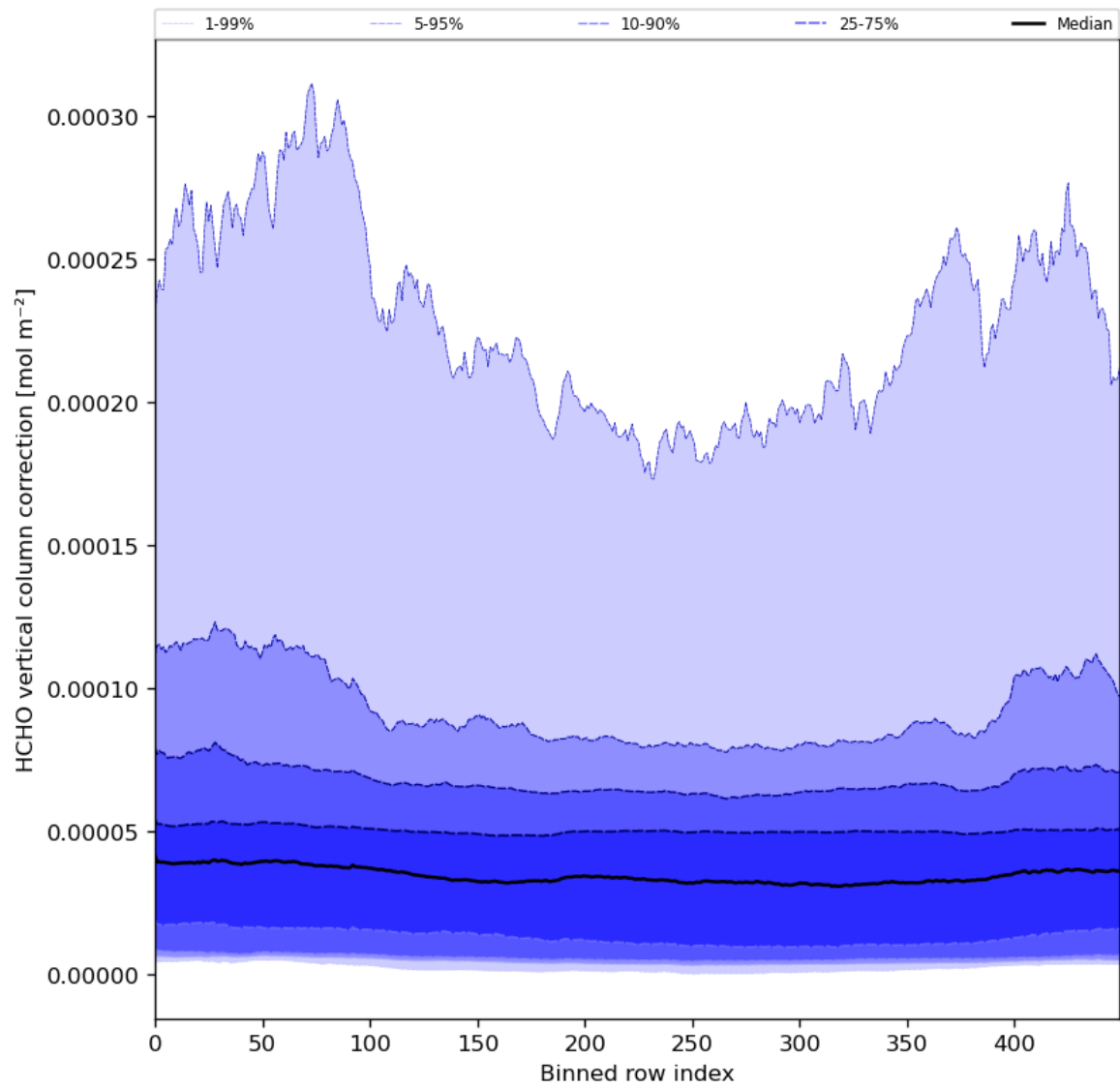
Figure 51: Along track statistics of “HCHO vertical column correction” for 2024-05-02 to 2024-05-04
