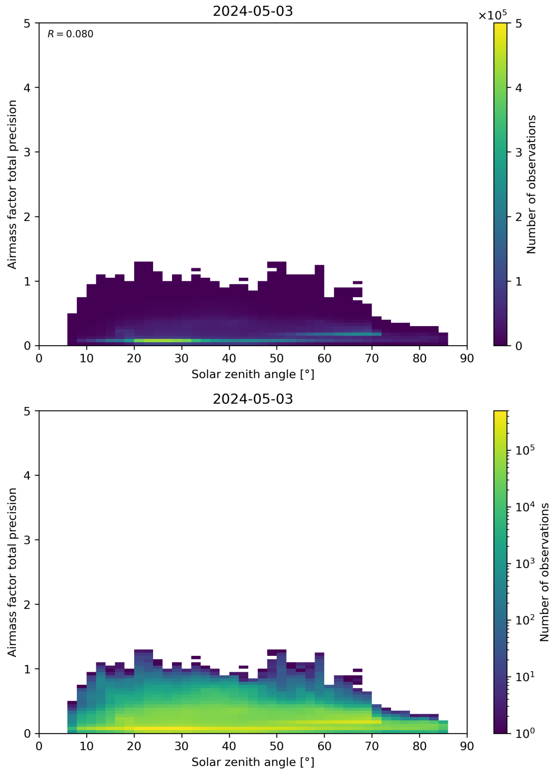
Figure 176: Scatter density plot of “Solar zenith angle” against “Airmass factor total precision” for 2024-05-02 to 2024-05-04.
