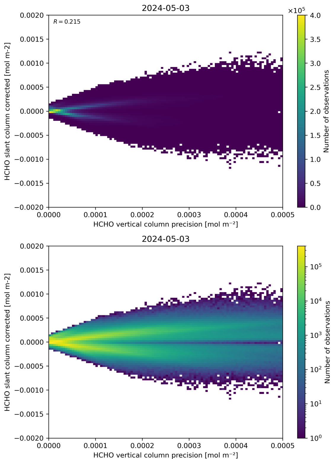
Figure 140: Scatter density plot of “HCHO vertical column precision” against “HCHO slant column corrected” for 2024-05-02 to 2024-05-04.
