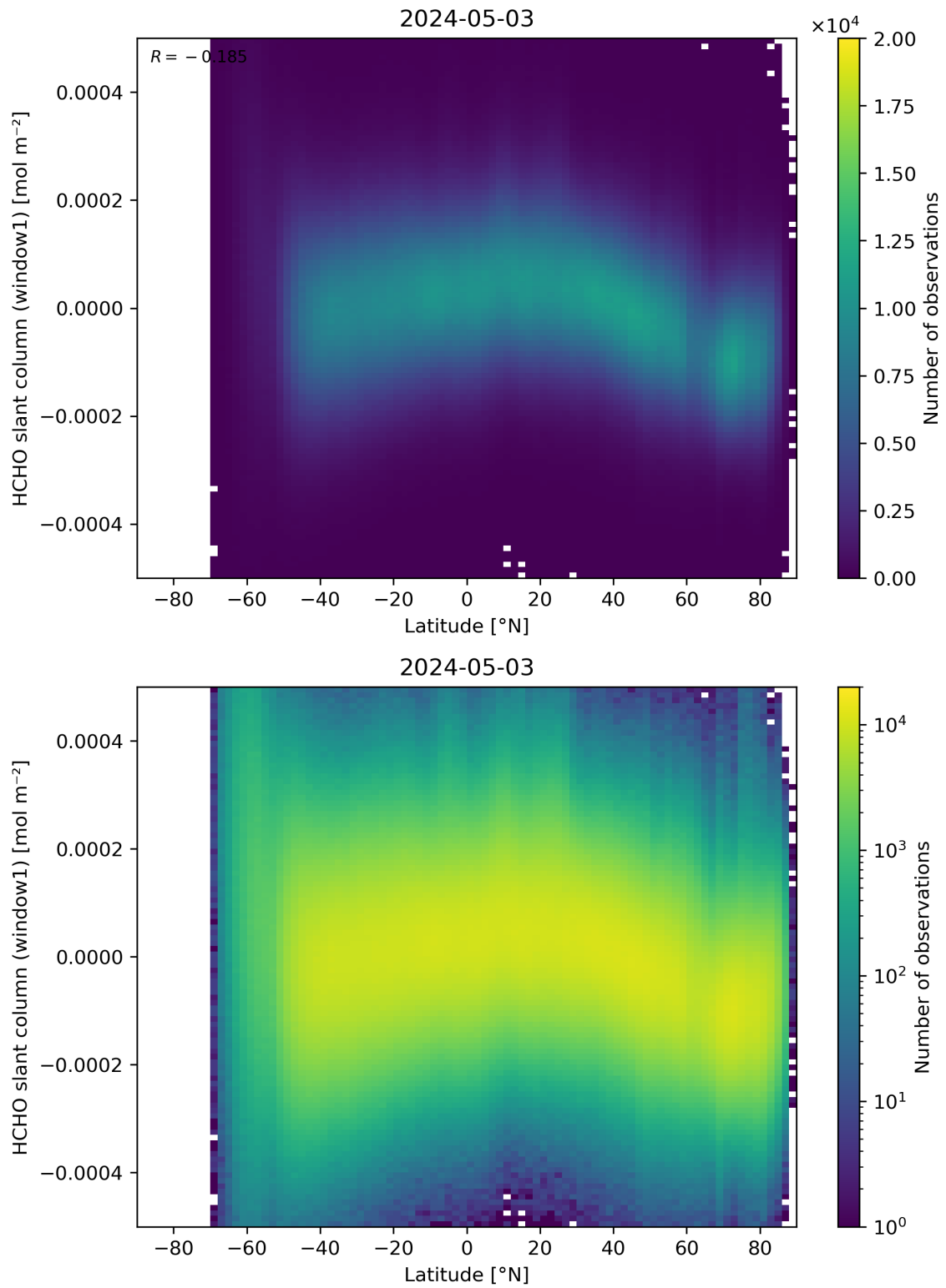
Figure 159: Scatter density plot of “Latitude” against “HCHO slant column (window1)” for 2024-05-02 to 2024-05-04.
