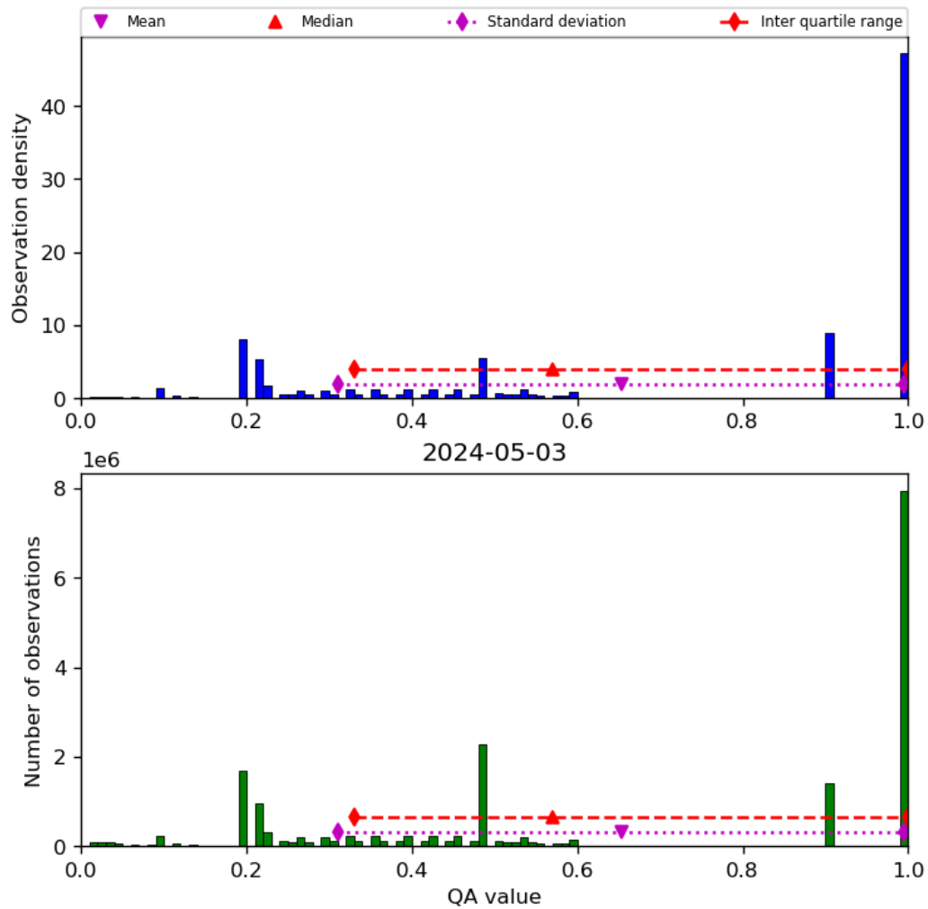
Figure 34: Histogram of “QA value” for 2024-05-02 to 2024-05-04
