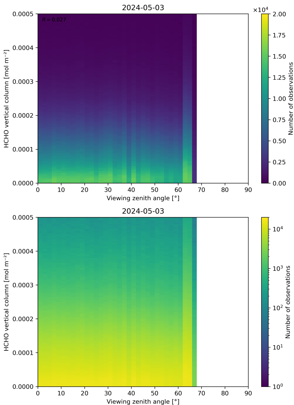
Figure 192: Scatter density plot of “Viewing zenith angle” against “HCHO vertical column” for 2024-05-02 to 2024-05-04.
