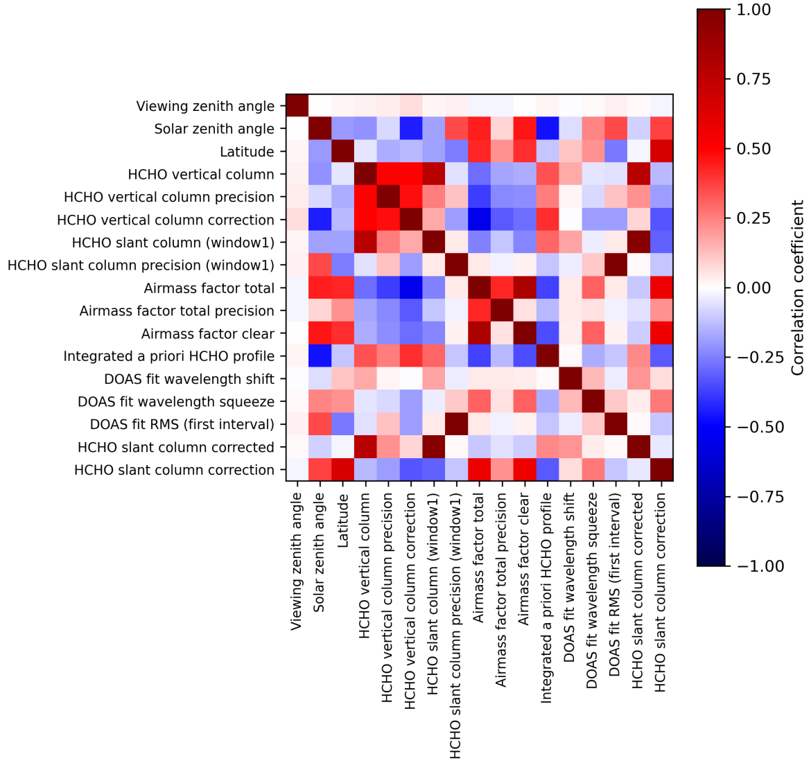
Figure 2: Map of correlation matrix for 2024-05-02 to 2024-05-04.
