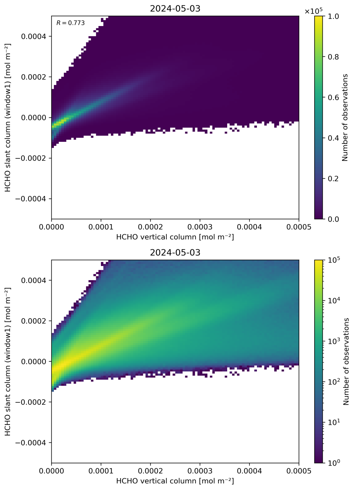
Figure 129: Scatter density plot of “HCHO vertical column” against “HCHO slant column (window1)” for 2024-05-02 to 2024-05-04.
