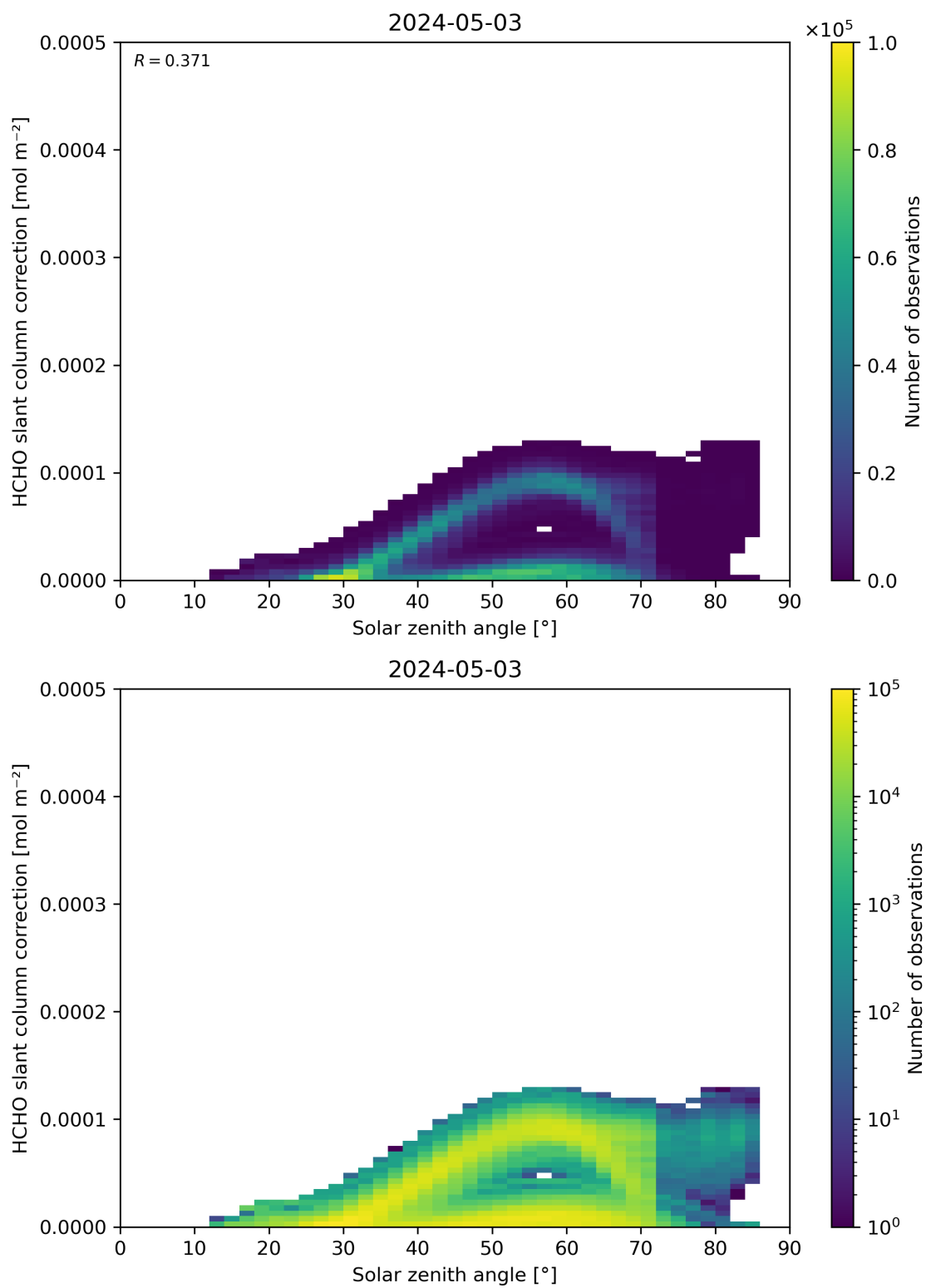
Figure 172: Scatter density plot of “Solar zenith angle” against “HCHO slant column correction” for 2024-05-02 to 2024-05-04.
