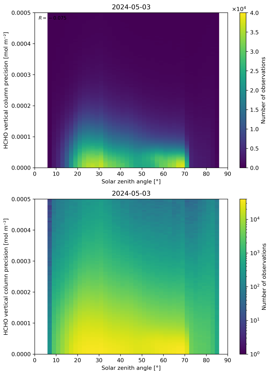
Figure 179: Scatter density plot of “Solar zenith angle” against “HCHO vertical column precision” for 2024-05-02 to 2024-05-04.
