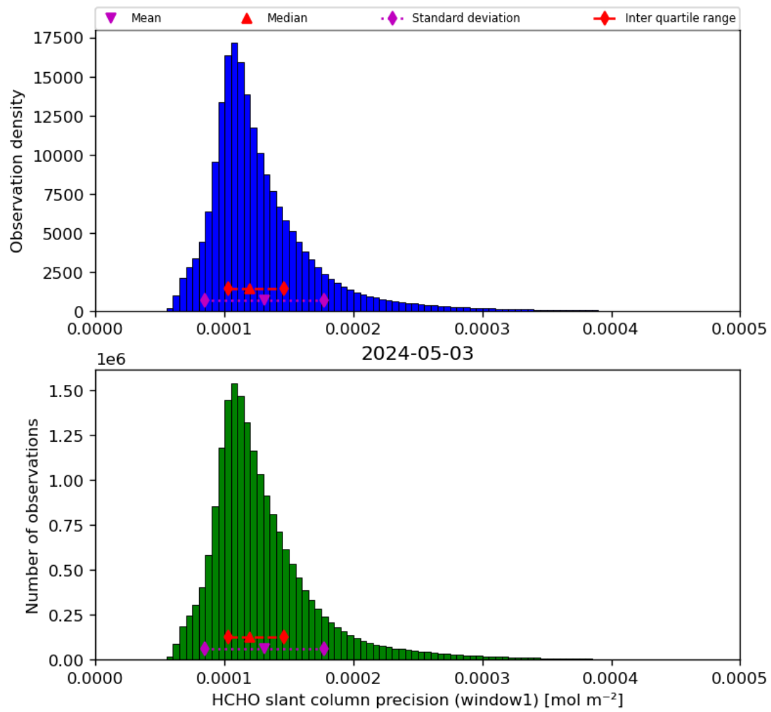
Figure 39: Histogram of “HCHO slant column precision (window1)” for 2024-05-02 to 2024-05-04
