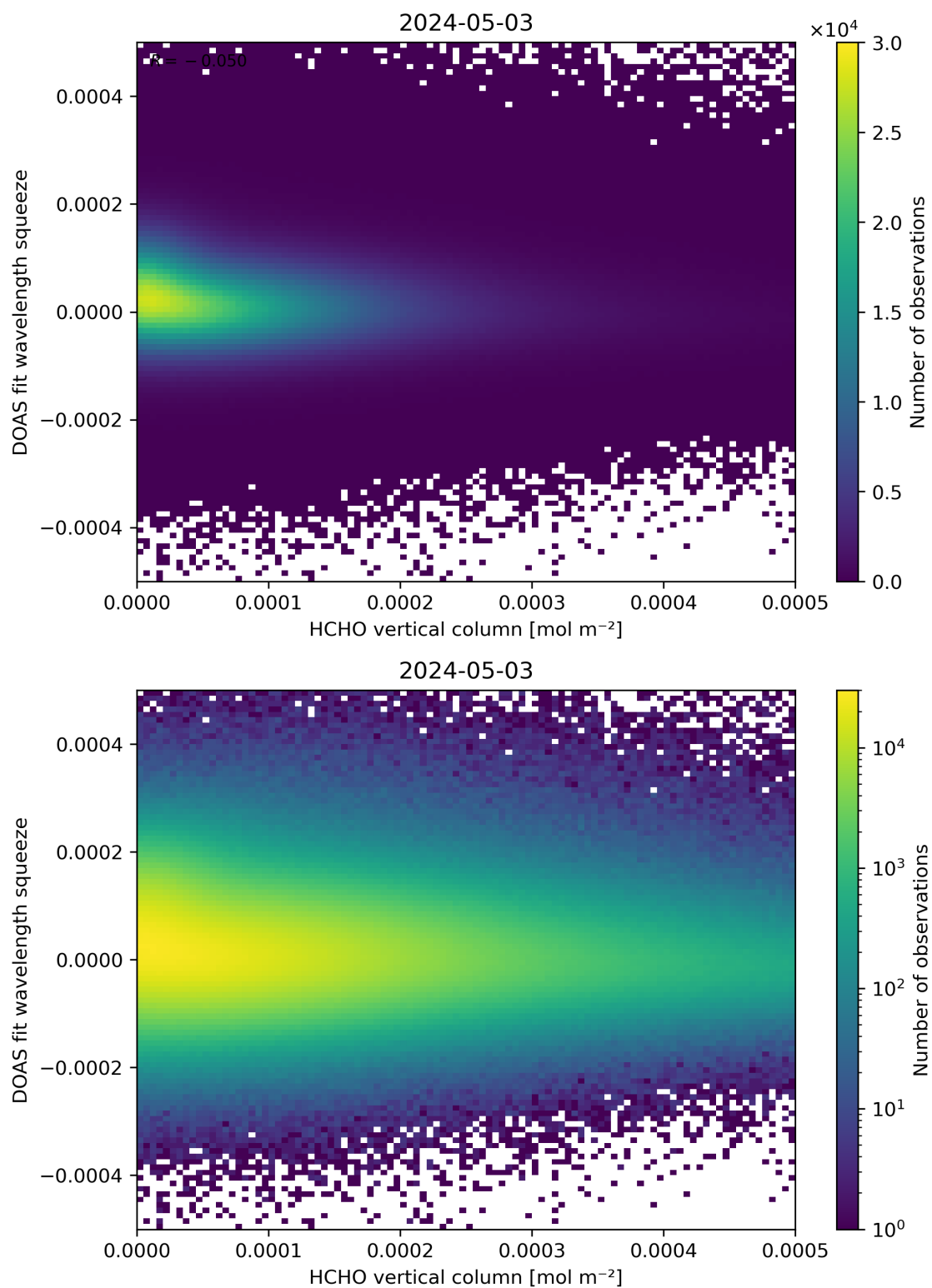
Figure 125: Scatter density plot of “HCHO vertical column” against “DOAS fit wavelength squeeze” for 2024-05-02 to 2024-05-04.
