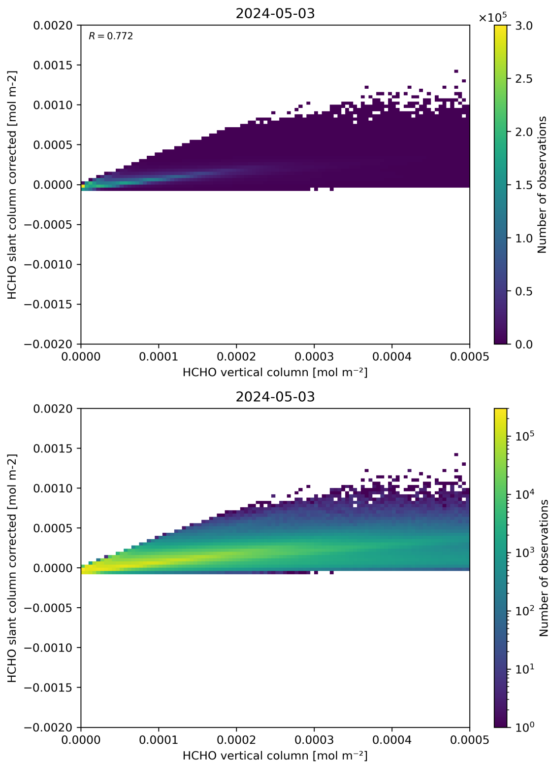
Figure 127: Scatter density plot of “HCHO vertical column” against “HCHO slant column corrected” for 2024-05-02 to 2024-05-04.
