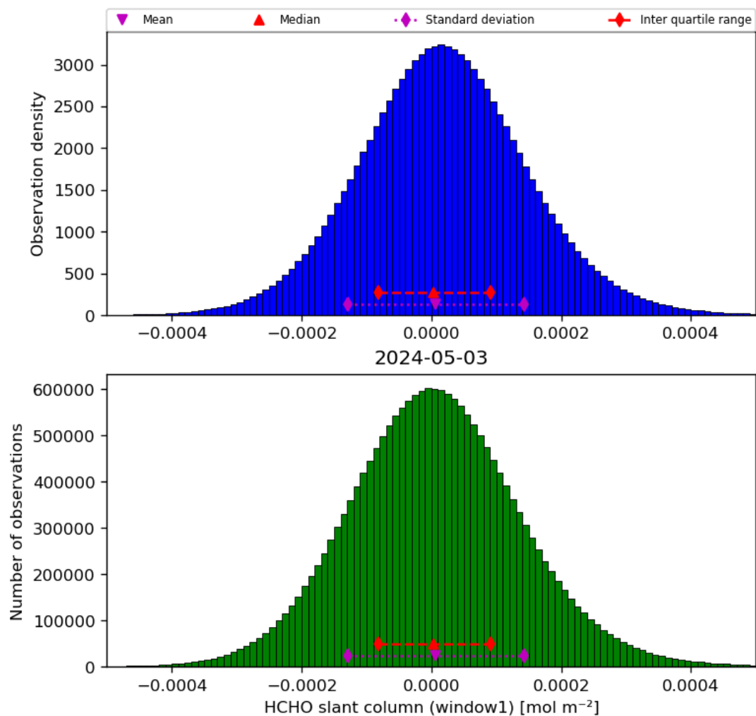
Figure 38: Histogram of “HCHO slant column (window1)” for 2024-05-02 to 2024-05-04
