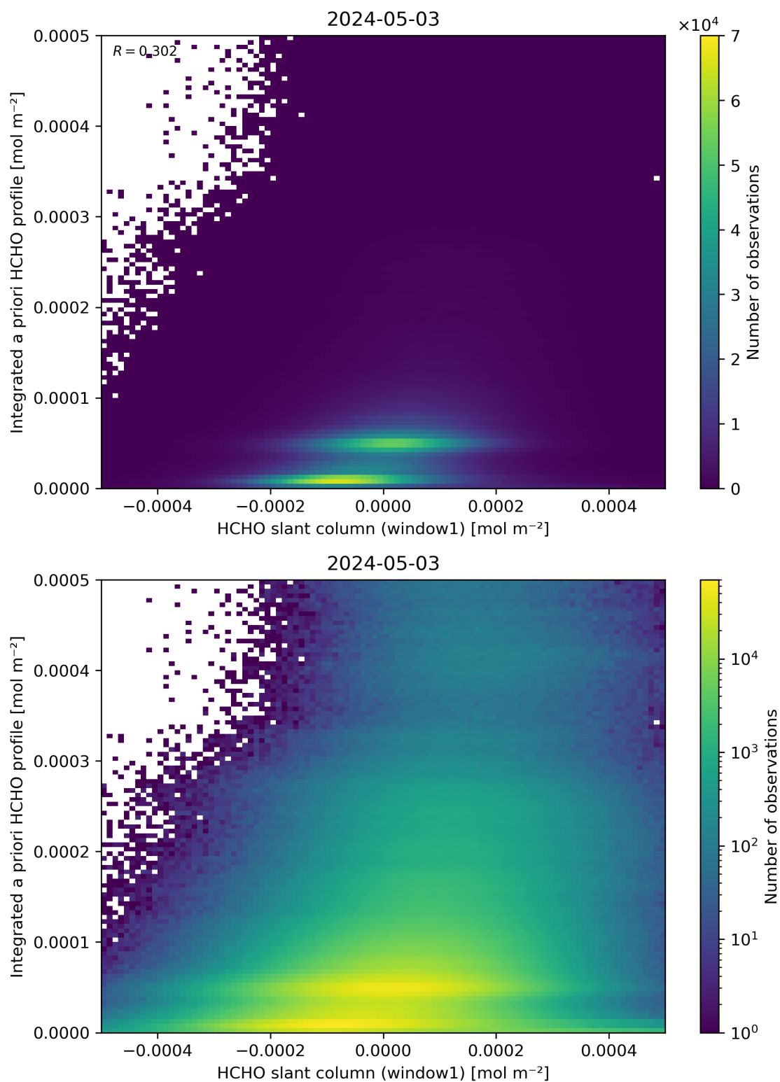
Figure 87: Scatter density plot of “HCHO slant column (window1)” against “Integrated a priori HCHO profile” for 2024-05-02 to 2024-05-04.
