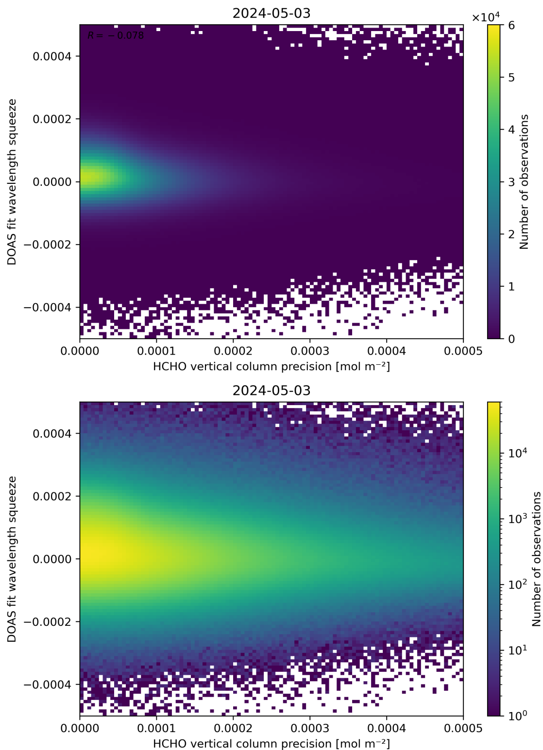
Figure 138: Scatter density plot of “HCHO vertical column precision” against “DOAS fit wavelength squeeze” for 2024-05-02 to 2024-05-04.
