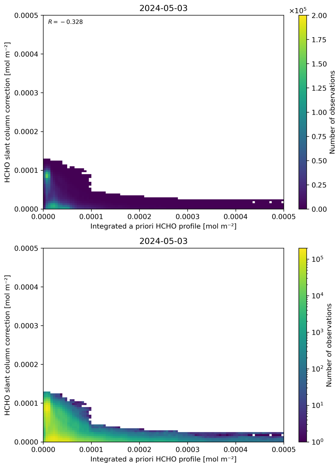
Figure 152: Scatter density plot of “Integrated a priori HCHO profile” against “HCHO slant column correction” for 2024-05-02 to 2024-05-04.
