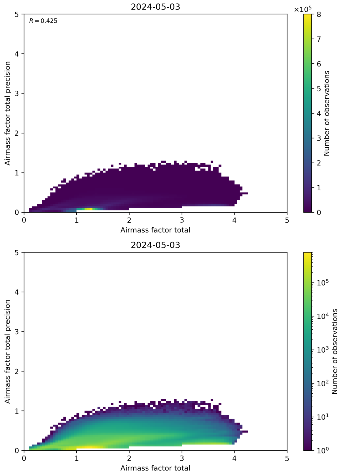
Figure 103: Scatter density plot of “Airmass factor total” against “Airmass factor total precision” for 2024-05-02 to 2024-05-04.
