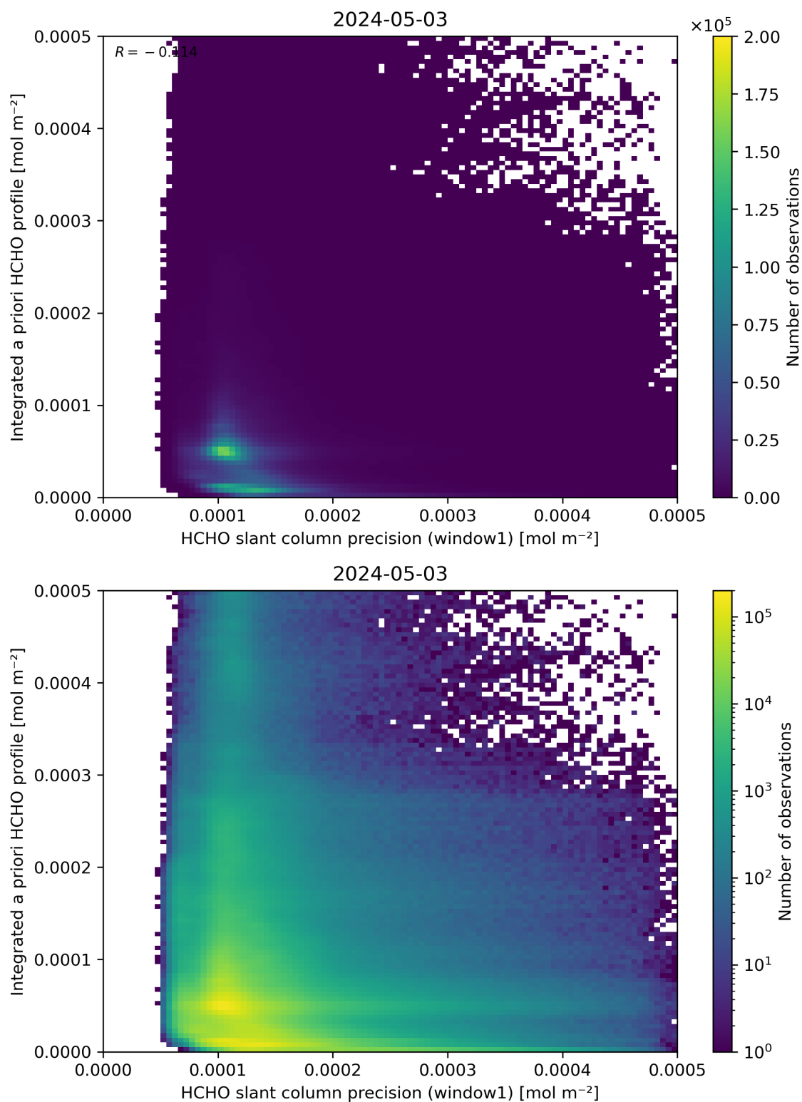
Figure 96: Scatter density plot of “HCHO slant column precision (window1)” against “Integrated a priori HCHO profile” for 2024-05-02 to 2024-05-04.
