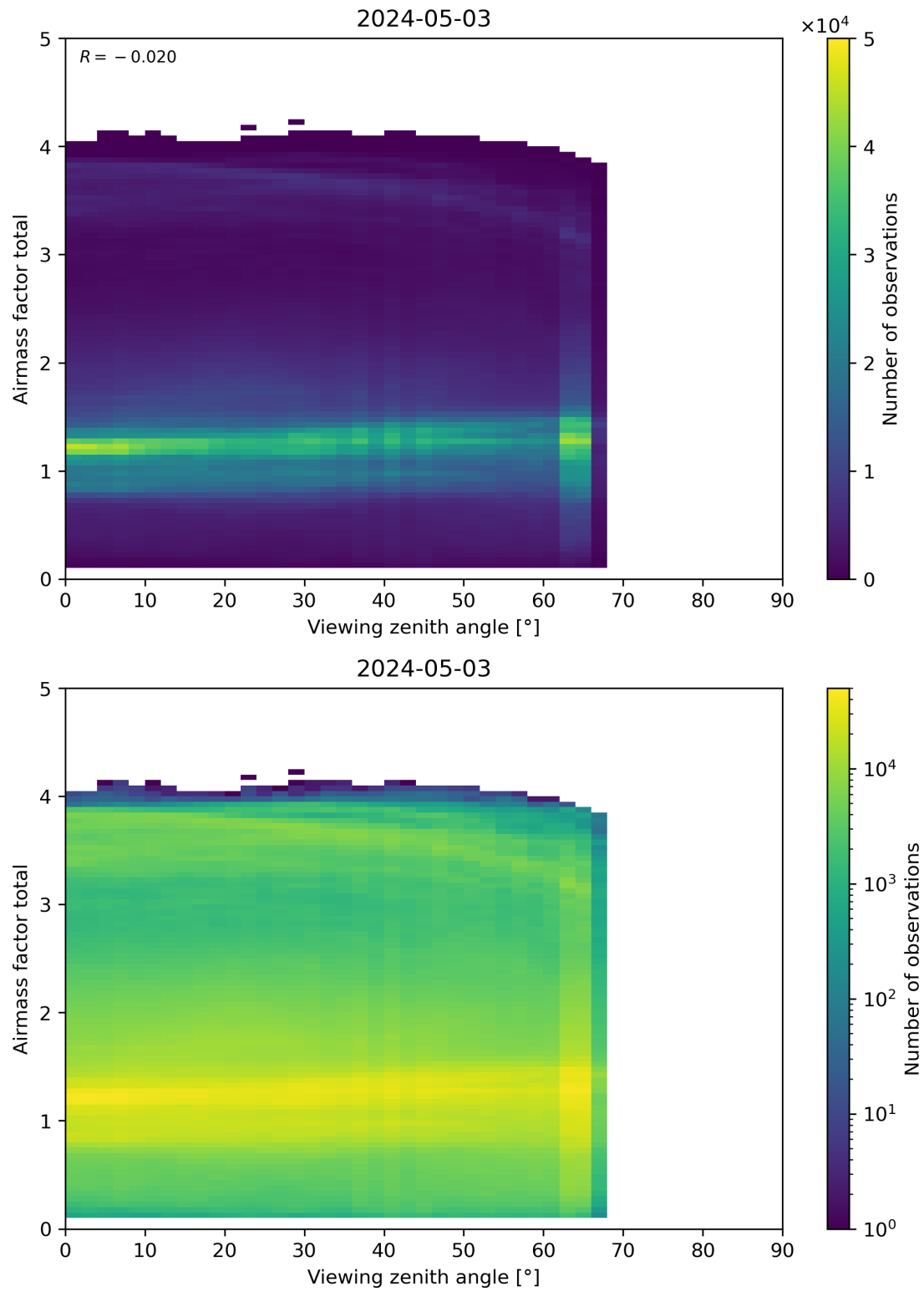
Figure 190: Scatter density plot of “Viewing zenith angle” against “Airmass factor total” for 2024-05-02 to 2024-05-04.
