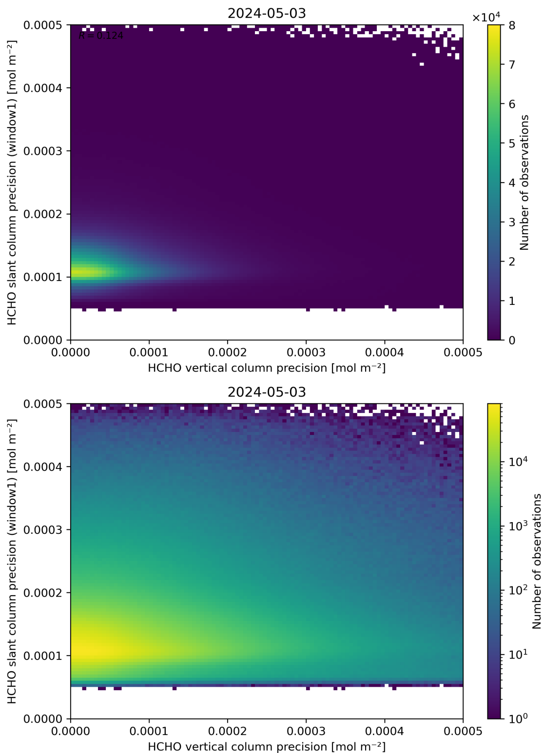
Figure 143: Scatter density plot of “HCHO vertical column precision” against “HCHO slant column precision (window1)” for 2024-05-02 to 2024-05-04.
