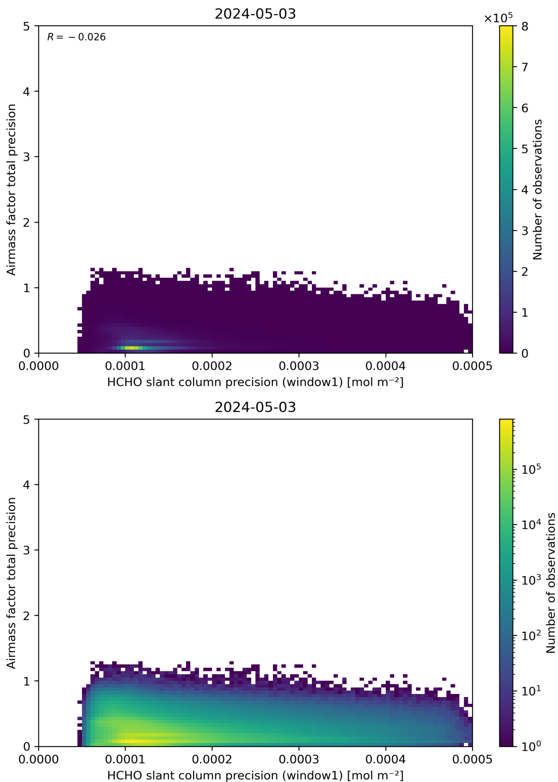
Figure 95: Scatter density plot of “HCHO slant column precision (window1)” against “Airmass factor total precision” for 2024-05-02 to 2024-05-04.
