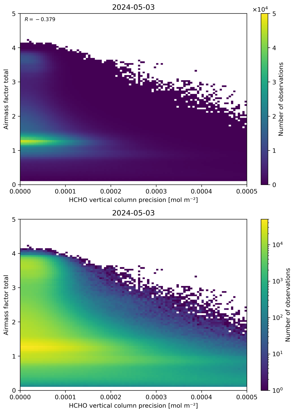
Figure 144: Scatter density plot of “HCHO vertical column precision” against “Airmass factor total” for 2024-05-02 to 2024-05-04.
