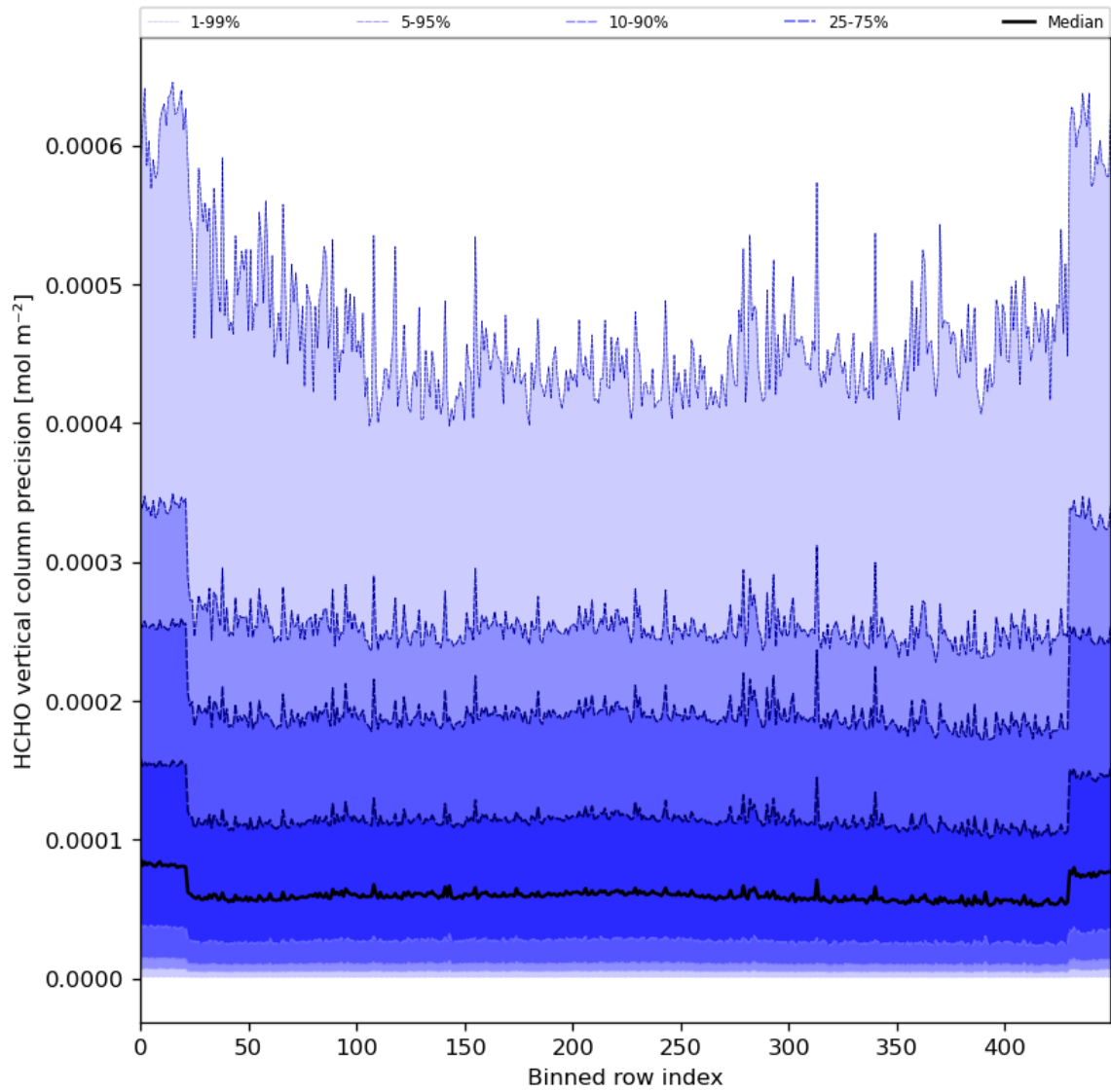
Figure 50: Along track statistics of “HCHO vertical column precision” for 2024-05-02 to 2024-05-04
