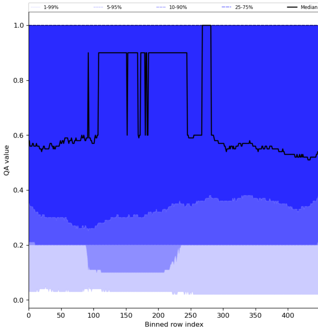
Figure 48: Along track statistics of “QA value” for 2024-05-02 to 2024-05-04
