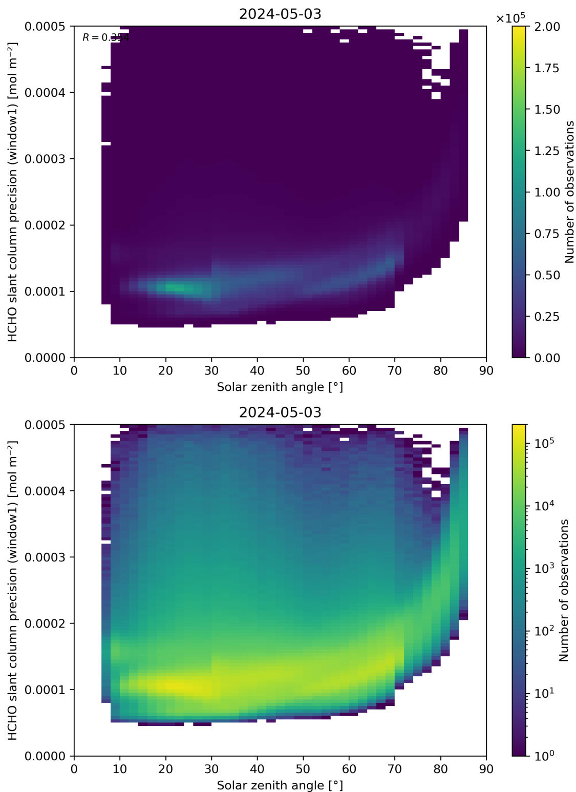
Figure 174: Scatter density plot of “Solar zenith angle” against “HCHO slant column precision (window1)” for 2024-05-02 to 2024-05-04.
