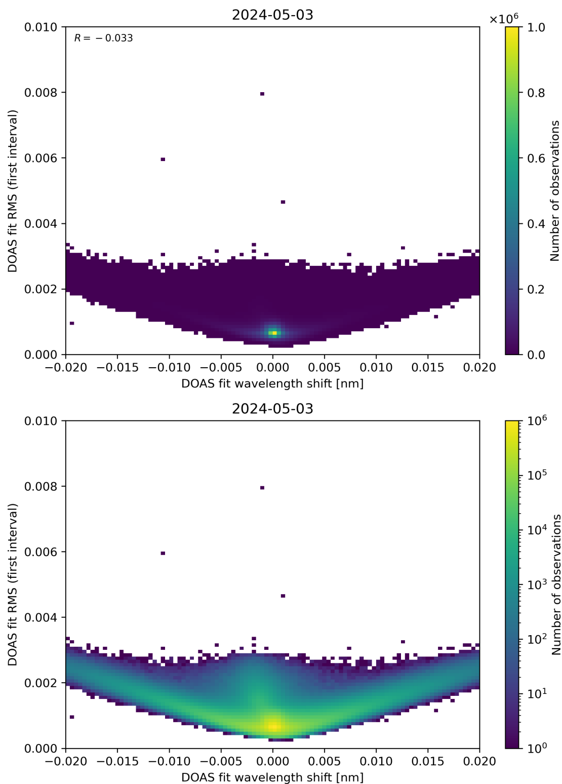
Figure 64: Scatter density plot of “DOAS fit wavelength shift” against “DOAS fit RMS (first interval)” for 2024-05-02 to 2024-05-04.
