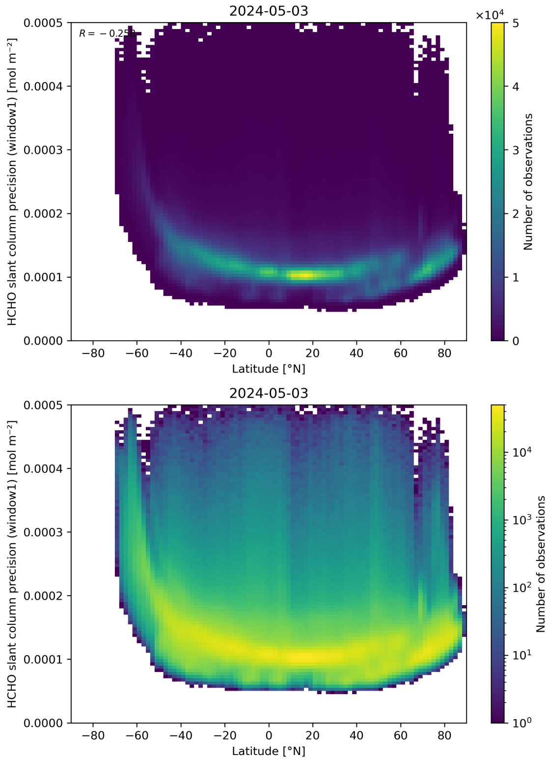
Figure 160: Scatter density plot of “Latitude” against “HCHO slant column precision (window1)” for 2024-05-02 to 2024-05-04.
