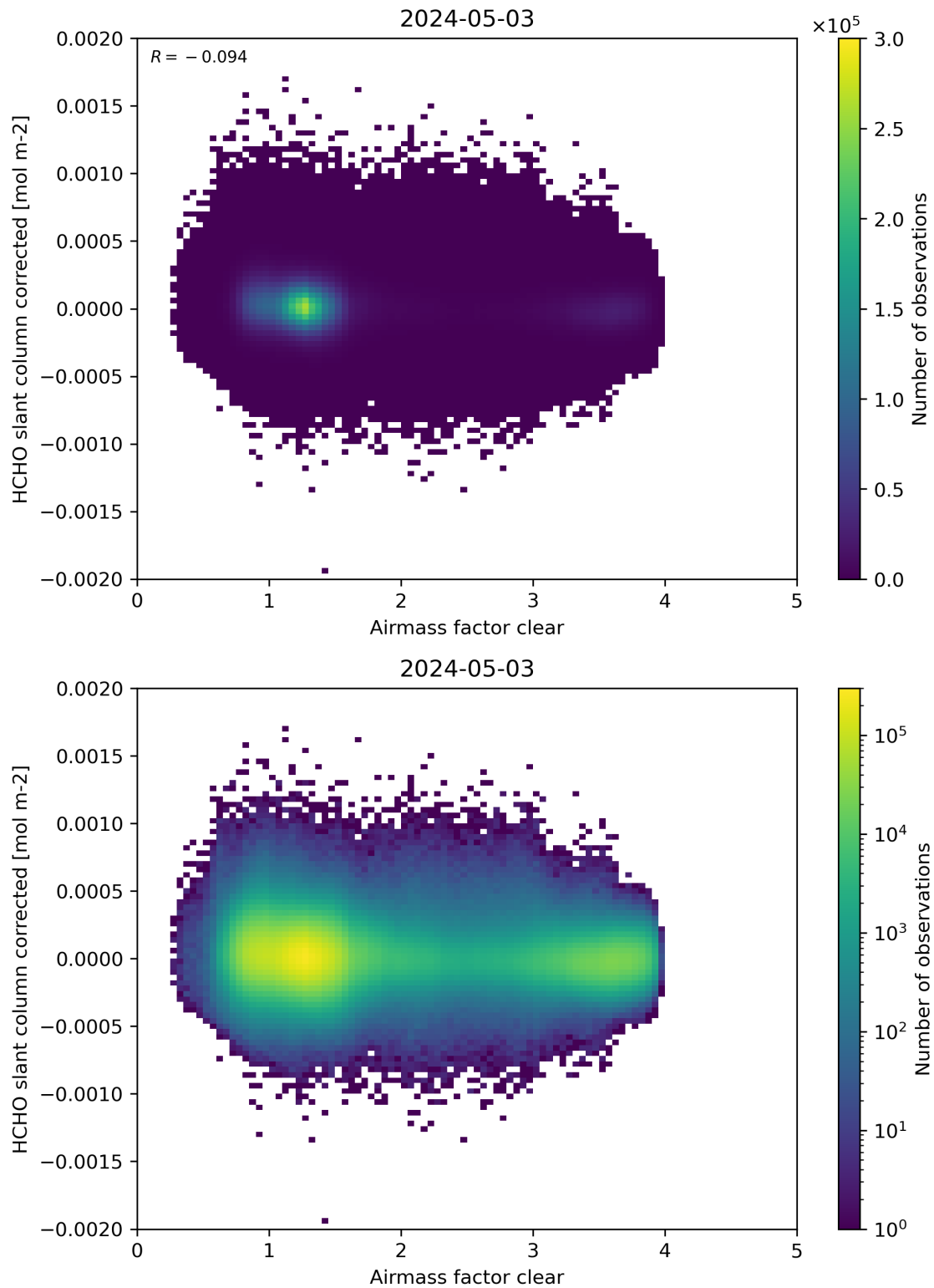
Figure 74: Scatter density plot of “Airmass factor clear” against “HCHO slant column corrected” for 2024-05-02 to 2024-05-04.
