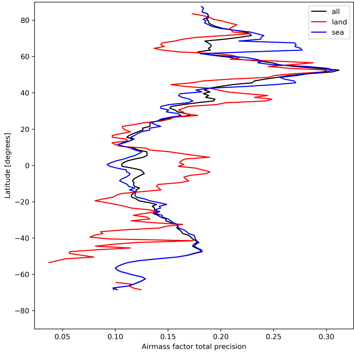
Figure 27: Zonal average of “Airmass factor total precision” for 2024-05-02 to 2024-05-04.
