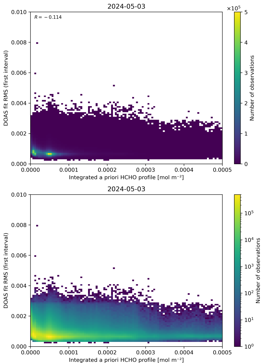
Figure 148: Scatter density plot of “Integrated a priori HCHO profile” against “DOAS fit RMS (first interval)” for 2024-05-02 to 2024-05-04.
