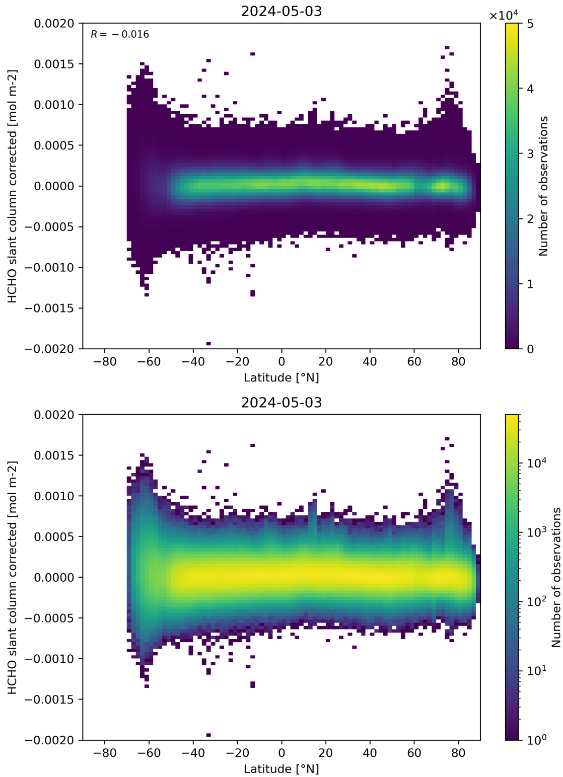
Figure 157: Scatter density plot of “Latitude” against “HCHO slant column corrected” for 2024-05-02 to 2024-05-04.
