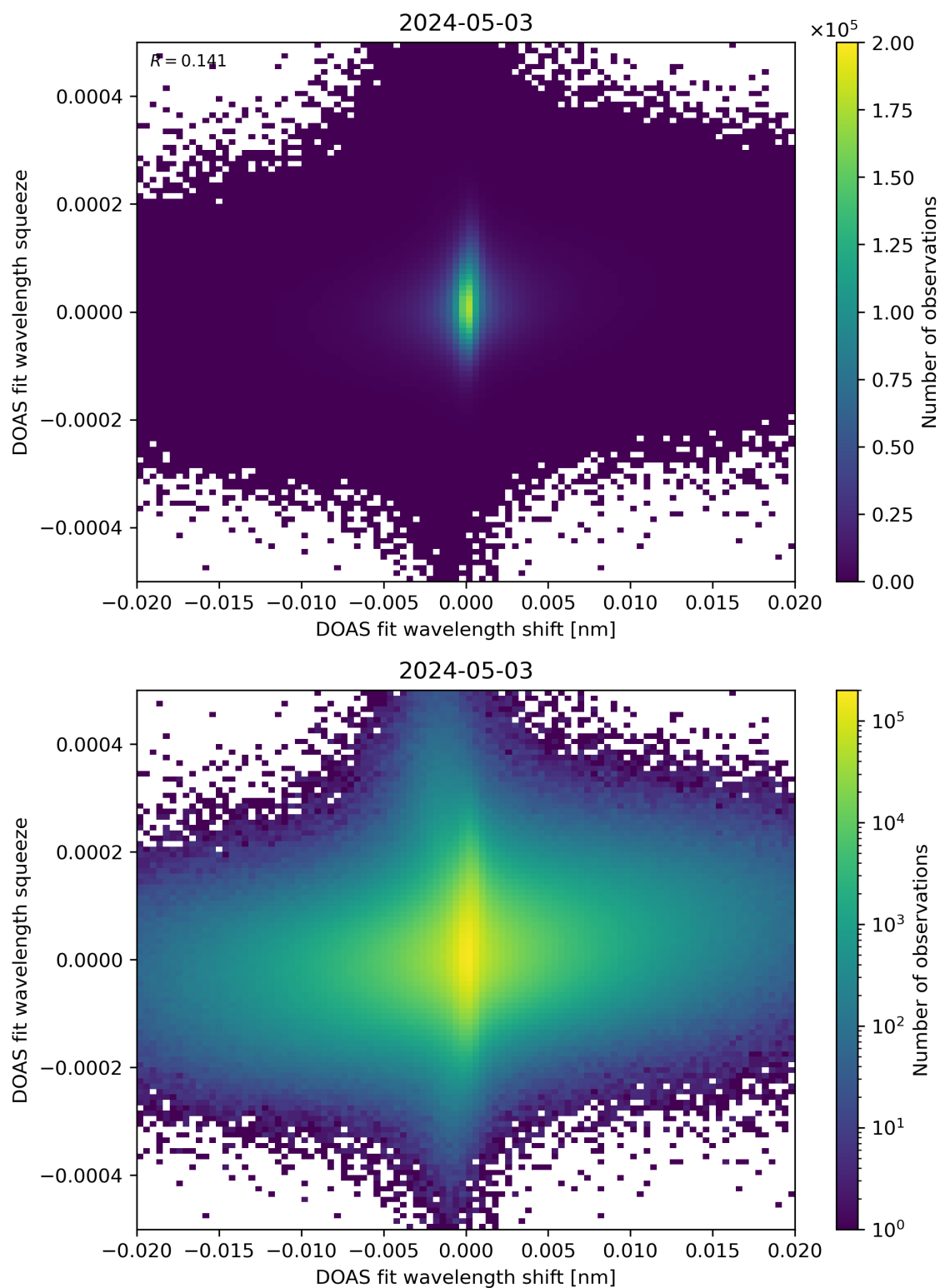
Figure 65: Scatter density plot of “DOAS fit wavelength shift” against “DOAS fit wavelength squeeze” for 2024-05-02 to 2024-05-04.
