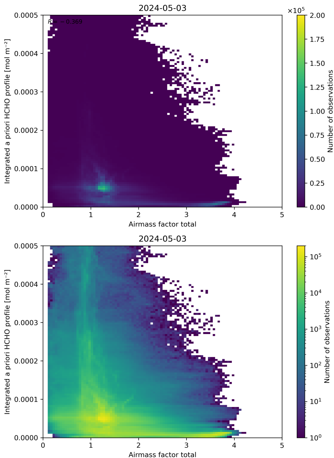
Figure 104: Scatter density plot of “Air mass factor total” against “Integrated a priori HCHO profile” for 2024-05-02 to 2024-05-04.
