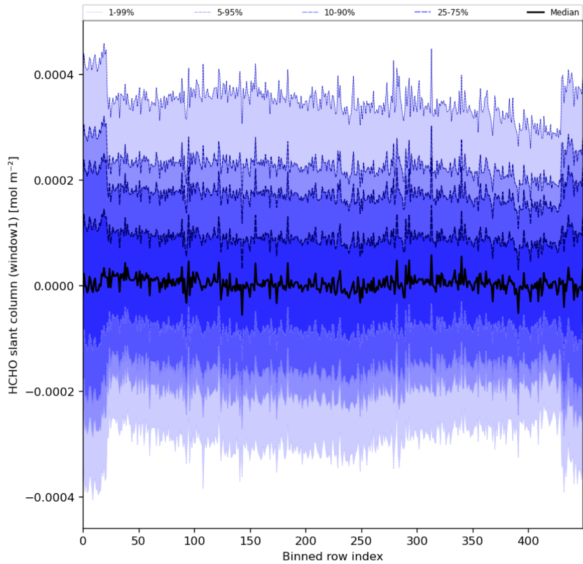
Figure 52: Along track statistics of “HCHO slant column (window1)” for 2024-05-02 to 2024-05-04
