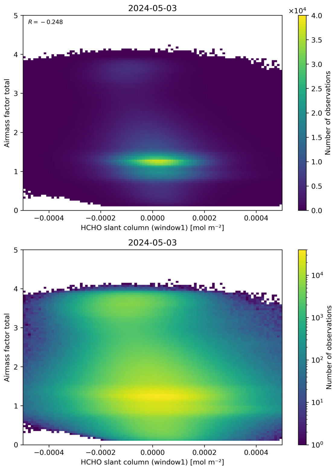
Figure 85: Scatter density plot of “HCHO slant column (window1)” against “Airmass factor total” for 2024-05-02 to 2024-05-04.
