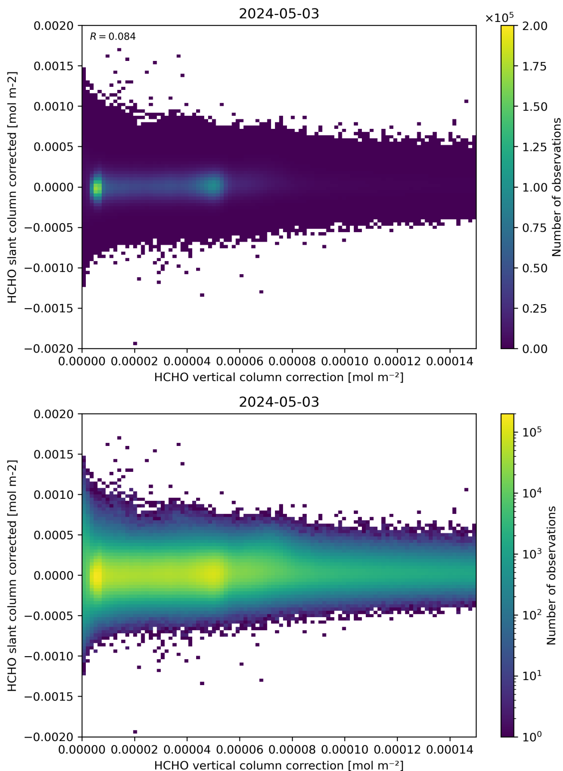
Figure 116: Scatter density plot of “HCHO vertical column correction” against “HCHO slant column corrected” for 2024-05-02 to 2024-05-04.
