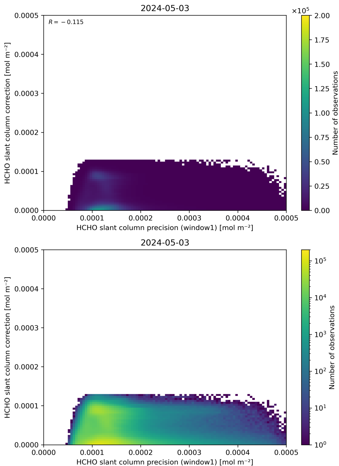
Figure 93: Scatter density plot of “HCHO slant column precision (window1)” against “HCHO slant column correction” for 2024-05-02 to 2024-05-04.
