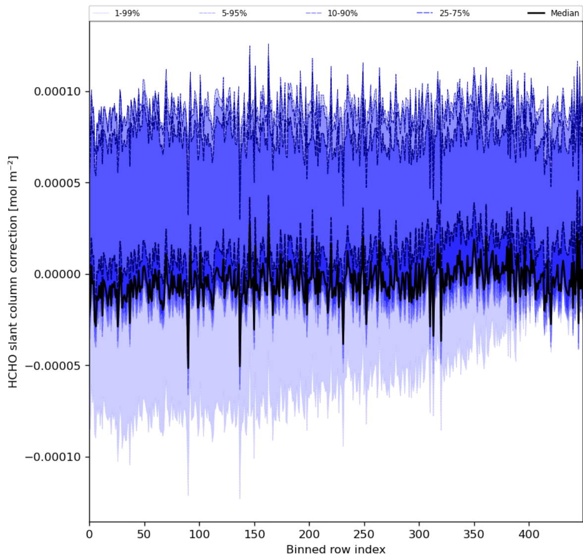
Figure 61: Along track statistics of “HCHO slant column correction” for 2024-05-02 to 2024-05-04
