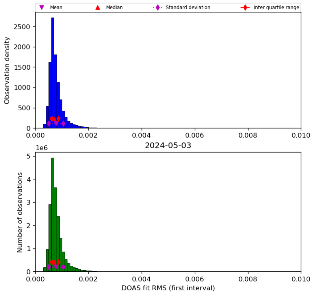
Figure 46: Histogram of “DOAS fit RMS (first interval)” for 2024-05-02 to 2024-05-04
