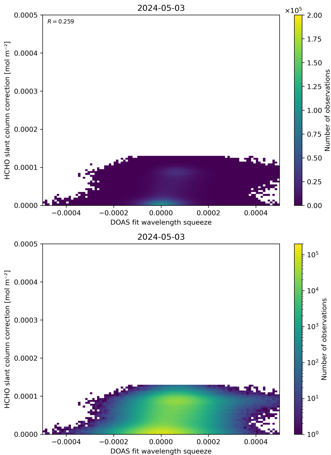
Figure 70: Scatter density plot of “DOAS fit wavelength squeeze” against “HCHO slant column correction” for 2024-05-02 to 2024-05-04.
