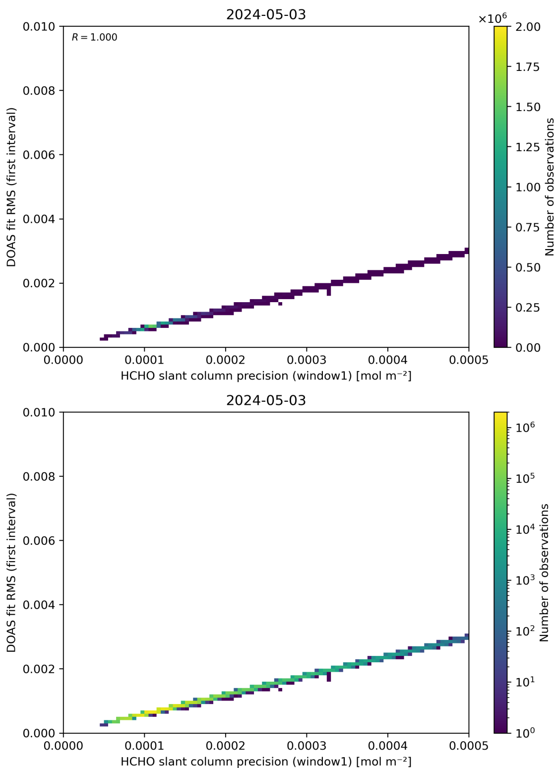
Figure 88: Scatter density plot of “HCHO slant column precision (window1)” against “DOAS fit RMS (first interval)” for 2024-05-02 to 2024-05-04.
