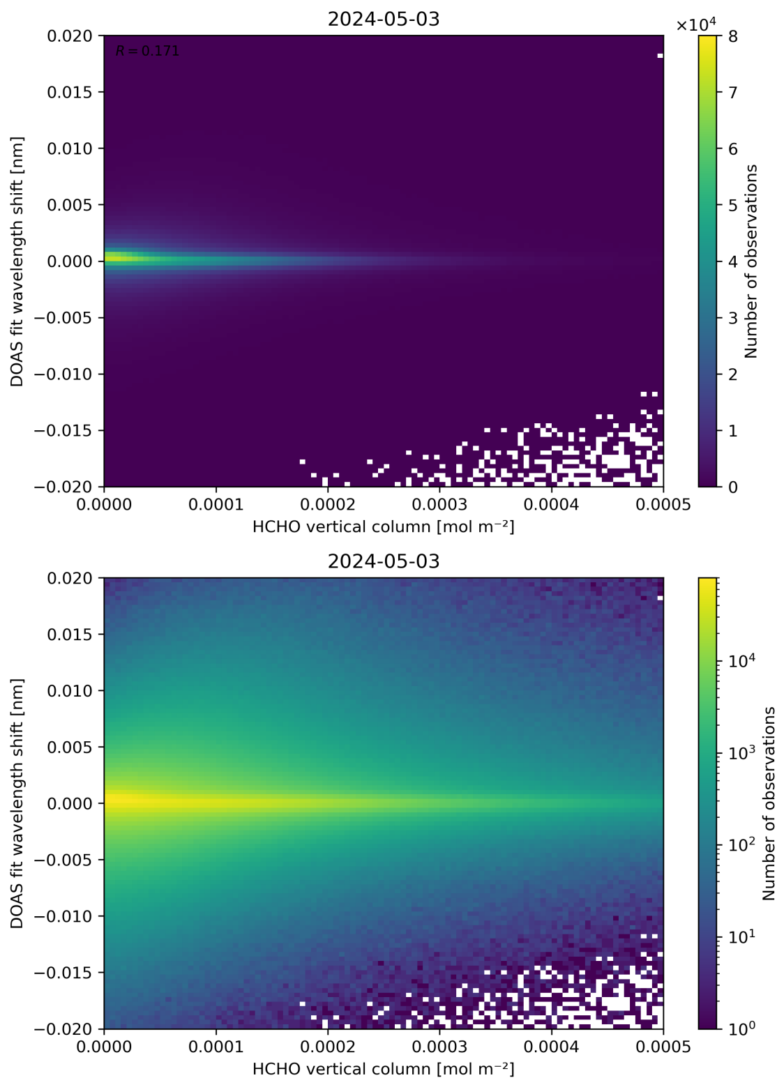
Figure 124: Scatter density plot of “HCHO vertical column” against “DOAS fit wavelength shift” for 2024-05-02 to 2024-05-04.
