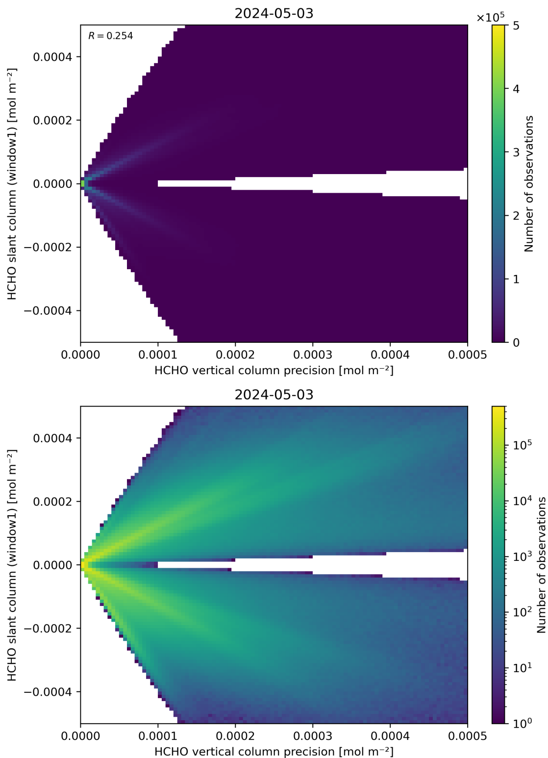
Figure 142: Scatter density plot of “HCHO vertical column precision” against “HCHO slant column (window1)” for 2024-05-02 to 2024-05-04.
