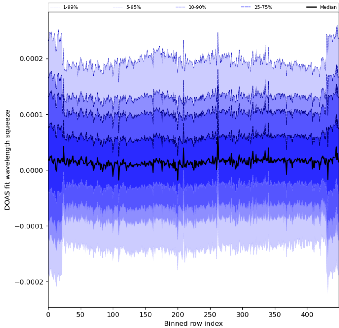
Figure 59: Along track statistics of “DOAS fit wavelength squeeze” for 2024-05-02 to 2024-05-04
