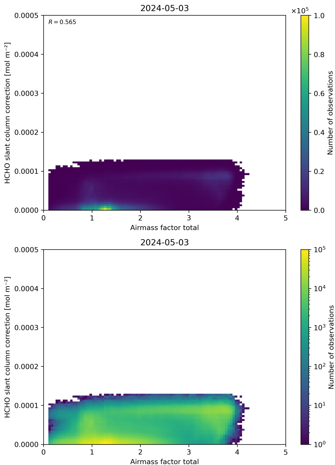
Figure 102: Scatter density plot of “Airmass factor total” against “HCHO slant column correction” for 2024-05-02 to 2024-05-04.
