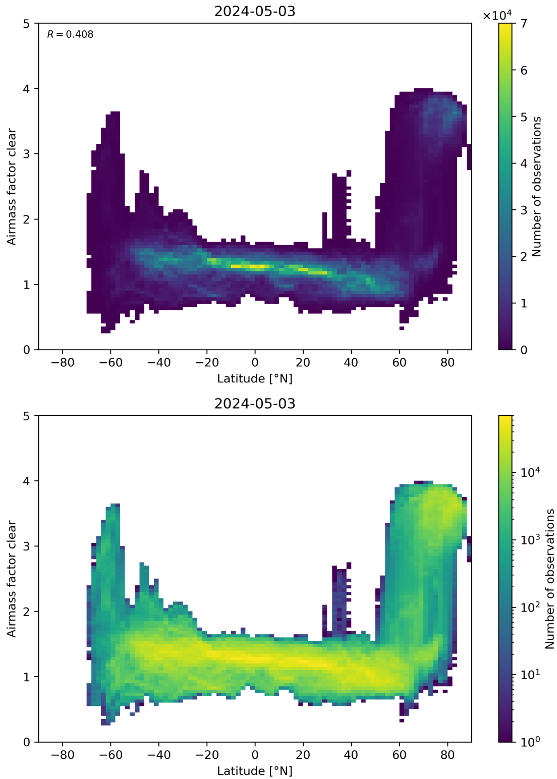
Figure 156: Scatter density plot of “Latitude” against “Airmass factor clear” for 2024-05-02 to 2024-05-04.
