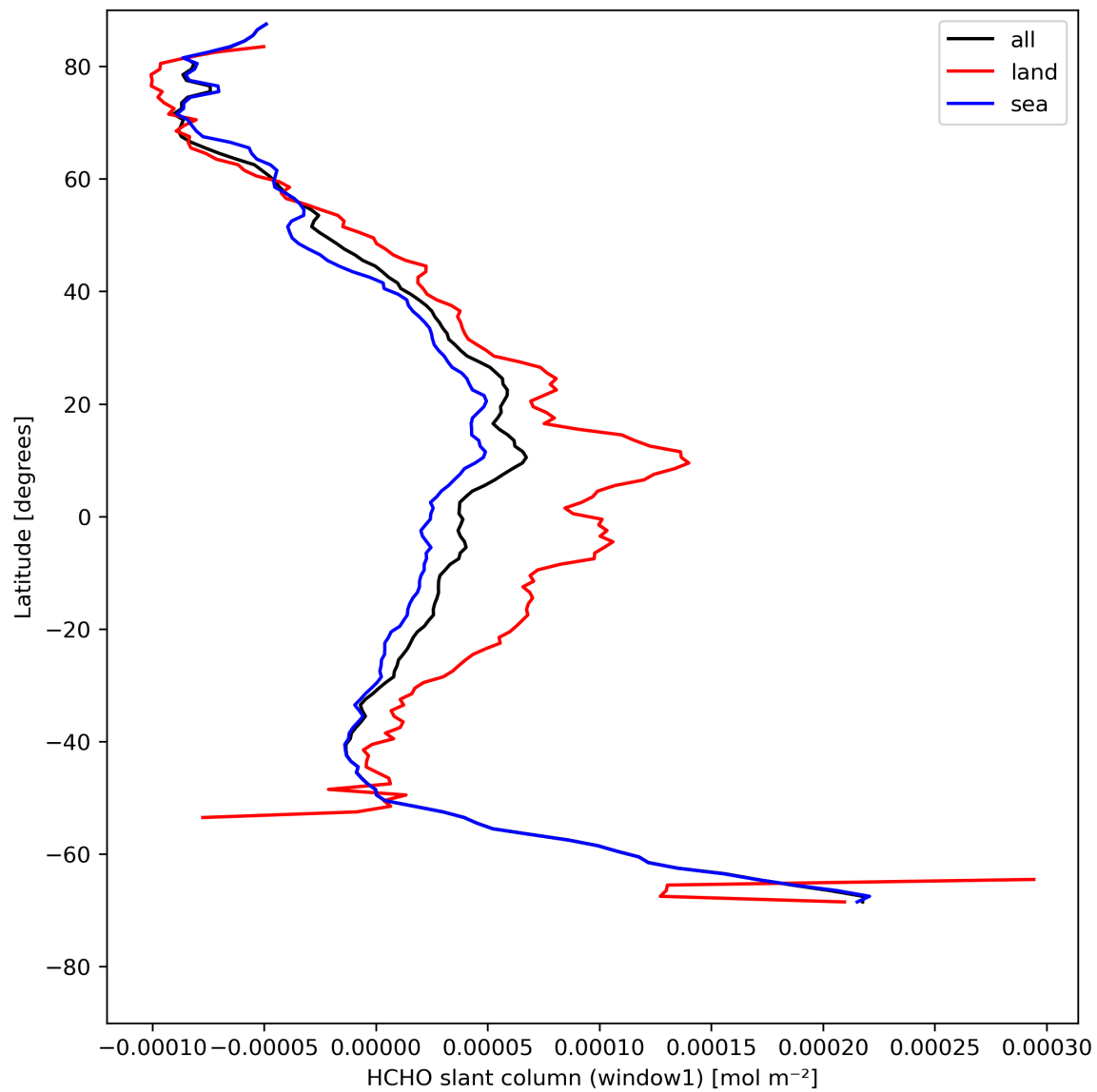
Figure 24: Zonal average of “HCHO slant column (window1)” for 2024-05-02 to 2024-05-04.
