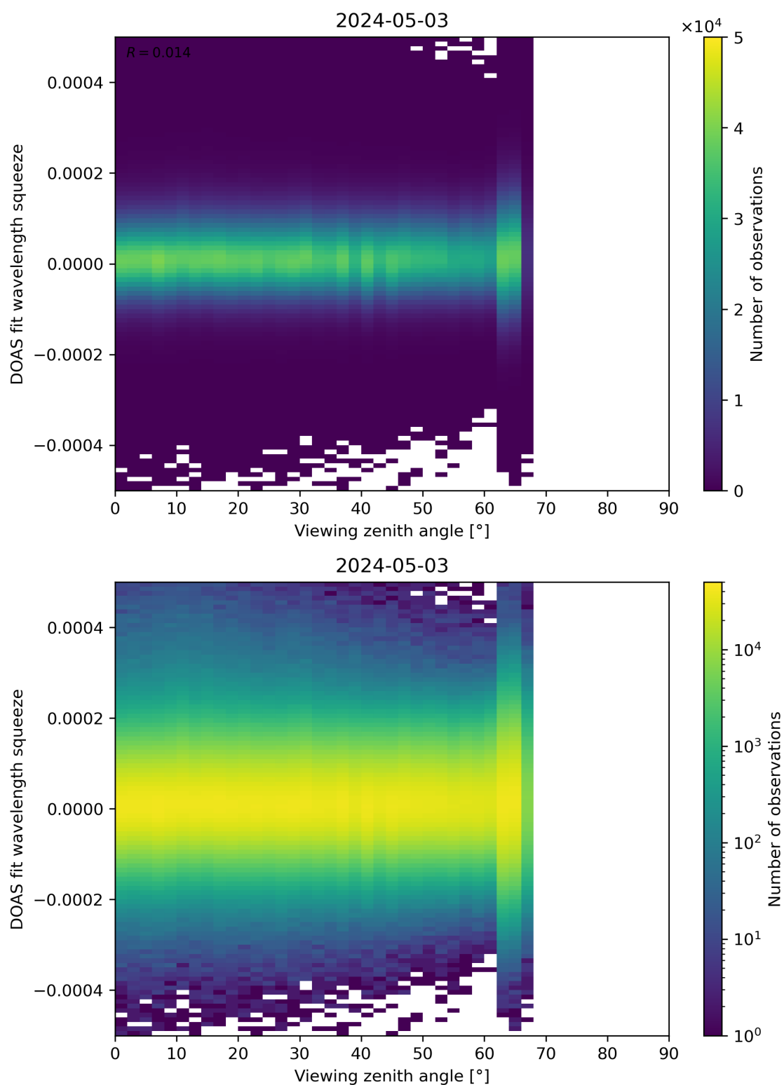
Figure 184: Scatter density plot of “Viewing zenith angle” against “DOAS fit wavelength squeeze” for 2024-05-02 to 2024-05-04.
