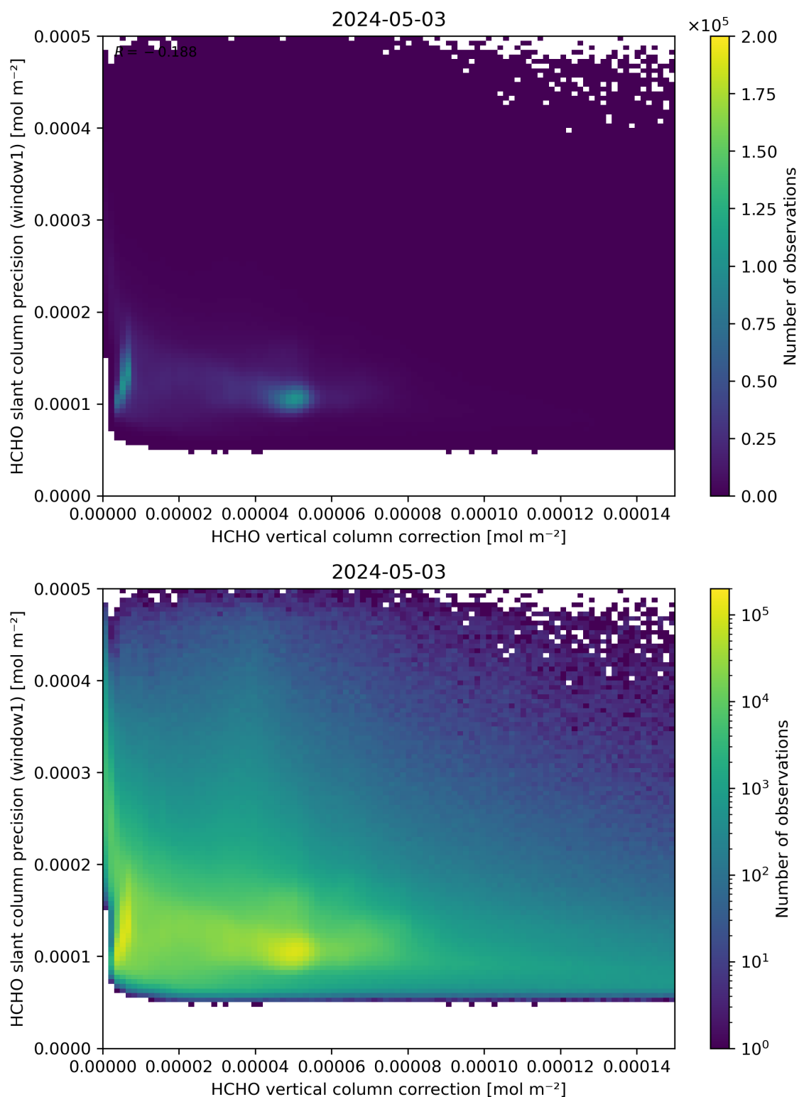
Figure 119: Scatter density plot of “HCHO vertical column correction” against “HCHO slant column precision (window1)” for 2024-05-02 to 2024-05-04.
