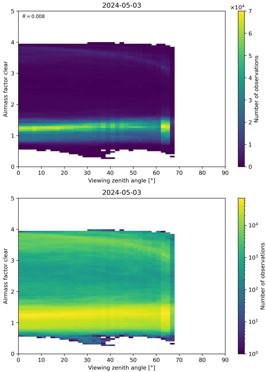
Figure 185: Scatter density plot of “Viewing zenith angle” against “Airmass factor clear” for 2024-05-02 to 2024-05-04.
