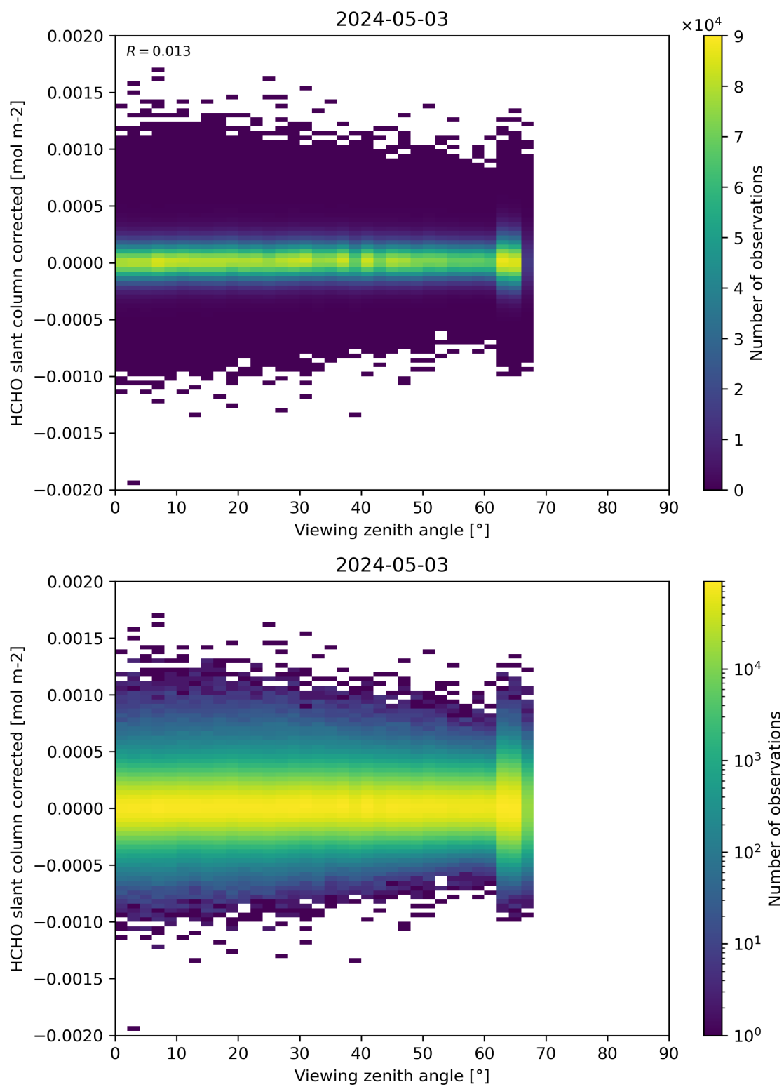
Figure 186: Scatter density plot of “Viewing zenith angle” against “HCHO slant column corrected” for 2024-05-02 to 2024-05-04.
