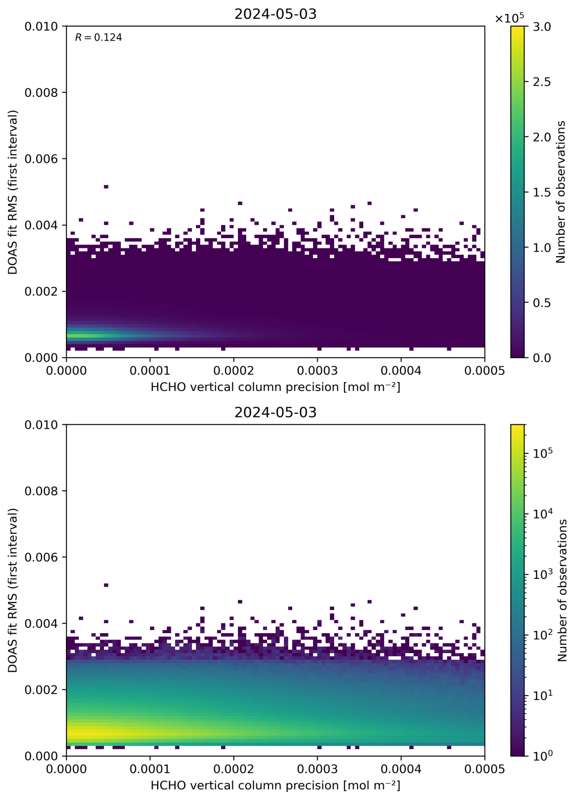
Figure 136: Scatter density plot of “HCHO vertical column precision” against “DOAS fit RMS (first interval)” for 2024-05-02 to 2024-05-04.
