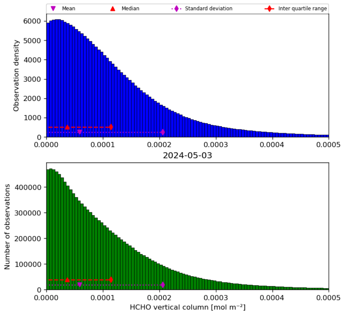
Figure 35: Histogram of “HCHO vertical column” for 2024-05-02 to 2024-05-04
