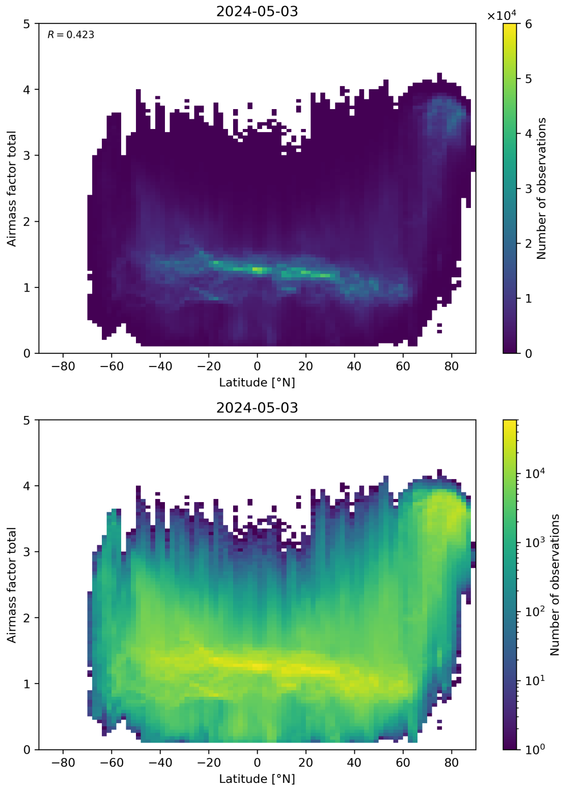
Figure 161: Scatter density plot of “Latitude” against “Airmass factor total” for 2024-05-02 to 2024-05-04.
