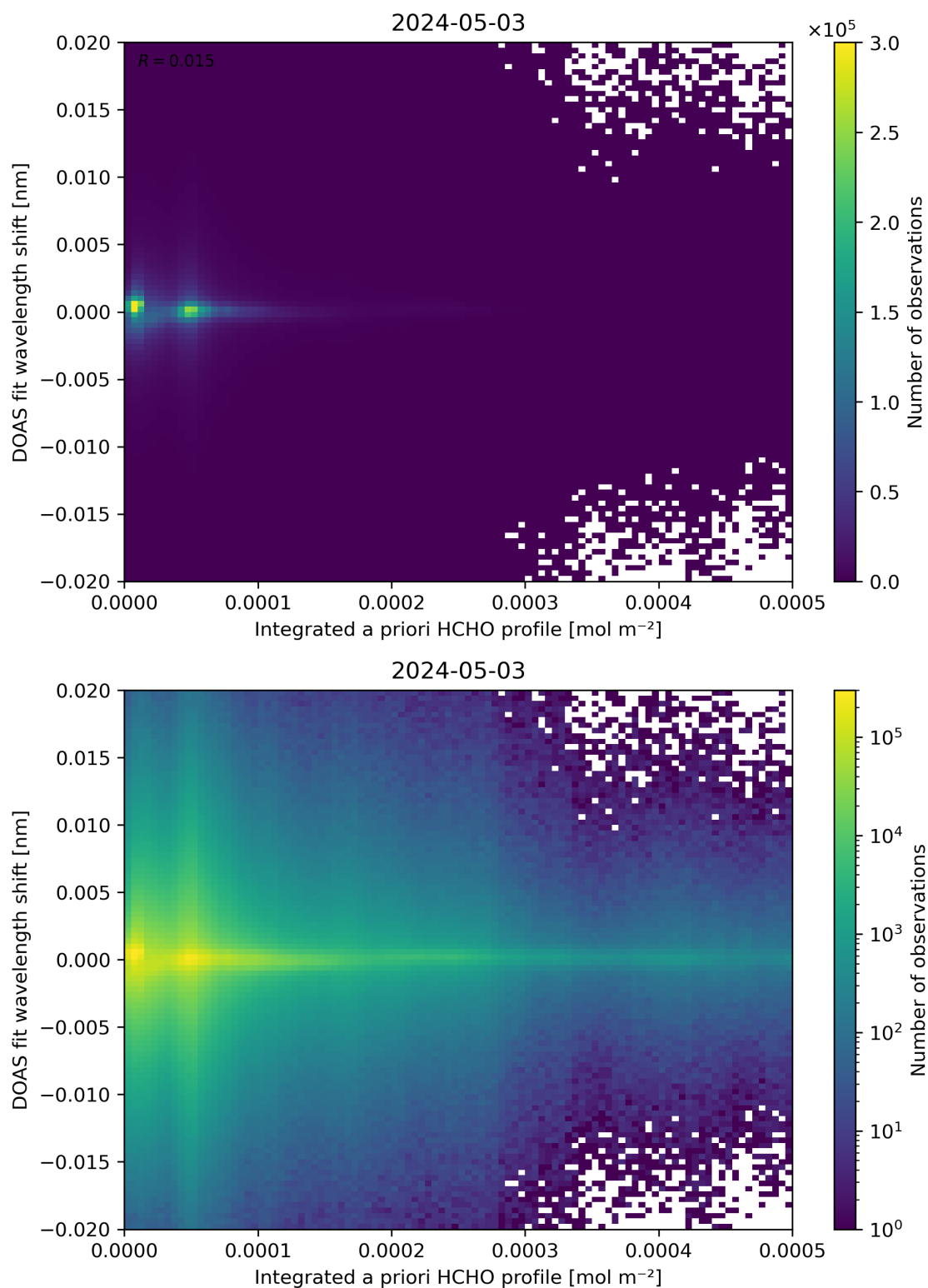
Figure 149: Scatter density plot of “Integrated a priori HCHO profile” against “DOAS fit wavelength shift” for 2024-05-02 to 2024-05-04.
