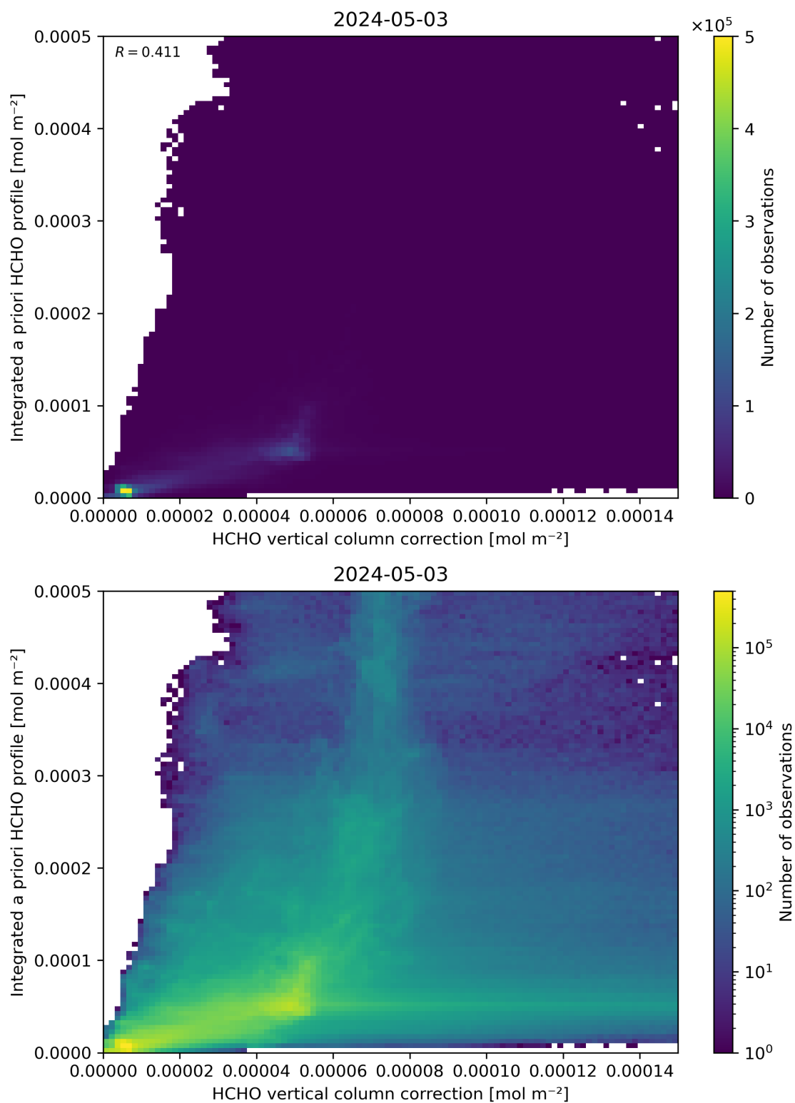
Figure 122: Scatter density plot of “HCHO vertical column correction” against “Integrated a priori HCHO profile” for 2024-05-02 to 2024-05-04.
