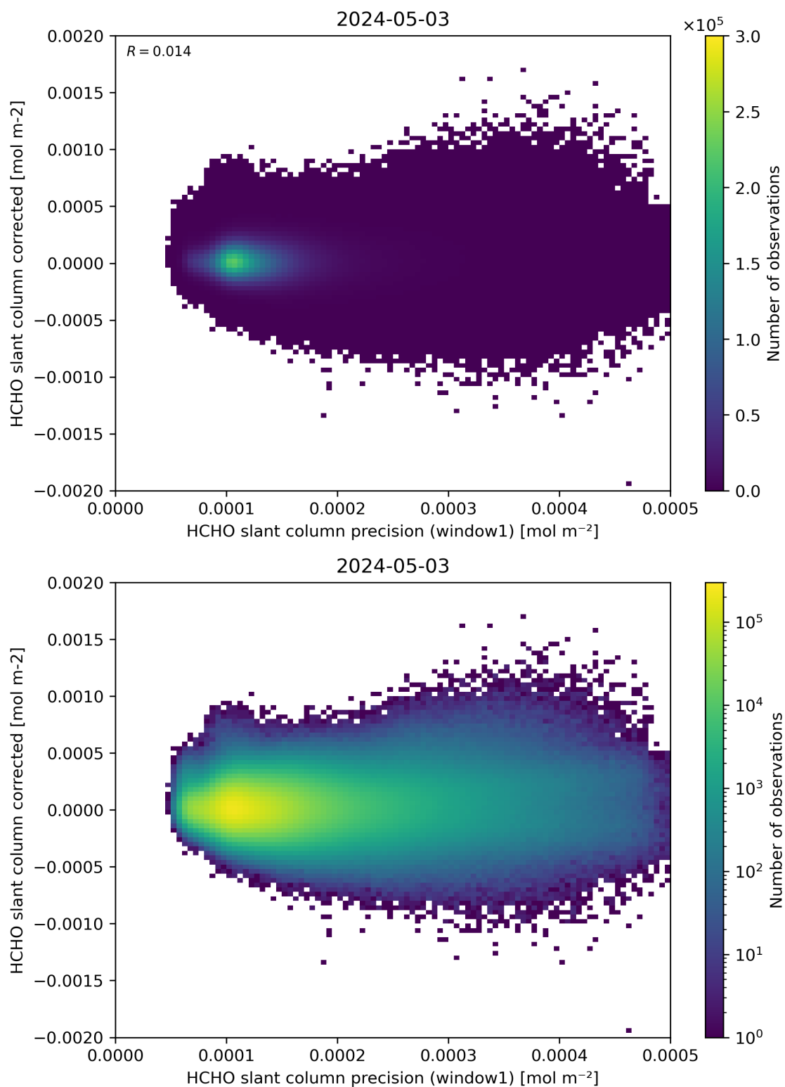
Figure 92: Scatter density plot of “HCHO slant column precision (window1)” against “HCHO slant column corrected” for 2024-05-02 to 2024-05-04.
