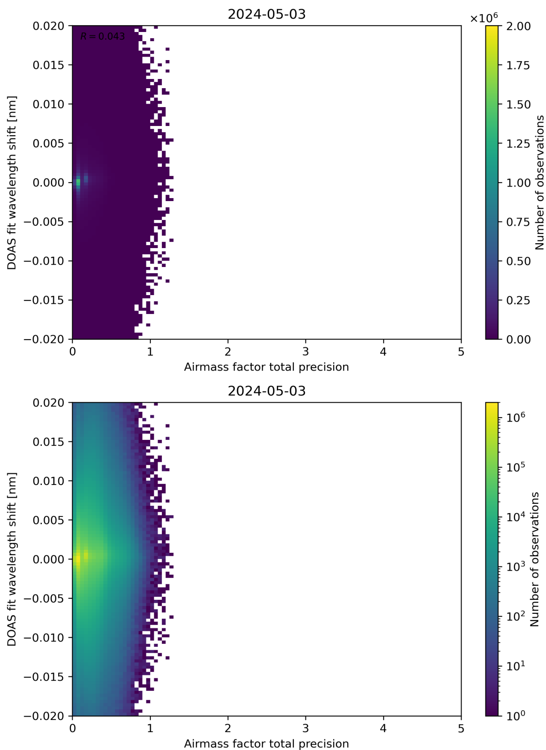
Figure 106: Scatter density plot of “Airmass factor total precision” against “DOAS fit wavelength shift” for 2024-05-02 to 2024-05-04.
