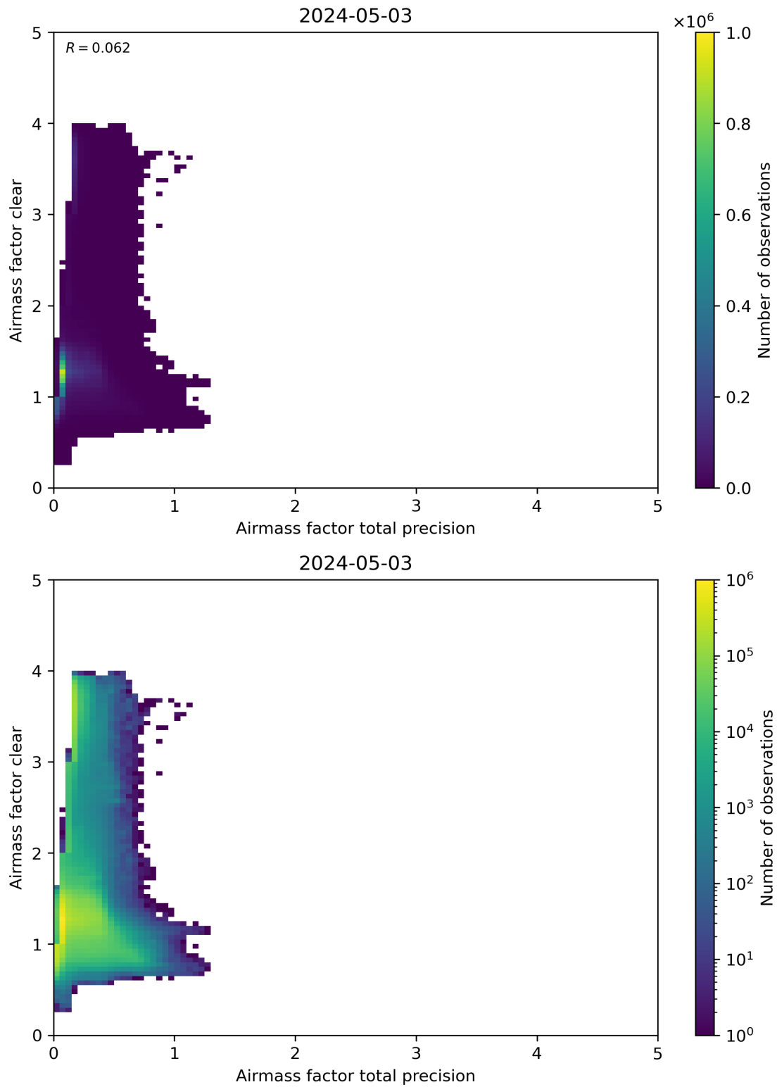
Figure 108: Scatter density plot of “Airmass factor total precision” against “Airmass factor clear” for 2024-05-02 to 2024-05-04.
