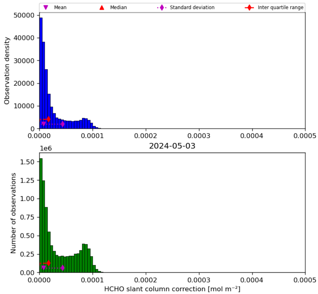
Figure 47: Histogram of “HCHO slant column correction” for 2024-05-02 to 2024-05-04
