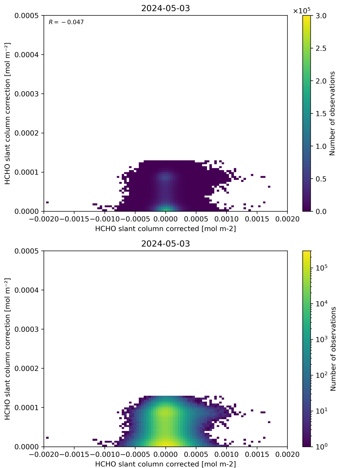
Figure 77: Scatter density plot of “HCHO slant column corrected” against “HCHO slant column correction” for 2024-05-02 to 2024-05-04.
