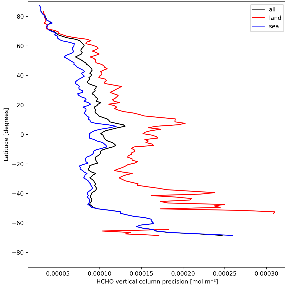
Figure 22: Zonal average of “HCHO vertical column precision” for 2024-05-02 to 2024-05-04.
