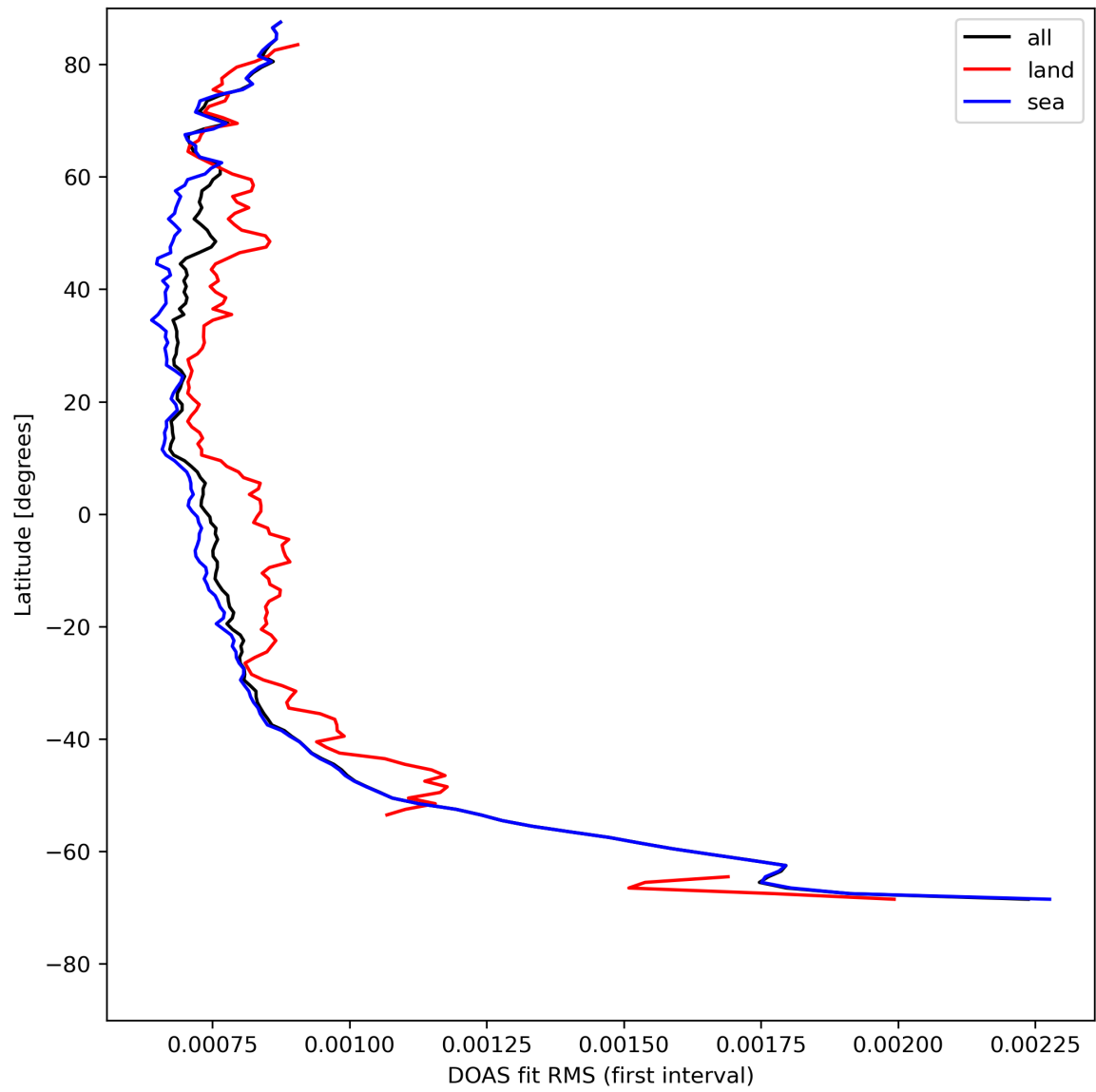
Figure 32: Zonal average of “DOAS fit RMS (first interval)” for 2024-05-02 to 2024-05-04.
