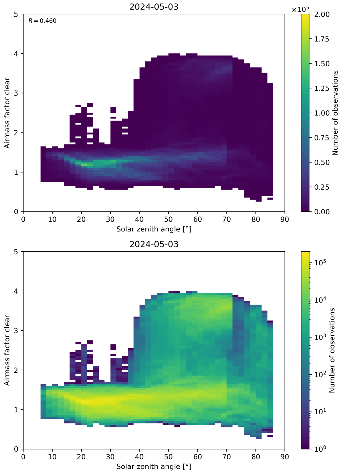
Figure 170: Scatter density plot of “Solar zenith angle” against “Airmass factor clear” for 2024-05-02 to 2024-05-04.
