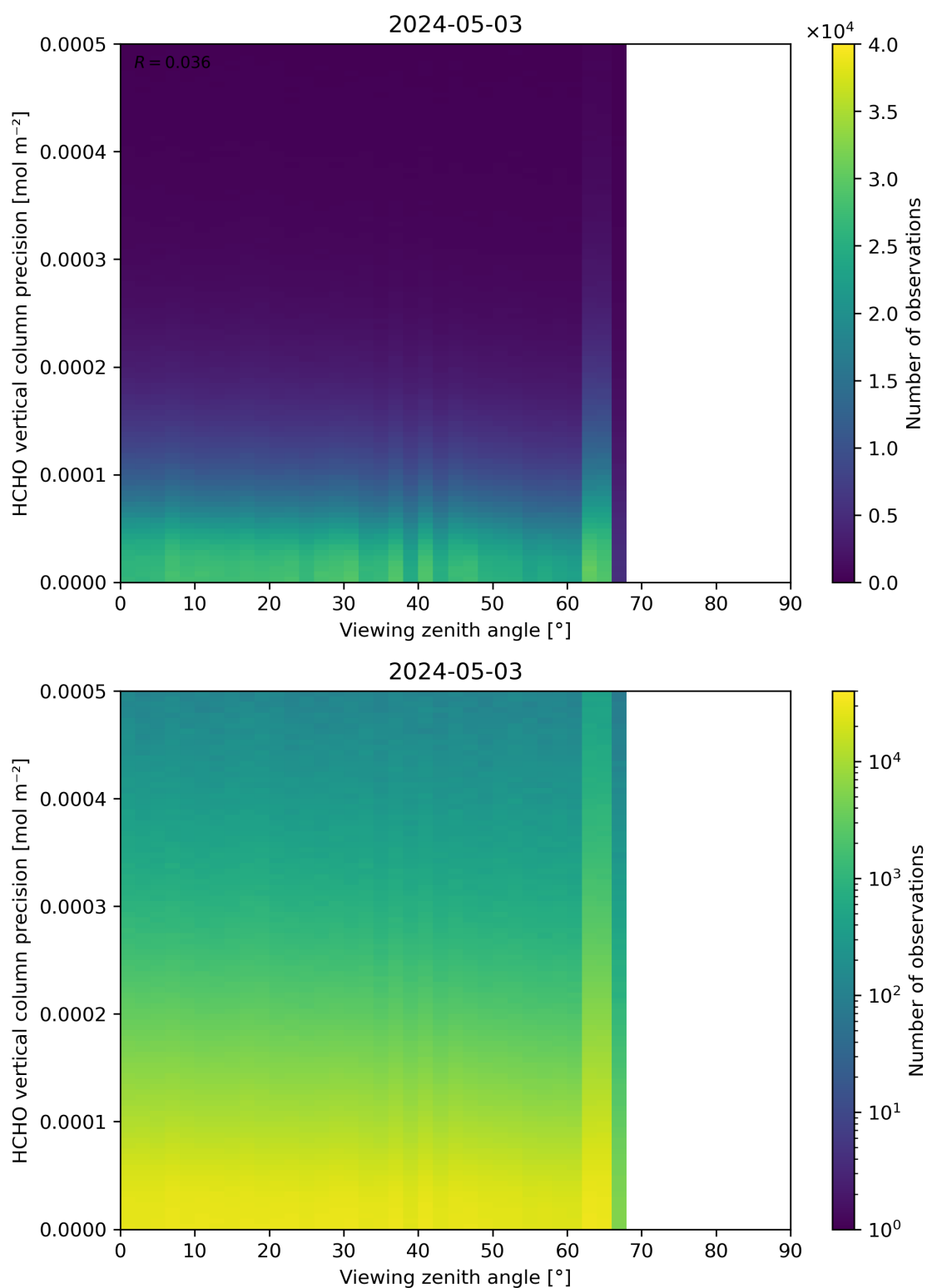
Figure 194: Scatter density plot of “Viewing zenith angle” against “HCHO vertical column precision” for 2024-05-02 to 2024-05-04.
