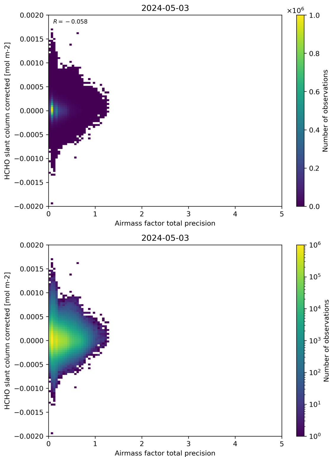
Figure 109: Scatter density plot of “Airmass factor total precision” against “HCHO slant column corrected” for 2024-05-02 to 2024-05-04.
