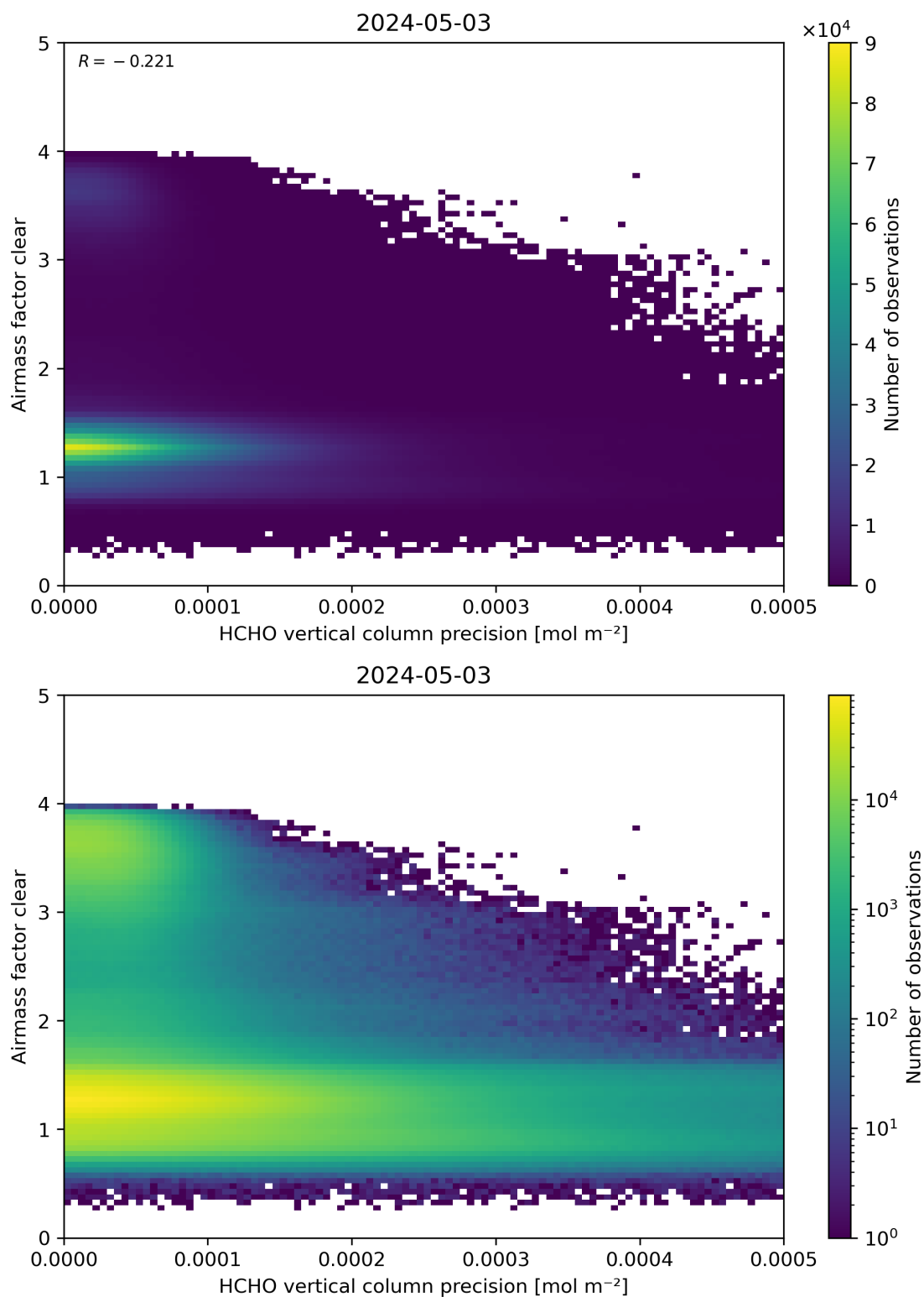
Figure 139: Scatter density plot of “HCHO vertical column precision” against “Airmass factor clear” for 2024-05-02 to 2024-05-04.
