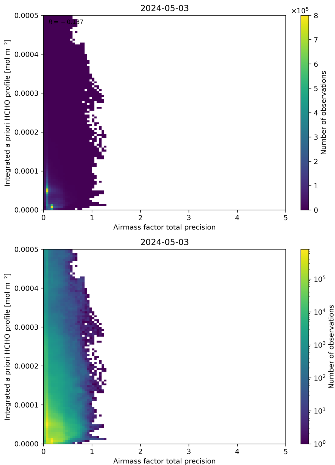
Figure 111: Scatter density plot of “Airmass factor total precision” against “Integrated a priori HCHO profile” for 2024-05-02 to 2024-05-04.
