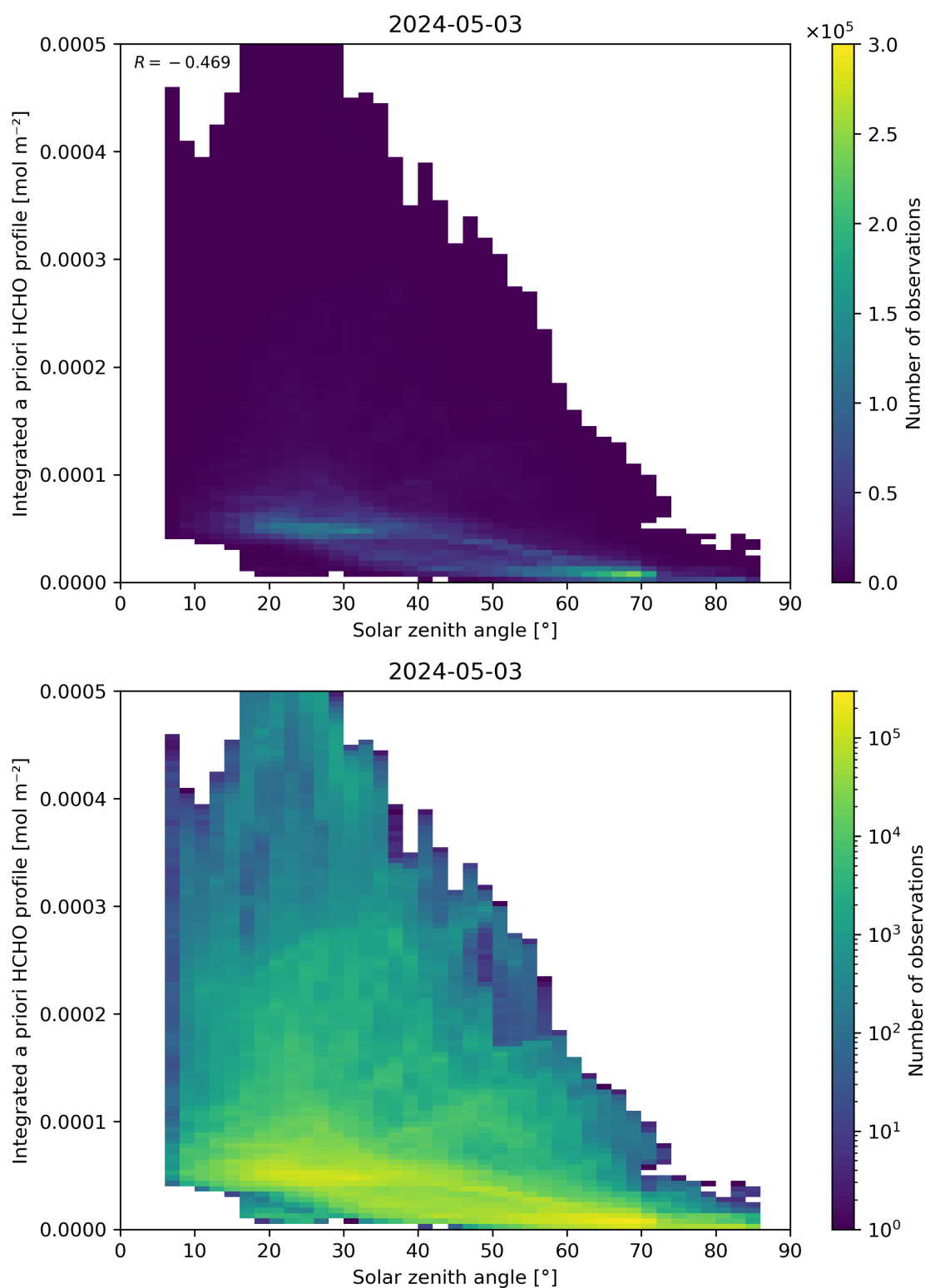
Figure 180: Scatter density plot of “Solar zenith angle” against “Integrated a priori HCHO profile” for 2024-05-02 to 2024-05-04.
