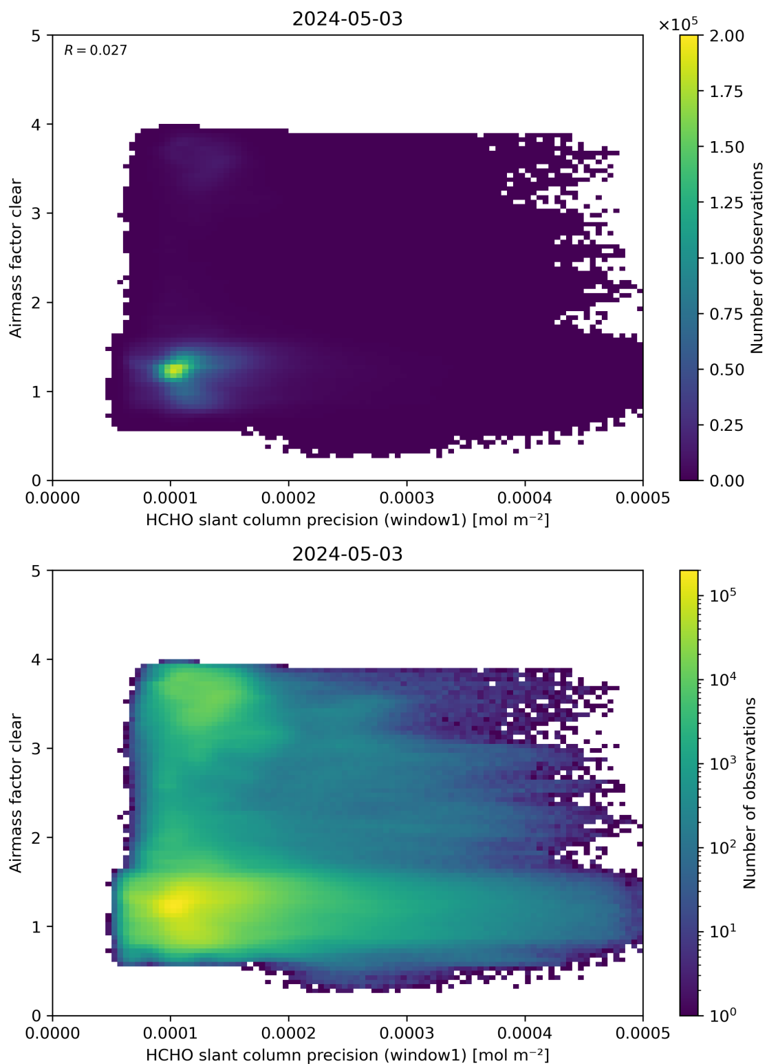
Figure 91: Scatter density plot of “HCHO slant column precision (window1)” against “Airmass factor clear” for 2024-05-02 to 2024-05-04.
