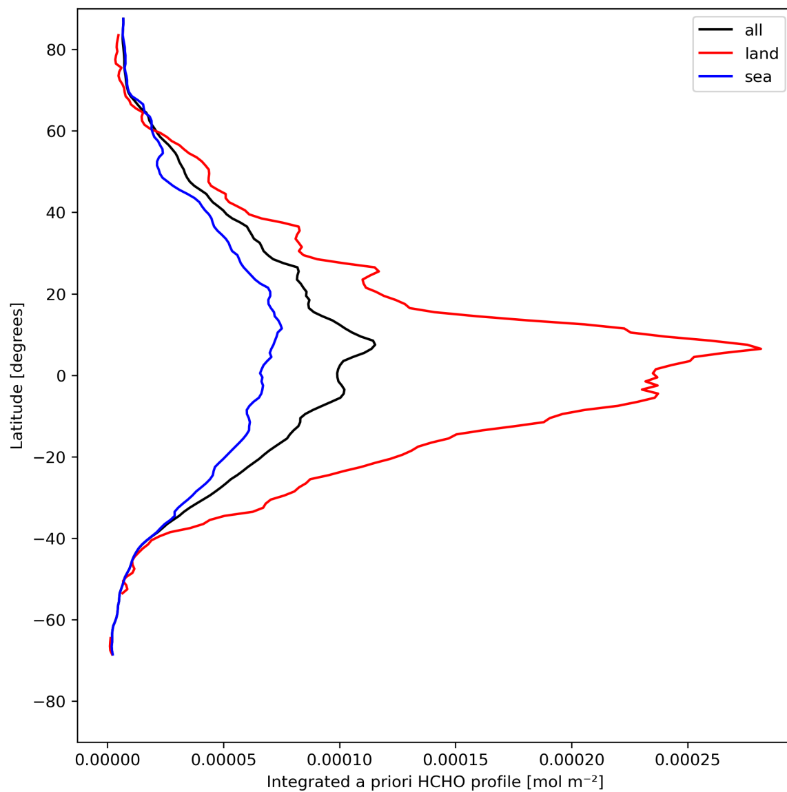
Figure 29: Zonal average of “Integrated a priori HCHO profile” for 2024-05-02 to 2024-05-04.
