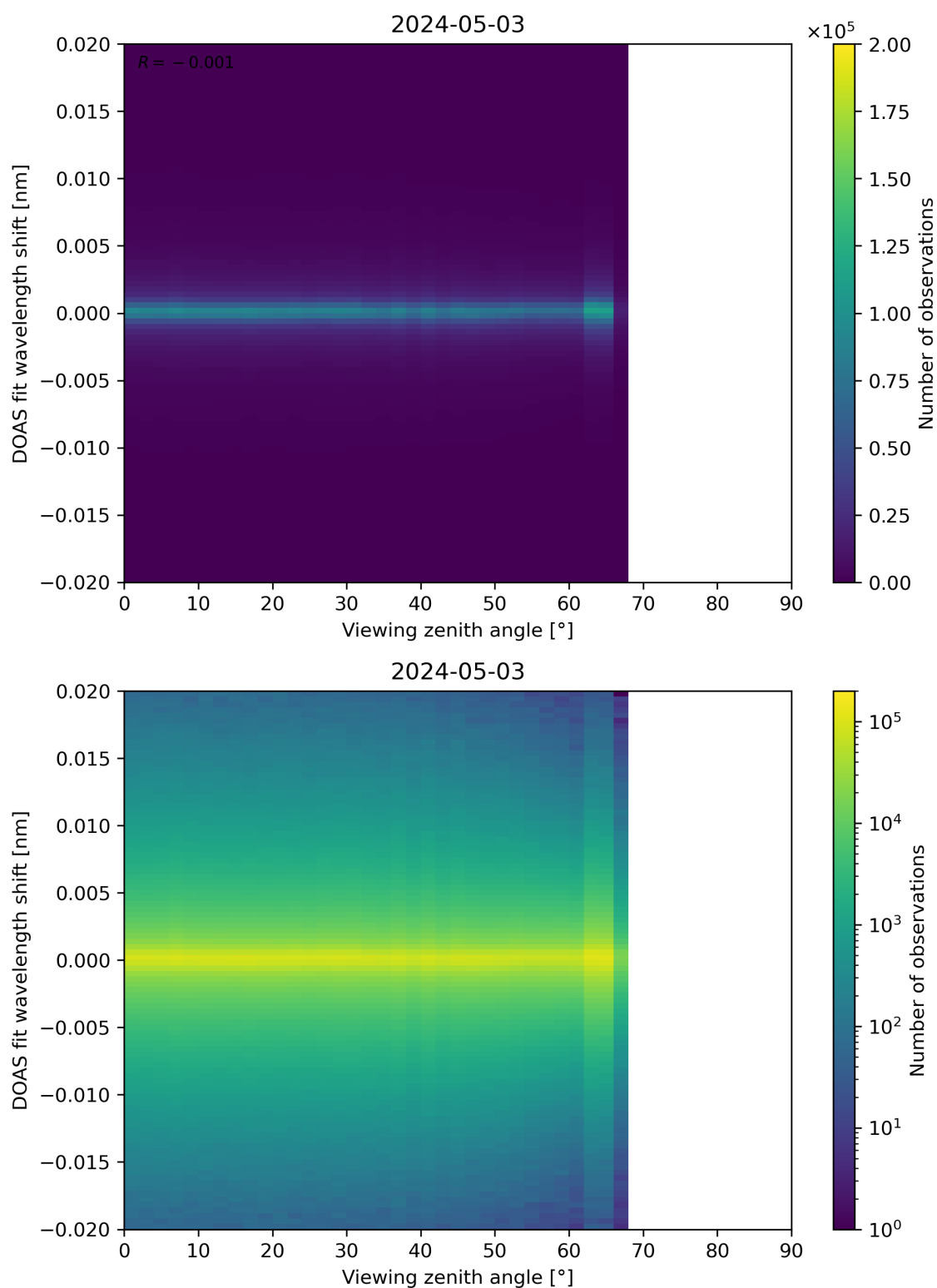
Figure 183: Scatter density plot of “Viewing zenith angle” against “DOAS fit wavelength shift” for 2024-05-02 to 2024-05-04.
