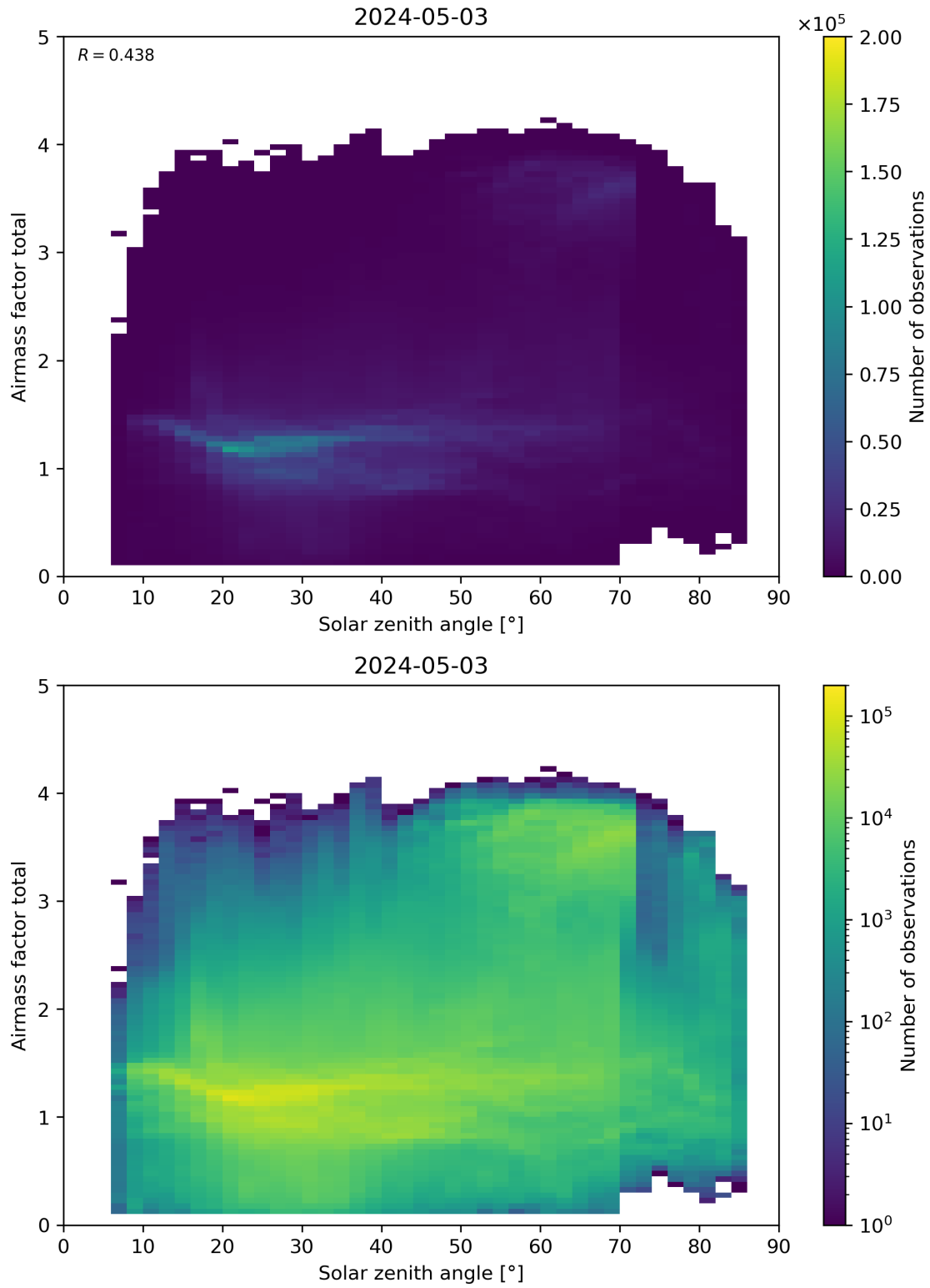
Figure 175: Scatter density plot of “Solar zenith angle” against “Airmass factor total” for 2024-05-02 to 2024-05-04.
