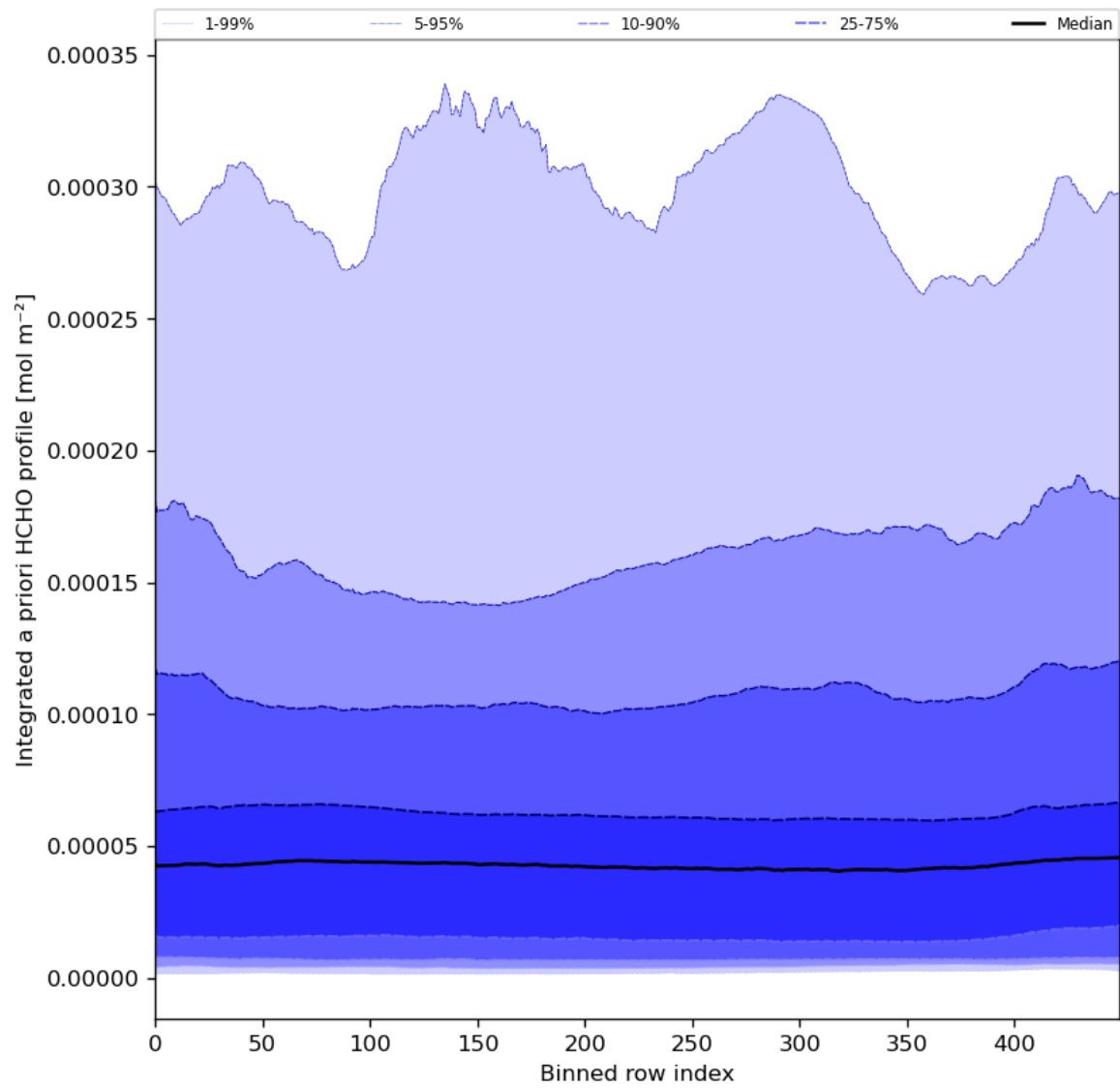
Figure 57: Along track statistics of “Integrated a priori HCHO profile” for 2024-05-02 to 2024-05-04
