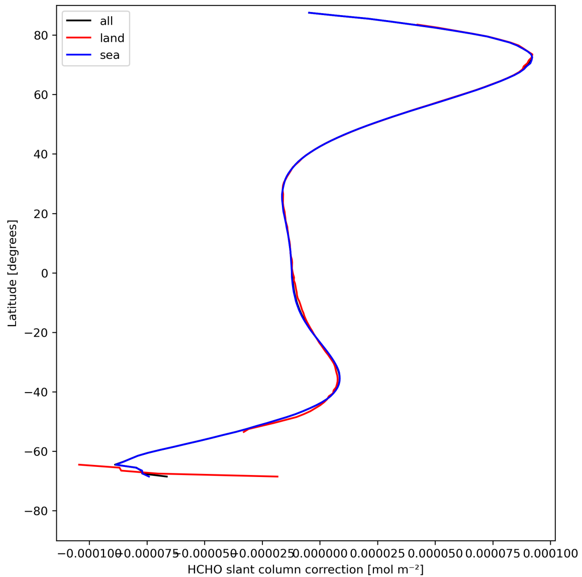
Figure 33: Zonal average of “HCHO slant column correction” for 2024-05-02 to 2024-05-04.
