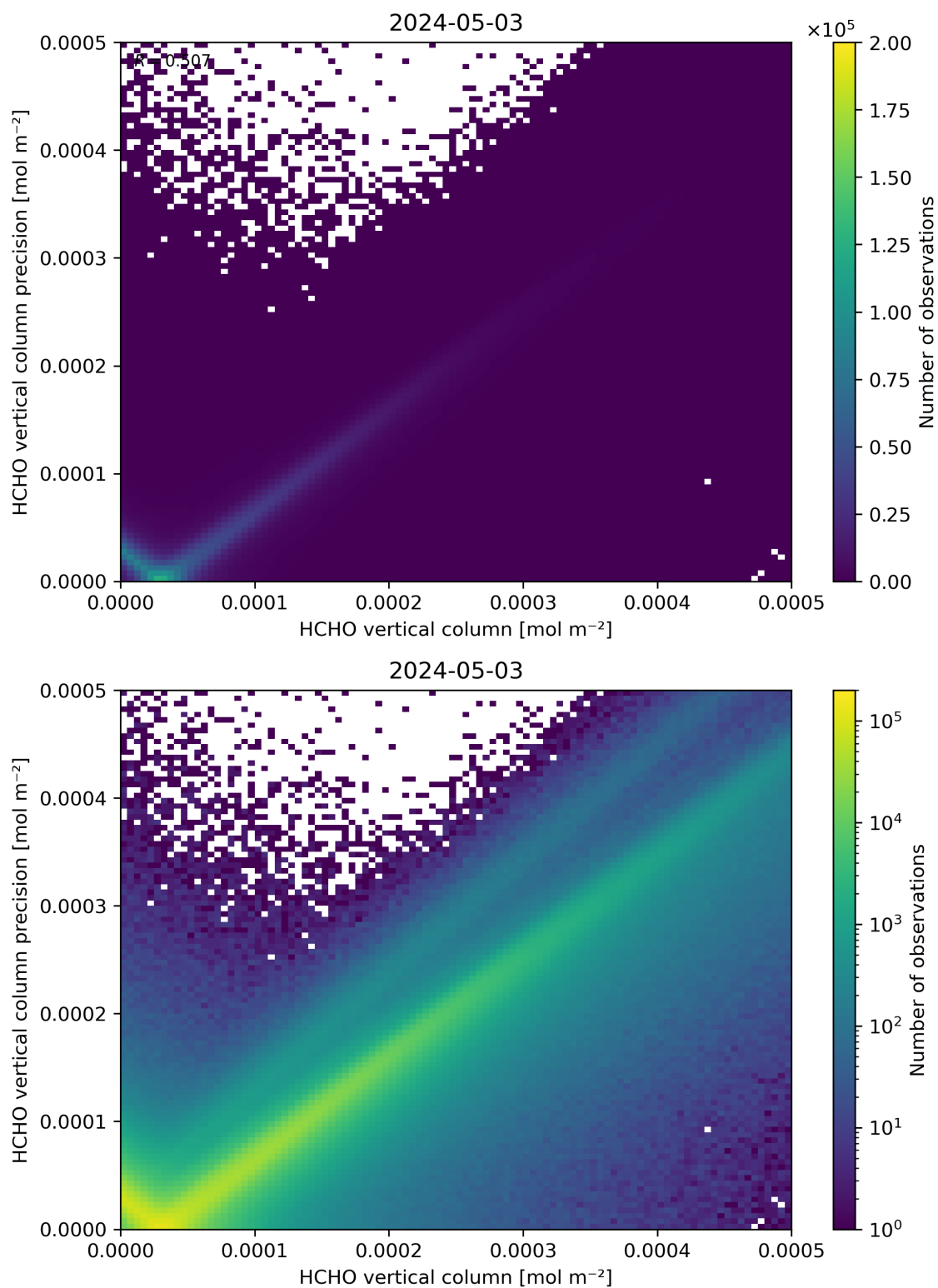
Figure 134: Scatter density plot of “HCHO vertical column” against “HCHO vertical column precision” for 2024-05-02 to 2024-05-04.
