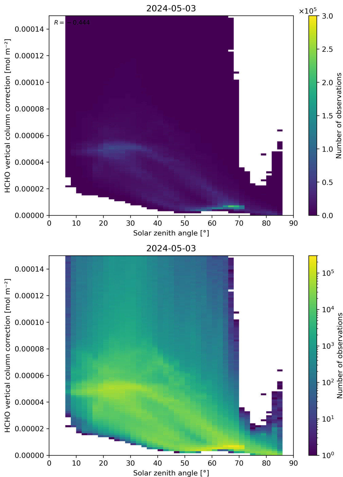
Figure 178: Scatter density plot of “Solar zenith angle” against “HCHO vertical column correction” for 2024-05-02 to 2024-05-04.
