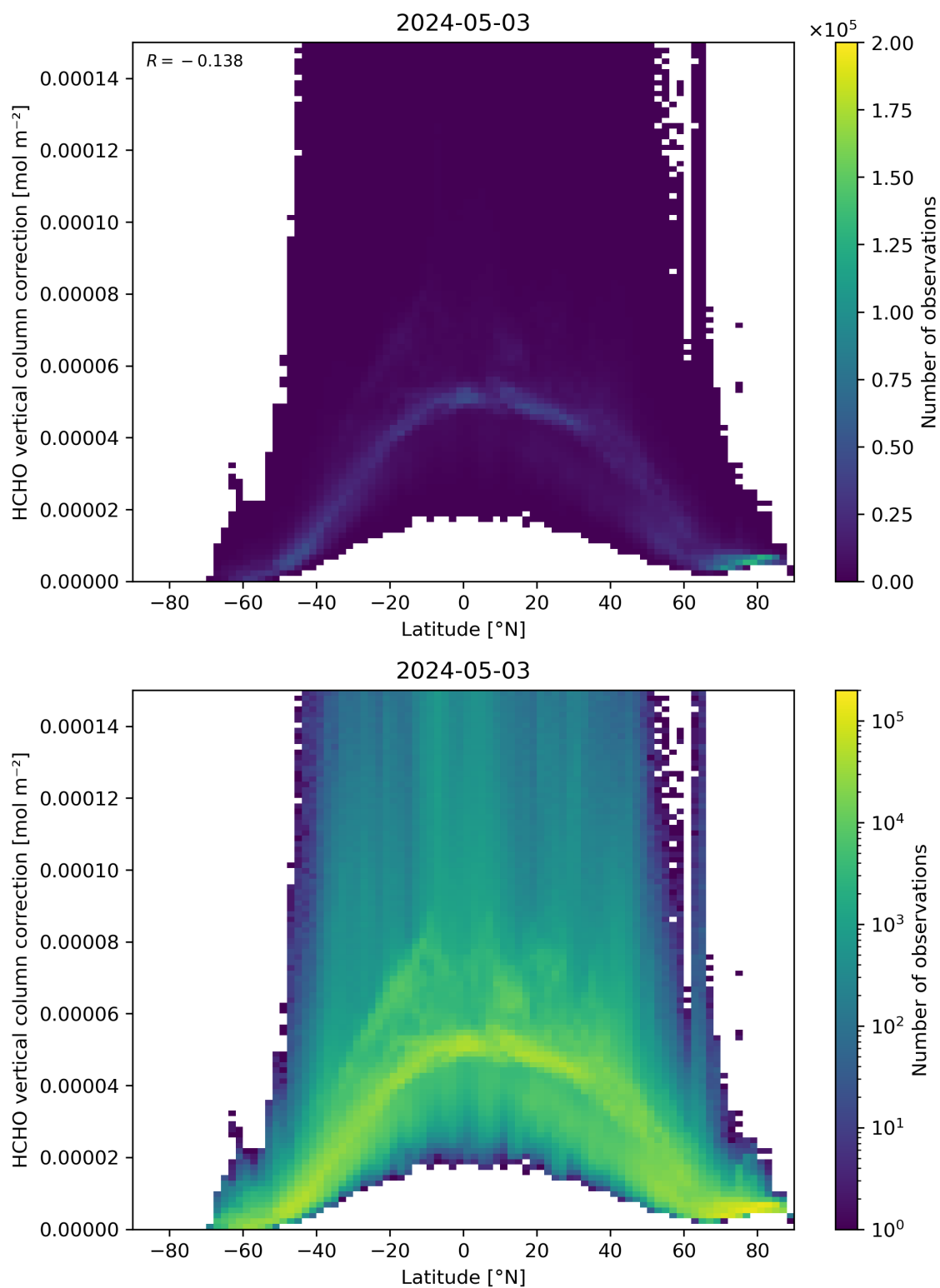
Figure 164: Scatter density plot of “Latitude” against “HCHO vertical column correction” for 2024-05-02 to 2024-05-04.
