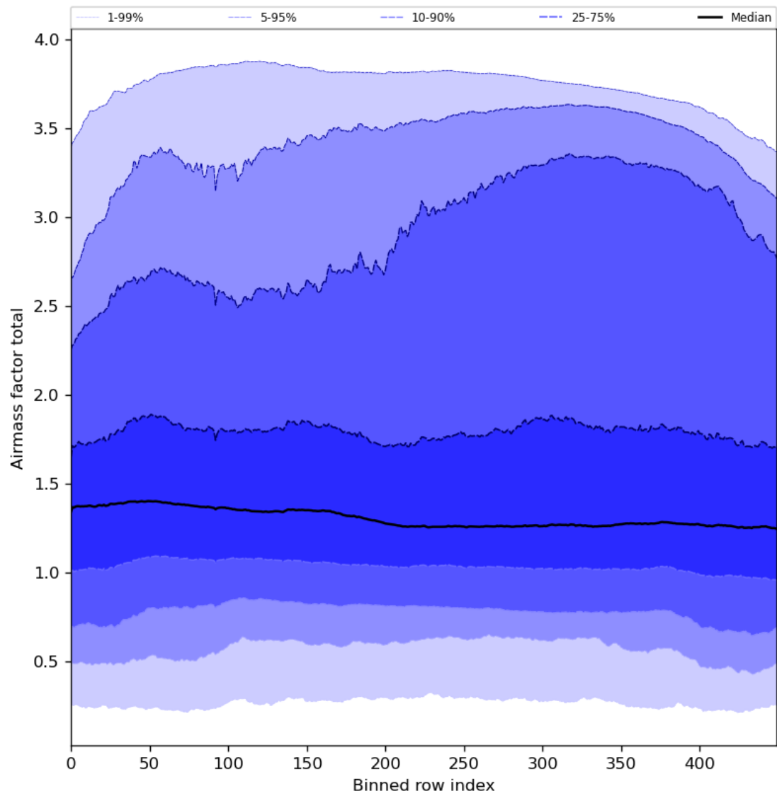
Figure 54: Along track statistics of “Airmass factor total” for 2024-05-02 to 2024-05-04
