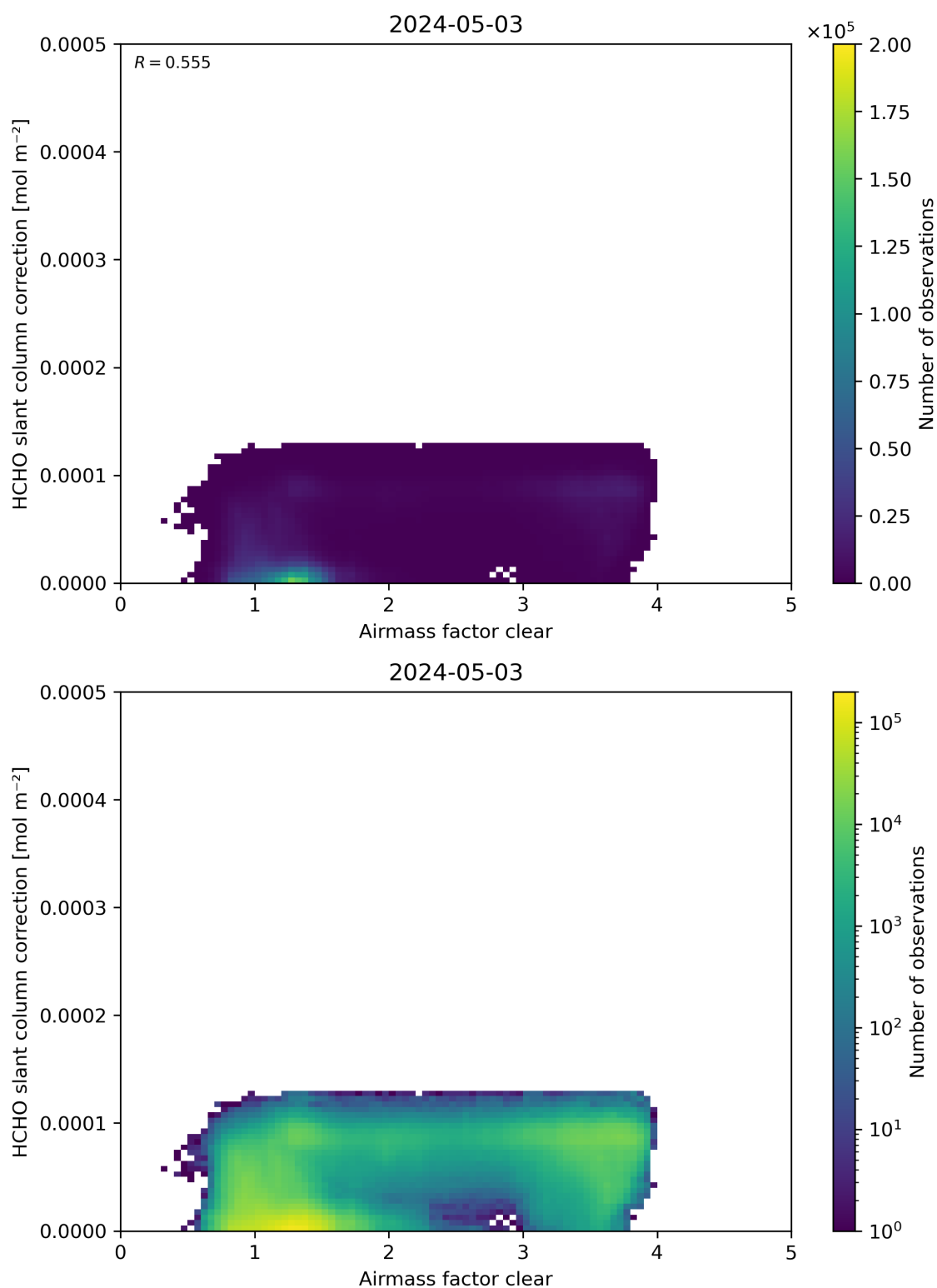
Figure 75: Scatter density plot of “Airmass factor clear” against “HCHO slant column correction” for 2024-05-02 to 2024-05-04.
