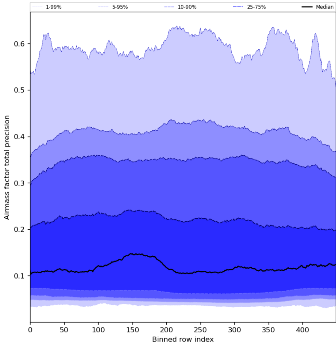
Figure 55: Along track statistics of “Airmass factor total precision” for 2024-05-02 to 2024-05-04
