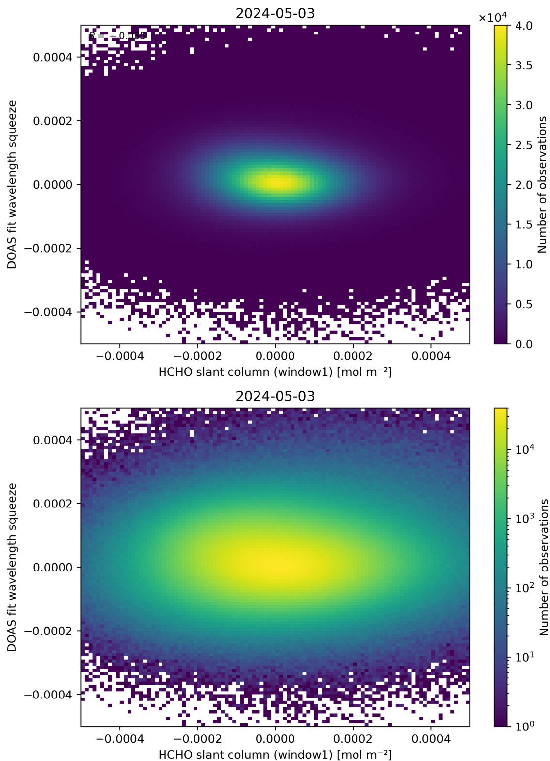
Figure 80: Scatter density plot of “HCHO slant column (window1)” against “DOAS fit wavelength squeeze” for 2024-05-02 to 2024-05-04.
