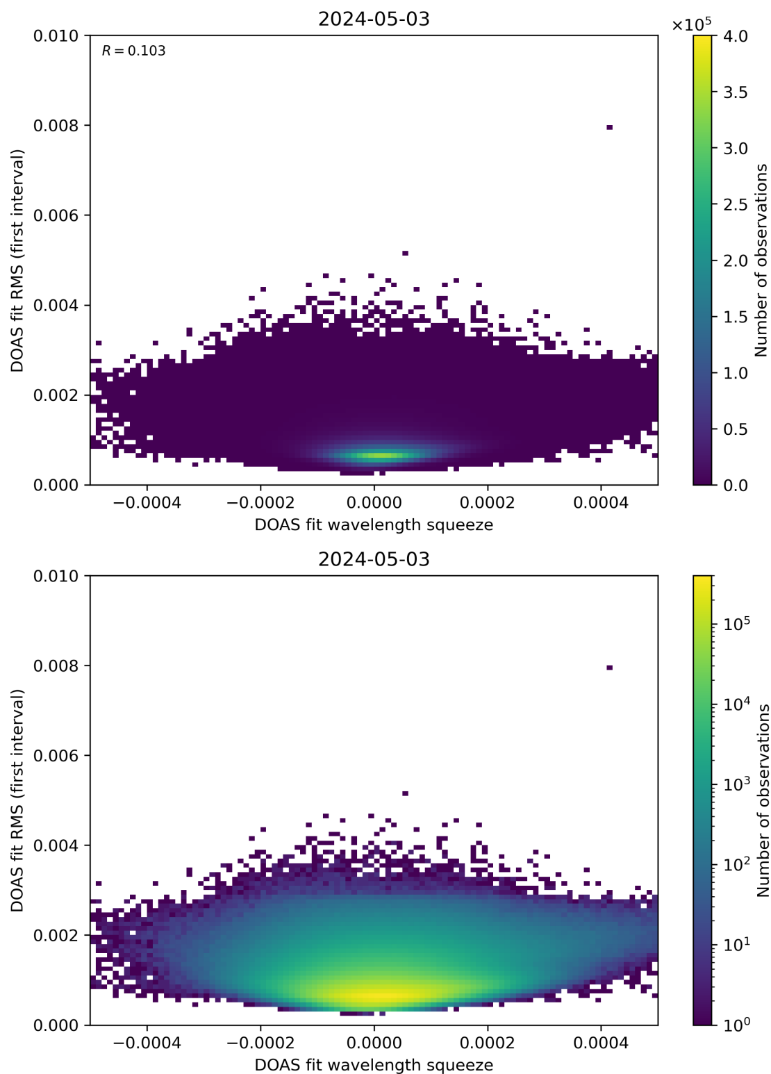
Figure 68: Scatter density plot of “DOAS fit wavelength squeeze” against “DOAS fit RMS (first interval)” for 2024-05-02 to 2024-05-04.
