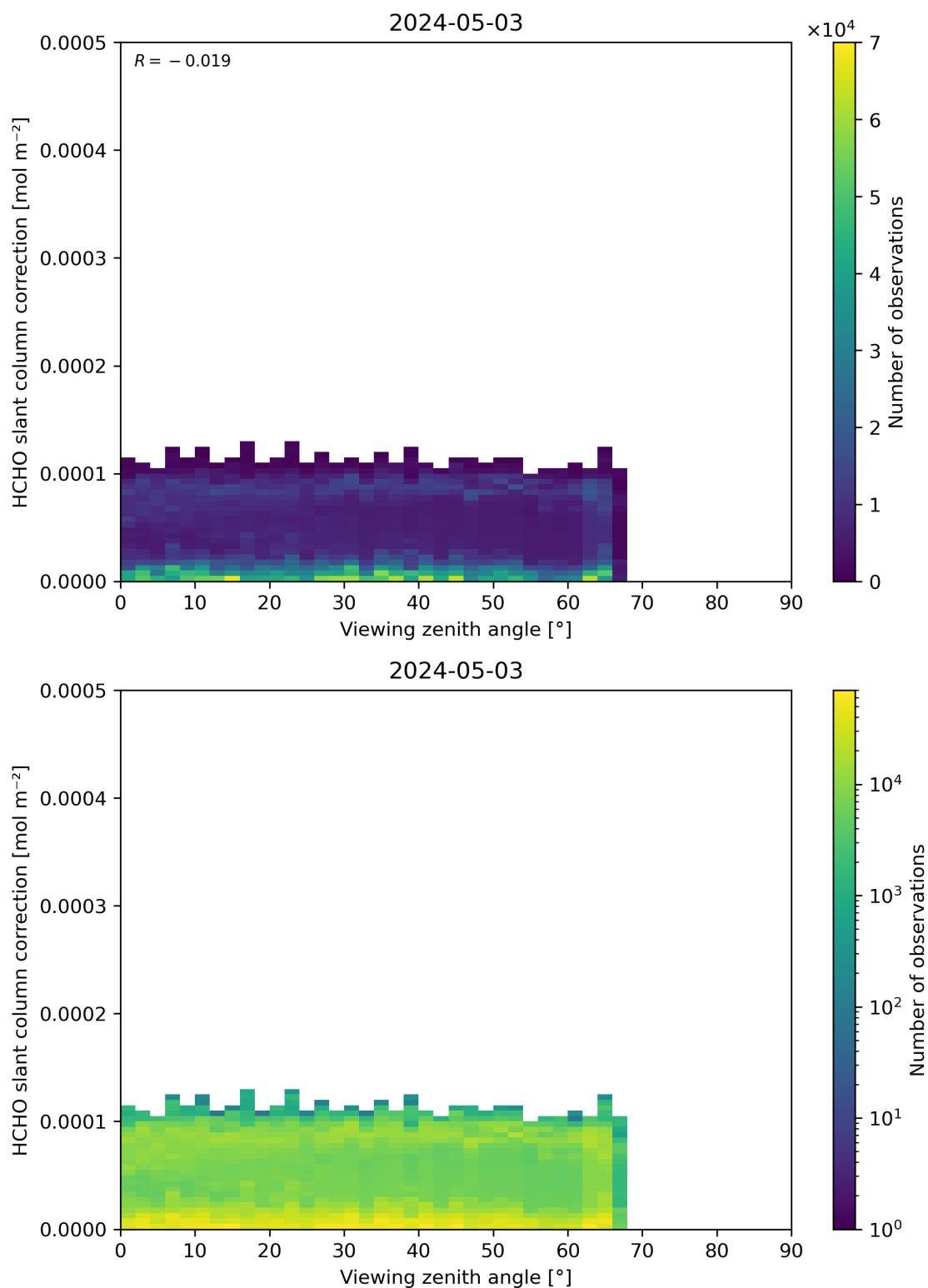
Figure 187: Scatter density plot of “Viewing zenith angle” against “HCHO slant column correction” for 2024-05-02 to 2024-05-04.
