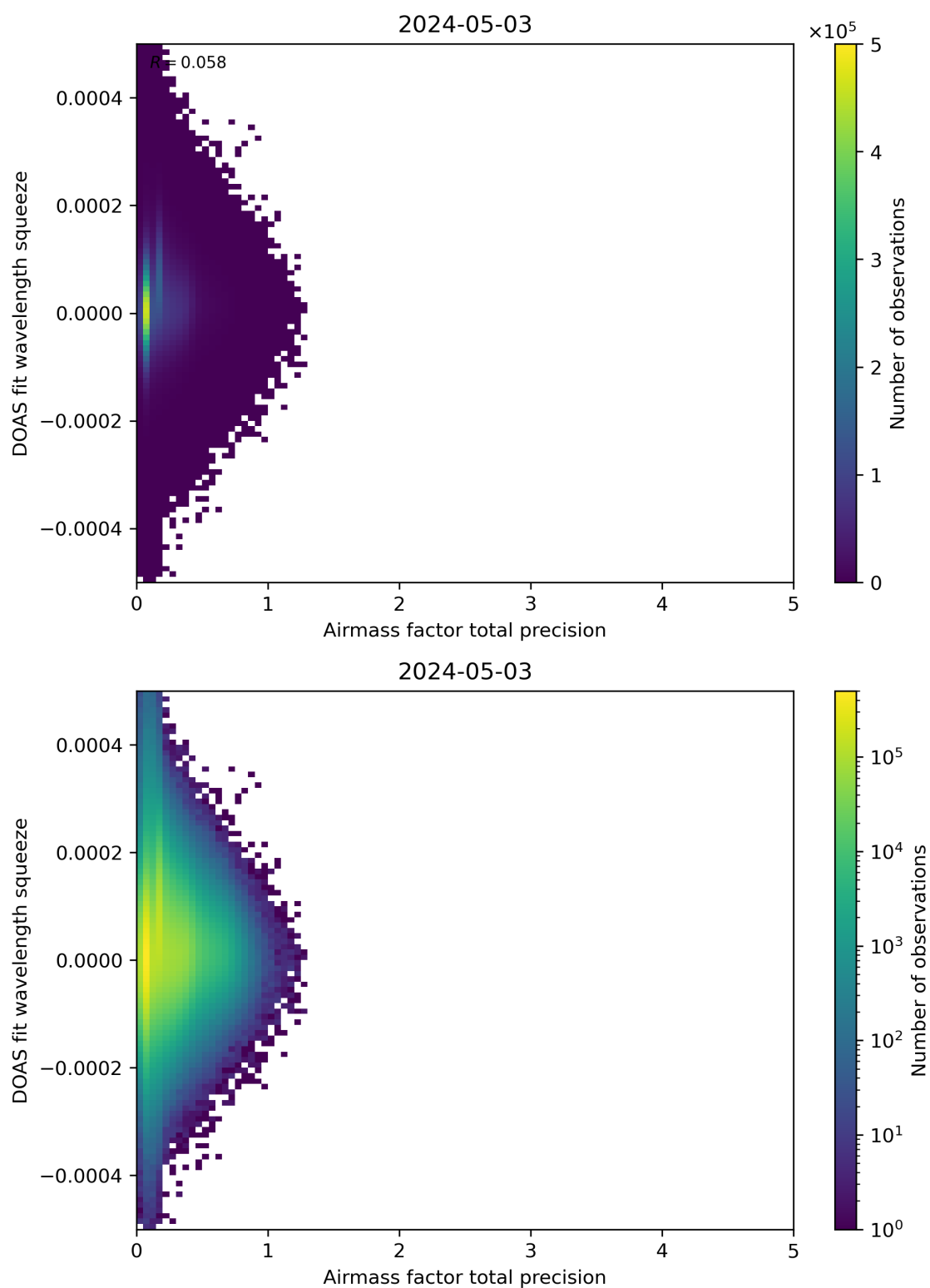
Figure 107: Scatter density plot of “Airmass factor total precision” against “DOAS fit wavelength squeeze” for 2024-05-02 to 2024-05-04.
