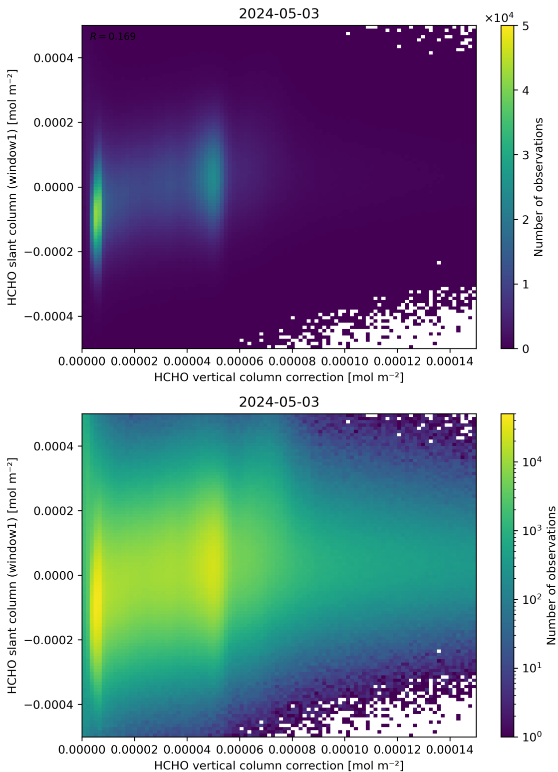
Figure 118: Scatter density plot of “HCHO vertical column correction” against “HCHO slant column (window1)” for 2024-05-02 to 2024-05-04.
