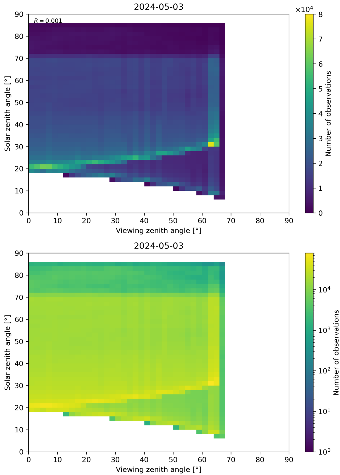
Figure 197: Scatter density plot of “Viewing zenith angle” against “Solar zenith angle” for 2024-05-02 to 2024-05-04.
