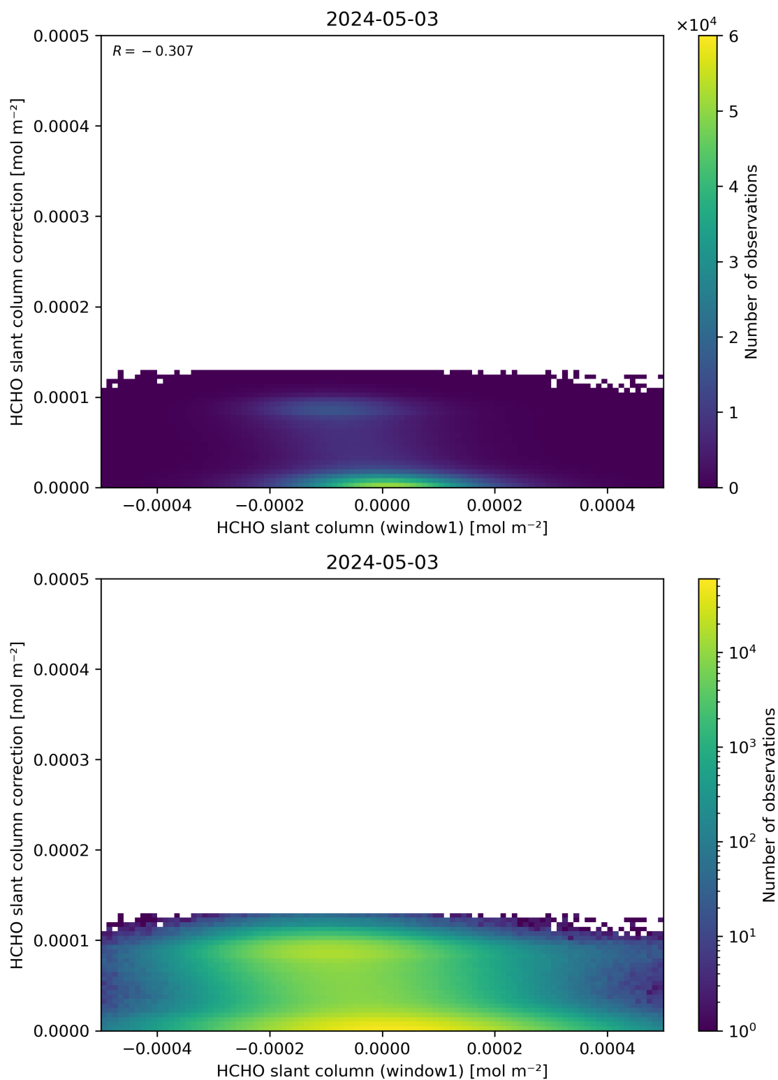
Figure 83: Scatter density plot of “HCHO slant column (window1)” against “HCHO slant column correction” for 2024-05-02 to 2024-05-04.
