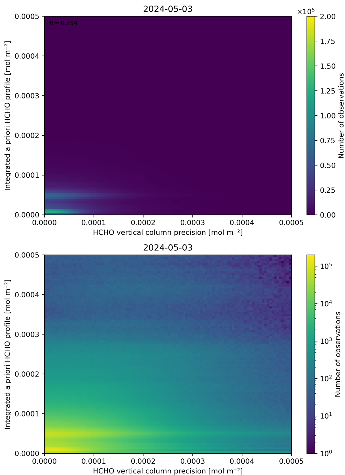
Figure 147: Scatter density plot of “HCHO vertical column precision” against “Integrated a priori HCHO profile” for 2024-05-02 to 2024-05-04.
