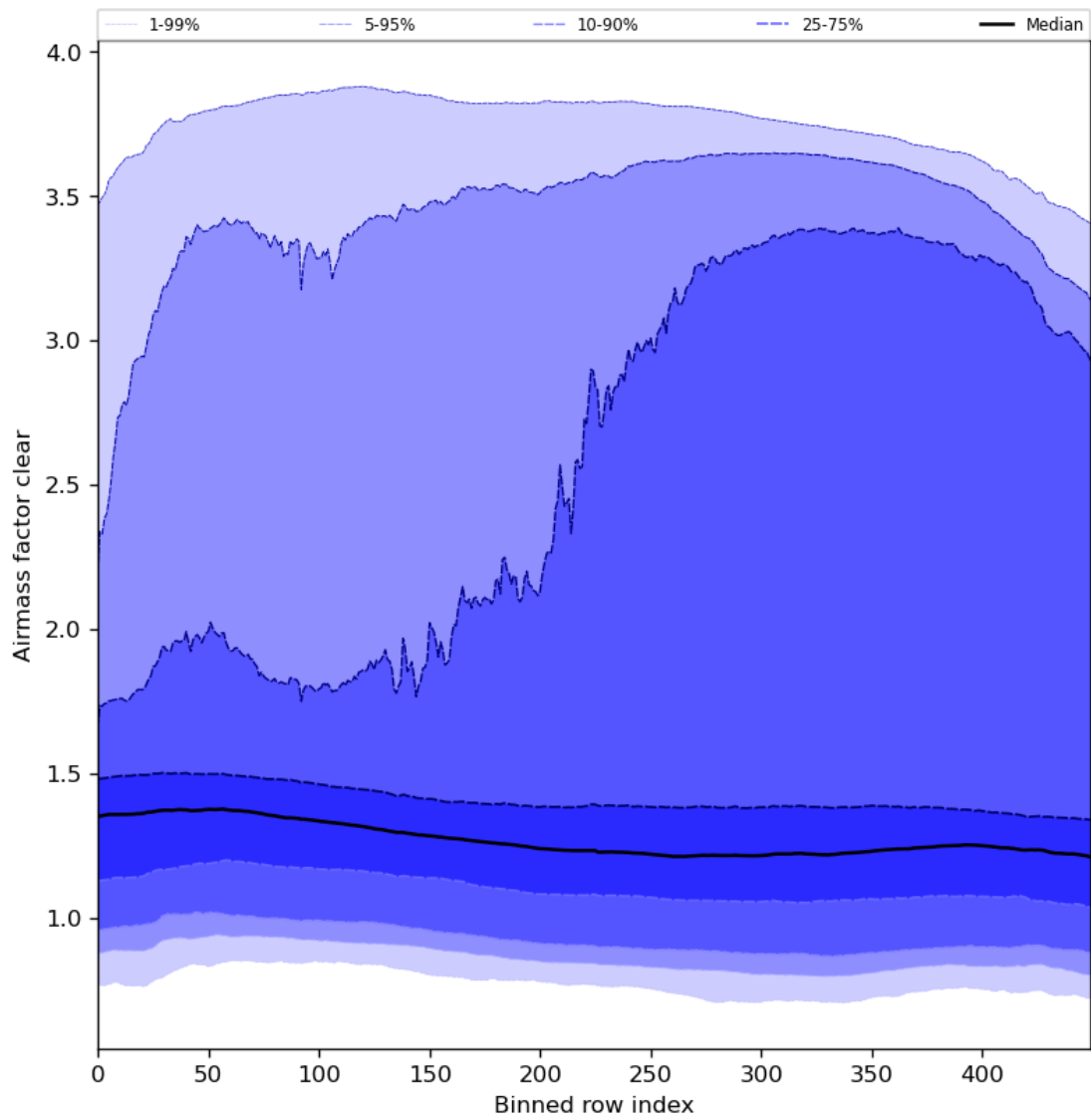
Figure 56: Along track statistics of “Airmass factor clear” for 2024-05-02 to 2024-05-04
