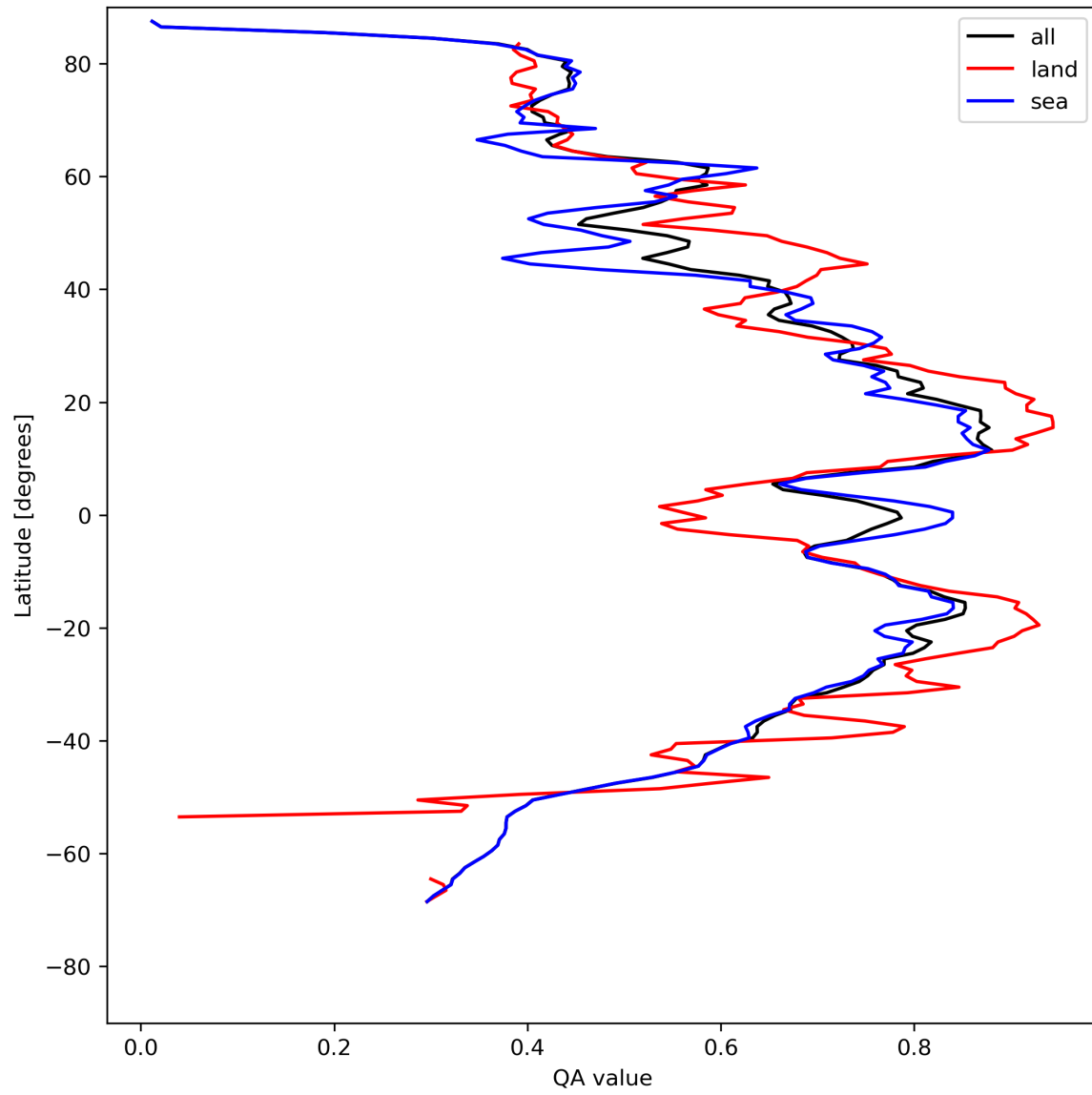
Figure 20: Zonal average of “QA value” for 2024-05-02 to 2024-05-04.
