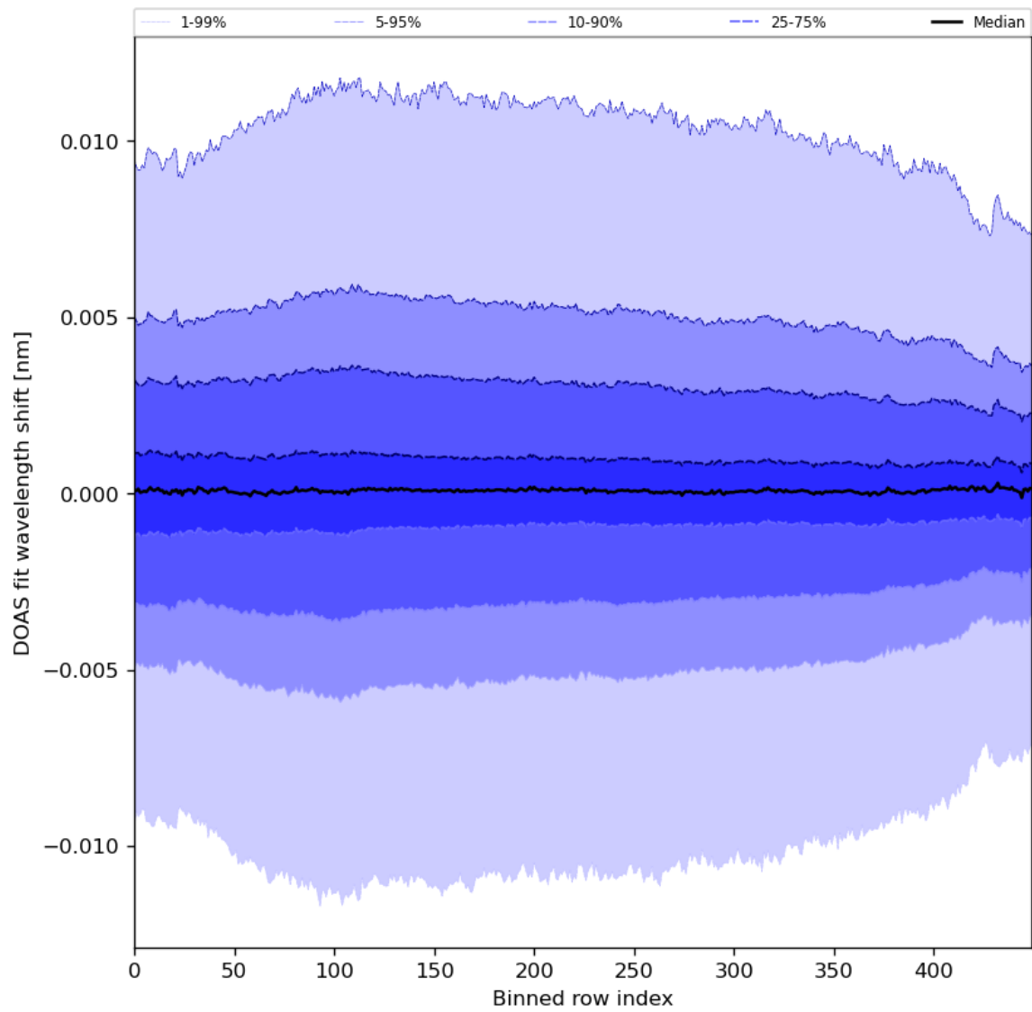
Figure 58: Along track statistics of “DOAS fit wavelength shift” for 2024-05-02 to 2024-05-04
