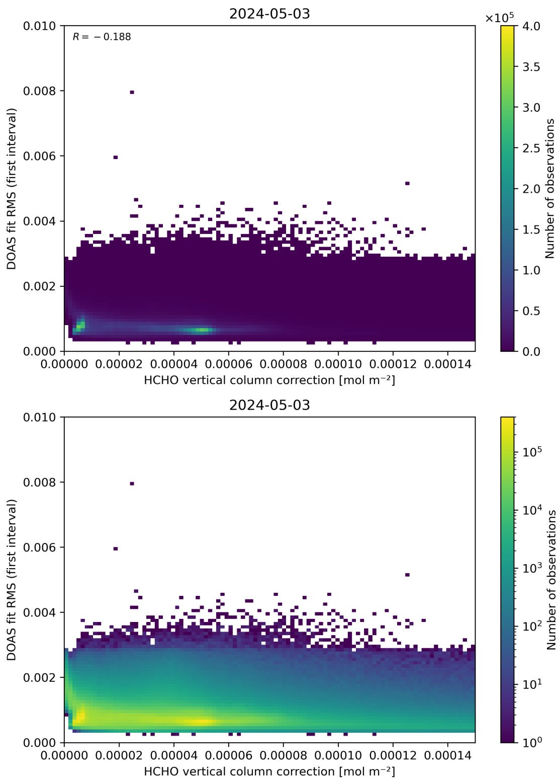
Figure 112: Scatter density plot of “HCHO vertical column correction” against “DOAS fit RMS (first interval)” for 2024-05-02 to 2024-05-04.
