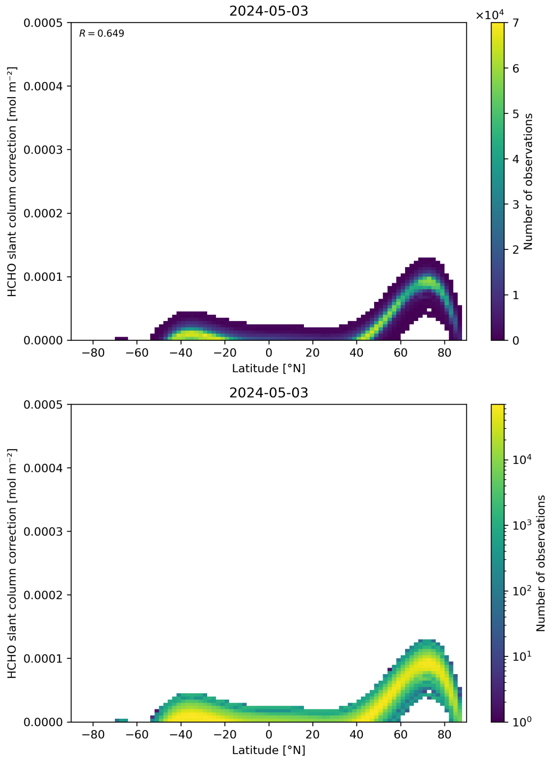
Figure 158: Scatter density plot of “Latitude” against “HCHO slant column correction” for 2024-05-02 to 2024-05-04.
