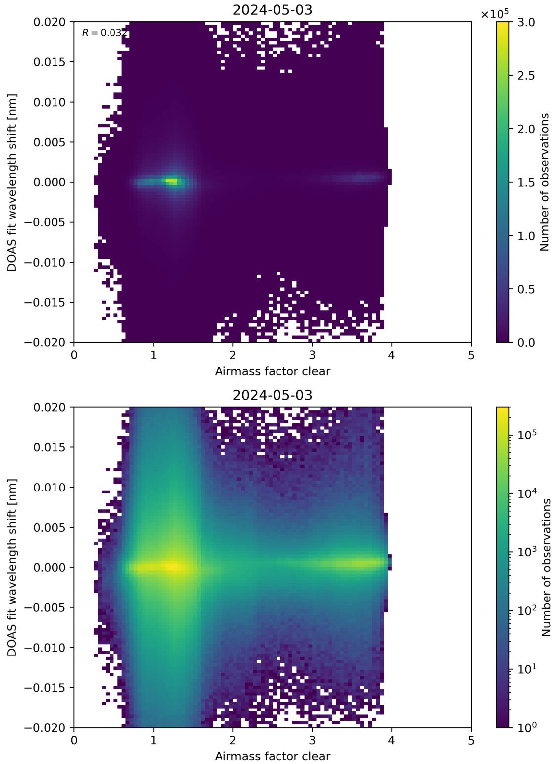
Figure 72: Scatter density plot of “Airmass factor clear” against “DOAS fit wavelength shift” for 2024-05-02 to 2024-05-04.
