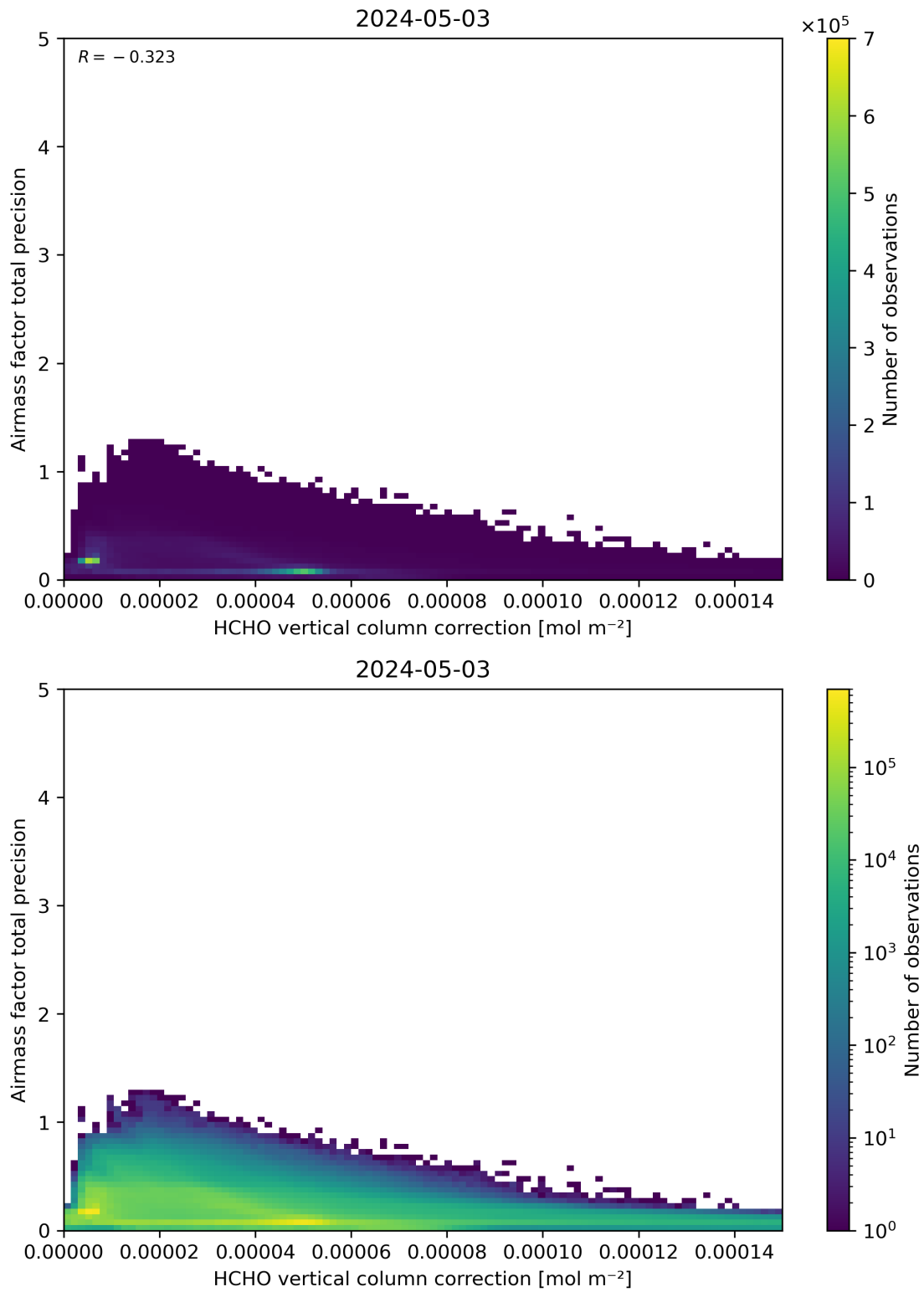
Figure 121: Scatter density plot of “HCHO vertical column correction” against “Airmass factor total precision” for 2024-05-02 to 2024-05-04.
