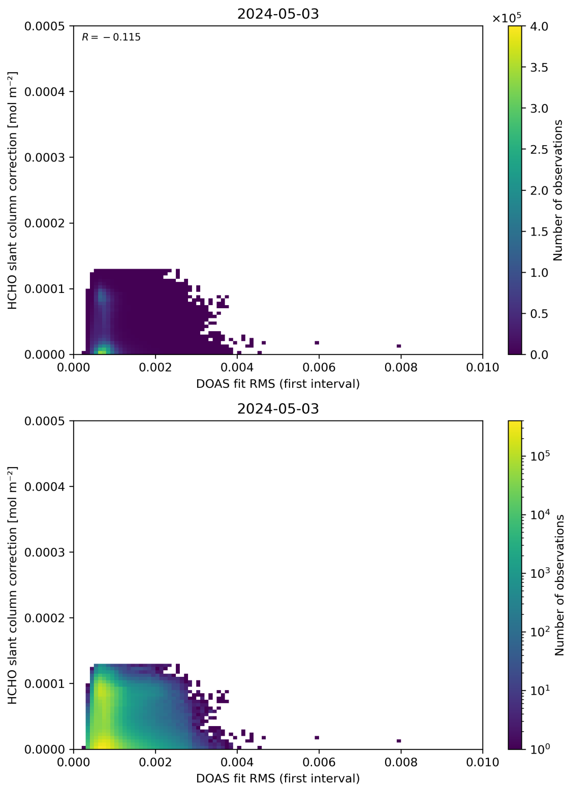
Figure 63: Scatter density plot of “DOAS fit RMS (first interval)” against “HCHO slant column correction” for 2024-05-02 to 2024-05-04.
