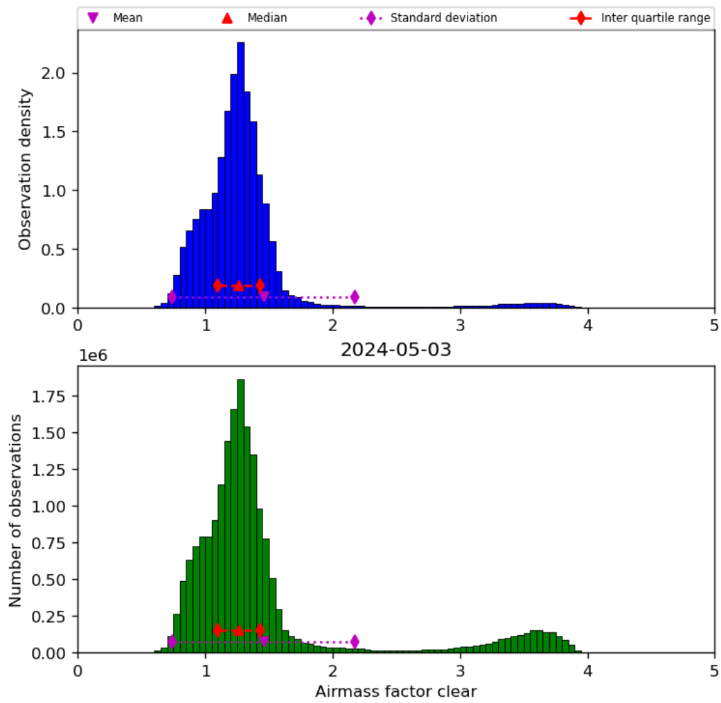
Figure 42: Histogram of “Airmass factor clear” for 2024-05-02 to 2024-05-04
