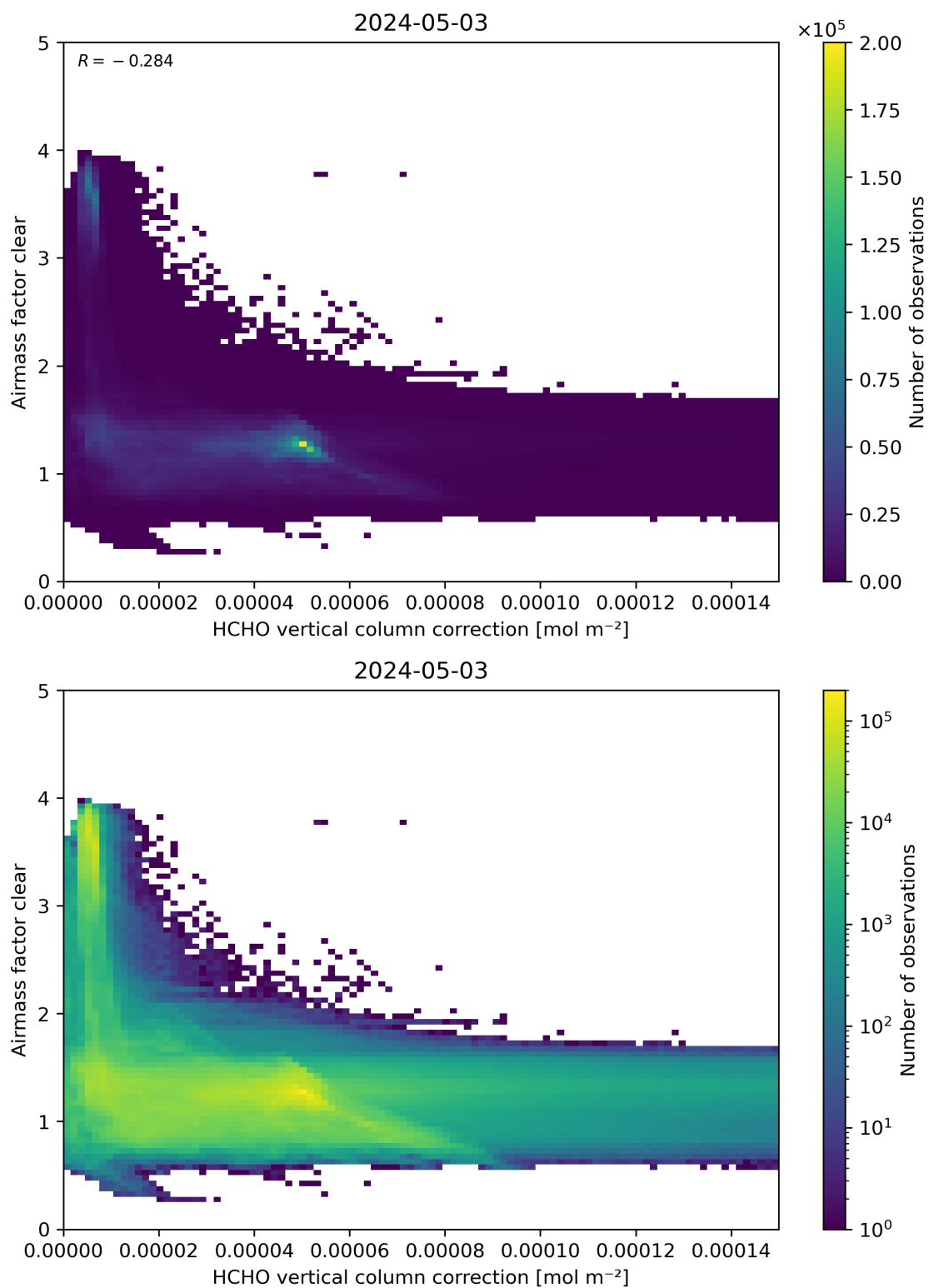
Figure 115: Scatter density plot of “HCHO vertical column correction” against “Airmass factor clear” for 2024-05-02 to 2024-05-04.
