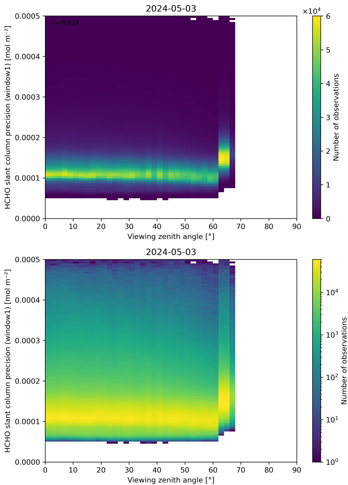
Figure 189: Scatter density plot of “Viewing zenith angle” against “HCHO slant column precision (window1)” for 2024-05-02 to 2024-05-04.
