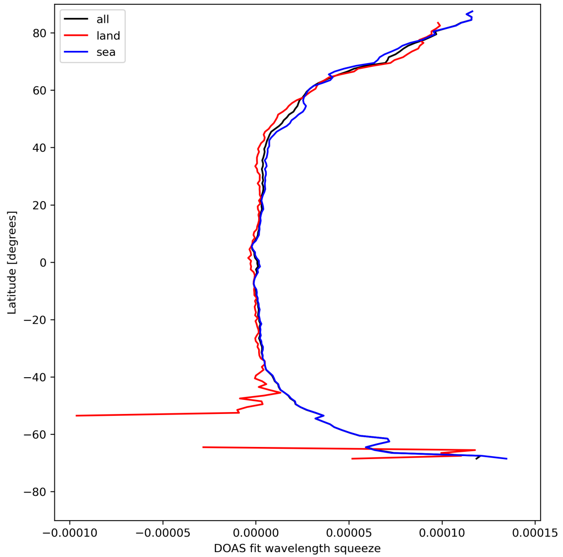
Figure 31: Zonal average of “DOAS fit wavelength squeeze” for 2024-05-02 to 2024-05-04.
