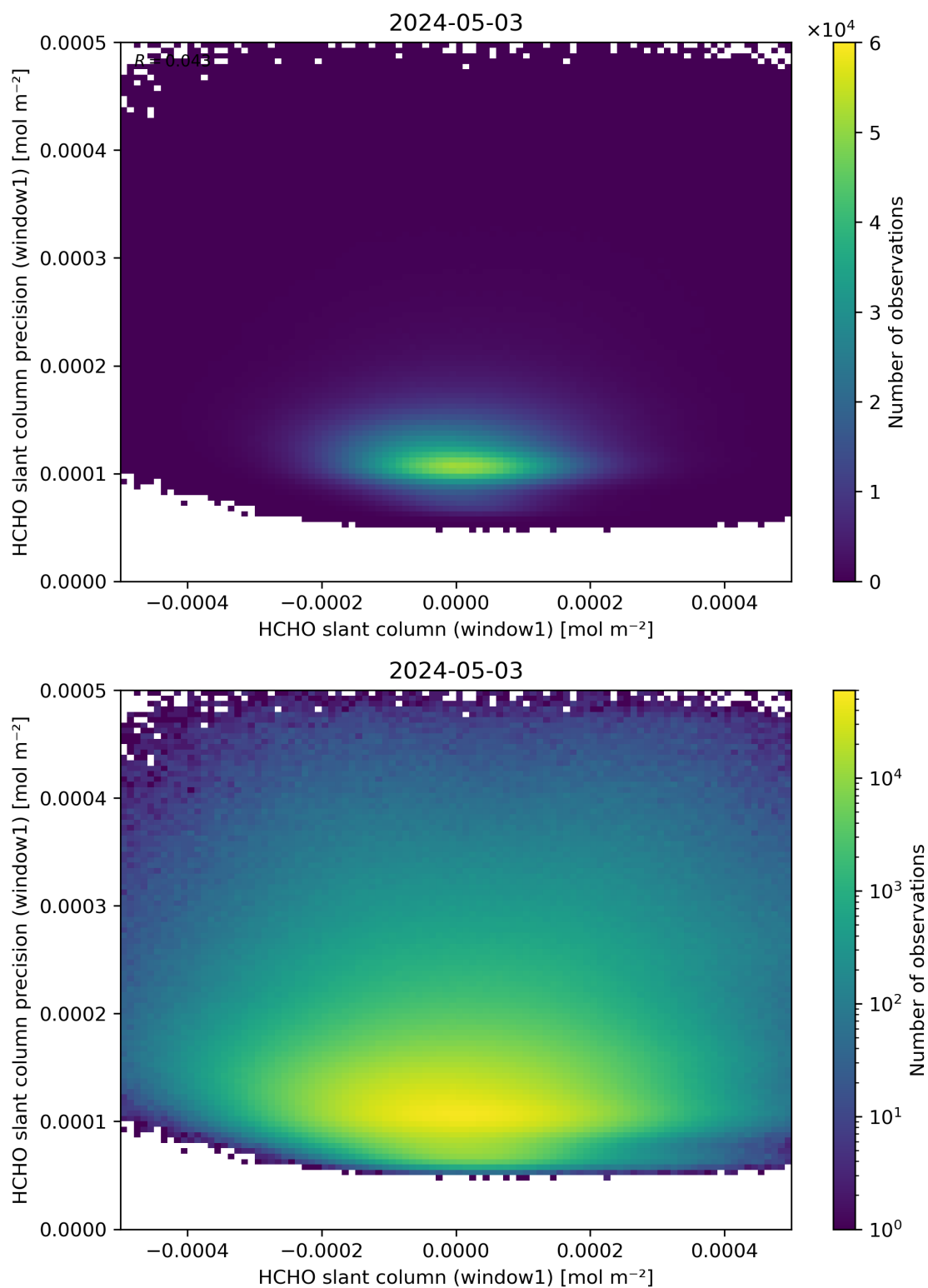
Figure 84: Scatter density plot of “HCHO slant column (window1)” against “HCHO slant column precision (window1)” for 2024-05-02 to 2024-05-04.
