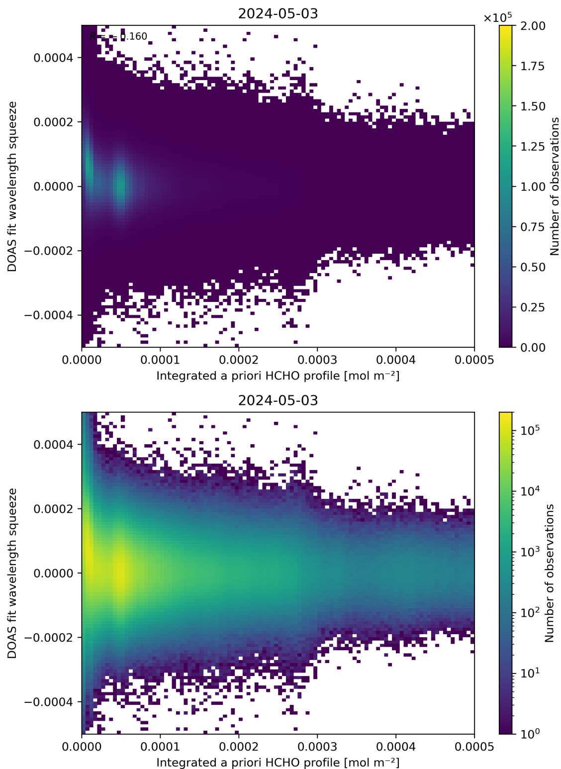
Figure 150: Scatter density plot of “Integrated a priori HCHO profile” against “DOAS fit wavelength squeeze” for 2024-05-02 to 2024-05-04.
