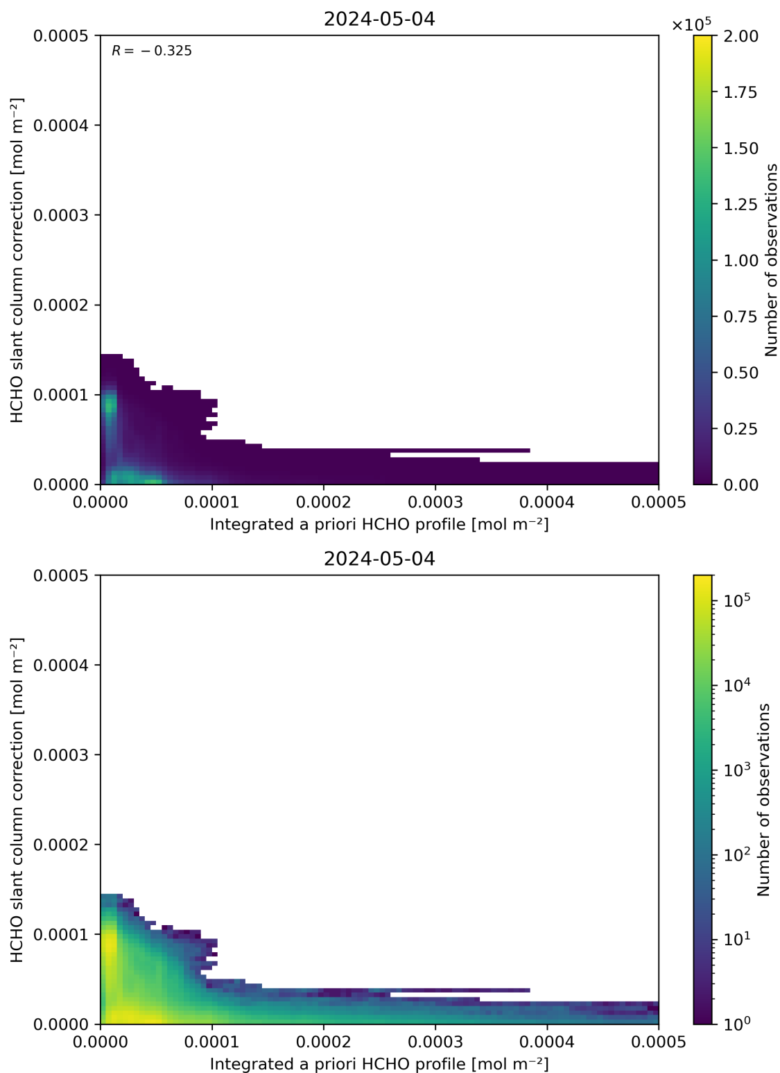
Figure 152: Scatter density plot of “Integrated a priori HCHO profile” against “HCHO slant column correction” for 2024-05-03 to 2024-05-05.
