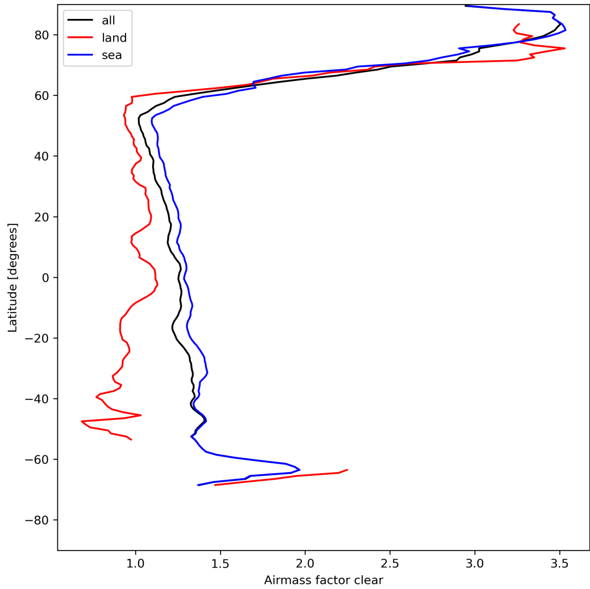
Figure 28: Zonal average of “Airmass factor clear” for 2024-05-03 to 2024-05-05.
