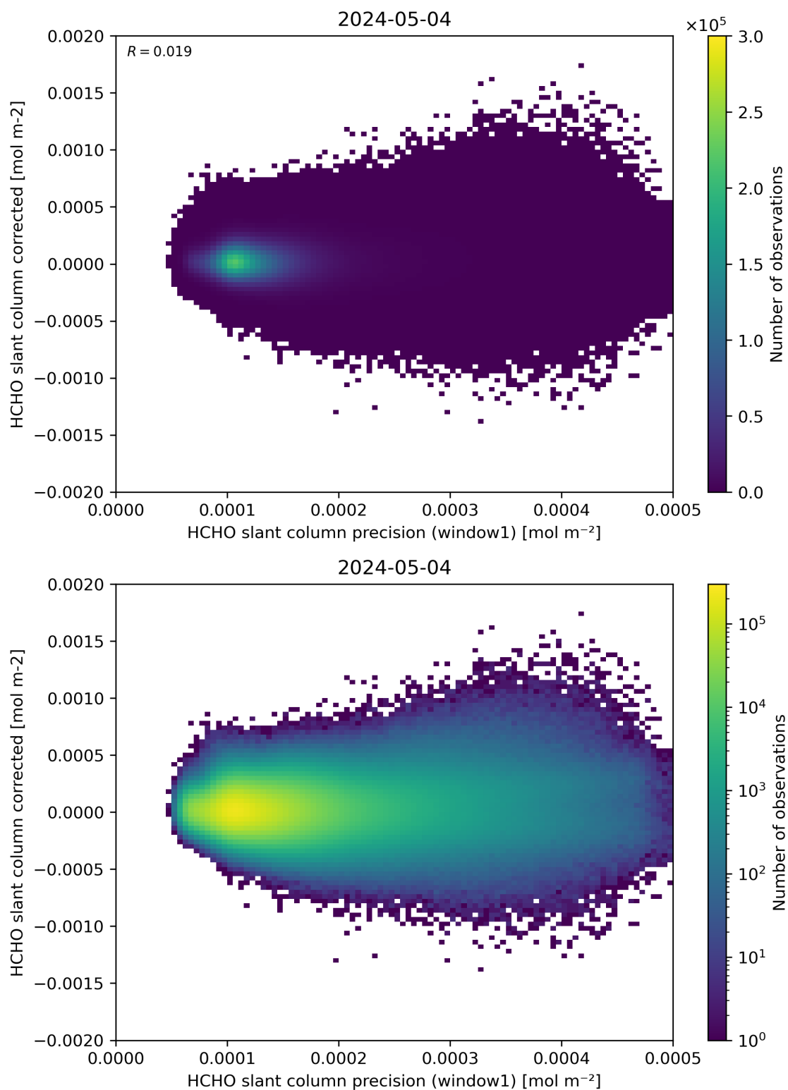
Figure 92: Scatter density plot of “HCHO slant column precision (window1)” against “HCHO slant column corrected” for 2024-05-03 to 2024-05-05.
