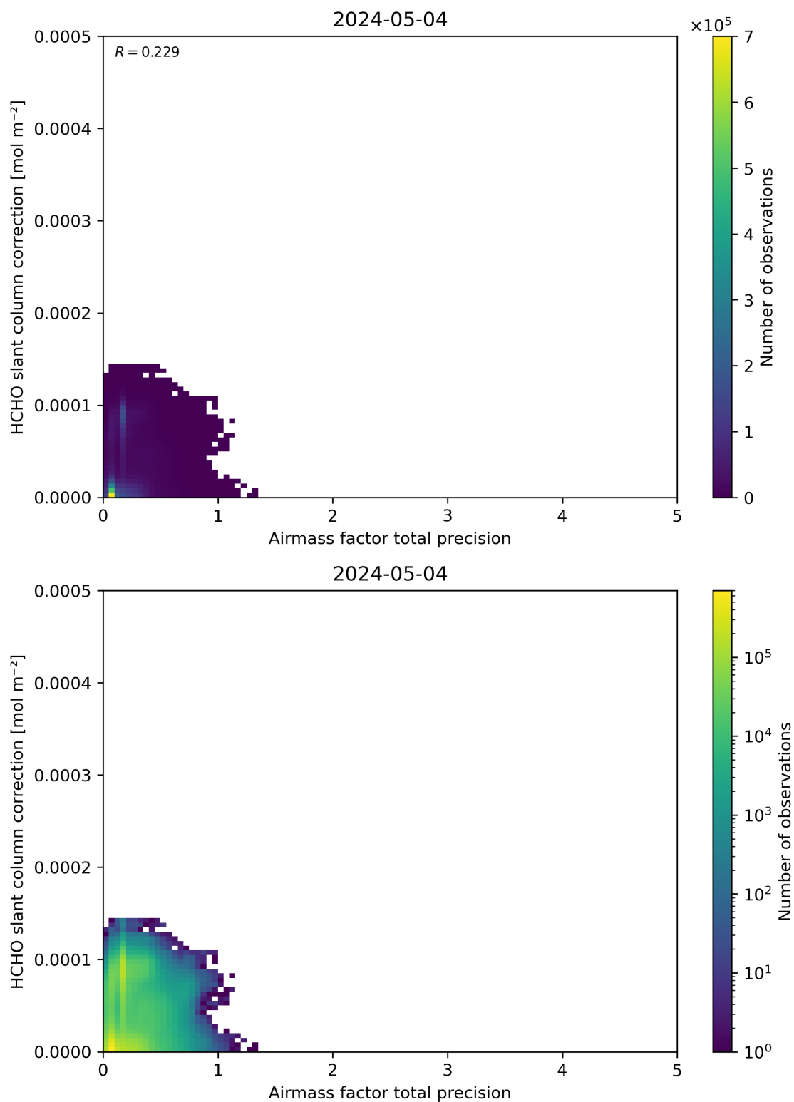
Figure 110: Scatter density plot of “Airmass factor total precision” against “HCHO slant column correction” for 2024-05-03 to 2024-05-05.
