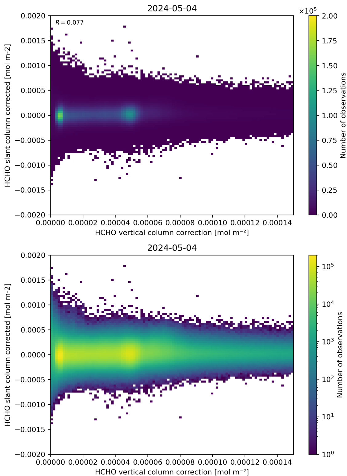
Figure 116: Scatter density plot of “HCHO vertical column correction” against “HCHO slant column corrected” for 2024-05-03 to 2024-05-05.
