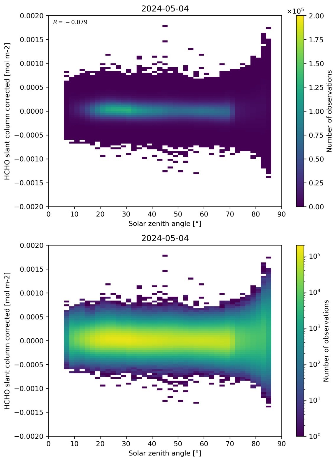
Figure 171: Scatter density plot of “Solar zenith angle” against “HCHO slant column corrected” for 2024-05-03 to 2024-05-05.
