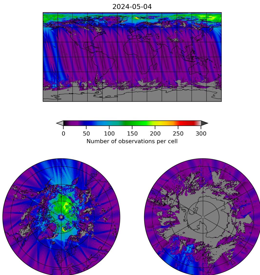
Figure 19: Map of the number of observations for 2024-05-03 to 2024-05-05
