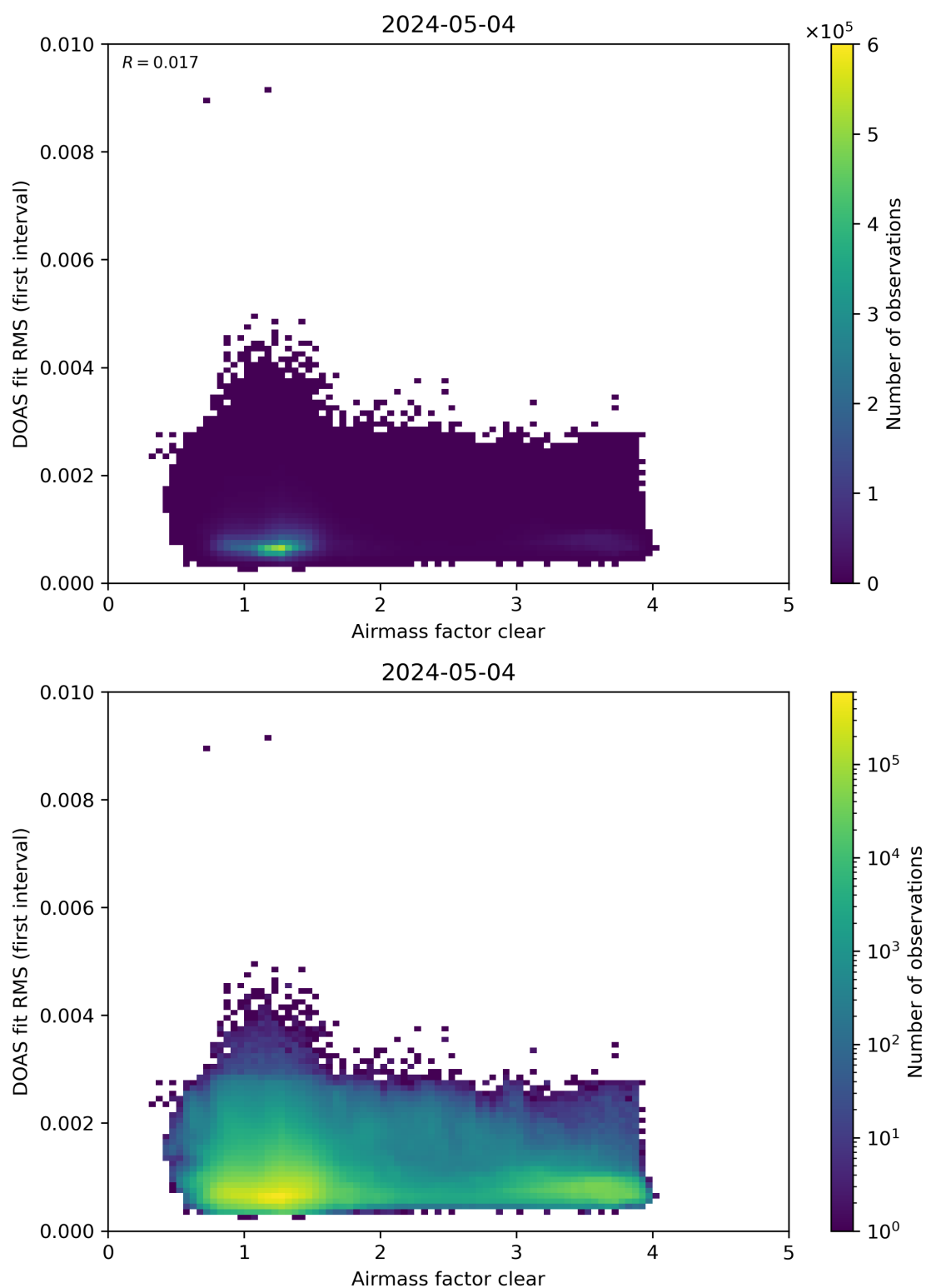
Figure 71: Scatter density plot of “Airmass factor clear” against “DOAS fit RMS (first interval)” for 2024-05-03 to 2024-05-05.
