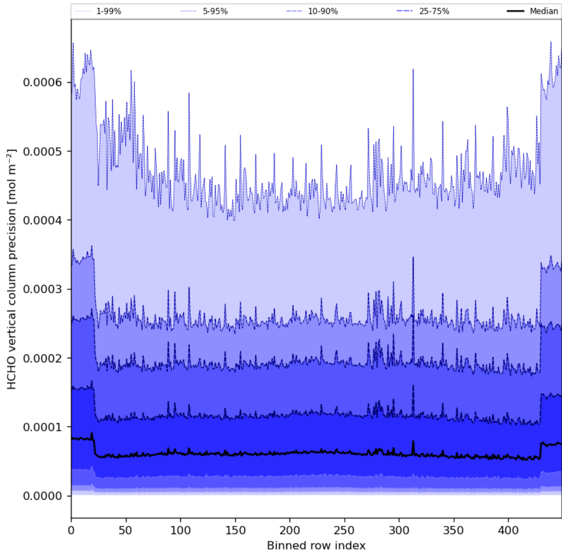
Figure 50: Along track statistics of “HCHO vertical column precision” for 2024-05-03 to 2024-05-05
