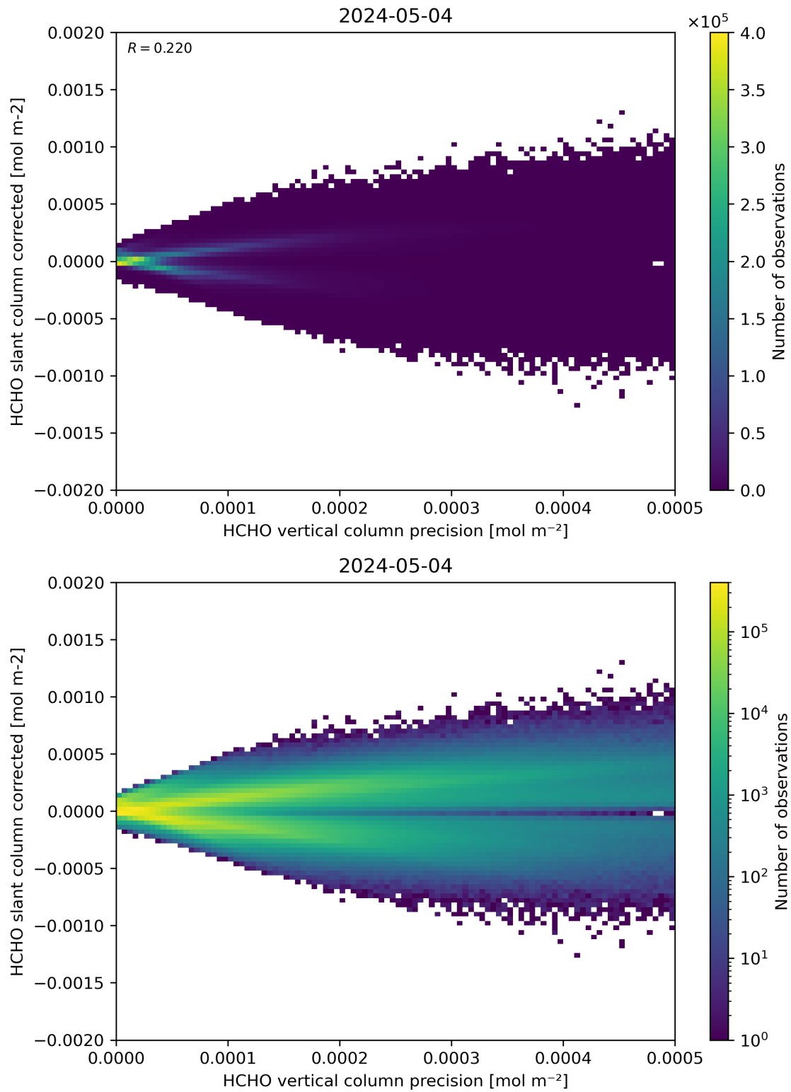
Figure 140: Scatter density plot of “HCHO vertical column precision” against “HCHO slant column corrected” for 2024-05-03 to 2024-05-05.
