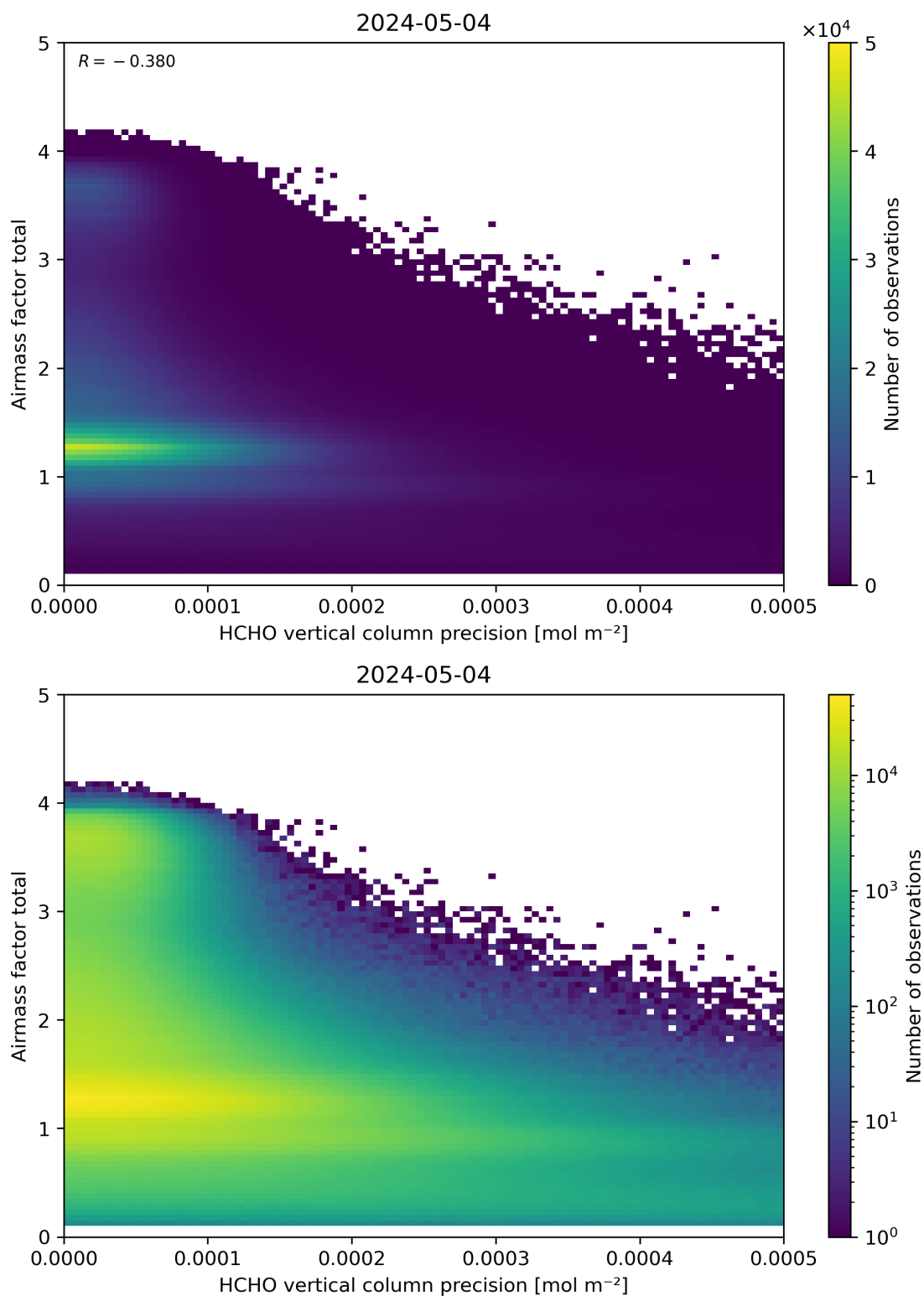
Figure 144: Scatter density plot of “HCHO vertical column precision” against “Airmass factor total” for 2024-05-03 to 2024-05-05.
