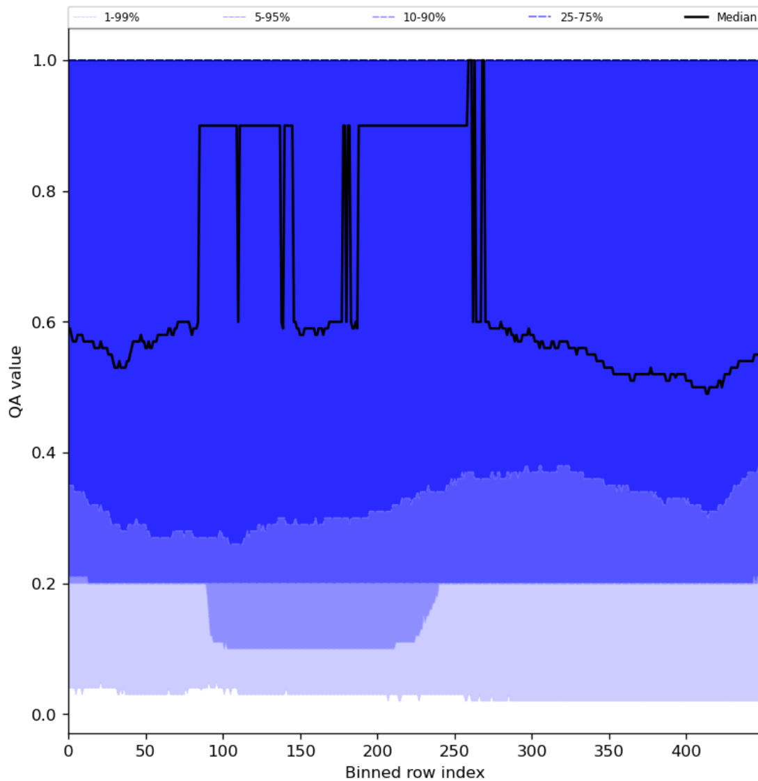
Figure 48: Along track statistics of “QA value” for 2024-05-03 to 2024-05-05
