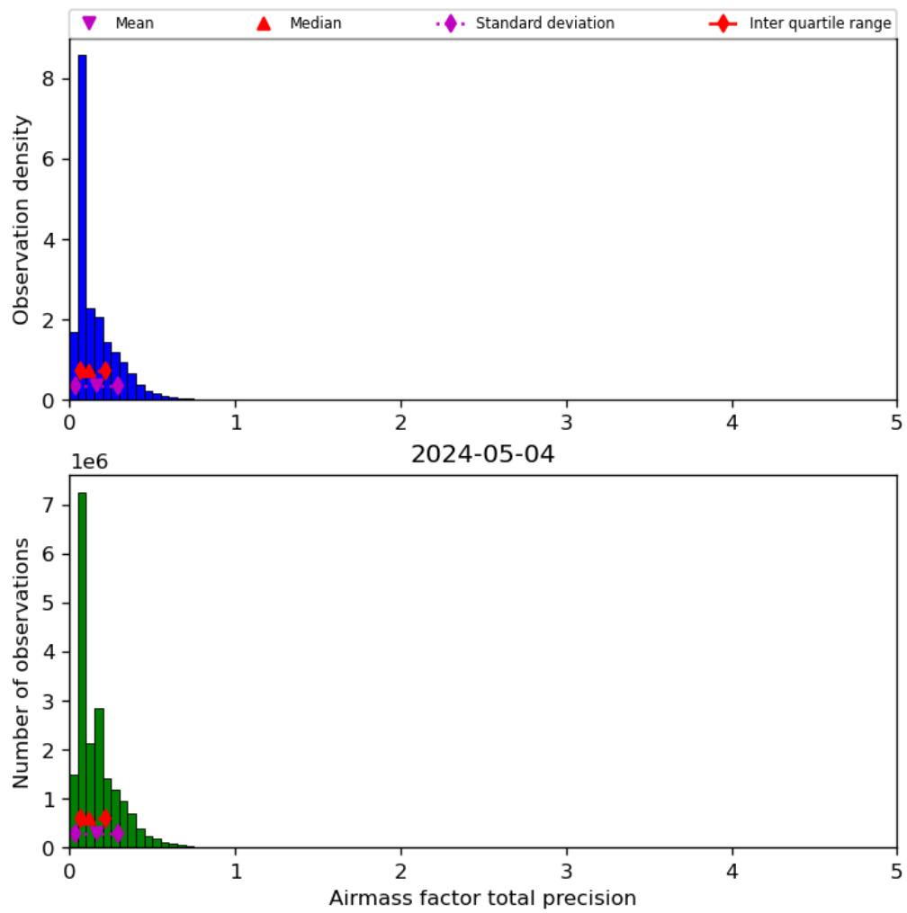
Figure 41: Histogram of “Airmass factor total precision” for 2024-05-03 to 2024-05-05
