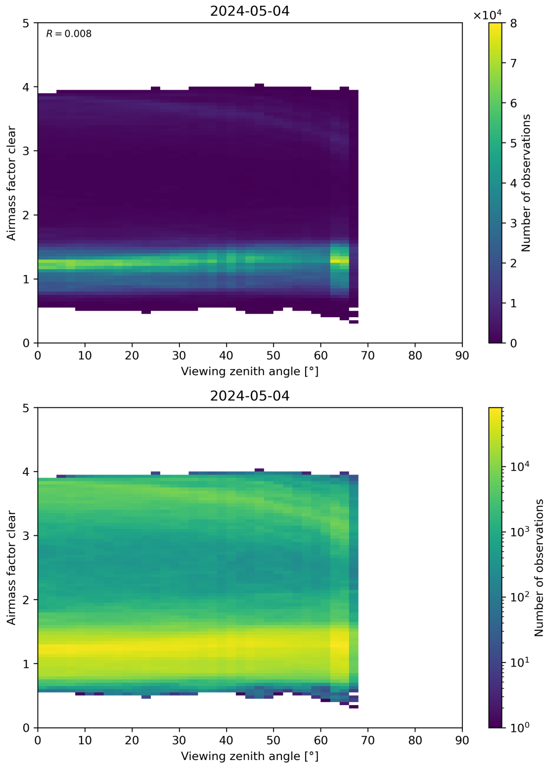
Figure 185: Scatter density plot of “Viewing zenith angle” against “Airmass factor clear” for 2024-05-03 to 2024-05-05.
