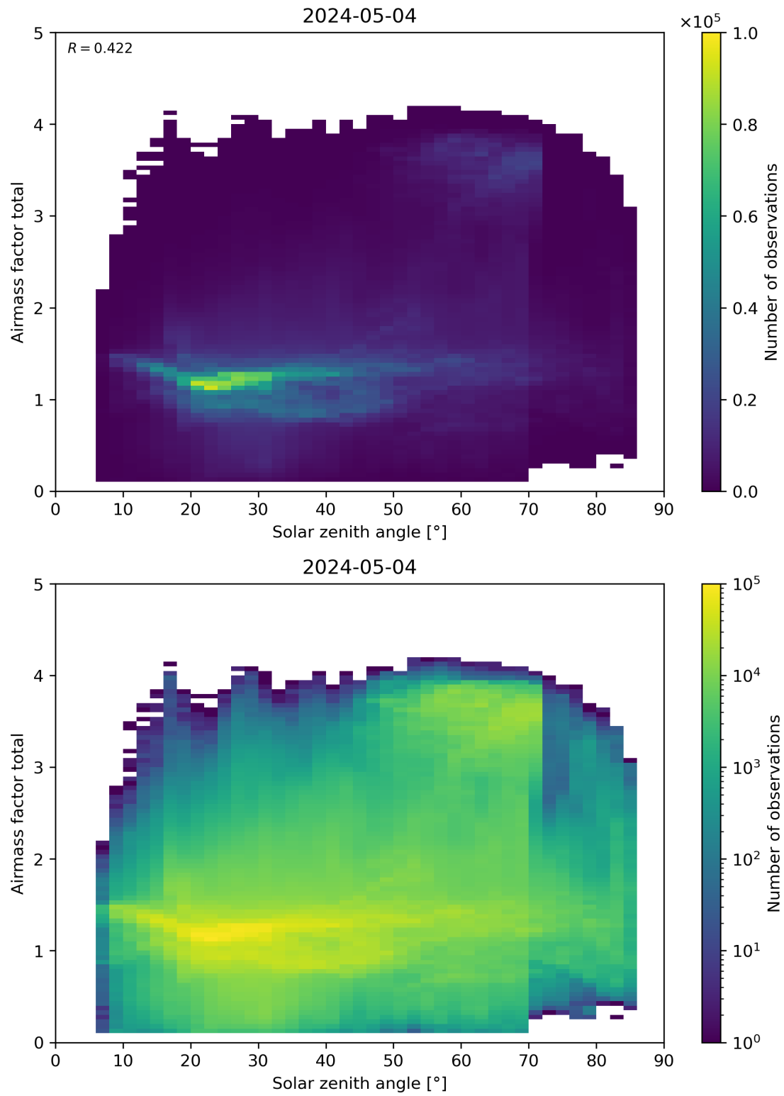
Figure 175: Scatter density plot of “Solar zenith angle” against “Airmass factor total” for 2024-05-03 to 2024-05-05.
