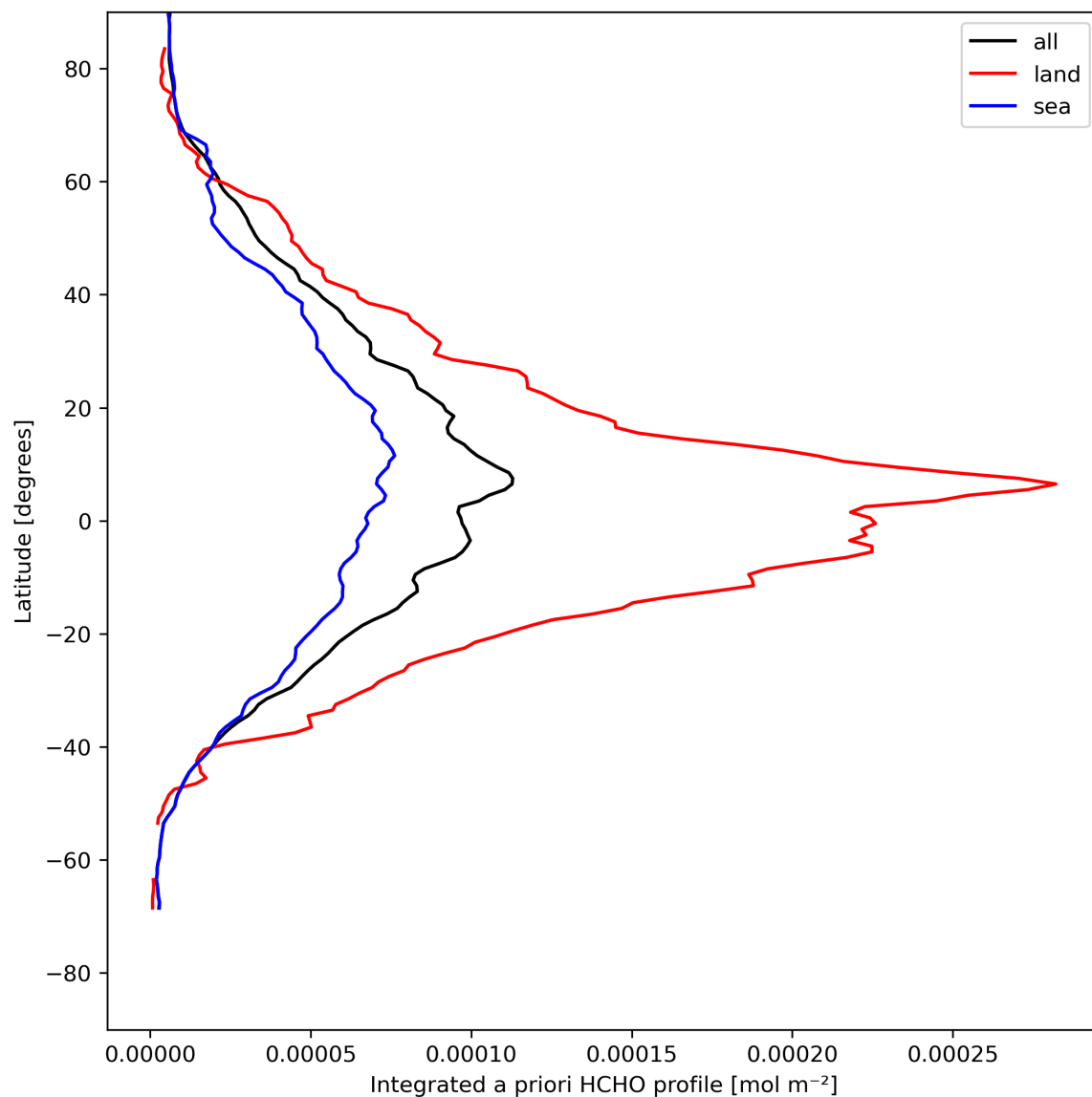
Figure 29: Zonal average of “Integrated a priori HCHO profile” for 2024-05-03 to 2024-05-05.
