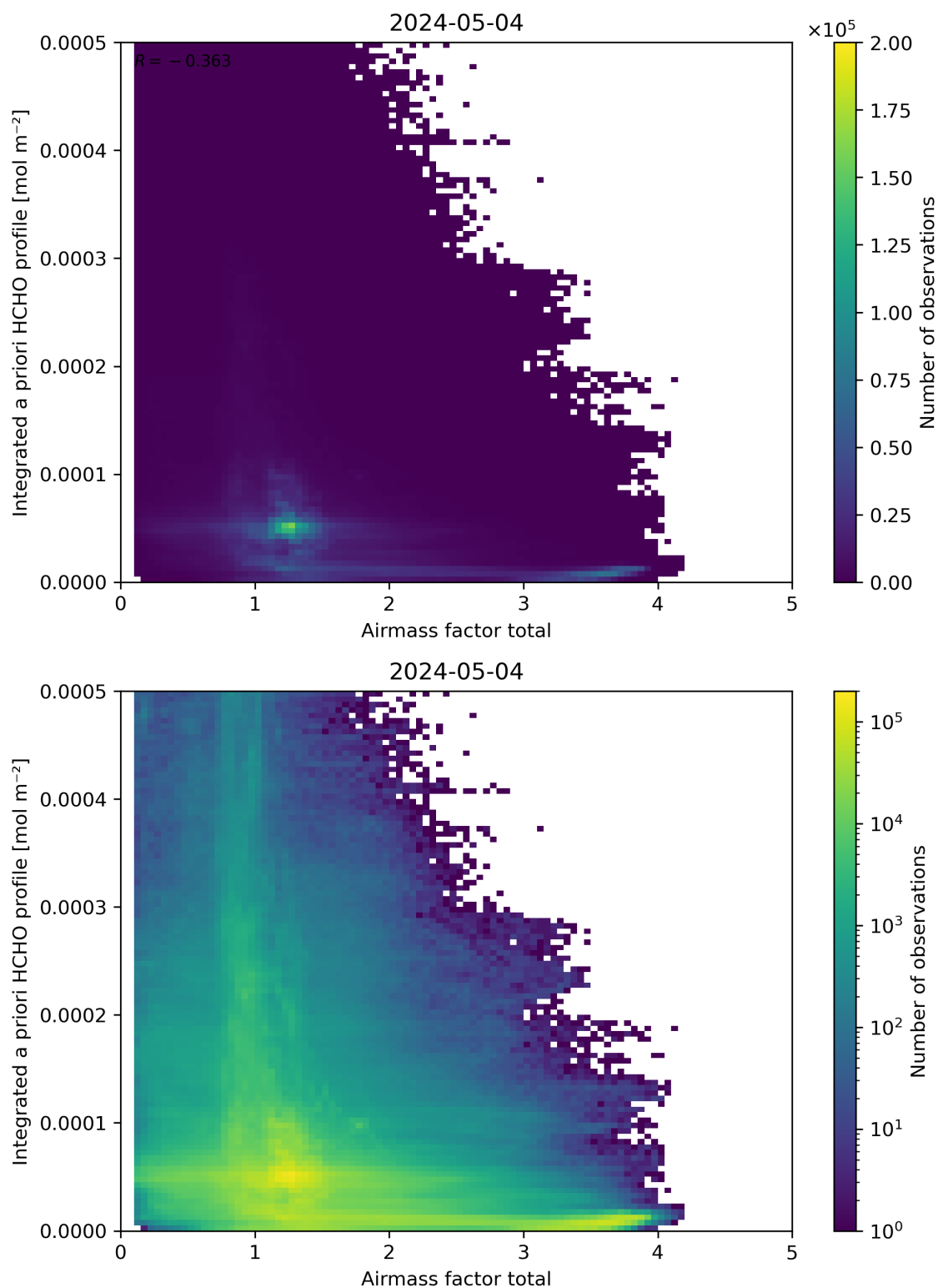
Figure 104: Scatter density plot of “Airmass factor total” against “Integrated a priori HCHO profile” for 2024-05-03 to 2024-05-05.
