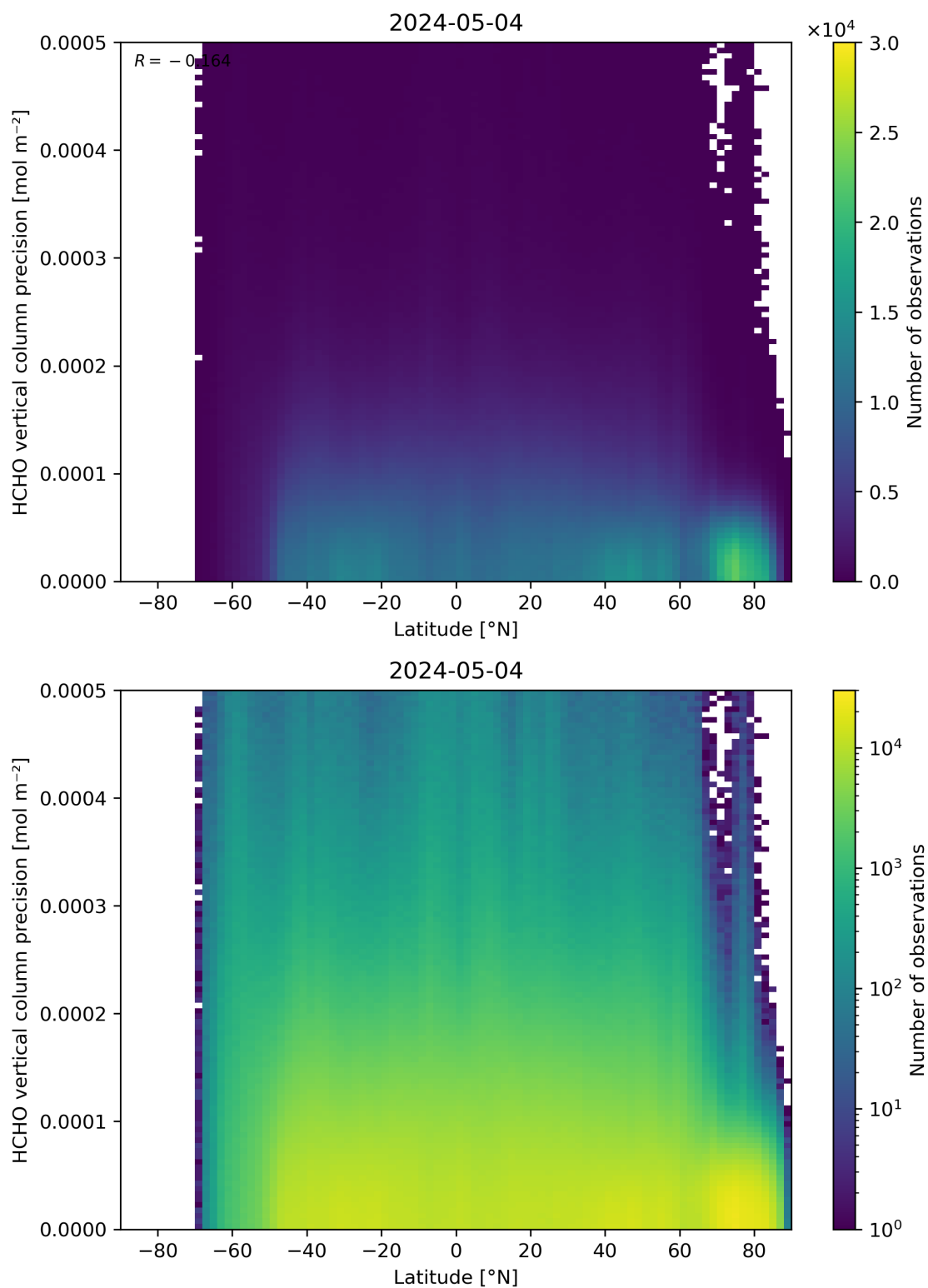
Figure 165: Scatter density plot of “Latitude” against “HCHO vertical column precision” for 2024-05-03 to 2024-05-05.
