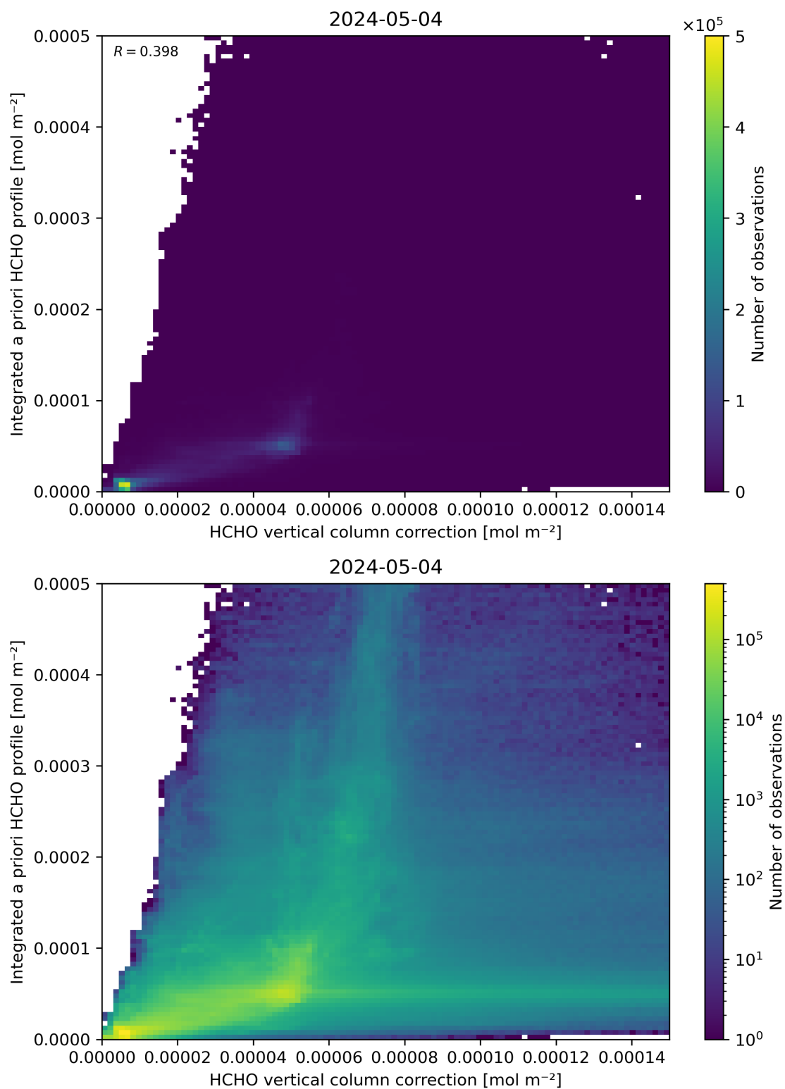
Figure 122: Scatter density plot of “HCHO vertical column correction” against “Integrated a priori HCHO profile” for 2024-05-03 to 2024-05-05.
