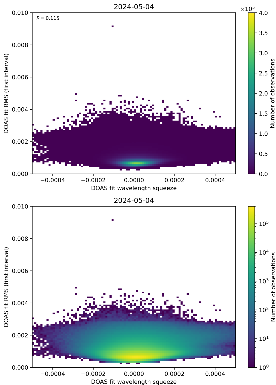
Figure 68: Scatter density plot of “DOAS fit wavelength squeeze” against “DOAS fit RMS (first interval)” for 2024-05-03 to 2024-05-05.
