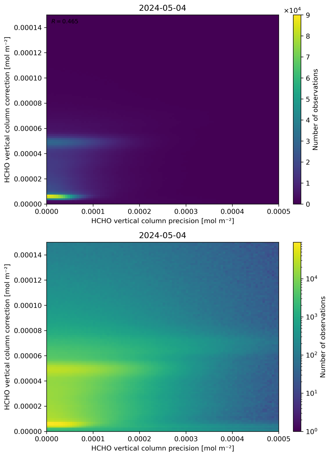
Figure 146: Scatter density plot of “HCHO vertical column precision” against “HCHO vertical column correction” for 2024-05-03 to 2024-05-05.
