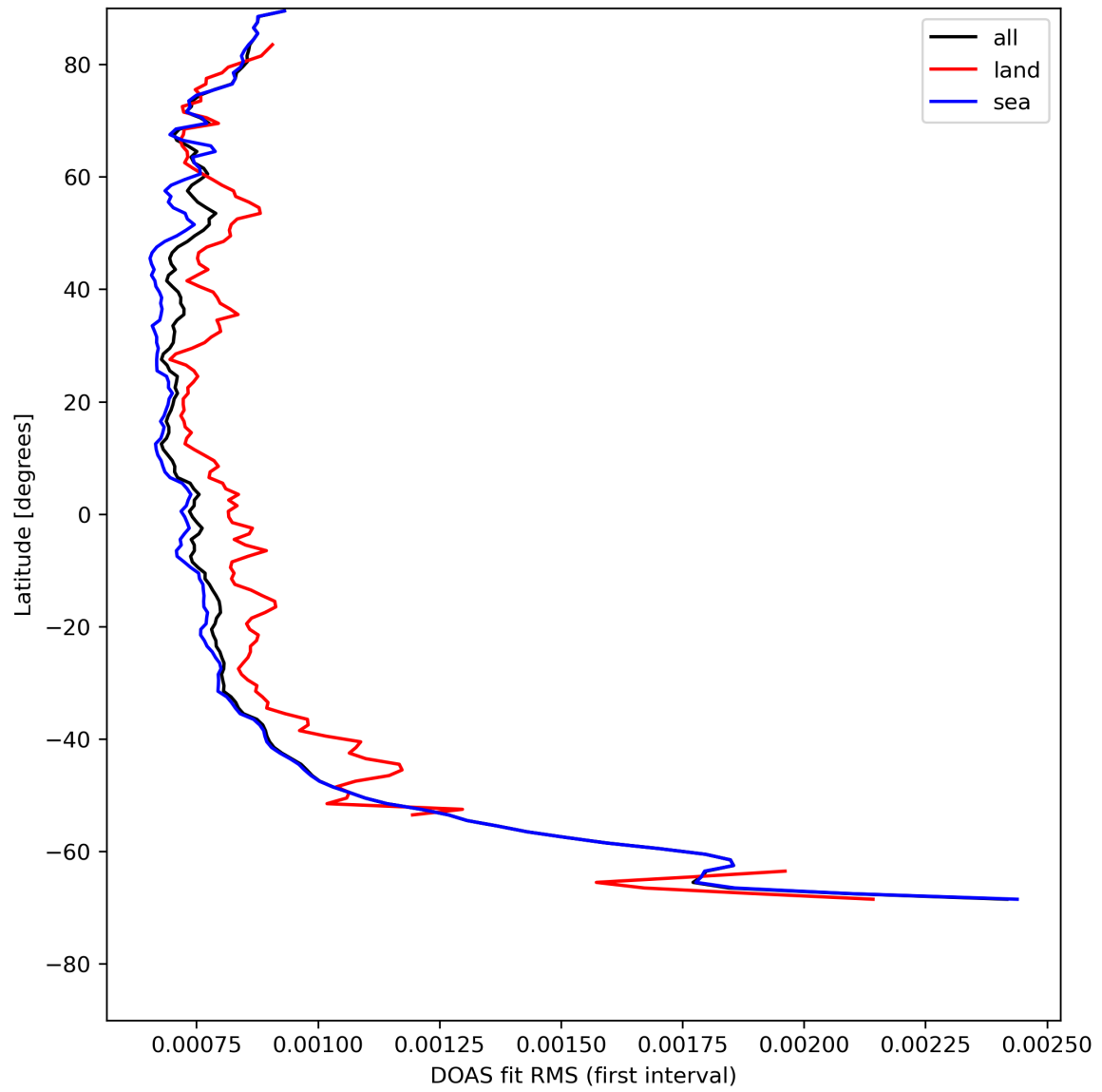
Figure 32: Zonal average of “DOAS fit RMS (first interval)” for 2024-05-03 to 2024-05-05.
