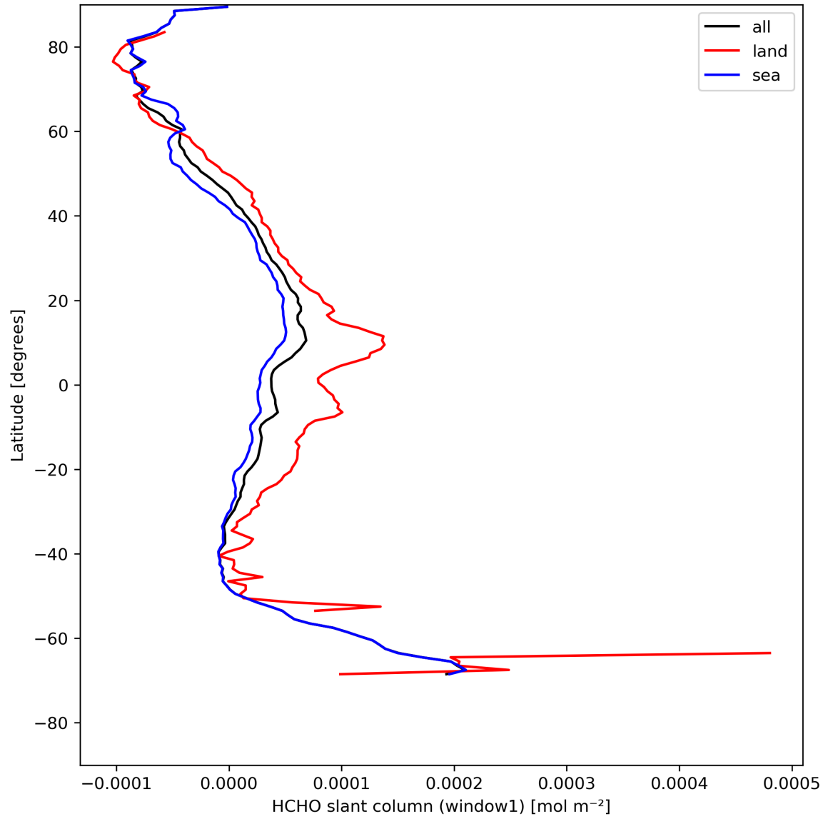
Figure 24: Zonal average of “HCHO slant column (window1)” for 2024-05-03 to 2024-05-05.
