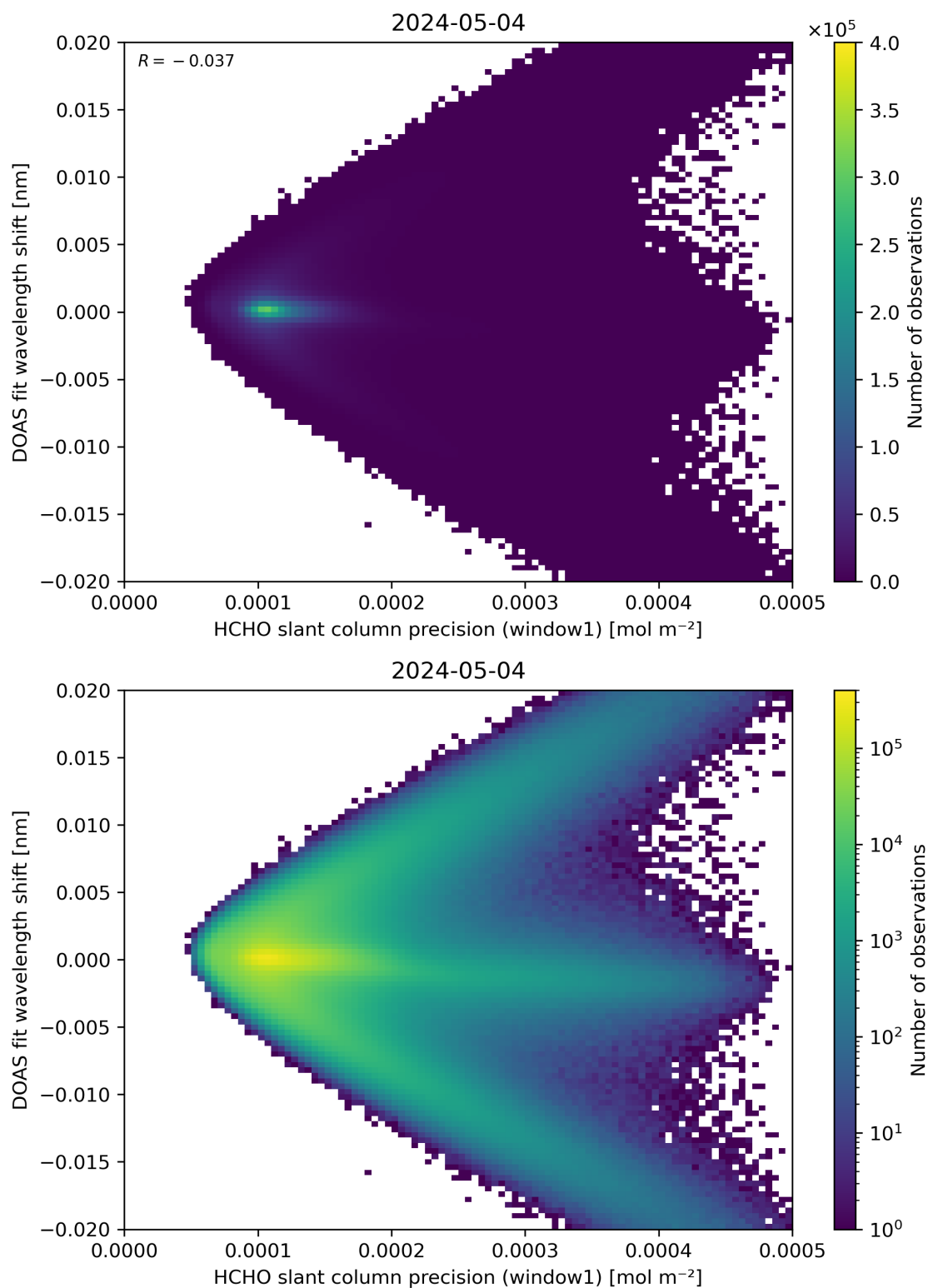
Figure 89: Scatter density plot of “HCHO slant column precision (window1)” against “DOAS fit wavelength shift” for 2024-05-03 to 2024-05-05.
