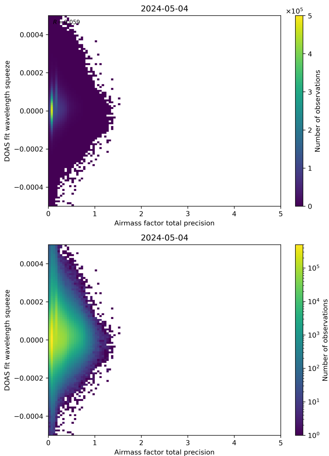
Figure 107: Scatter density plot of “Airmass factor total precision” against “DOAS fit wavelength squeeze” for 2024-05-03 to 2024-05-05.
