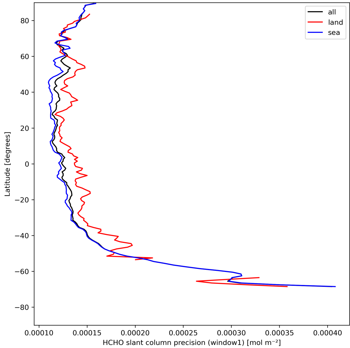
Figure 25: Zonal average of "HCHO slant column precision (window1)" for 2024-05-03 to 2024-05-05.
