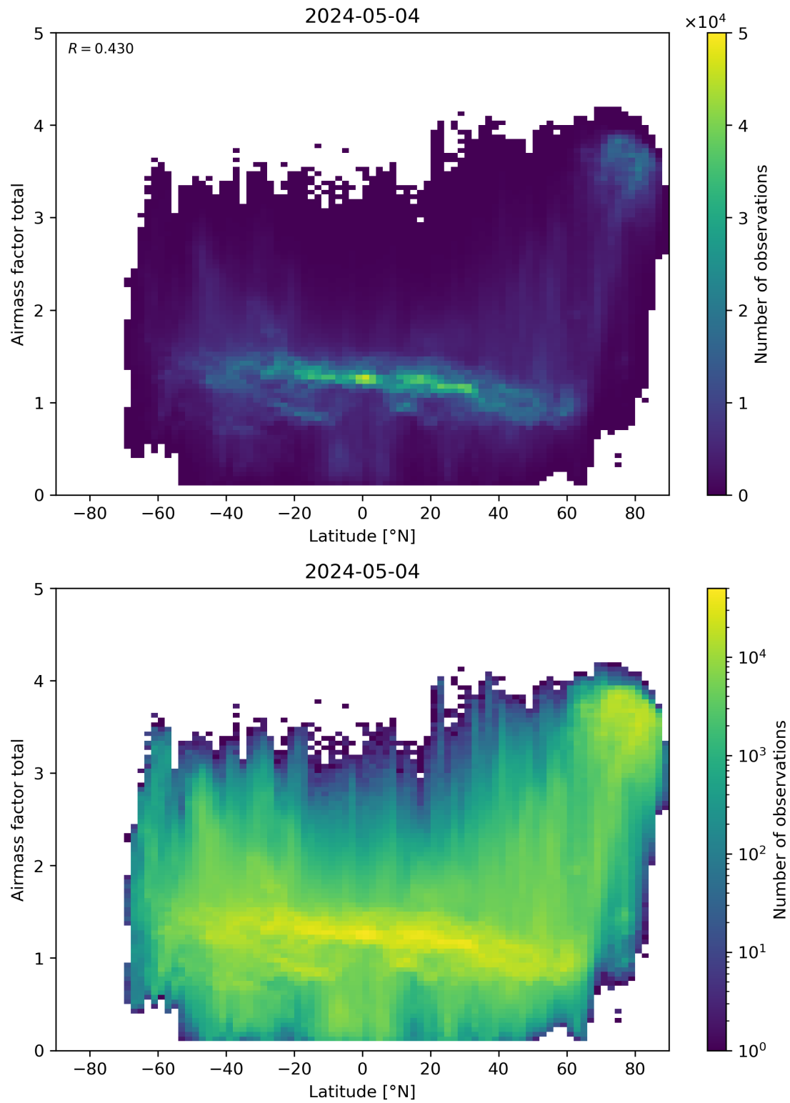
Figure 161: Scatter density plot of “Latitude” against “Airmass factor total” for 2024-05-03 to 2024-05-05.
