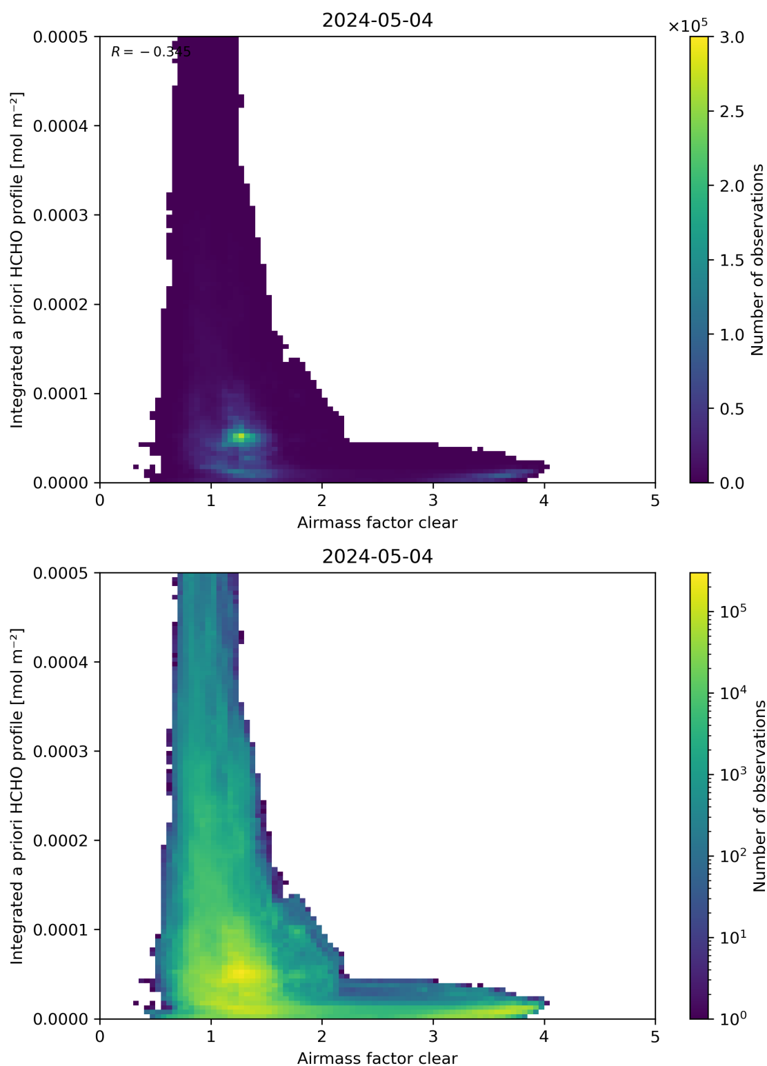
Figure 76: Scatter density plot of “Airmass factor clear” against “Integrated a priori HCHO profile” for 2024-05-03 to 2024-05-05.
