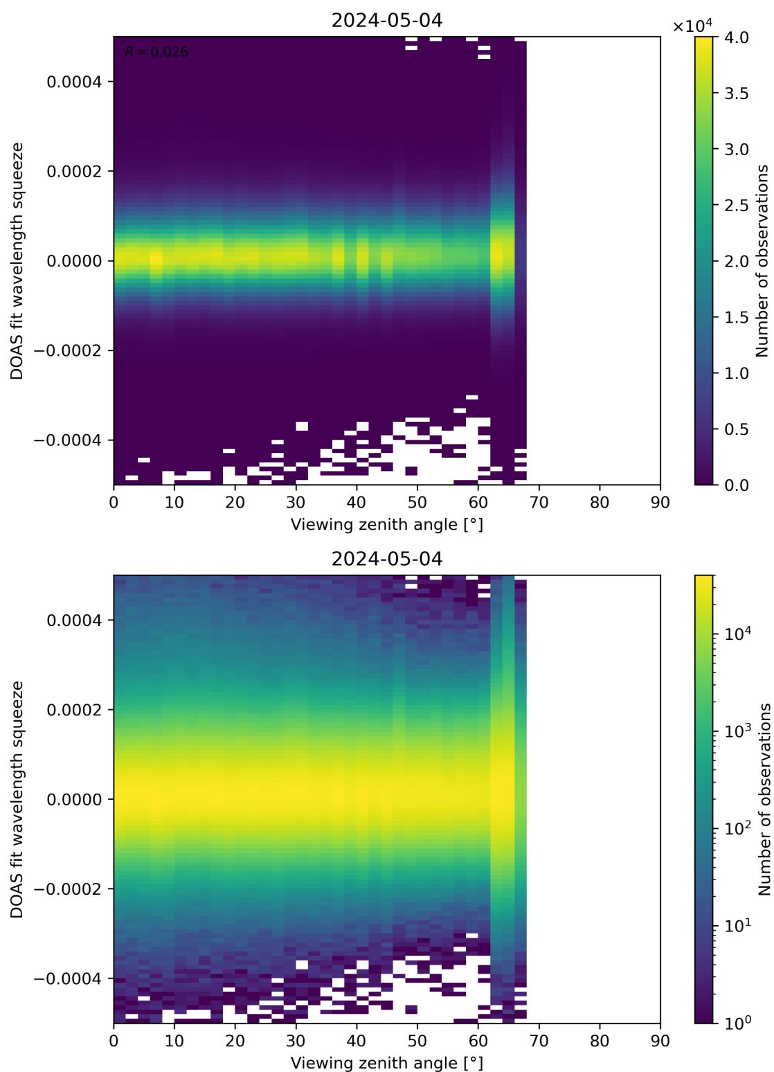
Figure 184: Scatter density plot of “Viewing zenith angle” against “DOAS fit wavelength squeeze” for 2024-05-03 to 2024-05-05.
