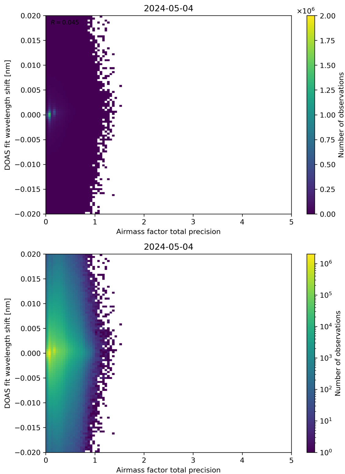
Figure 106: Scatter density plot of “Airmass factor total precision” against “DOAS fit wavelength shift” for 2024-05-03 to 2024-05-05.
