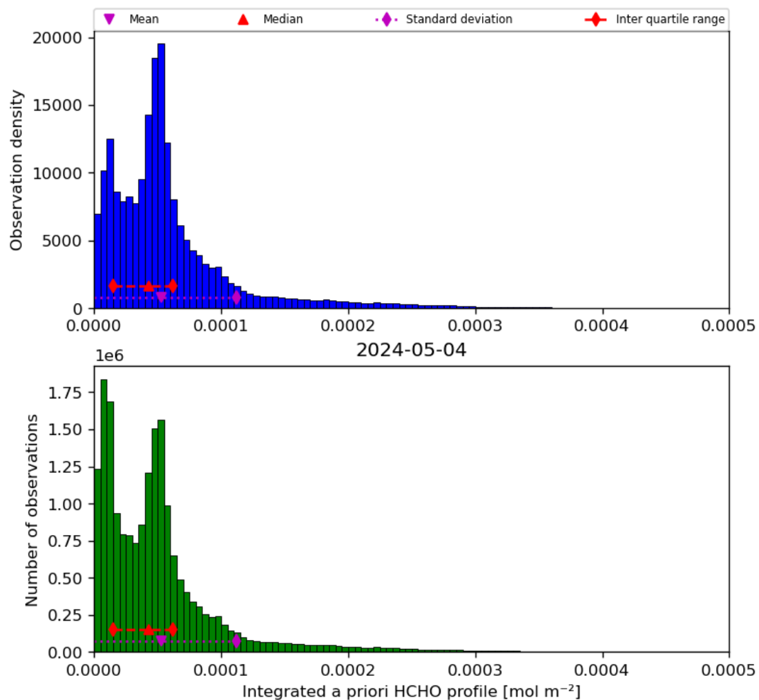
Figure 43: Histogram of “Integrated a priori HCHO profile” for 2024-05-03 to 2024-05-05
