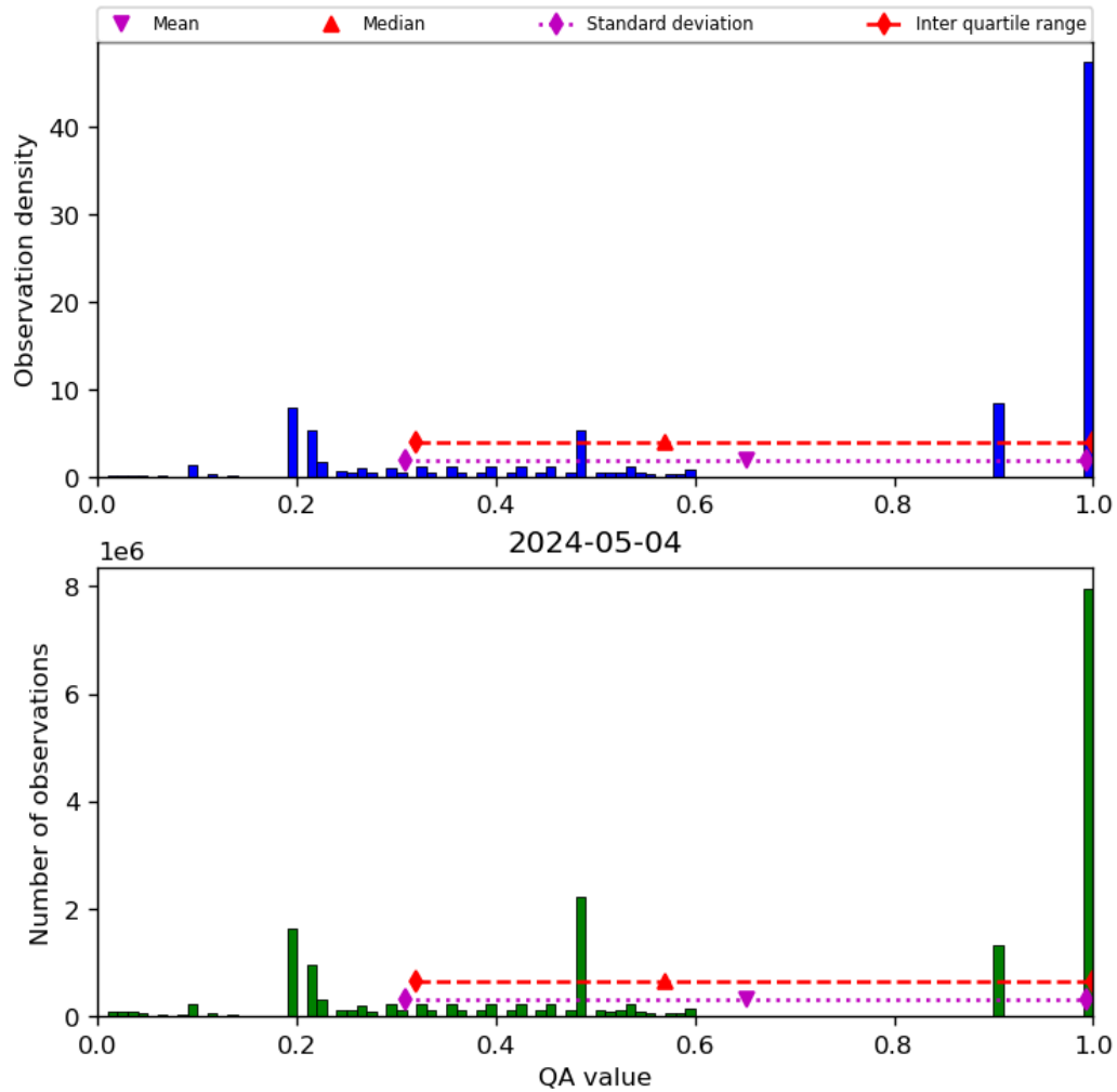
Figure 34: Histogram of “QA value” for 2024-05-03 to 2024-05-05
