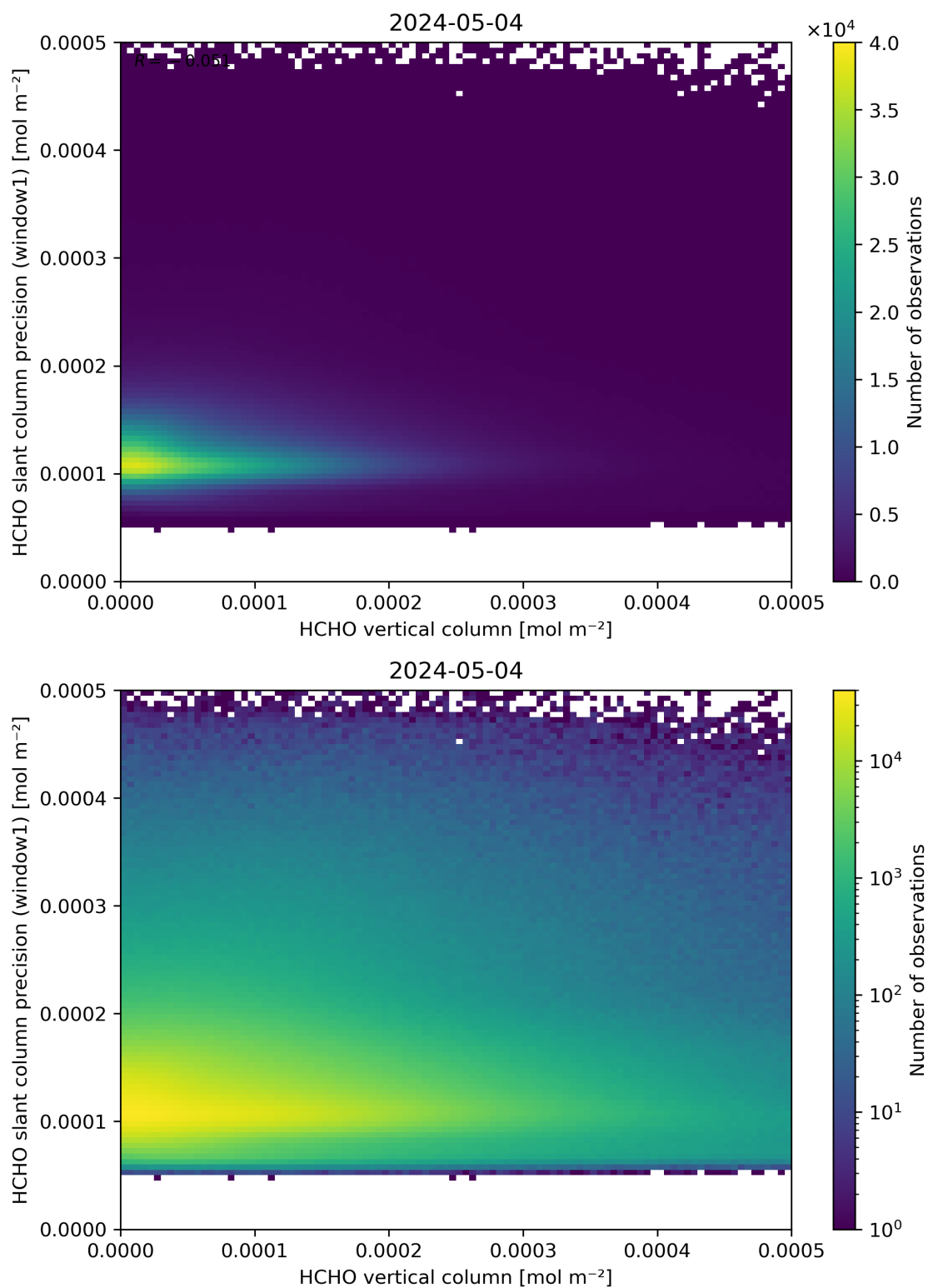
Figure 130: Scatter density plot of “HCHO vertical column” against “HCHO slant column precision (window1)” for 2024-05-03 to 2024-05-05.
