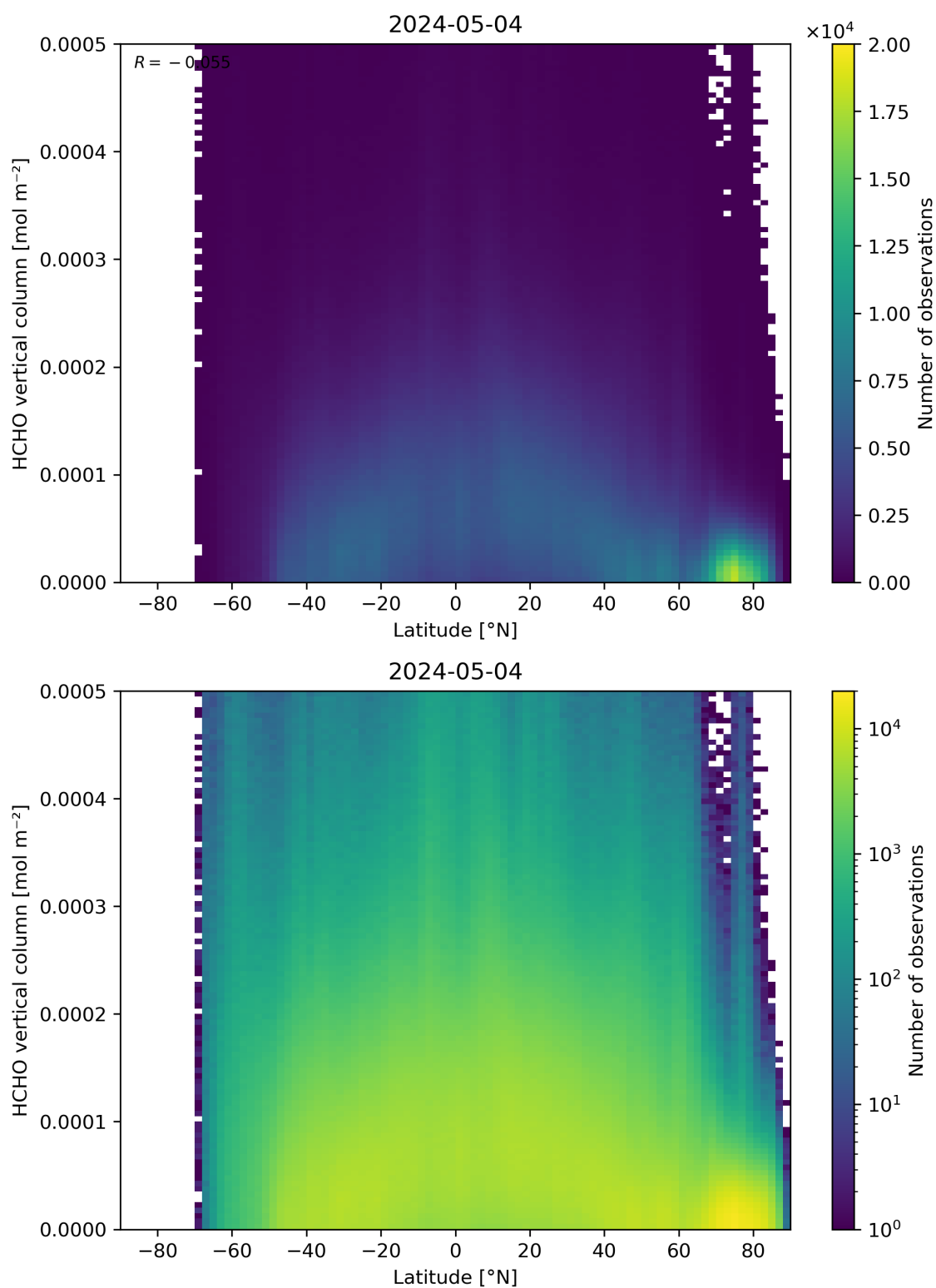
Figure 163: Scatter density plot of “Latitude” against “HCHO vertical column” for 2024-05-03 to 2024-05-05.
