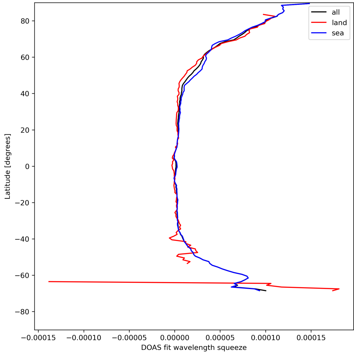
Figure 31: Zonal average of “DOAS fit wavelength squeeze” for 2024-05-03 to 2024-05-05.
