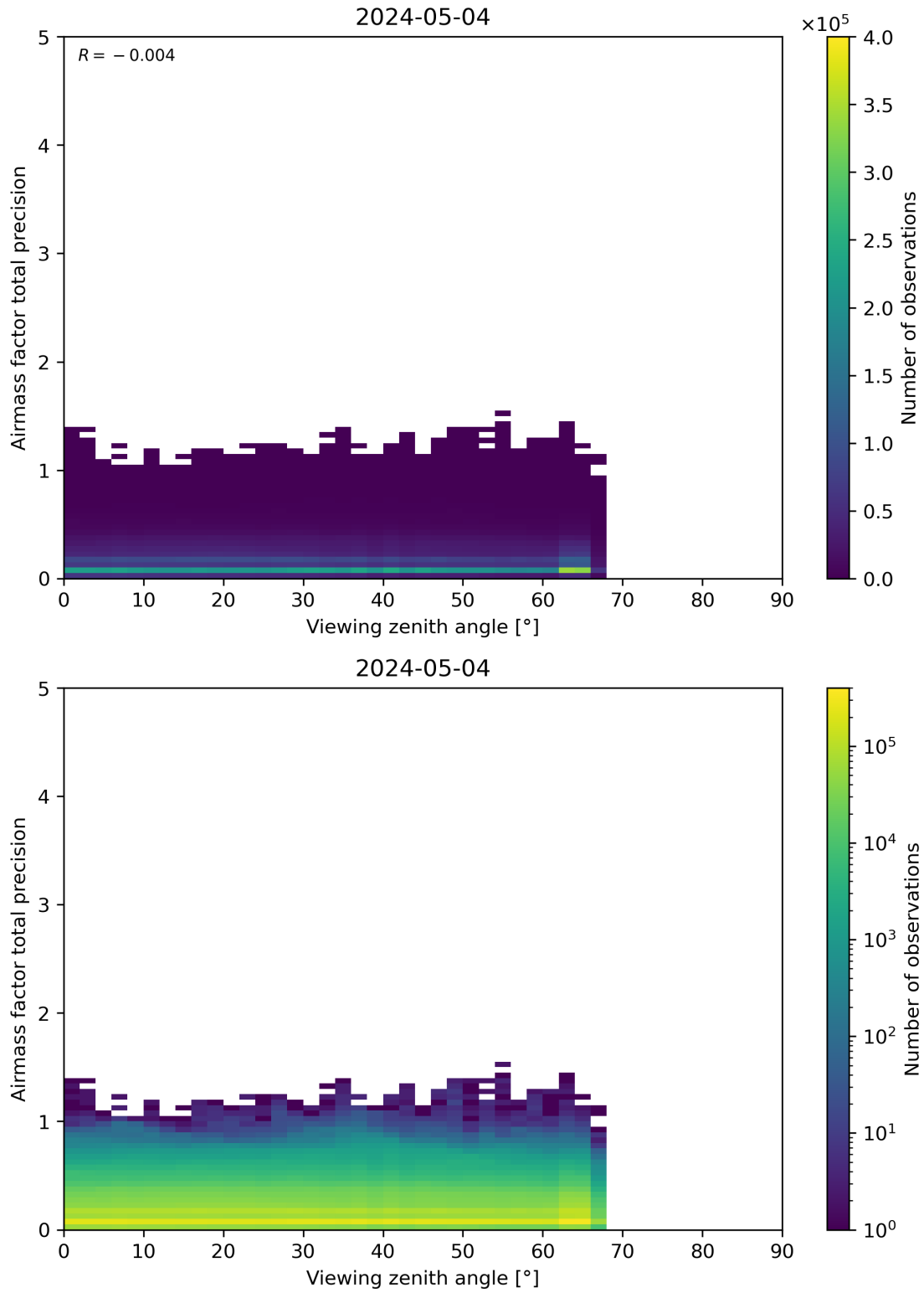
Figure 191: Scatter density plot of “Viewing zenith angle” against “Airmass factor total precision” for 2024-05-03 to 2024-05-05.
