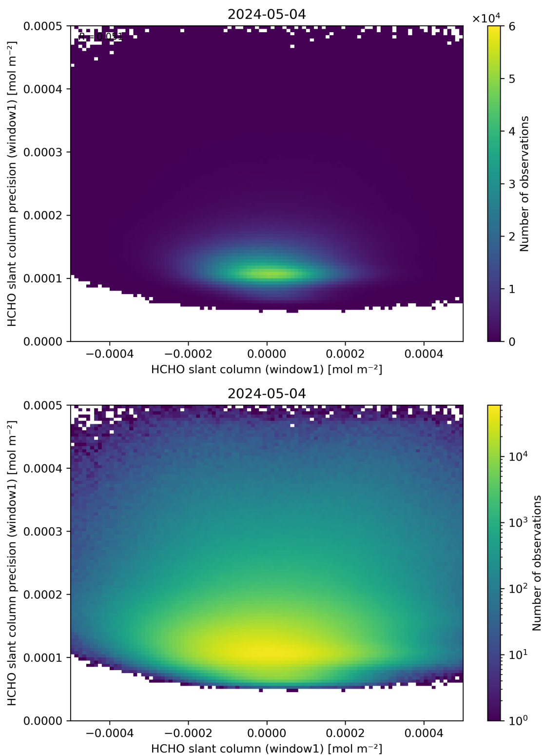
Figure 84: Scatter density plot of “HCHO slant column (window1)” against “HCHO slant column precision (window1)” for 2024-05-03 to 2024-05-05.
