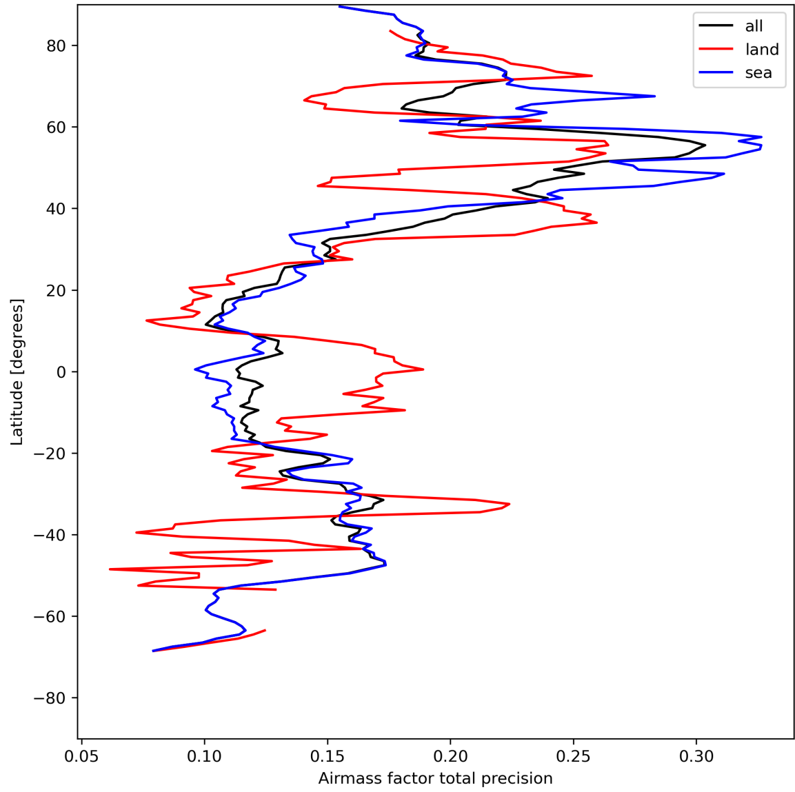
Figure 27: Zonal average of “Airmass factor total precision” for 2024-05-03 to 2024-05-05.
