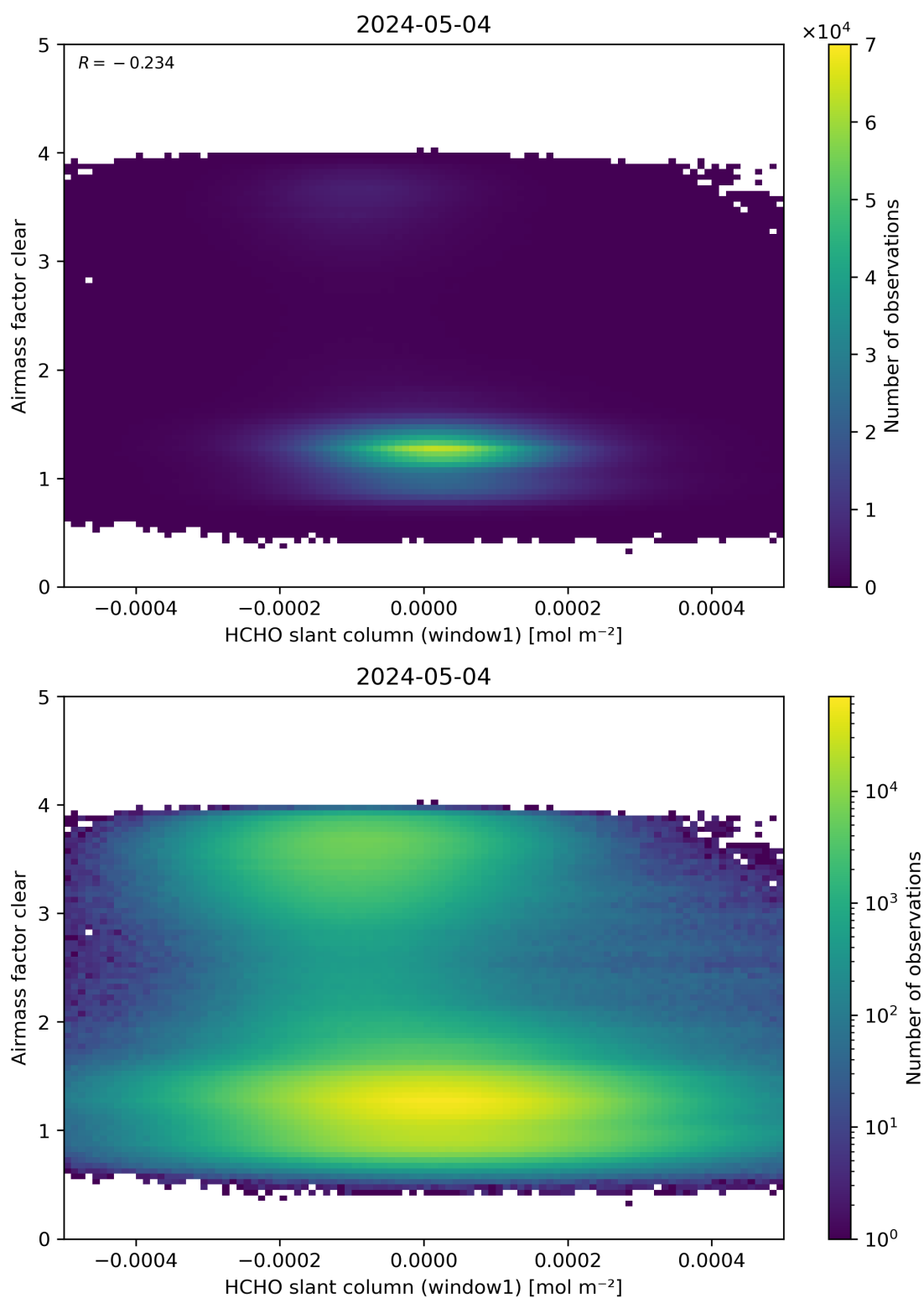
Figure 81: Scatter density plot of “HCHO slant column (window1)” against “Airmass factor clear” for 2024-05-03 to 2024-05-05.
