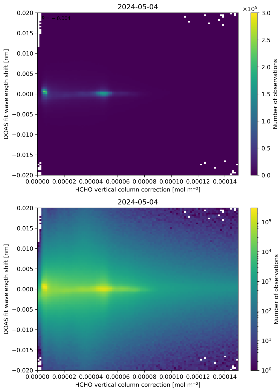
Figure 113: Scatter density plot of “HCHO vertical column correction” against “DOAS fit wavelength shift” for 2024-05-03 to 2024-05-05.
