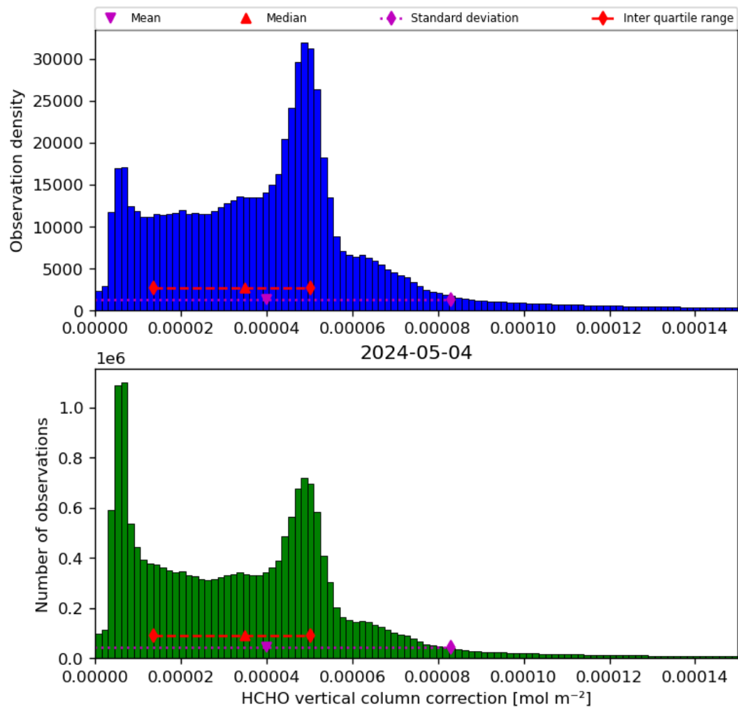
Figure 37: Histogram of “HCHO vertical column correction” for 2024-05-03 to 2024-05-05
