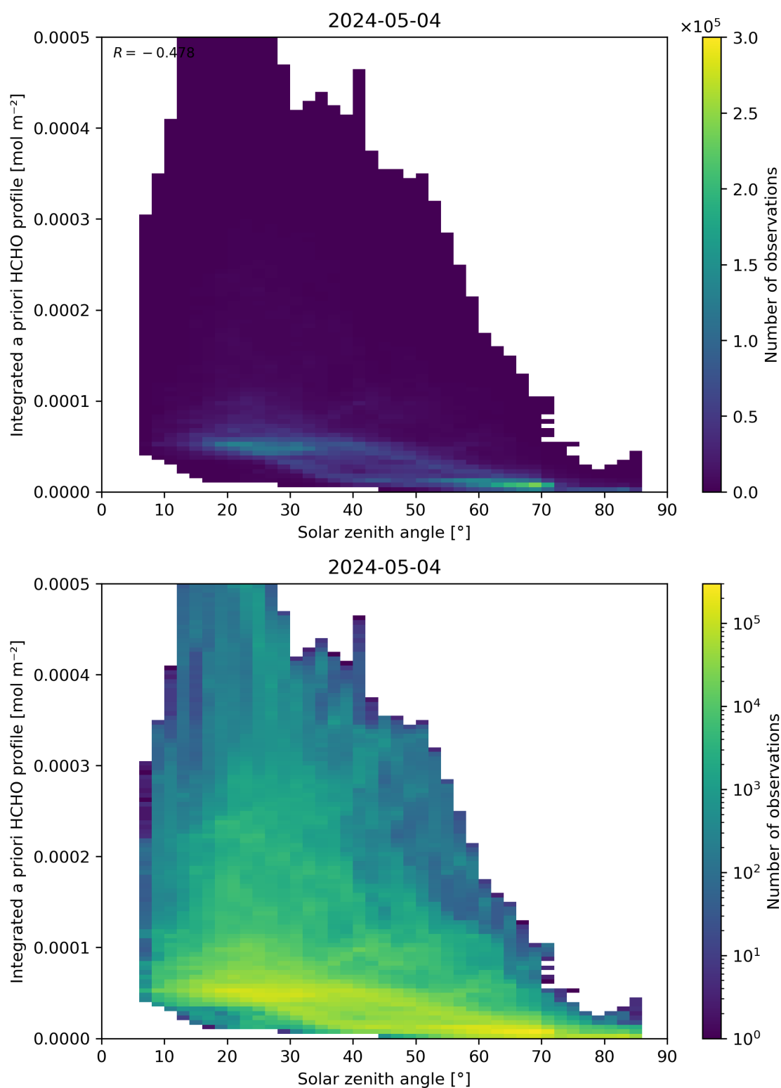
Figure 180: Scatter density plot of “Solar zenith angle” against “Integrated a priori HCHO profile” for 2024-05-03 to 2024-05-05.
