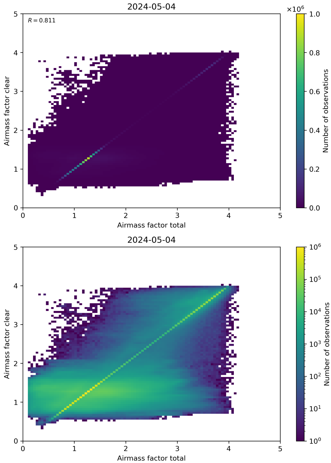
Figure 100: Scatter density plot of “Airmass factor total” against “Airmass factor clear” for 2024-05-03 to 2024-05-05.
