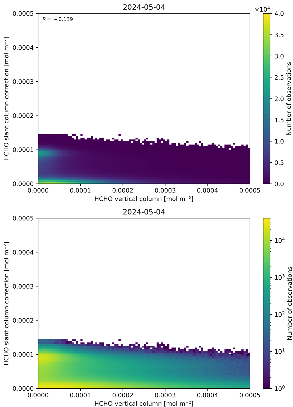
Figure 128: Scatter density plot of “HCHO vertical column” against “HCHO slant column correction” for 2024-05-03 to 2024-05-05.
