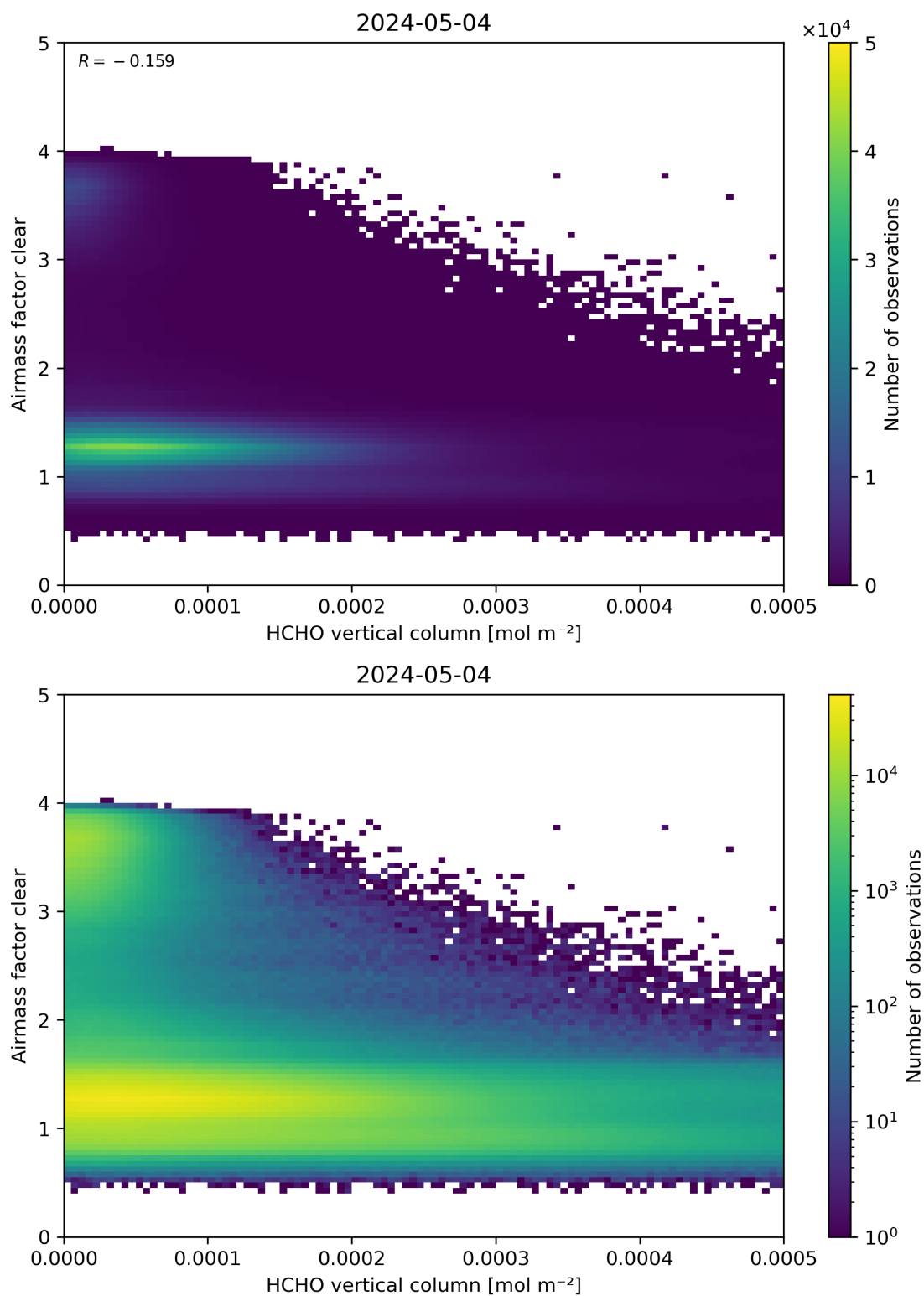
Figure 126: Scatter density plot of “HCHO vertical column” against “Airmass factor clear” for 2024-05-03 to 2024-05-05.
