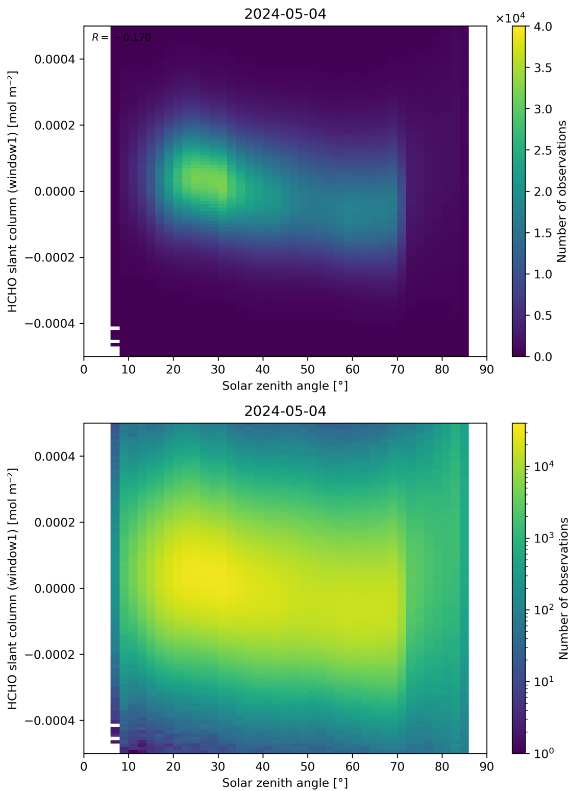
Figure 173: Scatter density plot of “Solar zenith angle” against “HCHO slant column (window1)” for 2024-05-03 to 2024-05-05.
