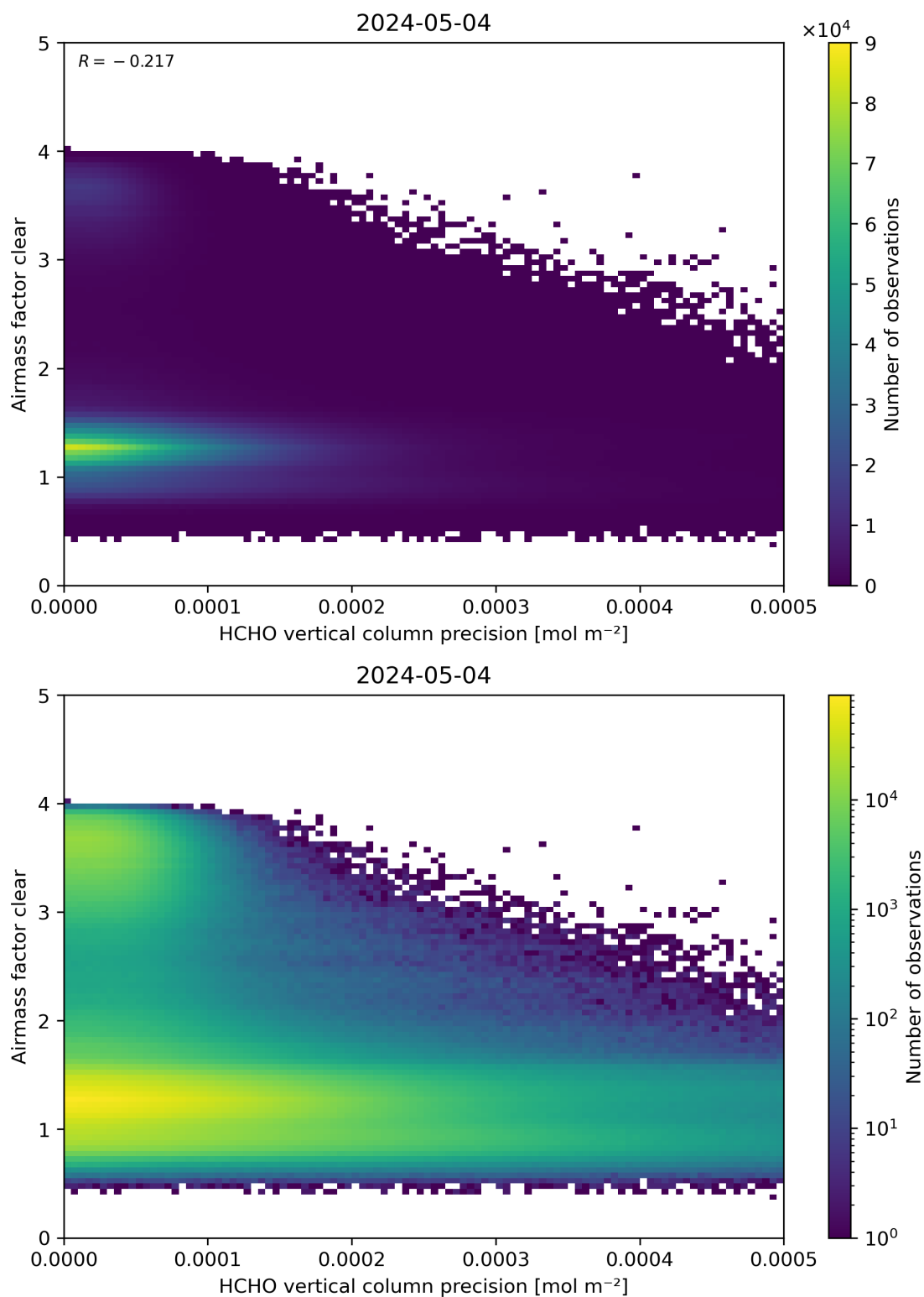
Figure 139: Scatter density plot of “HCHO vertical column precision” against “Airmass factor clear” for 2024-05-03 to 2024-05-05.
