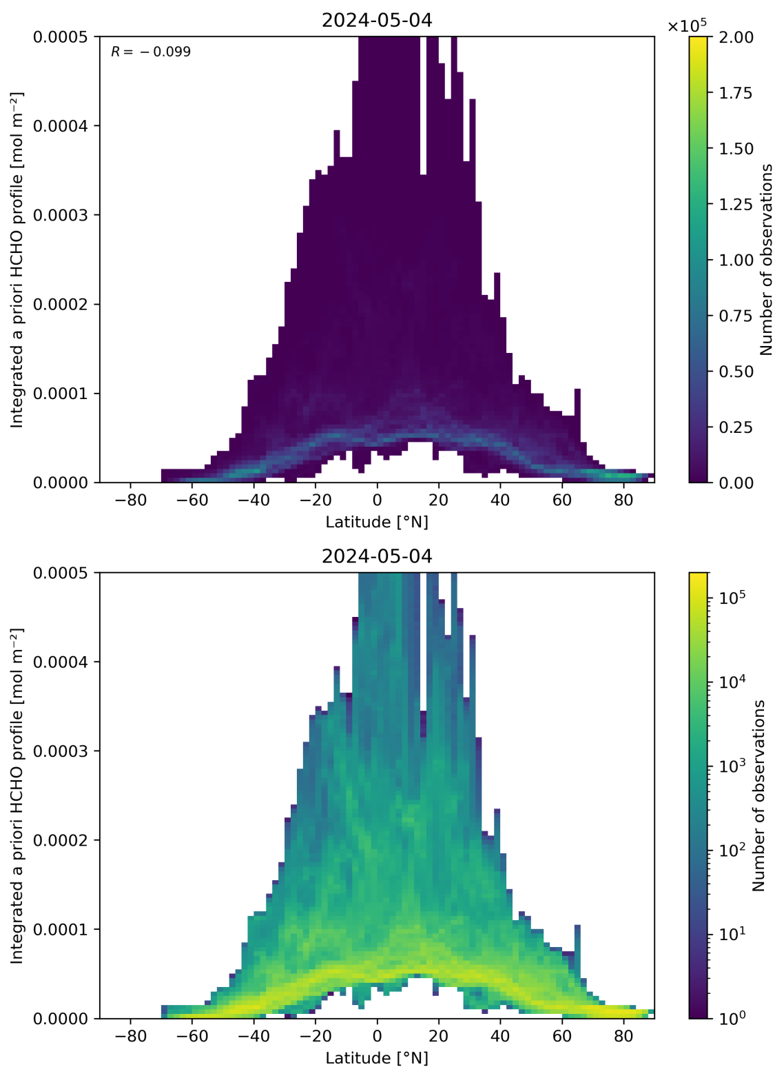
Figure 166: Scatter density plot of “Latitude” against “Integrated a priori HCHO profile” for 2024-05-03 to 2024-05-05.
