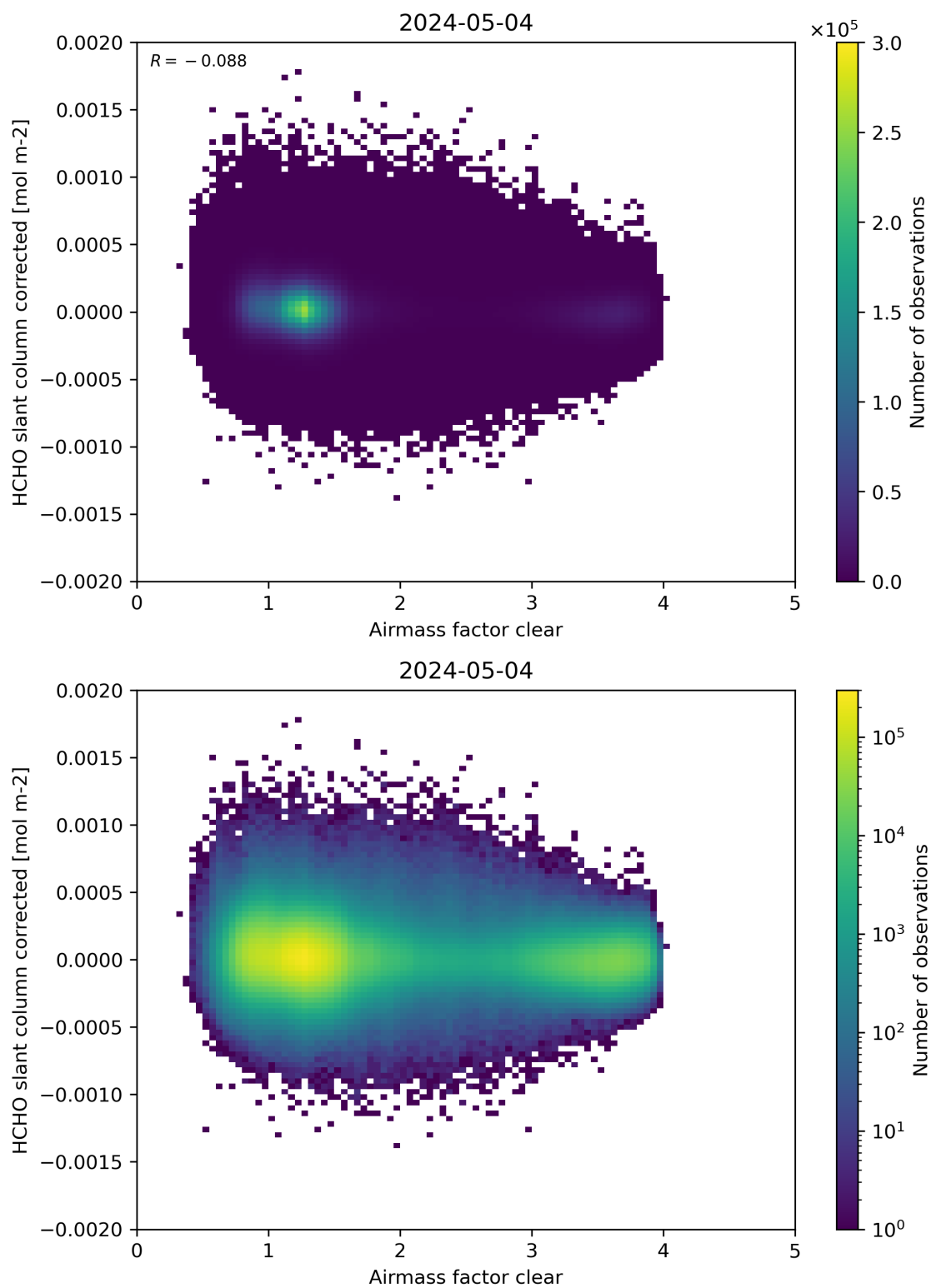
Figure 74: Scatter density plot of “Airmass factor clear” against “HCHO slant column corrected” for 2024-05-03 to 2024-05-05.
