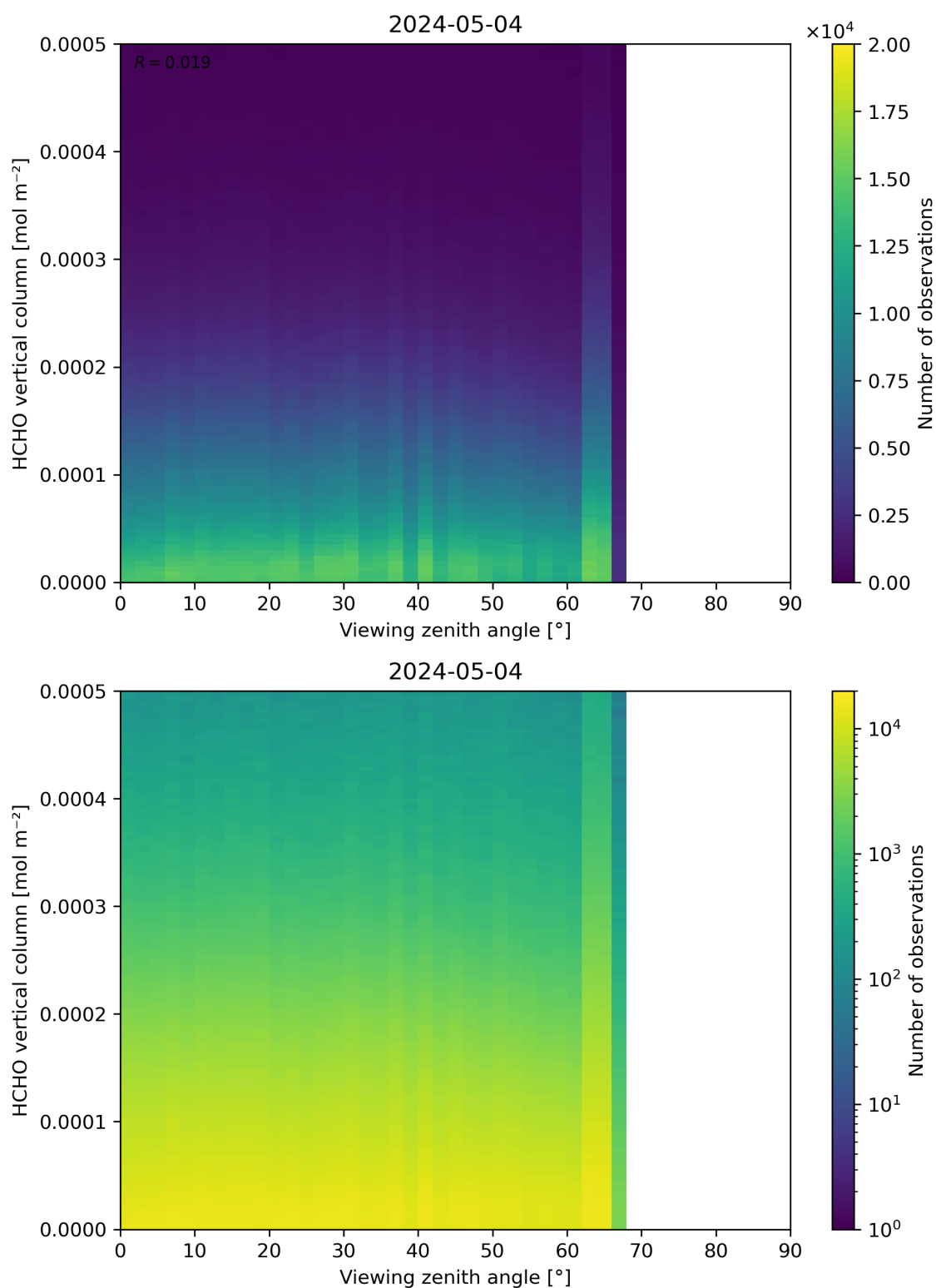
Figure 192: Scatter density plot of “Viewing zenith angle” against “HCHO vertical column” for 2024-05-03 to 2024-05-05.
