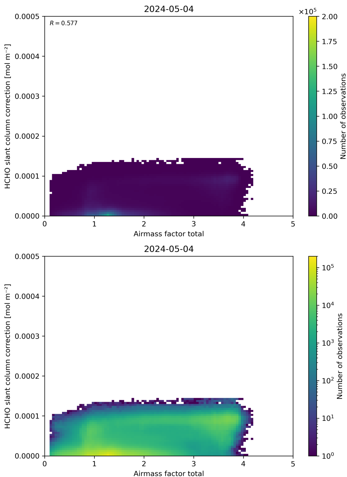
Figure 102: Scatter density plot of “Airmass factor total” against “HCHO slant column correction” for 2024-05-03 to 2024-05-05.
