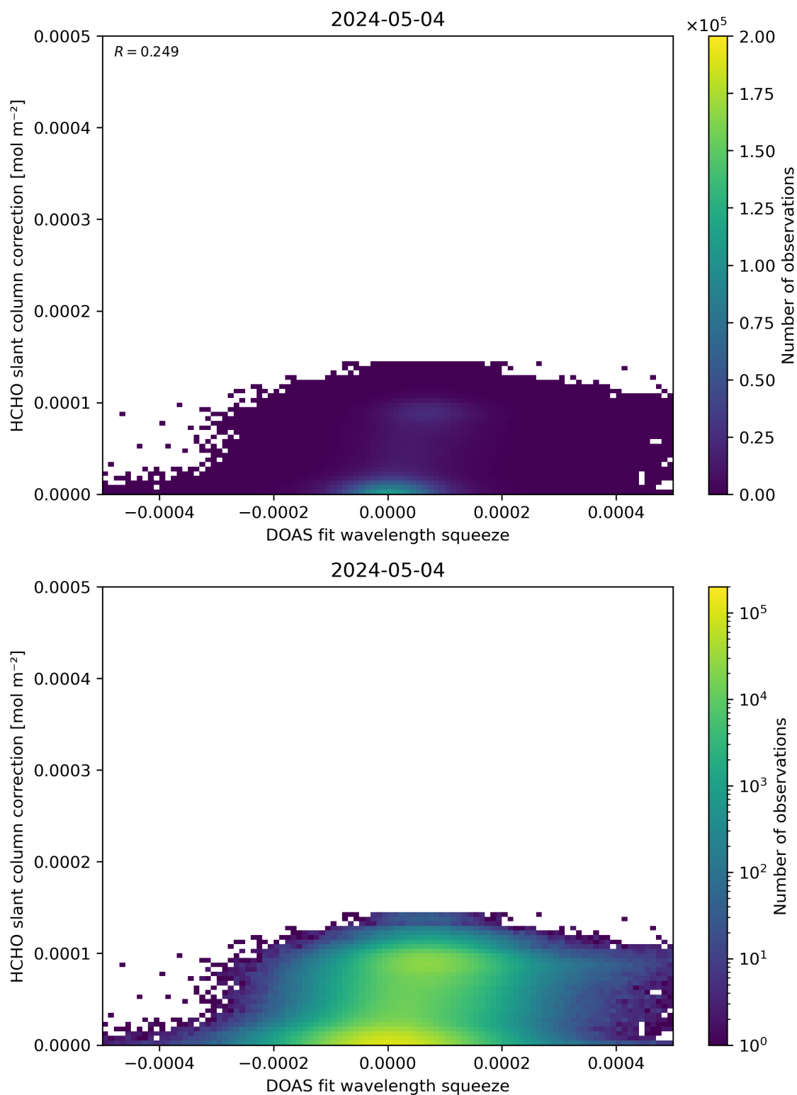
Figure 70: Scatter density plot of “DOAS fit wavelength squeeze” against “HCHO slant column correction” for 2024-05-03 to 2024-05-05.
