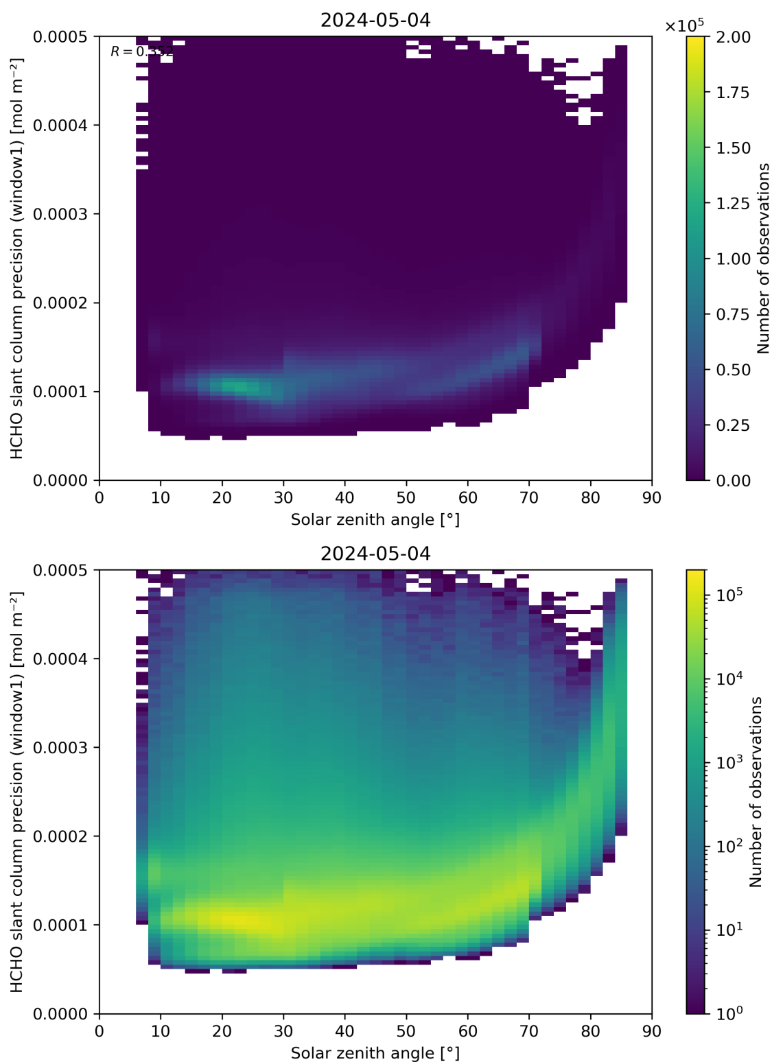
Figure 174: Scatter density plot of “Solar zenith angle” against “HCHO slant column precision (window1)” for 2024-05-03 to 2024-05-05.
