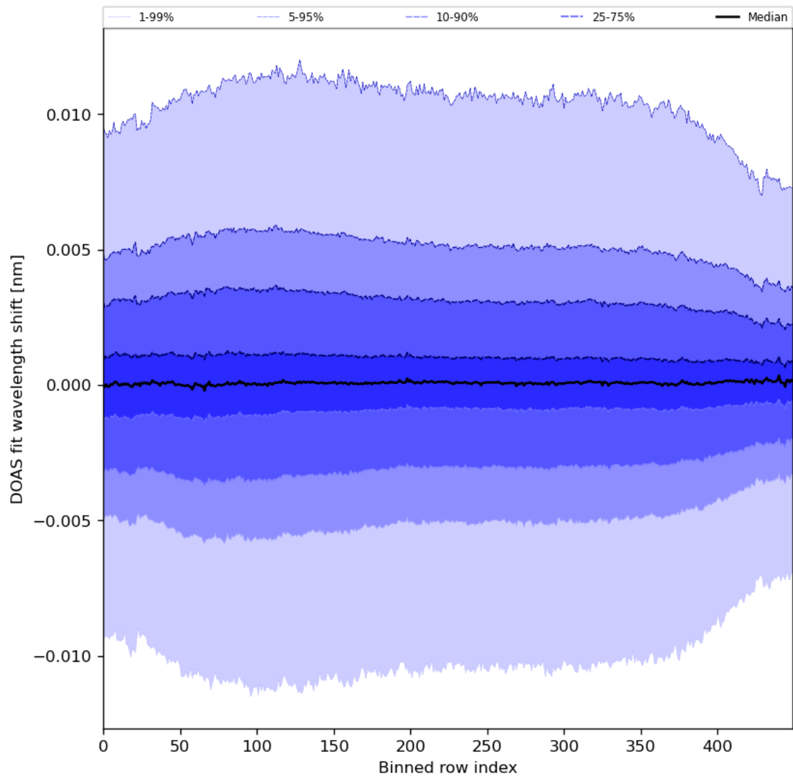
Figure 58: Along track statistics of “DOAS fit wavelength shift” for 2024-05-03 to 2024-05-05
