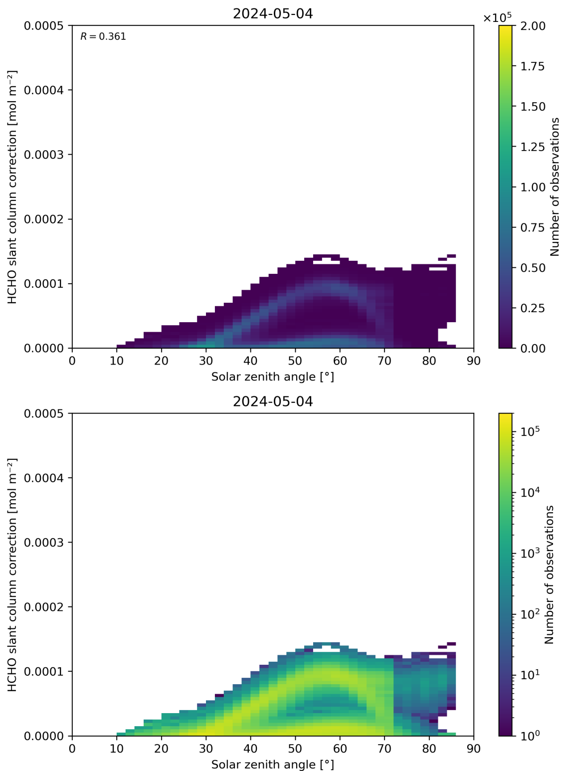
Figure 172: Scatter density plot of “Solar zenith angle” against “HCHO slant column correction” for 2024-05-03 to 2024-05-05.
