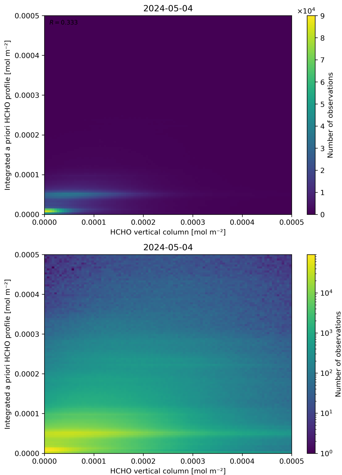
Figure 135: Scatter density plot of “HCHO vertical column” against “Integrated a priori HCHO profile” for 2024-05-03 to 2024-05-05.
