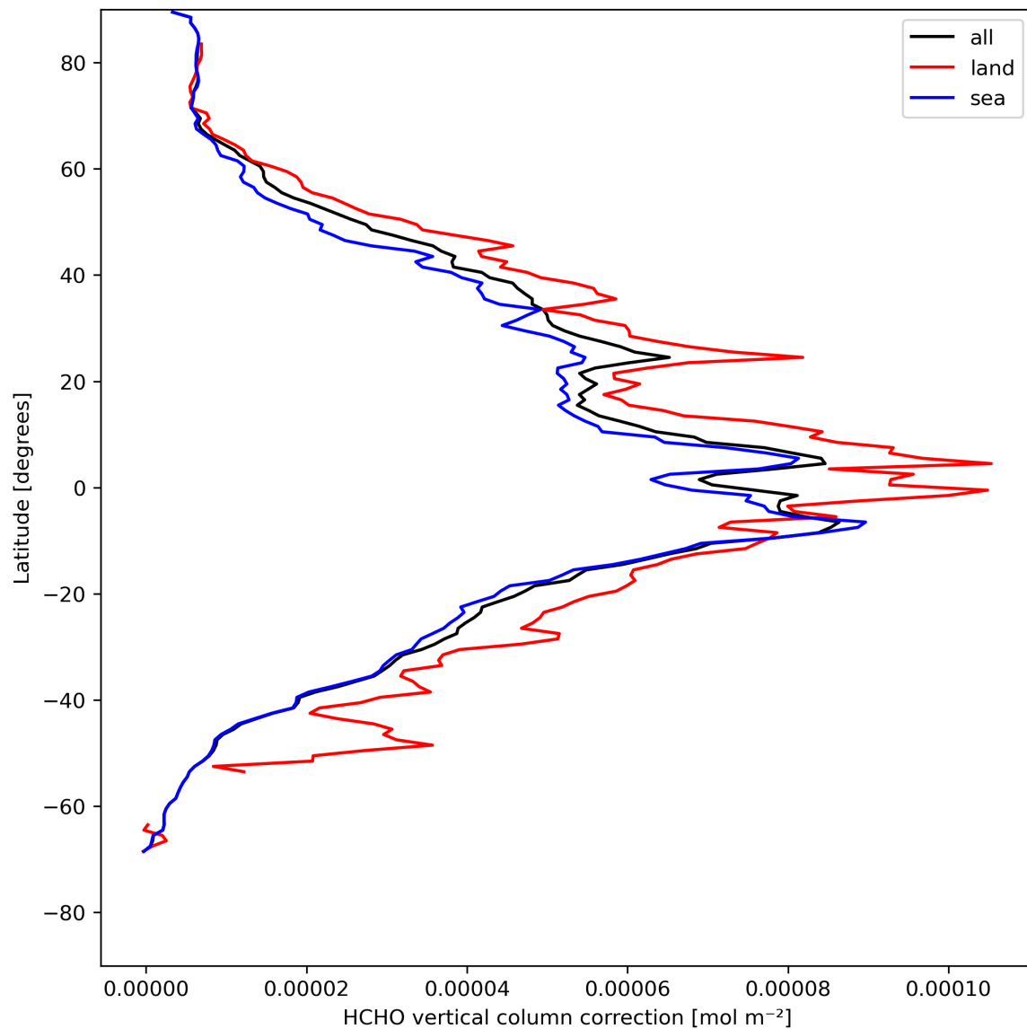
Figure 23: Zonal average of “HCHO vertical column correction” for 2024-05-03 to 2024-05-05.
