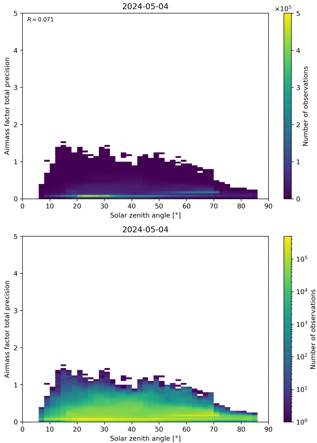
Figure 176: Scatter density plot of “Solar zenith angle” against “Airmass factor total precision” for 2024-05-03 to 2024-05-05.
