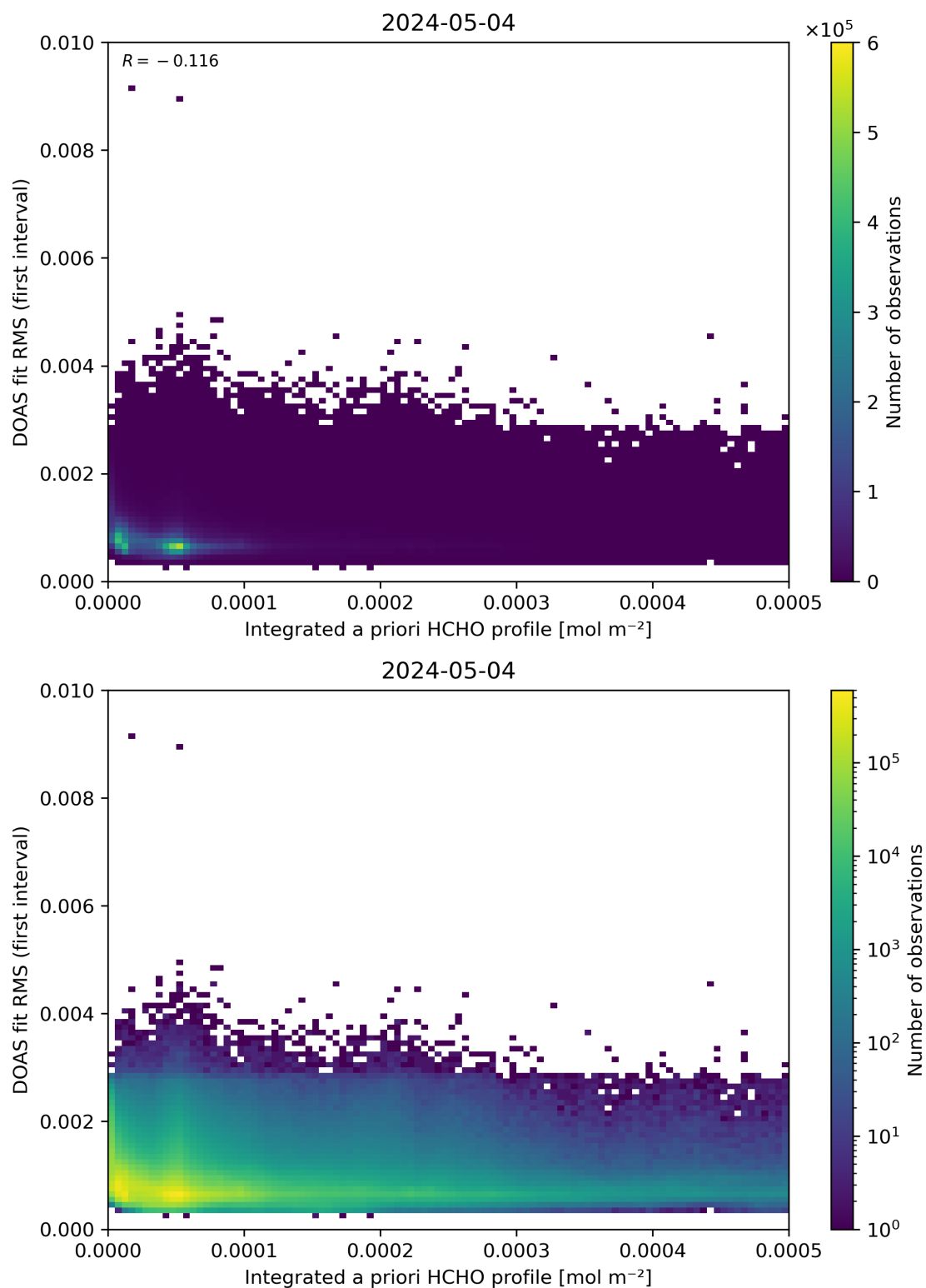
Figure 148: Scatter density plot of “Integrated a priori HCHO profile” against “DOAS fit RMS (first interval)” for 2024-05-03 to 2024-05-05.
