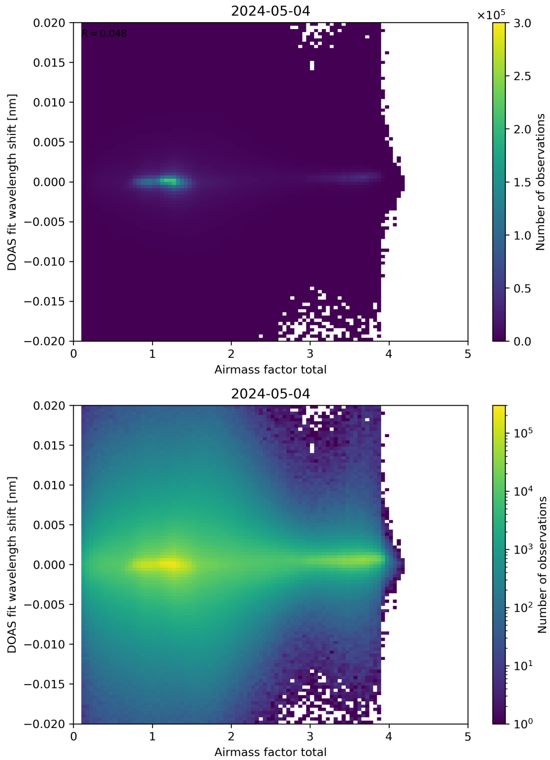
Figure 98: Scatter density plot of “Airmass factor total” against “DOAS fit wavelength shift” for 2024-05-03 to 2024-05-05.
