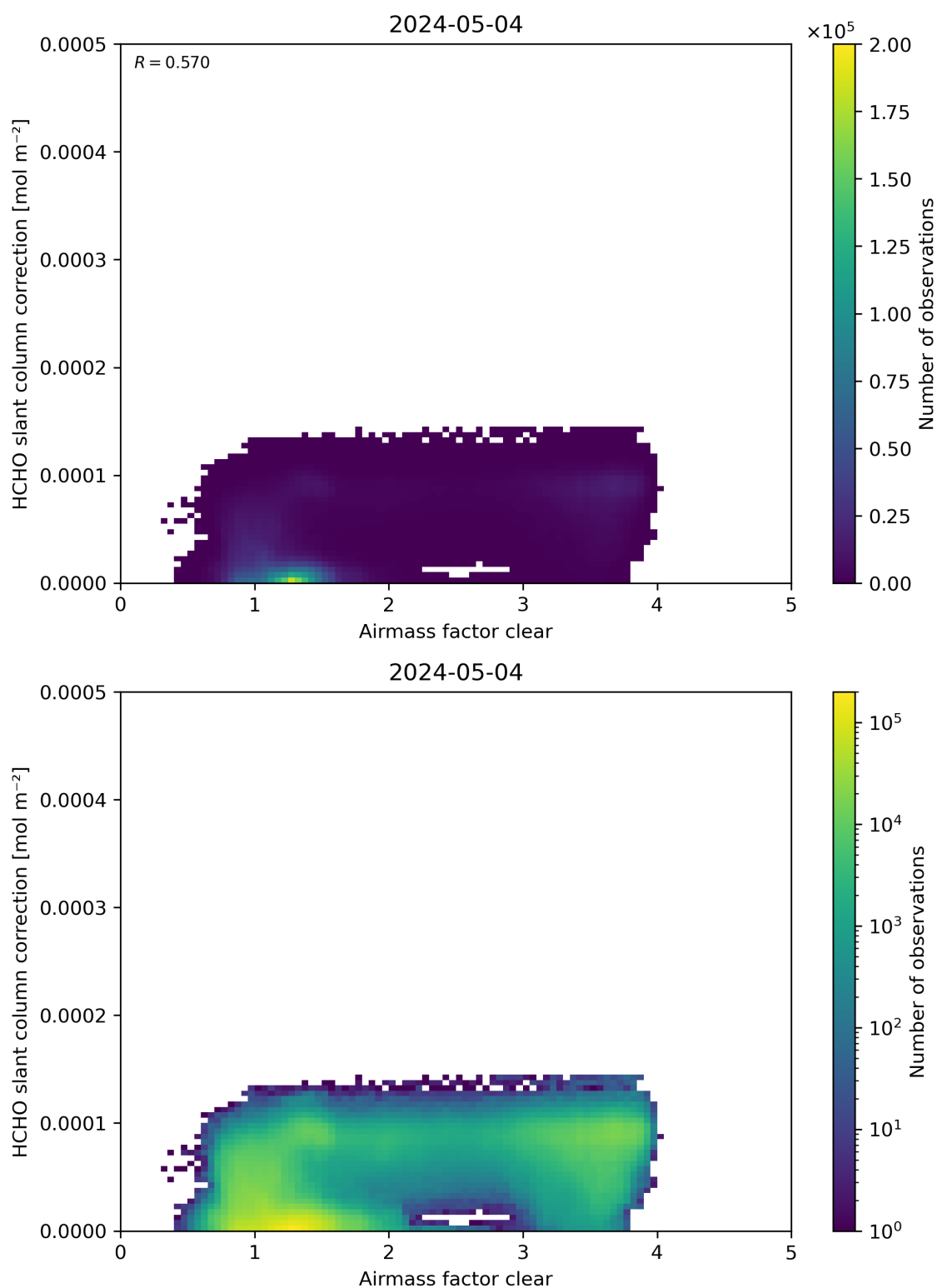
Figure 75: Scatter density plot of “Airmass factor clear” against “HCHO slant column correction” for 2024-05-03 to 2024-05-05.
