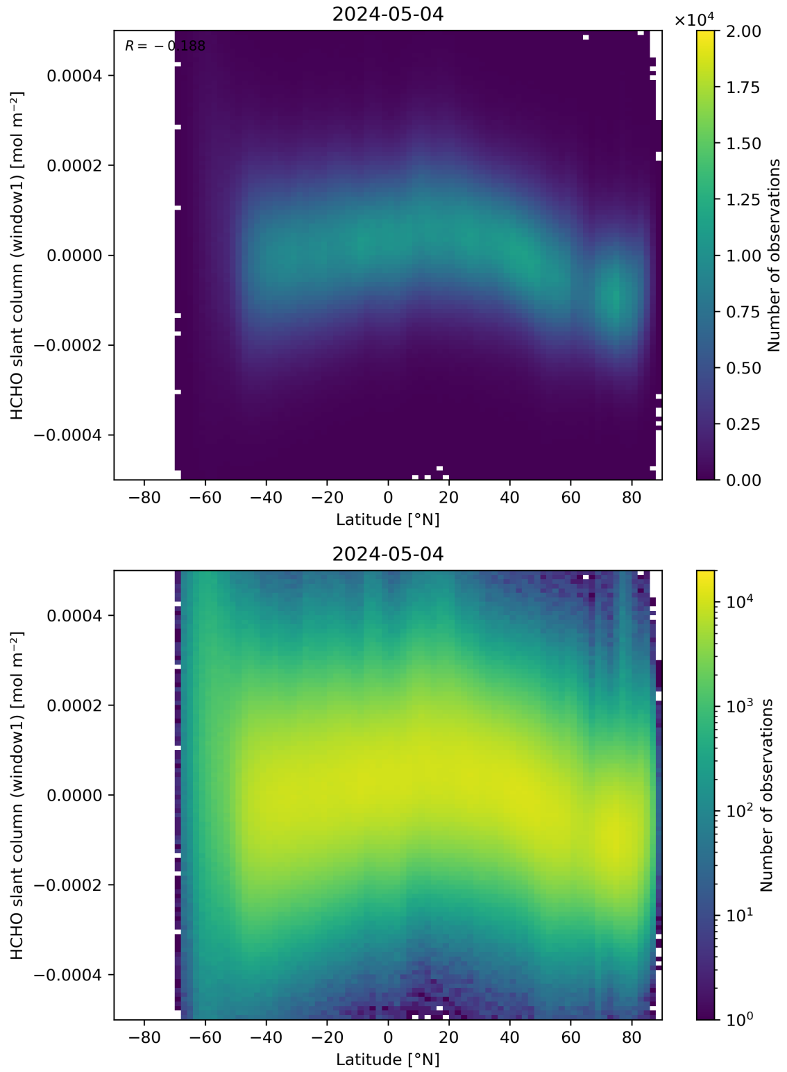
Figure 159: Scatter density plot of “Latitude” against “HCHO slant column (window1)” for 2024-05-03 to 2024-05-05.
