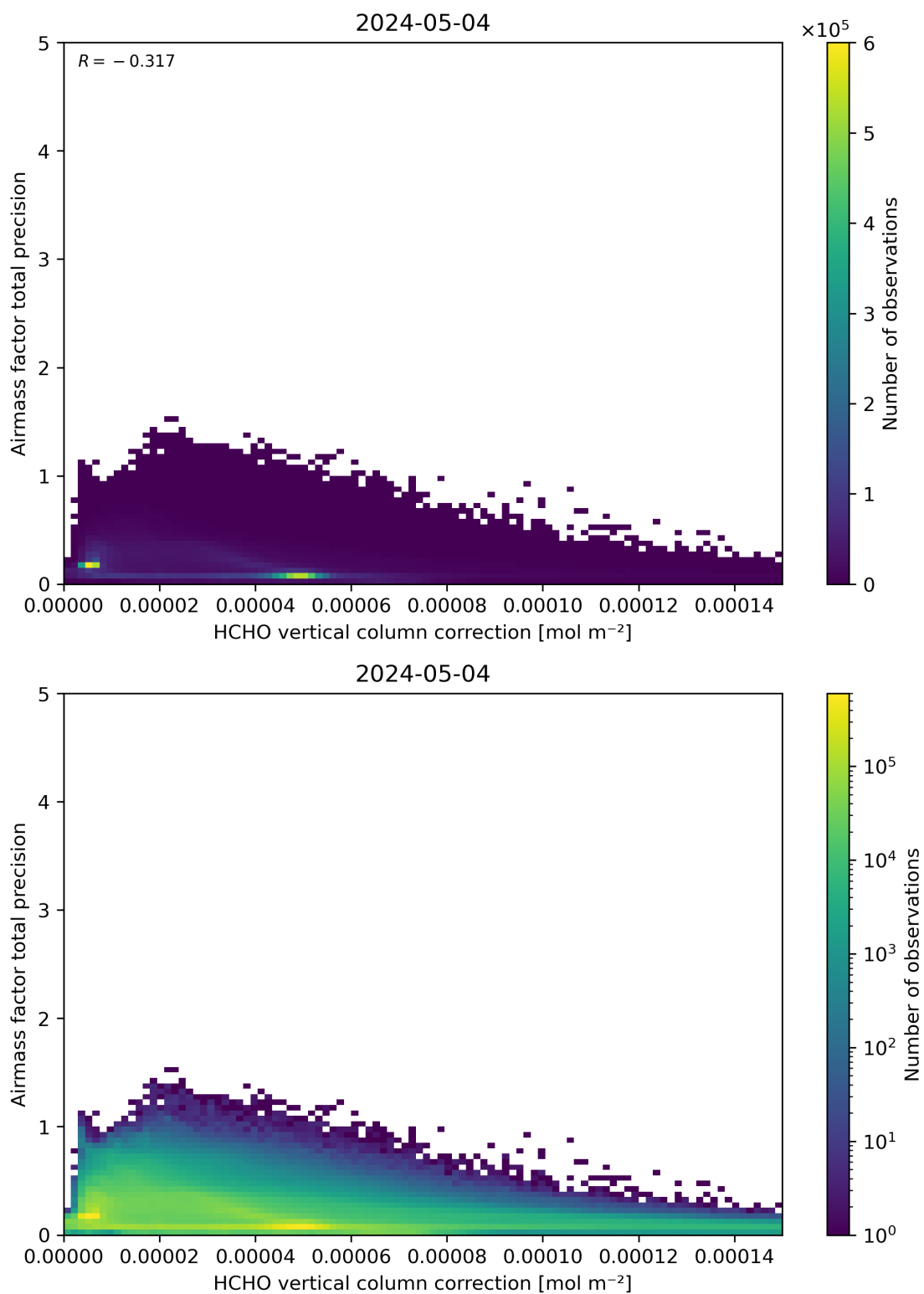
Figure 121: Scatter density plot of “HCHO vertical column correction” against “Airmass factor total precision” for 2024-05-03 to 2024-05-05.
