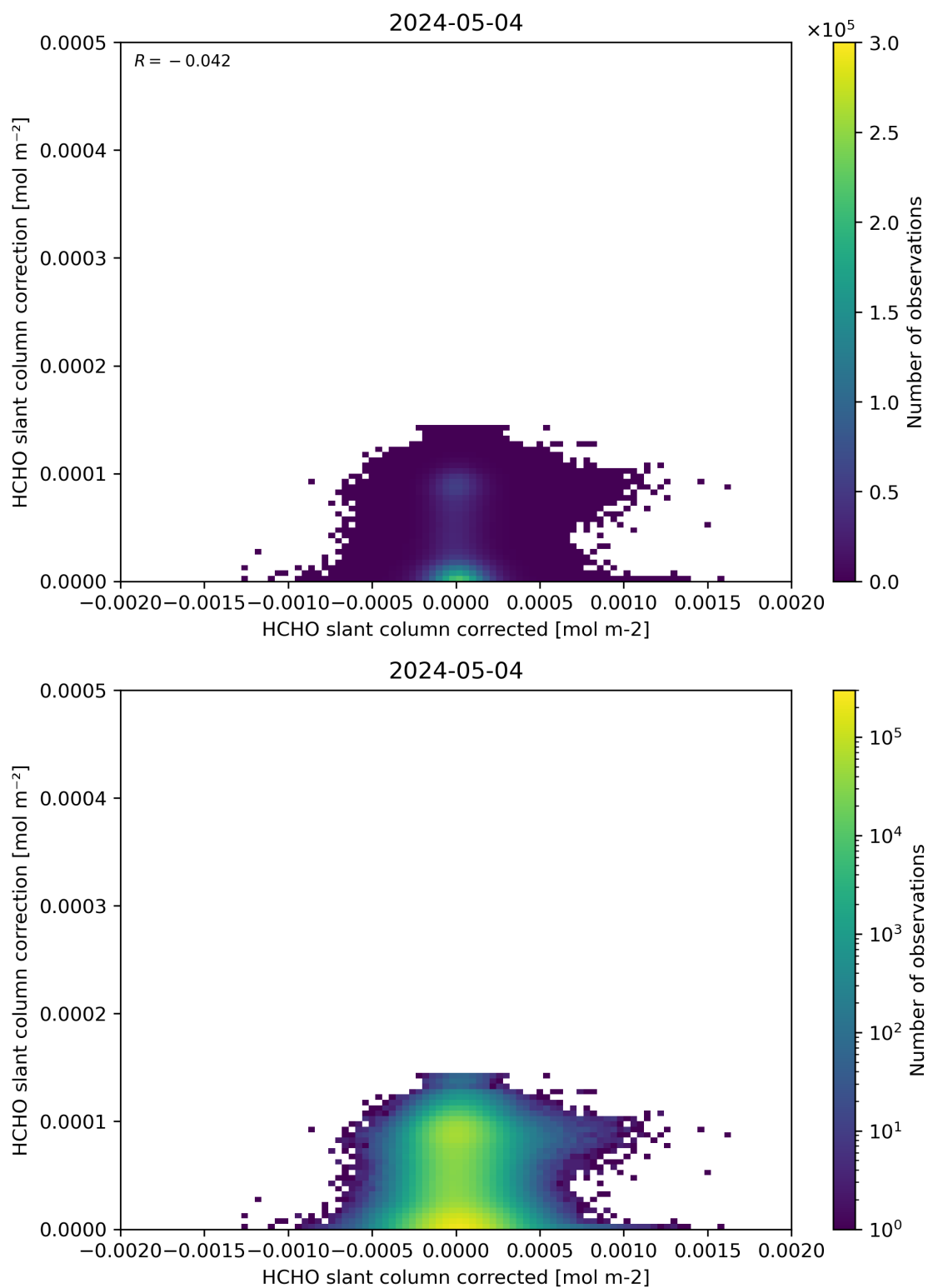
Figure 77: Scatter density plot of “HCHO slant column corrected” against “HCHO slant column correction” for 2024-05-03 to 2024-05-05.
