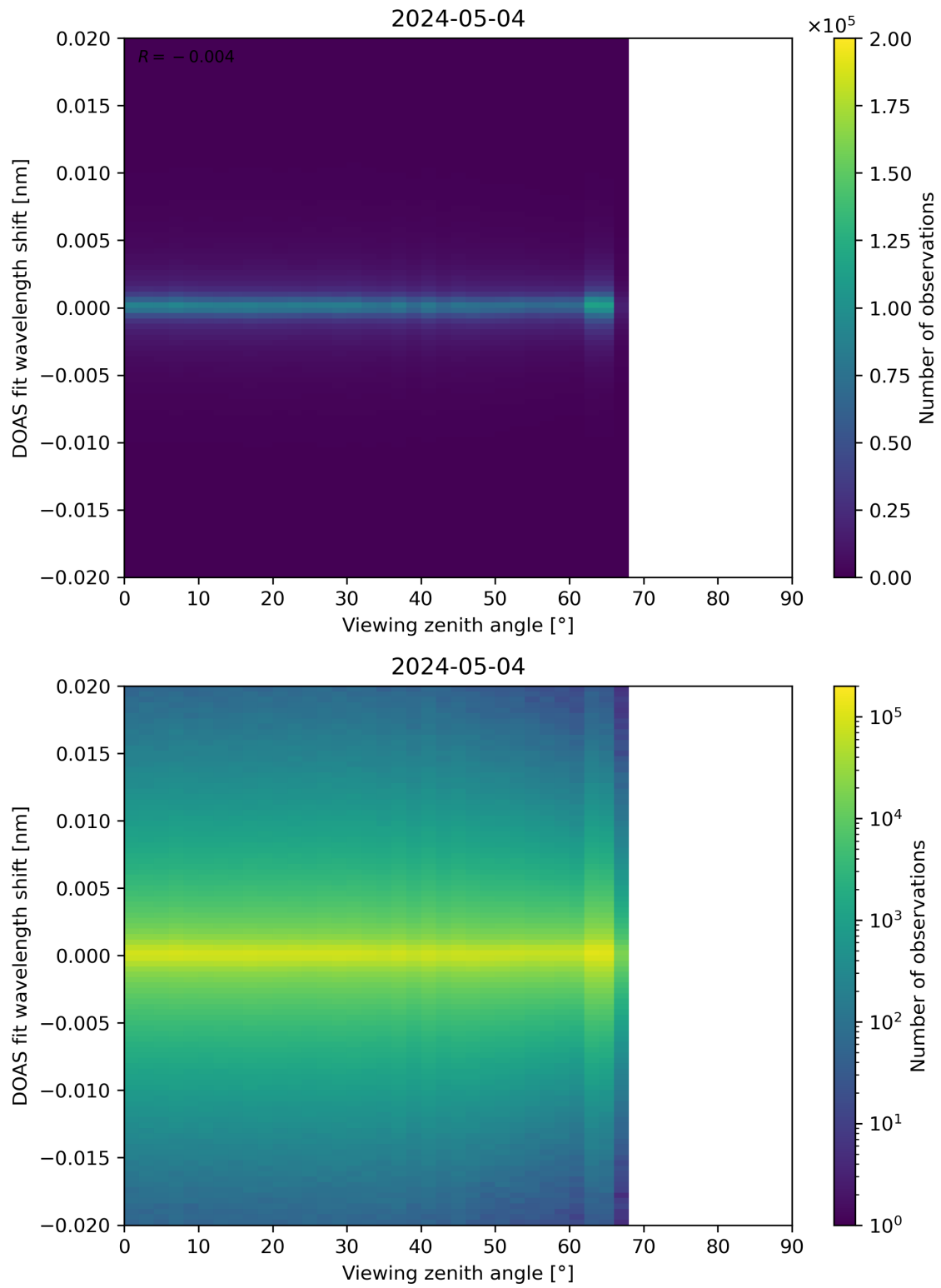
Figure 183: Scatter density plot of “Viewing zenith angle” against “DOAS fit wavelength shift” for 2024-05-03 to 2024-05-05.
