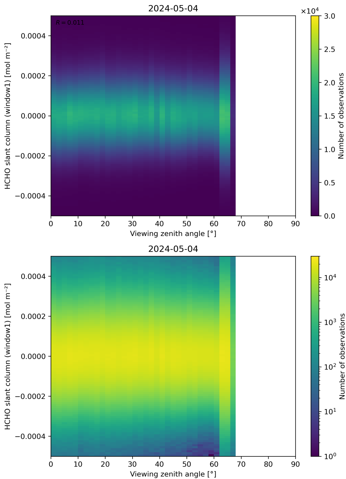
Figure 188: Scatter density plot of “Viewing zenith angle” against “HCHO slant column (window1)” for 2024-05-03 to 2024-05-05.
