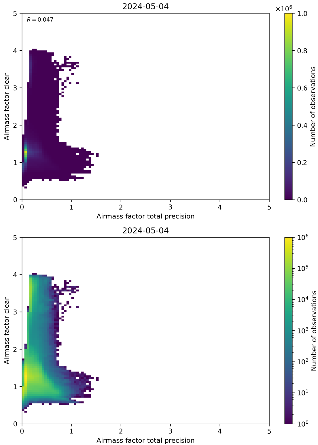
Figure 108: Scatter density plot of “Airmass factor total precision” against “Airmass factor clear” for 2024-05-03 to 2024-05-05.
