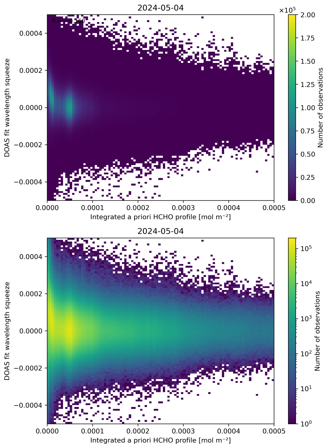
Figure 150: Scatter density plot of “Integrated a priori HCHO profile” against “DOAS fit wavelength squeeze” for 2024-05-03 to 2024-05-05.
