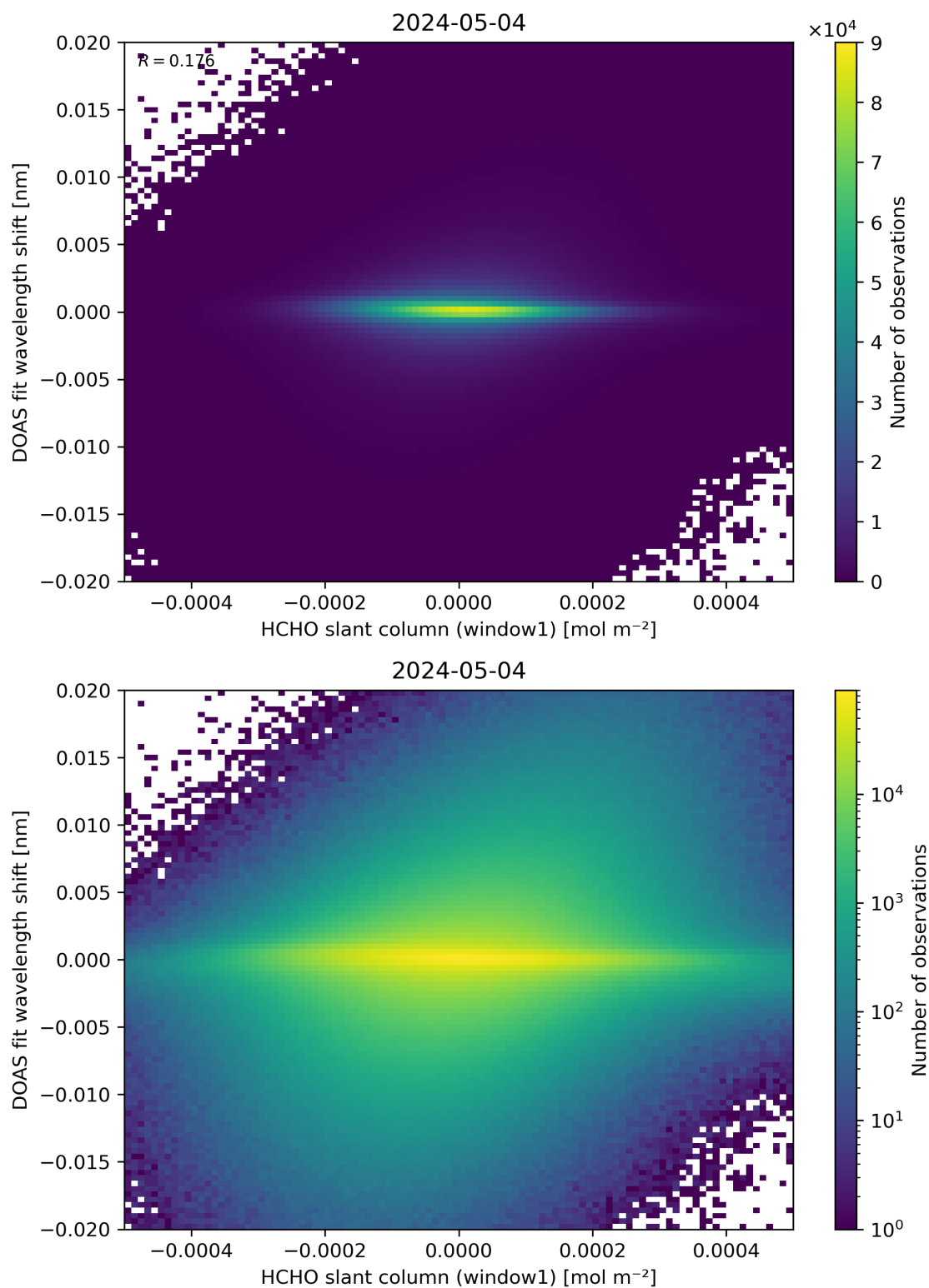
Figure 79: Scatter density plot of “HCHO slant column (window1)” against “DOAS fit wavelength shift” for 2024-05-03 to 2024-05-05.
