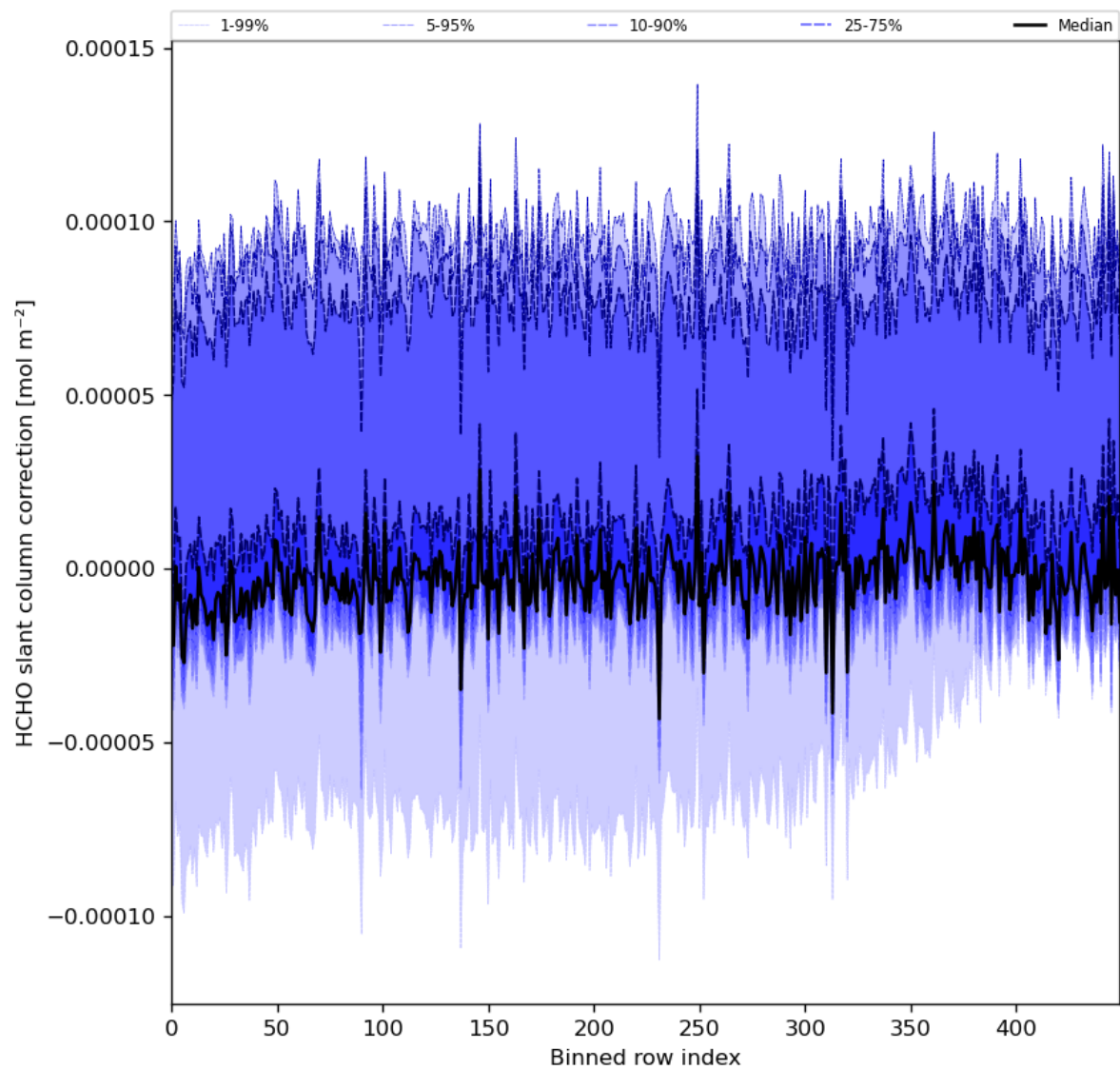
Figure 61: Along track statistics of “HCHO slant column correction” for 2024-05-03 to 2024-05-05
