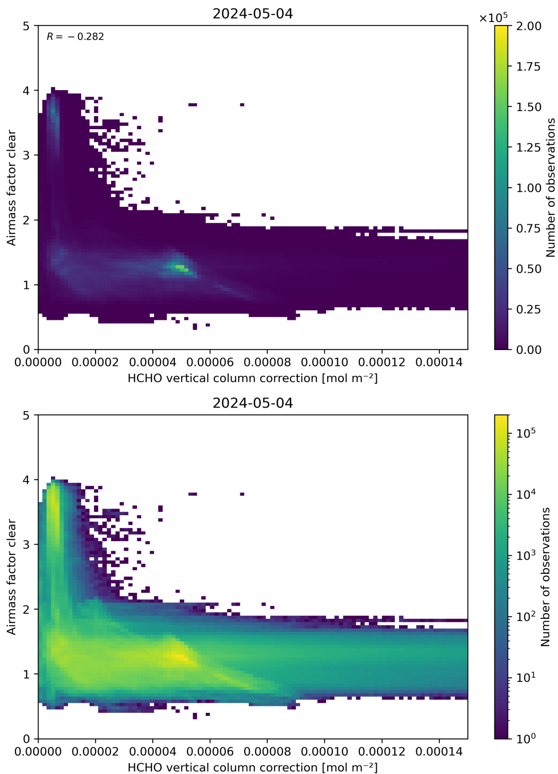
Figure 115: Scatter density plot of “HCHO vertical column correction” against “Airmass factor clear” for 2024-05-03 to 2024-05-05.
