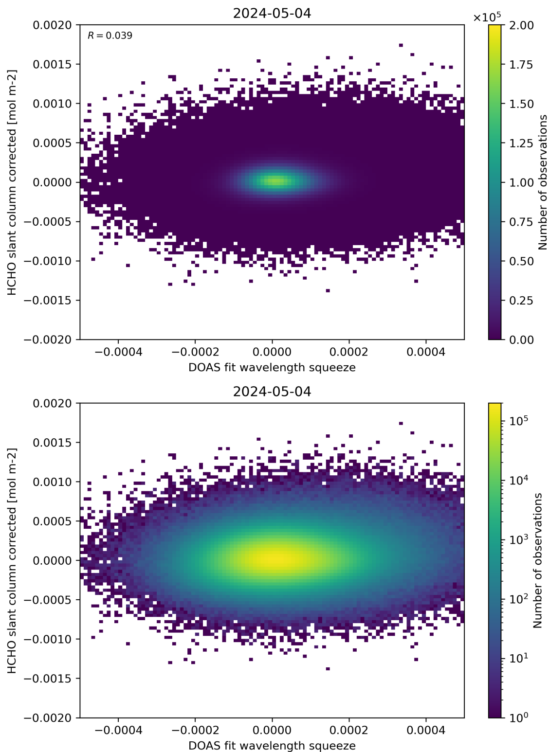
Figure 69: Scatter density plot of “DOAS fit wavelength squeeze” against “HCHO slant column corrected” for 2024-05-03 to 2024-05-05.
