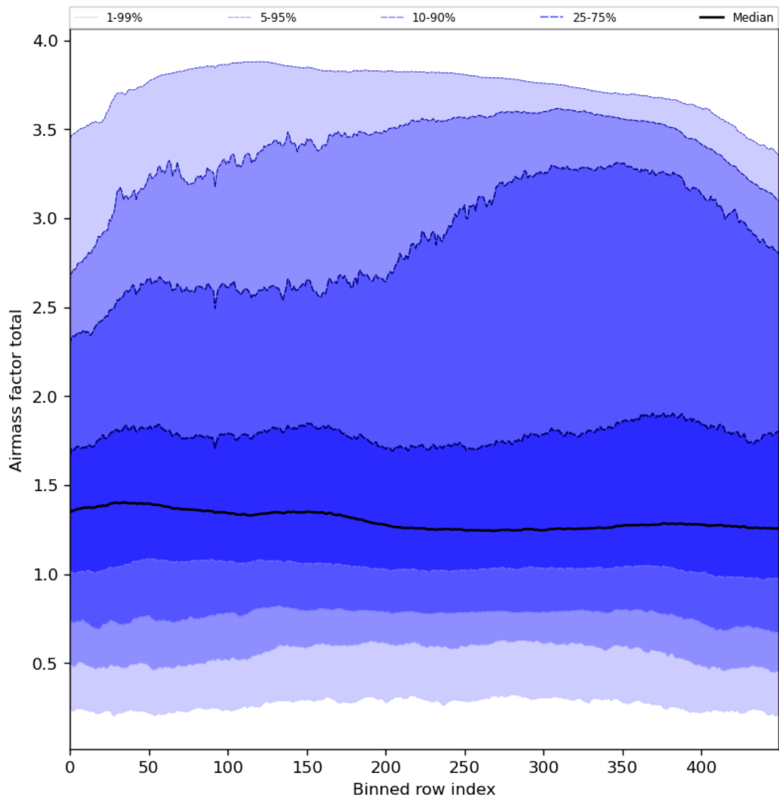
Figure 54: Along track statistics of “Airmass factor total” for 2024-05-03 to 2024-05-05
