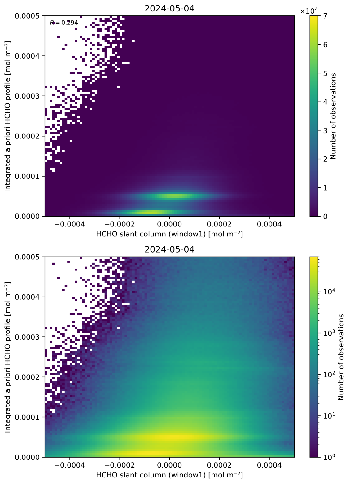
Figure 87: Scatter density plot of “HCHO slant column (window1)” against “Integrated a priori HCHO profile” for 2024-05-03 to 2024-05-05.
