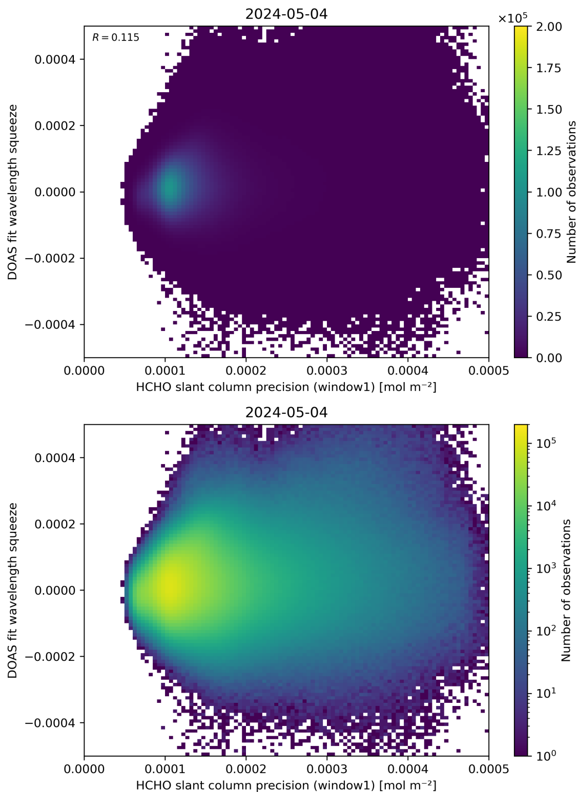
Figure 90: Scatter density plot of “HCHO slant column precision (window1)” against “DOAS fit wavelength squeeze” for 2024-05-03 to 2024-05-05.
