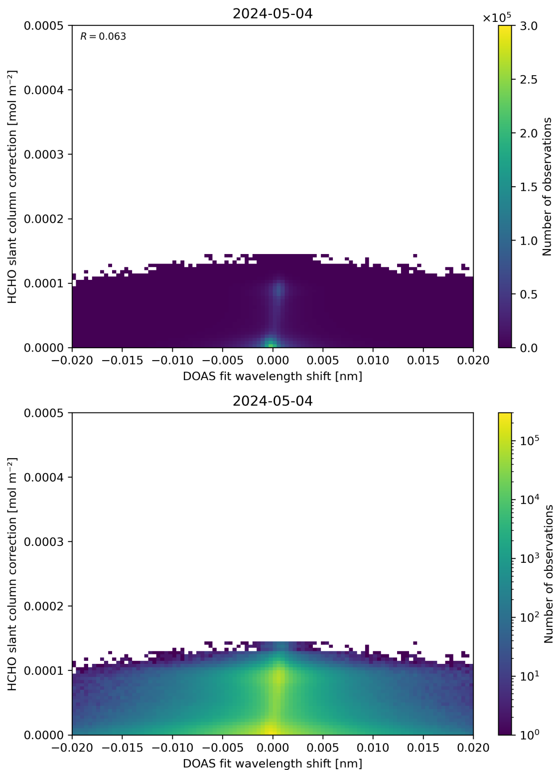
Figure 67: Scatter density plot of “DOAS fit wavelength shift” against “HCHO slant column correction” for 2024-05-03 to 2024-05-05.
