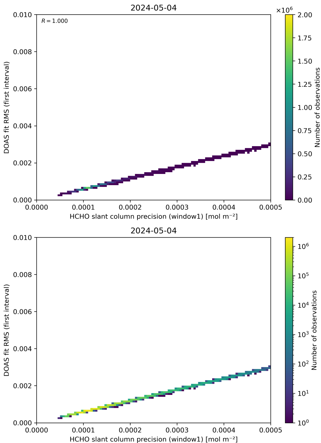
Figure 88: Scatter density plot of “HCHO slant column precision (window1)” against “DOAS fit RMS (first interval)” for 2024-05-03 to 2024-05-05.
