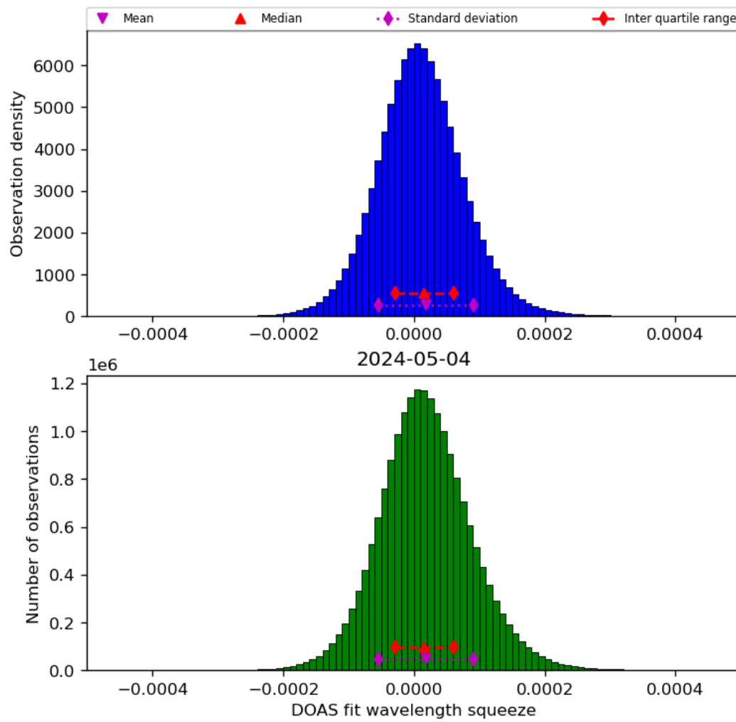
Figure 45: Histogram of “DOAS fit wavelength squeeze” for 2024-05-03 to 2024-05-05
