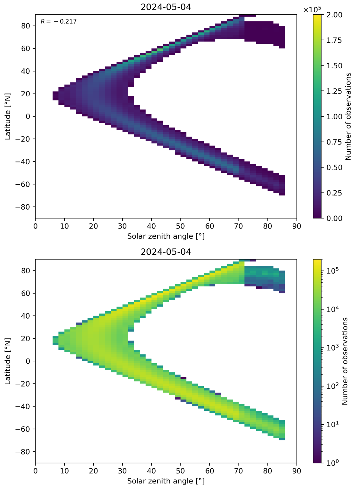
Figure 181: Scatter density plot of “Solar zenith angle” against “Latitude” for 2024-05-03 to 2024-05-05.
