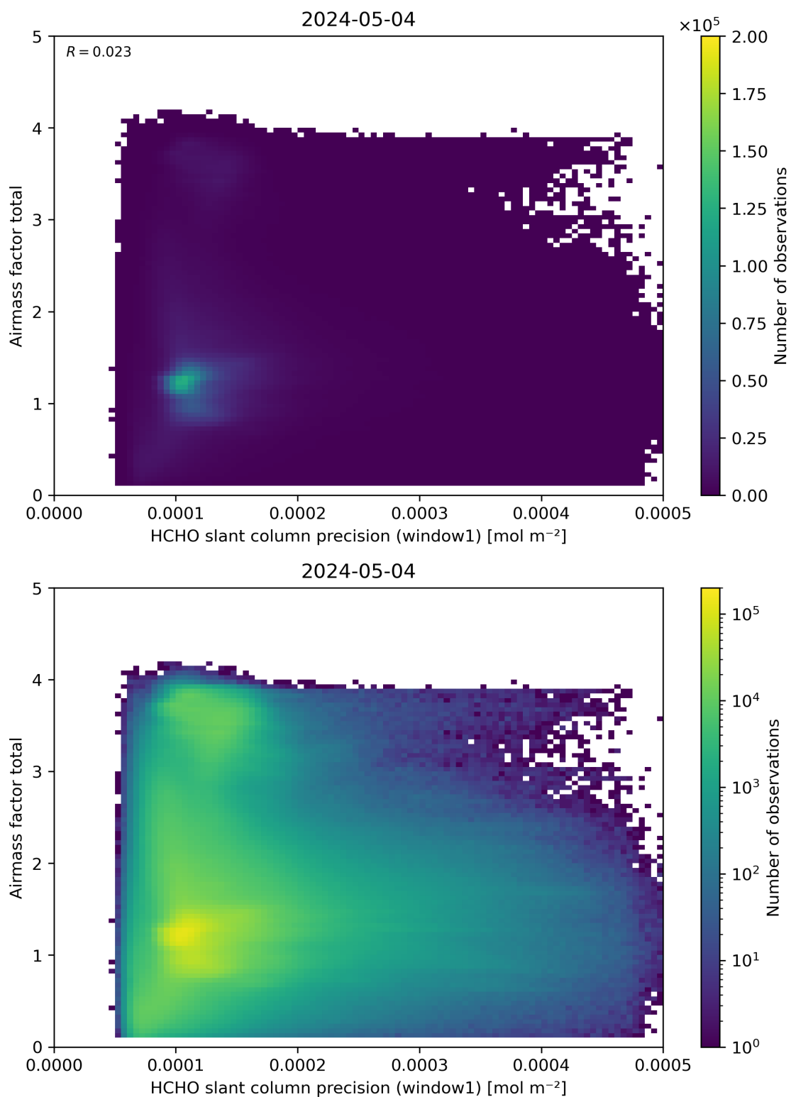
Figure 94: Scatter density plot of “HCHO slant column precision (window1)” against “Airmass factor total” for 2024-05-03 to 2024-05-05.
