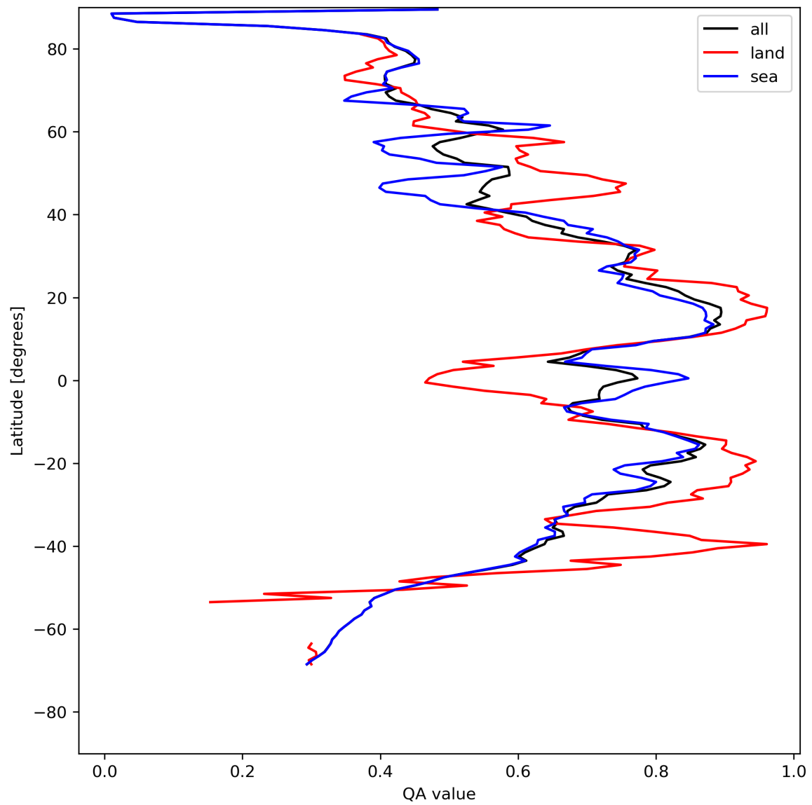
Figure 20: Zonal average of “QA value” for 2024-05-03 to 2024-05-05.
