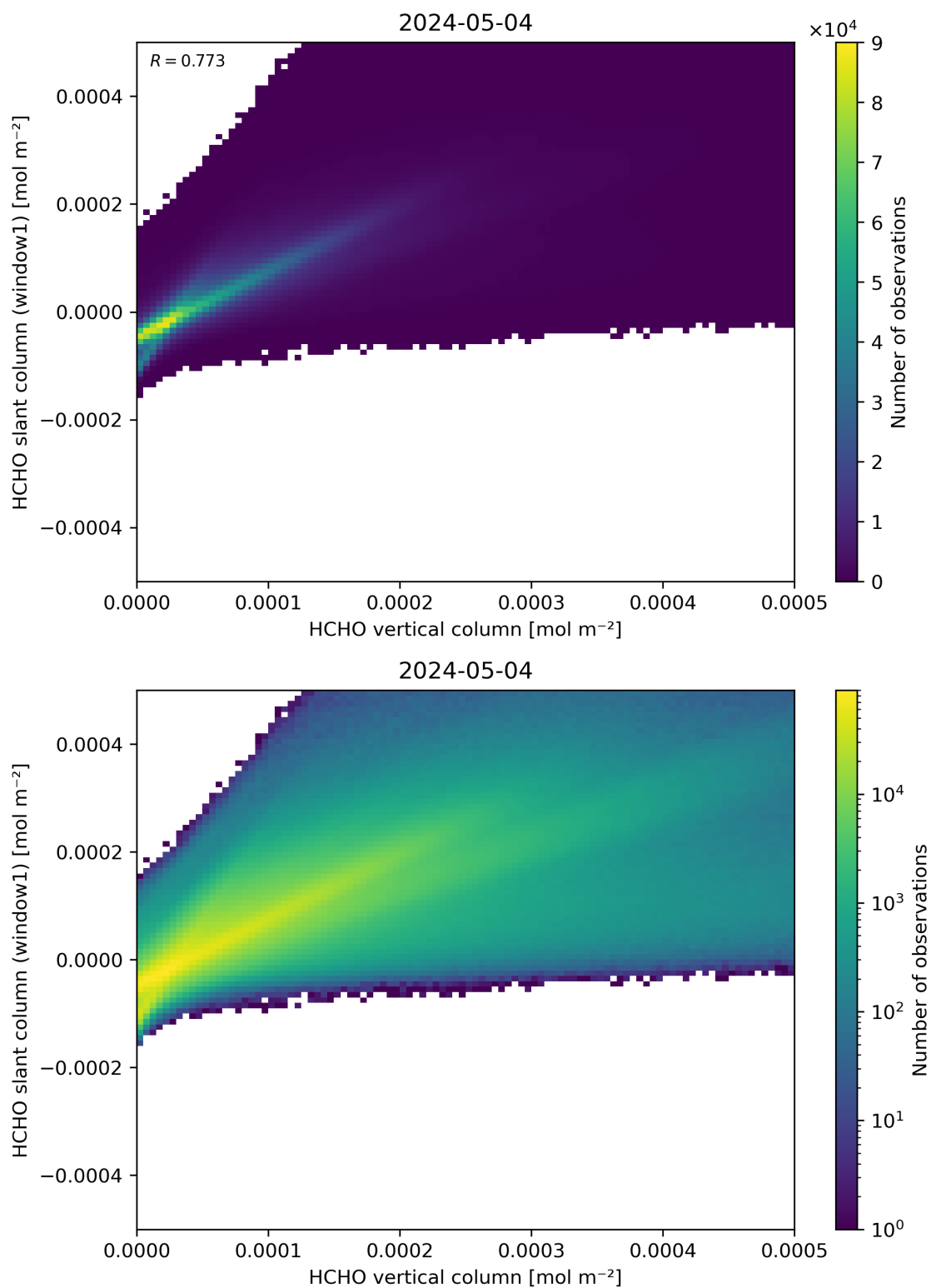
Figure 129: Scatter density plot of “HCHO vertical column” against “HCHO slant column (window1)” for 2024-05-03 to 2024-05-05.
