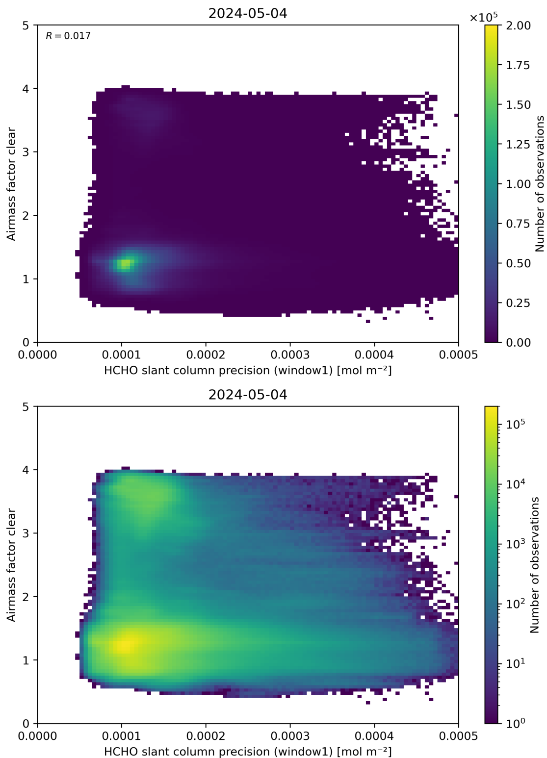
Figure 91: Scatter density plot of “HCHO slant column precision (window1)” against “Airmass factor clear” for 2024-05-03 to 2024-05-05.
