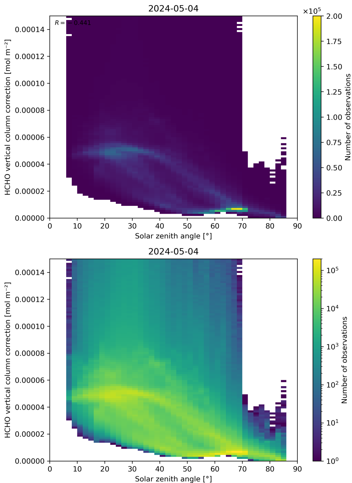
Figure 178: Scatter density plot of “Solar zenith angle” against “HCHO vertical column correction” for 2024-05-03 to 2024-05-05.
