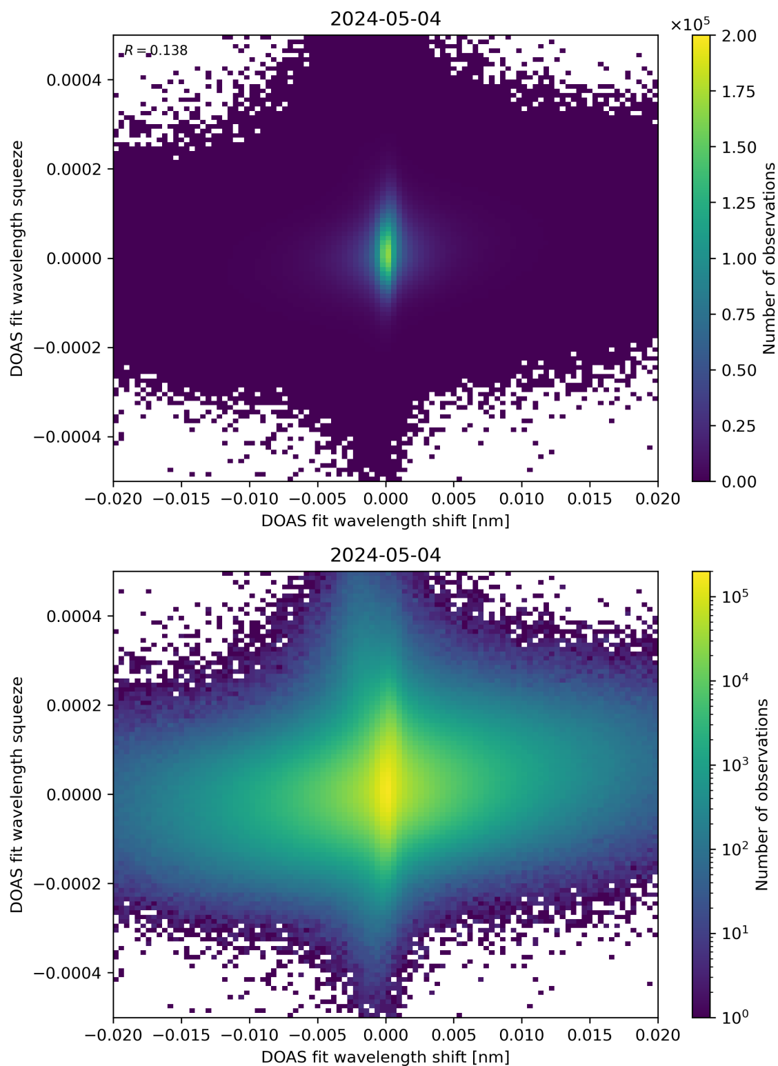
Figure 65: Scatter density plot of “DOAS fit wavelength shift” against “DOAS fit wavelength squeeze” for 2024-05-03 to 2024-05-05.
