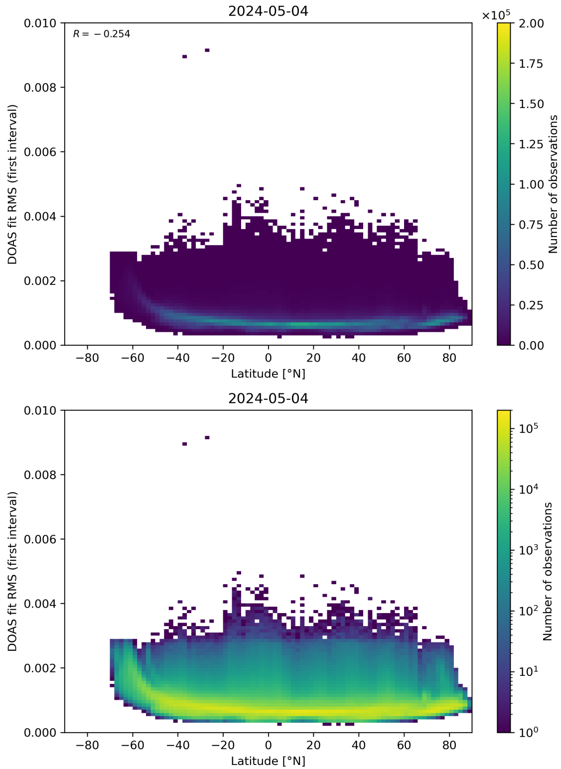
Figure 153: Scatter density plot of “Latitude” against “DOAS fit RMS (first interval)” for 2024-05-03 to 2024-05-05.
