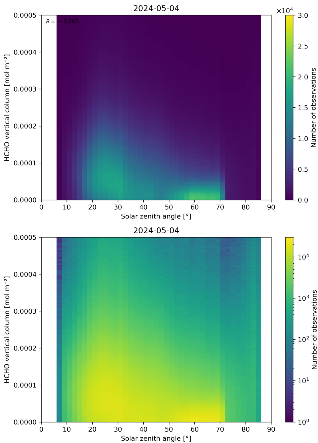
Figure 177: Scatter density plot of “Solar zenith angle” against “HCHO vertical column” for 2024-05-03 to 2024-05-05.
