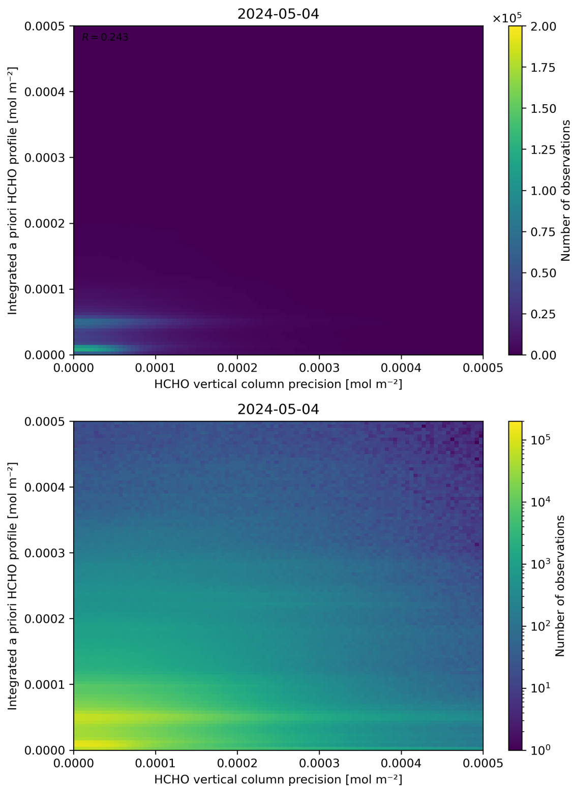
Figure 147: Scatter density plot of “HCHO vertical column precision” against “Integrated a priori HCHO profile” for 2024-05-03 to 2024-05-05.
