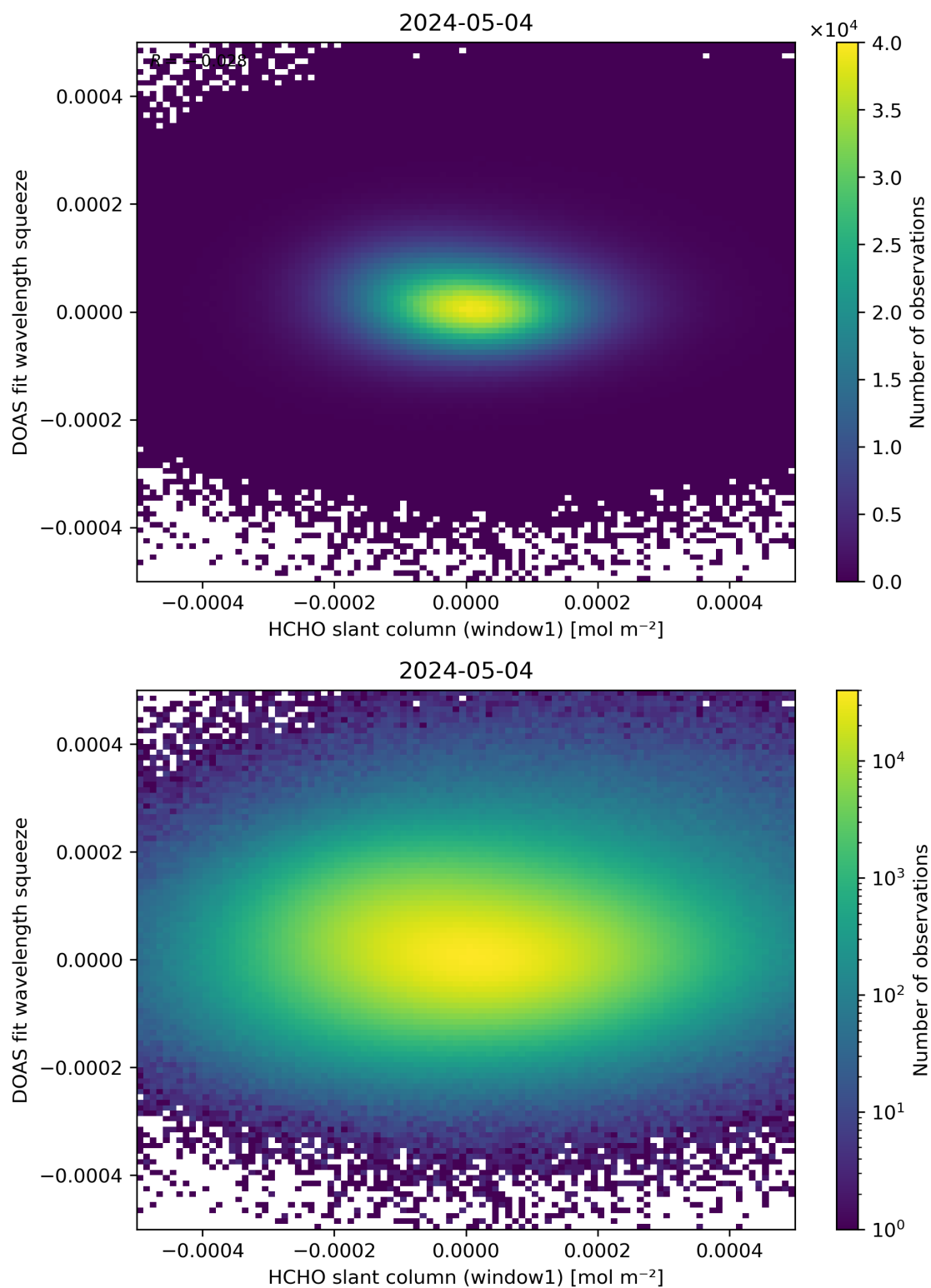
Figure 80: Scatter density plot of “HCHO slant column (window1)” against “DOAS fit wavelength squeeze” for 2024-05-03 to 2024-05-05.
