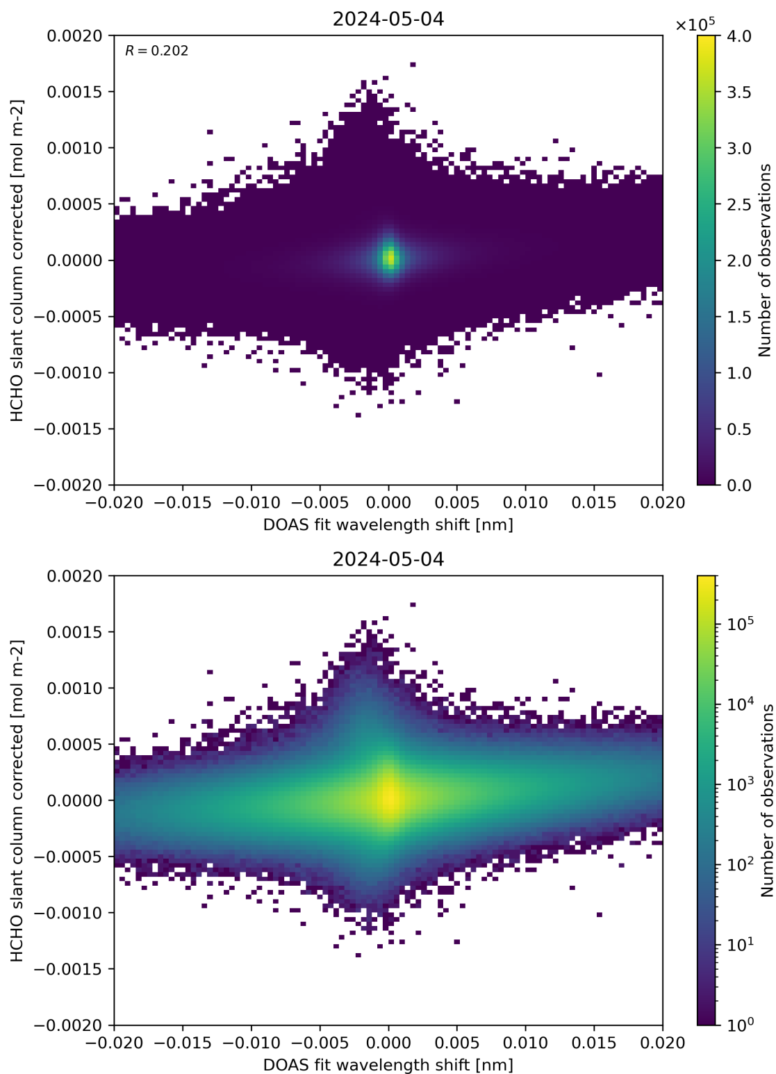
Figure 66: Scatter density plot of “DOAS fit wavelength shift” against “HCHO slant column corrected” for 2024-05-03 to 2024-05-05.
