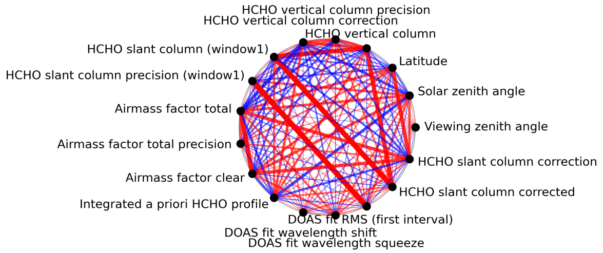
Figure 1: Map of correlation graph for 2024-05-03 to 2024-05-05.
