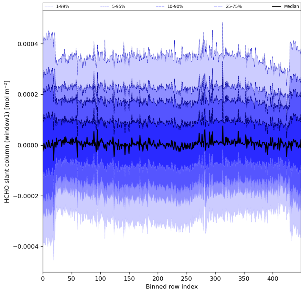
Figure 52: Along track statistics of “HCHO slant column (window1)” for 2024-05-03 to 2024-05-05
