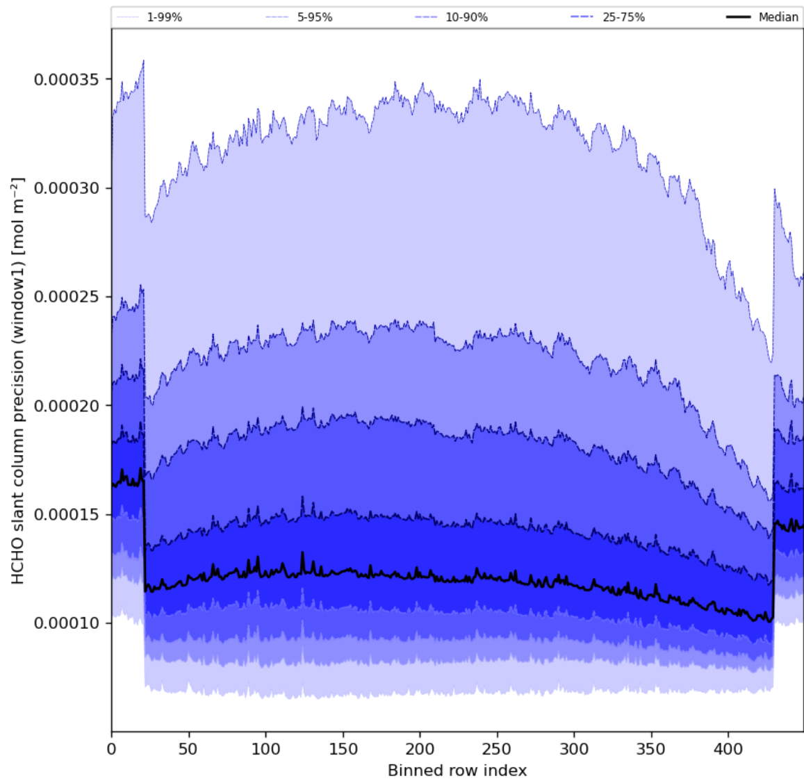
Figure 53: Along track statistics of “HCHO slant column precision (window1)” for 2024-05-03 to 2024-05-05
