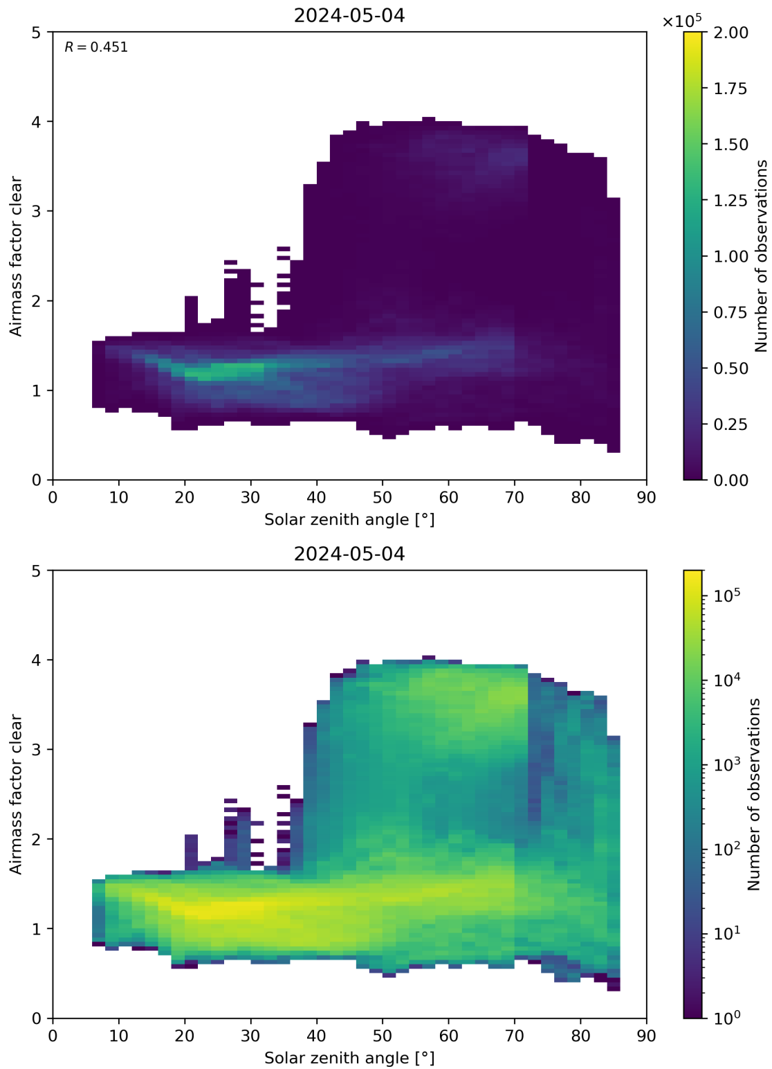
Figure 170: Scatter density plot of “Solar zenith angle” against “Airmass factor clear” for 2024-05-03 to 2024-05-05.
