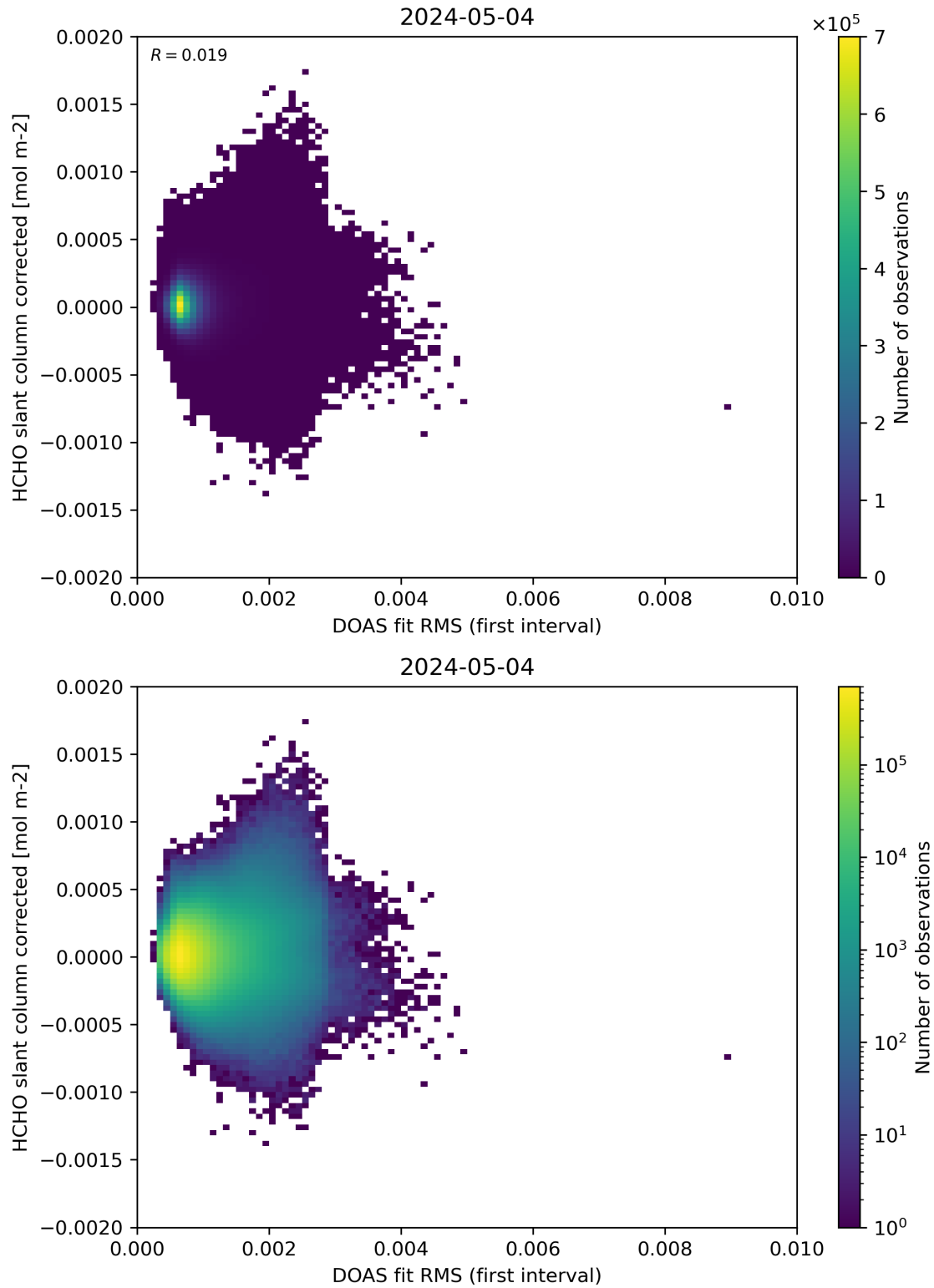
Figure 62: Scatter density plot of “DOAS fit RMS (first interval)” against “HCHO slant column corrected” for 2024-05-03 to 2024-05-05.
