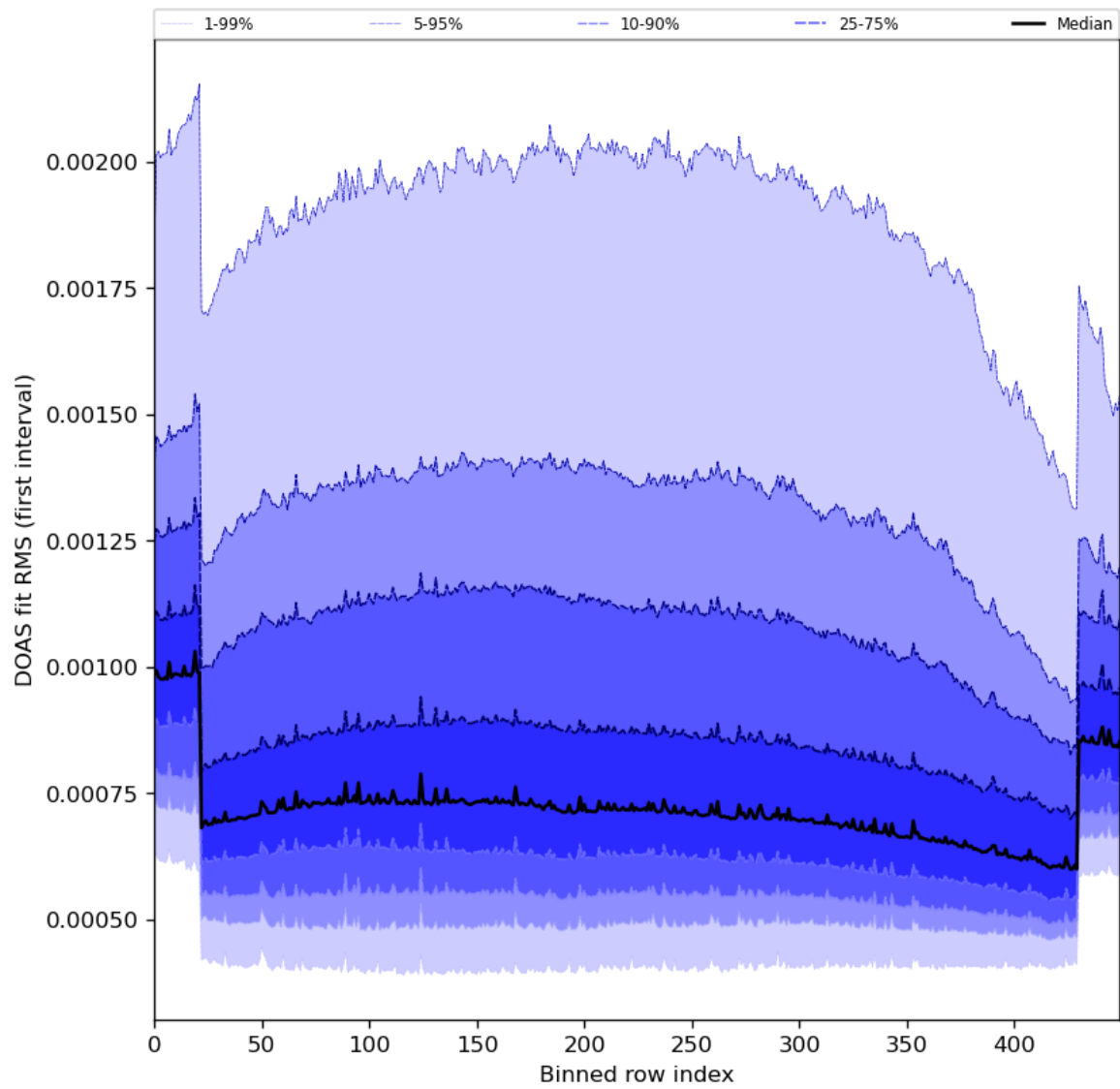
Figure 60: Along track statistics of “DOAS fit RMS (first interval)” for 2024-05-03 to 2024-05-05
