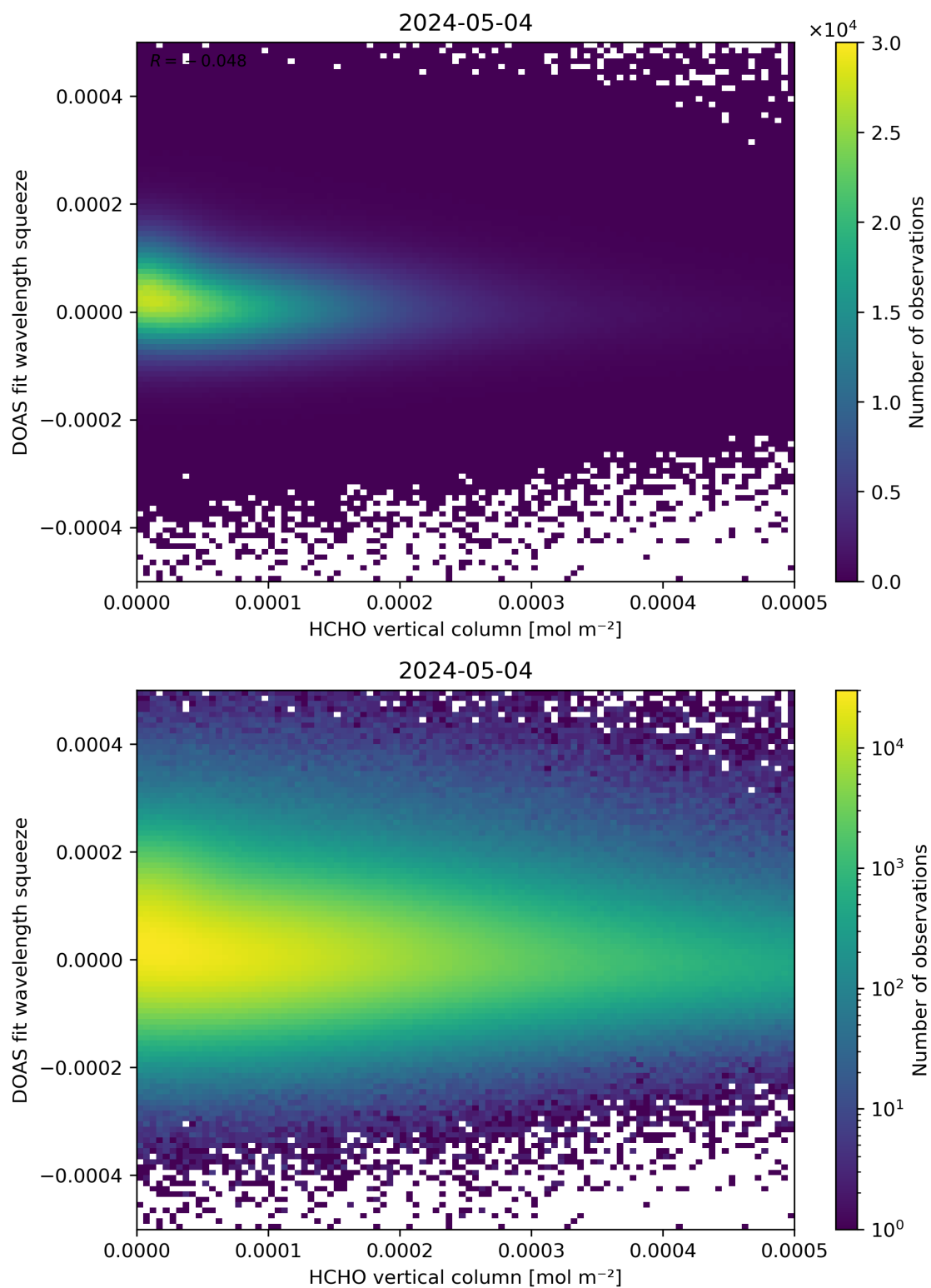
Figure 125: Scatter density plot of “HCHO vertical column” against “DOAS fit wavelength squeeze” for 2024-05-03 to 2024-05-05.
