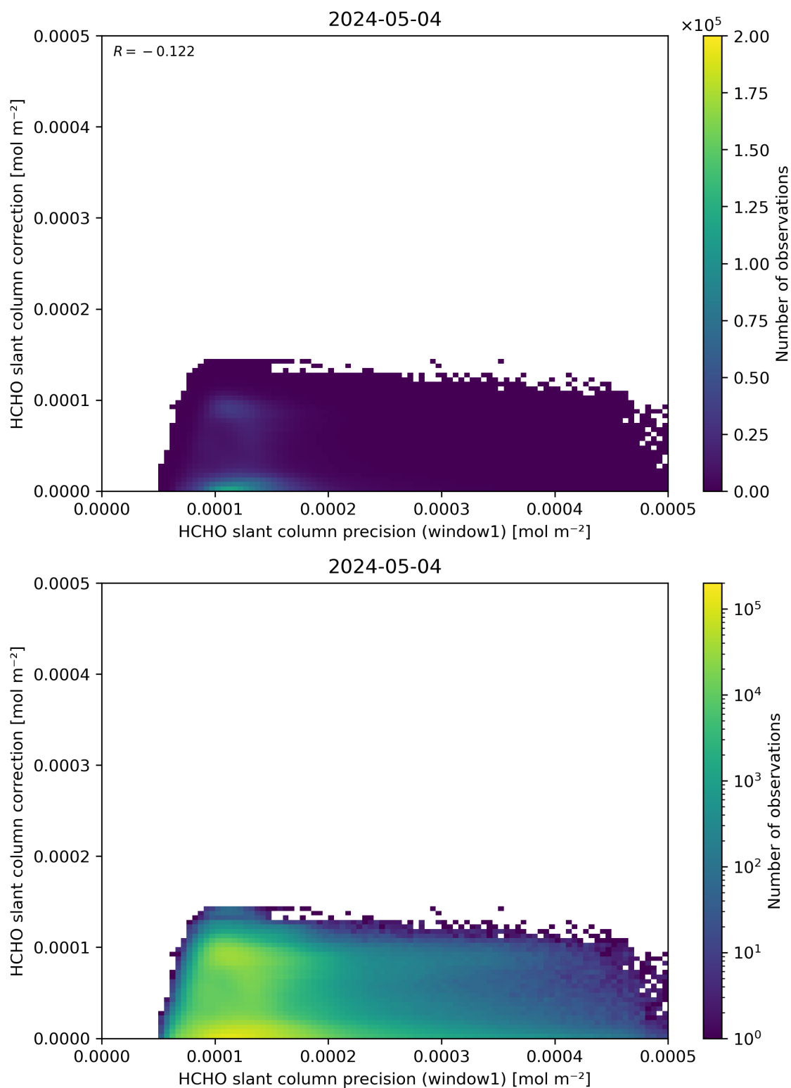
Figure 93: Scatter density plot of “HCHO slant column precision (window1)” against “HCHO slant column correction” for 2024-05-03 to 2024-05-05.
