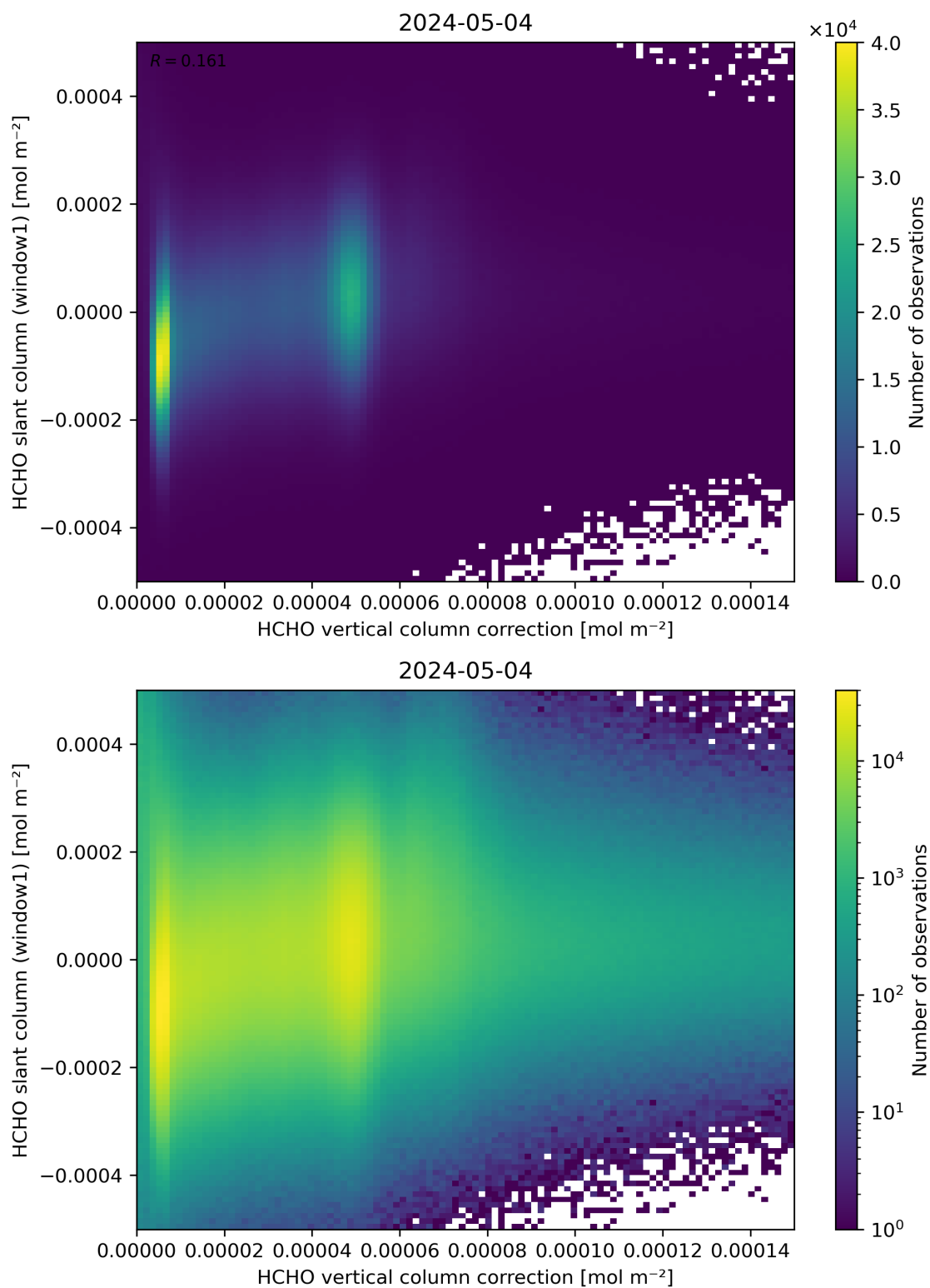
Figure 118: Scatter density plot of “HCHO vertical column correction” against “HCHO slant column (window1)” for 2024-05-03 to 2024-05-05.
