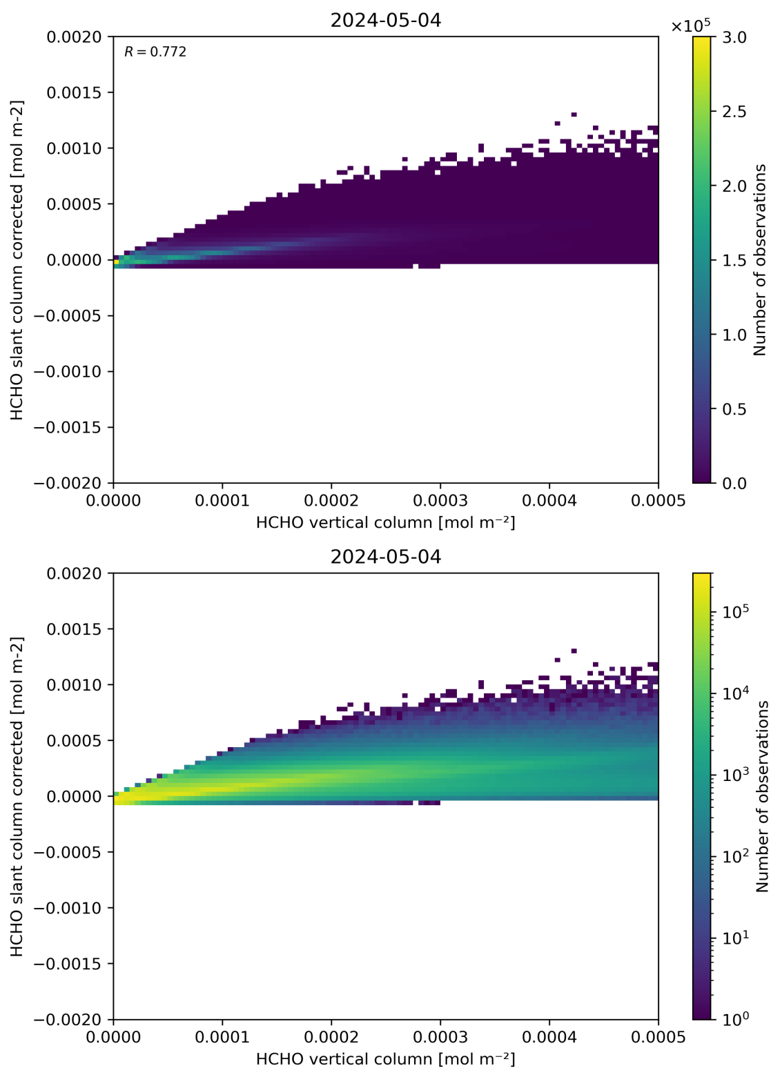
Figure 127: Scatter density plot of “HCHO vertical column” against “HCHO slant column corrected” for 2024-05-03 to 2024-05-05.
