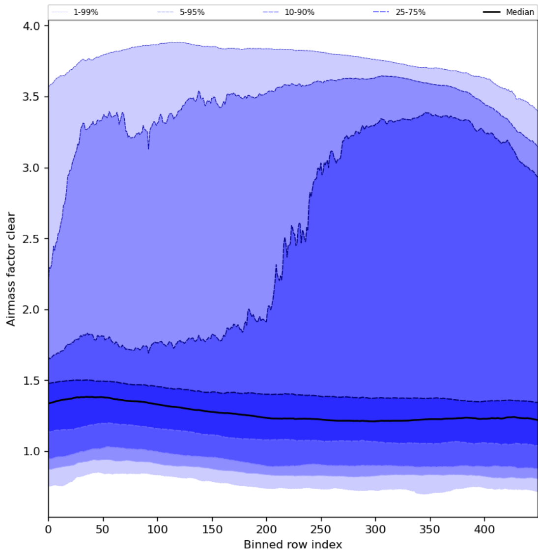
Figure 56: Along track statistics of “Airmass factor clear” for 2024-05-03 to 2024-05-05
