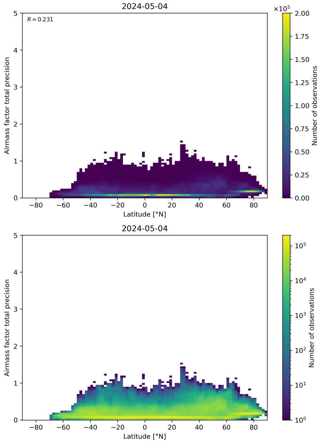
Figure 162: Scatter density plot of “Latitude” against “Airmass factor total precision” for 2024-05-03 to 2024-05-05.
