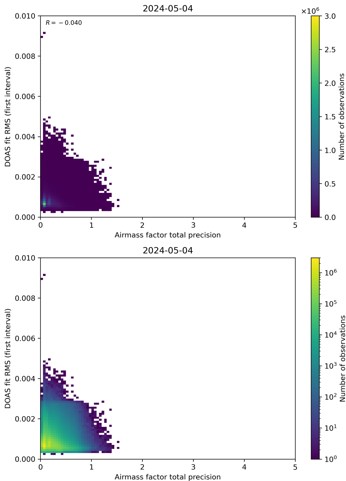
Figure 105: Scatter density plot of “Airmass factor total precision” against “DOAS fit RMS (first interval)” for 2024-05-03 to 2024-05-05.
