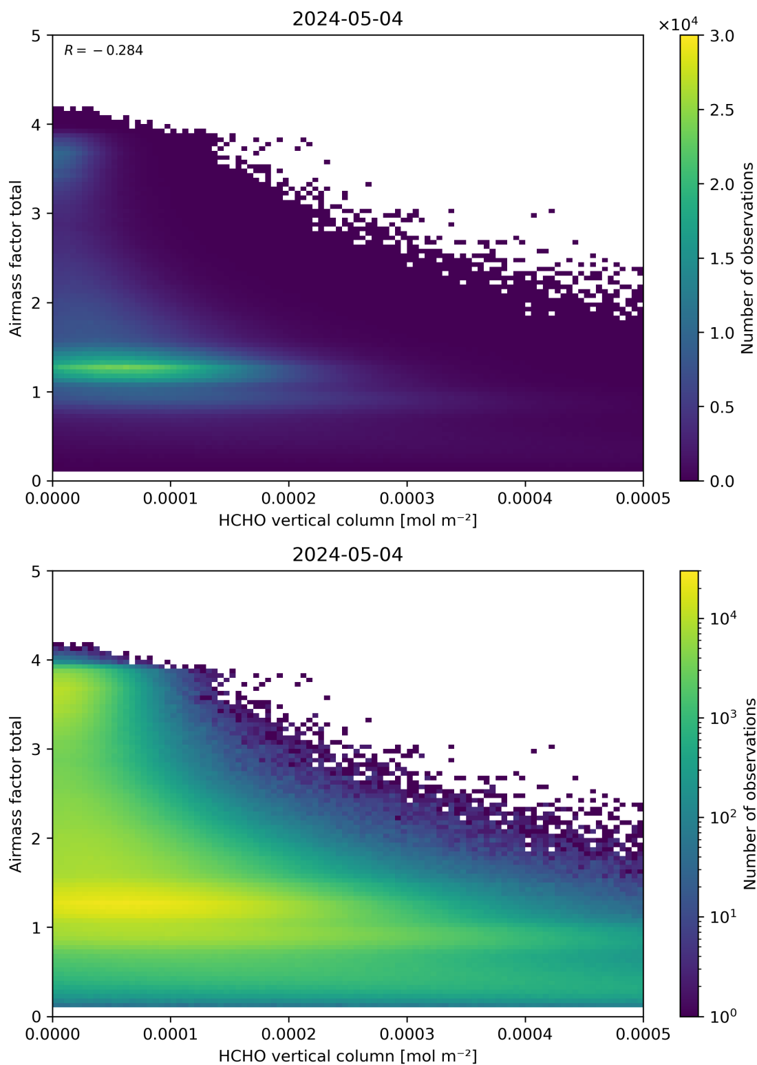
Figure 131: Scatter density plot of “HCHO vertical column” against “Airmass factor total” for 2024-05-03 to 2024-05-05.
