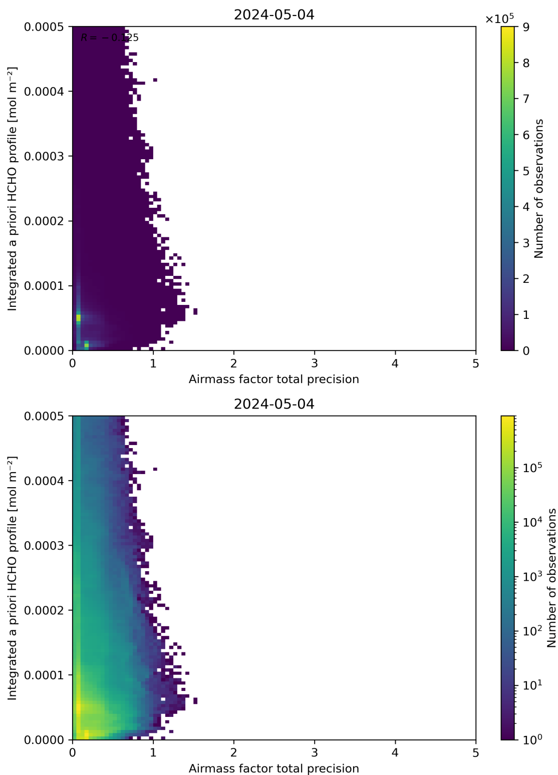
Figure 111: Scatter density plot of “Airmass factor total precision” against “Integrated a priori HCHO profile” for 2024-05-03 to 2024-05-05.
