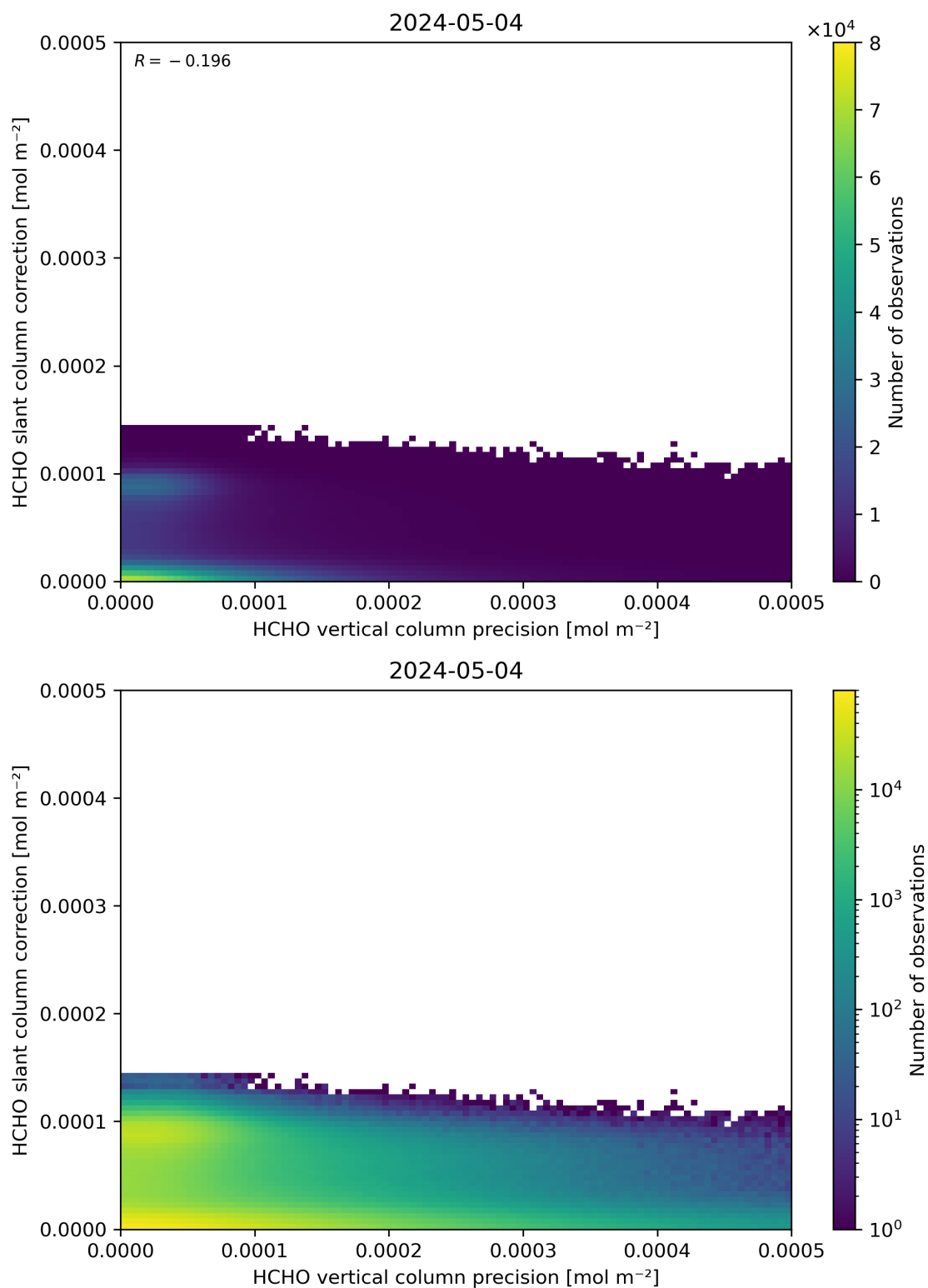
Figure 141: Scatter density plot of “HCHO vertical column precision” against “HCHO slant column correction” for 2024-05-03 to 2024-05-05.
