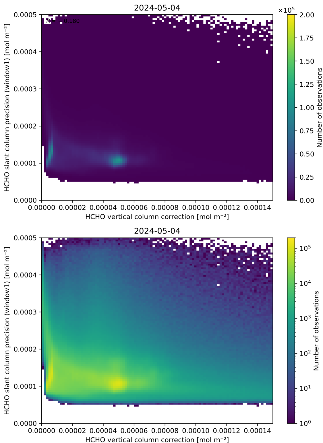
Figure 119: Scatter density plot of “HCHO vertical column correction” against “HCHO slant column precision (window1)” for 2024-05-03 to 2024-05-05.
