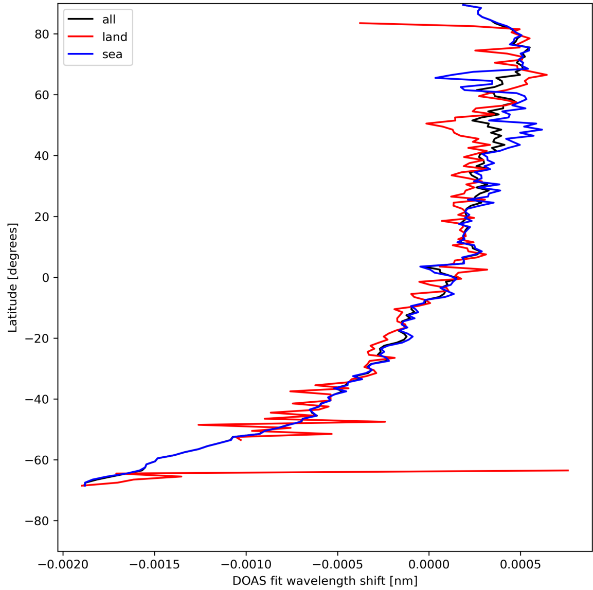
Figure 30: Zonal average of "DOAS fit wavelength shift" for 2024-05-03 to 2024-05-05.
