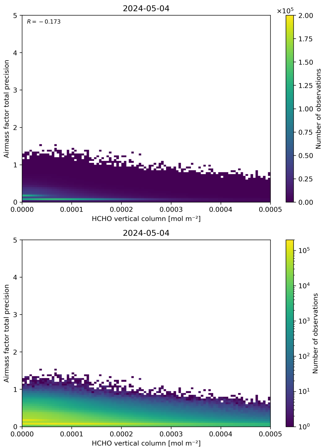
Figure 132: Scatter density plot of “HCHO vertical column” against “Airmass factor total precision” for 2024-05-03 to 2024-05-05.
