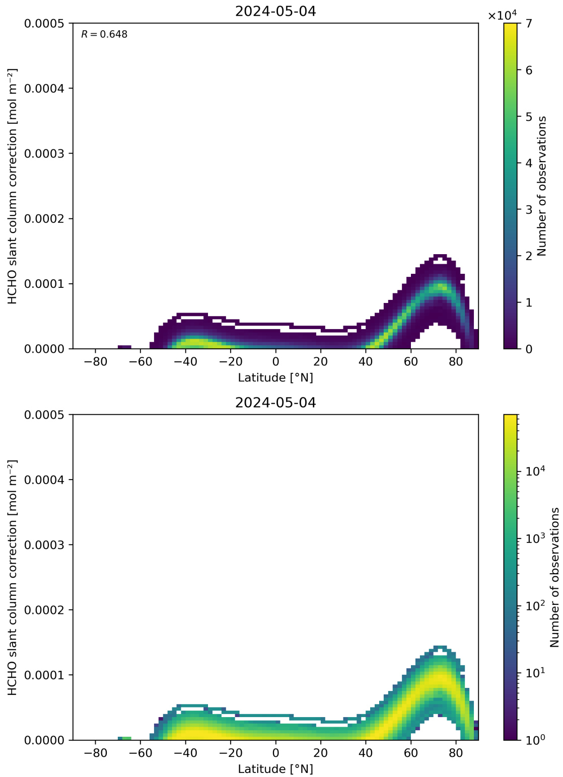
Figure 158: Scatter density plot of “Latitude” against “HCHO slant column correction” for 2024-05-03 to 2024-05-05.
