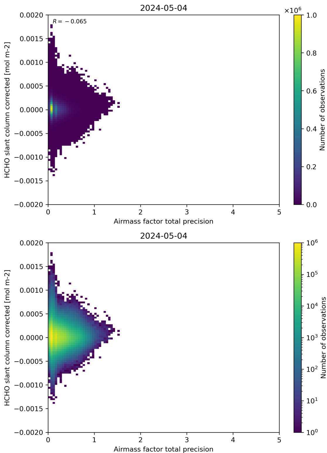
Figure 109: Scatter density plot of “Airmass factor total precision” against “HCHO slant column corrected” for 2024-05-03 to 2024-05-05.
