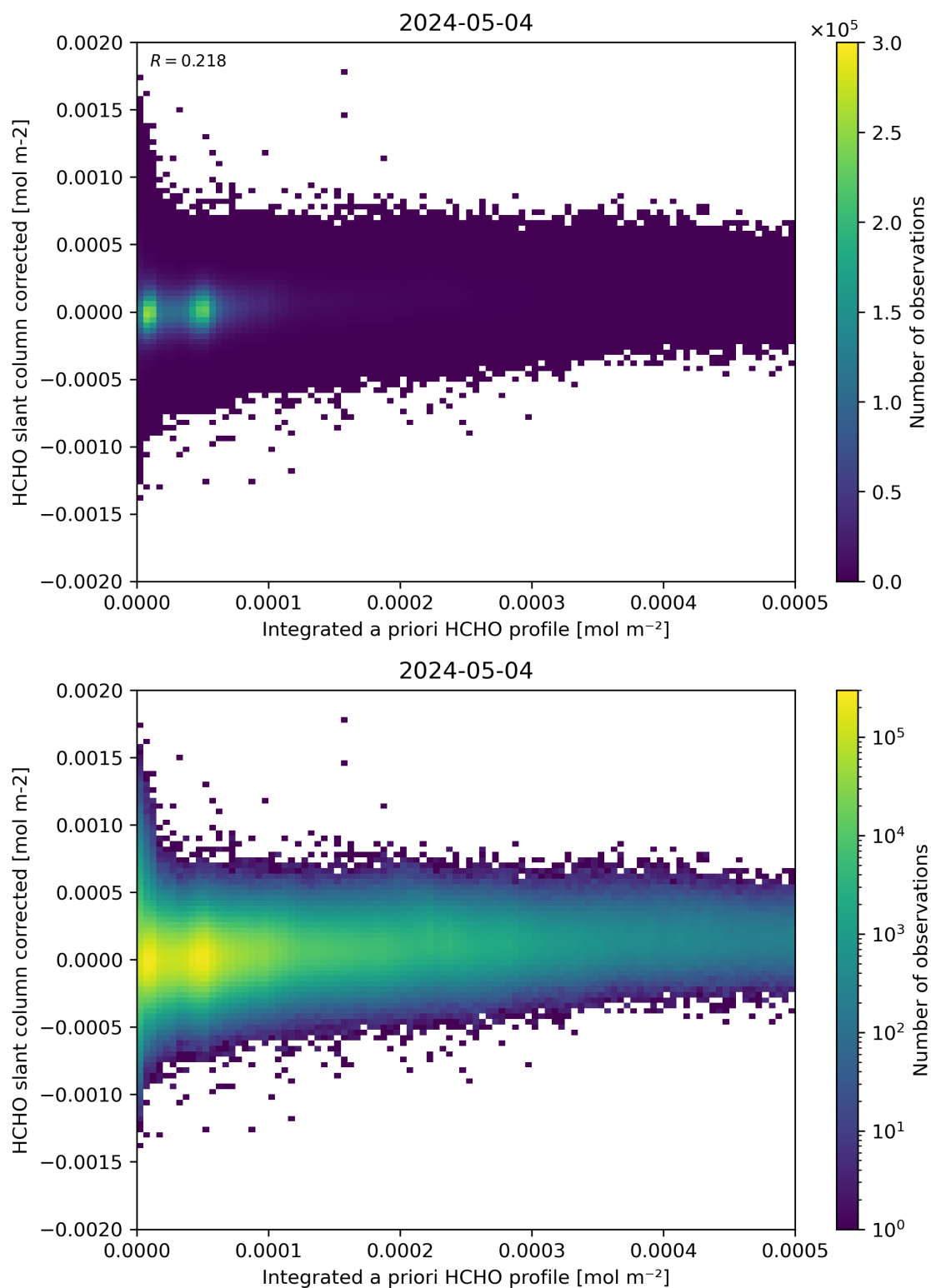
Figure 151: Scatter density plot of “Integrated a priori HCHO profile” against “HCHO slant column corrected” for 2024-05-03 to 2024-05-05.
