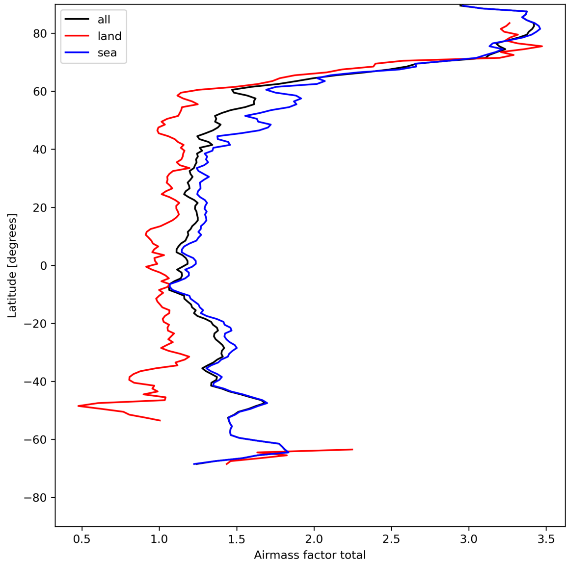
Figure 26: Zonal average of “Airmass factor total” for 2024-05-03 to 2024-05-05.
