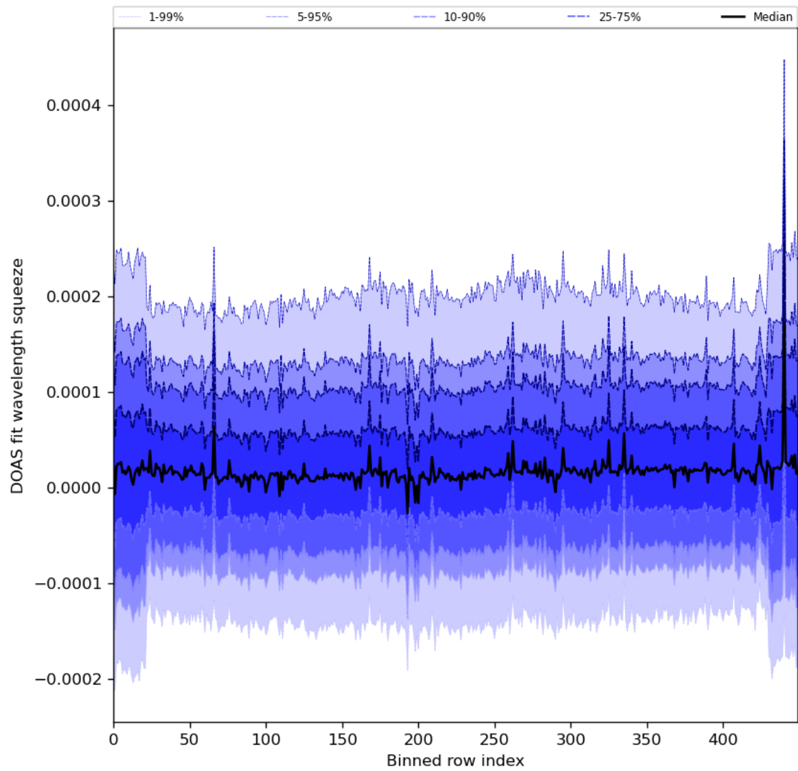
Figure 59: Along track statistics of “DOAS fit wavelength squeeze” for 2024-05-03 to 2024-05-05
