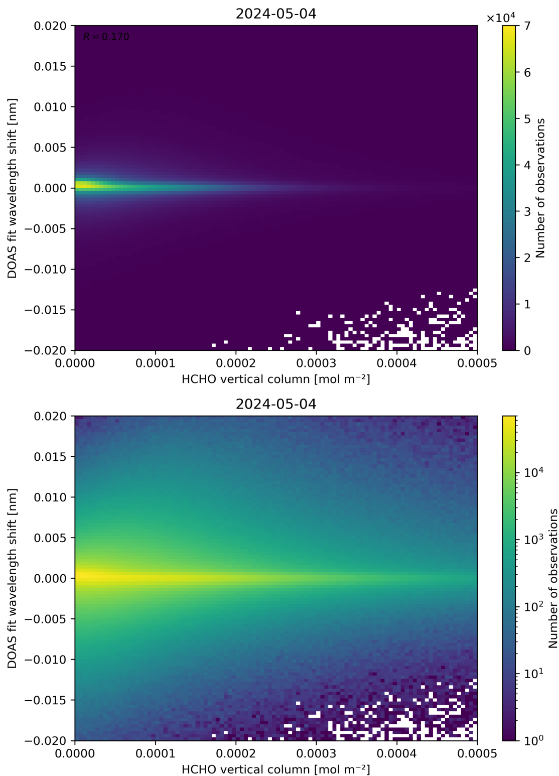
Figure 124: Scatter density plot of “HCHO vertical column” against “DOAS fit wavelength shift” for 2024-05-03 to 2024-05-05.
