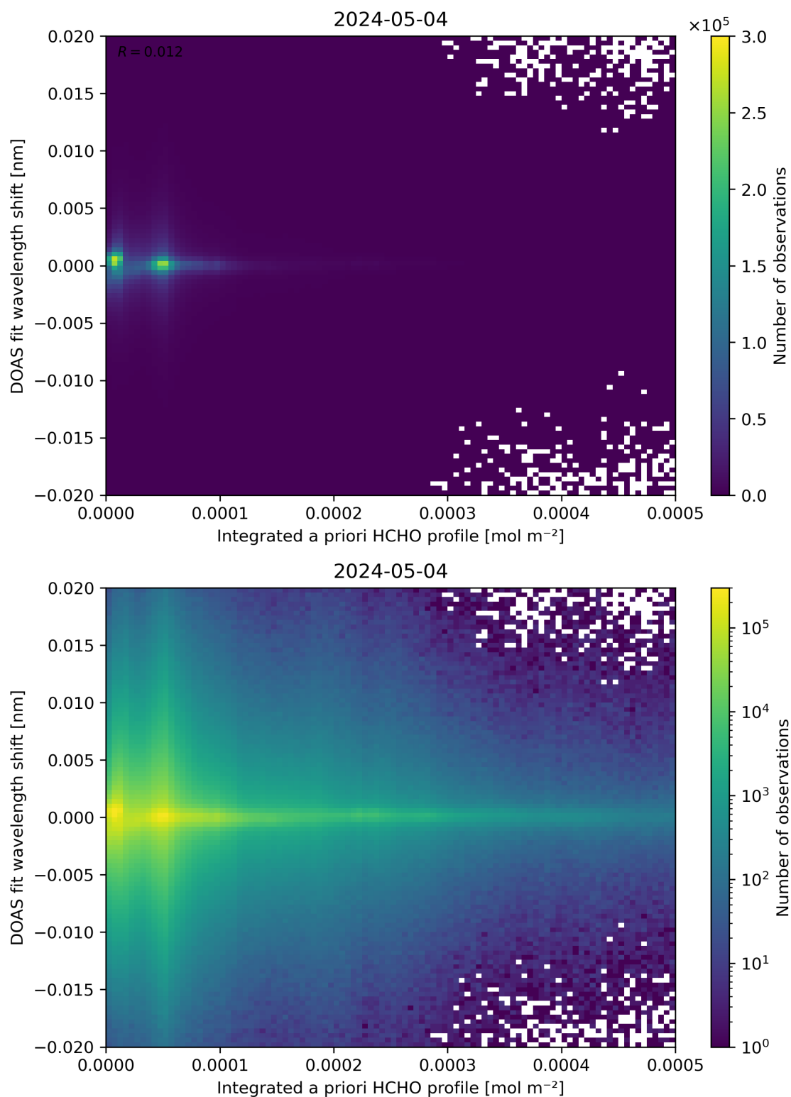
Figure 149: Scatter density plot of “Integrated a priori HCHO profile” against “DOAS fit wavelength shift” for 2024-05-03 to 2024-05-05.
