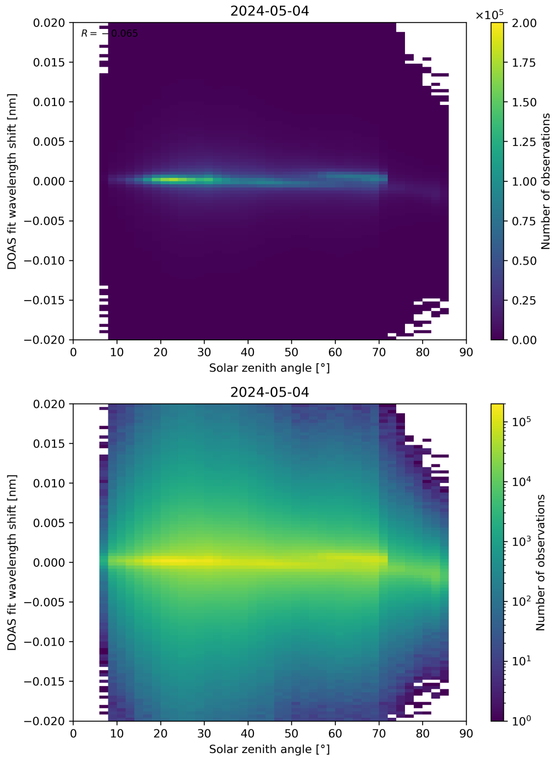
Figure 168: Scatter density plot of “Solar zenith angle” against “DOAS fit wavelength shift” for 2024-05-03 to 2024-05-05.
