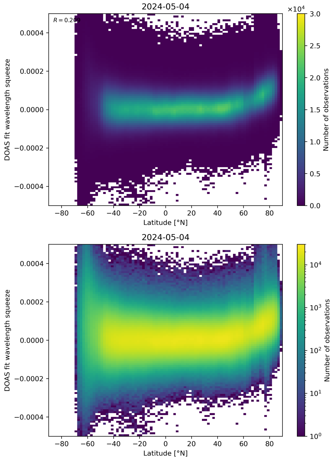
Figure 155: Scatter density plot of “Latitude” against “DOAS fit wavelength squeeze” for 2024-05-03 to 2024-05-05.
