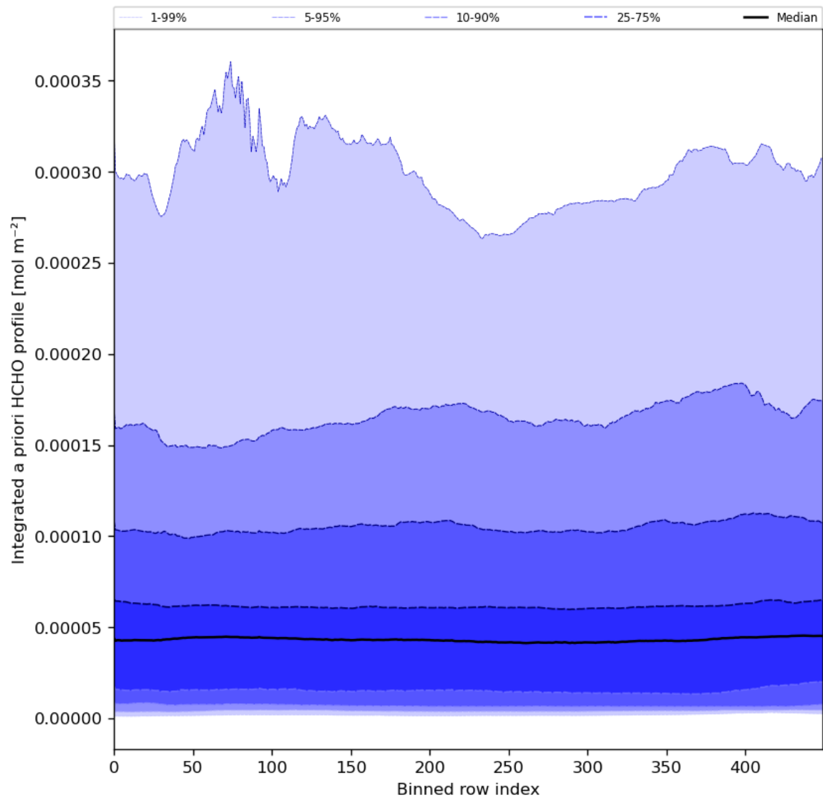
Figure 57: Along track statistics of "Integrated a priori HCHO profile" for 2024-05-03 to 2024-05-05
