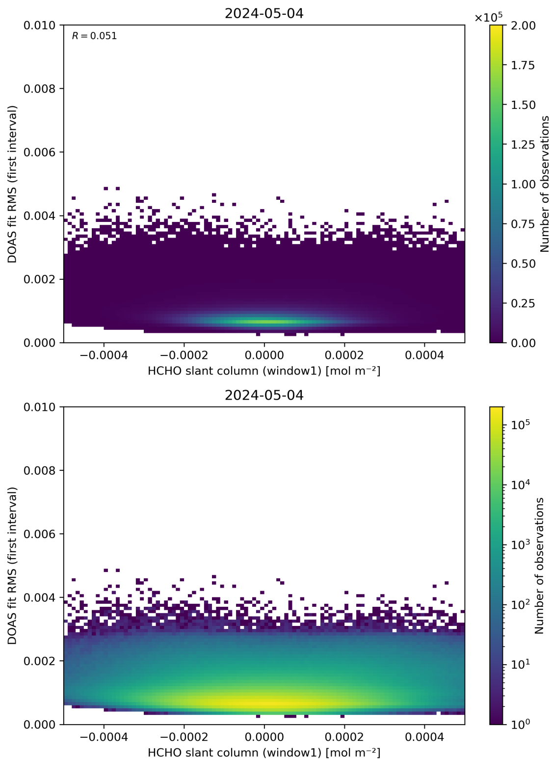
Figure 78: Scatter density plot of “HCHO slant column (window1)” against “DOAS fit RMS (first interval)” for 2024-05-03 to 2024-05-05.
