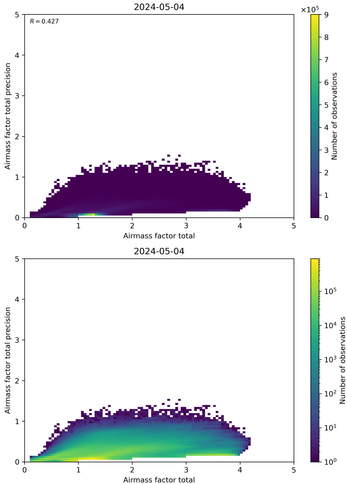
Figure 103: Scatter density plot of “Airmass factor total” against “Airmass factor total precision” for 2024-05-03 to 2024-05-05.
