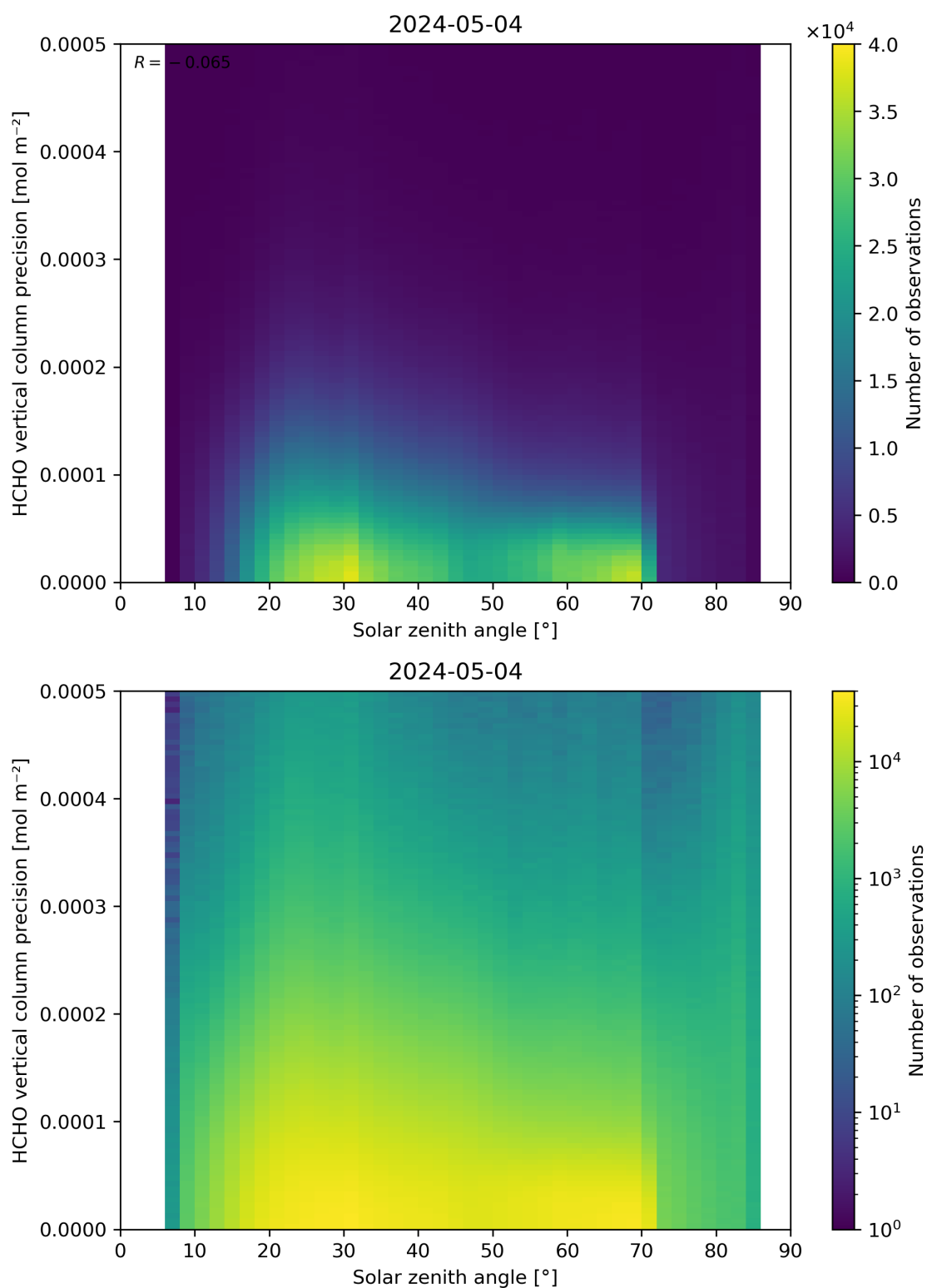
Figure 179: Scatter density plot of “Solar zenith angle” against “HCHO vertical column precision” for 2024-05-03 to 2024-05-05.
