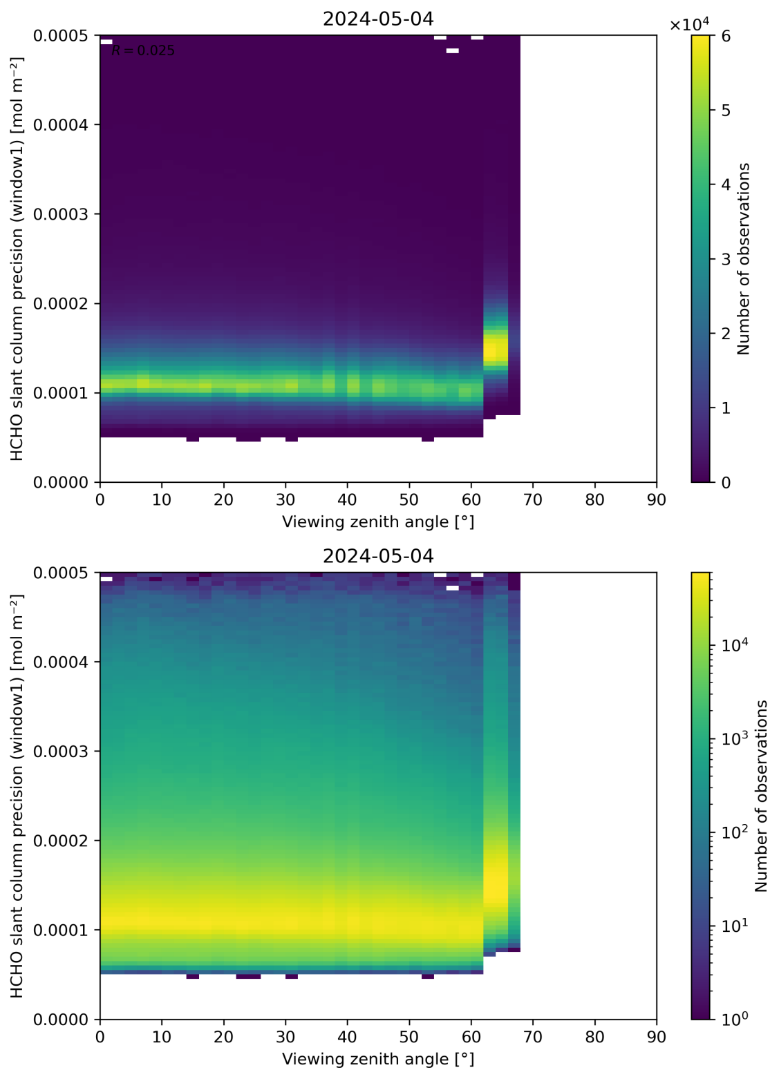
Figure 189: Scatter density plot of “Viewing zenith angle” against “HCHO slant column precision (window1)” for 2024-05-03 to 2024-05-05.
