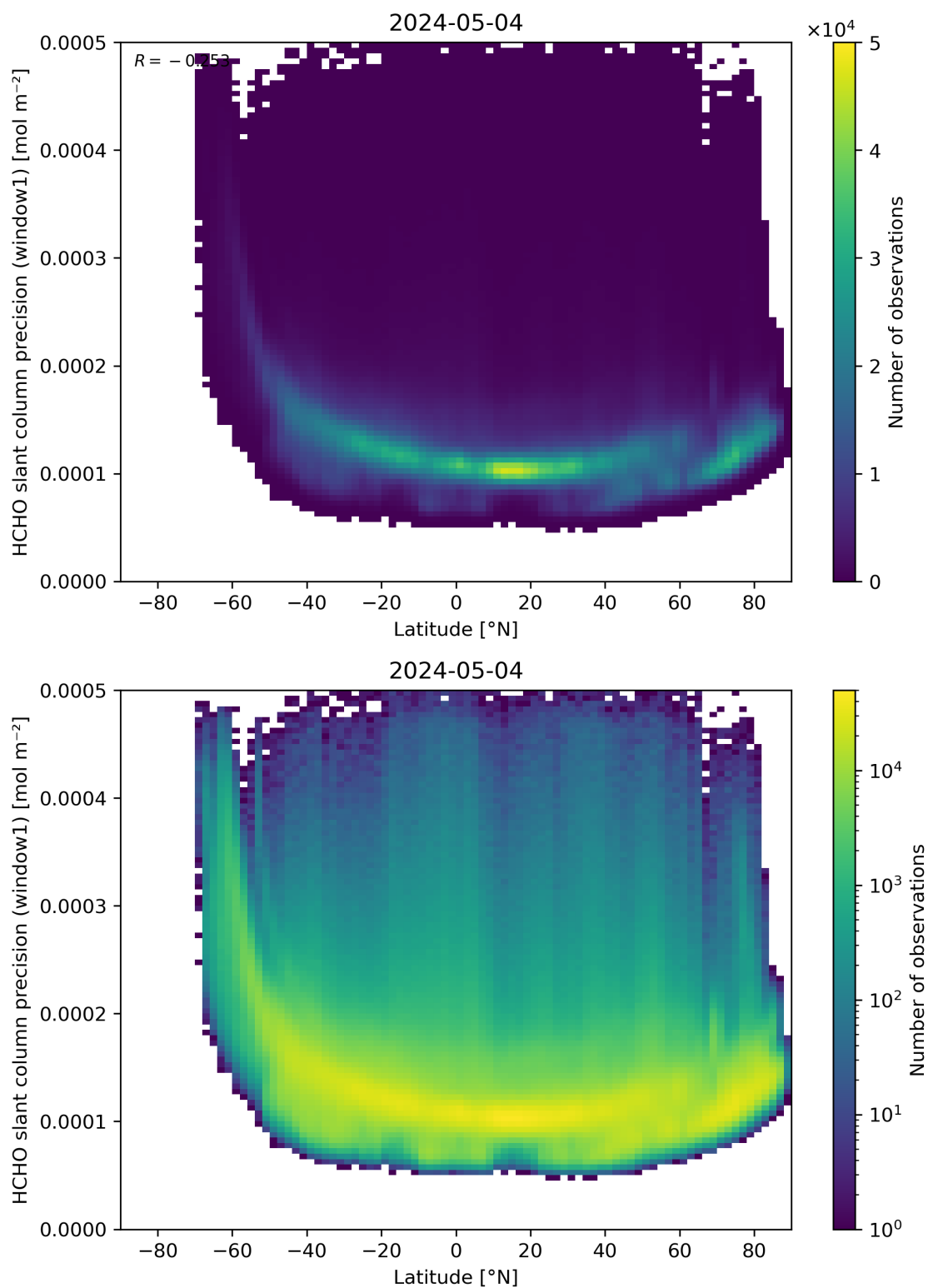
Figure 160: Scatter density plot of “Latitude” against “HCHO slant column precision (window1)” for 2024-05-03 to 2024-05-05.
