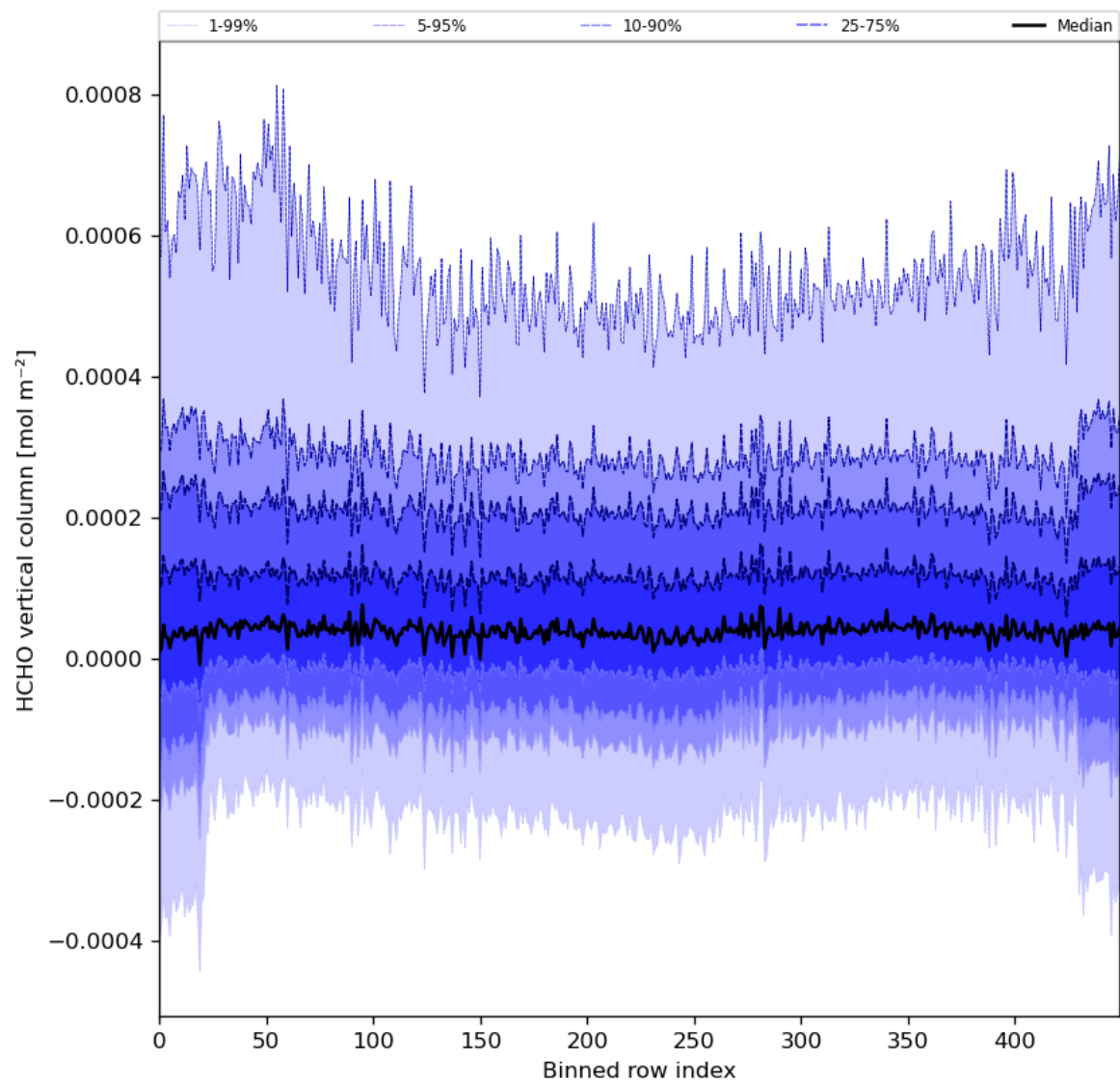
Figure 49: Along track statistics of “HCHO vertical column” for 2024-05-03 to 2024-05-05
