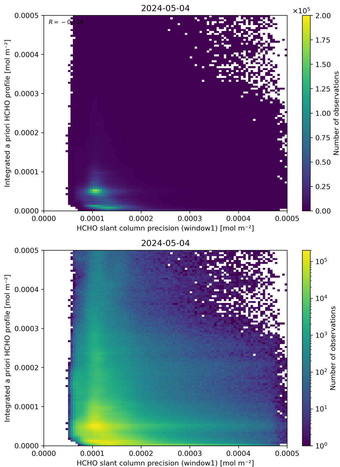
Figure 96: Scatter density plot of “HCHO slant column precision (window1)” against “Integrated a priori HCHO profile” for 2024-05-03 to 2024-05-05.
