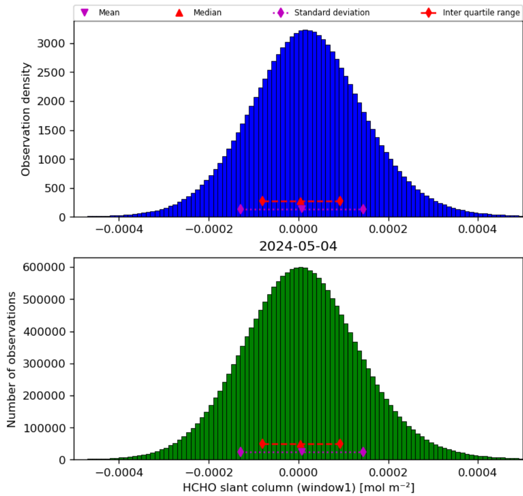
Figure 38: Histogram of “HCHO slant column (window1)” for 2024-05-03 to 2024-05-05
