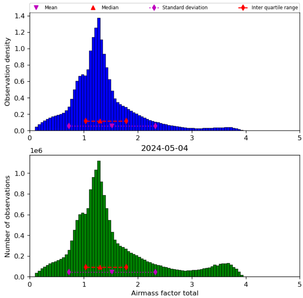
Figure 40: Histogram of “Airmass factor total” for 2024-05-03 to 2024-05-05
