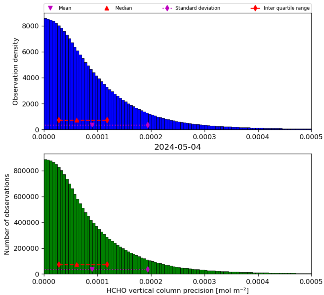
Figure 36: Histogram of “HCHO vertical column precision” for 2024-05-03 to 2024-05-05
