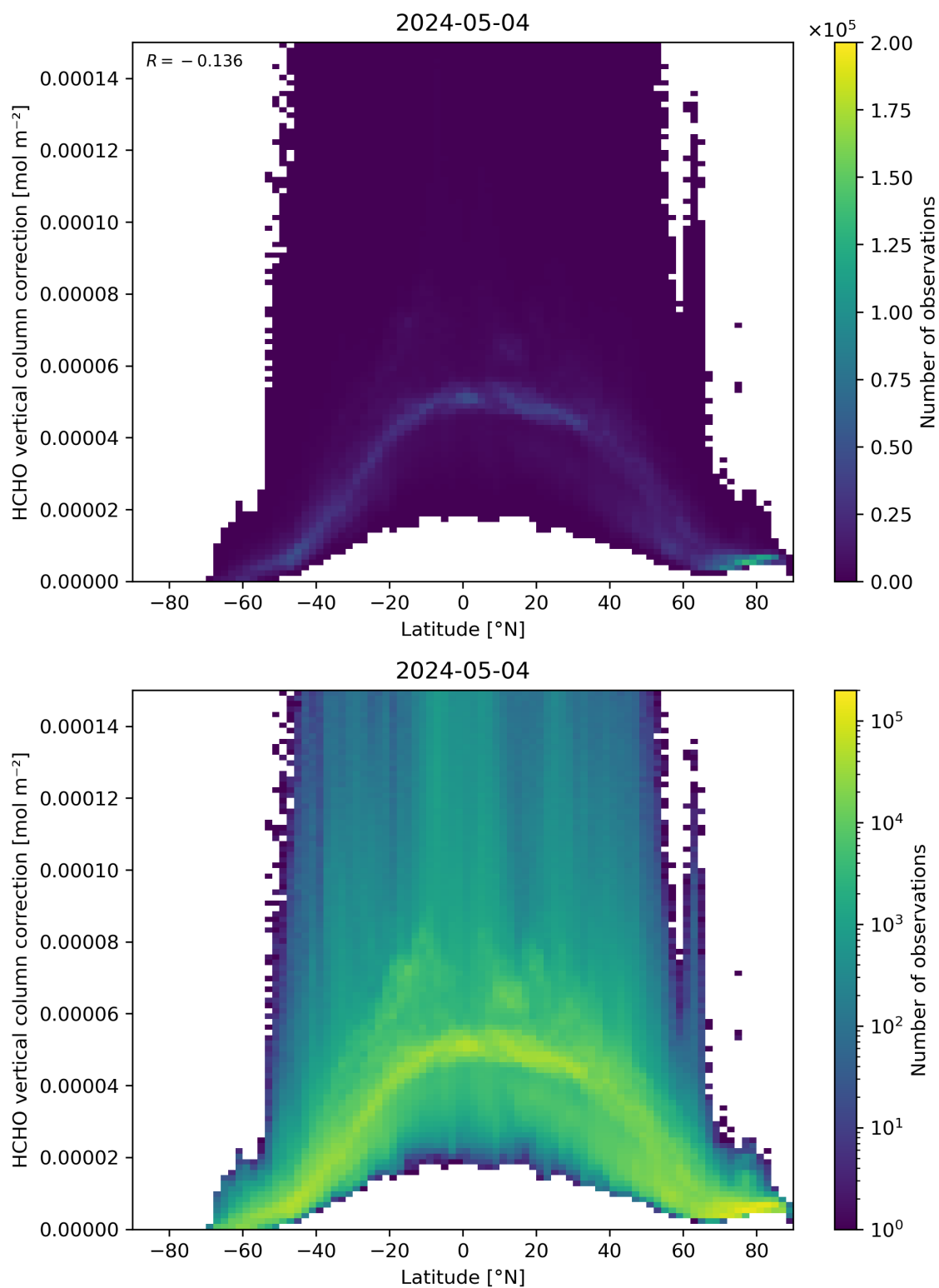
Figure 164: Scatter density plot of “Latitude” against “HCHO vertical column correction” for 2024-05-03 to 2024-05-05.
