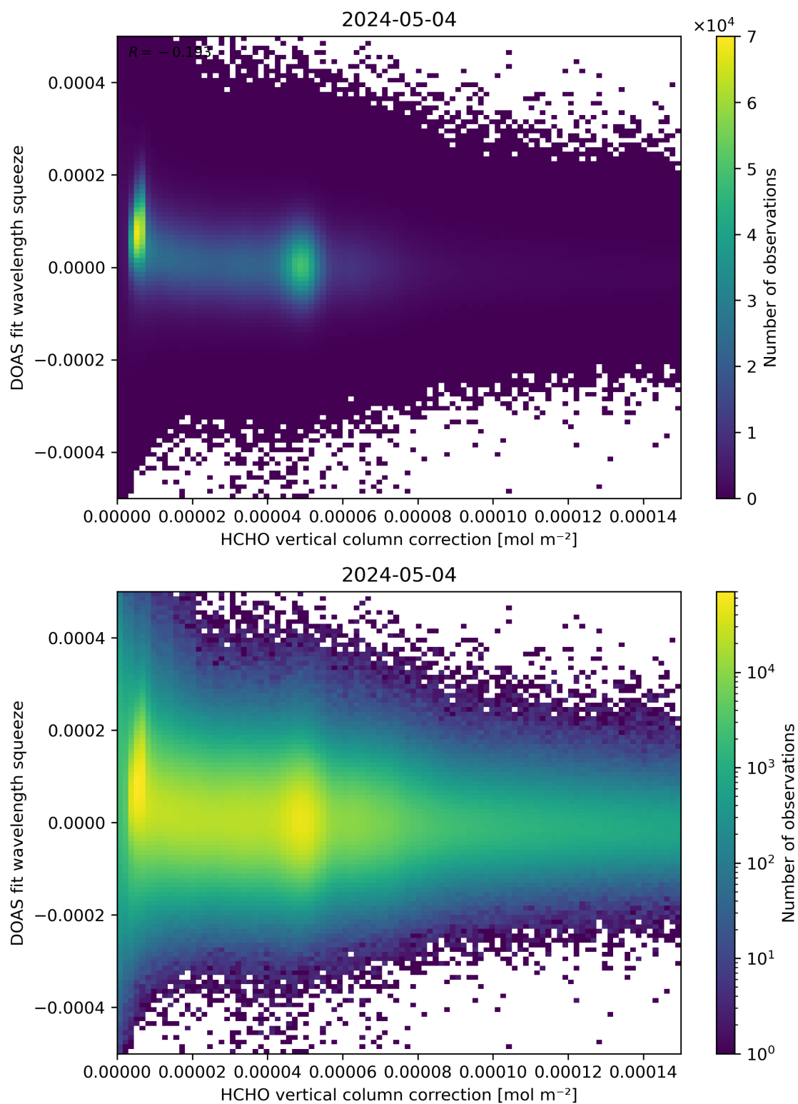
Figure 114: Scatter density plot of “HCHO vertical column correction” against “DOAS fit wavelength squeeze” for 2024-05-03 to 2024-05-05.
