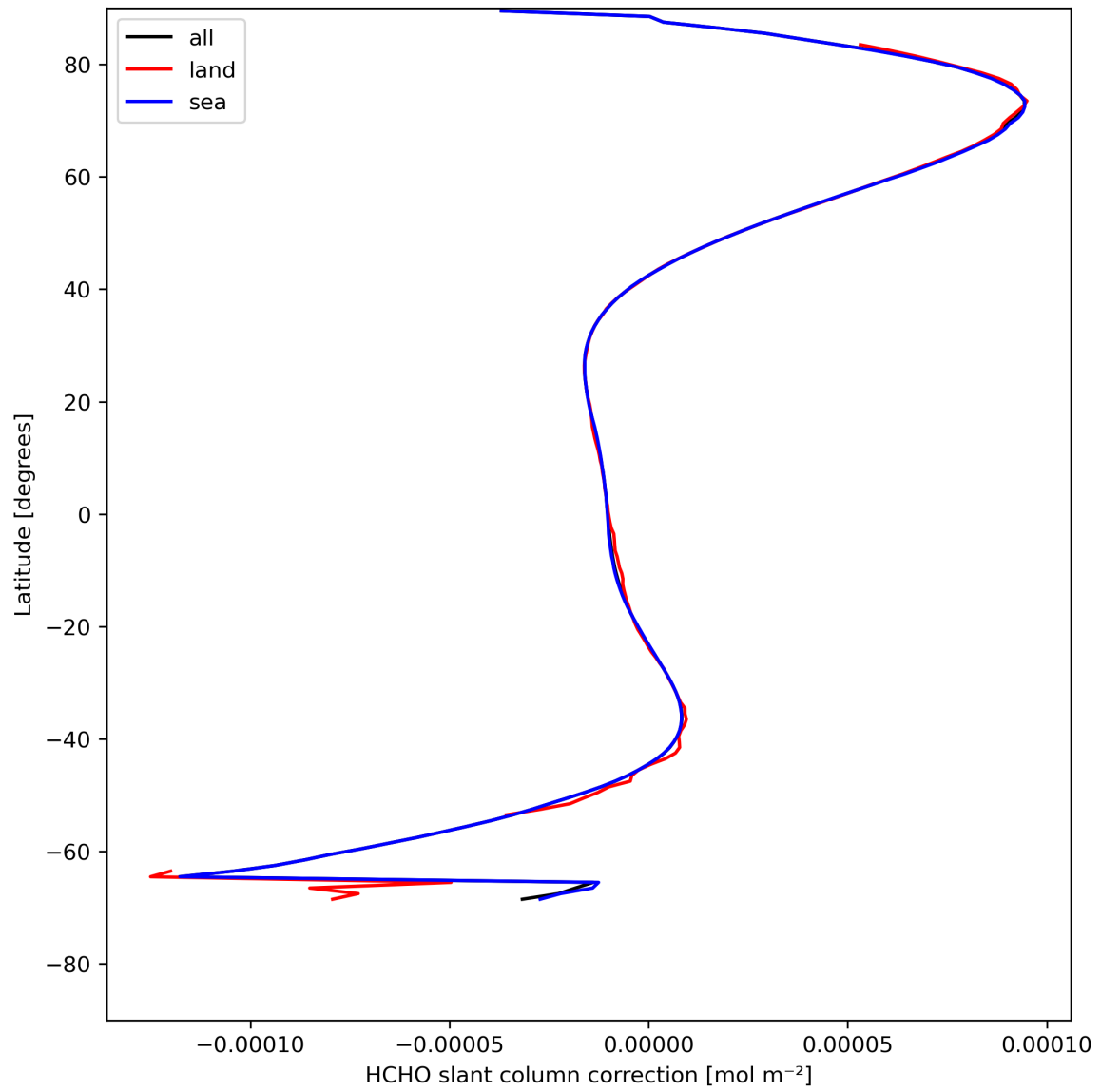
Figure 33: Zonal average of “HCHO slant column correction” for 2024-05-03 to 2024-05-05.
