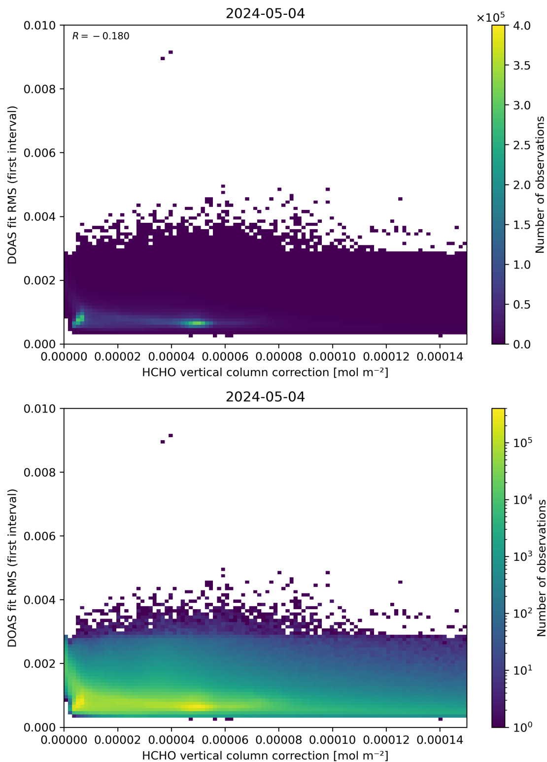
Figure 112: Scatter density plot of “HCHO vertical column correction” against “DOAS fit RMS (first interval)” for 2024-05-03 to 2024-05-05.
