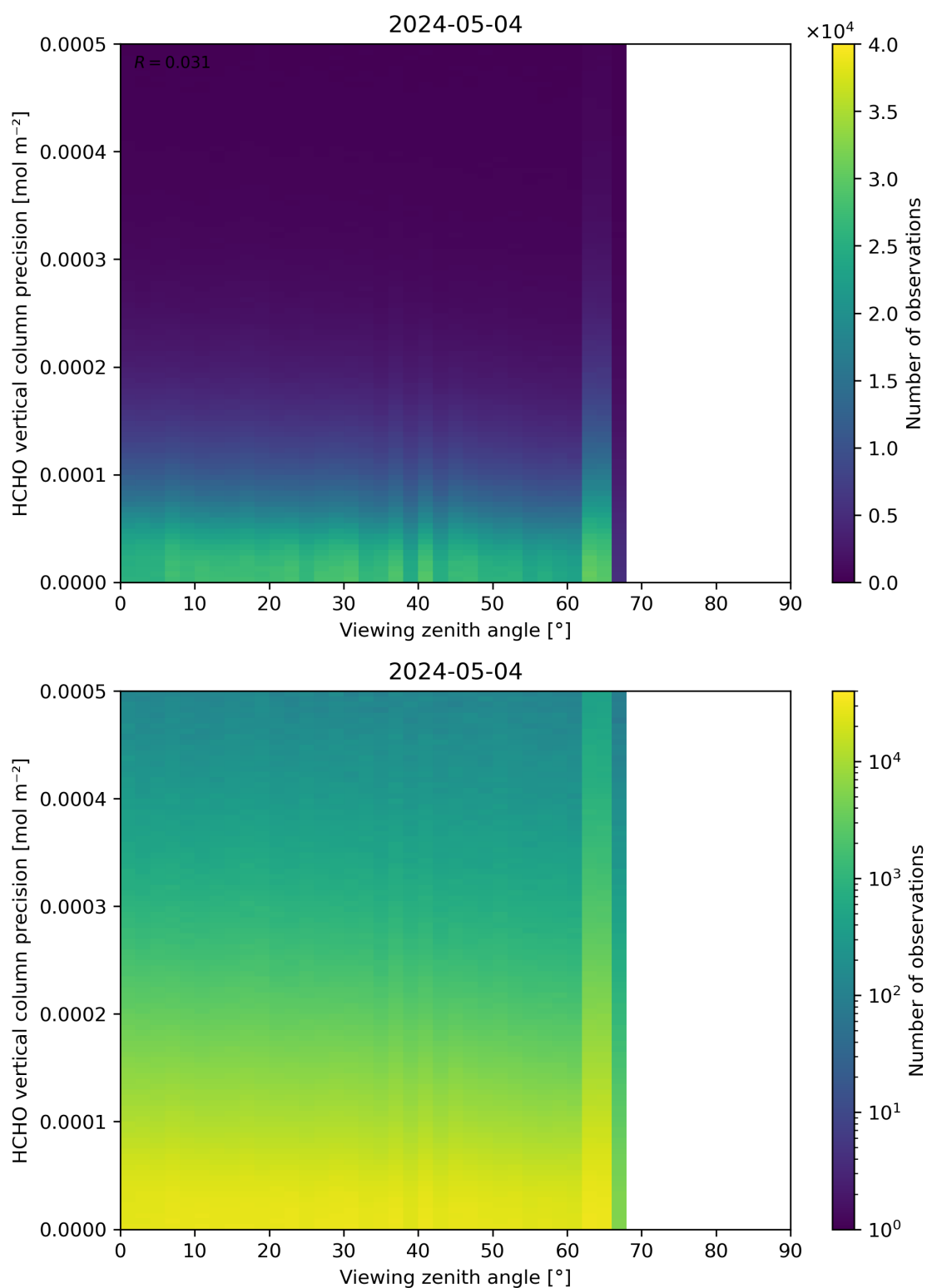
Figure 194: Scatter density plot of “Viewing zenith angle” against “HCHO vertical column precision” for 2024-05-03 to 2024-05-05.
