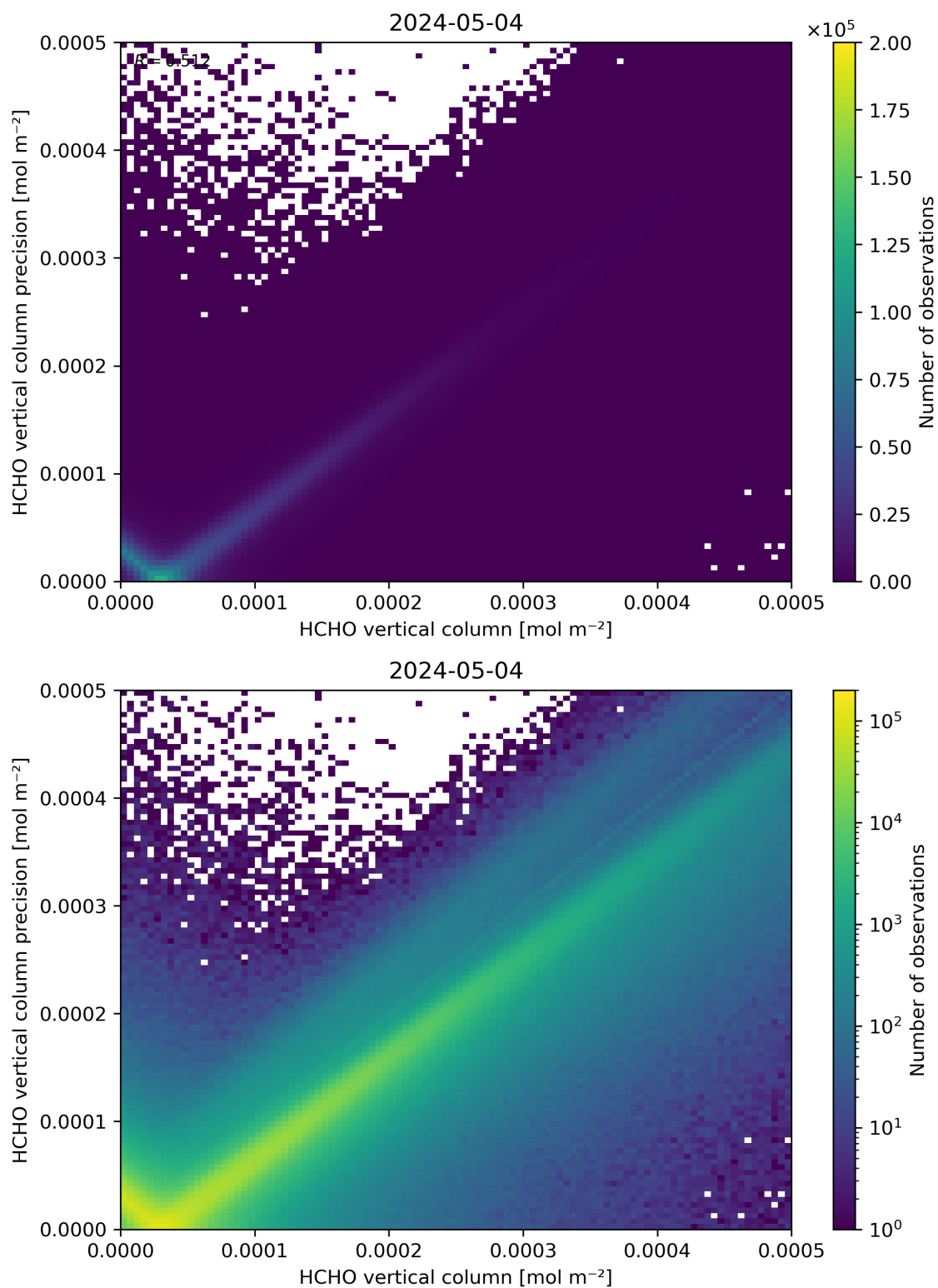
Figure 134: Scatter density plot of “HCHO vertical column” against “HCHO vertical column precision” for 2024-05-03 to 2024-05-05.
