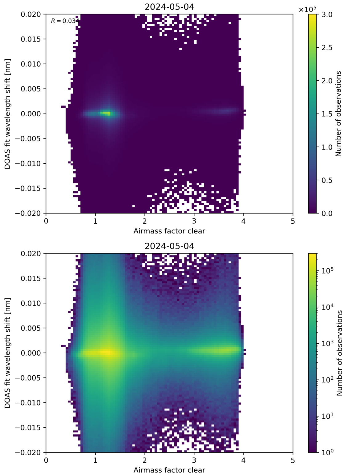
Figure 72: Scatter density plot of “Airmass factor clear” against “DOAS fit wavelength shift” for 2024-05-03 to 2024-05-05.
