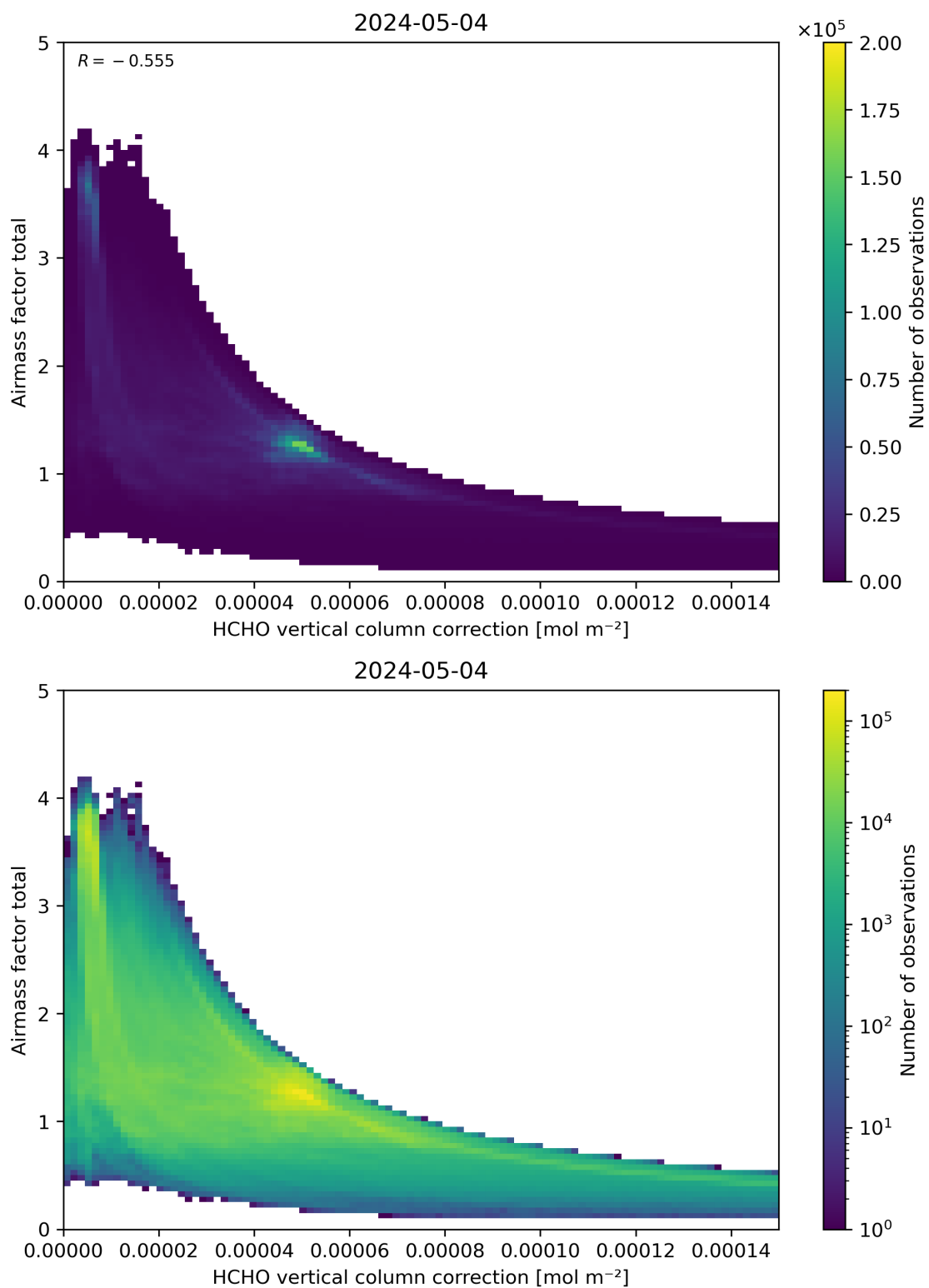
Figure 120: Scatter density plot of “HCHO vertical column correction” against “Airmass factor total” for 2024-05-03 to 2024-05-05.
