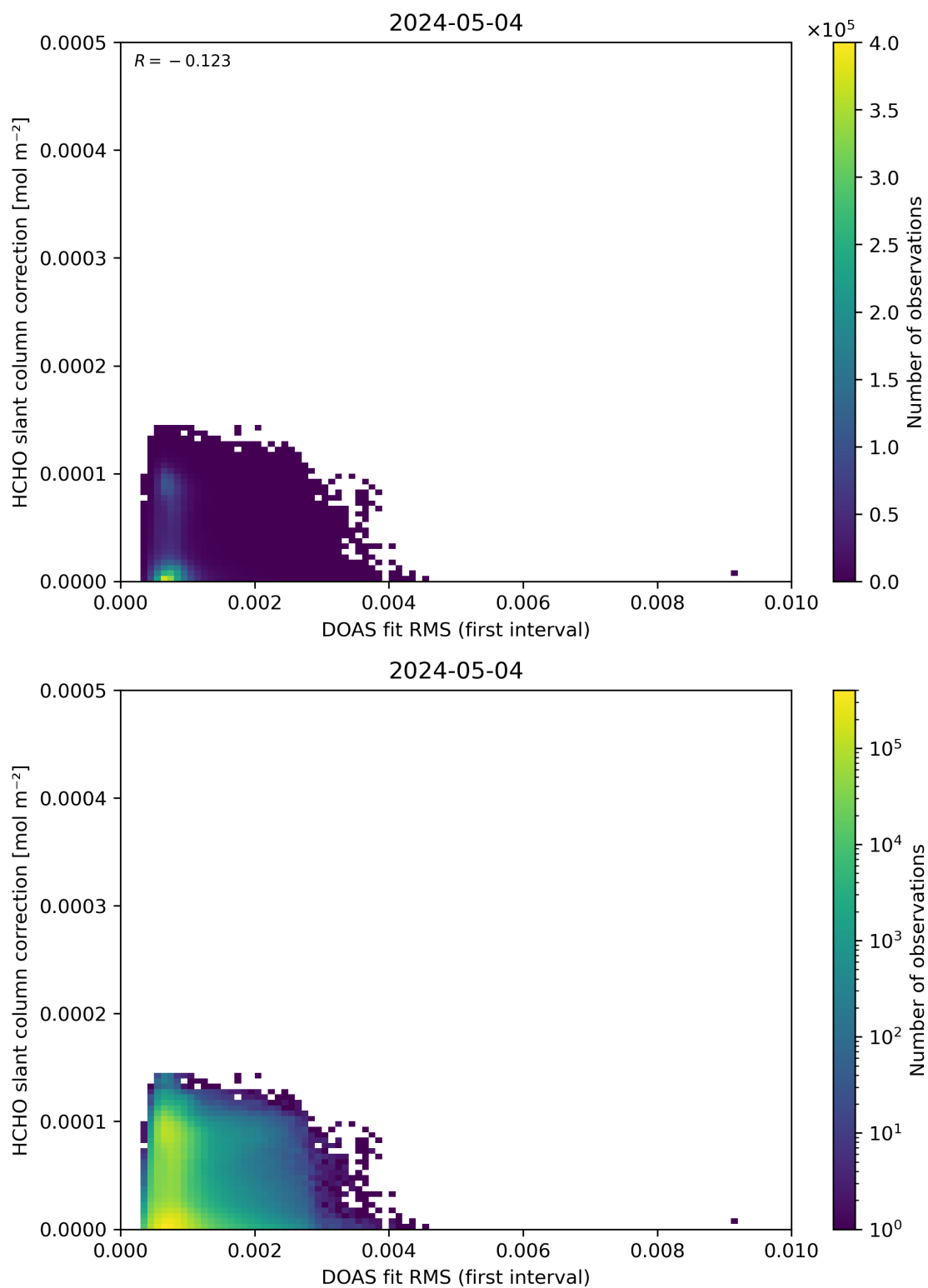
Figure 63: Scatter density plot of “DOAS fit RMS (first interval)” against “HCHO slant column correction” for 2024-05-03 to 2024-05-05.
