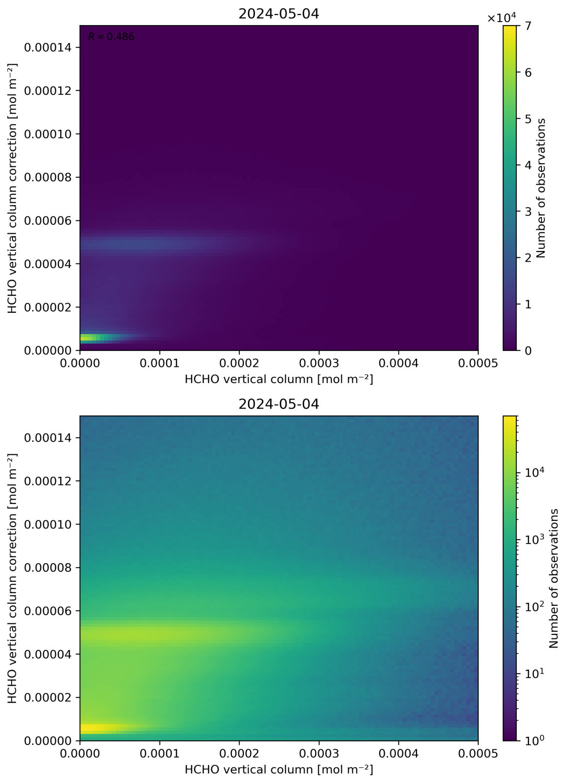
Figure 133: Scatter density plot of “HCHO vertical column” against “HCHO vertical column correction” for 2024-05-03 to 2024-05-05.
