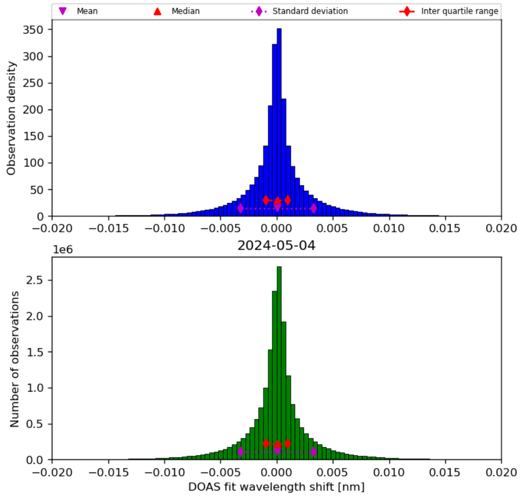
Figure 44: Histogram of “DOAS fit wavelength shift” for 2024-05-03 to 2024-05-05
