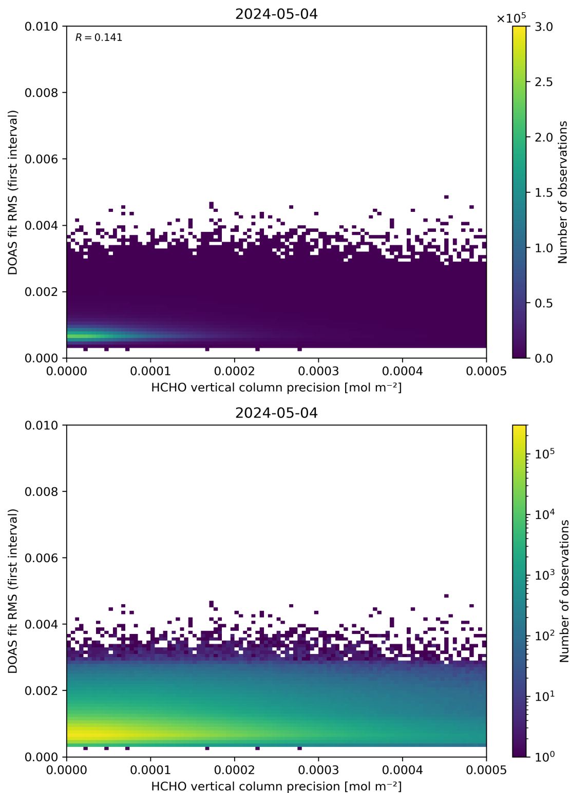
Figure 136: Scatter density plot of “HCHO vertical column precision” against “DOAS fit RMS (first interval)” for 2024-05-03 to 2024-05-05.
