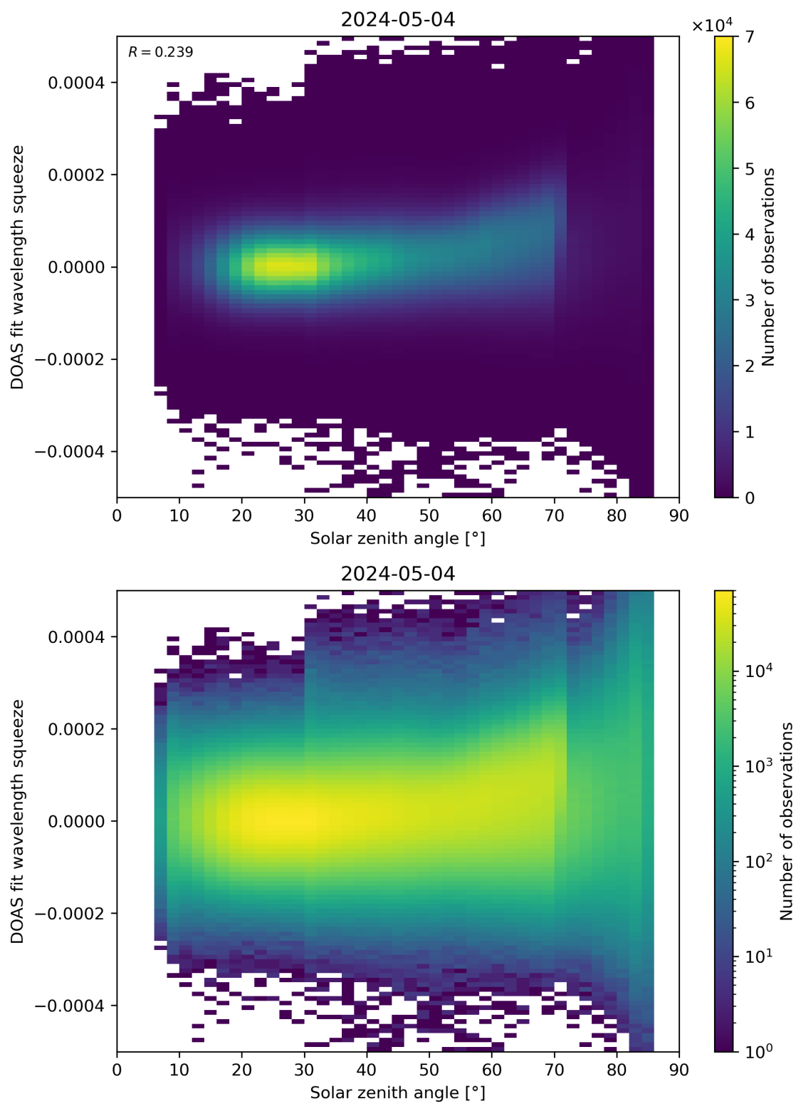
Figure 169: Scatter density plot of “Solar zenith angle” against “DOAS fit wavelength squeeze” for 2024-05-03 to 2024-05-05.
