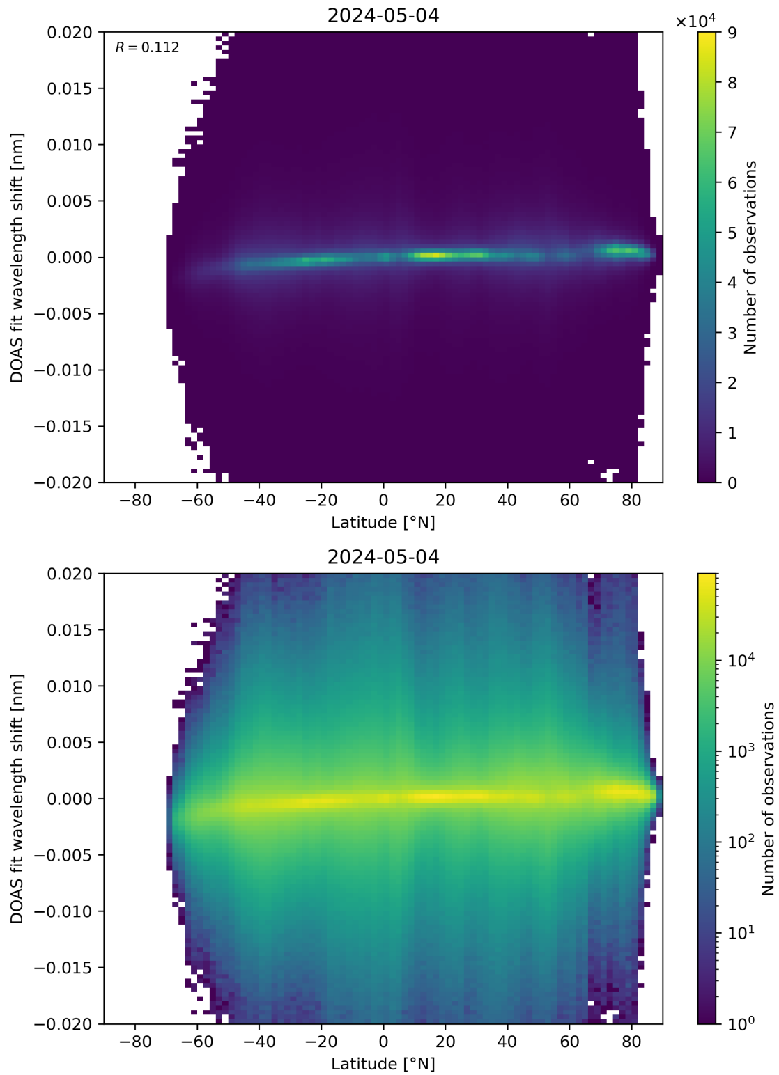
Figure 154: Scatter density plot of “Latitude” against “DOAS fit wavelength shift” for 2024-05-03 to 2024-05-05.
