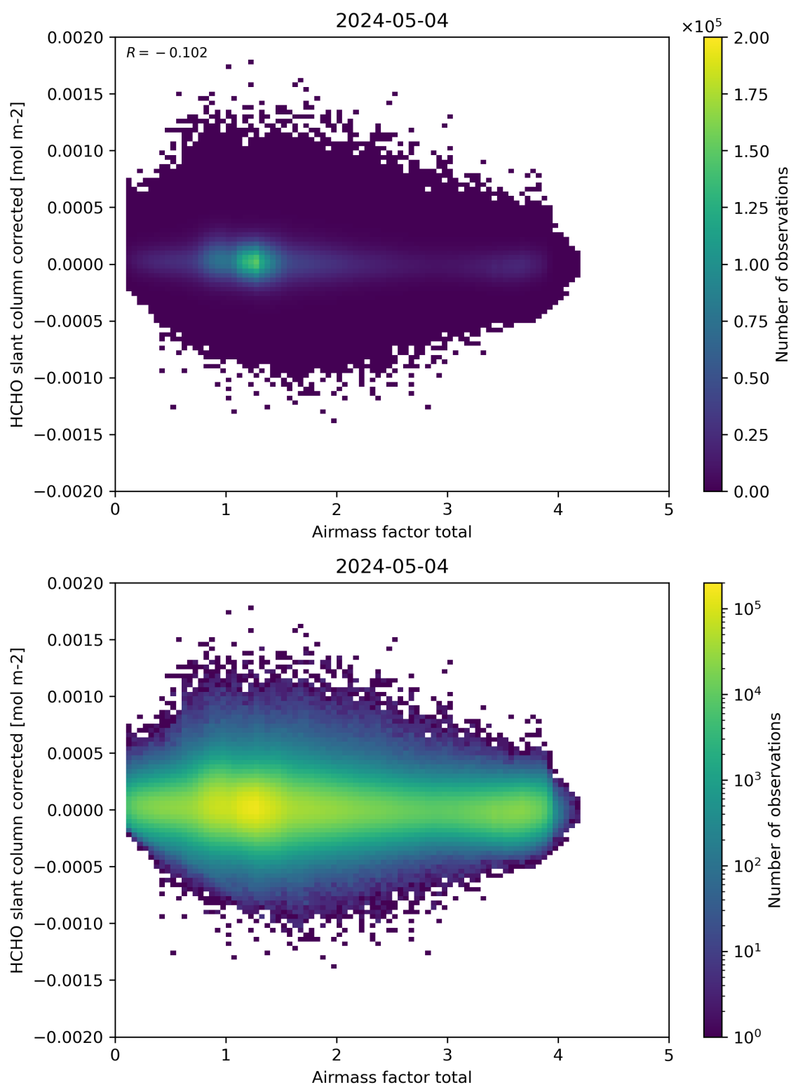
Figure 101: Scatter density plot of “Airmass factor total” against “HCHO slant column corrected” for 2024-05-03 to 2024-05-05.
