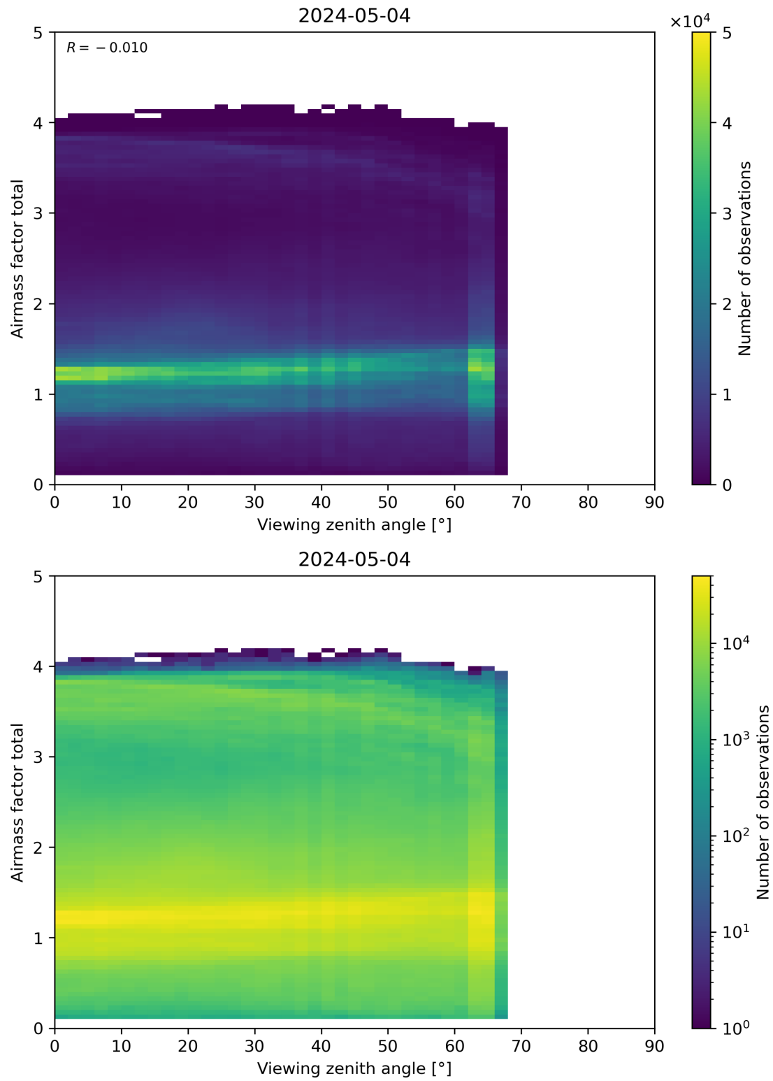
Figure 190: Scatter density plot of “Viewing zenith angle” against “Airmass factor total” for 2024-05-03 to 2024-05-05.
