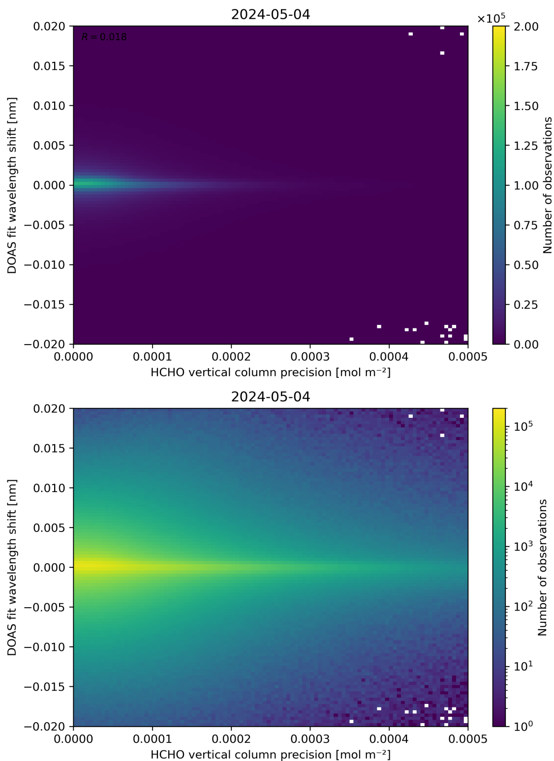
Figure 137: Scatter density plot of “HCHO vertical column precision” against “DOAS fit wavelength shift” for 2024-05-03 to 2024-05-05.
