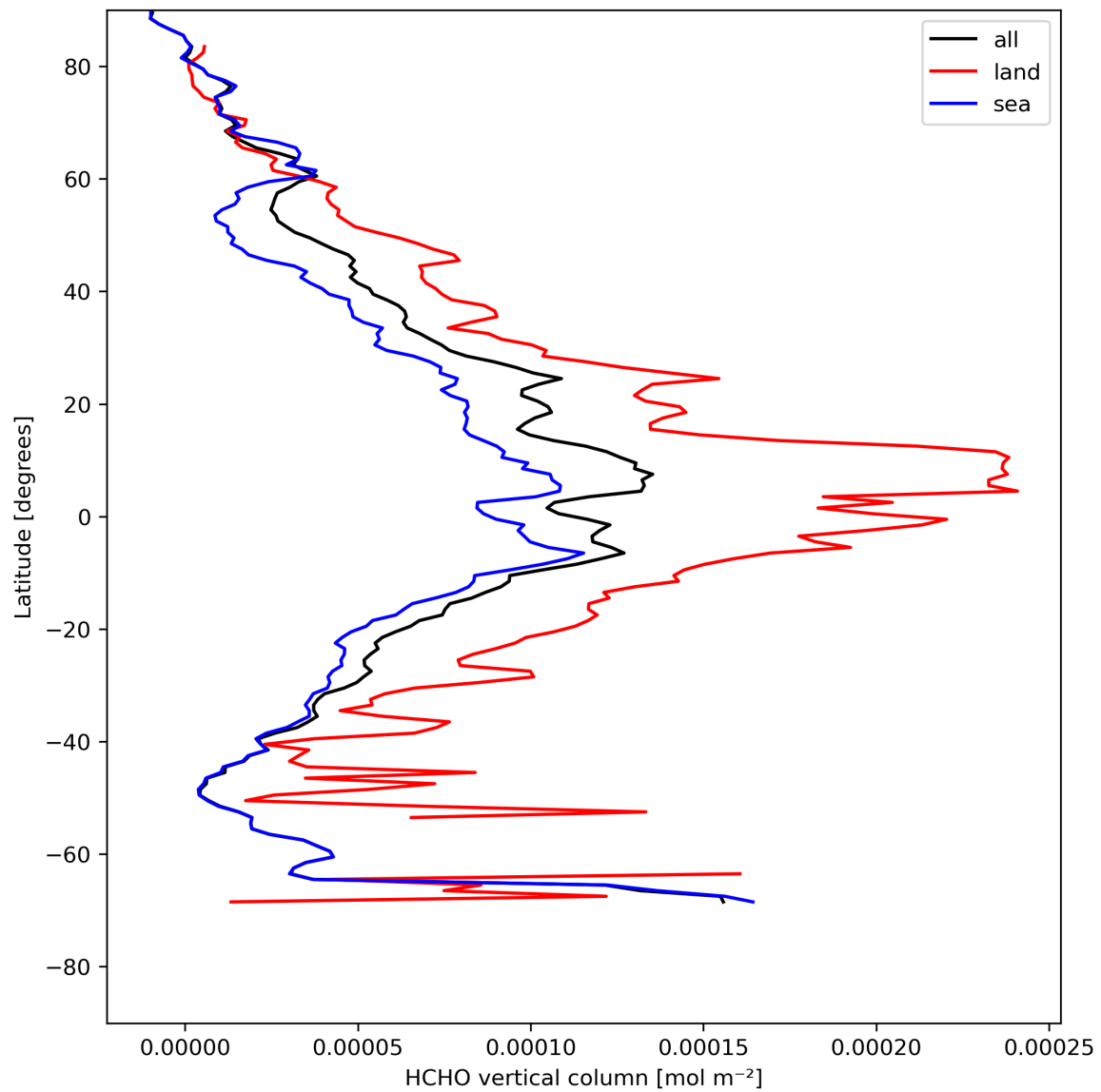
Figure 21: Zonal average of “HCHO vertical column” for 2024-05-03 to 2024-05-05.
