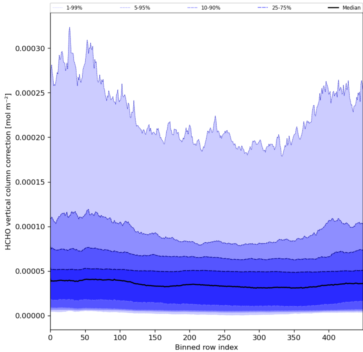
Figure 51: Along track statistics of “HCHO vertical column correction” for 2024-05-03 to 2024-05-05
