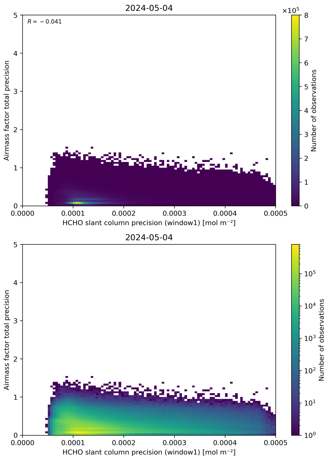
Figure 95: Scatter density plot of “HCHO slant column precision (window1)” against “Airmass factor total precision” for 2024-05-03 to 2024-05-05.
