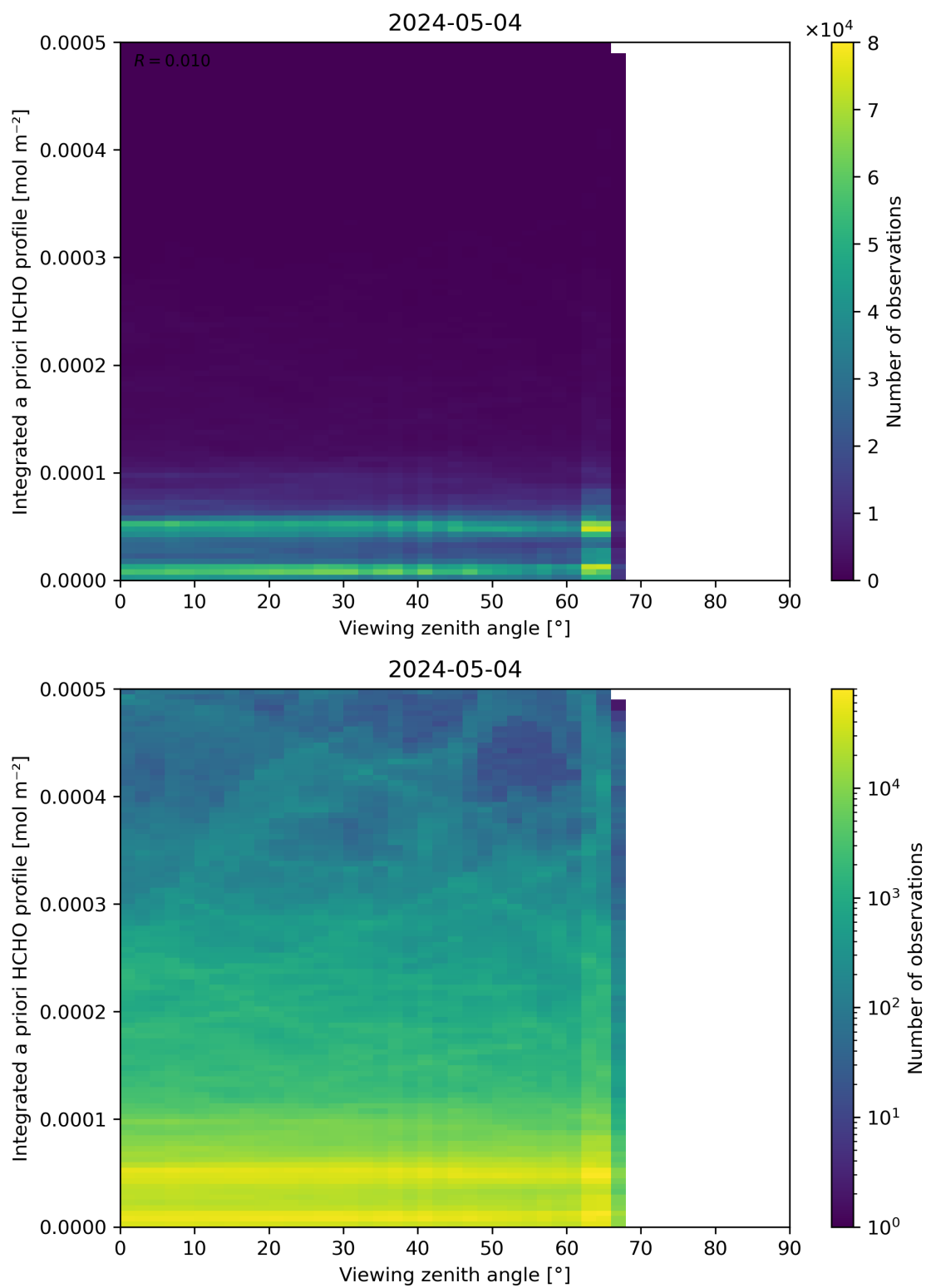
Figure 195: Scatter density plot of “Viewing zenith angle” against “Integrated a priori HCHO profile” for 2024-05-03 to 2024-05-05.
