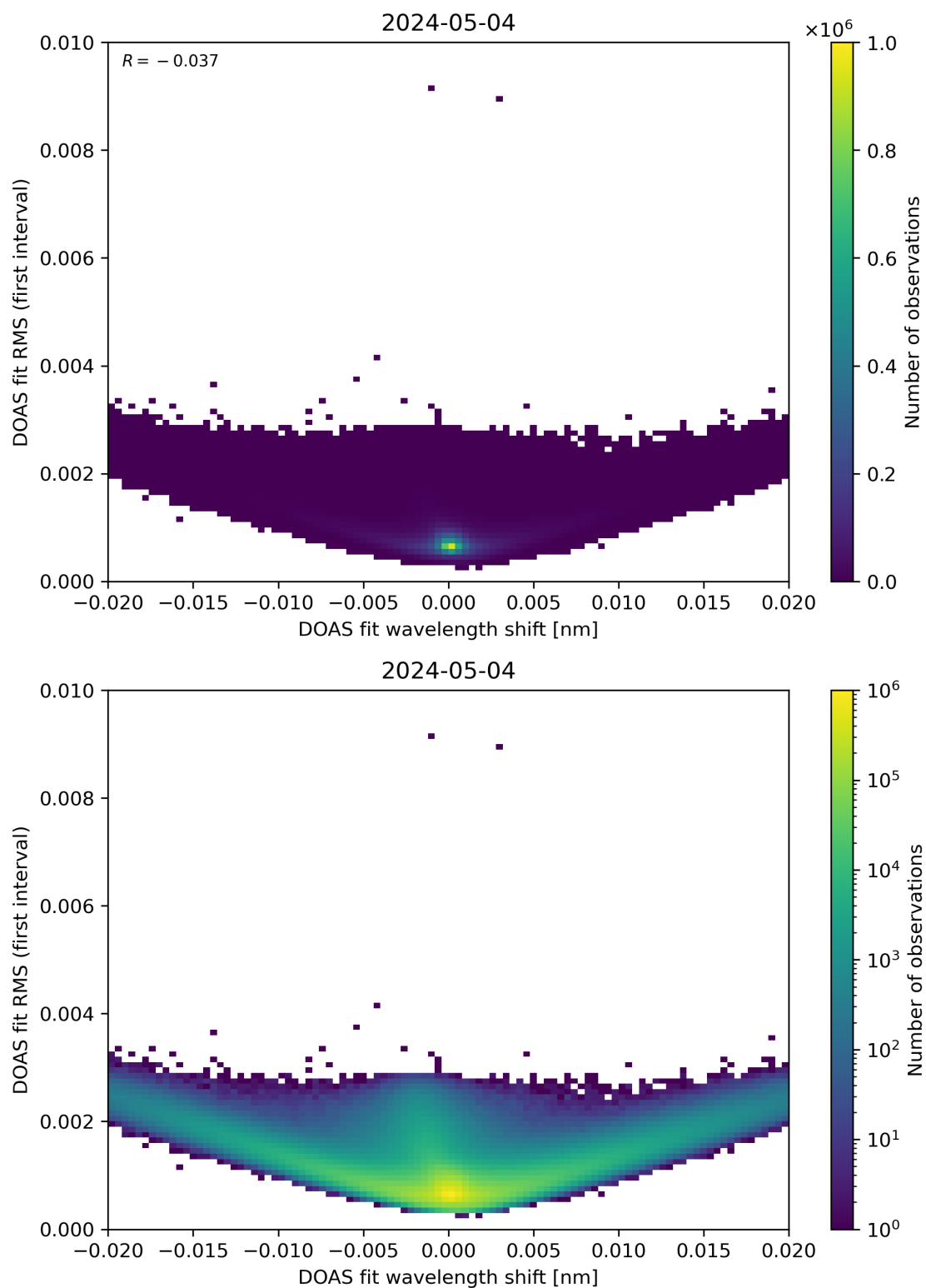
Figure 64: Scatter density plot of “DOAS fit wavelength shift” against “DOAS fit RMS (first interval)” for 2024-05-03 to 2024-05-05.
