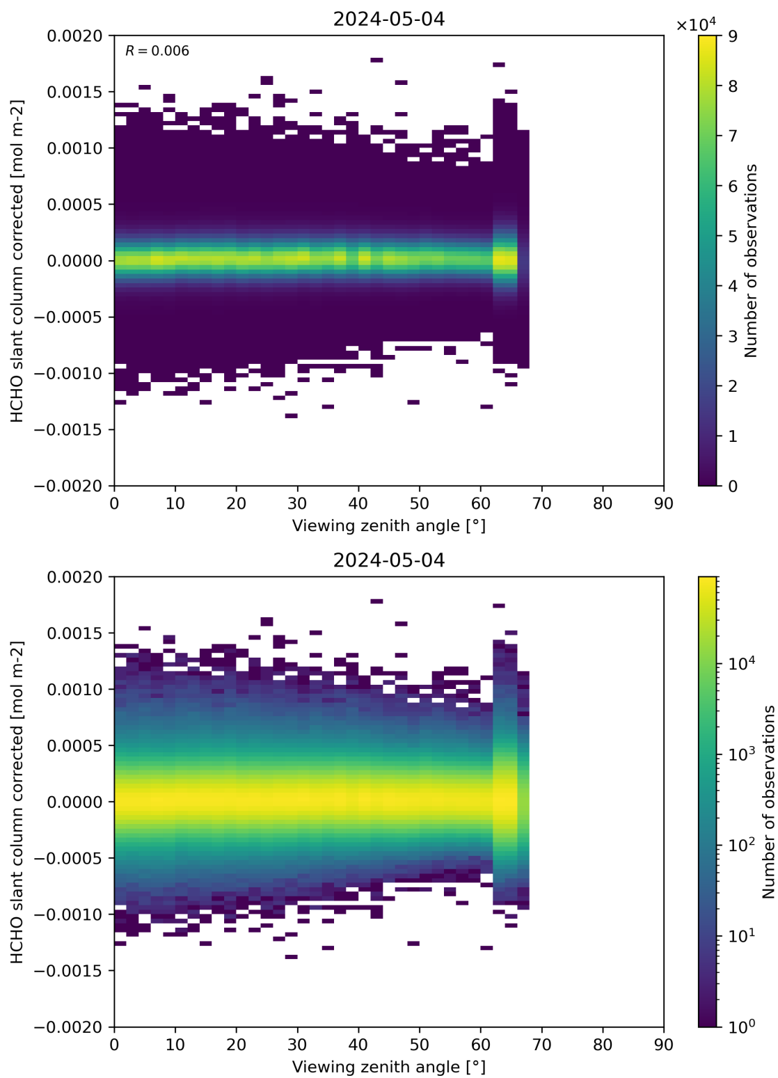
Figure 186: Scatter density plot of “Viewing zenith angle” against “HCHO slant column corrected” for 2024-05-03 to 2024-05-05.
