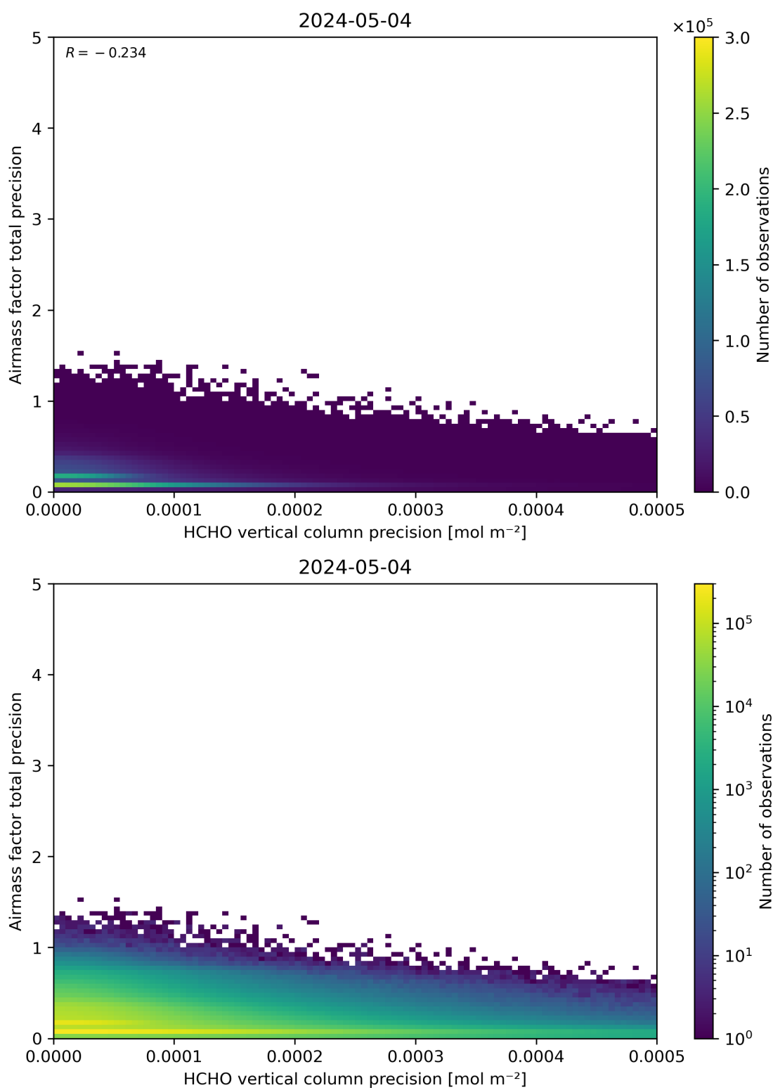
Figure 145: Scatter density plot of “HCHO vertical column precision” against “Airmass factor total precision” for 2024-05-03 to 2024-05-05.
