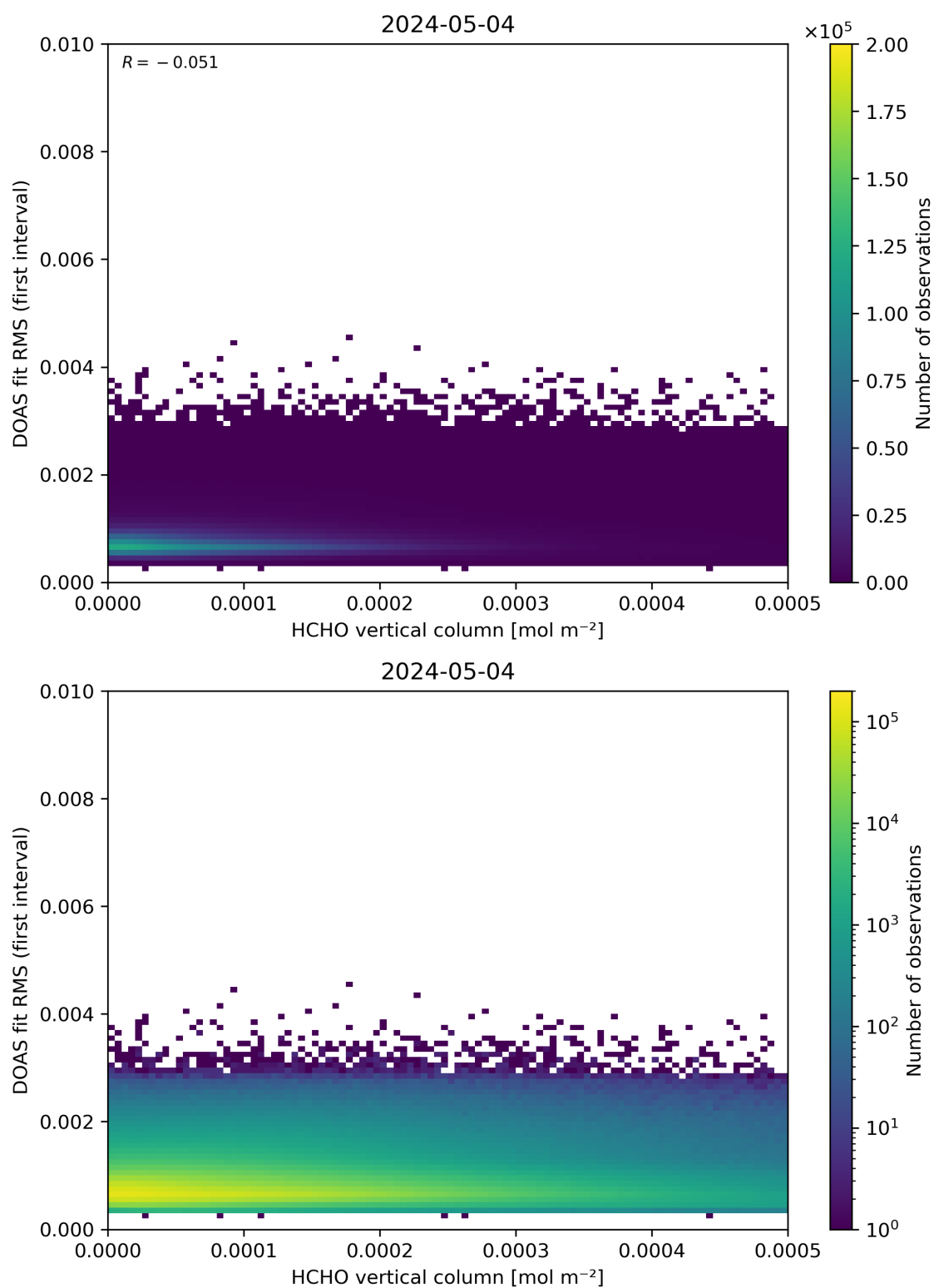
Figure 123: Scatter density plot of “HCHO vertical column” against “DOAS fit RMS (first interval)” for 2024-05-03 to 2024-05-05.
