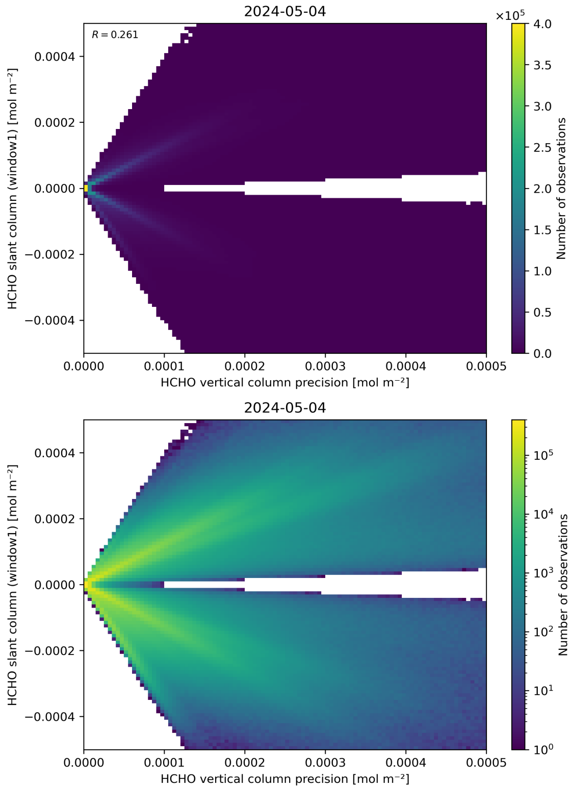
Figure 142: Scatter density plot of “HCHO vertical column precision” against “HCHO slant column (window1)” for 2024-05-03 to 2024-05-05.
