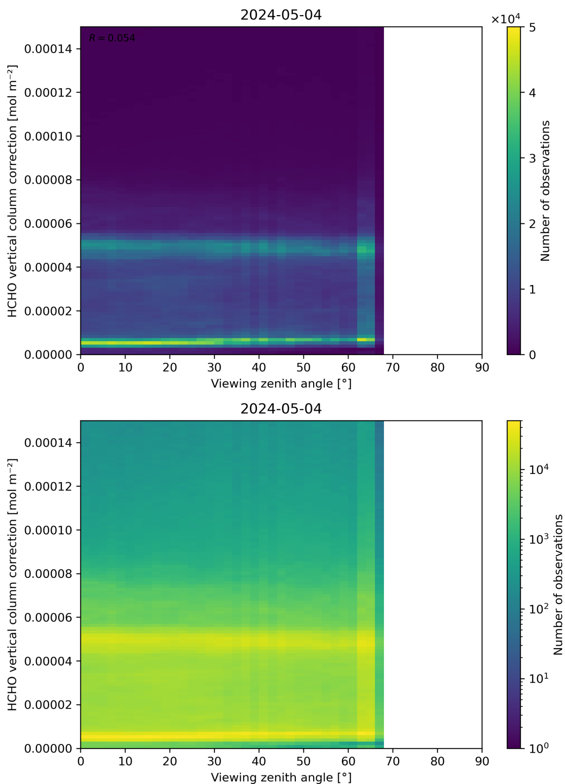
Figure 193: Scatter density plot of “Viewing zenith angle” against “HCHO vertical column correction” for 2024-05-03 to 2024-05-05.
