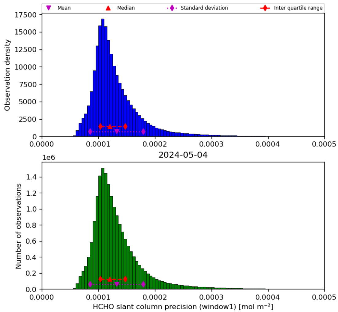
Figure 39: Histogram of “HCHO slant column precision (window1)” for 2024-05-03 to 2024-05-05
