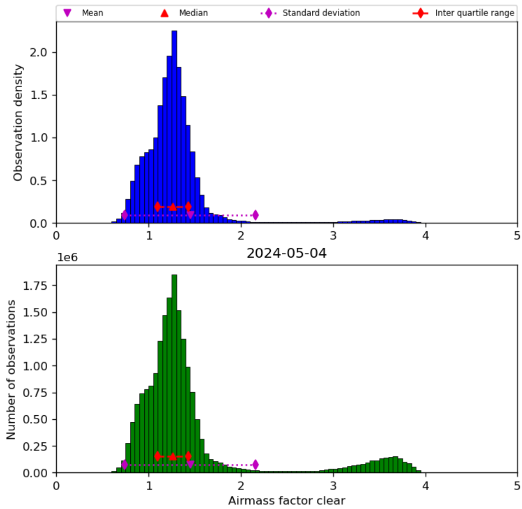
Figure 42: Histogram of “Airmass factor clear” for 2024-05-03 to 2024-05-05
