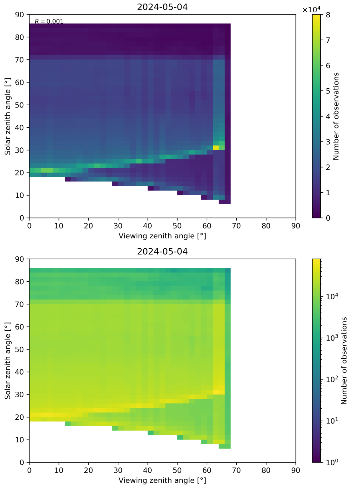
Figure 197: Scatter density plot of “Viewing zenith angle” against “Solar zenith angle” for 2024-05-03 to 2024-05-05.
