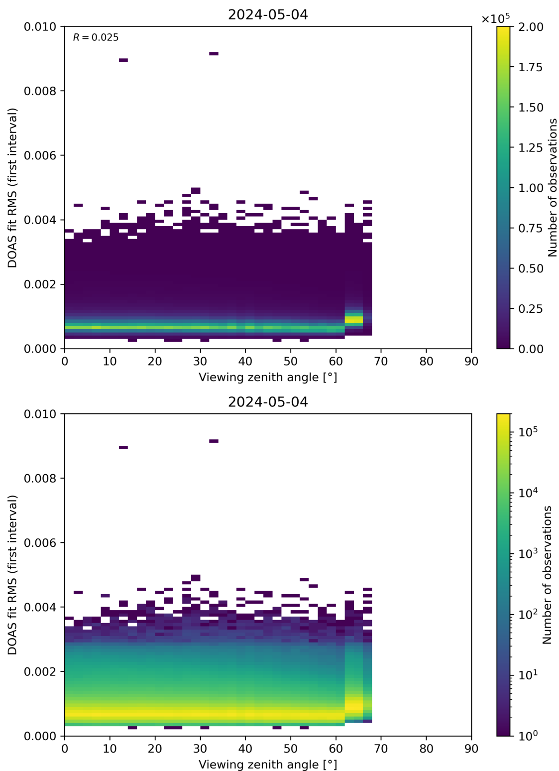
Figure 182: Scatter density plot of “Viewing zenith angle” against “DOAS fit RMS (first interval)” for 2024-05-03 to 2024-05-05.
