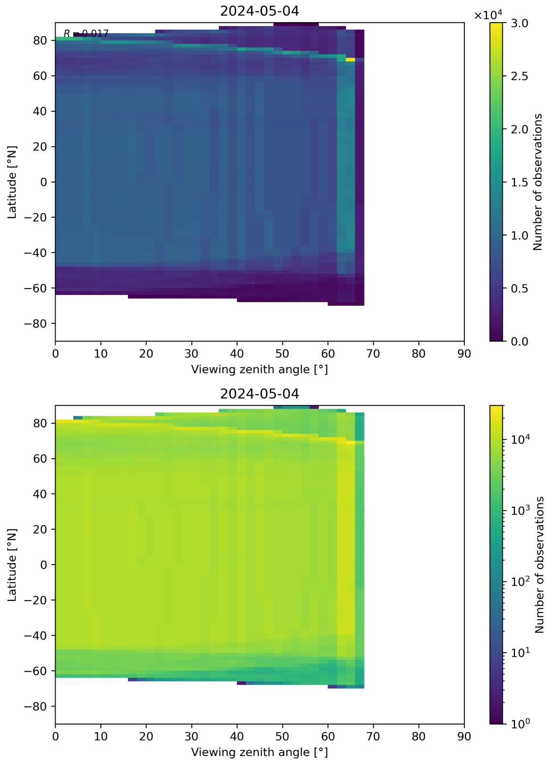
Figure 196: Scatter density plot of “Viewing zenith angle” against “Latitude” for 2024-05-03 to 2024-05-05.
