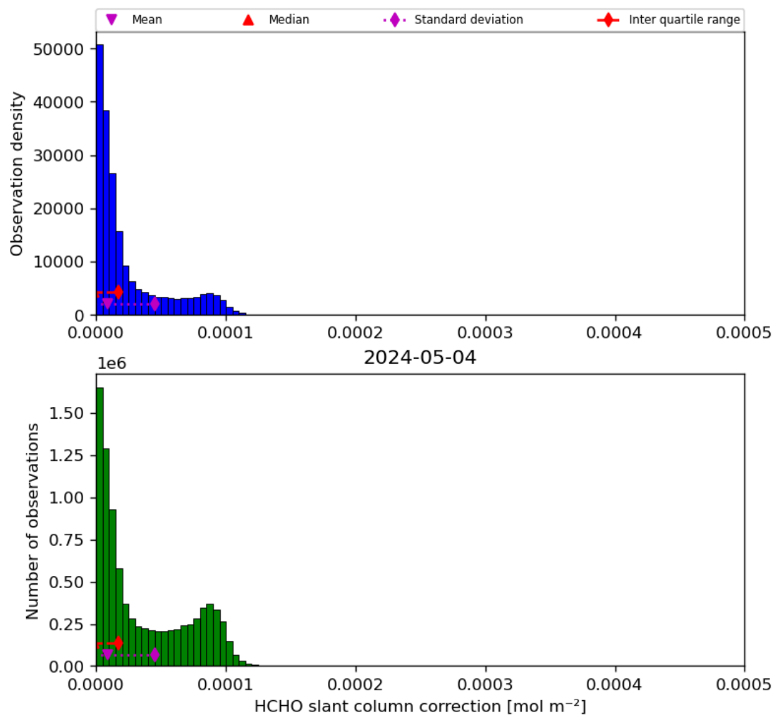
Figure 47: Histogram of “HCHO slant column correction” for 2024-05-03 to 2024-05-05
