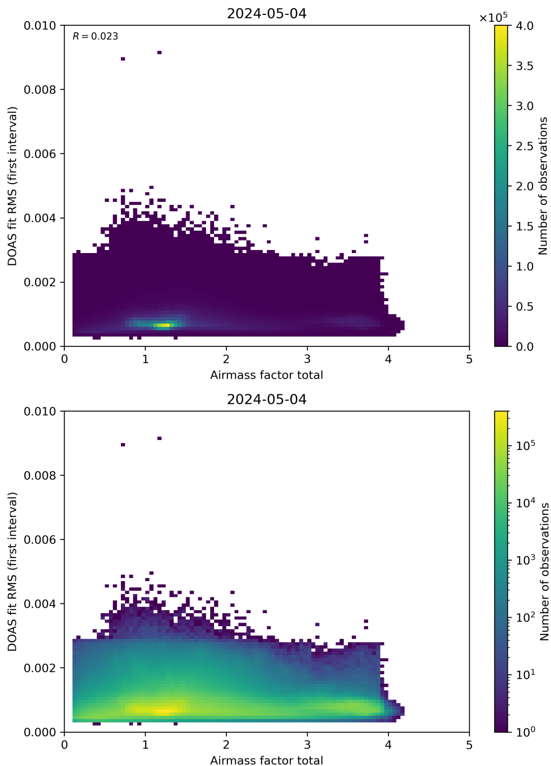
Figure 97: Scatter density plot of “Airmass factor total” against “DOAS fit RMS (first interval)” for 2024-05-03 to 2024-05-05.
