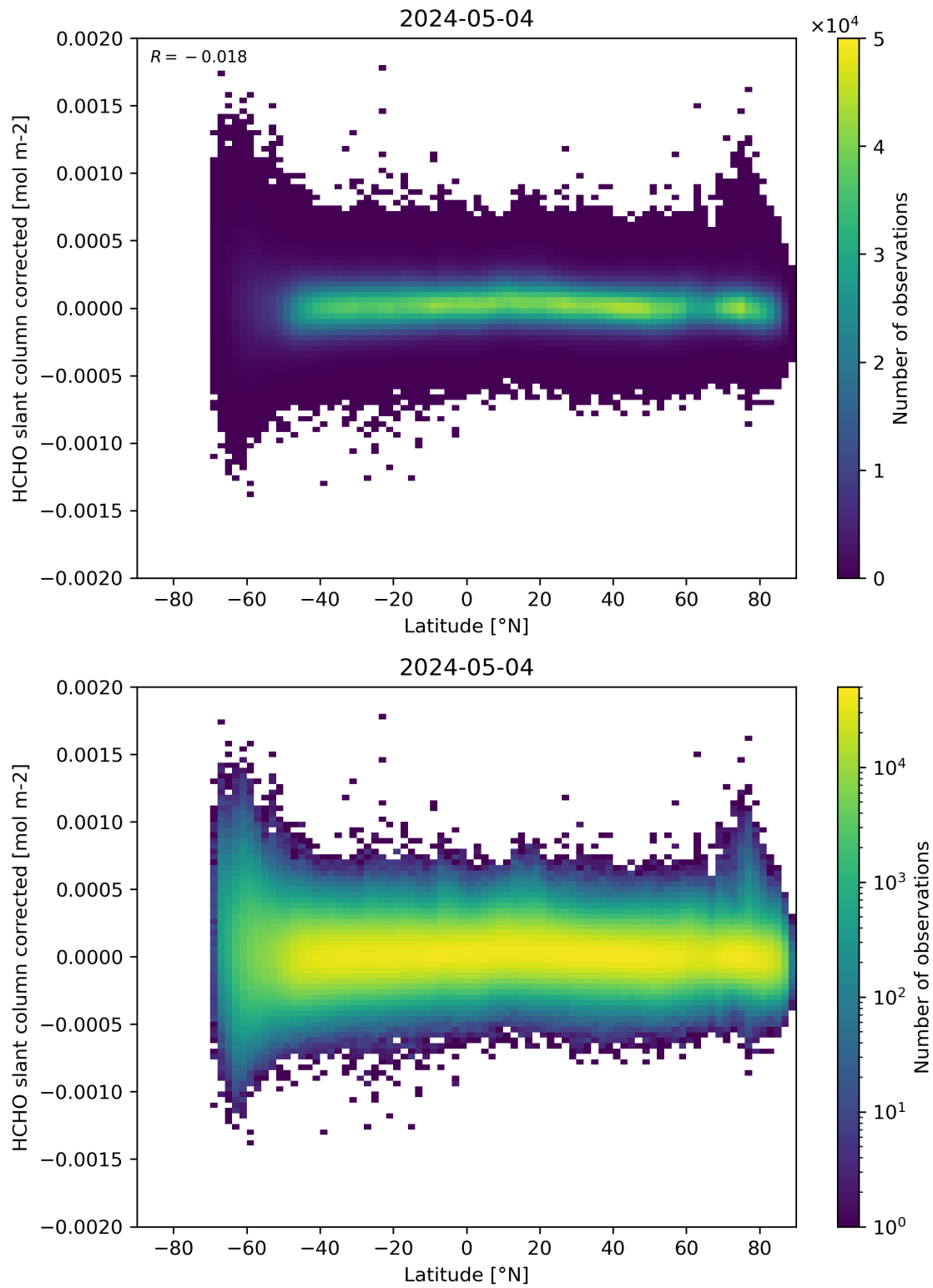
Figure 157: Scatter density plot of “Latitude” against “HCHO slant column corrected” for 2024-05-03 to 2024-05-05.
