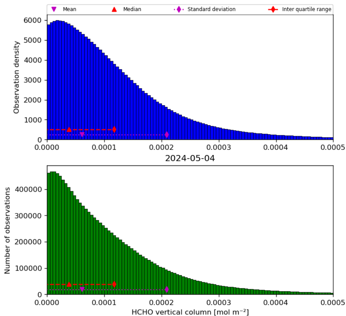
Figure 35: Histogram of “HCHO vertical column” for 2024-05-03 to 2024-05-05
