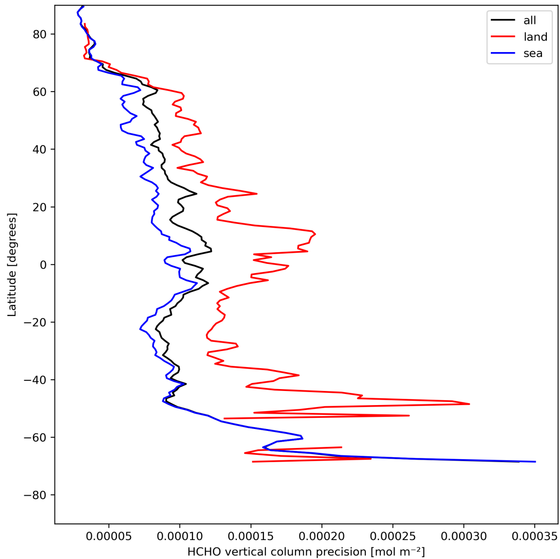
Figure 22: Zonal average of “HCHO vertical column precision” for 2024-05-03 to 2024-05-05.
