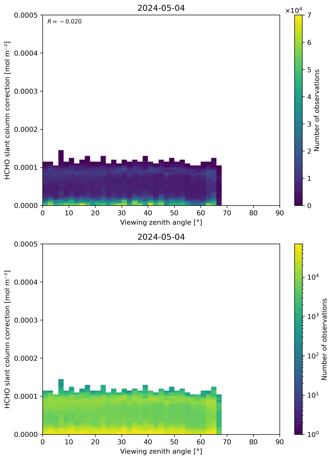
Figure 187: Scatter density plot of “Viewing zenith angle” against “HCHO slant column correction” for 2024-05-03 to 2024-05-05.
