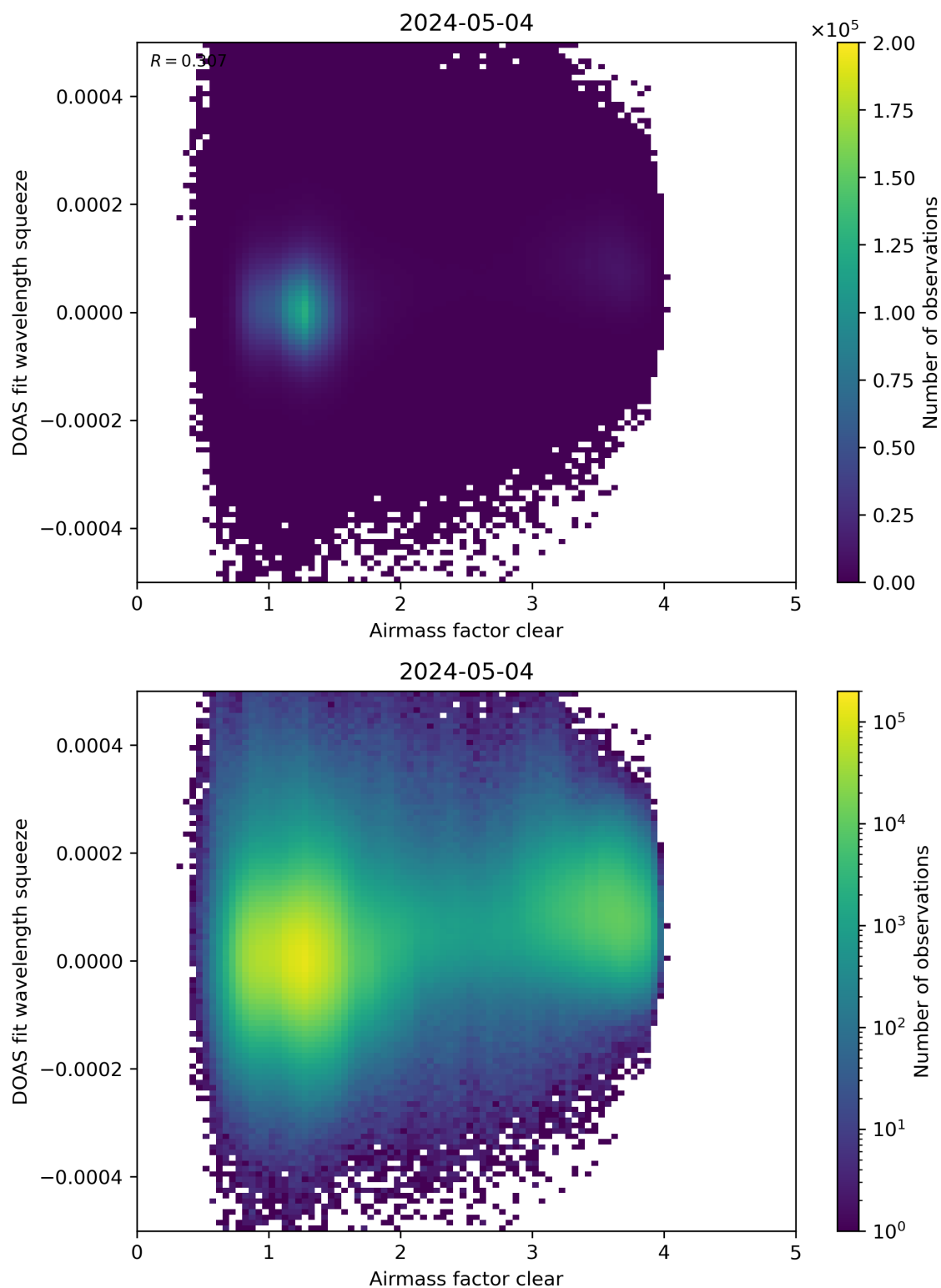
Figure 73: Scatter density plot of “Airmass factor clear” against “DOAS fit wavelength squeeze” for 2024-05-03 to 2024-05-05.
