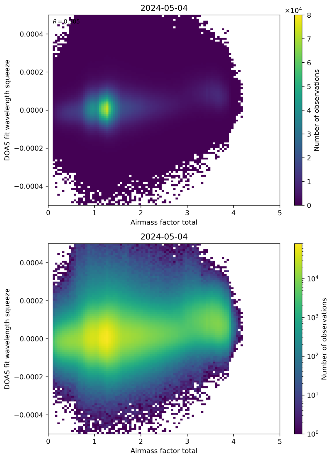
Figure 99: Scatter density plot of “Airmass factor total” against “DOAS fit wavelength squeeze” for 2024-05-03 to 2024-05-05.
