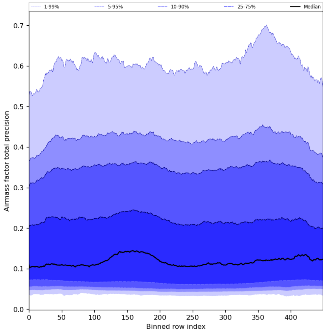
Figure 55: Along track statistics of “Airmass factor total precision” for 2024-05-03 to 2024-05-05
