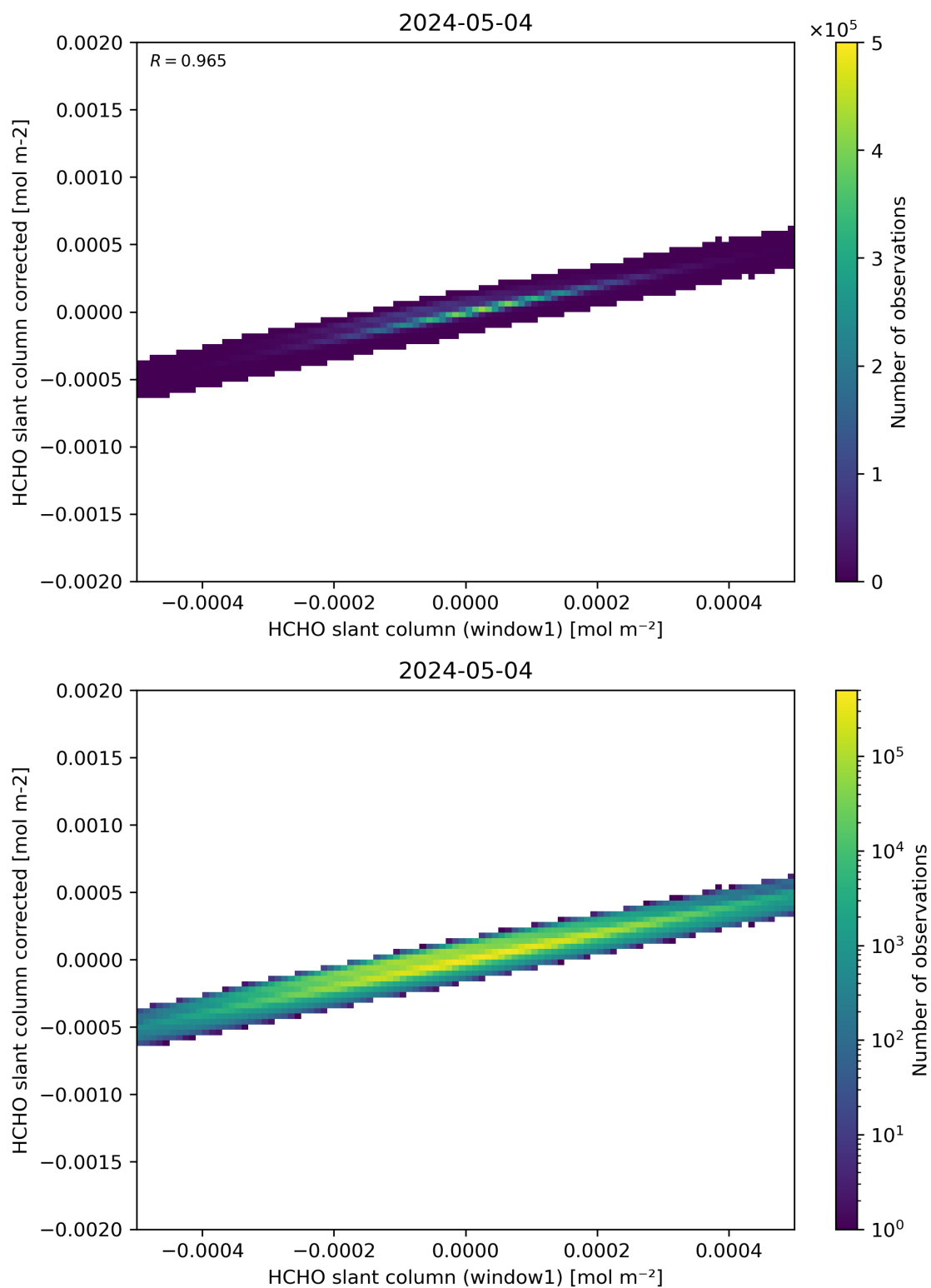
Figure 82: Scatter density plot of “HCHO slant column (window1)” against “HCHO slant column corrected” for 2024-05-03 to 2024-05-05.
