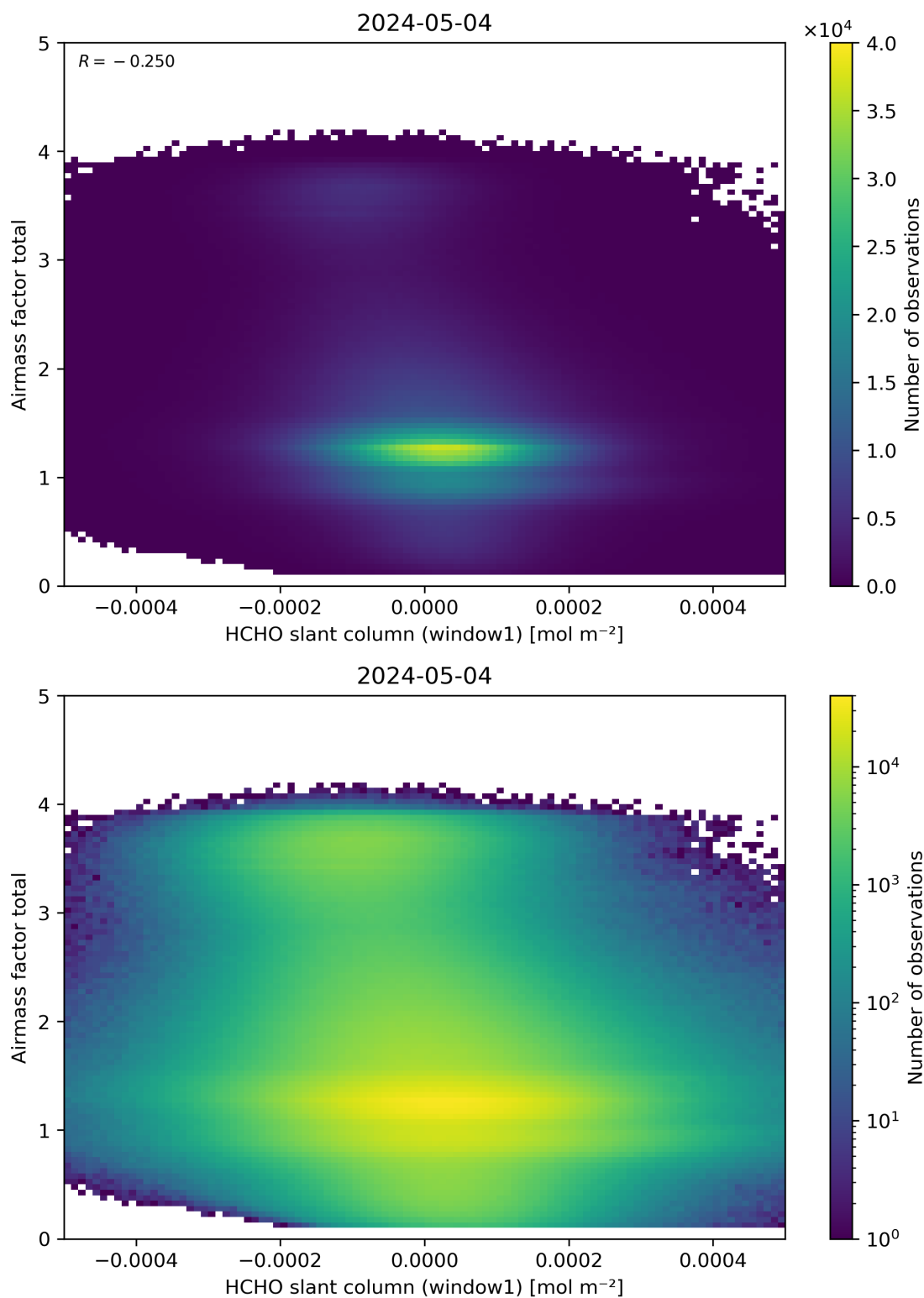
Figure 85: Scatter density plot of “HCHO slant column (window1)” against “Airmass factor total” for 2024-05-03 to 2024-05-05.
