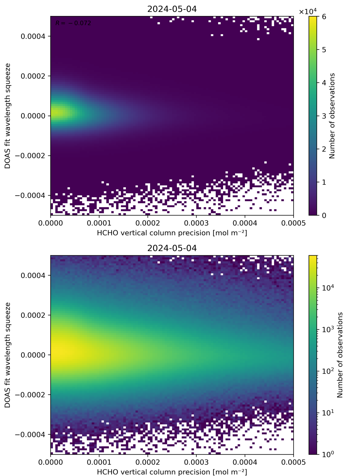
Figure 138: Scatter density plot of “HCHO vertical column precision” against “DOAS fit wavelength squeeze” for 2024-05-03 to 2024-05-05.
