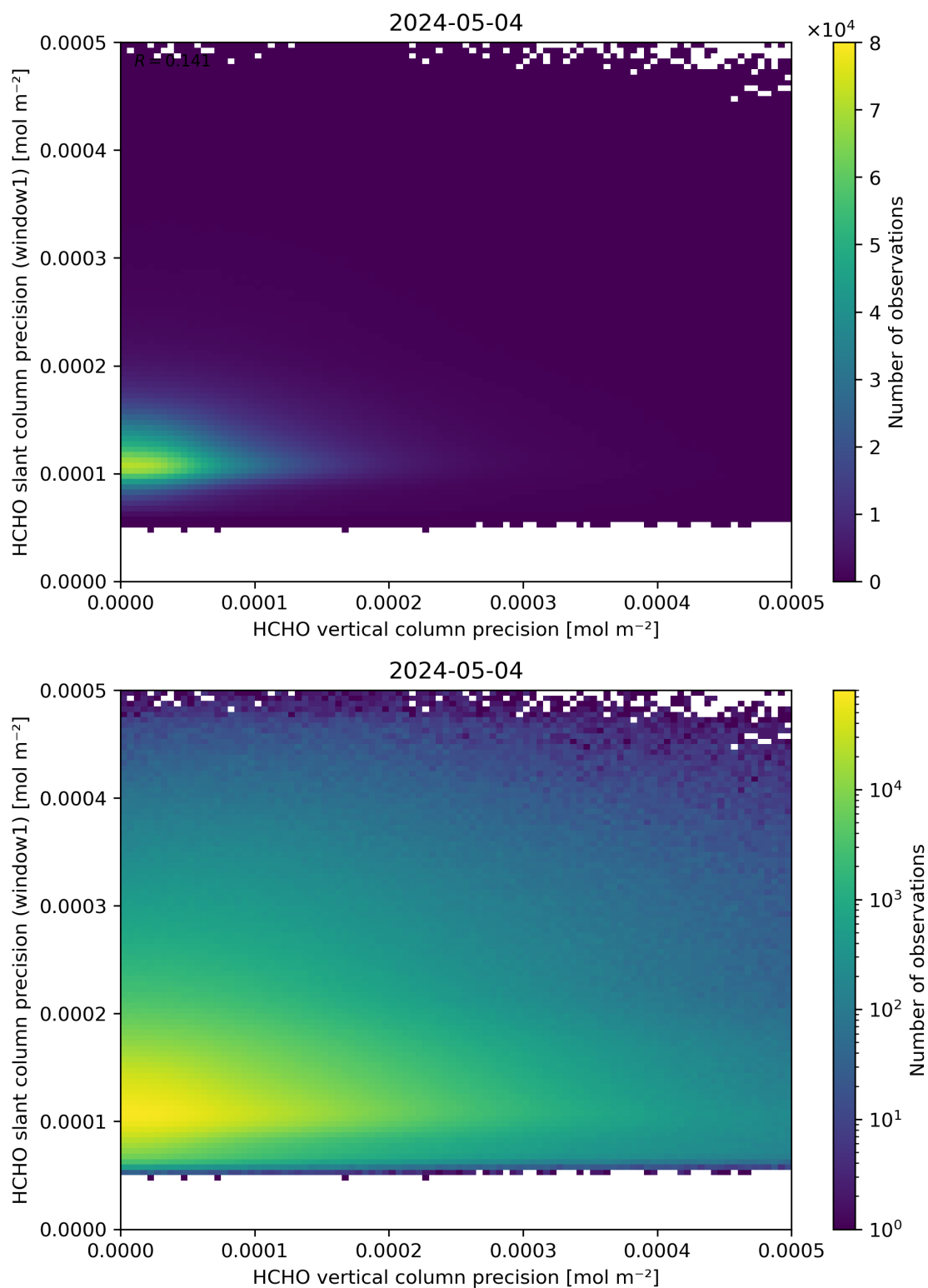
Figure 143: Scatter density plot of “HCHO vertical column precision” against “HCHO slant column precision (window1)” for 2024-05-03 to 2024-05-05.
