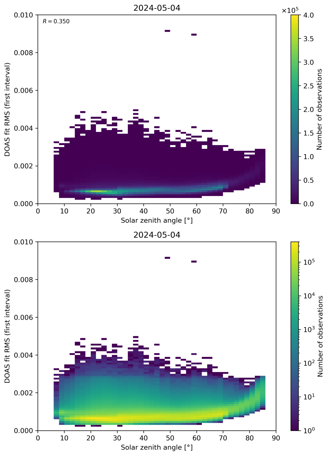
Figure 167: Scatter density plot of “Solar zenith angle” against “DOAS fit RMS (first interval)” for 2024-05-03 to 2024-05-05.
