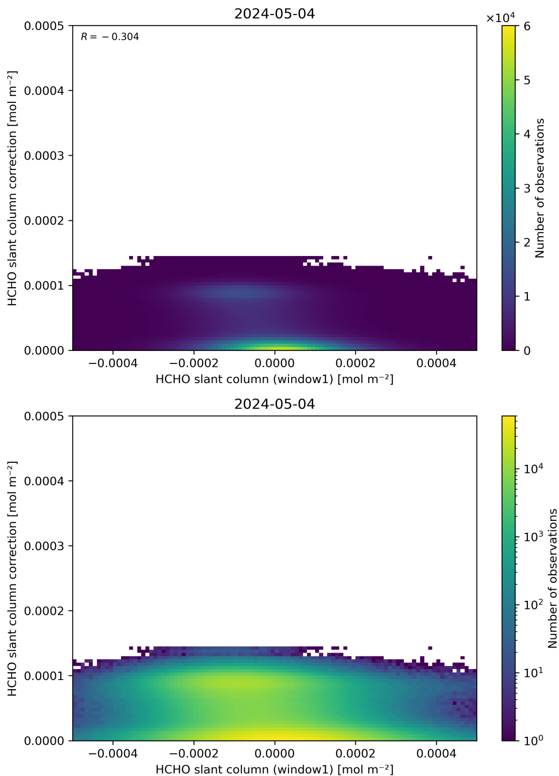
Figure 83: Scatter density plot of “HCHO slant column (window1)” against “HCHO slant column correction” for 2024-05-03 to 2024-05-05.
