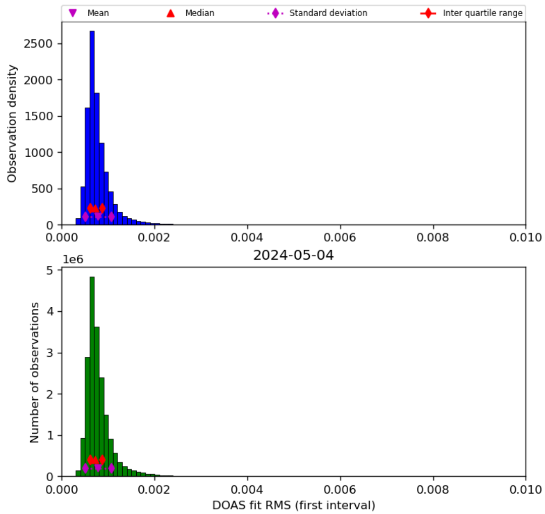
Figure 46: Histogram of “DOAS fit RMS (first interval)” for 2024-05-03 to 2024-05-05
