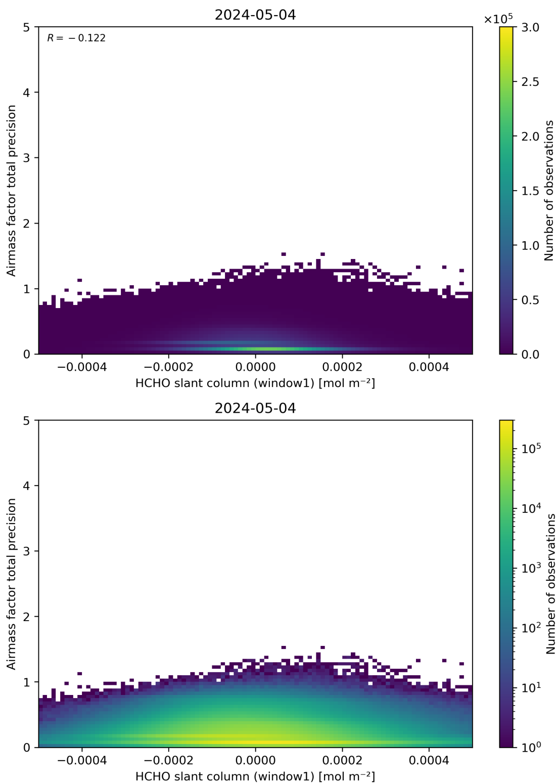
Figure 86: Scatter density plot of “HCHO slant column (window1)” against “Airmass factor total precision” for 2024-05-03 to 2024-05-05.
