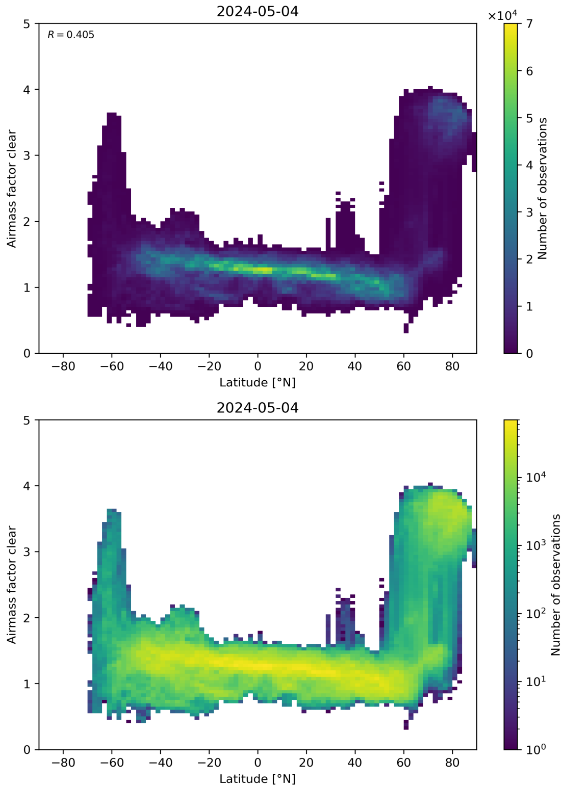
Figure 156: Scatter density plot of “Latitude” against “Airmass factor clear” for 2024-05-03 to 2024-05-05.
