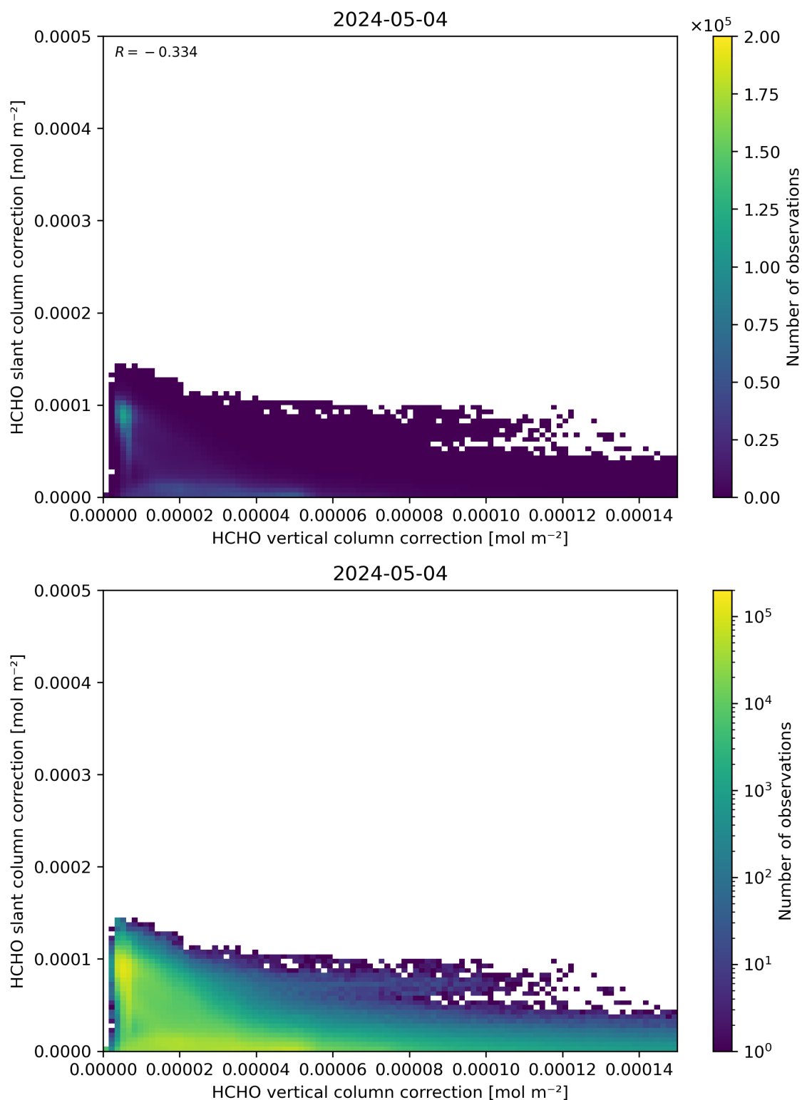
Figure 117: Scatter density plot of “HCHO vertical column correction” against “HCHO slant column correction” for 2024-05-03 to 2024-05-05.
