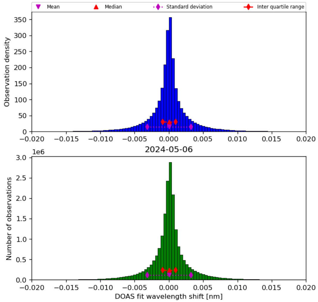
Figure 44: Histogram of “DOAS fit wavelength shift” for 2024-05-05 to 2024-05-07
