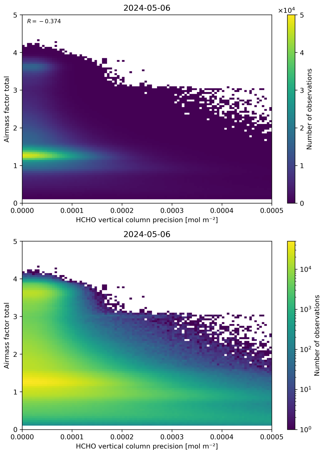
Figure 144: Scatter density plot of “HCHO vertical column precision” against “Airmass factor total” for 2024-05-05 to 2024-05-07.
