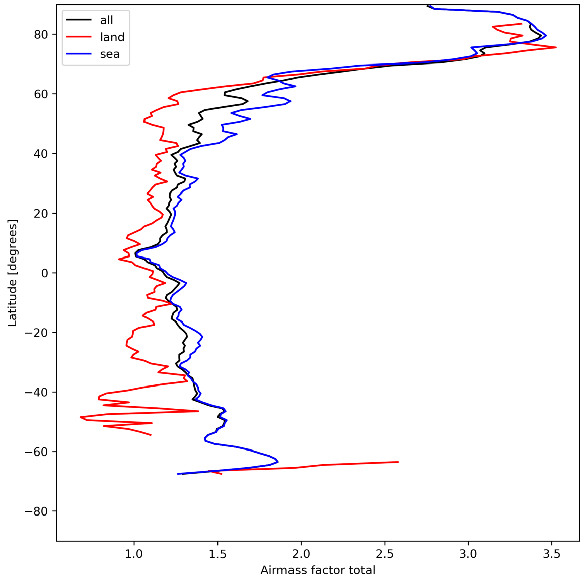
Figure 26: Zonal average of “Airmass factor total” for 2024-05-05 to 2024-05-07.
