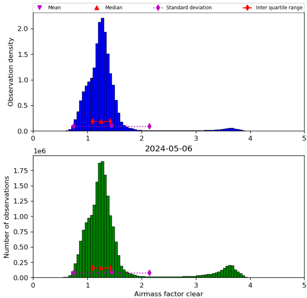
Figure 42: Histogram of “Airmass factor clear” for 2024-05-05 to 2024-05-07
