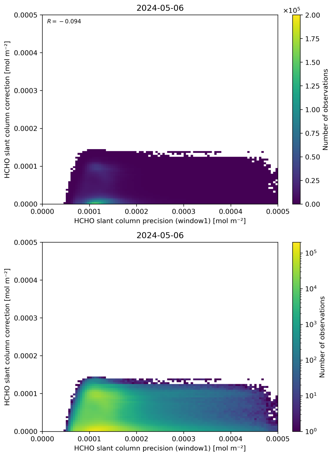
Figure 93: Scatter density plot of “HCHO slant column precision (window1)” against “HCHO slant column correction” for 2024-05-05 to 2024-05-07.
