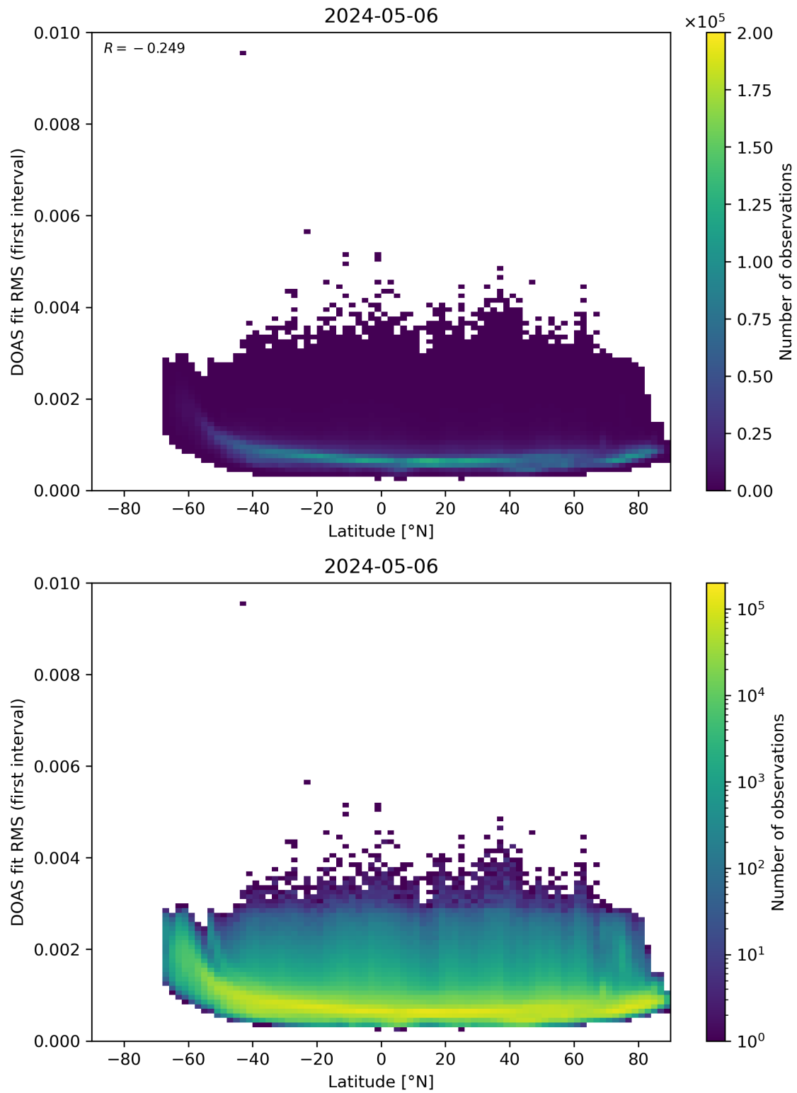
Figure 153: Scatter density plot of “Latitude” against “DOAS fit RMS (first interval)” for 2024-05-05 to 2024-05-07.
