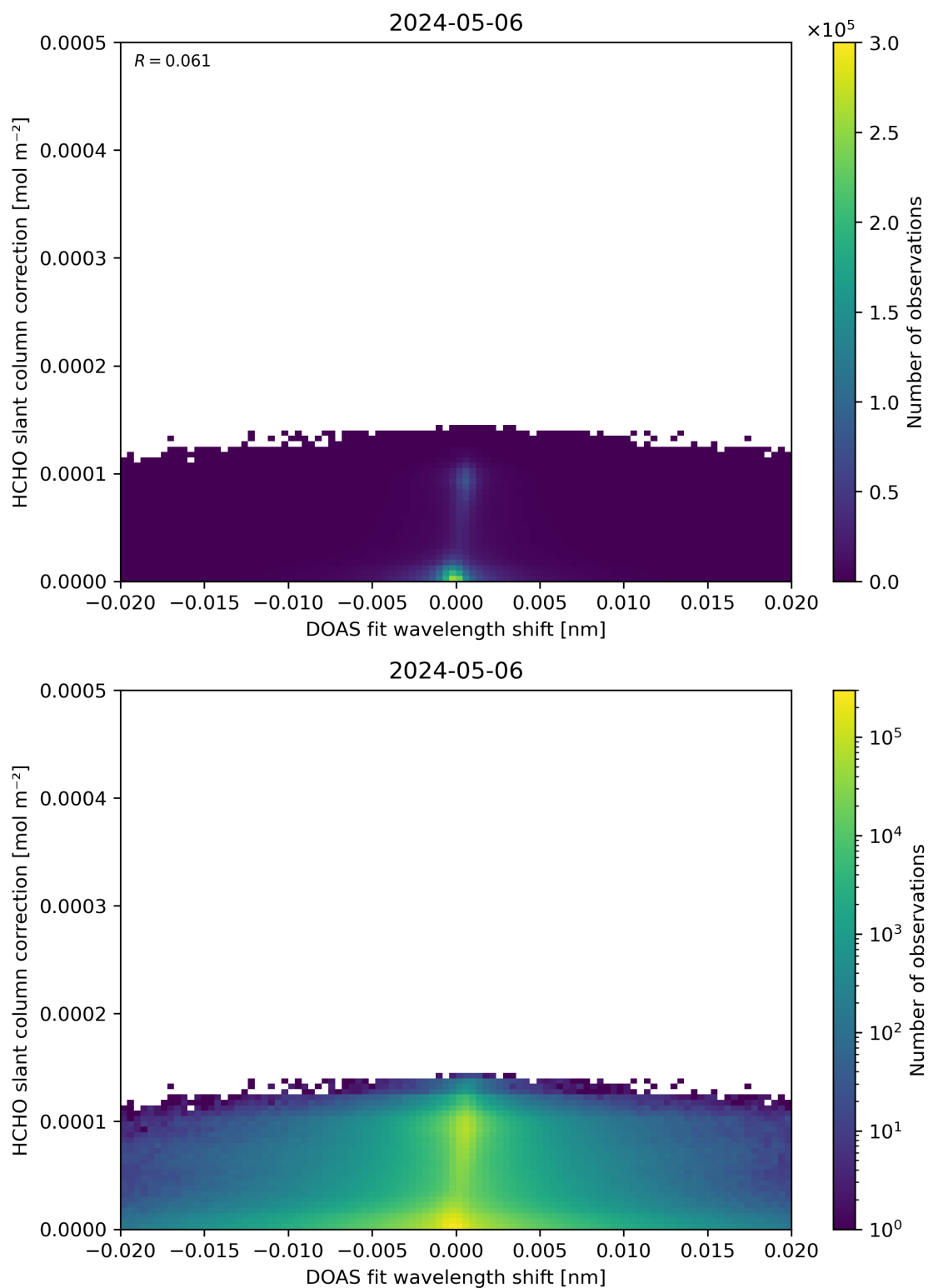
Figure 67: Scatter density plot of “DOAS fit wavelength shift” against “HCHO slant column correction” for 2024-05-05 to 2024-05-07.
