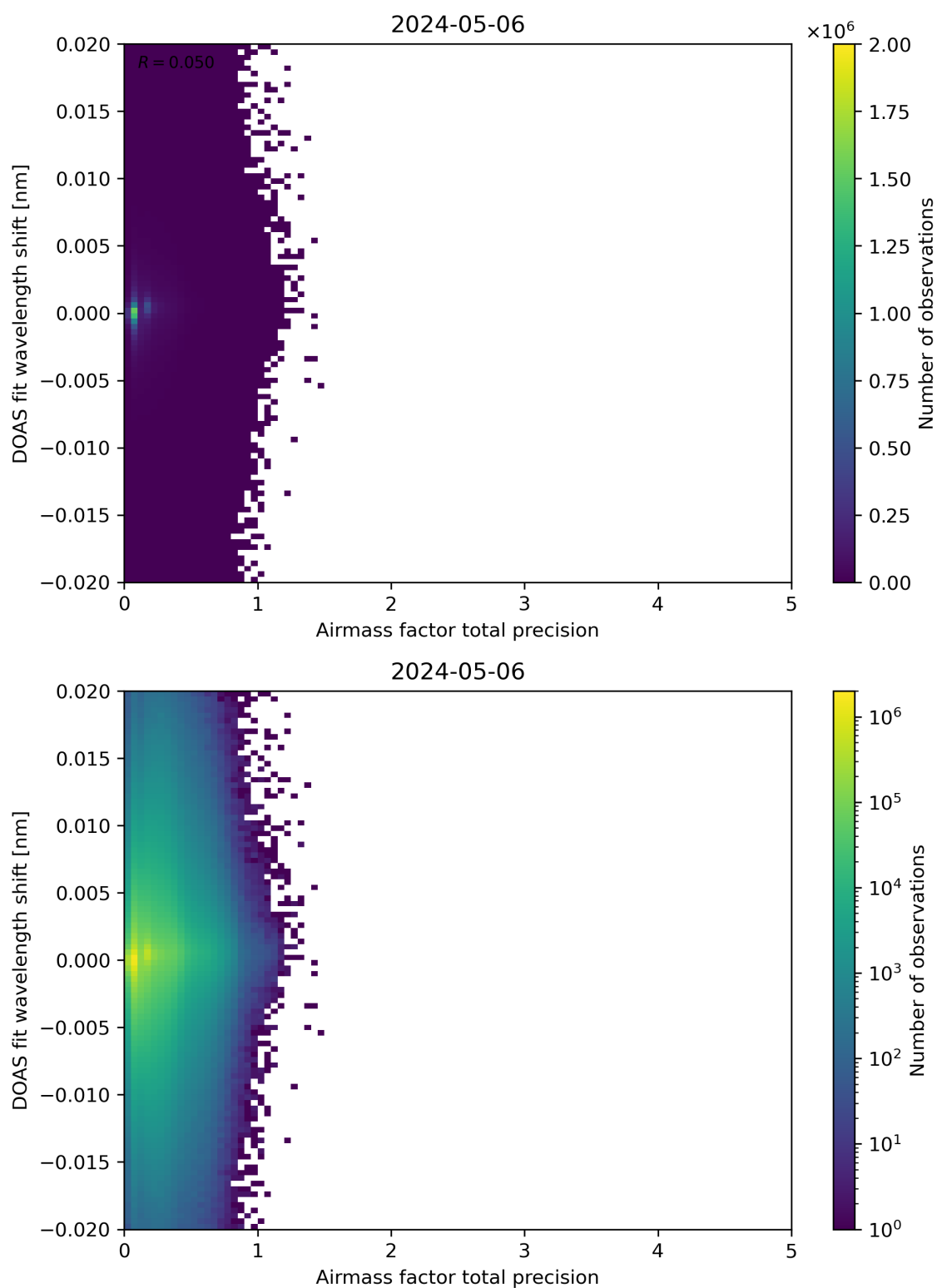
Figure 106: Scatter density plot of “Airmass factor total precision” against “DOAS fit wavelength shift” for 2024-05-05 to 2024-05-07.
