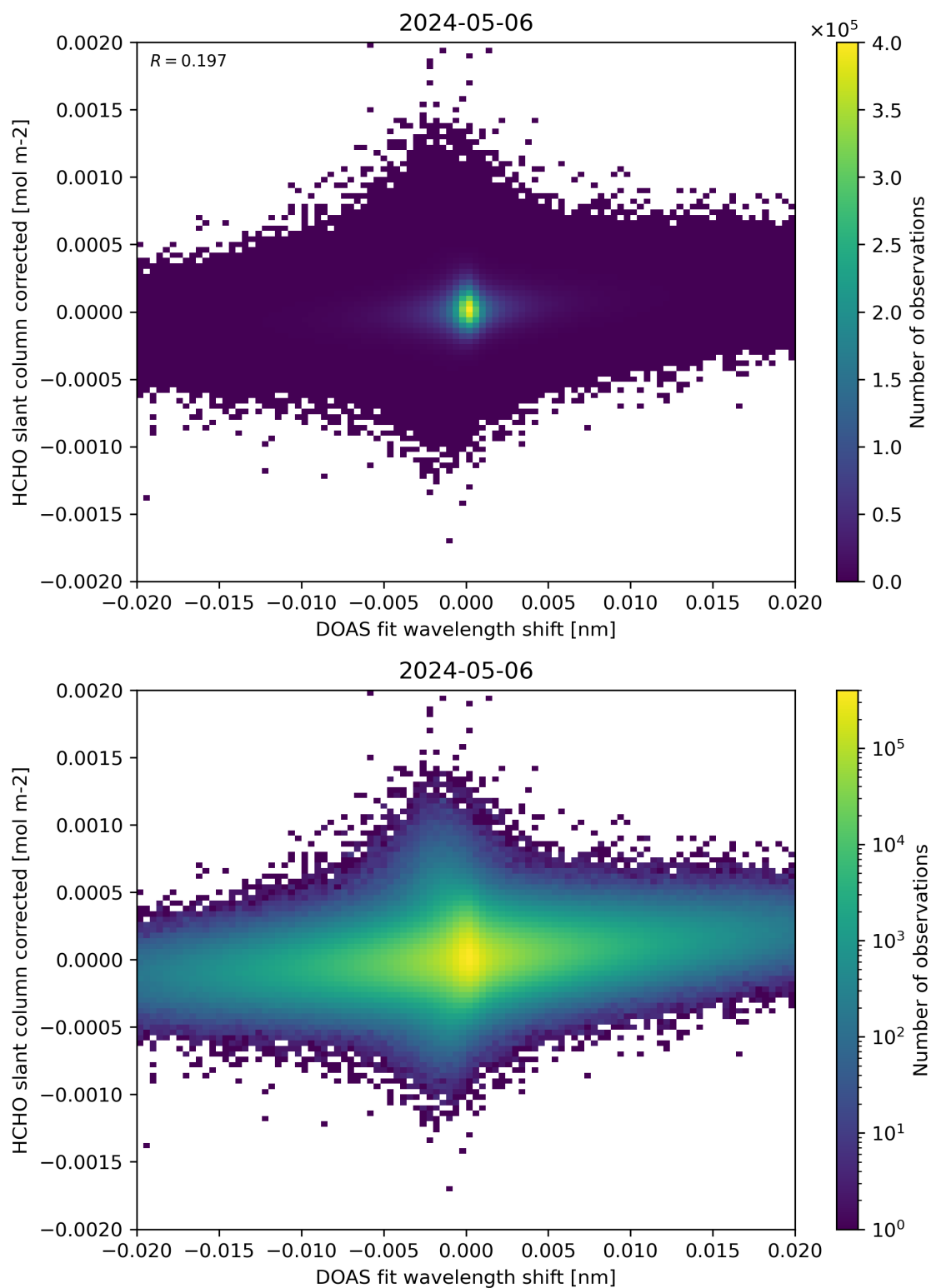
Figure 66: Scatter density plot of “DOAS fit wavelength shift” against “HCHO slant column corrected” for 2024-05-05 to 2024-05-07.
