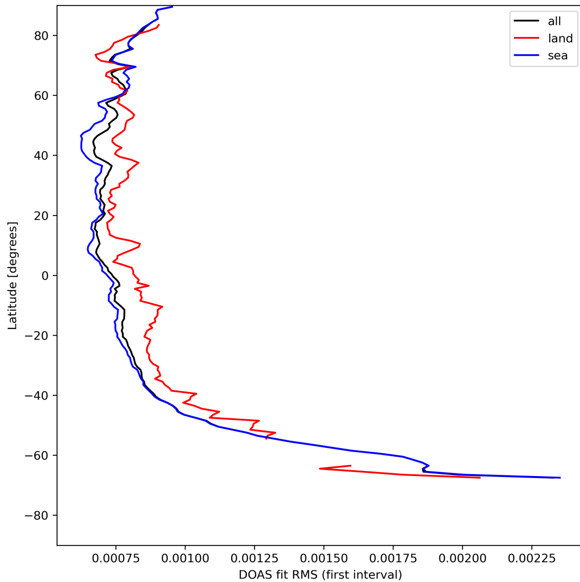
Figure 32: Zonal average of “DOAS fit RMS (first interval)” for 2024-05-05 to 2024-05-07.
