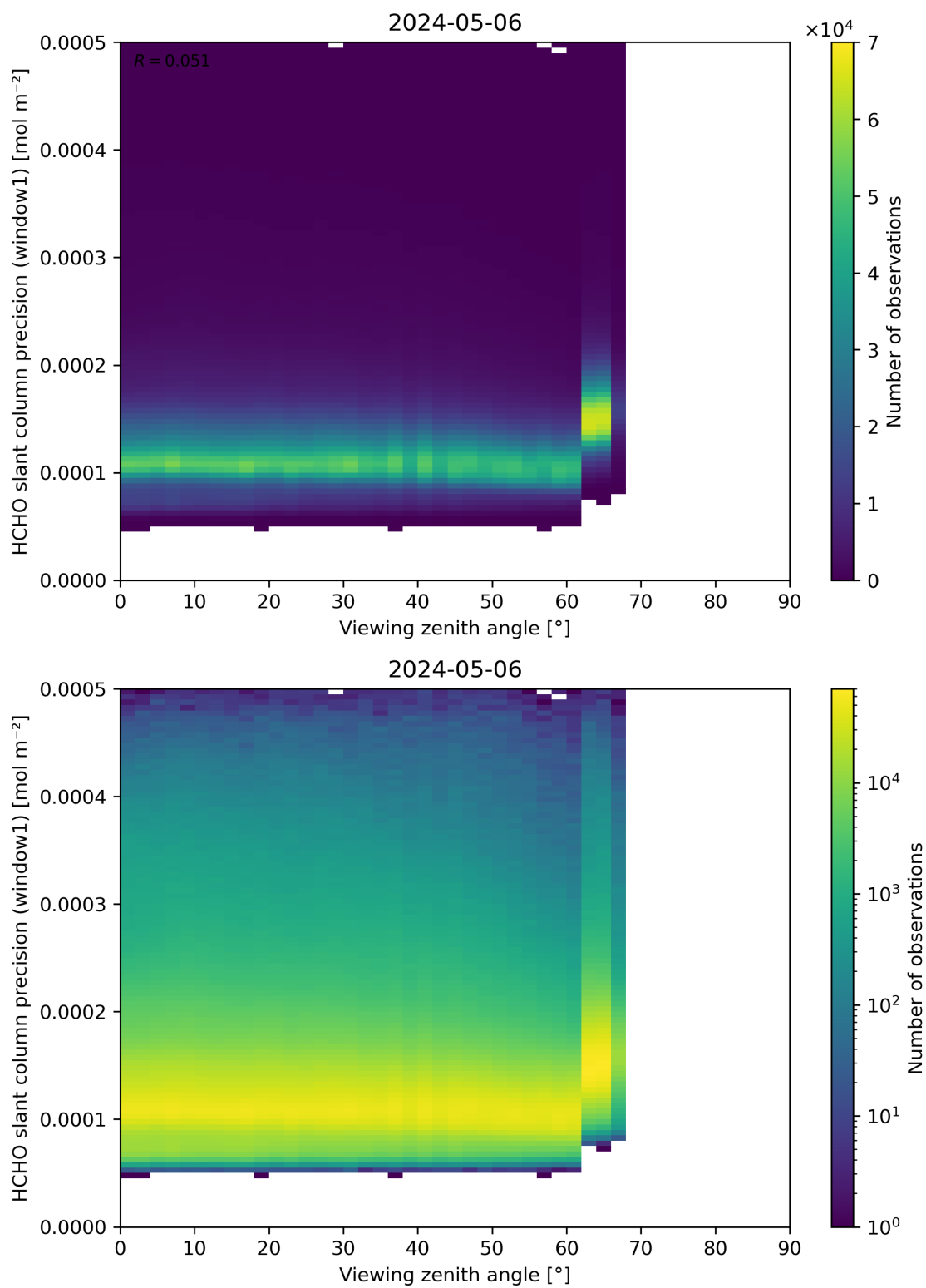
Figure 189: Scatter density plot of “Viewing zenith angle” against “HCHO slant column precision (window1)” for 2024-05-05 to 2024-05-07.
