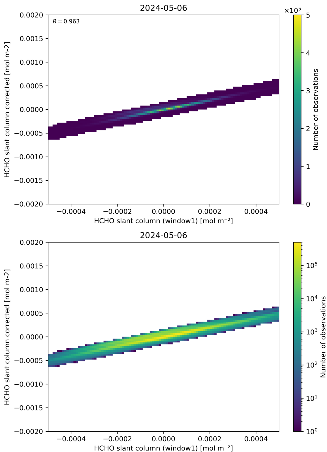
Figure 82: Scatter density plot of “HCHO slant column (window1)” against “HCHO slant column corrected” for 2024-05-05 to 2024-05-07.
