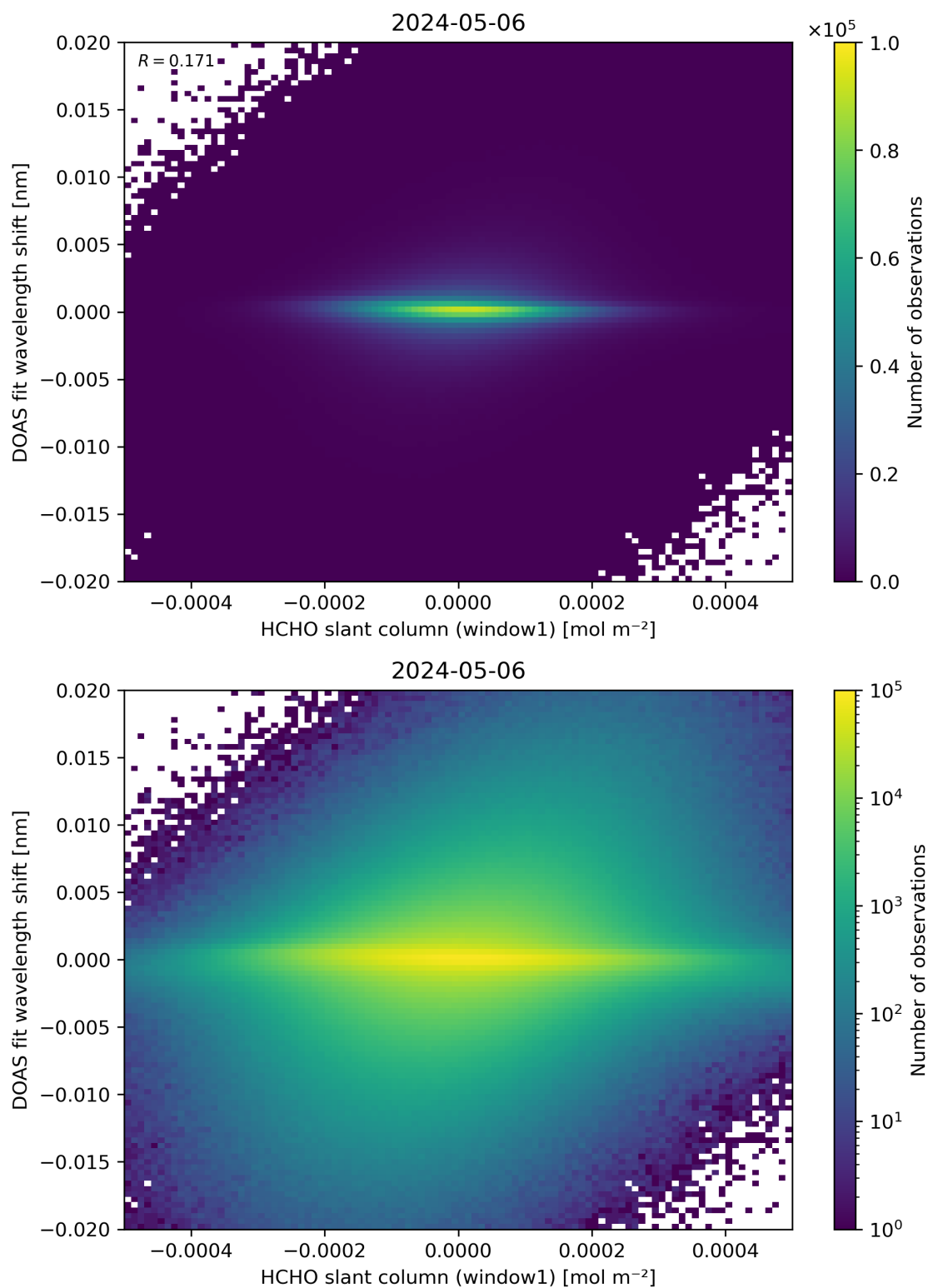
Figure 79: Scatter density plot of “HCHO slant column (window1)” against “DOAS fit wavelength shift” for 2024-05-05 to 2024-05-07.
