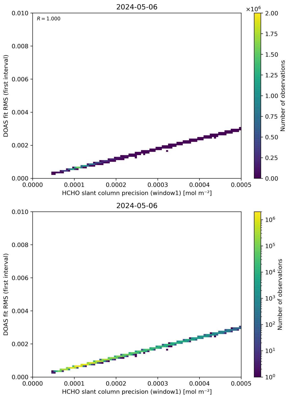
Figure 88: Scatter density plot of “HCHO slant column precision (window1)” against “DOAS fit RMS (first interval)” for 2024-05-05 to 2024-05-07.
