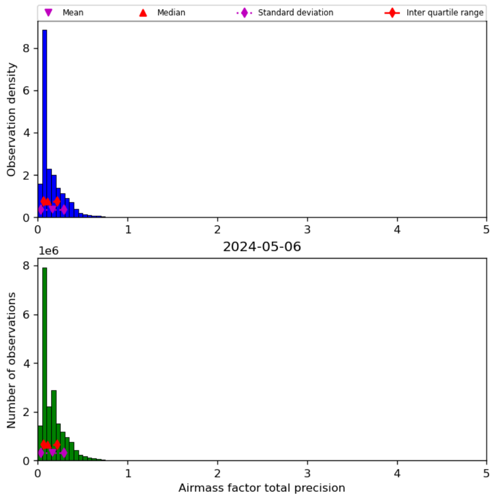
Figure 41: Histogram of “Airmass factor total precision” for 2024-05-05 to 2024-05-07
