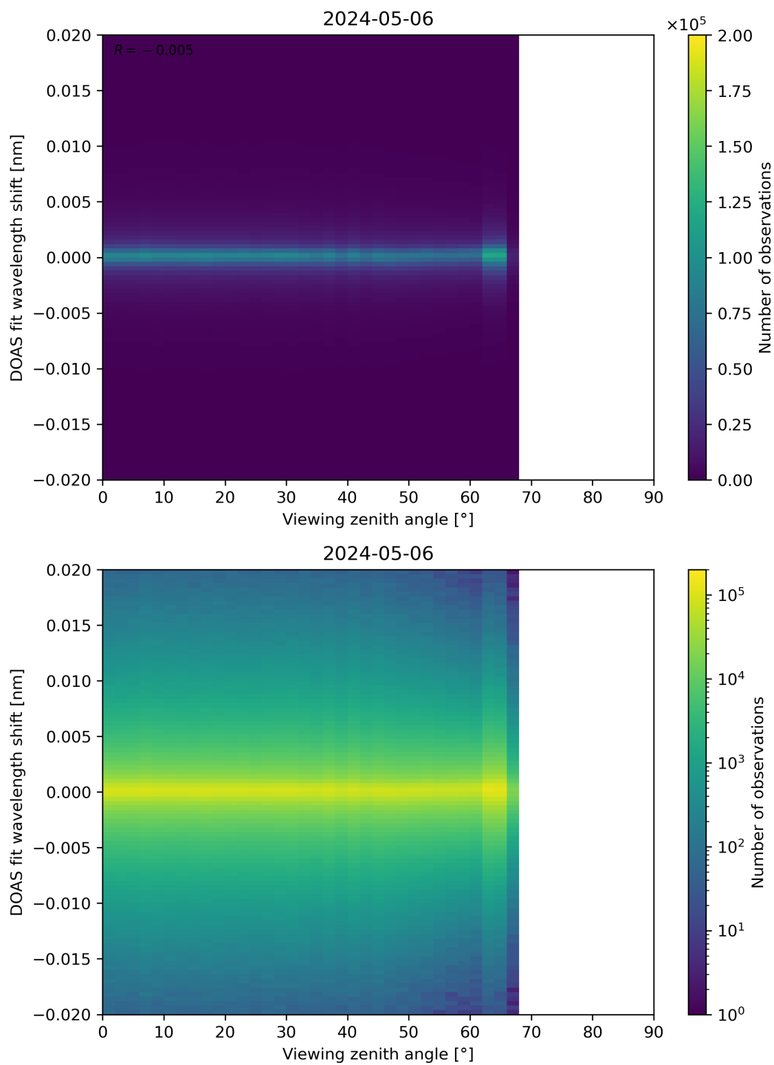
Figure 183: Scatter density plot of “Viewing zenith angle” against “DOAS fit wavelength shift” for 2024-05-05 to 2024-05-07.
