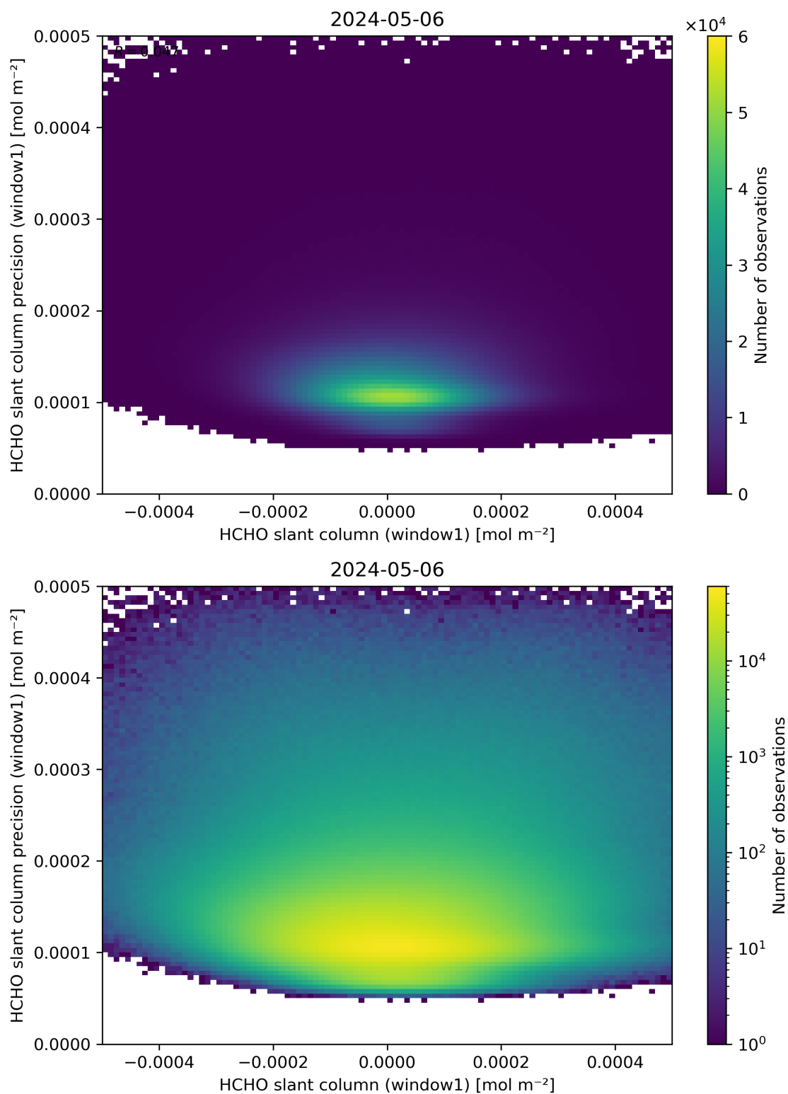
Figure 84: Scatter density plot of “HCHO slant column (window1)” against “HCHO slant column precision (window1)” for 2024-05-05 to 2024-05-07.
