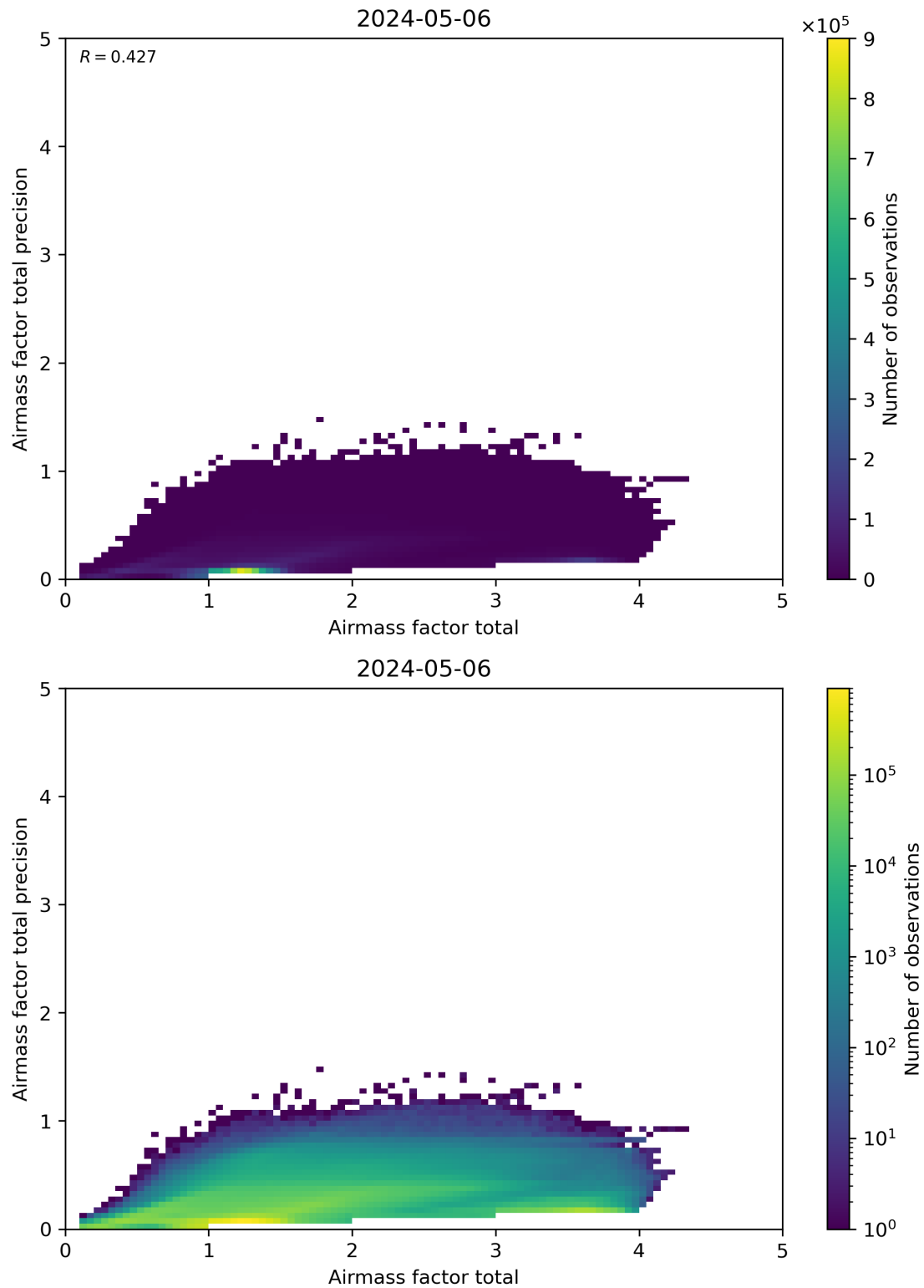
Figure 103: Scatter density plot of “Airmass factor total” against “Airmass factor total precision” for 2024-05-05 to 2024-05-07.
