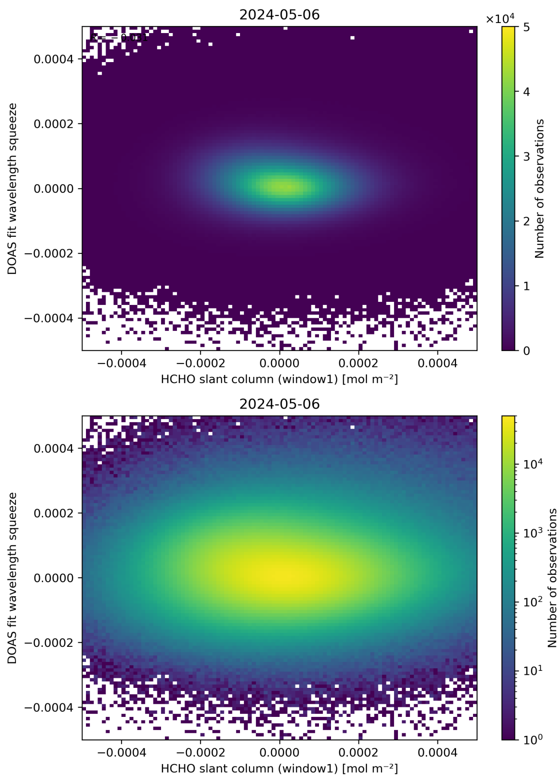
Figure 80: Scatter density plot of “HCHO slant column (window1)” against “DOAS fit wavelength squeeze” for 2024-05-05 to 2024-05-07.
