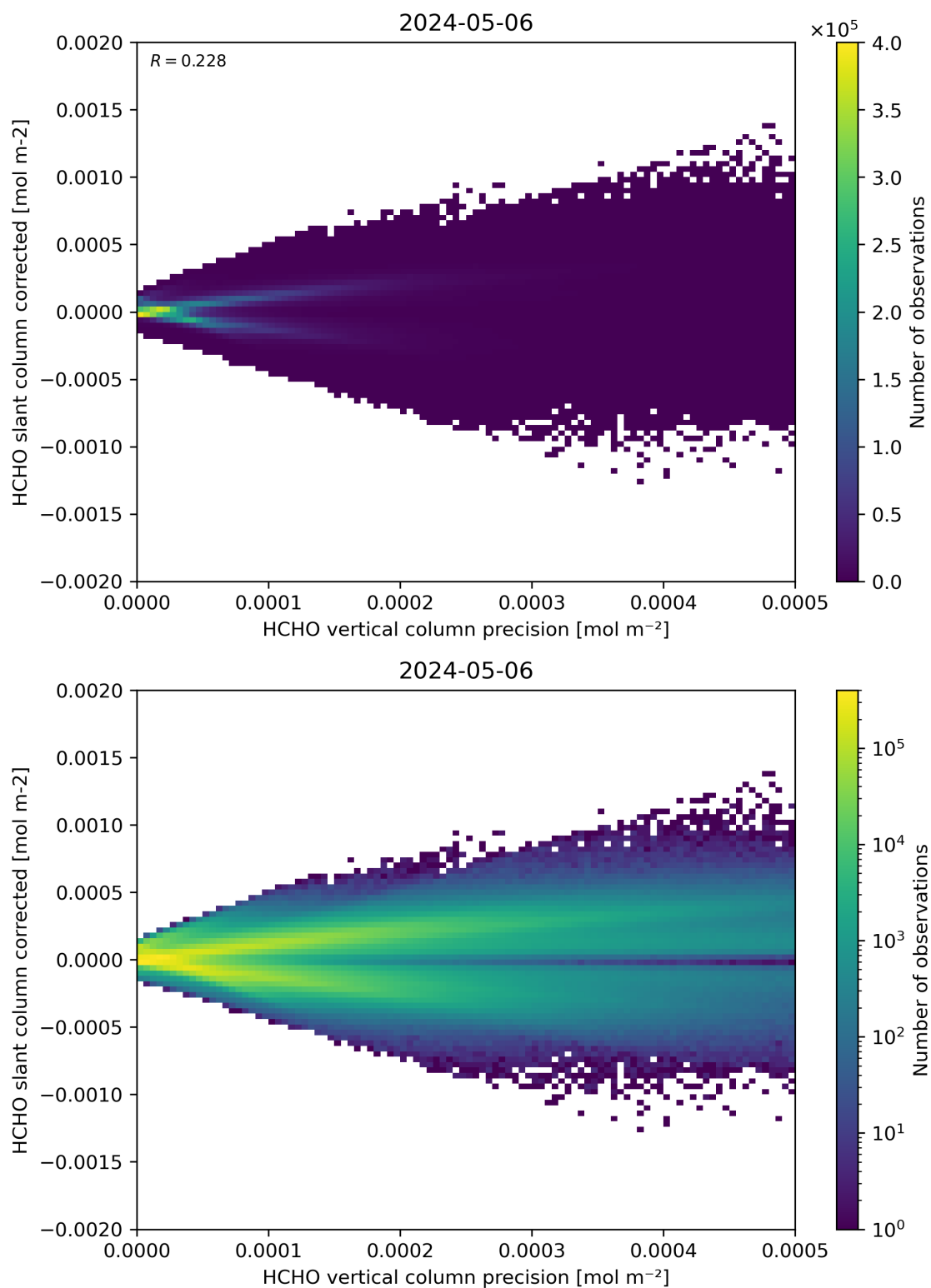
Figure 140: Scatter density plot of “HCHO vertical column precision” against “HCHO slant column corrected” for 2024-05-05 to 2024-05-07.
