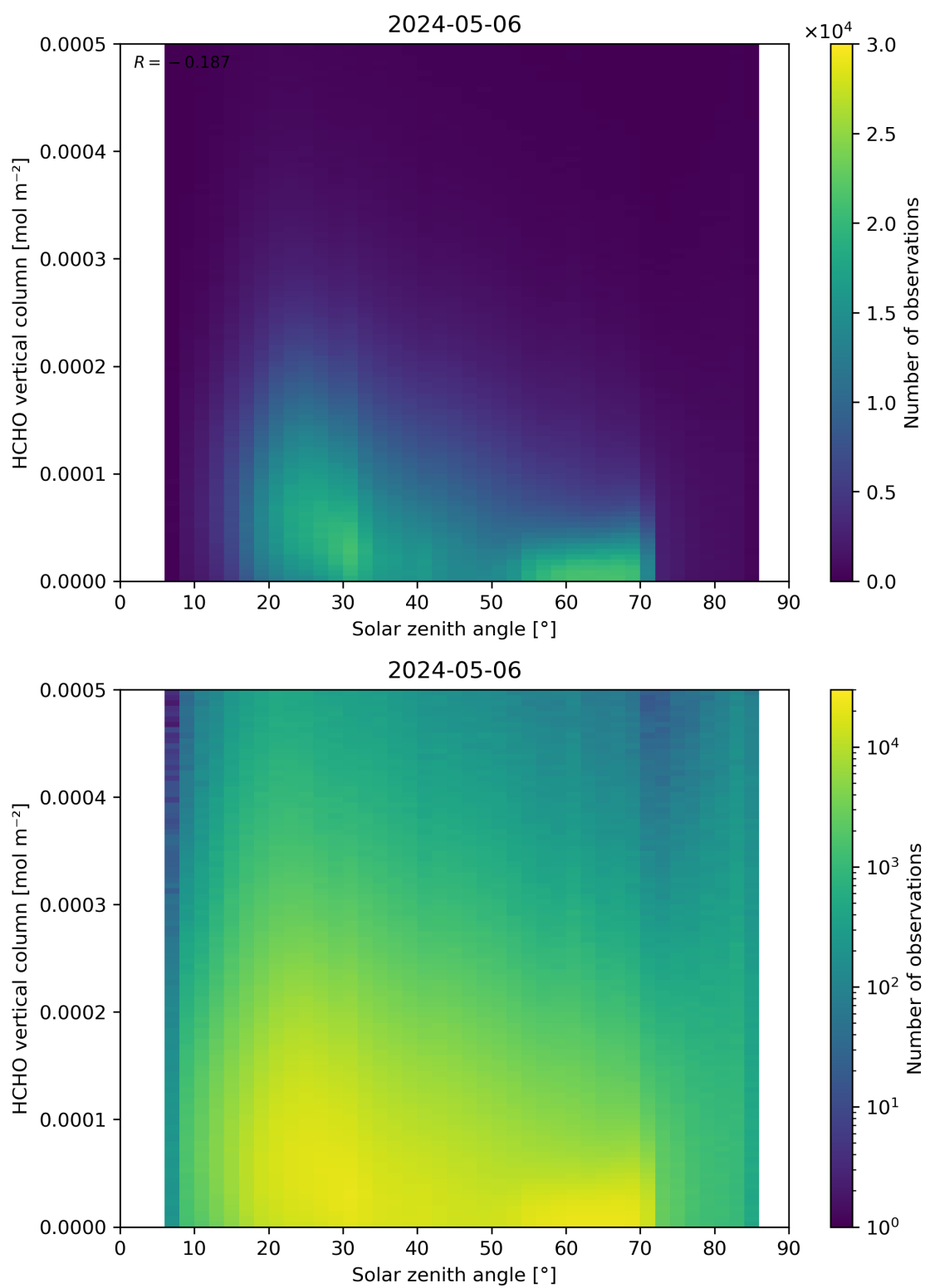
Figure 177: Scatter density plot of “Solar zenith angle” against “HCHO vertical column” for 2024-05-05 to 2024-05-07.
