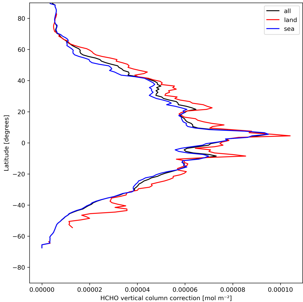
Figure 23: Zonal average of “HCHO vertical column correction” for 2024-05-05 to 2024-05-07.
