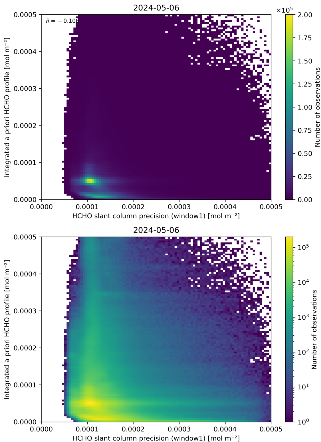
Figure 96: Scatter density plot of “HCHO slant column precision (window1)” against “Integrated a priori HCHO profile” for 2024-05-05 to 2024-05-07.
