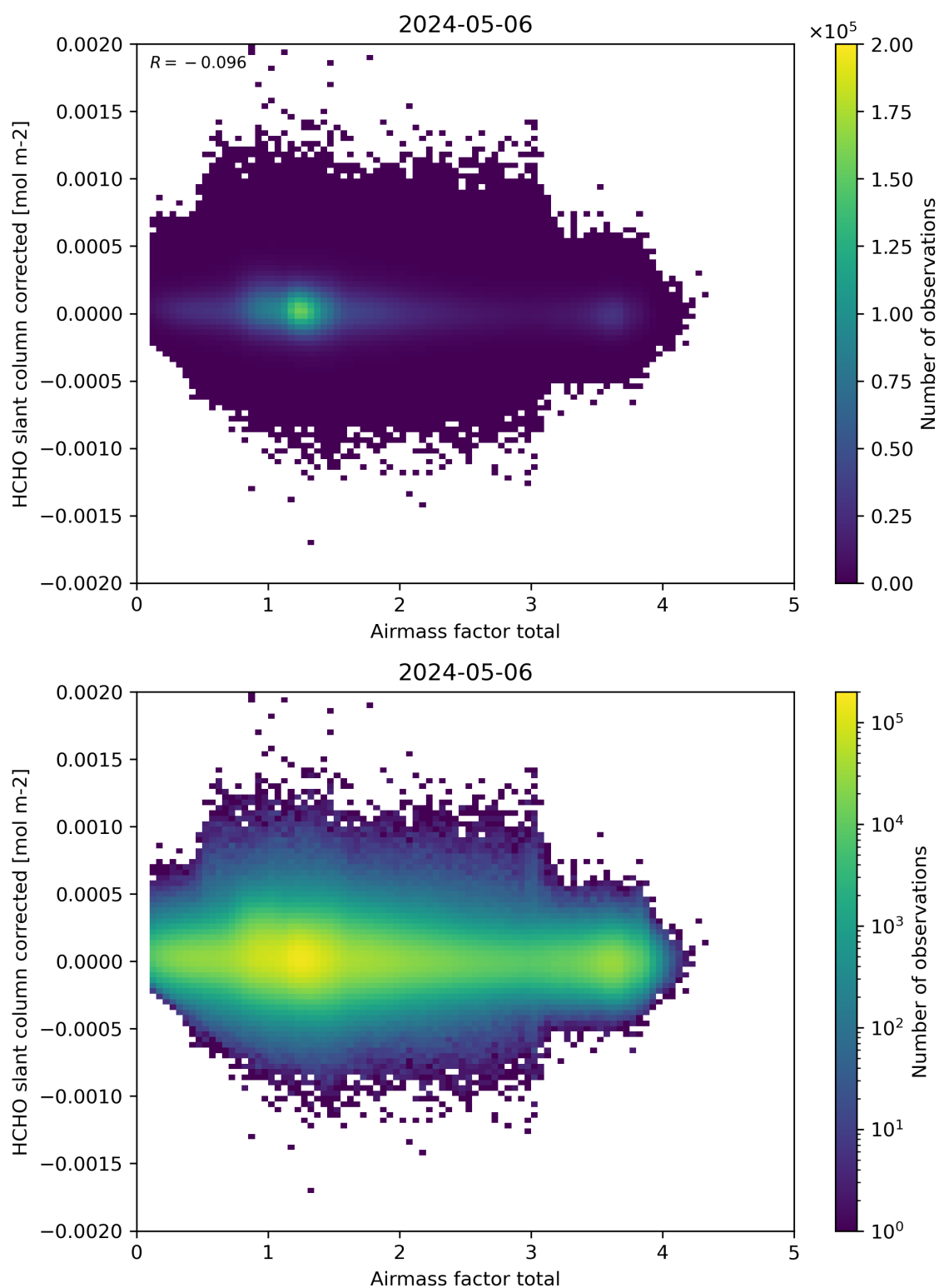
Figure 101: Scatter density plot of “Airmass factor total” against “HCHO slant column corrected” for 2024-05-05 to 2024-05-07.
