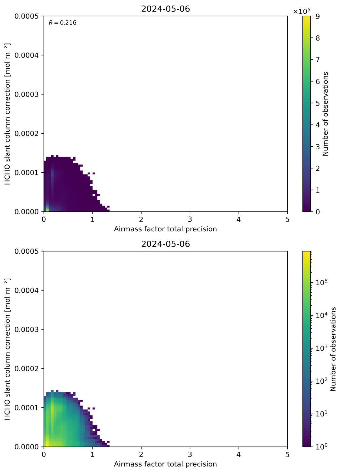
Figure 110: Scatter density plot of “Airmass factor total precision” against “HCHO slant column correction” for 2024-05-05 to 2024-05-07.
