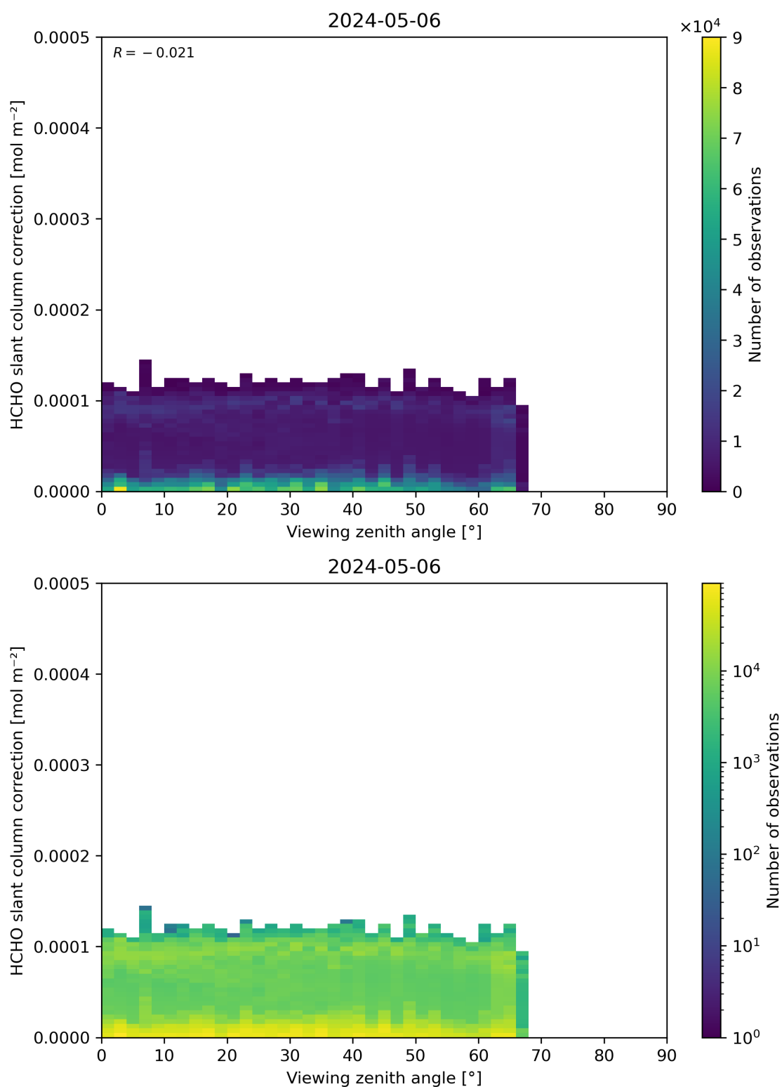
Figure 187: Scatter density plot of “Viewing zenith angle” against “HCHO slant column correction” for 2024-05-05 to 2024-05-07.
