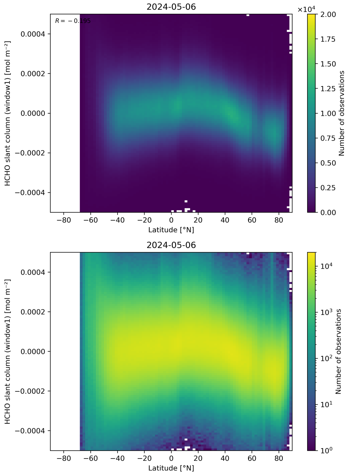
Figure 159: Scatter density plot of “Latitude” against “HCHO slant column (window1)” for 2024-05-05 to 2024-05-07.
