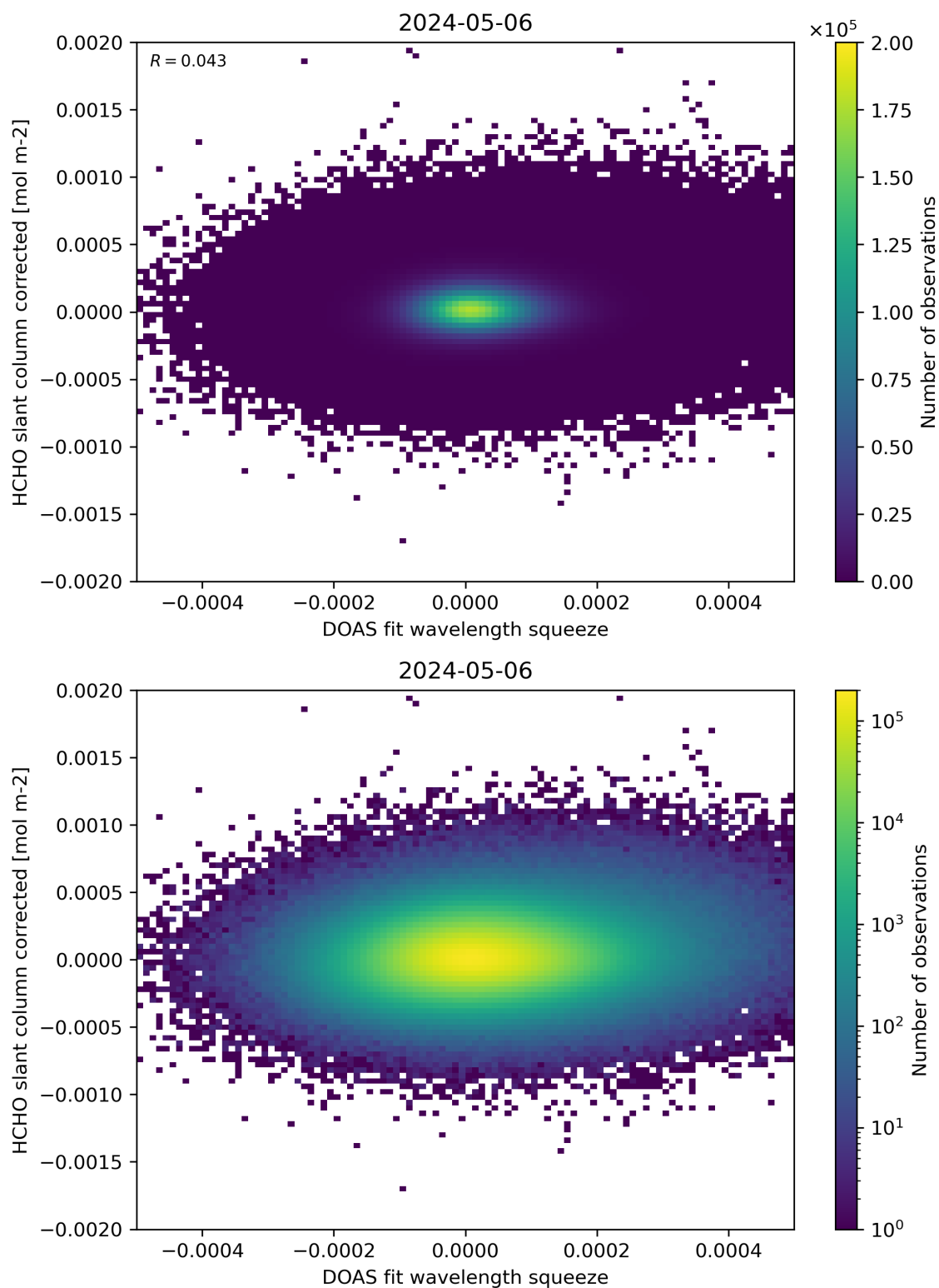
Figure 69: Scatter density plot of “DOAS fit wavelength squeeze” against “HCHO slant column corrected” for 2024-05-05 to 2024-05-07.
