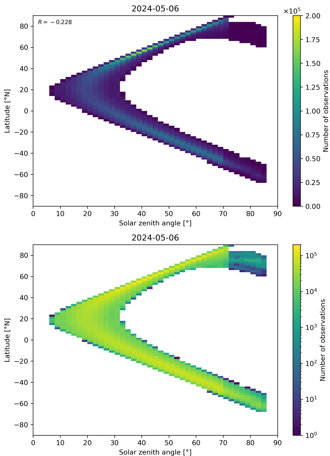
Figure 181: Scatter density plot of “Solar zenith angle” against “Latitude” for 2024-05-05 to 2024-05-07.
