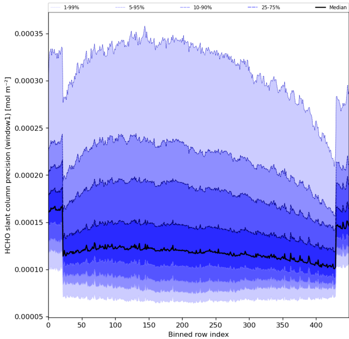
Figure 53: Along track statistics of “HCHO slant column precision (window1)” for 2024-05-05 to 2024-05-07
