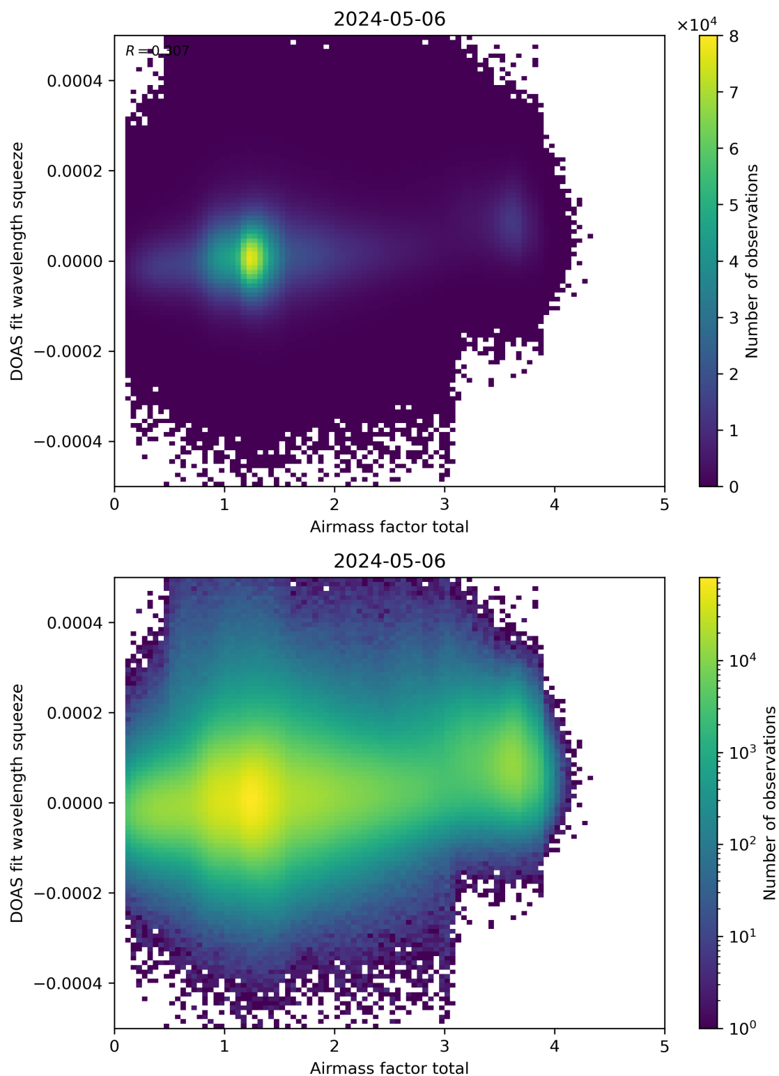
Figure 99: Scatter density plot of “Airmass factor total” against “DOAS fit wavelength squeeze” for 2024-05-05 to 2024-05-07.
