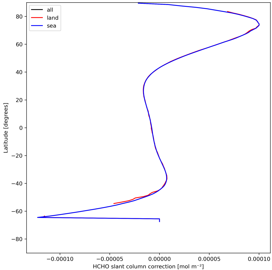
Figure 33: Zonal average of “HCHO slant column correction” for 2024-05-05 to 2024-05-07.
