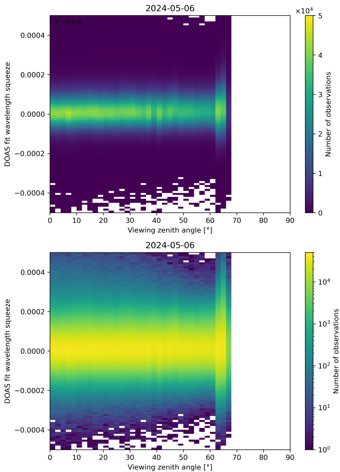
Figure 184: Scatter density plot of “Viewing zenith angle” against “DOAS fit wavelength squeeze” for 2024-05-05 to 2024-05-07.
