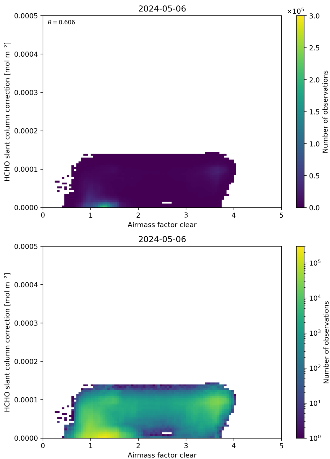
Figure 75: Scatter density plot of “Airmass factor clear” against “HCHO slant column correction” for 2024-05-05 to 2024-05-07.
