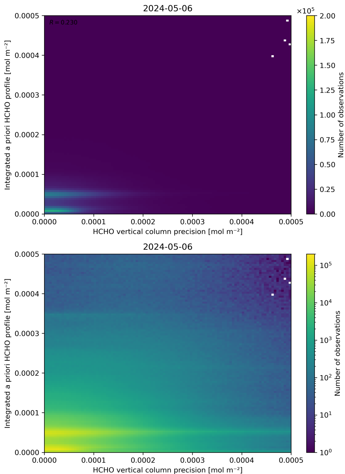
Figure 147: Scatter density plot of “HCHO vertical column precision” against “Integrated a priori HCHO profile” for 2024-05-05 to 2024-05-07.
