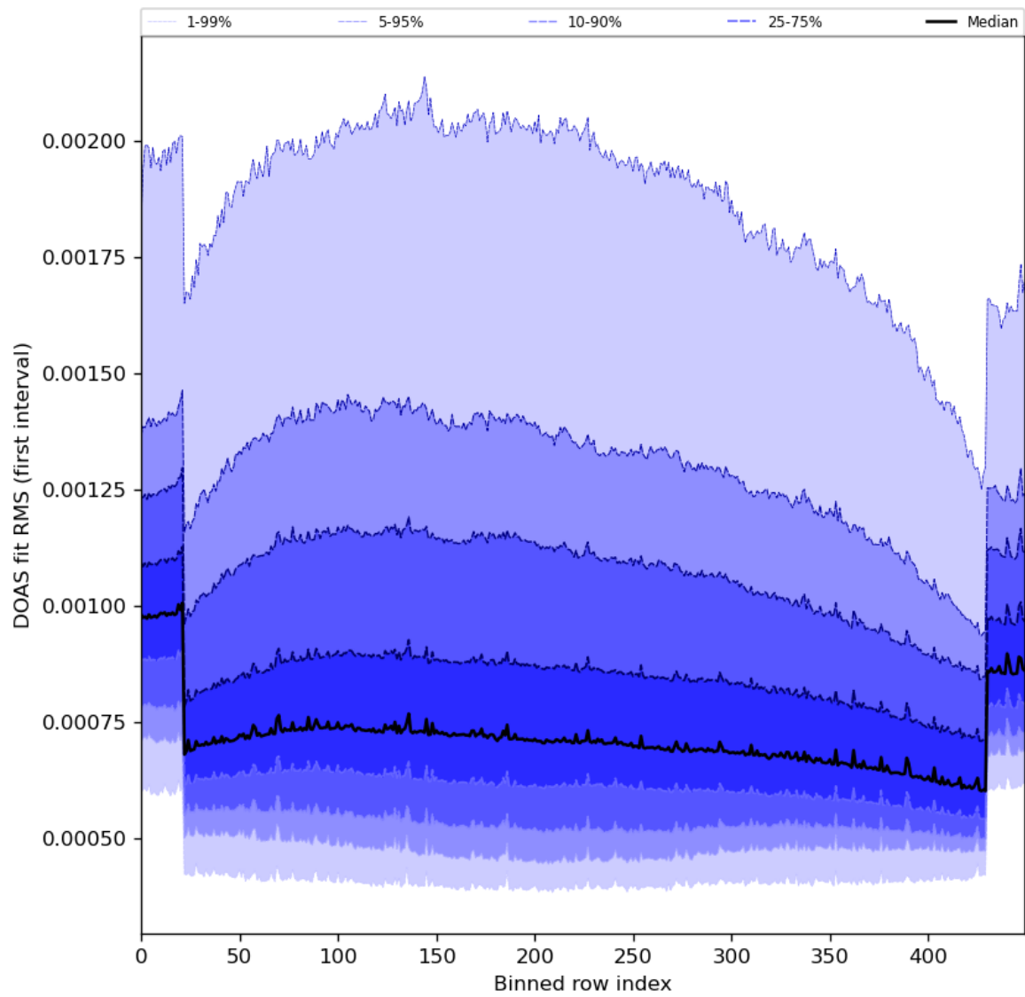
Figure 60: Along track statistics of “DOAS fit RMS (first interval)” for 2024-05-05 to 2024-05-07
