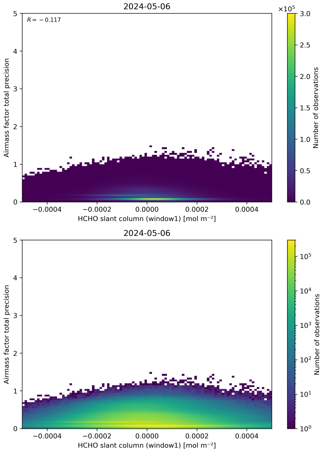
Figure 86: Scatter density plot of “HCHO slant column (window1)” against “Airmass factor total precision” for 2024-05-05 to 2024-05-07.
