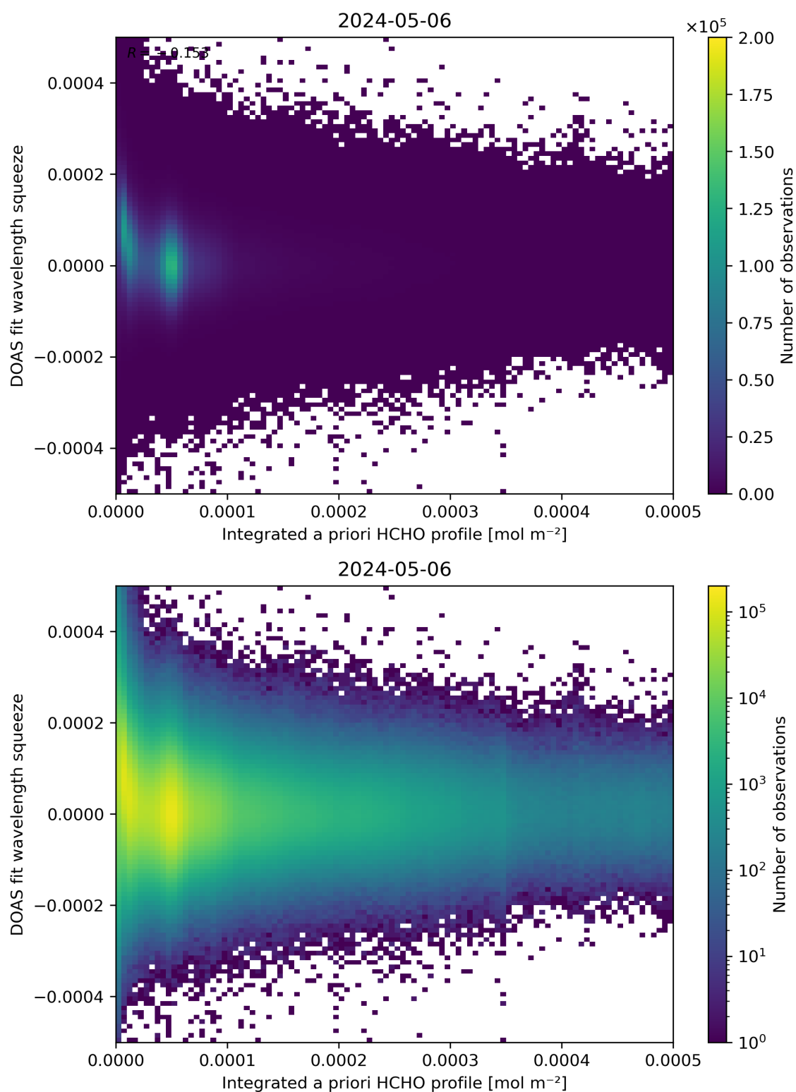
Figure 150: Scatter density plot of “Integrated a priori HCHO profile” against “DOAS fit wavelength squeeze” for 2024-05-05 to 2024-05-07.
