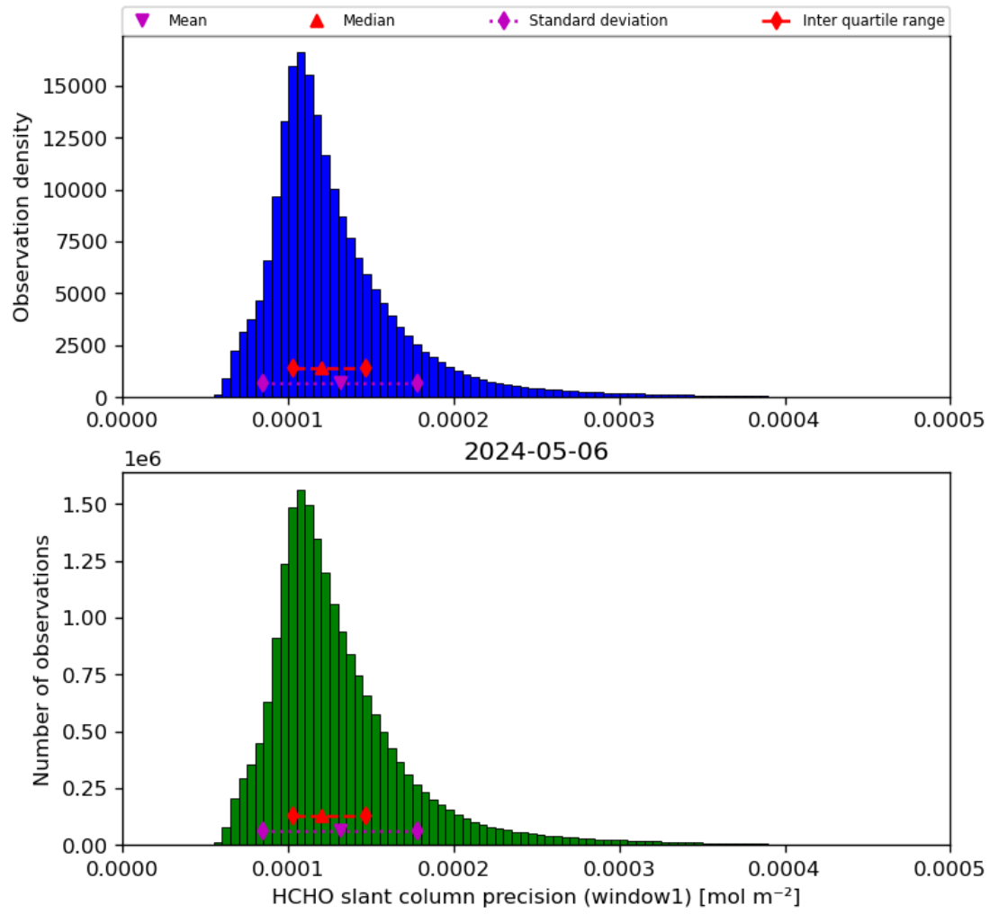
Figure 39: Histogram of “HCHO slant column precision (window1)” for 2024-05-05 to 2024-05-07
