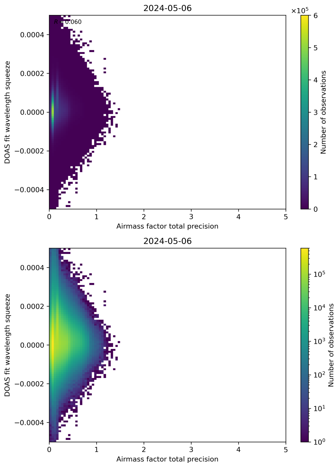
Figure 107: Scatter density plot of “Airmass factor total precision” against “DOAS fit wavelength squeeze” for 2024-05-05 to 2024-05-07.
