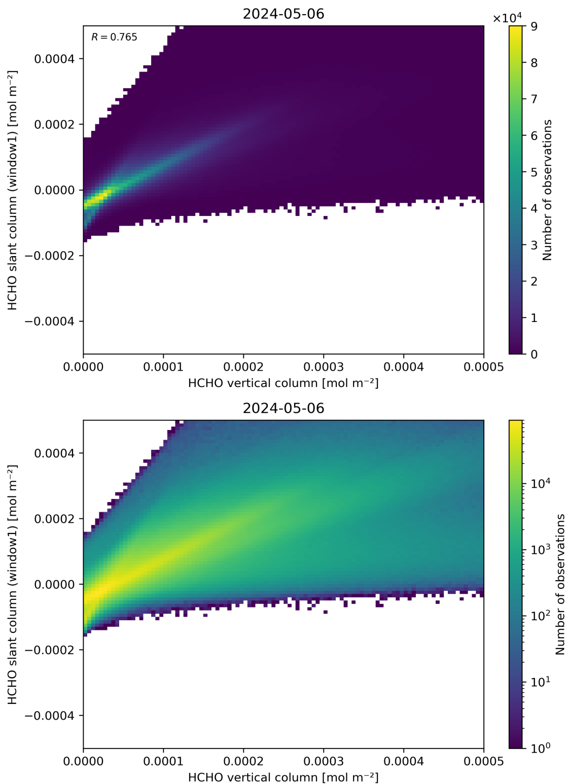
Figure 129: Scatter density plot of “HCHO vertical column” against “HCHO slant column (window1)” for 2024-05-05 to 2024-05-07.
