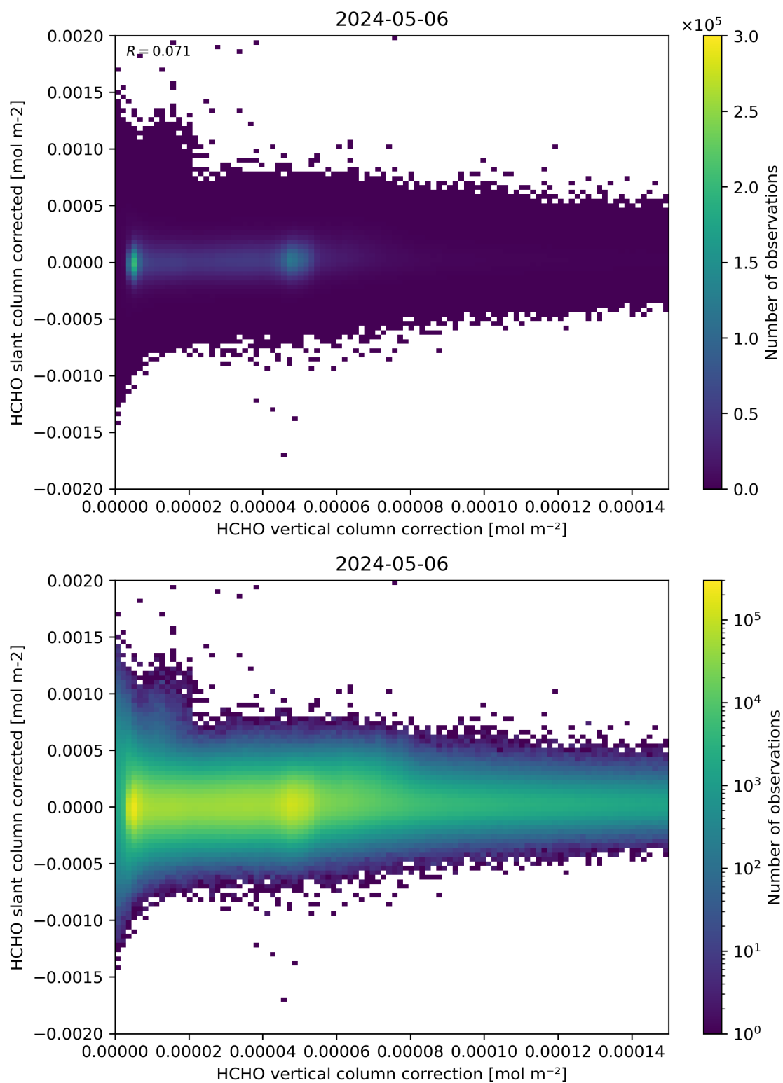
Figure 116: Scatter density plot of “HCHO vertical column correction” against “HCHO slant column corrected” for 2024-05-05 to 2024-05-07.
