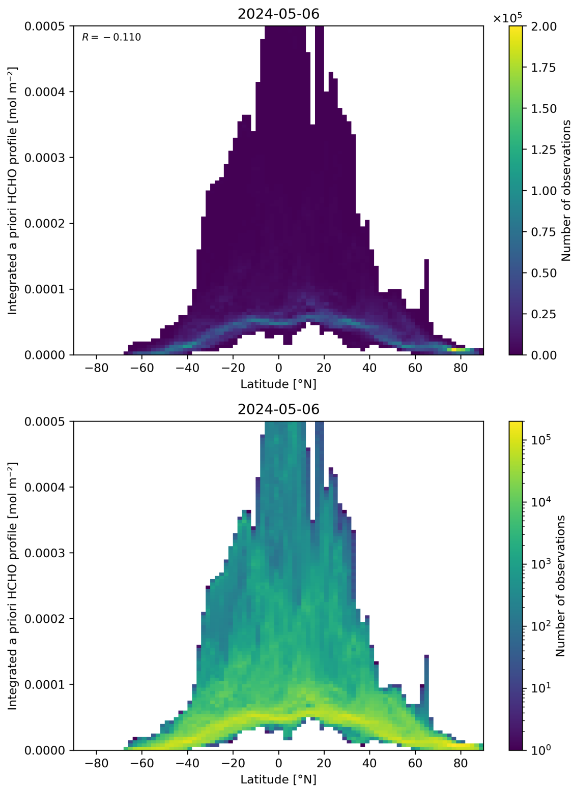
Figure 166: Scatter density plot of “Latitude” against “Integrated a priori HCHO profile” for 2024-05-05 to 2024-05-07.
