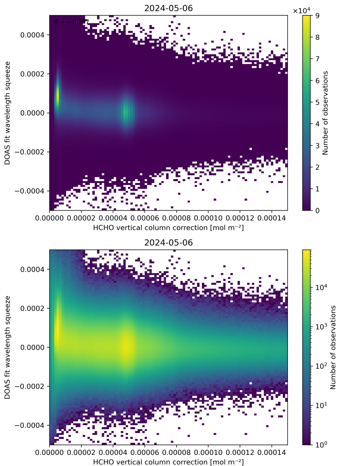
Figure 114: Scatter density plot of “HCHO vertical column correction” against “DOAS fit wavelength squeeze” for 2024-05-05 to 2024-05-07.
