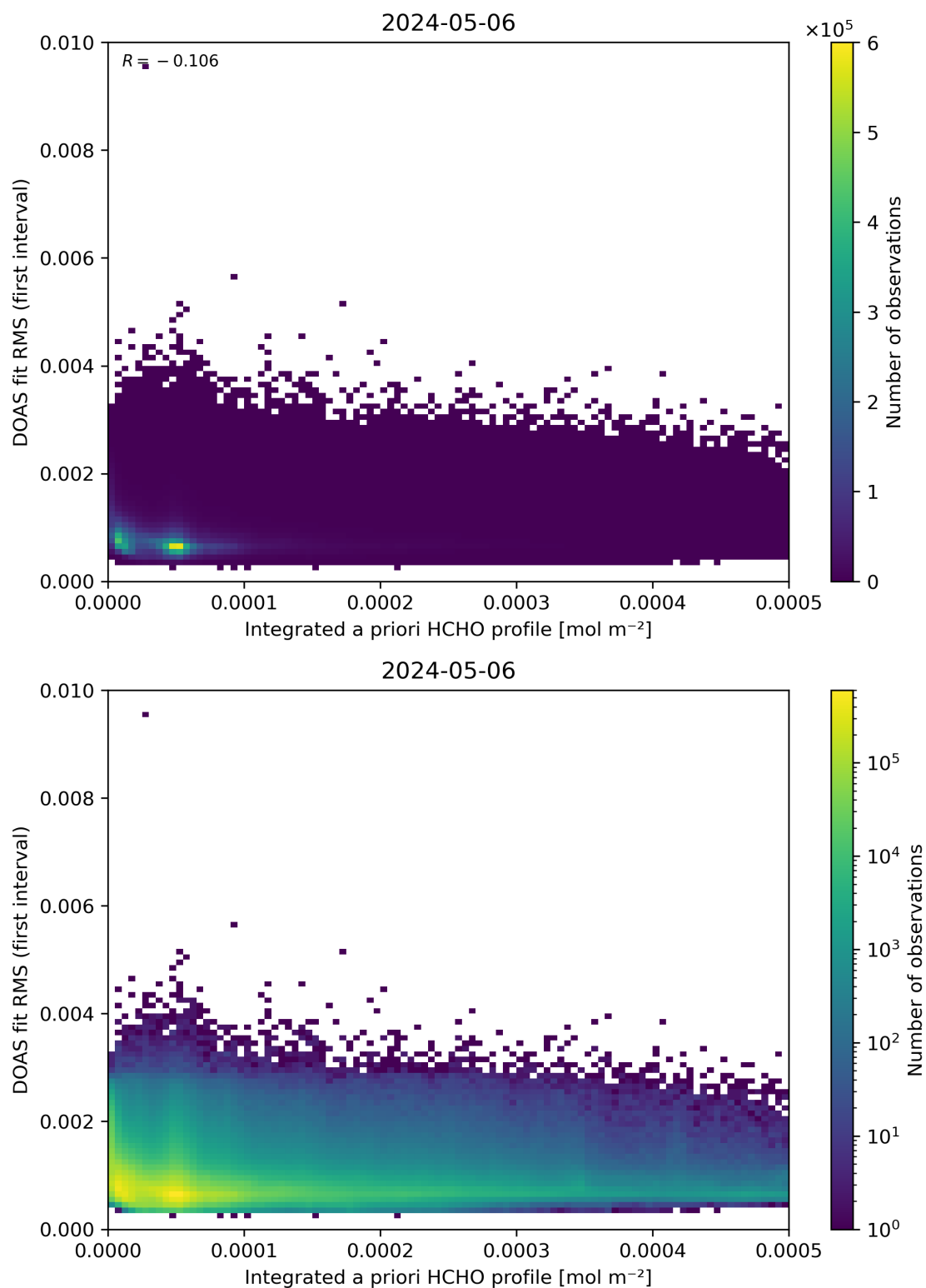
Figure 148: Scatter density plot of “Integrated a priori HCHO profile” against “DOAS fit RMS (first interval)” for 2024-05-05 to 2024-05-07.
