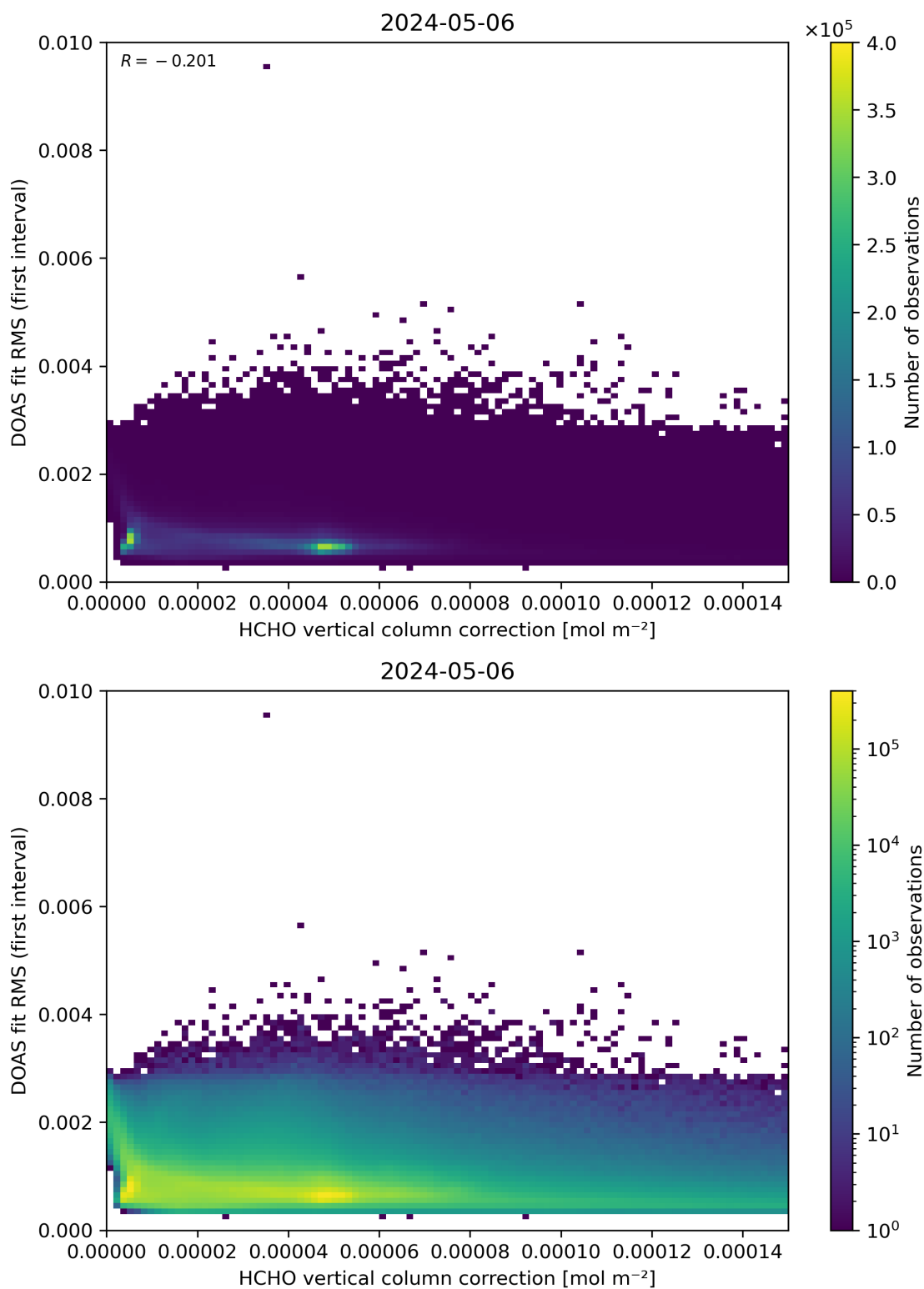
Figure 112: Scatter density plot of “HCHO vertical column correction” against “DOAS fit RMS (first interval)” for 2024-05-05 to 2024-05-07.
