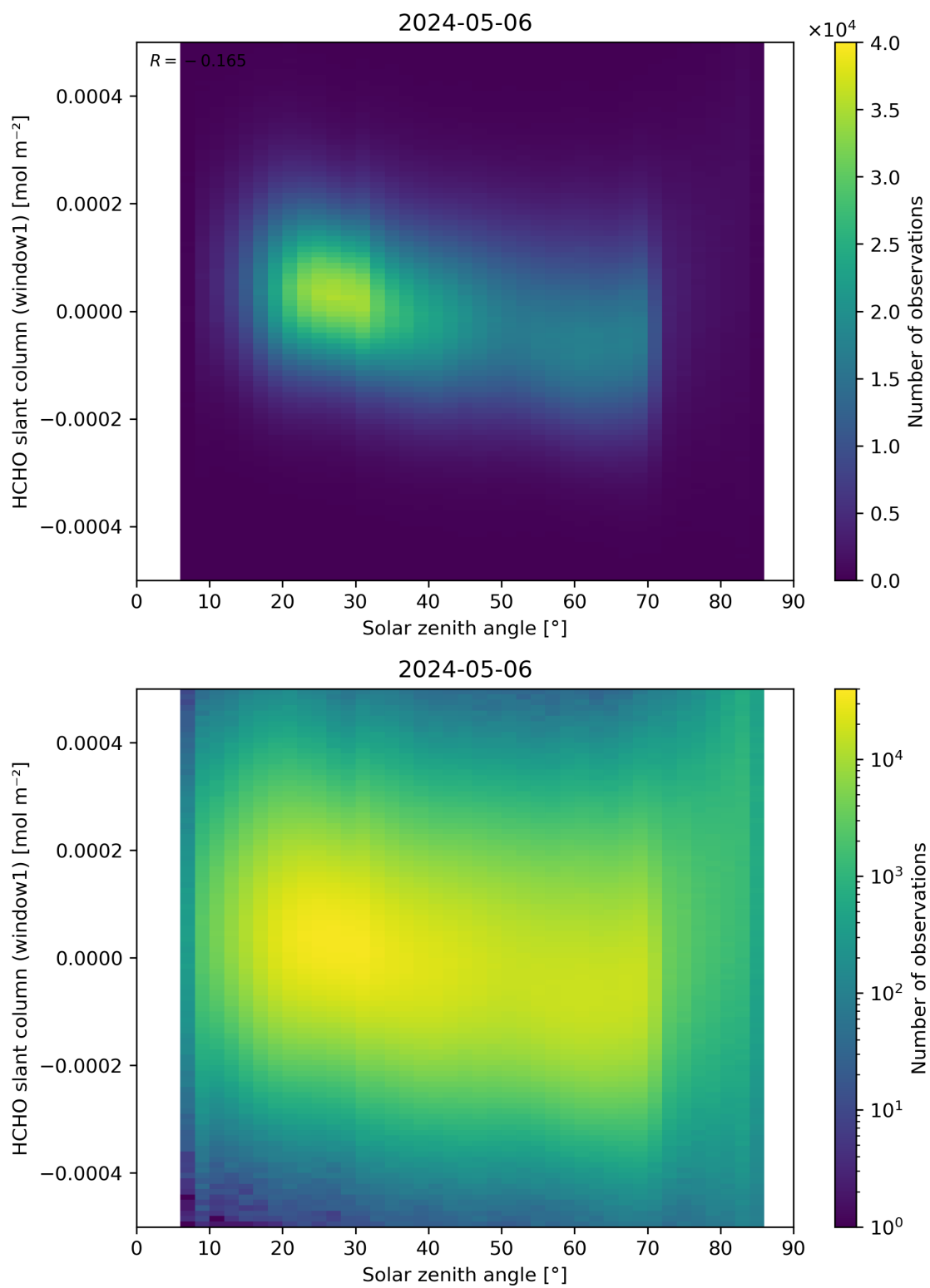
Figure 173: Scatter density plot of “Solar zenith angle” against “HCHO slant column (window1)” for 2024-05-05 to 2024-05-07.
