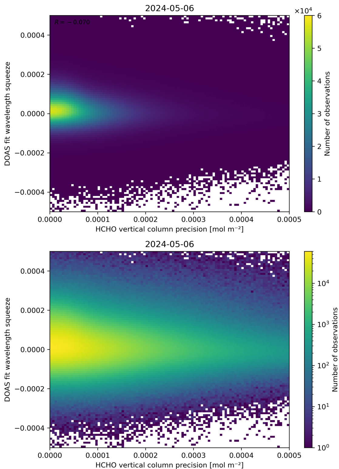
Figure 138: Scatter density plot of “HCHO vertical column precision” against “DOAS fit wavelength squeeze” for 2024-05-05 to 2024-05-07.
