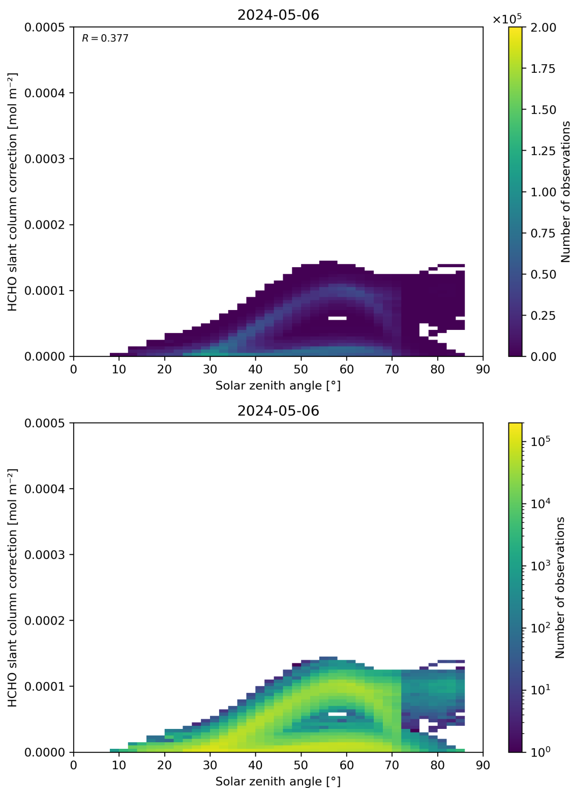
Figure 172: Scatter density plot of “Solar zenith angle” against “HCHO slant column correction” for 2024-05-05 to 2024-05-07.
