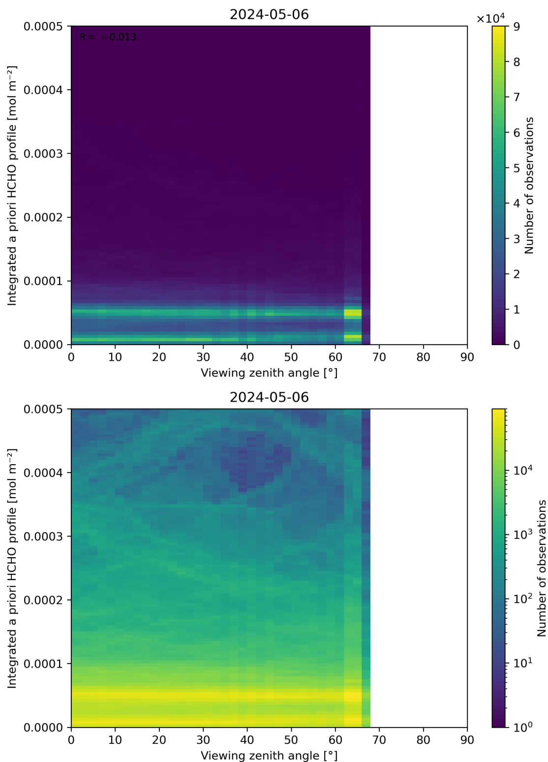
Figure 195: Scatter density plot of “Viewing zenith angle” against “Integrated a priori HCHO profile” for 2024-05-05 to 2024-05-07.
