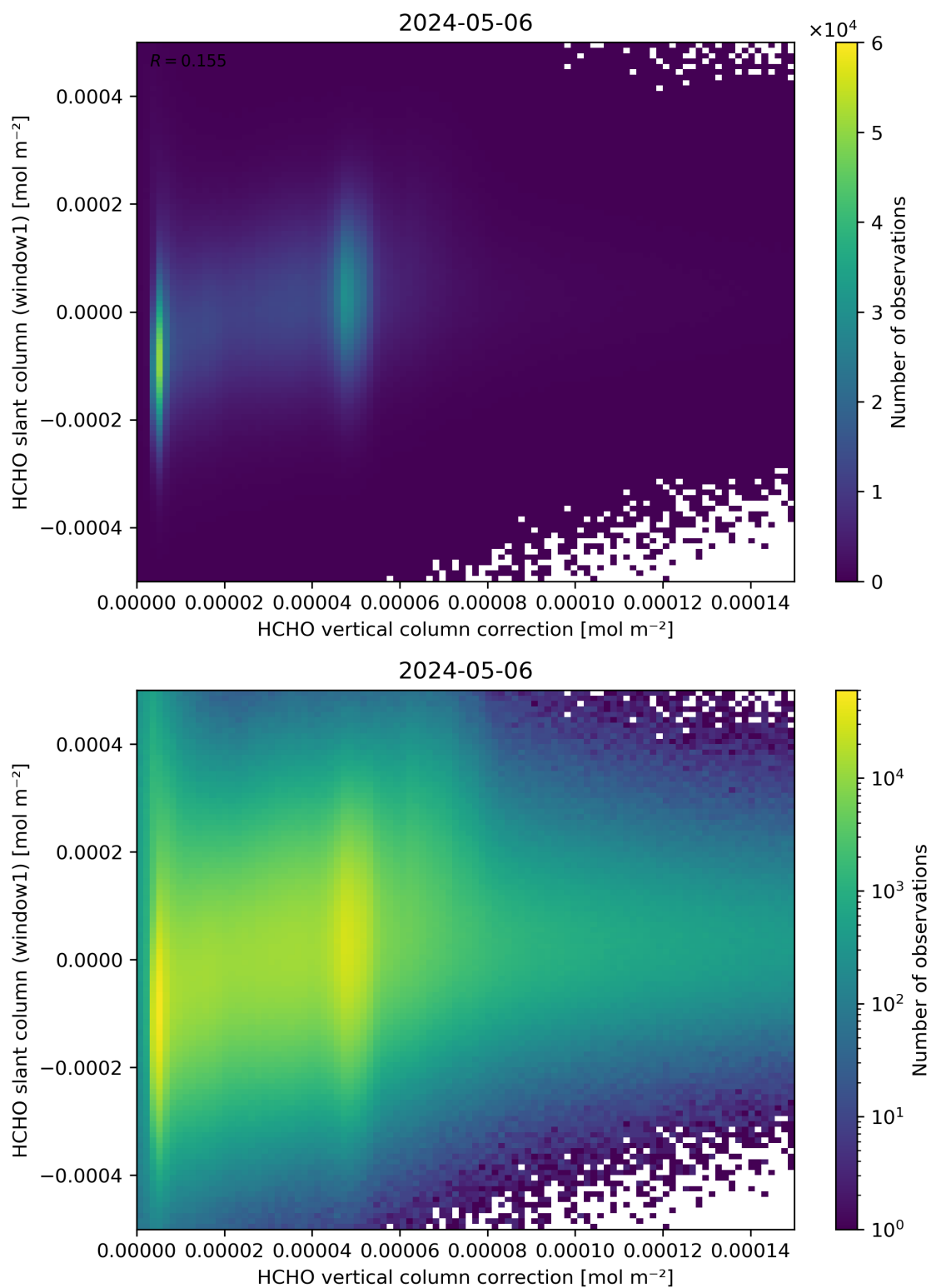
Figure 118: Scatter density plot of “HCHO vertical column correction” against “HCHO slant column (window1)” for 2024-05-05 to 2024-05-07.
