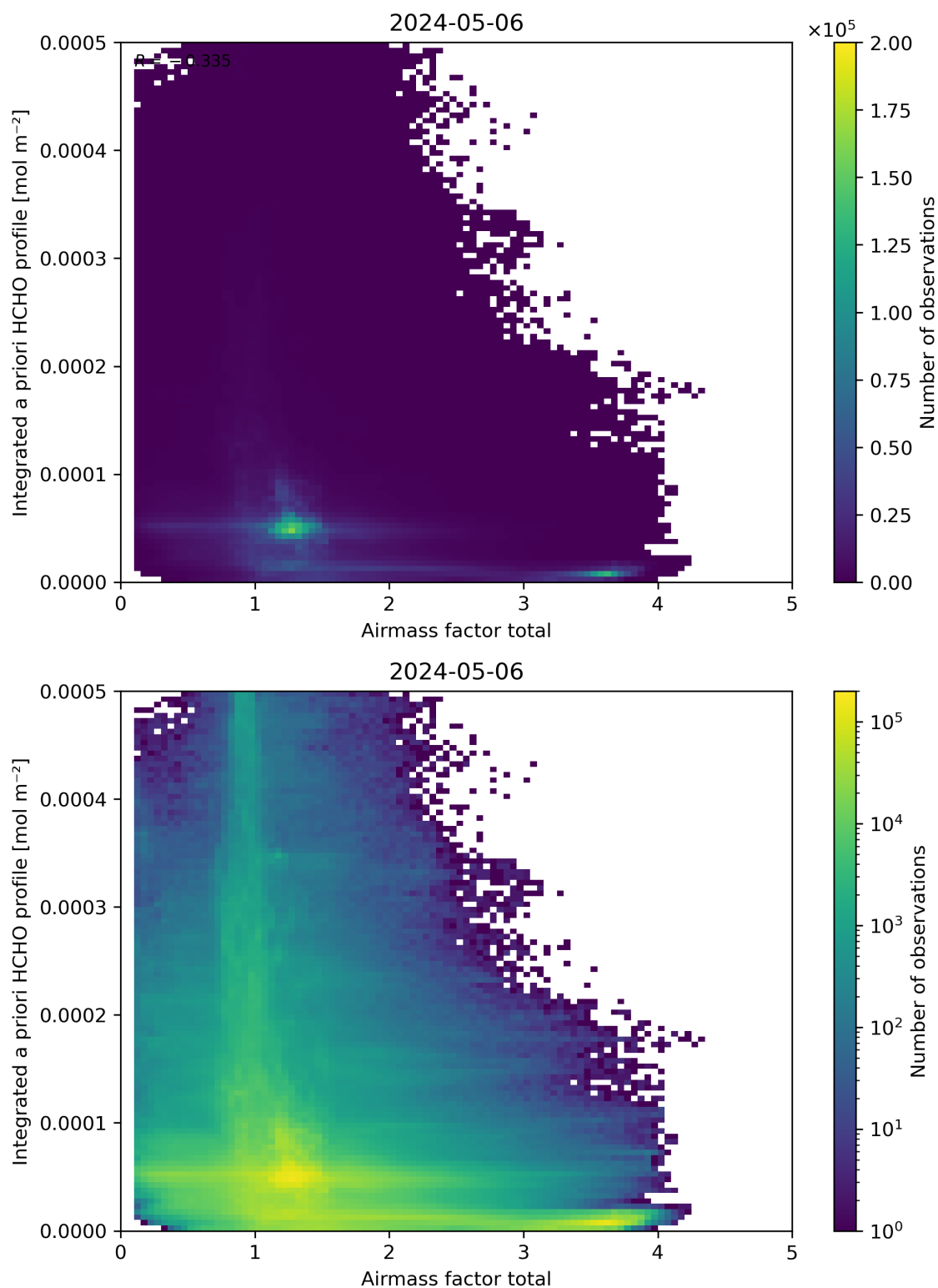
Figure 104: Scatter density plot of “Air mass factor total” against “Integrated a priori HCHO profile” for 2024-05-05 to 2024-05-07.
