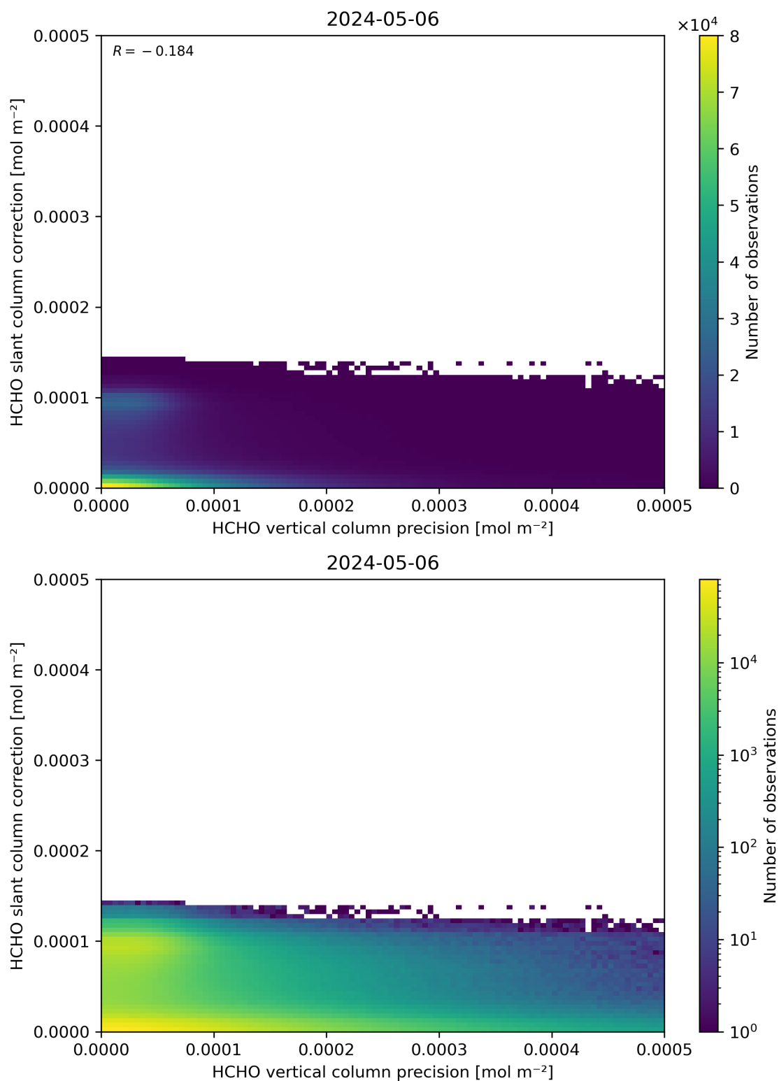
Figure 141: Scatter density plot of “HCHO vertical column precision” against “HCHO slant column correction” for 2024-05-05 to 2024-05-07.
