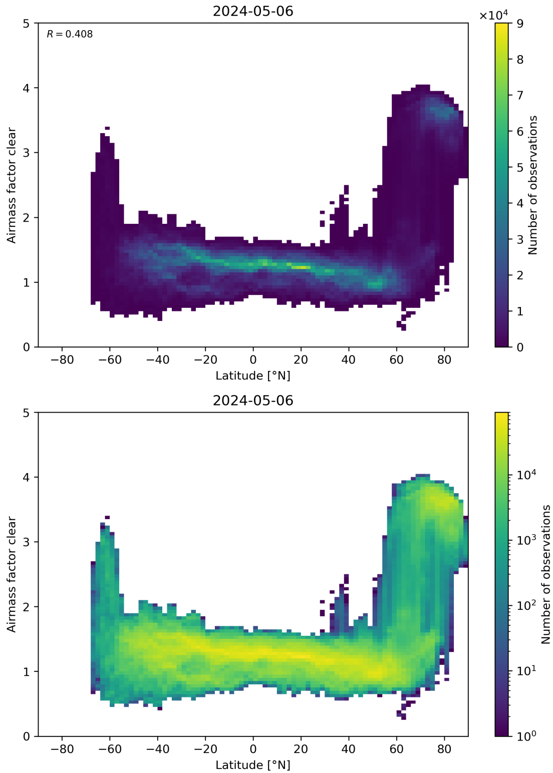
Figure 156: Scatter density plot of “Latitude” against “Airmass factor clear” for 2024-05-05 to 2024-05-07.
