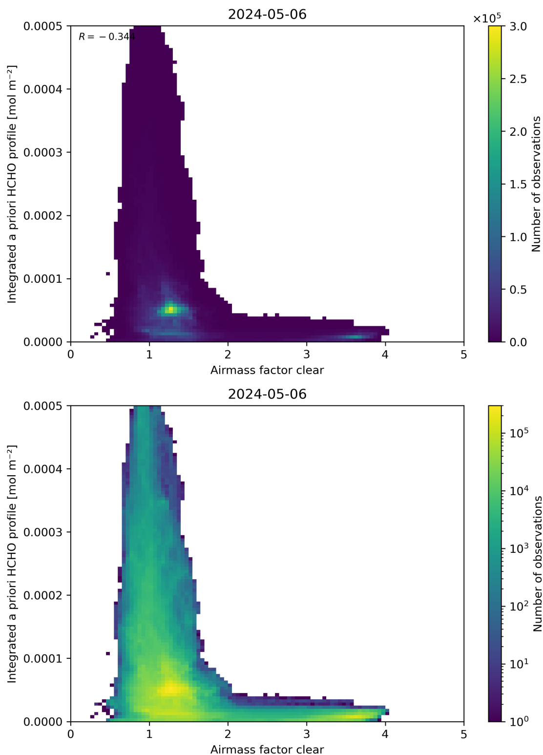
Figure 76: Scatter density plot of “Airmass factor clear” against “Integrated a priori HCHO profile” for 2024-05-05 to 2024-05-07.
