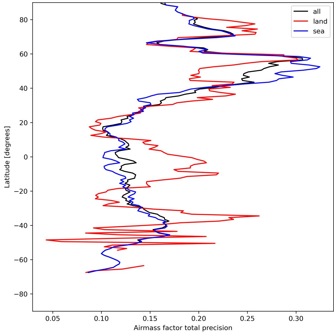
Figure 27: Zonal average of “Airmass factor total precision” for 2024-05-05 to 2024-05-07.
