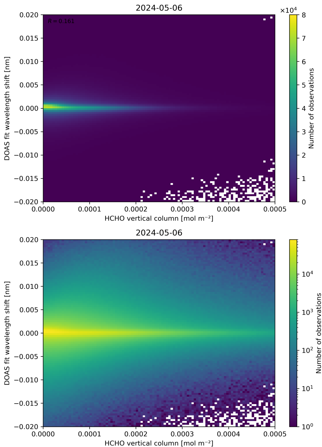
Figure 124: Scatter density plot of “HCHO vertical column” against “DOAS fit wavelength shift” for 2024-05-05 to 2024-05-07.
