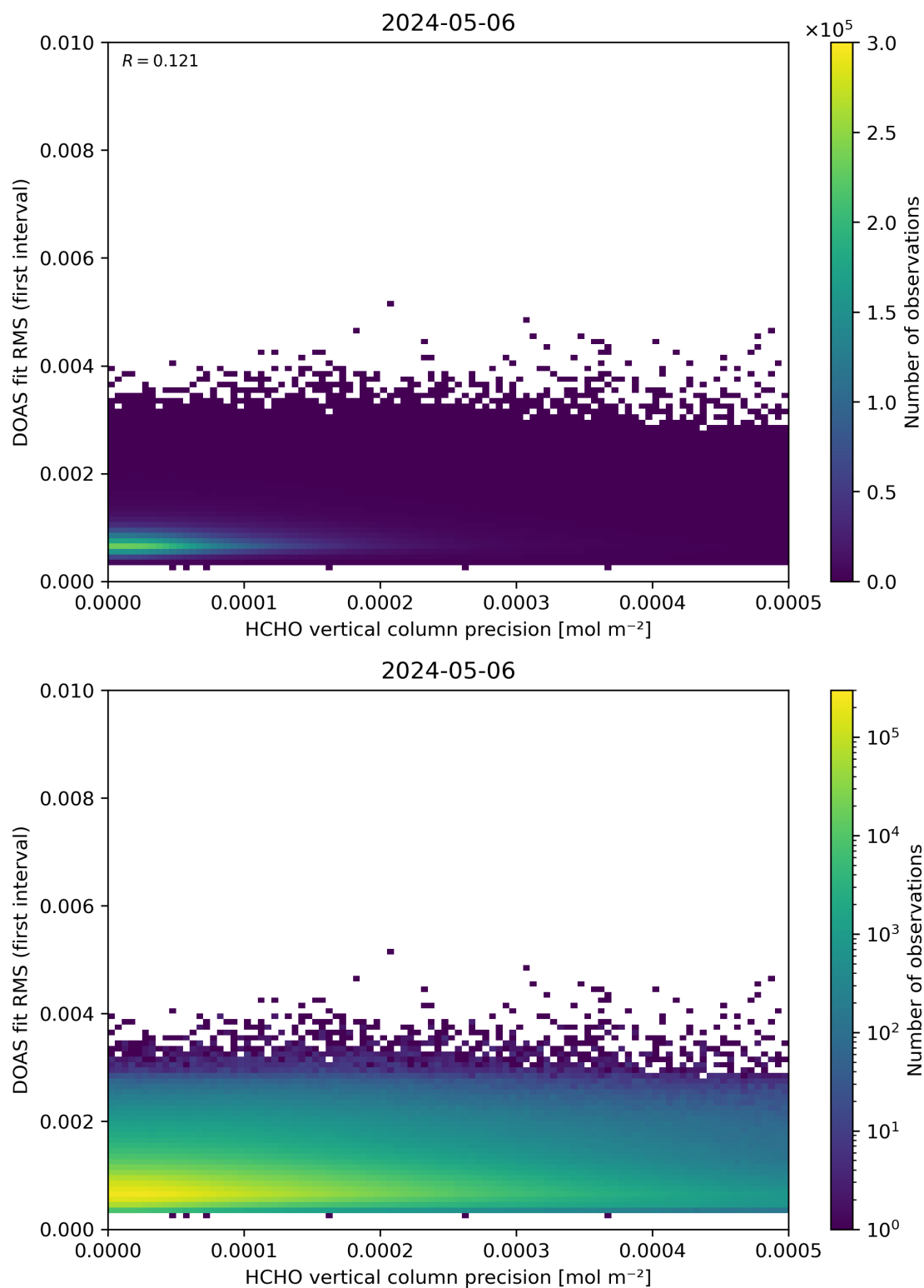
Figure 136: Scatter density plot of “HCHO vertical column precision” against “DOAS fit RMS (first interval)” for 2024-05-05 to 2024-05-07.
