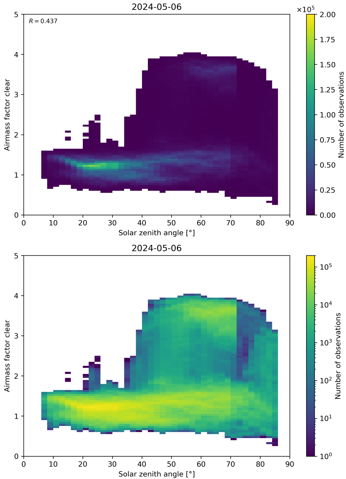
Figure 170: Scatter density plot of “Solar zenith angle” against “Airmass factor clear” for 2024-05-05 to 2024-05-07.
