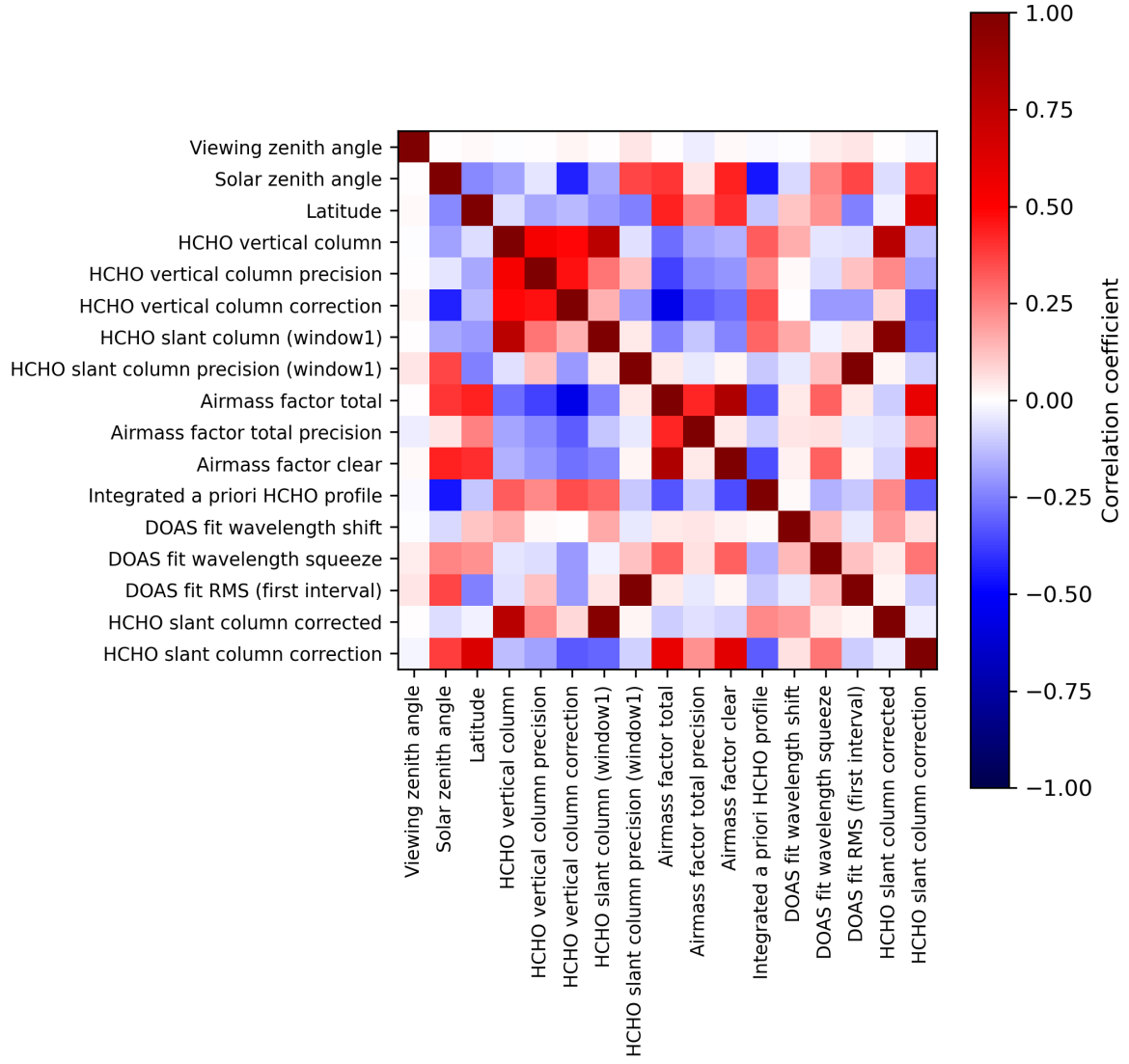
Figure 2: Map of correlation matrix for 2024-05-05 to 2024-05-07.
