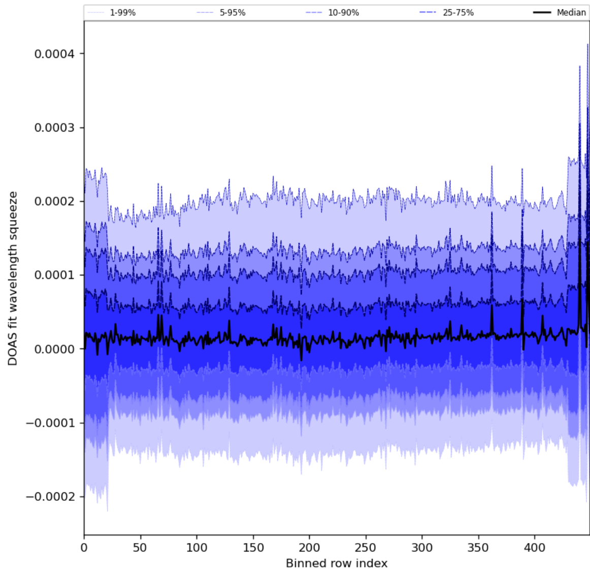
Figure 59: Along track statistics of “DOAS fit wavelength squeeze” for 2024-05-05 to 2024-05-07
