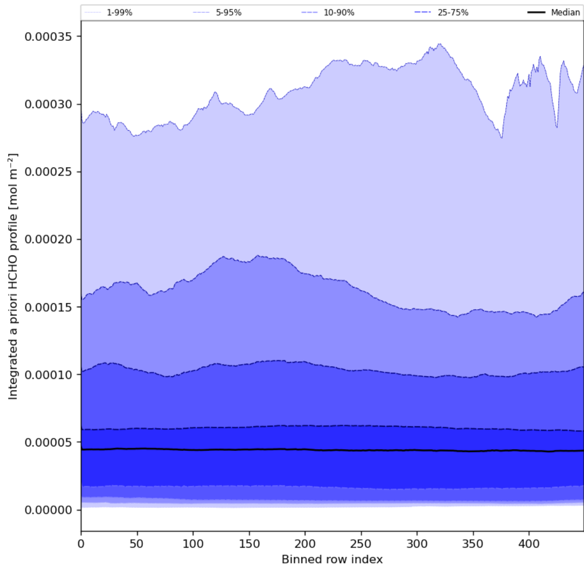
Figure 57: Along track statistics of "Integrated a priori HCHO profile" for 2024-05-05 to 2024-05-07
