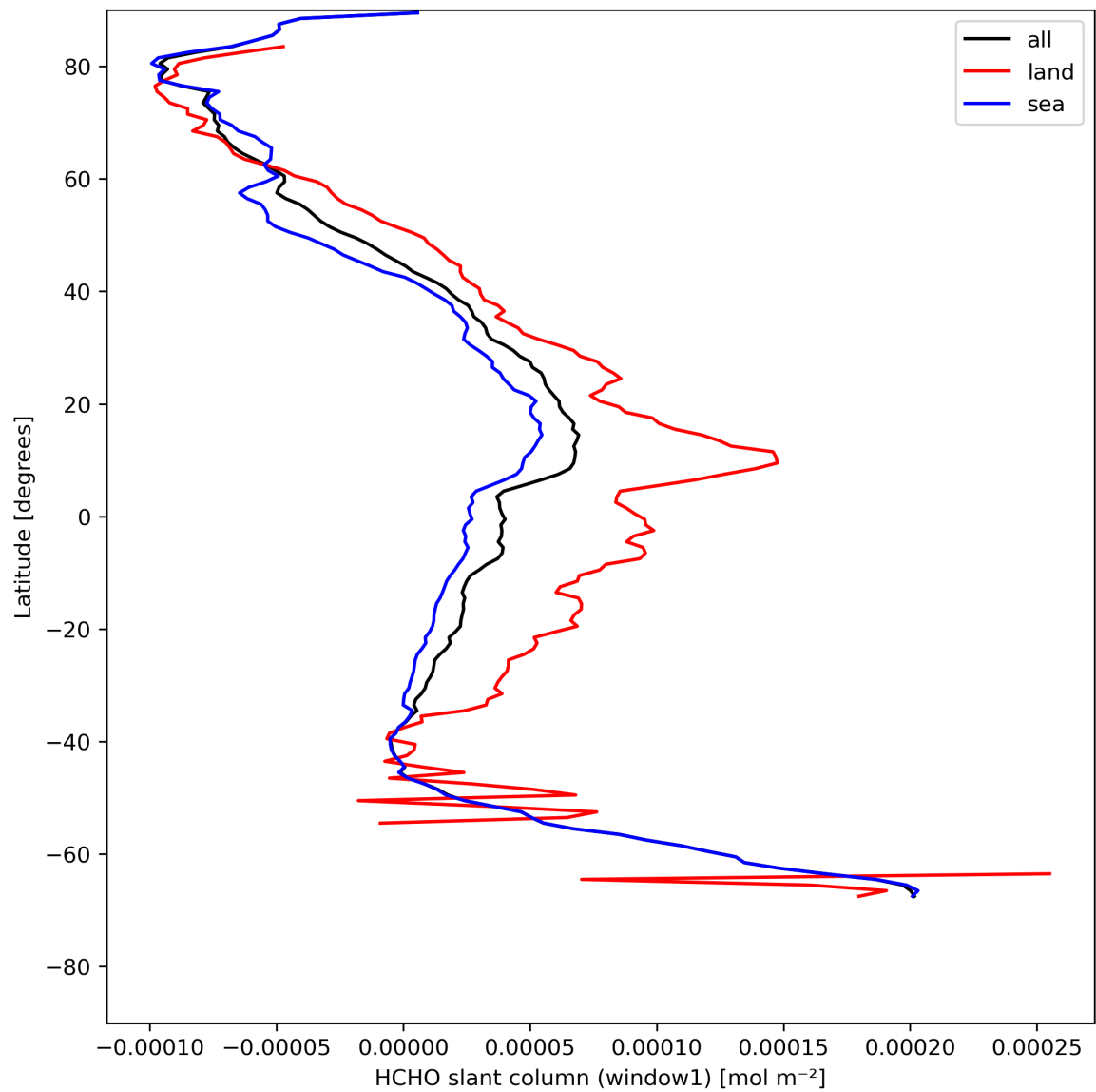
Figure 24: Zonal average of “HCHO slant column (window1)” for 2024-05-05 to 2024-05-07.
