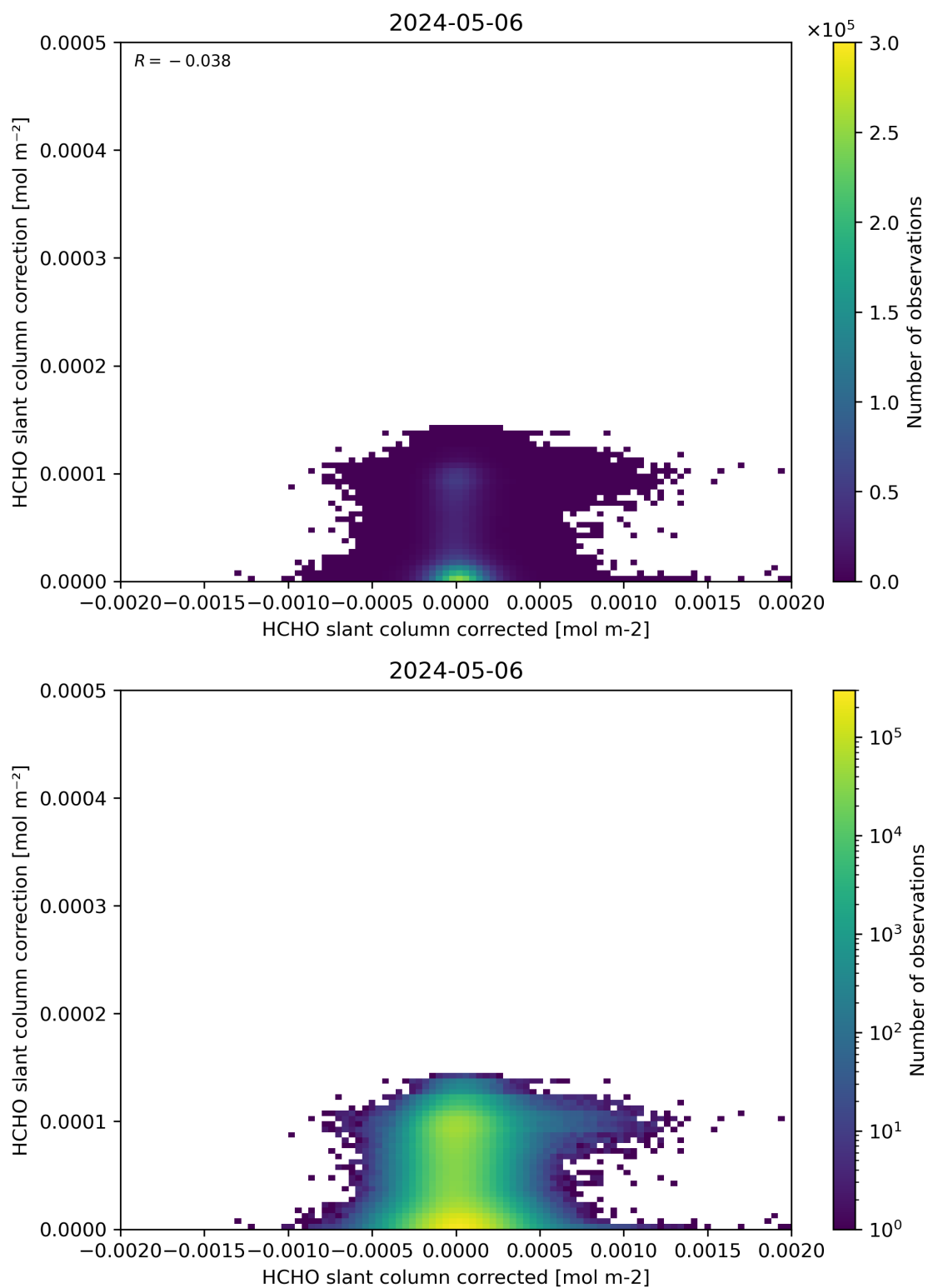
Figure 77: Scatter density plot of “HCHO slant column corrected” against “HCHO slant column correction” for 2024-05-05 to 2024-05-07.
