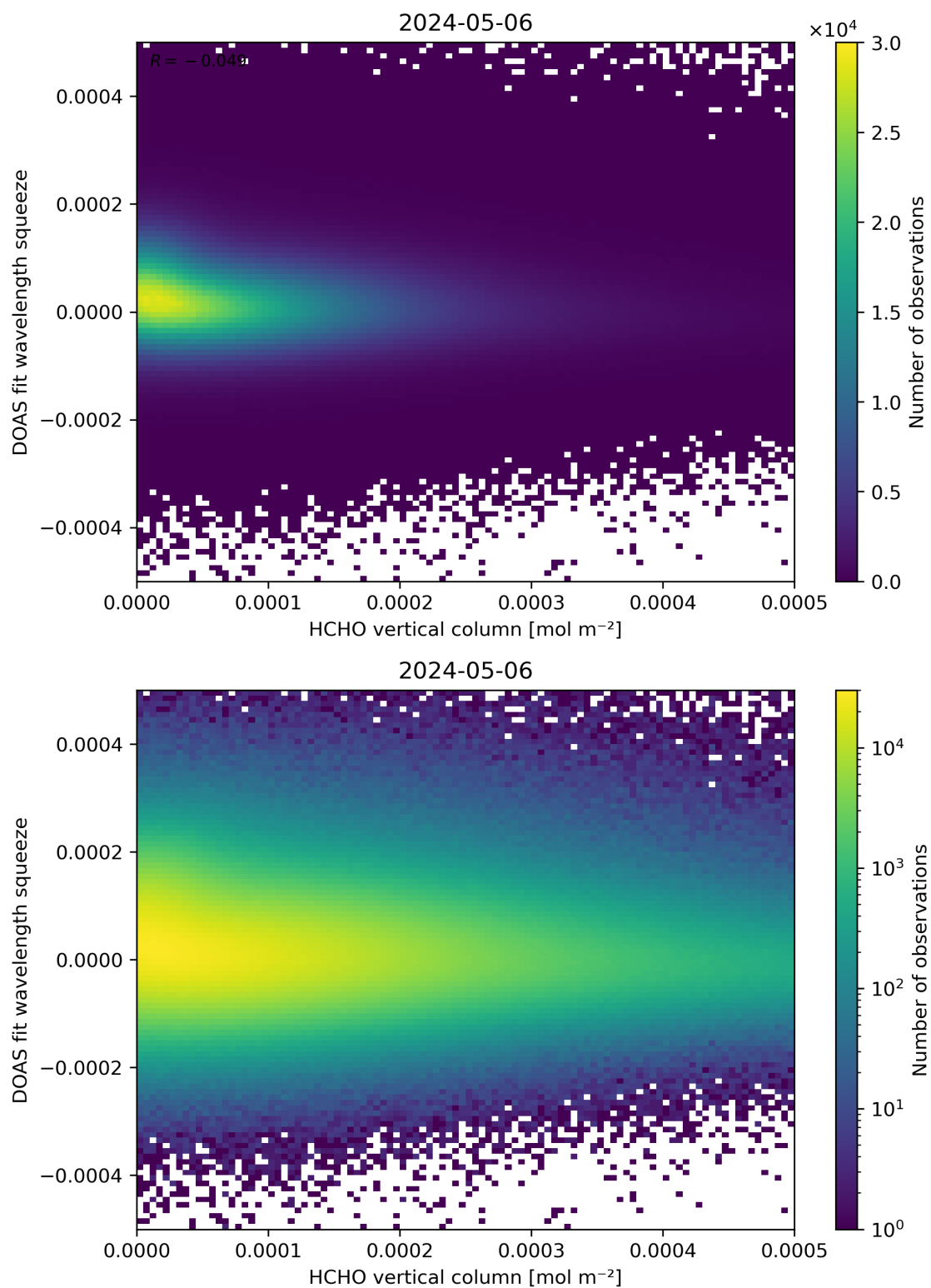
Figure 125: Scatter density plot of “HCHO vertical column” against “DOAS fit wavelength squeeze” for 2024-05-05 to 2024-05-07.
