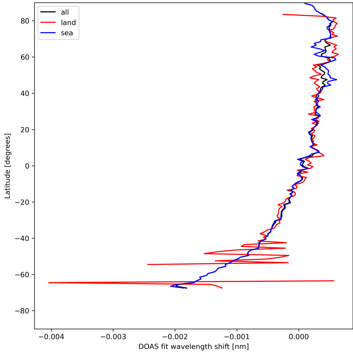
Figure 30: Zonal average of “DOAS fit wavelength shift” for 2024-05-05 to 2024-05-07.
