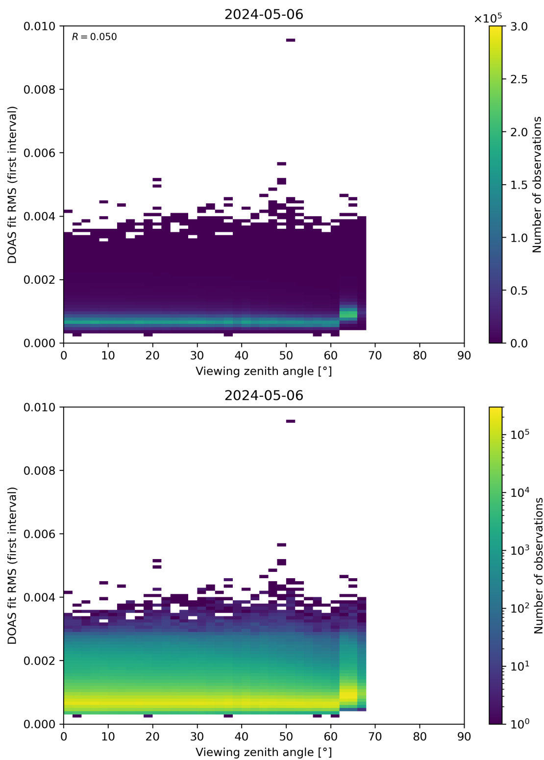
Figure 182: Scatter density plot of “Viewing zenith angle” against “DOAS fit RMS (first interval)” for 2024-05-05 to 2024-05-07.
