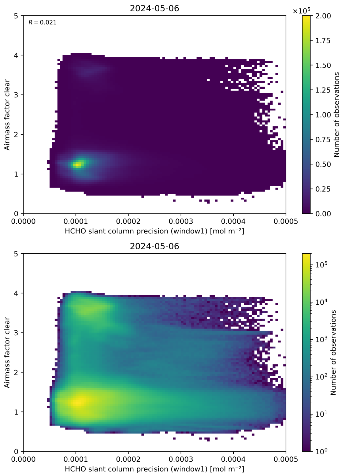
Figure 91: Scatter density plot of “HCHO slant column precision (window1)” against “Airmass factor clear” for 2024-05-05 to 2024-05-07.
