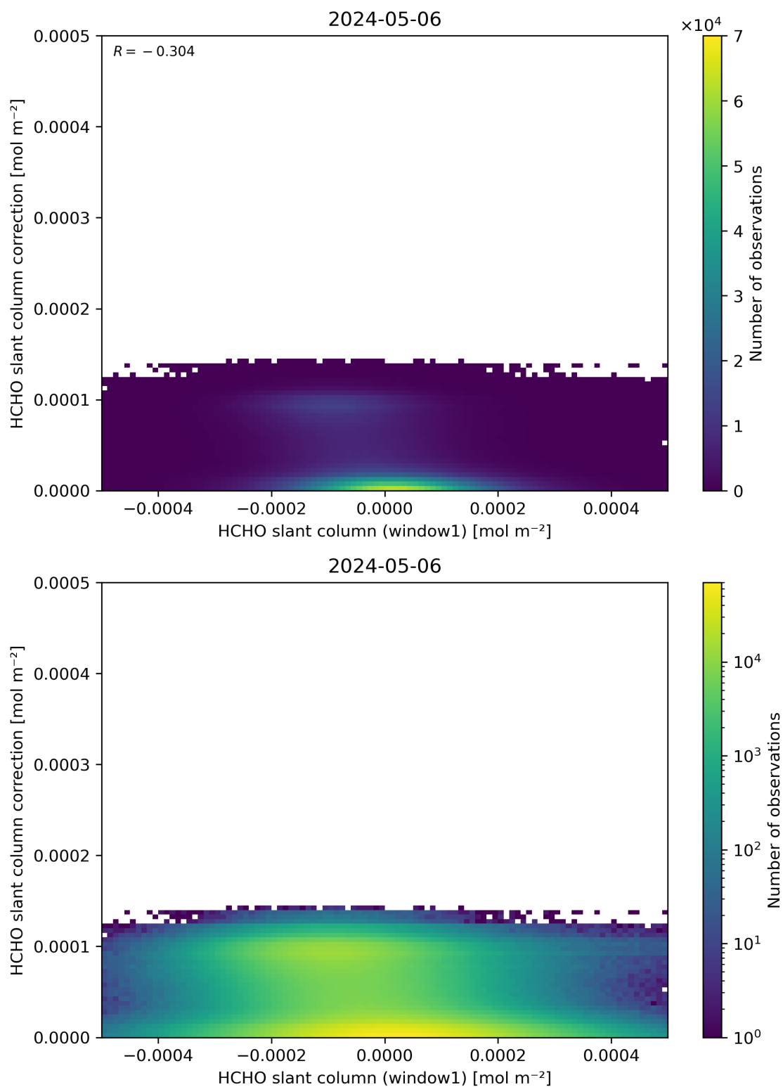
Figure 83: Scatter density plot of “HCHO slant column (window1)” against “HCHO slant column correction” for 2024-05-05 to 2024-05-07.
