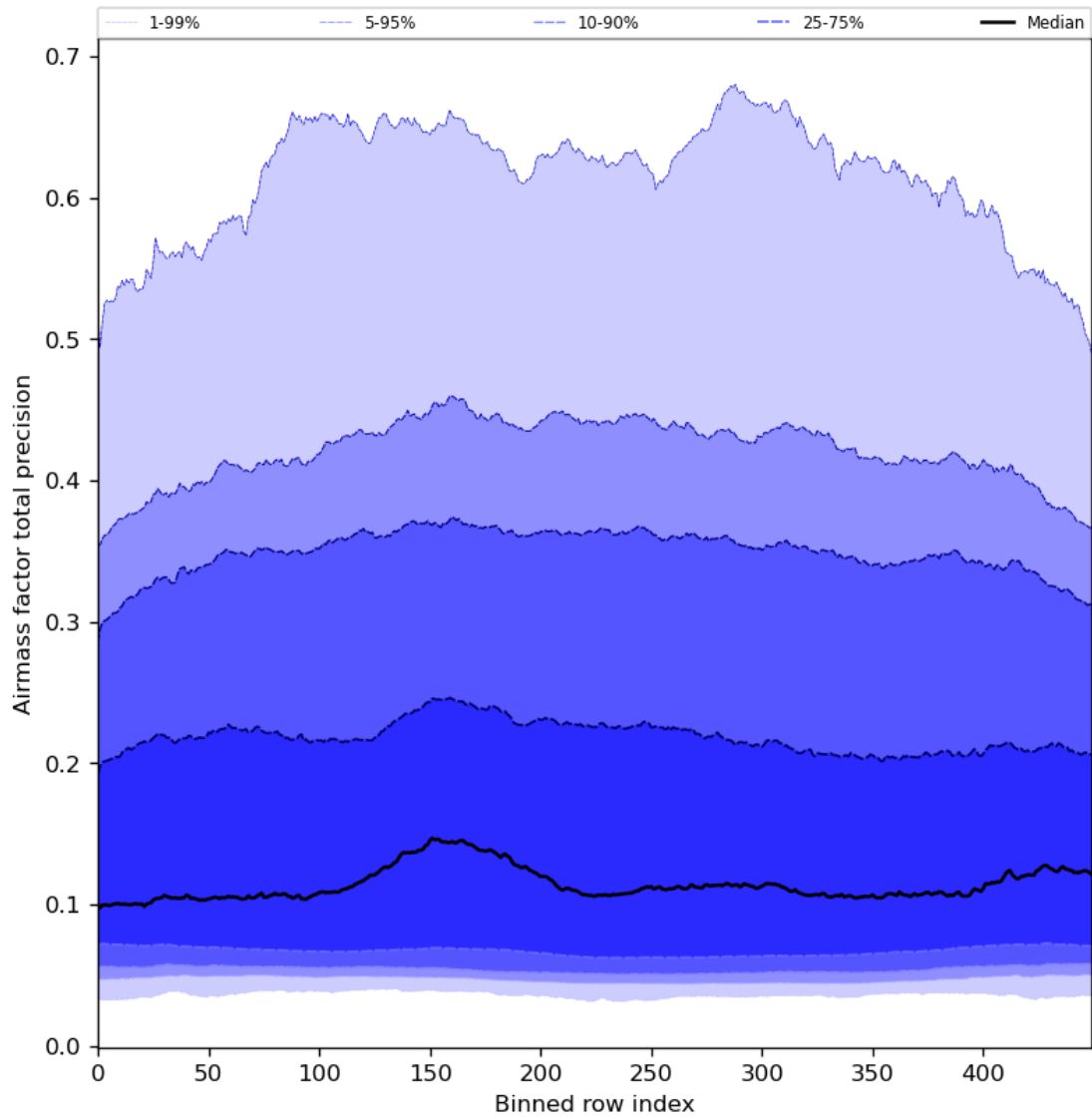
Figure 55: Along track statistics of “Airmass factor total precision” for 2024-05-05 to 2024-05-07
