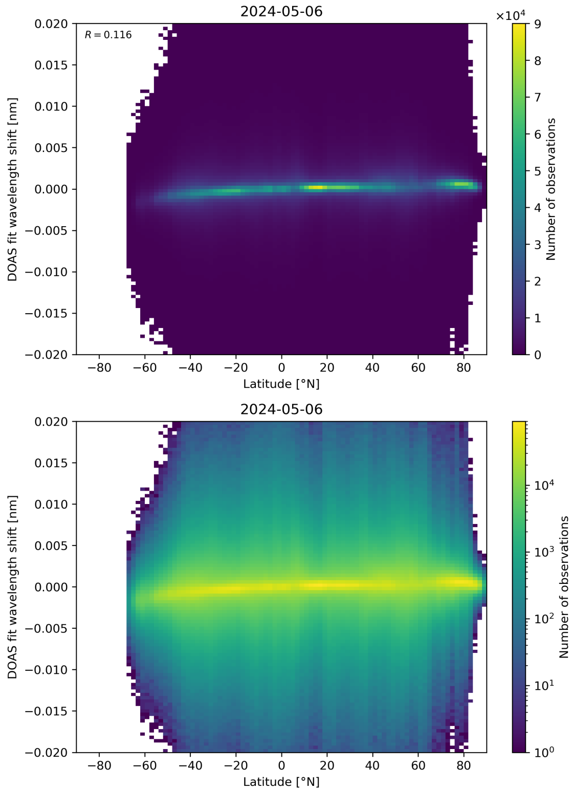
Figure 154: Scatter density plot of “Latitude” against “DOAS fit wavelength shift” for 2024-05-05 to 2024-05-07.
