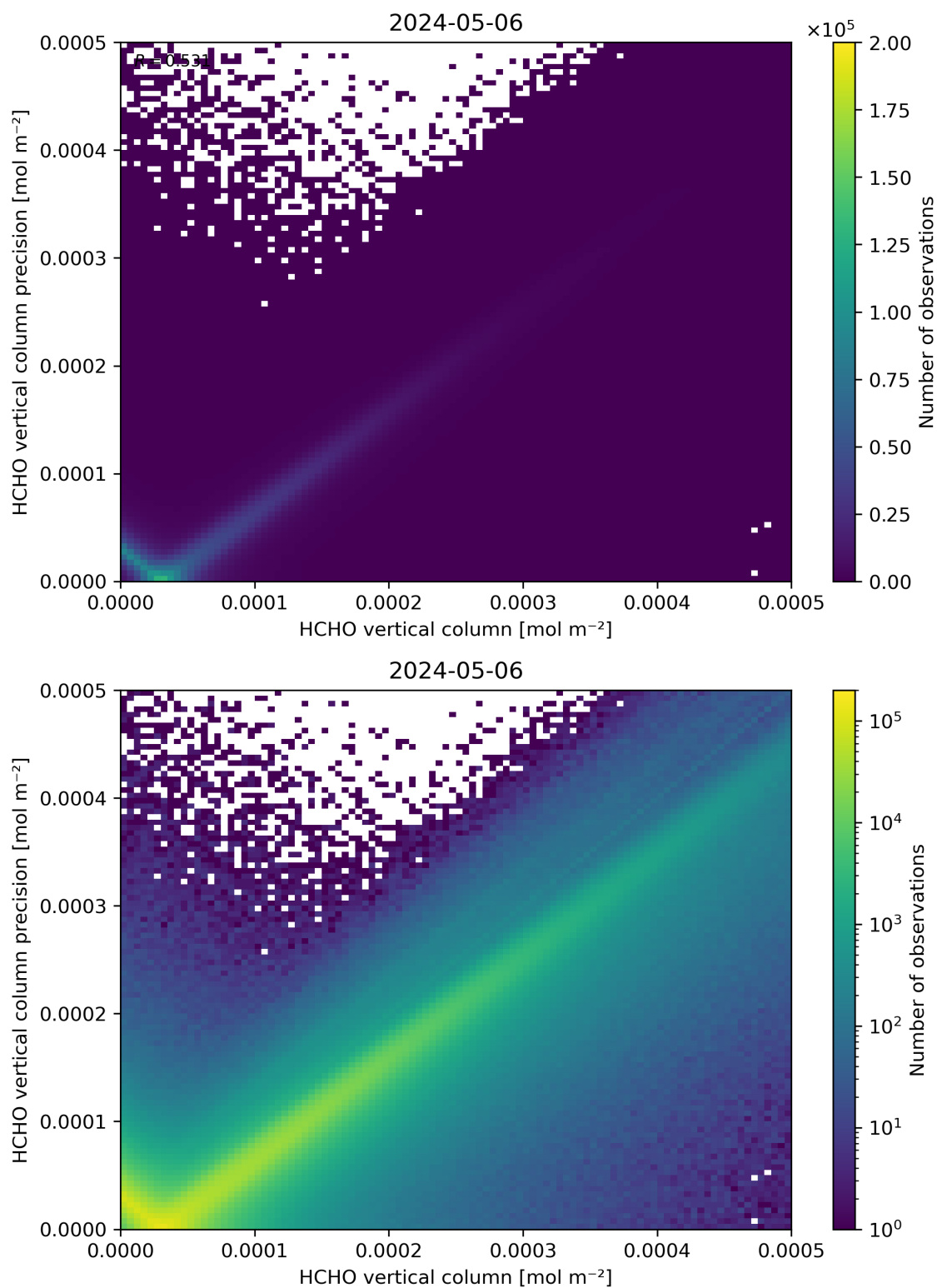
Figure 134: Scatter density plot of “HCHO vertical column” against “HCHO vertical column precision” for 2024-05-05 to 2024-05-07.
