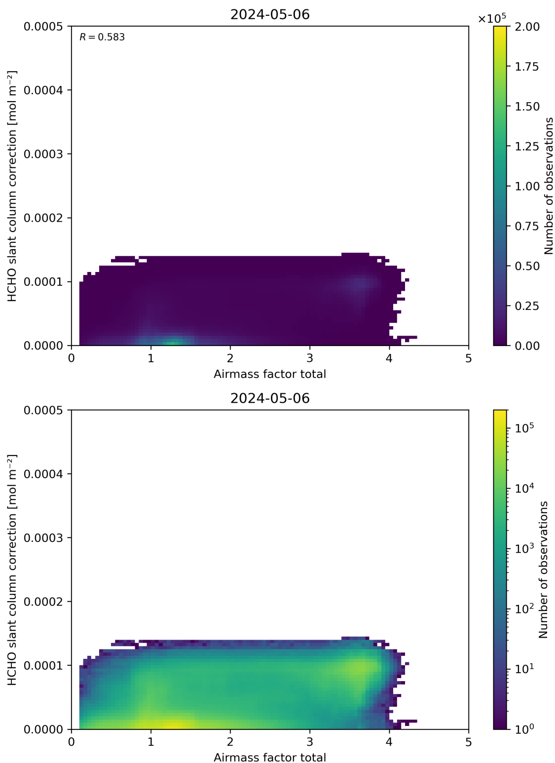
Figure 102: Scatter density plot of “Airmass factor total” against “HCHO slant column correction” for 2024-05-05 to 2024-05-07.
