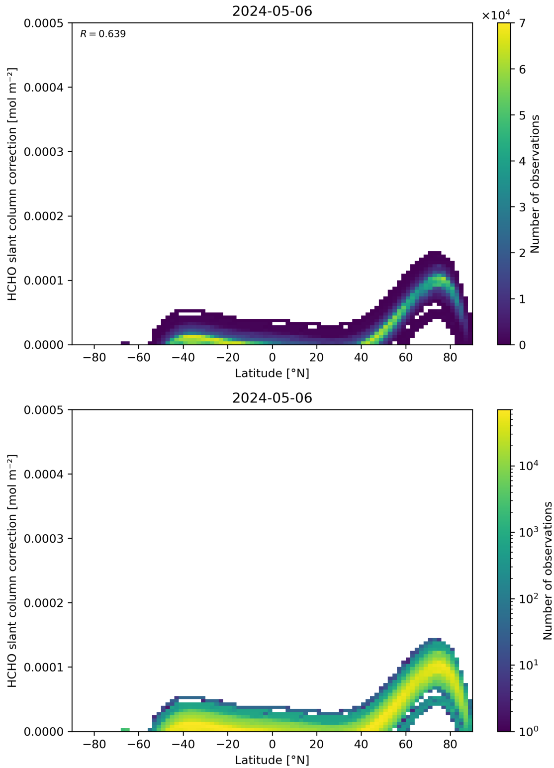
Figure 158: Scatter density plot of “Latitude” against “HCHO slant column correction” for 2024-05-05 to 2024-05-07.
