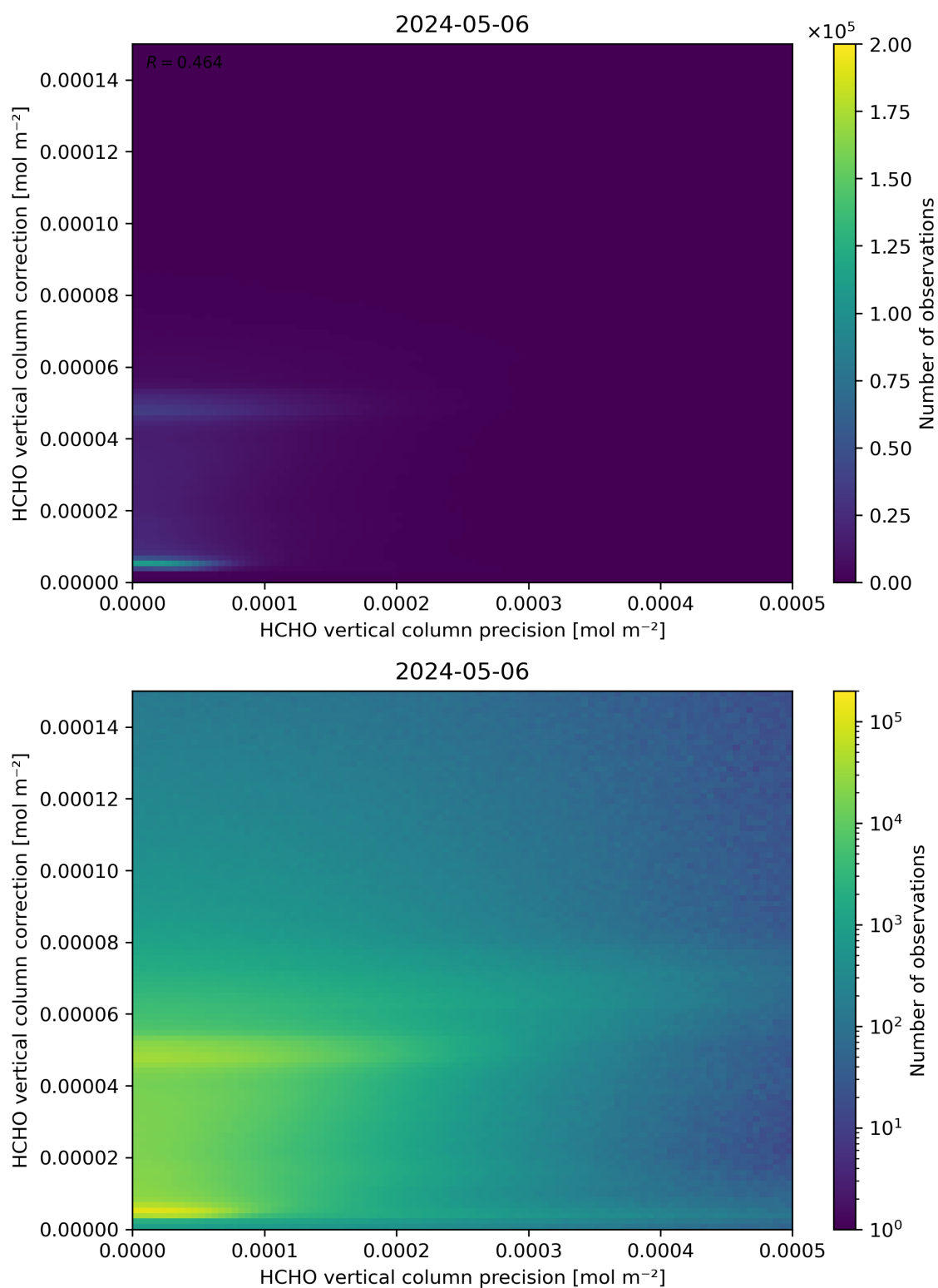
Figure 146: Scatter density plot of “HCHO vertical column precision” against “HCHO vertical column correction” for 2024-05-05 to 2024-05-07.
