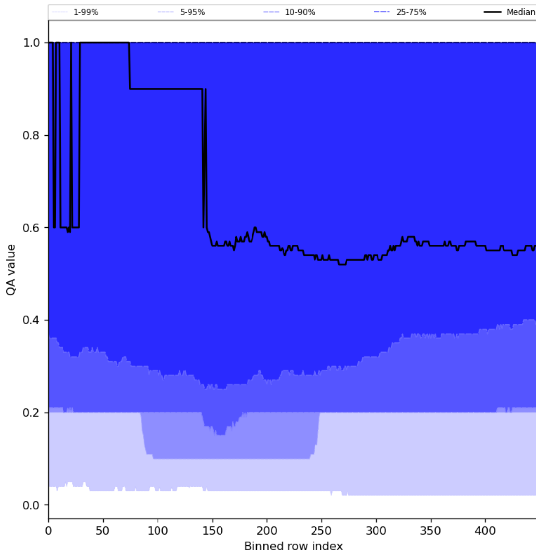
Figure 48: Along track statistics of “QA value” for 2024-05-05 to 2024-05-07
