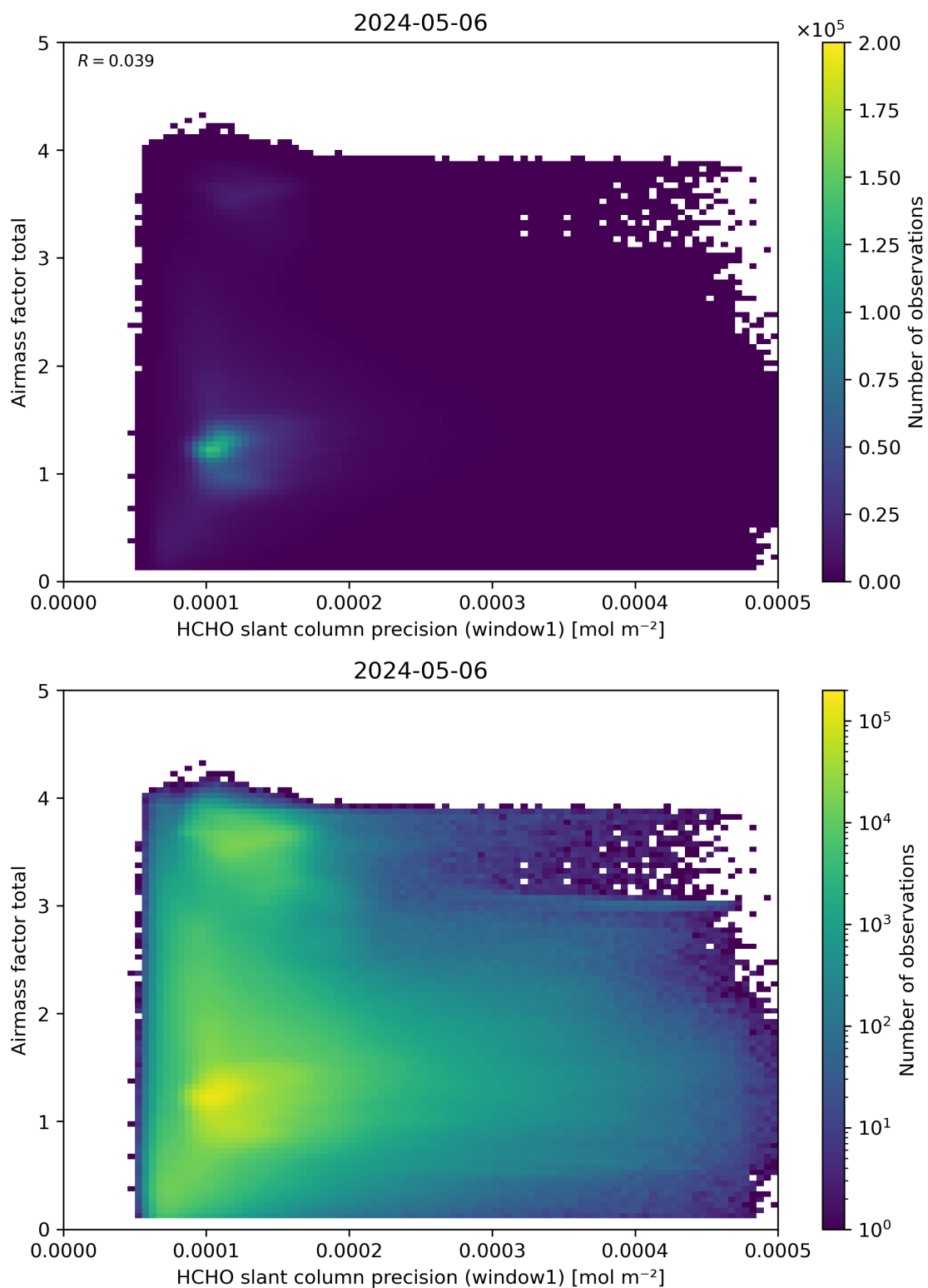
Figure 94: Scatter density plot of “HCHO slant column precision (window1)” against “Airmass factor total” for 2024-05-05 to 2024-05-07.
