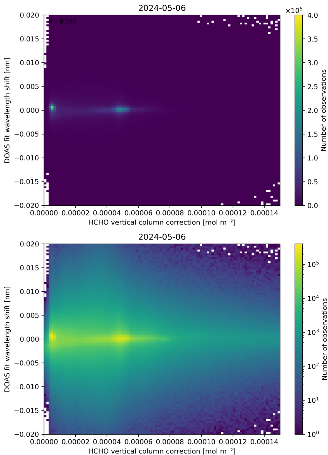
Figure 113: Scatter density plot of “HCHO vertical column correction” against “DOAS fit wavelength shift” for 2024-05-05 to 2024-05-07.
