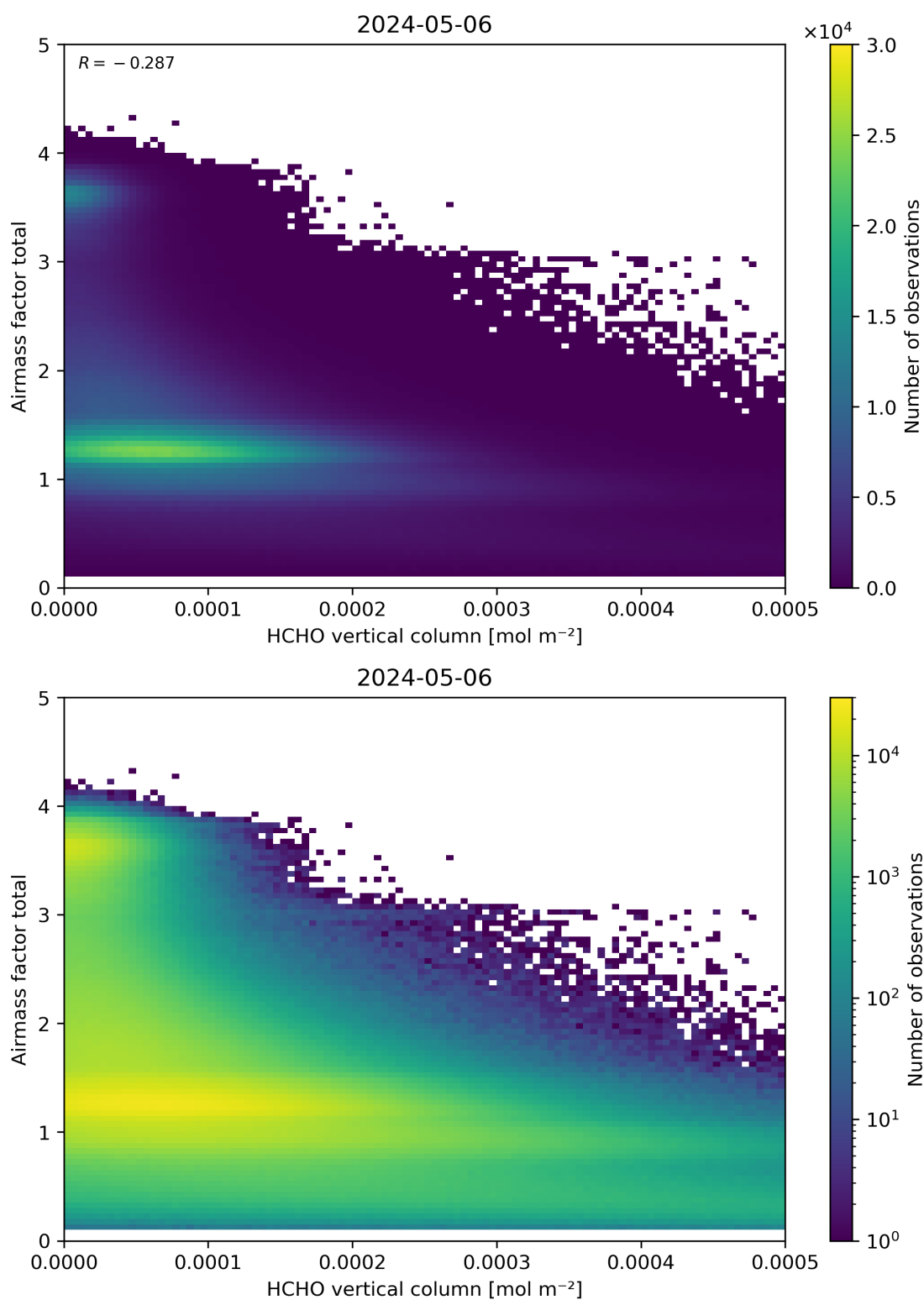
Figure 131: Scatter density plot of “HCHO vertical column” against “Airmass factor total” for 2024-05-05 to 2024-05-07.
