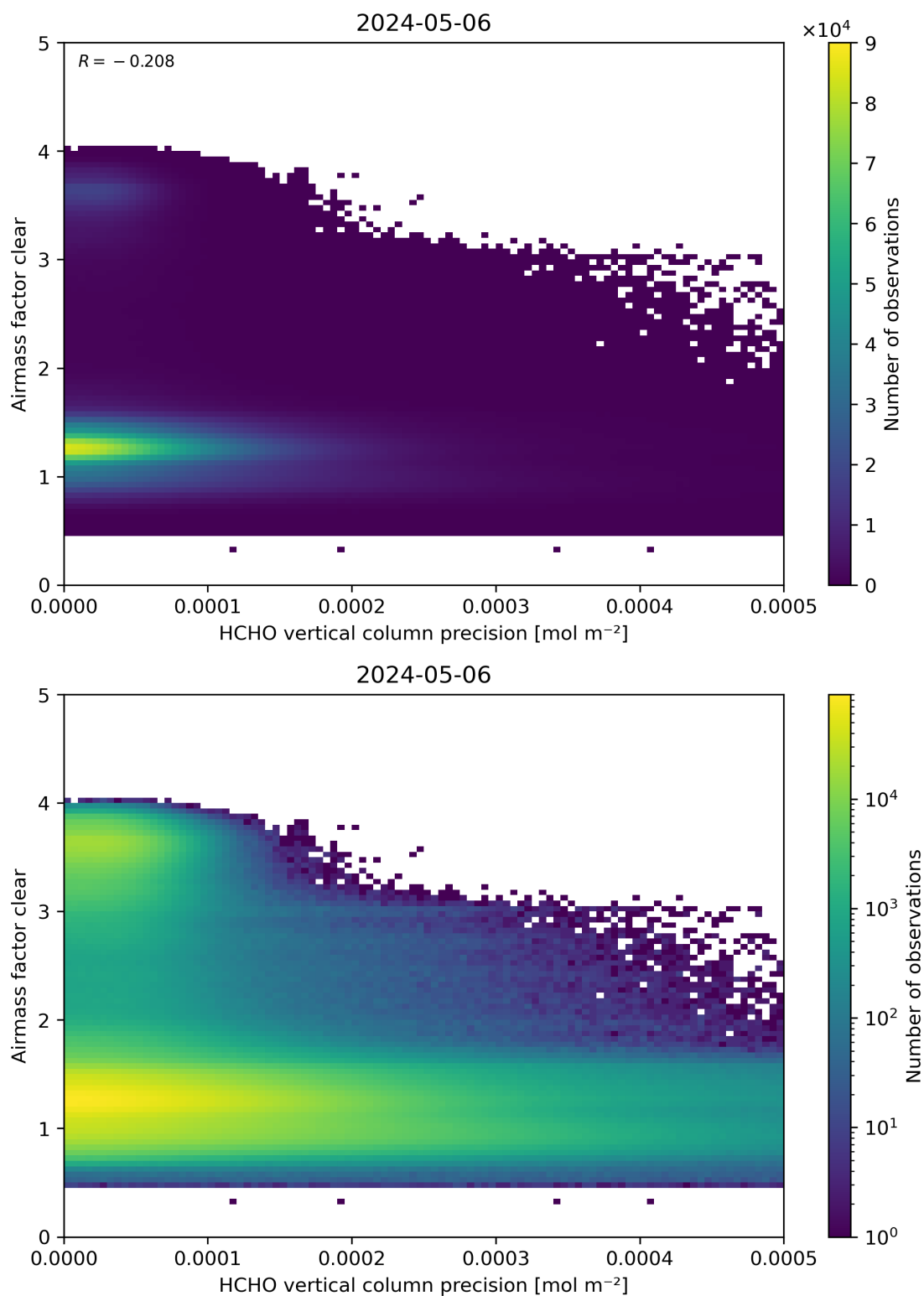
Figure 139: Scatter density plot of “HCHO vertical column precision” against “Airmass factor clear” for 2024-05-05 to 2024-05-07.
