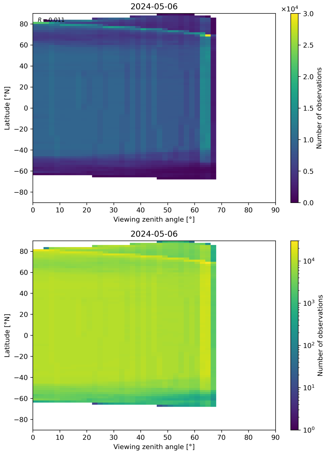
Figure 196: Scatter density plot of “Viewing zenith angle” against “Latitude” for 2024-05-05 to 2024-05-07.
