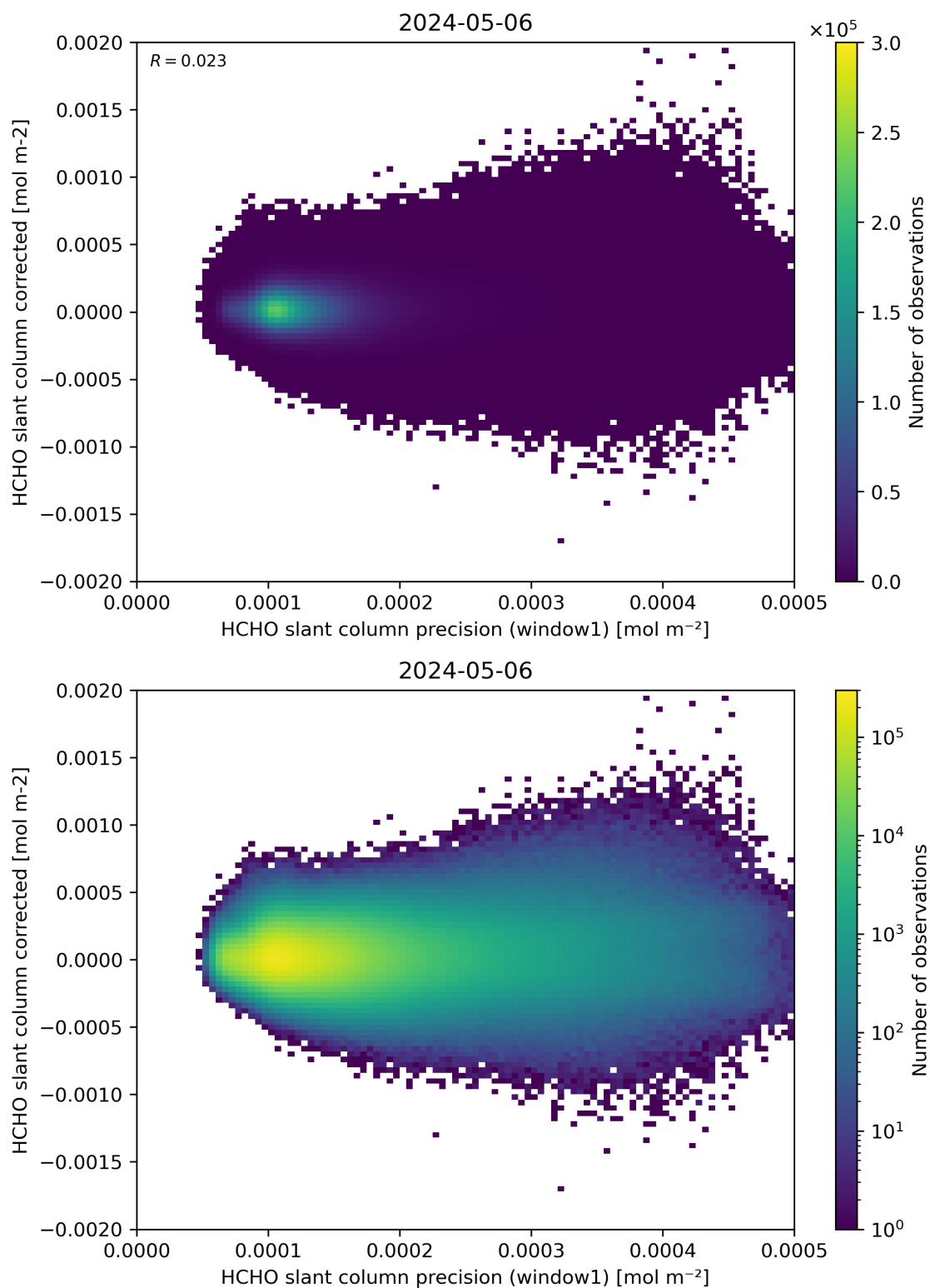
Figure 92: Scatter density plot of “HCHO slant column precision (window1)” against “HCHO slant column corrected” for 2024-05-05 to 2024-05-07.
