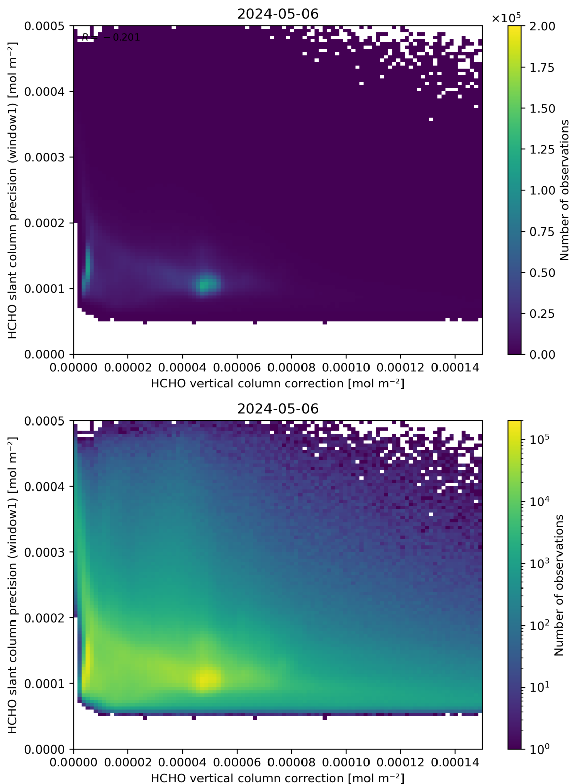
Figure 119: Scatter density plot of “HCHO vertical column correction” against “HCHO slant column precision (window1)” for 2024-05-05 to 2024-05-07.
