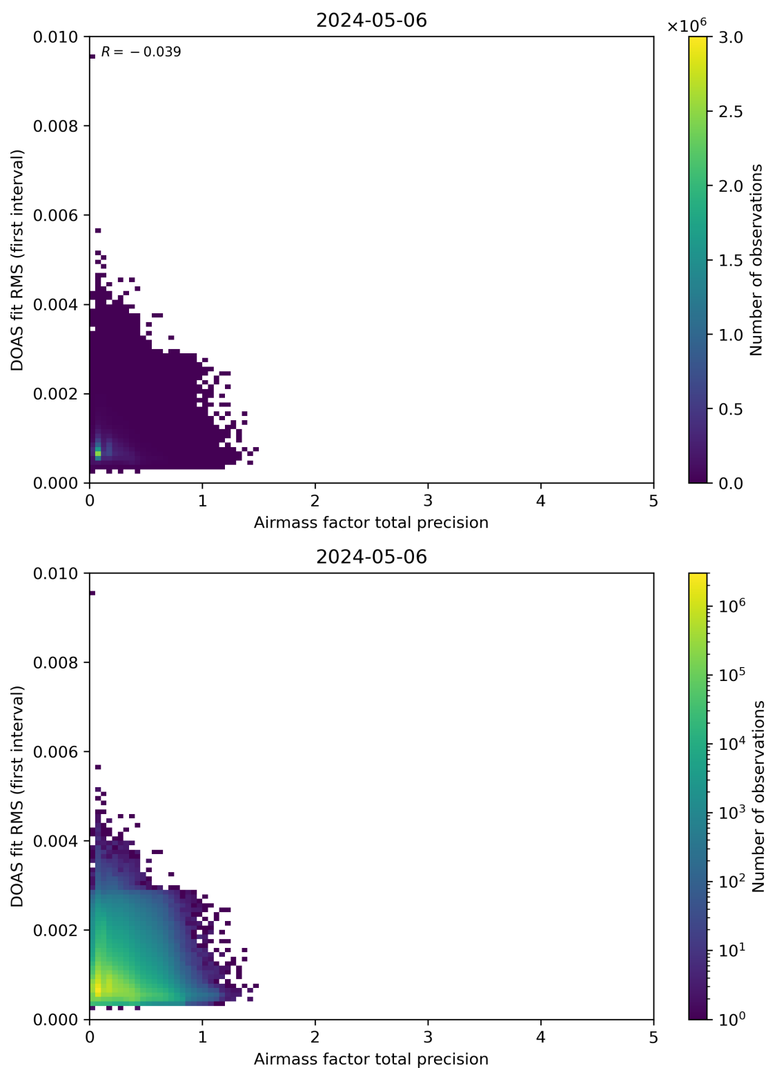
Figure 105: Scatter density plot of “Airmass factor total precision” against “DOAS fit RMS (first interval)” for 2024-05-05 to 2024-05-07.
