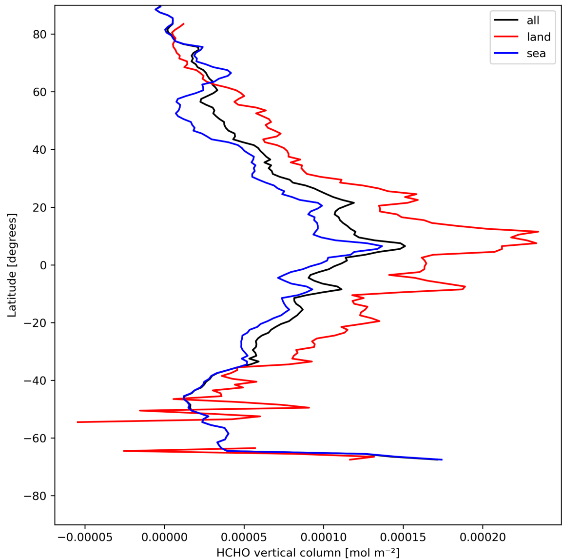
Figure 21: Zonal average of “HCHO vertical column” for 2024-05-05 to 2024-05-07.
