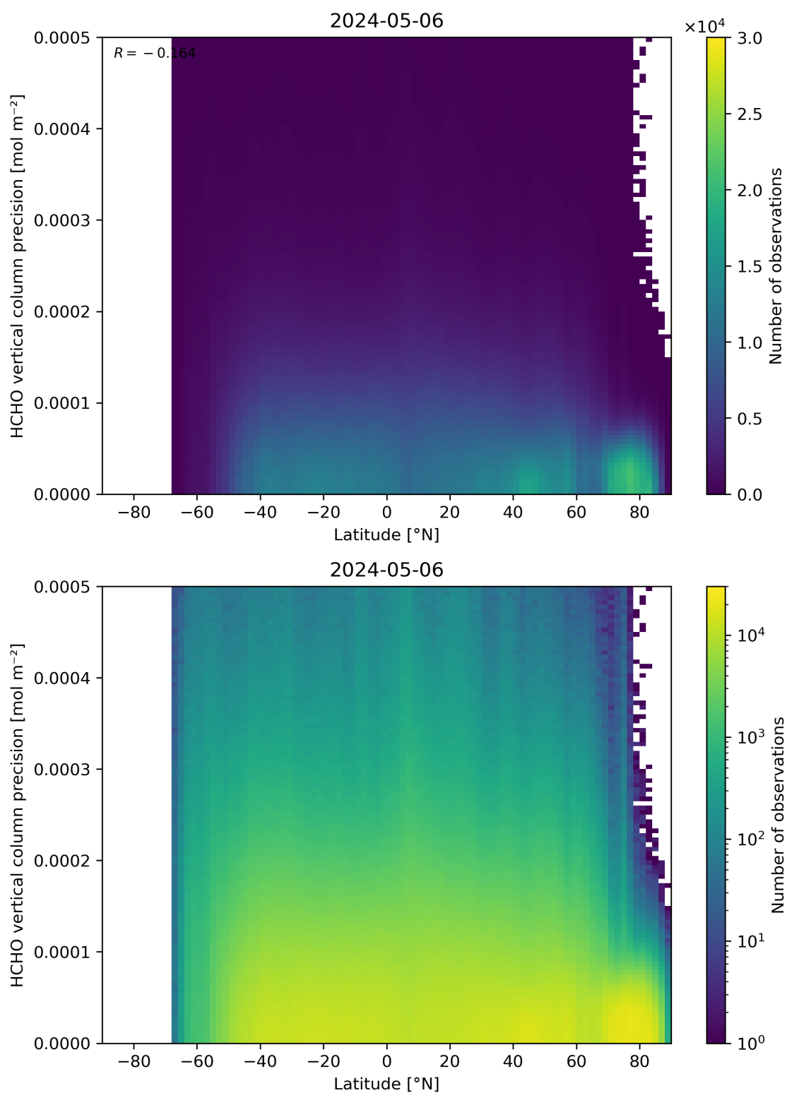
Figure 165: Scatter density plot of “Latitude” against “HCHO vertical column precision” for 2024-05-05 to 2024-05-07.
