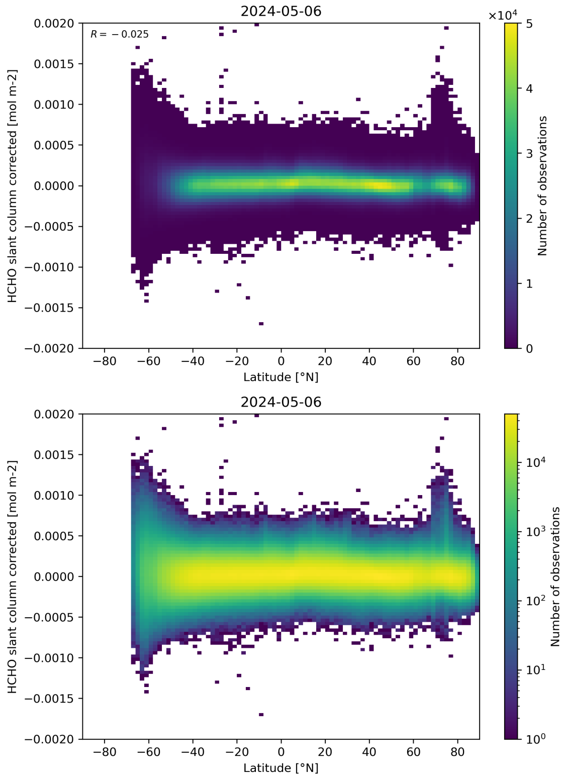
Figure 157: Scatter density plot of “Latitude” against “HCHO slant column corrected” for 2024-05-05 to 2024-05-07.
