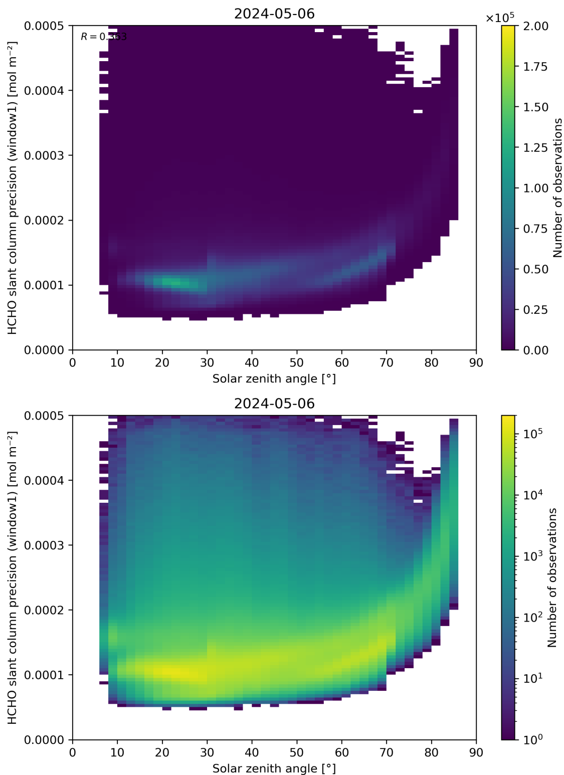
Figure 174: Scatter density plot of “Solar zenith angle” against “HCHO slant column precision (window1)” for 2024-05-05 to 2024-05-07.
