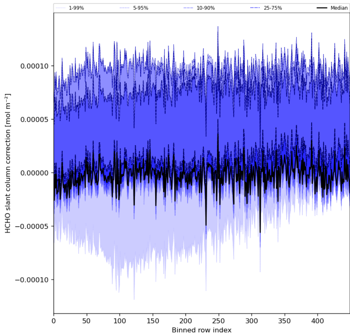
Figure 61: Along track statistics of “HCHO slant column correction” for 2024-05-05 to 2024-05-07
