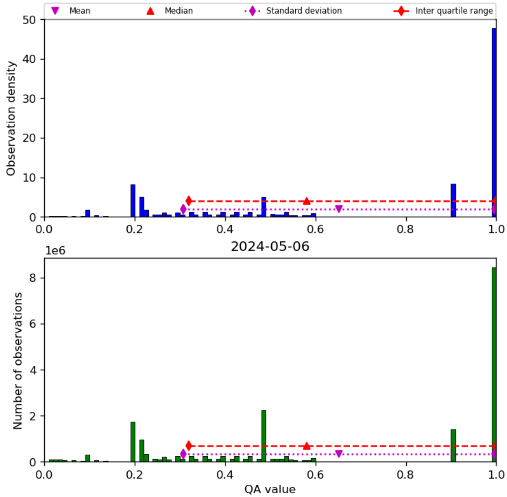
Figure 34: Histogram of “QA value” for 2024-05-05 to 2024-05-07
