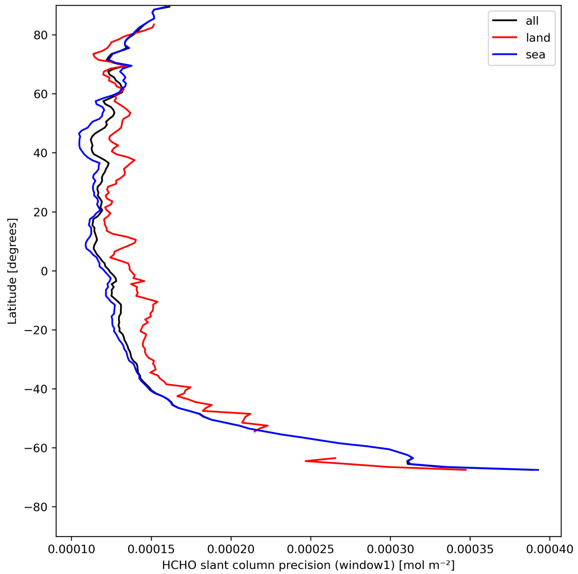
Figure 25: Zonal average of “HCHO slant column precision (window1)” for 2024-05-05 to 2024-05-07.
