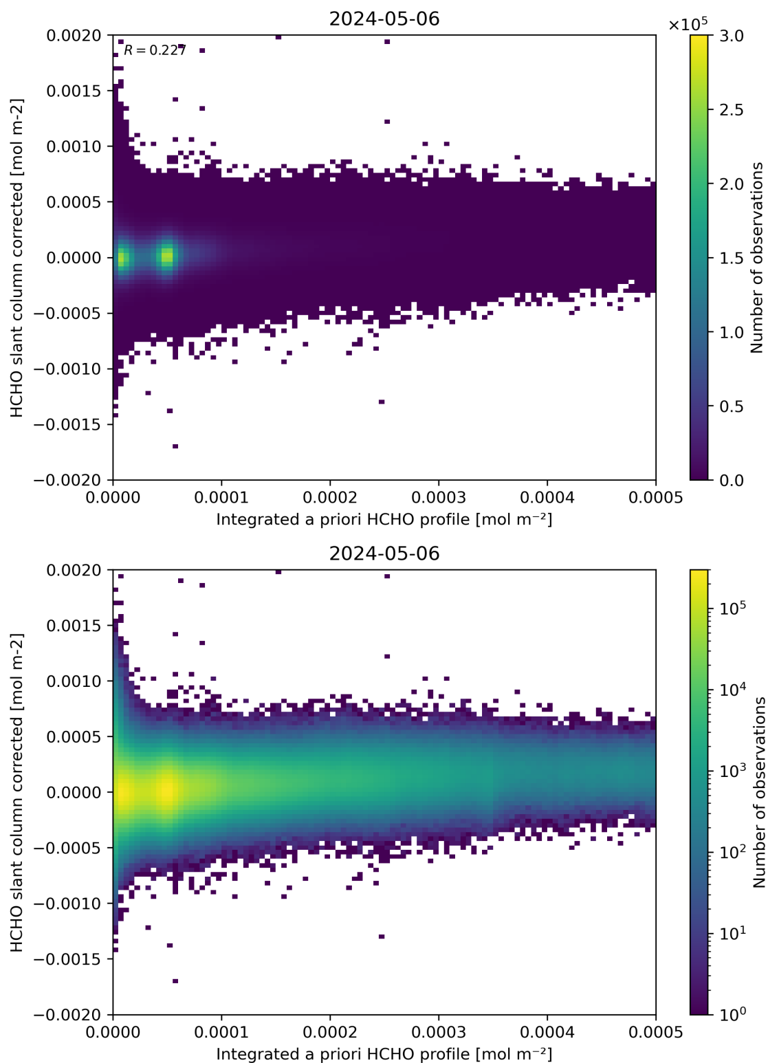
Figure 151: Scatter density plot of “Integrated a priori HCHO profile” against “HCHO slant column corrected” for 2024-05-05 to 2024-05-07.
