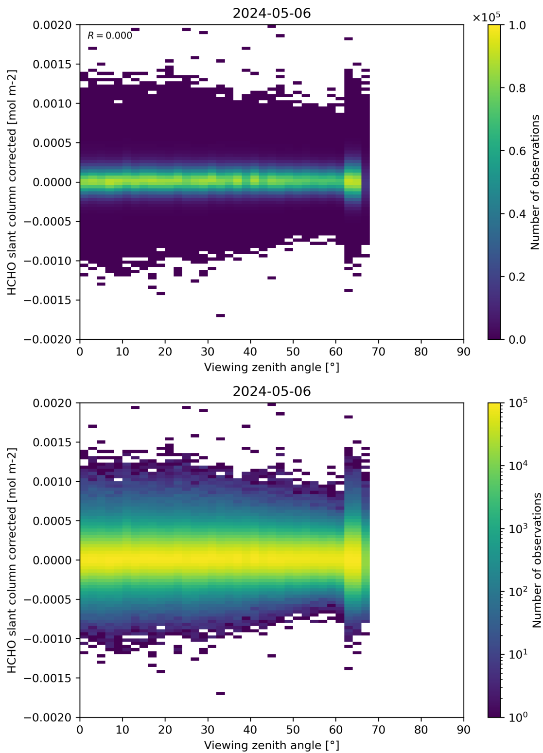
Figure 186: Scatter density plot of “Viewing zenith angle” against “HCHO slant column corrected” for 2024-05-05 to 2024-05-07.
