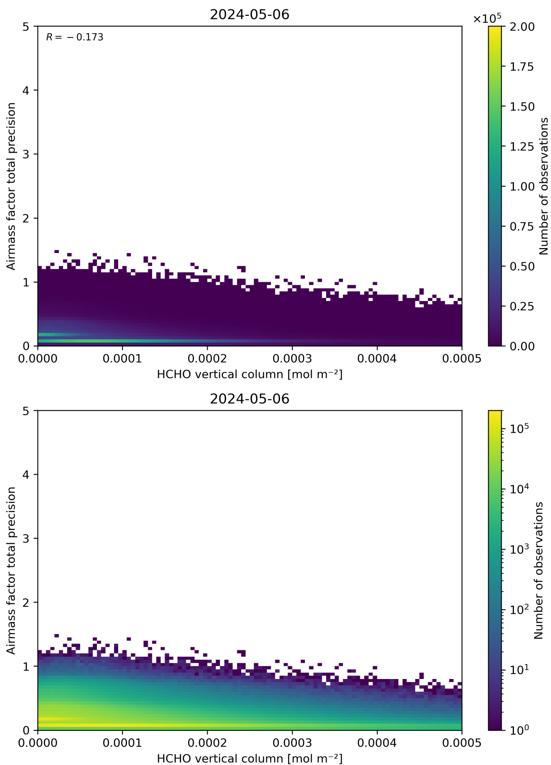
Figure 132: Scatter density plot of “HCHO vertical column” against “Airmass factor total precision” for 2024-05-05 to 2024-05-07.
