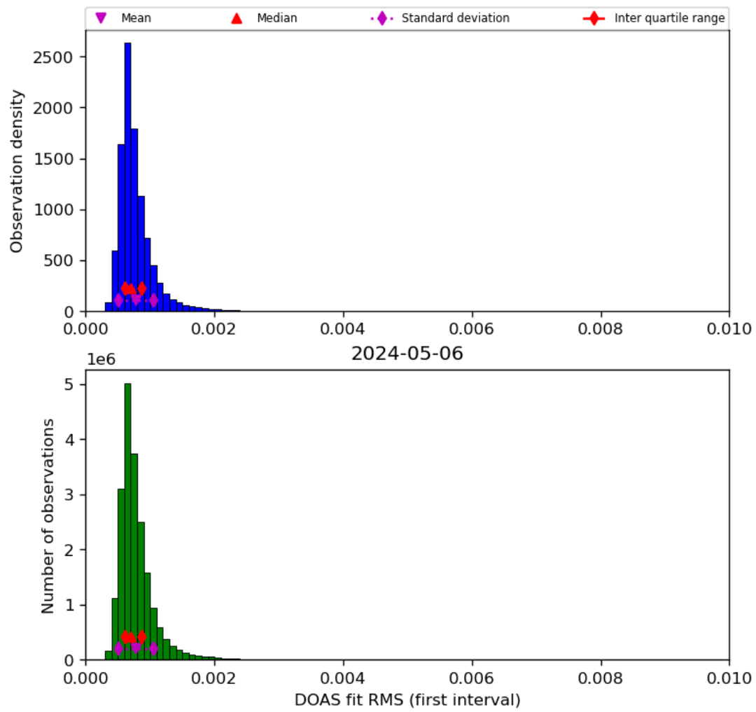
Figure 46: Histogram of “DOAS fit RMS (first interval)” for 2024-05-05 to 2024-05-07
