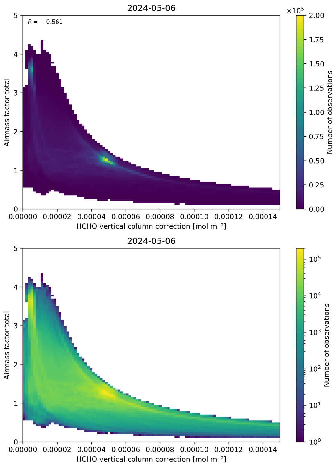
Figure 120: Scatter density plot of “HCHO vertical column correction” against “Airmass factor total” for 2024-05-05 to 2024-05-07.
