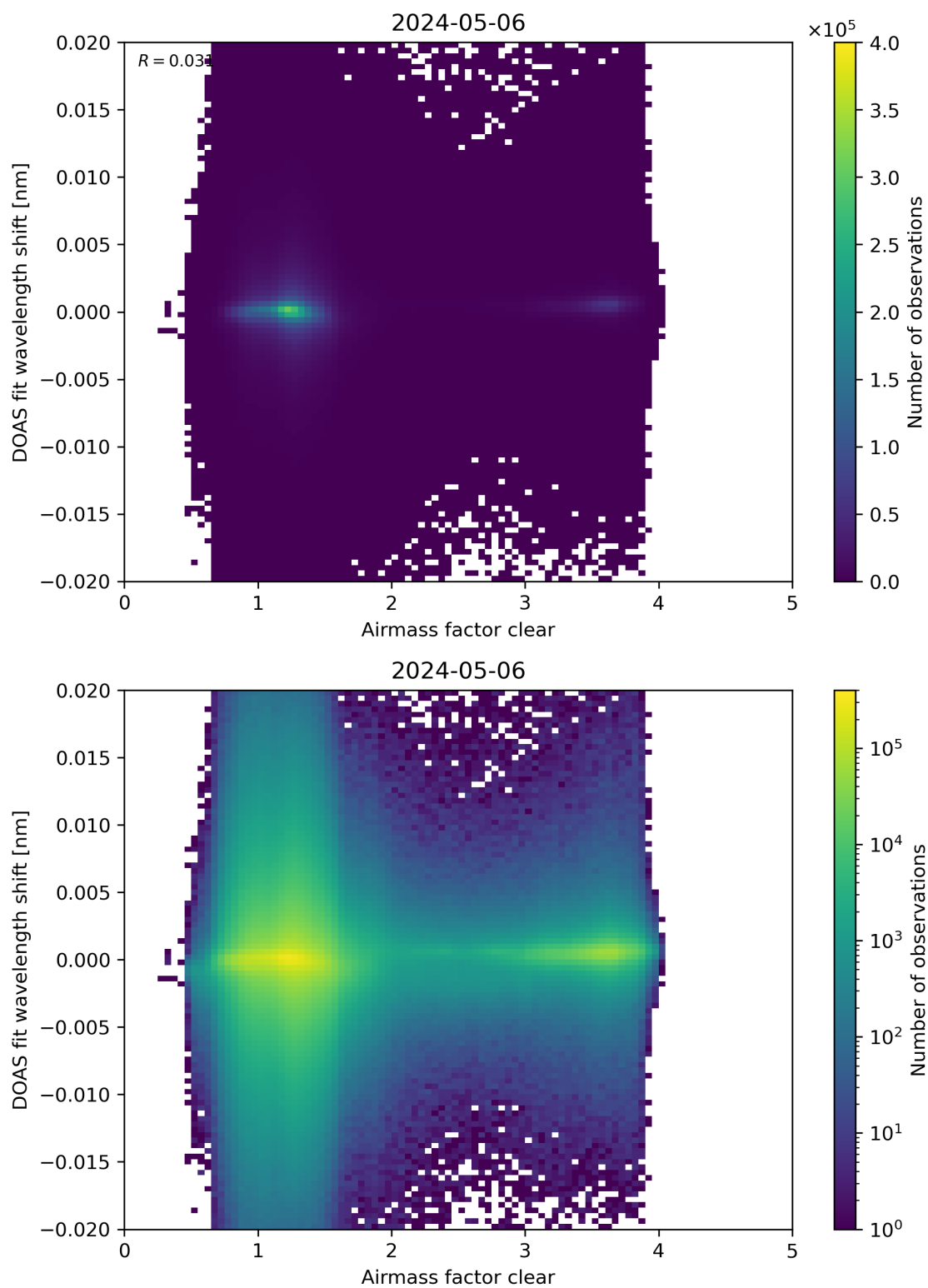
Figure 72: Scatter density plot of “Airmass factor clear” against “DOAS fit wavelength shift” for 2024-05-05 to 2024-05-07.
