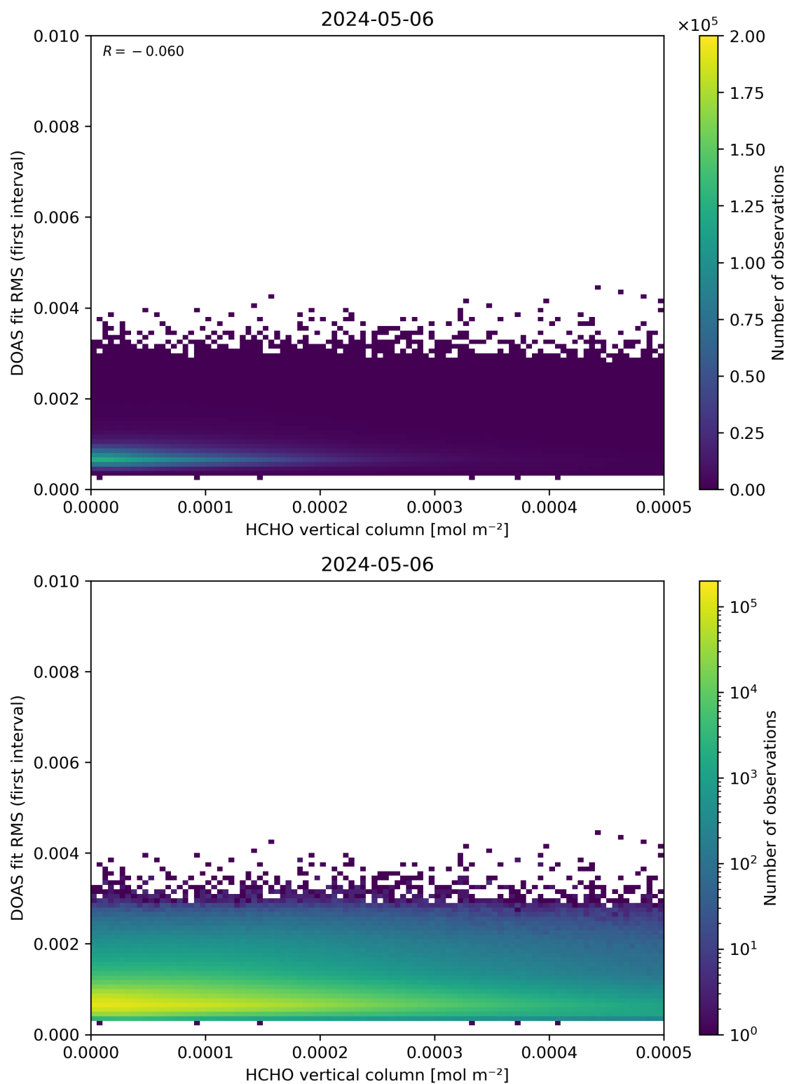
Figure 123: Scatter density plot of “HCHO vertical column” against “DOAS fit RMS (first interval)” for 2024-05-05 to 2024-05-07.
