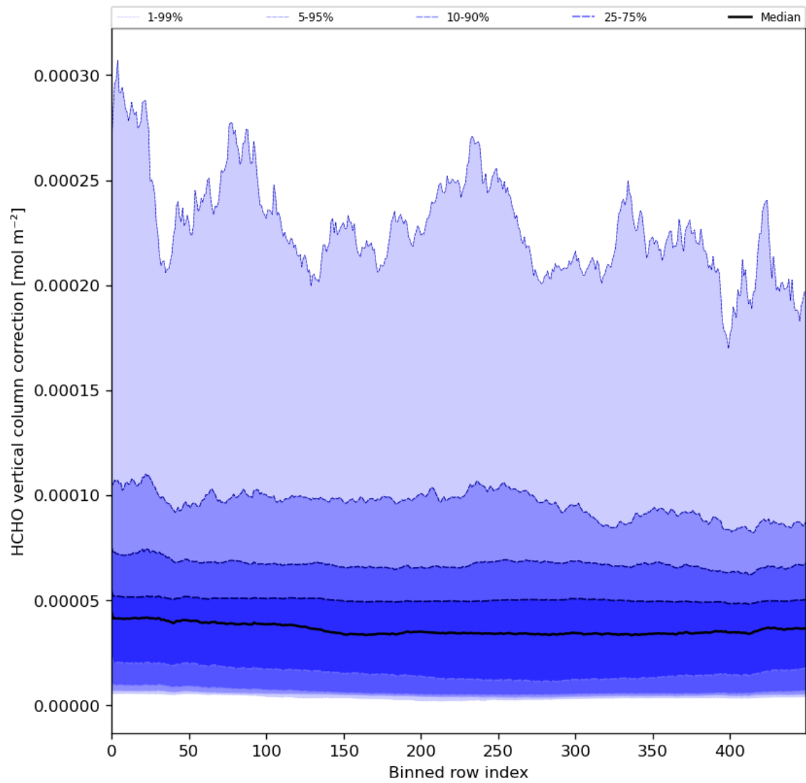
Figure 51: Along track statistics of “HCHO vertical column correction” for 2024-05-05 to 2024-05-07
