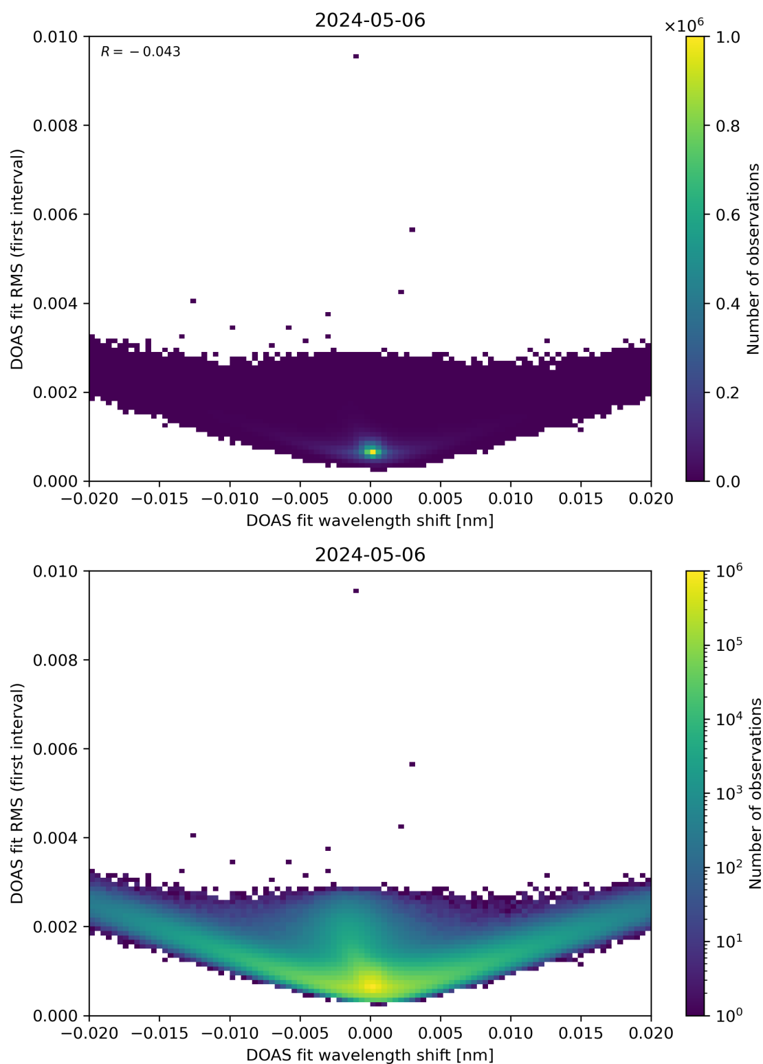
Figure 64: Scatter density plot of “DOAS fit wavelength shift” against “DOAS fit RMS (first interval)” for 2024-05-05 to 2024-05-07.
