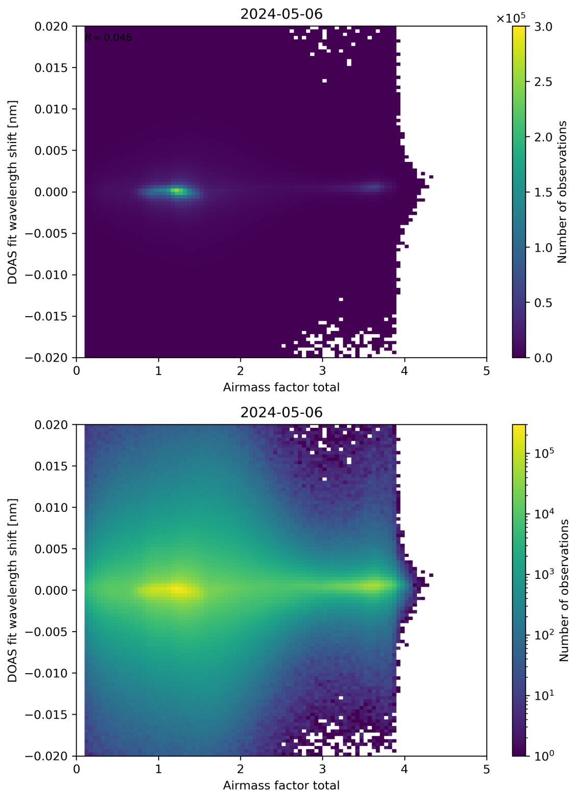
Figure 98: Scatter density plot of “Airmass factor total” against “DOAS fit wavelength shift” for 2024-05-05 to 2024-05-07.
