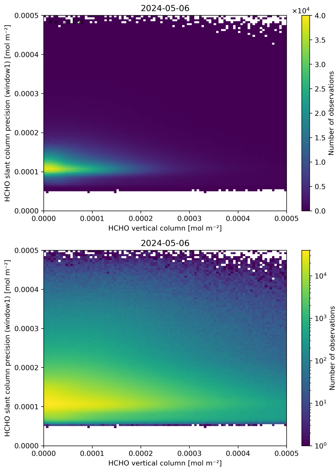
Figure 130: Scatter density plot of “HCHO vertical column” against “HCHO slant column precision (window1)” for 2024-05-05 to 2024-05-07.
