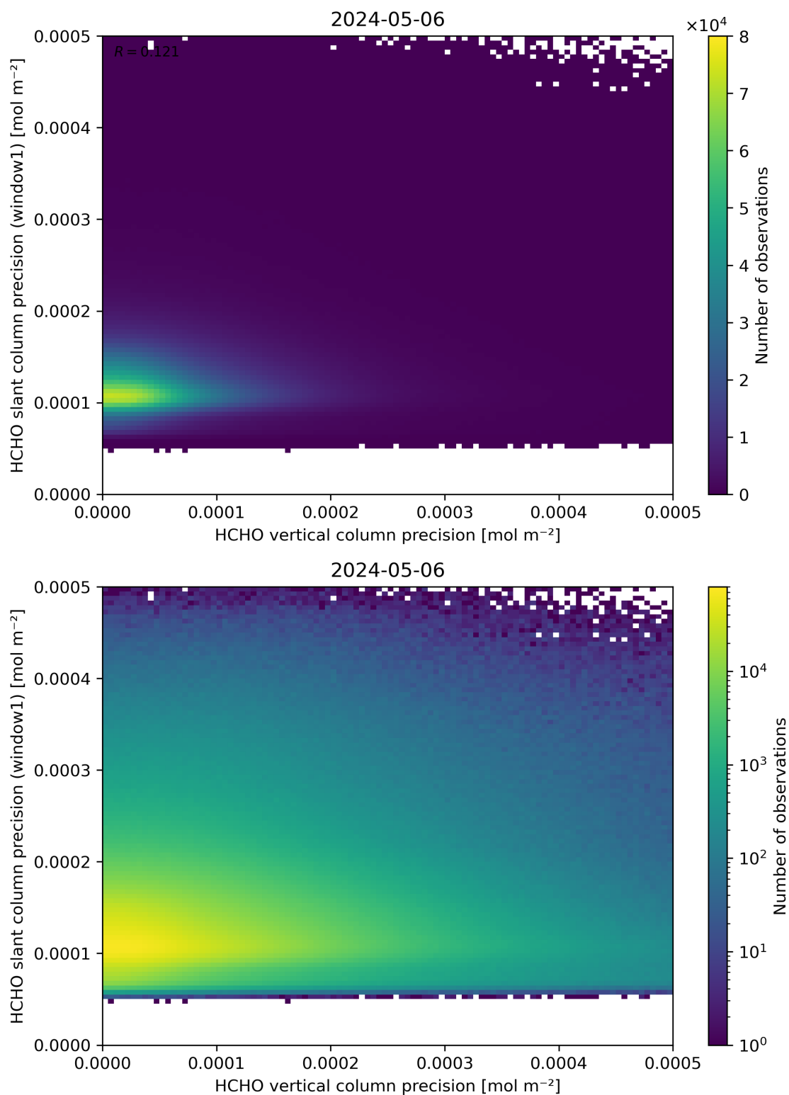
Figure 143: Scatter density plot of “HCHO vertical column precision” against “HCHO slant column precision (window1)” for 2024-05-05 to 2024-05-07.
