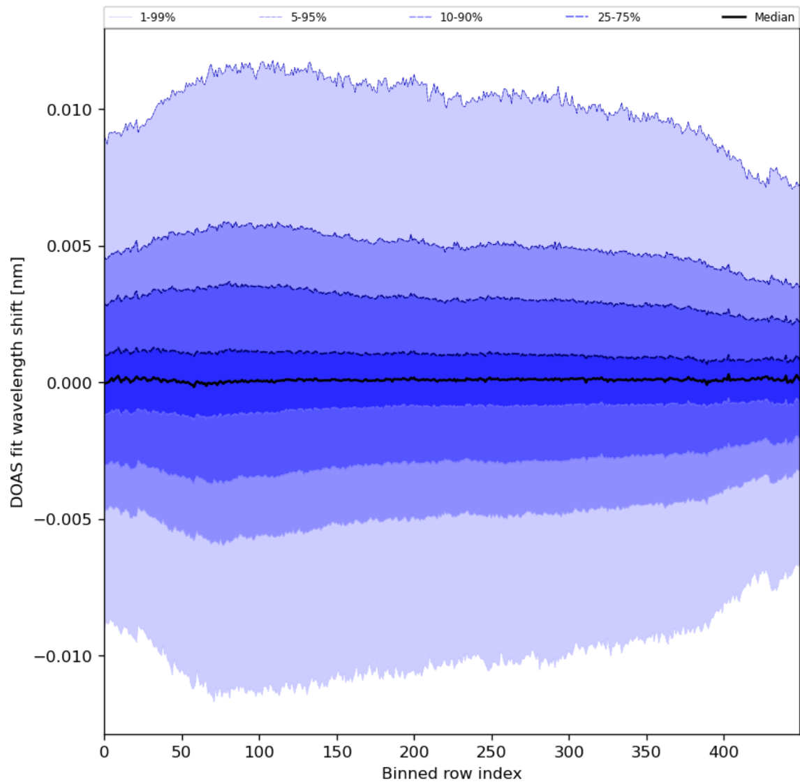
Figure 58: Along track statistics of “DOAS fit wavelength shift” for 2024-05-05 to 2024-05-07
