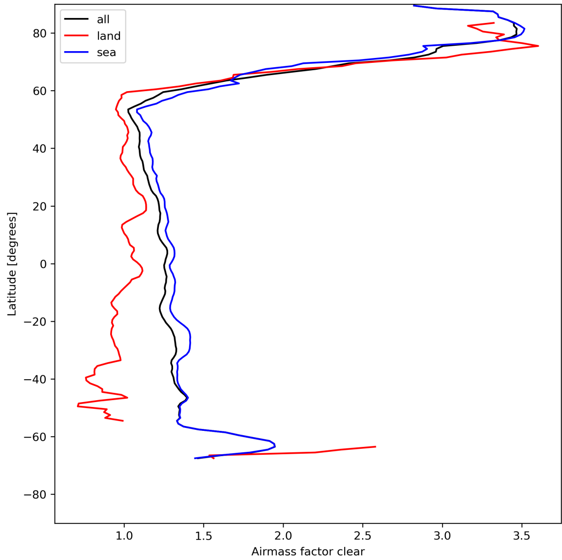
Figure 28: Zonal average of “Airmass factor clear” for 2024-05-05 to 2024-05-07.
