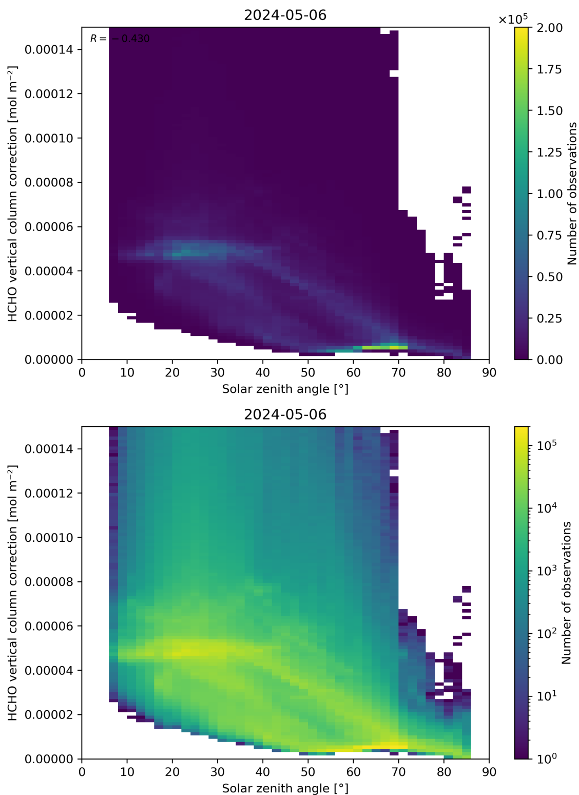
Figure 178: Scatter density plot of “Solar zenith angle” against “HCHO vertical column correction” for 2024-05-05 to 2024-05-07.
