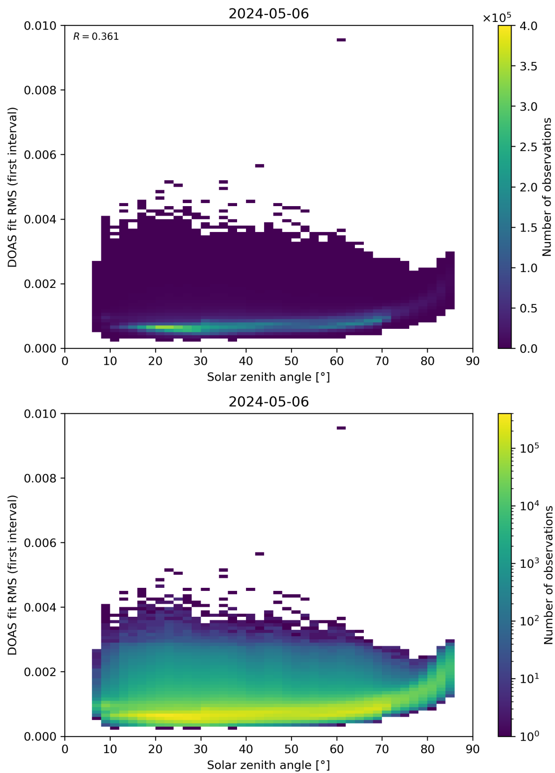
Figure 167: Scatter density plot of “Solar zenith angle” against “DOAS fit RMS (first interval)” for 2024-05-05 to 2024-05-07.
