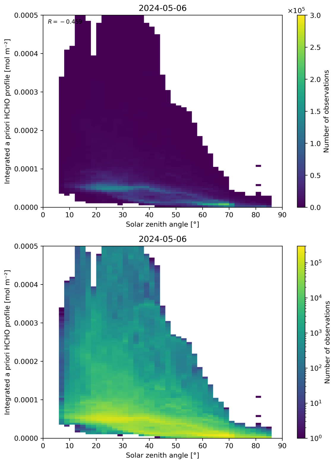
Figure 180: Scatter density plot of “Solar zenith angle” against “Integrated a priori HCHO profile” for 2024-05-05 to 2024-05-07.
