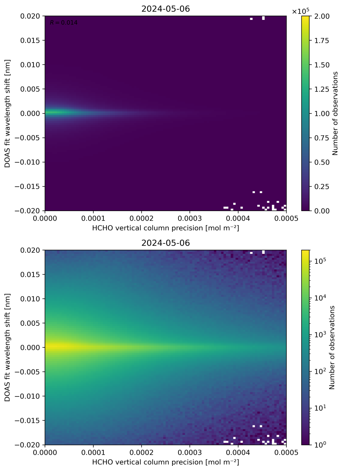
Figure 137: Scatter density plot of “HCHO vertical column precision” against “DOAS fit wavelength shift” for 2024-05-05 to 2024-05-07.
