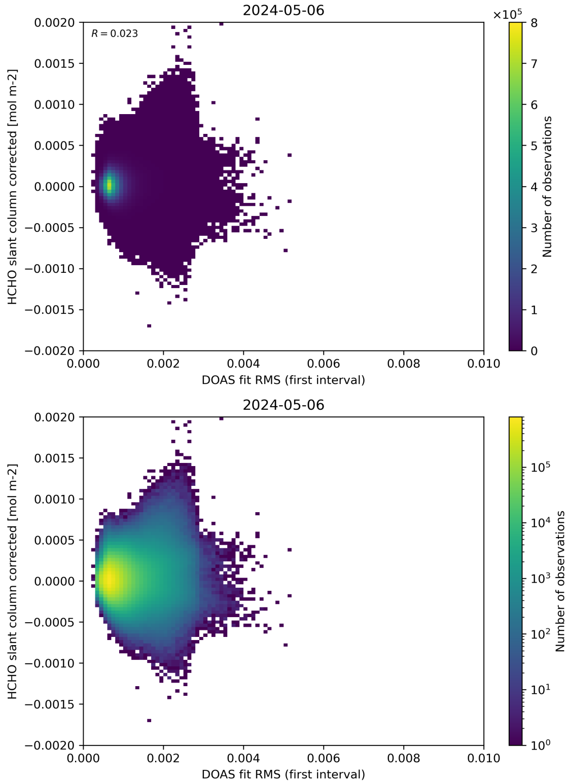
Figure 62: Scatter density plot of “DOAS fit RMS (first interval)” against “HCHO slant column corrected” for 2024-05-05 to 2024-05-07.
