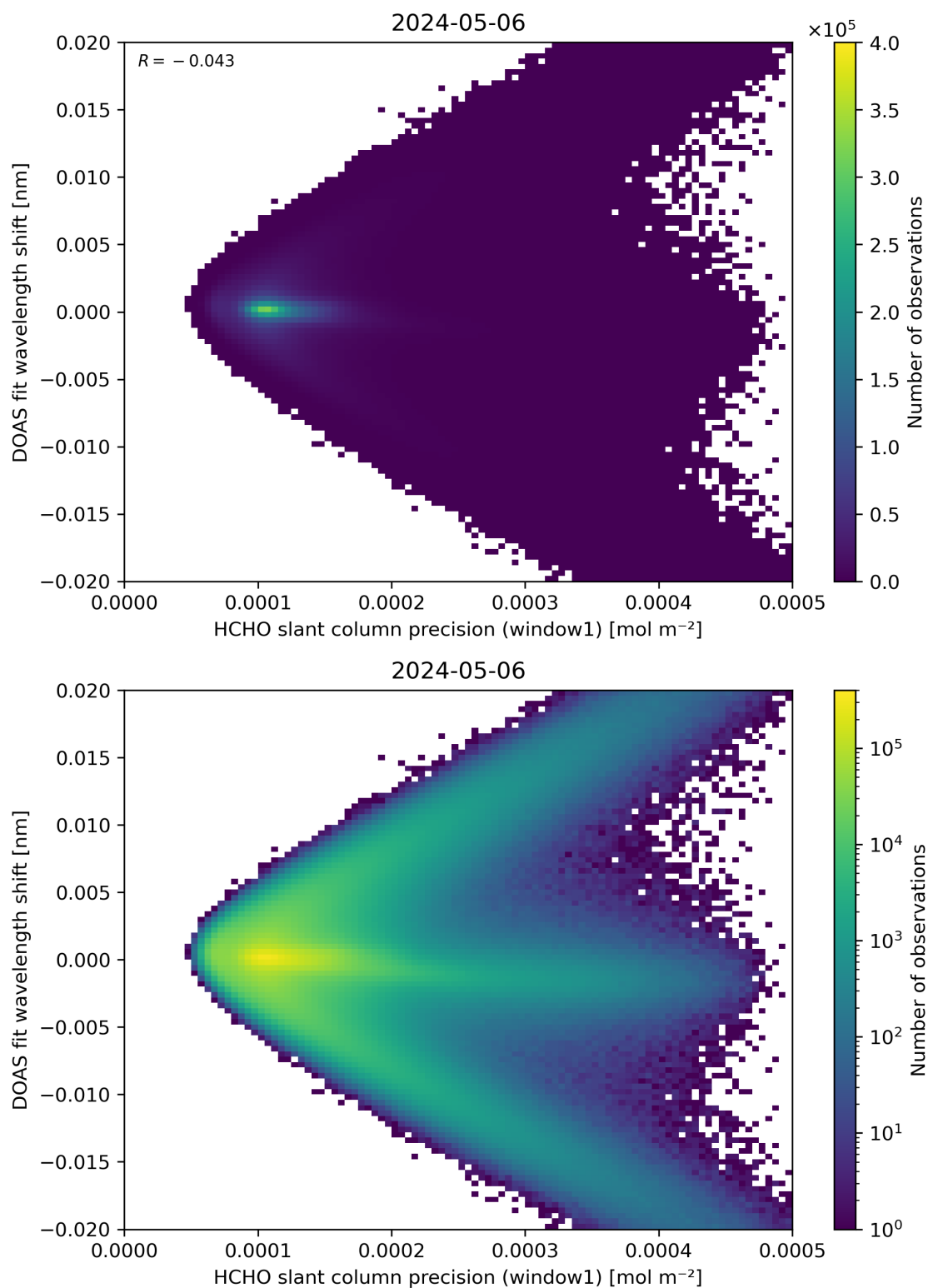
Figure 89: Scatter density plot of “HCHO slant column precision (window1)” against “DOAS fit wavelength shift” for 2024-05-05 to 2024-05-07.
