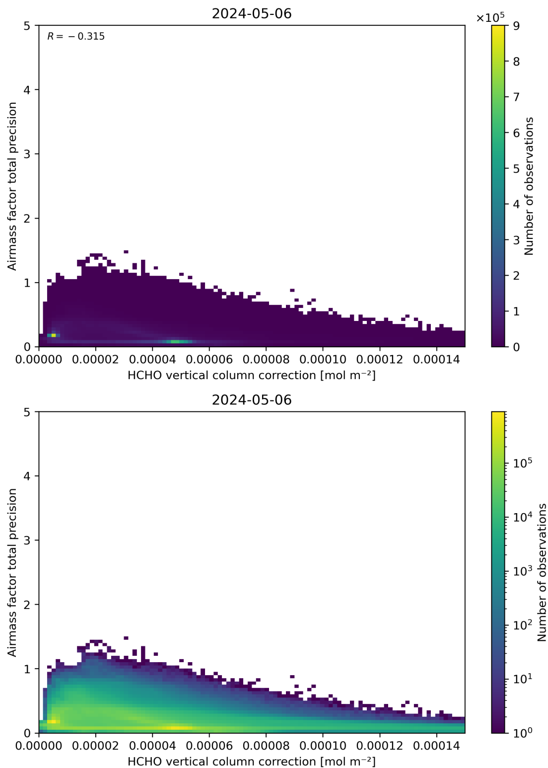
Figure 121: Scatter density plot of “HCHO vertical column correction” against “Airmass factor total precision” for 2024-05-05 to 2024-05-07.
