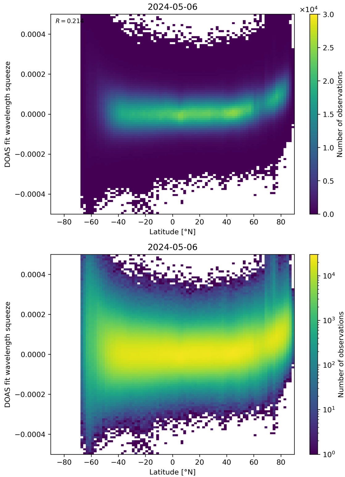
Figure 155: Scatter density plot of “Latitude” against “DOAS fit wavelength squeeze” for 2024-05-05 to 2024-05-07.
