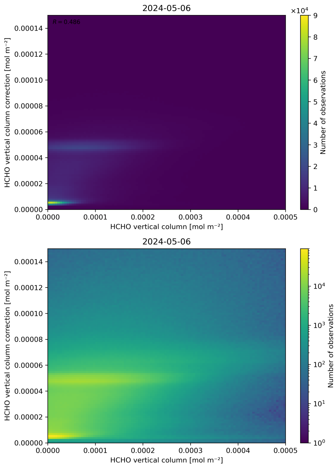
Figure 133: Scatter density plot of “HCHO vertical column” against “HCHO vertical column correction” for 2024-05-05 to 2024-05-07.
