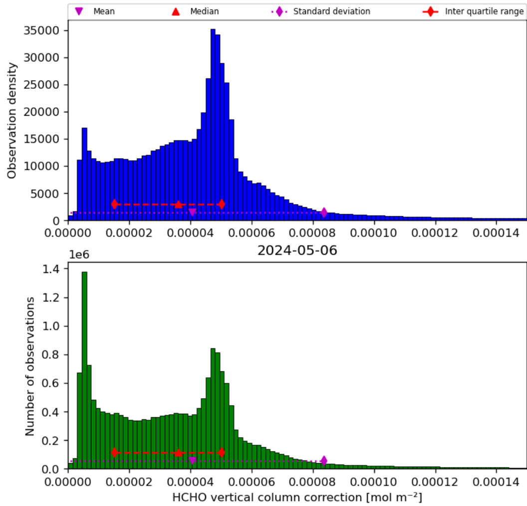
Figure 37: Histogram of “HCHO vertical column correction” for 2024-05-05 to 2024-05-07
