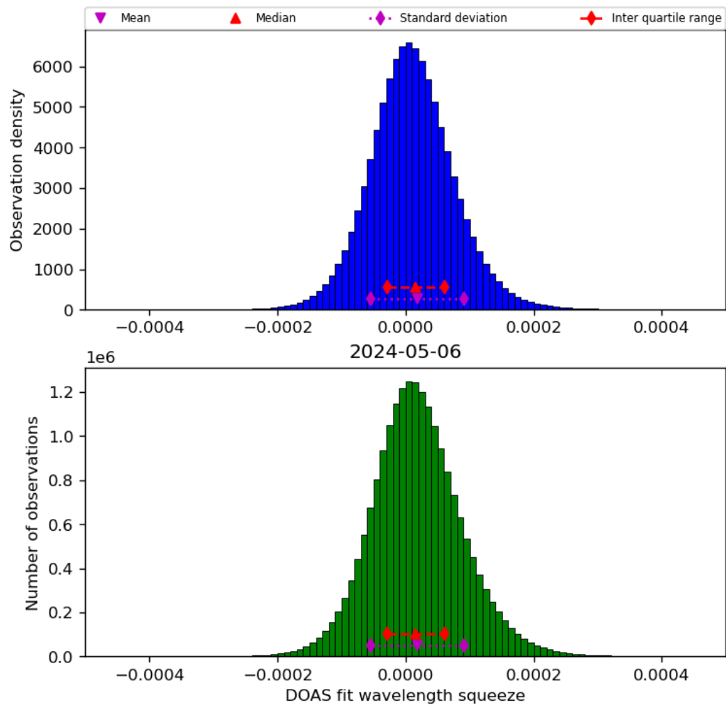
Figure 45: Histogram of “DOAS fit wavelength squeeze” for 2024-05-05 to 2024-05-07
