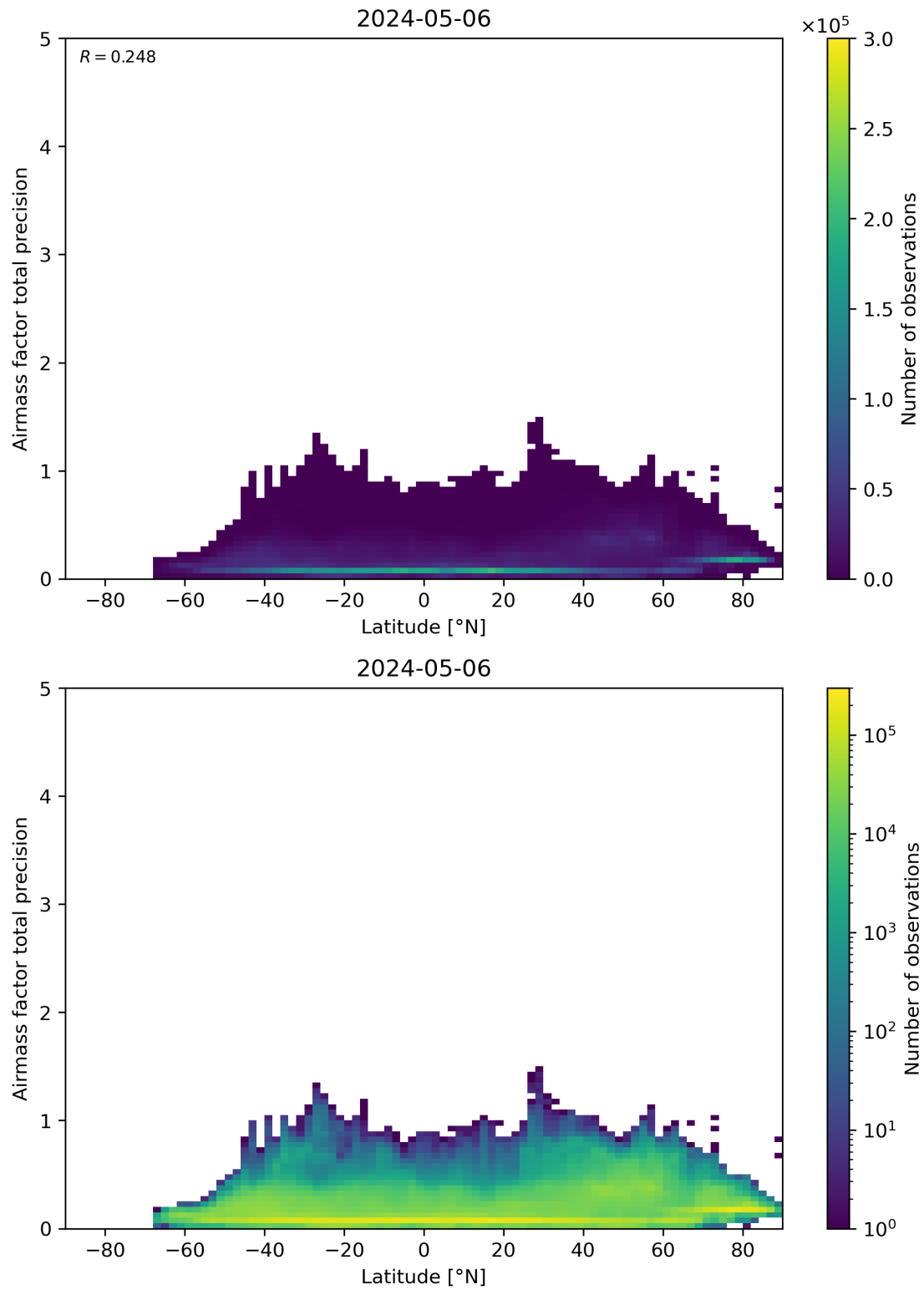
Figure 162: Scatter density plot of “Latitude” against “Airmass factor total precision” for 2024-05-05 to 2024-05-07.
