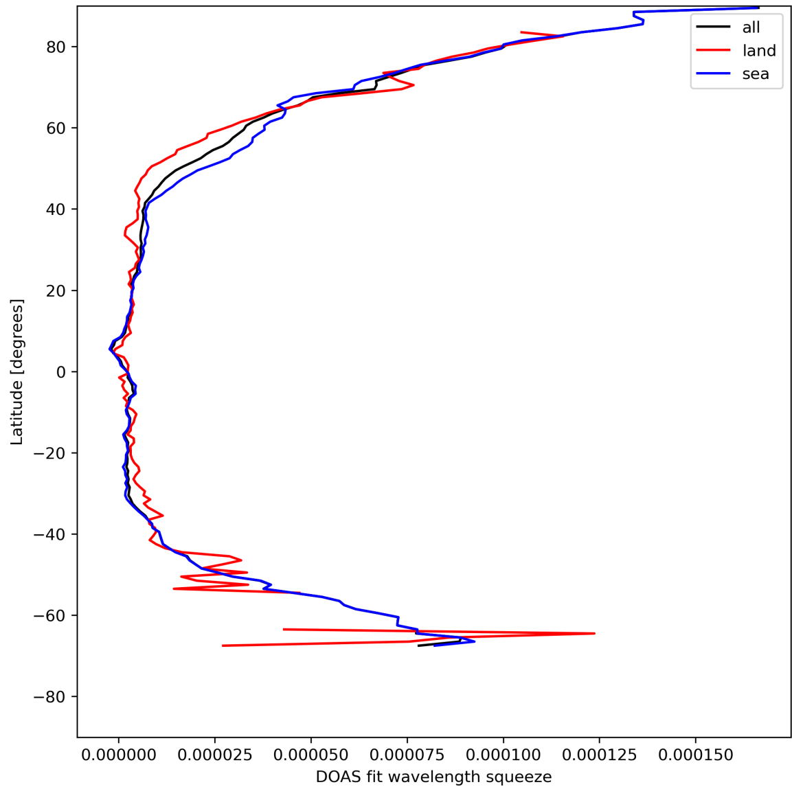
Figure 31: Zonal average of “DOAS fit wavelength squeeze” for 2024-05-05 to 2024-05-07.
