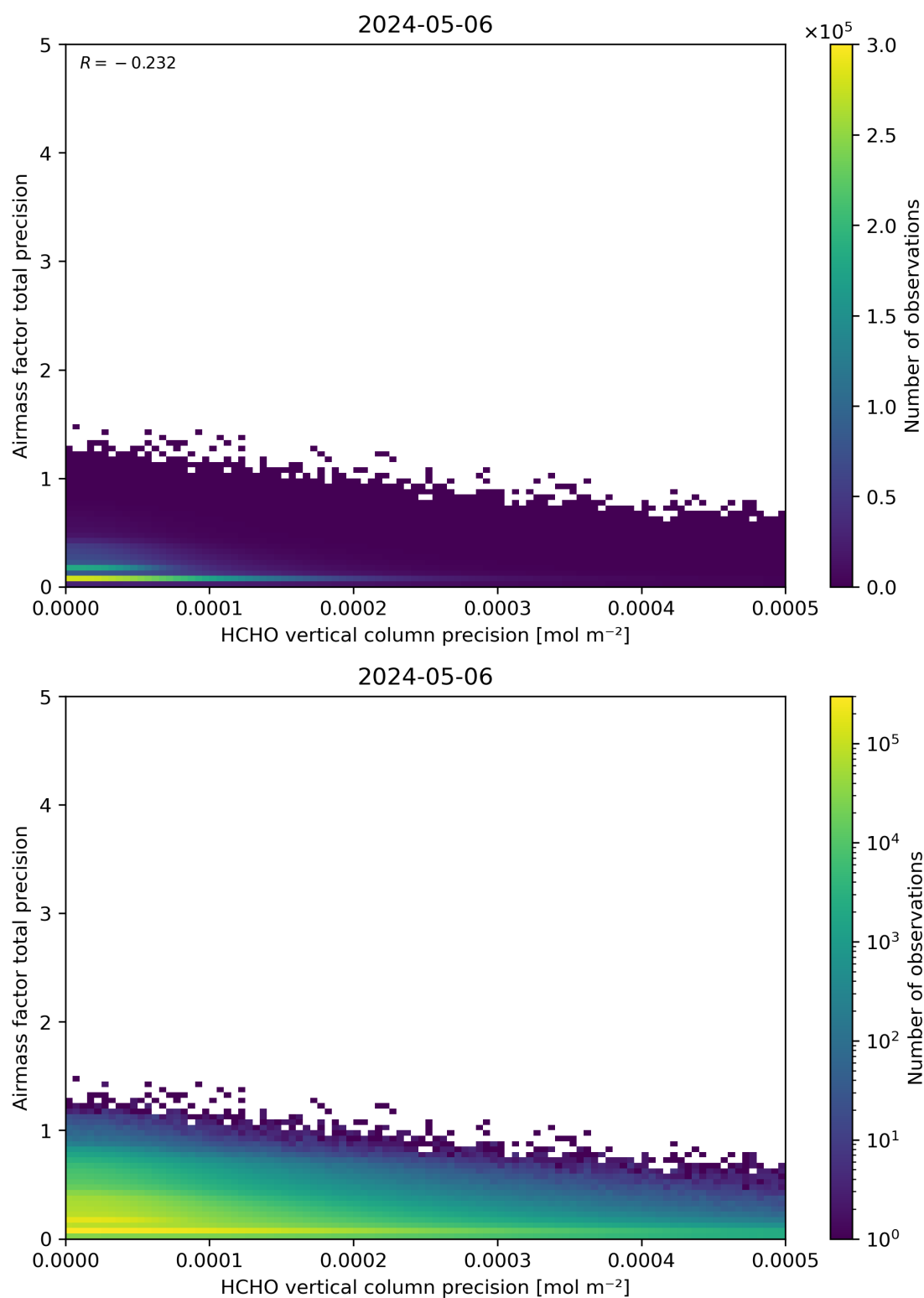
Figure 145: Scatter density plot of “HCHO vertical column precision” against “Airmass factor total precision” for 2024-05-05 to 2024-05-07.
