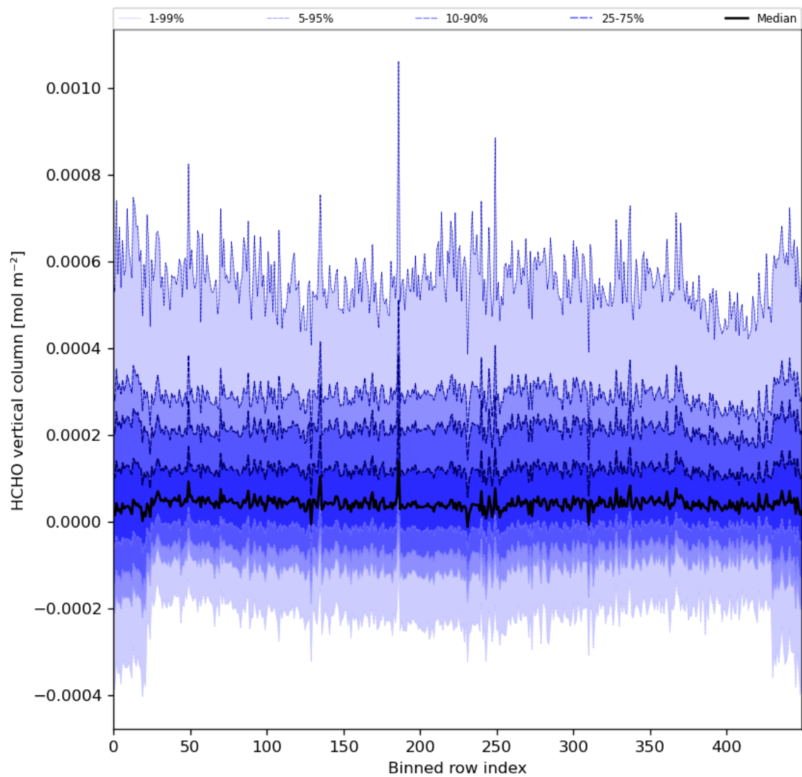
Figure 49: Along track statistics of “HCHO vertical column” for 2024-05-05 to 2024-05-07
