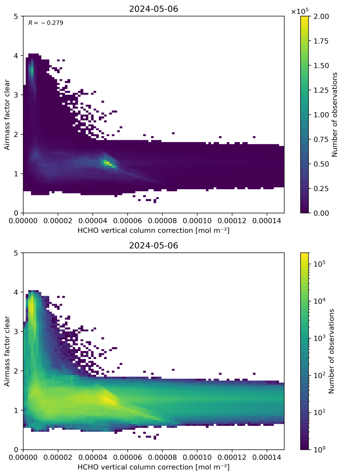
Figure 115: Scatter density plot of “HCHO vertical column correction” against “Airmass factor clear” for 2024-05-05 to 2024-05-07.
