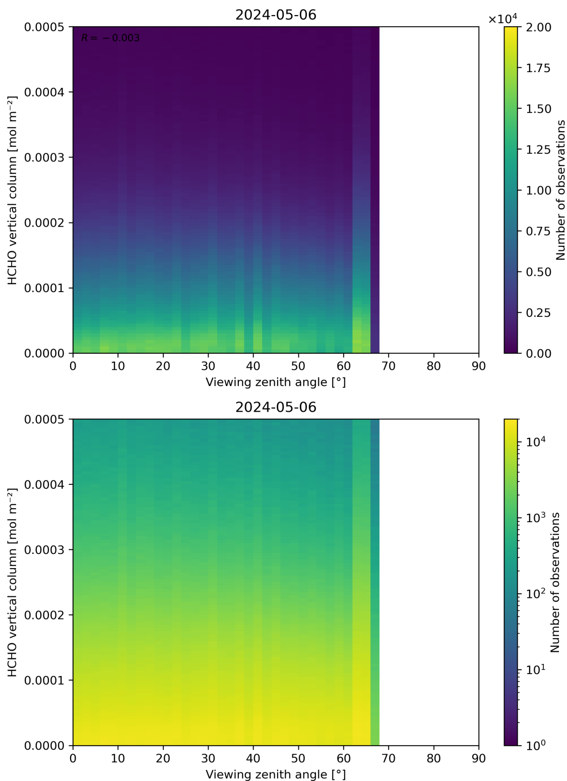
Figure 192: Scatter density plot of “Viewing zenith angle” against “HCHO vertical column” for 2024-05-05 to 2024-05-07.
