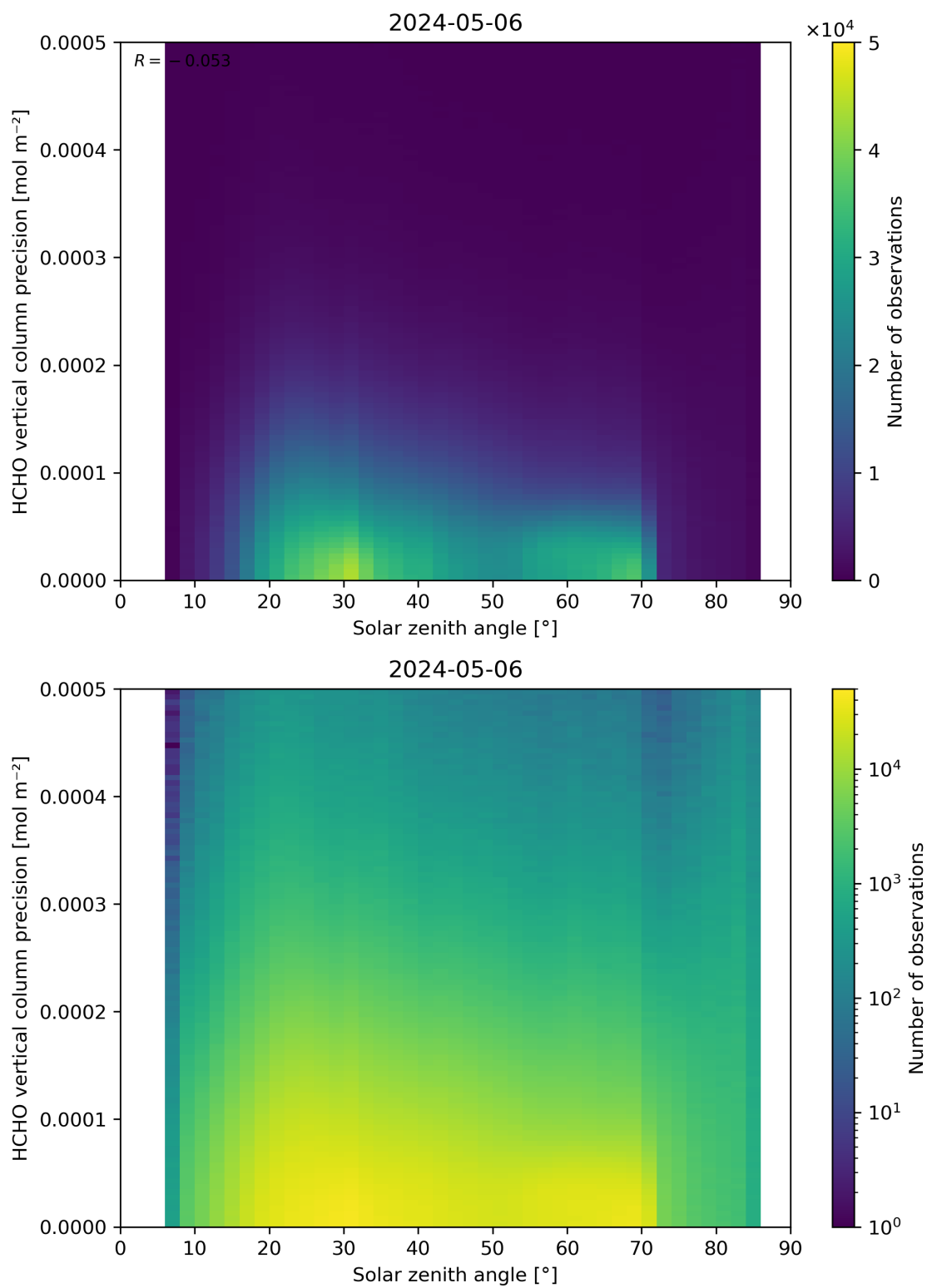
Figure 179: Scatter density plot of “Solar zenith angle” against “HCHO vertical column precision” for 2024-05-05 to 2024-05-07.
