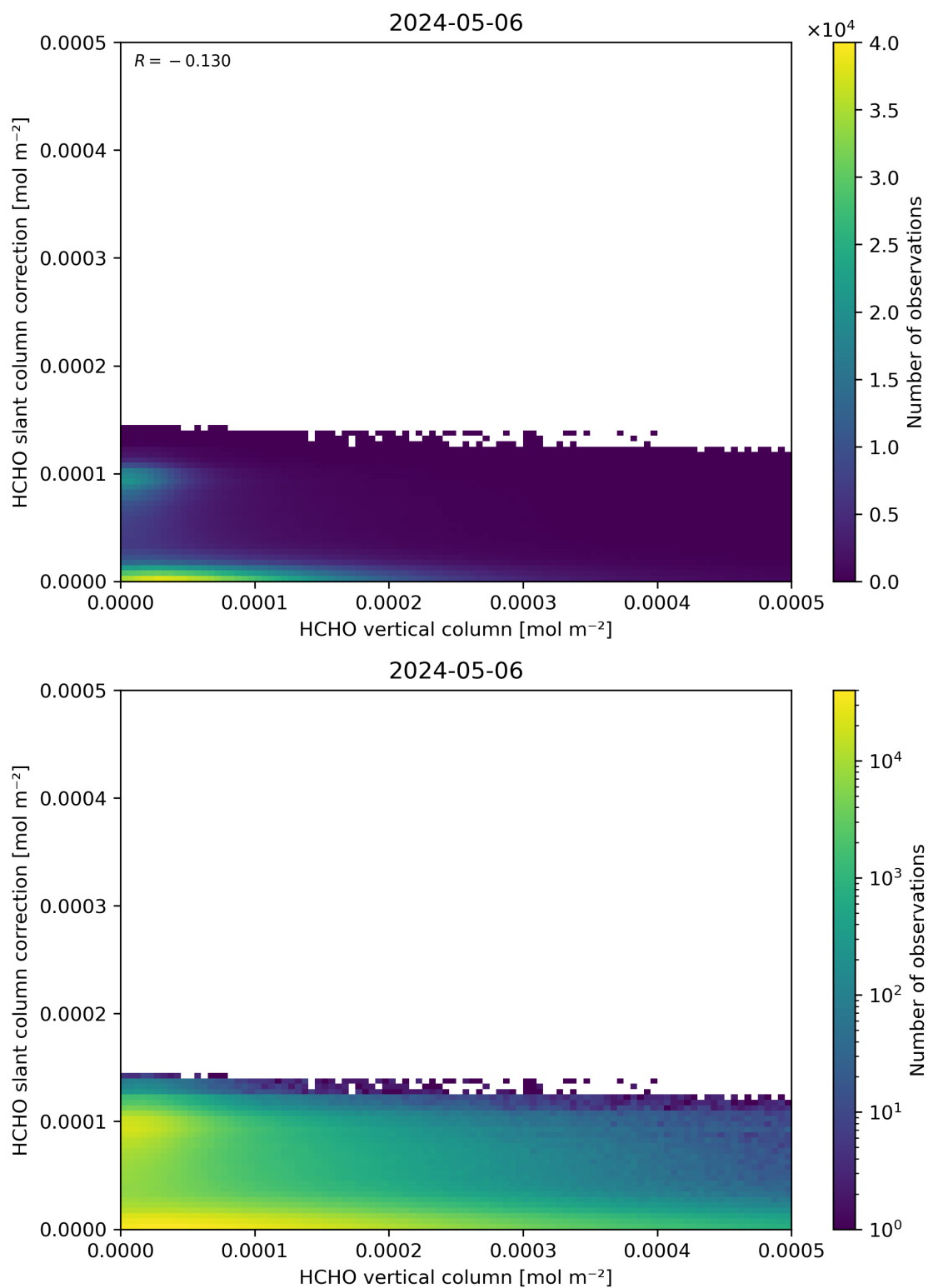
Figure 128: Scatter density plot of “HCHO vertical column” against “HCHO slant column correction” for 2024-05-05 to 2024-05-07.
