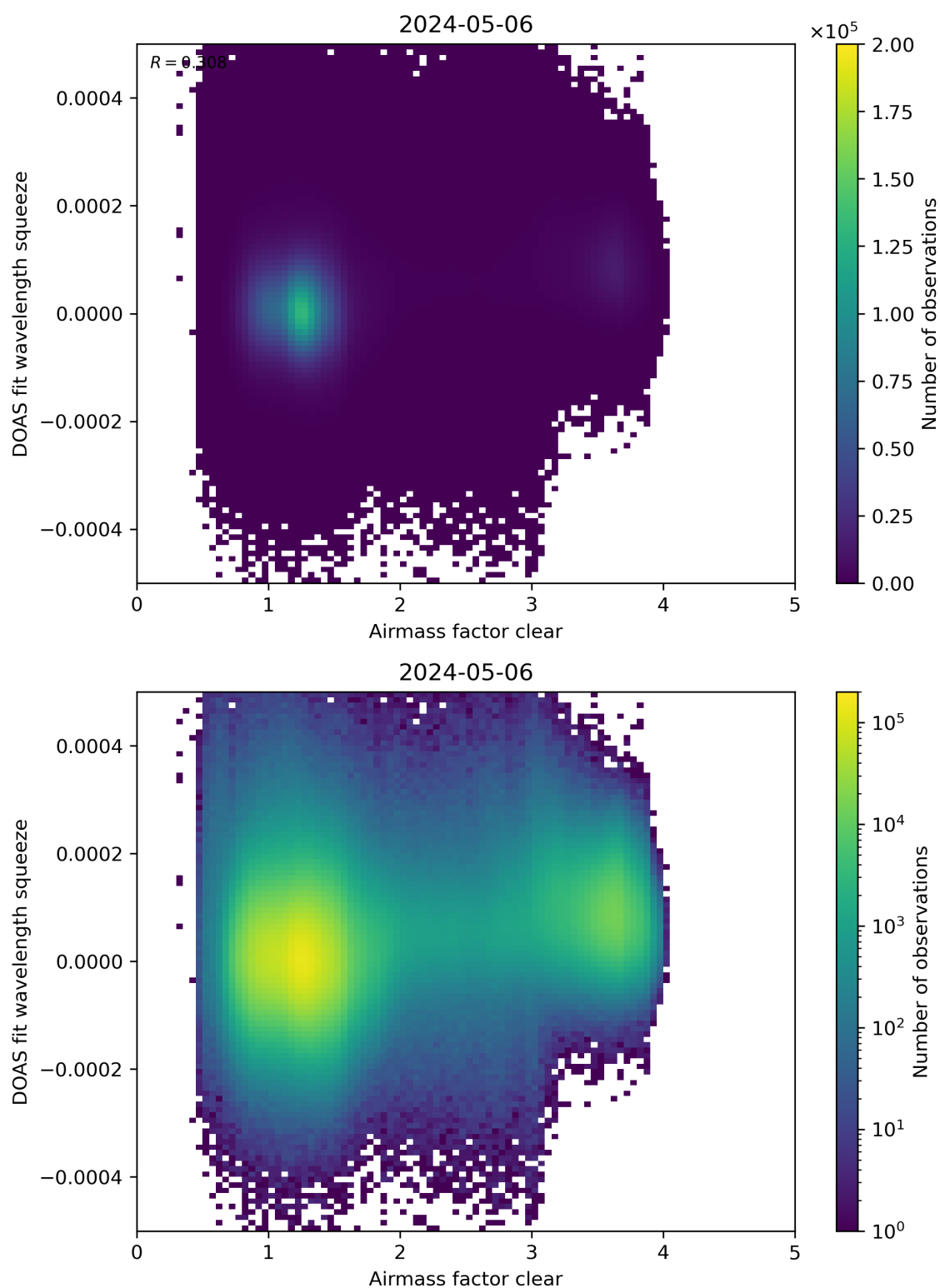
Figure 73: Scatter density plot of “Airmass factor clear” against “DOAS fit wavelength squeeze” for 2024-05-05 to 2024-05-07.
