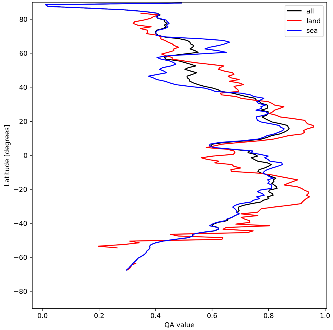
Figure 20: Zonal average of “QA value” for 2024-05-05 to 2024-05-07.
