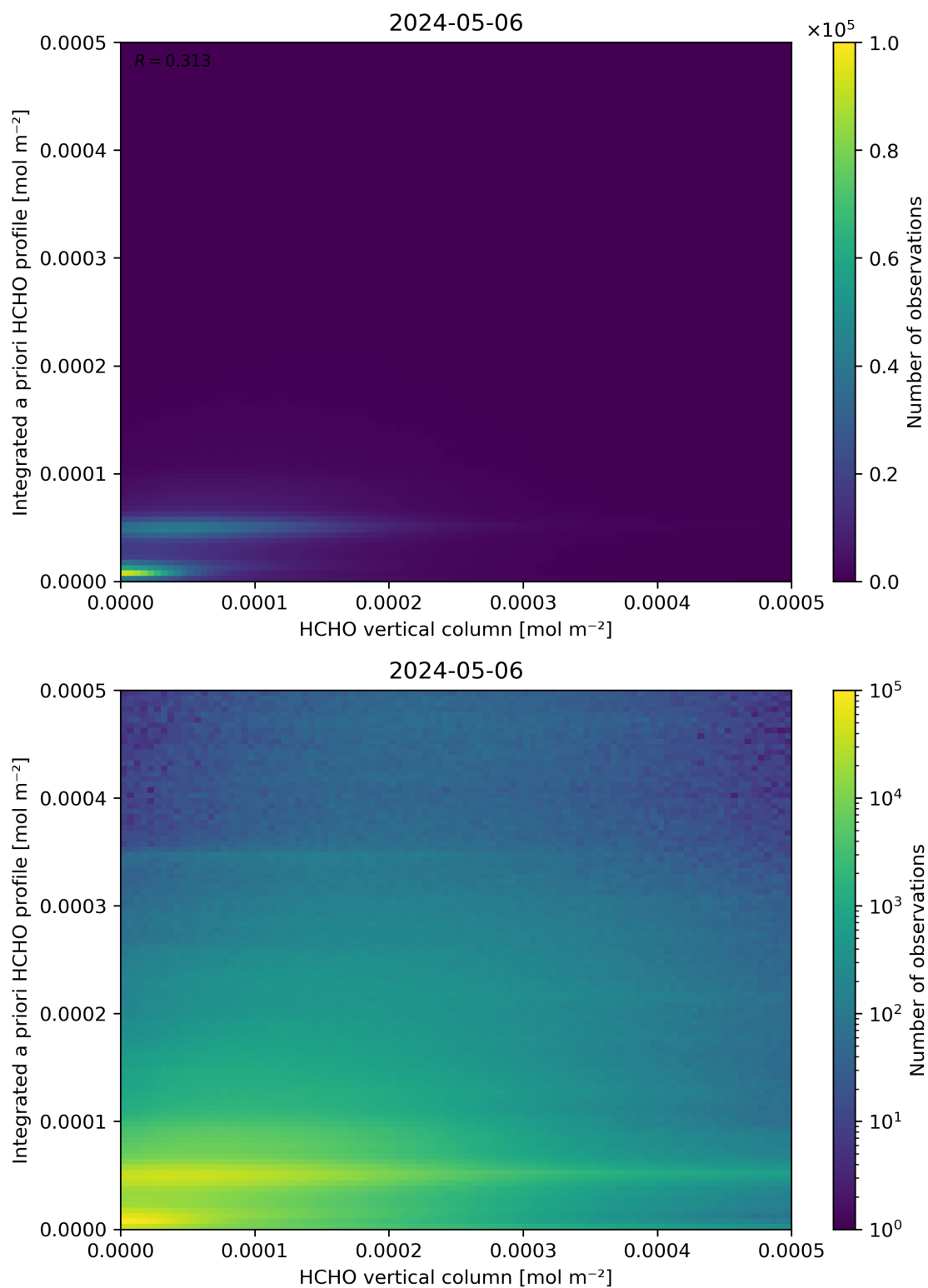
Figure 135: Scatter density plot of “HCHO vertical column” against “Integrated a priori HCHO profile” for 2024-05-05 to 2024-05-07.
