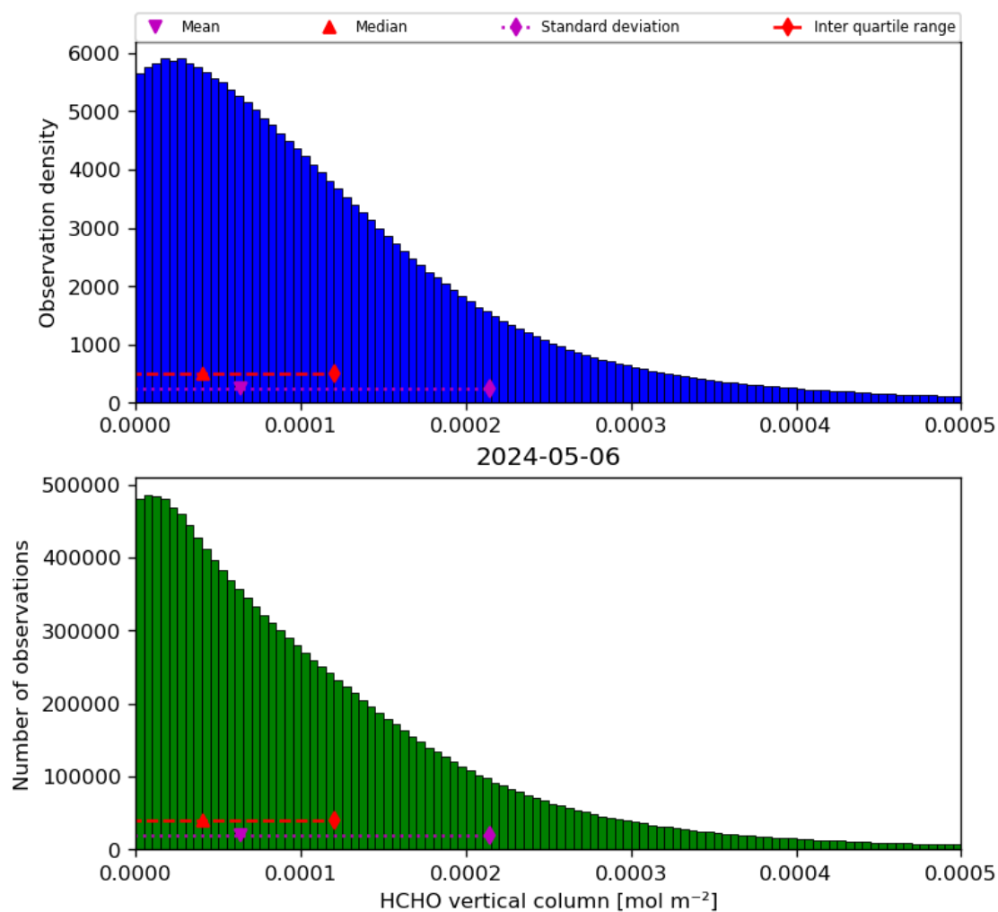
Figure 35: Histogram of “HCHO vertical column” for 2024-05-05 to 2024-05-07
