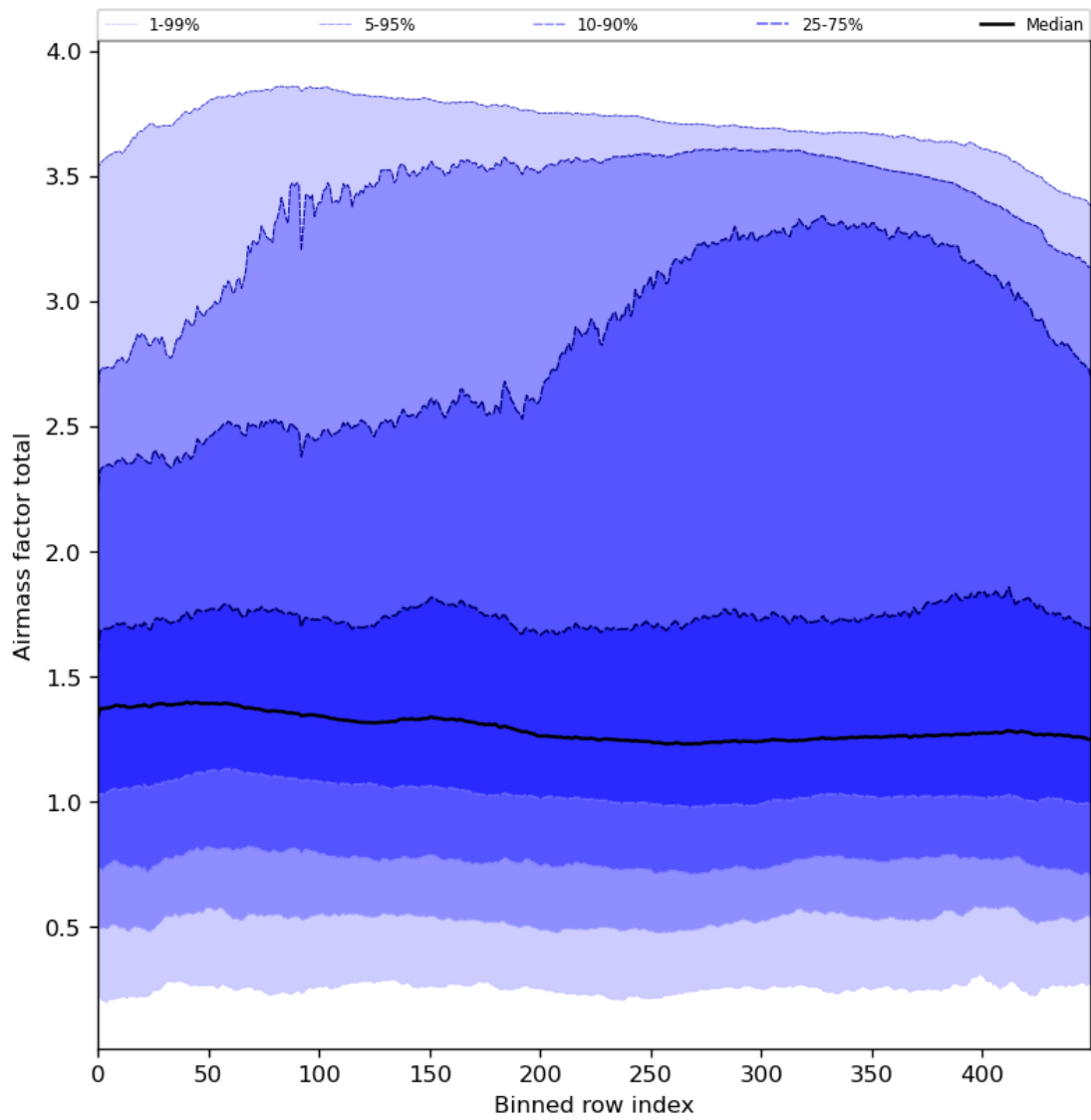
Figure 54: Along track statistics of “Airmass factor total” for 2024-05-05 to 2024-05-07
