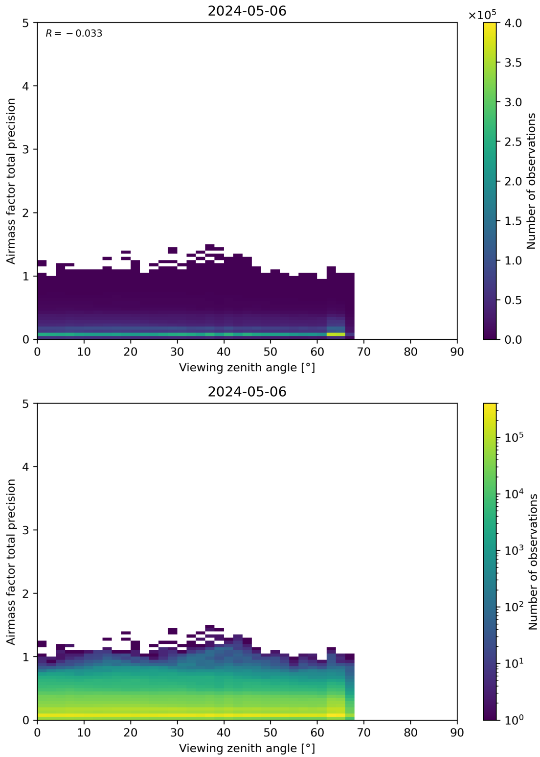
Figure 191: Scatter density plot of “Viewing zenith angle” against “Airmass factor total precision” for 2024-05-05 to 2024-05-07.
