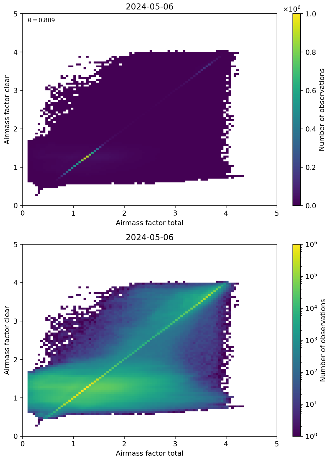
Figure 100: Scatter density plot of “Airmass factor total” against “Airmass factor clear” for 2024-05-05 to 2024-05-07.
