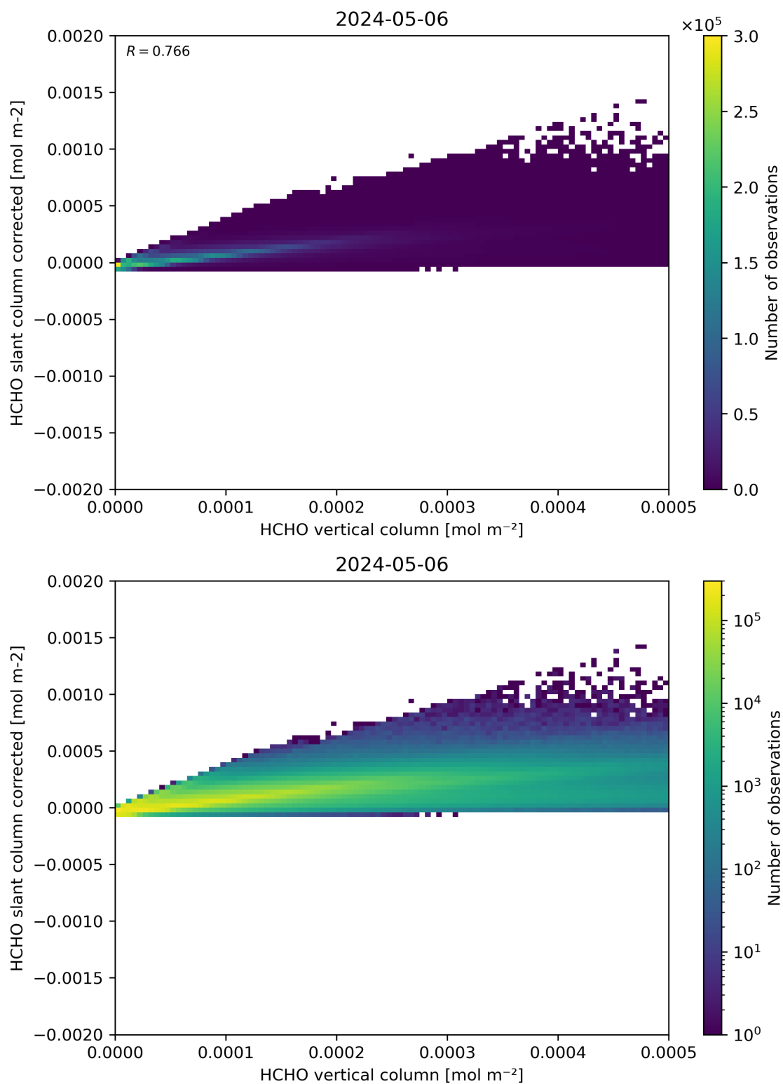
Figure 127: Scatter density plot of “HCHO vertical column” against “HCHO slant column corrected” for 2024-05-05 to 2024-05-07.
