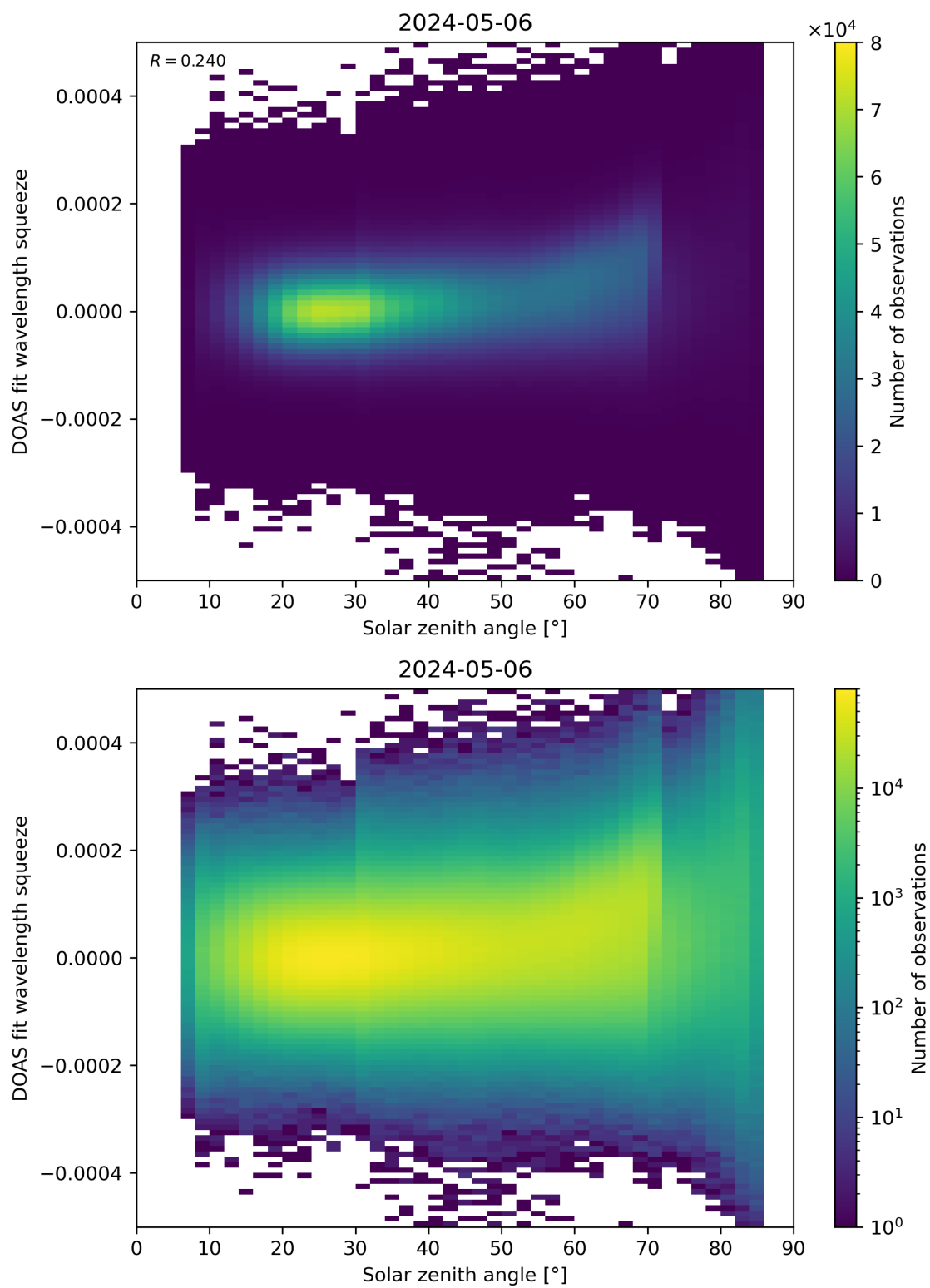
Figure 169: Scatter density plot of “Solar zenith angle” against “DOAS fit wavelength squeeze” for 2024-05-05 to 2024-05-07.
