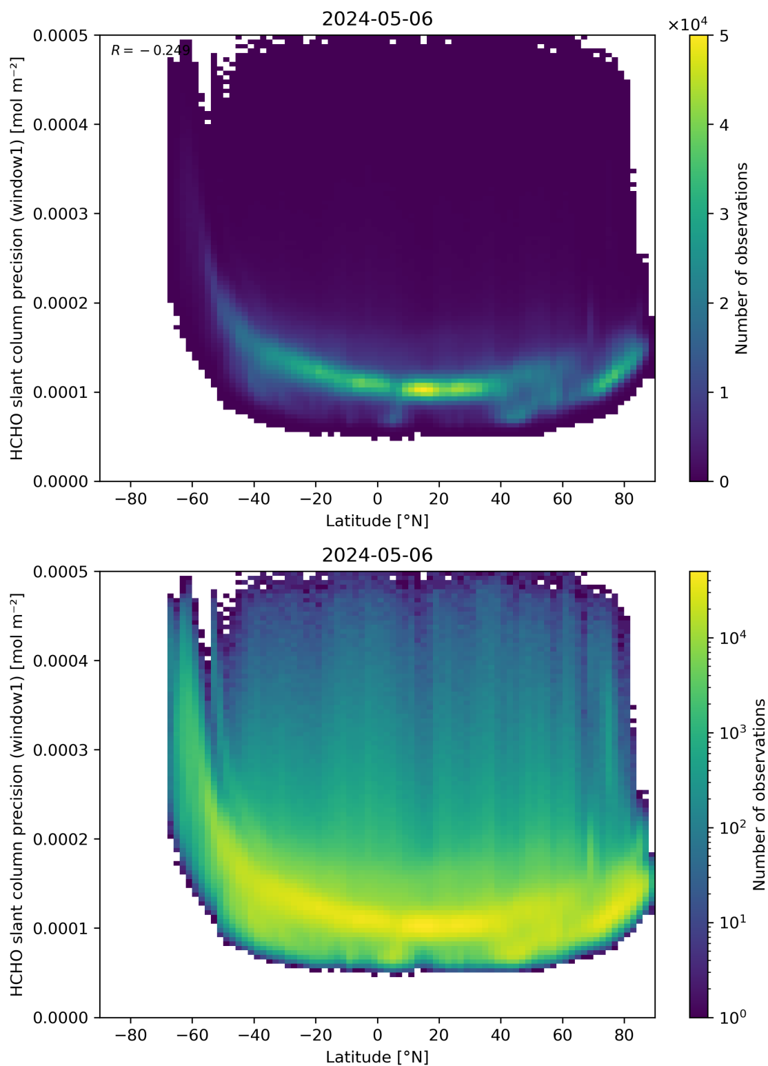
Figure 160: Scatter density plot of “Latitude” against “HCHO slant column precision (window1)” for 2024-05-05 to 2024-05-07.
