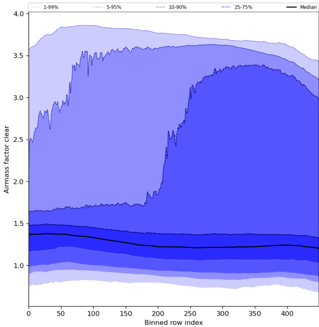
Figure 56: Along track statistics of “Airmass factor clear” for 2024-05-05 to 2024-05-07
