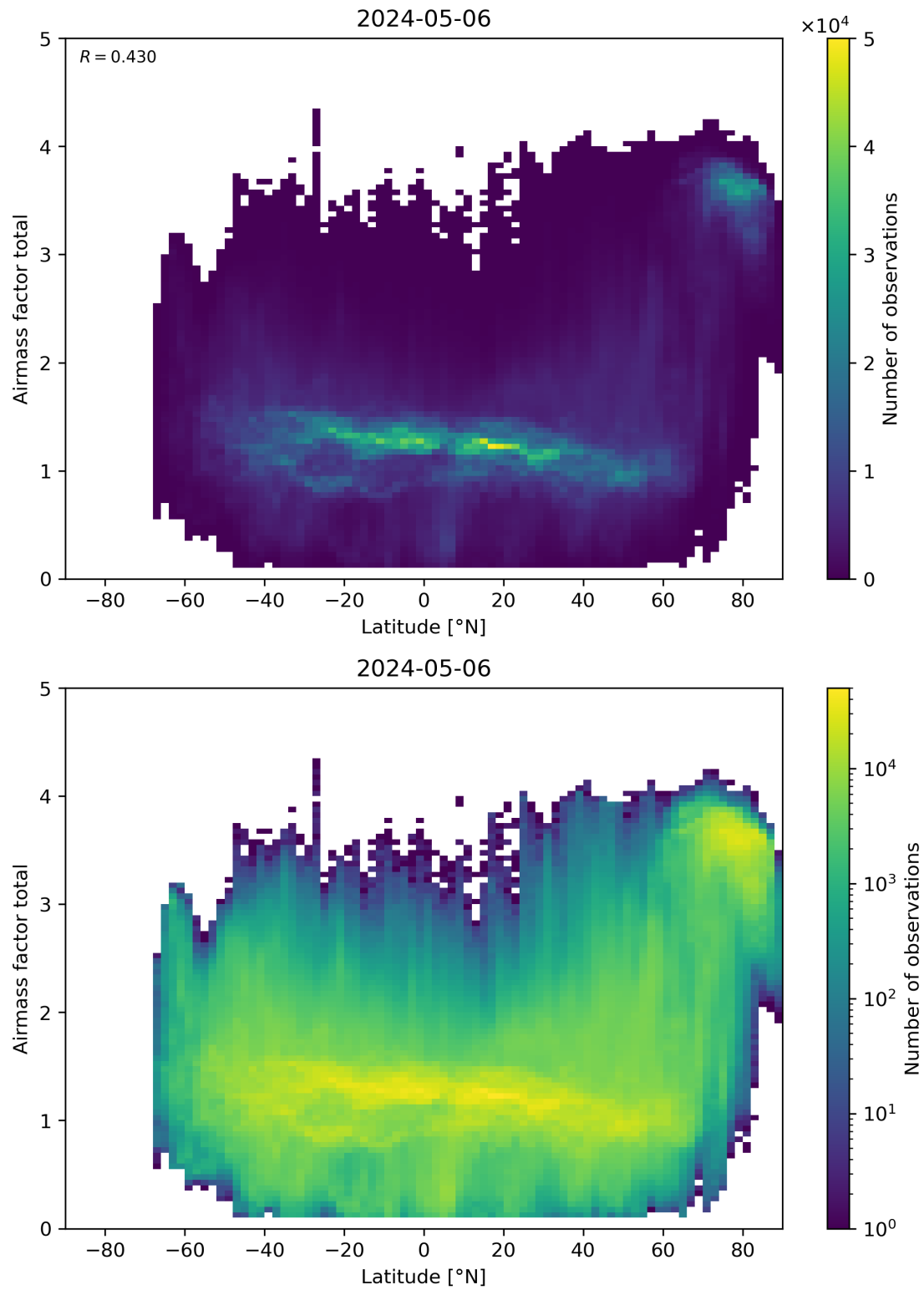
Figure 161: Scatter density plot of “Latitude” against “Airmass factor total” for 2024-05-05 to 2024-05-07.
