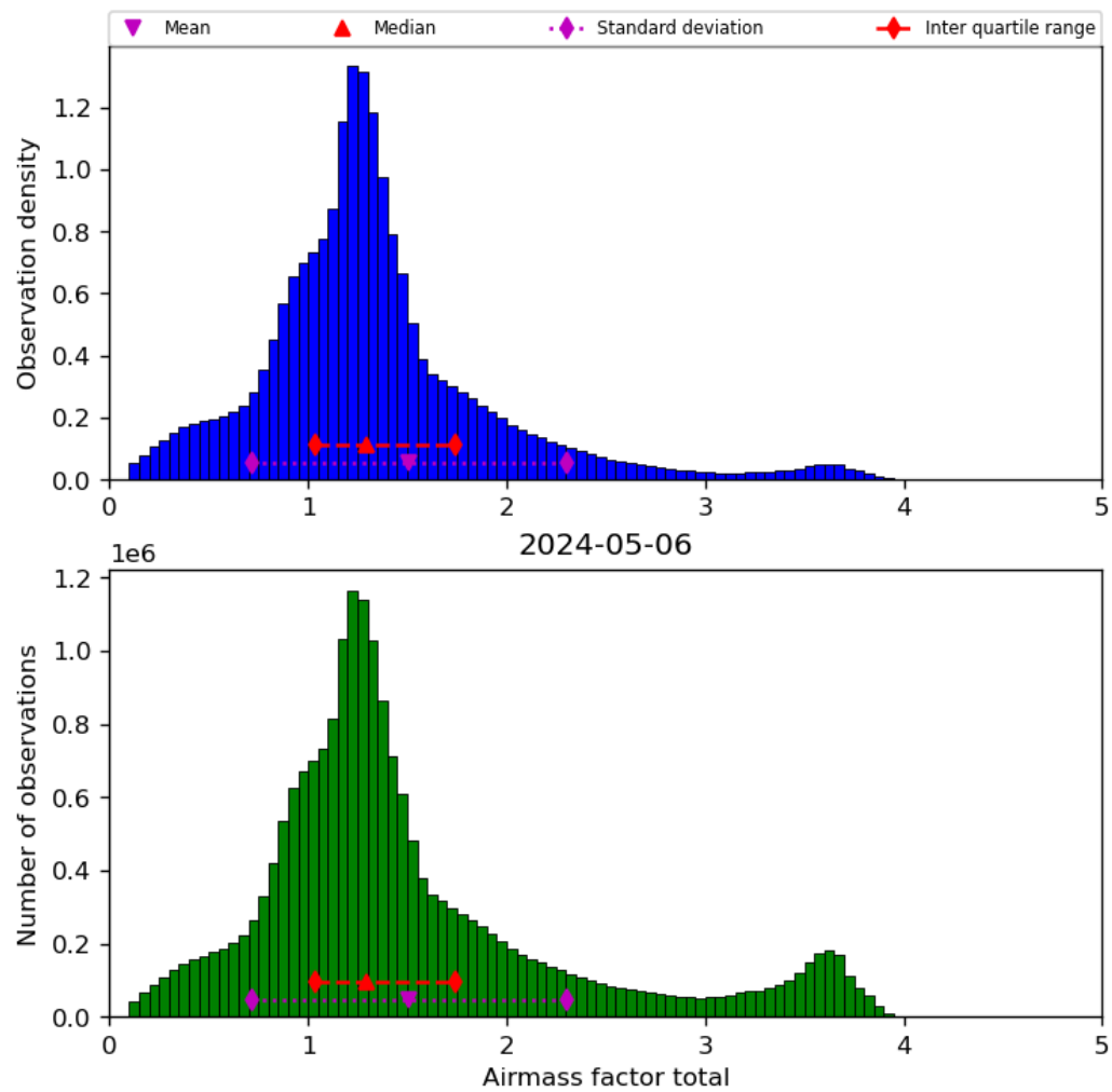
Figure 40: Histogram of “Airmass factor total” for 2024-05-05 to 2024-05-07
