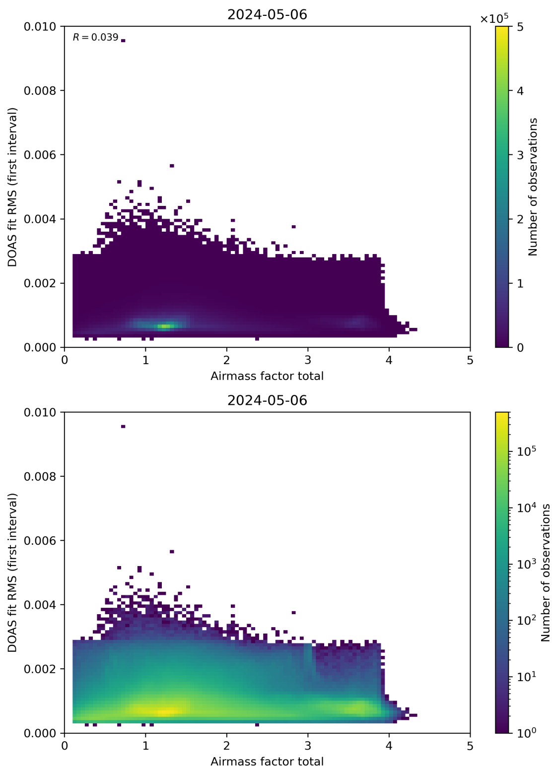
Figure 97: Scatter density plot of “Airmass factor total” against “DOAS fit RMS (first interval)” for 2024-05-05 to 2024-05-07.
