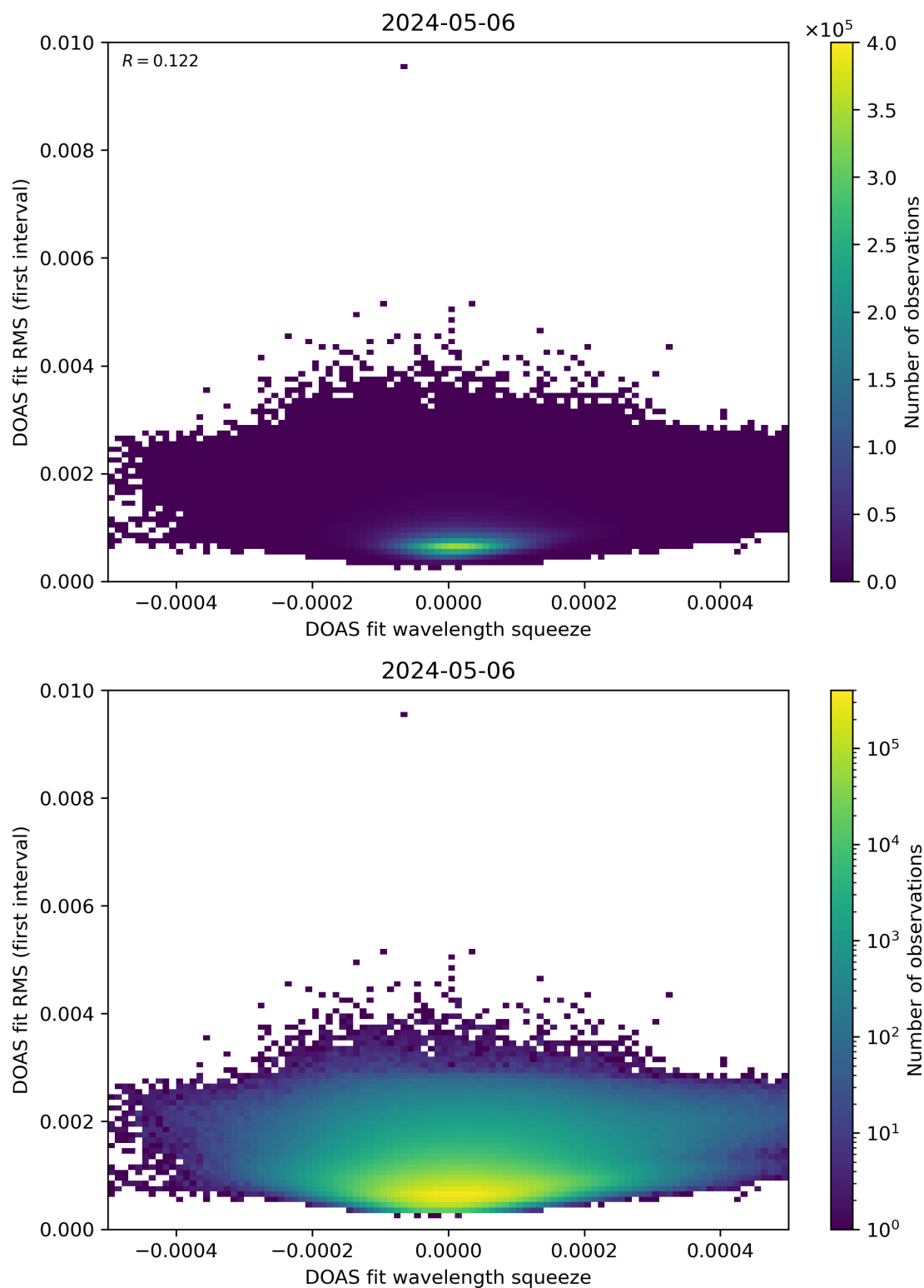
Figure 68: Scatter density plot of “DOAS fit wavelength squeeze” against “DOAS fit RMS (first interval)” for 2024-05-05 to 2024-05-07.
