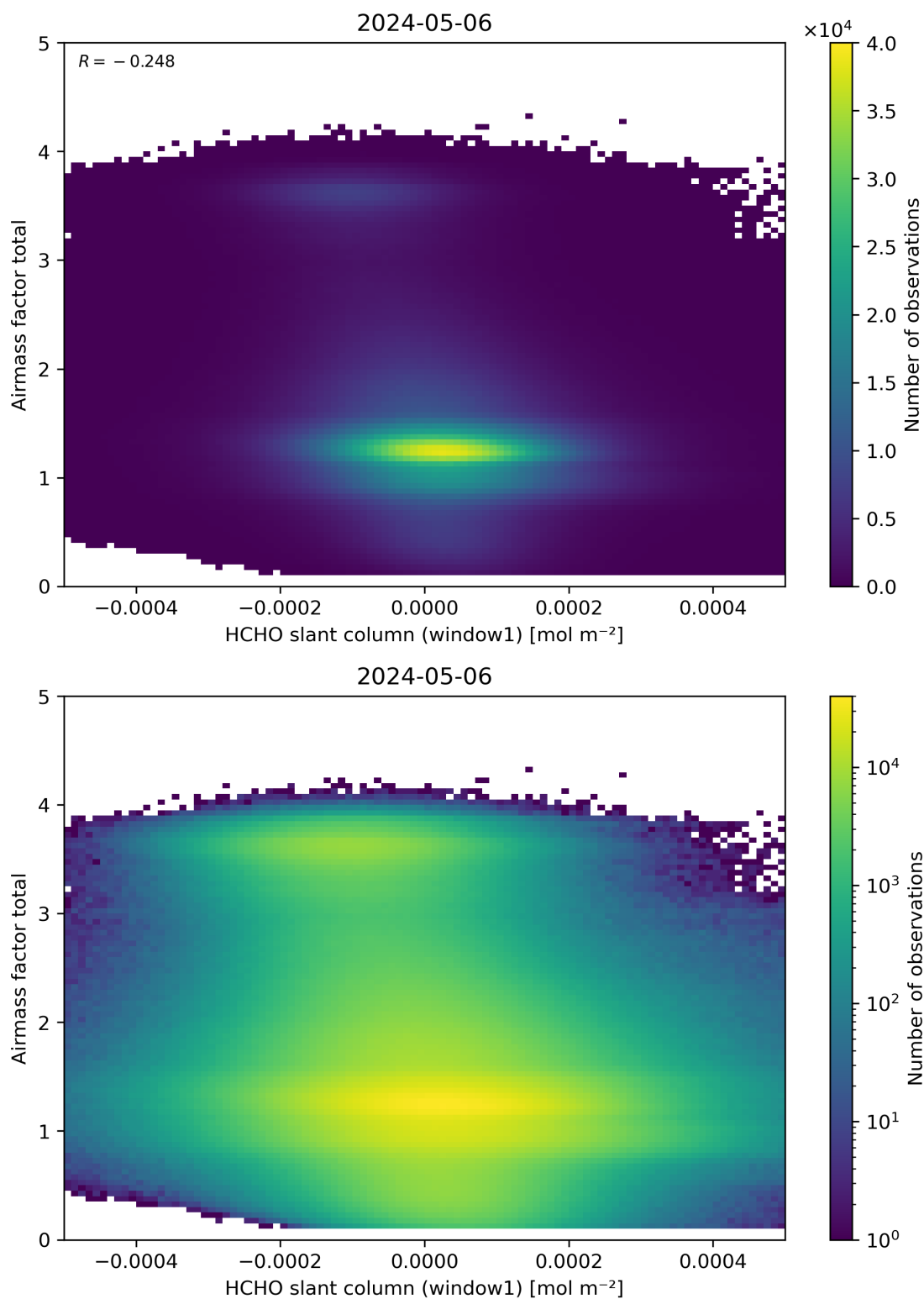
Figure 85: Scatter density plot of “HCHO slant column (window1)” against “Airmass factor total” for 2024-05-05 to 2024-05-07.
