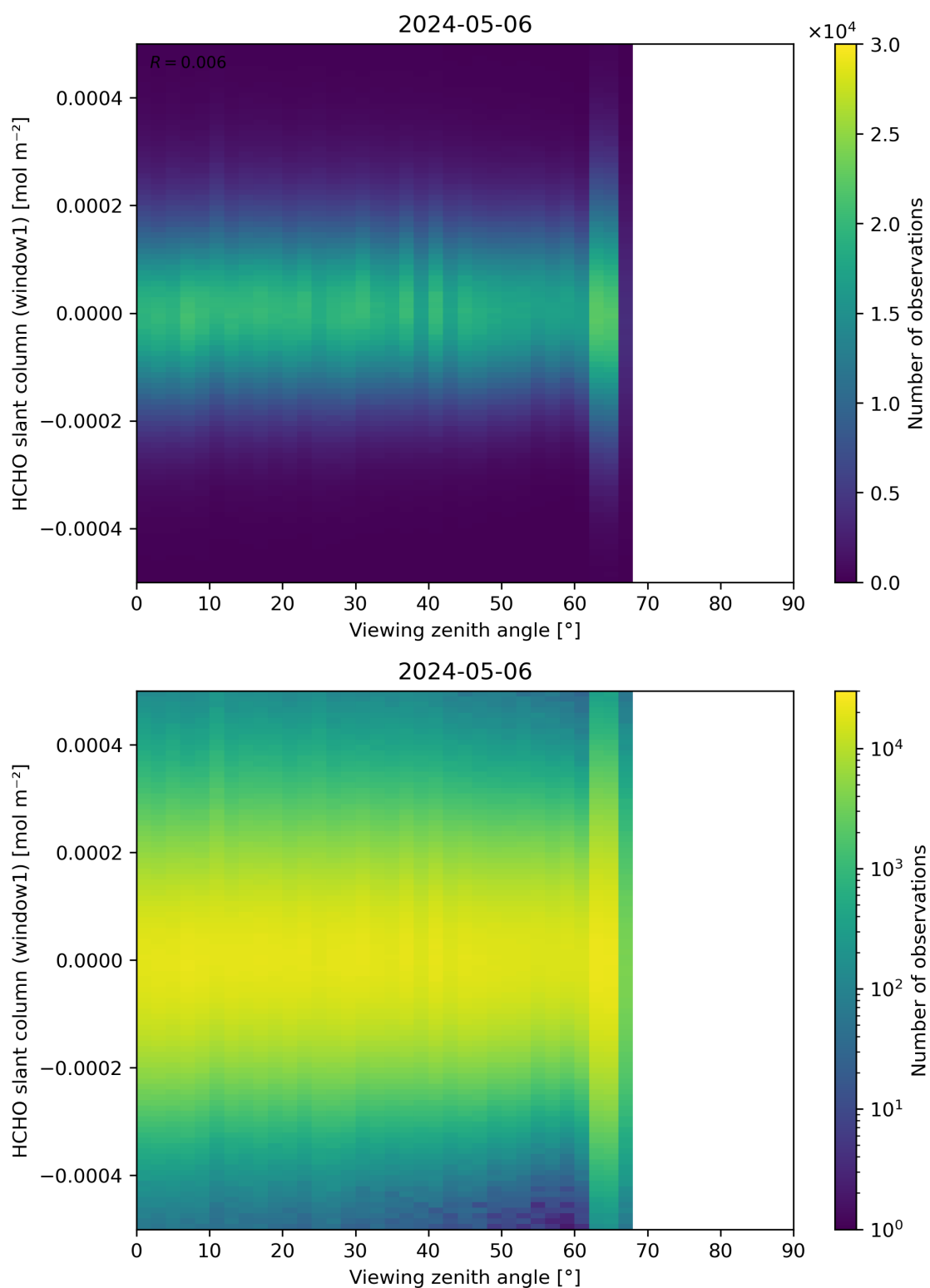
Figure 188: Scatter density plot of “Viewing zenith angle” against “HCHO slant column (window1)” for 2024-05-05 to 2024-05-07.
