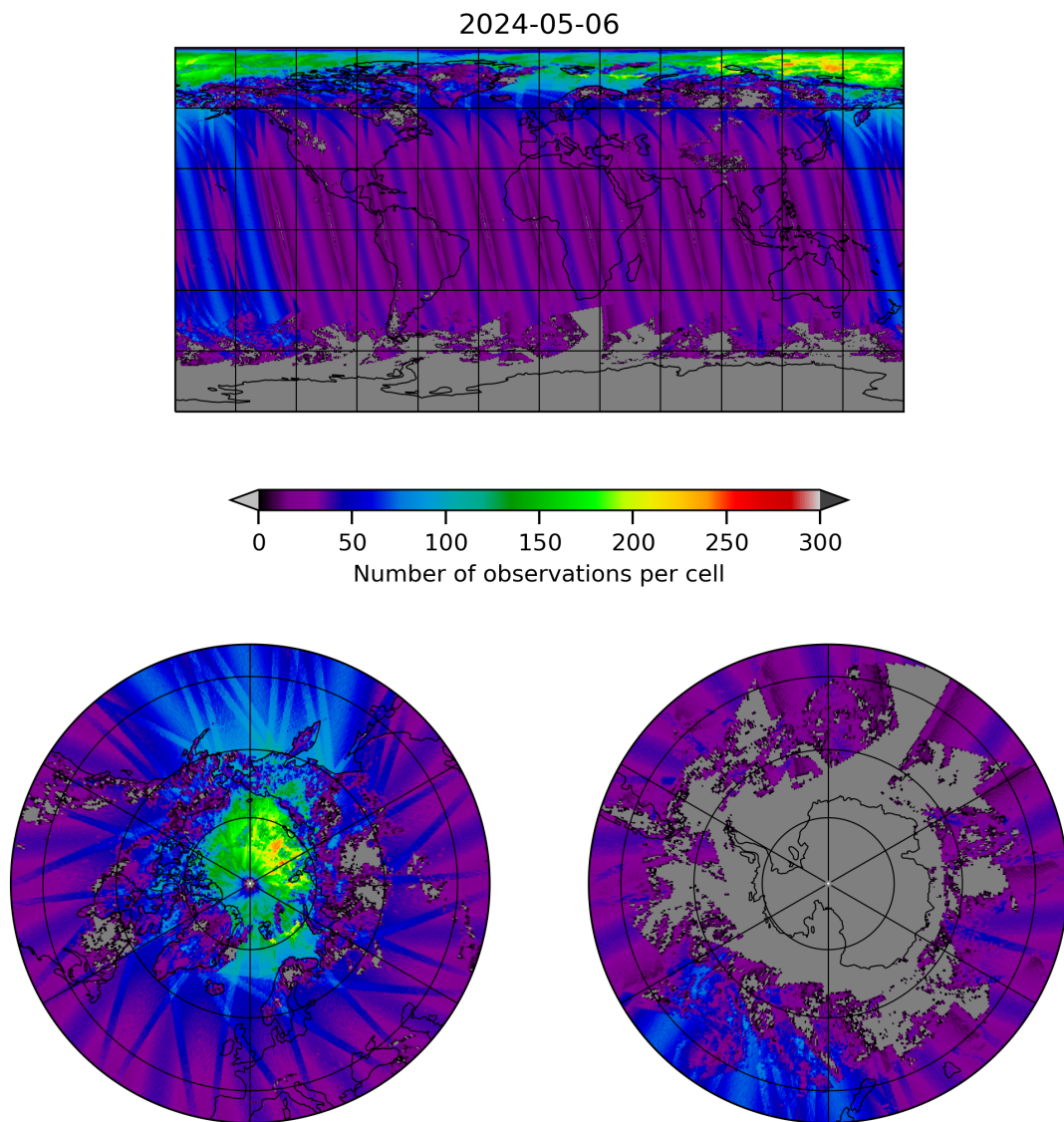
Figure 19: Map of the number of observations for 2024-05-05 to 2024-05-07
