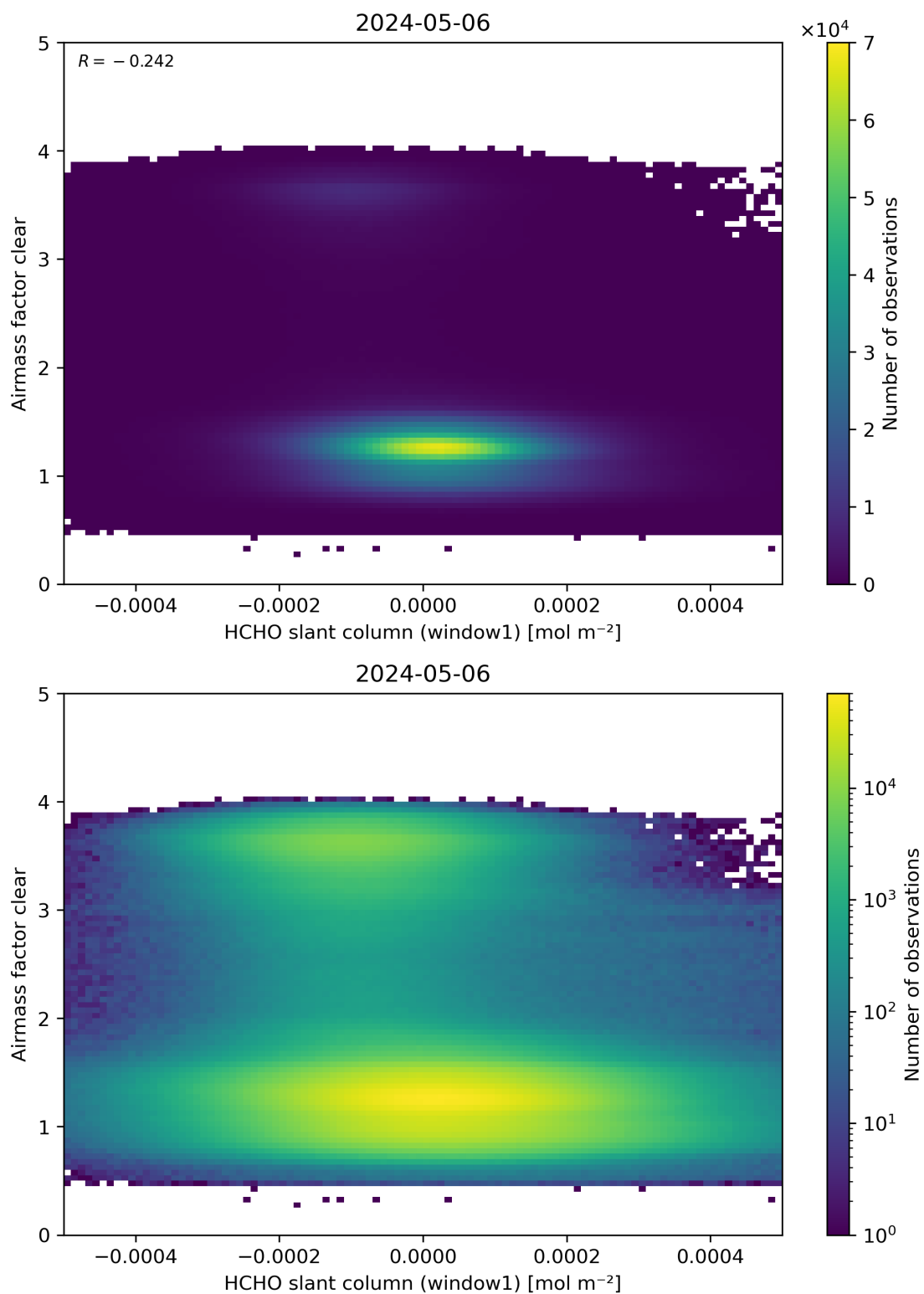
Figure 81: Scatter density plot of “HCHO slant column (window1)” against “Airmass factor clear” for 2024-05-05 to 2024-05-07.
