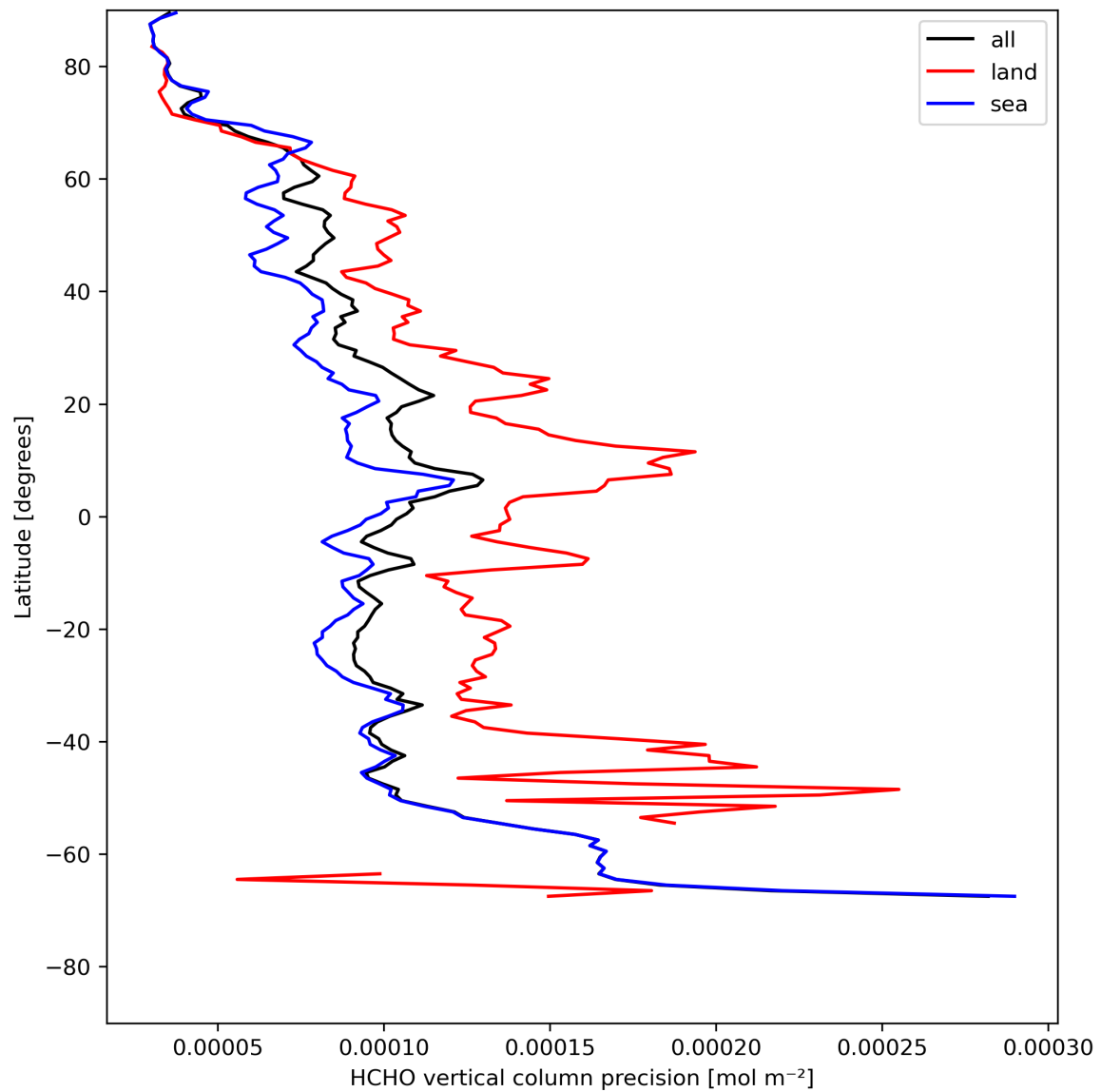
Figure 22: Zonal average of “HCHO vertical column precision” for 2024-05-05 to 2024-05-07.
