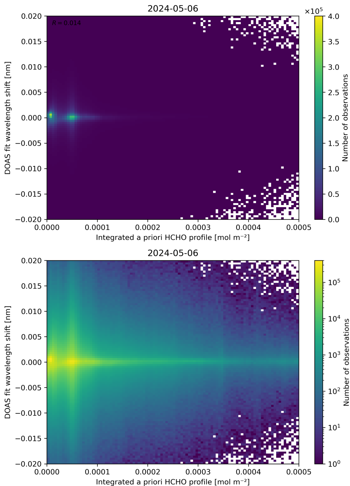
Figure 149: Scatter density plot of “Integrated a priori HCHO profile” against “DOAS fit wavelength shift” for 2024-05-05 to 2024-05-07.
