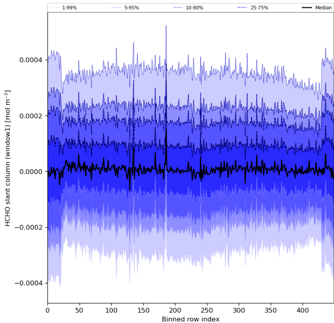
Figure 52: Along track statistics of “HCHO slant column (window1)” for 2024-05-05 to 2024-05-07
