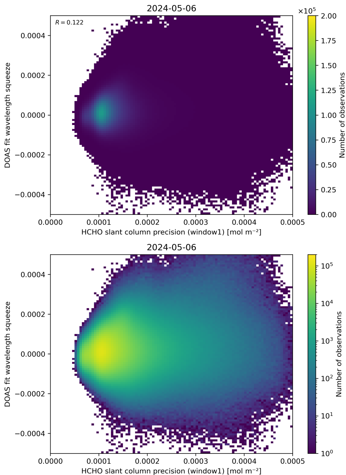
Figure 90: Scatter density plot of “HCHO slant column precision (window1)” against “DOAS fit wavelength squeeze” for 2024-05-05 to 2024-05-07.
