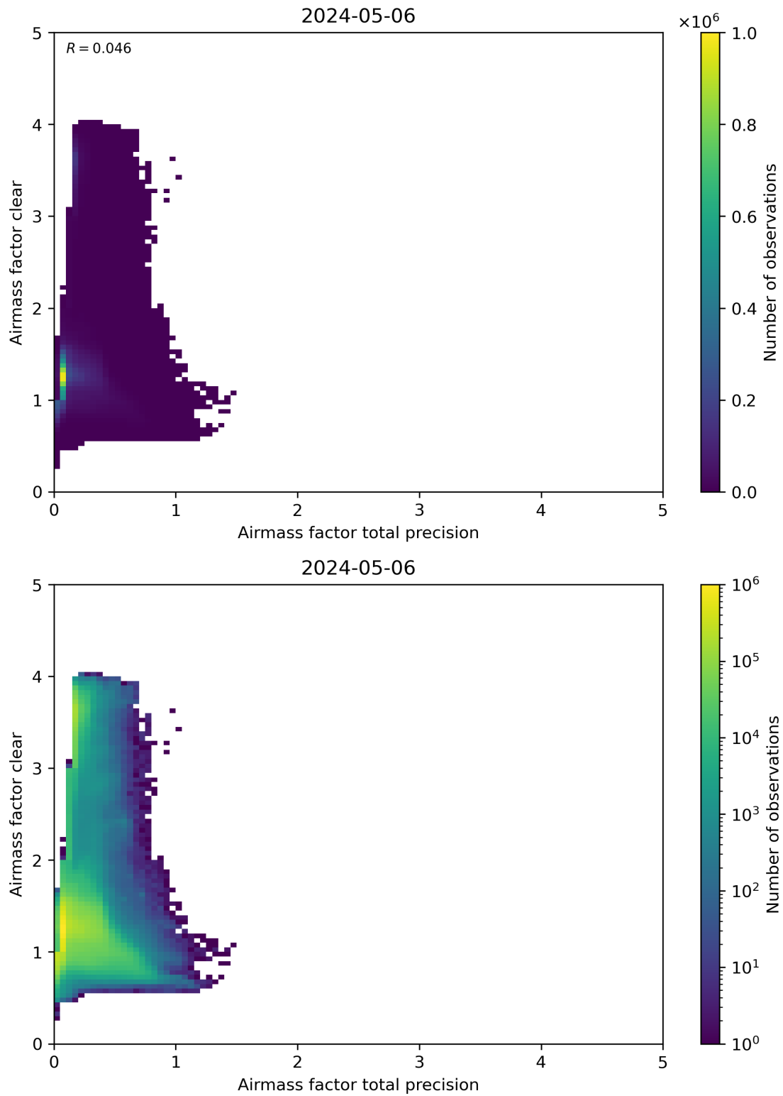
Figure 108: Scatter density plot of “Airmass factor total precision” against “Airmass factor clear” for 2024-05-05 to 2024-05-07.
