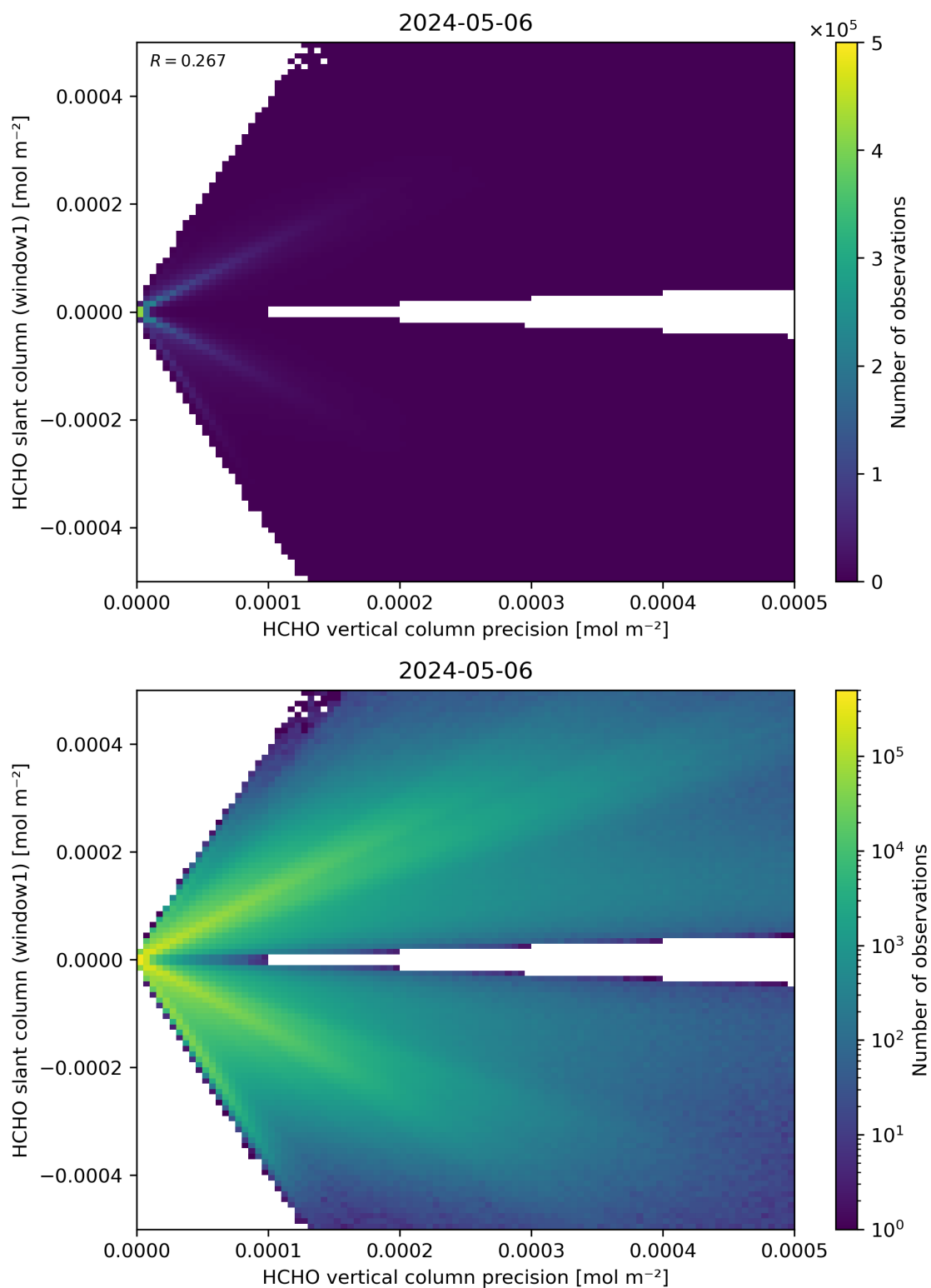
Figure 142: Scatter density plot of “HCHO vertical column precision” against “HCHO slant column (window1)” for 2024-05-05 to 2024-05-07.
