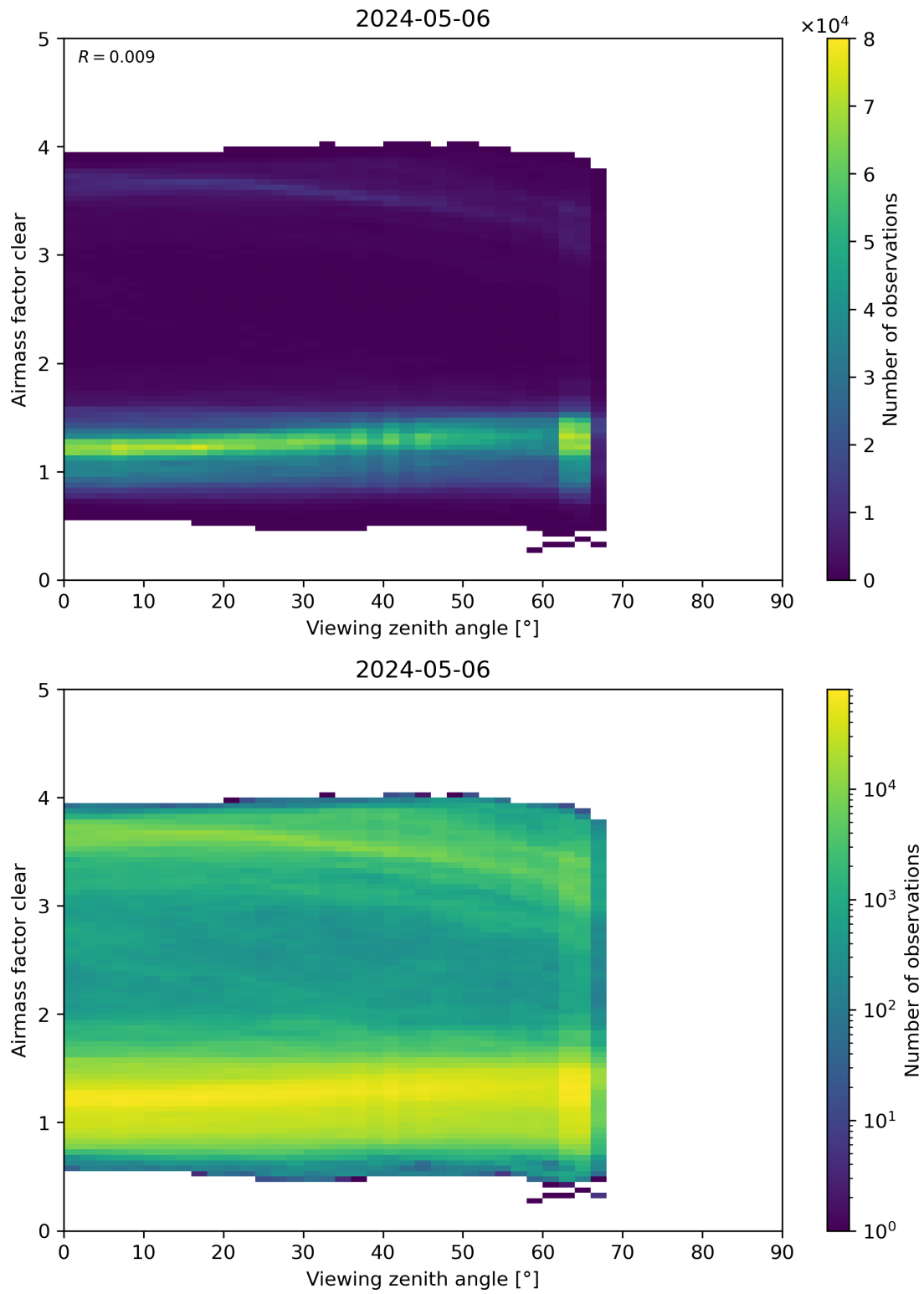
Figure 185: Scatter density plot of “Viewing zenith angle” against “Airmass factor clear” for 2024-05-05 to 2024-05-07.
