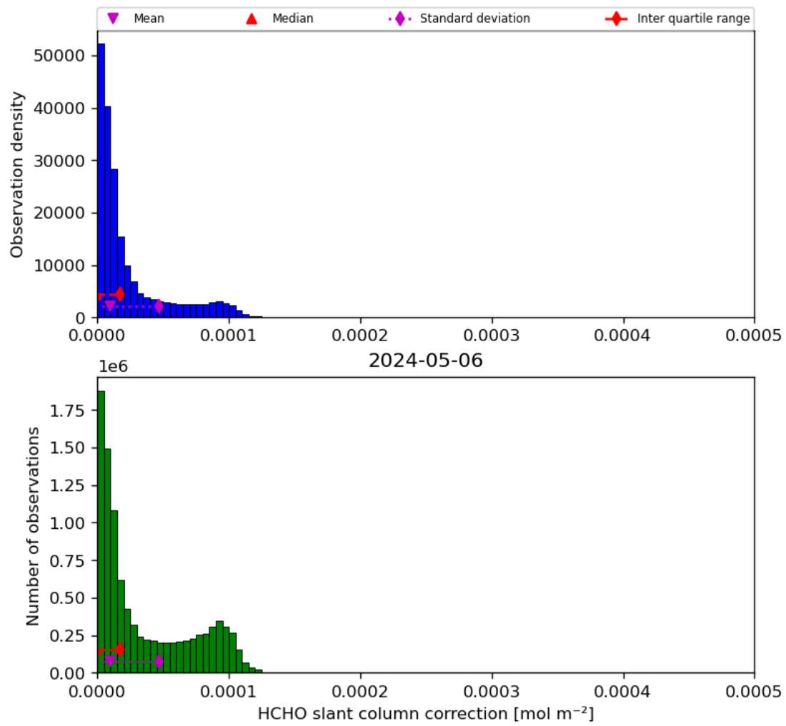
Figure 47: Histogram of “HCHO slant column correction” for 2024-05-05 to 2024-05-07
