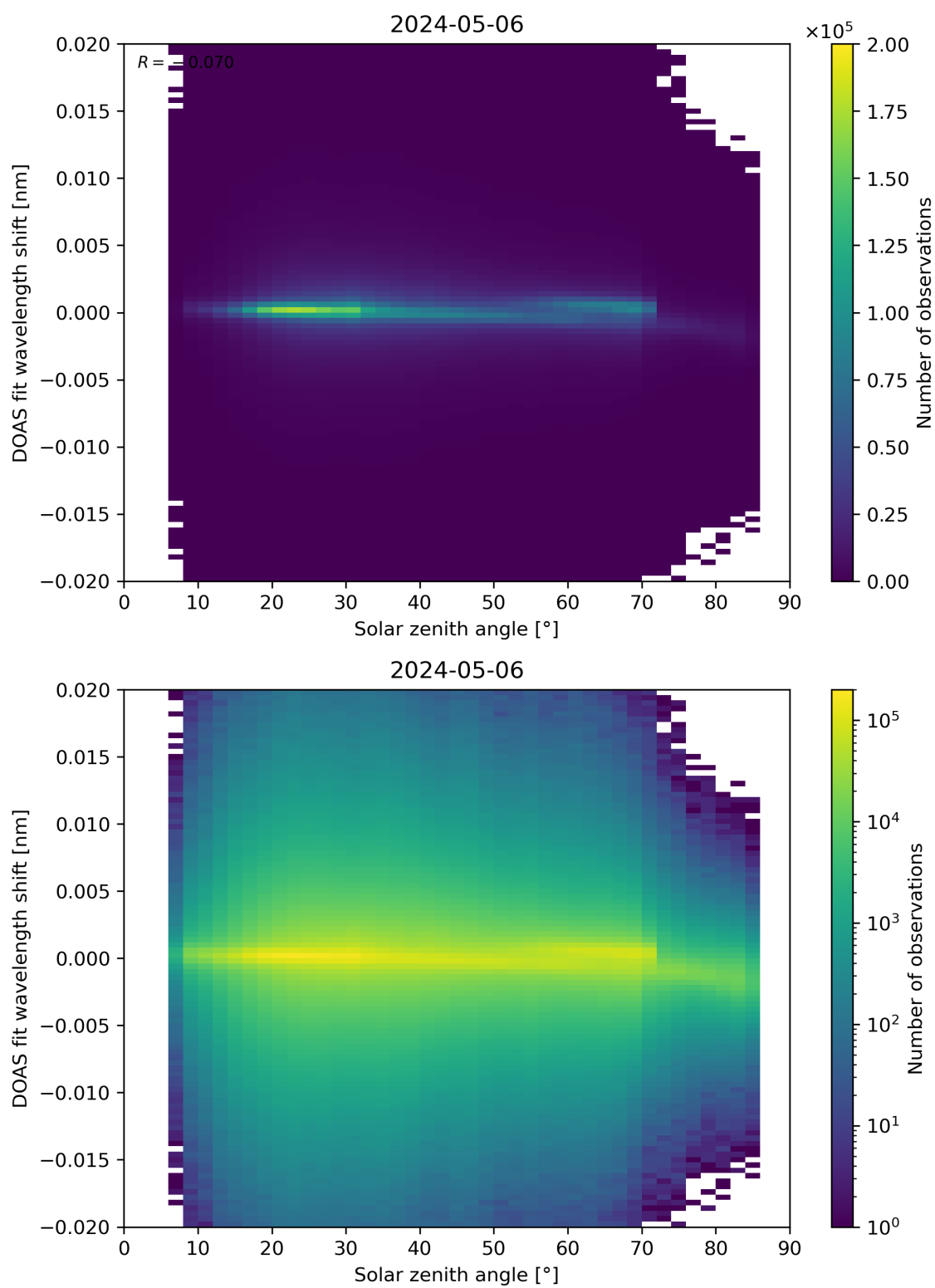
Figure 168: Scatter density plot of “Solar zenith angle” against “DOAS fit wavelength shift” for 2024-05-05 to 2024-05-07.
