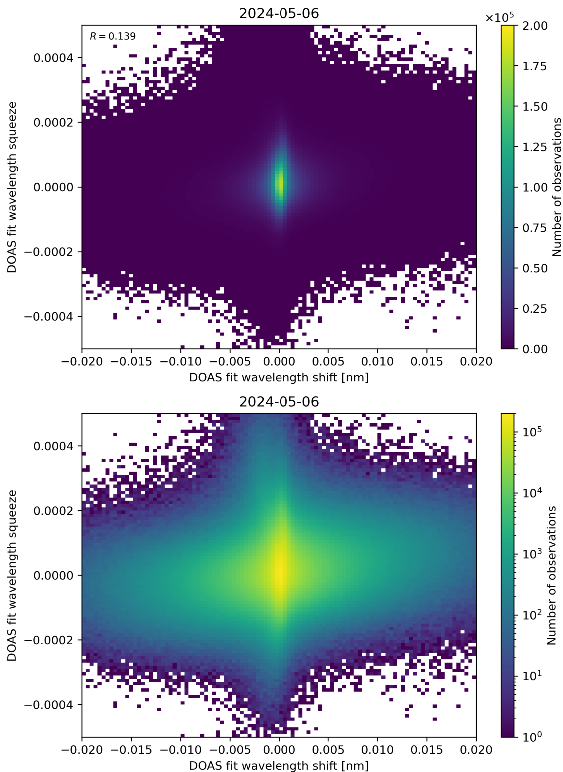
Figure 65: Scatter density plot of “DOAS fit wavelength shift” against “DOAS fit wavelength squeeze” for 2024-05-05 to 2024-05-07.
