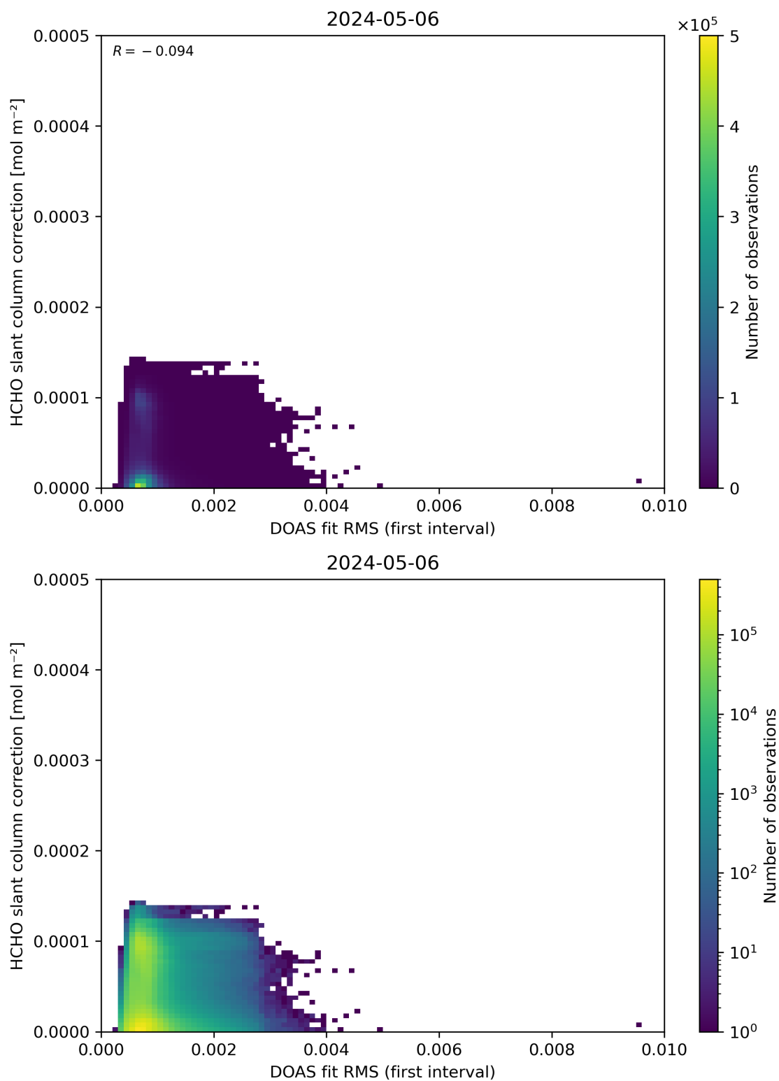
Figure 63: Scatter density plot of “DOAS fit RMS (first interval)” against “HCHO slant column correction” for 2024-05-05 to 2024-05-07.
