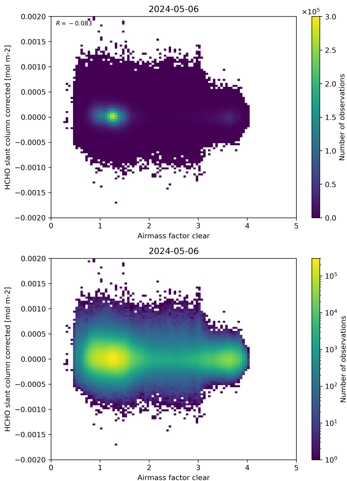
Figure 74: Scatter density plot of “Airmass factor clear” against “HCHO slant column corrected” for 2024-05-05 to 2024-05-07.
