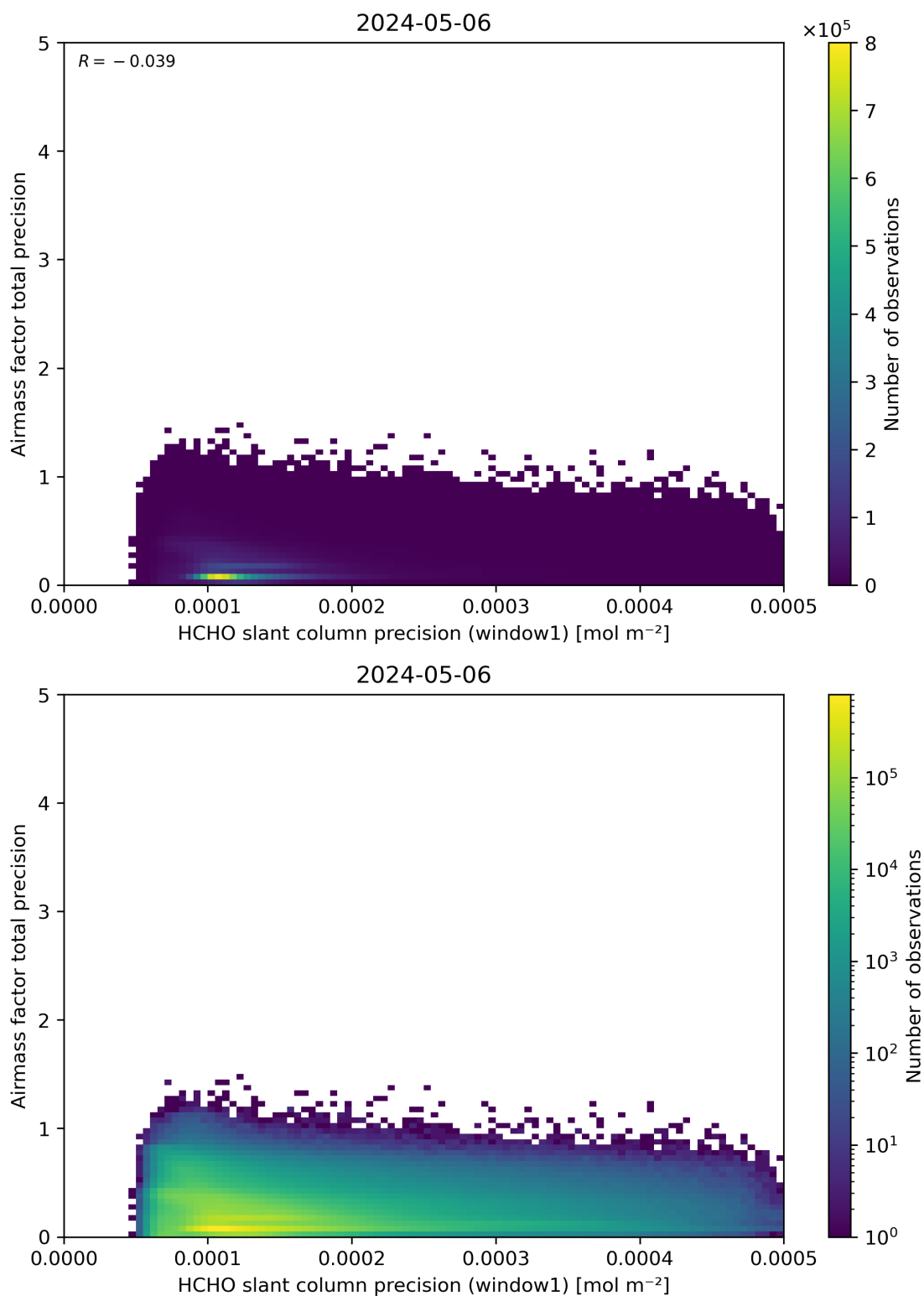
Figure 95: Scatter density plot of “HCHO slant column precision (window1)” against “Airmass factor total precision” for 2024-05-05 to 2024-05-07.
