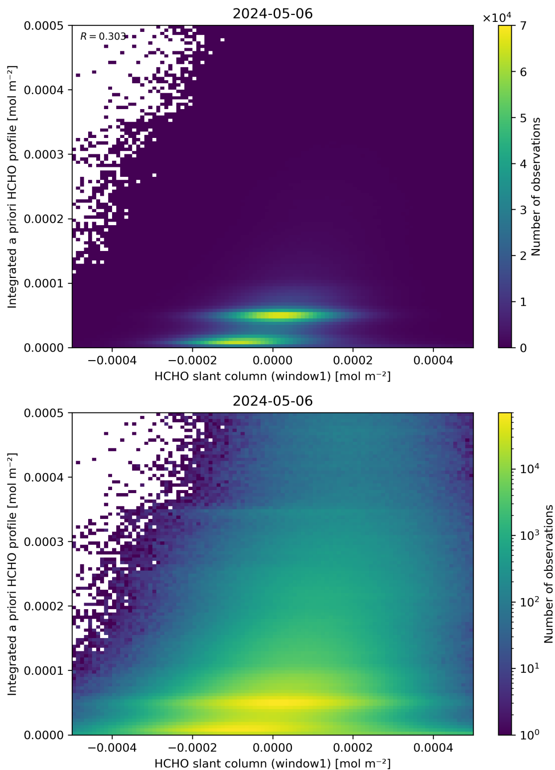
Figure 87: Scatter density plot of “HCHO slant column (window1)” against “Integrated a priori HCHO profile” for 2024-05-05 to 2024-05-07.
