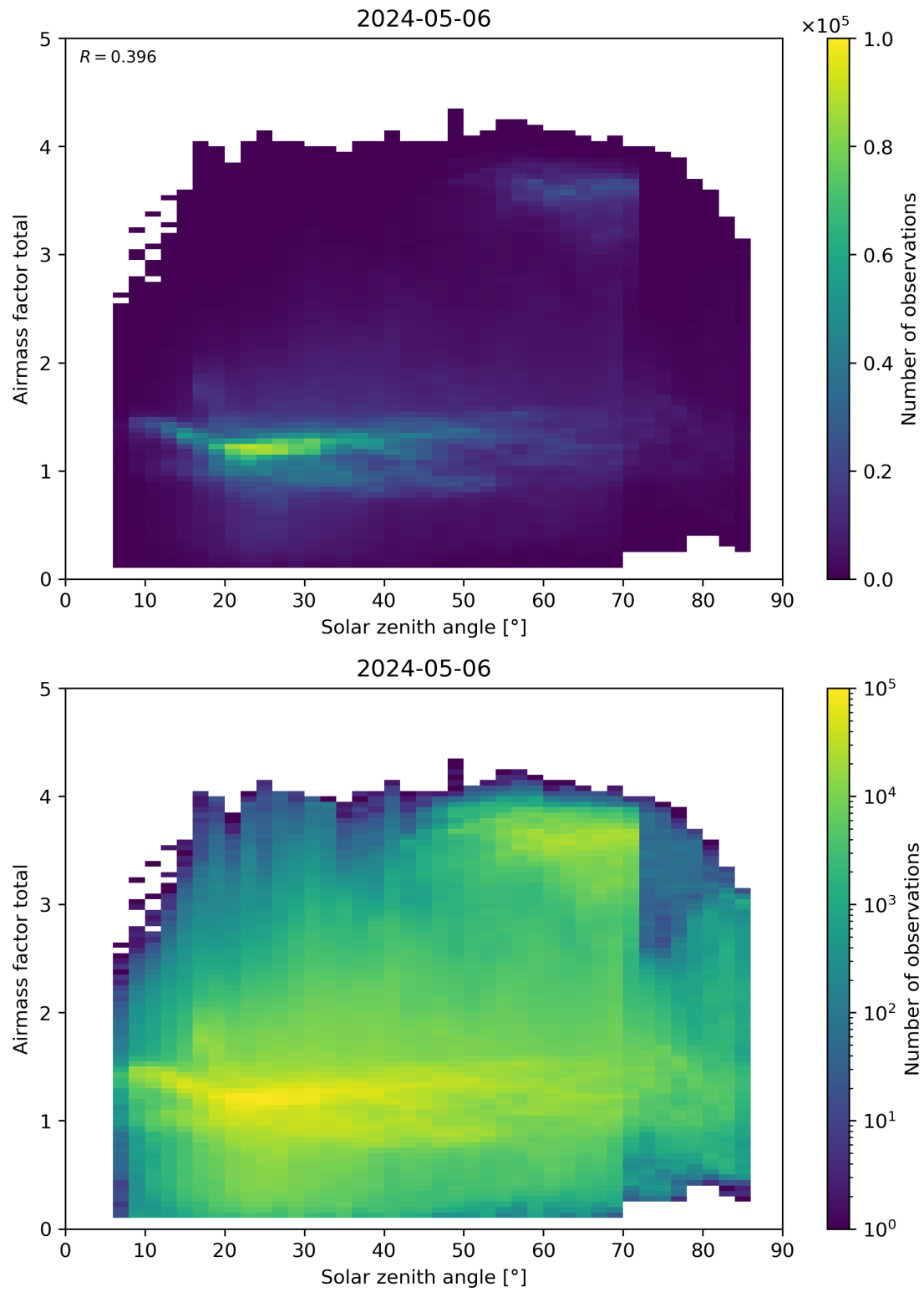
Figure 175: Scatter density plot of “Solar zenith angle” against “Airmass factor total” for 2024-05-05 to 2024-05-07.
