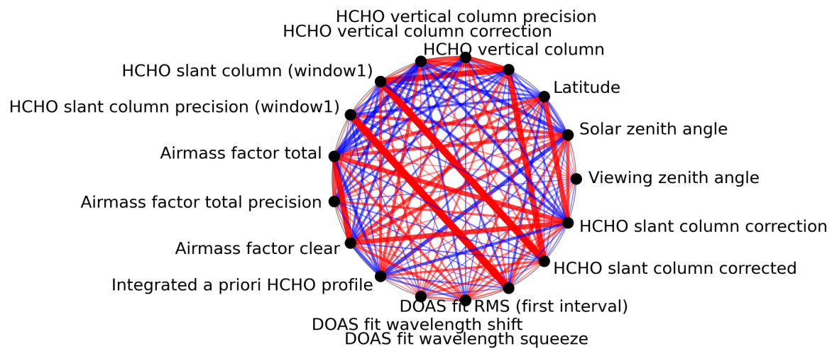
Figure 1: Map of correlation graph for 2024-05-05 to 2024-05-07.
