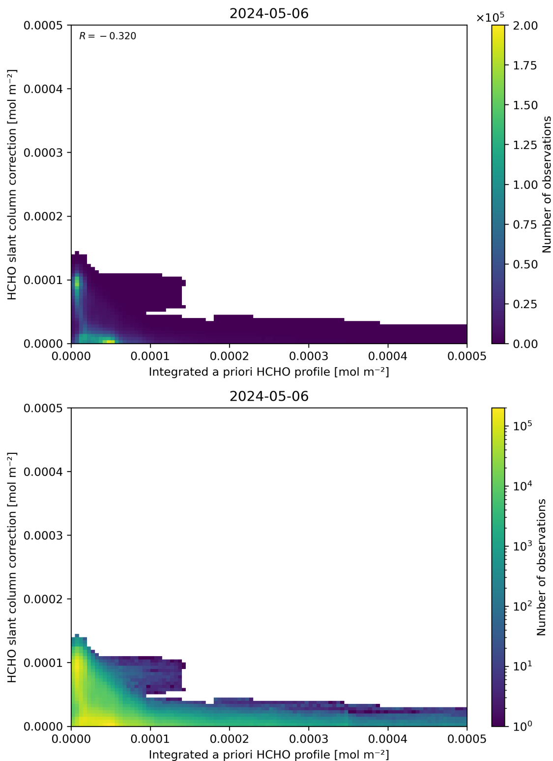
Figure 152: Scatter density plot of “Integrated a priori HCHO profile” against “HCHO slant column correction” for 2024-05-05 to 2024-05-07.
