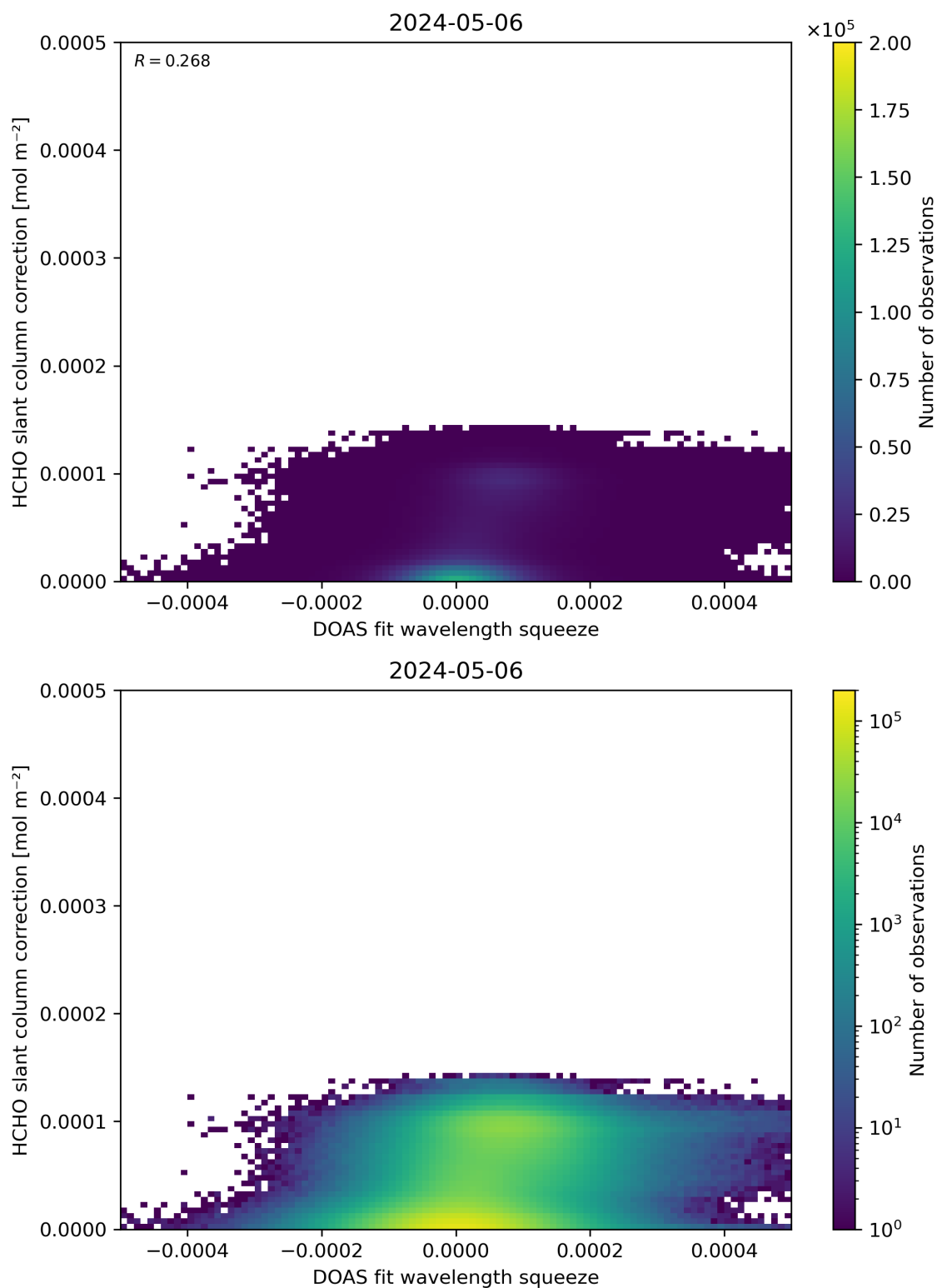
Figure 70: Scatter density plot of “DOAS fit wavelength squeeze” against “HCHO slant column correction” for 2024-05-05 to 2024-05-07.
