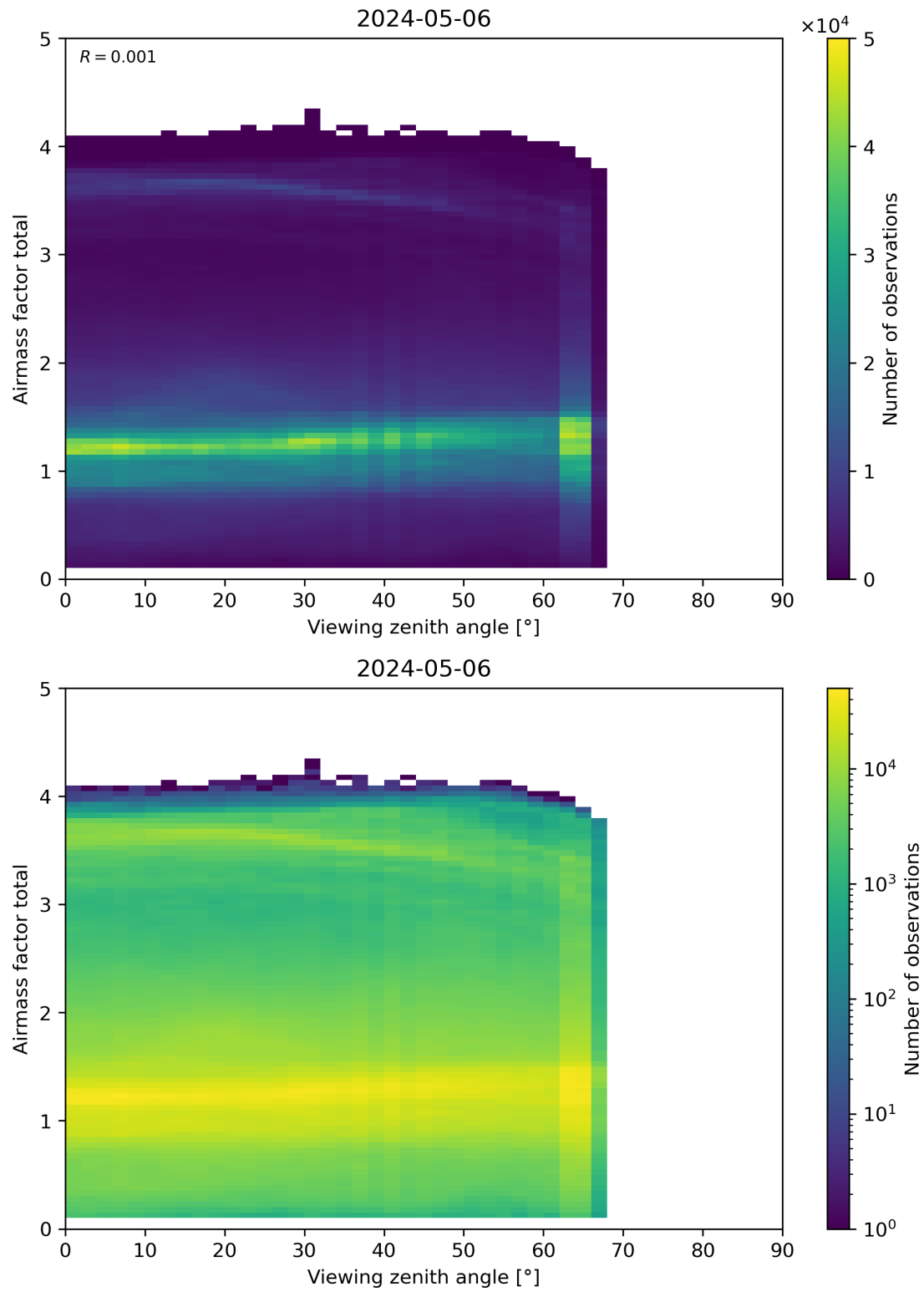
Figure 190: Scatter density plot of “Viewing zenith angle” against “Airmass factor total” for 2024-05-05 to 2024-05-07.
