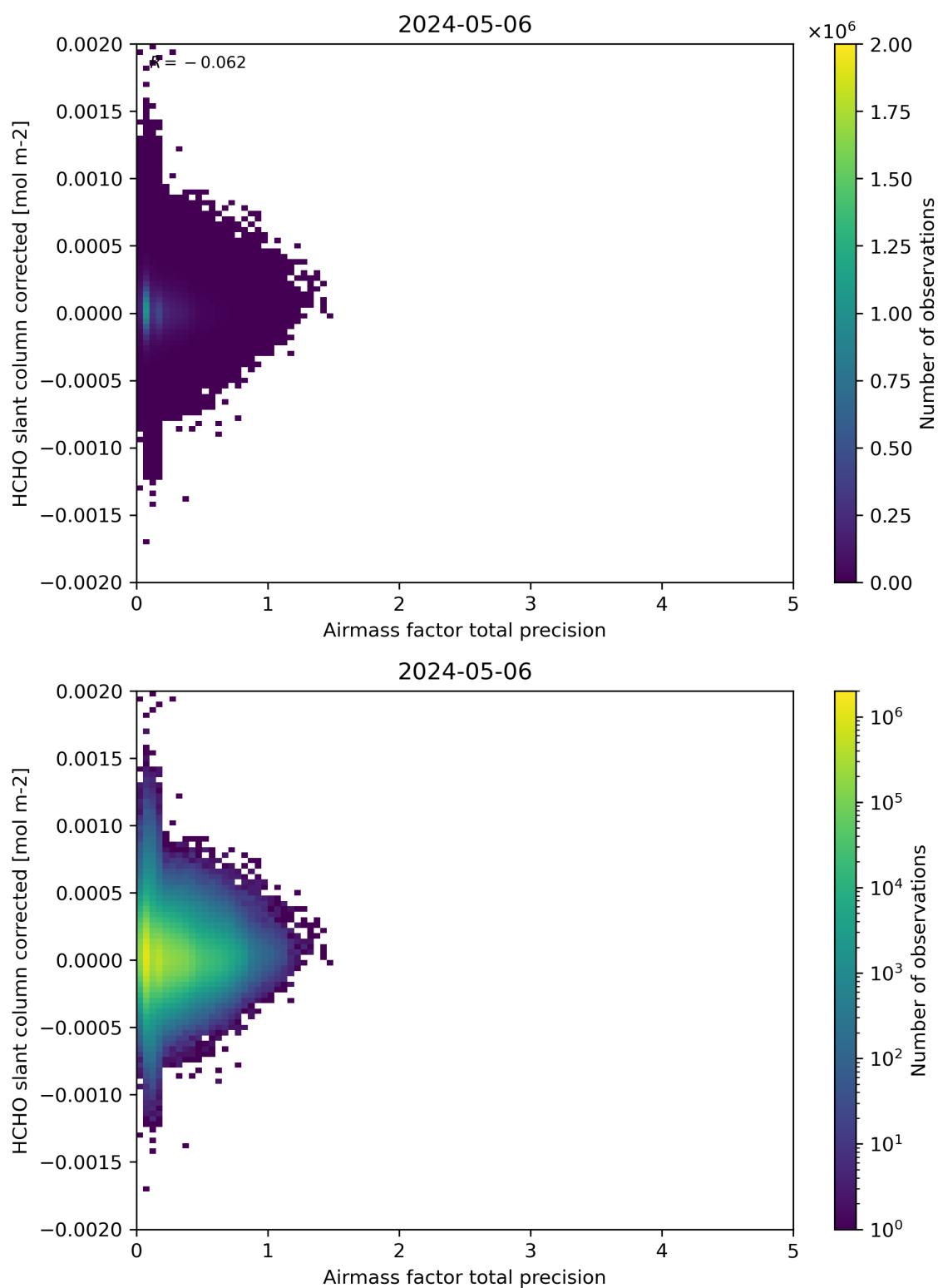
Figure 109: Scatter density plot of “Airmass factor total precision” against “HCHO slant column corrected” for 2024-05-05 to 2024-05-07.
