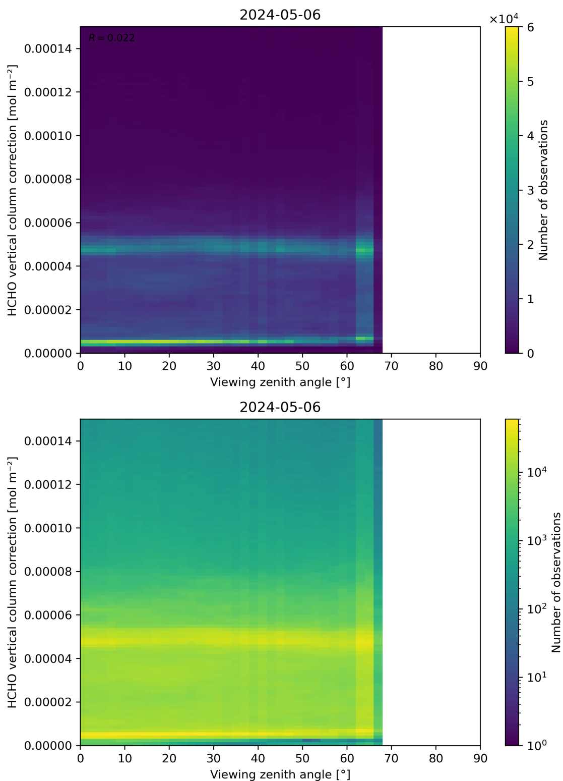
Figure 193: Scatter density plot of “Viewing zenith angle” against “HCHO vertical column correction” for 2024-05-05 to 2024-05-07.
