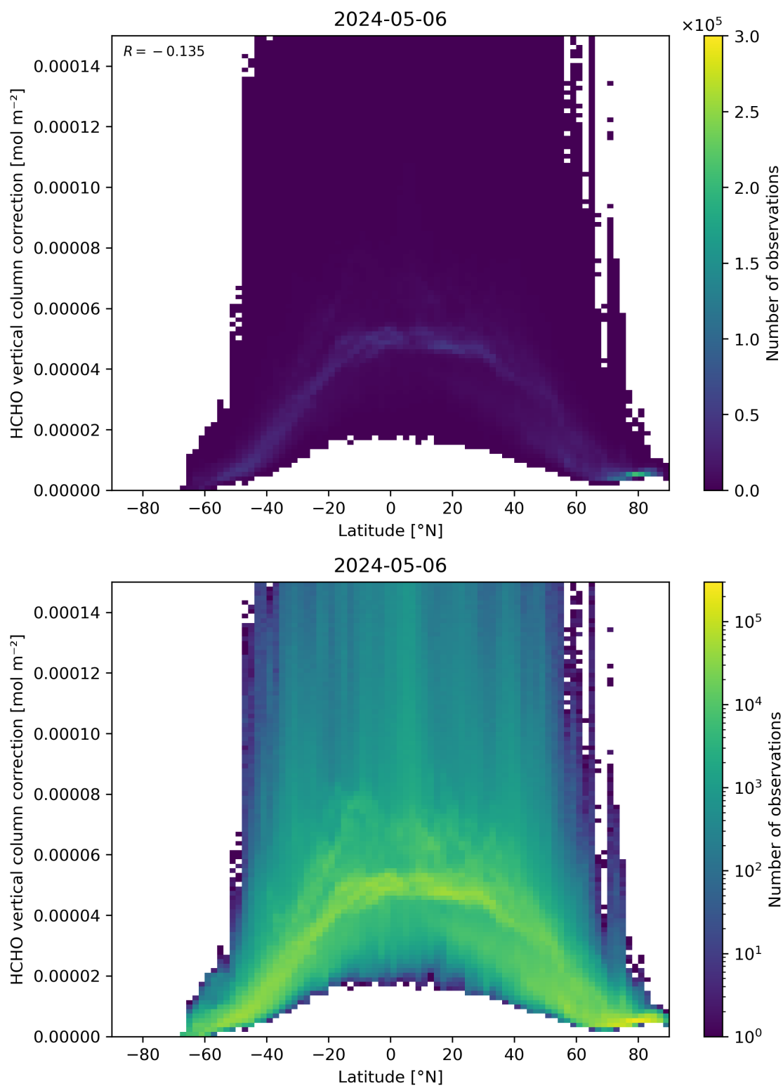
Figure 164: Scatter density plot of “Latitude” against “HCHO vertical column correction” for 2024-05-05 to 2024-05-07.
