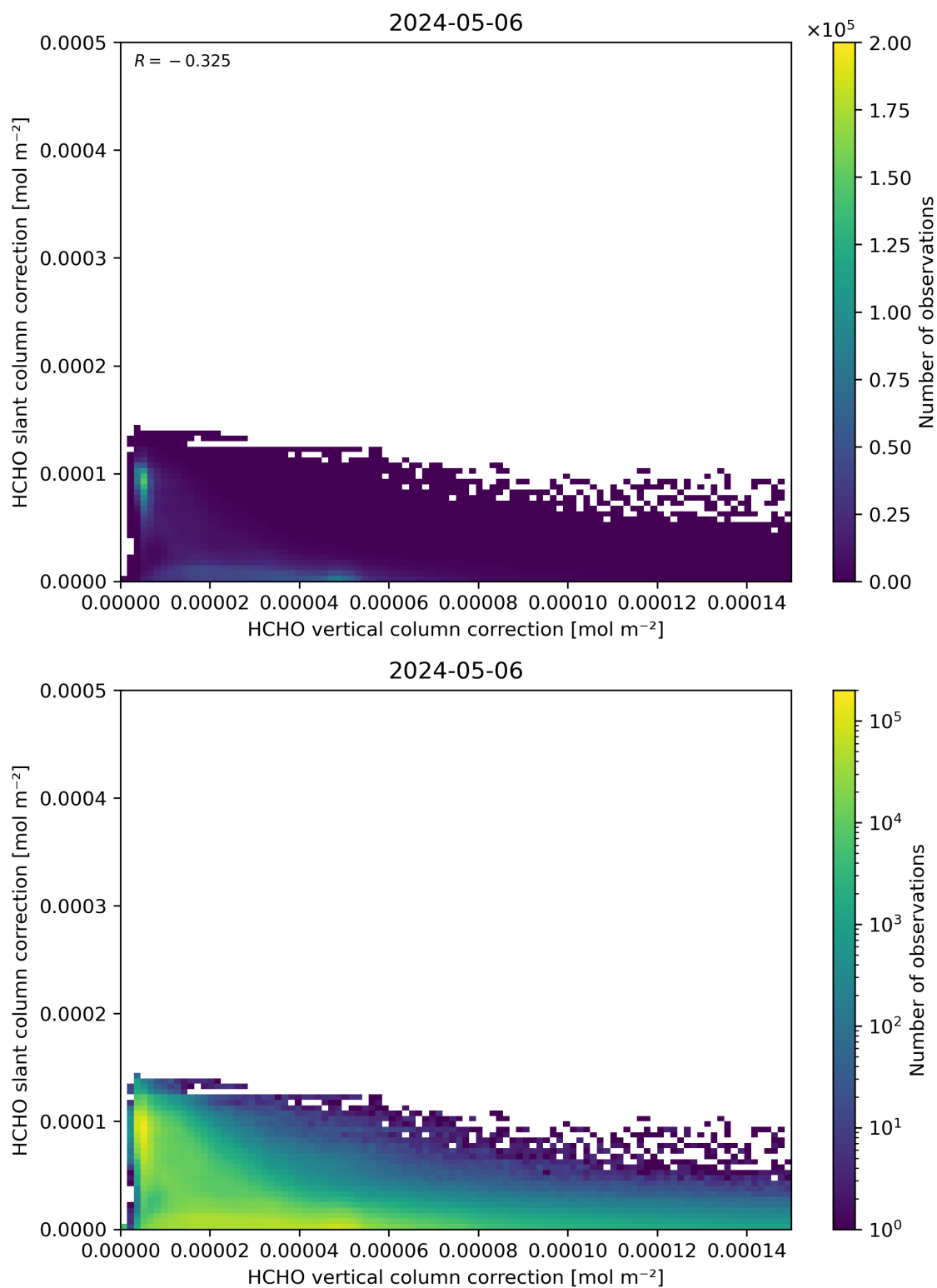
Figure 117: Scatter density plot of “HCHO vertical column correction” against “HCHO slant column correction” for 2024-05-05 to 2024-05-07.
