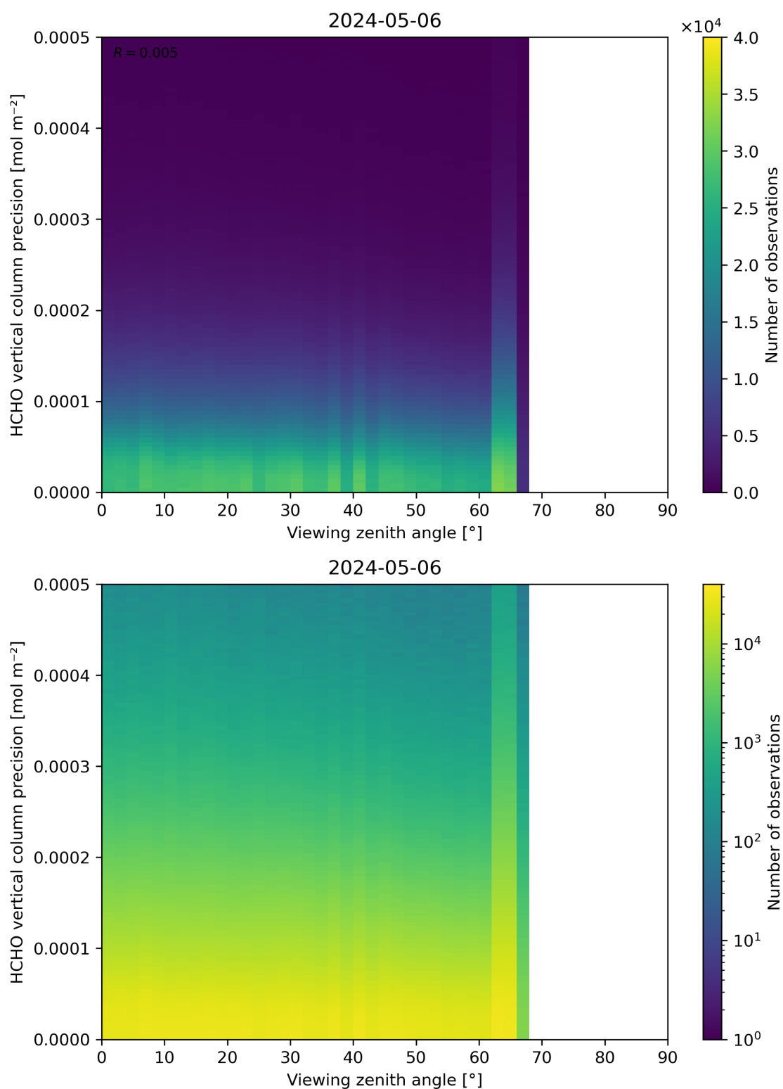
Figure 194: Scatter density plot of “Viewing zenith angle” against “HCHO vertical column precision” for 2024-05-05 to 2024-05-07.
