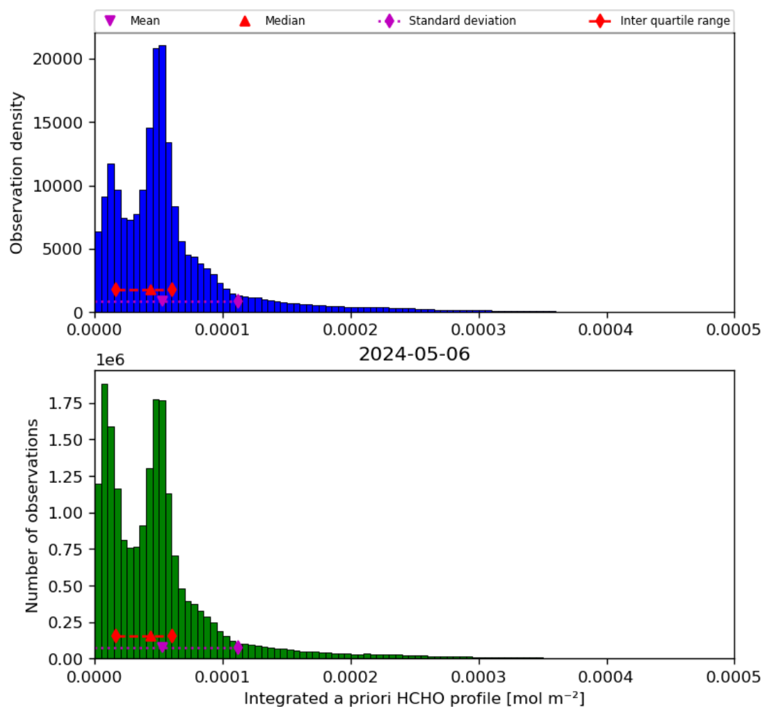
Figure 43: Histogram of “Integrated a priori HCHO profile” for 2024-05-05 to 2024-05-07
