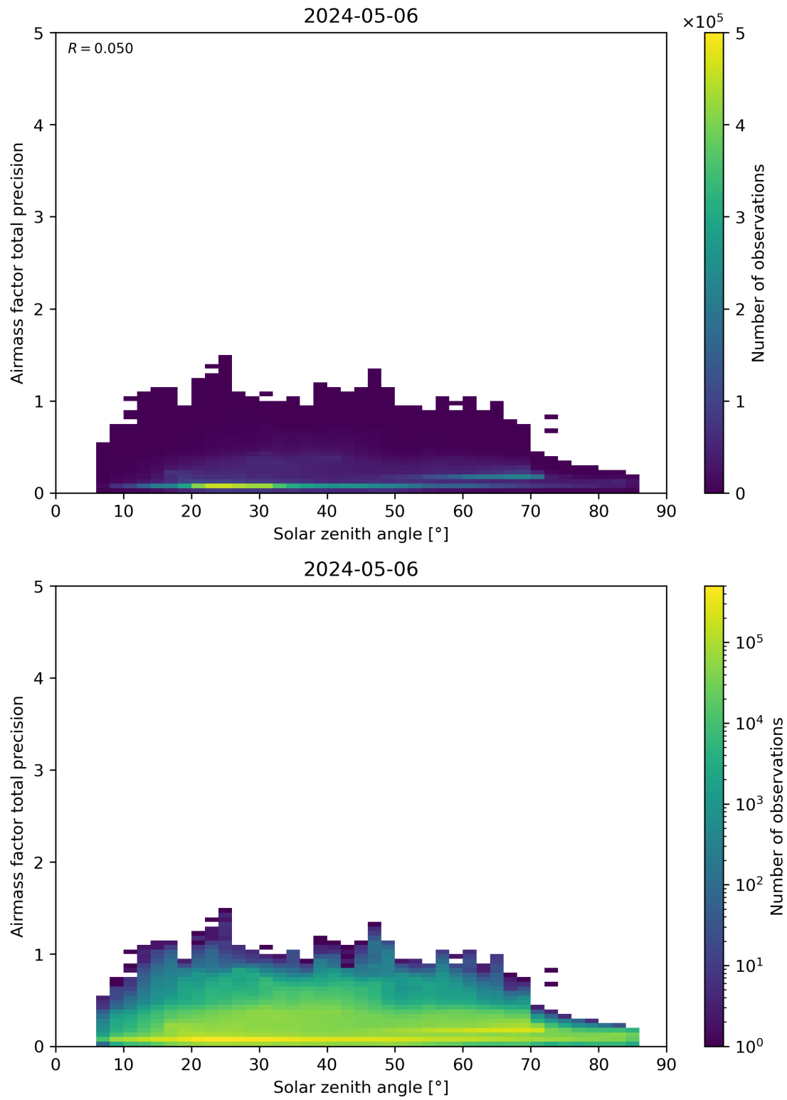
Figure 176: Scatter density plot of “Solar zenith angle” against “Airmass factor total precision” for 2024-05-05 to 2024-05-07.
