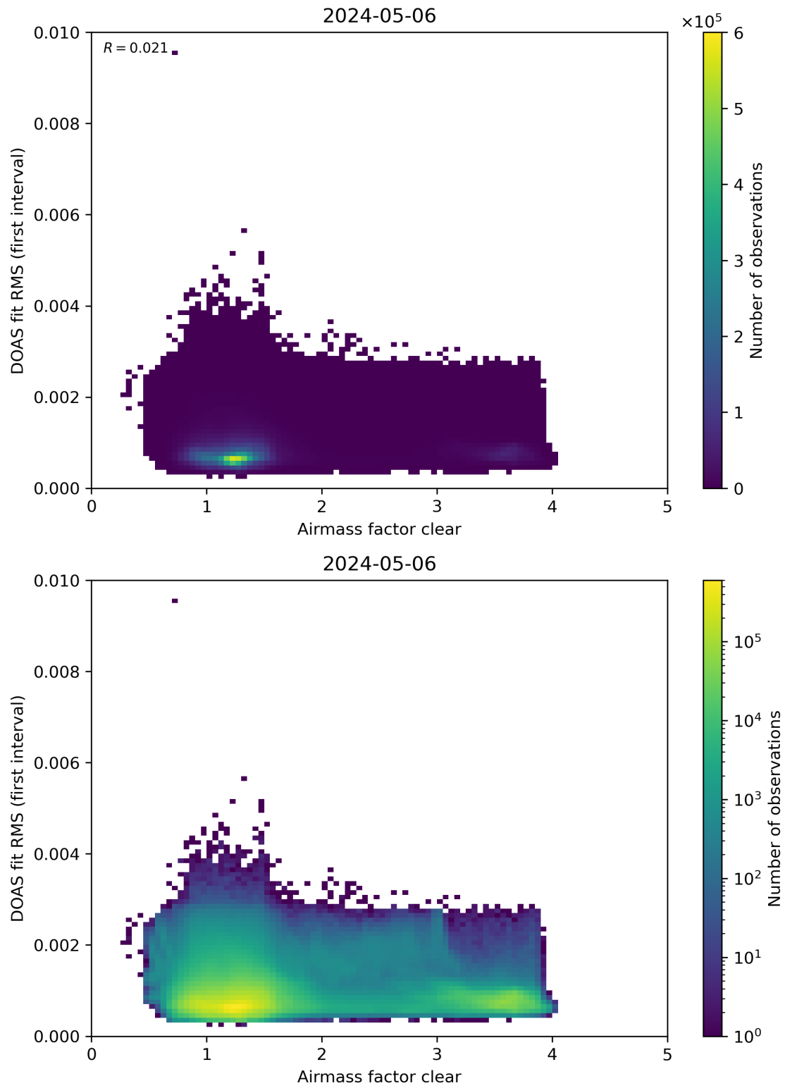
Figure 71: Scatter density plot of “Airmass factor clear” against “DOAS fit RMS (first interval)” for 2024-05-05 to 2024-05-07.
