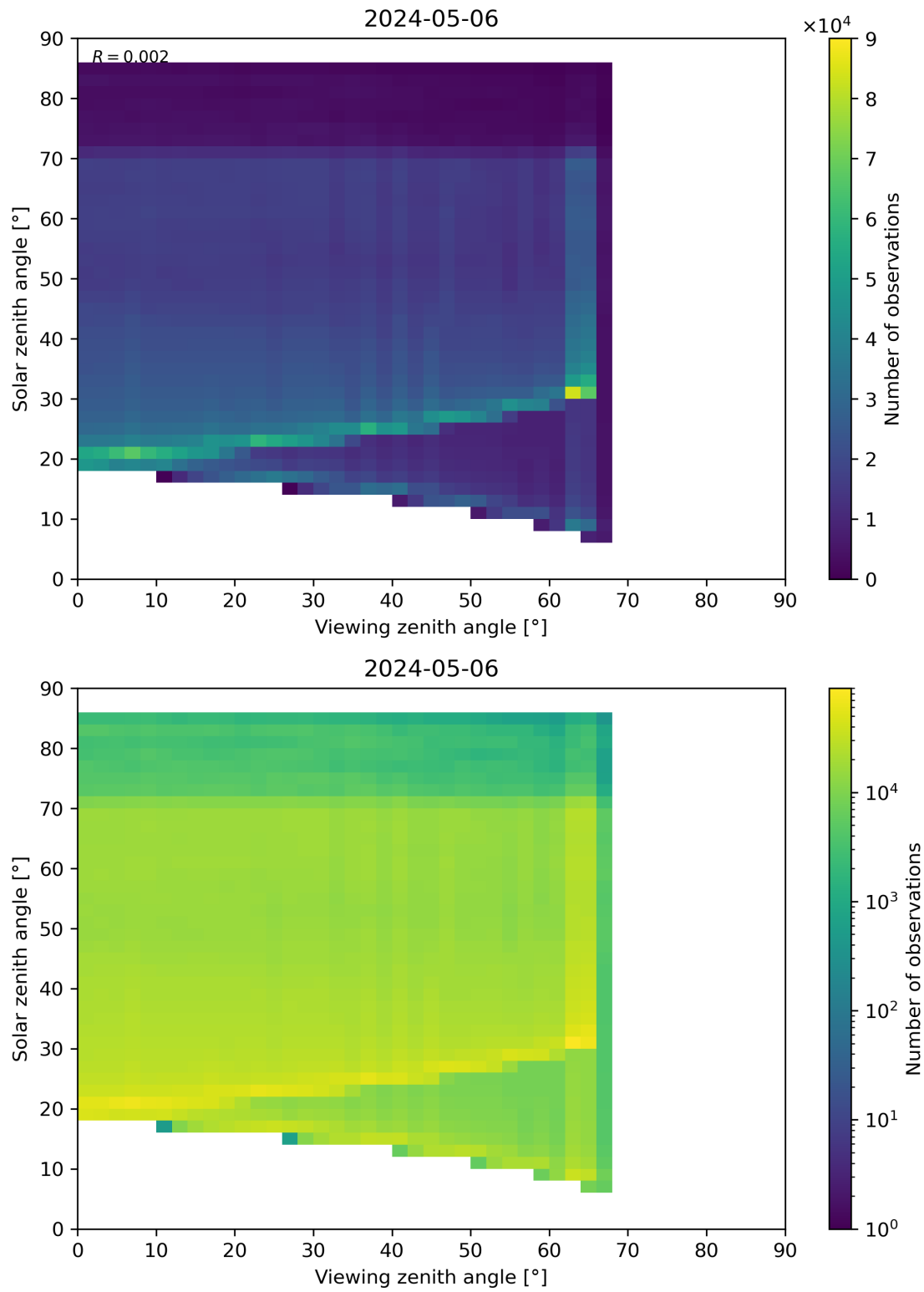
Figure 197: Scatter density plot of “Viewing zenith angle” against “Solar zenith angle” for 2024-05-05 to 2024-05-07.
