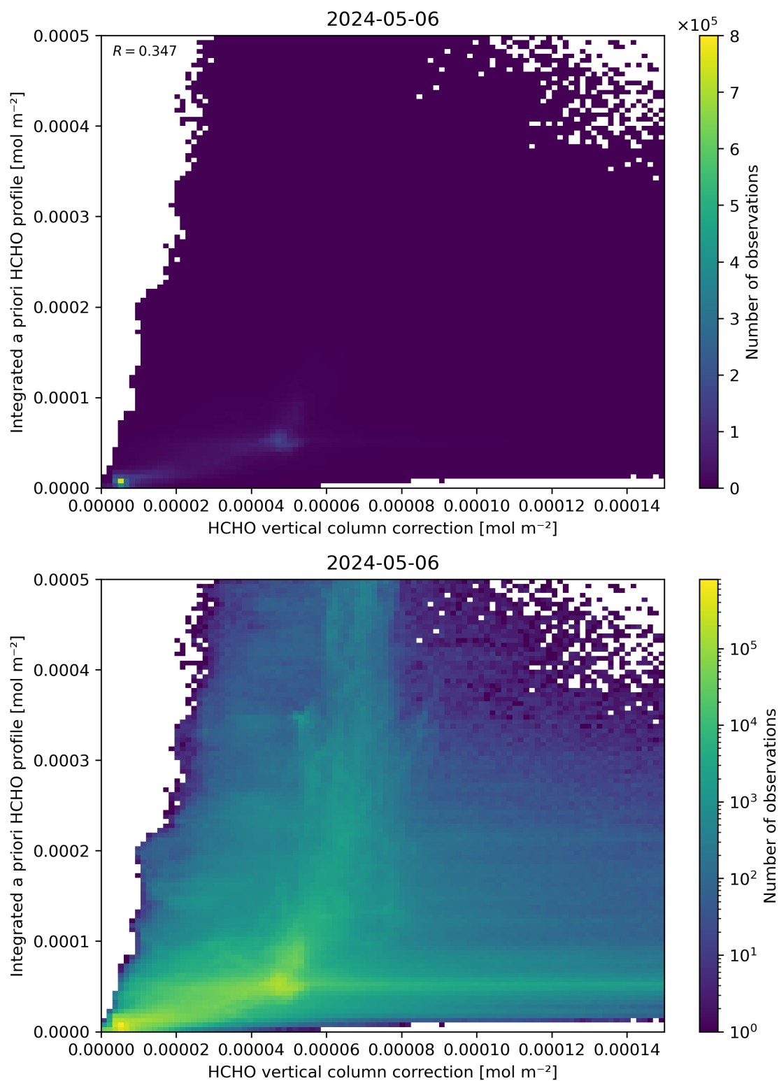
Figure 122: Scatter density plot of “HCHO vertical column correction” against “Integrated a priori HCHO profile” for 2024-05-05 to 2024-05-07.
