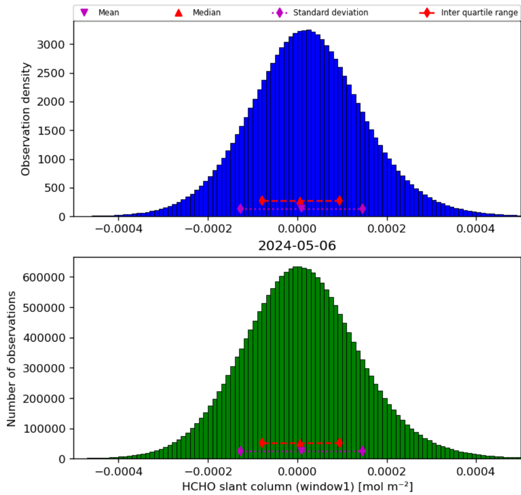
Figure 38: Histogram of “HCHO slant column (window1)” for 2024-05-05 to 2024-05-07
