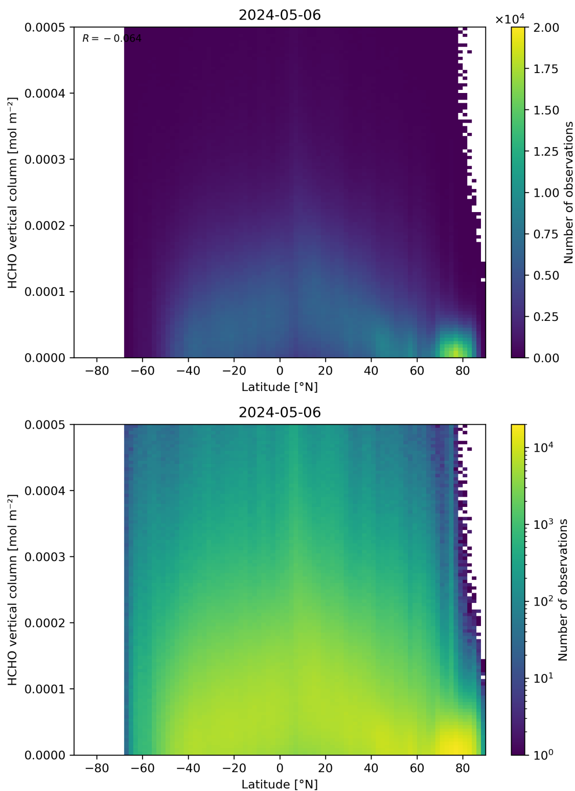
Figure 163: Scatter density plot of “Latitude” against “HCHO vertical column” for 2024-05-05 to 2024-05-07.
