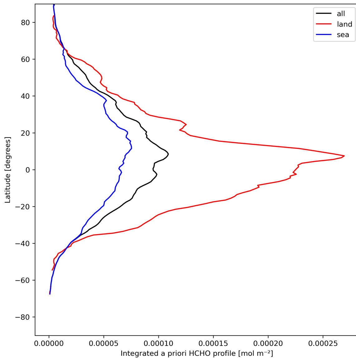
Figure 29: Zonal average of “Integrated a priori HCHO profile” for 2024-05-05 to 2024-05-07.
