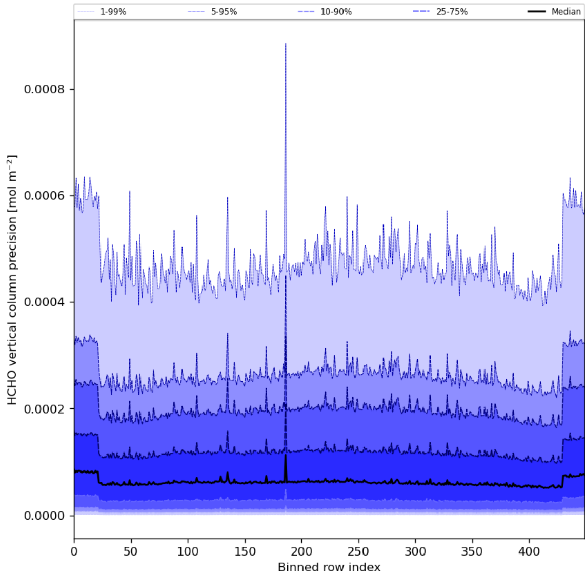
Figure 50: Along track statistics of “HCHO vertical column precision” for 2024-05-05 to 2024-05-07
