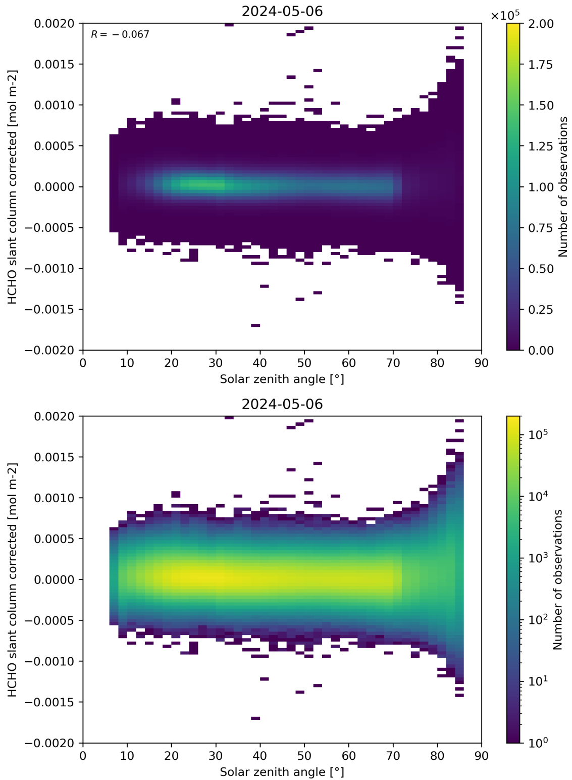
Figure 171: Scatter density plot of “Solar zenith angle” against “HCHO slant column corrected” for 2024-05-05 to 2024-05-07.
