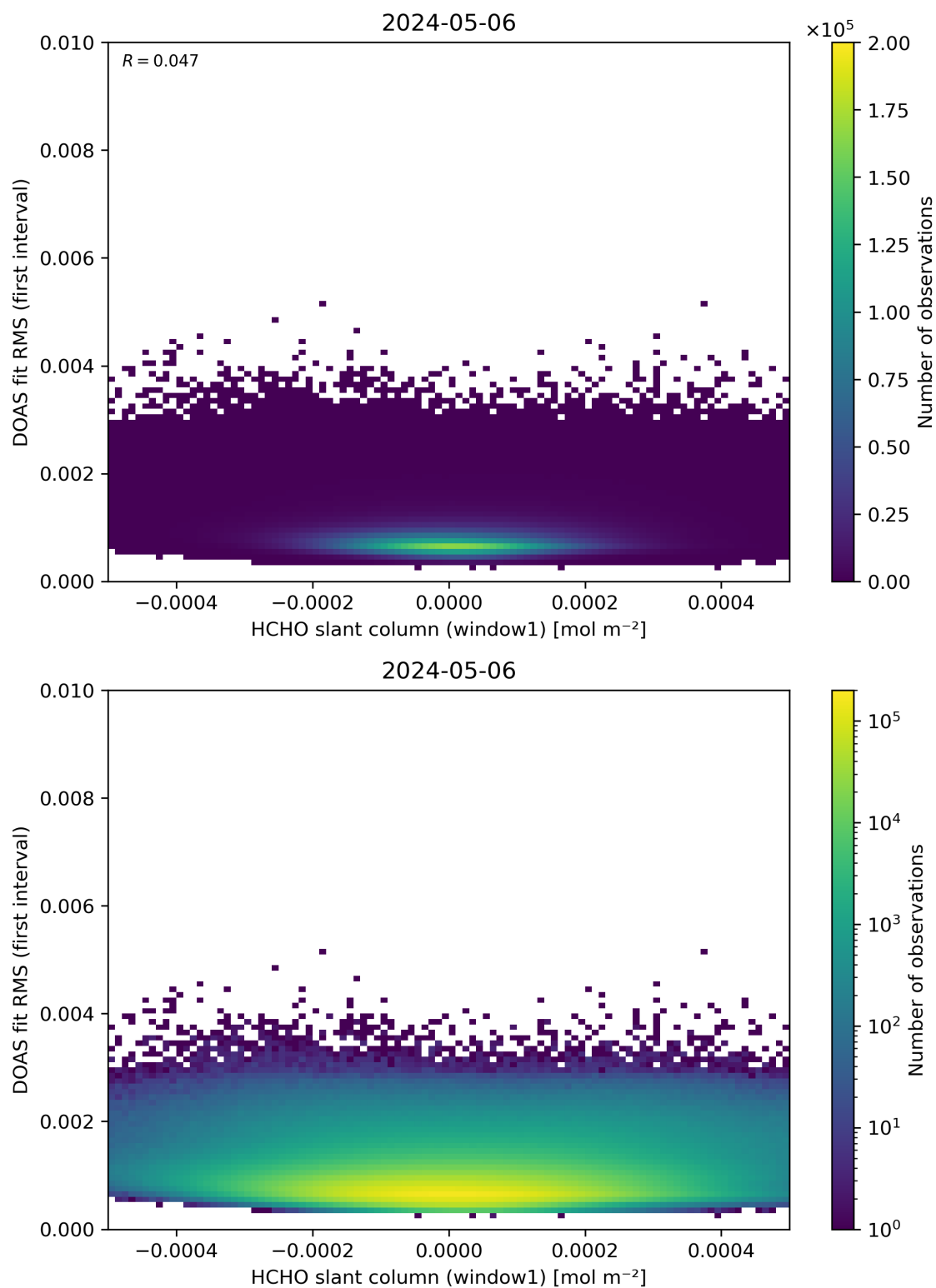
Figure 78: Scatter density plot of “HCHO slant column (window1)” against “DOAS fit RMS (first interval)” for 2024-05-05 to 2024-05-07.
