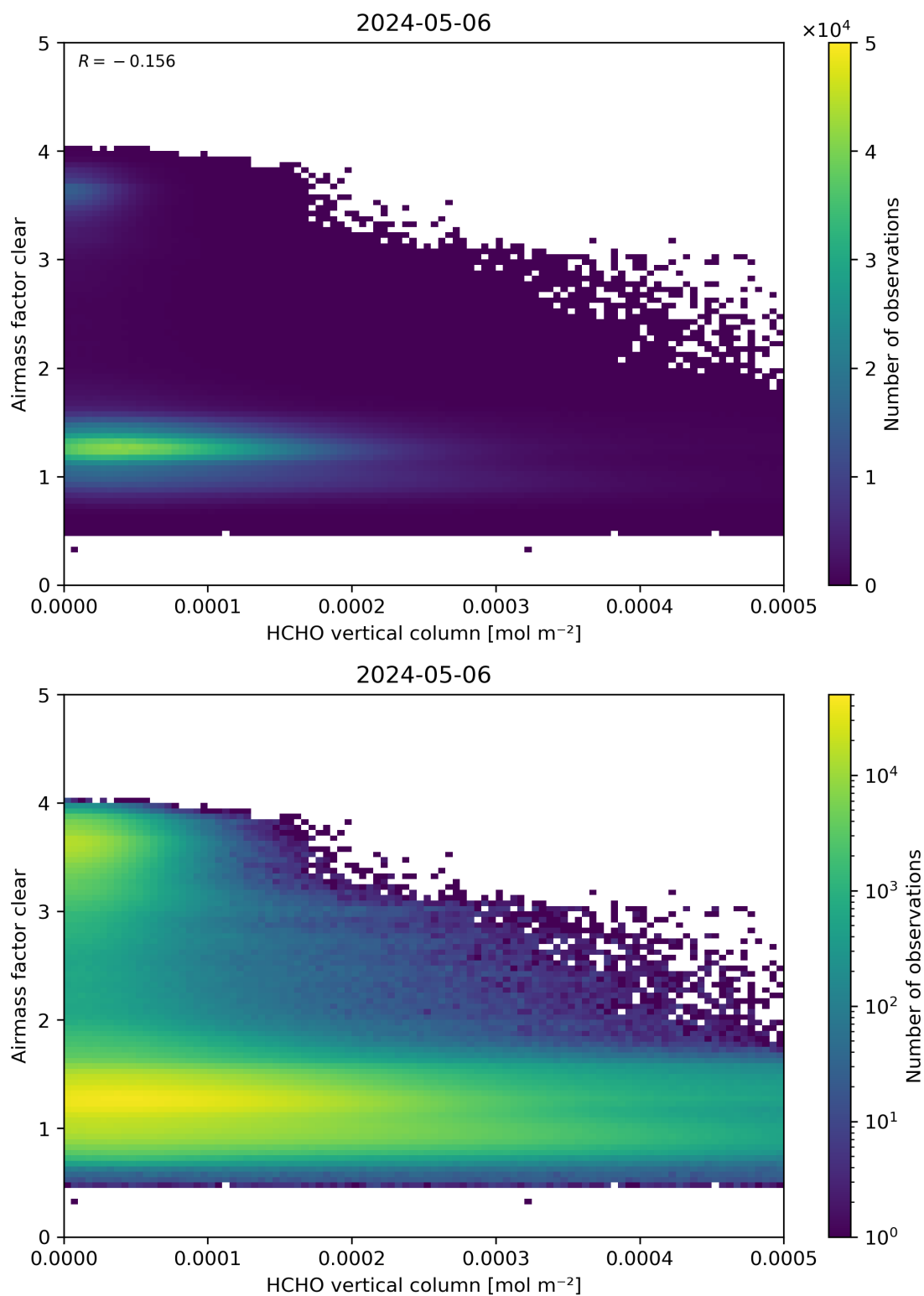
Figure 126: Scatter density plot of “HCHO vertical column” against “Airmass factor clear” for 2024-05-05 to 2024-05-07.
