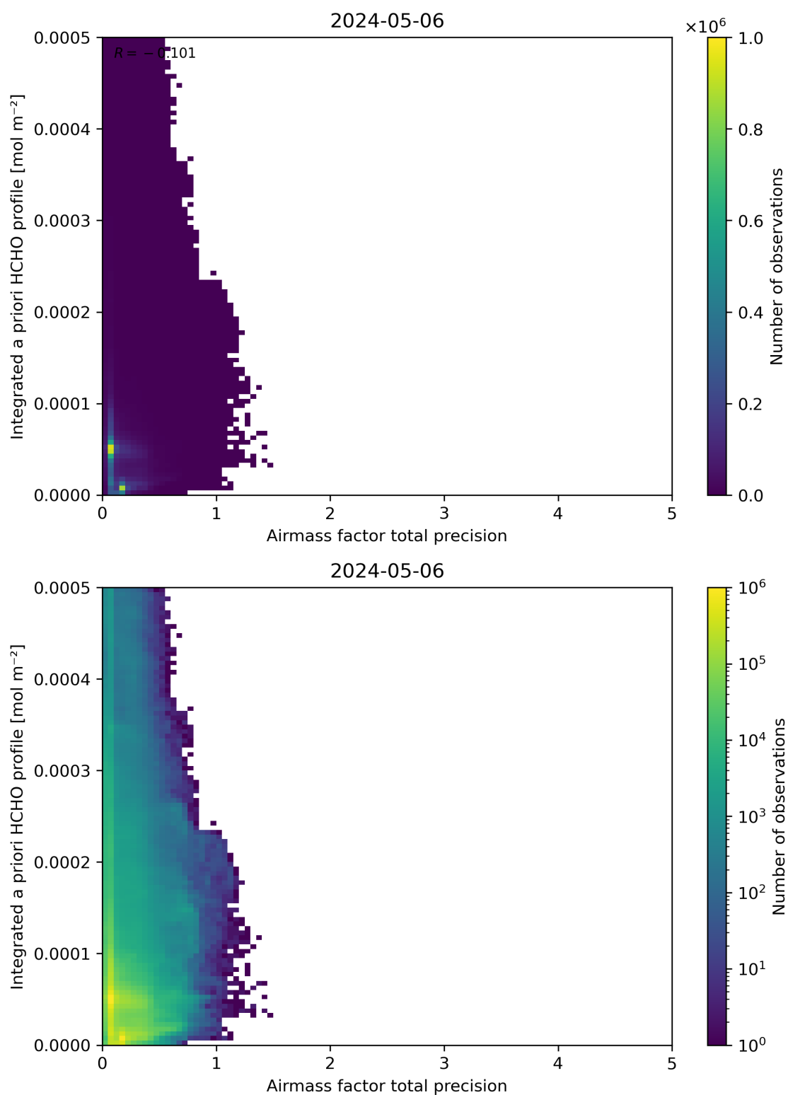
Figure 111: Scatter density plot of “Airmass factor total precision” against “Integrated a priori HCHO profile” for 2024-05-05 to 2024-05-07.
