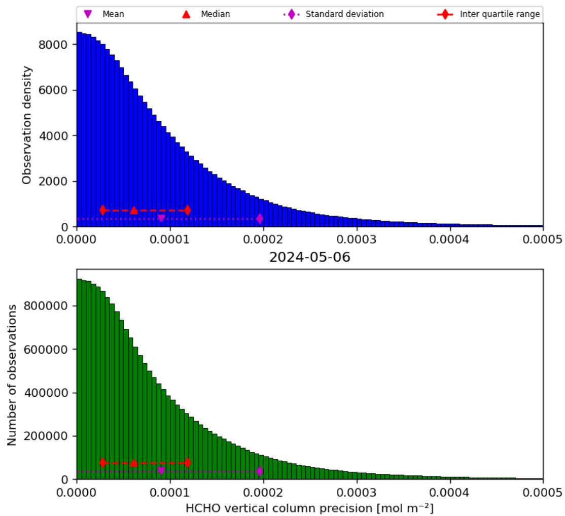
Figure 36: Histogram of “HCHO vertical column precision” for 2024-05-05 to 2024-05-07
