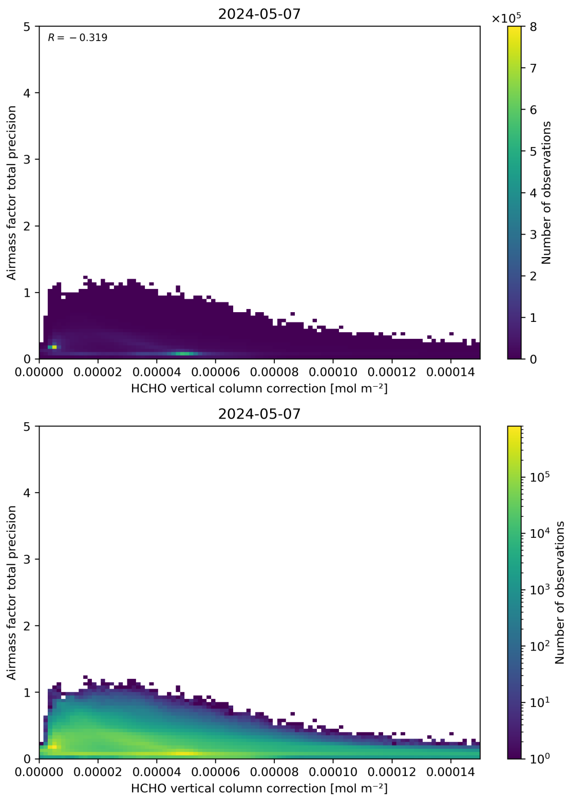
Figure 121: Scatter density plot of “HCHO vertical column correction” against “Airmass factor total precision” for 2024-05-07 to 2024-05-08.
