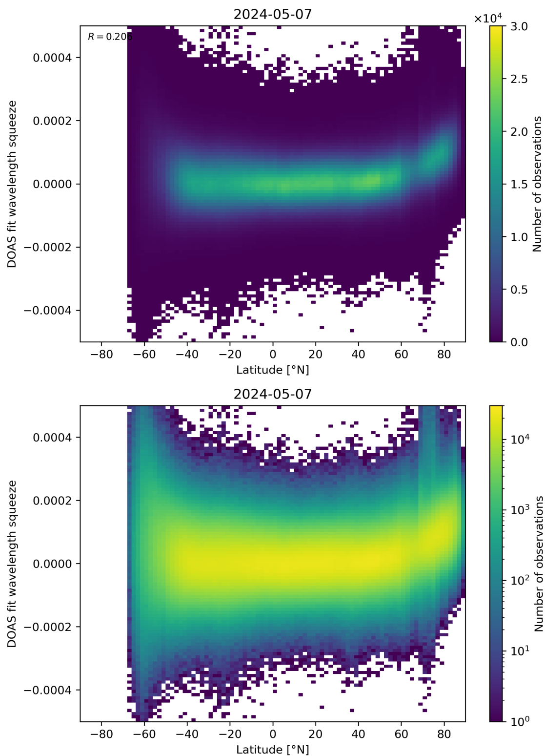
Figure 155: Scatter density plot of “Latitude” against “DOAS fit wavelength squeeze” for 2024-05-07 to 2024-05-08.
