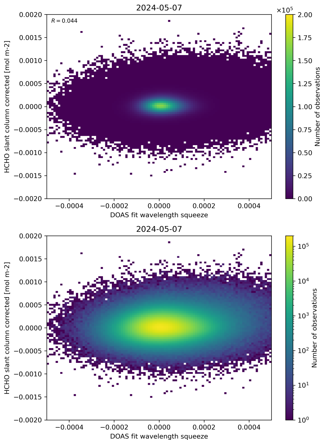
Figure 69: Scatter density plot of “DOAS fit wavelength squeeze” against “HCHO slant column corrected” for 2024-05-07 to 2024-05-08.
