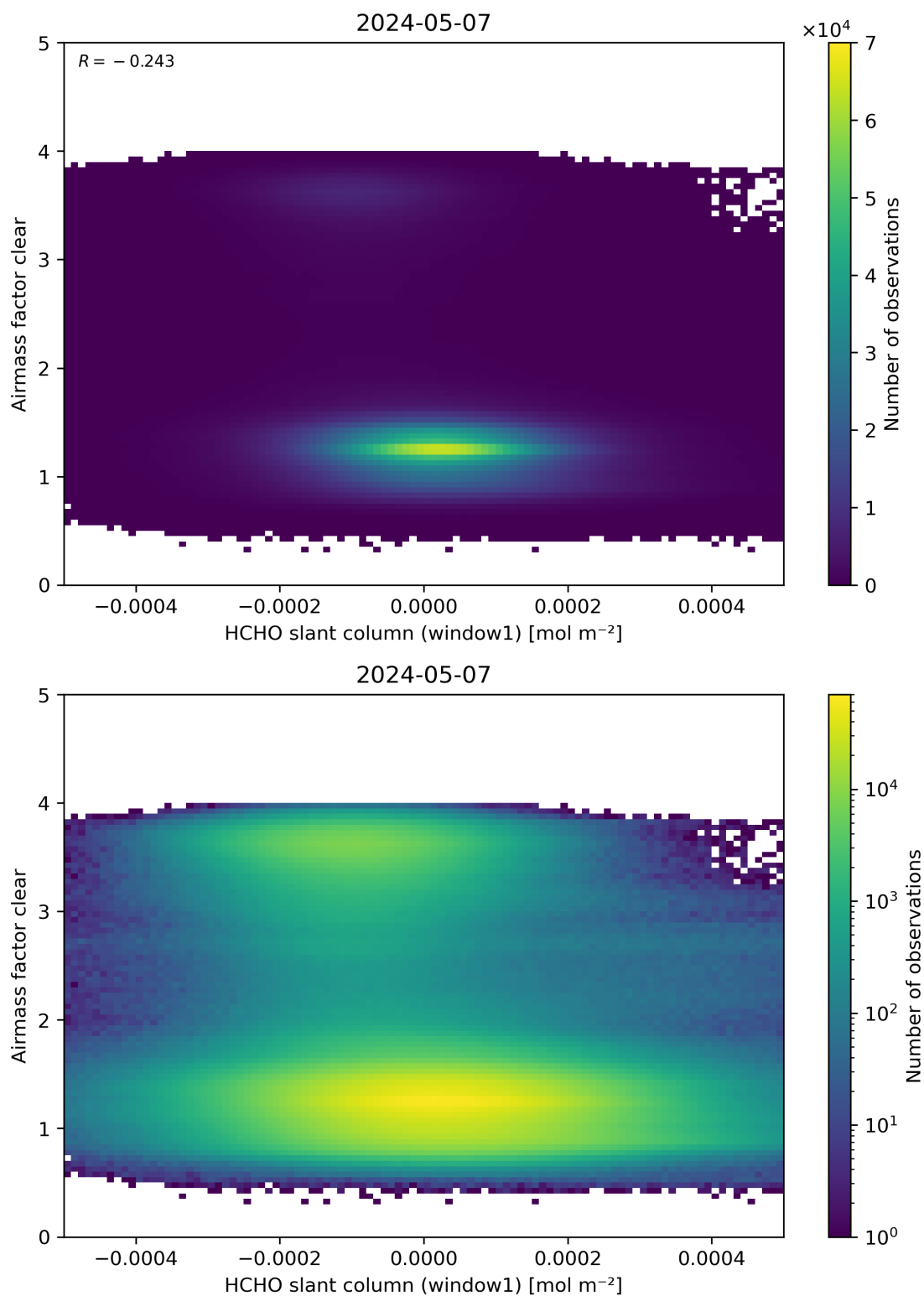
Figure 81: Scatter density plot of “HCHO slant column (window1)” against “Airmass factor clear” for 2024-05-07 to 2024-05-08.
