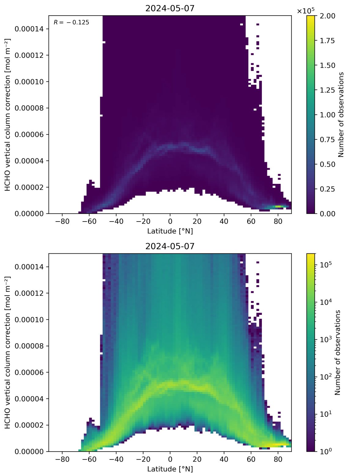
Figure 164: Scatter density plot of “Latitude” against “HCHO vertical column correction” for 2024-05-07 to 2024-05-08.
