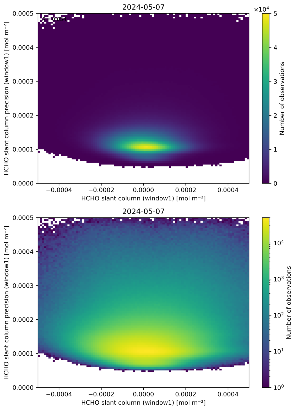
Figure 84: Scatter density plot of “HCHO slant column (window1)” against “HCHO slant column precision (window1)” for 2024-05-07 to 2024-05-08.
