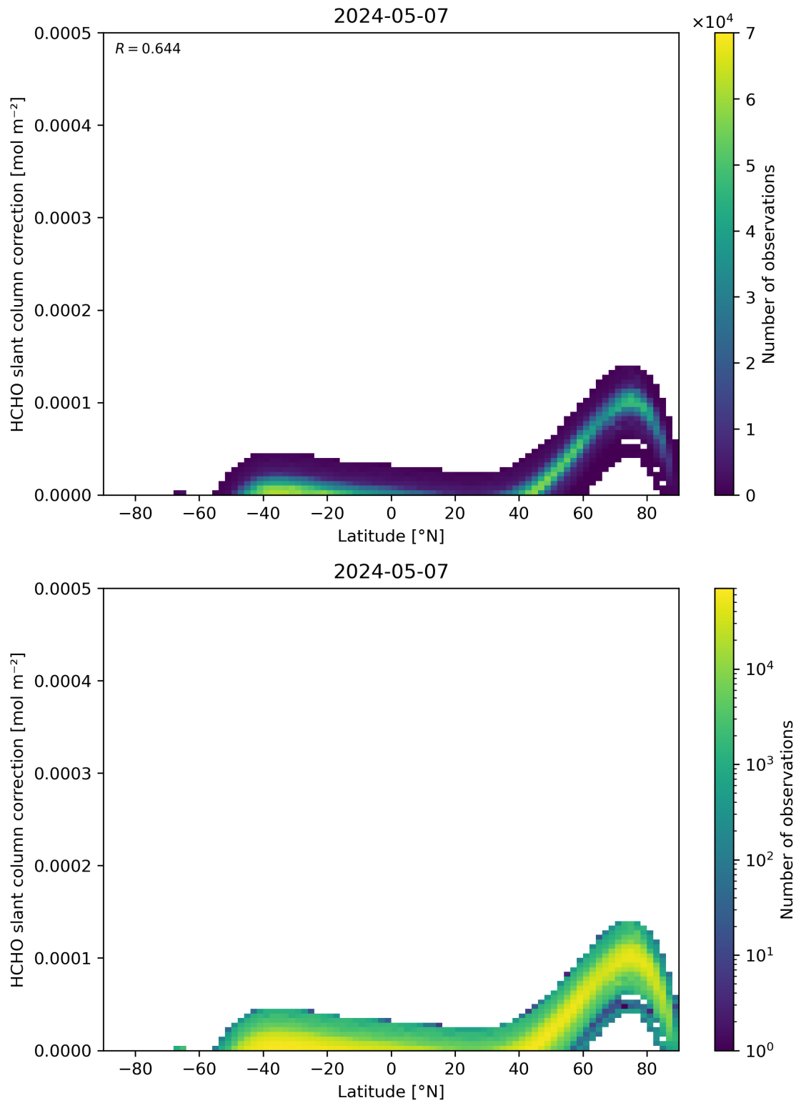
Figure 158: Scatter density plot of “Latitude” against “HCHO slant column correction” for 2024-05-07 to 2024-05-08.
