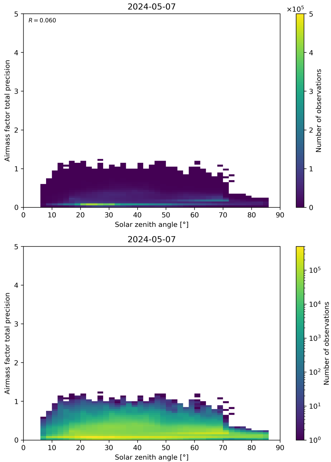
Figure 176: Scatter density plot of “Solar zenith angle” against “Airmass factor total precision” for 2024-05-07 to 2024-05-08.
