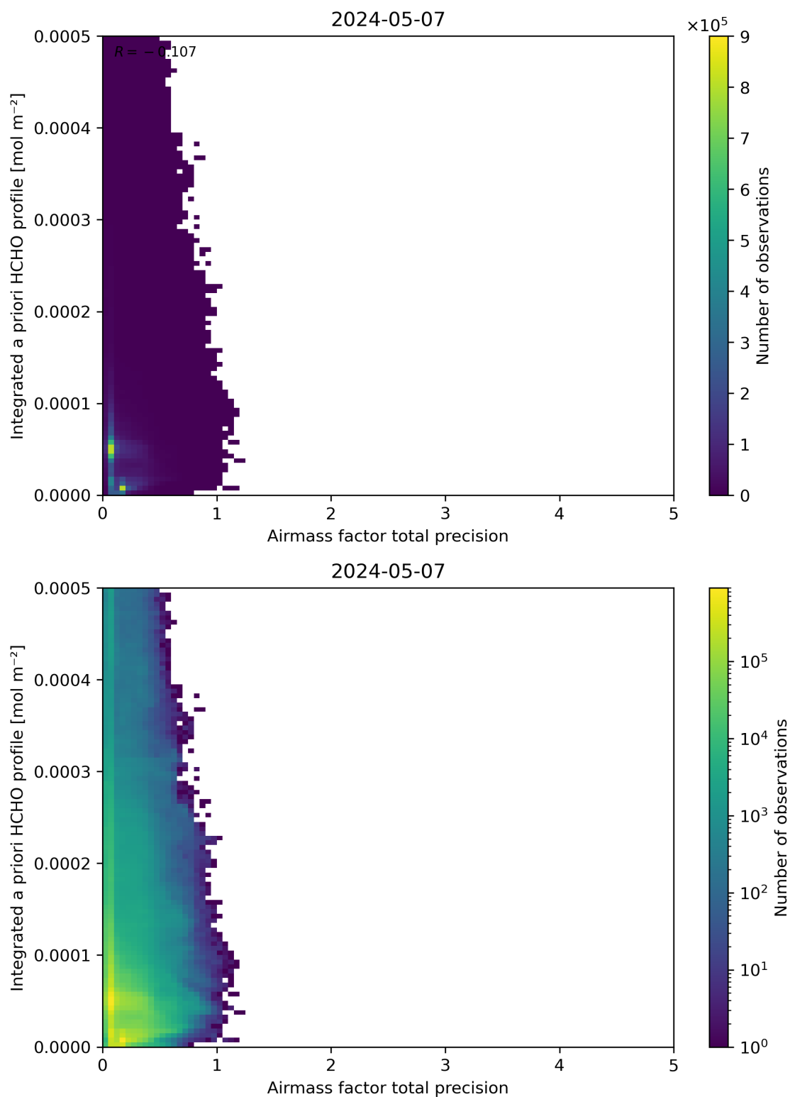
Figure 111: Scatter density plot of “Airmass factor total precision” against “Integrated a priori HCHO profile” for 2024-05-07 to 2024-05-08.
