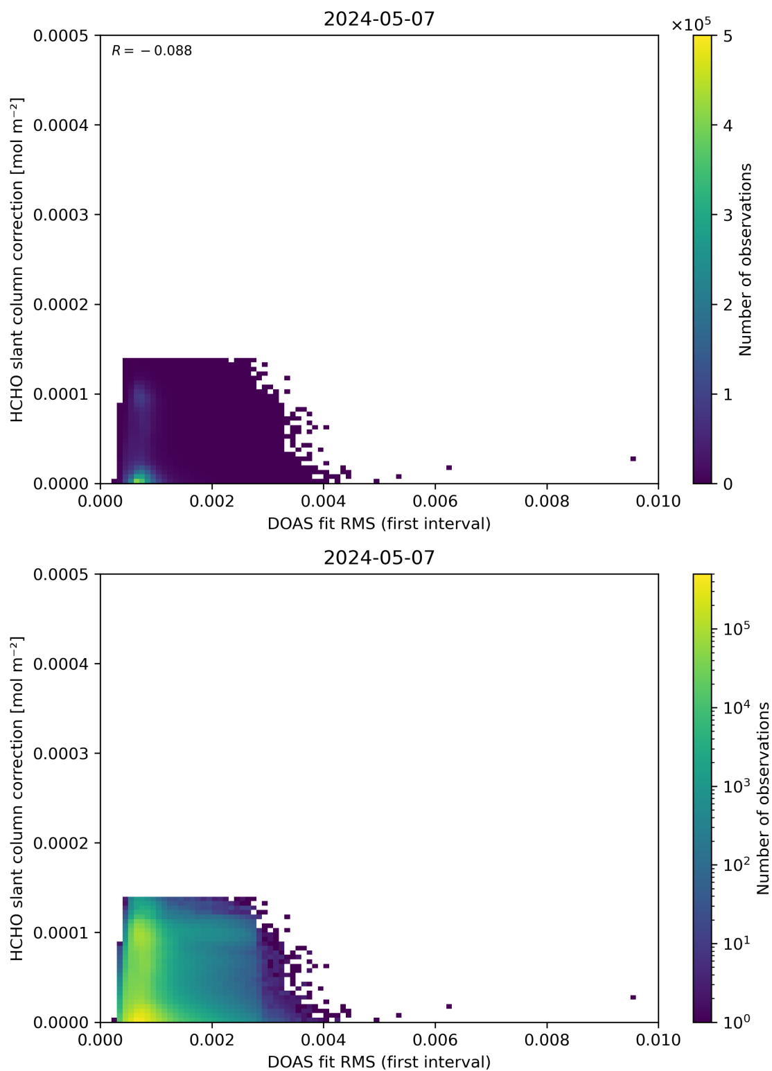
Figure 63: Scatter density plot of “DOAS fit RMS (first interval)” against “HCHO slant column correction” for 2024-05-07 to 2024-05-08.
