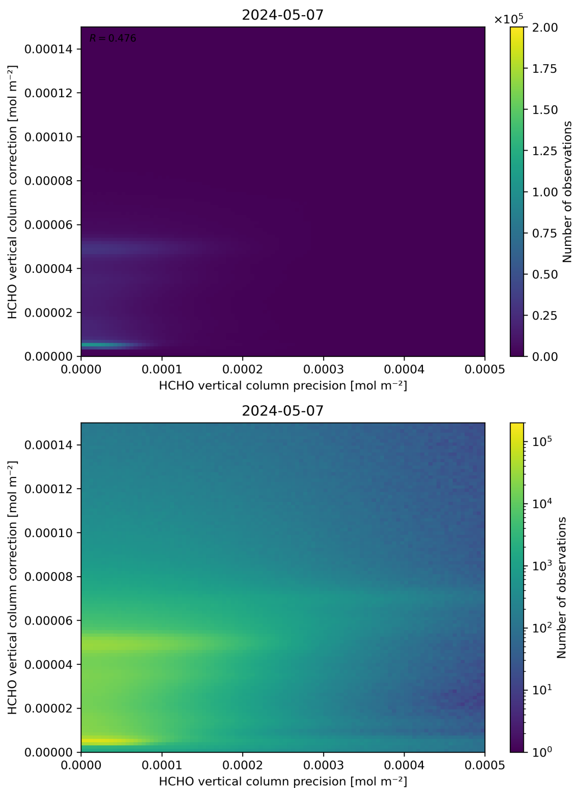
Figure 146: Scatter density plot of “HCHO vertical column precision” against “HCHO vertical column correction” for 2024-05-07 to 2024-05-08.
