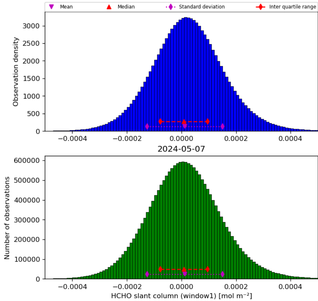
Figure 38: Histogram of “HCHO slant column (window1)” for 2024-05-07 to 2024-05-08
