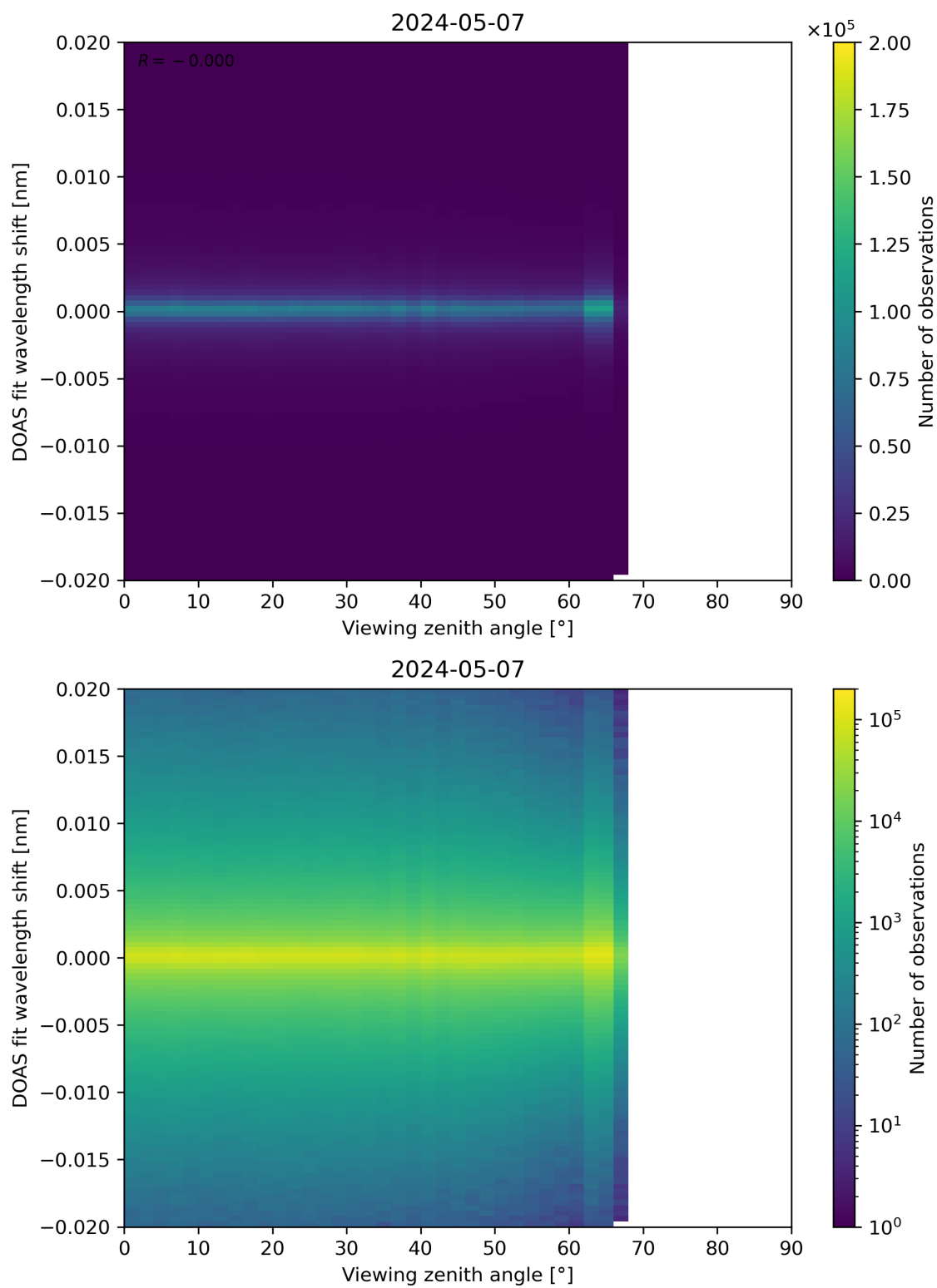
Figure 183: Scatter density plot of “Viewing zenith angle” against “DOAS fit wavelength shift” for 2024-05-07 to 2024-05-08.
