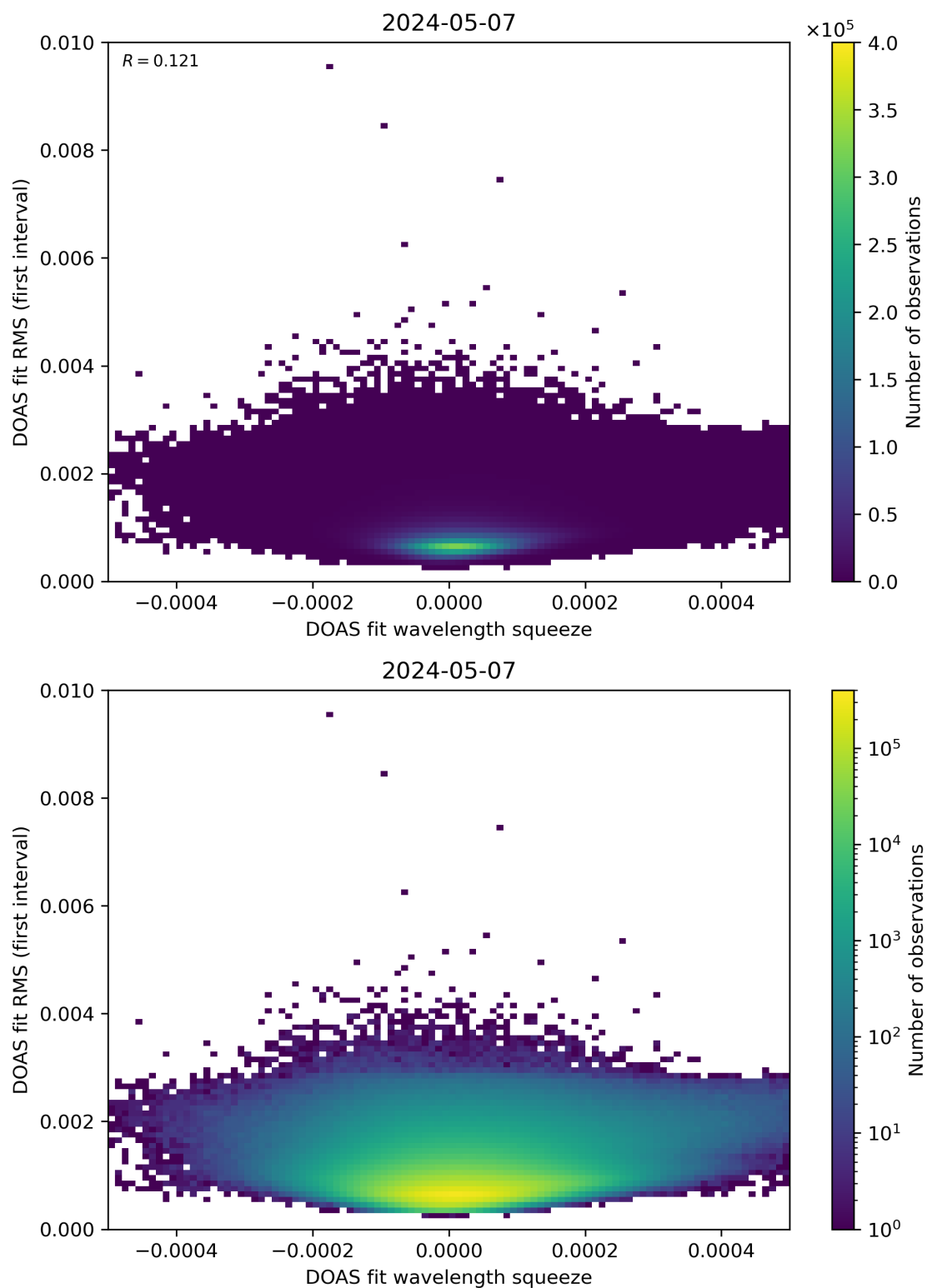
Figure 68: Scatter density plot of “DOAS fit wavelength squeeze” against “DOAS fit RMS (first interval)” for 2024-05-07 to 2024-05-08.
