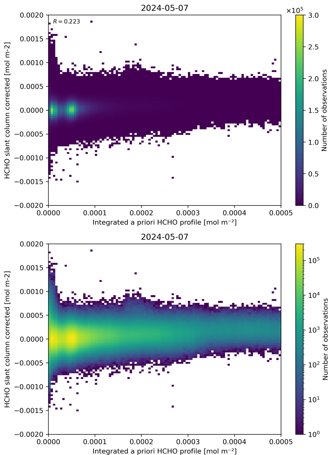
Figure 151: Scatter density plot of “Integrated a priori HCHO profile” against “HCHO slant column corrected” for 2024-05-07 to 2024-05-08.
