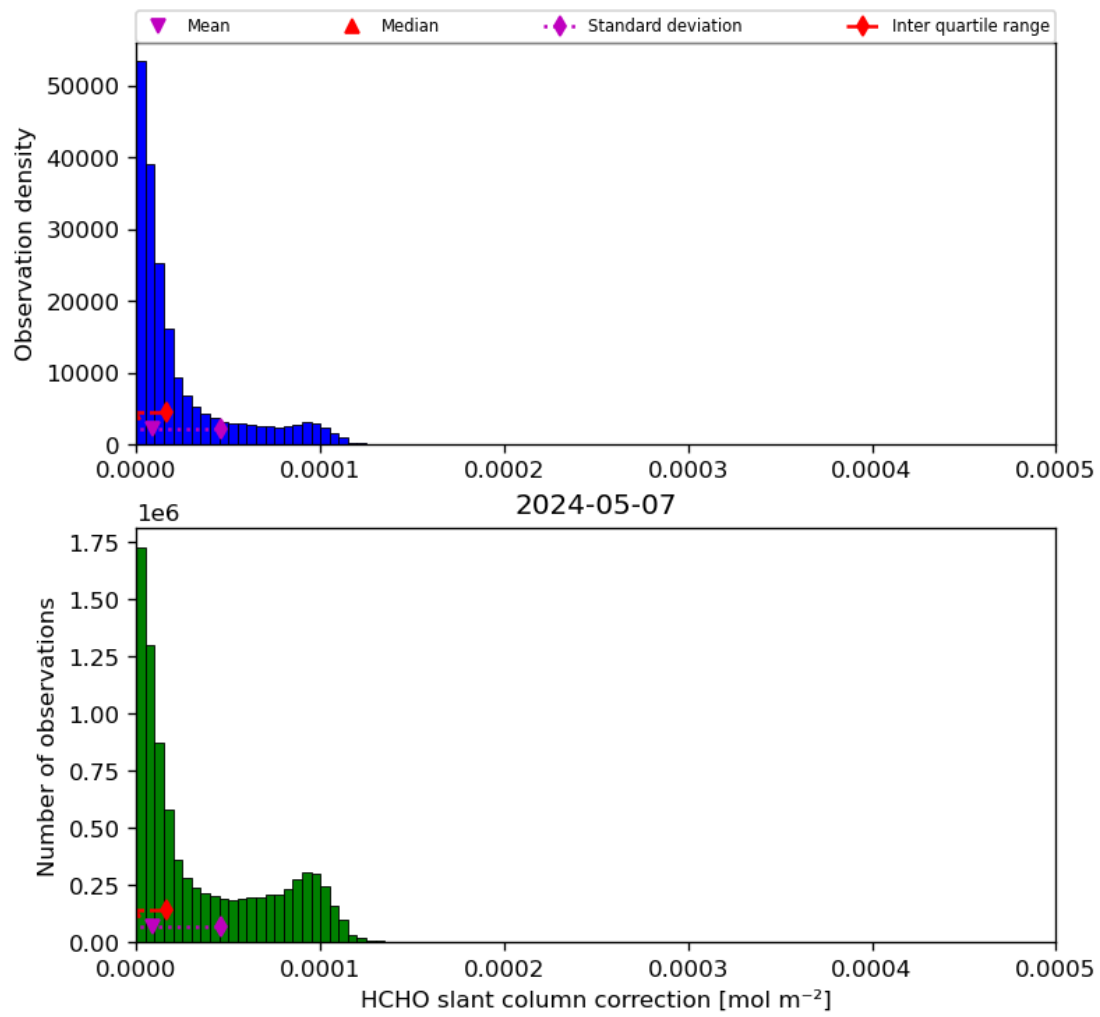
Figure 47: Histogram of “HCHO slant column correction” for 2024-05-07 to 2024-05-08
