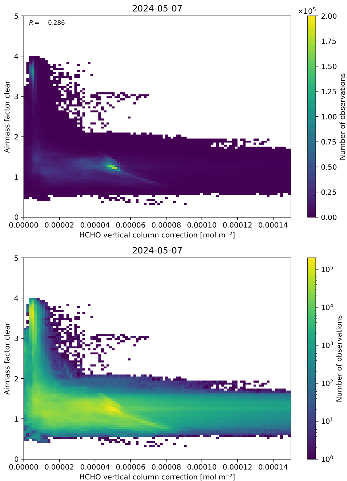
Figure 115: Scatter density plot of “HCHO vertical column correction” against “Airmass factor clear” for 2024-05-07 to 2024-05-08.
