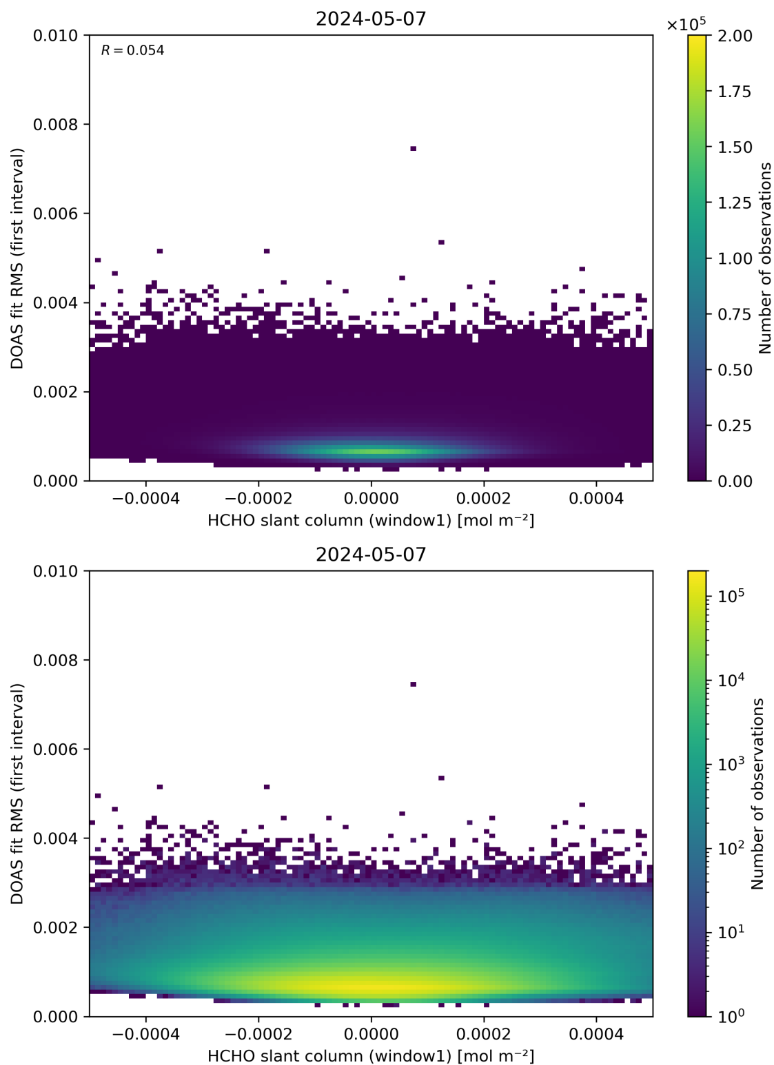
Figure 78: Scatter density plot of “HCHO slant column (window1)” against “DOAS fit RMS (first interval)” for 2024-05-07 to 2024-05-08.
