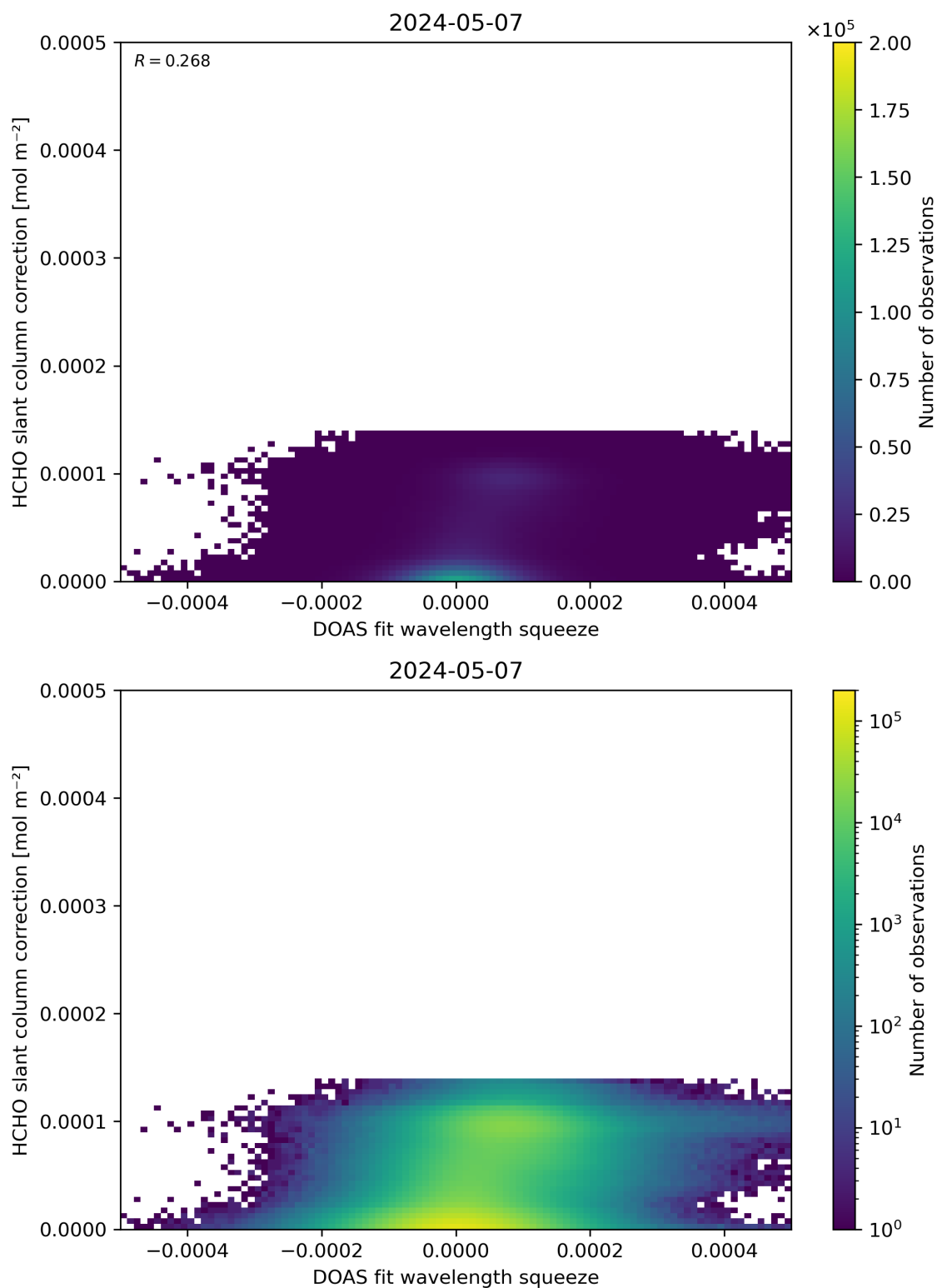
Figure 70: Scatter density plot of “DOAS fit wavelength squeeze” against “HCHO slant column correction” for 2024-05-07 to 2024-05-08.
