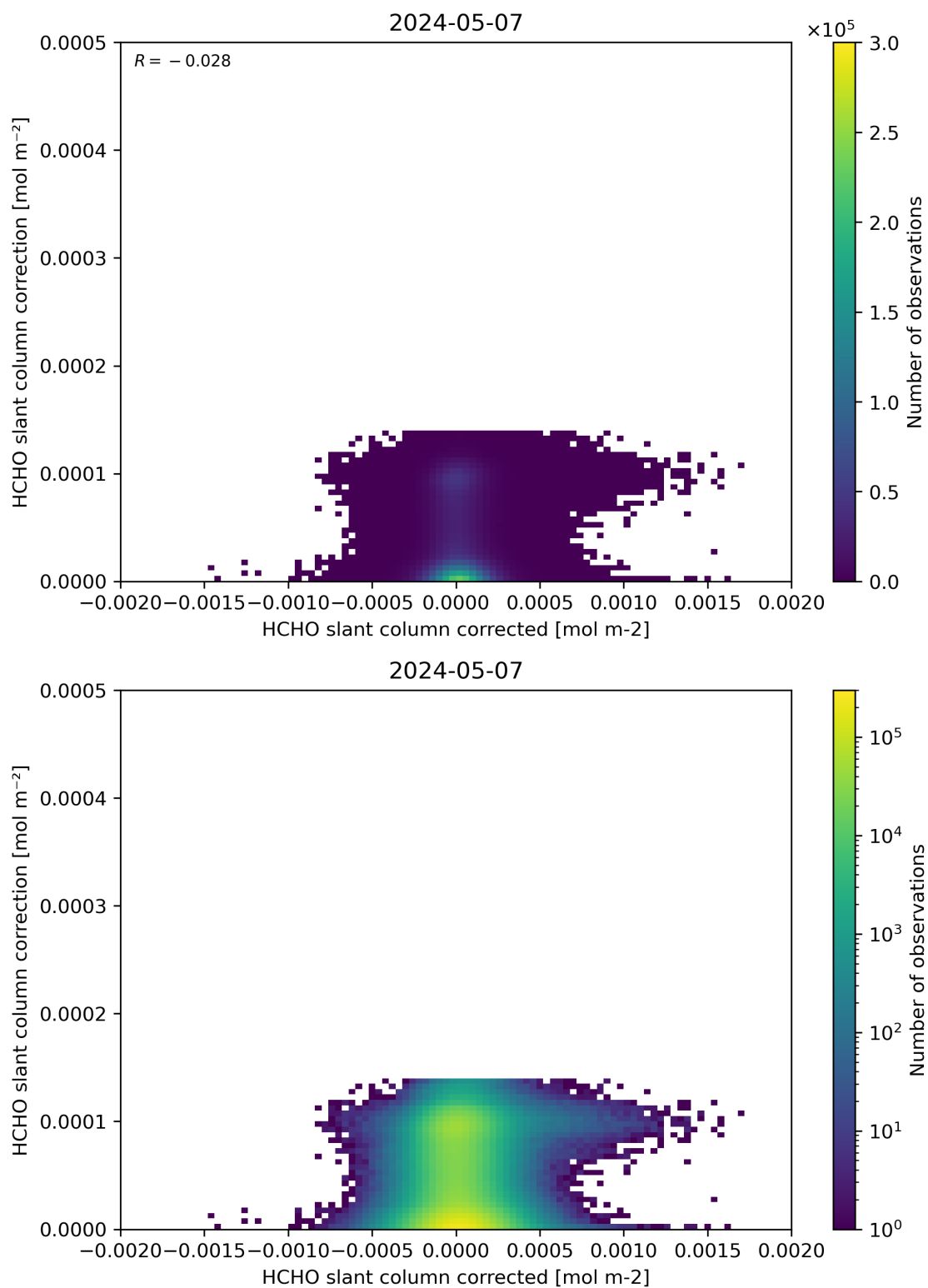
Figure 77: Scatter density plot of “HCHO slant column corrected” against “HCHO slant column correction” for 2024-05-07 to 2024-05-08.
