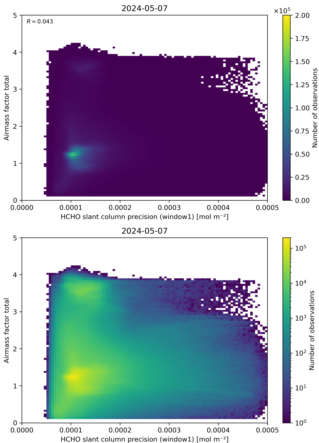
Figure 94: Scatter density plot of “HCHO slant column precision (window1)” against “Airmass factor total” for 2024-05-07 to 2024-05-08.
