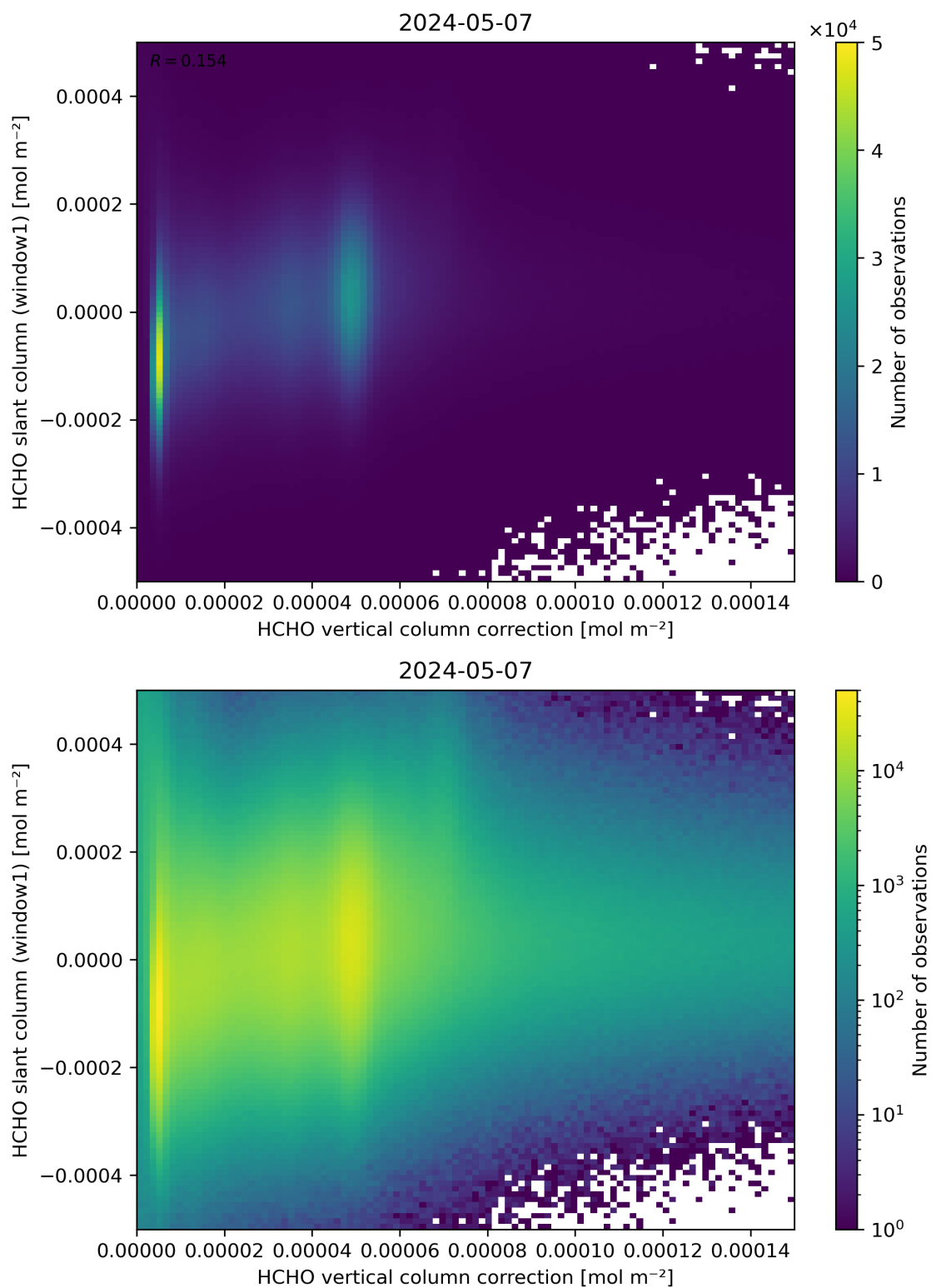
Figure 118: Scatter density plot of “HCHO vertical column correction” against “HCHO slant column (window1)” for 2024-05-07 to 2024-05-08.
