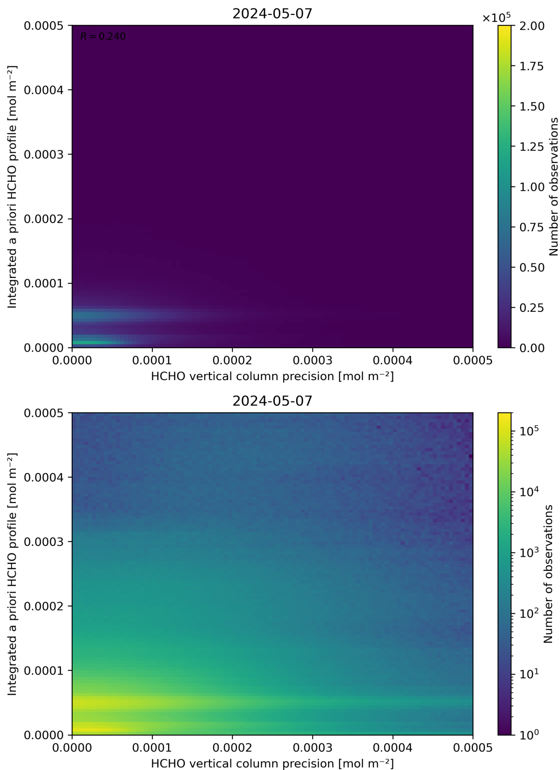
Figure 147: Scatter density plot of “HCHO vertical column precision” against “Integrated a priori HCHO profile” for 2024-05-07 to 2024-05-08.
