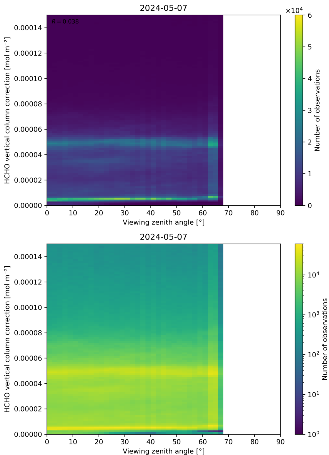
Figure 193: Scatter density plot of “Viewing zenith angle” against “HCHO vertical column correction” for 2024-05-07 to 2024-05-08.
