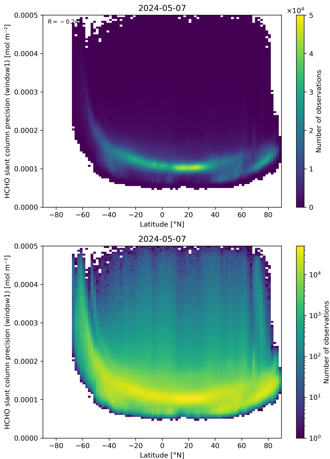
Figure 160: Scatter density plot of “Latitude” against “HCHO slant column precision (window1)” for 2024-05-07 to 2024-05-08.
