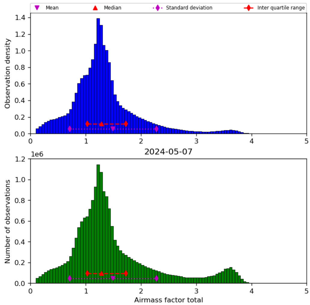
Figure 40: Histogram of “Airmass factor total” for 2024-05-07 to 2024-05-08
