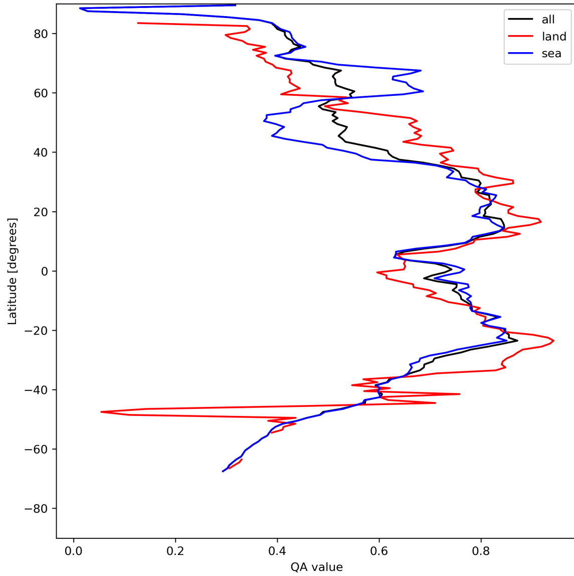
Figure 20: Zonal average of “QA value” for 2024-05-07 to 2024-05-08.
