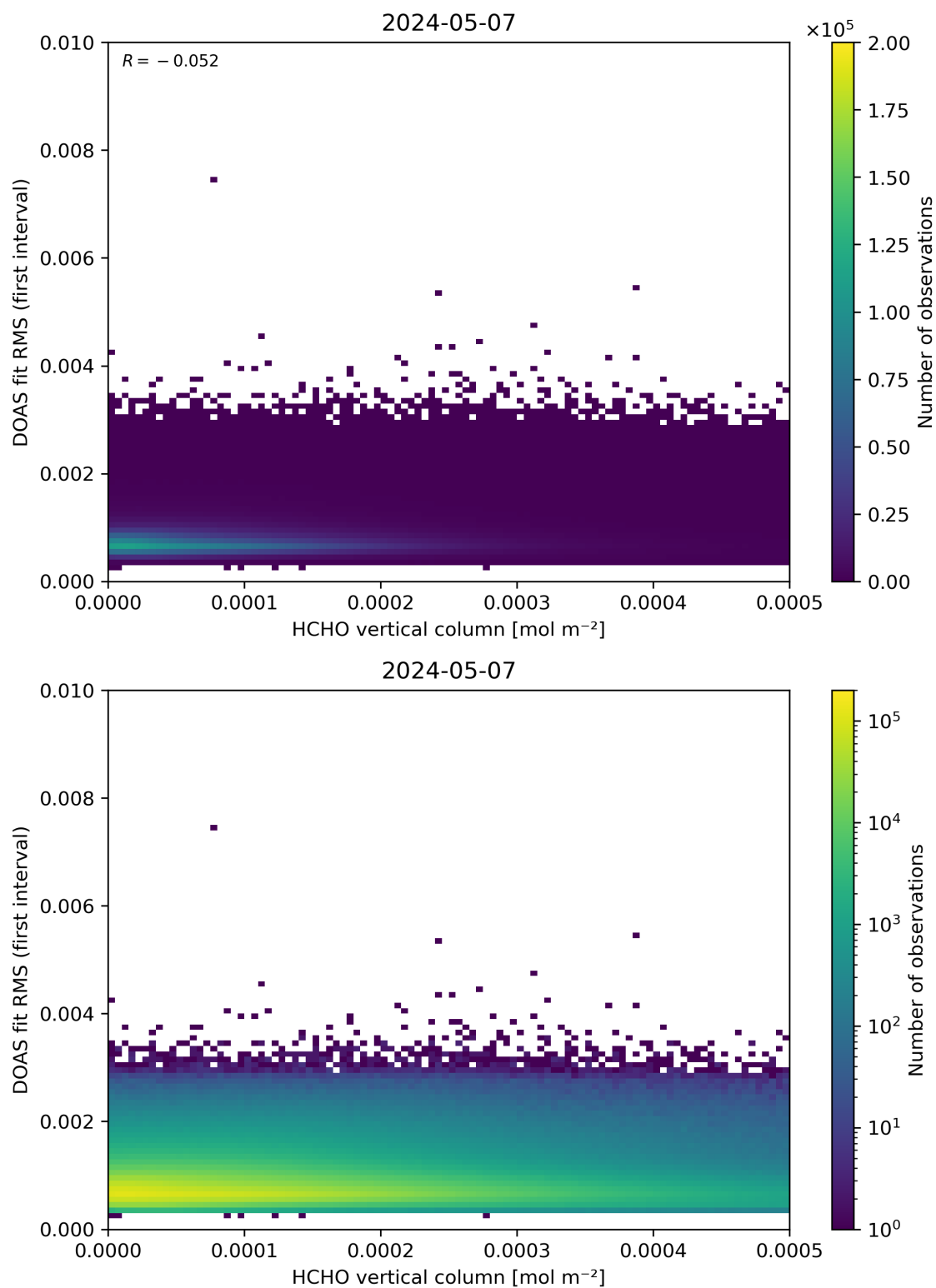
Figure 123: Scatter density plot of “HCHO vertical column” against “DOAS fit RMS (first interval)” for 2024-05-07 to 2024-05-08.
