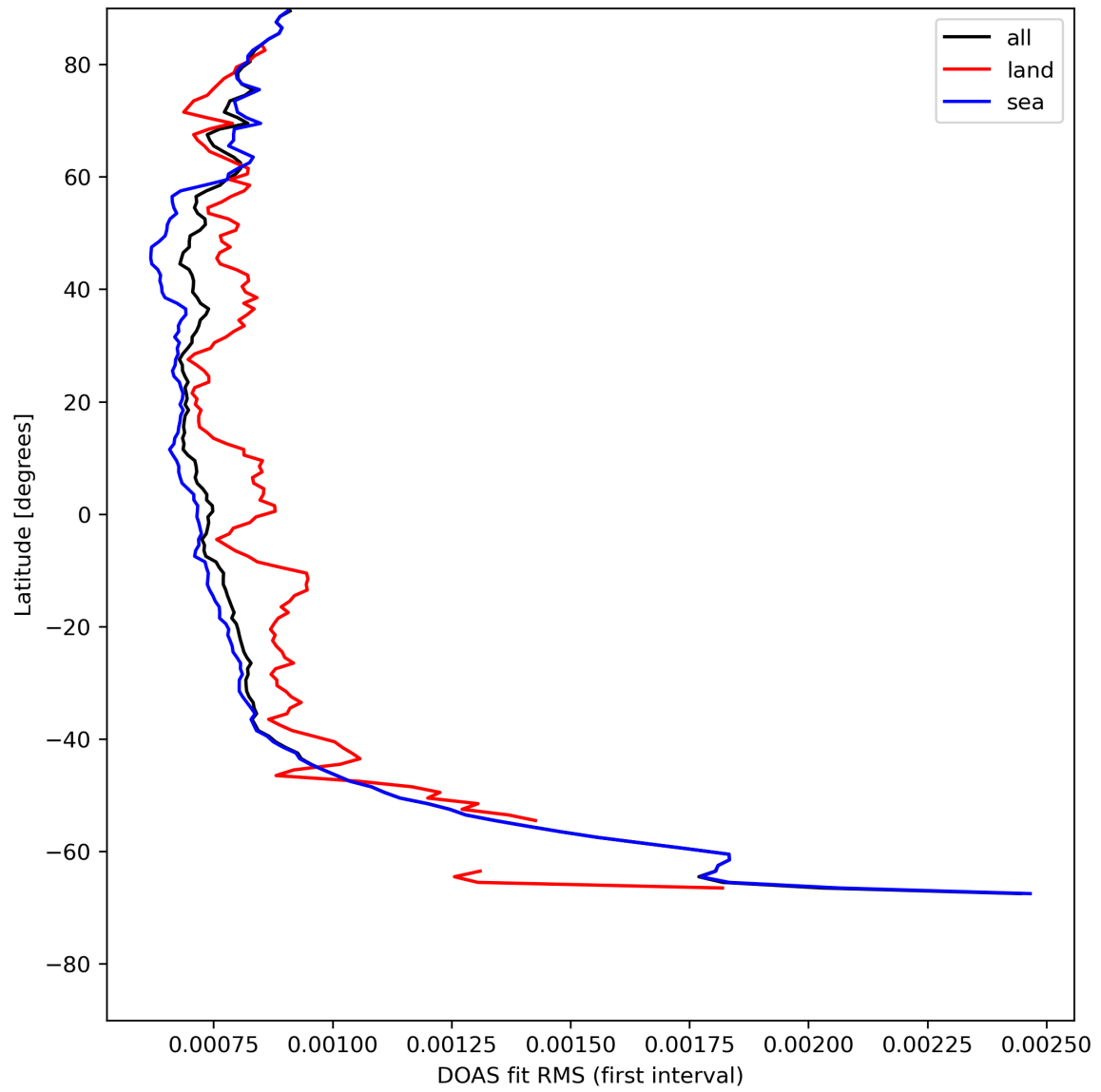
Figure 32: Zonal average of “DOAS fit RMS (first interval)” for 2024-05-07 to 2024-05-08.
