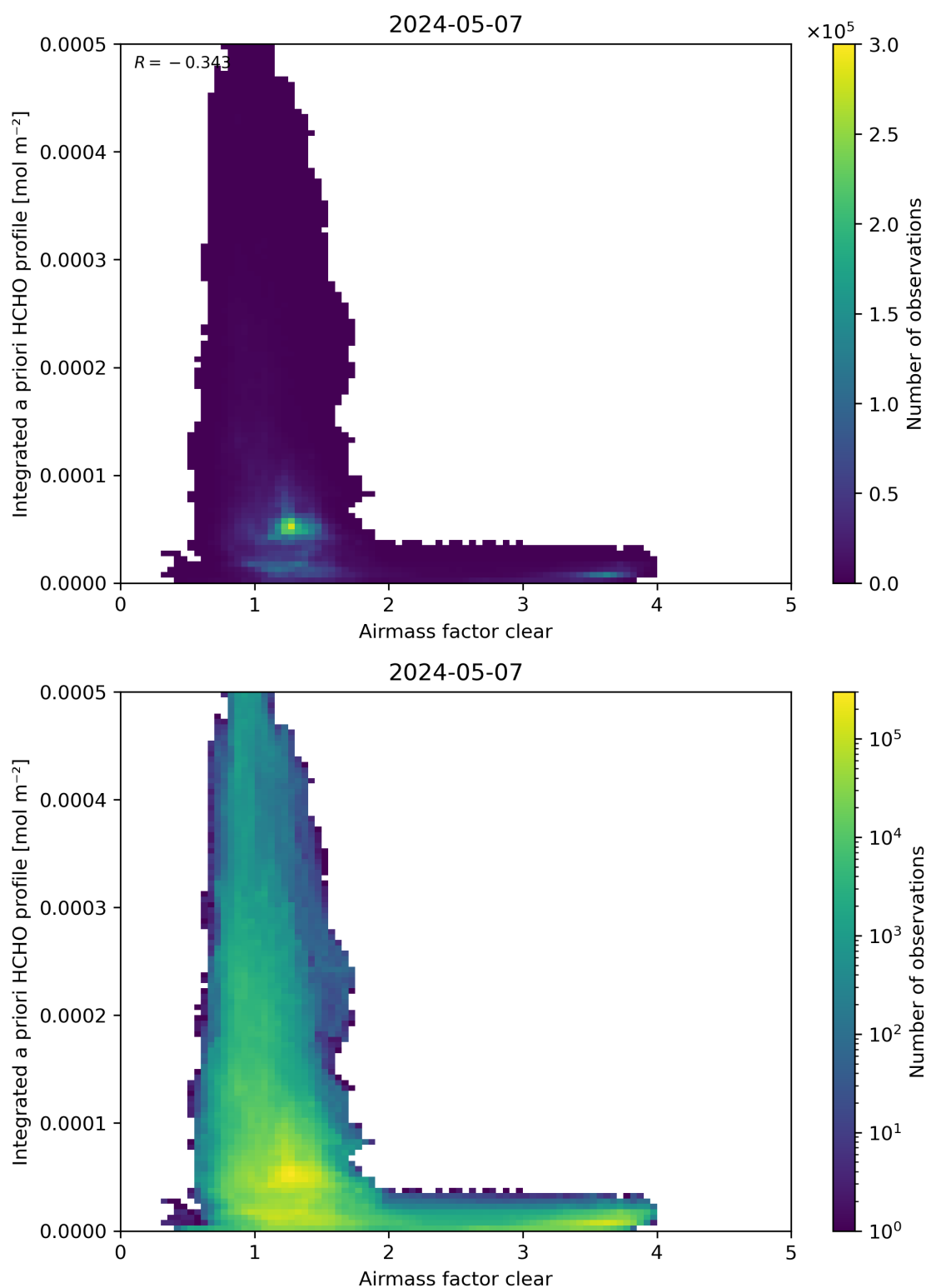
Figure 76: Scatter density plot of “Airmass factor clear” against “Integrated a priori HCHO profile” for 2024-05-07 to 2024-05-08.
