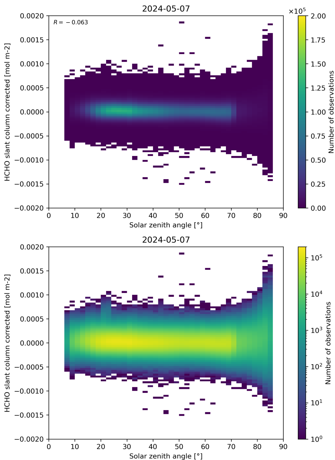
Figure 171: Scatter density plot of “Solar zenith angle” against “HCHO slant column corrected” for 2024-05-07 to 2024-05-08.
