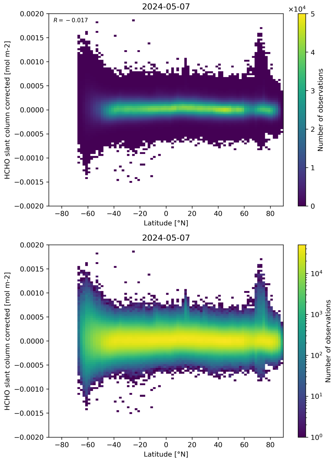
Figure 157: Scatter density plot of “Latitude” against “HCHO slant column corrected” for 2024-05-07 to 2024-05-08.
