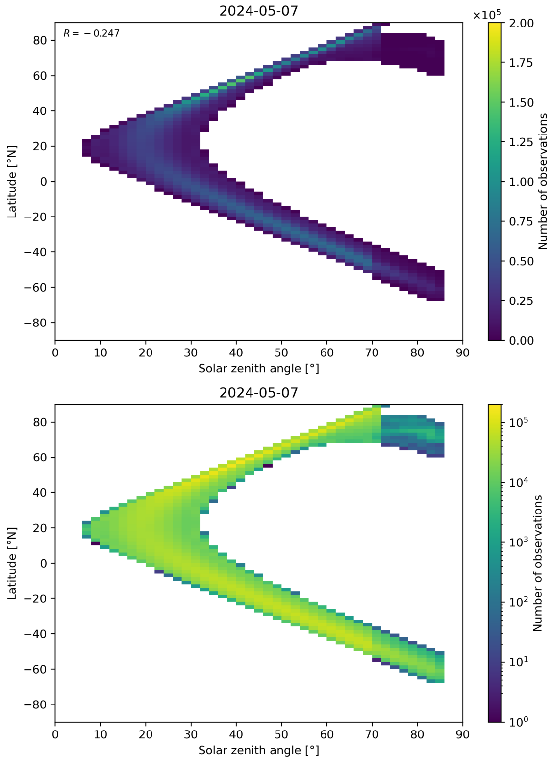
Figure 181: Scatter density plot of “Solar zenith angle” against “Latitude” for 2024-05-07 to 2024-05-08.
