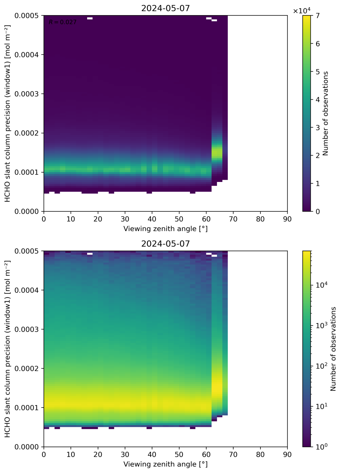
Figure 189: Scatter density plot of “Viewing zenith angle” against “HCHO slant column precision (window1)” for 2024-05-07 to 2024-05-08.
