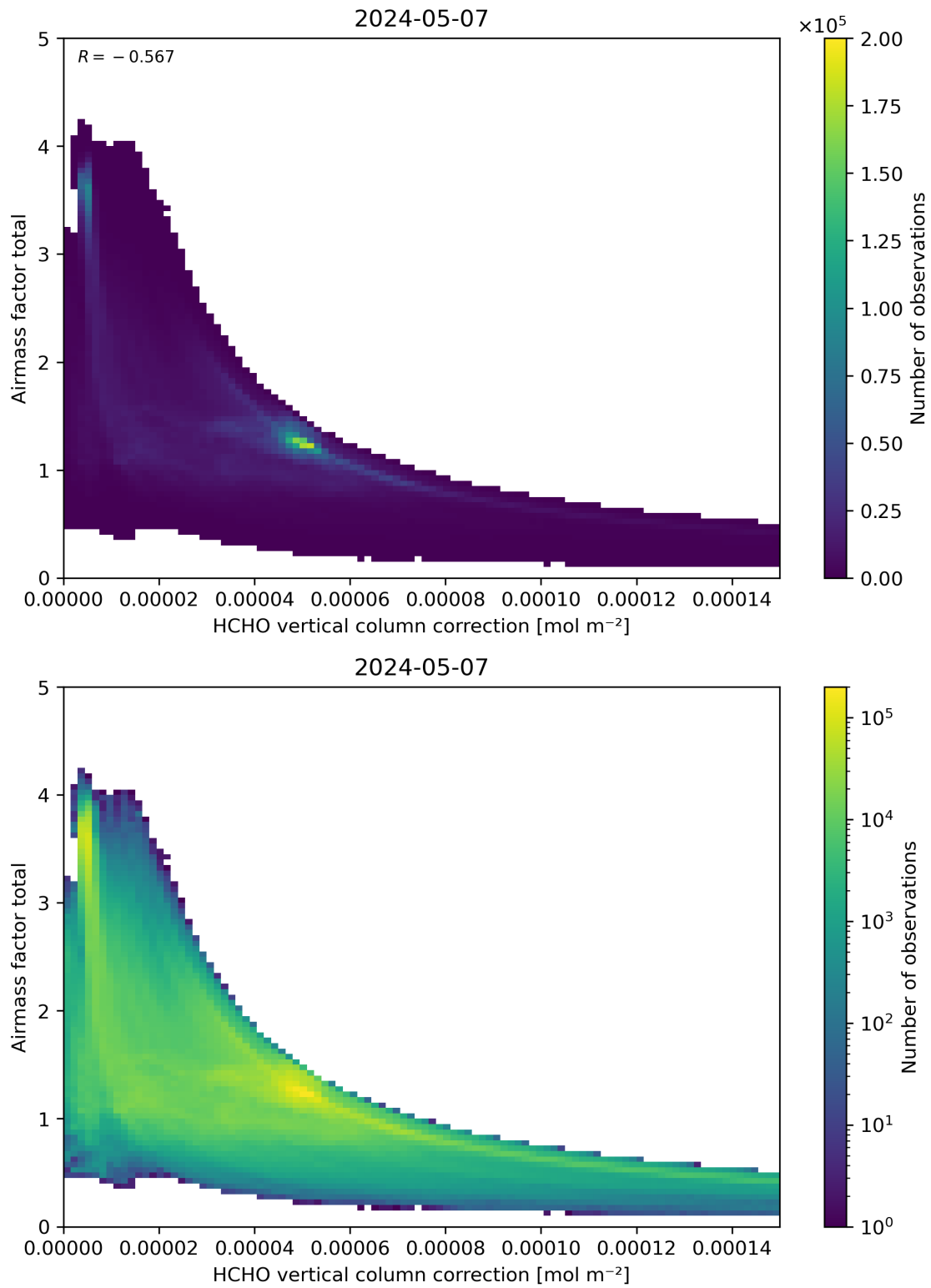
Figure 120: Scatter density plot of “HCHO vertical column correction” against “Airmass factor total” for 2024-05-07 to 2024-05-08.
