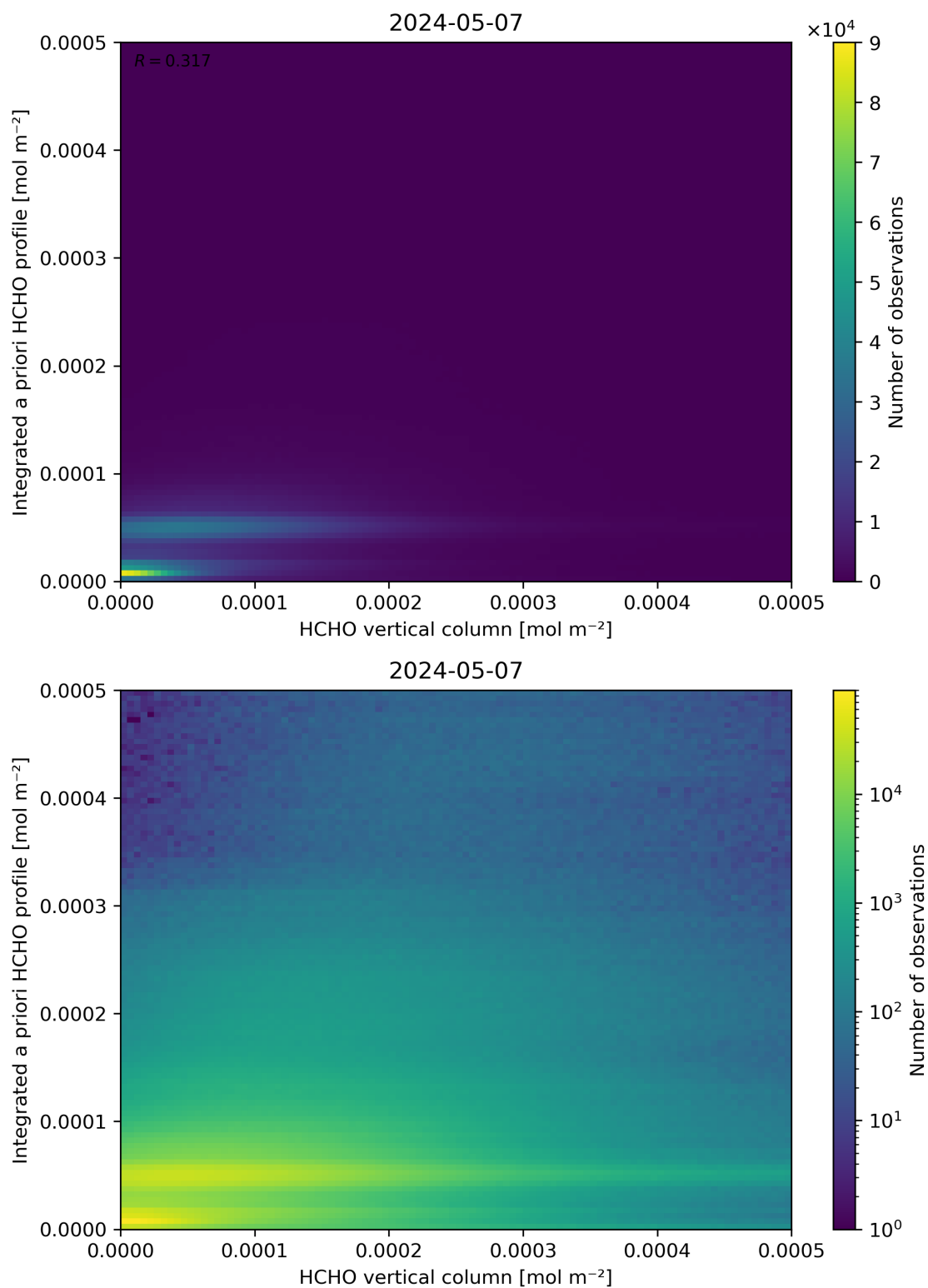
Figure 135: Scatter density plot of “HCHO vertical column” against “Integrated a priori HCHO profile” for 2024-05-07 to 2024-05-08.
