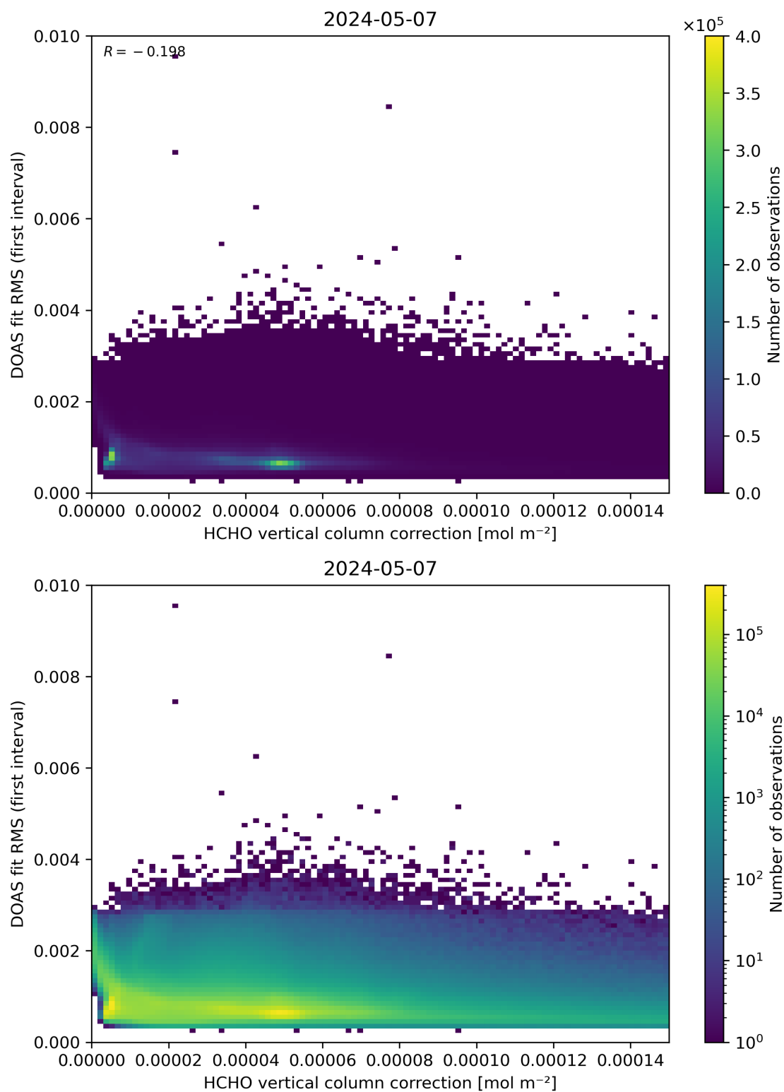
Figure 112: Scatter density plot of “HCHO vertical column correction” against “DOAS fit RMS (first interval)” for 2024-05-07 to 2024-05-08.
