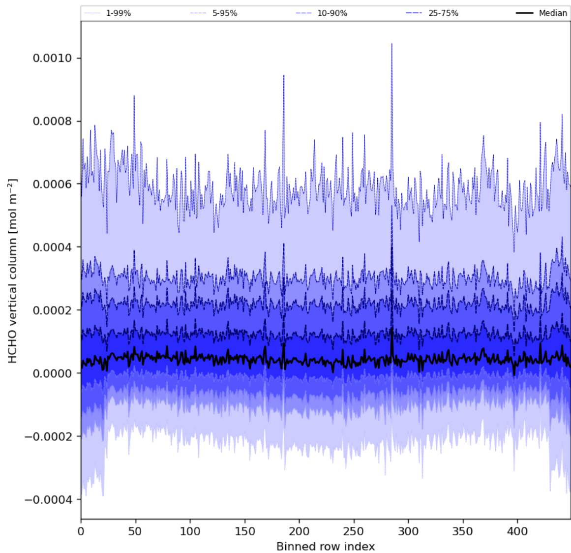
Figure 49: Along track statistics of “HCHO vertical column” for 2024-05-07 to 2024-05-08
