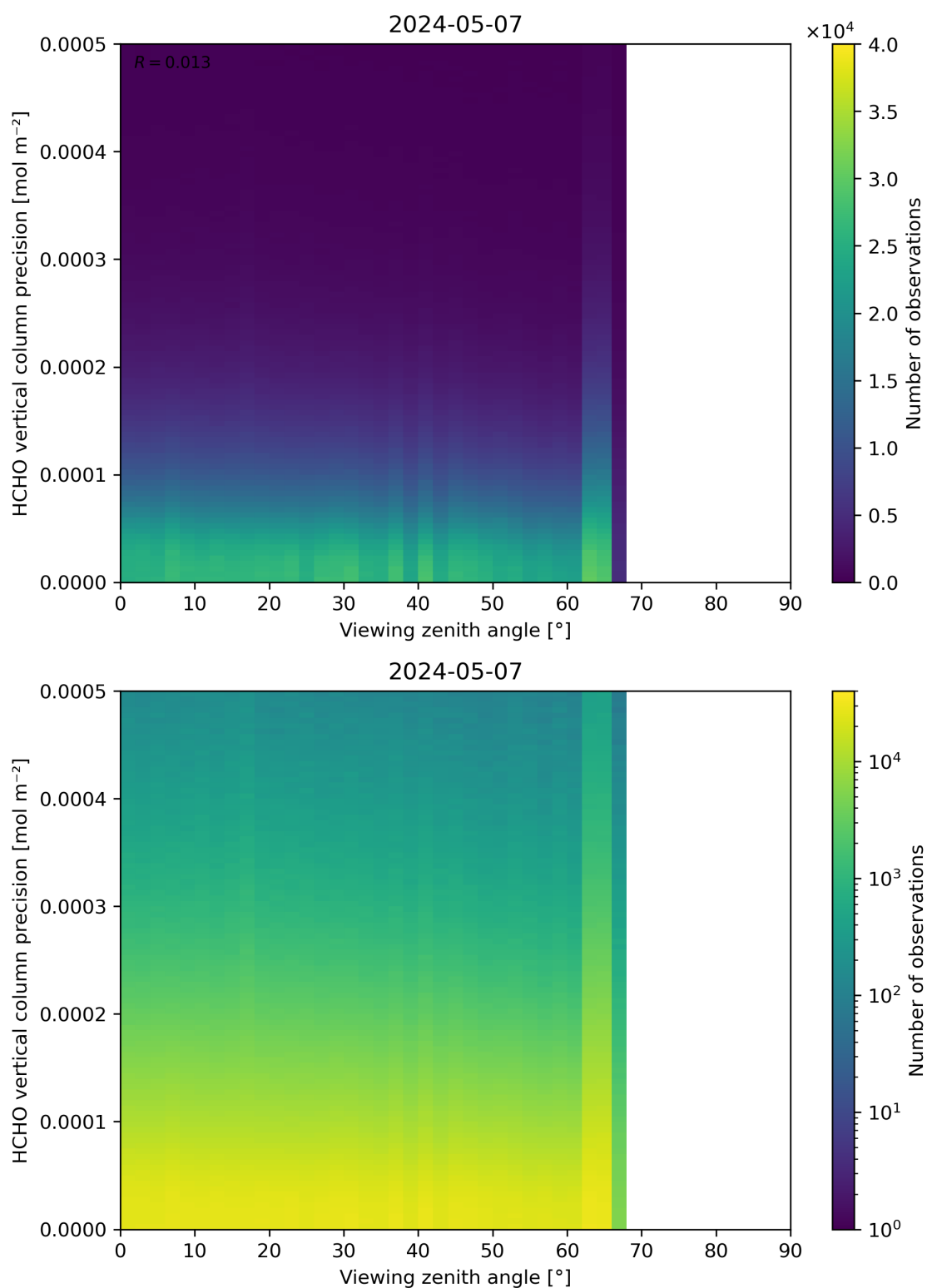
Figure 194: Scatter density plot of “Viewing zenith angle” against “HCHO vertical column precision” for 2024-05-07 to 2024-05-08.
