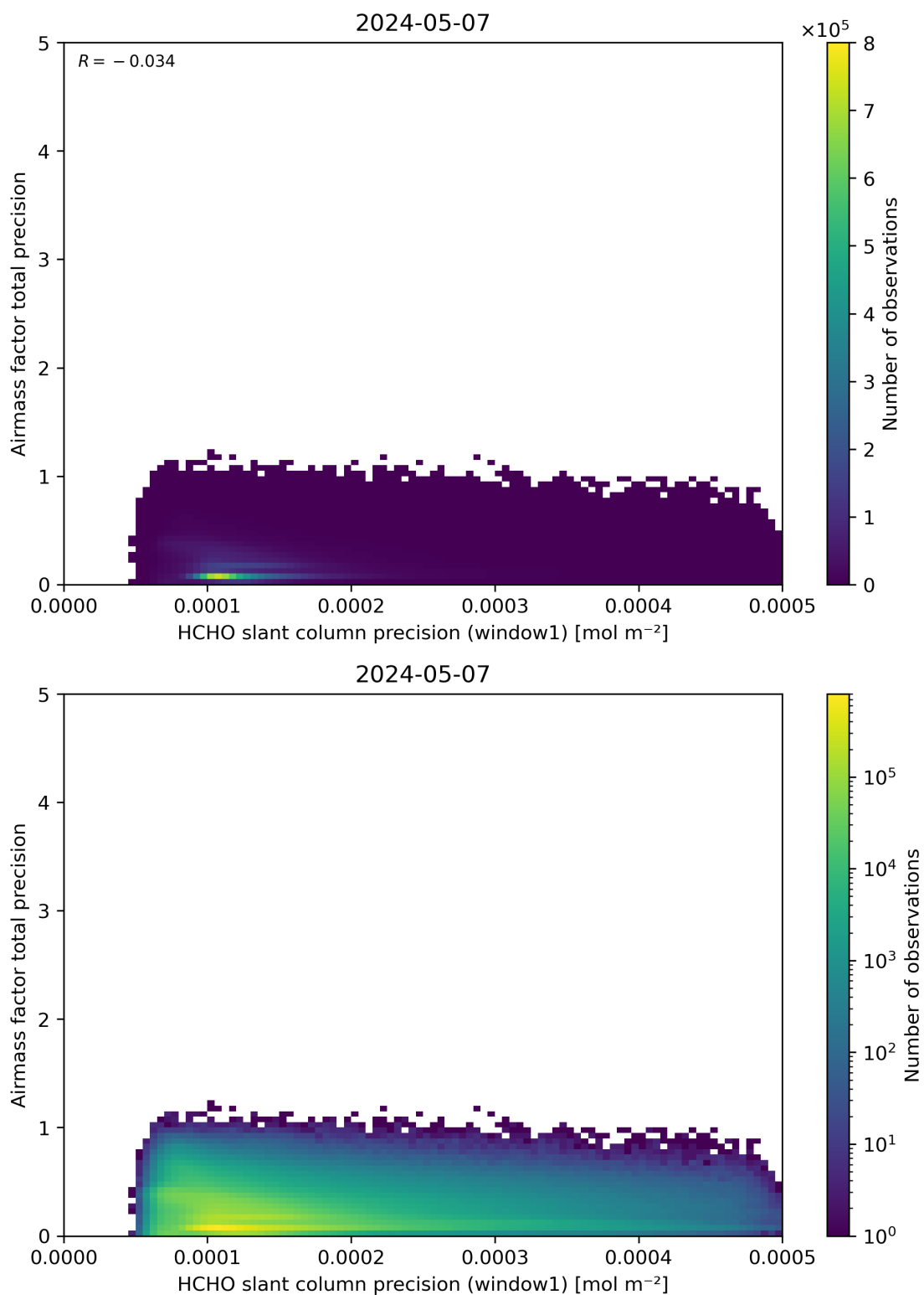
Figure 95: Scatter density plot of “HCHO slant column precision (window1)” against “Airmass factor total precision” for 2024-05-07 to 2024-05-08.
