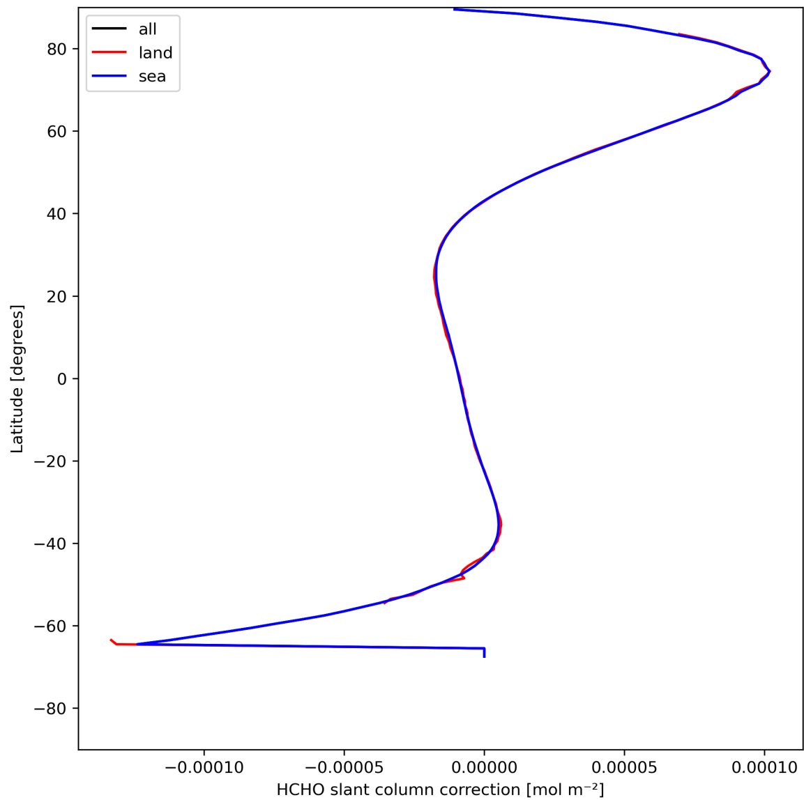
Figure 33: Zonal average of “HCHO slant column correction” for 2024-05-07 to 2024-05-08.
