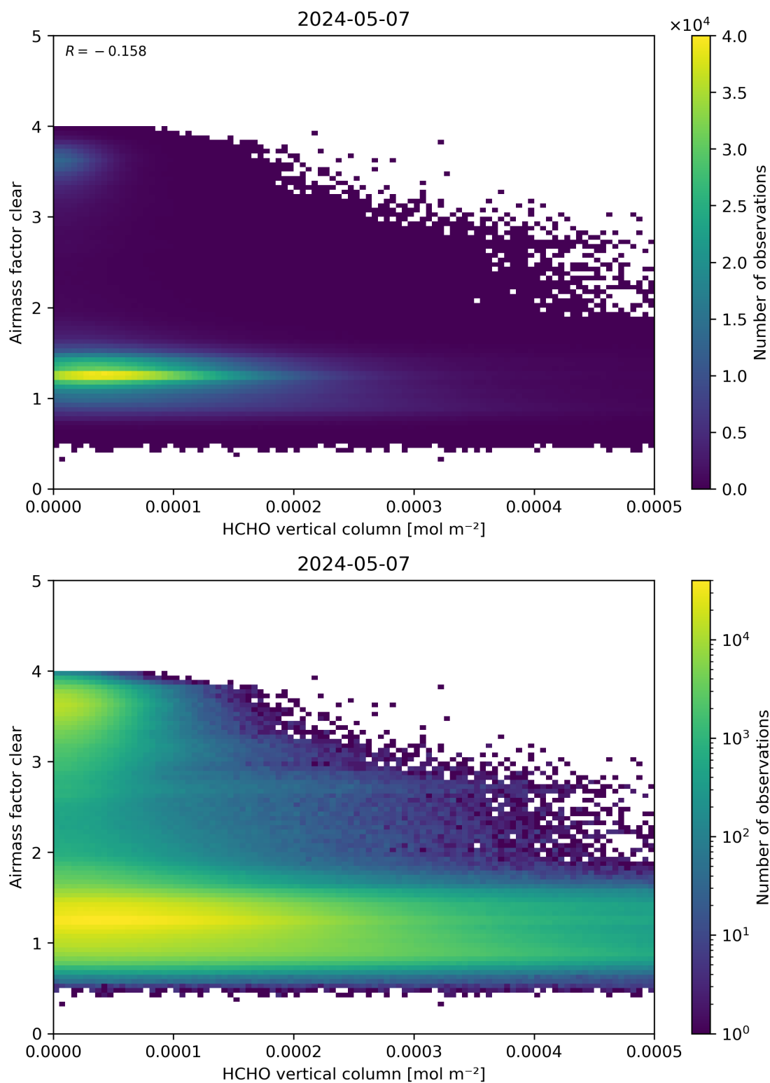
Figure 126: Scatter density plot of “HCHO vertical column” against “Airmass factor clear” for 2024-05-07 to 2024-05-08.
