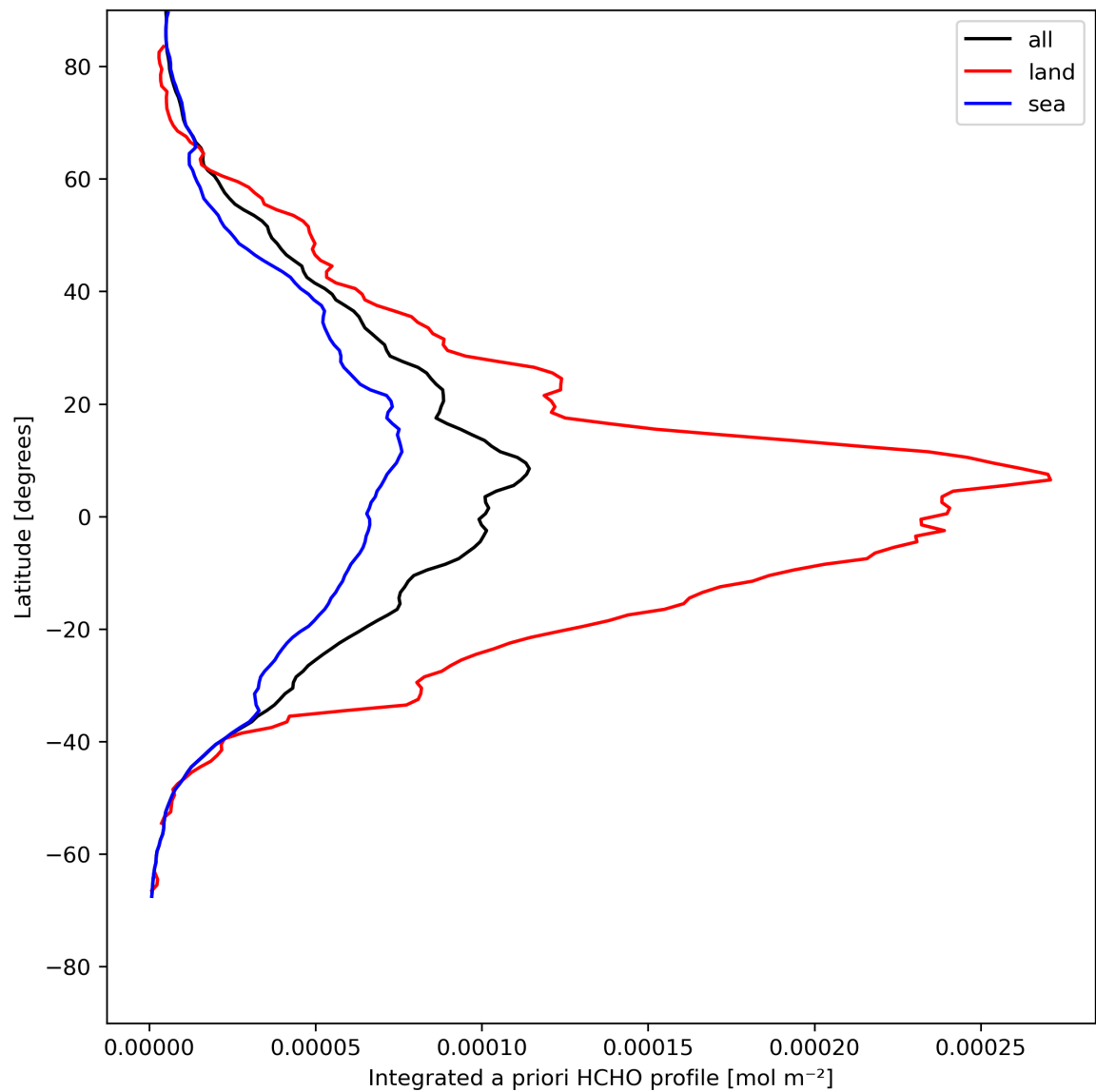
Figure 29: Zonal average of “Integrated a priori HCHO profile” for 2024-05-07 to 2024-05-08.
