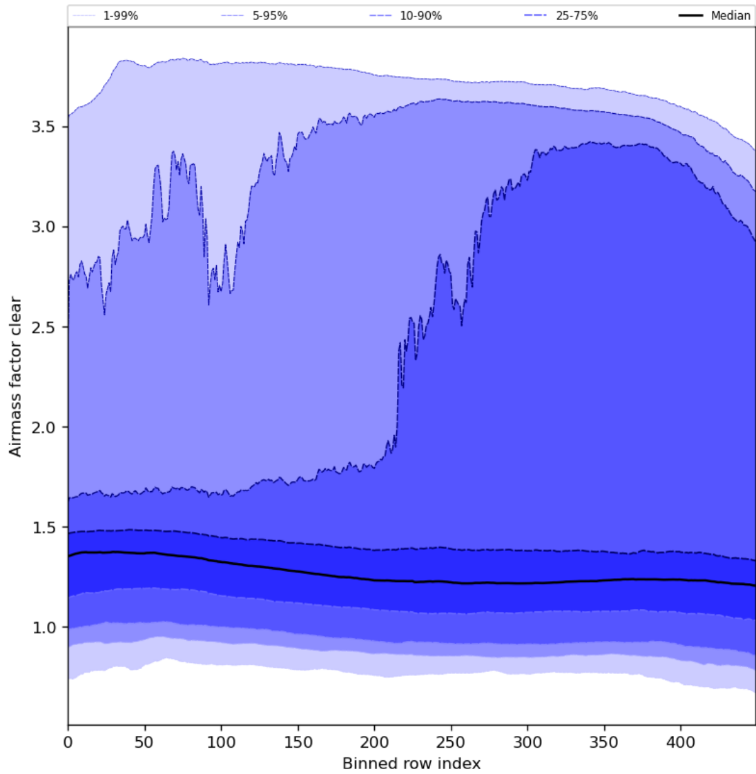
Figure 56: Along track statistics of “Airmass factor clear” for 2024-05-07 to 2024-05-08
