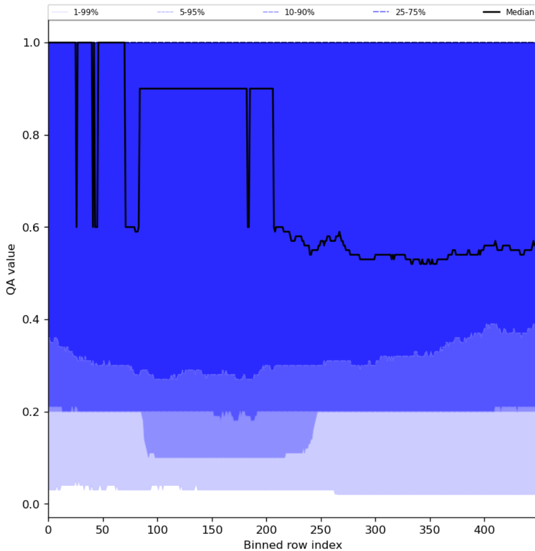
Figure 48: Along track statistics of “QA value” for 2024-05-07 to 2024-05-08
