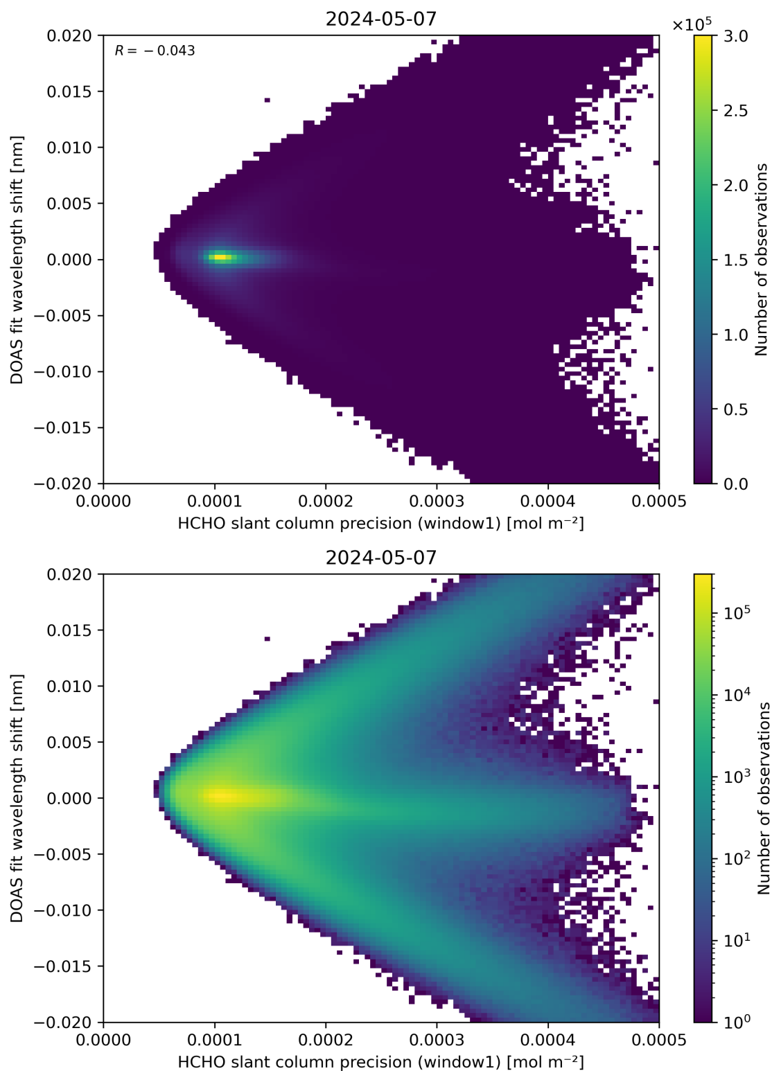
Figure 89: Scatter density plot of “HCHO slant column precision (window1)” against “DOAS fit wavelength shift” for 2024-05-07 to 2024-05-08.
