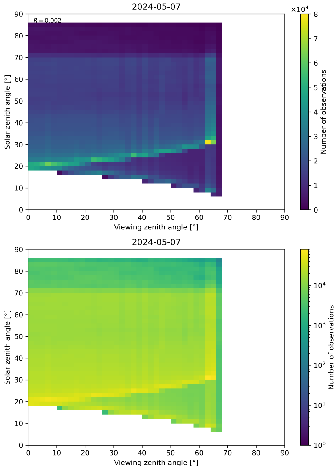
Figure 197: Scatter density plot of “Viewing zenith angle” against “Solar zenith angle” for 2024-05-07 to 2024-05-08.
