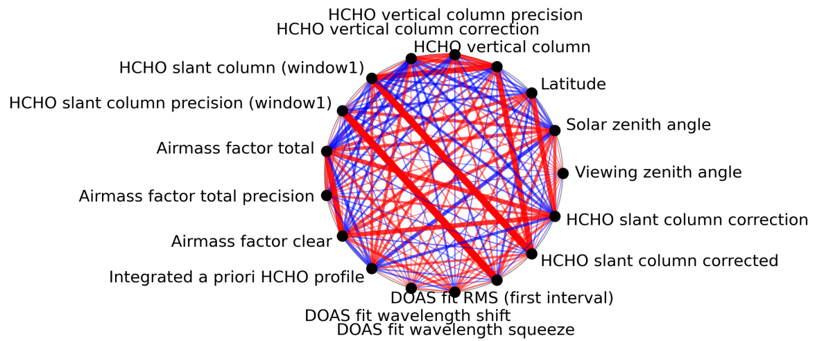
Figure 1: Map of correlation graph for 2024-05-07 to 2024-05-08.
