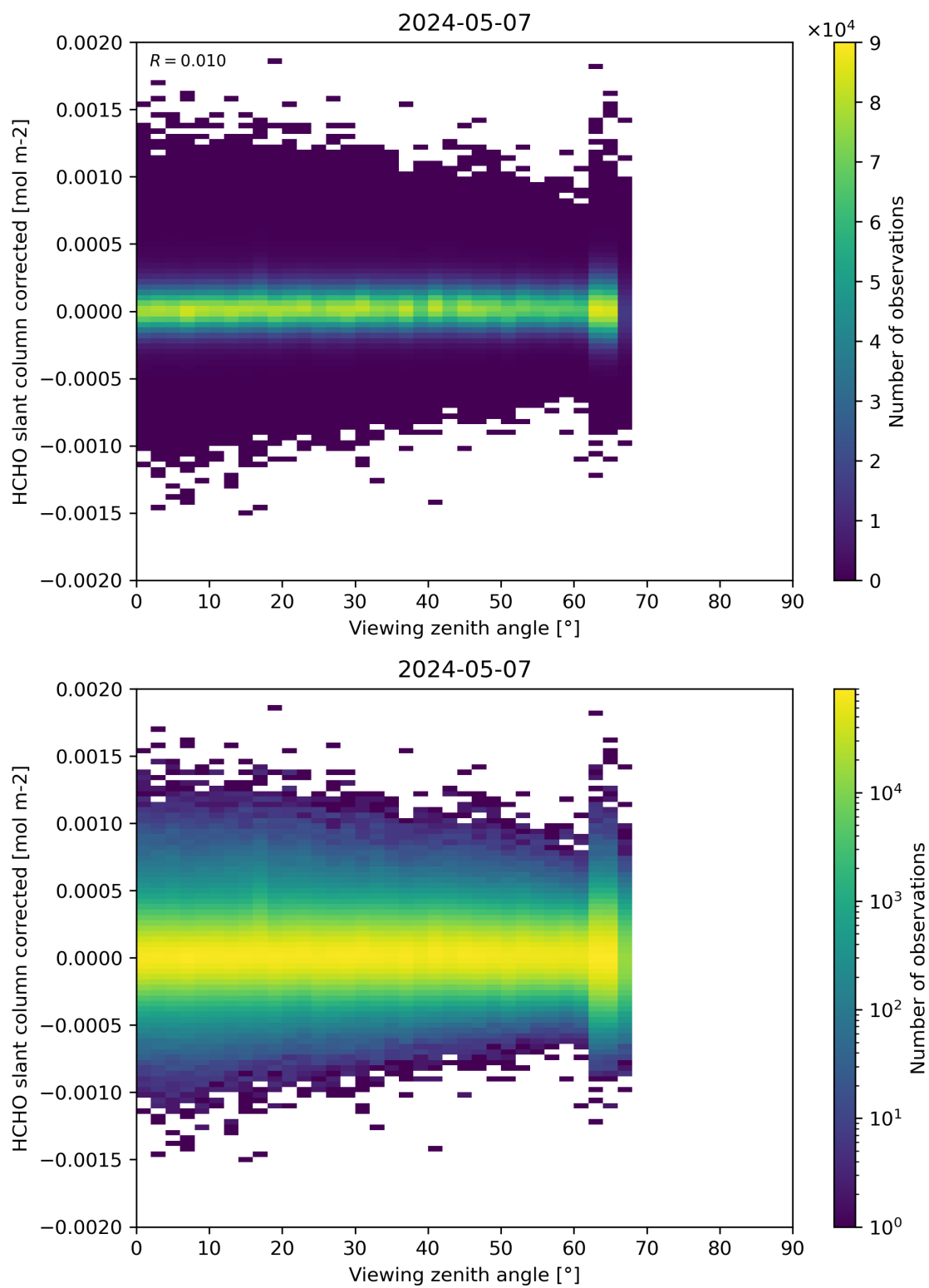
Figure 186: Scatter density plot of “Viewing zenith angle” against “HCHO slant column corrected” for 2024-05-07 to 2024-05-08.
