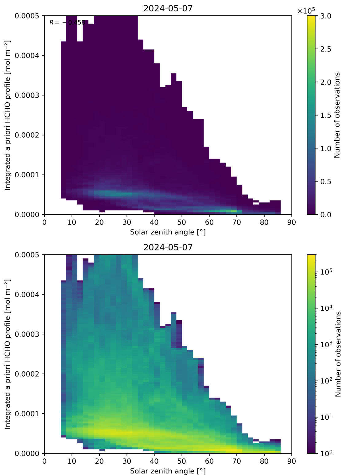
Figure 180: Scatter density plot of “Solar zenith angle” against “Integrated a priori HCHO profile” for 2024-05-07 to 2024-05-08.
