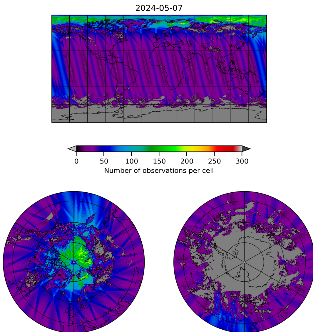
Figure 19: Map of the number of observations for 2024-05-07 to 2024-05-08
