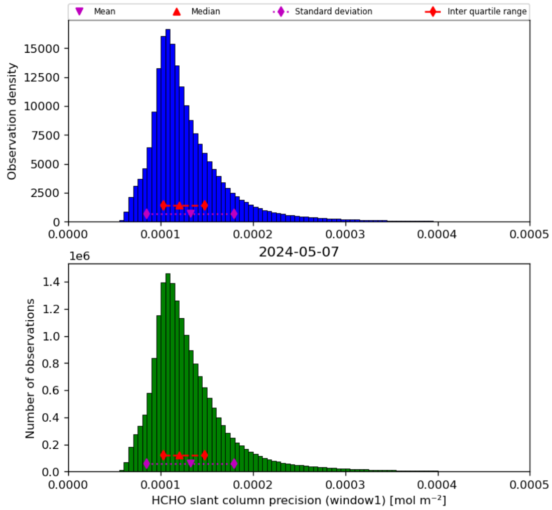
Figure 39: Histogram of “HCHO slant column precision (window1)” for 2024-05-07 to 2024-05-08
