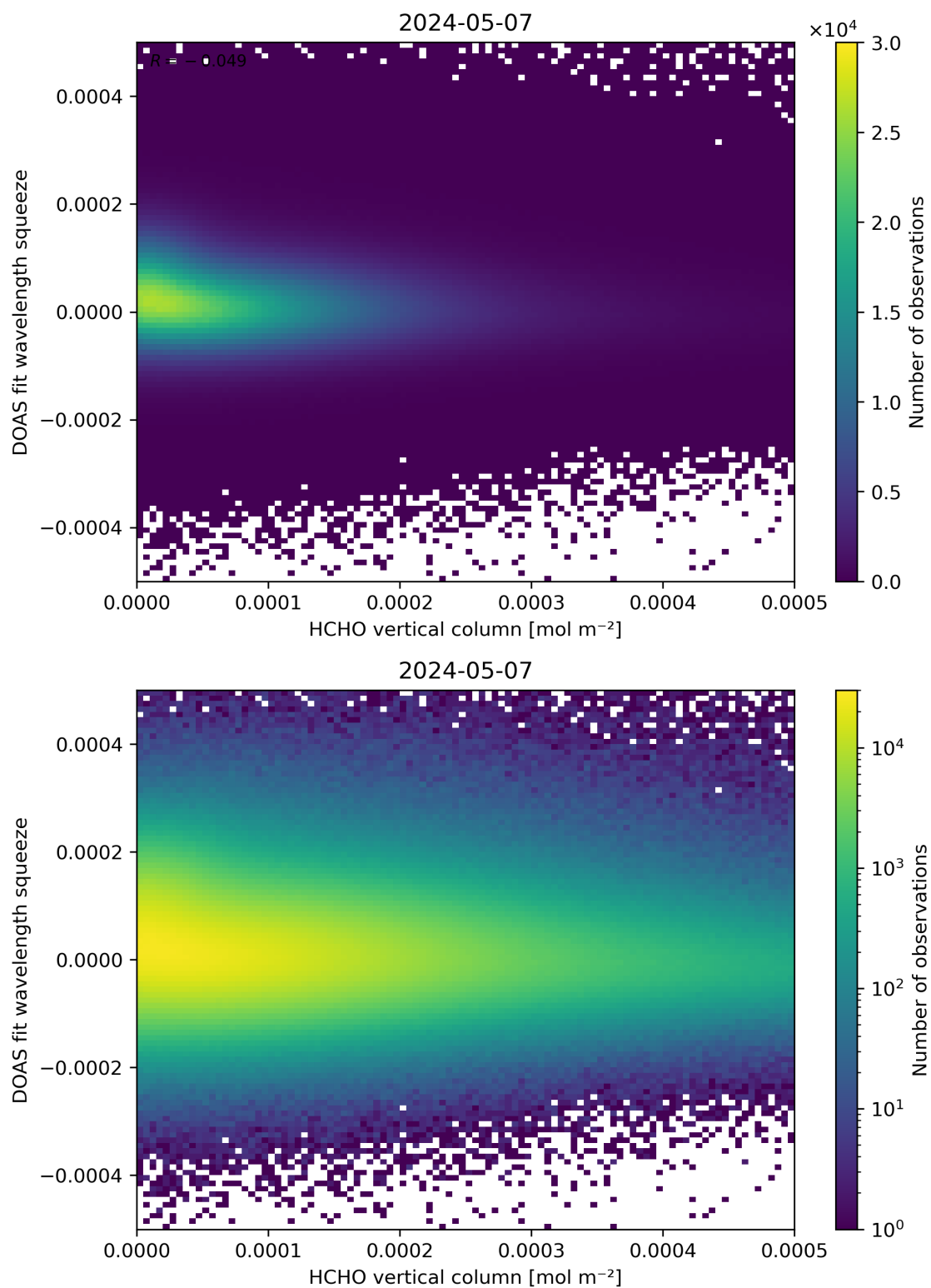
Figure 125: Scatter density plot of “HCHO vertical column” against “DOAS fit wavelength squeeze” for 2024-05-07 to 2024-05-08.
