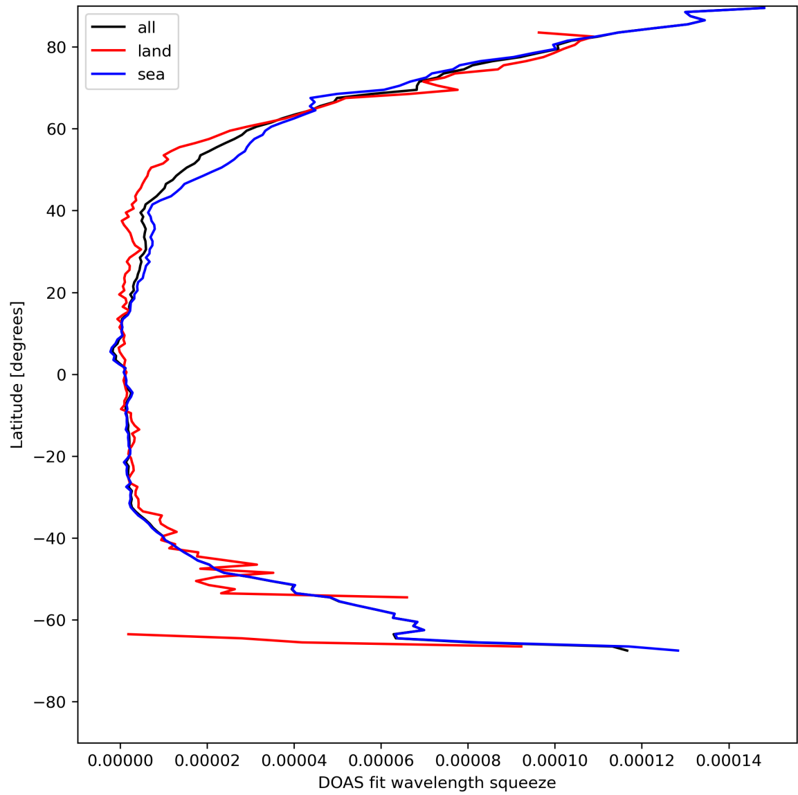
Figure 31: Zonal average of “DOAS fit wavelength squeeze” for 2024-05-07 to 2024-05-08.
