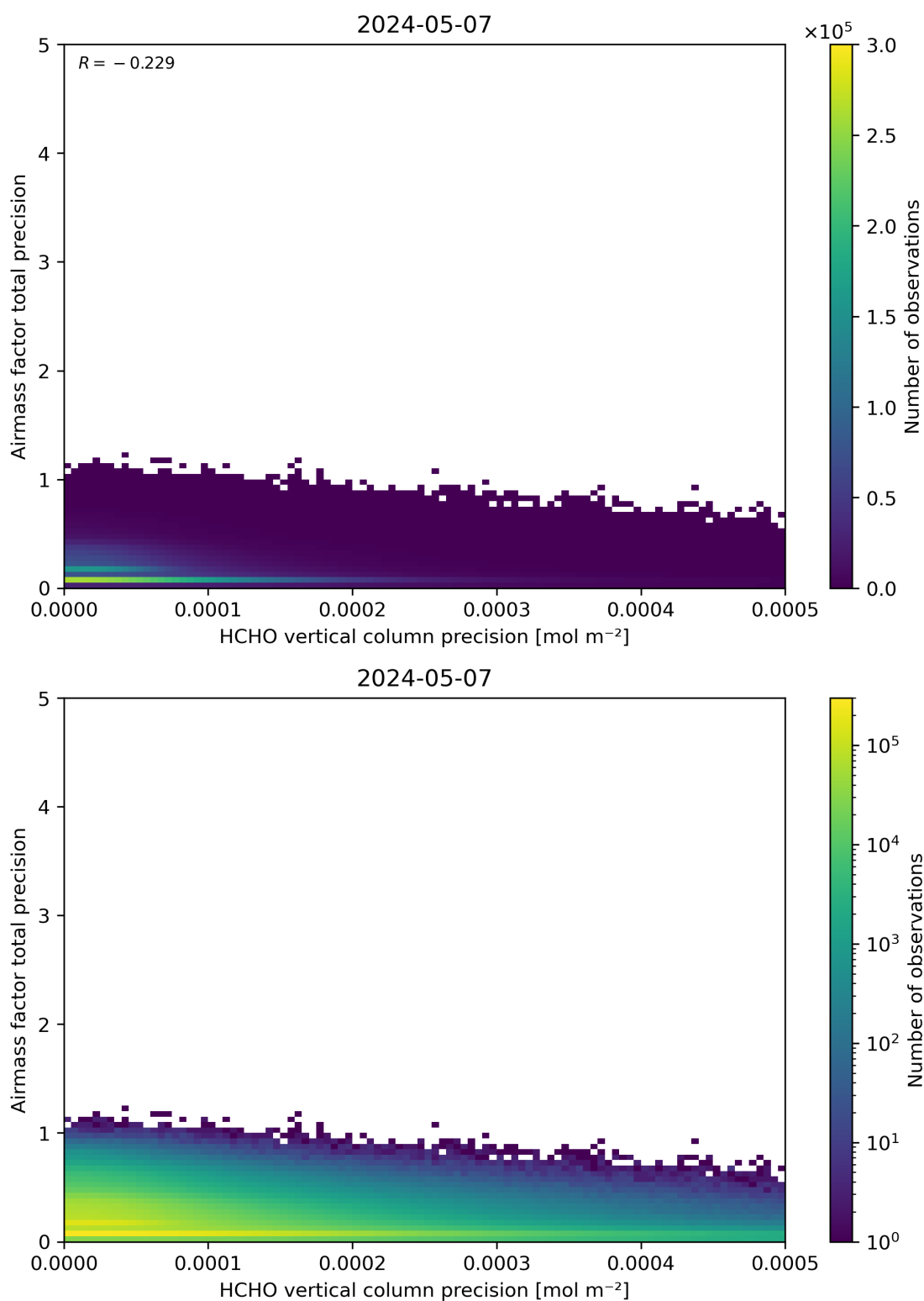
Figure 145: Scatter density plot of “HCHO vertical column precision” against “Airmass factor total precision” for 2024-05-07 to 2024-05-08.
