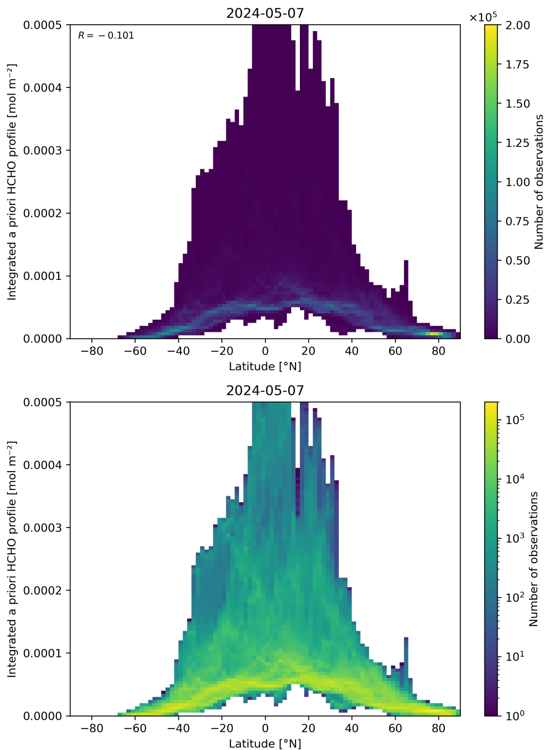
Figure 166: Scatter density plot of “Latitude” against “Integrated a priori HCHO profile” for 2024-05-07 to 2024-05-08.
