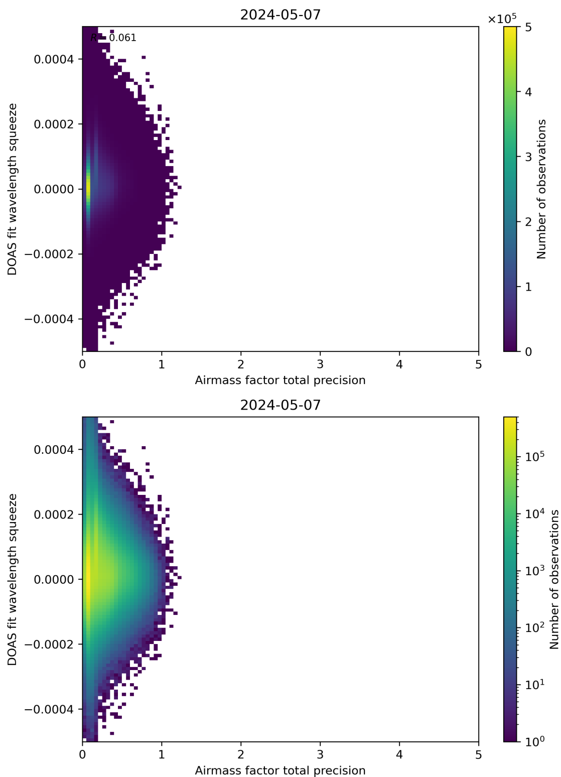
Figure 107: Scatter density plot of “Airmass factor total precision” against “DOAS fit wavelength squeeze” for 2024-05-07 to 2024-05-08.
