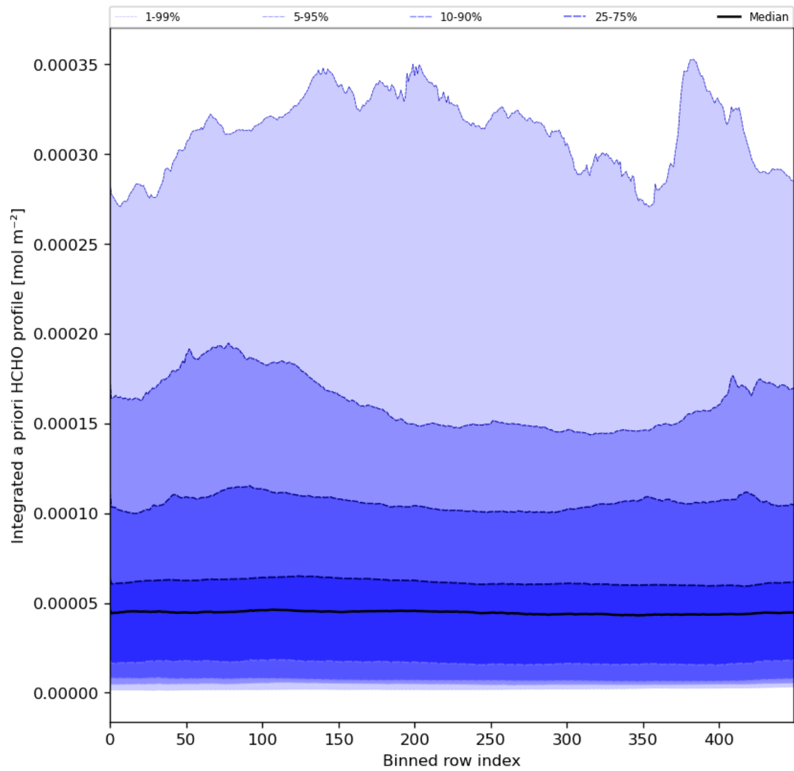
Figure 57: Along track statistics of “Integrated a priori HCHO profile” for 2024-05-07 to 2024-05-08
