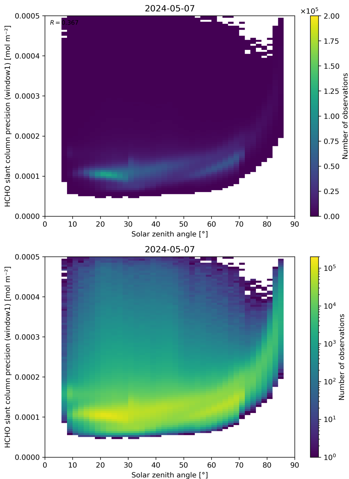
Figure 174: Scatter density plot of “Solar zenith angle” against “HCHO slant column precision (window1)” for 2024-05-07 to 2024-05-08.
