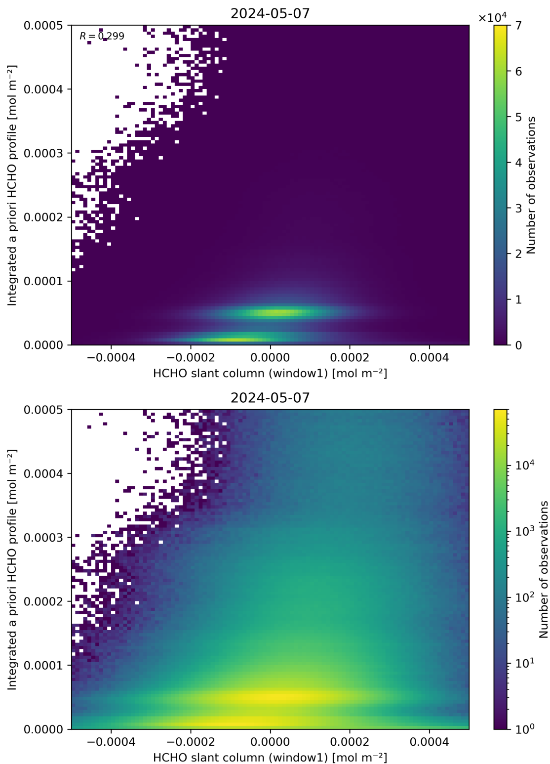
Figure 87: Scatter density plot of “HCHO slant column (window1)” against “Integrated a priori HCHO profile” for 2024-05-07 to 2024-05-08.
