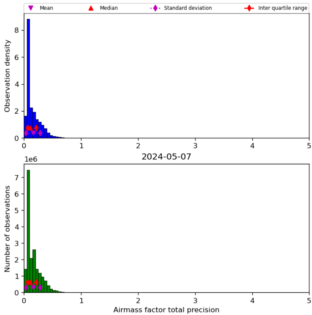
Figure 41: Histogram of “Airmass factor total precision” for 2024-05-07 to 2024-05-08
