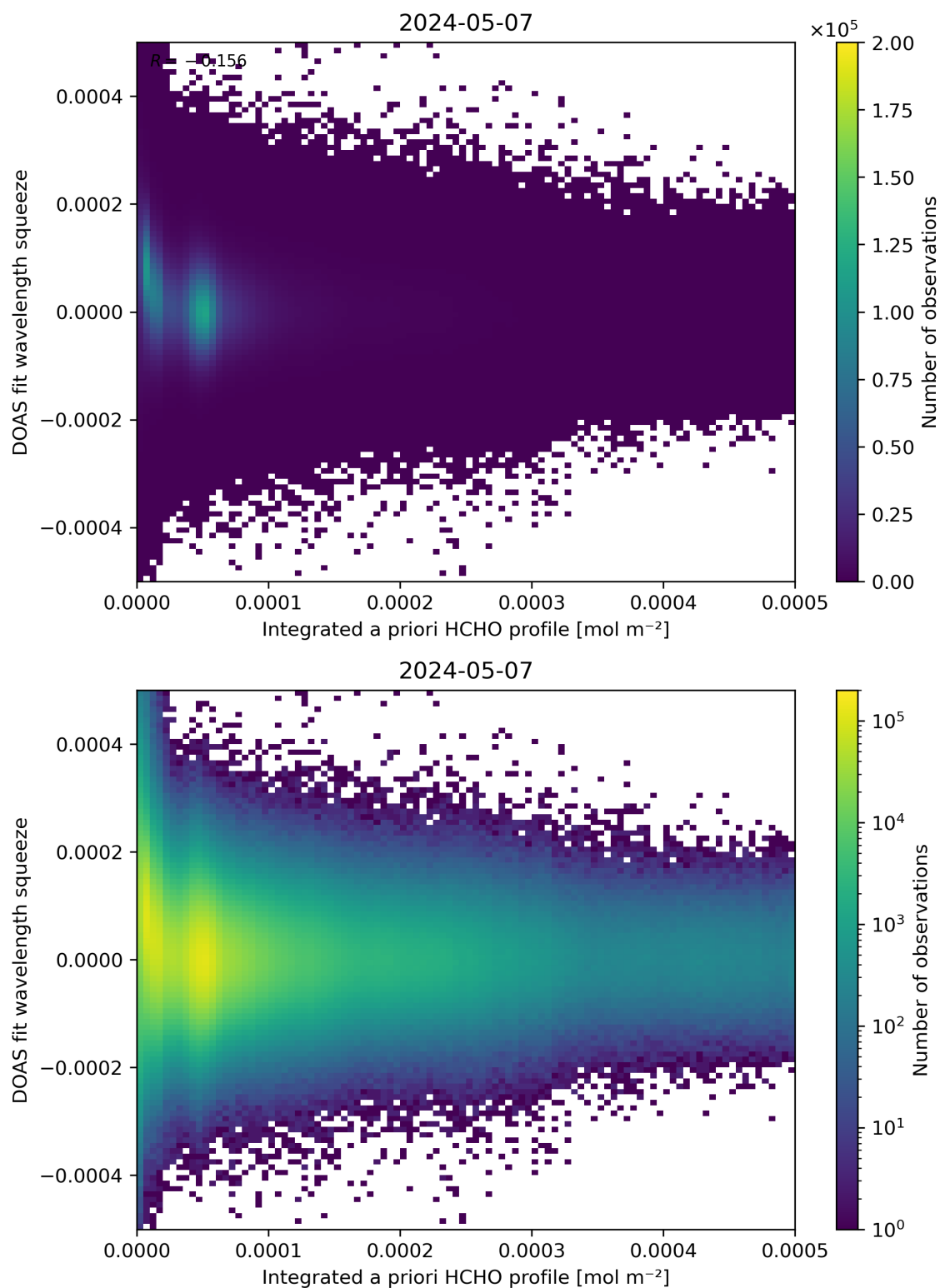
Figure 150: Scatter density plot of “Integrated a priori HCHO profile” against “DOAS fit wavelength squeeze” for 2024-05-07 to 2024-05-08.
