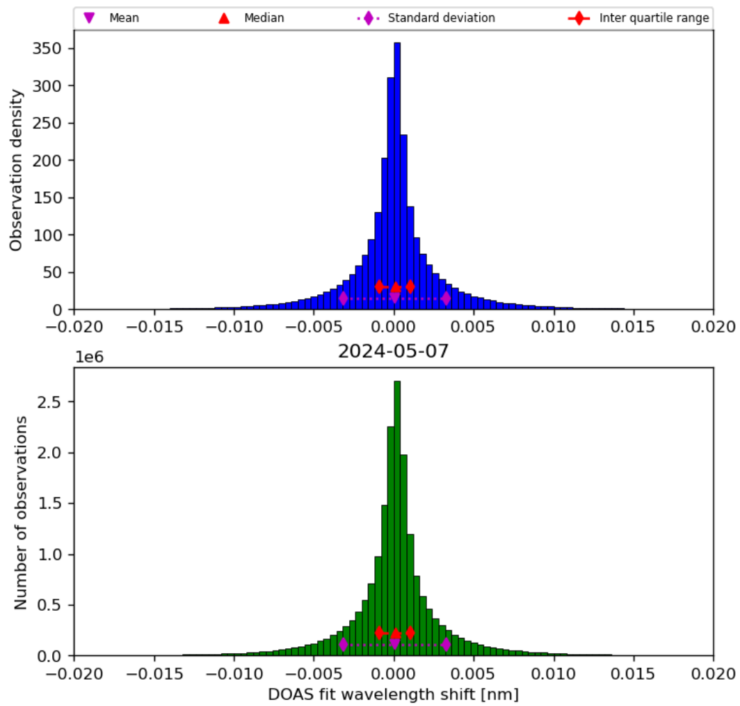
Figure 44: Histogram of “DOAS fit wavelength shift” for 2024-05-07 to 2024-05-08
