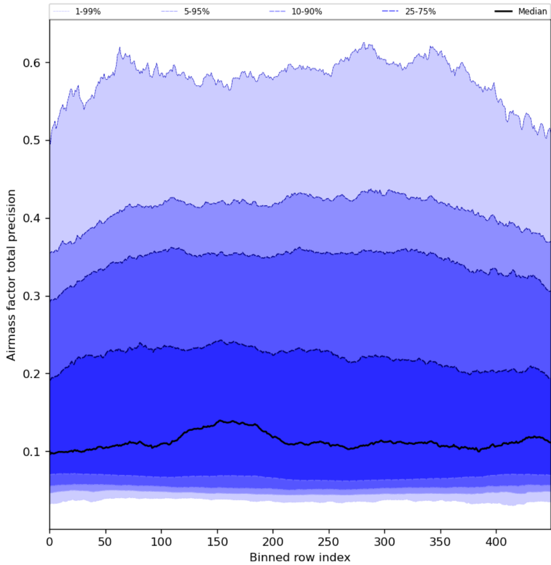
Figure 55: Along track statistics of “Airmass factor total precision” for 2024-05-07 to 2024-05-08
