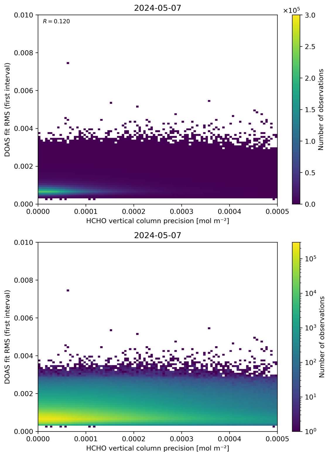
Figure 136: Scatter density plot of “HCHO vertical column precision” against “DOAS fit RMS (first interval)” for 2024-05-07 to 2024-05-08.
