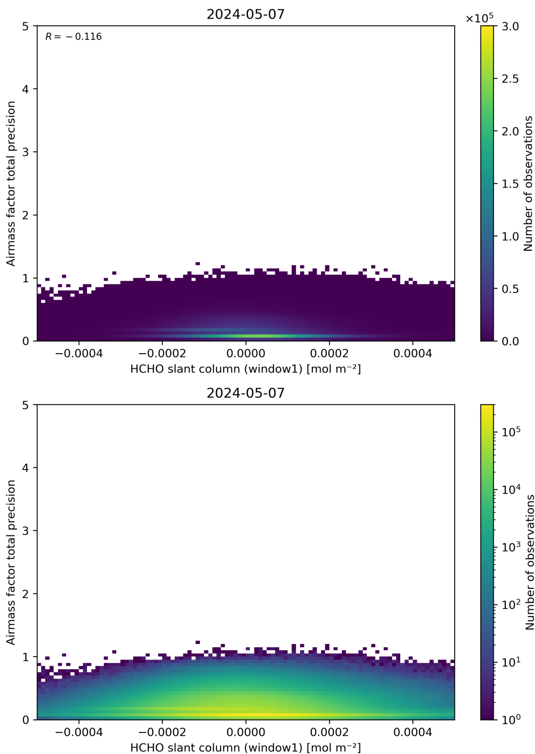
Figure 86: Scatter density plot of “HCHO slant column (window1)” against “Airmass factor total precision” for 2024-05-07 to 2024-05-08.
