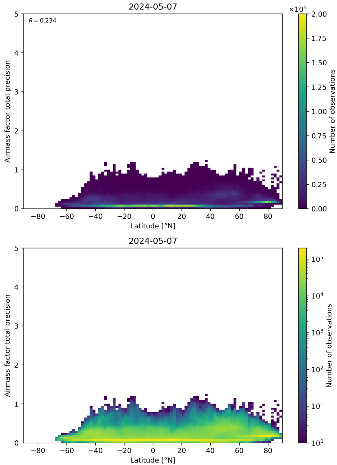
Figure 162: Scatter density plot of “Latitude” against “Airmass factor total precision” for 2024-05-07 to 2024-05-08.
