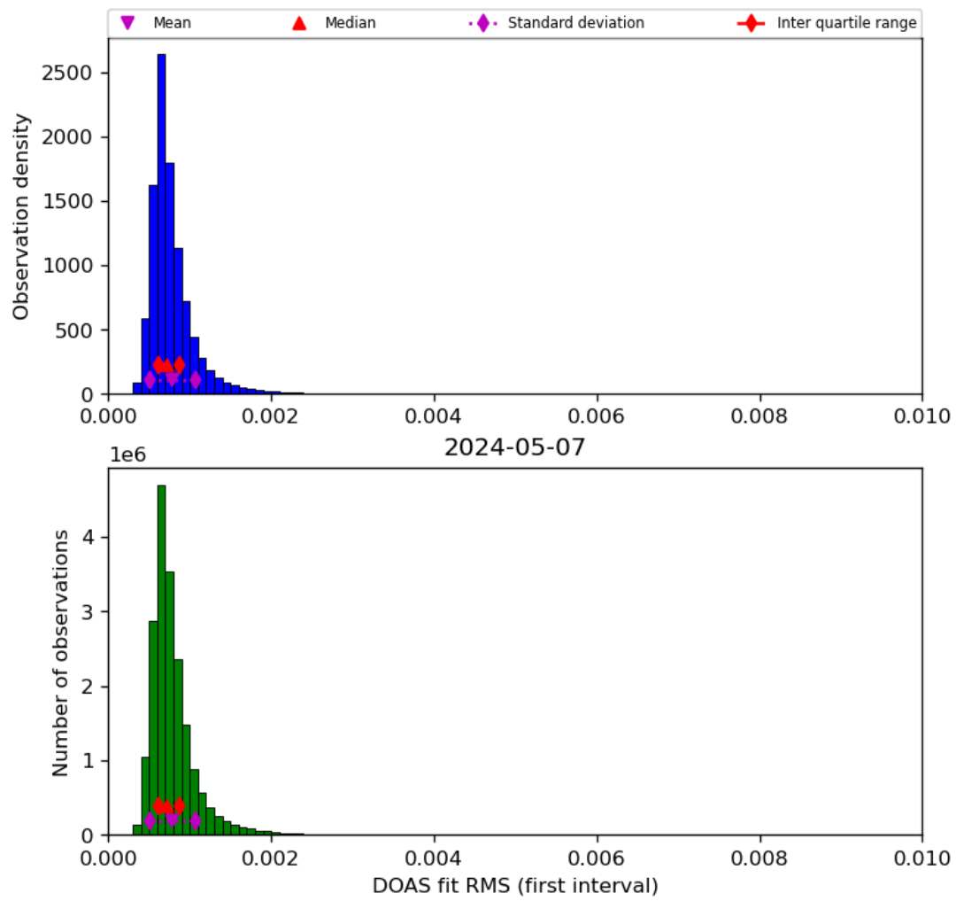
Figure 46: Histogram of “DOAS fit RMS (first interval)” for 2024-05-07 to 2024-05-08
