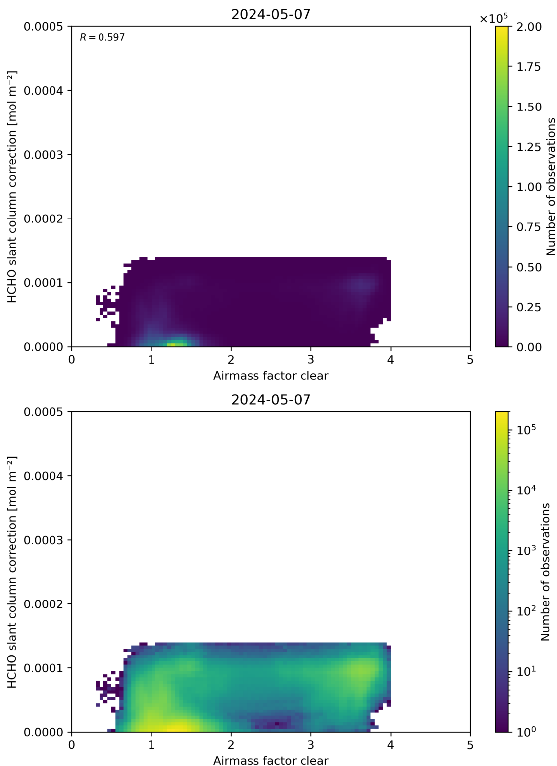
Figure 75: Scatter density plot of “Airmass factor clear” against “HCHO slant column correction” for 2024-05-07 to 2024-05-08.
