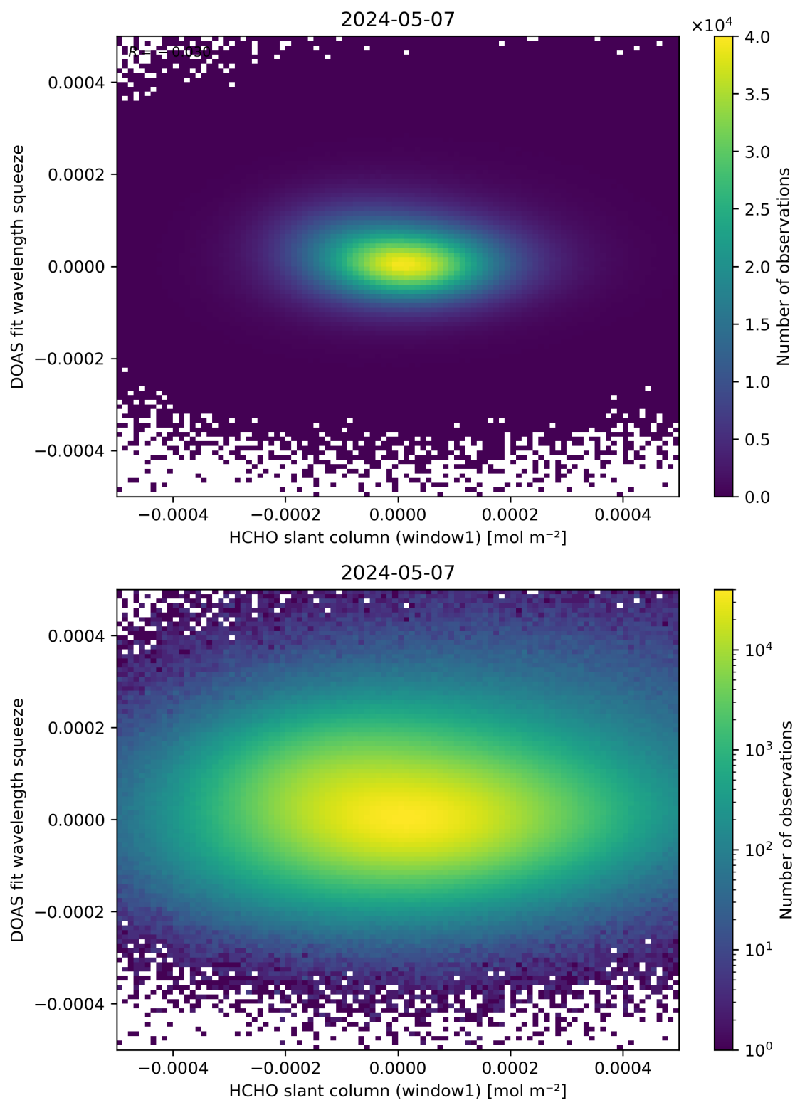
Figure 80: Scatter density plot of “HCHO slant column (window1)” against “DOAS fit wavelength squeeze” for 2024-05-07 to 2024-05-08.
