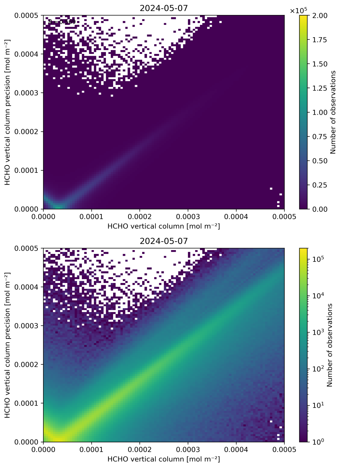
Figure 134: Scatter density plot of “HCHO vertical column” against “HCHO vertical column precision” for 2024-05-07 to 2024-05-08.
