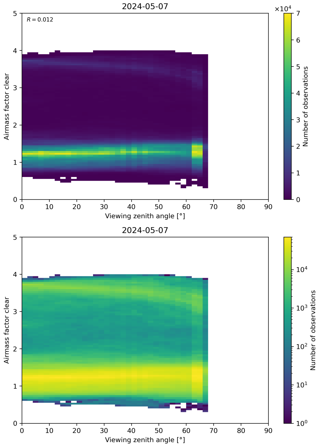
Figure 185: Scatter density plot of “Viewing zenith angle” against “Airmass factor clear” for 2024-05-07 to 2024-05-08.
