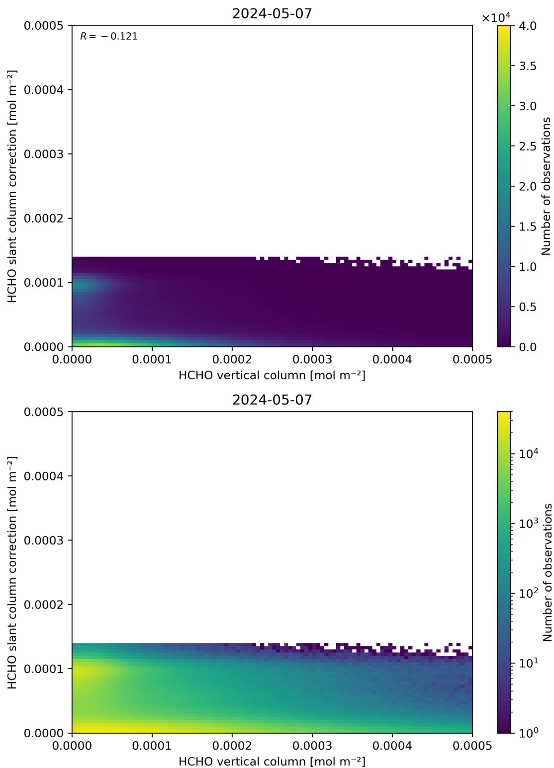
Figure 128: Scatter density plot of “HCHO vertical column” against “HCHO slant column correction” for 2024-05-07 to 2024-05-08.
