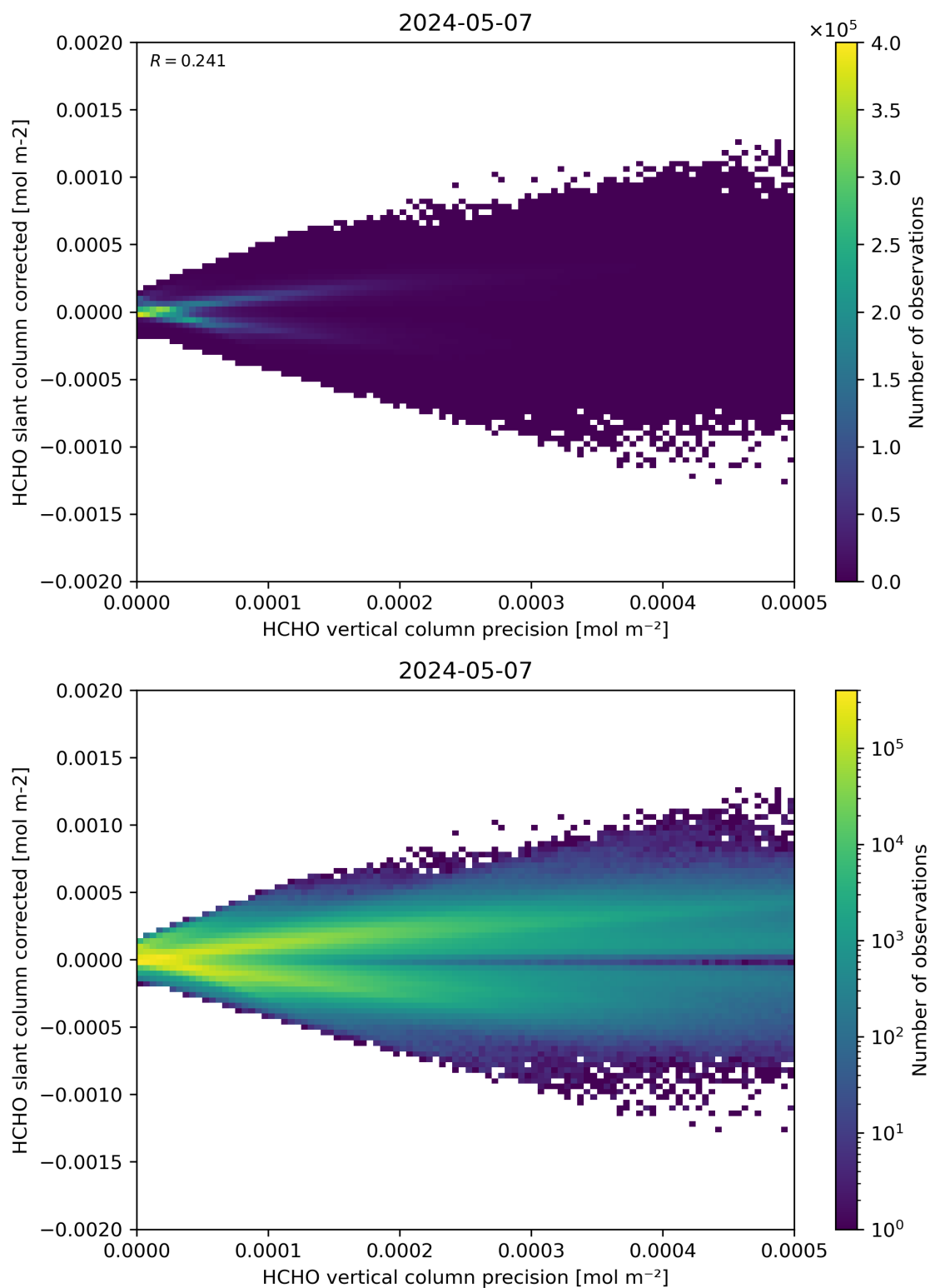
Figure 140: Scatter density plot of “HCHO vertical column precision” against “HCHO slant column corrected” for 2024-05-07 to 2024-05-08.
