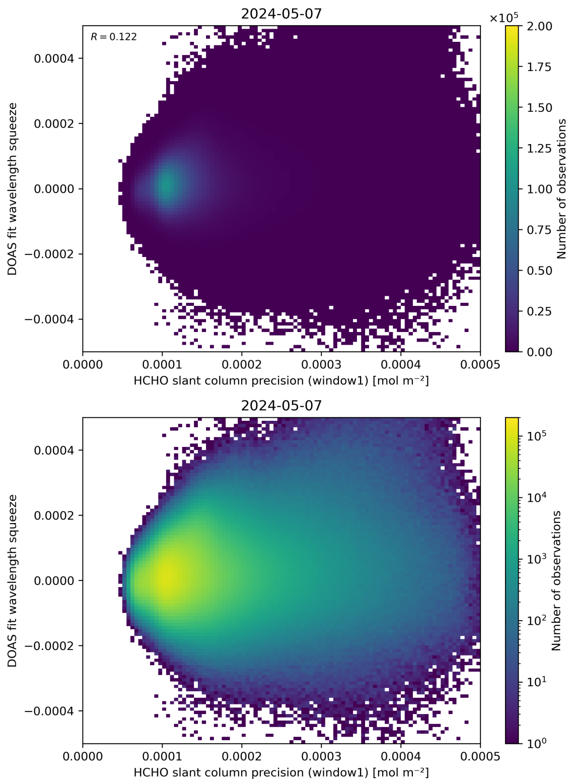
Figure 90: Scatter density plot of “HCHO slant column precision (window1)” against “DOAS fit wavelength squeeze” for 2024-05-07 to 2024-05-08.
