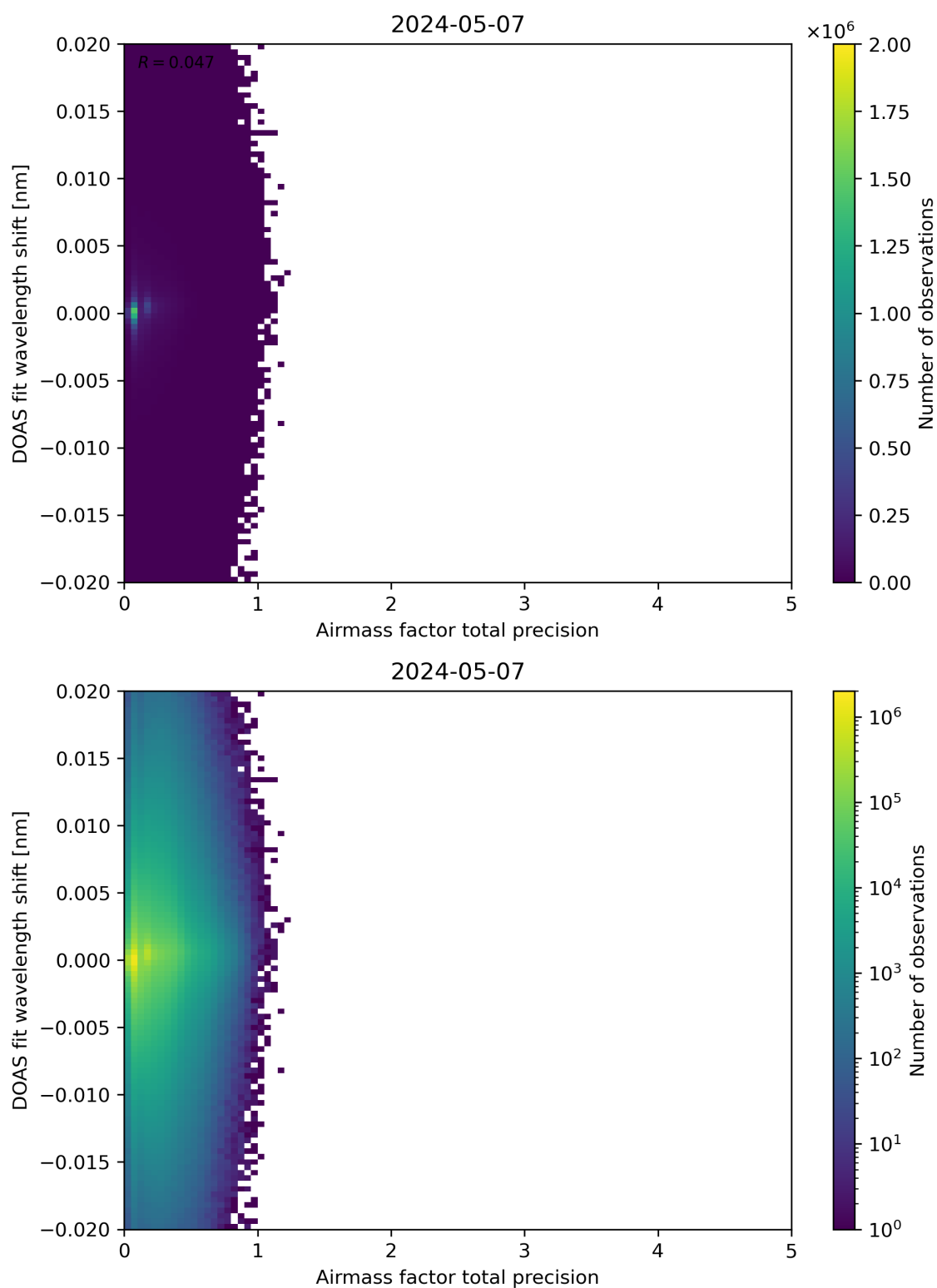
Figure 106: Scatter density plot of “Airmass factor total precision” against “DOAS fit wavelength shift” for 2024-05-07 to 2024-05-08.
