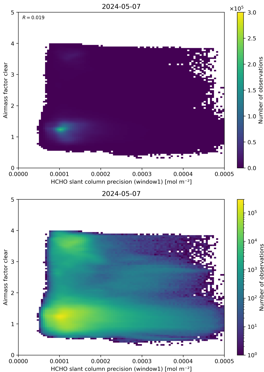
Figure 91: Scatter density plot of “HCHO slant column precision (window1)” against “Airmass factor clear” for 2024-05-07 to 2024-05-08.
