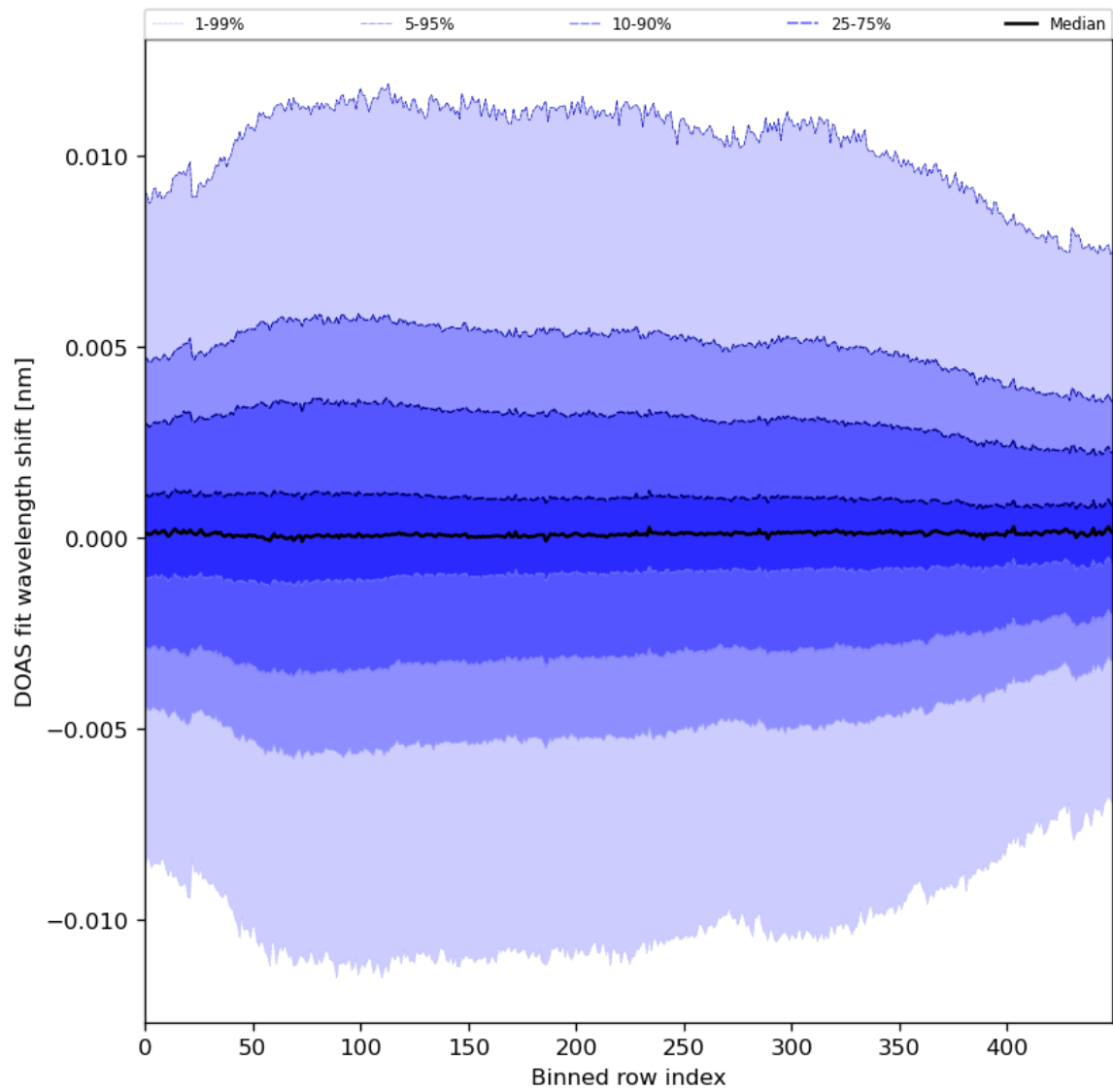
Figure 58: Along track statistics of “DOAS fit wavelength shift” for 2024-05-07 to 2024-05-08
