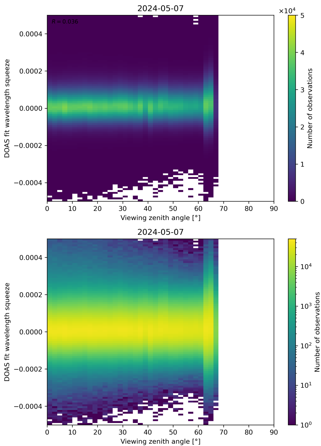
Figure 184: Scatter density plot of “Viewing zenith angle” against “DOAS fit wavelength squeeze” for 2024-05-07 to 2024-05-08.
