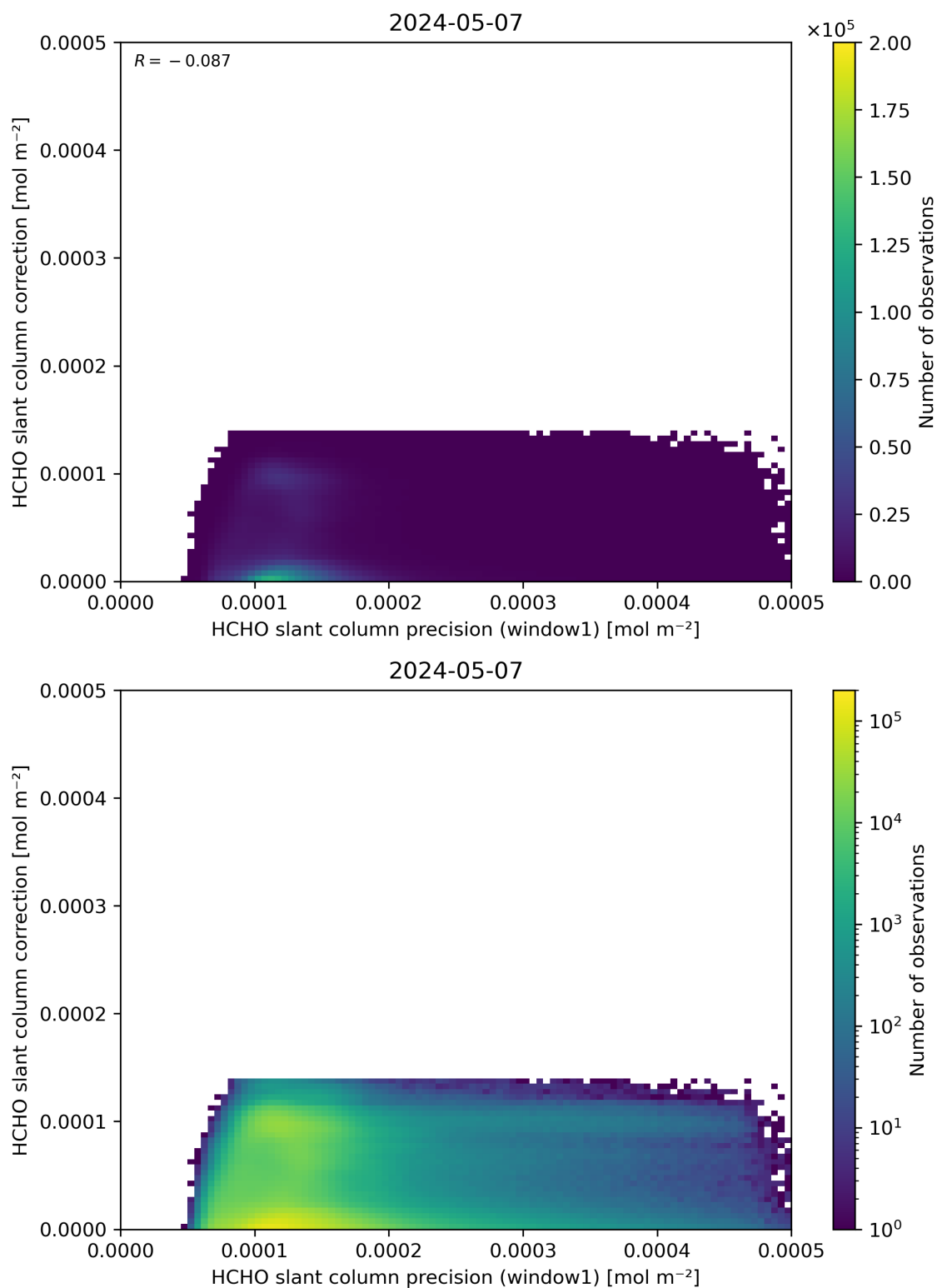
Figure 93: Scatter density plot of “HCHO slant column precision (window1)” against “HCHO slant column correction” for 2024-05-07 to 2024-05-08.
