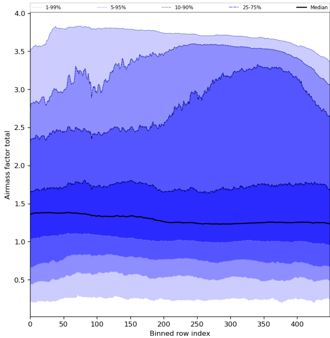
Figure 54: Along track statistics of “Airmass factor total” for 2024-05-07 to 2024-05-08
