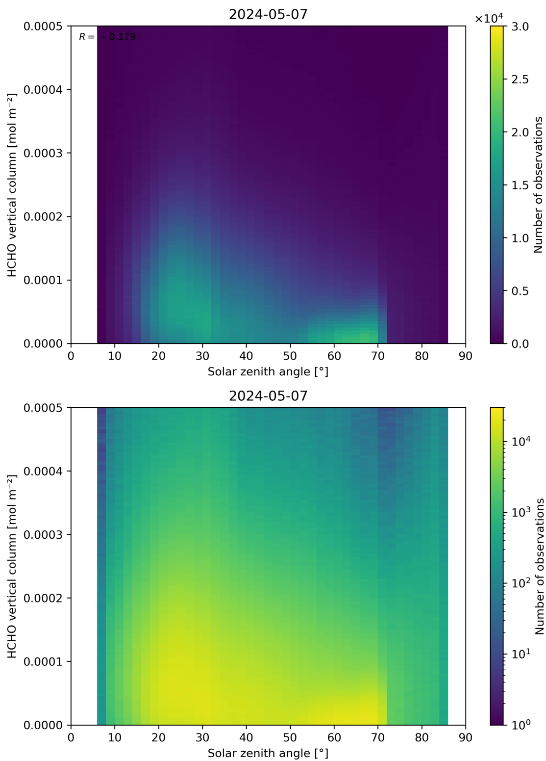
Figure 177: Scatter density plot of “Solar zenith angle” against “HCHO vertical column” for 2024-05-07 to 2024-05-08.
