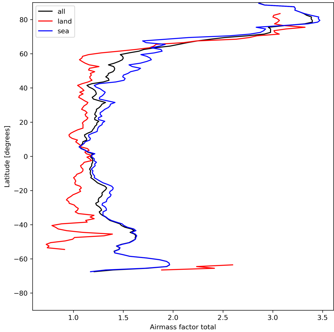
Figure 26: Zonal average of “Airmass factor total” for 2024-05-07 to 2024-05-08.
