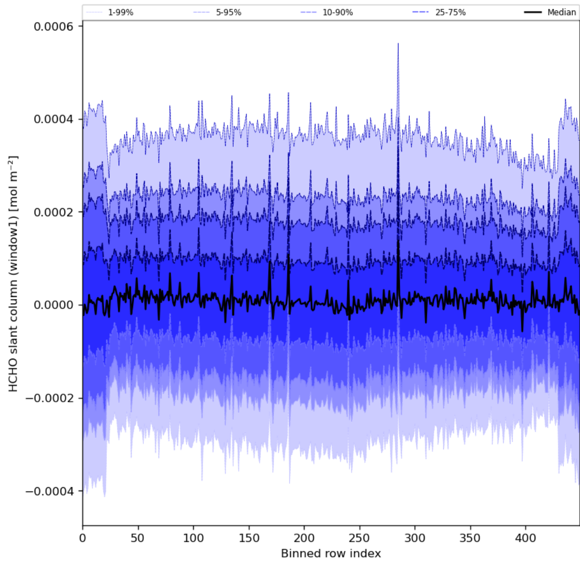
Figure 52: Along track statistics of “HCHO slant column (window1)” for 2024-05-07 to 2024-05-08
