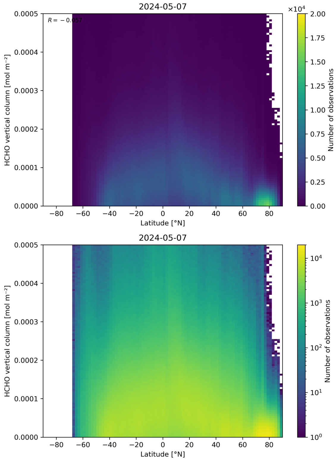
Figure 163: Scatter density plot of “Latitude” against “HCHO vertical column” for 2024-05-07 to 2024-05-08.
