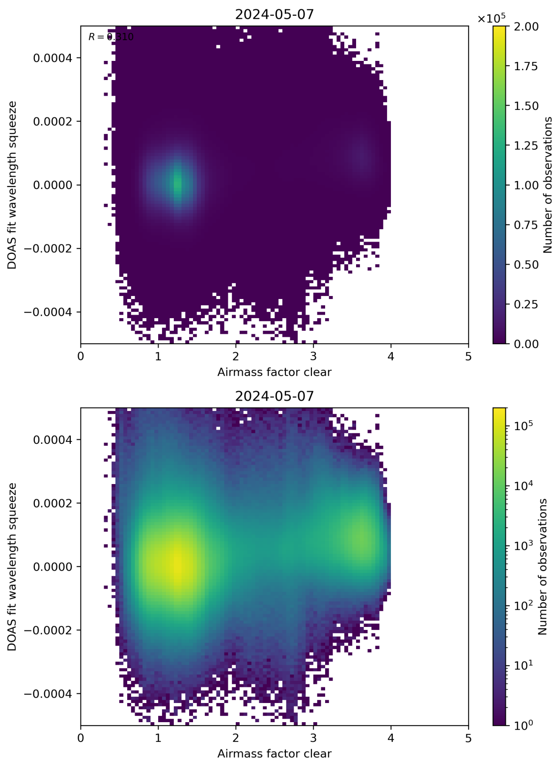
Figure 73: Scatter density plot of “Airmass factor clear” against “DOAS fit wavelength squeeze” for 2024-05-07 to 2024-05-08.
