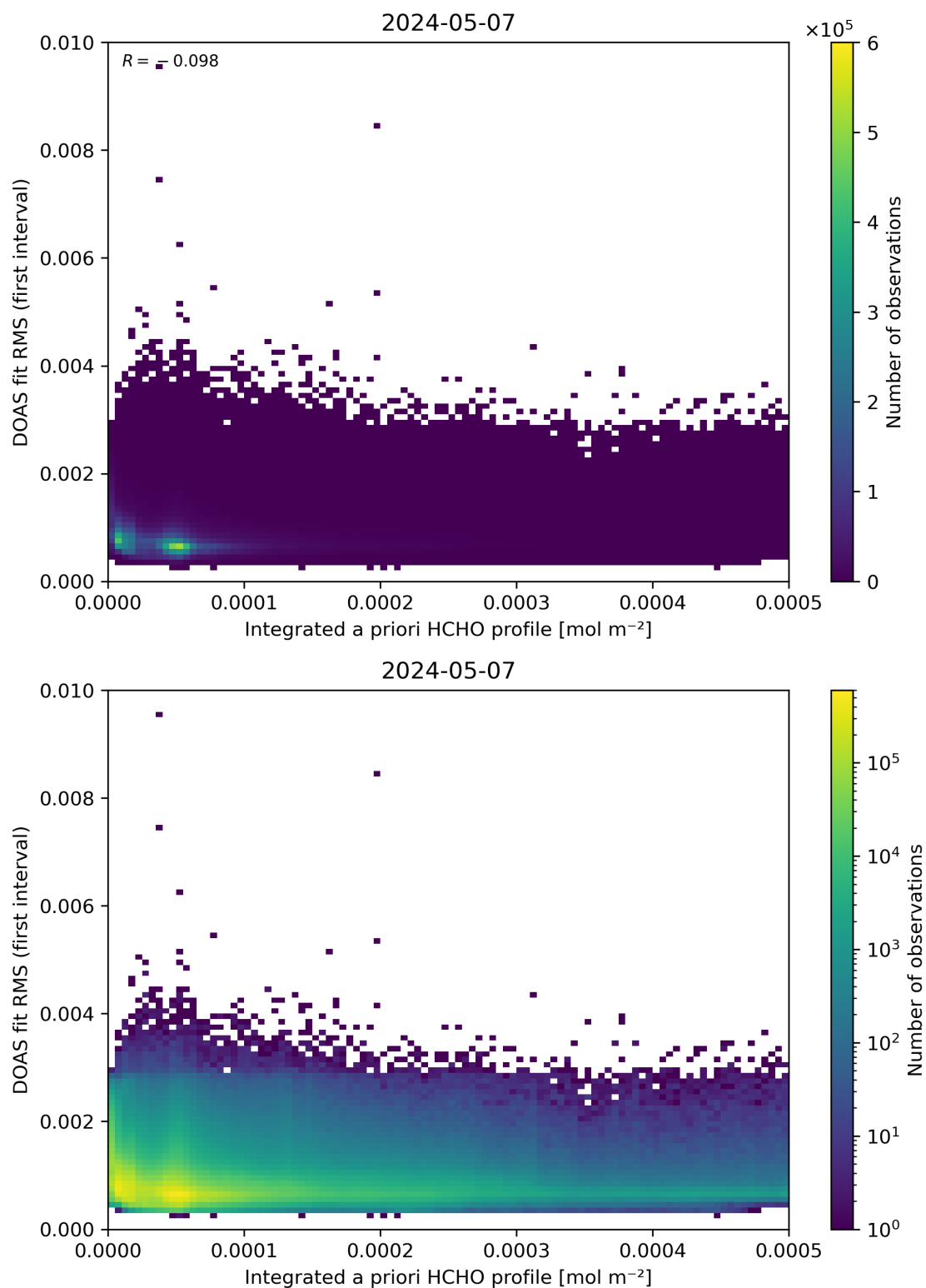
Figure 148: Scatter density plot of “Integrated a priori HCHO profile” against “DOAS fit RMS (first interval)” for 2024-05-07 to 2024-05-08.
