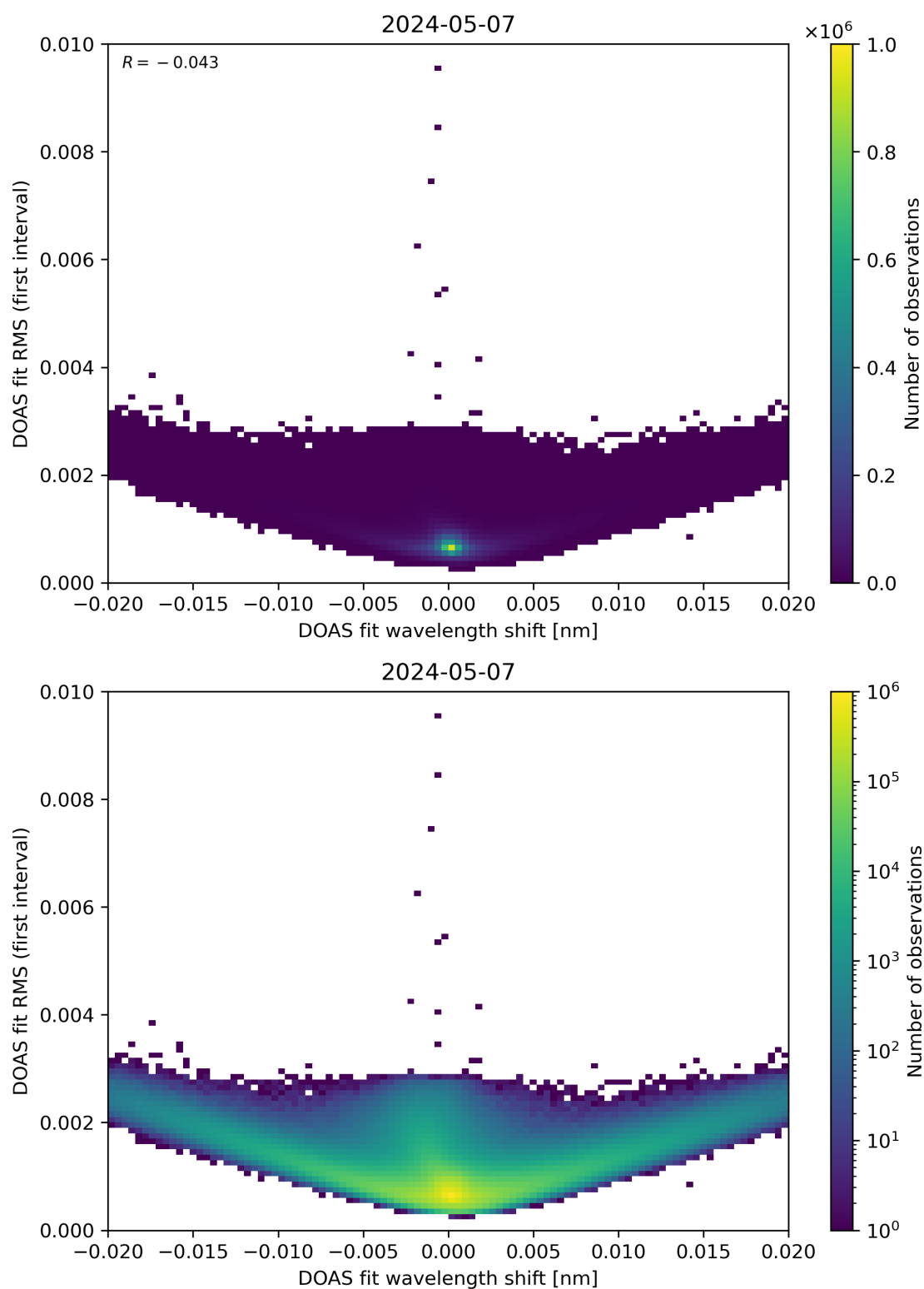
Figure 64: Scatter density plot of “DOAS fit wavelength shift” against “DOAS fit RMS (first interval)” for 2024-05-07 to 2024-05-08.
