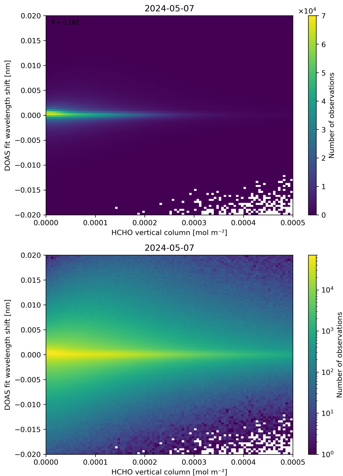
Figure 124: Scatter density plot of “HCHO vertical column” against “DOAS fit wavelength shift” for 2024-05-07 to 2024-05-08.
