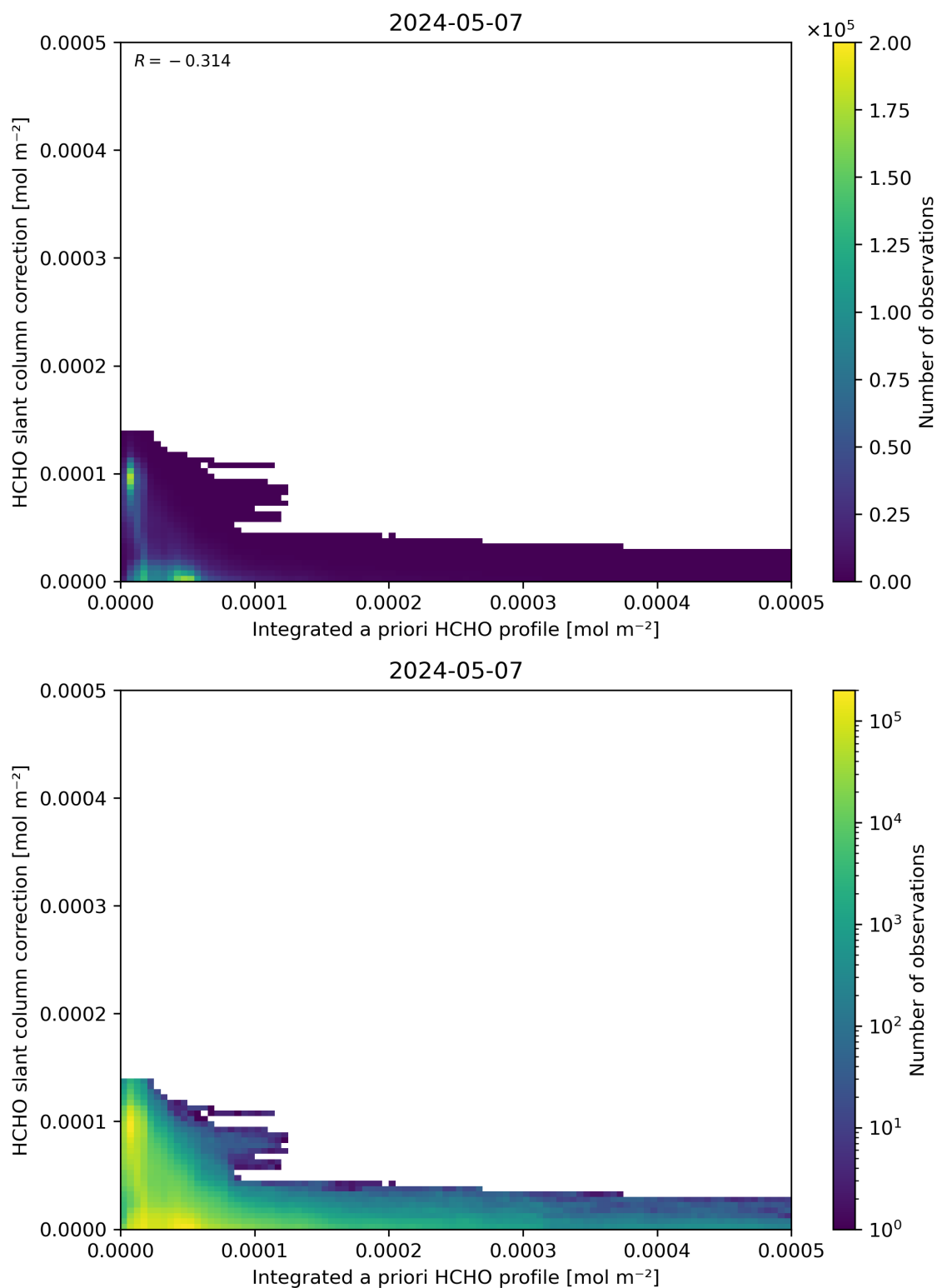
Figure 152: Scatter density plot of “Integrated a priori HCHO profile” against “HCHO slant column correction” for 2024-05-07 to 2024-05-08.
