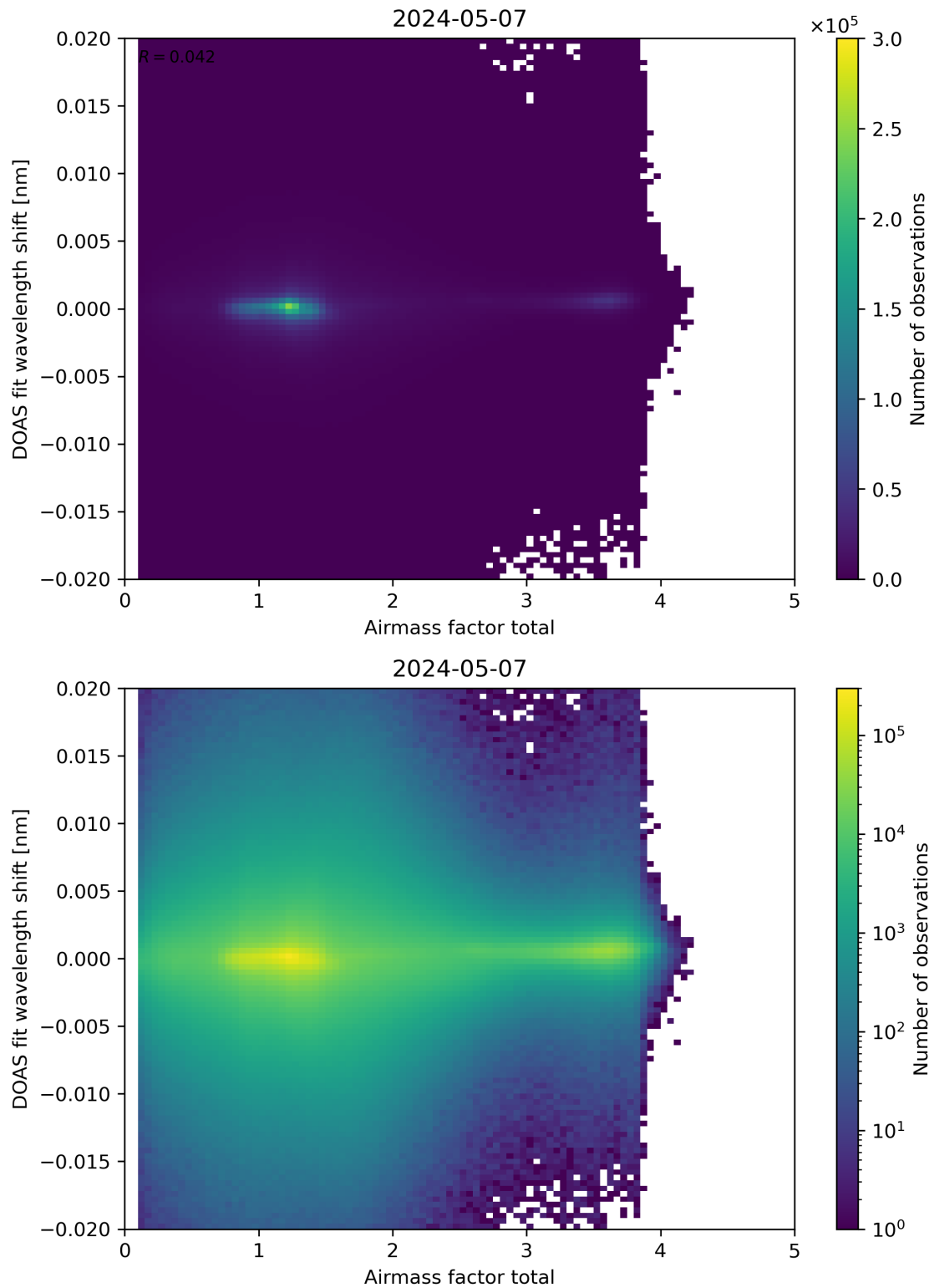
Figure 98: Scatter density plot of “Airmass factor total” against “DOAS fit wavelength shift” for 2024-05-07 to 2024-05-08.
