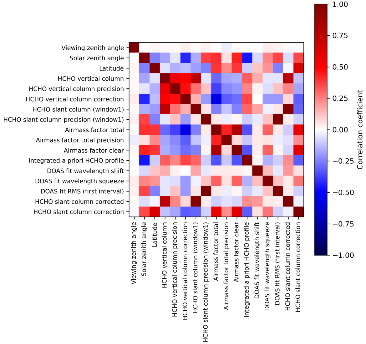
Figure 2: Map of correlation matrix for 2024-05-07 to 2024-05-08.
