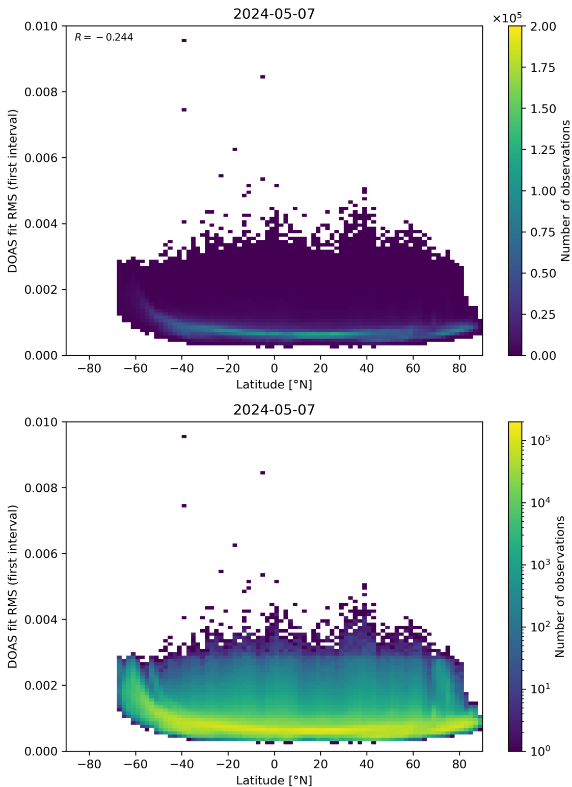
Figure 153: Scatter density plot of “Latitude” against “DOAS fit RMS (first interval)” for 2024-05-07 to 2024-05-08.
