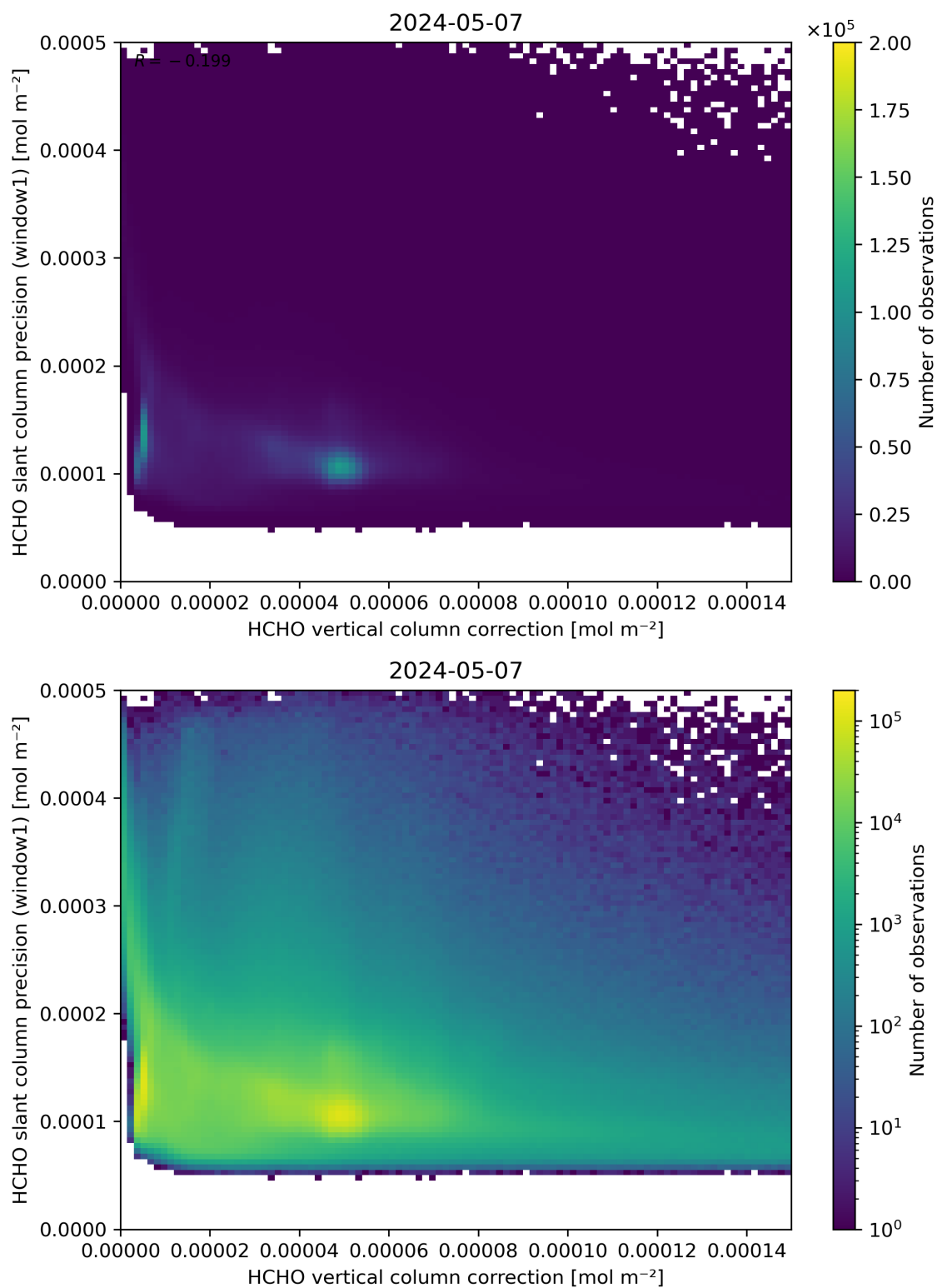
Figure 119: Scatter density plot of “HCHO vertical column correction” against “HCHO slant column precision (window1)” for 2024-05-07 to 2024-05-08.
