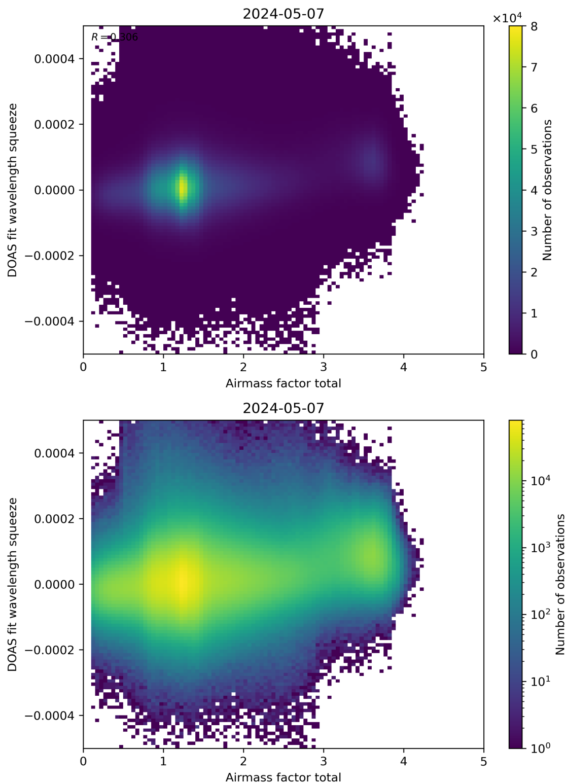
Figure 99: Scatter density plot of “Airmass factor total” against “DOAS fit wavelength squeeze” for 2024-05-07 to 2024-05-08.
