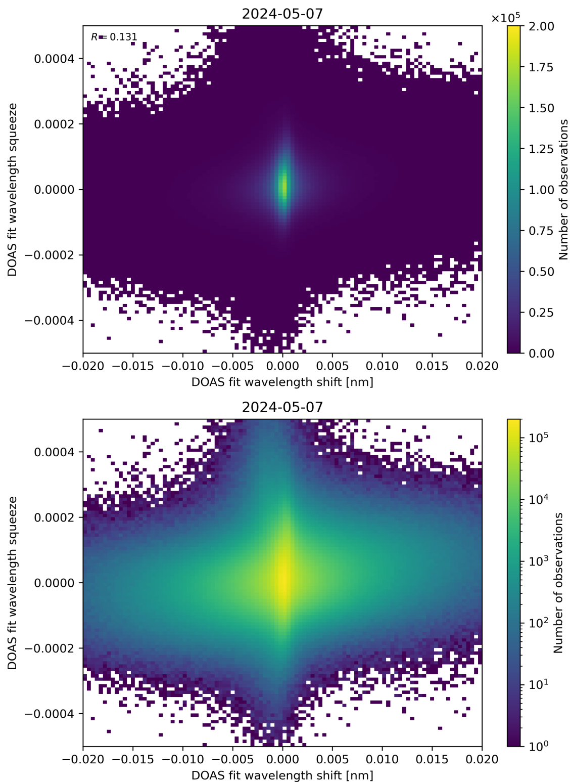
Figure 65: Scatter density plot of “DOAS fit wavelength shift” against “DOAS fit wavelength squeeze” for 2024-05-07 to 2024-05-08.
