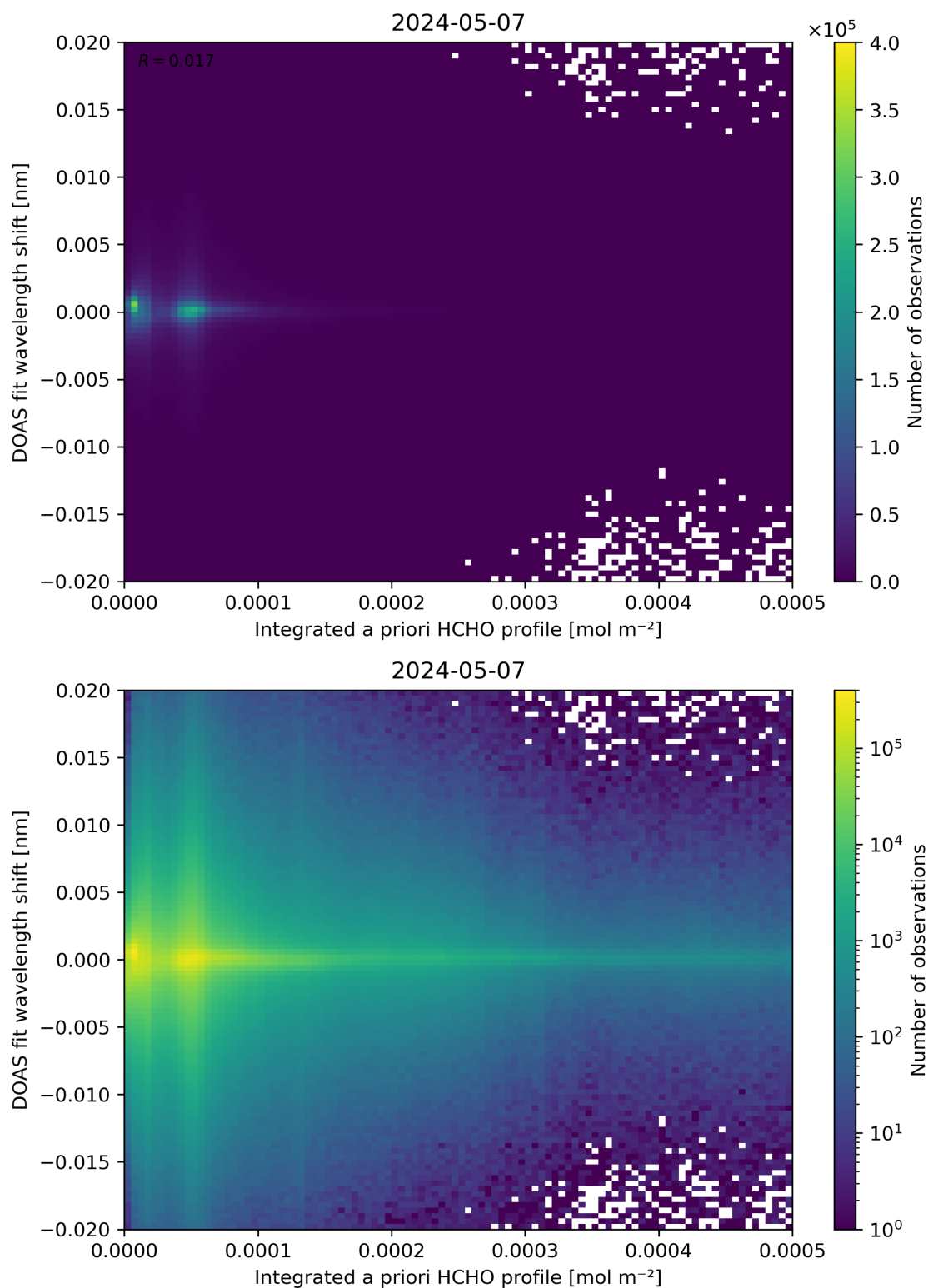
Figure 149: Scatter density plot of “Integrated a priori HCHO profile” against “DOAS fit wavelength shift” for 2024-05-07 to 2024-05-08.
