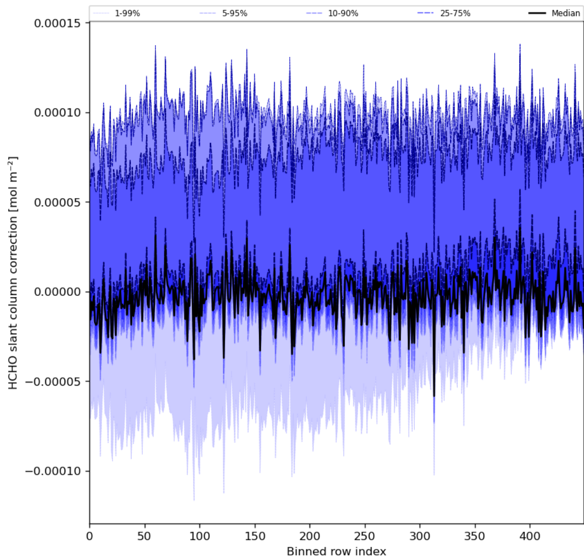
Figure 61: Along track statistics of “HCHO slant column correction” for 2024-05-07 to 2024-05-08
