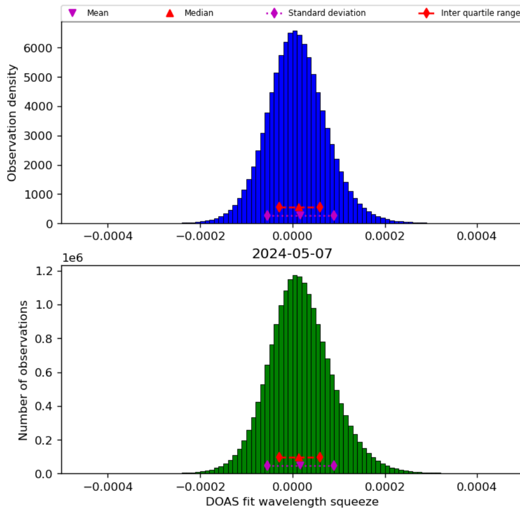
Figure 45: Histogram of “DOAS fit wavelength squeeze” for 2024-05-07 to 2024-05-08
