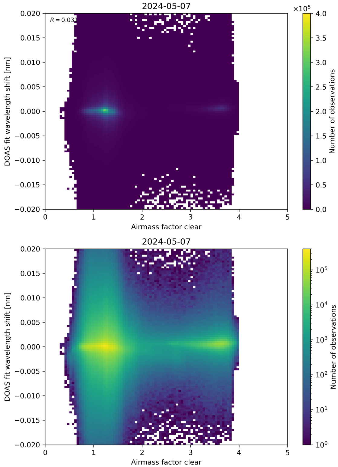
Figure 72: Scatter density plot of “Airmass factor clear” against “DOAS fit wavelength shift” for 2024-05-07 to 2024-05-08.
