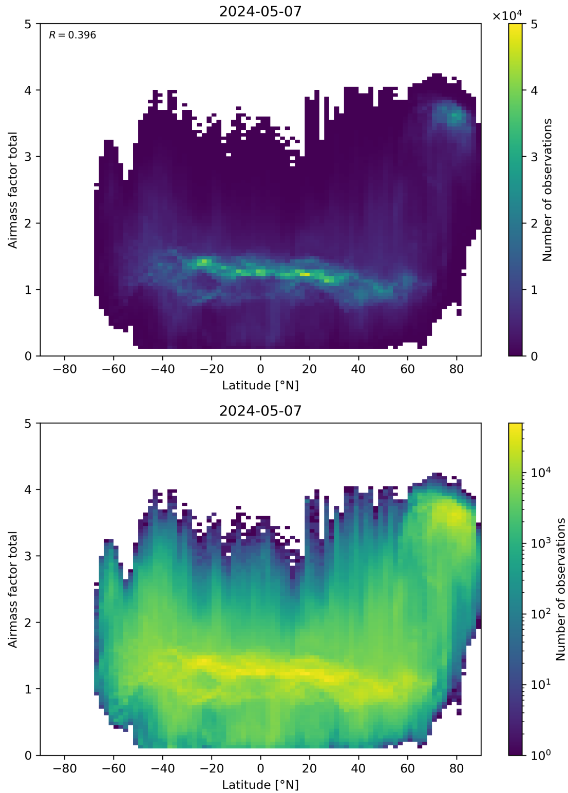
Figure 161: Scatter density plot of “Latitude” against “Airmass factor total” for 2024-05-07 to 2024-05-08.
