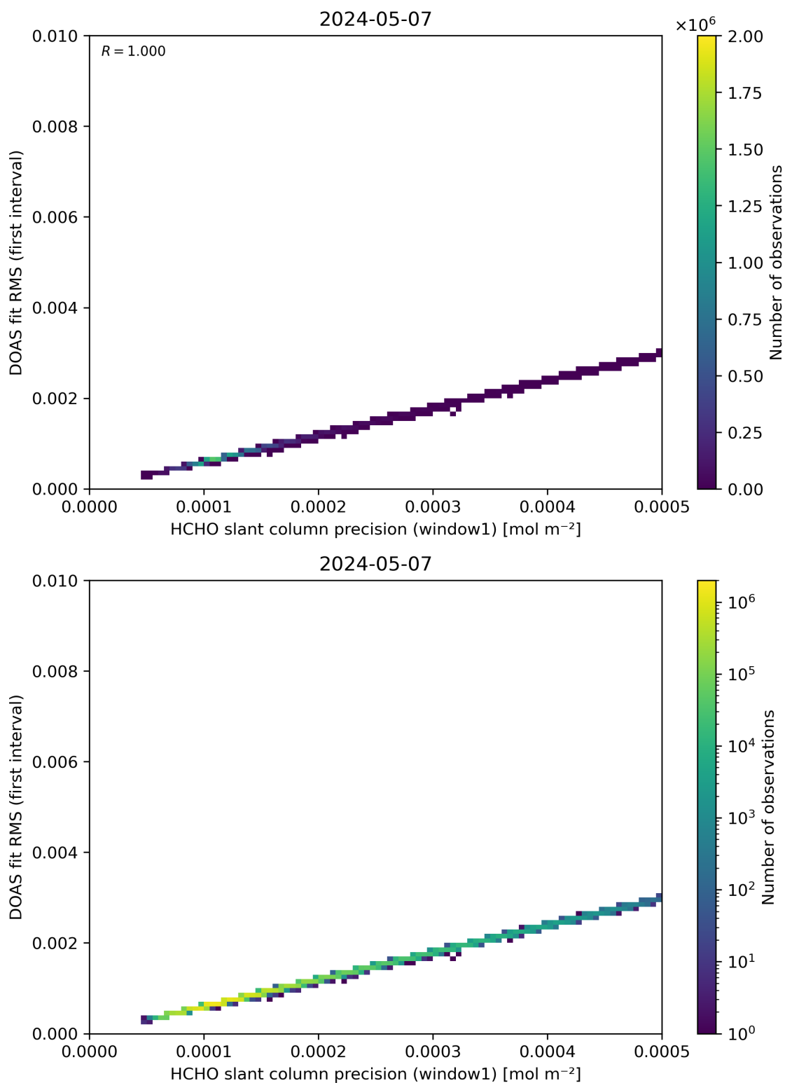
Figure 88: Scatter density plot of “HCHO slant column precision (window1)” against “DOAS fit RMS (first interval)” for 2024-05-07 to 2024-05-08.
