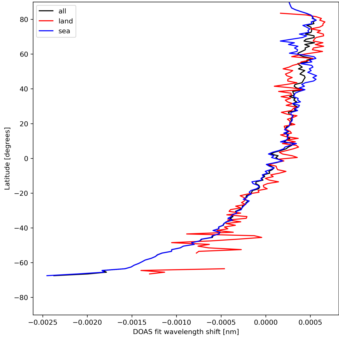
Figure 30: Zonal average of “DOAS fit wavelength shift” for 2024-05-07 to 2024-05-08.
