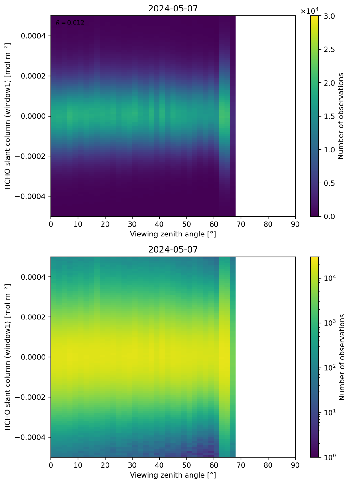
Figure 188: Scatter density plot of “Viewing zenith angle” against “HCHO slant column (window1)” for 2024-05-07 to 2024-05-08.
