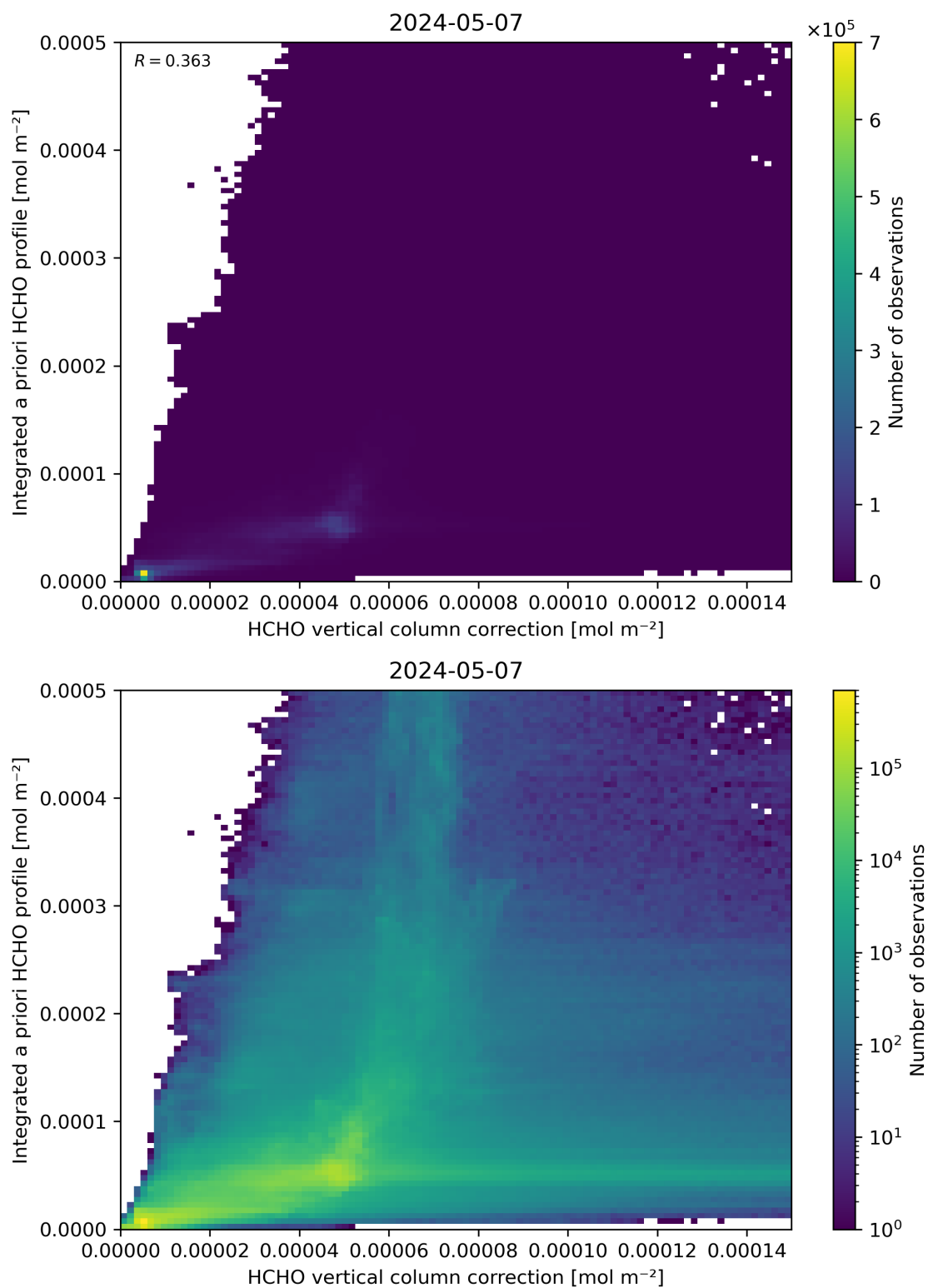
Figure 122: Scatter density plot of “HCHO vertical column correction” against “Integrated a priori HCHO profile” for 2024-05-07 to 2024-05-08.
