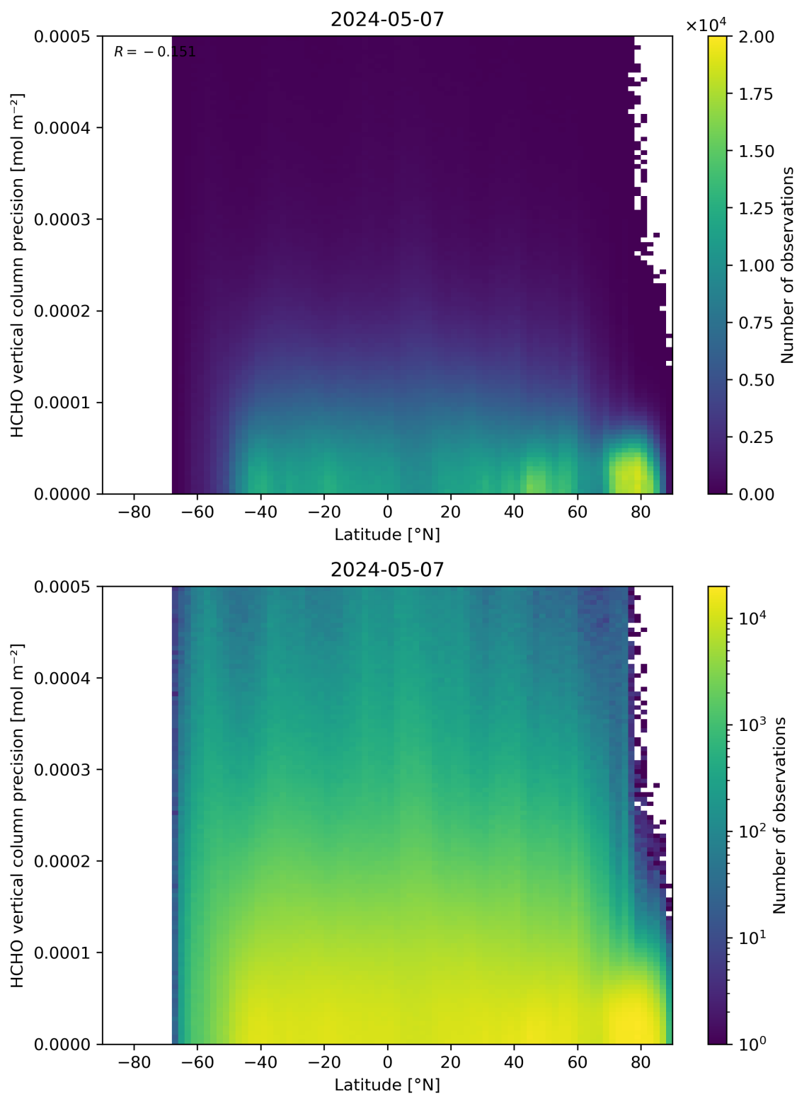
Figure 165: Scatter density plot of “Latitude” against “HCHO vertical column precision” for 2024-05-07 to 2024-05-08.
