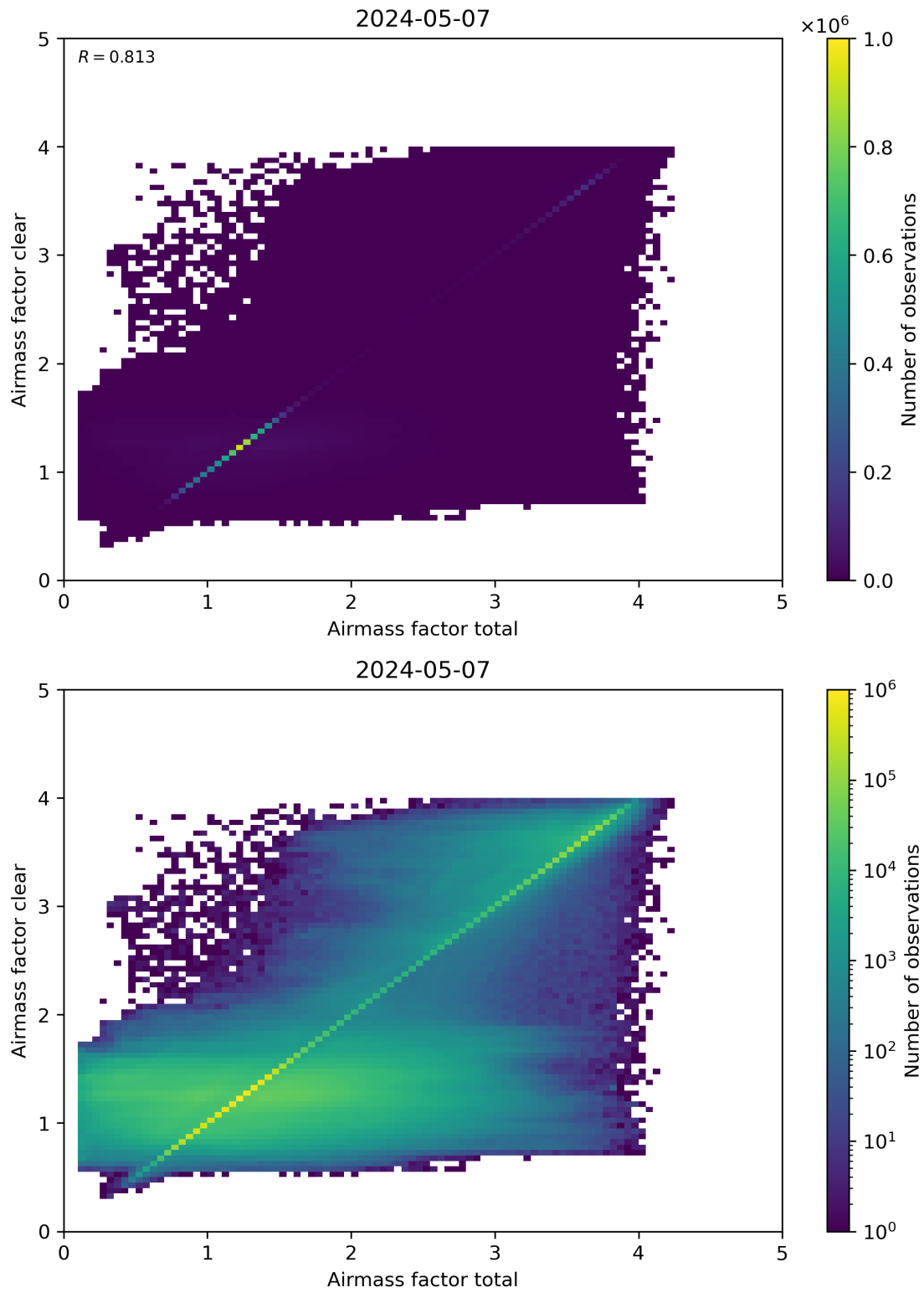
Figure 100: Scatter density plot of “Airmass factor total” against “Airmass factor clear” for 2024-05-07 to 2024-05-08.
