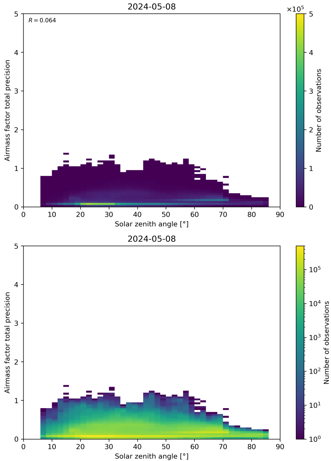
Figure 176: Scatter density plot of “Solar zenith angle” against “Airmass factor total precision” for 2024-05-07 to 2024-05-09.
