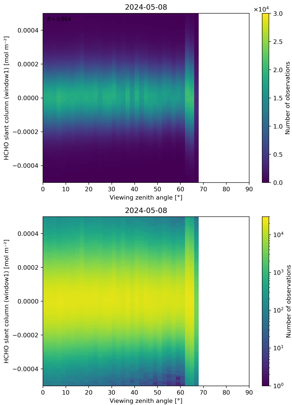
Figure 188: Scatter density plot of “Viewing zenith angle” against “HCHO slant column (window1)” for 2024-05-07 to 2024-05-09.
