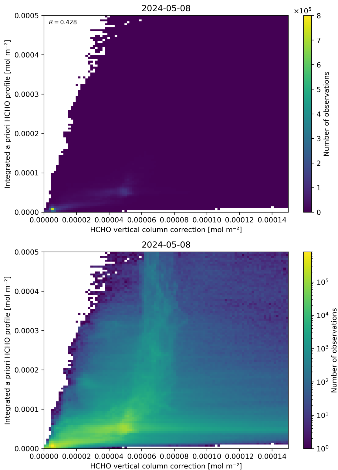
Figure 122: Scatter density plot of “HCHO vertical column correction” against “Integrated a priori HCHO profile” for 2024-05-07 to 2024-05-09.
