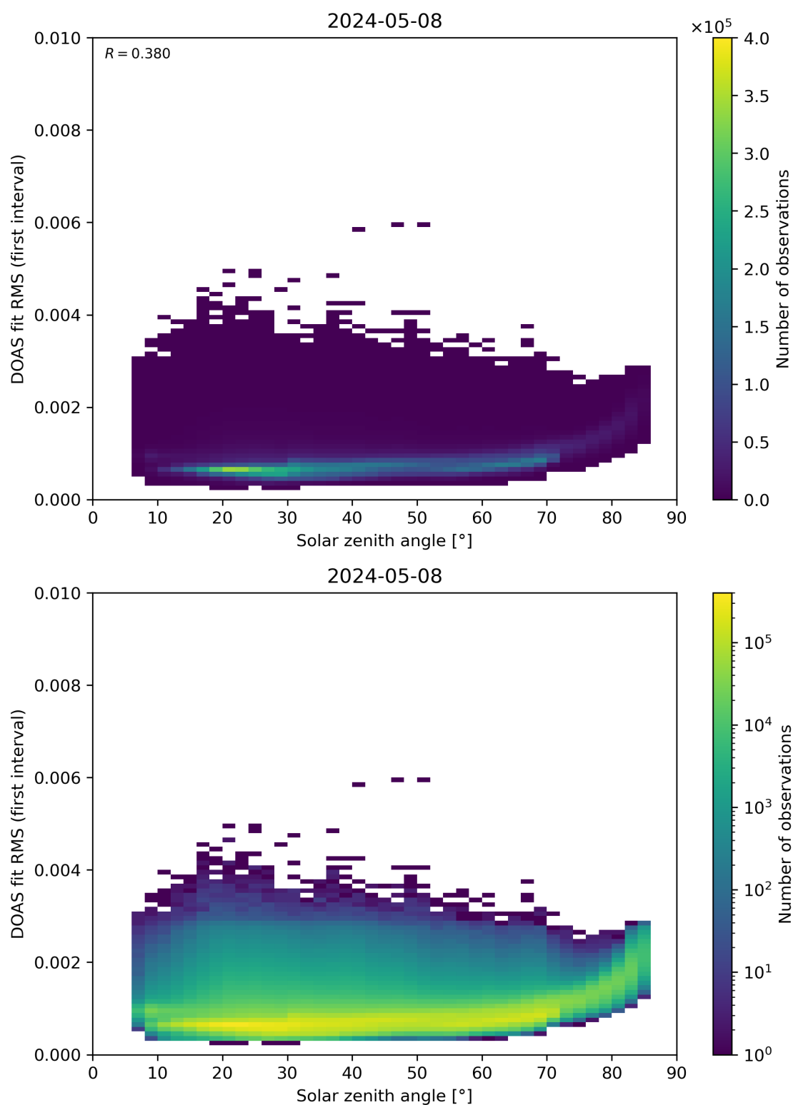
Figure 167: Scatter density plot of “Solar zenith angle” against “DOAS fit RMS (first interval)” for 2024-05-07 to 2024-05-09.
