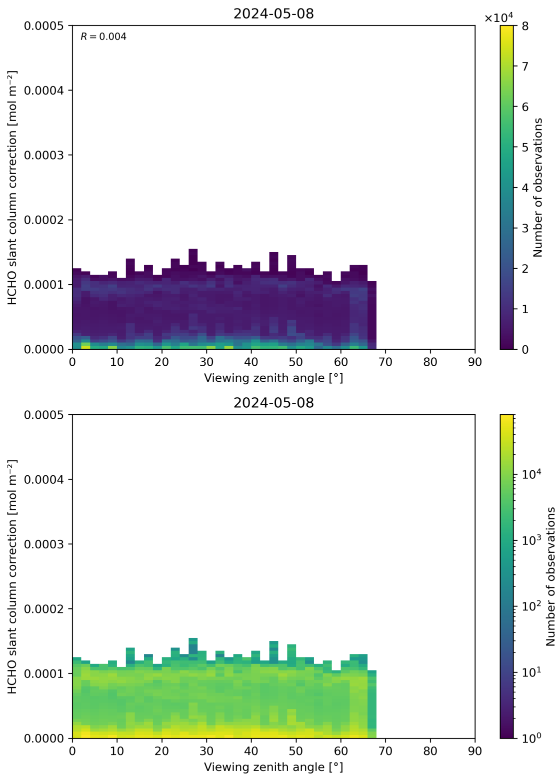
Figure 187: Scatter density plot of “Viewing zenith angle” against “HCHO slant column correction” for 2024-05-07 to 2024-05-09.
