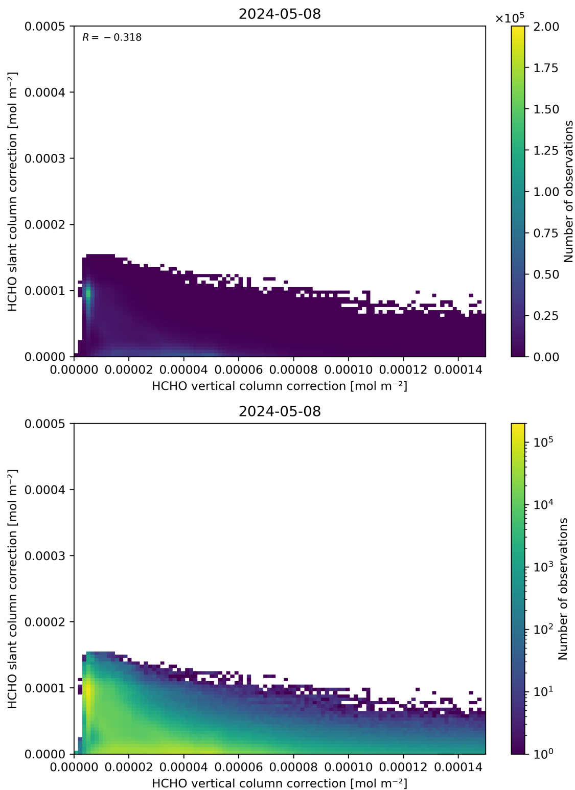
Figure 117: Scatter density plot of “HCHO vertical column correction” against “HCHO slant column correction” for 2024-05-07 to 2024-05-09.
