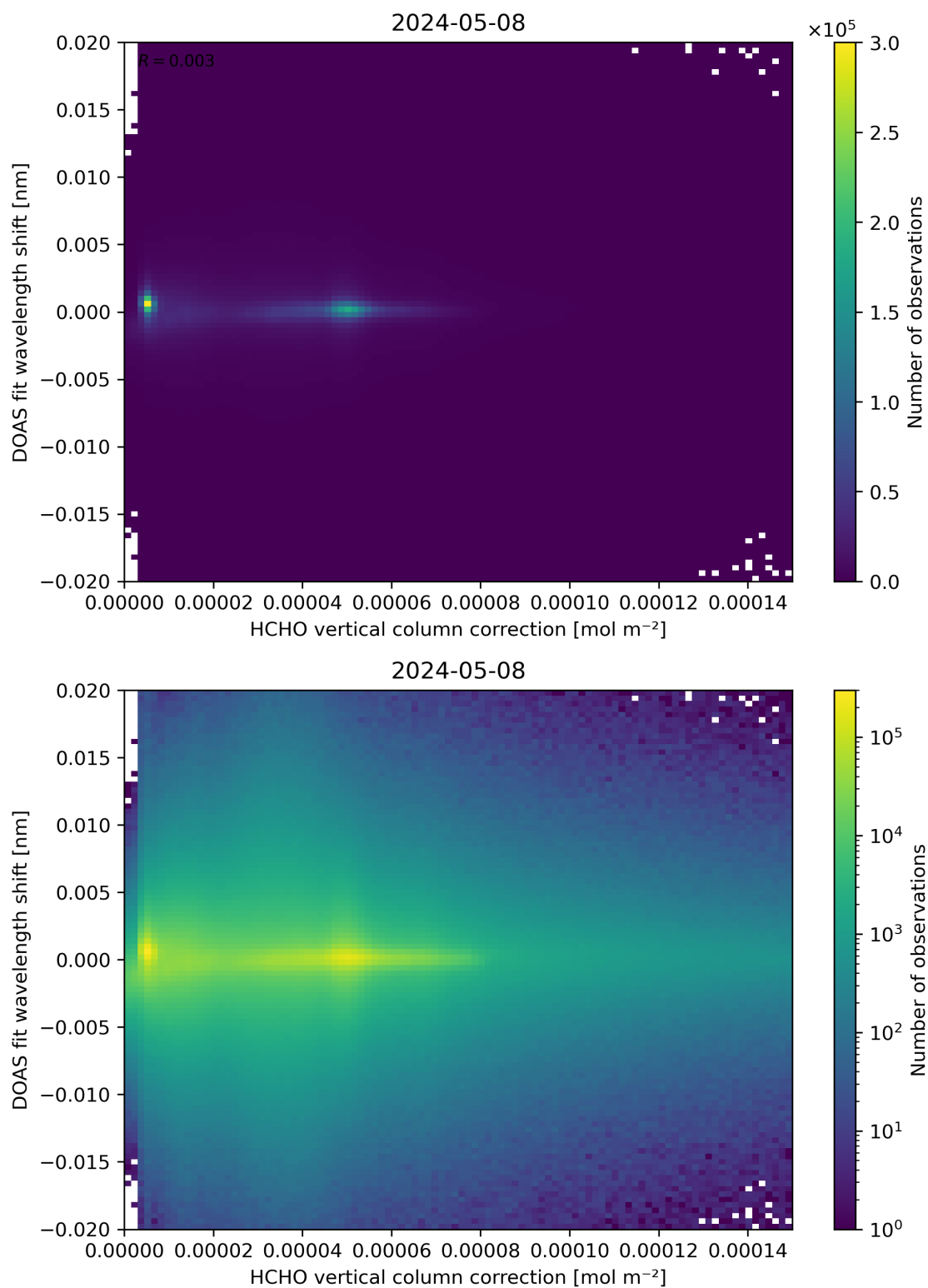
Figure 113: Scatter density plot of “HCHO vertical column correction” against “DOAS fit wavelength shift” for 2024-05-07 to 2024-05-09.
