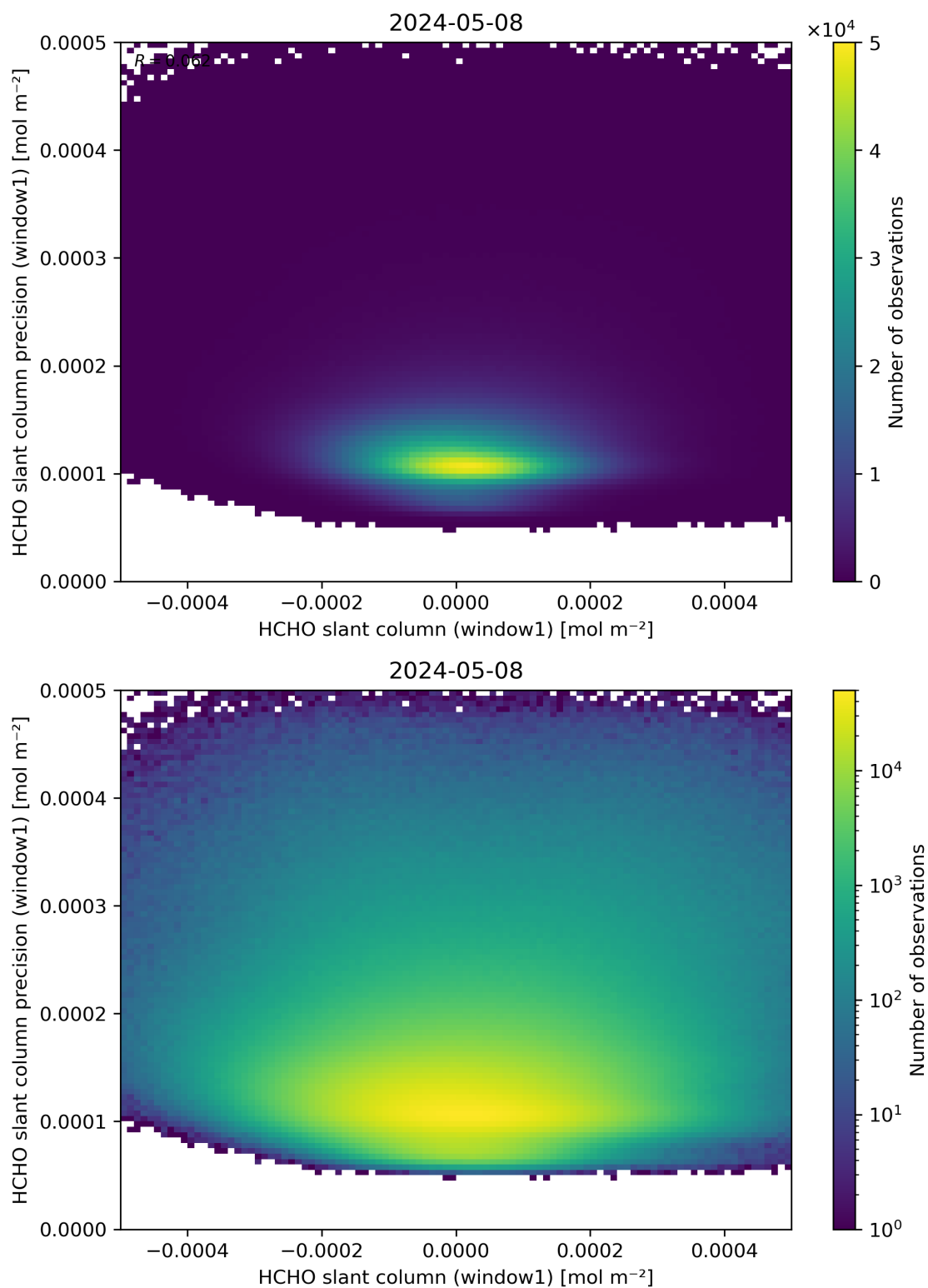
Figure 84: Scatter density plot of “HCHO slant column (window1)” against “HCHO slant column precision (window1)” for 2024-05-07 to 2024-05-09.
