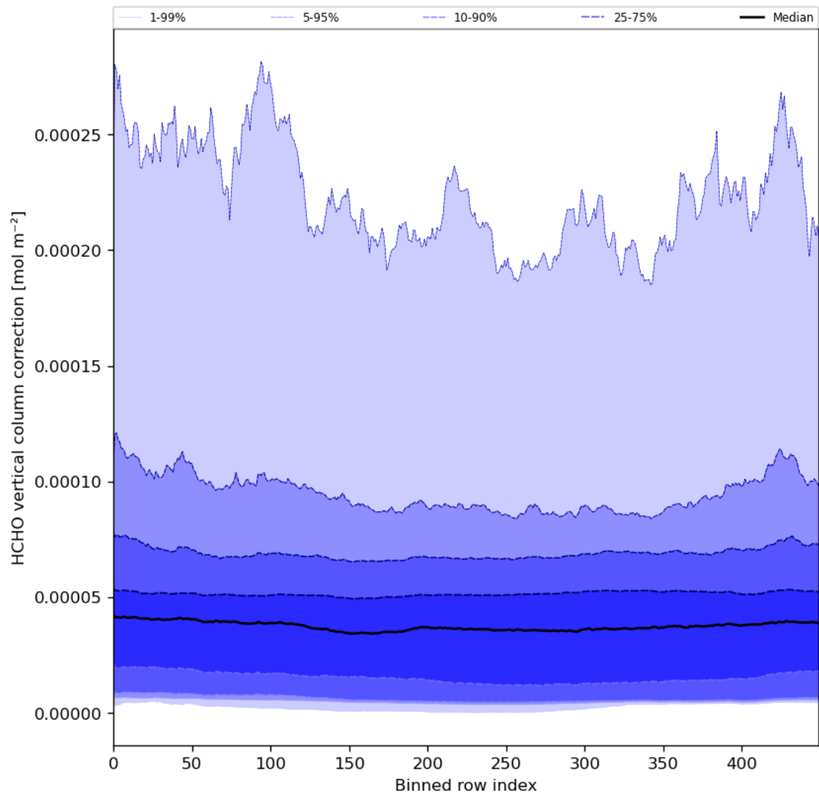
Figure 51: Along track statistics of “HCHO vertical column correction” for 2024-05-07 to 2024-05-09
