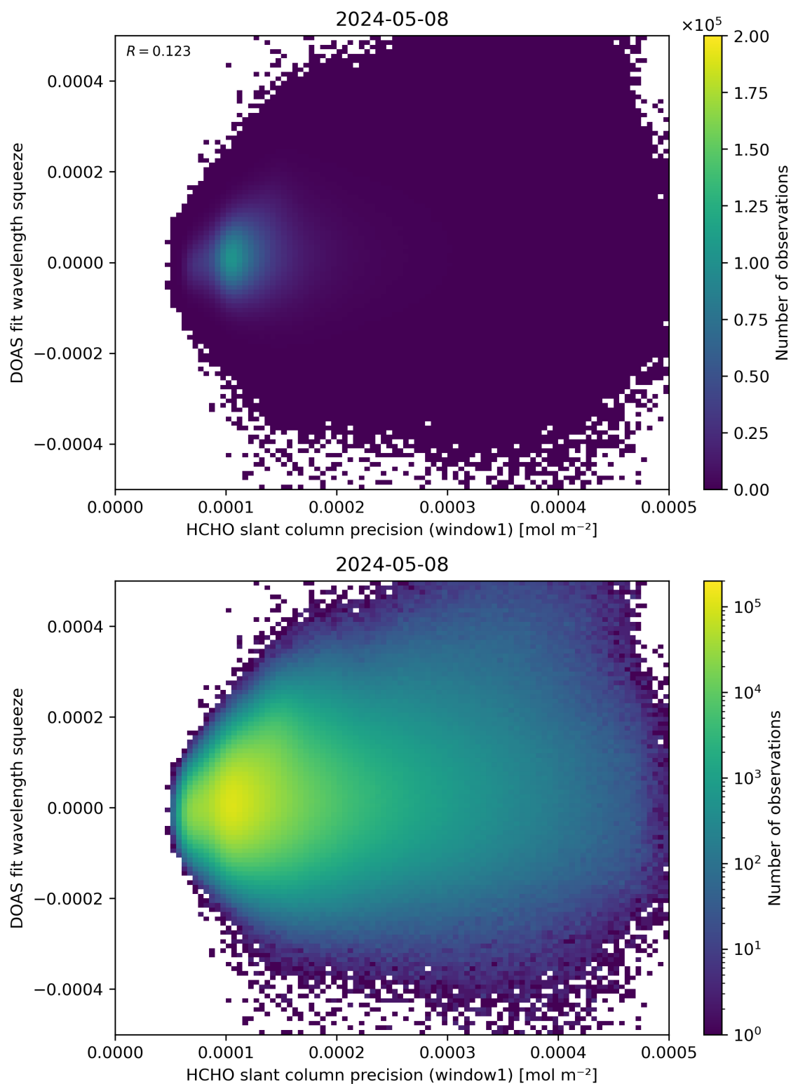
Figure 90: Scatter density plot of “HCHO slant column precision (window1)” against “DOAS fit wavelength squeeze” for 2024-05-07 to 2024-05-09.
