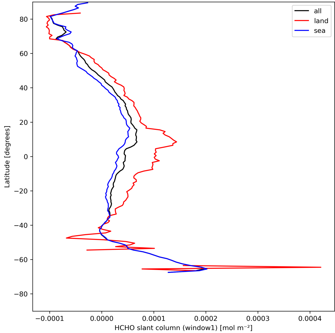
Figure 24: Zonal average of “HCHO slant column (window1)” for 2024-05-07 to 2024-05-09.
