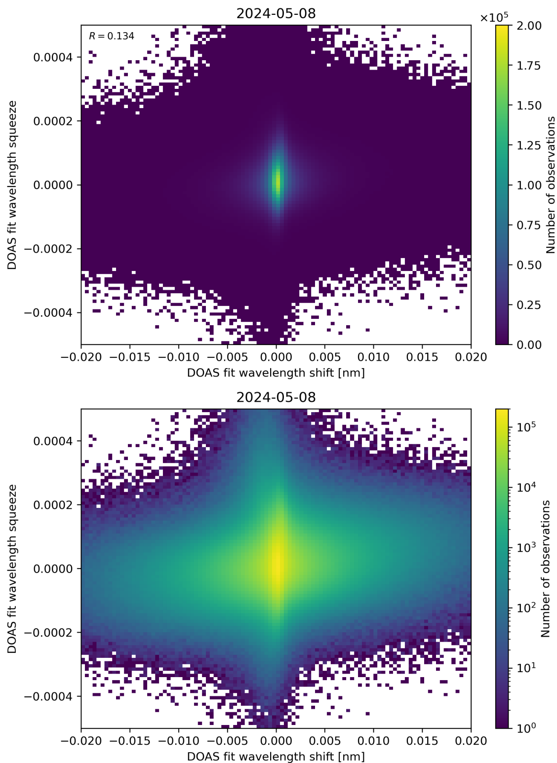
Figure 65: Scatter density plot of “DOAS fit wavelength shift” against “DOAS fit wavelength squeeze” for 2024-05-07 to 2024-05-09.
