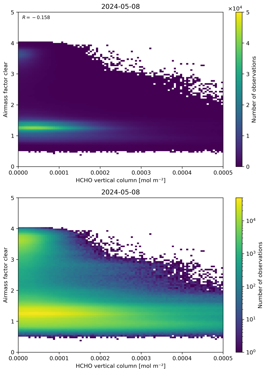
Figure 126: Scatter density plot of “HCHO vertical column” against “Airmass factor clear” for 2024-05-07 to 2024-05-09.
