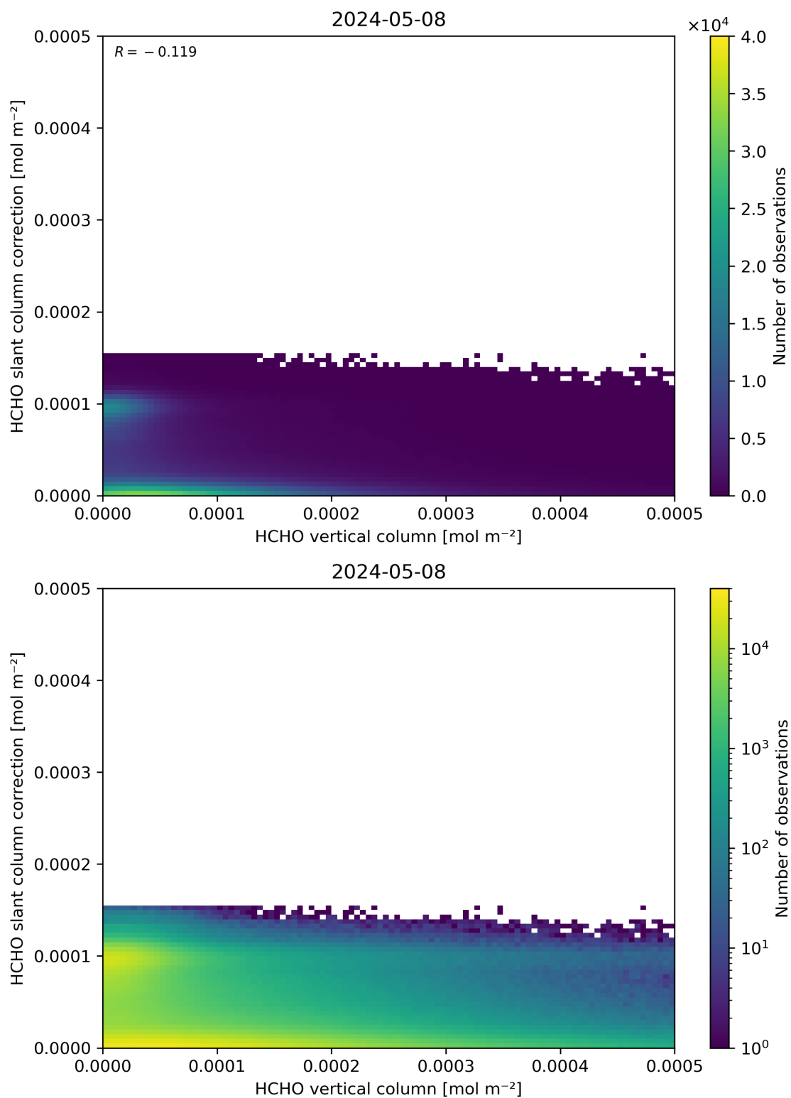
Figure 128: Scatter density plot of “HCHO vertical column” against “HCHO slant column correction” for 2024-05-07 to 2024-05-09.
