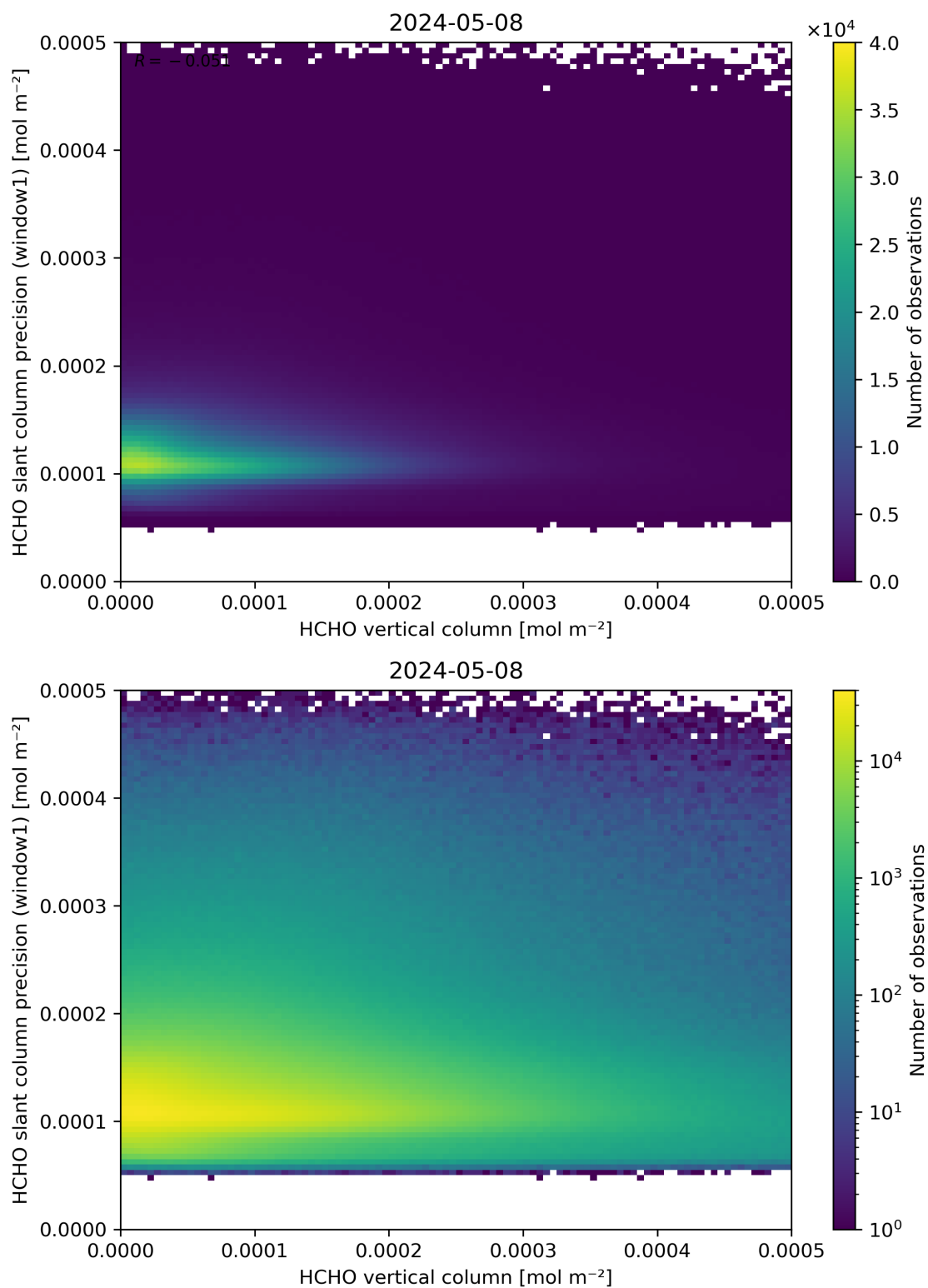
Figure 130: Scatter density plot of “HCHO vertical column” against “HCHO slant column precision (window1)” for 2024-05-07 to 2024-05-09.
