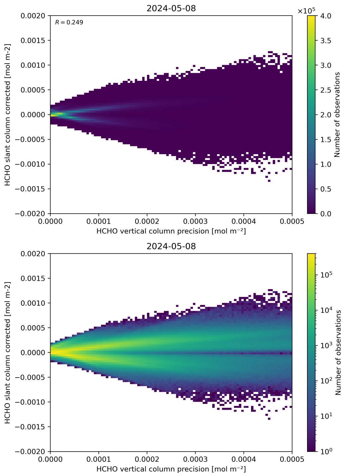
Figure 140: Scatter density plot of “HCHO vertical column precision” against “HCHO slant column corrected” for 2024-05-07 to 2024-05-09.
