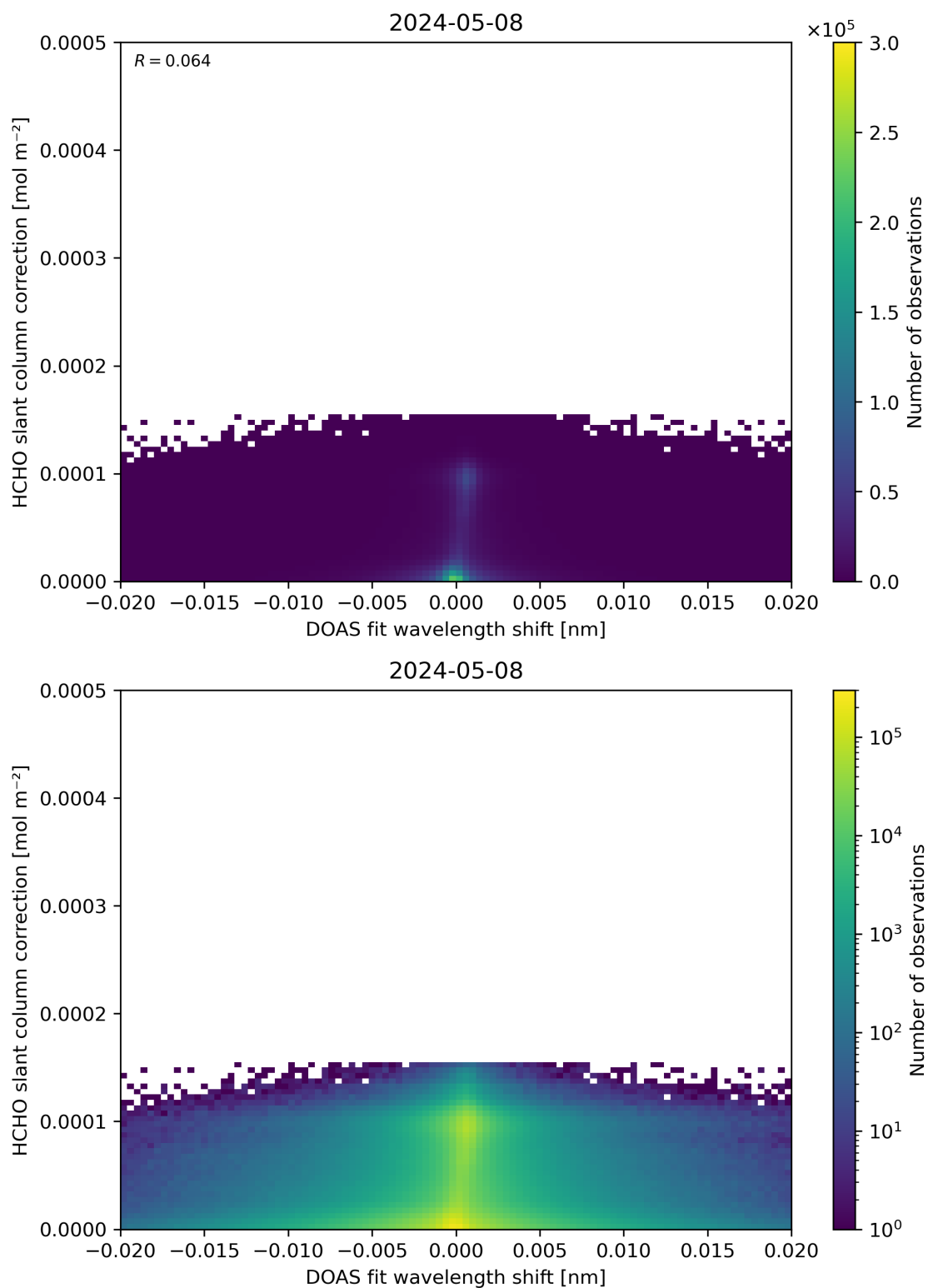
Figure 67: Scatter density plot of “DOAS fit wavelength shift” against “HCHO slant column correction” for 2024-05-07 to 2024-05-09.
