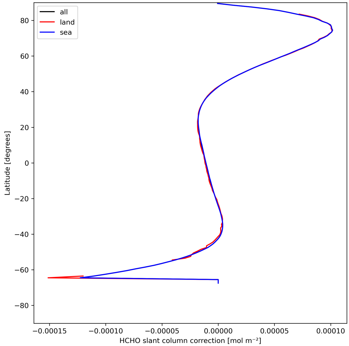
Figure 33: Zonal average of “HCHO slant column correction” for 2024-05-07 to 2024-05-09.
