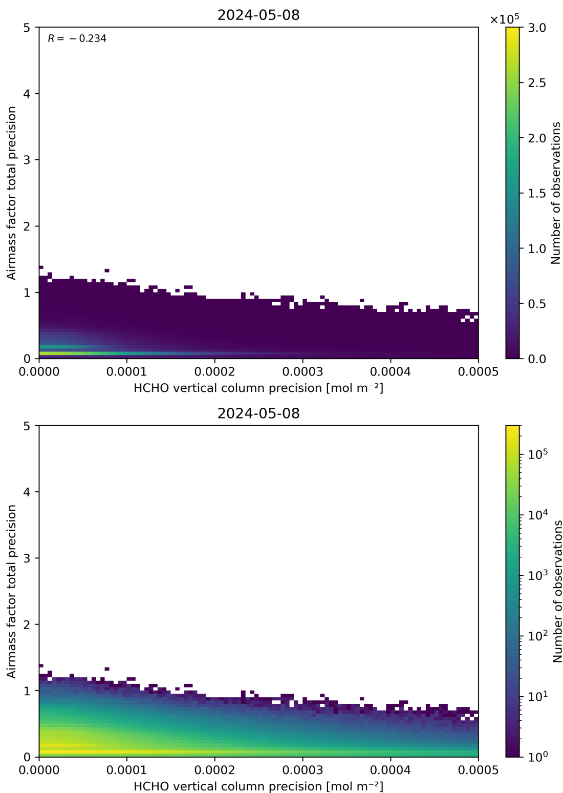
Figure 145: Scatter density plot of “HCHO vertical column precision” against “Airmass factor total precision” for 2024-05-07 to 2024-05-09.
