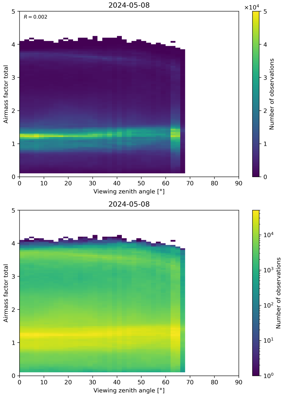
Figure 190: Scatter density plot of “Viewing zenith angle” against “Airmass factor total” for 2024-05-07 to 2024-05-09.
