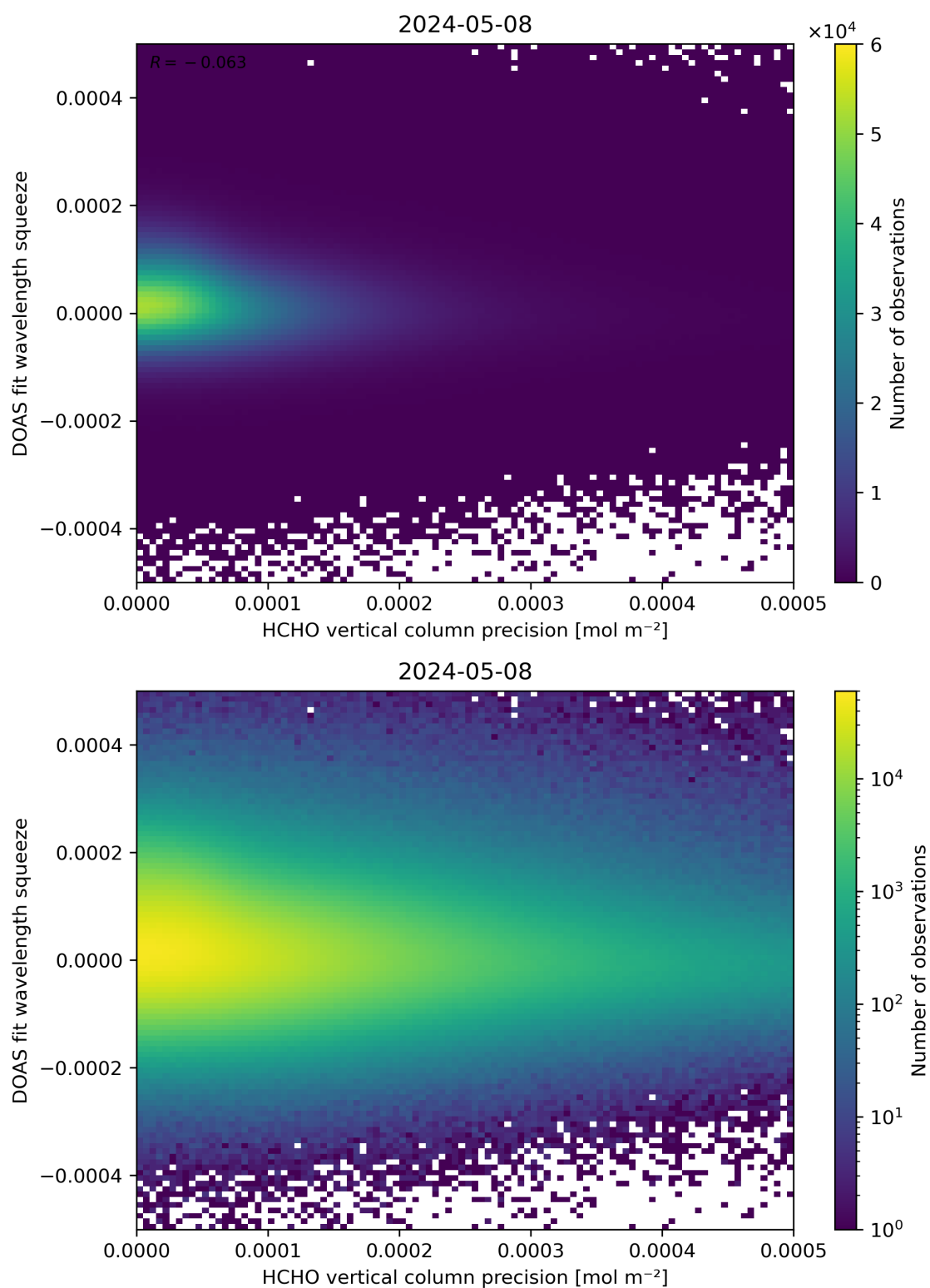
Figure 138: Scatter density plot of “HCHO vertical column precision” against “DOAS fit wavelength squeeze” for 2024-05-07 to 2024-05-09.
