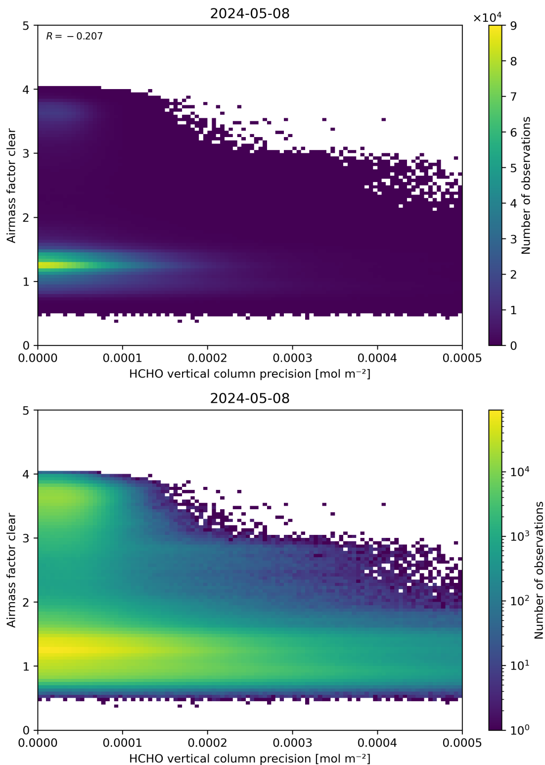
Figure 139: Scatter density plot of “HCHO vertical column precision” against “Airmass factor clear” for 2024-05-07 to 2024-05-09.
