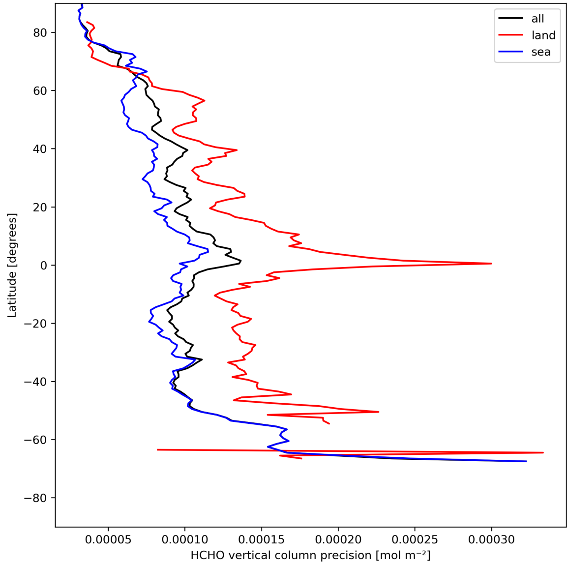
Figure 22: Zonal average of “HCHO vertical column precision” for 2024-05-07 to 2024-05-09.
