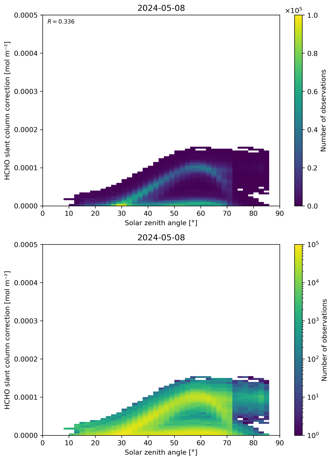
Figure 172: Scatter density plot of “Solar zenith angle” against “HCHO slant column correction” for 2024-05-07 to 2024-05-09.
