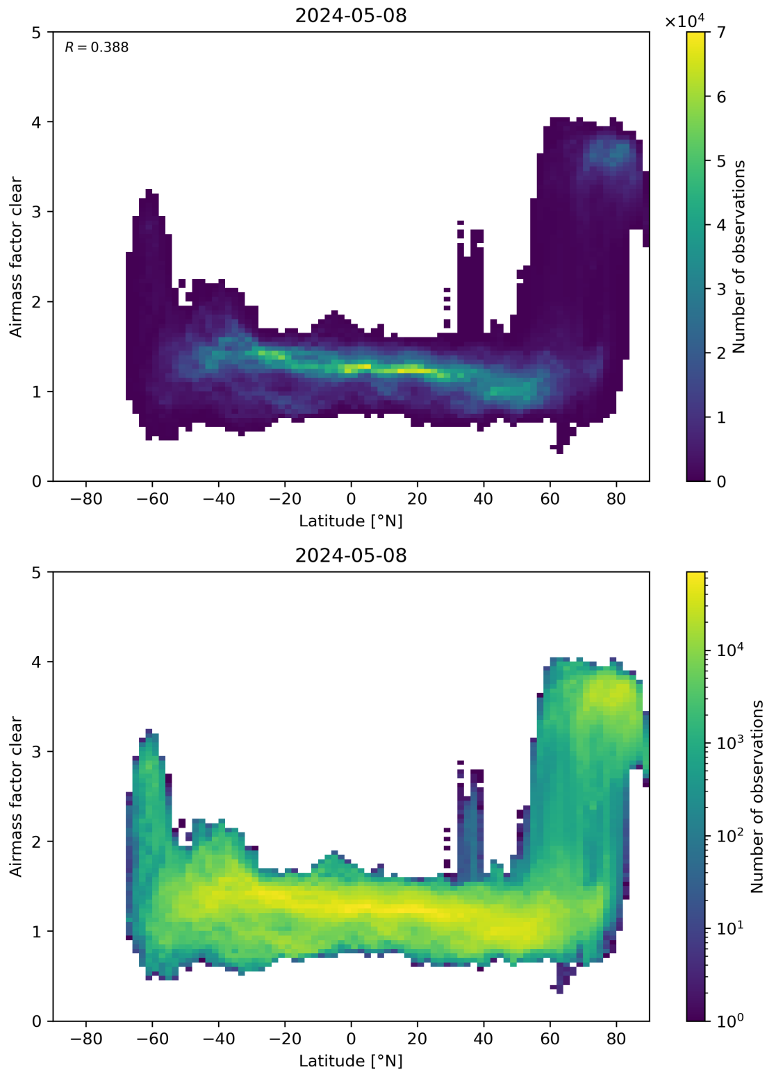
Figure 156: Scatter density plot of “Latitude” against “Airmass factor clear” for 2024-05-07 to 2024-05-09.
