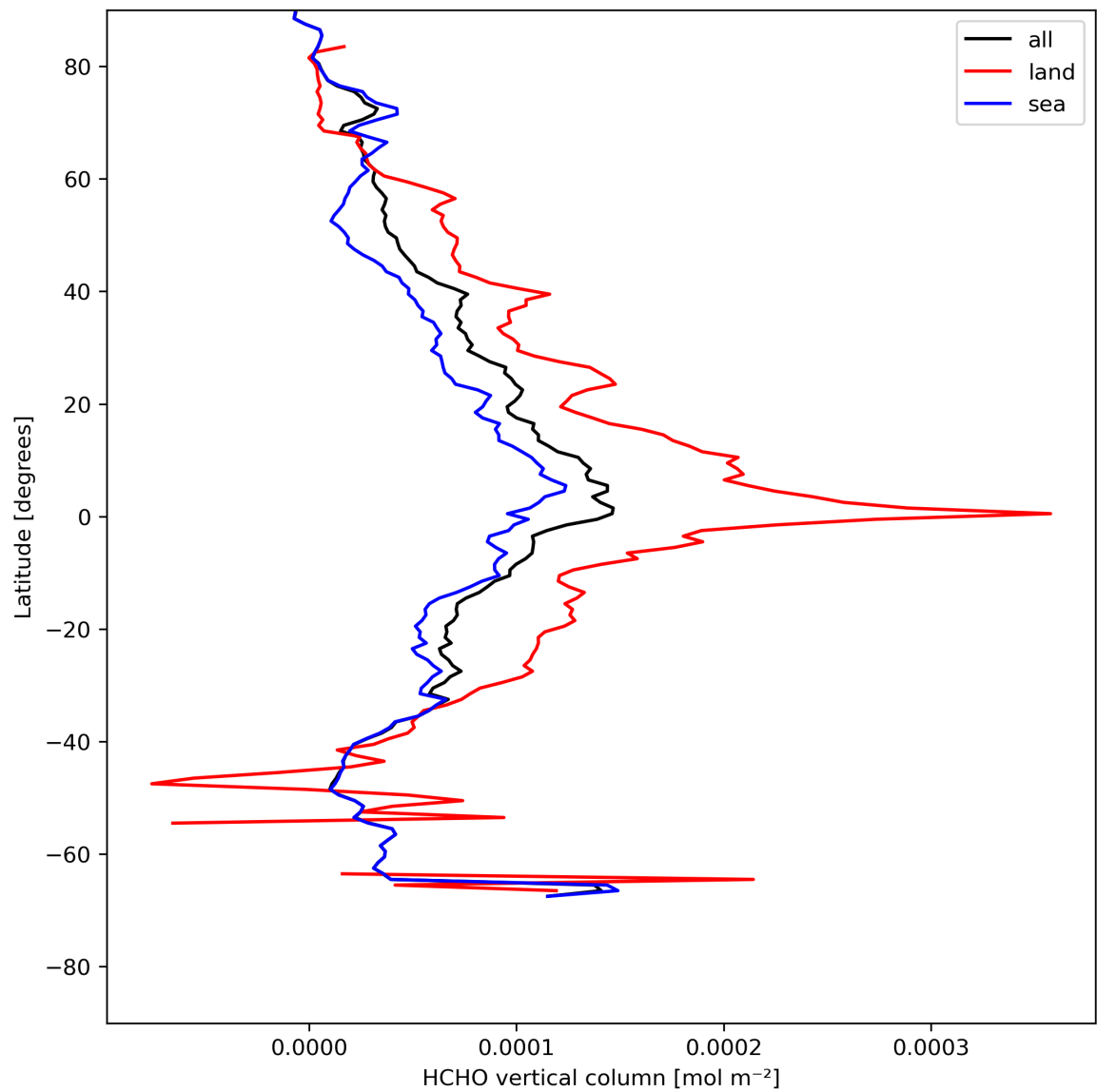
Figure 21: Zonal average of “HCHO vertical column” for 2024-05-07 to 2024-05-09.
