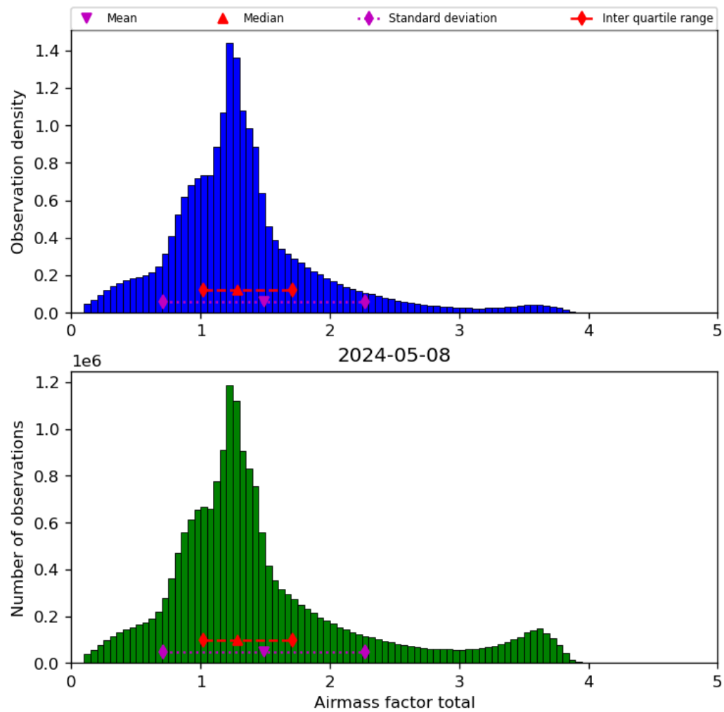
Figure 40: Histogram of “Airmass factor total” for 2024-05-07 to 2024-05-09
