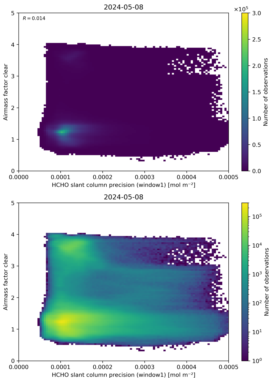
Figure 91: Scatter density plot of “HCHO slant column precision (window1)” against “Airmass factor clear” for 2024-05-07 to 2024-05-09.
