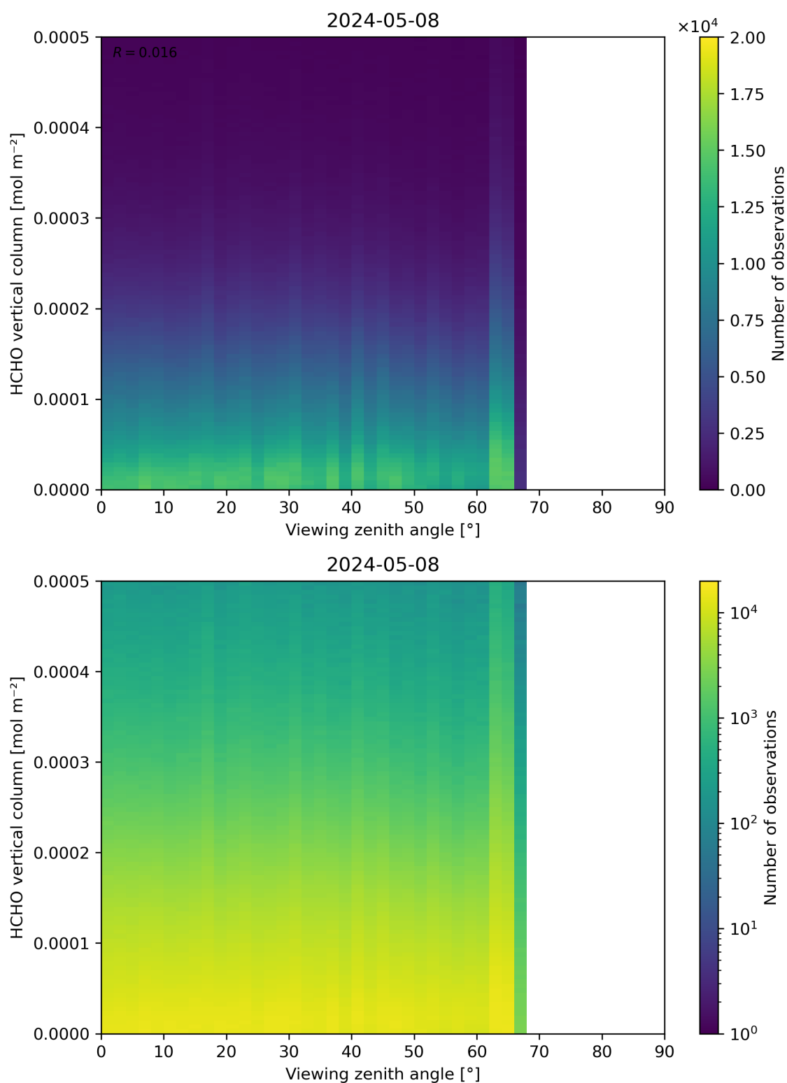
Figure 192: Scatter density plot of “Viewing zenith angle” against “HCHO vertical column” for 2024-05-07 to 2024-05-09.
