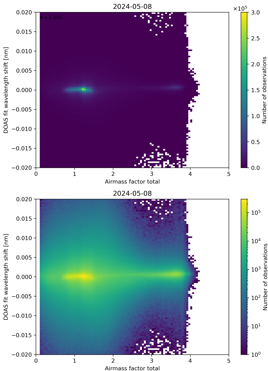
Figure 98: Scatter density plot of “Airmass factor total” against “DOAS fit wavelength shift” for 2024-05-07 to 2024-05-09.
