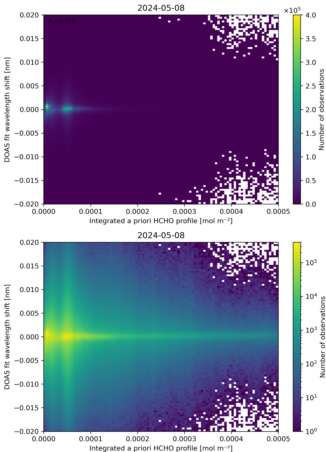
Figure 149: Scatter density plot of “Integrated a priori HCHO profile” against “DOAS fit wavelength shift” for 2024-05-07 to 2024-05-09.
