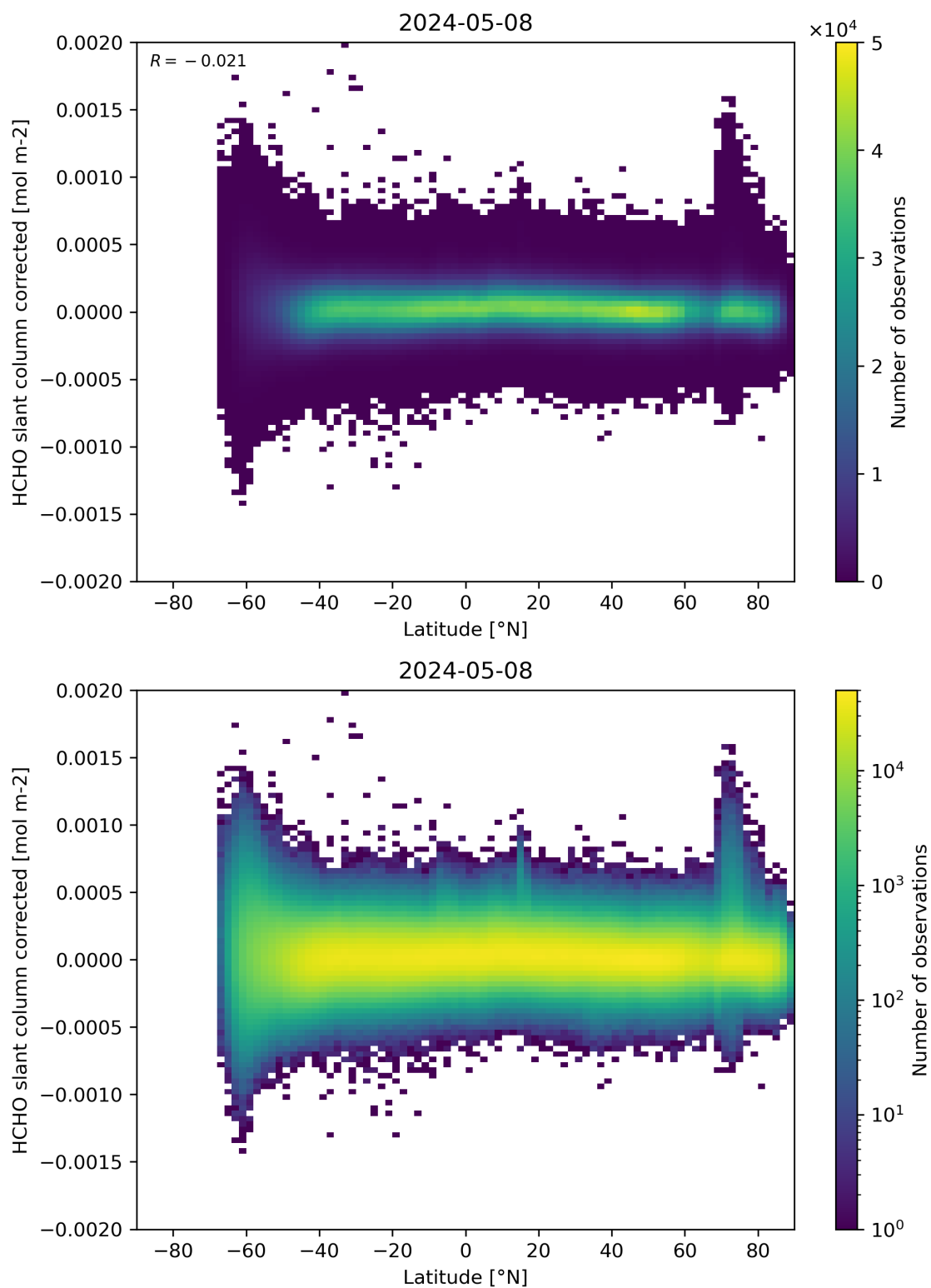
Figure 157: Scatter density plot of “Latitude” against “HCHO slant column corrected” for 2024-05-07 to 2024-05-09.
