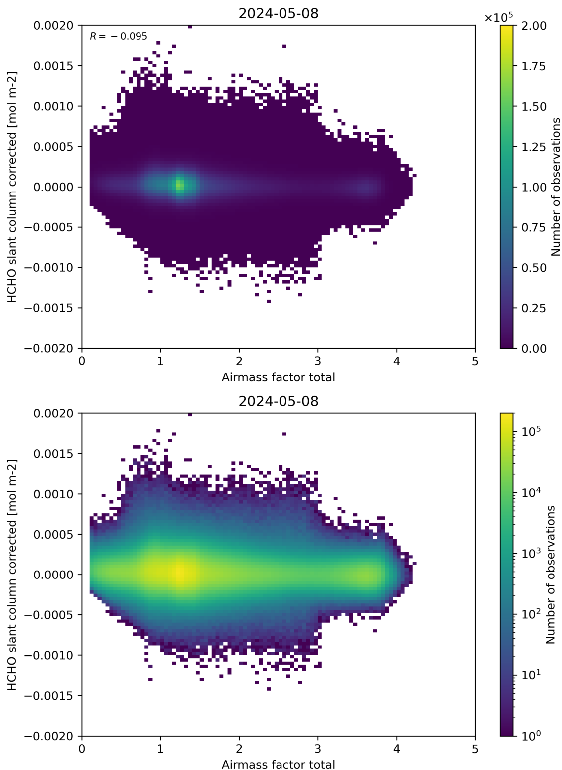
Figure 101: Scatter density plot of “Airmass factor total” against “HCHO slant column corrected” for 2024-05-07 to 2024-05-09.
