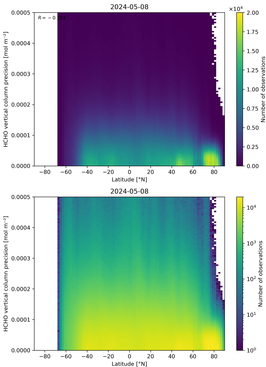
Figure 165: Scatter density plot of “Latitude” against “HCHO vertical column precision” for 2024-05-07 to 2024-05-09.
