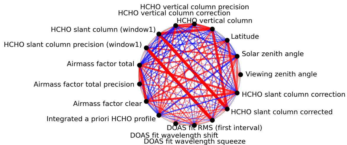
Figure 1: Map of correlation graph for 2024-05-07 to 2024-05-09.
