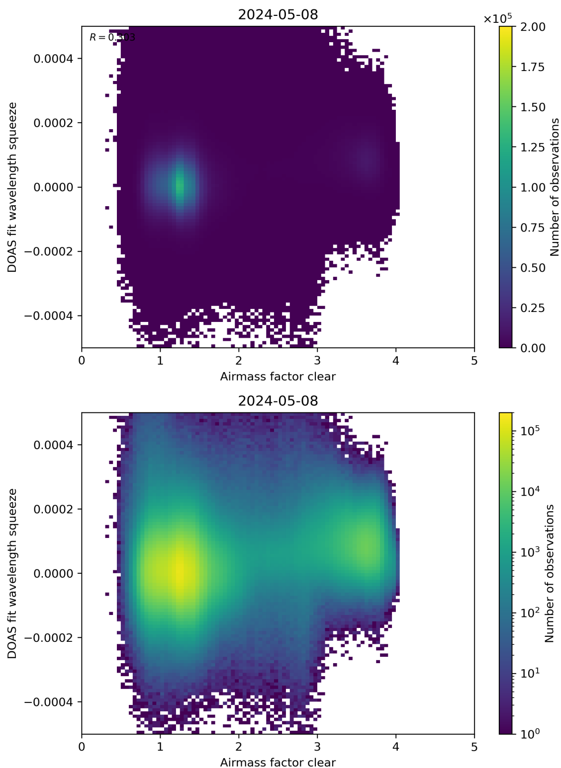
Figure 73: Scatter density plot of “Airmass factor clear” against “DOAS fit wavelength squeeze” for 2024-05-07 to 2024-05-09.
