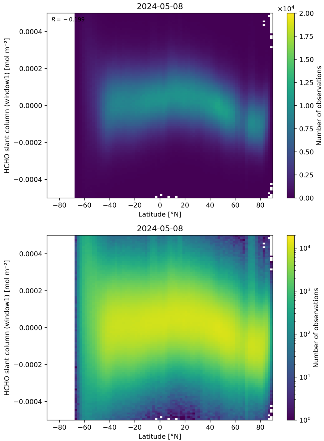
Figure 159: Scatter density plot of “Latitude” against “HCHO slant column (window1)” for 2024-05-07 to 2024-05-09.
