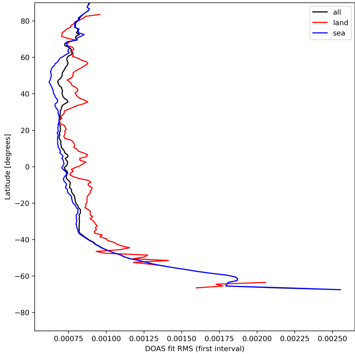
Figure 32: Zonal average of “DOAS fit RMS (first interval)” for 2024-05-07 to 2024-05-09.
