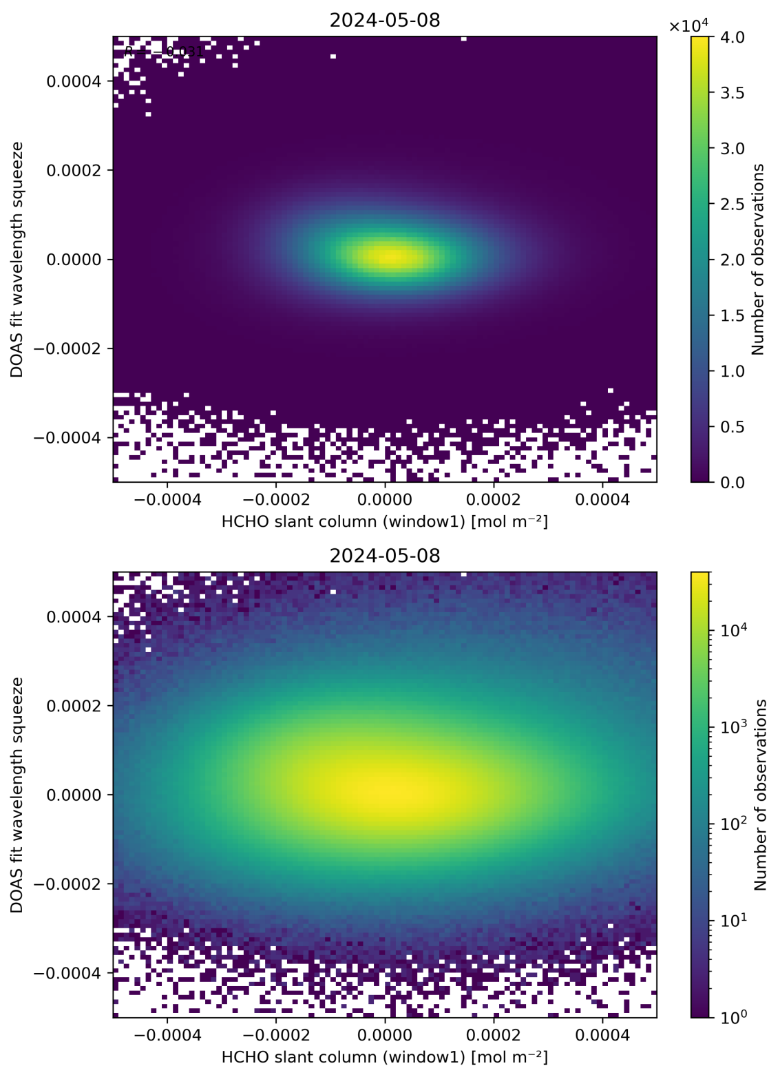
Figure 80: Scatter density plot of “HCHO slant column (window1)” against “DOAS fit wavelength squeeze” for 2024-05-07 to 2024-05-09.
