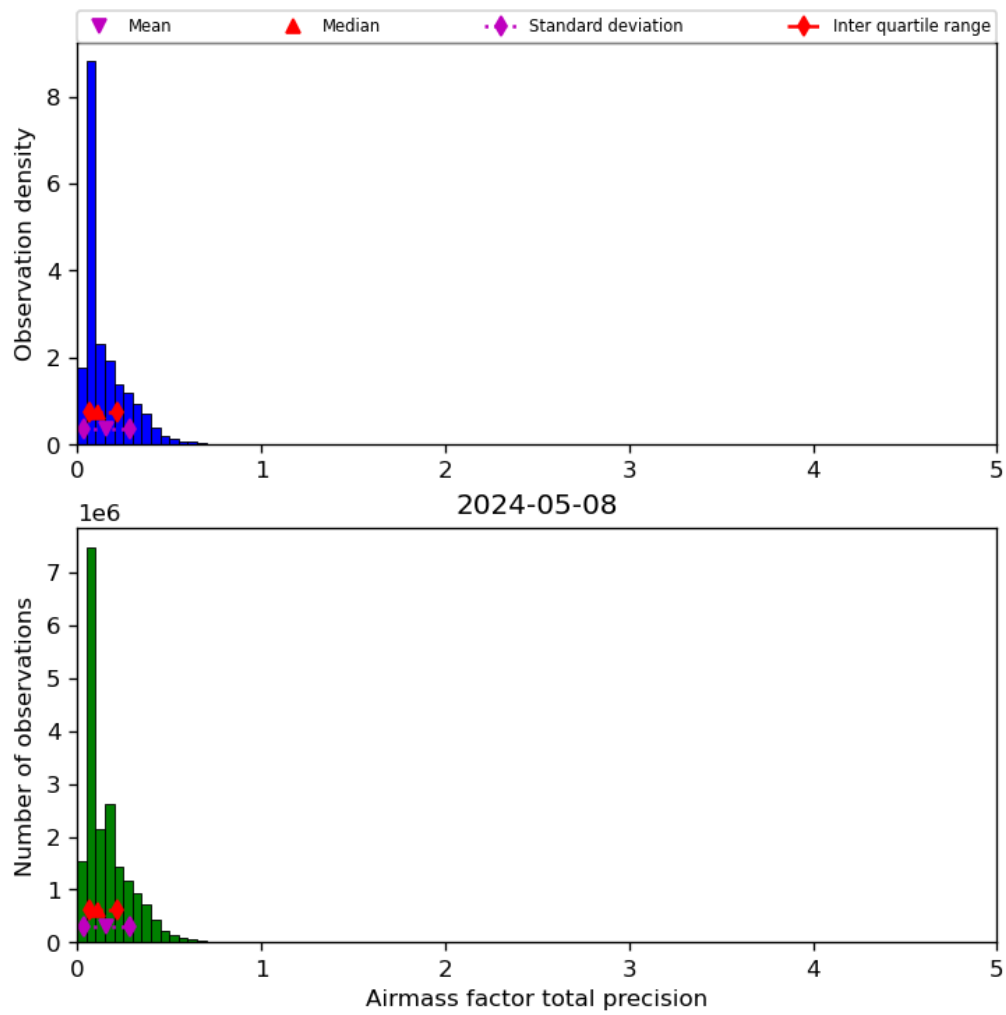
Figure 41: Histogram of “Airmass factor total precision” for 2024-05-07 to 2024-05-09
