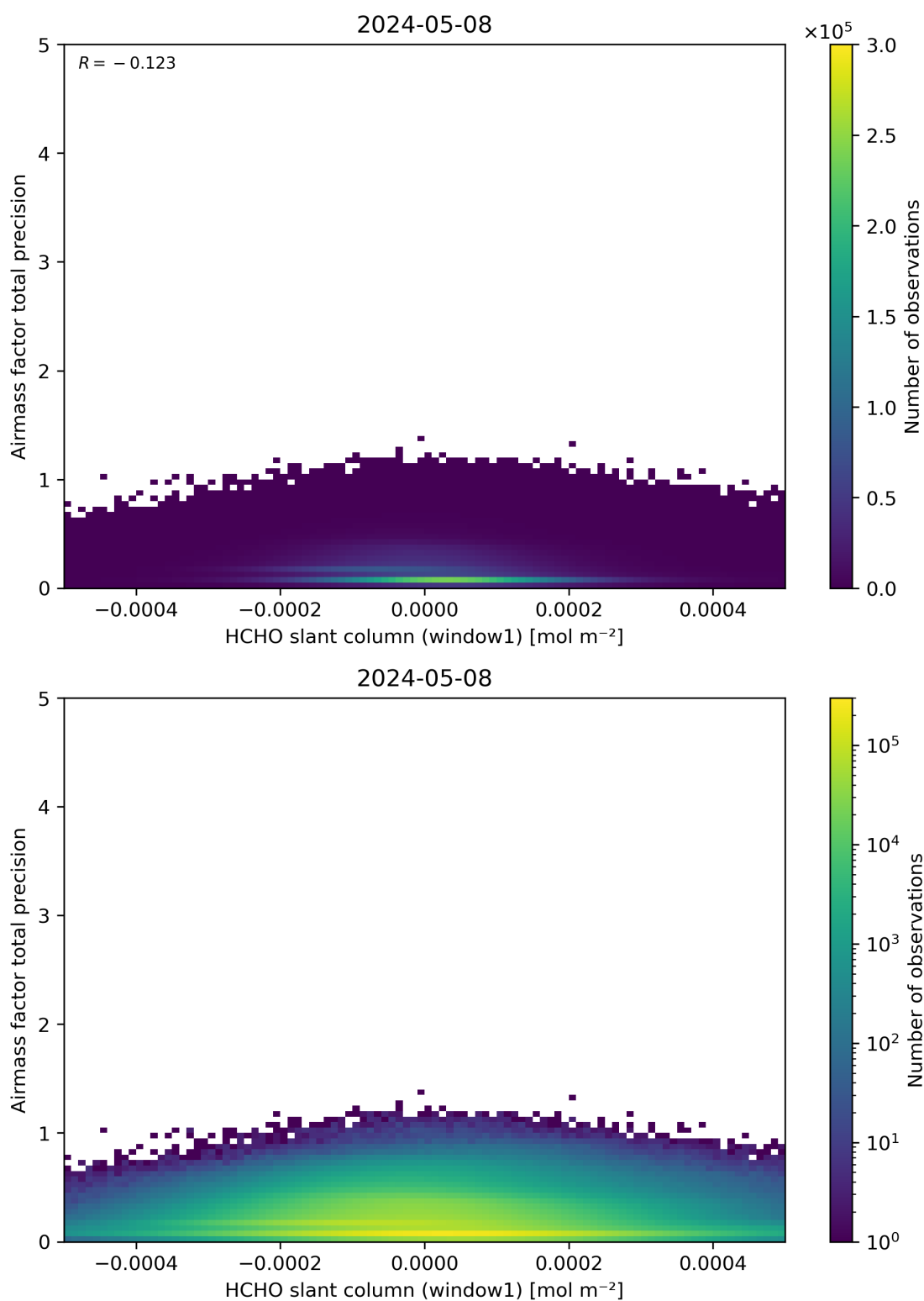
Figure 86: Scatter density plot of “HCHO slant column (window1)” against “Airmass factor total precision” for 2024-05-07 to 2024-05-09.
