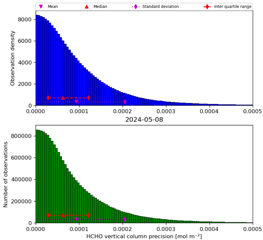
Figure 36: Histogram of “HCHO vertical column precision” for 2024-05-07 to 2024-05-09
