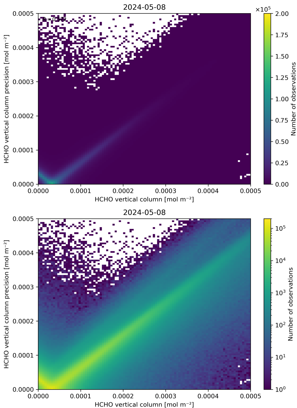
Figure 134: Scatter density plot of “HCHO vertical column” against “HCHO vertical column precision” for 2024-05-07 to 2024-05-09.
