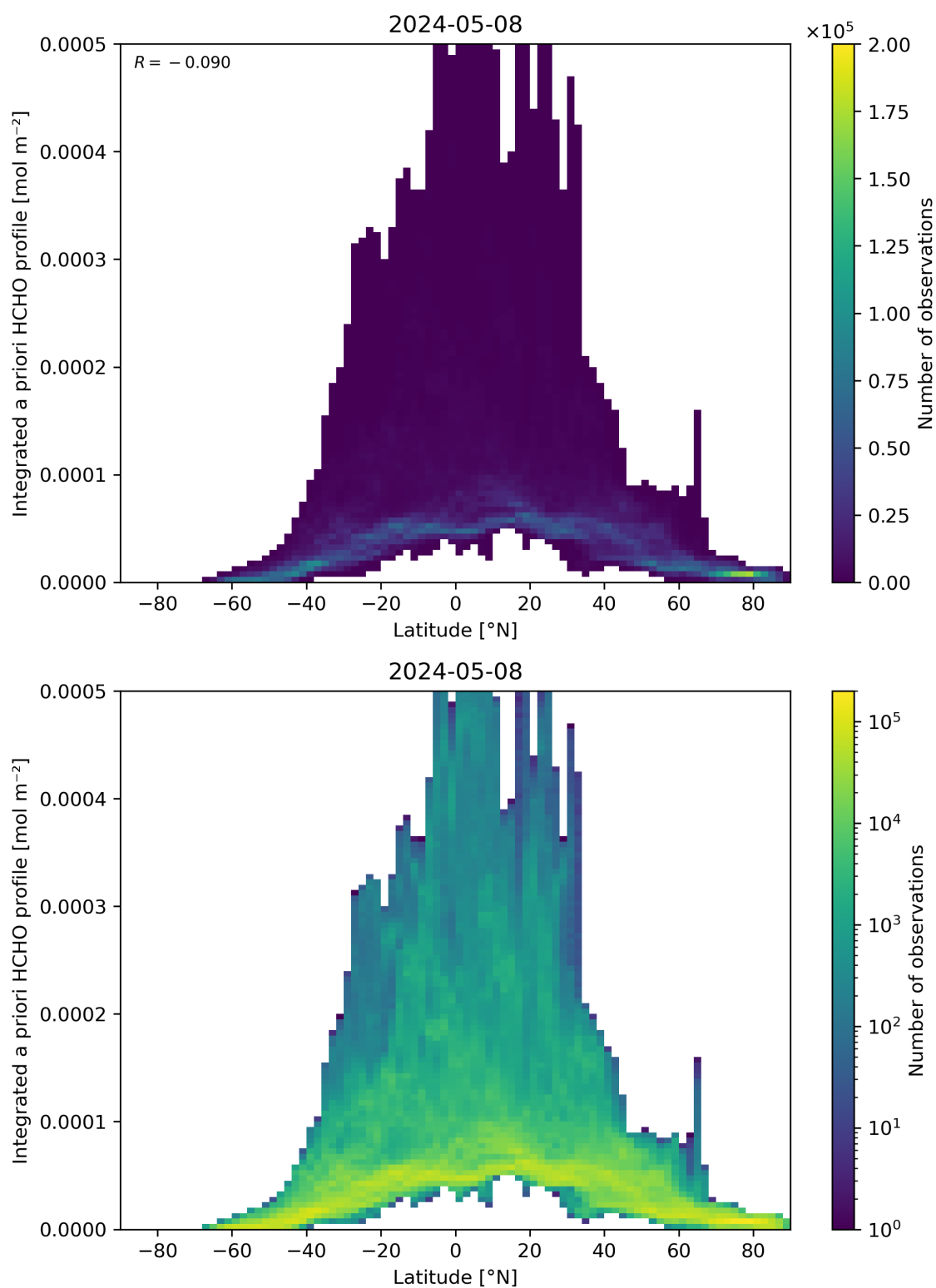
Figure 166: Scatter density plot of “Latitude” against “Integrated a priori HCHO profile” for 2024-05-07 to 2024-05-09.
