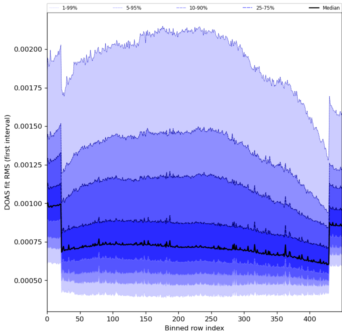
Figure 60: Along track statistics of “DOAS fit RMS (first interval)” for 2024-05-07 to 2024-05-09
