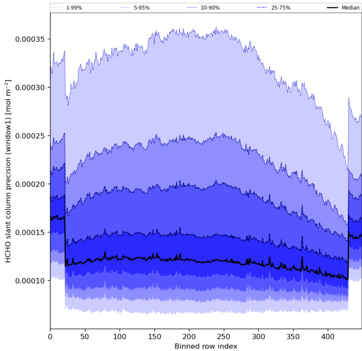
Figure 53: Along track statistics of “HCHO slant column precision (window1)” for 2024-05-07 to 2024-05-09
