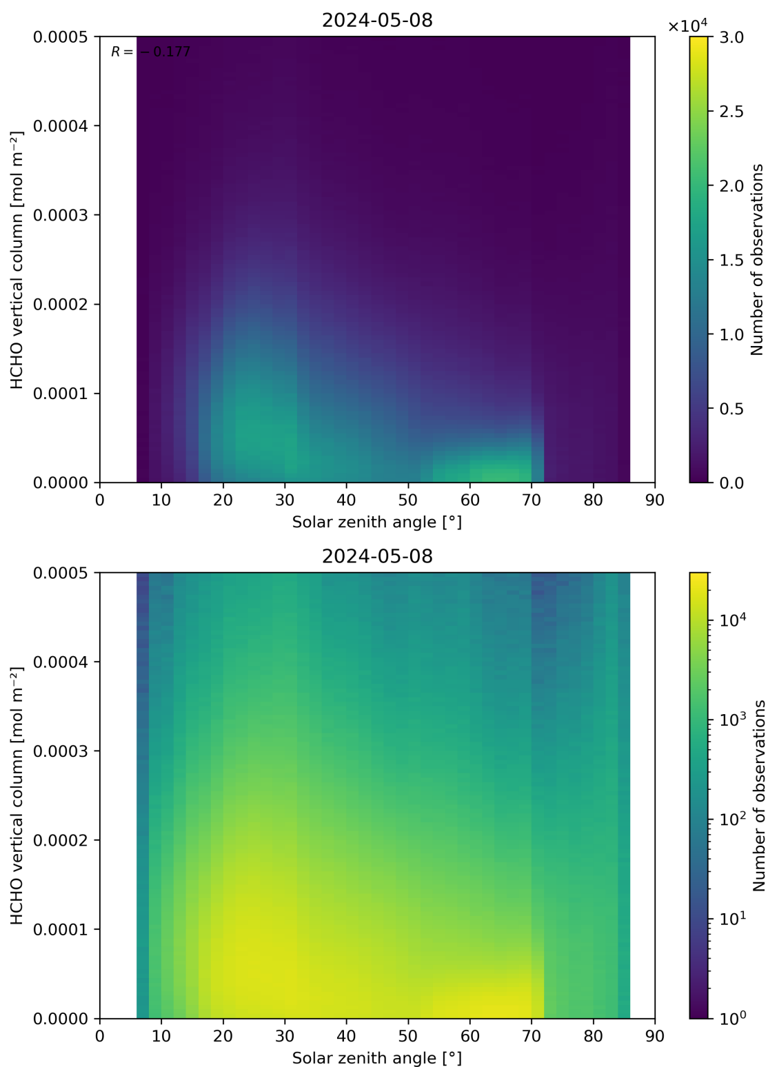
Figure 177: Scatter density plot of “Solar zenith angle” against “HCHO vertical column” for 2024-05-07 to 2024-05-09.
