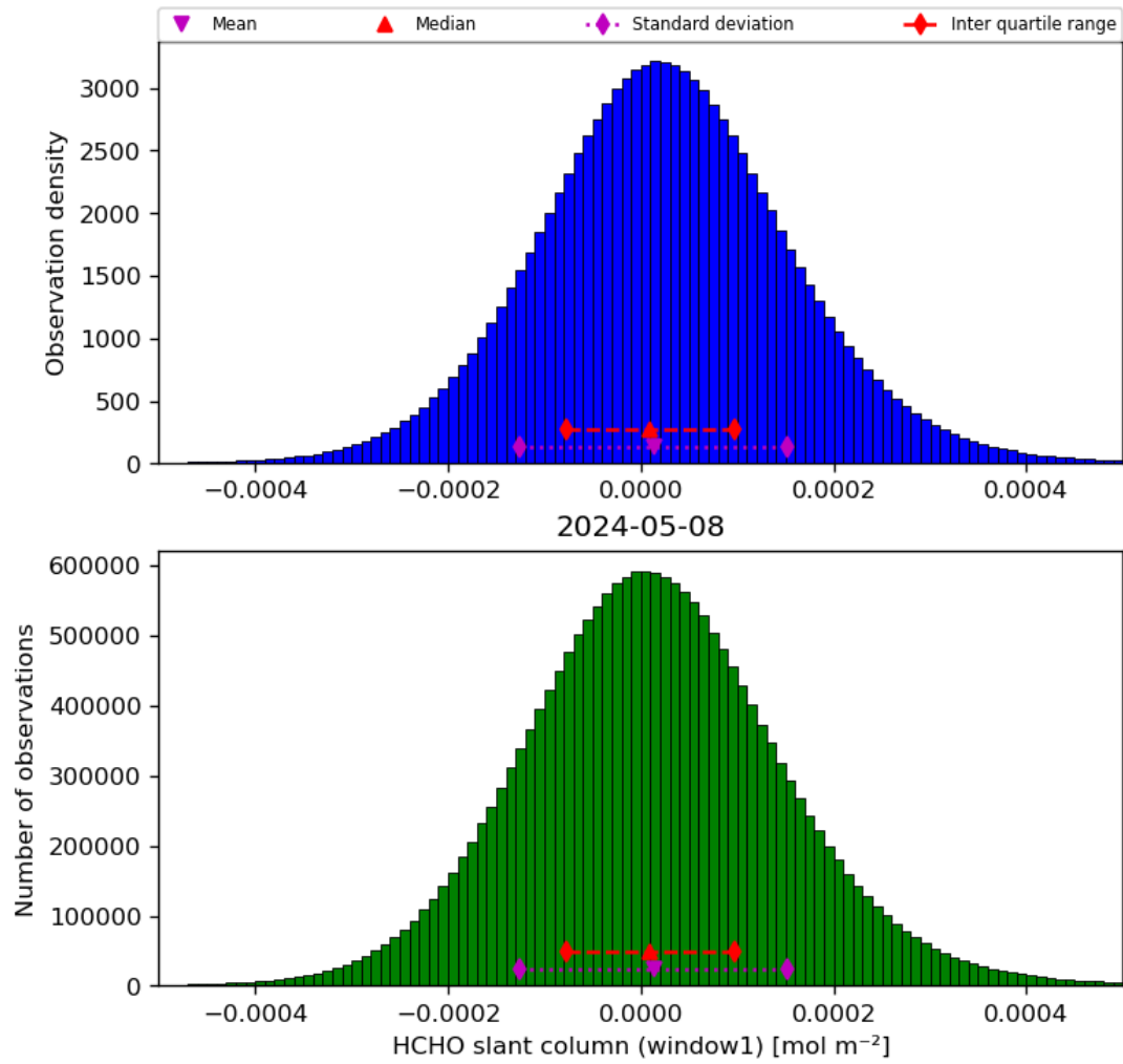
Figure 38: Histogram of “HCHO slant column (window1)” for 2024-05-07 to 2024-05-09
