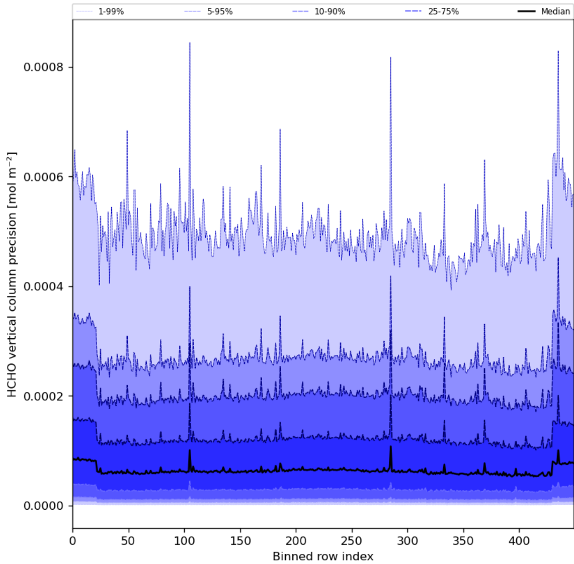
Figure 50: Along track statistics of “HCHO vertical column precision” for 2024-05-07 to 2024-05-09
