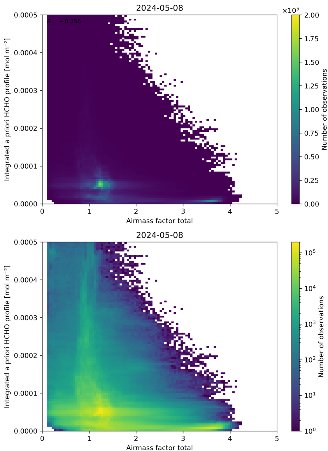
Figure 104: Scatter density plot of “Airmass factor total” against “Integrated a priori HCHO profile” for 2024-05-07 to 2024-05-09.
