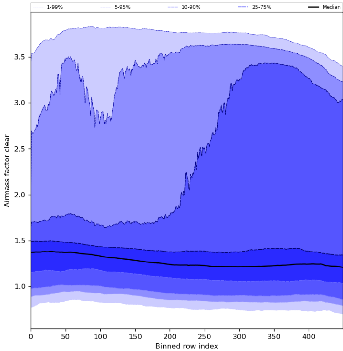
Figure 56: Along track statistics of “Airmass factor clear” for 2024-05-07 to 2024-05-09
