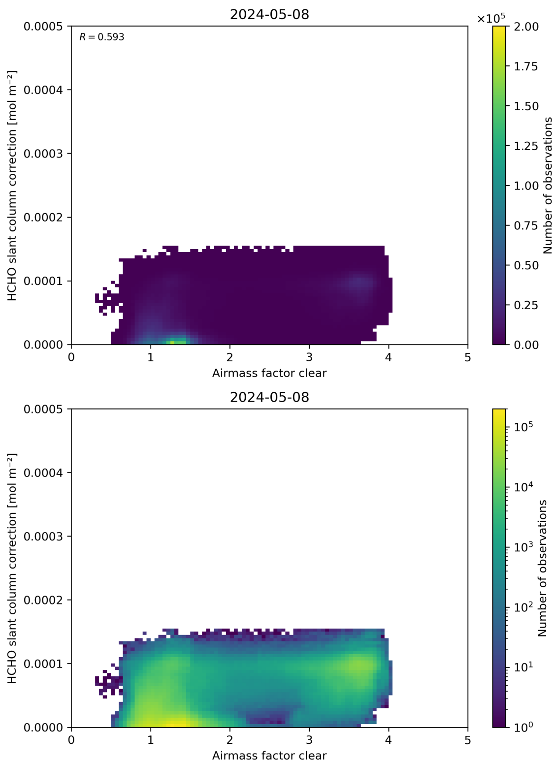
Figure 75: Scatter density plot of “Airmass factor clear” against “HCHO slant column correction” for 2024-05-07 to 2024-05-09.
