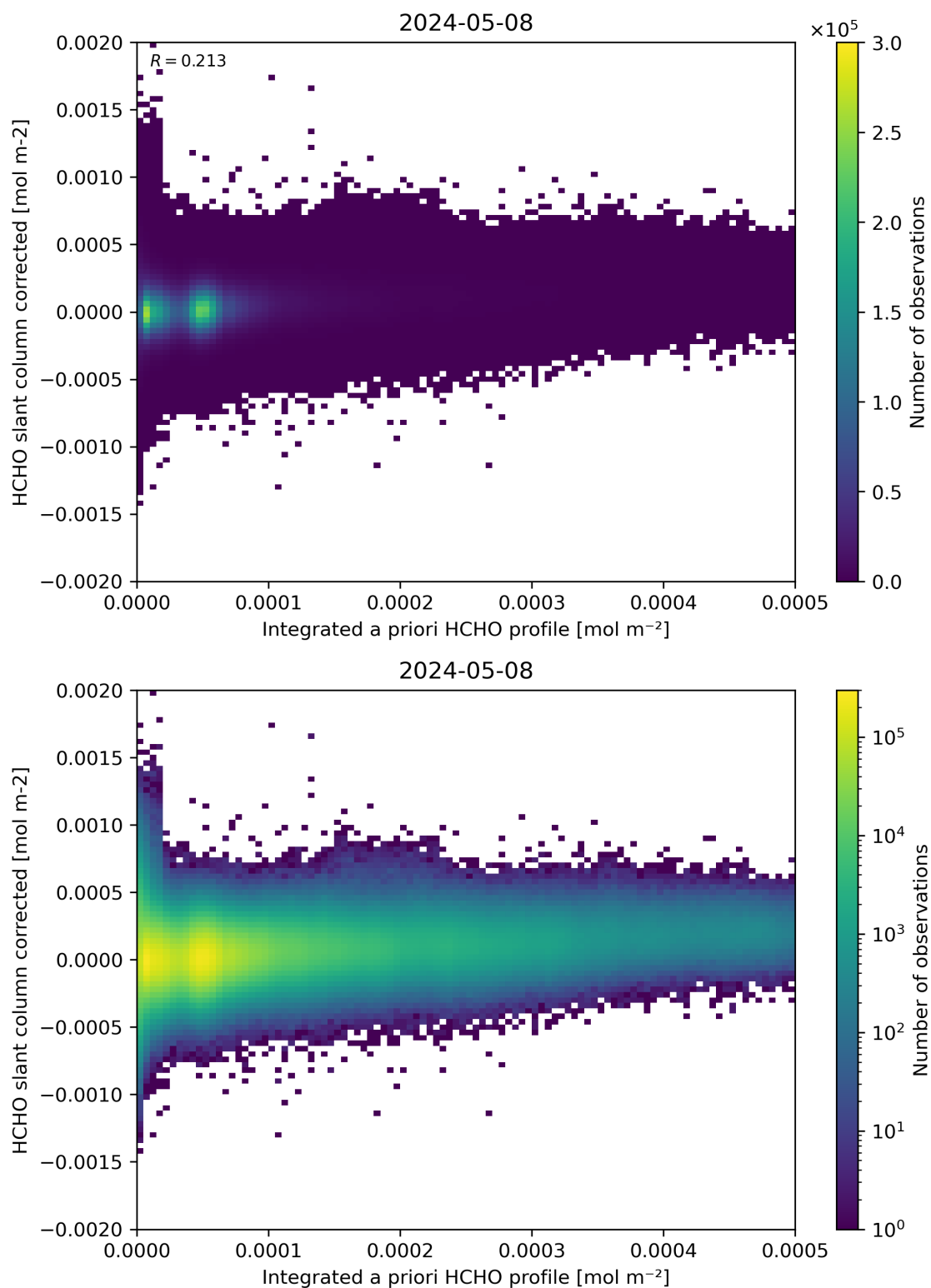
Figure 151: Scatter density plot of “Integrated a priori HCHO profile” against “HCHO slant column corrected” for 2024-05-07 to 2024-05-09.
