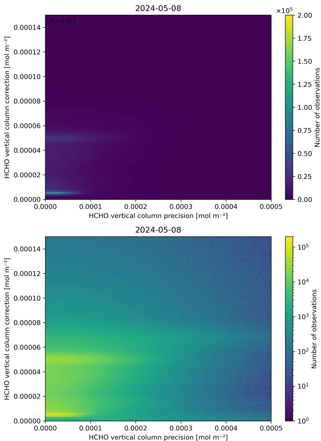
Figure 146: Scatter density plot of “HCHO vertical column precision” against “HCHO vertical column correction” for 2024-05-07 to 2024-05-09.
