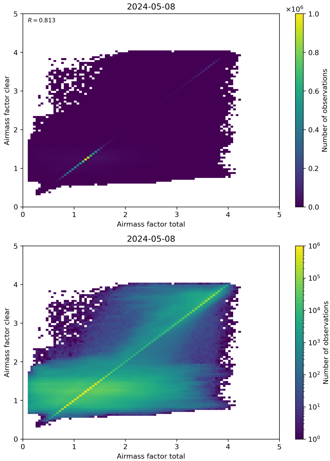
Figure 100: Scatter density plot of “Airmass factor total” against “Airmass factor clear” for 2024-05-07 to 2024-05-09.
