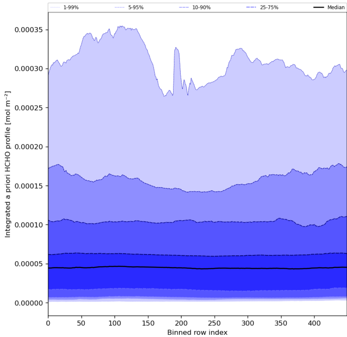
Figure 57: Along track statistics of “Integrated a priori HCHO profile” for 2024-05-07 to 2024-05-09
