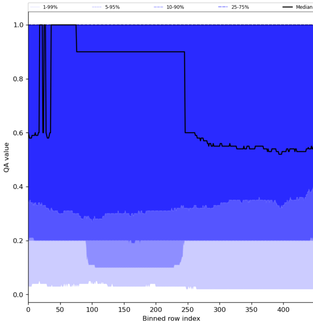
Figure 48: Along track statistics of “QA value” for 2024-05-07 to 2024-05-09
