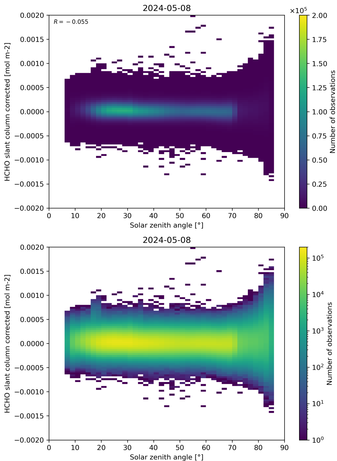
Figure 171: Scatter density plot of “Solar zenith angle” against “HCHO slant column corrected” for 2024-05-07 to 2024-05-09.
