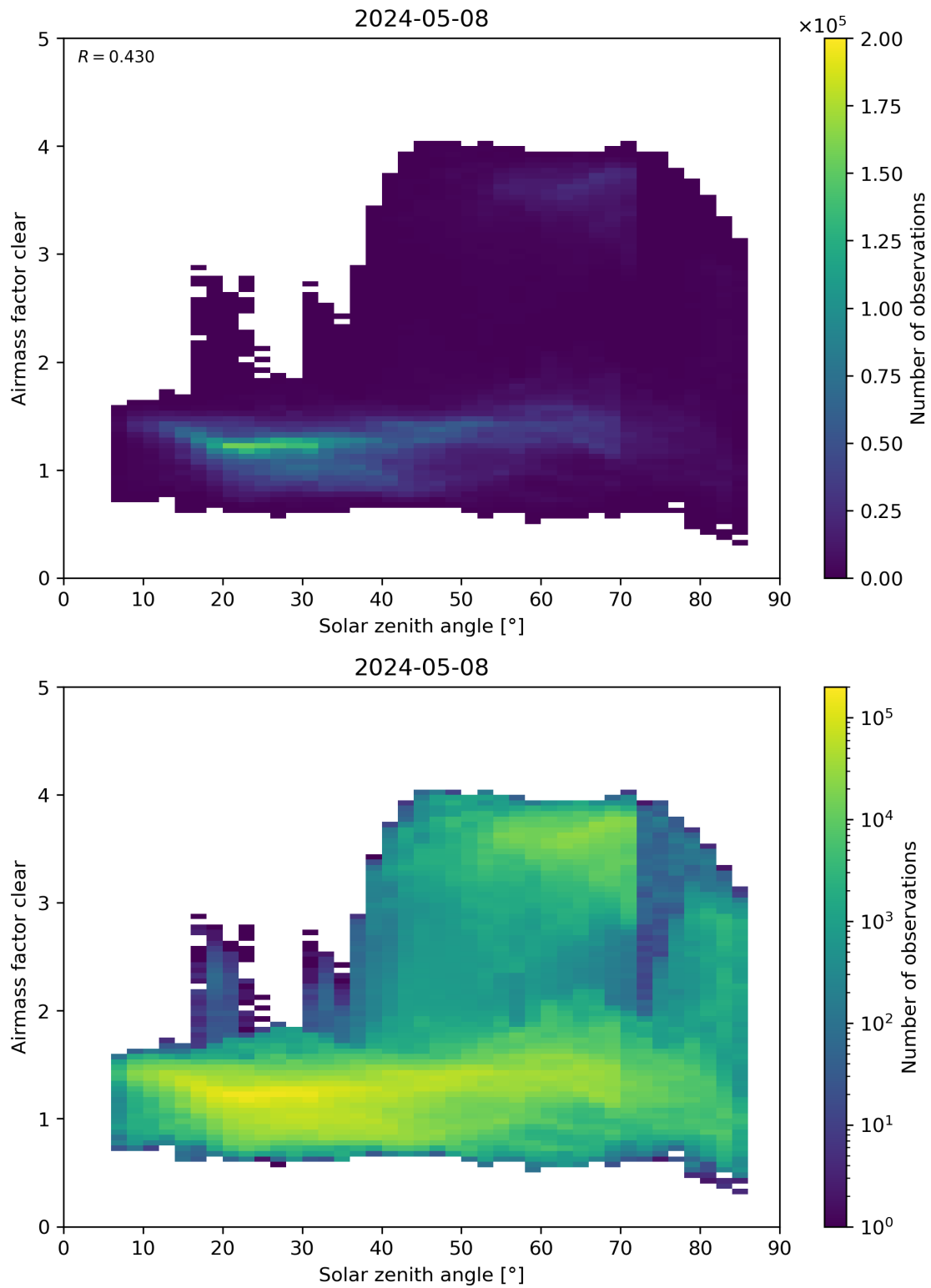
Figure 170: Scatter density plot of “Solar zenith angle” against “Airmass factor clear” for 2024-05-07 to 2024-05-09.
