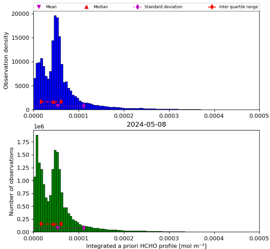
Figure 43: Histogram of “Integrated a priori HCHO profile” for 2024-05-07 to 2024-05-09
