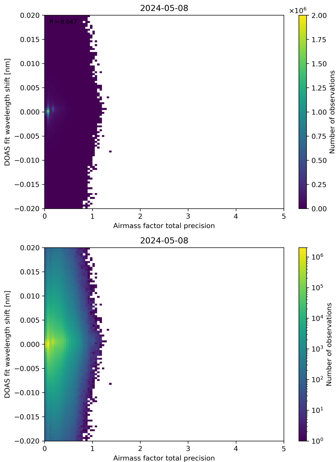
Figure 106: Scatter density plot of “Airmass factor total precision” against “DOAS fit wavelength shift” for 2024-05-07 to 2024-05-09.
