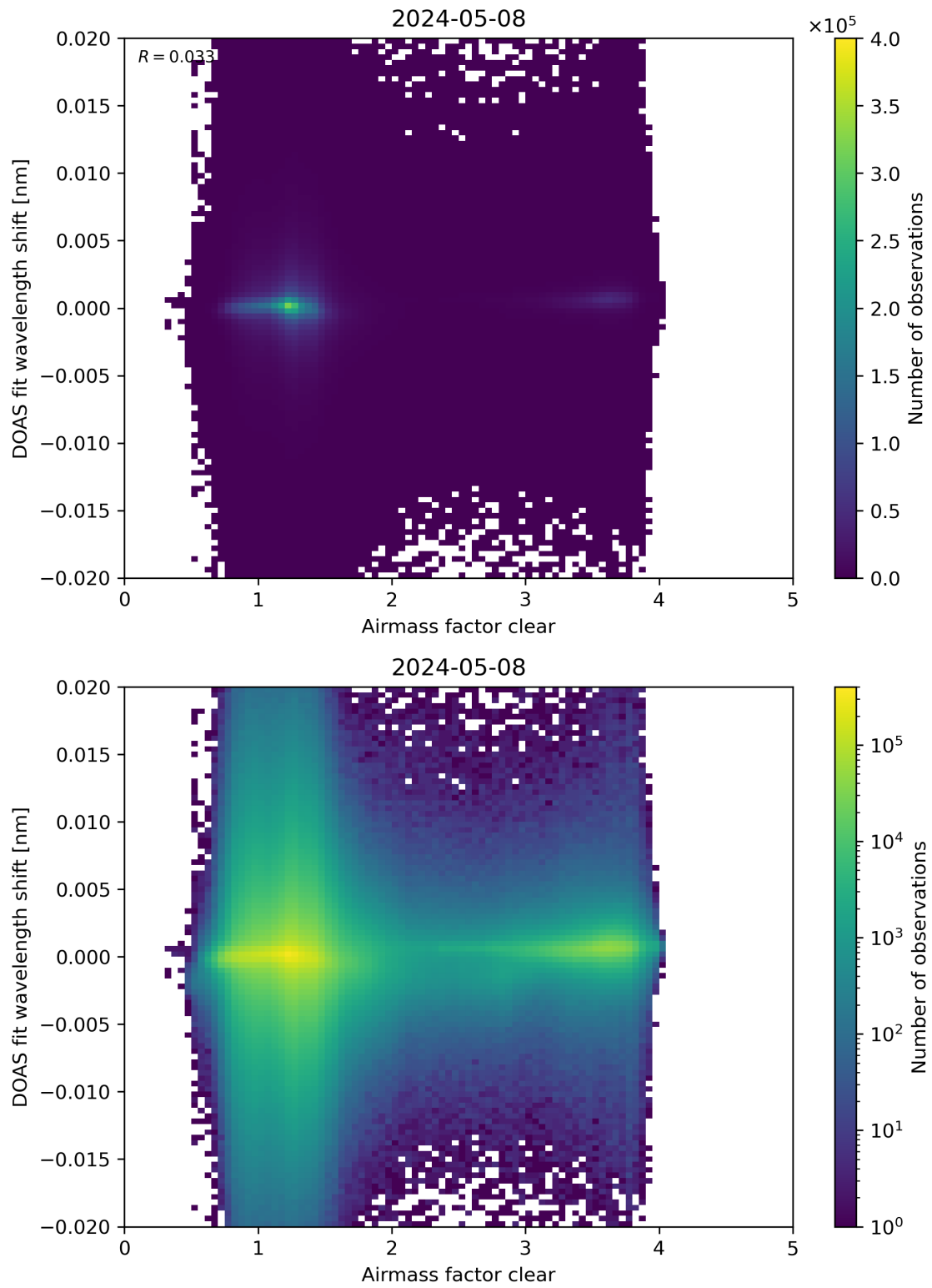
Figure 72: Scatter density plot of “Airmass factor clear” against “DOAS fit wavelength shift” for 2024-05-07 to 2024-05-09.
