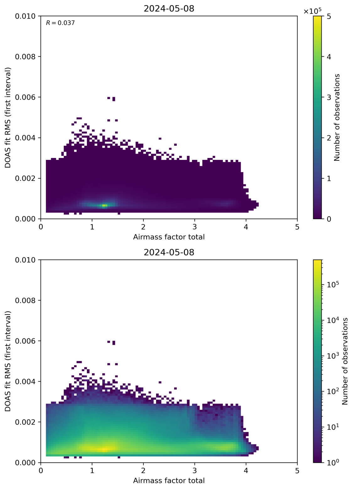
Figure 97: Scatter density plot of “Airmass factor total” against “DOAS fit RMS (first interval)” for 2024-05-07 to 2024-05-09.
