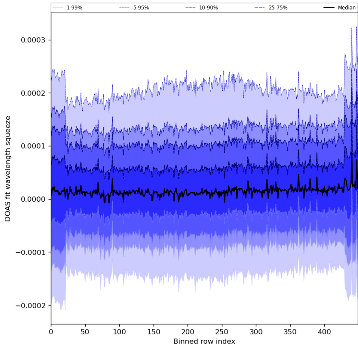
Figure 59: Along track statistics of “DOAS fit wavelength squeeze” for 2024-05-07 to 2024-05-09
