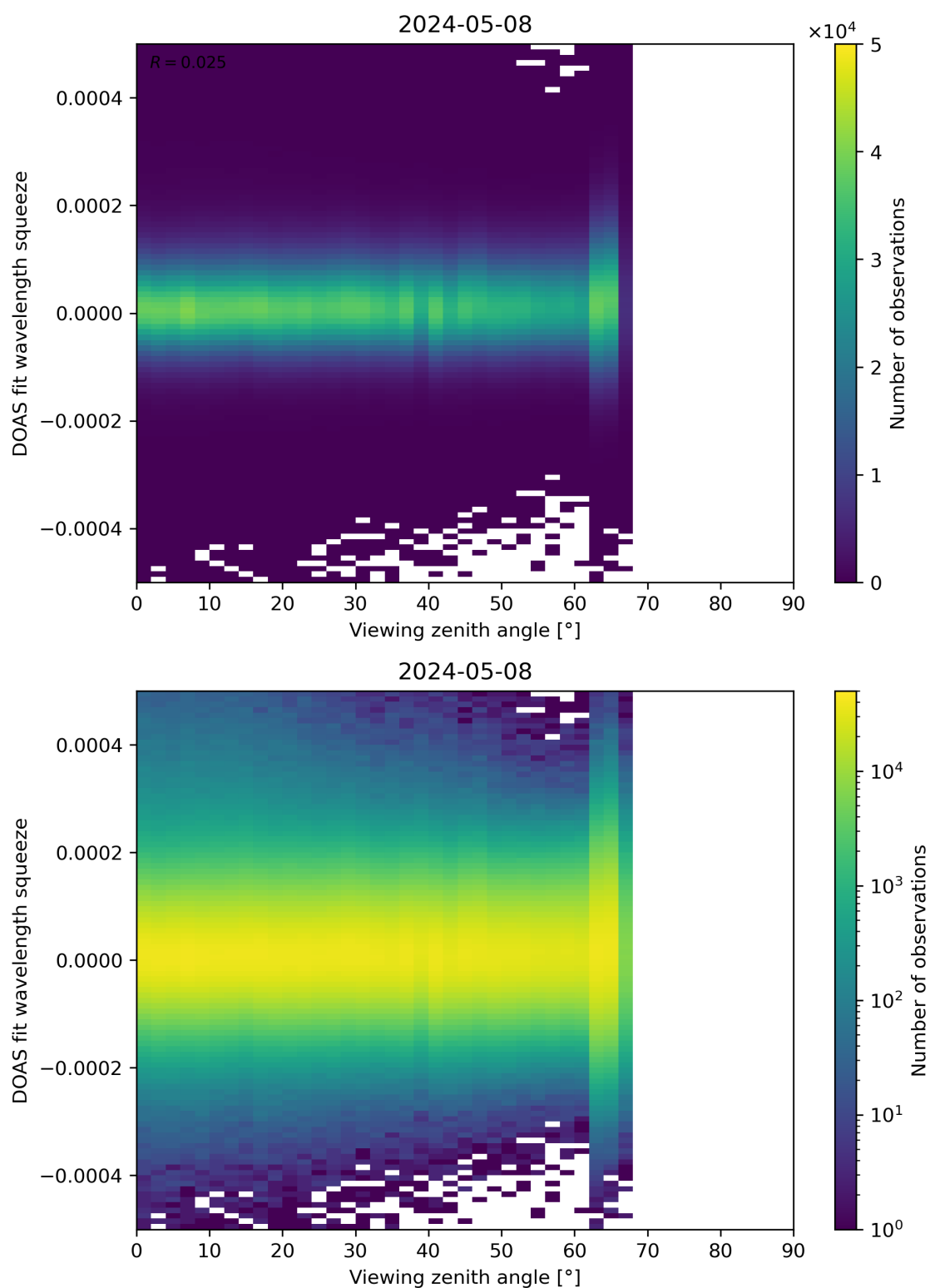
Figure 184: Scatter density plot of “Viewing zenith angle” against “DOAS fit wavelength squeeze” for 2024-05-07 to 2024-05-09.
