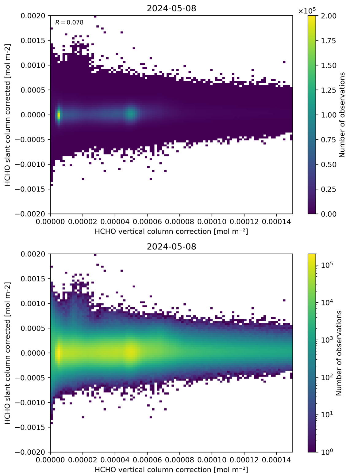
Figure 116: Scatter density plot of “HCHO vertical column correction” against “HCHO slant column corrected” for 2024-05-07 to 2024-05-09.
