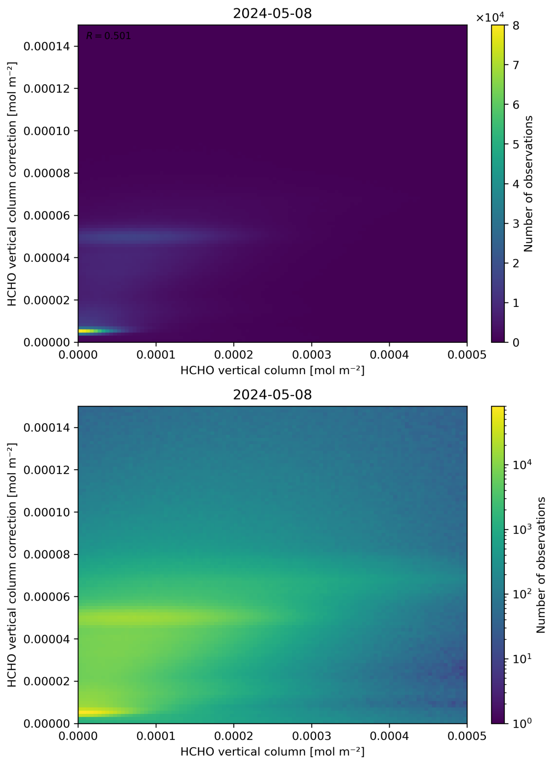
Figure 133: Scatter density plot of “HCHO vertical column” against “HCHO vertical column correction” for 2024-05-07 to 2024-05-09.
