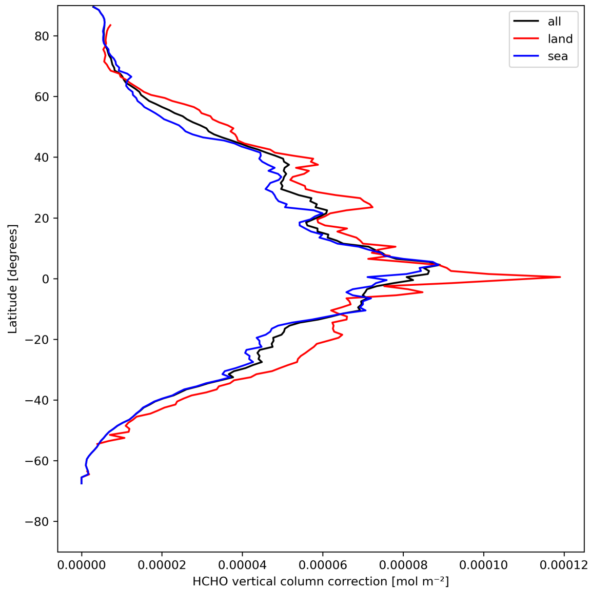
Figure 23: Zonal average of “HCHO vertical column correction” for 2024-05-07 to 2024-05-09.
