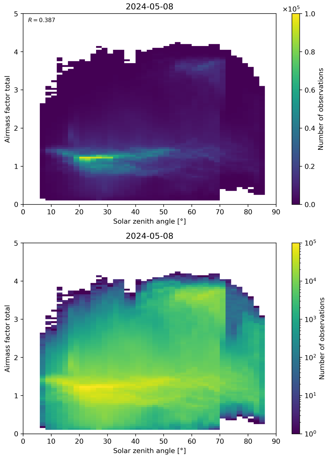
Figure 175: Scatter density plot of “Solar zenith angle” against “Airmass factor total” for 2024-05-07 to 2024-05-09.
