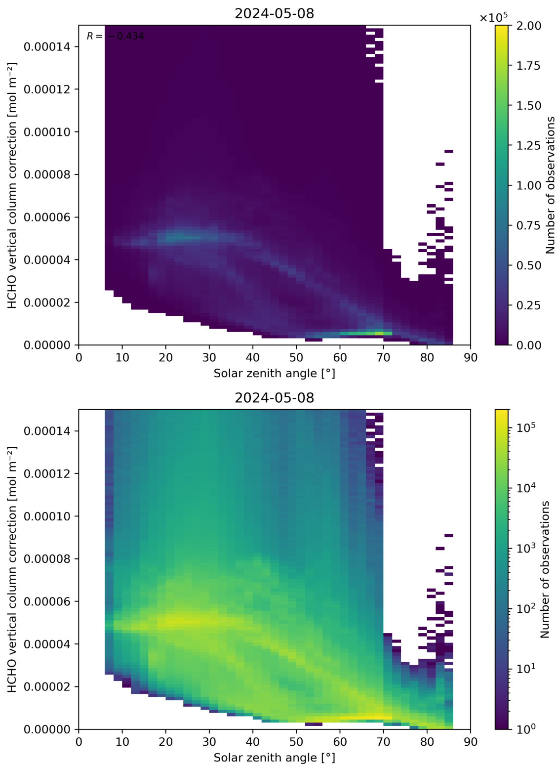
Figure 178: Scatter density plot of “Solar zenith angle” against “HCHO vertical column correction” for 2024-05-07 to 2024-05-09.
