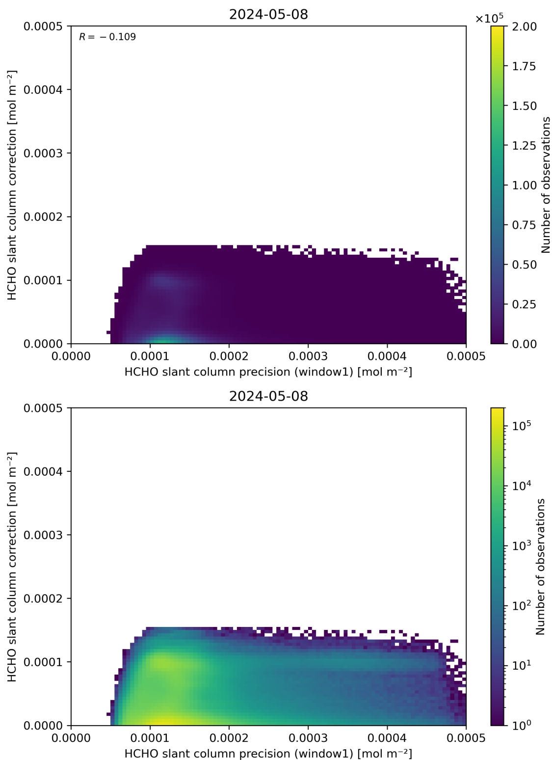
Figure 93: Scatter density plot of “HCHO slant column precision (window1)” against “HCHO slant column correction” for 2024-05-07 to 2024-05-09.
