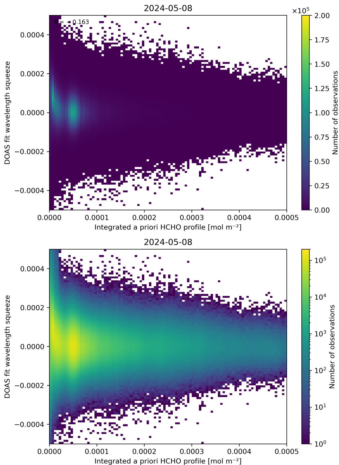
Figure 150: Scatter density plot of “Integrated a priori HCHO profile” against “DOAS fit wavelength squeeze” for 2024-05-07 to 2024-05-09.
