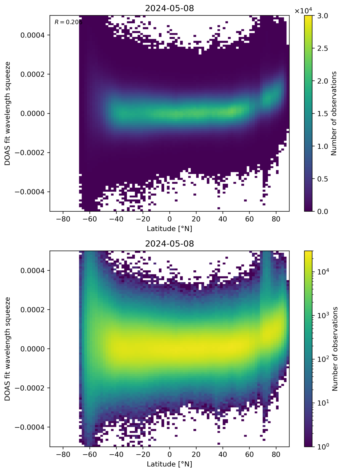
Figure 155: Scatter density plot of “Latitude” against “DOAS fit wavelength squeeze” for 2024-05-07 to 2024-05-09.
