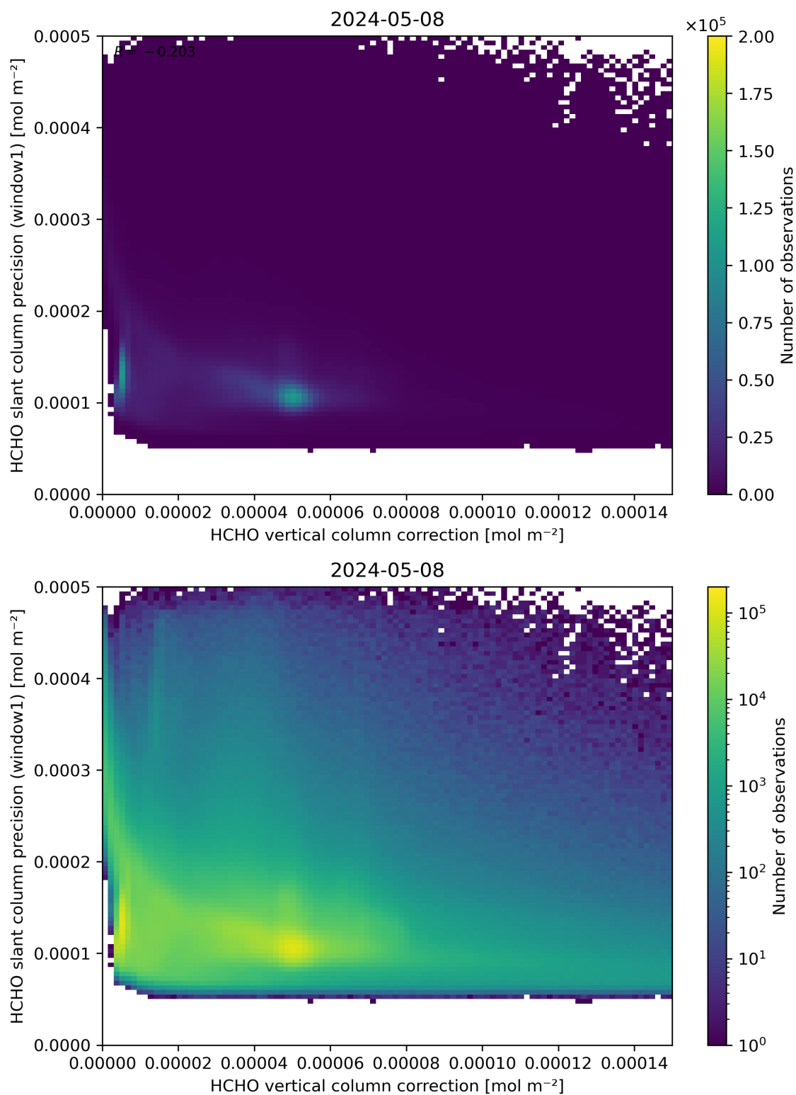
Figure 119: Scatter density plot of “HCHO vertical column correction” against “HCHO slant column precision (window1)” for 2024-05-07 to 2024-05-09.
