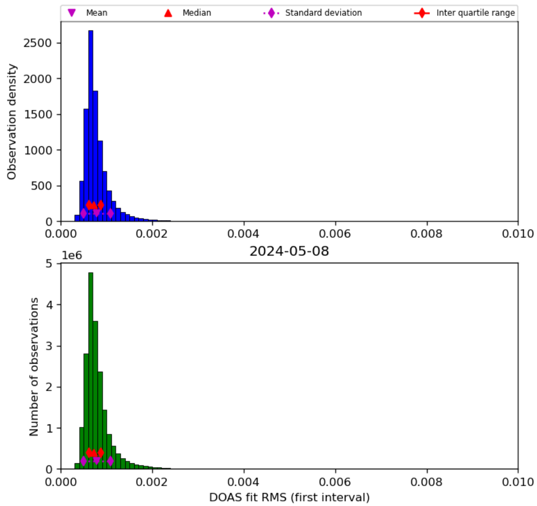
Figure 46: Histogram of “DOAS fit RMS (first interval)” for 2024-05-07 to 2024-05-09
