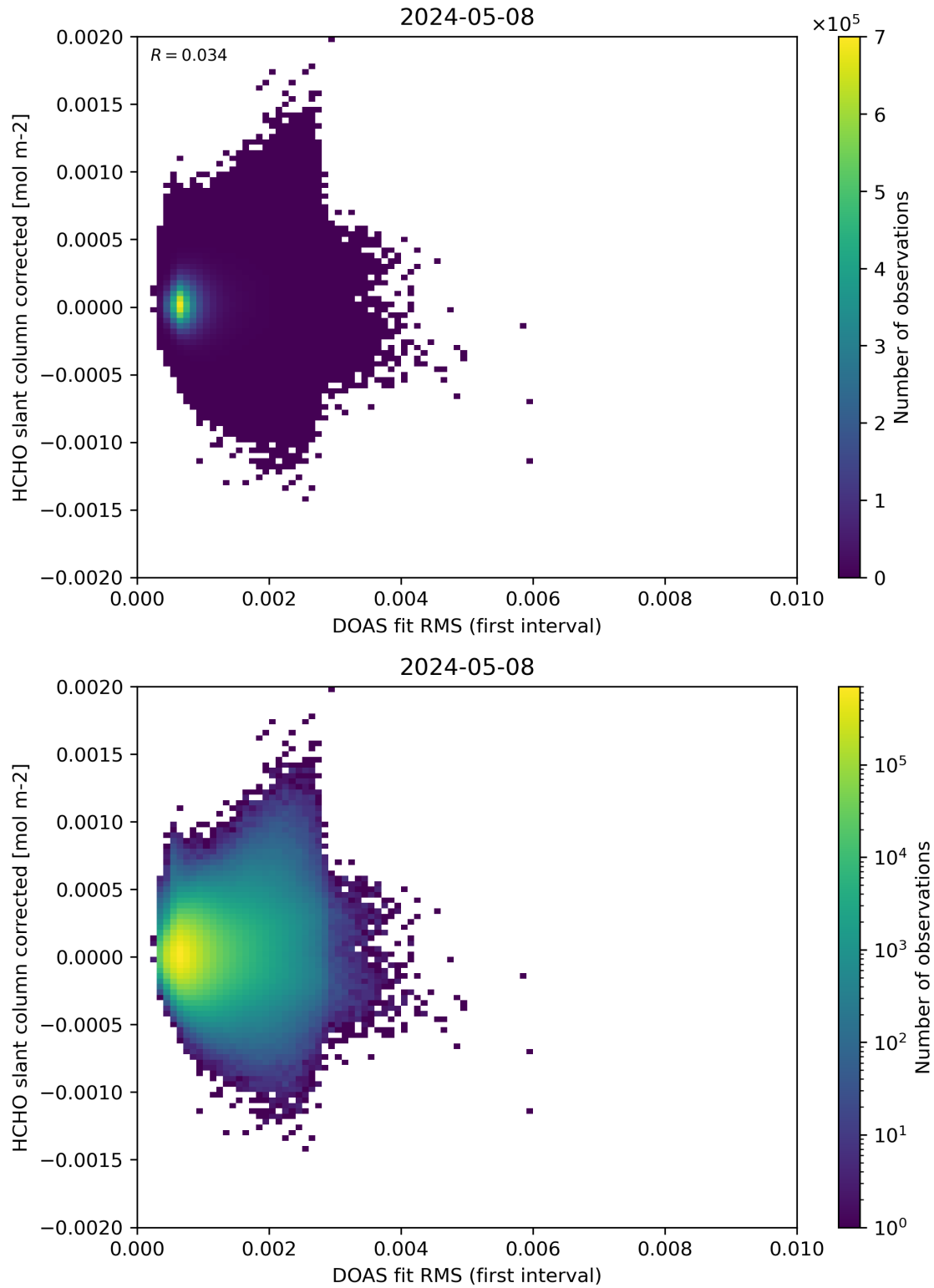
Figure 62: Scatter density plot of “DOAS fit RMS (first interval)” against “HCHO slant column corrected” for 2024-05-07 to 2024-05-09.
