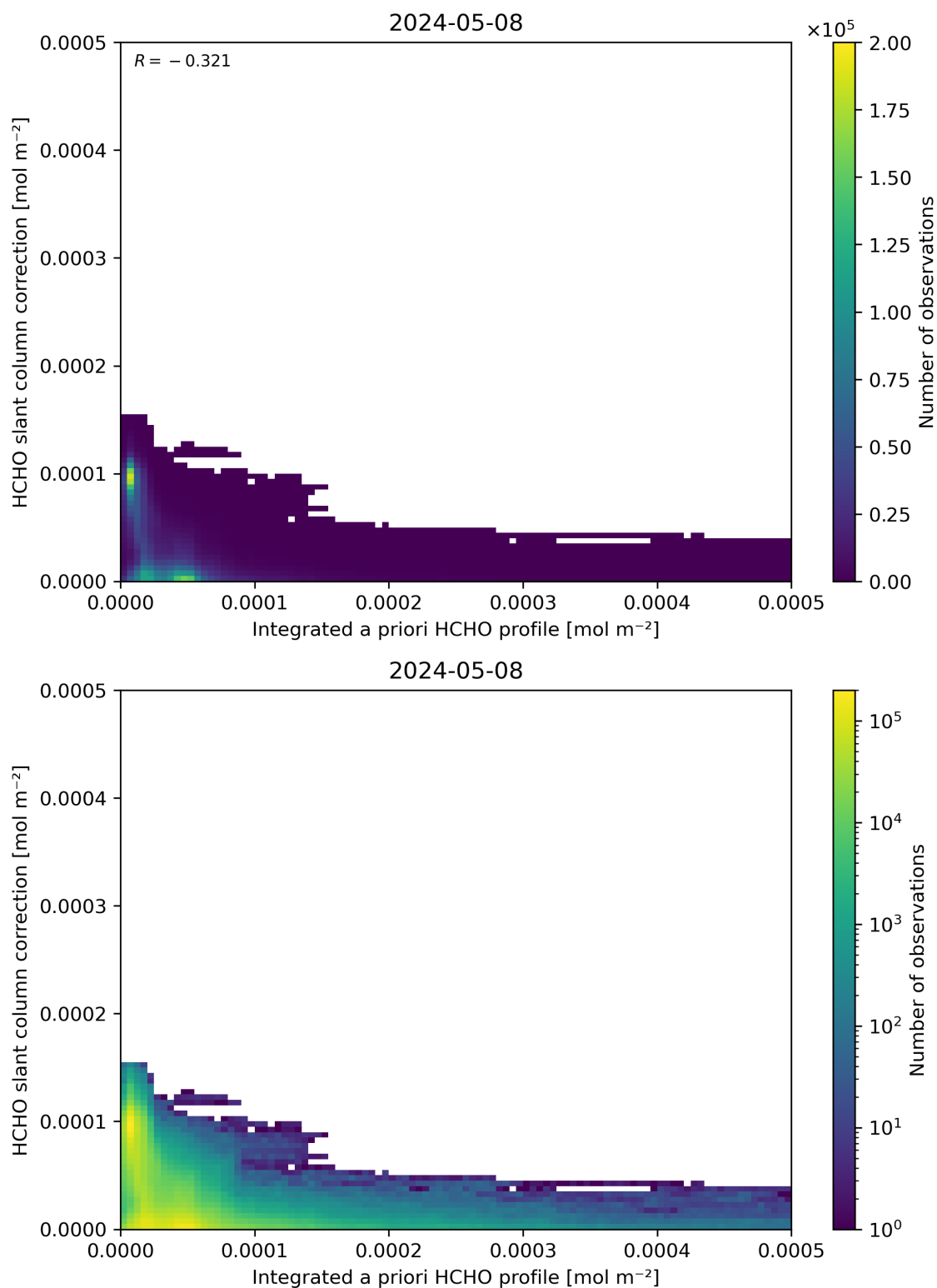
Figure 152: Scatter density plot of “Integrated a priori HCHO profile” against “HCHO slant column correction” for 2024-05-07 to 2024-05-09.
