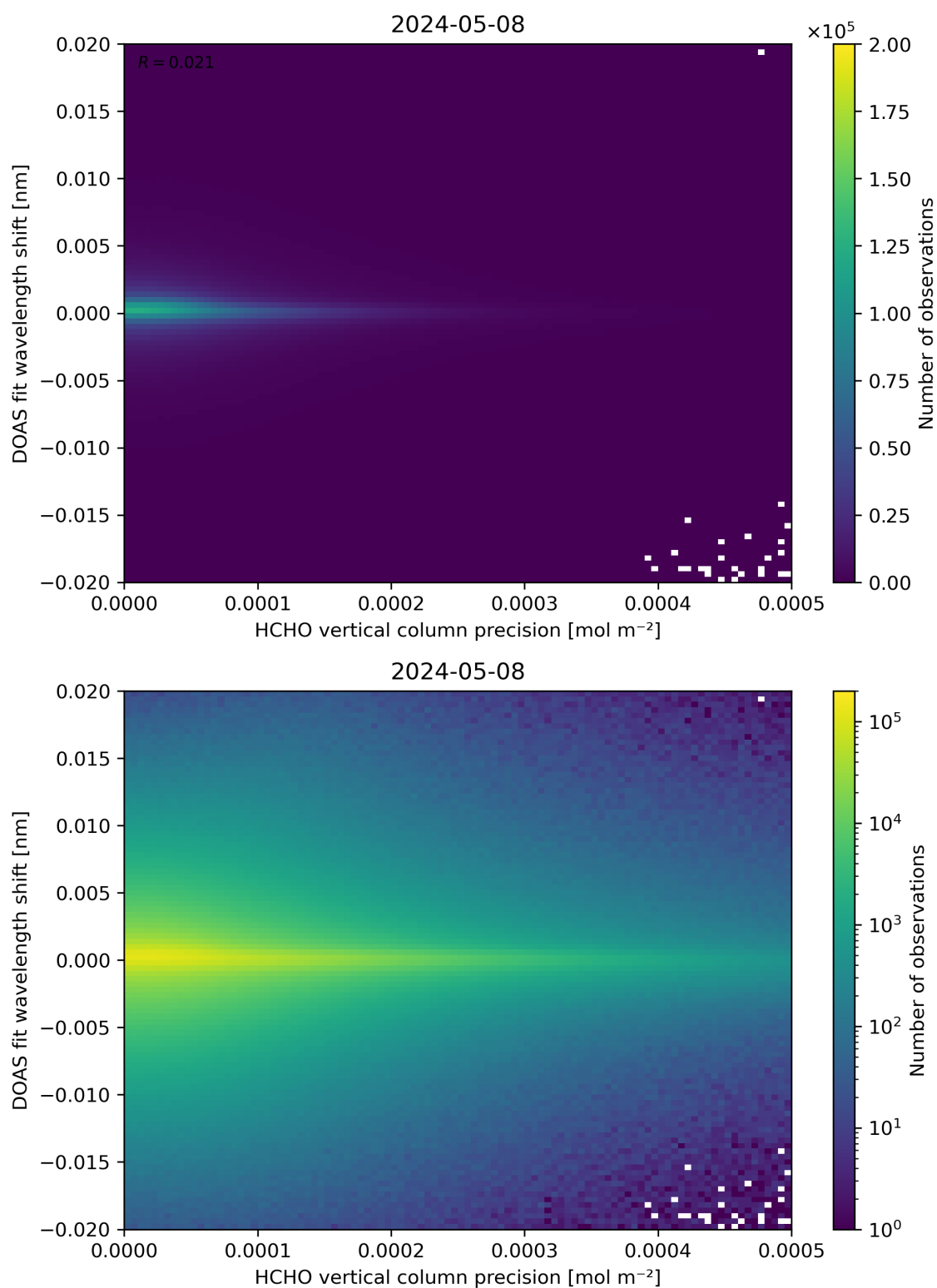
Figure 137: Scatter density plot of “HCHO vertical column precision” against “DOAS fit wavelength shift” for 2024-05-07 to 2024-05-09.
