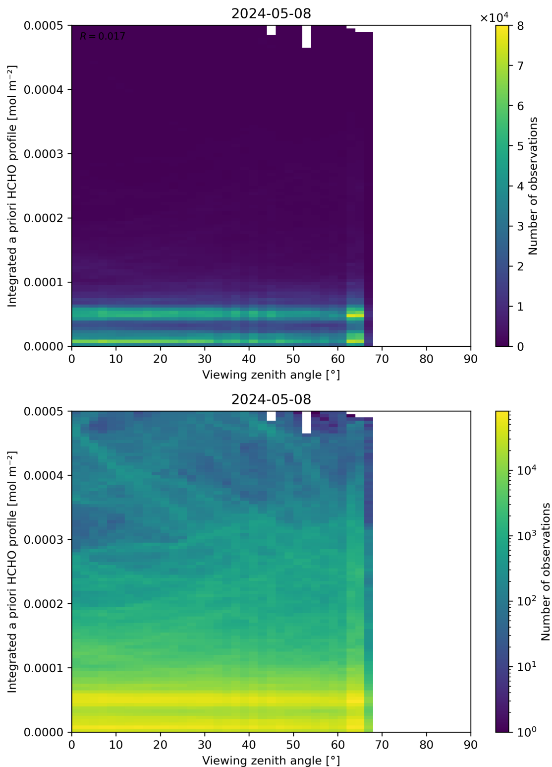
Figure 195: Scatter density plot of “Viewing zenith angle” against “Integrated a priori HCHO profile” for 2024-05-07 to 2024-05-09.
