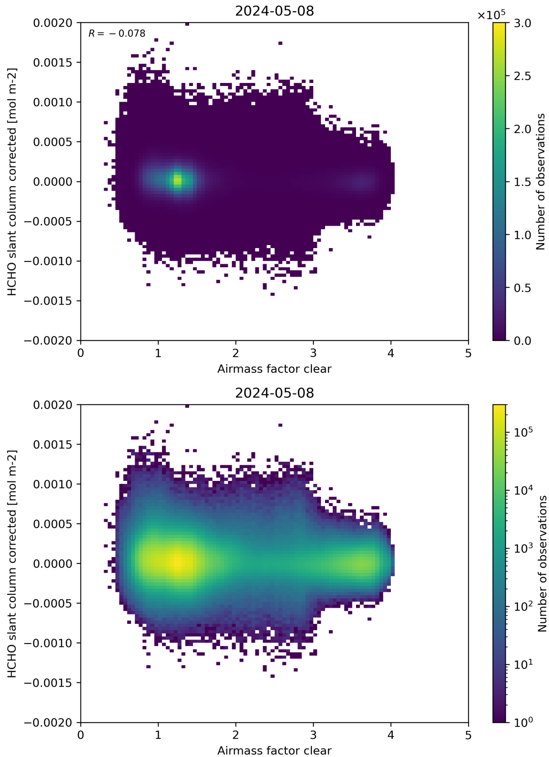
Figure 74: Scatter density plot of “Airmass factor clear” against “HCHO slant column corrected” for 2024-05-07 to 2024-05-09.
