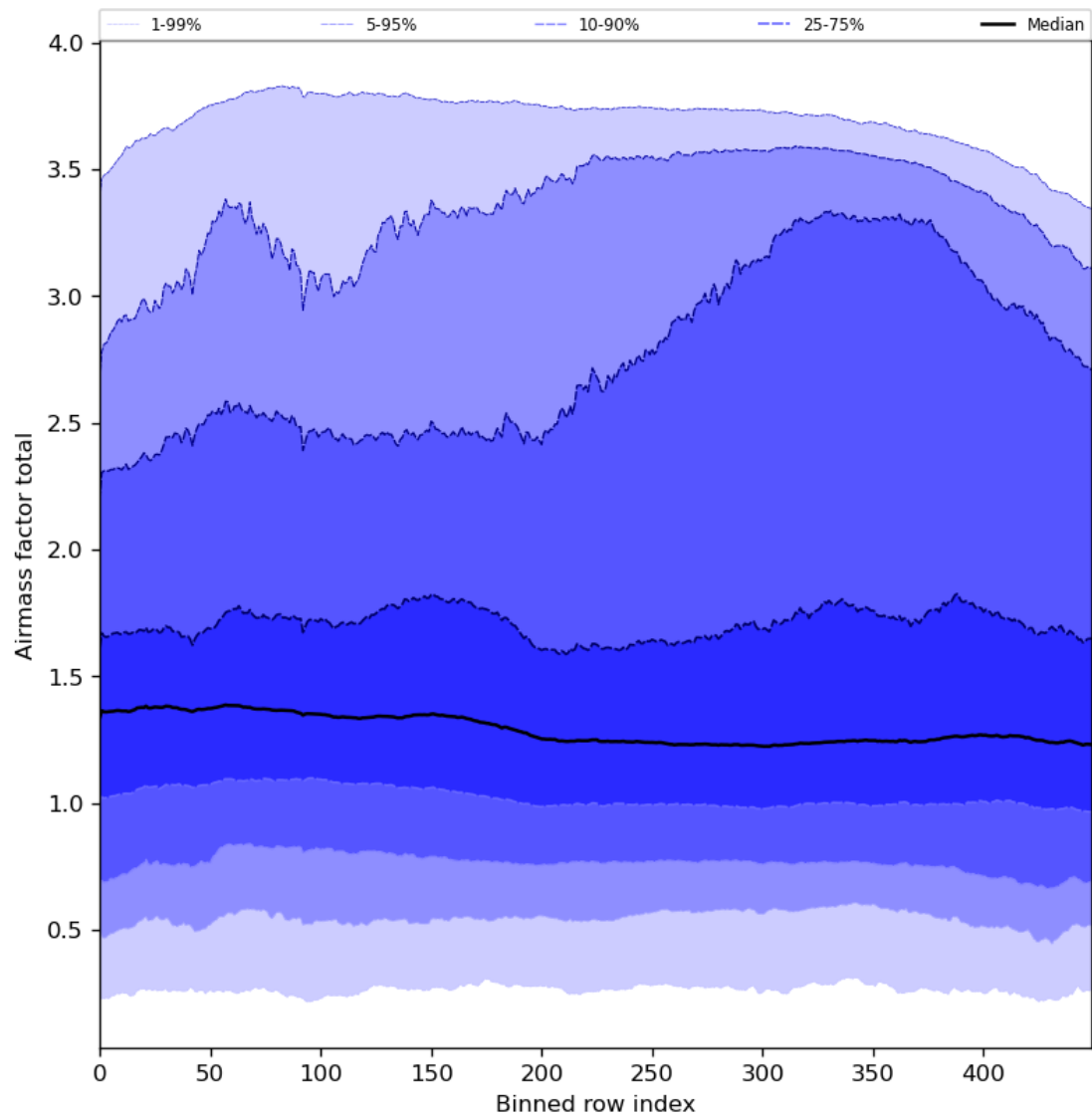
Figure 54: Along track statistics of “Airmass factor total” for 2024-05-07 to 2024-05-09
