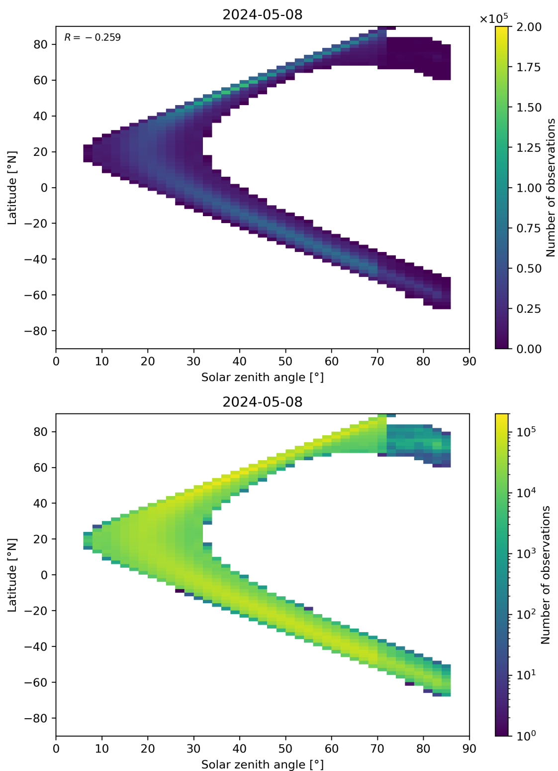
Figure 181: Scatter density plot of “Solar zenith angle” against “Latitude” for 2024-05-07 to 2024-05-09.
