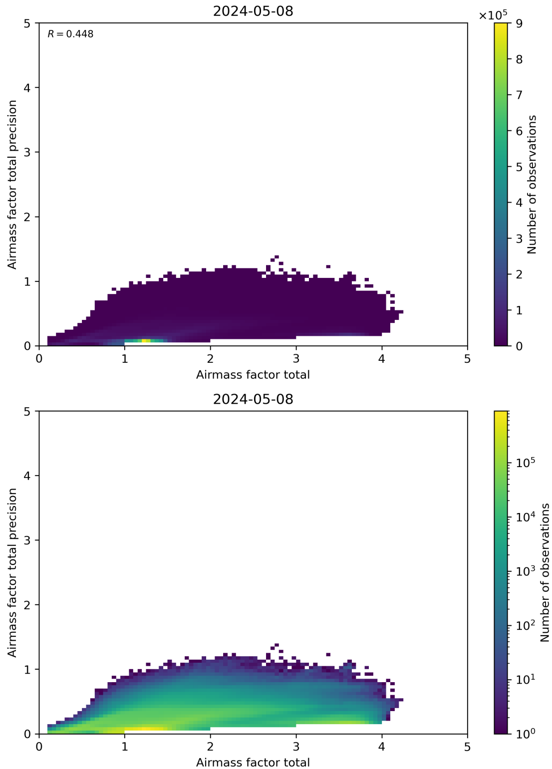
Figure 103: Scatter density plot of “Airmass factor total” against “Airmass factor total precision” for 2024-05-07 to 2024-05-09.
