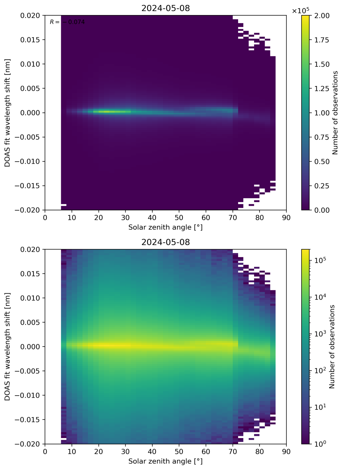
Figure 168: Scatter density plot of “Solar zenith angle” against “DOAS fit wavelength shift” for 2024-05-07 to 2024-05-09.
