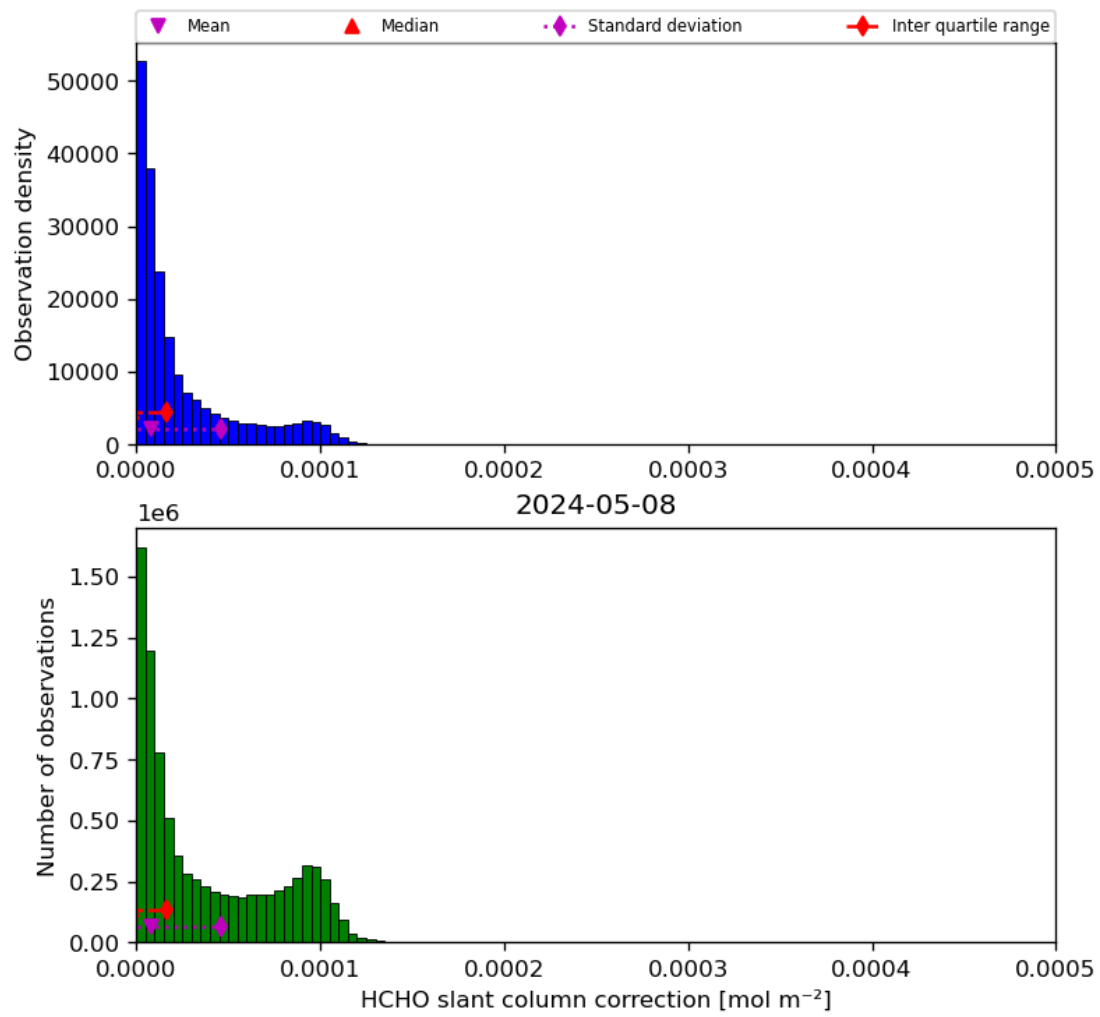
Figure 47: Histogram of “HCHO slant column correction” for 2024-05-07 to 2024-05-09
