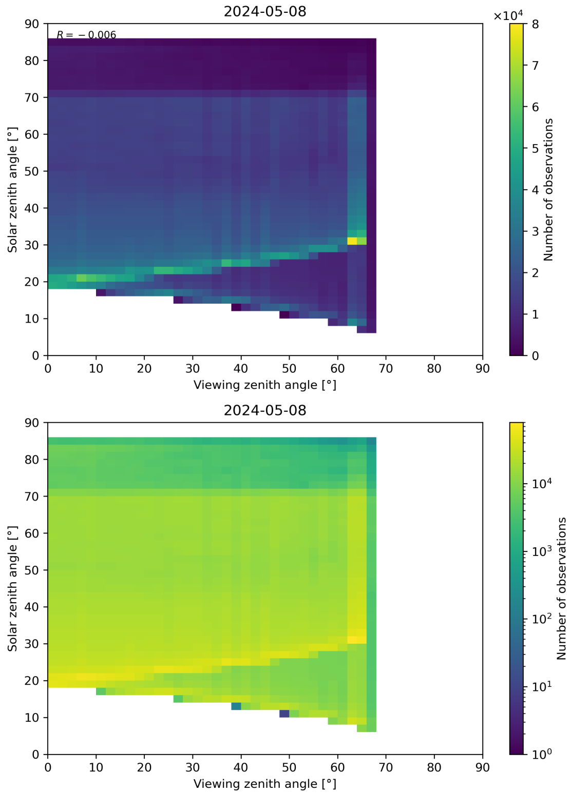
Figure 197: Scatter density plot of “Viewing zenith angle” against “Solar zenith angle” for 2024-05-07 to 2024-05-09.
