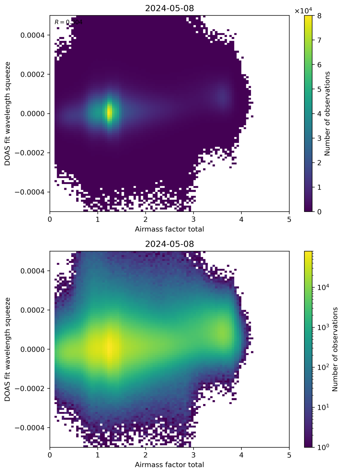
Figure 99: Scatter density plot of “Airmass factor total” against “DOAS fit wavelength squeeze” for 2024-05-07 to 2024-05-09.
