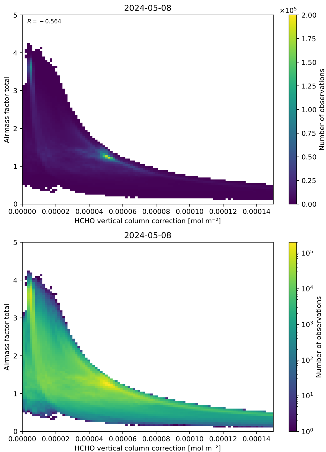
Figure 120: Scatter density plot of “HCHO vertical column correction” against “Airmass factor total” for 2024-05-07 to 2024-05-09.
