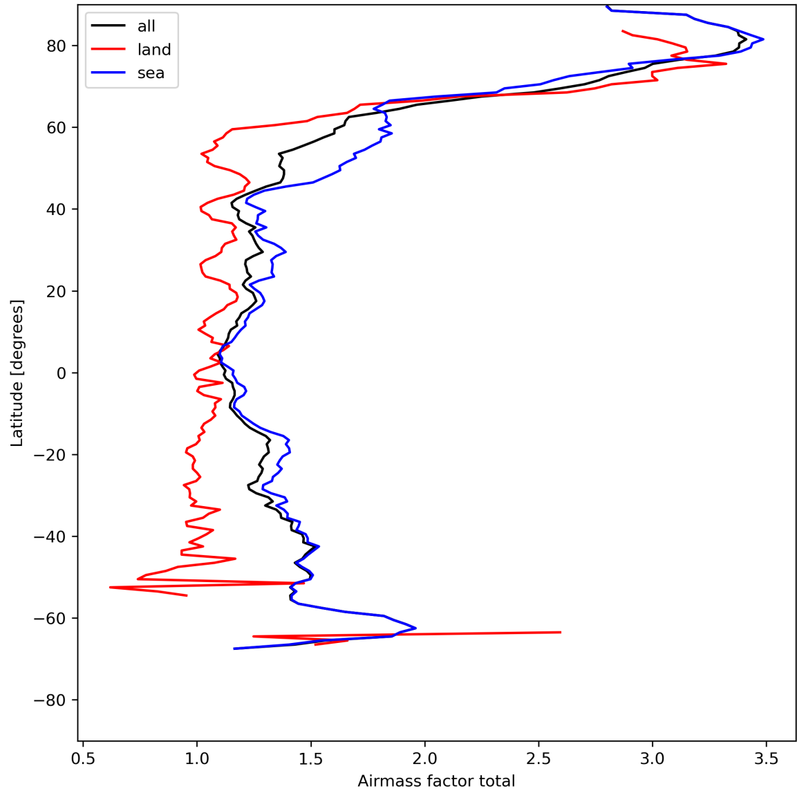
Figure 26: Zonal average of “Airmass factor total” for 2024-05-07 to 2024-05-09.
