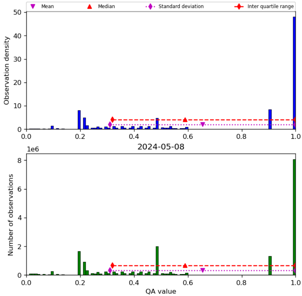
Figure 34: Histogram of “QA value” for 2024-05-07 to 2024-05-09
