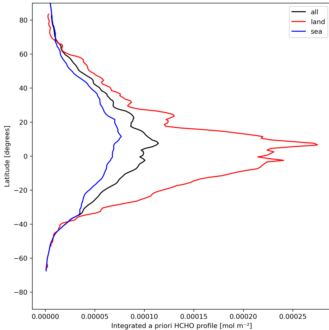
Figure 29: Zonal average of “Integrated a priori HCHO profile” for 2024-05-07 to 2024-05-09.
