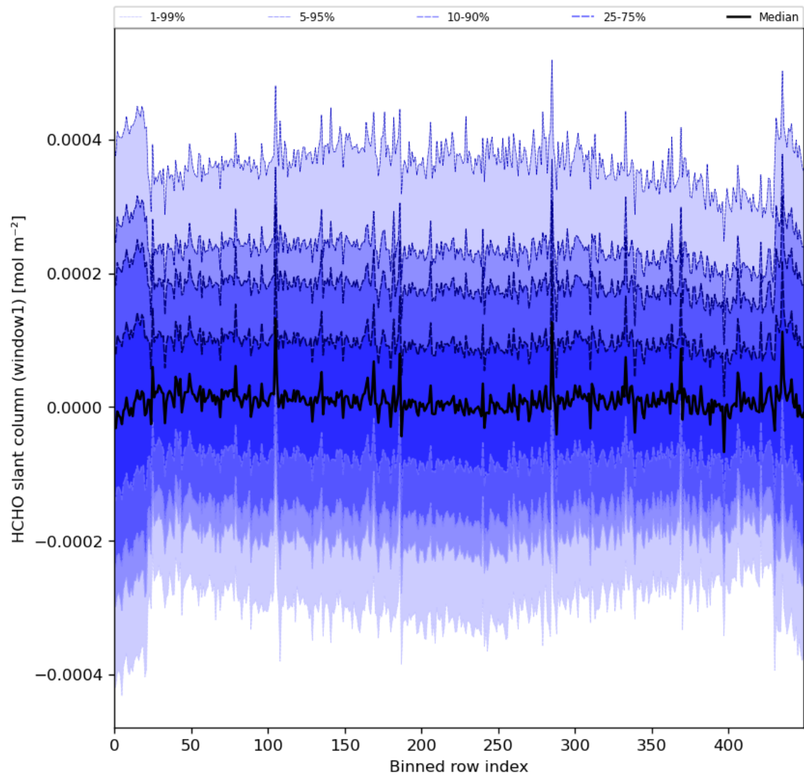
Figure 52: Along track statistics of “HCHO slant column (window1)” for 2024-05-07 to 2024-05-09
