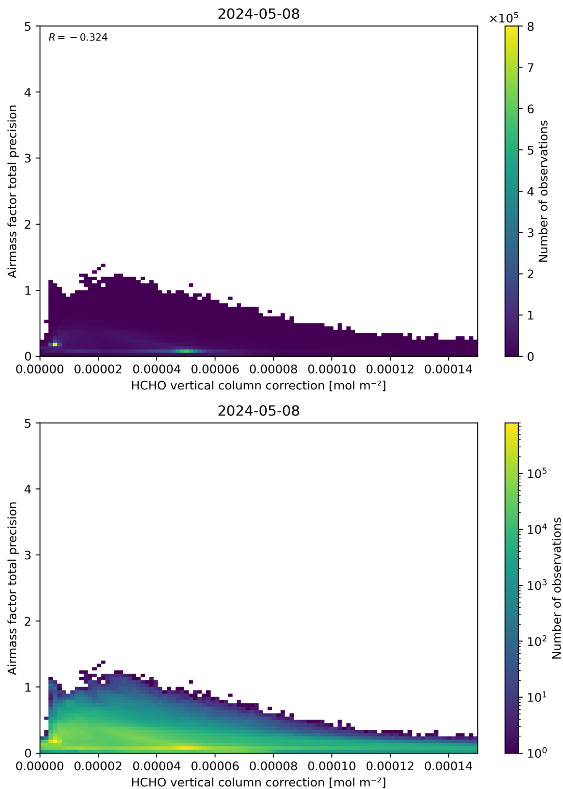
Figure 121: Scatter density plot of “HCHO vertical column correction” against “Airmass factor total precision” for 2024-05-07 to 2024-05-09.
