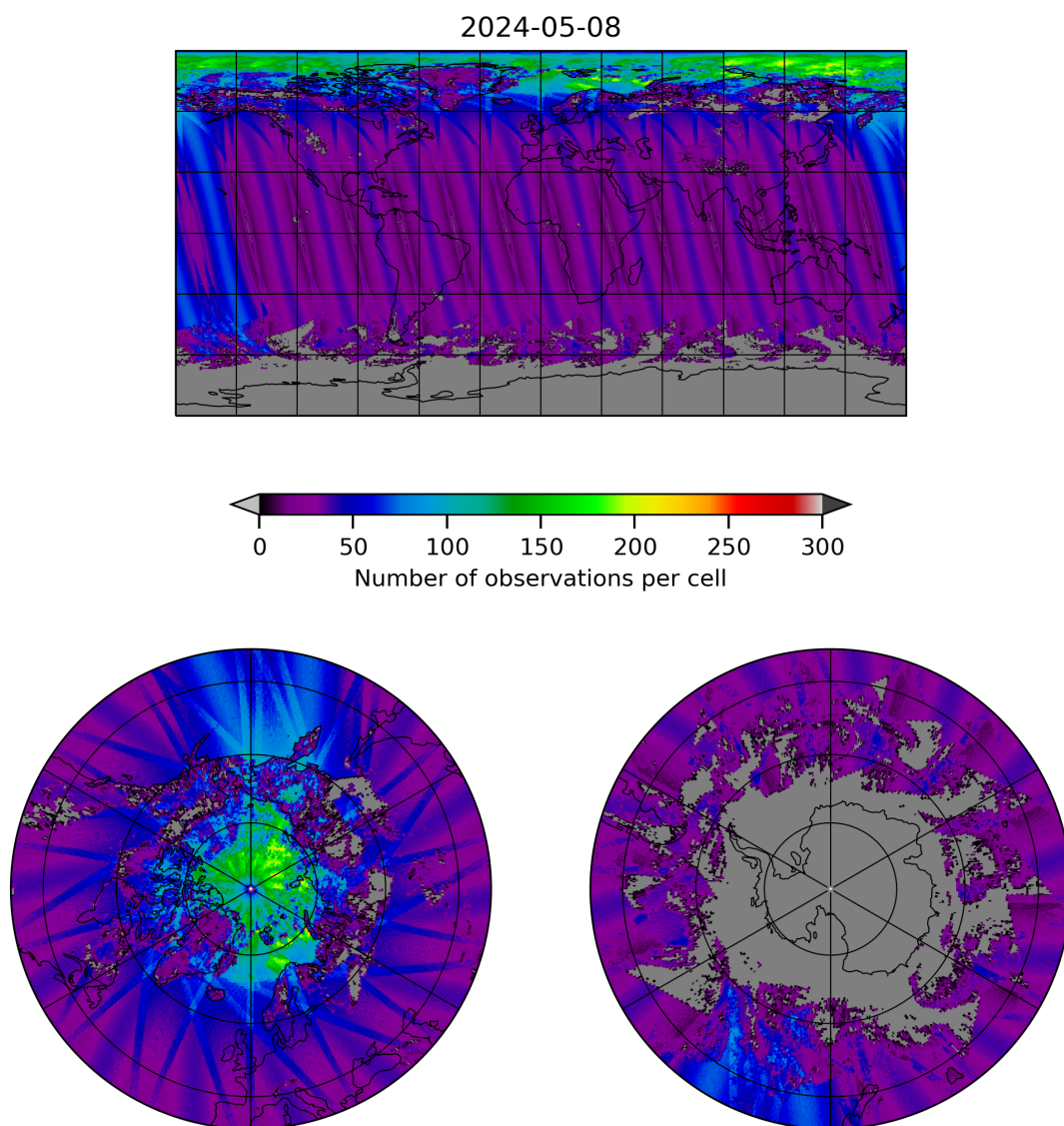
Figure 19: Map of the number of observations for 2024-05-07 to 2024-05-09
