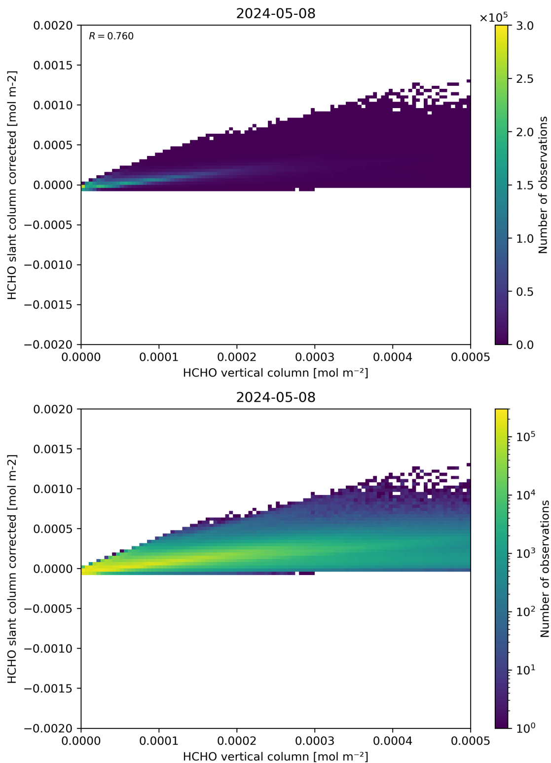
Figure 127: Scatter density plot of “HCHO vertical column” against “HCHO slant column corrected” for 2024-05-07 to 2024-05-09.
