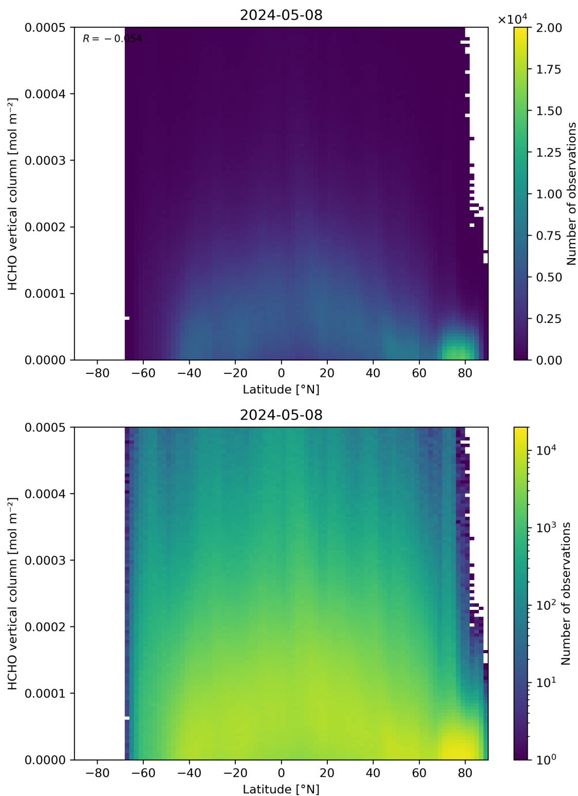
Figure 163: Scatter density plot of “Latitude” against “HCHO vertical column” for 2024-05-07 to 2024-05-09.
