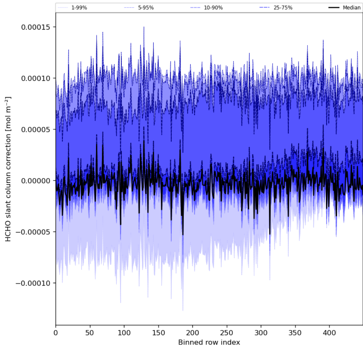
Figure 61: Along track statistics of “HCHO slant column correction” for 2024-05-07 to 2024-05-09
