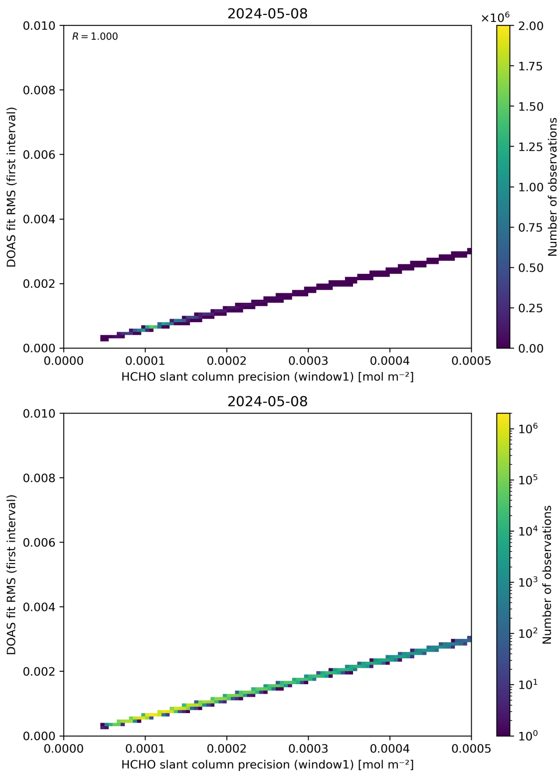
Figure 88: Scatter density plot of “HCHO slant column precision (window1)” against “DOAS fit RMS (first interval)” for 2024-05-07 to 2024-05-09.
