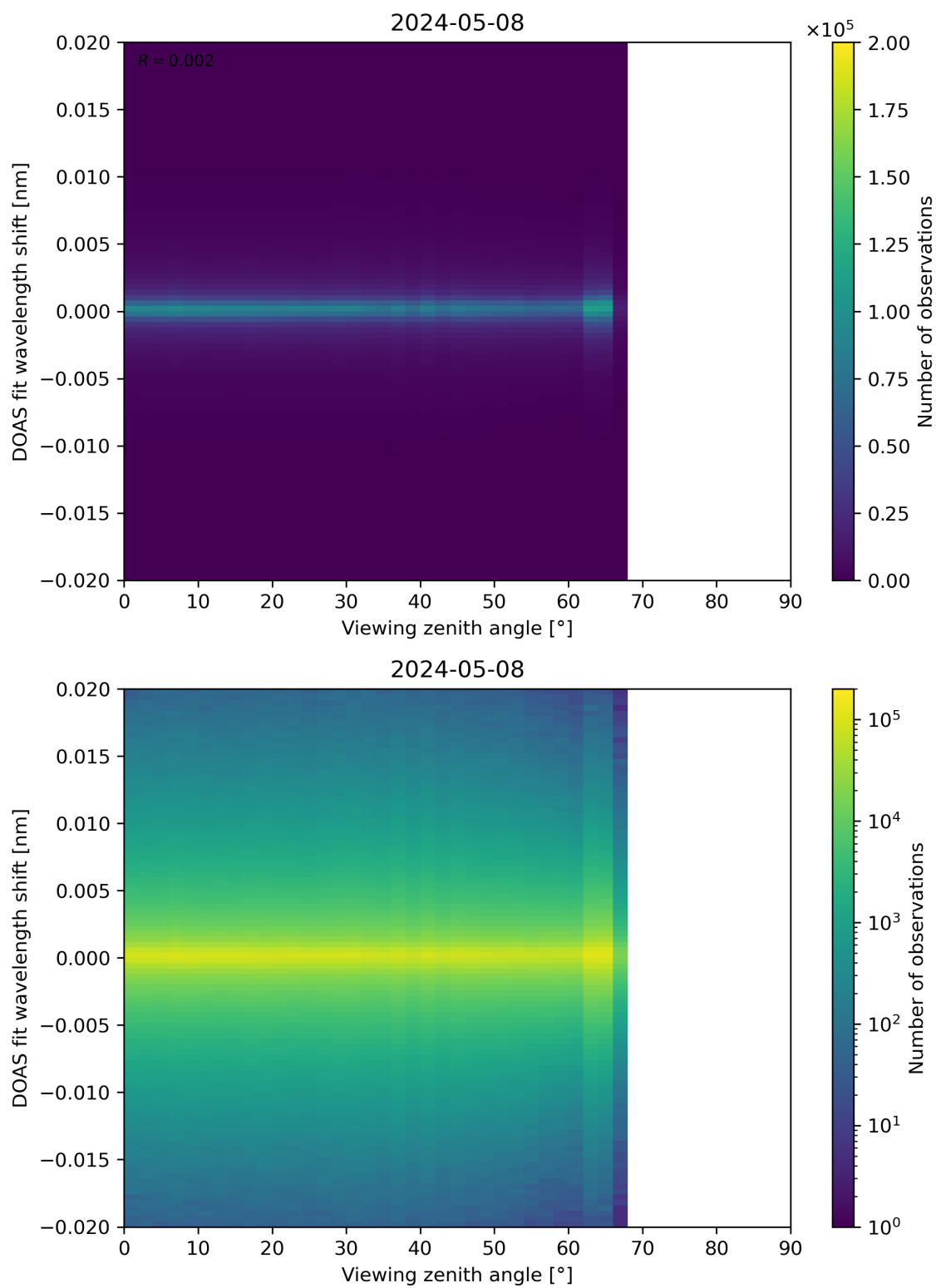
Figure 183: Scatter density plot of “Viewing zenith angle” against “DOAS fit wavelength shift” for 2024-05-07 to 2024-05-09.
