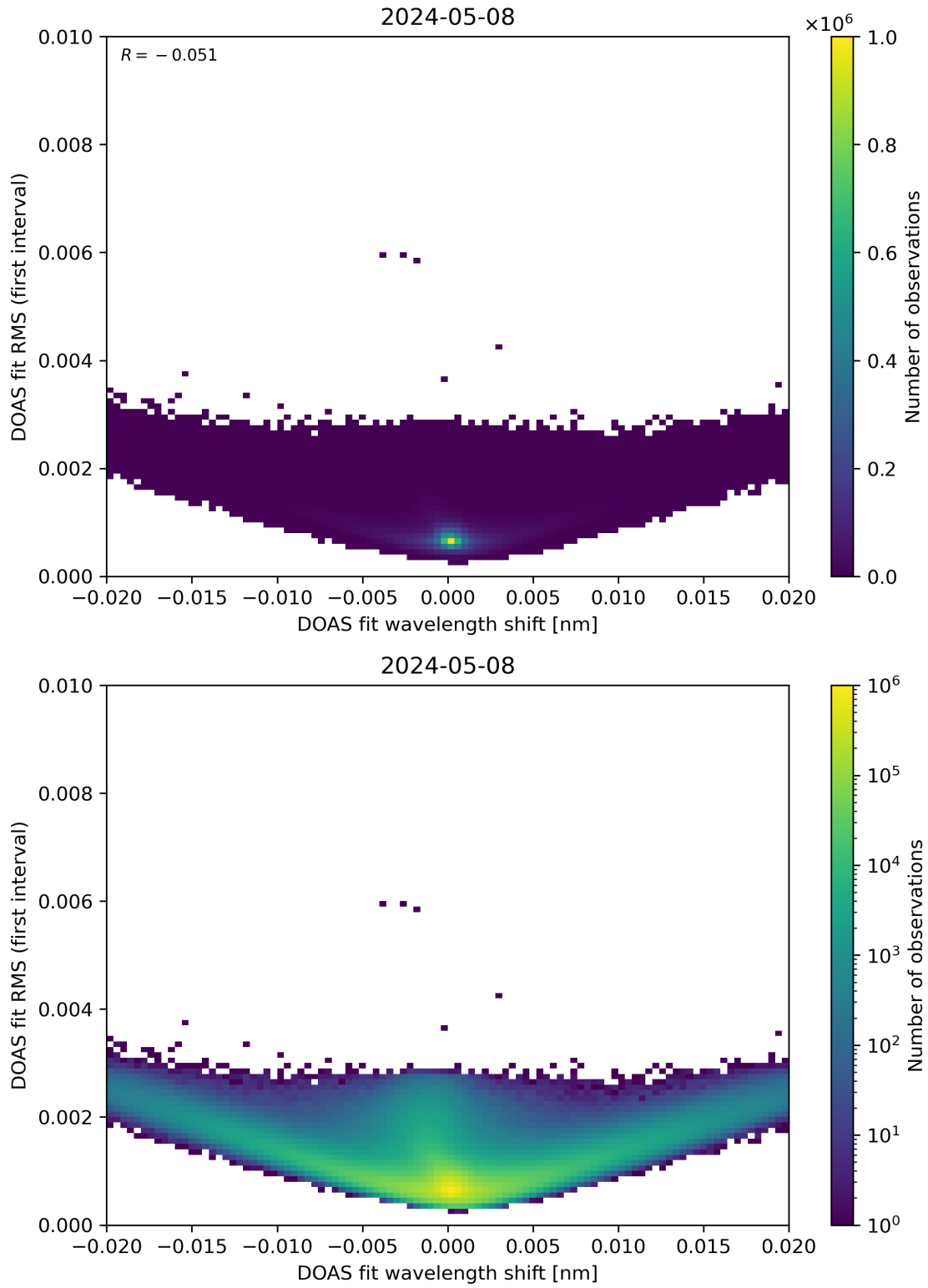
Figure 64: Scatter density plot of “DOAS fit wavelength shift” against “DOAS fit RMS (first interval)” for 2024-05-07 to 2024-05-09.
