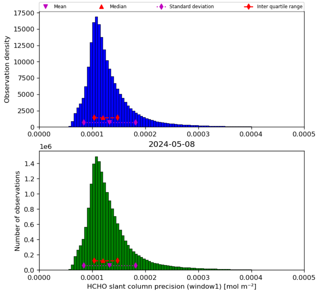
Figure 39: Histogram of “HCHO slant column precision (window1)” for 2024-05-07 to 2024-05-09
