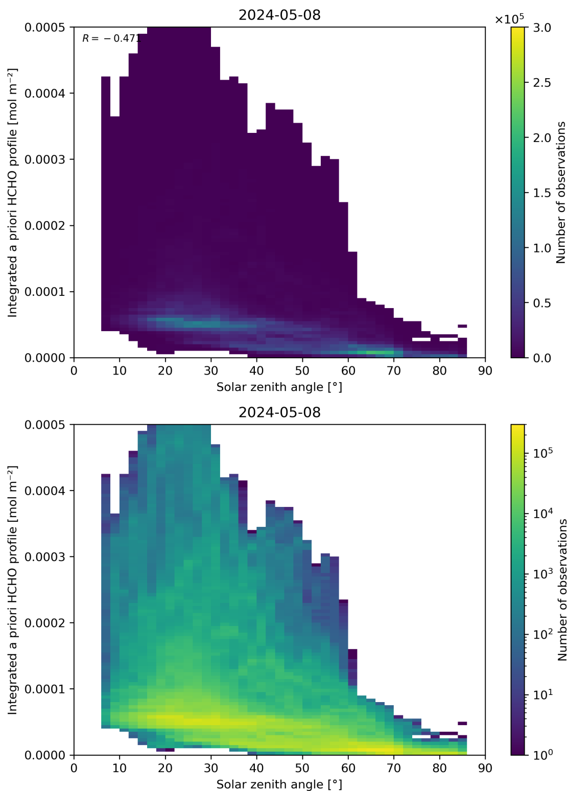
Figure 180: Scatter density plot of “Solar zenith angle” against “Integrated a priori HCHO profile” for 2024-05-07 to 2024-05-09.
