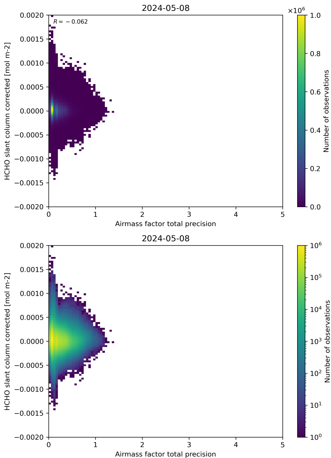
Figure 109: Scatter density plot of “Airmass factor total precision” against “HCHO slant column corrected” for 2024-05-07 to 2024-05-09.
