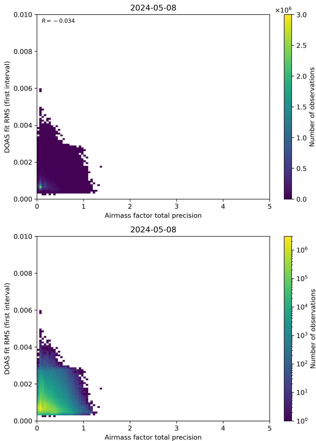
Figure 105: Scatter density plot of “Airmass factor total precision” against “DOAS fit RMS (first interval)” for 2024-05-07 to 2024-05-09.
