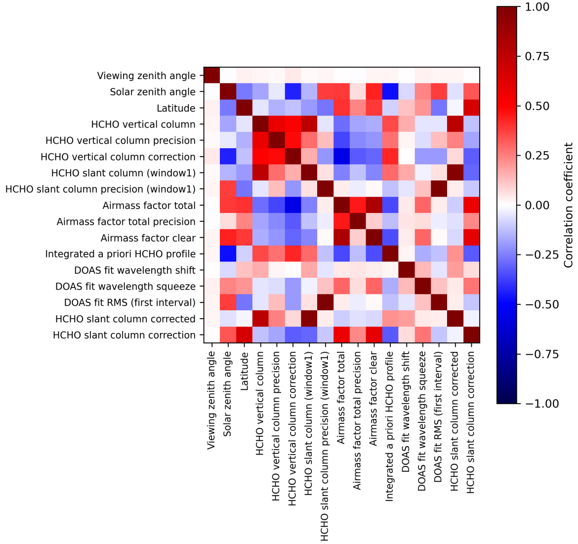
Figure 2: Map of correlation matrix for 2024-05-07 to 2024-05-09.
