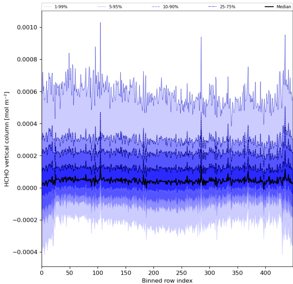
Figure 49: Along track statistics of “HCHO vertical column” for 2024-05-07 to 2024-05-09
