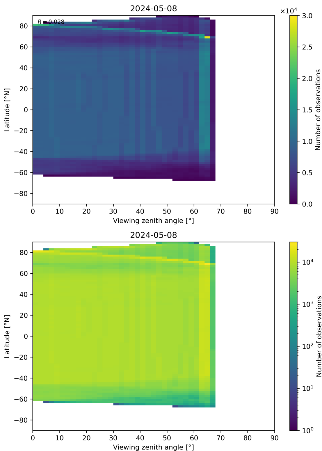
Figure 196: Scatter density plot of “Viewing zenith angle” against “Latitude” for 2024-05-07 to 2024-05-09.
