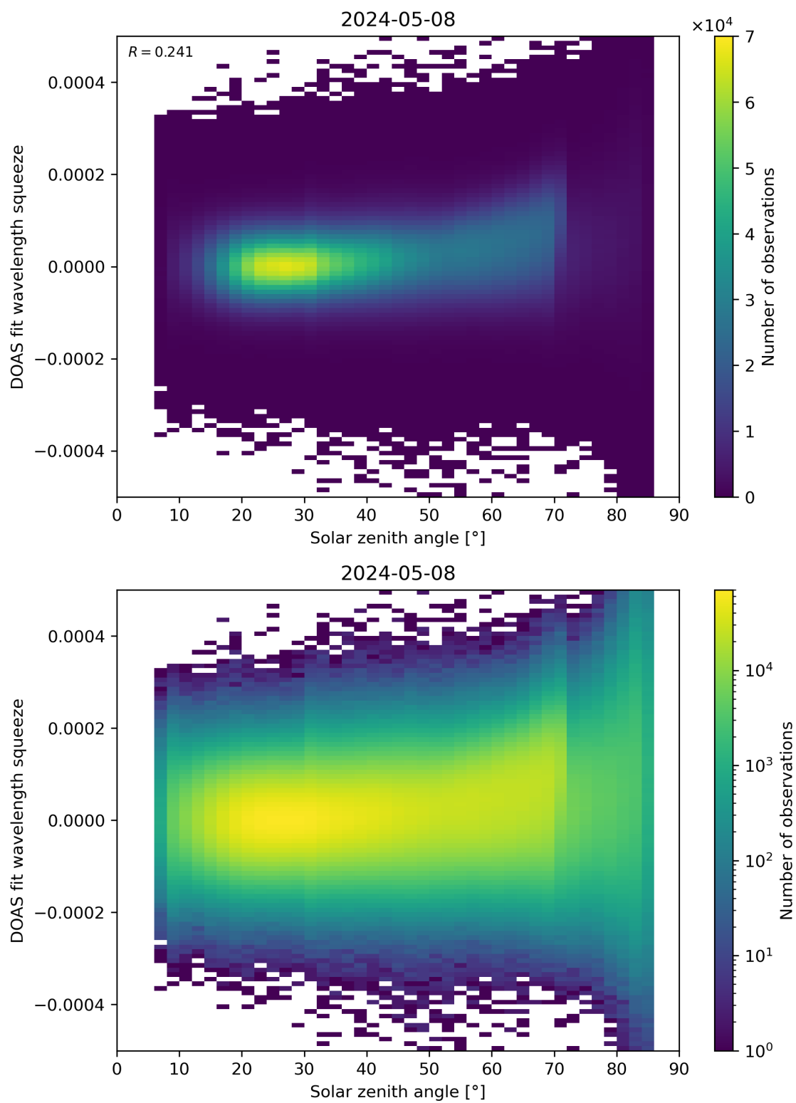
Figure 169: Scatter density plot of “Solar zenith angle” against “DOAS fit wavelength squeeze” for 2024-05-07 to 2024-05-09.
