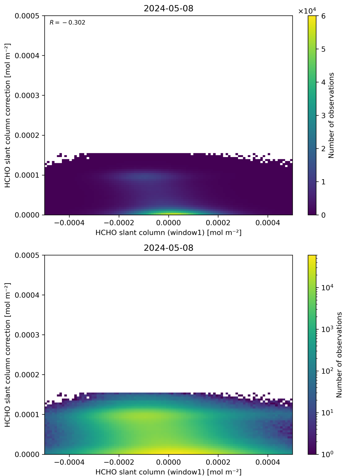
Figure 83: Scatter density plot of “HCHO slant column (window1)” against “HCHO slant column correction” for 2024-05-07 to 2024-05-09.
