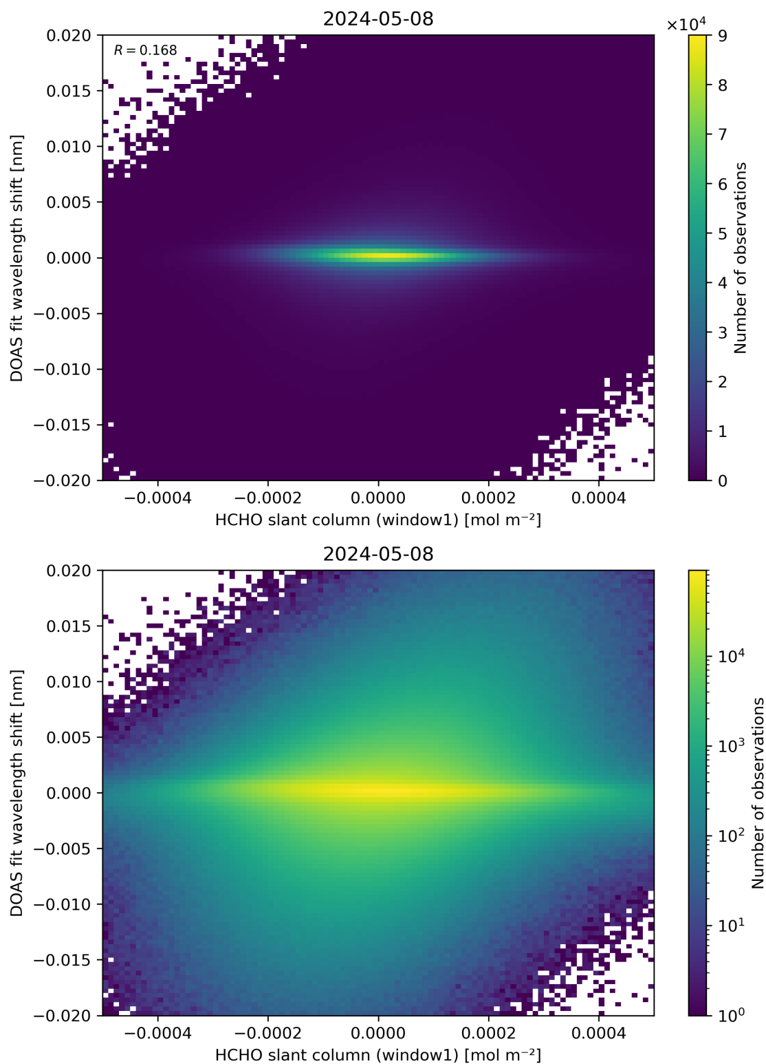
Figure 79: Scatter density plot of “HCHO slant column (window1)” against “DOAS fit wavelength shift” for 2024-05-07 to 2024-05-09.
