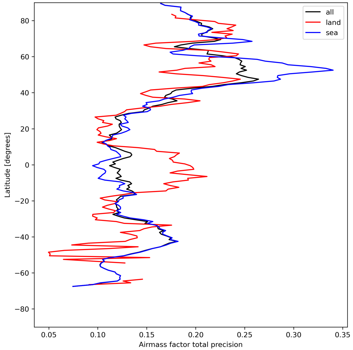
Figure 27: Zonal average of “Airmass factor total precision” for 2024-05-07 to 2024-05-09.
