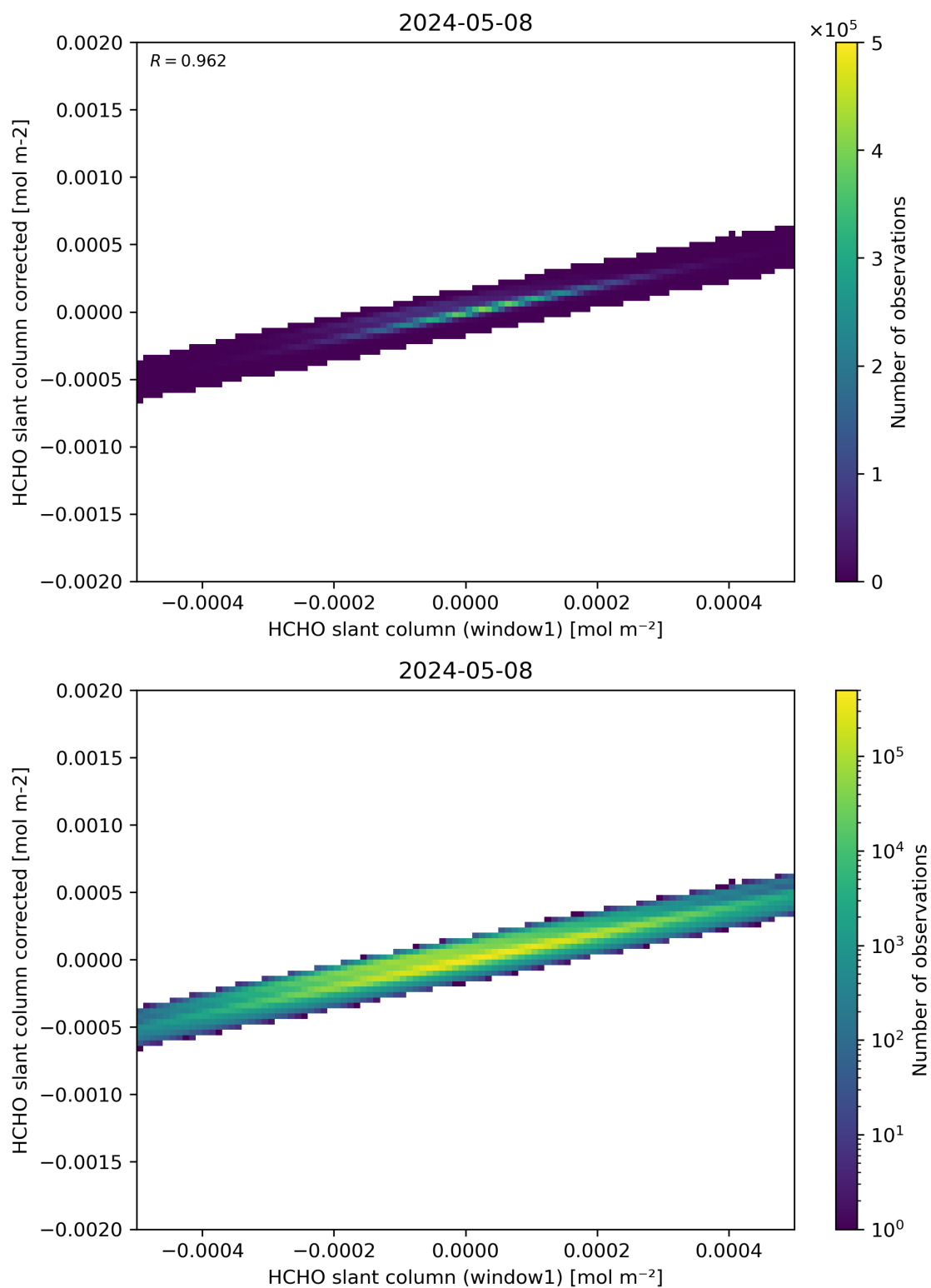
Figure 82: Scatter density plot of “HCHO slant column (window1)” against “HCHO slant column corrected” for 2024-05-07 to 2024-05-09.
