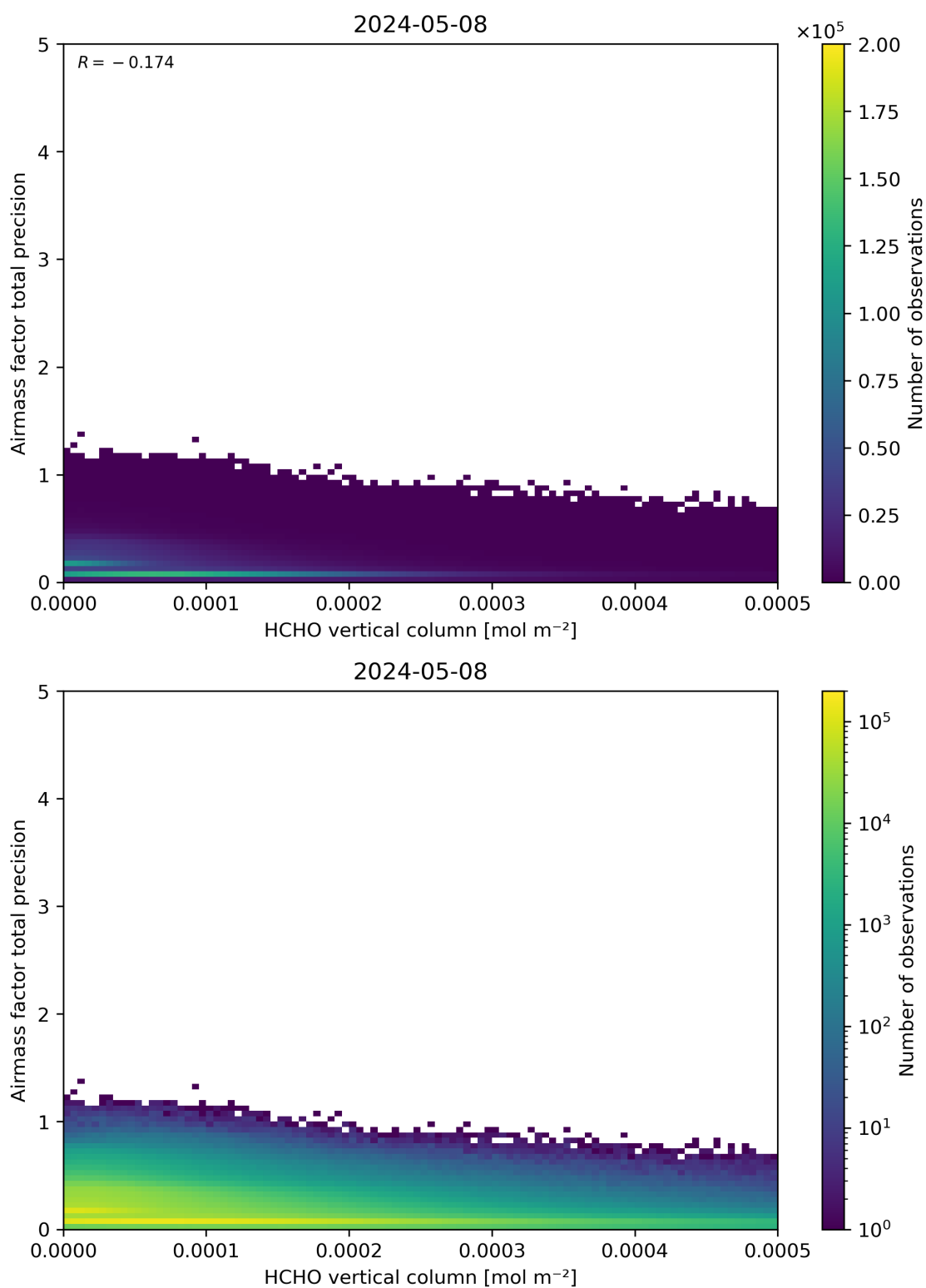
Figure 132: Scatter density plot of “HCHO vertical column” against “Airmass factor total precision” for 2024-05-07 to 2024-05-09.
