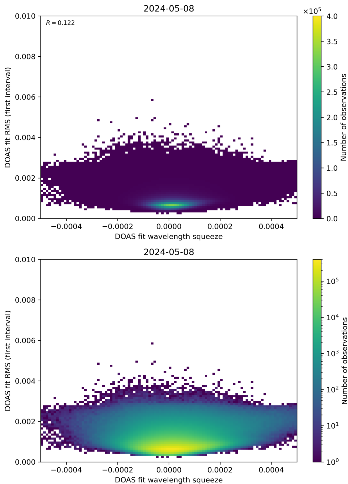
Figure 68: Scatter density plot of “DOAS fit wavelength squeeze” against “DOAS fit RMS (first interval)” for 2024-05-07 to 2024-05-09.
