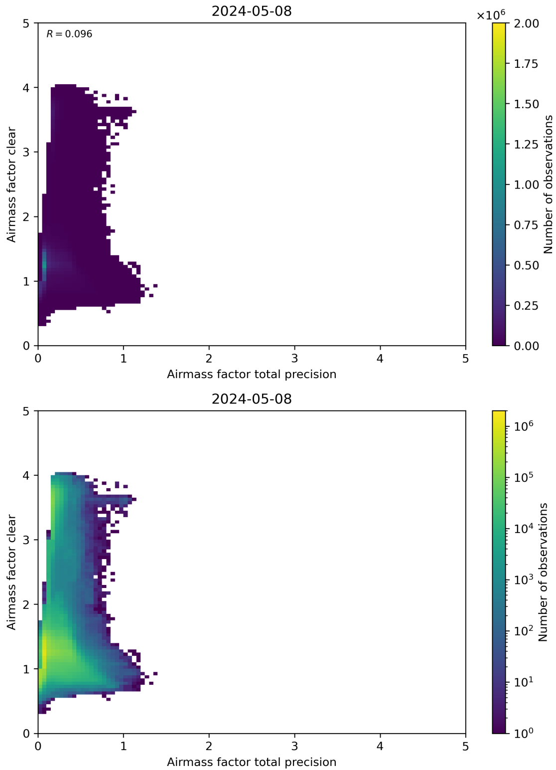
Figure 108: Scatter density plot of “Airmass factor total precision” against “Airmass factor clear” for 2024-05-07 to 2024-05-09.
