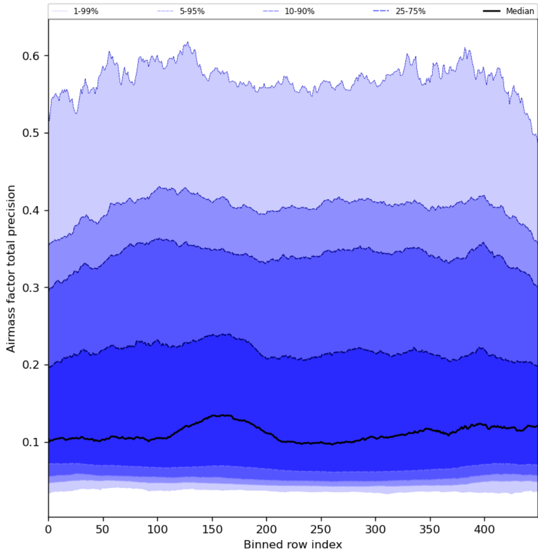
Figure 55: Along track statistics of “Airmass factor total precision” for 2024-05-07 to 2024-05-09
