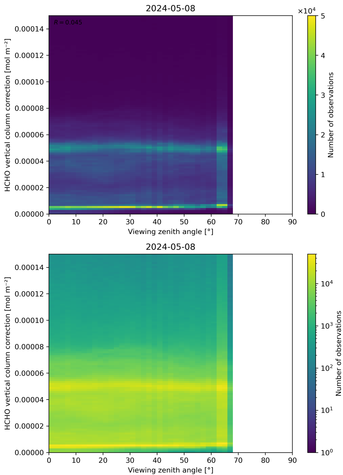
Figure 193: Scatter density plot of “Viewing zenith angle” against “HCHO vertical column correction” for 2024-05-07 to 2024-05-09.
