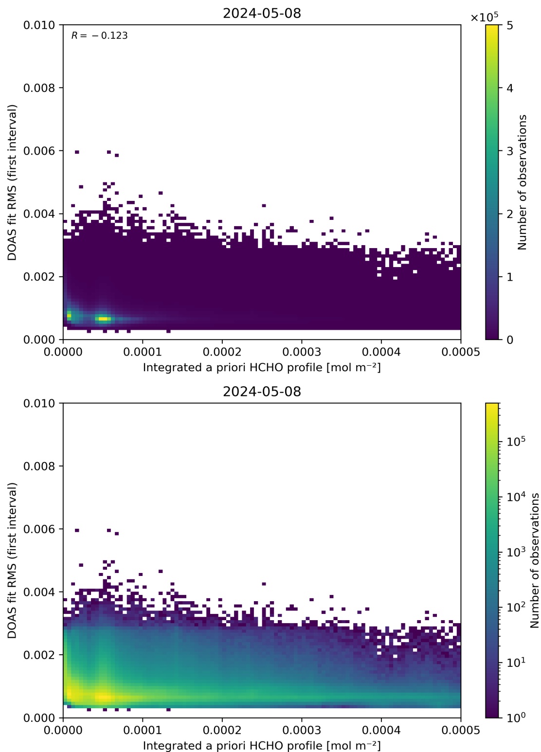
Figure 148: Scatter density plot of “Integrated a priori HCHO profile” against “DOAS fit RMS (first interval)” for 2024-05-07 to 2024-05-09.
