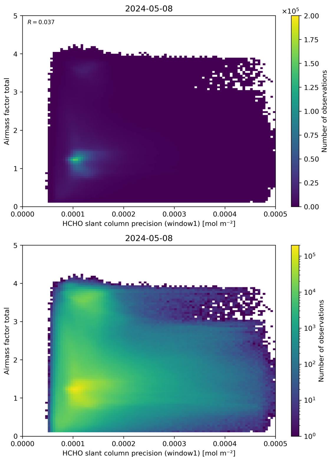
Figure 94: Scatter density plot of “HCHO slant column precision (window1)” against “Airmass factor total” for 2024-05-07 to 2024-05-09.
