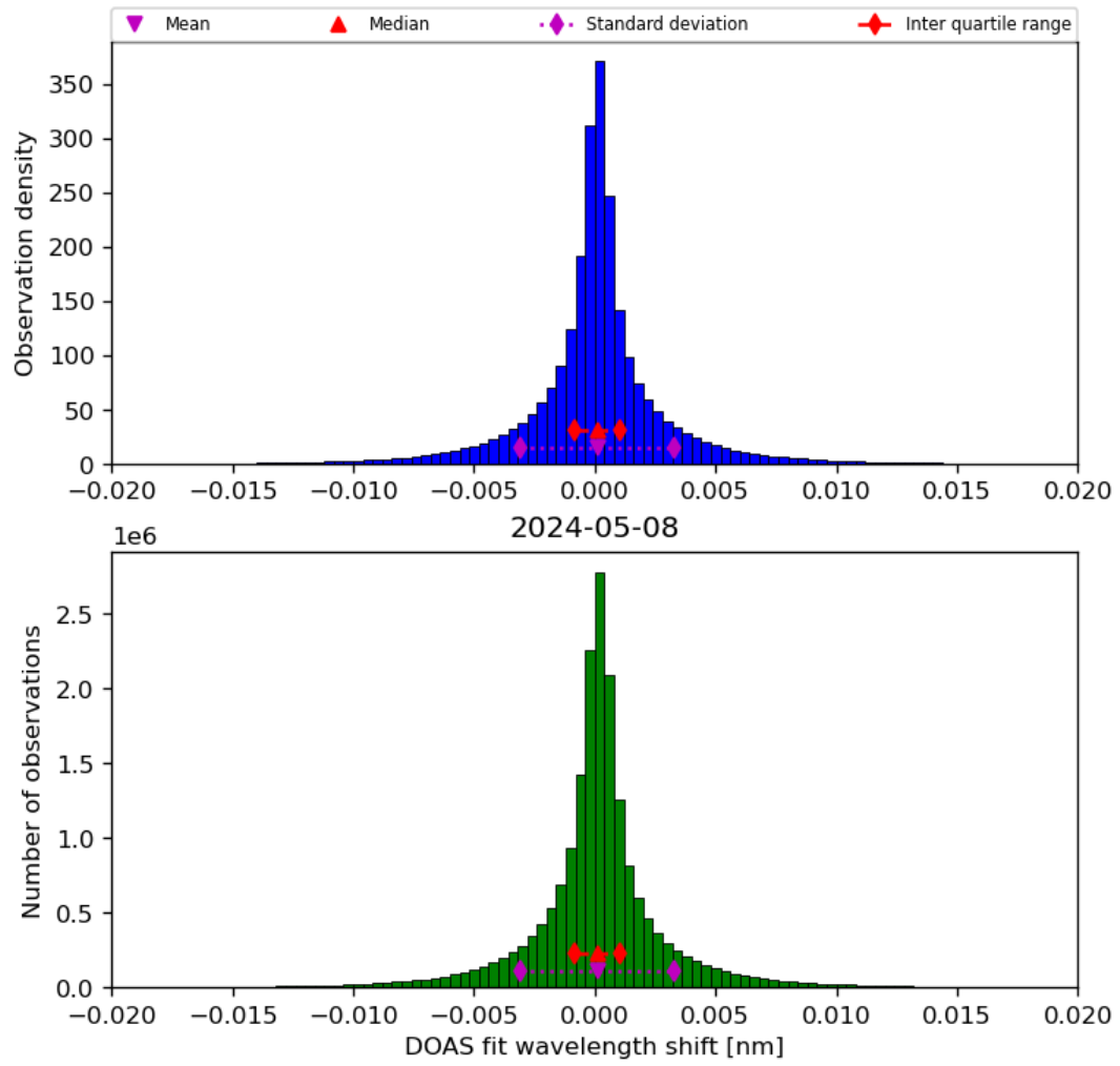
Figure 44: Histogram of “DOAS fit wavelength shift” for 2024-05-07 to 2024-05-09
