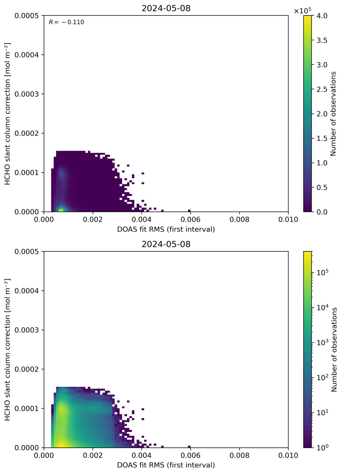
Figure 63: Scatter density plot of “DOAS fit RMS (first interval)” against “HCHO slant column correction” for 2024-05-07 to 2024-05-09.
