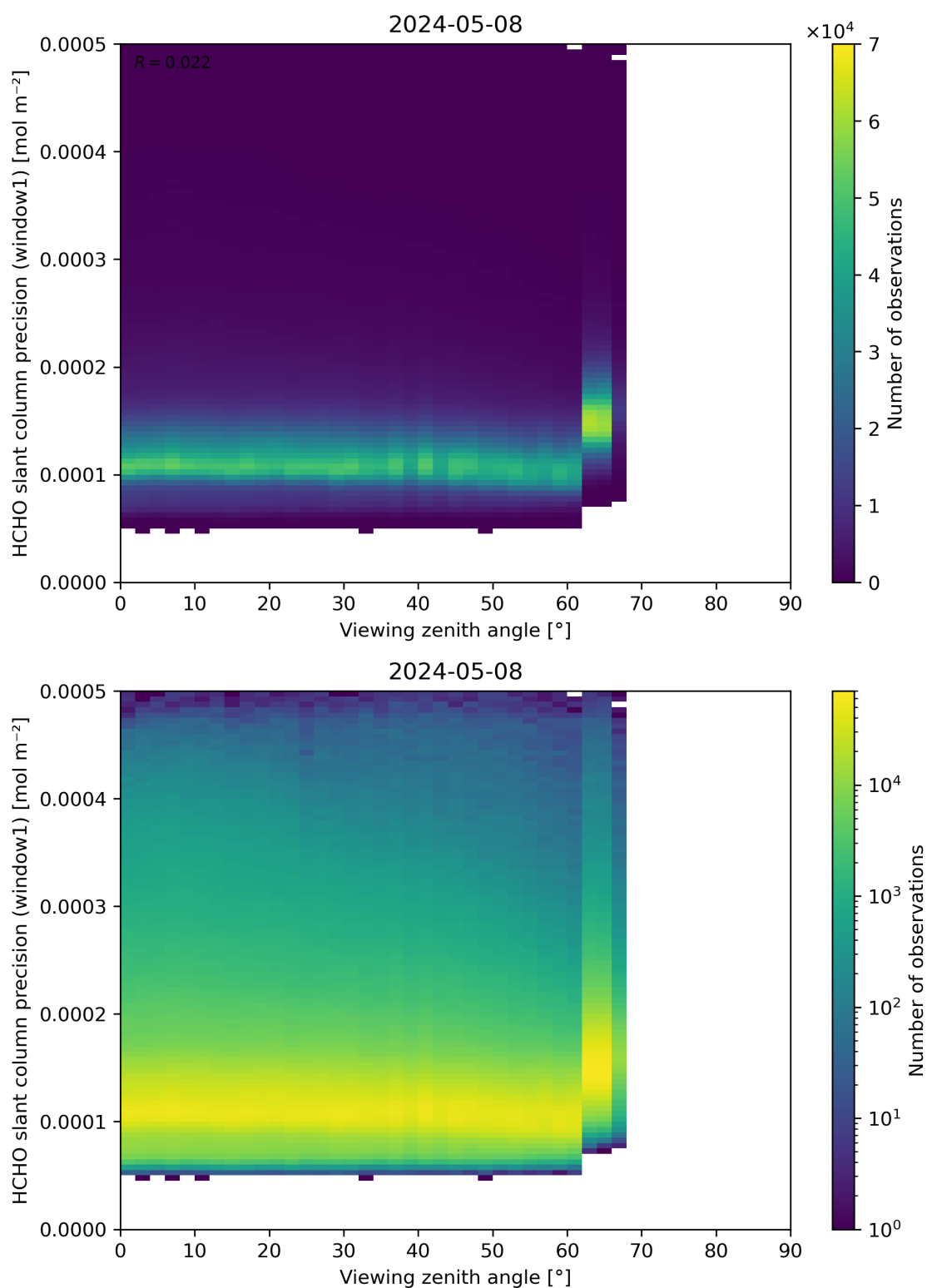
Figure 189: Scatter density plot of “Viewing zenith angle” against “HCHO slant column precision (window1)” for 2024-05-07 to 2024-05-09.
