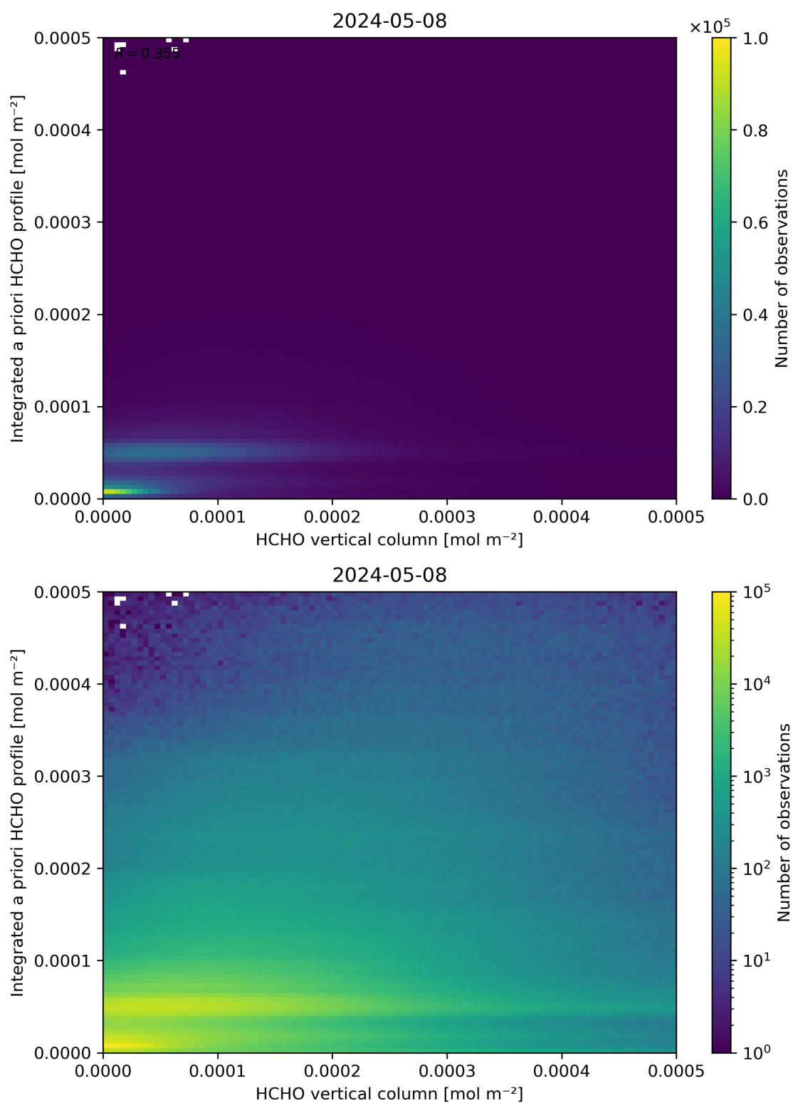
Figure 135: Scatter density plot of “HCHO vertical column” against “Integrated a priori HCHO profile” for 2024-05-07 to 2024-05-09.
