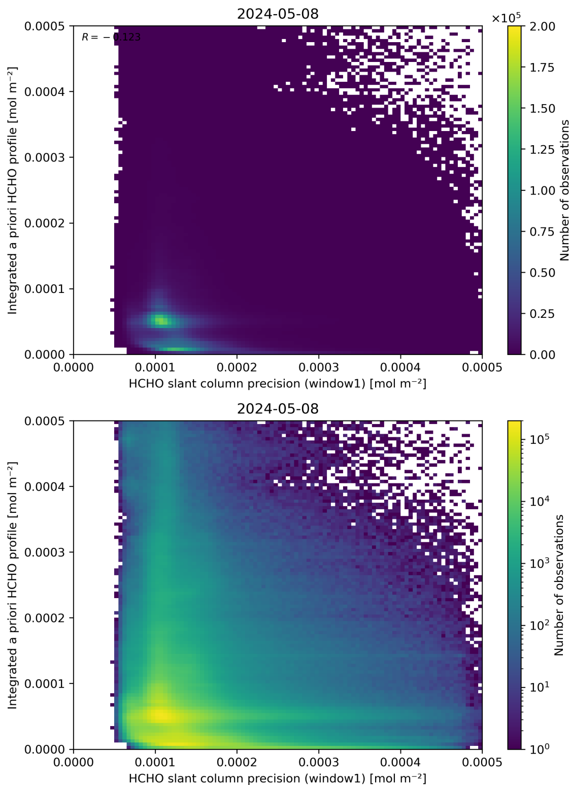
Figure 96: Scatter density plot of “HCHO slant column precision (window1)” against “Integrated a priori HCHO profile” for 2024-05-07 to 2024-05-09.
