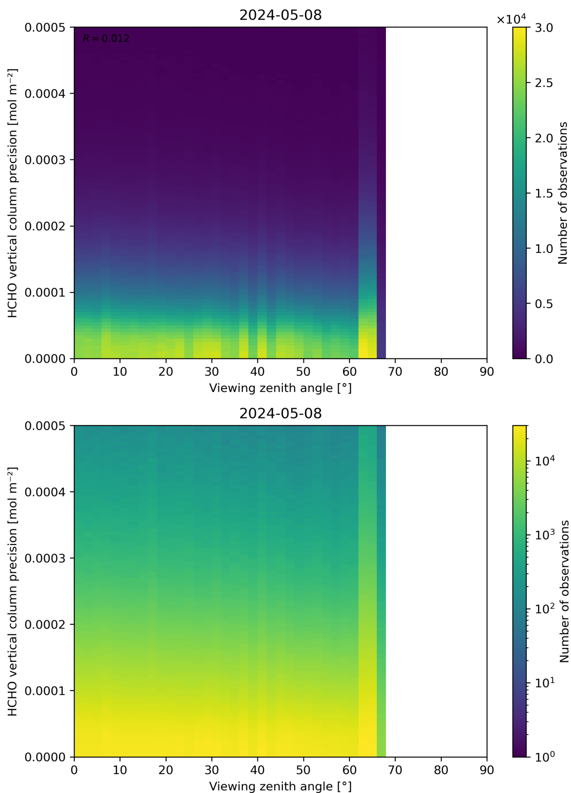
Figure 194: Scatter density plot of “Viewing zenith angle” against “HCHO vertical column precision” for 2024-05-07 to 2024-05-09.
