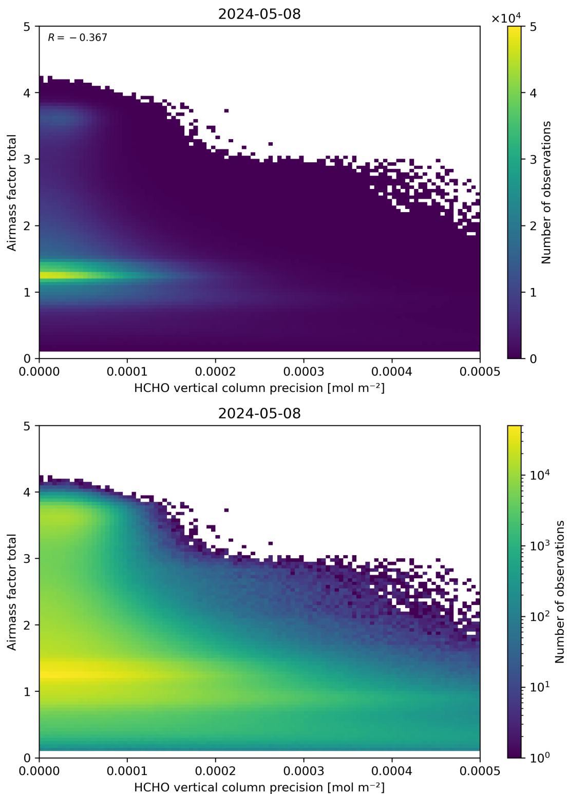
Figure 144: Scatter density plot of “HCHO vertical column precision” against “Airmass factor total” for 2024-05-07 to 2024-05-09.
