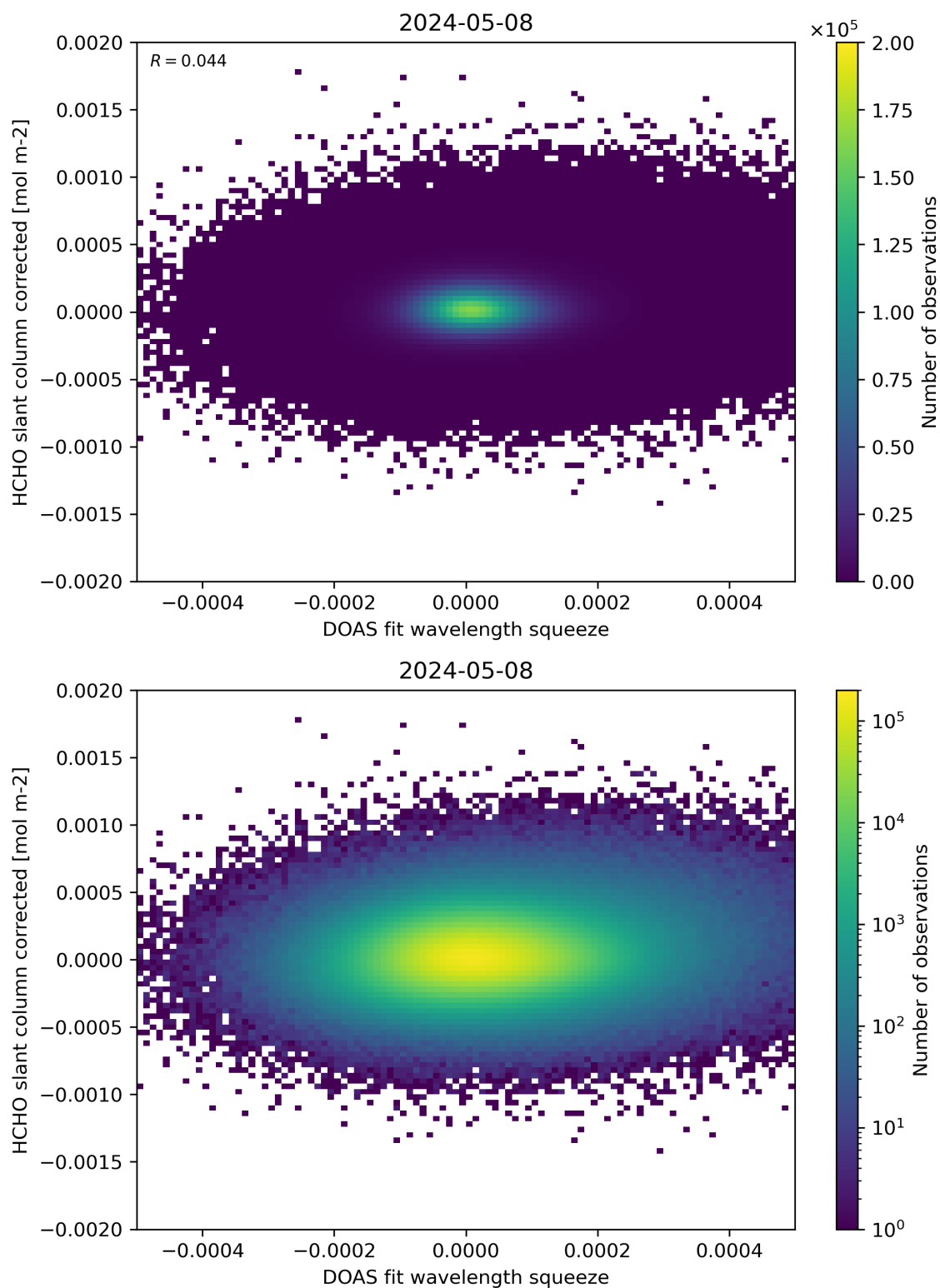
Figure 69: Scatter density plot of “DOAS fit wavelength squeeze” against “HCHO slant column corrected” for 2024-05-07 to 2024-05-09.
