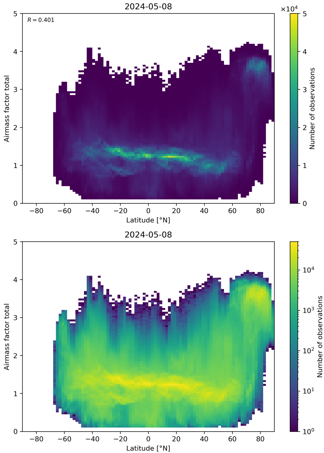
Figure 161: Scatter density plot of “Latitude” against “Airmass factor total” for 2024-05-07 to 2024-05-09.
