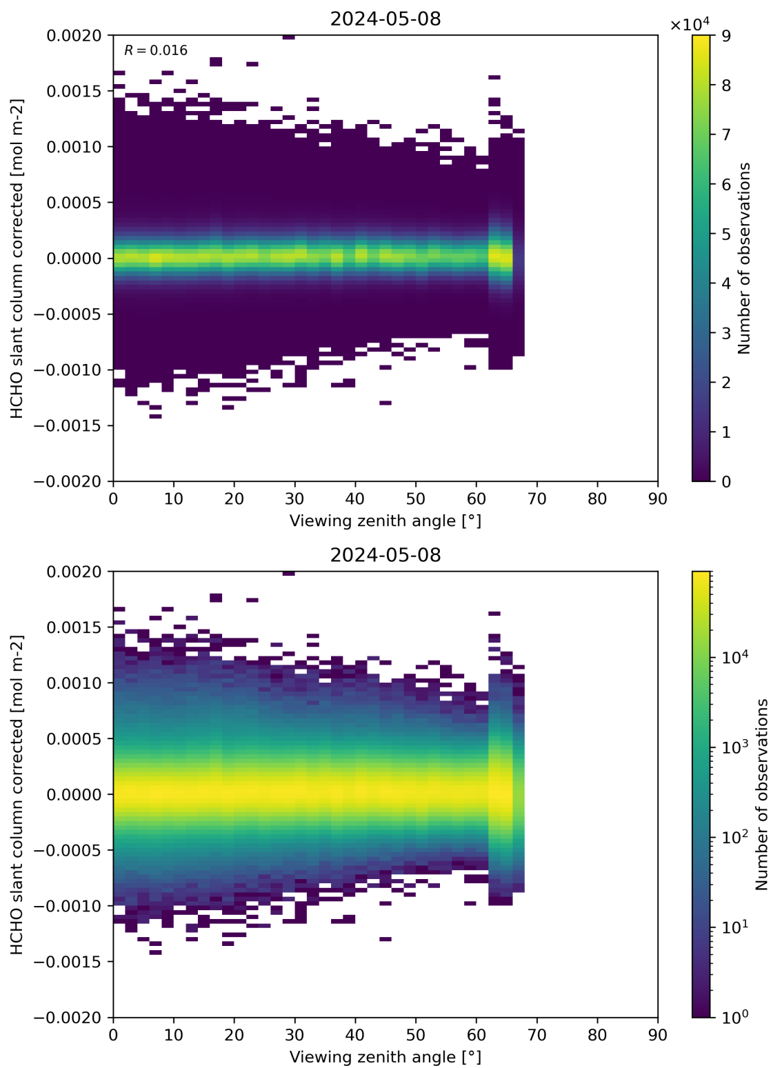
Figure 186: Scatter density plot of “Viewing zenith angle” against “HCHO slant column corrected” for 2024-05-07 to 2024-05-09.
