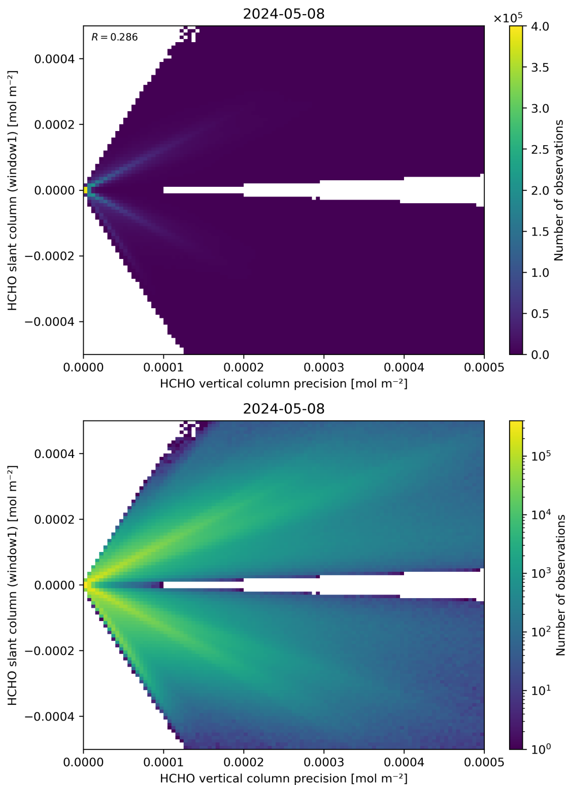
Figure 142: Scatter density plot of “HCHO vertical column precision” against “HCHO slant column (window1)” for 2024-05-07 to 2024-05-09.
