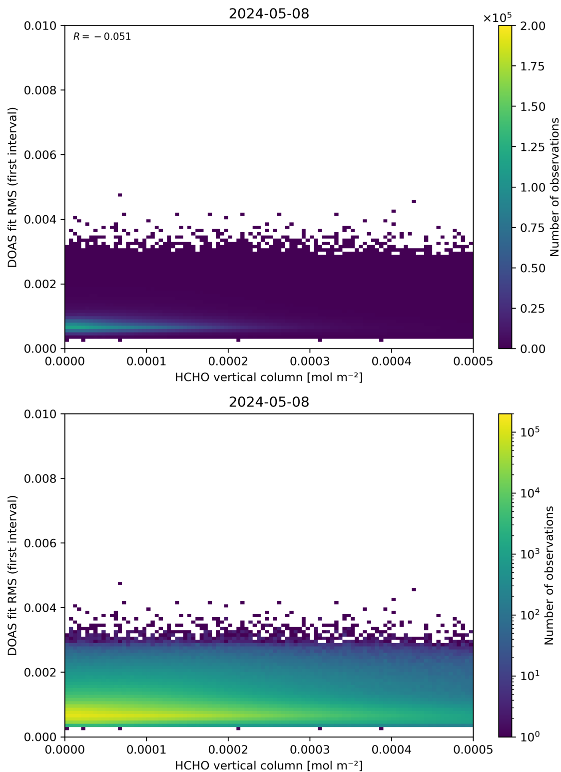
Figure 123: Scatter density plot of “HCHO vertical column” against “DOAS fit RMS (first interval)” for 2024-05-07 to 2024-05-09.
