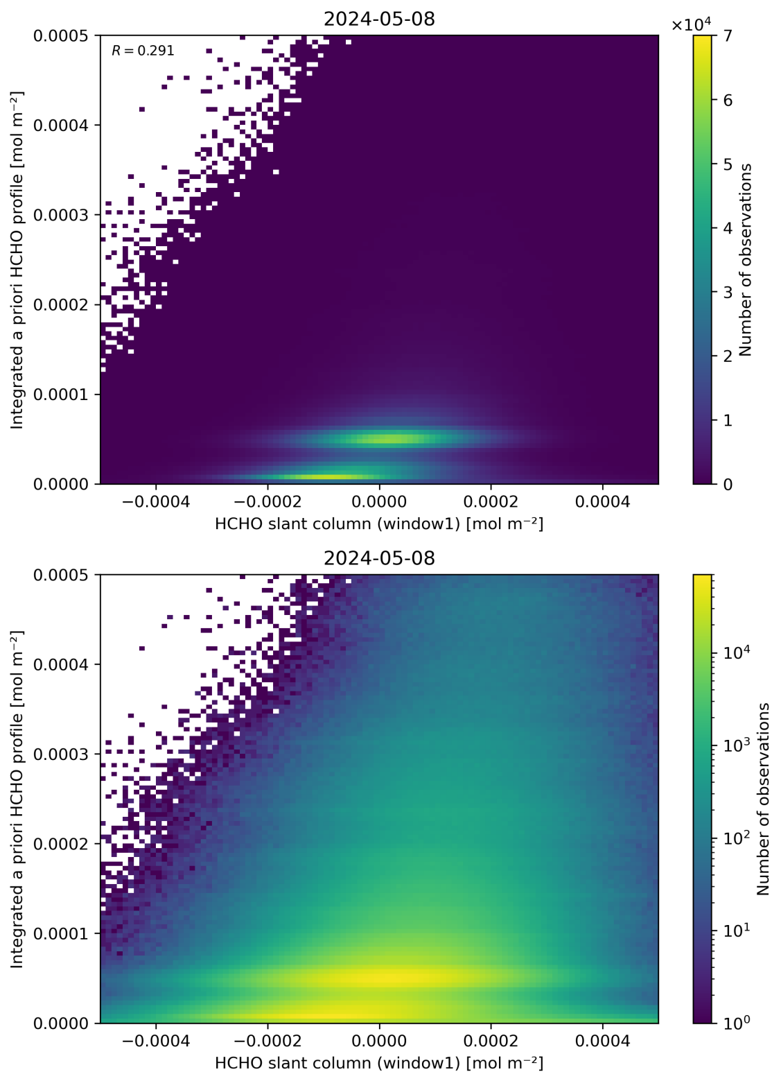
Figure 87: Scatter density plot of “HCHO slant column (window1)” against “Integrated a priori HCHO profile” for 2024-05-07 to 2024-05-09.
