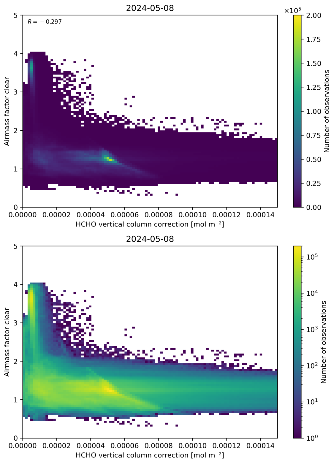
Figure 115: Scatter density plot of “HCHO vertical column correction” against “Airmass factor clear” for 2024-05-07 to 2024-05-09.
