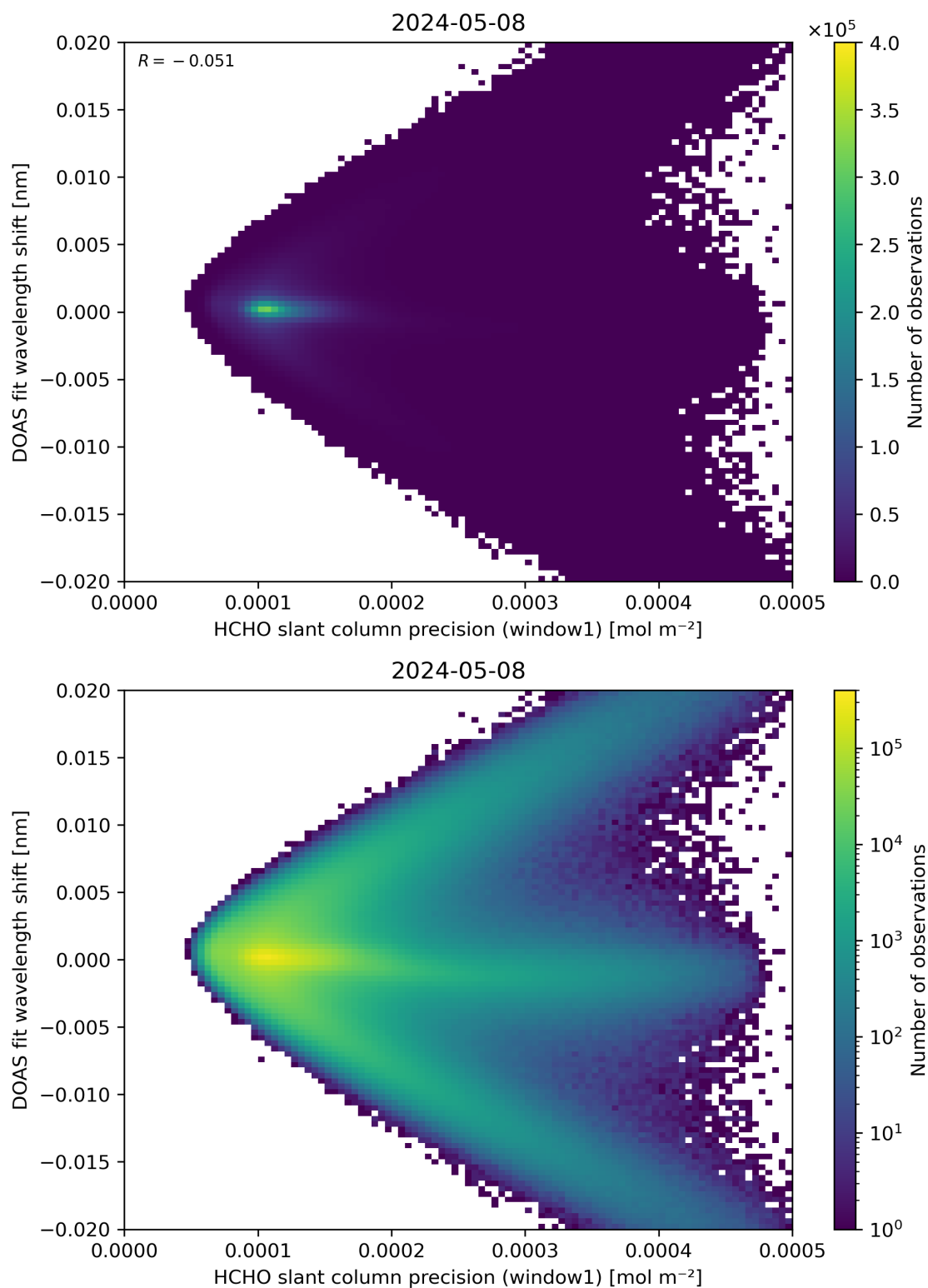
Figure 89: Scatter density plot of “HCHO slant column precision (window1)” against “DOAS fit wavelength shift” for 2024-05-07 to 2024-05-09.
