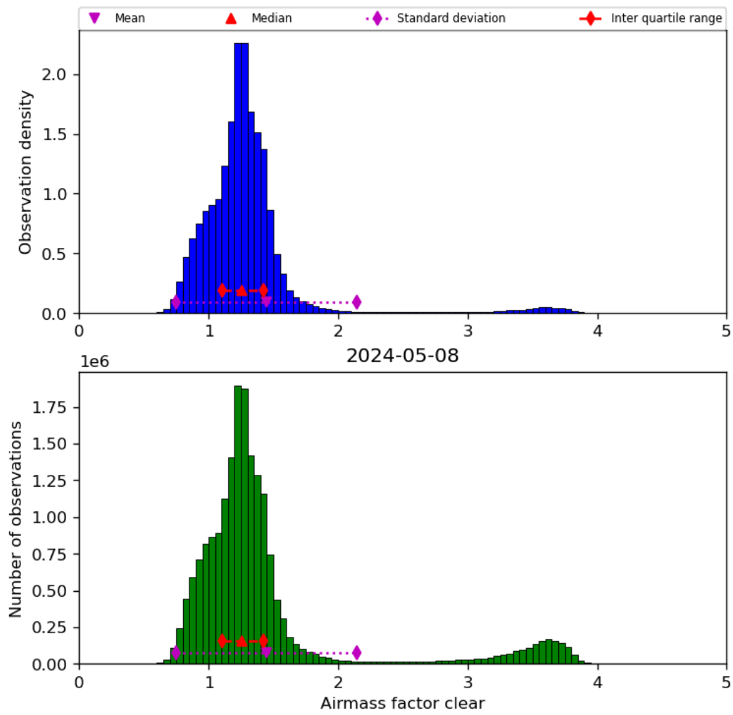
Figure 42: Histogram of “Airmass factor clear” for 2024-05-07 to 2024-05-09
