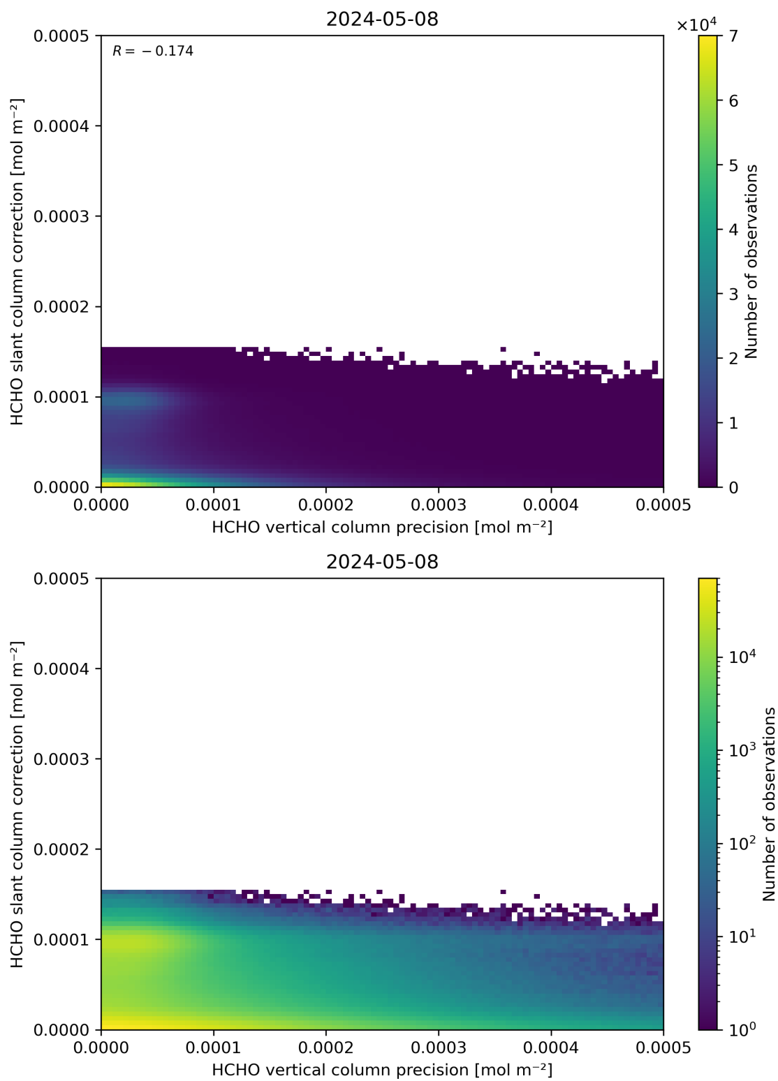
Figure 141: Scatter density plot of “HCHO vertical column precision” against “HCHO slant column correction” for 2024-05-07 to 2024-05-09.
