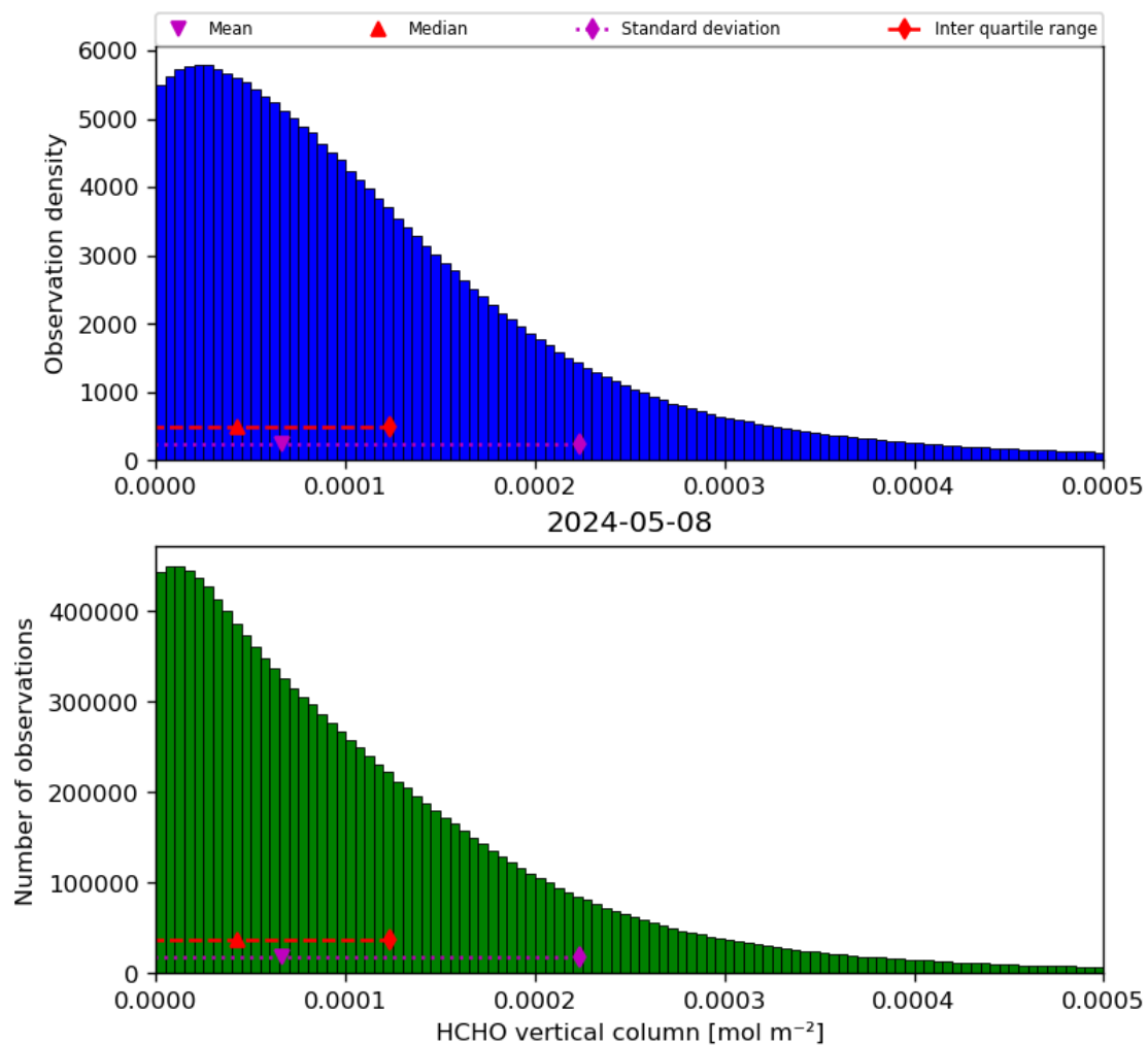
Figure 35: Histogram of “HCHO vertical column” for 2024-05-07 to 2024-05-09
