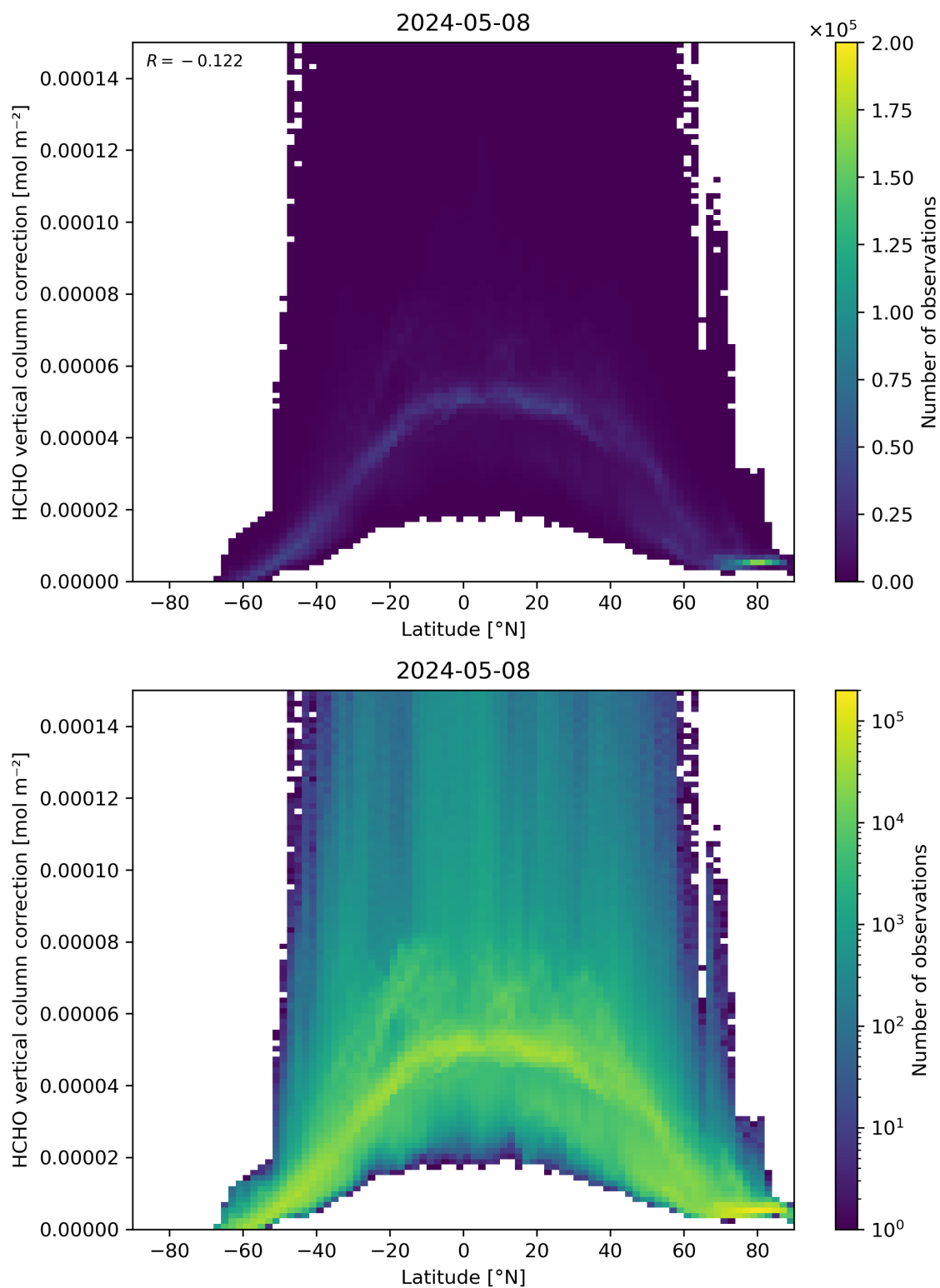
Figure 164: Scatter density plot of “Latitude” against “HCHO vertical column correction” for 2024-05-07 to 2024-05-09.
