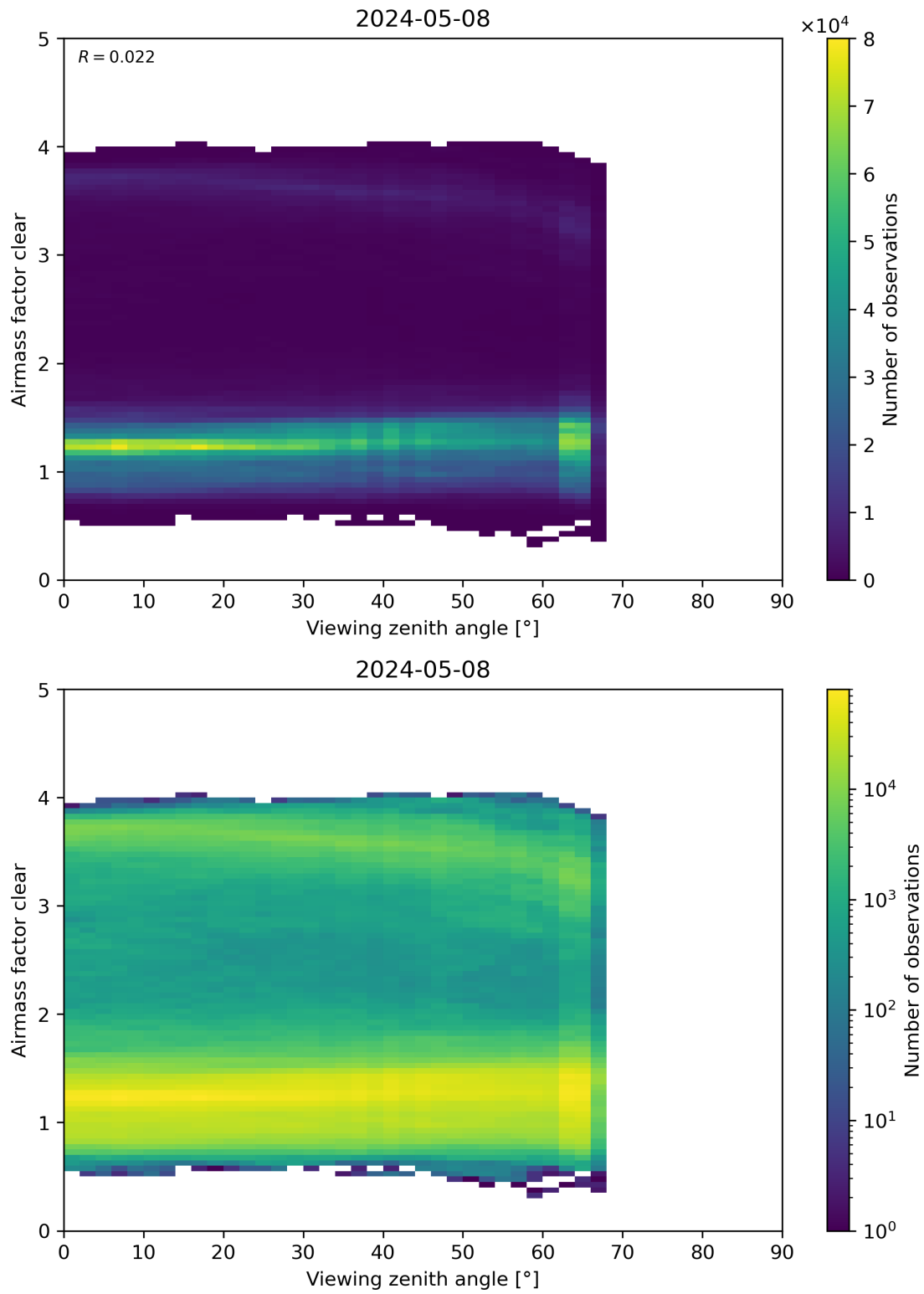
Figure 185: Scatter density plot of “Viewing zenith angle” against “Airmass factor clear” for 2024-05-07 to 2024-05-09.
