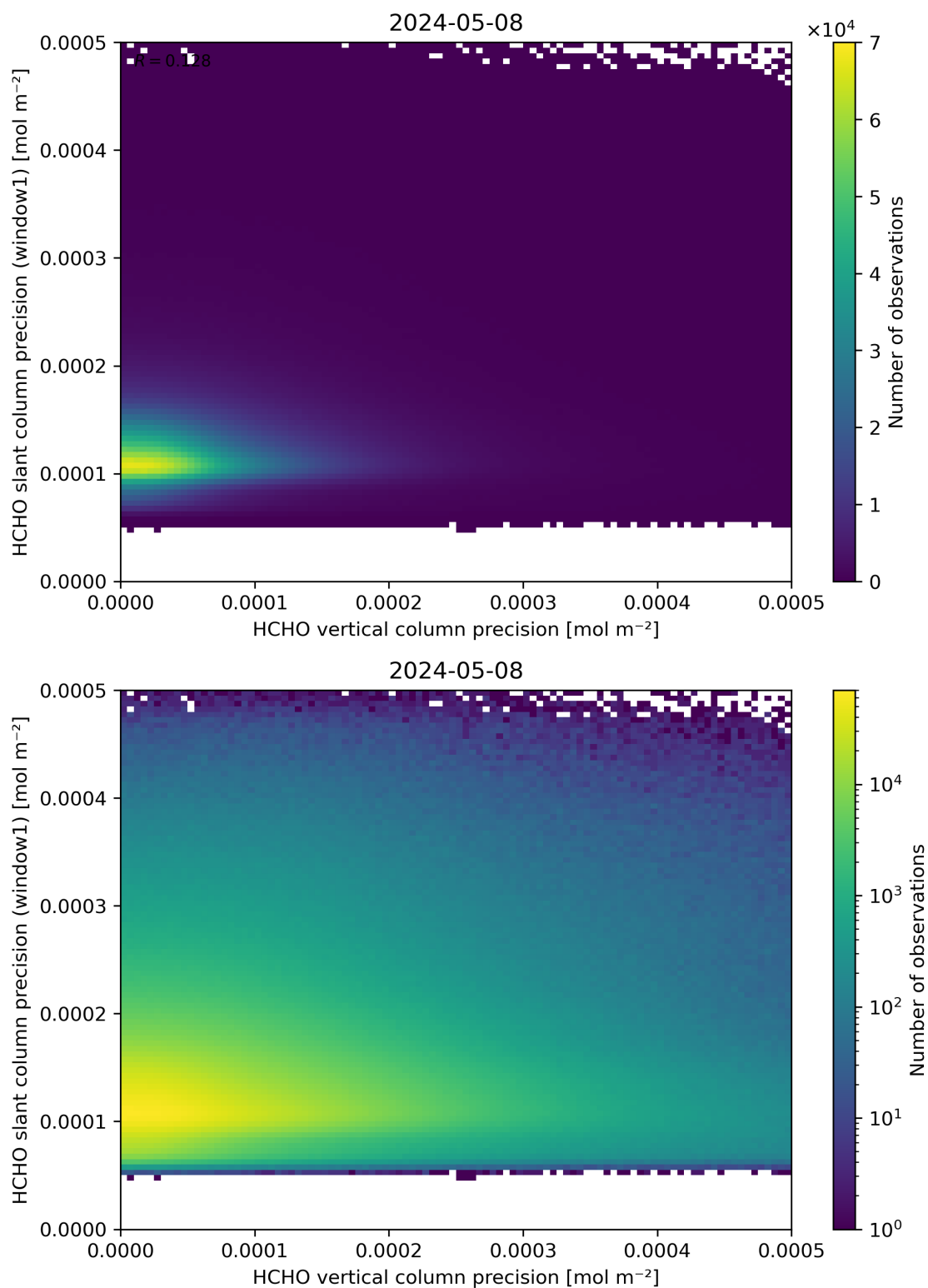
Figure 143: Scatter density plot of “HCHO vertical column precision” against “HCHO slant column precision (window1)” for 2024-05-07 to 2024-05-09.
