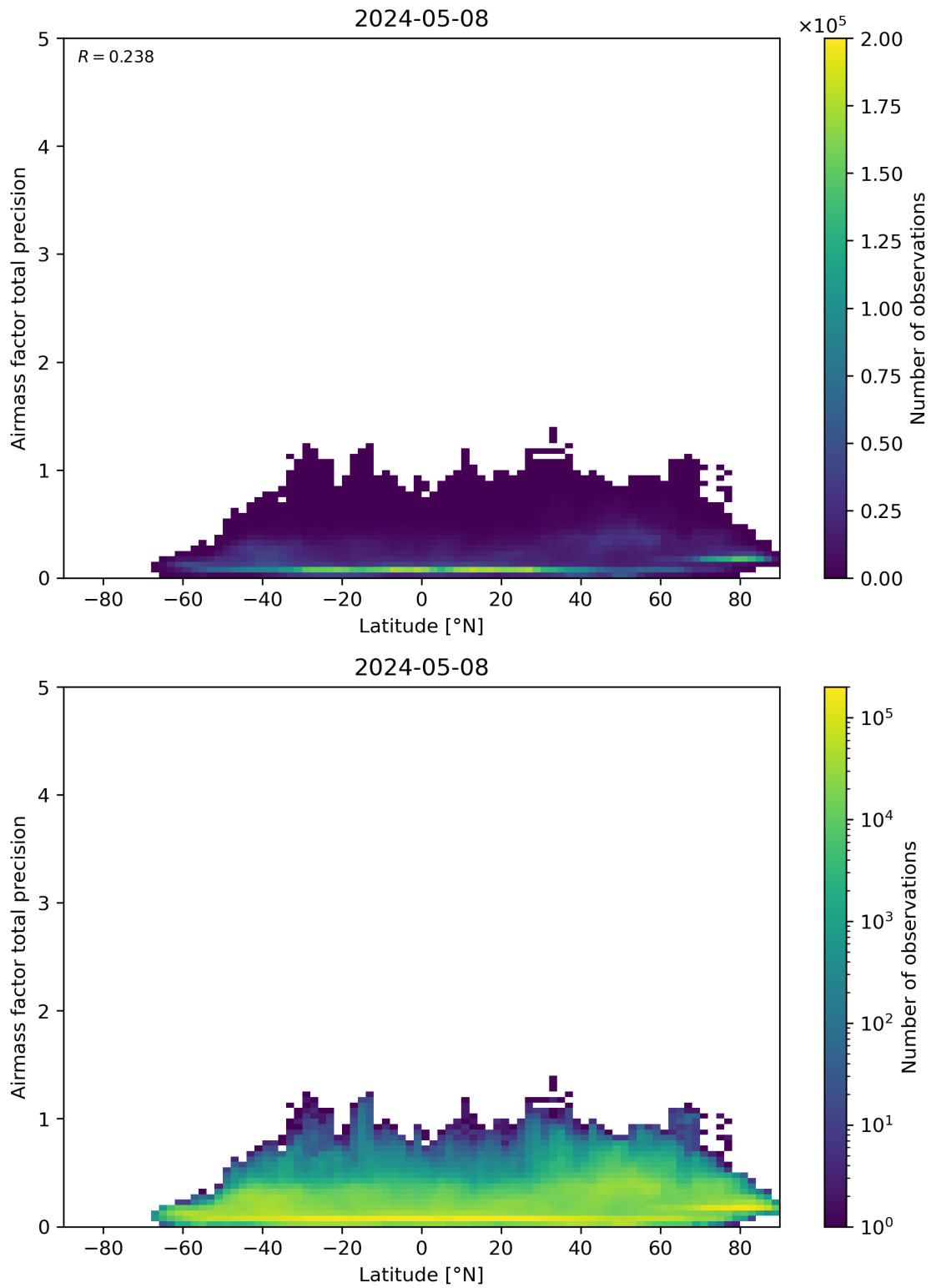
Figure 162: Scatter density plot of “Latitude” against “Airmass factor total precision” for 2024-05-07 to 2024-05-09.
