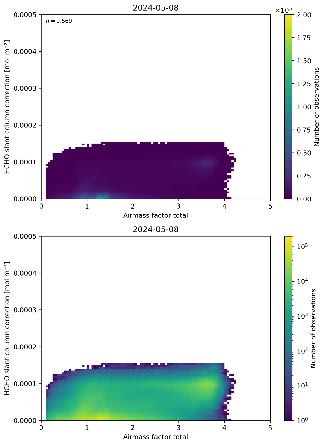
Figure 102: Scatter density plot of “Airmass factor total” against “HCHO slant column correction” for 2024-05-07 to 2024-05-09.
