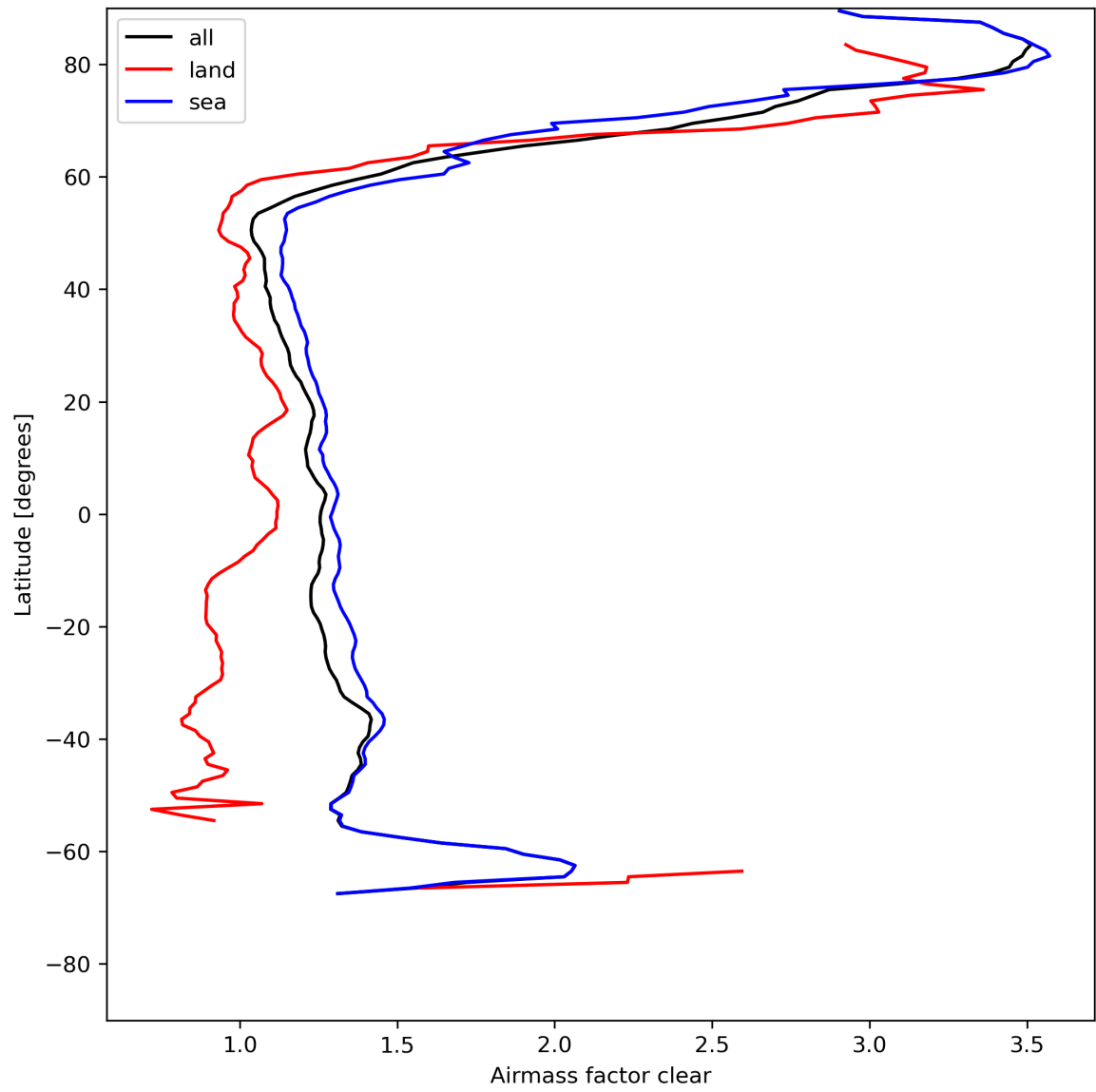
Figure 28: Zonal average of “Airmass factor clear” for 2024-05-07 to 2024-05-09.
