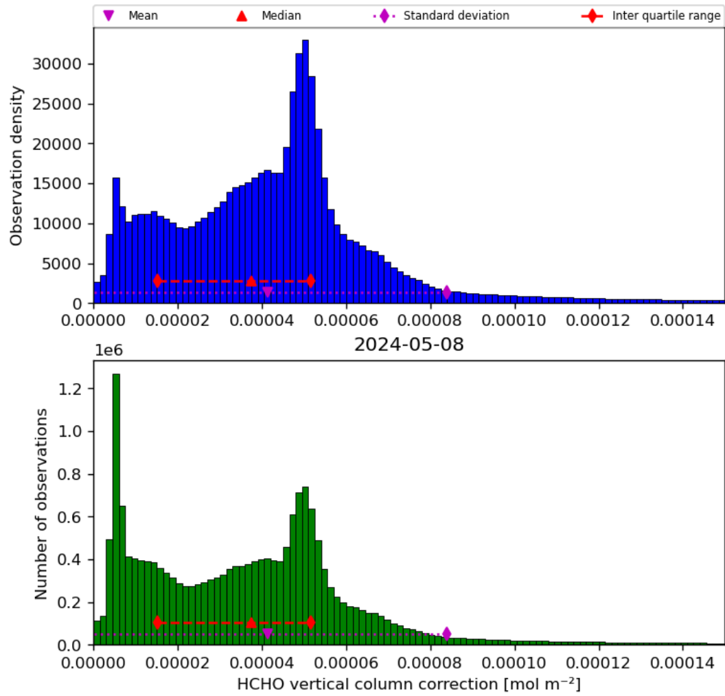
Figure 37: Histogram of “HCHO vertical column correction” for 2024-05-07 to 2024-05-09
