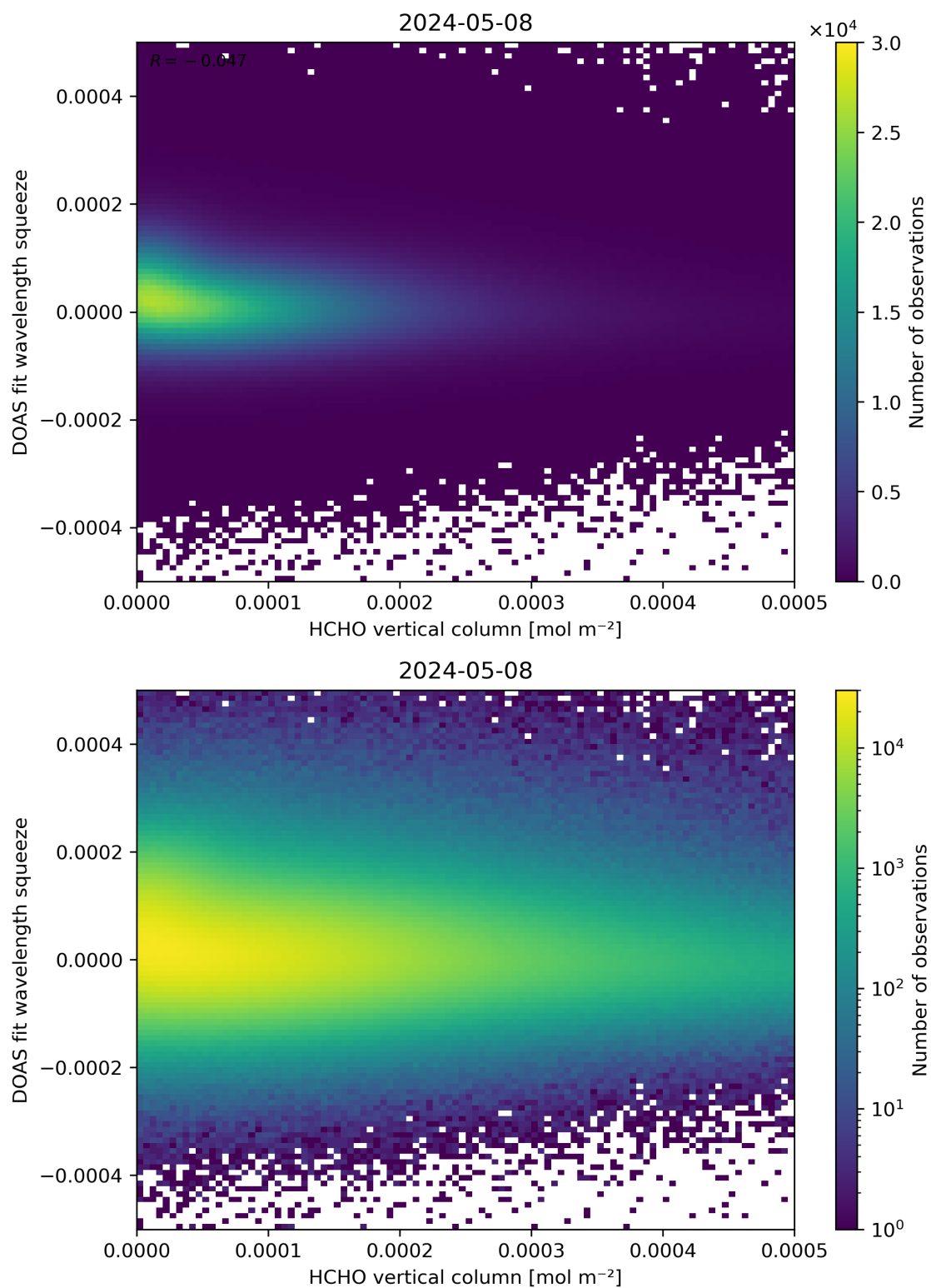
Figure 125: Scatter density plot of “HCHO vertical column” against “DOAS fit wavelength squeeze” for 2024-05-07 to 2024-05-09.
