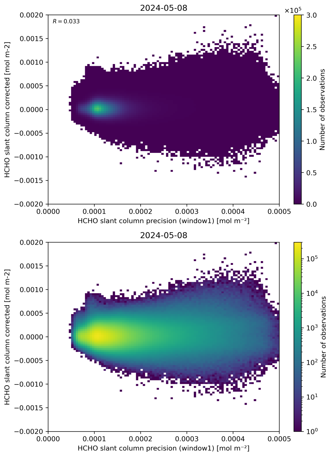
Figure 92: Scatter density plot of “HCHO slant column precision (window1)” against “HCHO slant column corrected” for 2024-05-07 to 2024-05-09.
