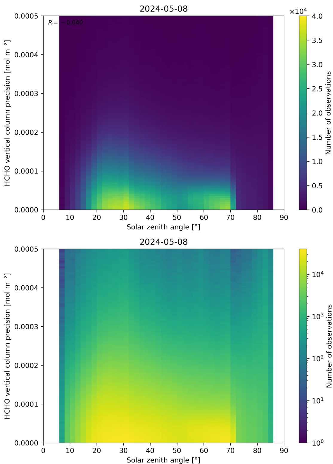
Figure 179: Scatter density plot of “Solar zenith angle” against “HCHO vertical column precision” for 2024-05-07 to 2024-05-09.
