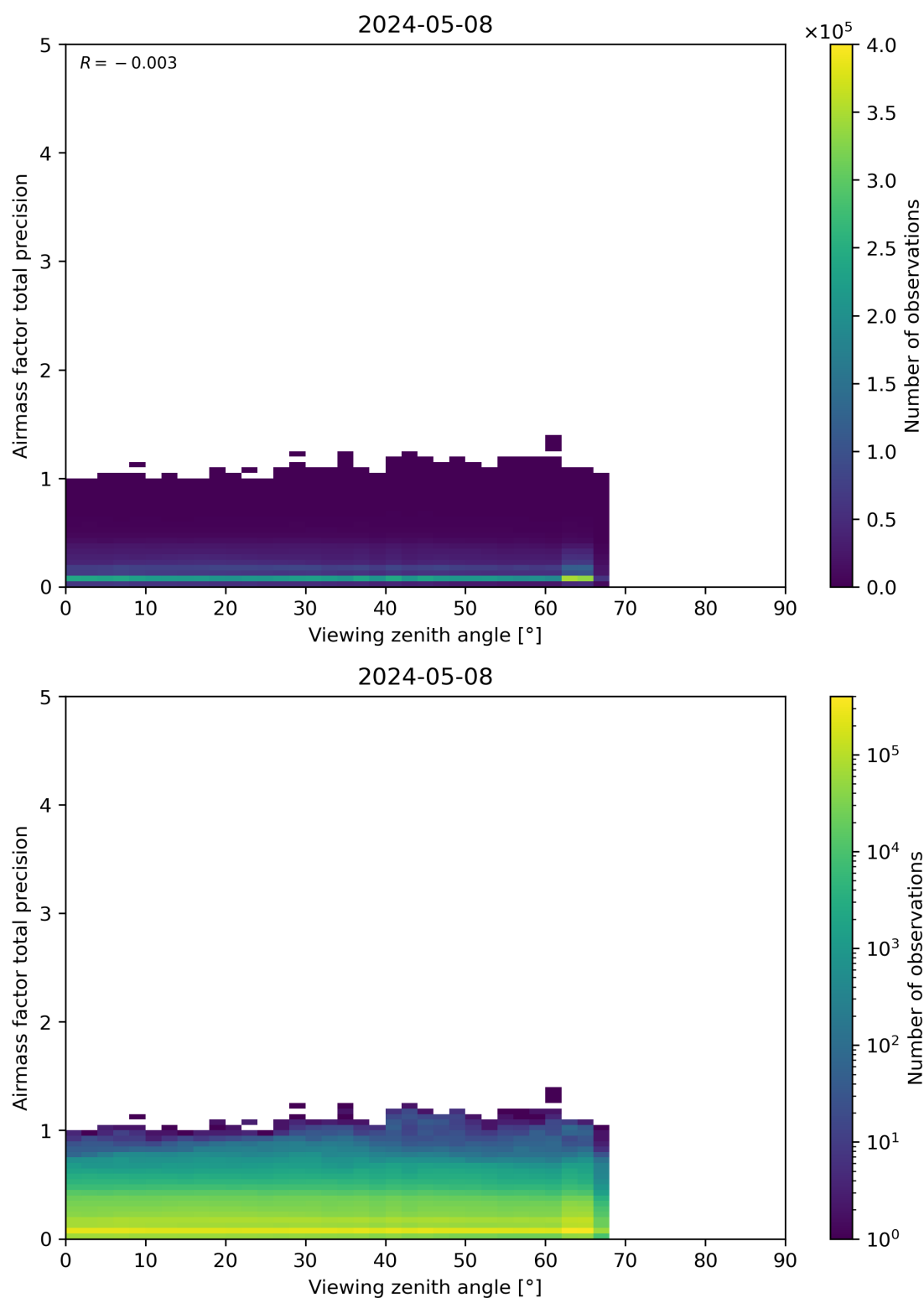
Figure 191: Scatter density plot of “Viewing zenith angle” against “Airmass factor total precision” for 2024-05-07 to 2024-05-09.
