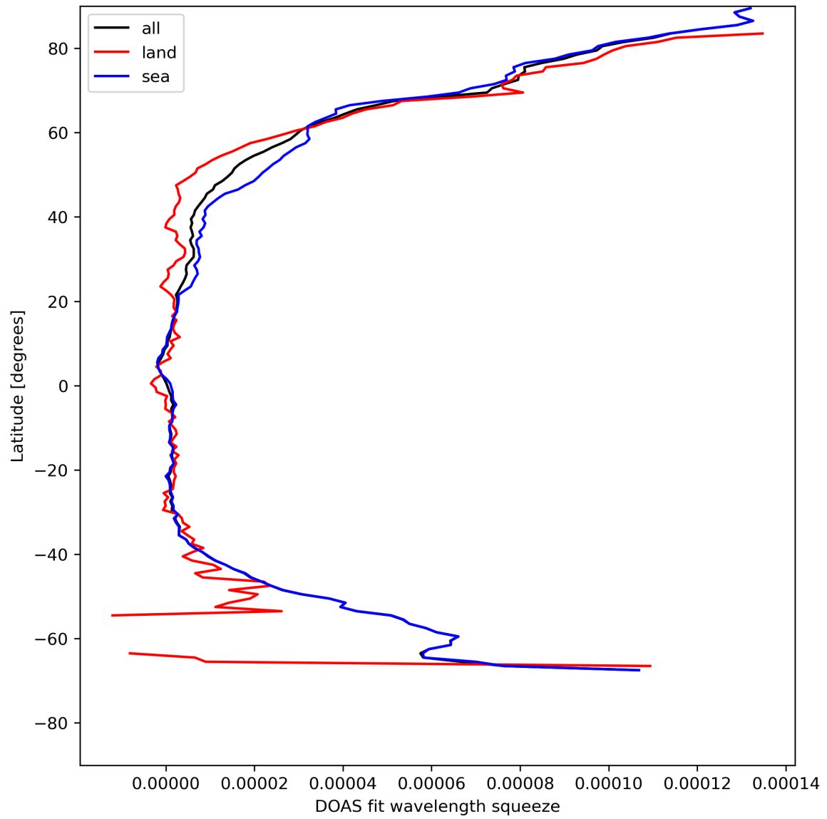
Figure 31: Zonal average of “DOAS fit wavelength squeeze” for 2024-05-07 to 2024-05-09.
