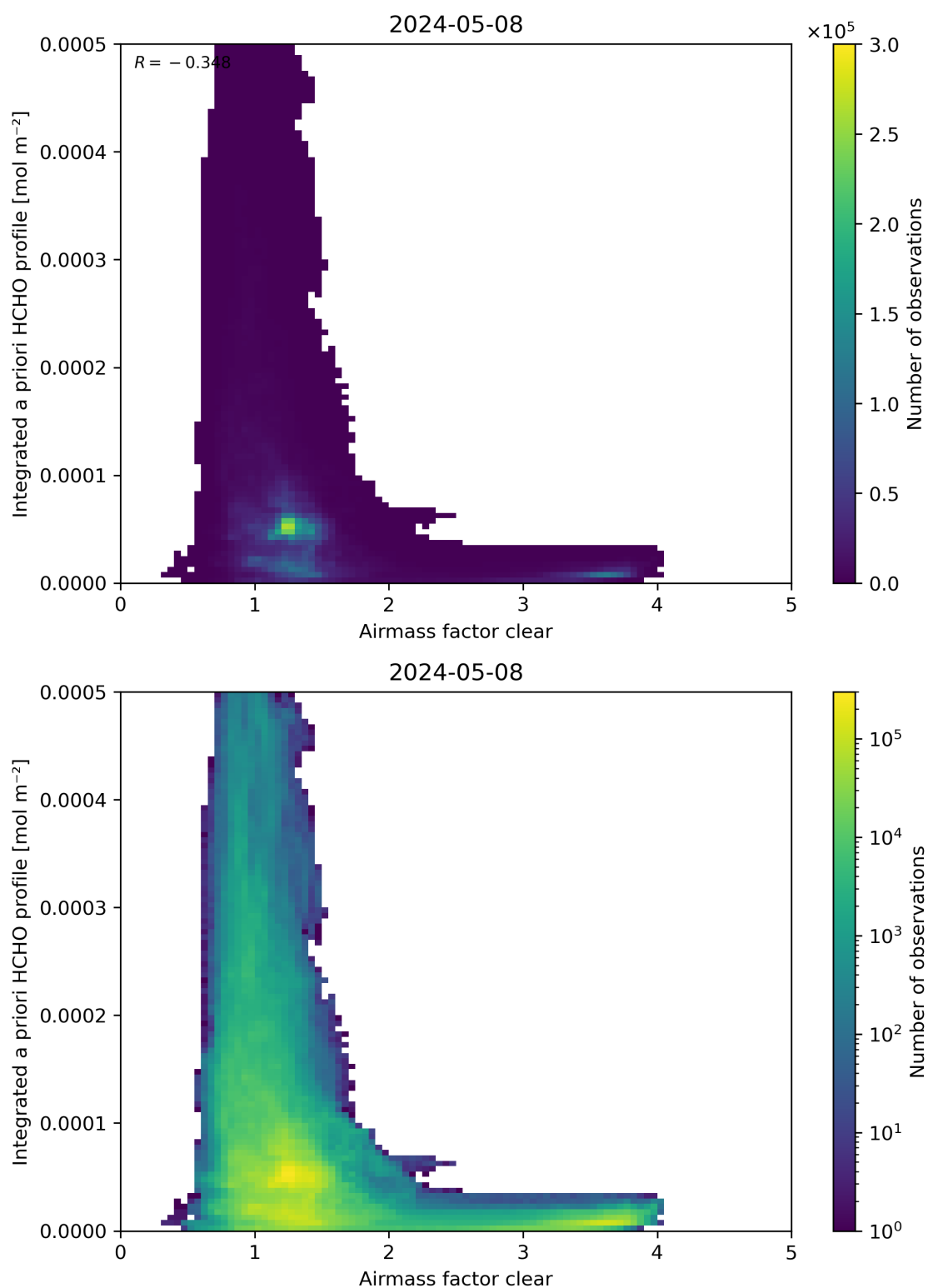
Figure 76: Scatter density plot of “Airmass factor clear” against “Integrated a priori HCHO profile” for 2024-05-07 to 2024-05-09.
