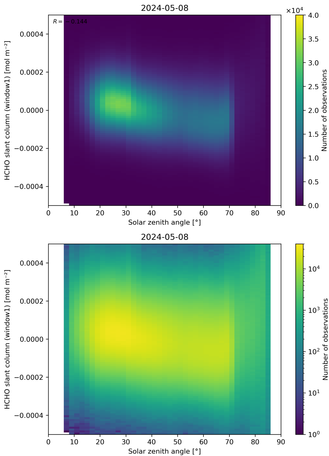
Figure 173: Scatter density plot of “Solar zenith angle” against “HCHO slant column (window1)” for 2024-05-07 to 2024-05-09.
