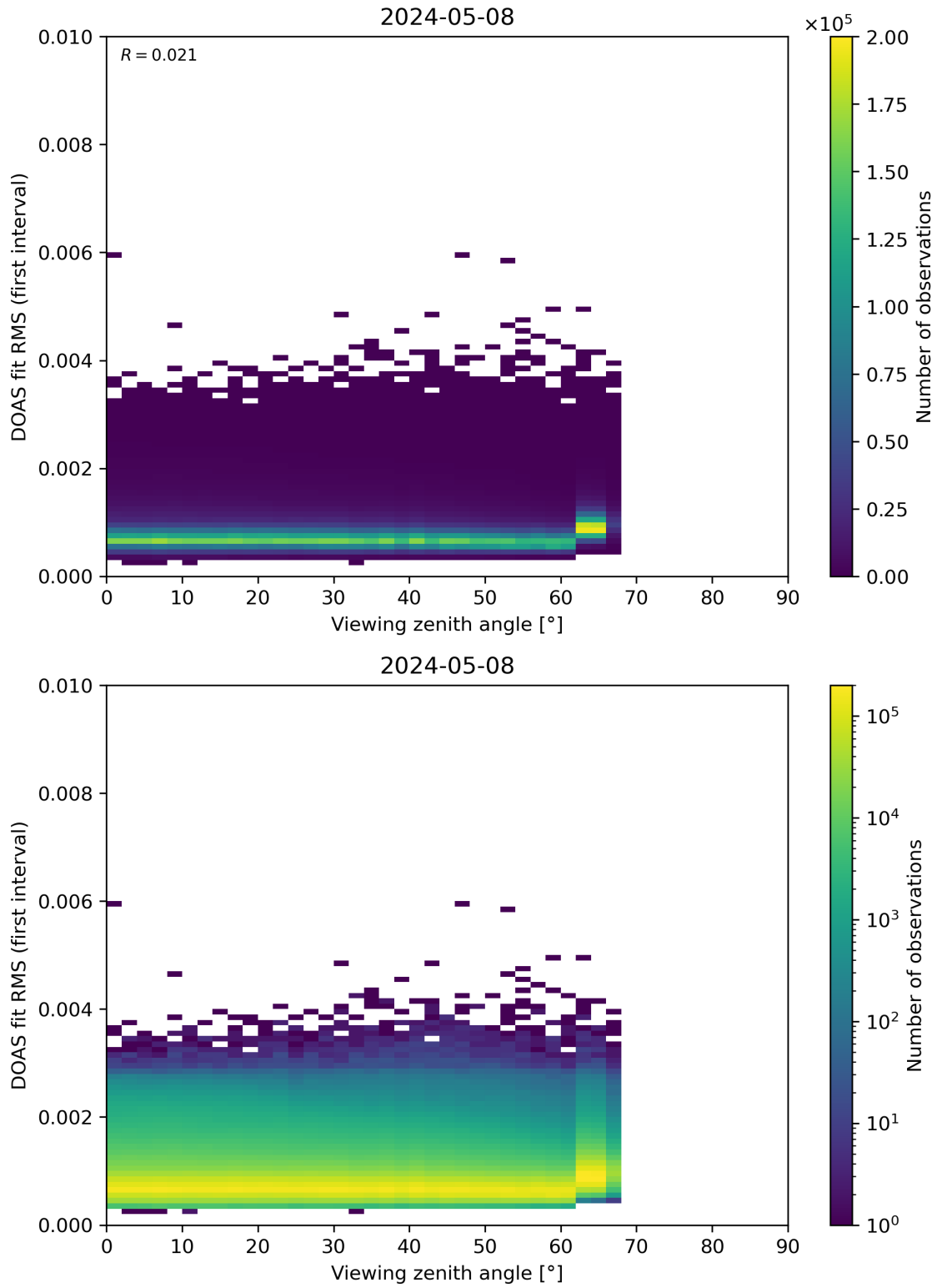
Figure 182: Scatter density plot of “Viewing zenith angle” against “DOAS fit RMS (first interval)” for 2024-05-07 to 2024-05-09.
