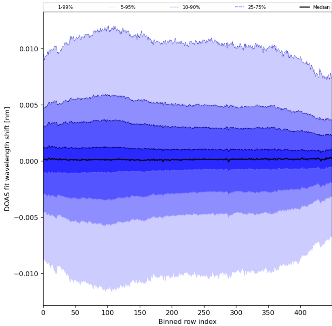
Figure 58: Along track statistics of “DOAS fit wavelength shift” for 2024-05-07 to 2024-05-09
