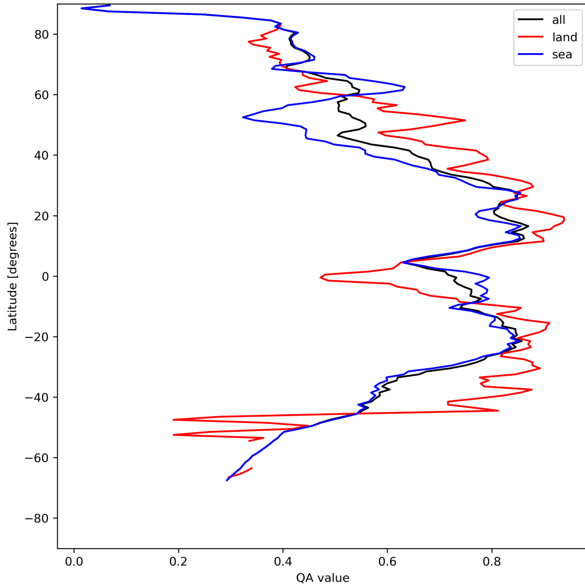
Figure 20: Zonal average of “QA value” for 2024-05-07 to 2024-05-09.
