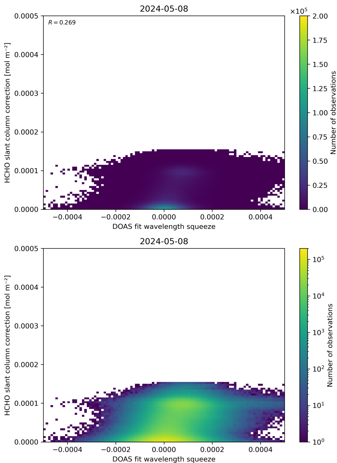
Figure 70: Scatter density plot of “DOAS fit wavelength squeeze” against “HCHO slant column correction” for 2024-05-07 to 2024-05-09.
