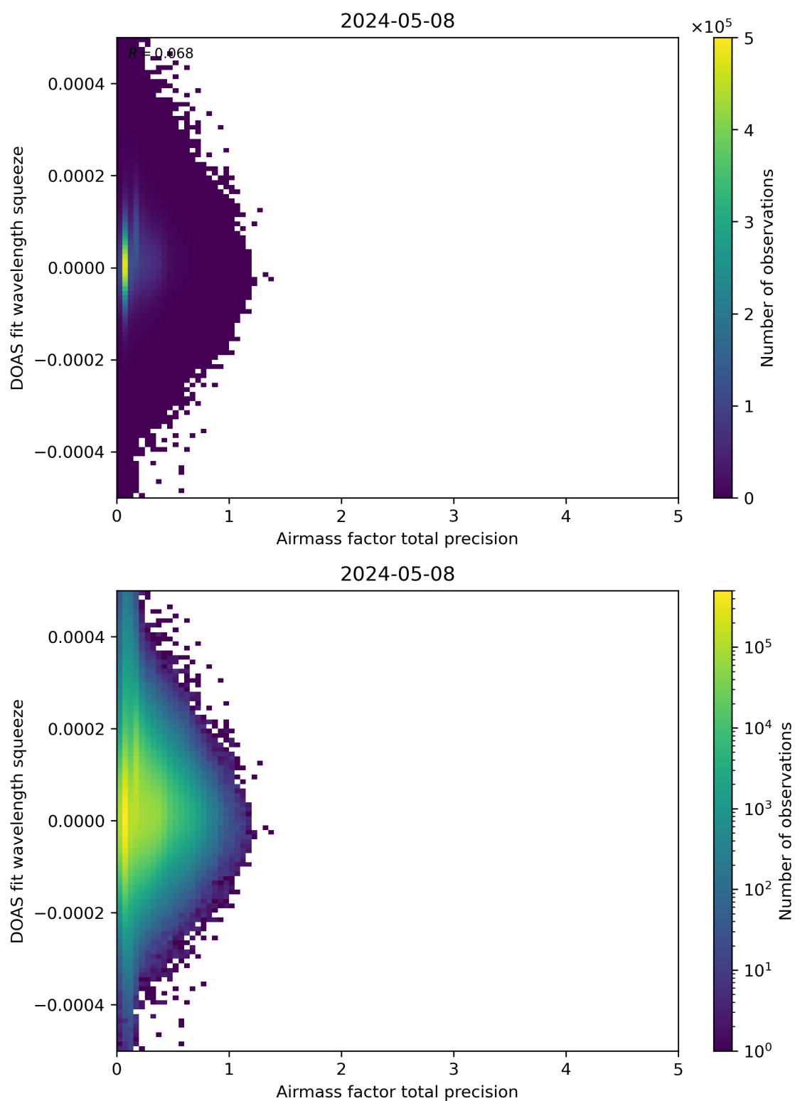
Figure 107: Scatter density plot of “Airmass factor total precision” against “DOAS fit wavelength squeeze” for 2024-05-07 to 2024-05-09.
