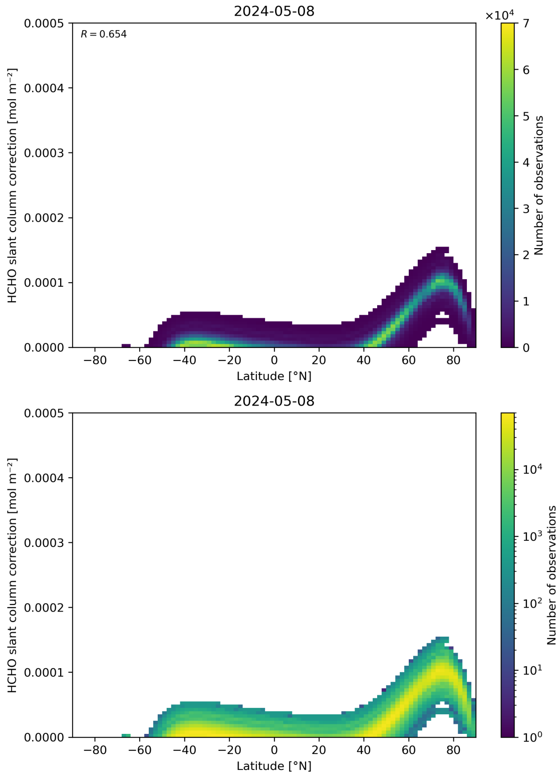
Figure 158: Scatter density plot of “Latitude” against “HCHO slant column correction” for 2024-05-07 to 2024-05-09.
