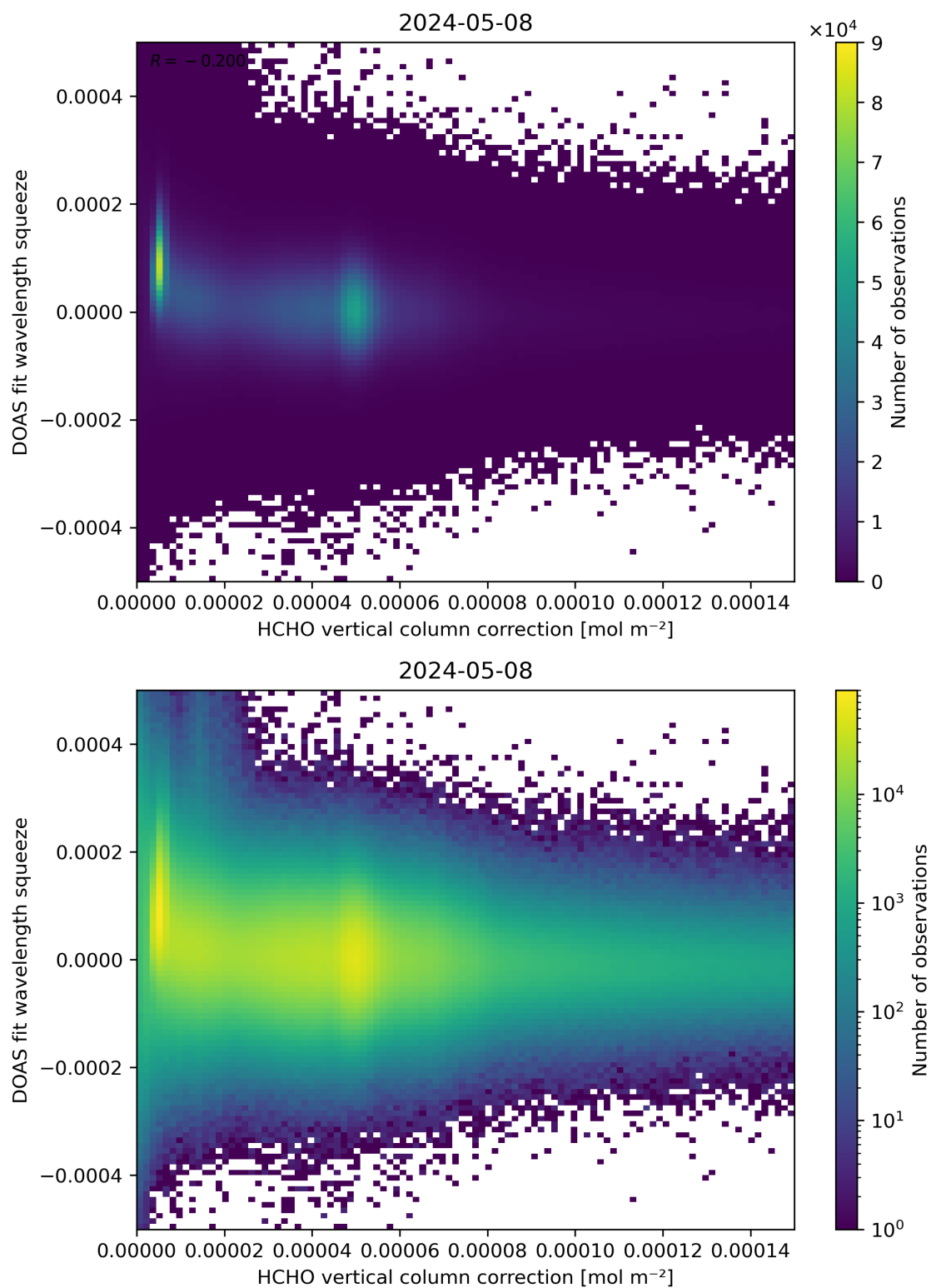
Figure 114: Scatter density plot of “HCHO vertical column correction” against “DOAS fit wavelength squeeze” for 2024-05-07 to 2024-05-09.
