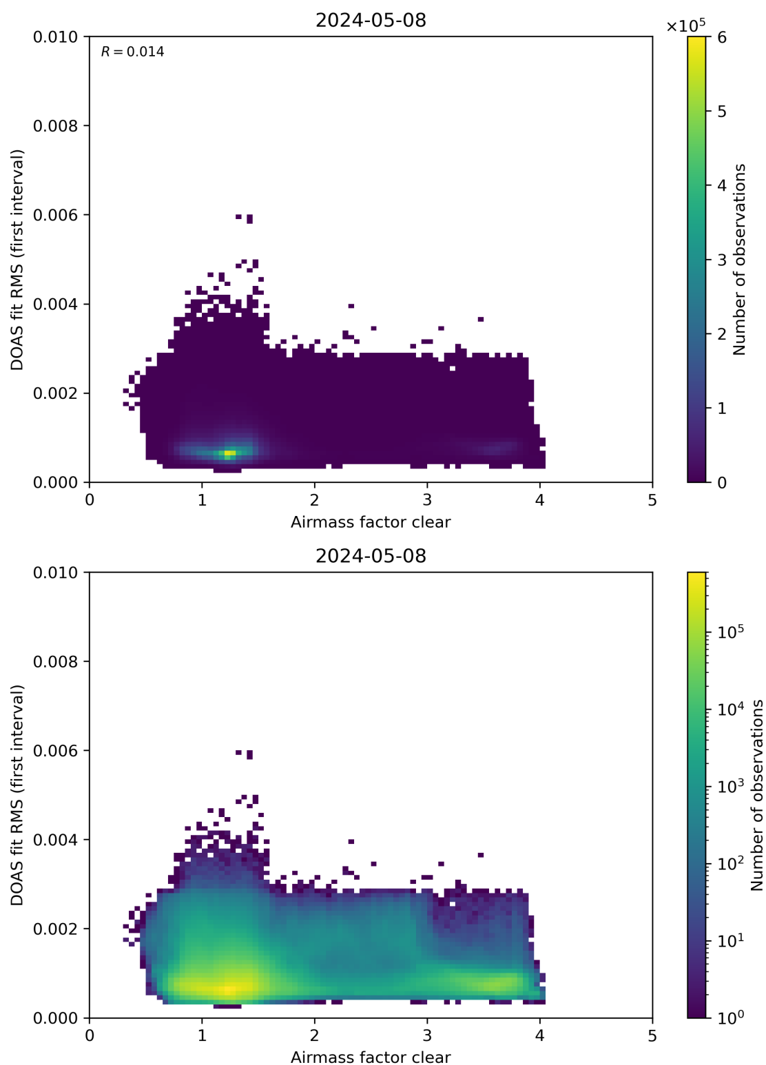
Figure 71: Scatter density plot of “Airmass factor clear” against “DOAS fit RMS (first interval)” for 2024-05-07 to 2024-05-09.
