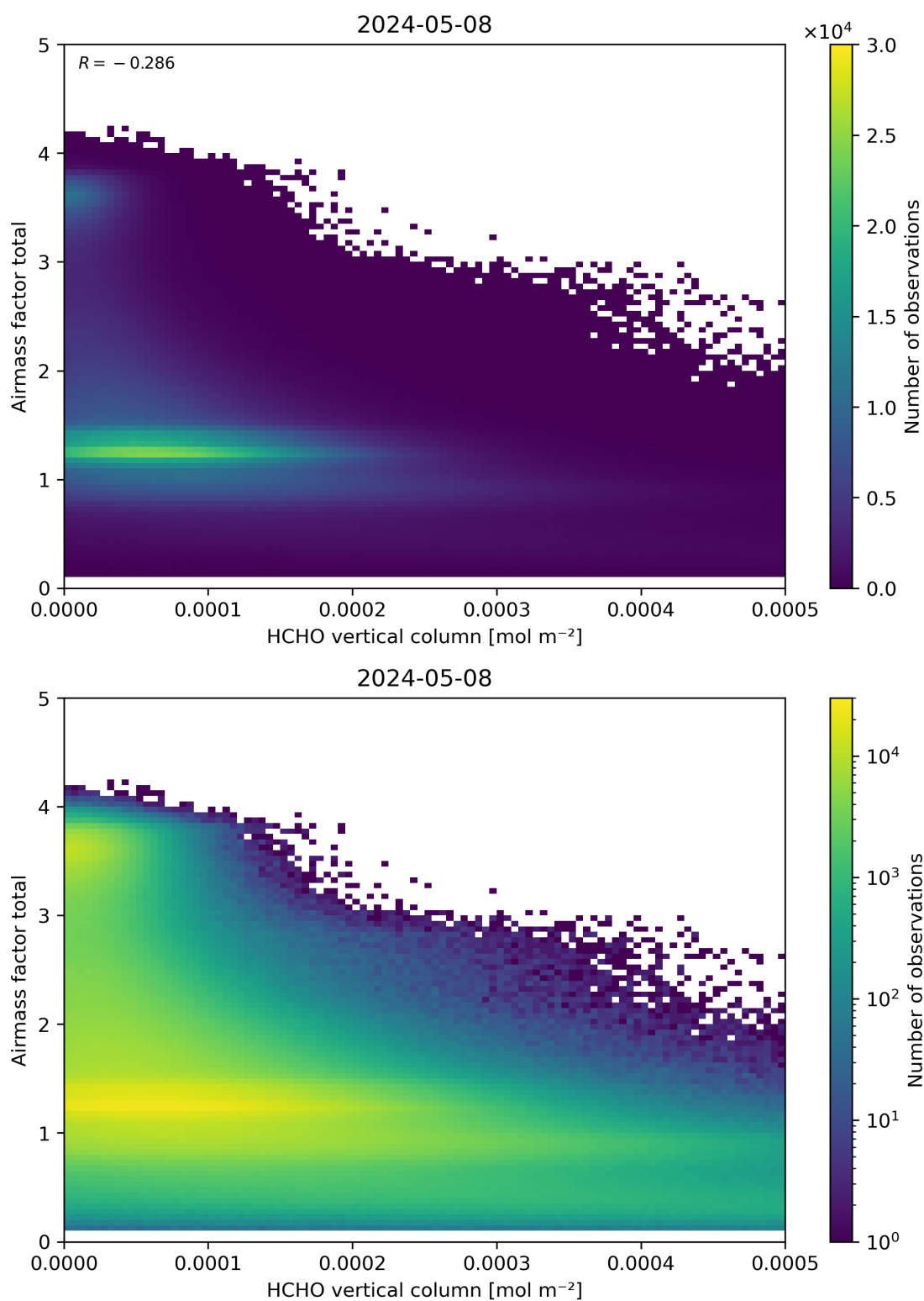
Figure 131: Scatter density plot of “HCHO vertical column” against “Airmass factor total” for 2024-05-07 to 2024-05-09.
