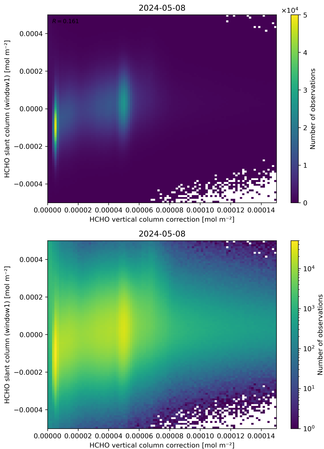
Figure 118: Scatter density plot of “HCHO vertical column correction” against “HCHO slant column (window1)” for 2024-05-07 to 2024-05-09.
