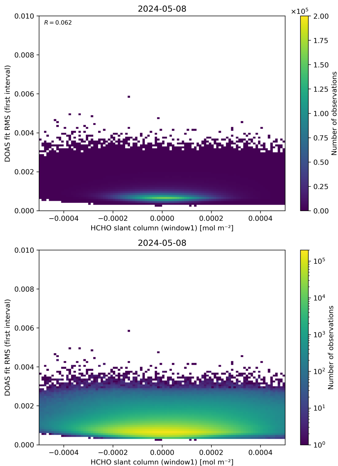
Figure 78: Scatter density plot of “HCHO slant column (window1)” against “DOAS fit RMS (first interval)” for 2024-05-07 to 2024-05-09.
