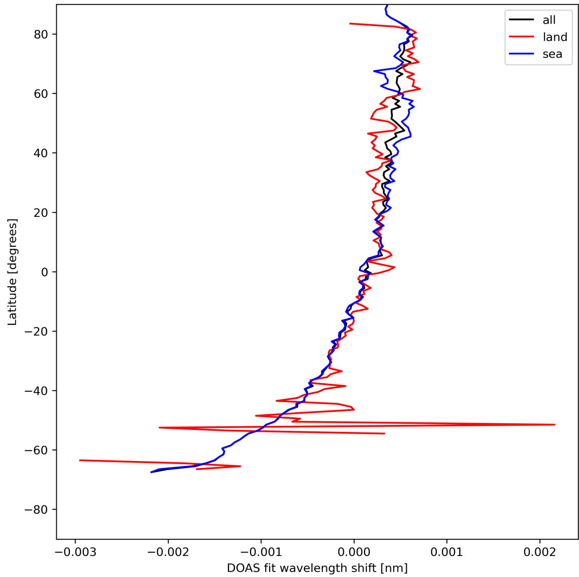
Figure 30: Zonal average of “DOAS fit wavelength shift” for 2024-05-07 to 2024-05-09.
