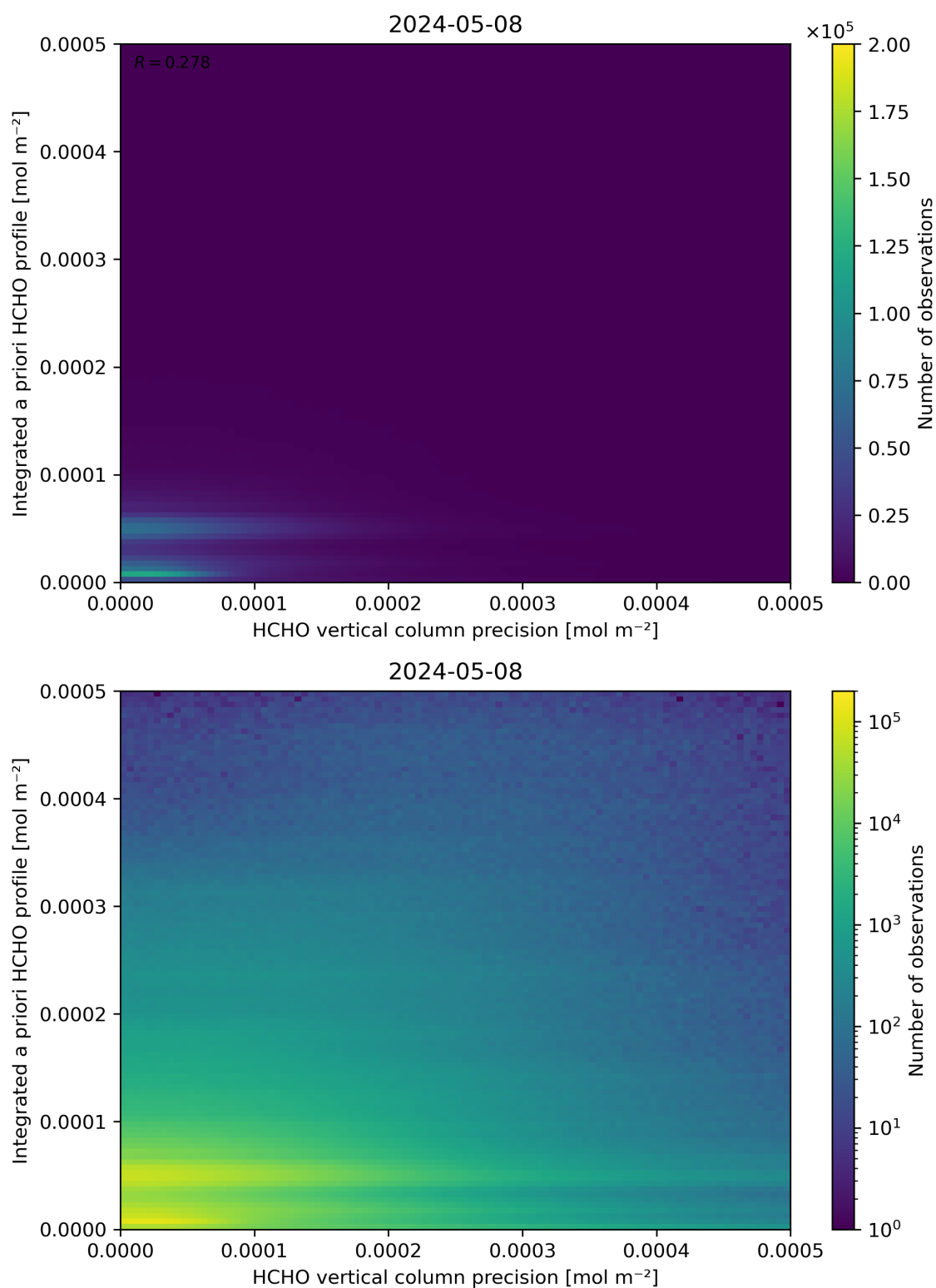
Figure 147: Scatter density plot of “HCHO vertical column precision” against “Integrated a priori HCHO profile” for 2024-05-07 to 2024-05-09.
