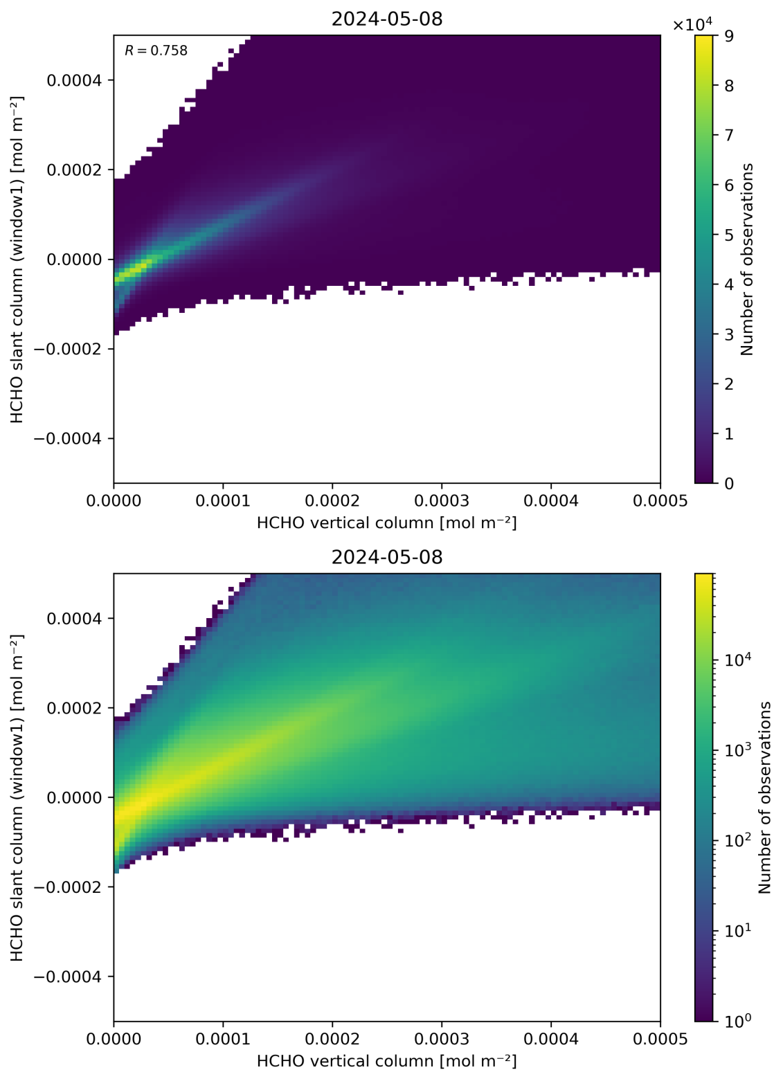
Figure 129: Scatter density plot of “HCHO vertical column” against “HCHO slant column (window1)” for 2024-05-07 to 2024-05-09.
