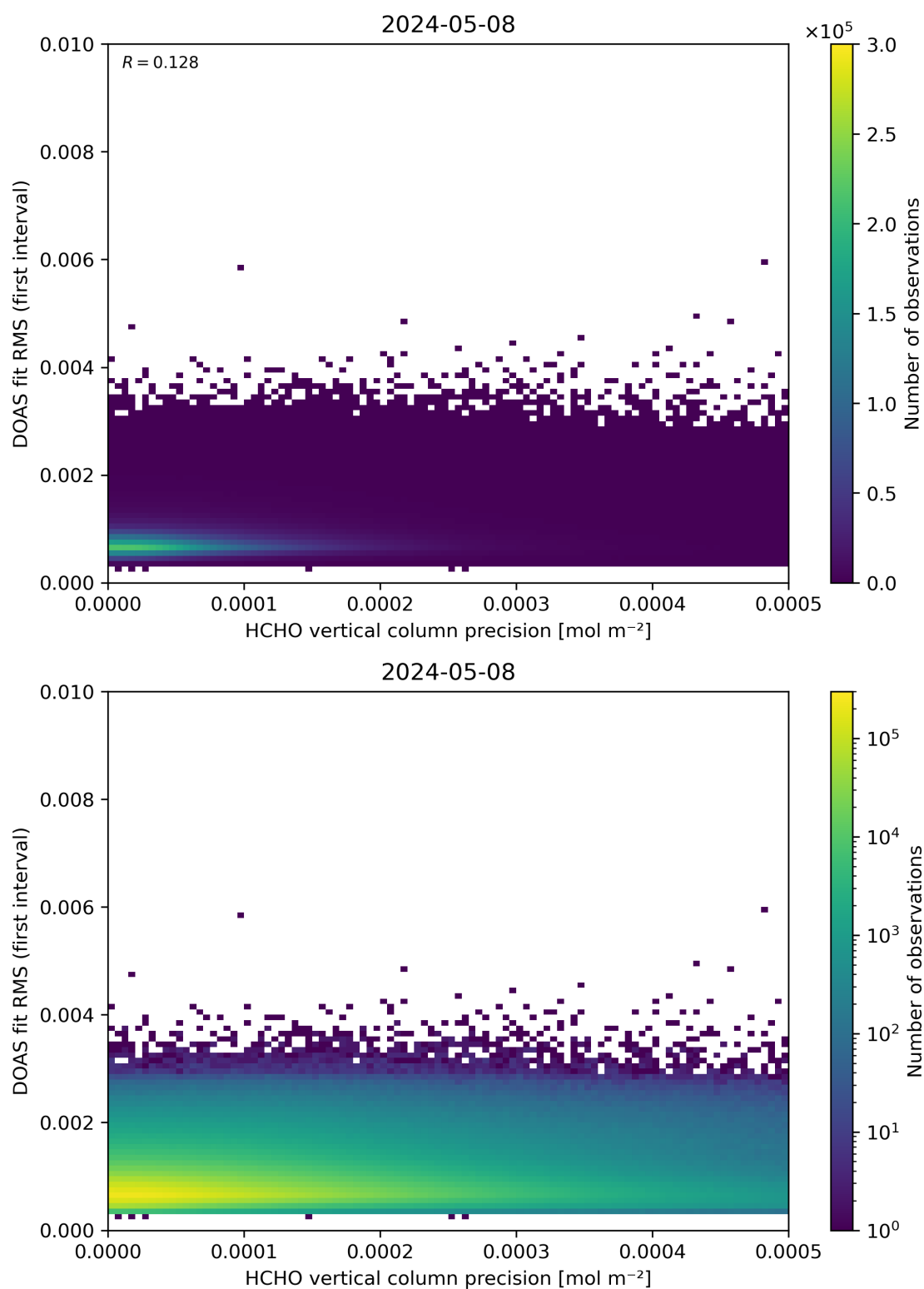
Figure 136: Scatter density plot of “HCHO vertical column precision” against “DOAS fit RMS (first interval)” for 2024-05-07 to 2024-05-09.
