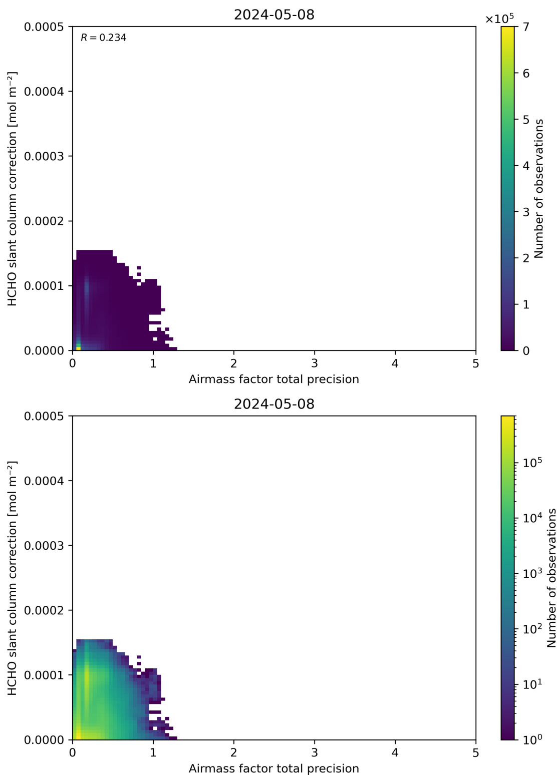
Figure 110: Scatter density plot of “Airmass factor total precision” against “HCHO slant column correction” for 2024-05-07 to 2024-05-09.
