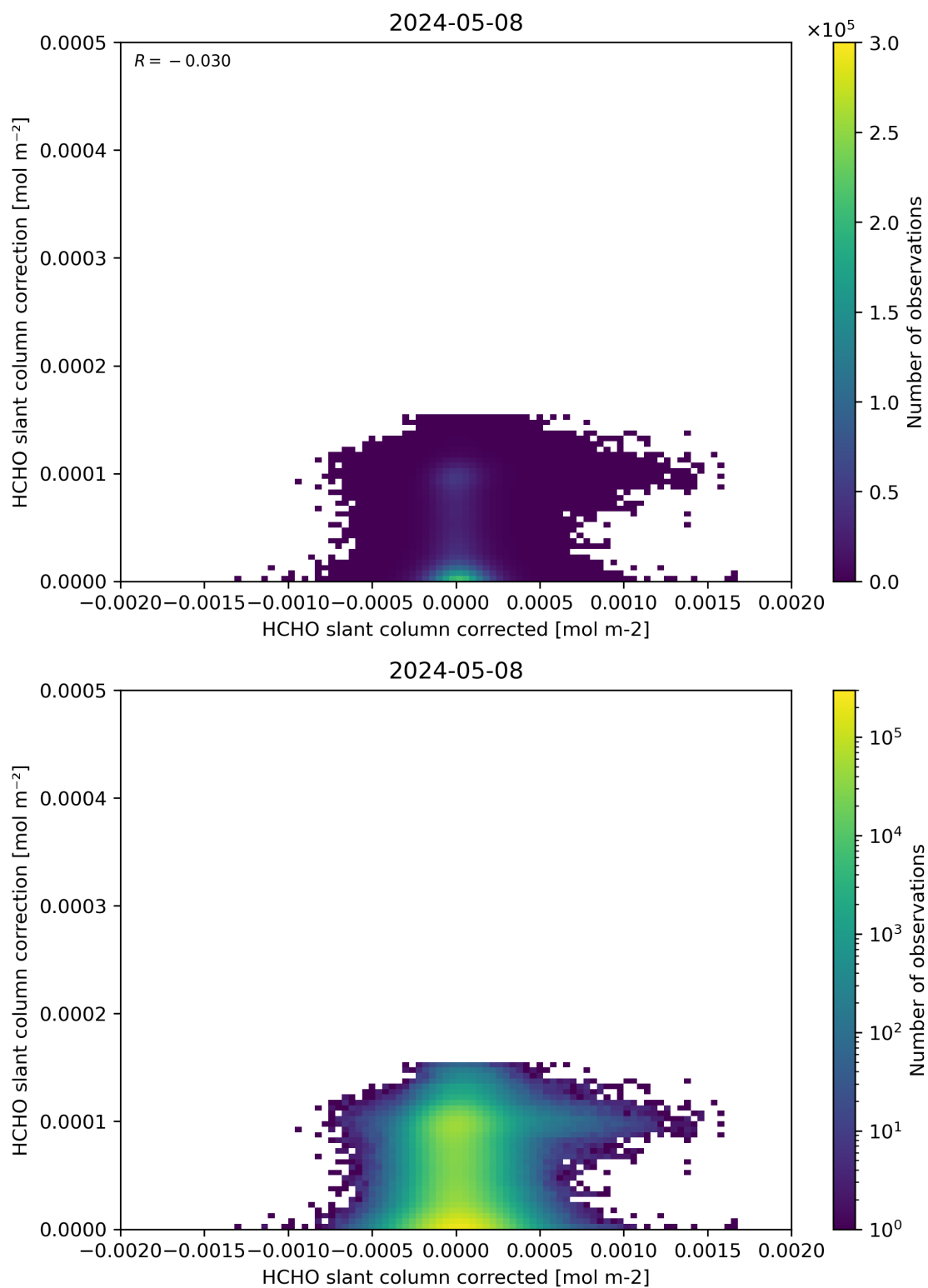
Figure 77: Scatter density plot of “HCHO slant column corrected” against “HCHO slant column correction” for 2024-05-07 to 2024-05-09.
