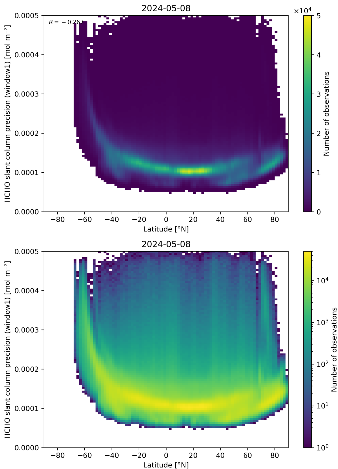
Figure 160: Scatter density plot of “Latitude” against “HCHO slant column precision (window1)” for 2024-05-07 to 2024-05-09.
