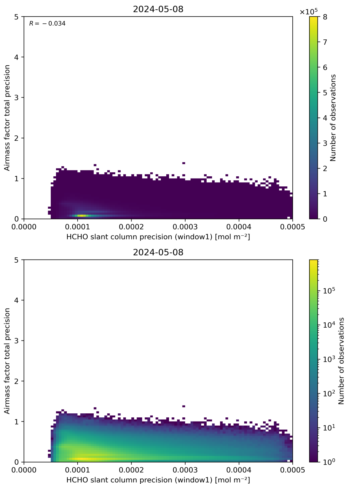
Figure 95: Scatter density plot of “HCHO slant column precision (window1)” against “Airmass factor total precision” for 2024-05-07 to 2024-05-09.
