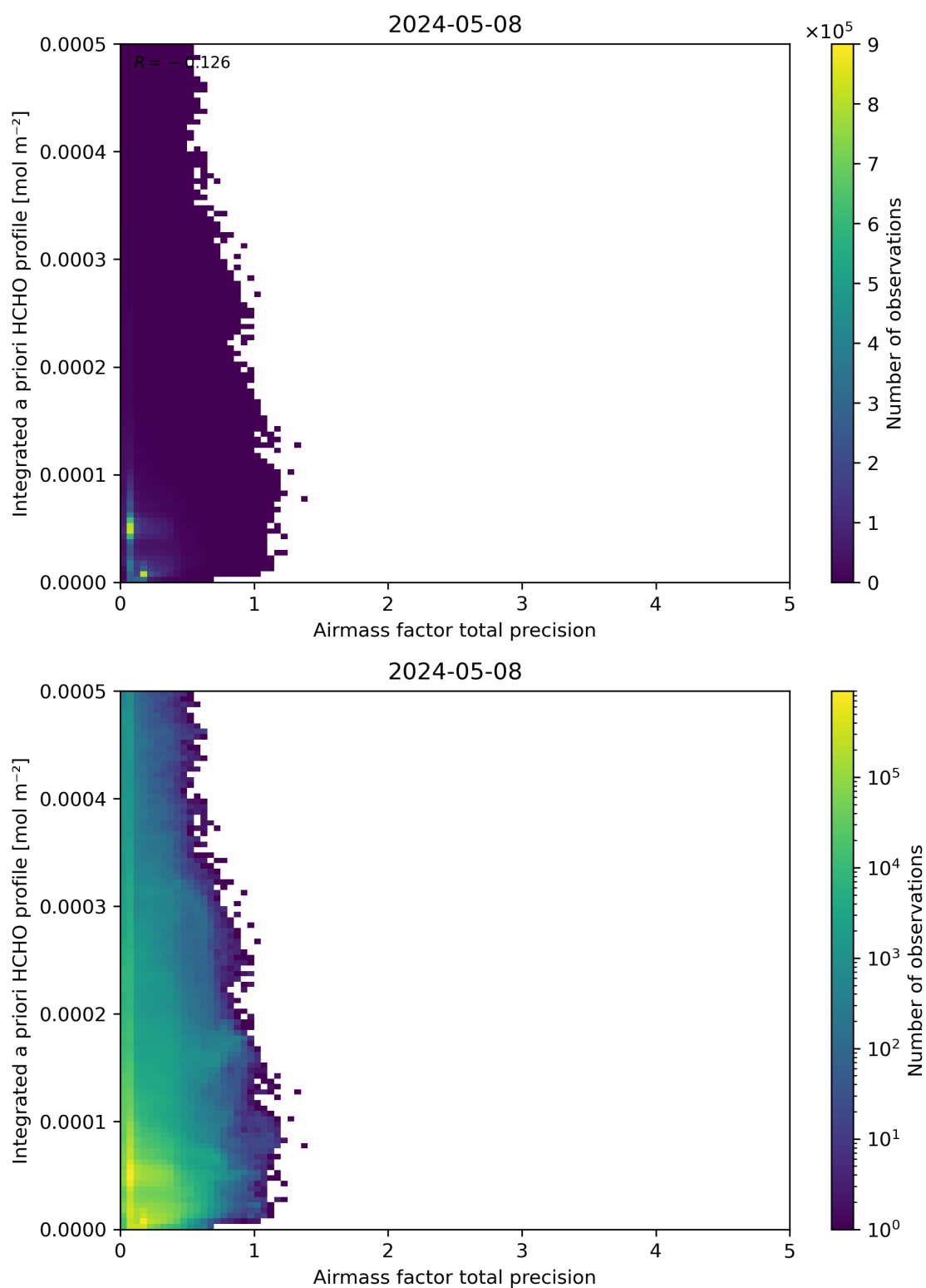
Figure 111: Scatter density plot of “Airmass factor total precision” against “Integrated a priori HCHO profile” for 2024-05-07 to 2024-05-09.
