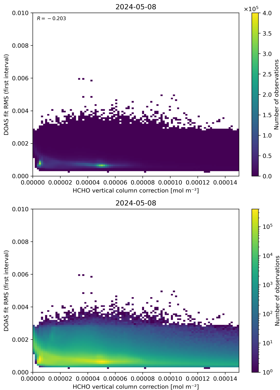
Figure 112: Scatter density plot of “HCHO vertical column correction” against “DOAS fit RMS (first interval)” for 2024-05-07 to 2024-05-09.
