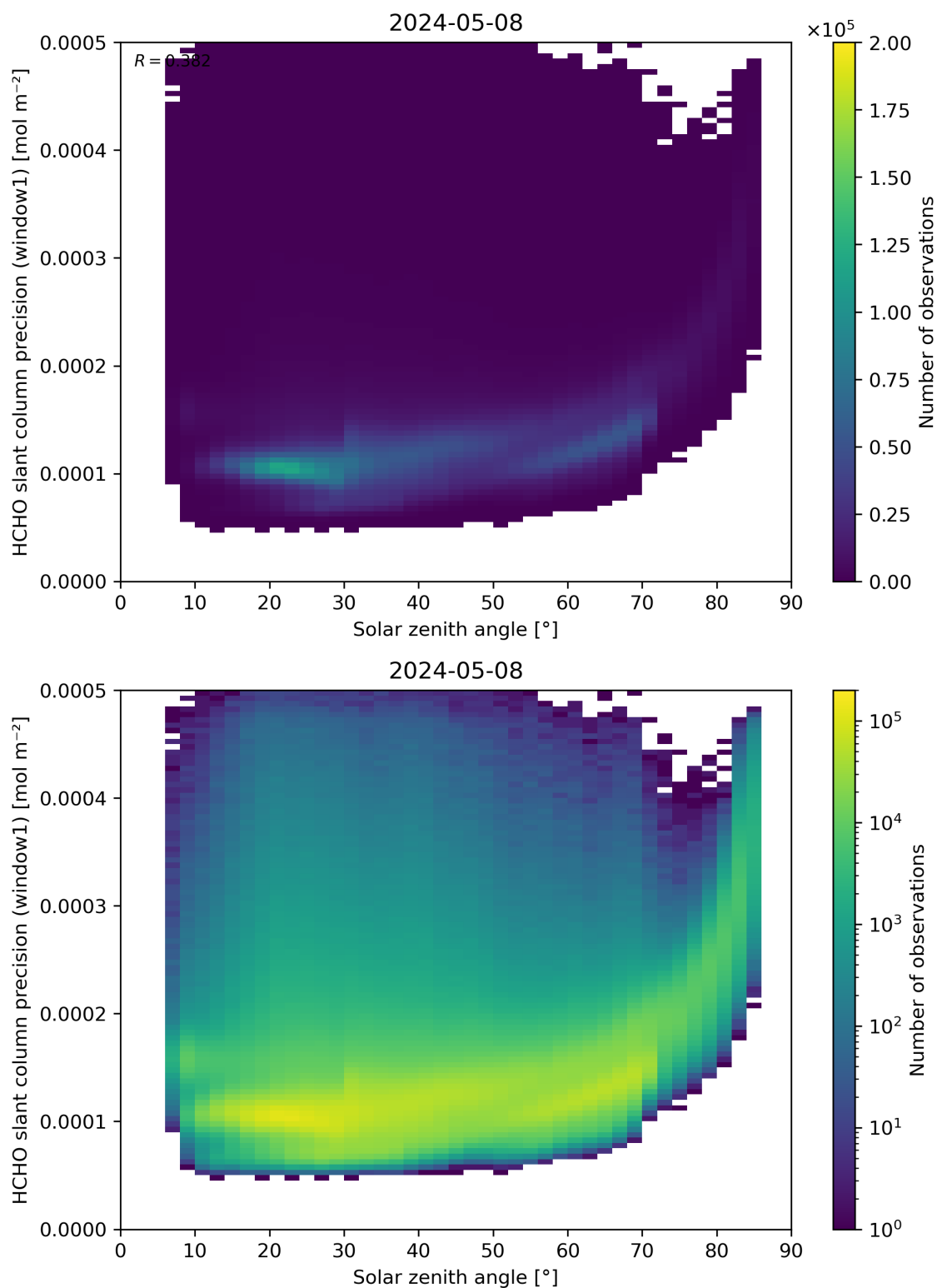
Figure 174: Scatter density plot of “Solar zenith angle” against “HCHO slant column precision (window1)” for 2024-05-07 to 2024-05-09.
