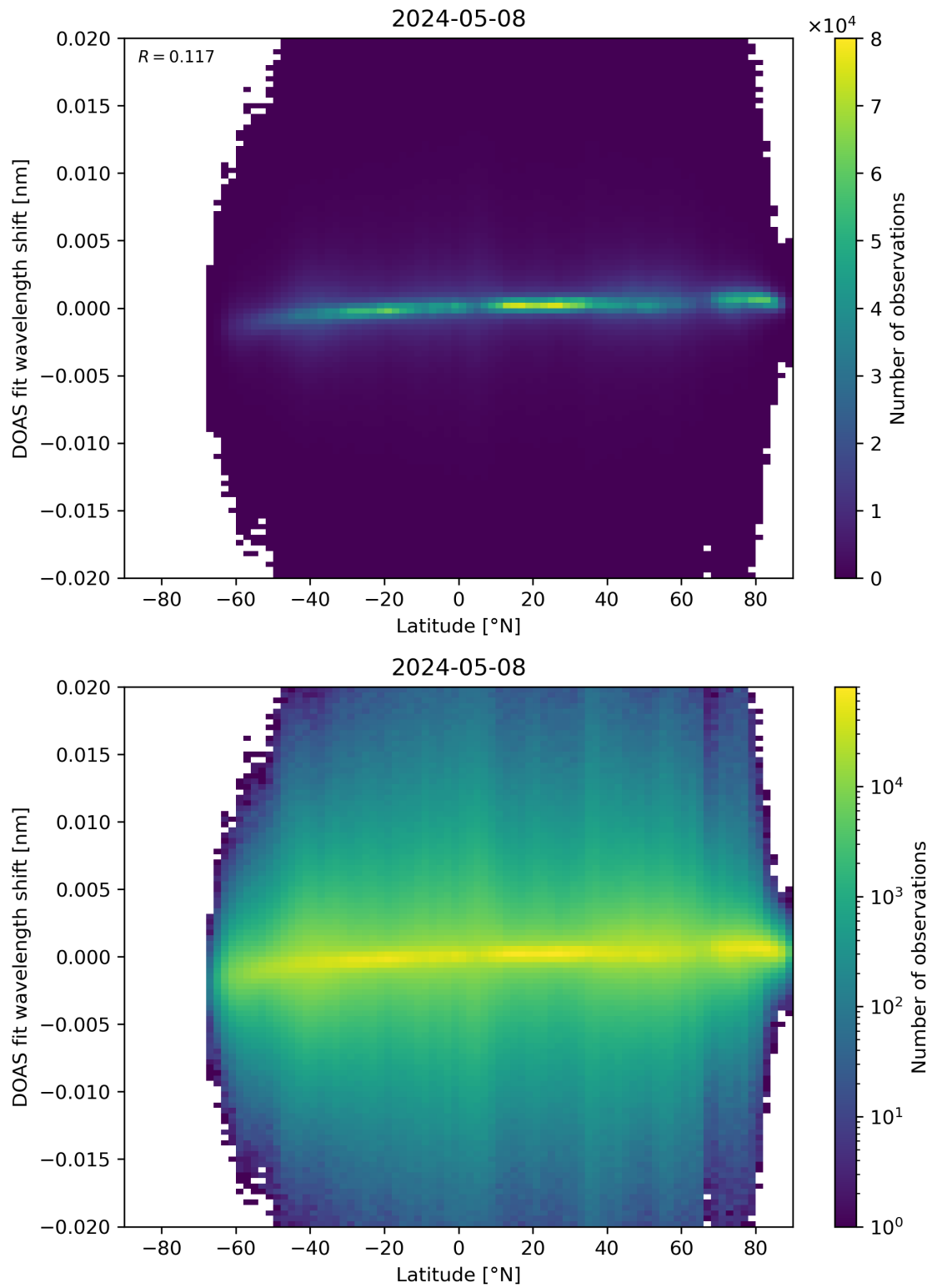
Figure 154: Scatter density plot of “Latitude” against “DOAS fit wavelength shift” for 2024-05-07 to 2024-05-09.
