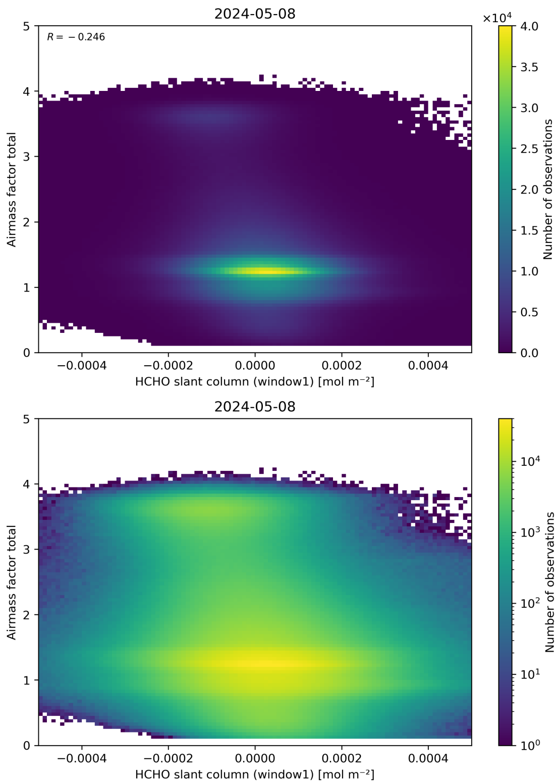
Figure 85: Scatter density plot of “HCHO slant column (window1)” against “Airmass factor total” for 2024-05-07 to 2024-05-09.
