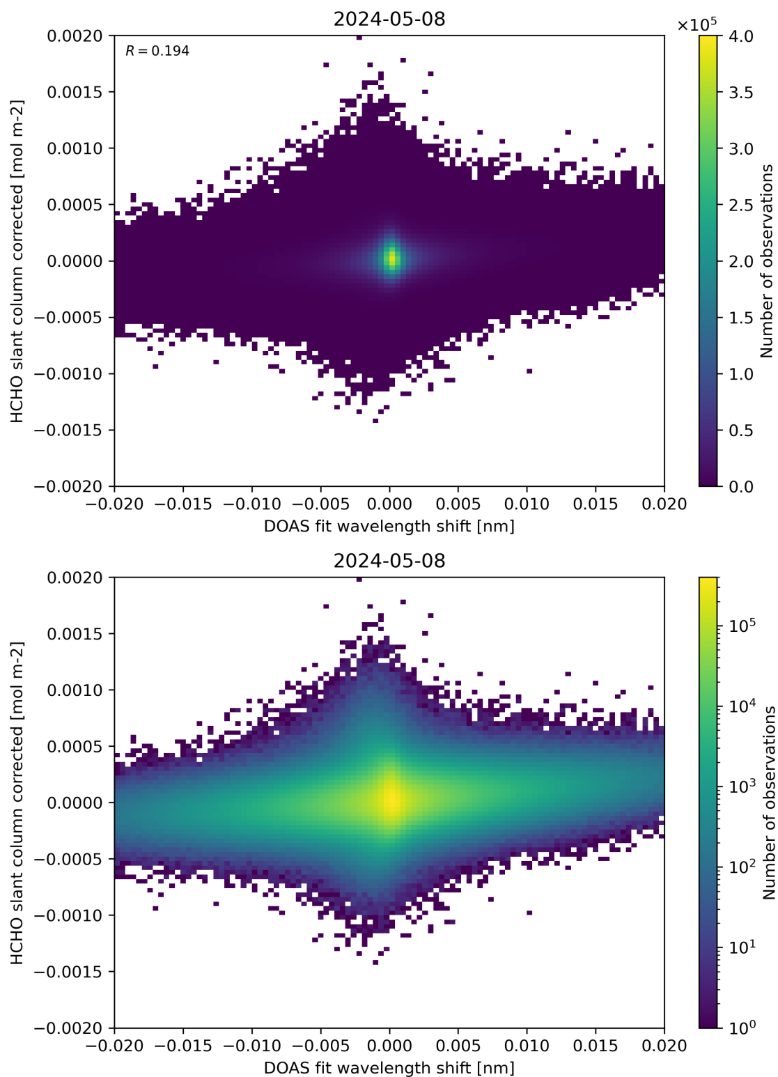
Figure 66: Scatter density plot of “DOAS fit wavelength shift” against “HCHO slant column corrected” for 2024-05-07 to 2024-05-09.
