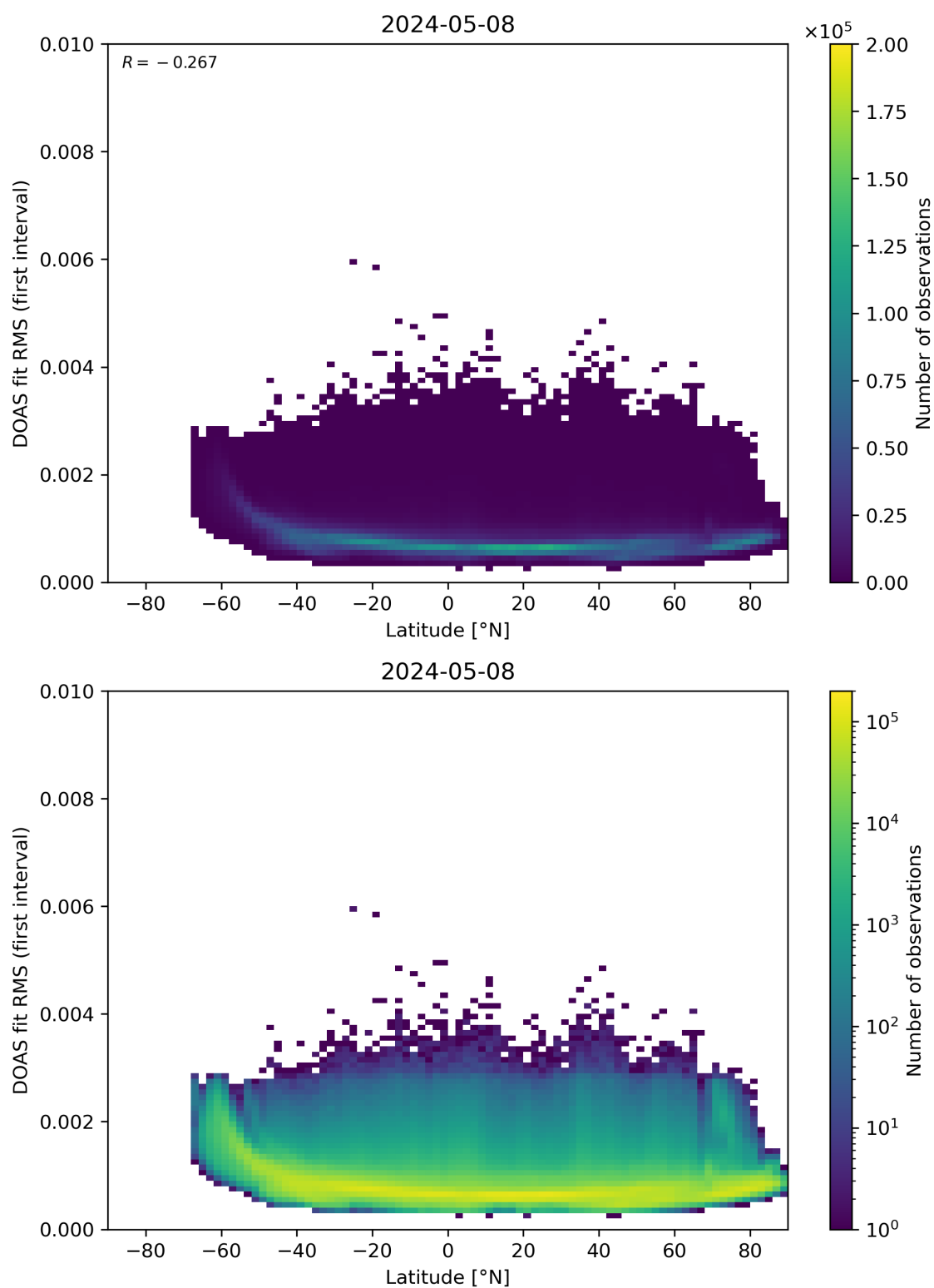
Figure 153: Scatter density plot of “Latitude” against “DOAS fit RMS (first interval)” for 2024-05-07 to 2024-05-09.
