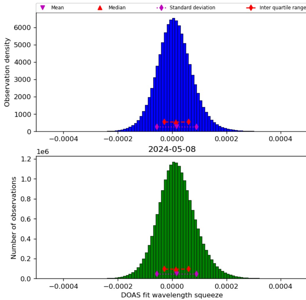
Figure 45: Histogram of “DOAS fit wavelength squeeze” for 2024-05-07 to 2024-05-09
