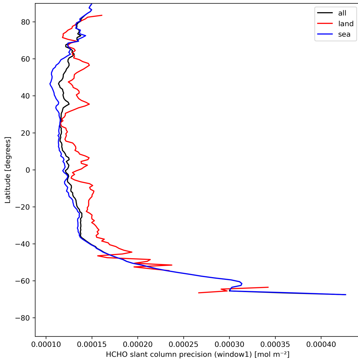
Figure 25: Zonal average of “HCHO slant column precision (window1)” for 2024-05-07 to 2024-05-09.
