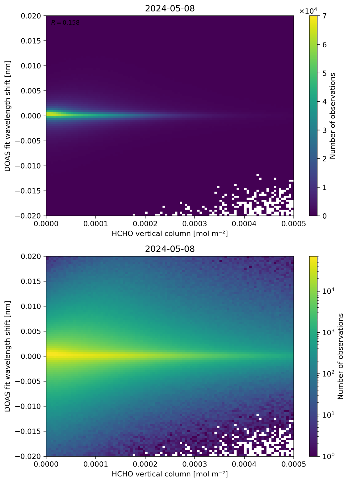
Figure 124: Scatter density plot of “HCHO vertical column” against “DOAS fit wavelength shift” for 2024-05-07 to 2024-05-09.
