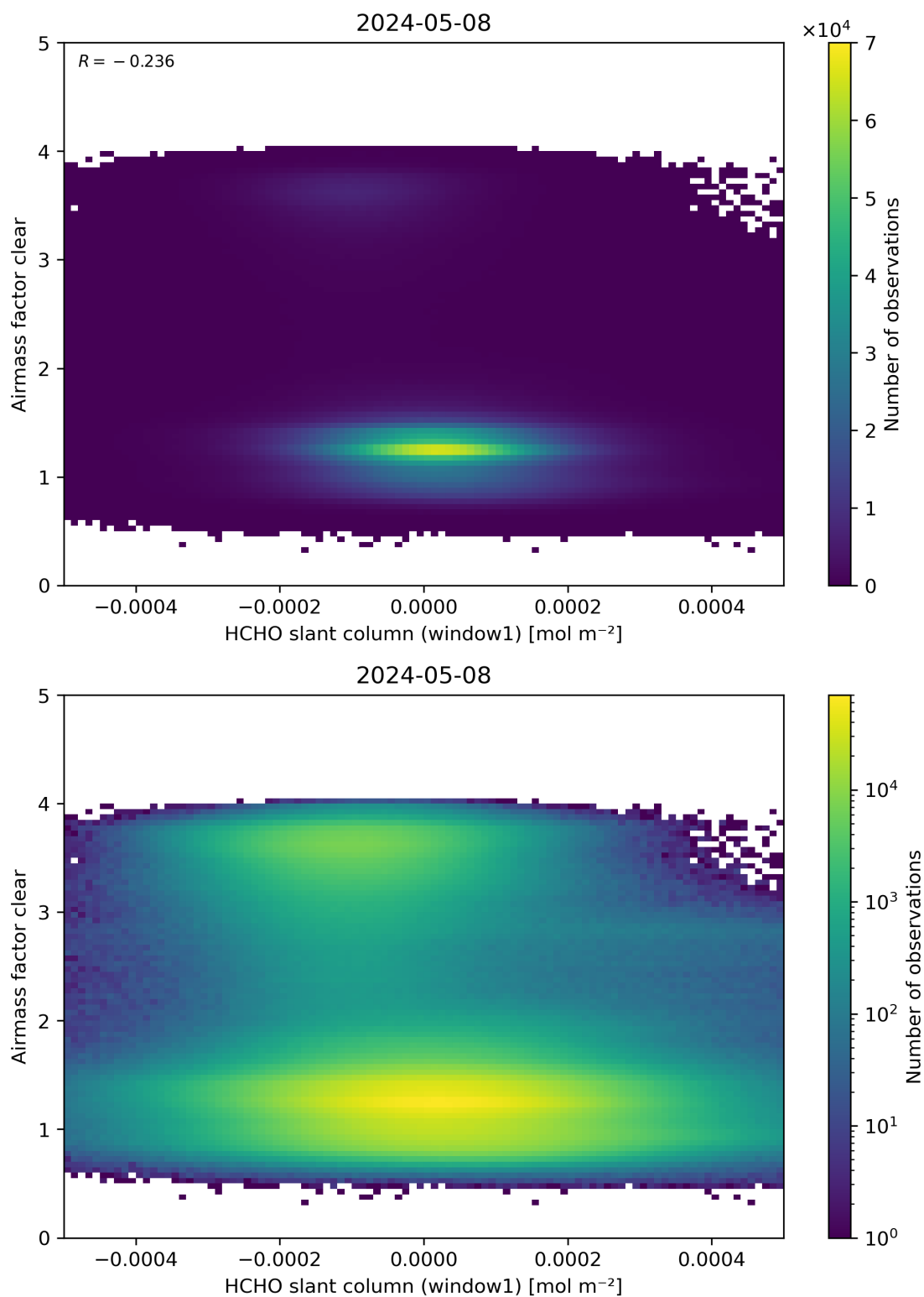
Figure 81: Scatter density plot of “HCHO slant column (window1)” against “Airmass factor clear” for 2024-05-07 to 2024-05-09.
