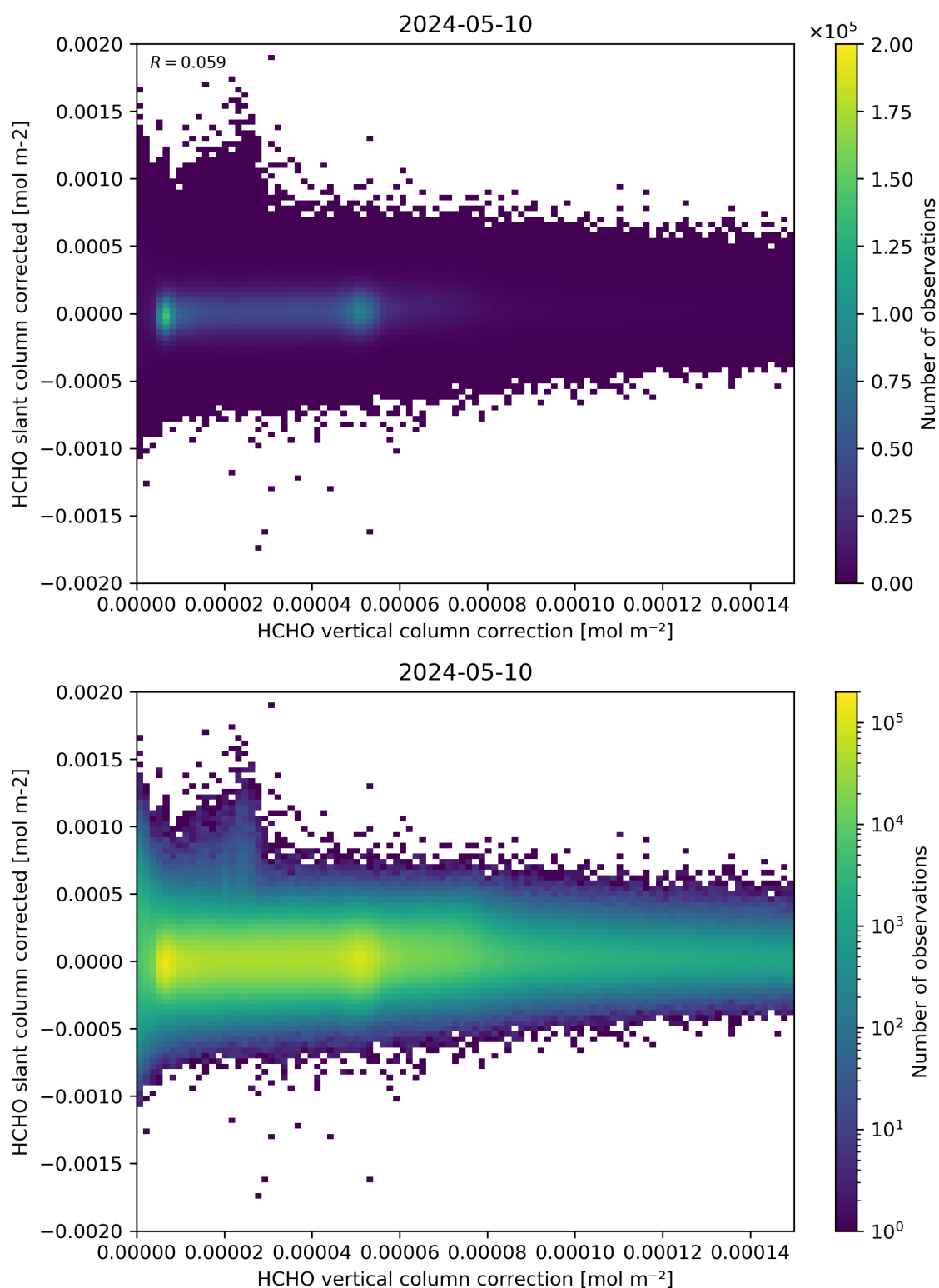
Figure 116: Scatter density plot of “HCHO vertical column correction” against “HCHO slant column corrected” for 2024-05-09 to 2024-05-11.
