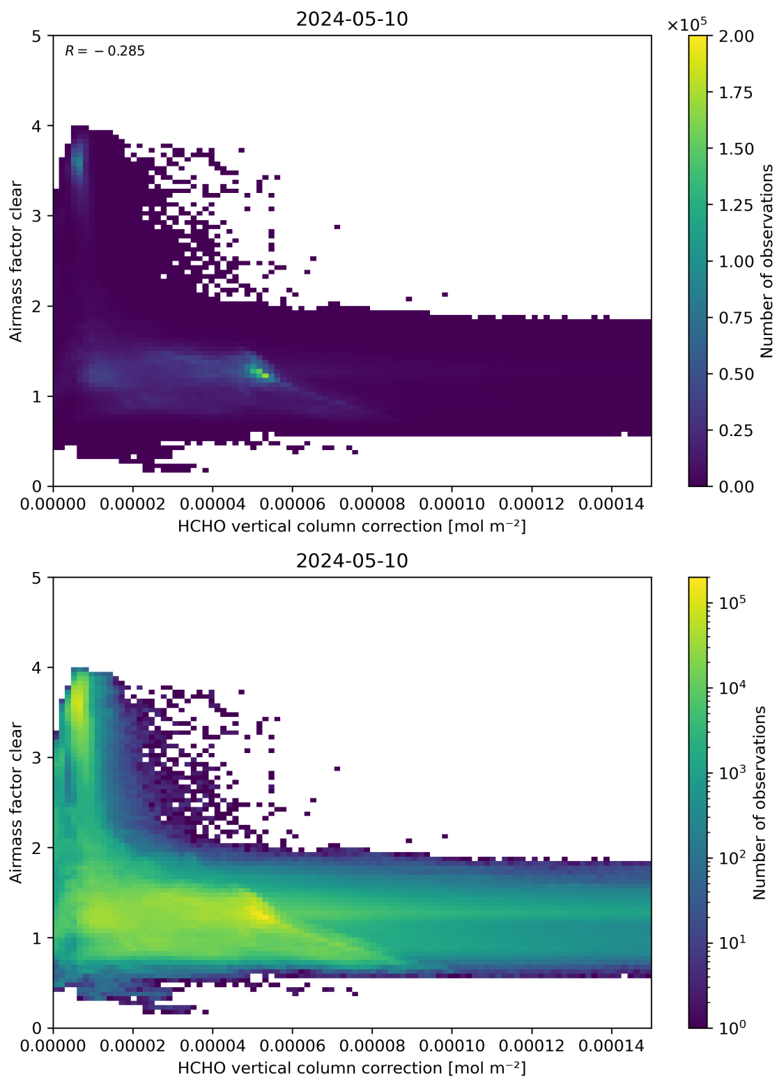
Figure 115: Scatter density plot of “HCHO vertical column correction” against “Airmass factor clear” for 2024-05-09 to 2024-05-11.
