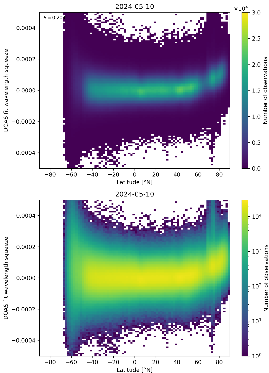
Figure 155: Scatter density plot of “Latitude” against “DOAS fit wavelength squeeze” for 2024-05-09 to 2024-05-11.
