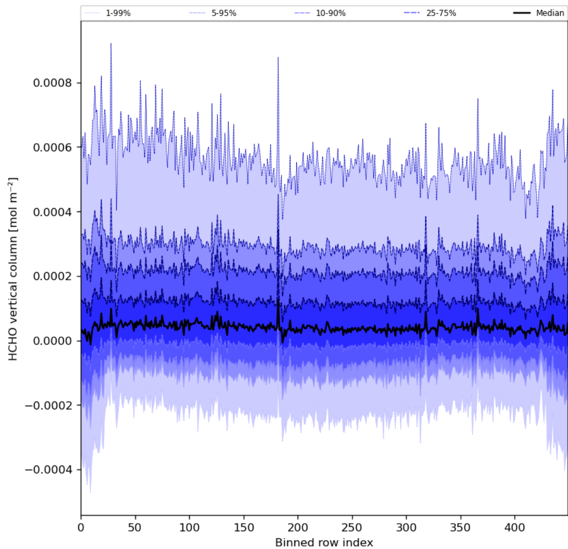
Figure 49: Along track statistics of “HCHO vertical column” for 2024-05-09 to 2024-05-11
