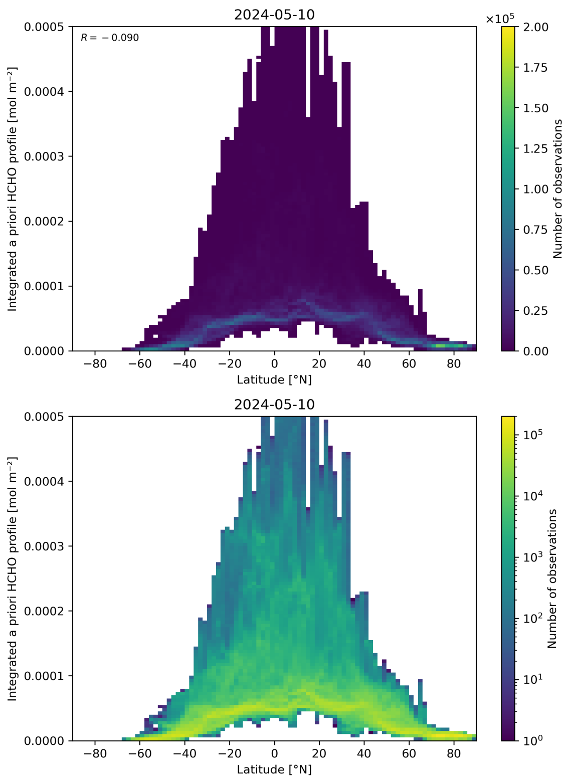
Figure 166: Scatter density plot of “Latitude” against “Integrated a priori HCHO profile” for 2024-05-09 to 2024-05-11.
