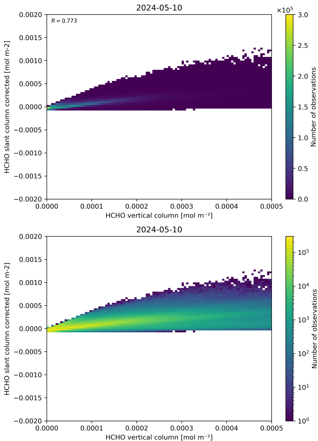
Figure 127: Scatter density plot of “HCHO vertical column” against “HCHO slant column corrected” for 2024-05-09 to 2024-05-11.
