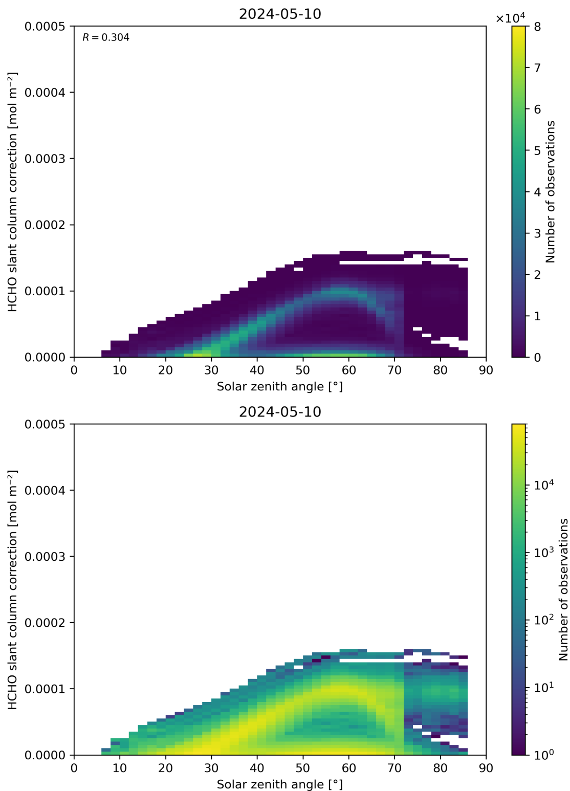
Figure 172: Scatter density plot of “Solar zenith angle” against “HCHO slant column correction” for 2024-05-09 to 2024-05-11.
