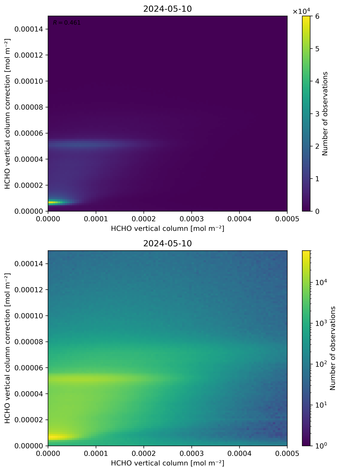
Figure 133: Scatter density plot of “HCHO vertical column” against “HCHO vertical column correction” for 2024-05-09 to 2024-05-11.
