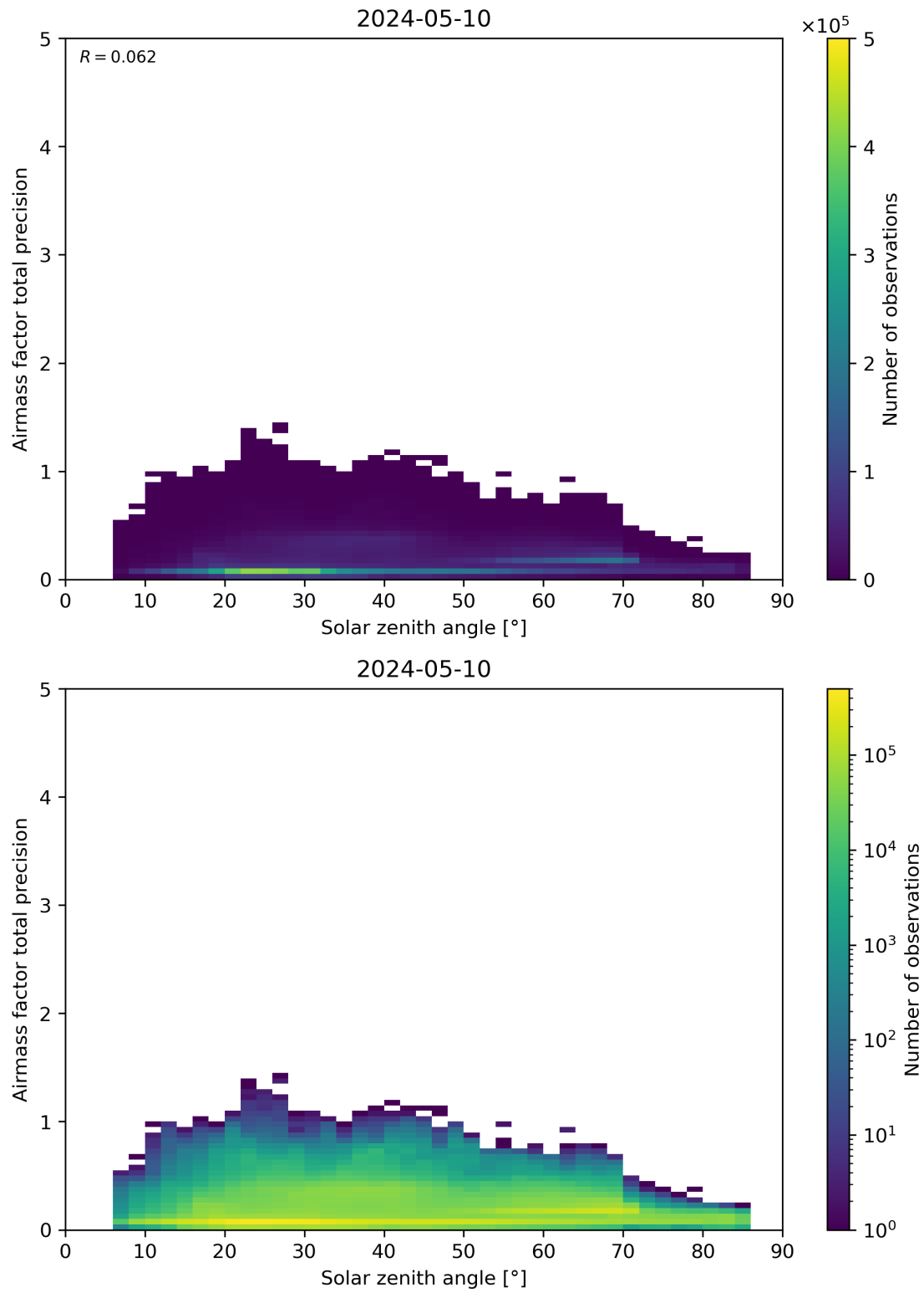
Figure 176: Scatter density plot of “Solar zenith angle” against “Airmass factor total precision” for 2024-05-09 to 2024-05-11.
