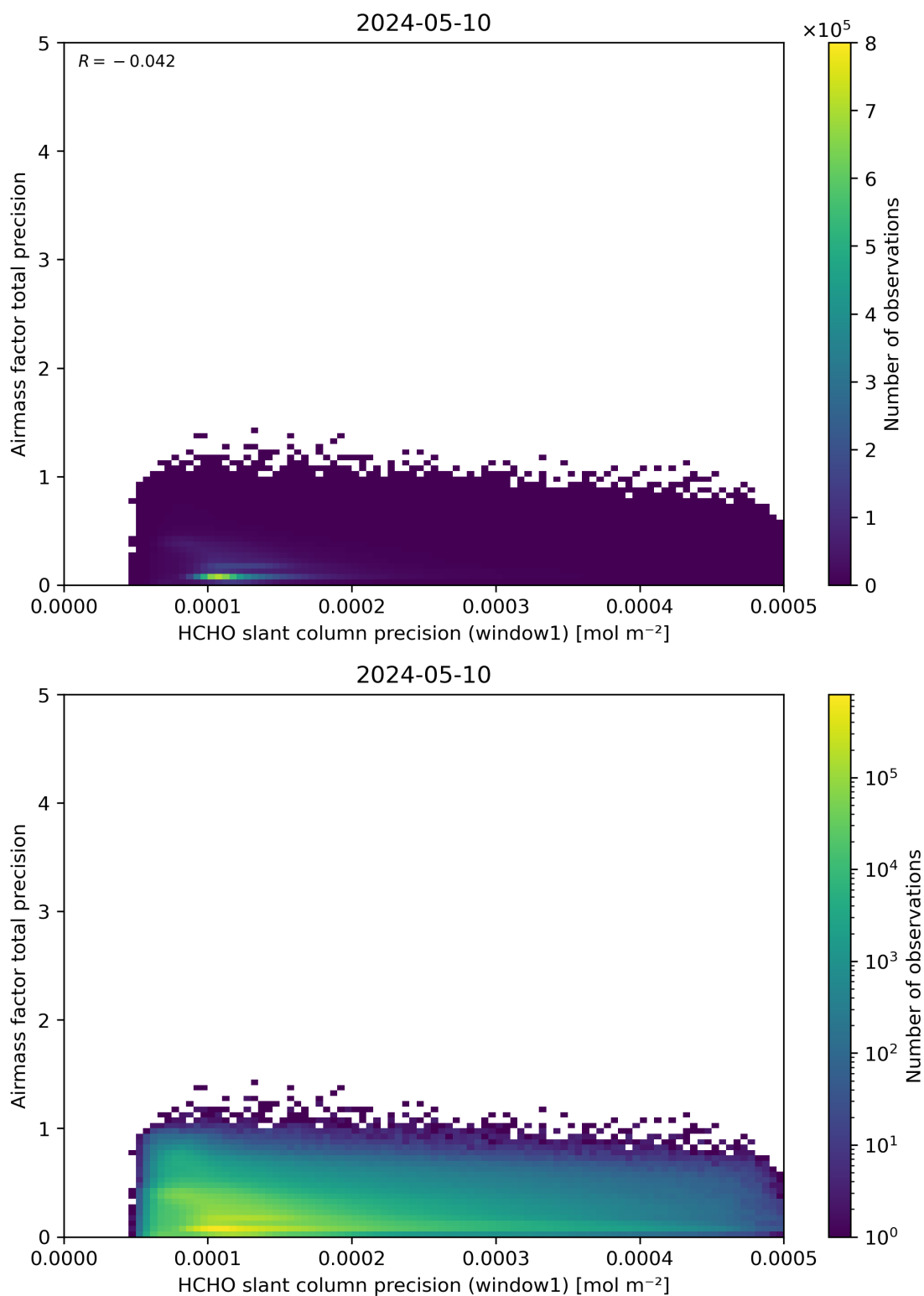
Figure 95: Scatter density plot of “HCHO slant column precision (window1)” against “Airmass factor total precision” for 2024-05-09 to 2024-05-11.
