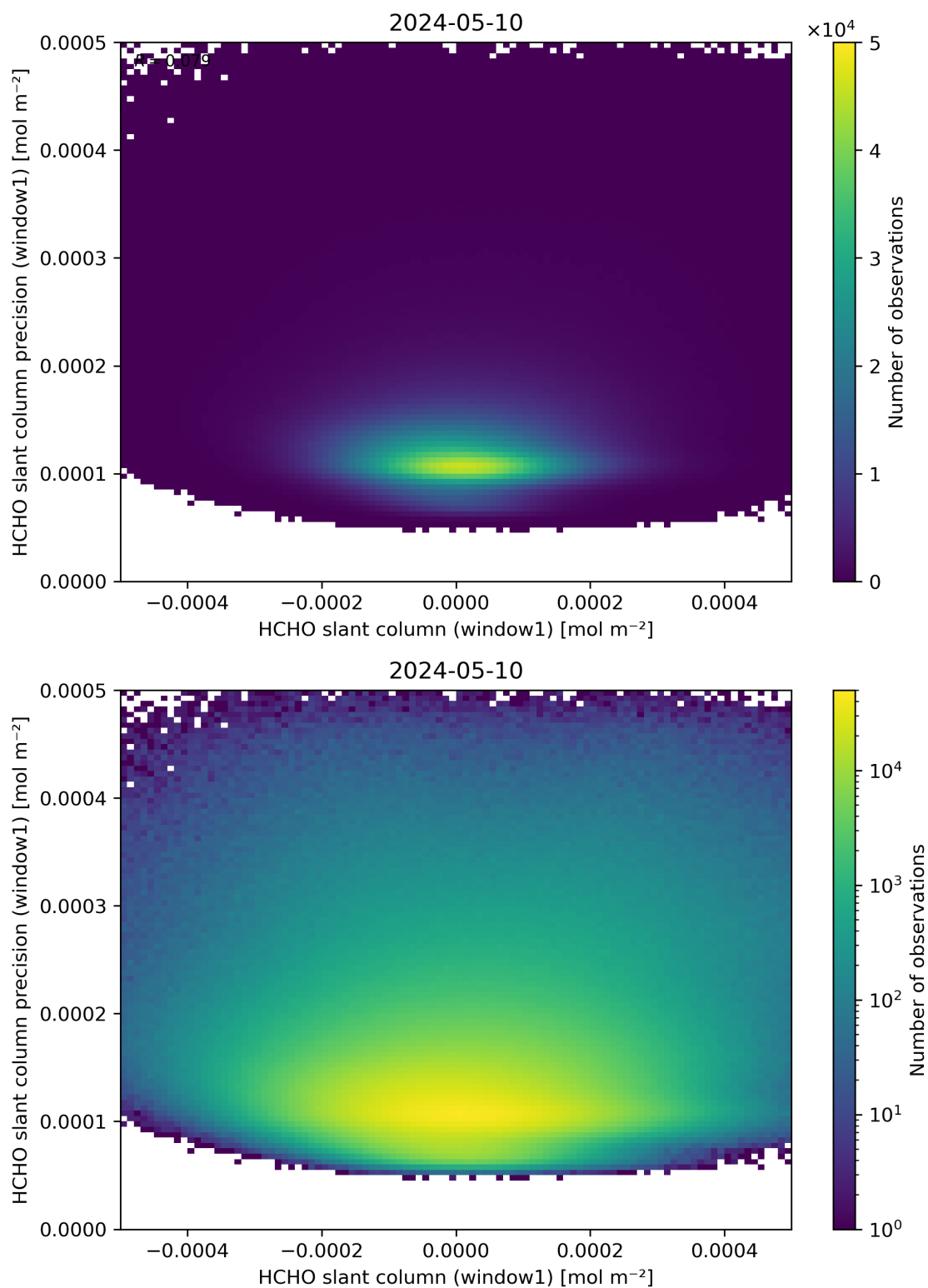
Figure 84: Scatter density plot of “HCHO slant column (window1)” against “HCHO slant column precision (window1)” for 2024-05-09 to 2024-05-11.
