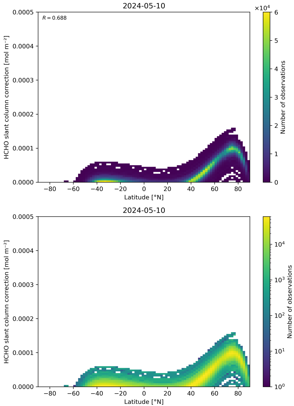
Figure 158: Scatter density plot of “Latitude” against “HCHO slant column correction” for 2024-05-09 to 2024-05-11.
