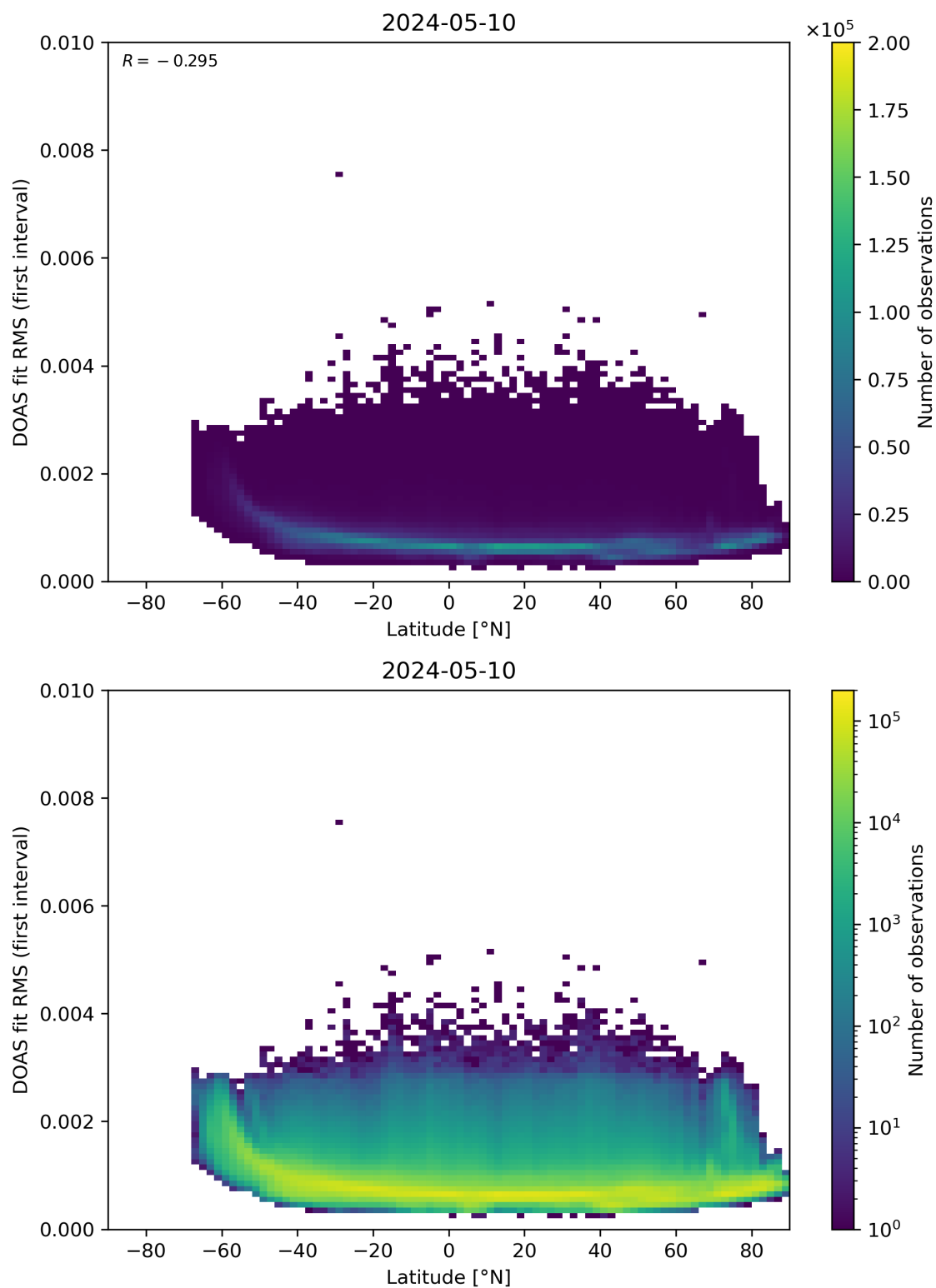
Figure 153: Scatter density plot of “Latitude” against “DOAS fit RMS (first interval)” for 2024-05-09 to 2024-05-11.
