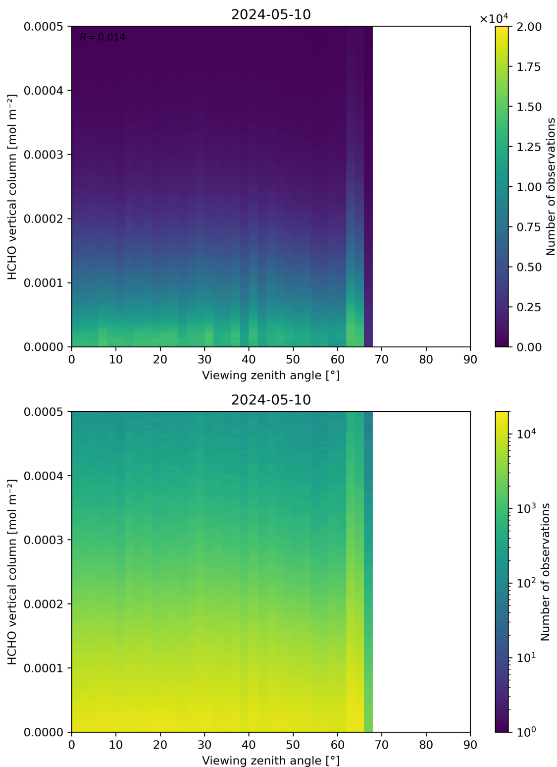
Figure 192: Scatter density plot of “Viewing zenith angle” against “HCHO vertical column” for 2024-05-09 to 2024-05-11.
