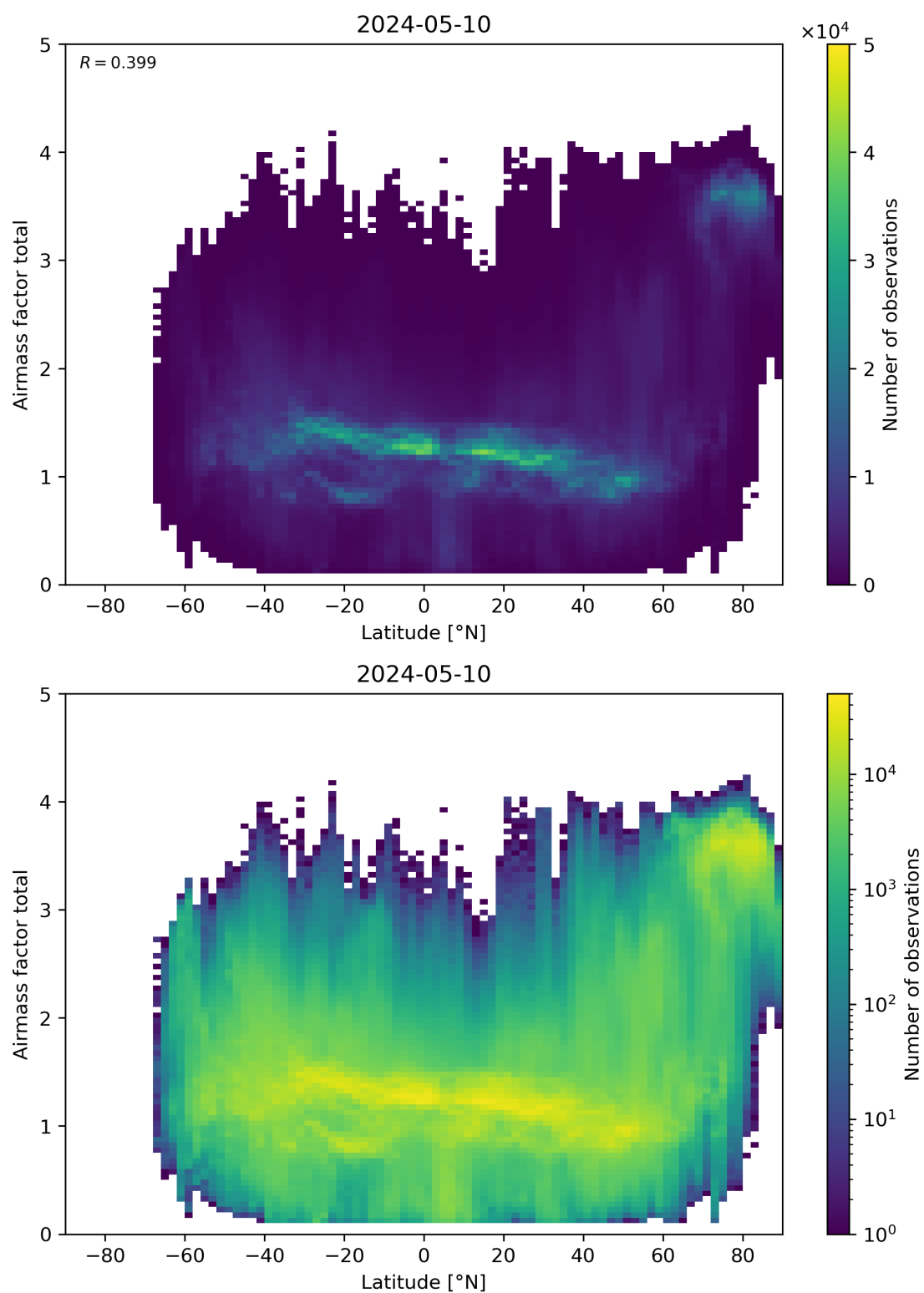
Figure 161: Scatter density plot of “Latitude” against “Airmass factor total” for 2024-05-09 to 2024-05-11.
