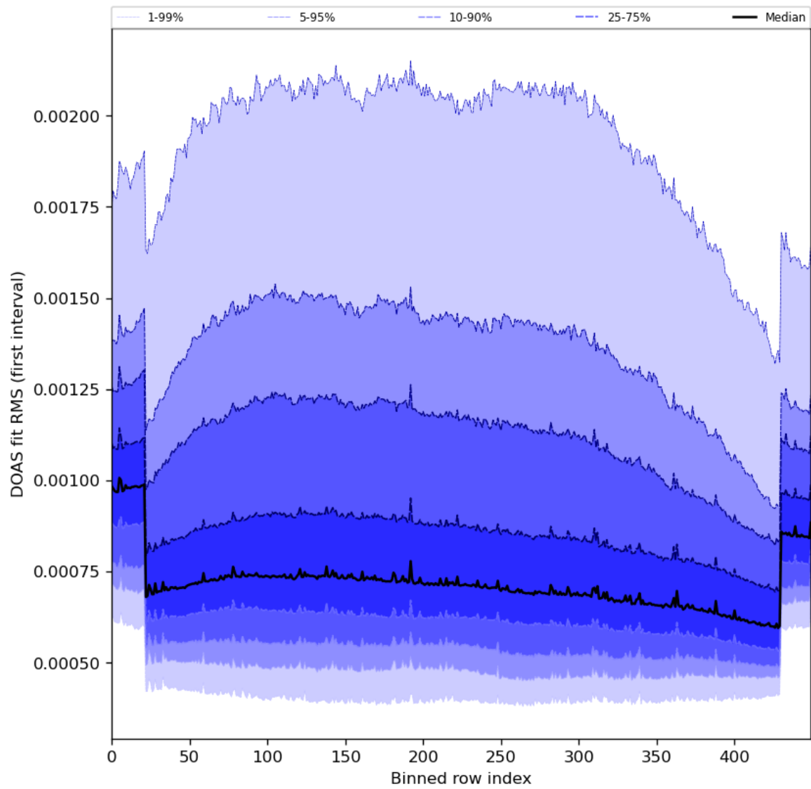
Figure 60: Along track statistics of “DOAS fit RMS (first interval)” for 2024-05-09 to 2024-05-11
