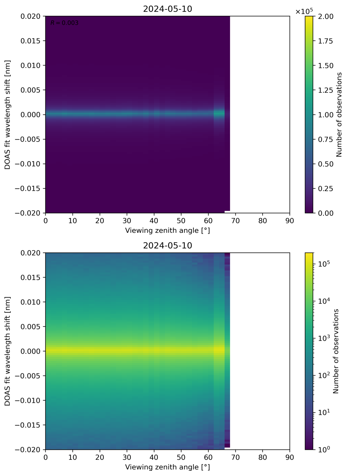
Figure 183: Scatter density plot of “Viewing zenith angle” against “DOAS fit wavelength shift” for 2024-05-09 to 2024-05-11.
