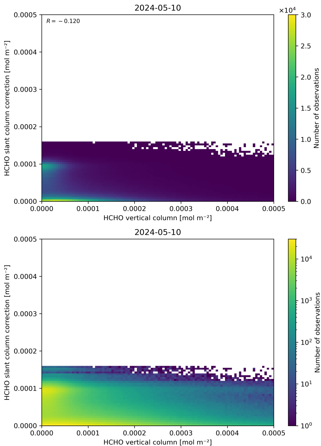
Figure 128: Scatter density plot of “HCHO vertical column” against “HCHO slant column correction” for 2024-05-09 to 2024-05-11.
