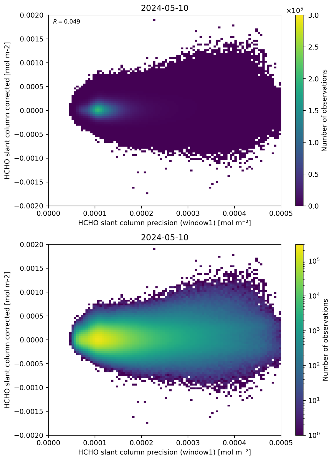
Figure 92: Scatter density plot of “HCHO slant column precision (window1)” against “HCHO slant column corrected” for 2024-05-09 to 2024-05-11.
