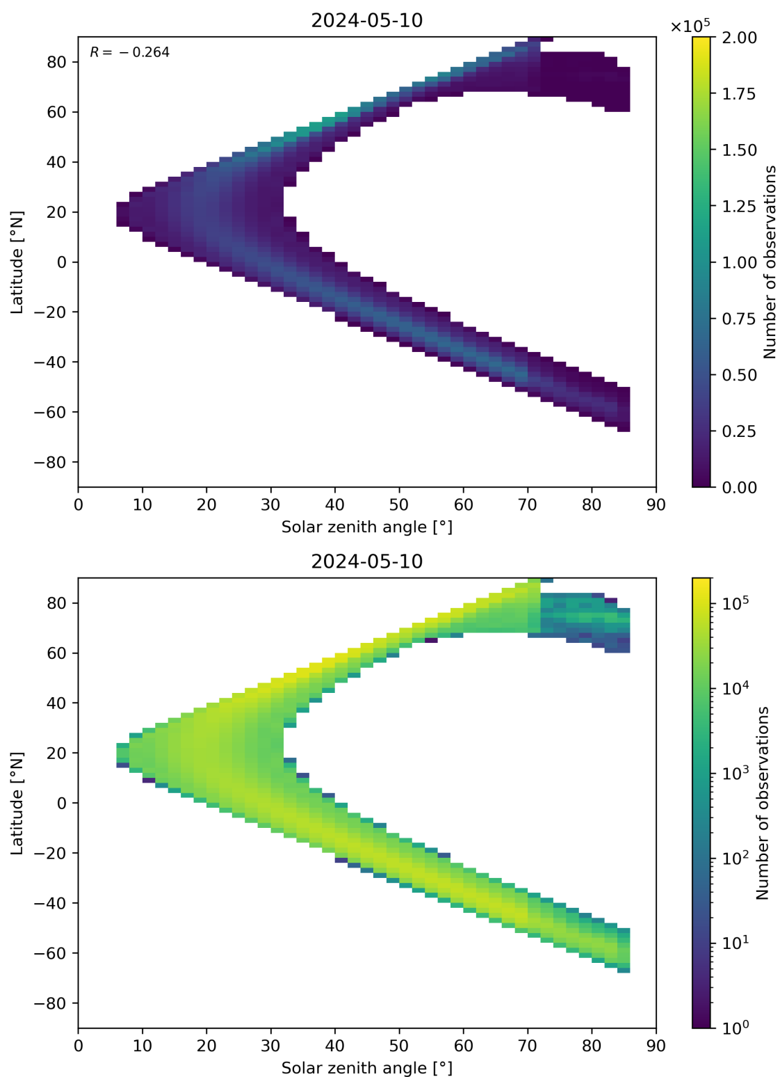
Figure 181: Scatter density plot of “Solar zenith angle” against “Latitude” for 2024-05-09 to 2024-05-11.
