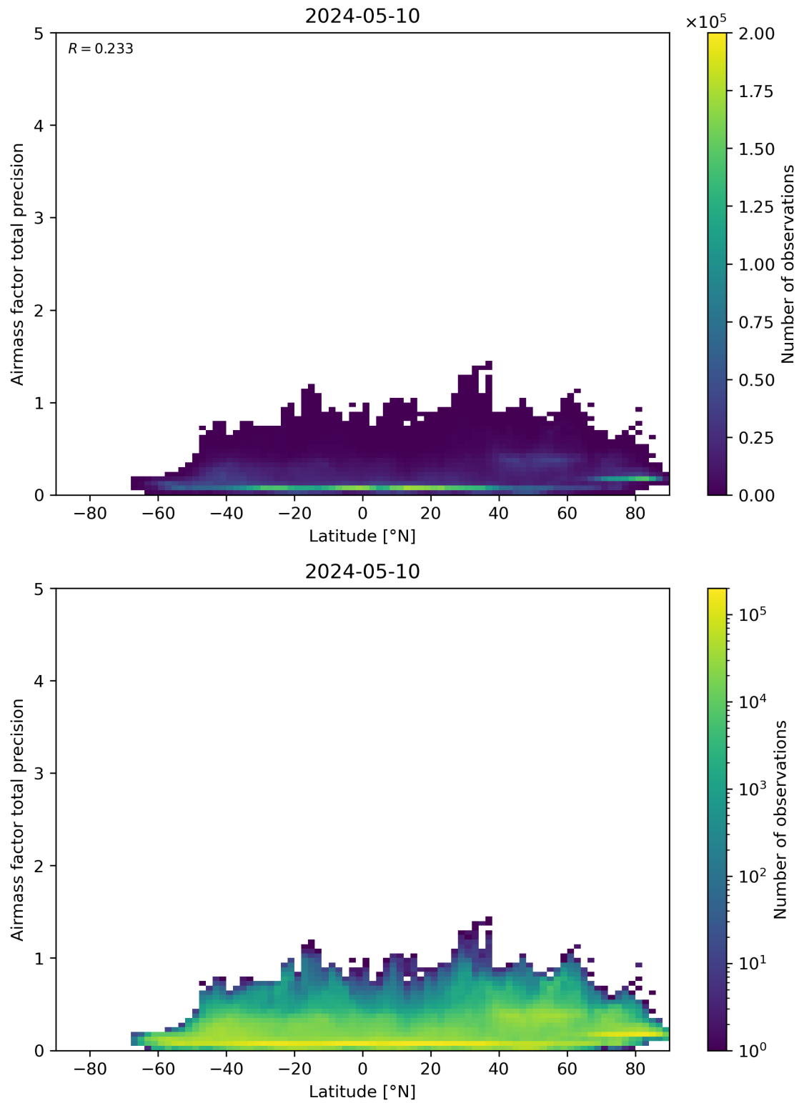
Figure 162: Scatter density plot of “Latitude” against “Airmass factor total precision” for 2024-05-09 to 2024-05-11.
