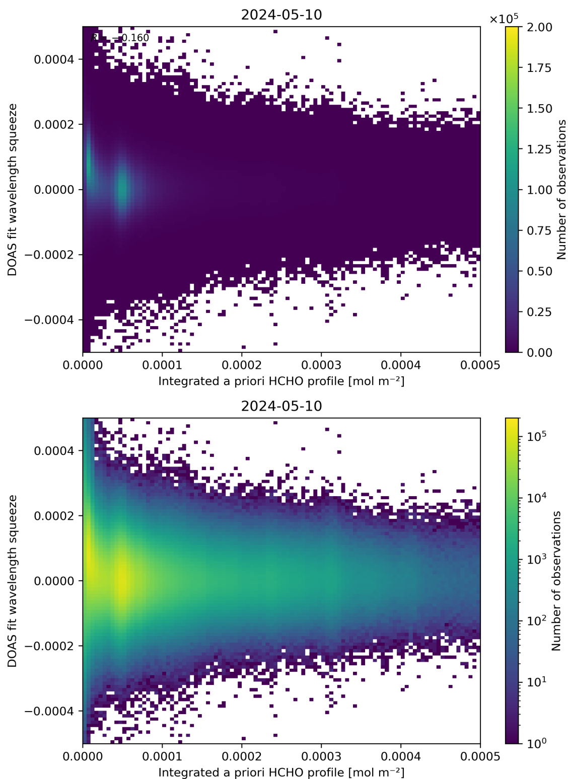
Figure 150: Scatter density plot of “Integrated a priori HCHO profile” against “DOAS fit wavelength squeeze” for 2024-05-09 to 2024-05-11.
