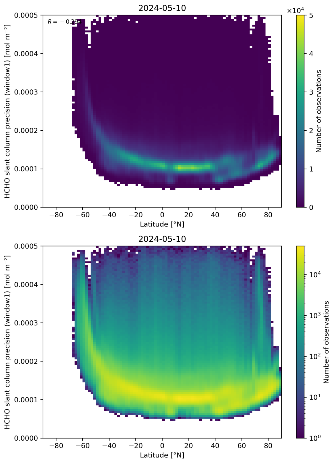
Figure 160: Scatter density plot of “Latitude” against “HCHO slant column precision (window1)” for 2024-05-09 to 2024-05-11.
