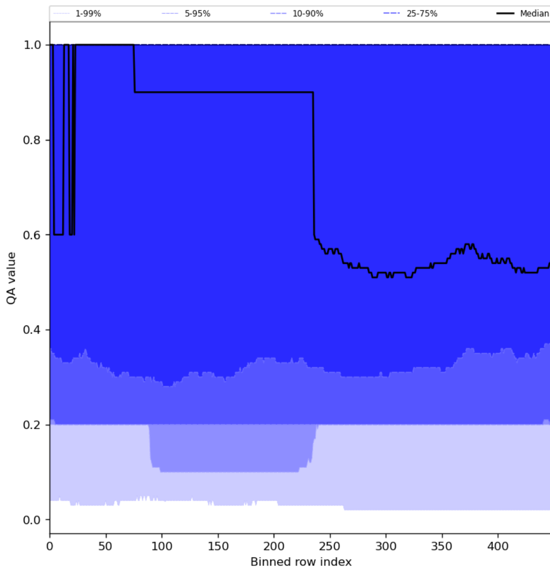
Figure 48: Along track statistics of “QA value” for 2024-05-09 to 2024-05-11
