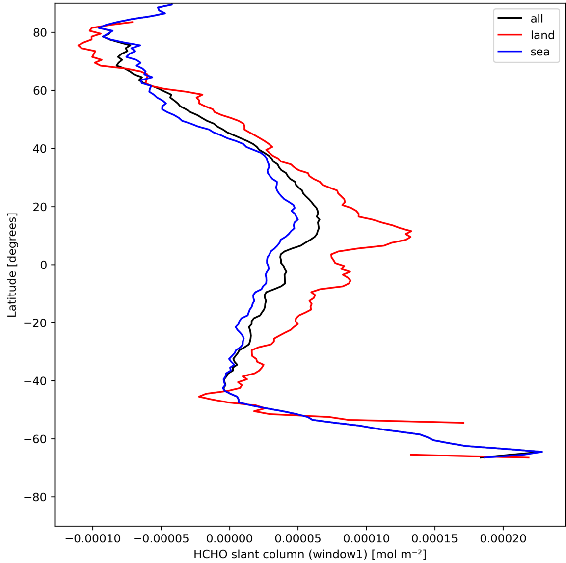
Figure 24: Zonal average of “HCHO slant column (window1)” for 2024-05-09 to 2024-05-11.
