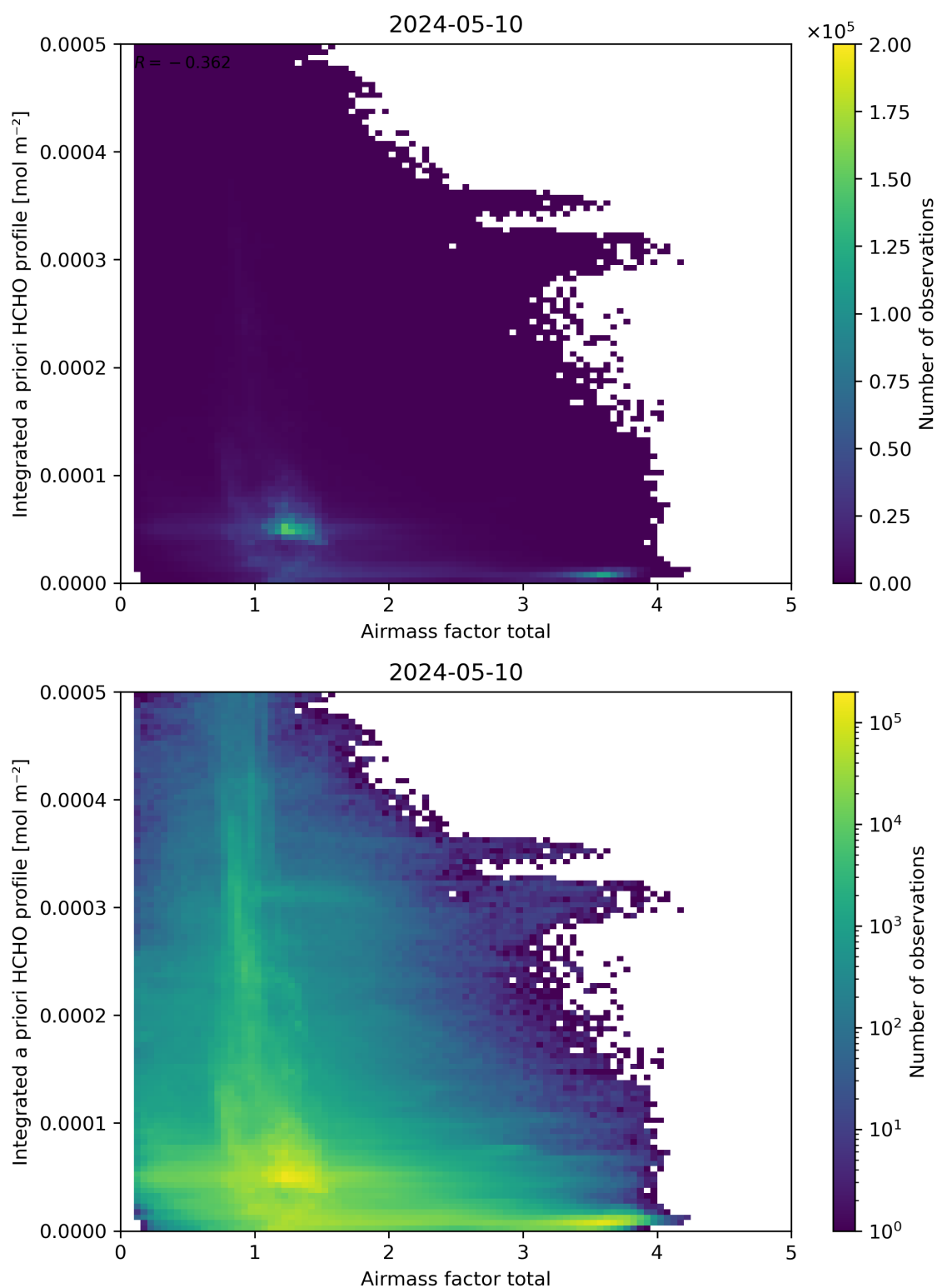
Figure 104: Scatter density plot of “Airmass factor total” against “Integrated a priori HCHO profile” for 2024-05-09 to 2024-05-11.
