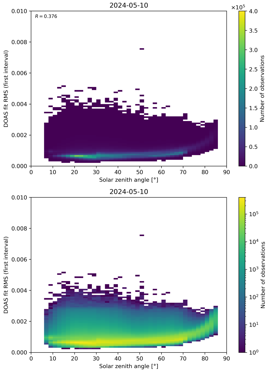
Figure 167: Scatter density plot of “Solar zenith angle” against “DOAS fit RMS (first interval)” for 2024-05-09 to 2024-05-11.
