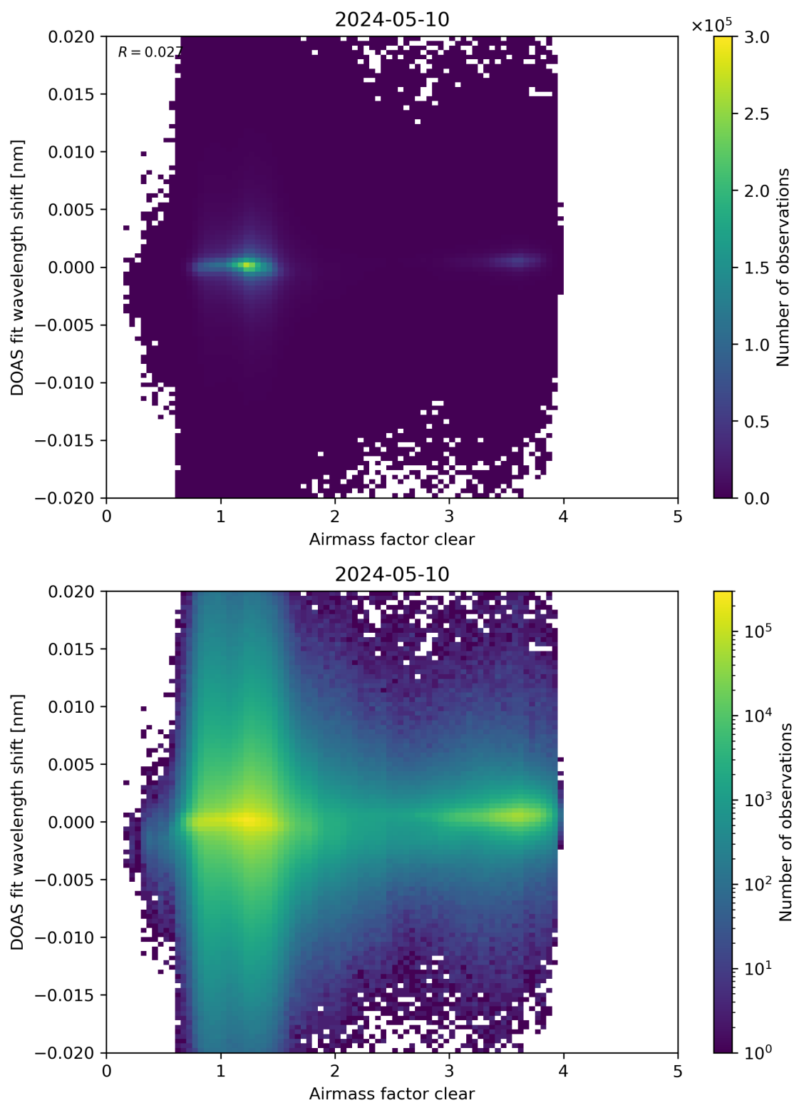
Figure 72: Scatter density plot of “Airmass factor clear” against “DOAS fit wavelength shift” for 2024-05-09 to 2024-05-11.
