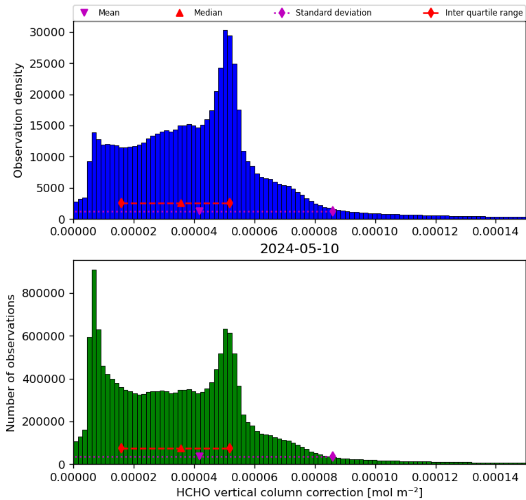
Figure 37: Histogram of “HCHO vertical column correction” for 2024-05-09 to 2024-05-11
