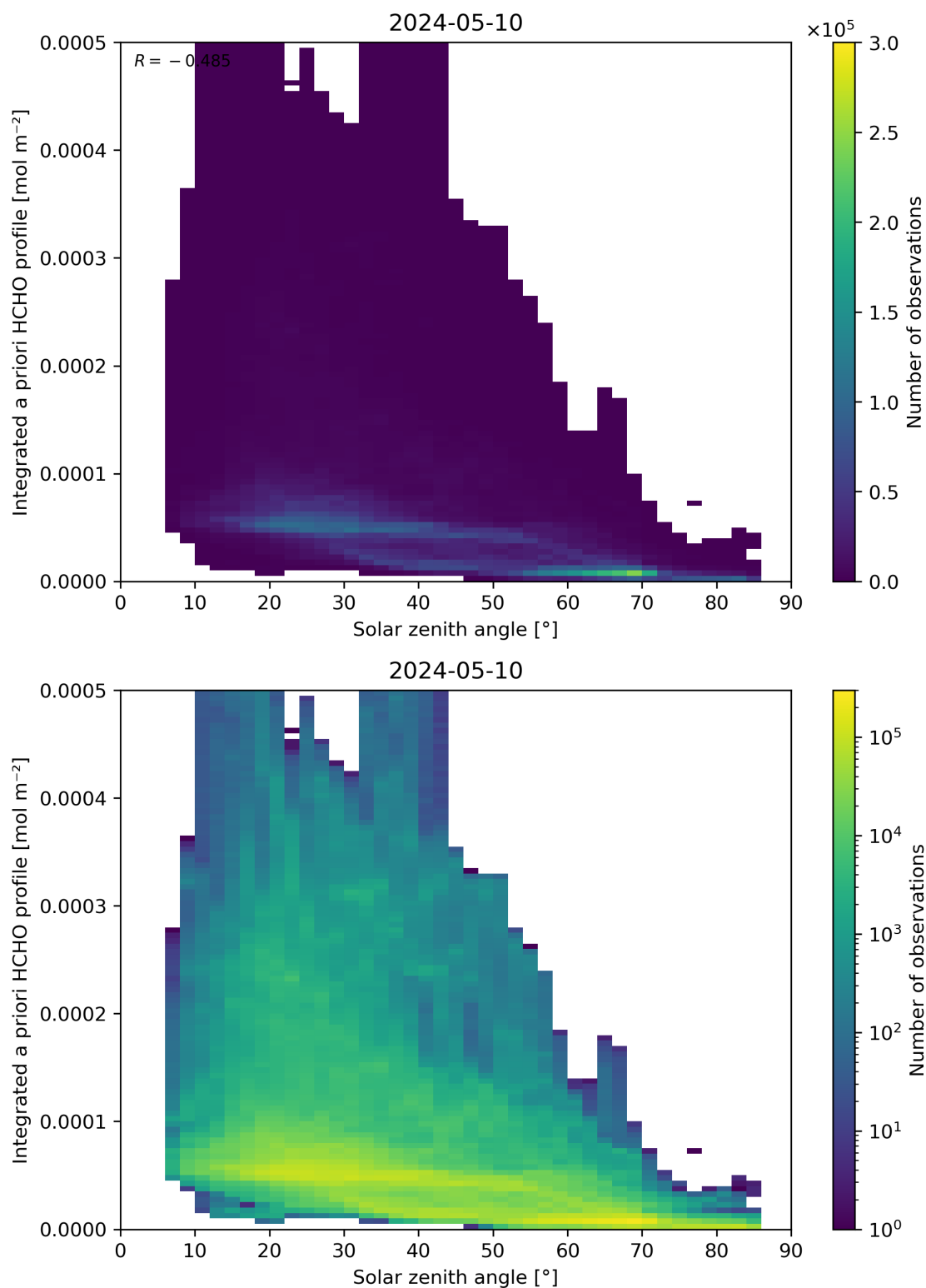
Figure 180: Scatter density plot of “Solar zenith angle” against “Integrated a priori HCHO profile” for 2024-05-09 to 2024-05-11.
