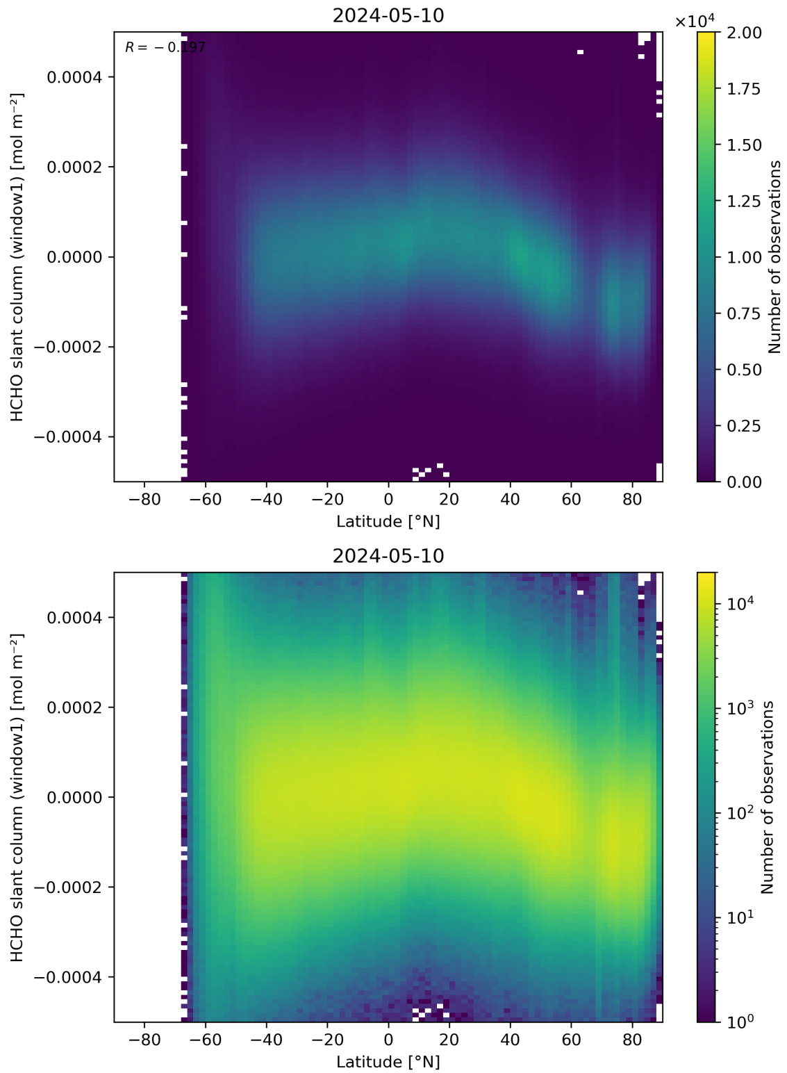
Figure 159: Scatter density plot of “Latitude” against “HCHO slant column (window1)” for 2024-05-09 to 2024-05-11.
