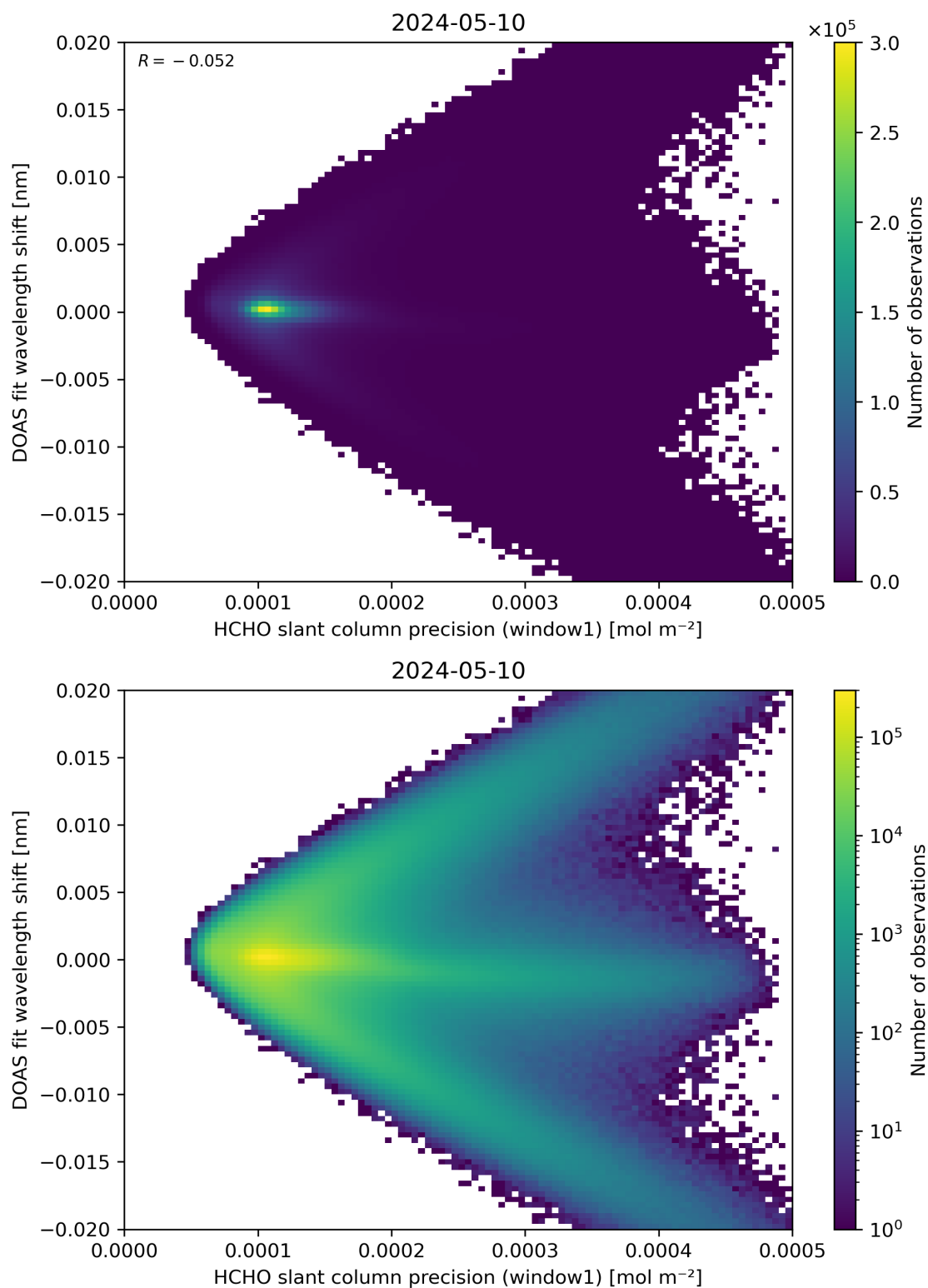
Figure 89: Scatter density plot of “HCHO slant column precision (window1)” against “DOAS fit wavelength shift” for 2024-05-09 to 2024-05-11.
