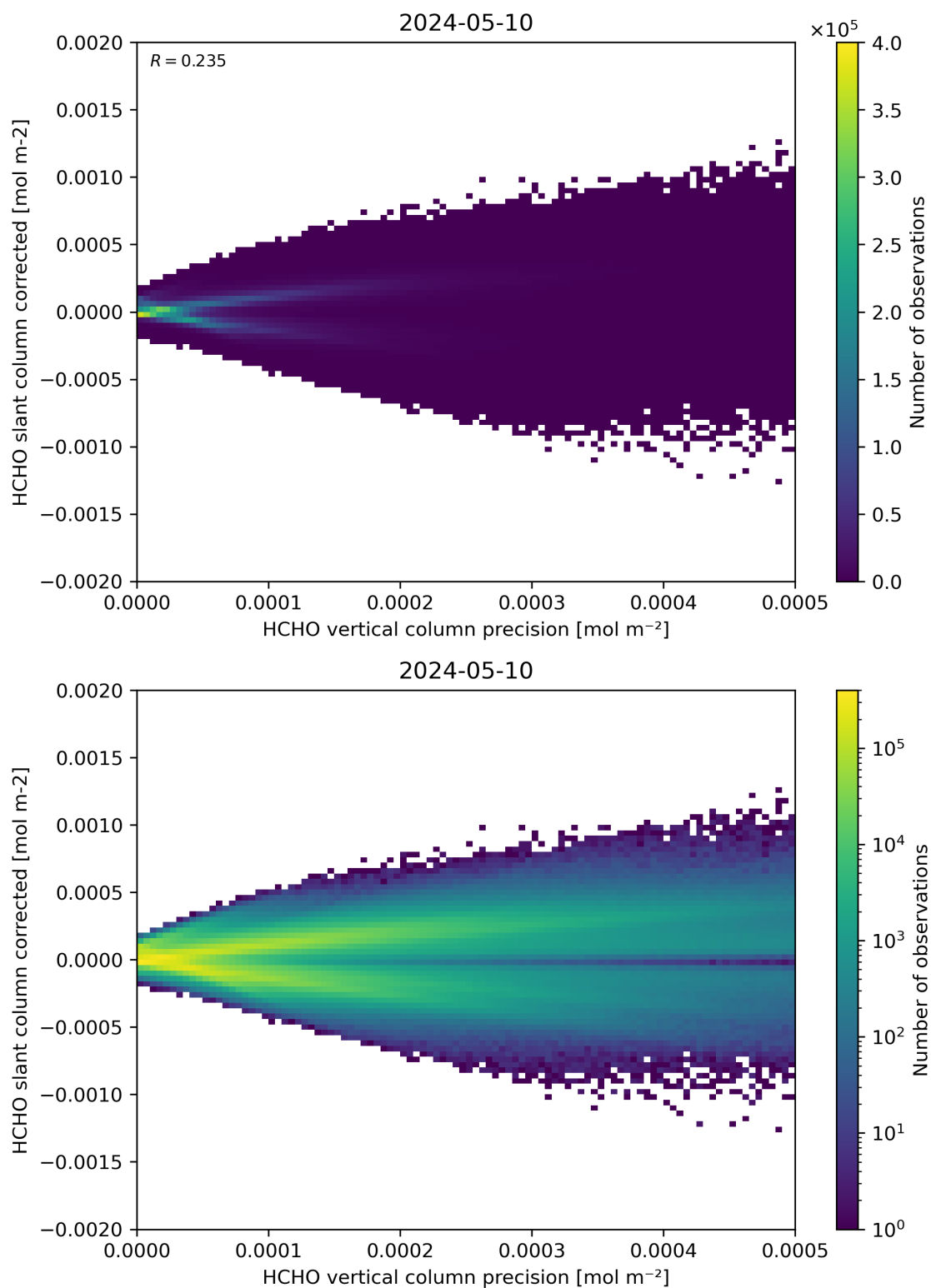
Figure 140: Scatter density plot of “HCHO vertical column precision” against “HCHO slant column corrected” for 2024-05-09 to 2024-05-11.
