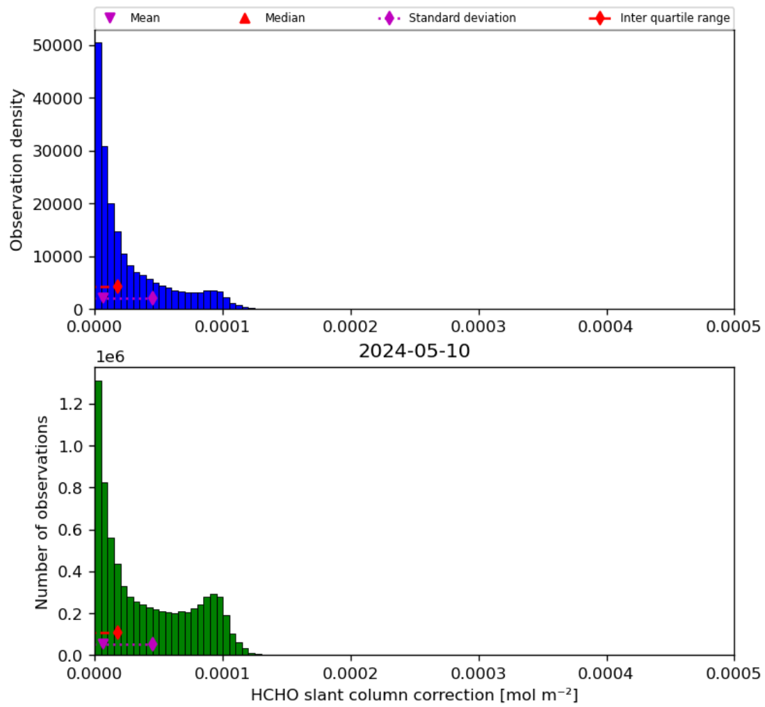
Figure 47: Histogram of “HCHO slant column correction” for 2024-05-09 to 2024-05-11
