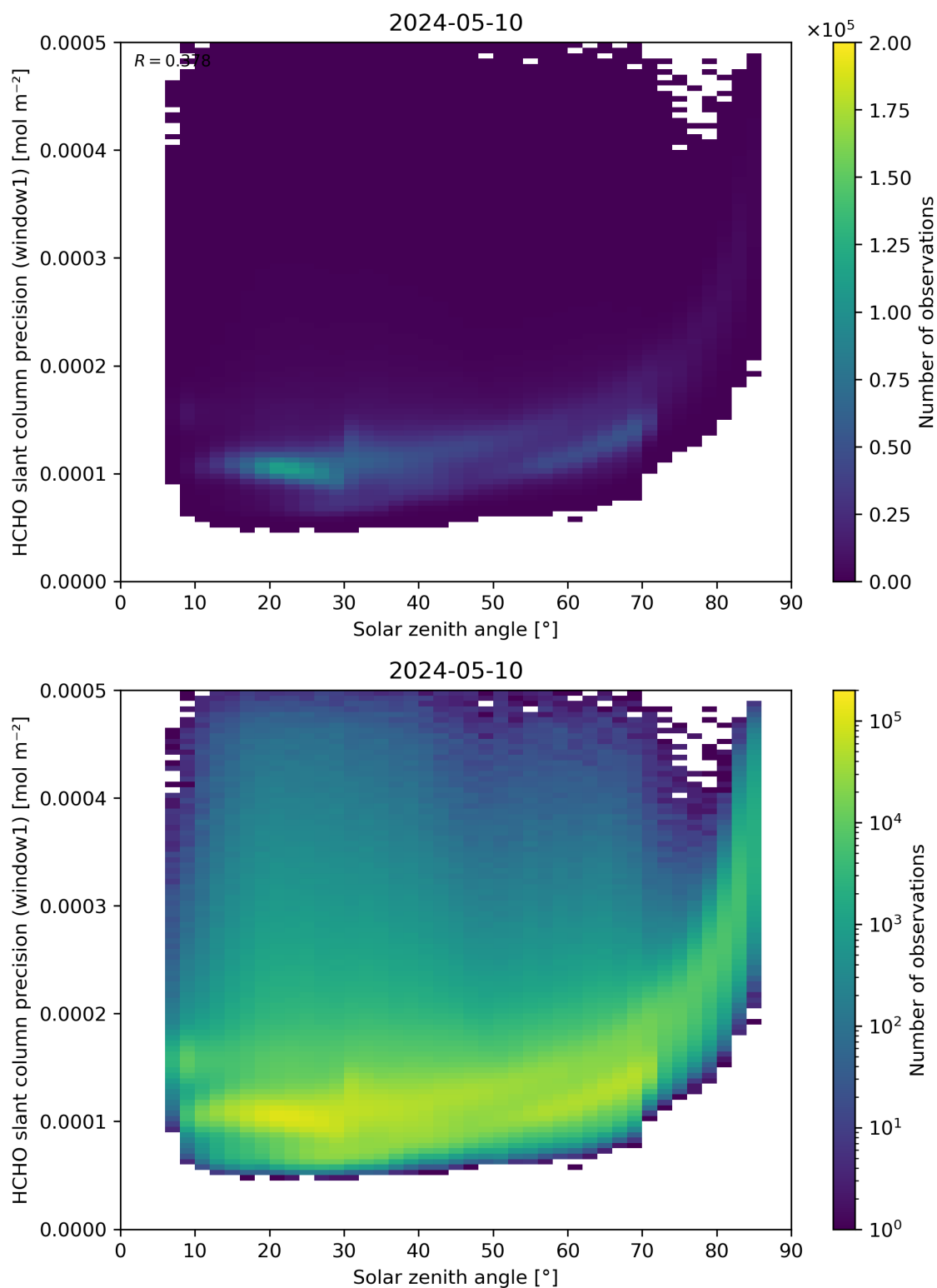
Figure 174: Scatter density plot of “Solar zenith angle” against “HCHO slant column precision (window1)” for 2024-05-09 to 2024-05-11.
