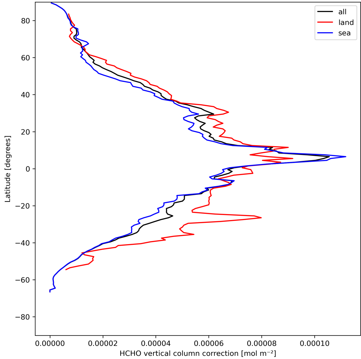
Figure 23: Zonal average of “HCHO vertical column correction” for 2024-05-09 to 2024-05-11.
