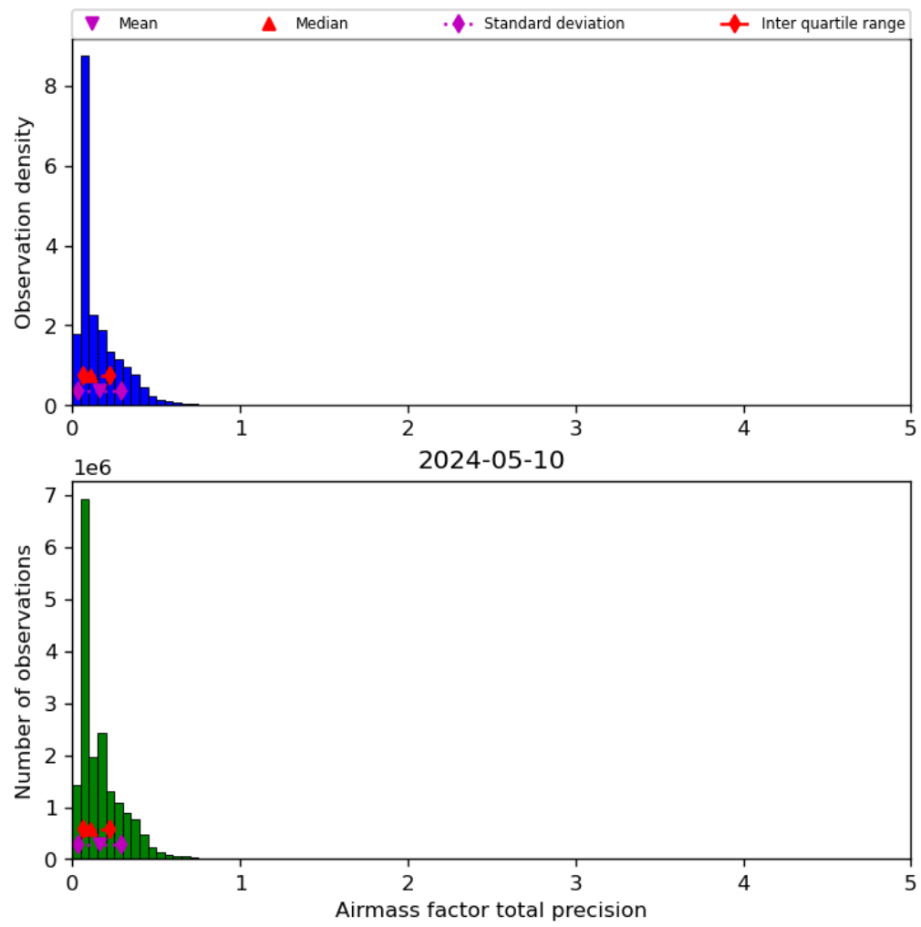
Figure 41: Histogram of “Airmass factor total precision” for 2024-05-09 to 2024-05-11
