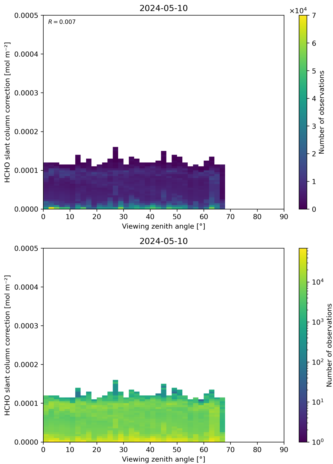
Figure 187: Scatter density plot of “Viewing zenith angle” against “HCHO slant column correction” for 2024-05-09 to 2024-05-11.
