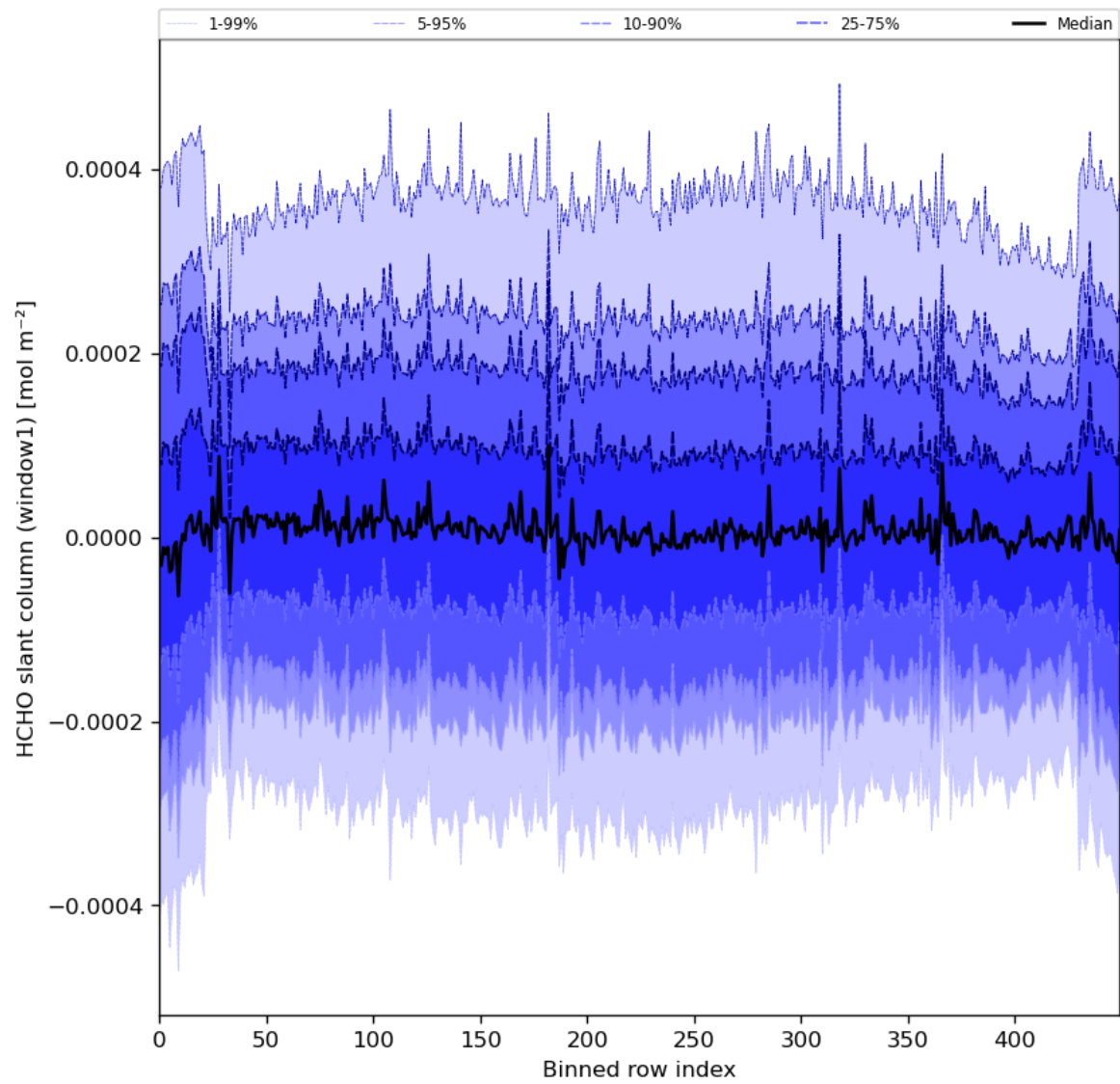
Figure 52: Along track statistics of "HCHO slant column (window1)" for 2024-05-09 to 2024-05-11
