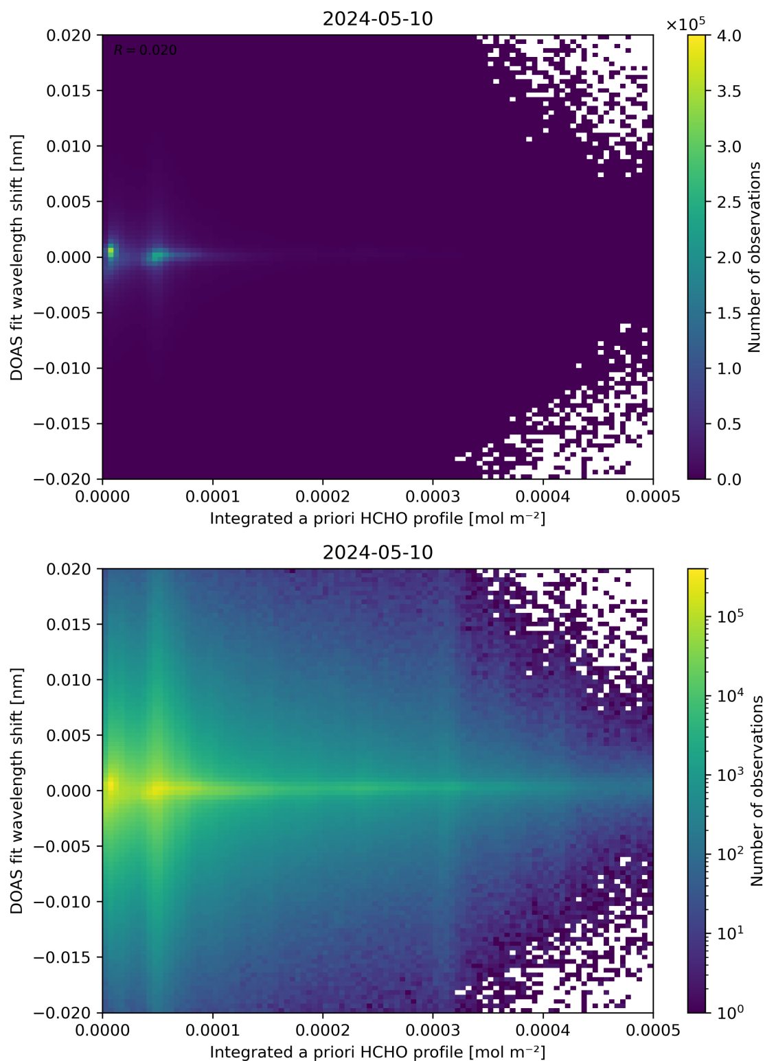
Figure 149: Scatter density plot of “Integrated a priori HCHO profile” against “DOAS fit wavelength shift” for 2024-05-09 to 2024-05-11.
