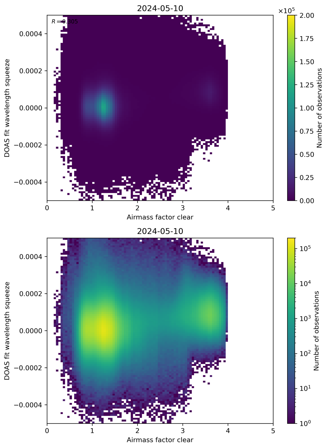
Figure 73: Scatter density plot of “Airmass factor clear” against “DOAS fit wavelength squeeze” for 2024-05-09 to 2024-05-11.
