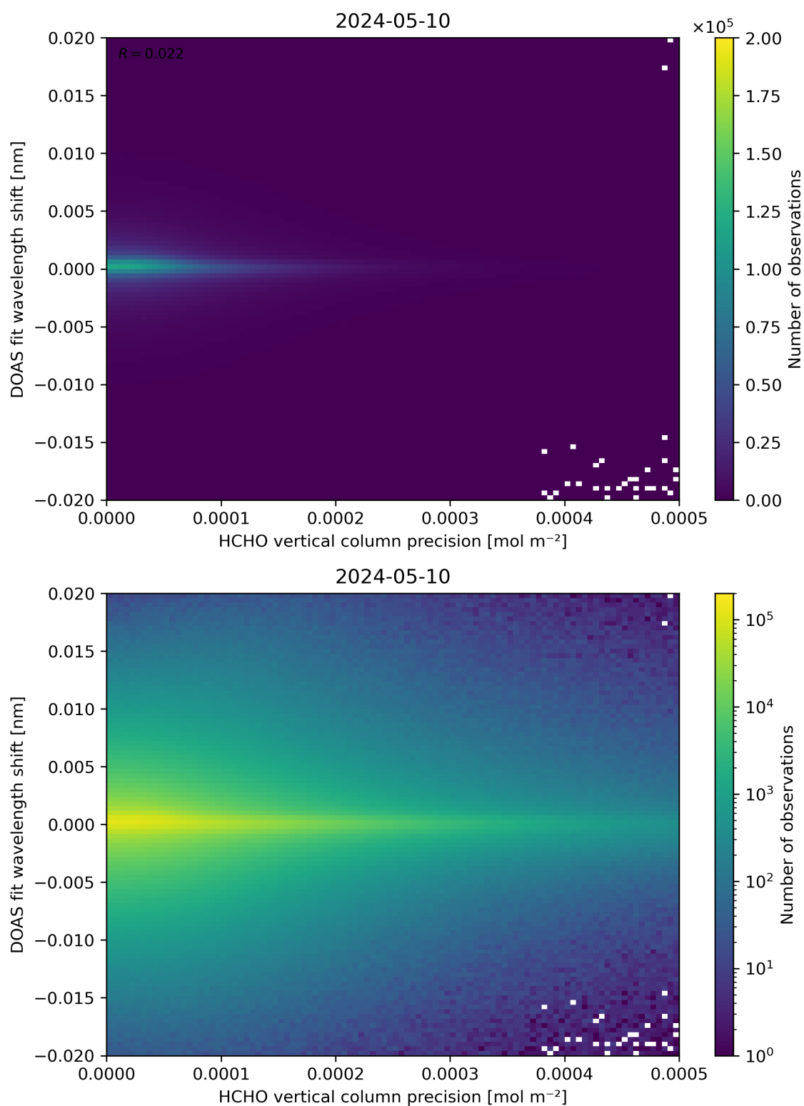
Figure 137: Scatter density plot of “HCHO vertical column precision” against “DOAS fit wavelength shift” for 2024-05-09 to 2024-05-11.
