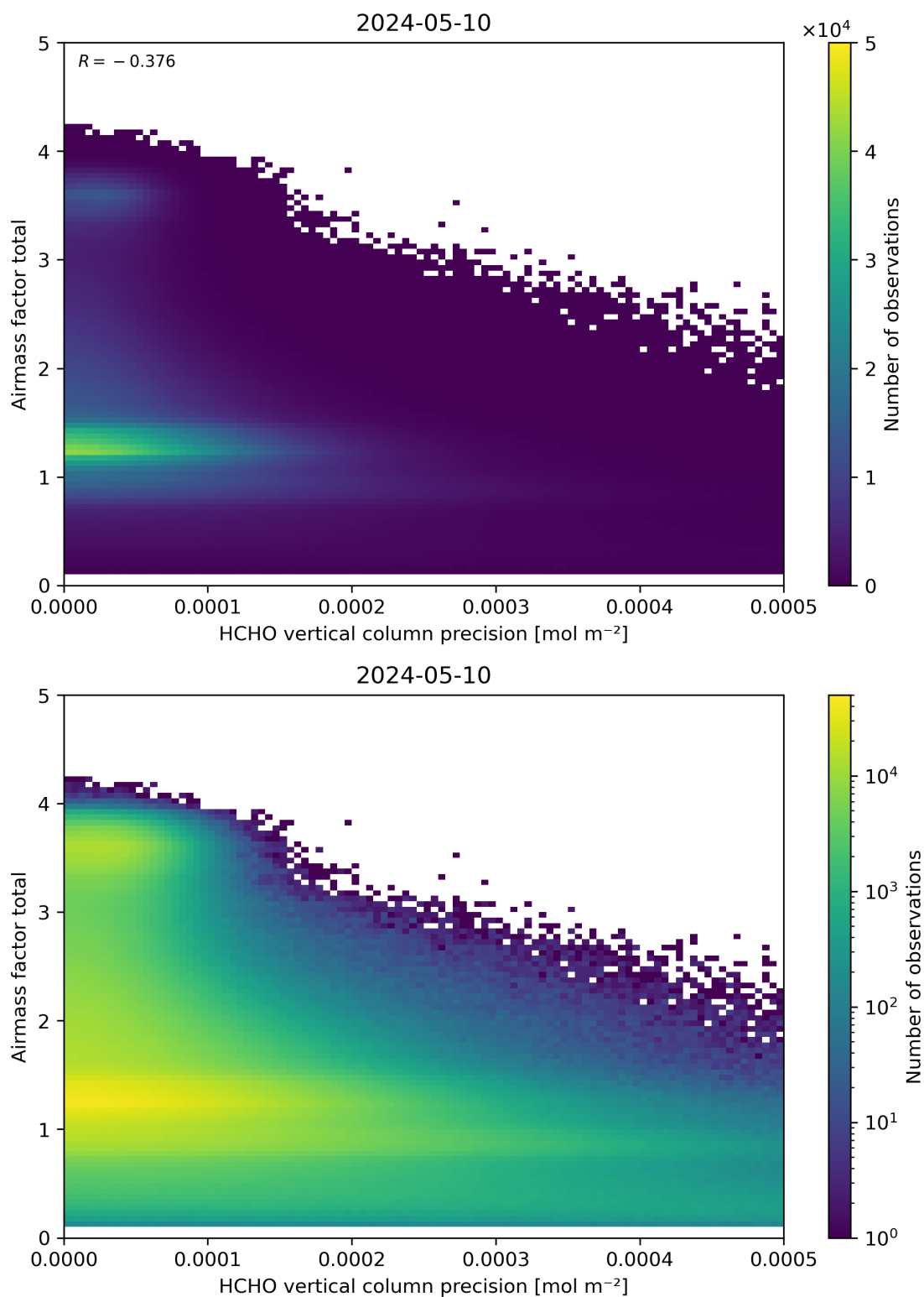
Figure 144: Scatter density plot of “HCHO vertical column precision” against “Airmass factor total” for 2024-05-09 to 2024-05-11.
