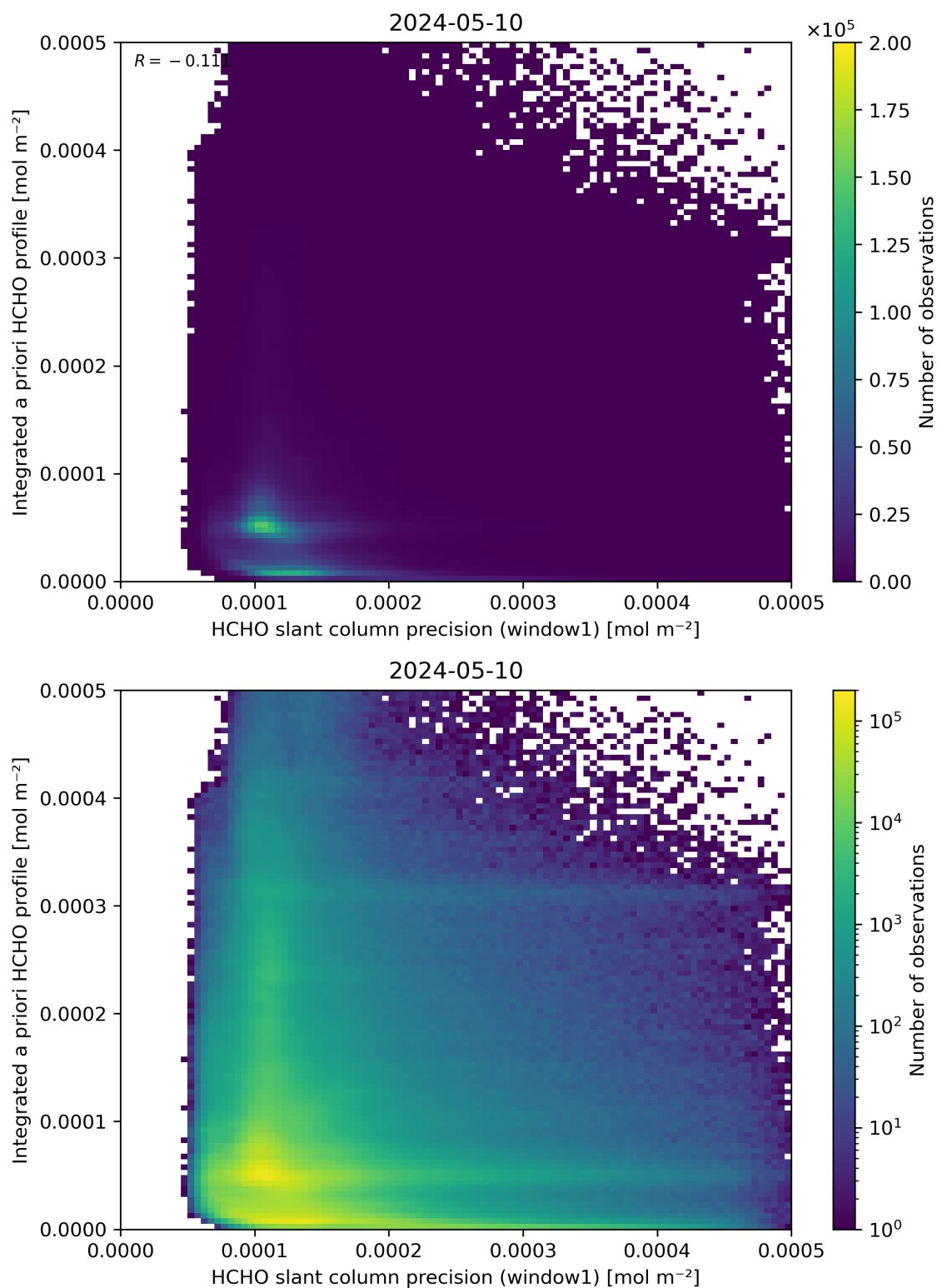
Figure 96: Scatter density plot of “HCHO slant column precision (window1)” against “Integrated a priori HCHO profile” for 2024-05-09 to 2024-05-11.
