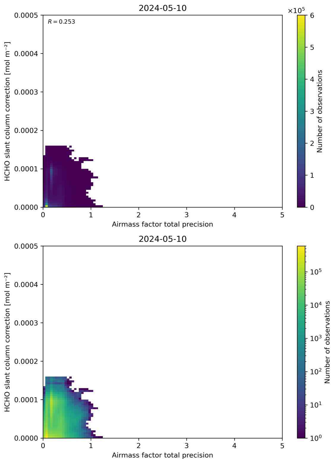
Figure 110: Scatter density plot of “Airmass factor total precision” against “HCHO slant column correction” for 2024-05-09 to 2024-05-11.
