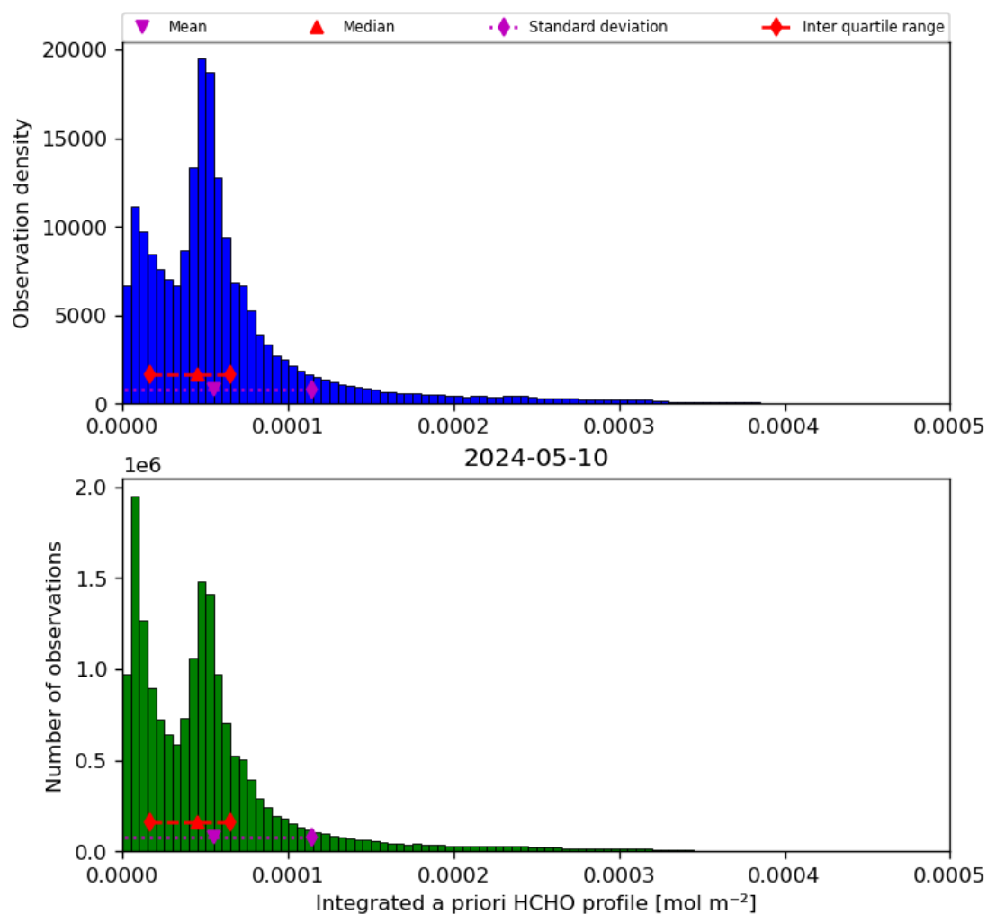
Figure 43: Histogram of “Integrated a priori HCHO profile” for 2024-05-09 to 2024-05-11
