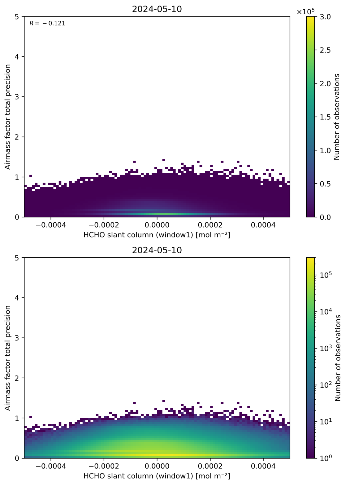
Figure 86: Scatter density plot of “HCHO slant column (window1)” against “Airmass factor total precision” for 2024-05-09 to 2024-05-11.
