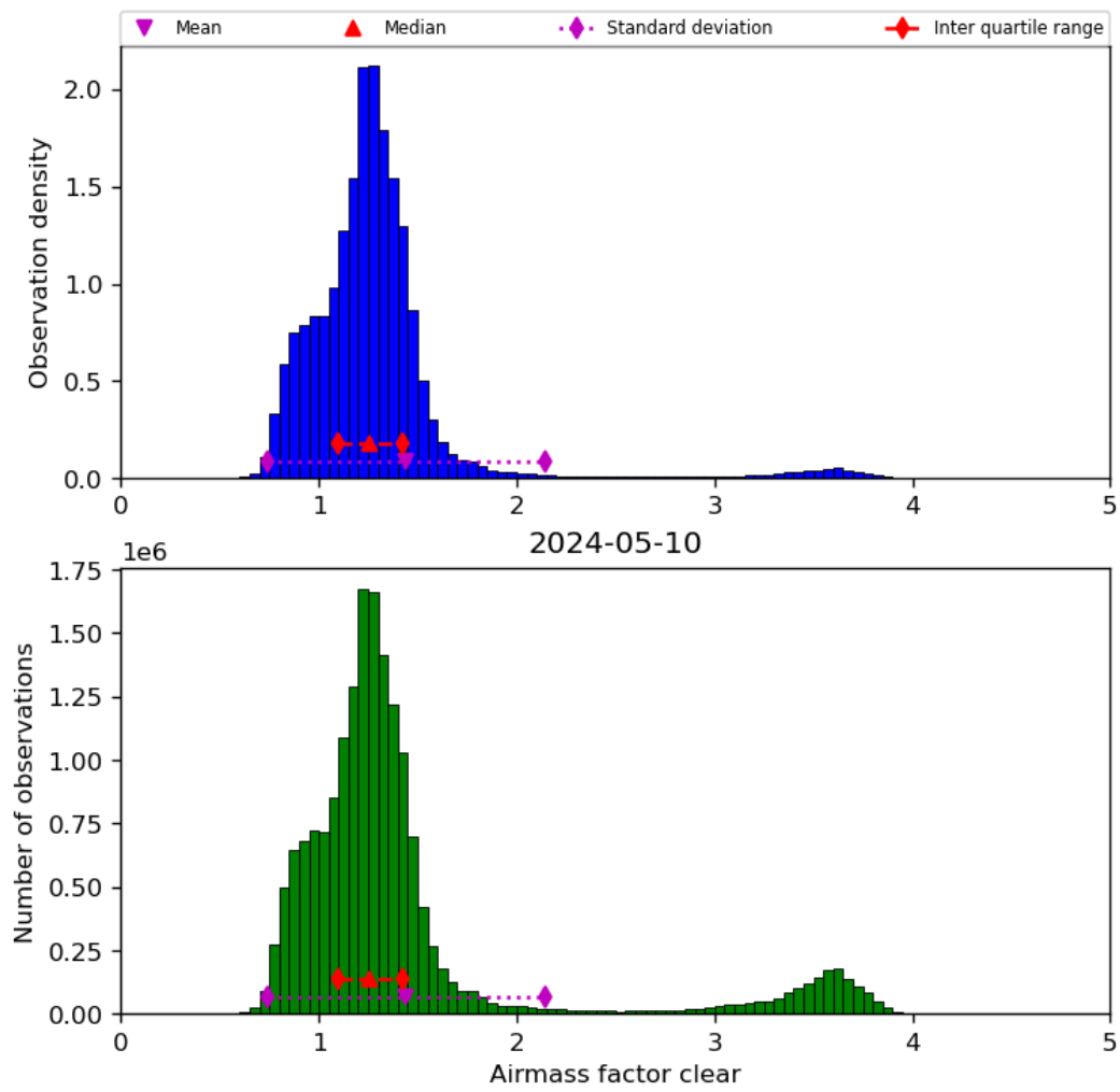
Figure 42: Histogram of “Airmass factor clear” for 2024-05-09 to 2024-05-11
