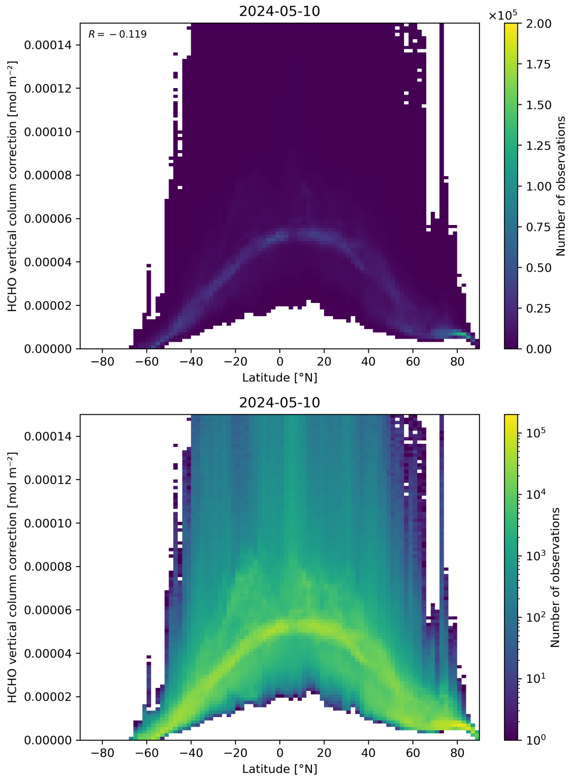
Figure 164: Scatter density plot of “Latitude” against “HCHO vertical column correction” for 2024-05-09 to 2024-05-11.
