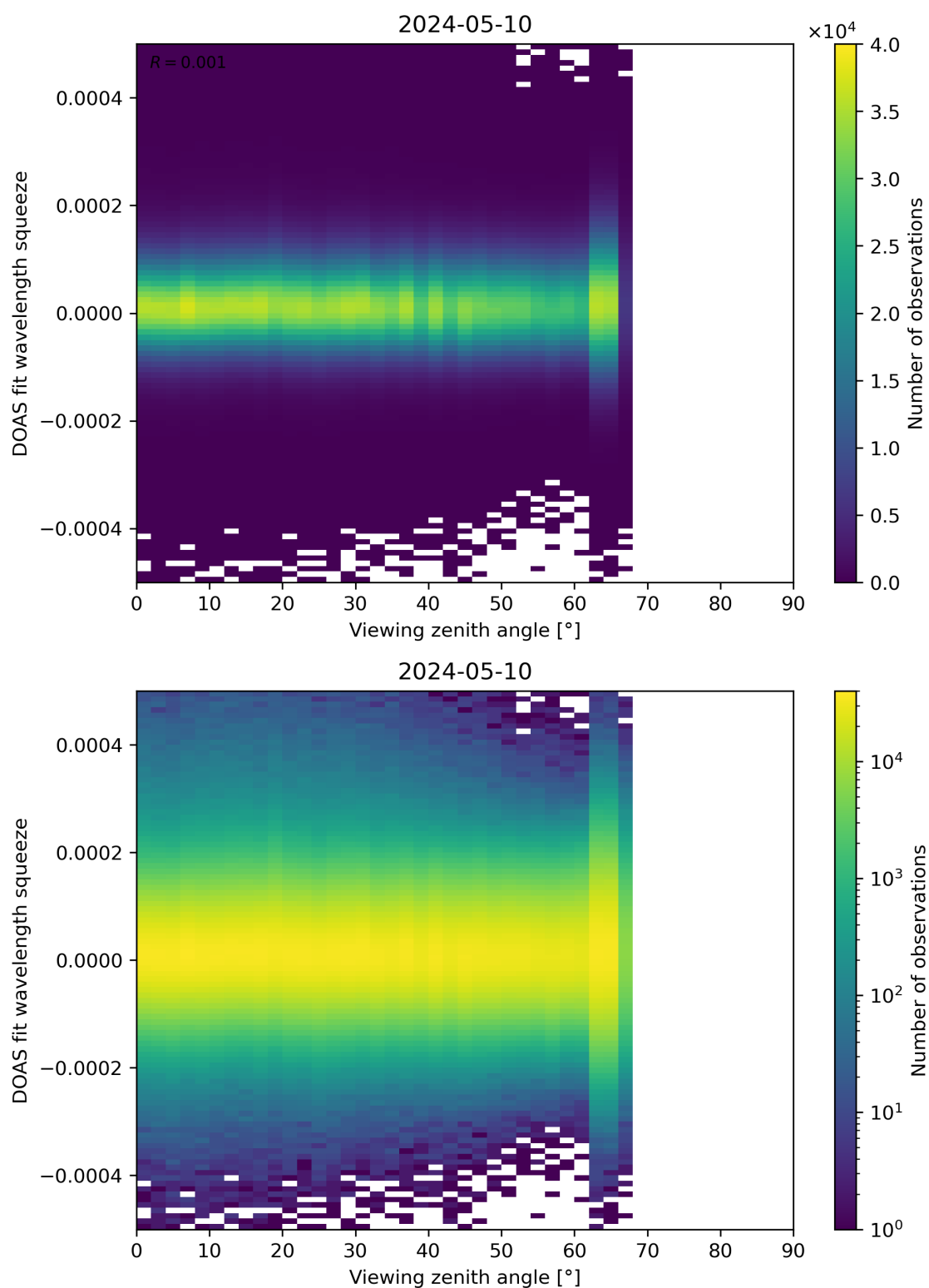
Figure 184: Scatter density plot of “Viewing zenith angle” against “DOAS fit wavelength squeeze” for 2024-05-09 to 2024-05-11.
