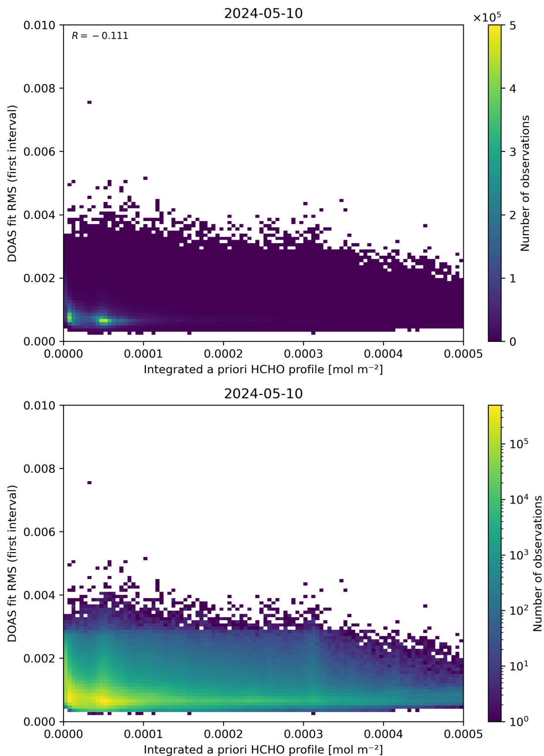
Figure 148: Scatter density plot of “Integrated a priori HCHO profile” against “DOAS fit RMS (first interval)” for 2024-05-09 to 2024-05-11.
