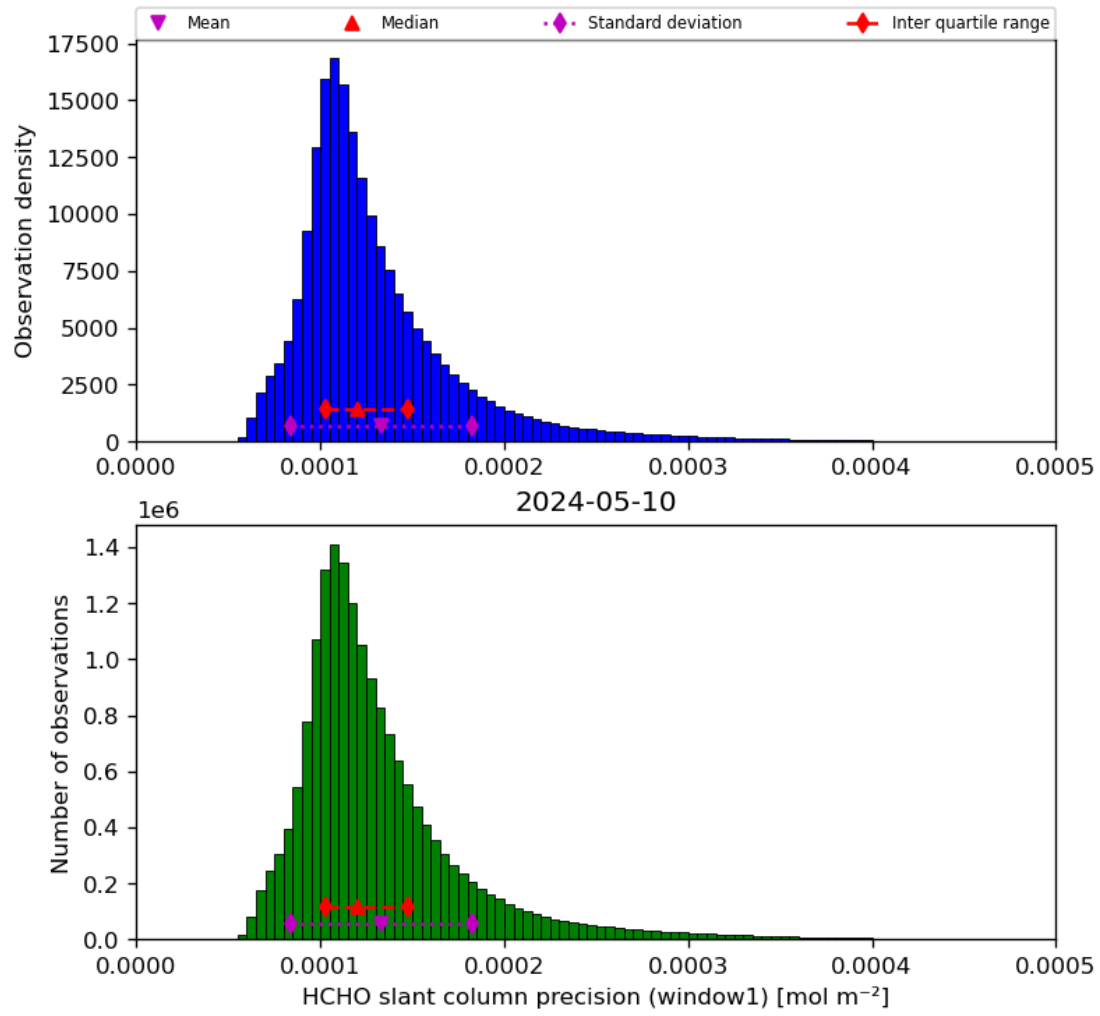
Figure 39: Histogram of “HCHO slant column precision (window1)” for 2024-05-09 to 2024-05-11
