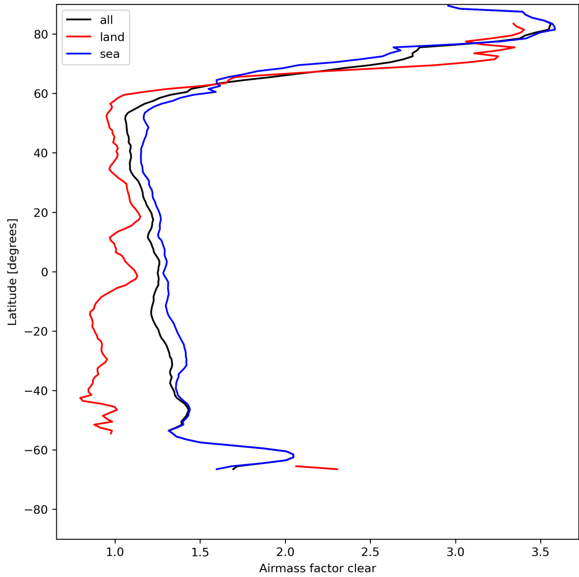
Figure 28: Zonal average of “Airmass factor clear” for 2024-05-09 to 2024-05-11.
