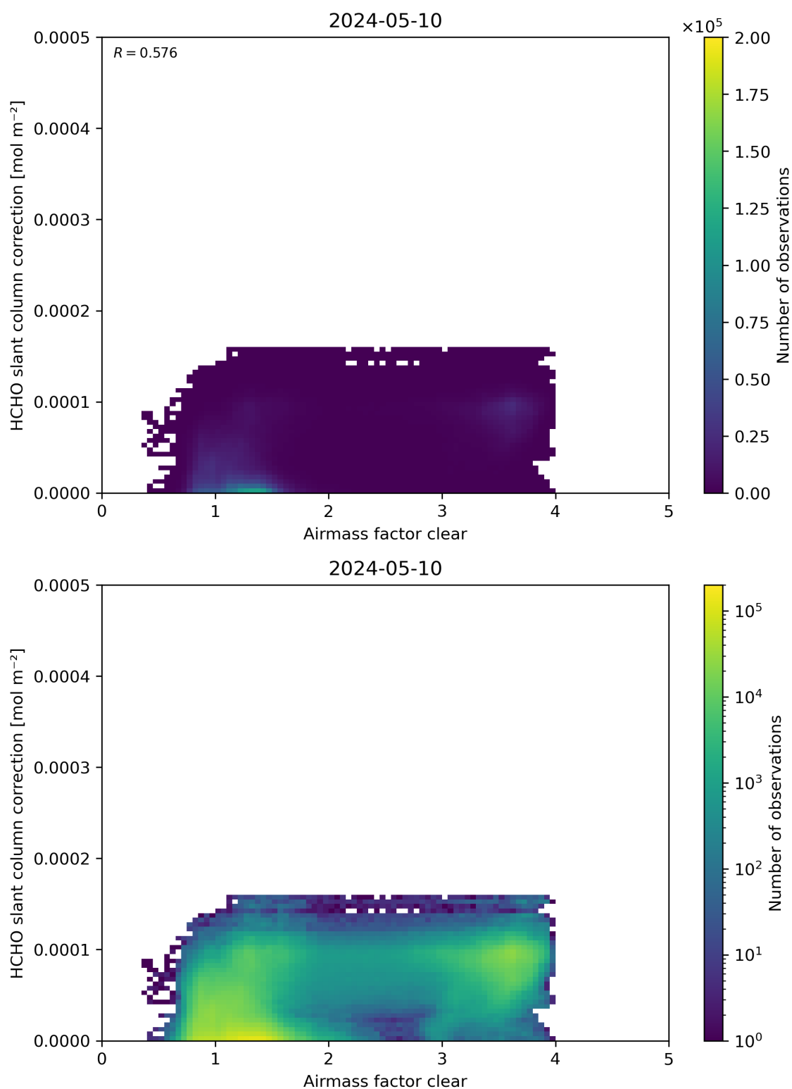
Figure 75: Scatter density plot of “Airmass factor clear” against “HCHO slant column correction” for 2024-05-09 to 2024-05-11.
