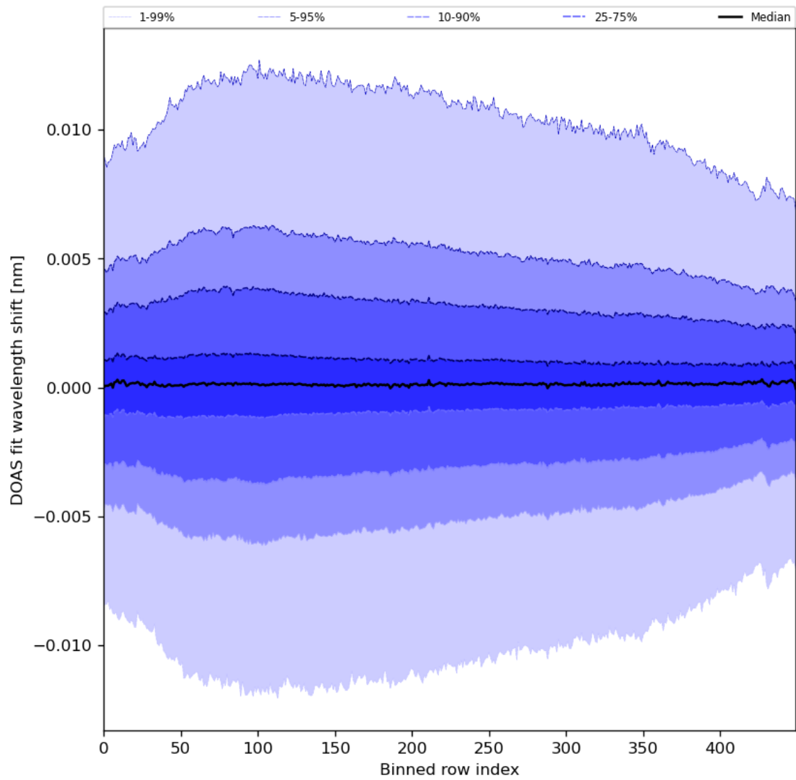
Figure 58: Along track statistics of “DOAS fit wavelength shift” for 2024-05-09 to 2024-05-11
