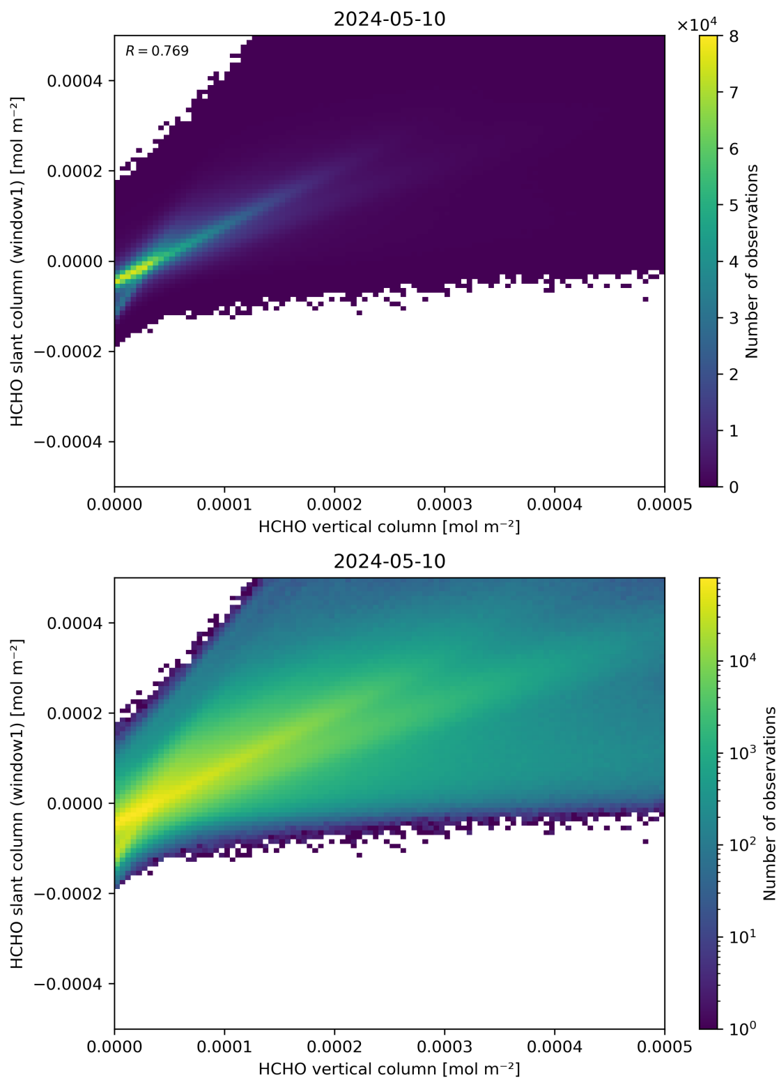
Figure 129: Scatter density plot of “HCHO vertical column” against “HCHO slant column (window1)” for 2024-05-09 to 2024-05-11.
