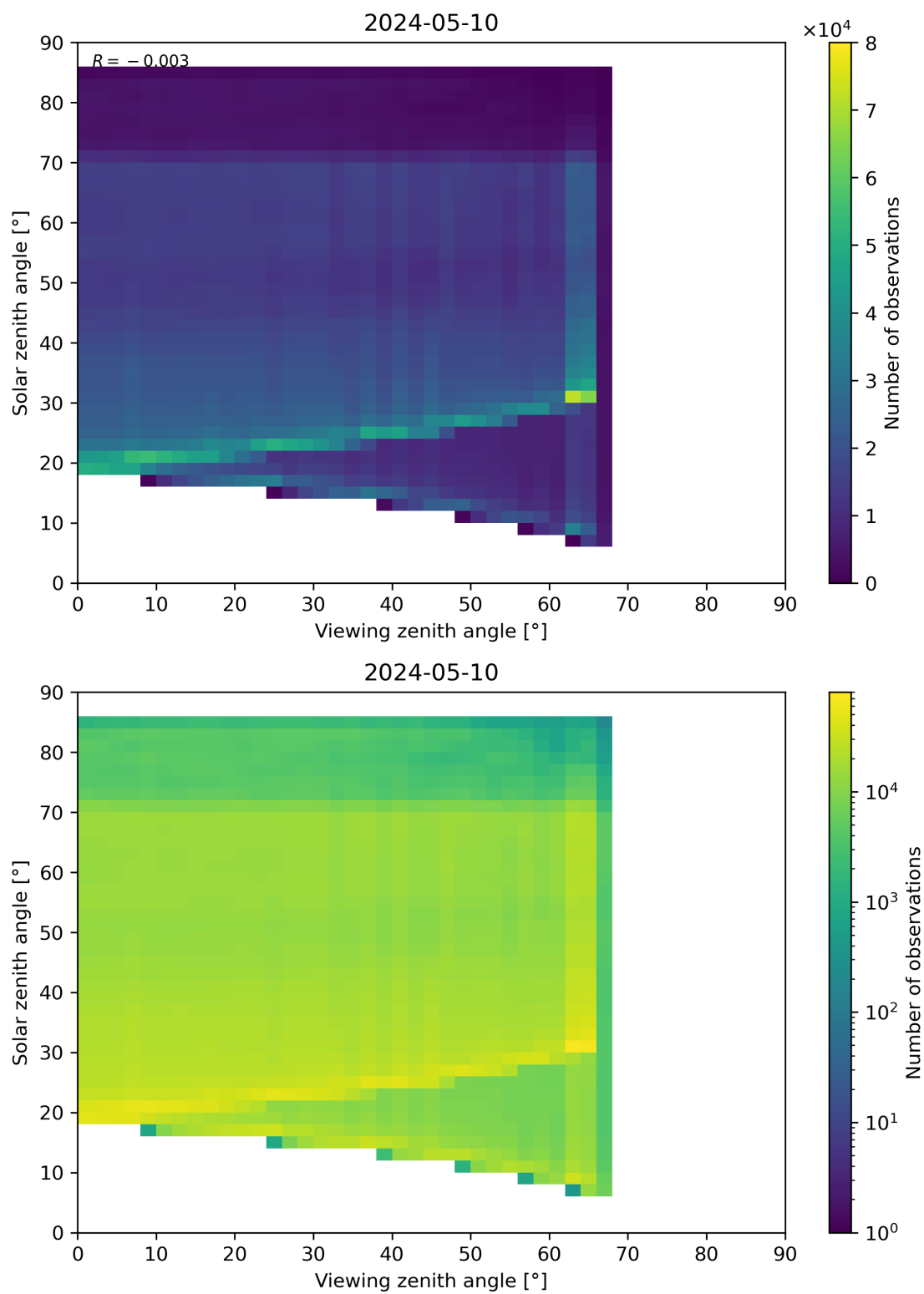
Figure 197: Scatter density plot of “Viewing zenith angle” against “Solar zenith angle” for 2024-05-09 to 2024-05-11.
