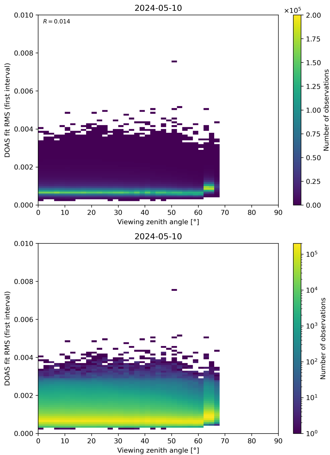
Figure 182: Scatter density plot of “Viewing zenith angle” against “DOAS fit RMS (first interval)” for 2024-05-09 to 2024-05-11.
