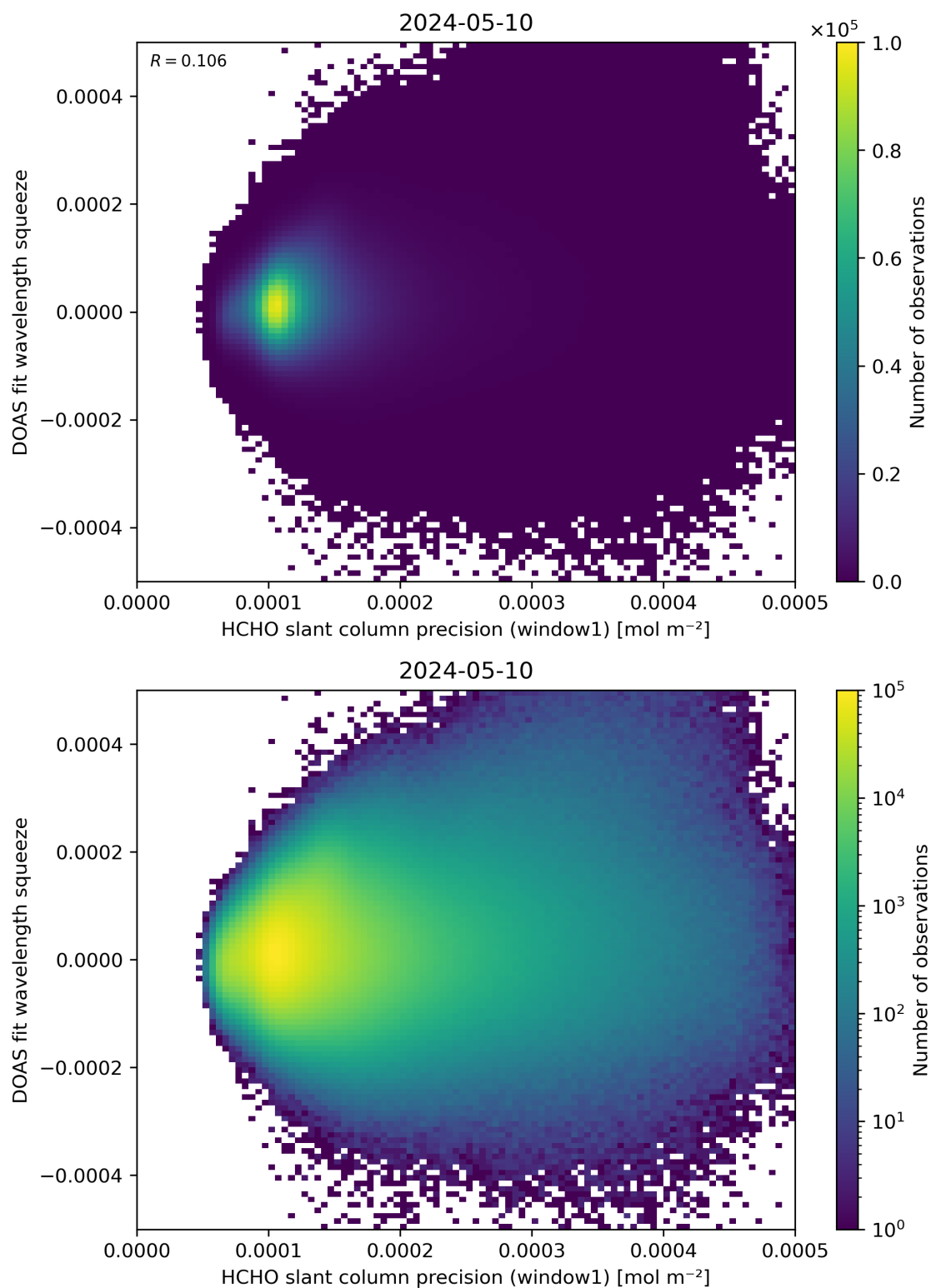
Figure 90: Scatter density plot of “HCHO slant column precision (window1)” against “DOAS fit wavelength squeeze” for 2024-05-09 to 2024-05-11.
