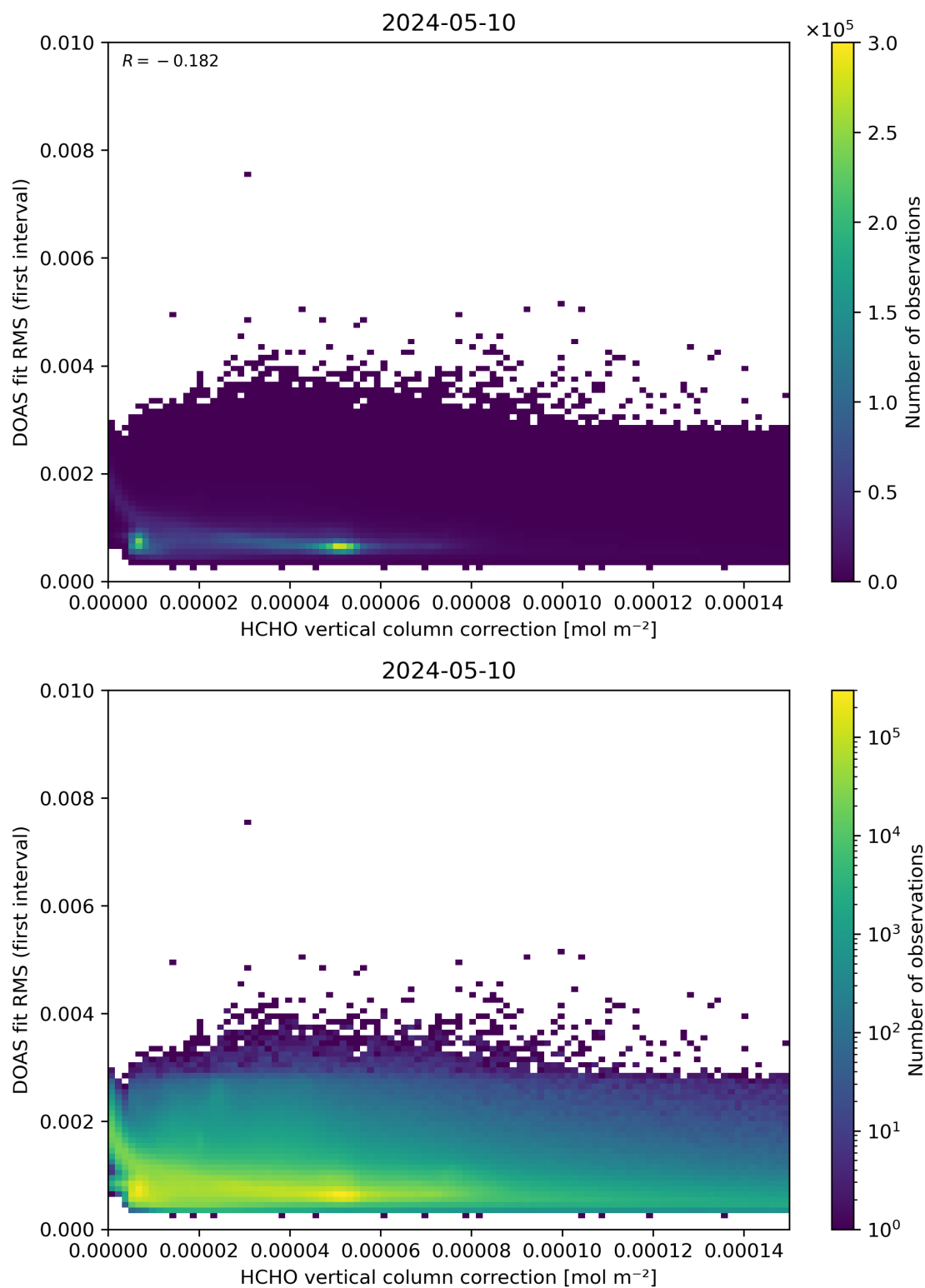
Figure 112: Scatter density plot of “HCHO vertical column correction” against “DOAS fit RMS (first interval)” for 2024-05-09 to 2024-05-11.
