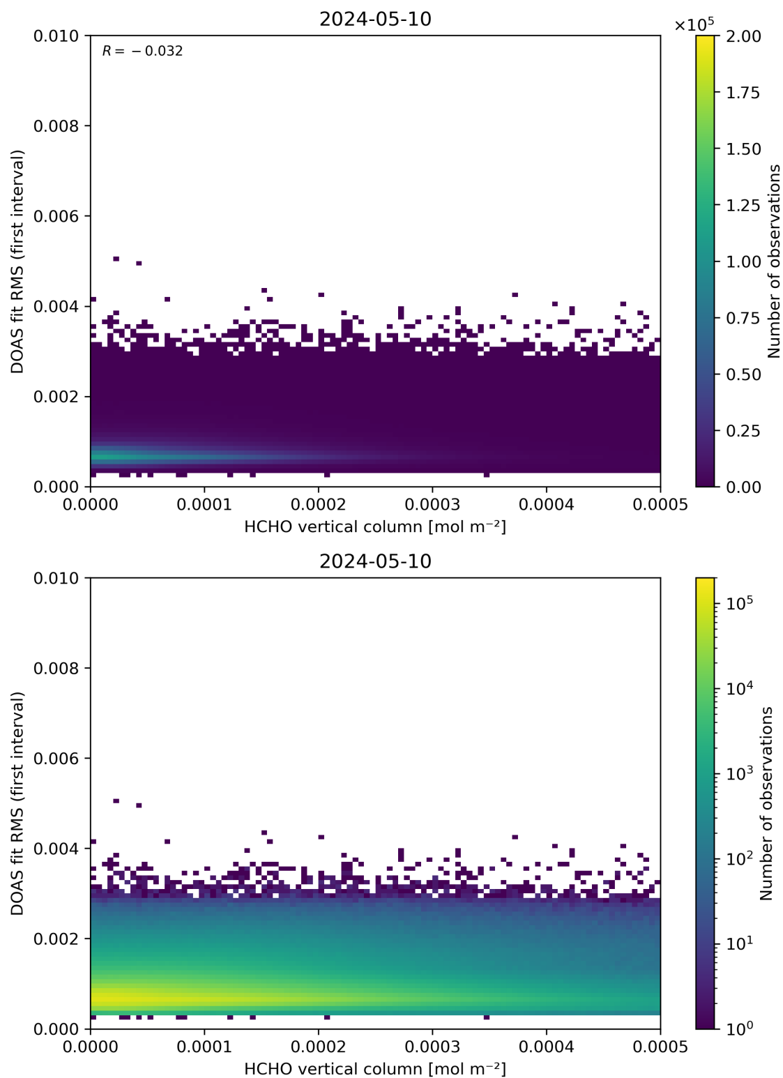
Figure 123: Scatter density plot of “HCHO vertical column” against “DOAS fit RMS (first interval)” for 2024-05-09 to 2024-05-11.
