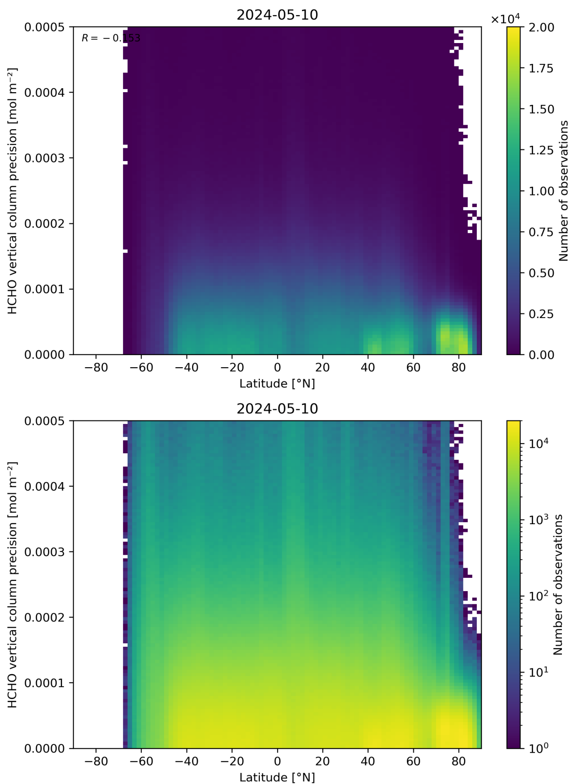
Figure 165: Scatter density plot of “Latitude” against “HCHO vertical column precision” for 2024-05-09 to 2024-05-11.
