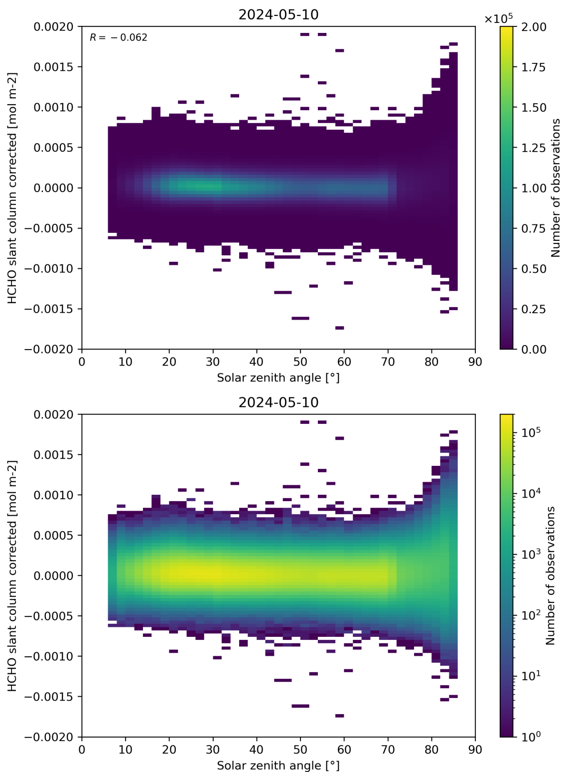
Figure 171: Scatter density plot of “Solar zenith angle” against “HCHO slant column corrected” for 2024-05-09 to 2024-05-11.
