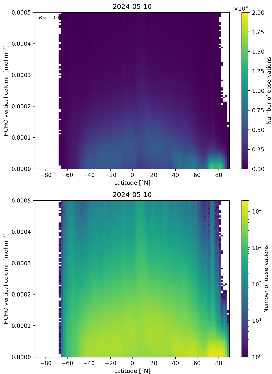
Figure 163: Scatter density plot of “Latitude” against “HCHO vertical column” for 2024-05-09 to 2024-05-11.
