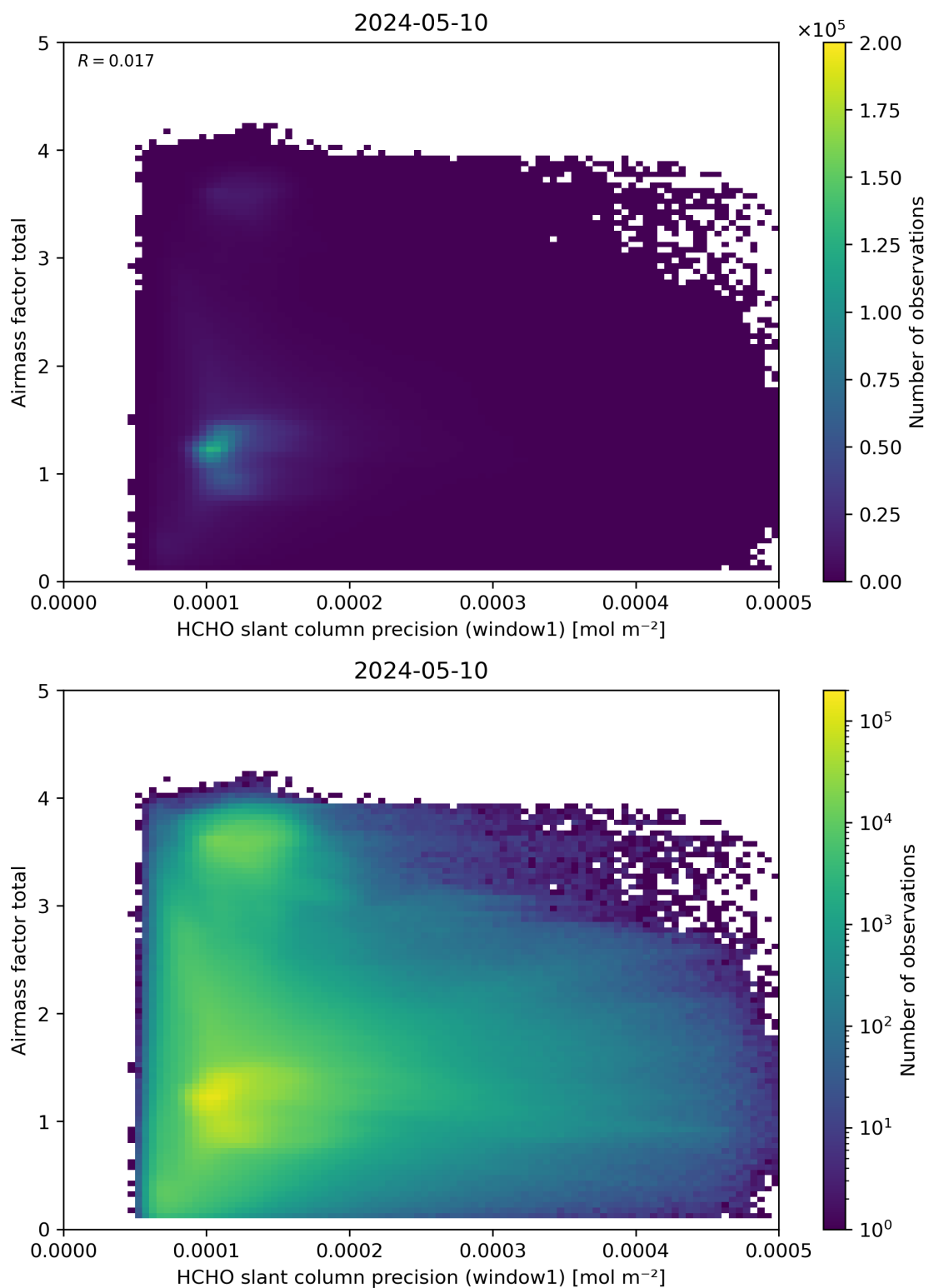
Figure 94: Scatter density plot of “HCHO slant column precision (window1)” against “Airmass factor total” for 2024-05-09 to 2024-05-11.
