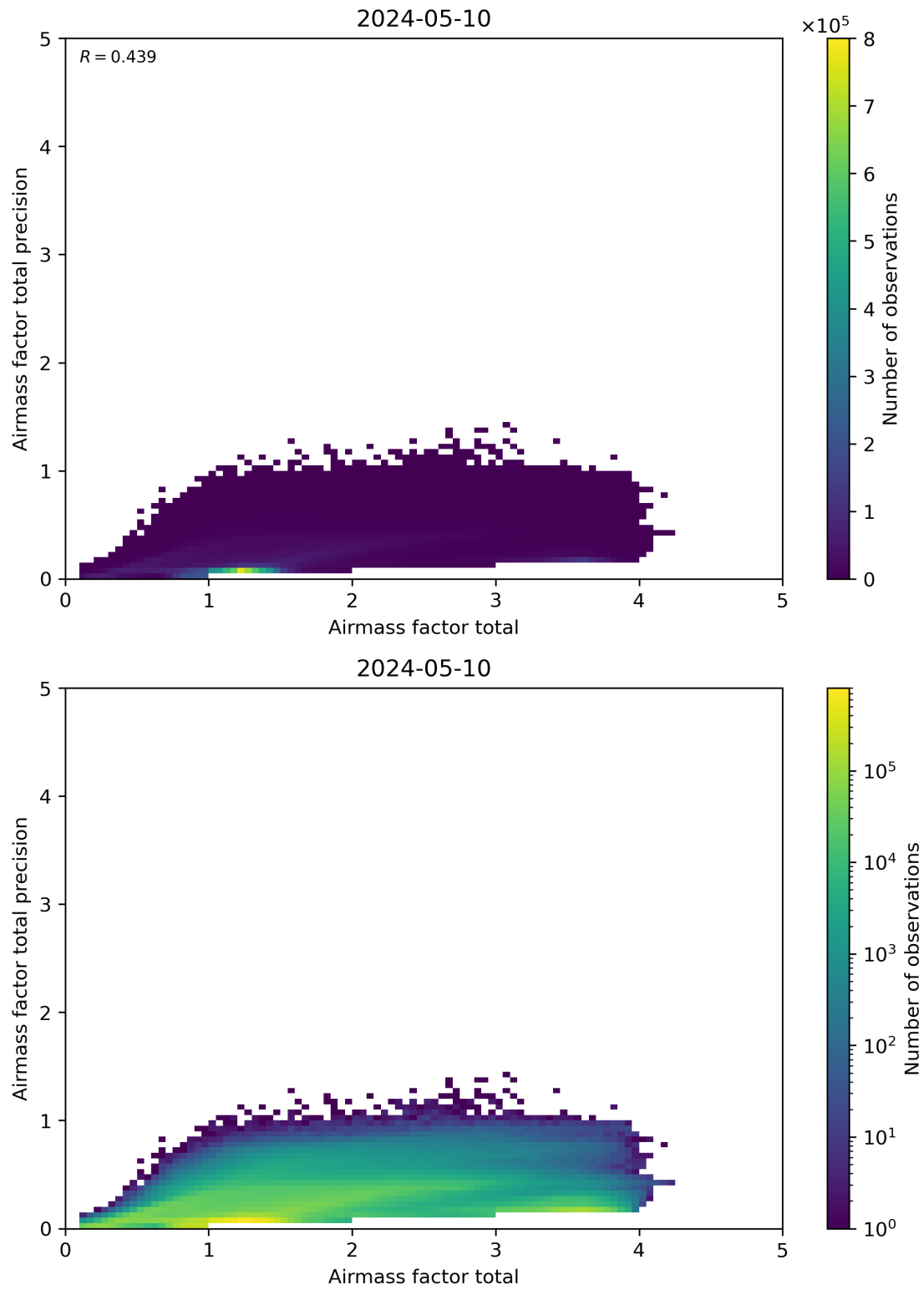
Figure 103: Scatter density plot of “Airmass factor total” against “Airmass factor total precision” for 2024-05-09 to 2024-05-11.
