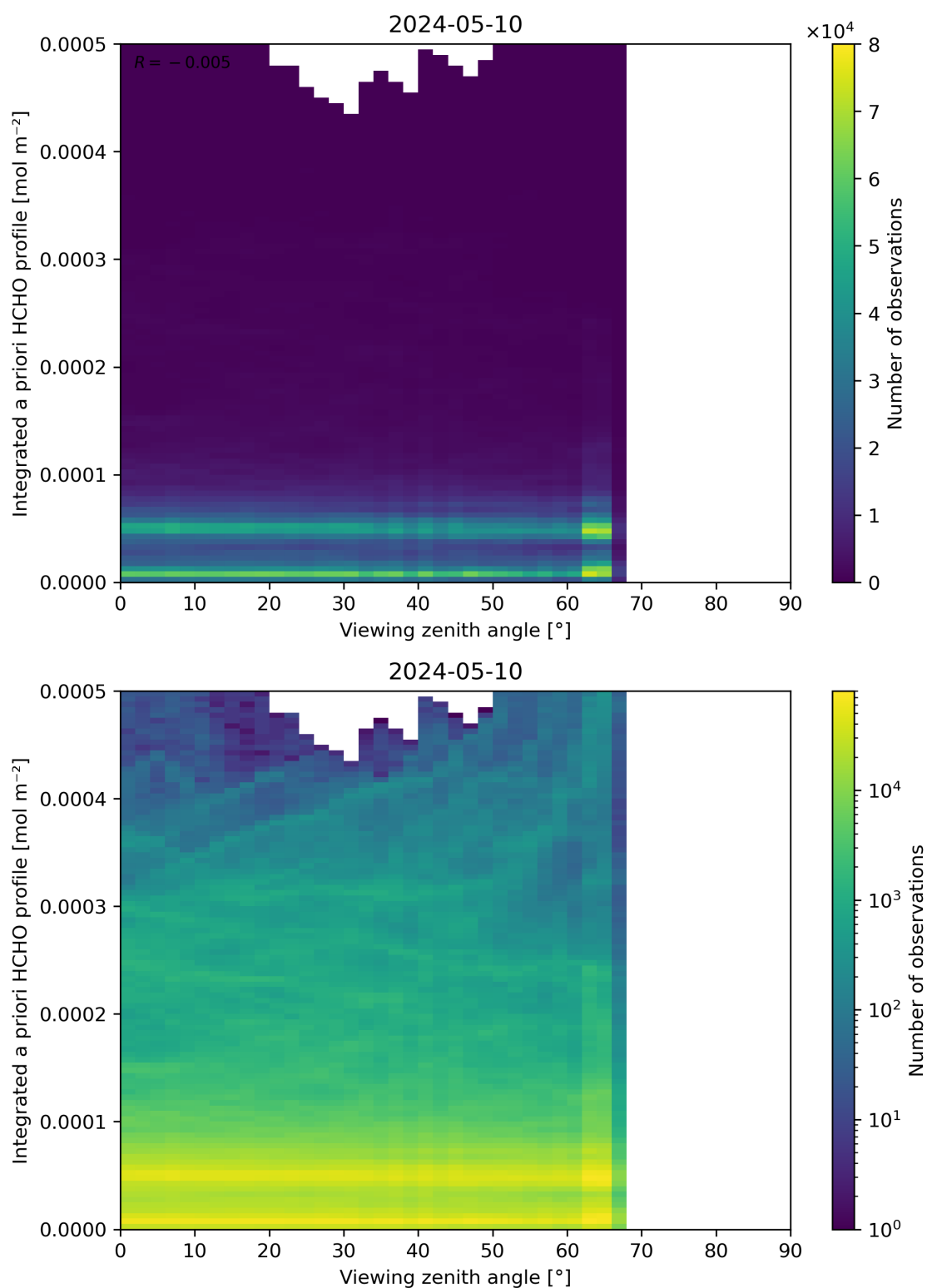
Figure 195: Scatter density plot of “Viewing zenith angle” against “Integrated a priori HCHO profile” for 2024-05-09 to 2024-05-11.
