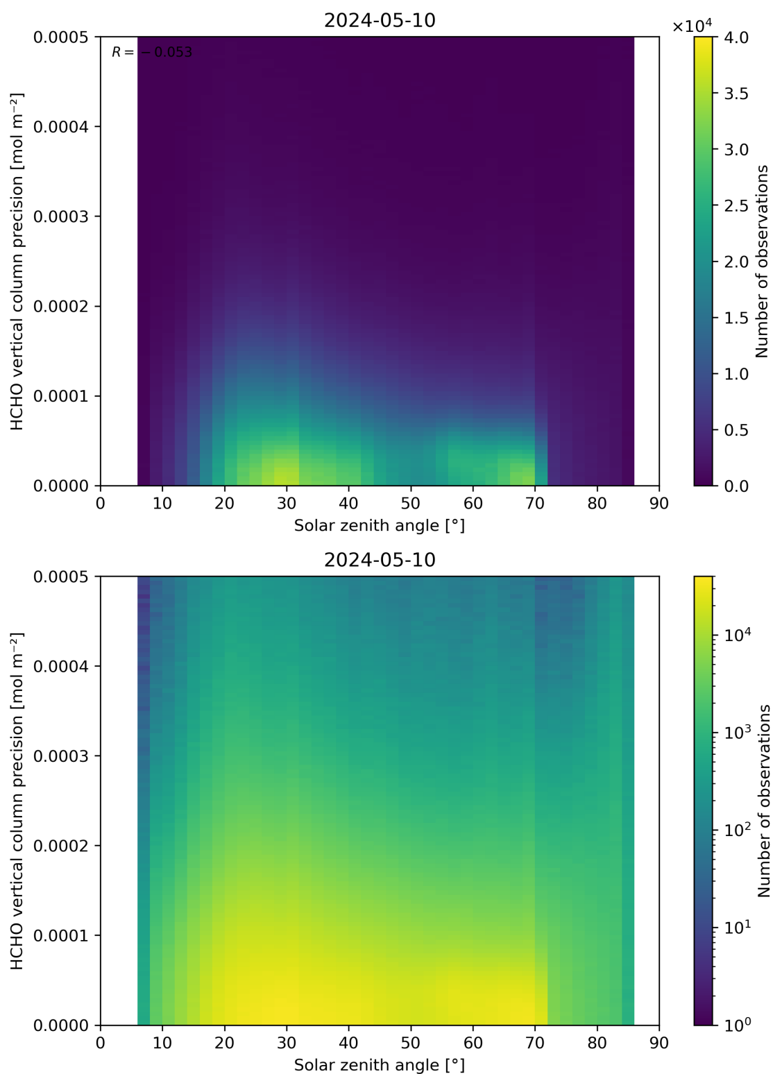
Figure 179: Scatter density plot of “Solar zenith angle” against “HCHO vertical column precision” for 2024-05-09 to 2024-05-11.
