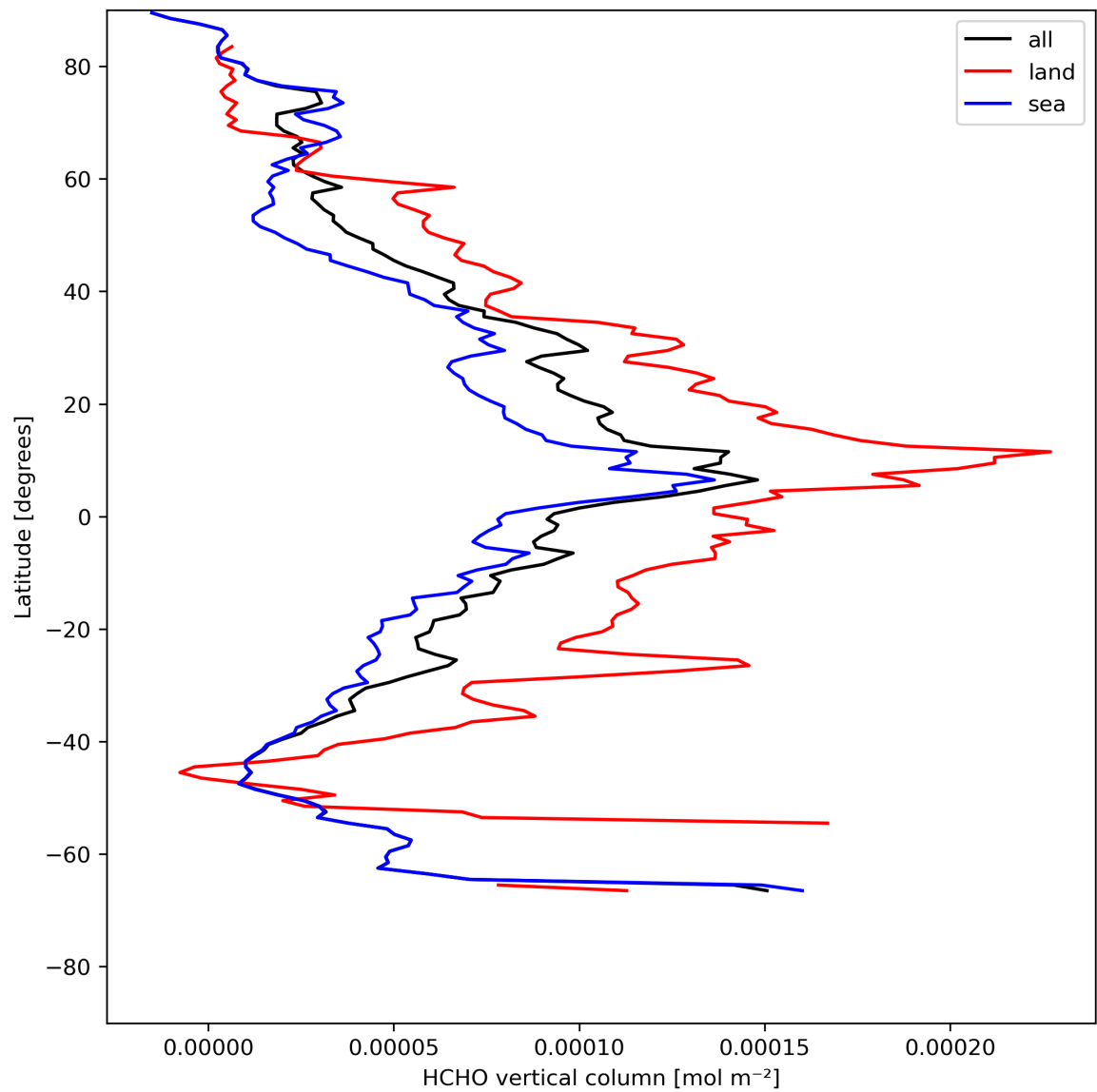
Figure 21: Zonal average of “HCHO vertical column” for 2024-05-09 to 2024-05-11.
