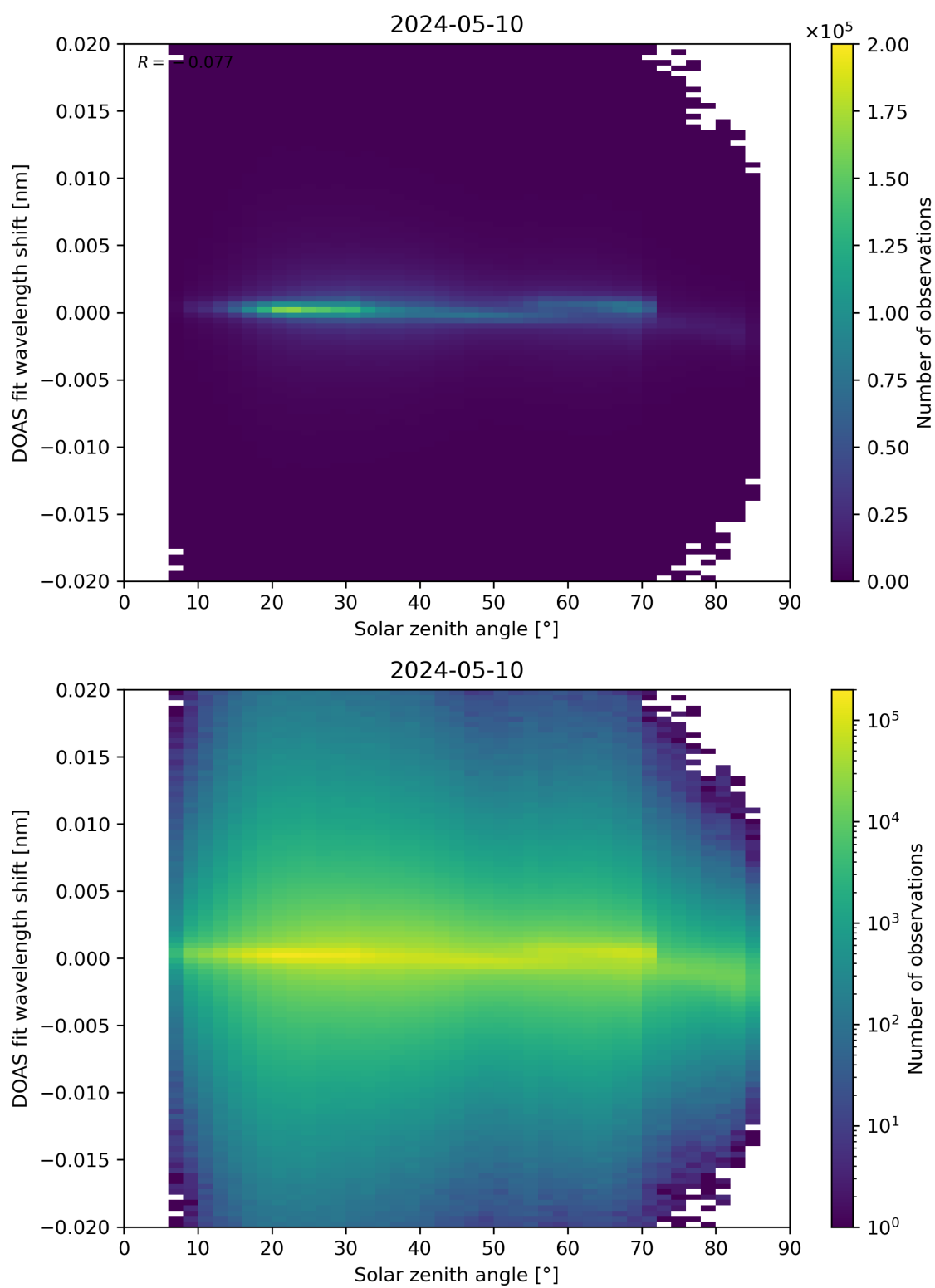
Figure 168: Scatter density plot of “Solar zenith angle” against “DOAS fit wavelength shift” for 2024-05-09 to 2024-05-11.
