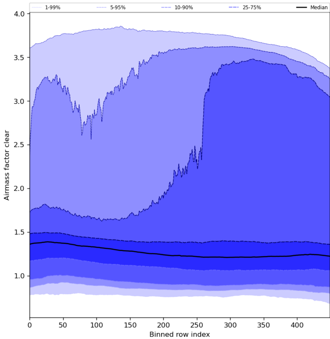
Figure 56: Along track statistics of “Airmass factor clear” for 2024-05-09 to 2024-05-11
