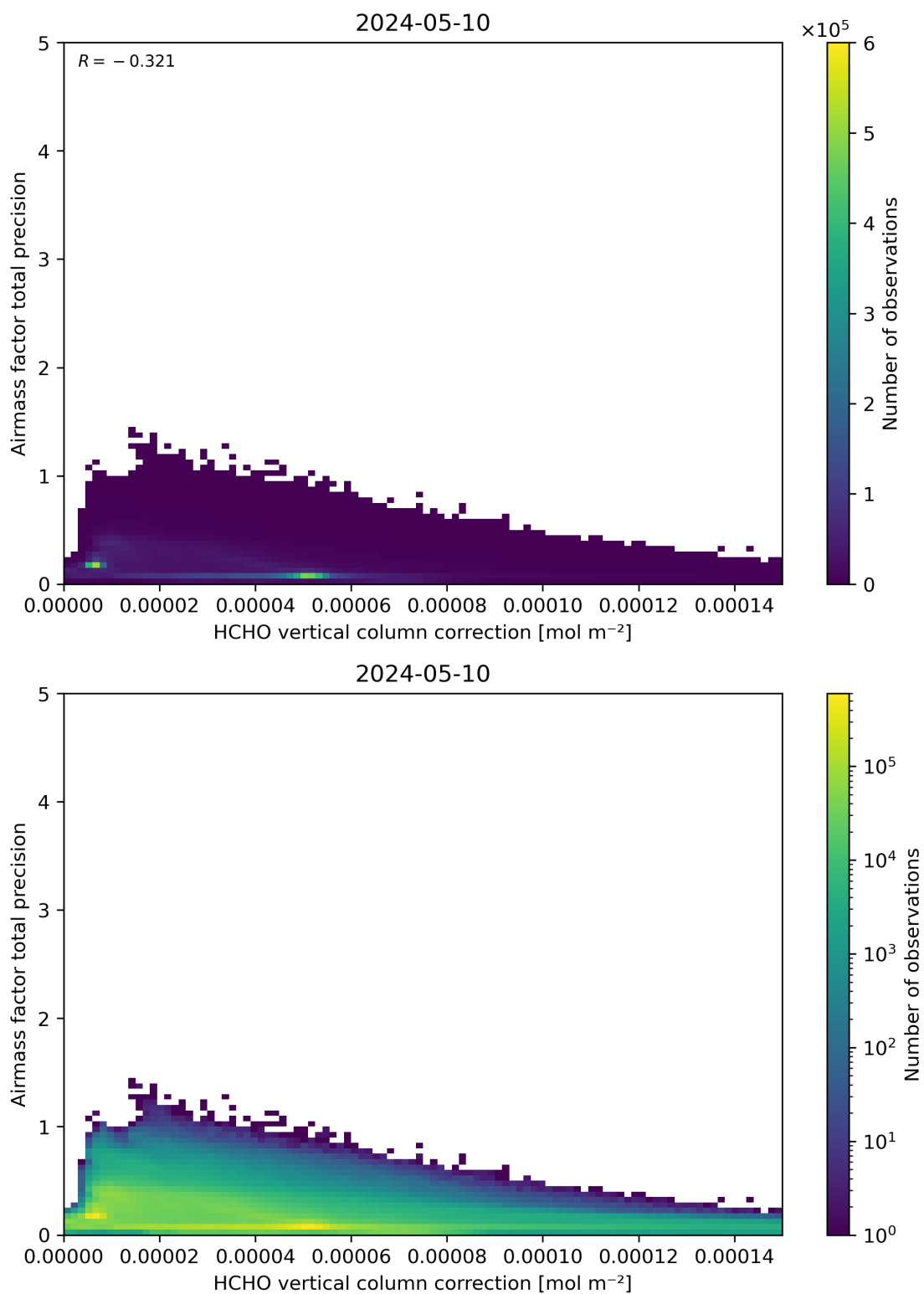
Figure 121: Scatter density plot of “HCHO vertical column correction” against “Airmass factor total precision” for 2024-05-09 to 2024-05-11.
