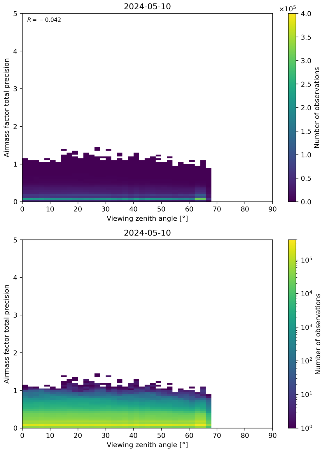
Figure 191: Scatter density plot of “Viewing zenith angle” against “Airmass factor total precision” for 2024-05-09 to 2024-05-11.
