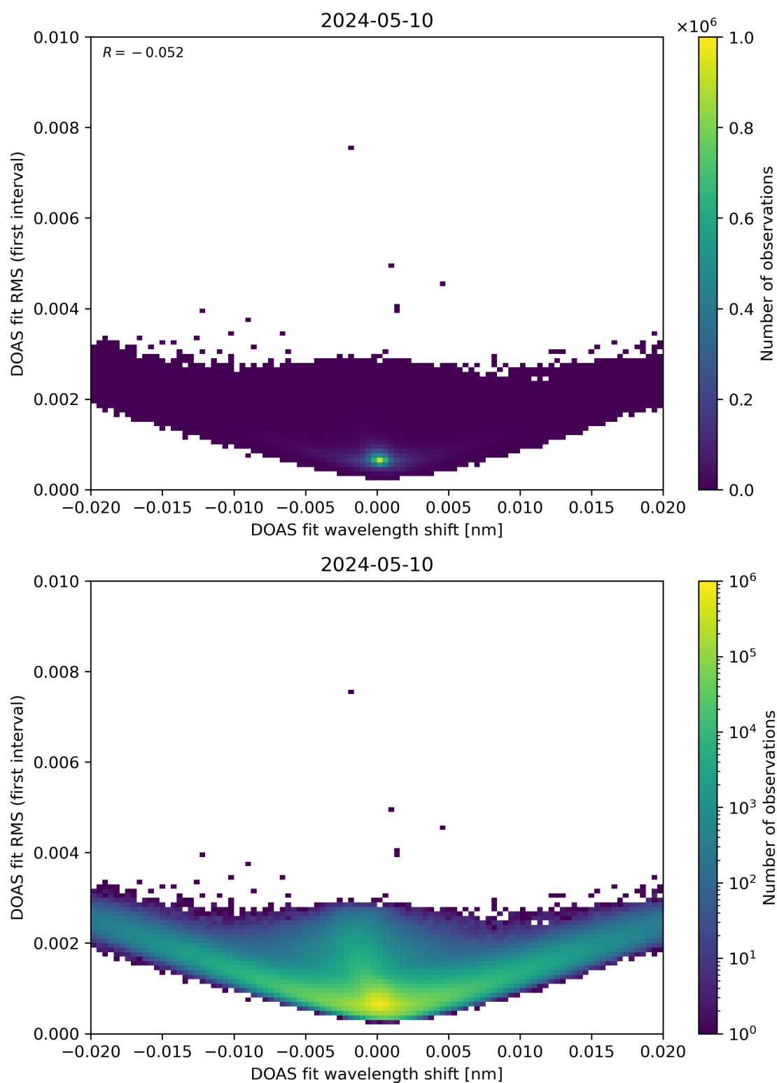
Figure 64: Scatter density plot of “DOAS fit wavelength shift” against “DOAS fit RMS (first interval)” for 2024-05-09 to 2024-05-11.
