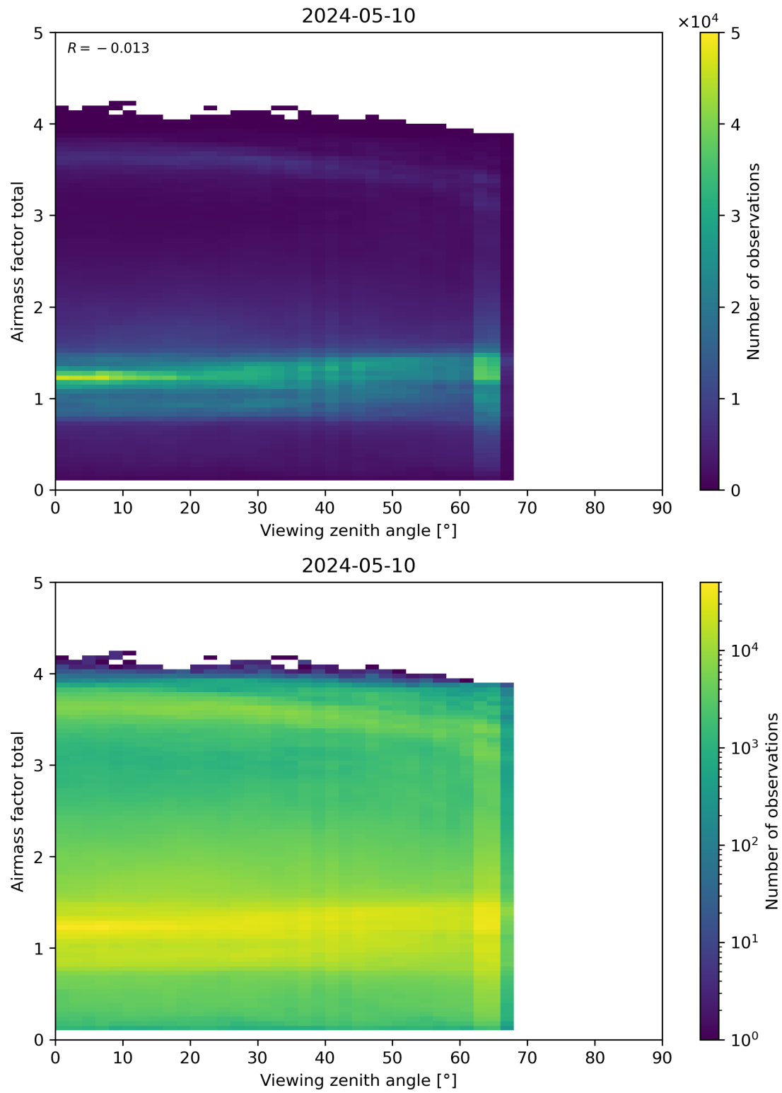
Figure 190: Scatter density plot of “Viewing zenith angle” against “Airmass factor total” for 2024-05-09 to 2024-05-11.
