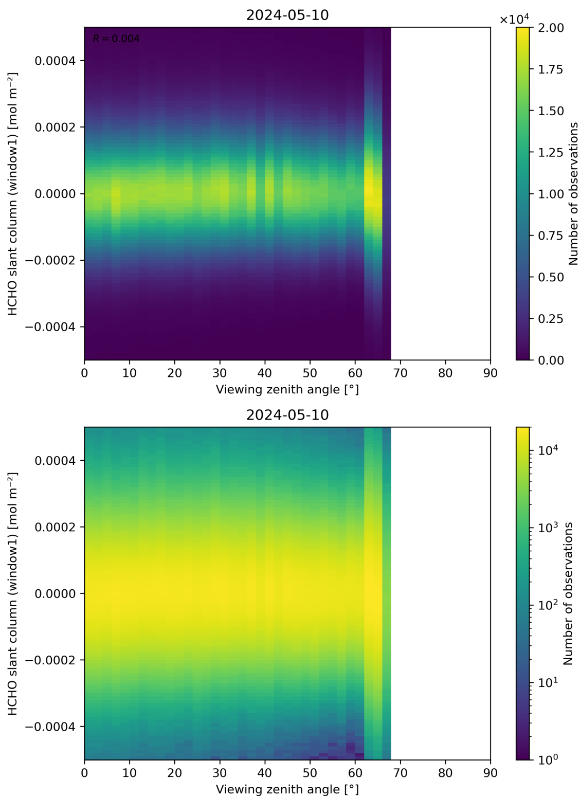
Figure 188: Scatter density plot of “Viewing zenith angle” against “HCHO slant column (window1)” for 2024-05-09 to 2024-05-11.
