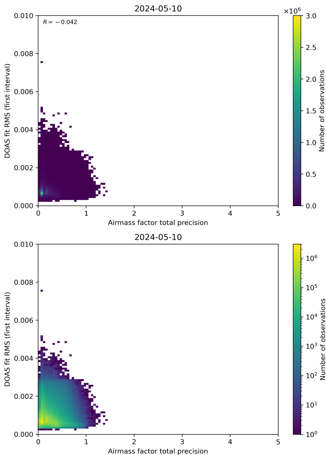
Figure 105: Scatter density plot of “Airmass factor total precision” against “DOAS fit RMS (first interval)” for 2024-05-09 to 2024-05-11.
