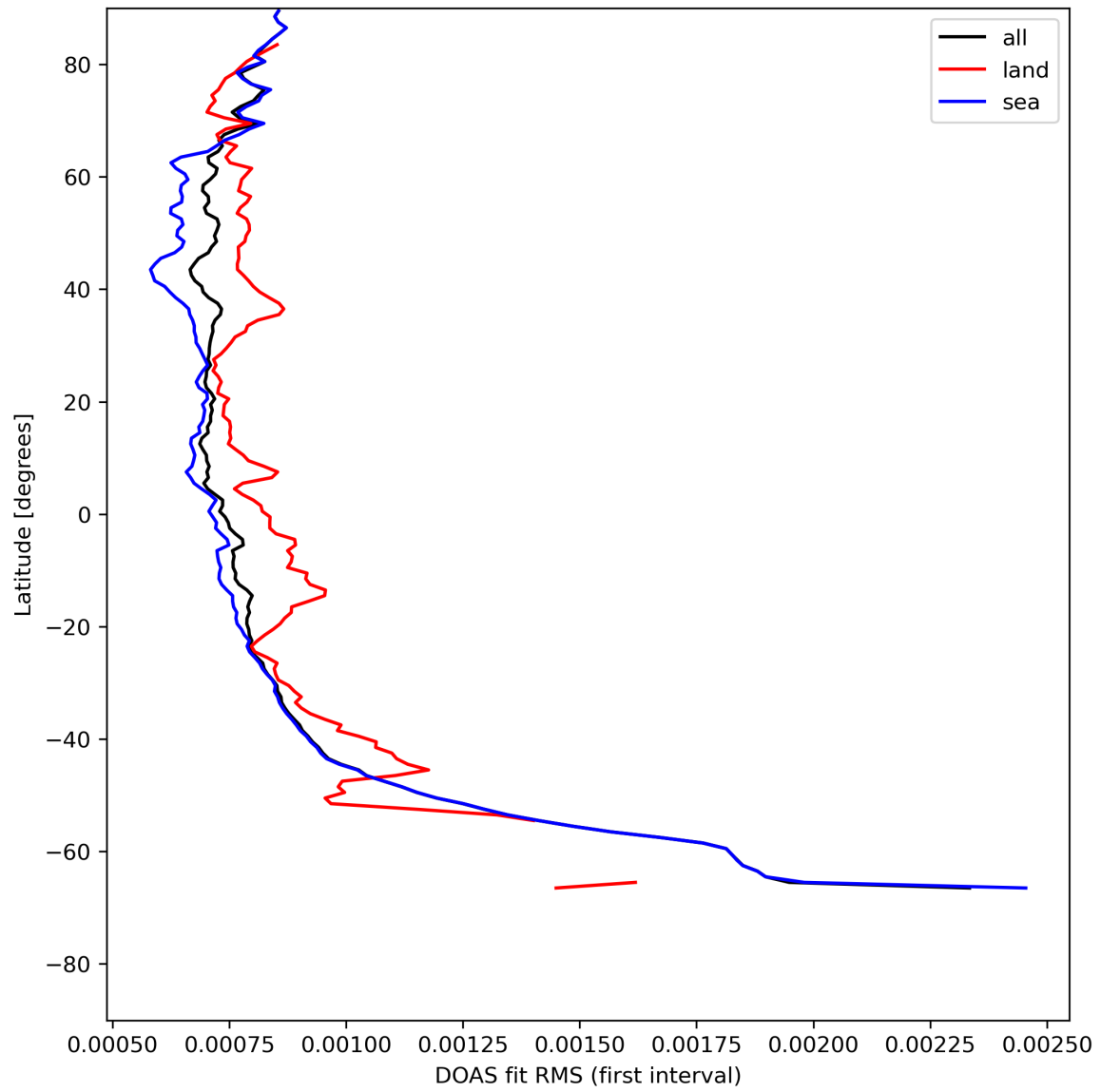
Figure 32: Zonal average of “DOAS fit RMS (first interval)” for 2024-05-09 to 2024-05-11.
