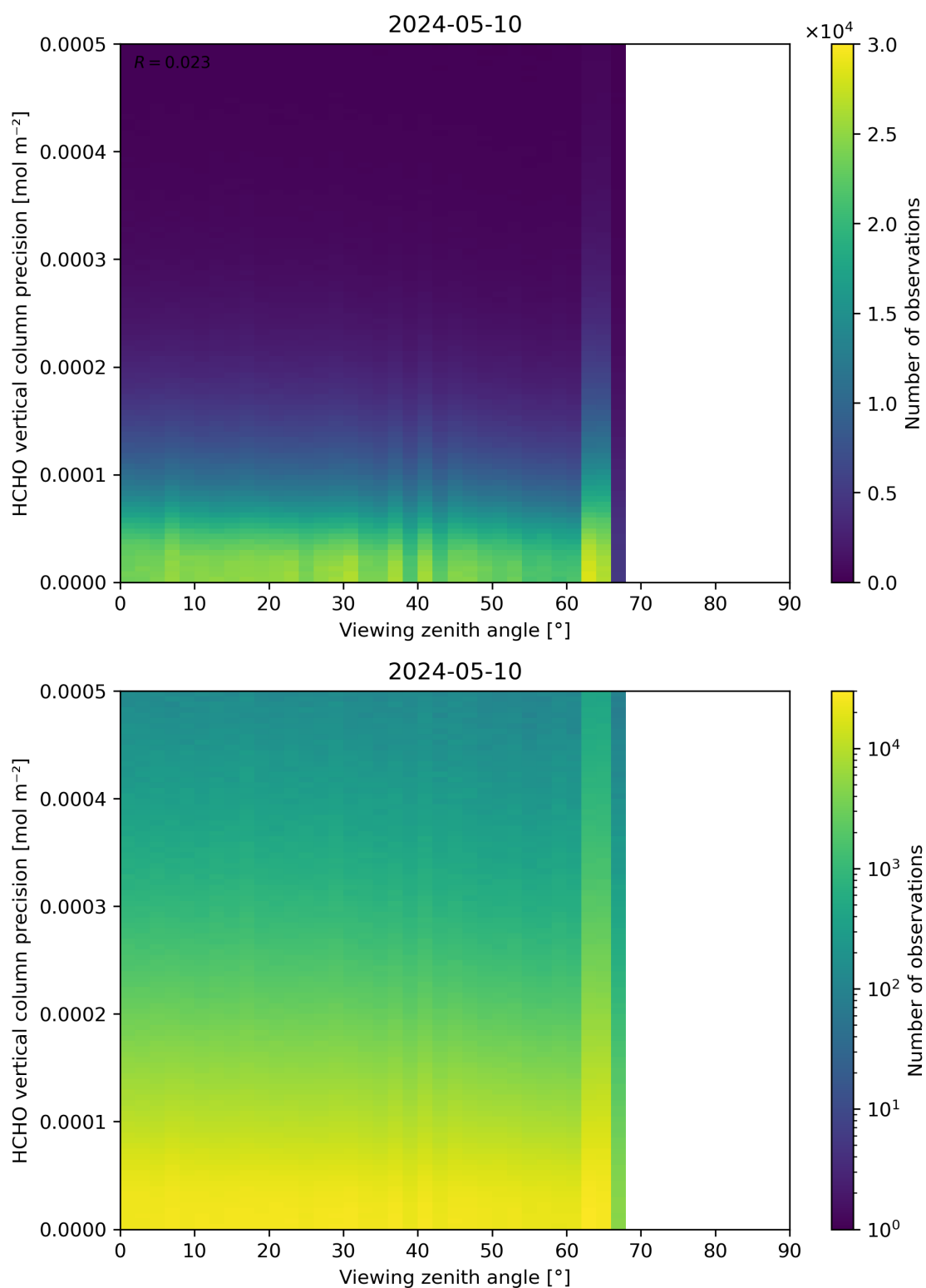
Figure 194: Scatter density plot of “Viewing zenith angle” against “HCHO vertical column precision” for 2024-05-09 to 2024-05-11.
