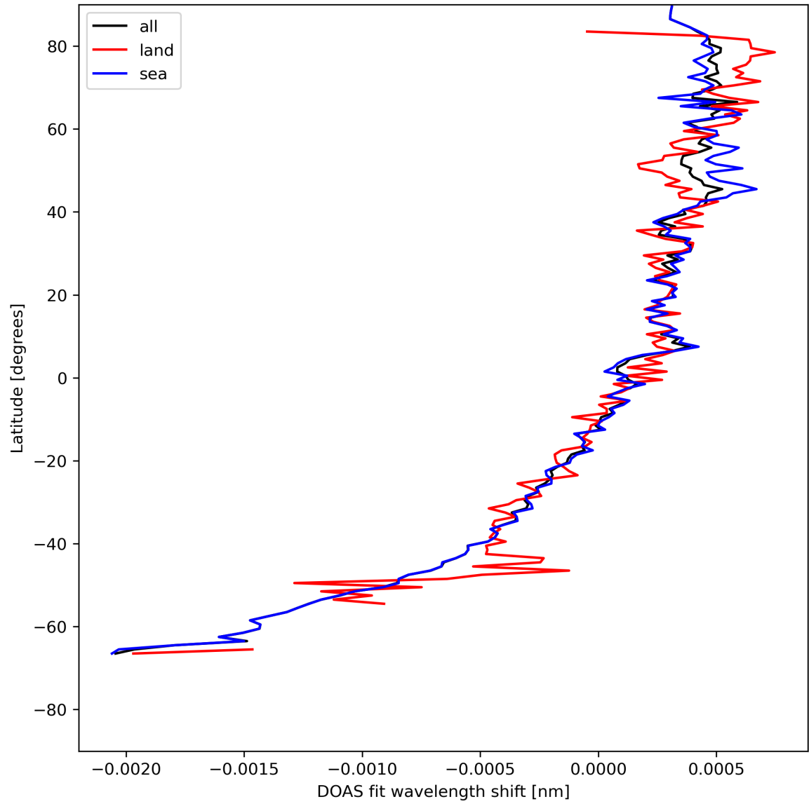
Figure 30: Zonal average of “DOAS fit wavelength shift” for 2024-05-09 to 2024-05-11.
