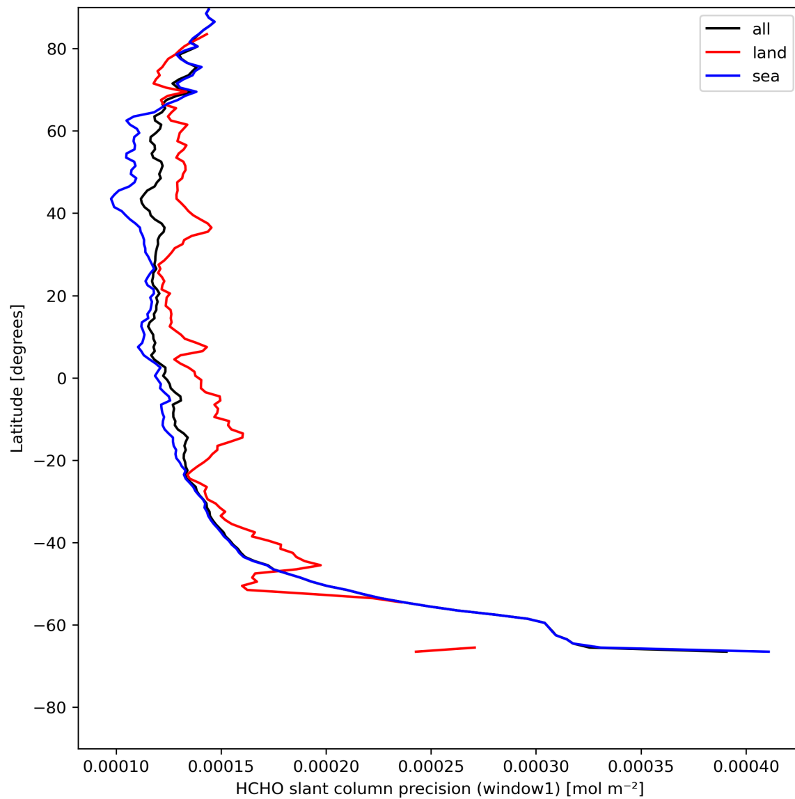
Figure 25: Zonal average of “HCHO slant column precision (window1)” for 2024-05-09 to 2024-05-11.
