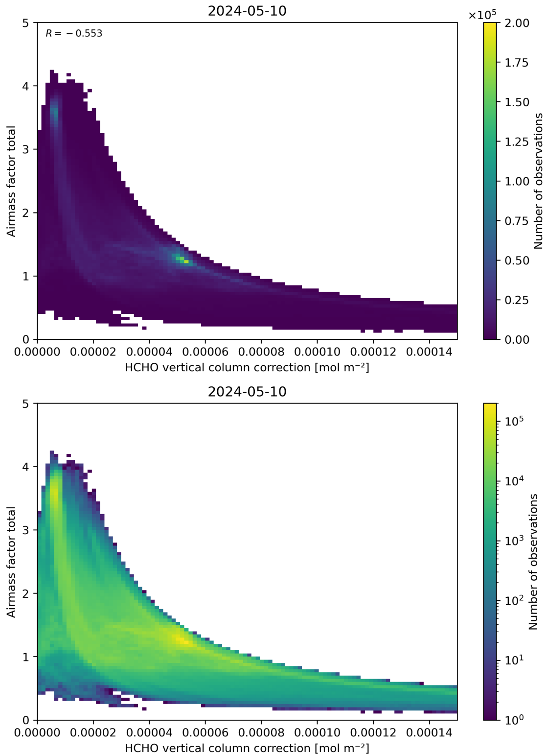
Figure 120: Scatter density plot of “HCHO vertical column correction” against “Airmass factor total” for 2024-05-09 to 2024-05-11.
