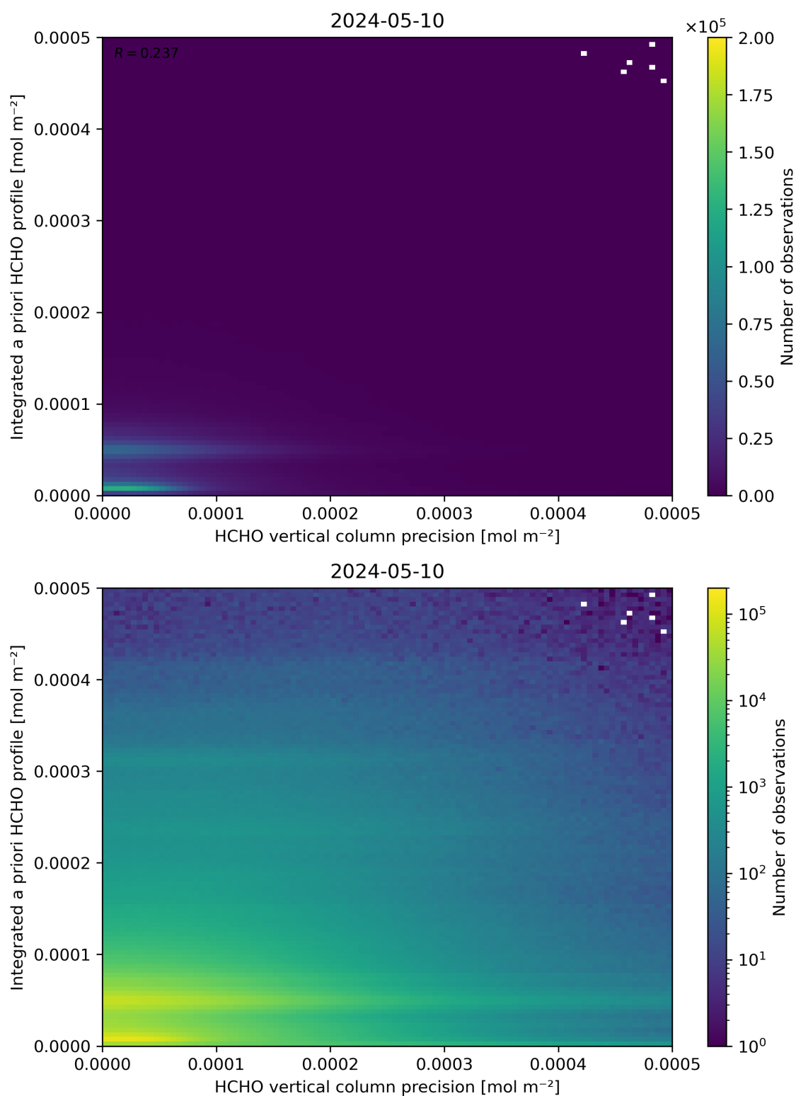
Figure 147: Scatter density plot of “HCHO vertical column precision” against “Integrated a priori HCHO profile” for 2024-05-09 to 2024-05-11.
