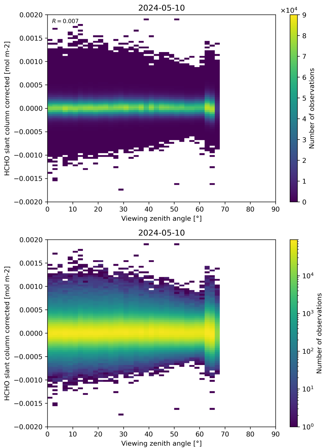
Figure 186: Scatter density plot of “Viewing zenith angle” against “HCHO slant column corrected” for 2024-05-09 to 2024-05-11.
