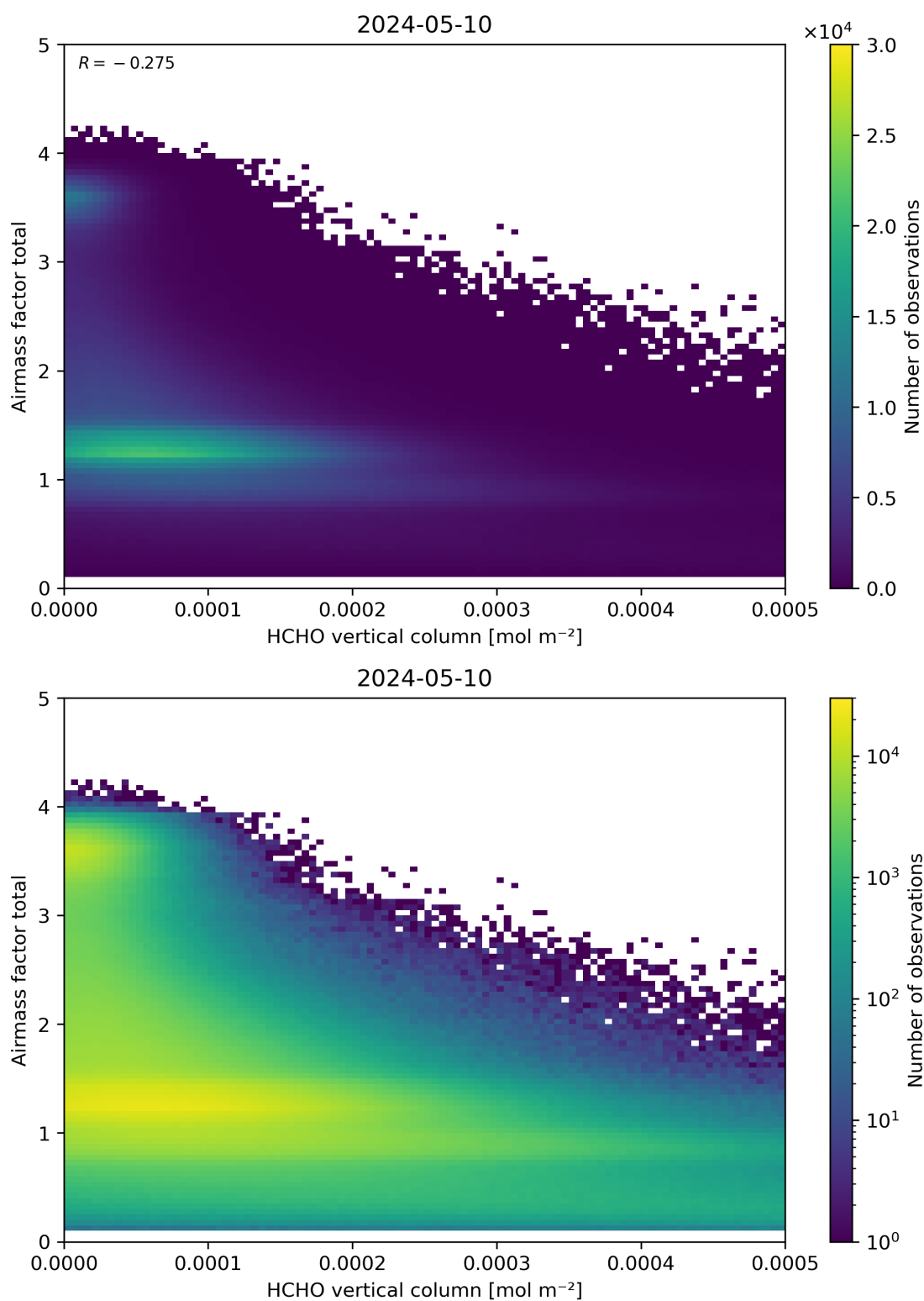
Figure 131: Scatter density plot of “HCHO vertical column” against “Airmass factor total” for 2024-05-09 to 2024-05-11.
