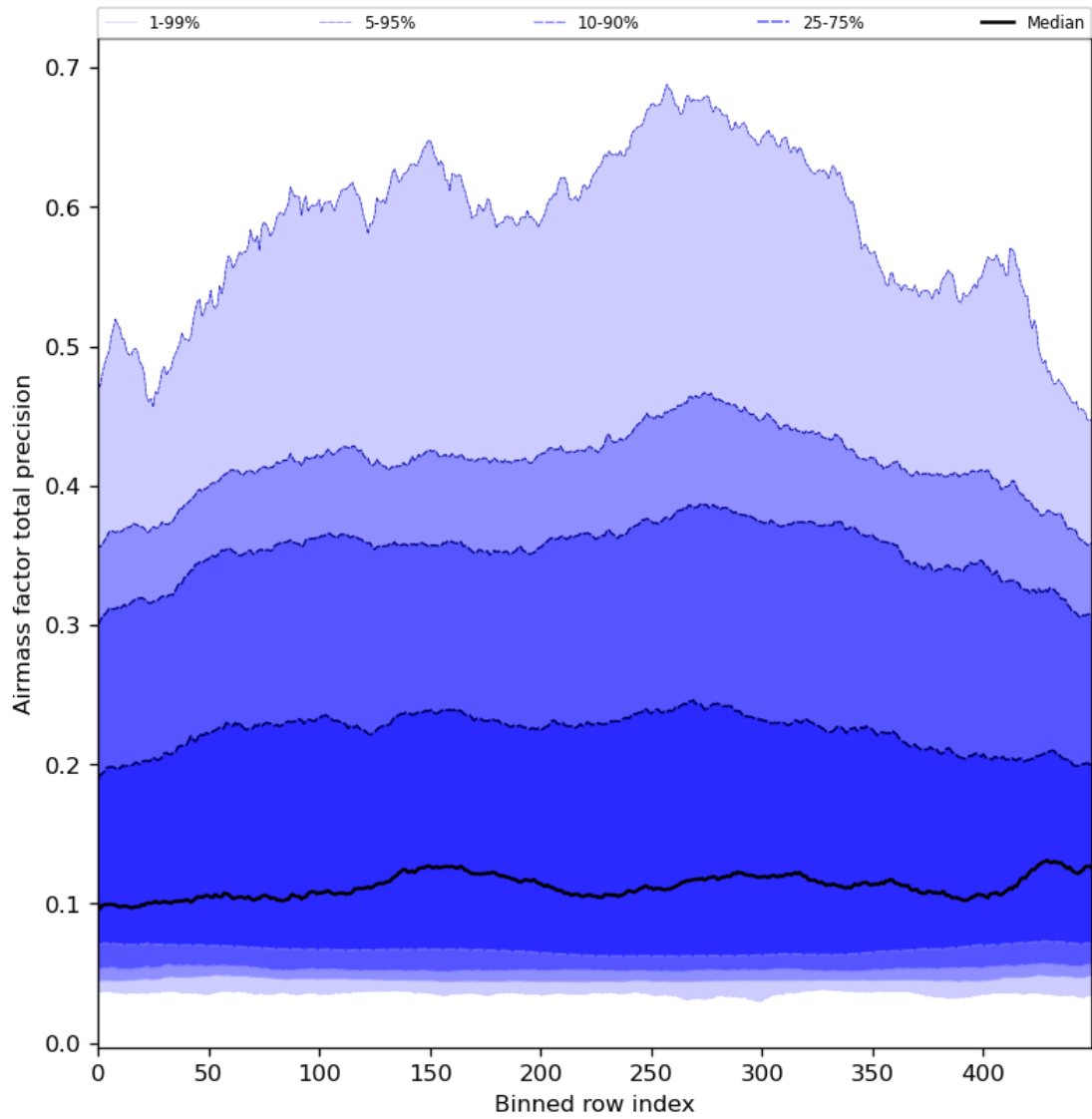
Figure 55: Along track statistics of “Airmass factor total precision” for 2024-05-09 to 2024-05-11
