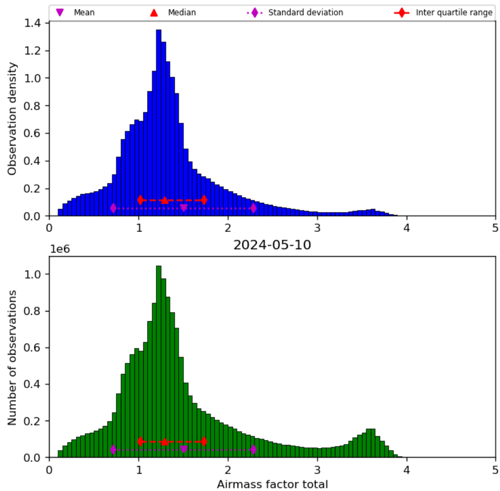
Figure 40: Histogram of “Airmass factor total” for 2024-05-09 to 2024-05-11
