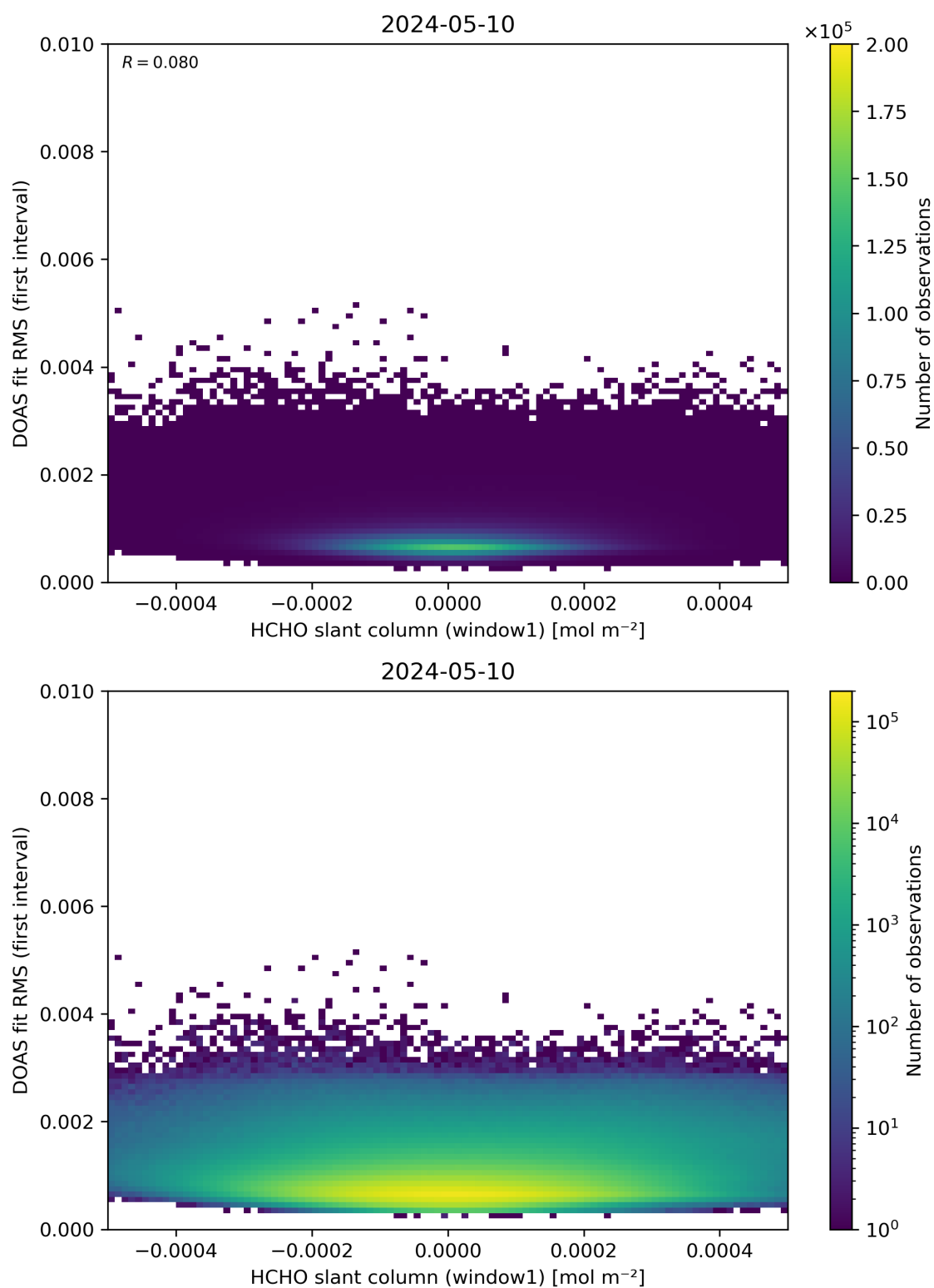
Figure 78: Scatter density plot of “HCHO slant column (window1)” against “DOAS fit RMS (first interval)” for 2024-05-09 to 2024-05-11.
