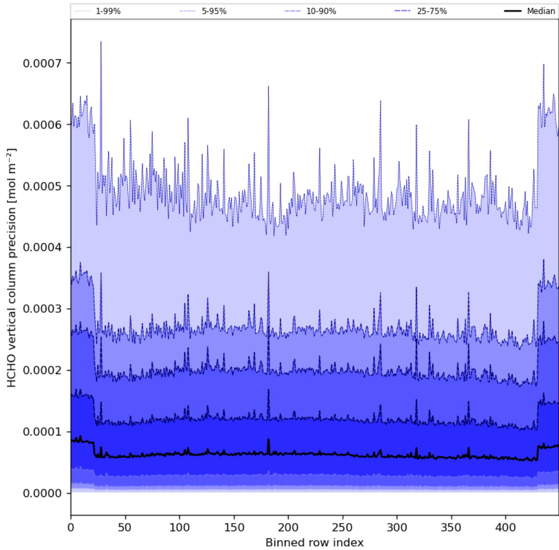
Figure 50: Along track statistics of "HCHO vertical column precision" for 2024-05-09 to 2024-05-11
