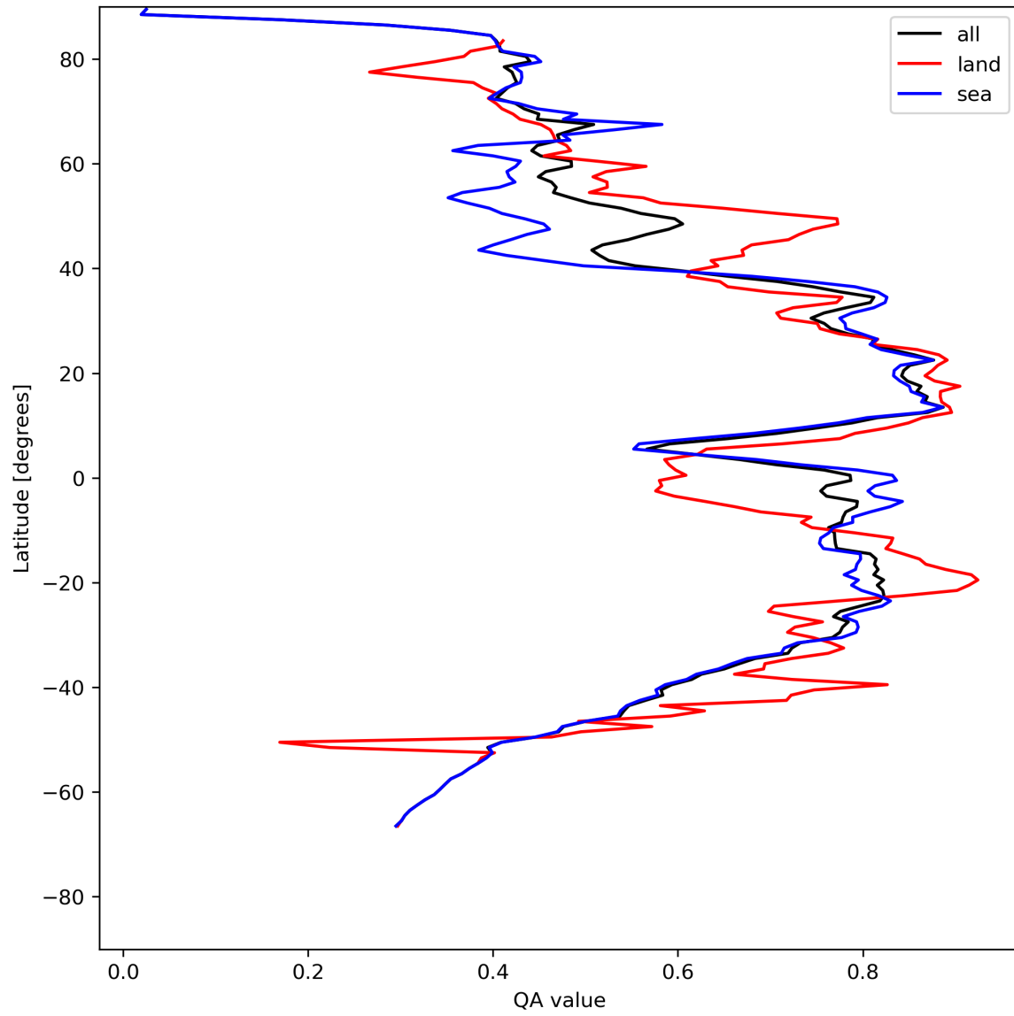
Figure 20: Zonal average of “QA value” for 2024-05-09 to 2024-05-11.
