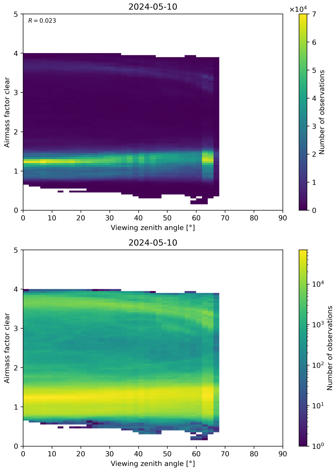
Figure 185: Scatter density plot of “Viewing zenith angle” against “Airmass factor clear” for 2024-05-09 to 2024-05-11.
