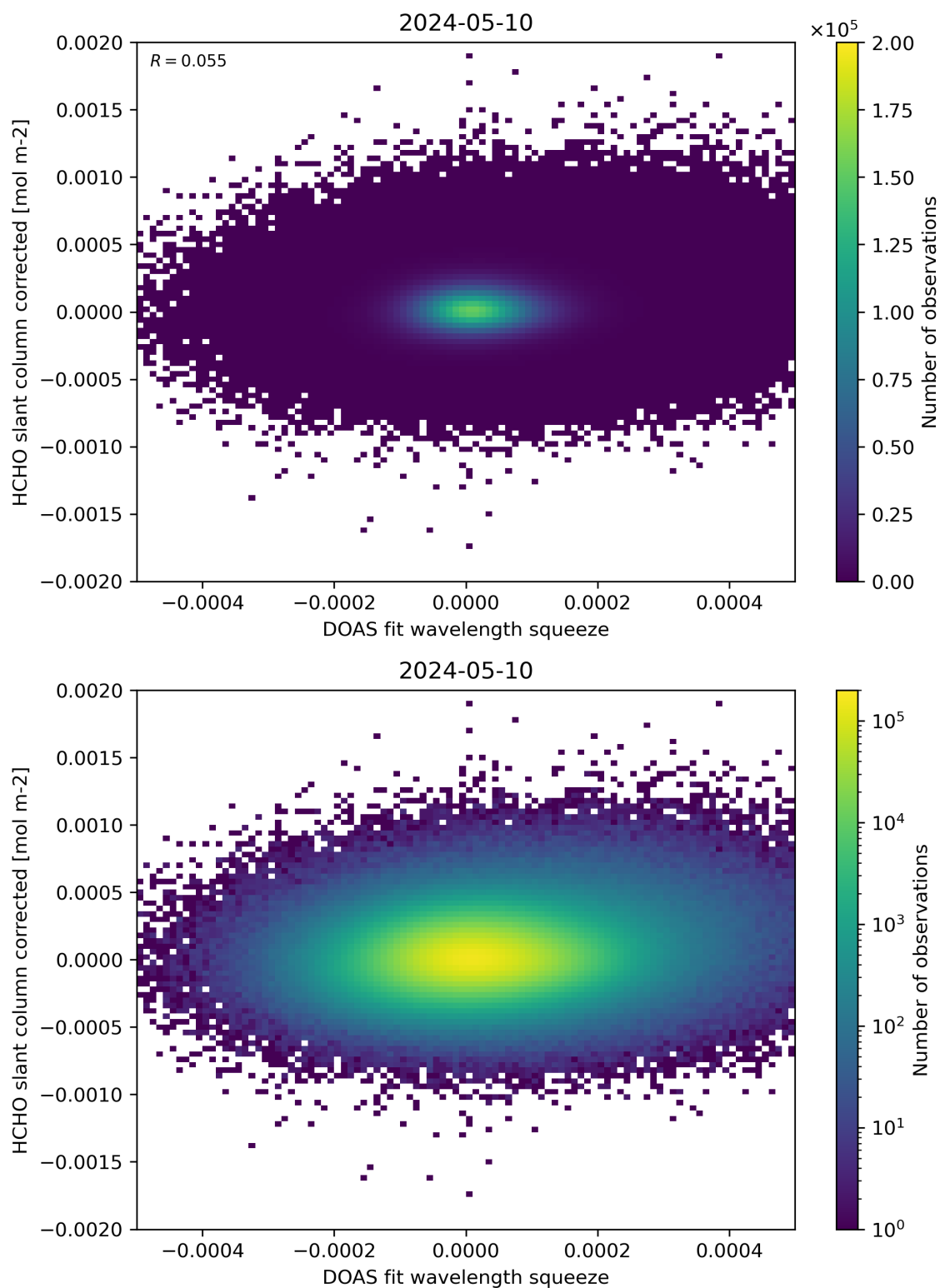
Figure 69: Scatter density plot of “DOAS fit wavelength squeeze” against “HCHO slant column corrected” for 2024-05-09 to 2024-05-11.
