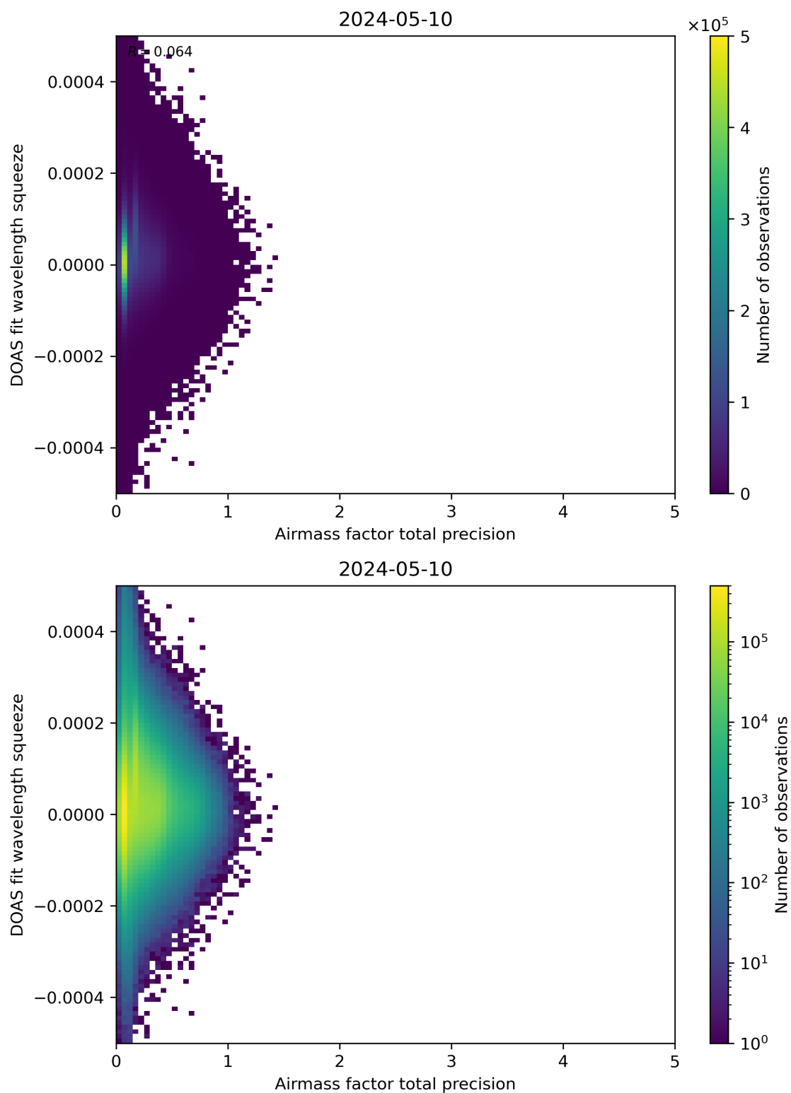
Figure 107: Scatter density plot of “Airmass factor total precision” against “DOAS fit wavelength squeeze” for 2024-05-09 to 2024-05-11.
