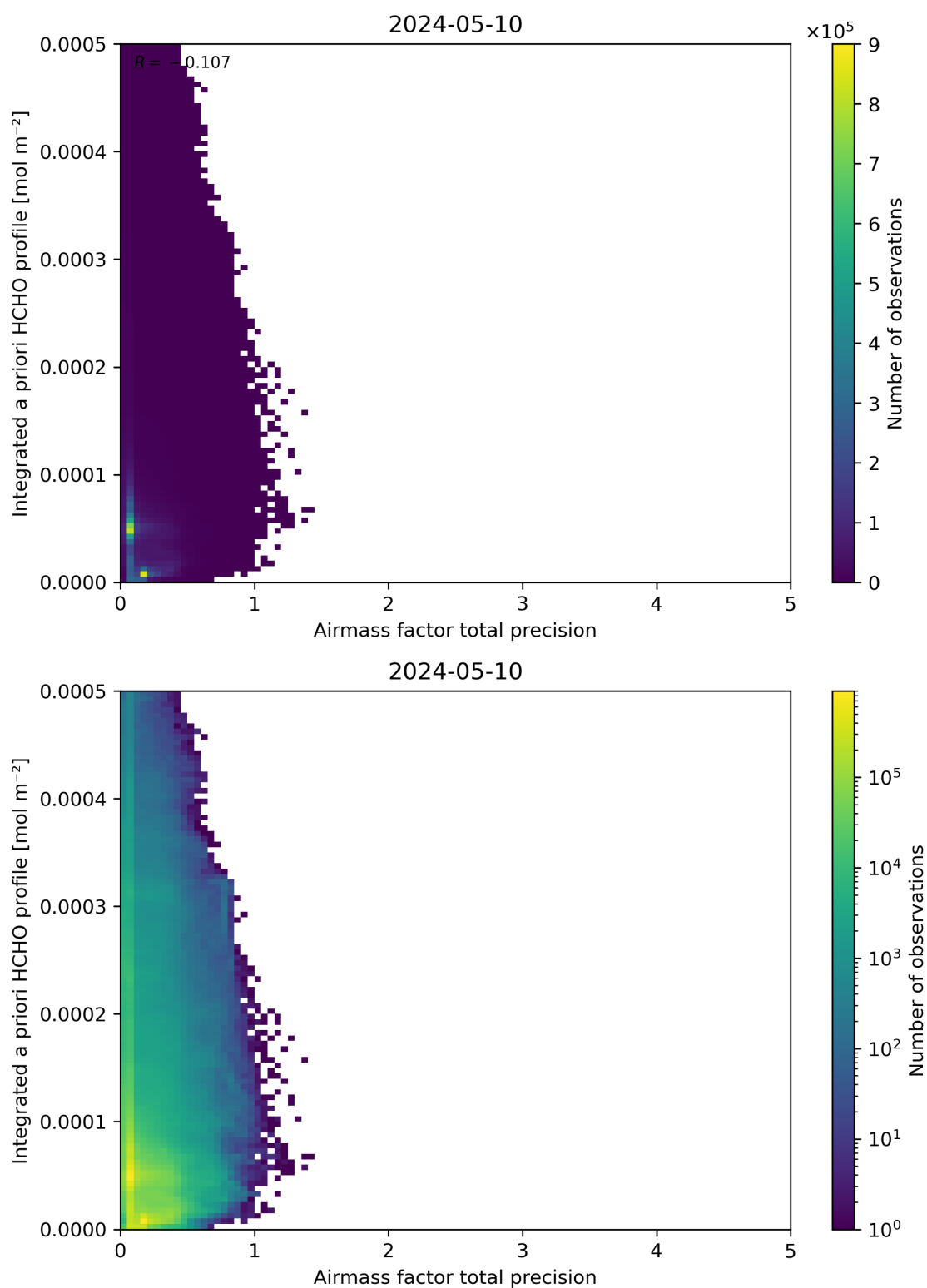
Figure 111: Scatter density plot of “Airmass factor total precision” against “Integrated a priori HCHO profile” for 2024-05-09 to 2024-05-11.
