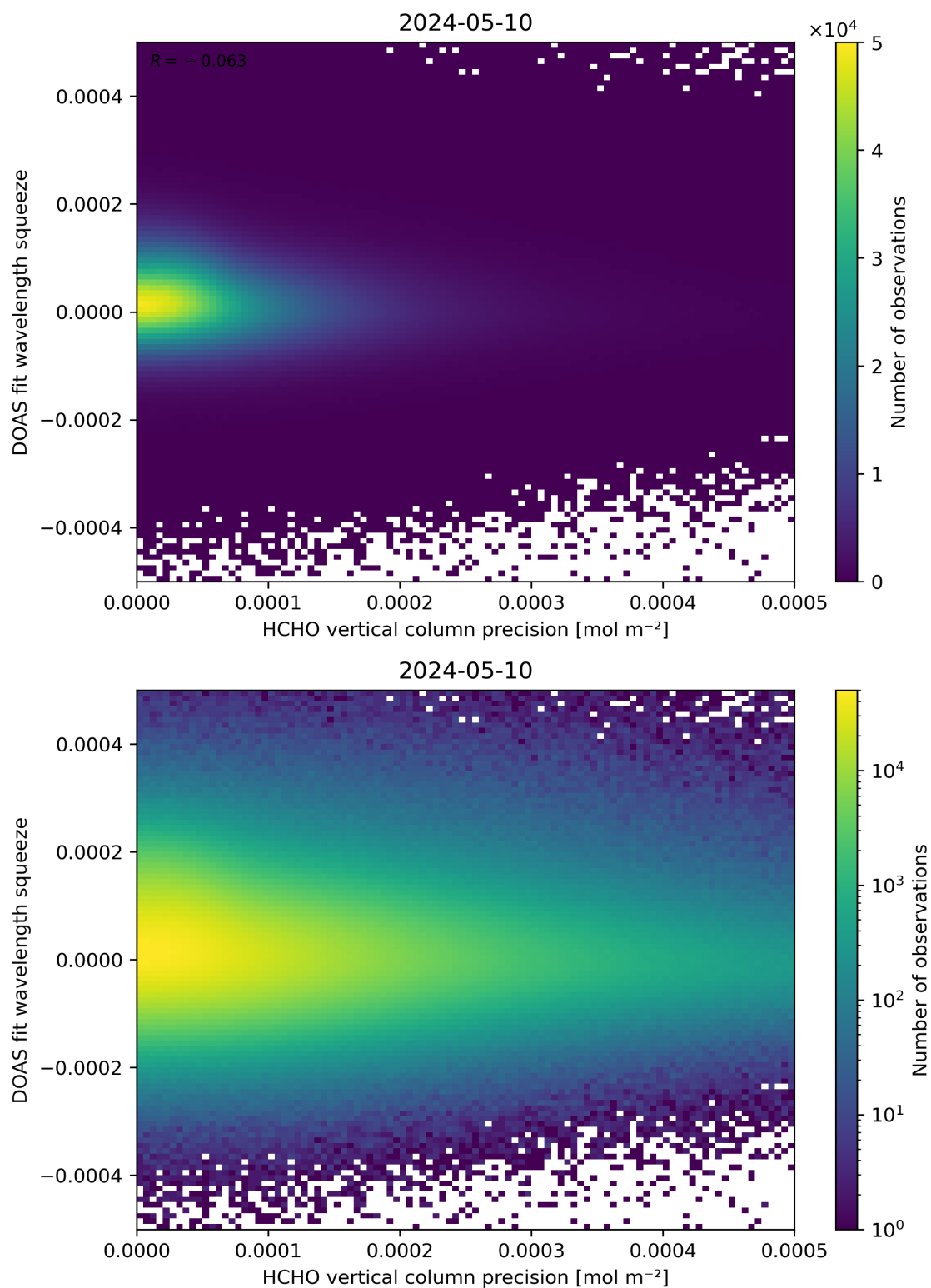
Figure 138: Scatter density plot of “HCHO vertical column precision” against “DOAS fit wavelength squeeze” for 2024-05-09 to 2024-05-11.
