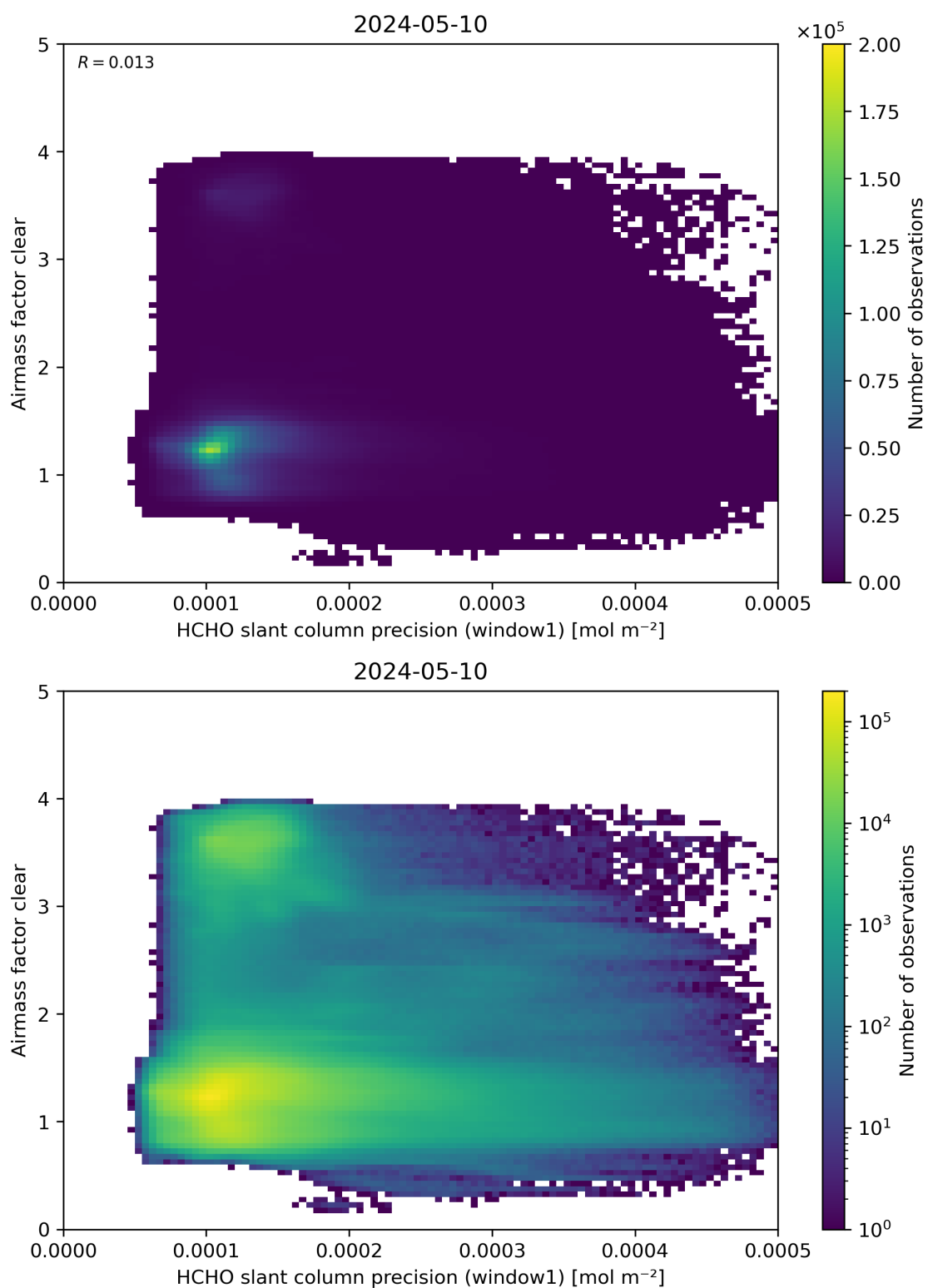
Figure 91: Scatter density plot of “HCHO slant column precision (window1)” against “Airmass factor clear” for 2024-05-09 to 2024-05-11.
