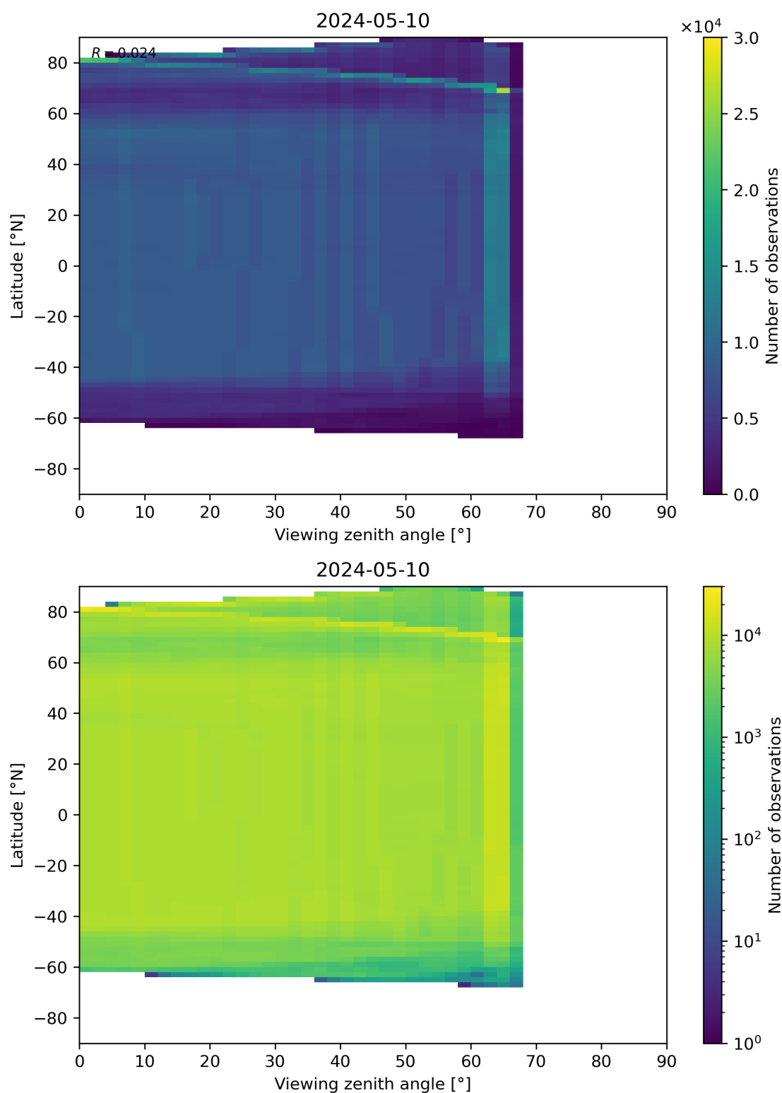
Figure 196: Scatter density plot of “Viewing zenith angle” against “Latitude” for 2024-05-09 to 2024-05-11.
