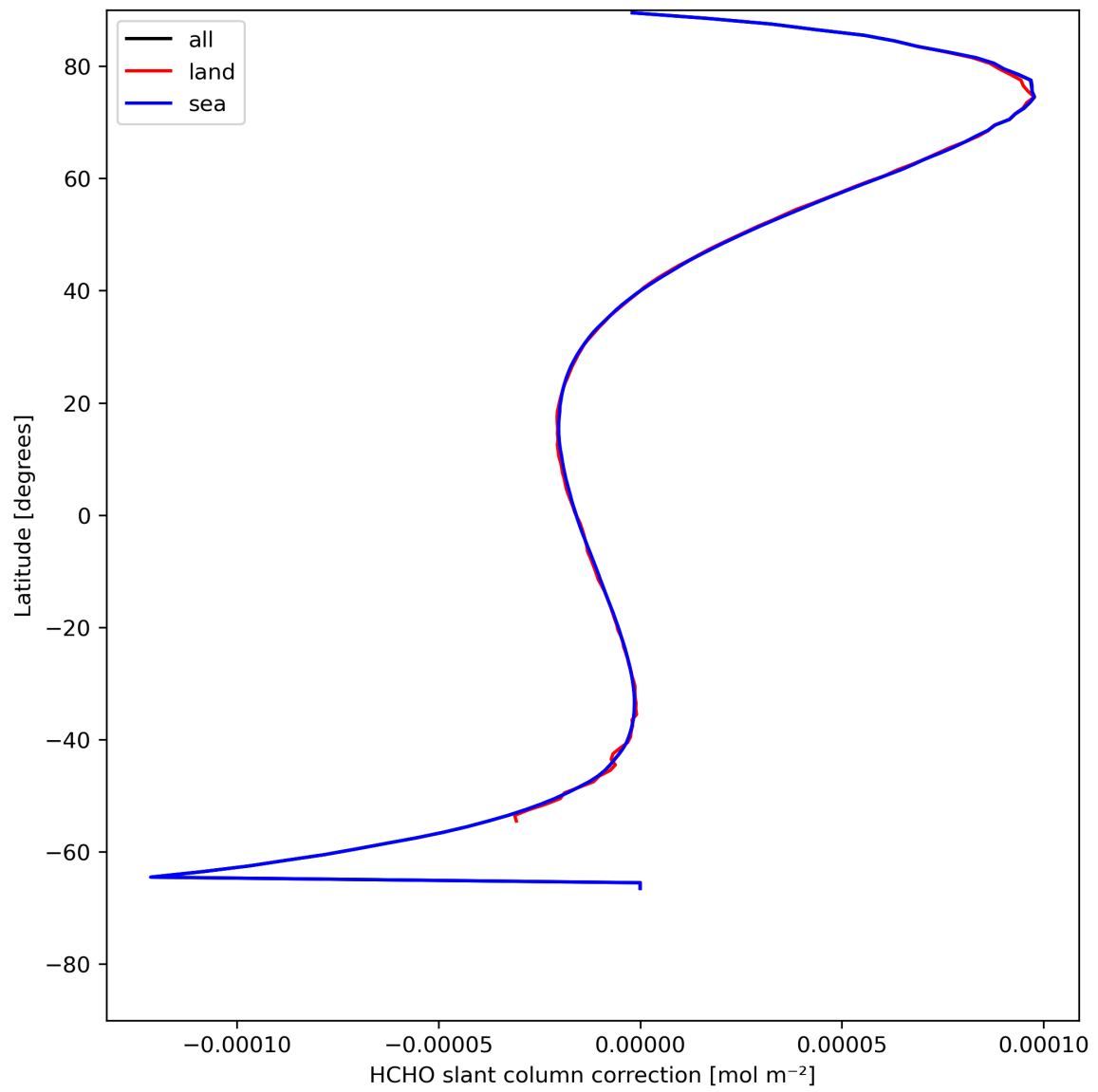
Figure 33: Zonal average of “HCHO slant column correction” for 2024-05-09 to 2024-05-11.
