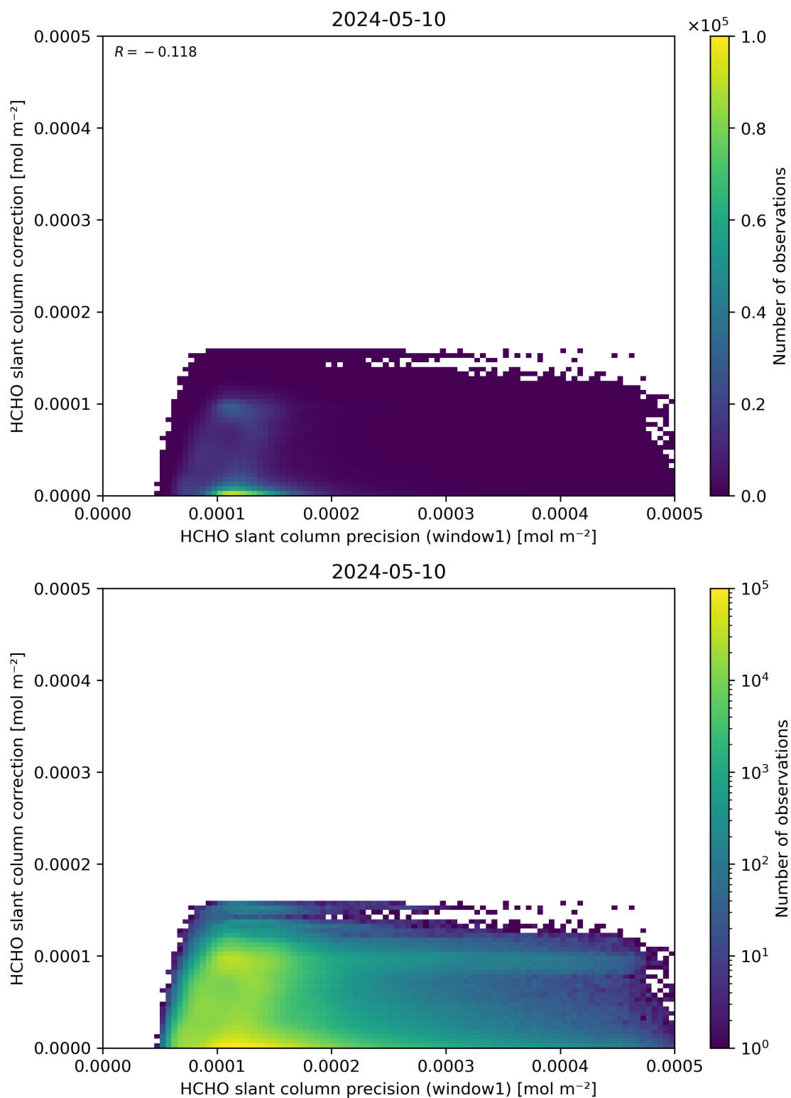
Figure 93: Scatter density plot of “HCHO slant column precision (window1)” against “HCHO slant column correction” for 2024-05-09 to 2024-05-11.
