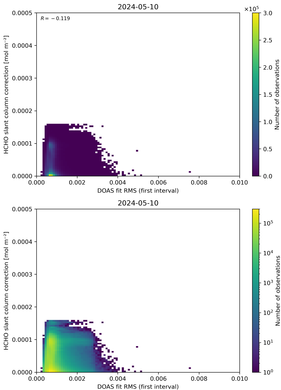
Figure 63: Scatter density plot of “DOAS fit RMS (first interval)” against “HCHO slant column correction” for 2024-05-09 to 2024-05-11.
