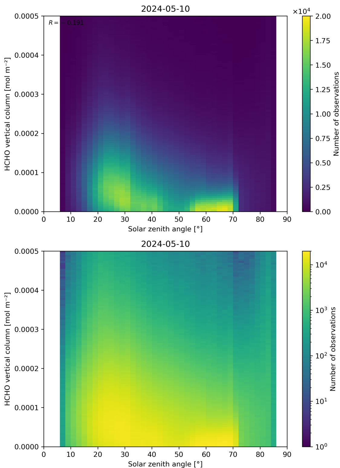
Figure 177: Scatter density plot of “Solar zenith angle” against “HCHO vertical column” for 2024-05-09 to 2024-05-11.
