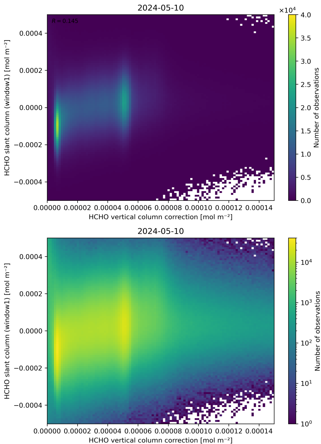
Figure 118: Scatter density plot of “HCHO vertical column correction” against “HCHO slant column (window1)” for 2024-05-09 to 2024-05-11.
