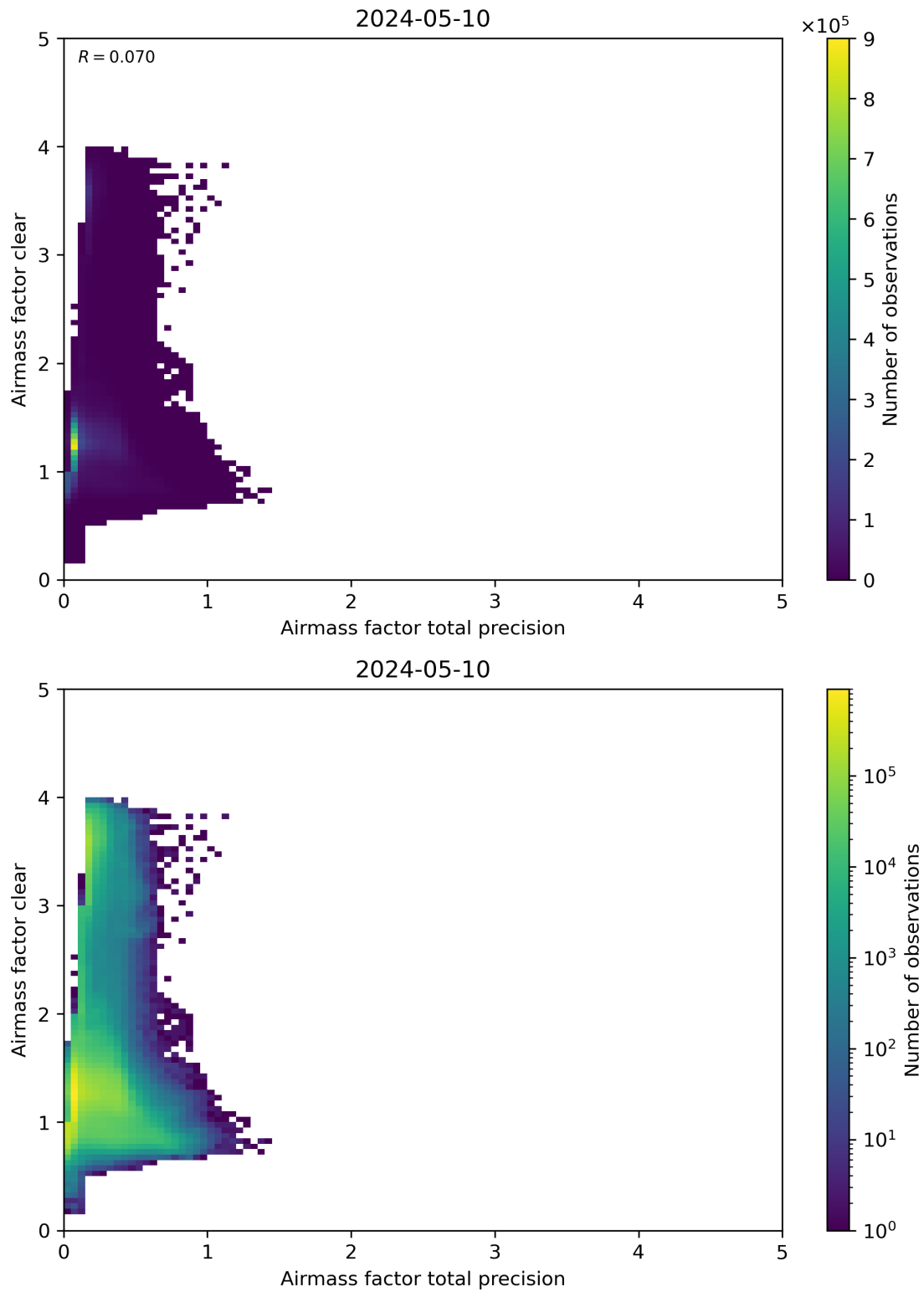
Figure 108: Scatter density plot of “Airmass factor total precision” against “Airmass factor clear” for 2024-05-09 to 2024-05-11.
