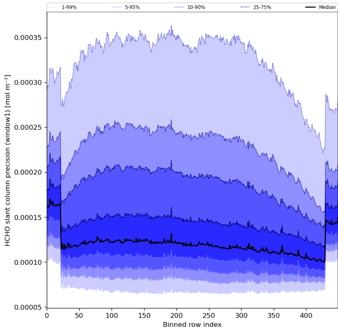
Figure 53: Along track statistics of “HCHO slant column precision (window1)” for 2024-05-09 to 2024-05-11
