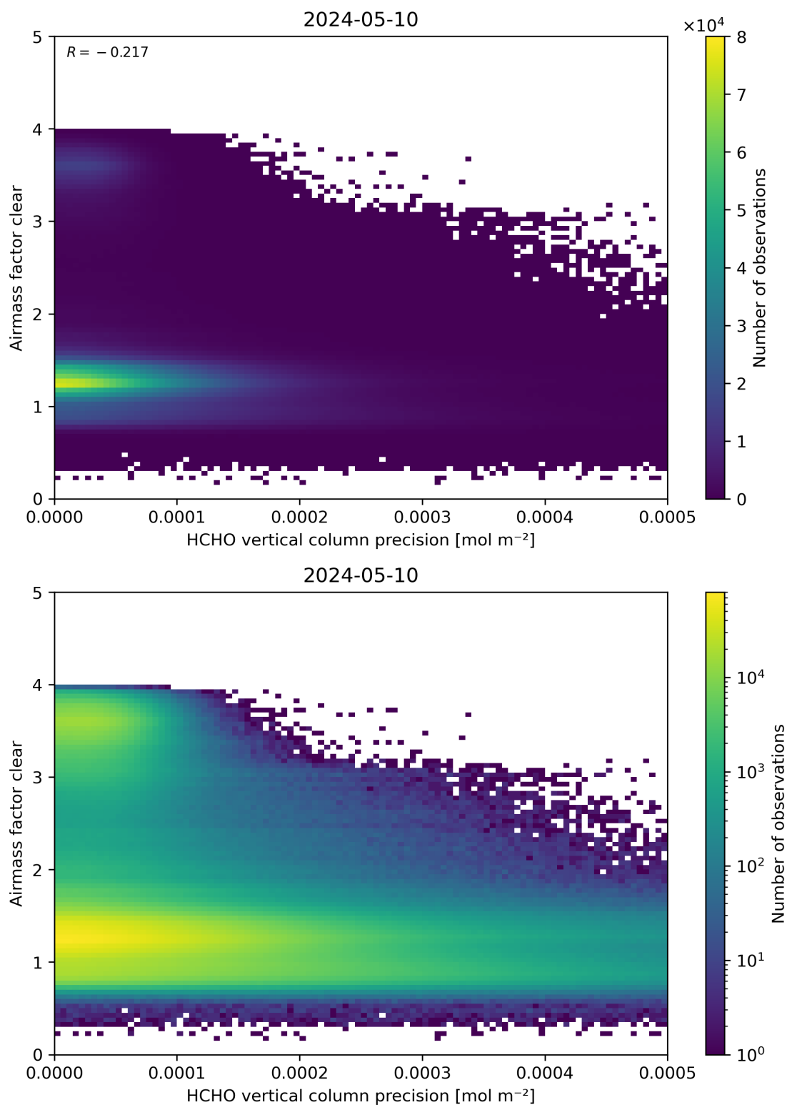
Figure 139: Scatter density plot of “HCHO vertical column precision” against “Airmass factor clear” for 2024-05-09 to 2024-05-11.
