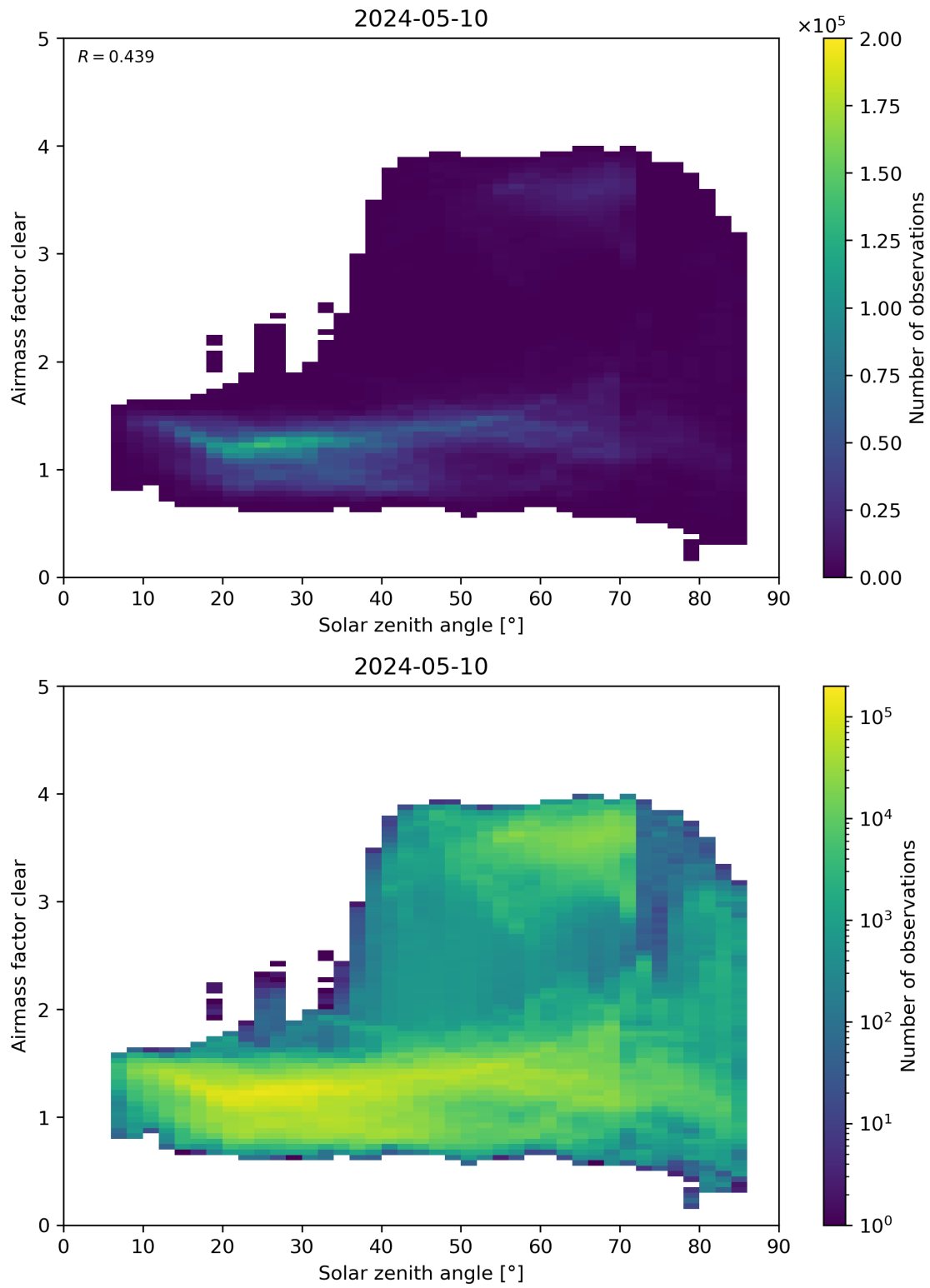
Figure 170: Scatter density plot of “Solar zenith angle” against “Airmass factor clear” for 2024-05-09 to 2024-05-11.
