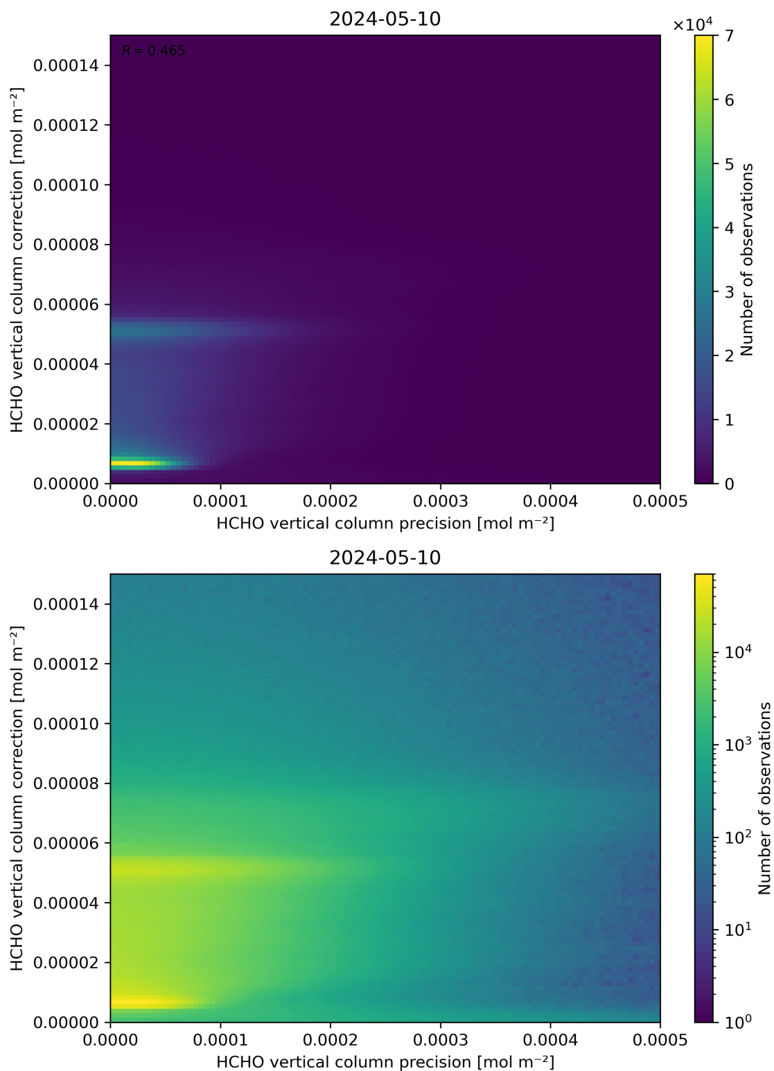
Figure 146: Scatter density plot of “HCHO vertical column precision” against “HCHO vertical column correction” for 2024-05-09 to 2024-05-11.
