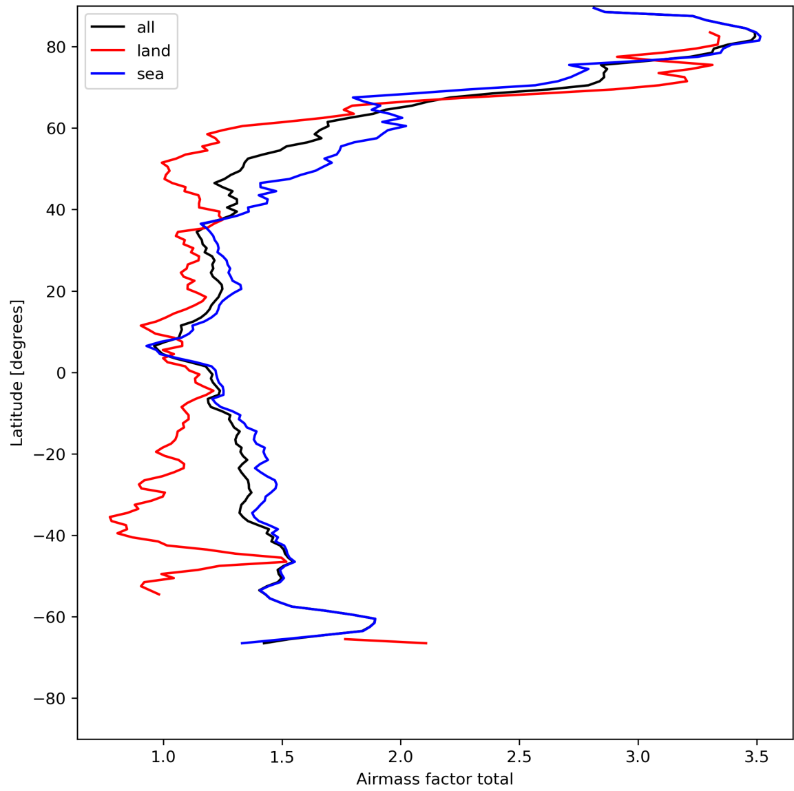
Figure 26: Zonal average of “Airmass factor total” for 2024-05-09 to 2024-05-11.
