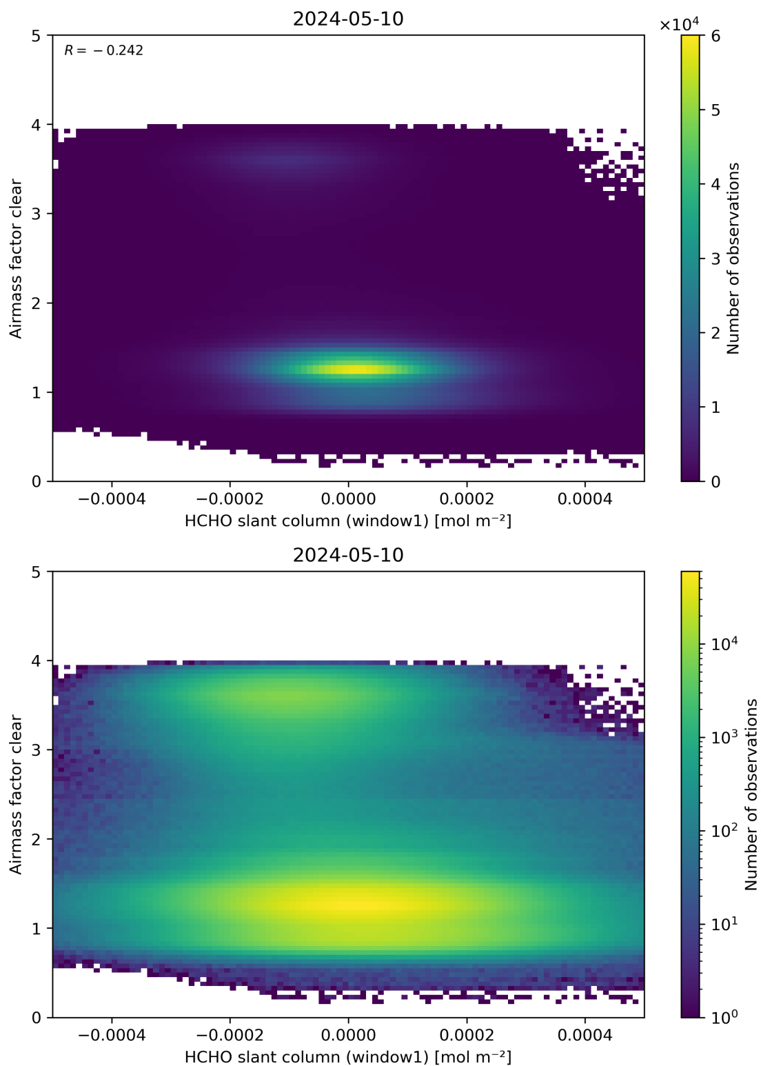
Figure 81: Scatter density plot of “HCHO slant column (window1)” against “Airmass factor clear” for 2024-05-09 to 2024-05-11.
