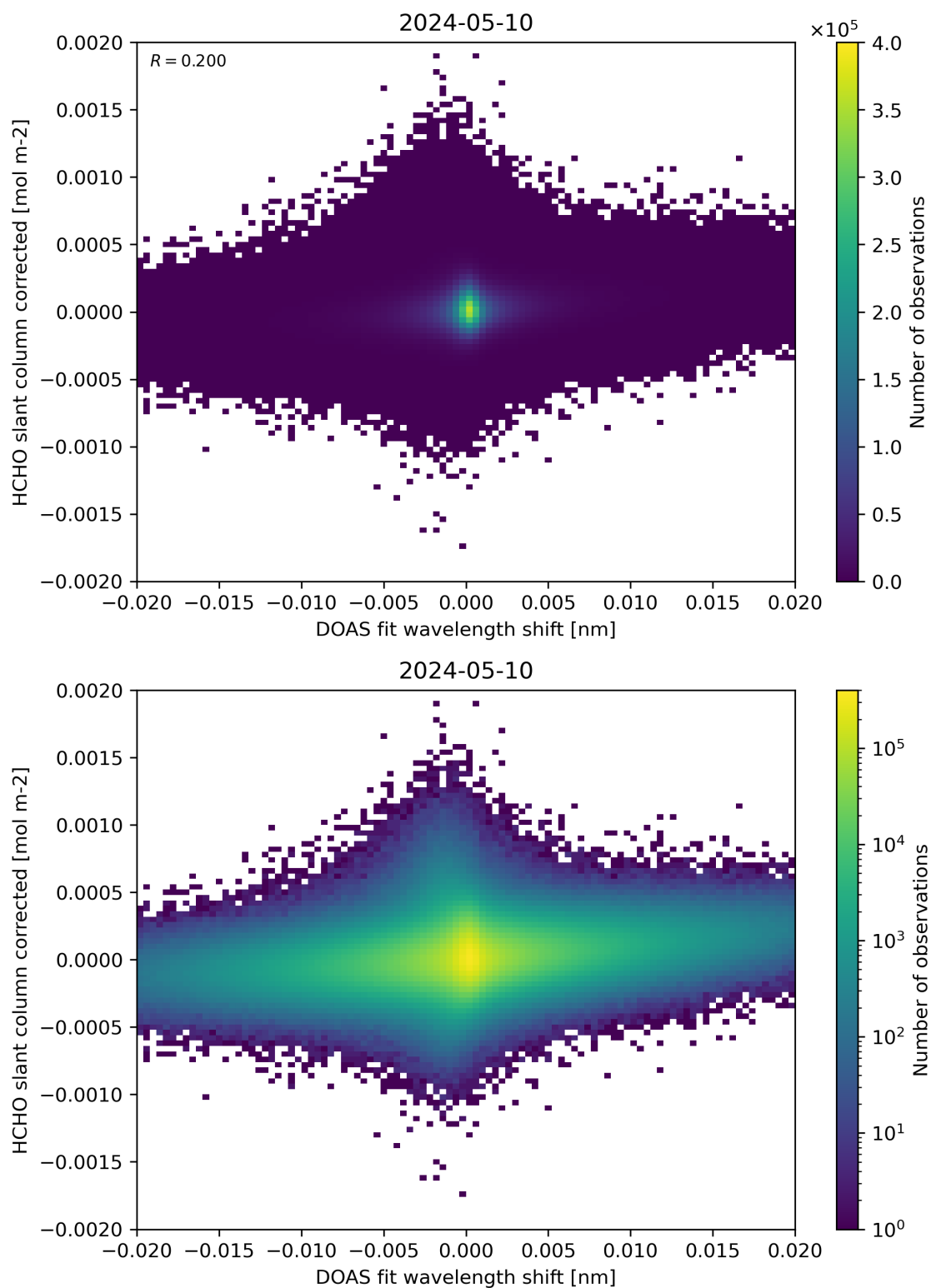
Figure 66: Scatter density plot of “DOAS fit wavelength shift” against “HCHO slant column corrected” for 2024-05-09 to 2024-05-11.
