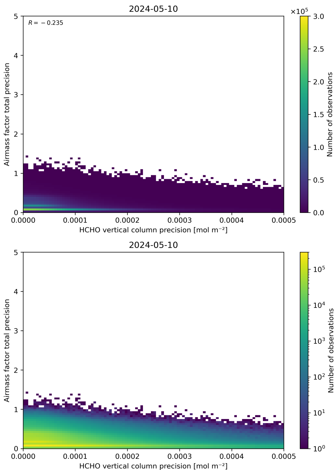
Figure 145: Scatter density plot of “HCHO vertical column precision” against “Airmass factor total precision” for 2024-05-09 to 2024-05-11.
