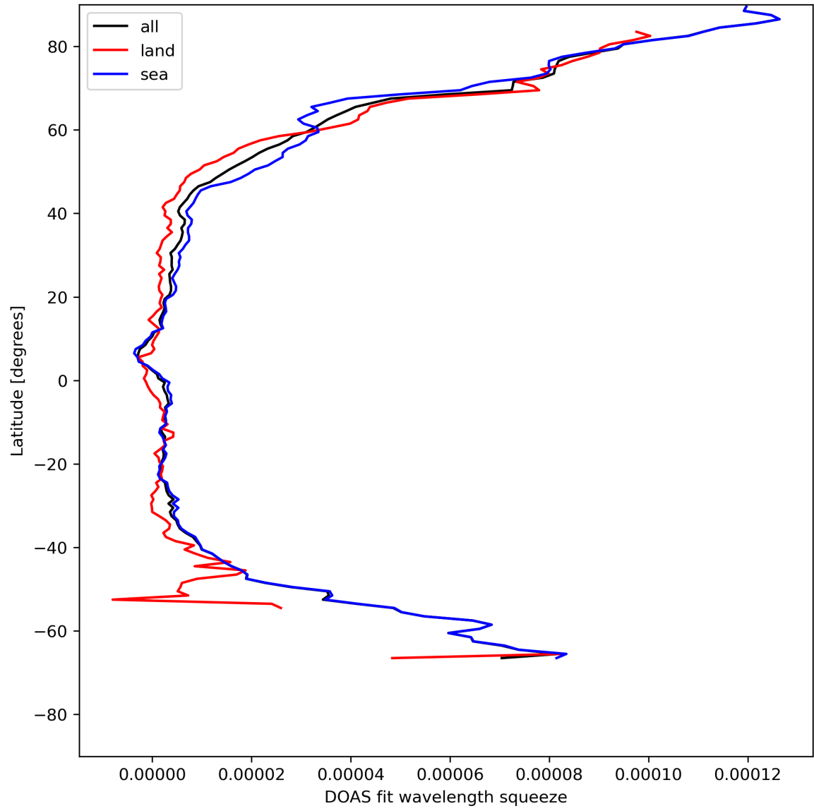
Figure 31: Zonal average of “DOAS fit wavelength squeeze” for 2024-05-09 to 2024-05-11.
