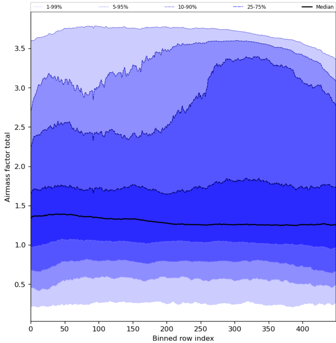
Figure 54: Along track statistics of “Airmass factor total” for 2024-05-09 to 2024-05-11
