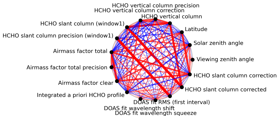
Figure 1: Map of correlation graph for 2024-05-09 to 2024-05-11.
