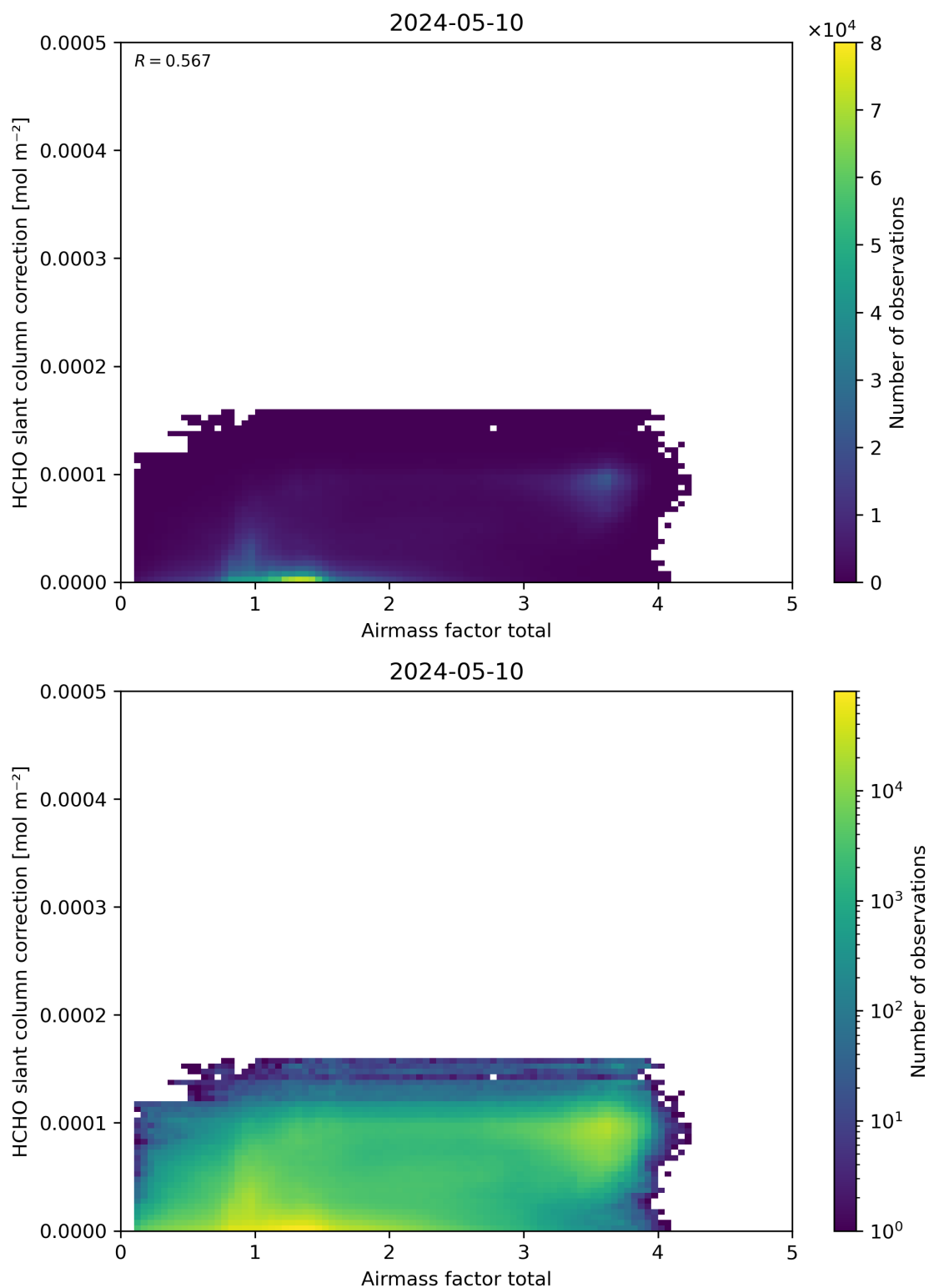
Figure 102: Scatter density plot of “Airmass factor total” against “HCHO slant column correction” for 2024-05-09 to 2024-05-11.
