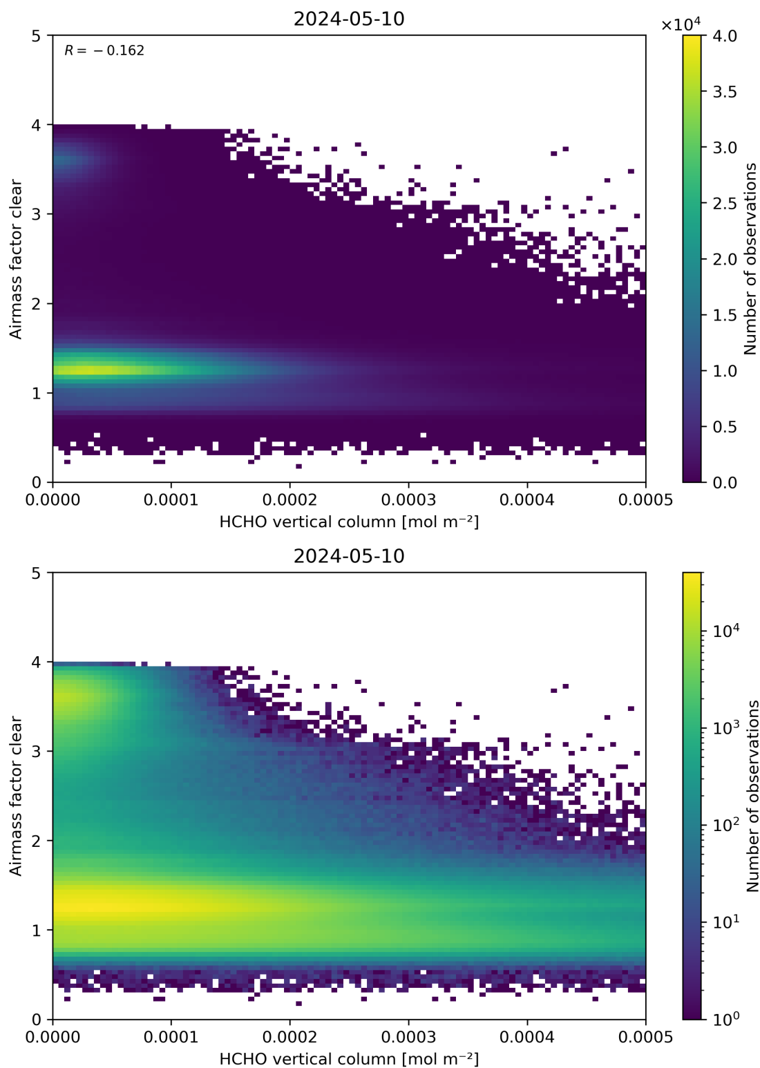
Figure 126: Scatter density plot of “HCHO vertical column” against “Airmass factor clear” for 2024-05-09 to 2024-05-11.
