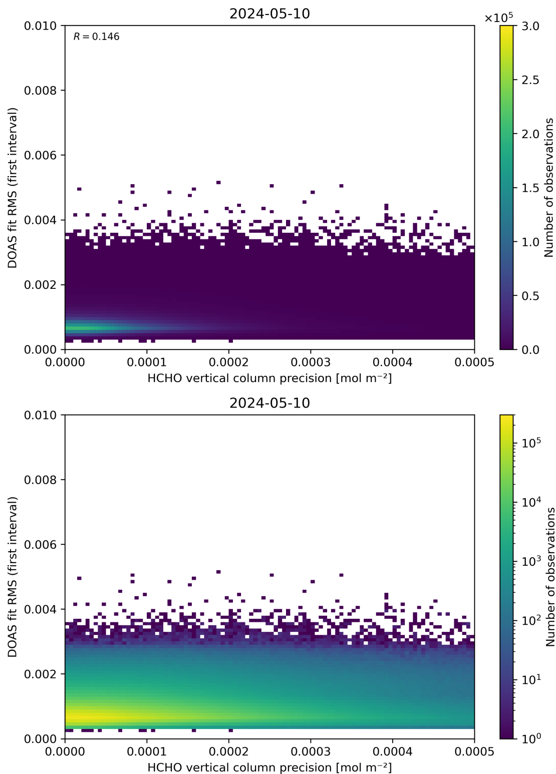
Figure 136: Scatter density plot of “HCHO vertical column precision” against “DOAS fit RMS (first interval)” for 2024-05-09 to 2024-05-11.
