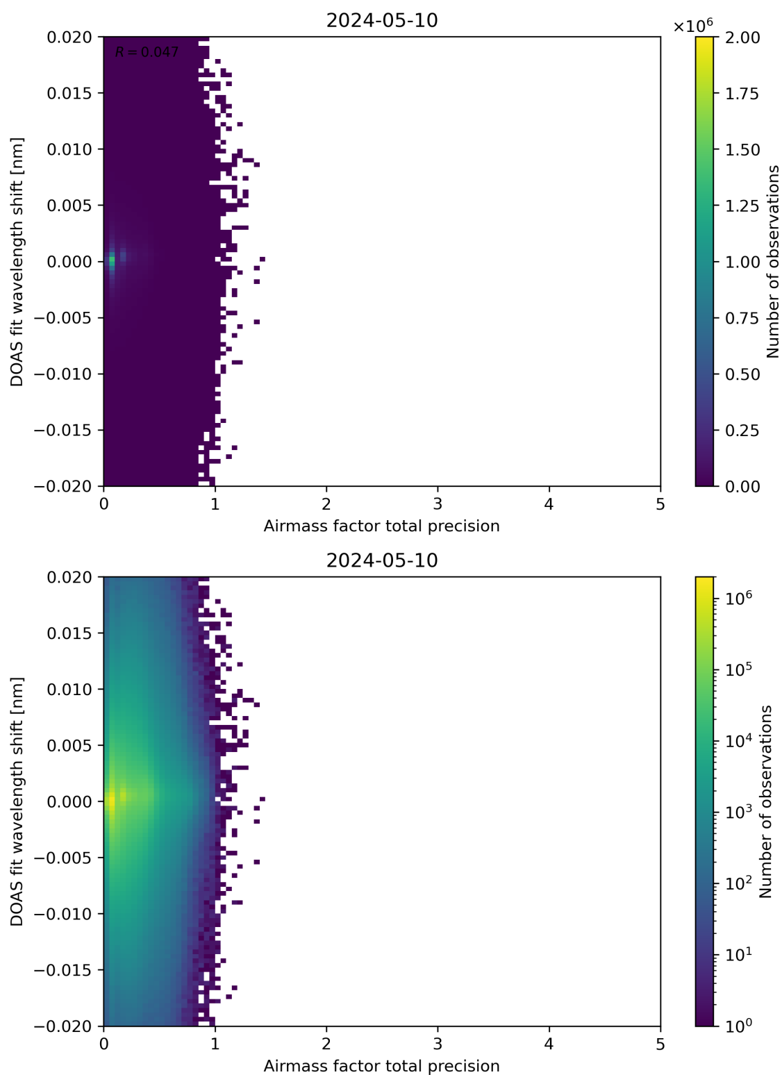
Figure 106: Scatter density plot of “Airmass factor total precision” against “DOAS fit wavelength shift” for 2024-05-09 to 2024-05-11.
