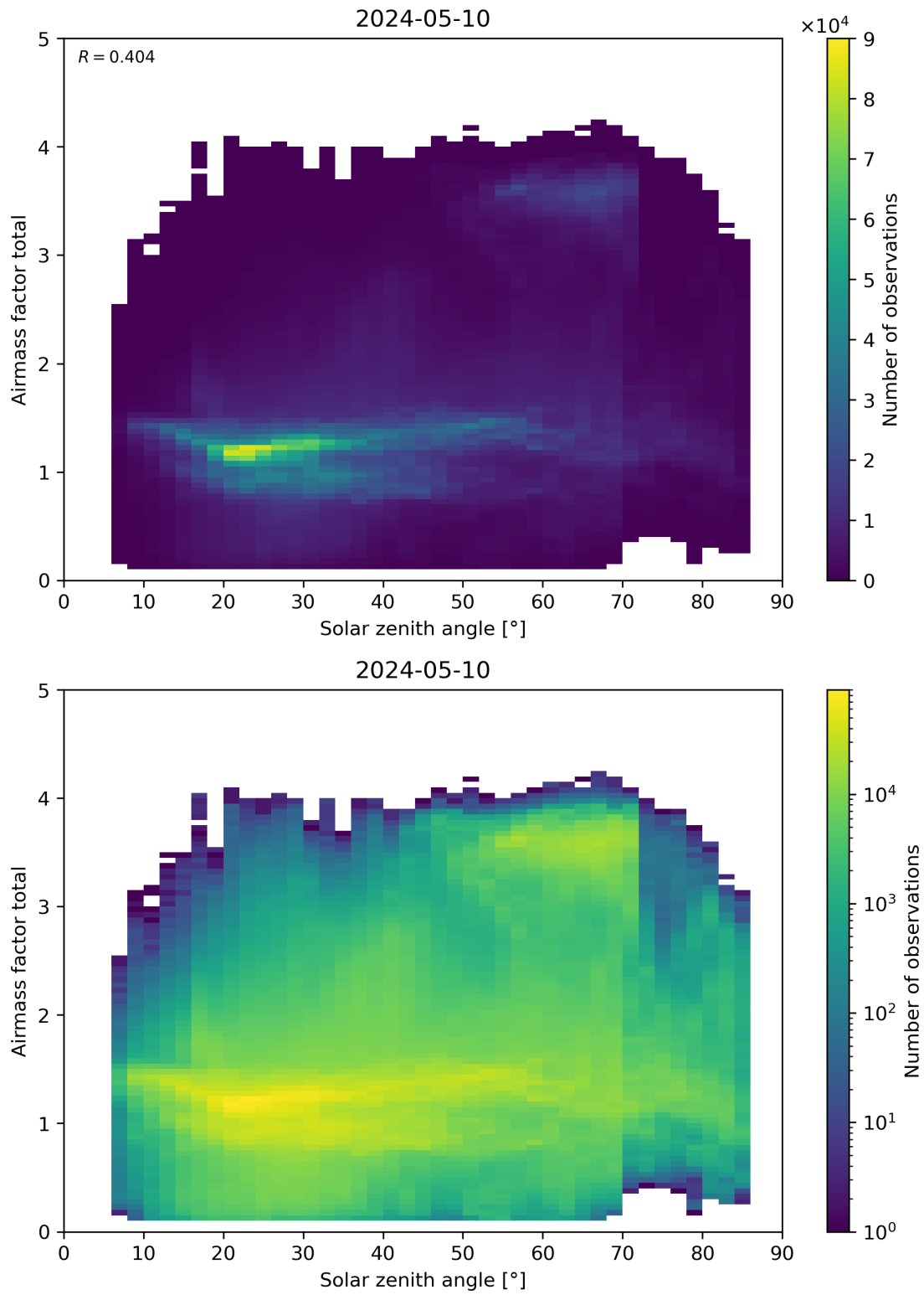
Figure 175: Scatter density plot of “Solar zenith angle” against “Airmass factor total” for 2024-05-09 to 2024-05-11.
