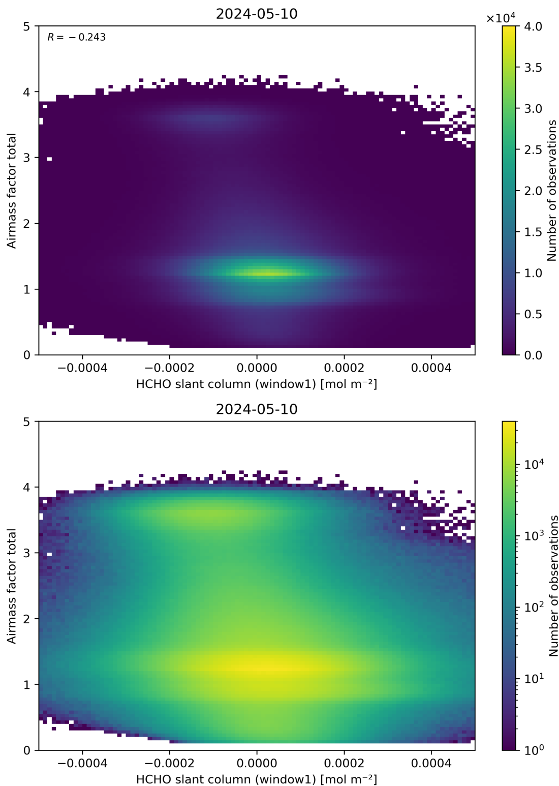
Figure 85: Scatter density plot of “HCHO slant column (window1)” against “Airmass factor total” for 2024-05-09 to 2024-05-11.
