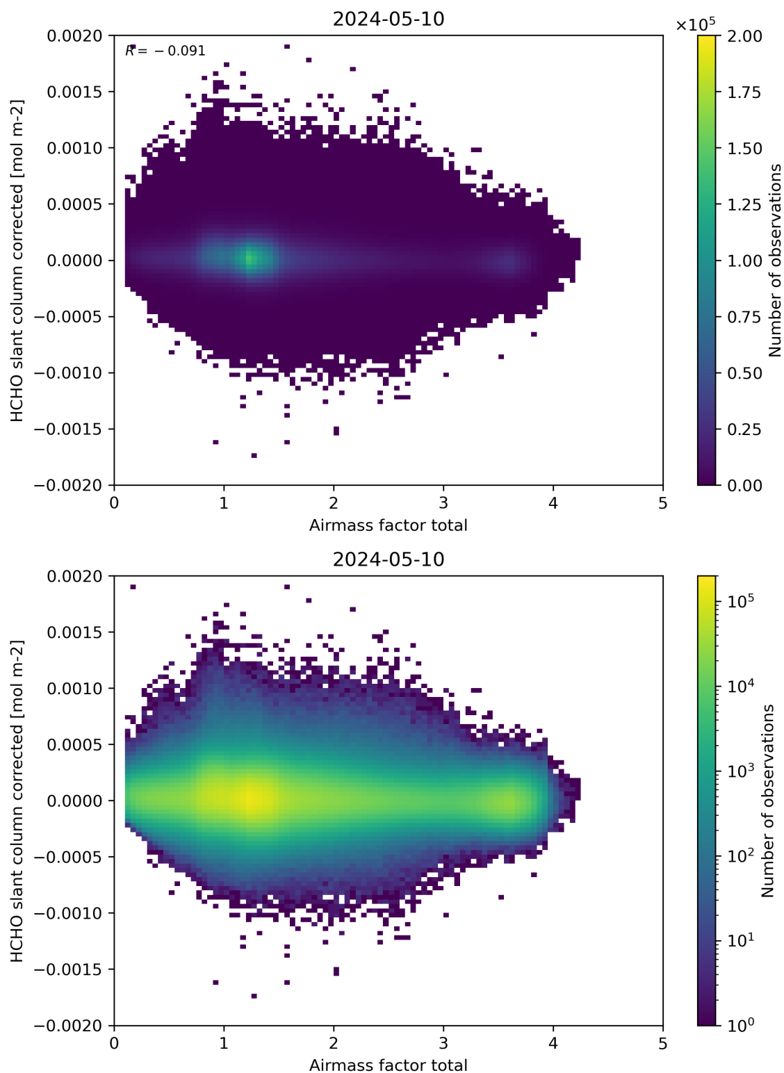
Figure 101: Scatter density plot of “Airmass factor total” against “HCHO slant column corrected” for 2024-05-09 to 2024-05-11.
