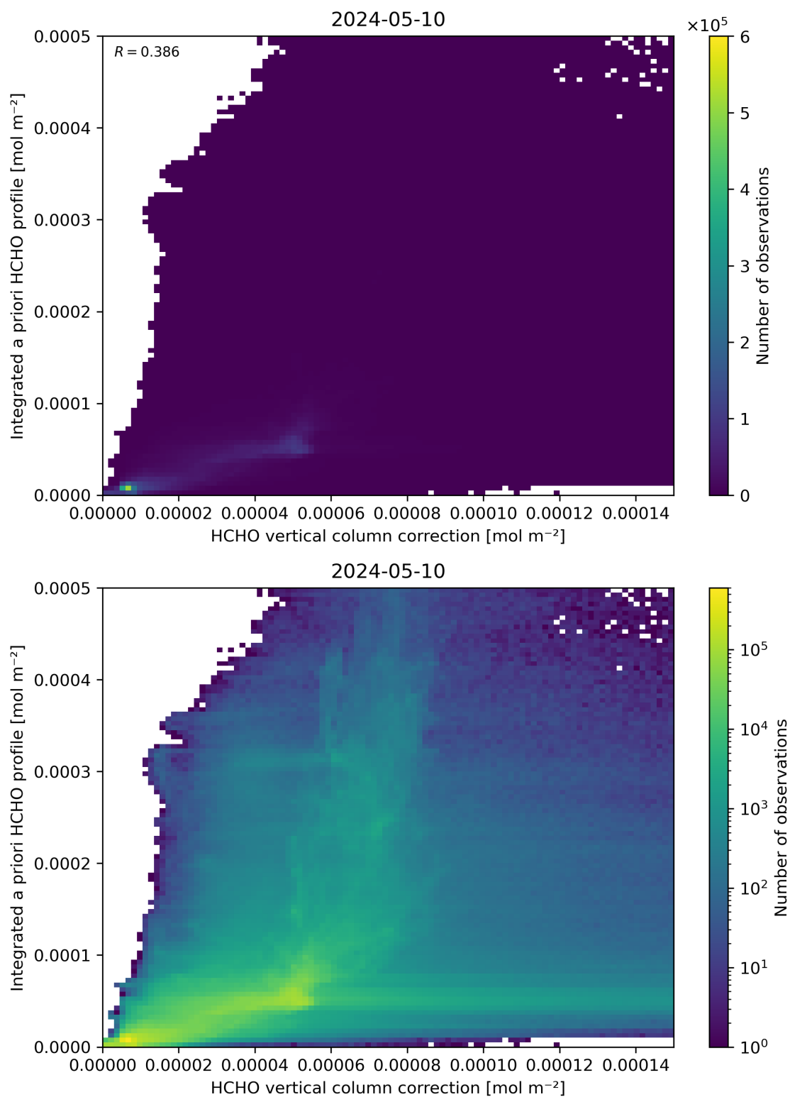
Figure 122: Scatter density plot of “HCHO vertical column correction” against “Integrated a priori HCHO profile” for 2024-05-09 to 2024-05-11.
