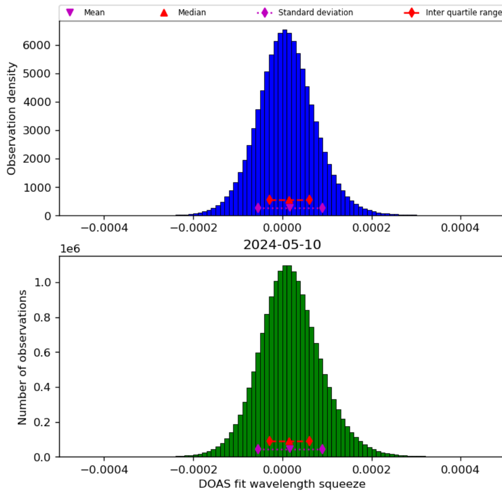
Figure 45: Histogram of “DOAS fit wavelength squeeze” for 2024-05-09 to 2024-05-11
