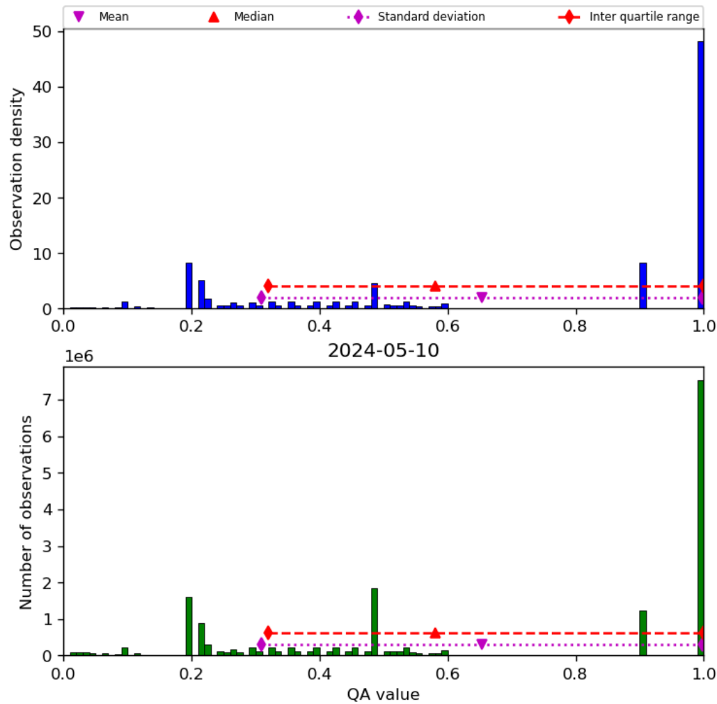
Figure 34: Histogram of “QA value” for 2024-05-09 to 2024-05-11
