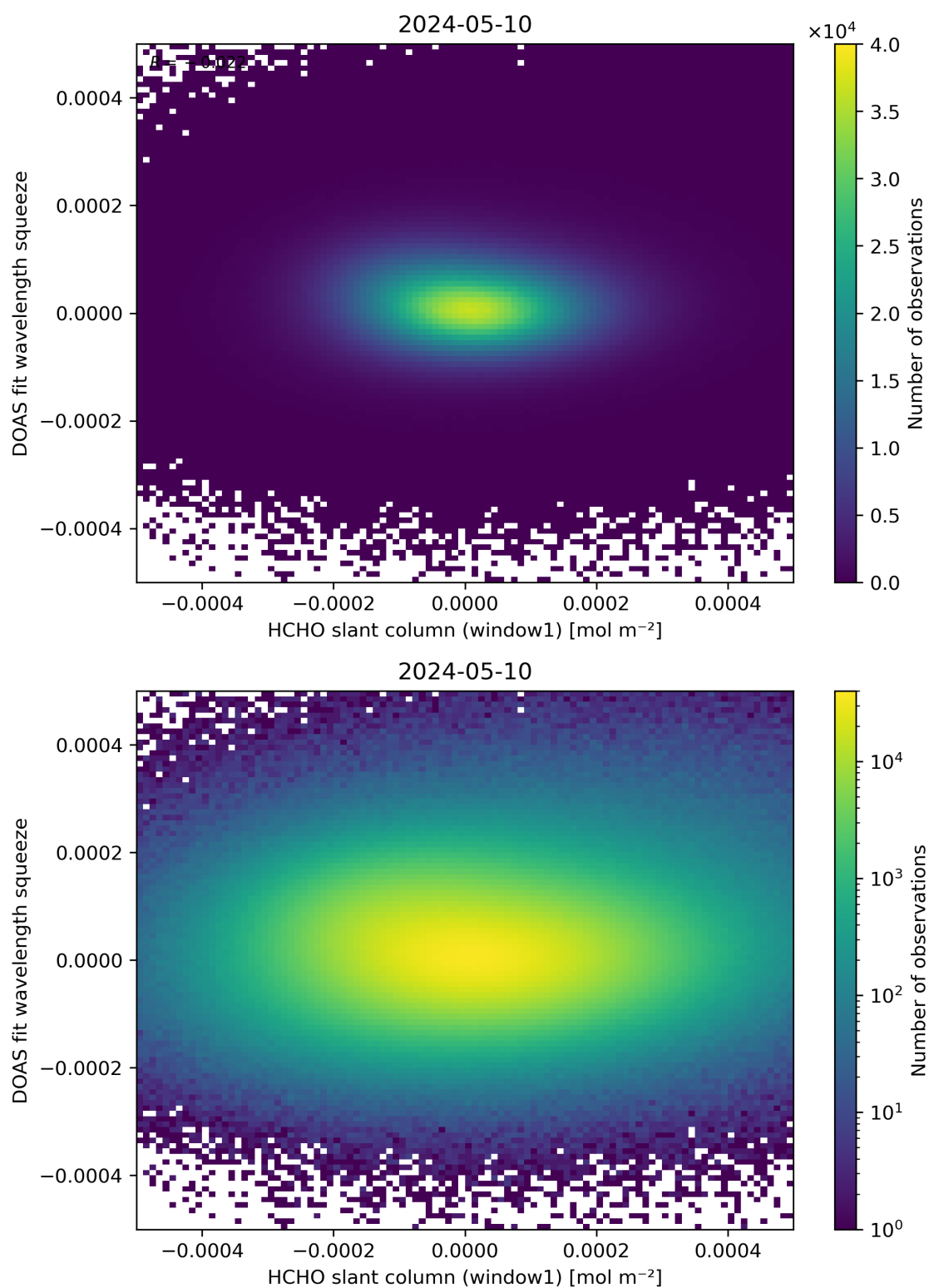
Figure 80: Scatter density plot of “HCHO slant column (window1)” against “DOAS fit wavelength squeeze” for 2024-05-09 to 2024-05-11.
