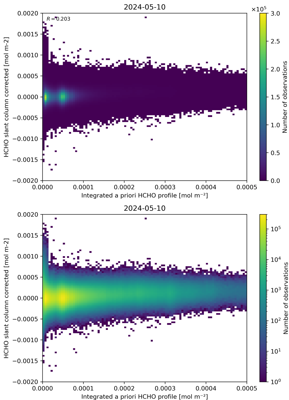
Figure 151: Scatter density plot of “Integrated a priori HCHO profile” against “HCHO slant column corrected” for 2024-05-09 to 2024-05-11.
