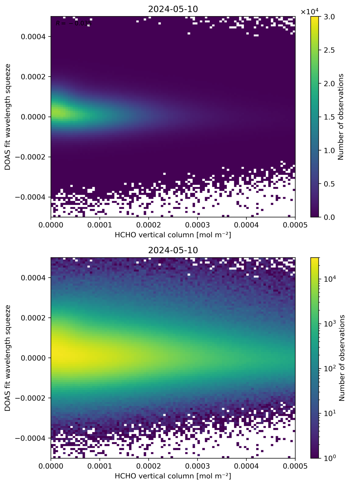
Figure 125: Scatter density plot of “HCHO vertical column” against “DOAS fit wavelength squeeze” for 2024-05-09 to 2024-05-11.
