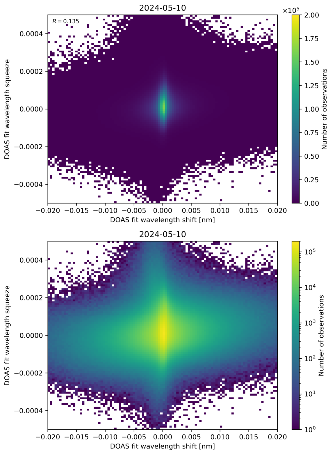
Figure 65: Scatter density plot of “DOAS fit wavelength shift” against “DOAS fit wavelength squeeze” for 2024-05-09 to 2024-05-11.
