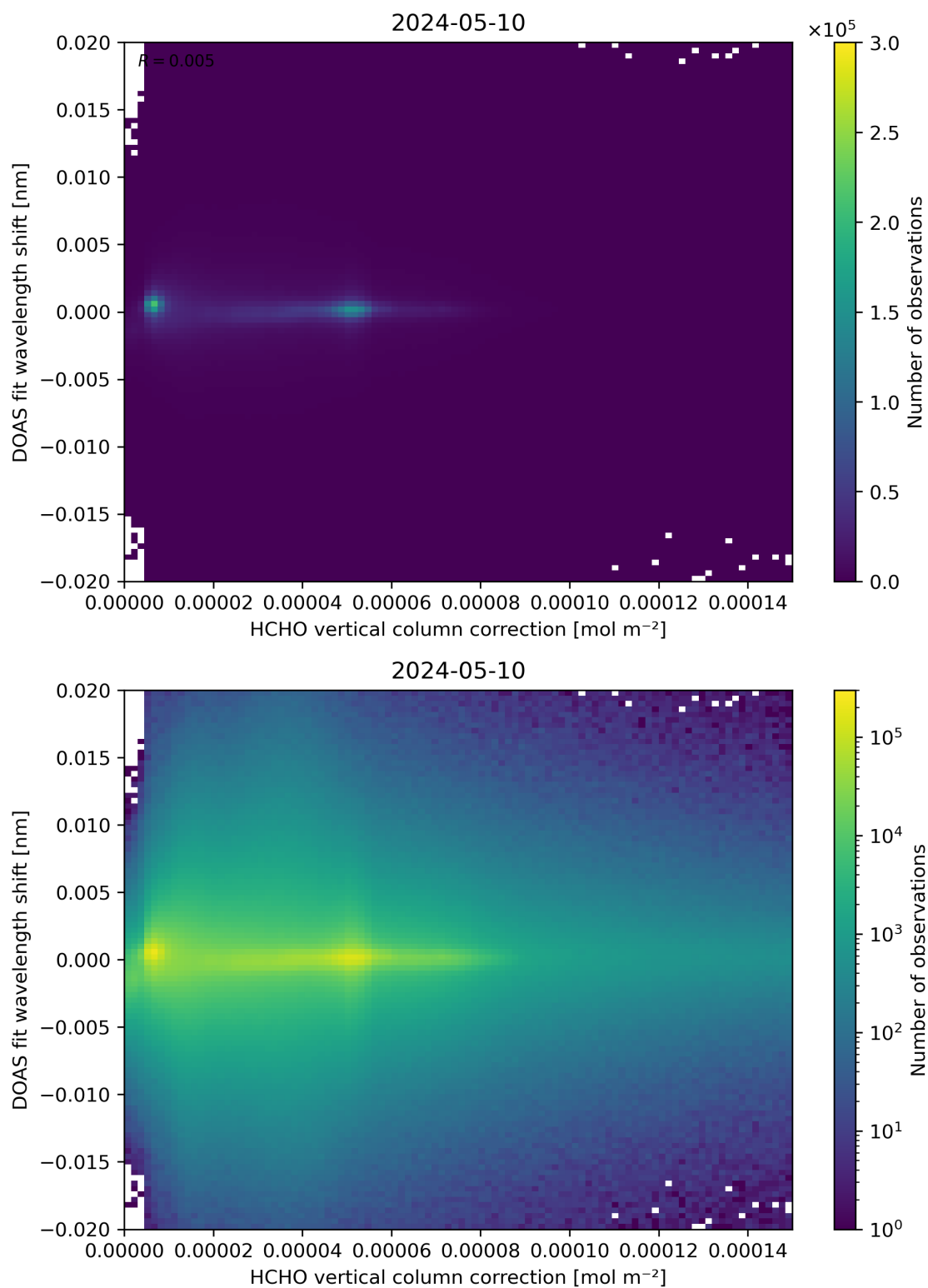
Figure 113: Scatter density plot of “HCHO vertical column correction” against “DOAS fit wavelength shift” for 2024-05-09 to 2024-05-11.
