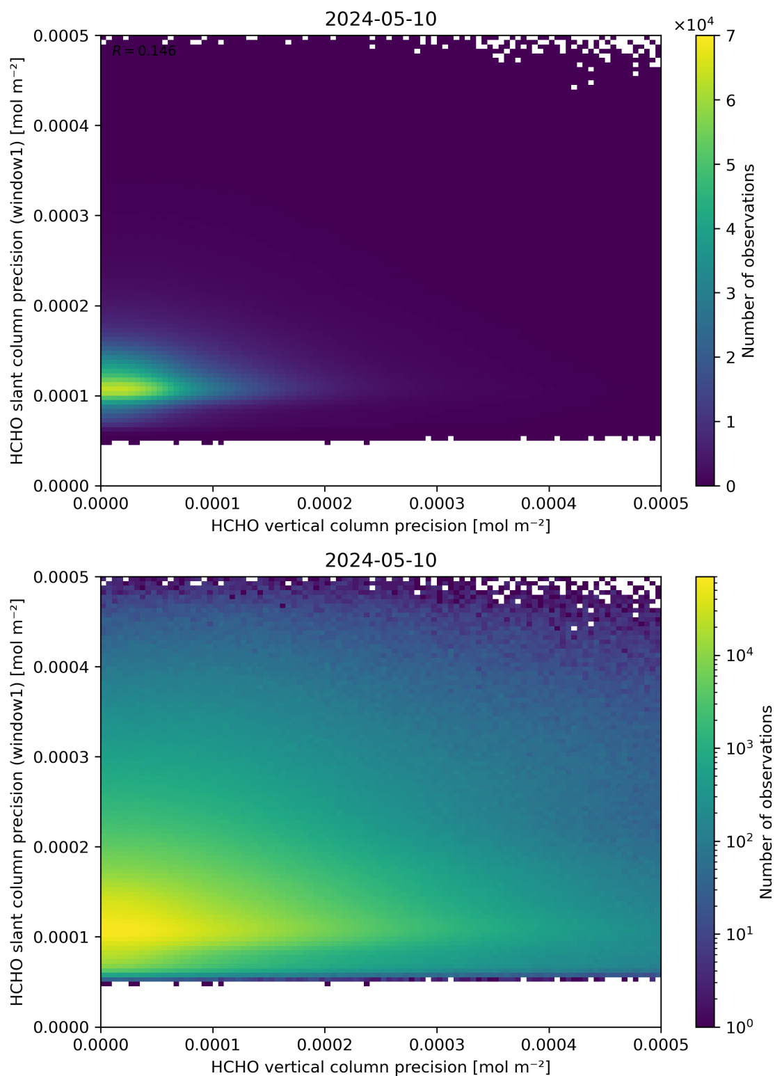
Figure 143: Scatter density plot of “HCHO vertical column precision” against “HCHO slant column precision (window1)” for 2024-05-09 to 2024-05-11.
