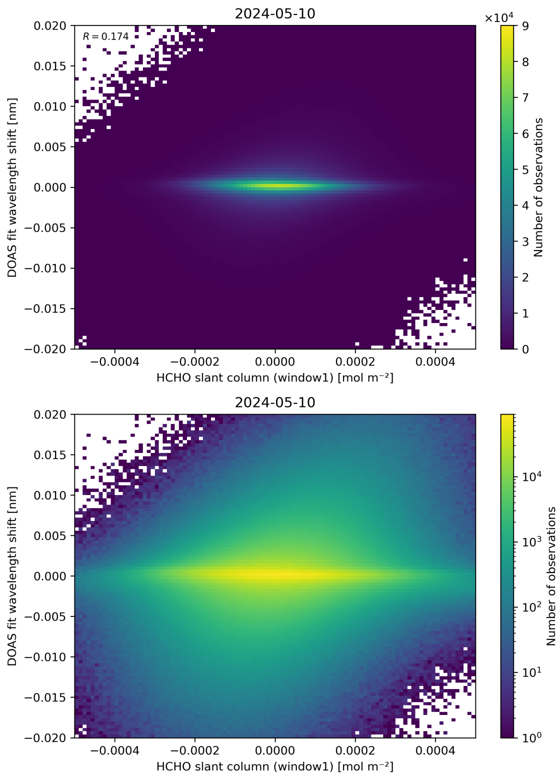
Figure 79: Scatter density plot of “HCHO slant column (window1)” against “DOAS fit wavelength shift” for 2024-05-09 to 2024-05-11.
