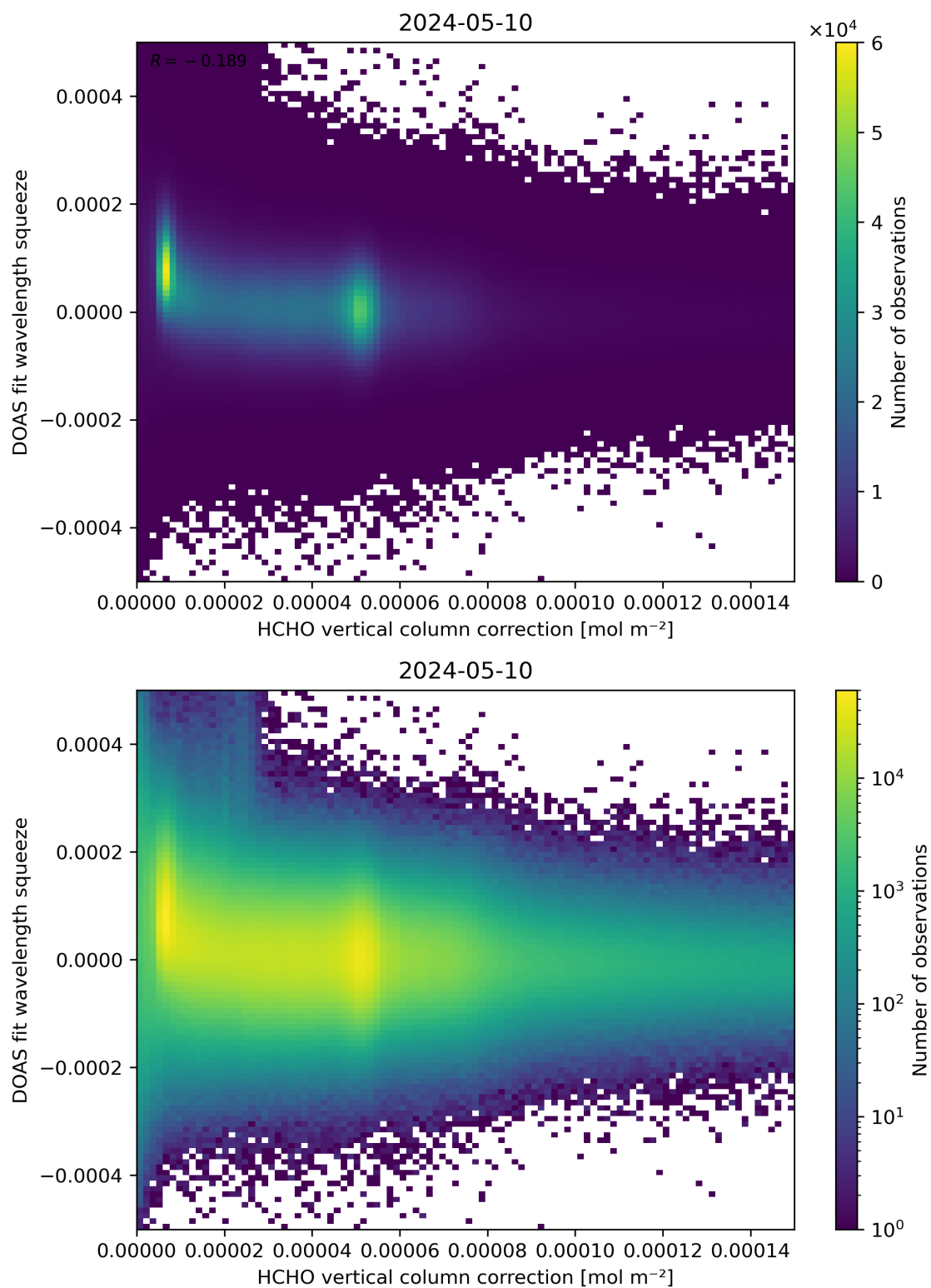
Figure 114: Scatter density plot of “HCHO vertical column correction” against “DOAS fit wavelength squeeze” for 2024-05-09 to 2024-05-11.
