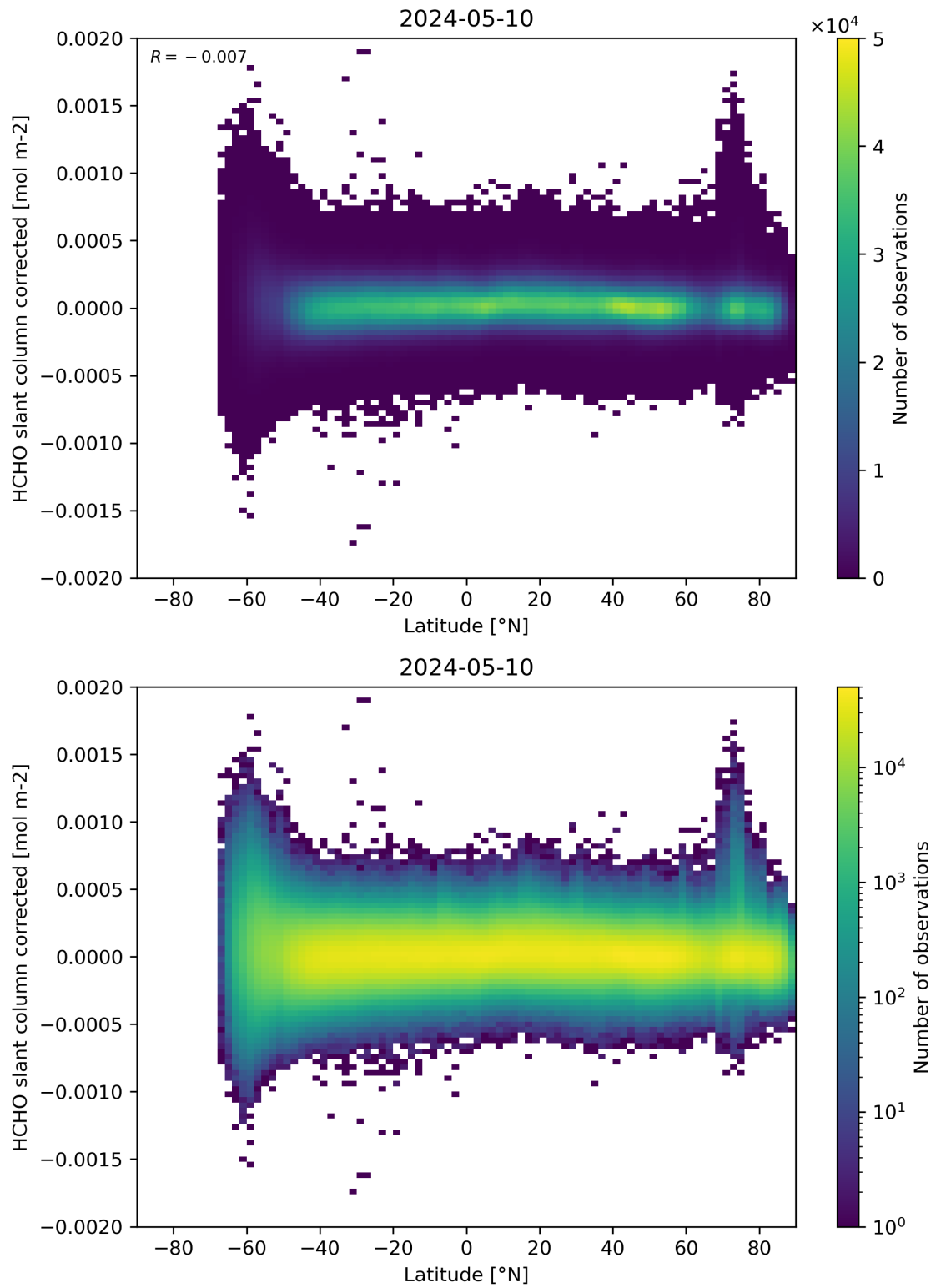
Figure 157: Scatter density plot of “Latitude” against “HCHO slant column corrected” for 2024-05-09 to 2024-05-11.
