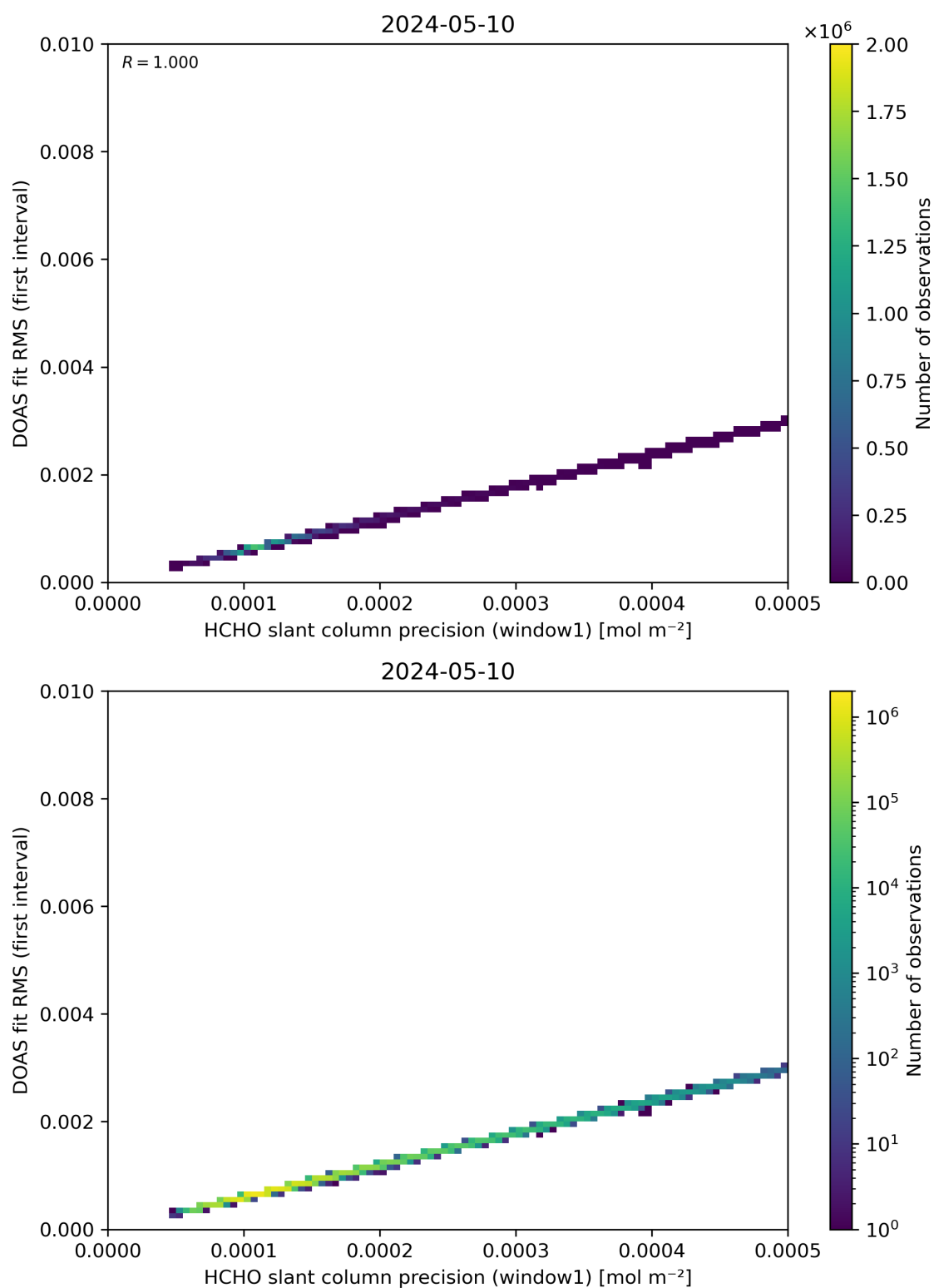
Figure 88: Scatter density plot of “HCHO slant column precision (window1)” against “DOAS fit RMS (first interval)” for 2024-05-09 to 2024-05-11.
