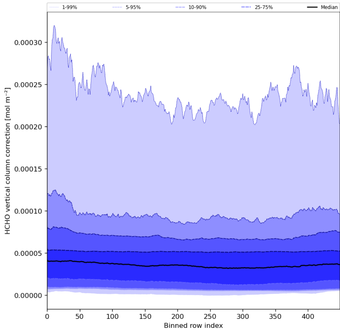
Figure 51: Along track statistics of “HCHO vertical column correction” for 2024-05-09 to 2024-05-11
