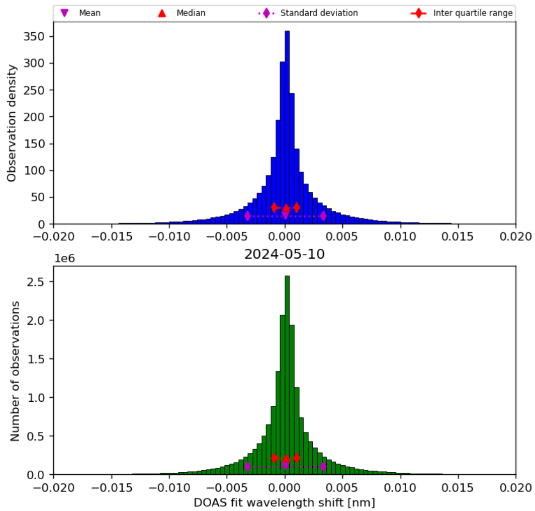
Figure 44: Histogram of “DOAS fit wavelength shift” for 2024-05-09 to 2024-05-11
