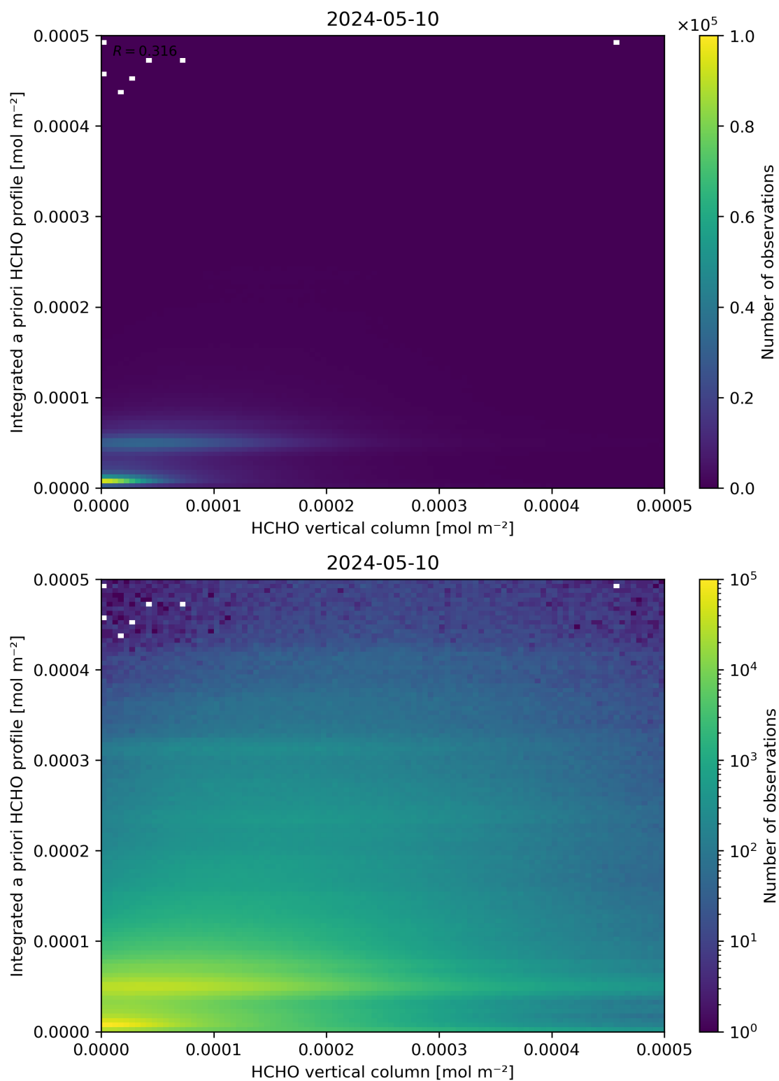
Figure 135: Scatter density plot of “HCHO vertical column” against “Integrated a priori HCHO profile” for 2024-05-09 to 2024-05-11.
