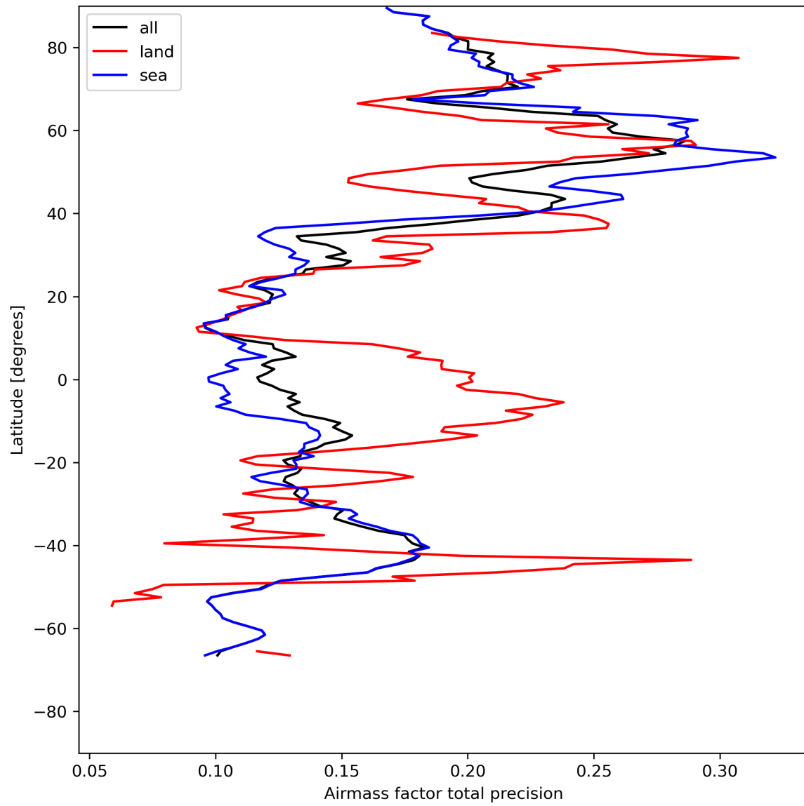
Figure 27: Zonal average of “Airmass factor total precision” for 2024-05-09 to 2024-05-11.
