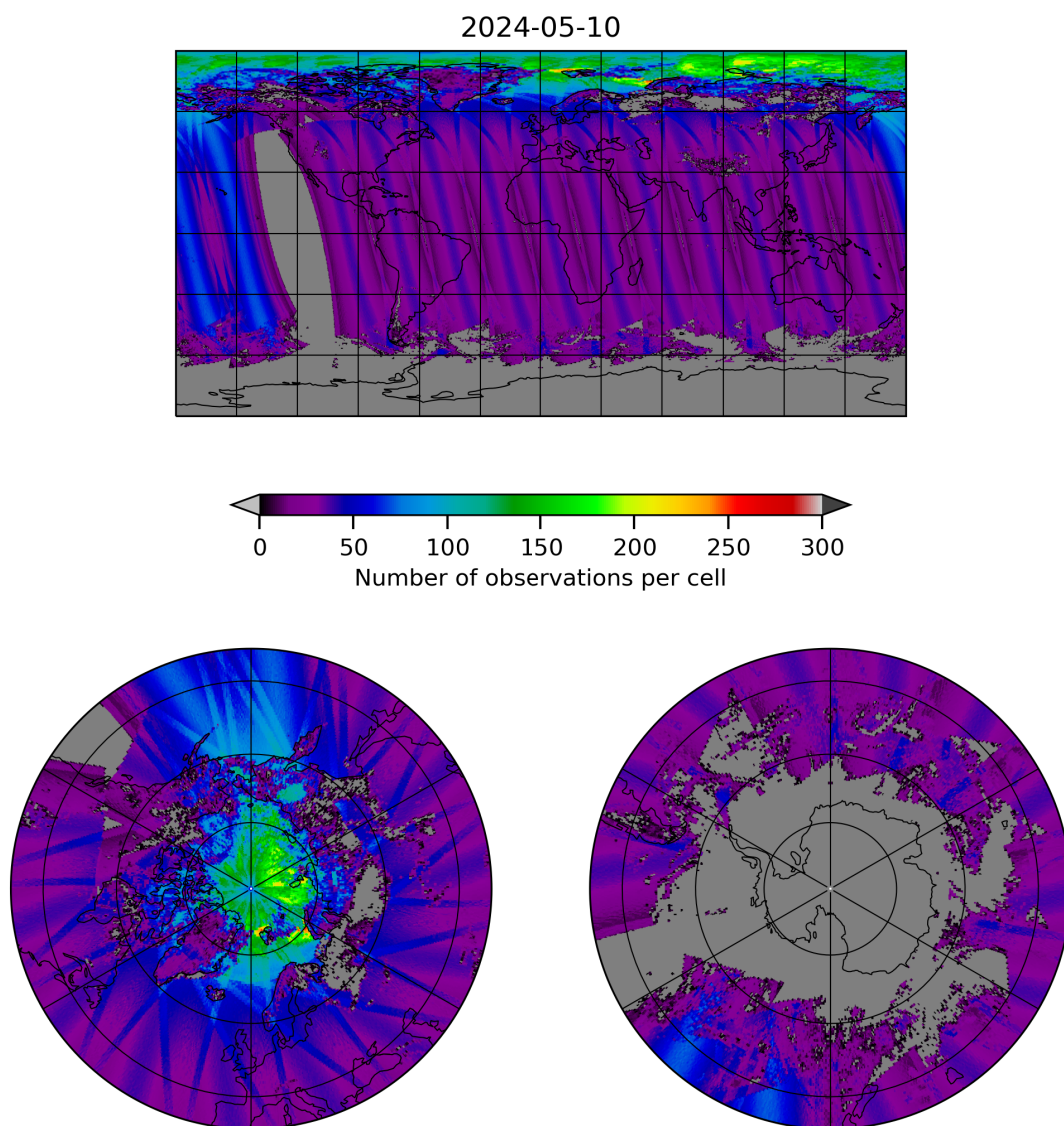
Figure 19: Map of the number of observations for 2024-05-09 to 2024-05-11
