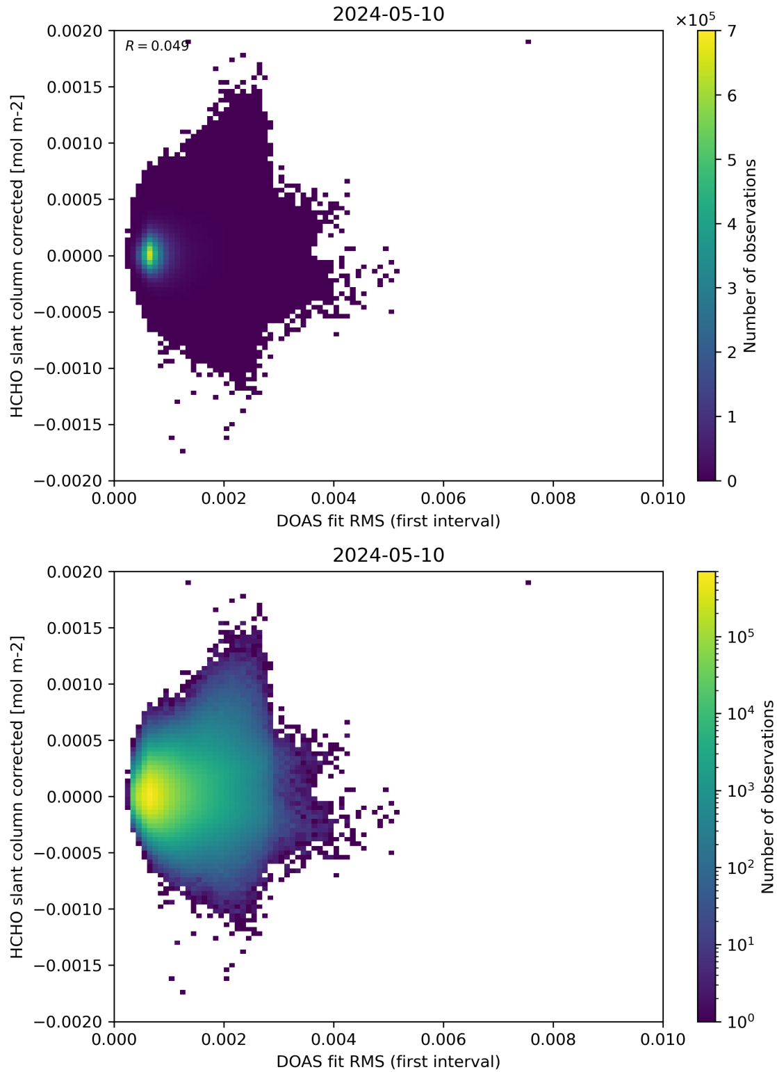
Figure 62: Scatter density plot of “DOAS fit RMS (first interval)” against “HCHO slant column corrected” for 2024-05-09 to 2024-05-11.
