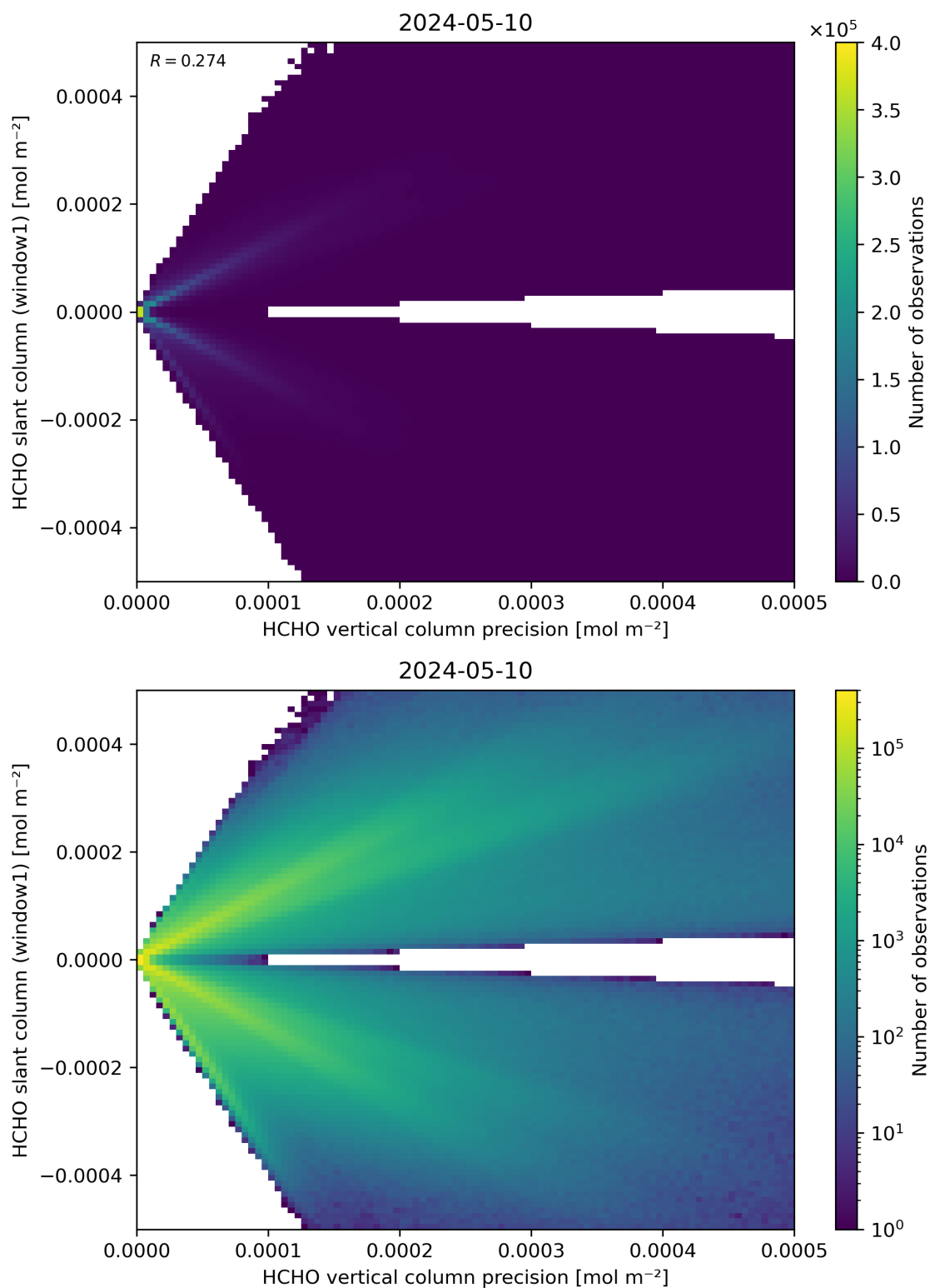
Figure 142: Scatter density plot of “HCHO vertical column precision” against “HCHO slant column (window1)” for 2024-05-09 to 2024-05-11.
