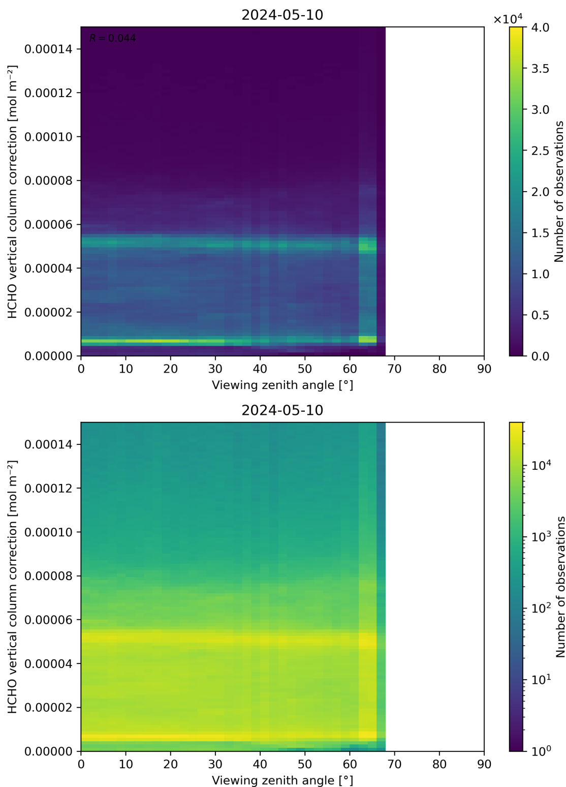
Figure 193: Scatter density plot of “Viewing zenith angle” against “HCHO vertical column correction” for 2024-05-09 to 2024-05-11.
