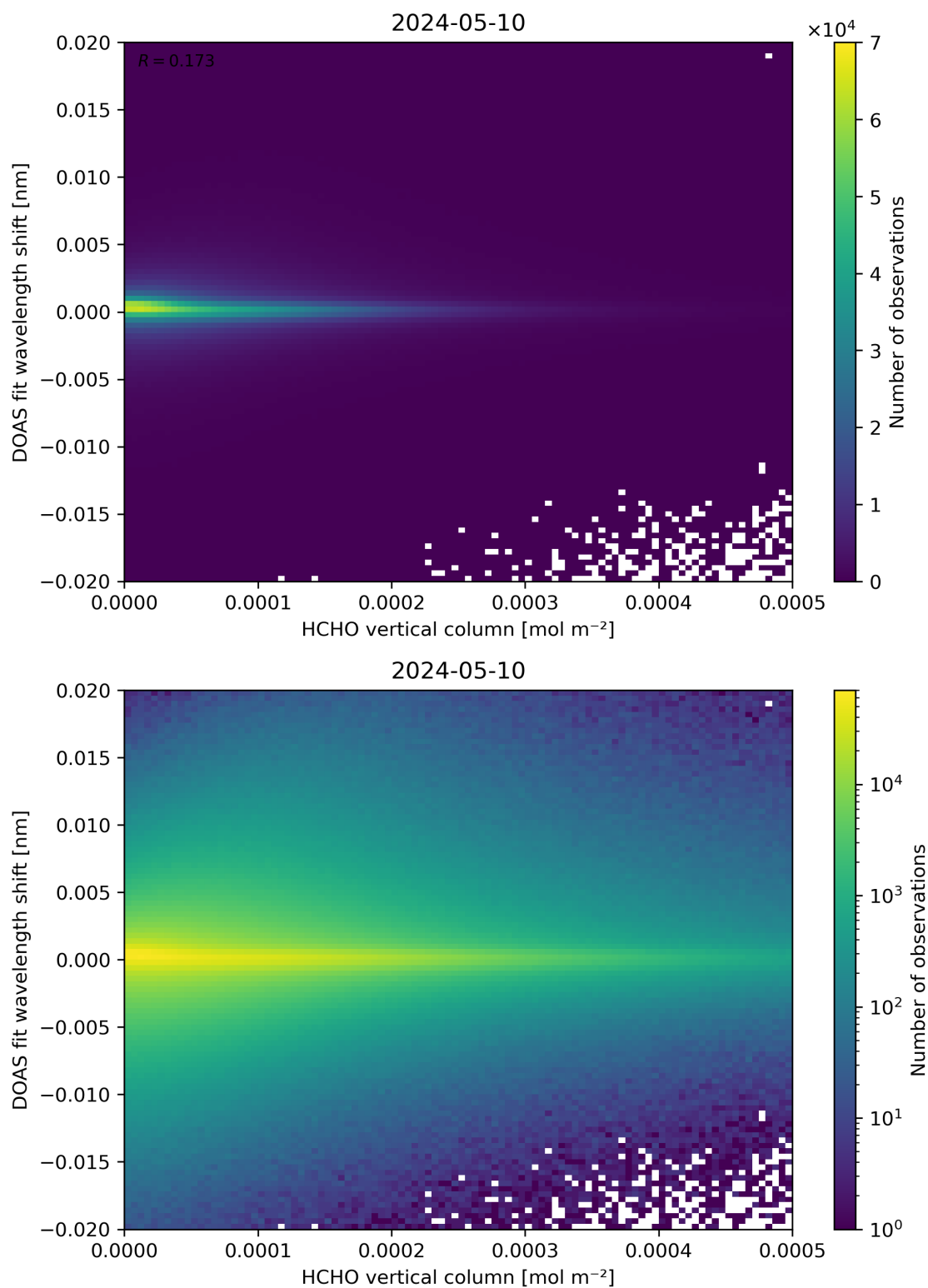
Figure 124: Scatter density plot of “HCHO vertical column” against “DOAS fit wavelength shift” for 2024-05-09 to 2024-05-11.
