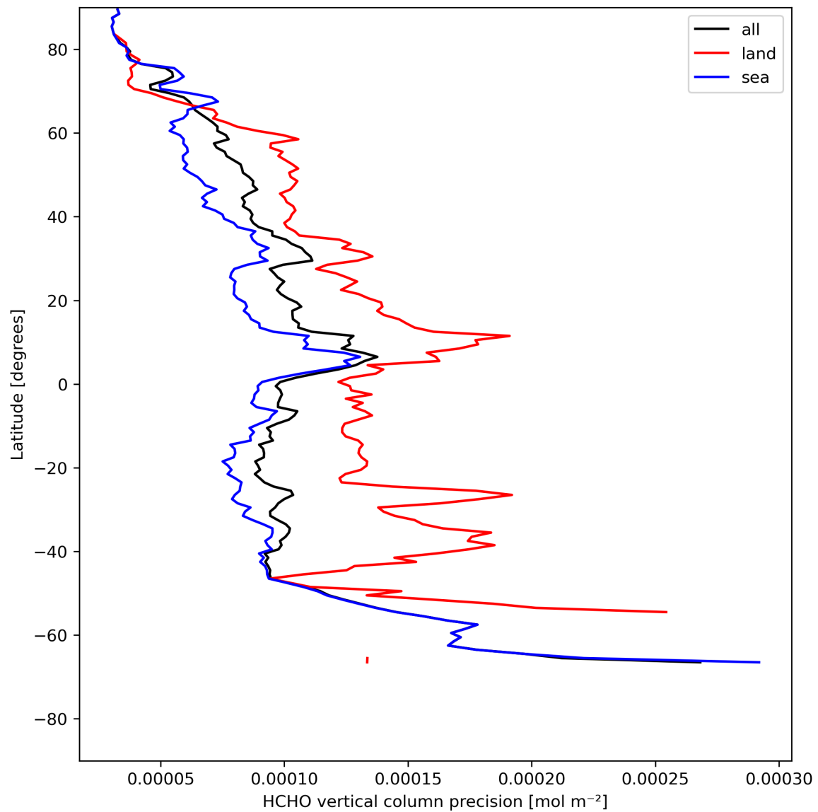
Figure 22: Zonal average of “HCHO vertical column precision” for 2024-05-09 to 2024-05-11.
