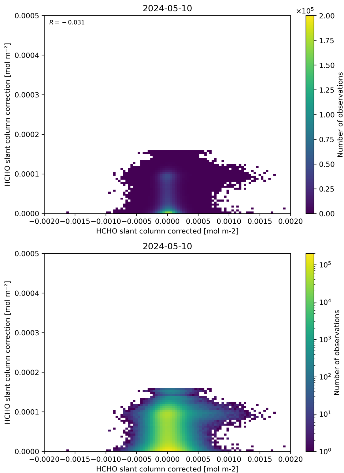
Figure 77: Scatter density plot of “HCHO slant column corrected” against “HCHO slant column correction” for 2024-05-09 to 2024-05-11.
