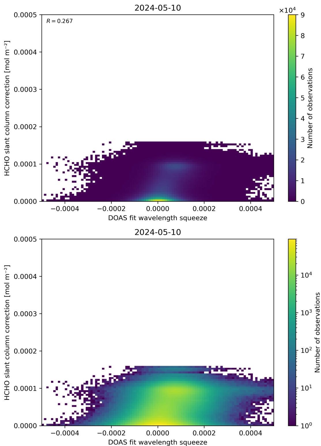
Figure 70: Scatter density plot of “DOAS fit wavelength squeeze” against “HCHO slant column correction” for 2024-05-09 to 2024-05-11.
