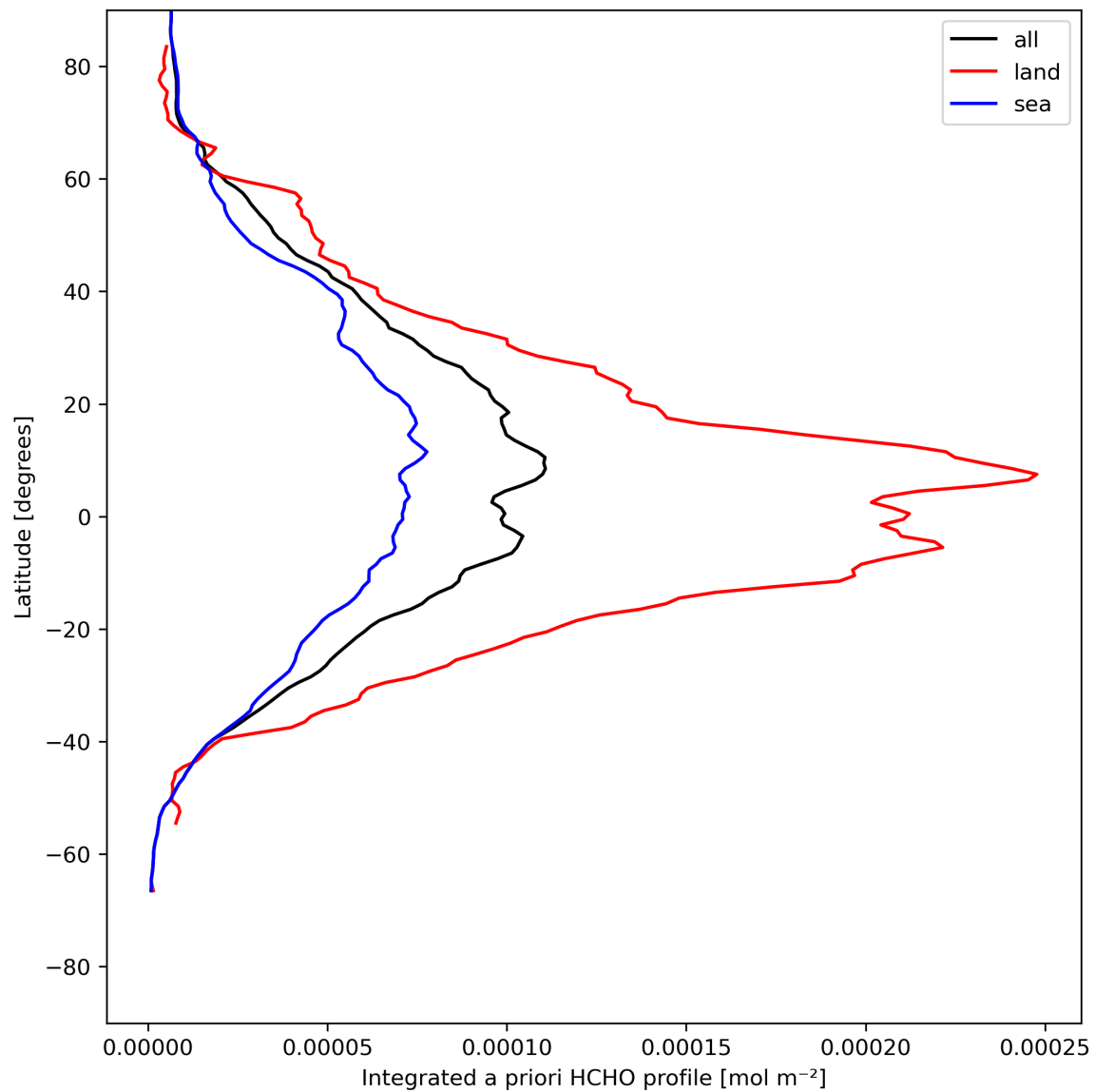
Figure 29: Zonal average of “Integrated a priori HCHO profile” for 2024-05-09 to 2024-05-11.
