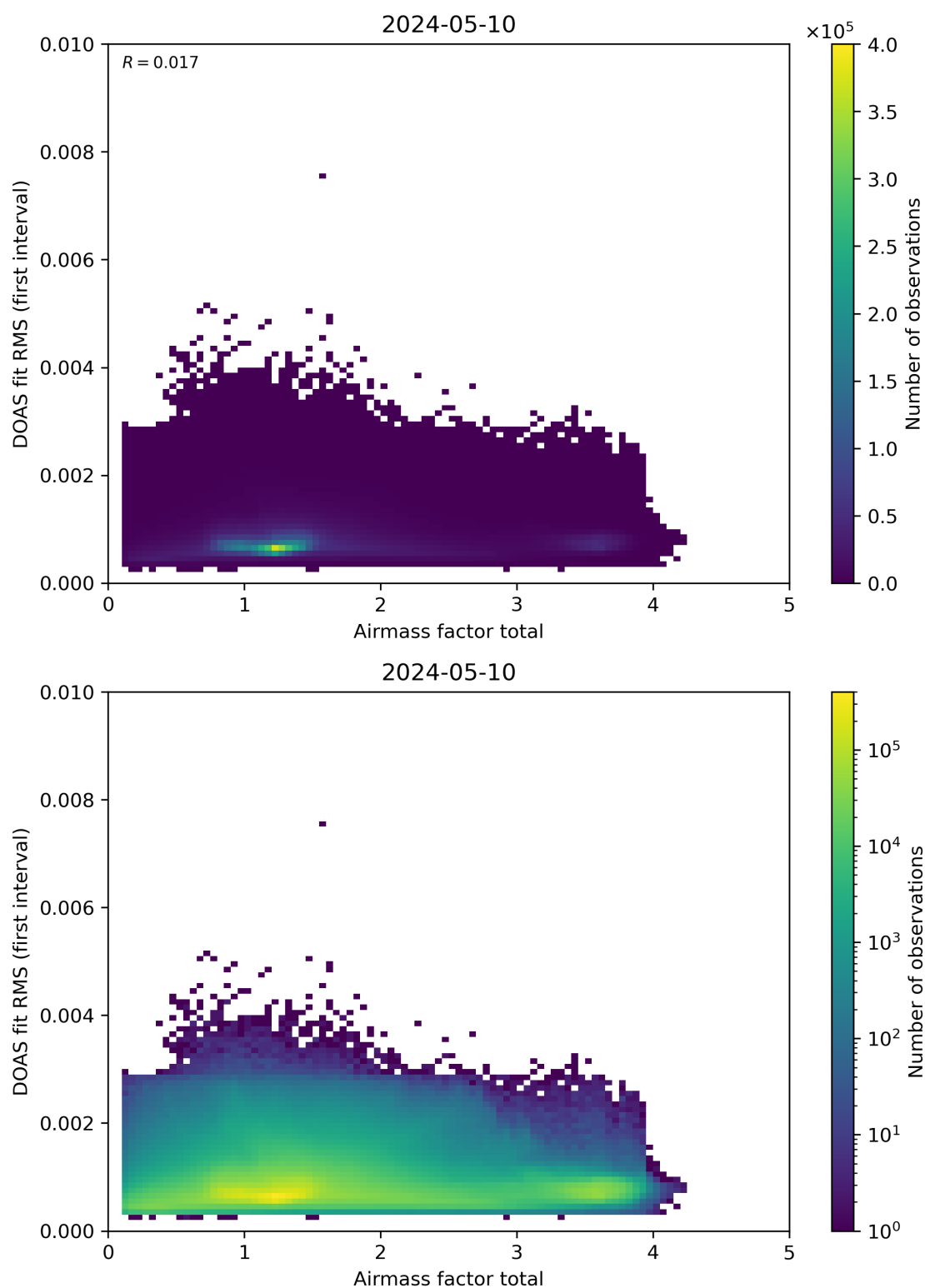
Figure 97: Scatter density plot of “Airmass factor total” against “DOAS fit RMS (first interval)” for 2024-05-09 to 2024-05-11.
