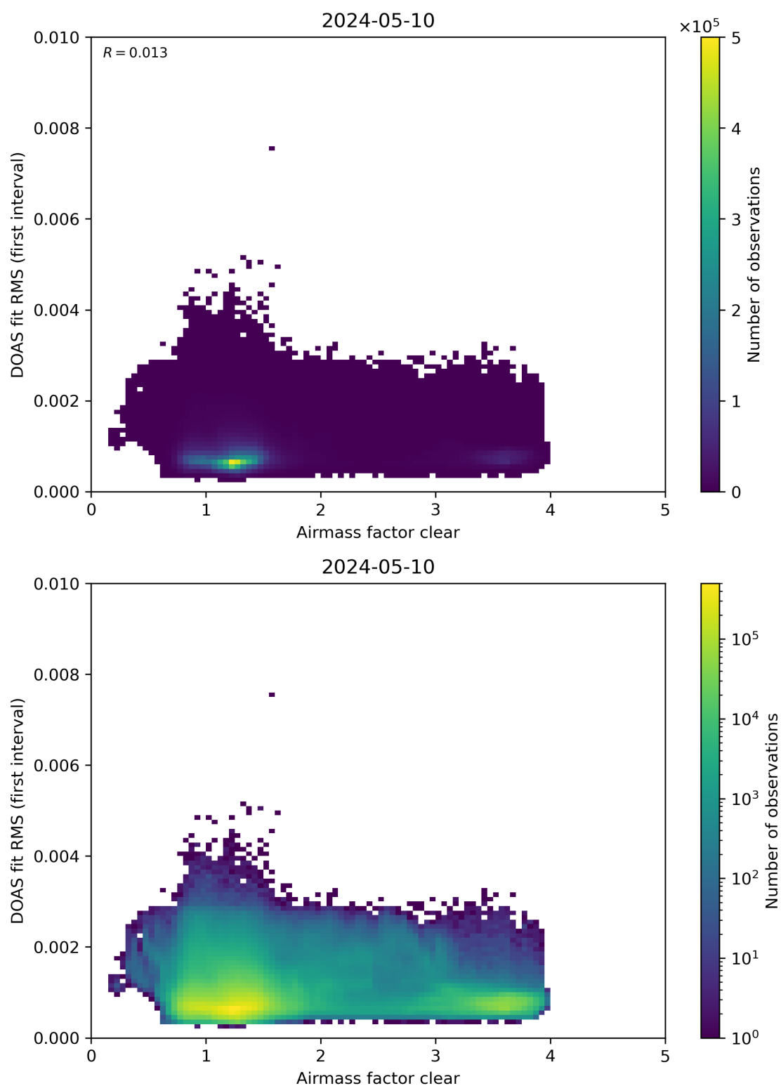
Figure 71: Scatter density plot of “Airmass factor clear” against “DOAS fit RMS (first interval)” for 2024-05-09 to 2024-05-11.
