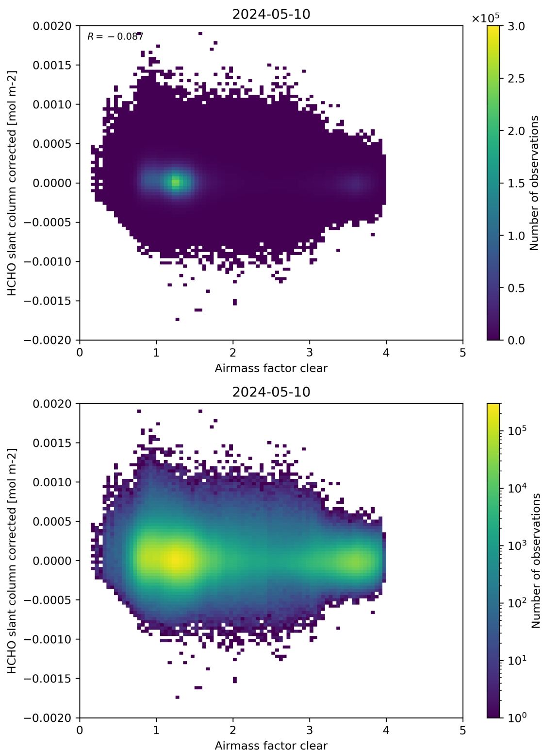
Figure 74: Scatter density plot of “Airmass factor clear” against “HCHO slant column corrected” for 2024-05-09 to 2024-05-11.
