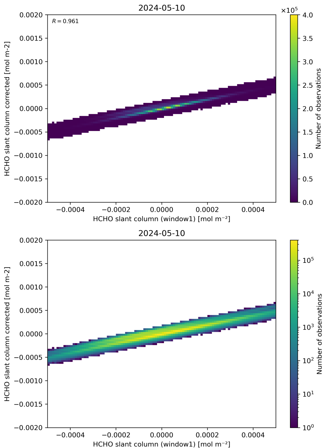
Figure 82: Scatter density plot of “HCHO slant column (window1)” against “HCHO slant column corrected” for 2024-05-09 to 2024-05-11.
