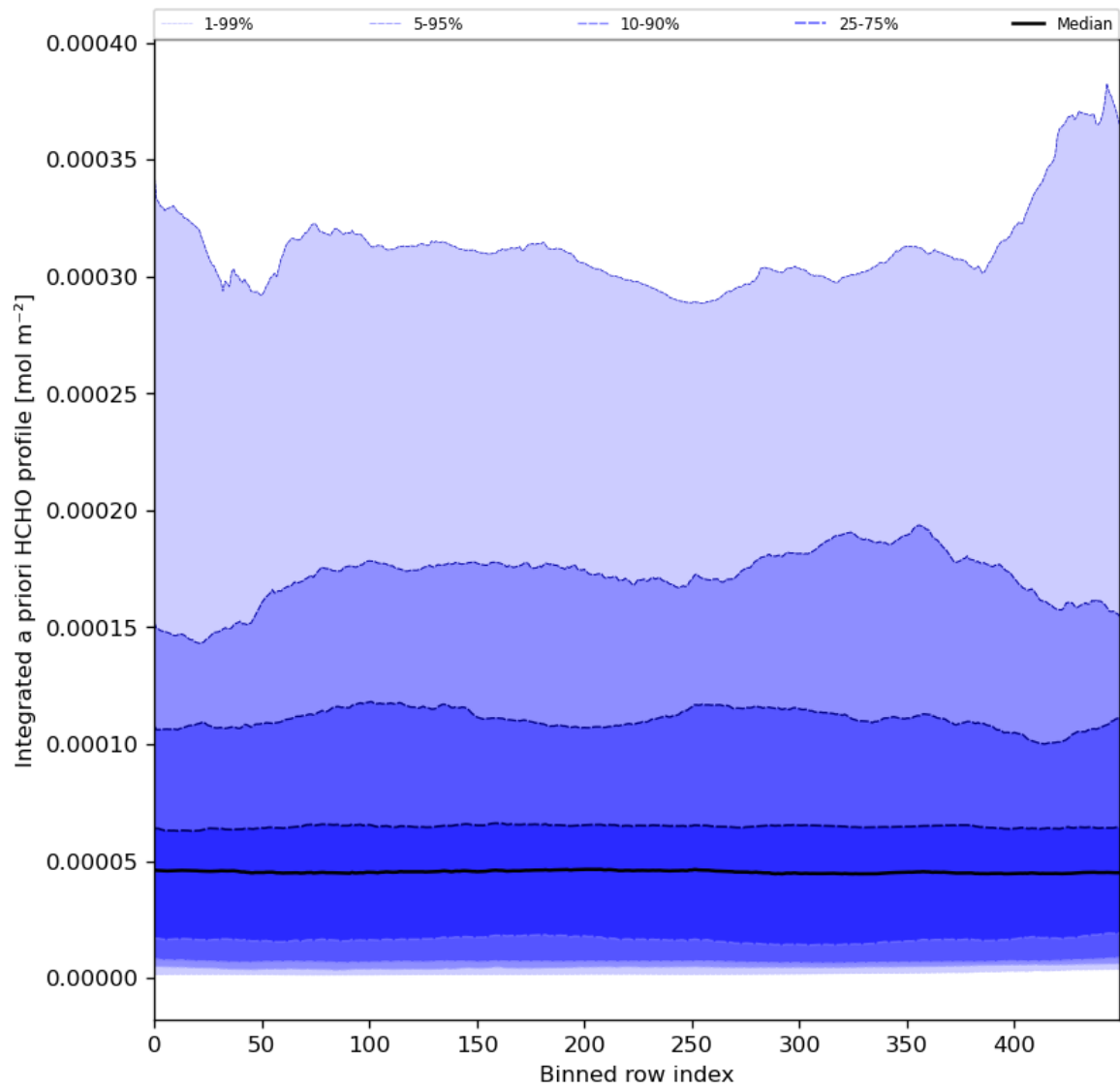
Figure 57: Along track statistics of "Integrated a priori HCHO profile" for 2024-05-09 to 2024-05-11
