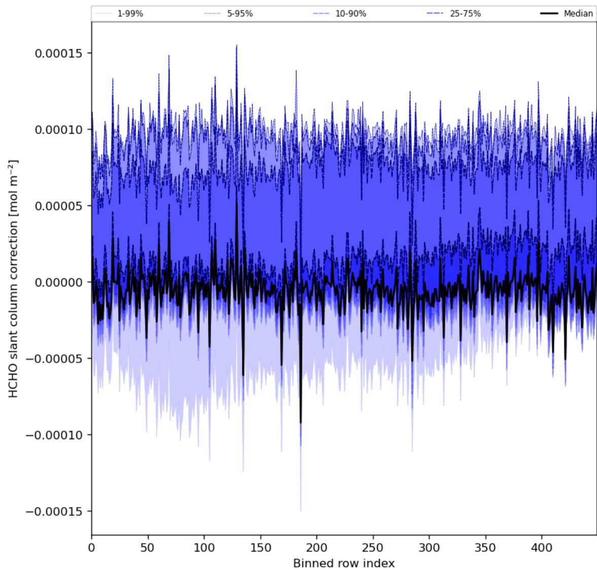
Figure 61: Along track statistics of “HCHO slant column correction” for 2024-05-09 to 2024-05-11
