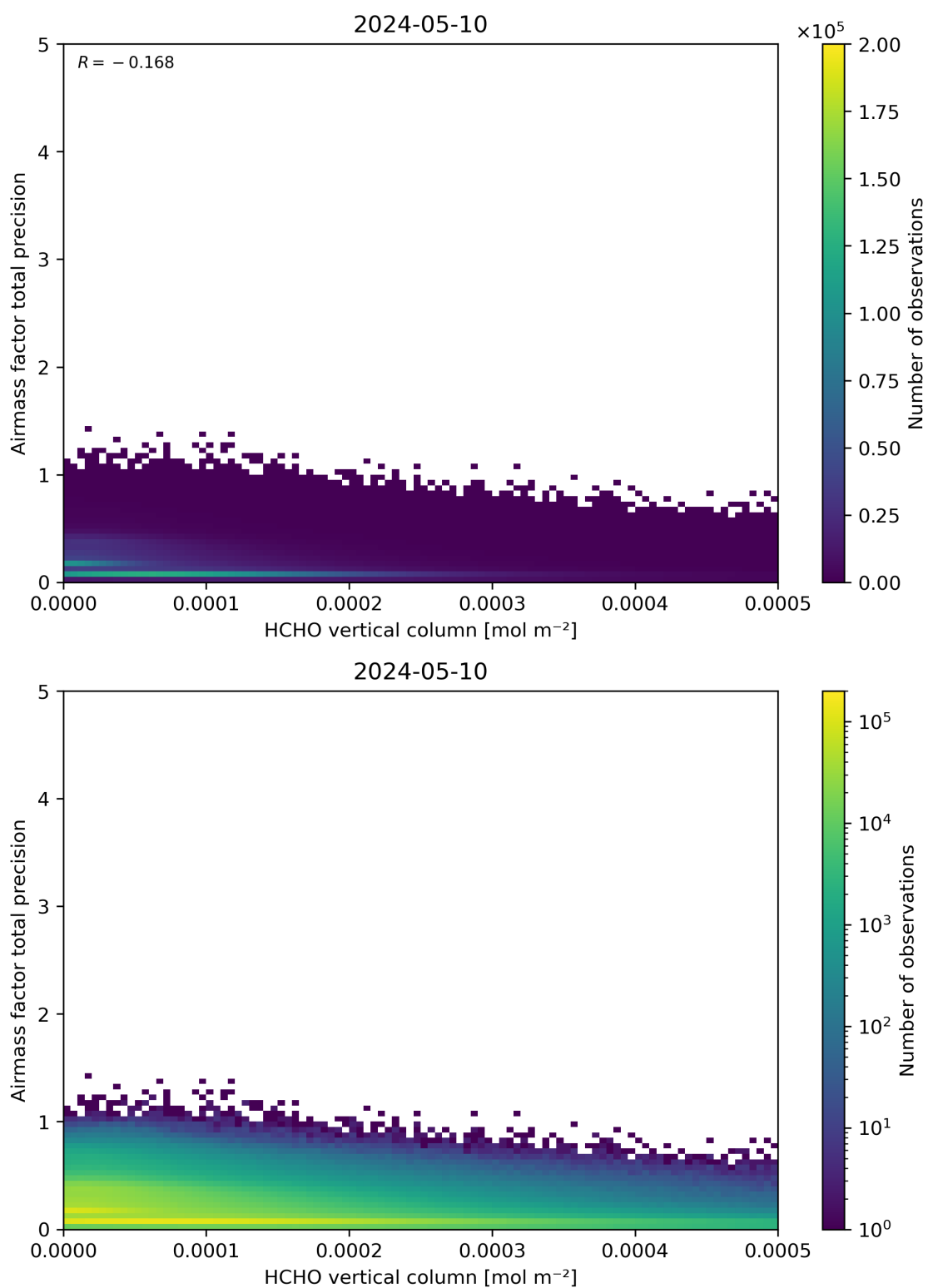
Figure 132: Scatter density plot of “HCHO vertical column” against “Airmass factor total precision” for 2024-05-09 to 2024-05-11.
