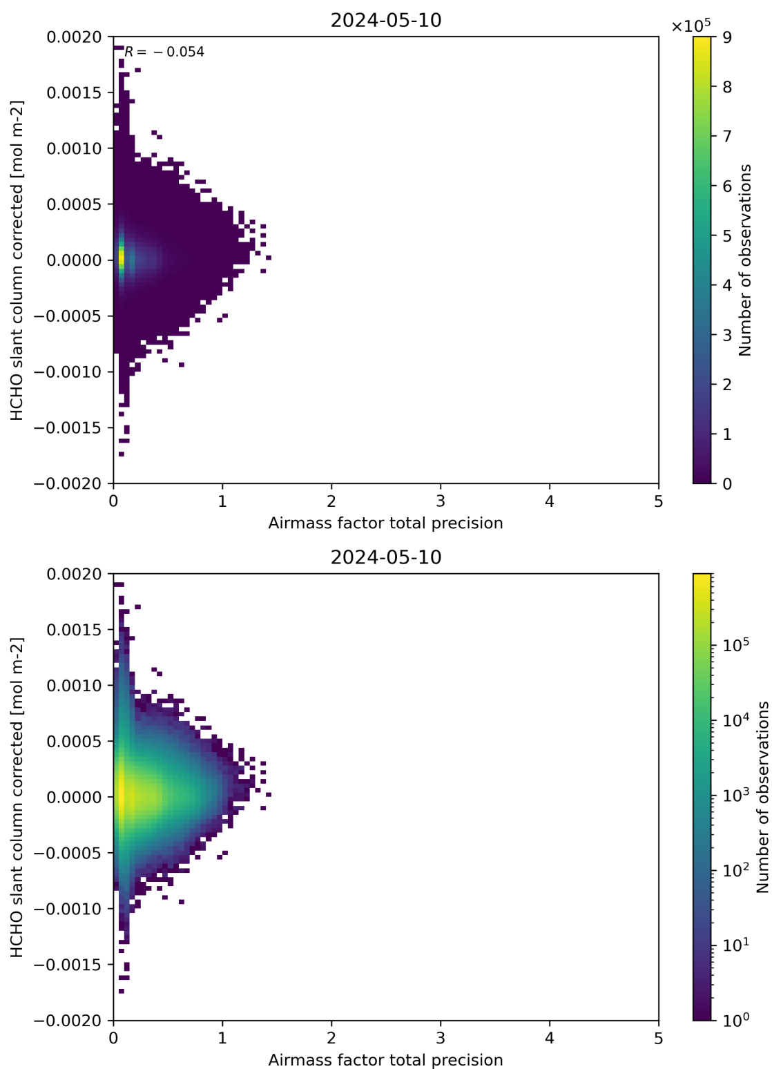
Figure 109: Scatter density plot of “Airmass factor total precision” against “HCHO slant column corrected” for 2024-05-09 to 2024-05-11.
