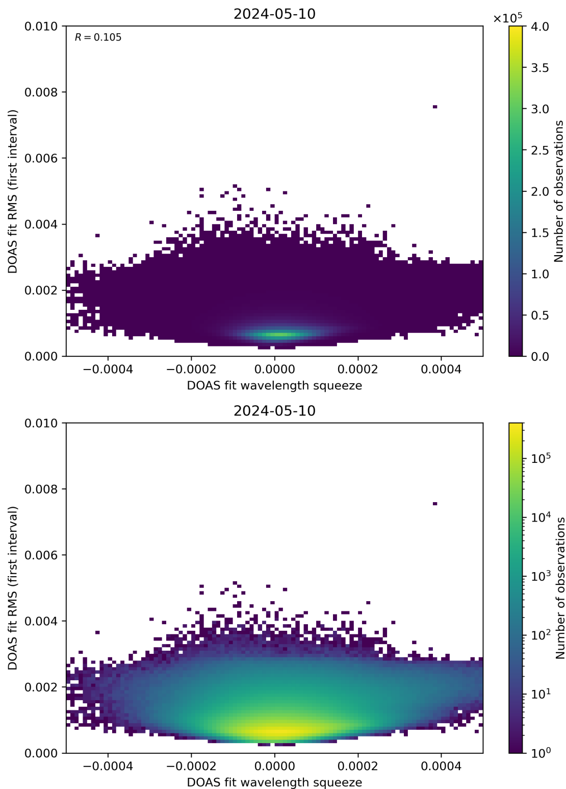
Figure 68: Scatter density plot of “DOAS fit wavelength squeeze” against “DOAS fit RMS (first interval)” for 2024-05-09 to 2024-05-11.
