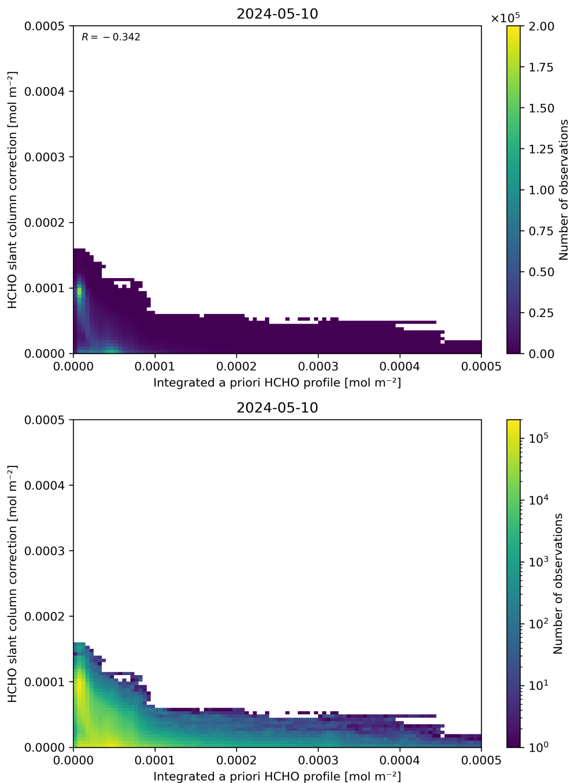
Figure 152: Scatter density plot of “Integrated a priori HCHO profile” against “HCHO slant column correction” for 2024-05-09 to 2024-05-11.
