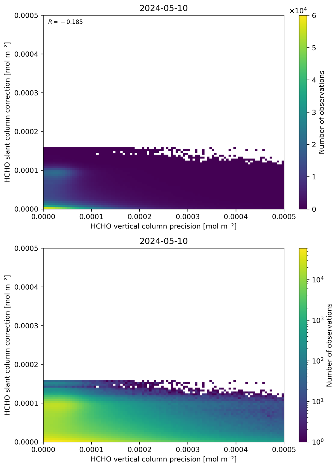
Figure 141: Scatter density plot of “HCHO vertical column precision” against “HCHO slant column correction” for 2024-05-09 to 2024-05-11.
