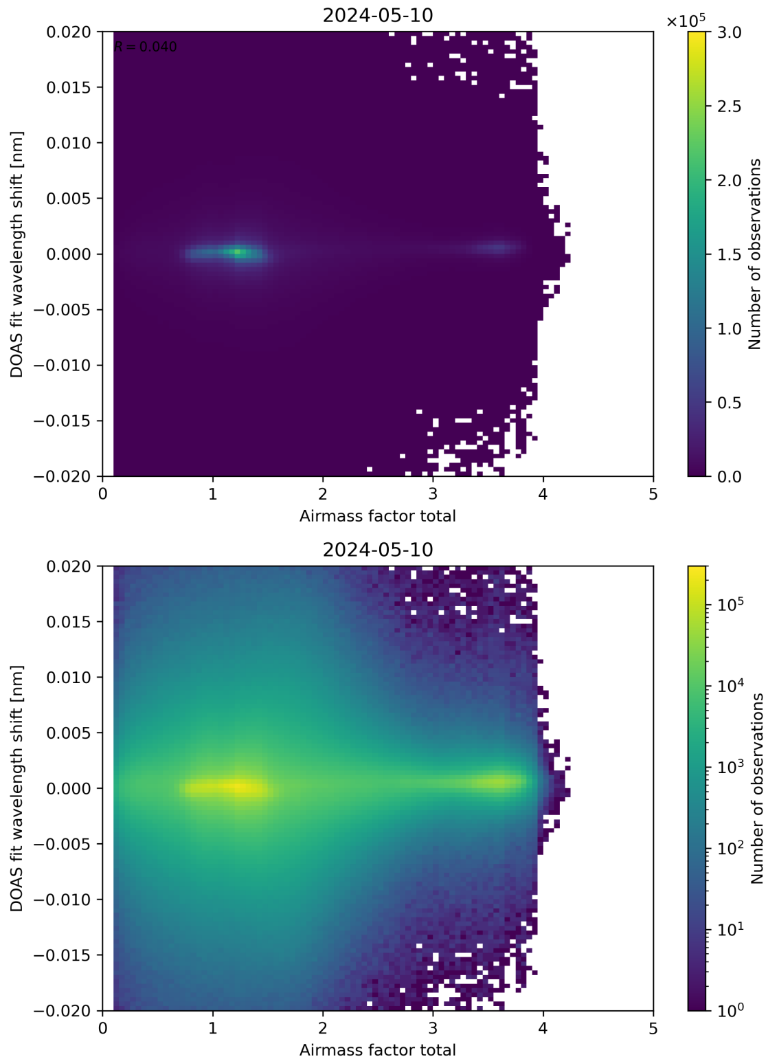
Figure 98: Scatter density plot of “Airmass factor total” against “DOAS fit wavelength shift” for 2024-05-09 to 2024-05-11.
