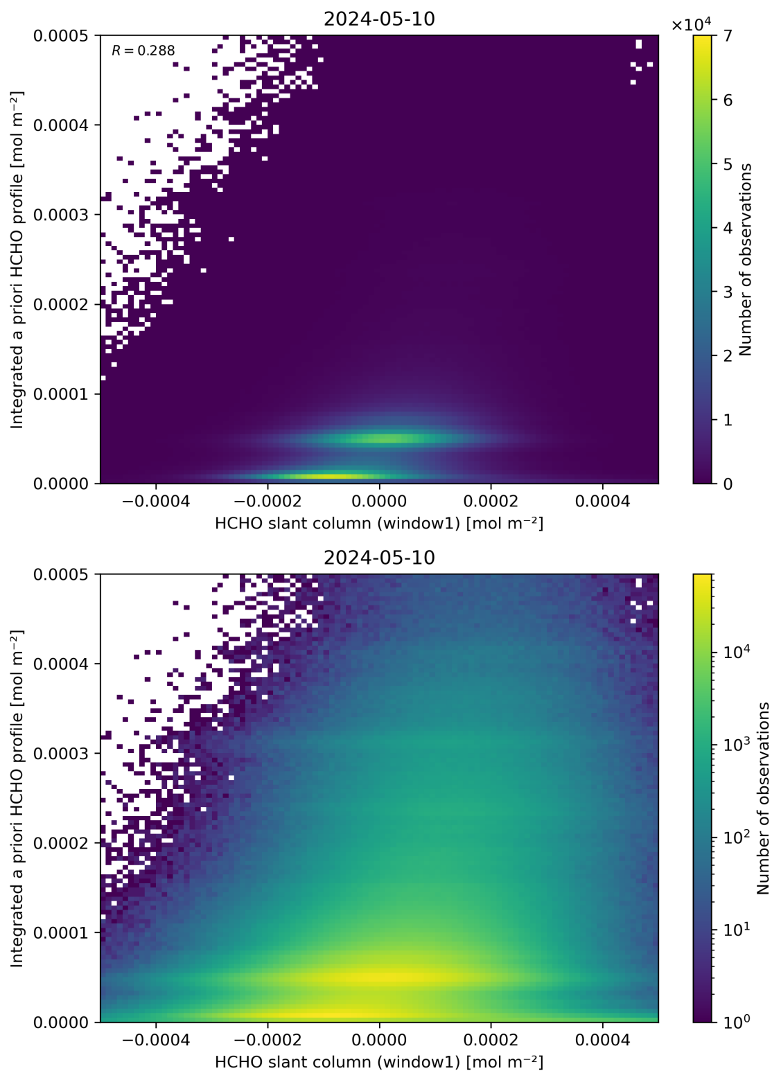
Figure 87: Scatter density plot of “HCHO slant column (window1)” against “Integrated a priori HCHO profile” for 2024-05-09 to 2024-05-11.
