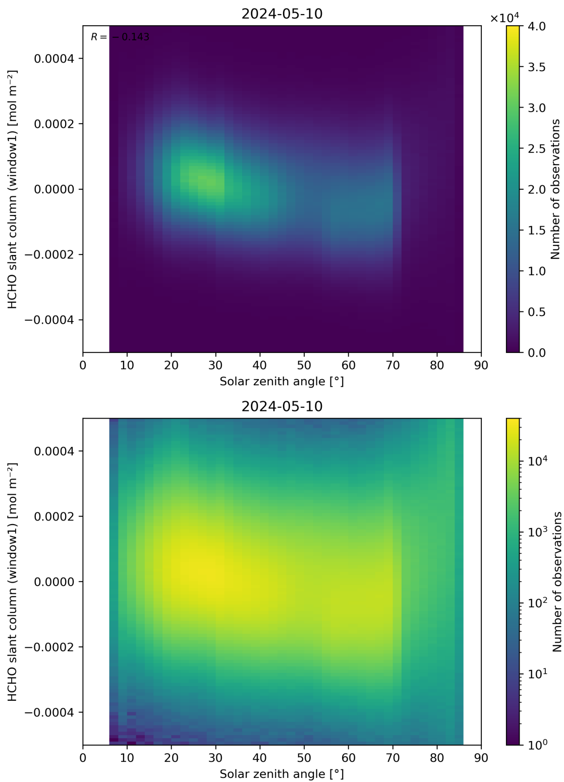
Figure 173: Scatter density plot of “Solar zenith angle” against “HCHO slant column (window1)” for 2024-05-09 to 2024-05-11.
