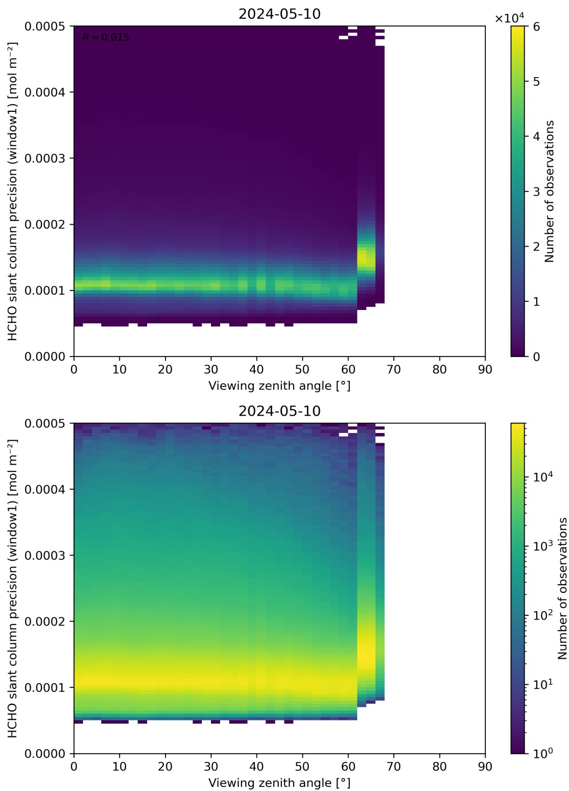
Figure 189: Scatter density plot of “Viewing zenith angle” against “HCHO slant column precision (window1)” for 2024-05-09 to 2024-05-11.
