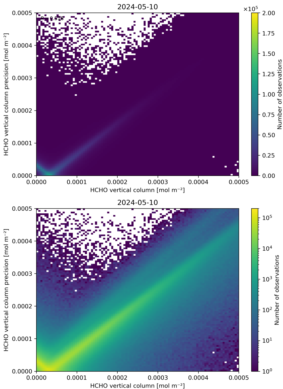
Figure 134: Scatter density plot of “HCHO vertical column” against “HCHO vertical column precision” for 2024-05-09 to 2024-05-11.
