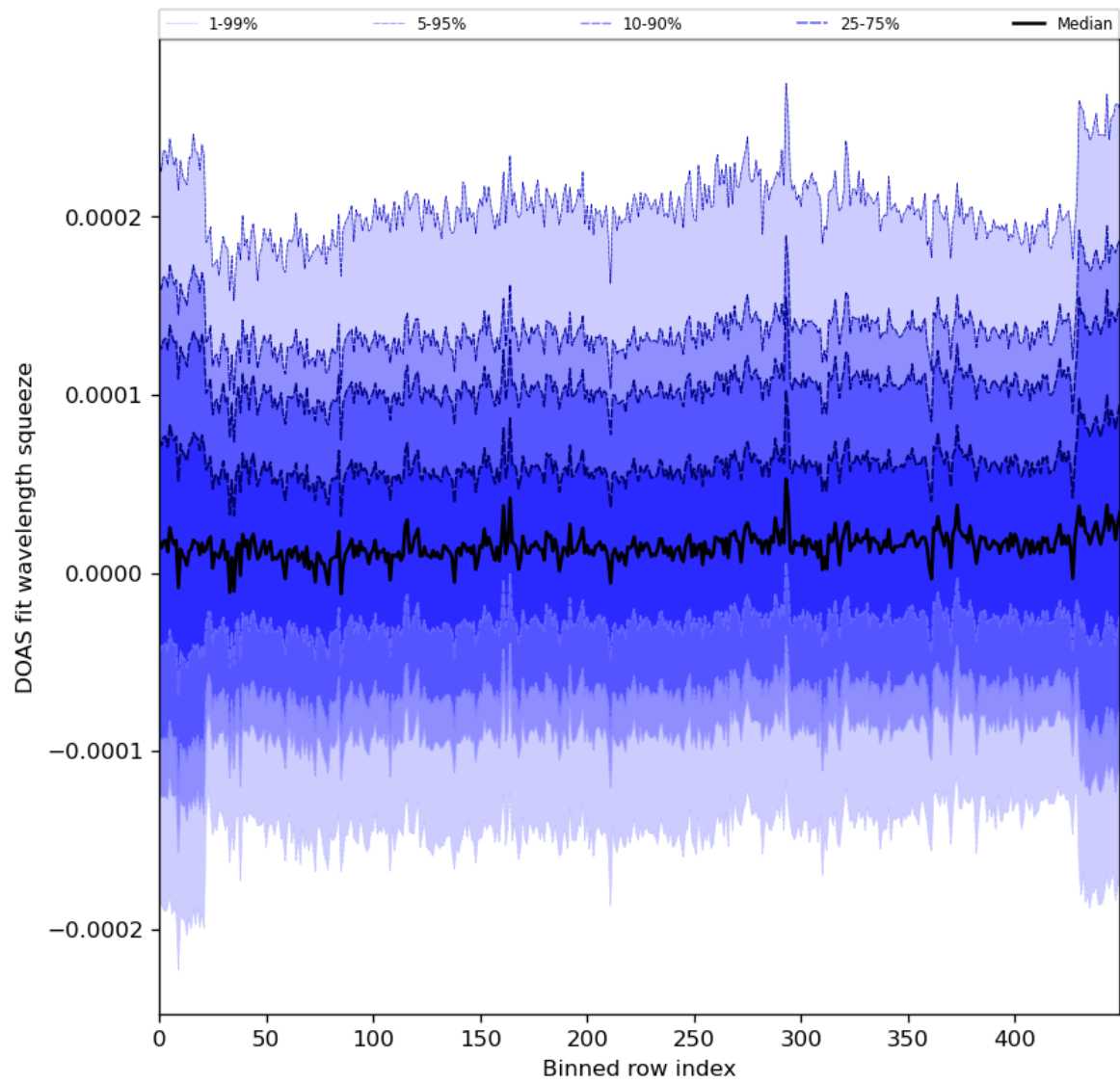
Figure 59: Along track statistics of “DOAS fit wavelength squeeze” for 2024-05-09 to 2024-05-11
