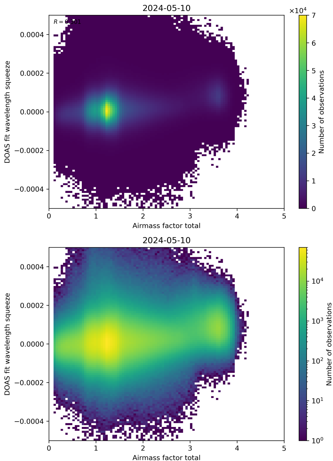
Figure 99: Scatter density plot of “Airmass factor total” against “DOAS fit wavelength squeeze” for 2024-05-09 to 2024-05-11.
