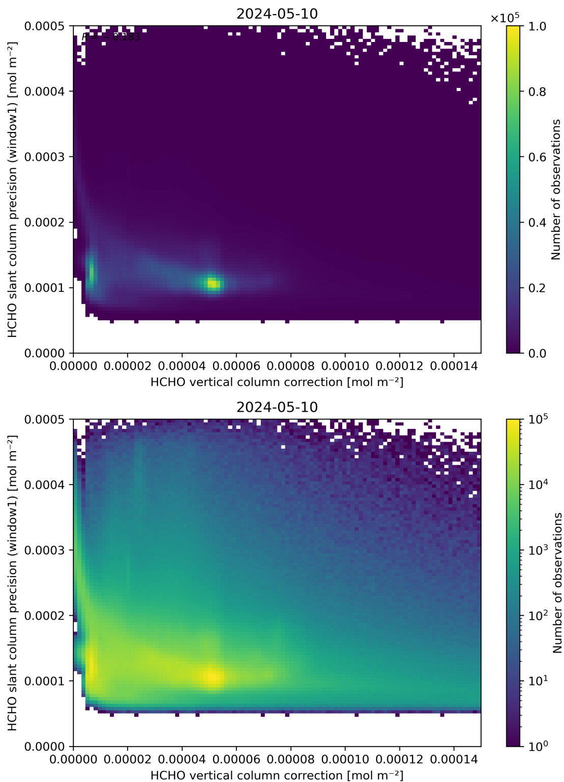
Figure 119: Scatter density plot of “HCHO vertical column correction” against “HCHO slant column precision (window1)” for 2024-05-09 to 2024-05-11.
