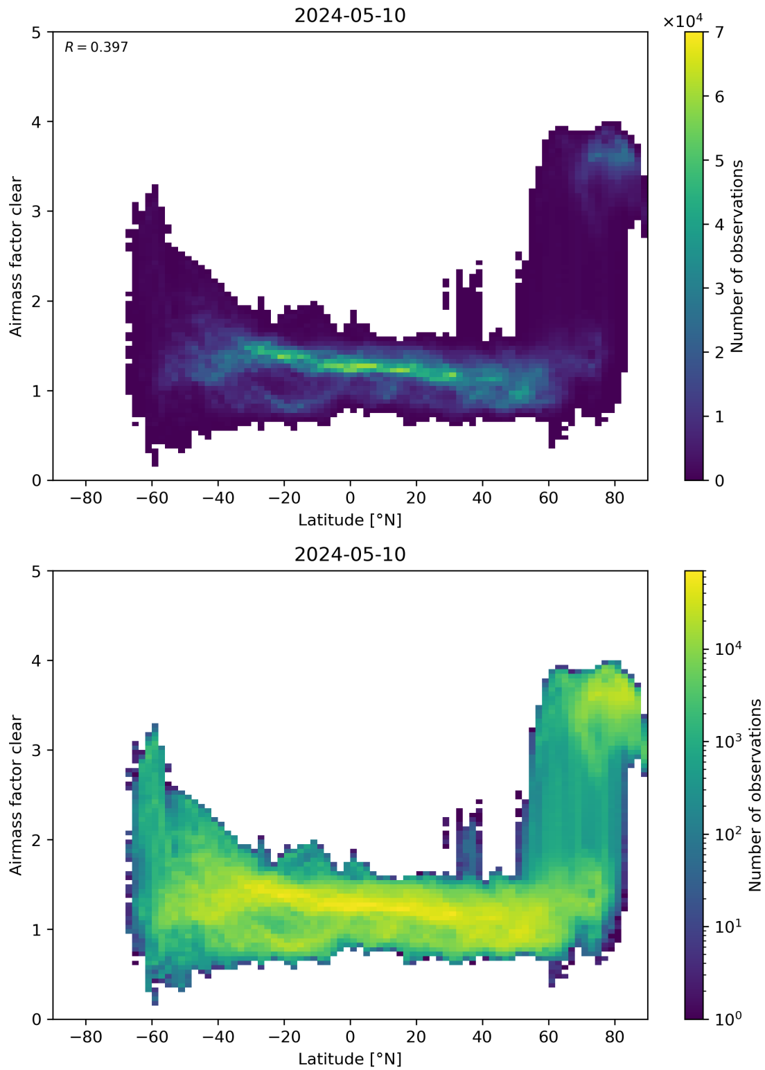
Figure 156: Scatter density plot of “Latitude” against “Airmass factor clear” for 2024-05-09 to 2024-05-11.
