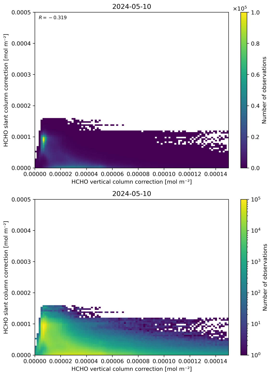
Figure 117: Scatter density plot of “HCHO vertical column correction” against “HCHO slant column correction” for 2024-05-09 to 2024-05-11.
