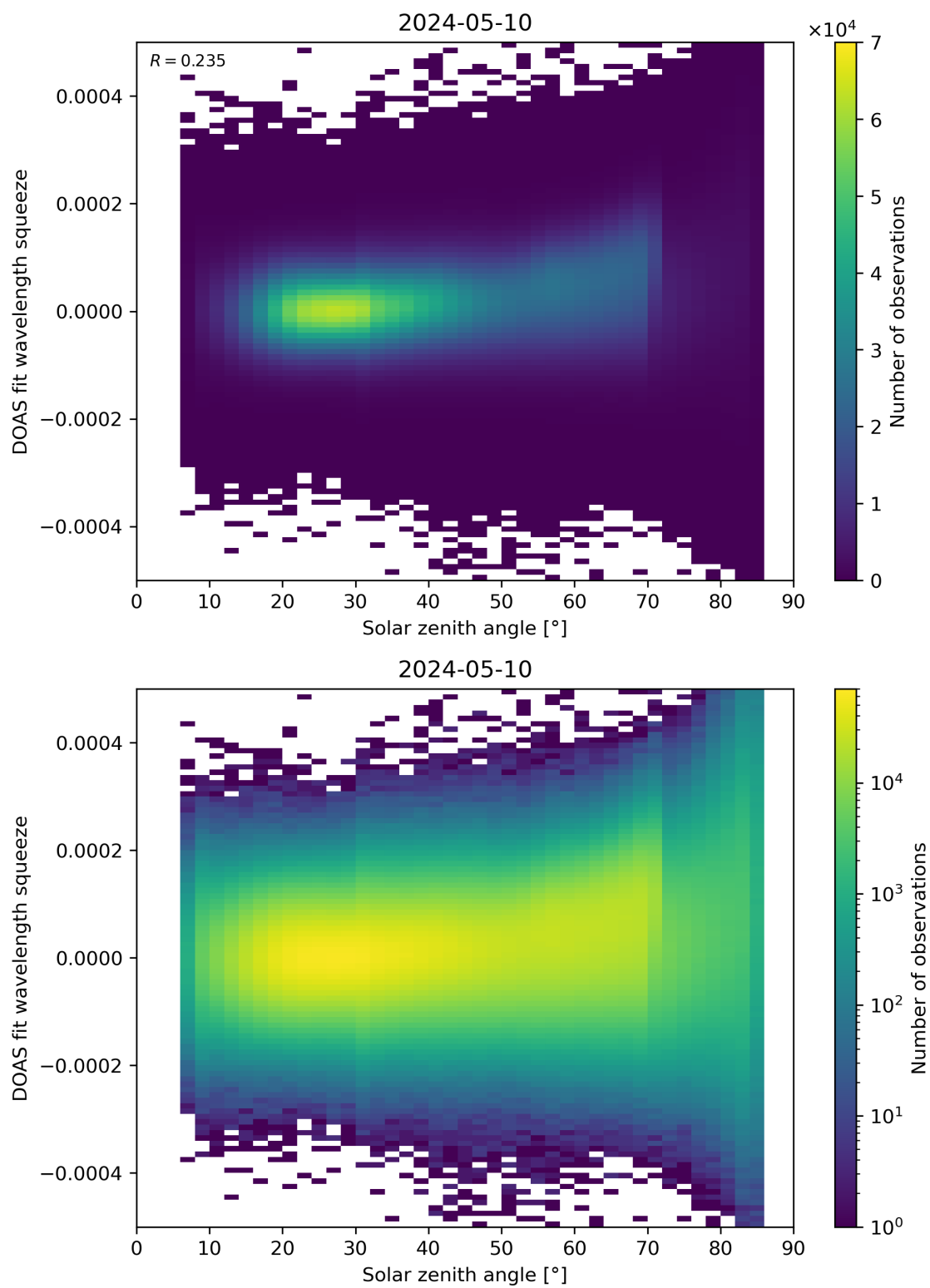
Figure 169: Scatter density plot of “Solar zenith angle” against “DOAS fit wavelength squeeze” for 2024-05-09 to 2024-05-11.
