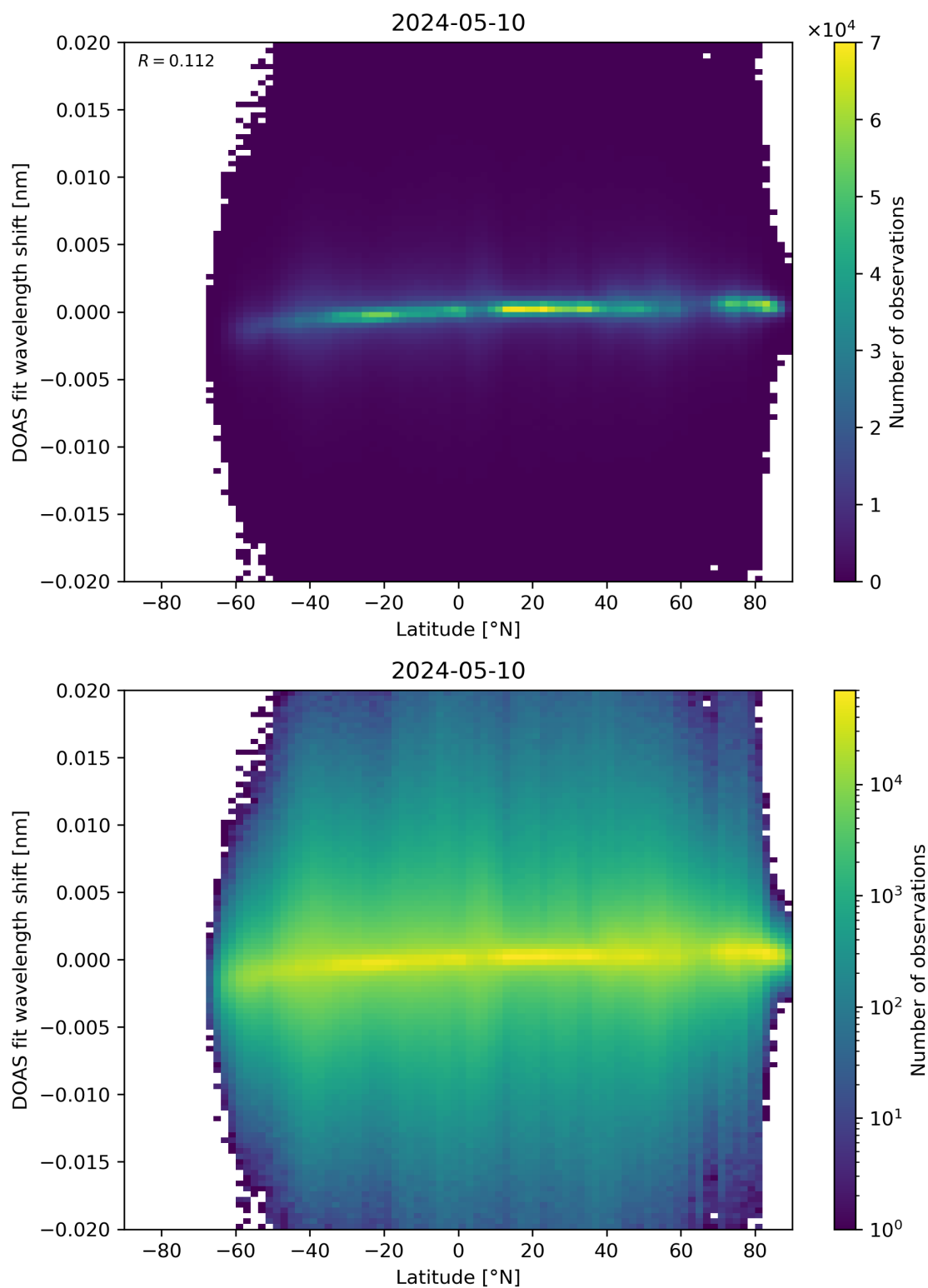
Figure 154: Scatter density plot of “Latitude” against “DOAS fit wavelength shift” for 2024-05-09 to 2024-05-11.
