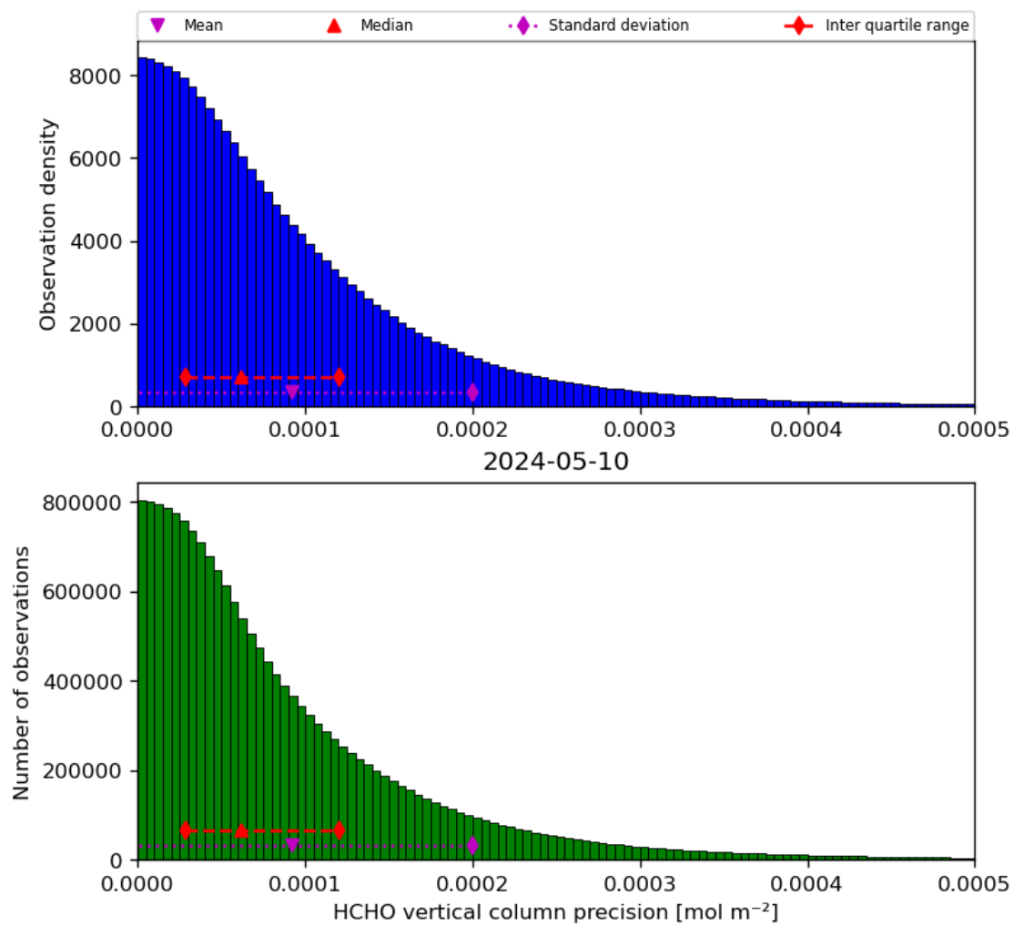
Figure 36: Histogram of “HCHO vertical column precision” for 2024-05-09 to 2024-05-11
