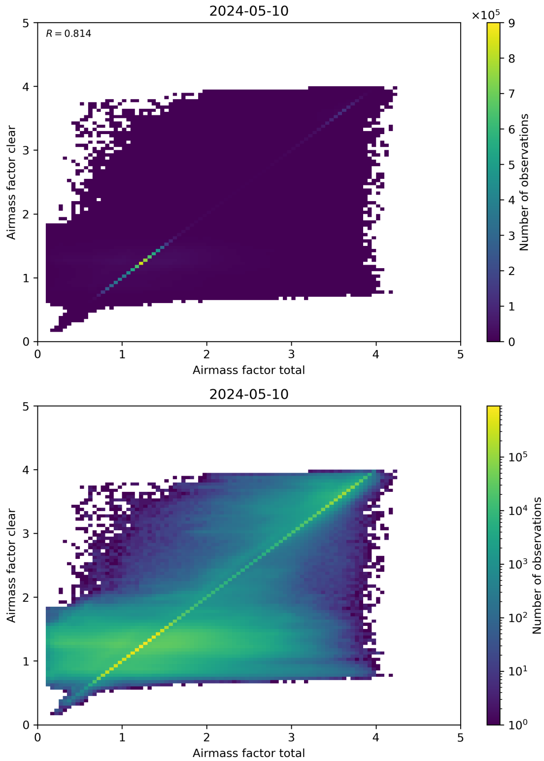
Figure 100: Scatter density plot of “Airmass factor total” against “Airmass factor clear” for 2024-05-09 to 2024-05-11.
