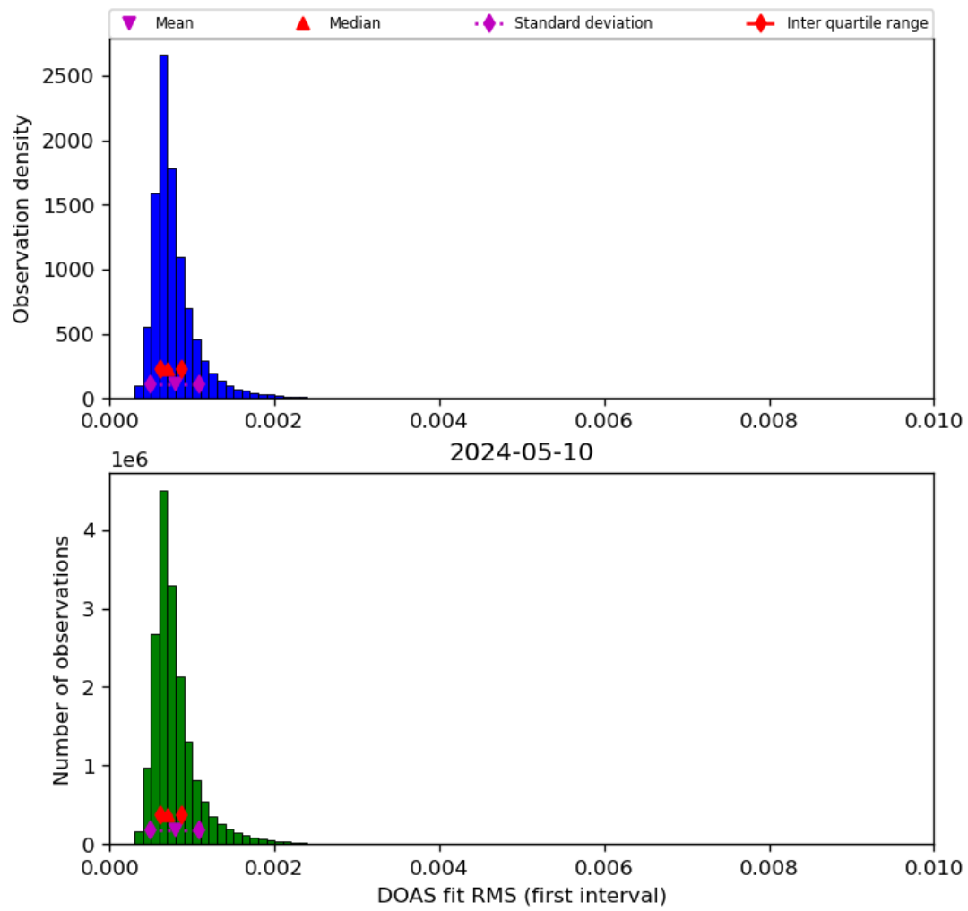
Figure 46: Histogram of “DOAS fit RMS (first interval)” for 2024-05-09 to 2024-05-11
