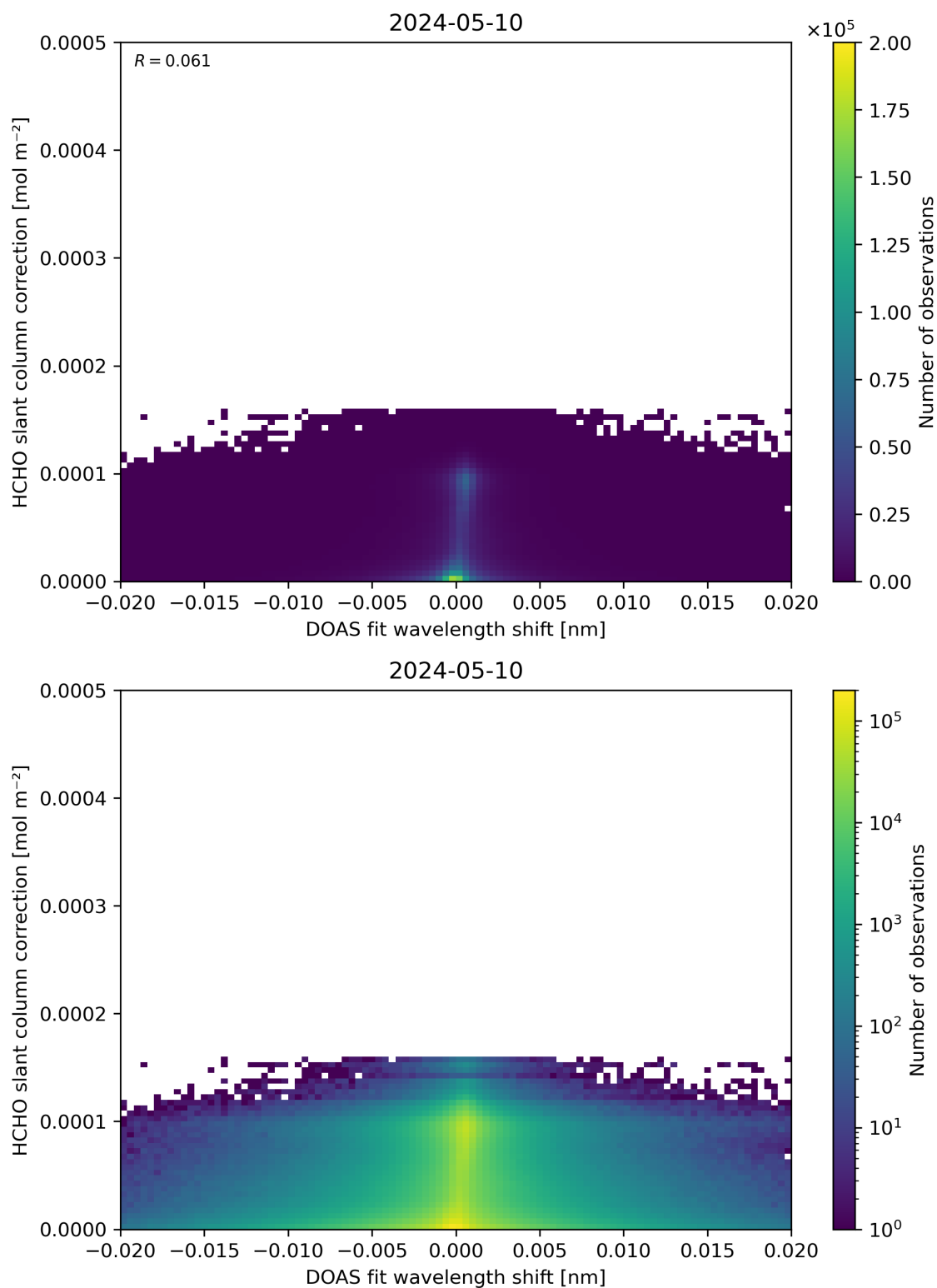
Figure 67: Scatter density plot of “DOAS fit wavelength shift” against “HCHO slant column correction” for 2024-05-09 to 2024-05-11.
