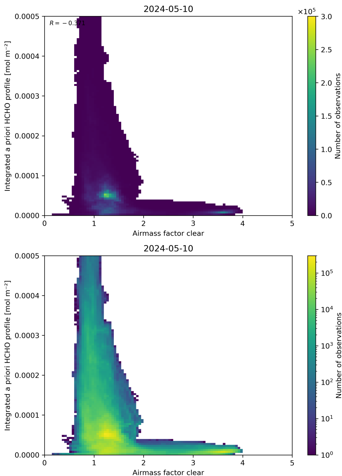
Figure 76: Scatter density plot of “Airmass factor clear” against “Integrated a priori HCHO profile” for 2024-05-09 to 2024-05-11.
