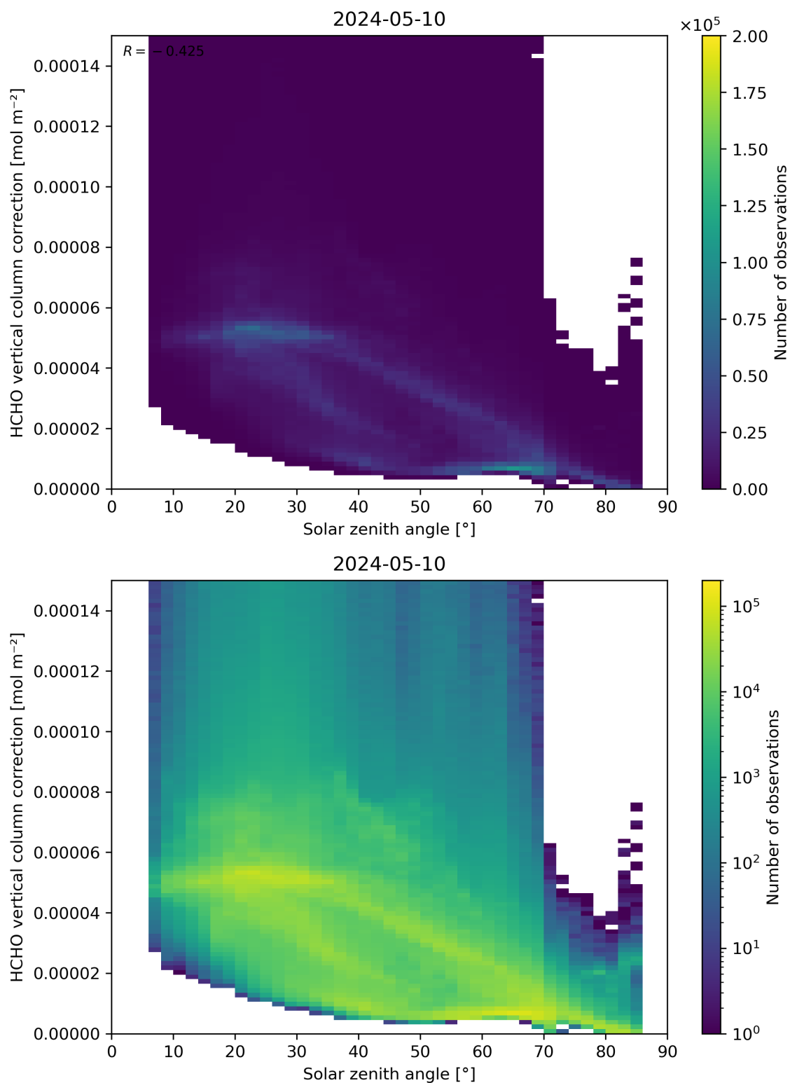
Figure 178: Scatter density plot of “Solar zenith angle” against “HCHO vertical column correction” for 2024-05-09 to 2024-05-11.
