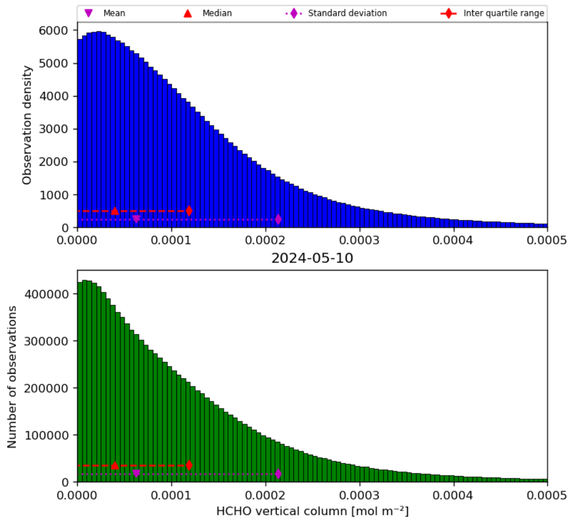
Figure 35: Histogram of “HCHO vertical column” for 2024-05-09 to 2024-05-11
