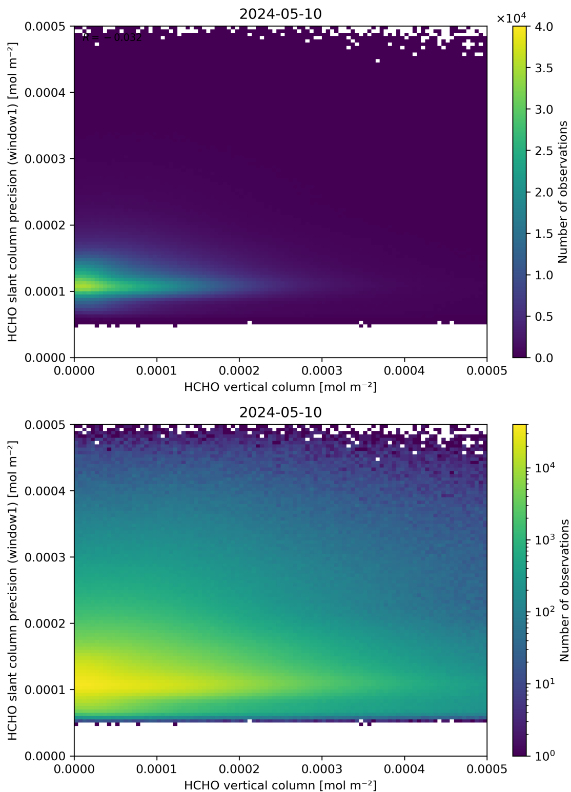
Figure 130: Scatter density plot of “HCHO vertical column” against “HCHO slant column precision (window1)” for 2024-05-09 to 2024-05-11.
