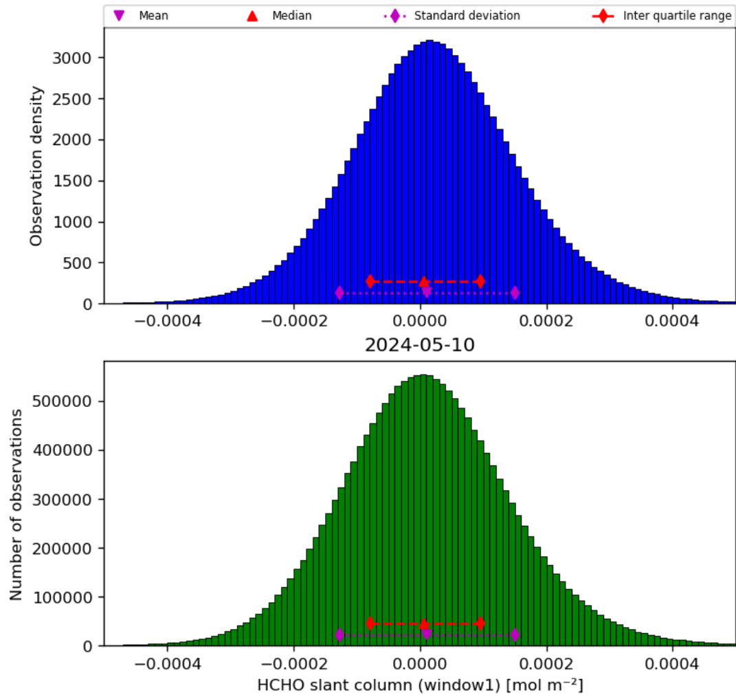
Figure 38: Histogram of “HCHO slant column (window1)” for 2024-05-09 to 2024-05-11
