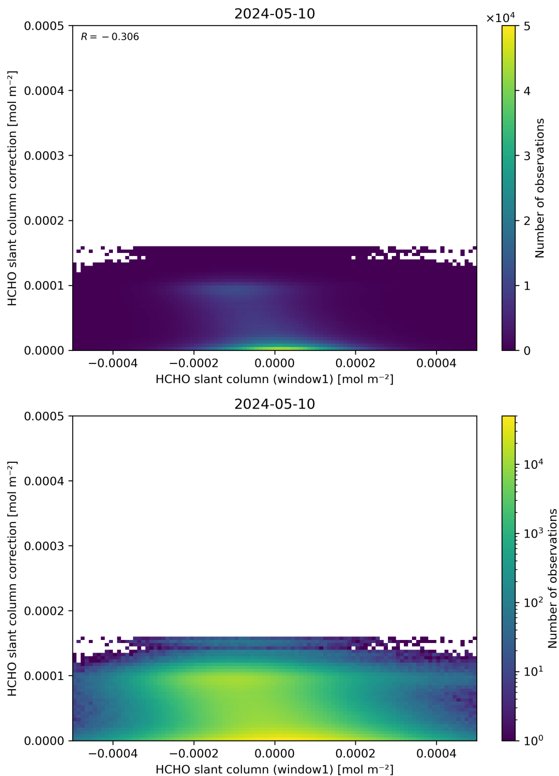
Figure 83: Scatter density plot of “HCHO slant column (window1)” against “HCHO slant column correction” for 2024-05-09 to 2024-05-11.
