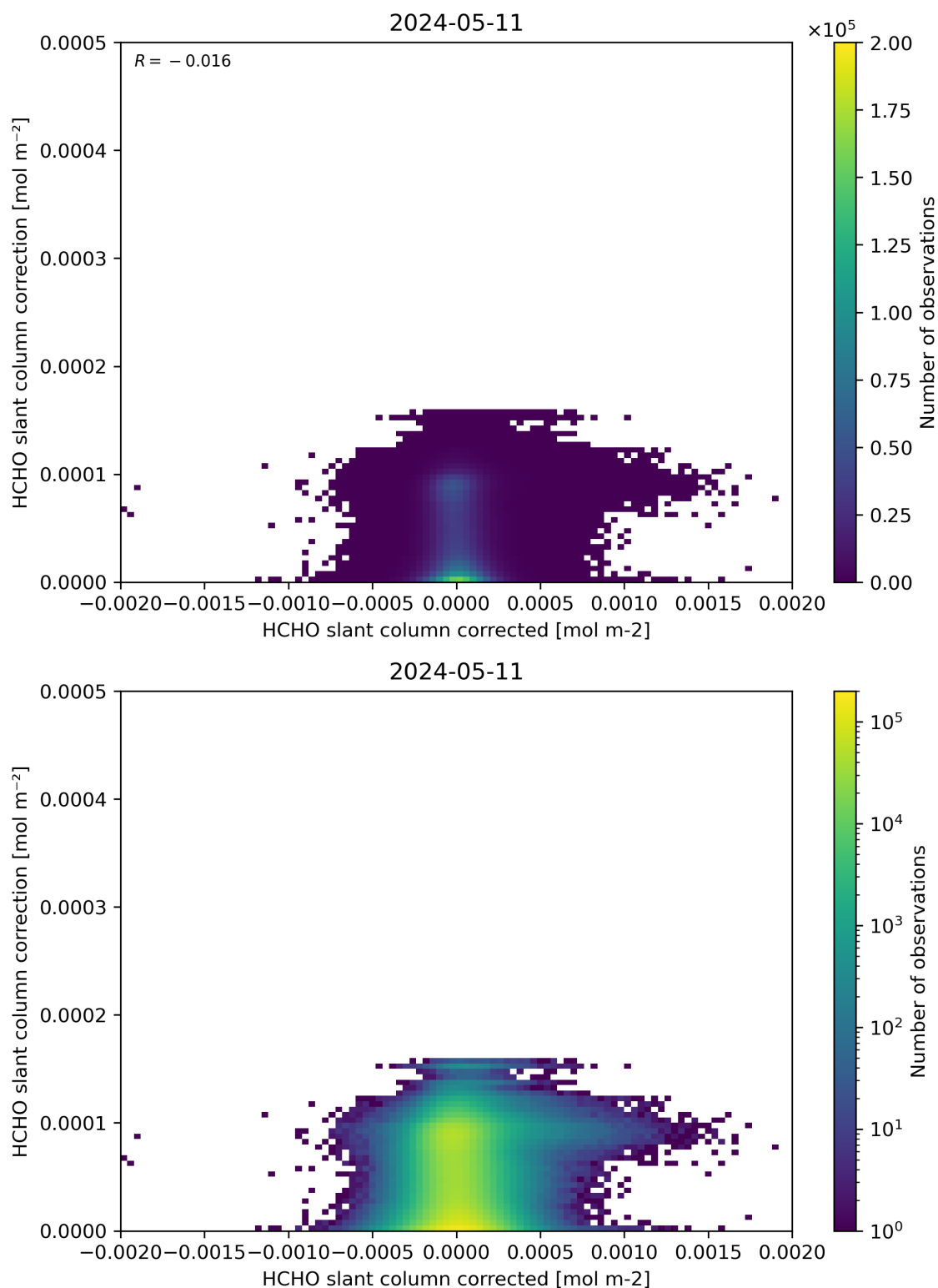
Figure 77: Scatter density plot of “HCHO slant column corrected” against “HCHO slant column correction” for 2024-05-10 to 2024-05-12.
