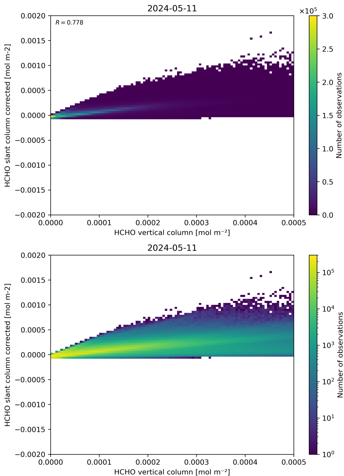
Figure 127: Scatter density plot of “HCHO vertical column” against “HCHO slant column corrected” for 2024-05-10 to 2024-05-12.
