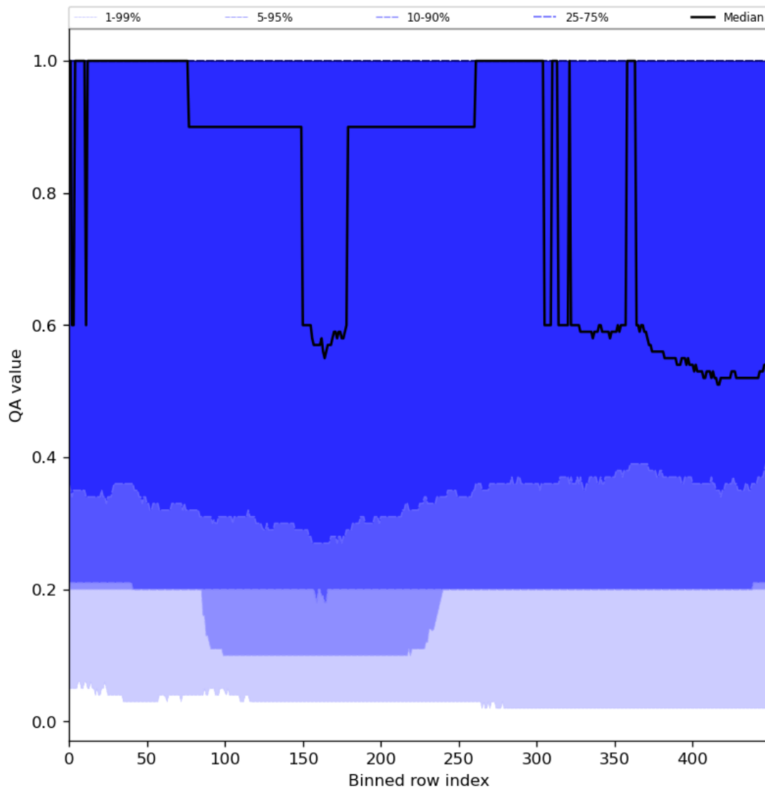
Figure 48: Along track statistics of “QA value” for 2024-05-10 to 2024-05-12
