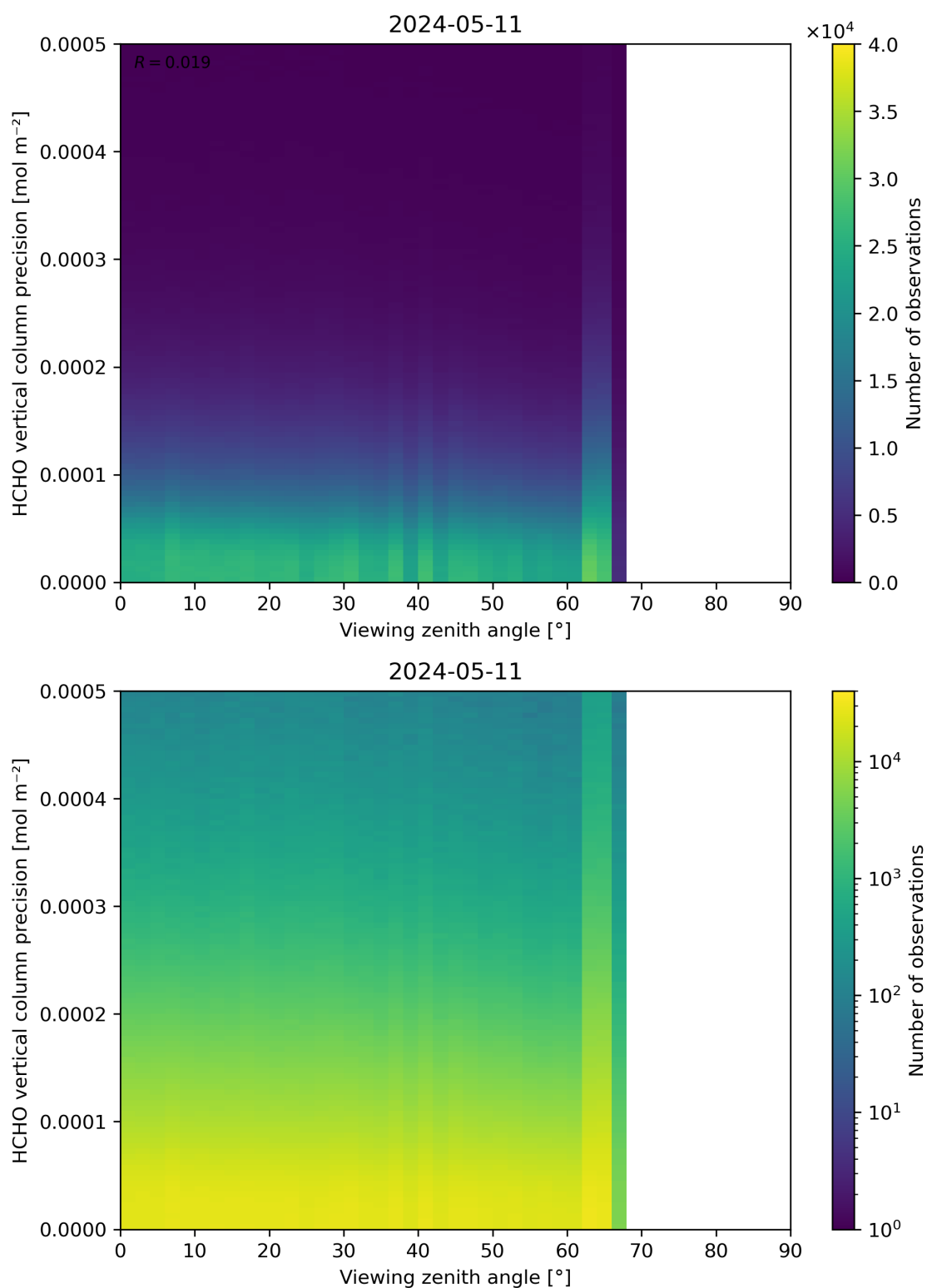
Figure 194: Scatter density plot of “Viewing zenith angle” against “HCHO vertical column precision” for 2024-05-10 to 2024-05-12.
