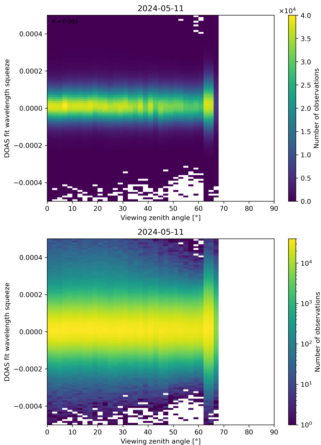
Figure 184: Scatter density plot of “Viewing zenith angle” against “DOAS fit wavelength squeeze” for 2024-05-10 to 2024-05-12.
