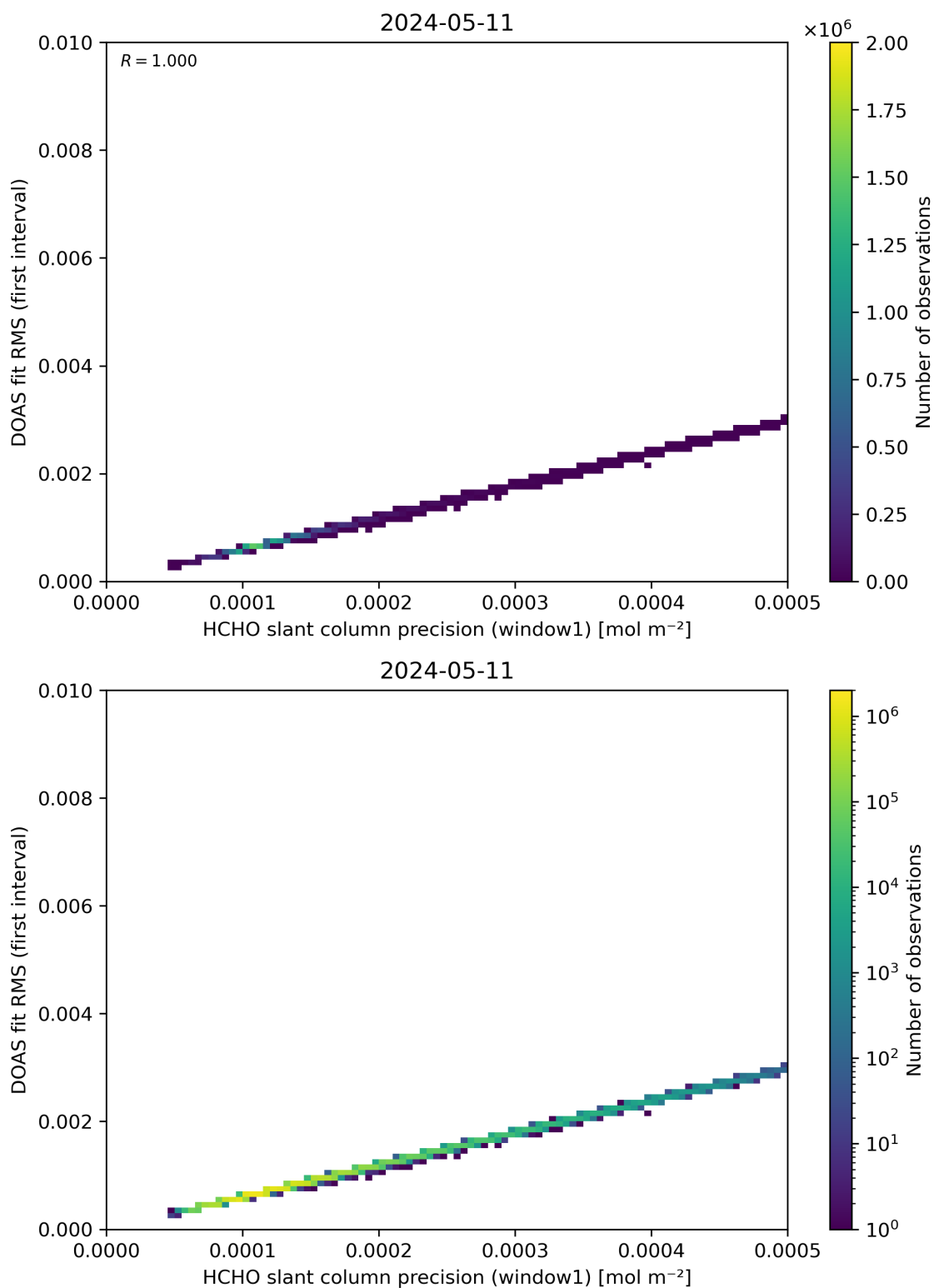
Figure 88: Scatter density plot of “HCHO slant column precision (window1)” against “DOAS fit RMS (first interval)” for 2024-05-10 to 2024-05-12.
