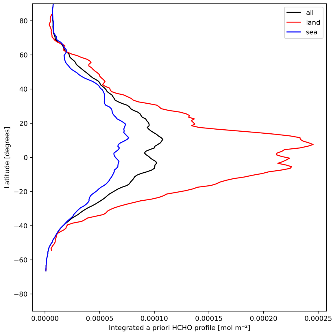
Figure 29: Zonal average of “Integrated a priori HCHO profile” for 2024-05-10 to 2024-05-12.
