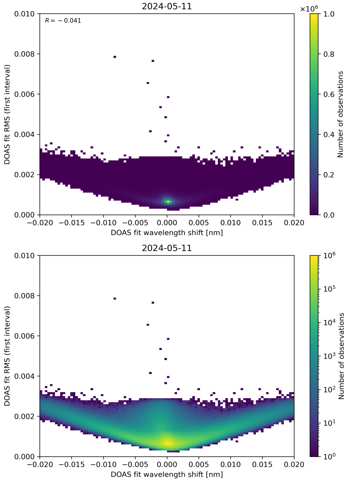
Figure 64: Scatter density plot of “DOAS fit wavelength shift” against “DOAS fit RMS (first interval)” for 2024-05-10 to 2024-05-12.
