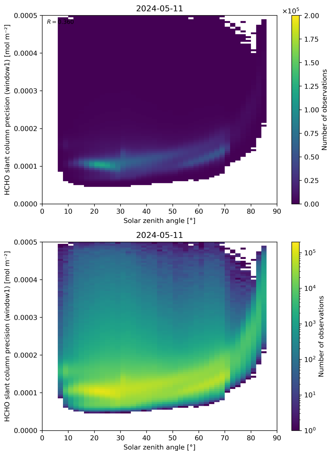
Figure 174: Scatter density plot of “Solar zenith angle” against “HCHO slant column precision (window1)” for 2024-05-10 to 2024-05-12.
