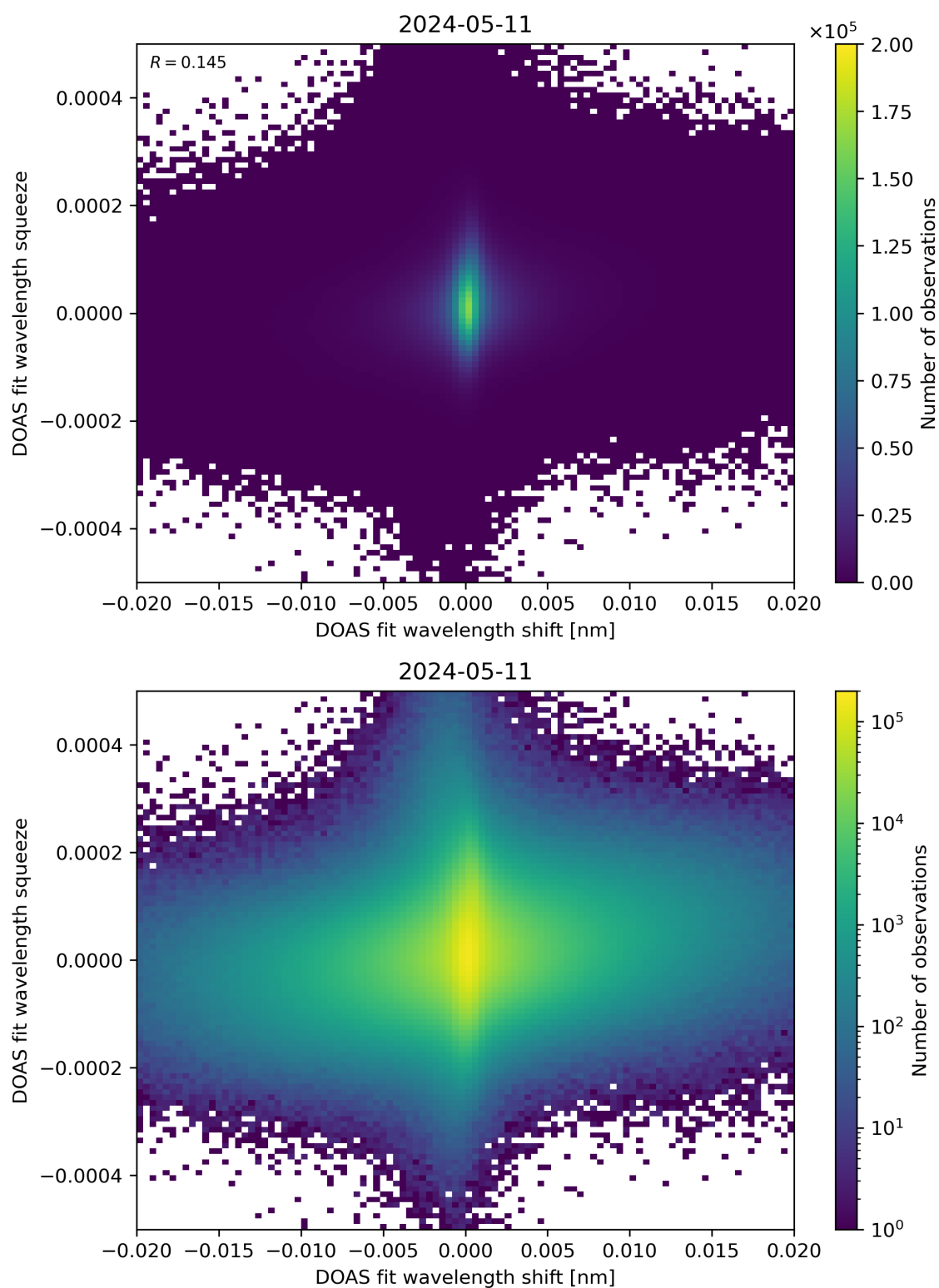
Figure 65: Scatter density plot of “DOAS fit wavelength shift” against “DOAS fit wavelength squeeze” for 2024-05-10 to 2024-05-12.
