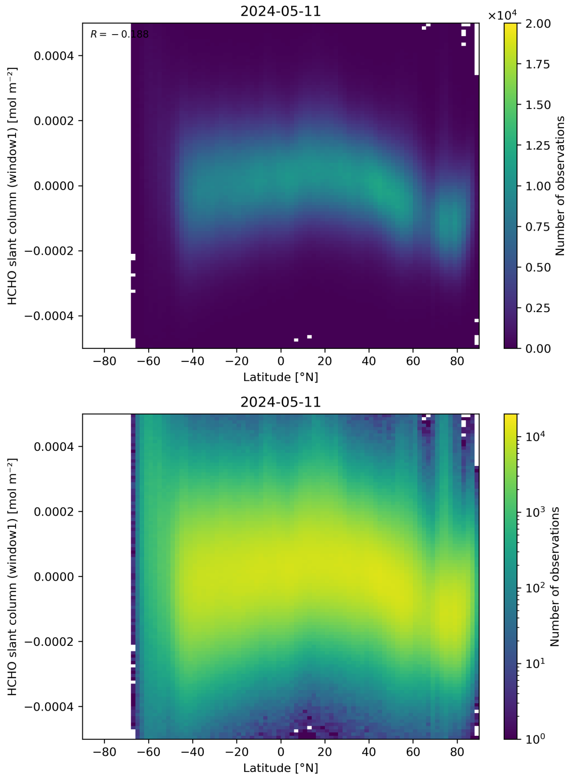
Figure 159: Scatter density plot of “Latitude” against “HCHO slant column (window1)” for 2024-05-10 to 2024-05-12.
