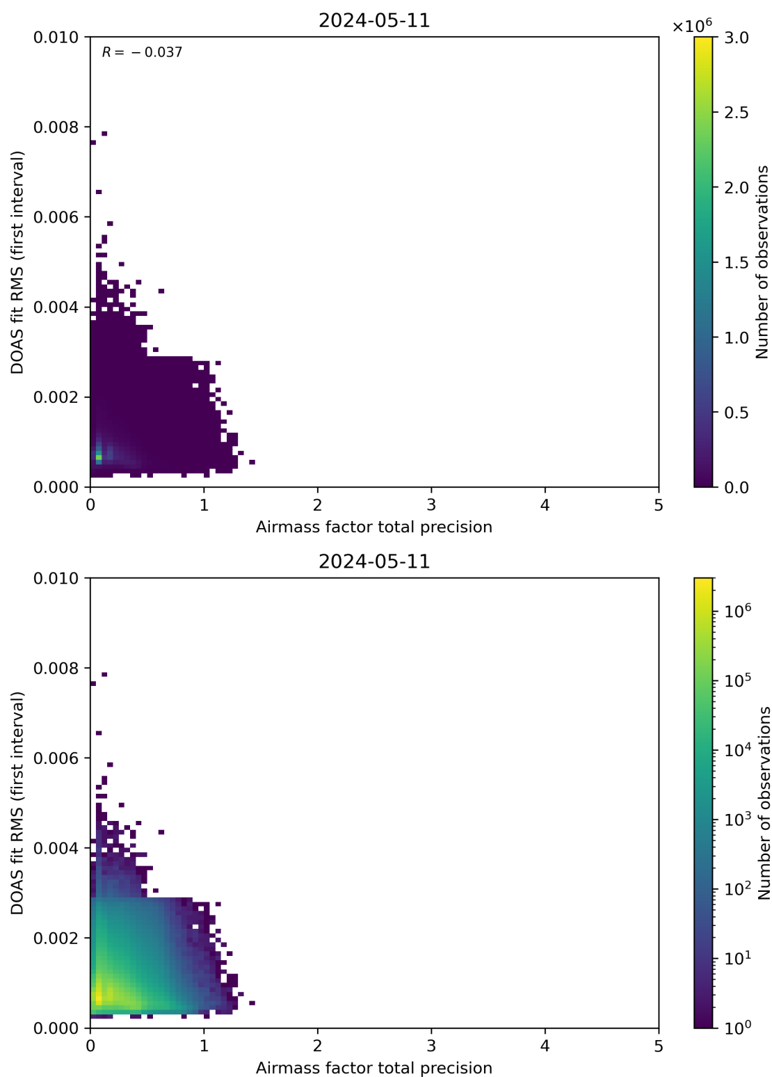
Figure 105: Scatter density plot of “Airmass factor total precision” against “DOAS fit RMS (first interval)” for 2024-05-10 to 2024-05-12.
