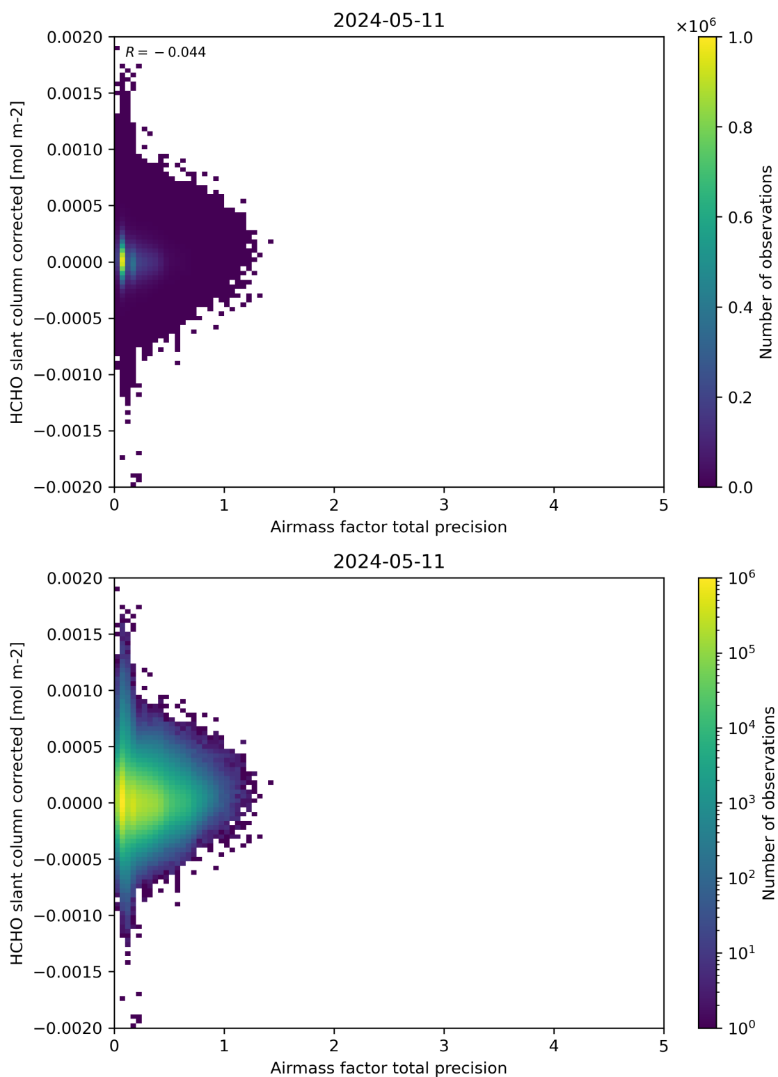
Figure 109: Scatter density plot of “Airmass factor total precision” against “HCHO slant column corrected” for 2024-05-10 to 2024-05-12.
