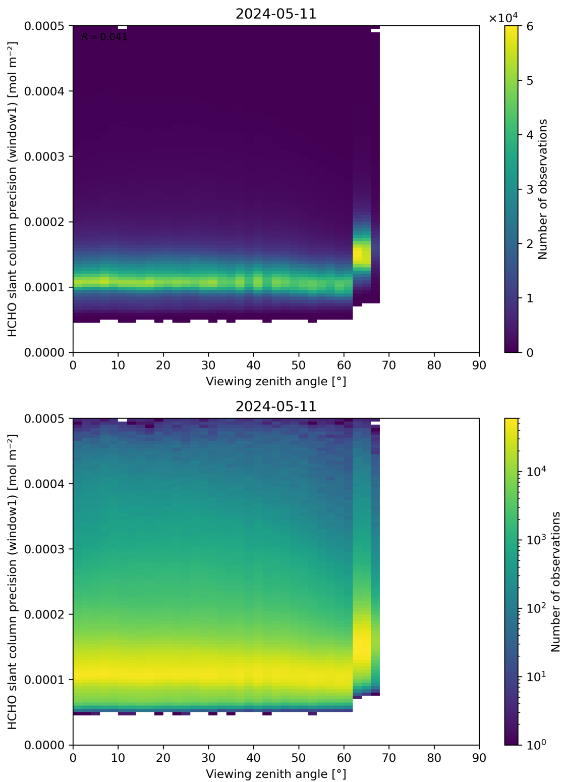
Figure 189: Scatter density plot of “Viewing zenith angle” against “HCHO slant column precision (window1)” for 2024-05-10 to 2024-05-12.
