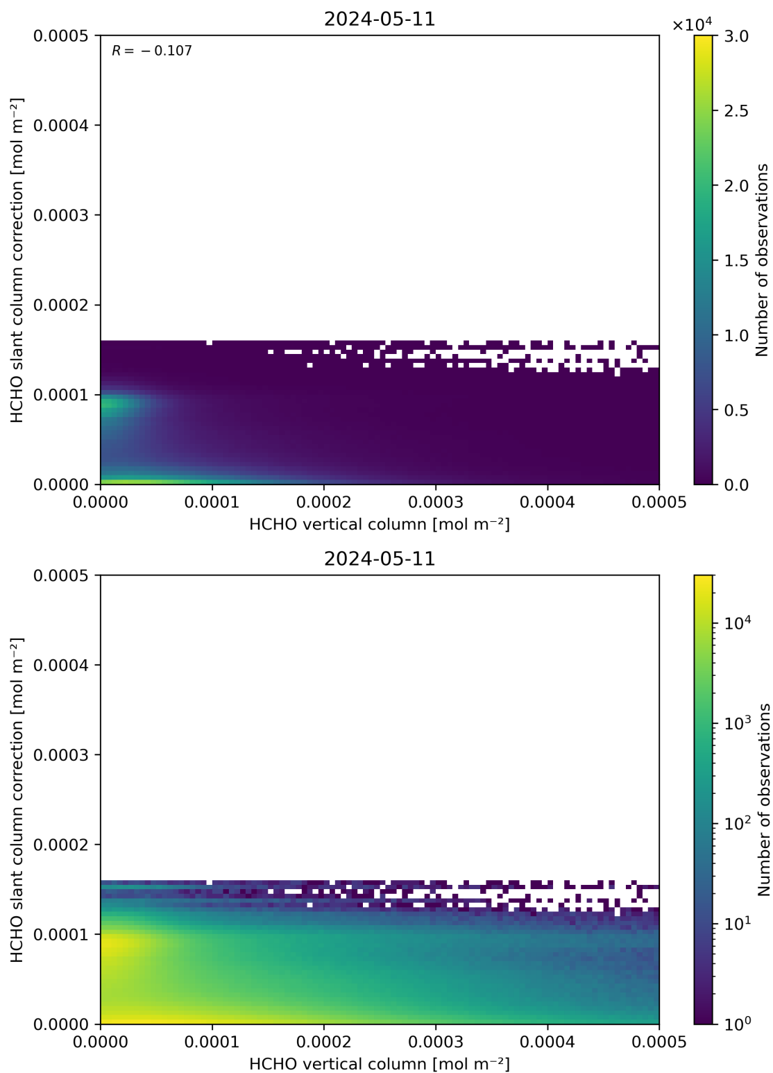
Figure 128: Scatter density plot of “HCHO vertical column” against “HCHO slant column correction” for 2024-05-10 to 2024-05-12.
