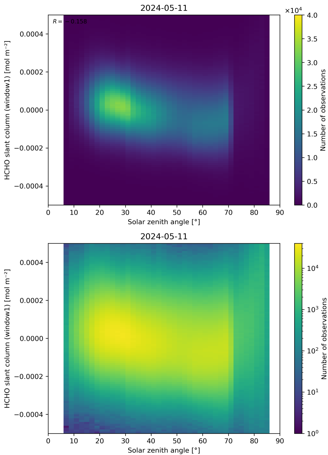
Figure 173: Scatter density plot of “Solar zenith angle” against “HCHO slant column (window1)” for 2024-05-10 to 2024-05-12.
