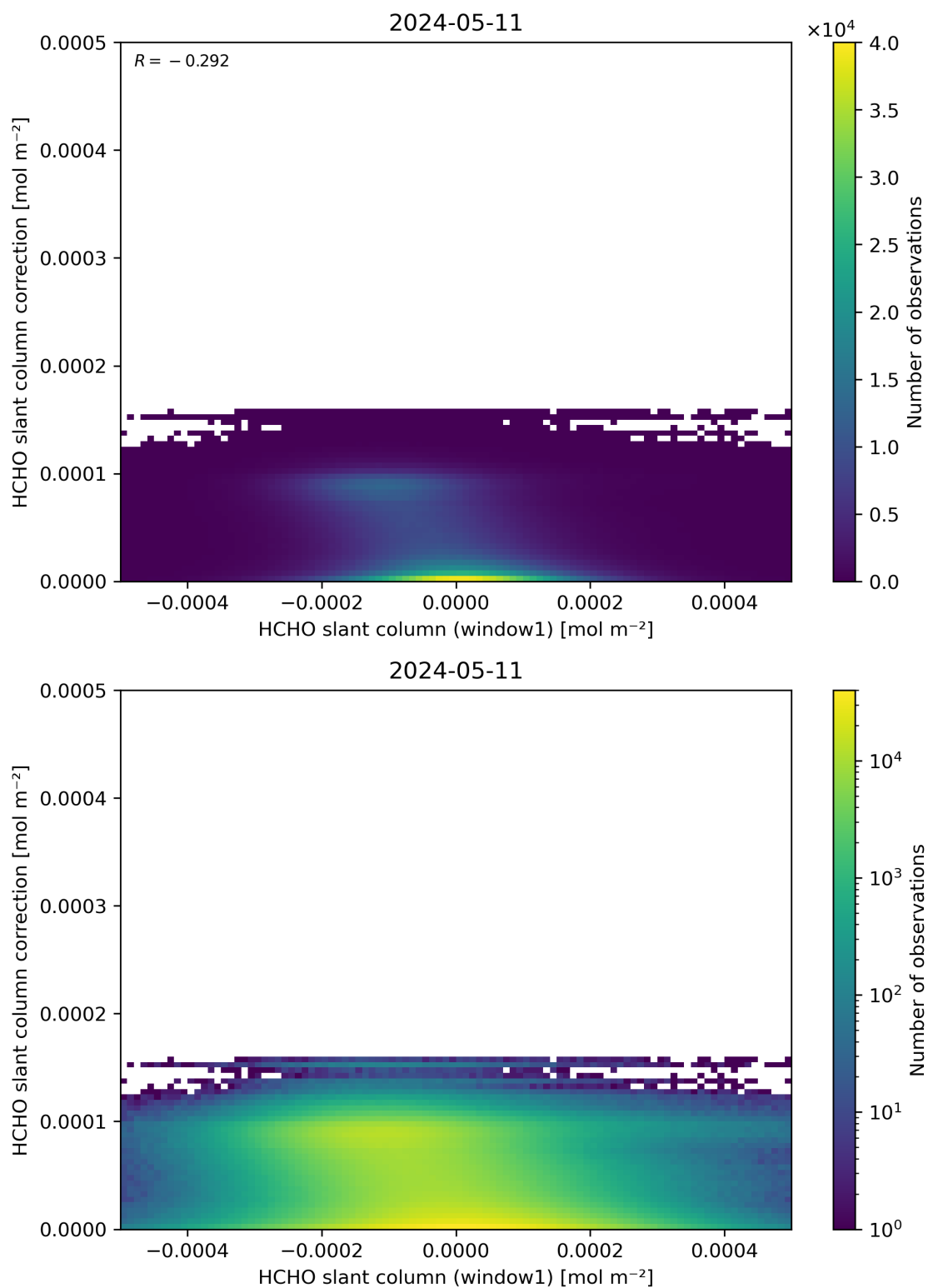
Figure 83: Scatter density plot of “HCHO slant column (window1)” against “HCHO slant column correction” for 2024-05-10 to 2024-05-12.
