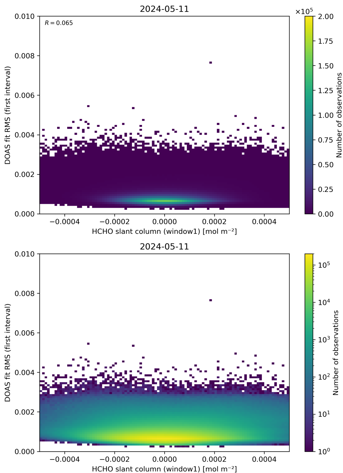
Figure 78: Scatter density plot of “HCHO slant column (window1)” against “DOAS fit RMS (first interval)” for 2024-05-10 to 2024-05-12.
