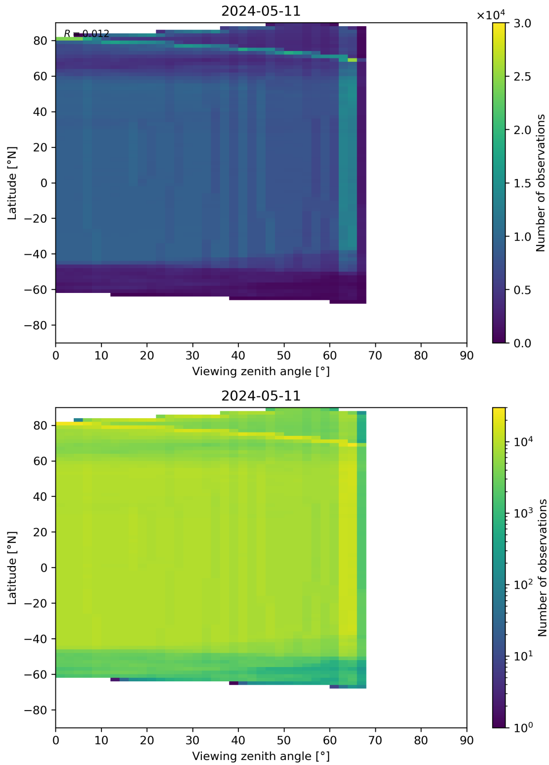
Figure 196: Scatter density plot of “Viewing zenith angle” against “Latitude” for 2024-05-10 to 2024-05-12.
