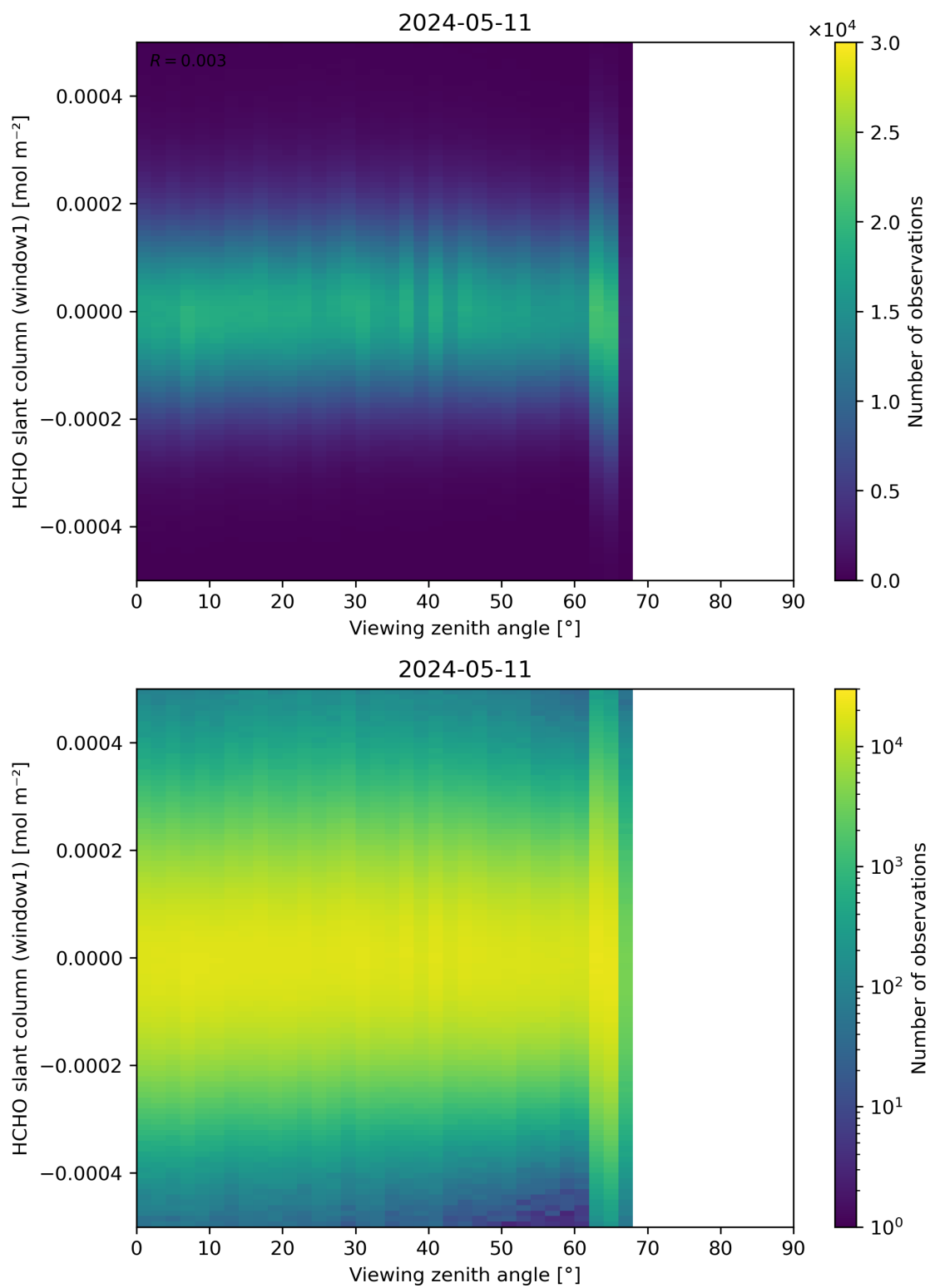
Figure 188: Scatter density plot of “Viewing zenith angle” against “HCHO slant column (window1)” for 2024-05-10 to 2024-05-12.
