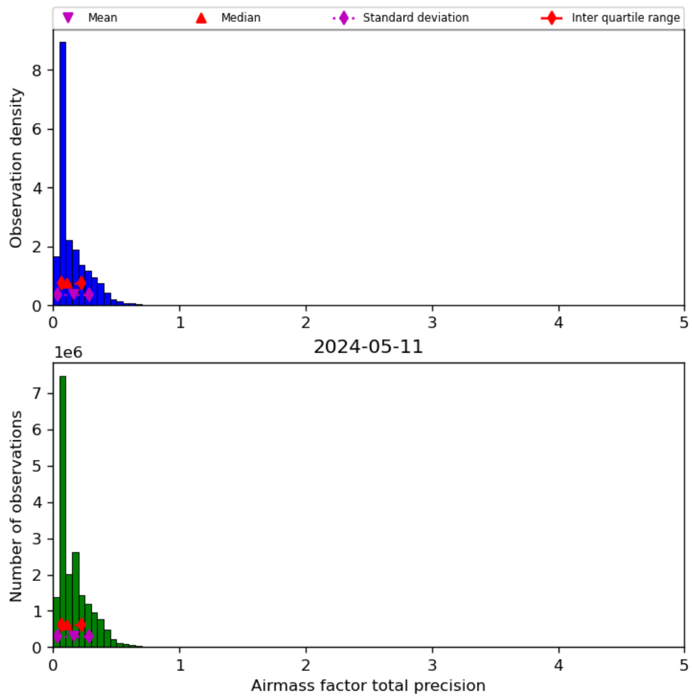
Figure 41: Histogram of “Airmass factor total precision” for 2024-05-10 to 2024-05-12
