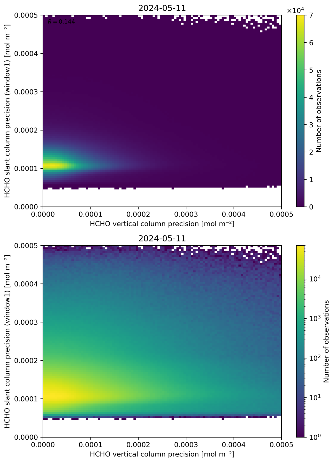
Figure 143: Scatter density plot of “HCHO vertical column precision” against “HCHO slant column precision (window1)” for 2024-05-10 to 2024-05-12.
