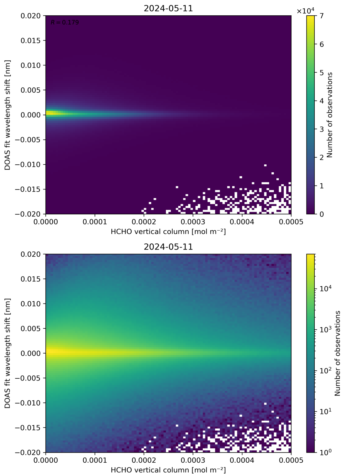
Figure 124: Scatter density plot of “HCHO vertical column” against “DOAS fit wavelength shift” for 2024-05-10 to 2024-05-12.
