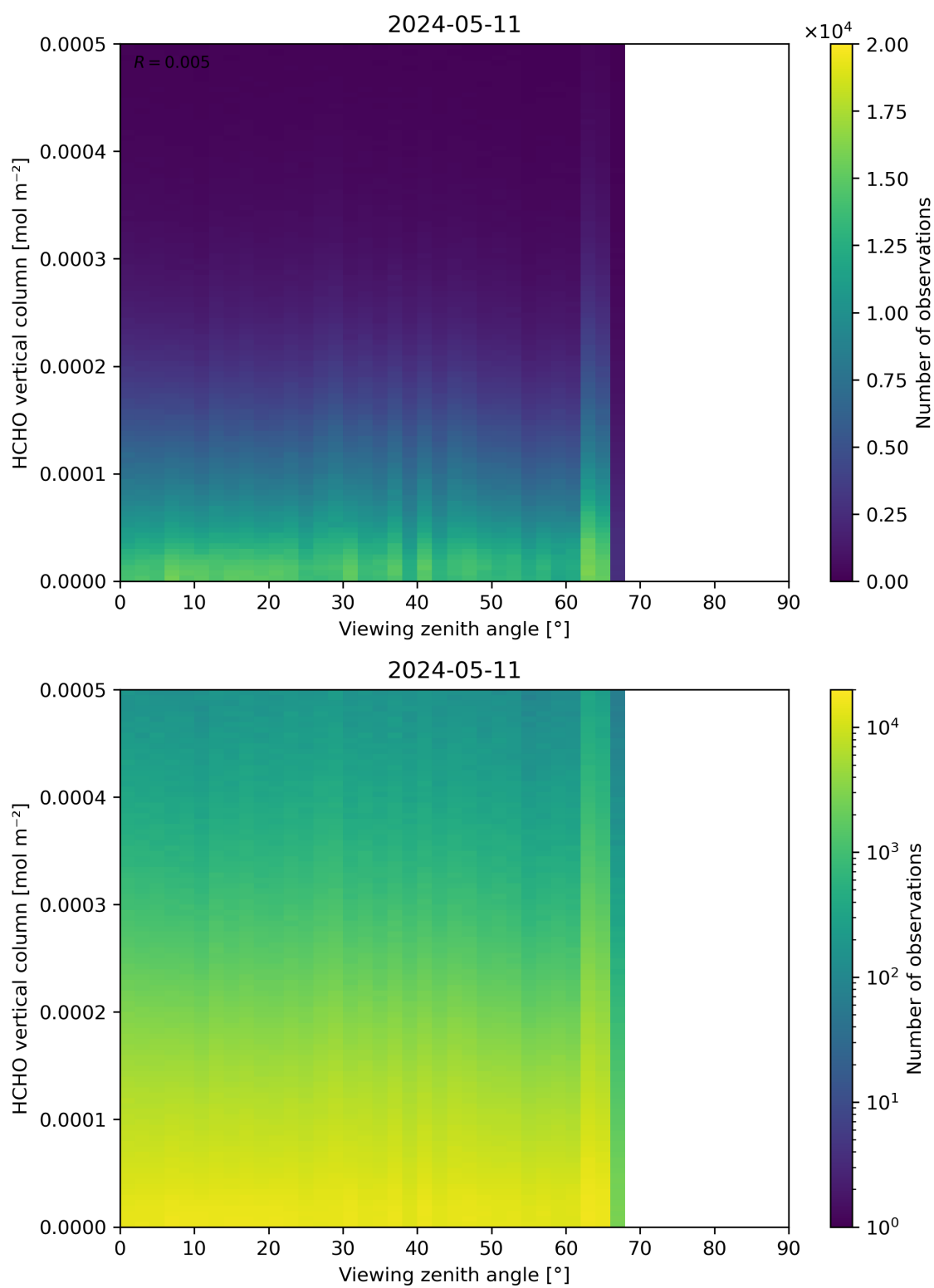
Figure 192: Scatter density plot of “Viewing zenith angle” against “HCHO vertical column” for 2024-05-10 to 2024-05-12.
