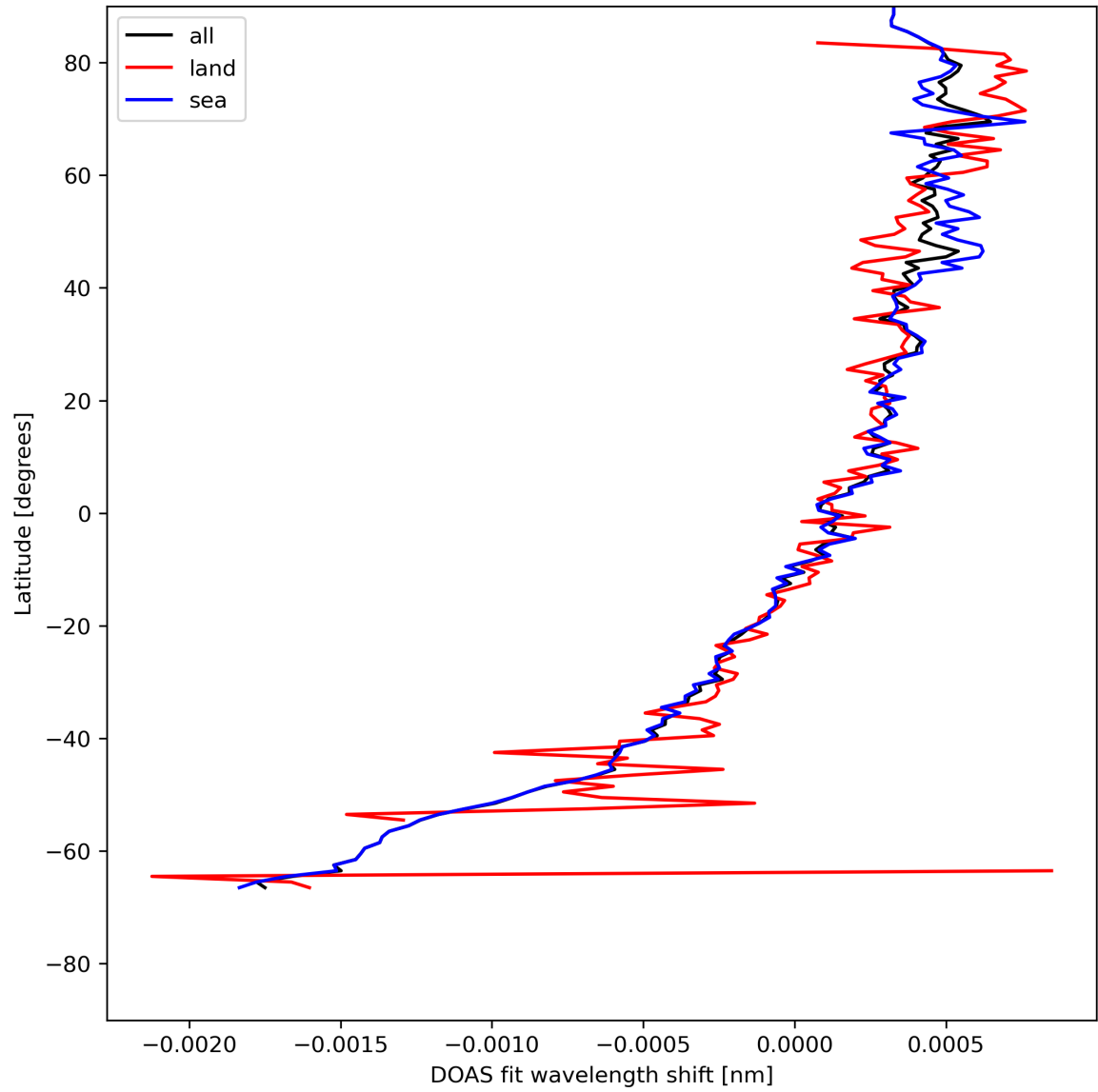
Figure 30: Zonal average of “DOAS fit wavelength shift” for 2024-05-10 to 2024-05-12.
