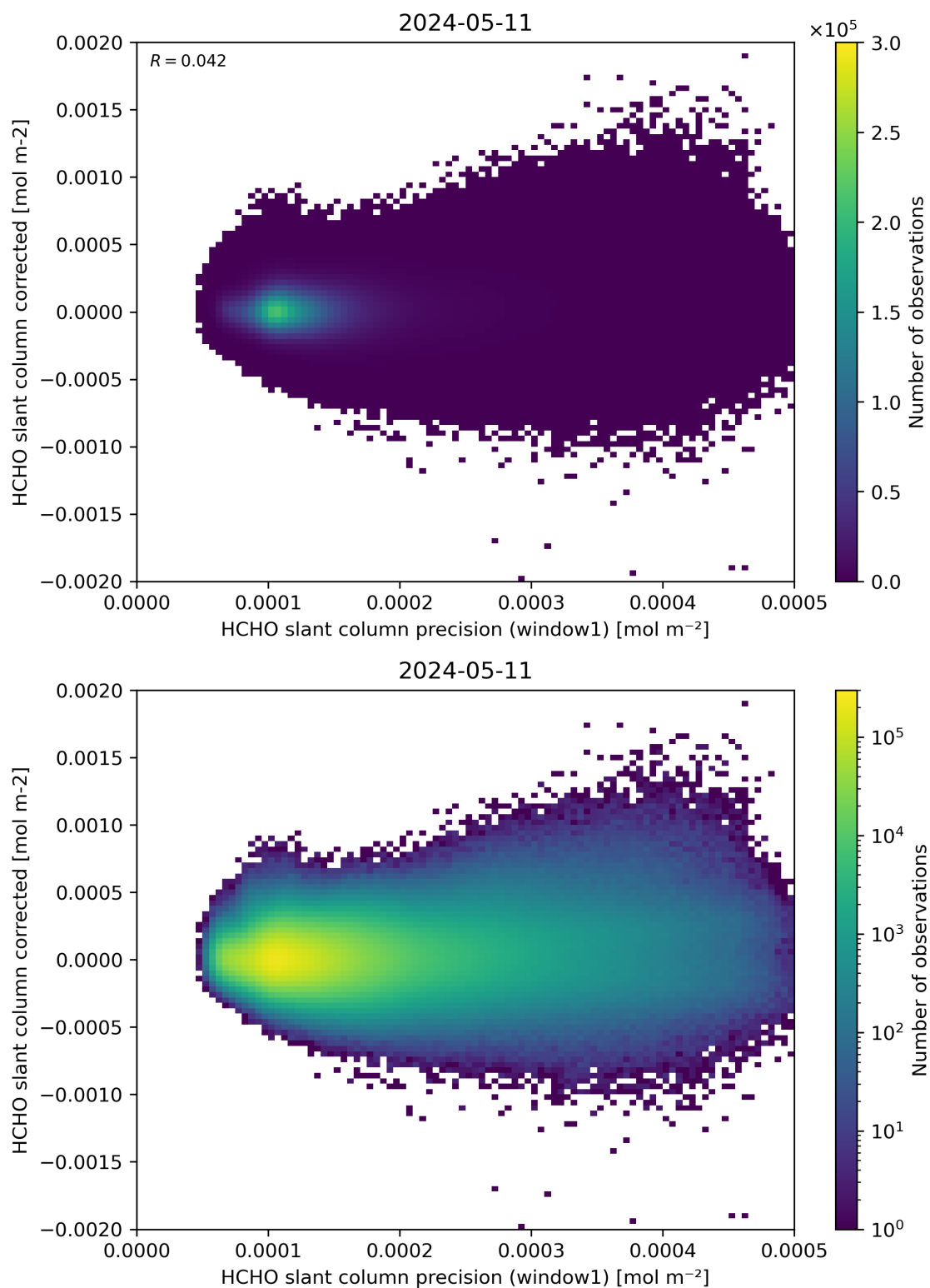
Figure 92: Scatter density plot of “HCHO slant column precision (window1)” against “HCHO slant column corrected” for 2024-05-10 to 2024-05-12.
