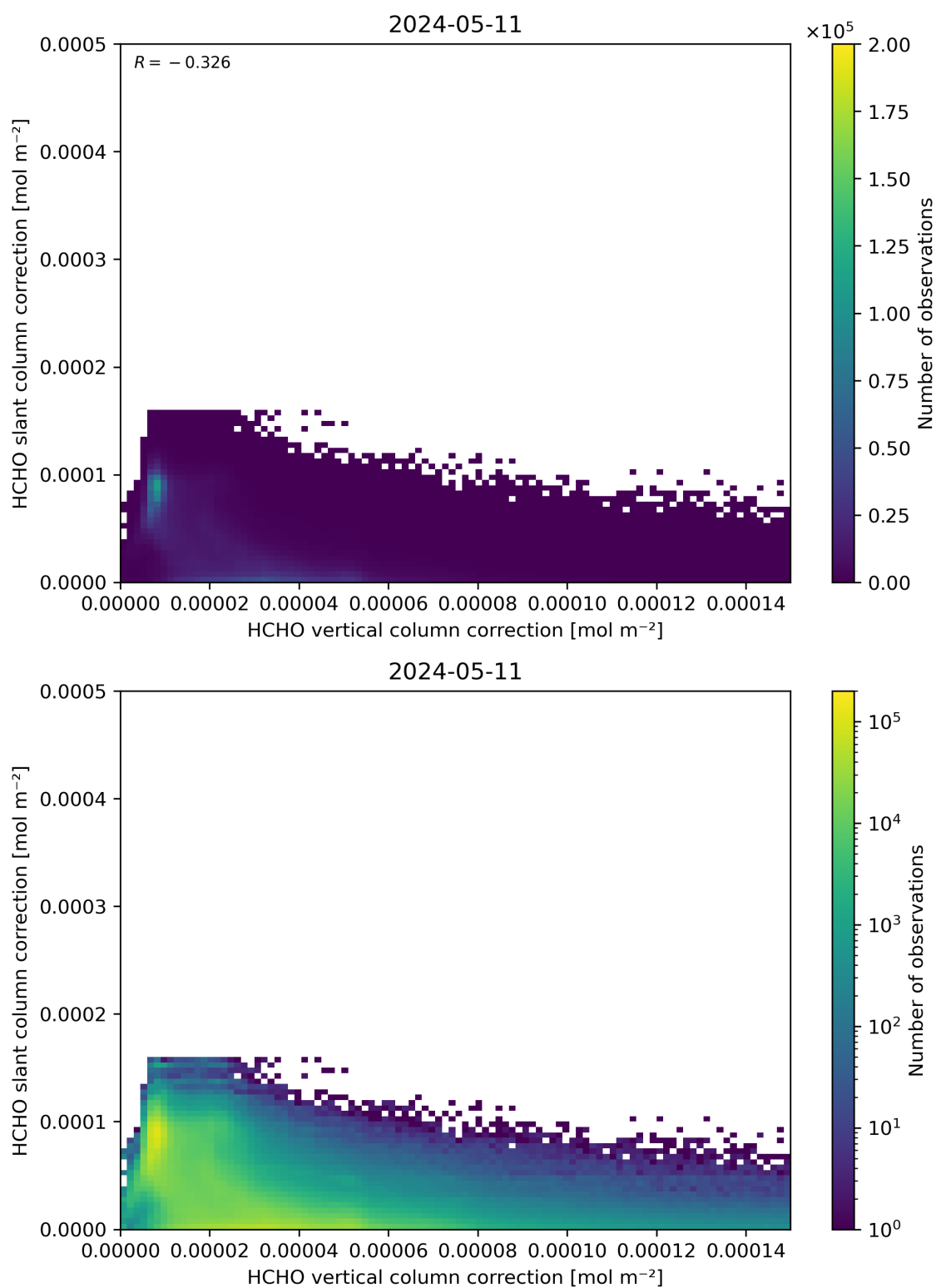
Figure 117: Scatter density plot of “HCHO vertical column correction” against “HCHO slant column correction” for 2024-05-10 to 2024-05-12.
