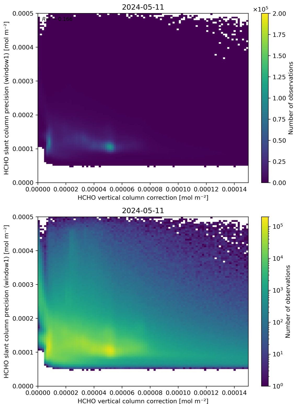
Figure 119: Scatter density plot of “HCHO vertical column correction” against “HCHO slant column precision (window1)” for 2024-05-10 to 2024-05-12.
