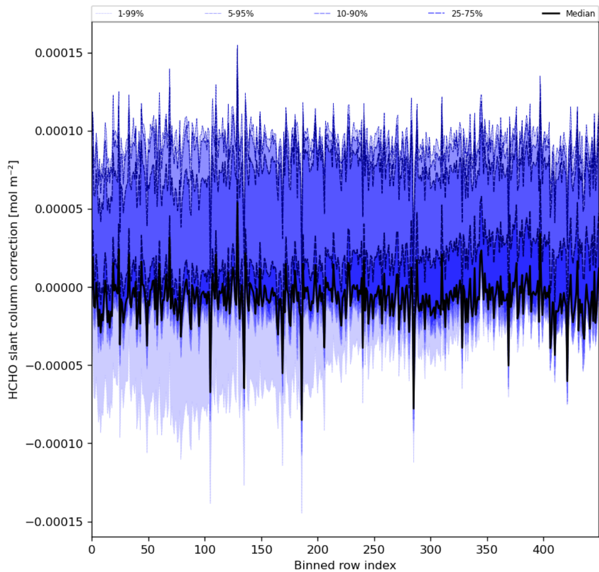
Figure 61: Along track statistics of “HCHO slant column correction” for 2024-05-10 to 2024-05-12
