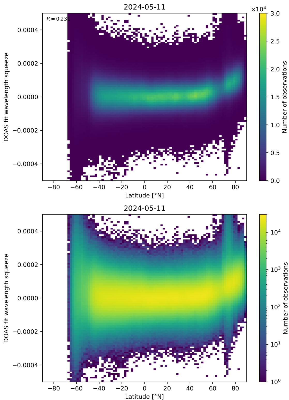
Figure 155: Scatter density plot of “Latitude” against “DOAS fit wavelength squeeze” for 2024-05-10 to 2024-05-12.
