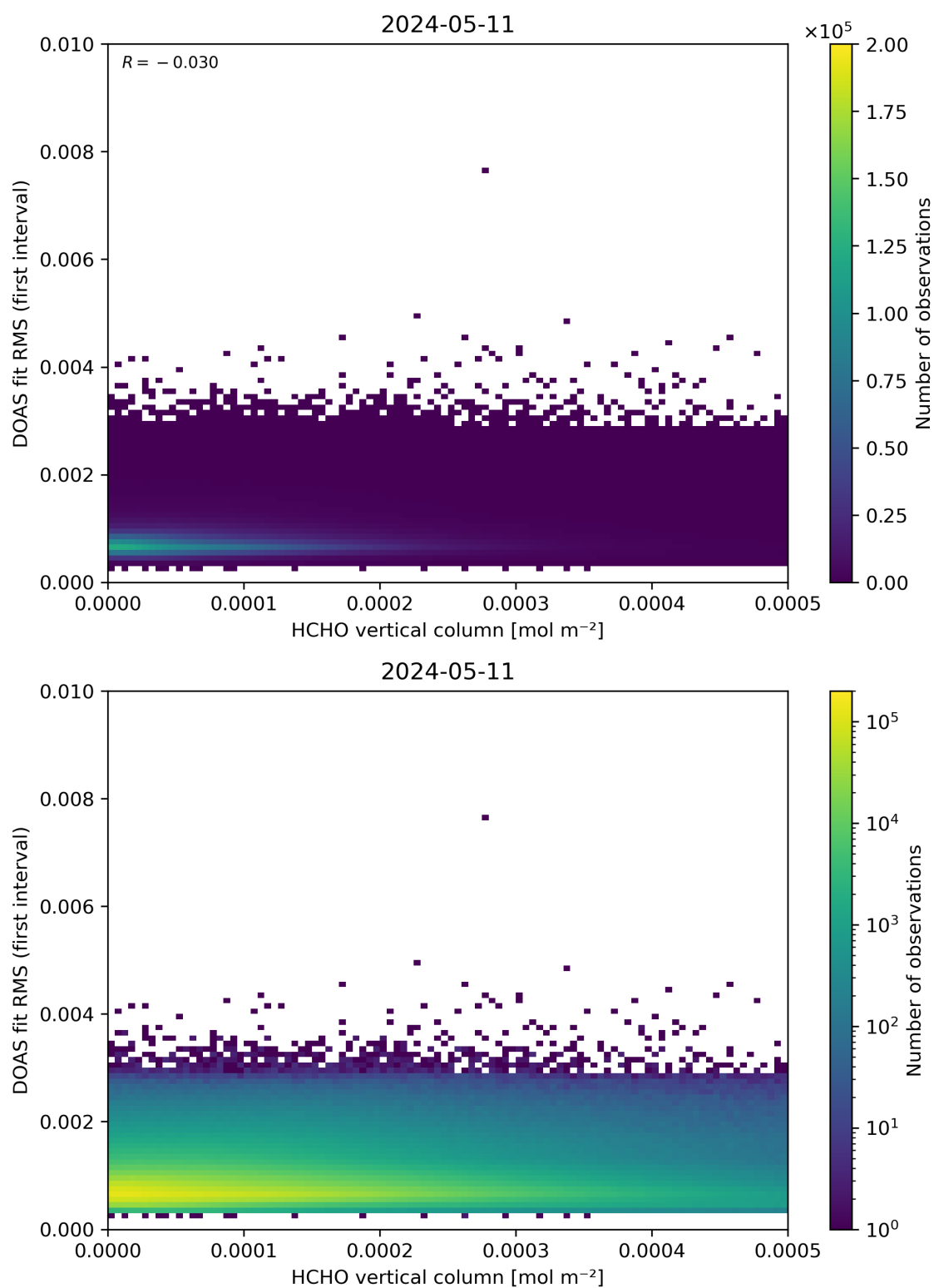
Figure 123: Scatter density plot of “HCHO vertical column” against “DOAS fit RMS (first interval)” for 2024-05-10 to 2024-05-12.
