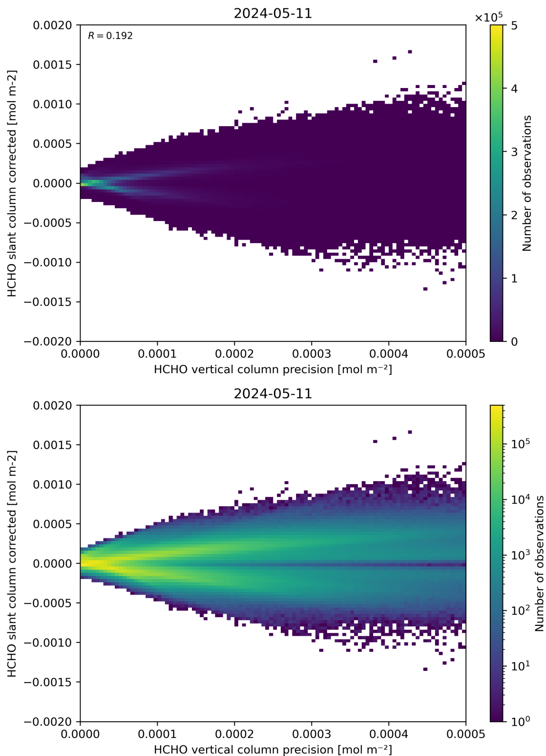
Figure 140: Scatter density plot of “HCHO vertical column precision” against “HCHO slant column corrected” for 2024-05-10 to 2024-05-12.
