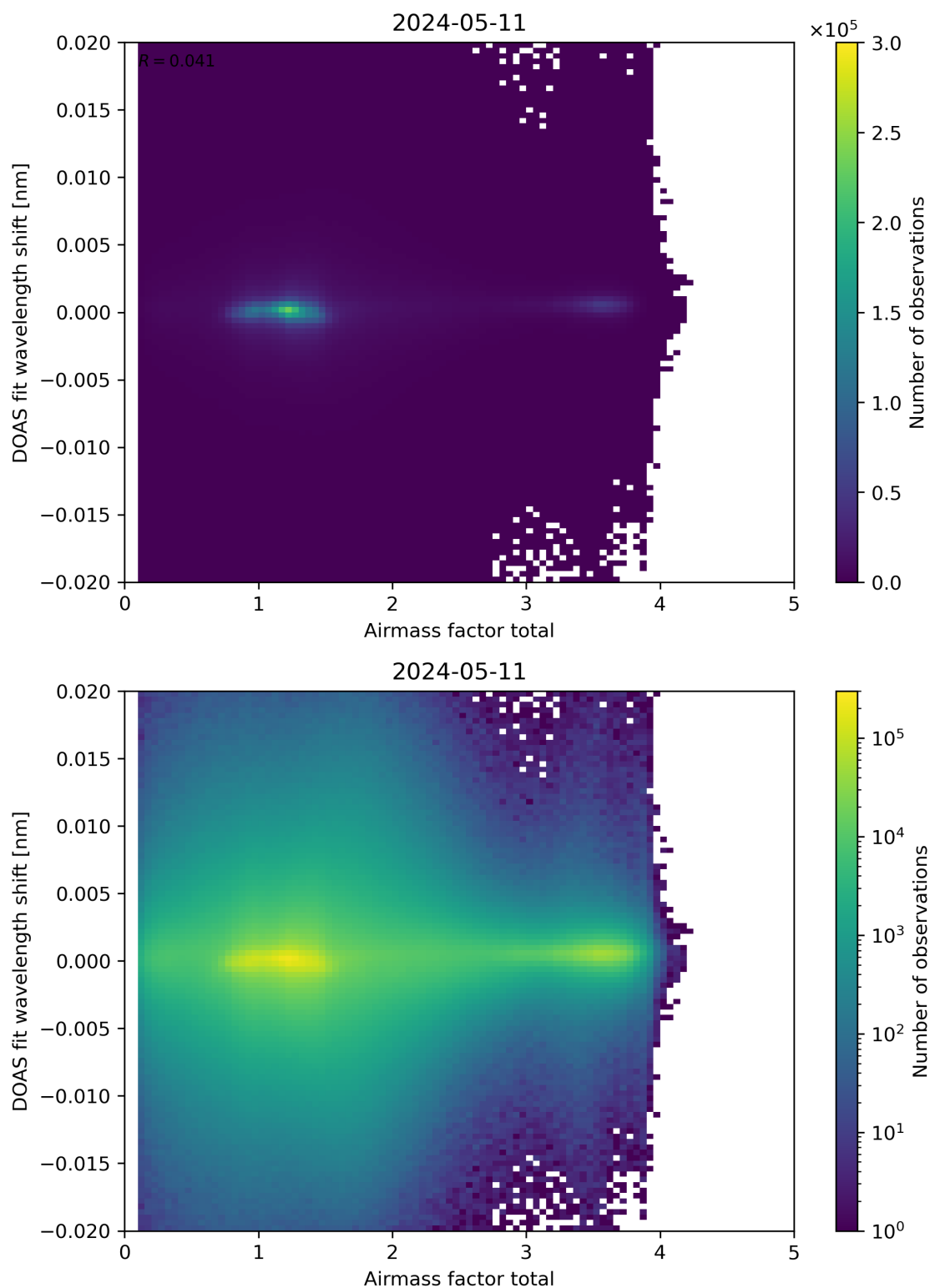
Figure 98: Scatter density plot of “Airmass factor total” against “DOAS fit wavelength shift” for 2024-05-10 to 2024-05-12.
