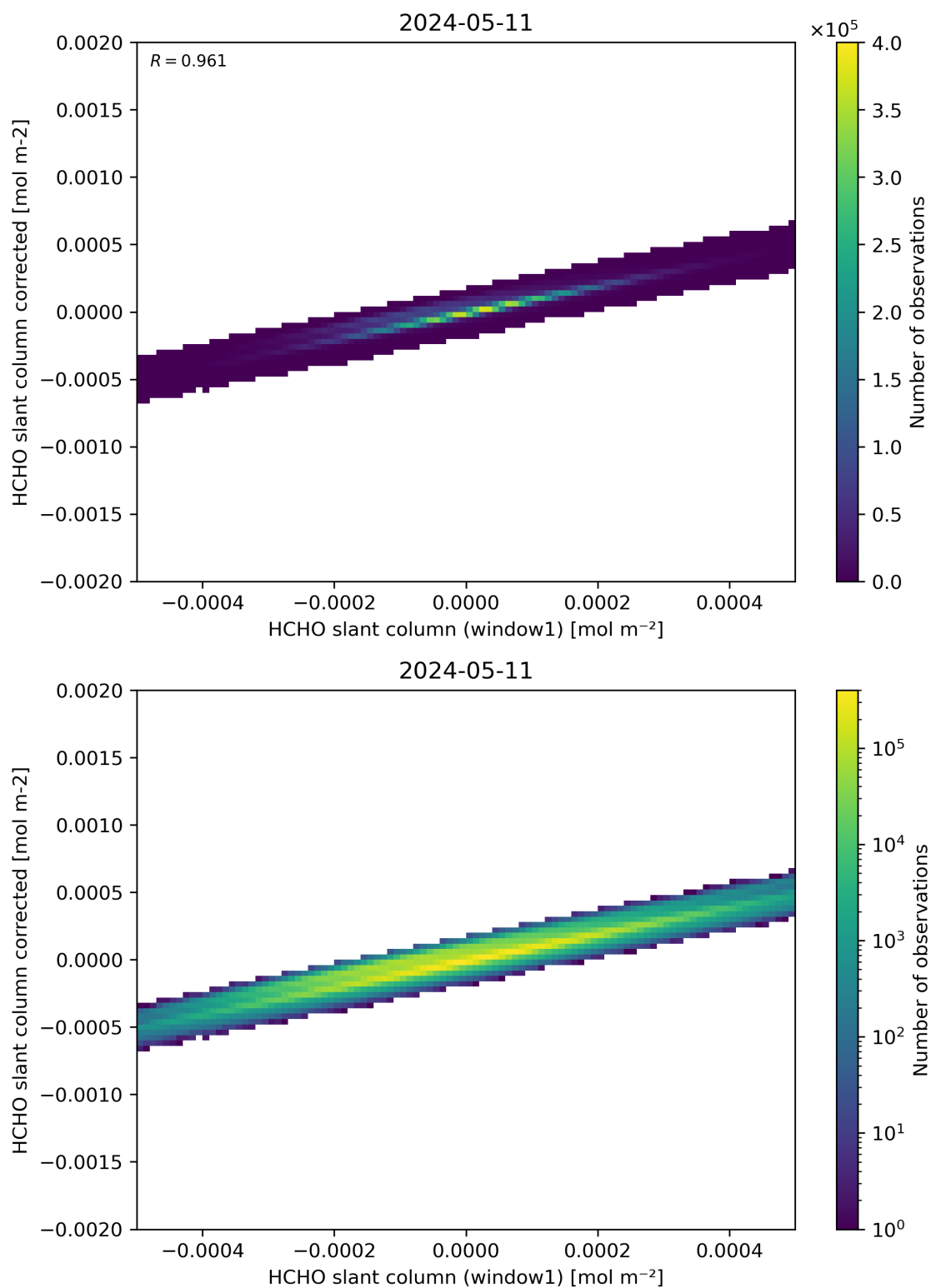
Figure 82: Scatter density plot of “HCHO slant column (window1)” against “HCHO slant column corrected” for 2024-05-10 to 2024-05-12.
