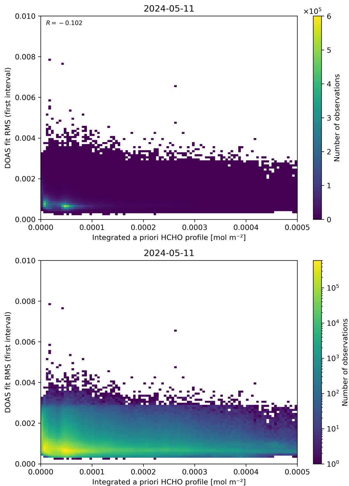
Figure 148: Scatter density plot of “Integrated a priori HCHO profile” against “DOAS fit RMS (first interval)” for 2024-05-10 to 2024-05-12.
