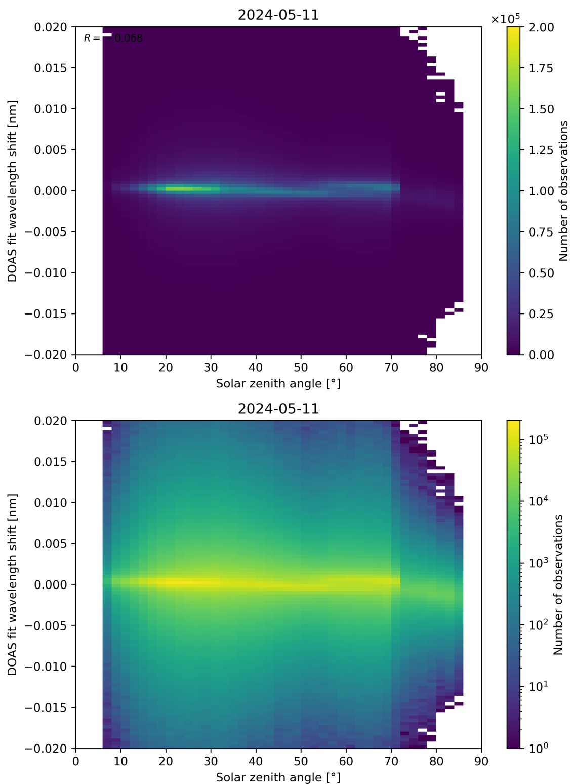
Figure 168: Scatter density plot of “Solar zenith angle” against “DOAS fit wavelength shift” for 2024-05-10 to 2024-05-12.
