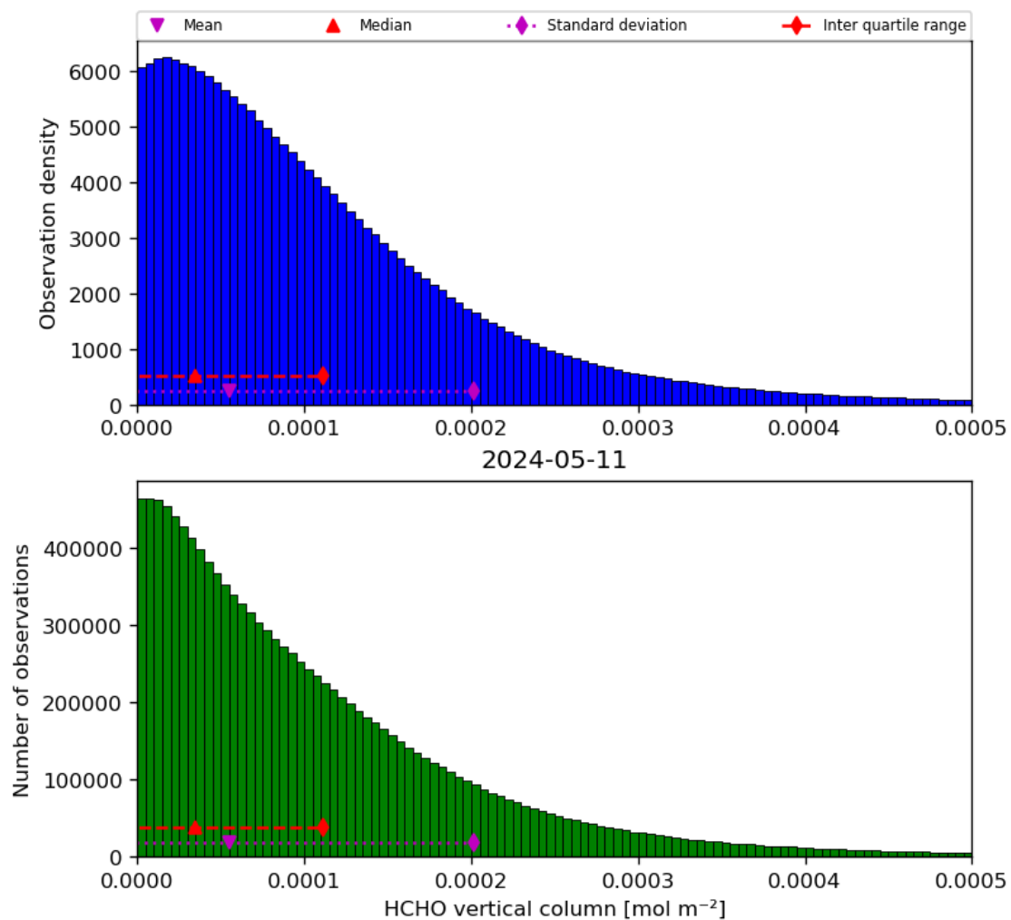
Figure 35: Histogram of “HCHO vertical column” for 2024-05-10 to 2024-05-12
