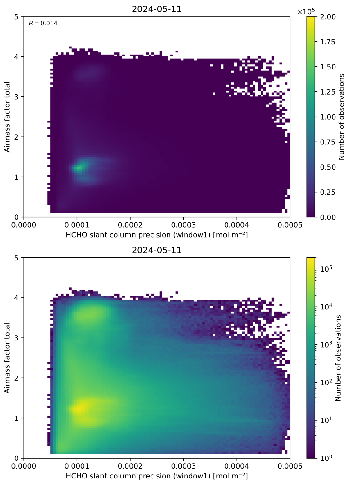
Figure 94: Scatter density plot of “HCHO slant column precision (window1)” against “Airmass factor total” for 2024-05-10 to 2024-05-12.
