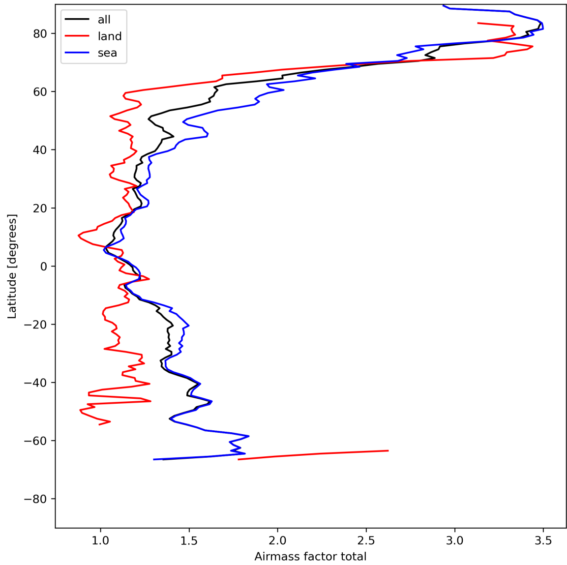
Figure 26: Zonal average of “Airmass factor total” for 2024-05-10 to 2024-05-12.
