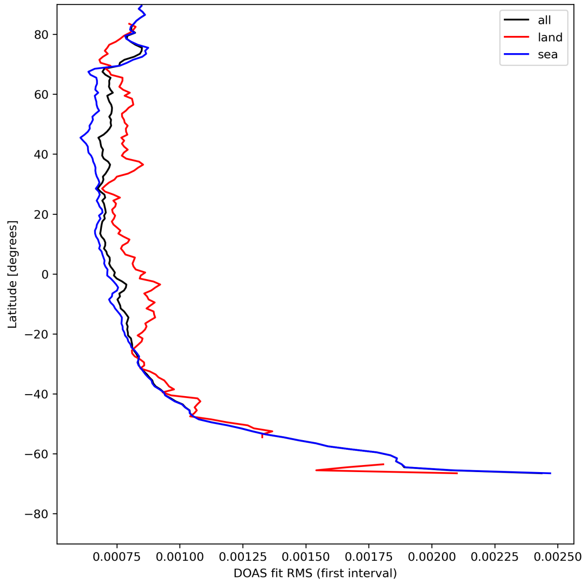
Figure 32: Zonal average of “DOAS fit RMS (first interval)” for 2024-05-10 to 2024-05-12.
