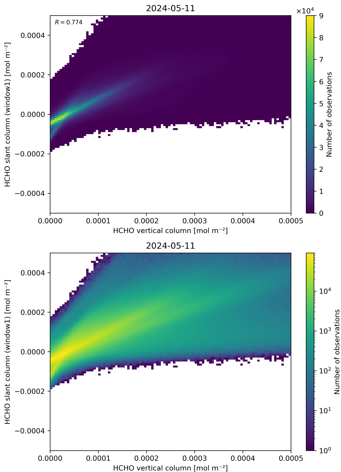
Figure 129: Scatter density plot of “HCHO vertical column” against “HCHO slant column (window1)” for 2024-05-10 to 2024-05-12.
