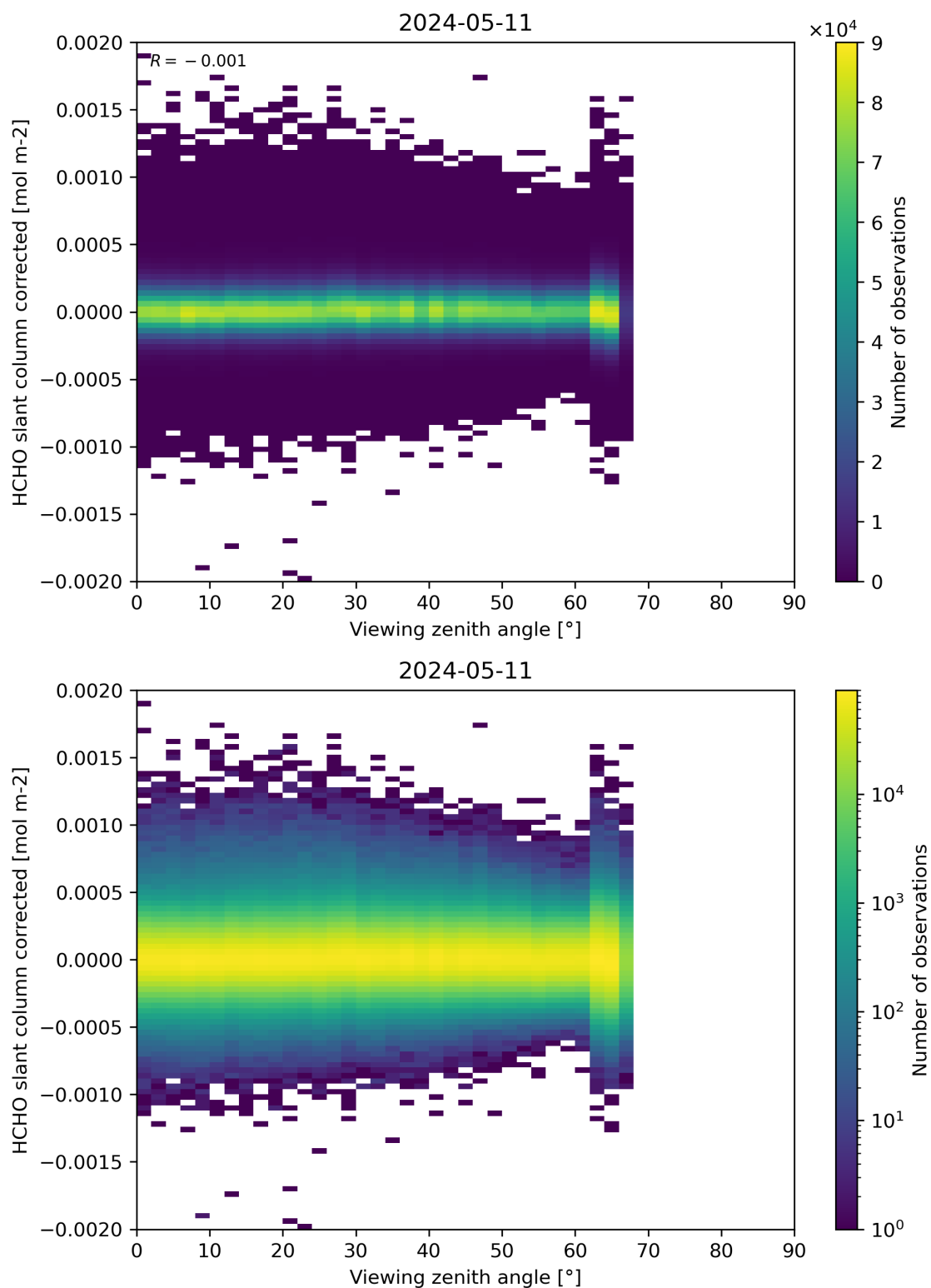
Figure 186: Scatter density plot of “Viewing zenith angle” against “HCHO slant column corrected” for 2024-05-10 to 2024-05-12.
