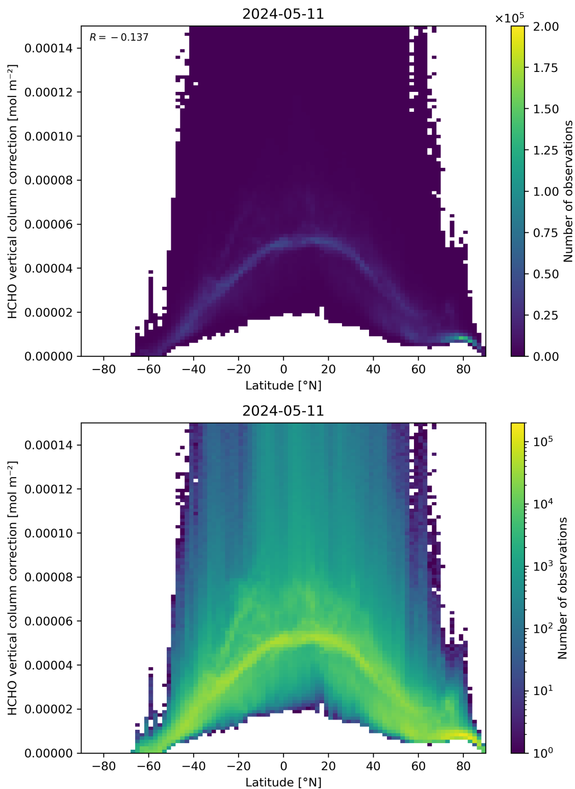
Figure 164: Scatter density plot of “Latitude” against “HCHO vertical column correction” for 2024-05-10 to 2024-05-12.
