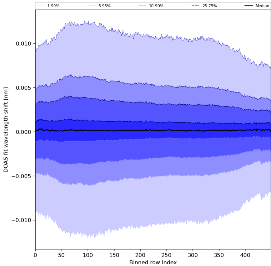
Figure 58: Along track statistics of “DOAS fit wavelength shift” for 2024-05-10 to 2024-05-12
