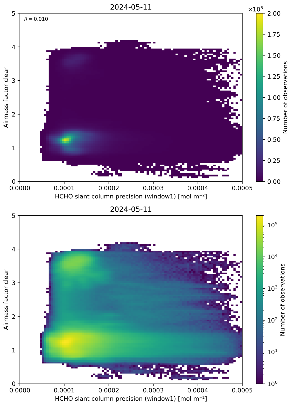
Figure 91: Scatter density plot of “HCHO slant column precision (window1)” against “Airmass factor clear” for 2024-05-10 to 2024-05-12.
