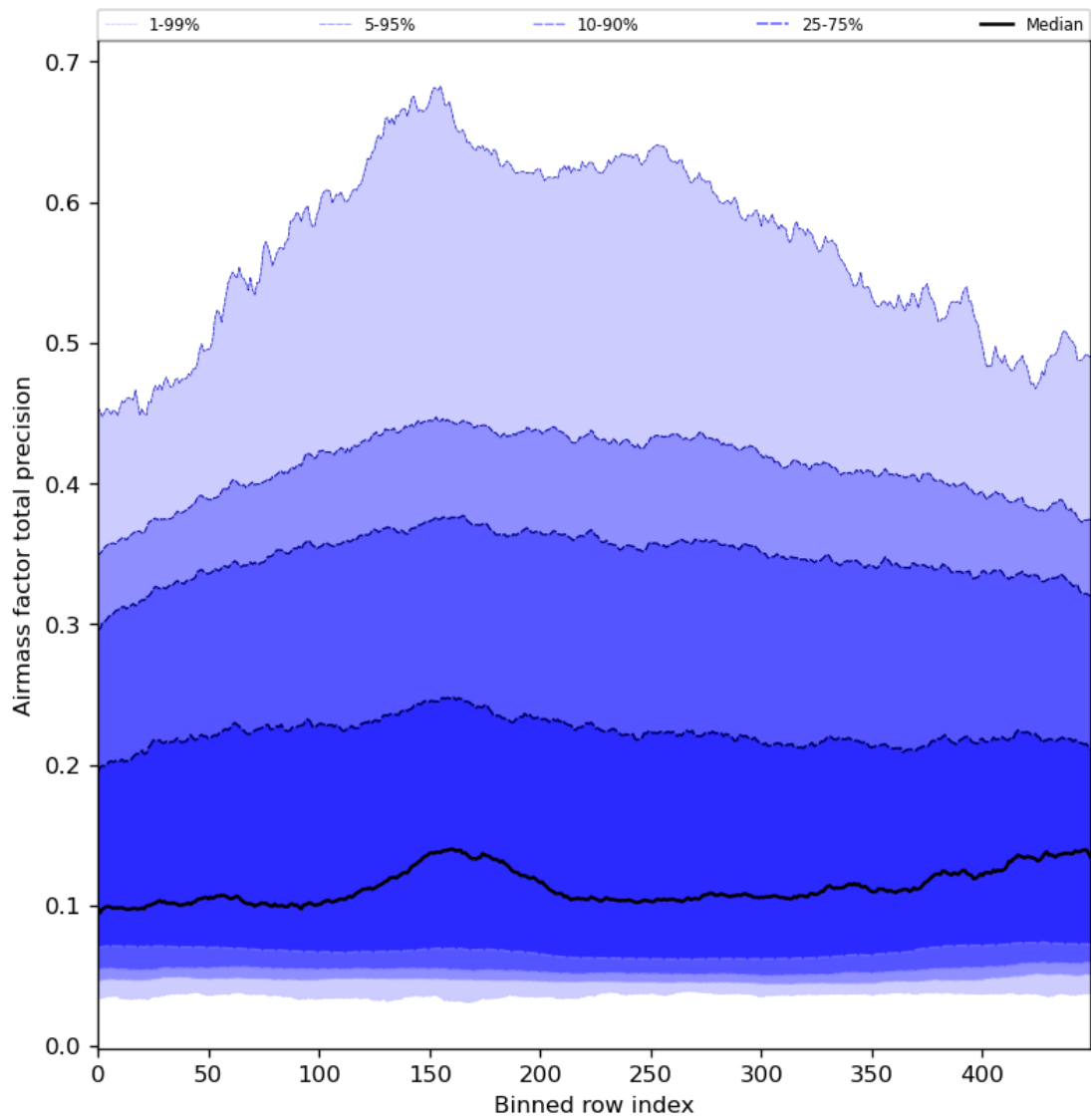
Figure 55: Along track statistics of “Airmass factor total precision” for 2024-05-10 to 2024-05-12
