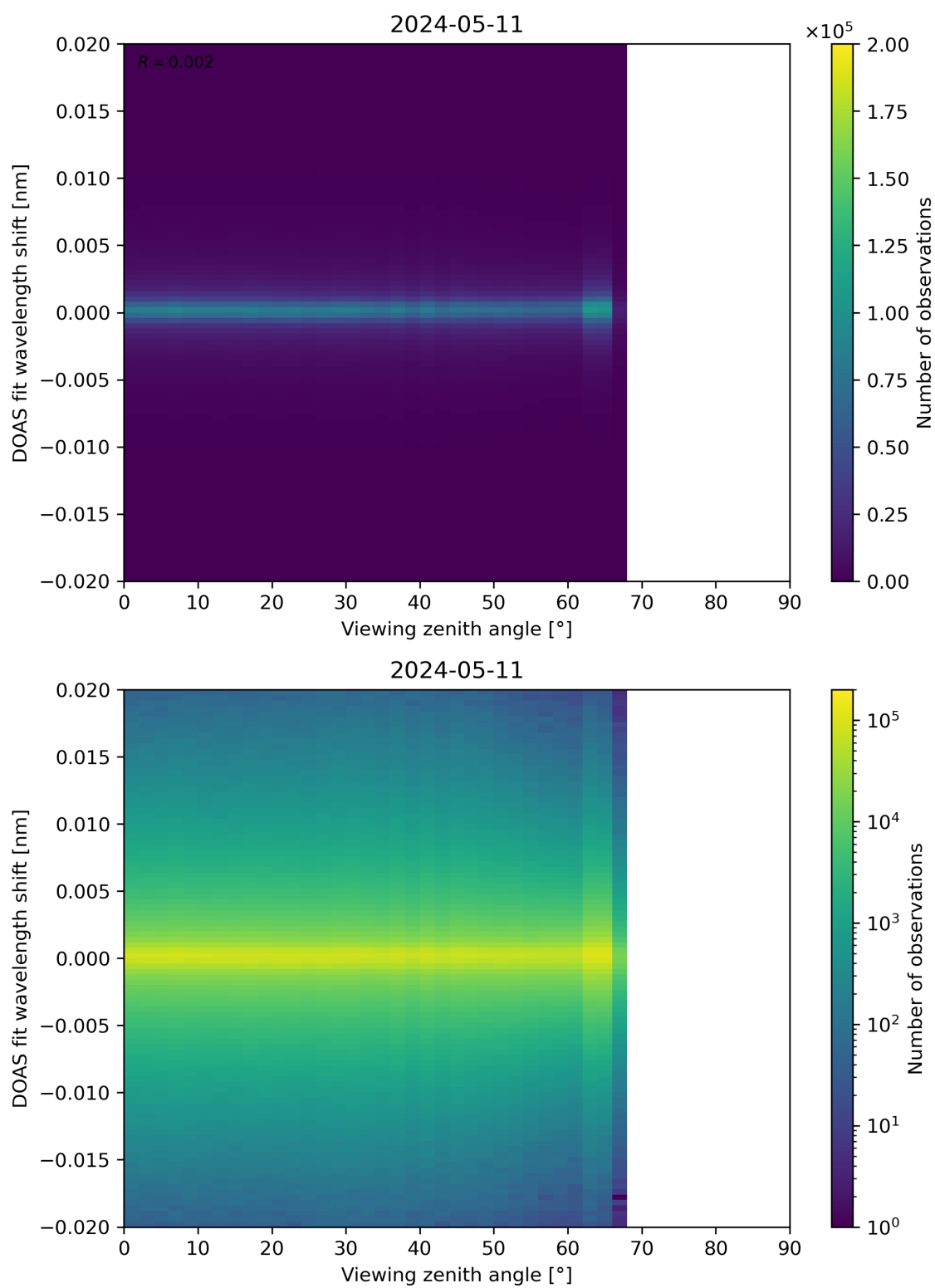
Figure 183: Scatter density plot of “Viewing zenith angle” against “DOAS fit wavelength shift” for 2024-05-10 to 2024-05-12.
