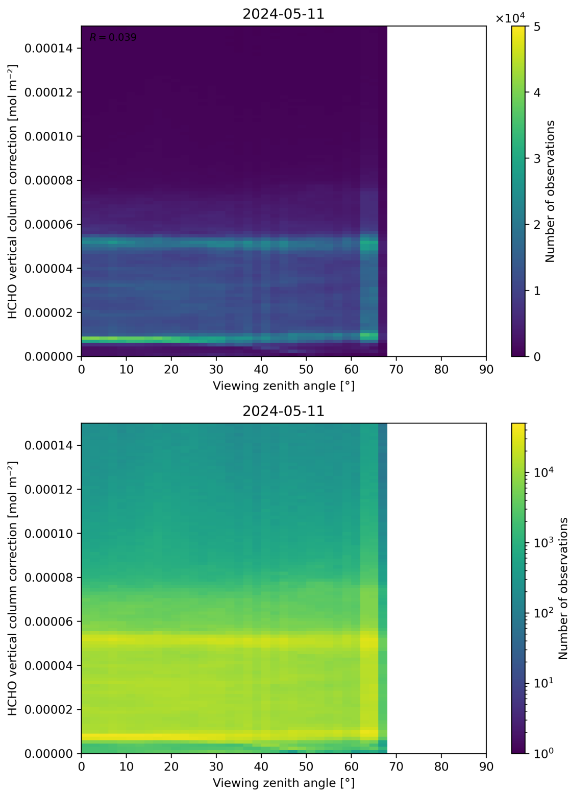
Figure 193: Scatter density plot of “Viewing zenith angle” against “HCHO vertical column correction” for 2024-05-10 to 2024-05-12.
