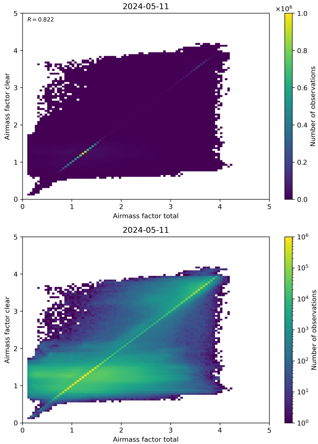
Figure 100: Scatter density plot of “Airmass factor total” against “Airmass factor clear” for 2024-05-10 to 2024-05-12.
