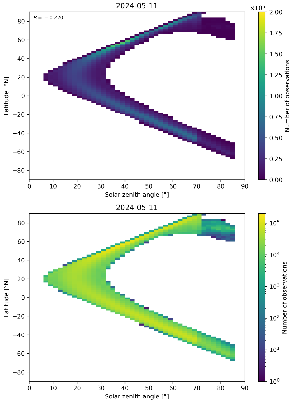
Figure 181: Scatter density plot of “Solar zenith angle” against “Latitude” for 2024-05-10 to 2024-05-12.
