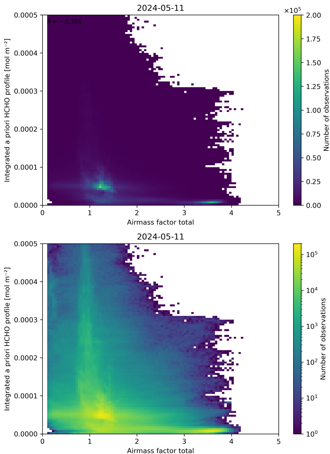
Figure 104: Scatter density plot of “Airmass factor total” against “Integrated a priori HCHO profile” for 2024-05-10 to 2024-05-12.
