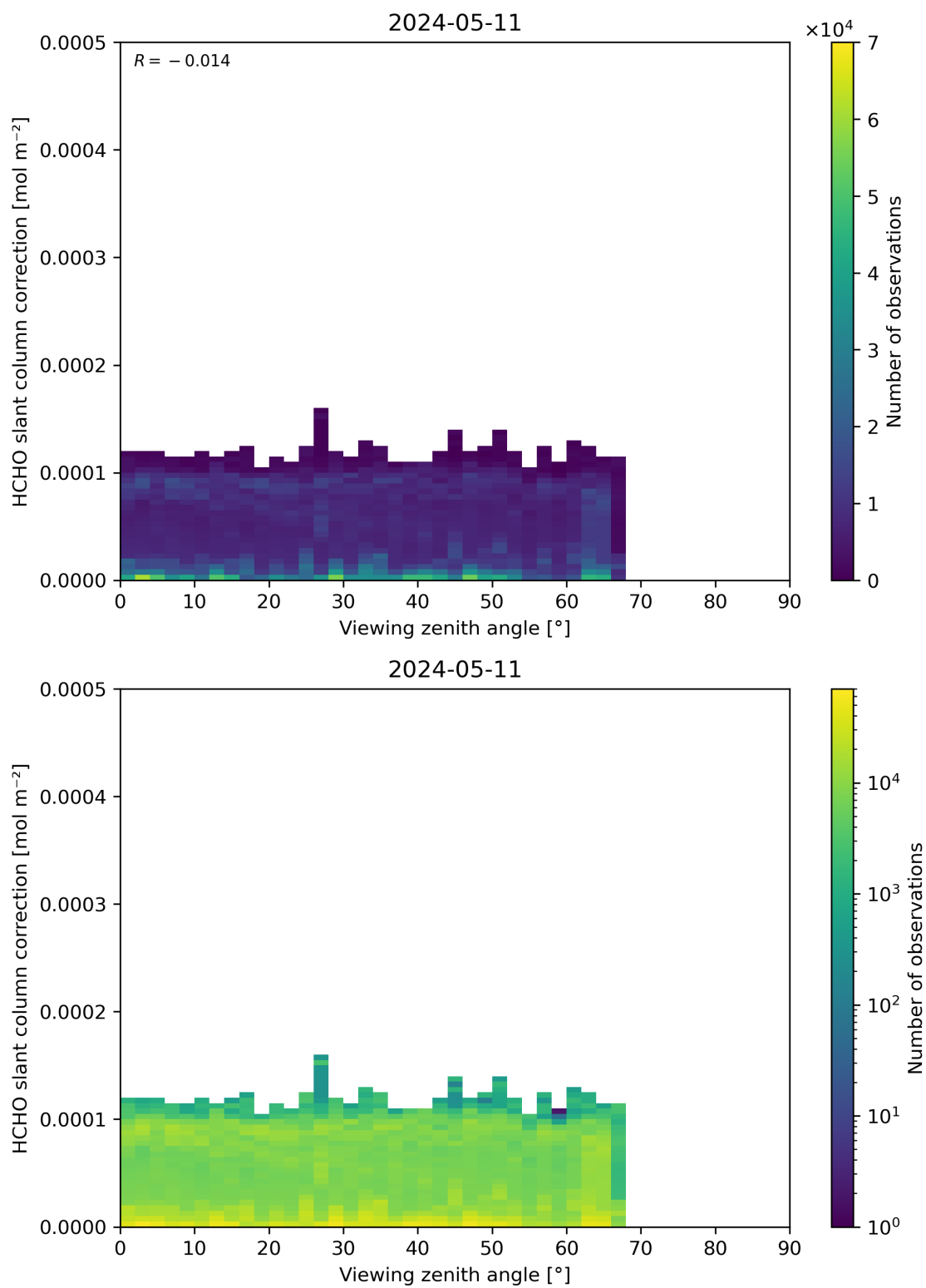
Figure 187: Scatter density plot of “Viewing zenith angle” against “HCHO slant column correction” for 2024-05-10 to 2024-05-12.
