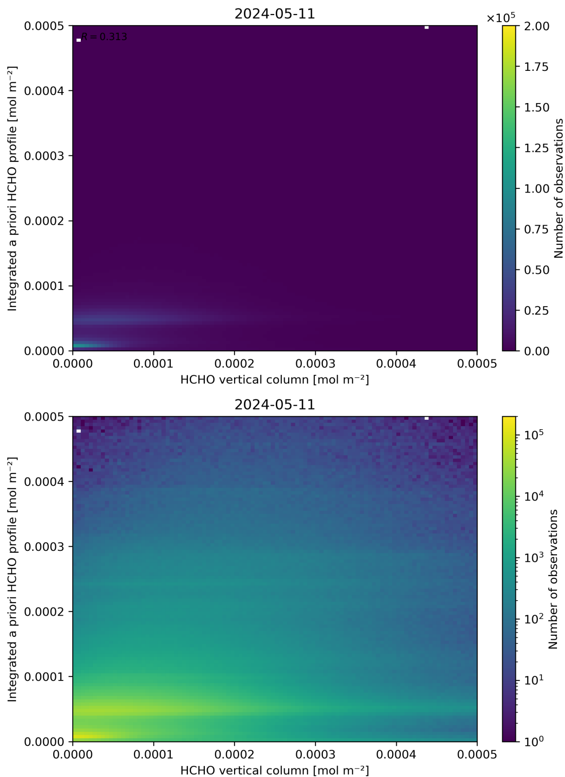
Figure 135: Scatter density plot of “HCHO vertical column” against “Integrated a priori HCHO profile” for 2024-05-10 to 2024-05-12.
