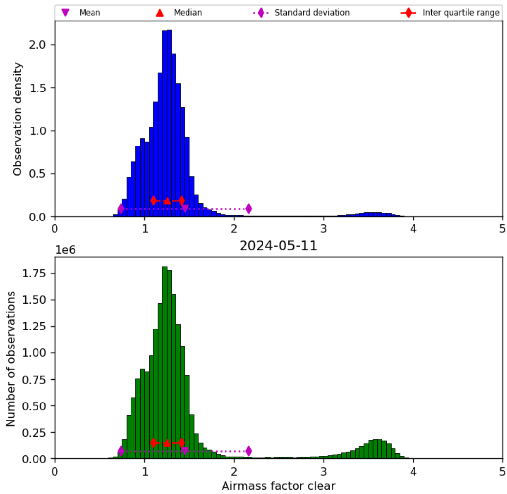
Figure 42: Histogram of “Airmass factor clear” for 2024-05-10 to 2024-05-12
