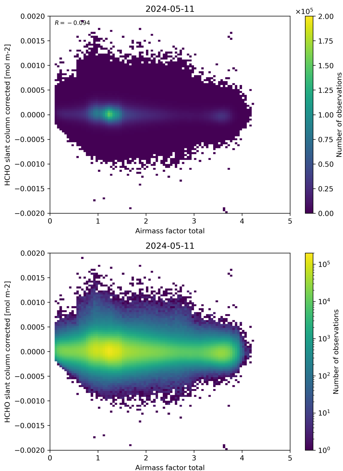
Figure 101: Scatter density plot of “Airmass factor total” against “HCHO slant column corrected” for 2024-05-10 to 2024-05-12.
