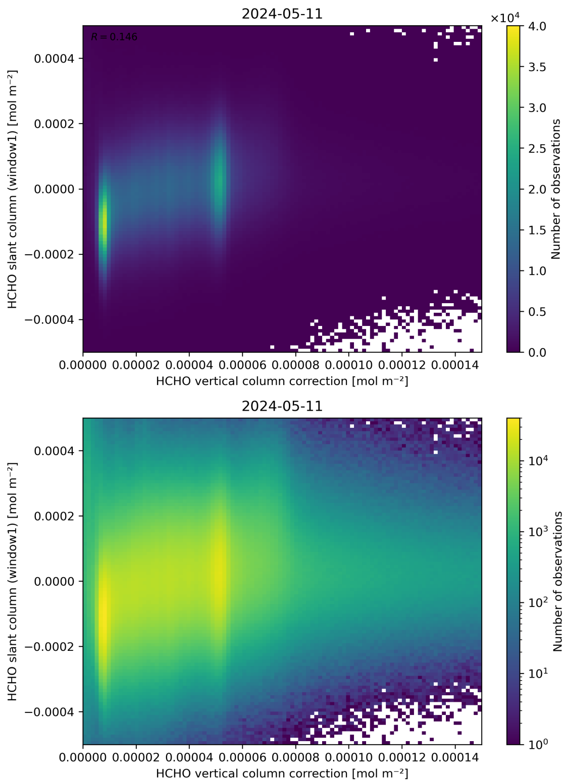
Figure 118: Scatter density plot of “HCHO vertical column correction” against “HCHO slant column (window1)” for 2024-05-10 to 2024-05-12.
