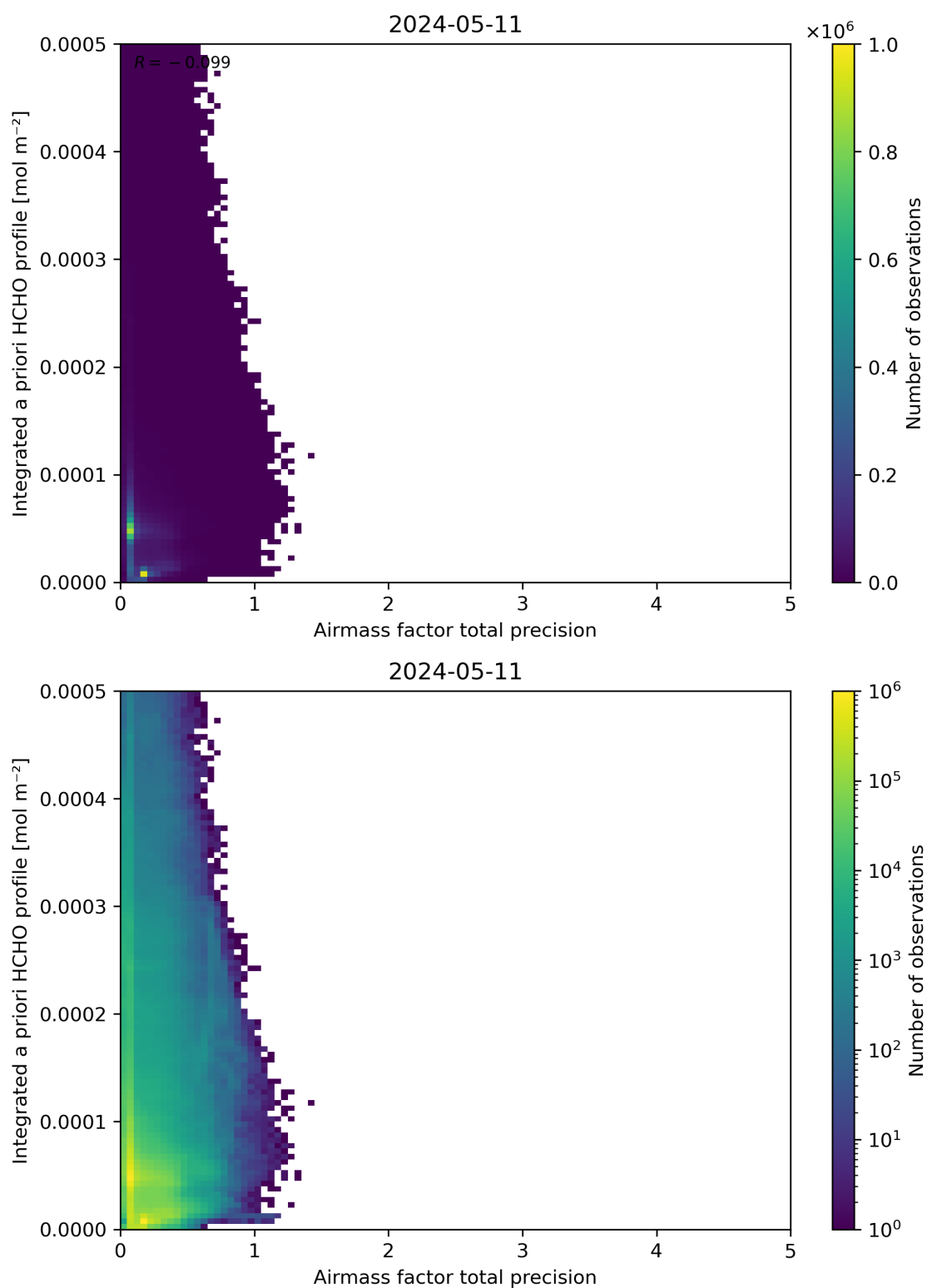
Figure 111: Scatter density plot of “Airmass factor total precision” against “Integrated a priori HCHO profile” for 2024-05-10 to 2024-05-12.
