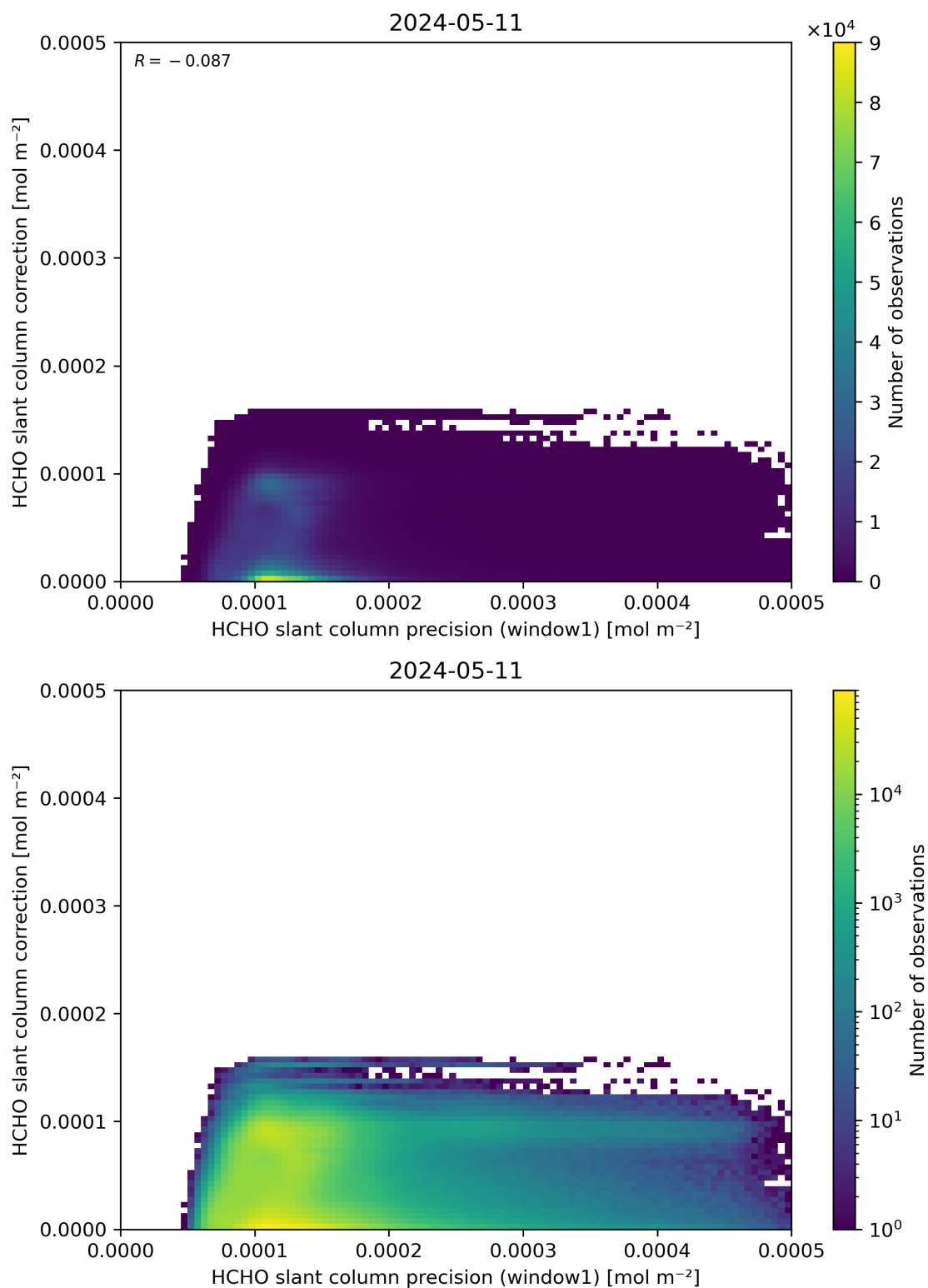
Figure 93: Scatter density plot of “HCHO slant column precision (window1)” against “HCHO slant column correction” for 2024-05-10 to 2024-05-12.
