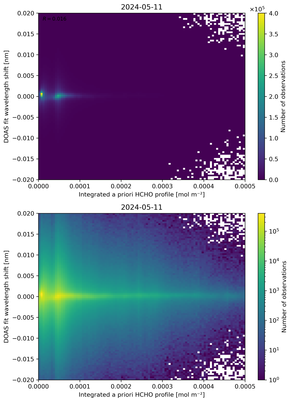
Figure 149: Scatter density plot of “Integrated a priori HCHO profile” against “DOAS fit wavelength shift” for 2024-05-10 to 2024-05-12.
