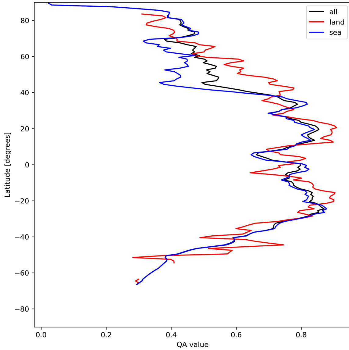
Figure 20: Zonal average of “QA value” for 2024-05-10 to 2024-05-12.
