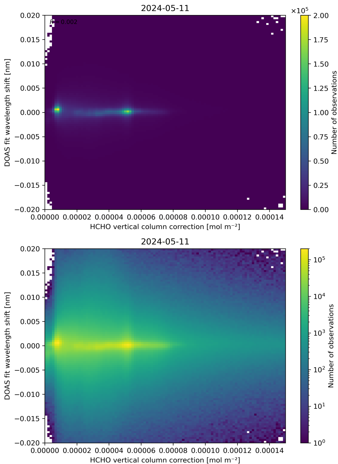
Figure 113: Scatter density plot of “HCHO vertical column correction” against “DOAS fit wavelength shift” for 2024-05-10 to 2024-05-12.
