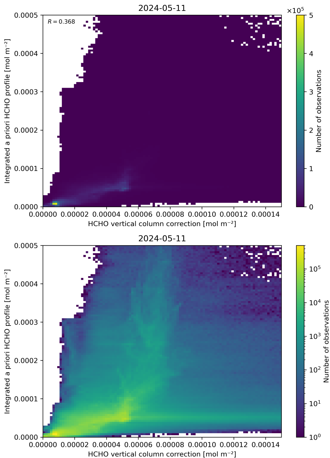
Figure 122: Scatter density plot of “HCHO vertical column correction” against “Integrated a priori HCHO profile” for 2024-05-10 to 2024-05-12.
