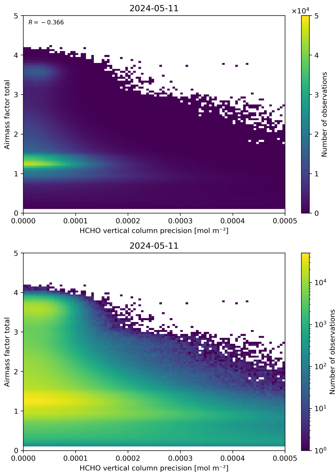
Figure 144: Scatter density plot of “HCHO vertical column precision” against “Airmass factor total” for 2024-05-10 to 2024-05-12.
