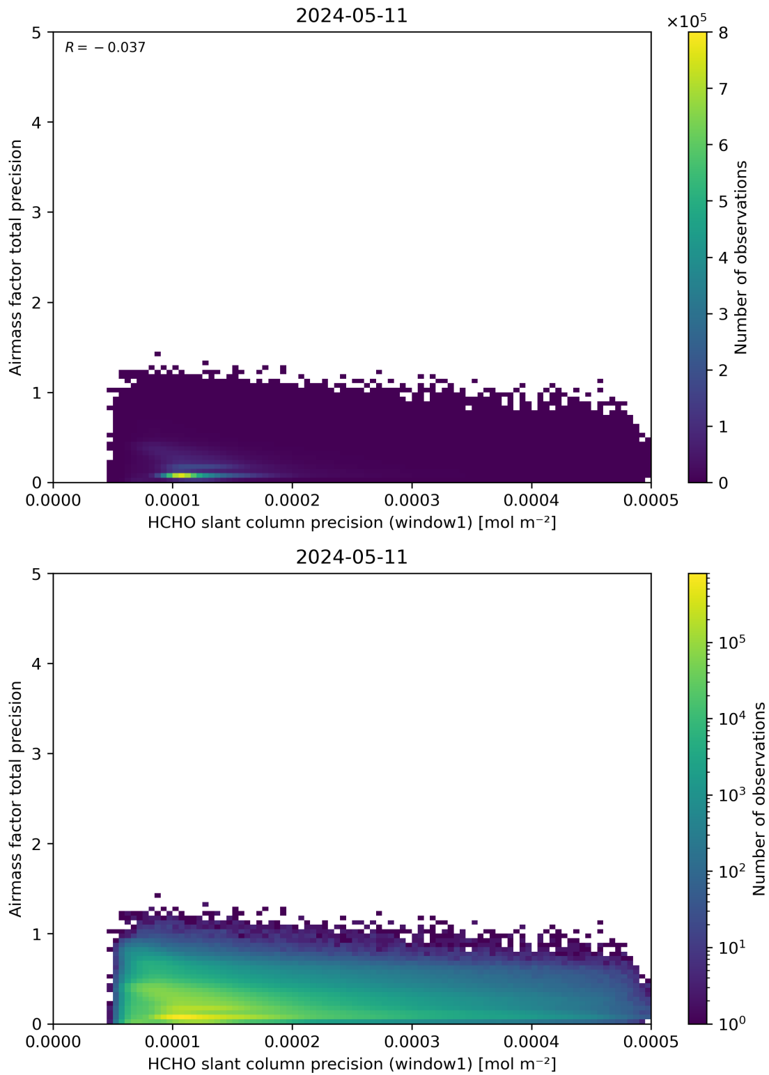
Figure 95: Scatter density plot of “HCHO slant column precision (window1)” against “Airmass factor total precision” for 2024-05-10 to 2024-05-12.
