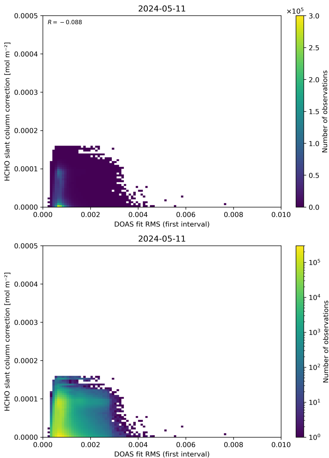
Figure 63: Scatter density plot of “DOAS fit RMS (first interval)” against “HCHO slant column correction” for 2024-05-10 to 2024-05-12.
