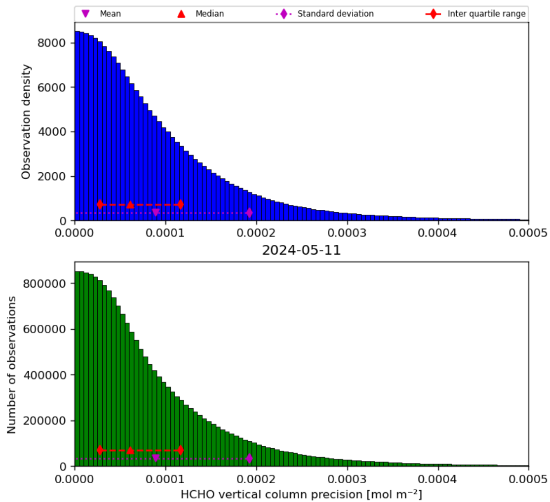
Figure 36: Histogram of “HCHO vertical column precision” for 2024-05-10 to 2024-05-12
