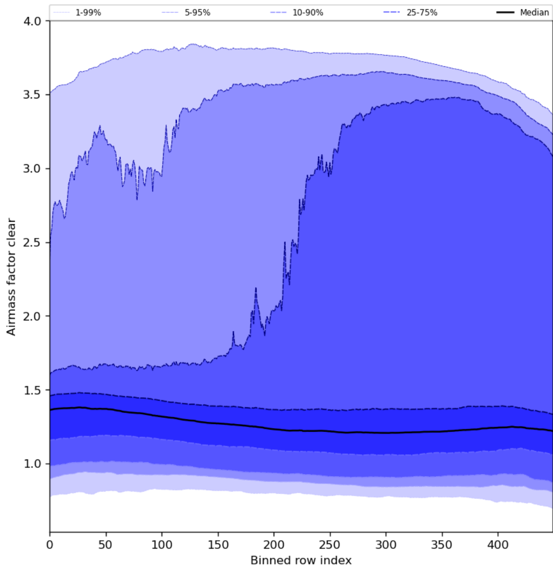
Figure 56: Along track statistics of “Airmass factor clear” for 2024-05-10 to 2024-05-12
