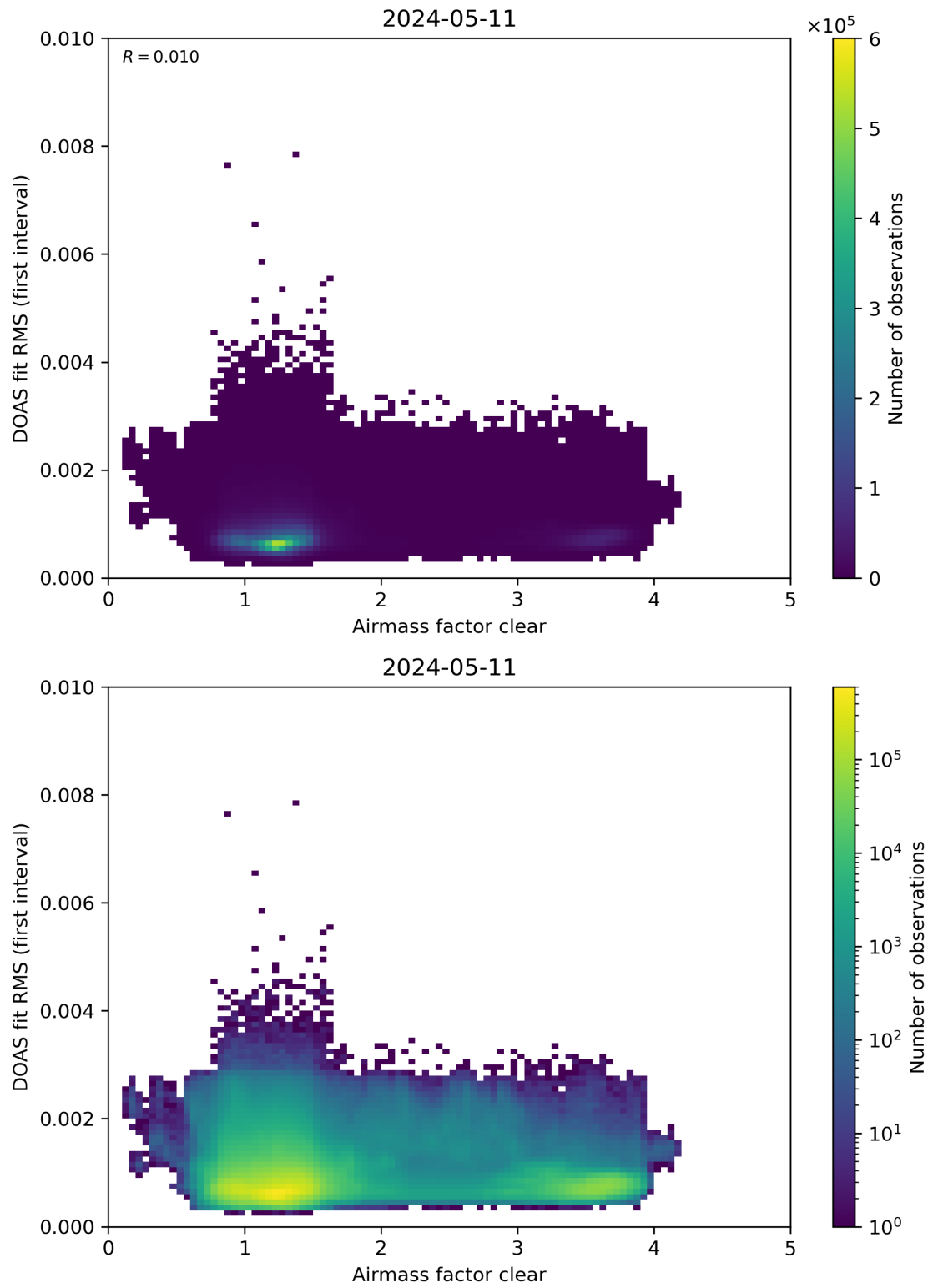
Figure 71: Scatter density plot of “Airmass factor clear” against “DOAS fit RMS (first interval)” for 2024-05-10 to 2024-05-12.
