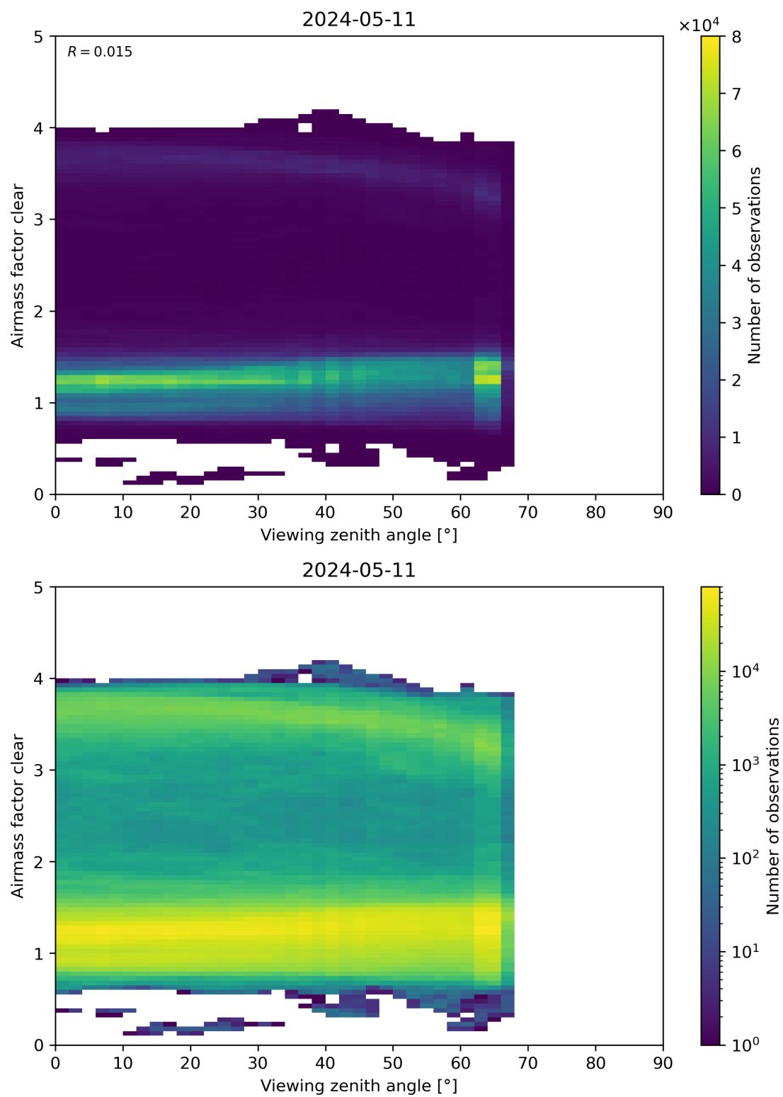
Figure 185: Scatter density plot of “Viewing zenith angle” against “Airmass factor clear” for 2024-05-10 to 2024-05-12.
