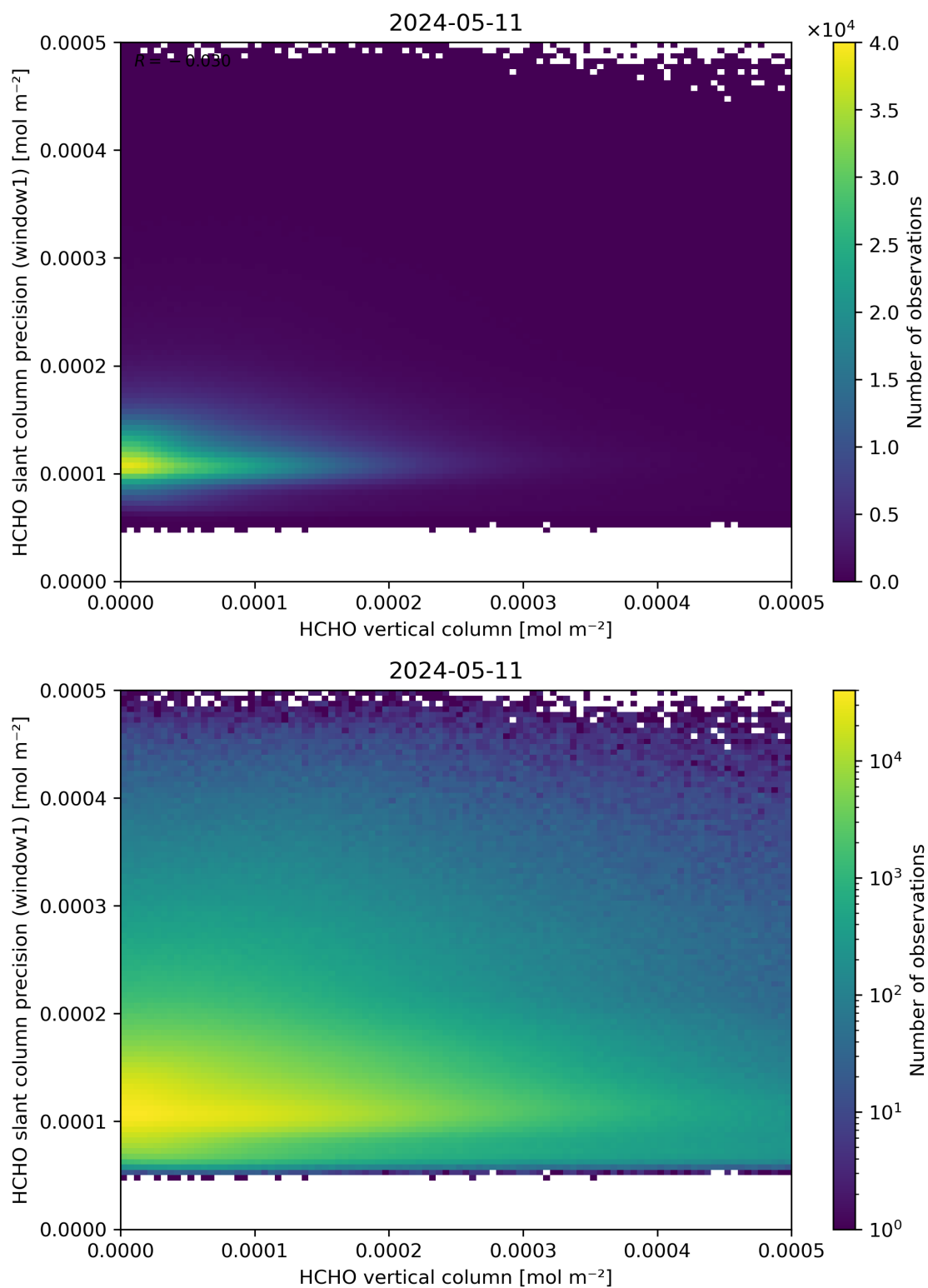
Figure 130: Scatter density plot of “HCHO vertical column” against “HCHO slant column precision (window1)” for 2024-05-10 to 2024-05-12.
