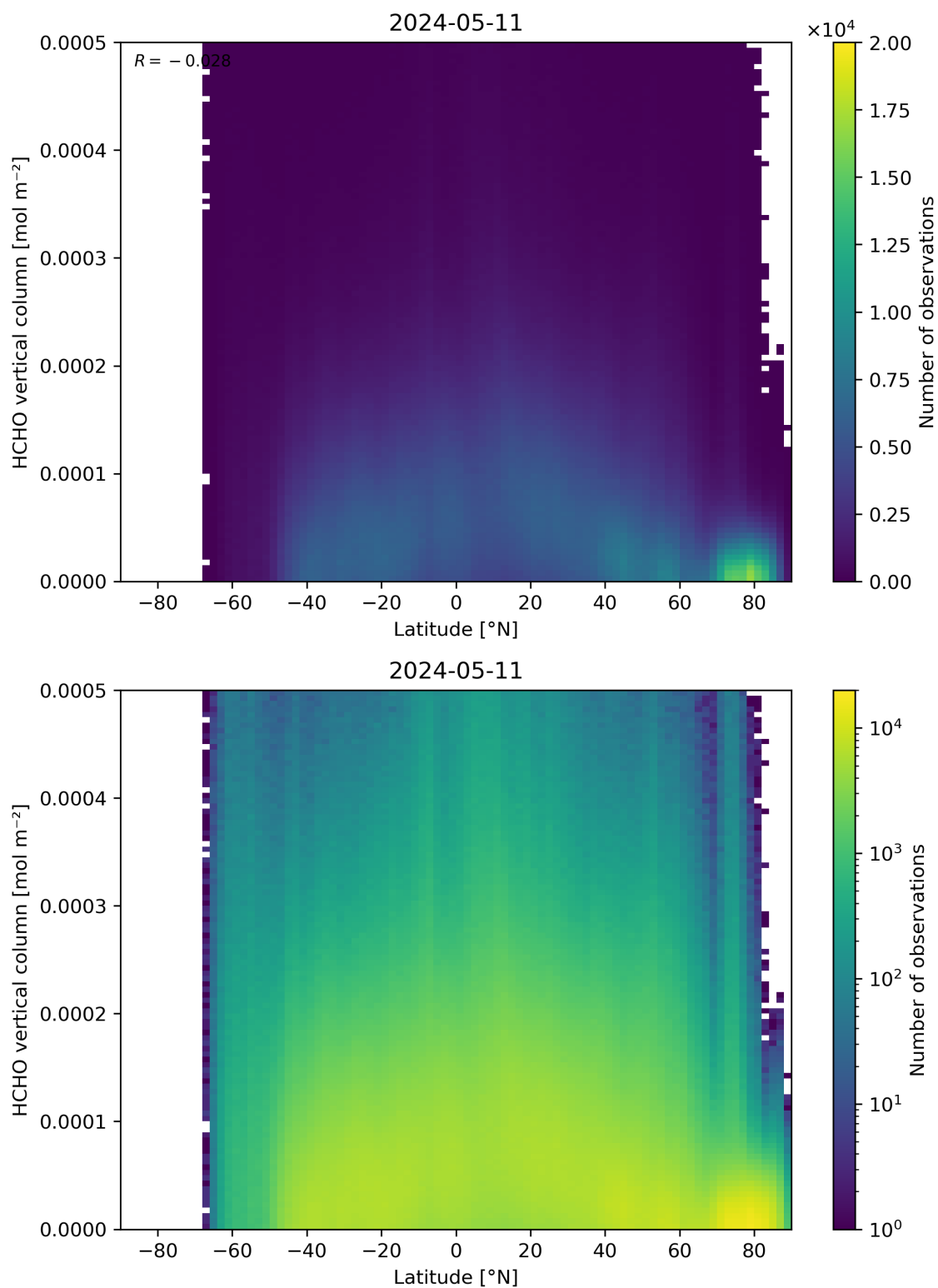
Figure 163: Scatter density plot of “Latitude” against “HCHO vertical column” for 2024-05-10 to 2024-05-12.
