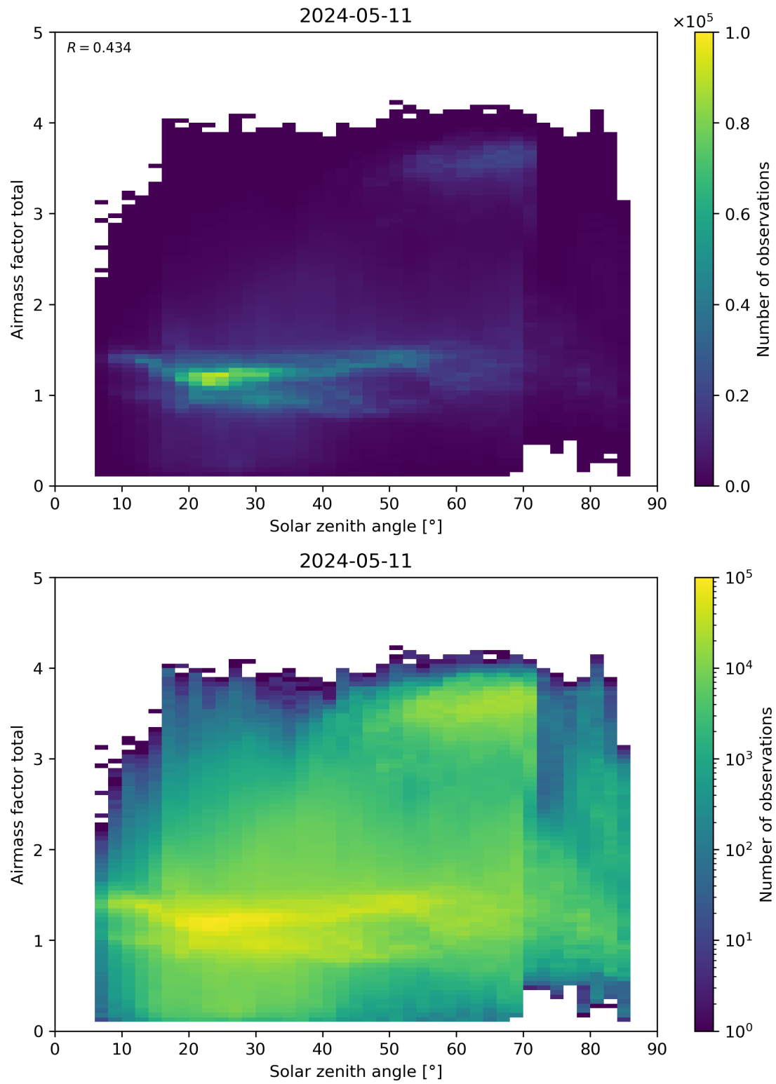
Figure 175: Scatter density plot of “Solar zenith angle” against “Airmass factor total” for 2024-05-10 to 2024-05-12.
