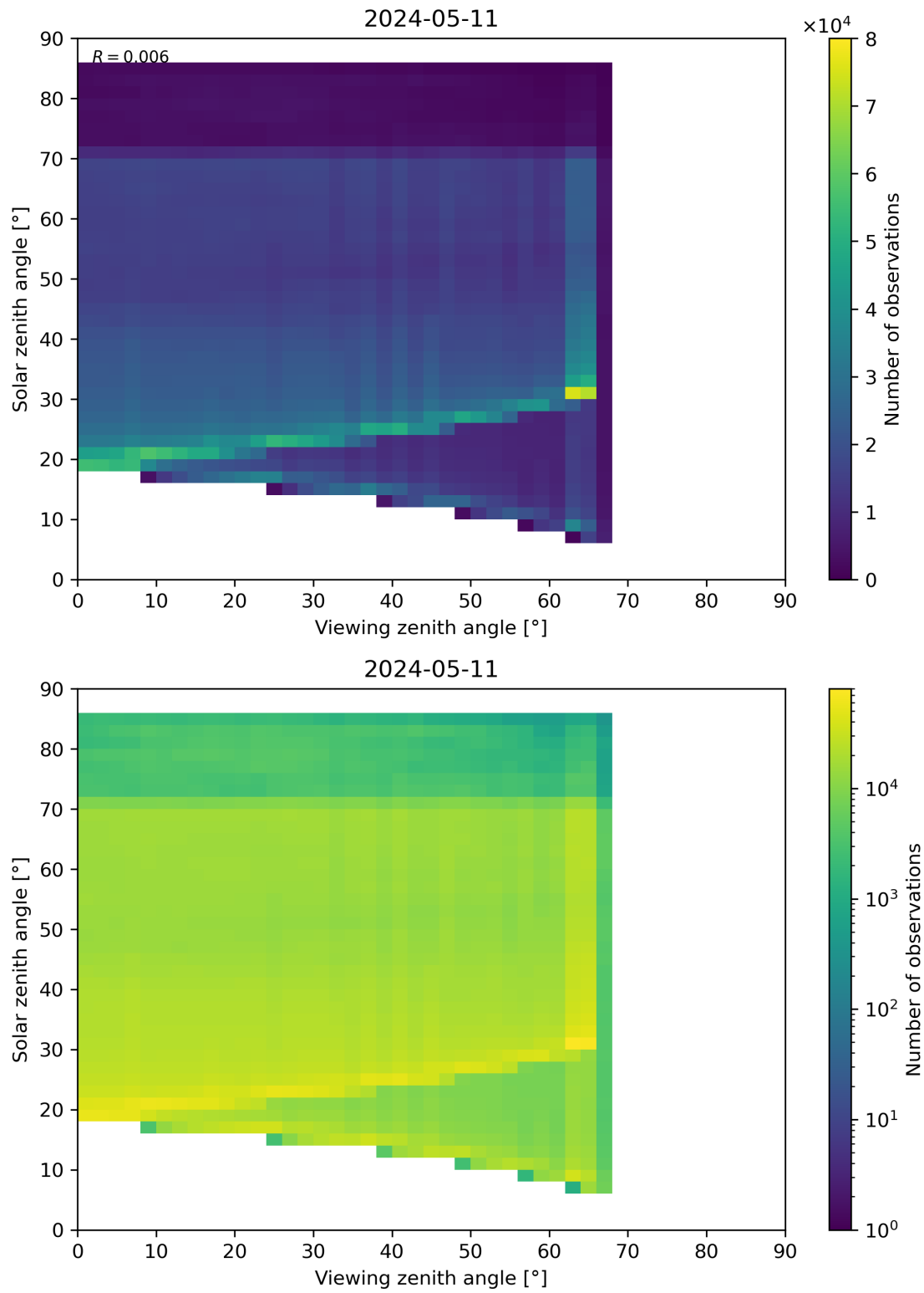
Figure 197: Scatter density plot of “Viewing zenith angle” against “Solar zenith angle” for 2024-05-10 to 2024-05-12.
