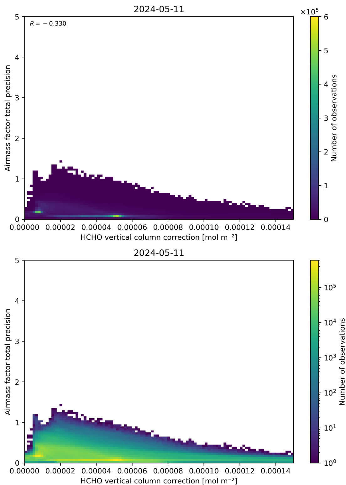
Figure 121: Scatter density plot of “HCHO vertical column correction” against “Airmass factor total precision” for 2024-05-10 to 2024-05-12.
