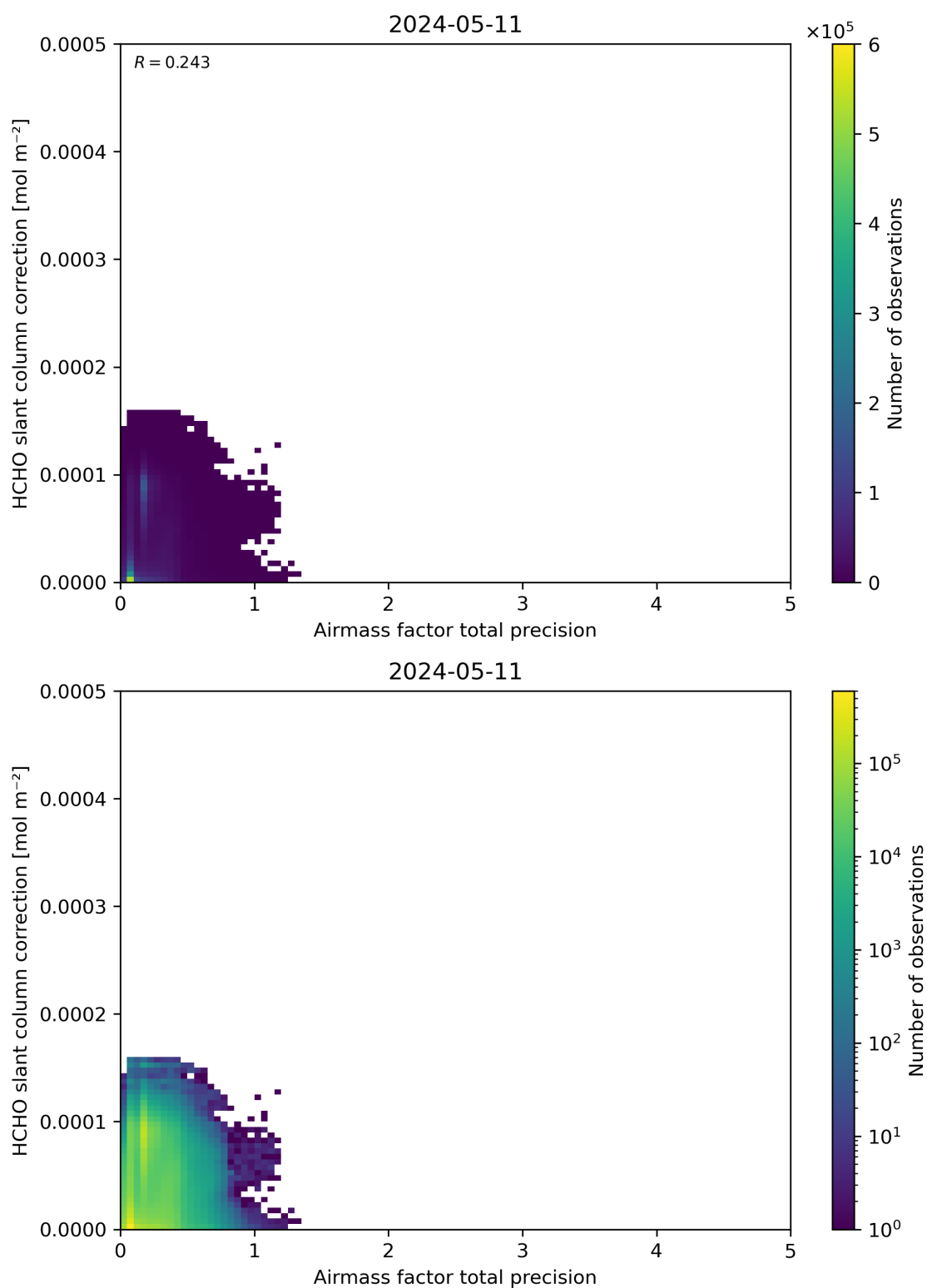
Figure 110: Scatter density plot of “Airmass factor total precision” against “HCHO slant column correction” for 2024-05-10 to 2024-05-12.
