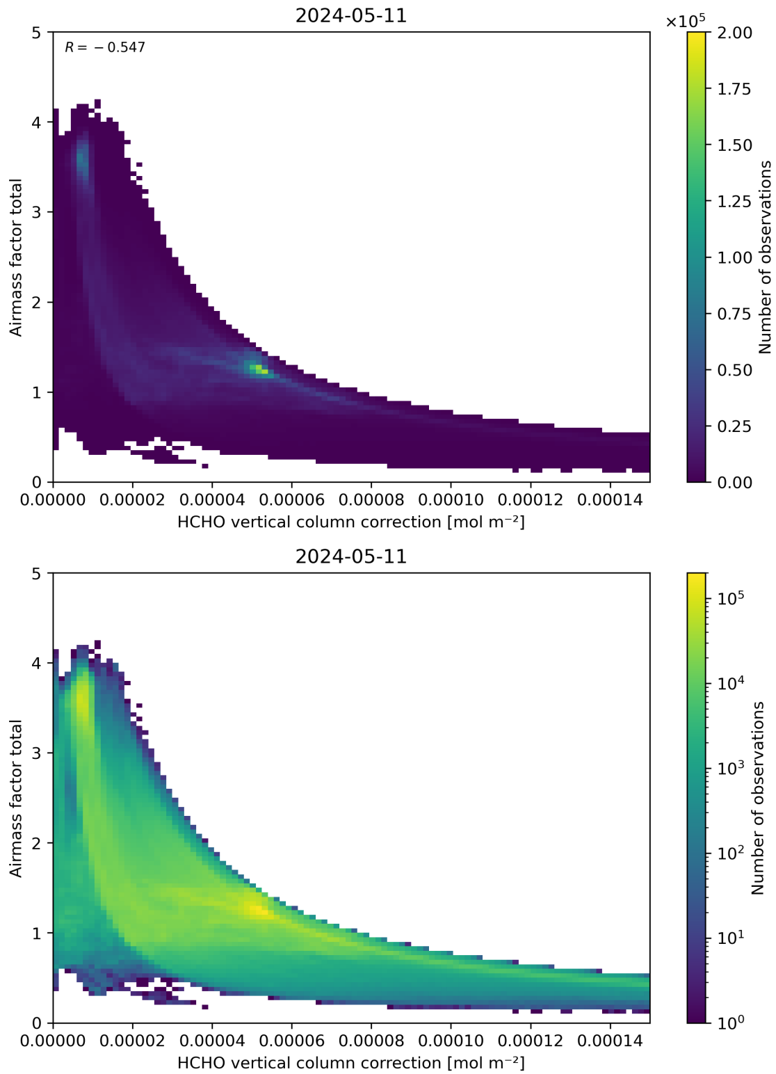
Figure 120: Scatter density plot of “HCHO vertical column correction” against “Airmass factor total” for 2024-05-10 to 2024-05-12.
