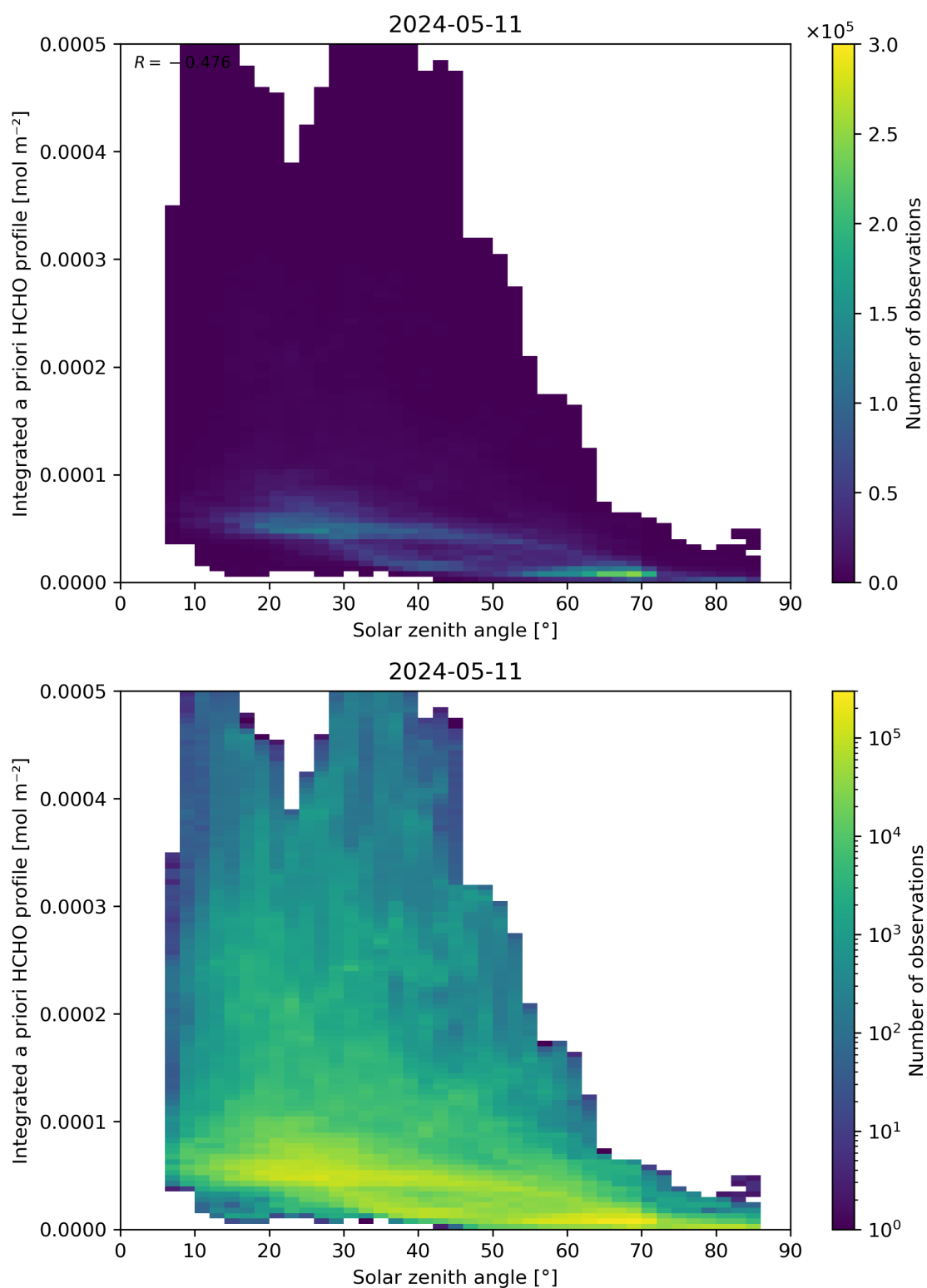
Figure 180: Scatter density plot of “Solar zenith angle” against “Integrated a priori HCHO profile” for 2024-05-10 to 2024-05-12.
