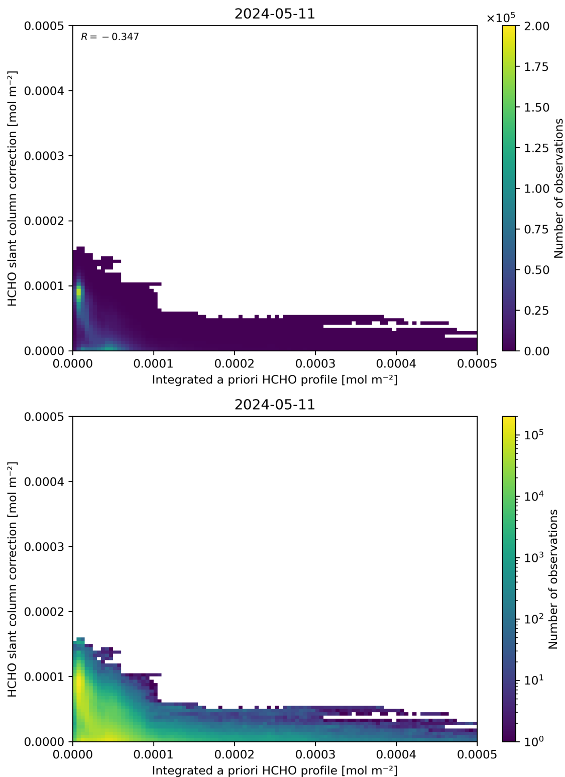
Figure 152: Scatter density plot of “Integrated a priori HCHO profile” against “HCHO slant column correction” for 2024-05-10 to 2024-05-12.
