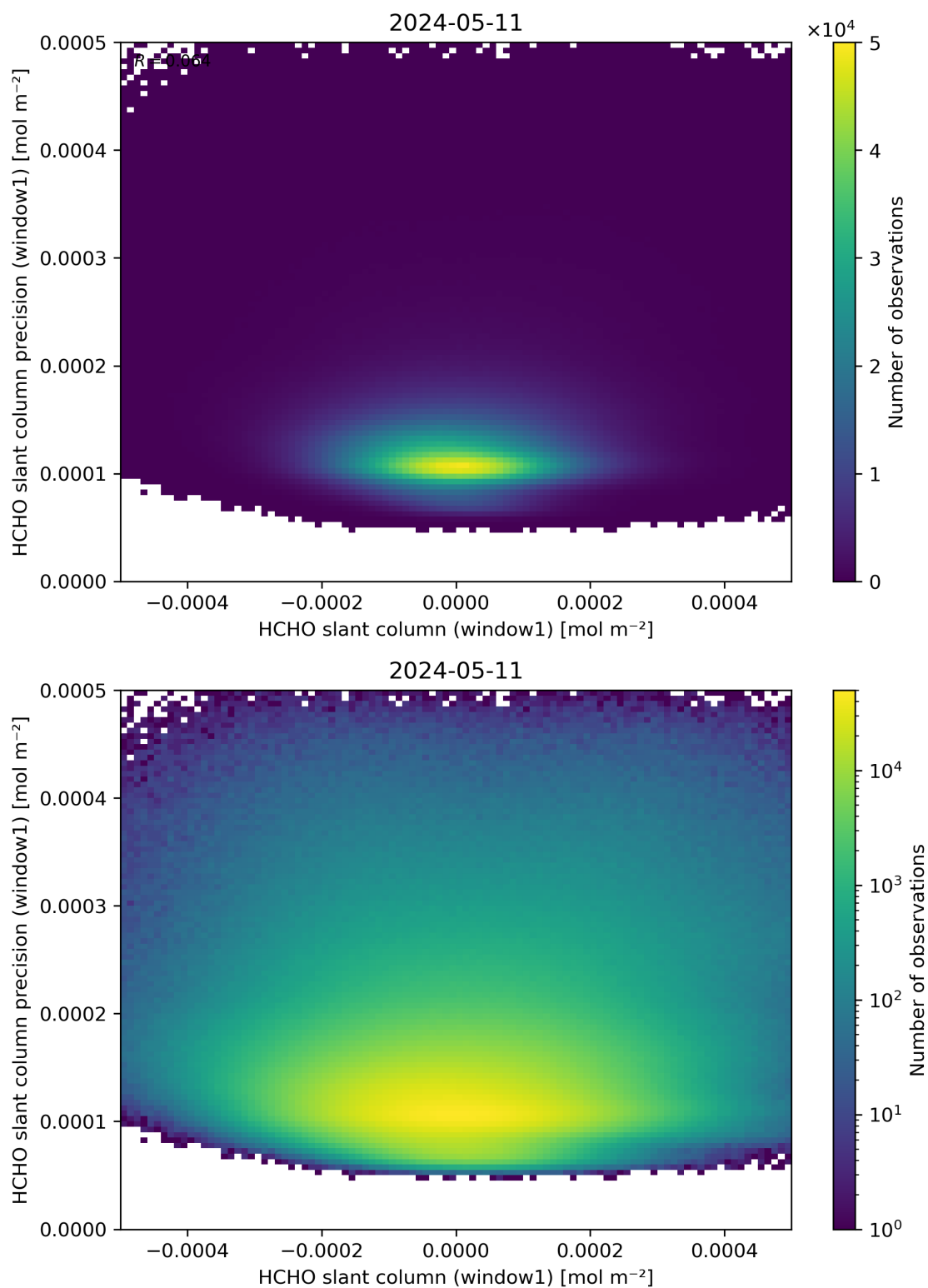
Figure 84: Scatter density plot of “HCHO slant column (window1)” against “HCHO slant column precision (window1)” for 2024-05-10 to 2024-05-12.
