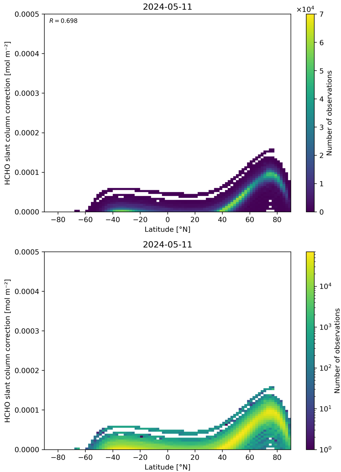
Figure 158: Scatter density plot of “Latitude” against “HCHO slant column correction” for 2024-05-10 to 2024-05-12.
