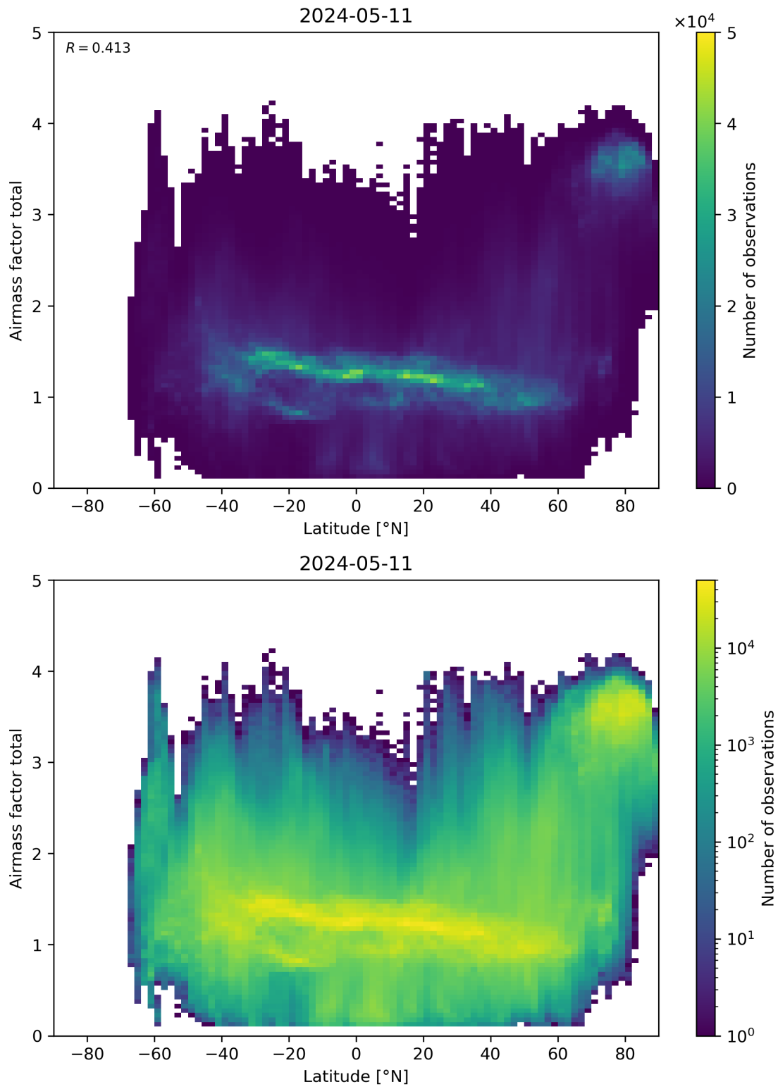
Figure 161: Scatter density plot of “Latitude” against “Airmass factor total” for 2024-05-10 to 2024-05-12.
