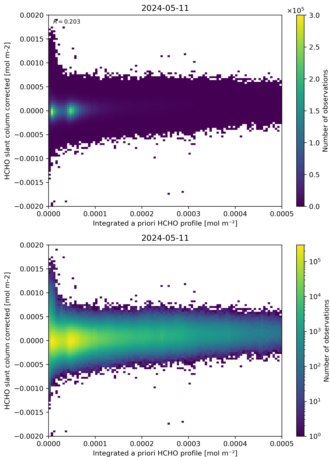
Figure 151: Scatter density plot of “Integrated a priori HCHO profile” against “HCHO slant column corrected” for 2024-05-10 to 2024-05-12.
