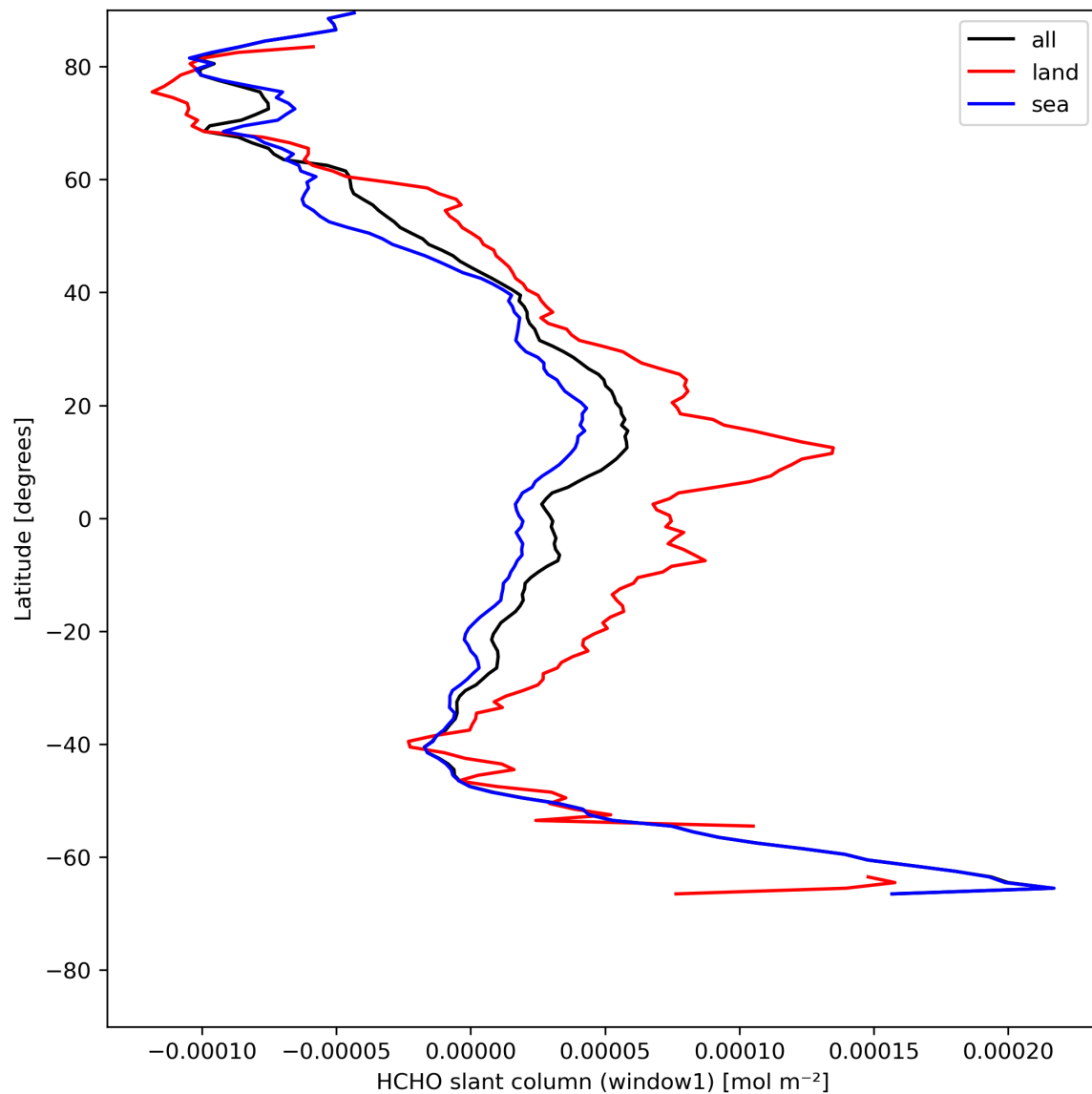
Figure 24: Zonal average of “HCHO slant column (window1)” for 2024-05-10 to 2024-05-12.
