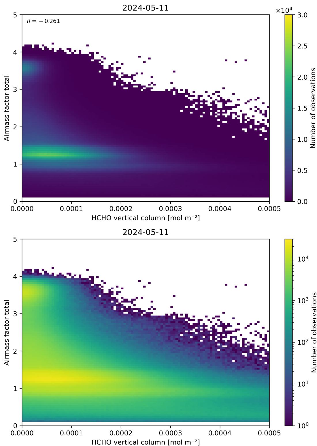
Figure 131: Scatter density plot of “HCHO vertical column” against “Airmass factor total” for 2024-05-10 to 2024-05-12.
