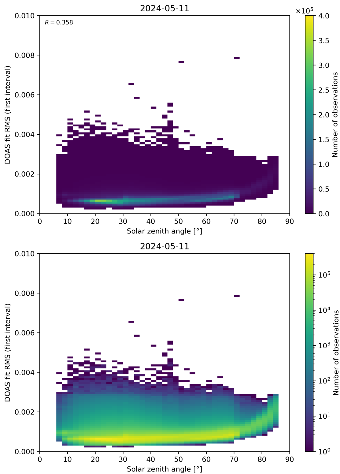
Figure 167: Scatter density plot of “Solar zenith angle” against “DOAS fit RMS (first interval)” for 2024-05-10 to 2024-05-12.
