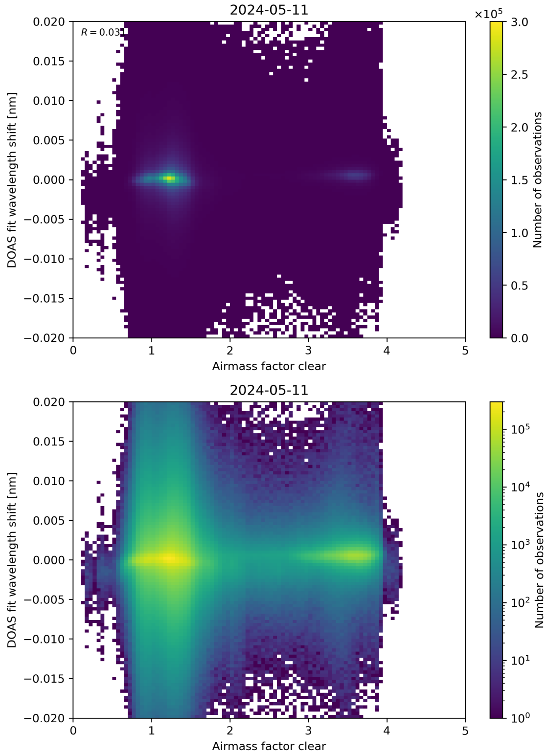
Figure 72: Scatter density plot of “Airmass factor clear” against “DOAS fit wavelength shift” for 2024-05-10 to 2024-05-12.
