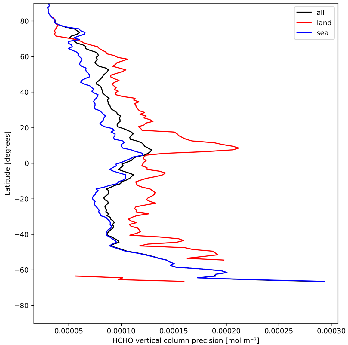
Figure 22: Zonal average of “HCHO vertical column precision” for 2024-05-10 to 2024-05-12.
