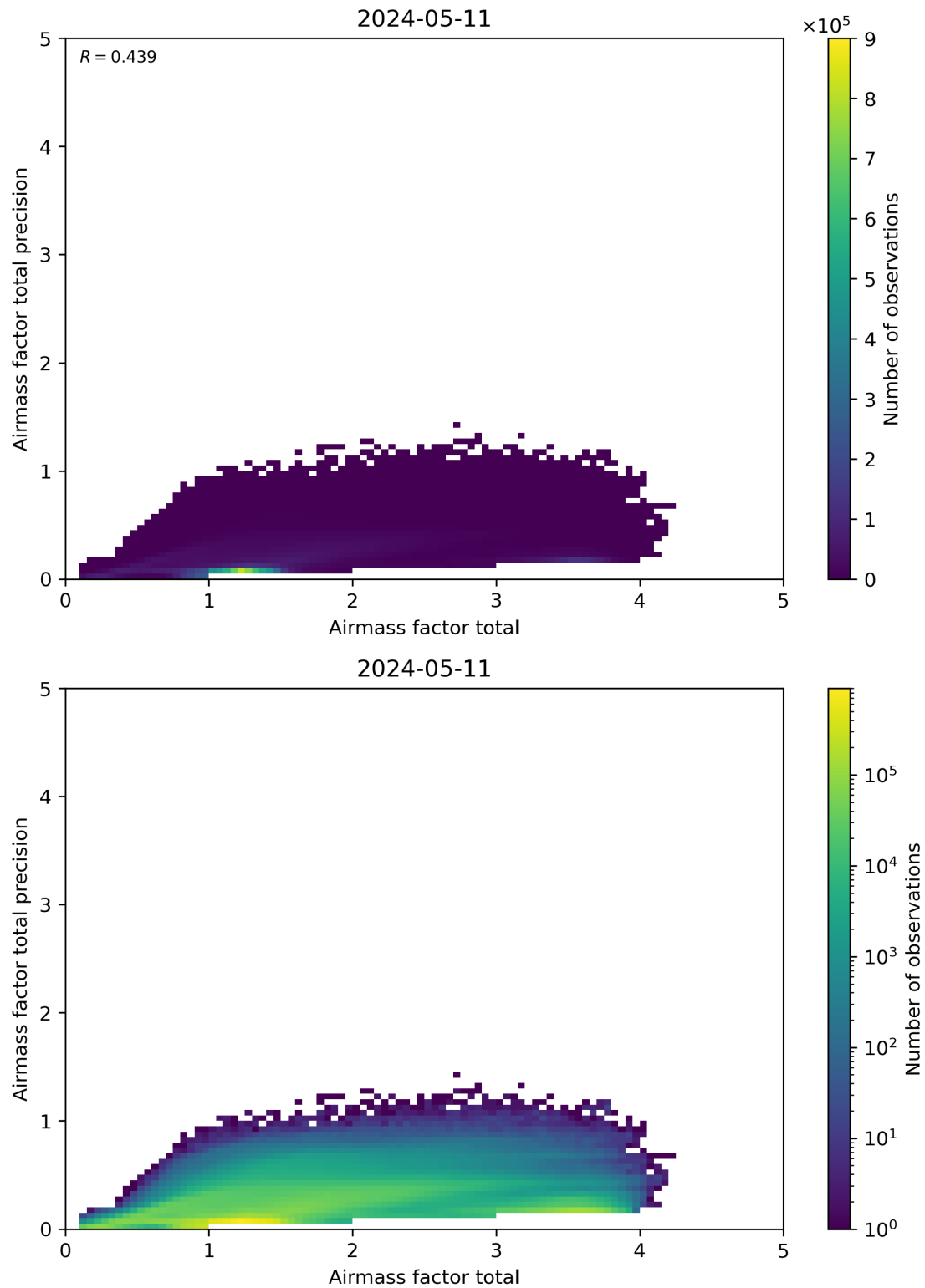
Figure 103: Scatter density plot of “Airmass factor total” against “Airmass factor total precision” for 2024-05-10 to 2024-05-12.
