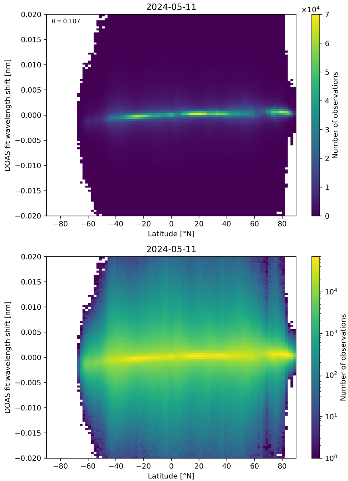
Figure 154: Scatter density plot of “Latitude” against “DOAS fit wavelength shift” for 2024-05-10 to 2024-05-12.
