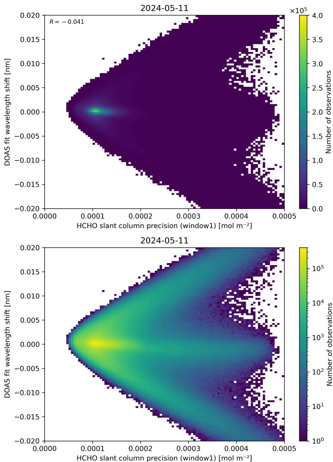
Figure 89: Scatter density plot of “HCHO slant column precision (window1)” against “DOAS fit wavelength shift” for 2024-05-10 to 2024-05-12.
