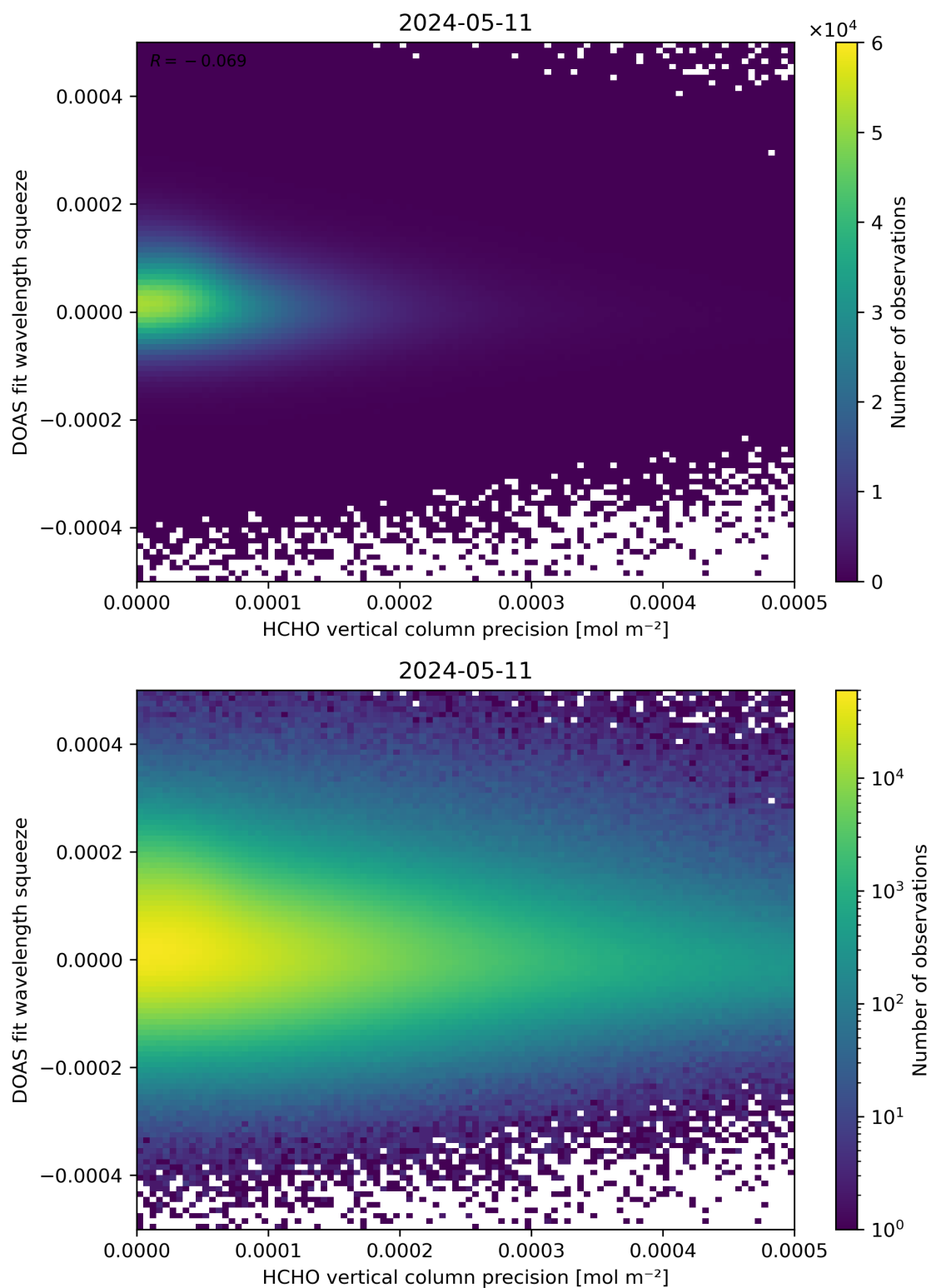
Figure 138: Scatter density plot of “HCHO vertical column precision” against “DOAS fit wavelength squeeze” for 2024-05-10 to 2024-05-12.
