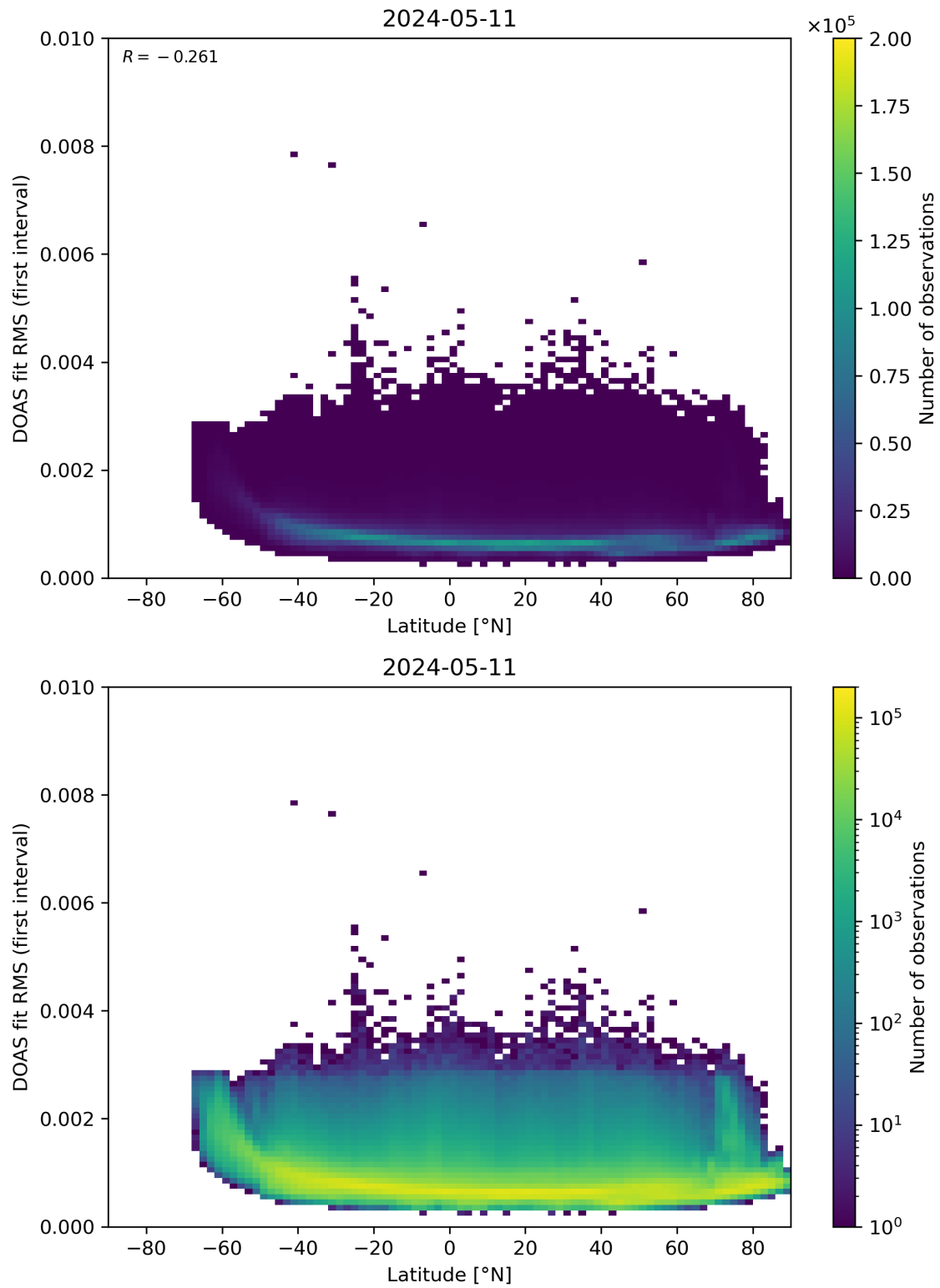
Figure 153: Scatter density plot of “Latitude” against “DOAS fit RMS (first interval)” for 2024-05-10 to 2024-05-12.
