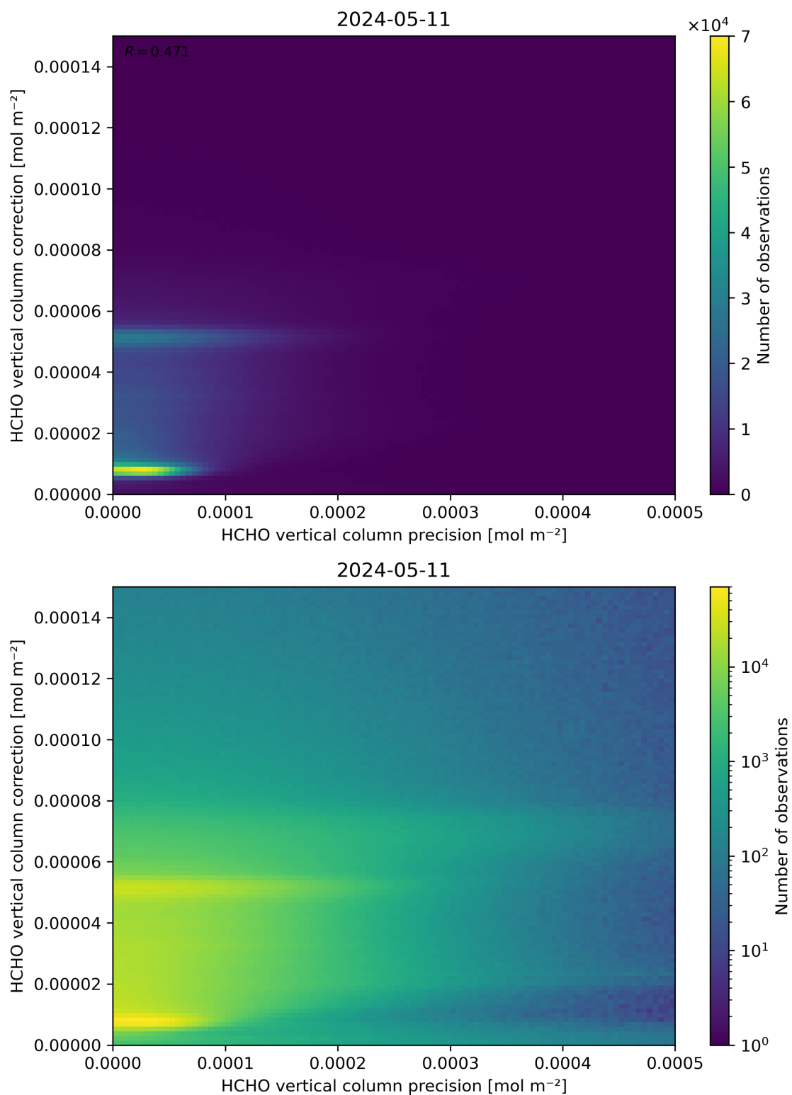
Figure 146: Scatter density plot of “HCHO vertical column precision” against “HCHO vertical column correction” for 2024-05-10 to 2024-05-12.
