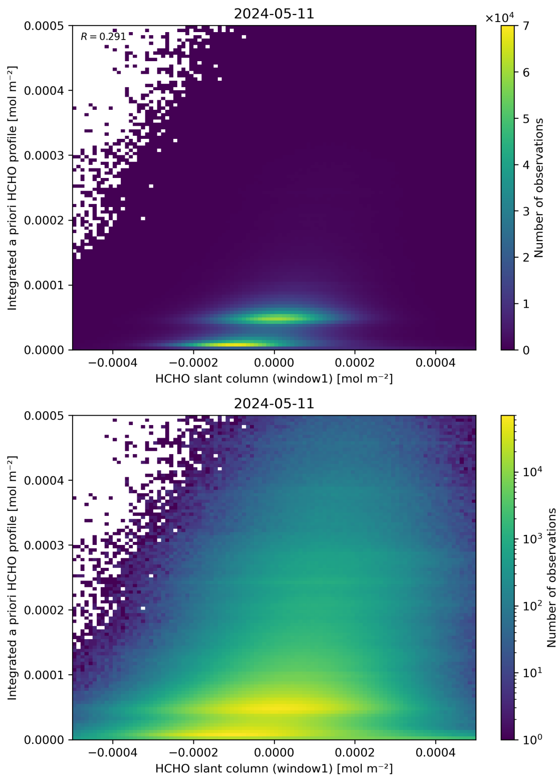
Figure 87: Scatter density plot of “HCHO slant column (window1)” against “Integrated a priori HCHO profile” for 2024-05-10 to 2024-05-12.
