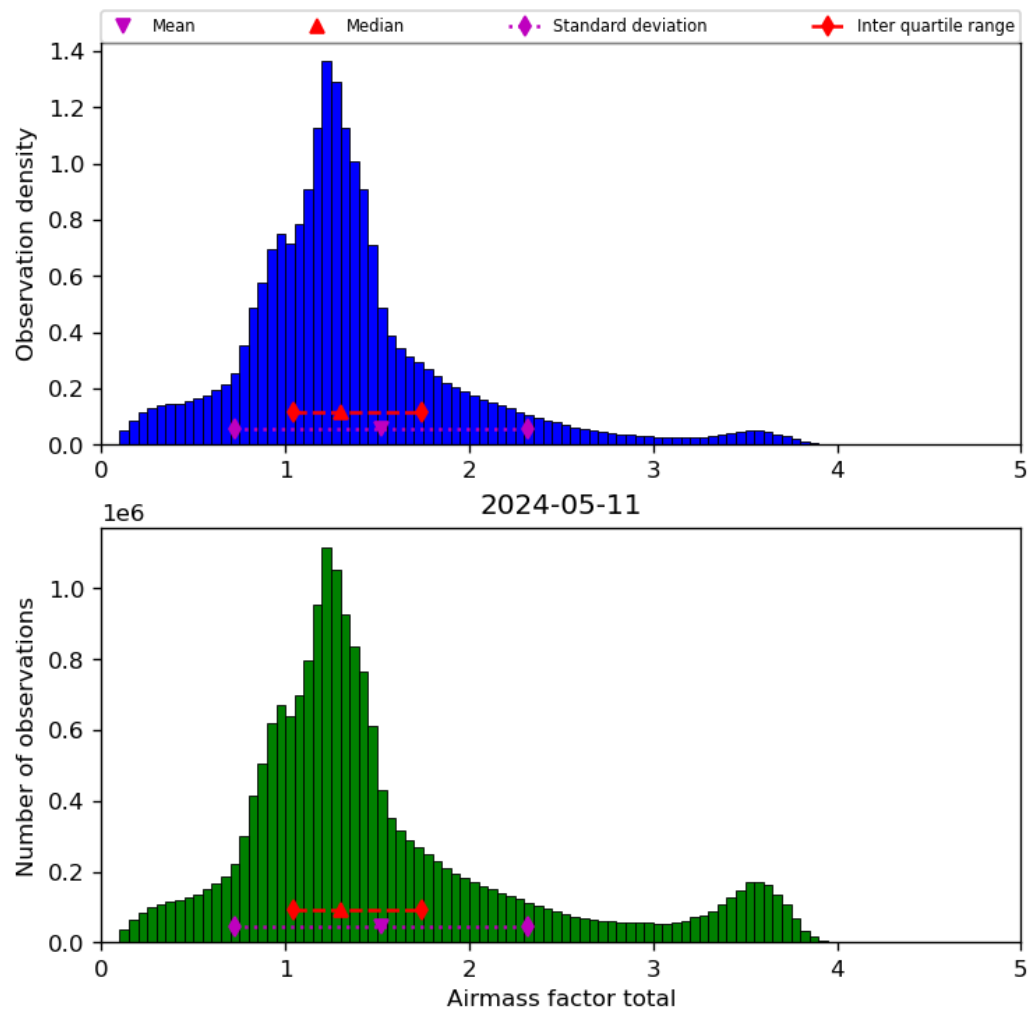
Figure 40: Histogram of “Airmass factor total” for 2024-05-10 to 2024-05-12
