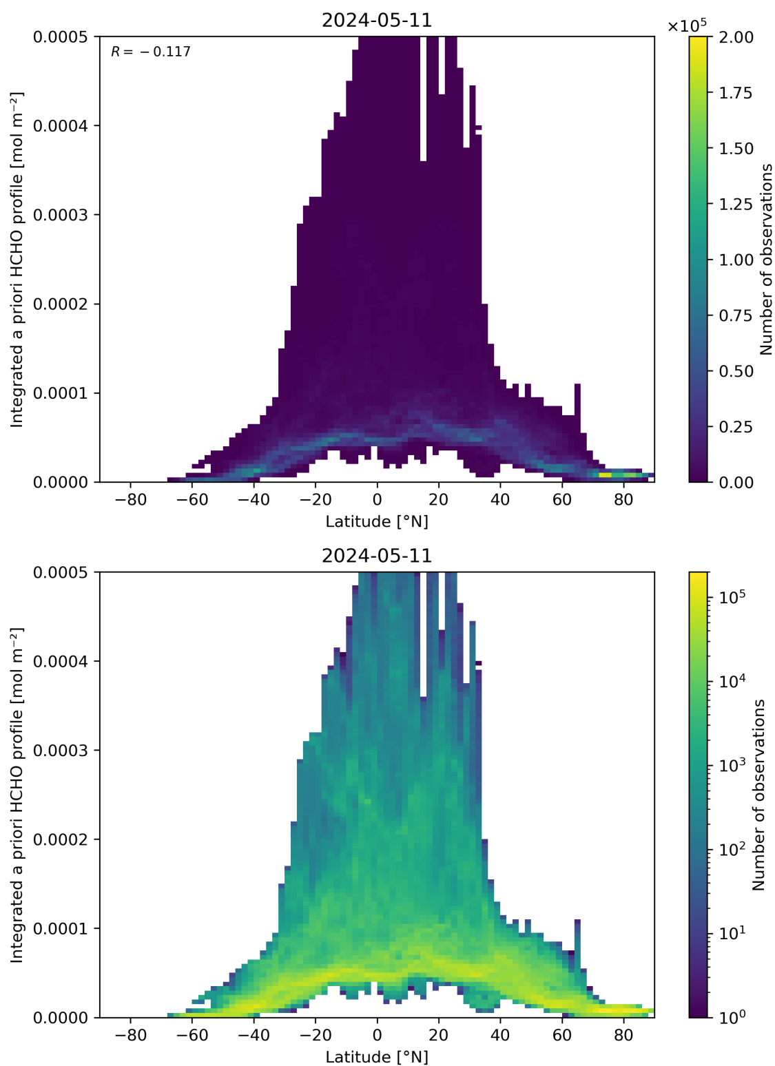
Figure 166: Scatter density plot of “Latitude” against “Integrated a priori HCHO profile” for 2024-05-10 to 2024-05-12.
