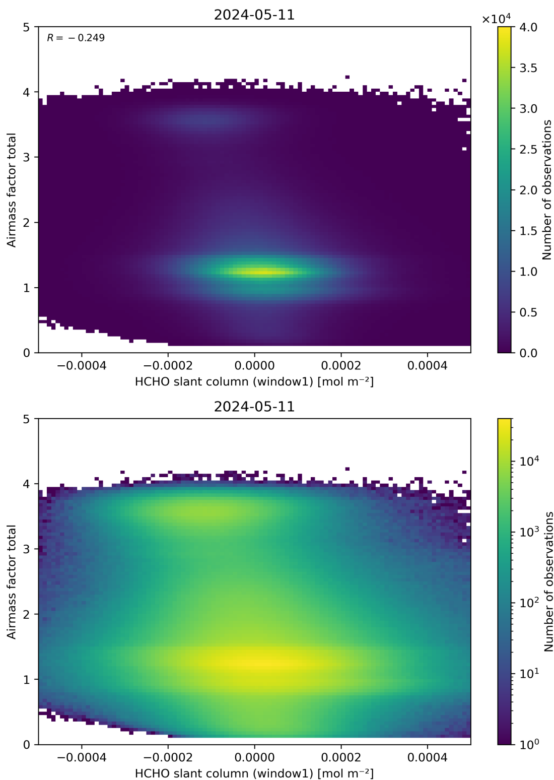
Figure 85: Scatter density plot of “HCHO slant column (window1)” against “Airmass factor total” for 2024-05-10 to 2024-05-12.
