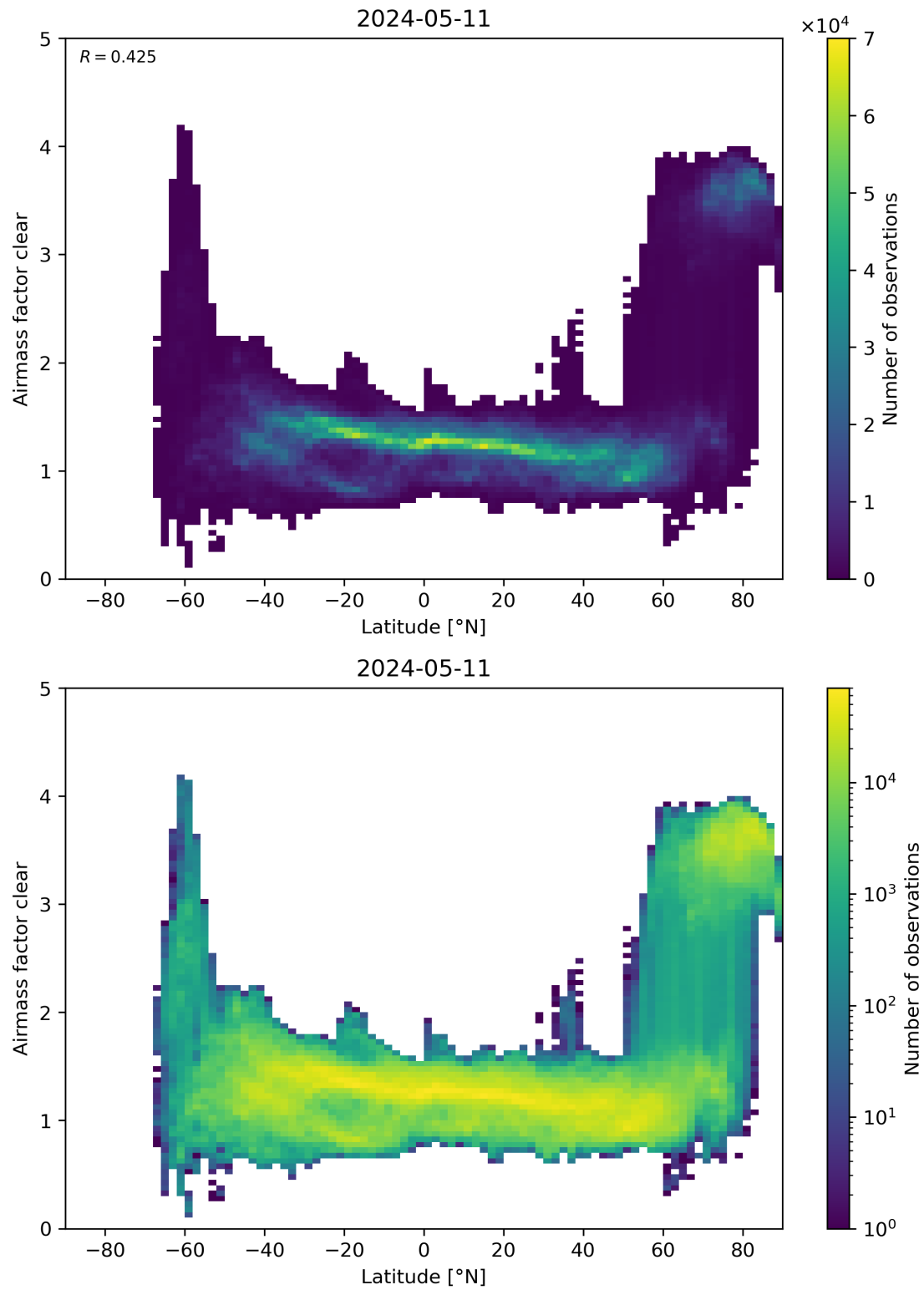
Figure 156: Scatter density plot of “Latitude” against “Airmass factor clear” for 2024-05-10 to 2024-05-12.
