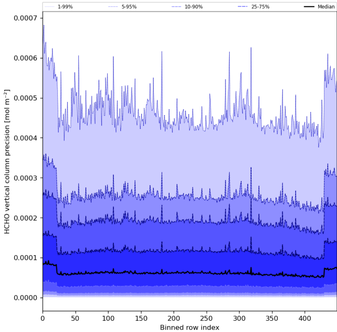
Figure 50: Along track statistics of “HCHO vertical column precision” for 2024-05-10 to 2024-05-12
