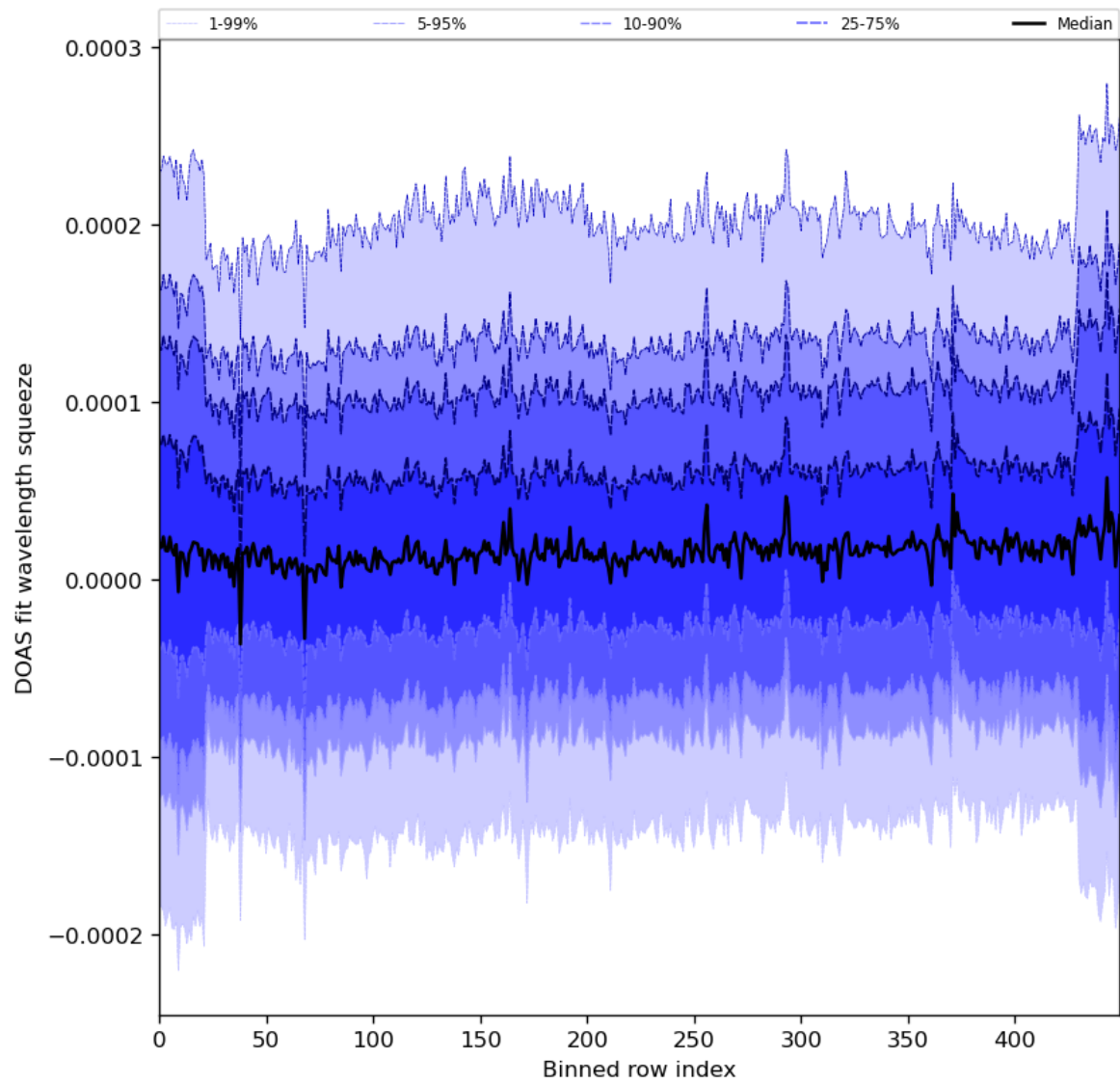
Figure 59: Along track statistics of “DOAS fit wavelength squeeze” for 2024-05-10 to 2024-05-12
