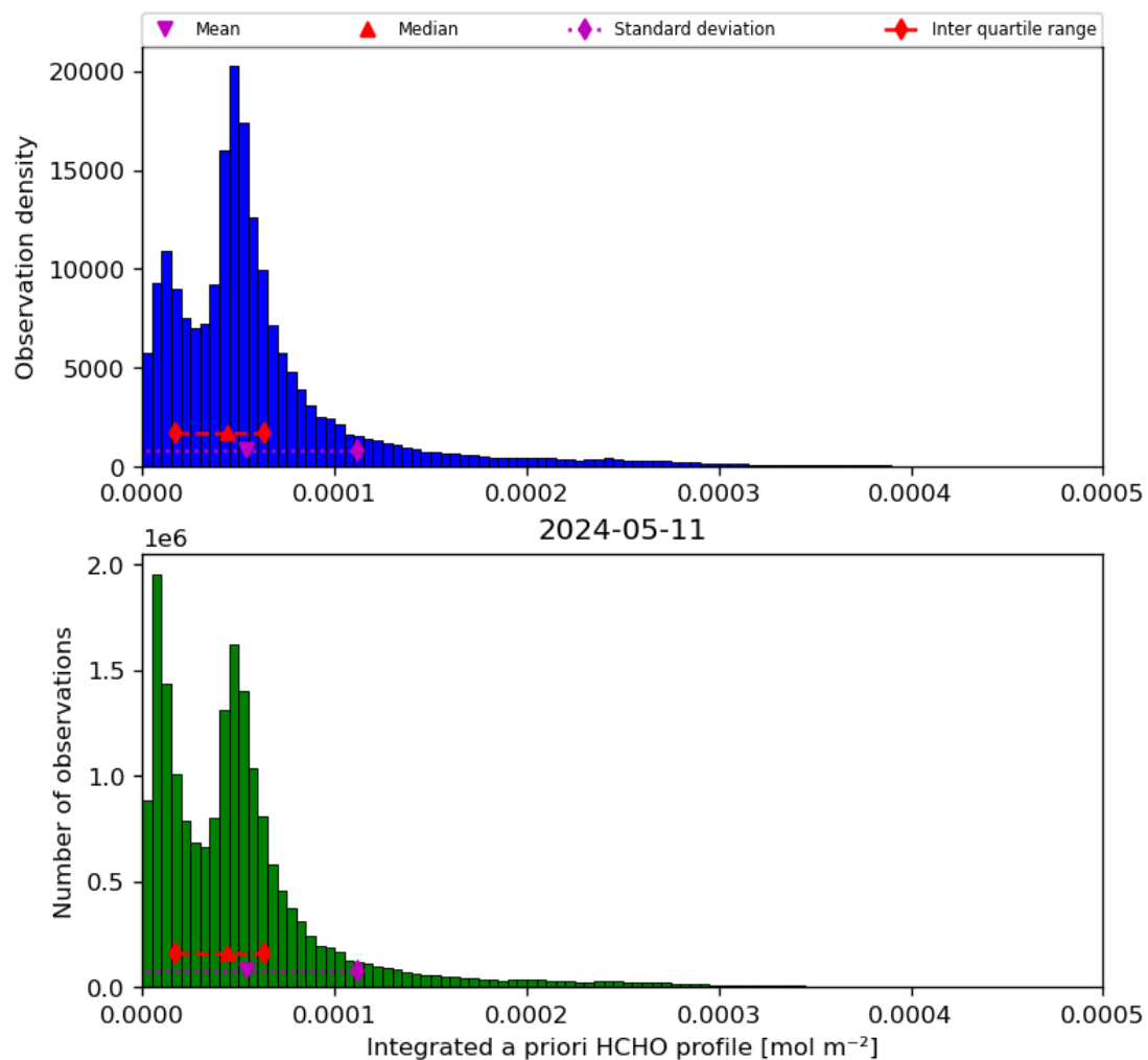
Figure 43: Histogram of “Integrated a priori HCHO profile” for 2024-05-10 to 2024-05-12
