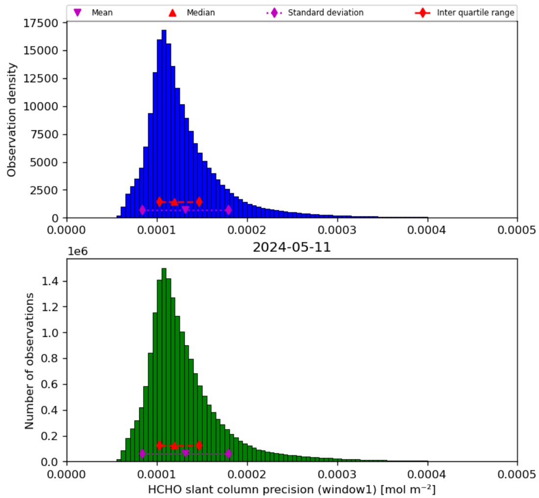
Figure 39: Histogram of “HCHO slant column precision (window1)” for 2024-05-10 to 2024-05-12
