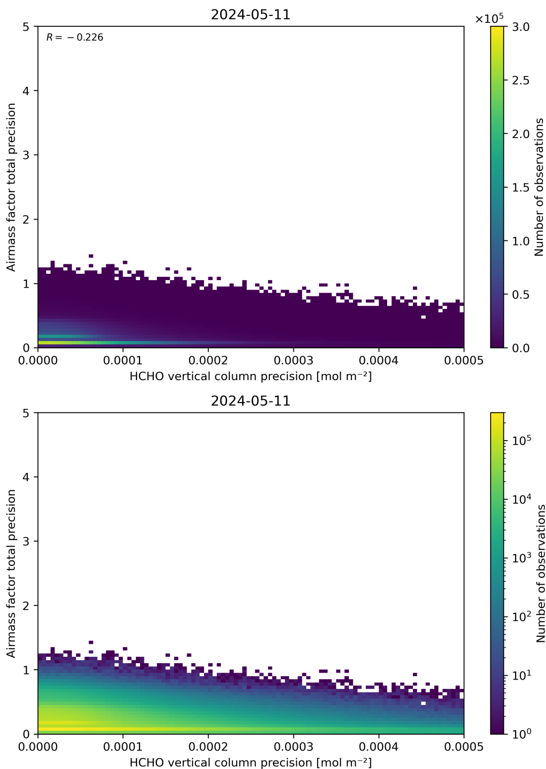
Figure 145: Scatter density plot of “HCHO vertical column precision” against “Airmass factor total precision” for 2024-05-10 to 2024-05-12.
