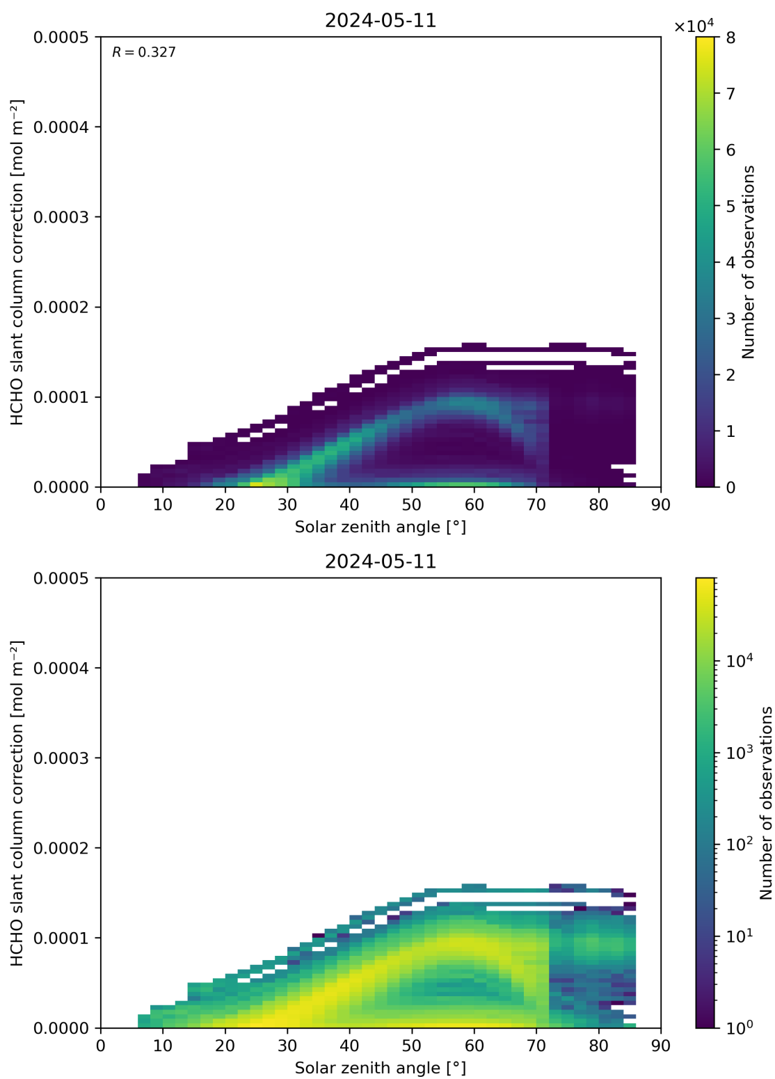
Figure 172: Scatter density plot of “Solar zenith angle” against “HCHO slant column correction” for 2024-05-10 to 2024-05-12.
