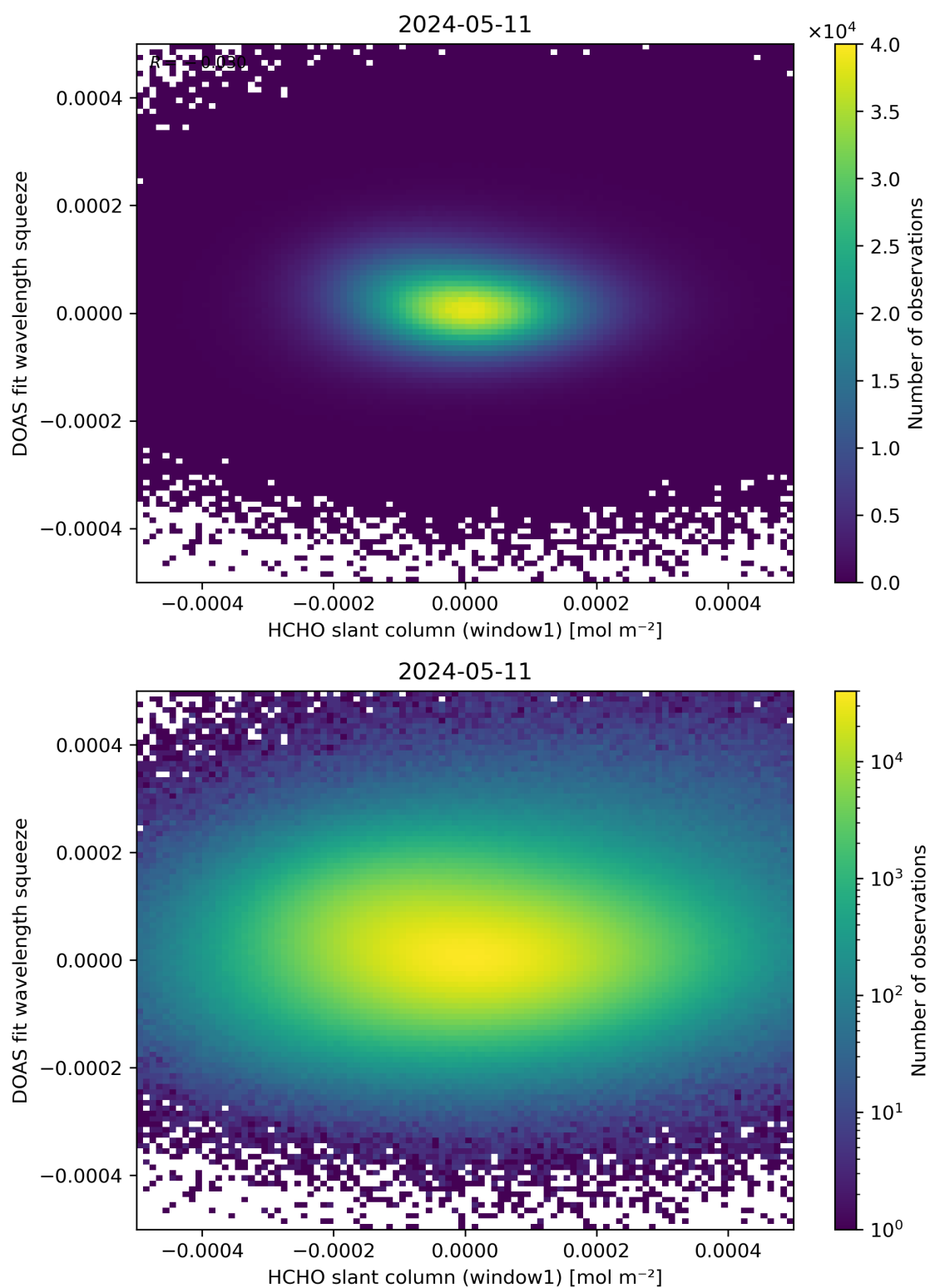
Figure 80: Scatter density plot of “HCHO slant column (window1)” against “DOAS fit wavelength squeeze” for 2024-05-10 to 2024-05-12.
