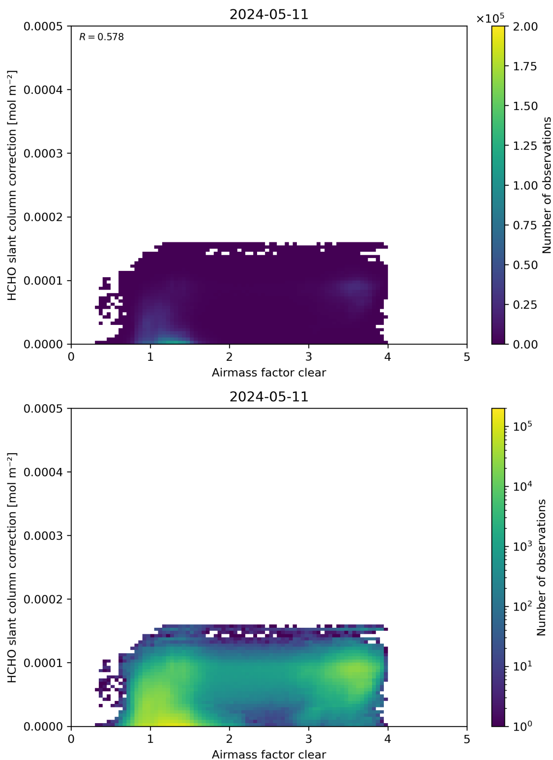
Figure 75: Scatter density plot of “Airmass factor clear” against “HCHO slant column correction” for 2024-05-10 to 2024-05-12.
