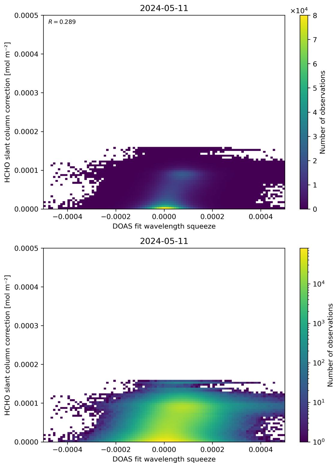
Figure 70: Scatter density plot of “DOAS fit wavelength squeeze” against “HCHO slant column correction” for 2024-05-10 to 2024-05-12.
