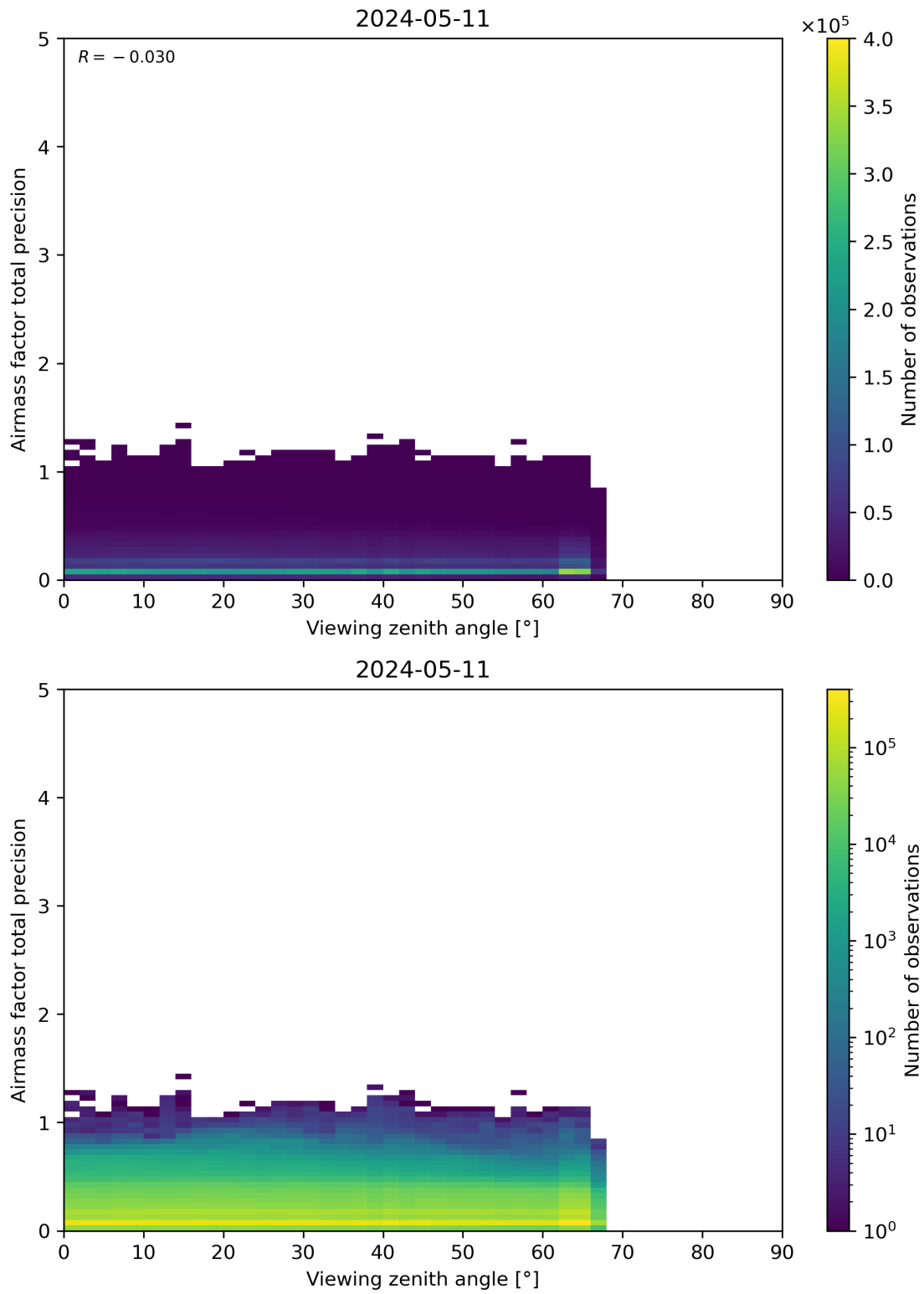
Figure 191: Scatter density plot of “Viewing zenith angle” against “Airmass factor total precision” for 2024-05-10 to 2024-05-12.
