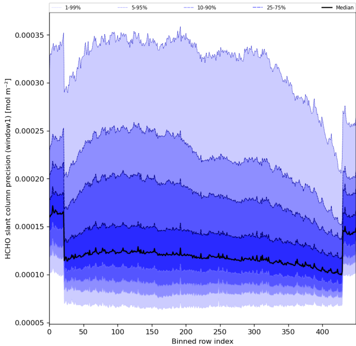
Figure 53: Along track statistics of “HCHO slant column precision (window1)” for 2024-05-10 to 2024-05-12
