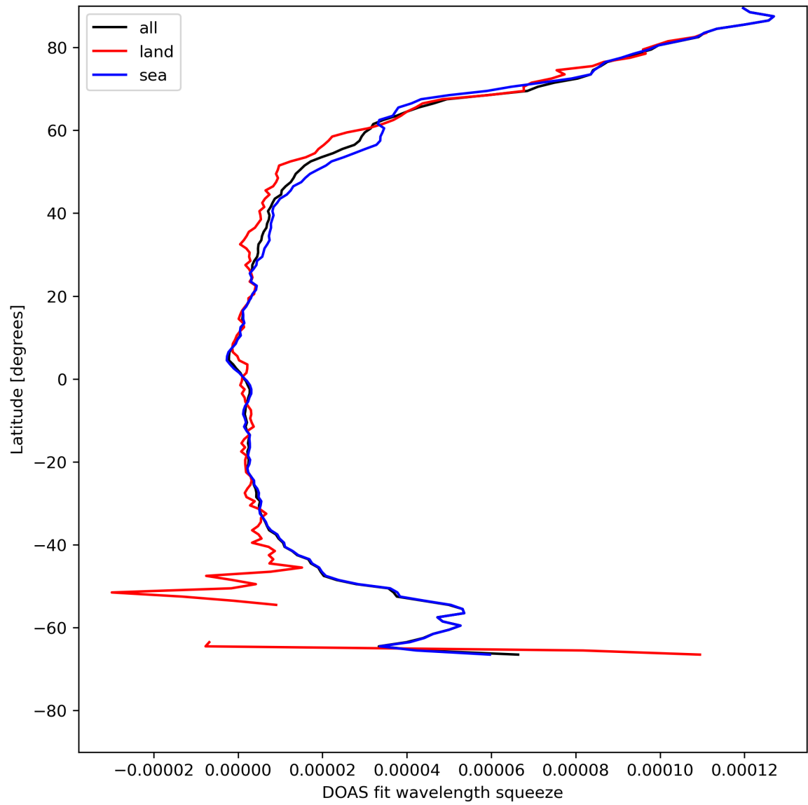
Figure 31: Zonal average of “DOAS fit wavelength squeeze” for 2024-05-10 to 2024-05-12.
