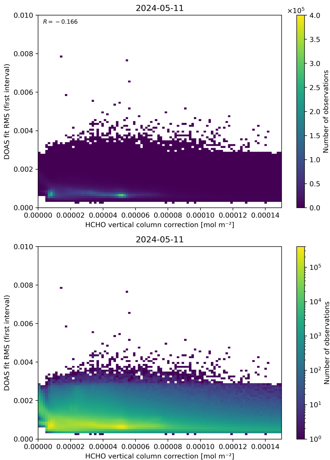
Figure 112: Scatter density plot of “HCHO vertical column correction” against “DOAS fit RMS (first interval)” for 2024-05-10 to 2024-05-12.
