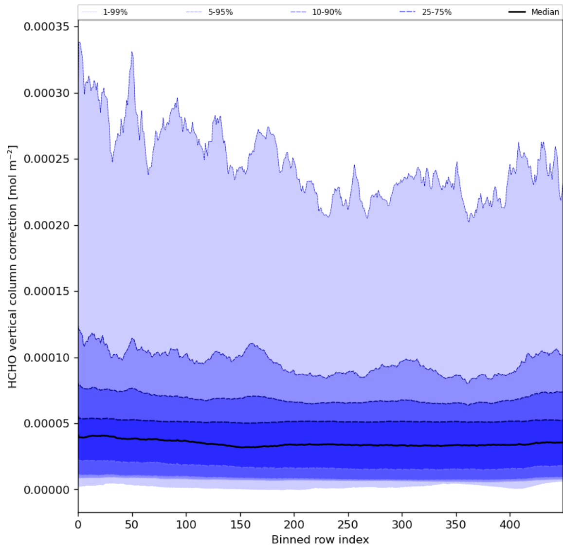
Figure 51: Along track statistics of “HCHO vertical column correction” for 2024-05-10 to 2024-05-12
