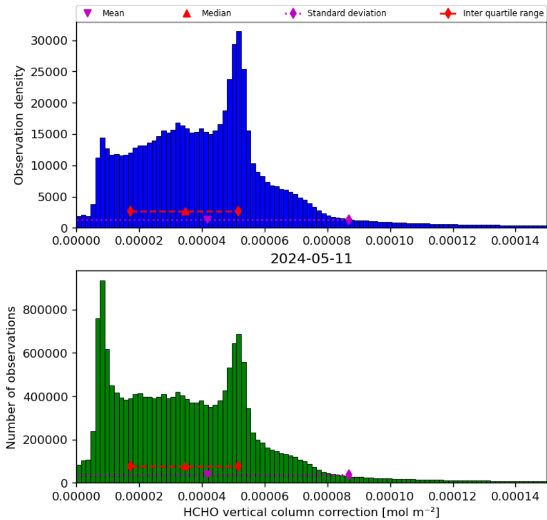
Figure 37: Histogram of “HCHO vertical column correction” for 2024-05-10 to 2024-05-12
