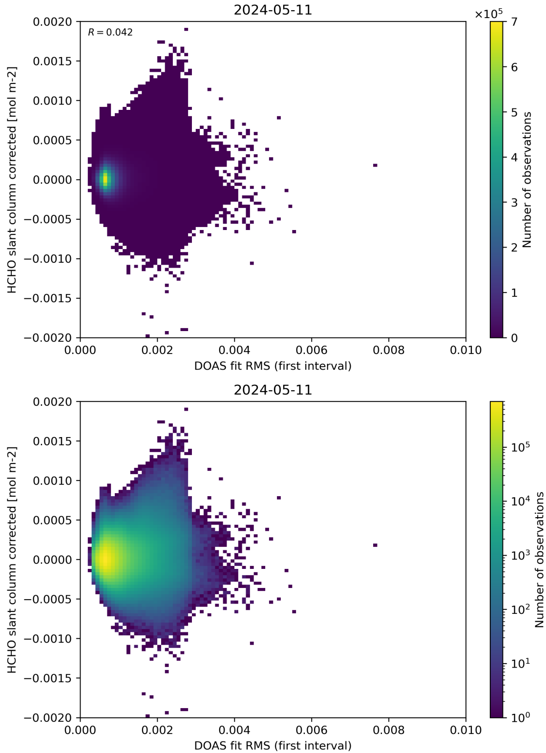
Figure 62: Scatter density plot of “DOAS fit RMS (first interval)” against “HCHO slant column corrected” for 2024-05-10 to 2024-05-12.
