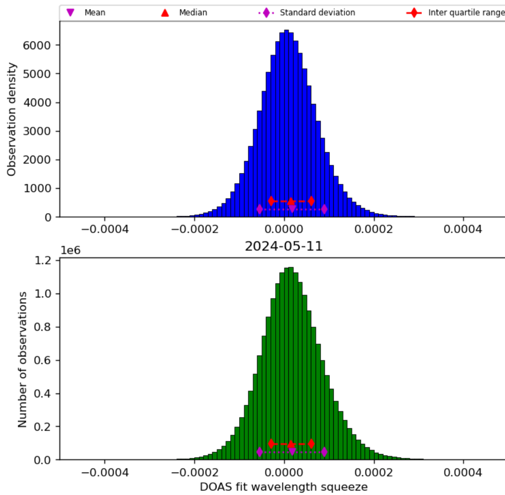
Figure 45: Histogram of “DOAS fit wavelength squeeze” for 2024-05-10 to 2024-05-12
