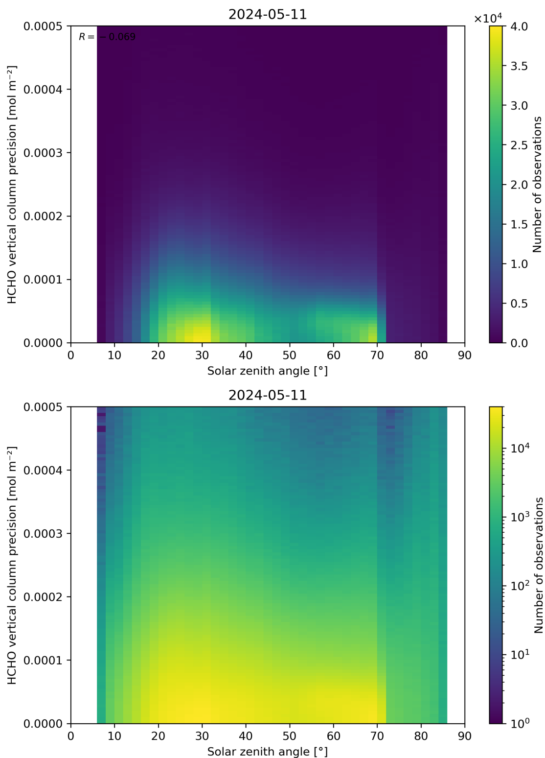
Figure 179: Scatter density plot of “Solar zenith angle” against “HCHO vertical column precision” for 2024-05-10 to 2024-05-12.
