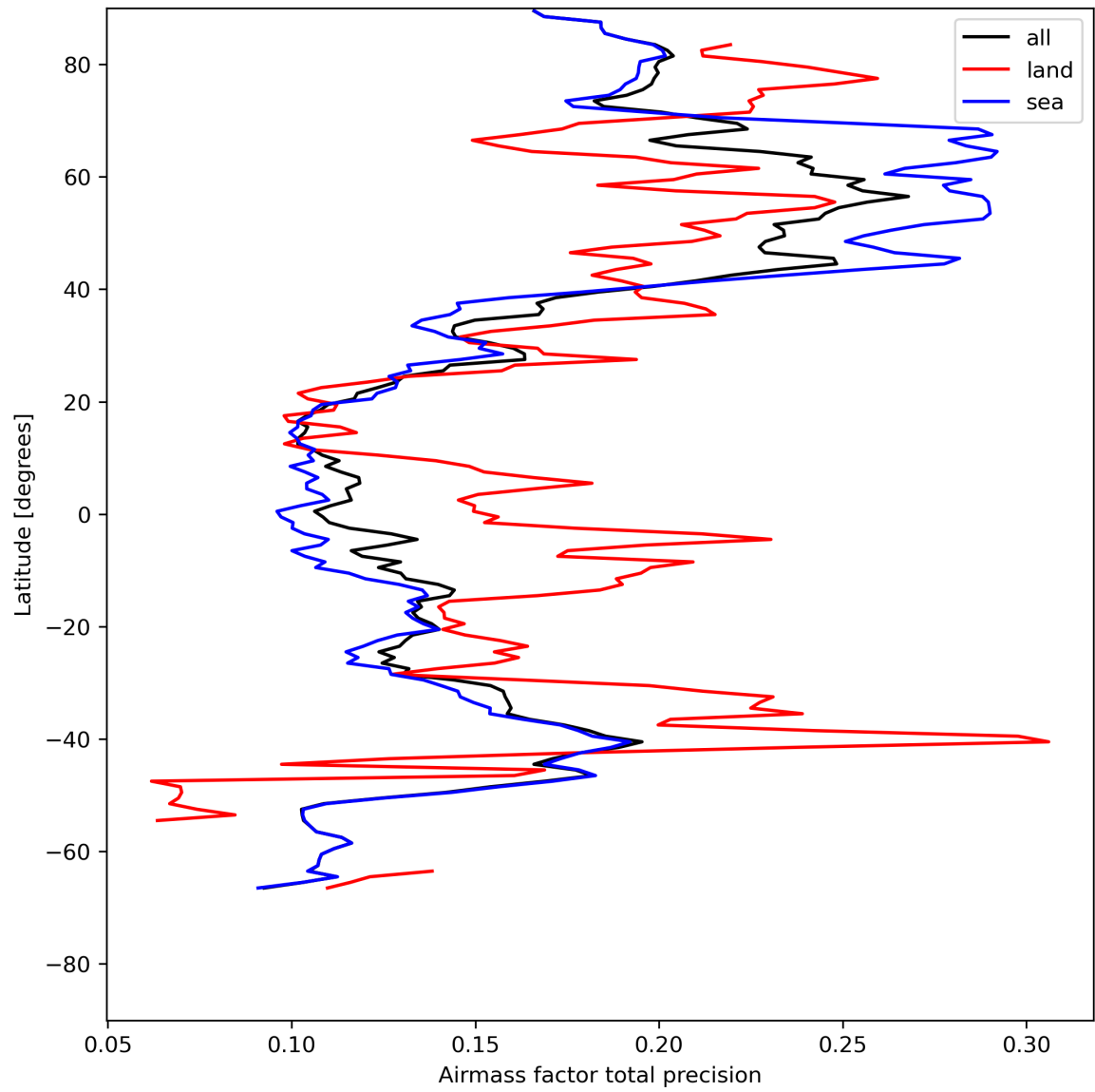
Figure 27: Zonal average of “Airmass factor total precision” for 2024-05-10 to 2024-05-12.
