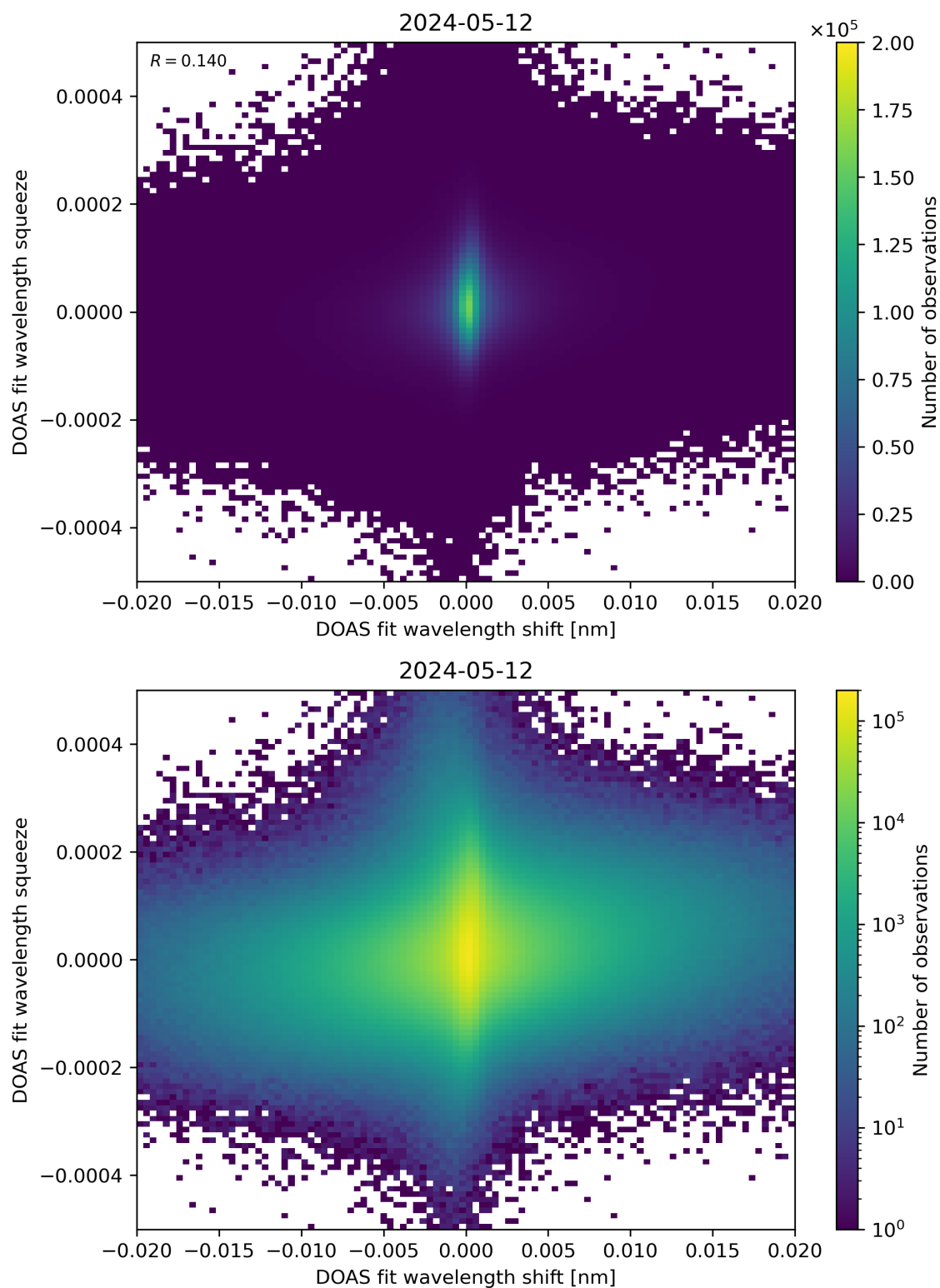
Figure 65: Scatter density plot of “DOAS fit wavelength shift” against “DOAS fit wavelength squeeze” for 2024-05-12 to 2024-05-13.
