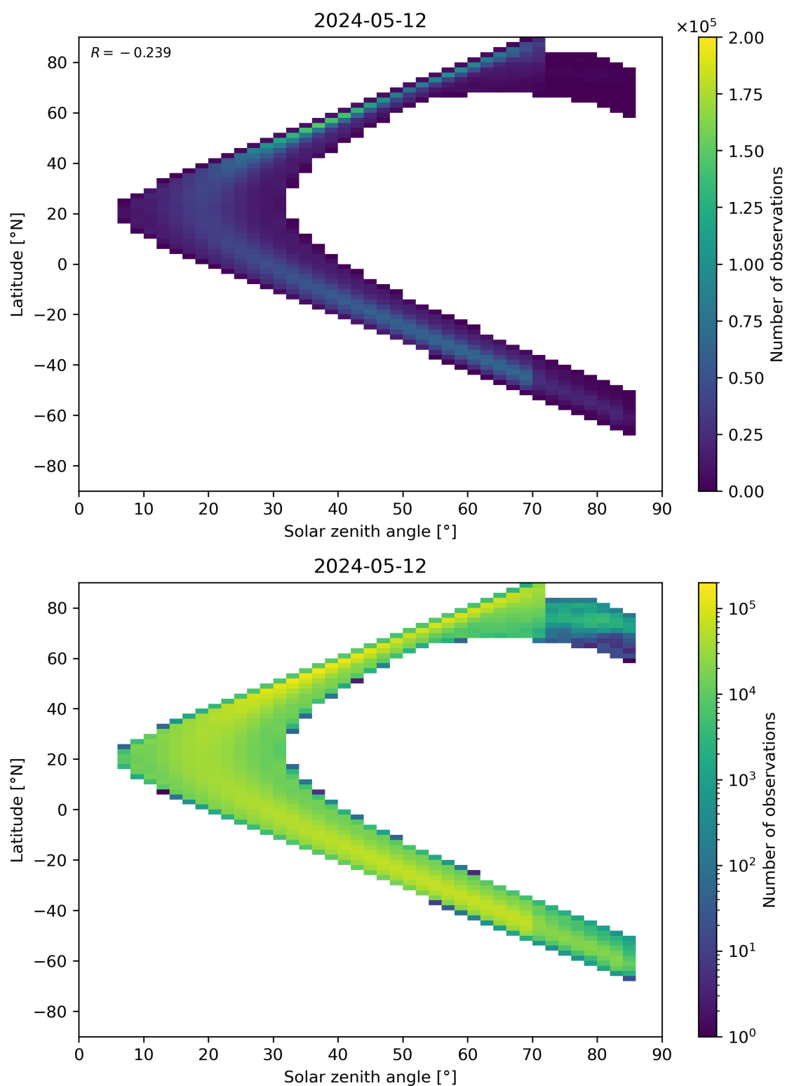
Figure 181: Scatter density plot of “Solar zenith angle” against “Latitude” for 2024-05-12 to 2024-05-13.
