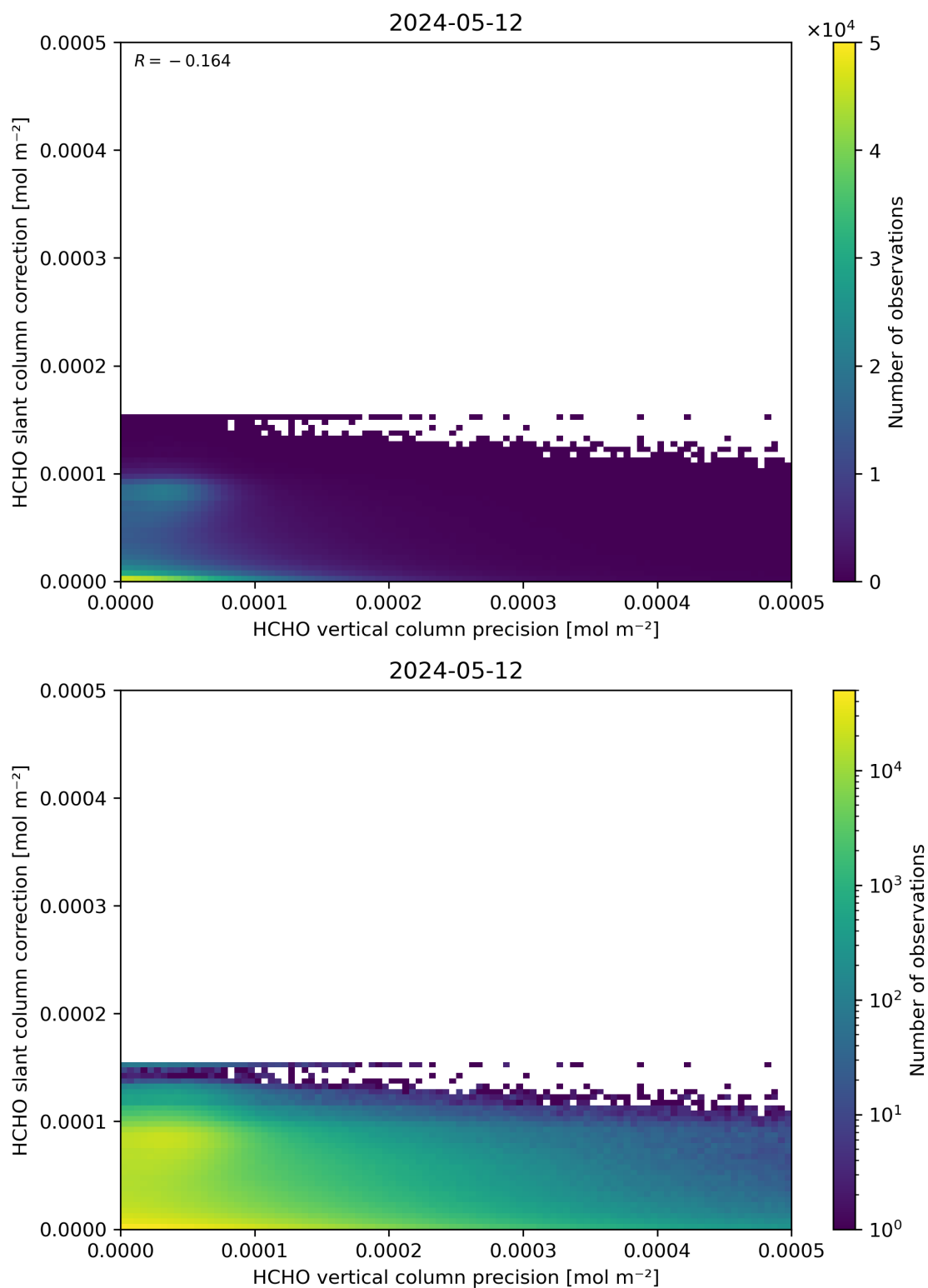
Figure 141: Scatter density plot of “HCHO vertical column precision” against “HCHO slant column correction” for 2024-05-12 to 2024-05-13.
