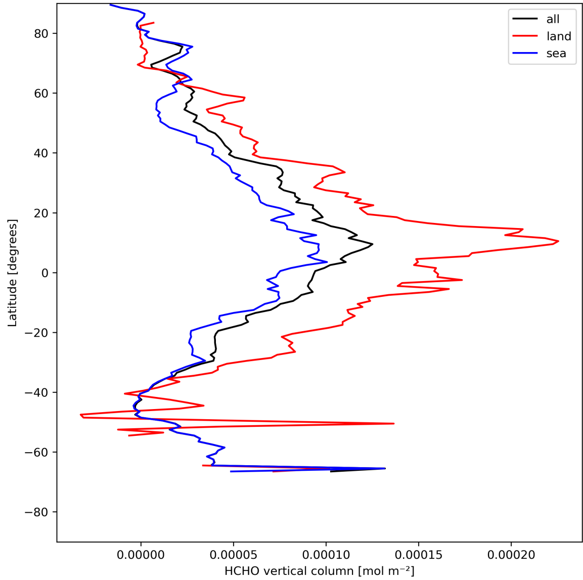
Figure 21: Zonal average of “HCHO vertical column” for 2024-05-12 to 2024-05-13.
