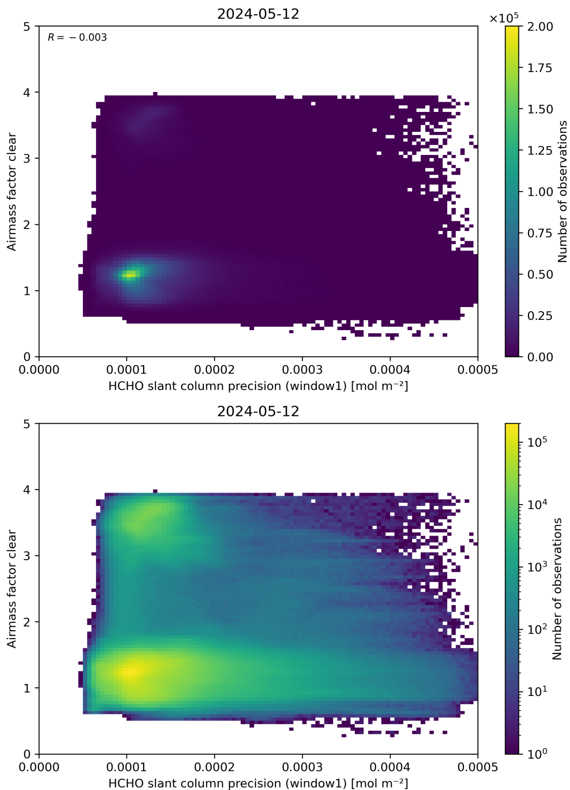
Figure 91: Scatter density plot of “HCHO slant column precision (window1)” against “Airmass factor clear” for 2024-05-12 to 2024-05-13.
