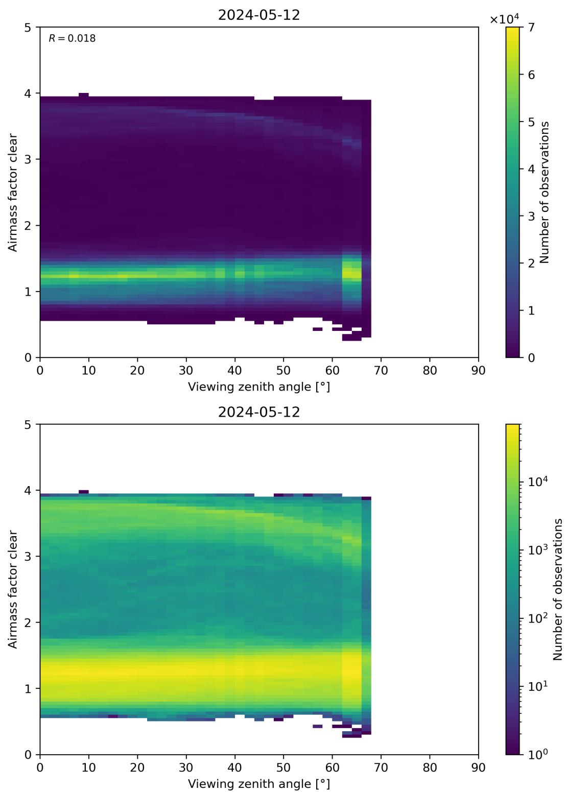
Figure 185: Scatter density plot of “Viewing zenith angle” against “Airmass factor clear” for 2024-05-12 to 2024-05-13.
