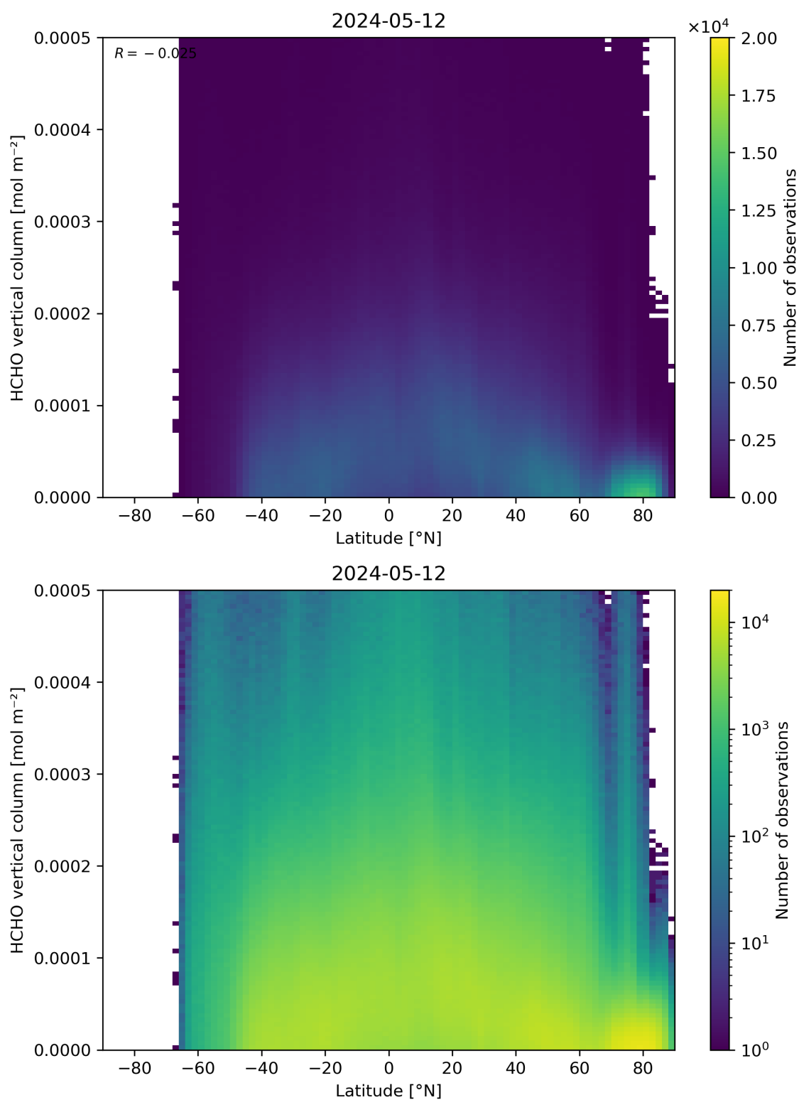
Figure 163: Scatter density plot of “Latitude” against “HCHO vertical column” for 2024-05-12 to 2024-05-13.
