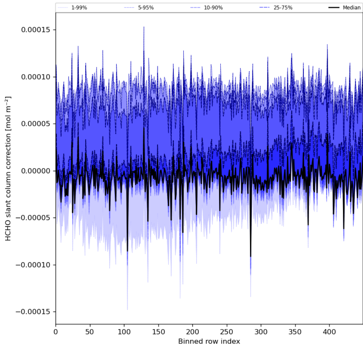
Figure 61: Along track statistics of “HCHO slant column correction” for 2024-05-12 to 2024-05-13
