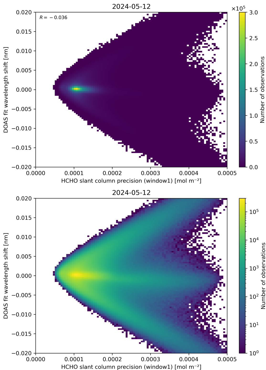
Figure 89: Scatter density plot of “HCHO slant column precision (window1)” against “DOAS fit wavelength shift” for 2024-05-12 to 2024-05-13.
