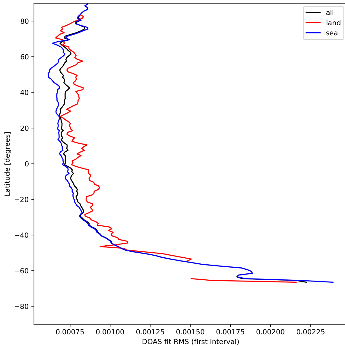
Figure 32: Zonal average of "DOAS fit RMS (first interval)" for 2024-05-12 to 2024-05-13.
