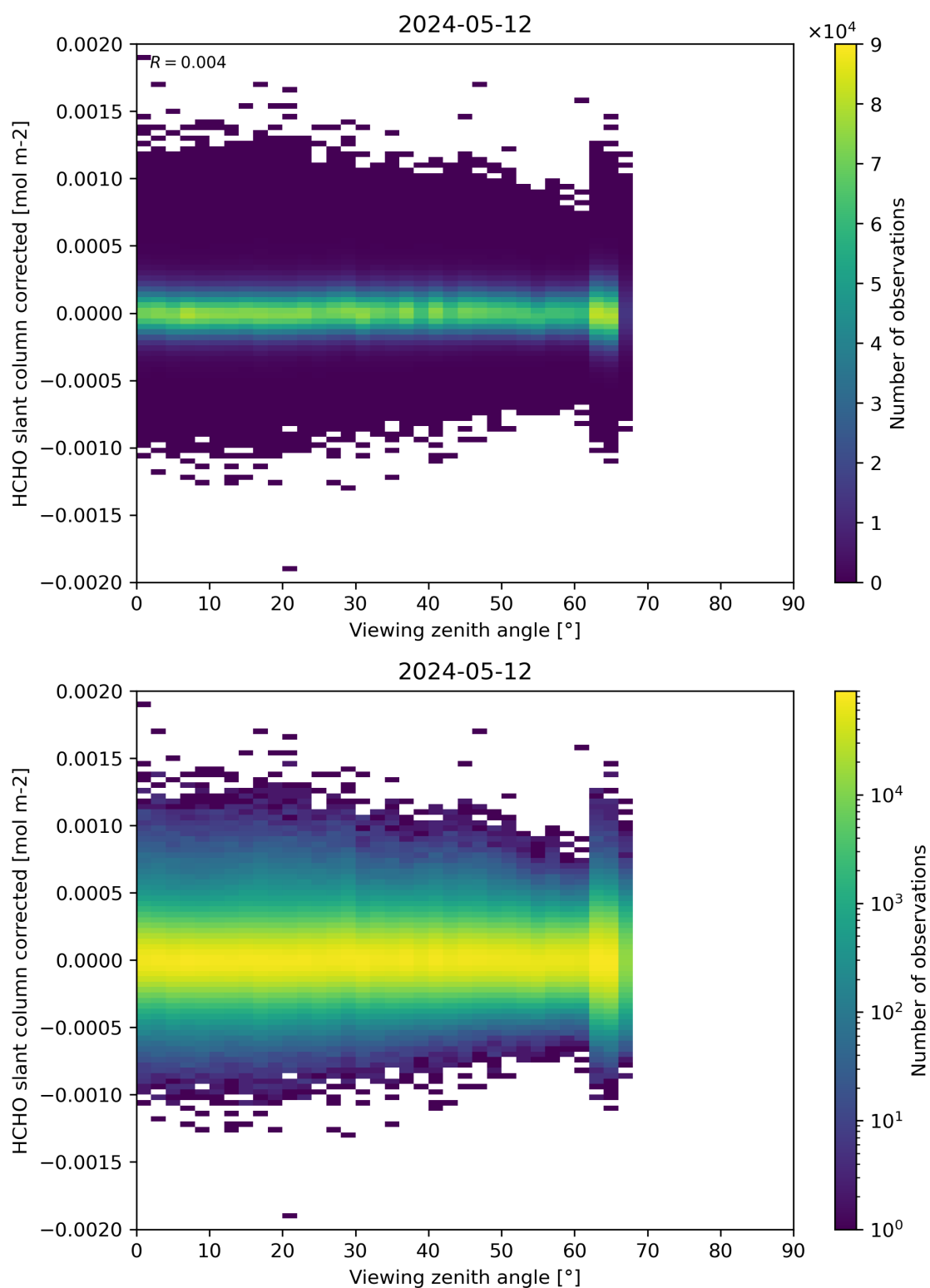
Figure 186: Scatter density plot of “Viewing zenith angle” against “HCHO slant column corrected” for 2024-05-12 to 2024-05-13.
