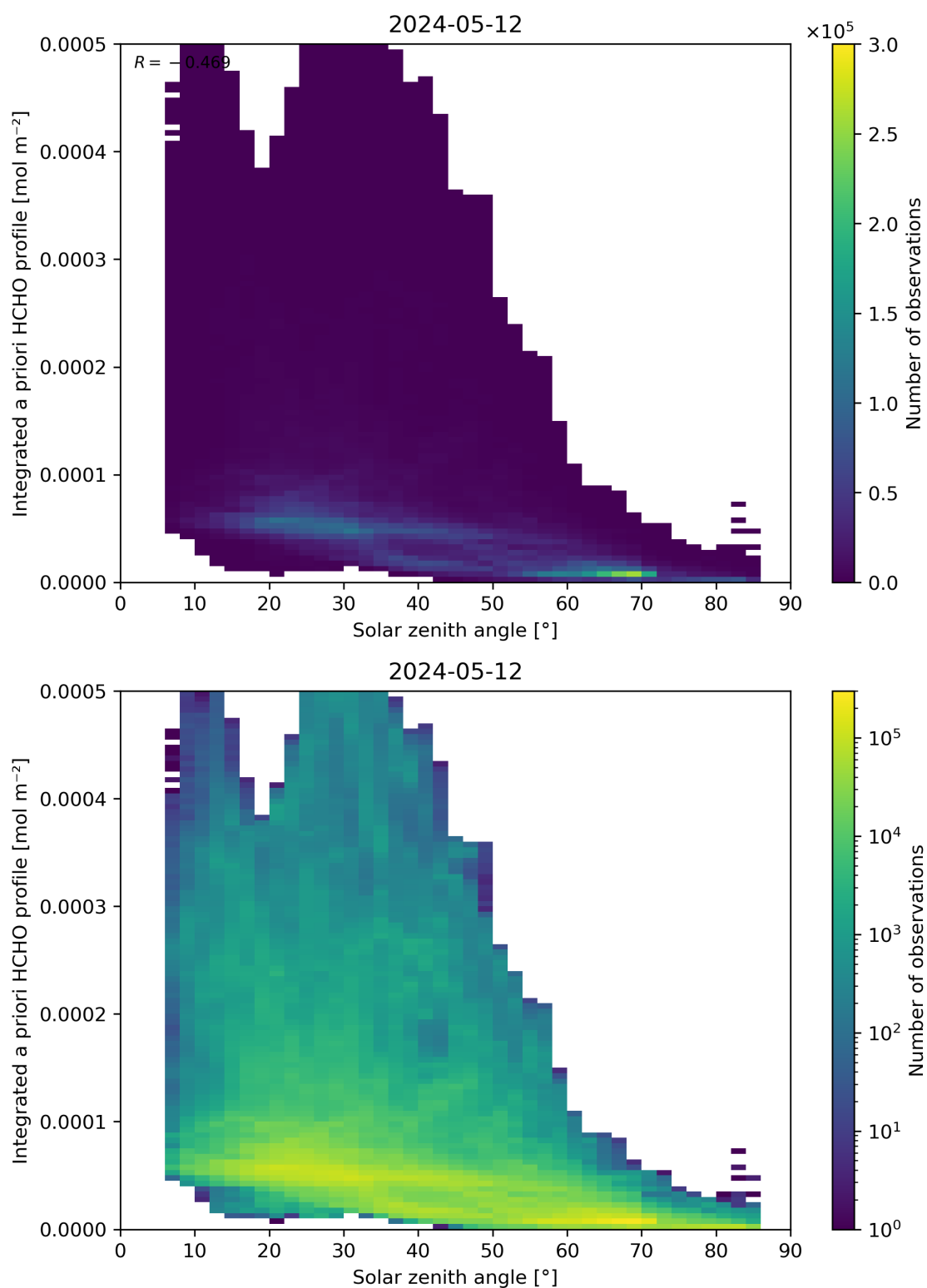
Figure 180: Scatter density plot of “Solar zenith angle” against “Integrated a priori HCHO profile” for 2024-05-12 to 2024-05-13.
