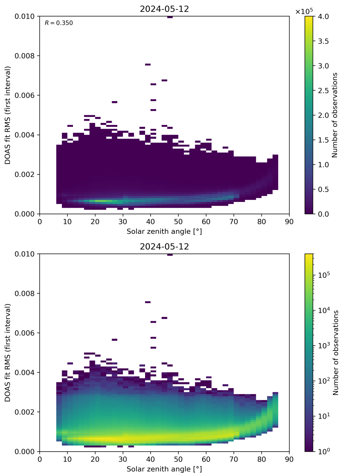
Figure 167: Scatter density plot of “Solar zenith angle” against “DOAS fit RMS (first interval)” for 2024-05-12 to 2024-05-13.
