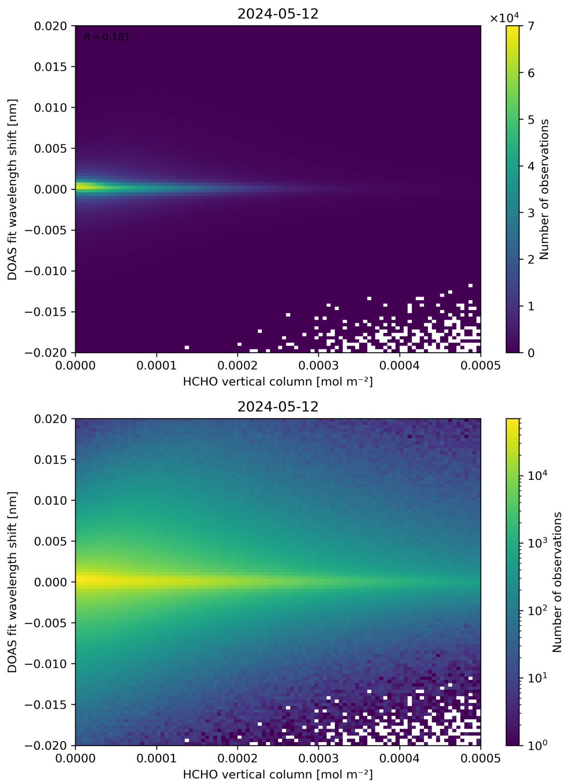
Figure 124: Scatter density plot of “HCHO vertical column” against “DOAS fit wavelength shift” for 2024-05-12 to 2024-05-13.
