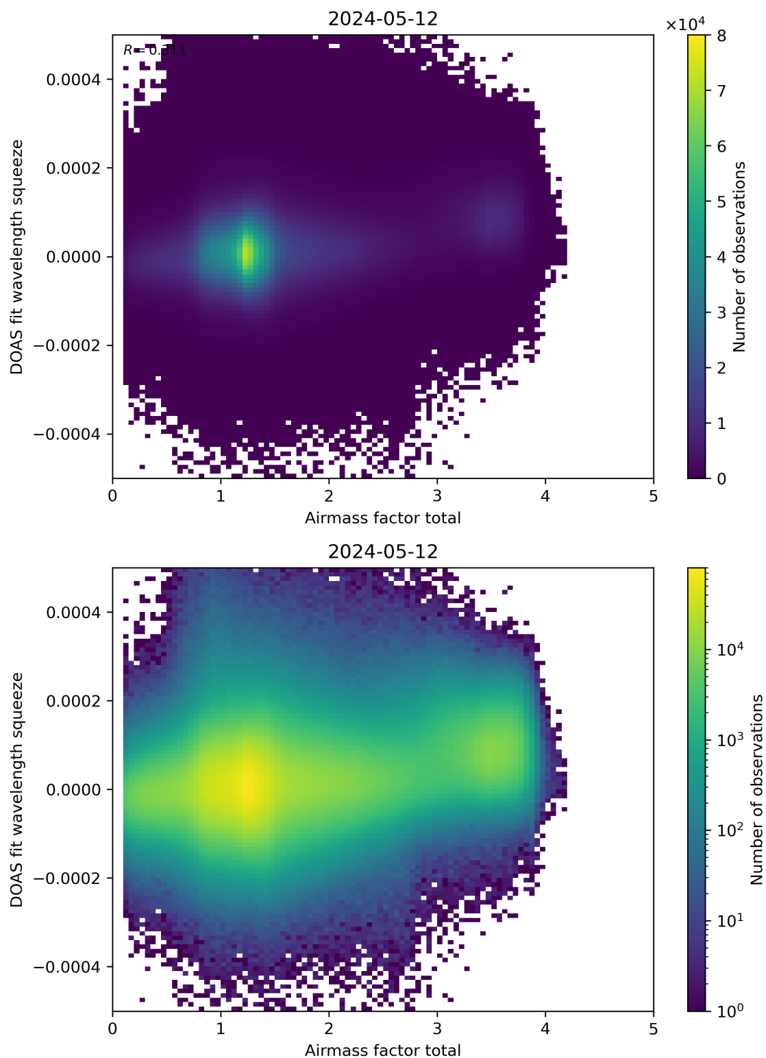
Figure 99: Scatter density plot of “Airmass factor total” against “DOAS fit wavelength squeeze” for 2024-05-12 to 2024-05-13.
