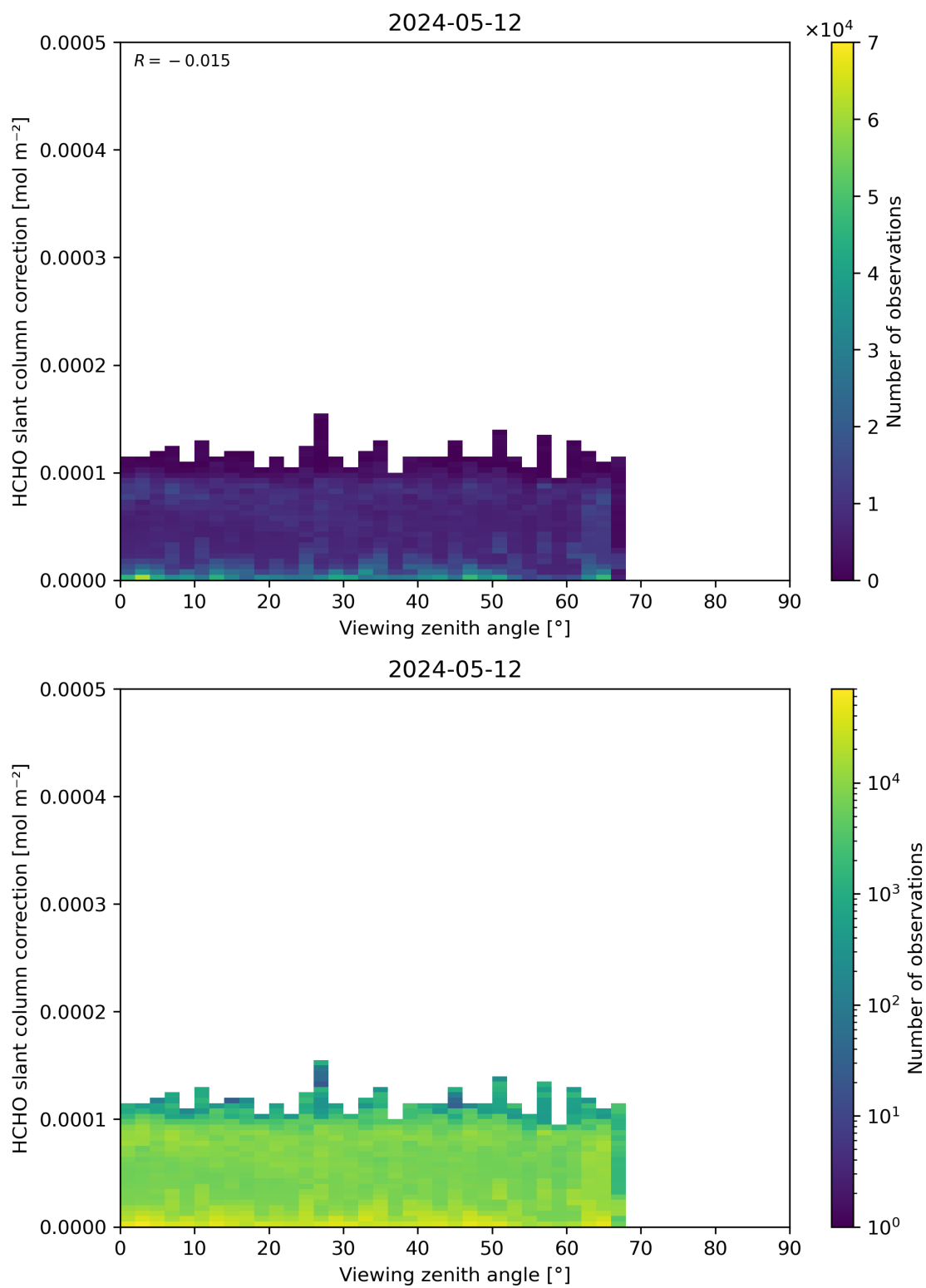
Figure 187: Scatter density plot of “Viewing zenith angle” against “HCHO slant column correction” for 2024-05-12 to 2024-05-13.
