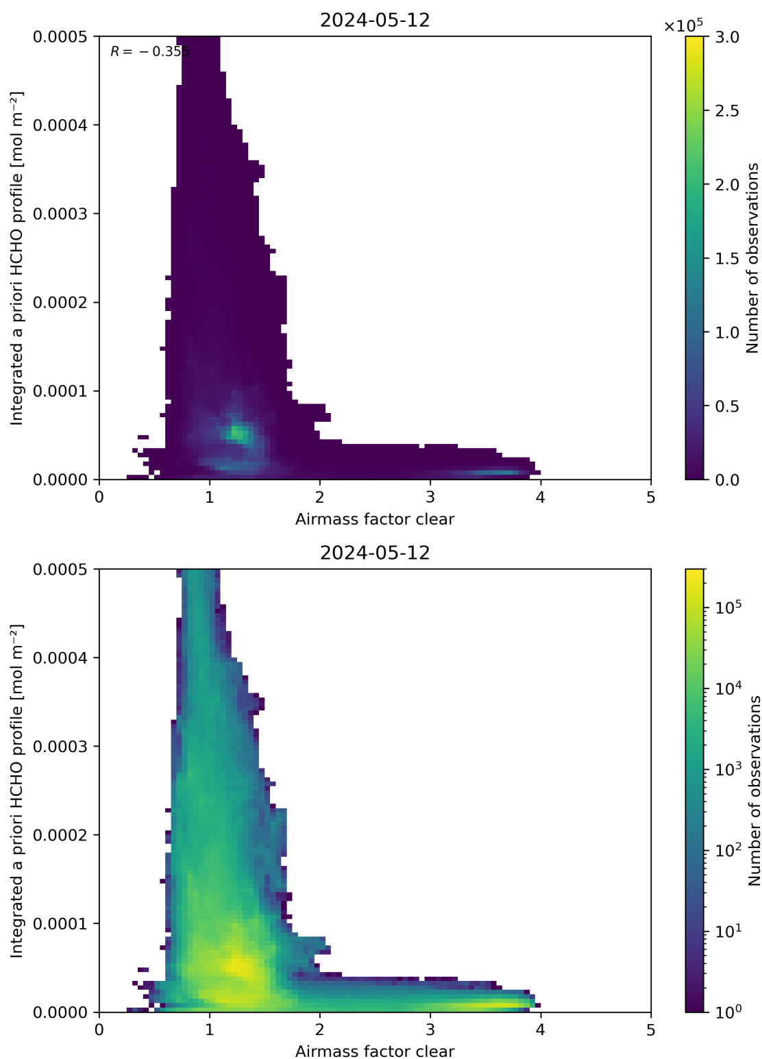
Figure 76: Scatter density plot of “Airmass factor clear” against “Integrated a priori HCHO profile” for 2024-05-12 to 2024-05-13.
