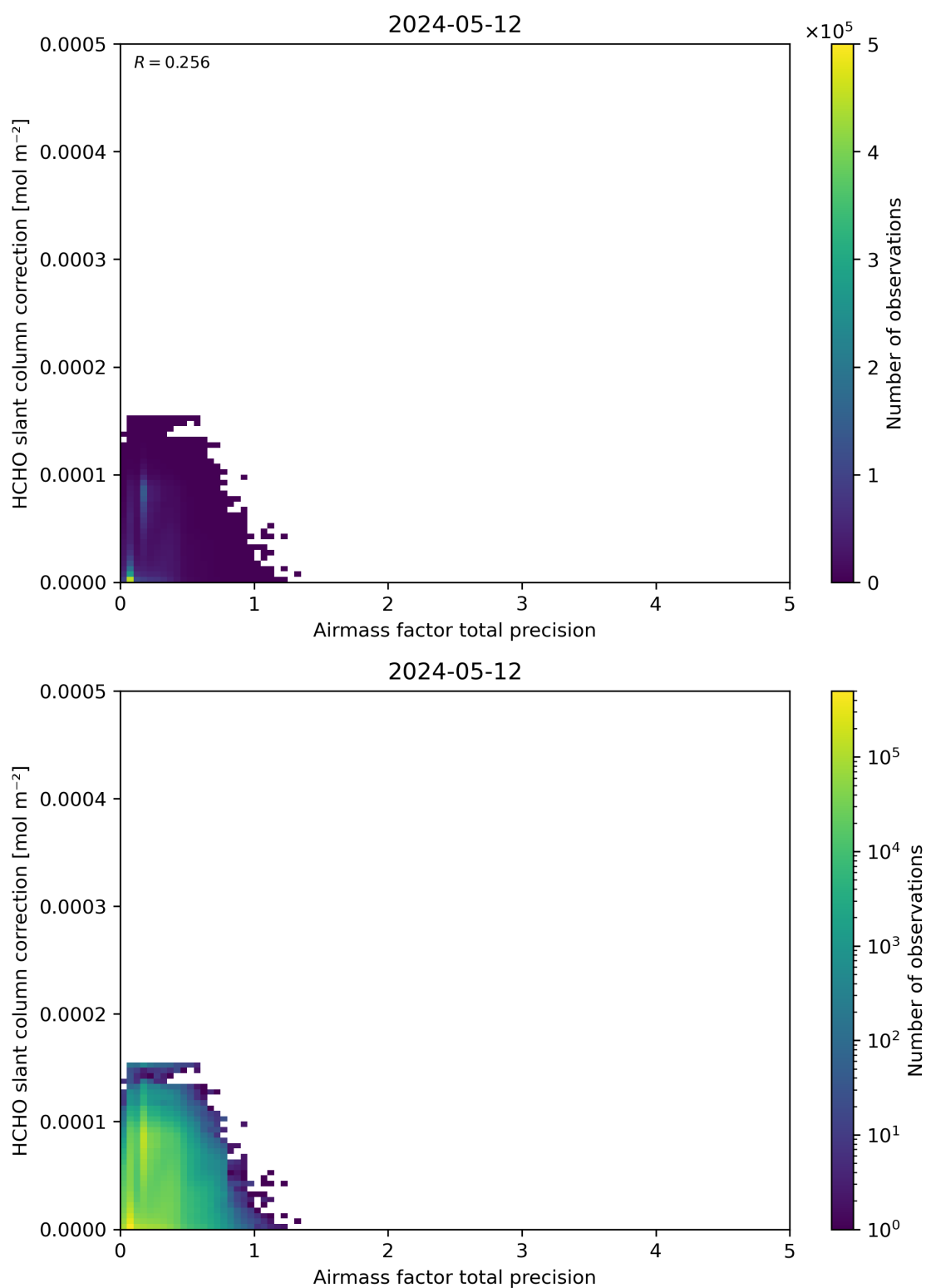
Figure 110: Scatter density plot of “Airmass factor total precision” against “HCHO slant column correction” for 2024-05-12 to 2024-05-13.
