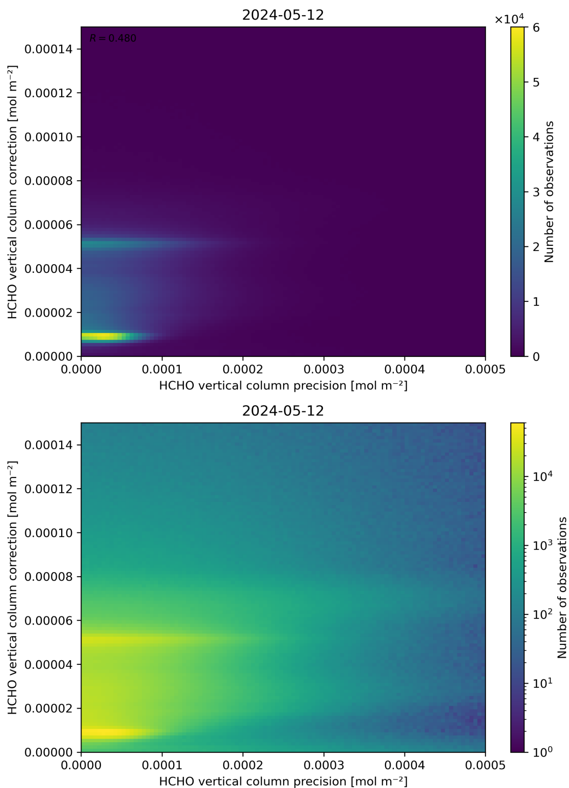
Figure 146: Scatter density plot of “HCHO vertical column precision” against “HCHO vertical column correction” for 2024-05-12 to 2024-05-13.
