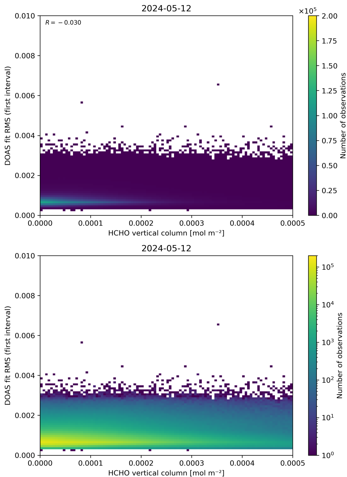
Figure 123: Scatter density plot of “HCHO vertical column” against “DOAS fit RMS (first interval)” for 2024-05-12 to 2024-05-13.
