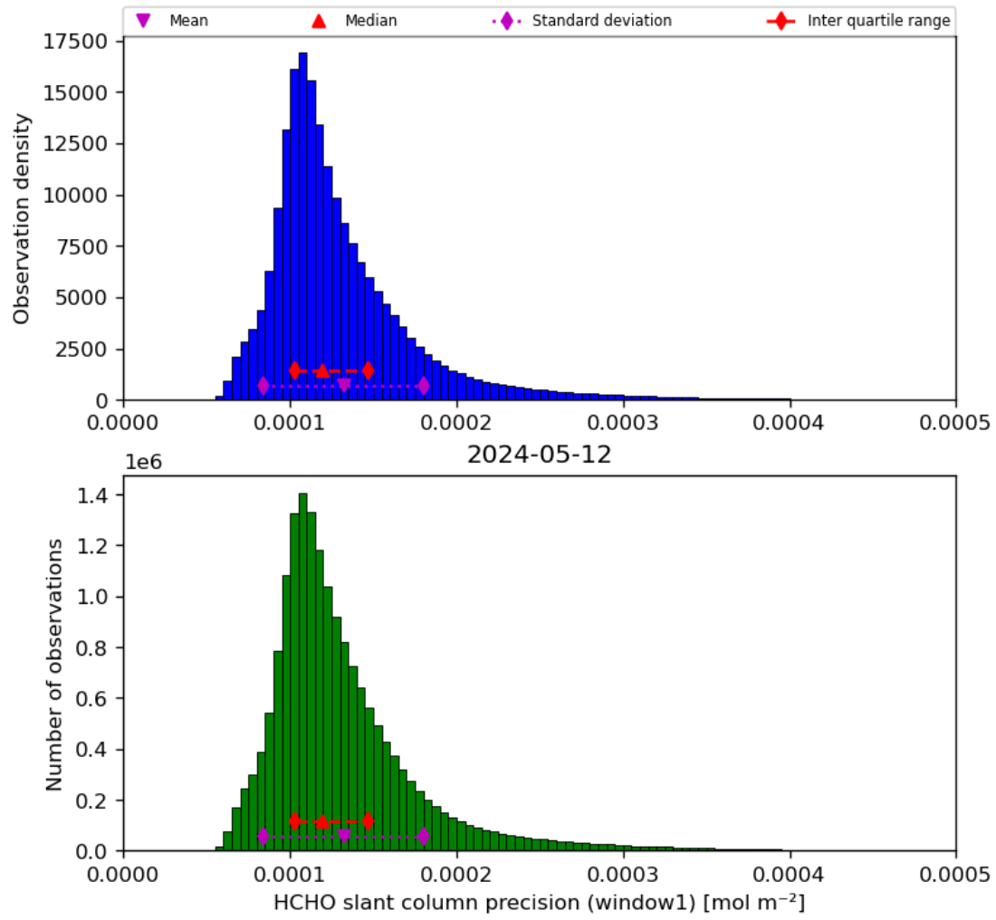
Figure 39: Histogram of “HCHO slant column precision (window1)” for 2024-05-12 to 2024-05-13
