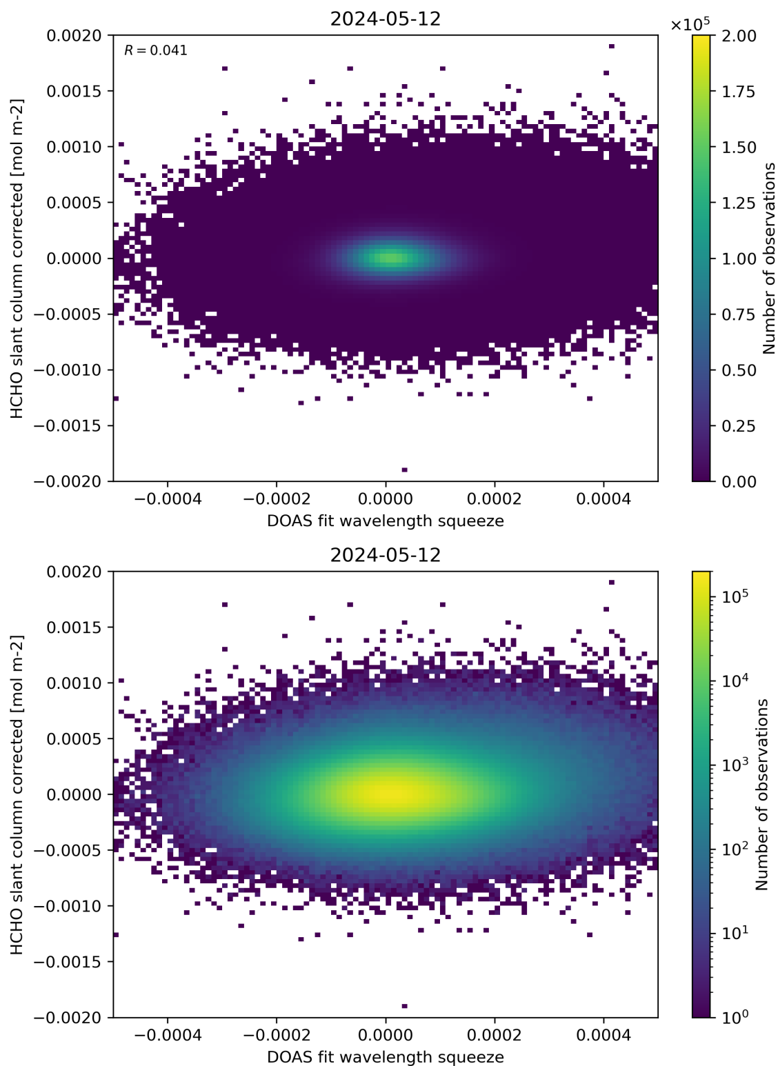
Figure 69: Scatter density plot of “DOAS fit wavelength squeeze” against “HCHO slant column corrected” for 2024-05-12 to 2024-05-13.
