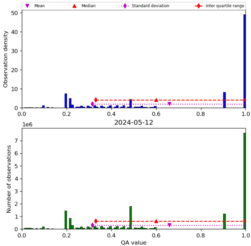
Figure 34: Histogram of “QA value” for 2024-05-12 to 2024-05-13
