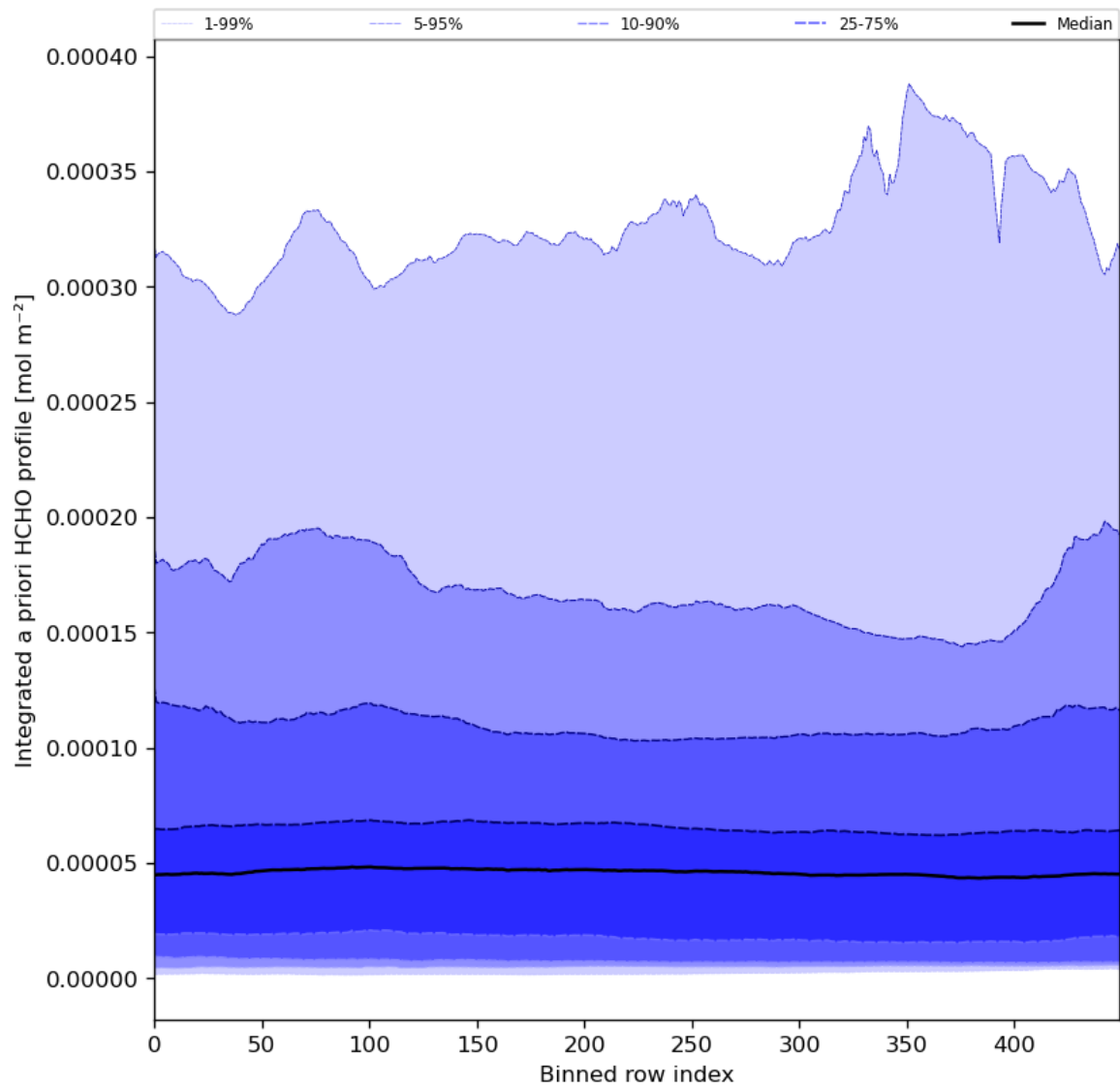
Figure 57: Along track statistics of “Integrated a priori HCHO profile” for 2024-05-12 to 2024-05-13
