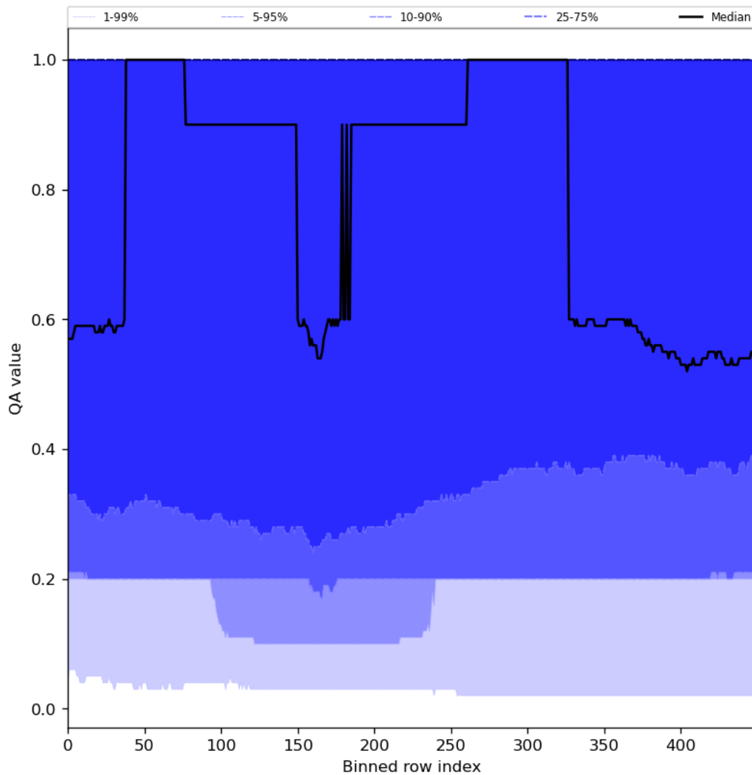
Figure 48: Along track statistics of “QA value” for 2024-05-12 to 2024-05-13
