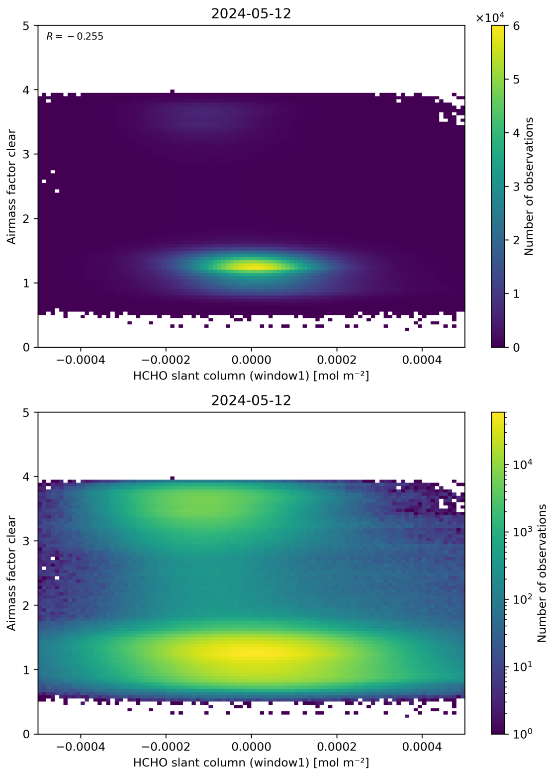
Figure 81: Scatter density plot of “HCHO slant column (window1)” against “Airmass factor clear” for 2024-05-12 to 2024-05-13.
