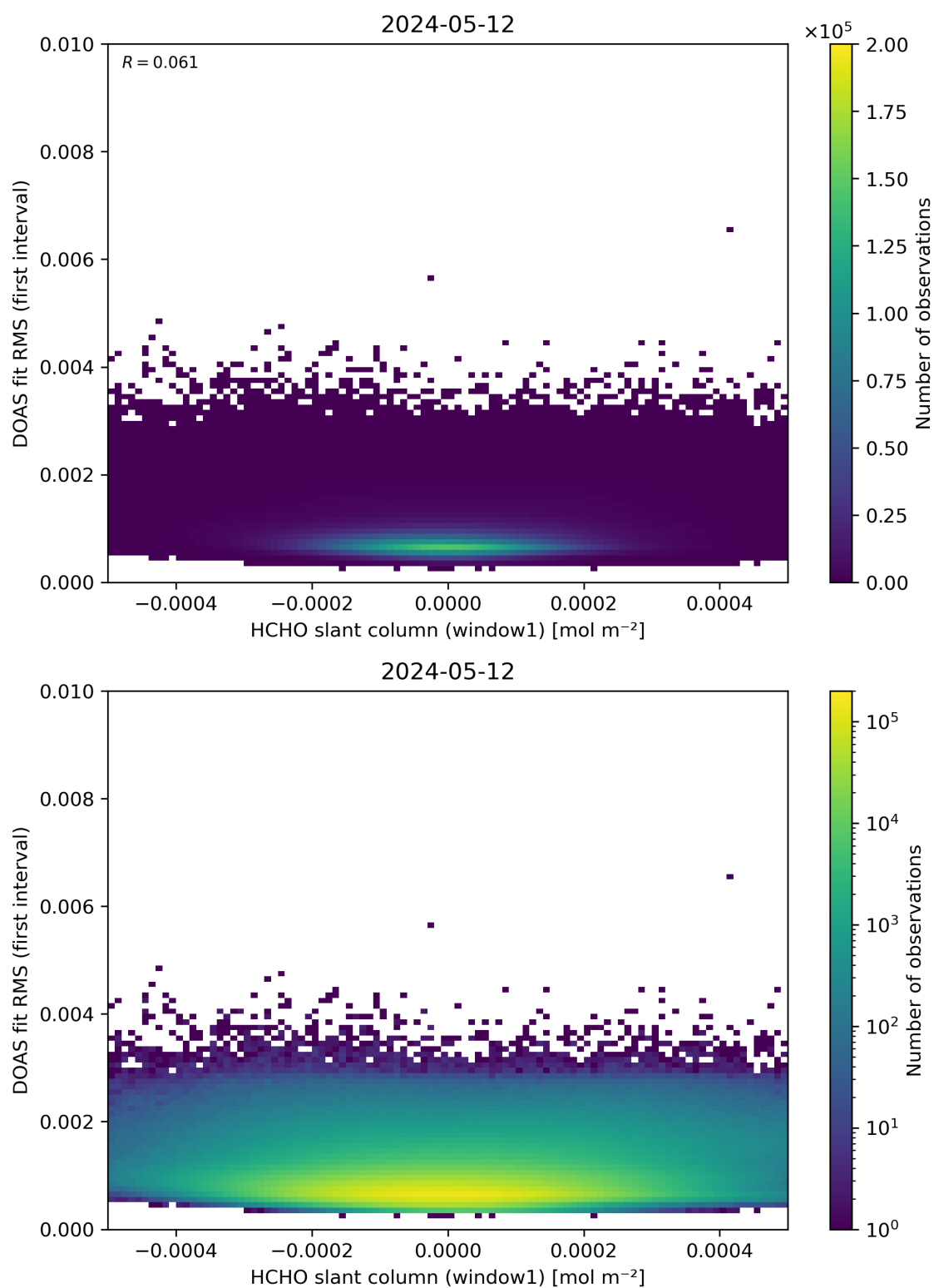
Figure 78: Scatter density plot of “HCHO slant column (window1)” against “DOAS fit RMS (first interval)” for 2024-05-12 to 2024-05-13.
