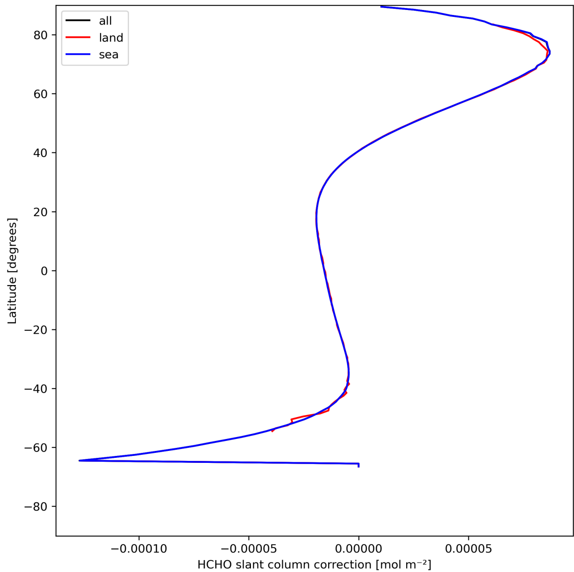
Figure 33: Zonal average of “HCHO slant column correction” for 2024-05-12 to 2024-05-13.
