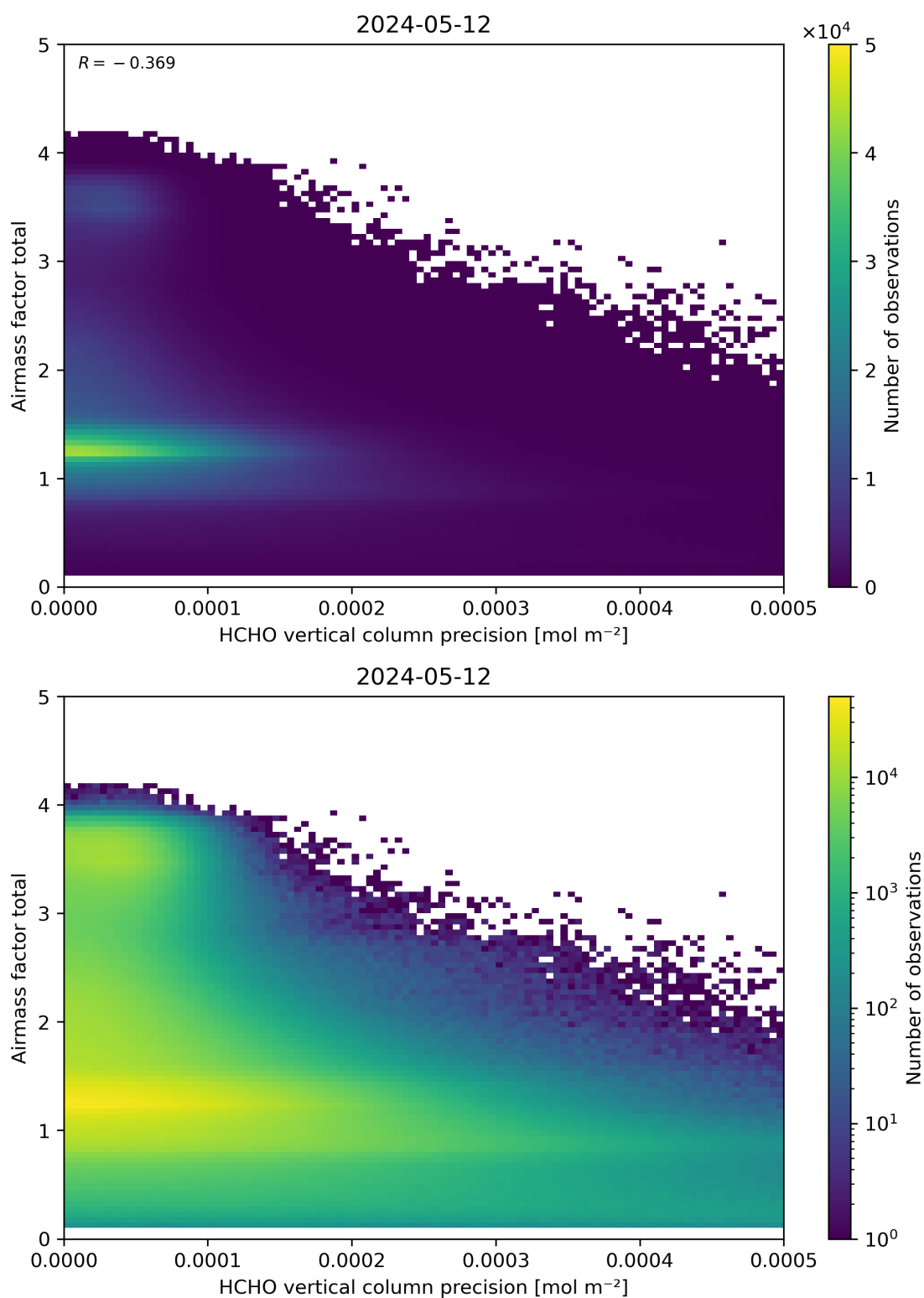
Figure 144: Scatter density plot of “HCHO vertical column precision” against “Airmass factor total” for 2024-05-12 to 2024-05-13.
