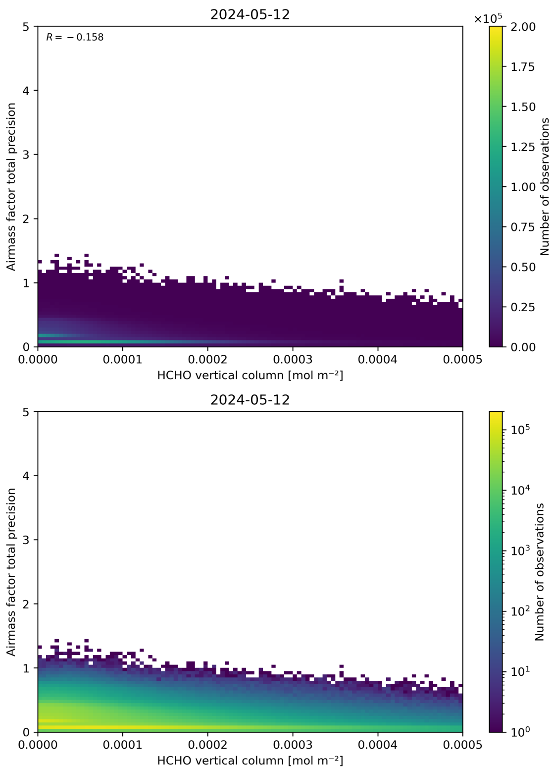
Figure 132: Scatter density plot of “HCHO vertical column” against “Airmass factor total precision” for 2024-05-12 to 2024-05-13.
