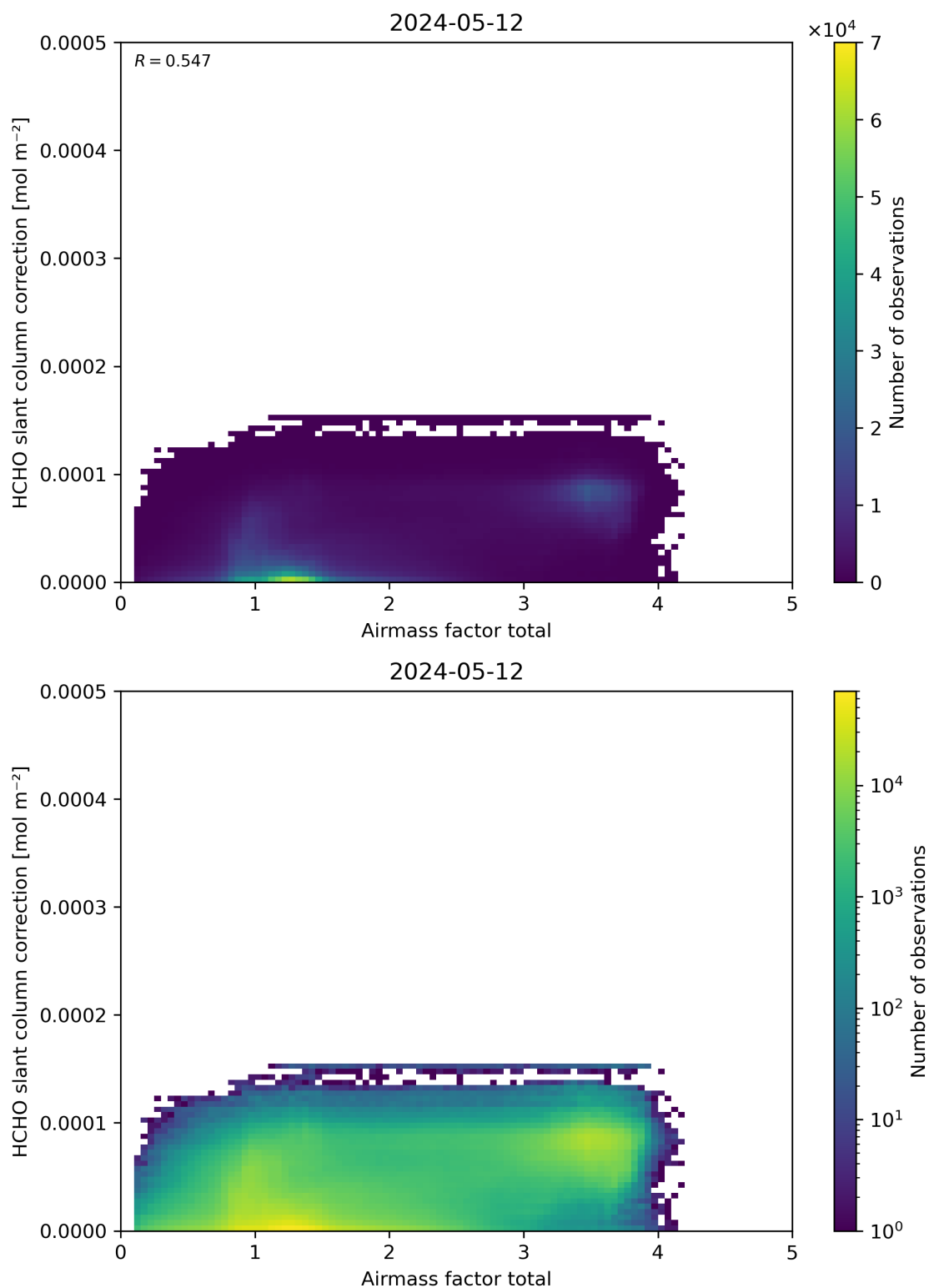
Figure 102: Scatter density plot of “Airmass factor total” against “HCHO slant column correction” for 2024-05-12 to 2024-05-13.
