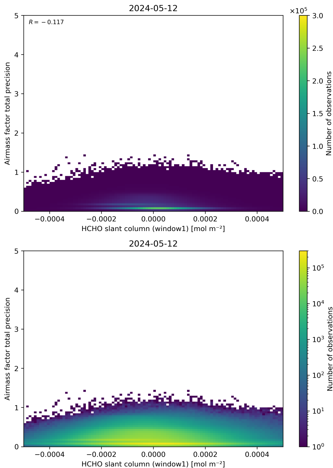
Figure 86: Scatter density plot of “HCHO slant column (window1)” against “Airmass factor total precision” for 2024-05-12 to 2024-05-13.
