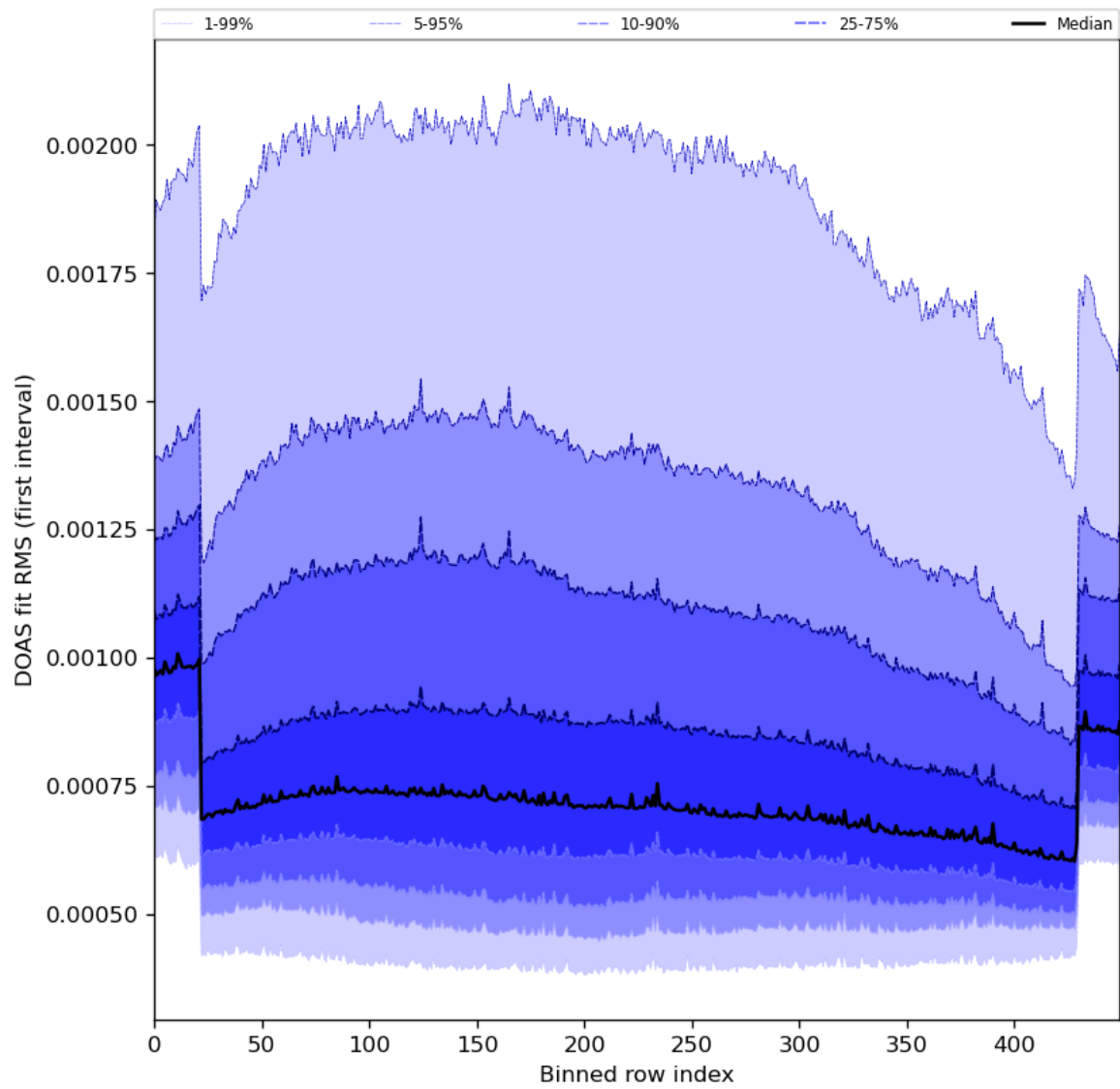
Figure 60: Along track statistics of “DOAS fit RMS (first interval)” for 2024-05-12 to 2024-05-13
