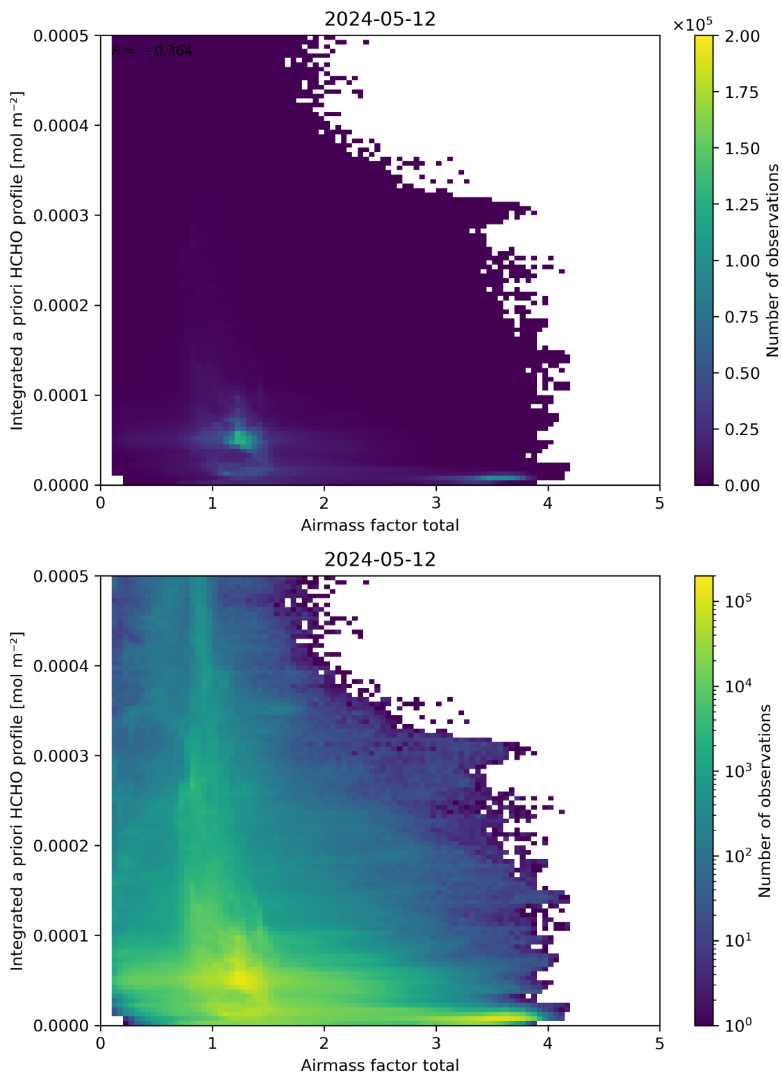
Figure 104: Scatter density plot of “Airmass factor total” against “Integrated a priori HCHO profile” for 2024-05-12 to 2024-05-13.
