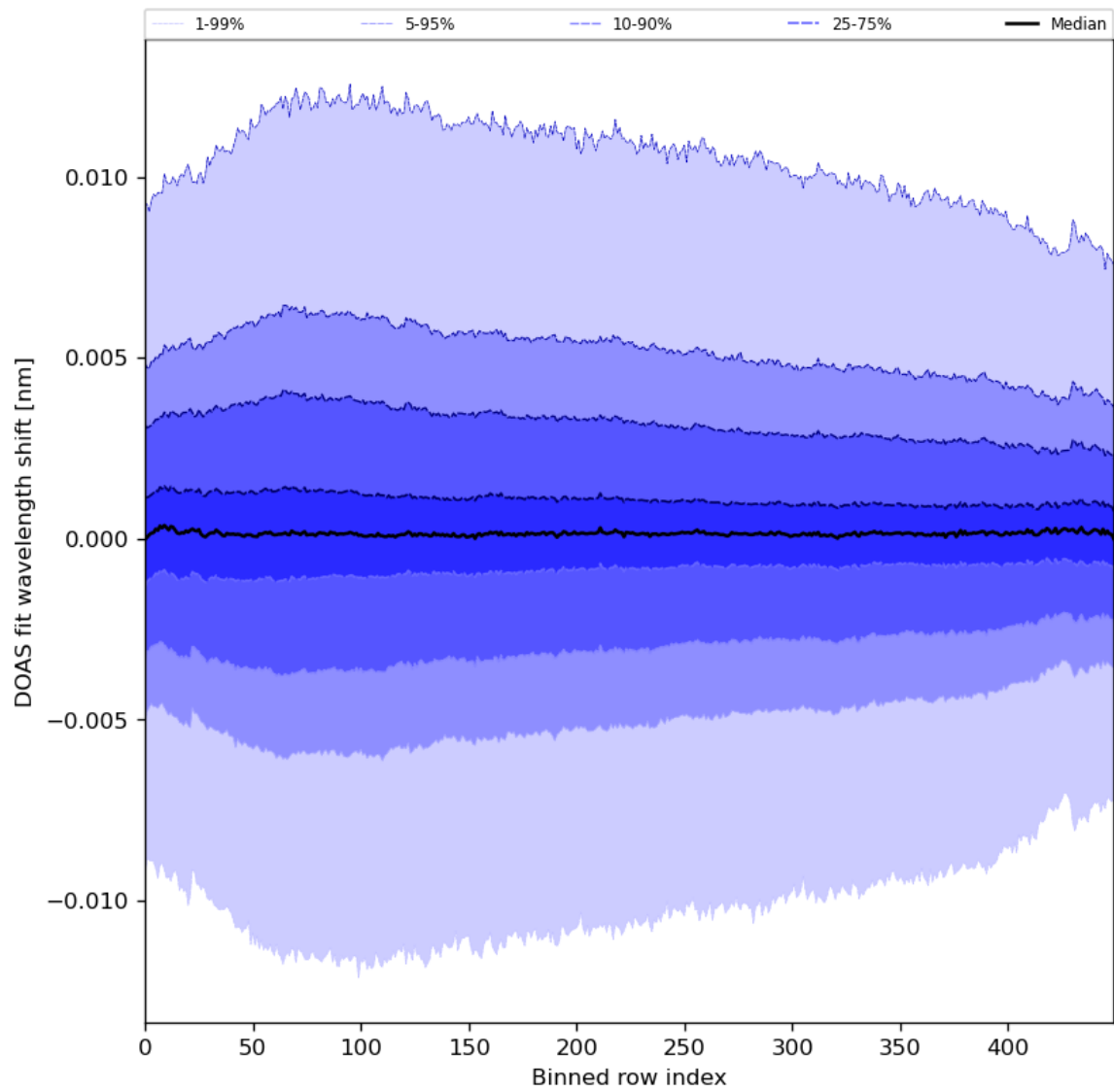
Figure 58: Along track statistics of “DOAS fit wavelength shift” for 2024-05-12 to 2024-05-13
