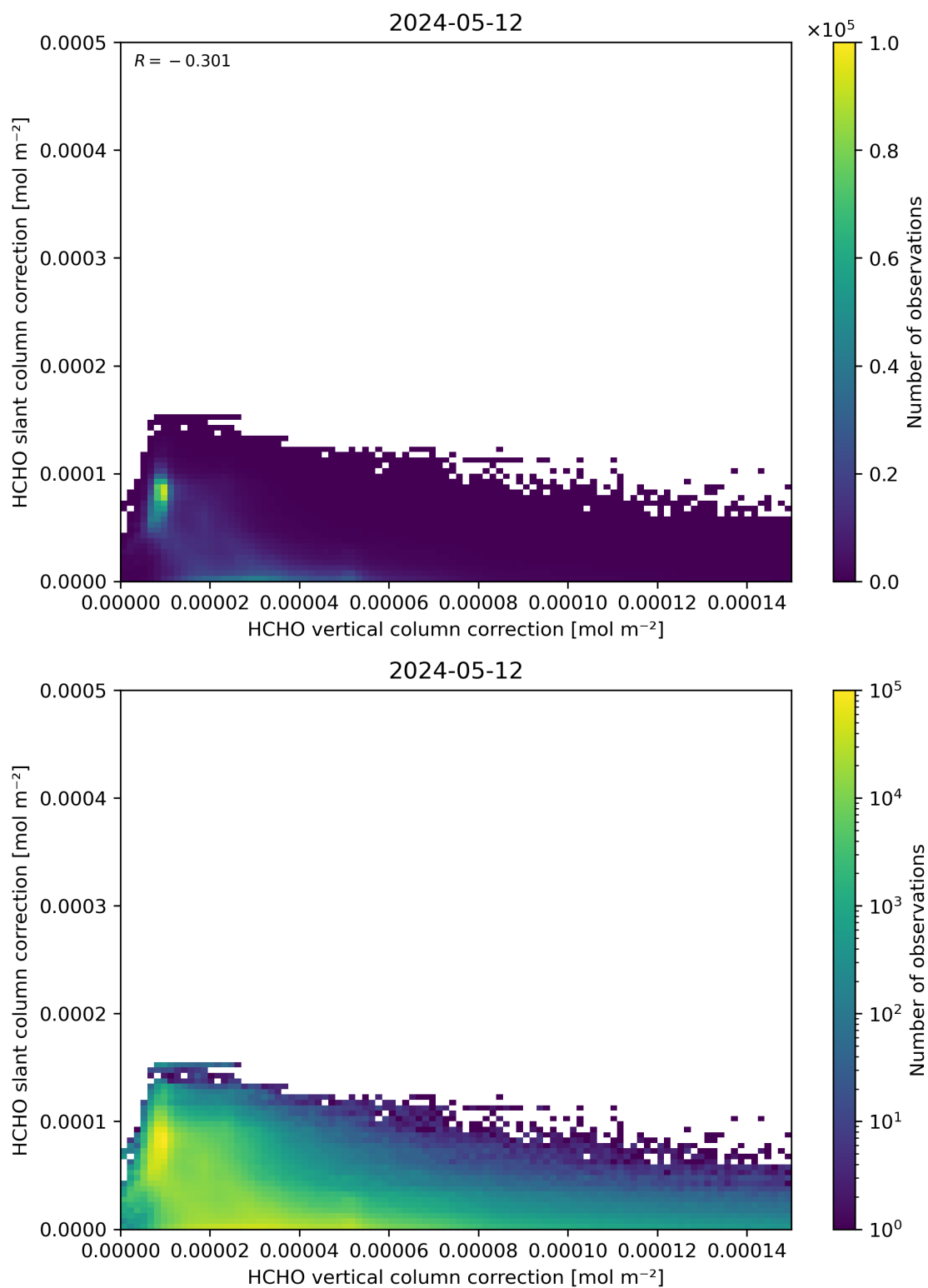
Figure 117: Scatter density plot of “HCHO vertical column correction” against “HCHO slant column correction” for 2024-05-12 to 2024-05-13.
