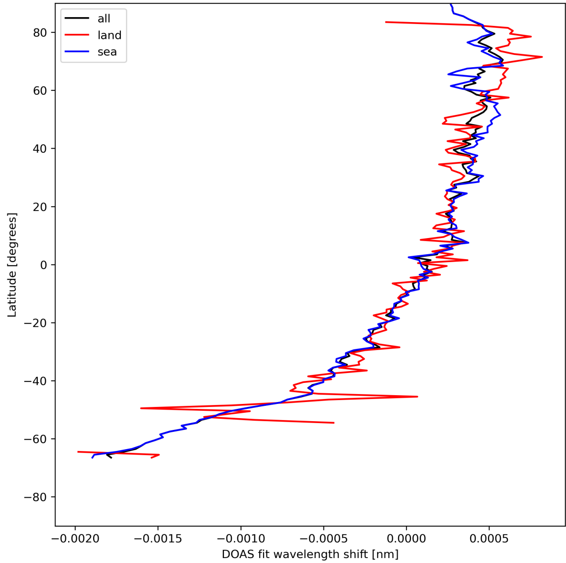
Figure 30: Zonal average of “DOAS fit wavelength shift” for 2024-05-12 to 2024-05-13.
