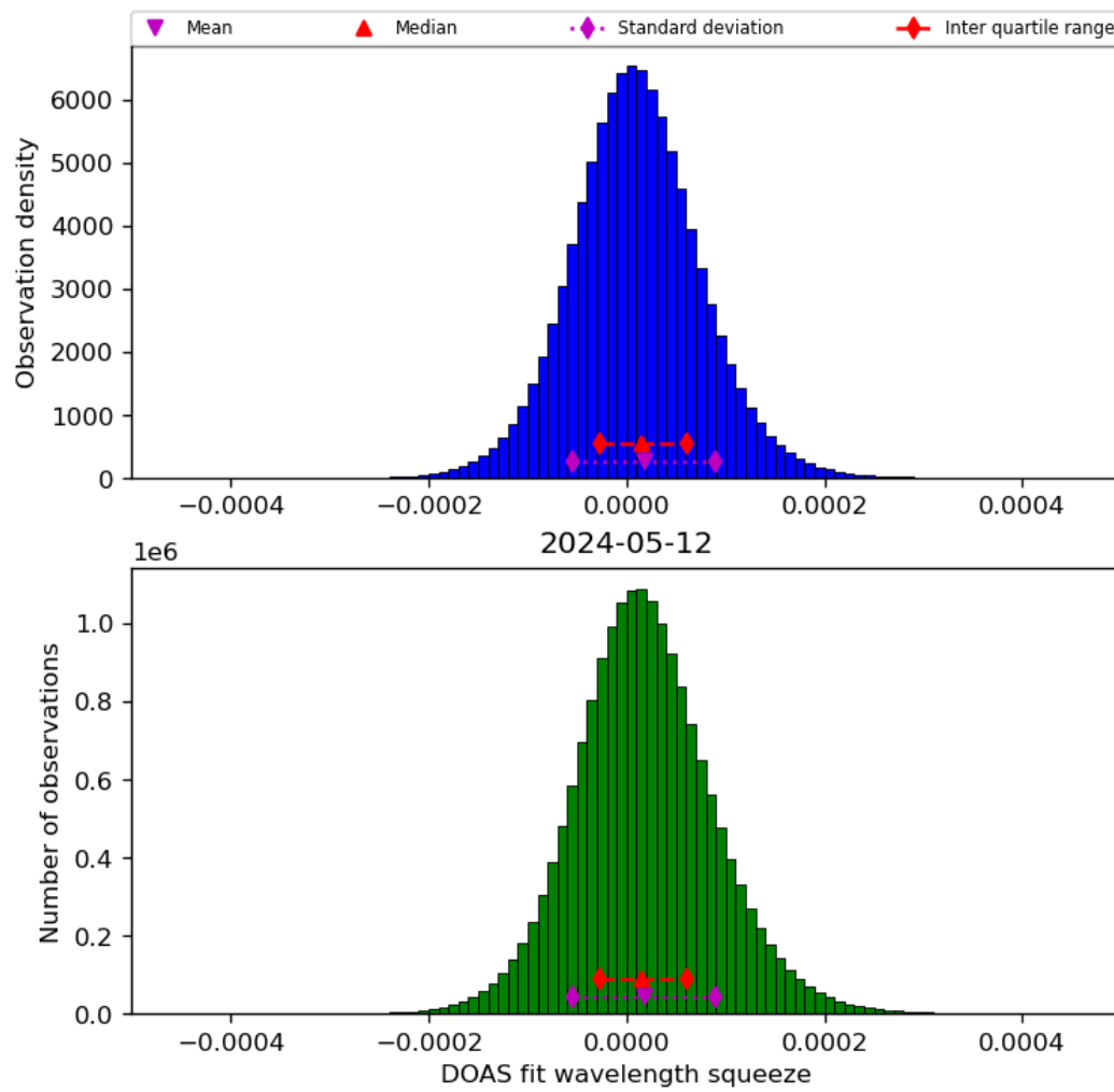
Figure 45: Histogram of “DOAS fit wavelength squeeze” for 2024-05-12 to 2024-05-13
