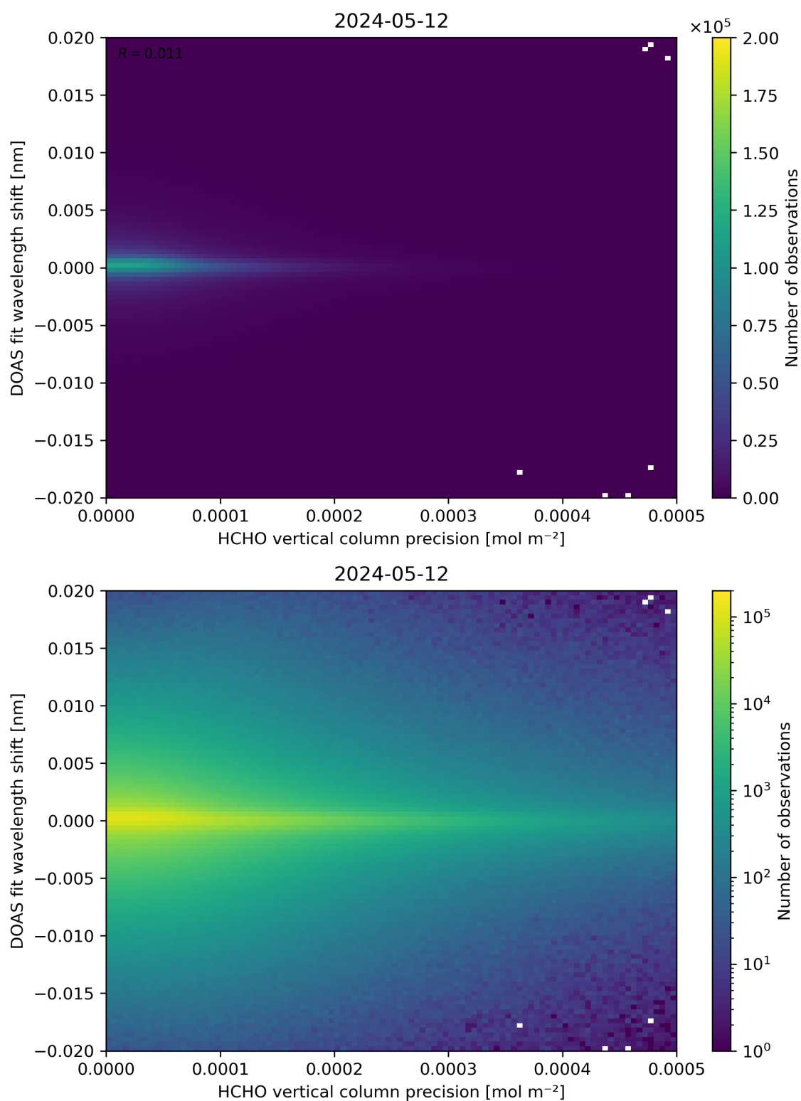
Figure 137: Scatter density plot of “HCHO vertical column precision” against “DOAS fit wavelength shift” for 2024-05-12 to 2024-05-13.
