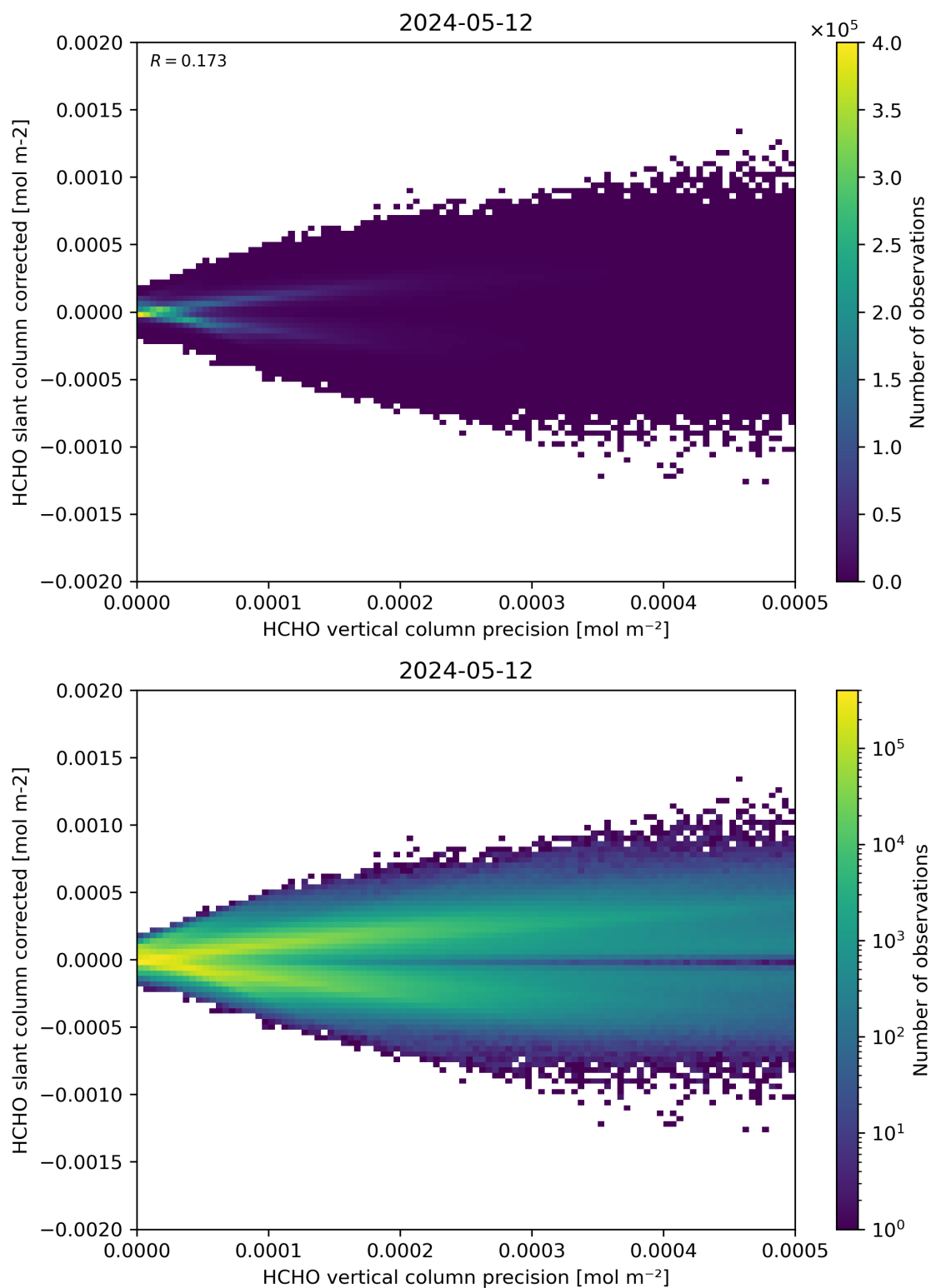
Figure 140: Scatter density plot of “HCHO vertical column precision” against “HCHO slant column corrected” for 2024-05-12 to 2024-05-13.
