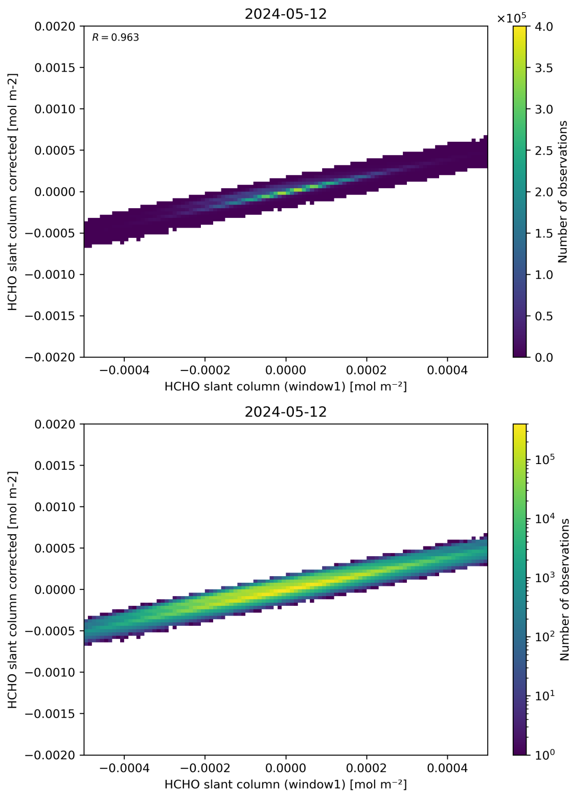
Figure 82: Scatter density plot of “HCHO slant column (window1)” against “HCHO slant column corrected” for 2024-05-12 to 2024-05-13.
