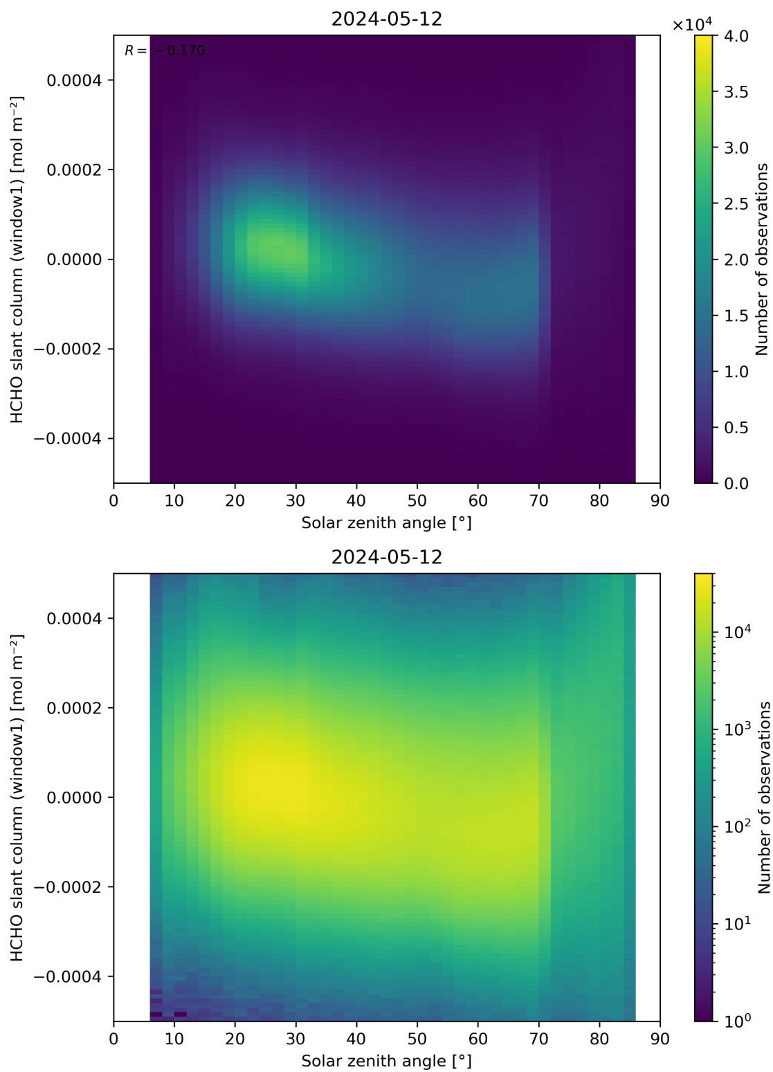
Figure 173: Scatter density plot of “Solar zenith angle” against “HCHO slant column (window1)” for 2024-05-12 to 2024-05-13.
