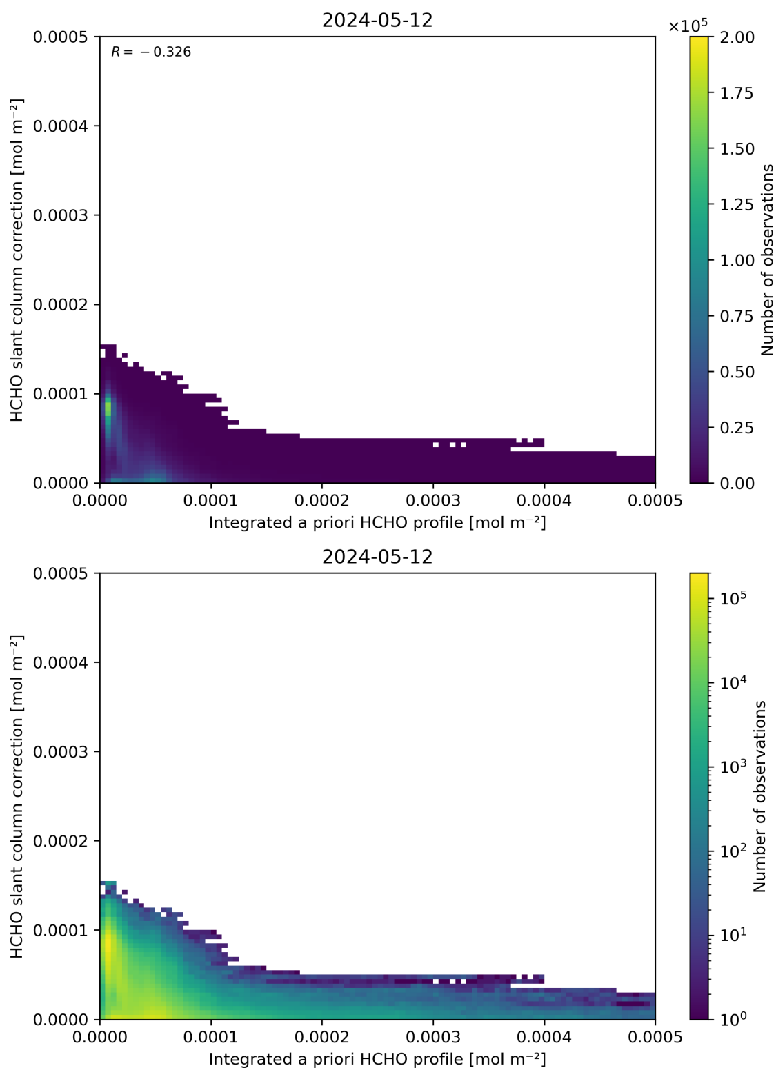
Figure 152: Scatter density plot of “Integrated a priori HCHO profile” against “HCHO slant column correction” for 2024-05-12 to 2024-05-13.
