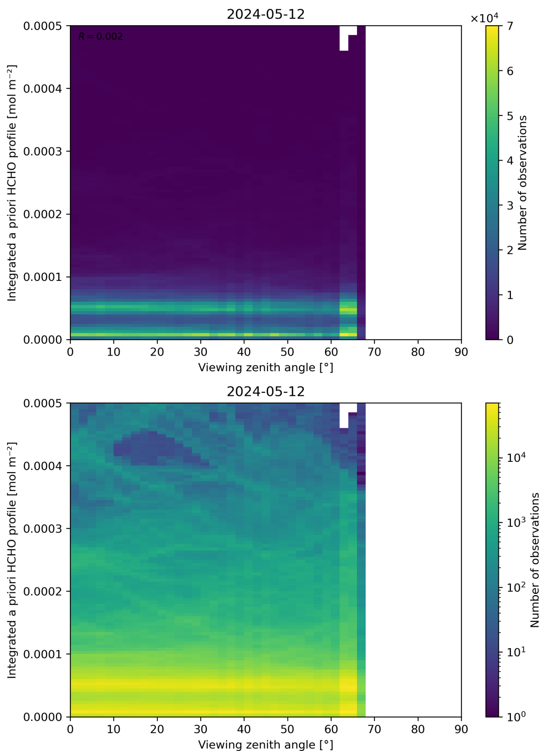
Figure 195: Scatter density plot of “Viewing zenith angle” against “Integrated a priori HCHO profile” for 2024-05-12 to 2024-05-13.
