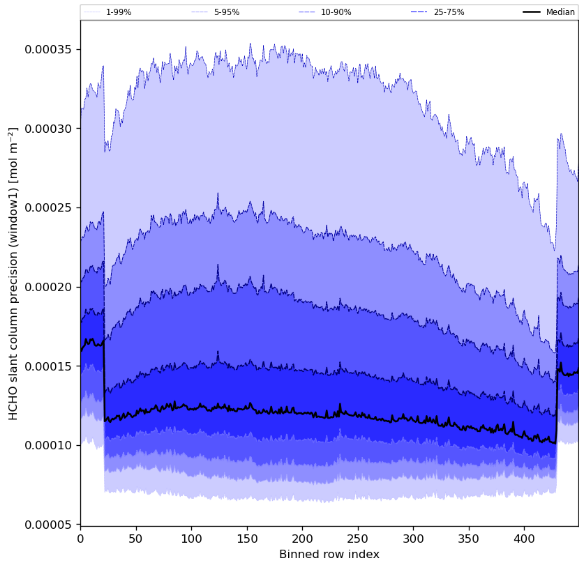
Figure 53: Along track statistics of “HCHO slant column precision (window1)” for 2024-05-12 to 2024-05-13
