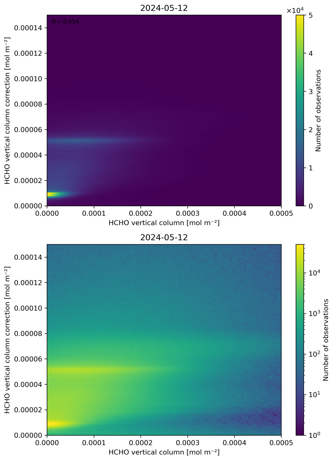
Figure 133: Scatter density plot of “HCHO vertical column” against “HCHO vertical column correction” for 2024-05-12 to 2024-05-13.
