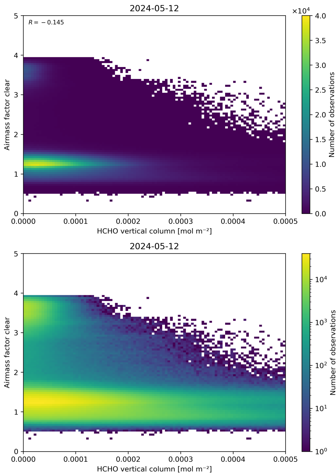
Figure 126: Scatter density plot of “HCHO vertical column” against “Airmass factor clear” for 2024-05-12 to 2024-05-13.
