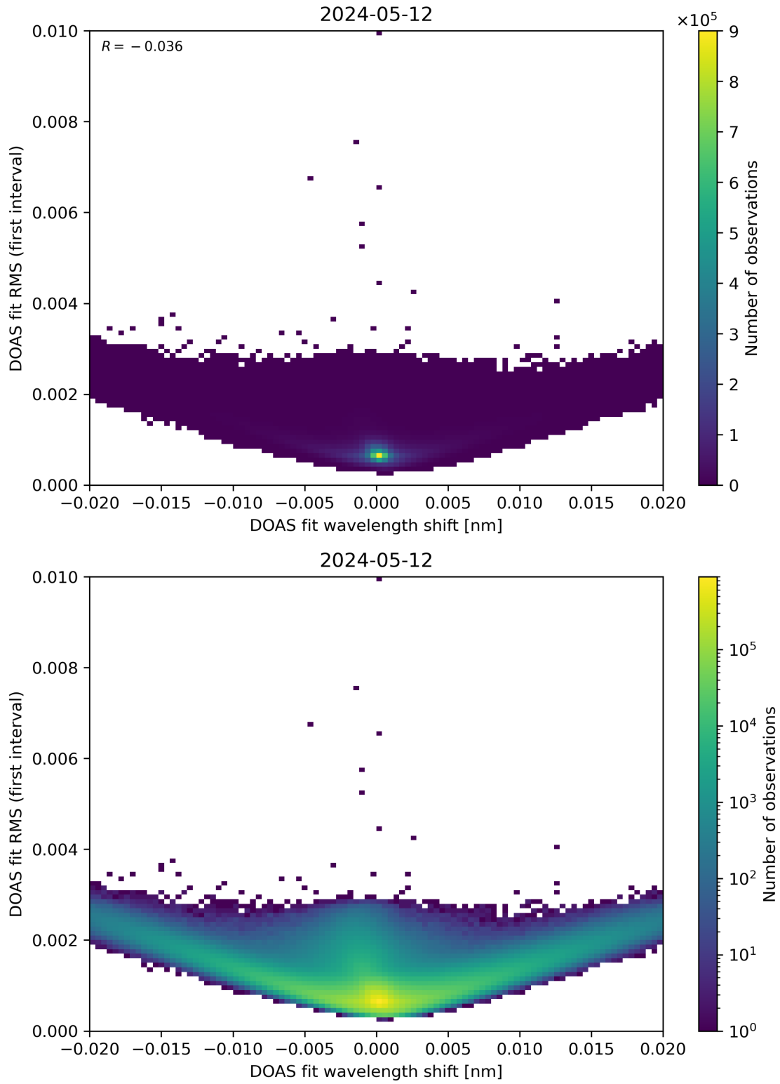
Figure 64: Scatter density plot of “DOAS fit wavelength shift” against “DOAS fit RMS (first interval)” for 2024-05-12 to 2024-05-13.
