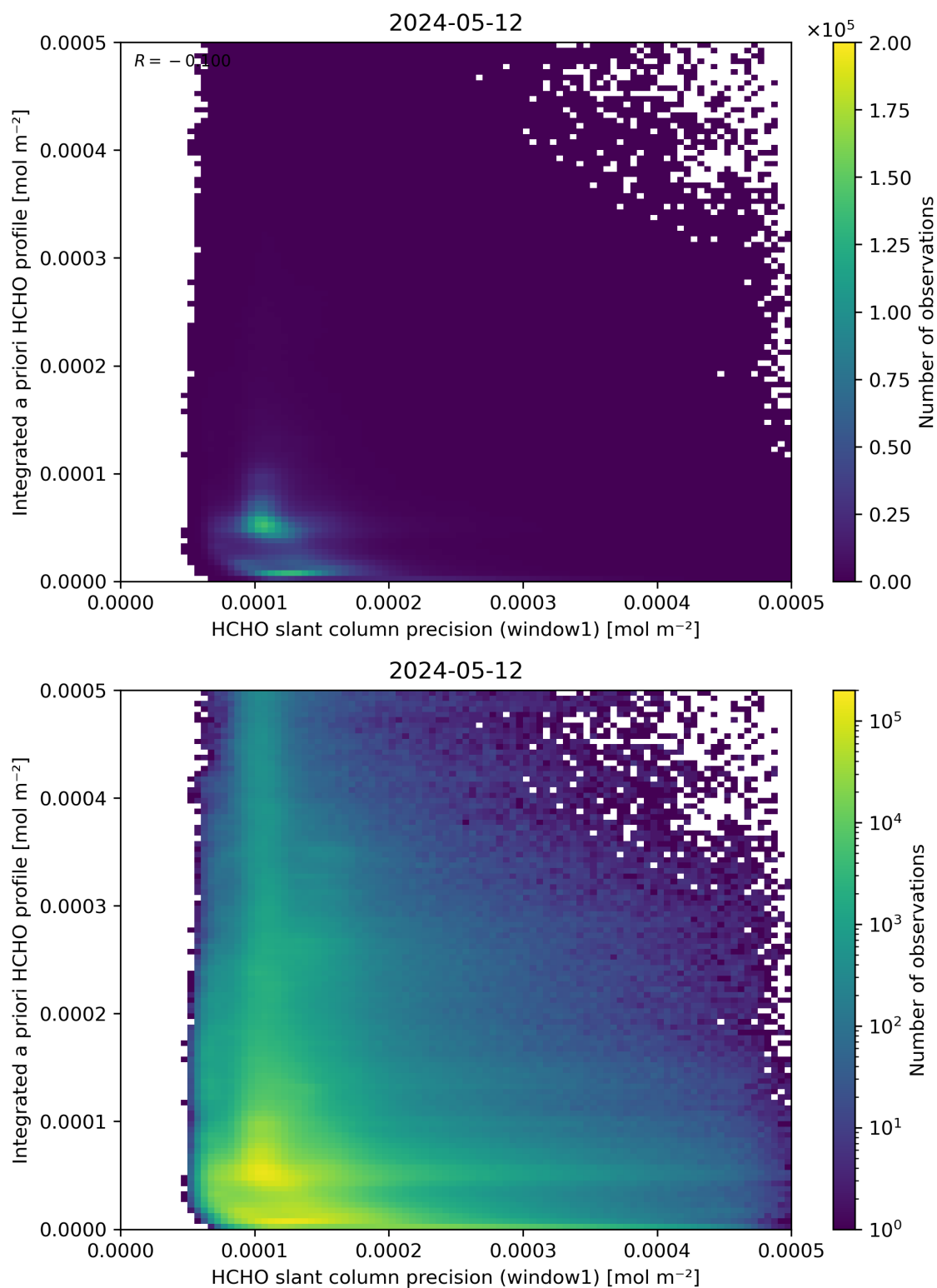
Figure 96: Scatter density plot of “HCHO slant column precision (window1)” against “Integrated a priori HCHO profile” for 2024-05-12 to 2024-05-13.
