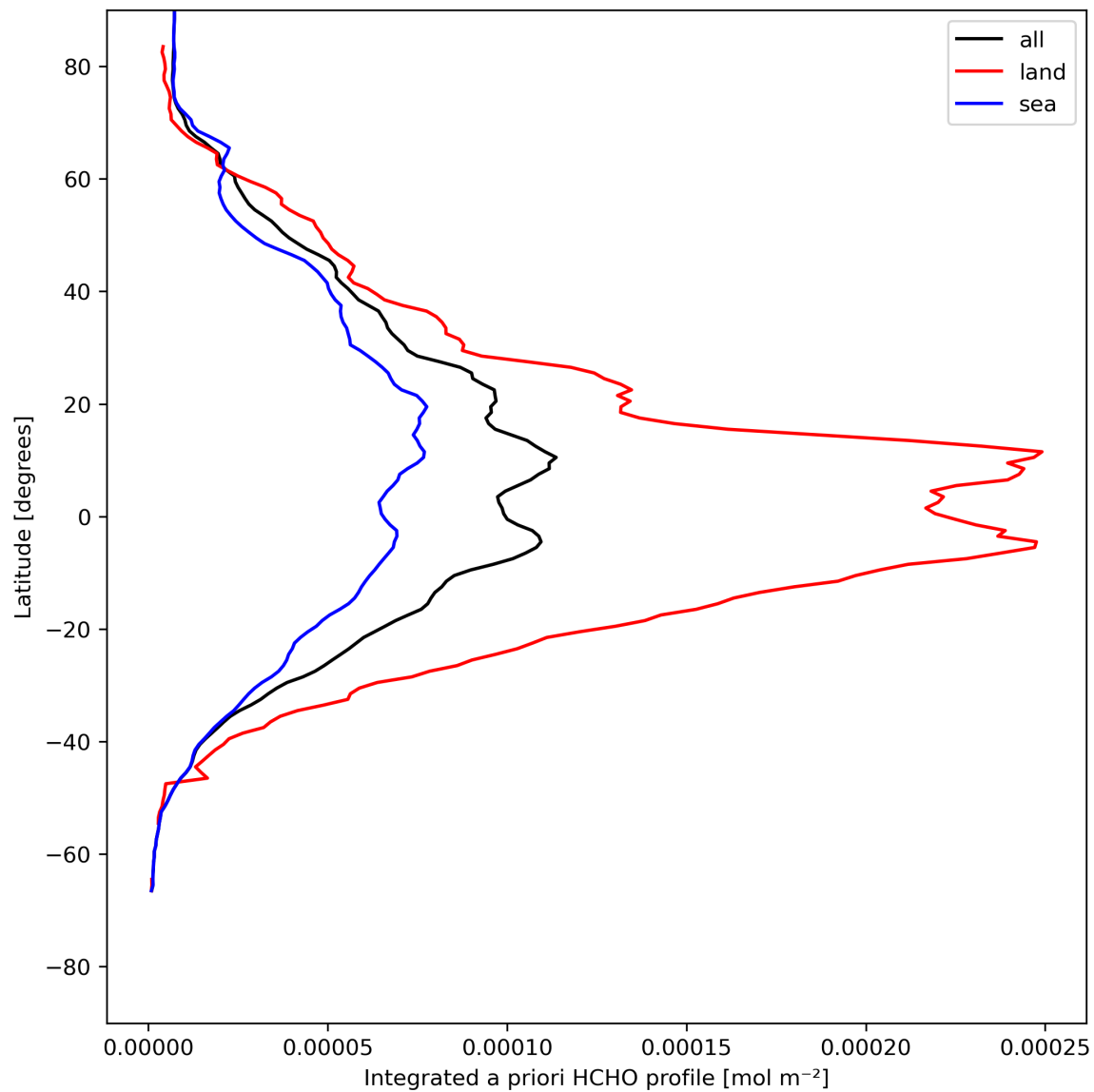
Figure 29: Zonal average of “Integrated a priori HCHO profile” for 2024-05-12 to 2024-05-13.
