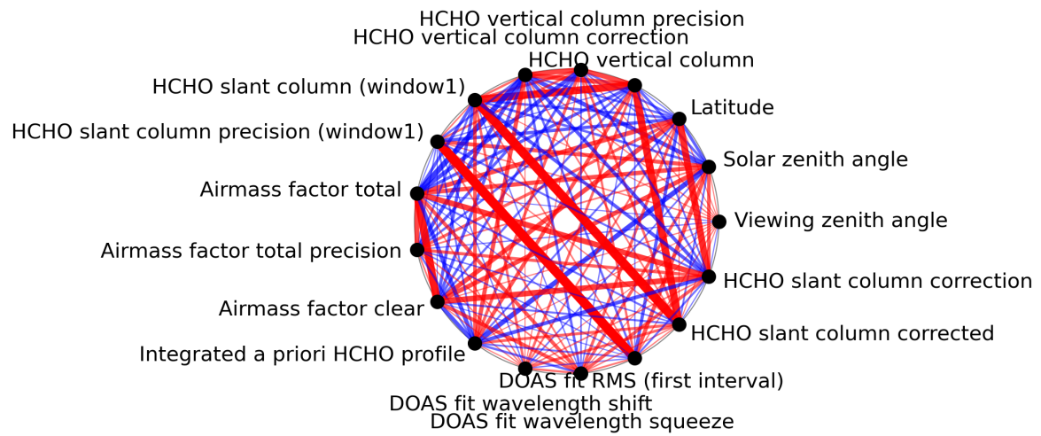
Figure 1: Map of correlation graph for 2024-05-12 to 2024-05-13.
