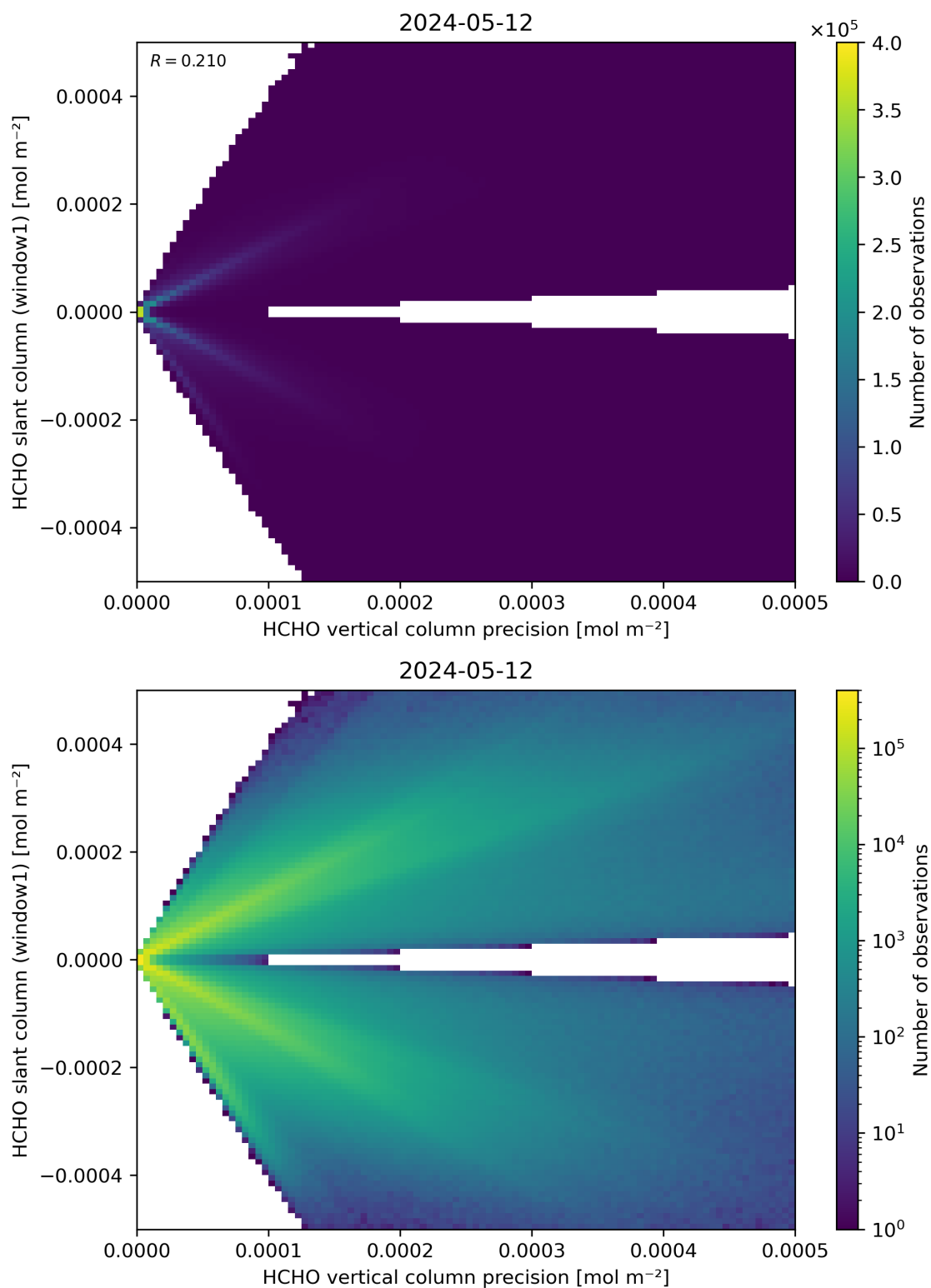
Figure 142: Scatter density plot of “HCHO vertical column precision” against “HCHO slant column (window1)” for 2024-05-12 to 2024-05-13.
