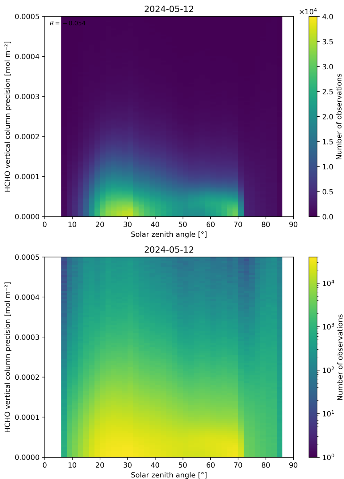
Figure 179: Scatter density plot of “Solar zenith angle” against “HCHO vertical column precision” for 2024-05-12 to 2024-05-13.
