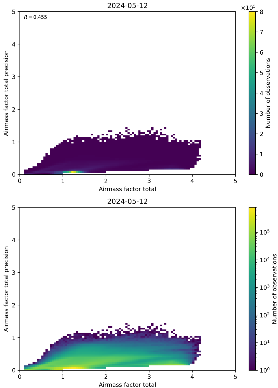
Figure 103: Scatter density plot of “Airmass factor total” against “Airmass factor total precision” for 2024-05-12 to 2024-05-13.
