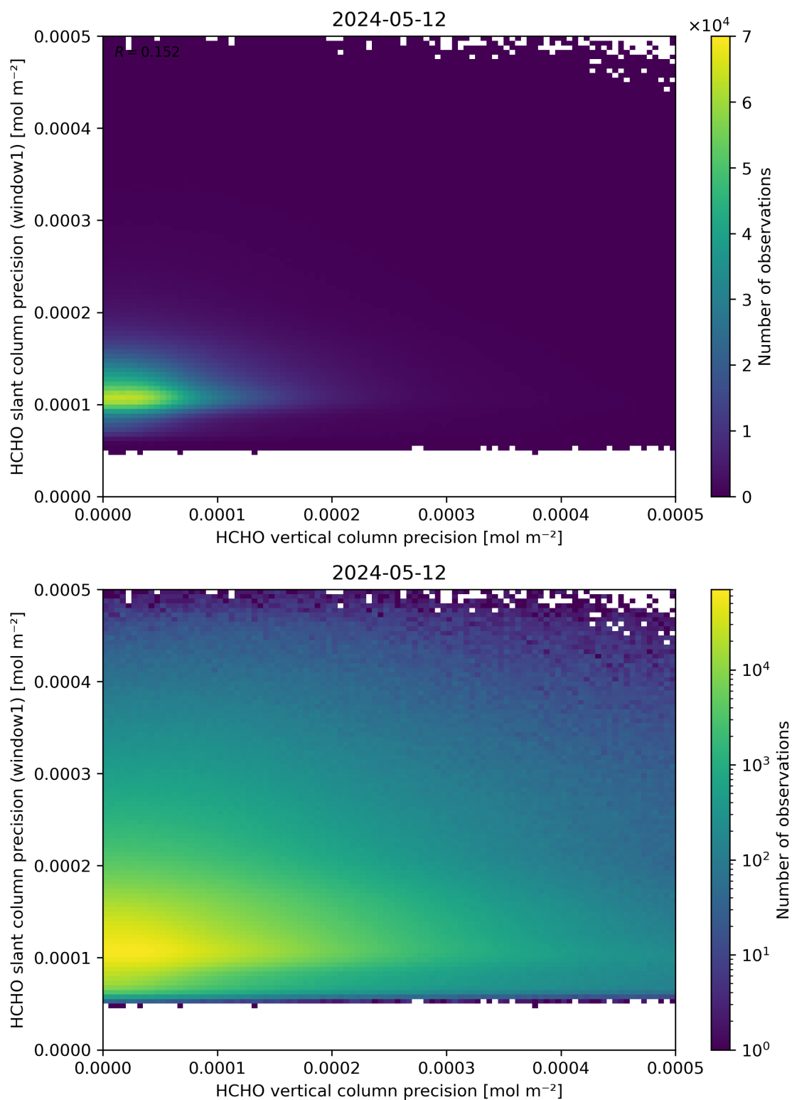
Figure 143: Scatter density plot of “HCHO vertical column precision” against “HCHO slant column precision (window1)” for 2024-05-12 to 2024-05-13.
