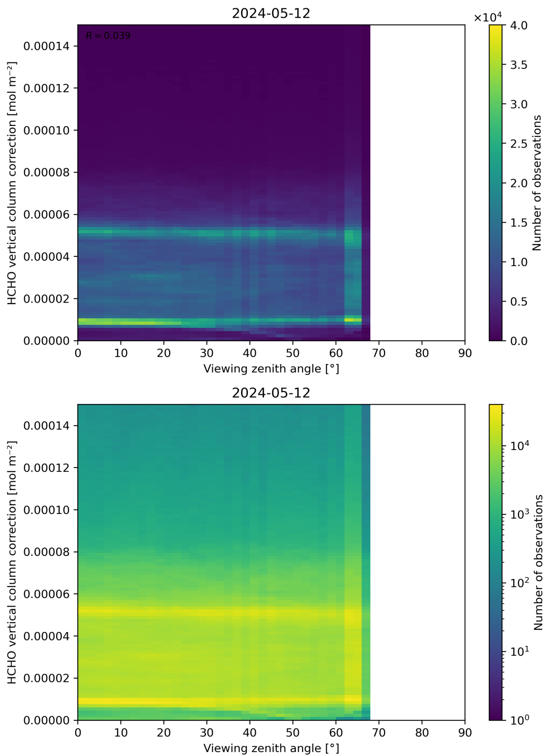
Figure 193: Scatter density plot of “Viewing zenith angle” against “HCHO vertical column correction” for 2024-05-12 to 2024-05-13.
