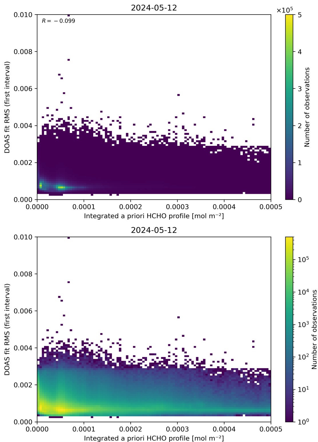
Figure 148: Scatter density plot of “Integrated a priori HCHO profile” against “DOAS fit RMS (first interval)” for 2024-05-12 to 2024-05-13.
