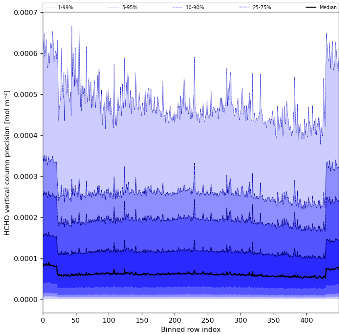
Figure 50: Along track statistics of “HCHO vertical column precision” for 2024-05-12 to 2024-05-13
