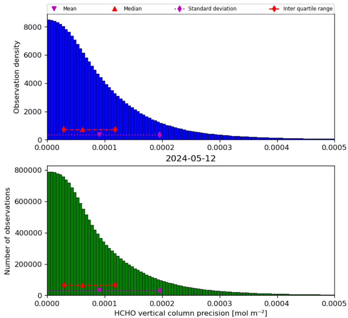
Figure 36: Histogram of “HCHO vertical column precision” for 2024-05-12 to 2024-05-13
