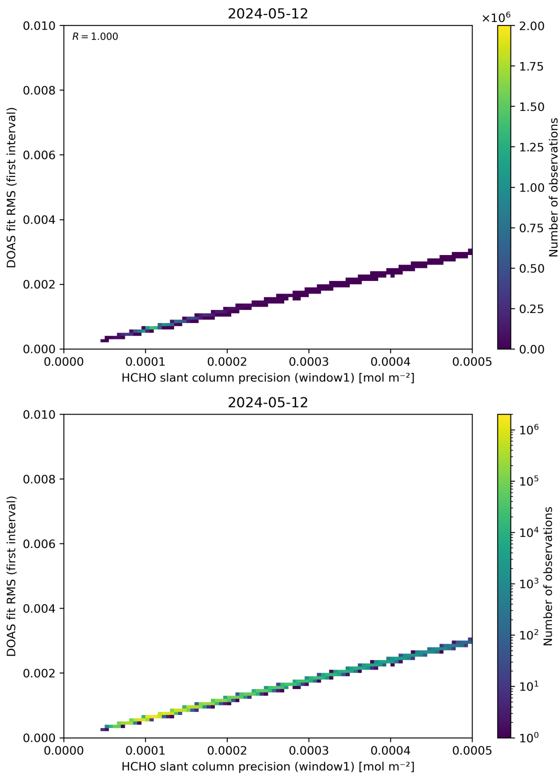
Figure 88: Scatter density plot of “HCHO slant column precision (window1)” against “DOAS fit RMS (first interval)” for 2024-05-12 to 2024-05-13.
