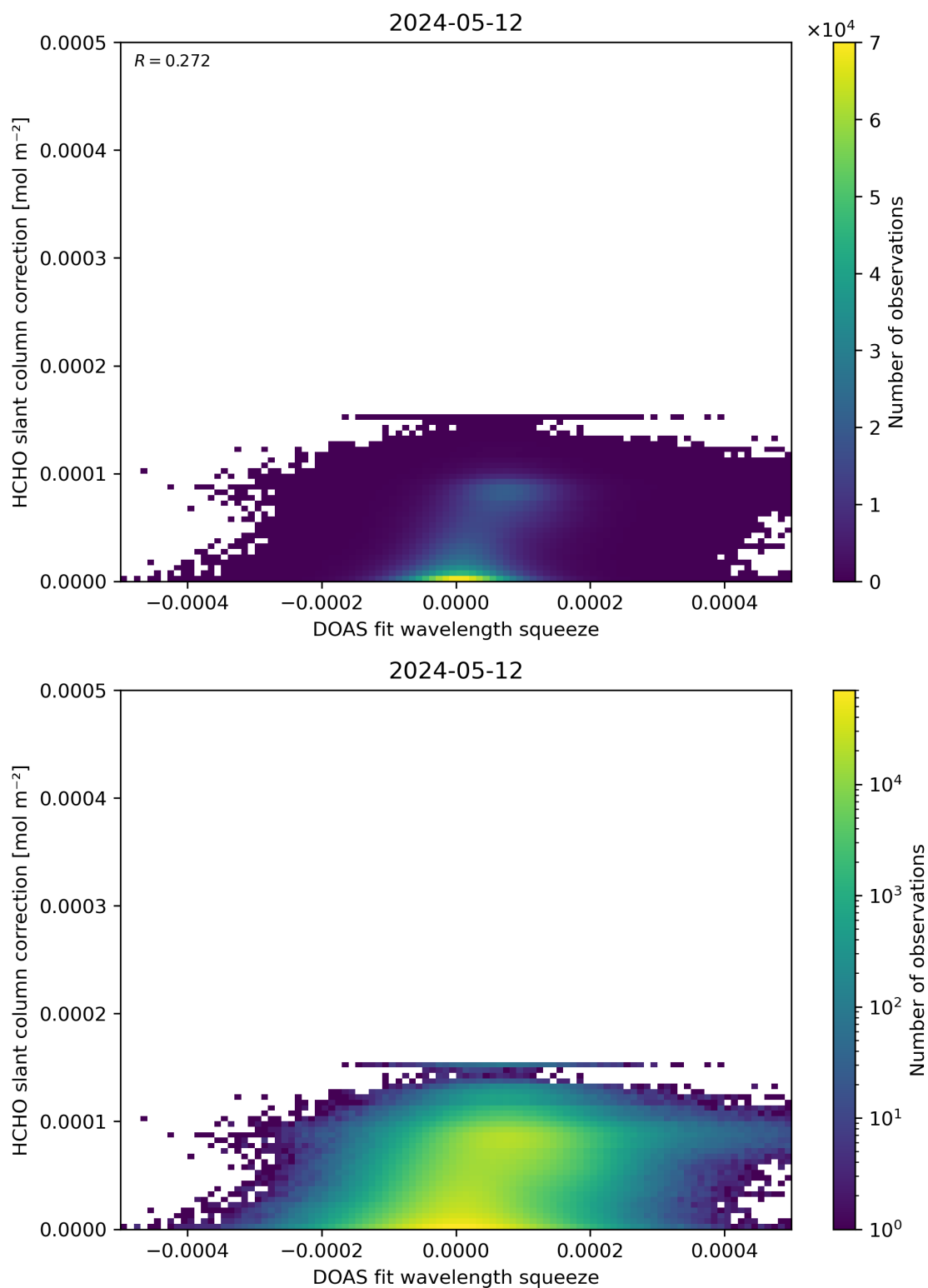
Figure 70: Scatter density plot of “DOAS fit wavelength squeeze” against “HCHO slant column correction” for 2024-05-12 to 2024-05-13.
