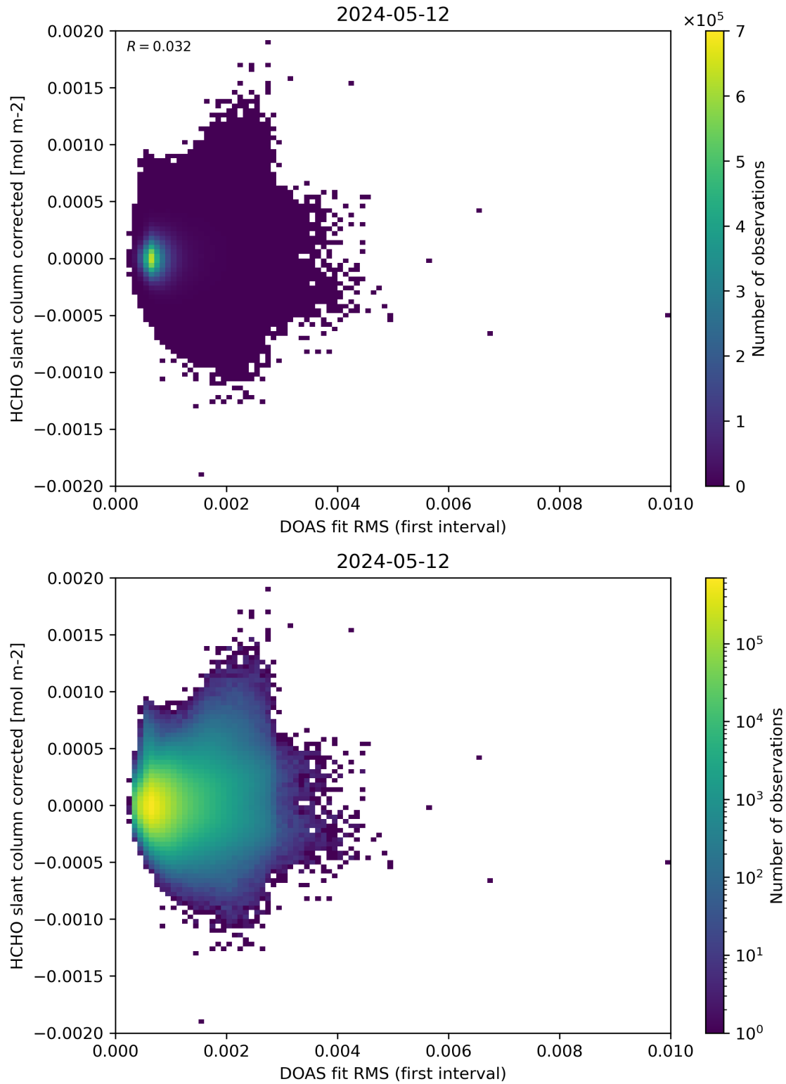
Figure 62: Scatter density plot of “DOAS fit RMS (first interval)” against “HCHO slant column corrected” for 2024-05-12 to 2024-05-13.
