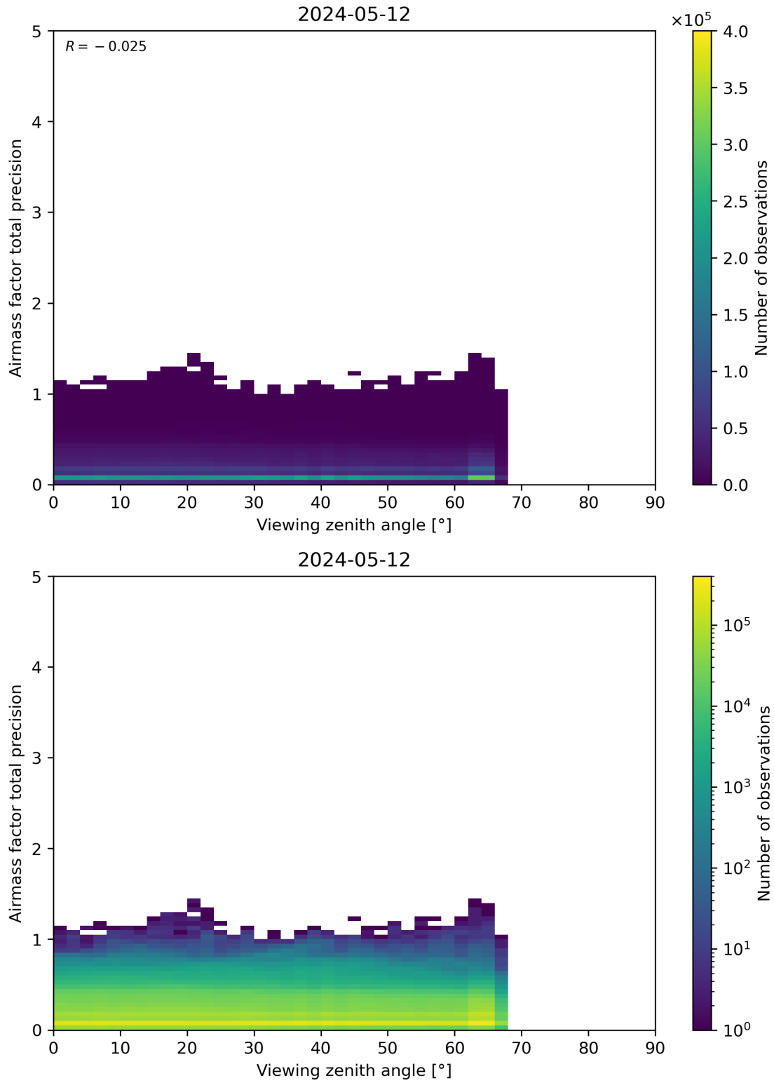
Figure 191: Scatter density plot of “Viewing zenith angle” against “Airmass factor total precision” for 2024-05-12 to 2024-05-13.
