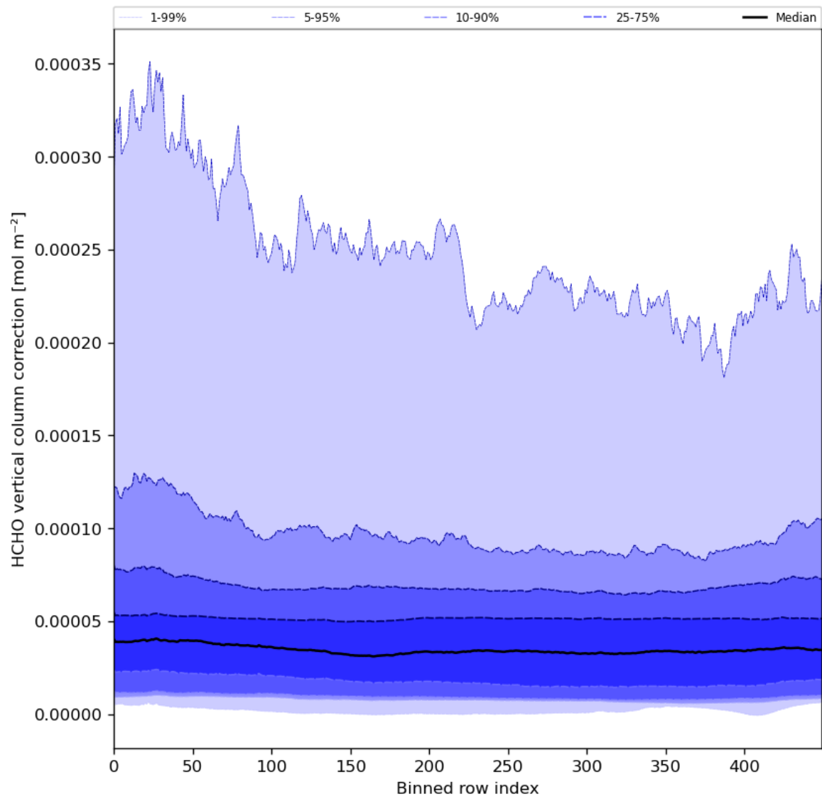
Figure 51: Along track statistics of “HCHO vertical column correction” for 2024-05-12 to 2024-05-13
