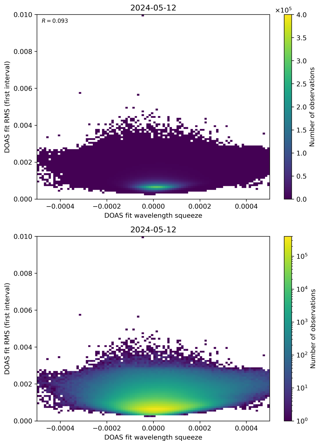
Figure 68: Scatter density plot of “DOAS fit wavelength squeeze” against “DOAS fit RMS (first interval)” for 2024-05-12 to 2024-05-13.
