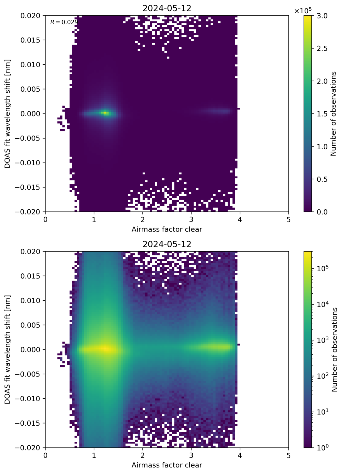
Figure 72: Scatter density plot of “Airmass factor clear” against “DOAS fit wavelength shift” for 2024-05-12 to 2024-05-13.
