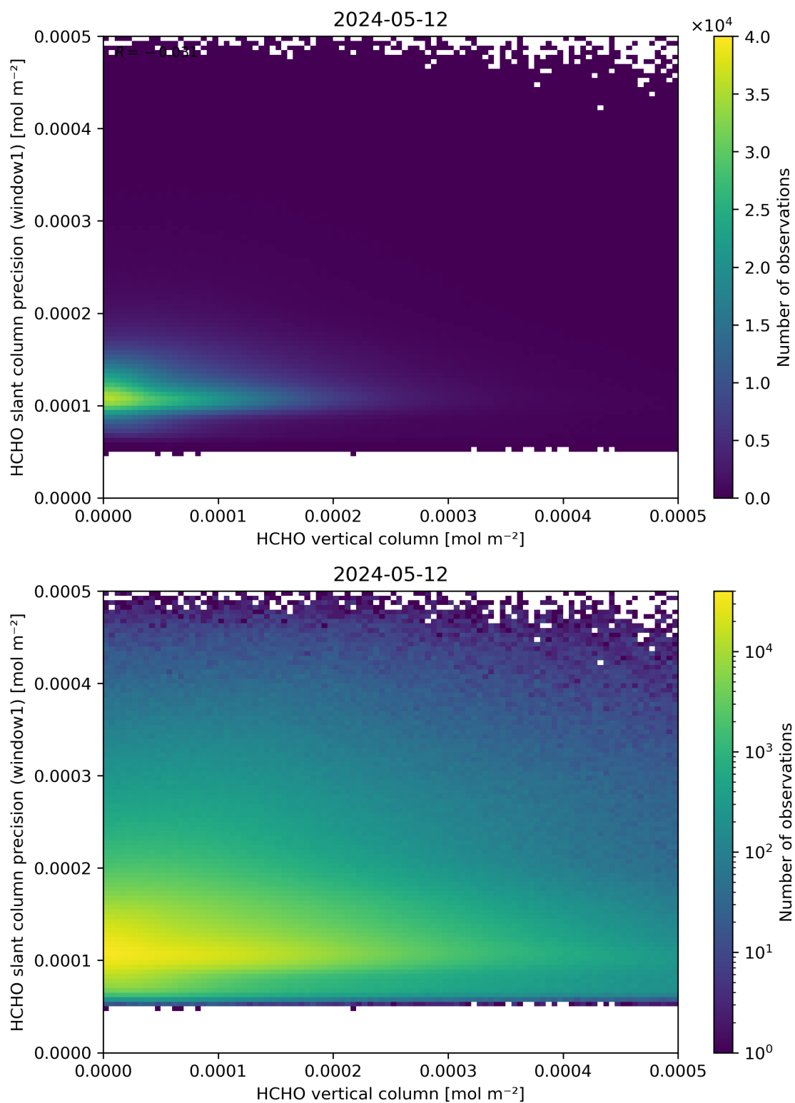
Figure 130: Scatter density plot of “HCHO vertical column” against “HCHO slant column precision (window1)” for 2024-05-12 to 2024-05-13.
