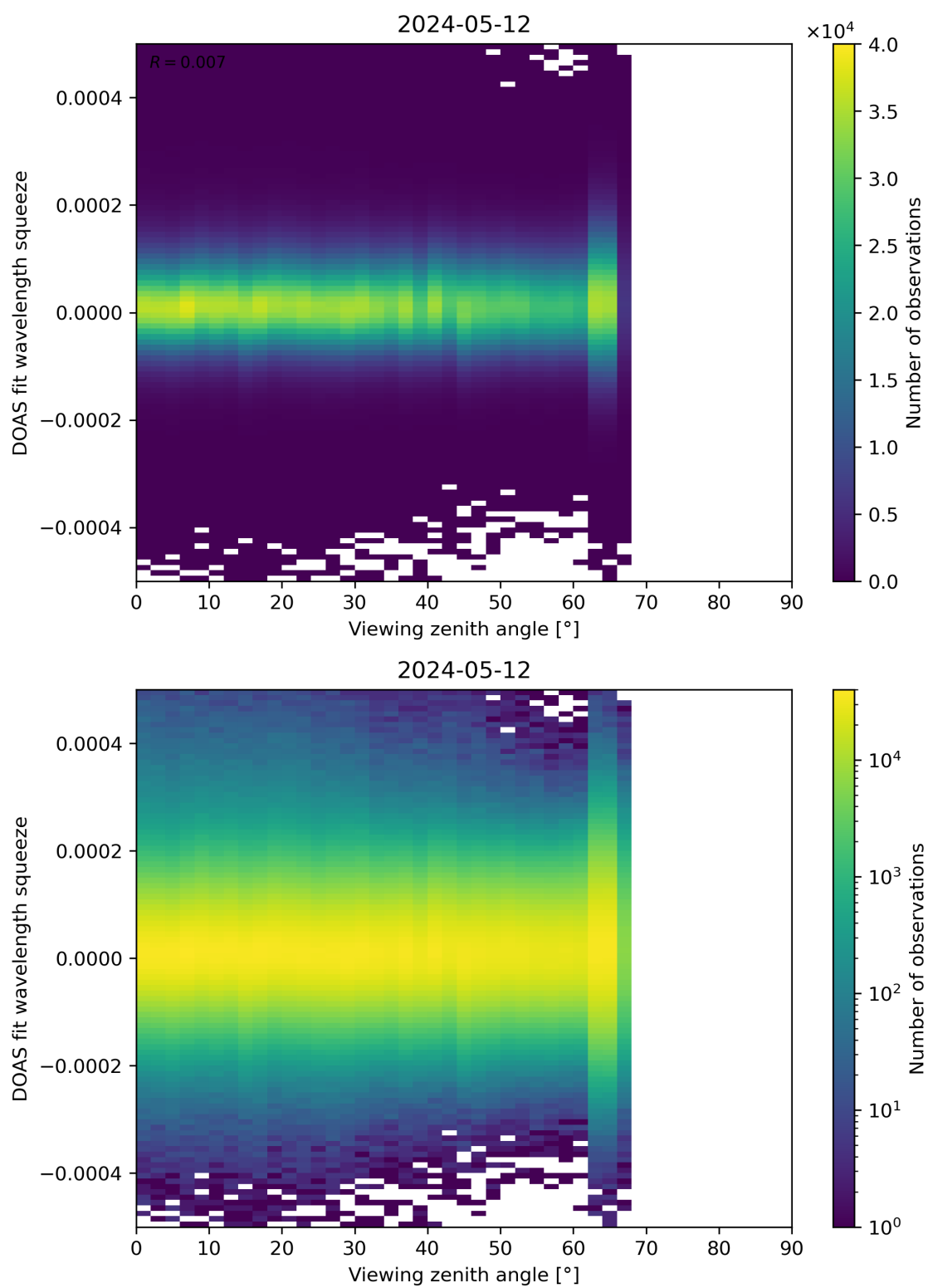
Figure 184: Scatter density plot of “Viewing zenith angle” against “DOAS fit wavelength squeeze” for 2024-05-12 to 2024-05-13.
