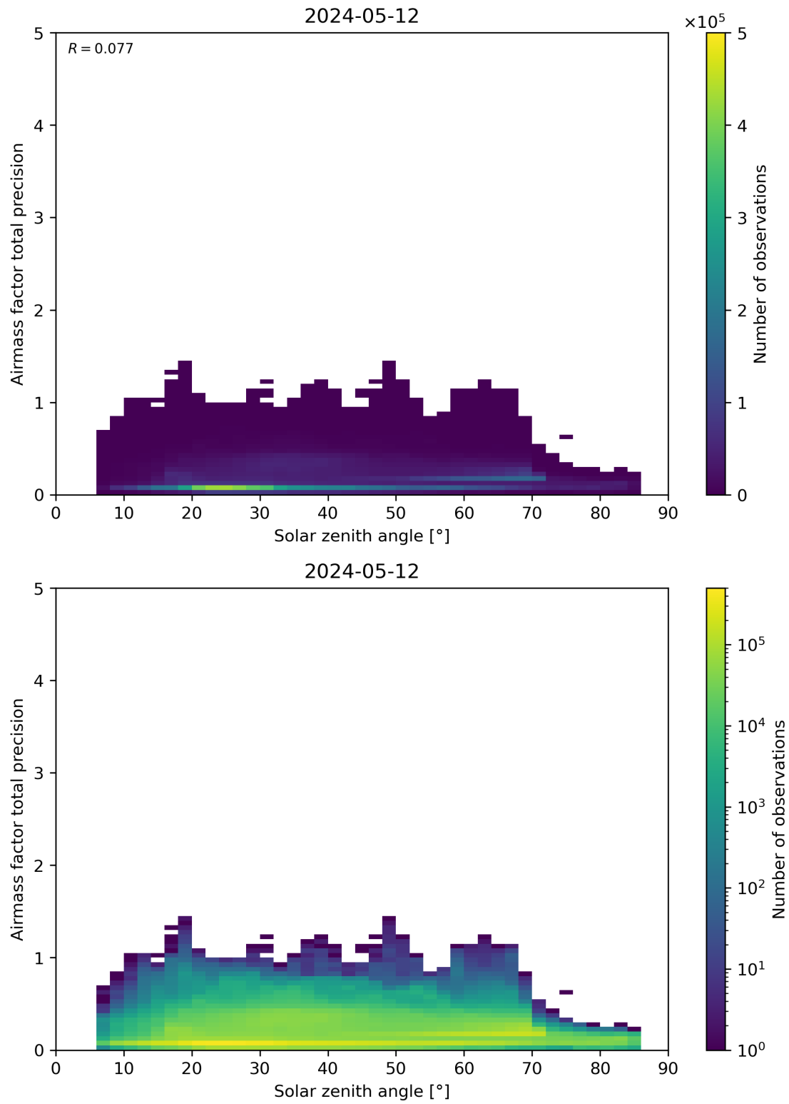
Figure 176: Scatter density plot of “Solar zenith angle” against “Airmass factor total precision” for 2024-05-12 to 2024-05-13.
