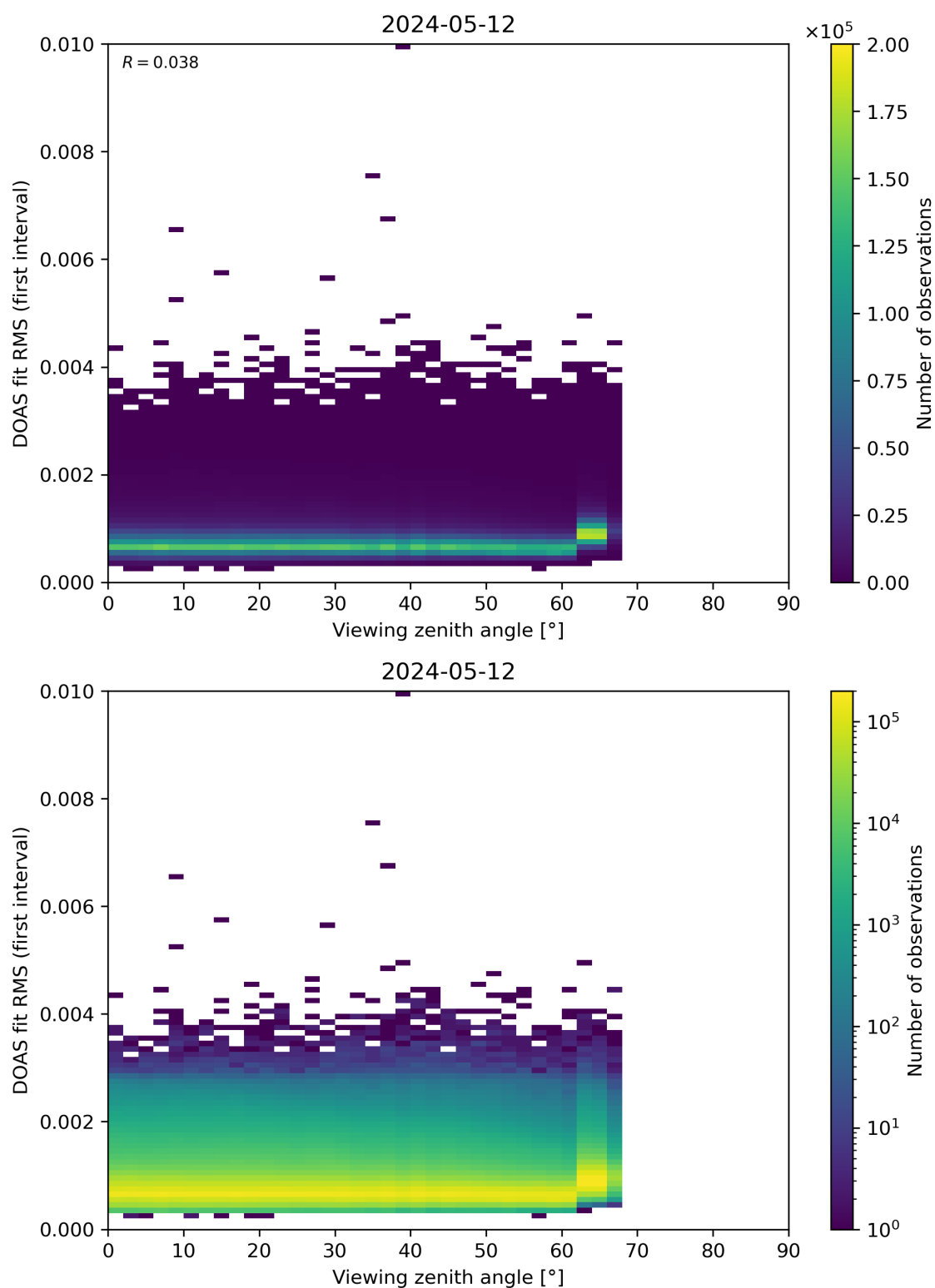
Figure 182: Scatter density plot of “Viewing zenith angle” against “DOAS fit RMS (first interval)” for 2024-05-12 to 2024-05-13.
