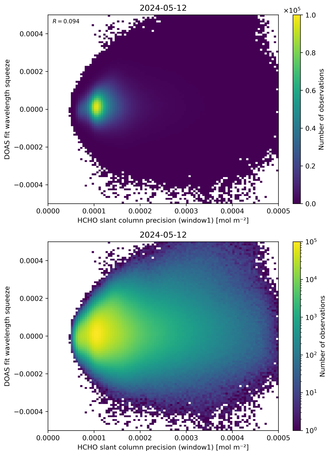
Figure 90: Scatter density plot of “HCHO slant column precision (window1)” against “DOAS fit wavelength squeeze” for 2024-05-12 to 2024-05-13.
