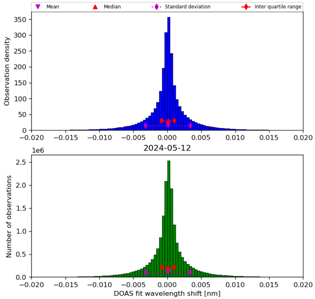
Figure 44: Histogram of “DOAS fit wavelength shift” for 2024-05-12 to 2024-05-13
