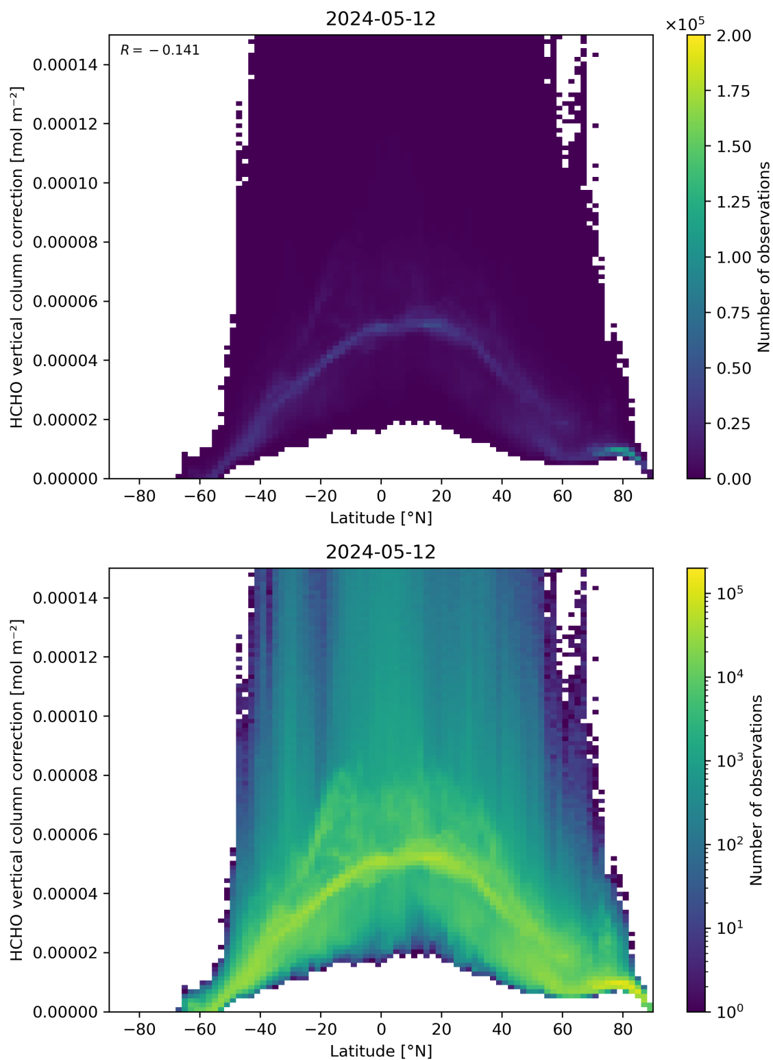
Figure 164: Scatter density plot of “Latitude” against “HCHO vertical column correction” for 2024-05-12 to 2024-05-13.
