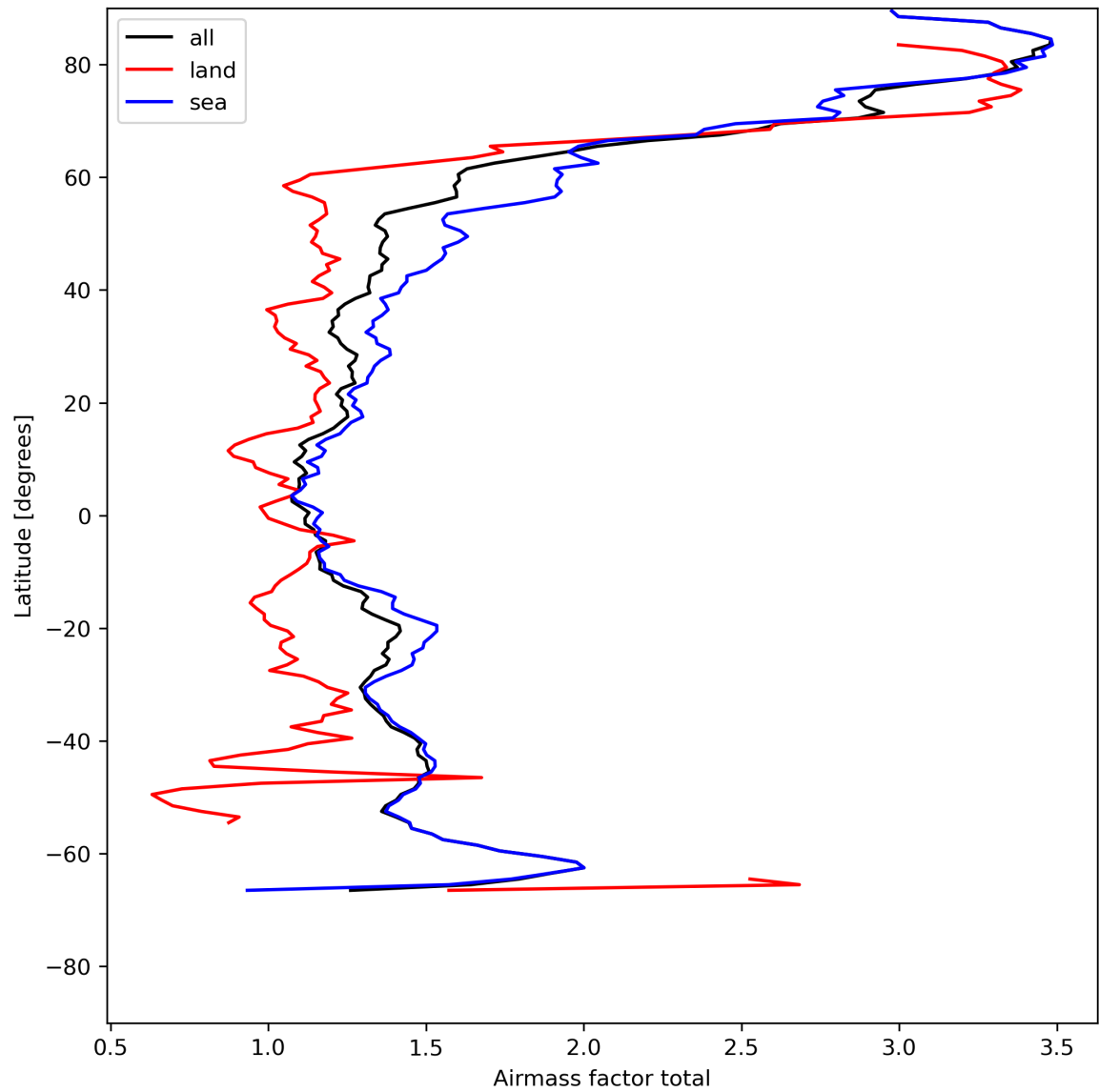
Figure 26: Zonal average of “Airmass factor total” for 2024-05-12 to 2024-05-13.
