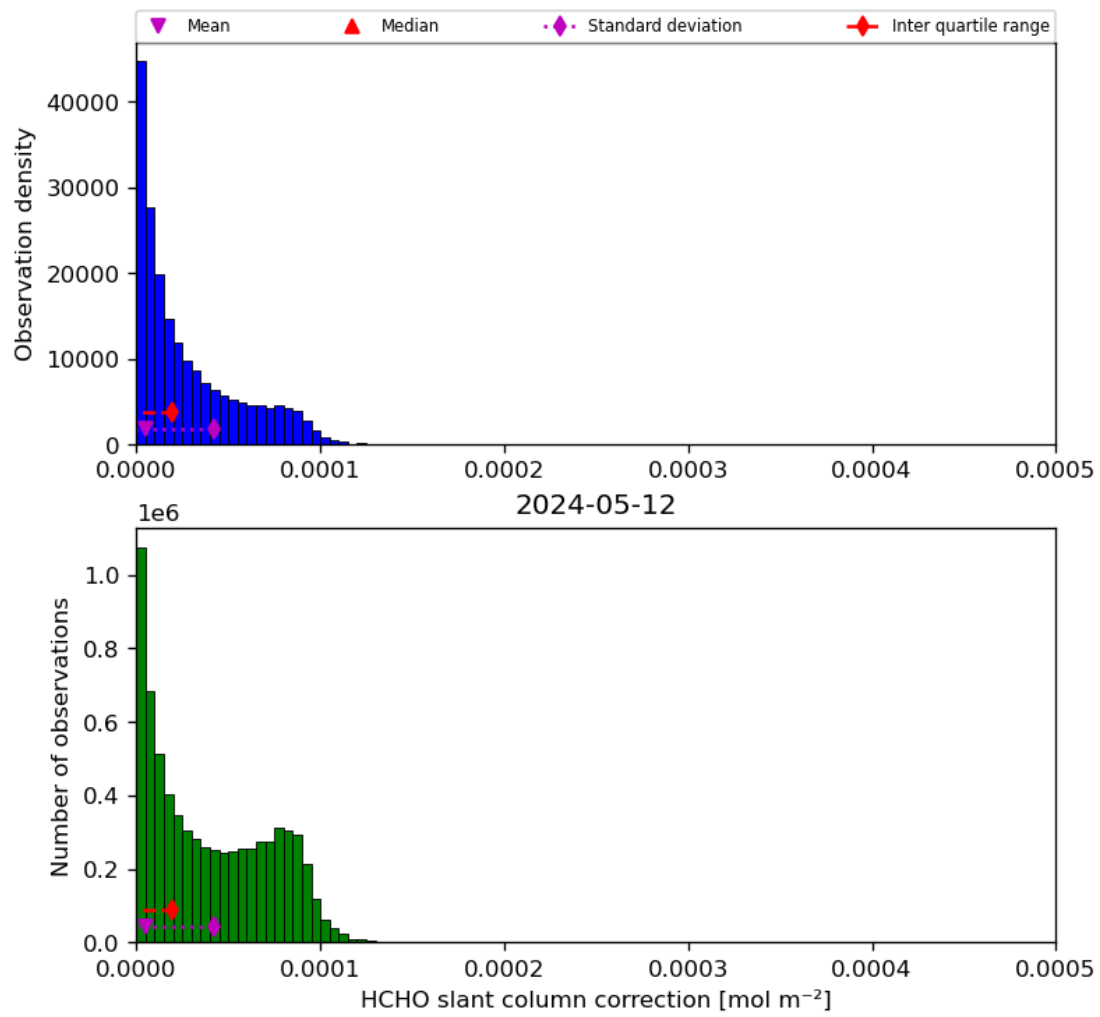
Figure 47: Histogram of “HCHO slant column correction” for 2024-05-12 to 2024-05-13
