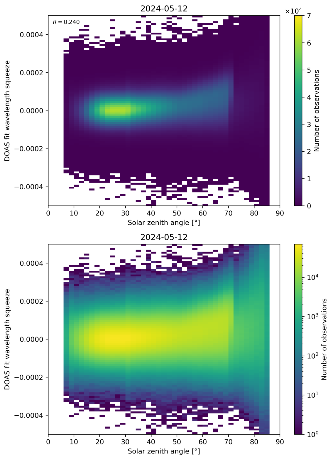
Figure 169: Scatter density plot of “Solar zenith angle” against “DOAS fit wavelength squeeze” for 2024-05-12 to 2024-05-13.
