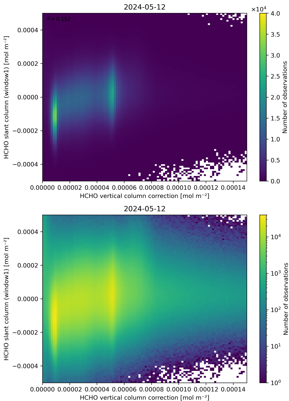
Figure 118: Scatter density plot of “HCHO vertical column correction” against “HCHO slant column (window1)” for 2024-05-12 to 2024-05-13.
