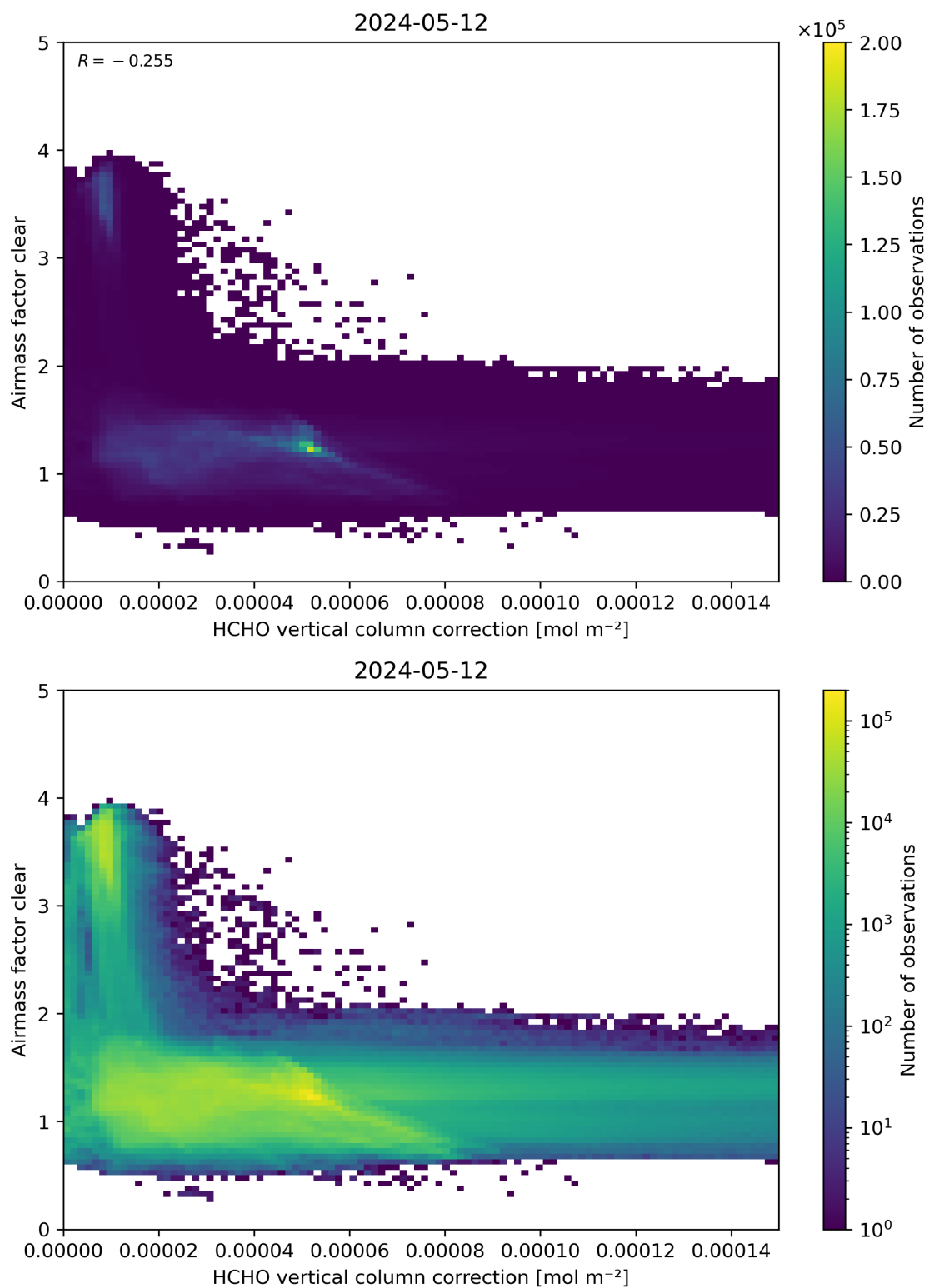
Figure 115: Scatter density plot of “HCHO vertical column correction” against “Airmass factor clear” for 2024-05-12 to 2024-05-13.
