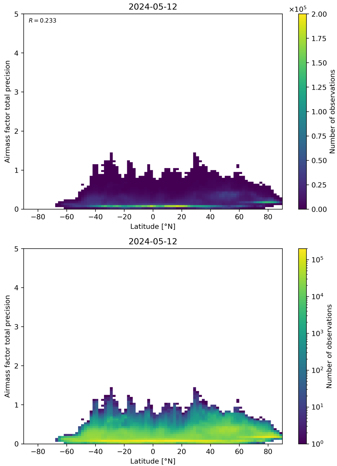
Figure 162: Scatter density plot of “Latitude” against “Airmass factor total precision” for 2024-05-12 to 2024-05-13.
