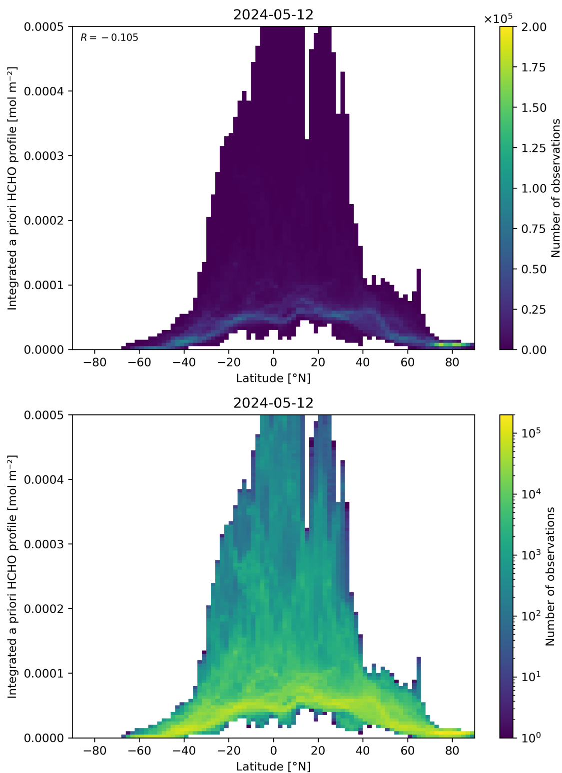
Figure 166: Scatter density plot of “Latitude” against “Integrated a priori HCHO profile” for 2024-05-12 to 2024-05-13.
