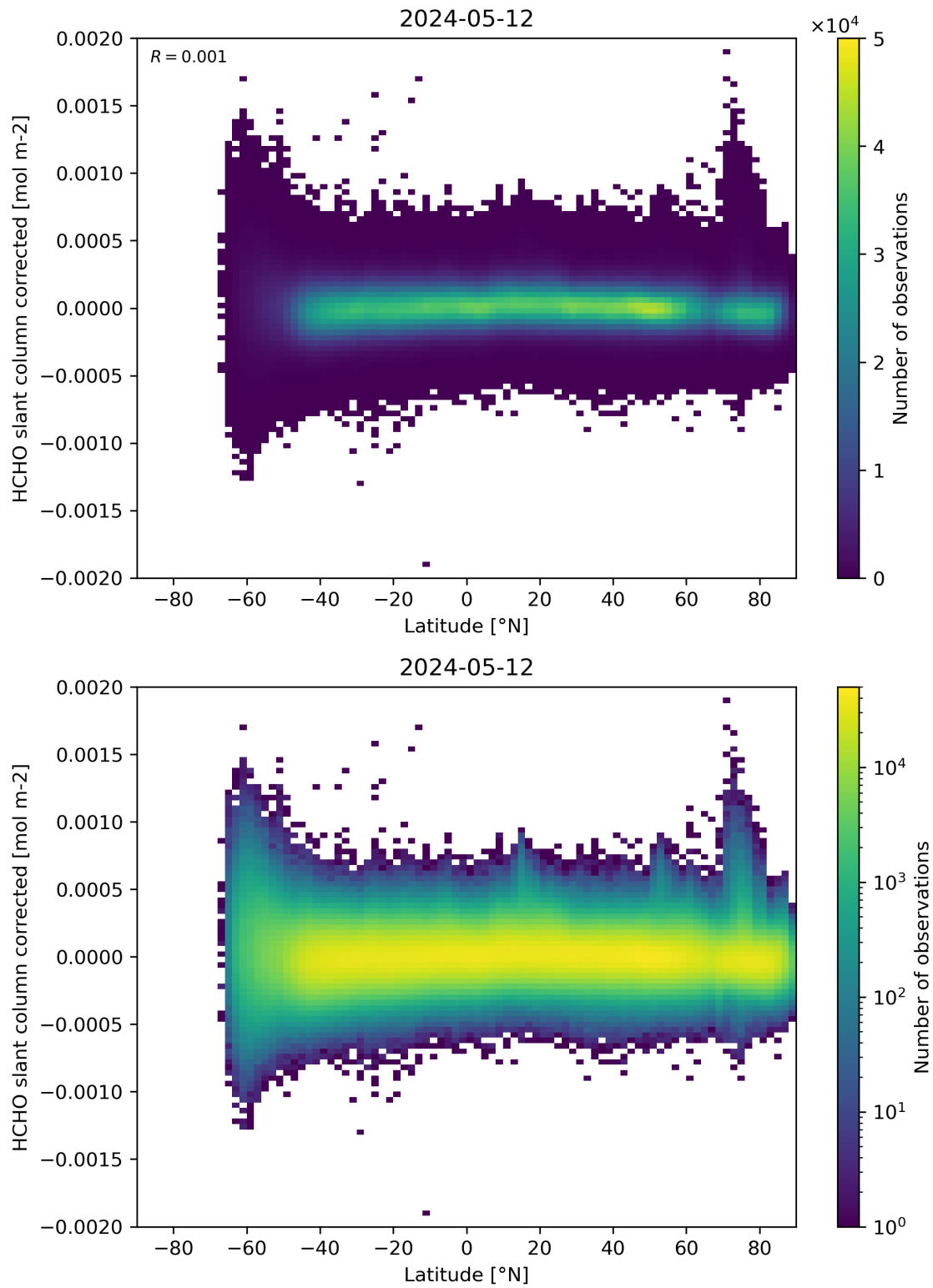
Figure 157: Scatter density plot of “Latitude” against “HCHO slant column corrected” for 2024-05-12 to 2024-05-13.
