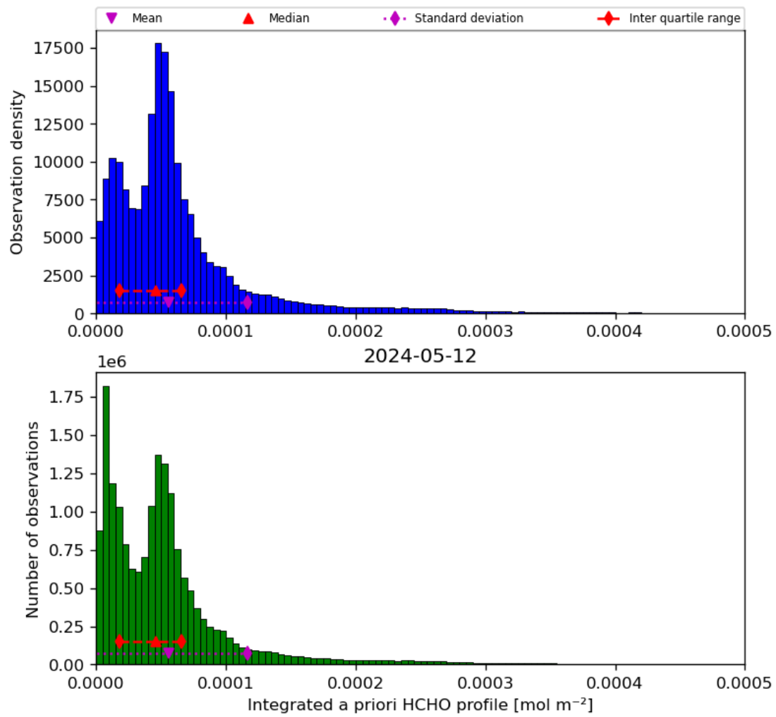
Figure 43: Histogram of “Integrated a priori HCHO profile” for 2024-05-12 to 2024-05-13
