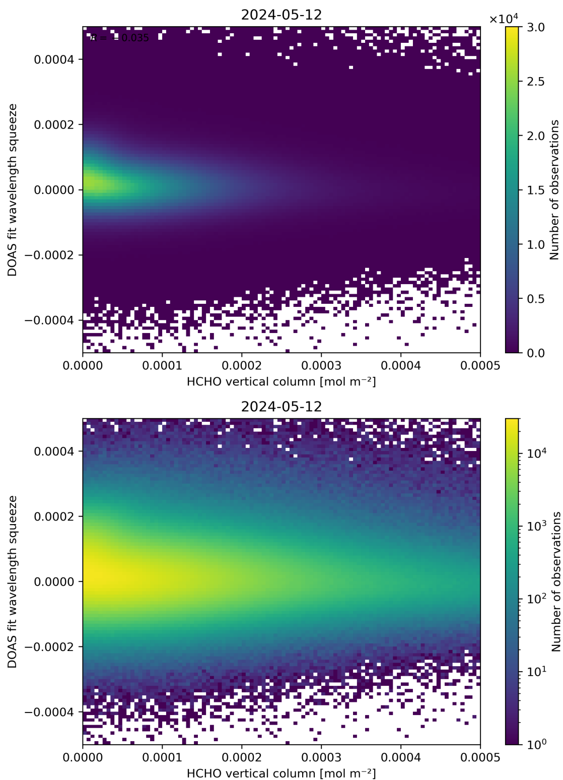
Figure 125: Scatter density plot of “HCHO vertical column” against “DOAS fit wavelength squeeze” for 2024-05-12 to 2024-05-13.
