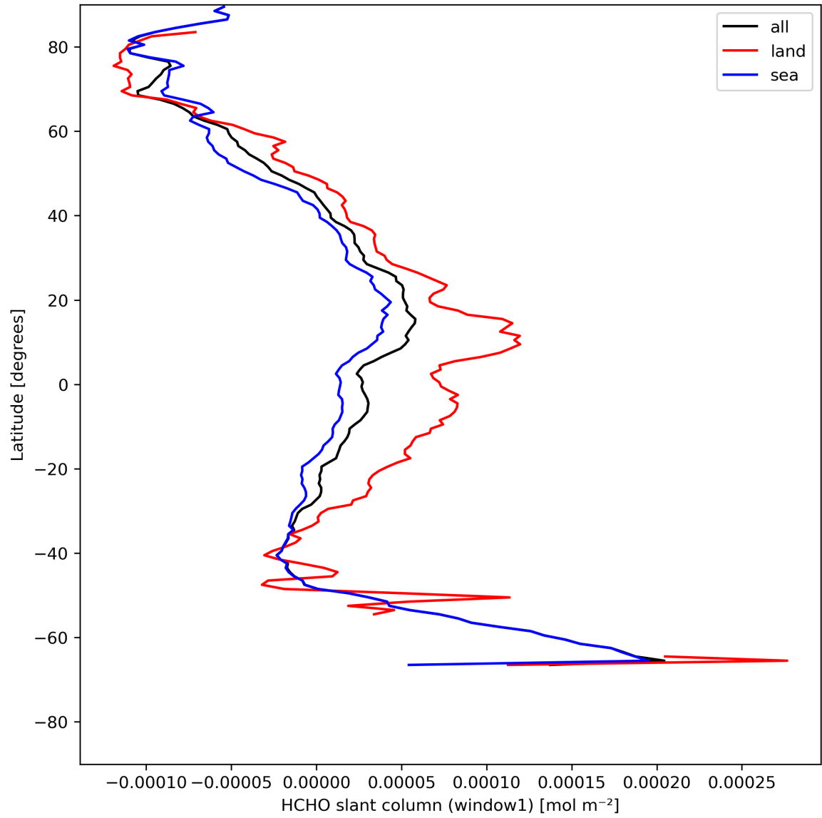
Figure 24: Zonal average of “HCHO slant column (window1)” for 2024-05-12 to 2024-05-13.
