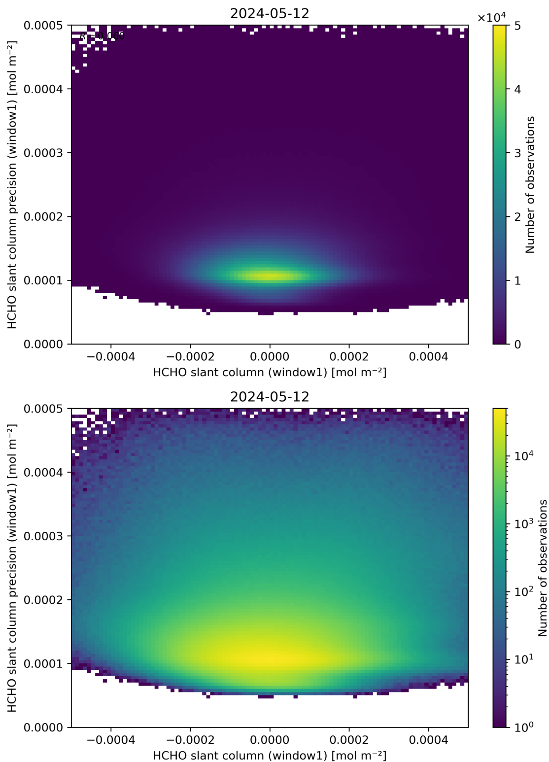
Figure 84: Scatter density plot of “HCHO slant column (window1)” against “HCHO slant column precision (window1)” for 2024-05-12 to 2024-05-13.
