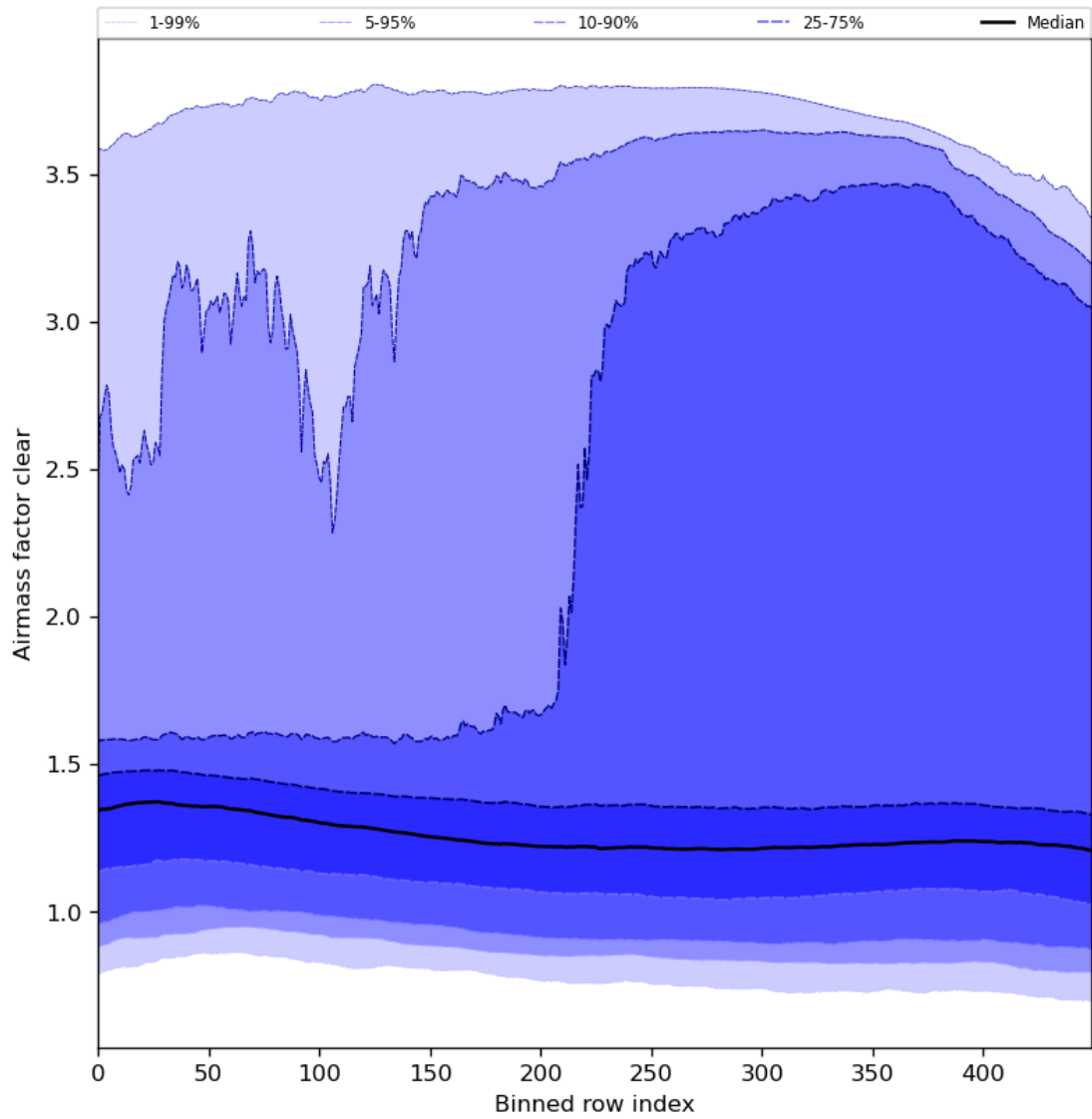
Figure 56: Along track statistics of “Airmass factor clear” for 2024-05-12 to 2024-05-13
