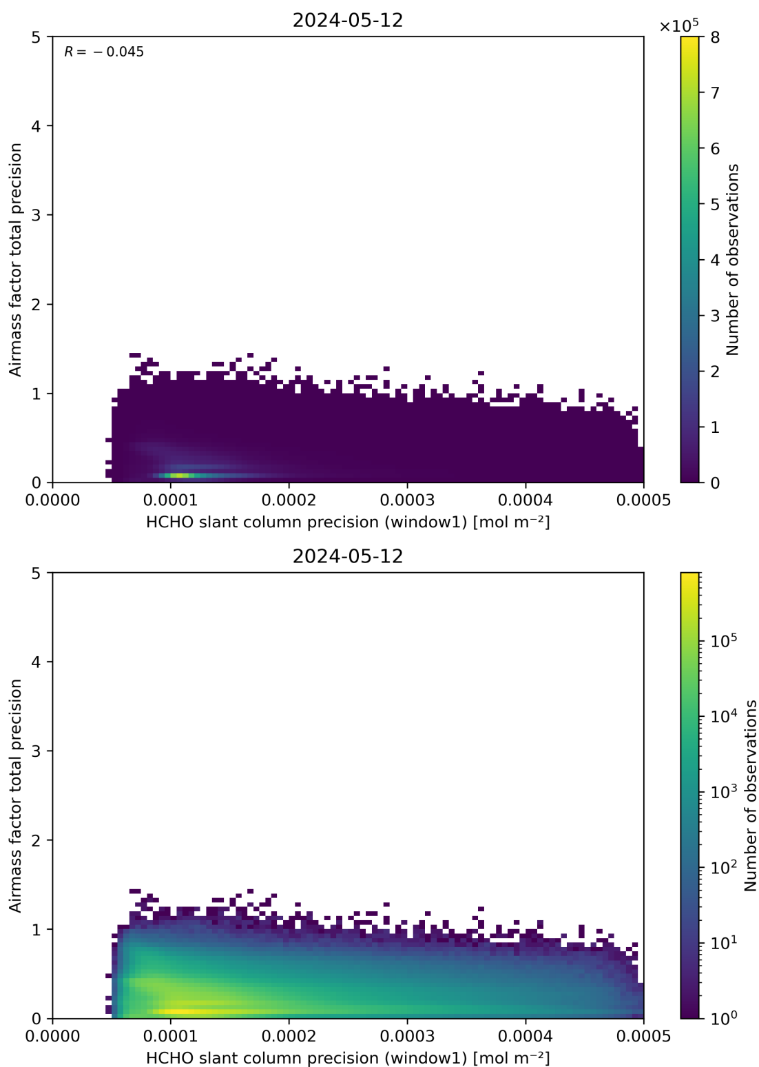
Figure 95: Scatter density plot of “HCHO slant column precision (window1)” against “Airmass factor total precision” for 2024-05-12 to 2024-05-13.
