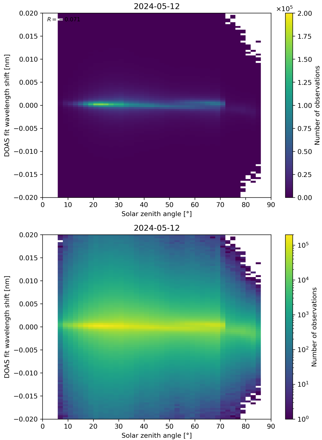
Figure 168: Scatter density plot of “Solar zenith angle” against “DOAS fit wavelength shift” for 2024-05-12 to 2024-05-13.
