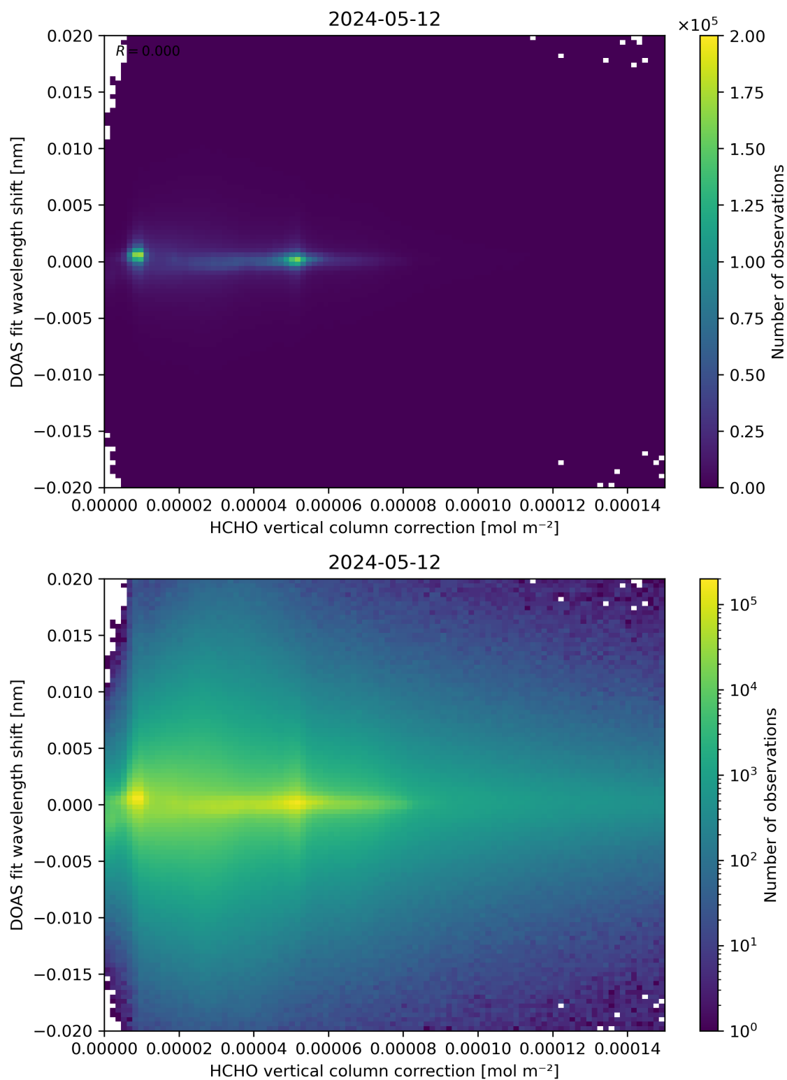
Figure 113: Scatter density plot of “HCHO vertical column correction” against “DOAS fit wavelength shift” for 2024-05-12 to 2024-05-13.
