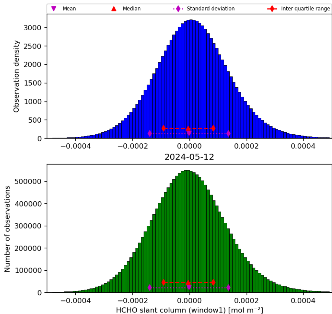
Figure 38: Histogram of “HCHO slant column (window1)” for 2024-05-12 to 2024-05-13
