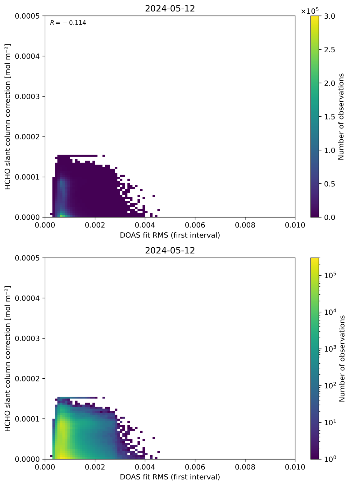
Figure 63: Scatter density plot of “DOAS fit RMS (first interval)” against “HCHO slant column correction” for 2024-05-12 to 2024-05-13.
