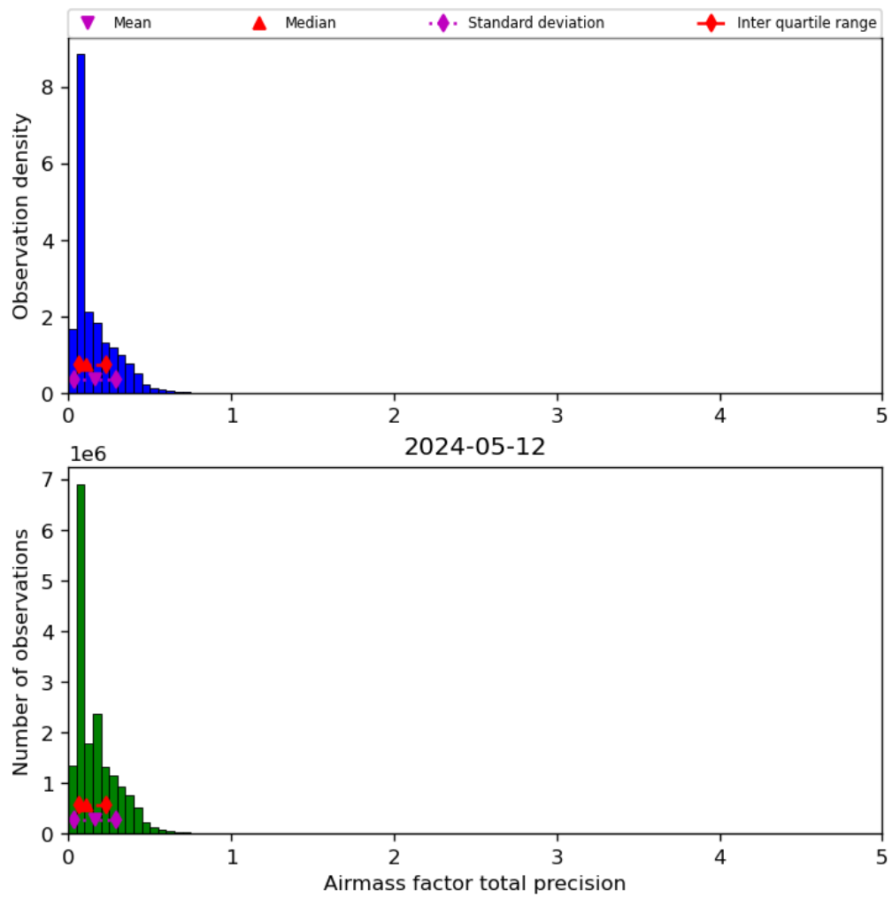
Figure 41: Histogram of “Airmass factor total precision” for 2024-05-12 to 2024-05-13
