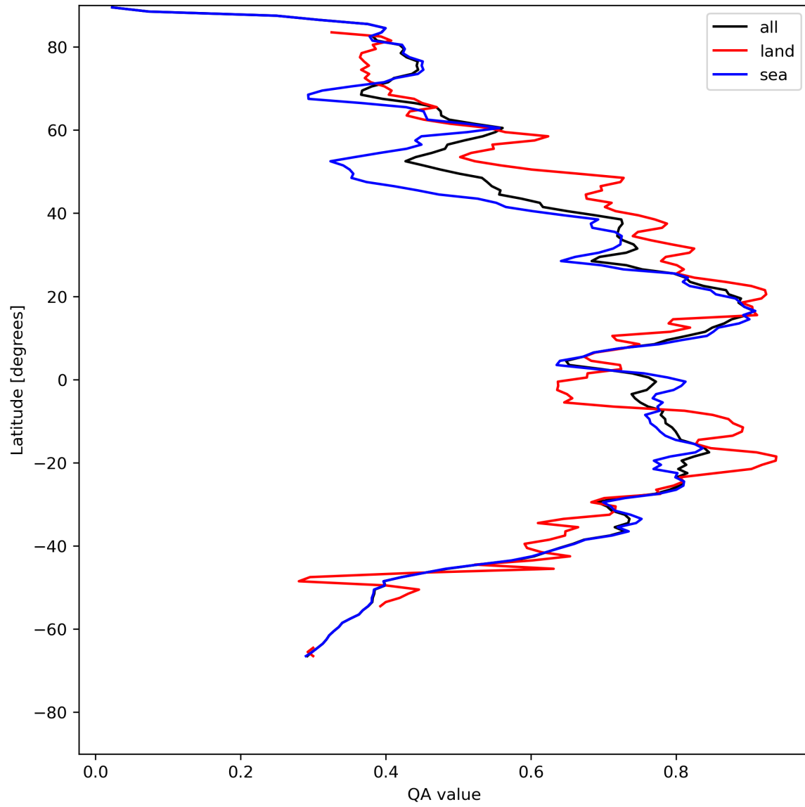
Figure 20: Zonal average of “QA value” for 2024-05-12 to 2024-05-13.
