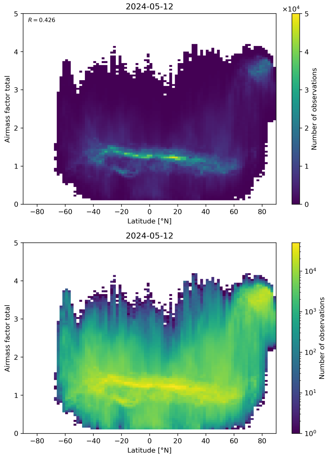
Figure 161: Scatter density plot of “Latitude” against “Airmass factor total” for 2024-05-12 to 2024-05-13.
