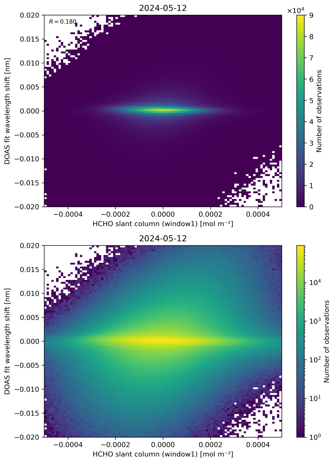
Figure 79: Scatter density plot of “HCHO slant column (window1)” against “DOAS fit wavelength shift” for 2024-05-12 to 2024-05-13.
