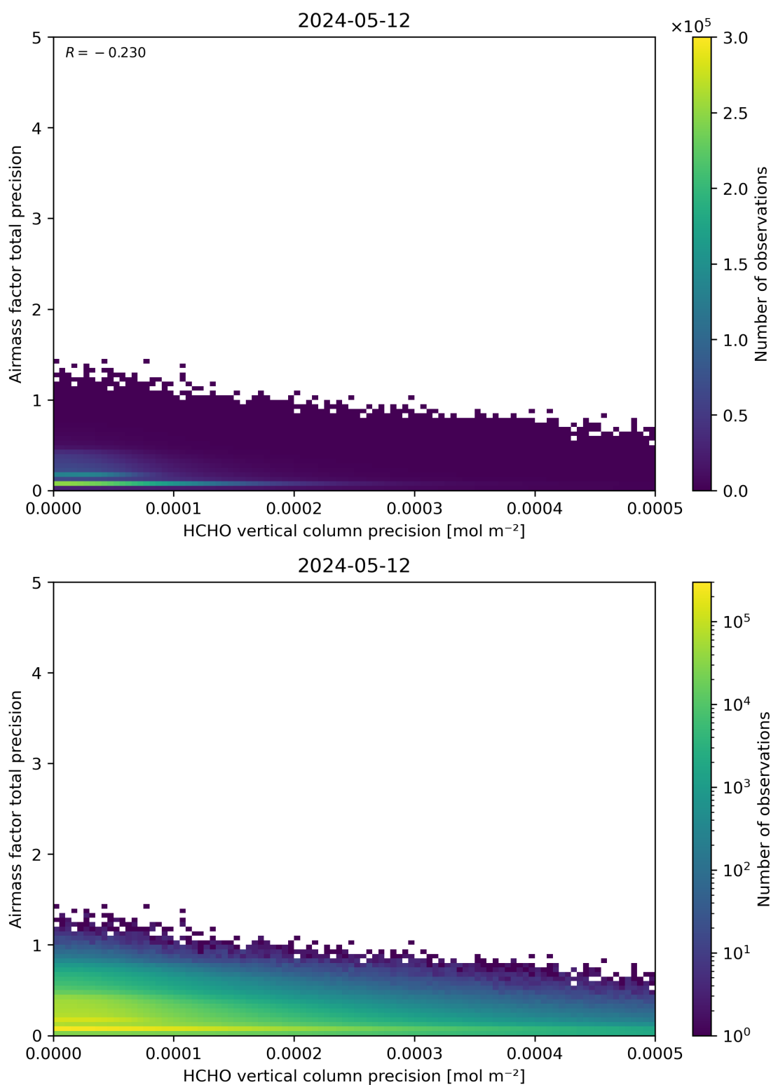
Figure 145: Scatter density plot of “HCHO vertical column precision” against “Airmass factor total precision” for 2024-05-12 to 2024-05-13.
