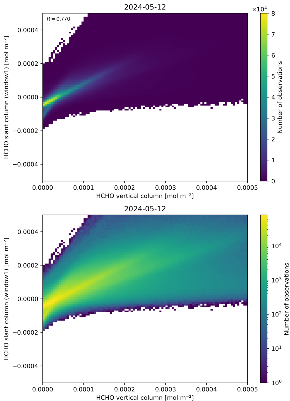
Figure 129: Scatter density plot of “HCHO vertical column” against “HCHO slant column (window1)” for 2024-05-12 to 2024-05-13.
