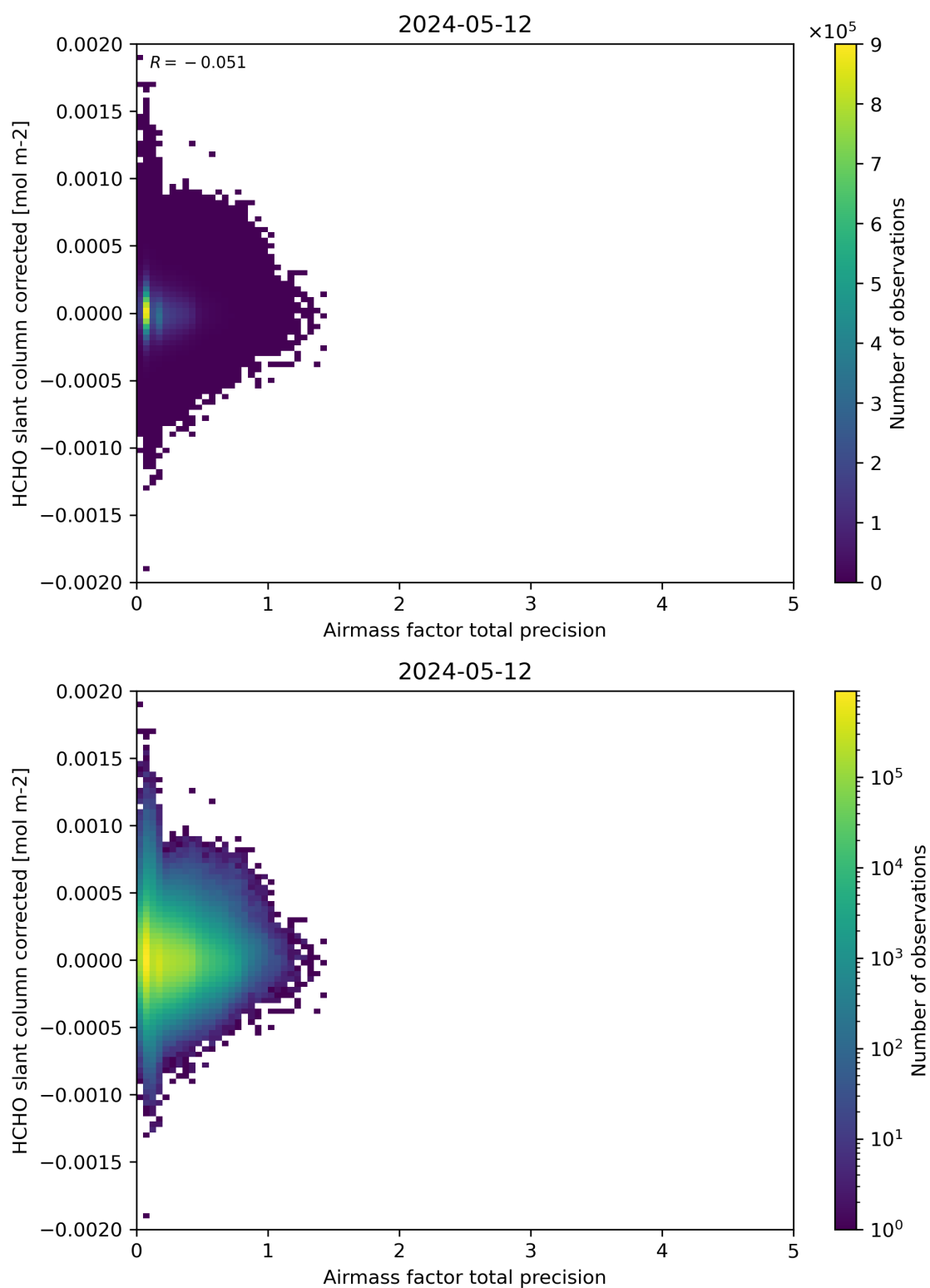
Figure 109: Scatter density plot of “Airmass factor total precision” against “HCHO slant column corrected” for 2024-05-12 to 2024-05-13.
