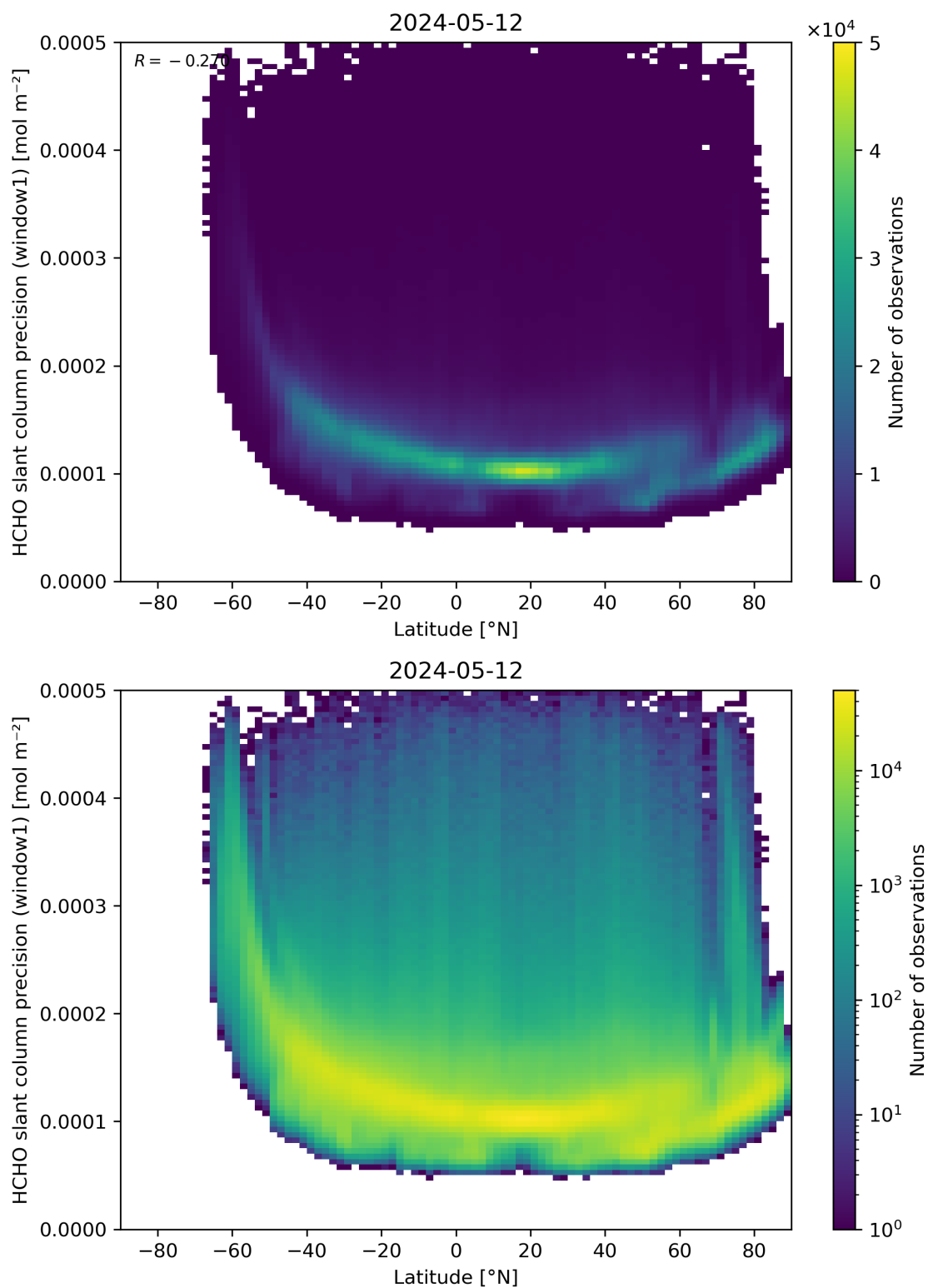
Figure 160: Scatter density plot of “Latitude” against “HCHO slant column precision (window1)” for 2024-05-12 to 2024-05-13.
