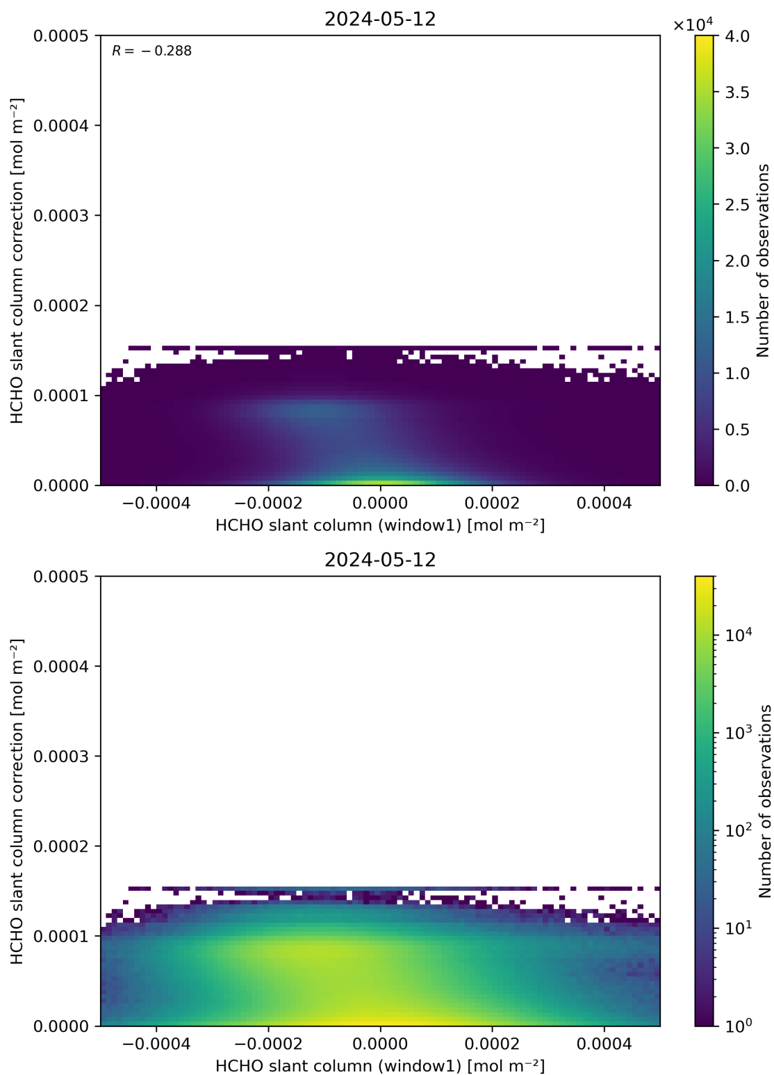
Figure 83: Scatter density plot of “HCHO slant column (window1)” against “HCHO slant column correction” for 2024-05-12 to 2024-05-13.
