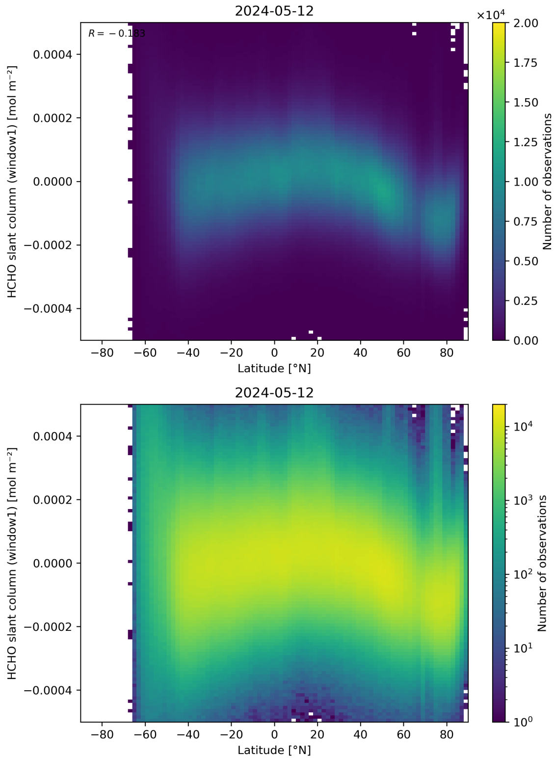
Figure 159: Scatter density plot of “Latitude” against “HCHO slant column (window1)” for 2024-05-12 to 2024-05-13.
