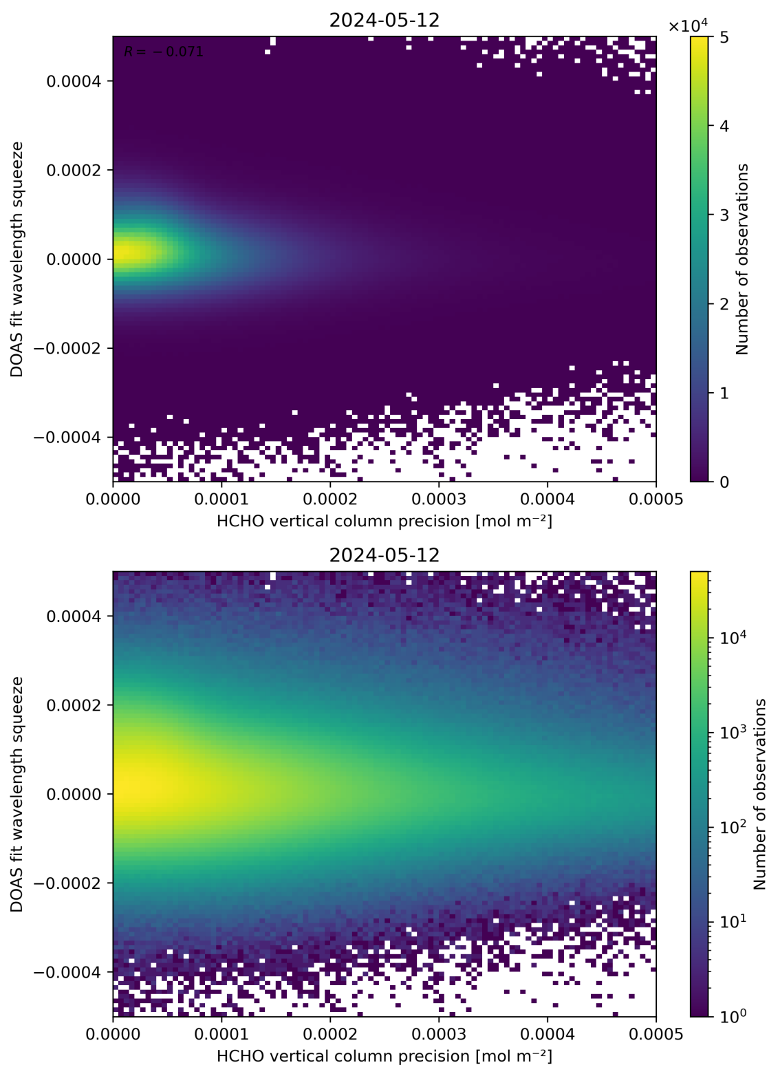
Figure 138: Scatter density plot of “HCHO vertical column precision” against “DOAS fit wavelength squeeze” for 2024-05-12 to 2024-05-13.
