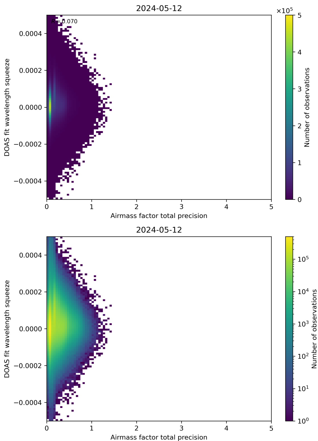
Figure 107: Scatter density plot of “Airmass factor total precision” against “DOAS fit wavelength squeeze” for 2024-05-12 to 2024-05-13.
