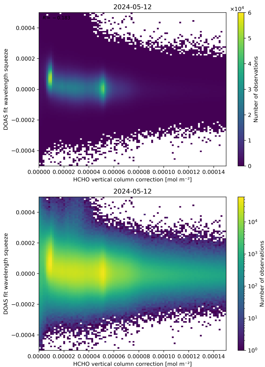
Figure 114: Scatter density plot of “HCHO vertical column correction” against “DOAS fit wavelength squeeze” for 2024-05-12 to 2024-05-13.
