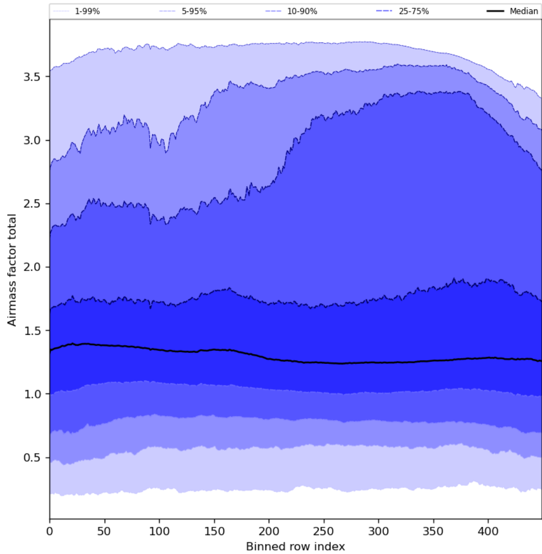
Figure 54: Along track statistics of “Airmass factor total” for 2024-05-12 to 2024-05-13
