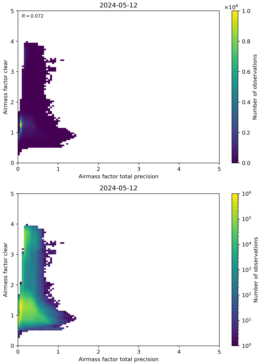
Figure 108: Scatter density plot of “Airmass factor total precision” against “Airmass factor clear” for 2024-05-12 to 2024-05-13.
