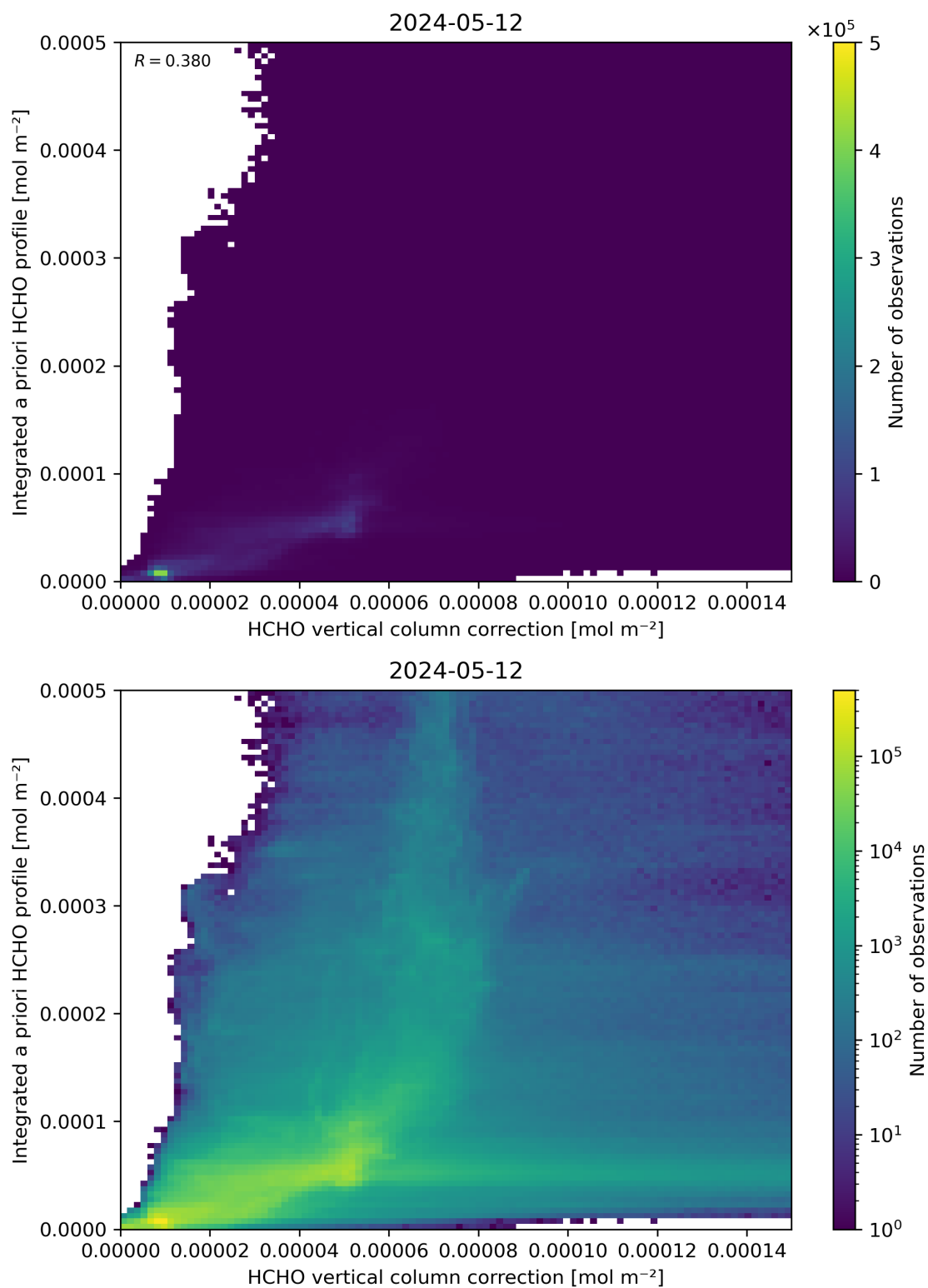
Figure 122: Scatter density plot of “HCHO vertical column correction” against “Integrated a priori HCHO profile” for 2024-05-12 to 2024-05-13.
