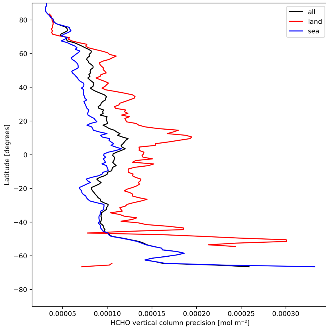
Figure 22: Zonal average of “HCHO vertical column precision” for 2024-05-12 to 2024-05-13.
