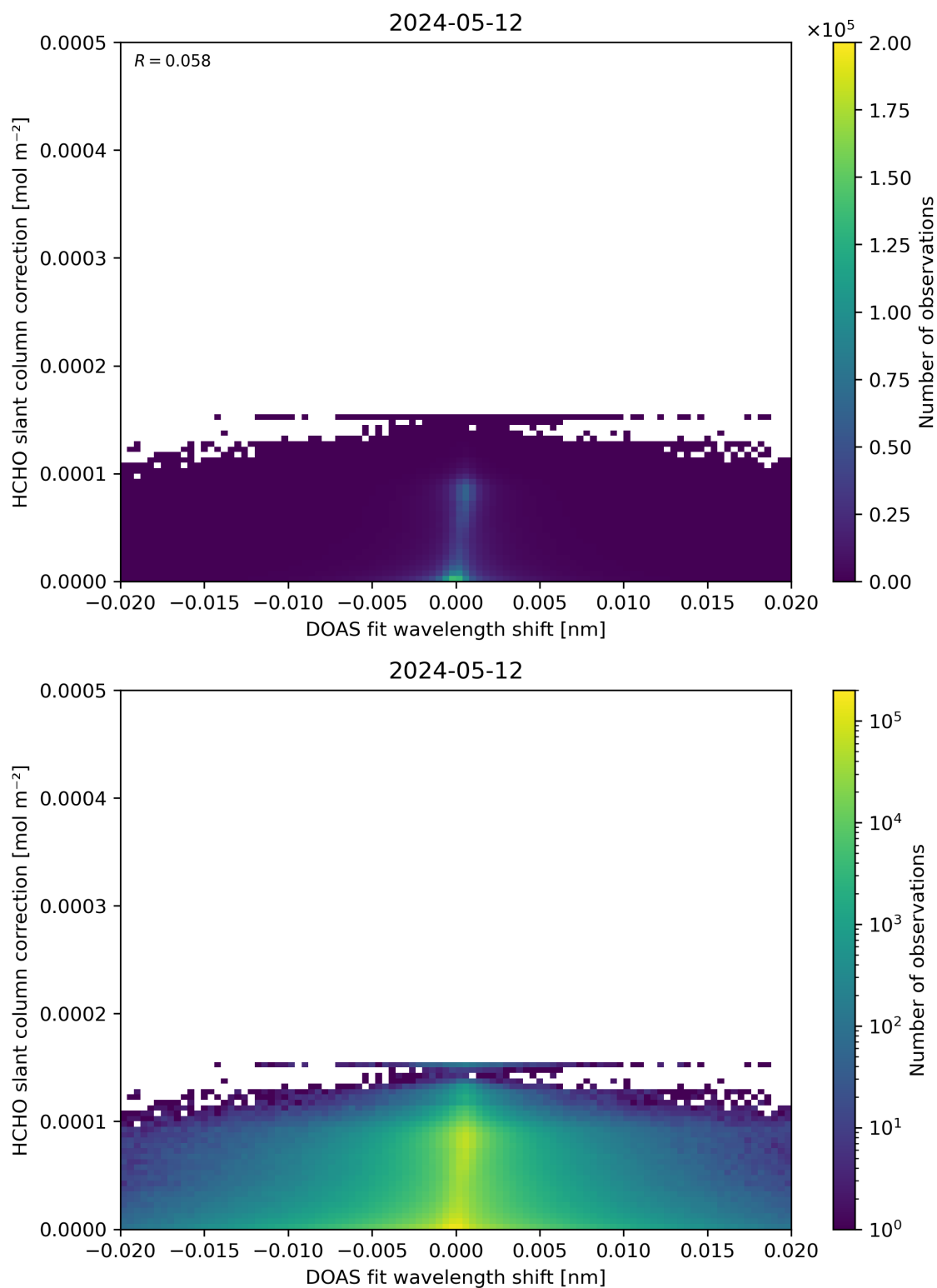
Figure 67: Scatter density plot of “DOAS fit wavelength shift” against “HCHO slant column correction” for 2024-05-12 to 2024-05-13.
