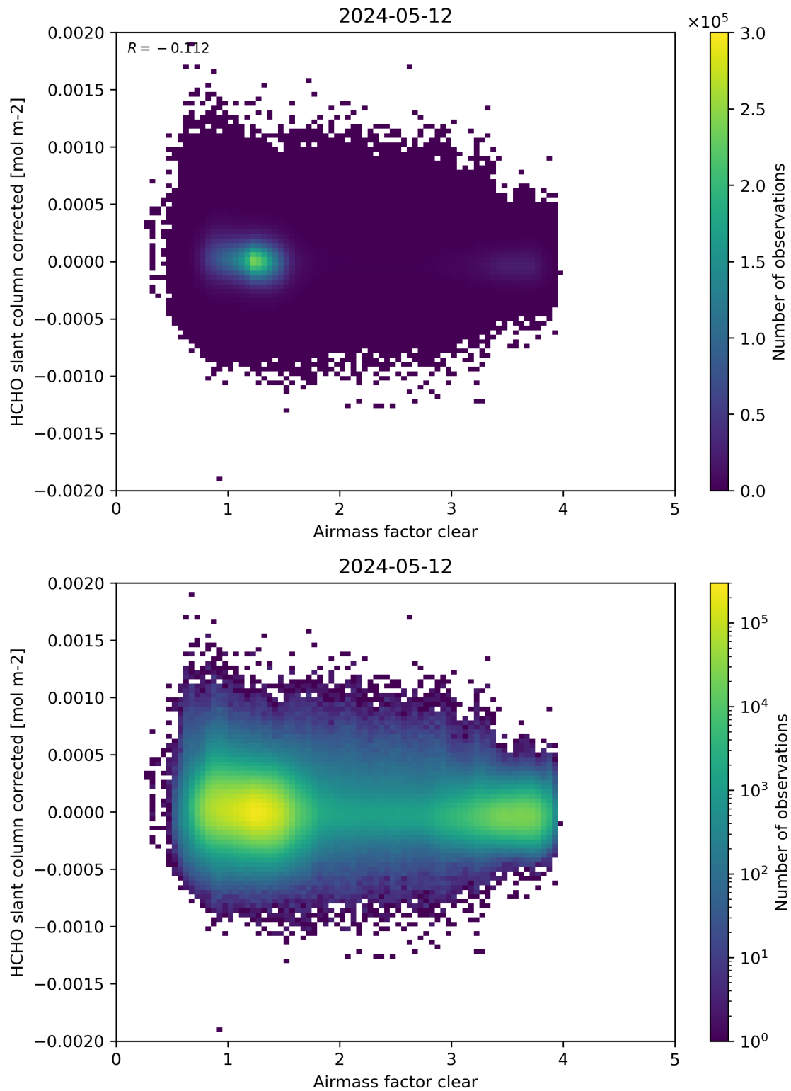
Figure 74: Scatter density plot of “Airmass factor clear” against “HCHO slant column corrected” for 2024-05-12 to 2024-05-13.
