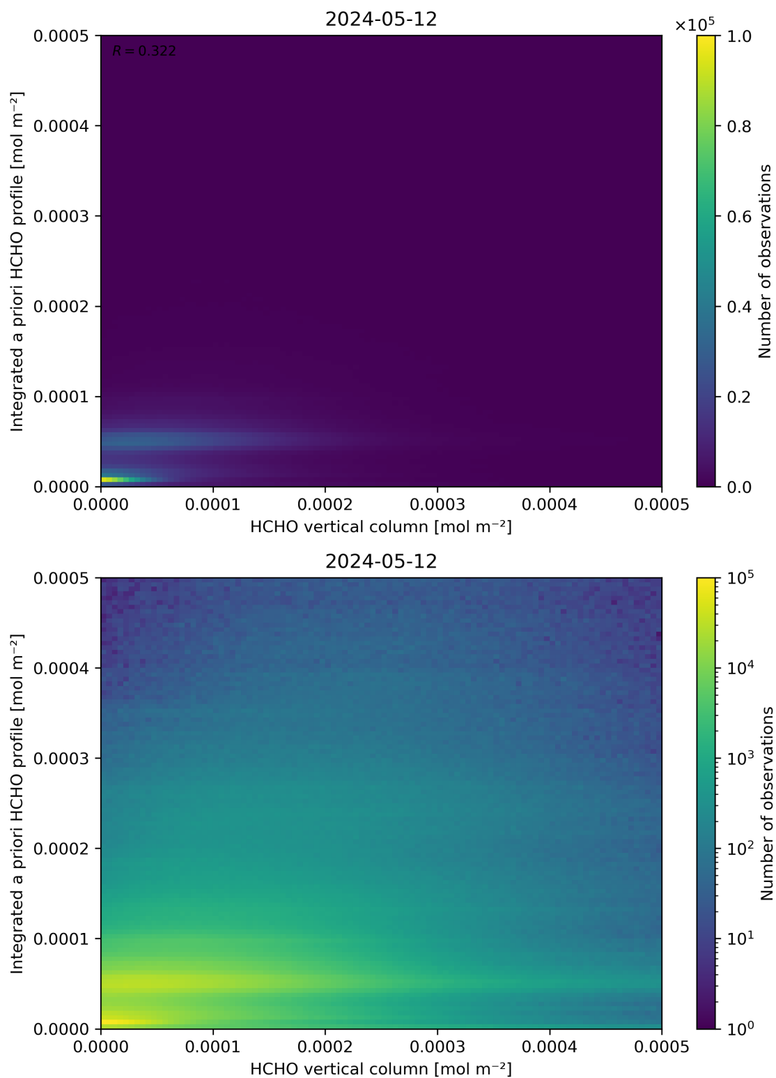
Figure 135: Scatter density plot of “HCHO vertical column” against “Integrated a priori HCHO profile” for 2024-05-12 to 2024-05-13.
