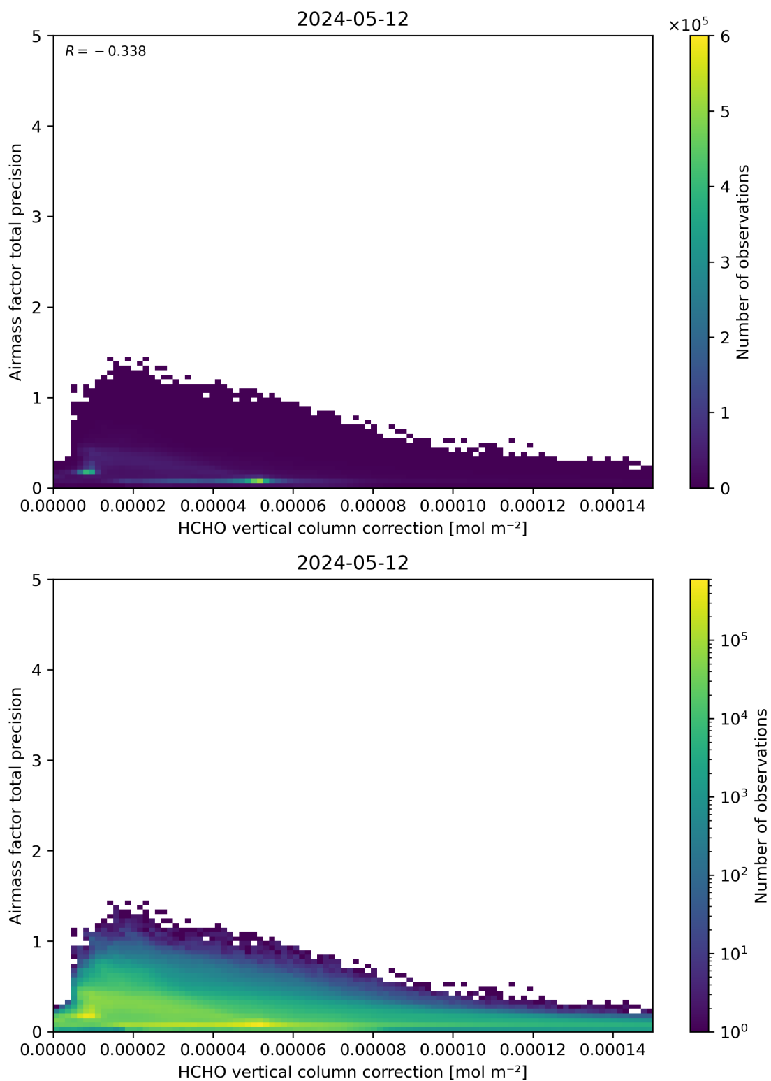
Figure 121: Scatter density plot of “HCHO vertical column correction” against “Airmass factor total precision” for 2024-05-12 to 2024-05-13.
