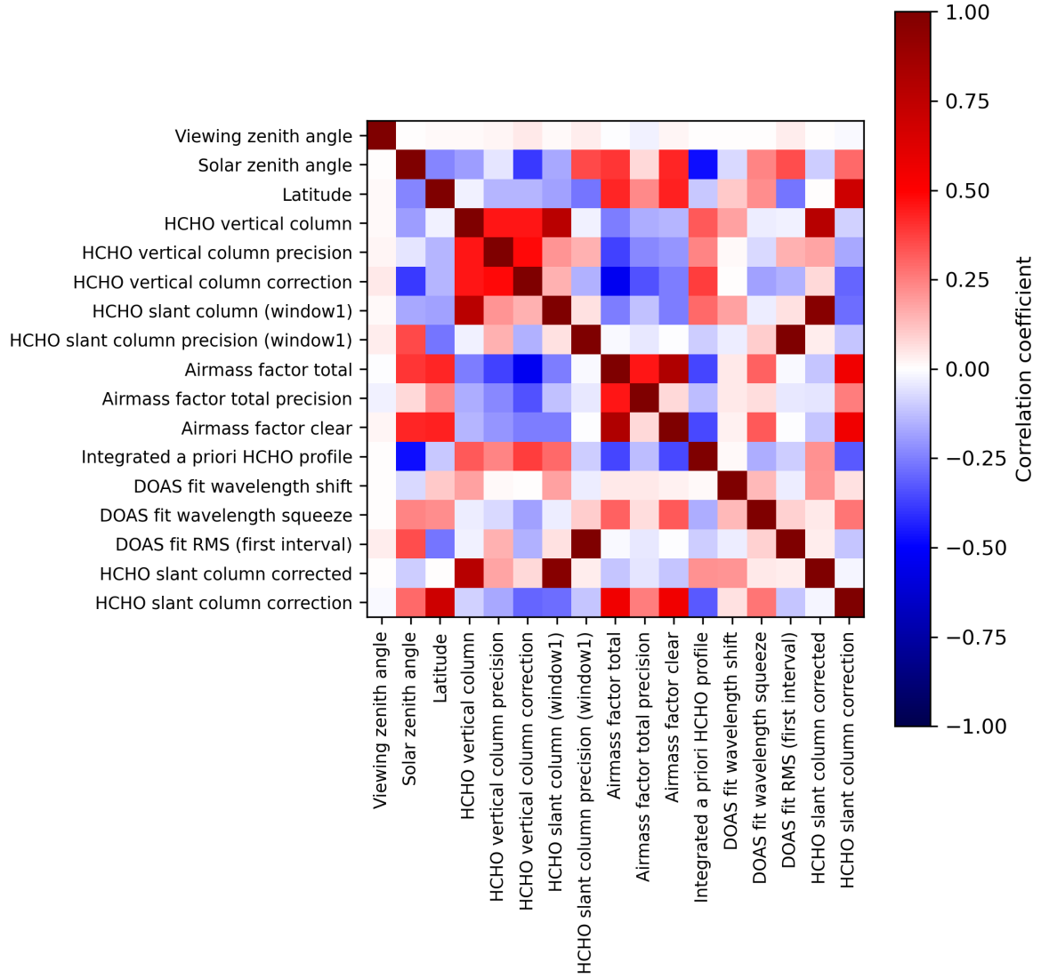
Figure 2: Map of correlation matrix for 2024-05-12 to 2024-05-13.
