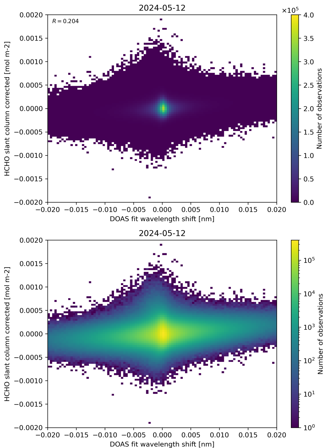
Figure 66: Scatter density plot of “DOAS fit wavelength shift” against “HCHO slant column corrected” for 2024-05-12 to 2024-05-13.
