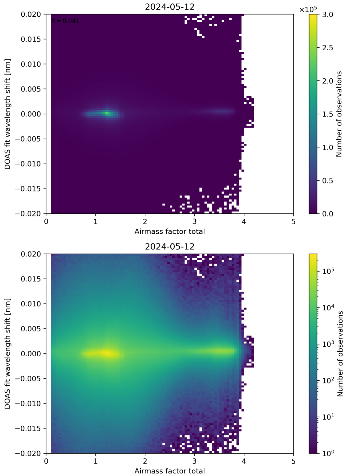
Figure 98: Scatter density plot of “Airmass factor total” against “DOAS fit wavelength shift” for 2024-05-12 to 2024-05-13.
