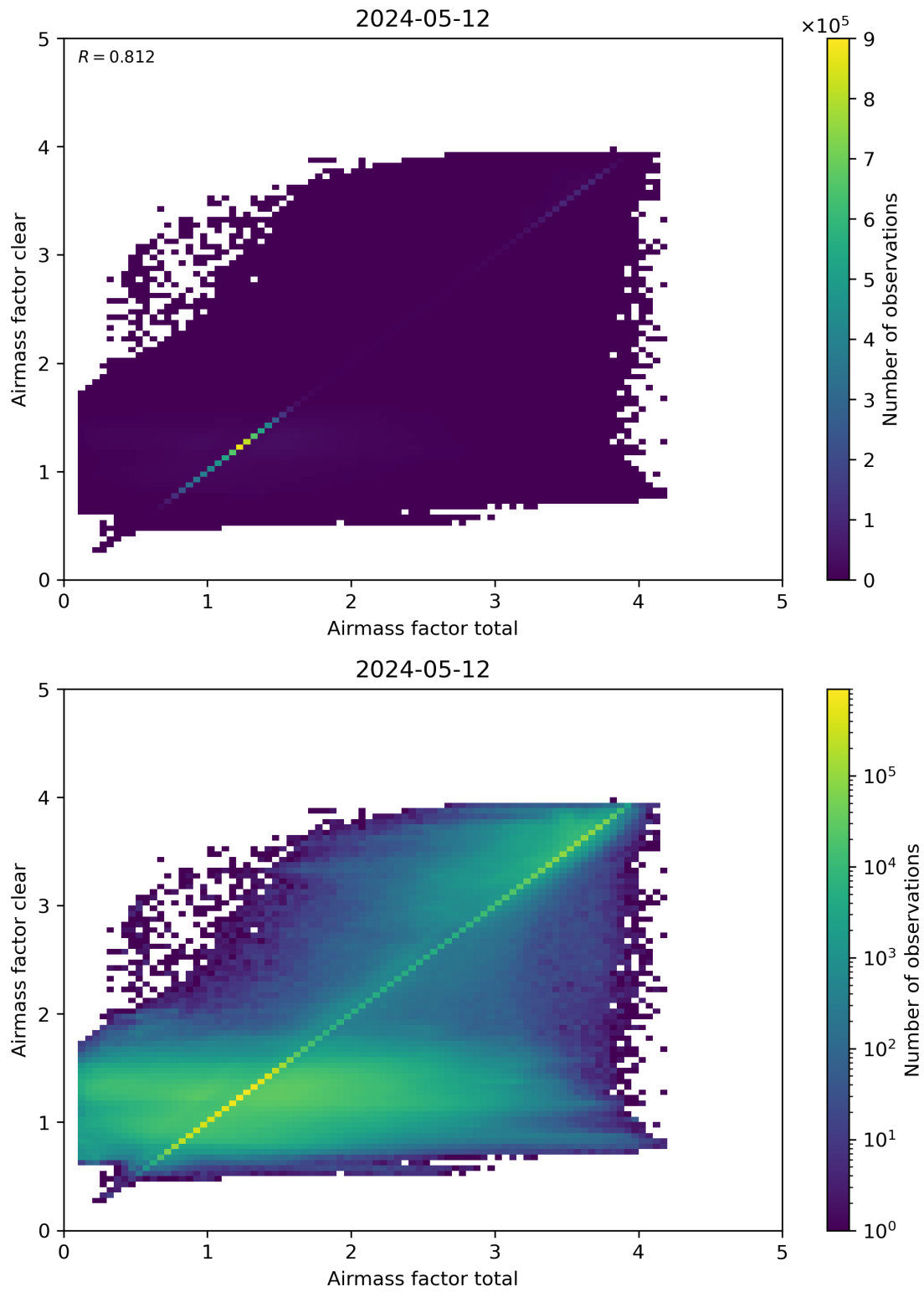
Figure 100: Scatter density plot of “Airmass factor total” against “Airmass factor clear” for 2024-05-12 to 2024-05-13.
