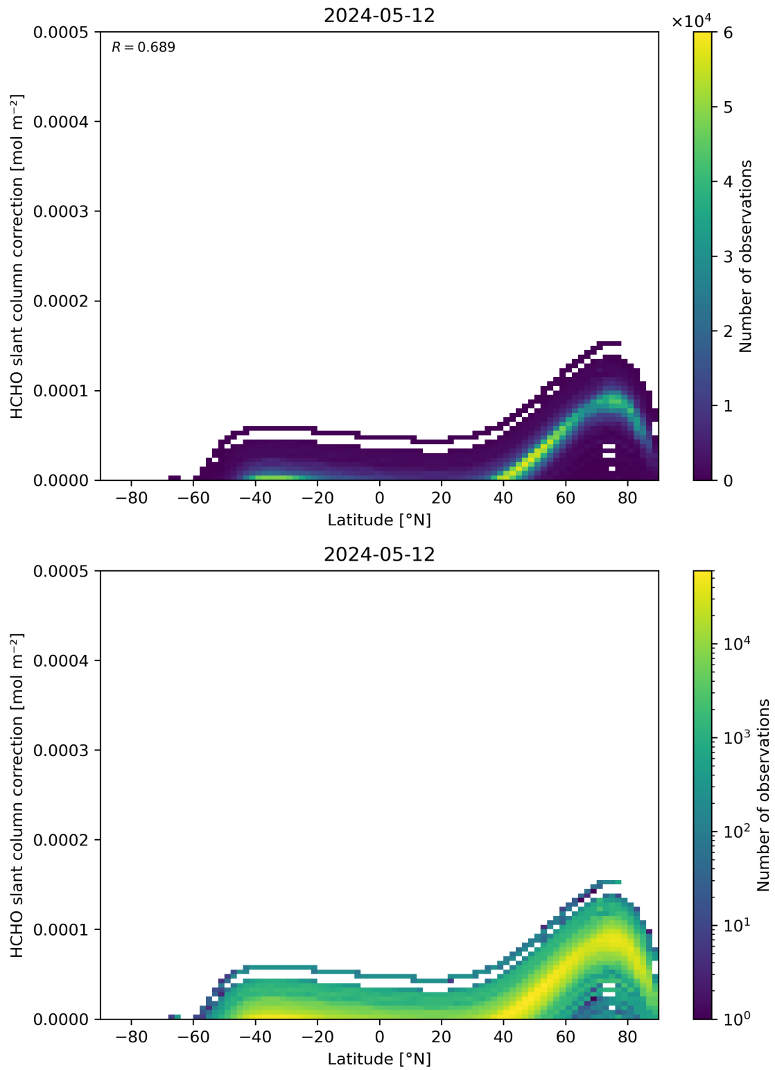
Figure 158: Scatter density plot of “Latitude” against “HCHO slant column correction” for 2024-05-12 to 2024-05-13.
