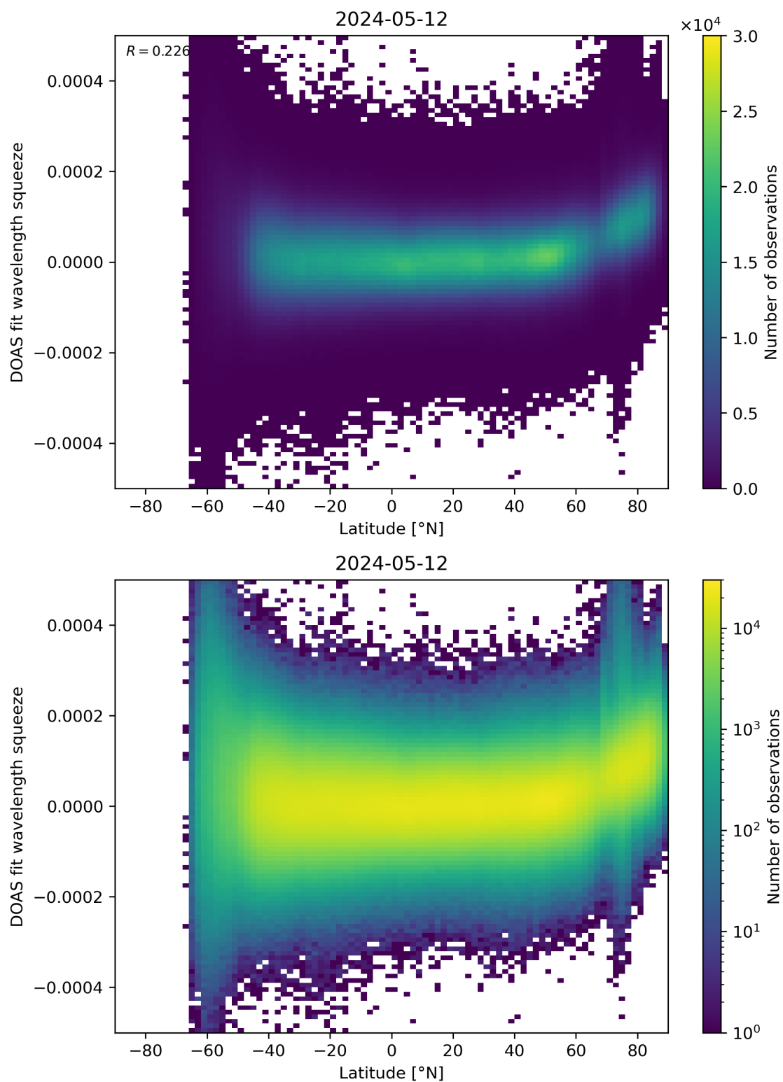
Figure 155: Scatter density plot of “Latitude” against “DOAS fit wavelength squeeze” for 2024-05-12 to 2024-05-13.
