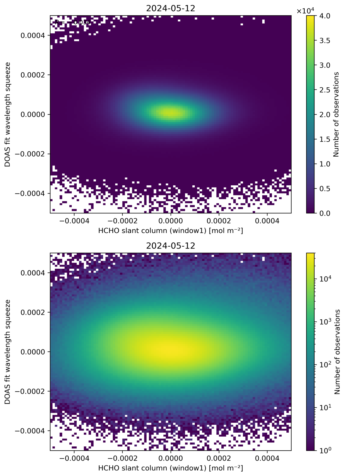
Figure 80: Scatter density plot of “HCHO slant column (window1)” against “DOAS fit wavelength squeeze” for 2024-05-12 to 2024-05-13.
