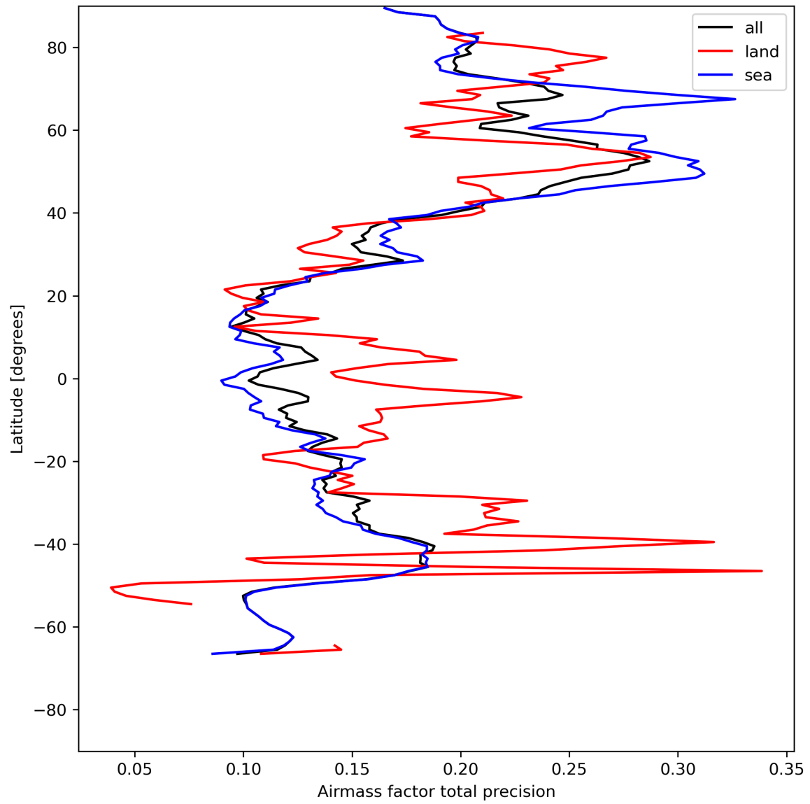
Figure 27: Zonal average of “Airmass factor total precision” for 2024-05-12 to 2024-05-13.
