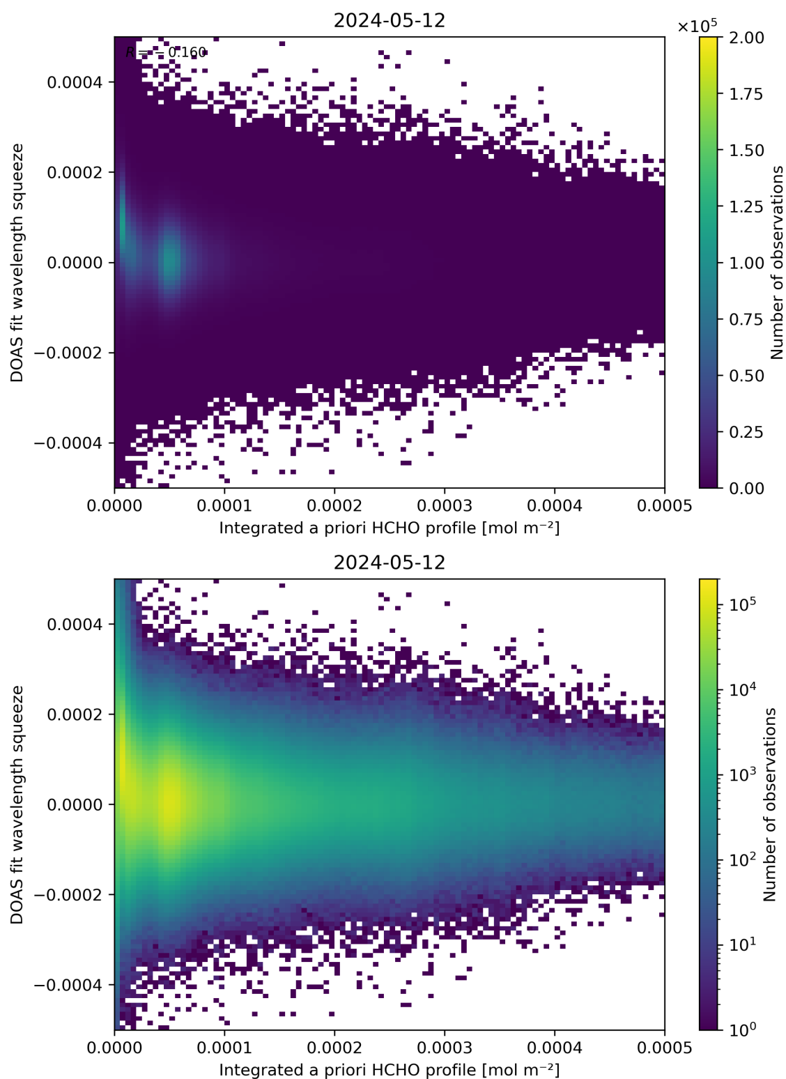
Figure 150: Scatter density plot of “Integrated a priori HCHO profile” against “DOAS fit wavelength squeeze” for 2024-05-12 to 2024-05-13.
