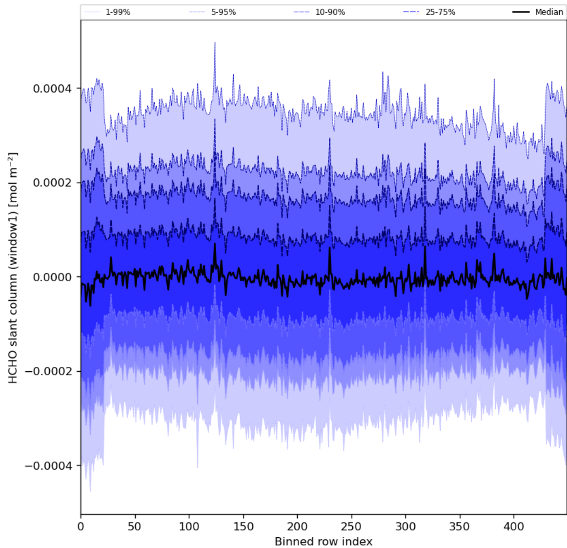
Figure 52: Along track statistics of “HCHO slant column (window1)” for 2024-05-12 to 2024-05-13
