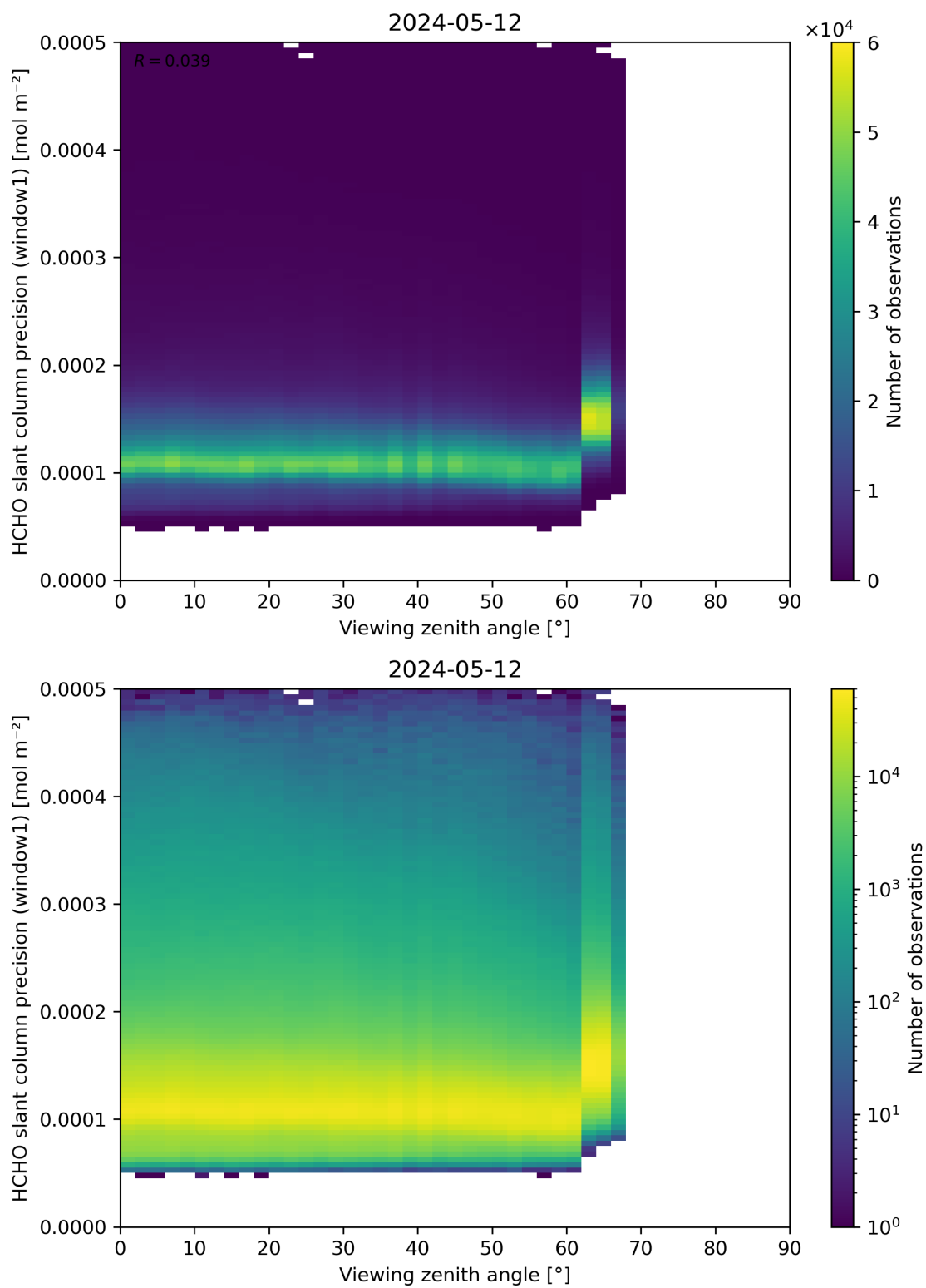
Figure 189: Scatter density plot of “Viewing zenith angle” against “HCHO slant column precision (window1)” for 2024-05-12 to 2024-05-13.
