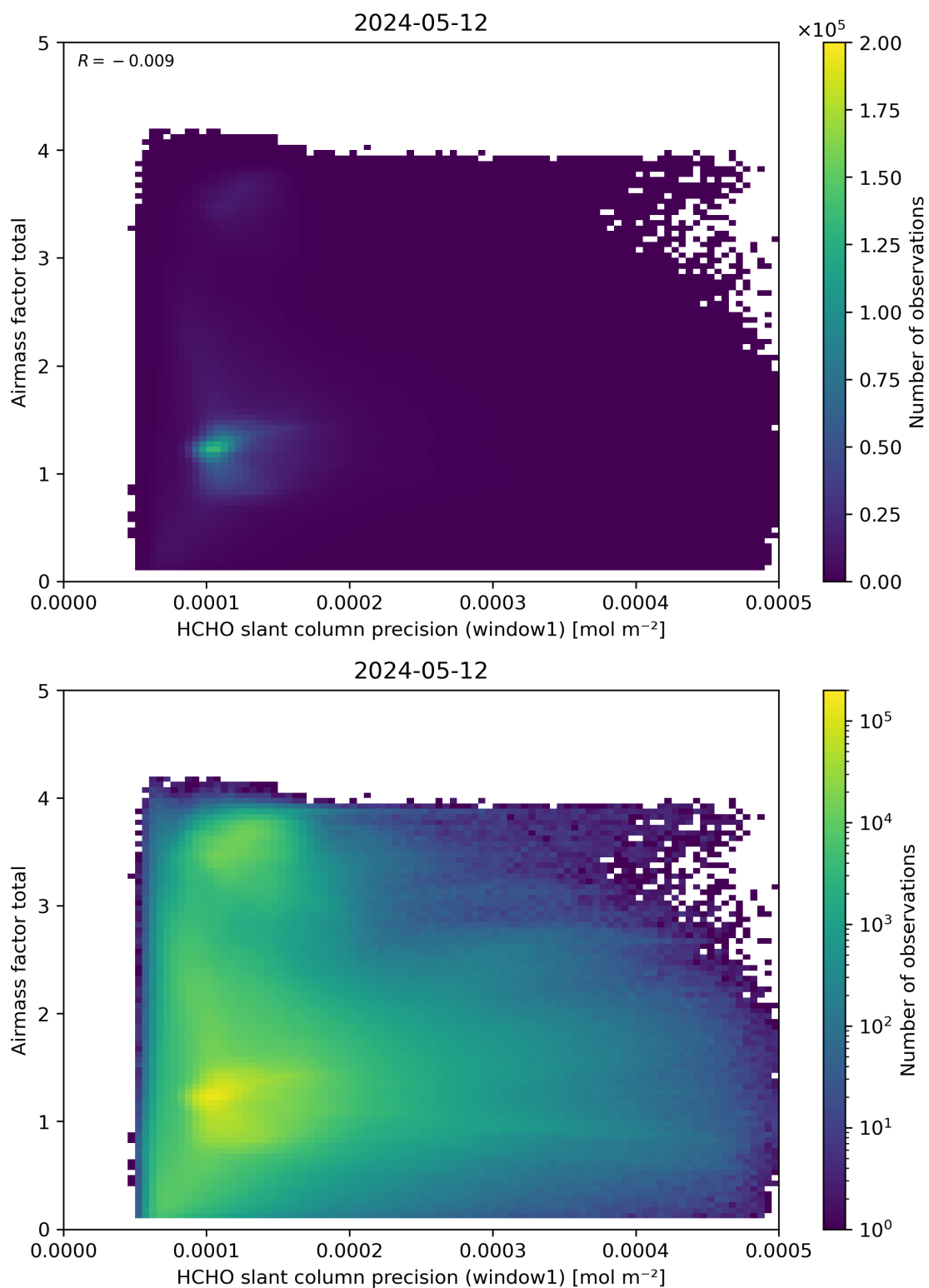
Figure 94: Scatter density plot of “HCHO slant column precision (window1)” against “Airmass factor total” for 2024-05-12 to 2024-05-13.
