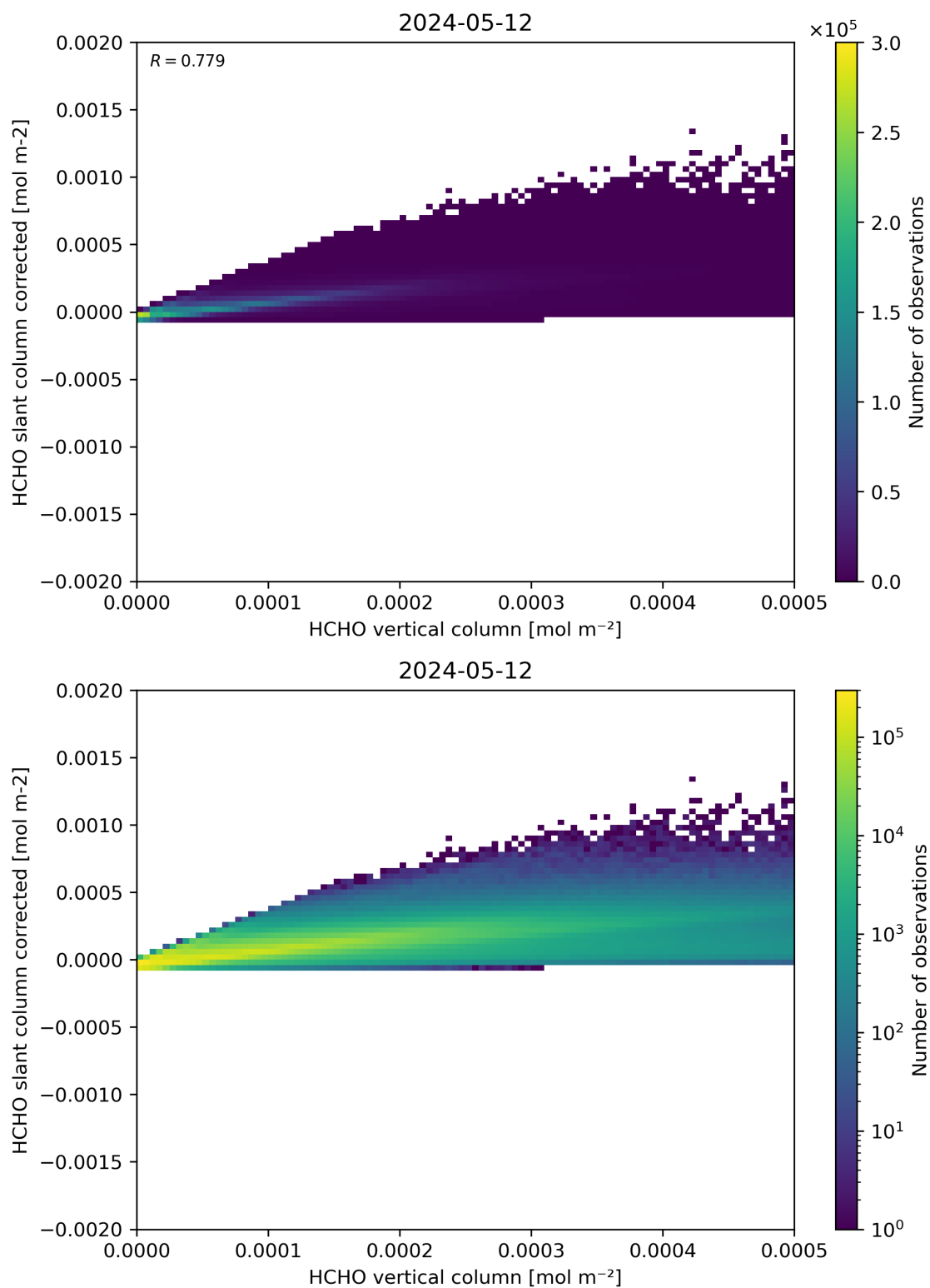
Figure 127: Scatter density plot of “HCHO vertical column” against “HCHO slant column corrected” for 2024-05-12 to 2024-05-13.
