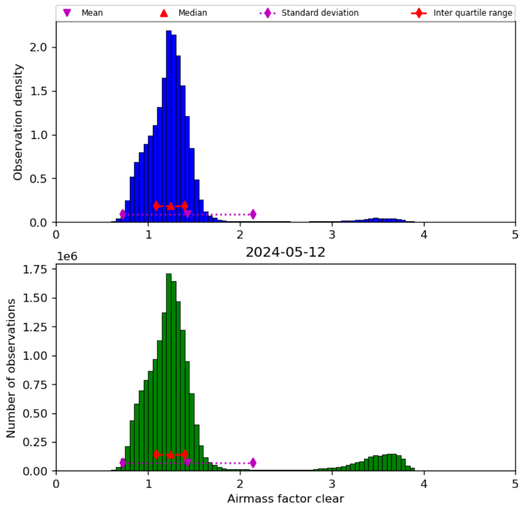
Figure 42: Histogram of “Airmass factor clear” for 2024-05-12 to 2024-05-13
