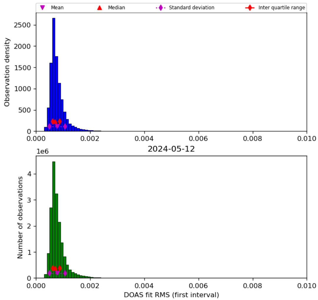
Figure 46: Histogram of “DOAS fit RMS (first interval)” for 2024-05-12 to 2024-05-13
