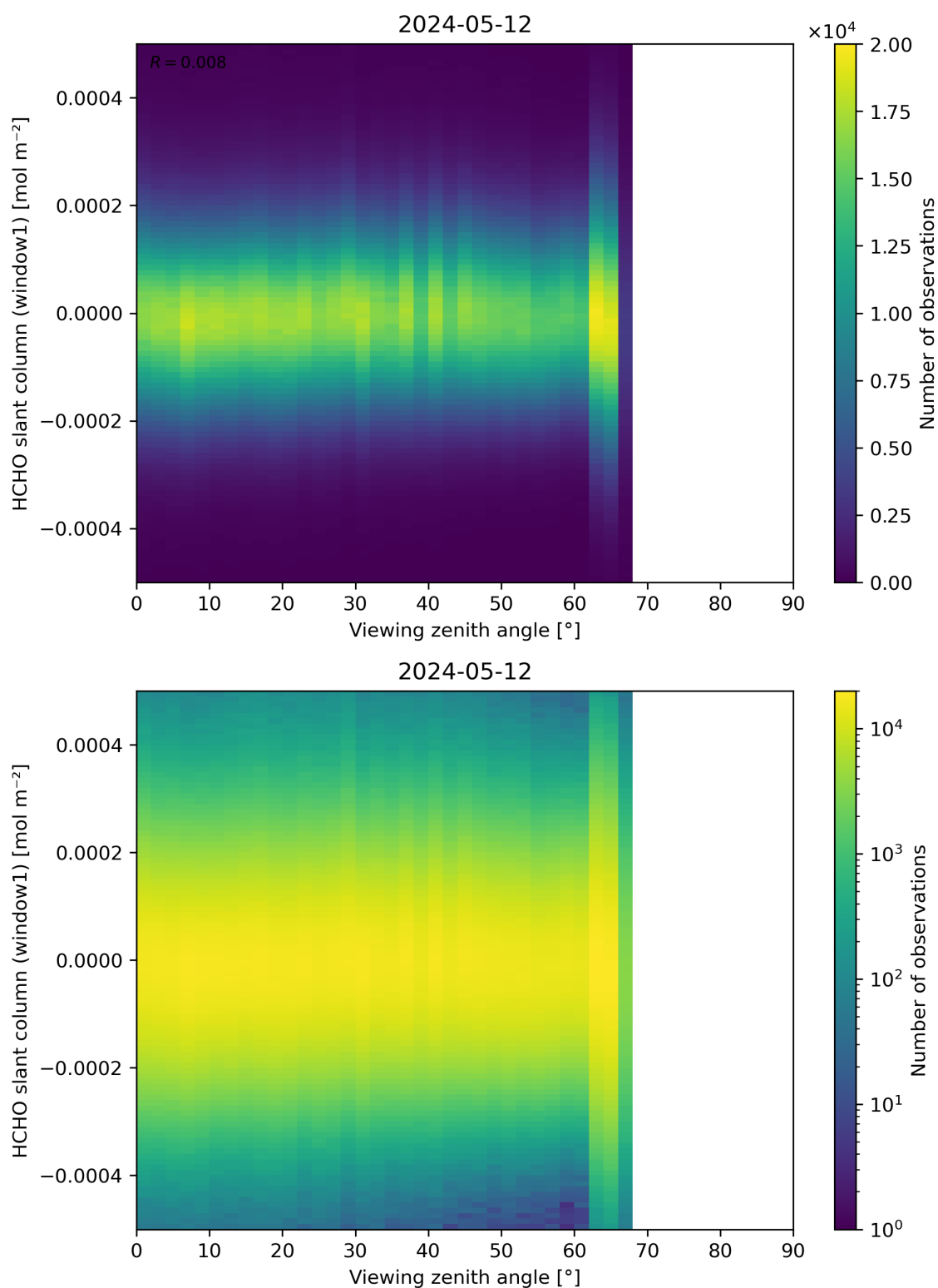
Figure 188: Scatter density plot of “Viewing zenith angle” against “HCHO slant column (window1)” for 2024-05-12 to 2024-05-13.
