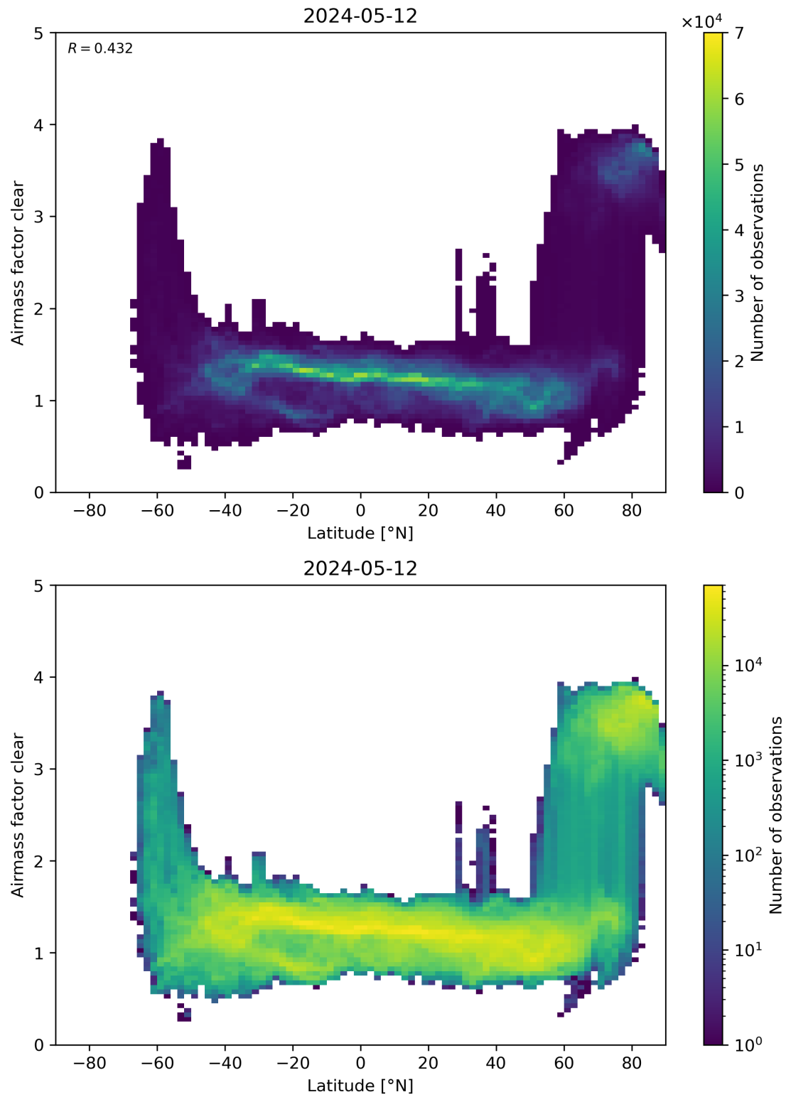
Figure 156: Scatter density plot of “Latitude” against “Airmass factor clear” for 2024-05-12 to 2024-05-13.
