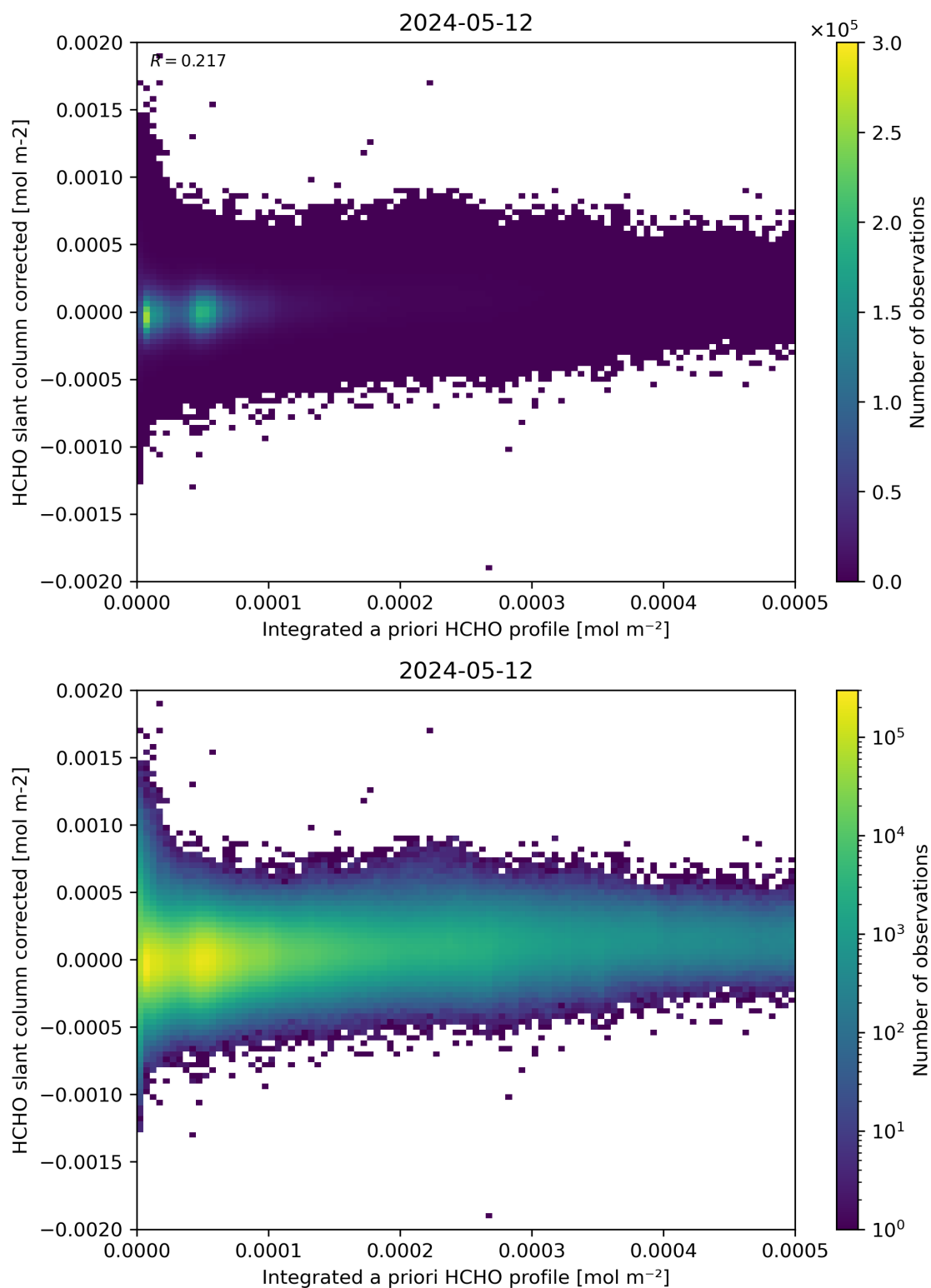
Figure 151: Scatter density plot of “Integrated a priori HCHO profile” against “HCHO slant column corrected” for 2024-05-12 to 2024-05-13.
