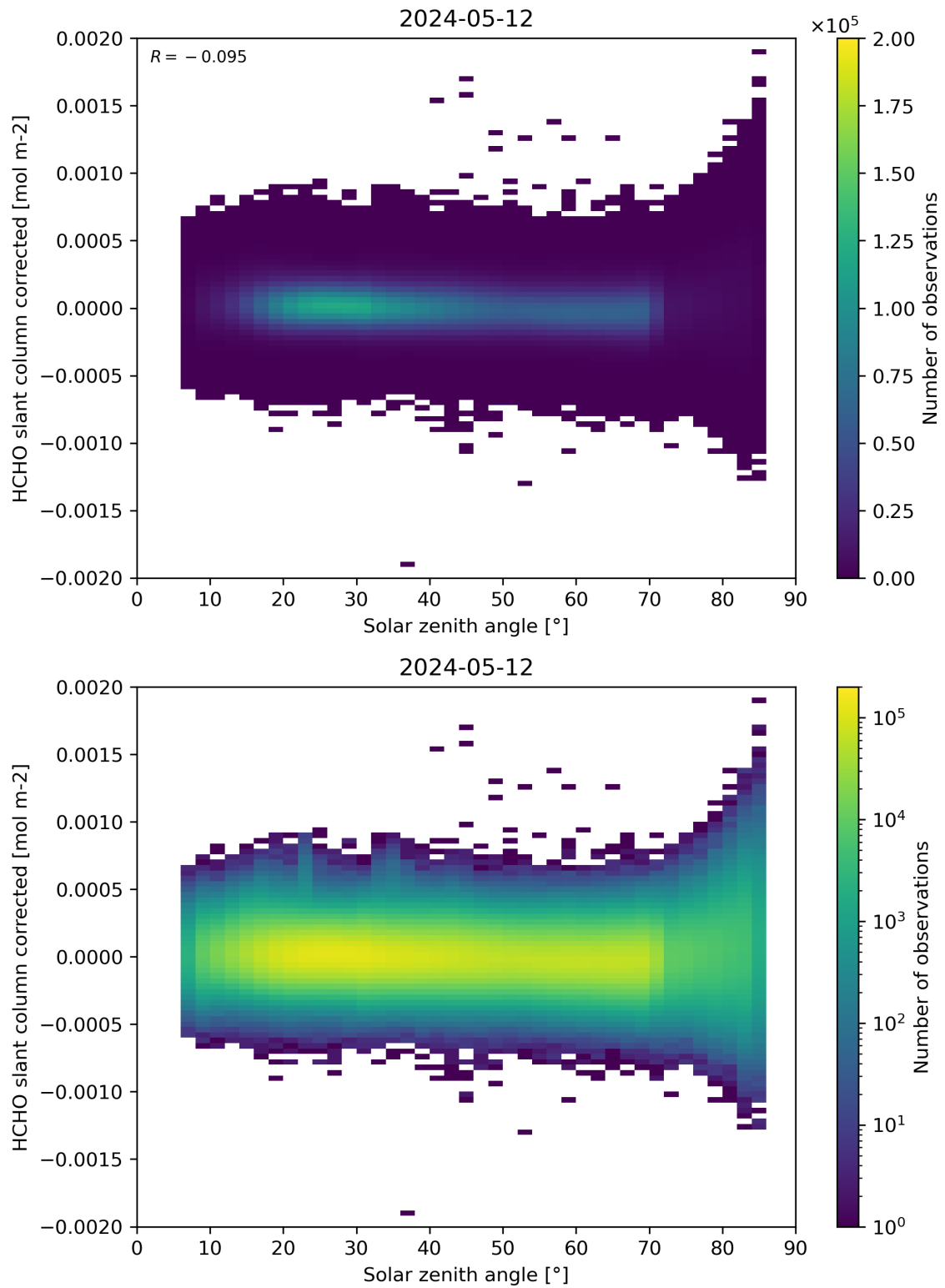
Figure 171: Scatter density plot of “Solar zenith angle” against “HCHO slant column corrected” for 2024-05-12 to 2024-05-13.
