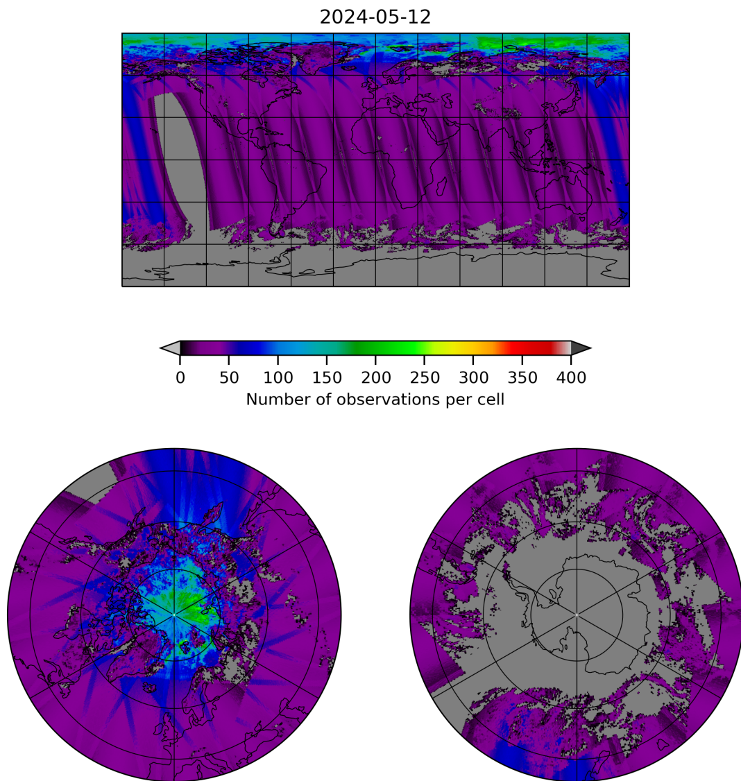
Figure 19: Map of the number of observations for 2024-05-12 to 2024-05-13
