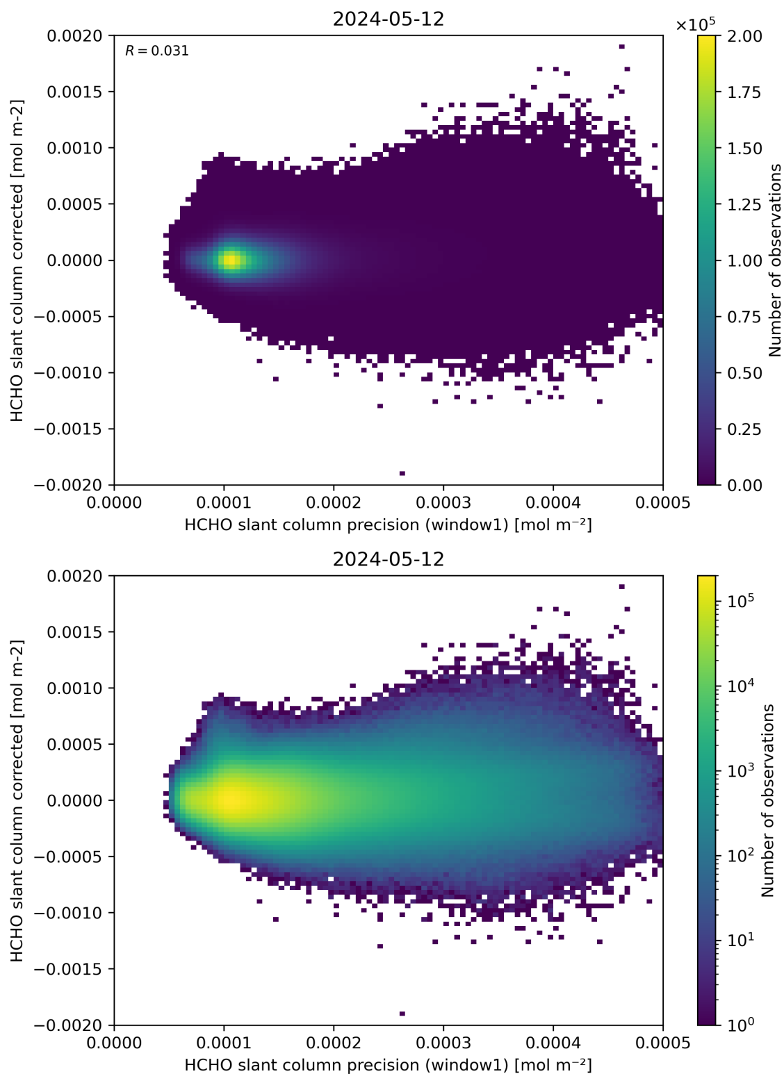
Figure 92: Scatter density plot of “HCHO slant column precision (window1)” against “HCHO slant column corrected” for 2024-05-12 to 2024-05-13.
