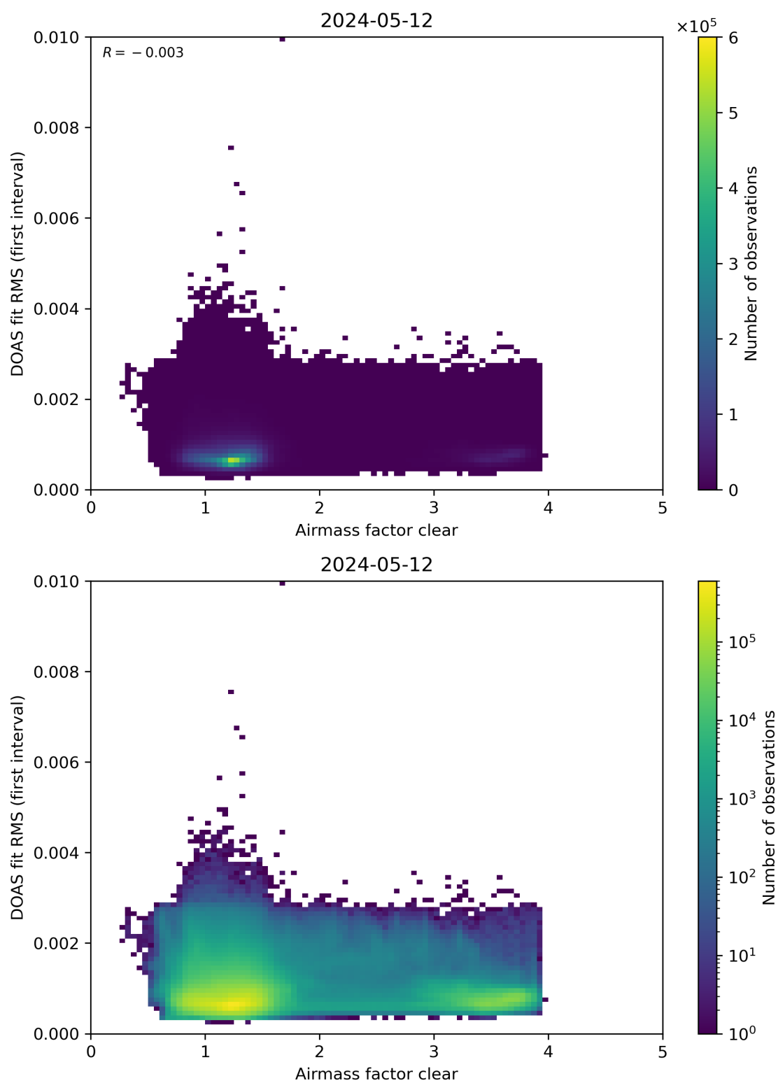
Figure 71: Scatter density plot of “Airmass factor clear” against “DOAS fit RMS (first interval)” for 2024-05-12 to 2024-05-13.
