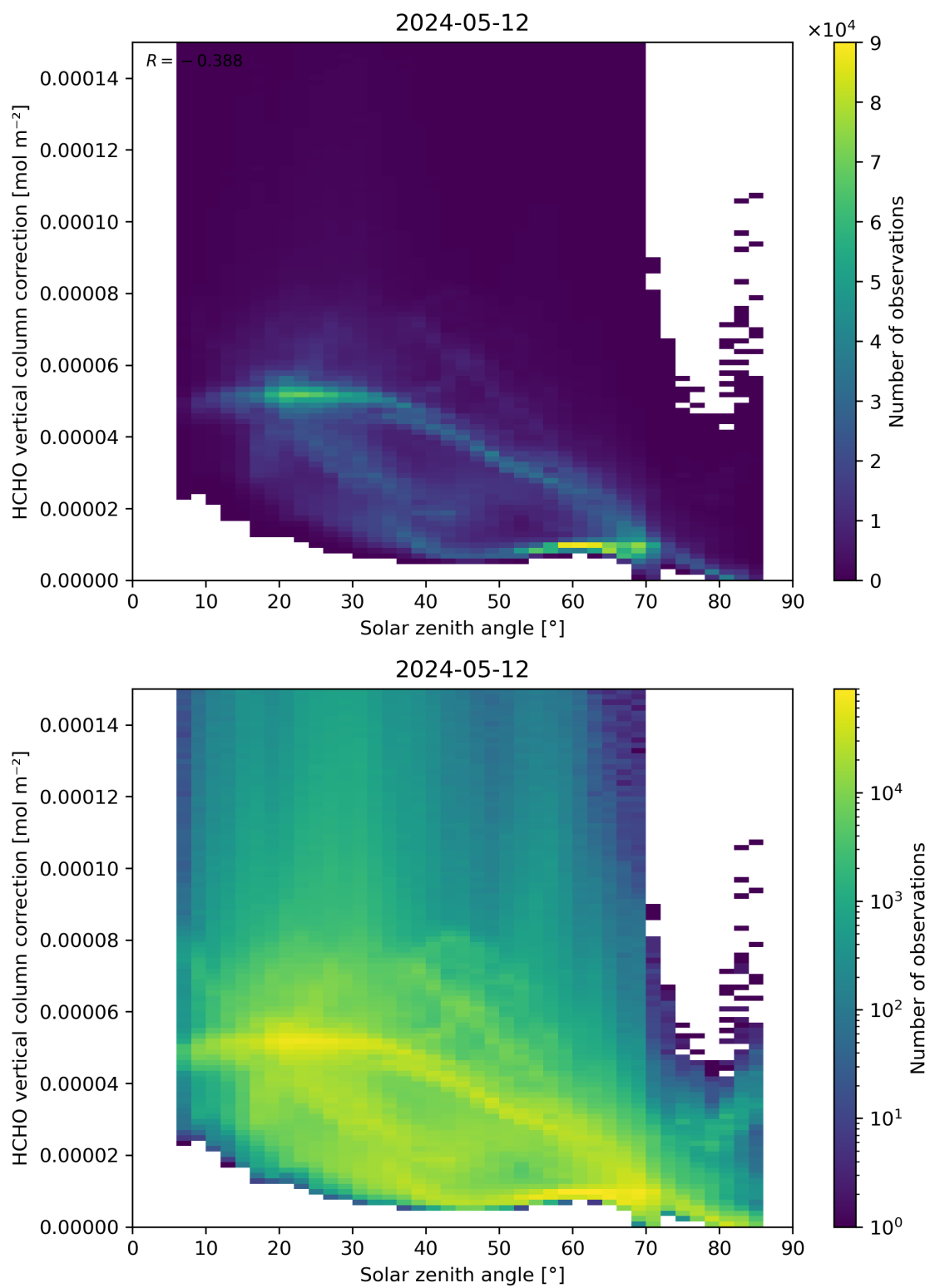
Figure 178: Scatter density plot of “Solar zenith angle” against “HCHO vertical column correction” for 2024-05-12 to 2024-05-13.
