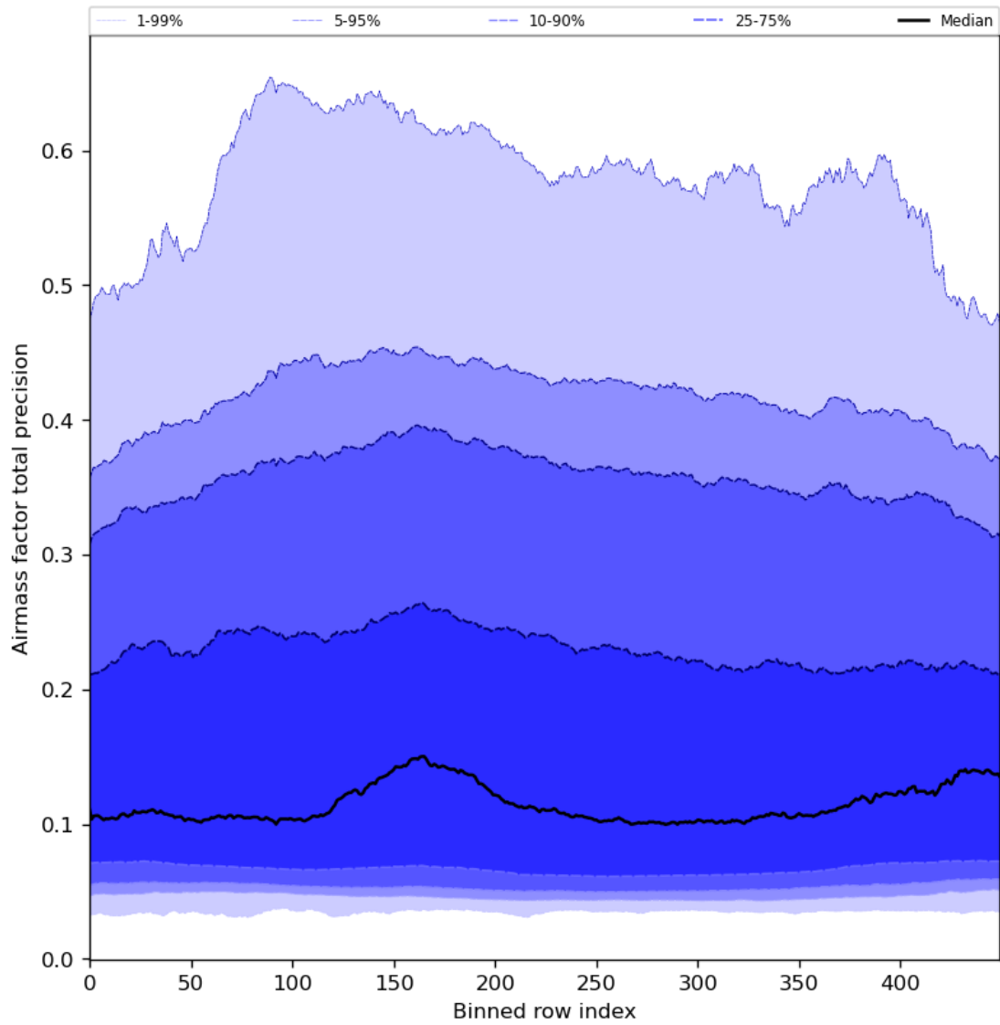
Figure 55: Along track statistics of “Airmass factor total precision” for 2024-05-12 to 2024-05-13
