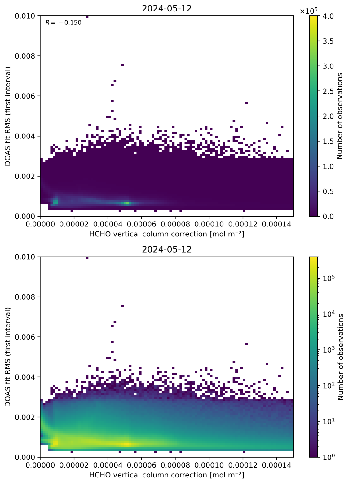
Figure 112: Scatter density plot of “HCHO vertical column correction” against “DOAS fit RMS (first interval)” for 2024-05-12 to 2024-05-13.
