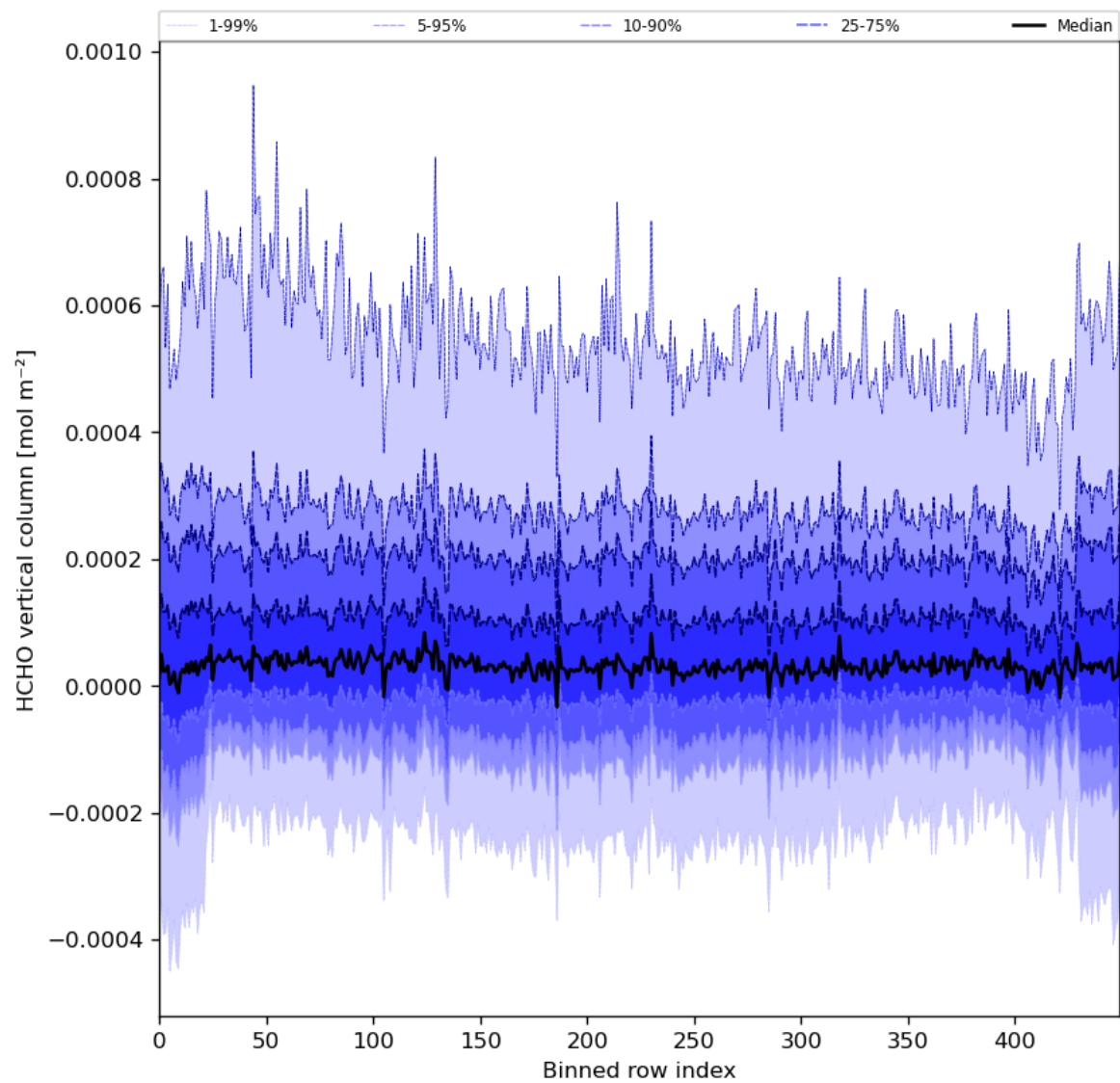
Figure 49: Along track statistics of “HCHO vertical column” for 2024-05-12 to 2024-05-13
