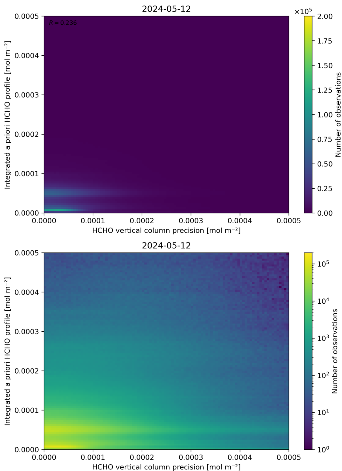
Figure 147: Scatter density plot of “HCHO vertical column precision” against “Integrated a priori HCHO profile” for 2024-05-12 to 2024-05-13.
