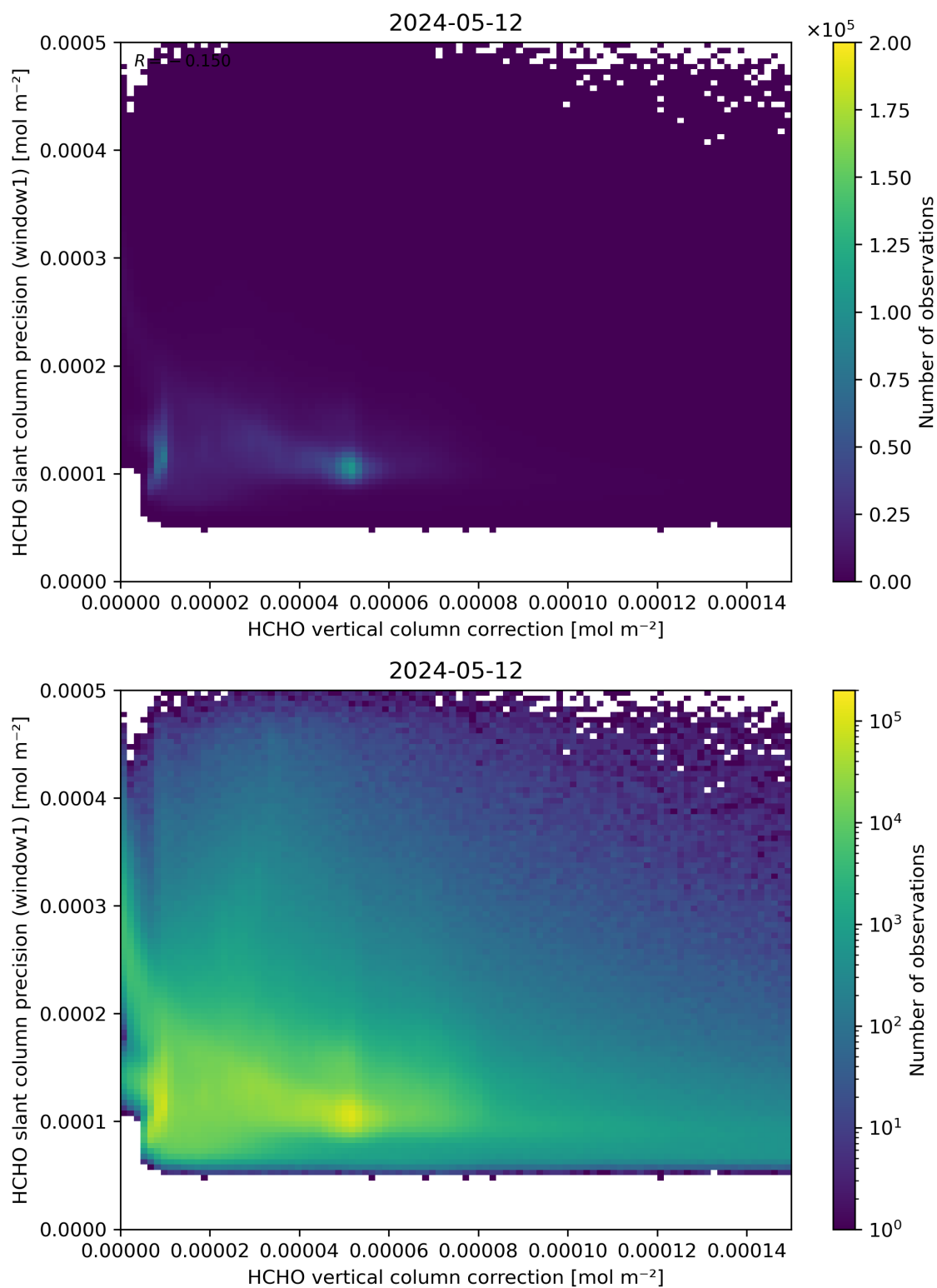
Figure 119: Scatter density plot of “HCHO vertical column correction” against “HCHO slant column precision (window1)” for 2024-05-12 to 2024-05-13.
