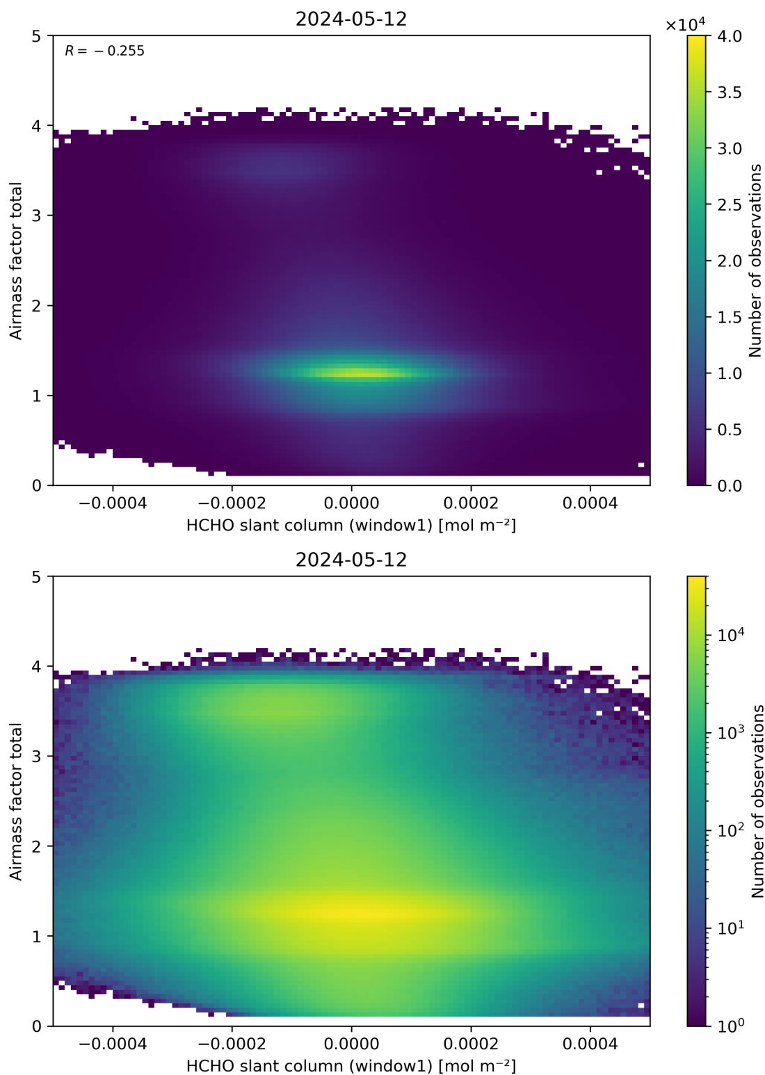
Figure 85: Scatter density plot of “HCHO slant column (window1)” against “Airmass factor total” for 2024-05-12 to 2024-05-13.
