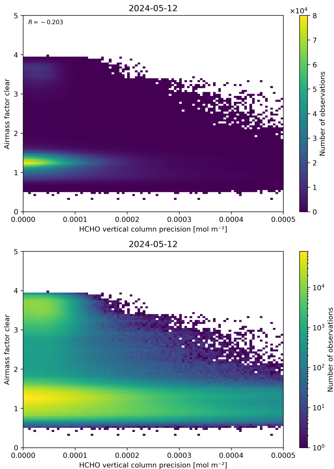
Figure 139: Scatter density plot of “HCHO vertical column precision” against “Airmass factor clear” for 2024-05-12 to 2024-05-13.
