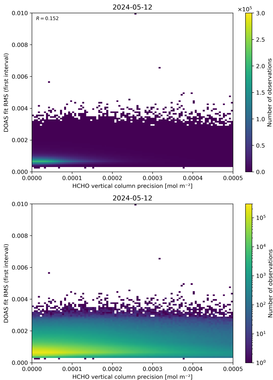
Figure 136: Scatter density plot of “HCHO vertical column precision” against “DOAS fit RMS (first interval)” for 2024-05-12 to 2024-05-13.
