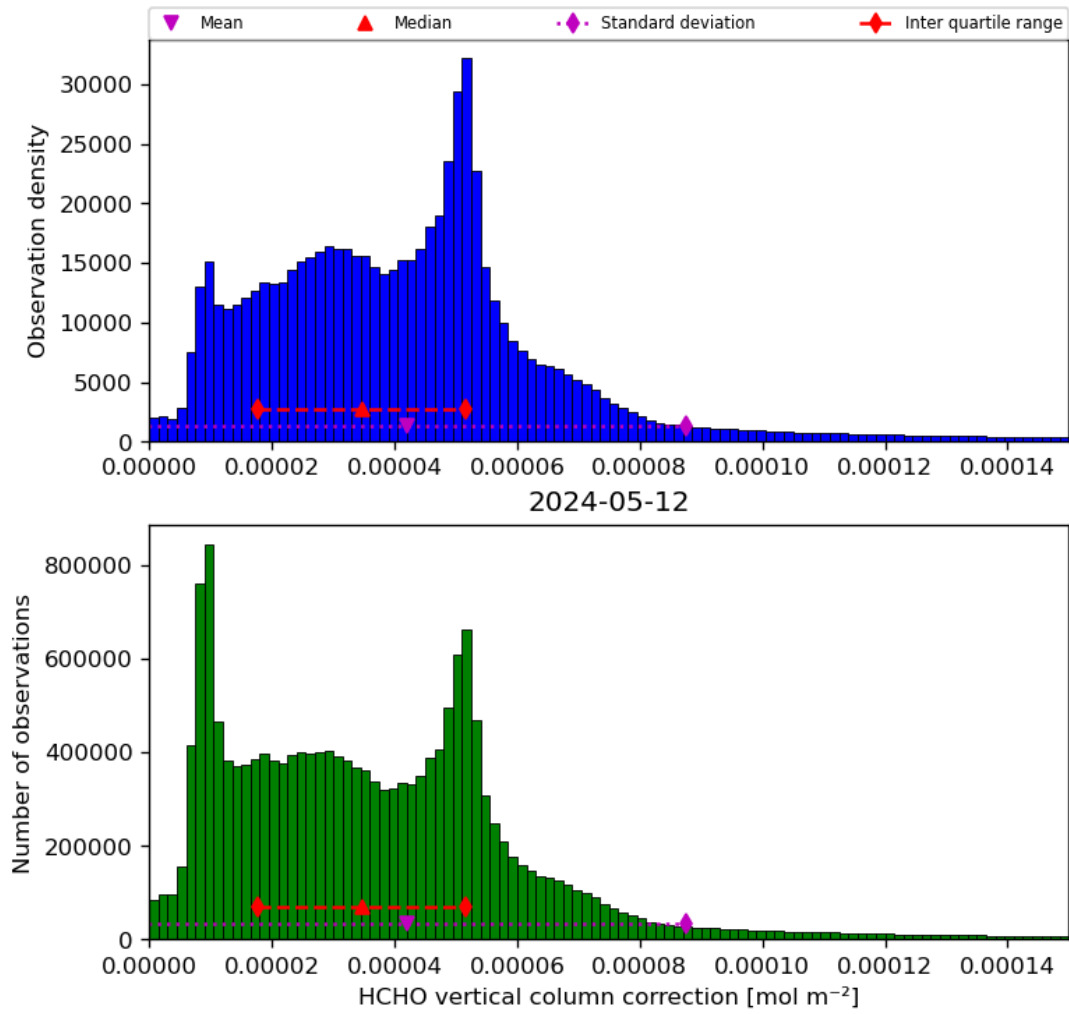
Figure 37: Histogram of “HCHO vertical column correction” for 2024-05-12 to 2024-05-13
