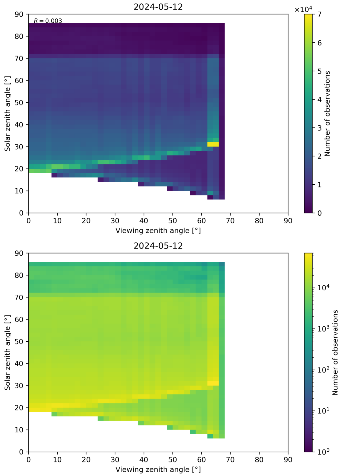
Figure 197: Scatter density plot of “Viewing zenith angle” against “Solar zenith angle” for 2024-05-12 to 2024-05-13.
