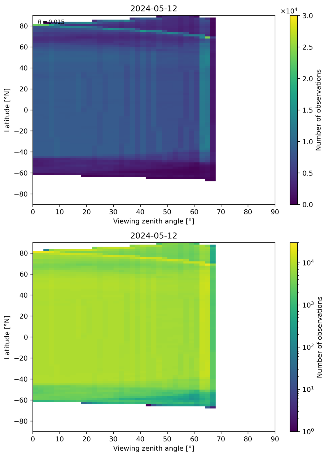
Figure 196: Scatter density plot of “Viewing zenith angle” against “Latitude” for 2024-05-12 to 2024-05-13.
