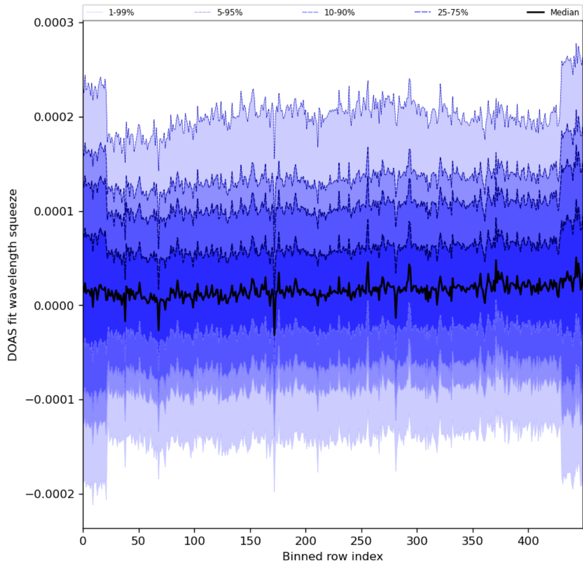
Figure 59: Along track statistics of “DOAS fit wavelength squeeze” for 2024-05-12 to 2024-05-13
