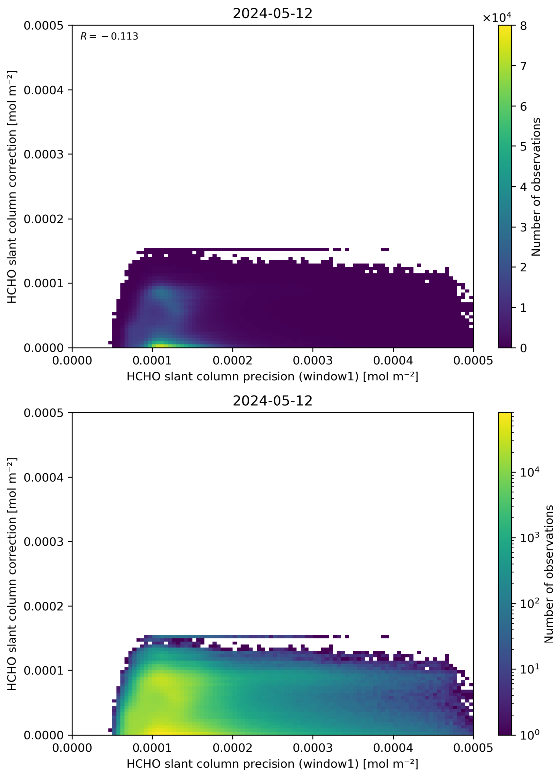
Figure 93: Scatter density plot of “HCHO slant column precision (window1)” against “HCHO slant column correction” for 2024-05-12 to 2024-05-13.
