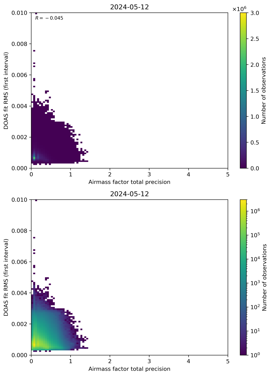
Figure 105: Scatter density plot of “Airmass factor total precision” against “DOAS fit RMS (first interval)” for 2024-05-12 to 2024-05-13.
