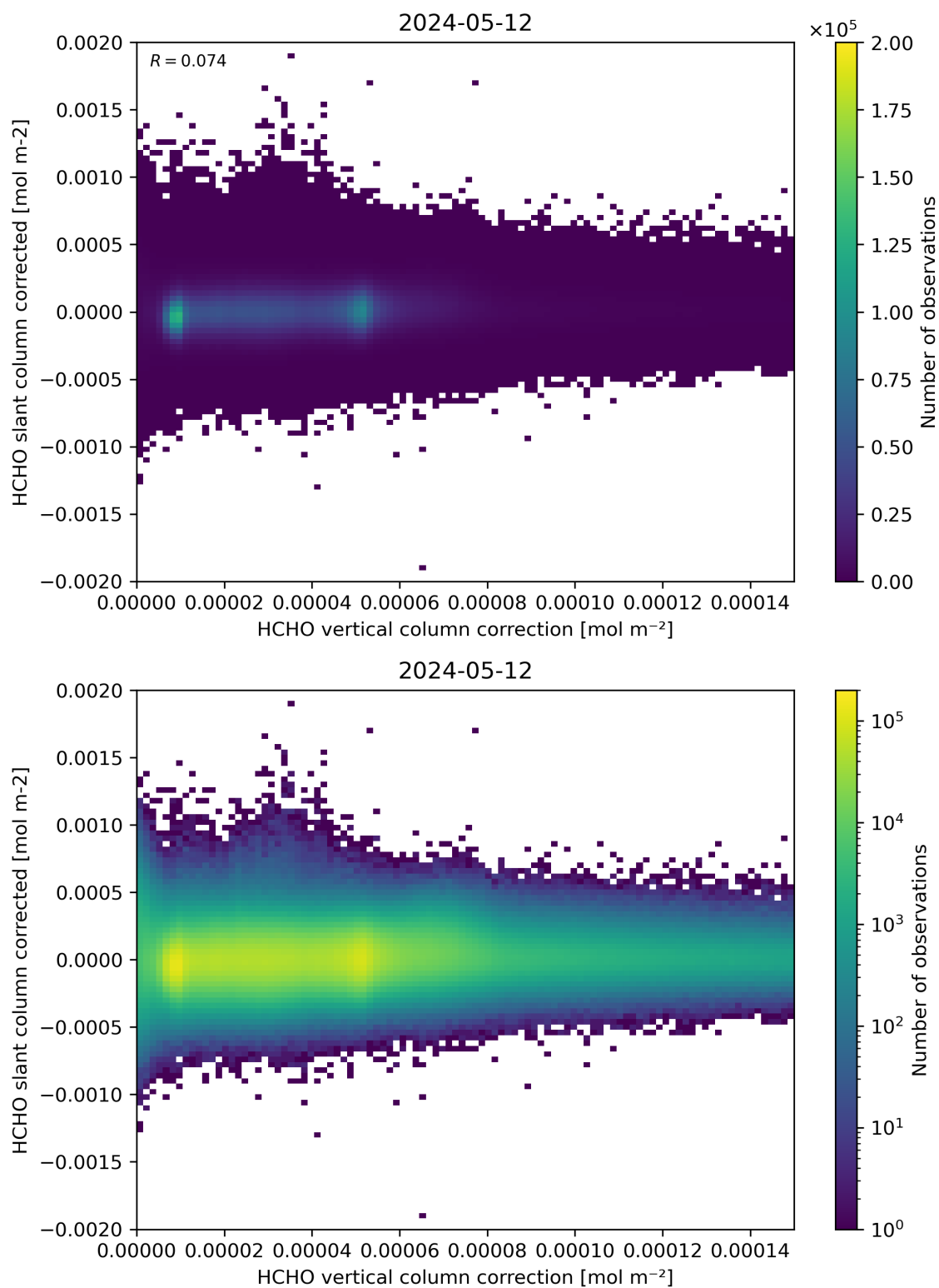
Figure 116: Scatter density plot of “HCHO vertical column correction” against “HCHO slant column corrected” for 2024-05-12 to 2024-05-13.
