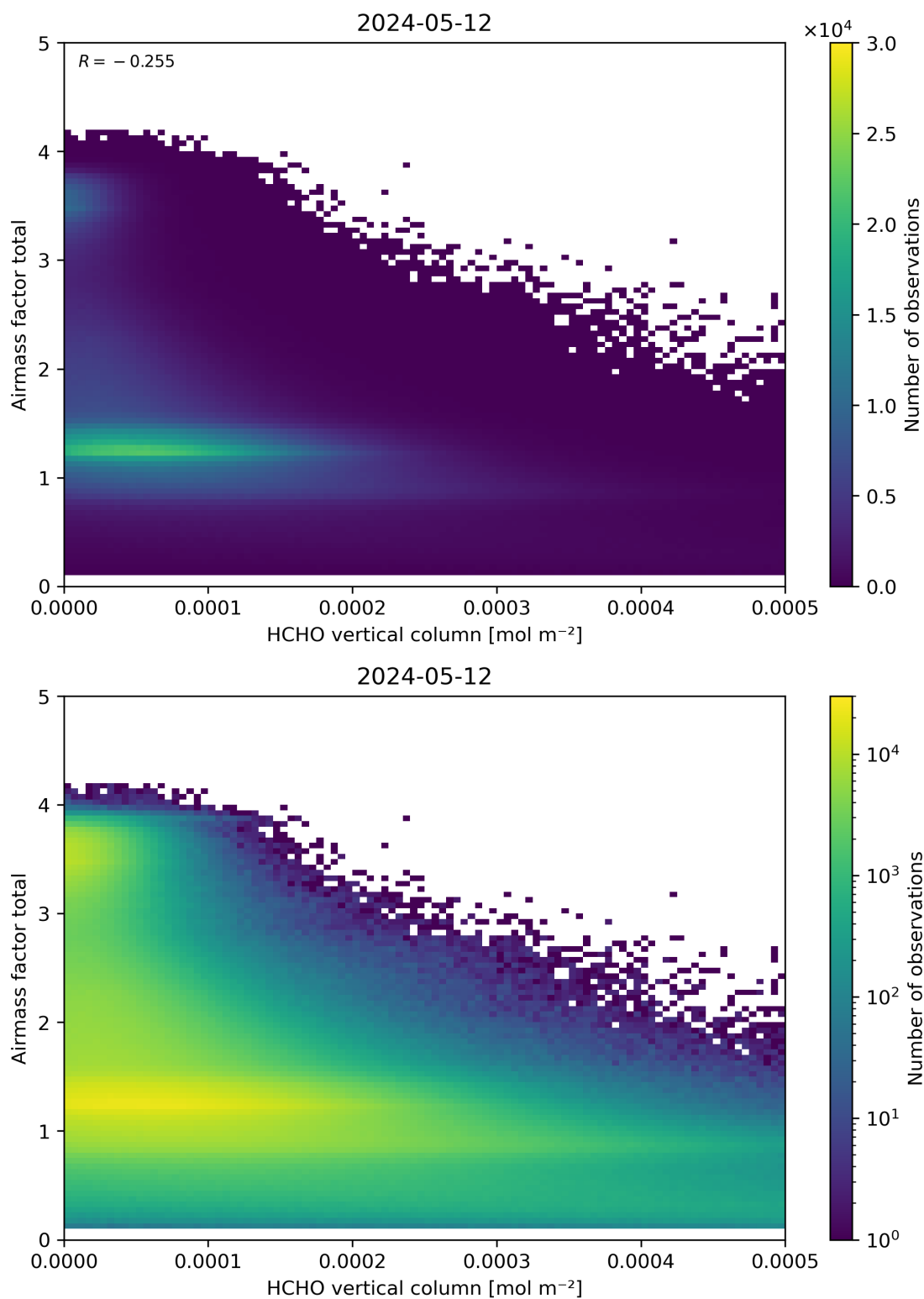
Figure 131: Scatter density plot of “HCHO vertical column” against “Airmass factor total” for 2024-05-12 to 2024-05-13.
