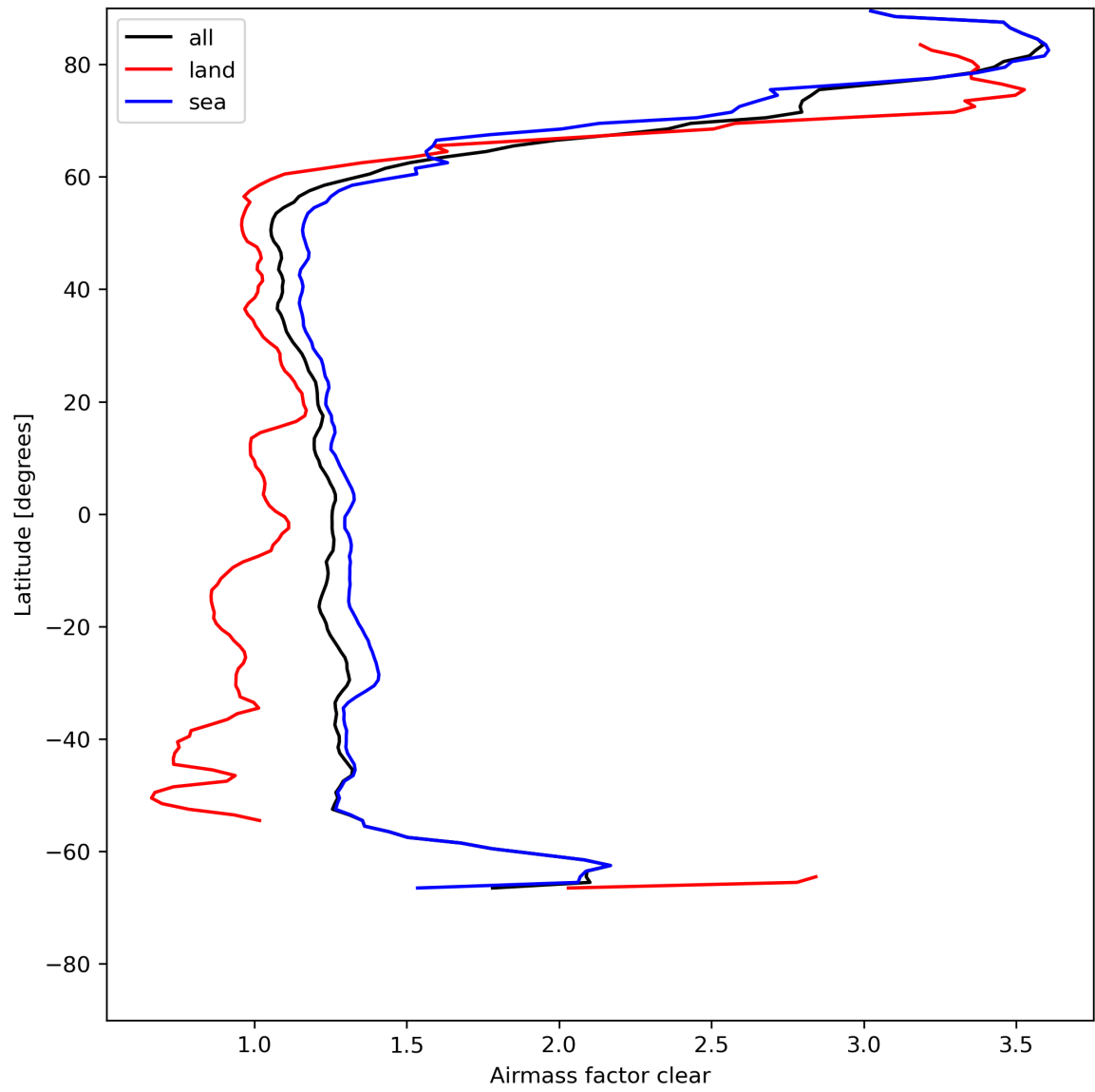
Figure 28: Zonal average of “Airmass factor clear” for 2024-05-12 to 2024-05-13.
