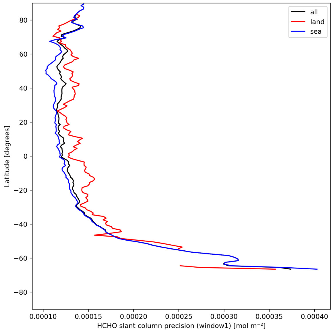
Figure 25: Zonal average of “HCHO slant column precision (window1)” for 2024-05-12 to 2024-05-13.
