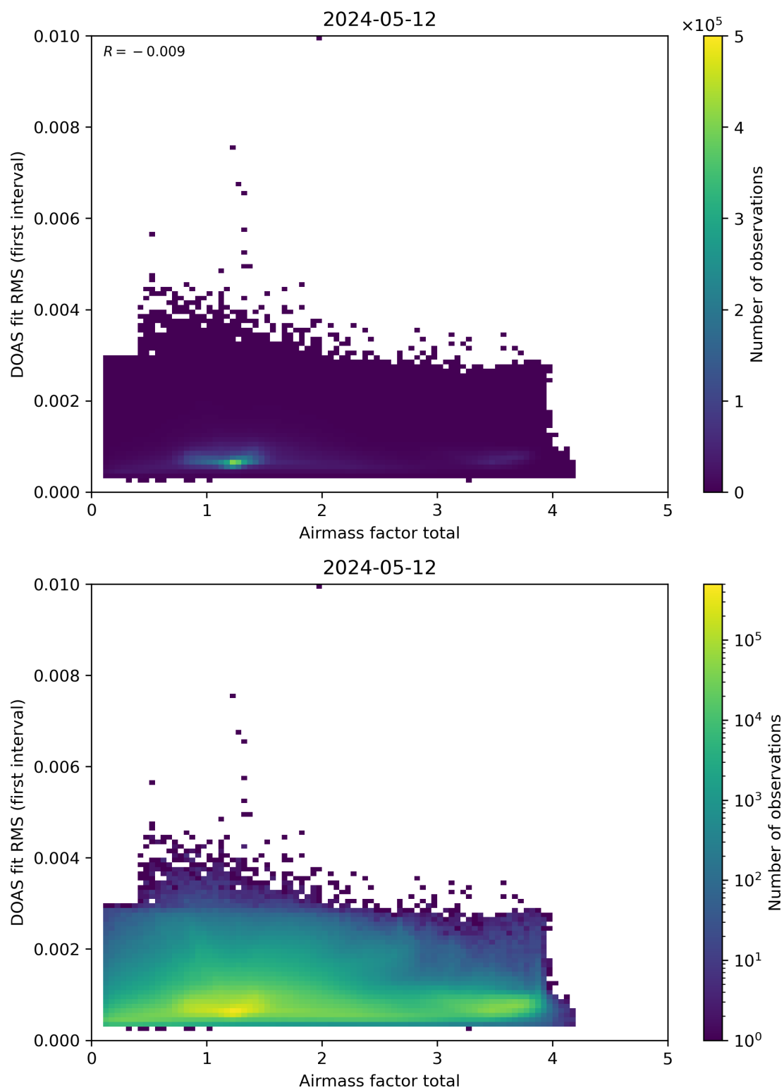
Figure 97: Scatter density plot of “Airmass factor total” against “DOAS fit RMS (first interval)” for 2024-05-12 to 2024-05-13.
