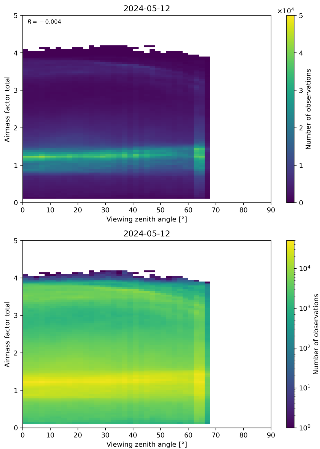
Figure 190: Scatter density plot of “Viewing zenith angle” against “Airmass factor total” for 2024-05-12 to 2024-05-13.
