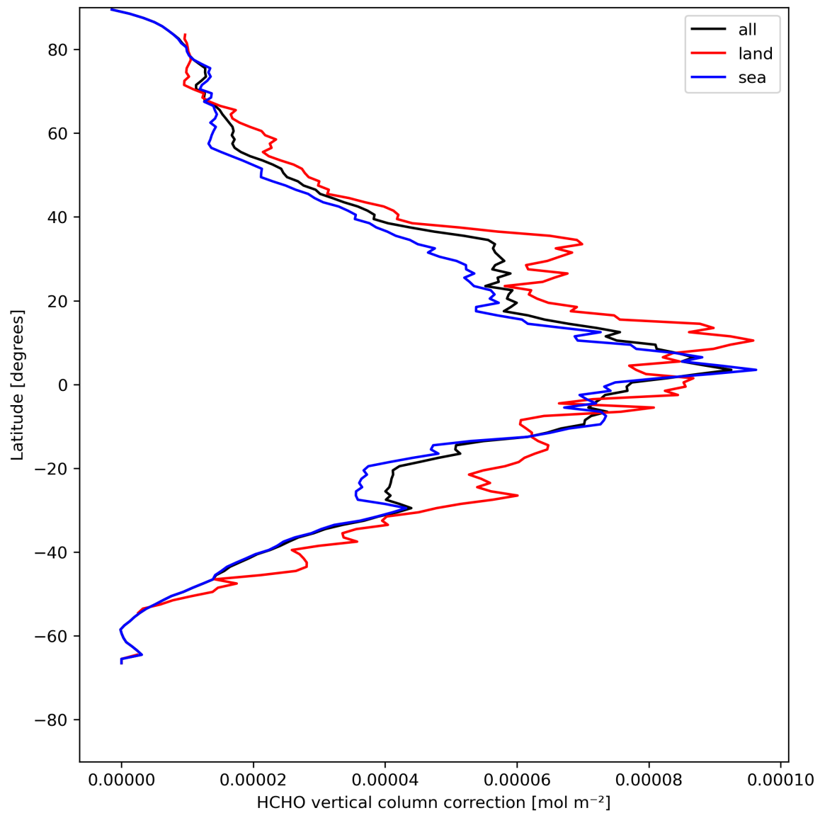
Figure 23: Zonal average of “HCHO vertical column correction” for 2024-05-12 to 2024-05-13.
