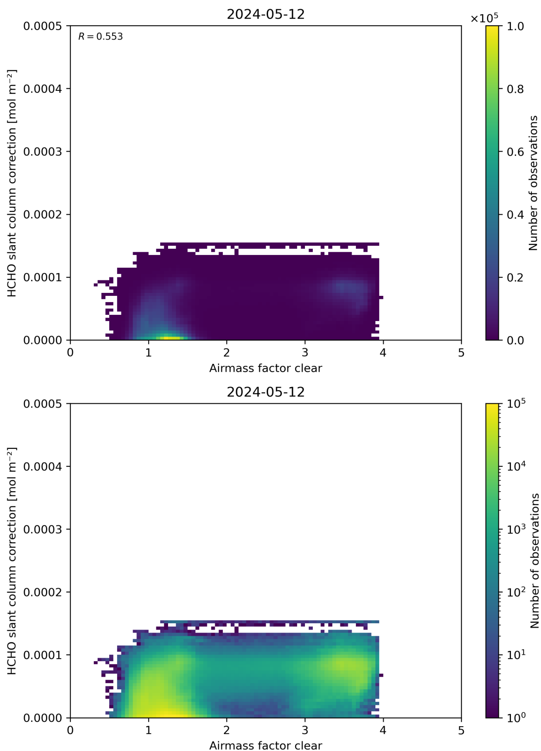
Figure 75: Scatter density plot of “Airmass factor clear” against “HCHO slant column correction” for 2024-05-12 to 2024-05-13.
