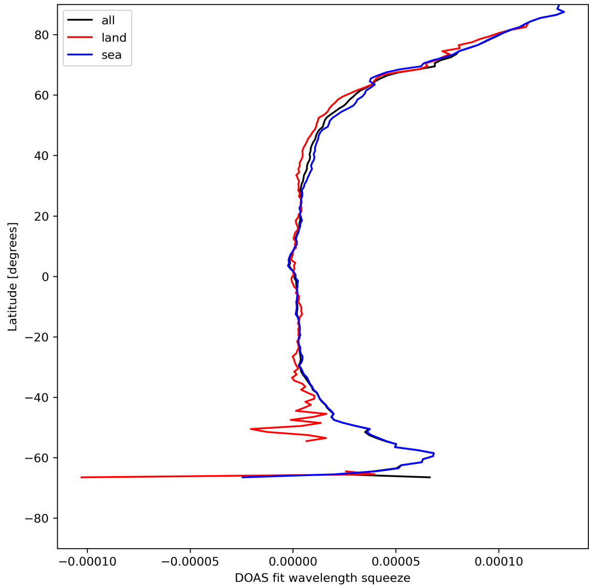
Figure 31: Zonal average of “DOAS fit wavelength squeeze” for 2024-05-12 to 2024-05-13.
