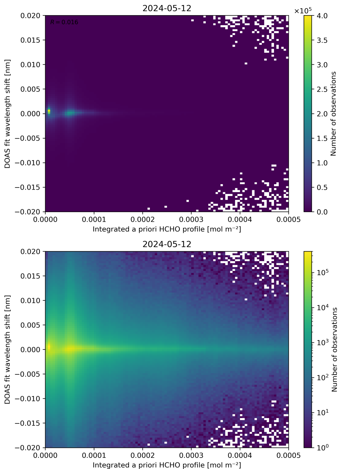
Figure 149: Scatter density plot of “Integrated a priori HCHO profile” against “DOAS fit wavelength shift” for 2024-05-12 to 2024-05-13.
