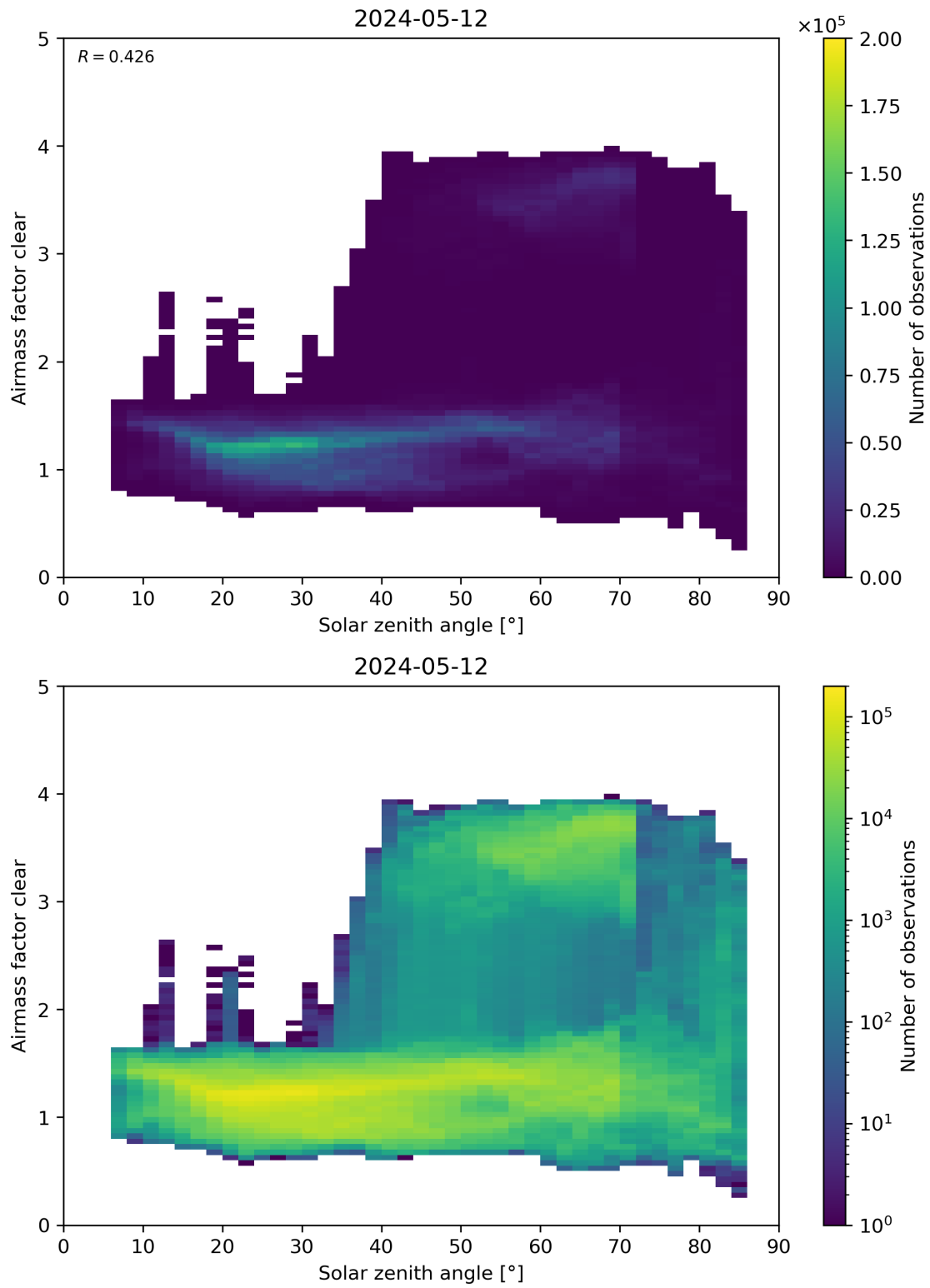
Figure 170: Scatter density plot of “Solar zenith angle” against “Airmass factor clear” for 2024-05-12 to 2024-05-13.
