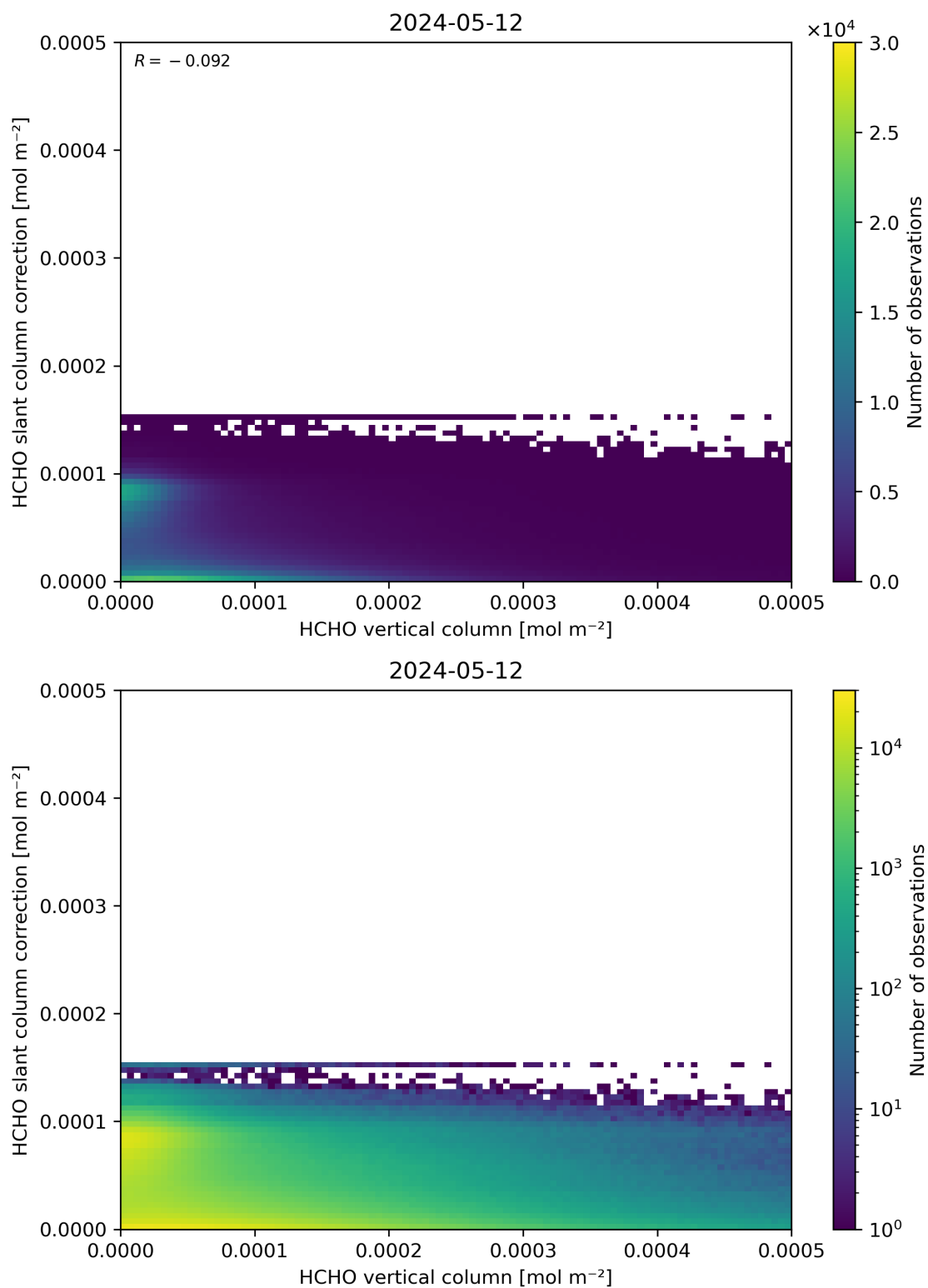
Figure 128: Scatter density plot of “HCHO vertical column” against “HCHO slant column correction” for 2024-05-12 to 2024-05-13.
