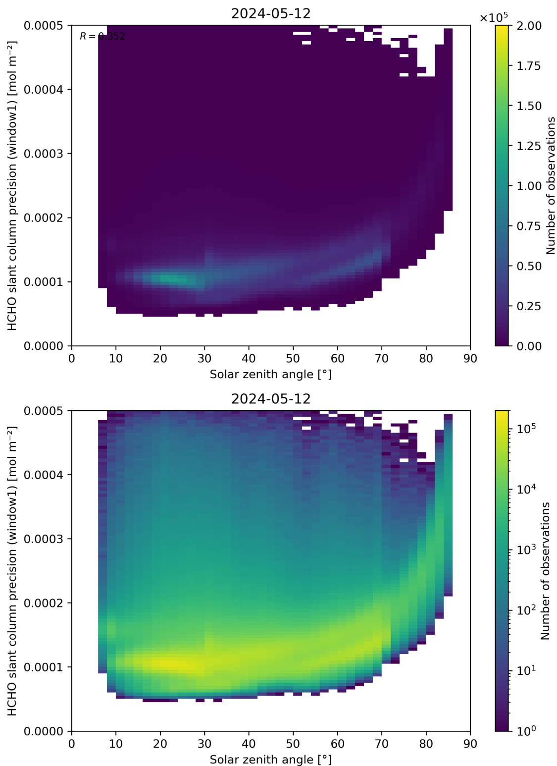
Figure 174: Scatter density plot of “Solar zenith angle” against “HCHO slant column precision (window1)” for 2024-05-12 to 2024-05-13.
