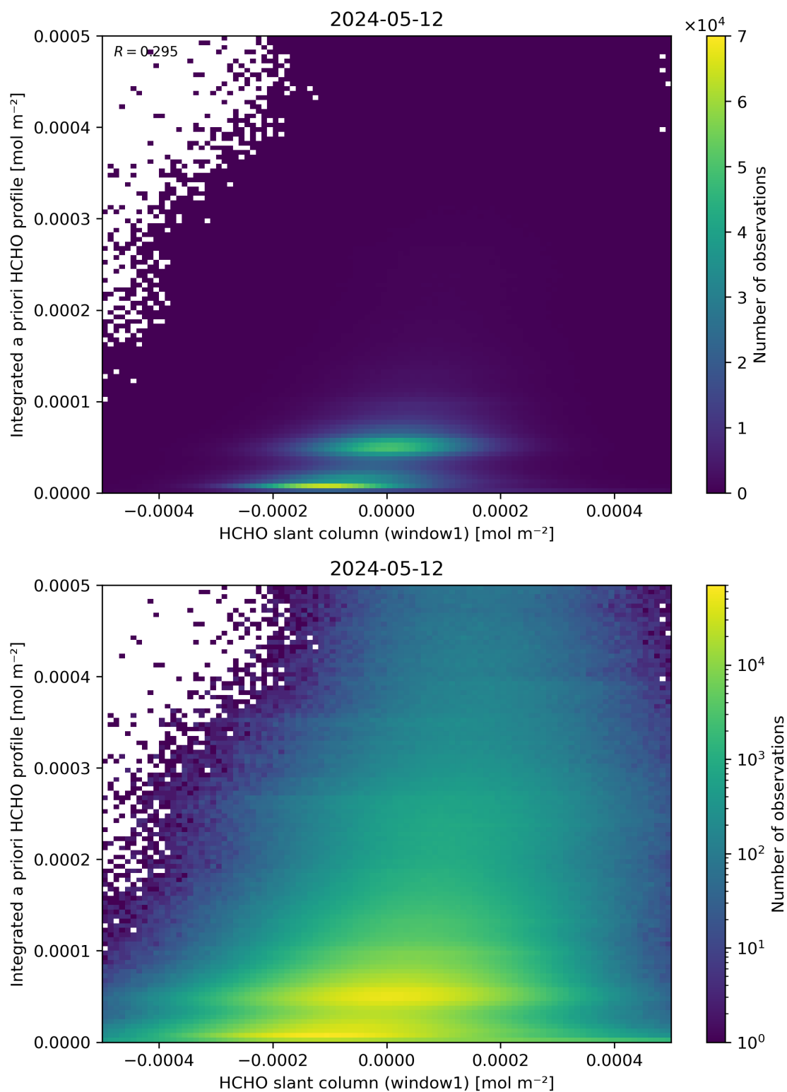
Figure 87: Scatter density plot of “HCHO slant column (window1)” against “Integrated a priori HCHO profile” for 2024-05-12 to 2024-05-13.
