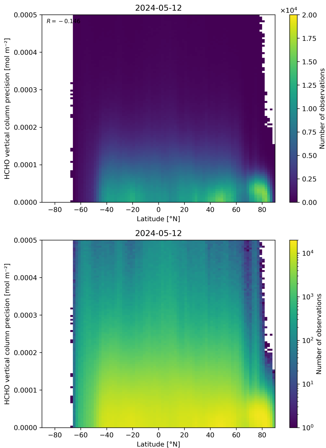
Figure 165: Scatter density plot of “Latitude” against “HCHO vertical column precision” for 2024-05-12 to 2024-05-13.
