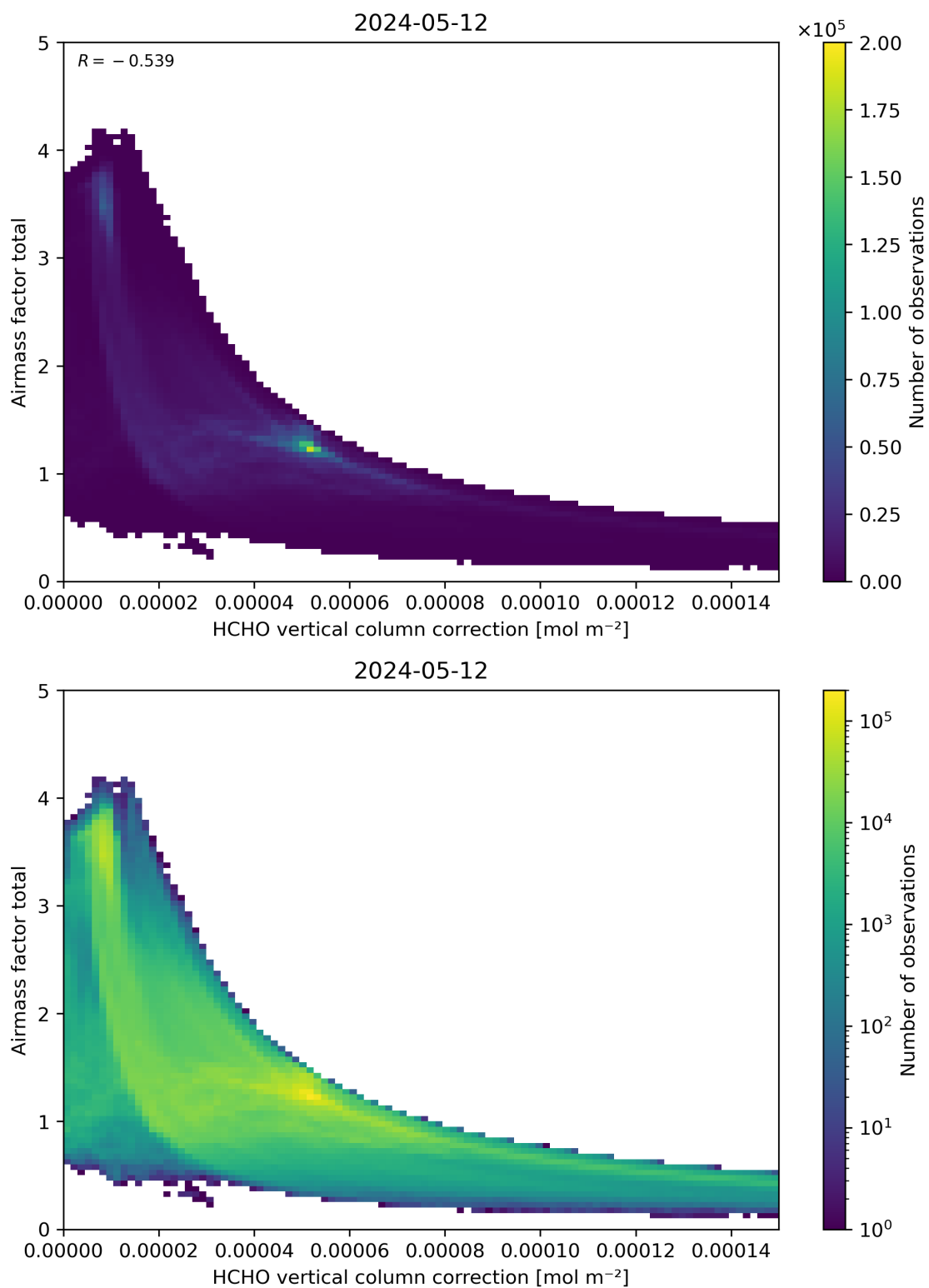
Figure 120: Scatter density plot of “HCHO vertical column correction” against “Airmass factor total” for 2024-05-12 to 2024-05-13.
