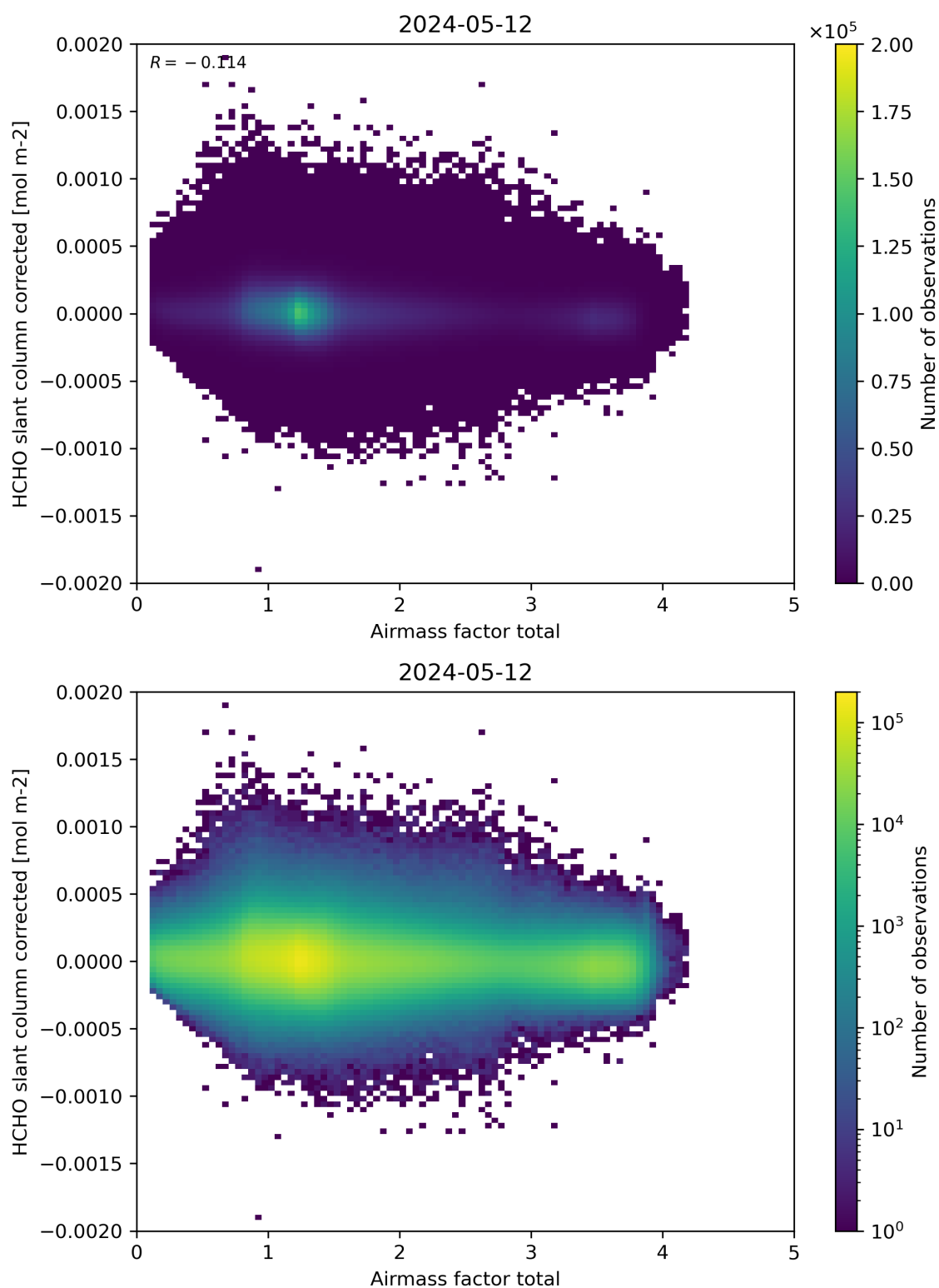
Figure 101: Scatter density plot of “Airmass factor total” against “HCHO slant column corrected” for 2024-05-12 to 2024-05-13.
