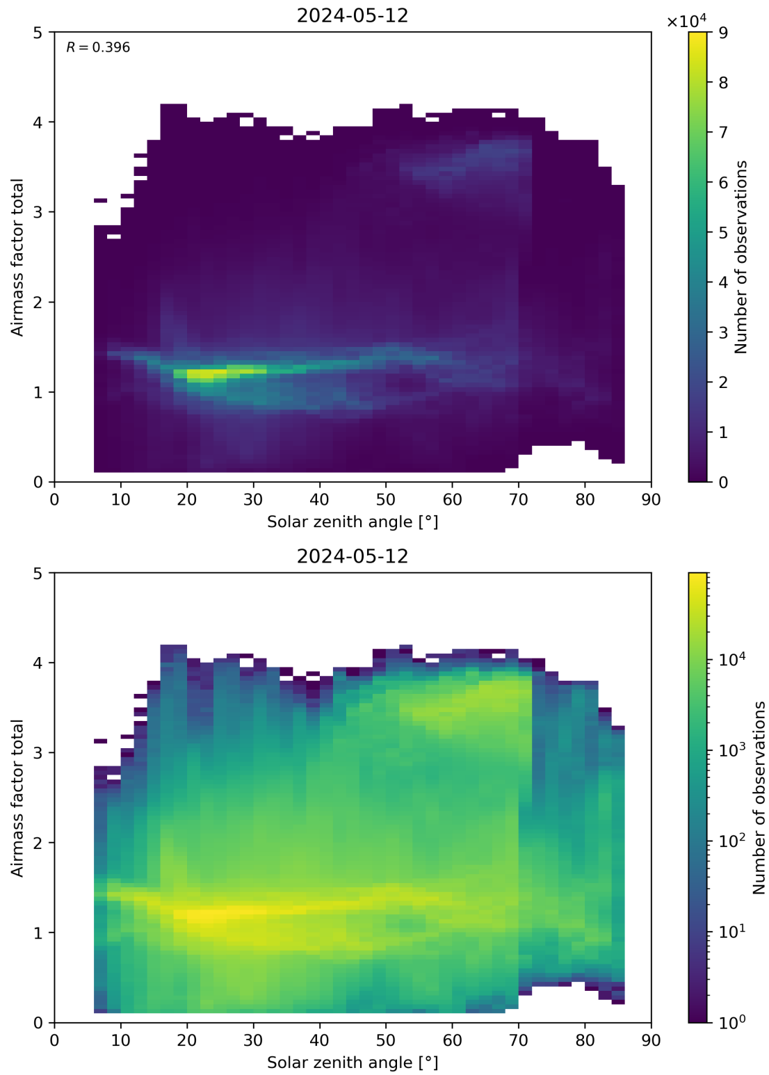
Figure 175: Scatter density plot of “Solar zenith angle” against “Airmass factor total” for 2024-05-12 to 2024-05-13.
