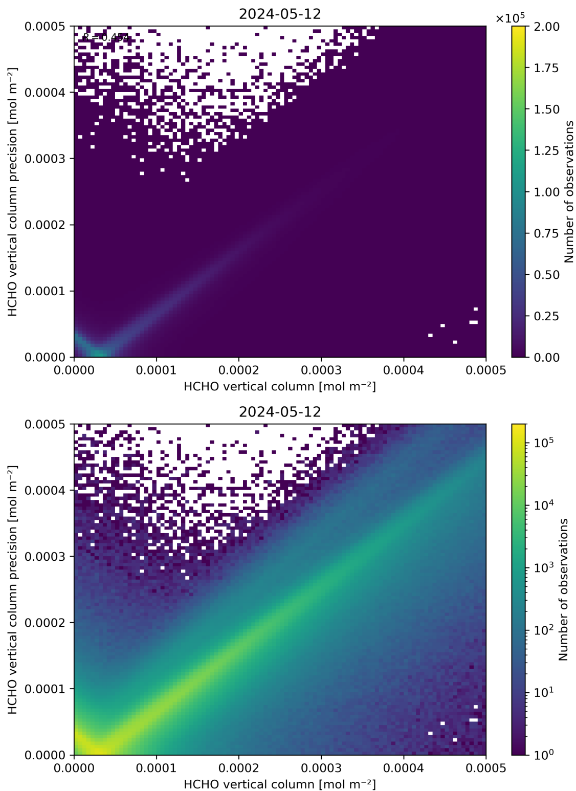
Figure 134: Scatter density plot of “HCHO vertical column” against “HCHO vertical column precision” for 2024-05-12 to 2024-05-13.
