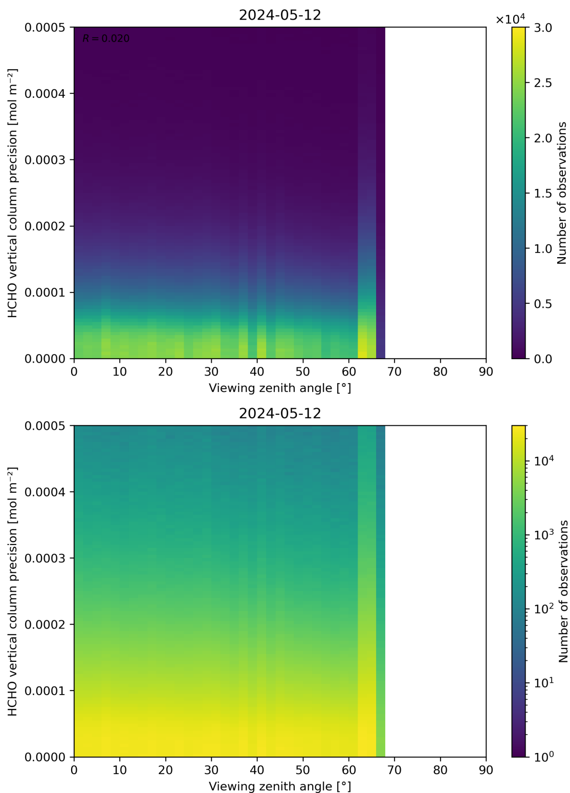
Figure 194: Scatter density plot of “Viewing zenith angle” against “HCHO vertical column precision” for 2024-05-12 to 2024-05-13.
