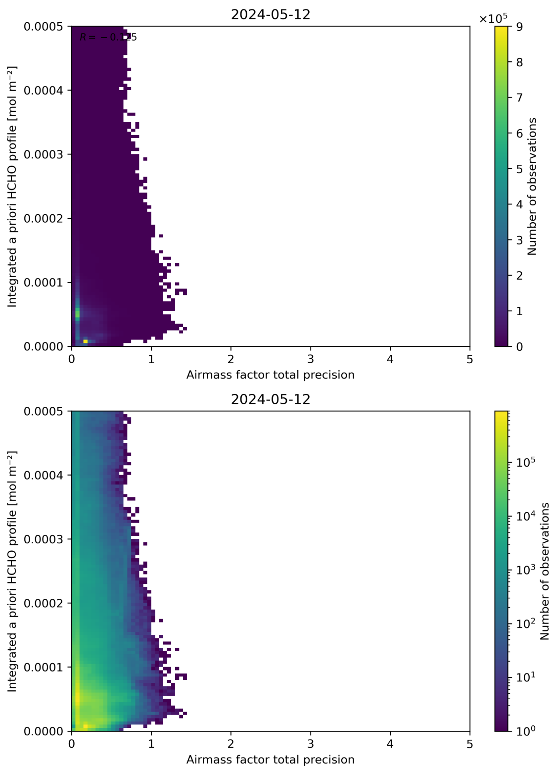
Figure 111: Scatter density plot of “Airmass factor total precision” against “Integrated a priori HCHO profile” for 2024-05-12 to 2024-05-13.
