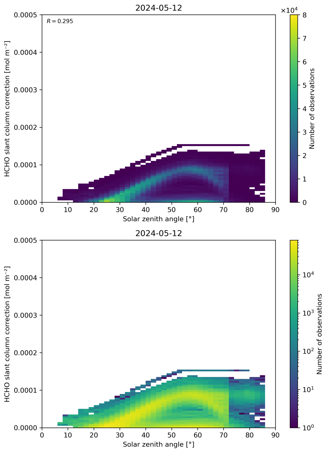
Figure 172: Scatter density plot of “Solar zenith angle” against “HCHO slant column correction” for 2024-05-12 to 2024-05-13.
