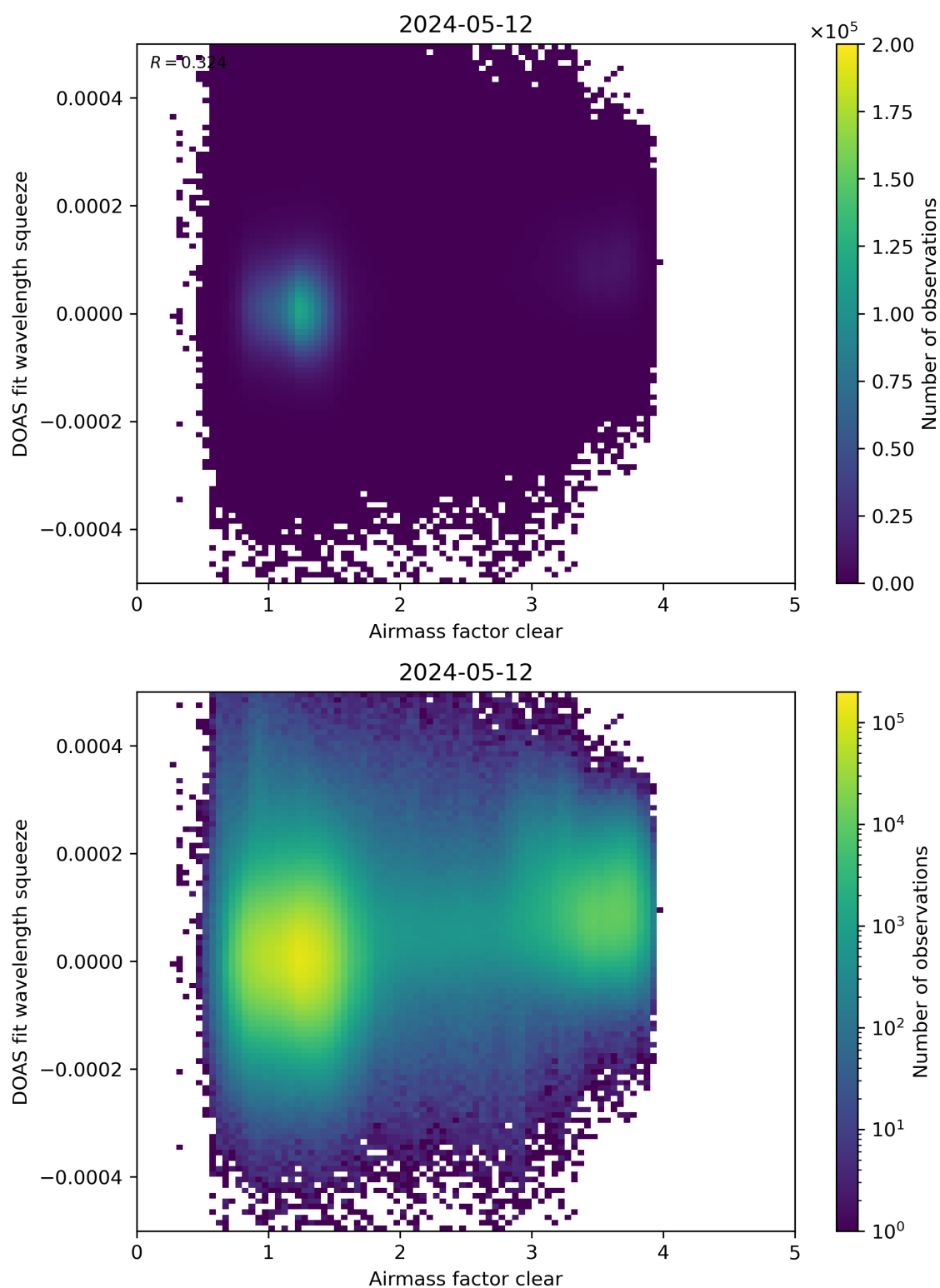
Figure 73: Scatter density plot of “Airmass factor clear” against “DOAS fit wavelength squeeze” for 2024-05-12 to 2024-05-13.
