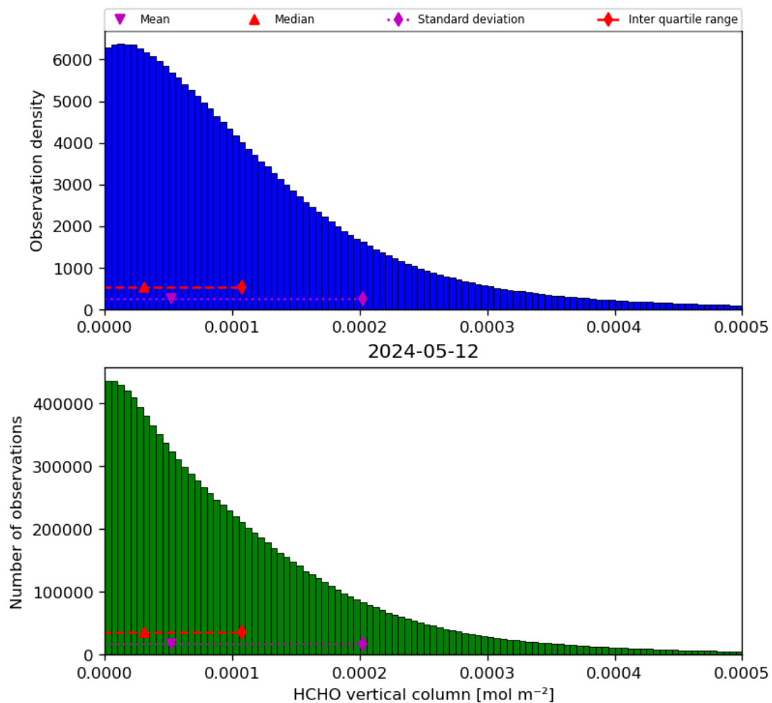
Figure 35: Histogram of “HCHO vertical column” for 2024-05-12 to 2024-05-13
