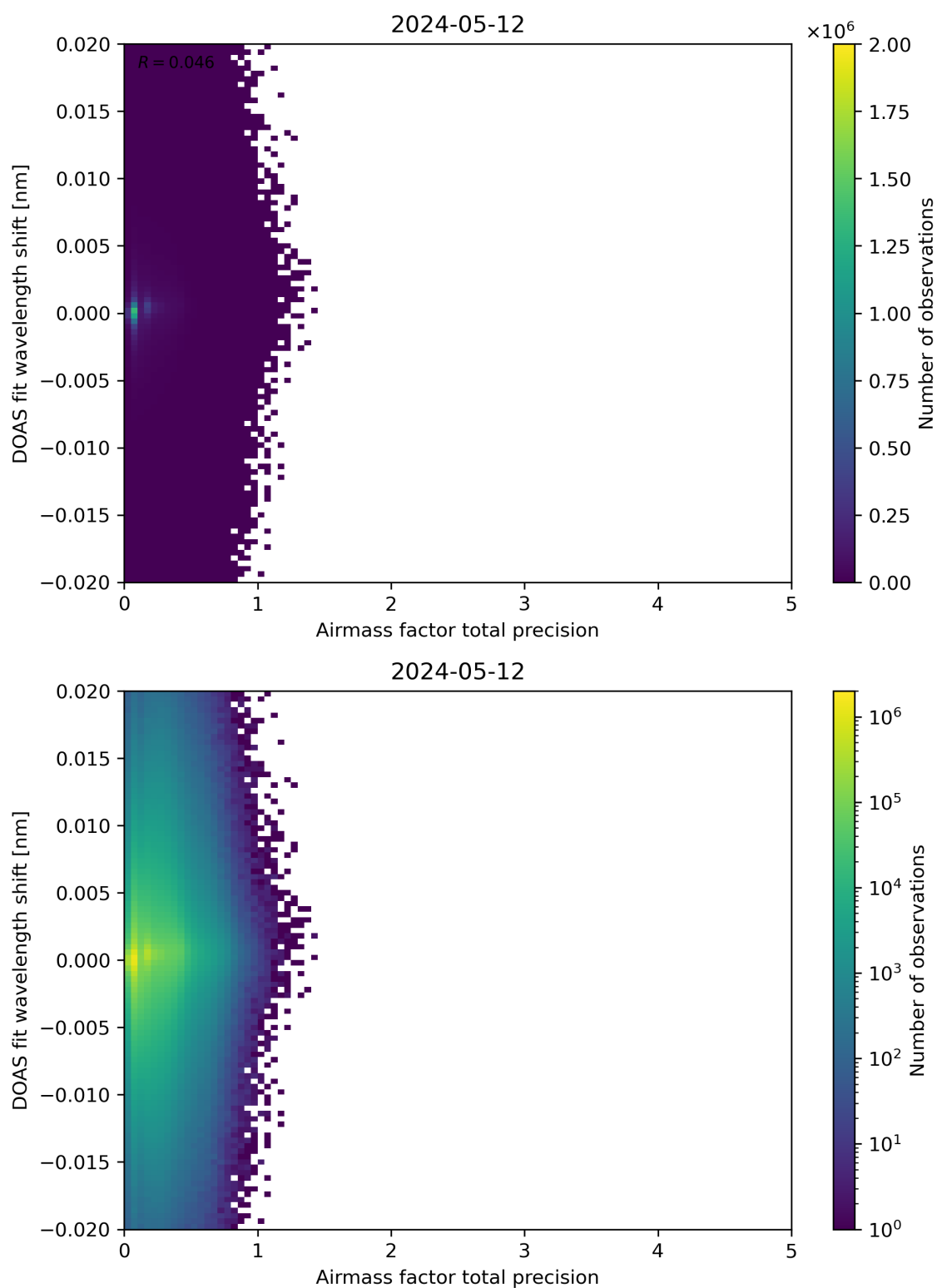
Figure 106: Scatter density plot of “Airmass factor total precision” against “DOAS fit wavelength shift” for 2024-05-12 to 2024-05-13.
