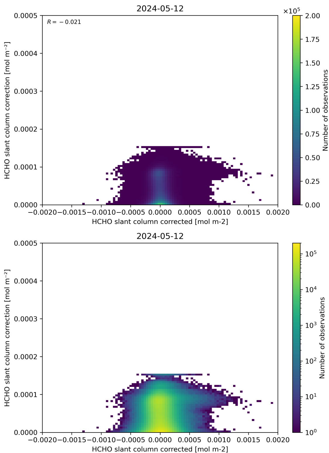
Figure 77: Scatter density plot of “HCHO slant column corrected” against “HCHO slant column correction” for 2024-05-12 to 2024-05-13.
