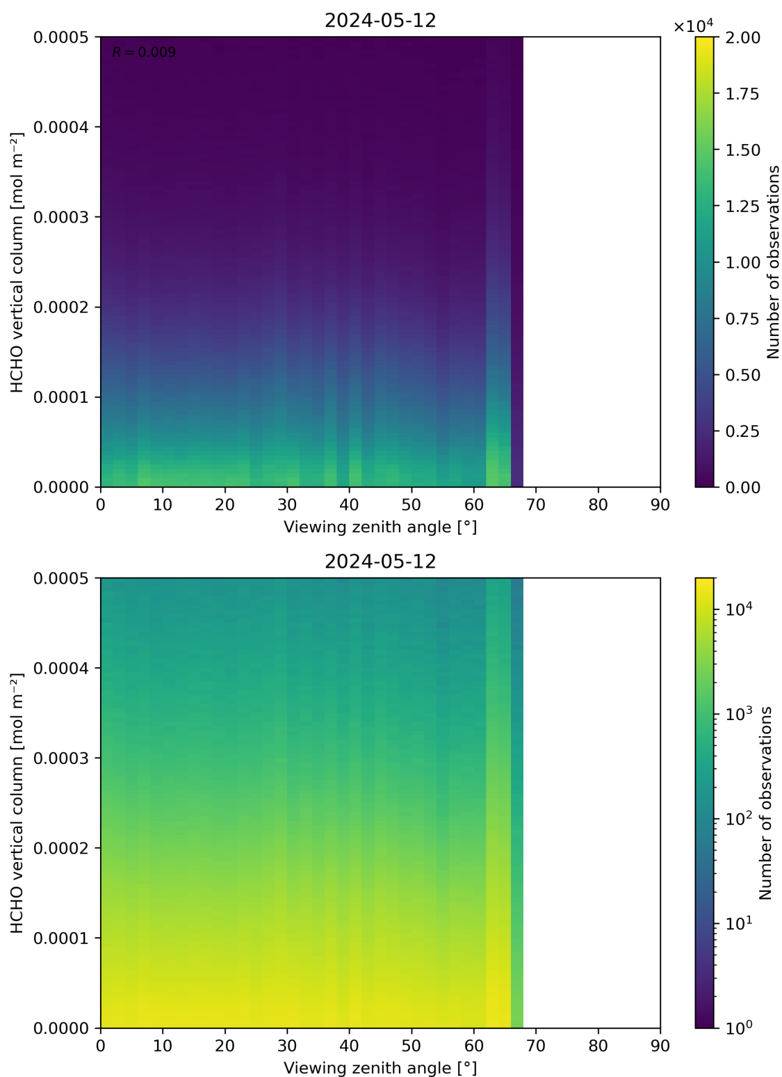
Figure 192: Scatter density plot of “Viewing zenith angle” against “HCHO vertical column” for 2024-05-12 to 2024-05-13.
