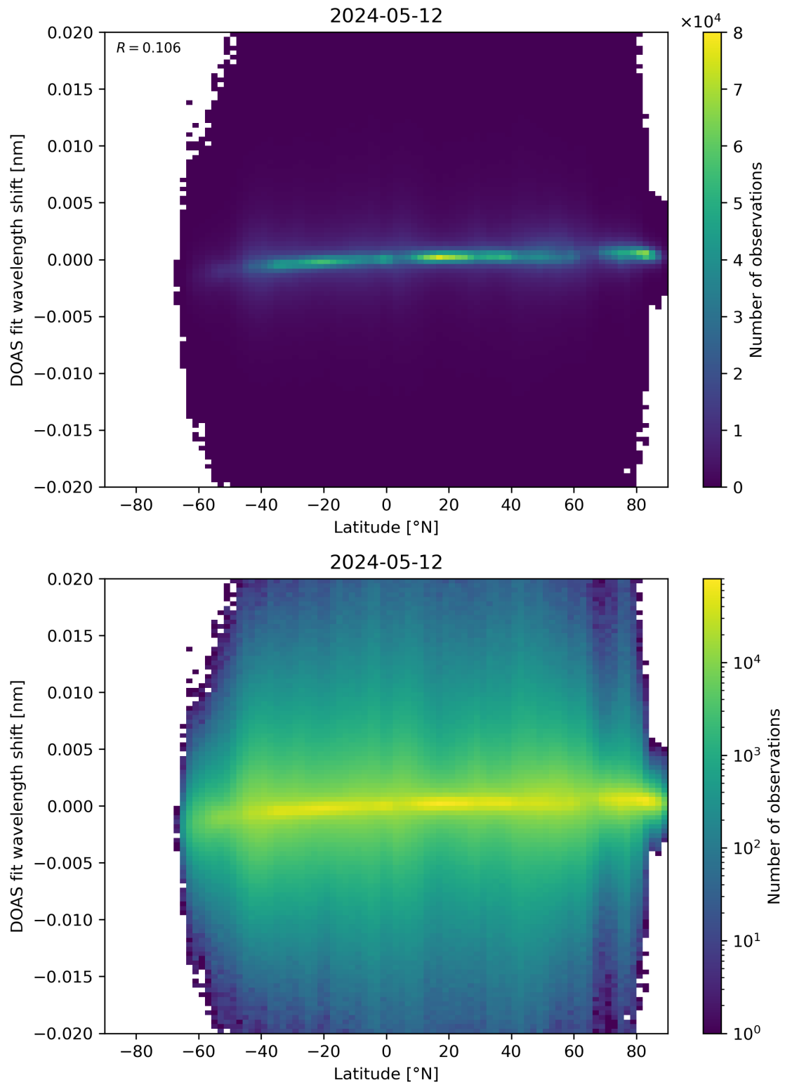
Figure 154: Scatter density plot of “Latitude” against “DOAS fit wavelength shift” for 2024-05-12 to 2024-05-13.
