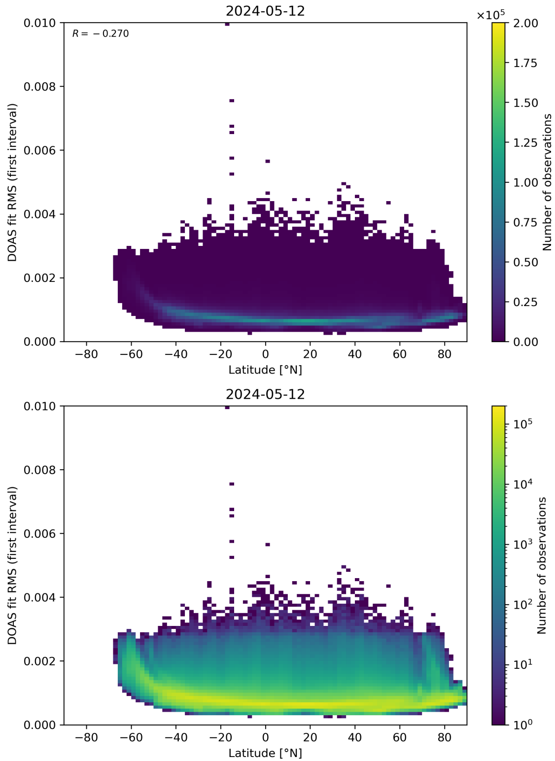
Figure 153: Scatter density plot of “Latitude” against “DOAS fit RMS (first interval)” for 2024-05-12 to 2024-05-13.
