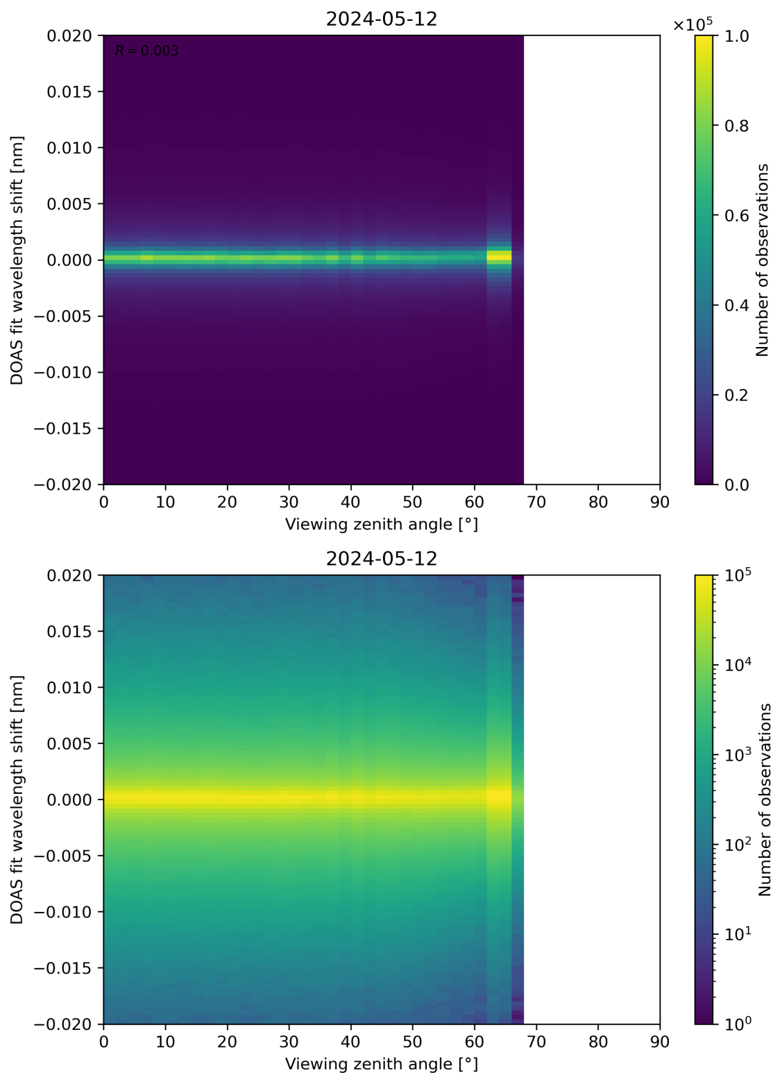
Figure 183: Scatter density plot of “Viewing zenith angle” against “DOAS fit wavelength shift” for 2024-05-12 to 2024-05-13.
