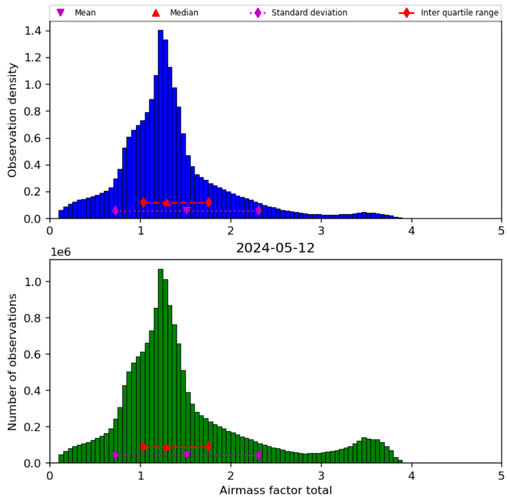
Figure 40: Histogram of “Airmass factor total” for 2024-05-12 to 2024-05-13
