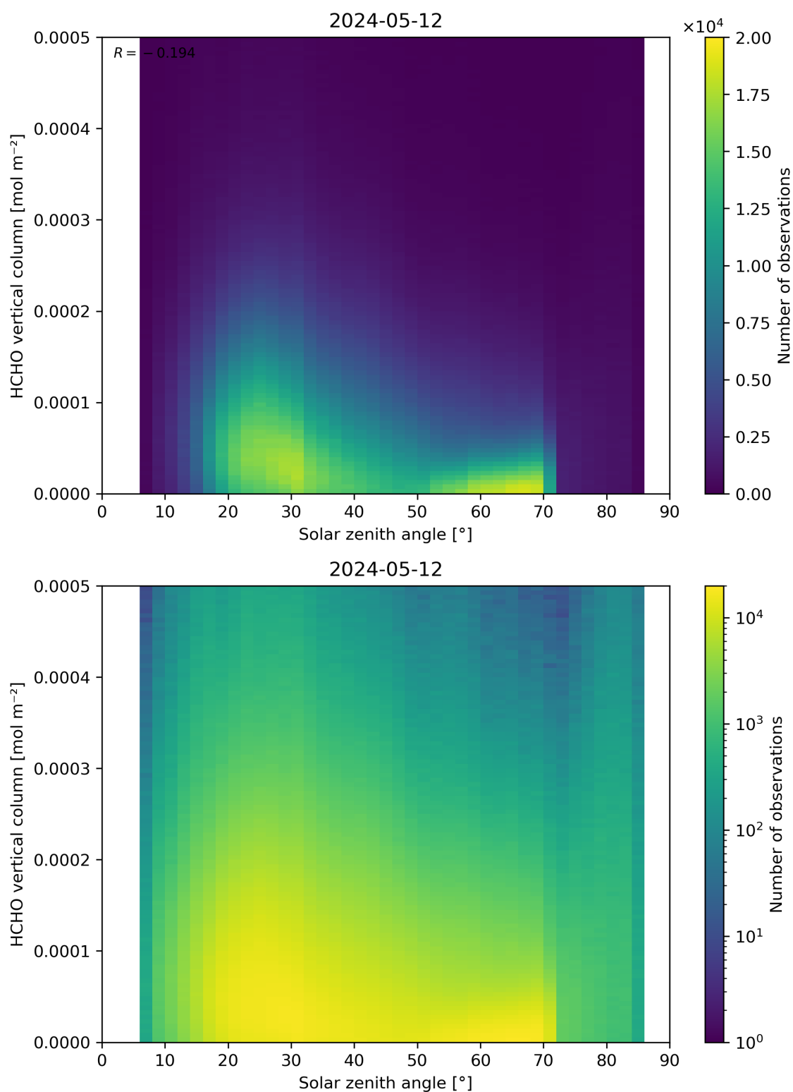
Figure 177: Scatter density plot of “Solar zenith angle” against “HCHO vertical column” for 2024-05-12 to 2024-05-13.
