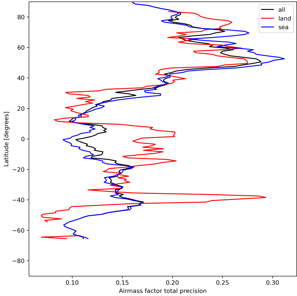
Figure 27: Zonal average of “Airmass factor total precision” for 2024-05-12 to 2024-05-14.
