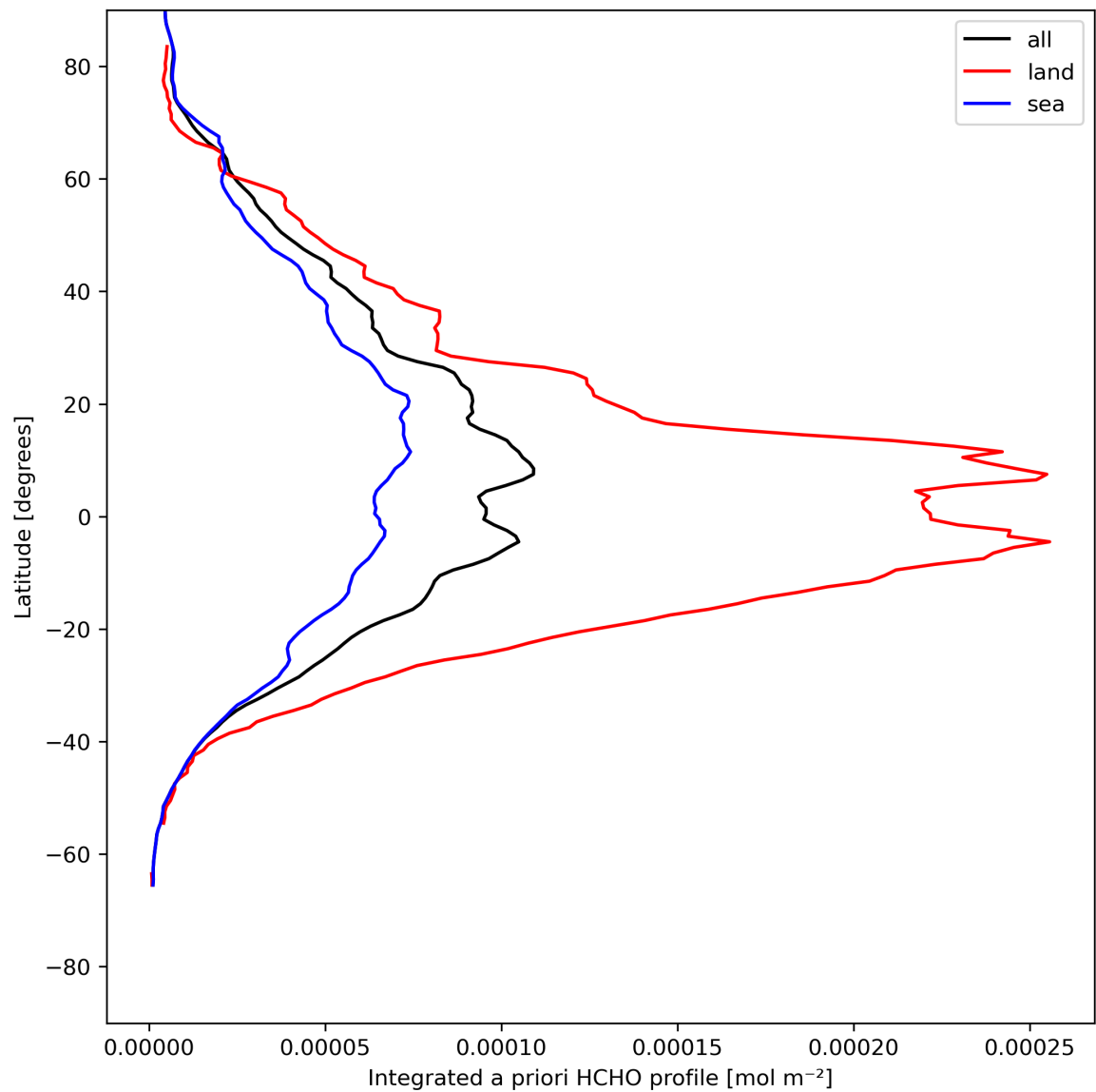
Figure 29: Zonal average of “Integrated a priori HCHO profile” for 2024-05-12 to 2024-05-14.
