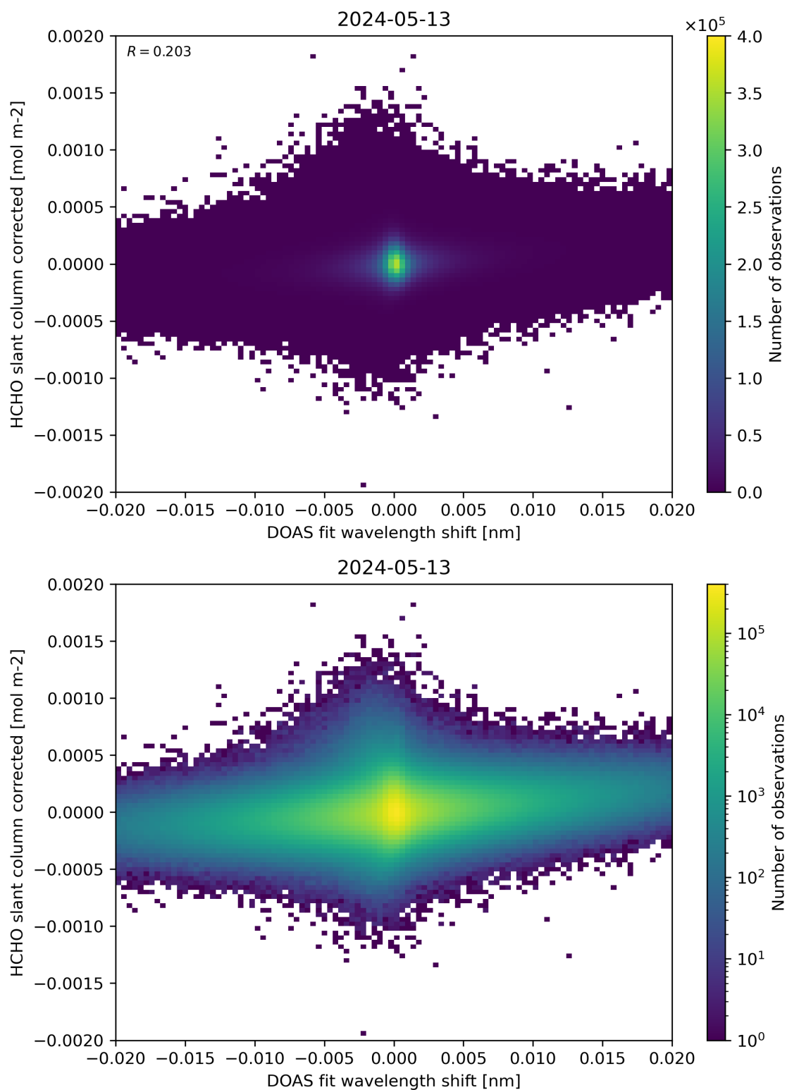
Figure 66: Scatter density plot of “DOAS fit wavelength shift” against “HCHO slant column corrected” for 2024-05-12 to 2024-05-14.
