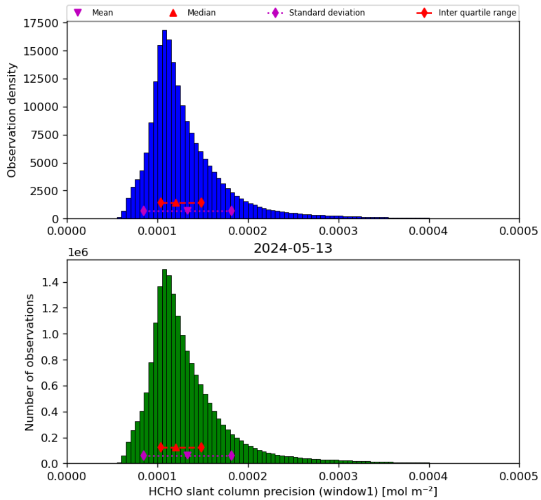
Figure 39: Histogram of “HCHO slant column precision (window1)” for 2024-05-12 to 2024-05-14
