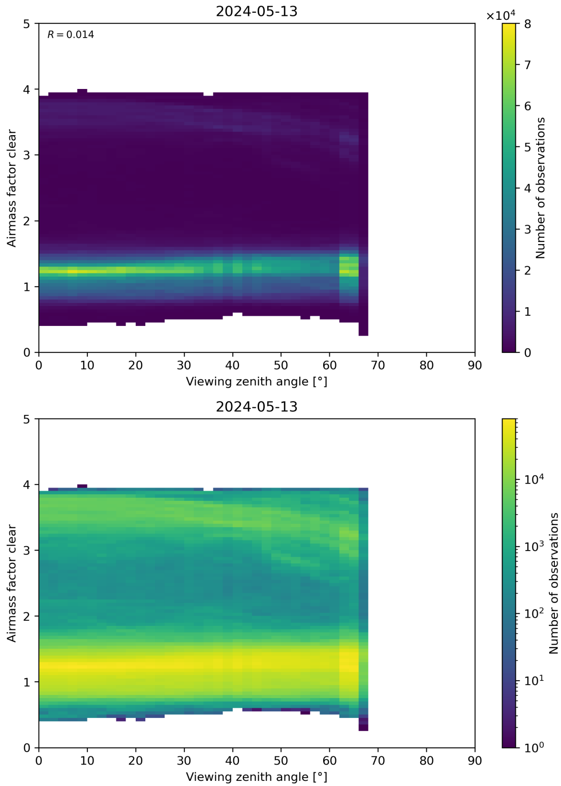
Figure 185: Scatter density plot of “Viewing zenith angle” against “Airmass factor clear” for 2024-05-12 to 2024-05-14.
