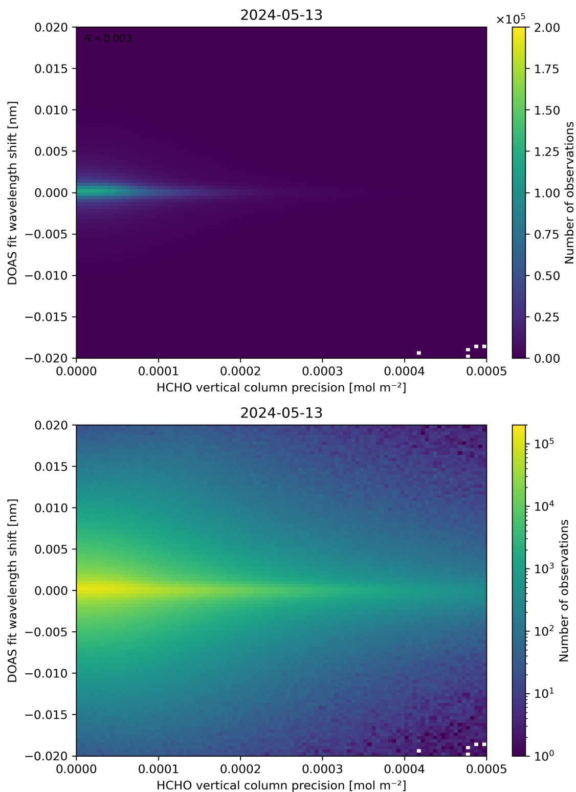
Figure 137: Scatter density plot of “HCHO vertical column precision” against “DOAS fit wavelength shift” for 2024-05-12 to 2024-05-14.
