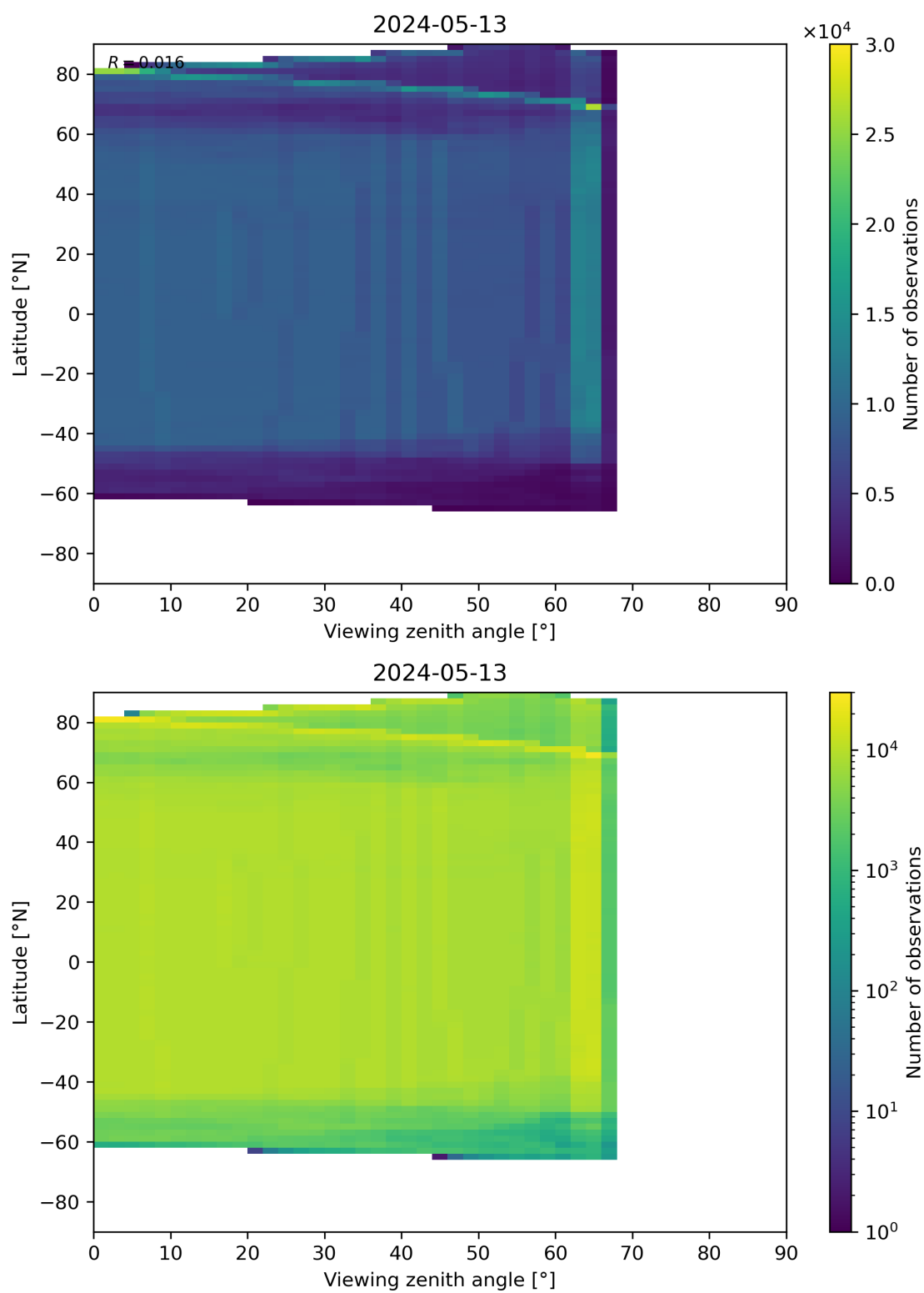
Figure 196: Scatter density plot of “Viewing zenith angle” against “Latitude” for 2024-05-12 to 2024-05-14.
