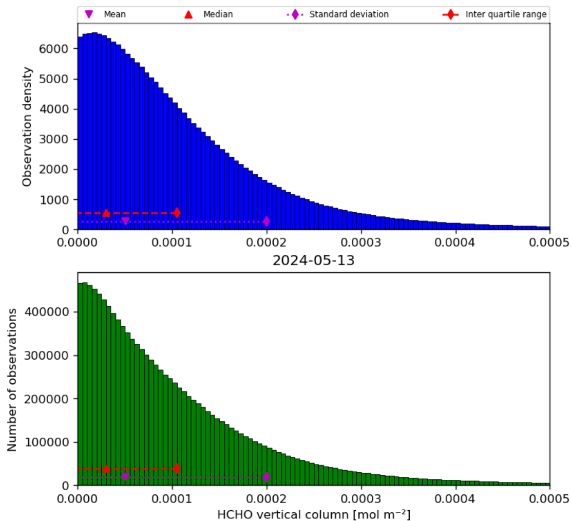
Figure 35: Histogram of “HCHO vertical column” for 2024-05-12 to 2024-05-14
