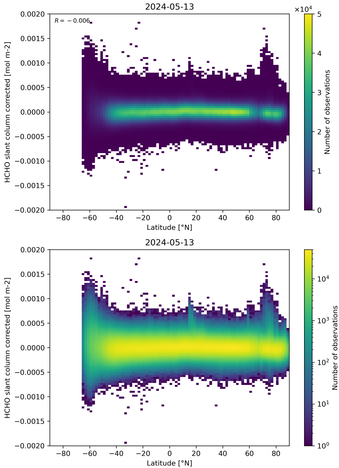
Figure 157: Scatter density plot of “Latitude” against “HCHO slant column corrected” for 2024-05-12 to 2024-05-14.
