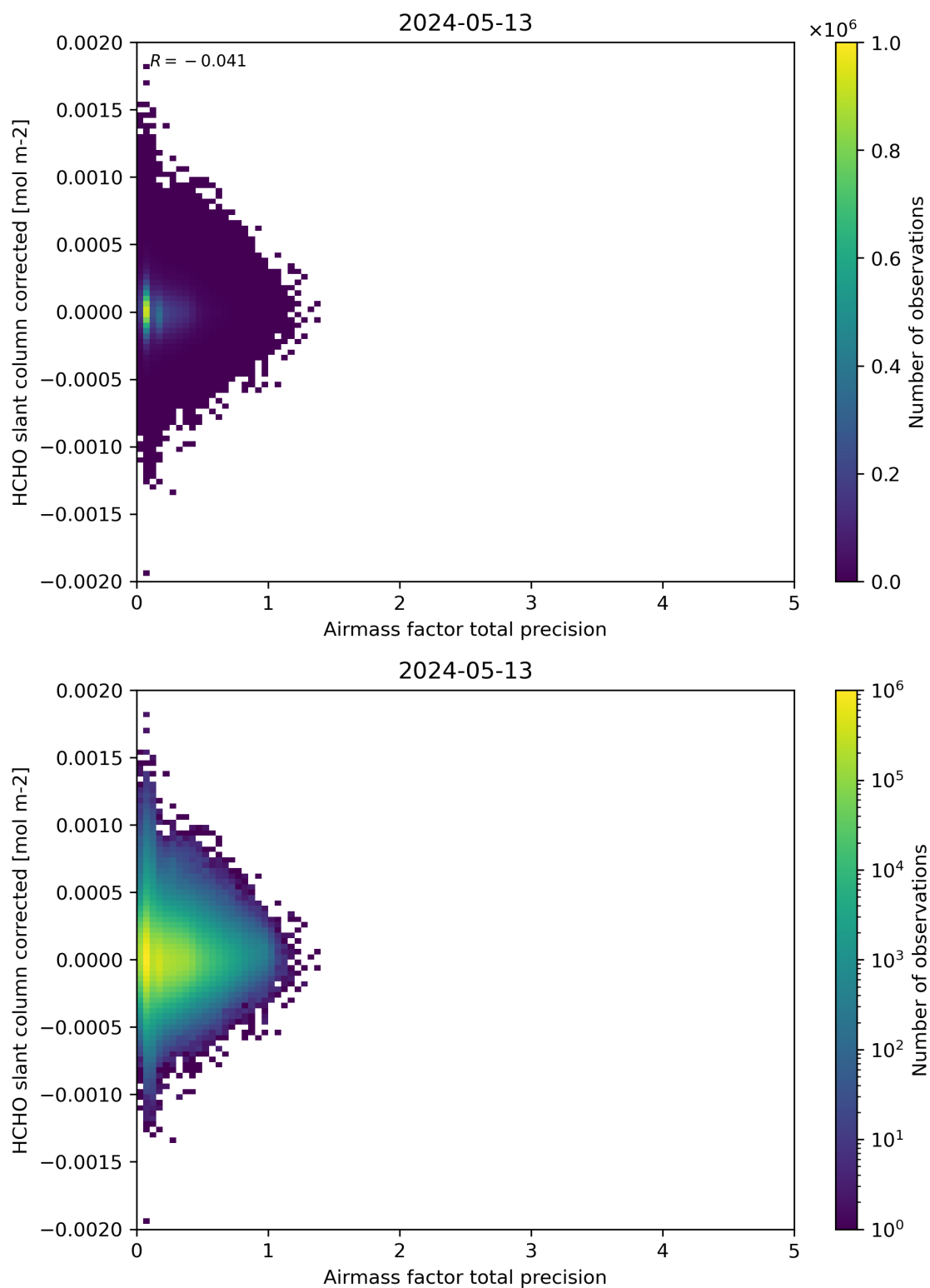
Figure 109: Scatter density plot of “Airmass factor total precision” against “HCHO slant column corrected” for 2024-05-12 to 2024-05-14.
