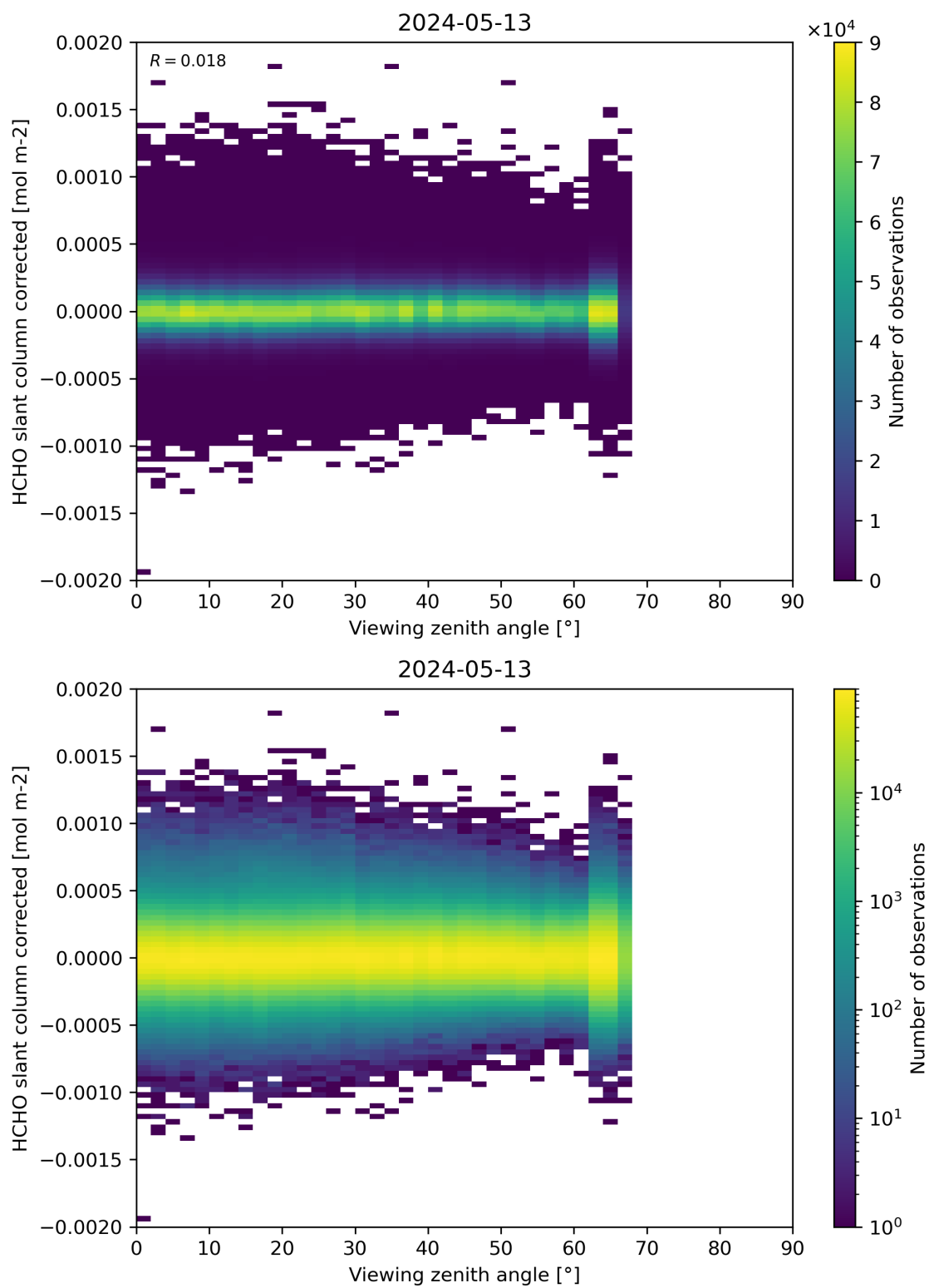
Figure 186: Scatter density plot of “Viewing zenith angle” against “HCHO slant column corrected” for 2024-05-12 to 2024-05-14.
