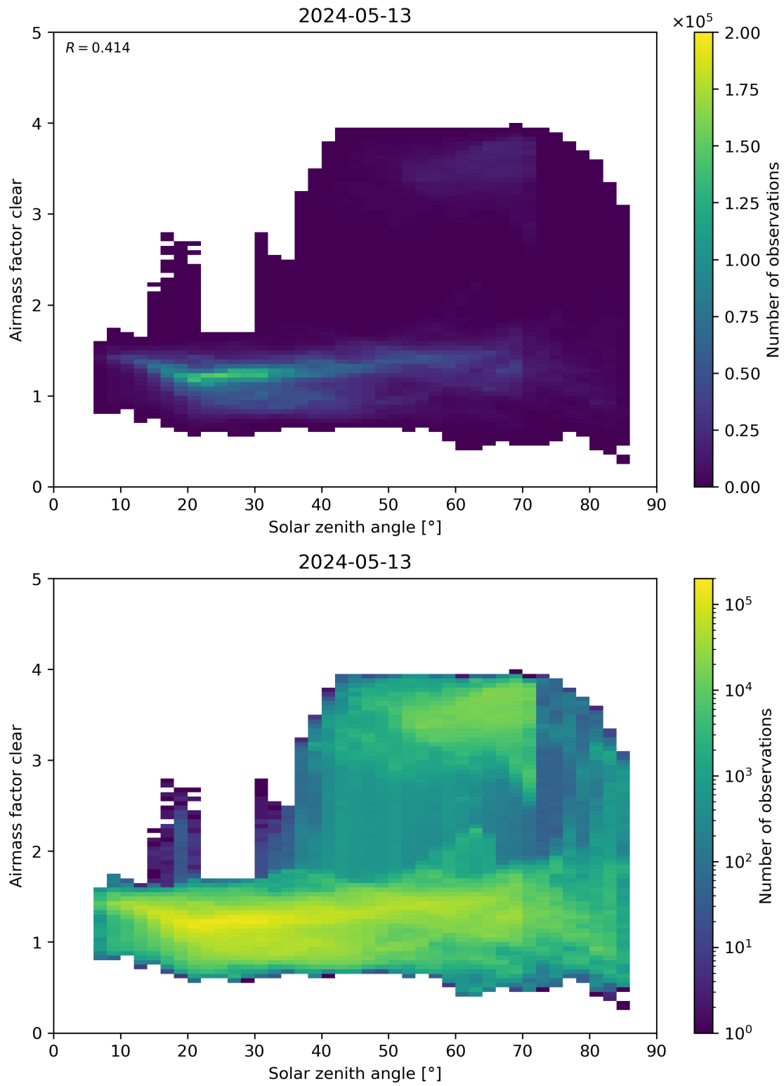
Figure 170: Scatter density plot of “Solar zenith angle” against “Airmass factor clear” for 2024-05-12 to 2024-05-14.
