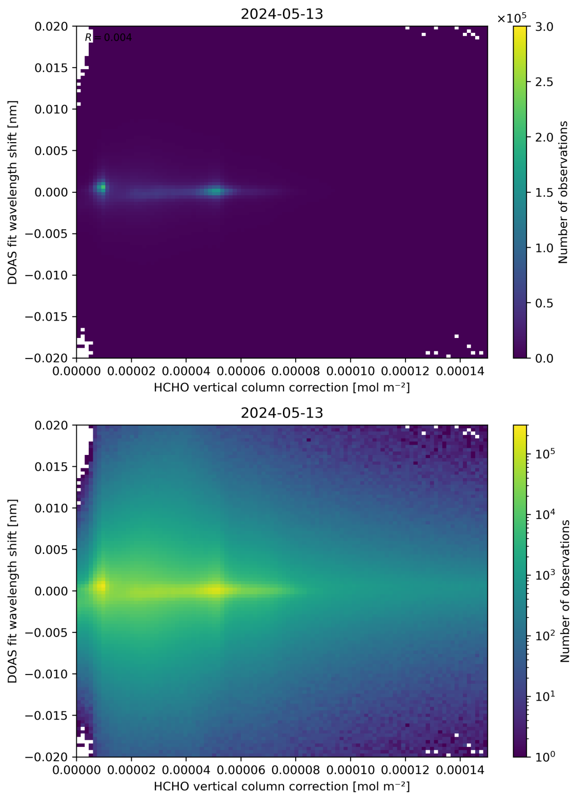
Figure 113: Scatter density plot of “HCHO vertical column correction” against “DOAS fit wavelength shift” for 2024-05-12 to 2024-05-14.
