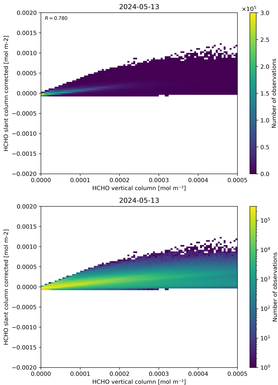
Figure 127: Scatter density plot of “HCHO vertical column” against “HCHO slant column corrected” for 2024-05-12 to 2024-05-14.
