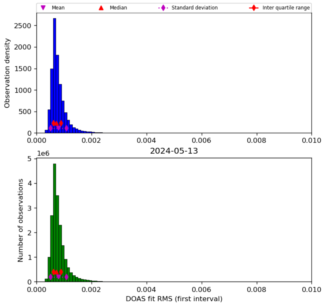
Figure 46: Histogram of “DOAS fit RMS (first interval)” for 2024-05-12 to 2024-05-14
