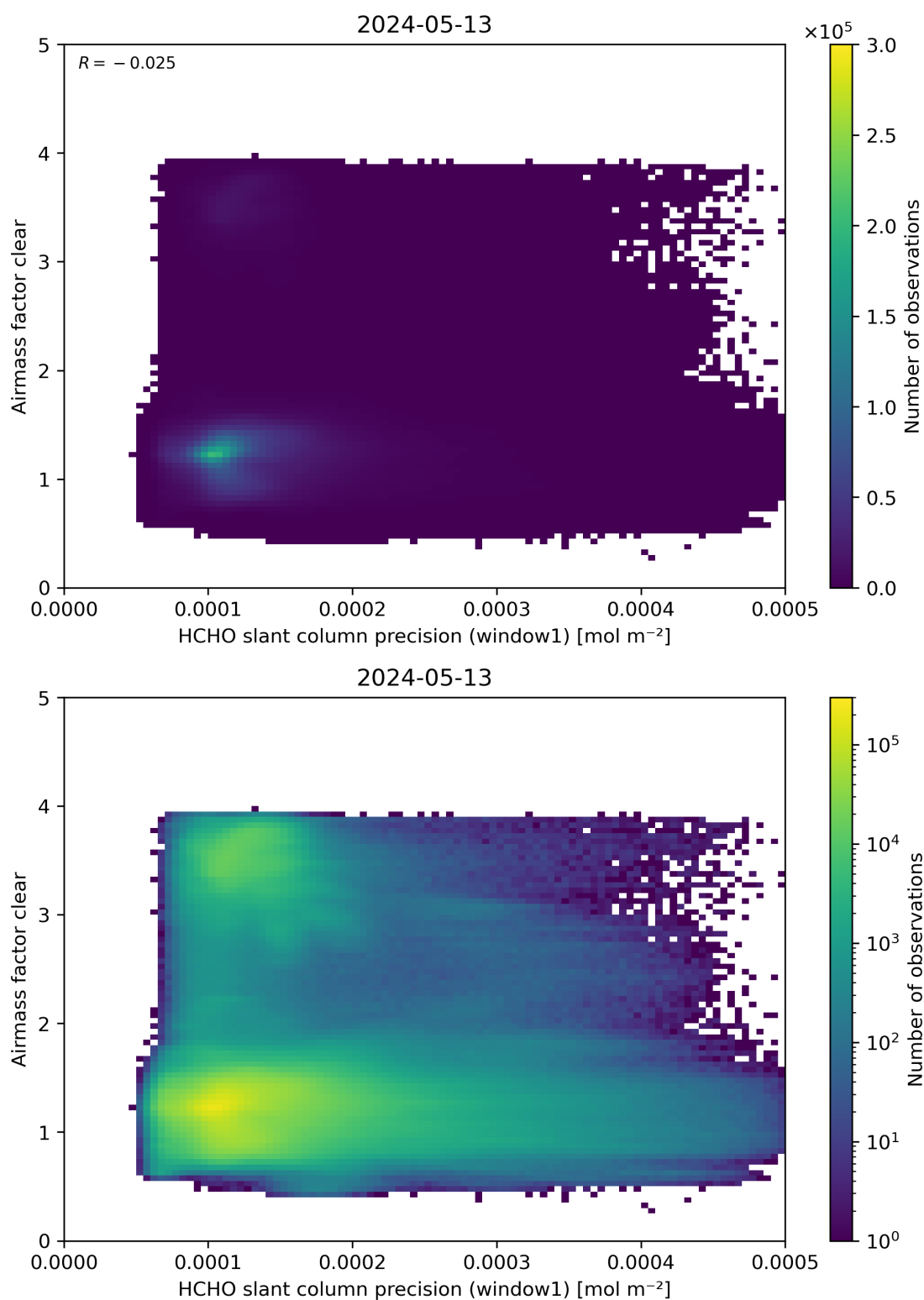
Figure 91: Scatter density plot of “HCHO slant column precision (window1)” against “Airmass factor clear” for 2024-05-12 to 2024-05-14.
