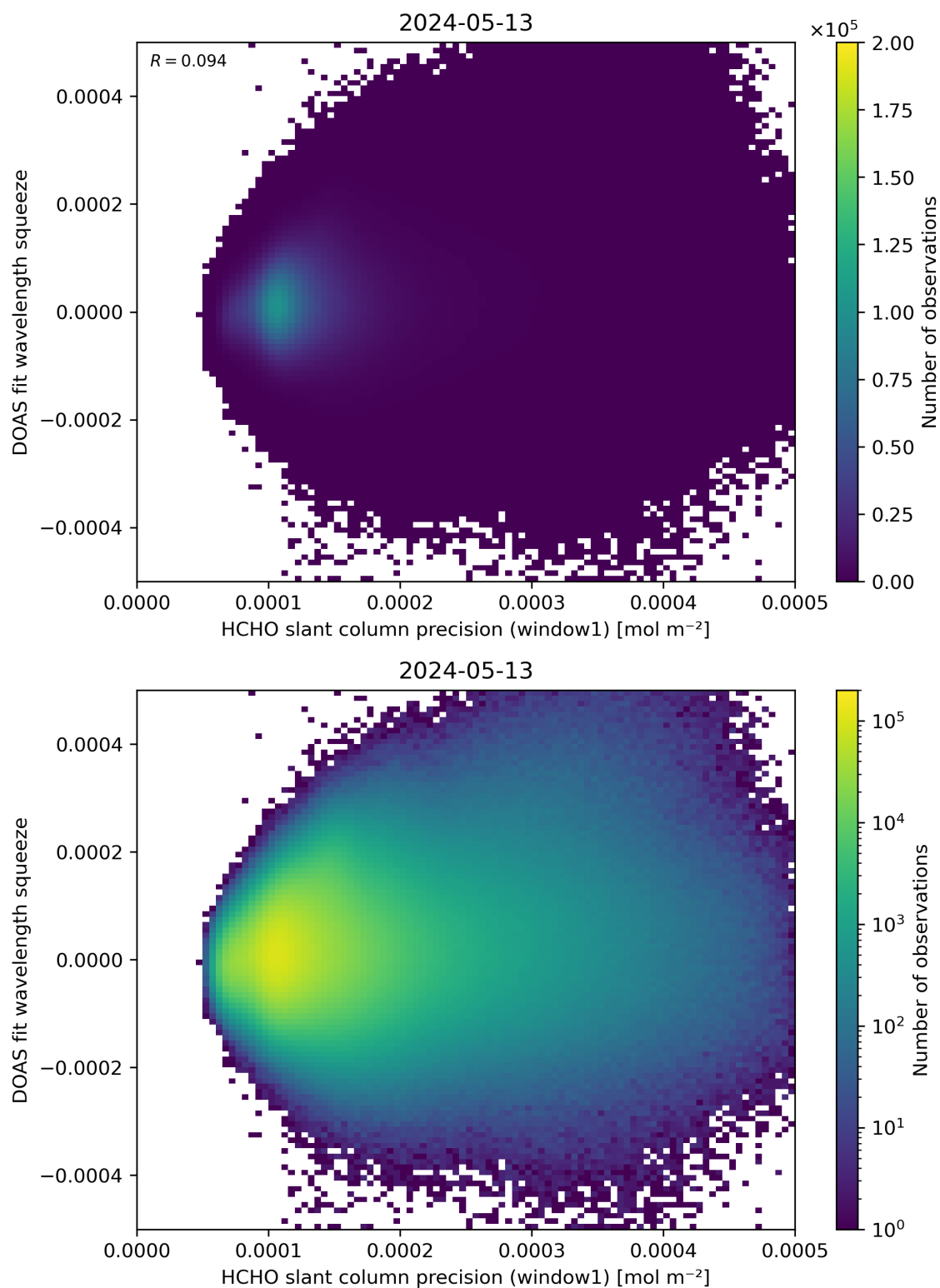
Figure 90: Scatter density plot of “HCHO slant column precision (window1)” against “DOAS fit wavelength squeeze” for 2024-05-12 to 2024-05-14.
