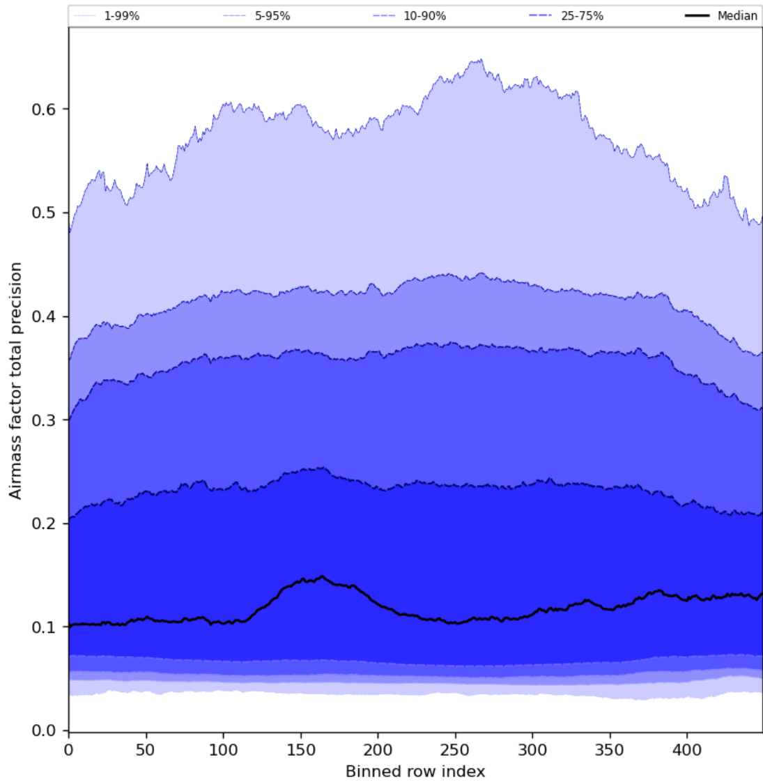
Figure 55: Along track statistics of “Airmass factor total precision” for 2024-05-12 to 2024-05-14
