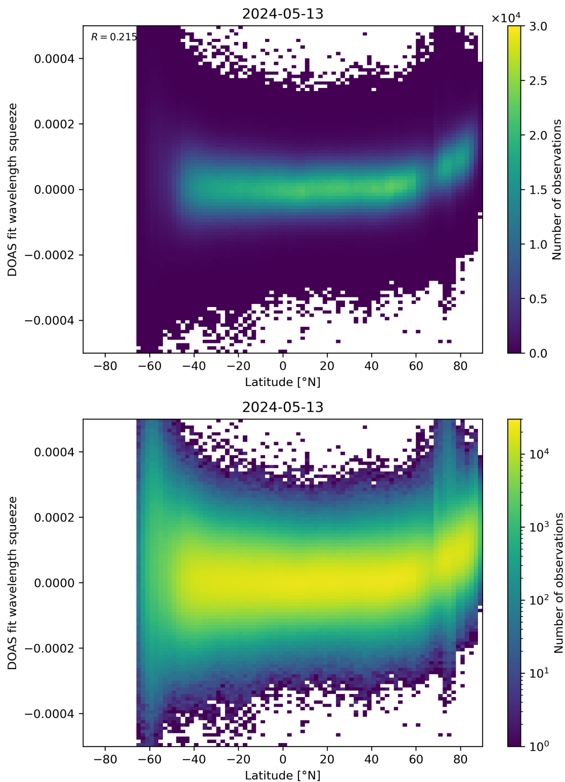
Figure 155: Scatter density plot of “Latitude” against “DOAS fit wavelength squeeze” for 2024-05-12 to 2024-05-14.
