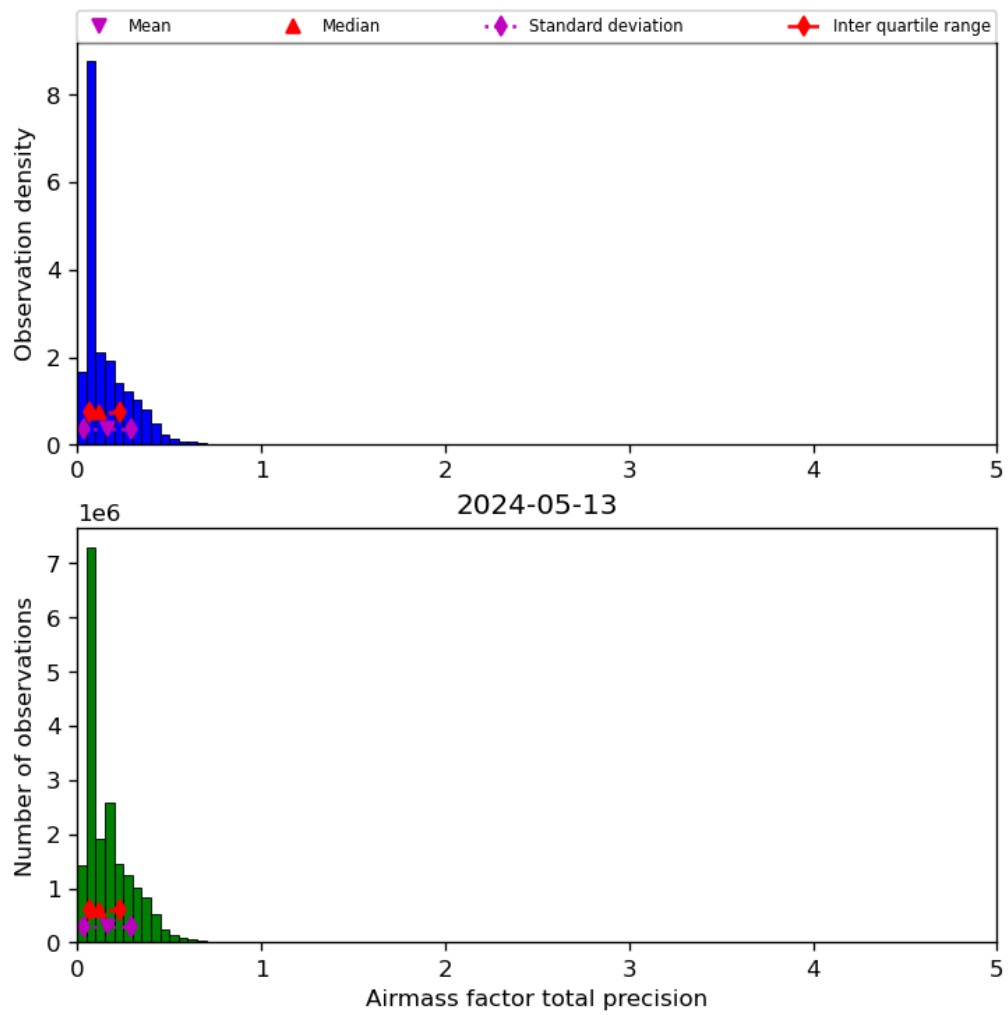
Figure 41: Histogram of “Airmass factor total precision” for 2024-05-12 to 2024-05-14
