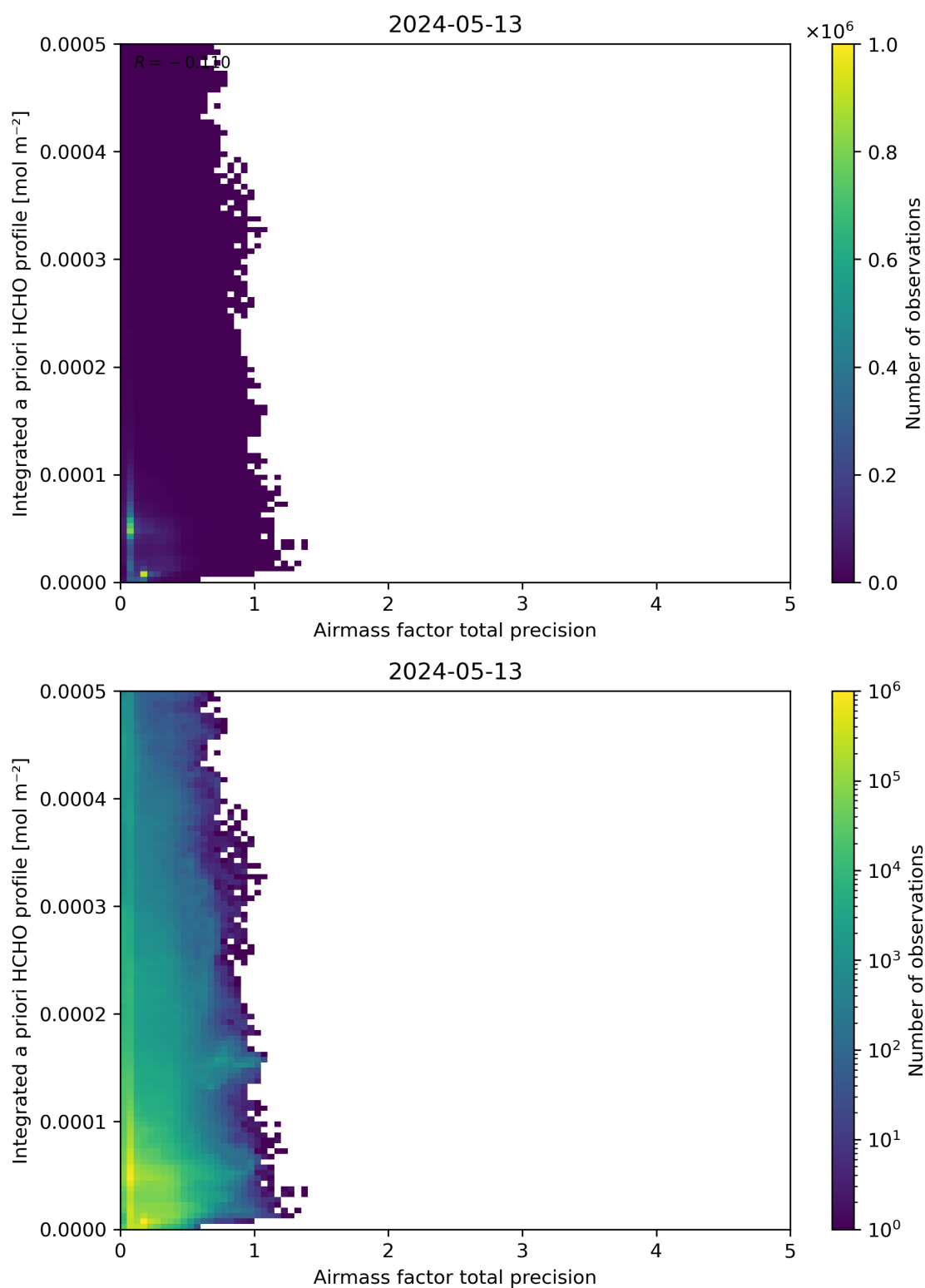
Figure 111: Scatter density plot of “Airmass factor total precision” against “Integrated a priori HCHO profile” for 2024-05-12 to 2024-05-14.
