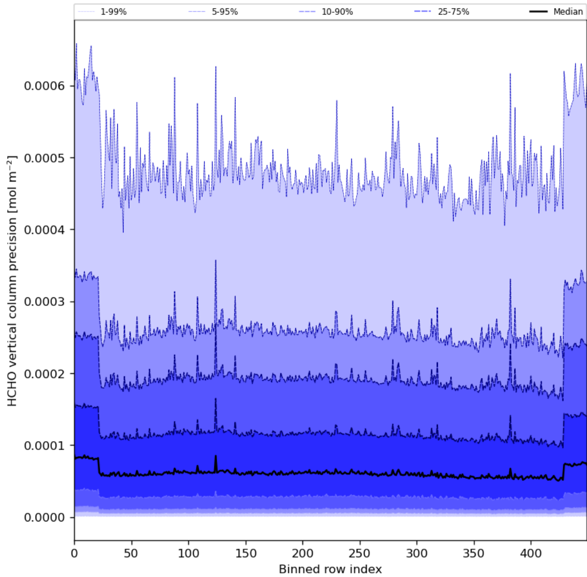
Figure 50: Along track statistics of “HCHO vertical column precision” for 2024-05-12 to 2024-05-14
