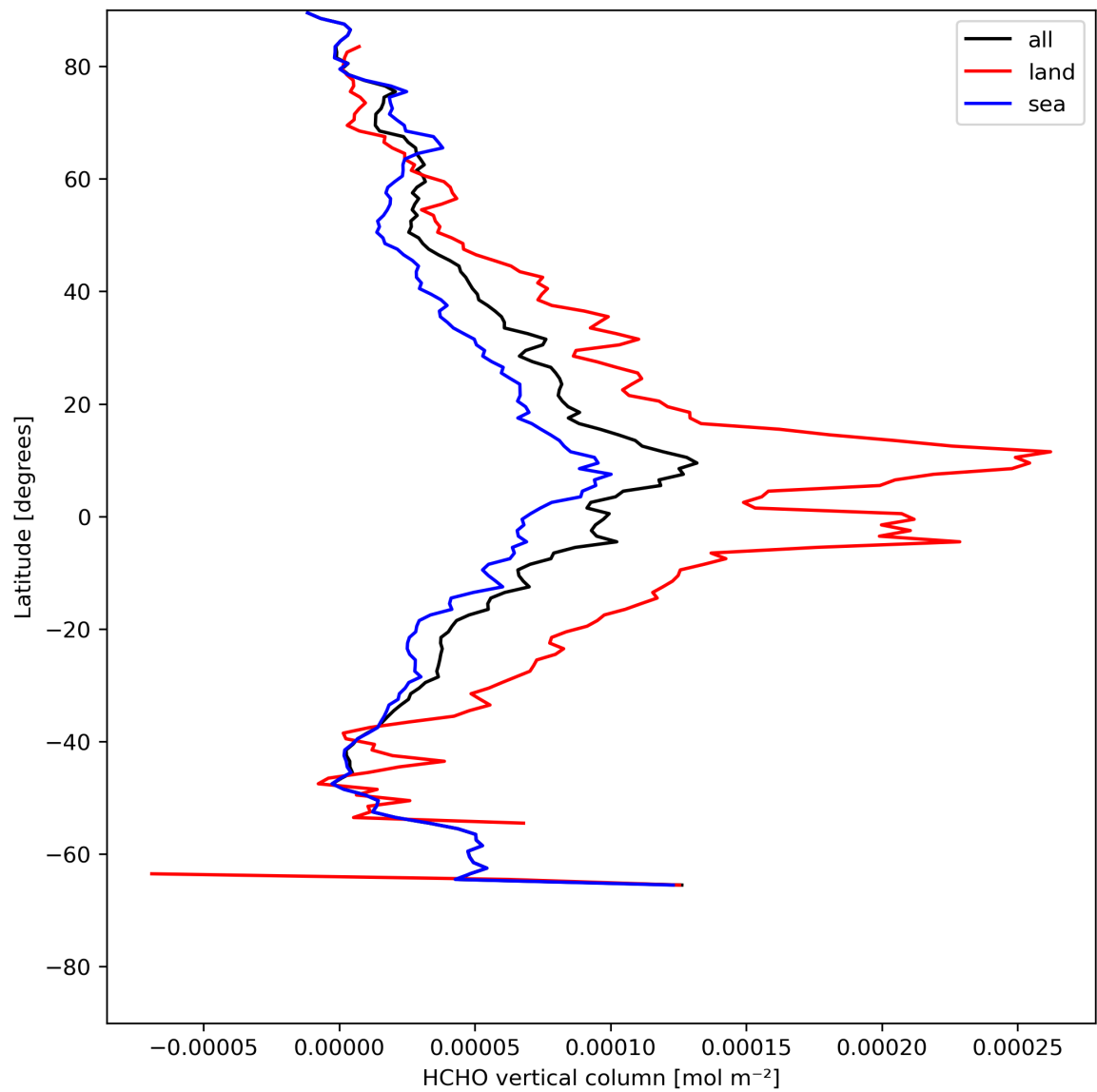
Figure 21: Zonal average of “HCHO vertical column” for 2024-05-12 to 2024-05-14.
