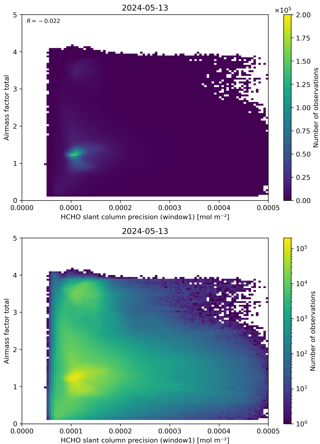
Figure 94: Scatter density plot of “HCHO slant column precision (window1)” against “Airmass factor total” for 2024-05-12 to 2024-05-14.
