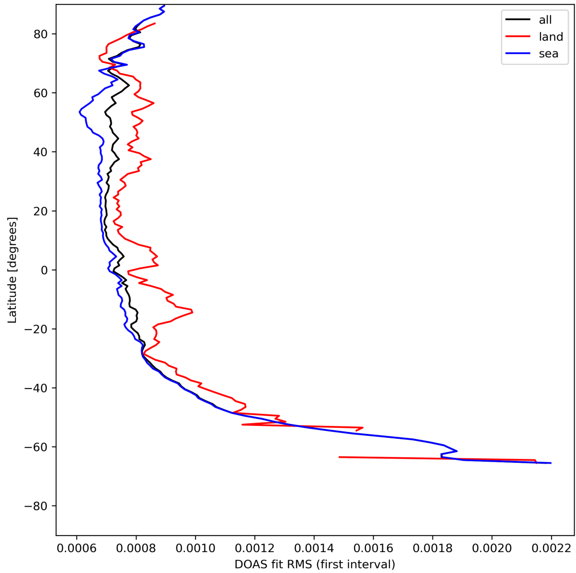
Figure 32: Zonal average of “DOAS fit RMS (first interval)” for 2024-05-12 to 2024-05-14.
