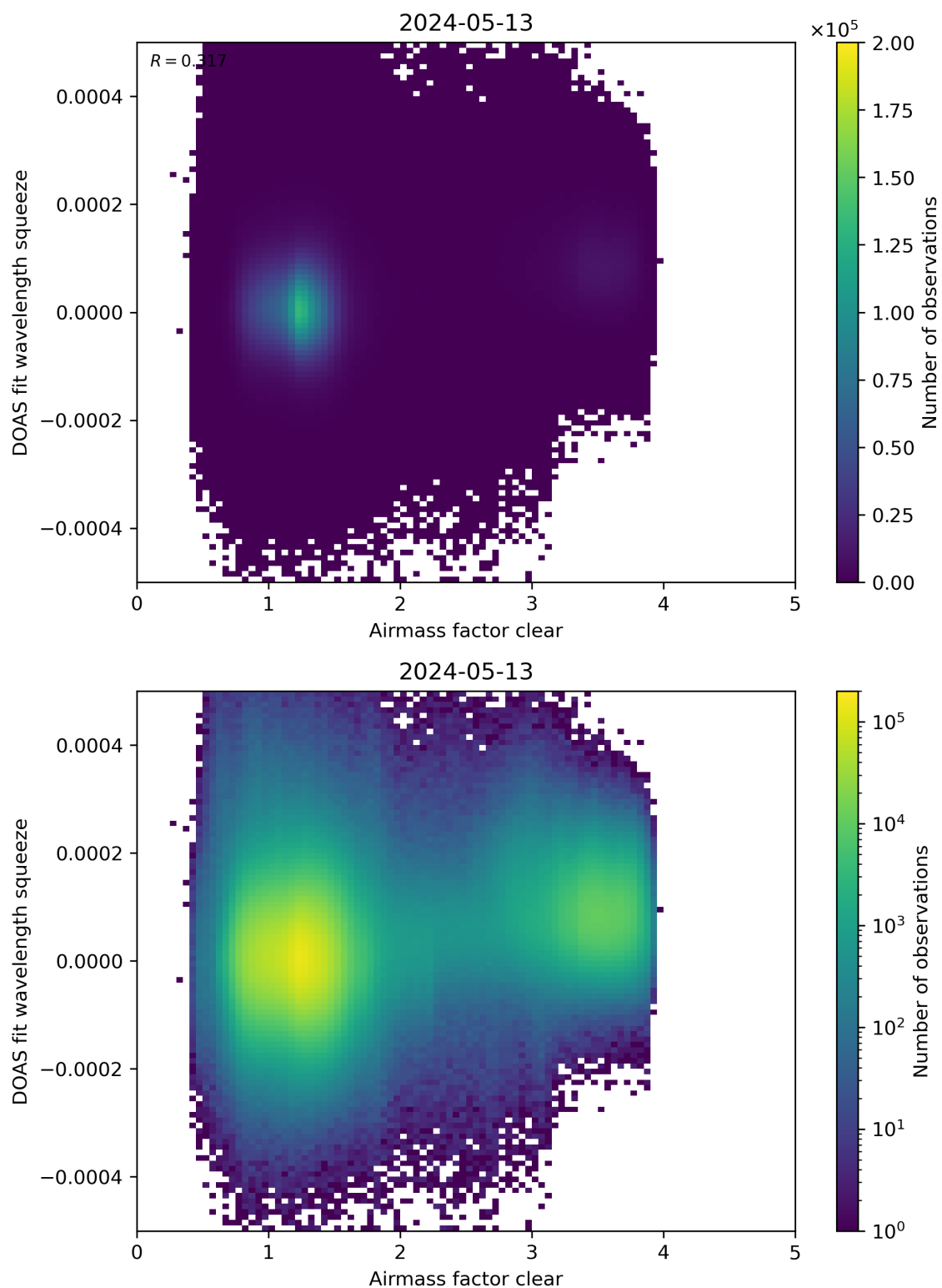
Figure 73: Scatter density plot of “Airmass factor clear” against “DOAS fit wavelength squeeze” for 2024-05-12 to 2024-05-14.
