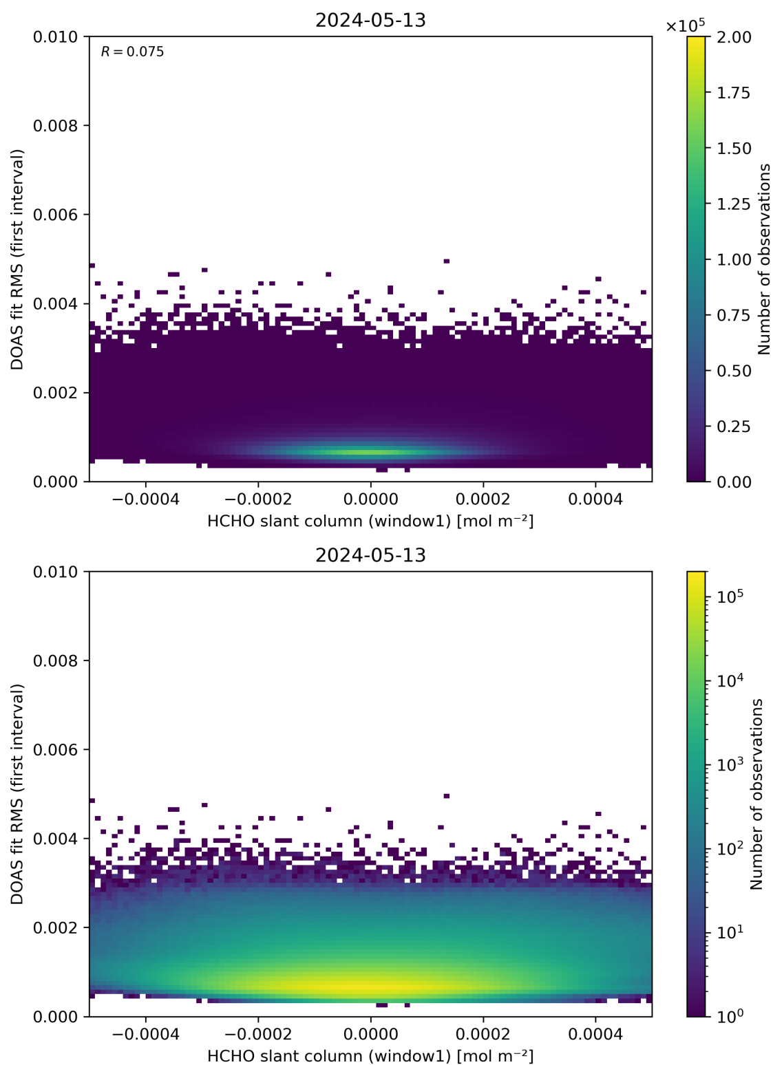
Figure 78: Scatter density plot of “HCHO slant column (window1)” against “DOAS fit RMS (first interval)” for 2024-05-12 to 2024-05-14.
