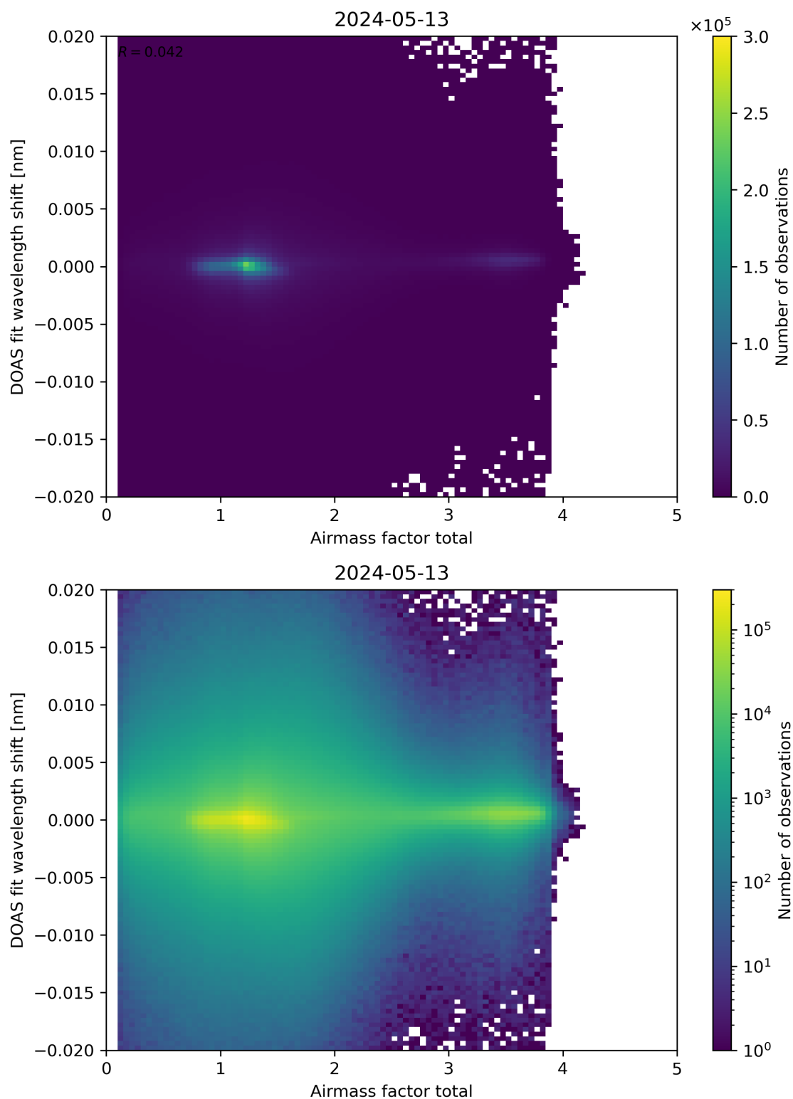
Figure 98: Scatter density plot of “Airmass factor total” against “DOAS fit wavelength shift” for 2024-05-12 to 2024-05-14.
