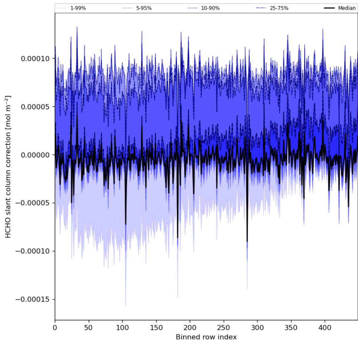
Figure 61: Along track statistics of “HCHO slant column correction” for 2024-05-12 to 2024-05-14
