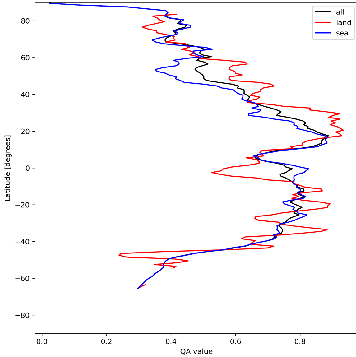
Figure 20: Zonal average of “QA value” for 2024-05-12 to 2024-05-14.
