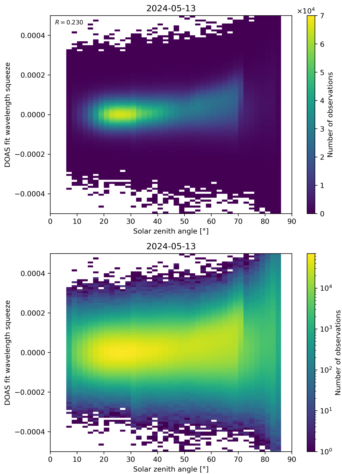
Figure 169: Scatter density plot of “Solar zenith angle” against “DOAS fit wavelength squeeze” for 2024-05-12 to 2024-05-14.
