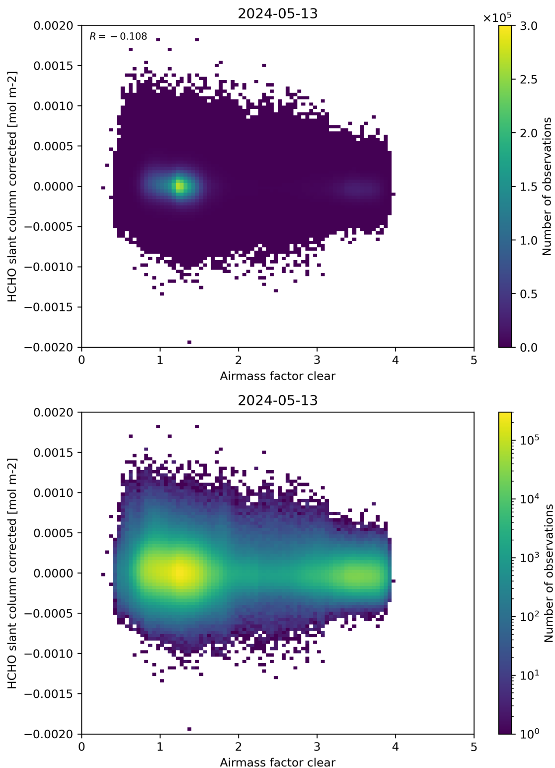
Figure 74: Scatter density plot of “Airmass factor clear” against “HCHO slant column corrected” for 2024-05-12 to 2024-05-14.
