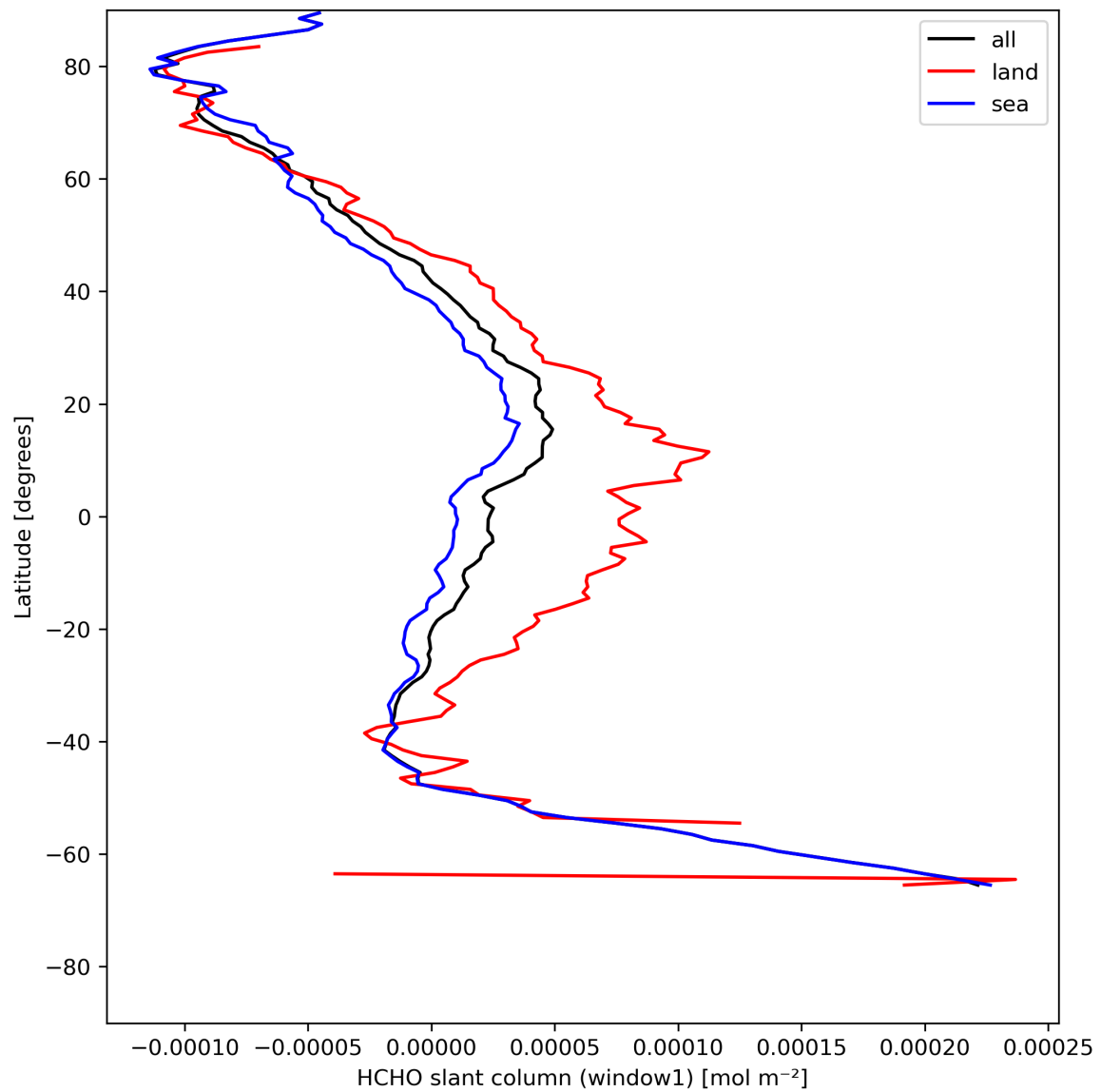
Figure 24: Zonal average of “HCHO slant column (window1)” for 2024-05-12 to 2024-05-14.
