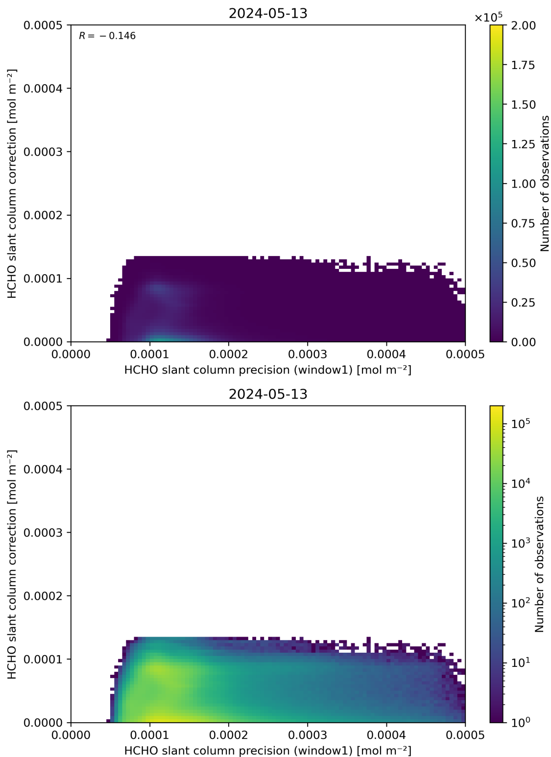
Figure 93: Scatter density plot of “HCHO slant column precision (window1)” against “HCHO slant column correction” for 2024-05-12 to 2024-05-14.
