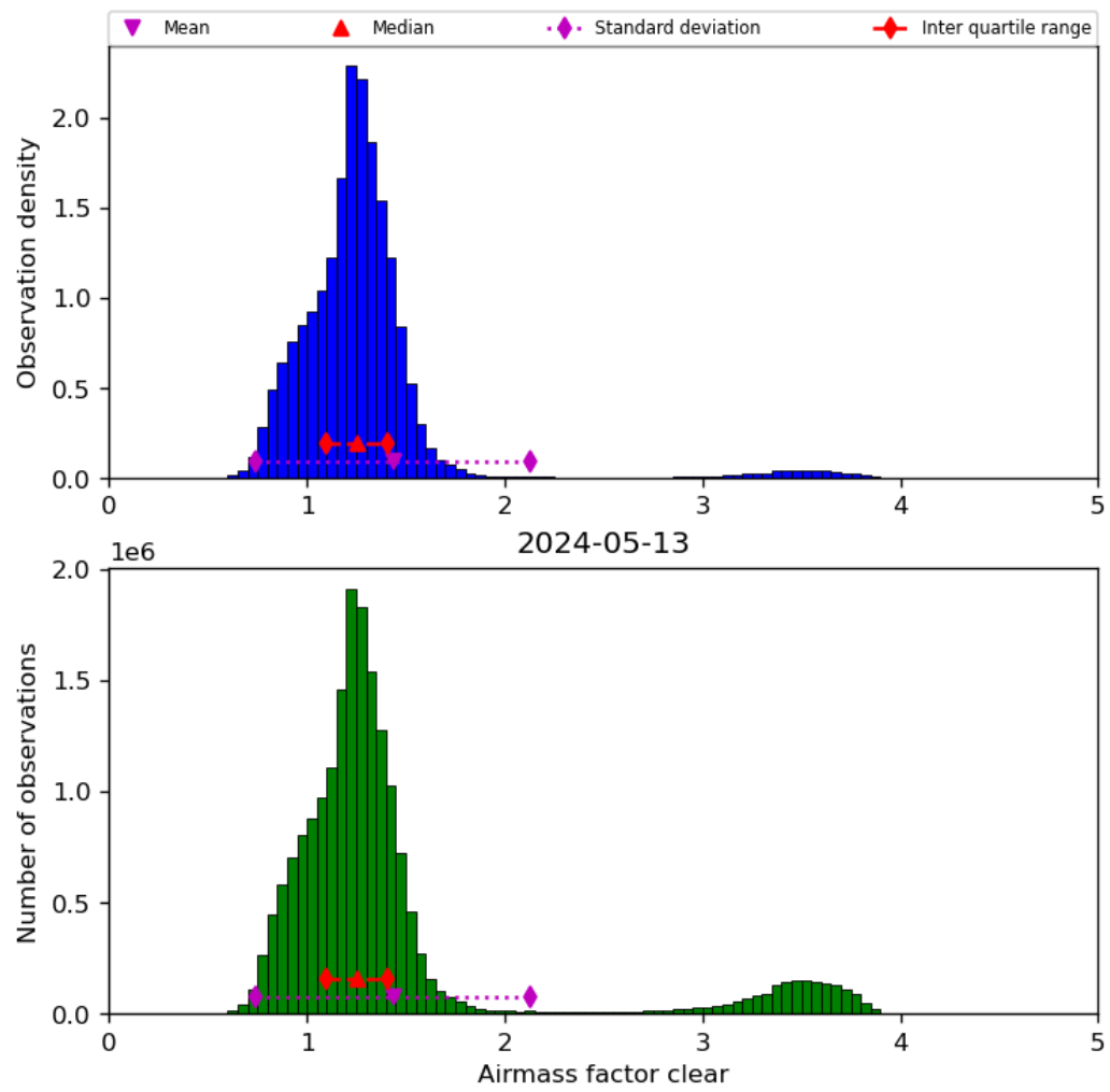
Figure 42: Histogram of “Airmass factor clear” for 2024-05-12 to 2024-05-14
