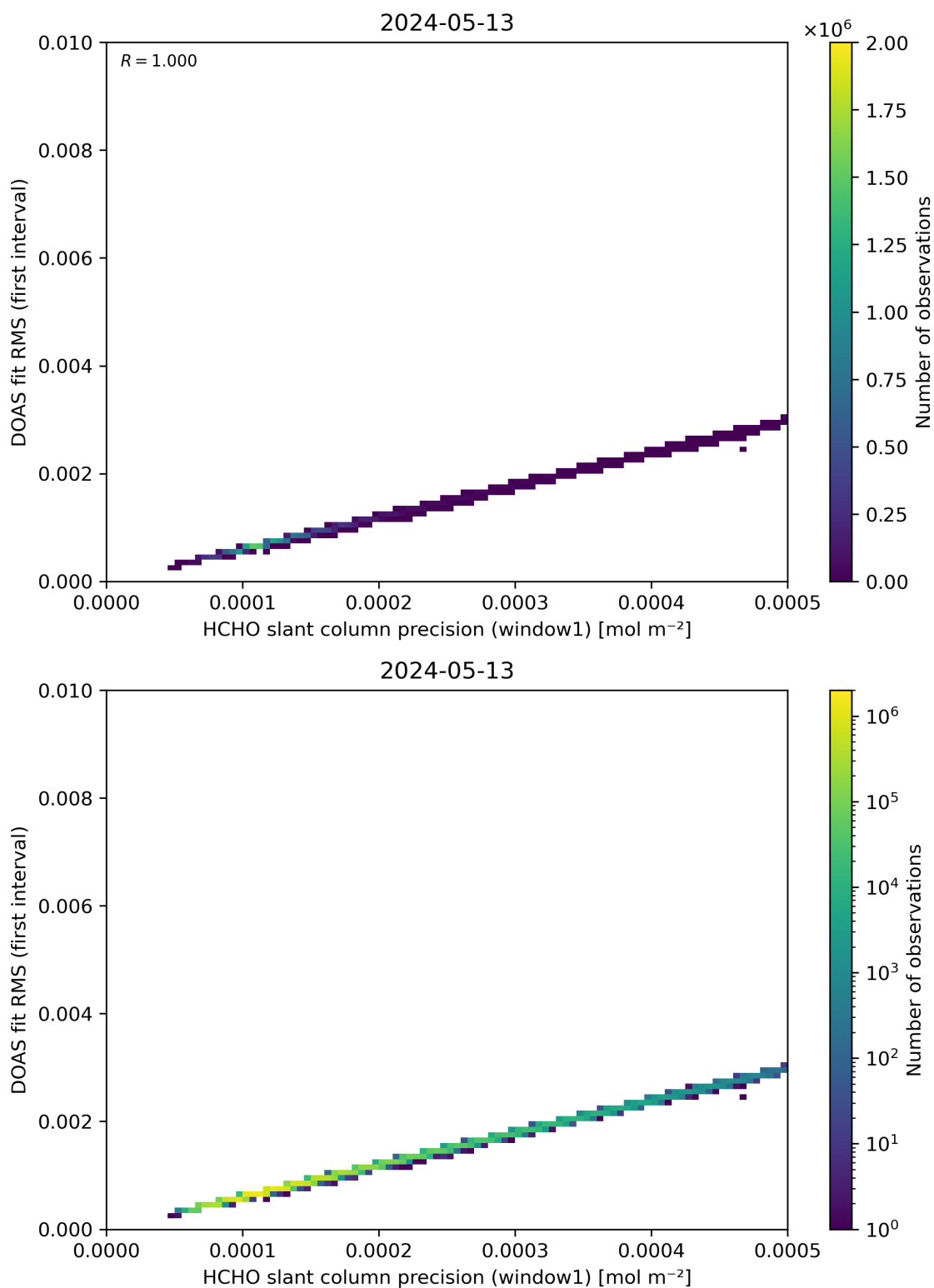
Figure 88: Scatter density plot of “HCHO slant column precision (window1)” against “DOAS fit RMS (first interval)” for 2024-05-12 to 2024-05-14.
