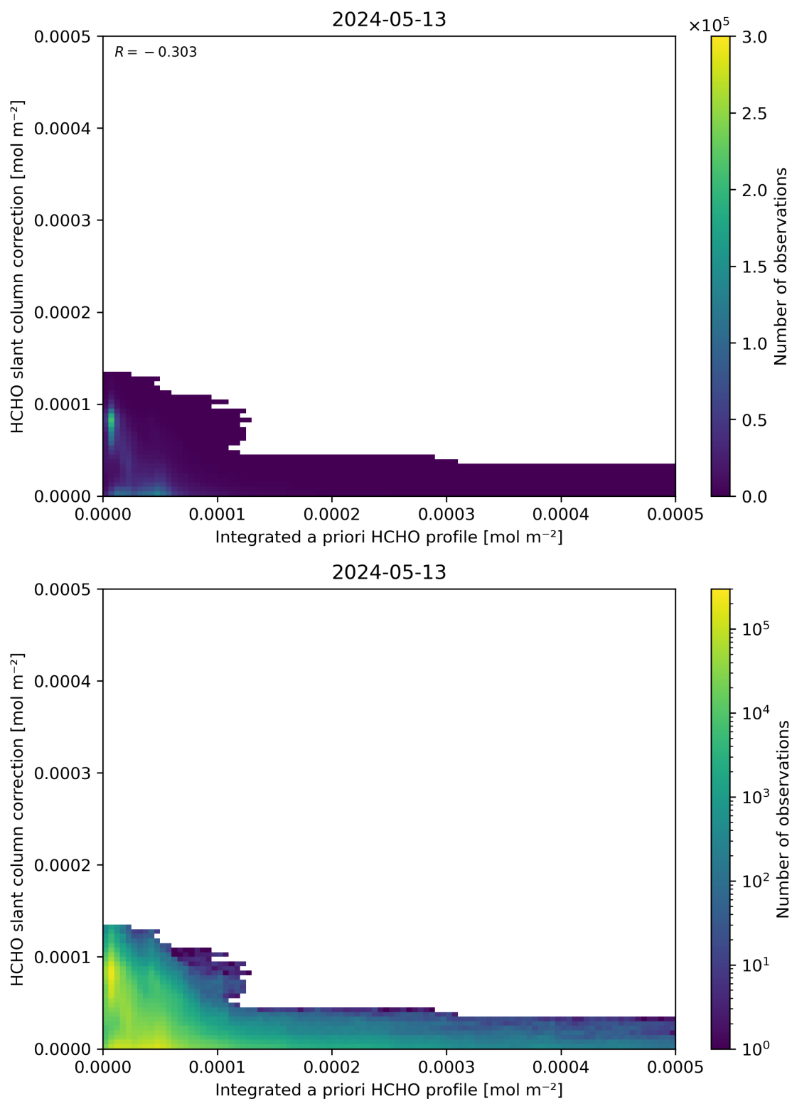
Figure 152: Scatter density plot of “Integrated a priori HCHO profile” against “HCHO slant column correction” for 2024-05-12 to 2024-05-14.
