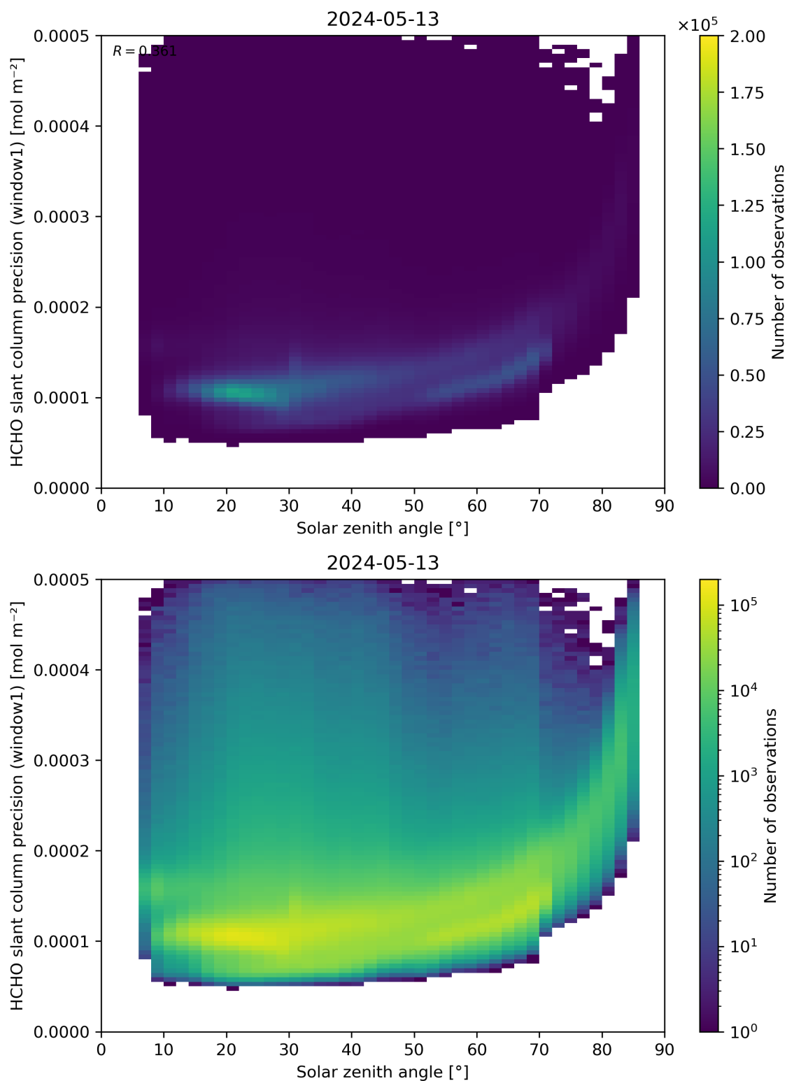
Figure 174: Scatter density plot of “Solar zenith angle” against “HCHO slant column precision (window1)” for 2024-05-12 to 2024-05-14.
