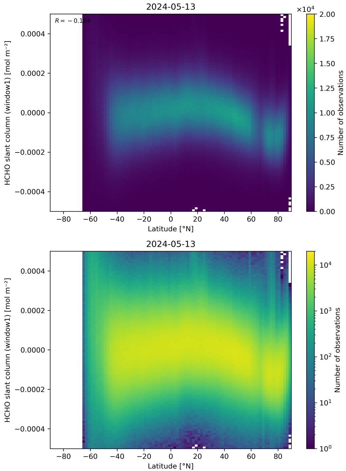
Figure 159: Scatter density plot of “Latitude” against “HCHO slant column (window1)” for 2024-05-12 to 2024-05-14.
