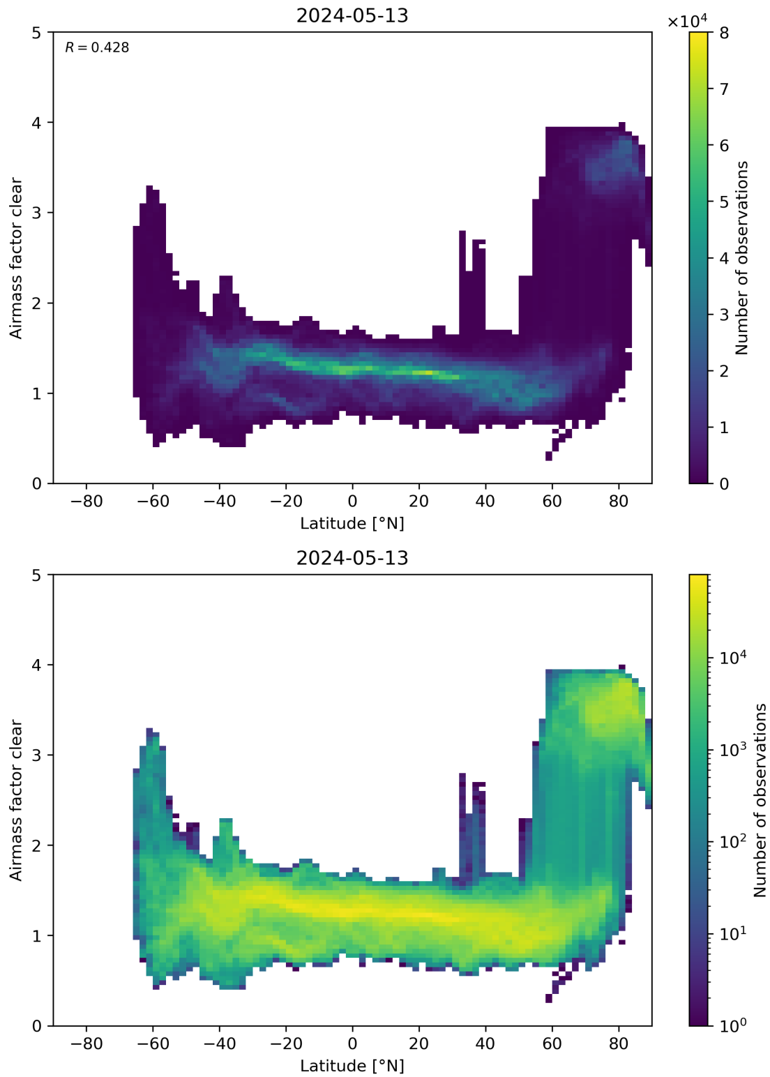
Figure 156: Scatter density plot of “Latitude” against “Airmass factor clear” for 2024-05-12 to 2024-05-14.
