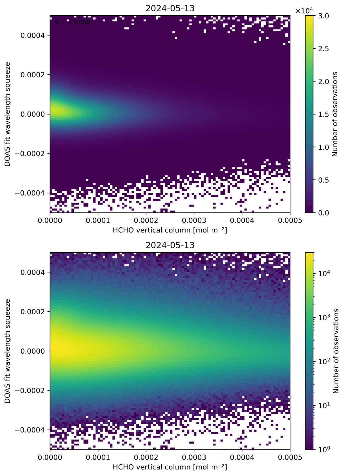
Figure 125: Scatter density plot of “HCHO vertical column” against “DOAS fit wavelength squeeze” for 2024-05-12 to 2024-05-14.
