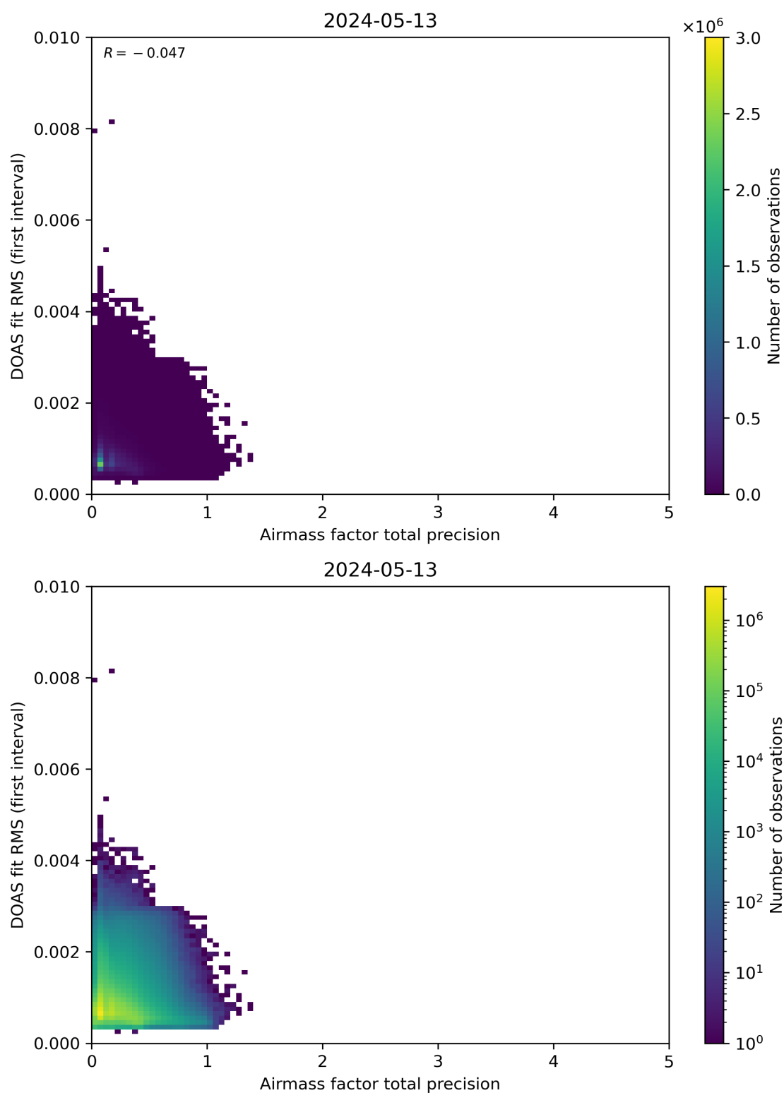
Figure 105: Scatter density plot of “Airmass factor total precision” against “DOAS fit RMS (first interval)” for 2024-05-12 to 2024-05-14.
