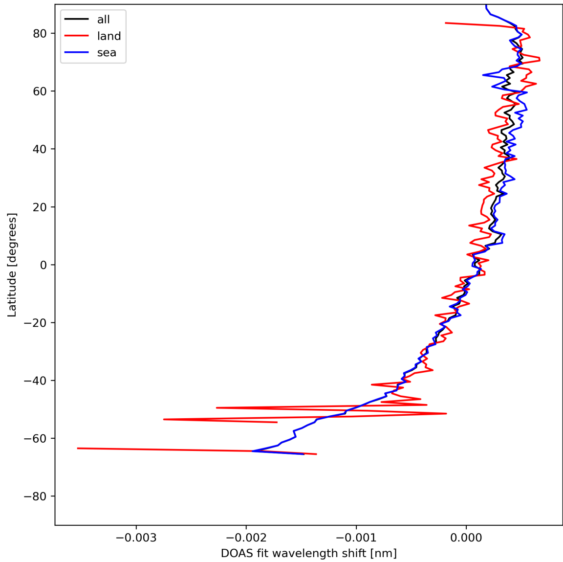
Figure 30: Zonal average of “DOAS fit wavelength shift” for 2024-05-12 to 2024-05-14.
