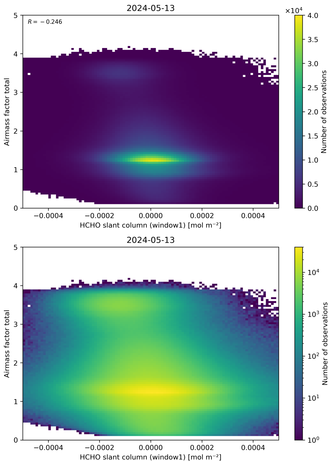
Figure 85: Scatter density plot of “HCHO slant column (window1)” against “Airmass factor total” for 2024-05-12 to 2024-05-14.
