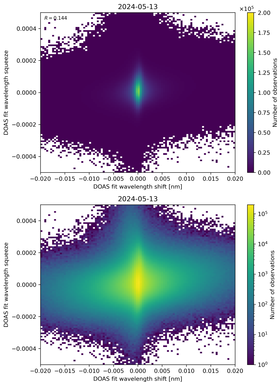
Figure 65: Scatter density plot of “DOAS fit wavelength shift” against “DOAS fit wavelength squeeze” for 2024-05-12 to 2024-05-14.
