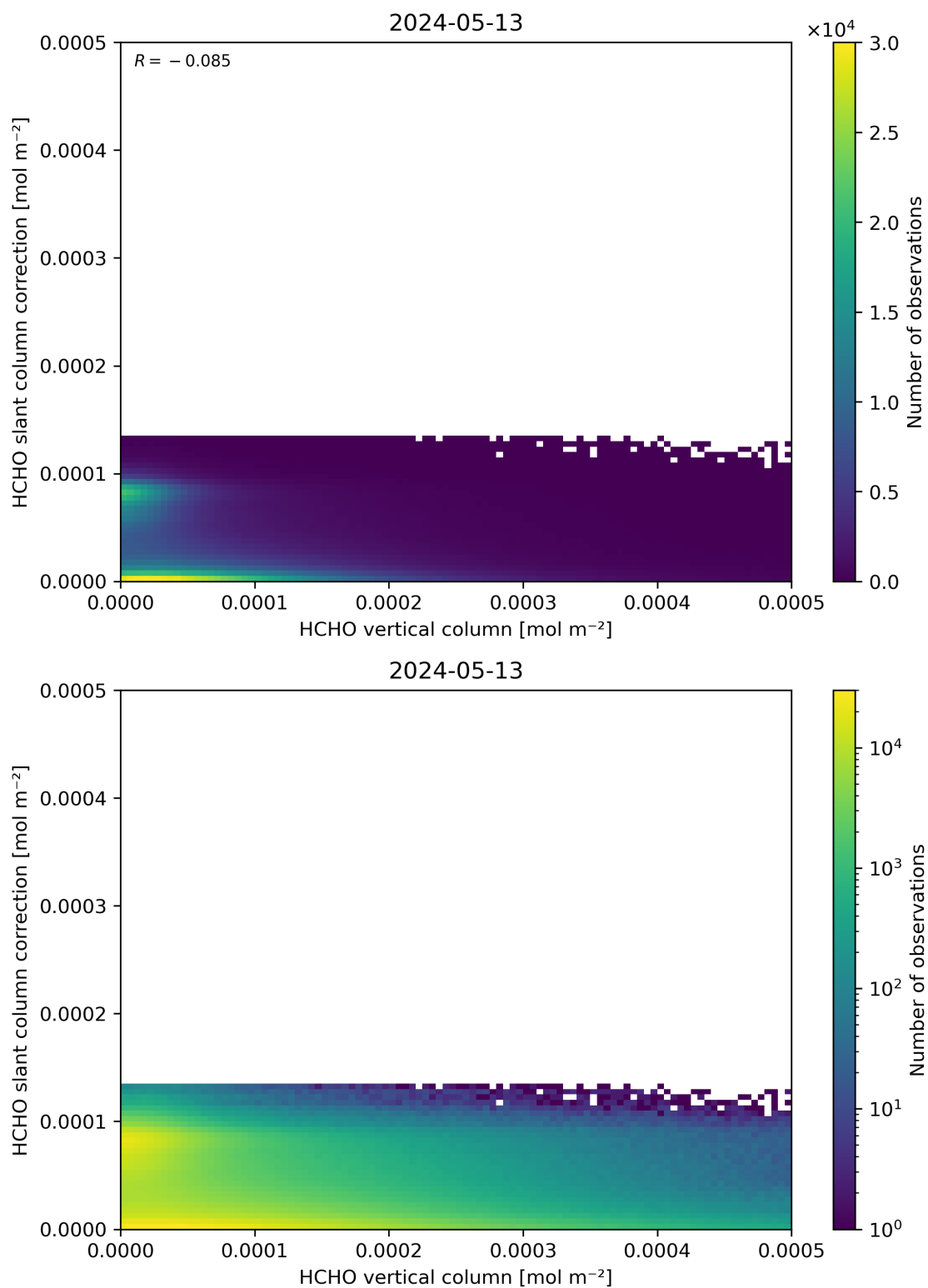
Figure 128: Scatter density plot of “HCHO vertical column” against “HCHO slant column correction” for 2024-05-12 to 2024-05-14.
