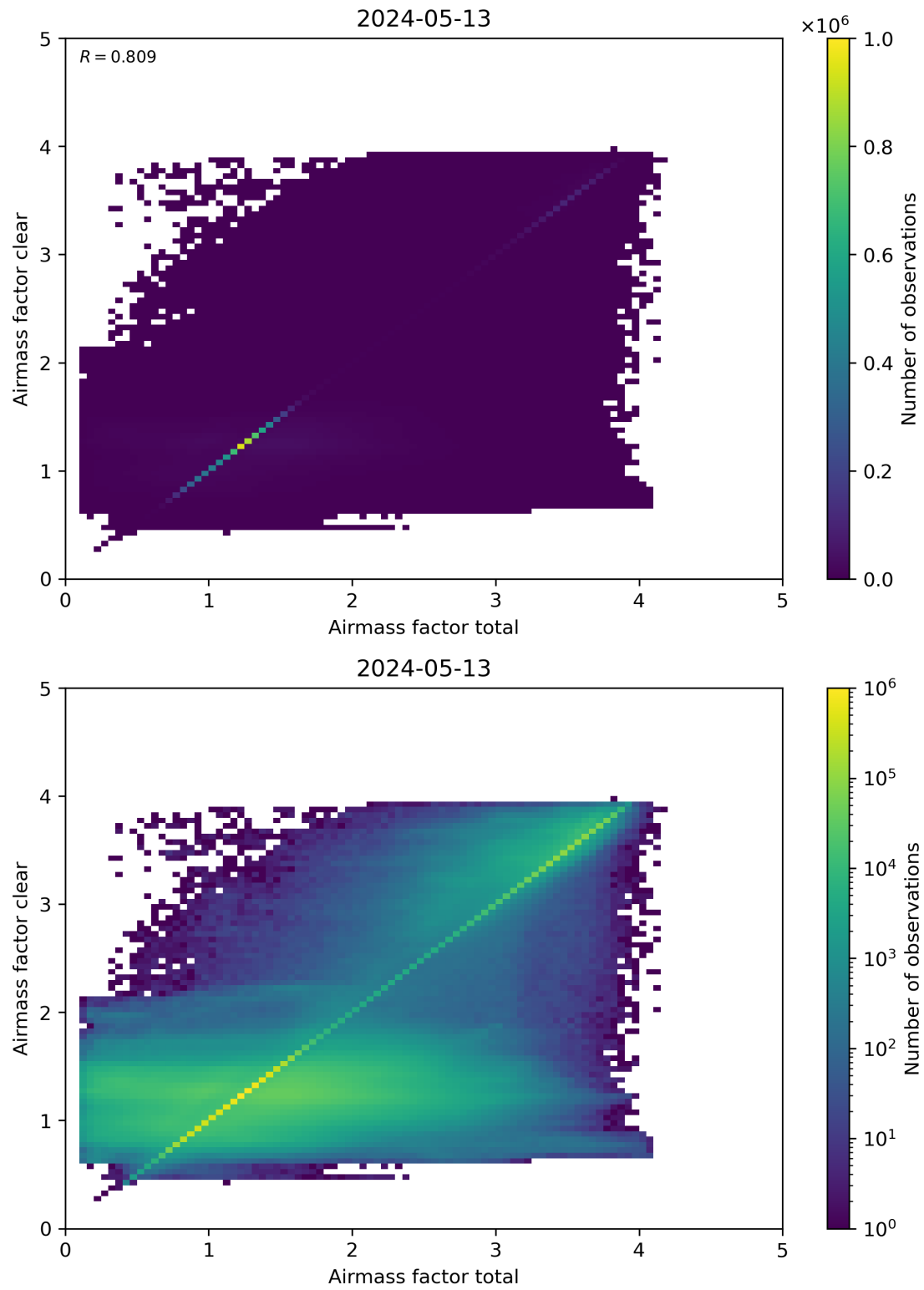
Figure 100: Scatter density plot of “Airmass factor total” against “Airmass factor clear” for 2024-05-12 to 2024-05-14.
