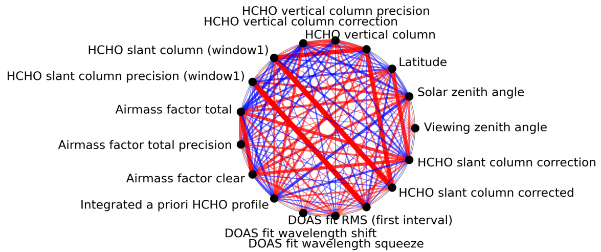
Figure 1: Map of correlation graph for 2024-05-12 to 2024-05-14.
