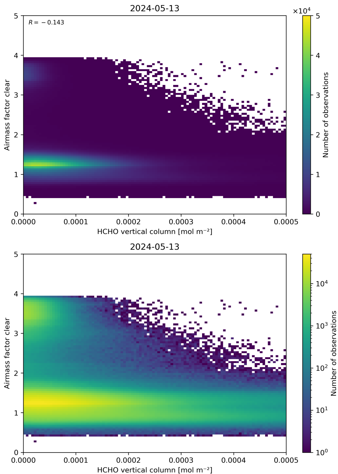
Figure 126: Scatter density plot of “HCHO vertical column” against “Airmass factor clear” for 2024-05-12 to 2024-05-14.
