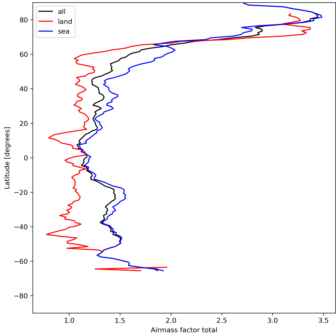
Figure 26: Zonal average of “Airmass factor total” for 2024-05-12 to 2024-05-14.
