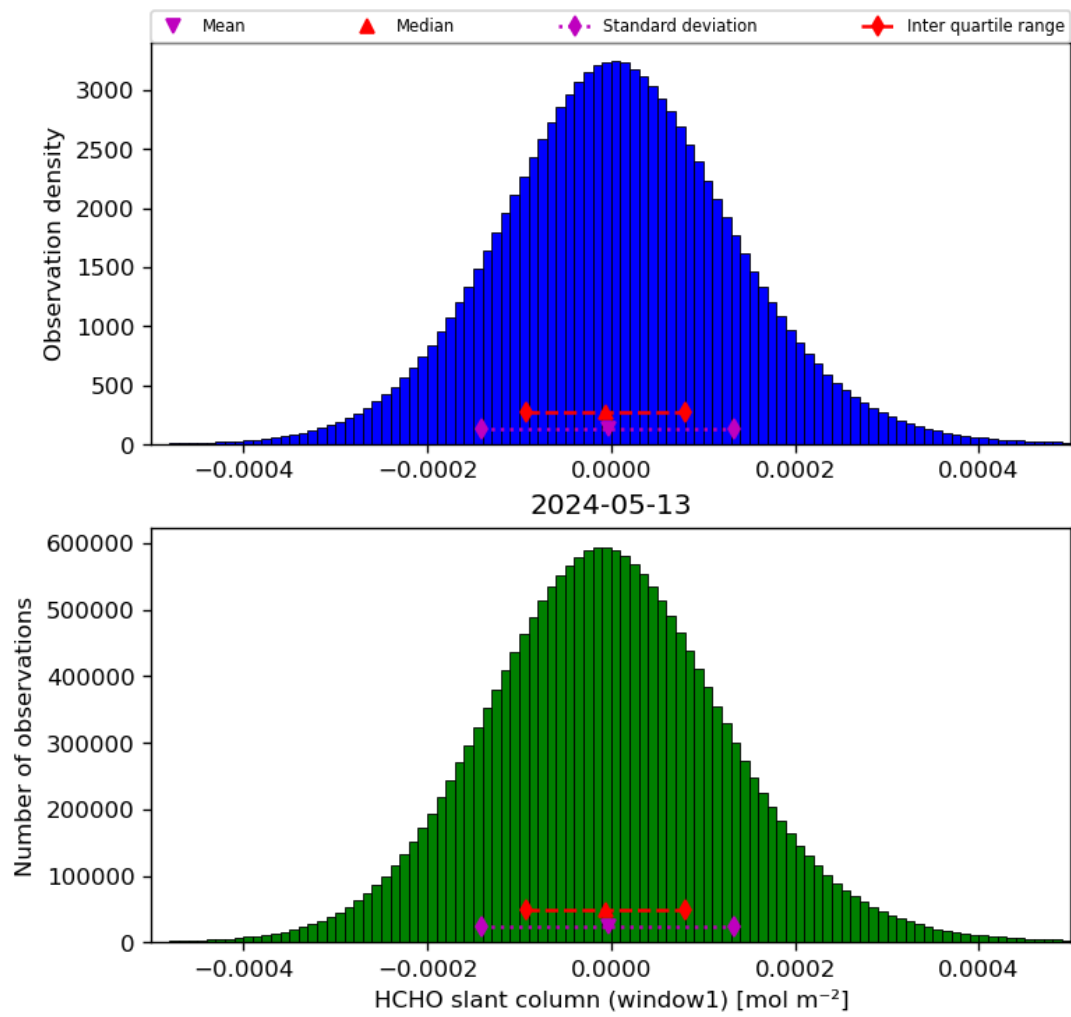
Figure 38: Histogram of “HCHO slant column (window1)” for 2024-05-12 to 2024-05-14
