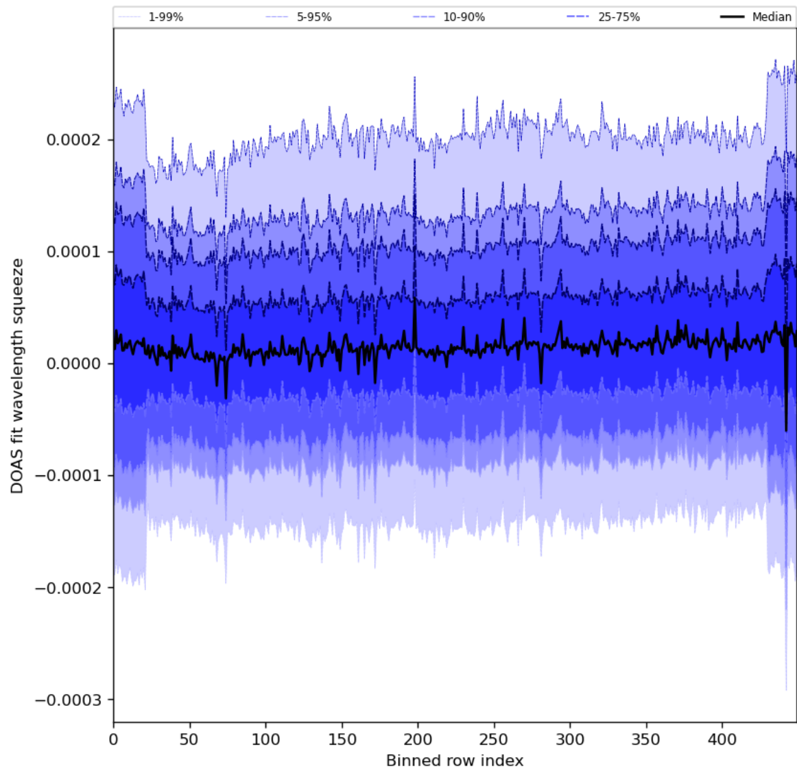
Figure 59: Along track statistics of “DOAS fit wavelength squeeze” for 2024-05-12 to 2024-05-14
