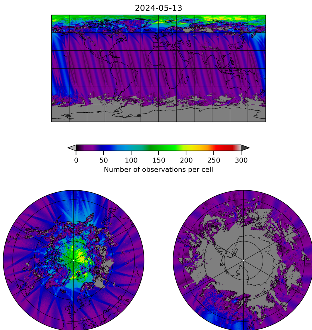
Figure 19: Map of the number of observations for 2024-05-12 to 2024-05-14
