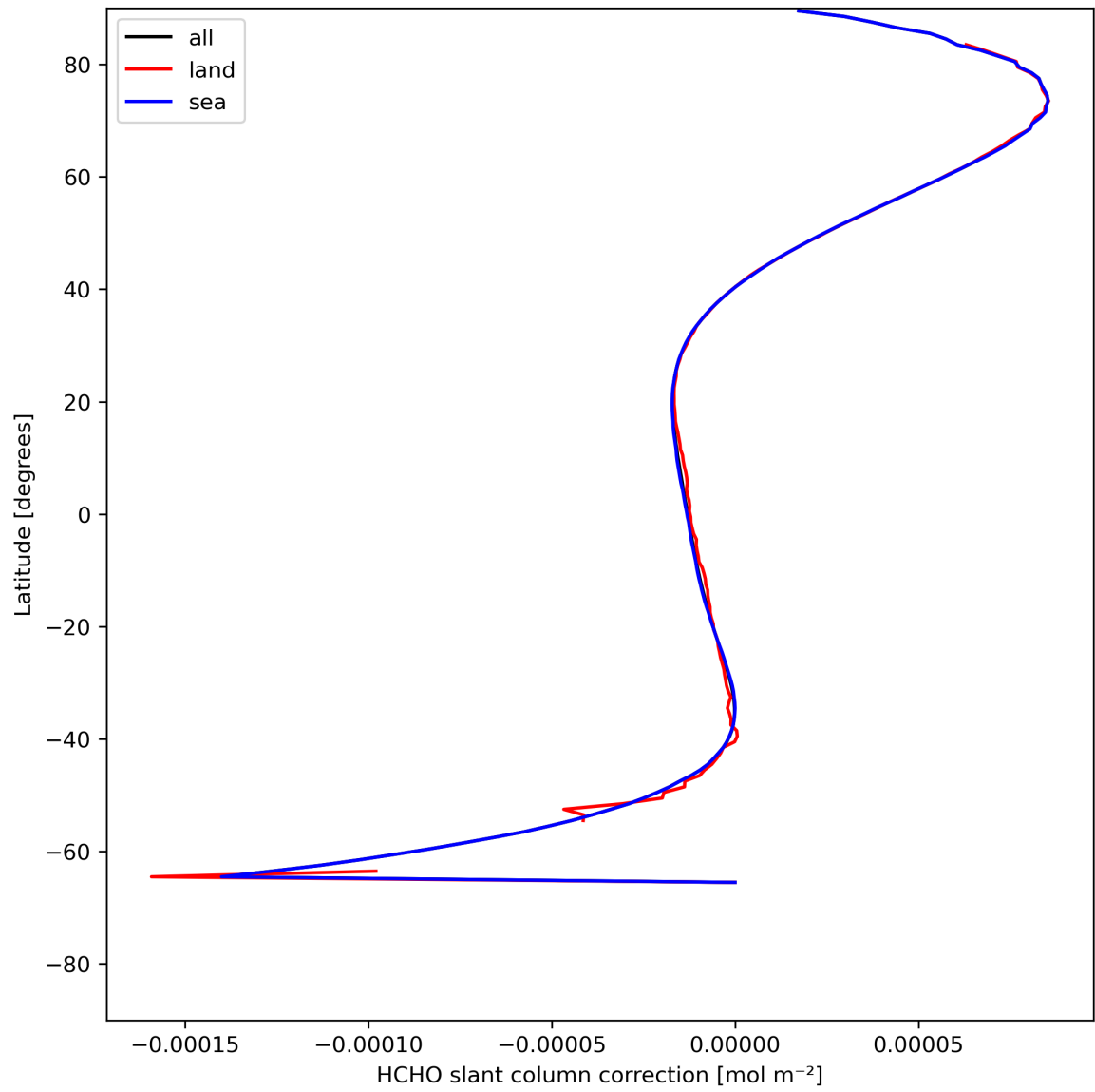
Figure 33: Zonal average of “HCHO slant column correction” for 2024-05-12 to 2024-05-14.
