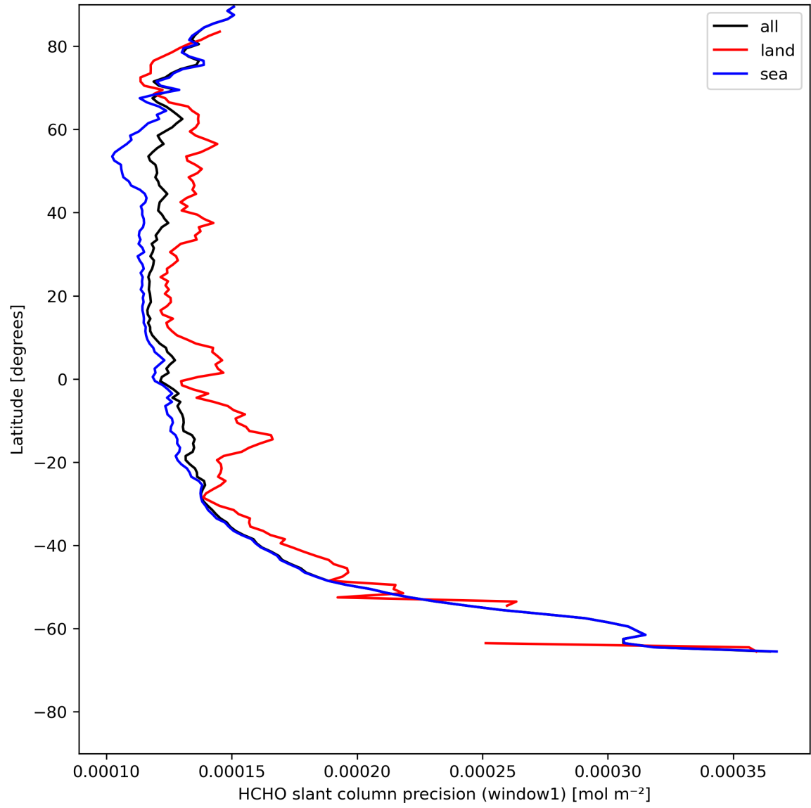
Figure 25: Zonal average of “HCHO slant column precision (window1)” for 2024-05-12 to 2024-05-14.
