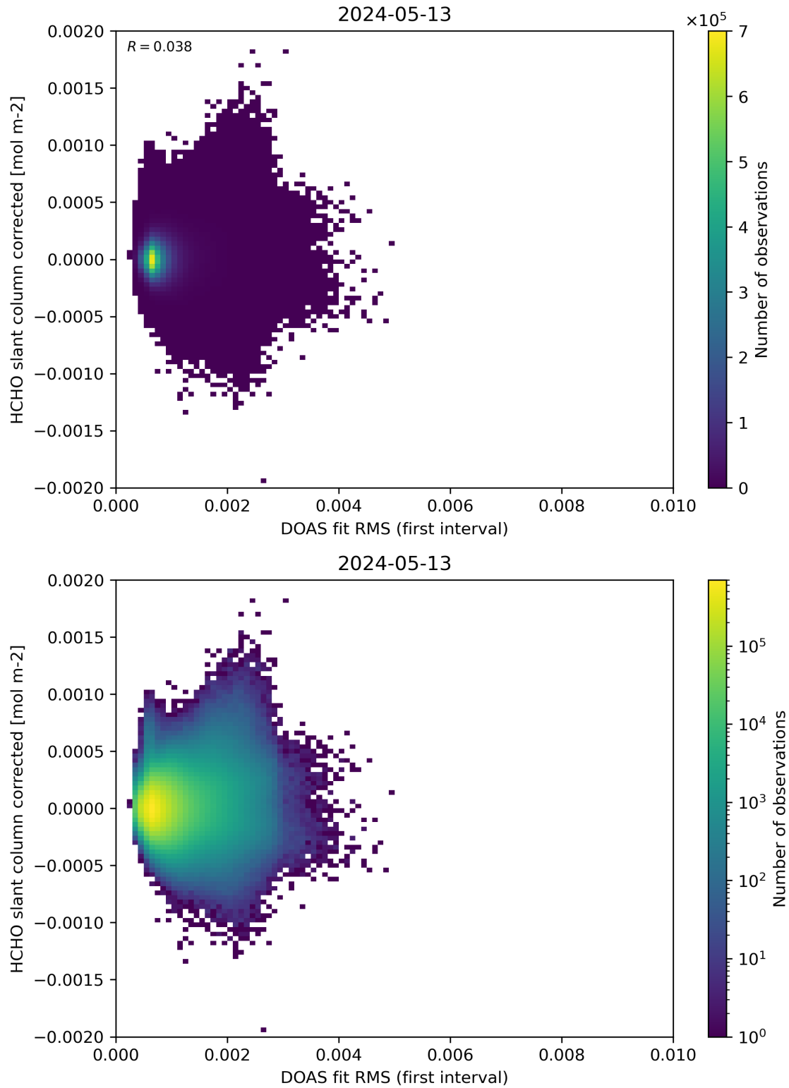
Figure 62: Scatter density plot of “DOAS fit RMS (first interval)” against “HCHO slant column corrected” for 2024-05-12 to 2024-05-14.
