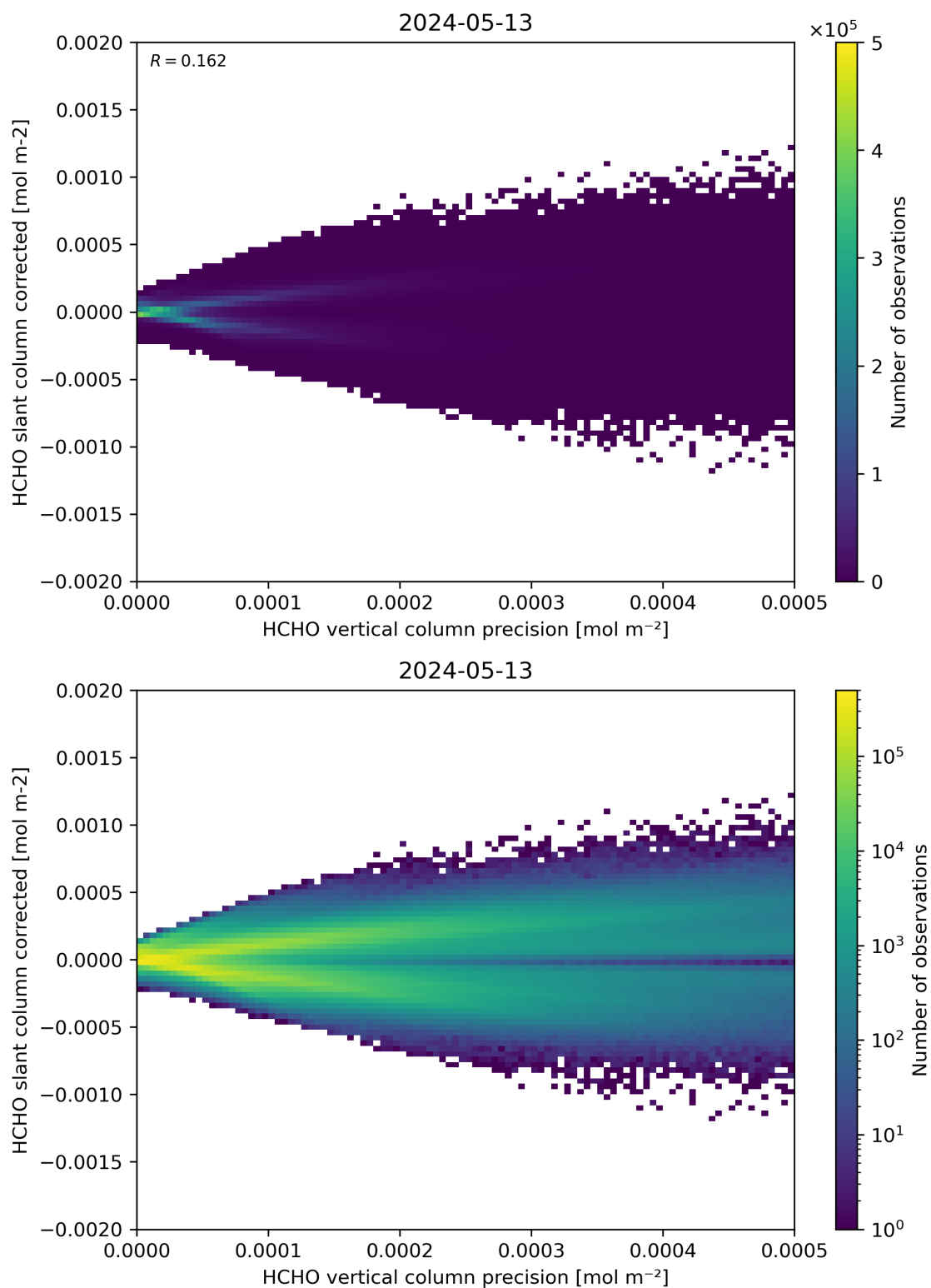
Figure 140: Scatter density plot of “HCHO vertical column precision” against “HCHO slant column corrected” for 2024-05-12 to 2024-05-14.
