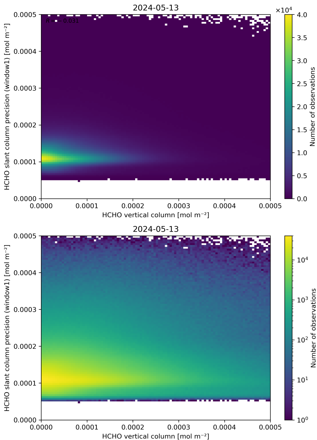
Figure 130: Scatter density plot of “HCHO vertical column” against “HCHO slant column precision (window1)” for 2024-05-12 to 2024-05-14.
