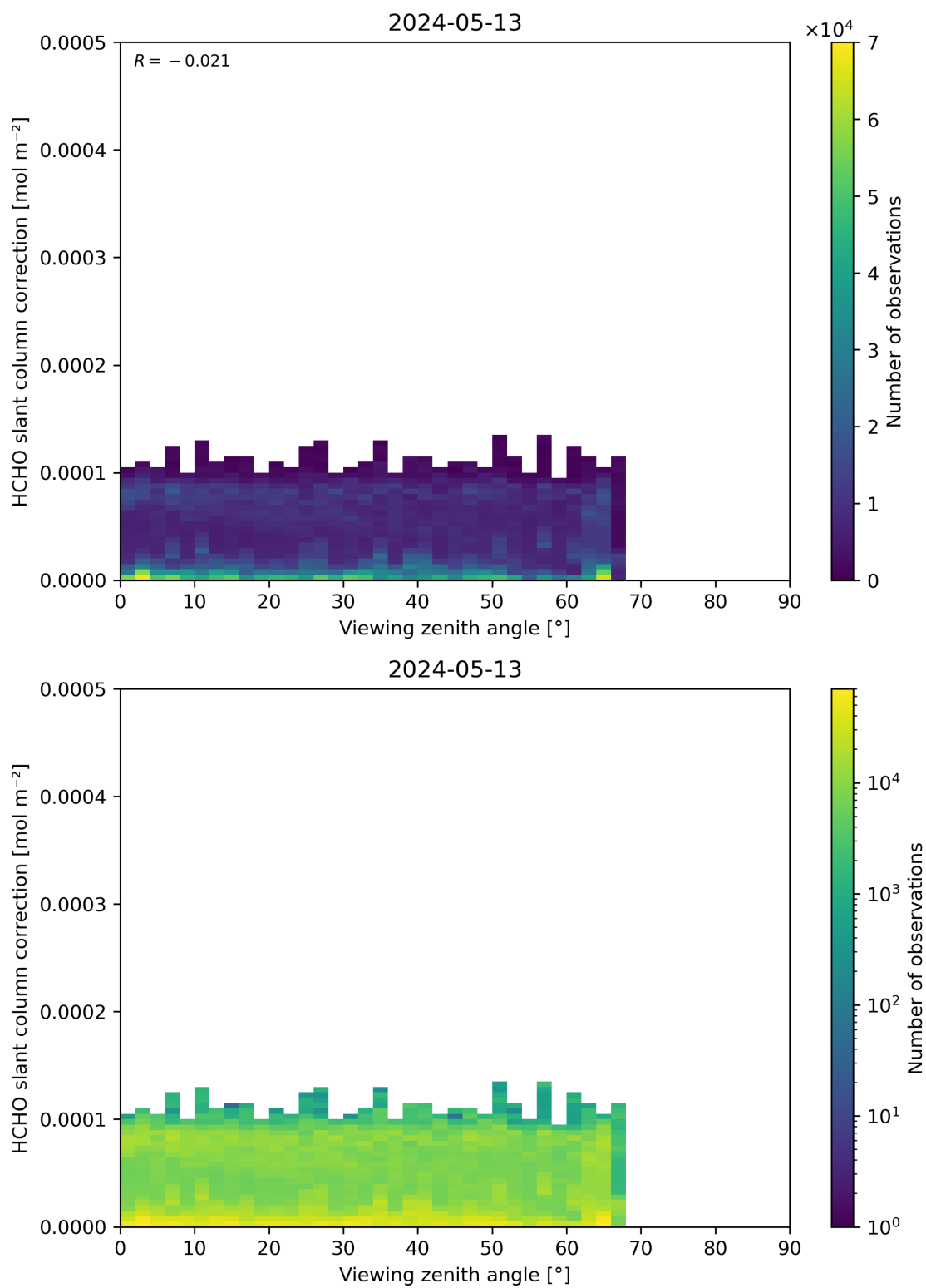
Figure 187: Scatter density plot of “Viewing zenith angle” against “HCHO slant column correction” for 2024-05-12 to 2024-05-14.
