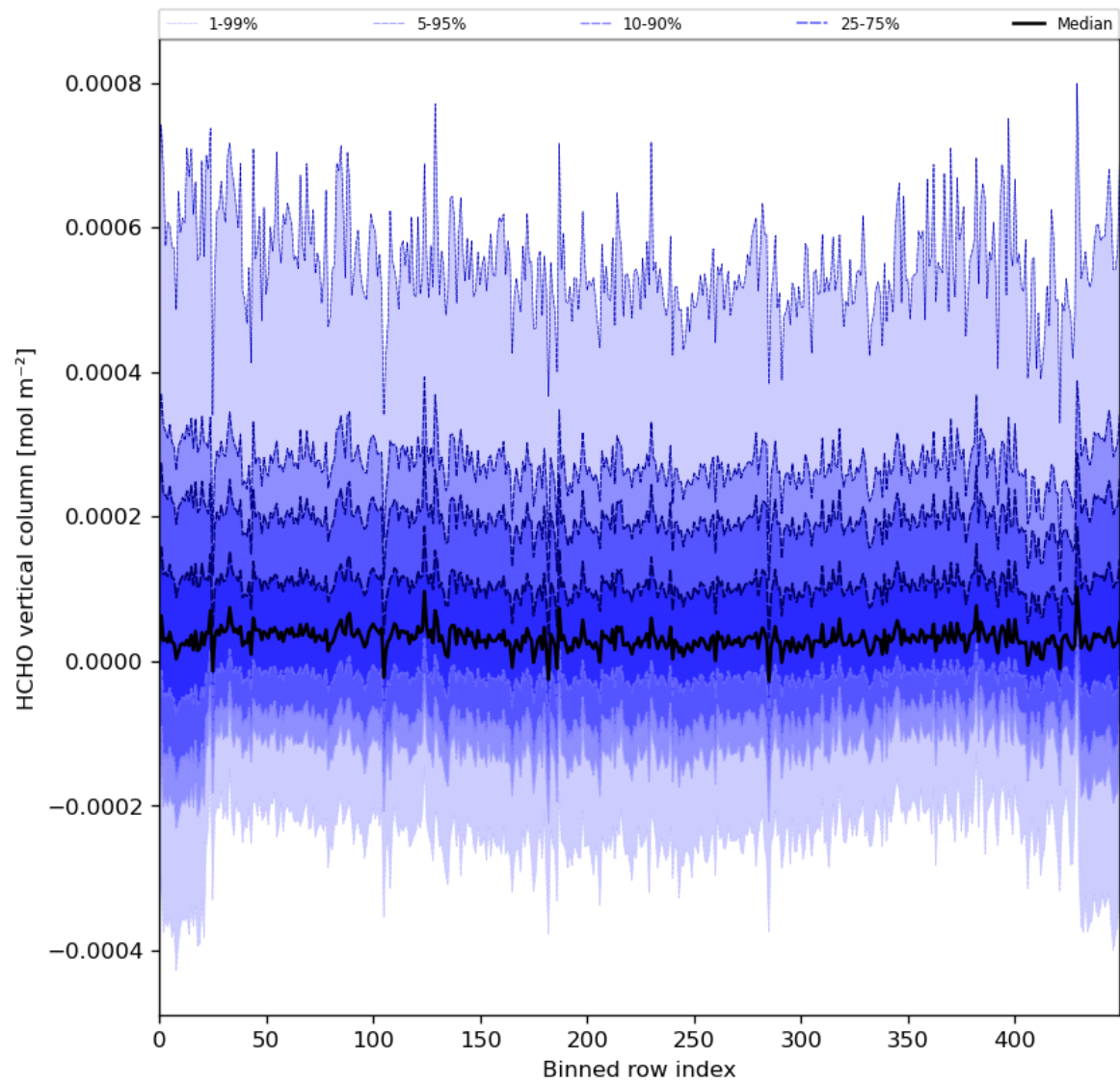
Figure 49: Along track statistics of “HCHO vertical column” for 2024-05-12 to 2024-05-14
