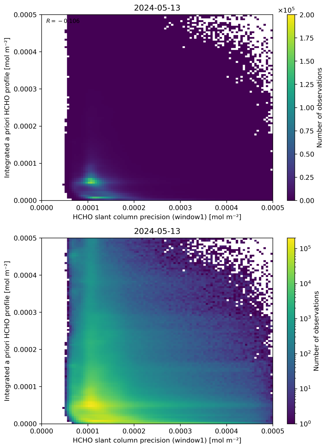
Figure 96: Scatter density plot of “HCHO slant column precision (window1)” against “Integrated a priori HCHO profile” for 2024-05-12 to 2024-05-14.
