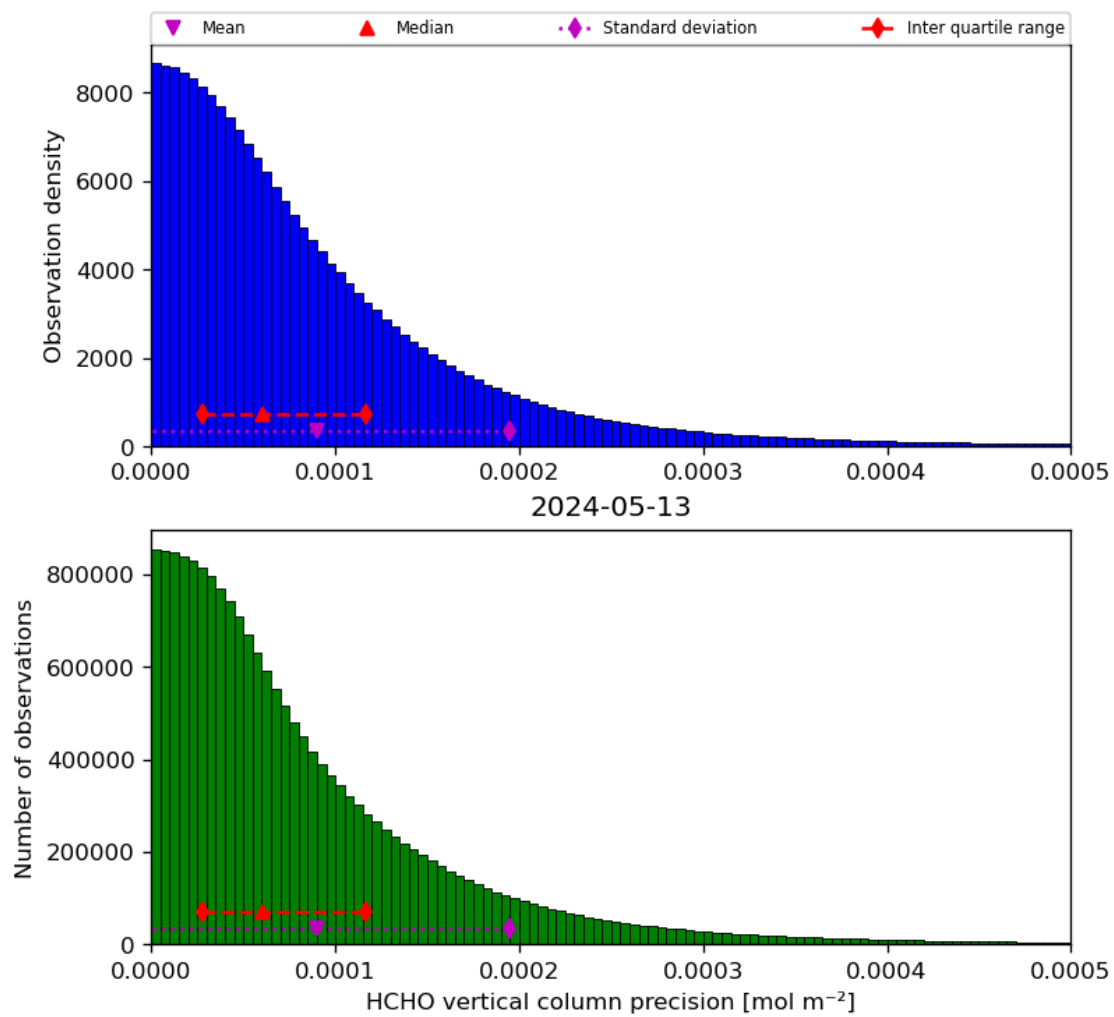
Figure 36: Histogram of “HCHO vertical column precision” for 2024-05-12 to 2024-05-14
