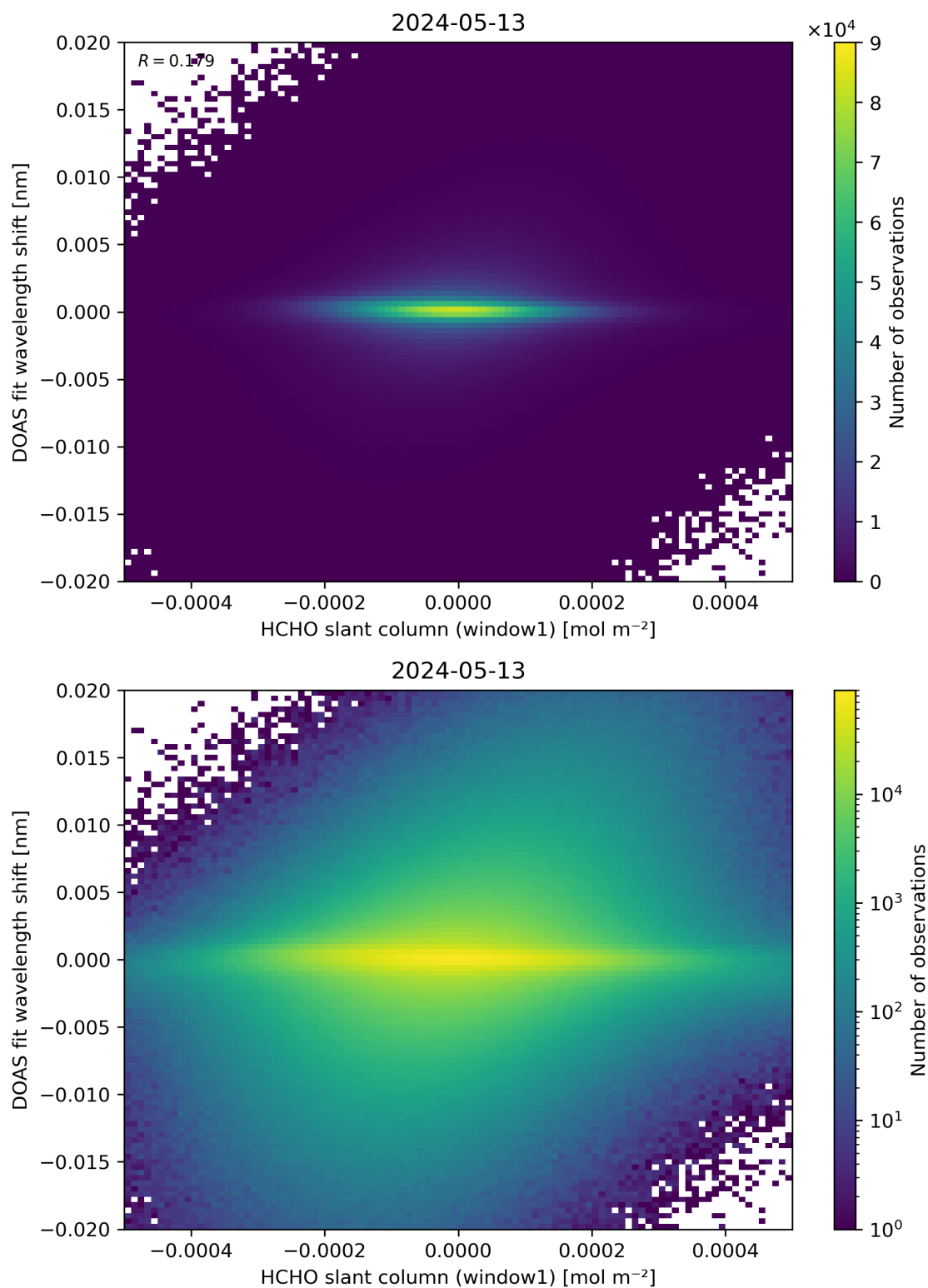
Figure 79: Scatter density plot of “HCHO slant column (window1)” against “DOAS fit wavelength shift” for 2024-05-12 to 2024-05-14.
