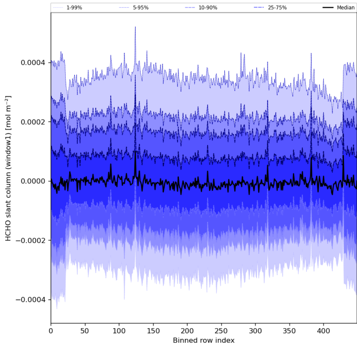
Figure 52: Along track statistics of “HCHO slant column (window1)” for 2024-05-12 to 2024-05-14
