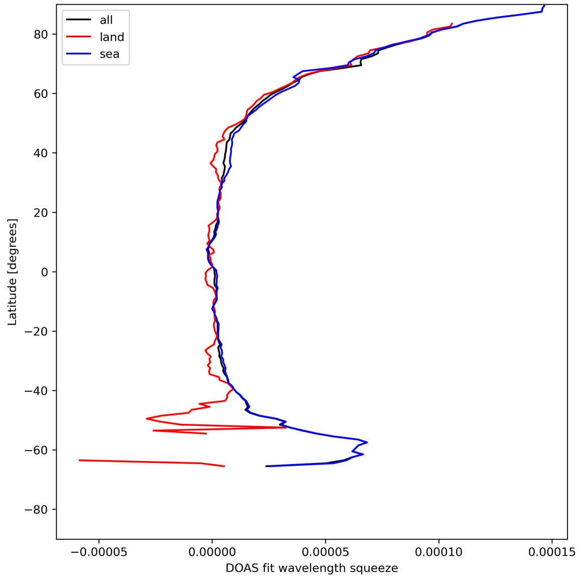
Figure 31: Zonal average of “DOAS fit wavelength squeeze” for 2024-05-12 to 2024-05-14.
