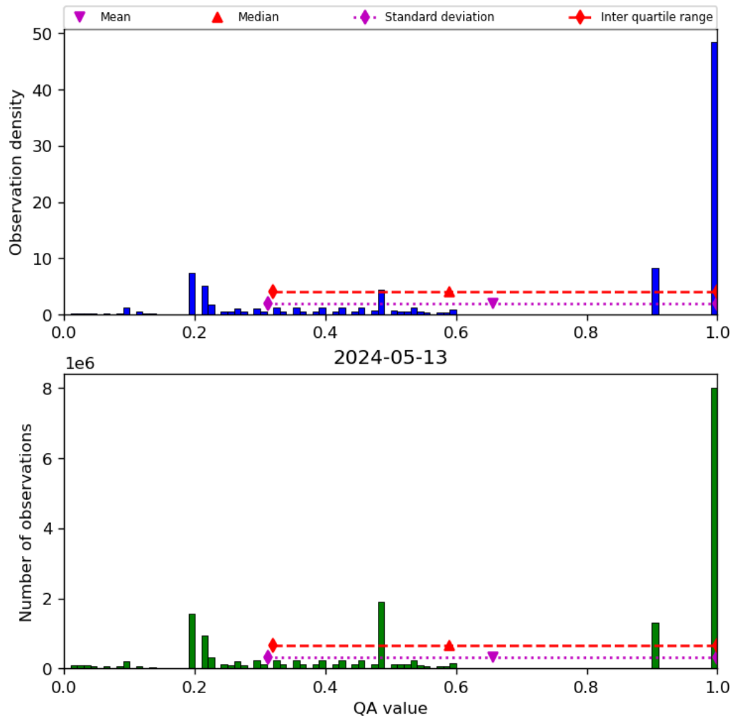
Figure 34: Histogram of “QA value” for 2024-05-12 to 2024-05-14
