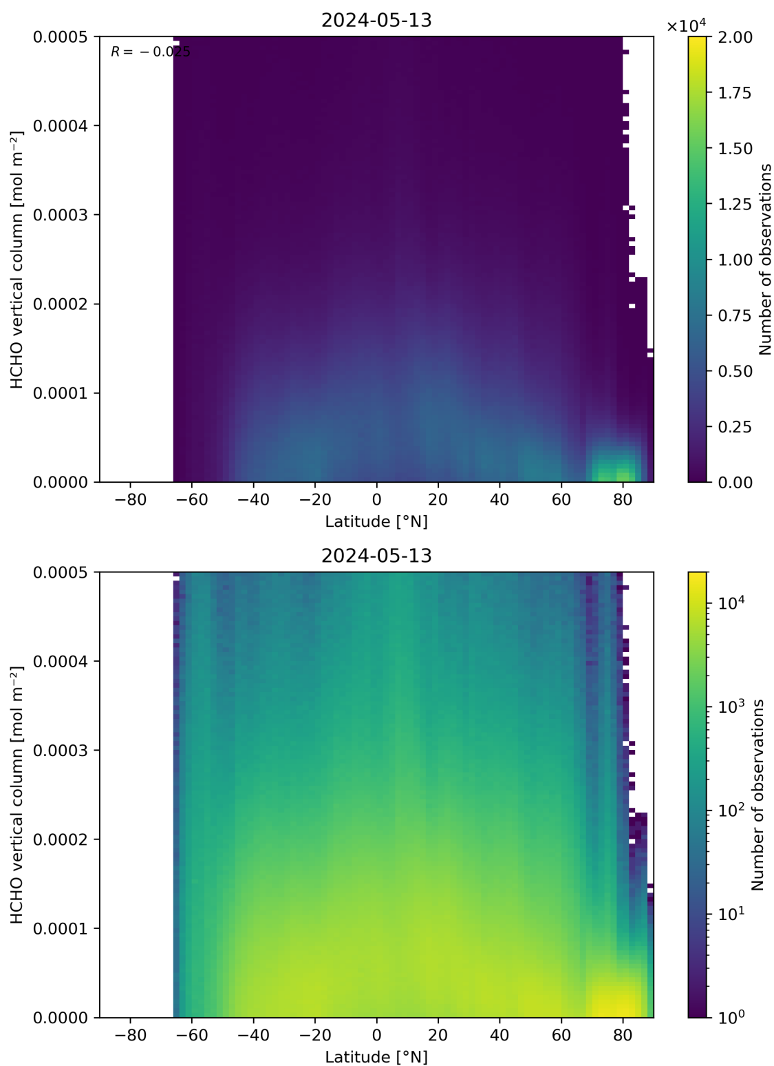
Figure 163: Scatter density plot of “Latitude” against “HCHO vertical column” for 2024-05-12 to 2024-05-14.
