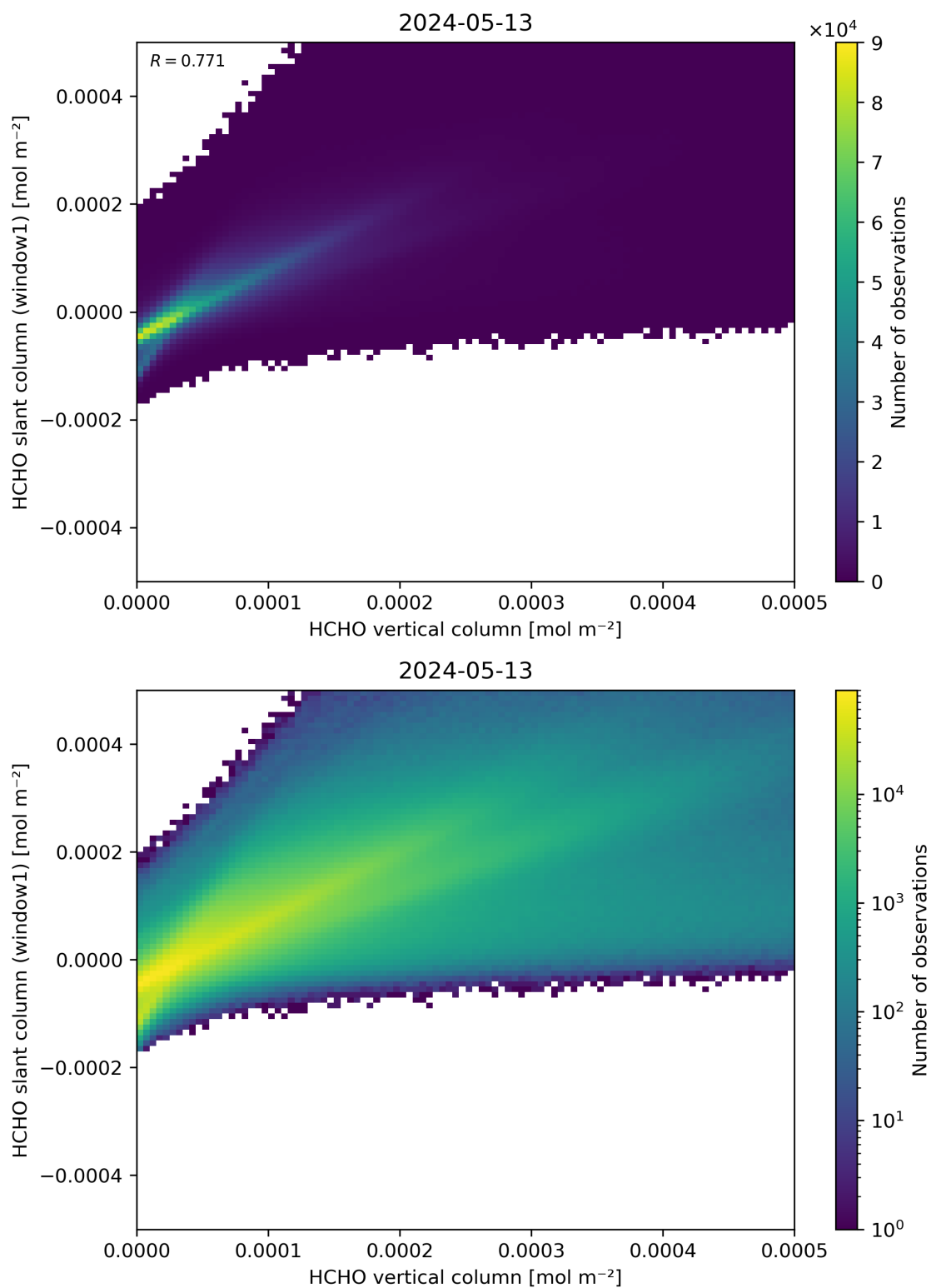
Figure 129: Scatter density plot of “HCHO vertical column” against “HCHO slant column (window1)” for 2024-05-12 to 2024-05-14.
