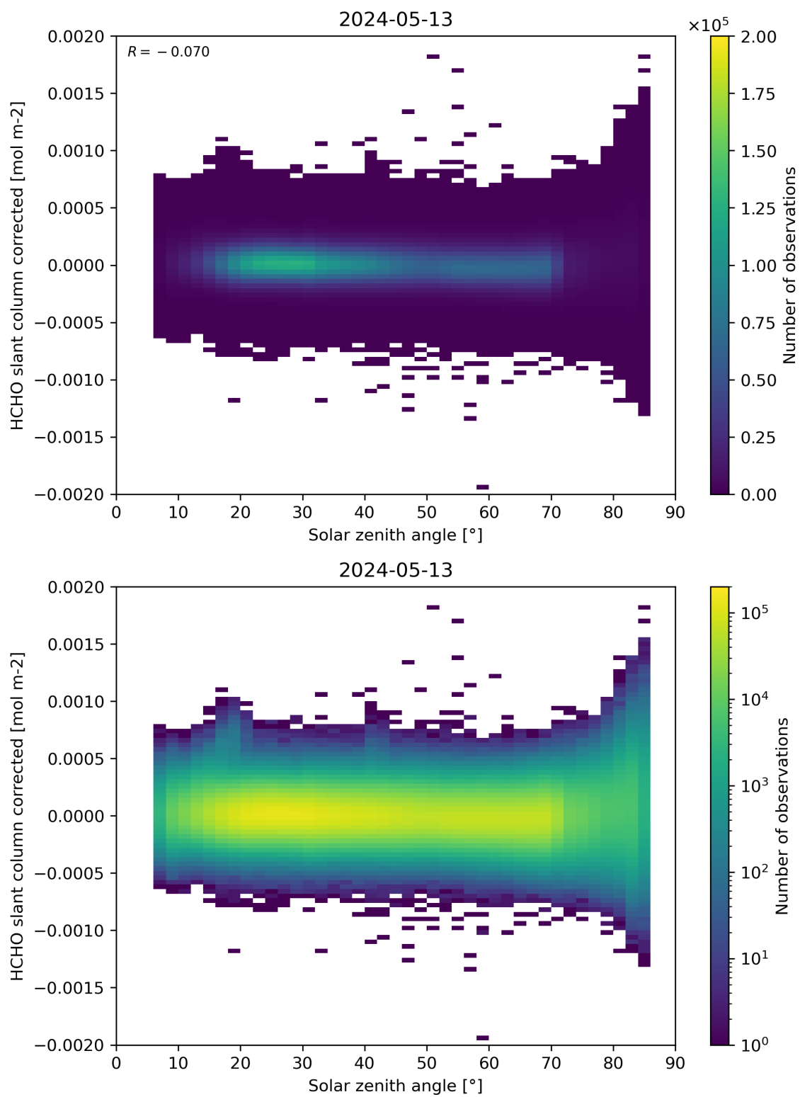
Figure 171: Scatter density plot of “Solar zenith angle” against “HCHO slant column corrected” for 2024-05-12 to 2024-05-14.
