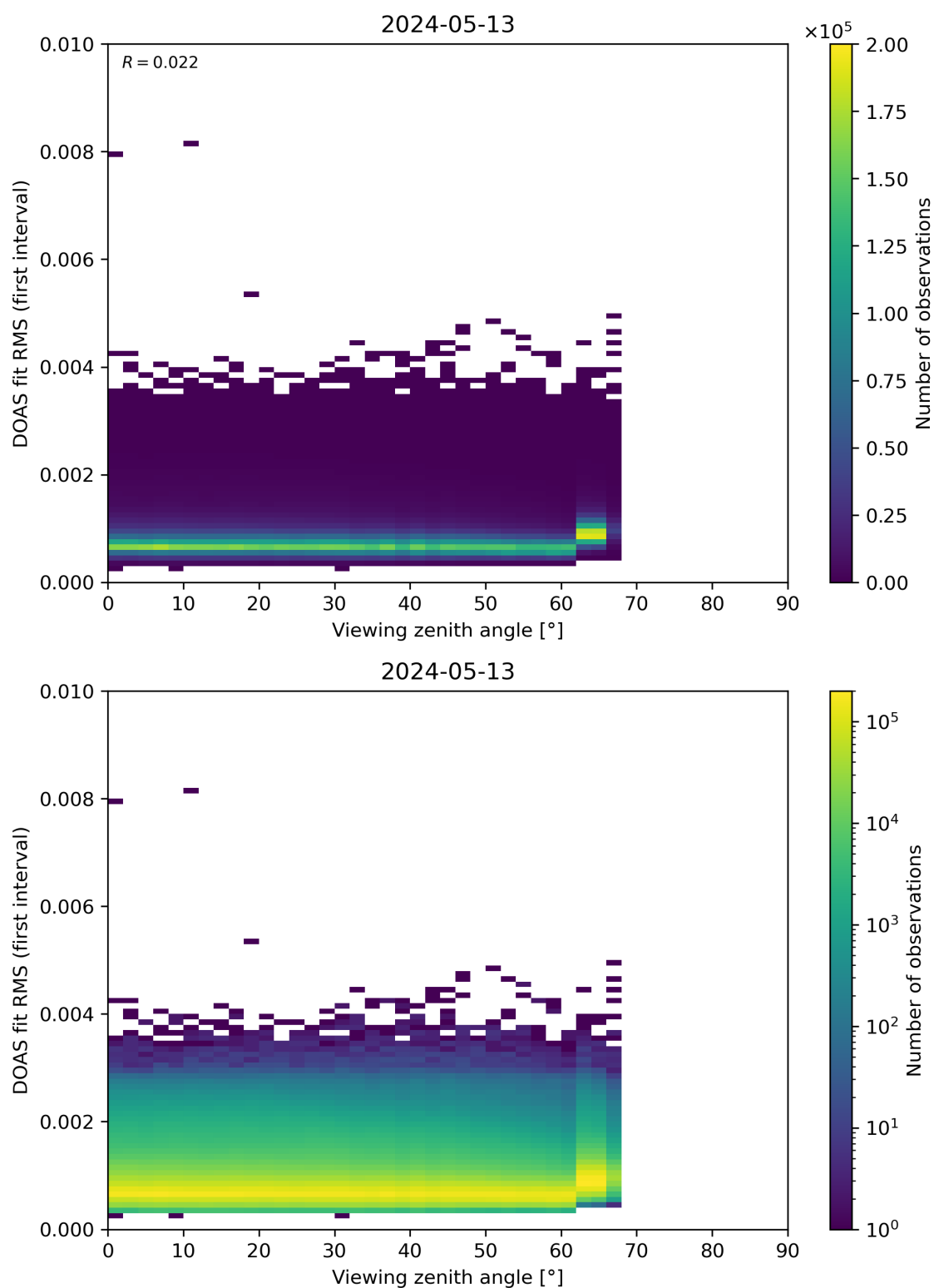
Figure 182: Scatter density plot of “Viewing zenith angle” against “DOAS fit RMS (first interval)” for 2024-05-12 to 2024-05-14.
