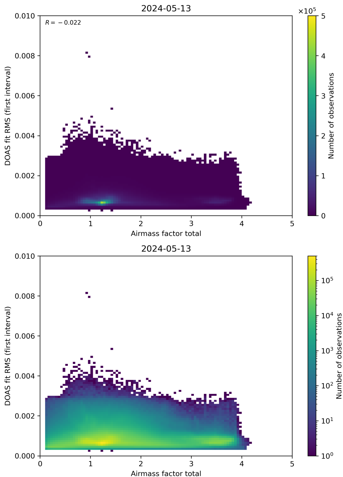
Figure 97: Scatter density plot of “Airmass factor total” against “DOAS fit RMS (first interval)” for 2024-05-12 to 2024-05-14.
