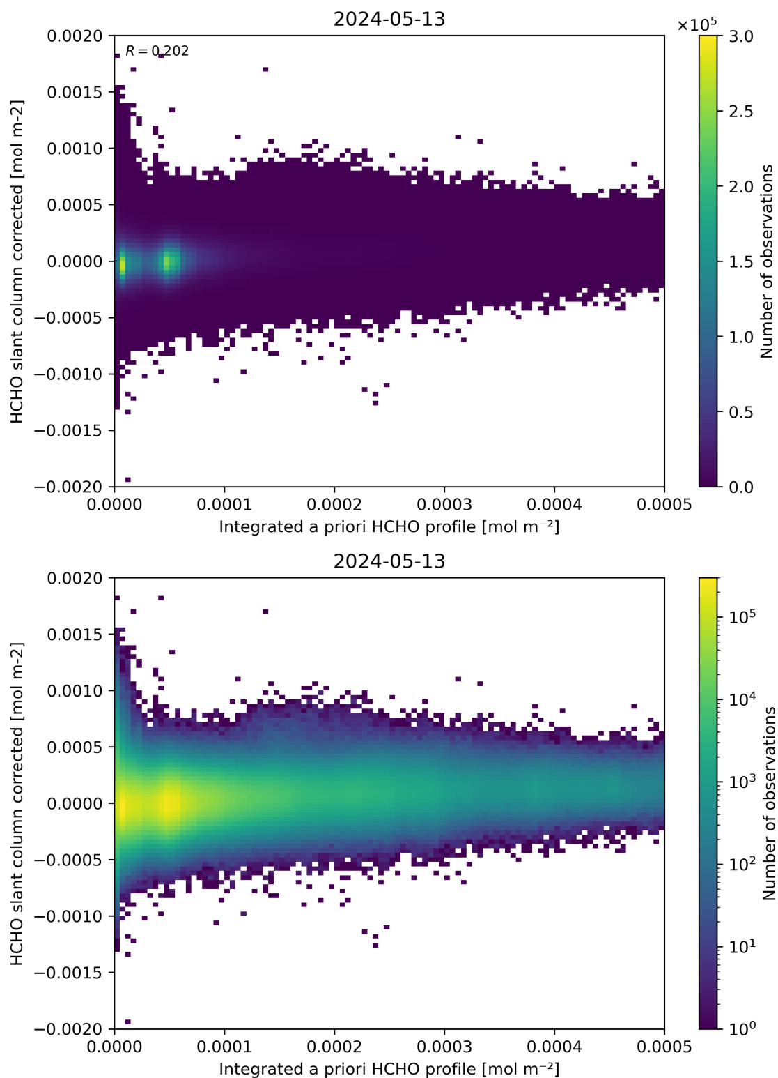
Figure 151: Scatter density plot of “Integrated a priori HCHO profile” against “HCHO slant column corrected” for 2024-05-12 to 2024-05-14.
