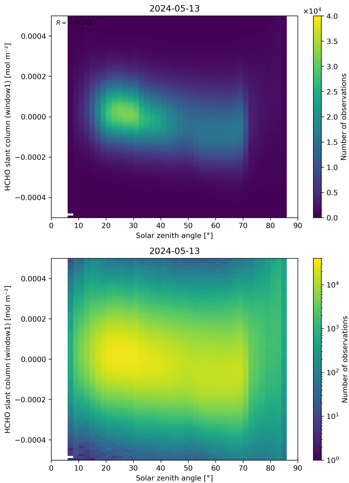
Figure 173: Scatter density plot of “Solar zenith angle” against “HCHO slant column (window1)” for 2024-05-12 to 2024-05-14.
