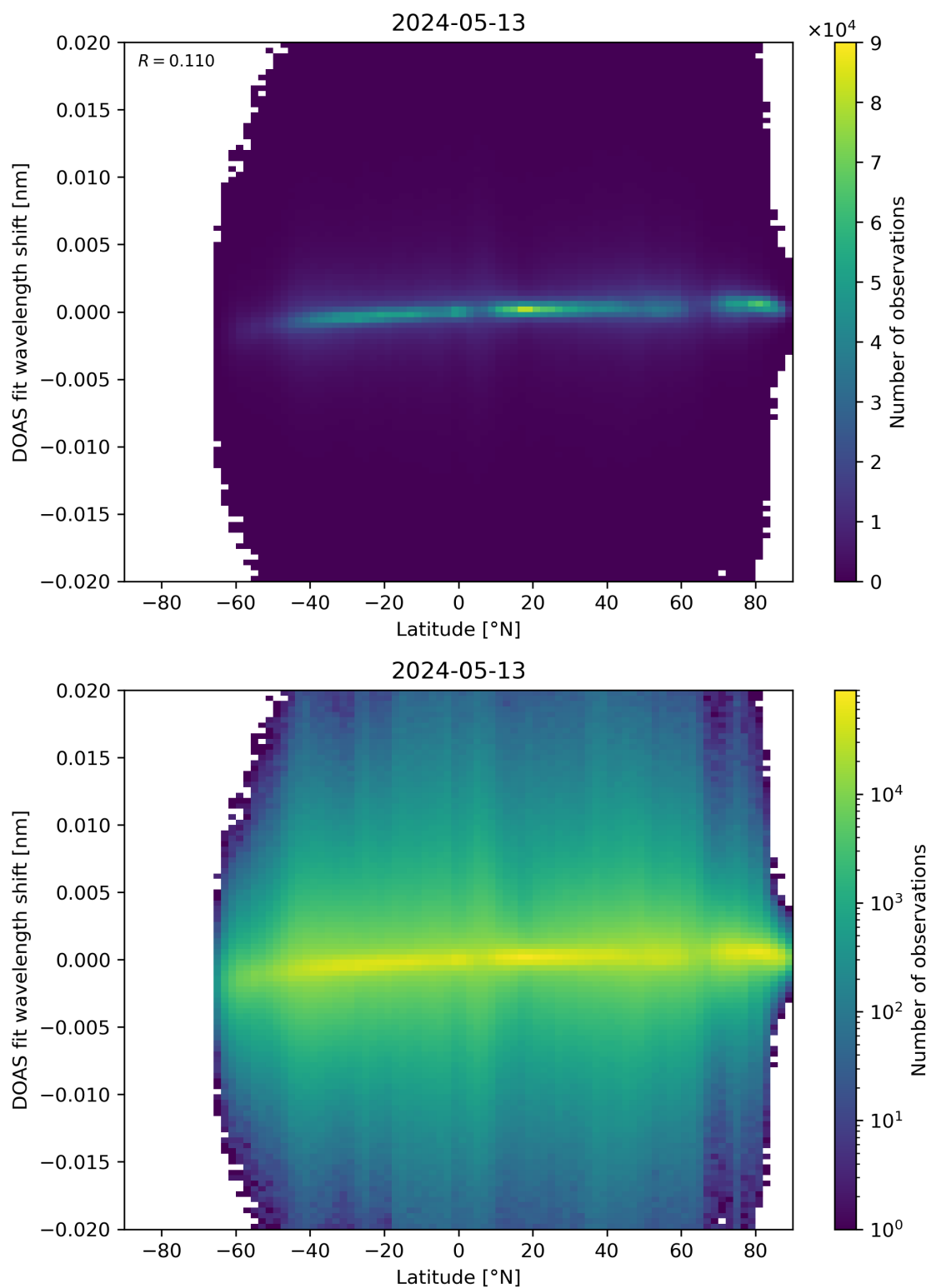
Figure 154: Scatter density plot of “Latitude” against “DOAS fit wavelength shift” for 2024-05-12 to 2024-05-14.
