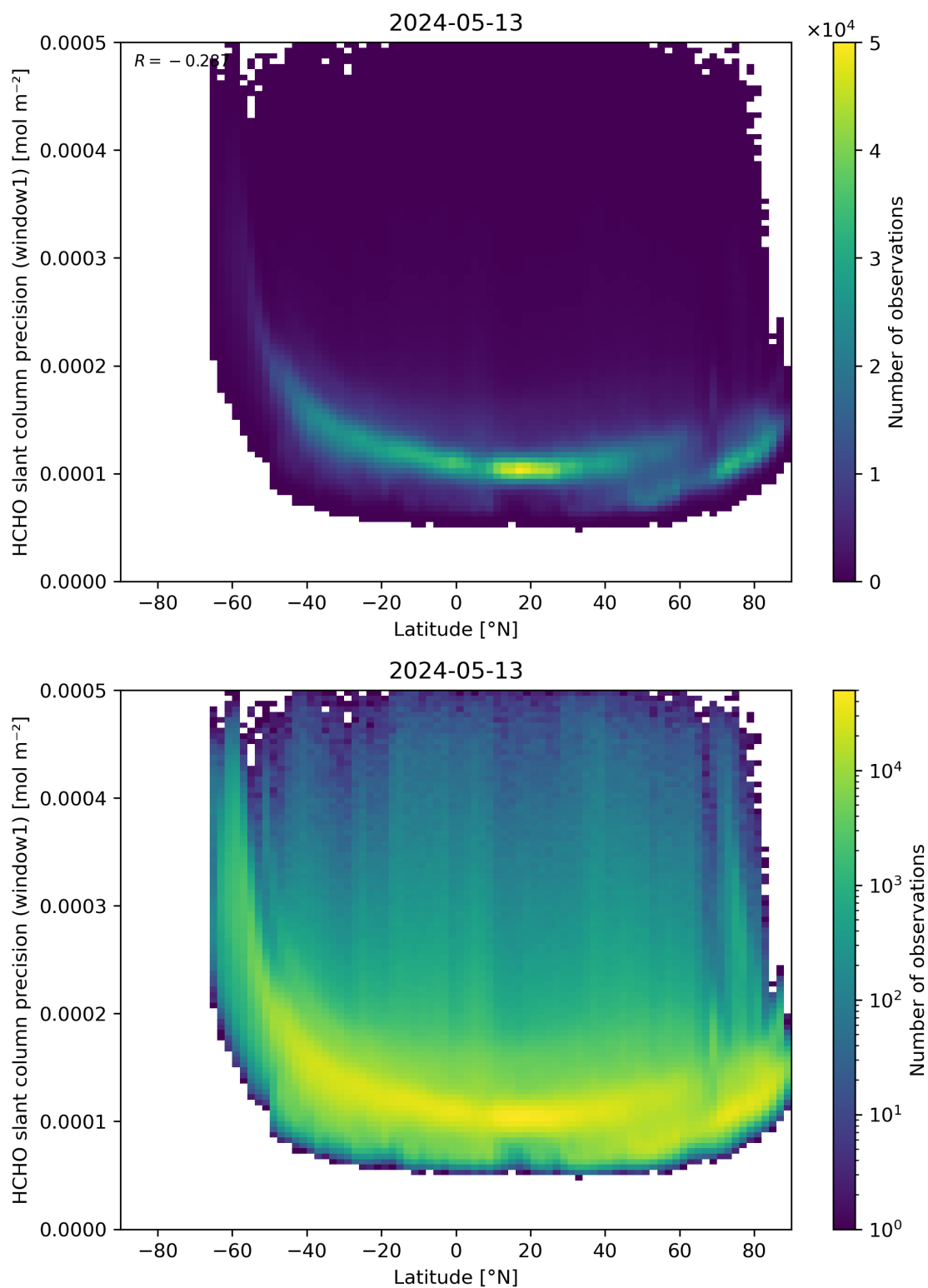
Figure 160: Scatter density plot of “Latitude” against “HCHO slant column precision (window1)” for 2024-05-12 to 2024-05-14.
