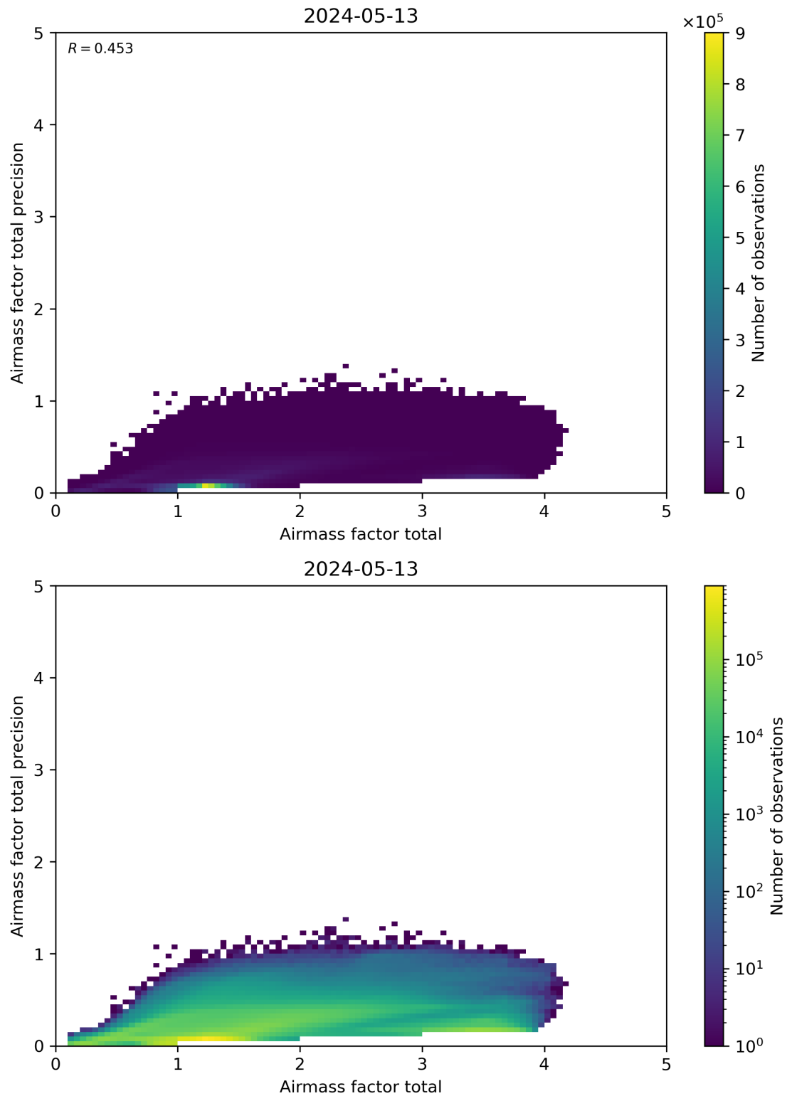
Figure 103: Scatter density plot of “Airmass factor total” against “Airmass factor total precision” for 2024-05-12 to 2024-05-14.
