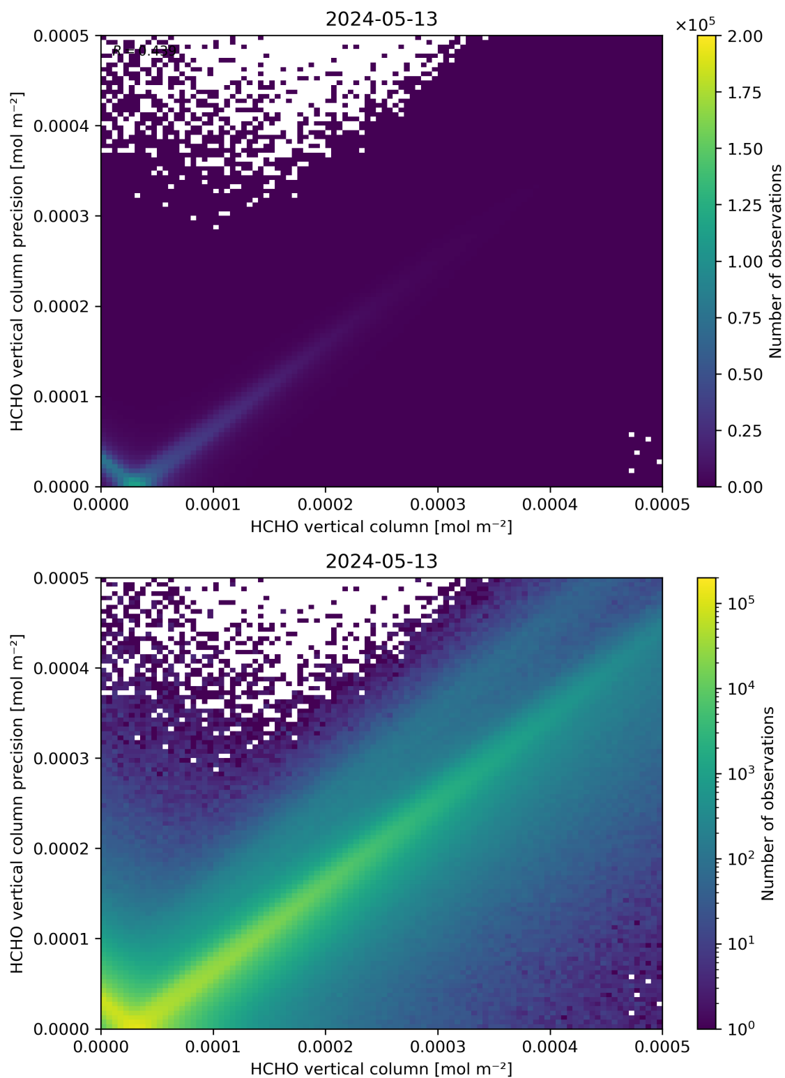
Figure 134: Scatter density plot of “HCHO vertical column” against “HCHO vertical column precision” for 2024-05-12 to 2024-05-14.
