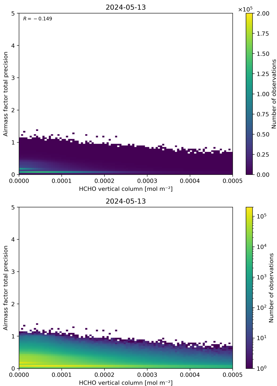
Figure 132: Scatter density plot of “HCHO vertical column” against “Airmass factor total precision” for 2024-05-12 to 2024-05-14.
