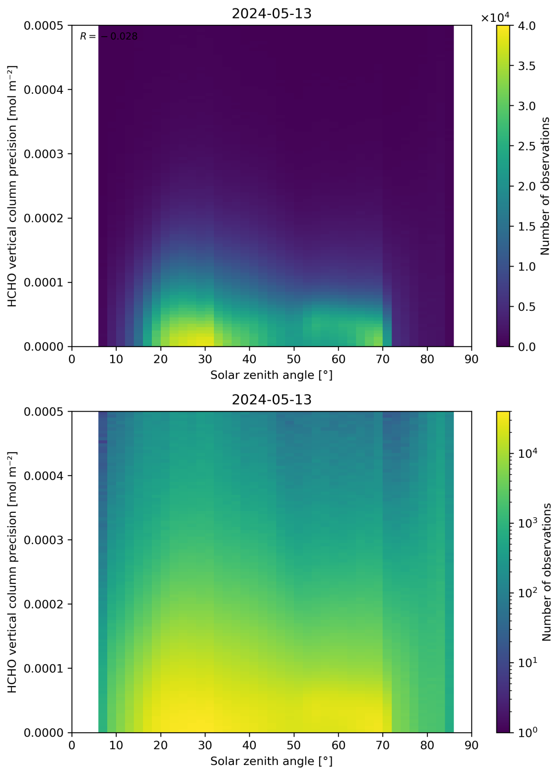
Figure 179: Scatter density plot of “Solar zenith angle” against “HCHO vertical column precision” for 2024-05-12 to 2024-05-14.
