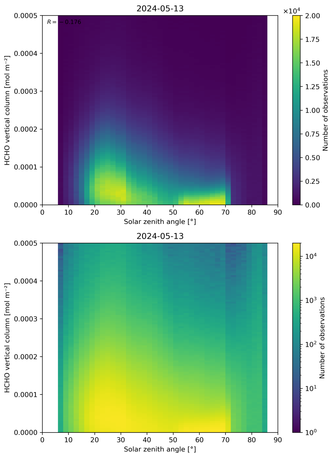
Figure 177: Scatter density plot of “Solar zenith angle” against “HCHO vertical column” for 2024-05-12 to 2024-05-14.
