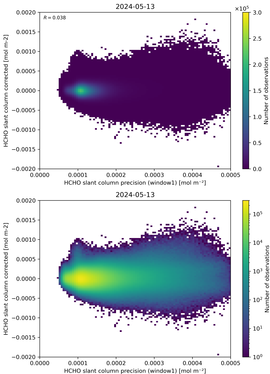
Figure 92: Scatter density plot of “HCHO slant column precision (window1)” against “HCHO slant column corrected” for 2024-05-12 to 2024-05-14.
