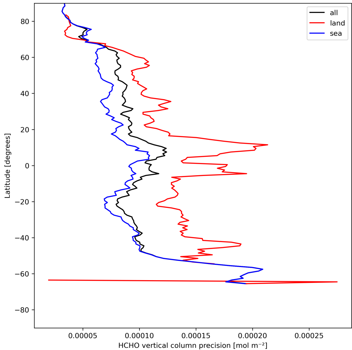
Figure 22: Zonal average of “HCHO vertical column precision” for 2024-05-12 to 2024-05-14.
