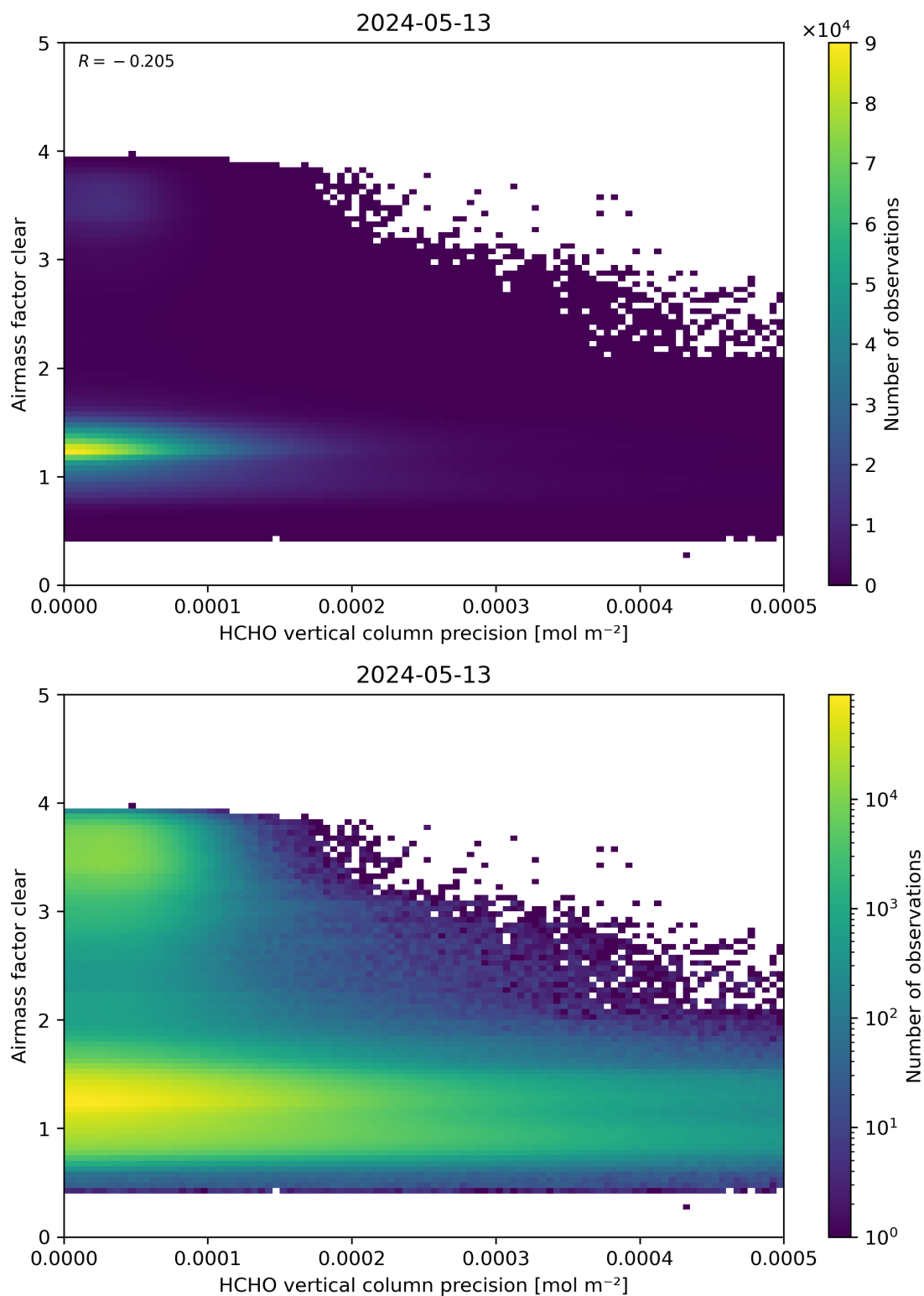
Figure 139: Scatter density plot of “HCHO vertical column precision” against “Airmass factor clear” for 2024-05-12 to 2024-05-14.
