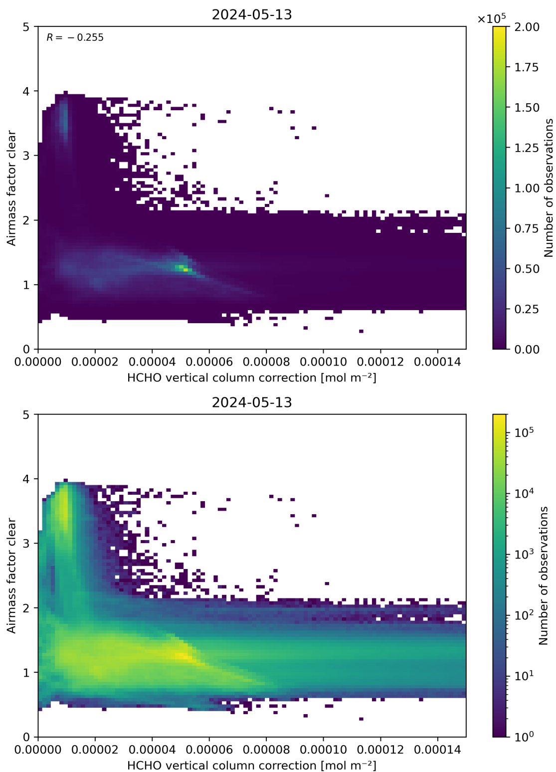
Figure 115: Scatter density plot of “HCHO vertical column correction” against “Airmass factor clear” for 2024-05-12 to 2024-05-14.
