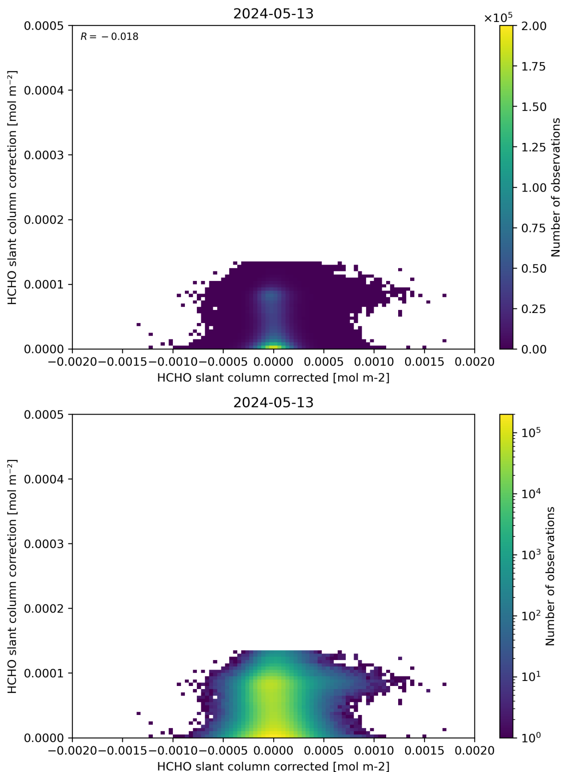
Figure 77: Scatter density plot of “HCHO slant column corrected” against “HCHO slant column correction” for 2024-05-12 to 2024-05-14.
