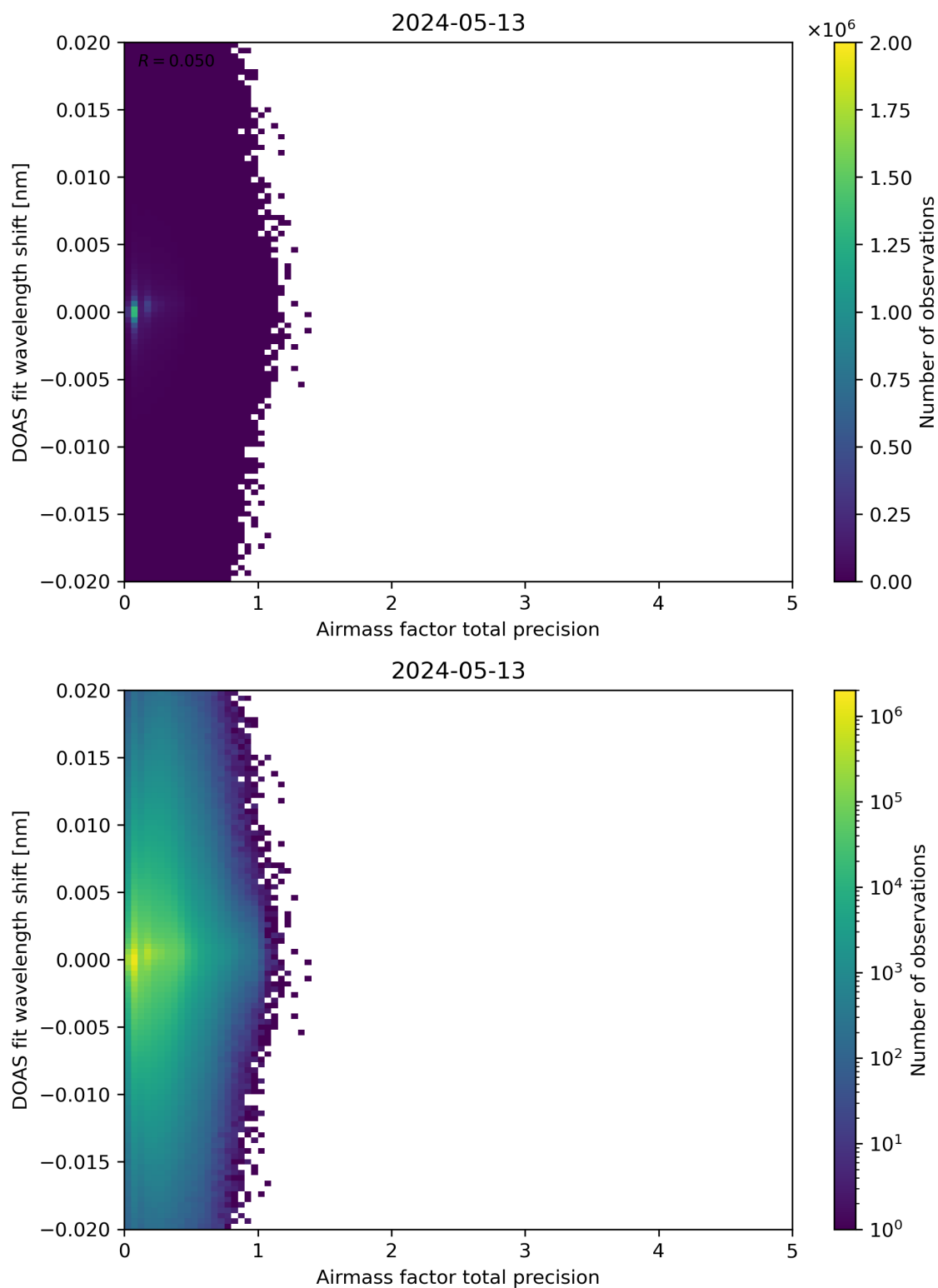
Figure 106: Scatter density plot of “Airmass factor total precision” against “DOAS fit wavelength shift” for 2024-05-12 to 2024-05-14.
