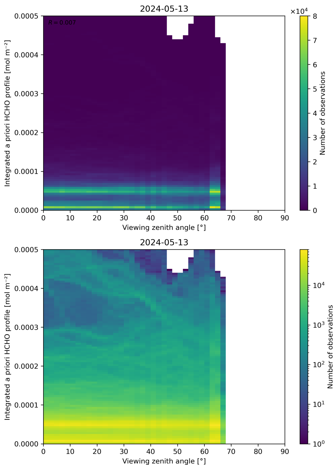
Figure 195: Scatter density plot of “Viewing zenith angle” against “Integrated a priori HCHO profile” for 2024-05-12 to 2024-05-14.
