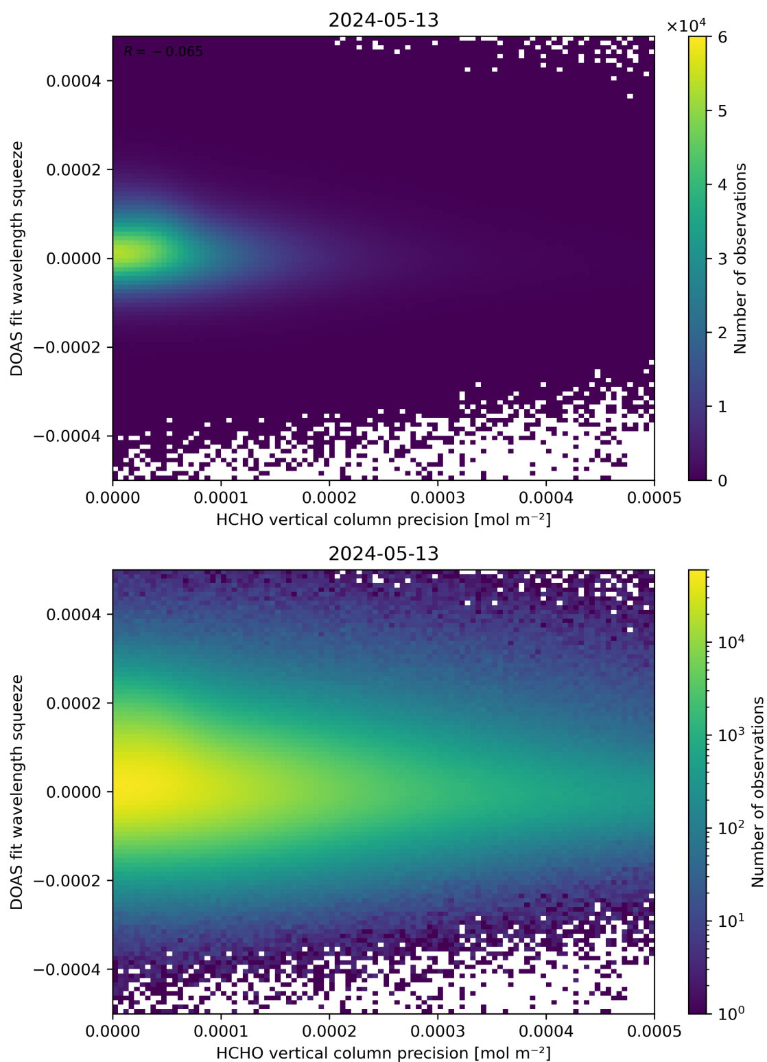
Figure 138: Scatter density plot of “HCHO vertical column precision” against “DOAS fit wavelength squeeze” for 2024-05-12 to 2024-05-14.
