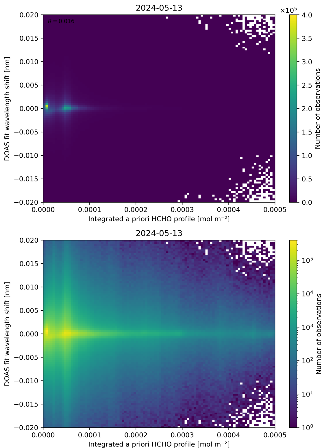
Figure 149: Scatter density plot of “Integrated a priori HCHO profile” against “DOAS fit wavelength shift” for 2024-05-12 to 2024-05-14.
