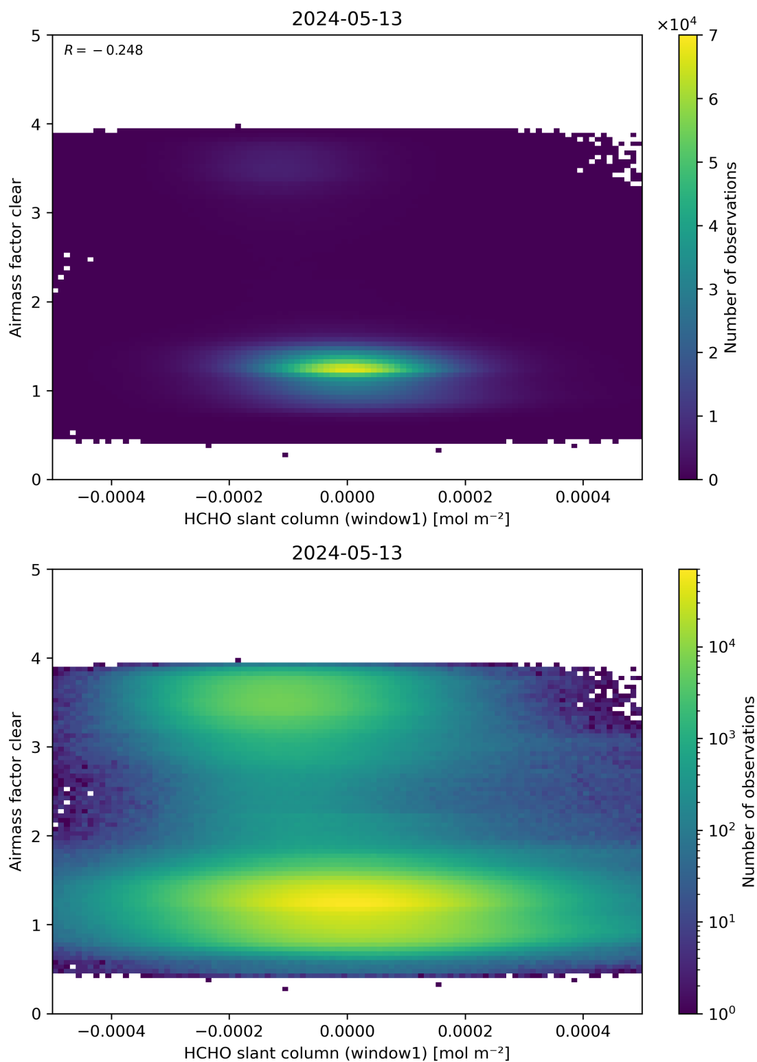
Figure 81: Scatter density plot of “HCHO slant column (window1)” against “Airmass factor clear” for 2024-05-12 to 2024-05-14.
