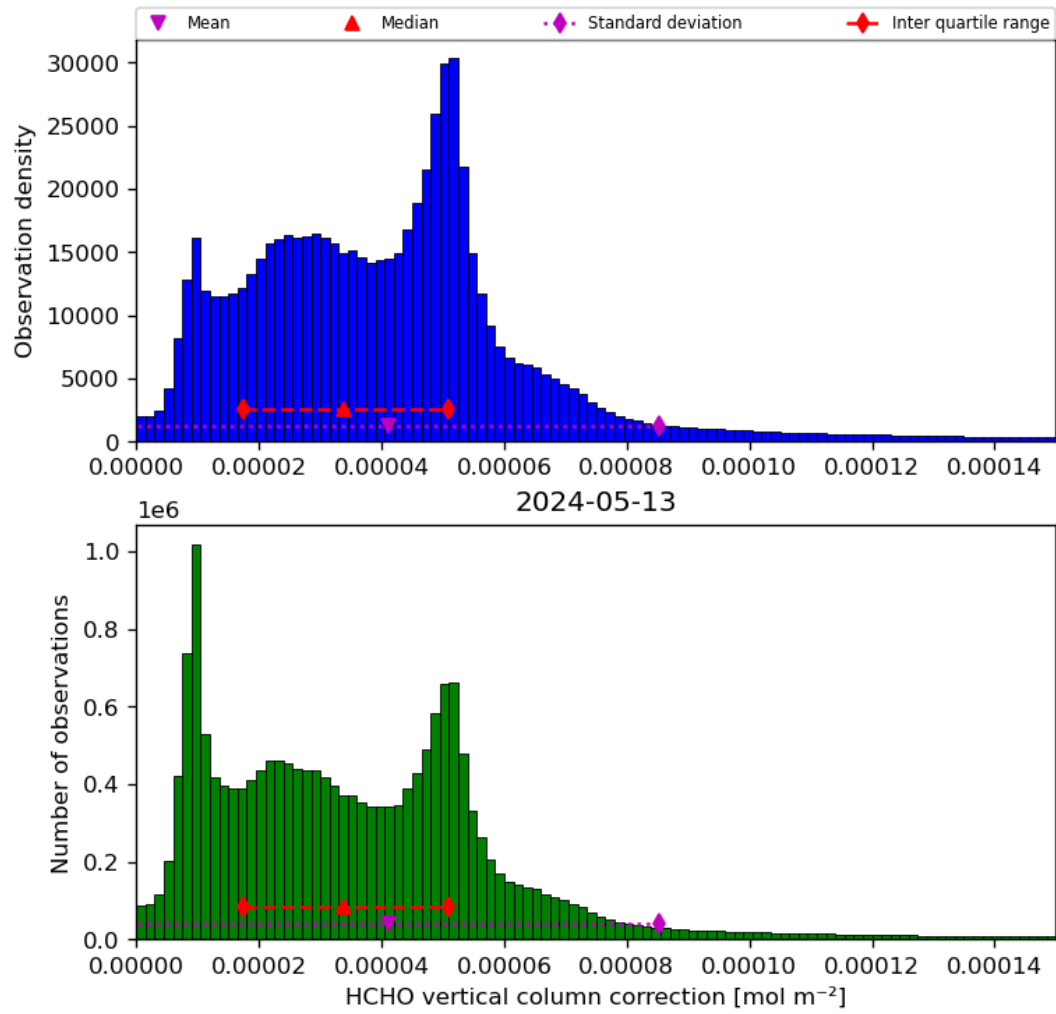
Figure 37: Histogram of “HCHO vertical column correction” for 2024-05-12 to 2024-05-14
