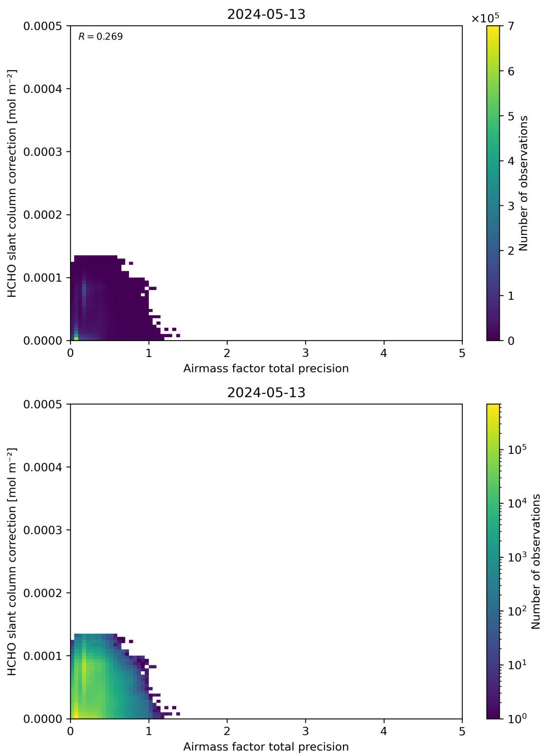
Figure 110: Scatter density plot of “Airmass factor total precision” against “HCHO slant column correction” for 2024-05-12 to 2024-05-14.
