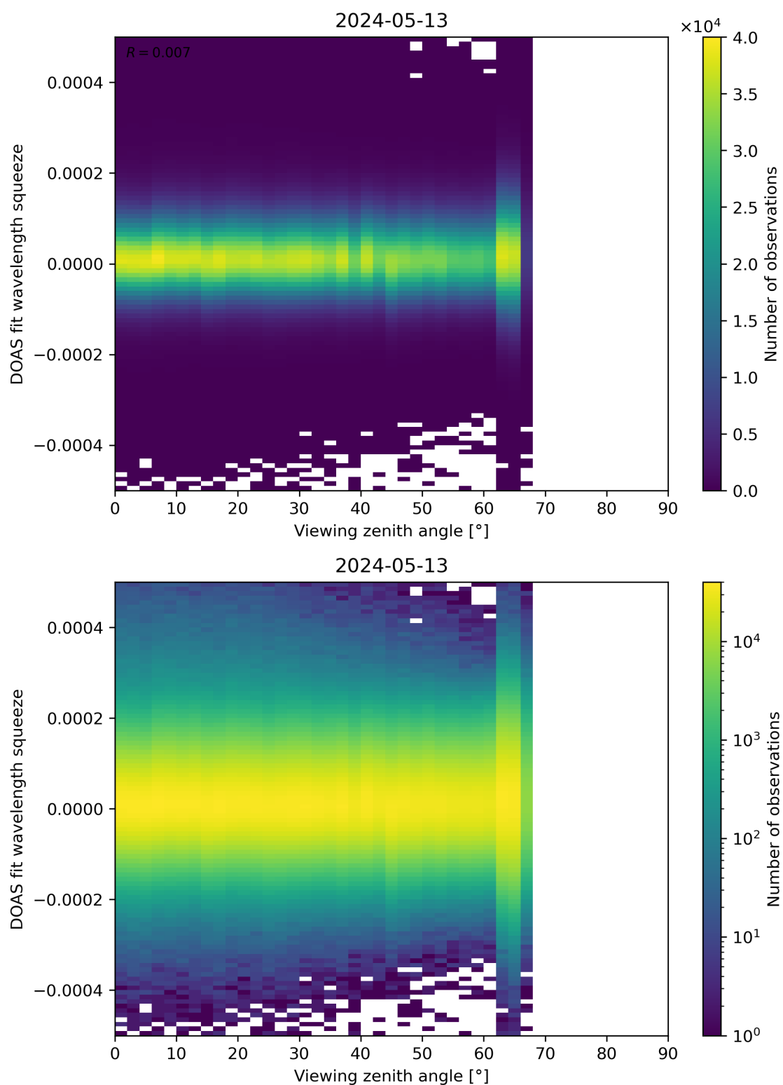
Figure 184: Scatter density plot of “Viewing zenith angle” against “DOAS fit wavelength squeeze” for 2024-05-12 to 2024-05-14.
