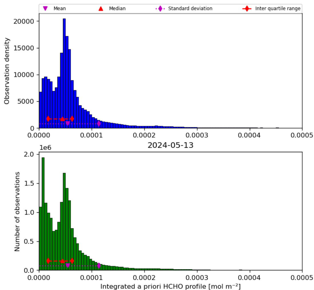
Figure 43: Histogram of “Integrated a priori HCHO profile” for 2024-05-12 to 2024-05-14
