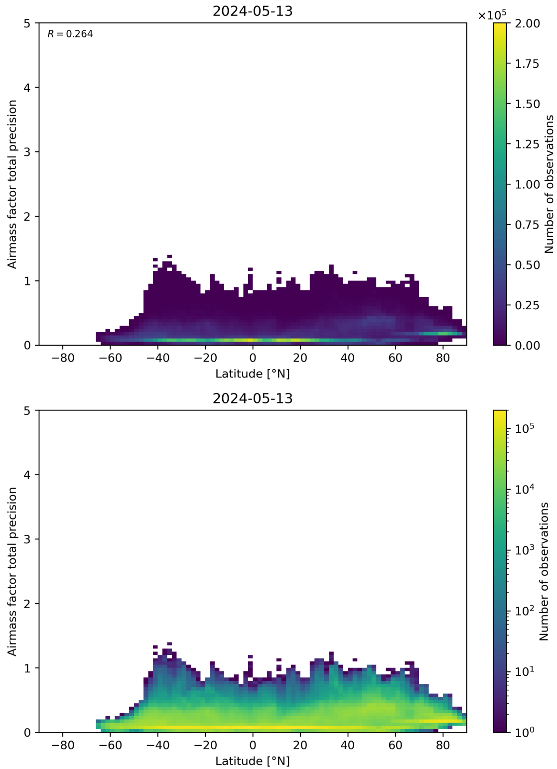
Figure 162: Scatter density plot of “Latitude” against “Airmass factor total precision” for 2024-05-12 to 2024-05-14.
