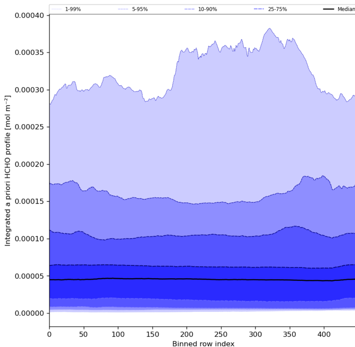
Figure 57: Along track statistics of "Integrated a priori HCHO profile" for 2024-05-12 to 2024-05-14
