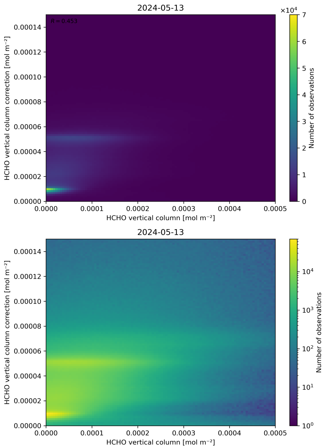
Figure 133: Scatter density plot of “HCHO vertical column” against “HCHO vertical column correction” for 2024-05-12 to 2024-05-14.
