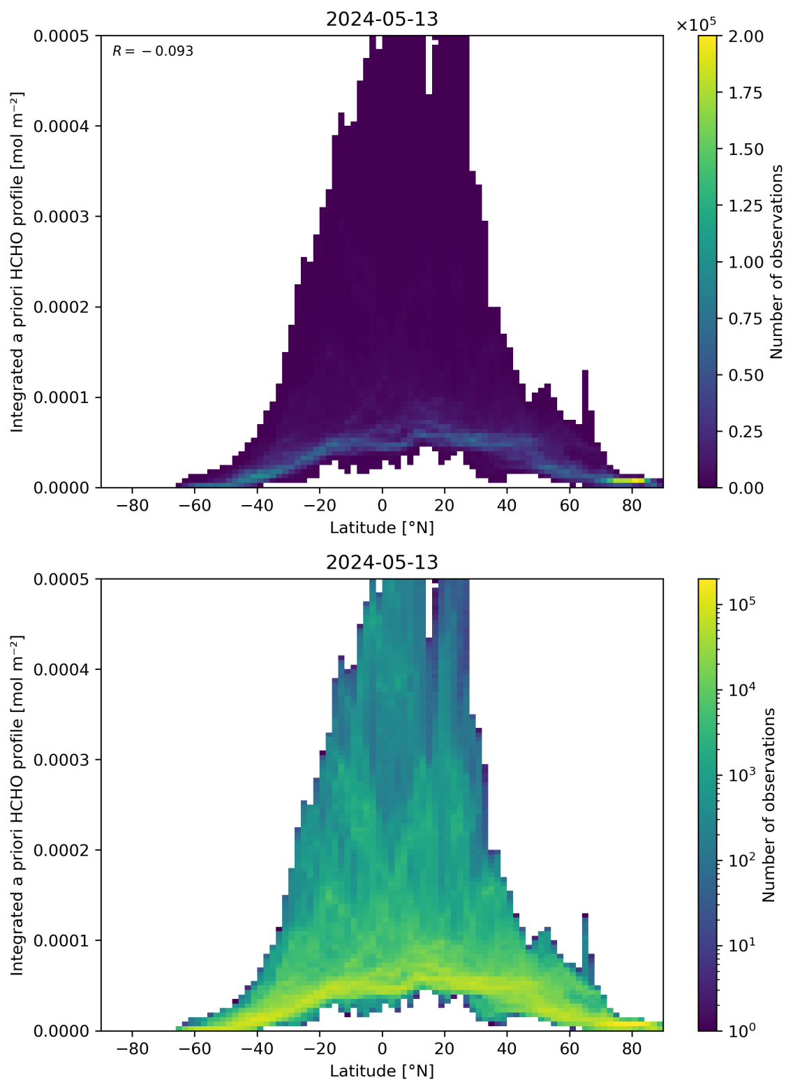
Figure 166: Scatter density plot of “Latitude” against “Integrated a priori HCHO profile” for 2024-05-12 to 2024-05-14.
