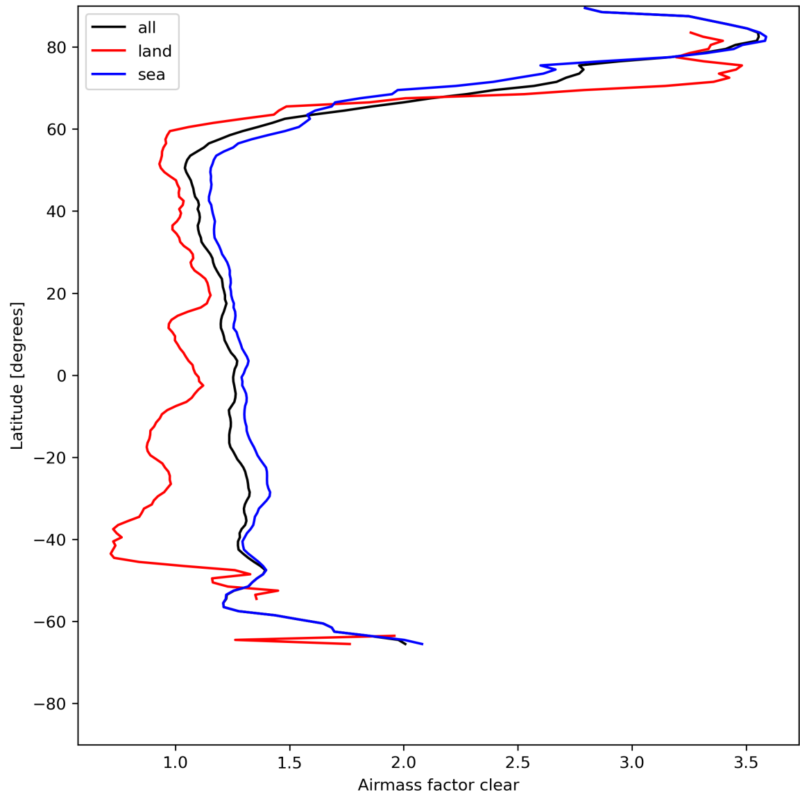
Figure 28: Zonal average of “Airmass factor clear” for 2024-05-12 to 2024-05-14.
