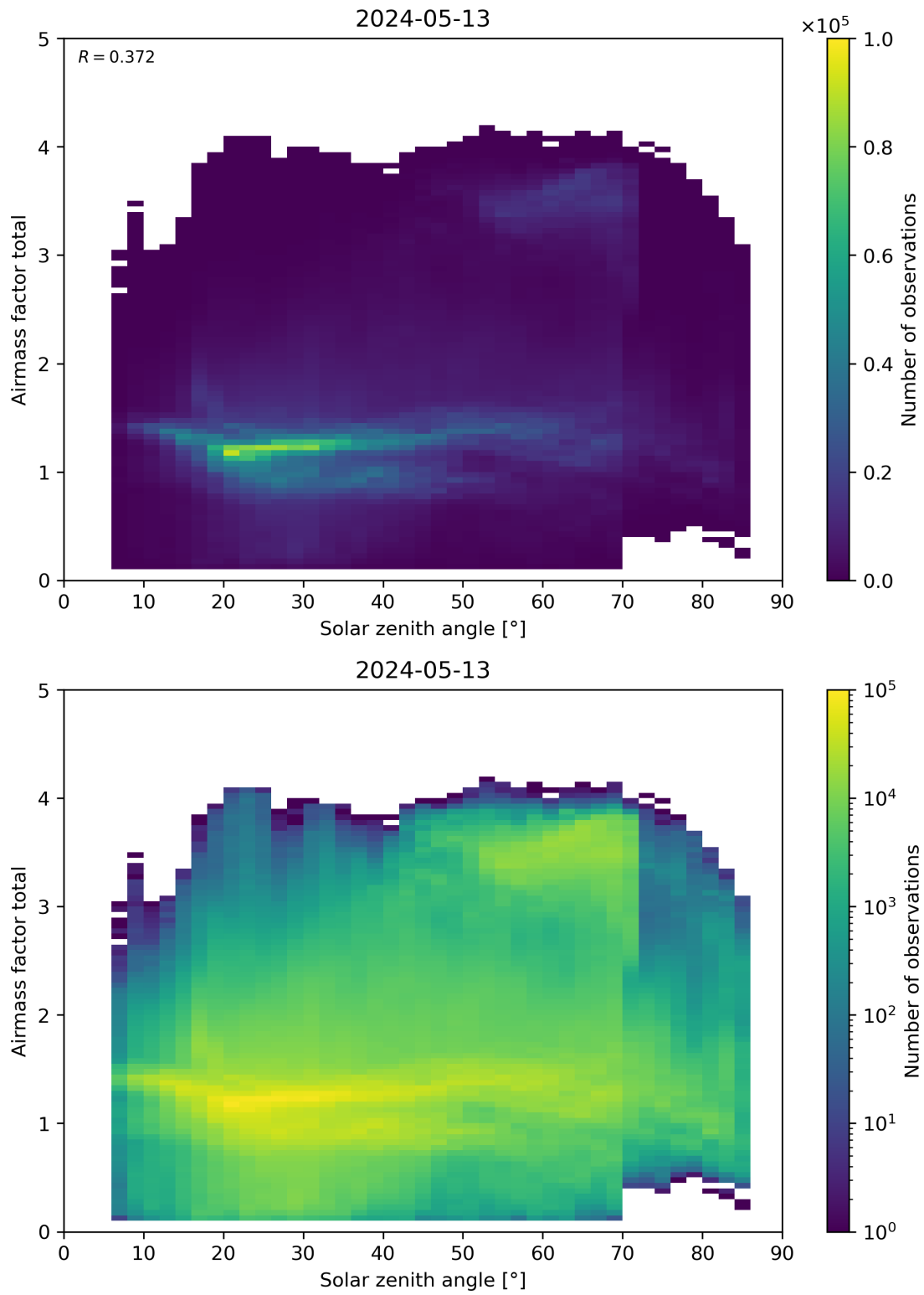
Figure 175: Scatter density plot of “Solar zenith angle” against “Airmass factor total” for 2024-05-12 to 2024-05-14.
