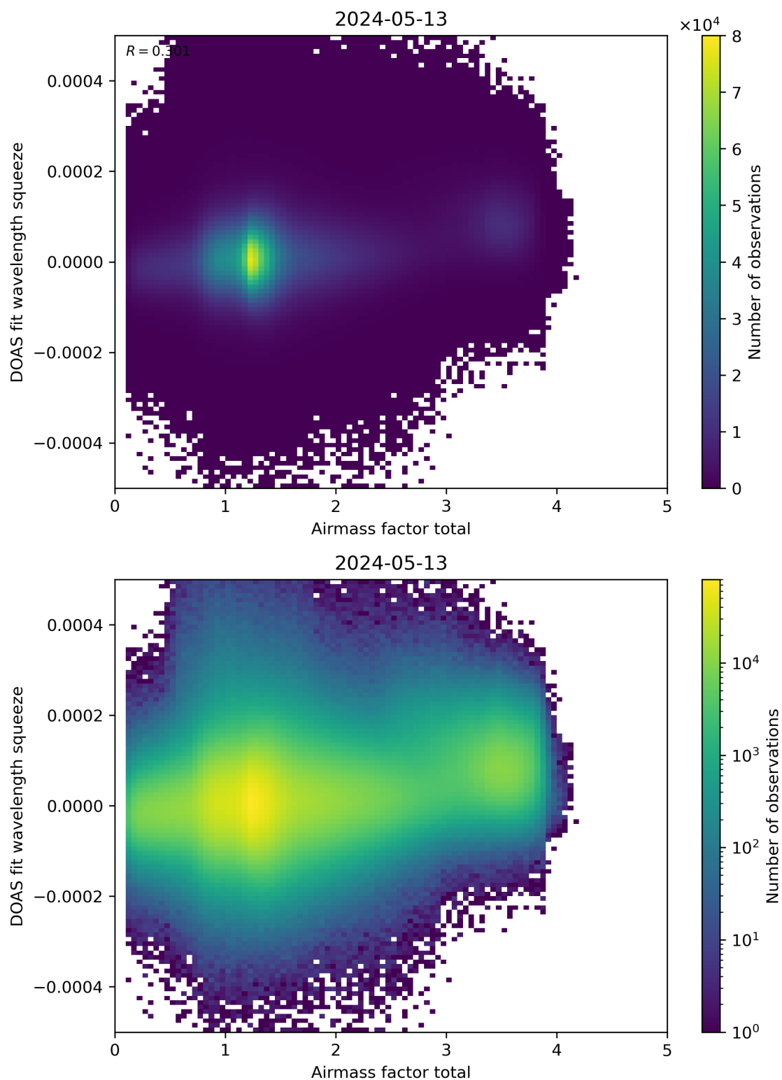
Figure 99: Scatter density plot of “Airmass factor total” against “DOAS fit wavelength squeeze” for 2024-05-12 to 2024-05-14.
