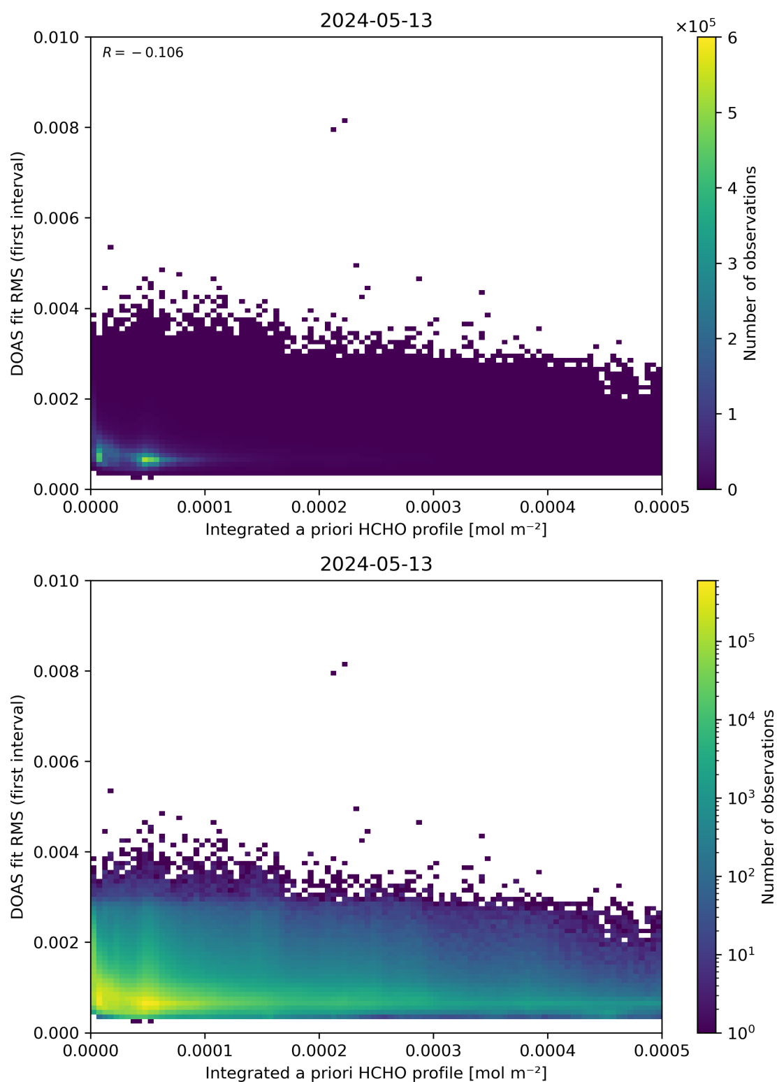
Figure 148: Scatter density plot of “Integrated a priori HCHO profile” against “DOAS fit RMS (first interval)” for 2024-05-12 to 2024-05-14.
