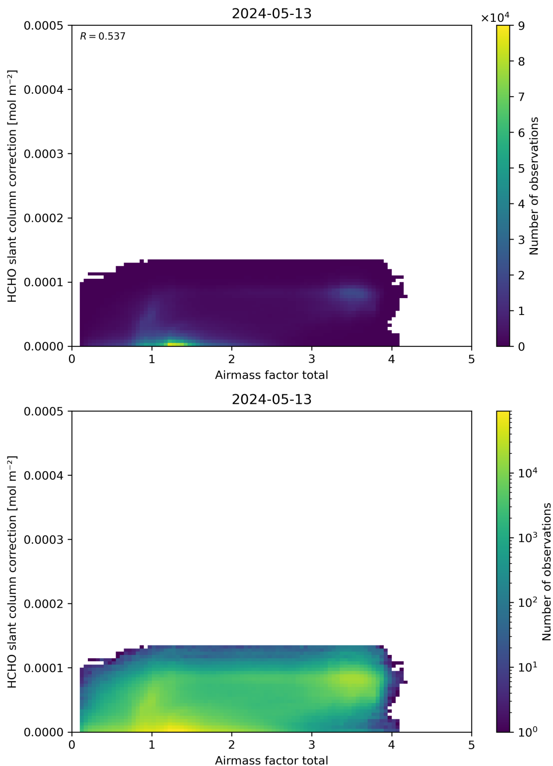
Figure 102: Scatter density plot of “Airmass factor total” against “HCHO slant column correction” for 2024-05-12 to 2024-05-14.
