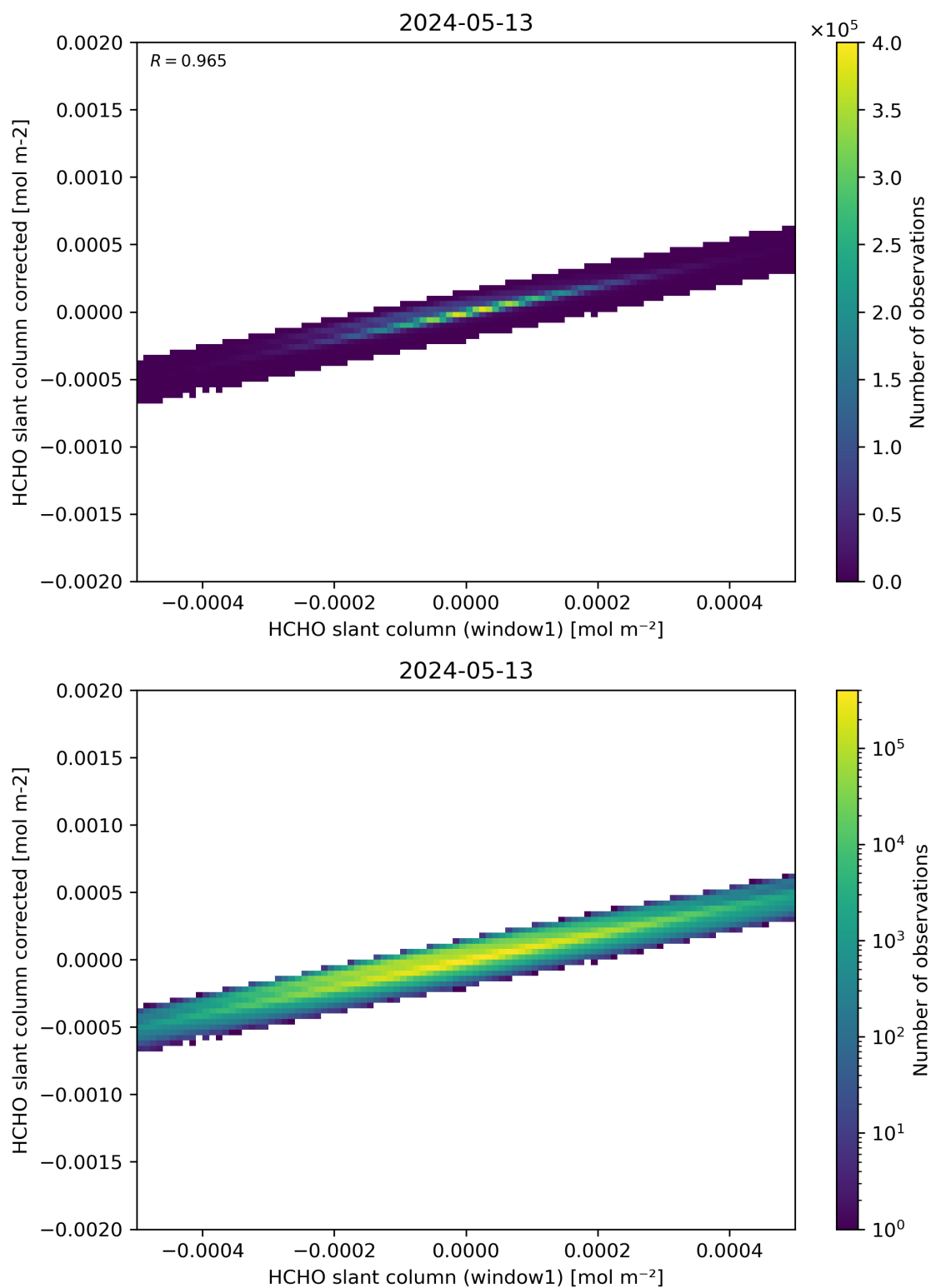
Figure 82: Scatter density plot of “HCHO slant column (window1)” against “HCHO slant column corrected” for 2024-05-12 to 2024-05-14.
