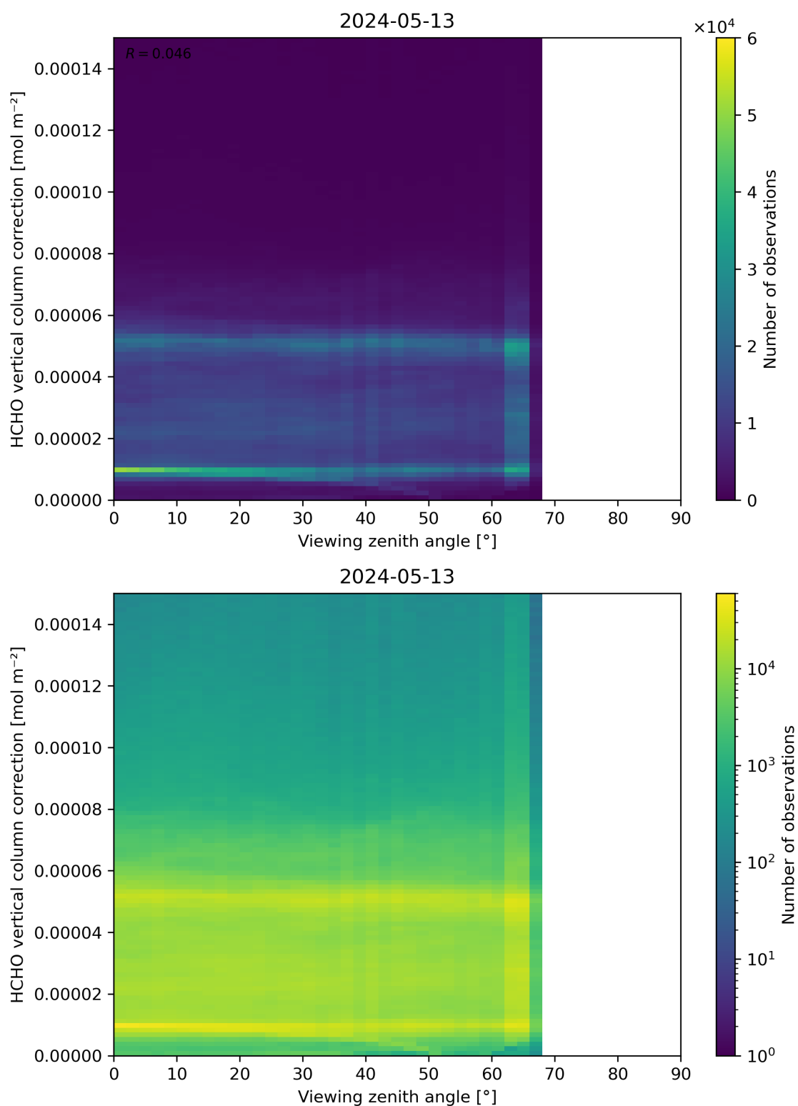
Figure 193: Scatter density plot of “Viewing zenith angle” against “HCHO vertical column correction” for 2024-05-12 to 2024-05-14.
