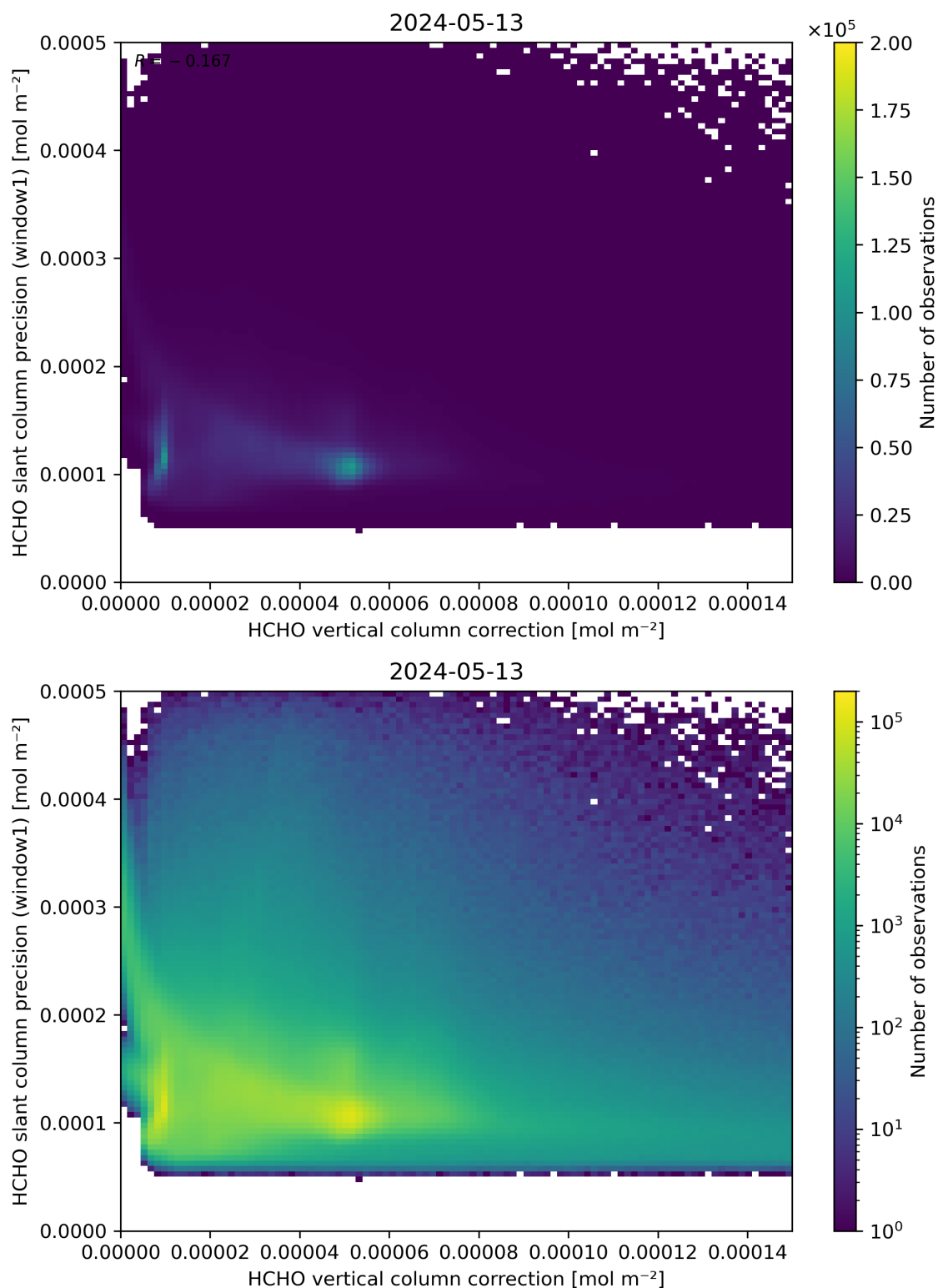
Figure 119: Scatter density plot of “HCHO vertical column correction” against “HCHO slant column precision (window1)” for 2024-05-12 to 2024-05-14.
