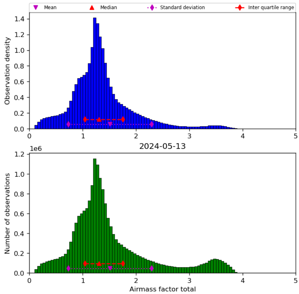
Figure 40: Histogram of “Airmass factor total” for 2024-05-12 to 2024-05-14
