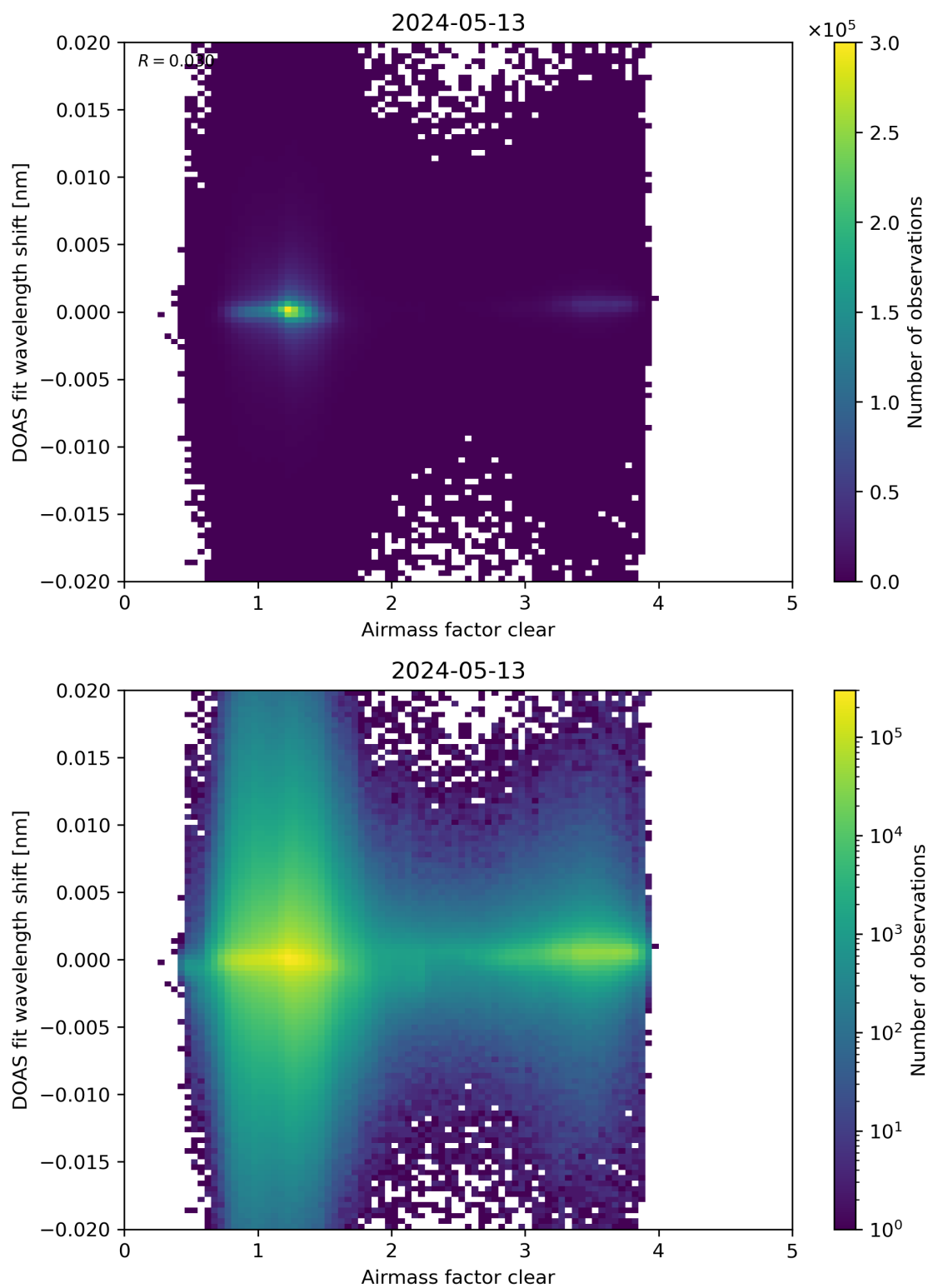
Figure 72: Scatter density plot of “Airmass factor clear” against “DOAS fit wavelength shift” for 2024-05-12 to 2024-05-14.
