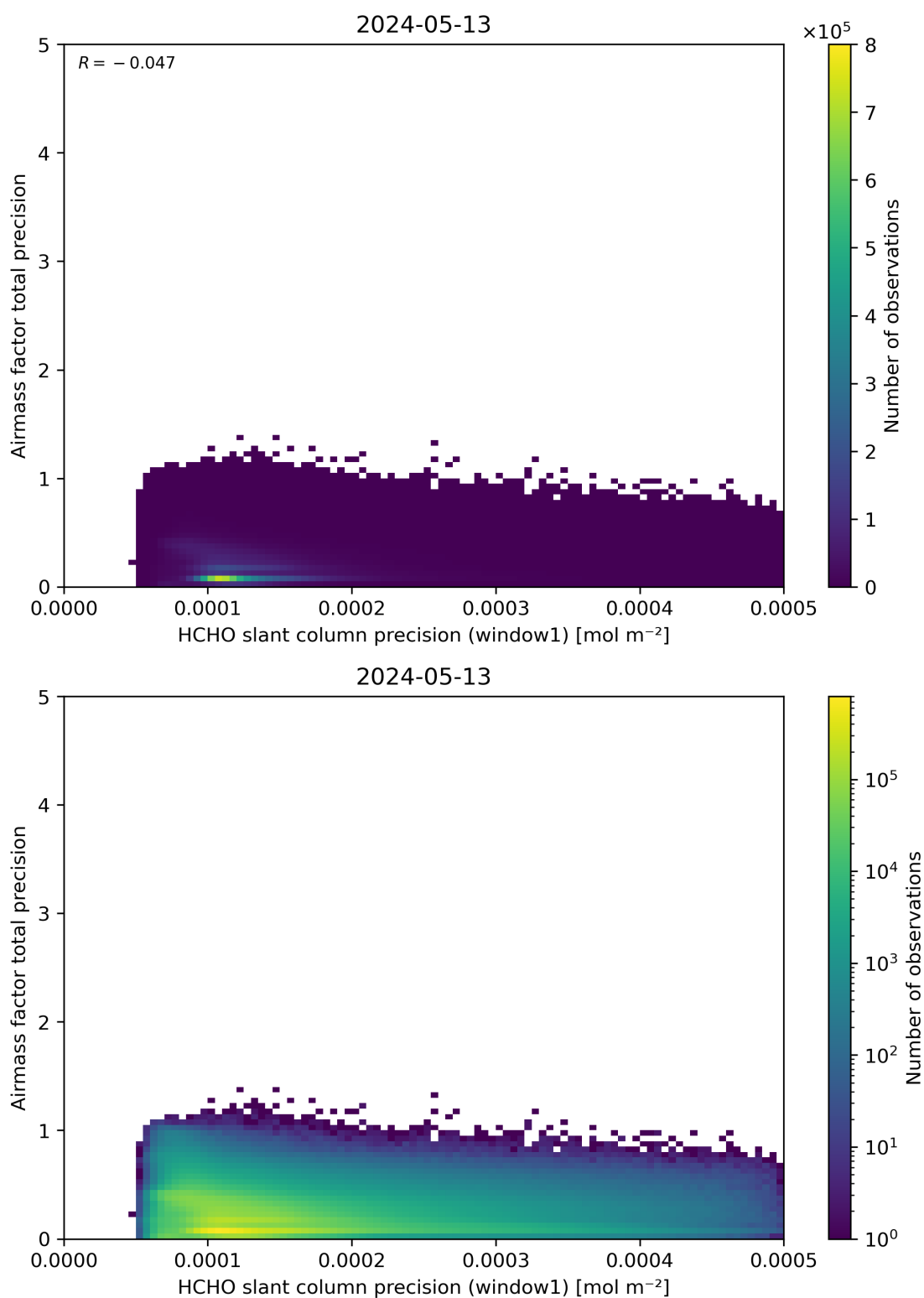
Figure 95: Scatter density plot of “HCHO slant column precision (window1)” against “Airmass factor total precision” for 2024-05-12 to 2024-05-14.
