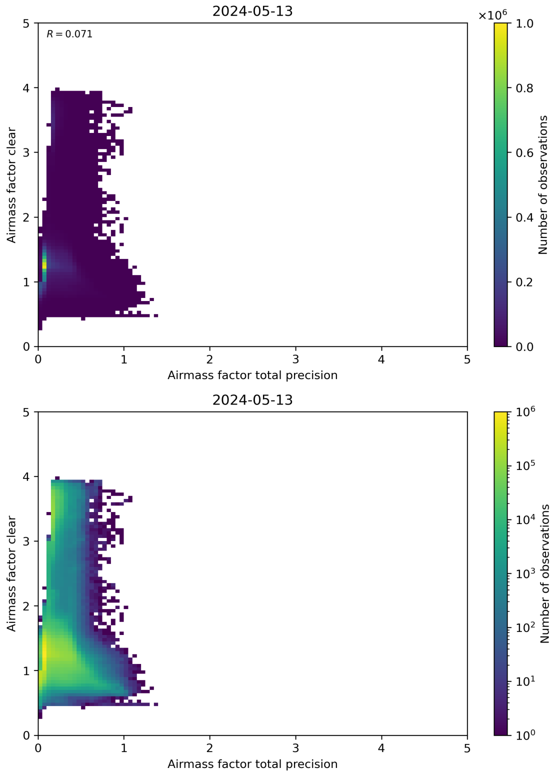
Figure 108: Scatter density plot of “Airmass factor total precision” against “Airmass factor clear” for 2024-05-12 to 2024-05-14.
