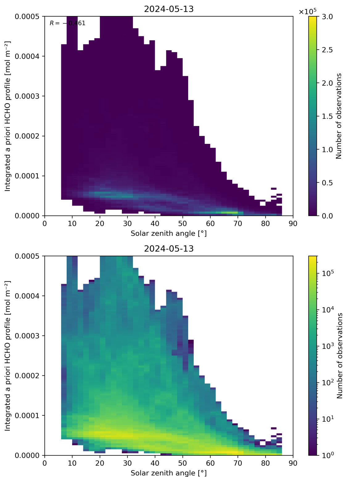
Figure 180: Scatter density plot of “Solar zenith angle” against “Integrated a priori HCHO profile” for 2024-05-12 to 2024-05-14.
