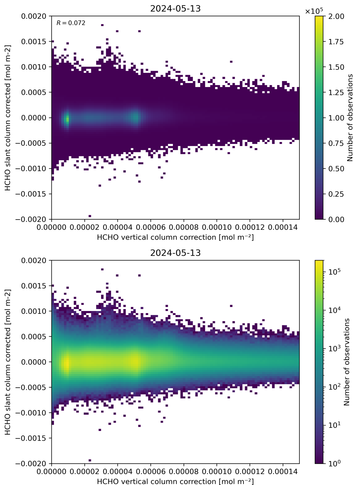
Figure 116: Scatter density plot of “HCHO vertical column correction” against “HCHO slant column corrected” for 2024-05-12 to 2024-05-14.
