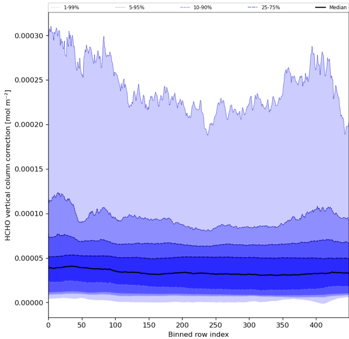
Figure 51: Along track statistics of “HCHO vertical column correction” for 2024-05-12 to 2024-05-14
