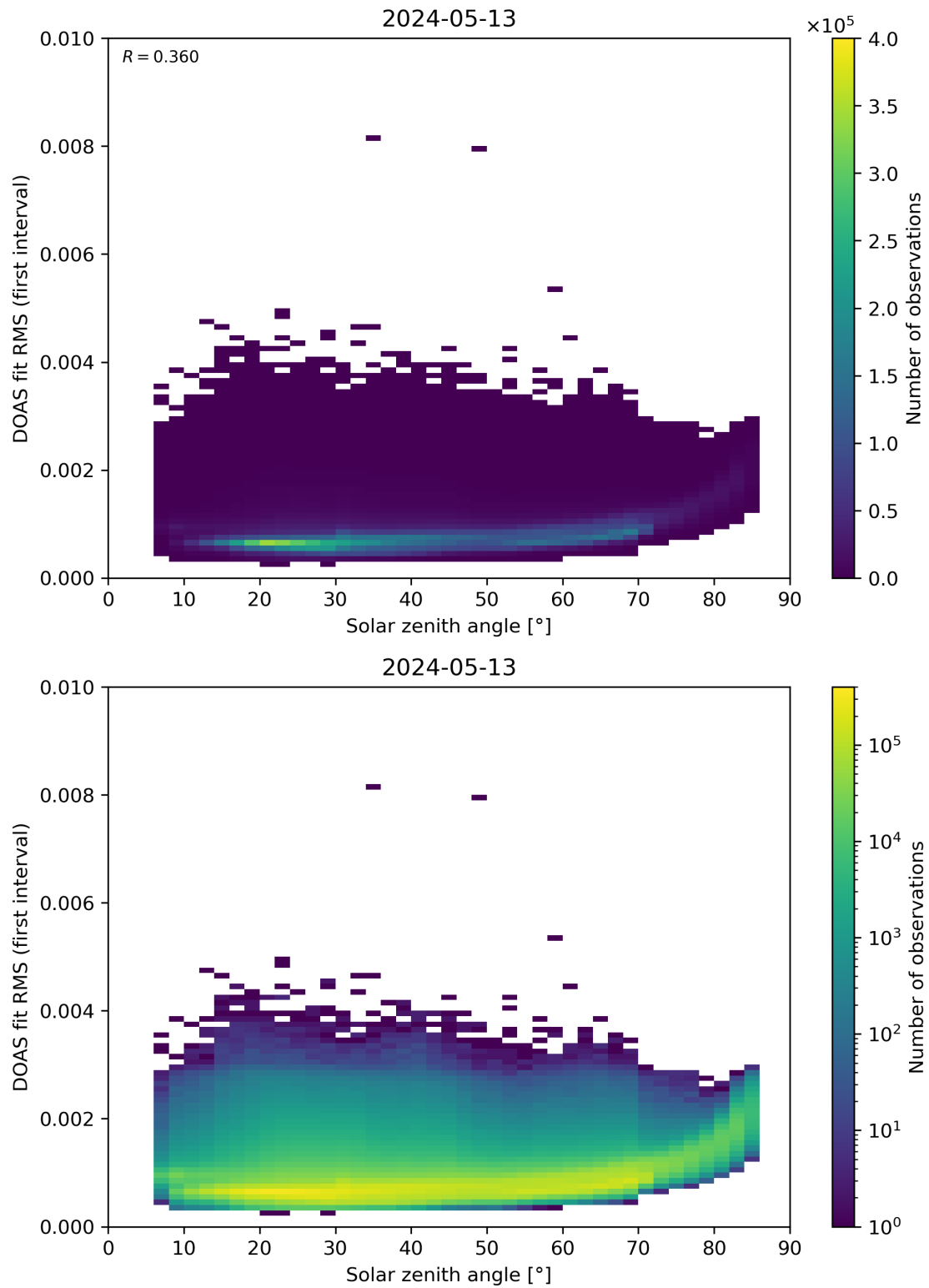
Figure 167: Scatter density plot of “Solar zenith angle” against “DOAS fit RMS (first interval)” for 2024-05-12 to 2024-05-14.
