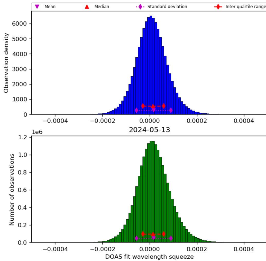
Figure 45: Histogram of “DOAS fit wavelength squeeze” for 2024-05-12 to 2024-05-14
