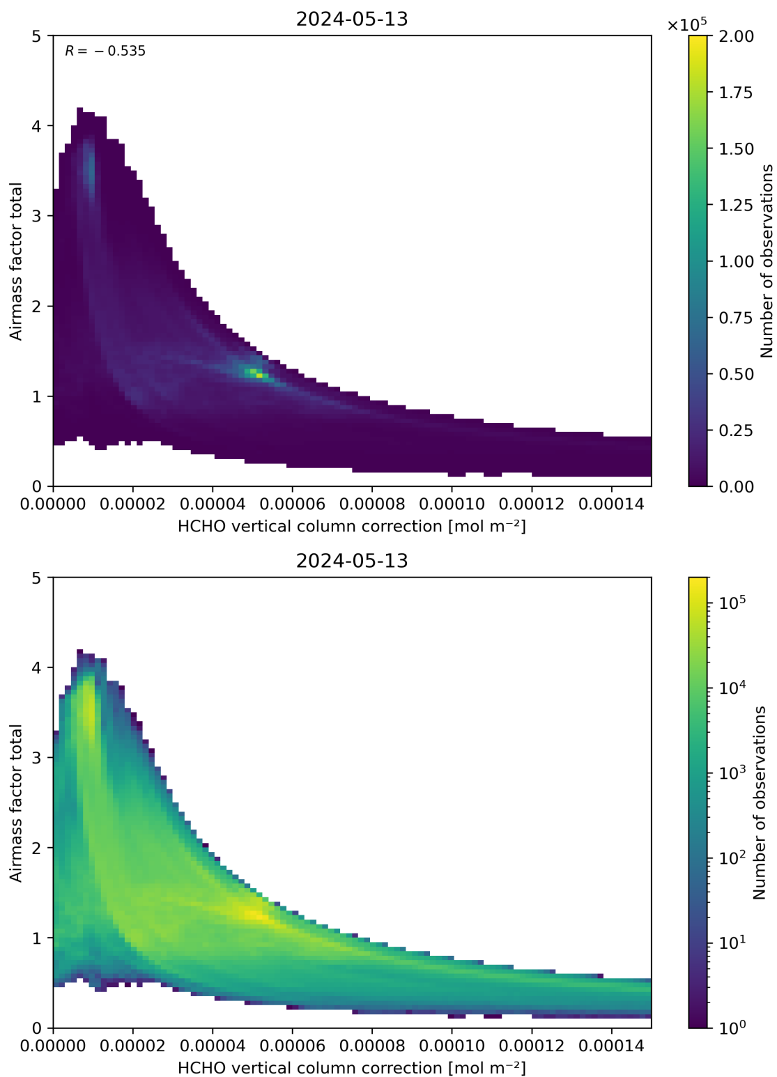
Figure 120: Scatter density plot of “HCHO vertical column correction” against “Airmass factor total” for 2024-05-12 to 2024-05-14.
