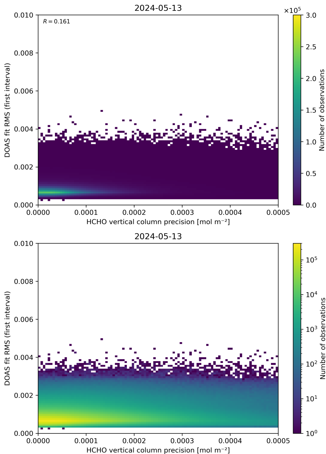
Figure 136: Scatter density plot of “HCHO vertical column precision” against “DOAS fit RMS (first interval)” for 2024-05-12 to 2024-05-14.
