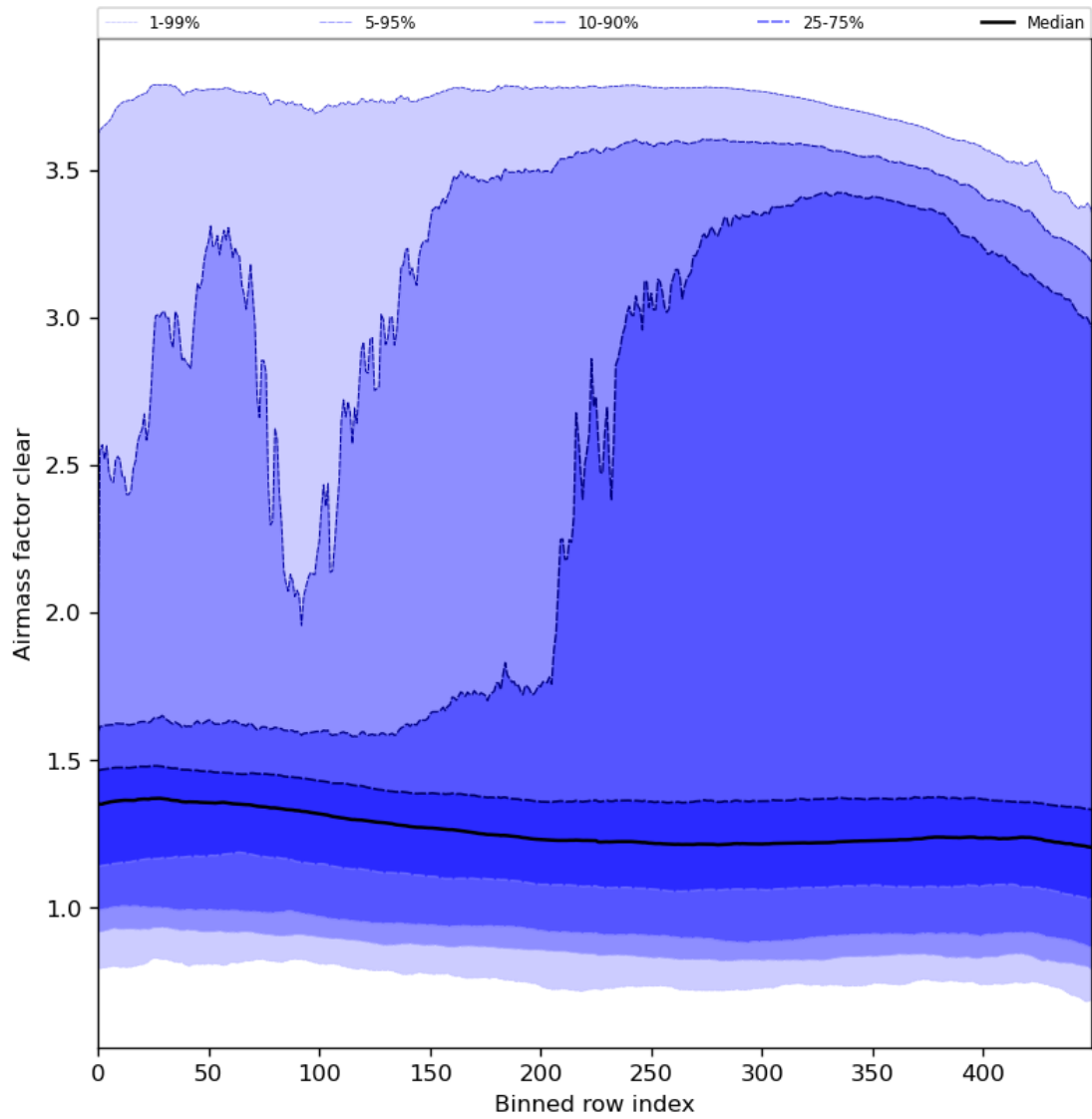
Figure 56: Along track statistics of “Airmass factor clear” for 2024-05-12 to 2024-05-14
