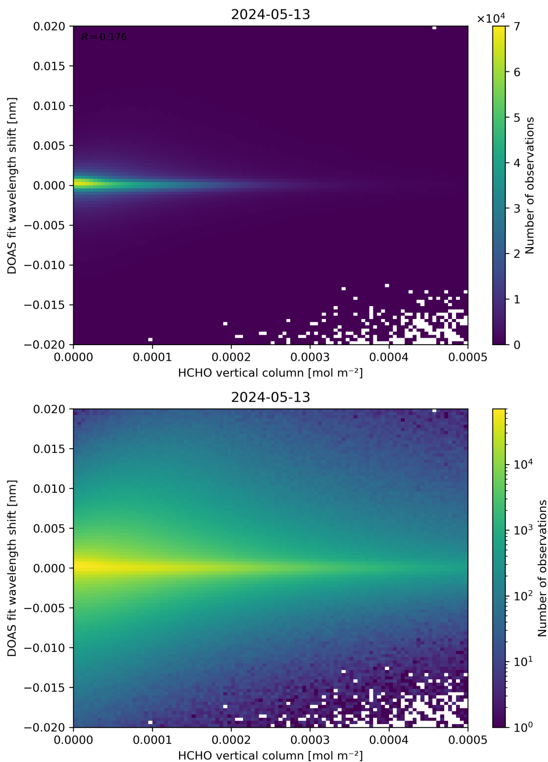
Figure 124: Scatter density plot of “HCHO vertical column” against “DOAS fit wavelength shift” for 2024-05-12 to 2024-05-14.
