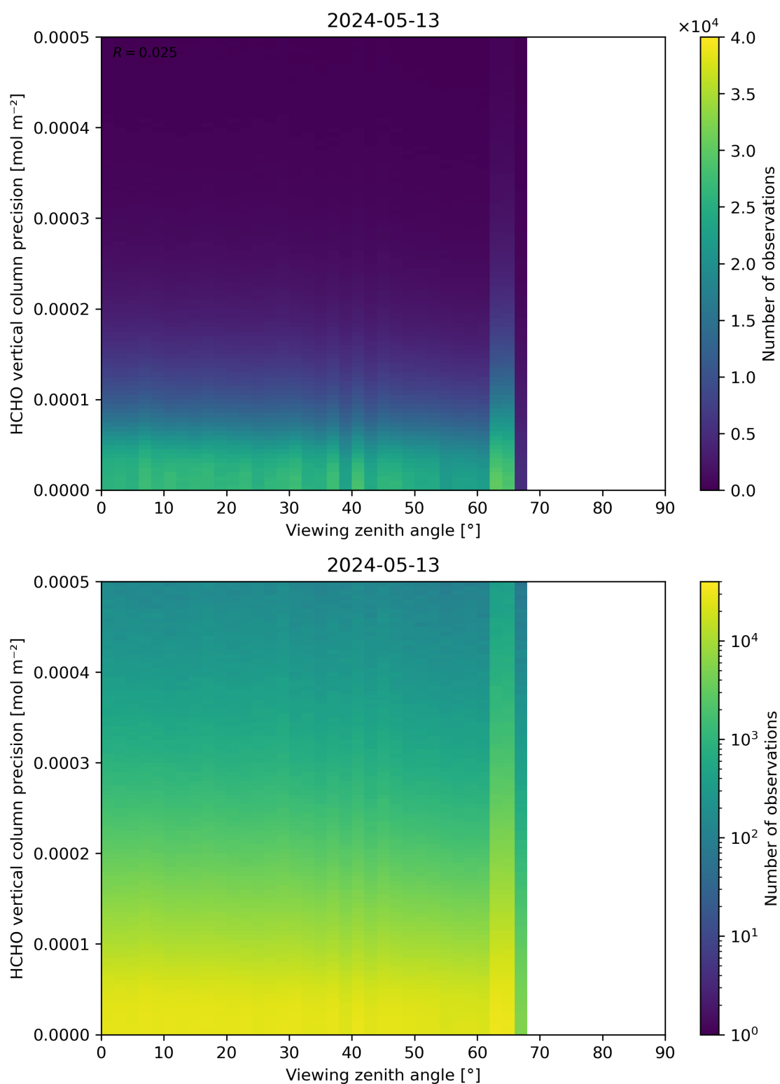
Figure 194: Scatter density plot of “Viewing zenith angle” against “HCHO vertical column precision” for 2024-05-12 to 2024-05-14.
