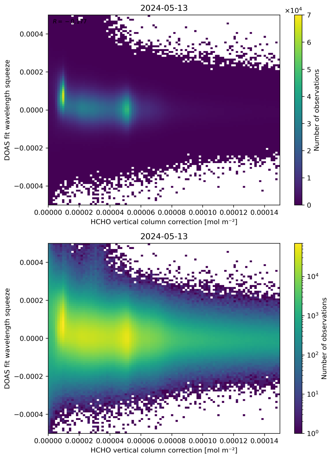
Figure 114: Scatter density plot of “HCHO vertical column correction” against “DOAS fit wavelength squeeze” for 2024-05-12 to 2024-05-14.
