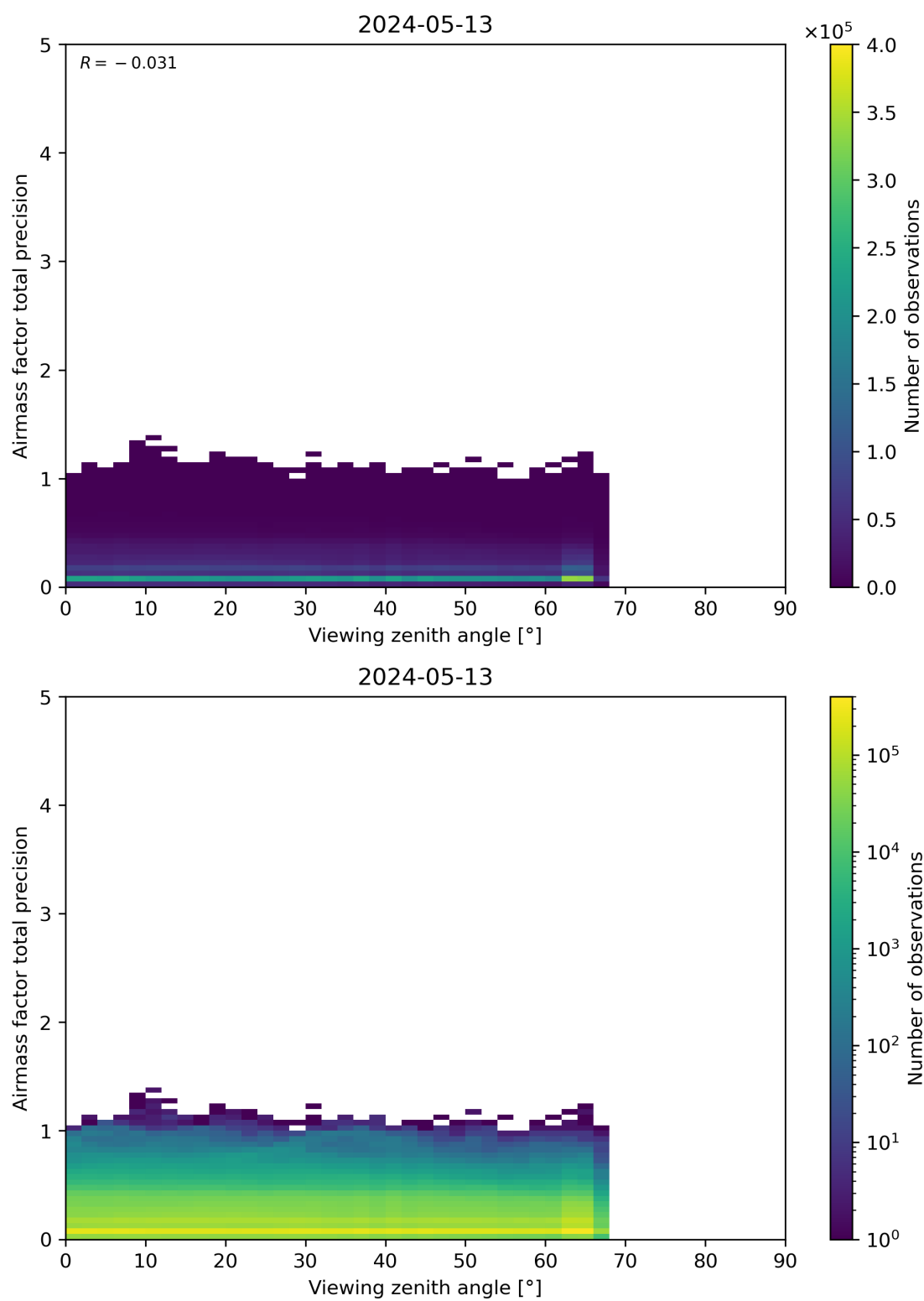
Figure 191: Scatter density plot of “Viewing zenith angle” against “Airmass factor total precision” for 2024-05-12 to 2024-05-14.
