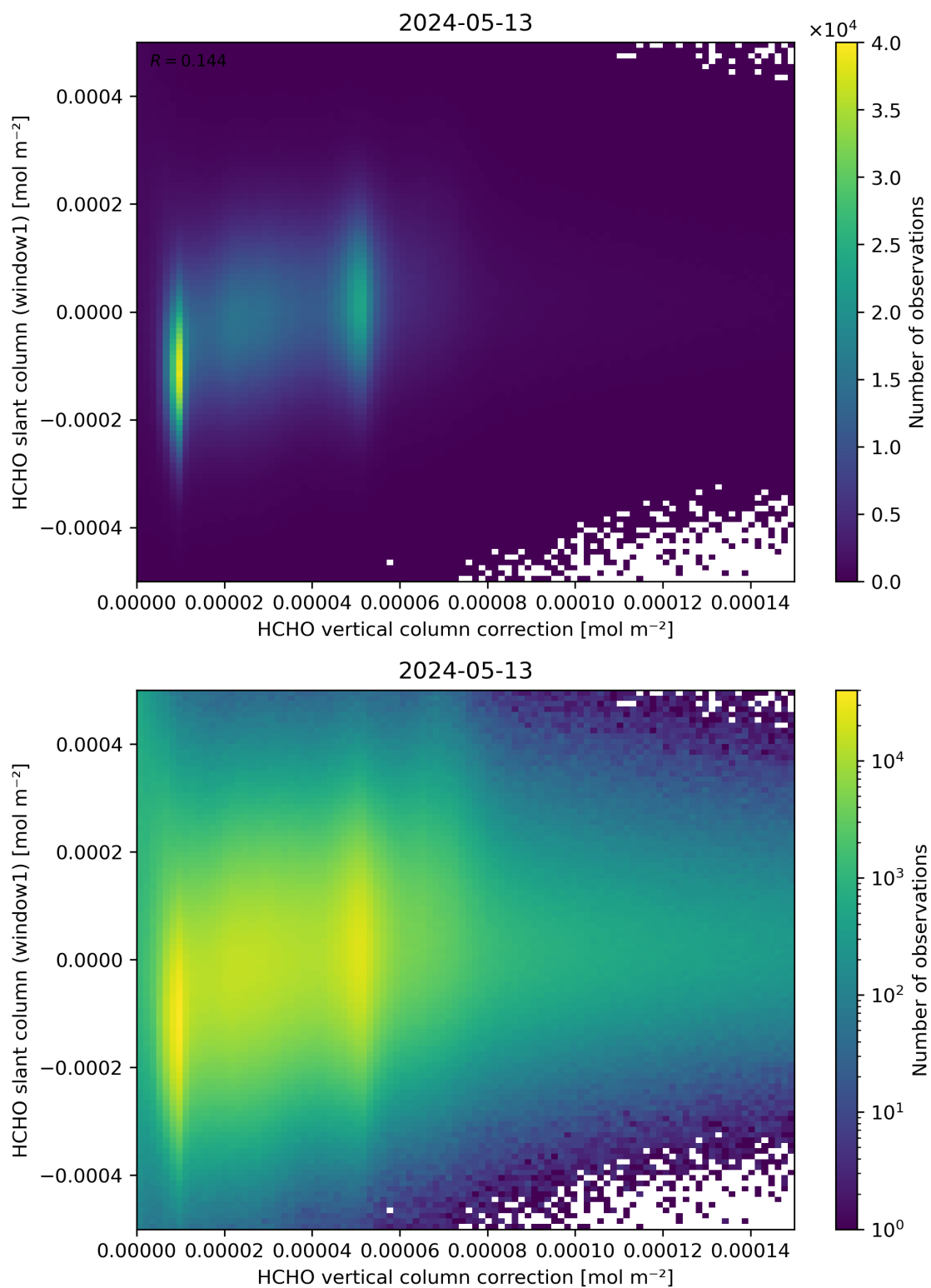
Figure 118: Scatter density plot of “HCHO vertical column correction” against “HCHO slant column (window1)” for 2024-05-12 to 2024-05-14.
