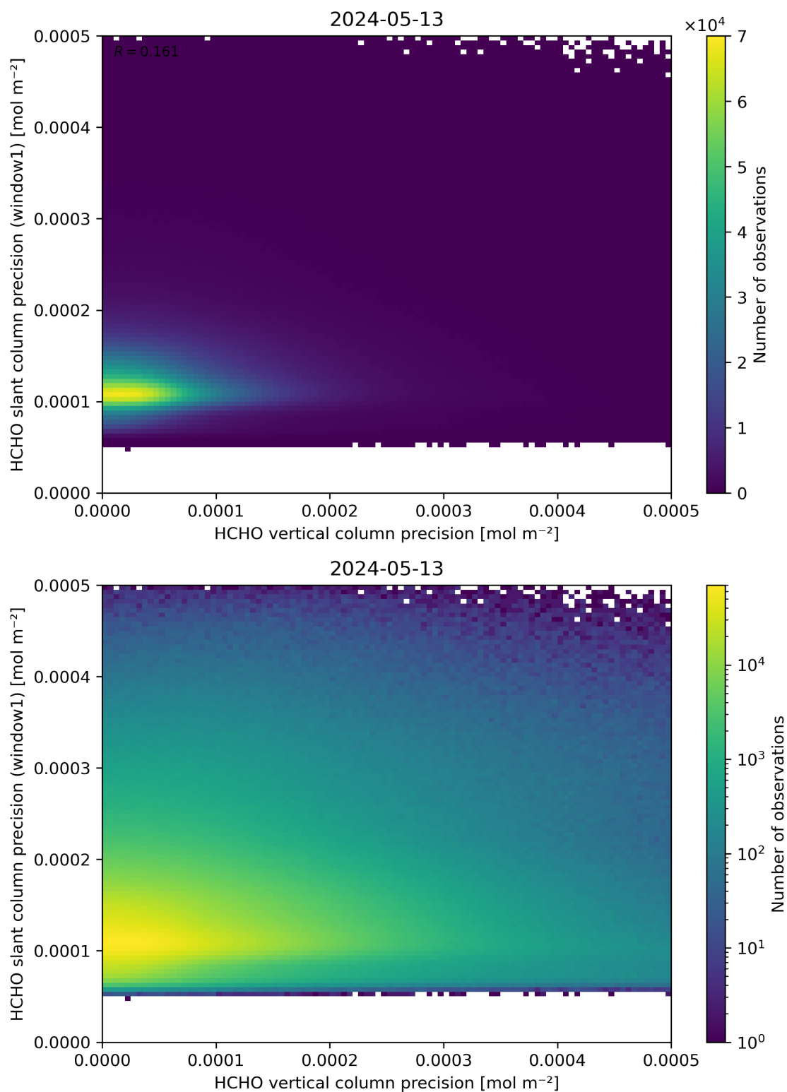
Figure 143: Scatter density plot of “HCHO vertical column precision” against “HCHO slant column precision (window1)” for 2024-05-12 to 2024-05-14.
