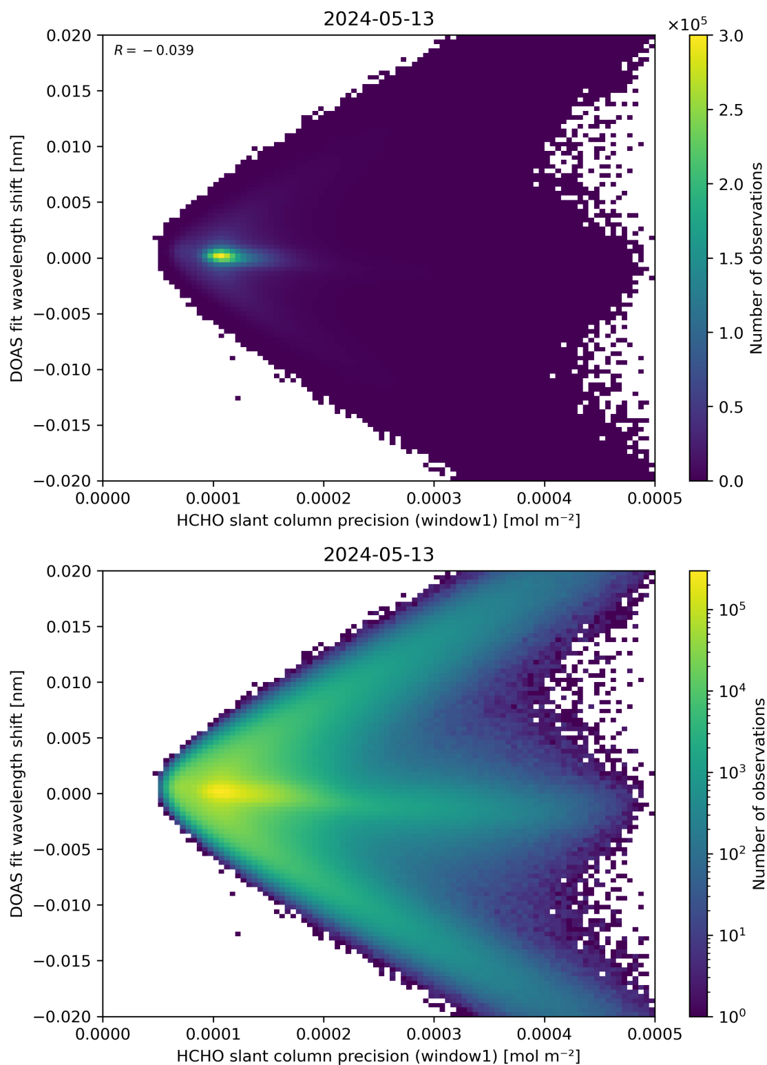
Figure 89: Scatter density plot of “HCHO slant column precision (window1)” against “DOAS fit wavelength shift” for 2024-05-12 to 2024-05-14.
