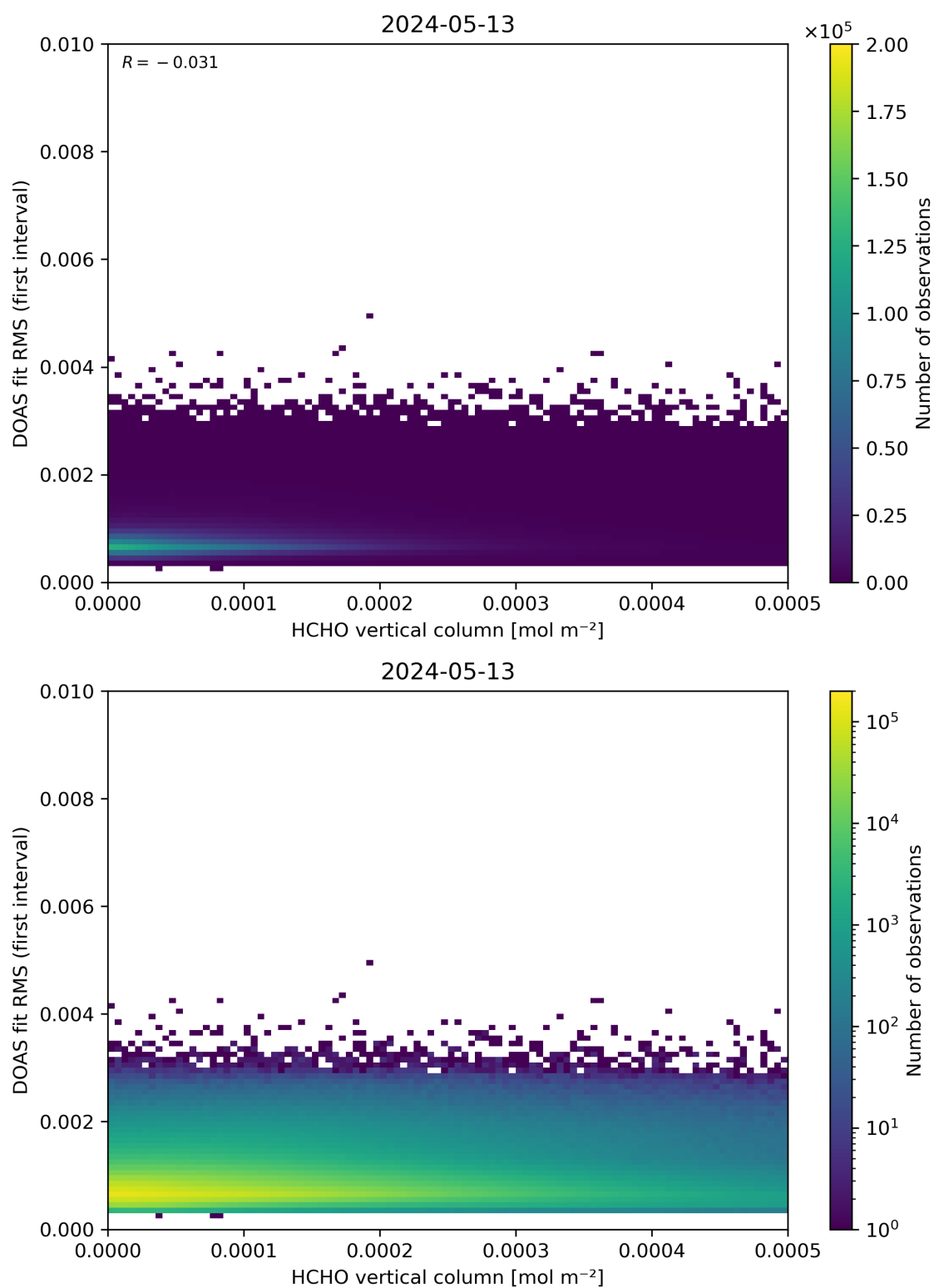
Figure 123: Scatter density plot of “HCHO vertical column” against “DOAS fit RMS (first interval)” for 2024-05-12 to 2024-05-14.
