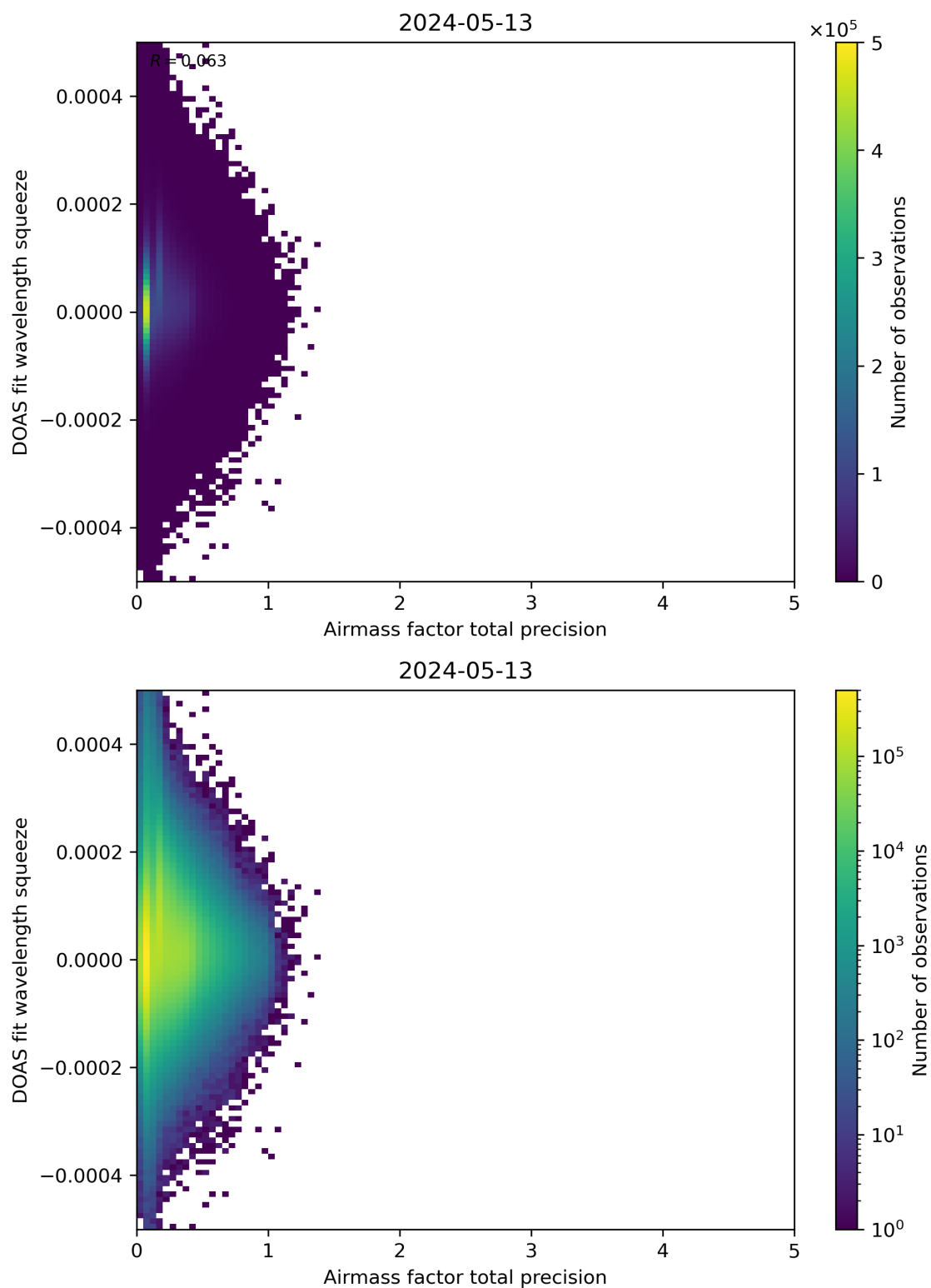
Figure 107: Scatter density plot of “Airmass factor total precision” against “DOAS fit wavelength squeeze” for 2024-05-12 to 2024-05-14.
