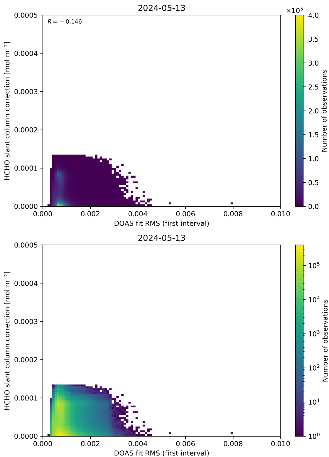
Figure 63: Scatter density plot of “DOAS fit RMS (first interval)” against “HCHO slant column correction” for 2024-05-12 to 2024-05-14.
