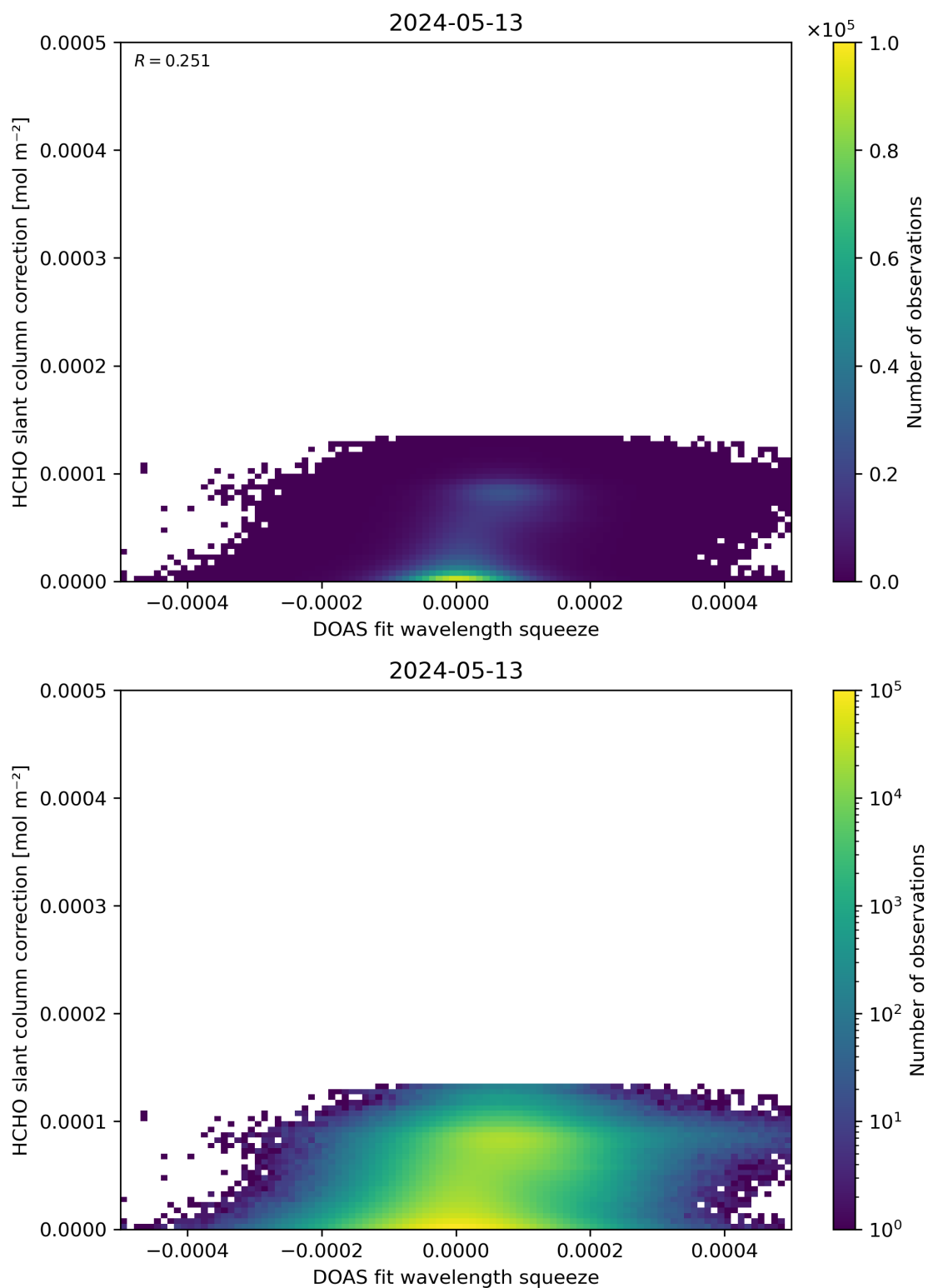
Figure 70: Scatter density plot of “DOAS fit wavelength squeeze” against “HCHO slant column correction” for 2024-05-12 to 2024-05-14.
