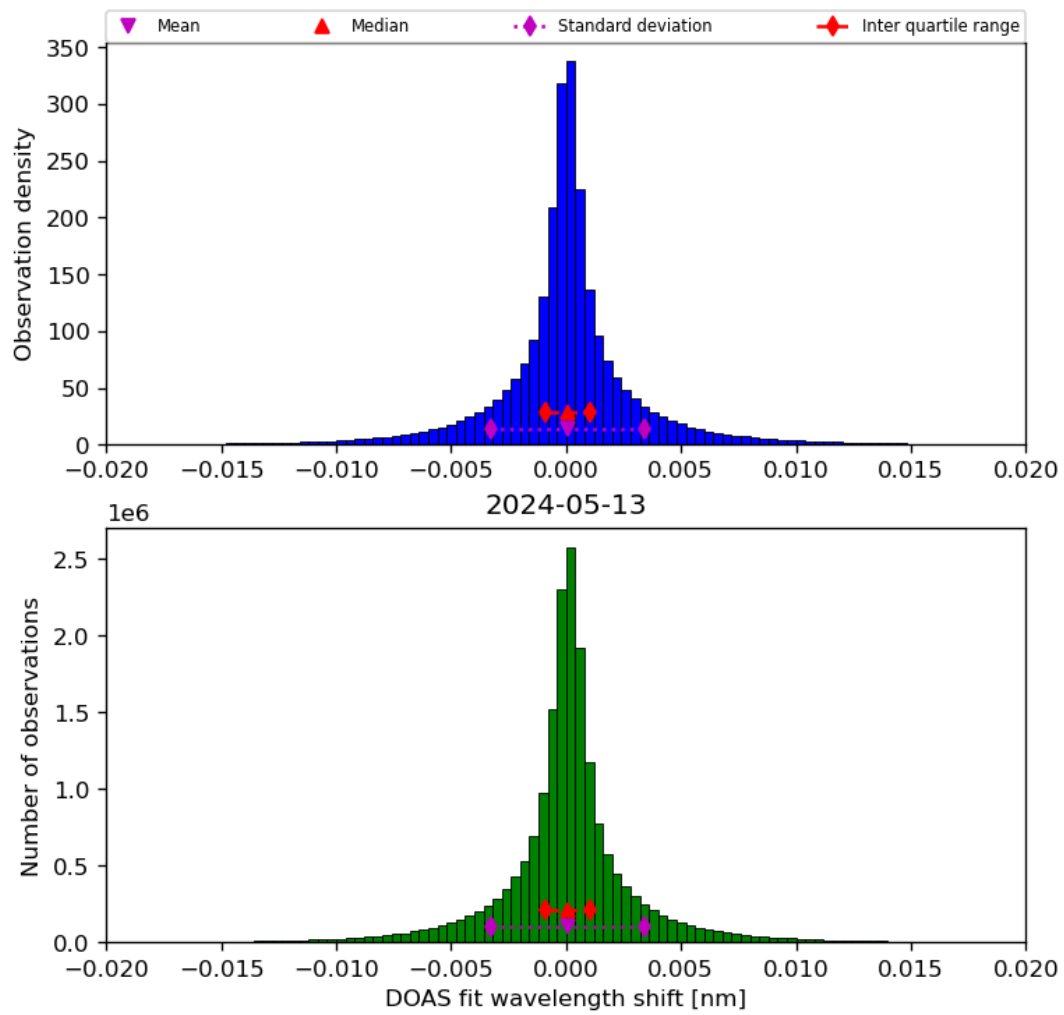
Figure 44: Histogram of “DOAS fit wavelength shift” for 2024-05-12 to 2024-05-14
