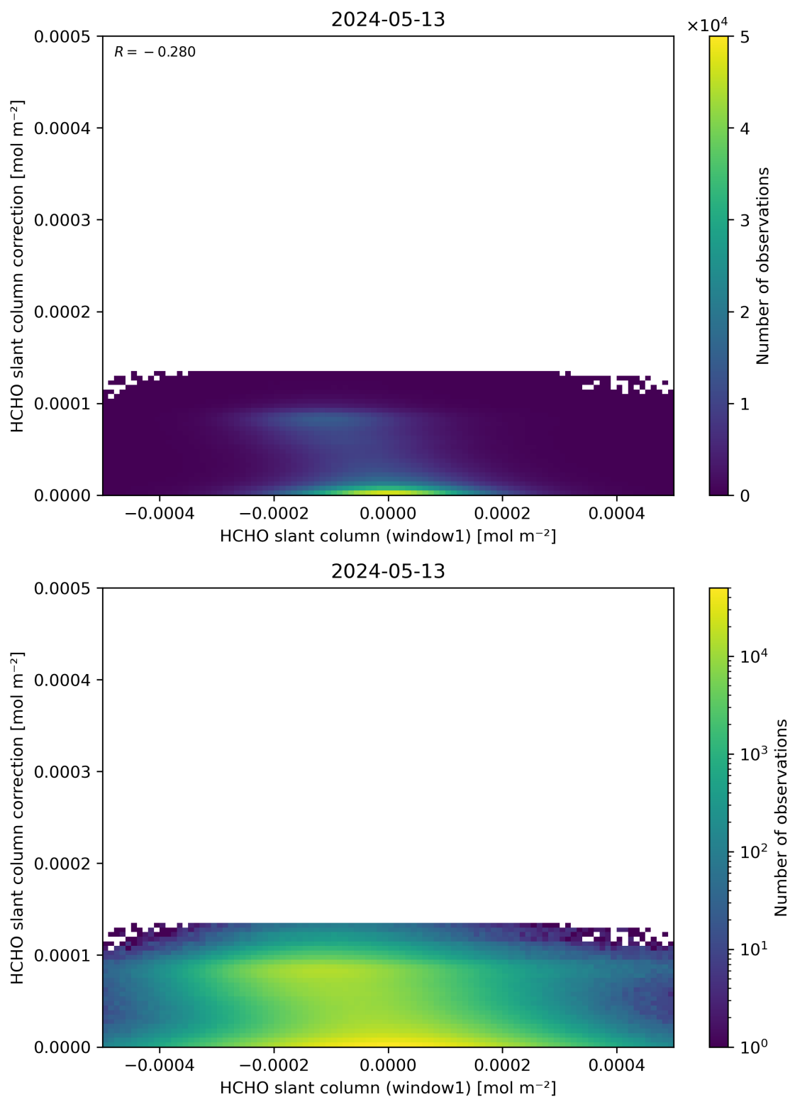
Figure 83: Scatter density plot of “HCHO slant column (window1)” against “HCHO slant column correction” for 2024-05-12 to 2024-05-14.
