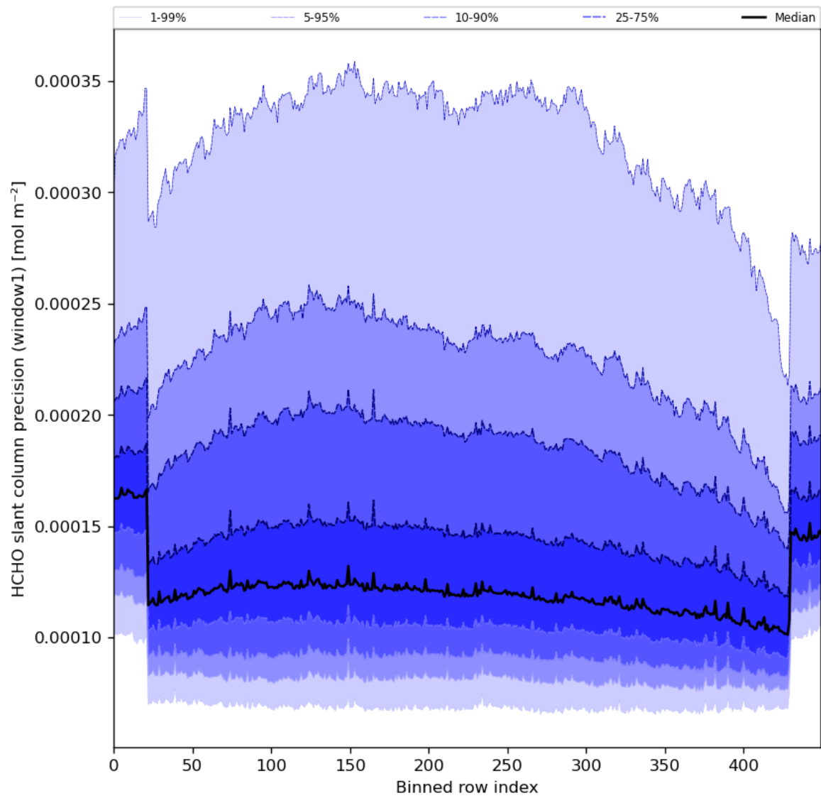
Figure 53: Along track statistics of “HCHO slant column precision (window1)” for 2024-05-12 to 2024-05-14
