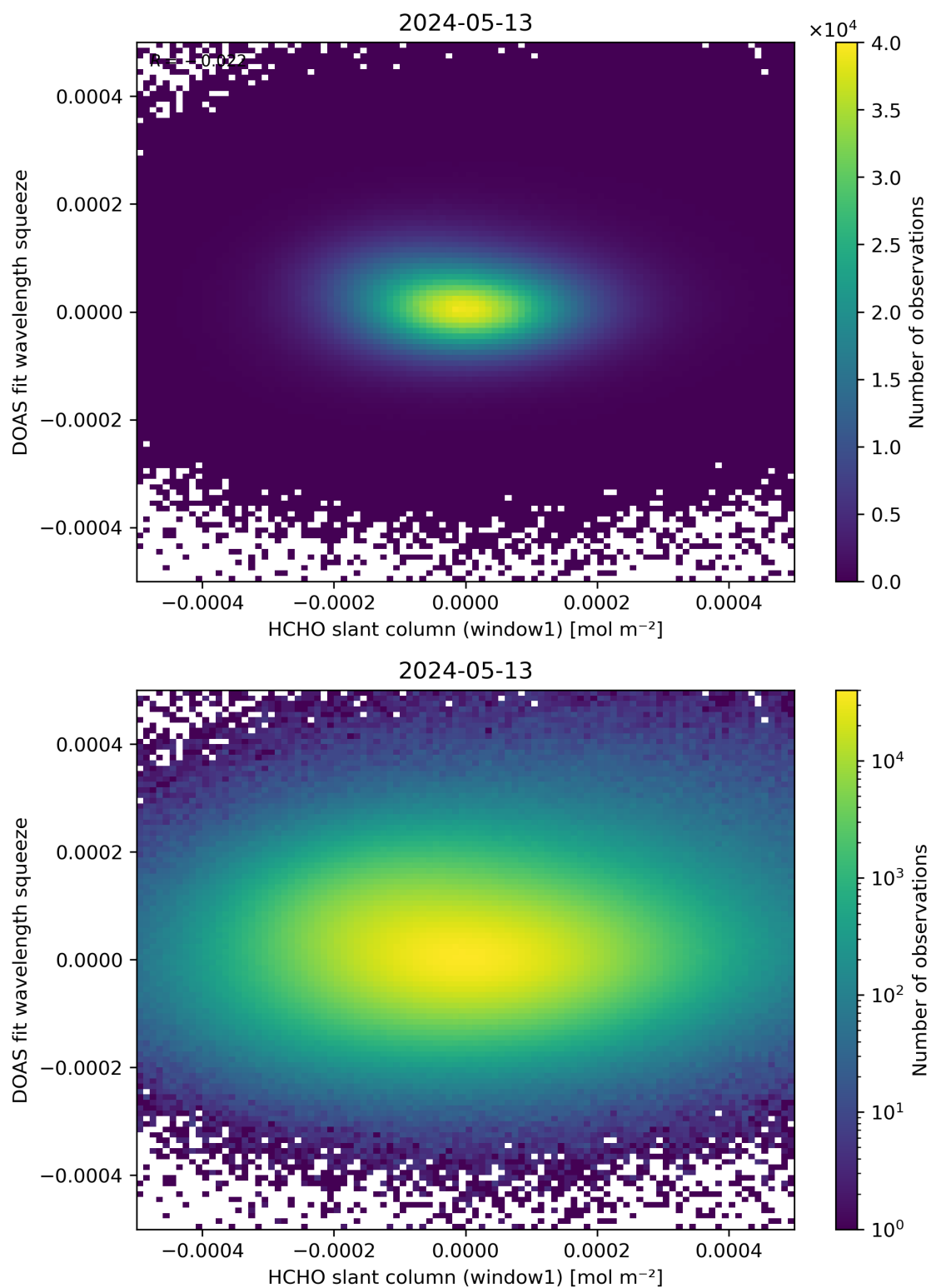
Figure 80: Scatter density plot of “HCHO slant column (window1)” against “DOAS fit wavelength squeeze” for 2024-05-12 to 2024-05-14.
