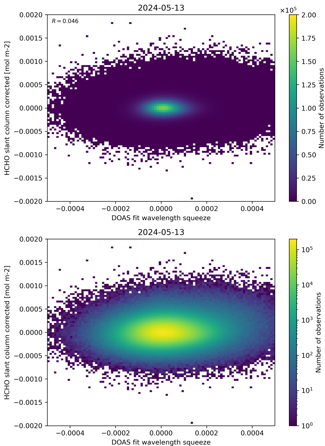
Figure 69: Scatter density plot of “DOAS fit wavelength squeeze” against “HCHO slant column corrected” for 2024-05-12 to 2024-05-14.
