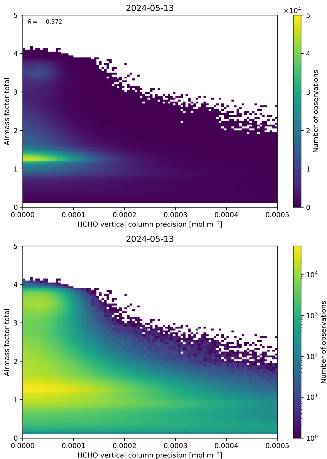
Figure 144: Scatter density plot of “HCHO vertical column precision” against “Airmass factor total” for 2024-05-12 to 2024-05-14.
