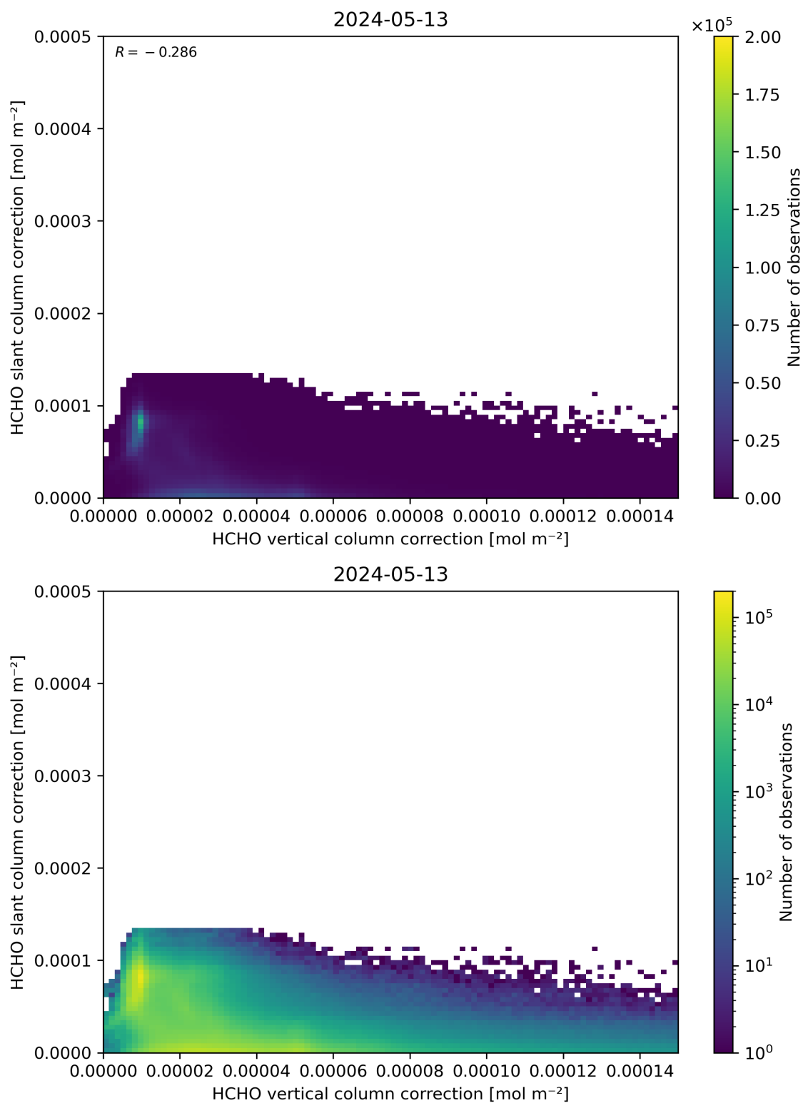
Figure 117: Scatter density plot of “HCHO vertical column correction” against “HCHO slant column correction” for 2024-05-12 to 2024-05-14.
