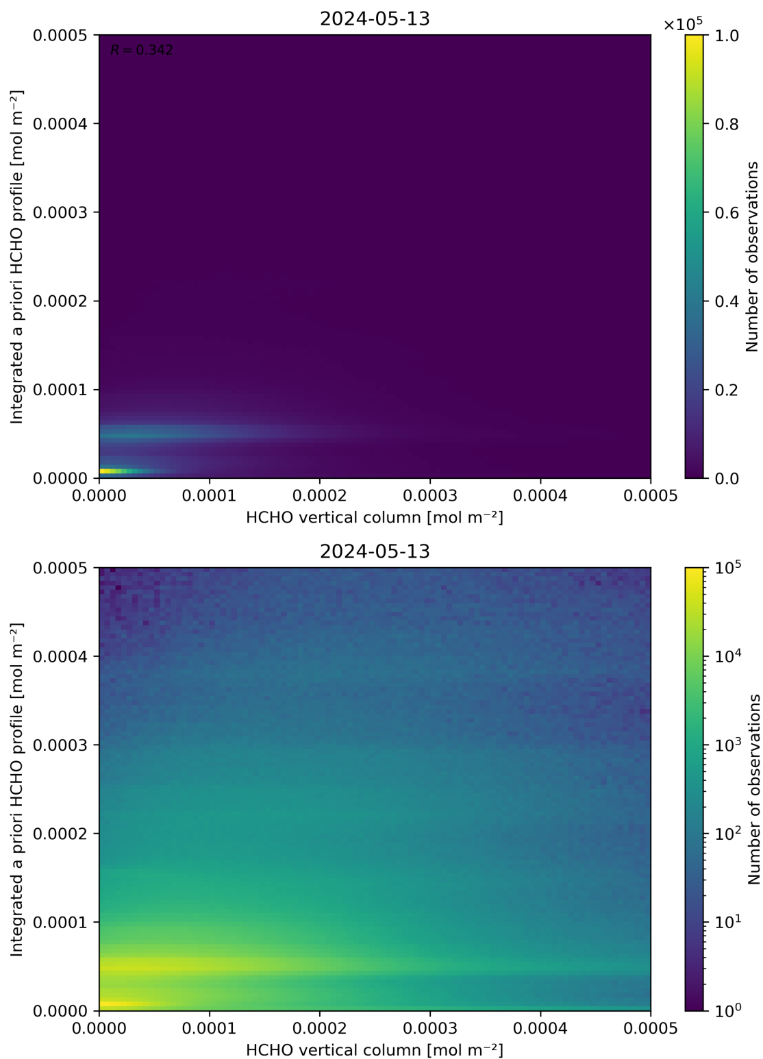
Figure 135: Scatter density plot of “HCHO vertical column” against “Integrated a priori HCHO profile” for 2024-05-12 to 2024-05-14.
