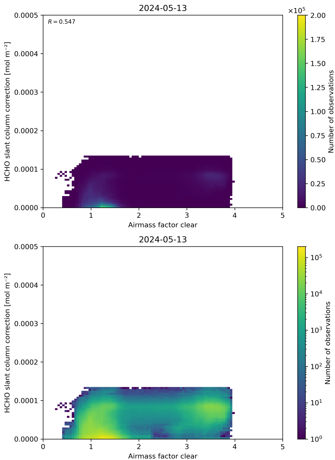
Figure 75: Scatter density plot of “Airmass factor clear” against “HCHO slant column correction” for 2024-05-12 to 2024-05-14.
