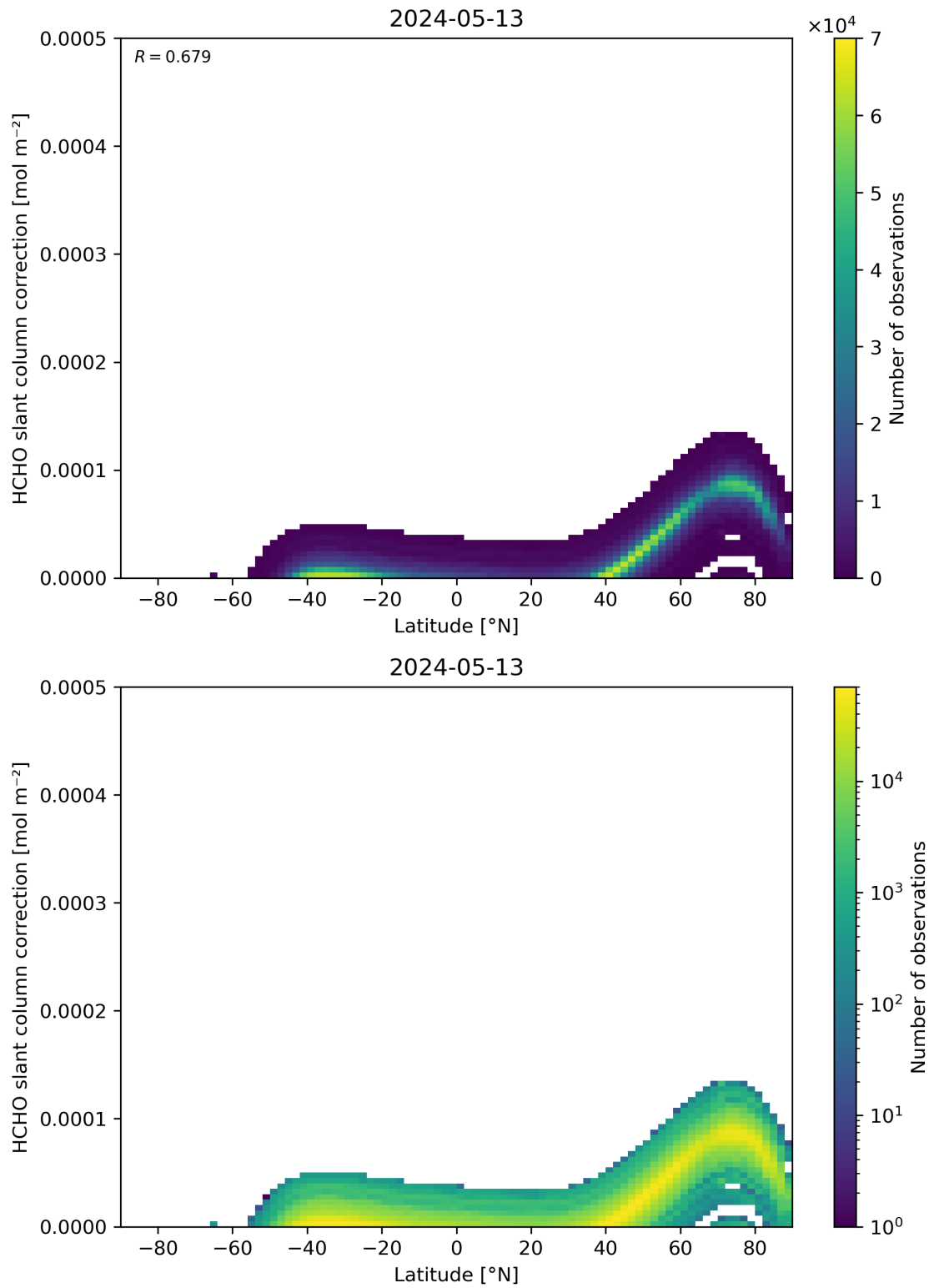
Figure 158: Scatter density plot of “Latitude” against “HCHO slant column correction” for 2024-05-12 to 2024-05-14.
