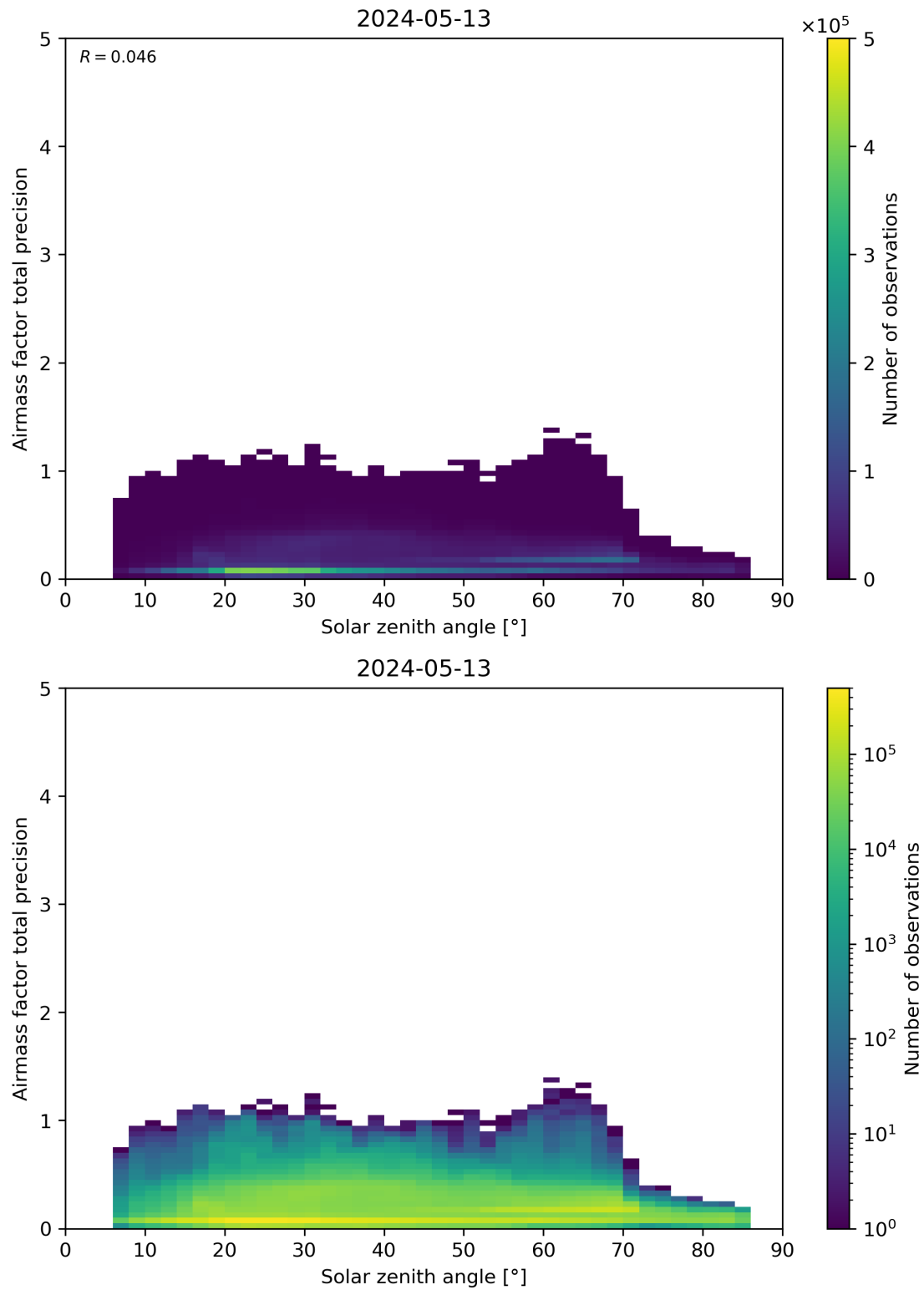
Figure 176: Scatter density plot of “Solar zenith angle” against “Airmass factor total precision” for 2024-05-12 to 2024-05-14.
