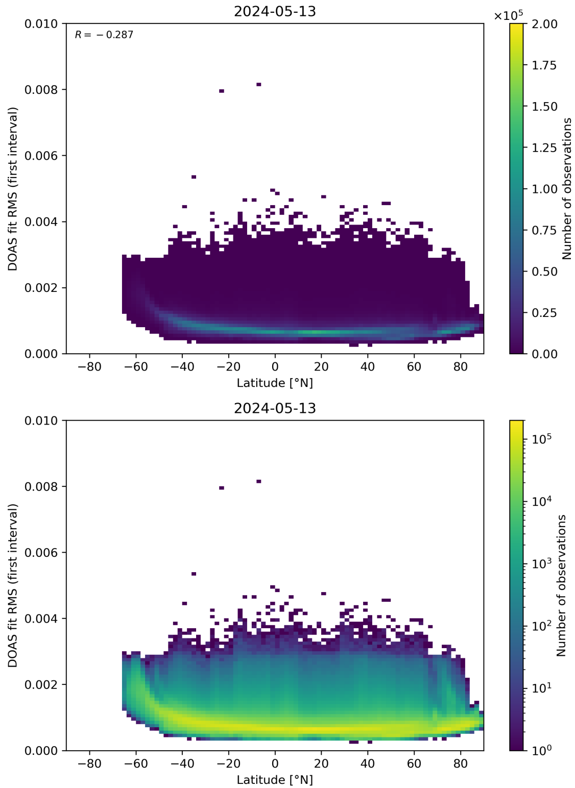
Figure 153: Scatter density plot of “Latitude” against “DOAS fit RMS (first interval)” for 2024-05-12 to 2024-05-14.
