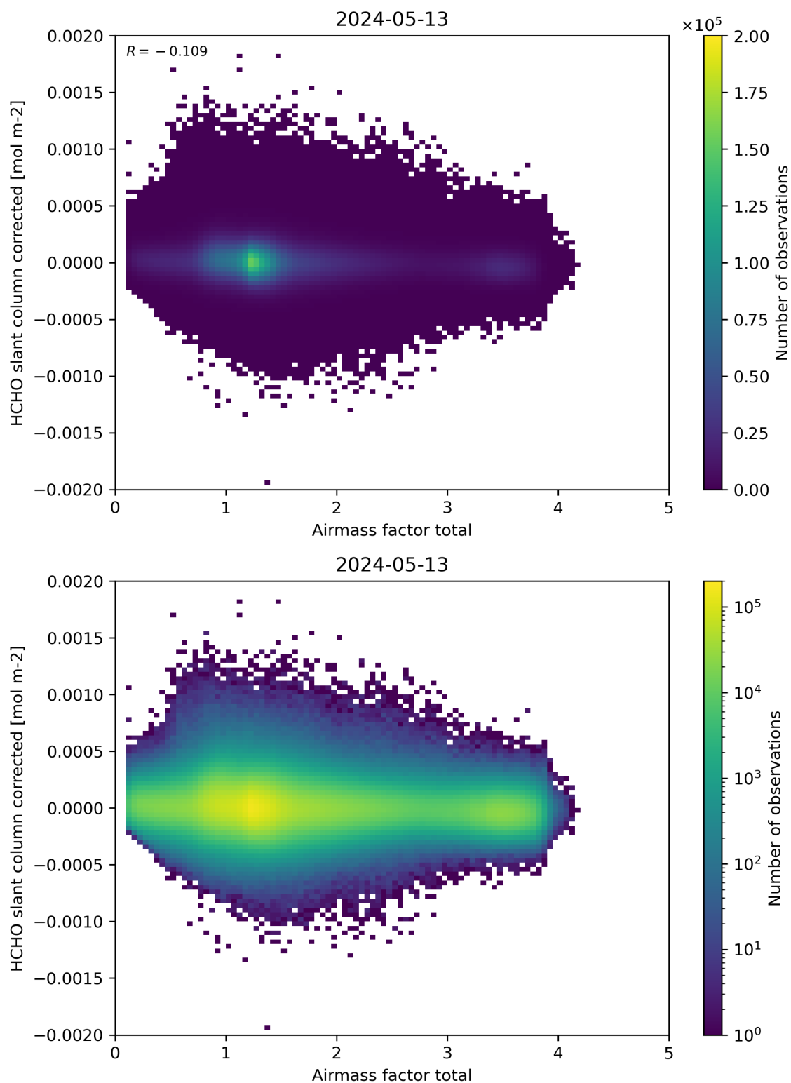
Figure 101: Scatter density plot of “Airmass factor total” against “HCHO slant column corrected” for 2024-05-12 to 2024-05-14.
