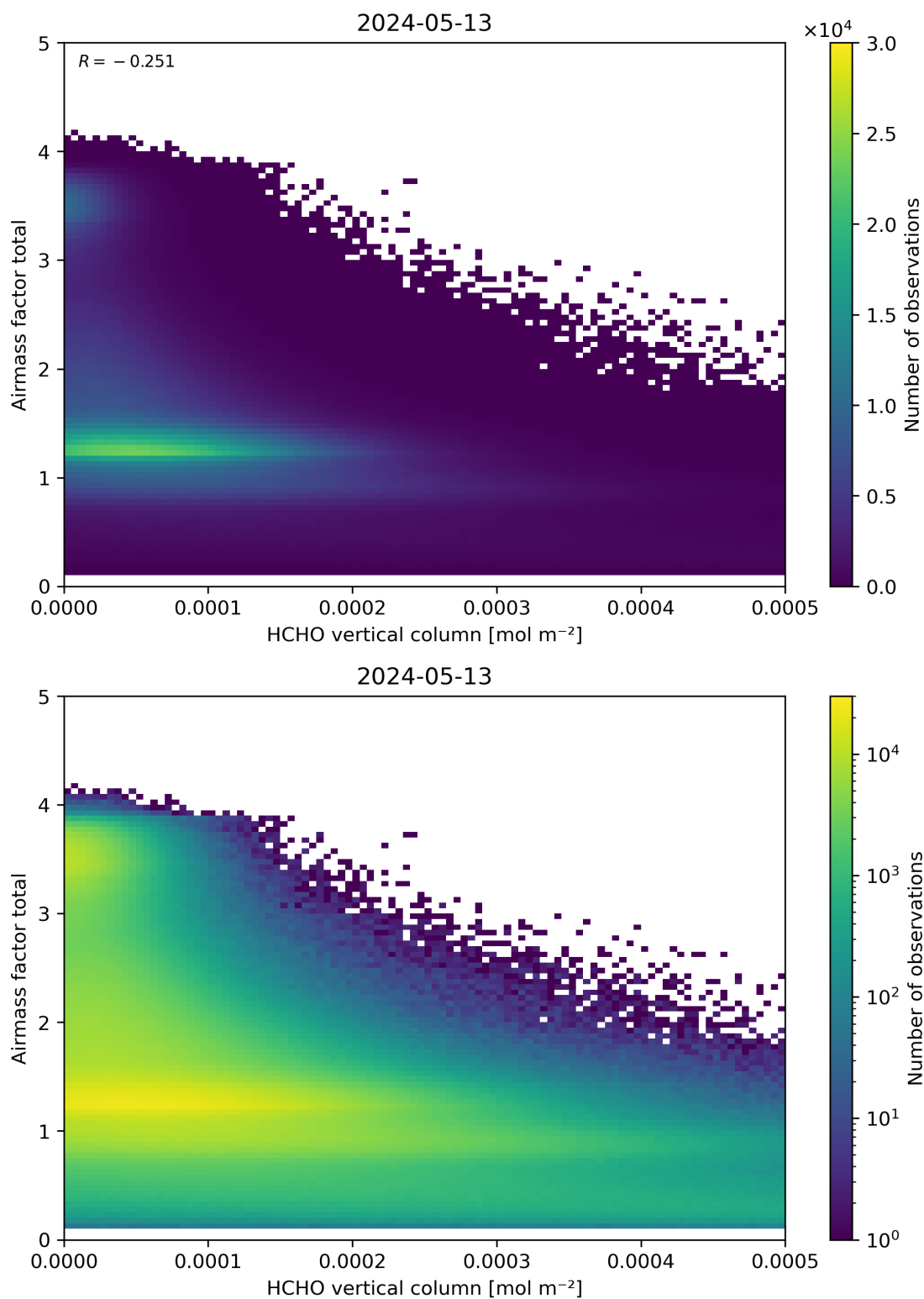
Figure 131: Scatter density plot of “HCHO vertical column” against “Airmass factor total” for 2024-05-12 to 2024-05-14.
