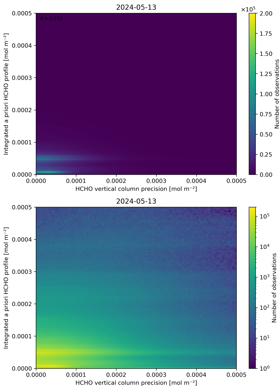
Figure 147: Scatter density plot of “HCHO vertical column precision” against “Integrated a priori HCHO profile” for 2024-05-12 to 2024-05-14.
