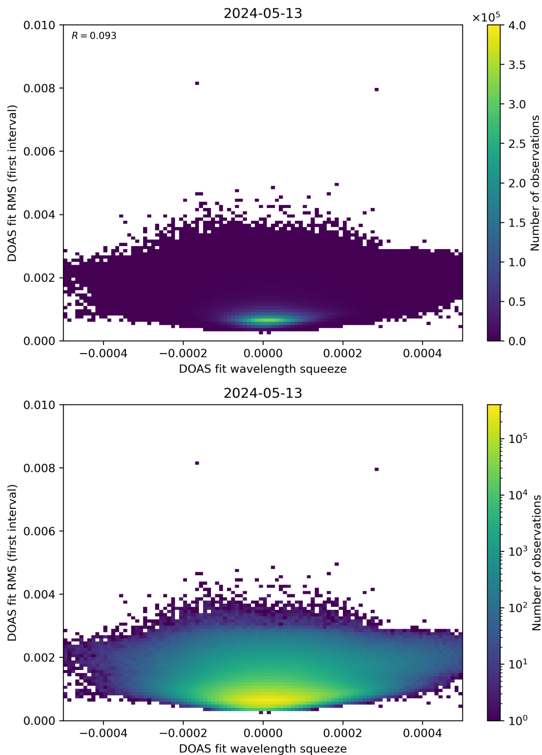
Figure 68: Scatter density plot of “DOAS fit wavelength squeeze” against “DOAS fit RMS (first interval)” for 2024-05-12 to 2024-05-14.
