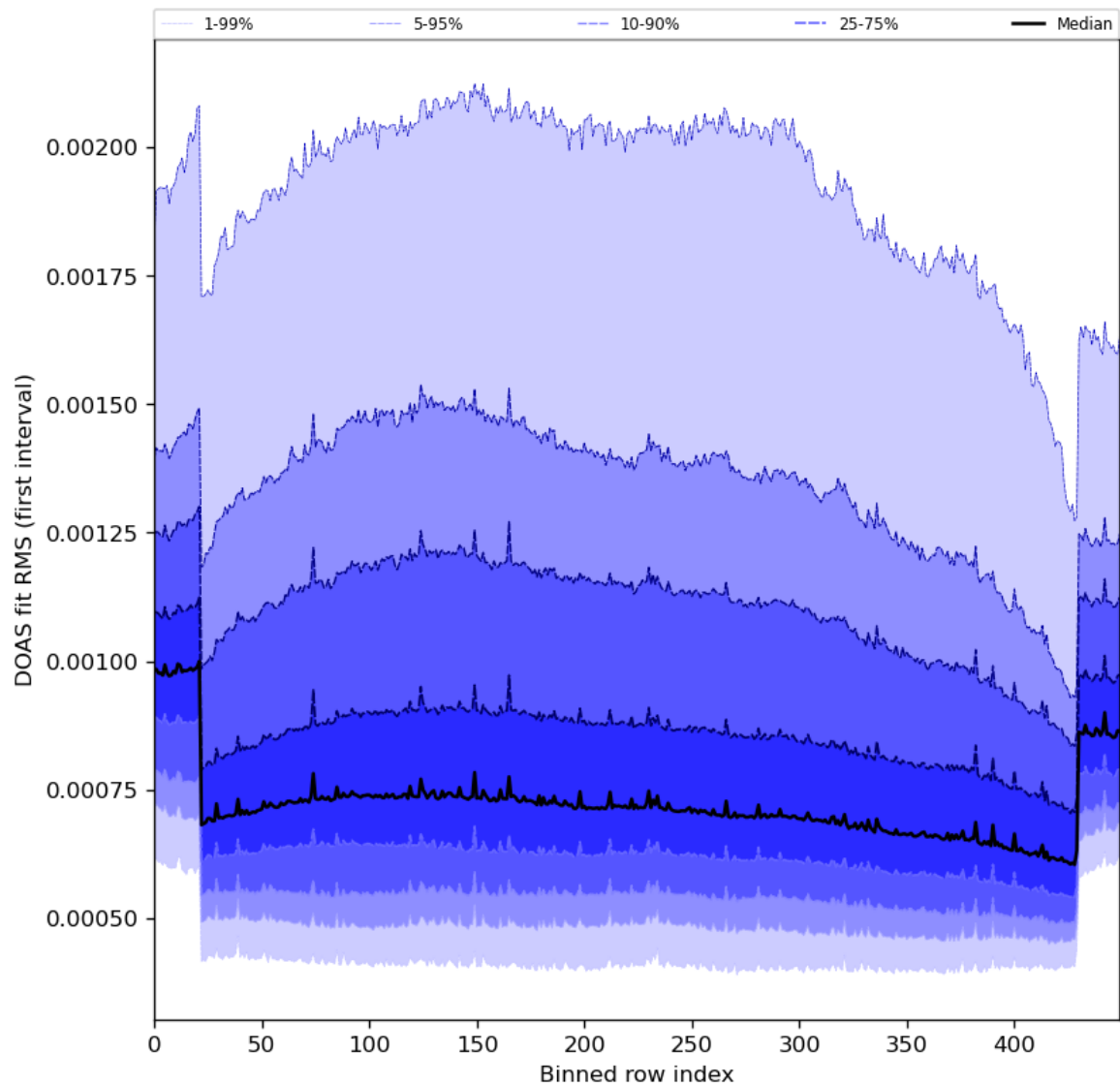
Figure 60: Along track statistics of “DOAS fit RMS (first interval)” for 2024-05-12 to 2024-05-14
