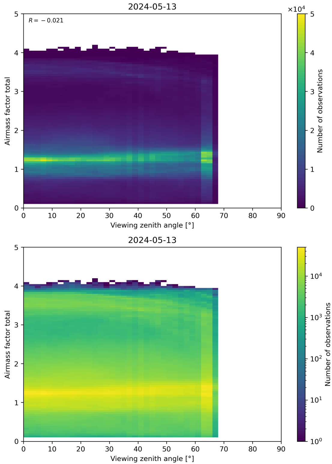
Figure 190: Scatter density plot of “Viewing zenith angle” against “Airmass factor total” for 2024-05-12 to 2024-05-14.
