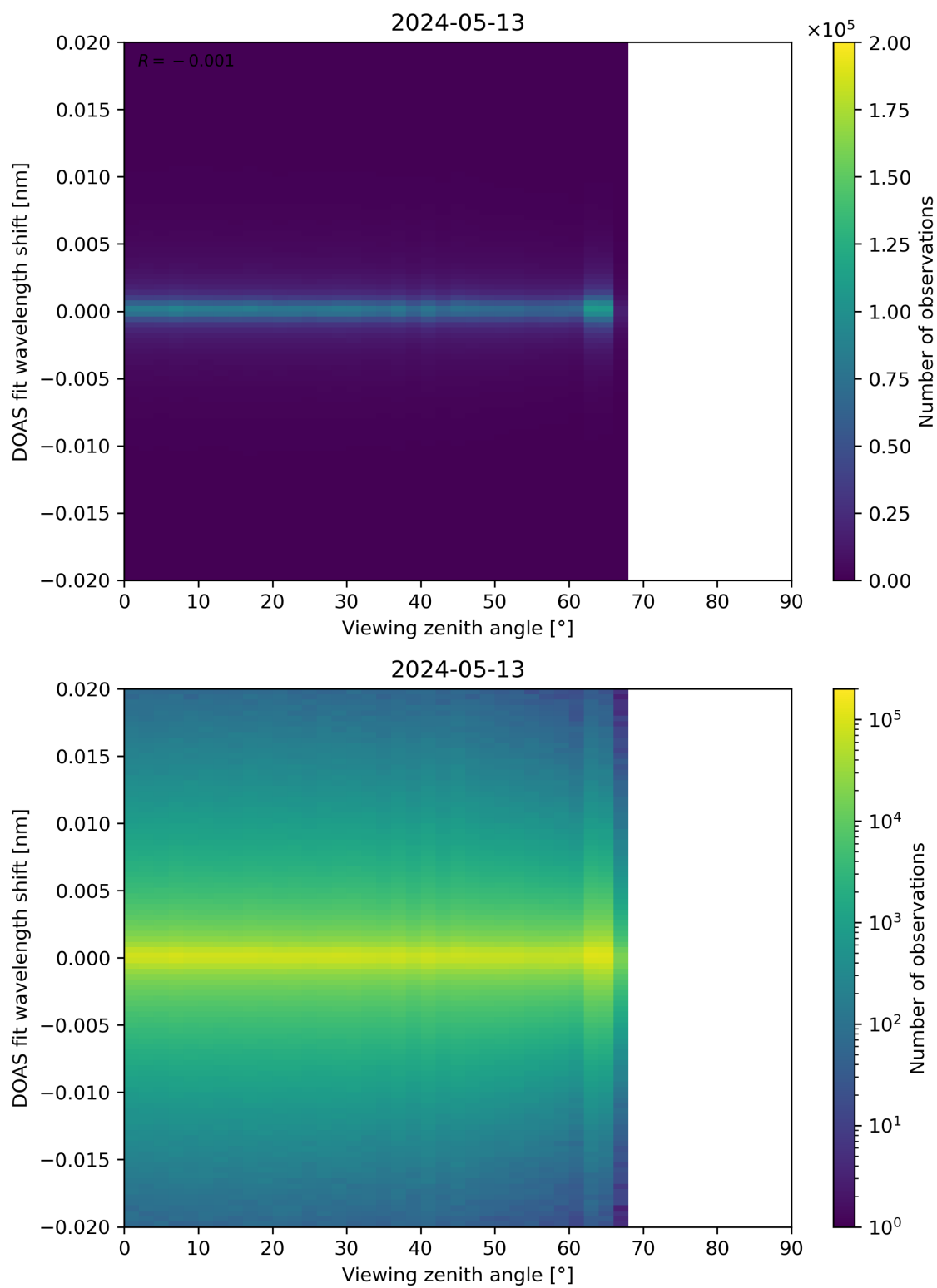
Figure 183: Scatter density plot of “Viewing zenith angle” against “DOAS fit wavelength shift” for 2024-05-12 to 2024-05-14.
