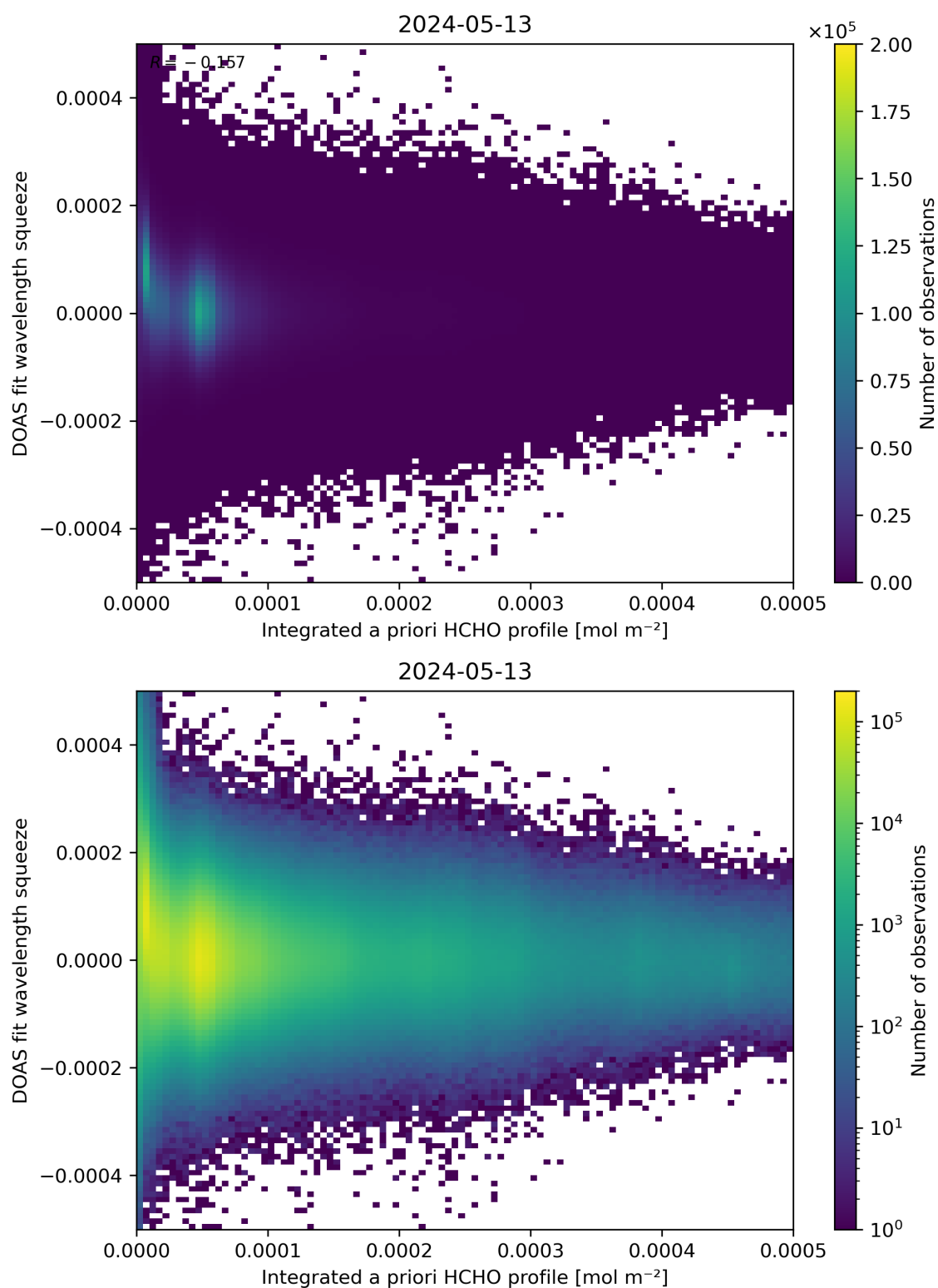
Figure 150: Scatter density plot of “Integrated a priori HCHO profile” against “DOAS fit wavelength squeeze” for 2024-05-12 to 2024-05-14.
