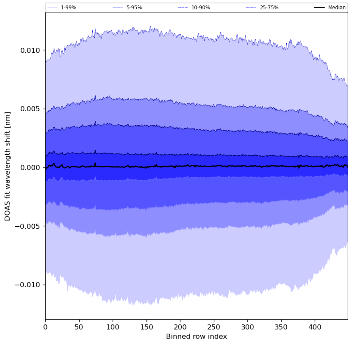
Figure 58: Along track statistics of “DOAS fit wavelength shift” for 2024-05-12 to 2024-05-14
