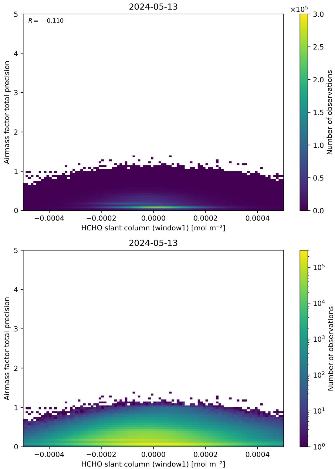
Figure 86: Scatter density plot of “HCHO slant column (window1)” against “Airmass factor total precision” for 2024-05-12 to 2024-05-14.
