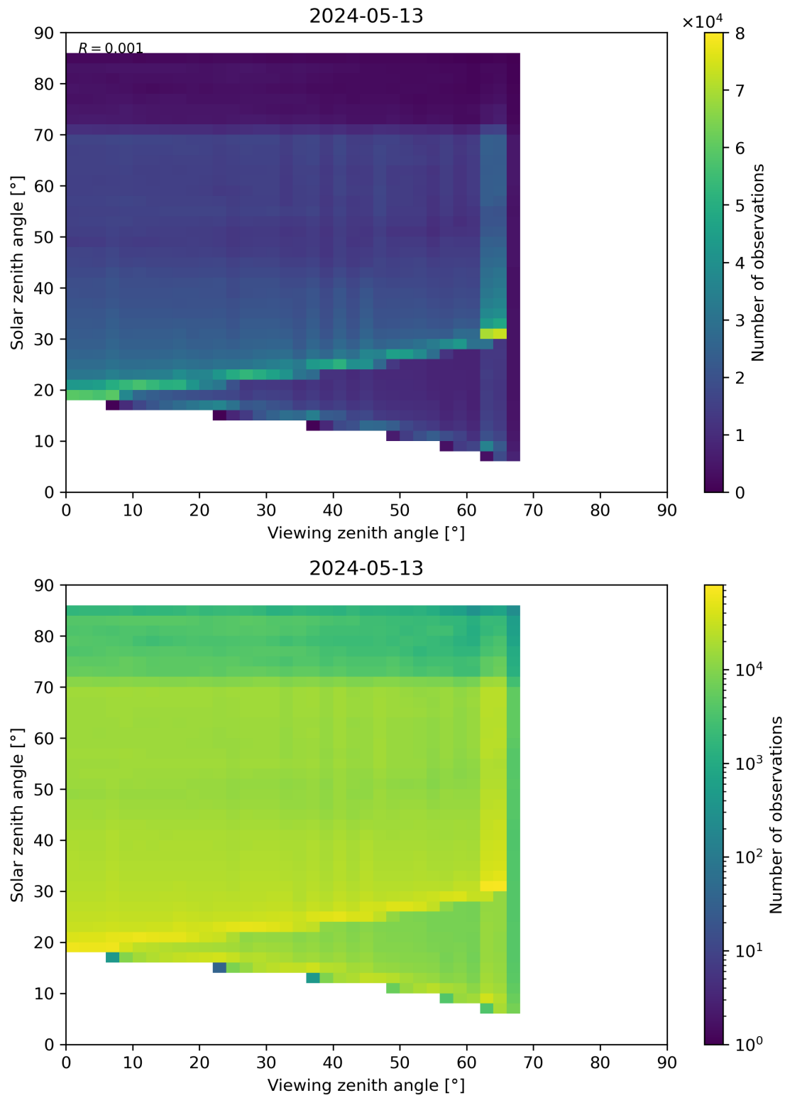
Figure 197: Scatter density plot of “Viewing zenith angle” against “Solar zenith angle” for 2024-05-12 to 2024-05-14.
