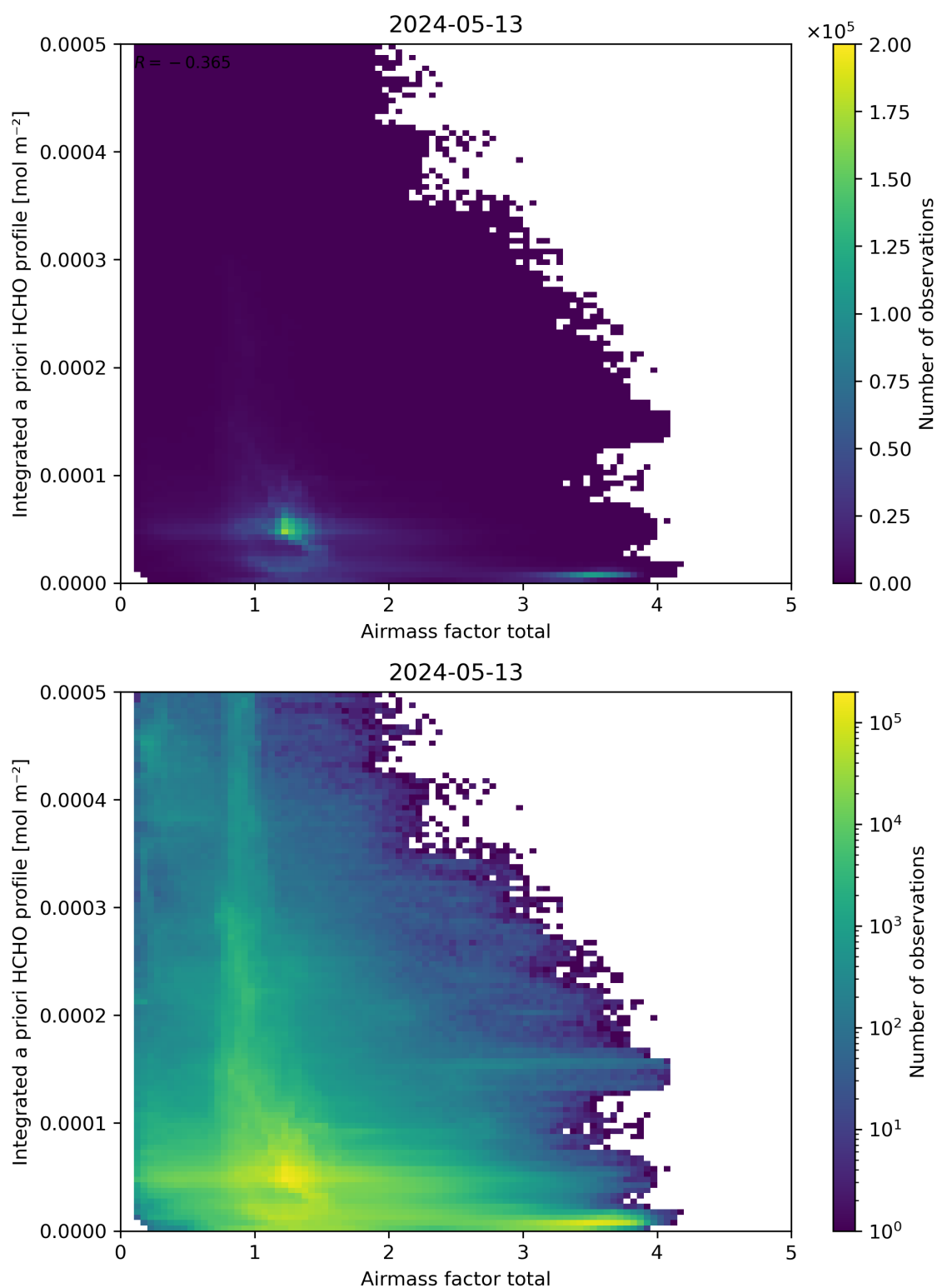
Figure 104: Scatter density plot of “Air mass factor total” against “Integrated a priori HCHO profile” for 2024-05-12 to 2024-05-14.
