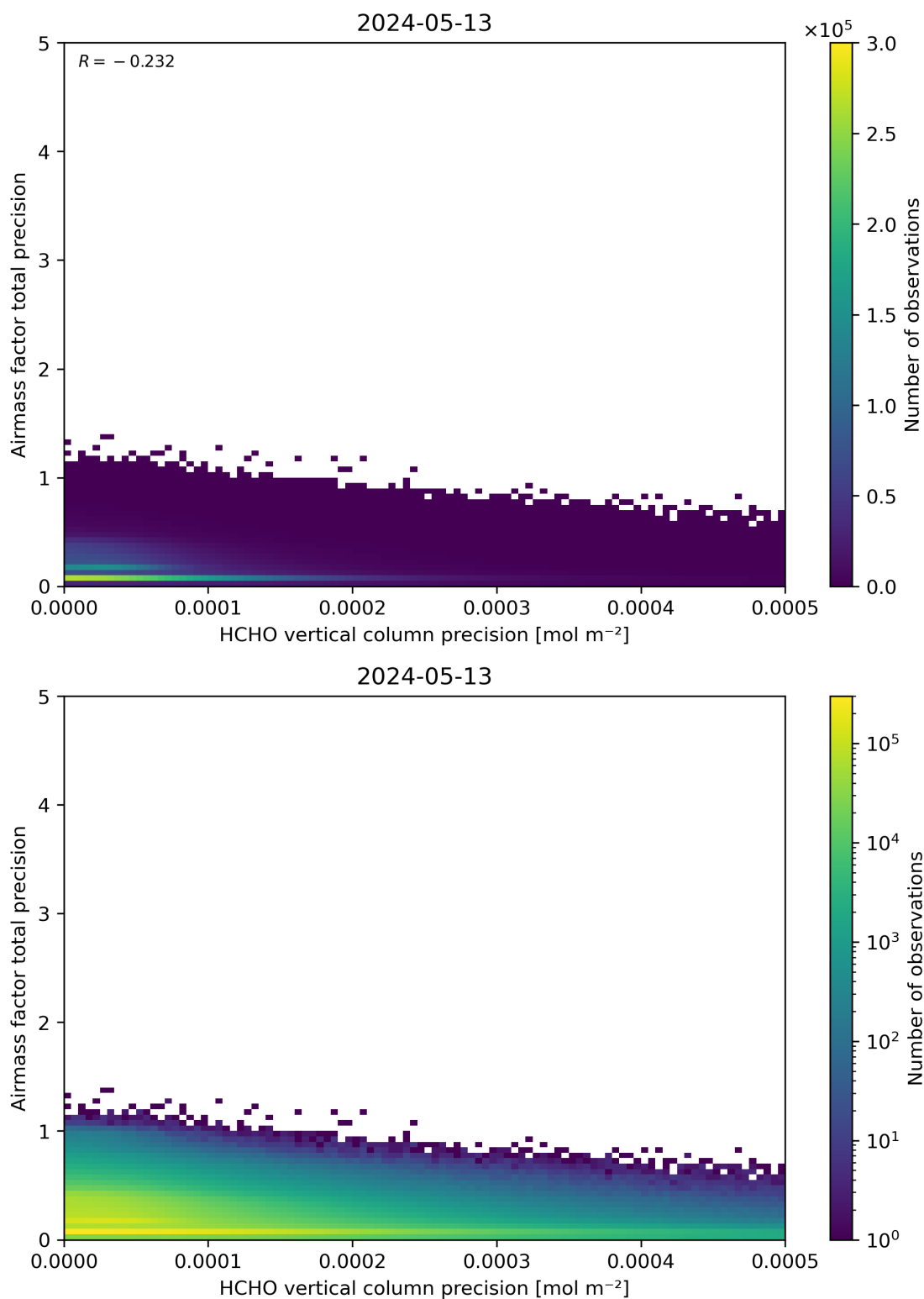
Figure 145: Scatter density plot of “HCHO vertical column precision” against “Airmass factor total precision” for 2024-05-12 to 2024-05-14.
