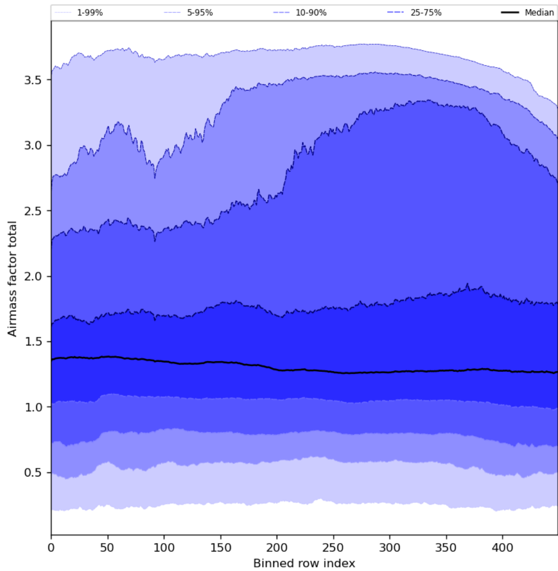
Figure 54: Along track statistics of “Airmass factor total” for 2024-05-12 to 2024-05-14
