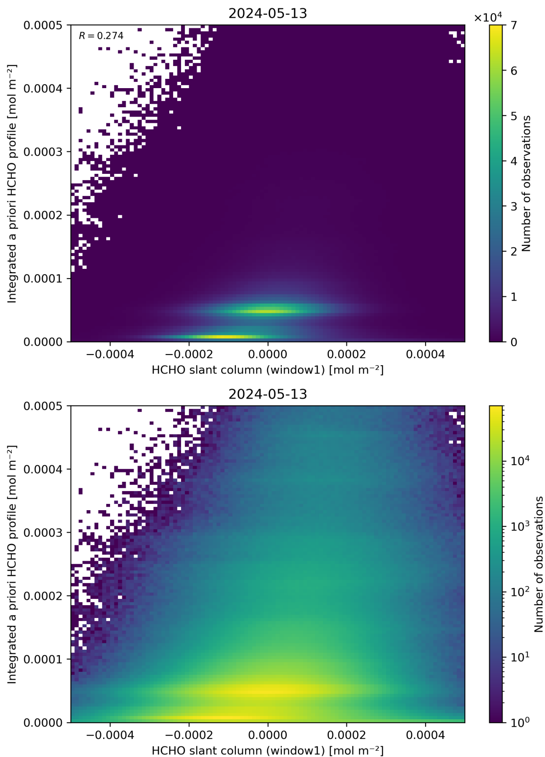
Figure 87: Scatter density plot of “HCHO slant column (window1)” against “Integrated a priori HCHO profile” for 2024-05-12 to 2024-05-14.
