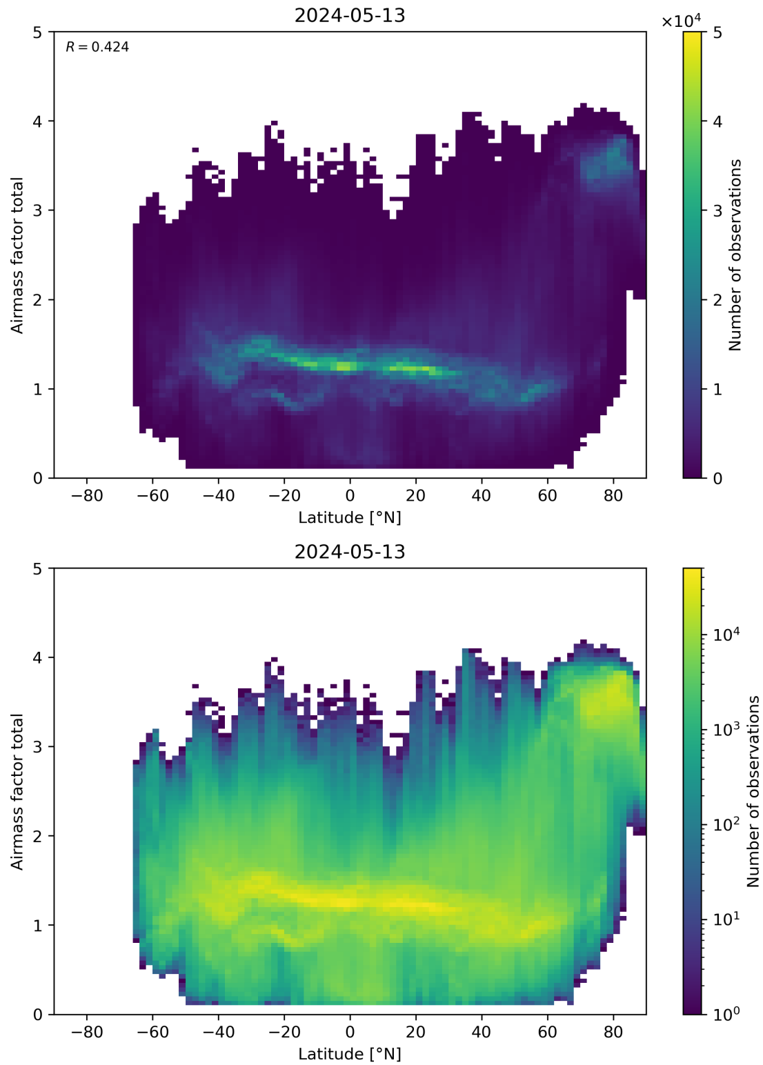
Figure 161: Scatter density plot of “Latitude” against “Airmass factor total” for 2024-05-12 to 2024-05-14.
