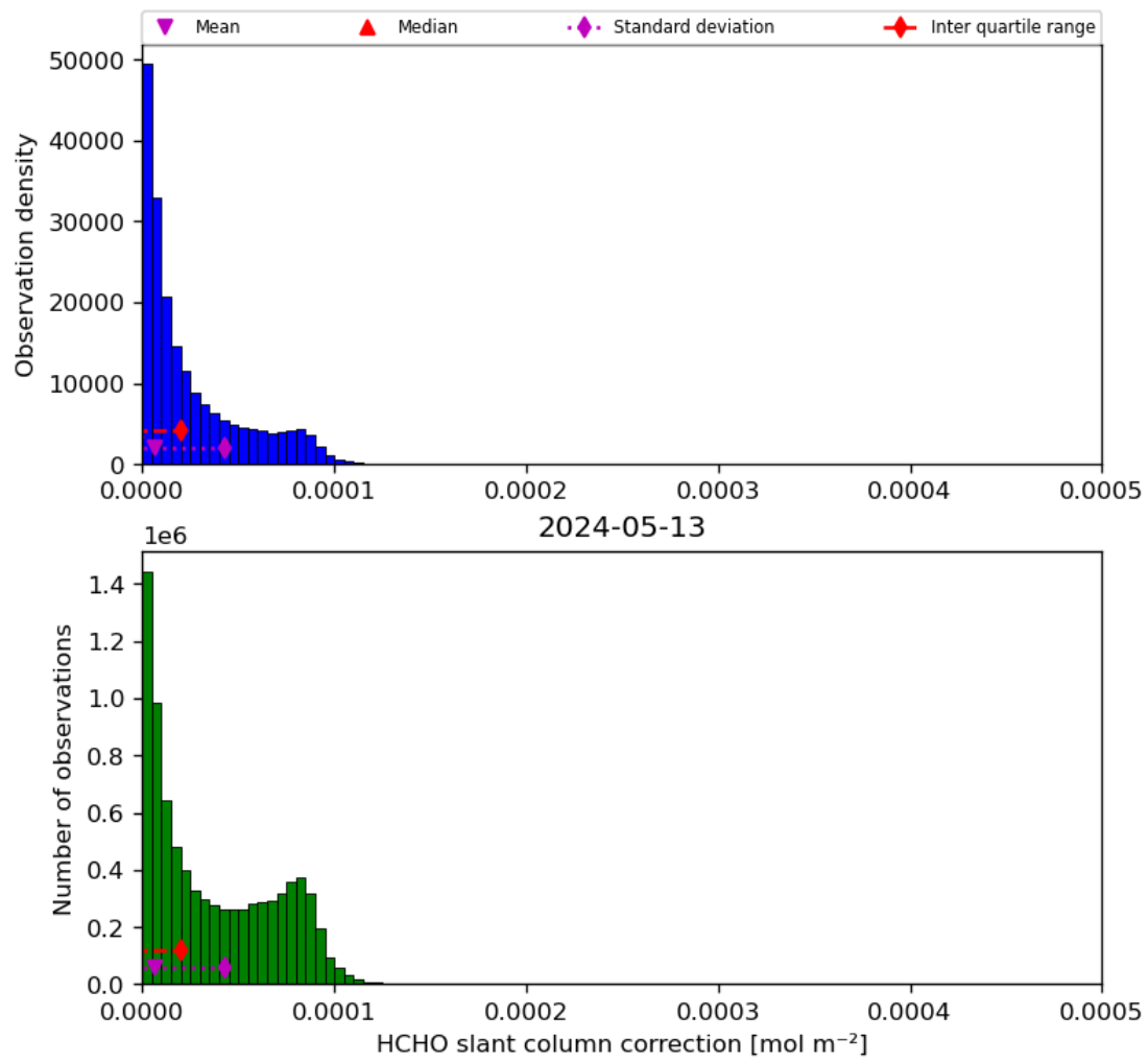
Figure 47: Histogram of “HCHO slant column correction” for 2024-05-12 to 2024-05-14
