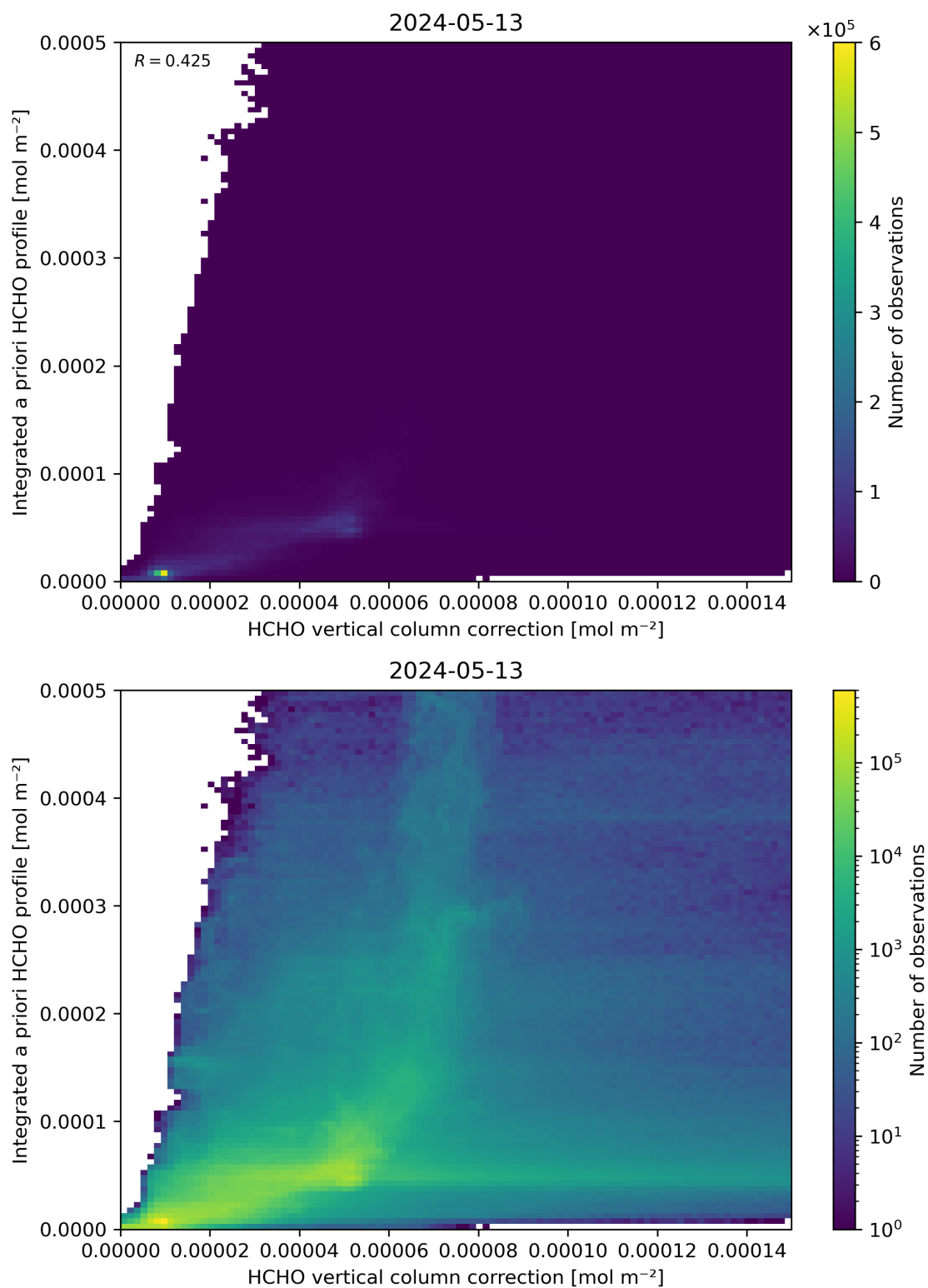
Figure 122: Scatter density plot of “HCHO vertical column correction” against “Integrated a priori HCHO profile” for 2024-05-12 to 2024-05-14.
