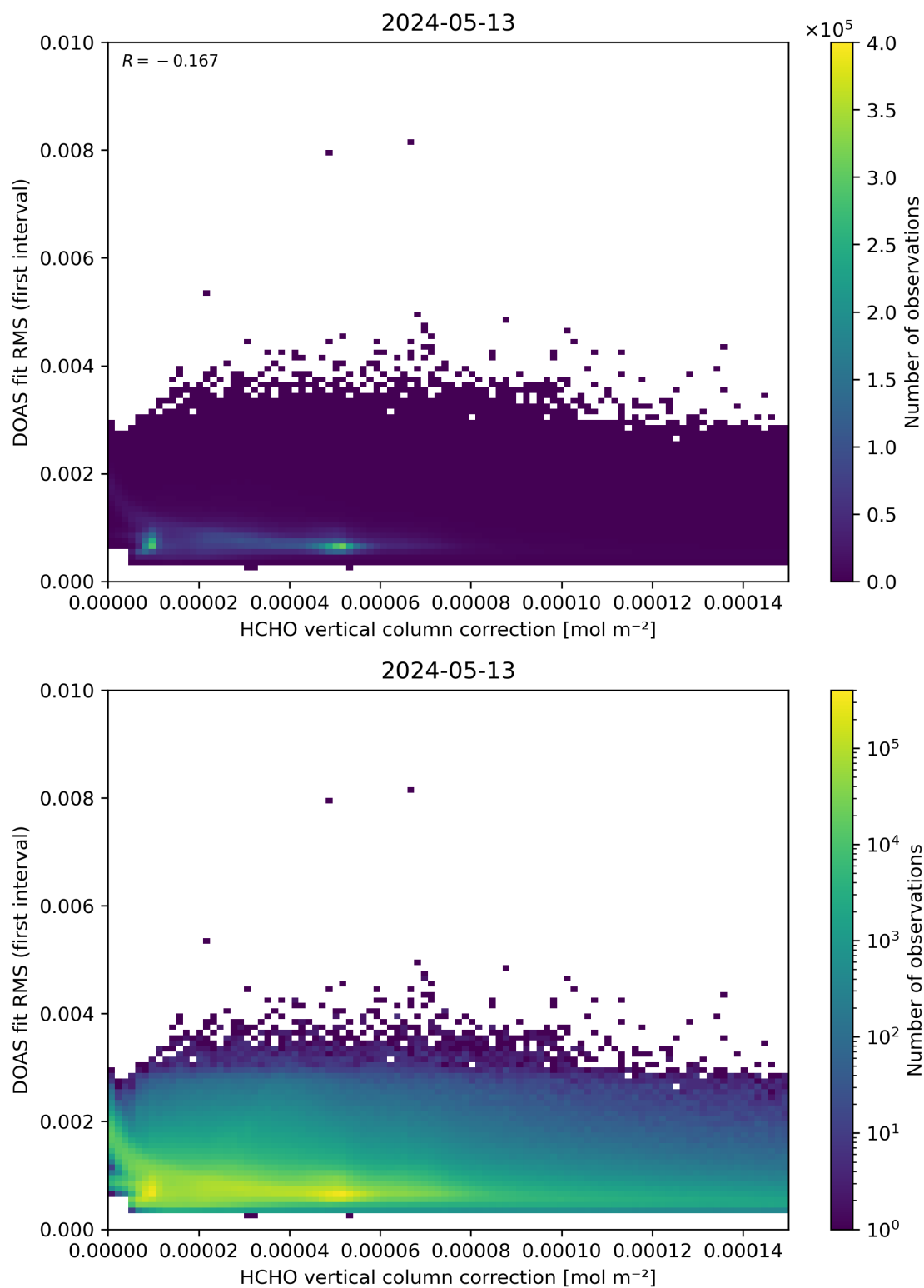
Figure 112: Scatter density plot of “HCHO vertical column correction” against “DOAS fit RMS (first interval)” for 2024-05-12 to 2024-05-14.
