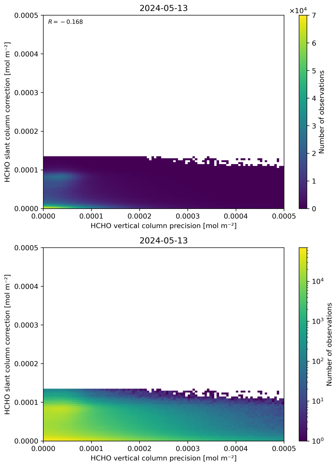
Figure 141: Scatter density plot of “HCHO vertical column precision” against “HCHO slant column correction” for 2024-05-12 to 2024-05-14.
