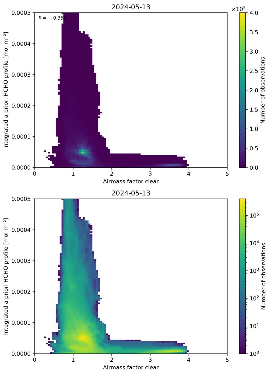
Figure 76: Scatter density plot of “Airmass factor clear” against “Integrated a priori HCHO profile” for 2024-05-12 to 2024-05-14.
