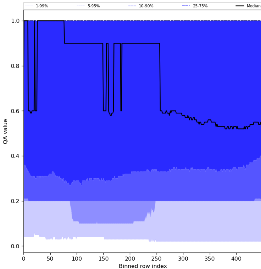
Figure 48: Along track statistics of “QA value” for 2024-05-12 to 2024-05-14
