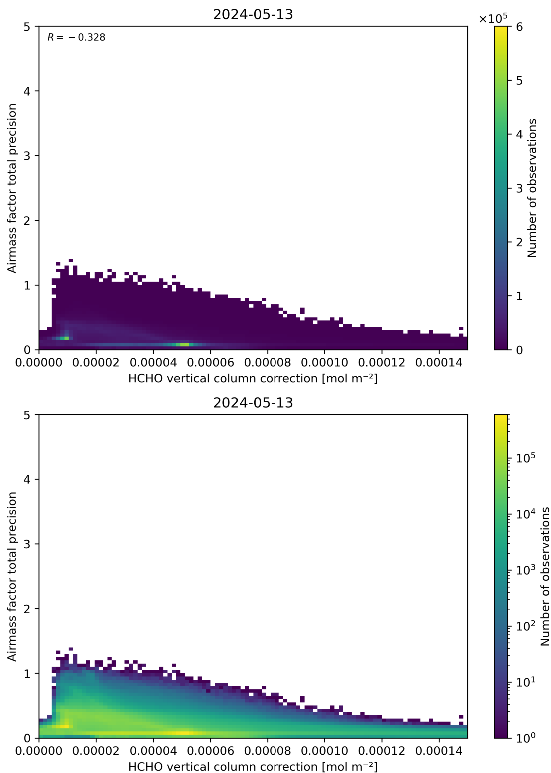
Figure 121: Scatter density plot of “HCHO vertical column correction” against “Airmass factor total precision” for 2024-05-12 to 2024-05-14.
