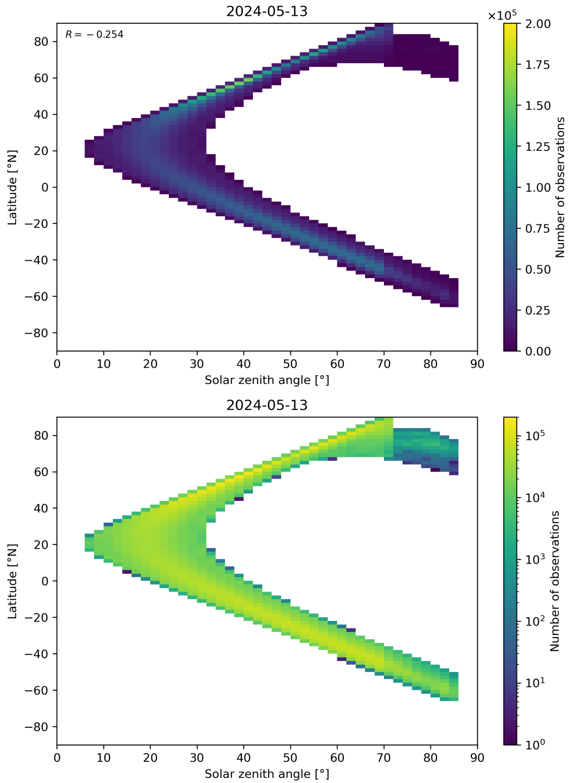
Figure 181: Scatter density plot of “Solar zenith angle” against “Latitude” for 2024-05-12 to 2024-05-14.
