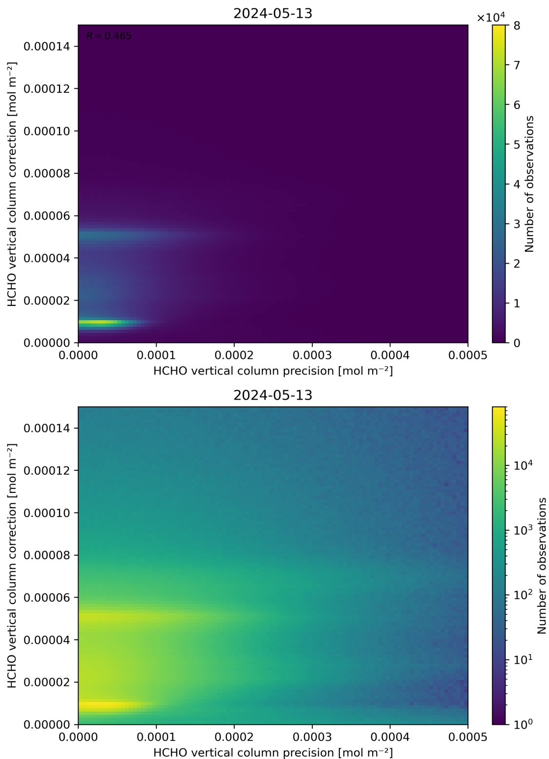
Figure 146: Scatter density plot of “HCHO vertical column precision” against “HCHO vertical column correction” for 2024-05-12 to 2024-05-14.
