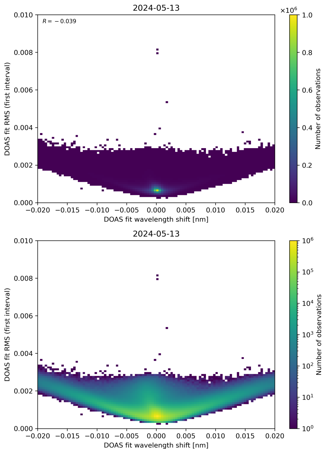
Figure 64: Scatter density plot of “DOAS fit wavelength shift” against “DOAS fit RMS (first interval)” for 2024-05-12 to 2024-05-14.
