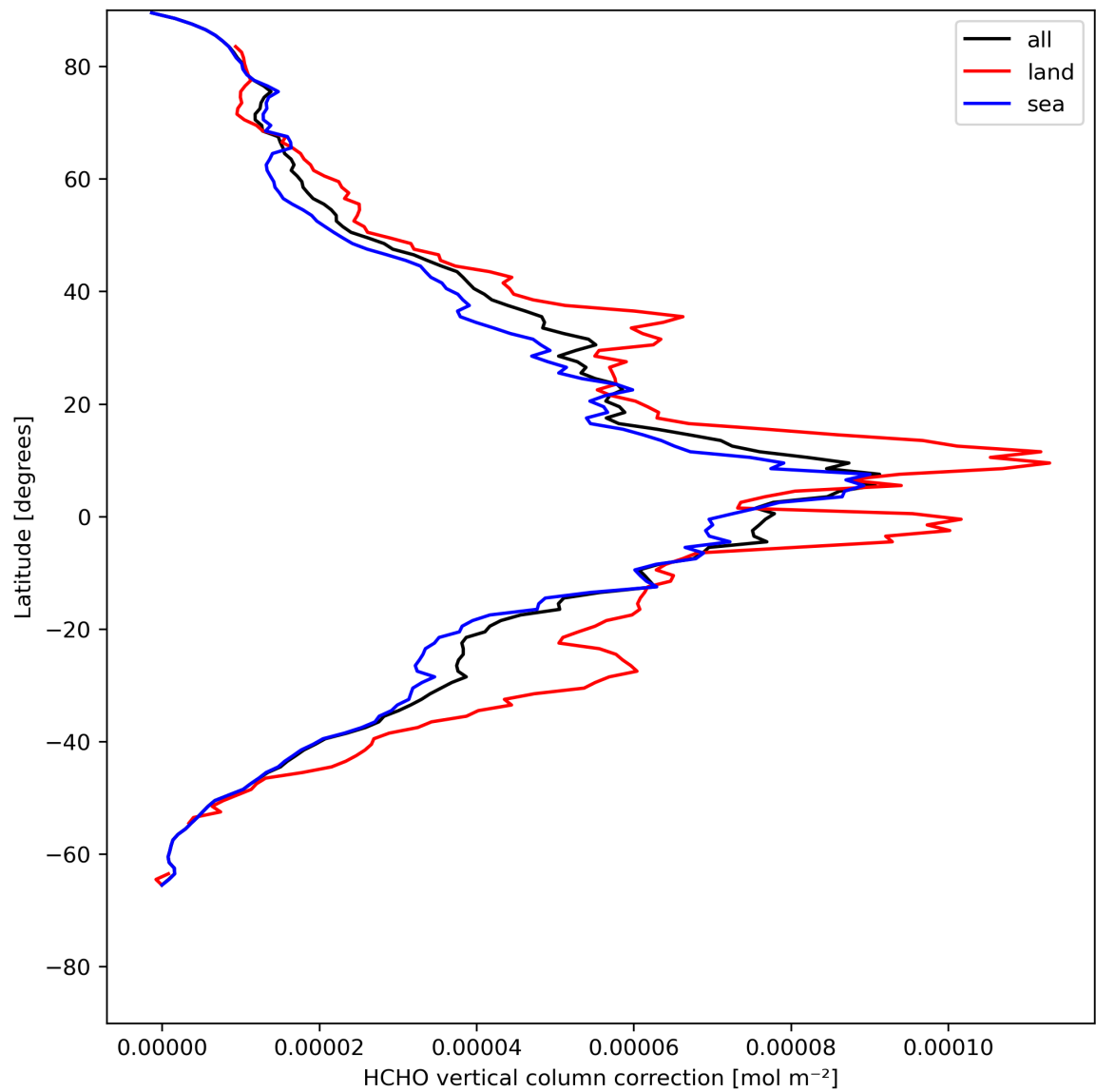
Figure 23: Zonal average of “HCHO vertical column correction” for 2024-05-12 to 2024-05-14.
