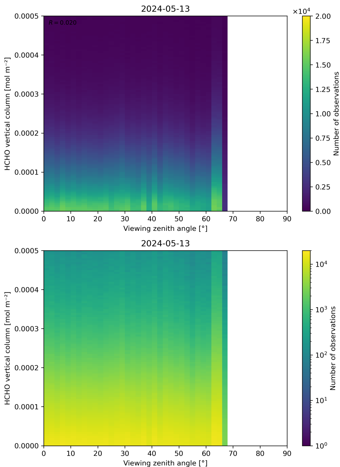
Figure 192: Scatter density plot of “Viewing zenith angle” against “HCHO vertical column” for 2024-05-12 to 2024-05-14.
