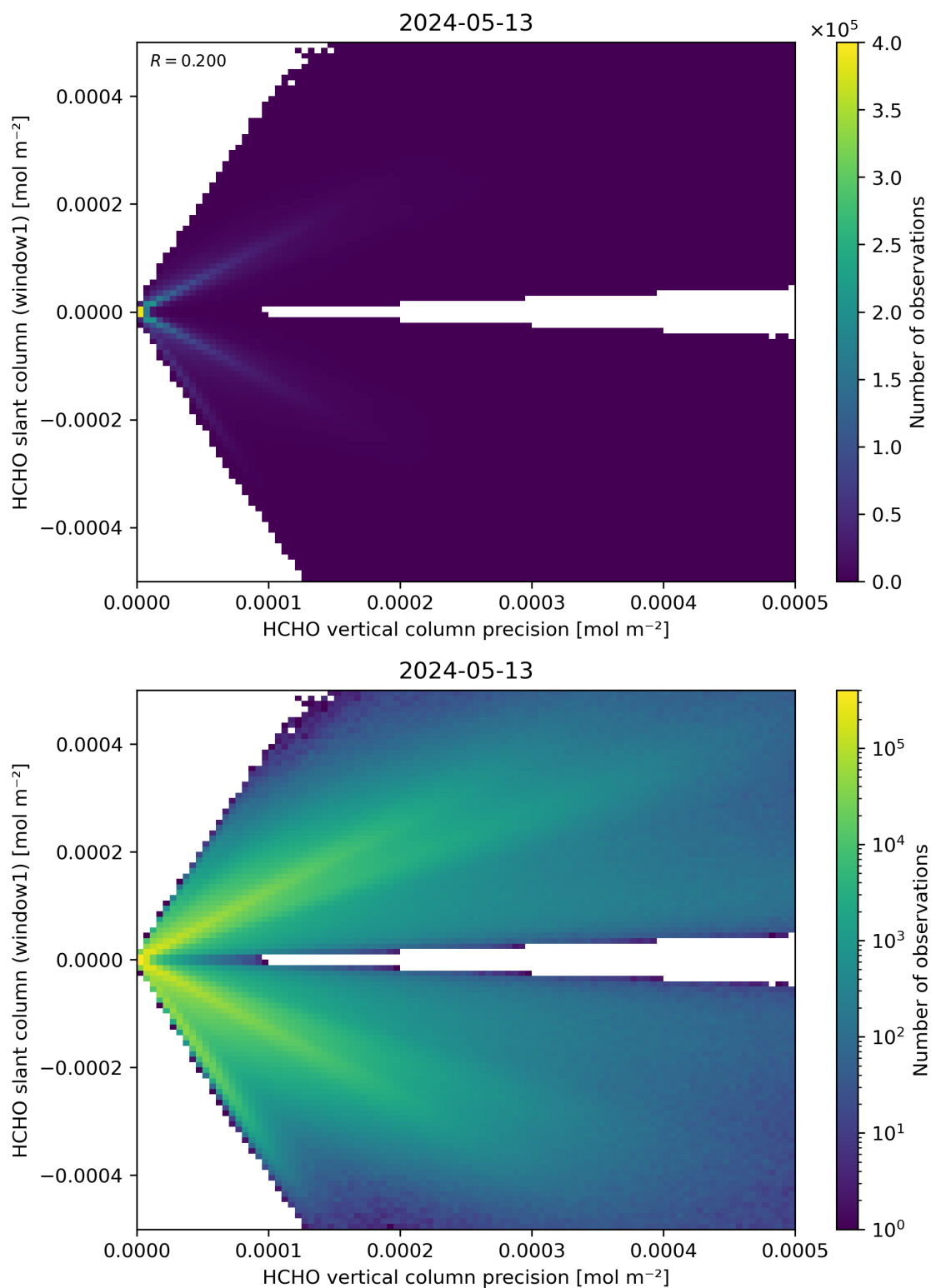
Figure 142: Scatter density plot of “HCHO vertical column precision” against “HCHO slant column (window1)” for 2024-05-12 to 2024-05-14.
