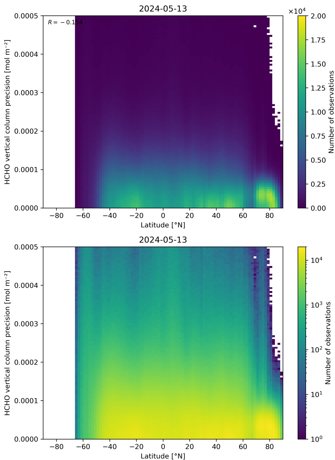
Figure 165: Scatter density plot of “Latitude” against “HCHO vertical column precision” for 2024-05-12 to 2024-05-14.
