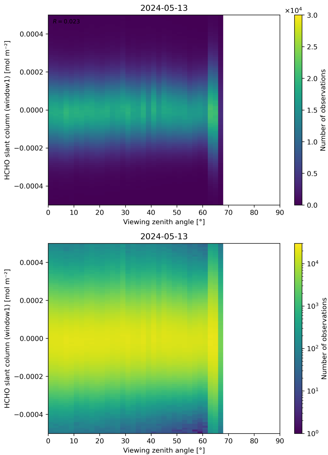
Figure 188: Scatter density plot of “Viewing zenith angle” against “HCHO slant column (window1)” for 2024-05-12 to 2024-05-14.
