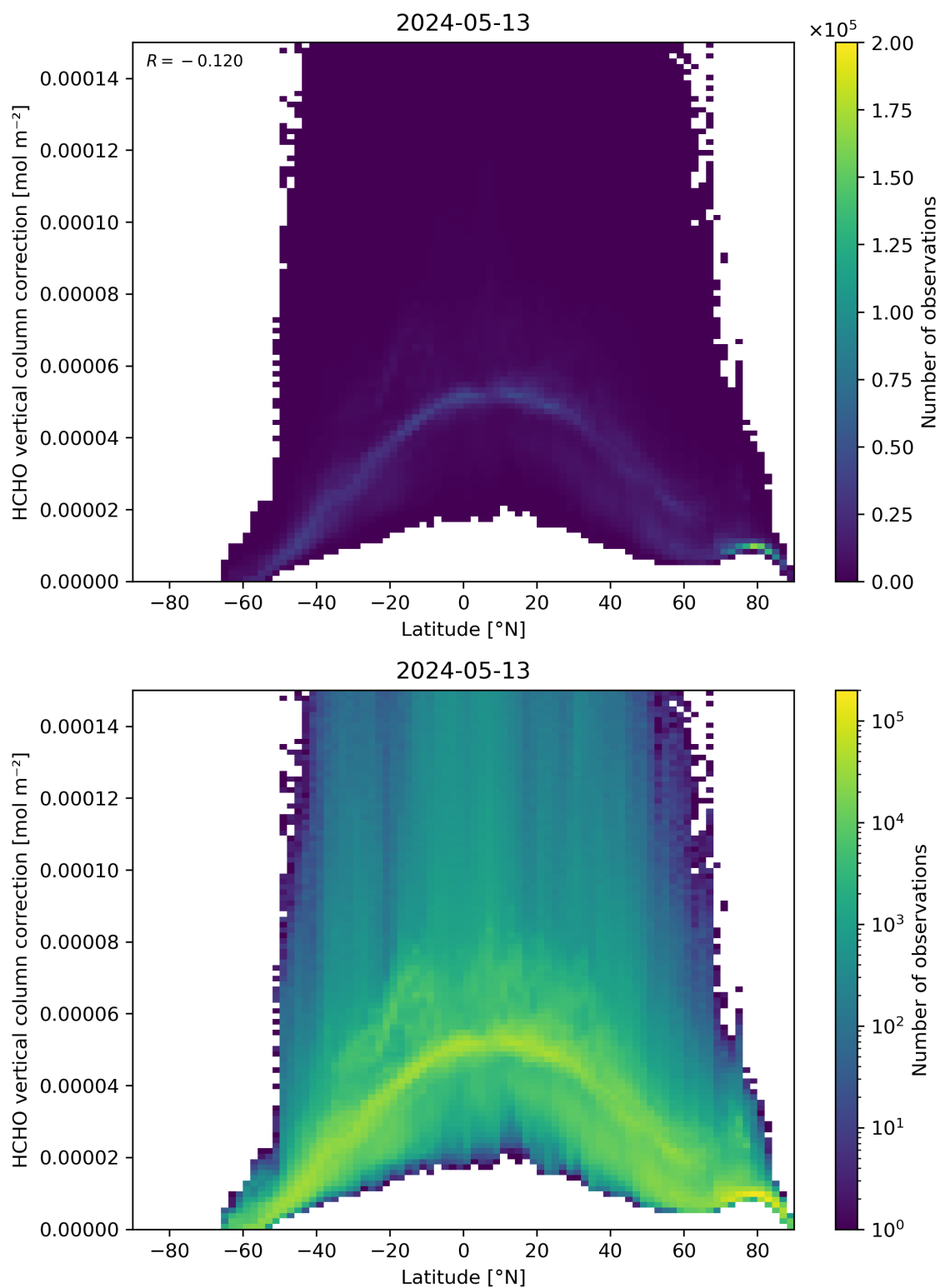
Figure 164: Scatter density plot of “Latitude” against “HCHO vertical column correction” for 2024-05-12 to 2024-05-14.
