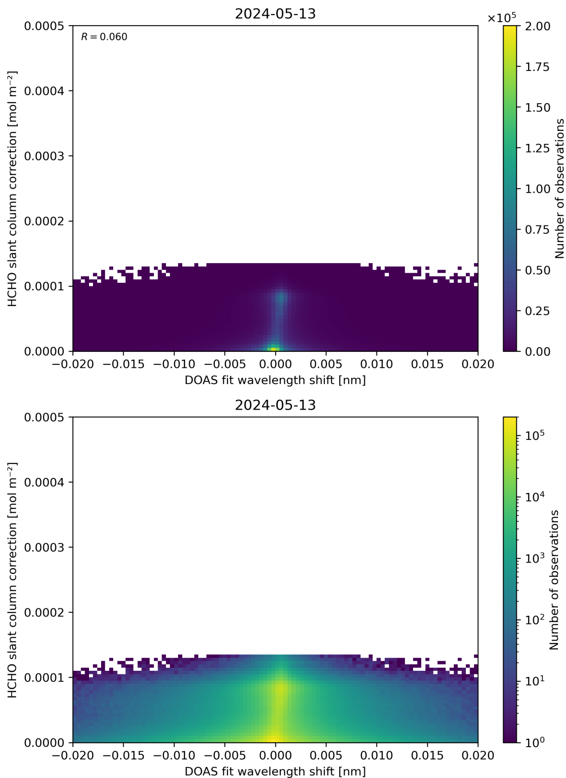
Figure 67: Scatter density plot of “DOAS fit wavelength shift” against “HCHO slant column correction” for 2024-05-12 to 2024-05-14.
