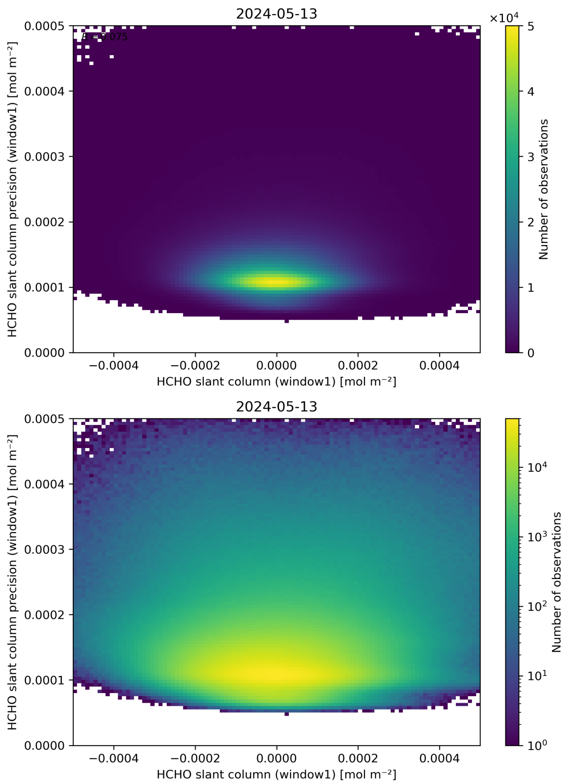
Figure 84: Scatter density plot of “HCHO slant column (window1)” against “HCHO slant column precision (window1)” for 2024-05-12 to 2024-05-14.
