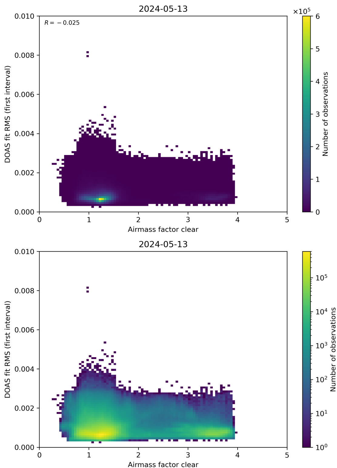
Figure 71: Scatter density plot of “Airmass factor clear” against “DOAS fit RMS (first interval)” for 2024-05-12 to 2024-05-14.
