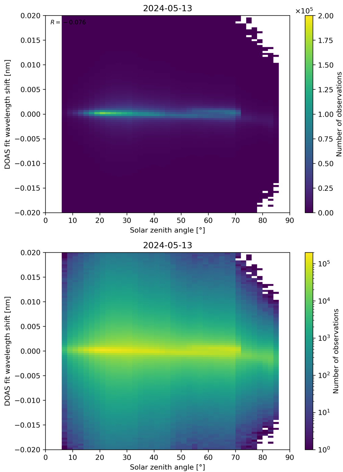
Figure 168: Scatter density plot of “Solar zenith angle” against “DOAS fit wavelength shift” for 2024-05-12 to 2024-05-14.
