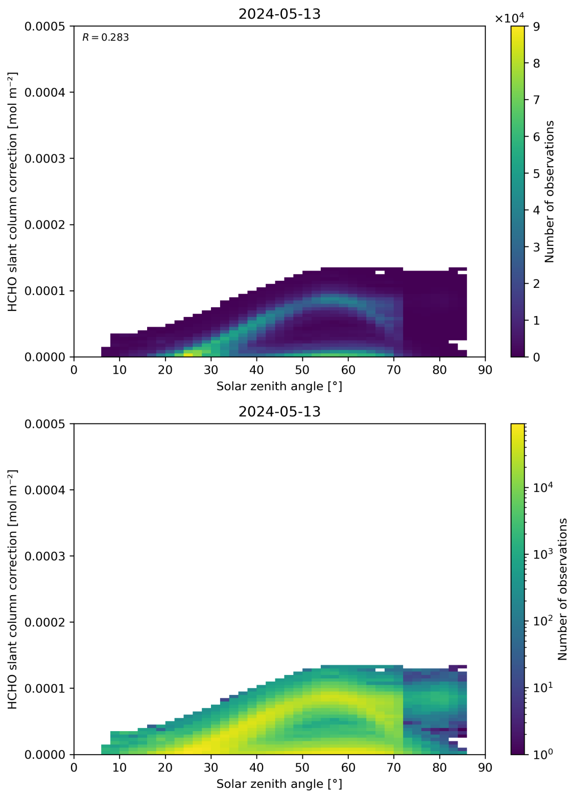
Figure 172: Scatter density plot of “Solar zenith angle” against “HCHO slant column correction” for 2024-05-12 to 2024-05-14.
