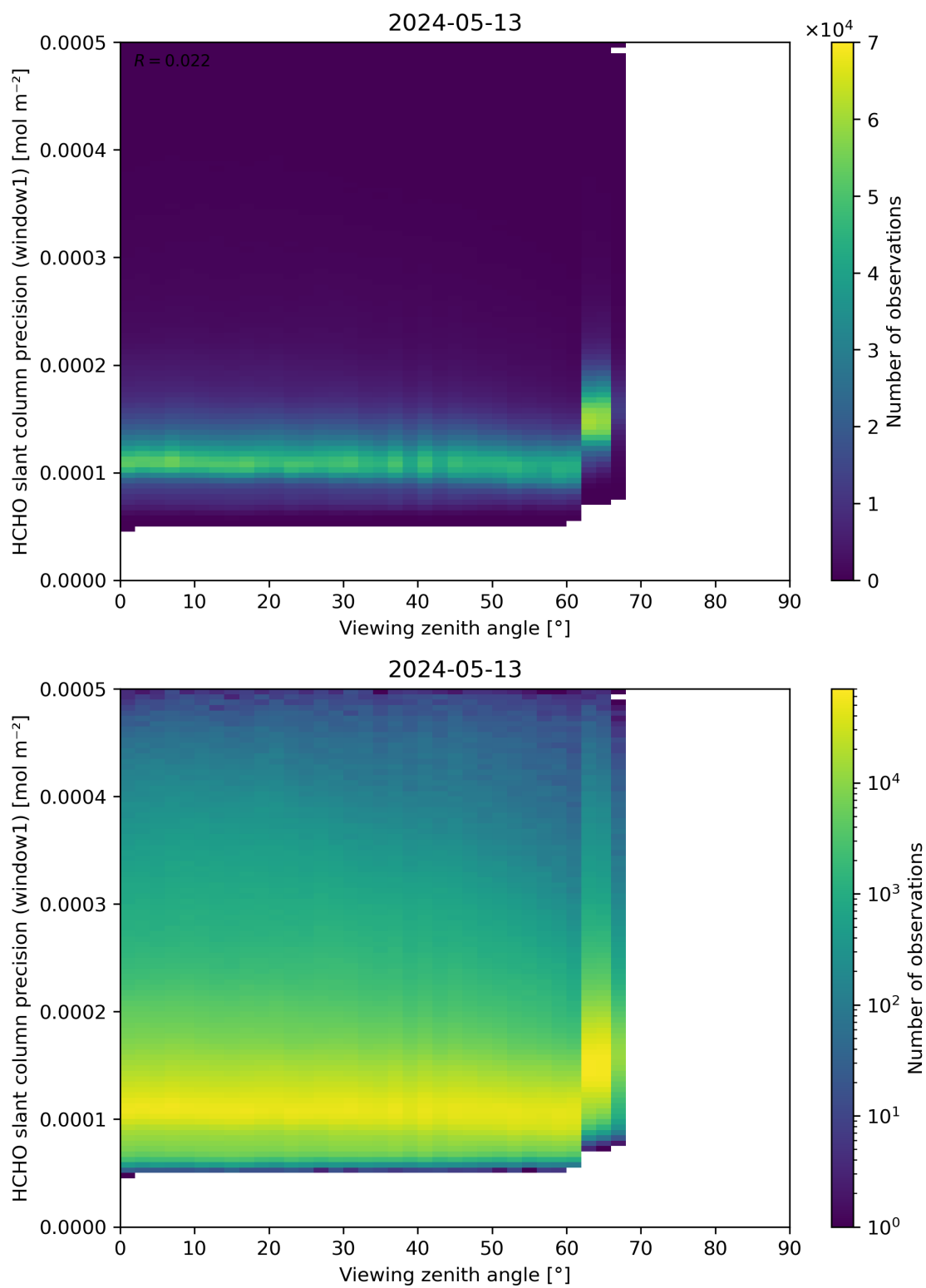
Figure 189: Scatter density plot of “Viewing zenith angle” against “HCHO slant column precision (window1)” for 2024-05-12 to 2024-05-14.
