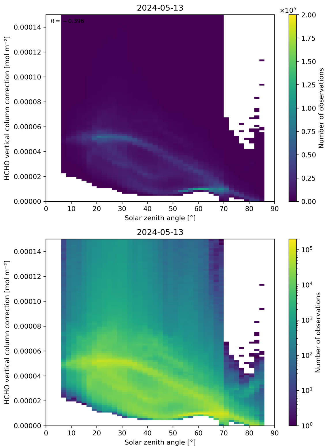
Figure 178: Scatter density plot of “Solar zenith angle” against “HCHO vertical column correction” for 2024-05-12 to 2024-05-14.
