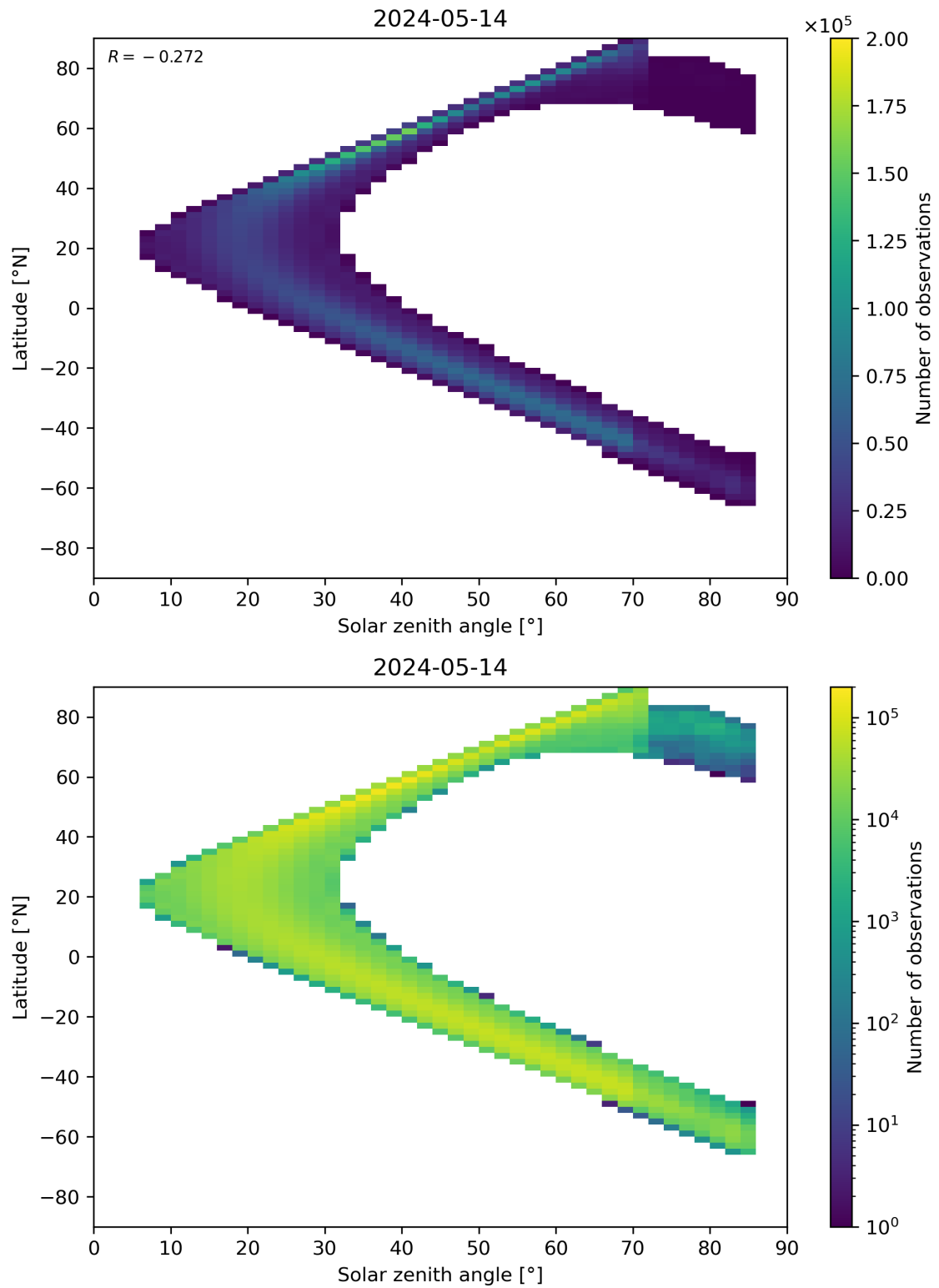
Figure 181: Scatter density plot of “Solar zenith angle” against “Latitude” for 2024-05-13 to 2024-05-15.
