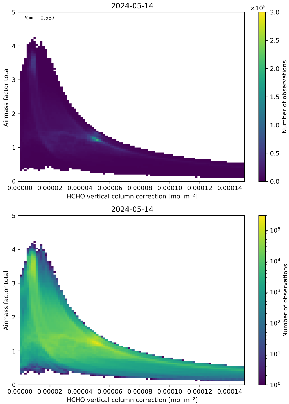
Figure 120: Scatter density plot of “HCHO vertical column correction” against “Airmass factor total” for 2024-05-13 to 2024-05-15.
