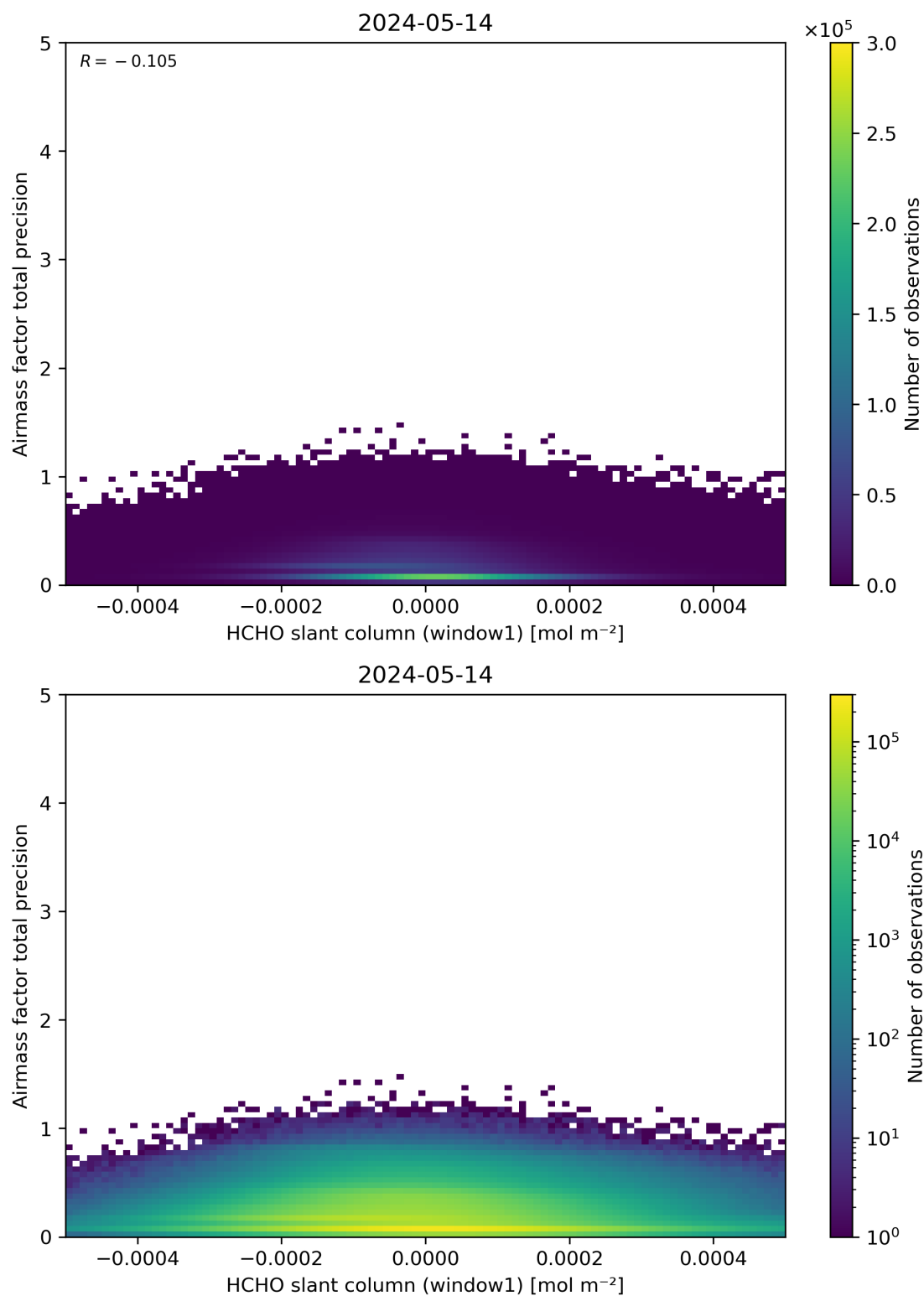
Figure 86: Scatter density plot of “HCHO slant column (window1)” against “Airmass factor total precision” for 2024-05-13 to 2024-05-15.
