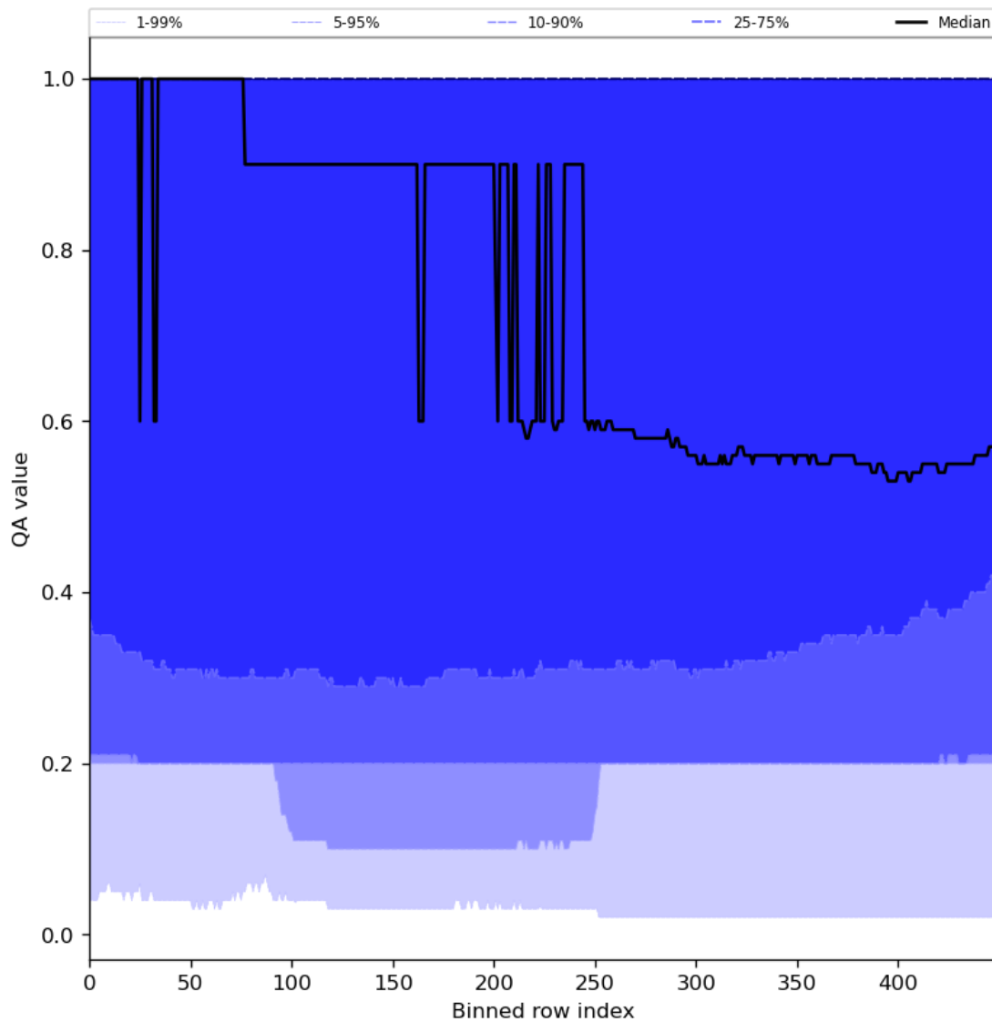
Figure 48: Along track statistics of “QA value” for 2024-05-13 to 2024-05-15
