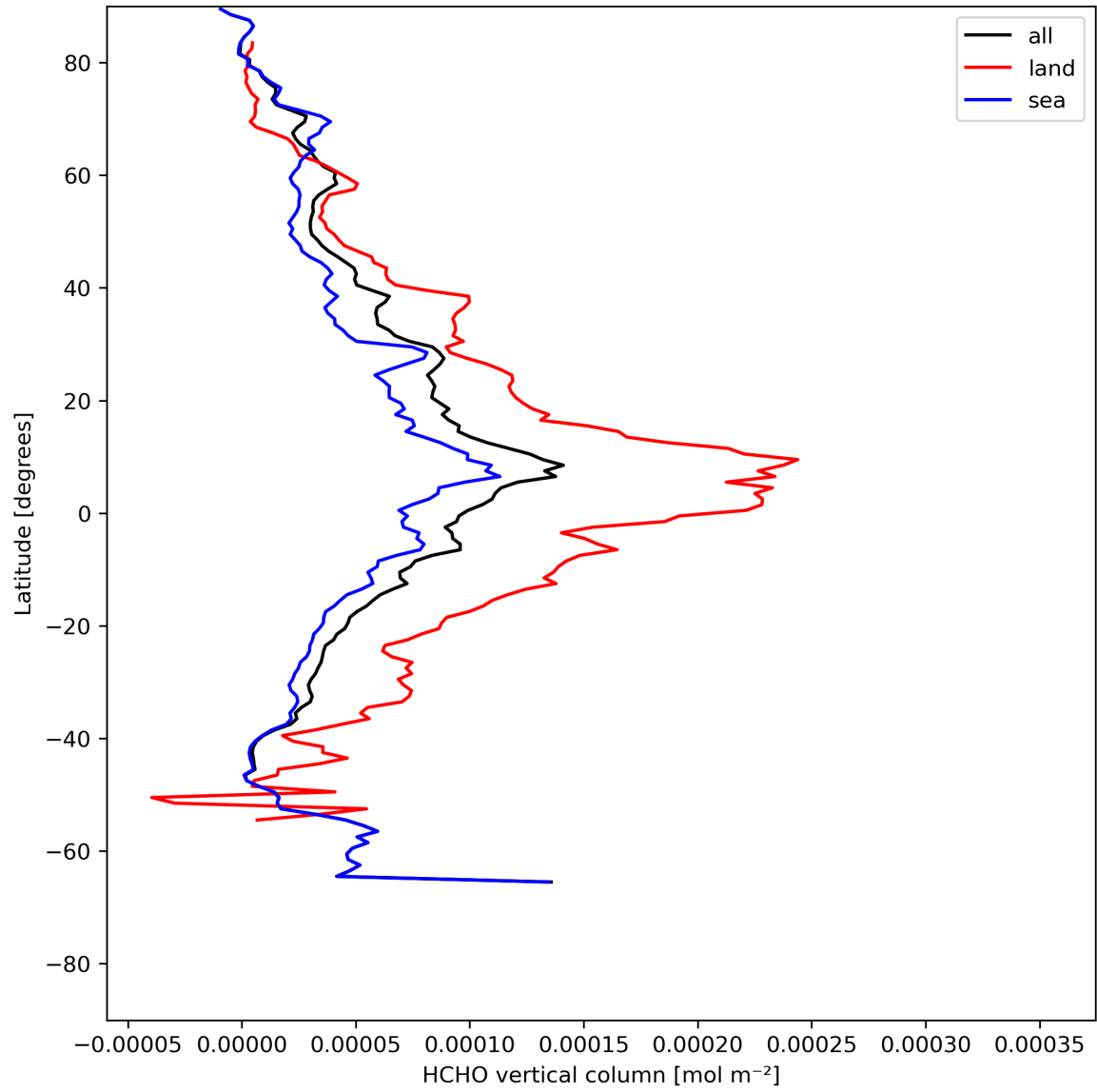
Figure 21: Zonal average of “HCHO vertical column” for 2024-05-13 to 2024-05-15.
