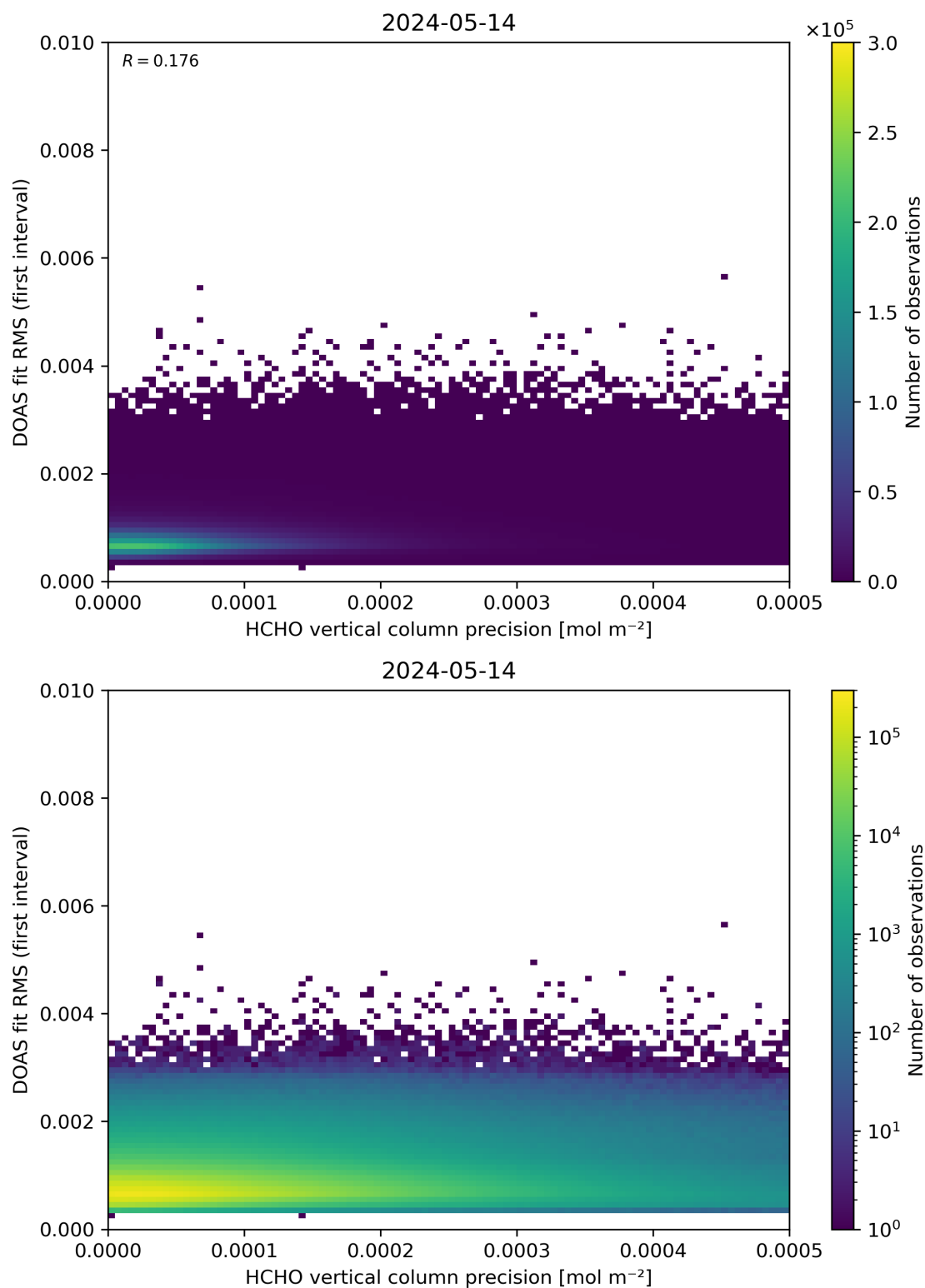
Figure 136: Scatter density plot of “HCHO vertical column precision” against “DOAS fit RMS (first interval)” for 2024-05-13 to 2024-05-15.
