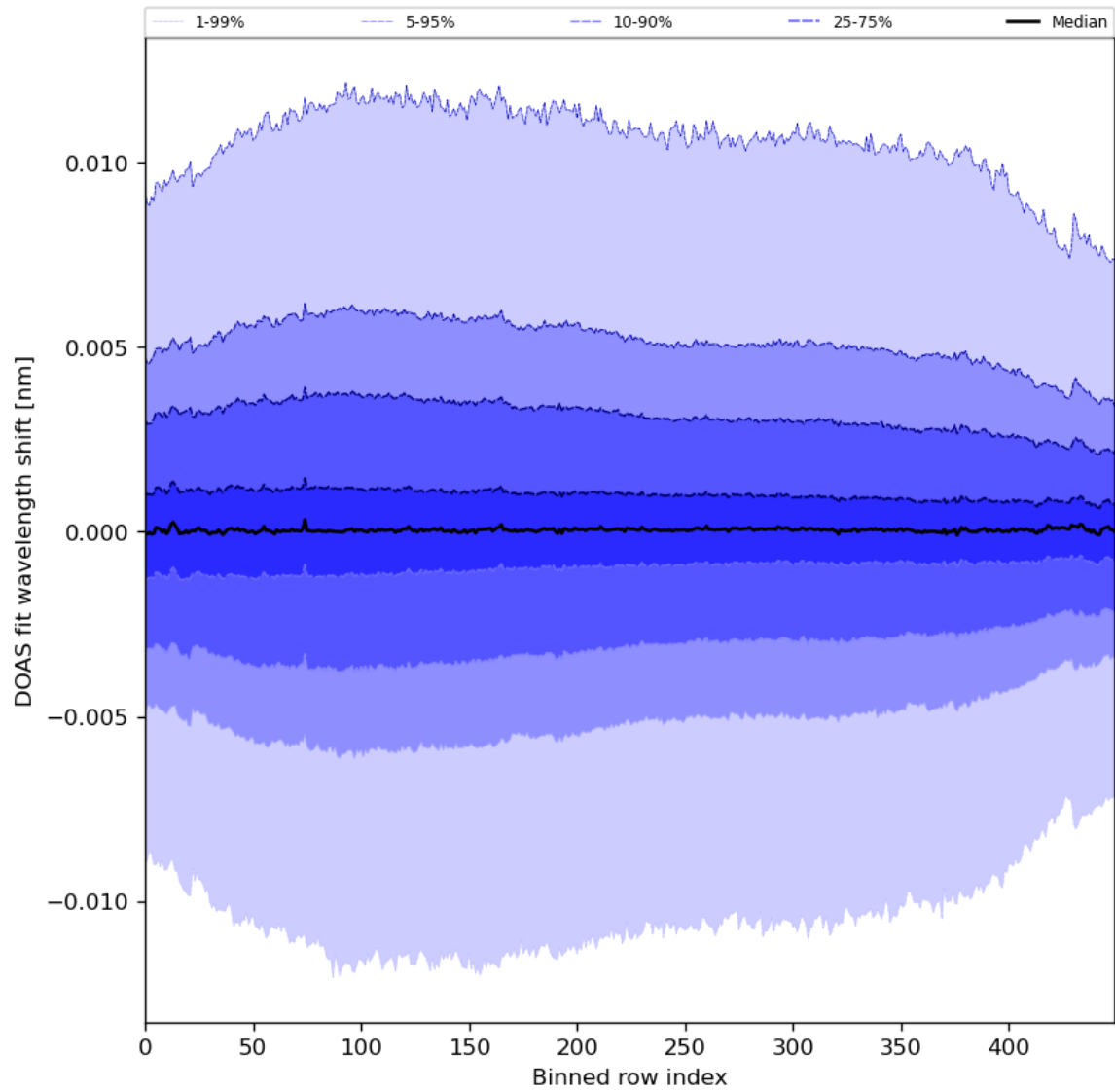
Figure 58: Along track statistics of “DOAS fit wavelength shift” for 2024-05-13 to 2024-05-15
