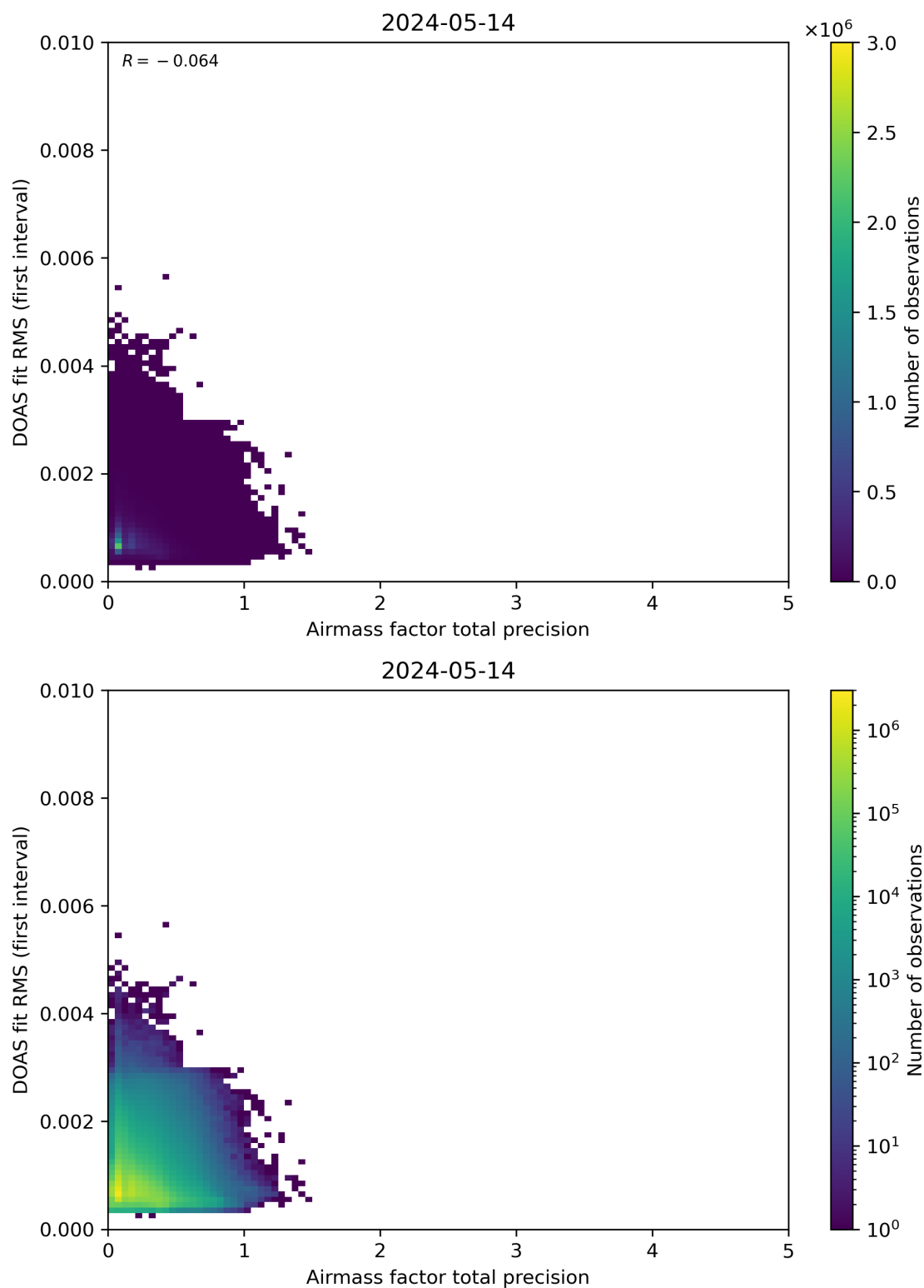
Figure 105: Scatter density plot of “Airmass factor total precision” against “DOAS fit RMS (first interval)” for 2024-05-13 to 2024-05-15.
