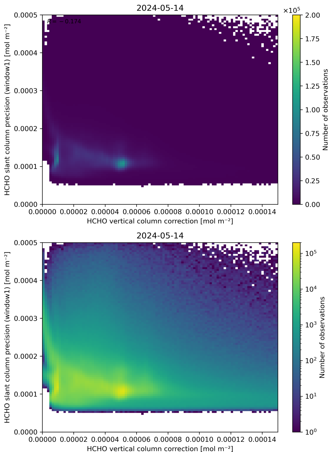
Figure 119: Scatter density plot of “HCHO vertical column correction” against “HCHO slant column precision (window1)” for 2024-05-13 to 2024-05-15.
