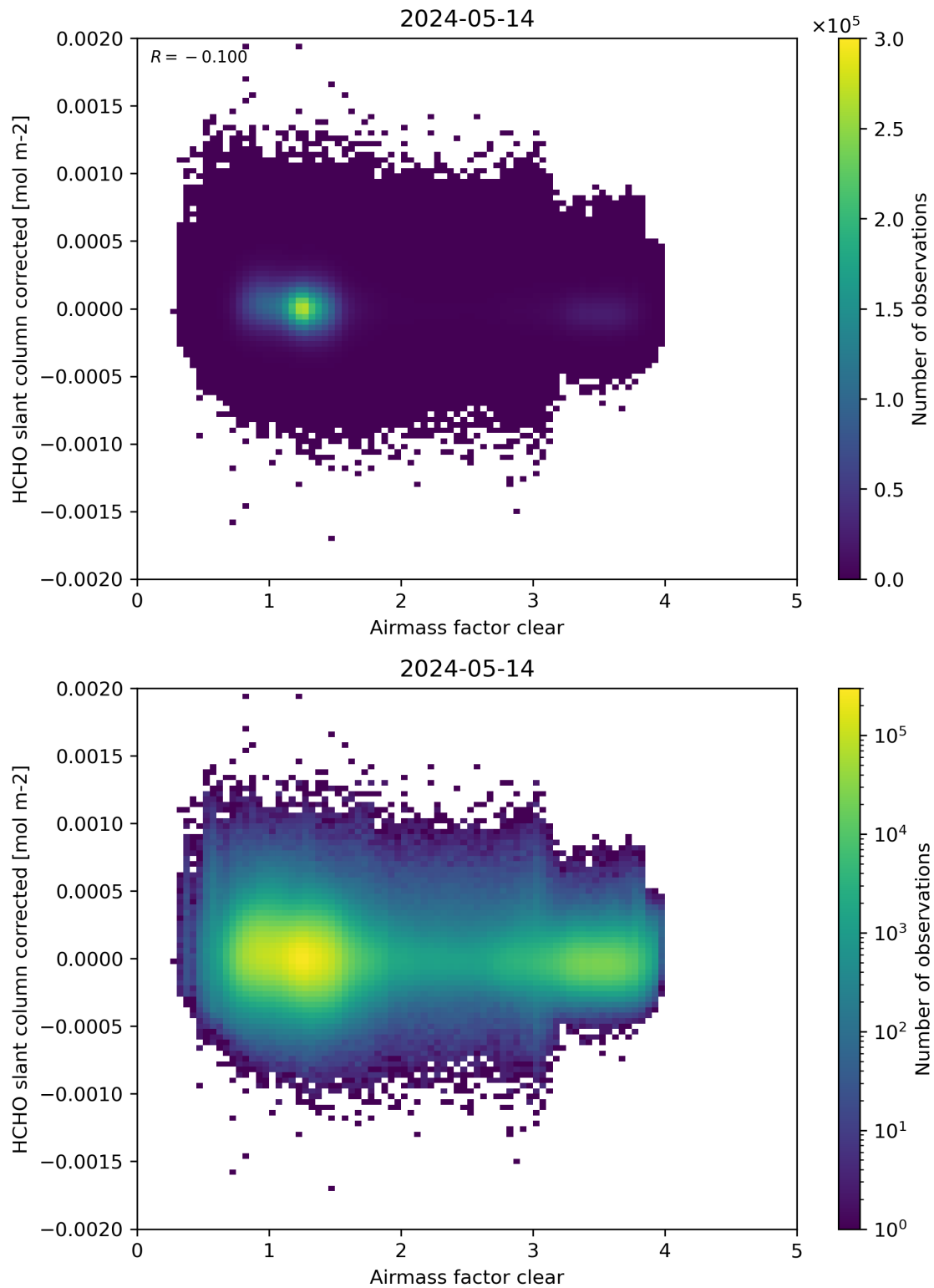
Figure 74: Scatter density plot of “Airmass factor clear” against “HCHO slant column corrected” for 2024-05-13 to 2024-05-15.
