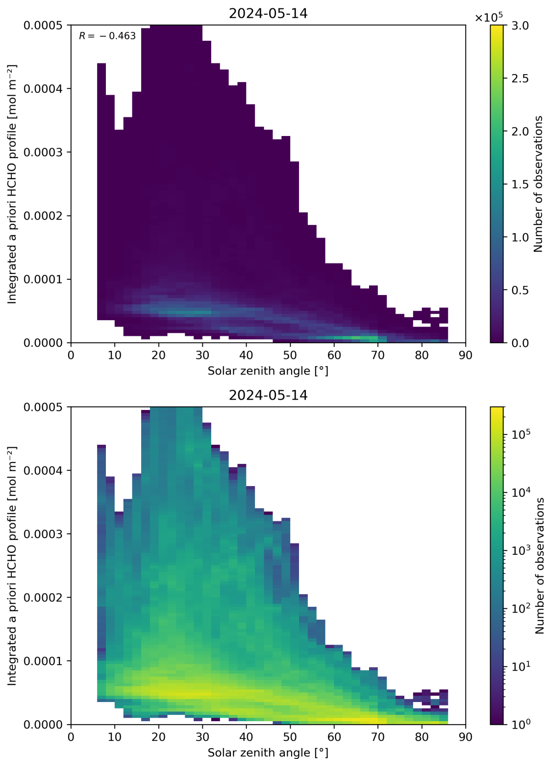
Figure 180: Scatter density plot of “Solar zenith angle” against “Integrated a priori HCHO profile” for 2024-05-13 to 2024-05-15.
