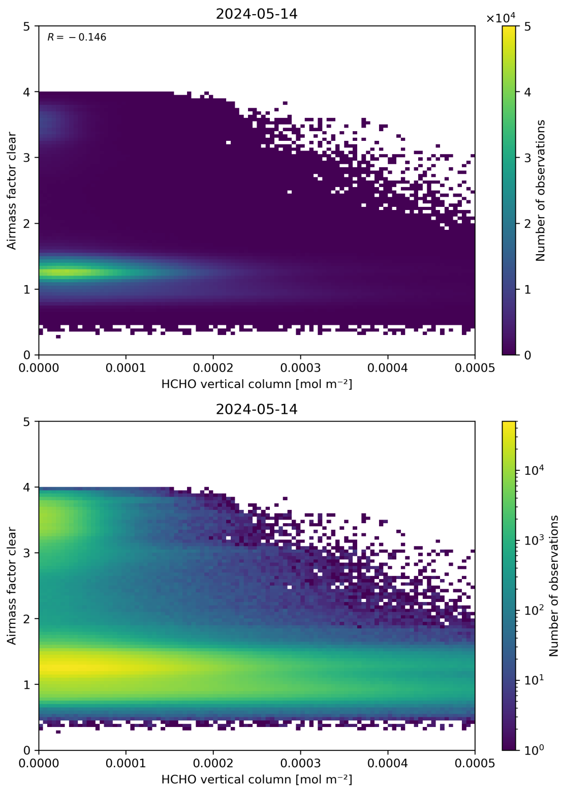
Figure 126: Scatter density plot of “HCHO vertical column” against “Airmass factor clear” for 2024-05-13 to 2024-05-15.
