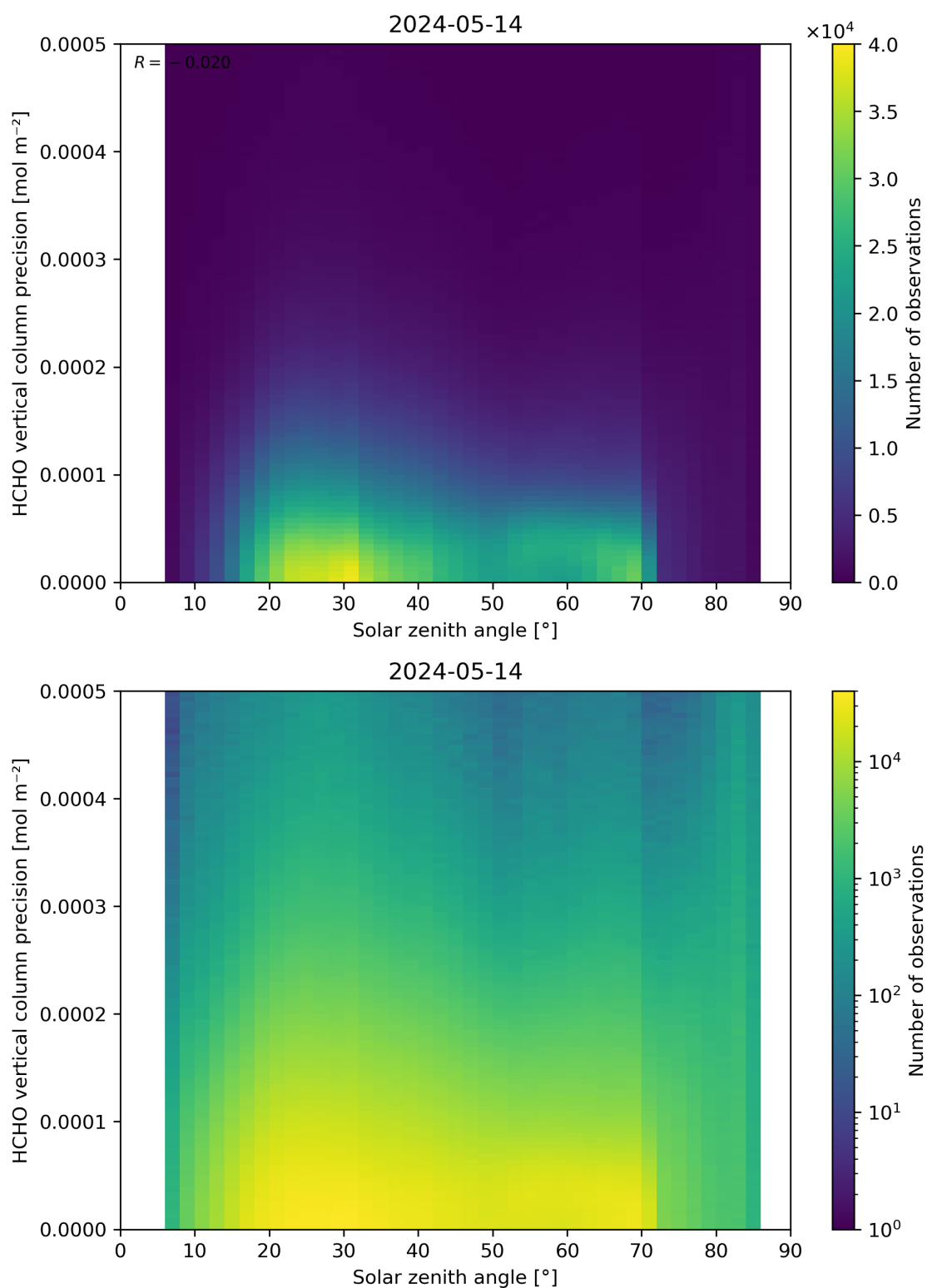
Figure 179: Scatter density plot of “Solar zenith angle” against “HCHO vertical column precision” for 2024-05-13 to 2024-05-15.
