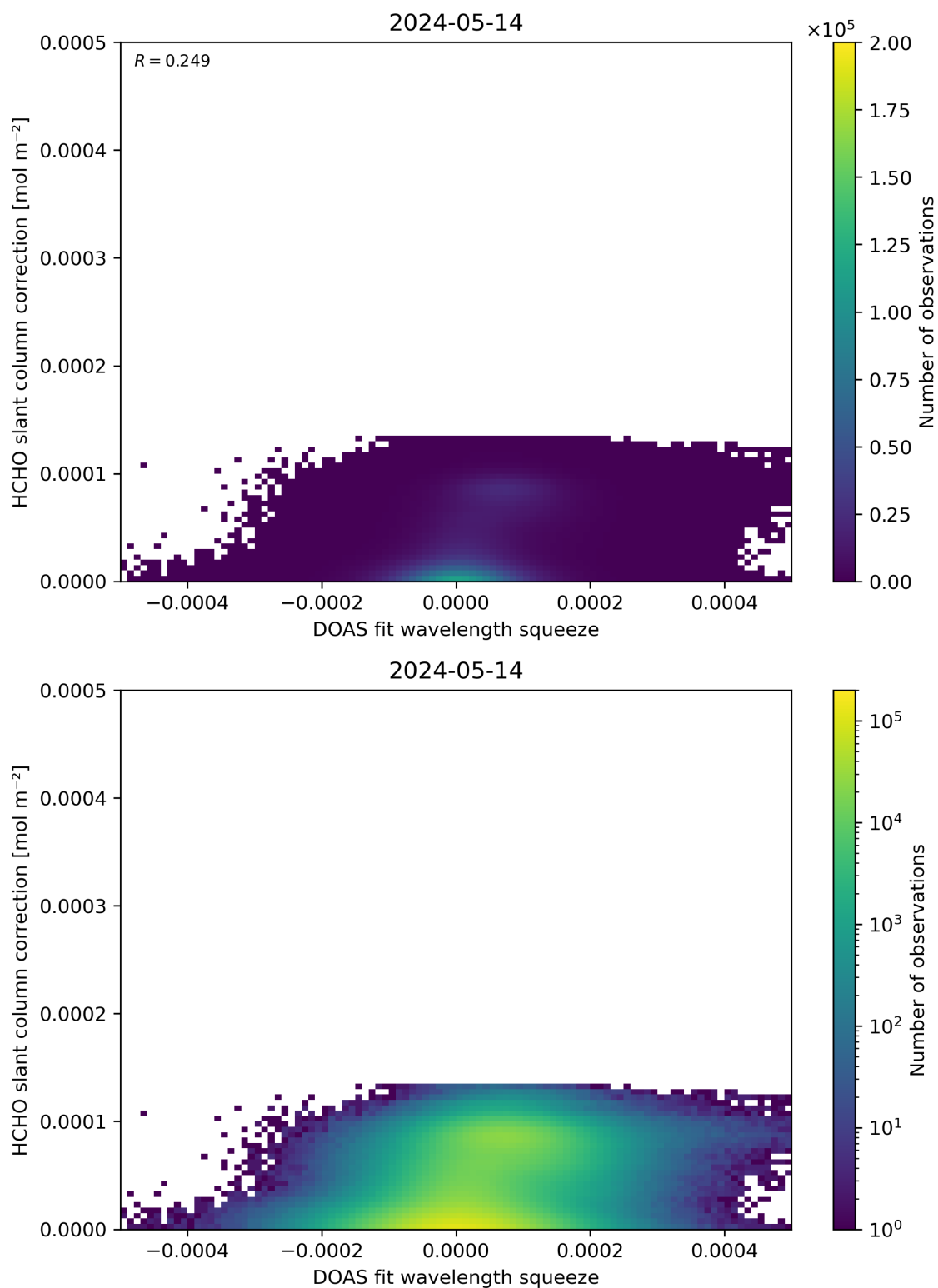
Figure 70: Scatter density plot of “DOAS fit wavelength squeeze” against “HCHO slant column correction” for 2024-05-13 to 2024-05-15.
