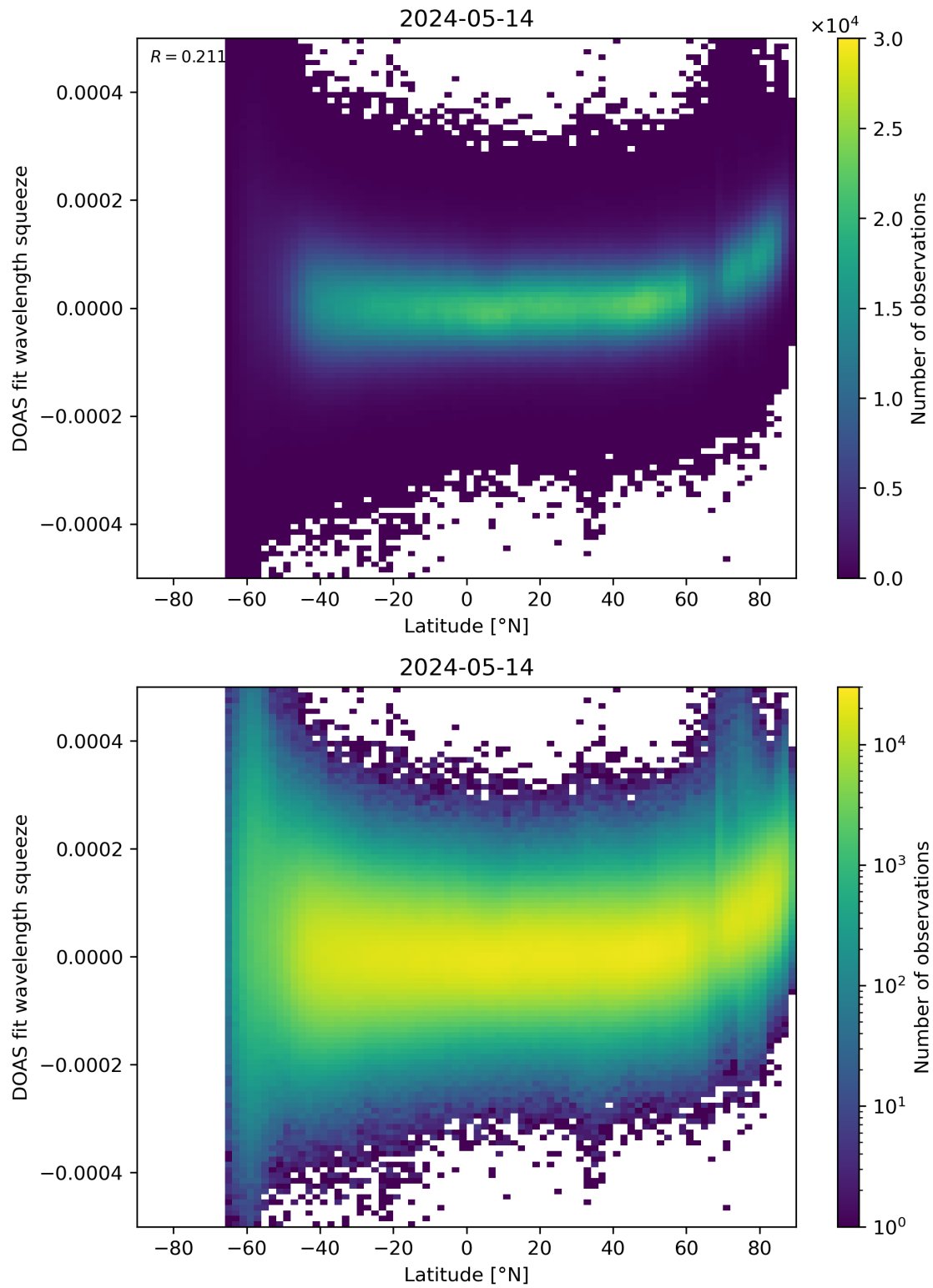
Figure 155: Scatter density plot of “Latitude” against “DOAS fit wavelength squeeze” for 2024-05-13 to 2024-05-15.
