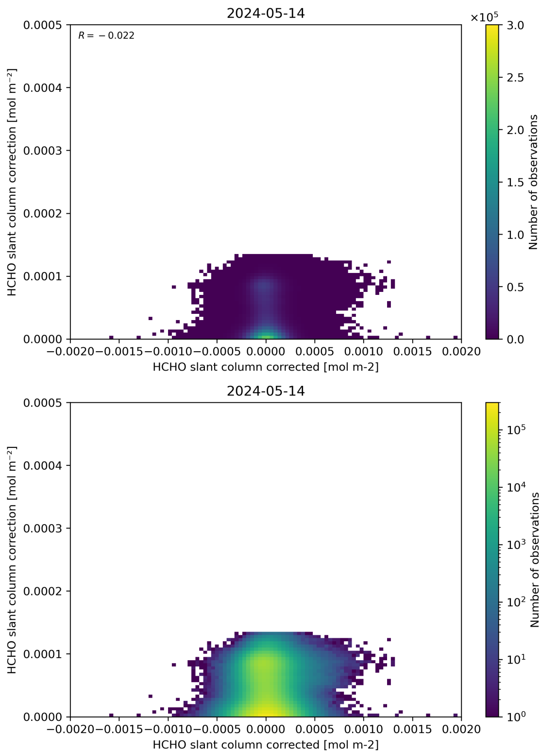
Figure 77: Scatter density plot of “HCHO slant column corrected” against “HCHO slant column correction” for 2024-05-13 to 2024-05-15.
