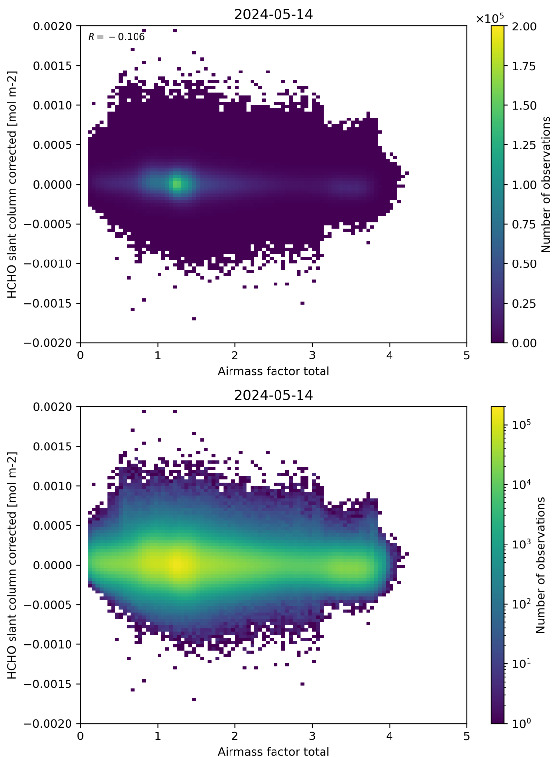
Figure 101: Scatter density plot of “Airmass factor total” against “HCHO slant column corrected” for 2024-05-13 to 2024-05-15.
