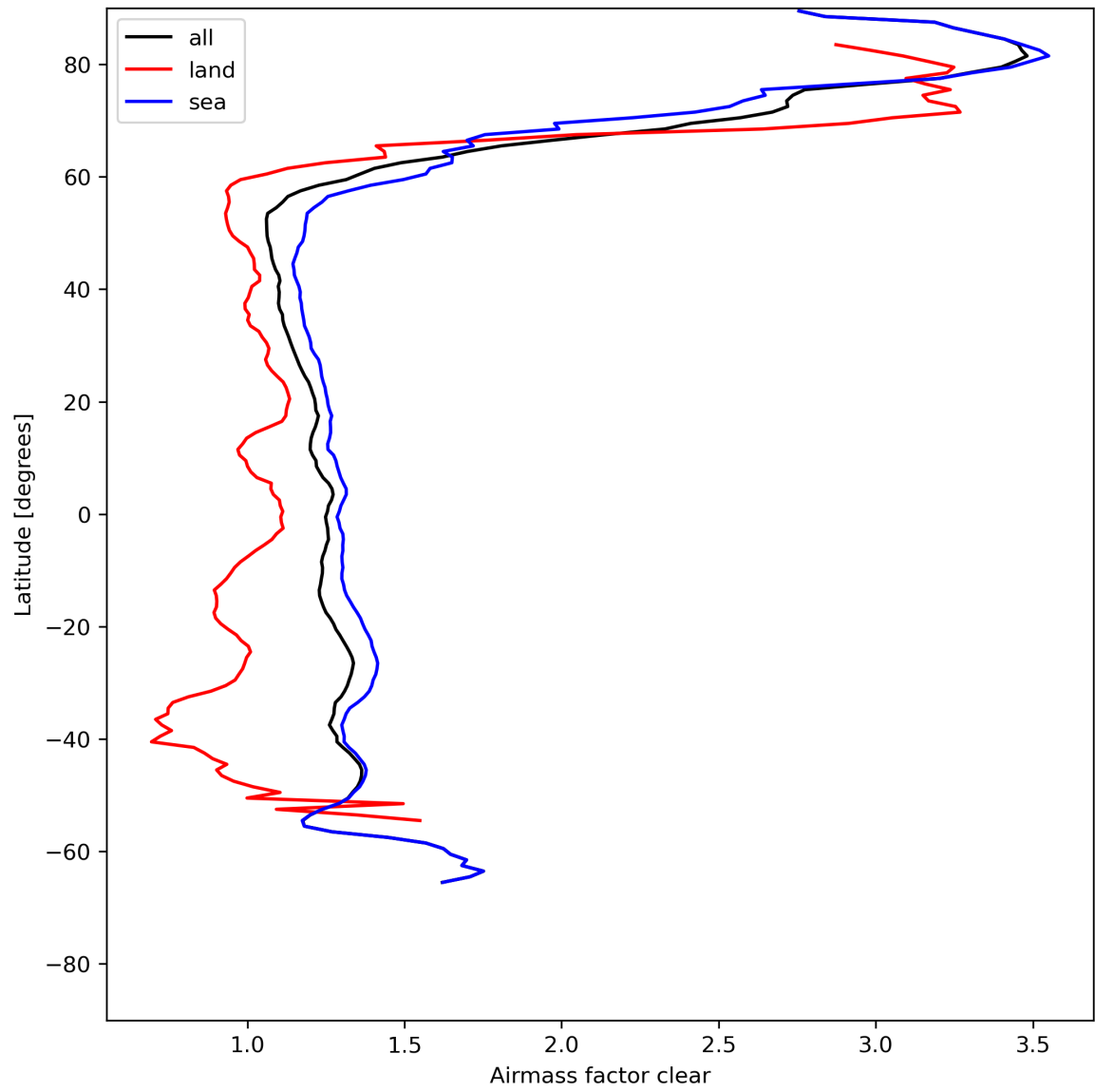
Figure 28: Zonal average of “Airmass factor clear” for 2024-05-13 to 2024-05-15.
