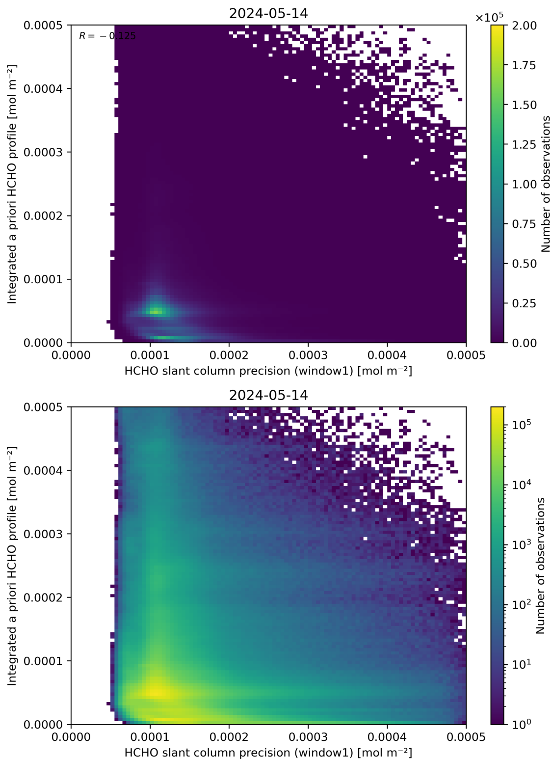
Figure 96: Scatter density plot of “HCHO slant column precision (window1)” against “Integrated a priori HCHO profile” for 2024-05-13 to 2024-05-15.
