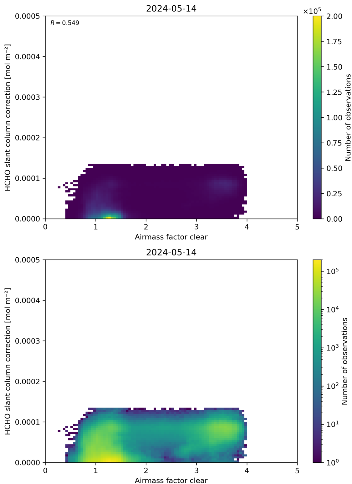
Figure 75: Scatter density plot of “Airmass factor clear” against “HCHO slant column correction” for 2024-05-13 to 2024-05-15.
