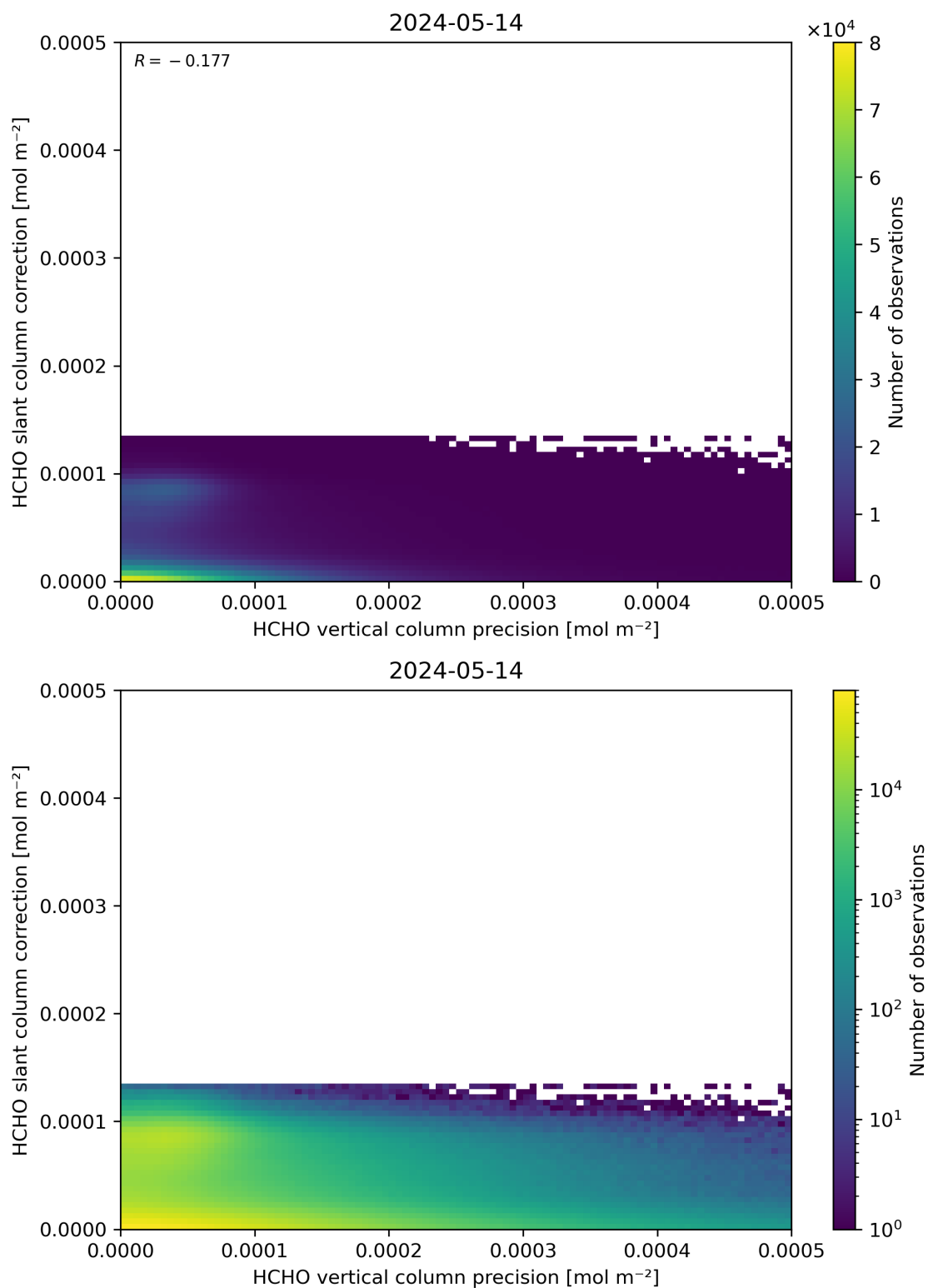
Figure 141: Scatter density plot of “HCHO vertical column precision” against “HCHO slant column correction” for 2024-05-13 to 2024-05-15.
