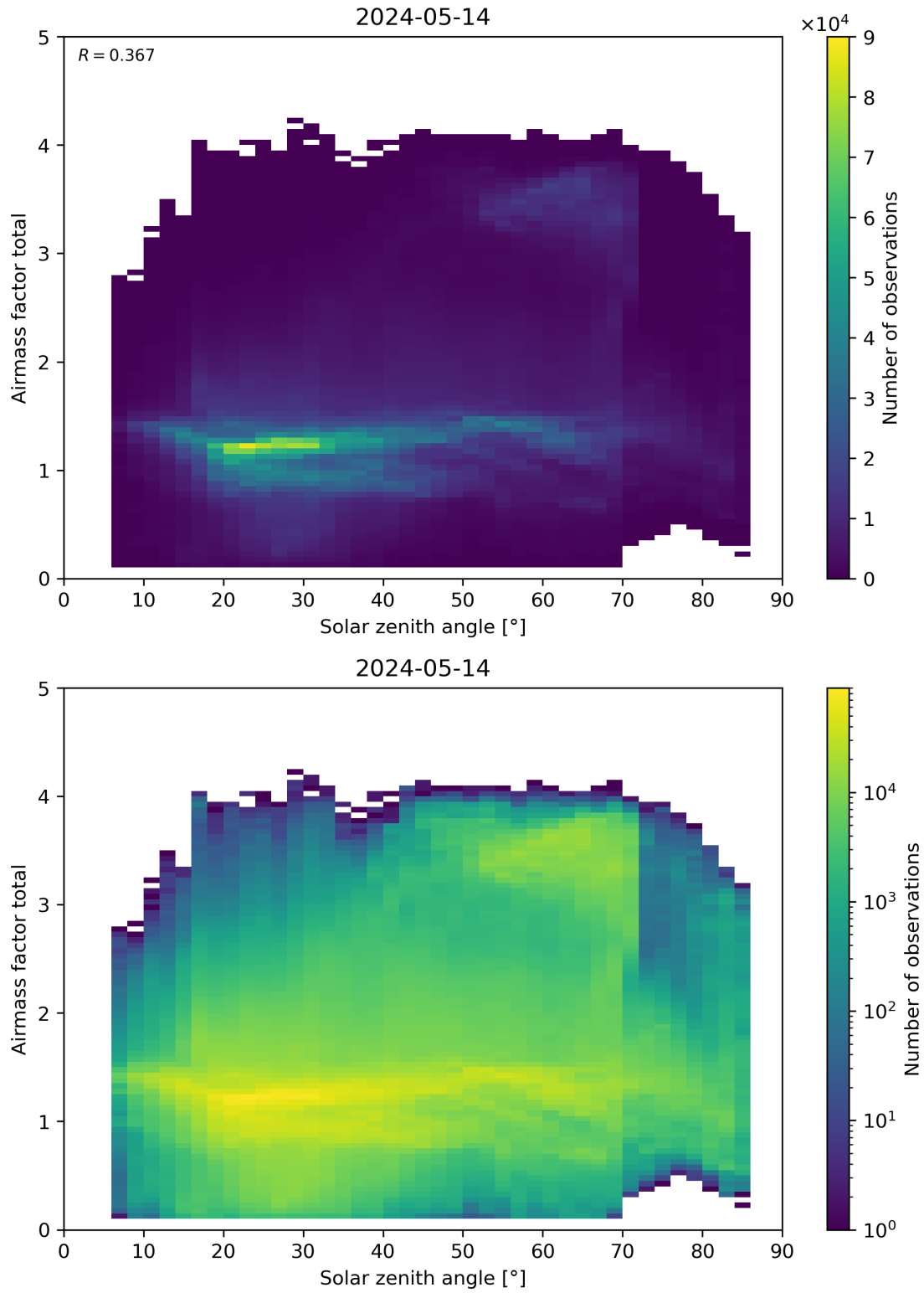
Figure 175: Scatter density plot of “Solar zenith angle” against “Airmass factor total” for 2024-05-13 to 2024-05-15.
