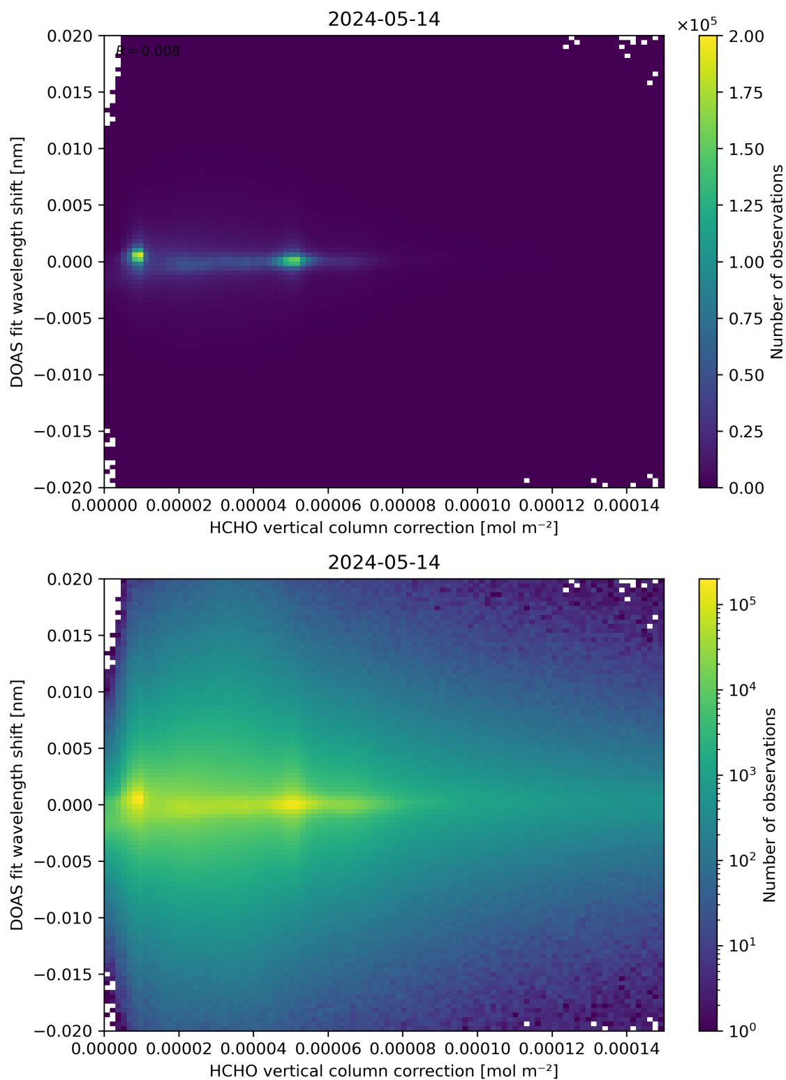
Figure 113: Scatter density plot of “HCHO vertical column correction” against “DOAS fit wavelength shift” for 2024-05-13 to 2024-05-15.
