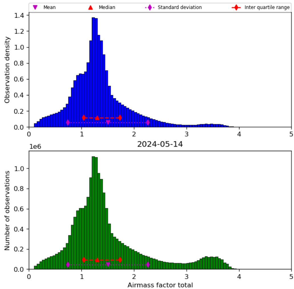
Figure 40: Histogram of “Airmass factor total” for 2024-05-13 to 2024-05-15
