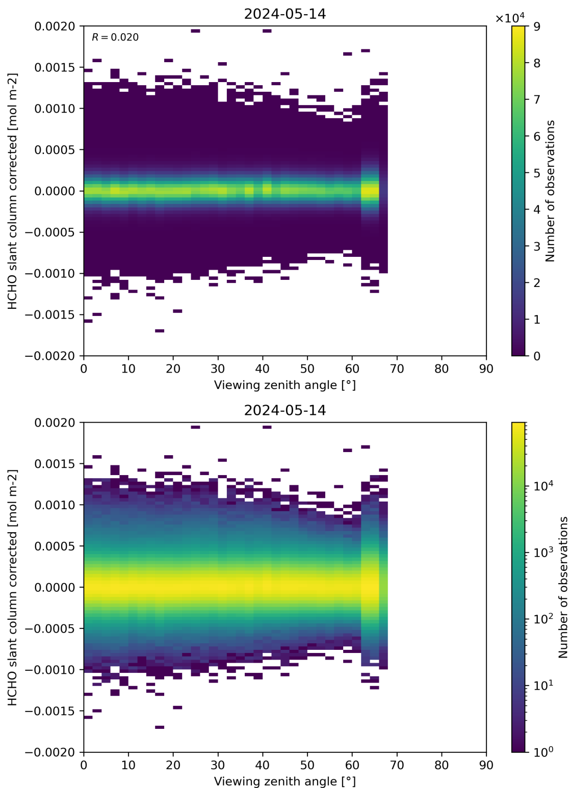
Figure 186: Scatter density plot of “Viewing zenith angle” against “HCHO slant column corrected” for 2024-05-13 to 2024-05-15.
