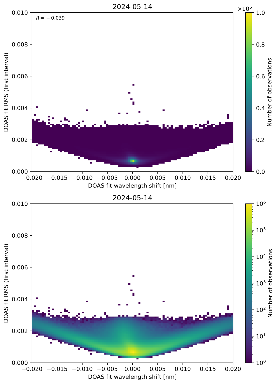
Figure 64: Scatter density plot of “DOAS fit wavelength shift” against “DOAS fit RMS (first interval)” for 2024-05-13 to 2024-05-15.
