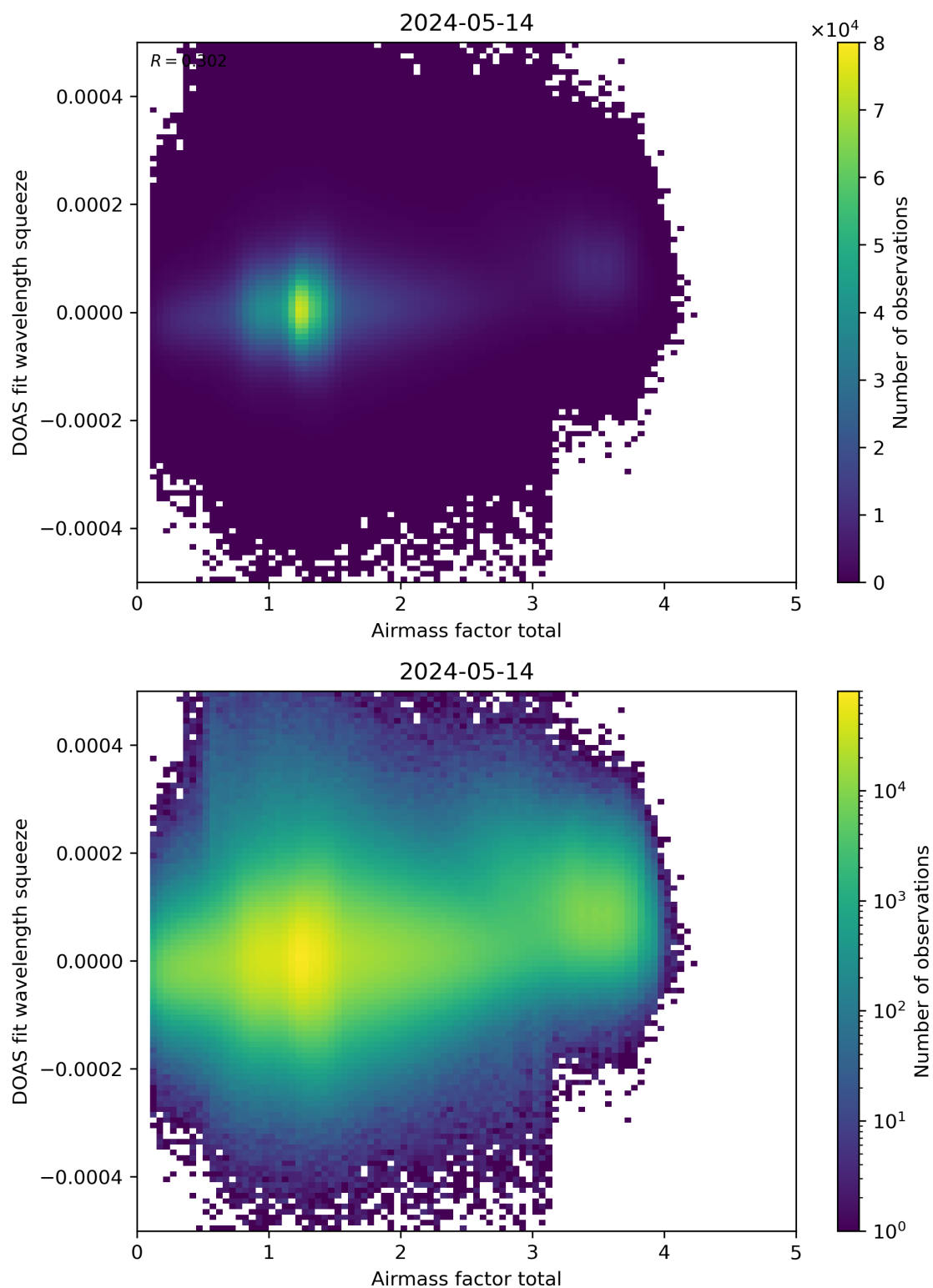
Figure 99: Scatter density plot of “Airmass factor total” against “DOAS fit wavelength squeeze” for 2024-05-13 to 2024-05-15.
