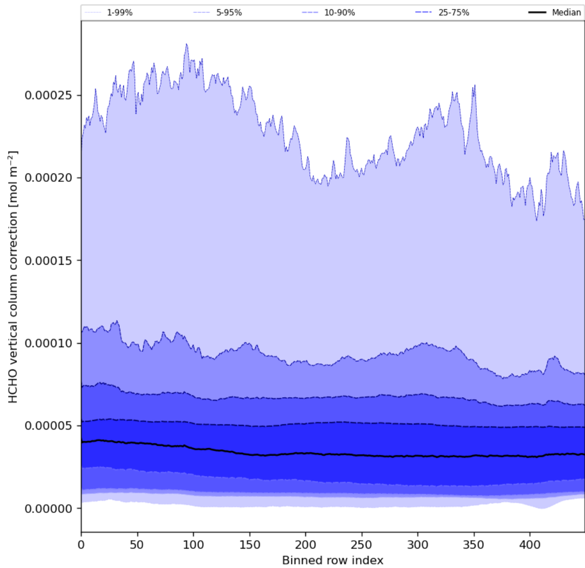
Figure 51: Along track statistics of “HCHO vertical column correction” for 2024-05-13 to 2024-05-15
