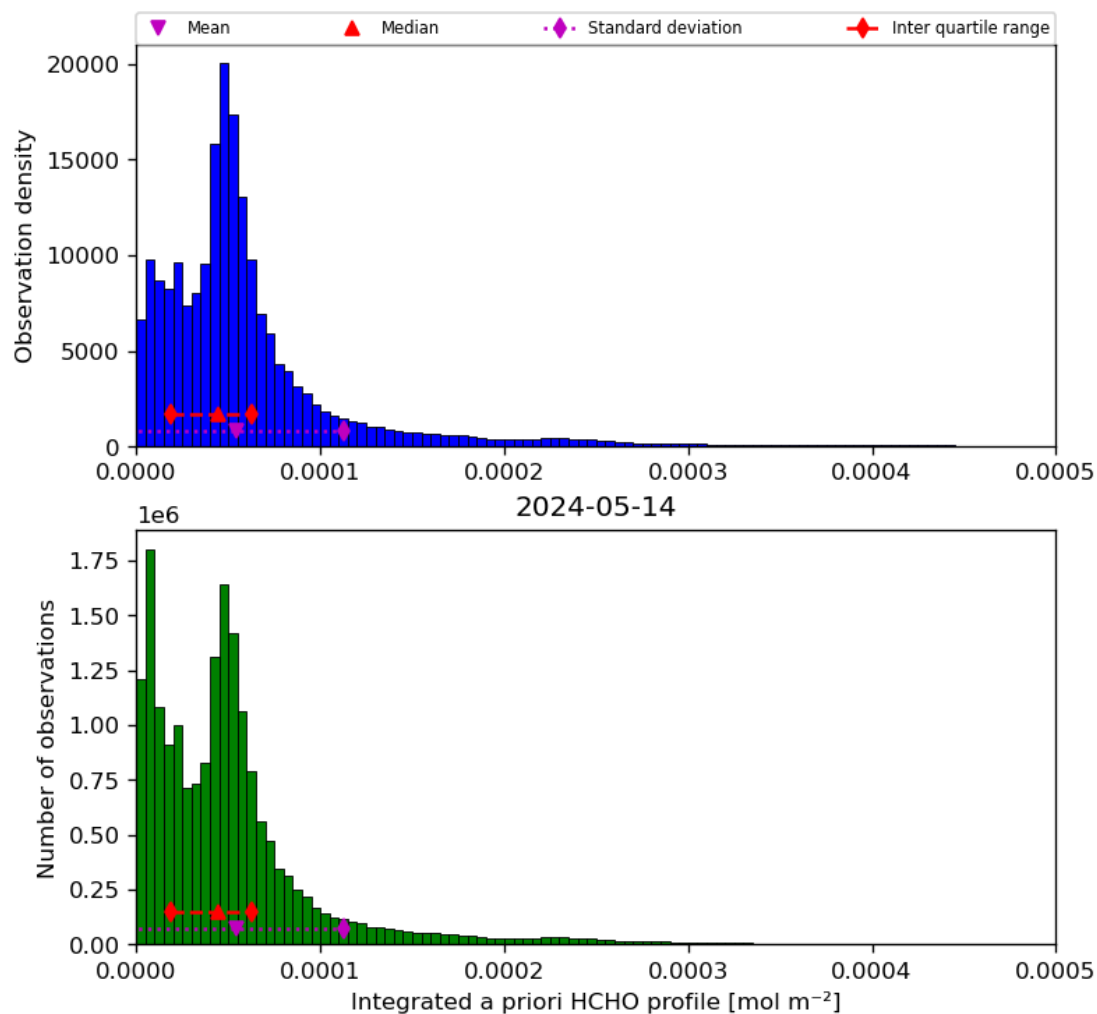
Figure 43: Histogram of “Integrated a priori HCHO profile” for 2024-05-13 to 2024-05-15
