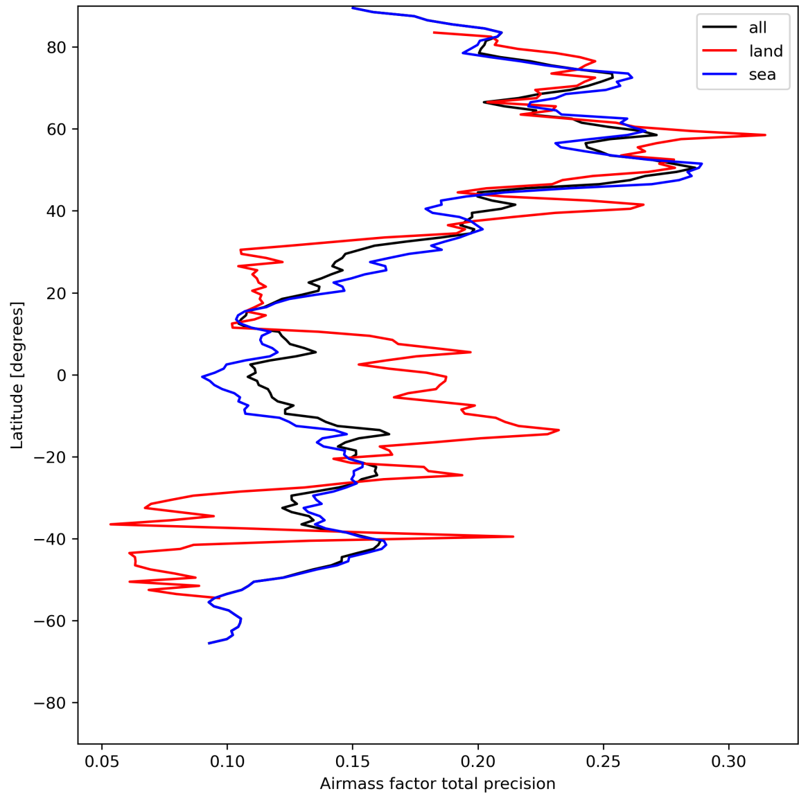
Figure 27: Zonal average of “Airmass factor total precision” for 2024-05-13 to 2024-05-15.
