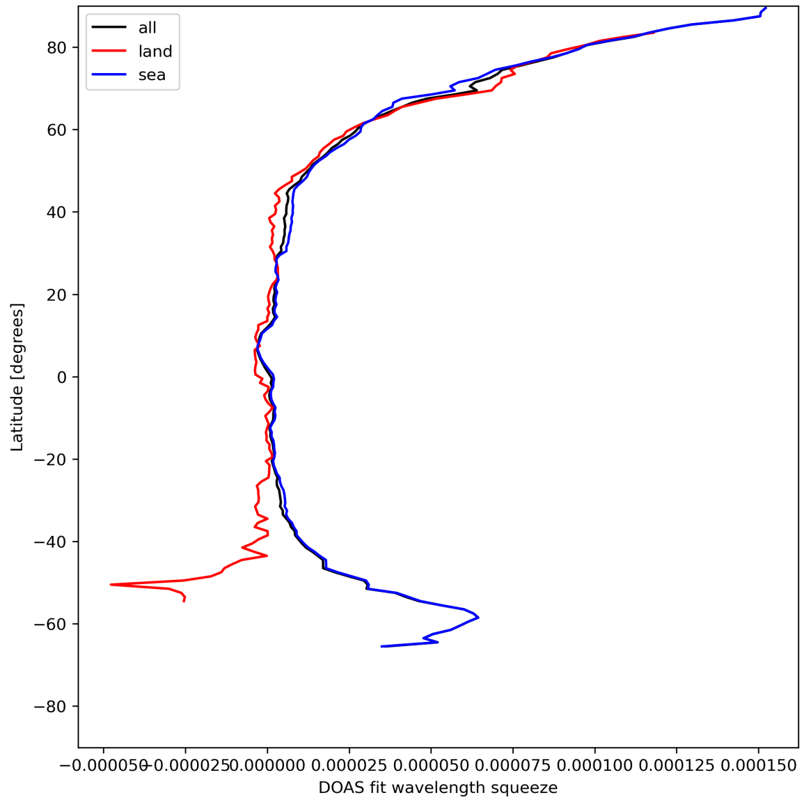
Figure 31: Zonal average of “DOAS fit wavelength squeeze” for 2024-05-13 to 2024-05-15.
