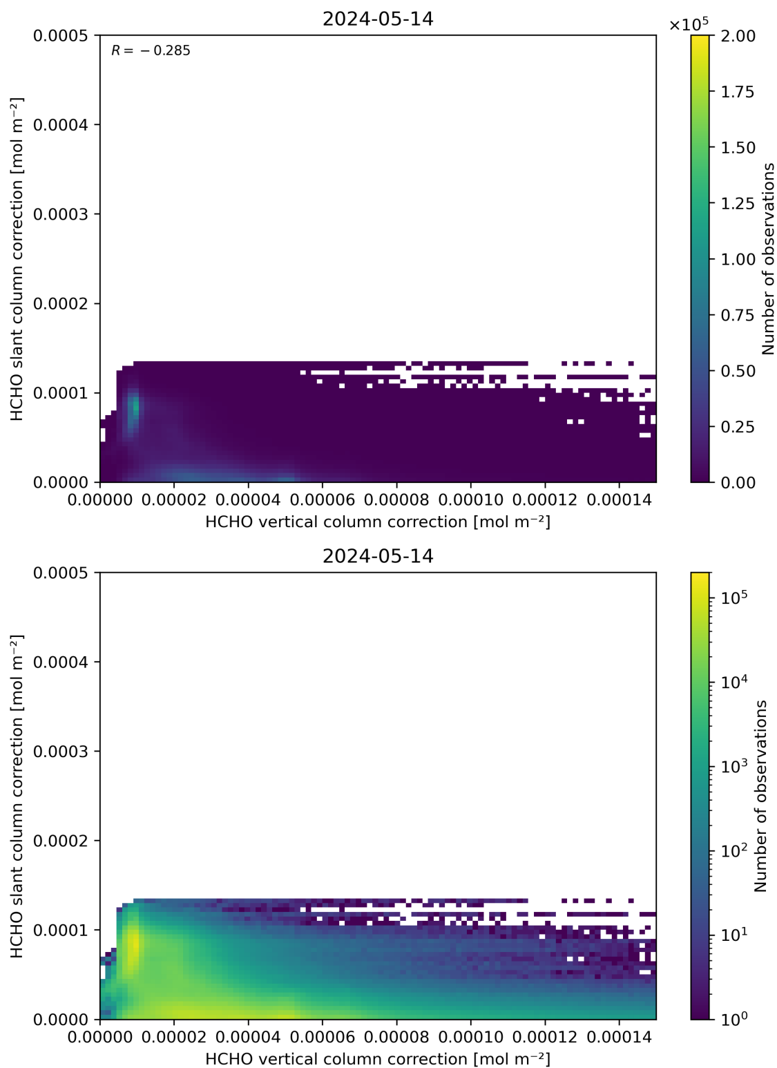
Figure 117: Scatter density plot of “HCHO vertical column correction” against “HCHO slant column correction” for 2024-05-13 to 2024-05-15.
