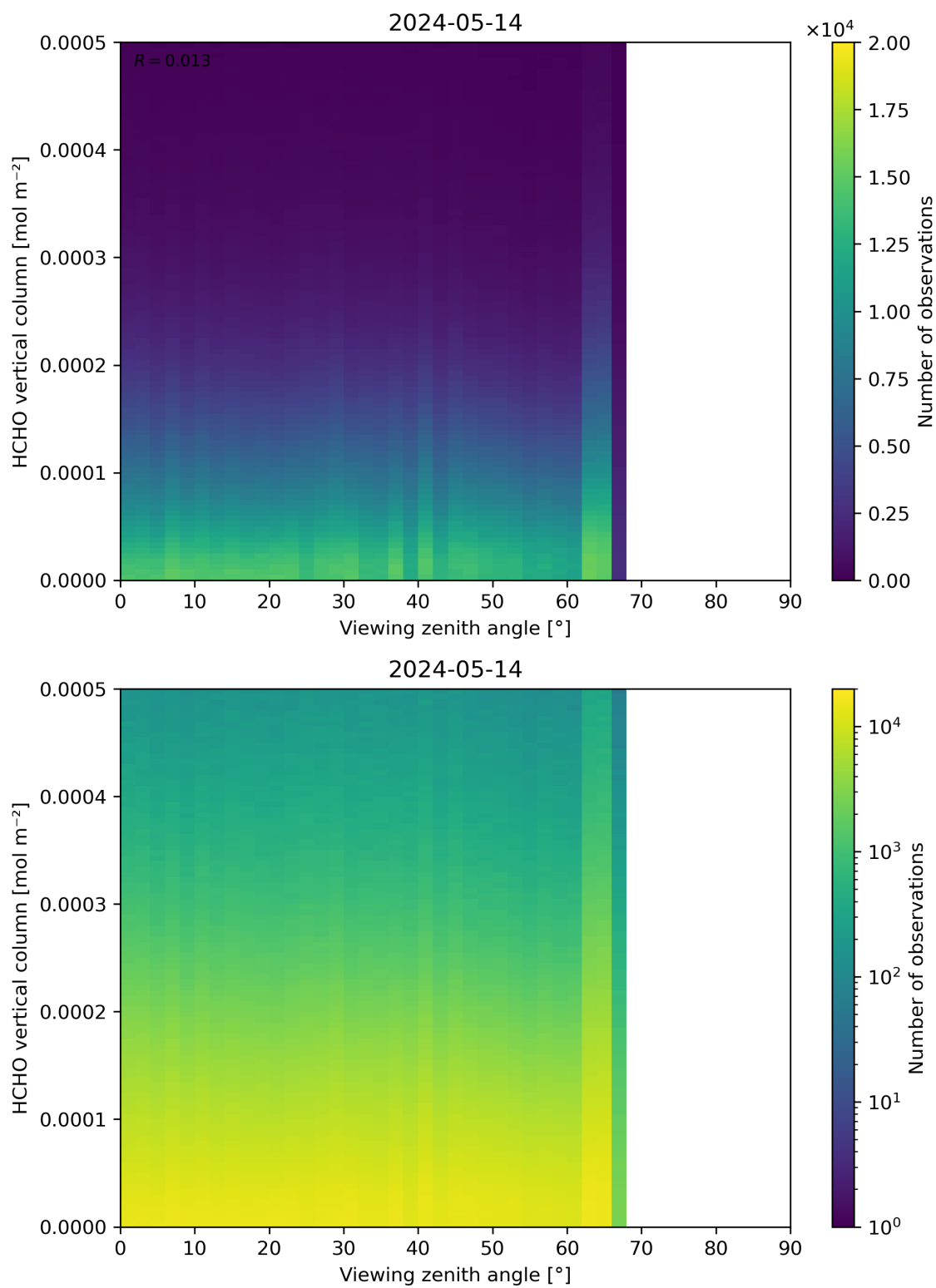
Figure 192: Scatter density plot of “Viewing zenith angle” against “HCHO vertical column” for 2024-05-13 to 2024-05-15.
