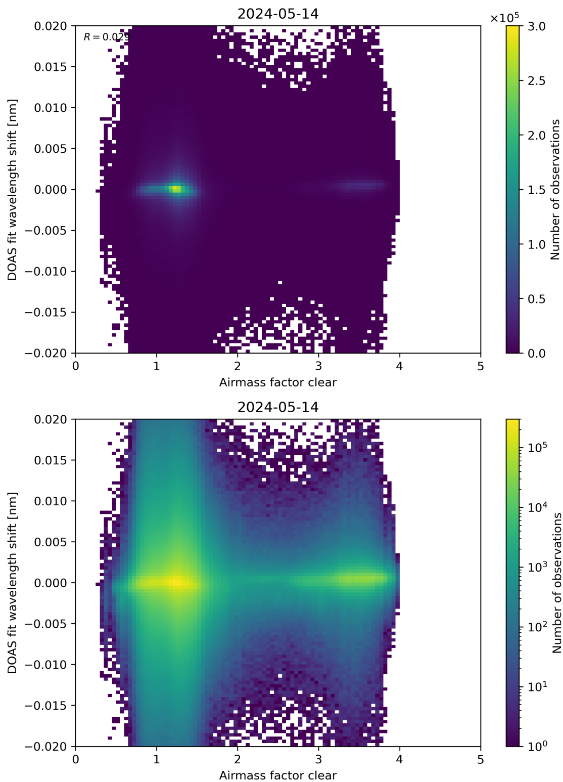
Figure 72: Scatter density plot of “Airmass factor clear” against “DOAS fit wavelength shift” for 2024-05-13 to 2024-05-15.
