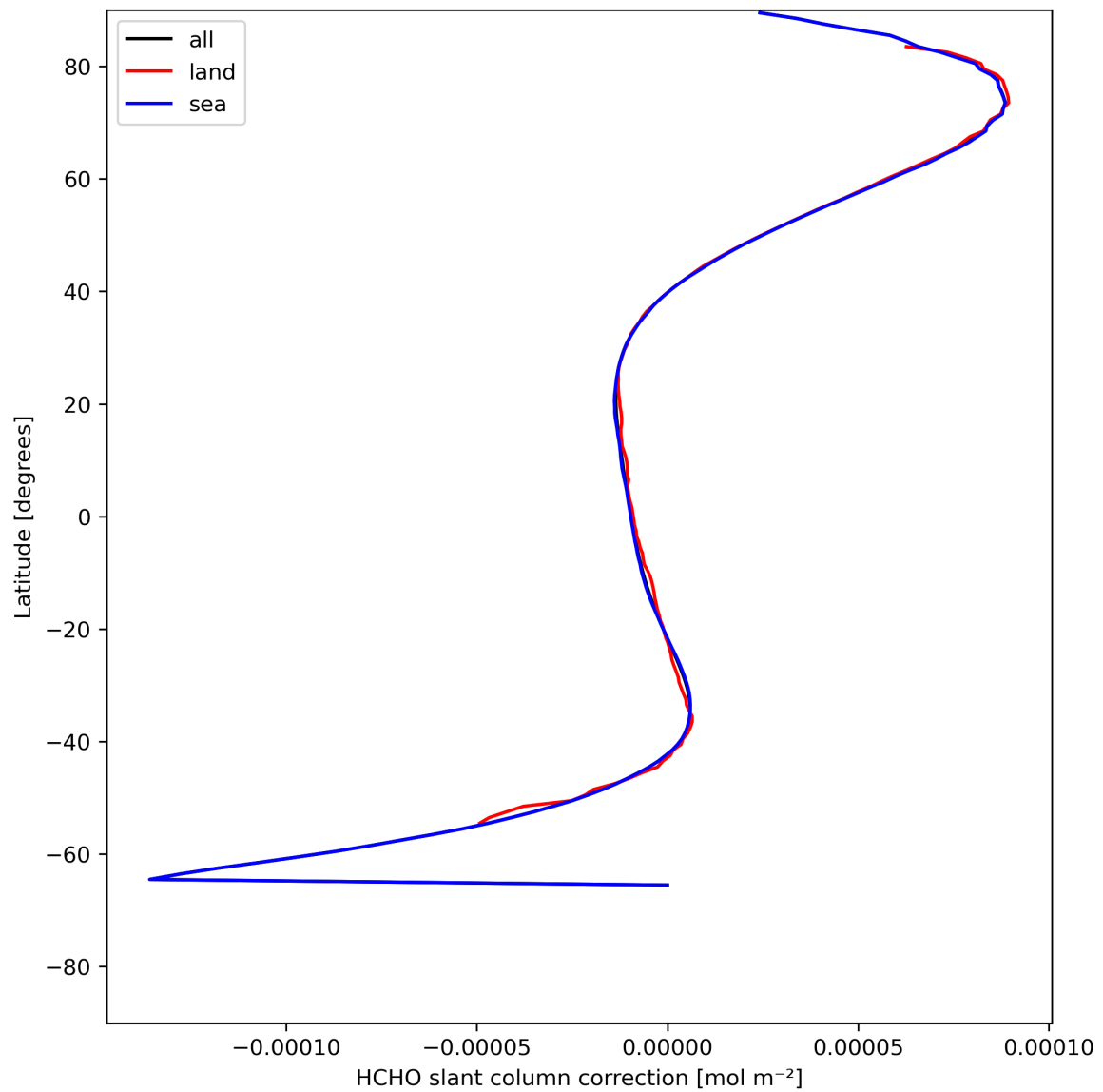
Figure 33: Zonal average of “HCHO slant column correction” for 2024-05-13 to 2024-05-15.
