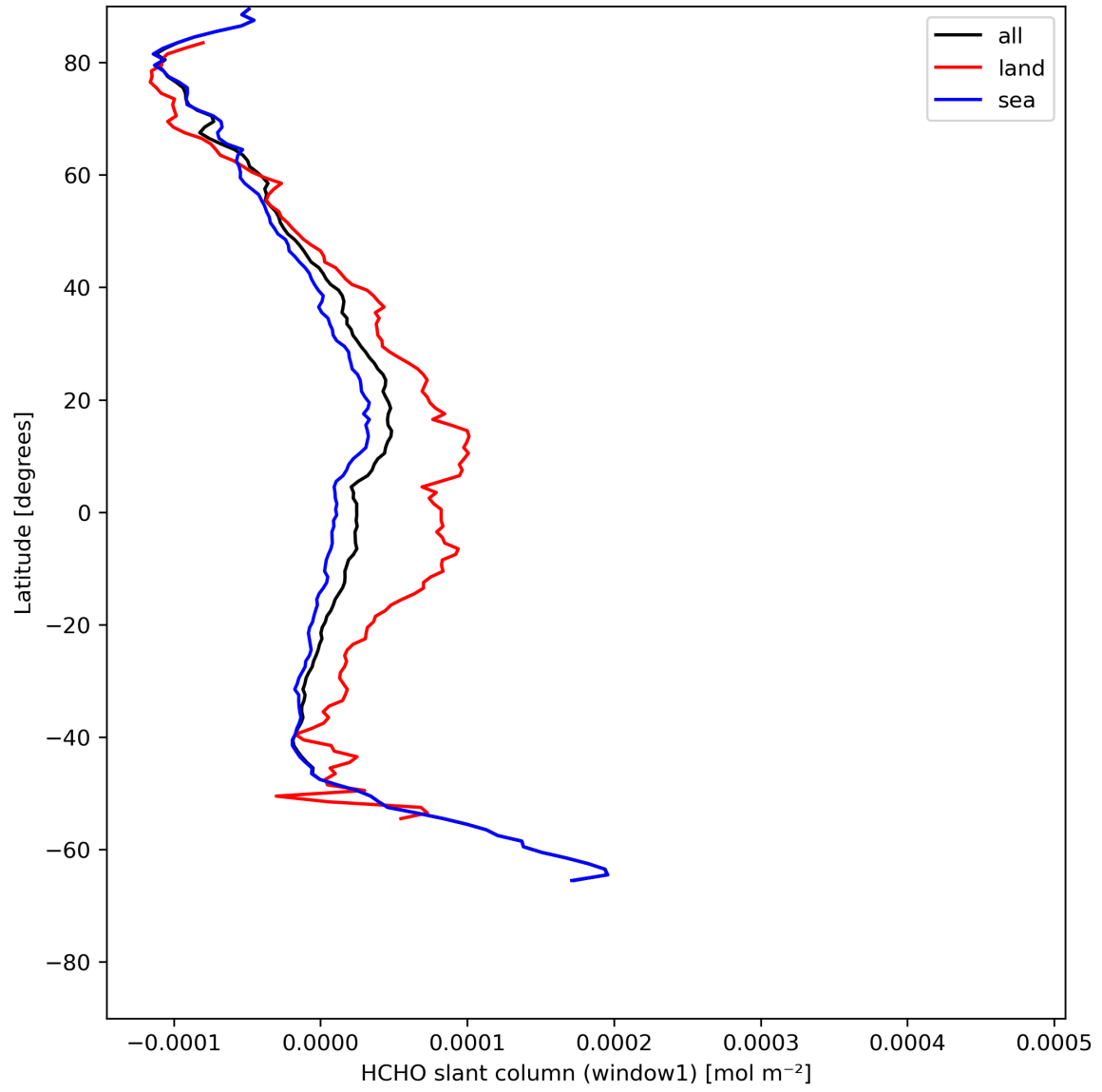
Figure 24: Zonal average of “HCHO slant column (window1)” for 2024-05-13 to 2024-05-15.
