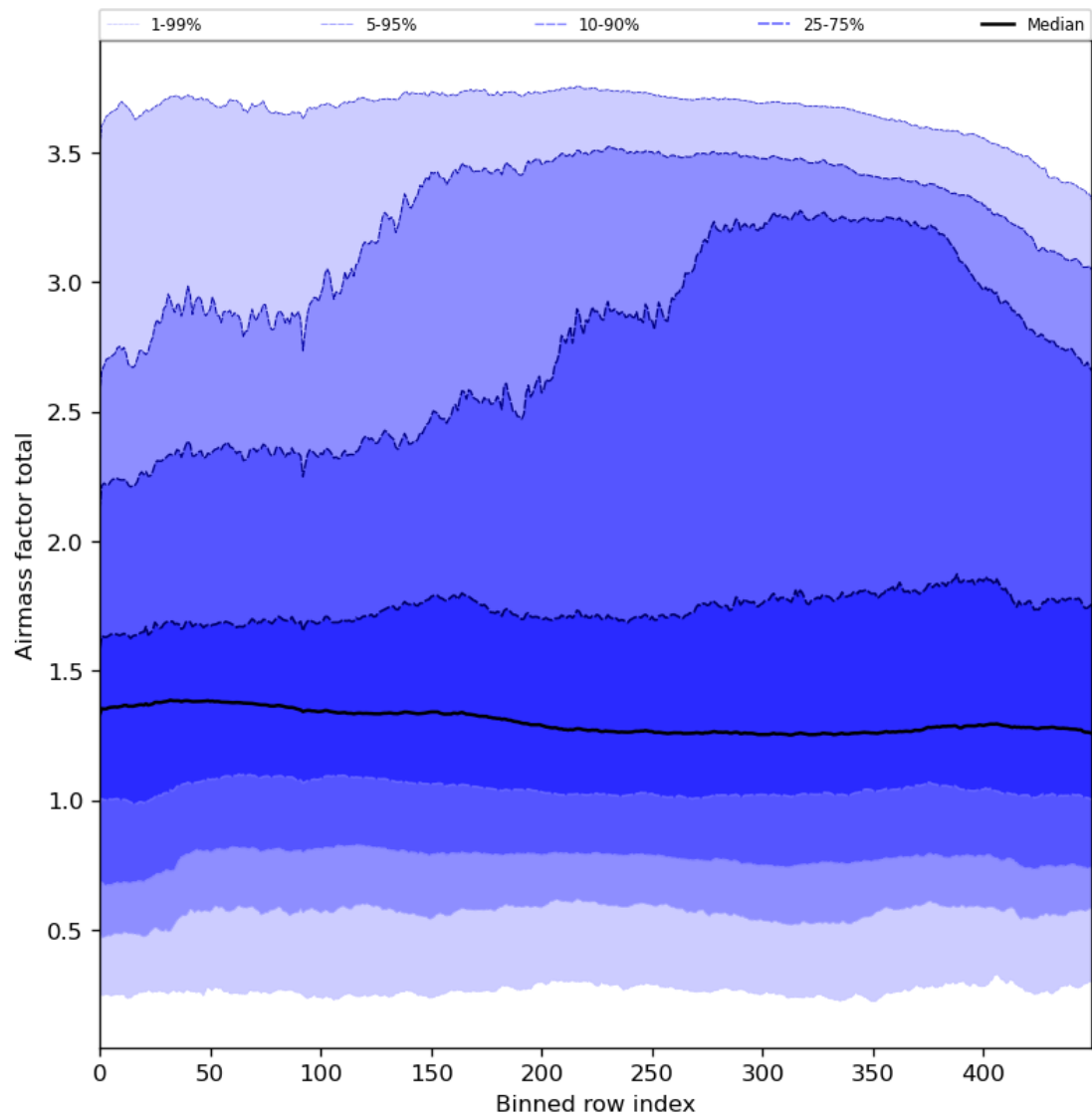
Figure 54: Along track statistics of “Airmass factor total” for 2024-05-13 to 2024-05-15
