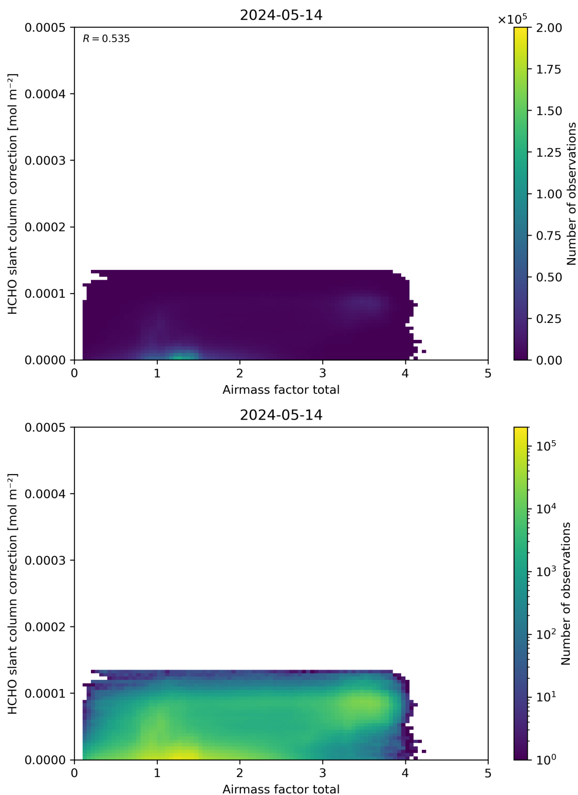
Figure 102: Scatter density plot of “Airmass factor total” against “HCHO slant column correction” for 2024-05-13 to 2024-05-15.
