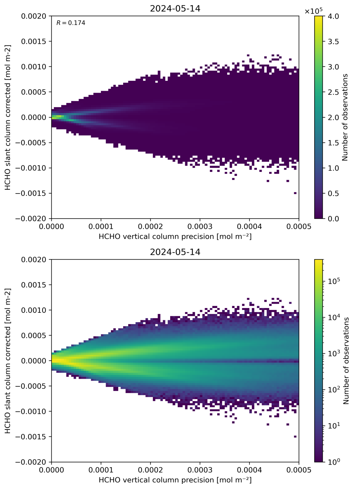
Figure 140: Scatter density plot of “HCHO vertical column precision” against “HCHO slant column corrected” for 2024-05-13 to 2024-05-15.
