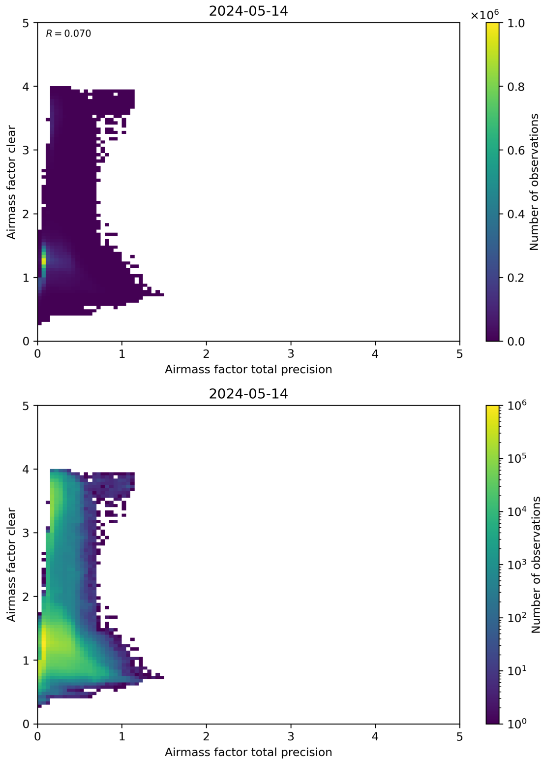
Figure 108: Scatter density plot of “Airmass factor total precision” against “Airmass factor clear” for 2024-05-13 to 2024-05-15.
