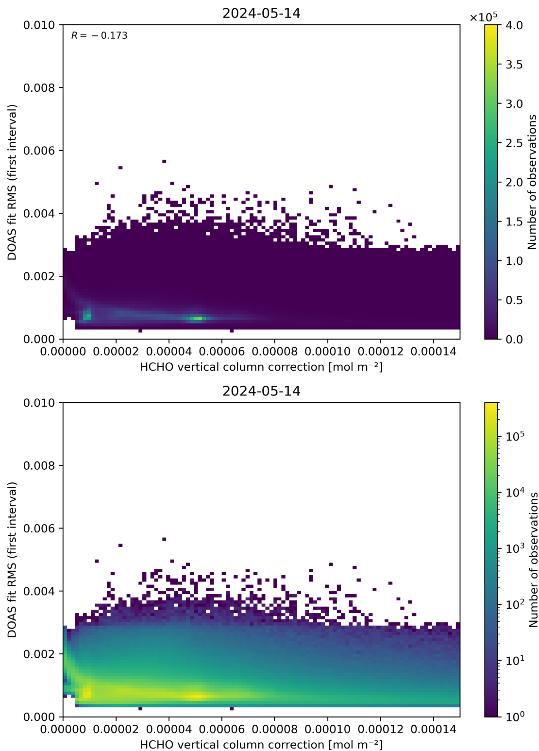
Figure 112: Scatter density plot of “HCHO vertical column correction” against “DOAS fit RMS (first interval)” for 2024-05-13 to 2024-05-15.
