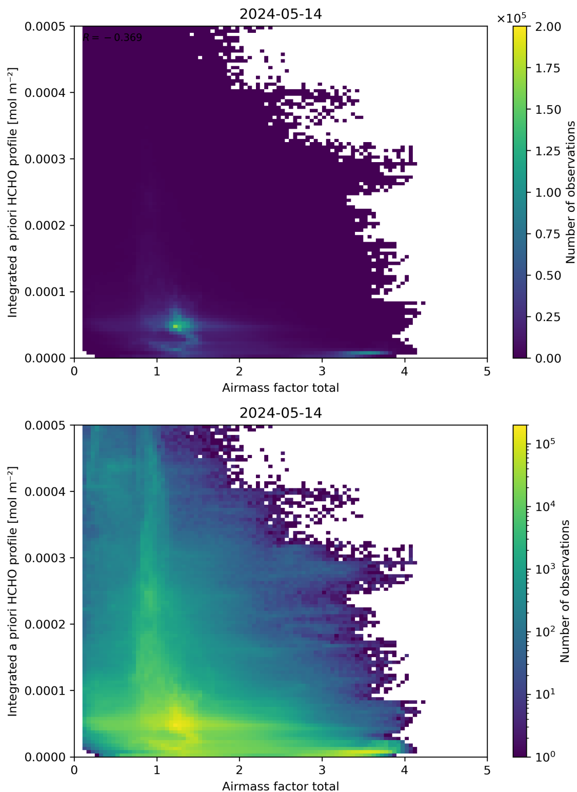
Figure 104: Scatter density plot of “Airmass factor total” against “Integrated a priori HCHO profile” for 2024-05-13 to 2024-05-15.
