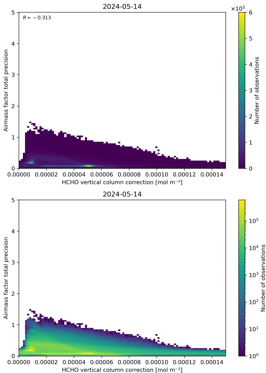
Figure 121: Scatter density plot of “HCHO vertical column correction” against “Airmass factor total precision” for 2024-05-13 to 2024-05-15.
