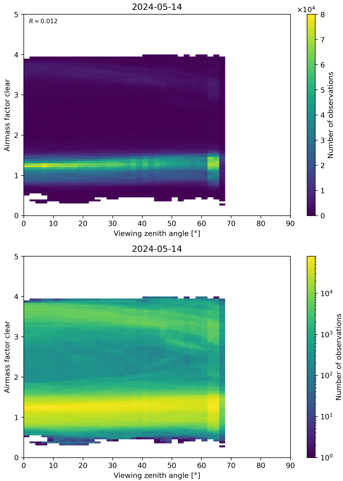
Figure 185: Scatter density plot of “Viewing zenith angle” against “Airmass factor clear” for 2024-05-13 to 2024-05-15.
