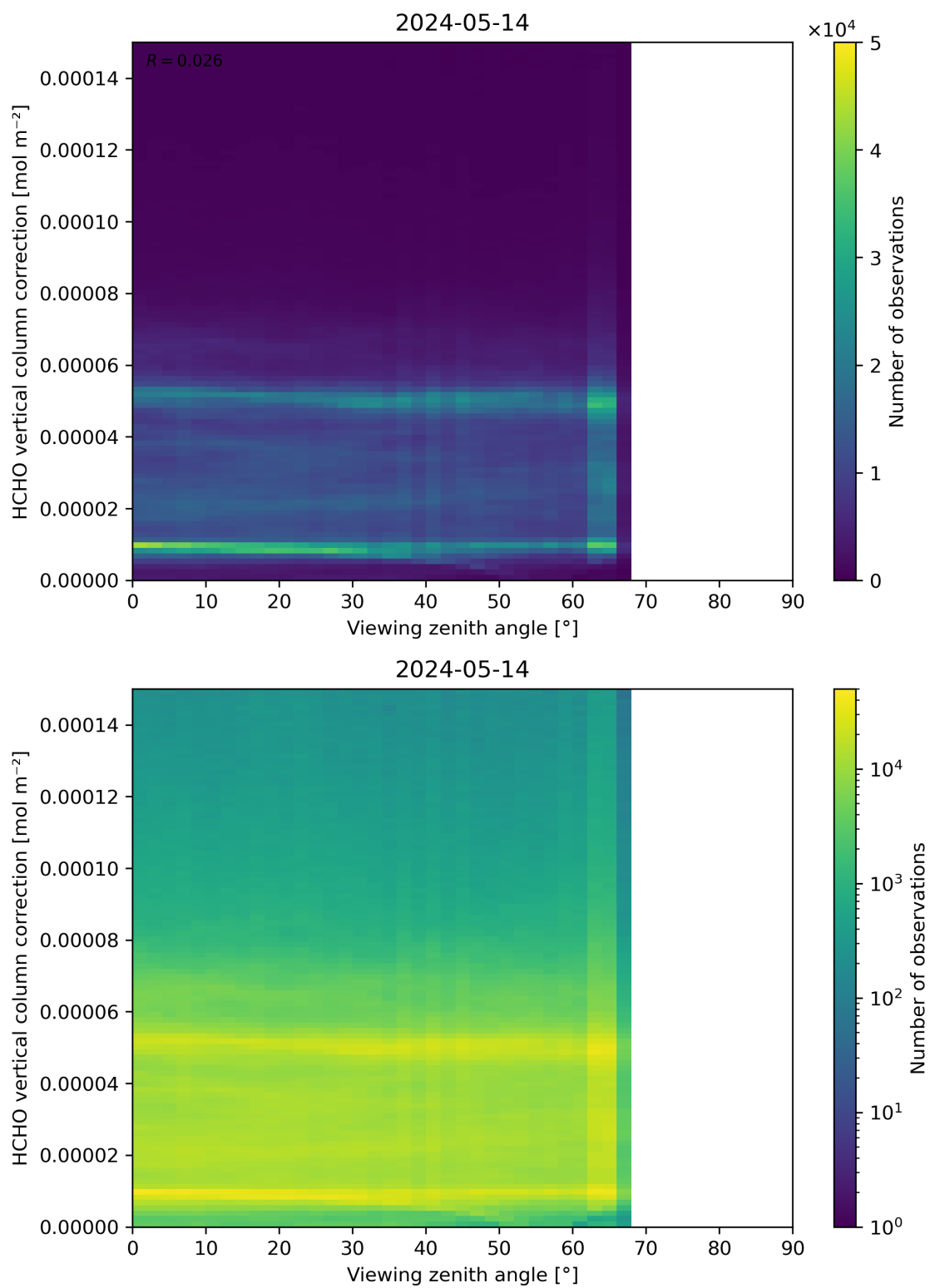
Figure 193: Scatter density plot of “Viewing zenith angle” against “HCHO vertical column correction” for 2024-05-13 to 2024-05-15.
