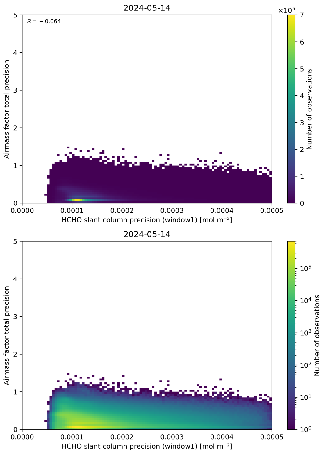
Figure 95: Scatter density plot of “HCHO slant column precision (window1)” against “Airmass factor total precision” for 2024-05-13 to 2024-05-15.
