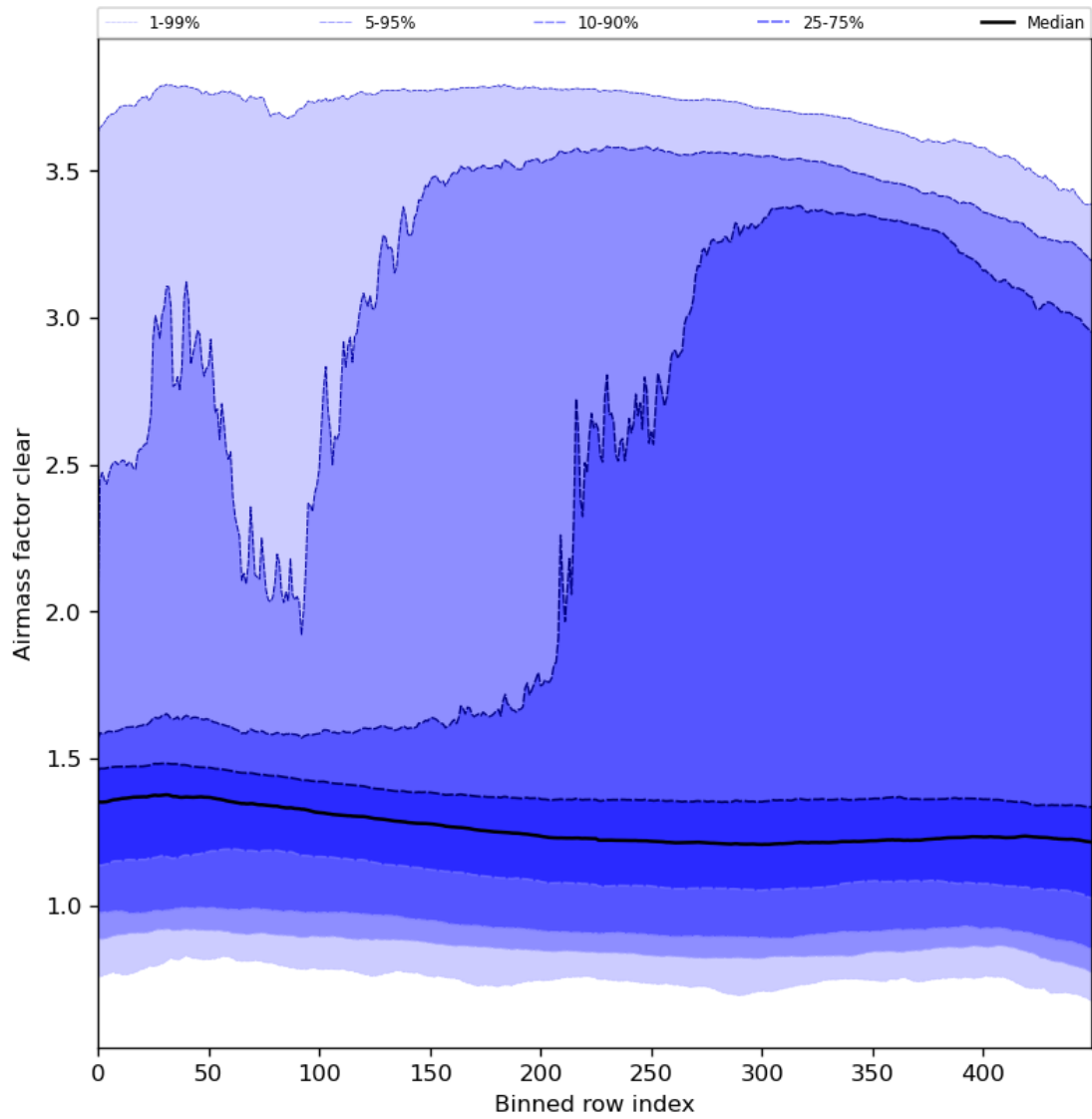
Figure 56: Along track statistics of “Airmass factor clear” for 2024-05-13 to 2024-05-15
