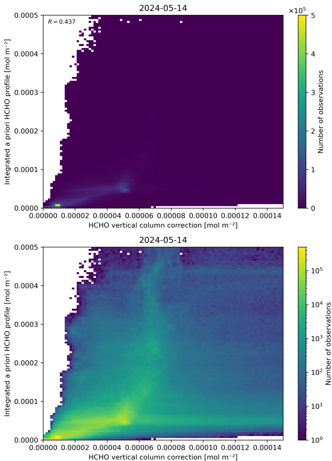
Figure 122: Scatter density plot of “HCHO vertical column correction” against “Integrated a priori HCHO profile” for 2024-05-13 to 2024-05-15.
