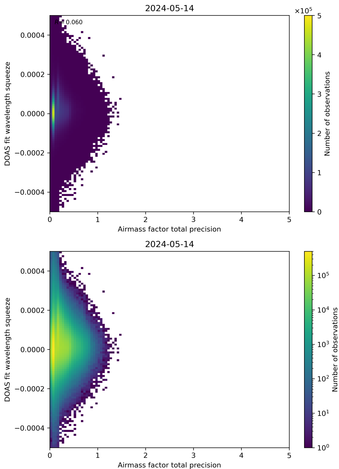
Figure 107: Scatter density plot of “Airmass factor total precision” against “DOAS fit wavelength squeeze” for 2024-05-13 to 2024-05-15.
