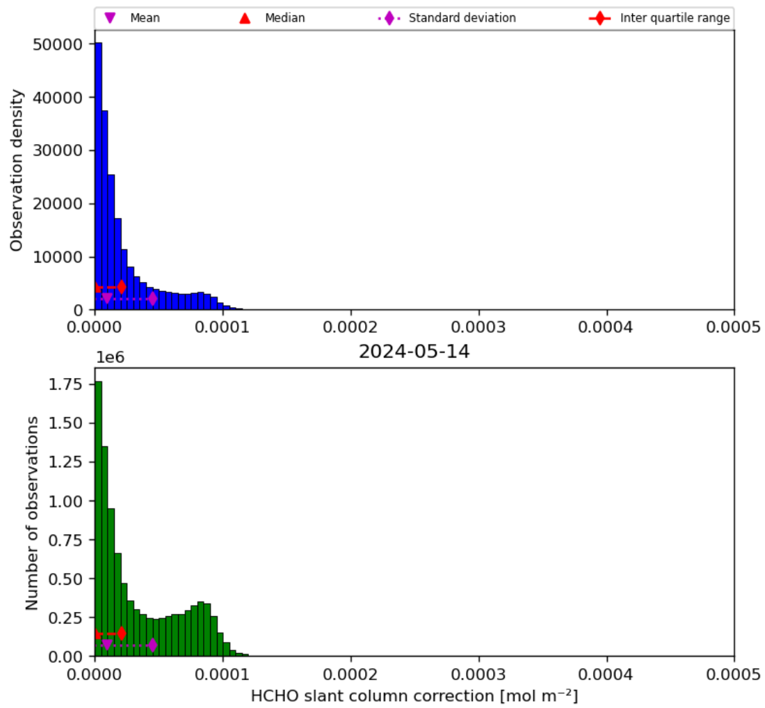
Figure 47: Histogram of “HCHO slant column correction” for 2024-05-13 to 2024-05-15
