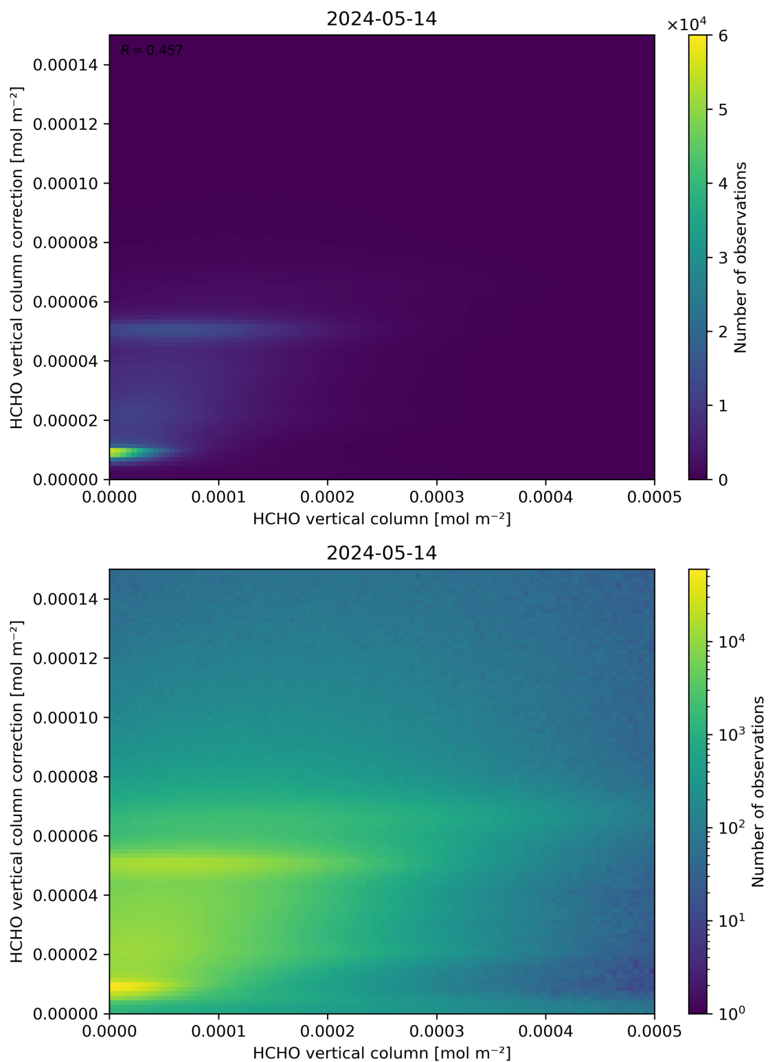
Figure 133: Scatter density plot of “HCHO vertical column” against “HCHO vertical column correction” for 2024-05-13 to 2024-05-15.
