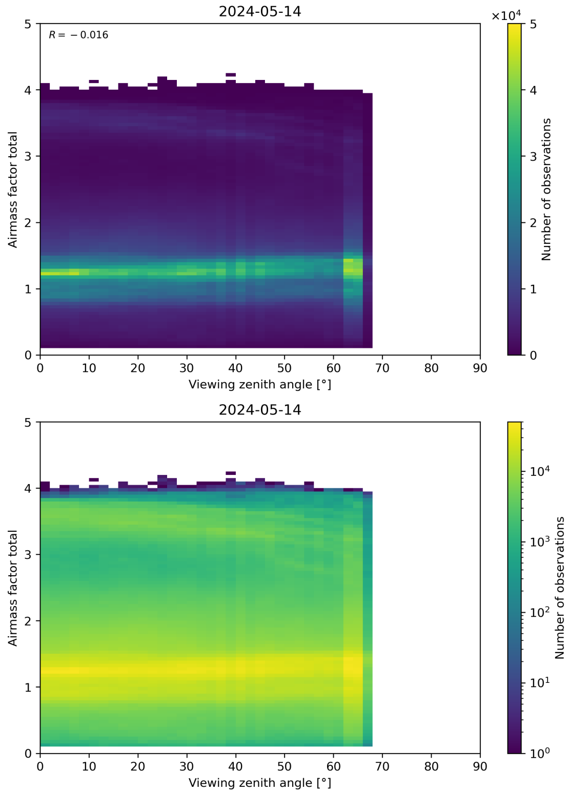
Figure 190: Scatter density plot of “Viewing zenith angle” against “Airmass factor total” for 2024-05-13 to 2024-05-15.
