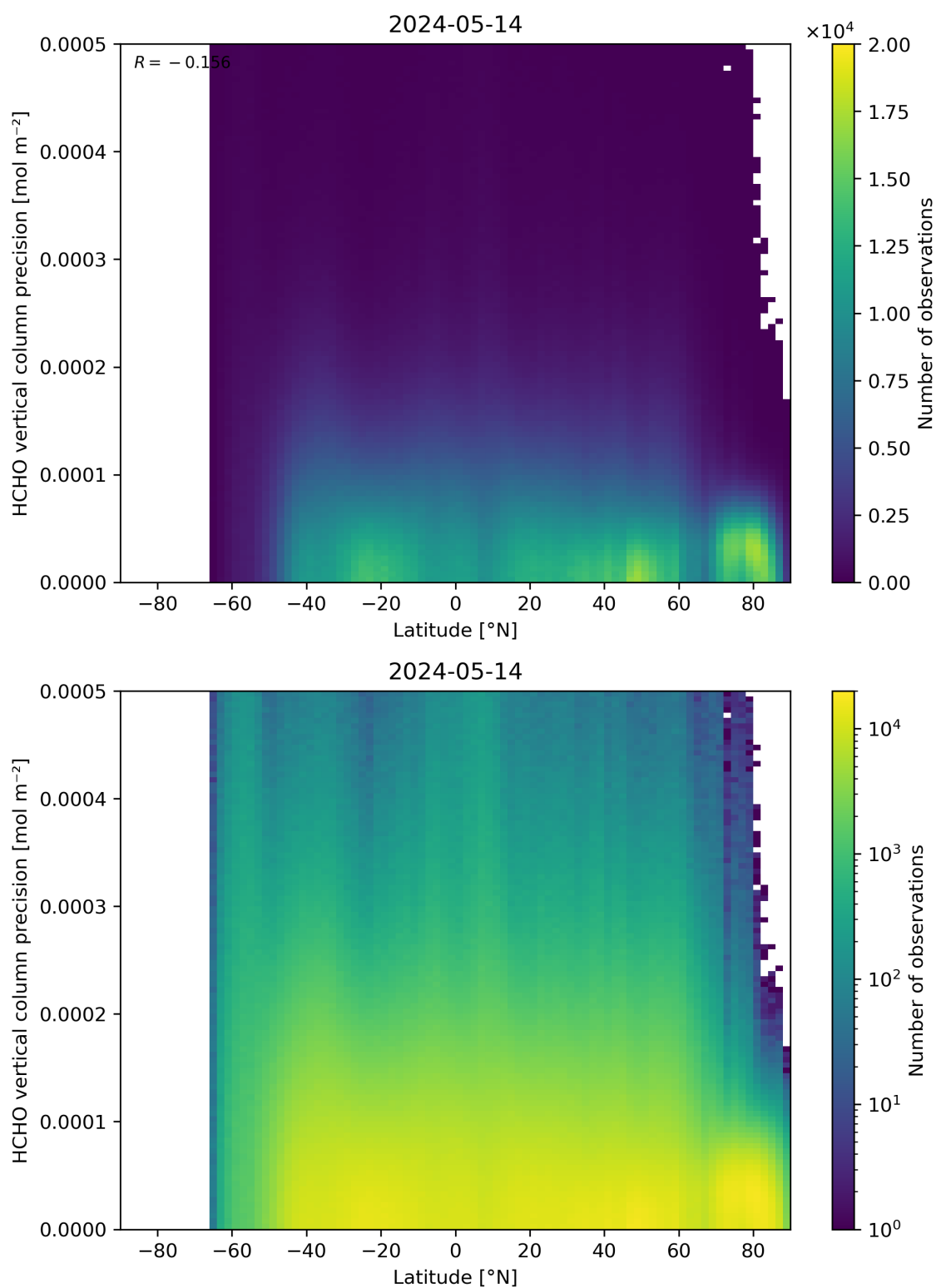
Figure 165: Scatter density plot of “Latitude” against “HCHO vertical column precision” for 2024-05-13 to 2024-05-15.
