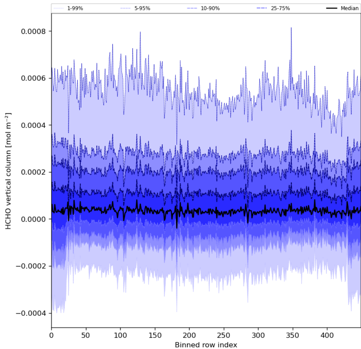
Figure 49: Along track statistics of “HCHO vertical column” for 2024-05-13 to 2024-05-15
