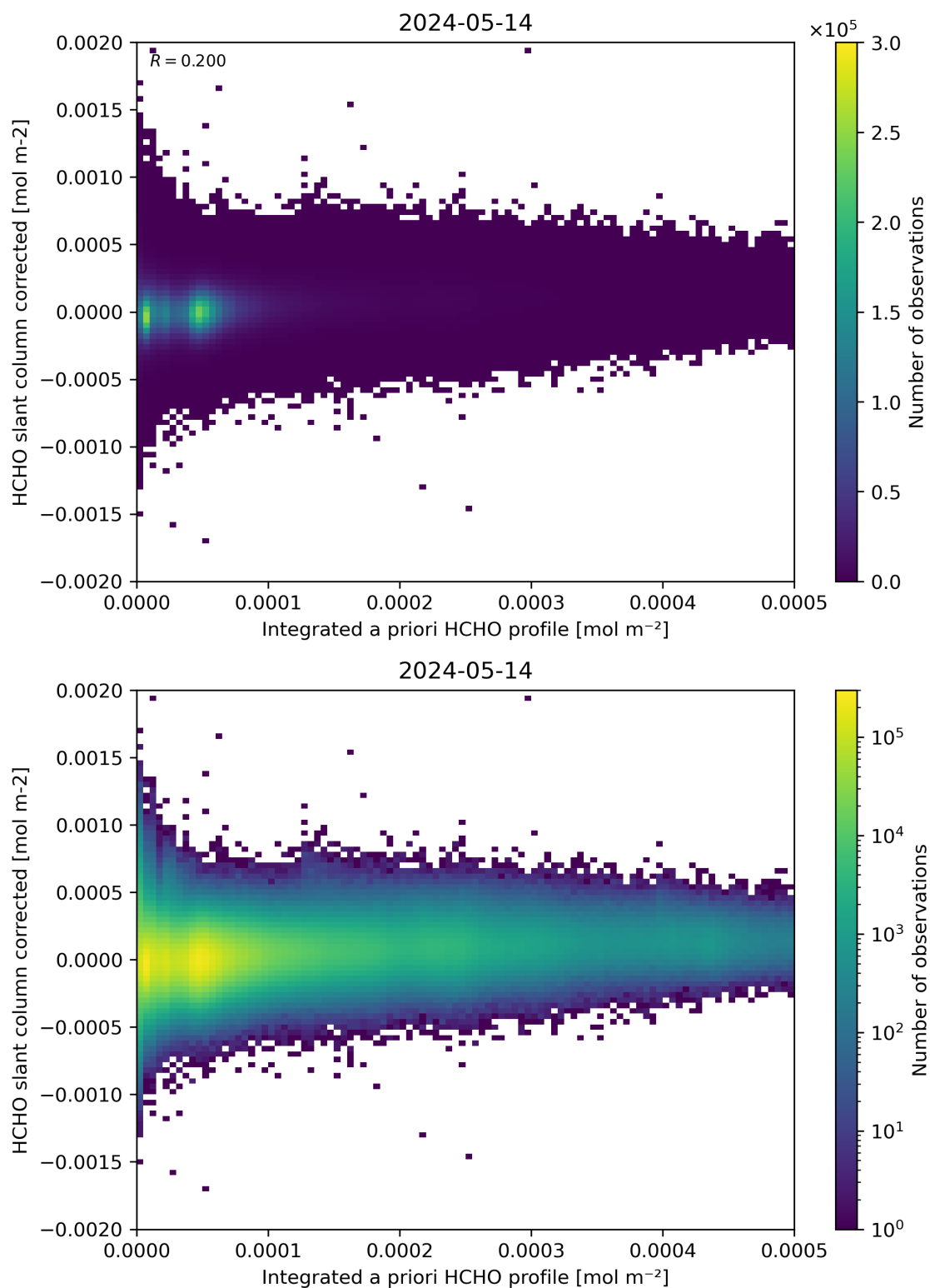
Figure 151: Scatter density plot of “Integrated a priori HCHO profile” against “HCHO slant column corrected” for 2024-05-13 to 2024-05-15.
