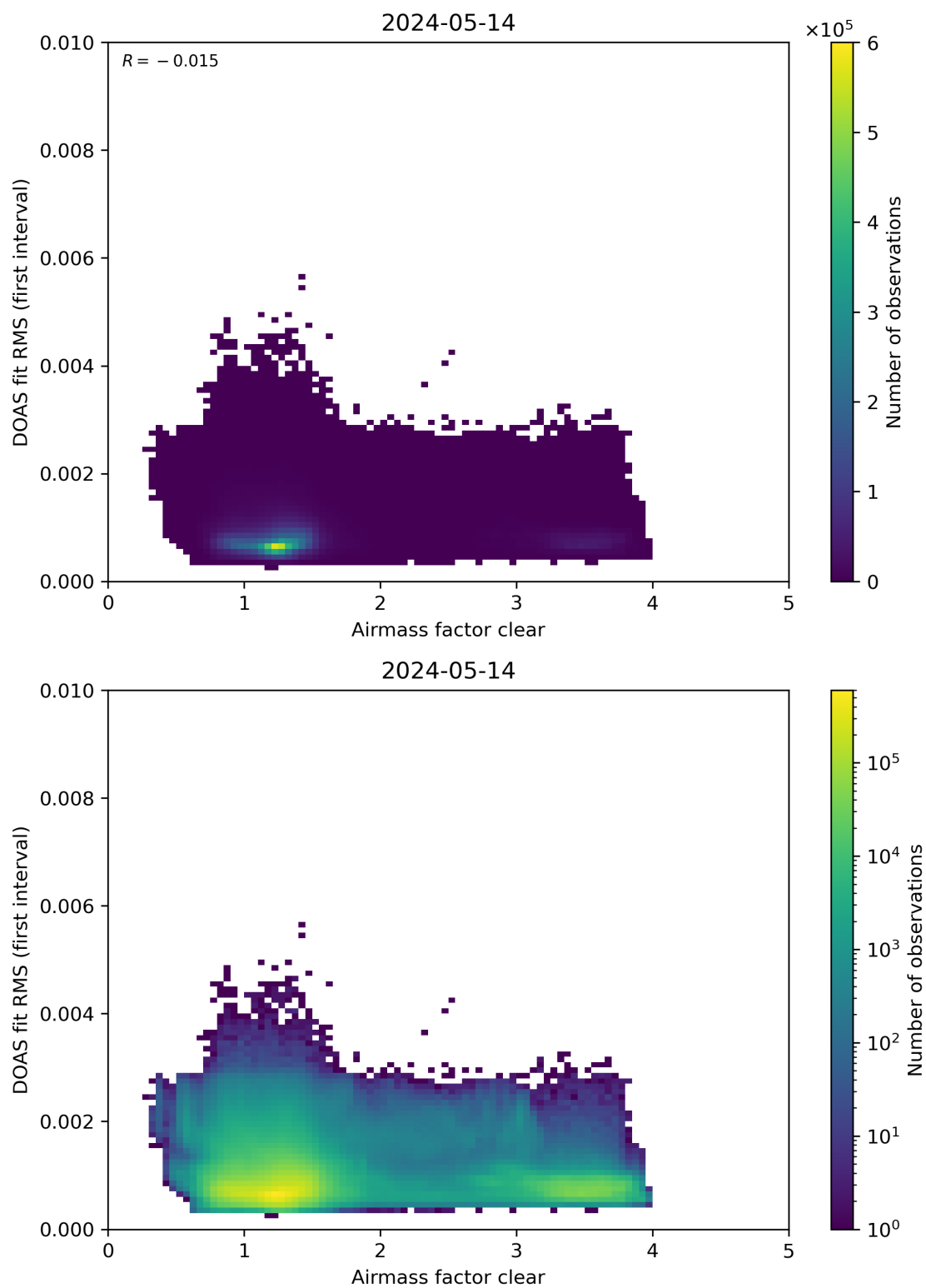
Figure 71: Scatter density plot of “Airmass factor clear” against “DOAS fit RMS (first interval)” for 2024-05-13 to 2024-05-15.
