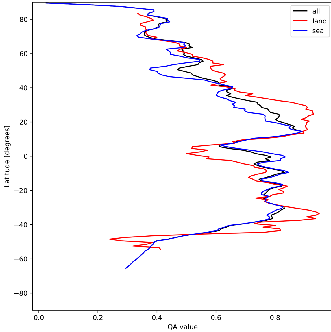
Figure 20: Zonal average of “QA value” for 2024-05-13 to 2024-05-15.
