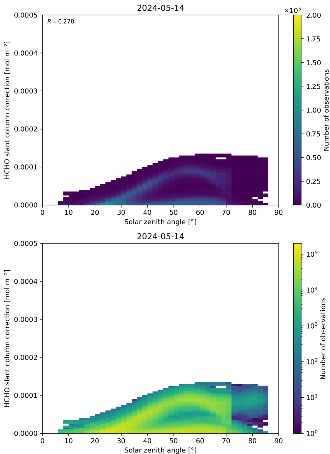
Figure 172: Scatter density plot of “Solar zenith angle” against “HCHO slant column correction” for 2024-05-13 to 2024-05-15.
