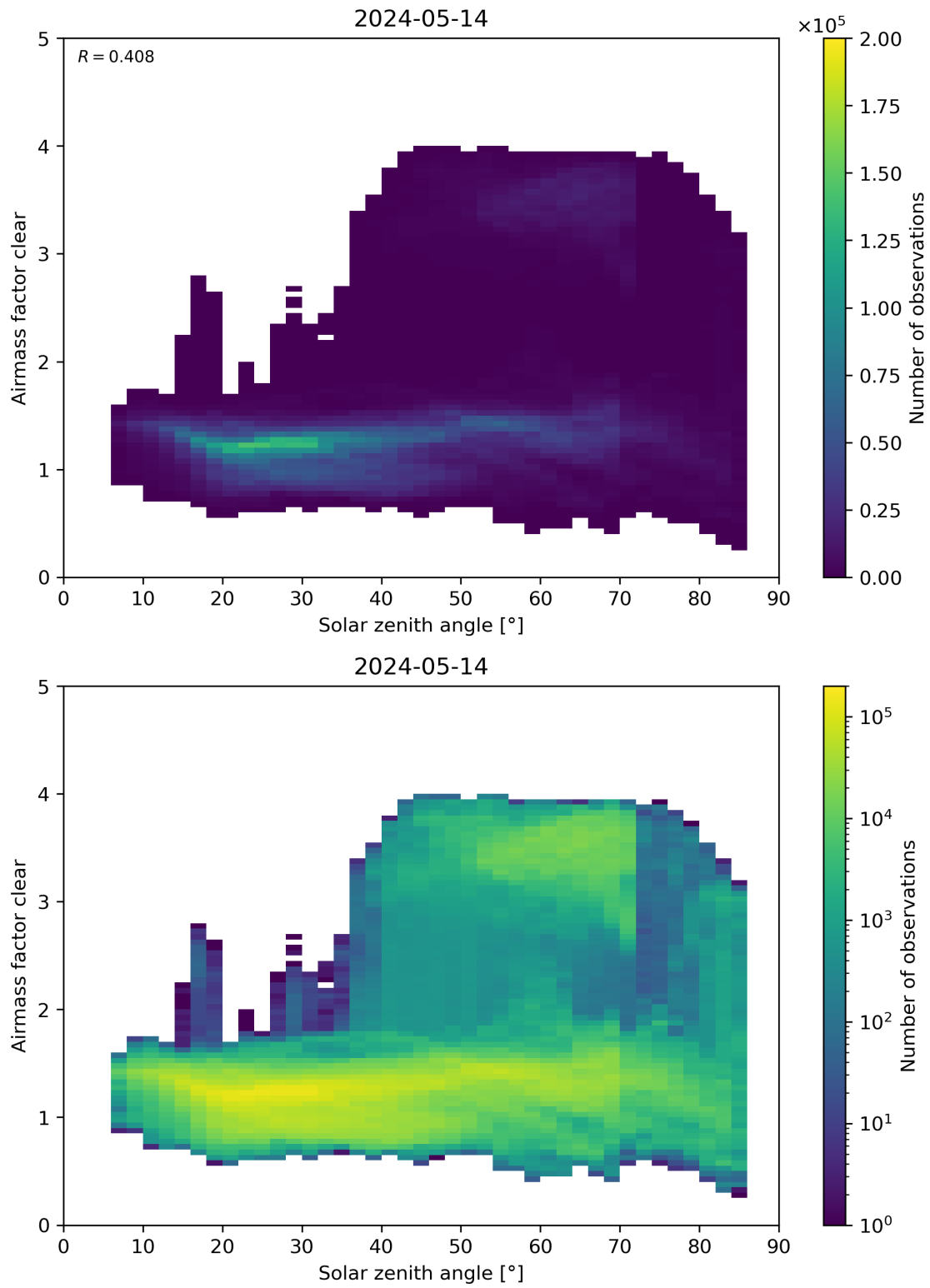
Figure 170: Scatter density plot of “Solar zenith angle” against “Airmass factor clear” for 2024-05-13 to 2024-05-15.
