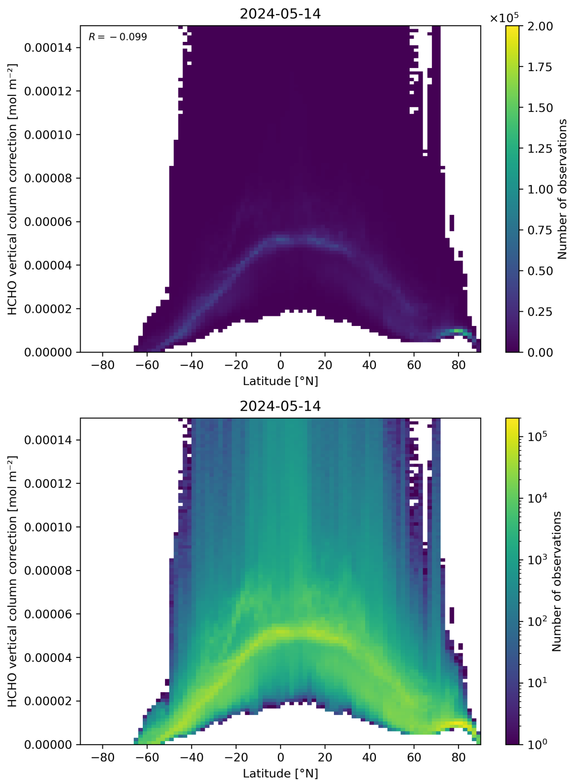
Figure 164: Scatter density plot of “Latitude” against “HCHO vertical column correction” for 2024-05-13 to 2024-05-15.
