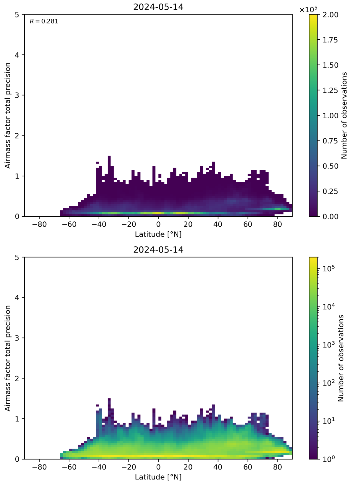
Figure 162: Scatter density plot of “Latitude” against “Airmass factor total precision” for 2024-05-13 to 2024-05-15.
