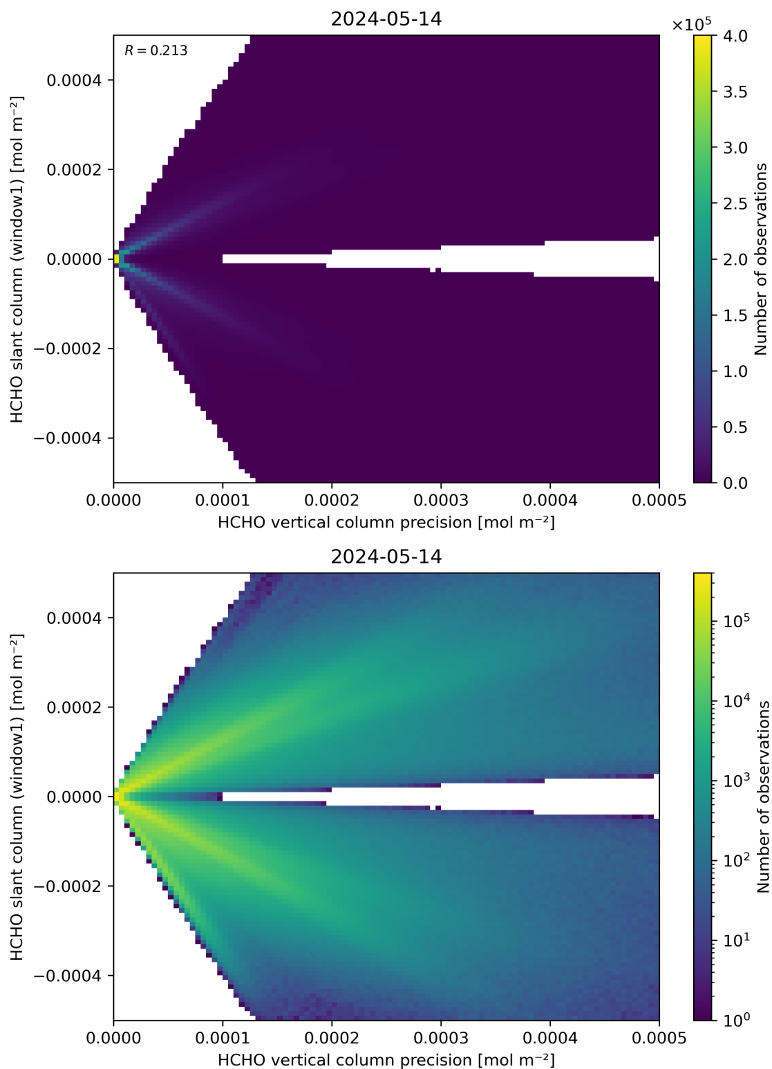
Figure 142: Scatter density plot of “HCHO vertical column precision” against “HCHO slant column (window1)” for 2024-05-13 to 2024-05-15.
