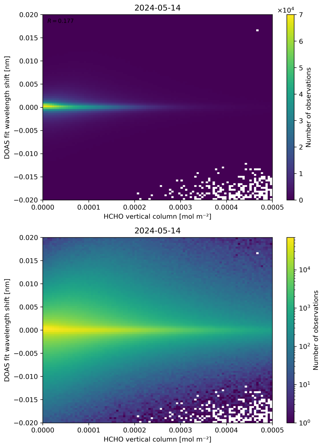
Figure 124: Scatter density plot of “HCHO vertical column” against “DOAS fit wavelength shift” for 2024-05-13 to 2024-05-15.
