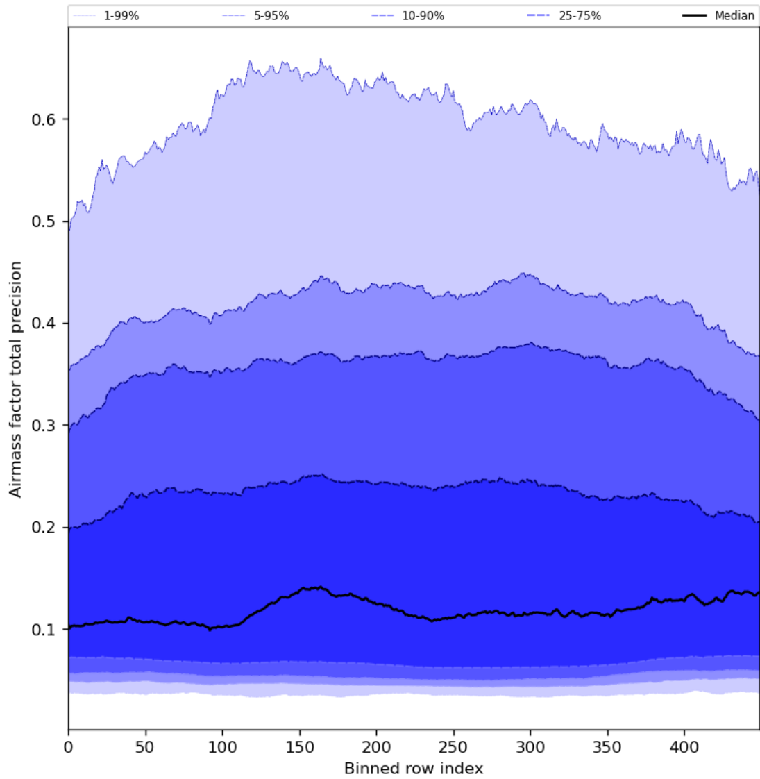
Figure 55: Along track statistics of “Airmass factor total precision” for 2024-05-13 to 2024-05-15
