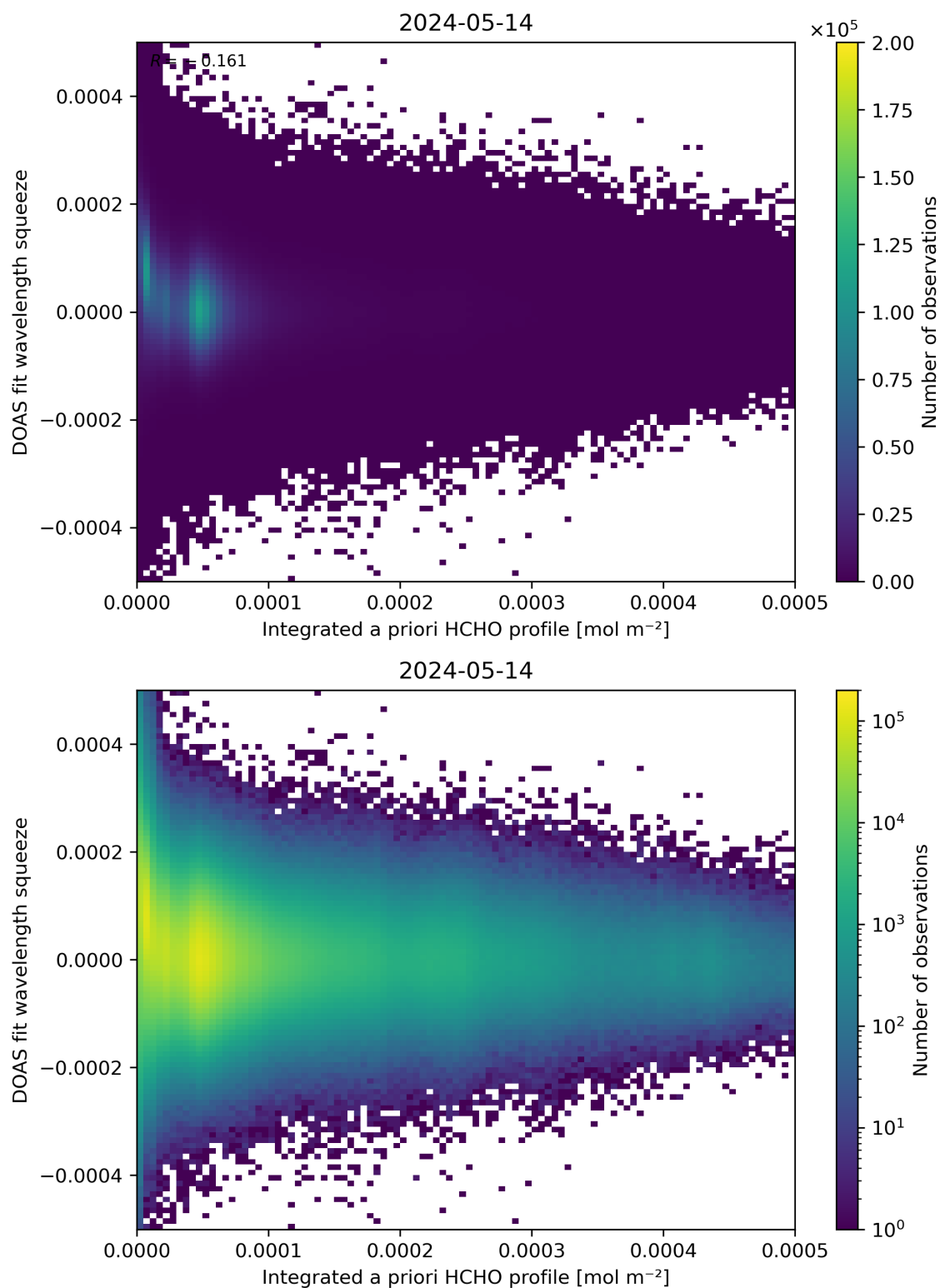
Figure 150: Scatter density plot of “Integrated a priori HCHO profile” against “DOAS fit wavelength squeeze” for 2024-05-13 to 2024-05-15.
