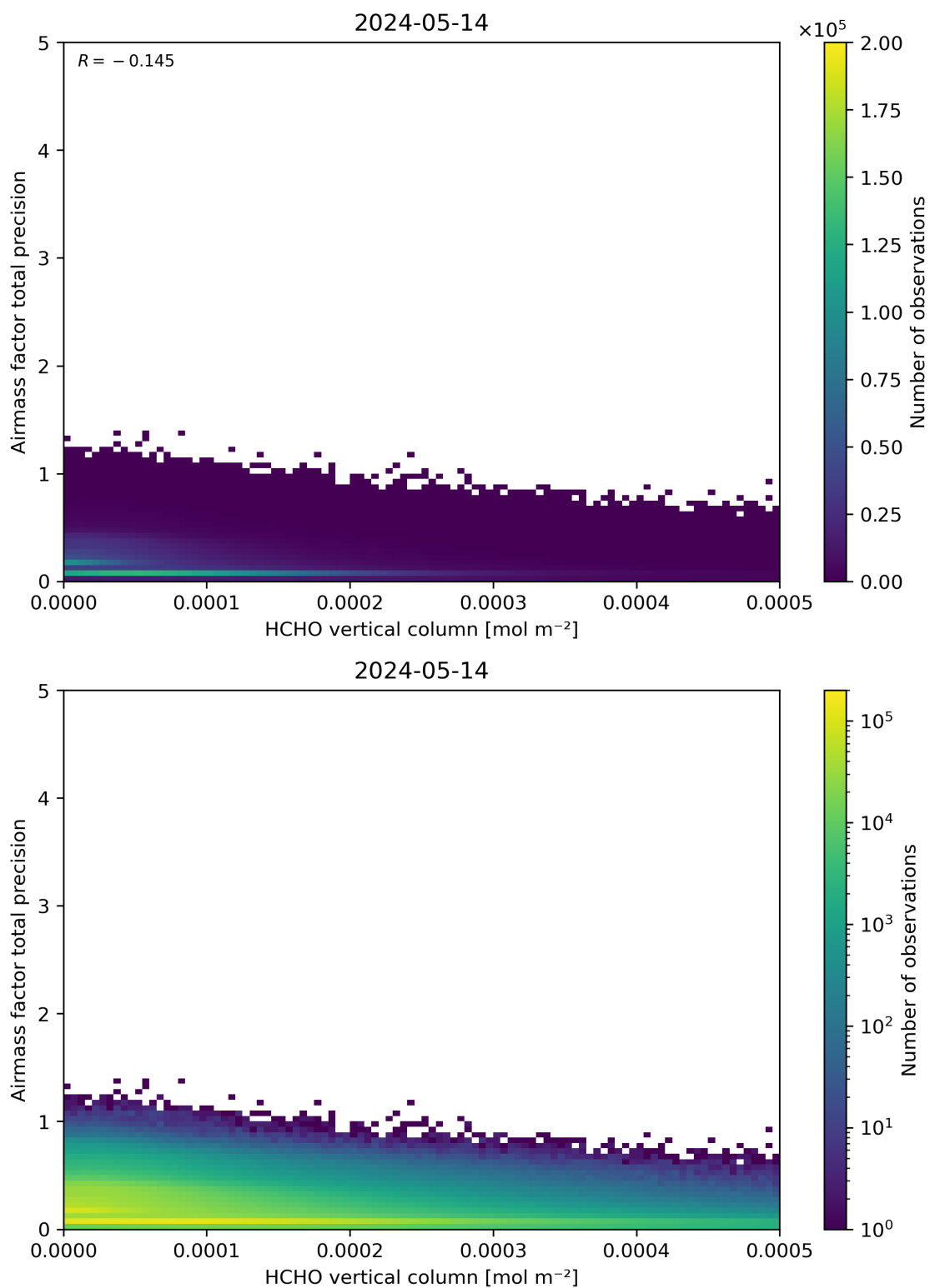
Figure 132: Scatter density plot of “HCHO vertical column” against “Airmass factor total precision” for 2024-05-13 to 2024-05-15.
