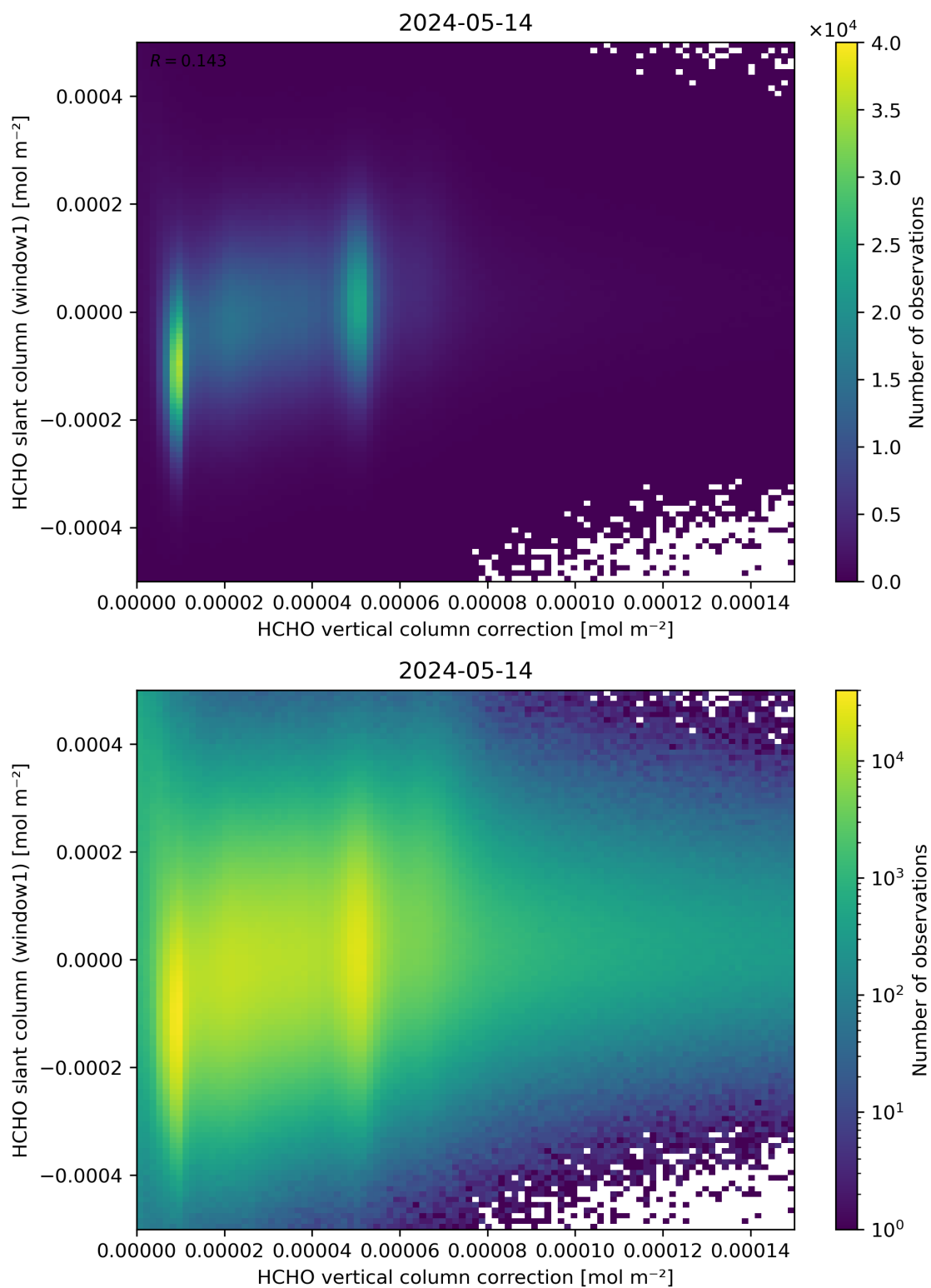
Figure 118: Scatter density plot of “HCHO vertical column correction” against “HCHO slant column (window1)” for 2024-05-13 to 2024-05-15.
