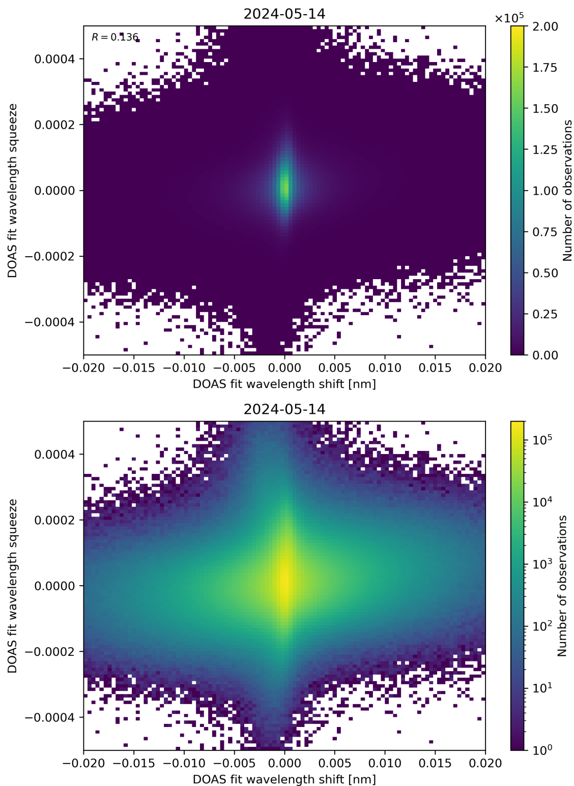
Figure 65: Scatter density plot of “DOAS fit wavelength shift” against “DOAS fit wavelength squeeze” for 2024-05-13 to 2024-05-15.
