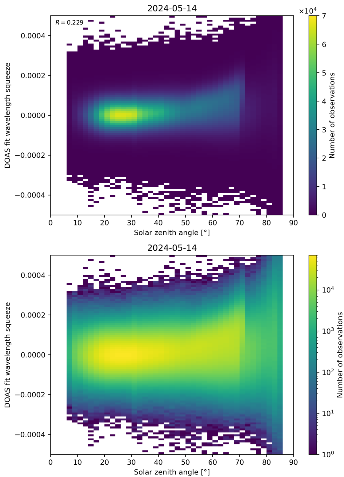
Figure 169: Scatter density plot of “Solar zenith angle” against “DOAS fit wavelength squeeze” for 2024-05-13 to 2024-05-15.
