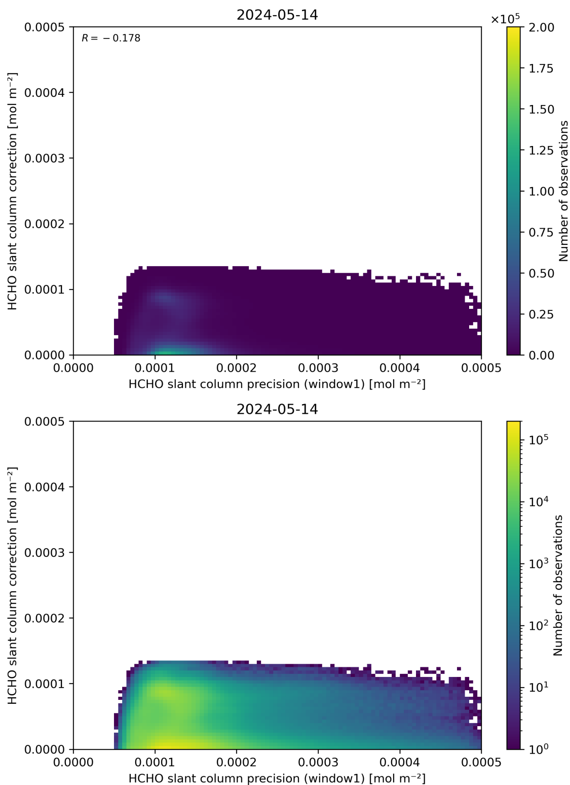
Figure 93: Scatter density plot of “HCHO slant column precision (window1)” against “HCHO slant column correction” for 2024-05-13 to 2024-05-15.
