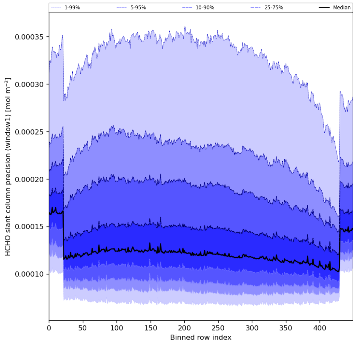
Figure 53: Along track statistics of “HCHO slant column precision (window1)” for 2024-05-13 to 2024-05-15
