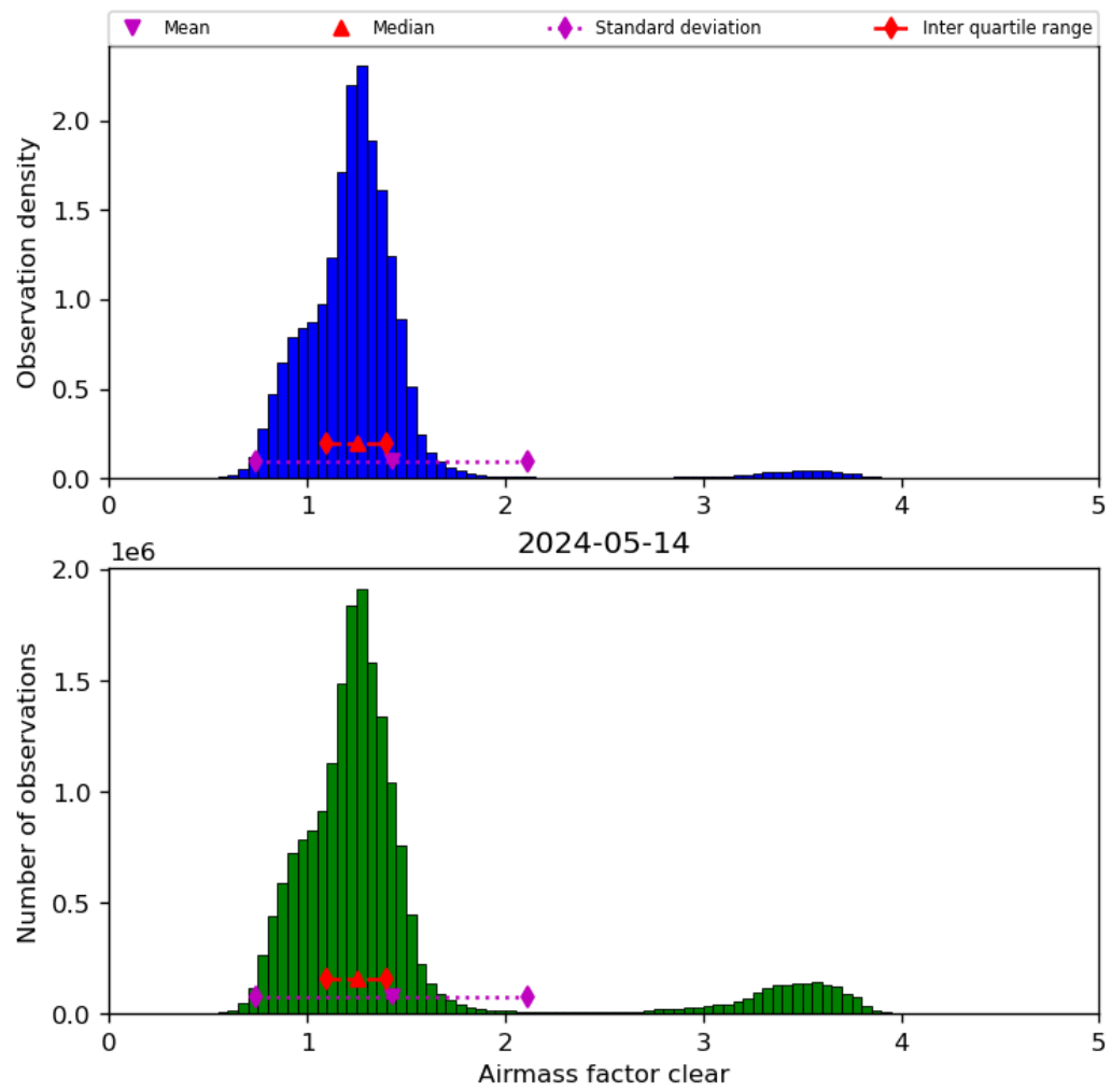
Figure 42: Histogram of “Airmass factor clear” for 2024-05-13 to 2024-05-15
