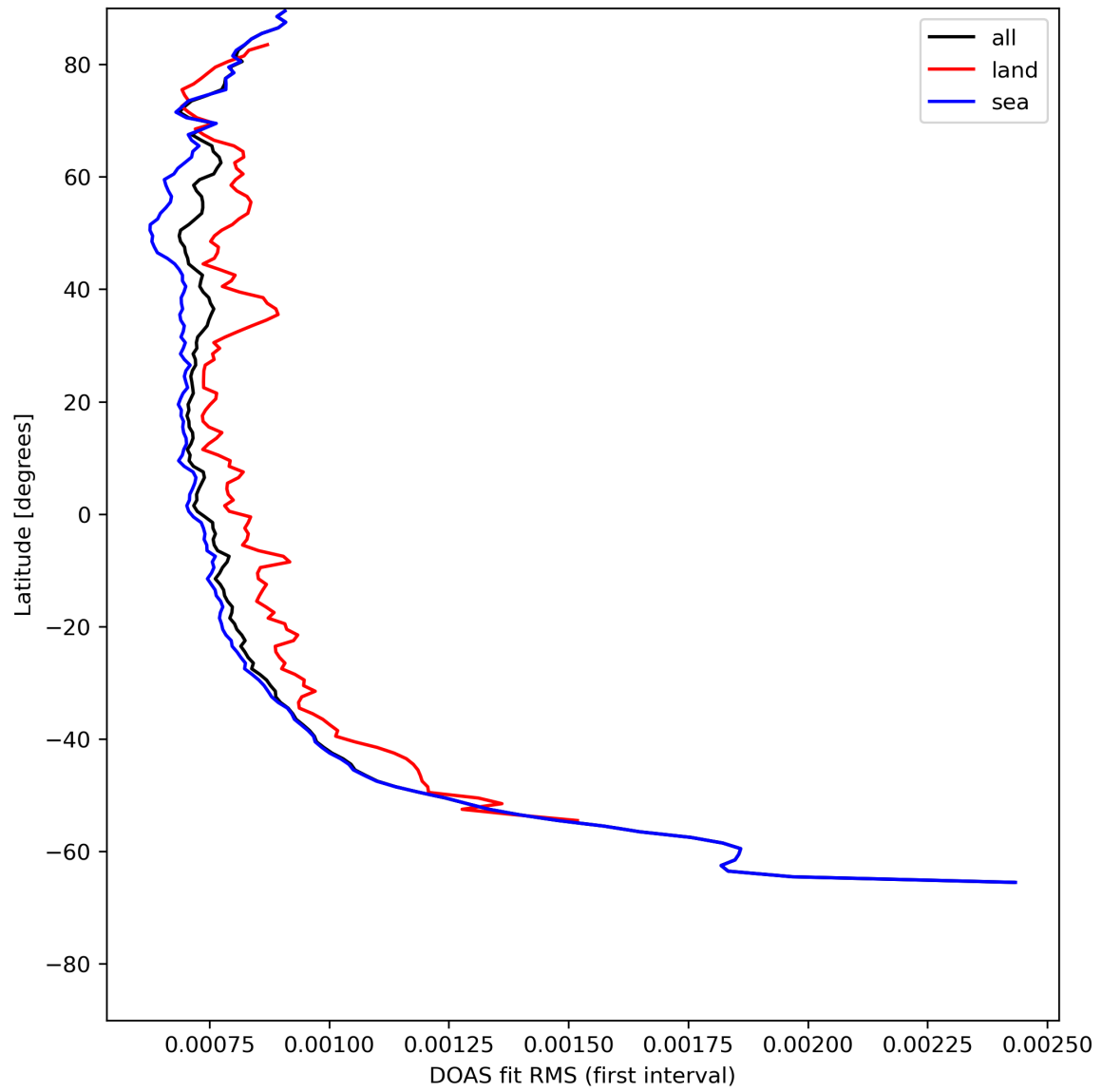
Figure 32: Zonal average of “DOAS fit RMS (first interval)” for 2024-05-13 to 2024-05-15.
