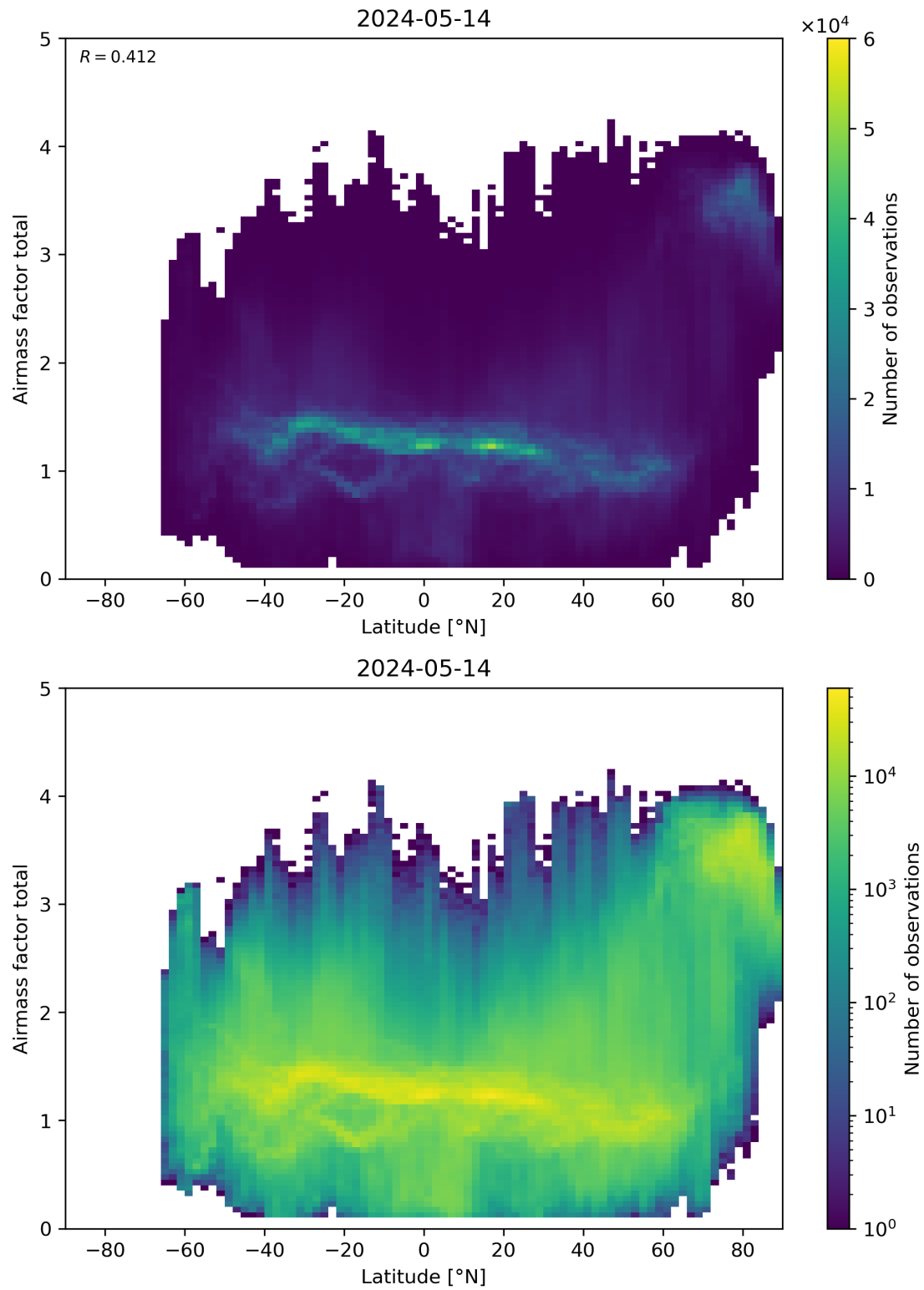
Figure 161: Scatter density plot of “Latitude” against “Airmass factor total” for 2024-05-13 to 2024-05-15.
