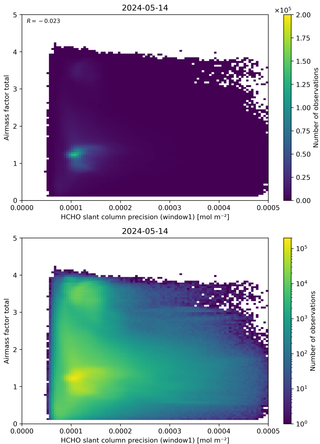
Figure 94: Scatter density plot of “HCHO slant column precision (window1)” against “Airmass factor total” for 2024-05-13 to 2024-05-15.
