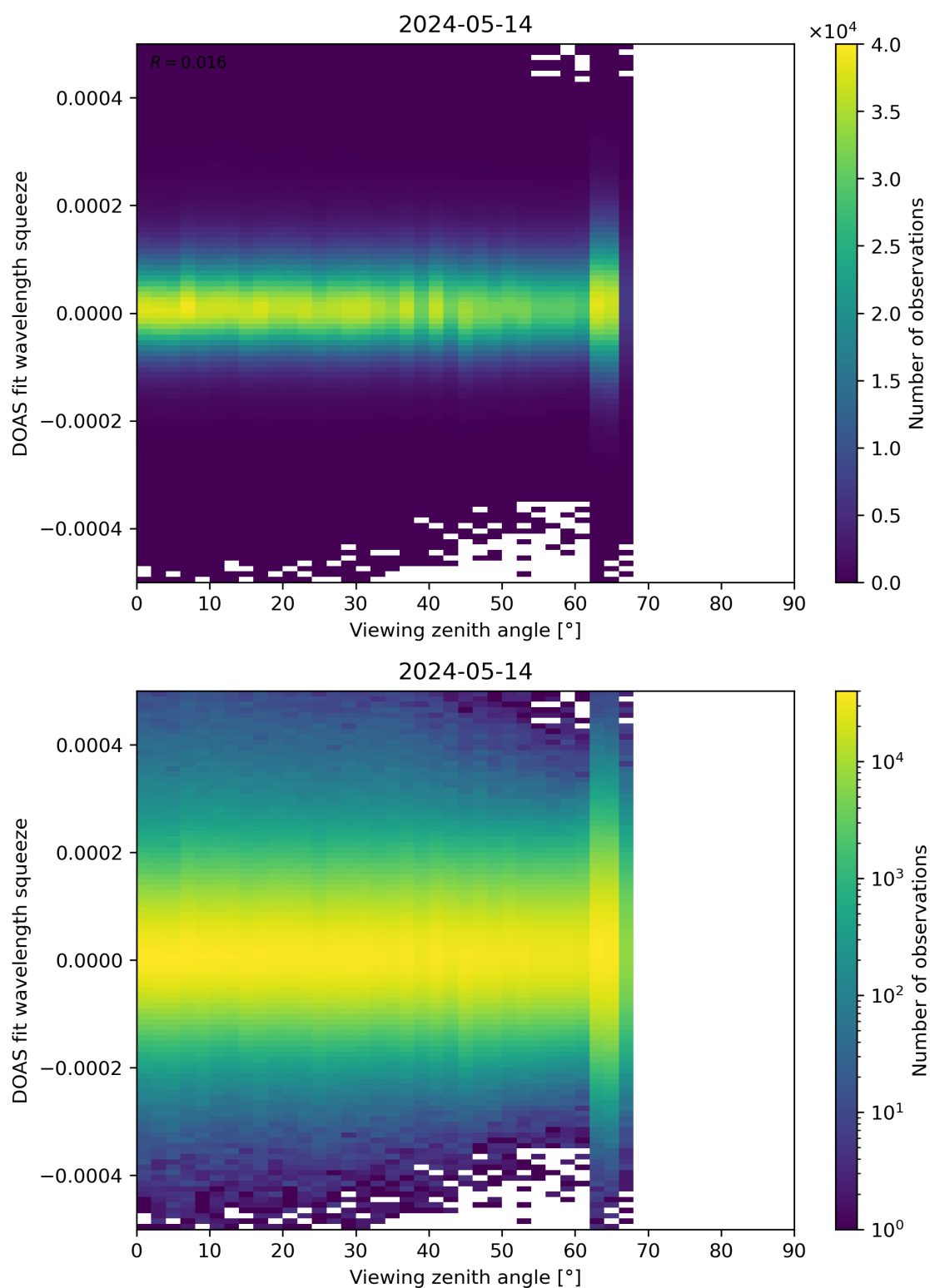
Figure 184: Scatter density plot of “Viewing zenith angle” against “DOAS fit wavelength squeeze” for 2024-05-13 to 2024-05-15.
