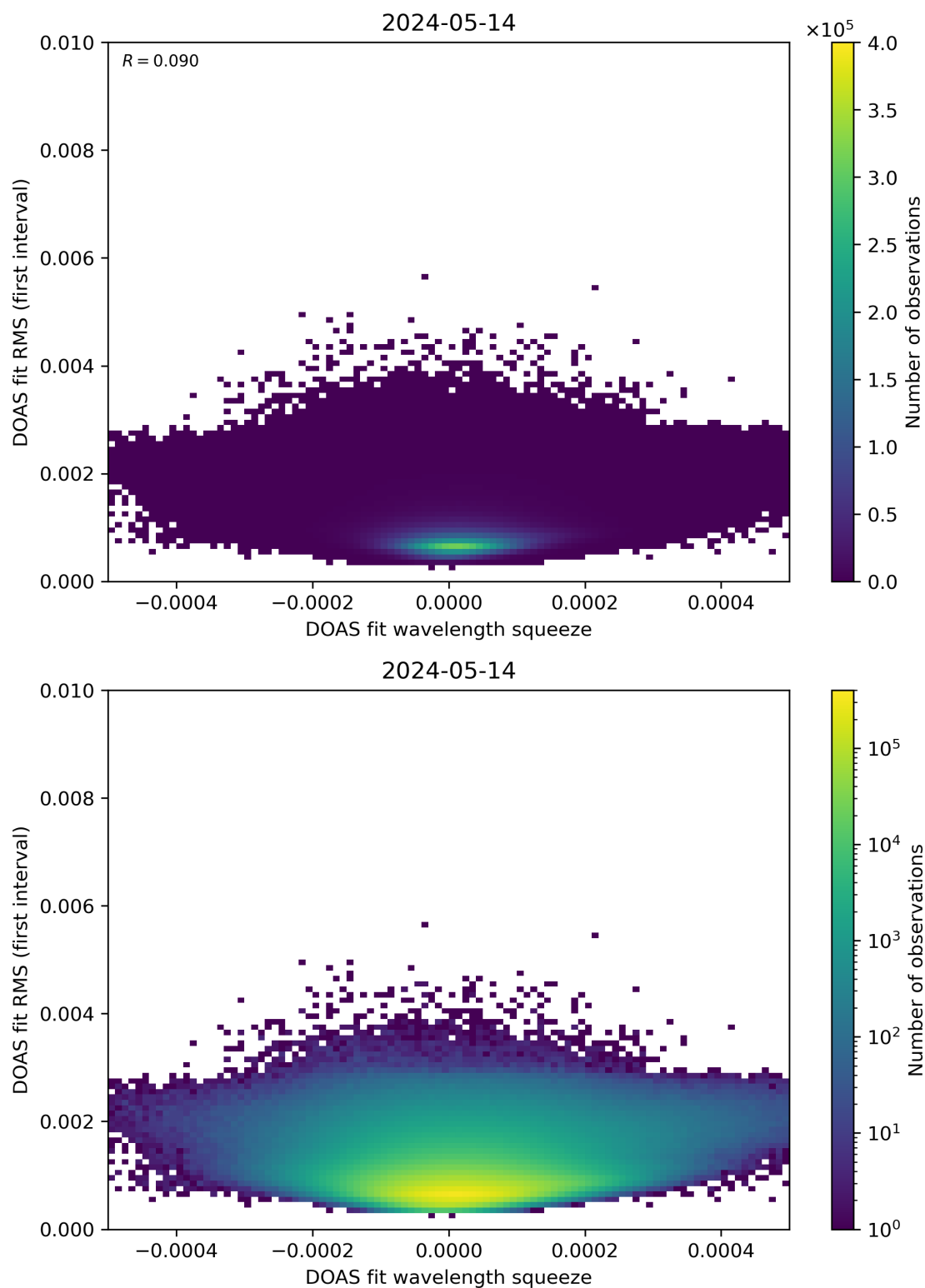
Figure 68: Scatter density plot of “DOAS fit wavelength squeeze” against “DOAS fit RMS (first interval)” for 2024-05-13 to 2024-05-15.
