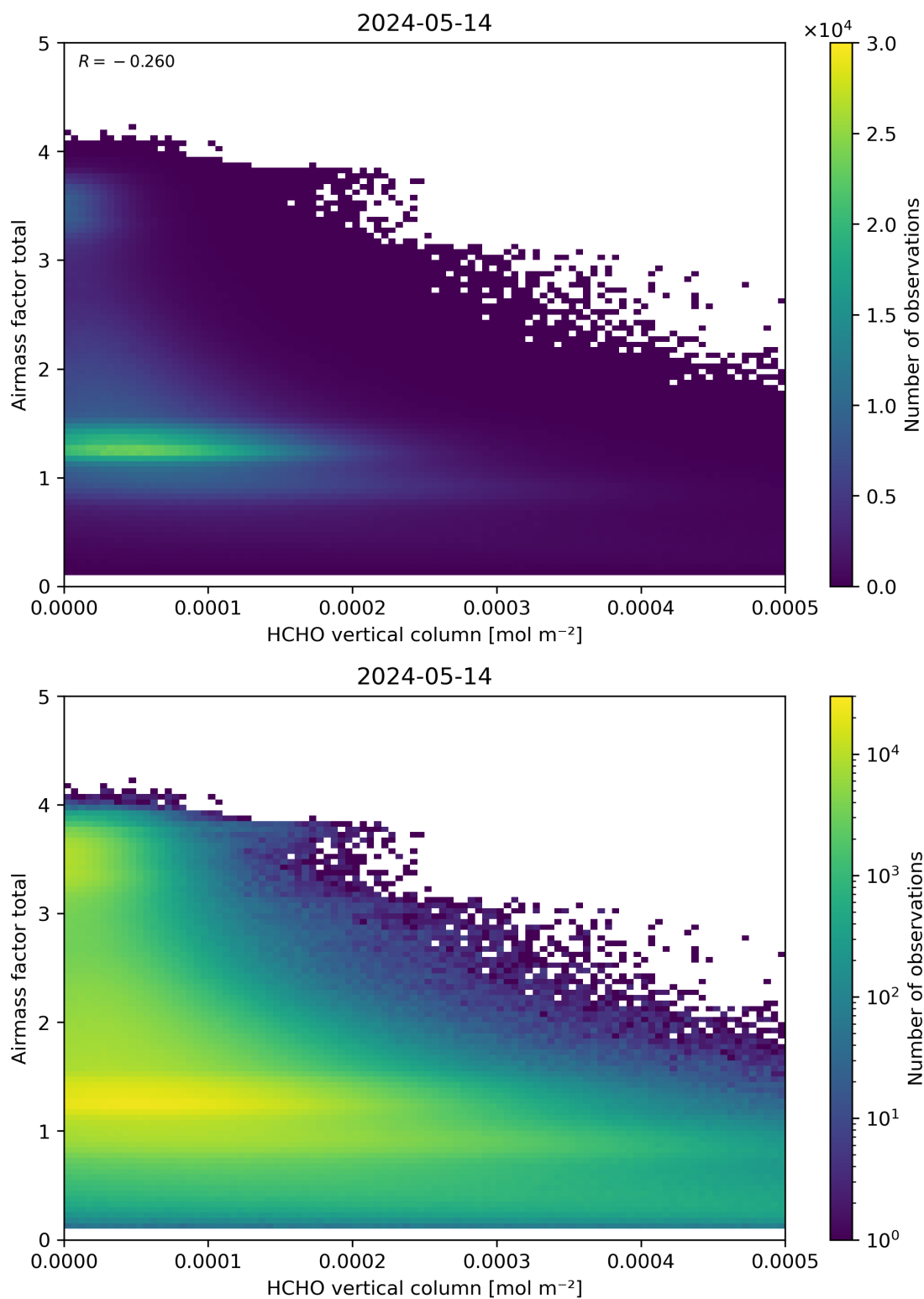
Figure 131: Scatter density plot of “HCHO vertical column” against “Airmass factor total” for 2024-05-13 to 2024-05-15.
