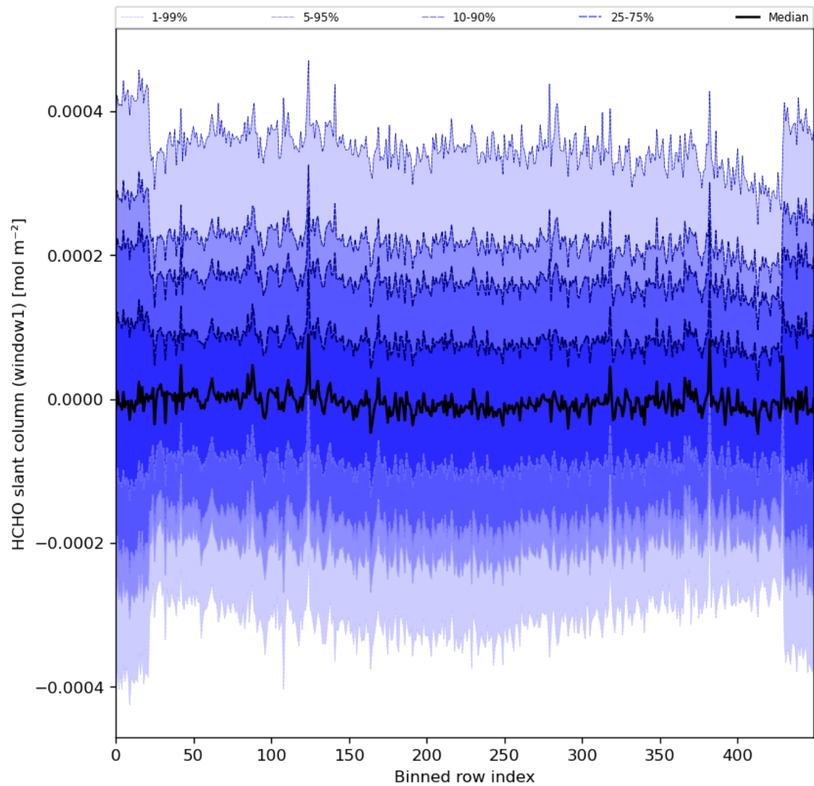
Figure 52: Along track statistics of “HCHO slant column (window1)” for 2024-05-13 to 2024-05-15
