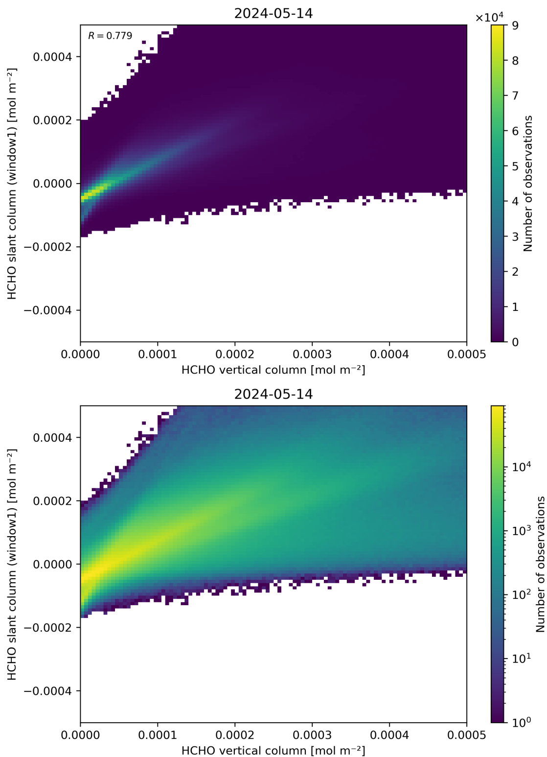
Figure 129: Scatter density plot of “HCHO vertical column” against “HCHO slant column (window1)” for 2024-05-13 to 2024-05-15.
