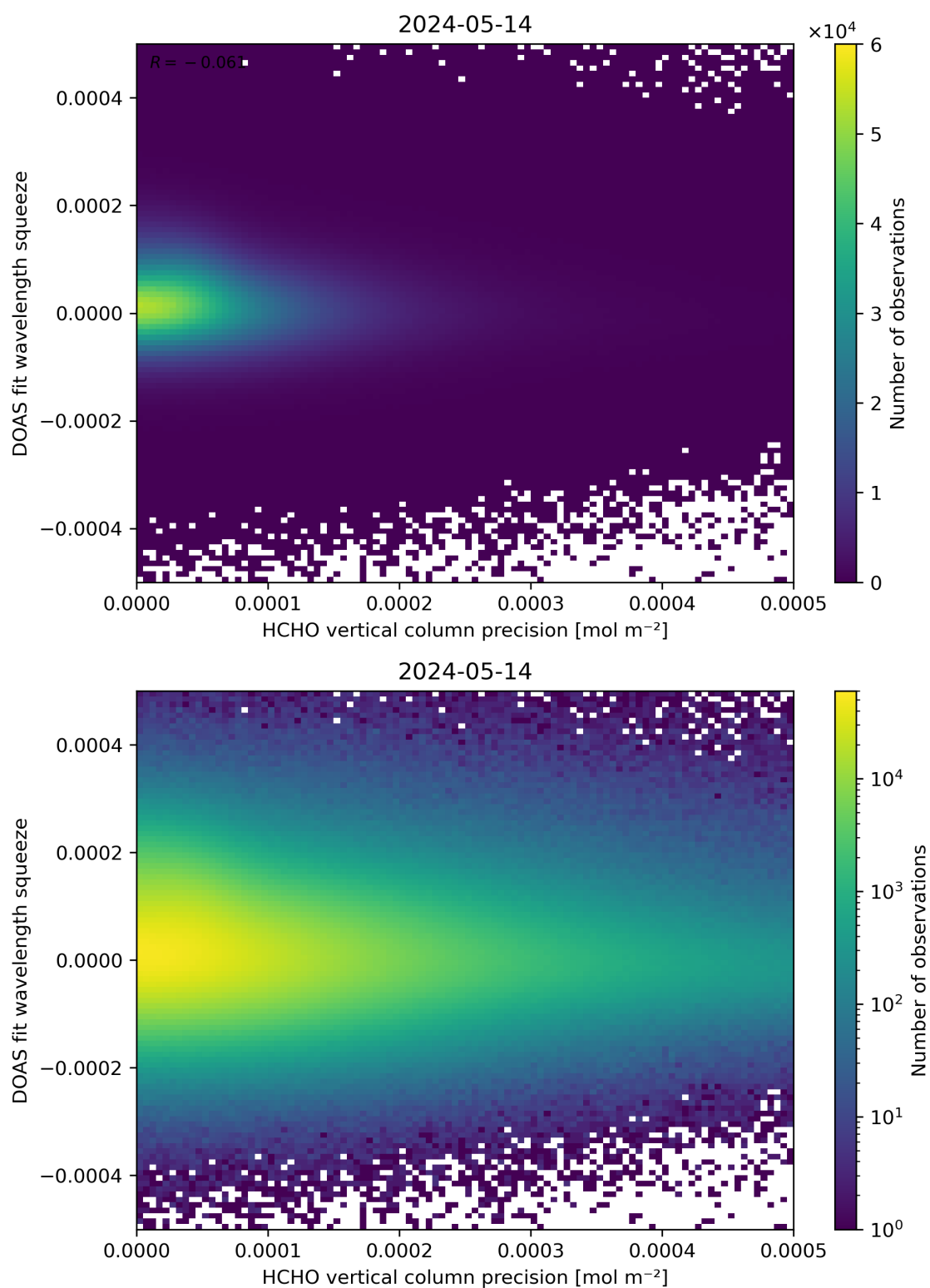
Figure 138: Scatter density plot of “HCHO vertical column precision” against “DOAS fit wavelength squeeze” for 2024-05-13 to 2024-05-15.
