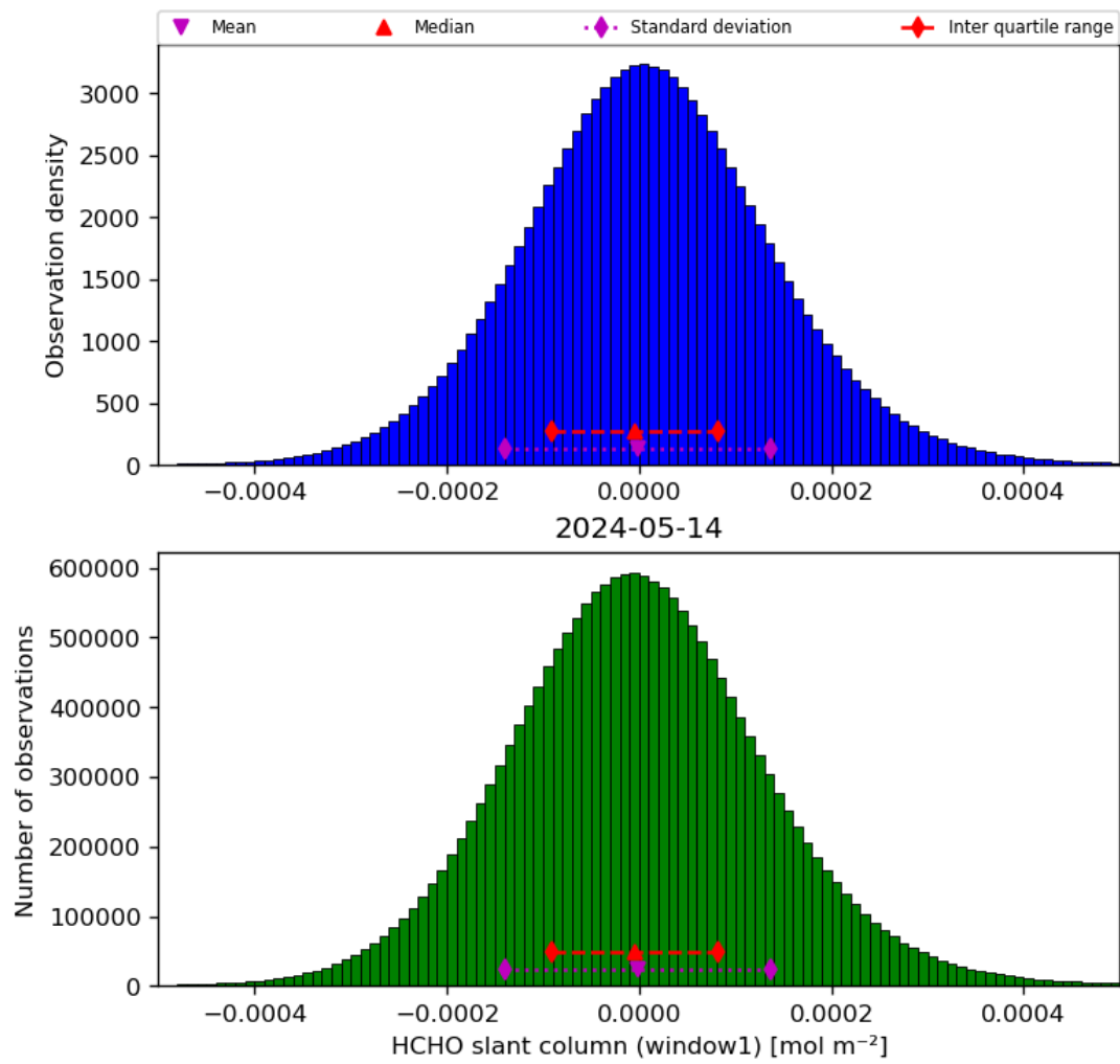
Figure 38: Histogram of “HCHO slant column (window1)” for 2024-05-13 to 2024-05-15
