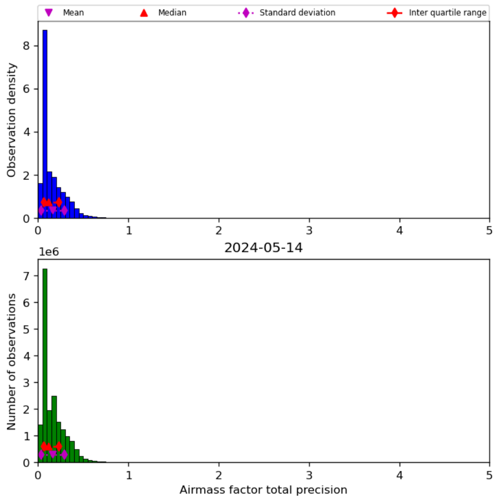
Figure 41: Histogram of “Airmass factor total precision” for 2024-05-13 to 2024-05-15
