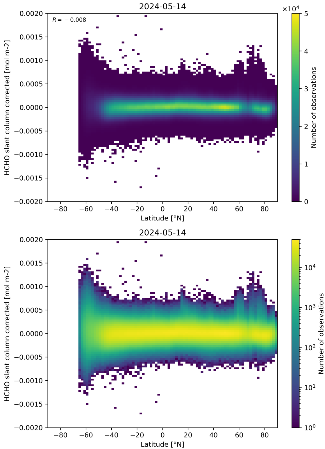
Figure 157: Scatter density plot of “Latitude” against “HCHO slant column corrected” for 2024-05-13 to 2024-05-15.
