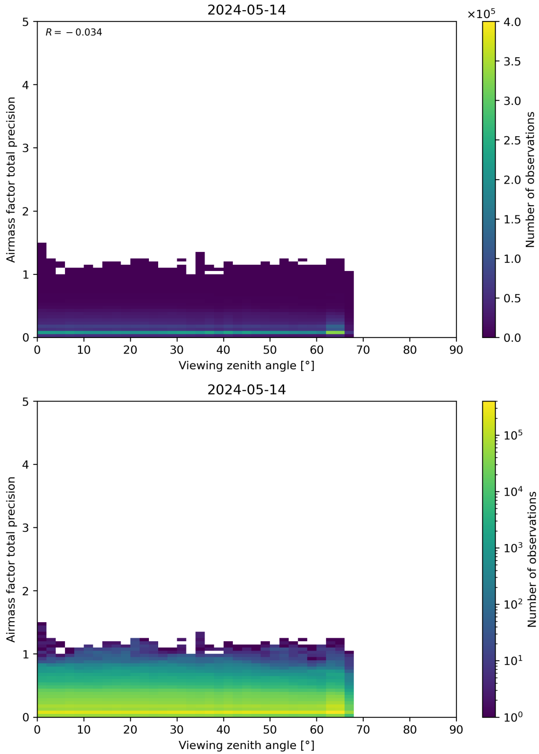
Figure 191: Scatter density plot of “Viewing zenith angle” against “Airmass factor total precision” for 2024-05-13 to 2024-05-15.
