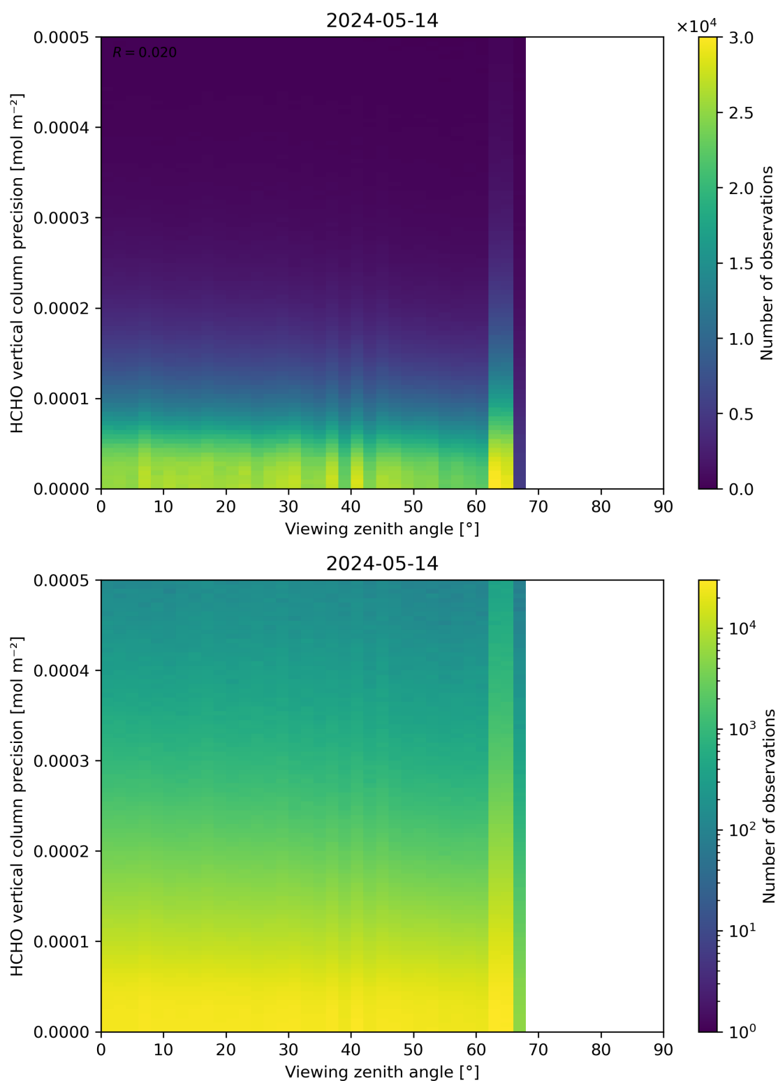
Figure 194: Scatter density plot of “Viewing zenith angle” against “HCHO vertical column precision” for 2024-05-13 to 2024-05-15.
