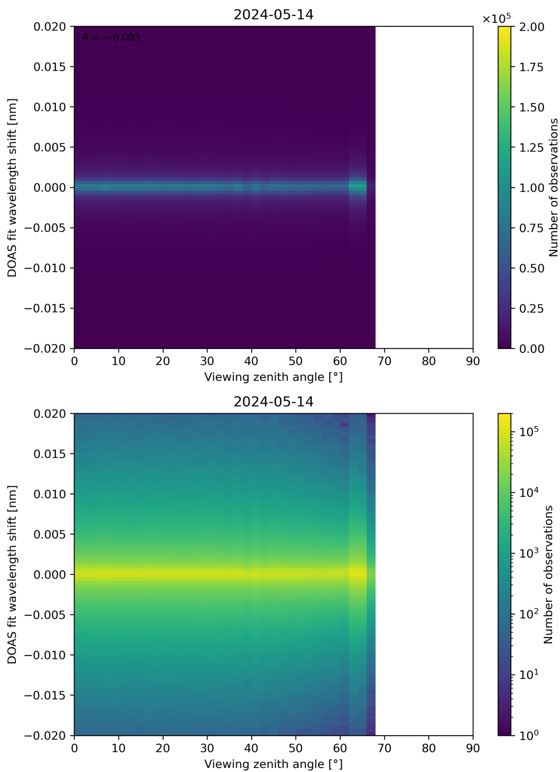
Figure 183: Scatter density plot of “Viewing zenith angle” against “DOAS fit wavelength shift” for 2024-05-13 to 2024-05-15.
