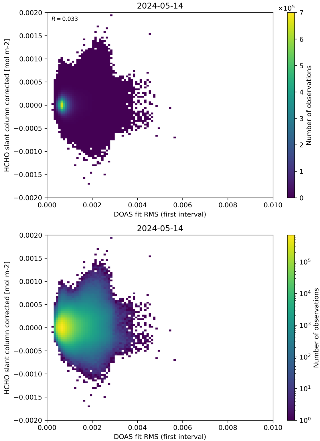
Figure 62: Scatter density plot of “DOAS fit RMS (first interval)” against “HCHO slant column corrected” for 2024-05-13 to 2024-05-15.
