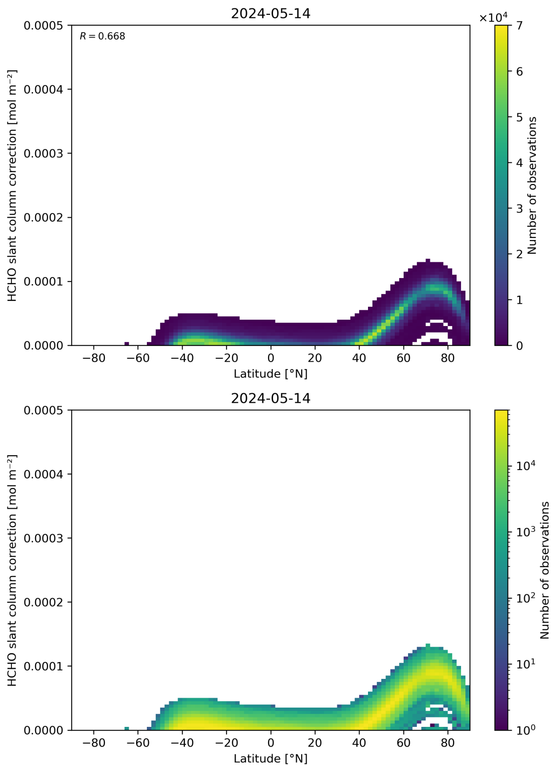
Figure 158: Scatter density plot of “Latitude” against “HCHO slant column correction” for 2024-05-13 to 2024-05-15.
