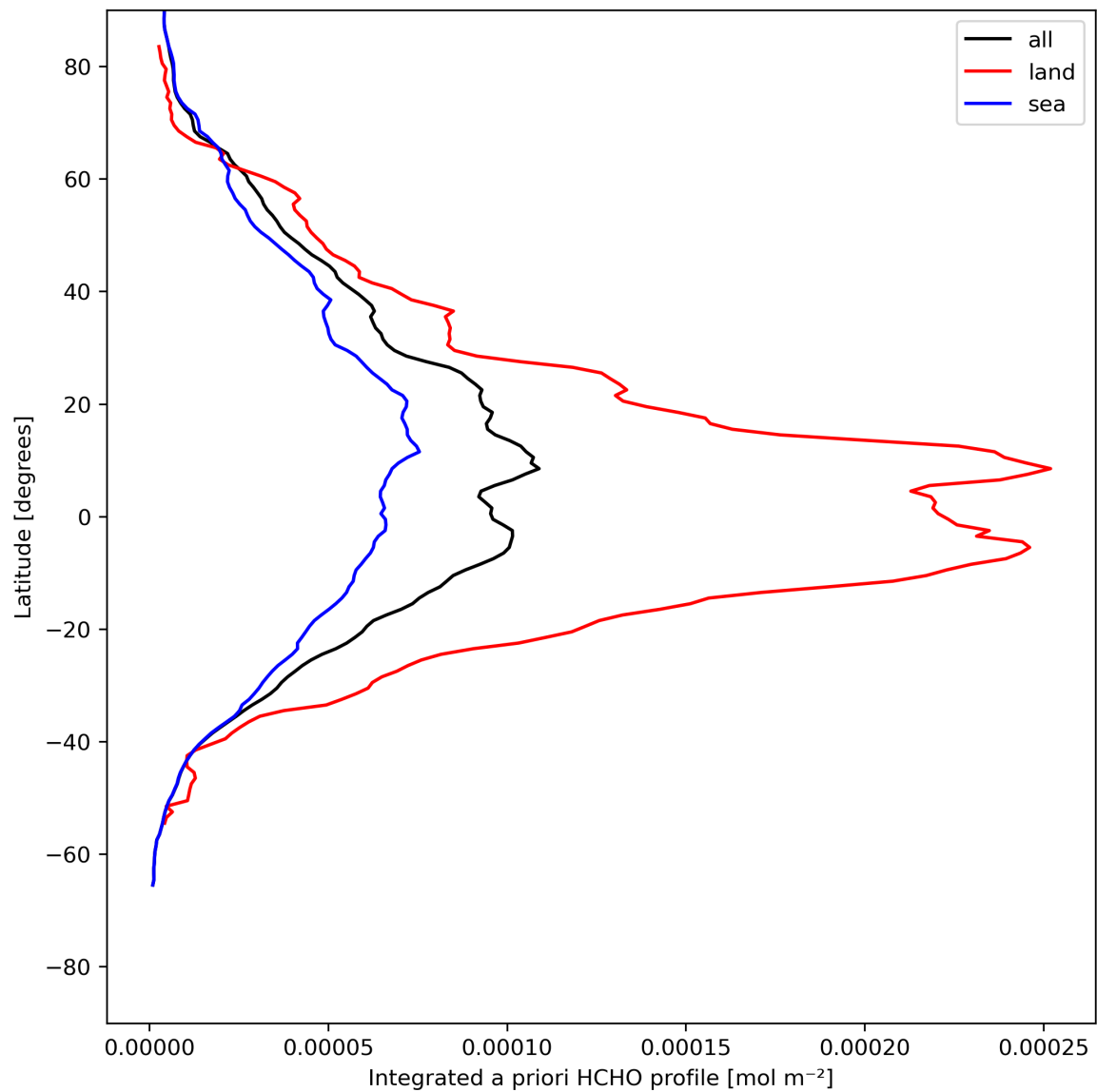
Figure 29: Zonal average of “Integrated a priori HCHO profile” for 2024-05-13 to 2024-05-15.
