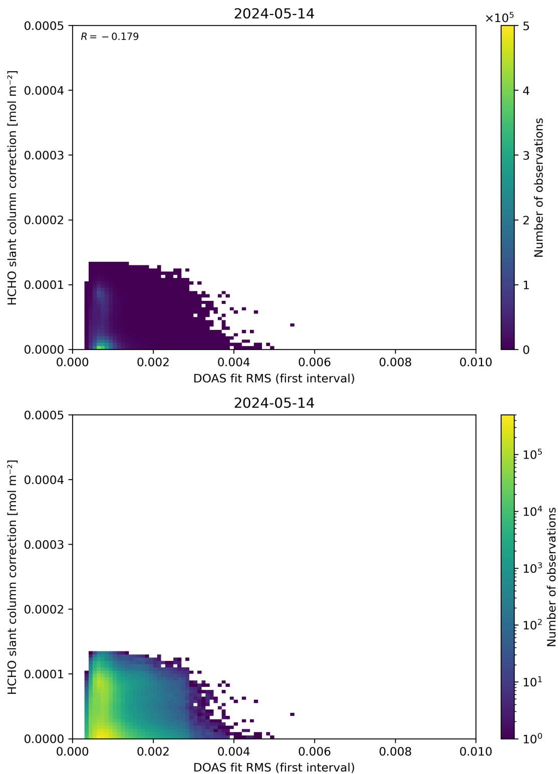
Figure 63: Scatter density plot of “DOAS fit RMS (first interval)” against “HCHO slant column correction” for 2024-05-13 to 2024-05-15.
