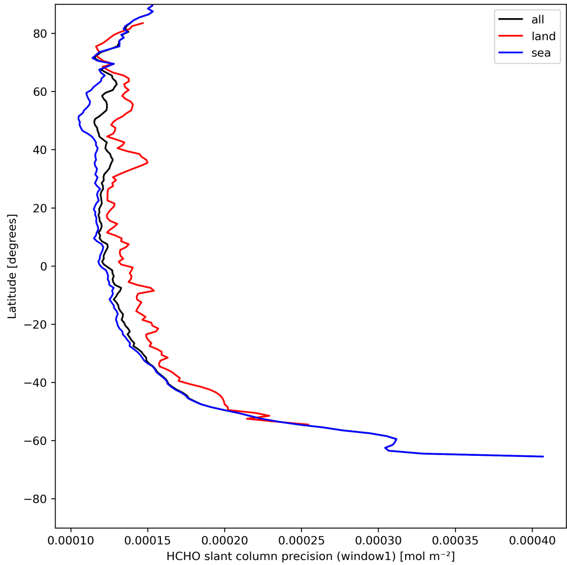
Figure 25: Zonal average of “HCHO slant column precision (window1)” for 2024-05-13 to 2024-05-15.
