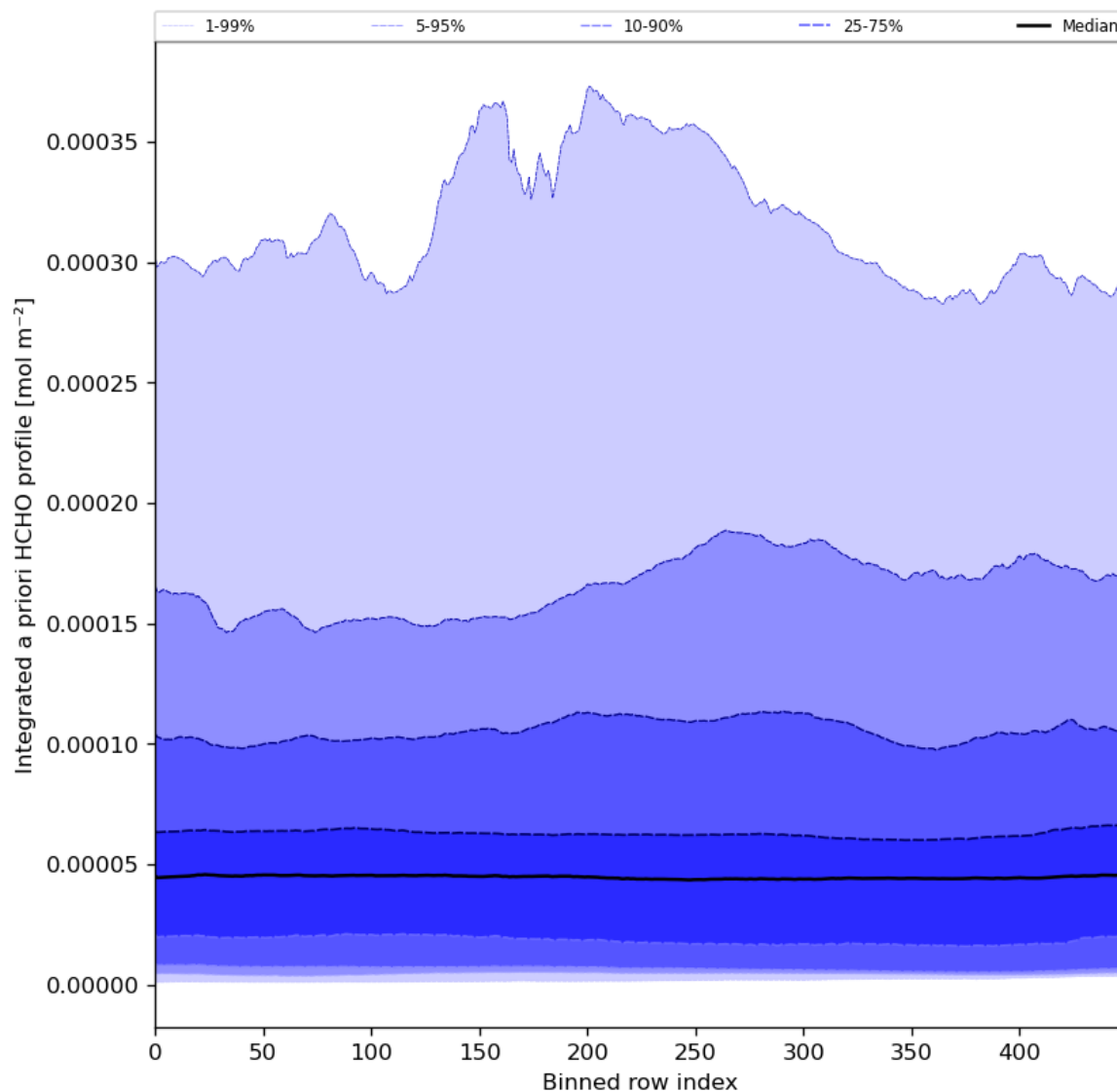
Figure 57: Along track statistics of “Integrated a priori HCHO profile” for 2024-05-13 to 2024-05-15
