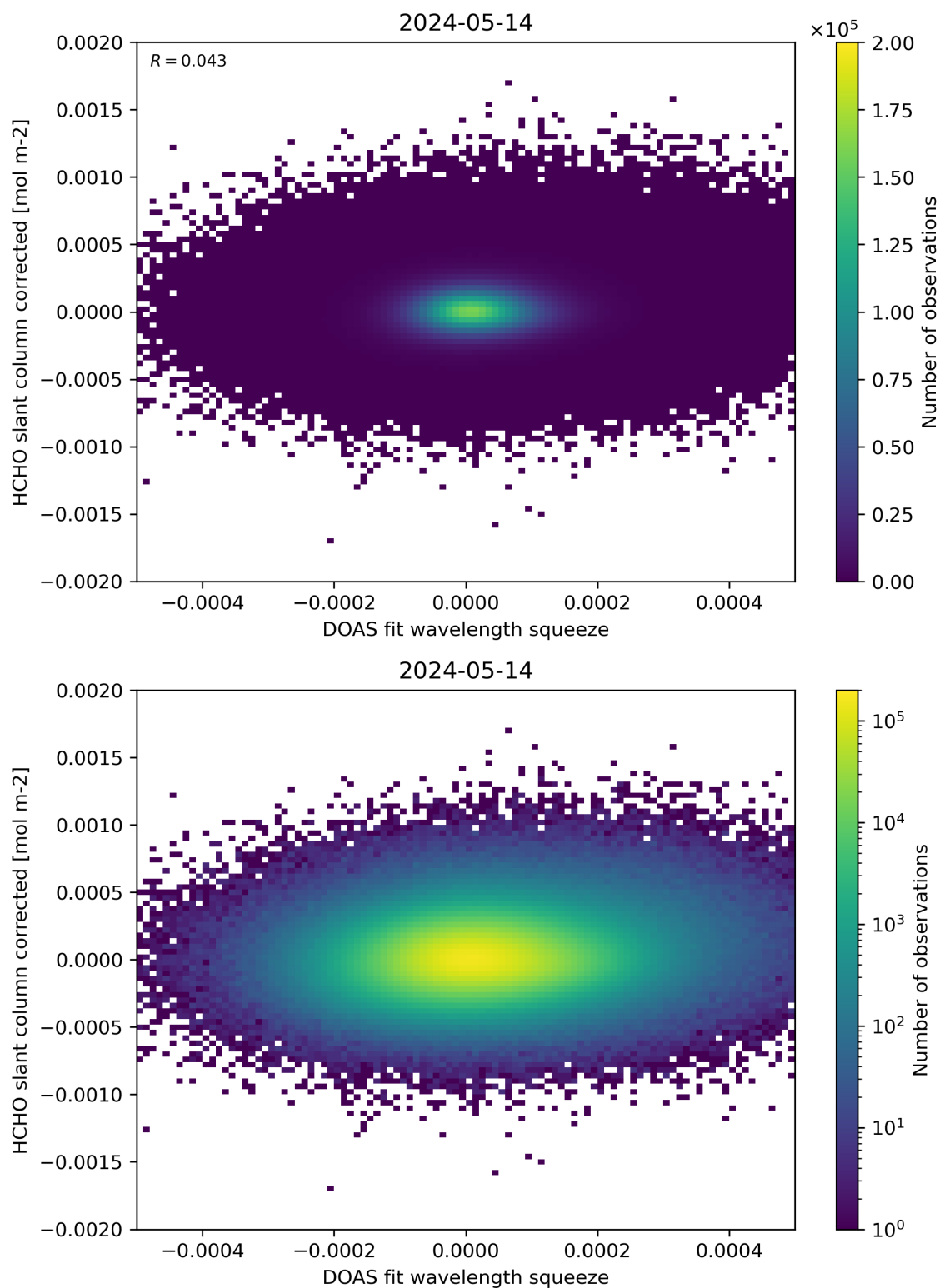
Figure 69: Scatter density plot of “DOAS fit wavelength squeeze” against “HCHO slant column corrected” for 2024-05-13 to 2024-05-15.
