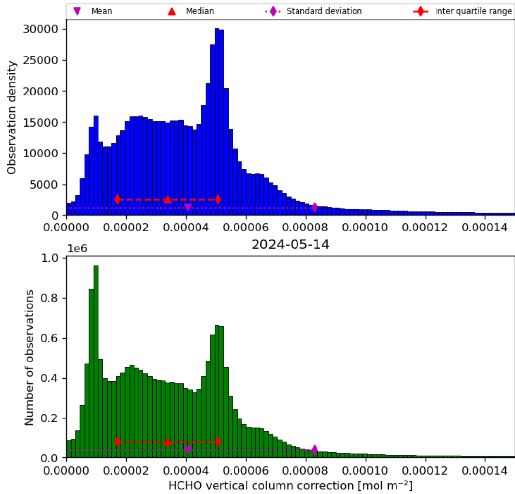
Figure 37: Histogram of “HCHO vertical column correction” for 2024-05-13 to 2024-05-15
