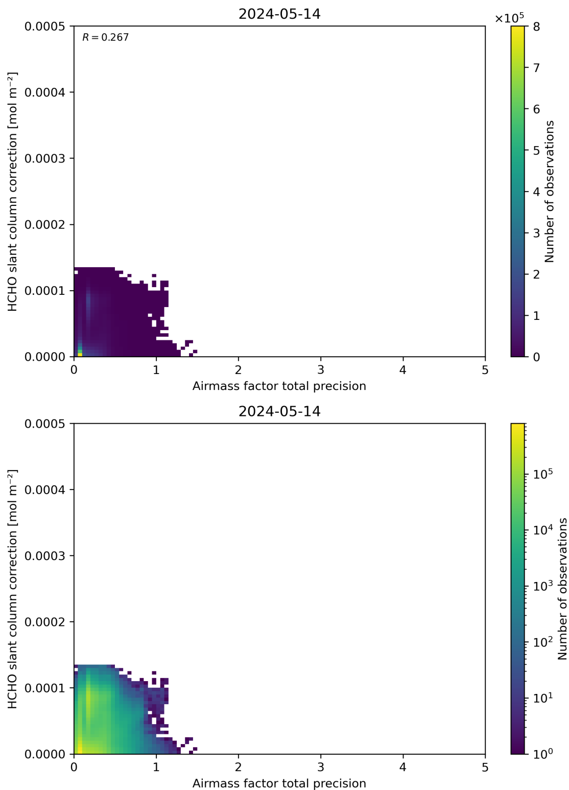
Figure 110: Scatter density plot of “Airmass factor total precision” against “HCHO slant column correction” for 2024-05-13 to 2024-05-15.
