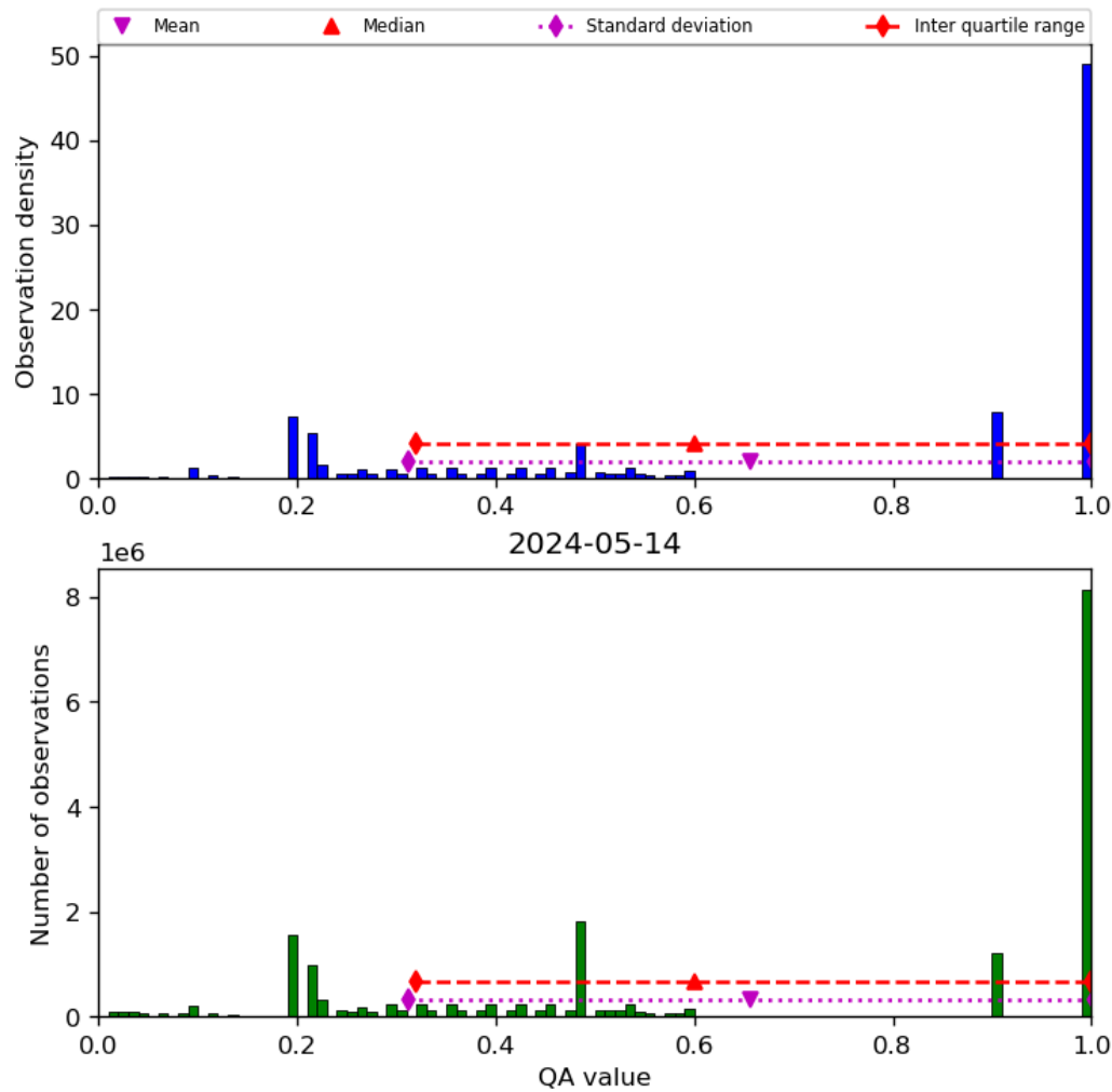
Figure 34: Histogram of “QA value” for 2024-05-13 to 2024-05-15
