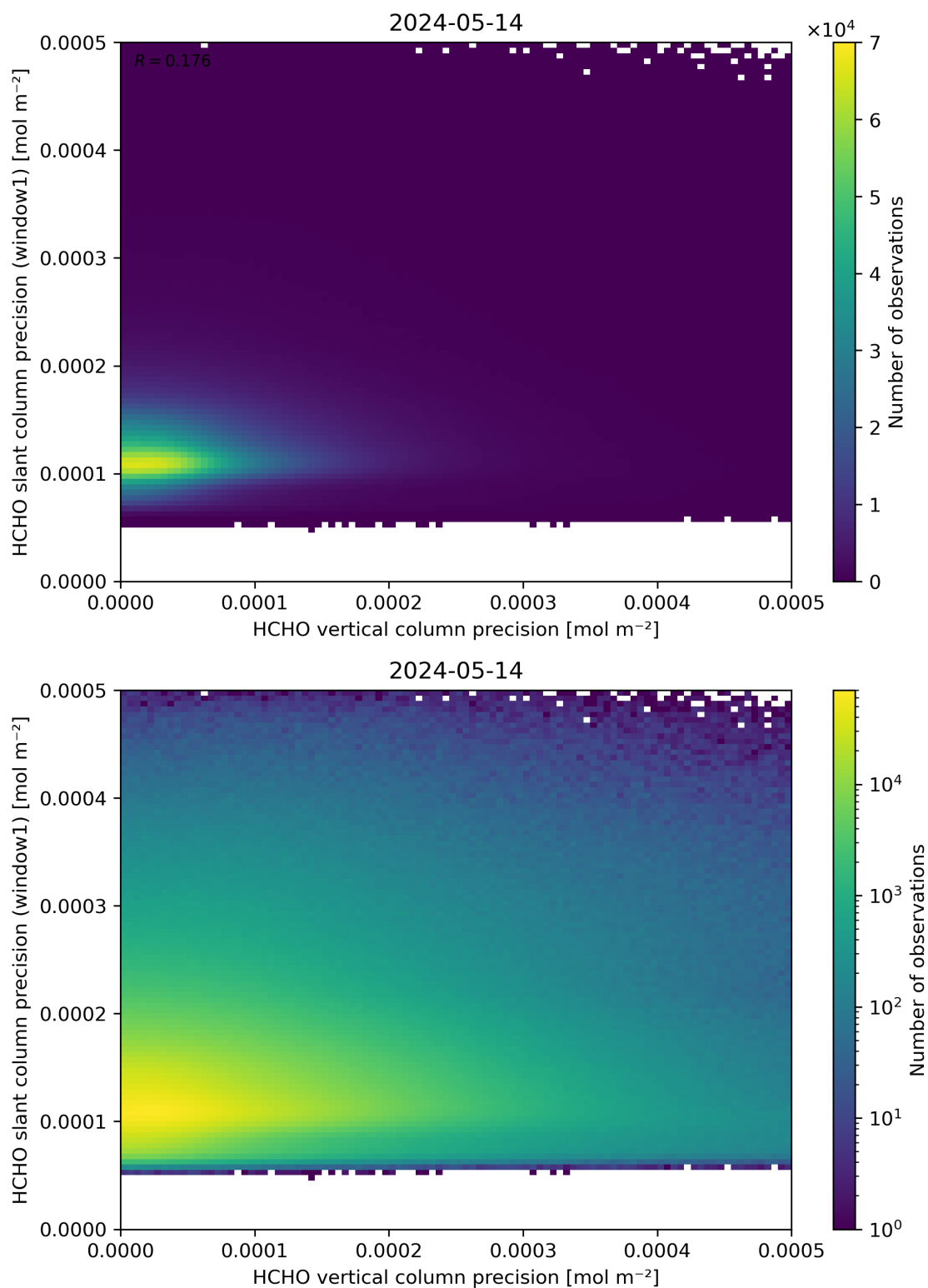
Figure 143: Scatter density plot of “HCHO vertical column precision” against “HCHO slant column precision (window1)” for 2024-05-13 to 2024-05-15.
