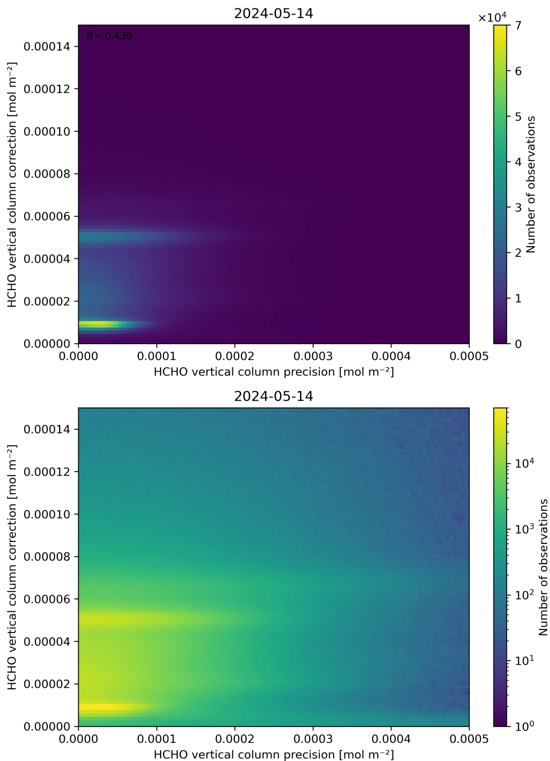
Figure 146: Scatter density plot of “HCHO vertical column precision” against “HCHO vertical column correction” for 2024-05-13 to 2024-05-15.
