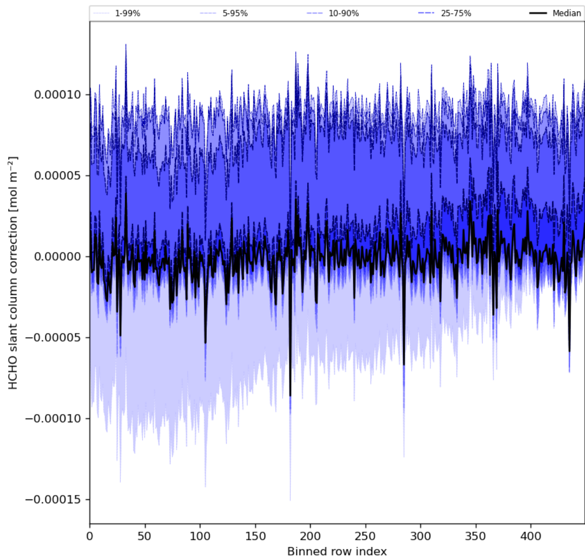
Figure 61: Along track statistics of “HCHO slant column correction” for 2024-05-13 to 2024-05-15
