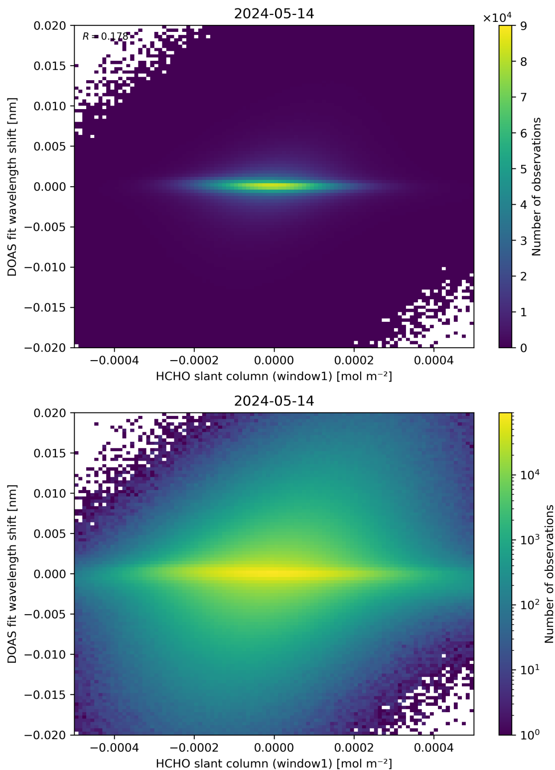
Figure 79: Scatter density plot of “HCHO slant column (window1)” against “DOAS fit wavelength shift” for 2024-05-13 to 2024-05-15.
