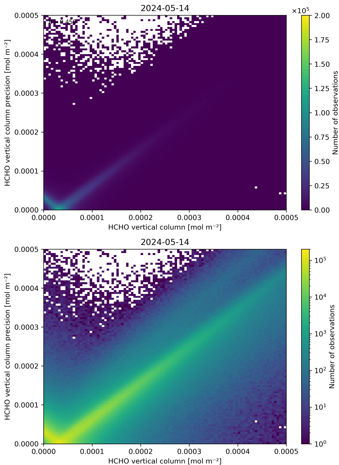
Figure 134: Scatter density plot of “HCHO vertical column” against “HCHO vertical column precision” for 2024-05-13 to 2024-05-15.
