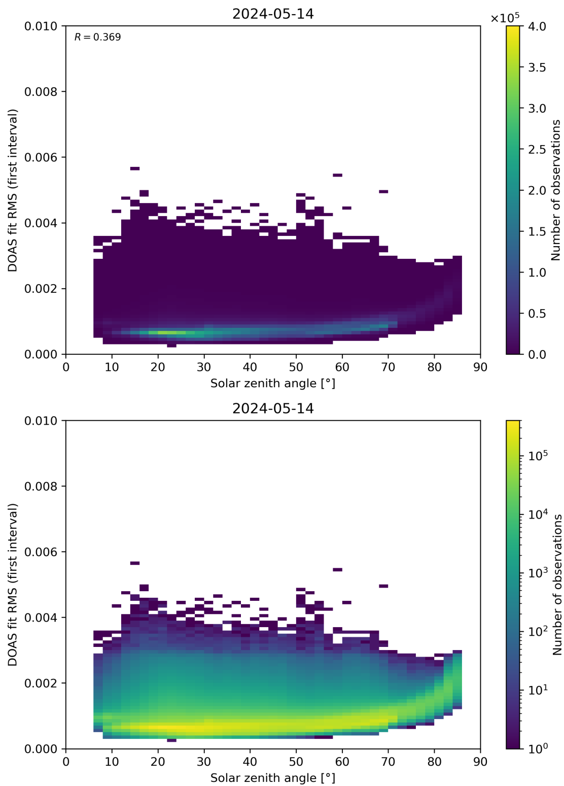
Figure 167: Scatter density plot of “Solar zenith angle” against “DOAS fit RMS (first interval)” for 2024-05-13 to 2024-05-15.
