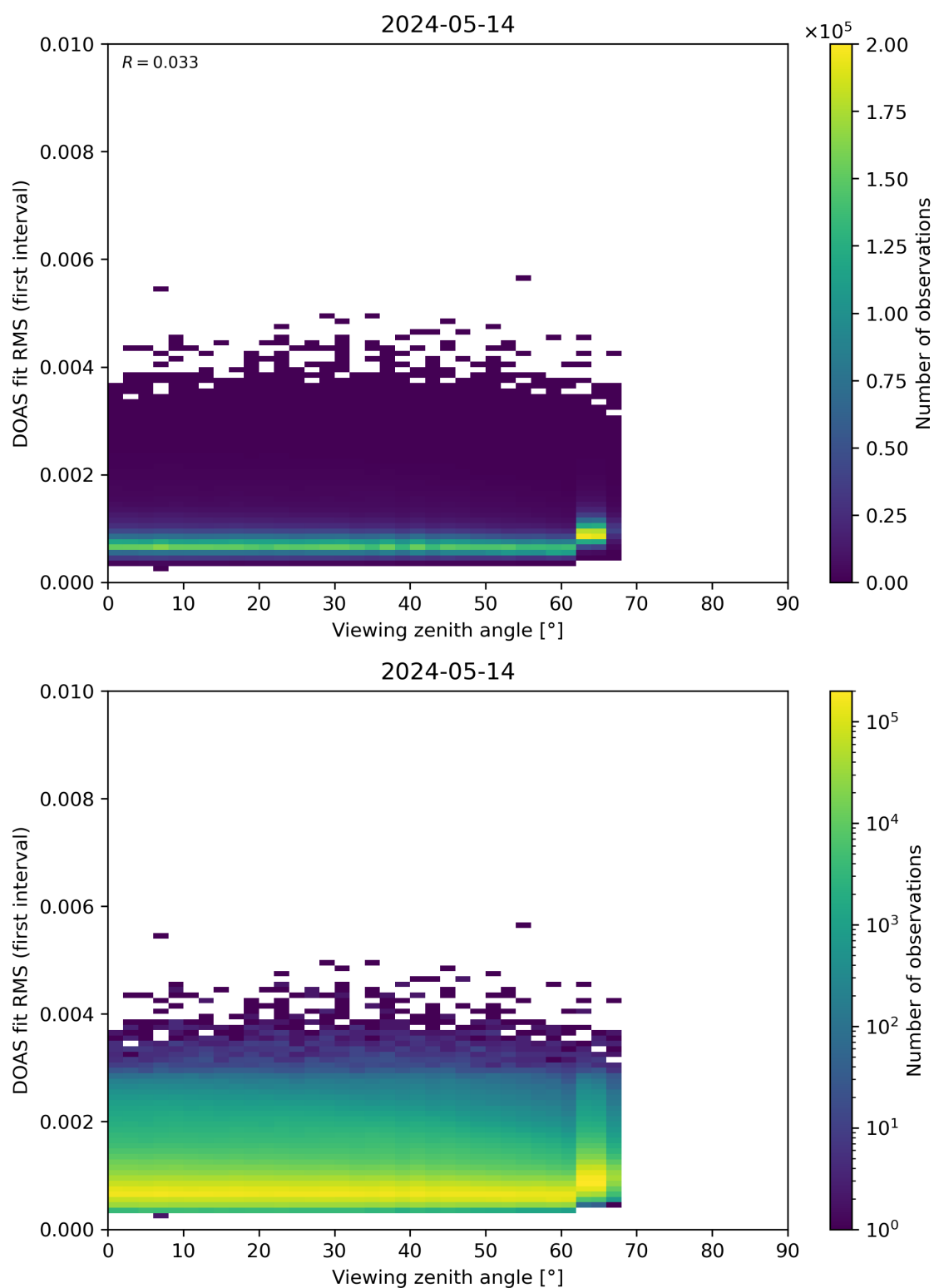
Figure 182: Scatter density plot of “Viewing zenith angle” against “DOAS fit RMS (first interval)” for 2024-05-13 to 2024-05-15.
