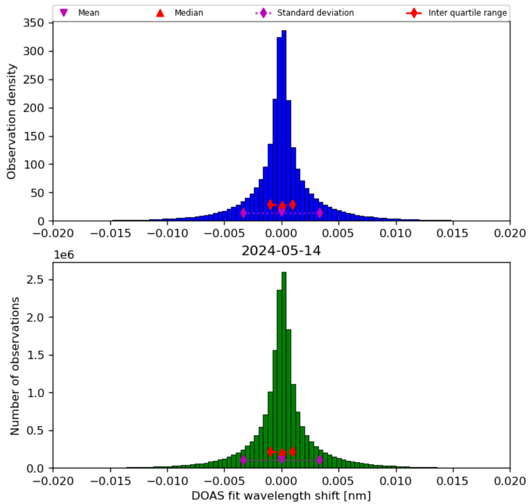
Figure 44: Histogram of “DOAS fit wavelength shift” for 2024-05-13 to 2024-05-15
