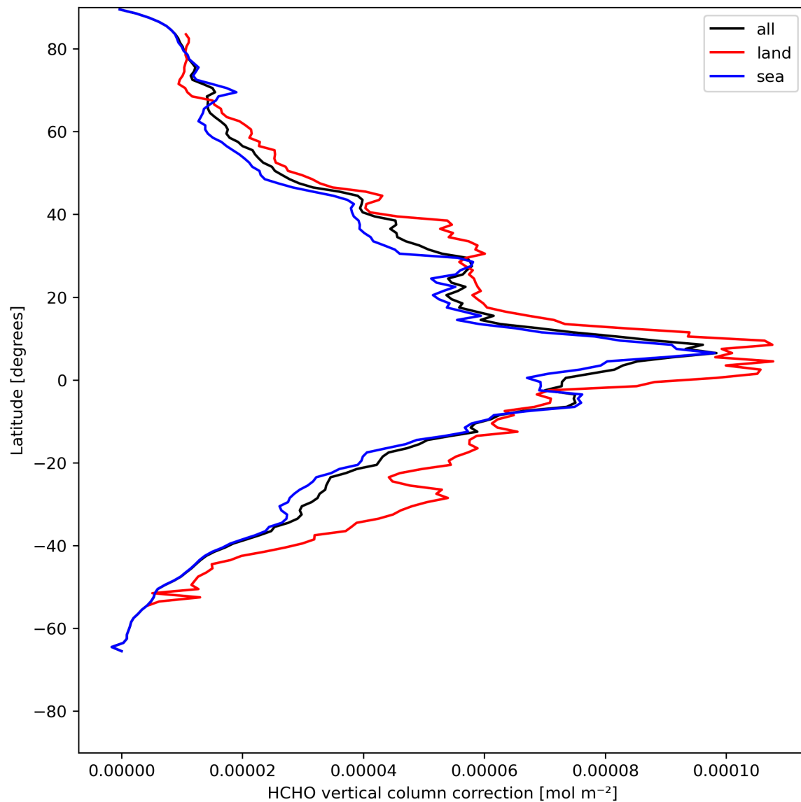
Figure 23: Zonal average of “HCHO vertical column correction” for 2024-05-13 to 2024-05-15.
