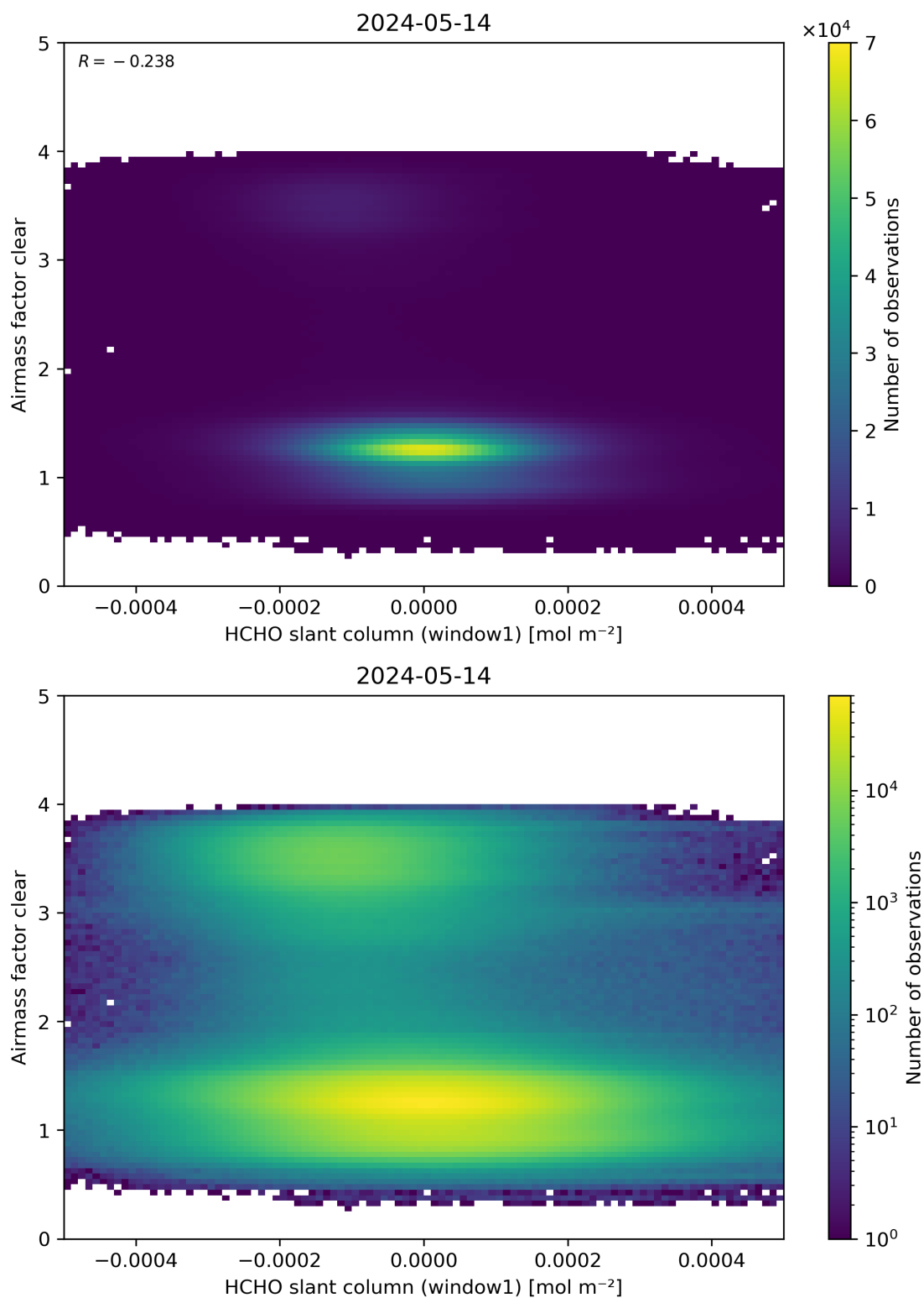
Figure 81: Scatter density plot of “HCHO slant column (window1)” against “Airmass factor clear” for 2024-05-13 to 2024-05-15.
