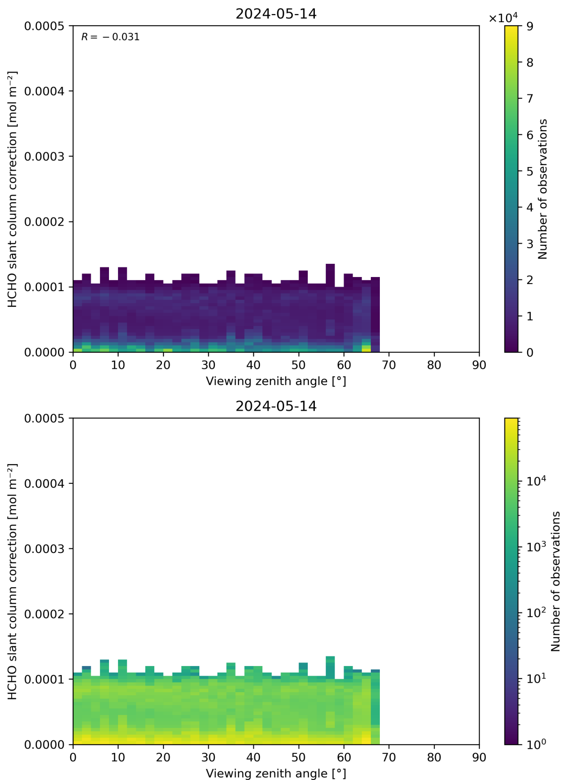
Figure 187: Scatter density plot of “Viewing zenith angle” against “HCHO slant column correction” for 2024-05-13 to 2024-05-15.
