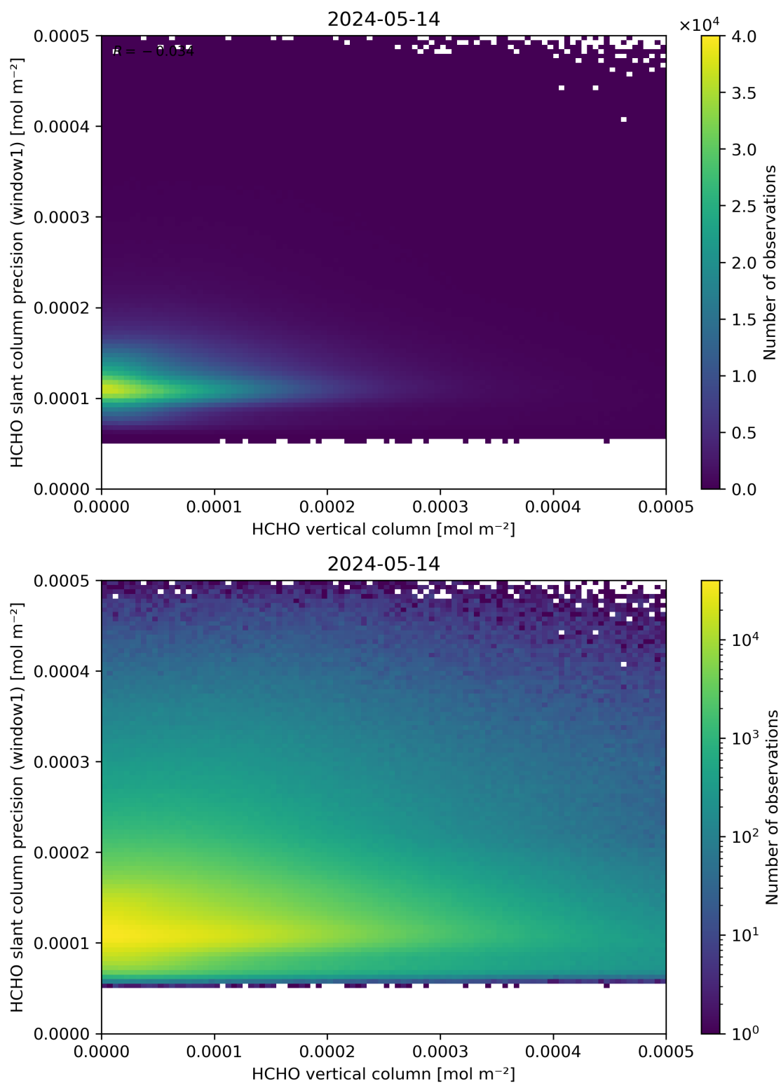
Figure 130: Scatter density plot of “HCHO vertical column” against “HCHO slant column precision (window1)” for 2024-05-13 to 2024-05-15.
