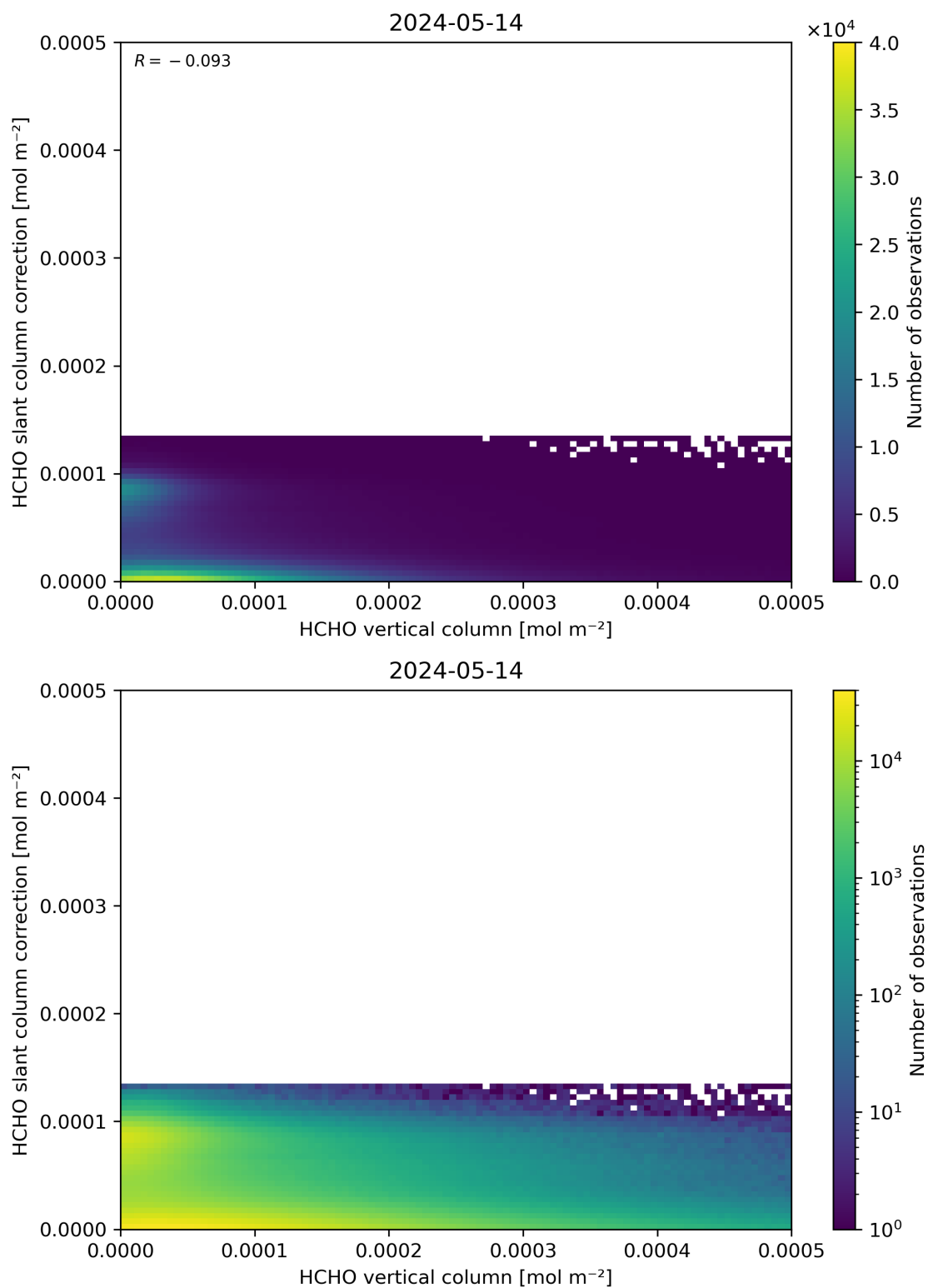
Figure 128: Scatter density plot of “HCHO vertical column” against “HCHO slant column correction” for 2024-05-13 to 2024-05-15.
