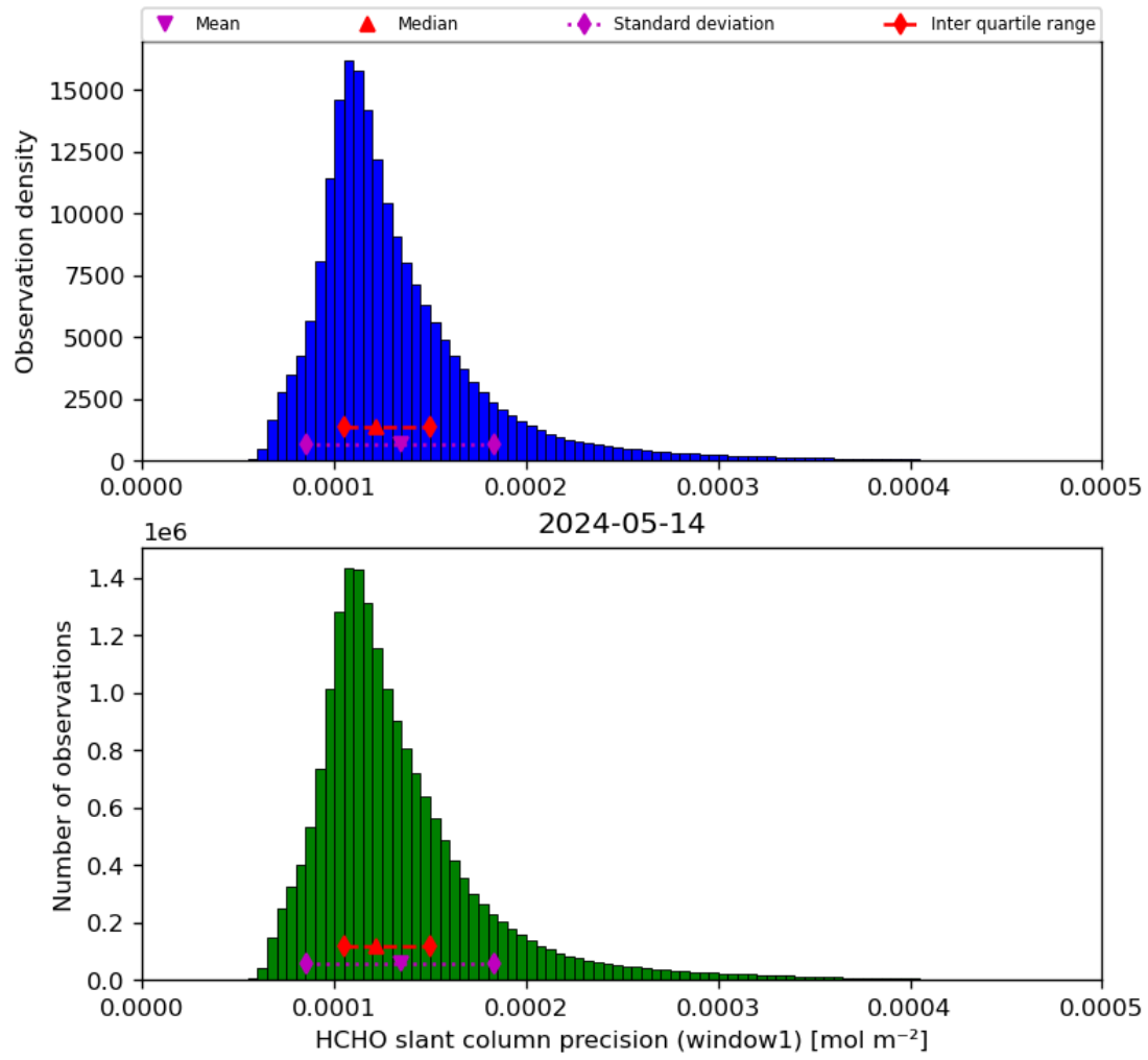
Figure 39: Histogram of “HCHO slant column precision (window1)” for 2024-05-13 to 2024-05-15
