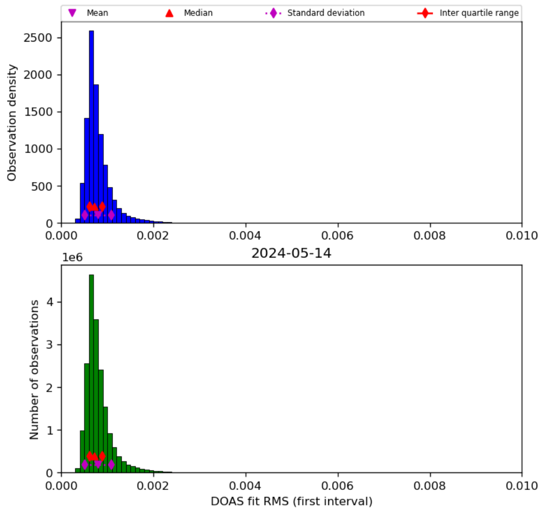
Figure 46: Histogram of “DOAS fit RMS (first interval)” for 2024-05-13 to 2024-05-15
