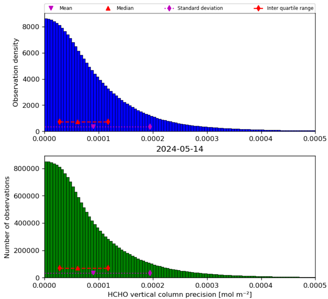
Figure 36: Histogram of “HCHO vertical column precision” for 2024-05-13 to 2024-05-15
