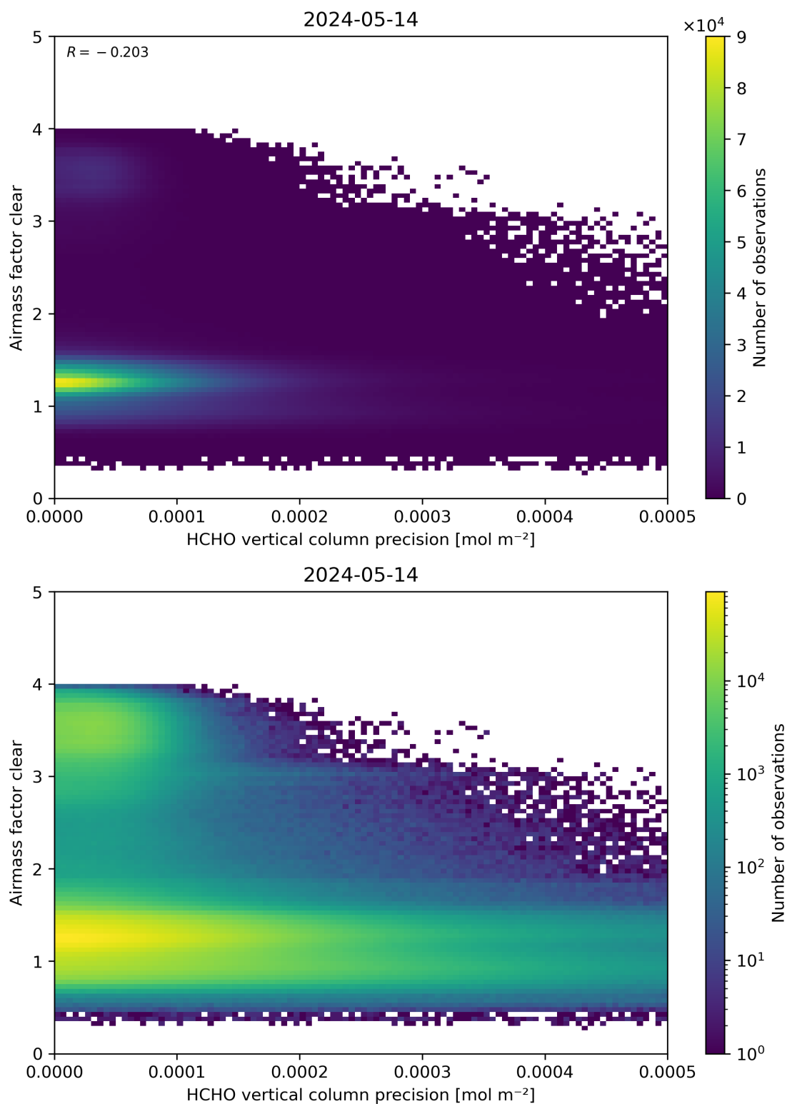
Figure 139: Scatter density plot of “HCHO vertical column precision” against “Airmass factor clear” for 2024-05-13 to 2024-05-15.
