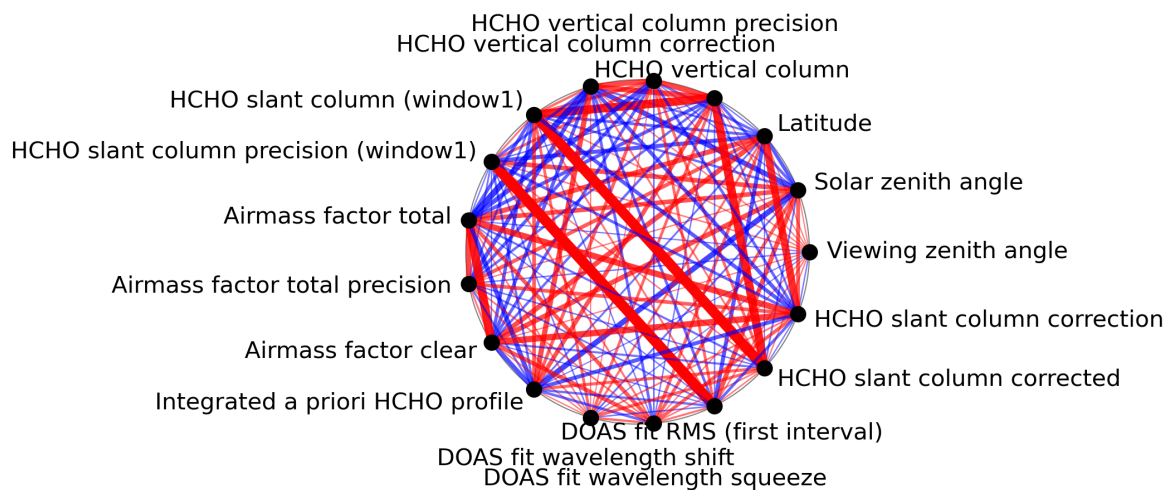
Figure 1: Map of correlation graph for 2024-05-13 to 2024-05-15.
