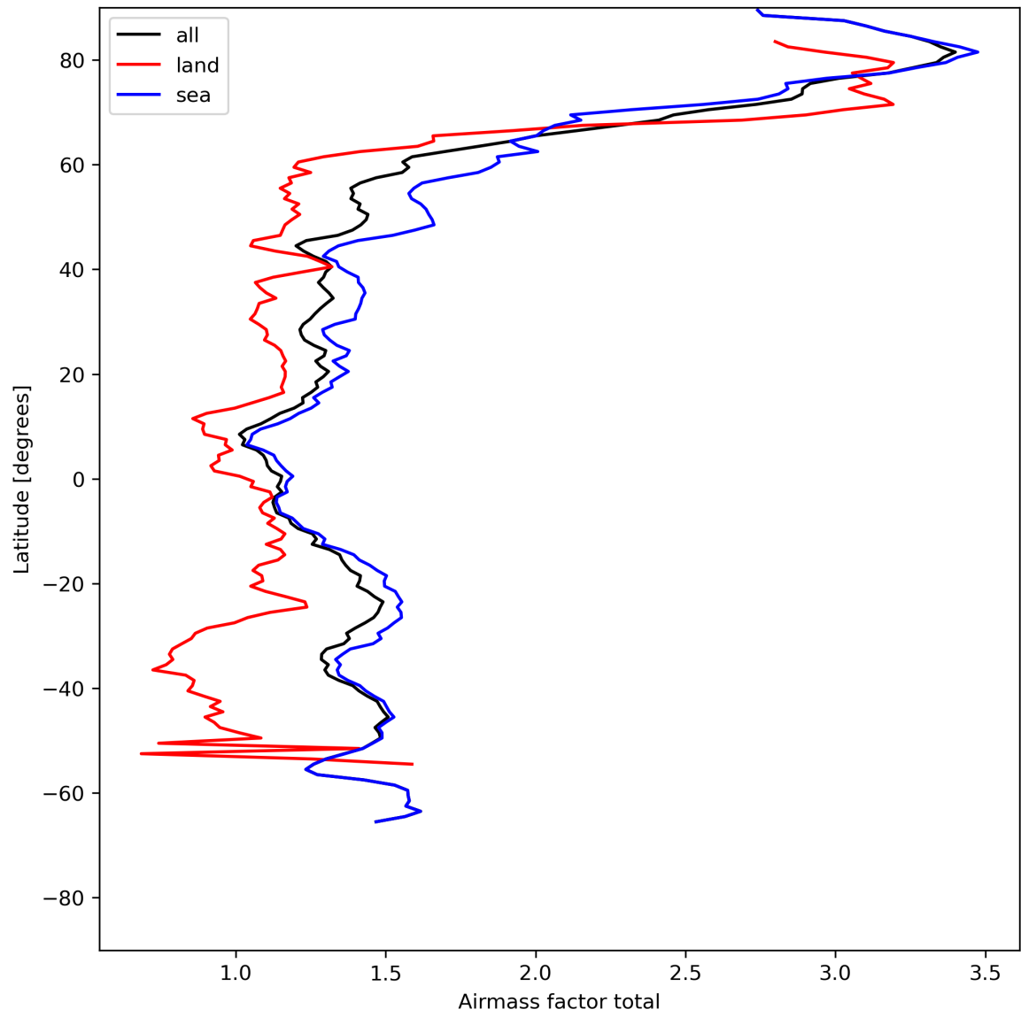
Figure 26: Zonal average of “Airmass factor total” for 2024-05-13 to 2024-05-15.
