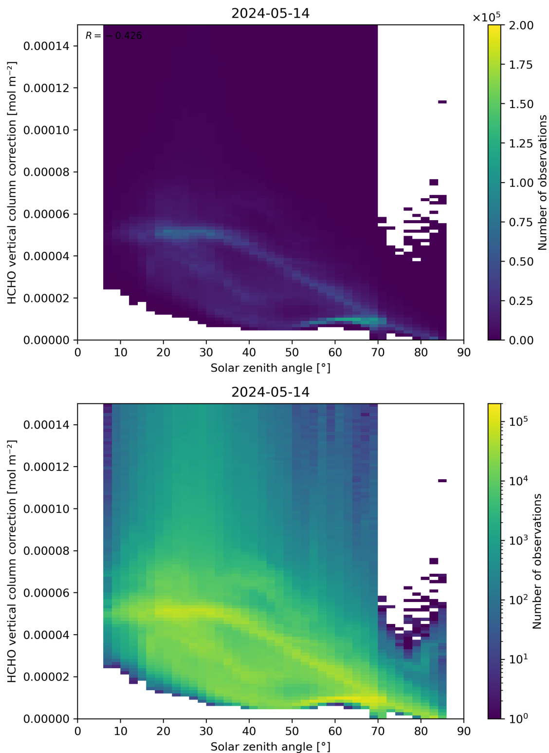
Figure 178: Scatter density plot of “Solar zenith angle” against “HCHO vertical column correction” for 2024-05-13 to 2024-05-15.
