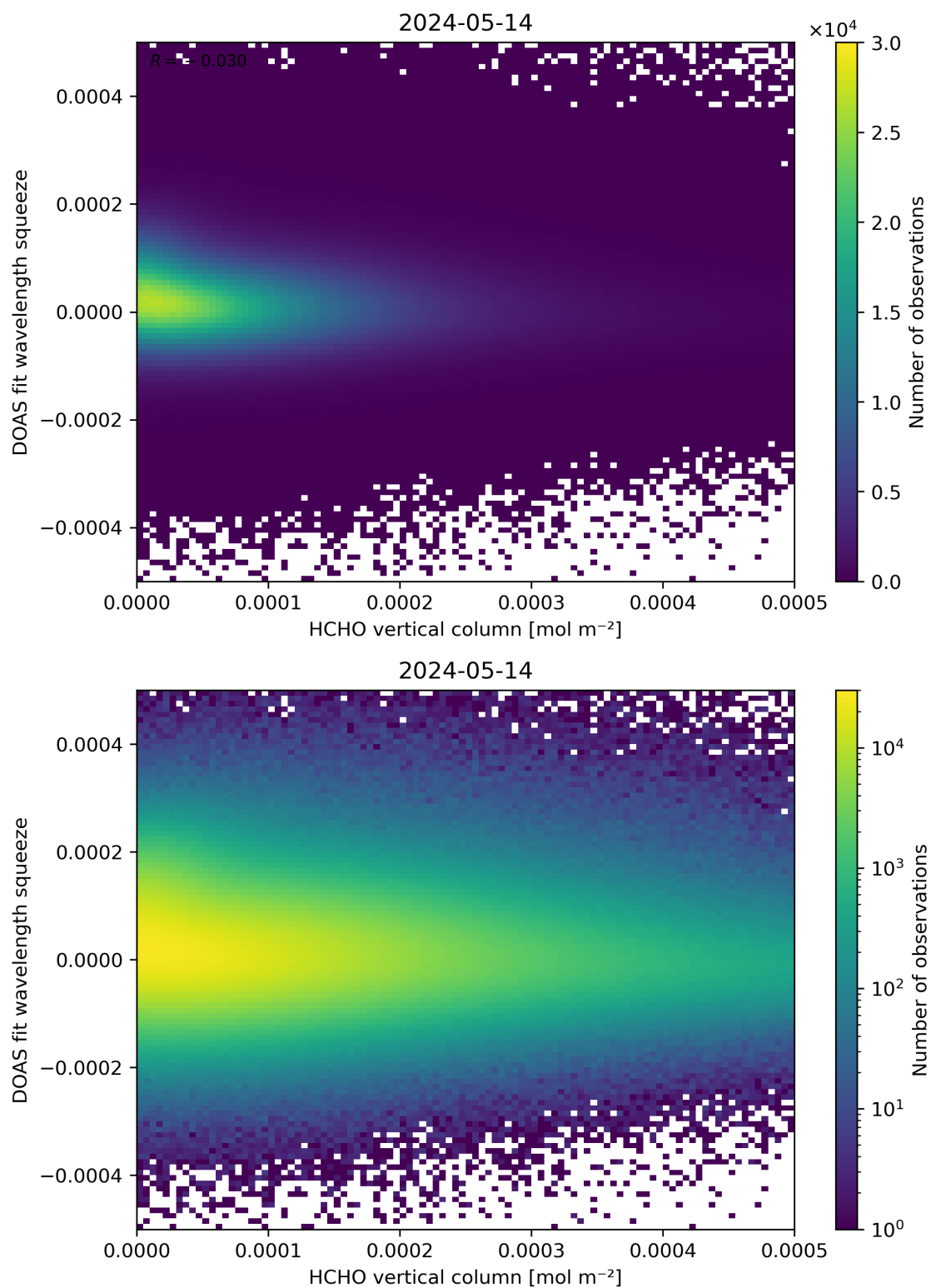
Figure 125: Scatter density plot of “HCHO vertical column” against “DOAS fit wavelength squeeze” for 2024-05-13 to 2024-05-15.
