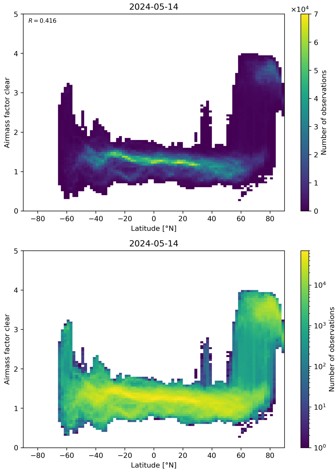
Figure 156: Scatter density plot of “Latitude” against “Airmass factor clear” for 2024-05-13 to 2024-05-15.
