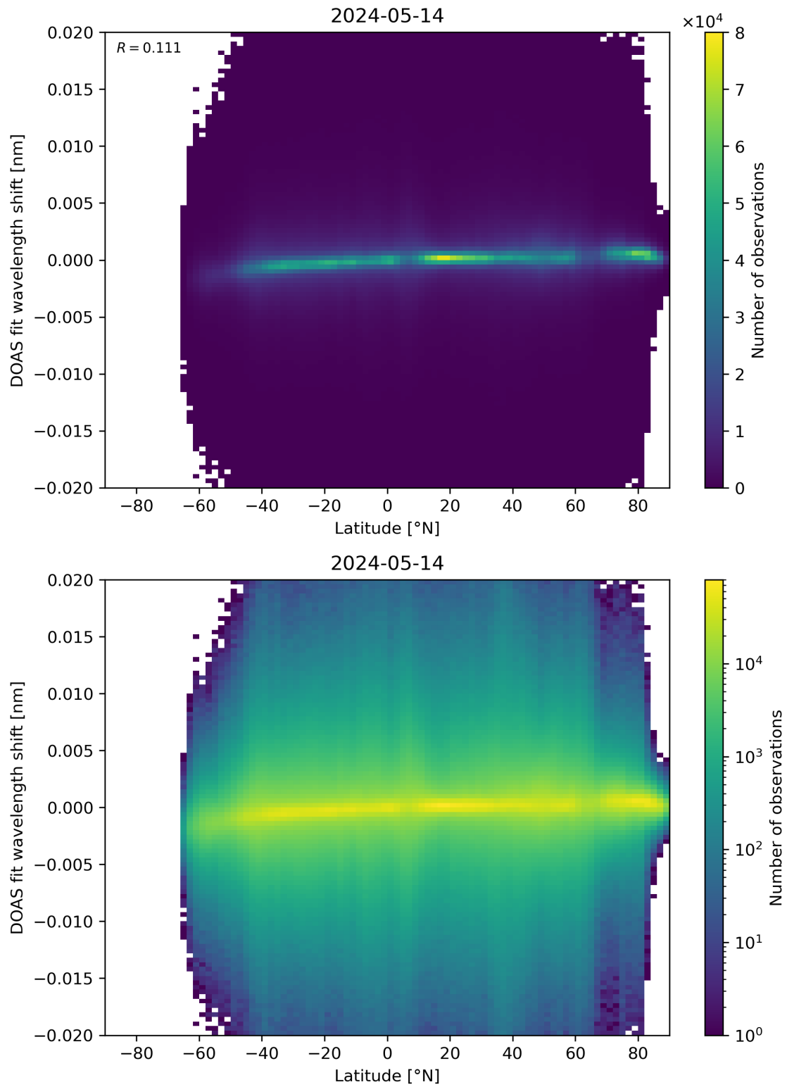
Figure 154: Scatter density plot of “Latitude” against “DOAS fit wavelength shift” for 2024-05-13 to 2024-05-15.
