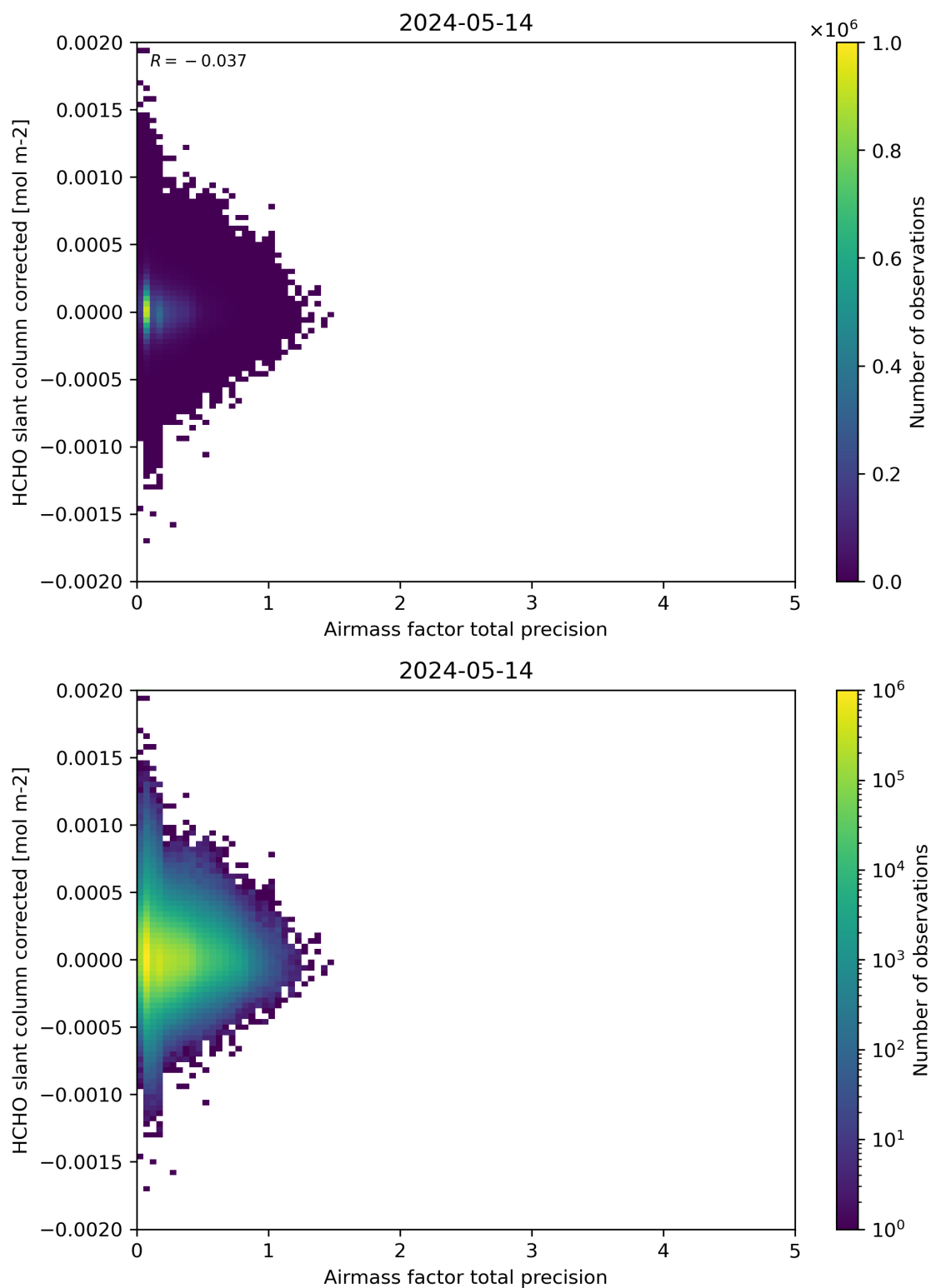
Figure 109: Scatter density plot of “Airmass factor total precision” against “HCHO slant column corrected” for 2024-05-13 to 2024-05-15.
