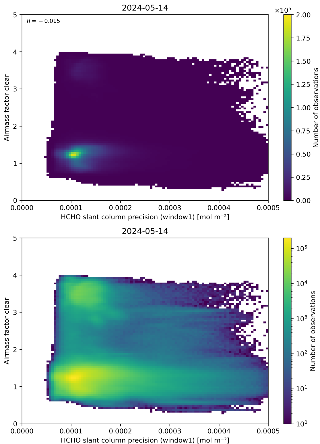
Figure 91: Scatter density plot of “HCHO slant column precision (window1)” against “Airmass factor clear” for 2024-05-13 to 2024-05-15.
