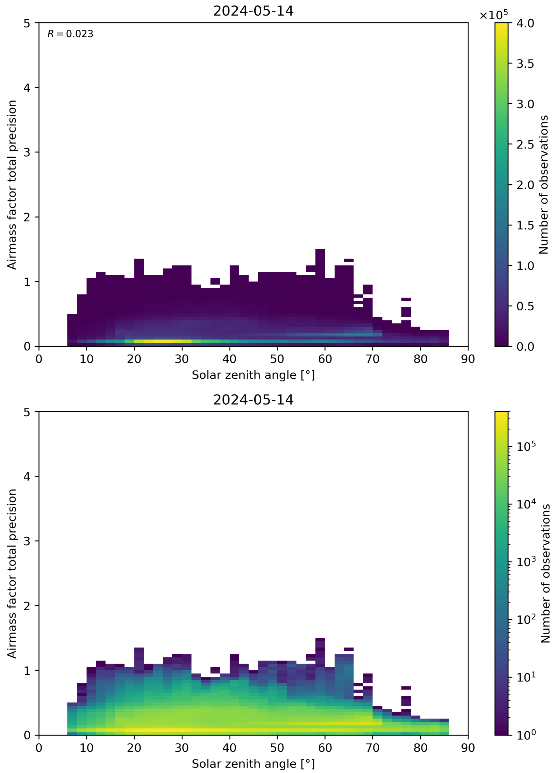
Figure 176: Scatter density plot of “Solar zenith angle” against “Airmass factor total precision” for 2024-05-13 to 2024-05-15.
