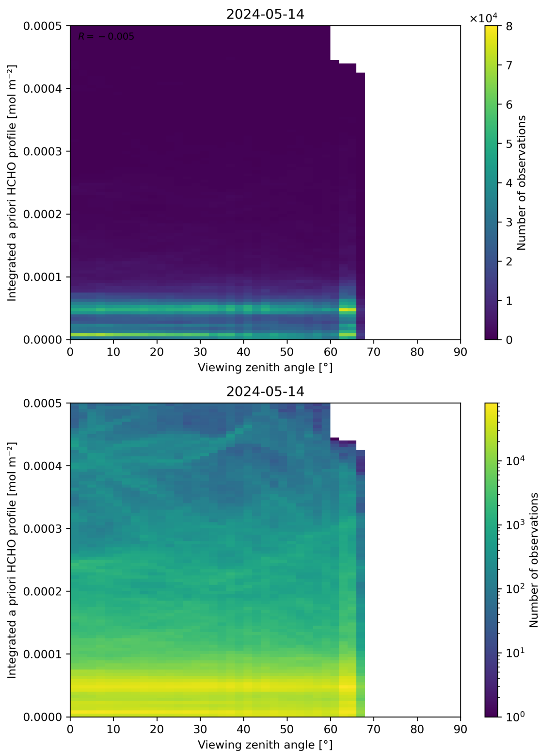
Figure 195: Scatter density plot of “Viewing zenith angle” against “Integrated a priori HCHO profile” for 2024-05-13 to 2024-05-15.
