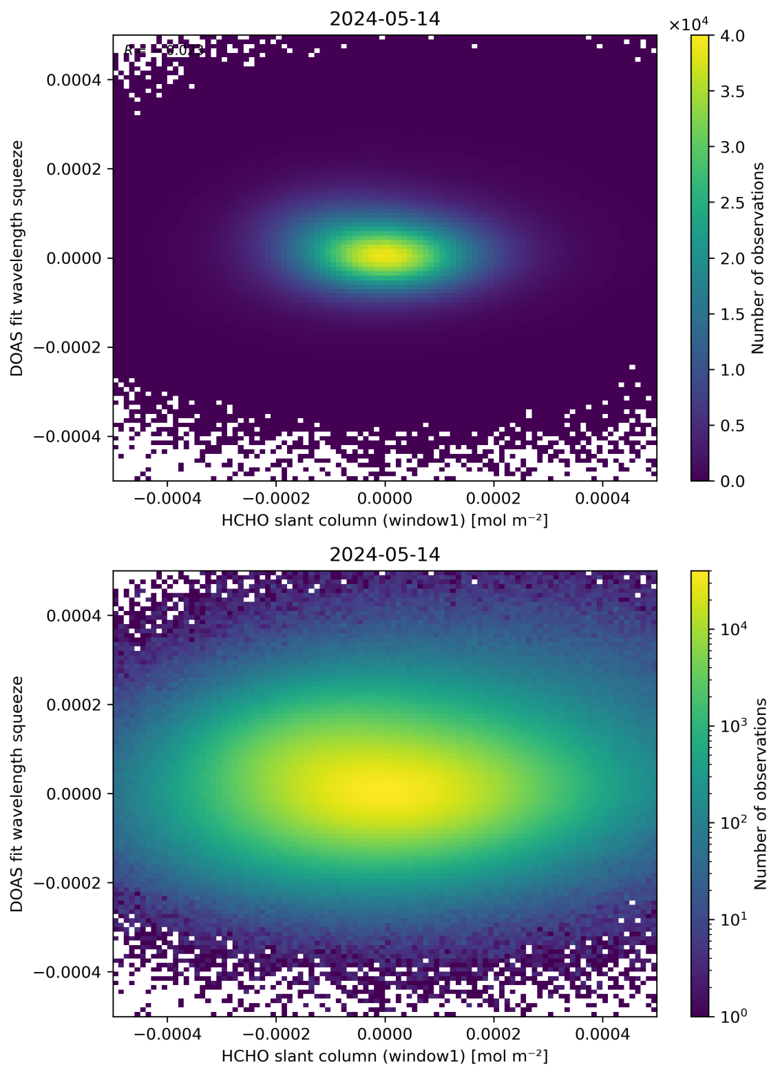
Figure 80: Scatter density plot of “HCHO slant column (window1)” against “DOAS fit wavelength squeeze” for 2024-05-13 to 2024-05-15.
