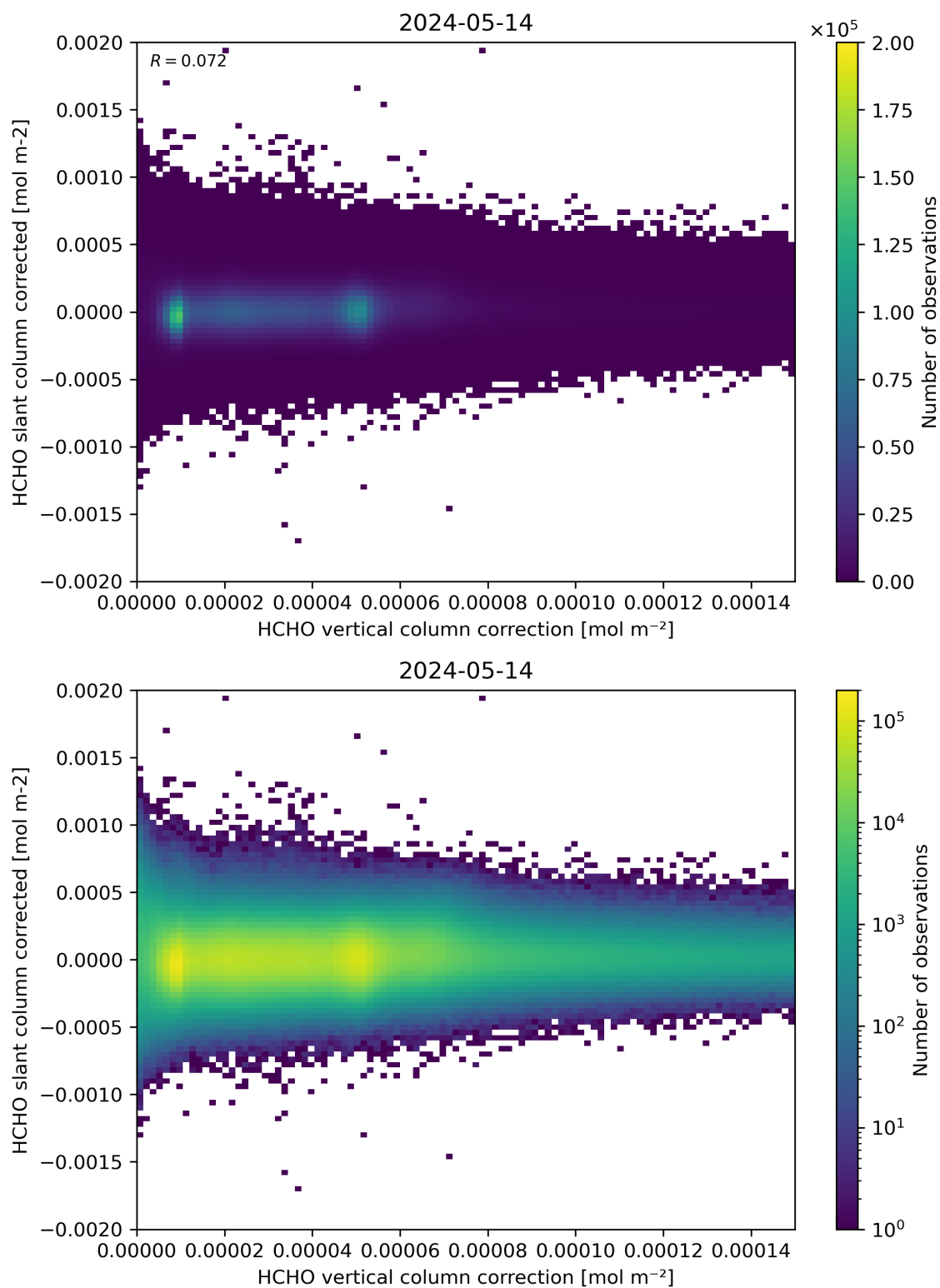
Figure 116: Scatter density plot of “HCHO vertical column correction” against “HCHO slant column corrected” for 2024-05-13 to 2024-05-15.
