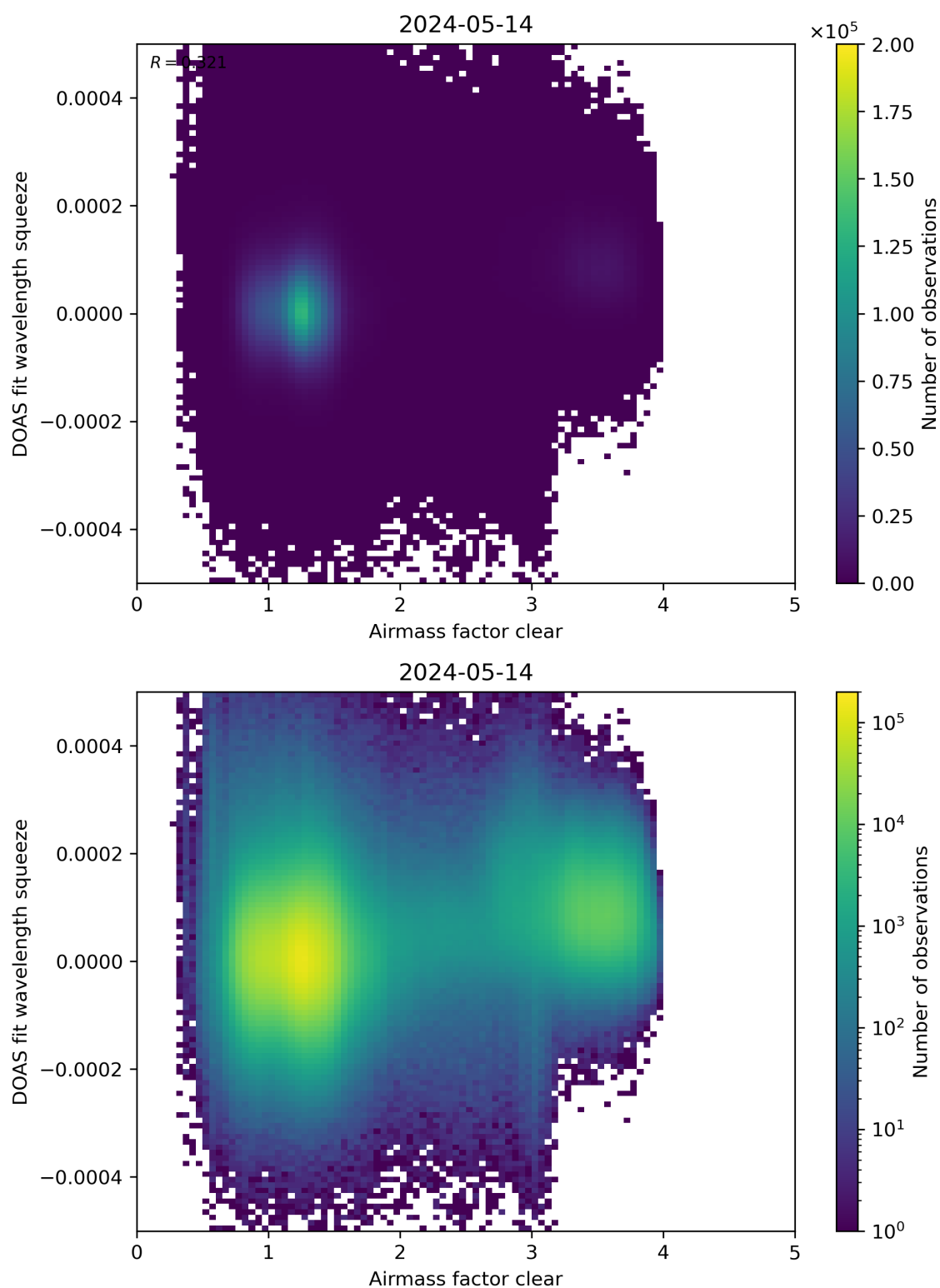
Figure 73: Scatter density plot of “Airmass factor clear” against “DOAS fit wavelength squeeze” for 2024-05-13 to 2024-05-15.
