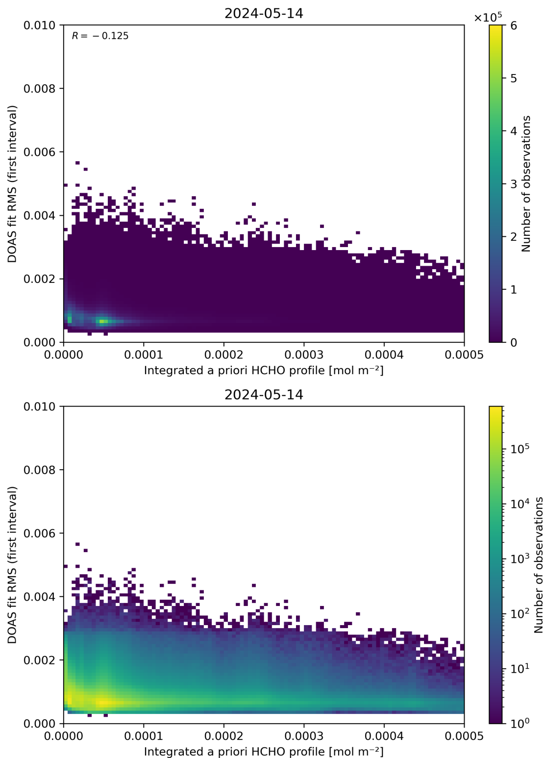
Figure 148: Scatter density plot of “Integrated a priori HCHO profile” against “DOAS fit RMS (first interval)” for 2024-05-13 to 2024-05-15.
