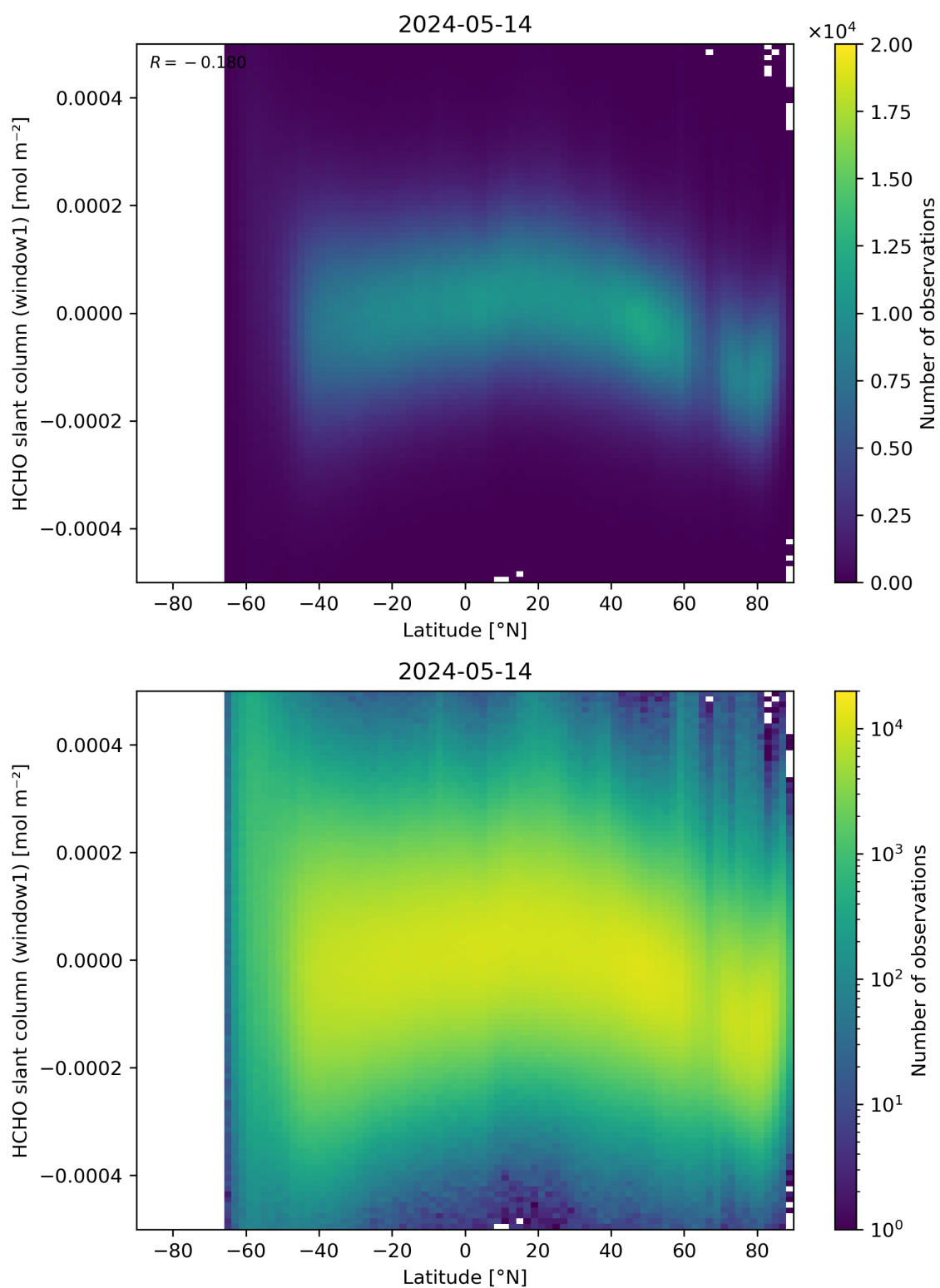
Figure 159: Scatter density plot of “Latitude” against “HCHO slant column (window1)” for 2024-05-13 to 2024-05-15.
