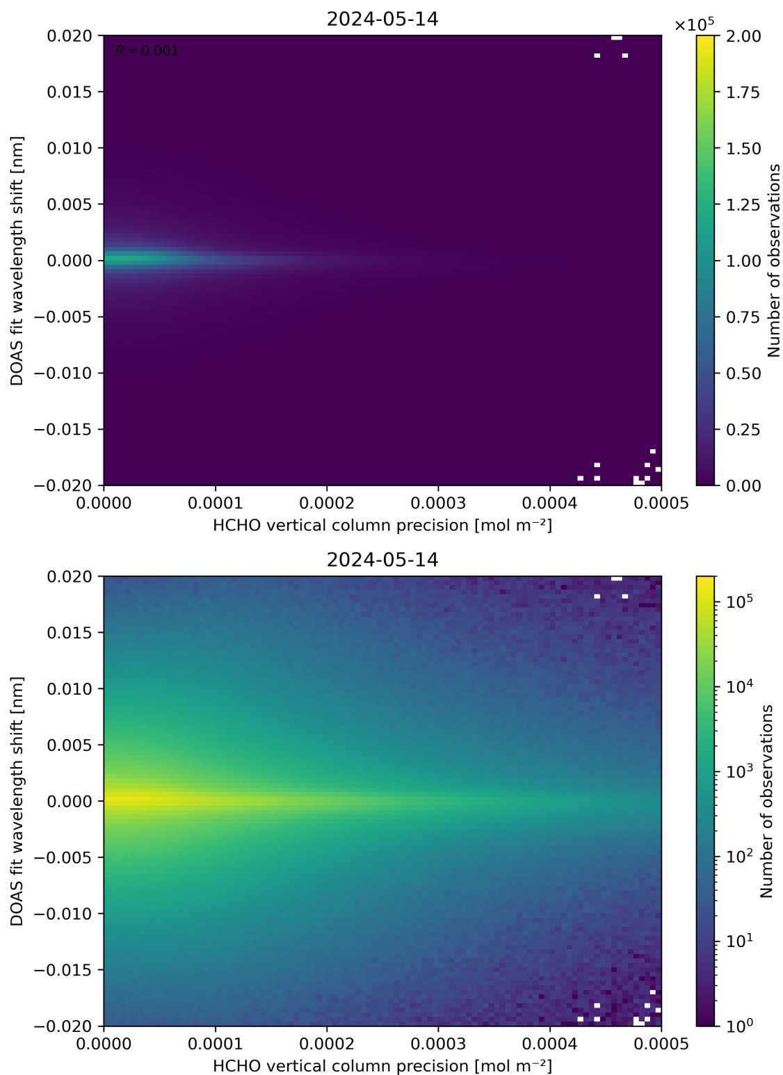
Figure 137: Scatter density plot of “HCHO vertical column precision” against “DOAS fit wavelength shift” for 2024-05-13 to 2024-05-15.
