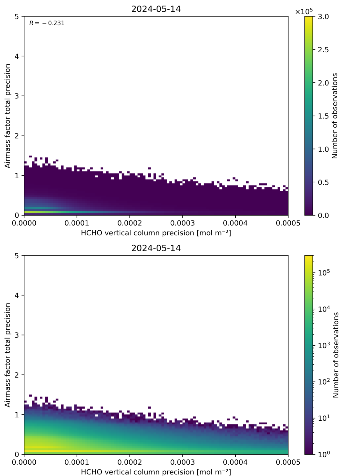
Figure 145: Scatter density plot of “HCHO vertical column precision” against “Airmass factor total precision” for 2024-05-13 to 2024-05-15.
