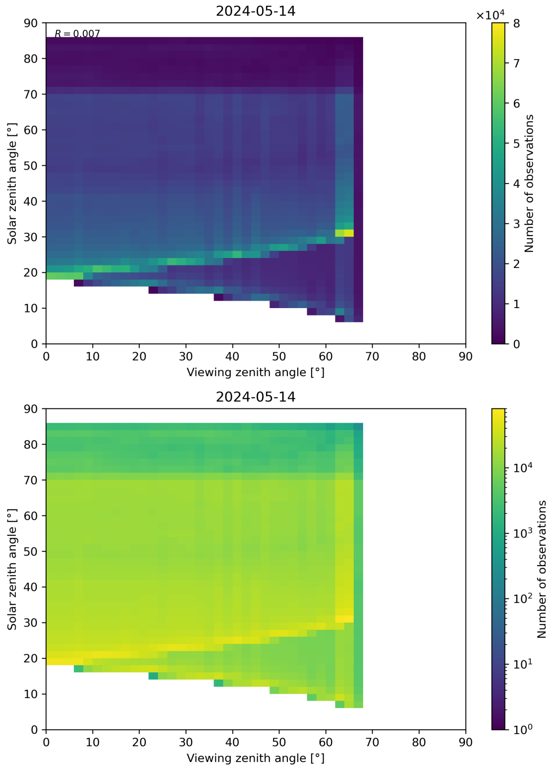
Figure 197: Scatter density plot of “Viewing zenith angle” against “Solar zenith angle” for 2024-05-13 to 2024-05-15.
