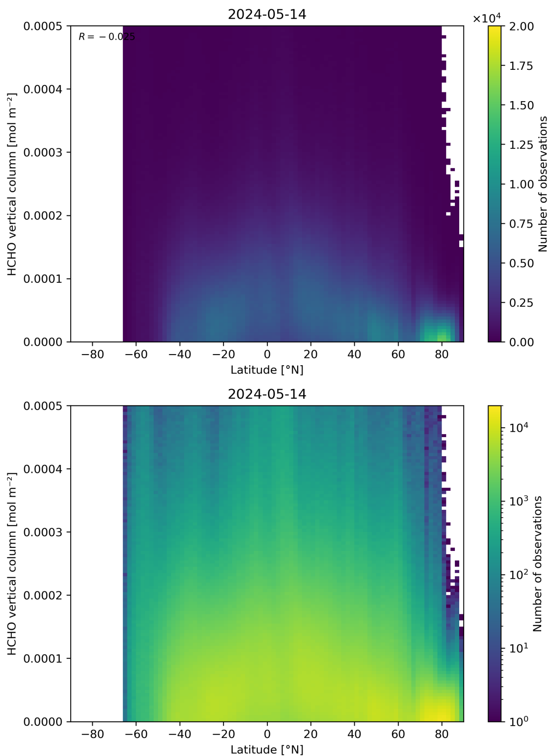
Figure 163: Scatter density plot of “Latitude” against “HCHO vertical column” for 2024-05-13 to 2024-05-15.
