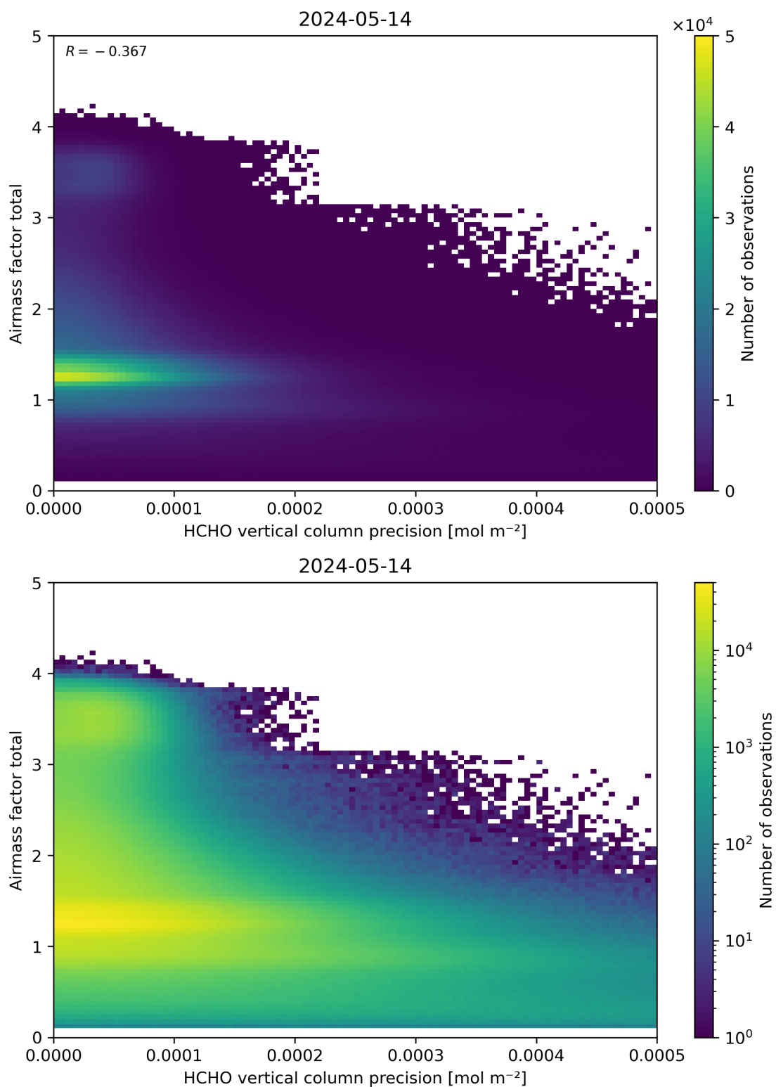
Figure 144: Scatter density plot of “HCHO vertical column precision” against “Airmass factor total” for 2024-05-13 to 2024-05-15.
