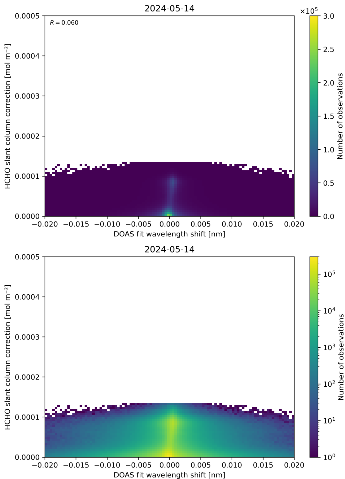
Figure 67: Scatter density plot of “DOAS fit wavelength shift” against “HCHO slant column correction” for 2024-05-13 to 2024-05-15.
