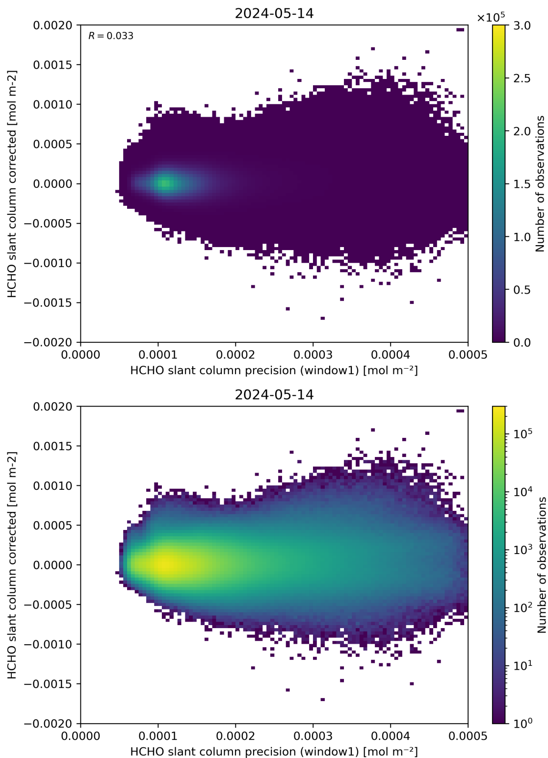
Figure 92: Scatter density plot of “HCHO slant column precision (window1)” against “HCHO slant column corrected” for 2024-05-13 to 2024-05-15.
