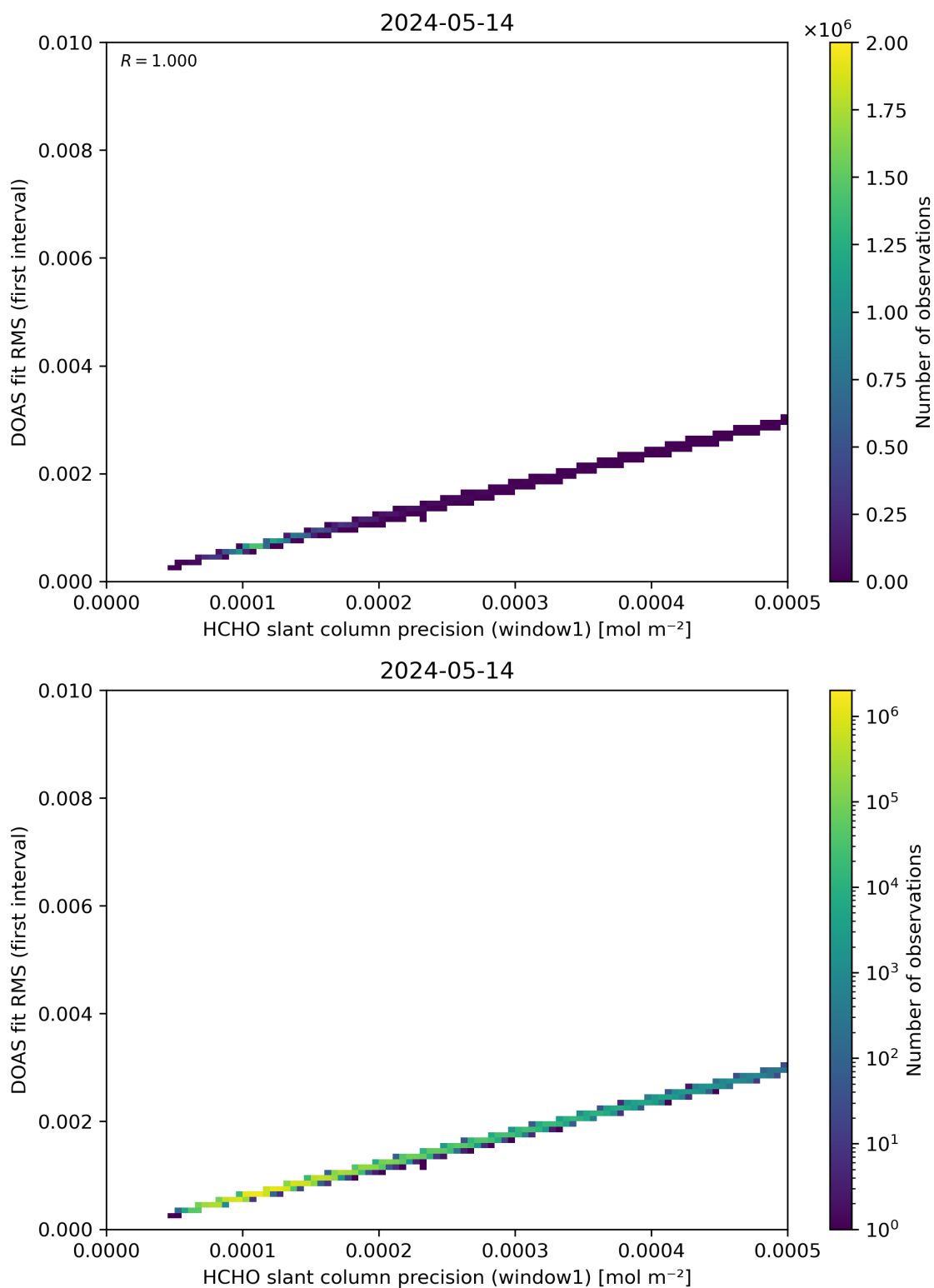
Figure 88: Scatter density plot of “HCHO slant column precision (window1)” against “DOAS fit RMS (first interval)” for 2024-05-13 to 2024-05-15.
