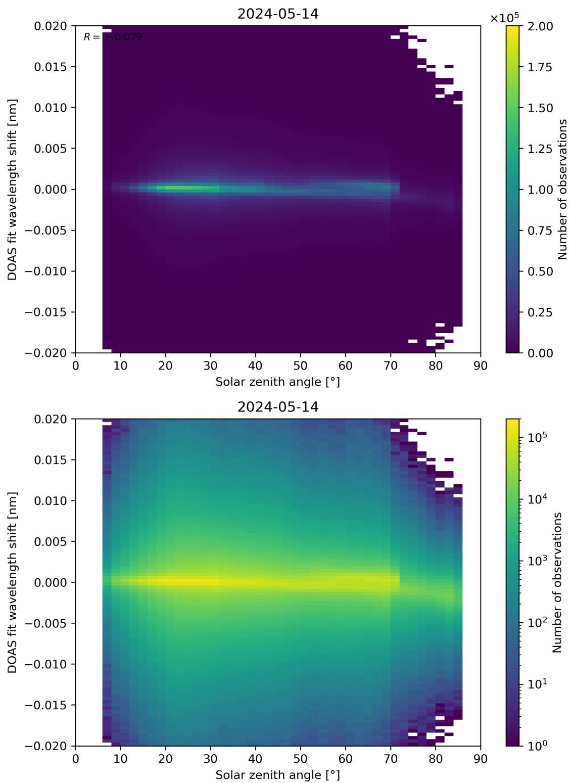
Figure 168: Scatter density plot of “Solar zenith angle” against “DOAS fit wavelength shift” for 2024-05-13 to 2024-05-15.
