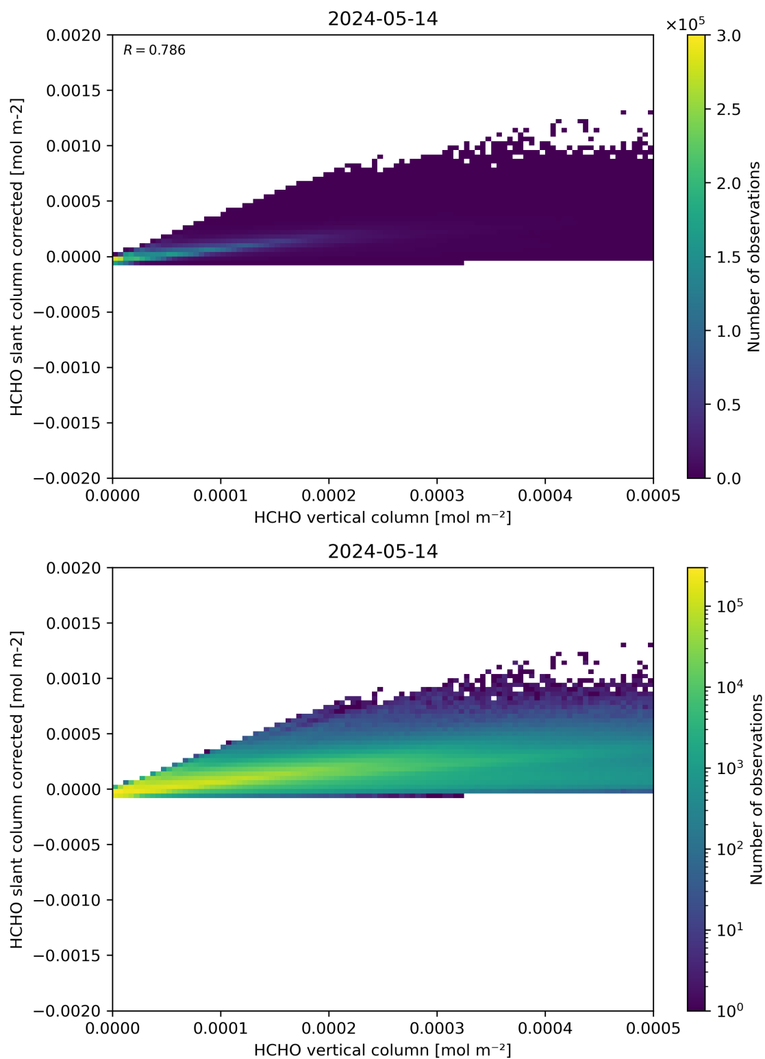
Figure 127: Scatter density plot of “HCHO vertical column” against “HCHO slant column corrected” for 2024-05-13 to 2024-05-15.
