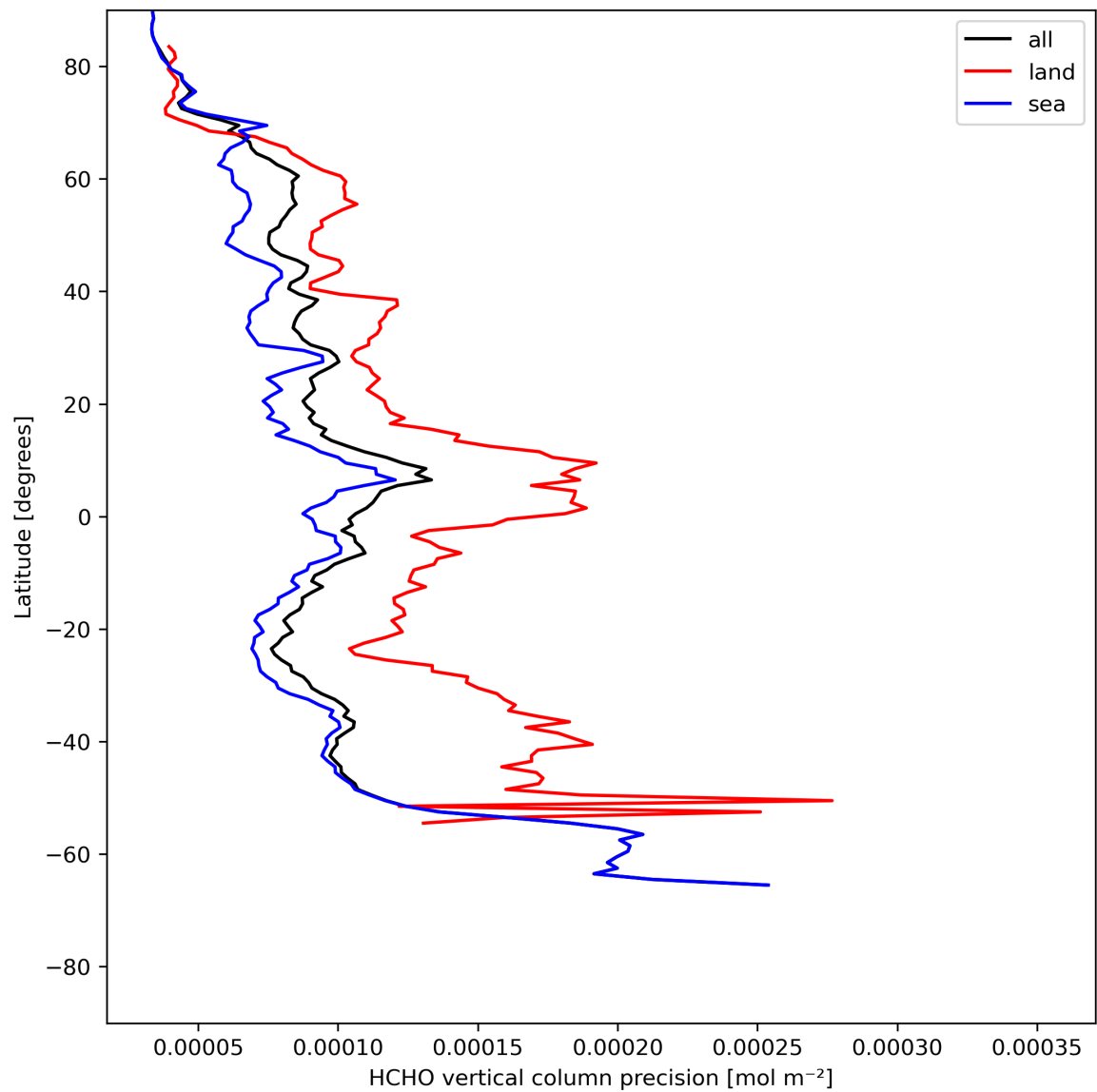
Figure 22: Zonal average of “HCHO vertical column precision” for 2024-05-13 to 2024-05-15.
