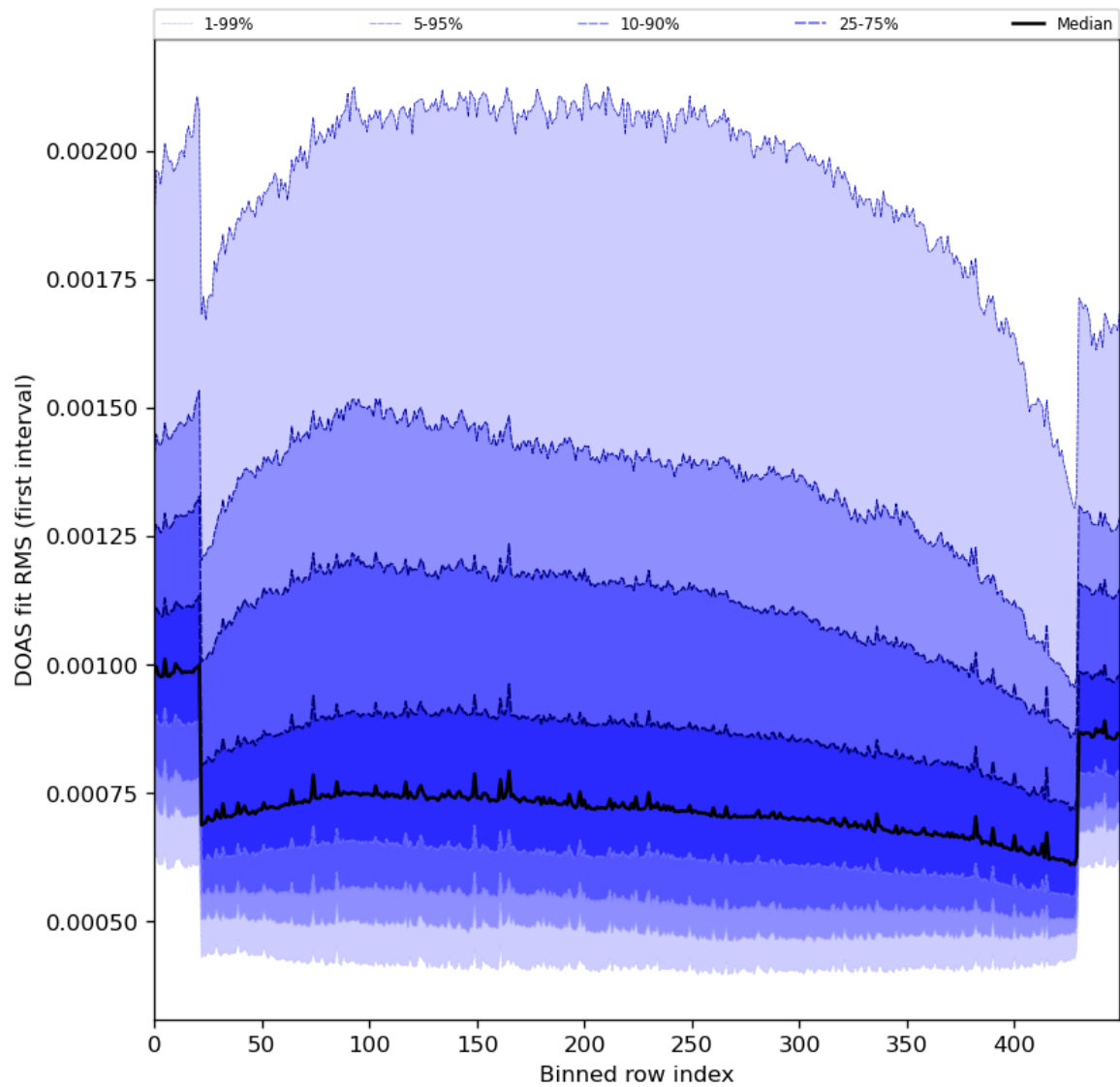
Figure 60: Along track statistics of “DOAS fit RMS (first interval)” for 2024-05-13 to 2024-05-15
