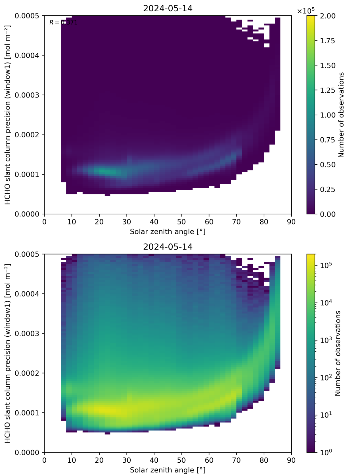
Figure 174: Scatter density plot of “Solar zenith angle” against “HCHO slant column precision (window1)” for 2024-05-13 to 2024-05-15.
