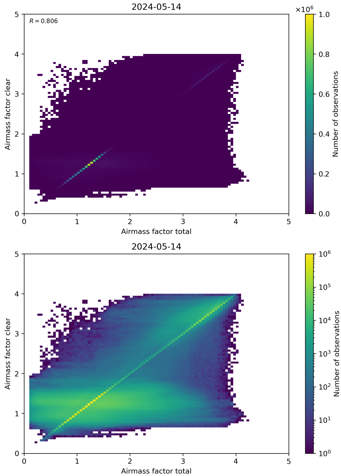
Figure 100: Scatter density plot of “Airmass factor total” against “Airmass factor clear” for 2024-05-13 to 2024-05-15.
