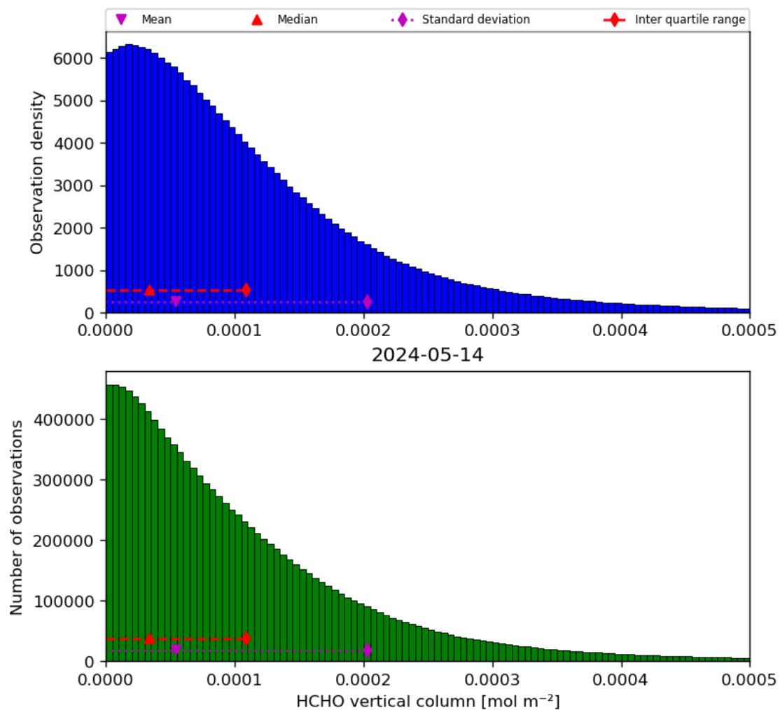
Figure 35: Histogram of “HCHO vertical column” for 2024-05-13 to 2024-05-15
