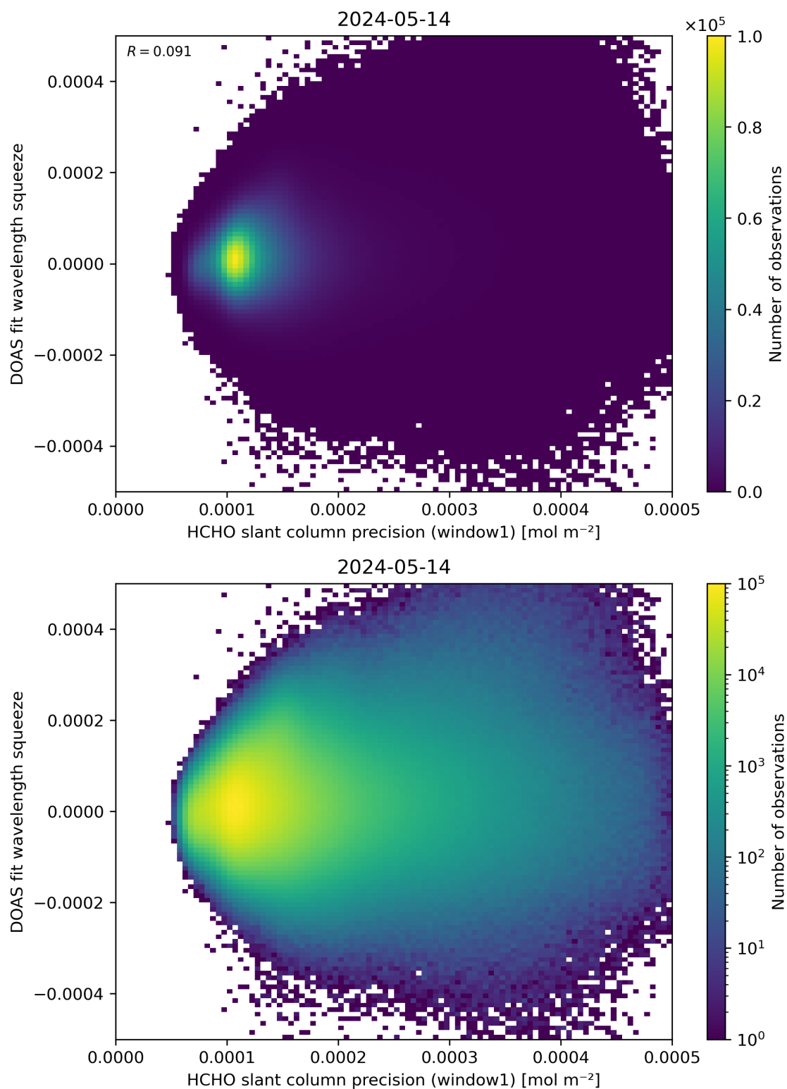
Figure 90: Scatter density plot of “HCHO slant column precision (window1)” against “DOAS fit wavelength squeeze” for 2024-05-13 to 2024-05-15.
