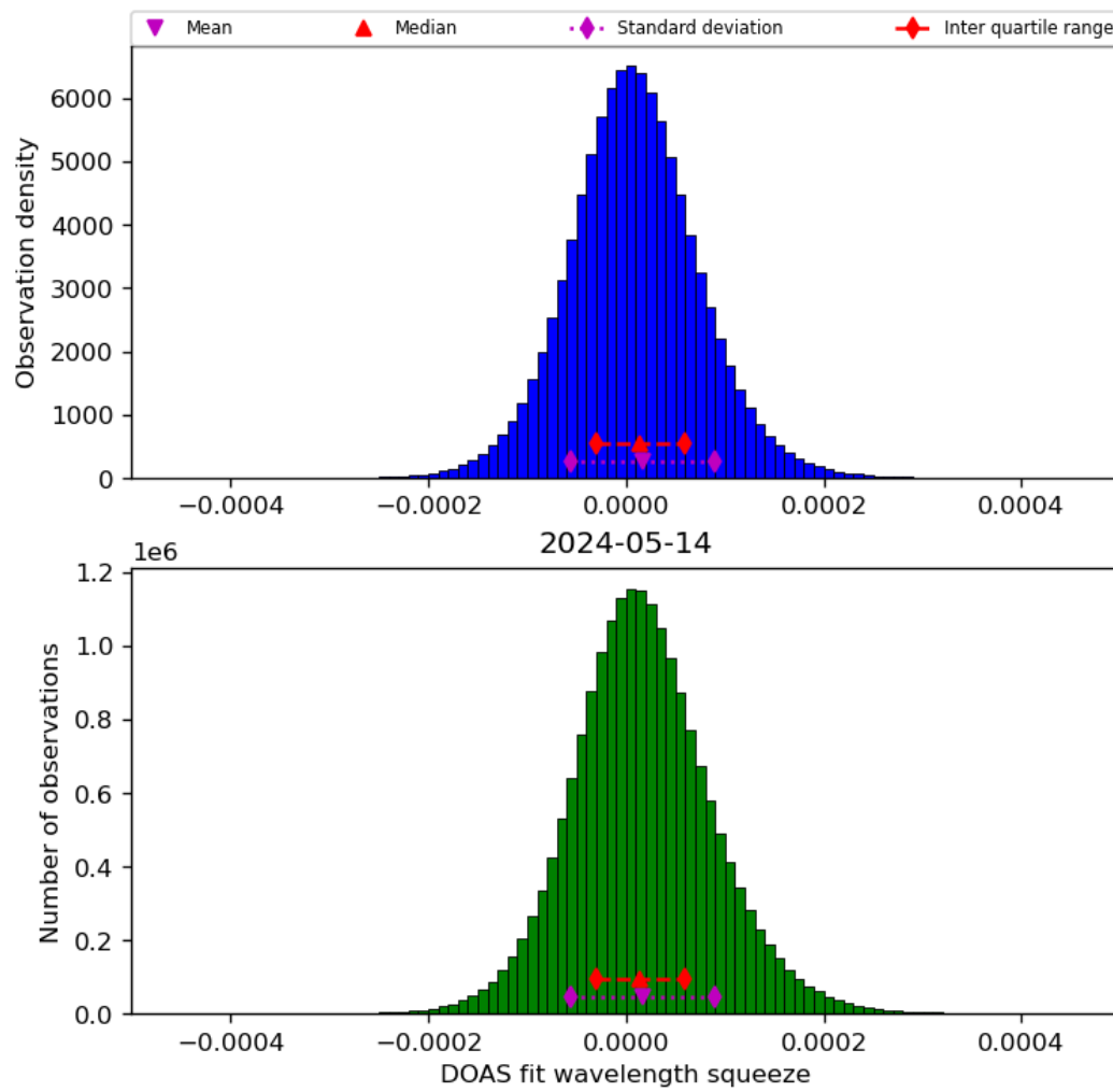
Figure 45: Histogram of "DOAS fit wavelength squeeze" for 2024-05-13 to 2024-05-15
