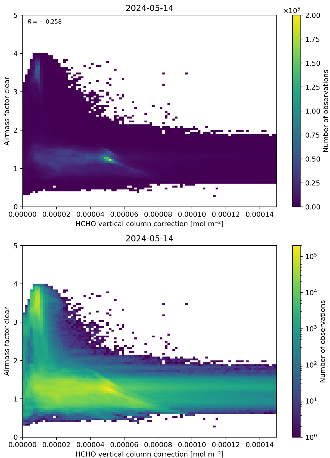
Figure 115: Scatter density plot of “HCHO vertical column correction” against “Airmass factor clear” for 2024-05-13 to 2024-05-15.
