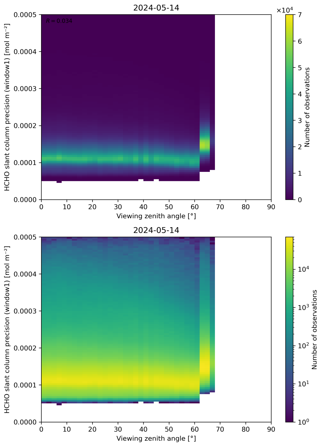
Figure 189: Scatter density plot of “Viewing zenith angle” against “HCHO slant column precision (window1)” for 2024-05-13 to 2024-05-15.
