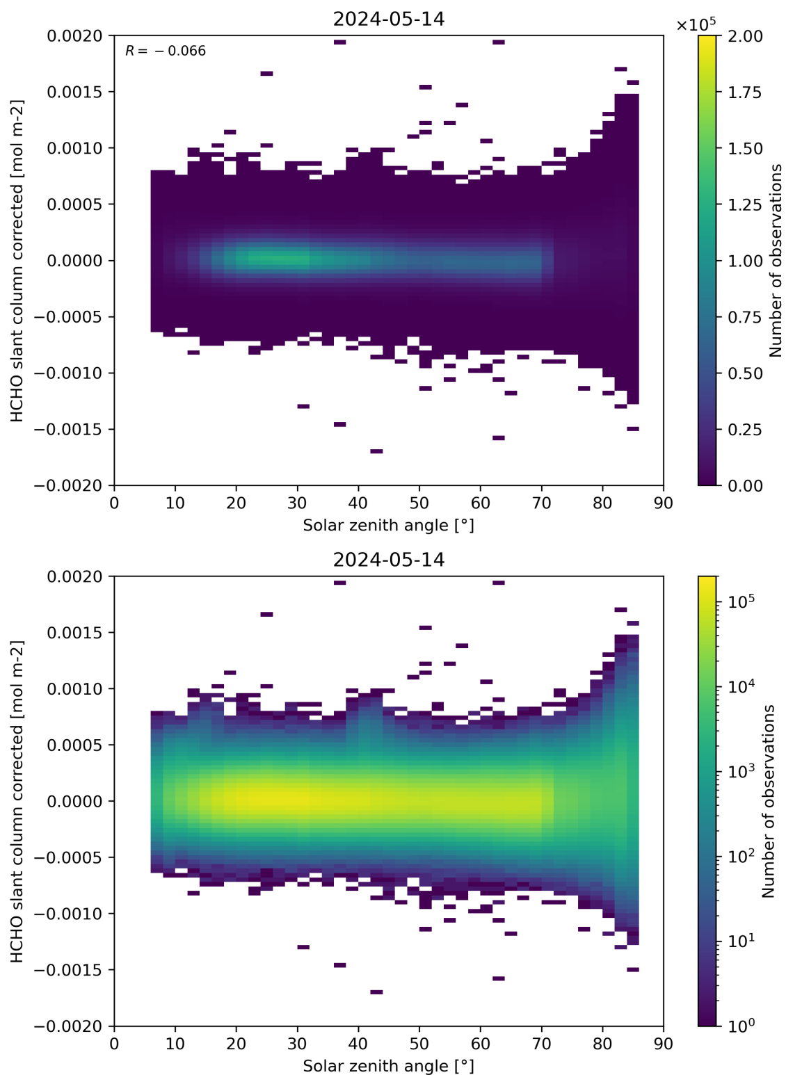
Figure 171: Scatter density plot of “Solar zenith angle” against “HCHO slant column corrected” for 2024-05-13 to 2024-05-15.
