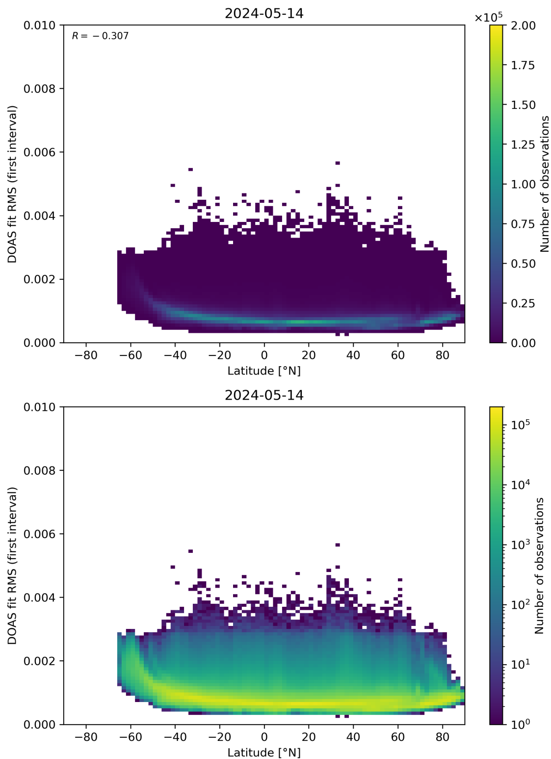
Figure 153: Scatter density plot of “Latitude” against “DOAS fit RMS (first interval)” for 2024-05-13 to 2024-05-15.
