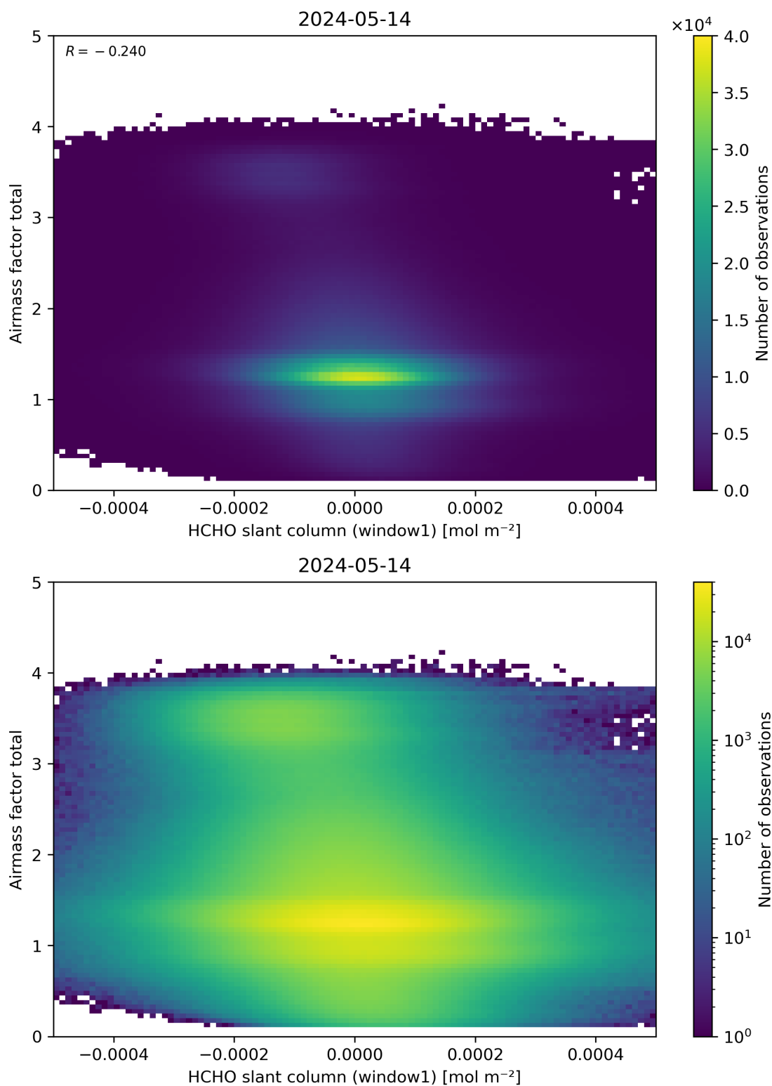
Figure 85: Scatter density plot of “HCHO slant column (window1)” against “Airmass factor total” for 2024-05-13 to 2024-05-15.
