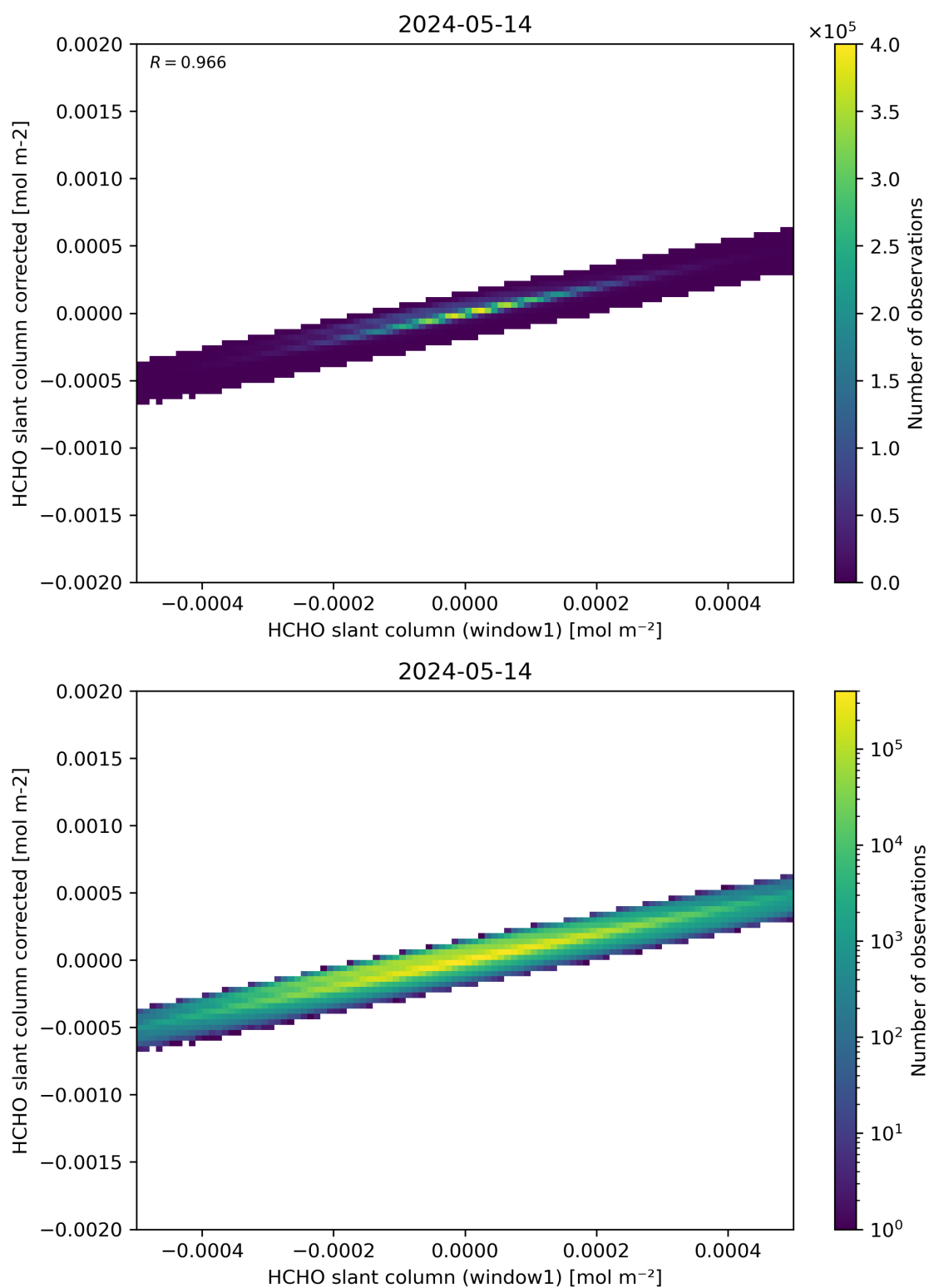
Figure 82: Scatter density plot of “HCHO slant column (window1)” against “HCHO slant column corrected” for 2024-05-13 to 2024-05-15.
