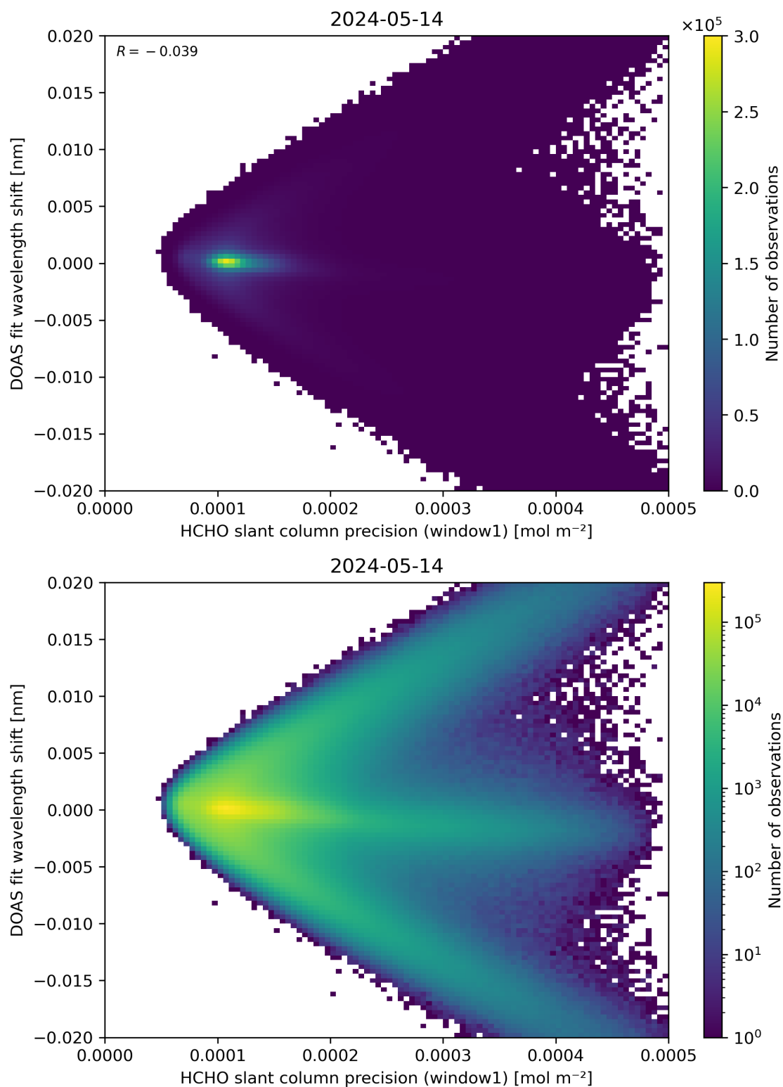
Figure 89: Scatter density plot of “HCHO slant column precision (window1)” against “DOAS fit wavelength shift” for 2024-05-13 to 2024-05-15.
