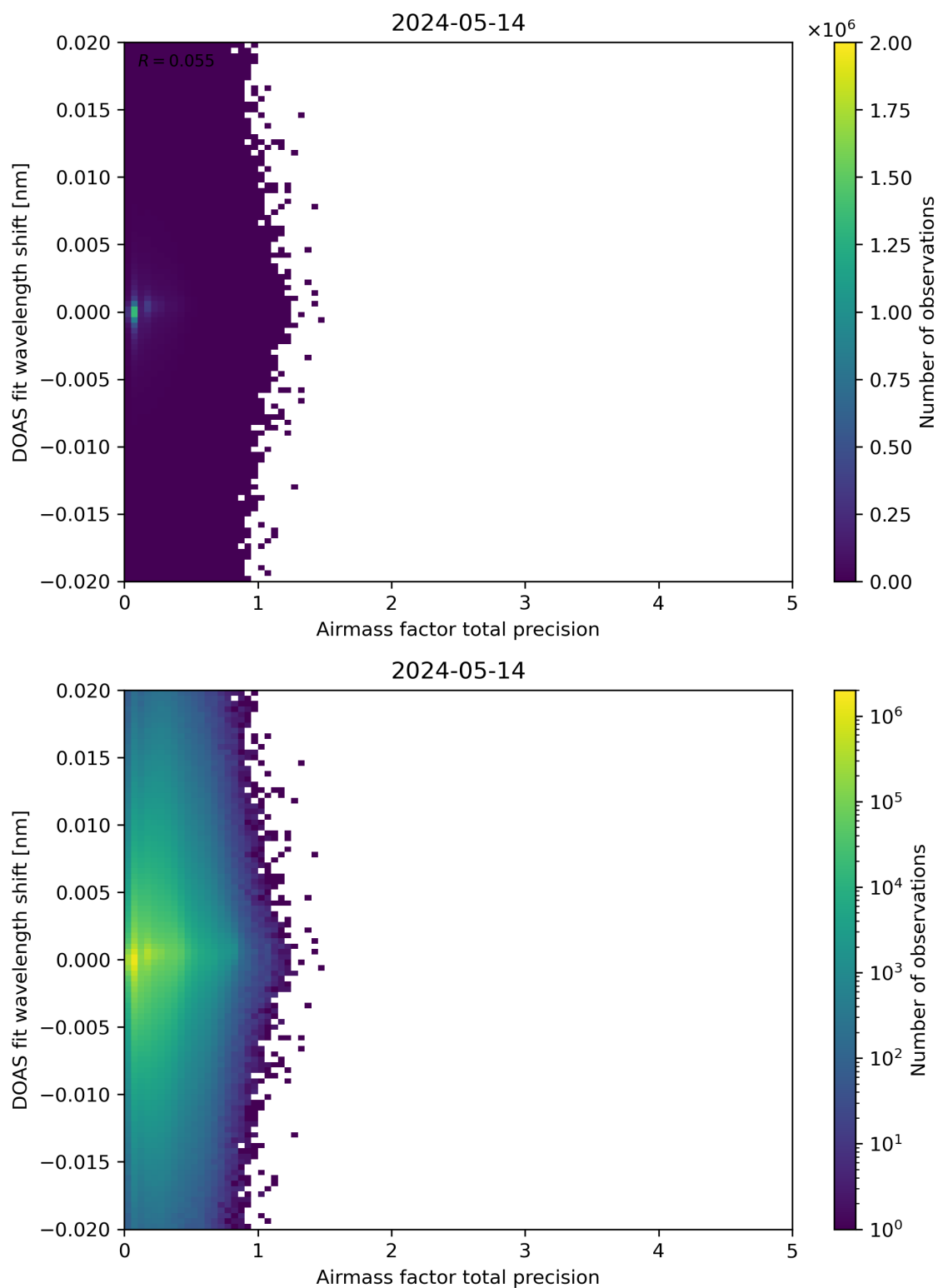
Figure 106: Scatter density plot of “Airmass factor total precision” against “DOAS fit wavelength shift” for 2024-05-13 to 2024-05-15.
