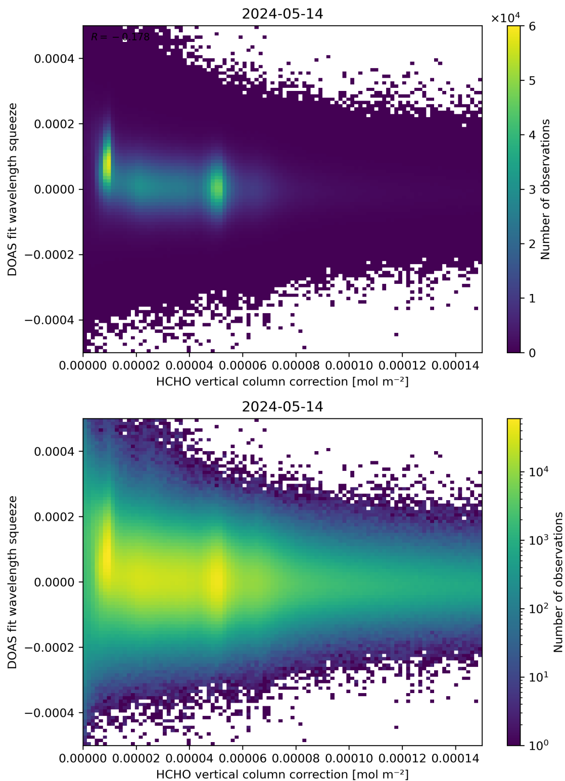
Figure 114: Scatter density plot of “HCHO vertical column correction” against “DOAS fit wavelength squeeze” for 2024-05-13 to 2024-05-15.
