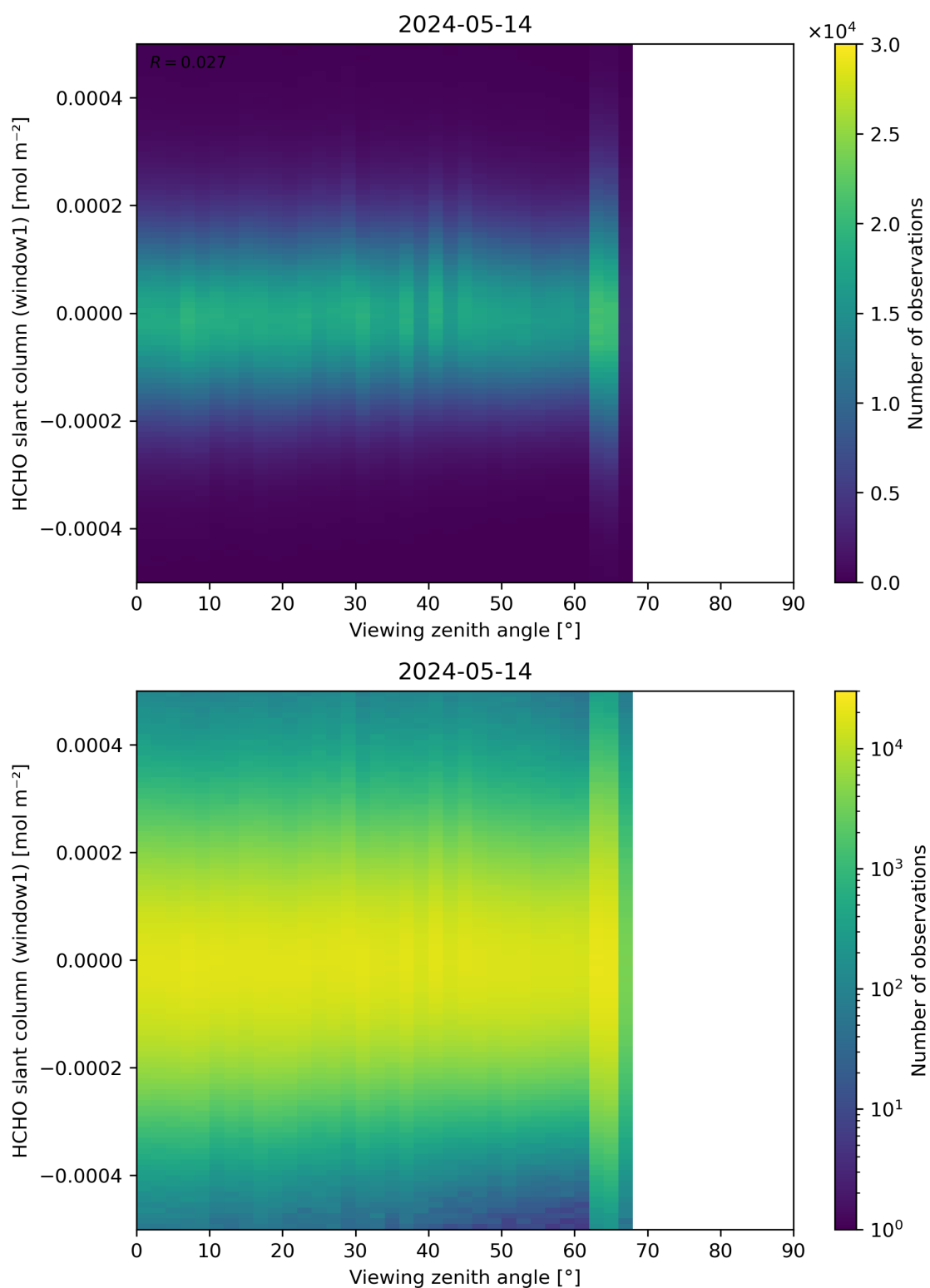
Figure 188: Scatter density plot of “Viewing zenith angle” against “HCHO slant column (window1)” for 2024-05-13 to 2024-05-15.
