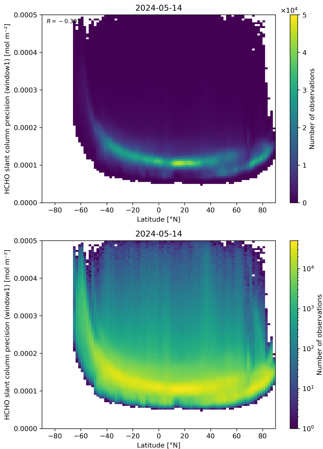
Figure 160: Scatter density plot of “Latitude” against “HCHO slant column precision (window1)” for 2024-05-13 to 2024-05-15.
