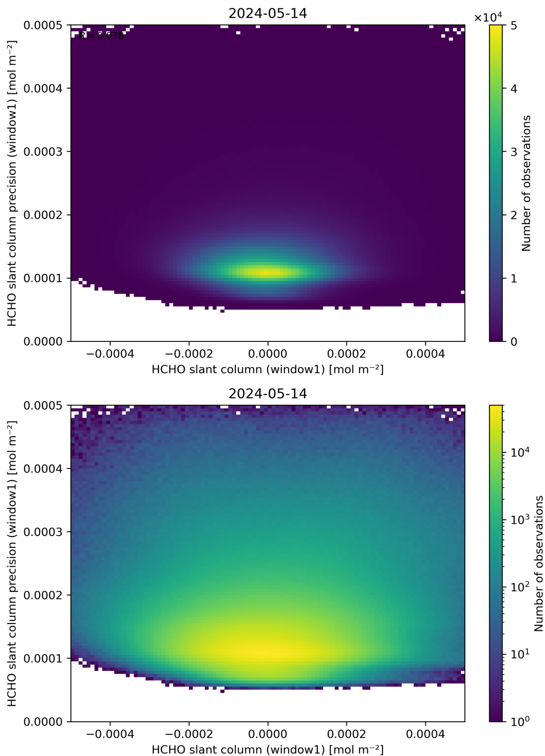
Figure 84: Scatter density plot of “HCHO slant column (window1)” against “HCHO slant column precision (window1)” for 2024-05-13 to 2024-05-15.
