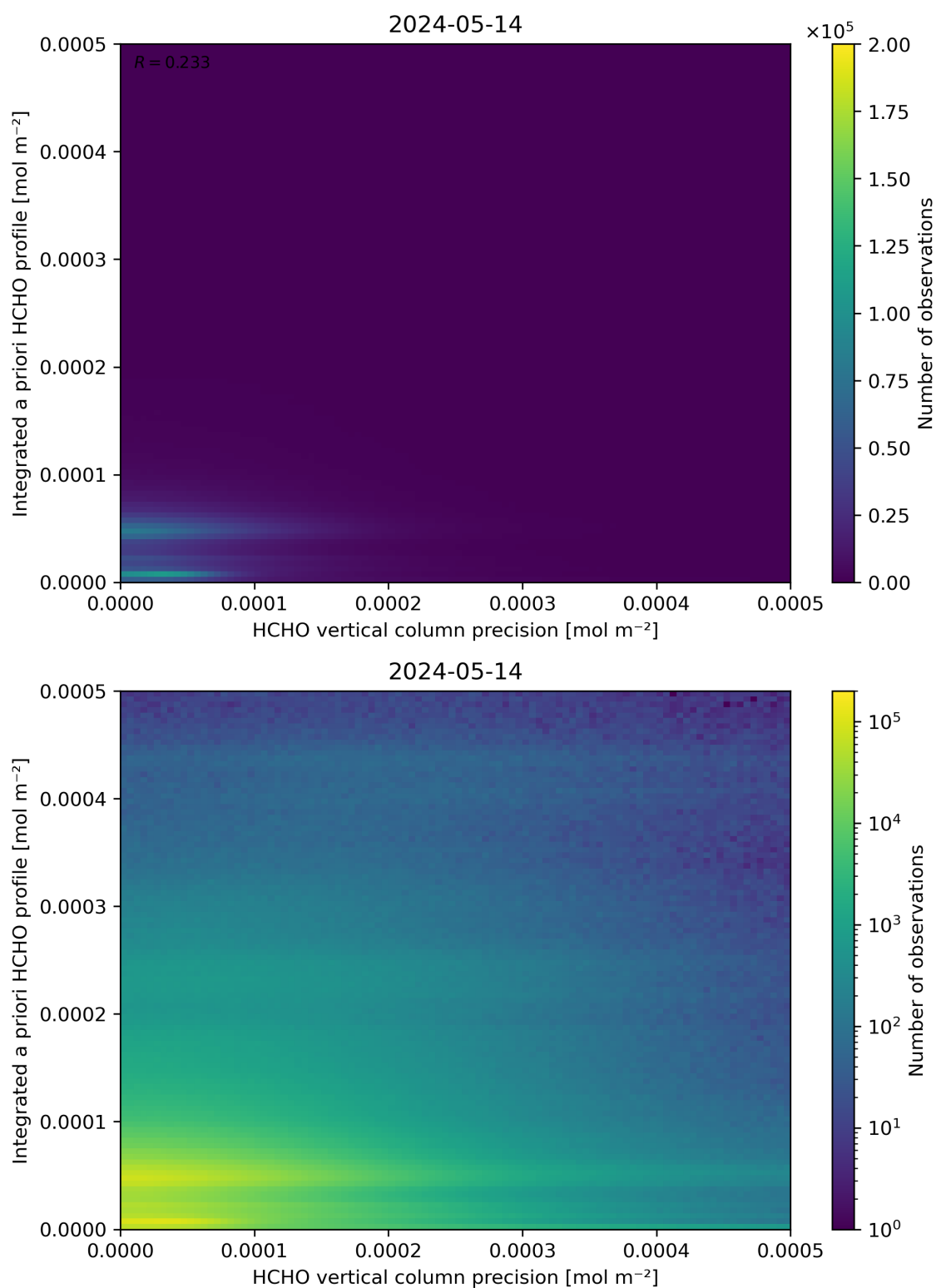
Figure 147: Scatter density plot of “HCHO vertical column precision” against “Integrated a priori HCHO profile” for 2024-05-13 to 2024-05-15.
