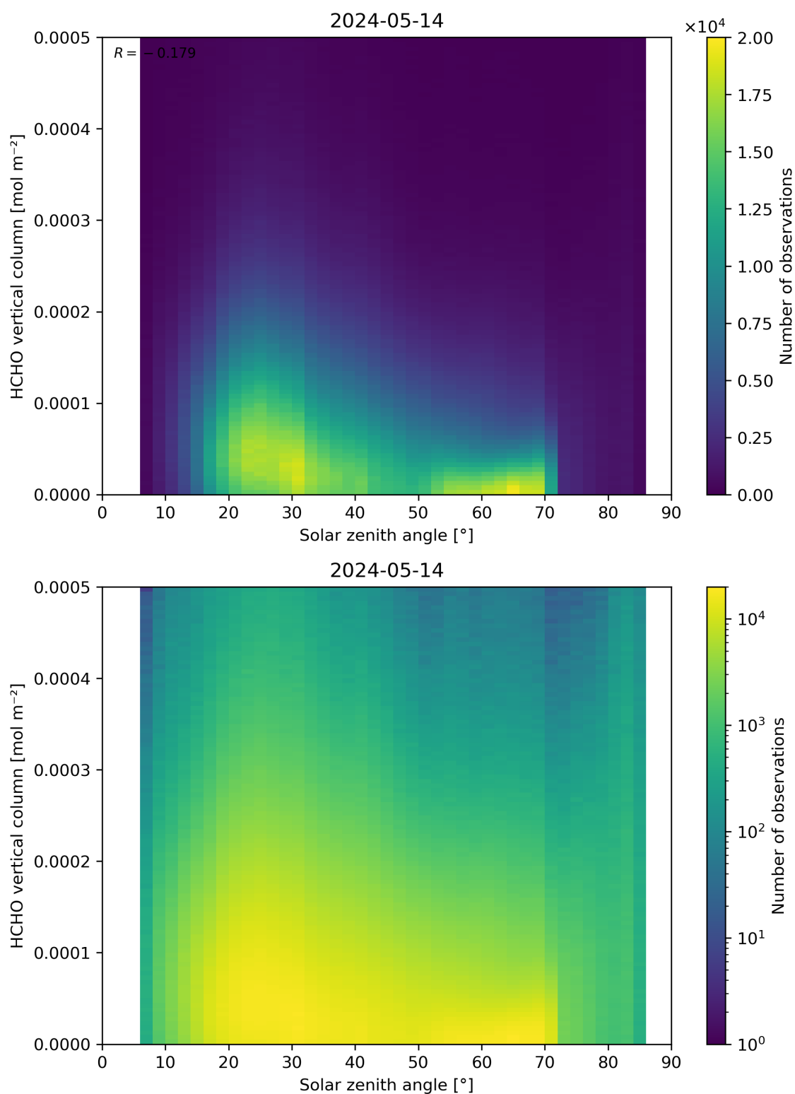
Figure 177: Scatter density plot of “Solar zenith angle” against “HCHO vertical column” for 2024-05-13 to 2024-05-15.
