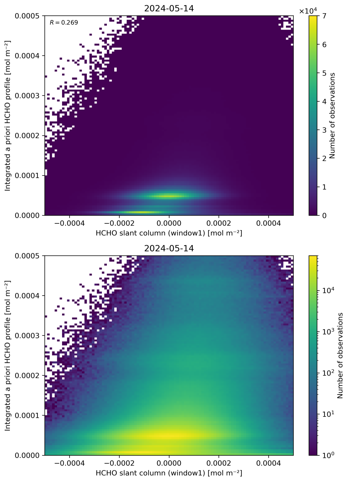
Figure 87: Scatter density plot of “HCHO slant column (window1)” against “Integrated a priori HCHO profile” for 2024-05-13 to 2024-05-15.
