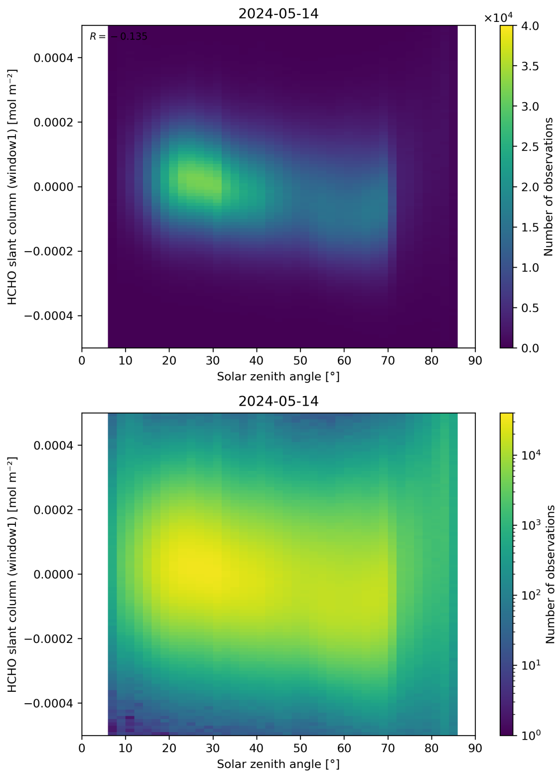
Figure 173: Scatter density plot of “Solar zenith angle” against “HCHO slant column (window1)” for 2024-05-13 to 2024-05-15.
