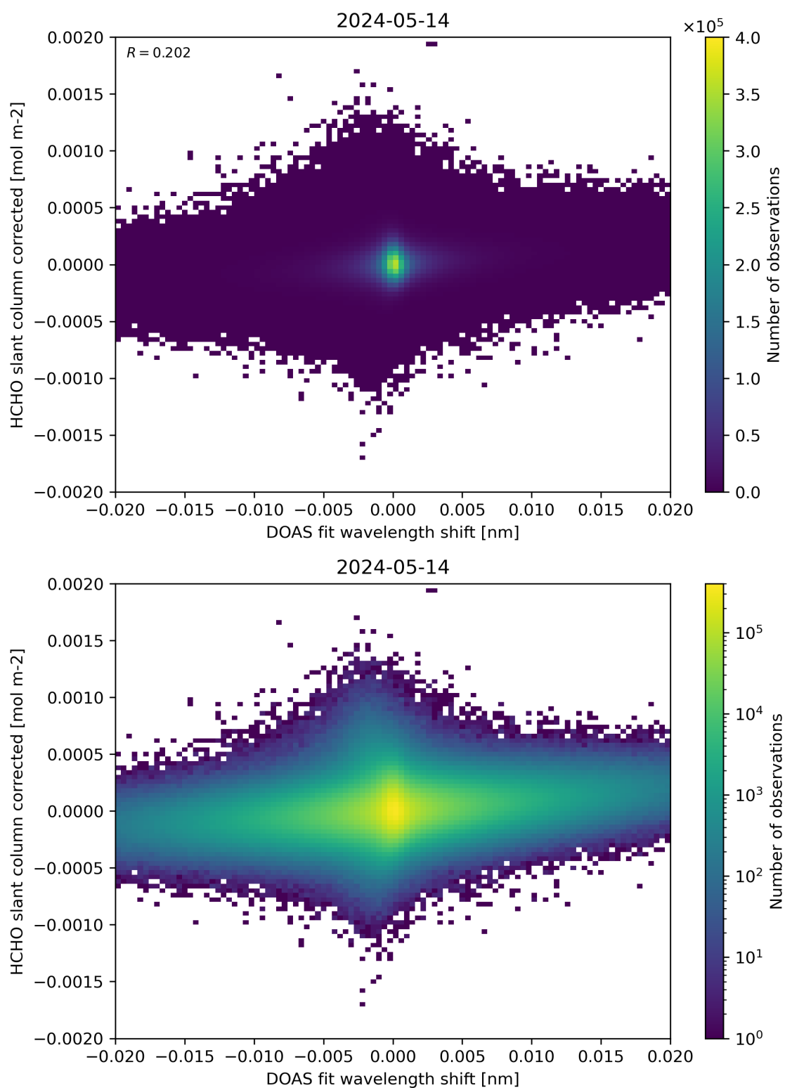
Figure 66: Scatter density plot of “DOAS fit wavelength shift” against “HCHO slant column corrected” for 2024-05-13 to 2024-05-15.
