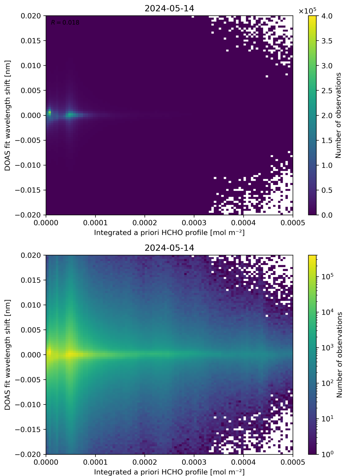
Figure 149: Scatter density plot of “Integrated a priori HCHO profile” against “DOAS fit wavelength shift” for 2024-05-13 to 2024-05-15.
