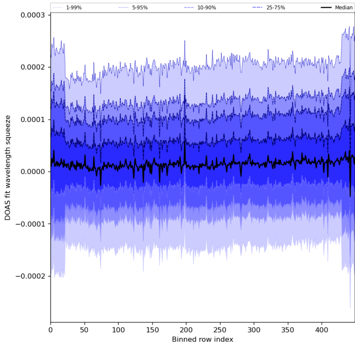
Figure 59: Along track statistics of “DOAS fit wavelength squeeze” for 2024-05-13 to 2024-05-15
