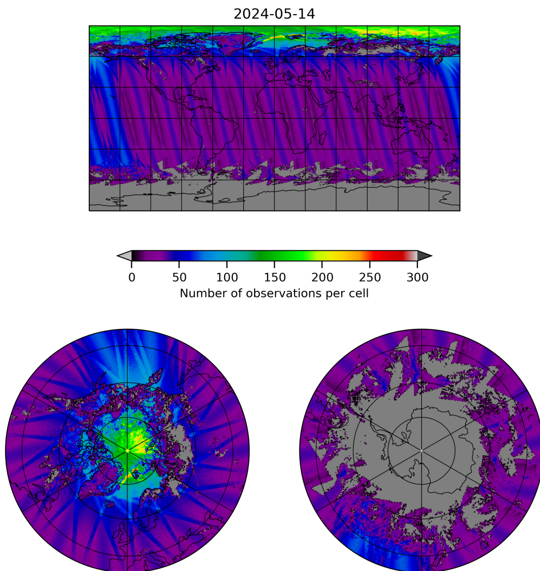
Figure 19: Map of the number of observations for 2024-05-13 to 2024-05-15
