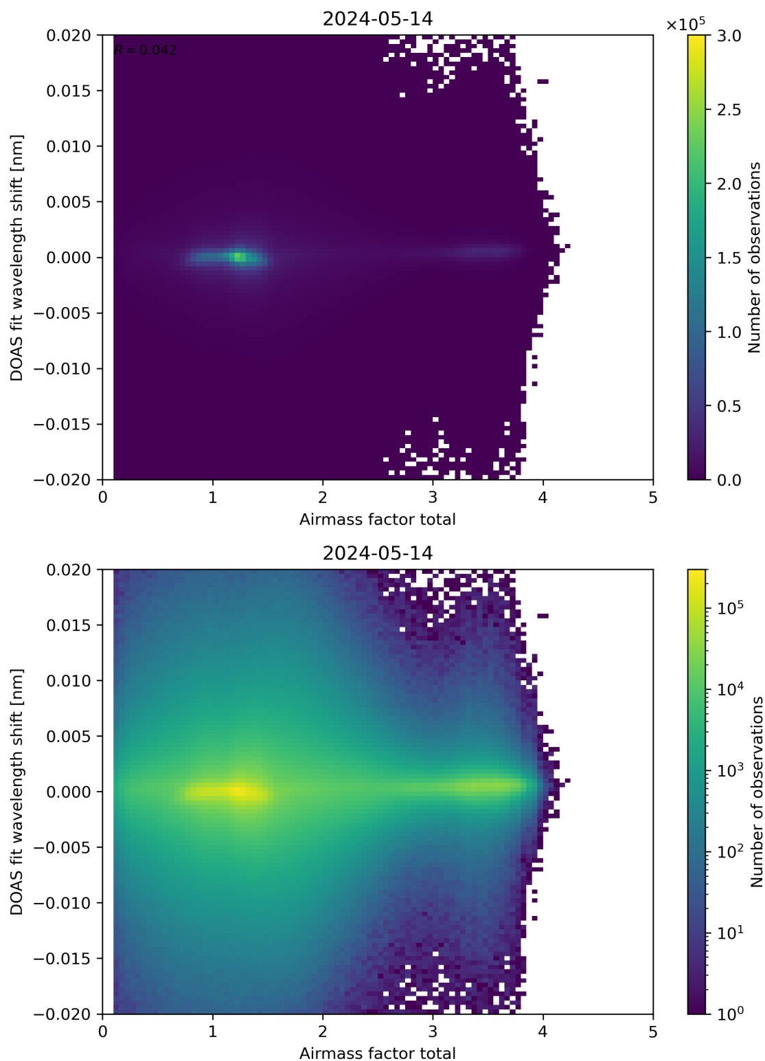
Figure 98: Scatter density plot of “Airmass factor total” against “DOAS fit wavelength shift” for 2024-05-13 to 2024-05-15.
