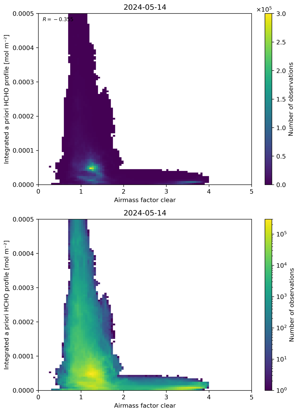
Figure 76: Scatter density plot of “Airmass factor clear” against “Integrated a priori HCHO profile” for 2024-05-13 to 2024-05-15.
