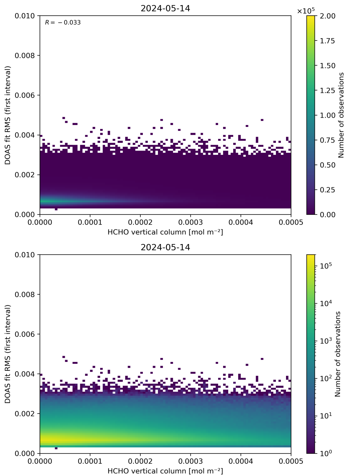
Figure 123: Scatter density plot of “HCHO vertical column” against “DOAS fit RMS (first interval)” for 2024-05-13 to 2024-05-15.
