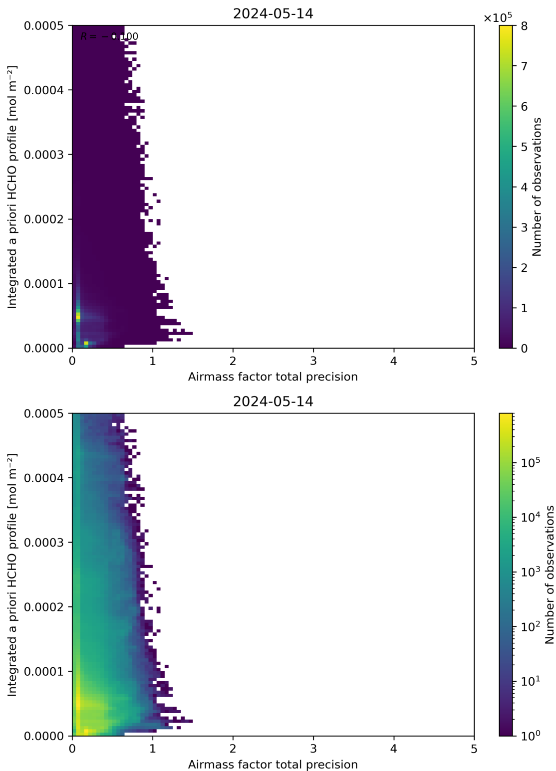
Figure 111: Scatter density plot of “Airmass factor total precision” against “Integrated a priori HCHO profile” for 2024-05-13 to 2024-05-15.
