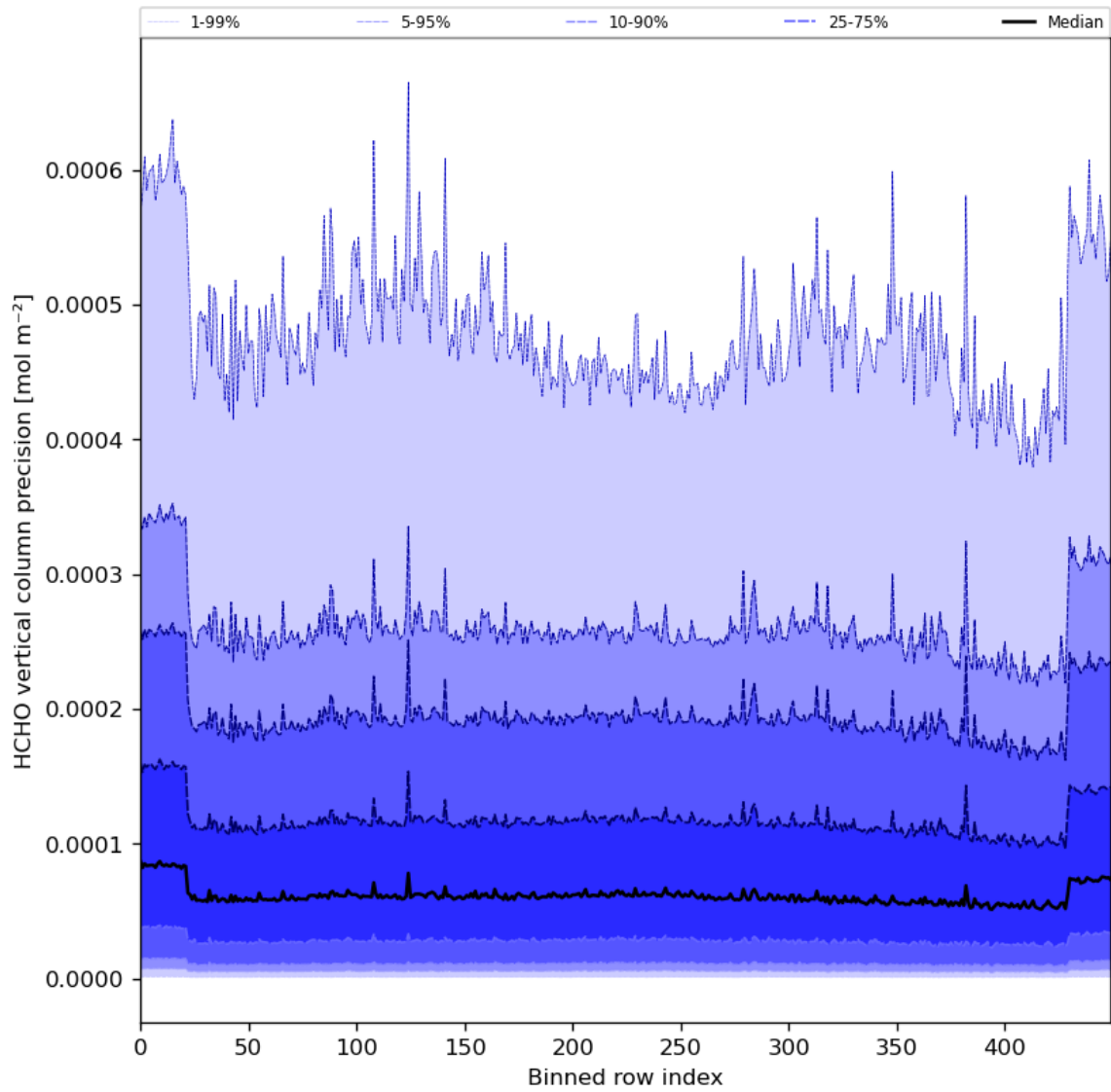
Figure 50: Along track statistics of “HCHO vertical column precision” for 2024-05-13 to 2024-05-15
