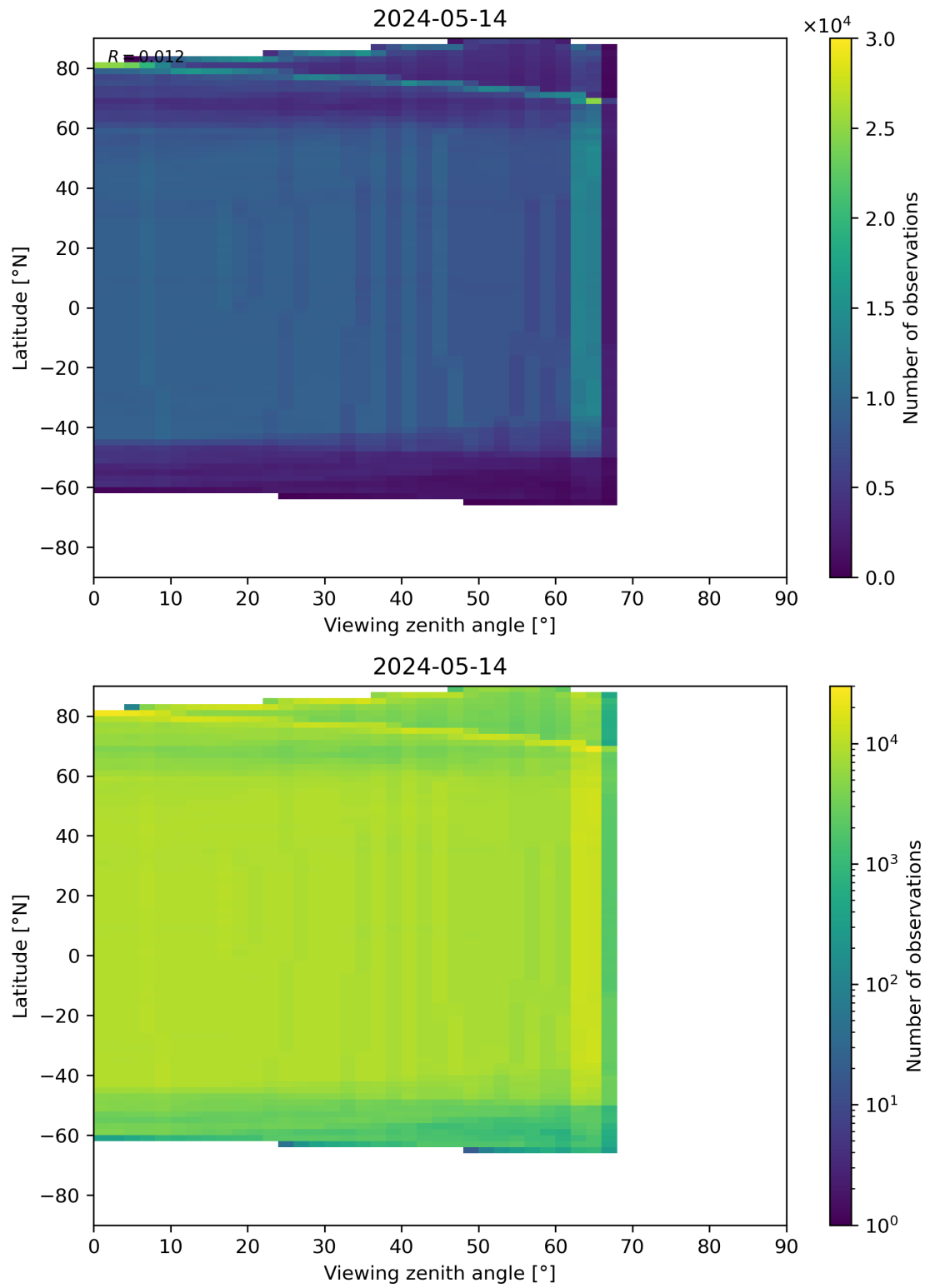
Figure 196: Scatter density plot of “Viewing zenith angle” against “Latitude” for 2024-05-13 to 2024-05-15.
