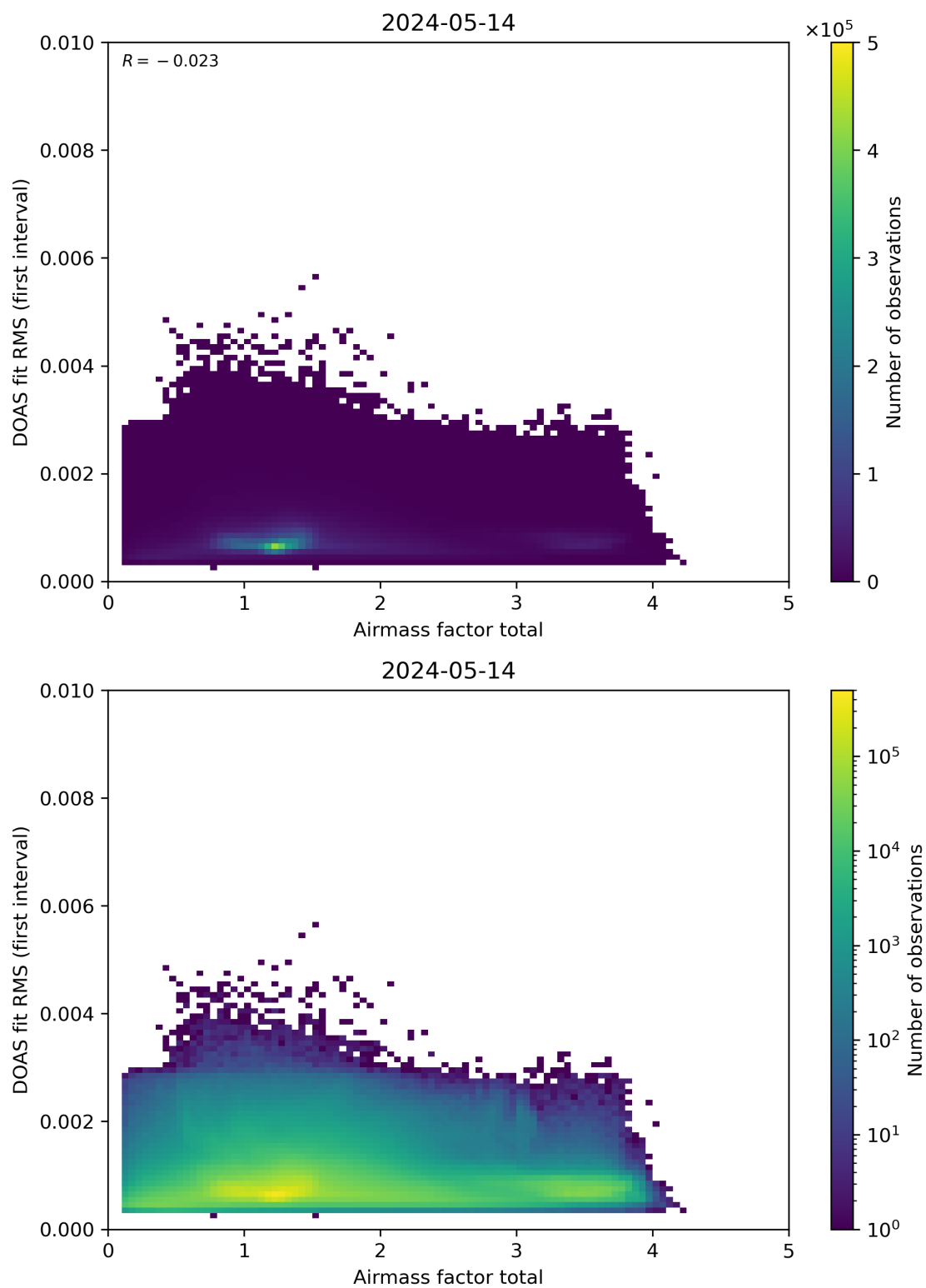
Figure 97: Scatter density plot of “Airmass factor total” against “DOAS fit RMS (first interval)” for 2024-05-13 to 2024-05-15.
