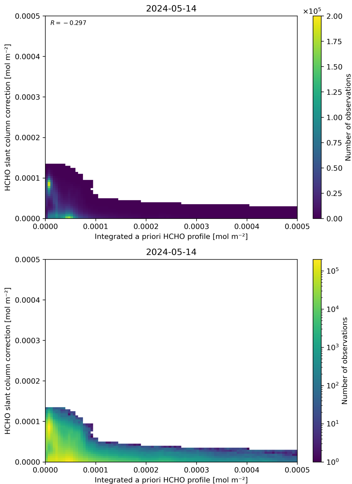
Figure 152: Scatter density plot of “Integrated a priori HCHO profile” against “HCHO slant column correction” for 2024-05-13 to 2024-05-15.
