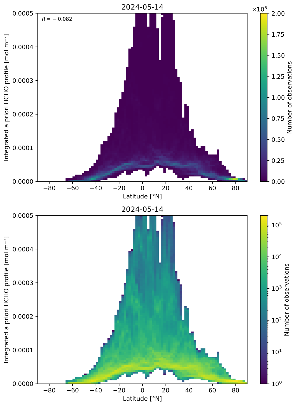
Figure 166: Scatter density plot of “Latitude” against “Integrated a priori HCHO profile” for 2024-05-13 to 2024-05-15.
