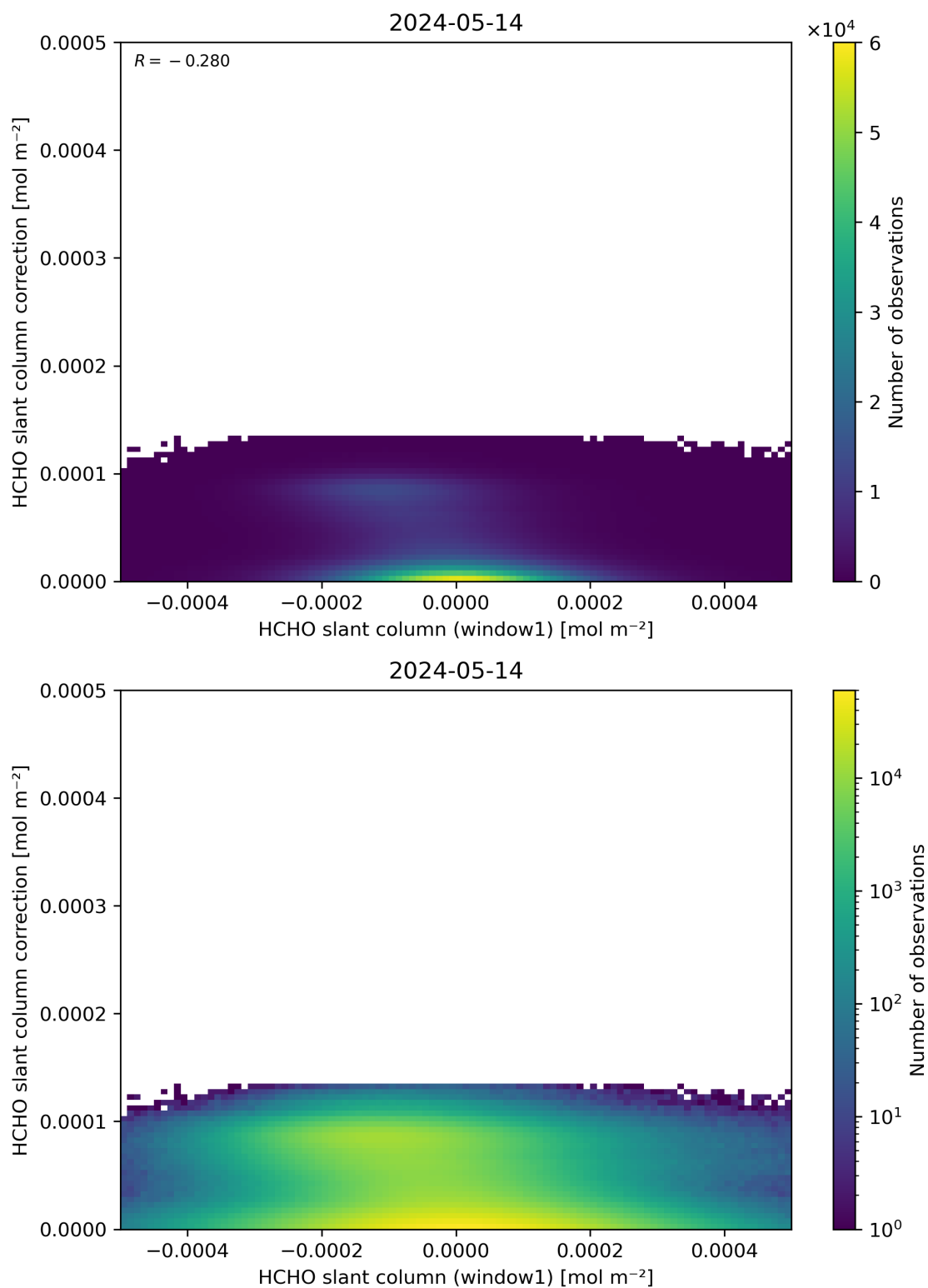
Figure 83: Scatter density plot of “HCHO slant column (window1)” against “HCHO slant column correction” for 2024-05-13 to 2024-05-15.
