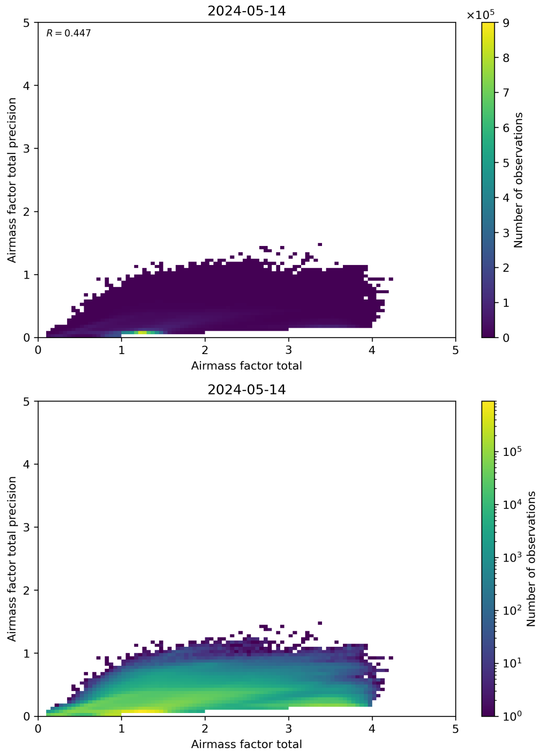
Figure 103: Scatter density plot of “Airmass factor total” against “Airmass factor total precision” for 2024-05-13 to 2024-05-15.
