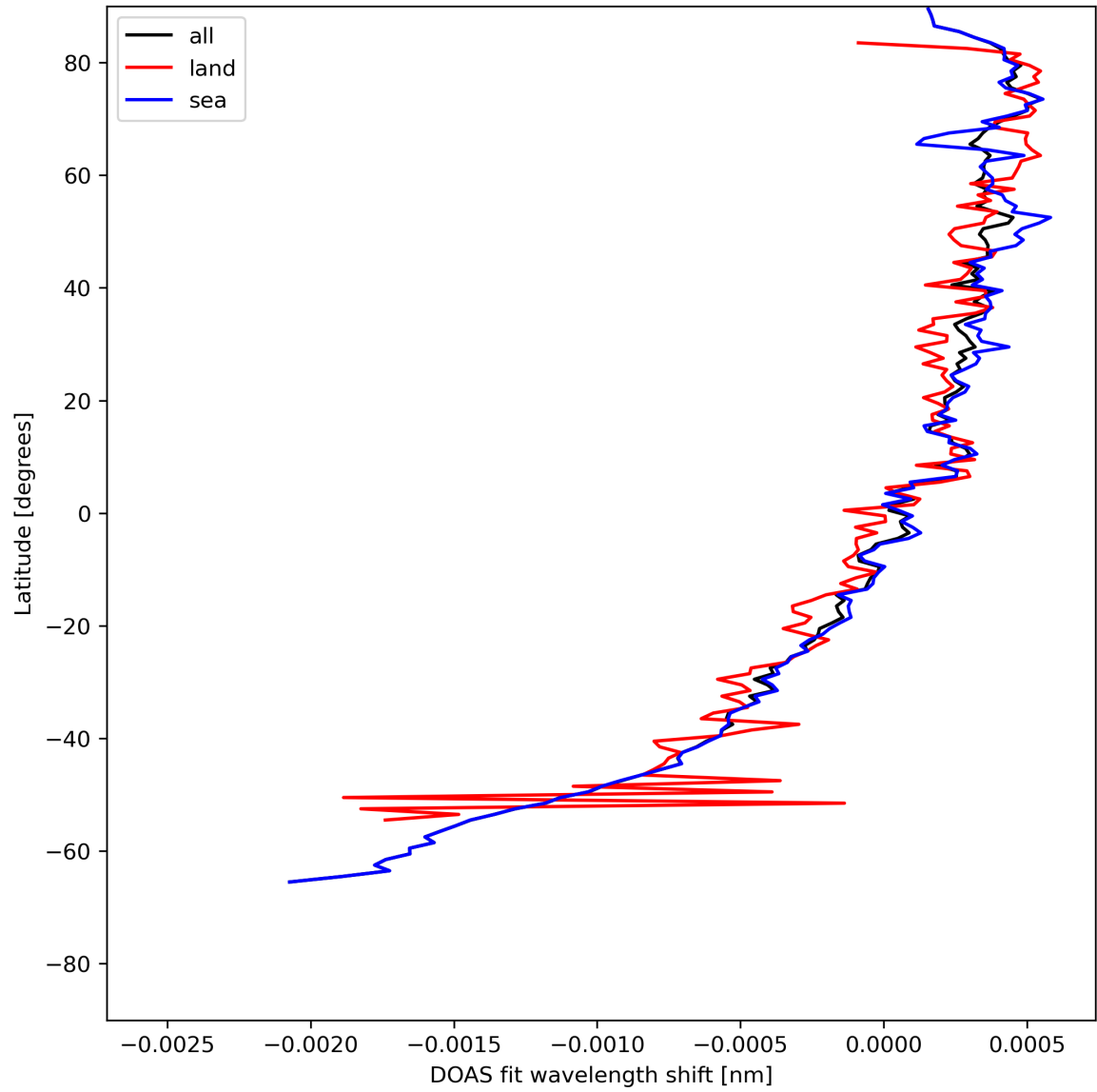
Figure 30: Zonal average of “DOAS fit wavelength shift” for 2024-05-13 to 2024-05-15.
