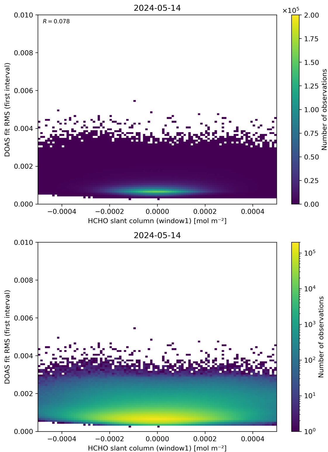
Figure 78: Scatter density plot of “HCHO slant column (window1)” against “DOAS fit RMS (first interval)” for 2024-05-13 to 2024-05-15.
