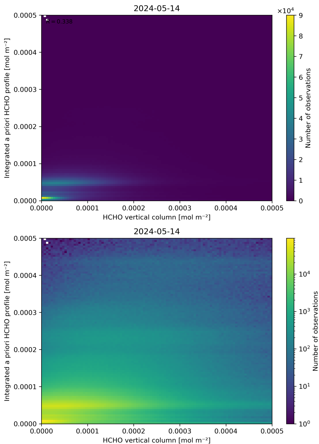
Figure 135: Scatter density plot of “HCHO vertical column” against “Integrated a priori HCHO profile” for 2024-05-13 to 2024-05-15.
