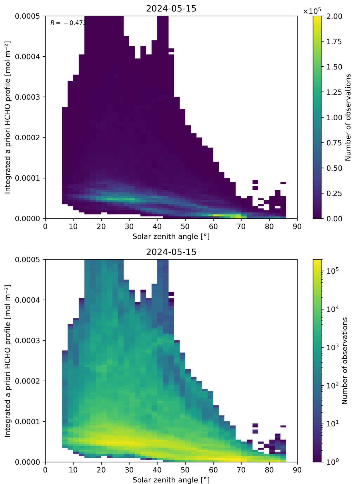
Figure 180: Scatter density plot of “Solar zenith angle” against “Integrated a priori HCHO profile” for 2024-05-14 to 2024-05-16.
