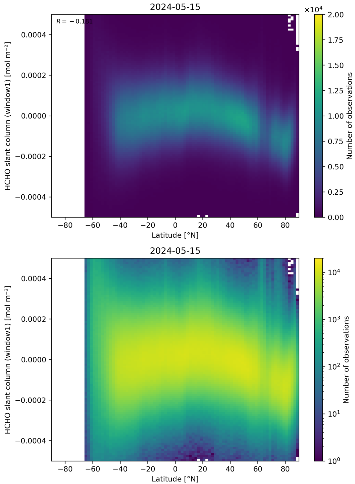
Figure 159: Scatter density plot of “Latitude” against “HCHO slant column (window1)” for 2024-05-14 to 2024-05-16.
