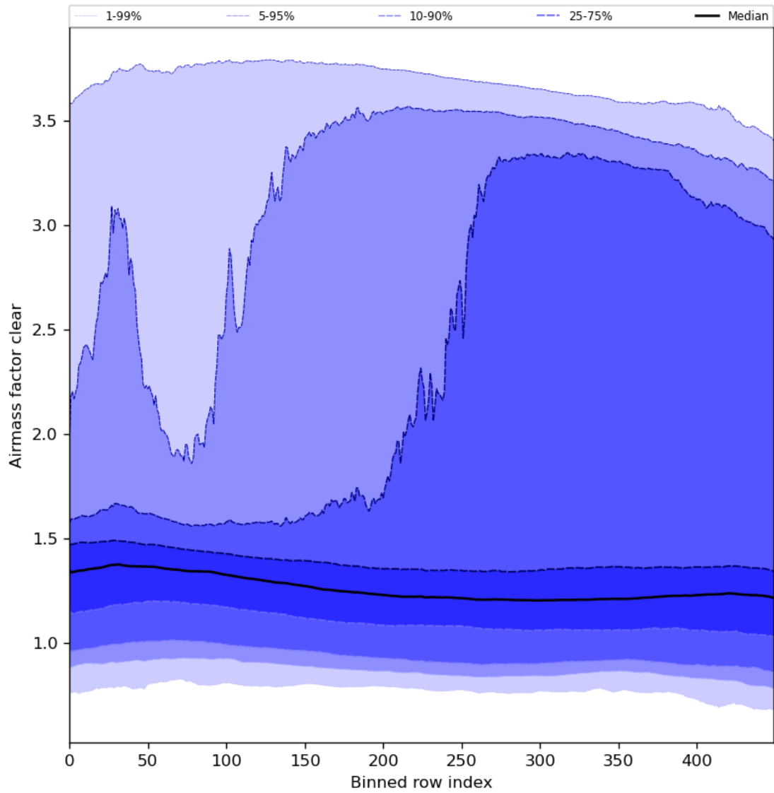
Figure 56: Along track statistics of “Airmass factor clear” for 2024-05-14 to 2024-05-16
