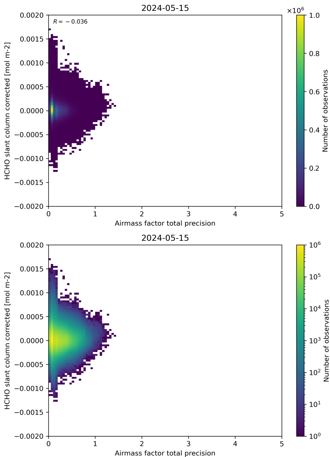
Figure 109: Scatter density plot of “Airmass factor total precision” against “HCHO slant column corrected” for 2024-05-14 to 2024-05-16.
