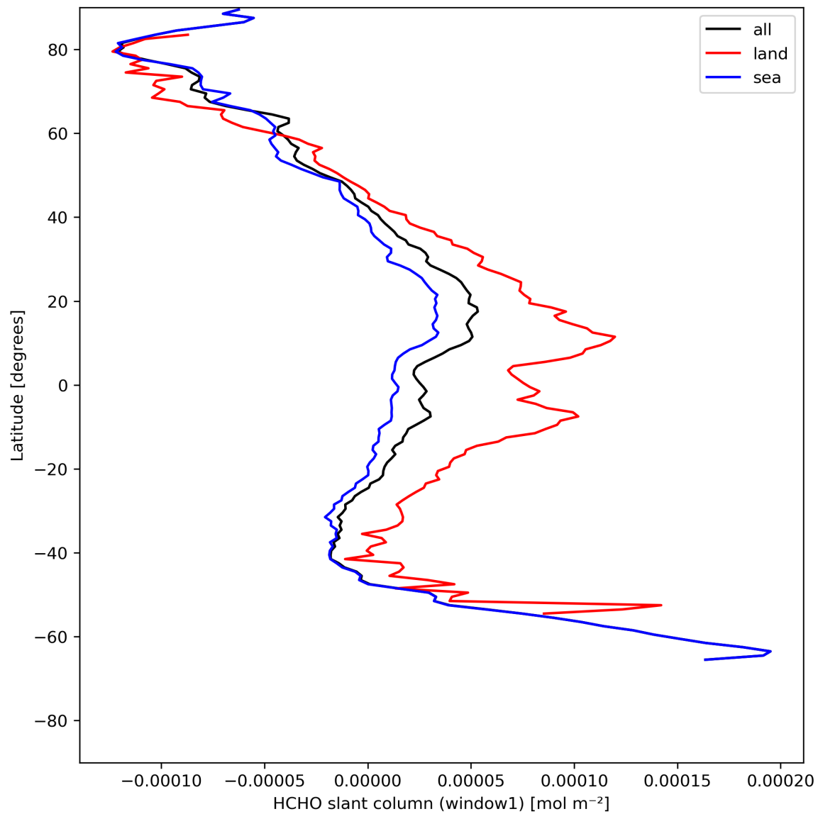
Figure 24: Zonal average of “HCHO slant column (window1)” for 2024-05-14 to 2024-05-16.
