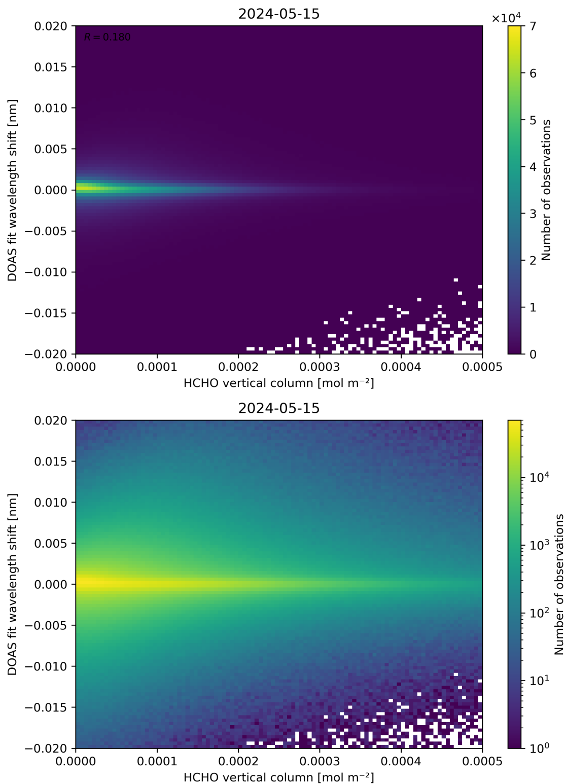
Figure 124: Scatter density plot of “HCHO vertical column” against “DOAS fit wavelength shift” for 2024-05-14 to 2024-05-16.
