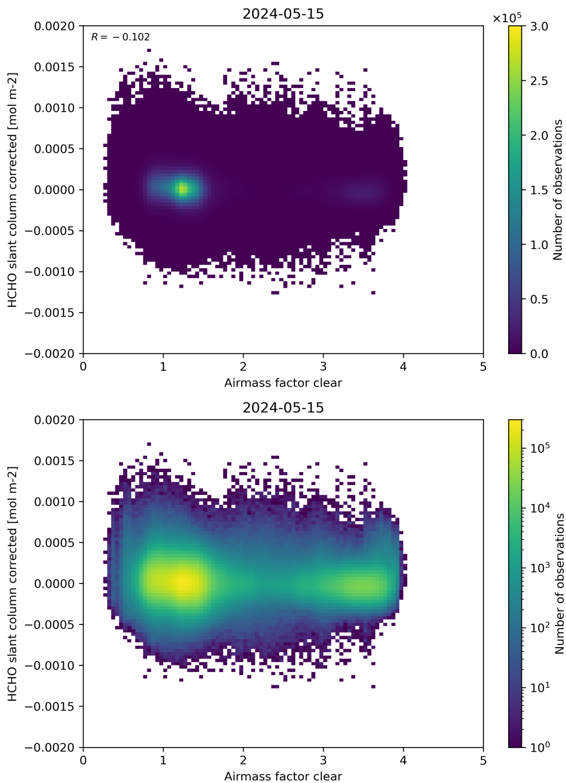
Figure 74: Scatter density plot of “Airmass factor clear” against “HCHO slant column corrected” for 2024-05-14 to 2024-05-16.
