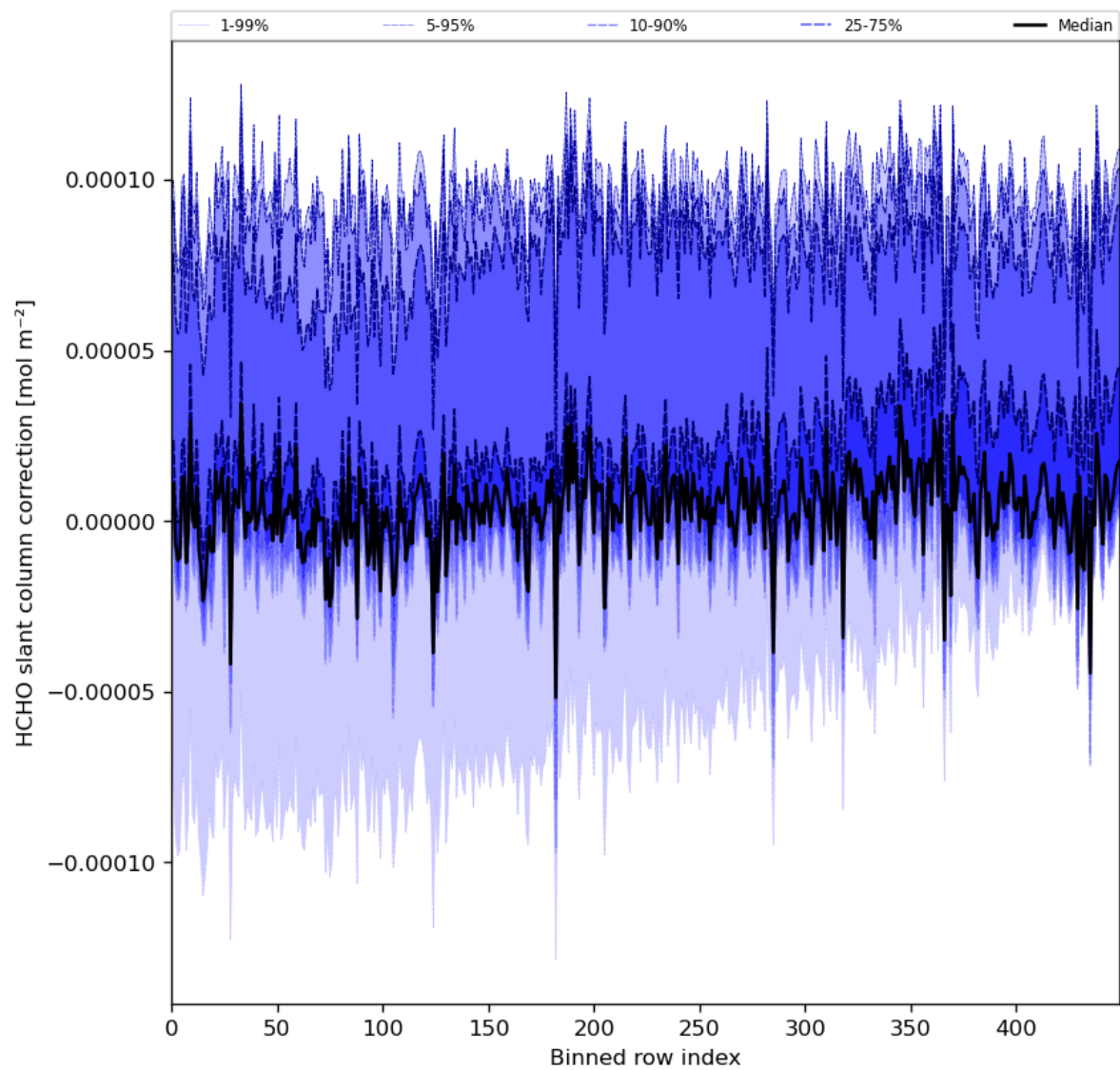
Figure 61: Along track statistics of “HCHO slant column correction” for 2024-05-14 to 2024-05-16
