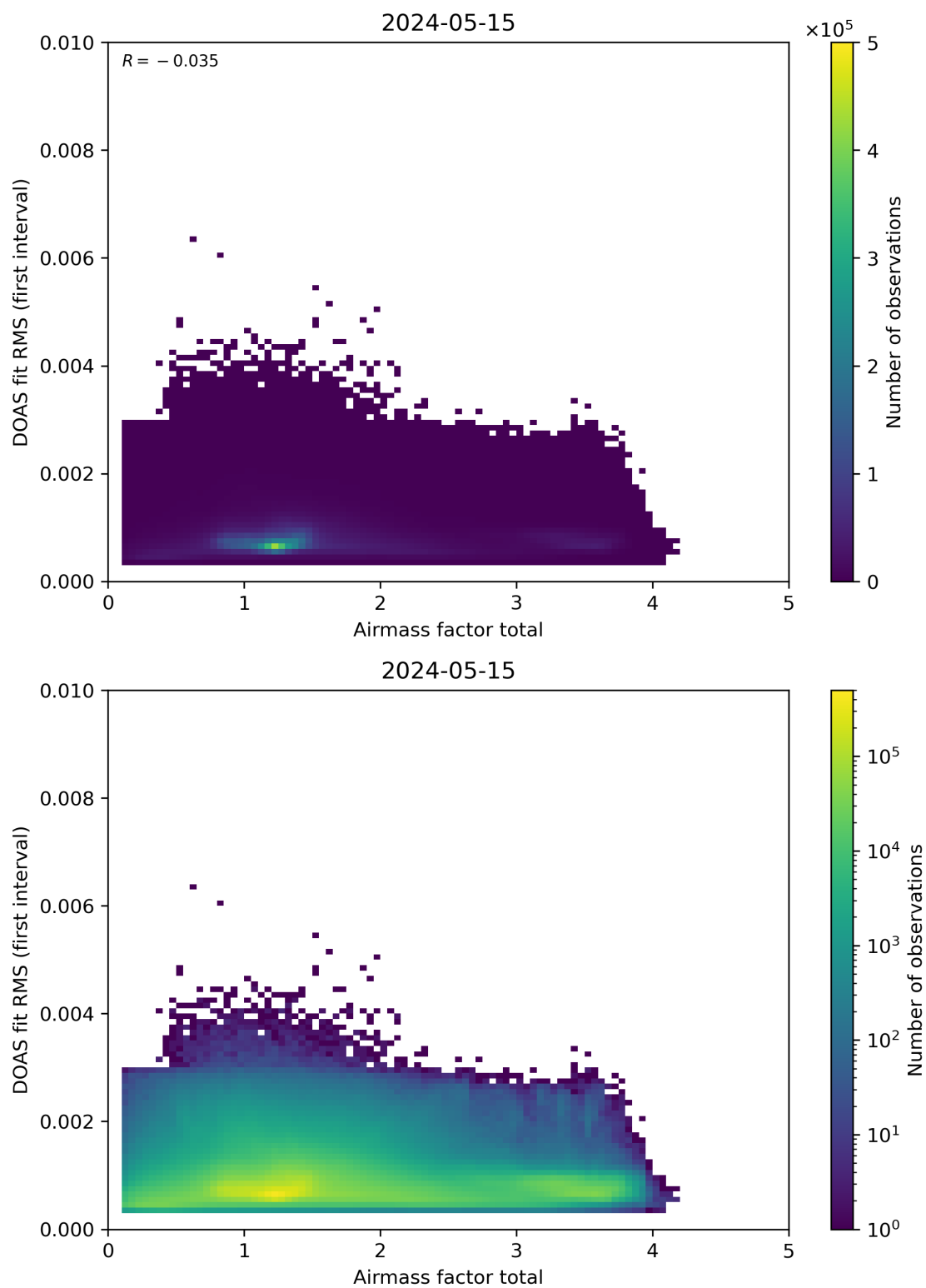
Figure 97: Scatter density plot of “Airmass factor total” against “DOAS fit RMS (first interval)” for 2024-05-14 to 2024-05-16.
