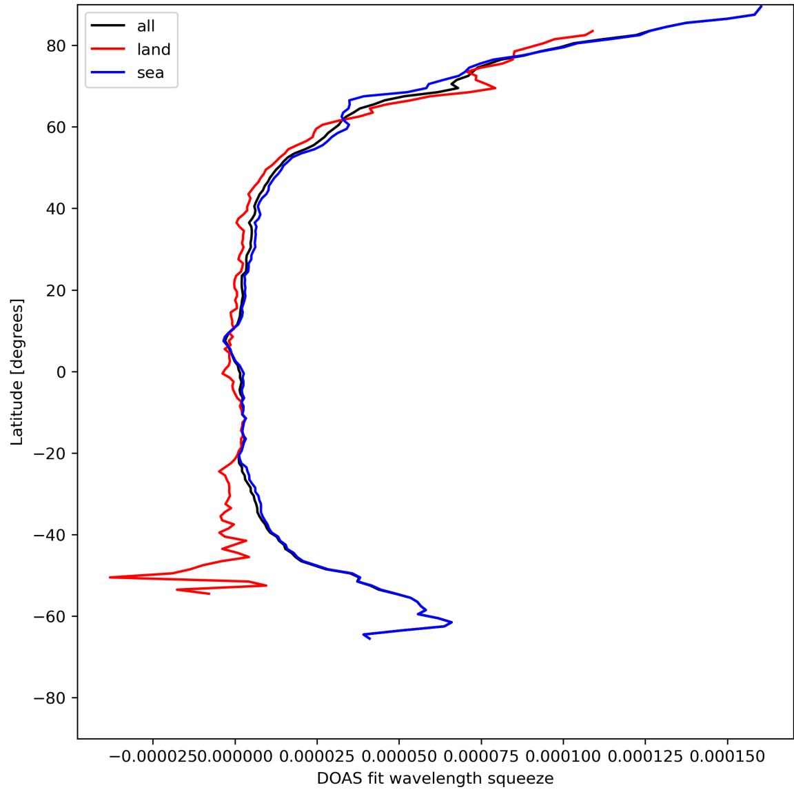
Figure 31: Zonal average of “DOAS fit wavelength squeeze” for 2024-05-14 to 2024-05-16.
