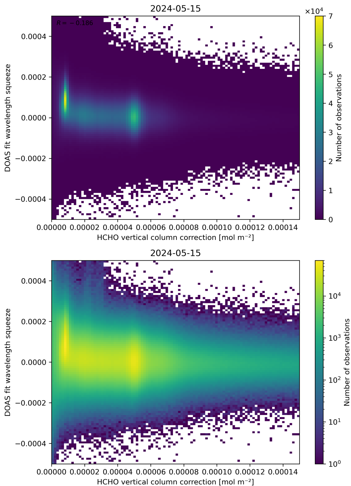
Figure 114: Scatter density plot of “HCHO vertical column correction” against “DOAS fit wavelength squeeze” for 2024-05-14 to 2024-05-16.
