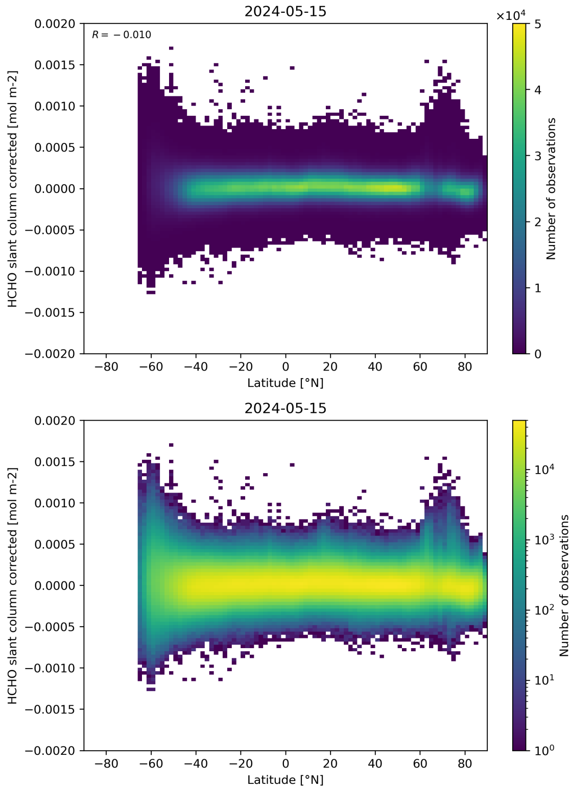
Figure 157: Scatter density plot of “Latitude” against “HCHO slant column corrected” for 2024-05-14 to 2024-05-16.
