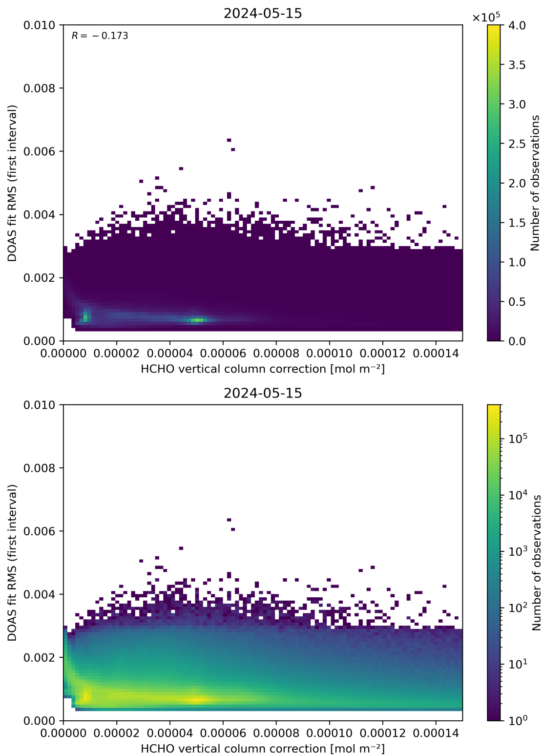
Figure 112: Scatter density plot of “HCHO vertical column correction” against “DOAS fit RMS (first interval)” for 2024-05-14 to 2024-05-16.
