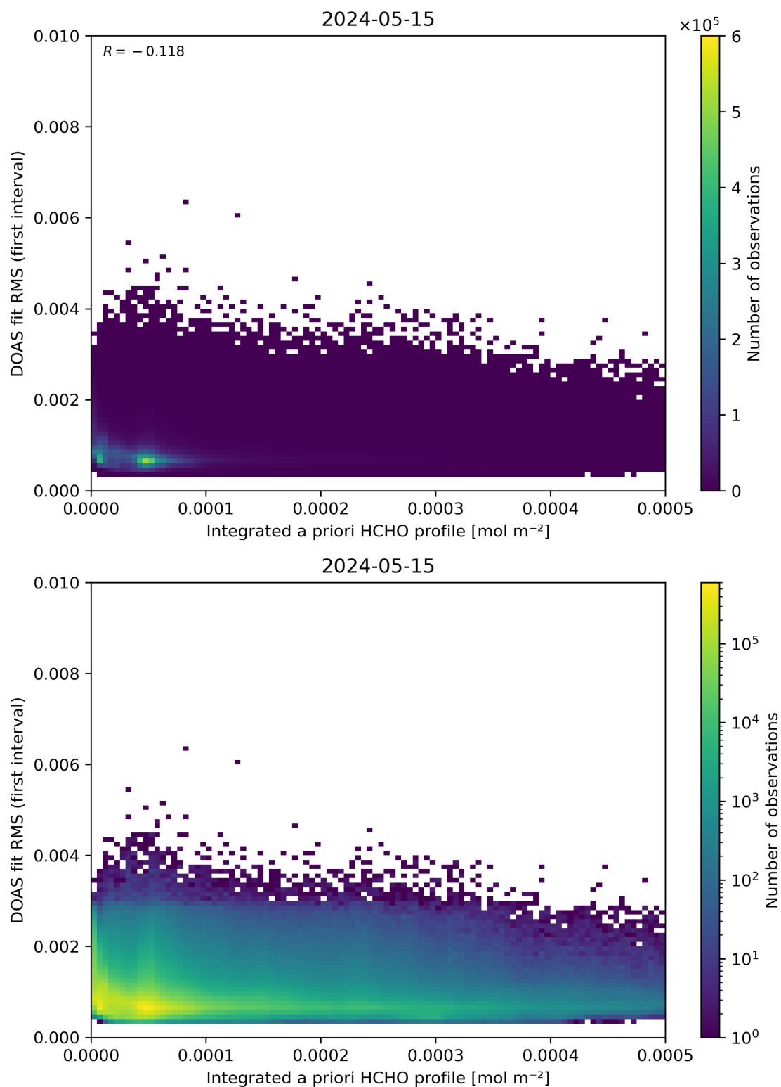
Figure 148: Scatter density plot of “Integrated a priori HCHO profile” against “DOAS fit RMS (first interval)” for 2024-05-14 to 2024-05-16.
