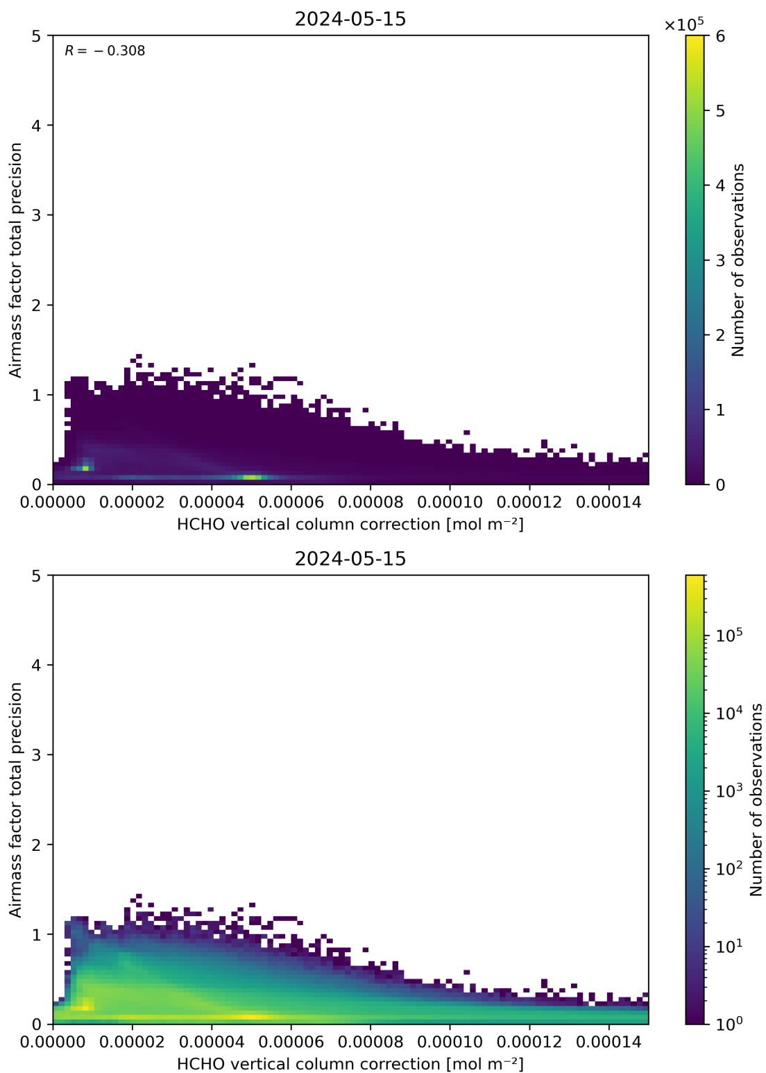
Figure 121: Scatter density plot of “HCHO vertical column correction” against “Airmass factor total precision” for 2024-05-14 to 2024-05-16.
