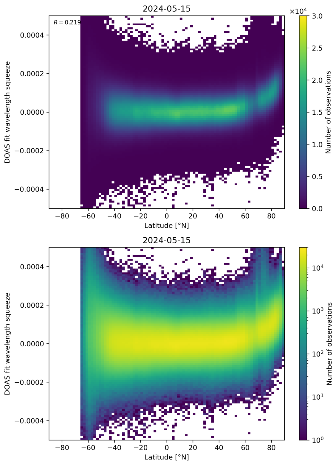
Figure 155: Scatter density plot of “Latitude” against “DOAS fit wavelength squeeze” for 2024-05-14 to 2024-05-16.
