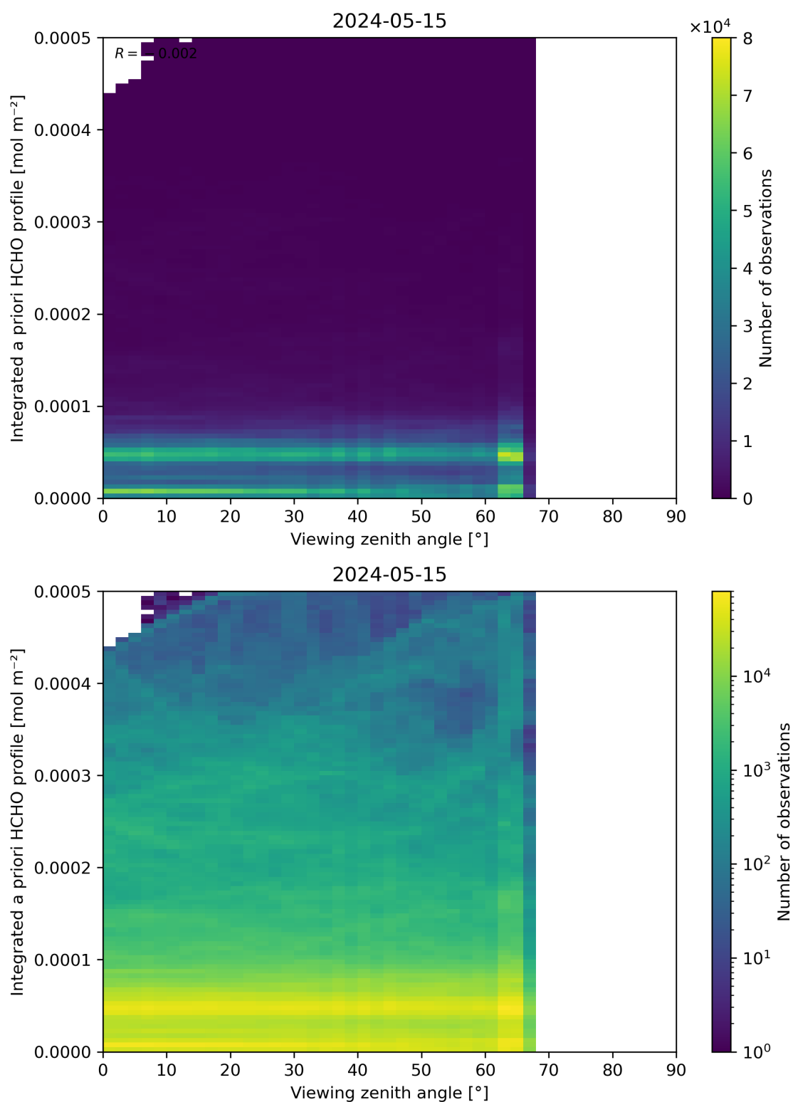
Figure 195: Scatter density plot of “Viewing zenith angle” against “Integrated a priori HCHO profile” for 2024-05-14 to 2024-05-16.
