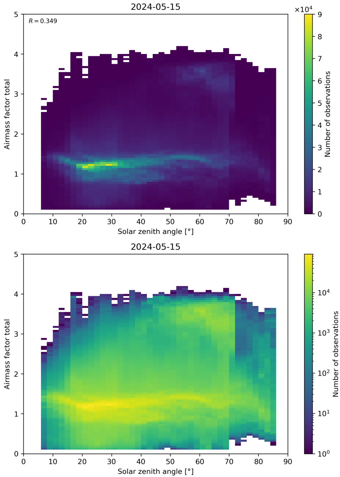
Figure 175: Scatter density plot of “Solar zenith angle” against “Airmass factor total” for 2024-05-14 to 2024-05-16.
