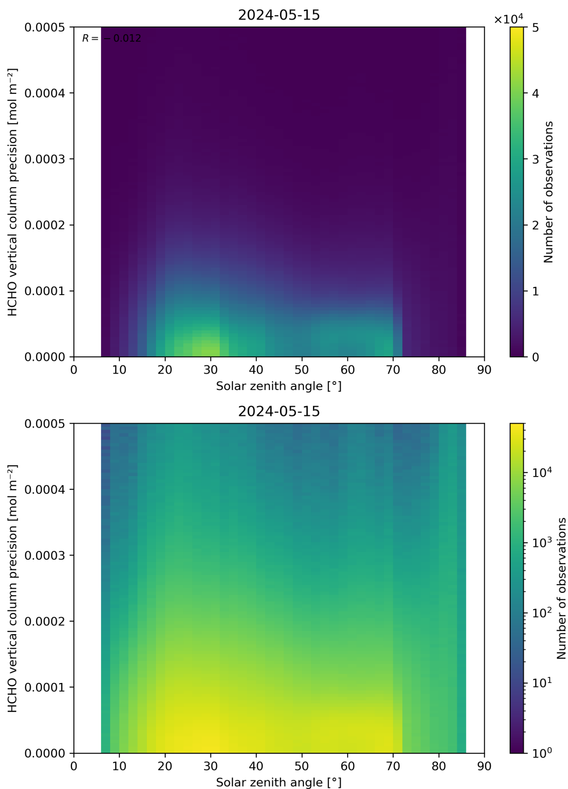
Figure 179: Scatter density plot of “Solar zenith angle” against “HCHO vertical column precision” for 2024-05-14 to 2024-05-16.
