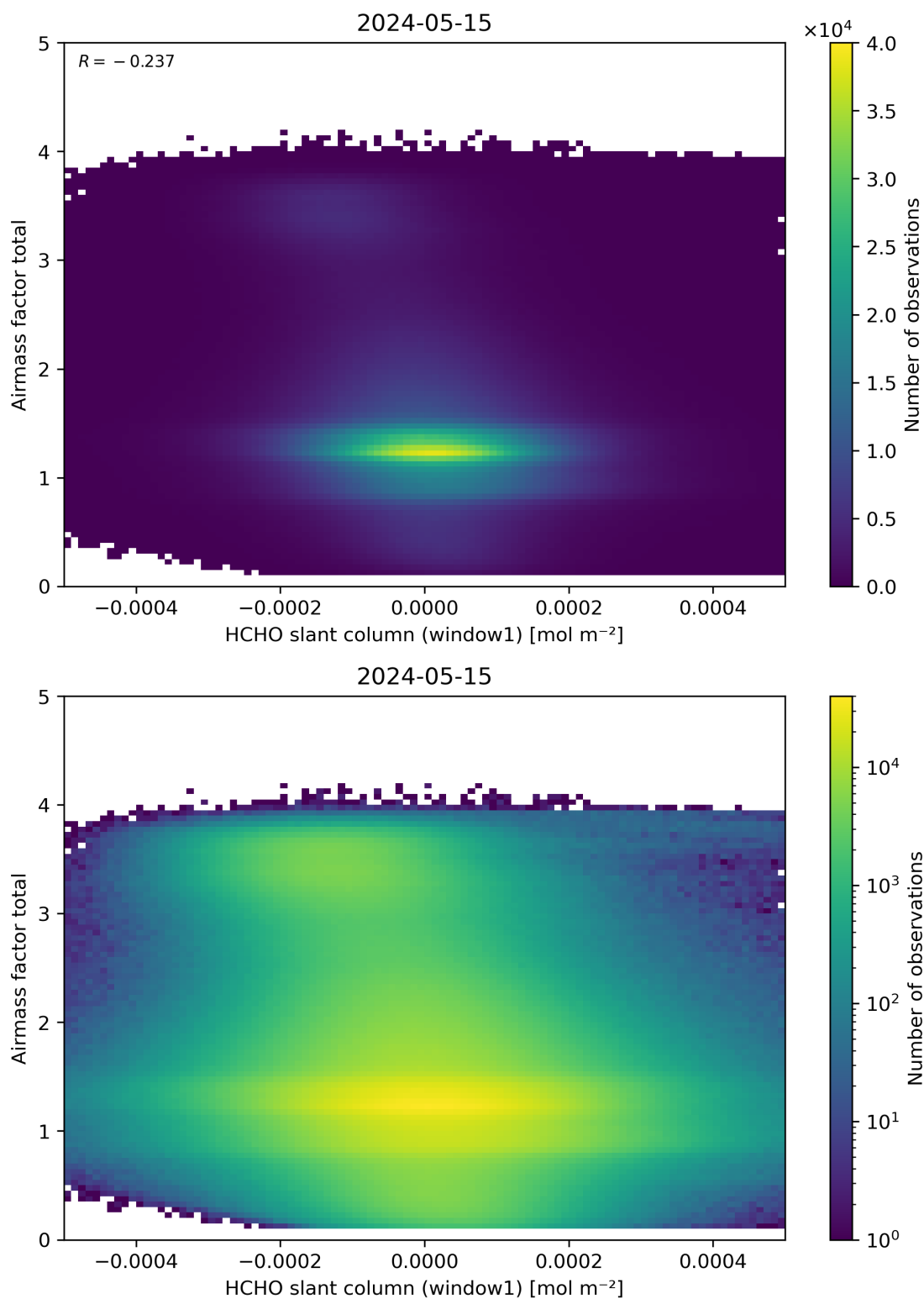
Figure 85: Scatter density plot of “HCHO slant column (window1)” against “Airmass factor total” for 2024-05-14 to 2024-05-16.
