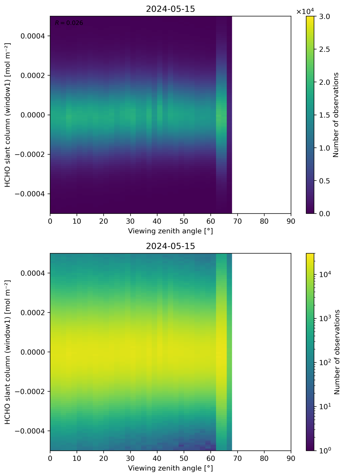
Figure 188: Scatter density plot of “Viewing zenith angle” against “HCHO slant column (window1)” for 2024-05-14 to 2024-05-16.
