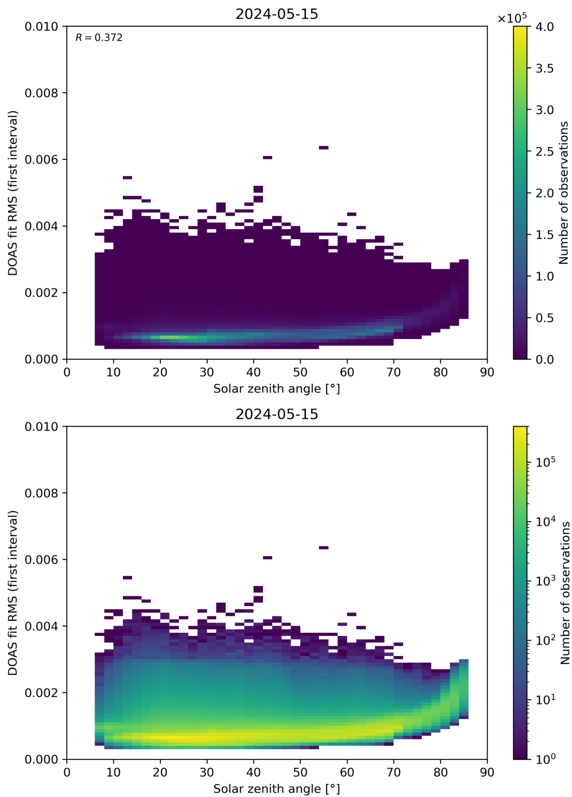
Figure 167: Scatter density plot of “Solar zenith angle” against “DOAS fit RMS (first interval)” for 2024-05-14 to 2024-05-16.
