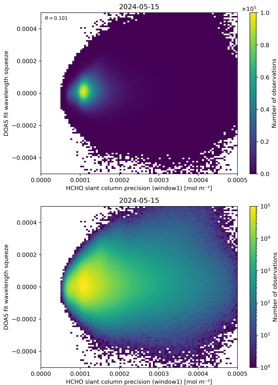
Figure 90: Scatter density plot of “HCHO slant column precision (window1)” against “DOAS fit wavelength squeeze” for 2024-05-14 to 2024-05-16.
