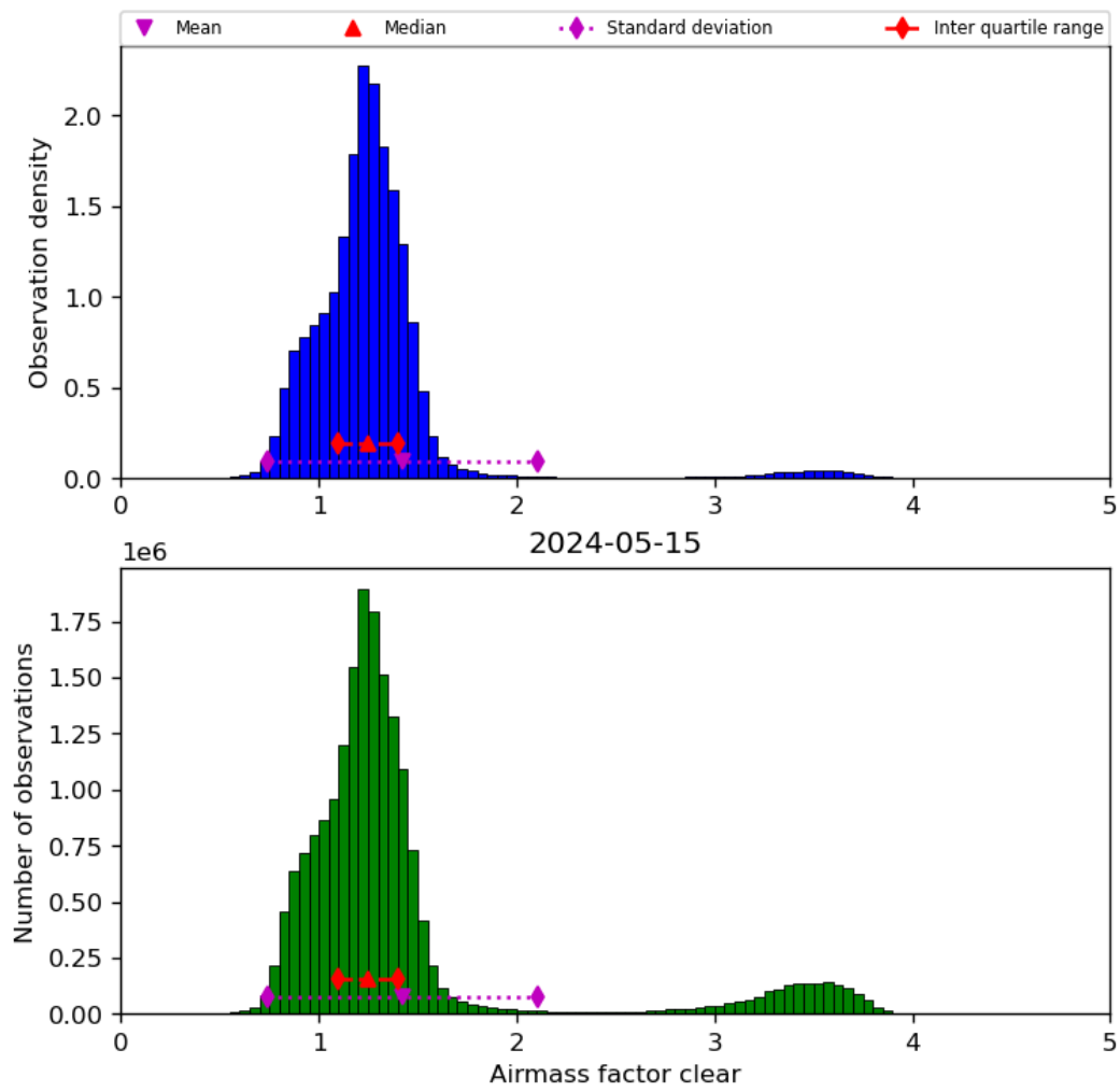
Figure 42: Histogram of “Airmass factor clear” for 2024-05-14 to 2024-05-16
