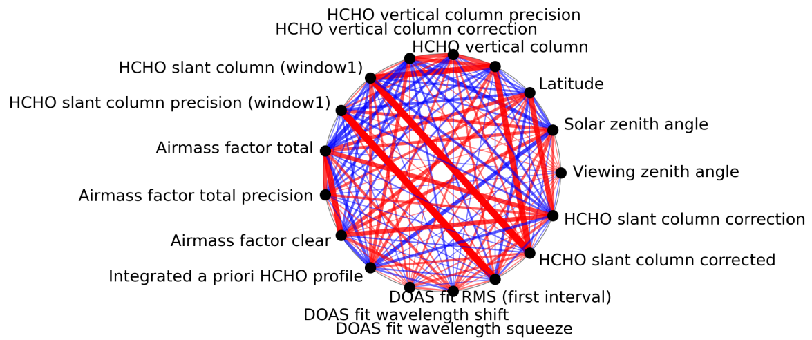
Figure 1: Map of correlation graph for 2024-05-14 to 2024-05-16.
