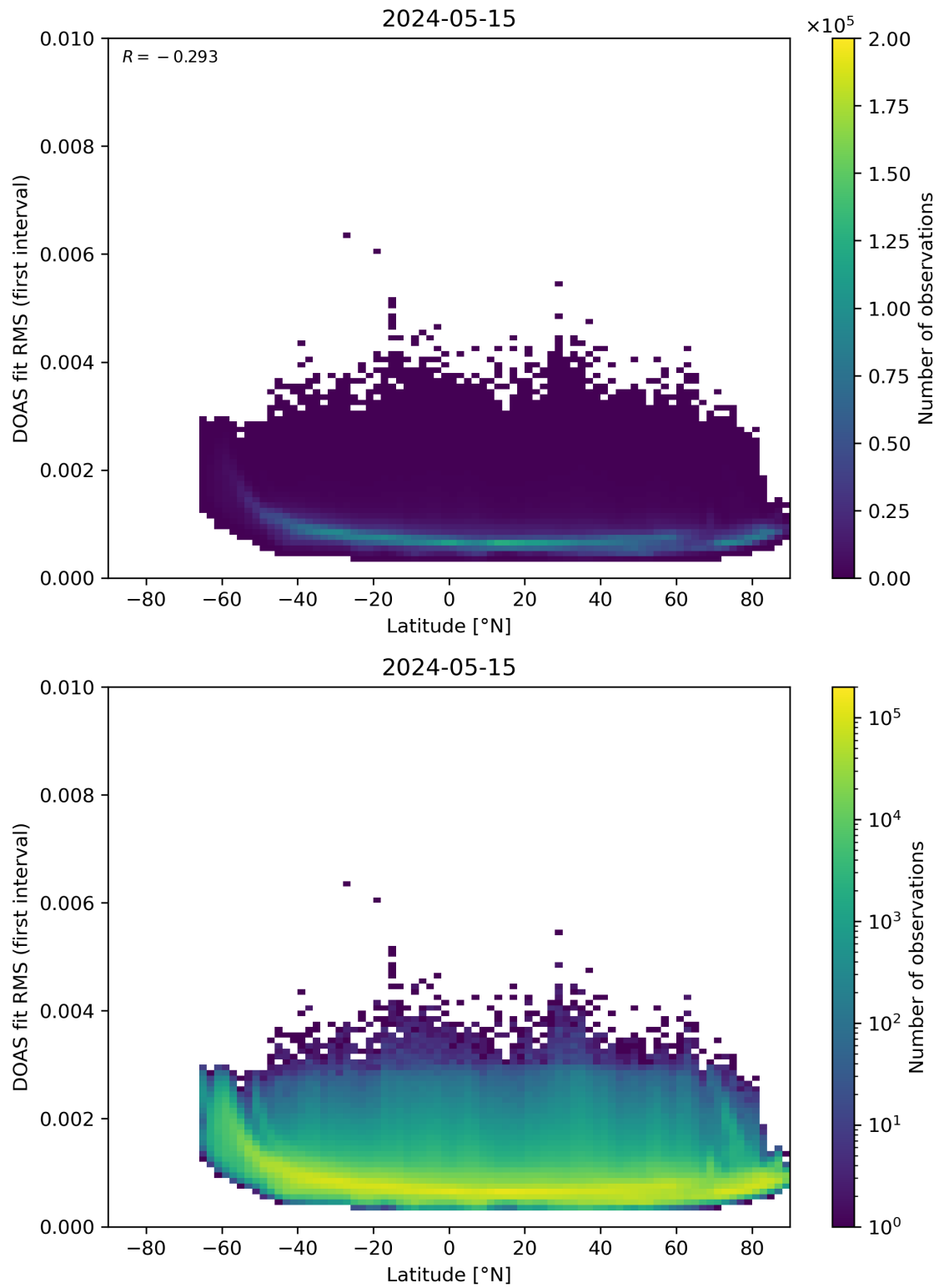
Figure 153: Scatter density plot of “Latitude” against “DOAS fit RMS (first interval)” for 2024-05-14 to 2024-05-16.
