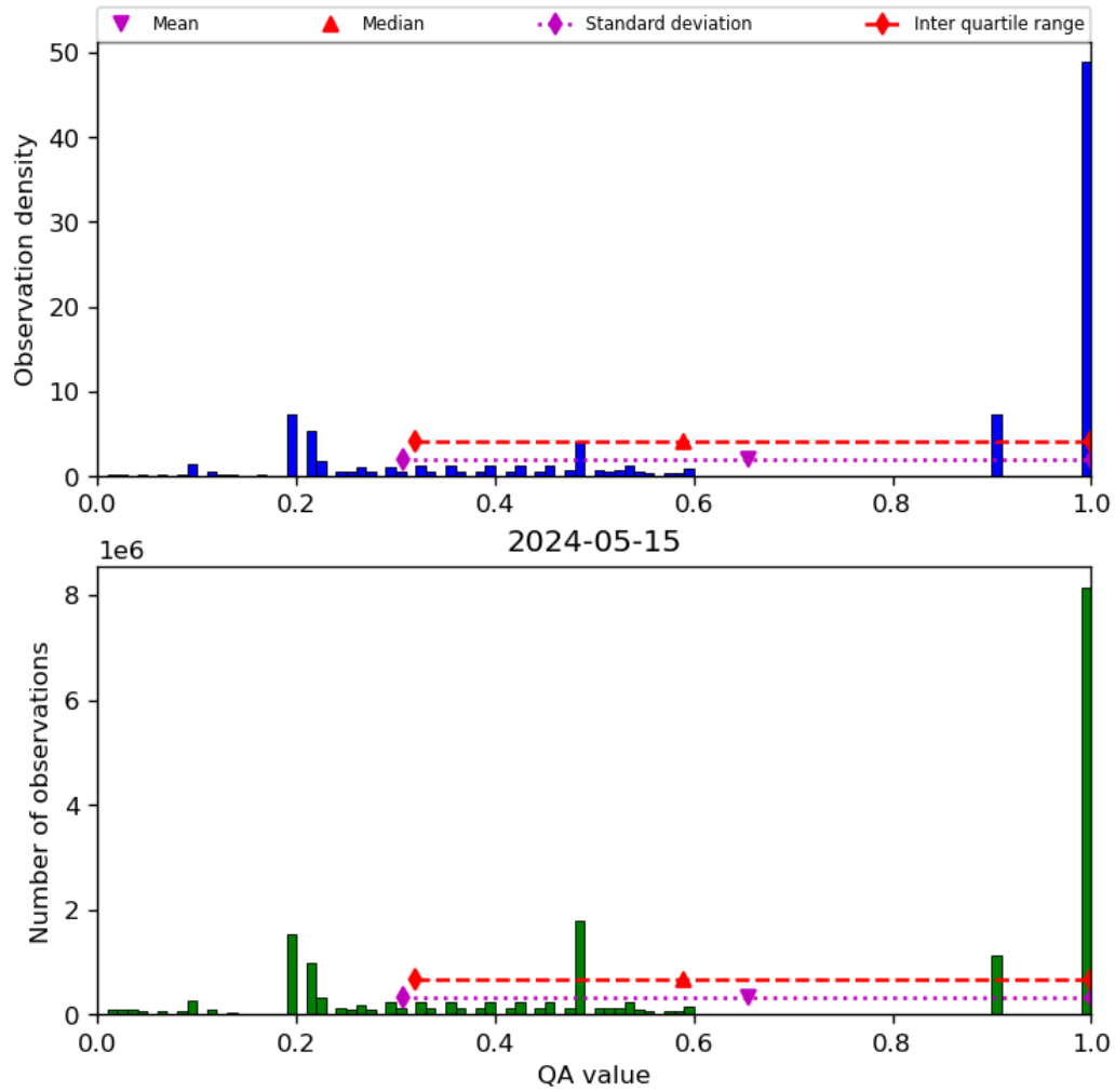
Figure 34: Histogram of “QA value” for 2024-05-14 to 2024-05-16
