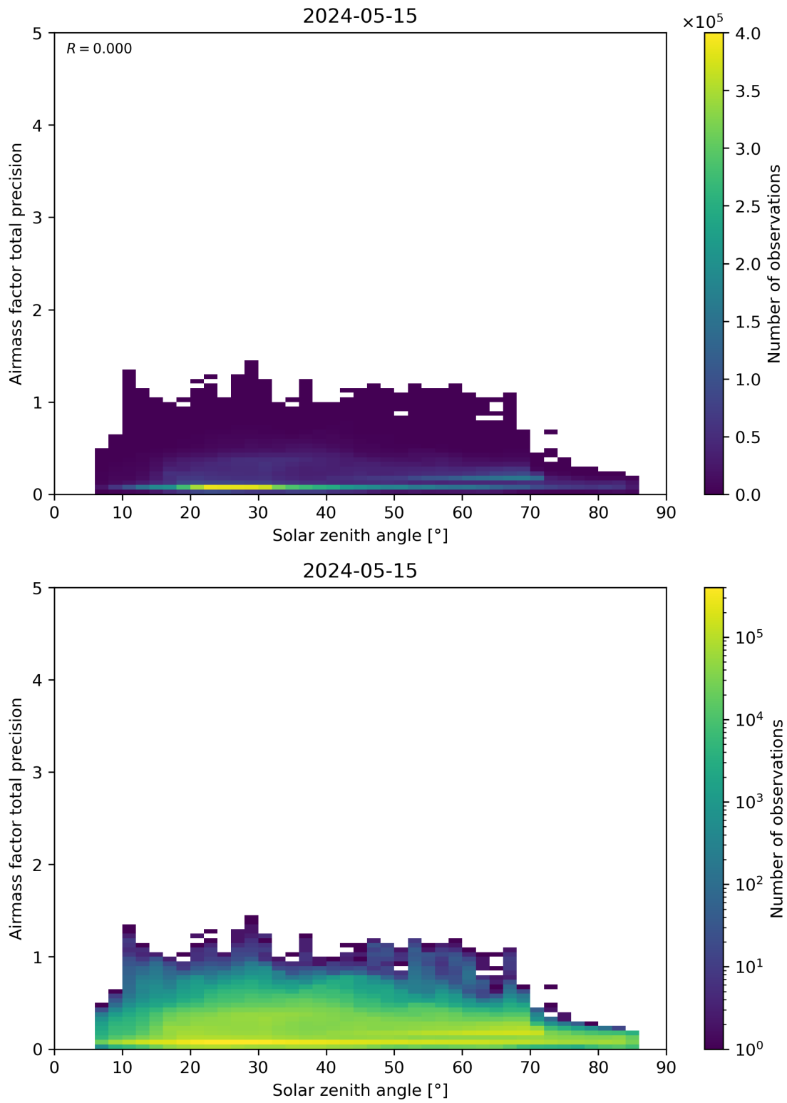
Figure 176: Scatter density plot of “Solar zenith angle” against “Airmass factor total precision” for 2024-05-14 to 2024-05-16.
