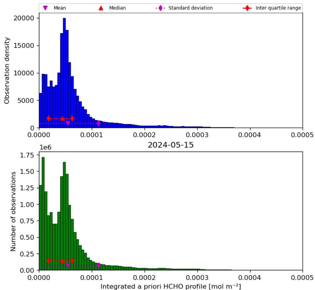
Figure 43: Histogram of “Integrated a priori HCHO profile” for 2024-05-14 to 2024-05-16
