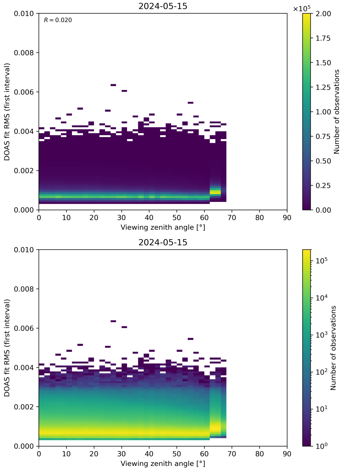
Figure 182: Scatter density plot of “Viewing zenith angle” against “DOAS fit RMS (first interval)” for 2024-05-14 to 2024-05-16.
