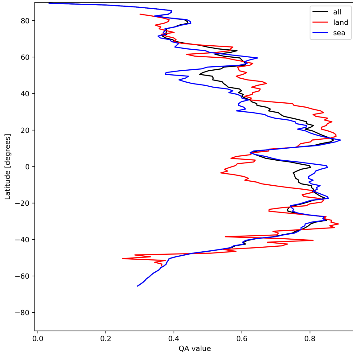
Figure 20: Zonal average of “QA value” for 2024-05-14 to 2024-05-16.
