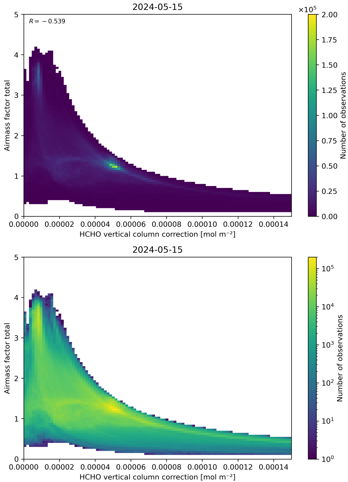
Figure 120: Scatter density plot of “HCHO vertical column correction” against “Airmass factor total” for 2024-05-14 to 2024-05-16.
