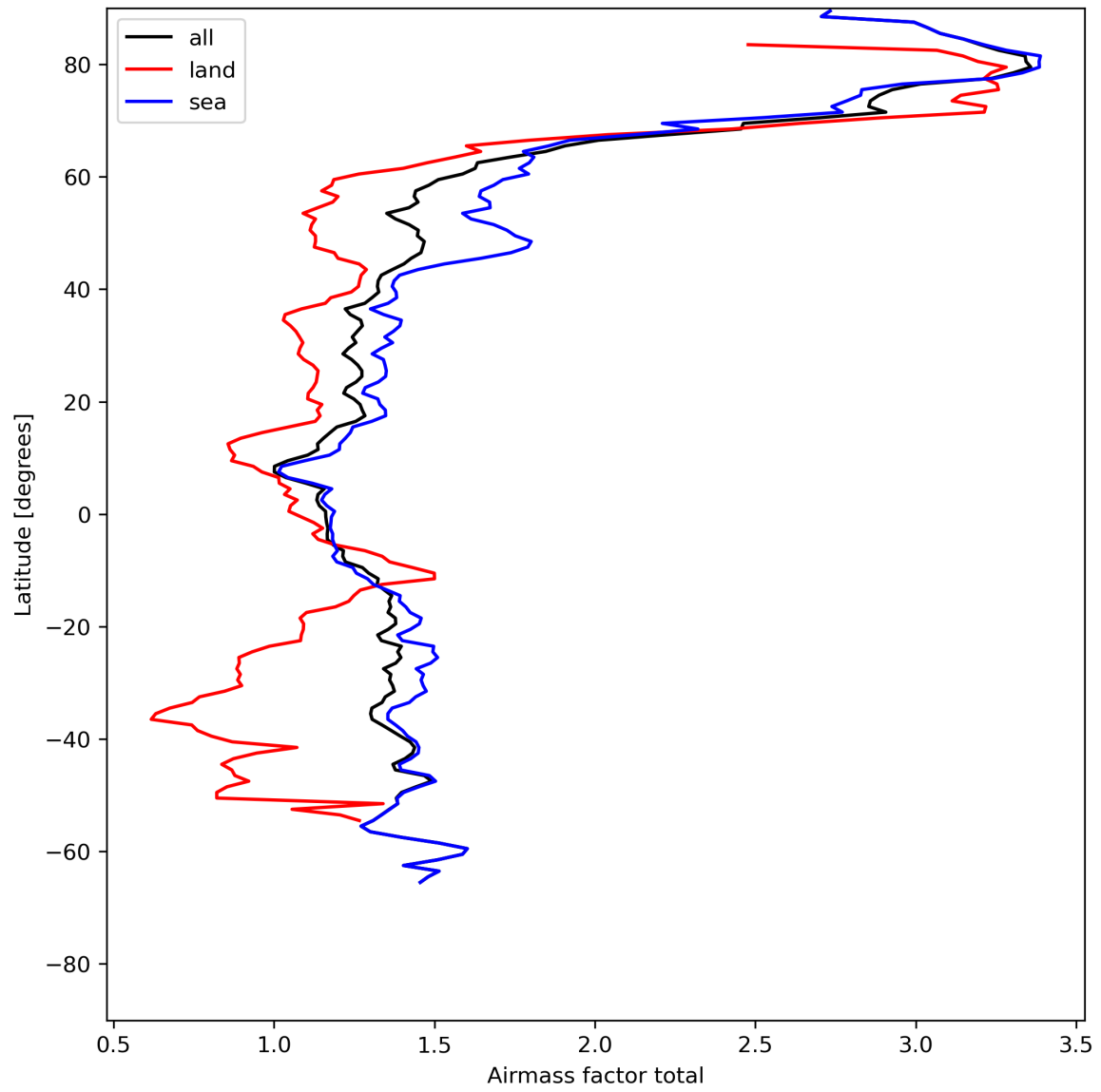
Figure 26: Zonal average of “Airmass factor total” for 2024-05-14 to 2024-05-16.
