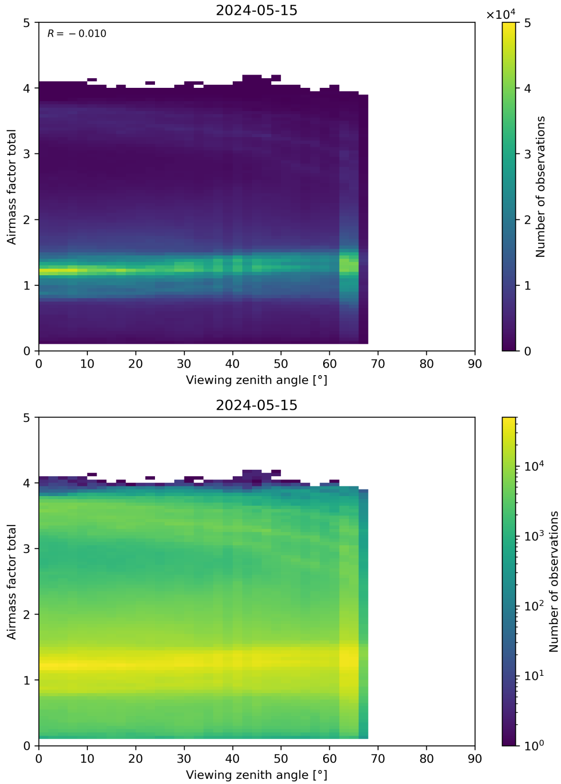
Figure 190: Scatter density plot of “Viewing zenith angle” against “Airmass factor total” for 2024-05-14 to 2024-05-16.
