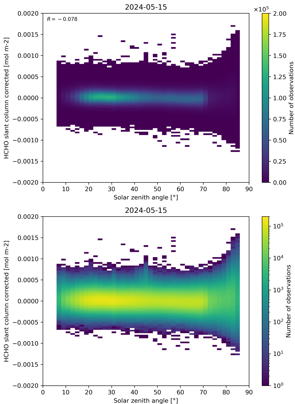
Figure 171: Scatter density plot of “Solar zenith angle” against “HCHO slant column corrected” for 2024-05-14 to 2024-05-16.
