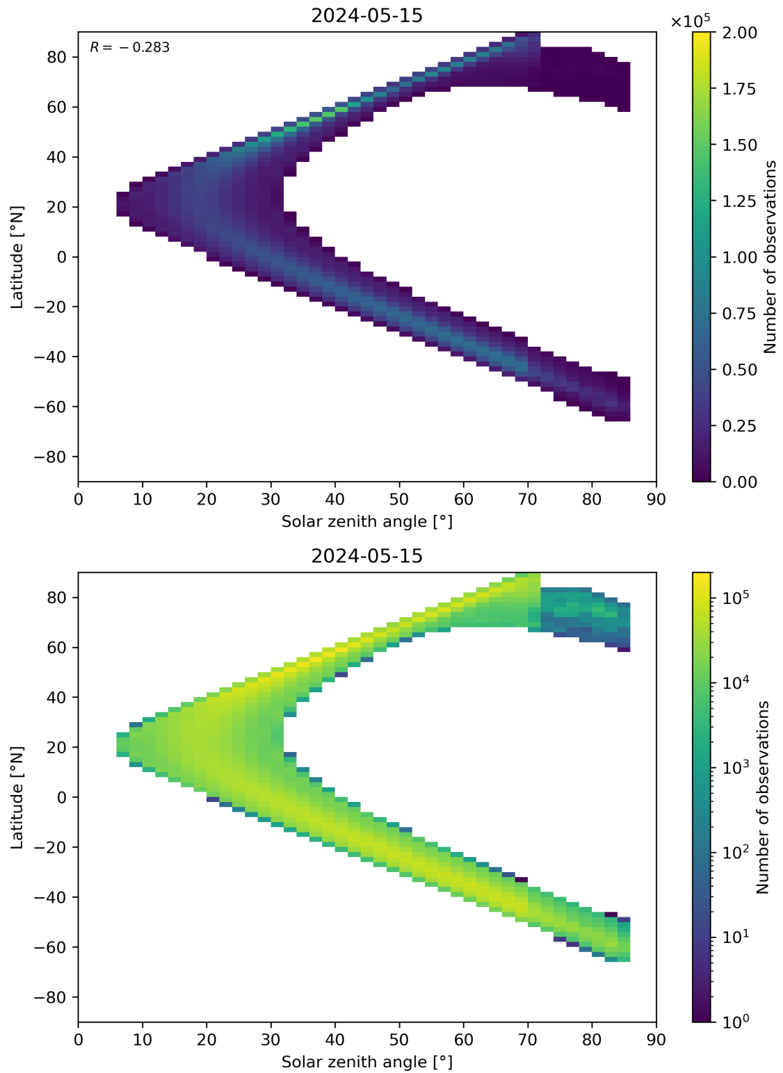
Figure 181: Scatter density plot of “Solar zenith angle” against “Latitude” for 2024-05-14 to 2024-05-16.
