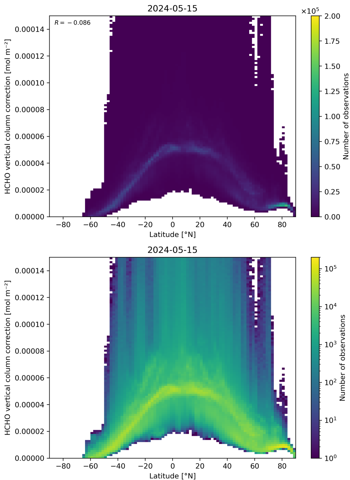
Figure 164: Scatter density plot of “Latitude” against “HCHO vertical column correction” for 2024-05-14 to 2024-05-16.
