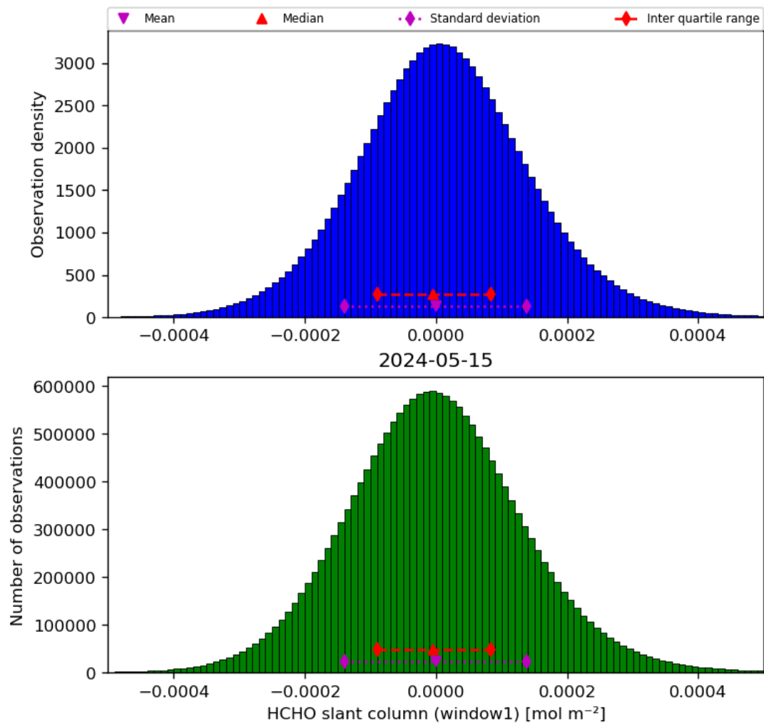
Figure 38: Histogram of “HCHO slant column (window1)” for 2024-05-14 to 2024-05-16
