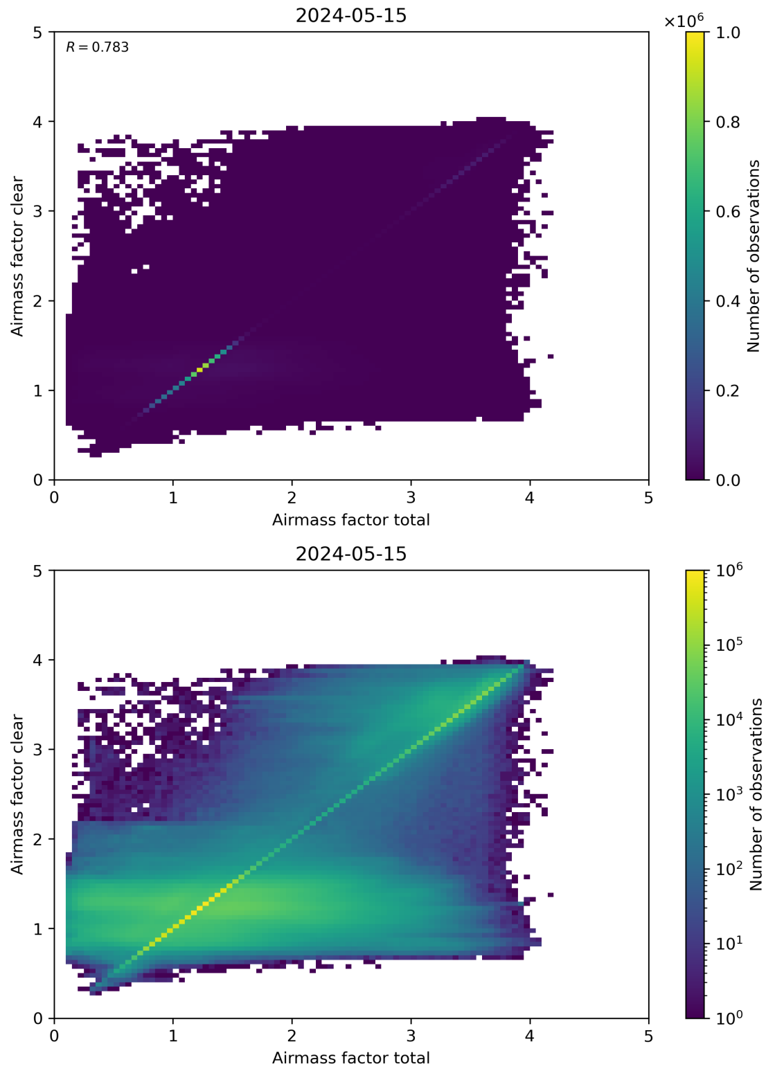
Figure 100: Scatter density plot of “Airmass factor total” against “Airmass factor clear” for 2024-05-14 to 2024-05-16.
