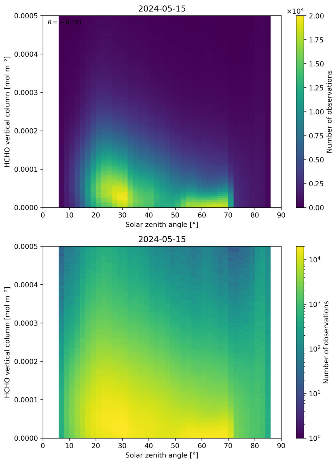
Figure 177: Scatter density plot of “Solar zenith angle” against “HCHO vertical column” for 2024-05-14 to 2024-05-16.
