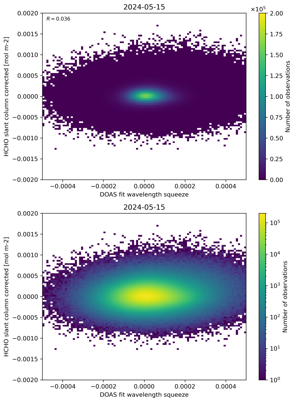
Figure 69: Scatter density plot of “DOAS fit wavelength squeeze” against “HCHO slant column corrected” for 2024-05-14 to 2024-05-16.
