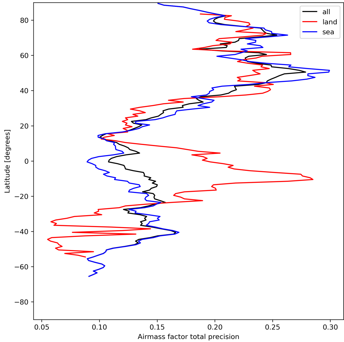
Figure 27: Zonal average of “Airmass factor total precision” for 2024-05-14 to 2024-05-16.
