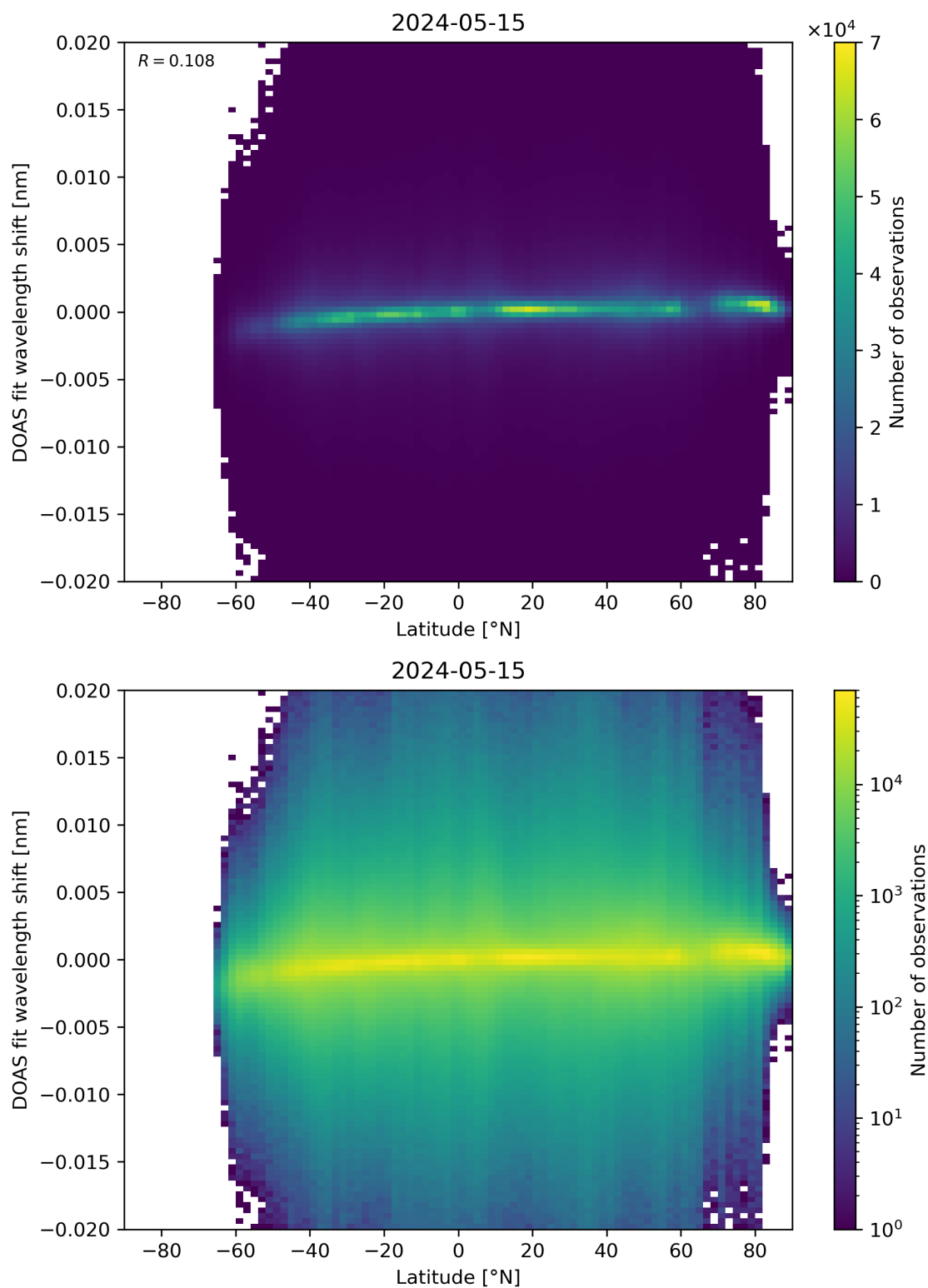
Figure 154: Scatter density plot of “Latitude” against “DOAS fit wavelength shift” for 2024-05-14 to 2024-05-16.
