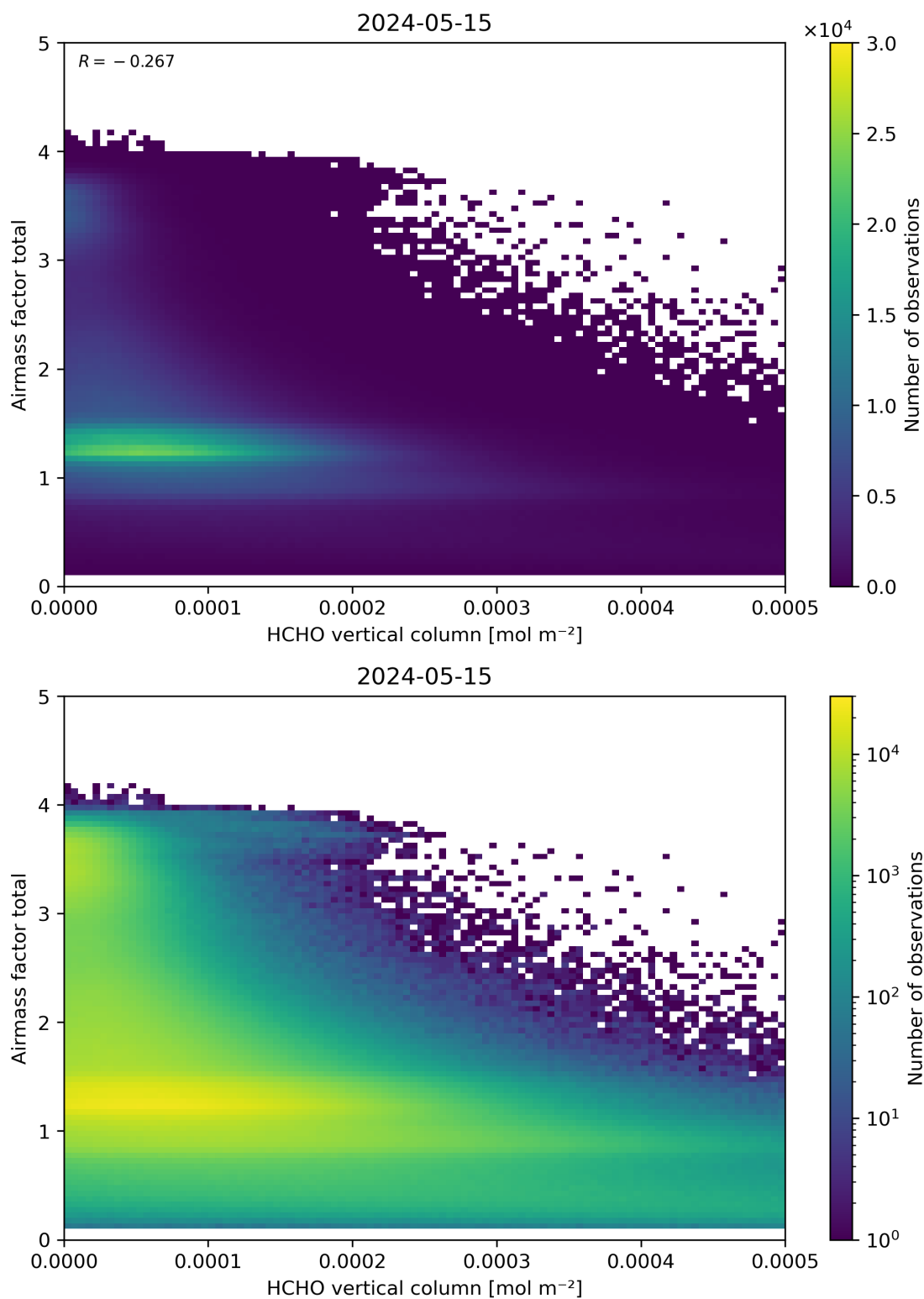
Figure 131: Scatter density plot of “HCHO vertical column” against “Airmass factor total” for 2024-05-14 to 2024-05-16.
