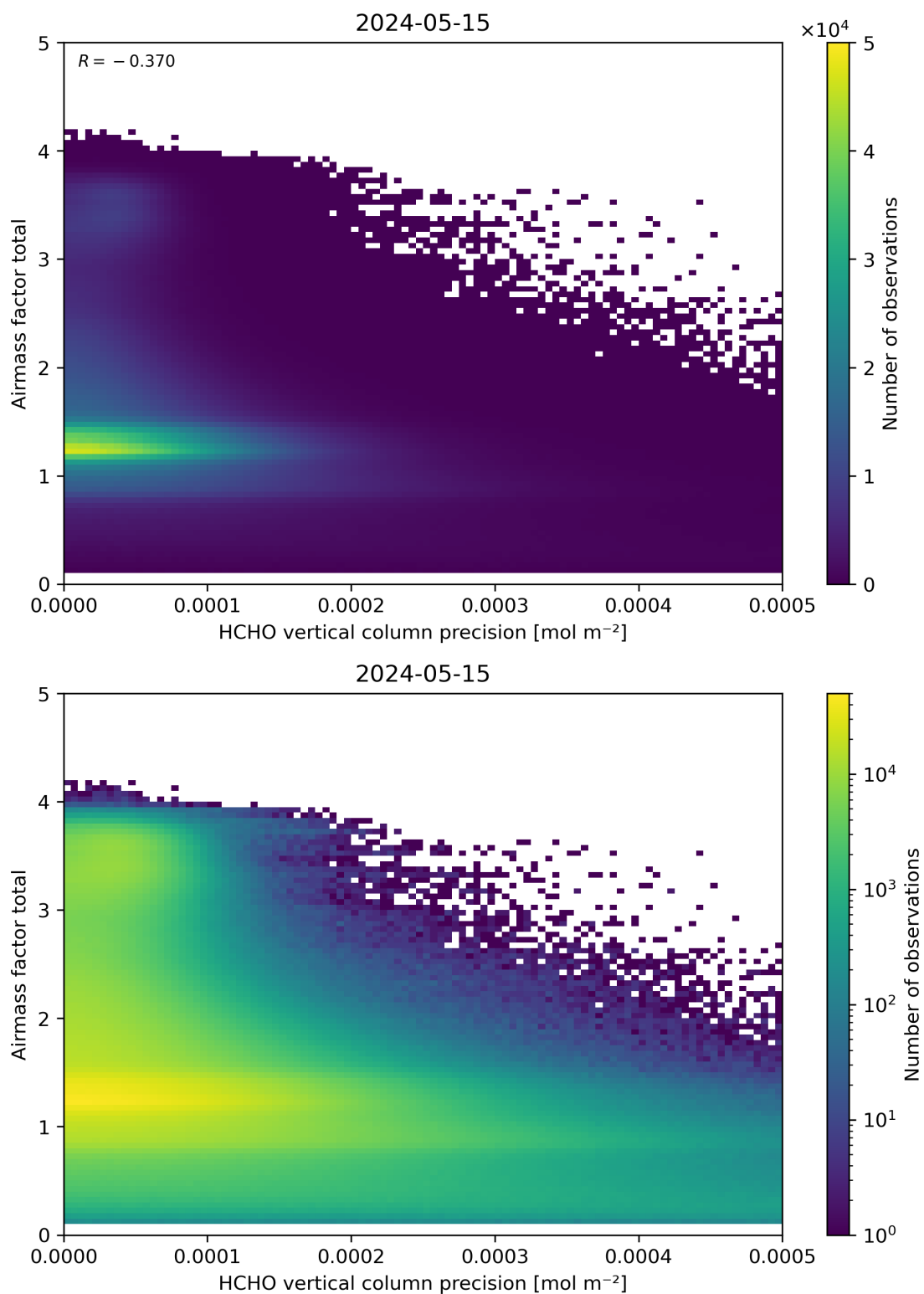
Figure 144: Scatter density plot of “HCHO vertical column precision” against “Airmass factor total” for 2024-05-14 to 2024-05-16.
