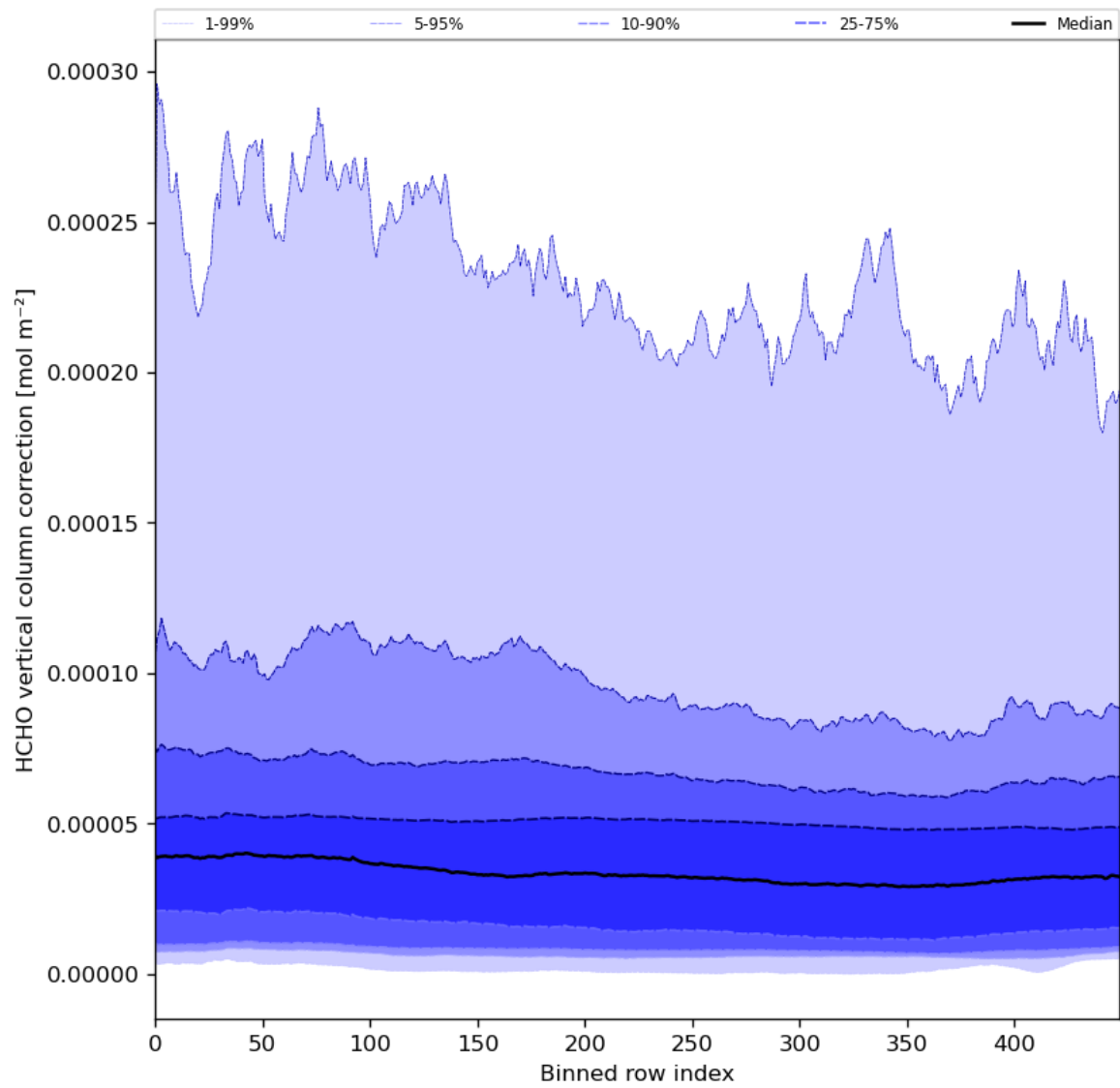
Figure 51: Along track statistics of “HCHO vertical column correction” for 2024-05-14 to 2024-05-16
