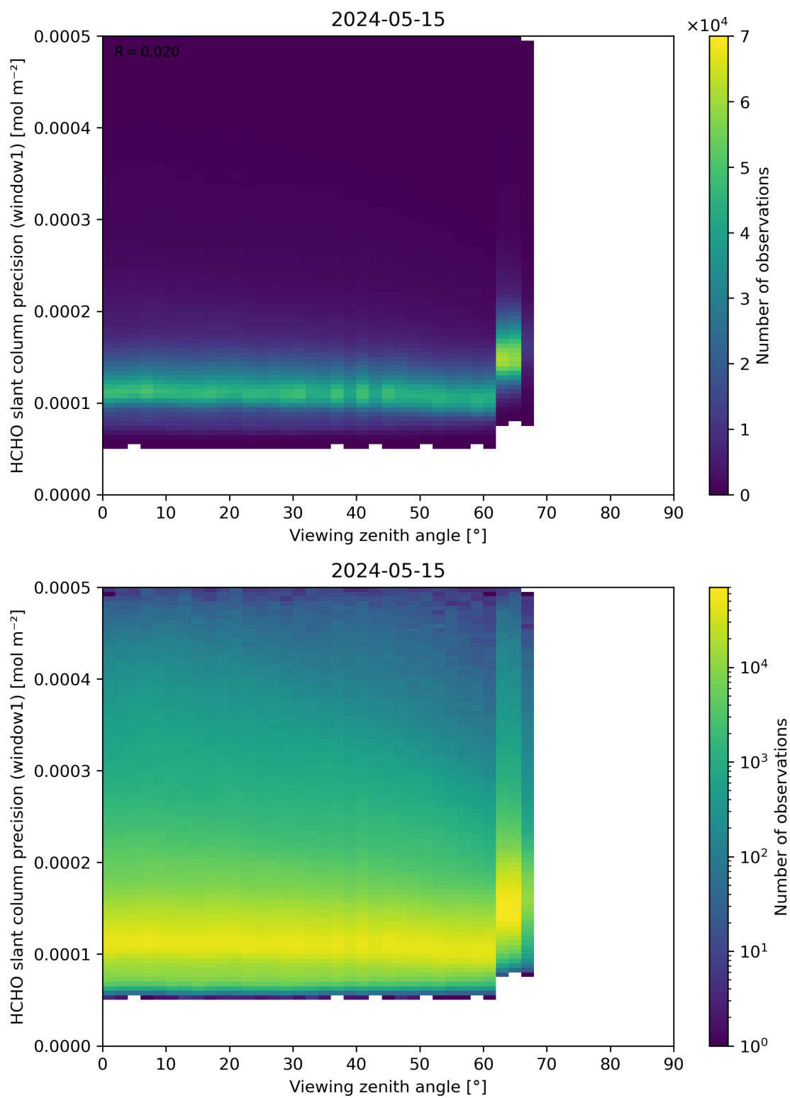
Figure 189: Scatter density plot of “Viewing zenith angle” against “HCHO slant column precision (window1)” for 2024-05-14 to 2024-05-16.
