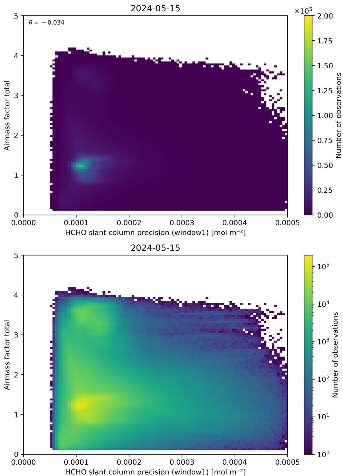
Figure 94: Scatter density plot of “HCHO slant column precision (window1)” against “Airmass factor total” for 2024-05-14 to 2024-05-16.
