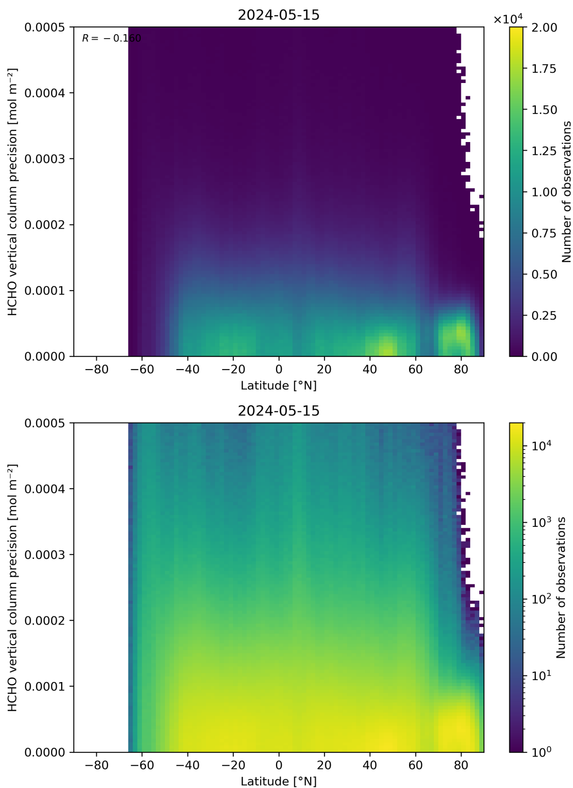
Figure 165: Scatter density plot of “Latitude” against “HCHO vertical column precision” for 2024-05-14 to 2024-05-16.
