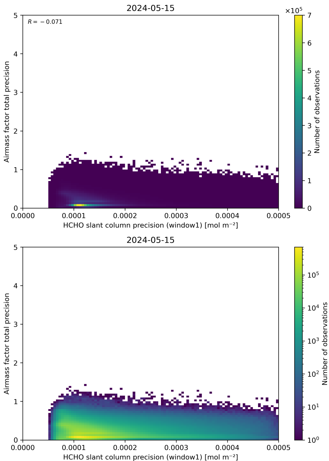
Figure 95: Scatter density plot of “HCHO slant column precision (window1)” against “Airmass factor total precision” for 2024-05-14 to 2024-05-16.
