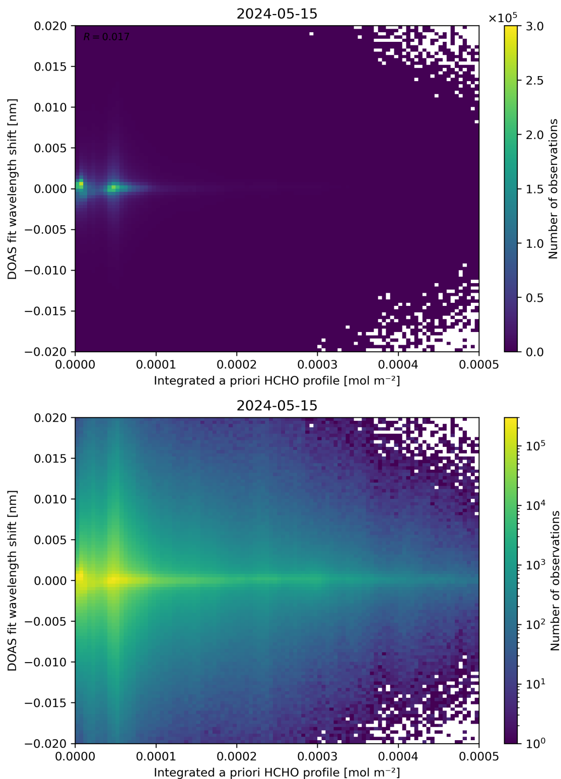
Figure 149: Scatter density plot of “Integrated a priori HCHO profile” against “DOAS fit wavelength shift” for 2024-05-14 to 2024-05-16.
