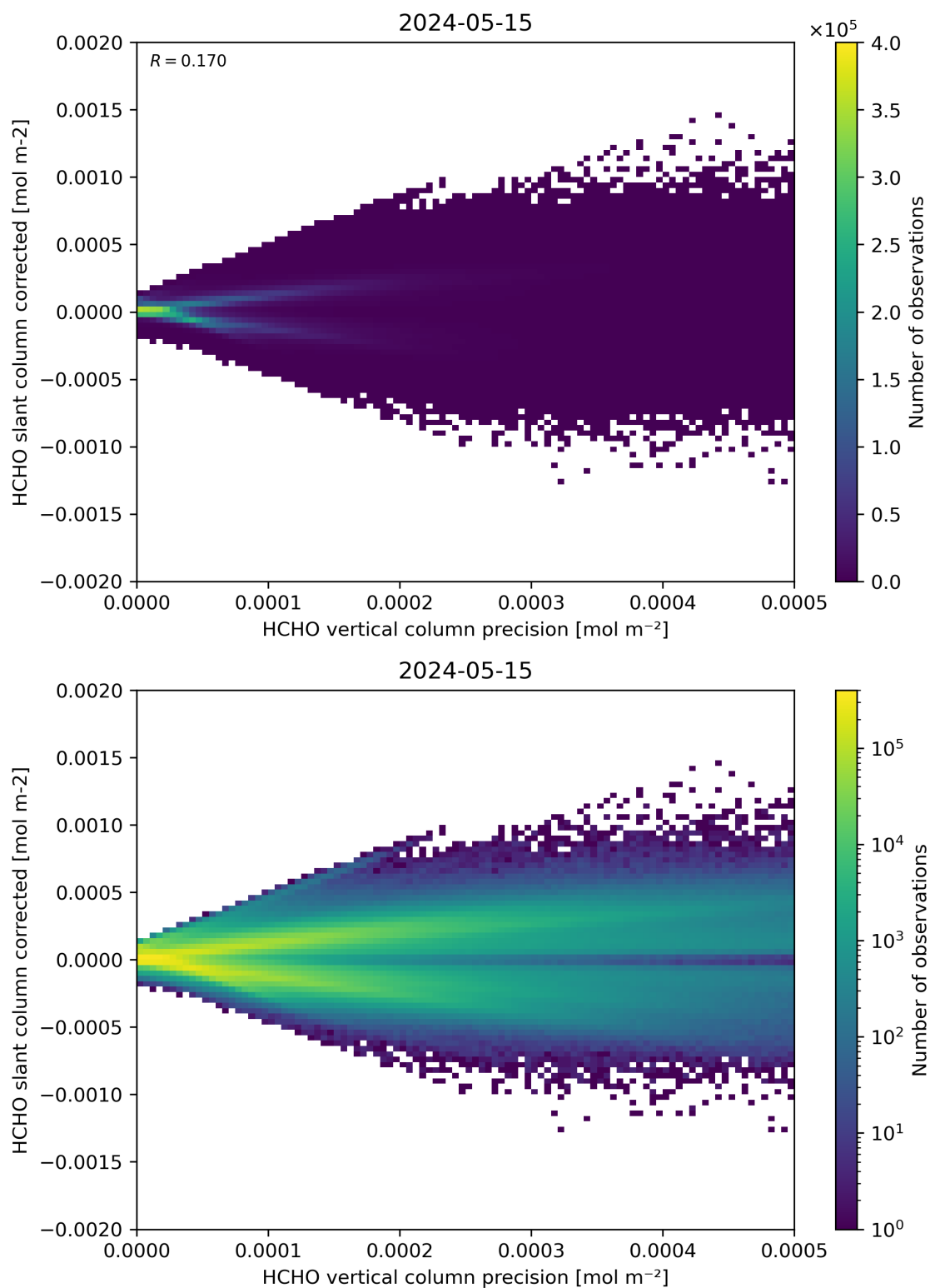
Figure 140: Scatter density plot of “HCHO vertical column precision” against “HCHO slant column corrected” for 2024-05-14 to 2024-05-16.
