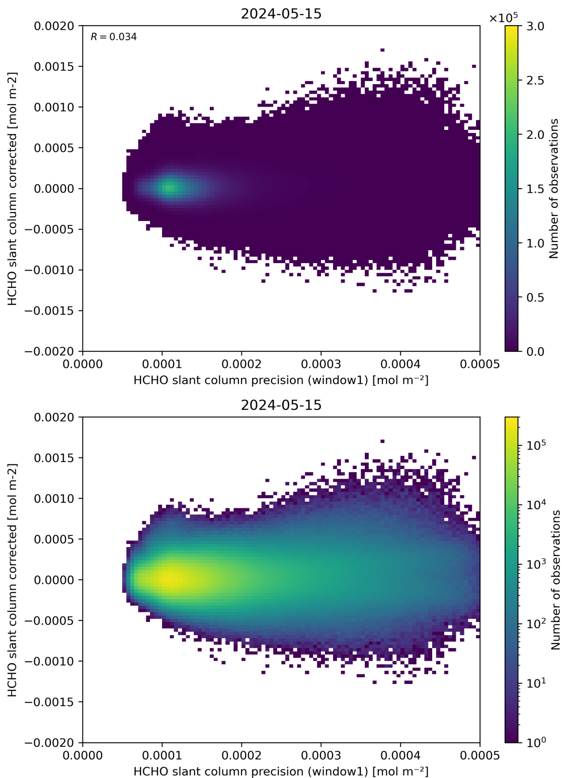
Figure 92: Scatter density plot of “HCHO slant column precision (window1)” against “HCHO slant column corrected” for 2024-05-14 to 2024-05-16.
