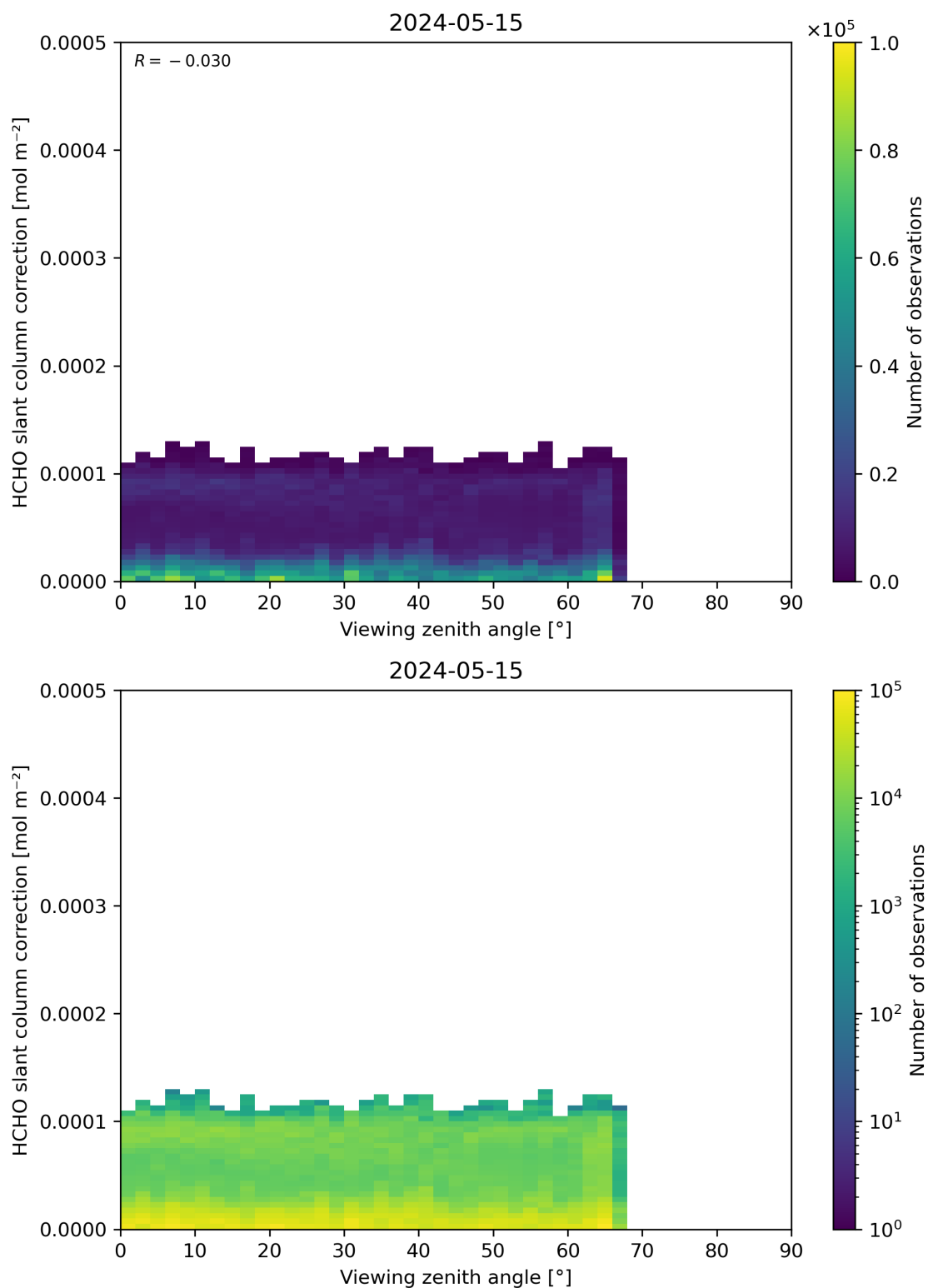
Figure 187: Scatter density plot of “Viewing zenith angle” against “HCHO slant column correction” for 2024-05-14 to 2024-05-16.
