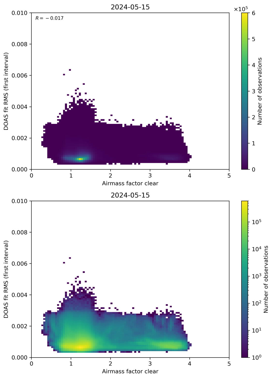
Figure 71: Scatter density plot of “Airmass factor clear” against “DOAS fit RMS (first interval)” for 2024-05-14 to 2024-05-16.
