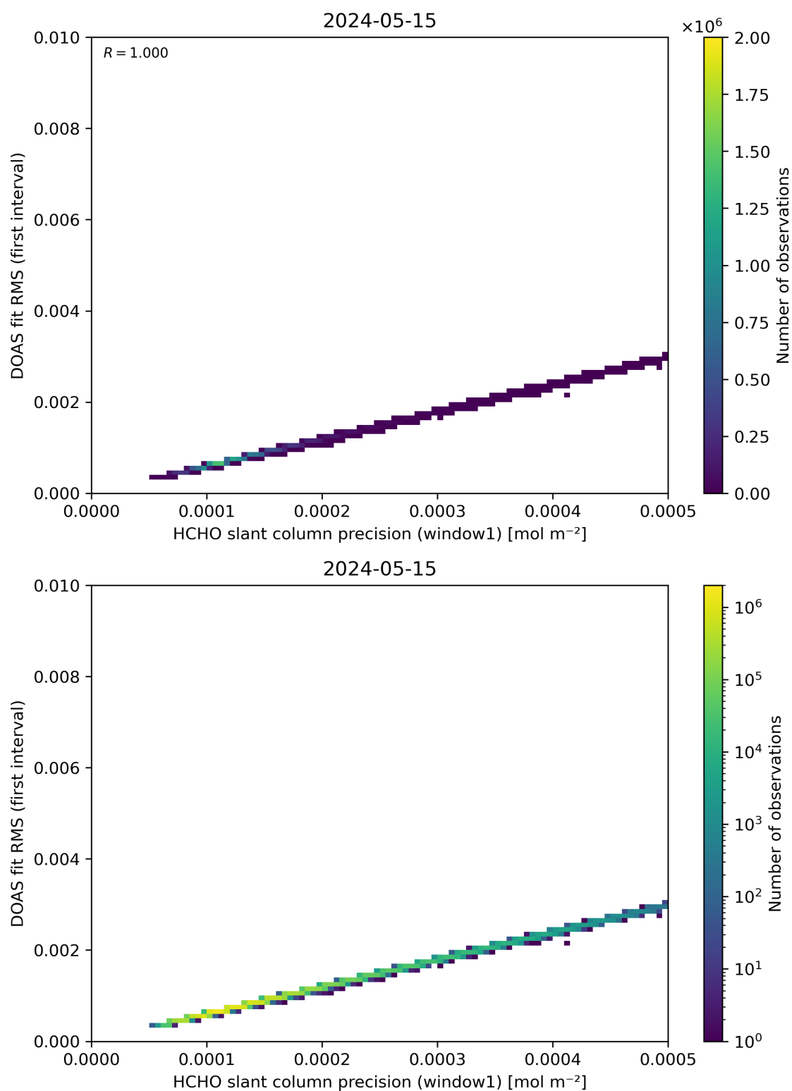
Figure 88: Scatter density plot of “HCHO slant column precision (window1)” against “DOAS fit RMS (first interval)” for 2024-05-14 to 2024-05-16.
