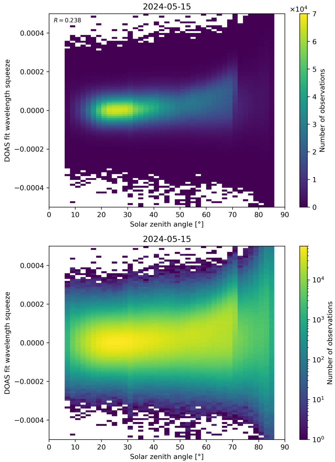
Figure 169: Scatter density plot of “Solar zenith angle” against “DOAS fit wavelength squeeze” for 2024-05-14 to 2024-05-16.
