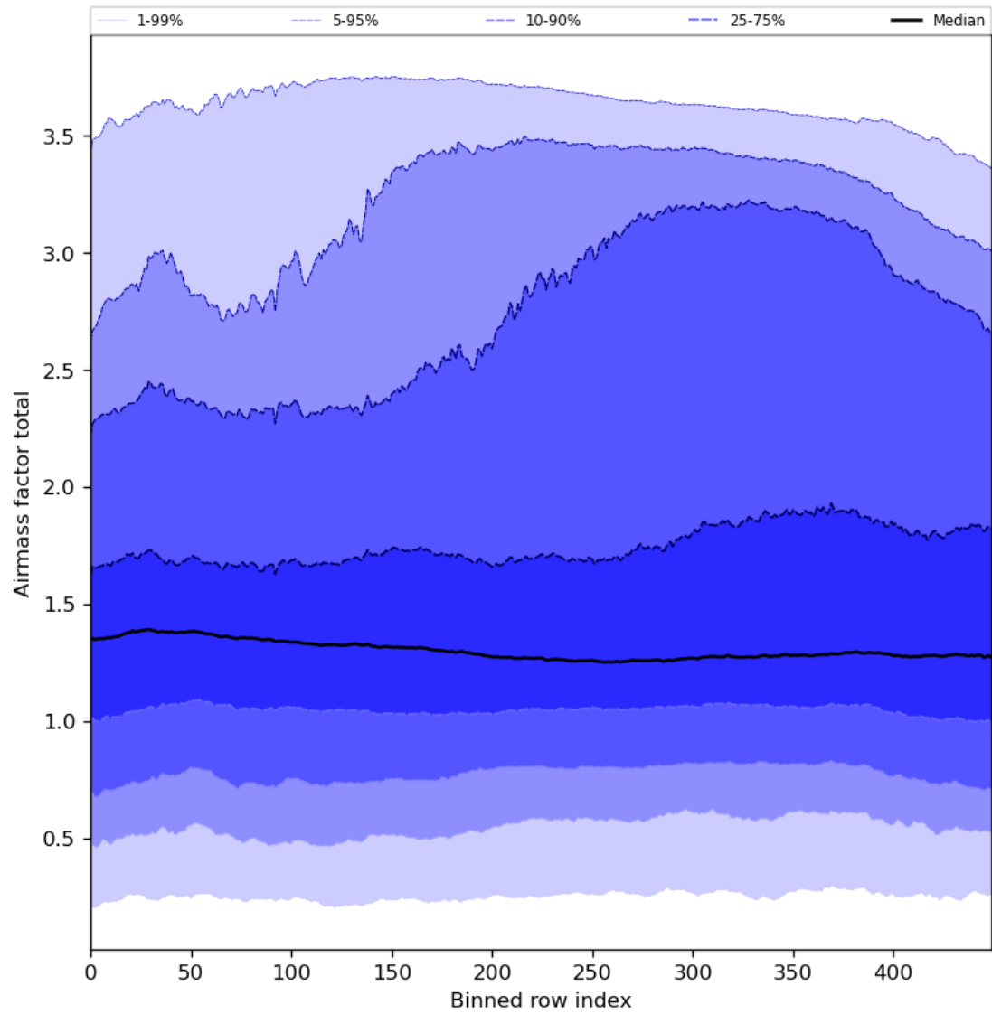
Figure 54: Along track statistics of “Airmass factor total” for 2024-05-14 to 2024-05-16
