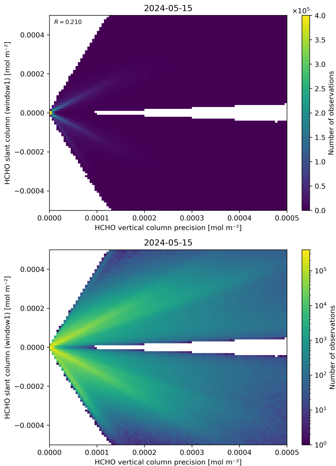
Figure 142: Scatter density plot of “HCHO vertical column precision” against “HCHO slant column (window1)” for 2024-05-14 to 2024-05-16.
