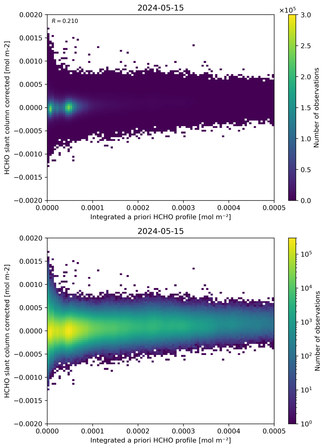
Figure 151: Scatter density plot of “Integrated a priori HCHO profile” against “HCHO slant column corrected” for 2024-05-14 to 2024-05-16.
