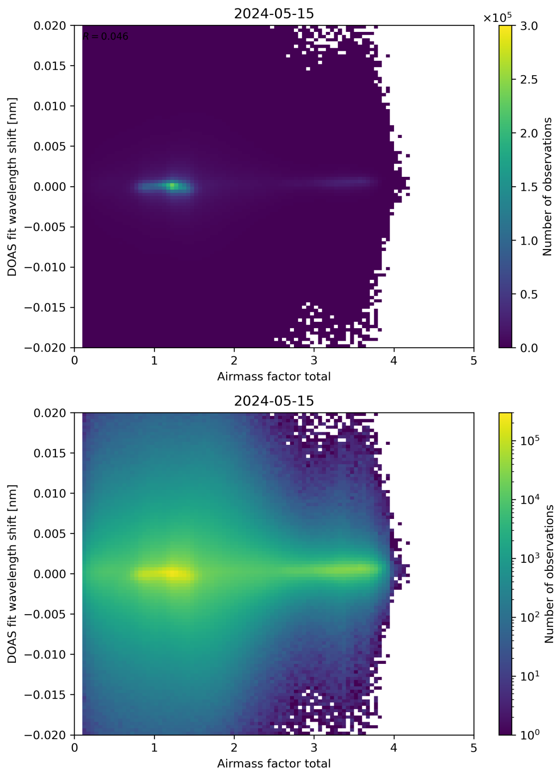
Figure 98: Scatter density plot of “Airmass factor total” against “DOAS fit wavelength shift” for 2024-05-14 to 2024-05-16.
