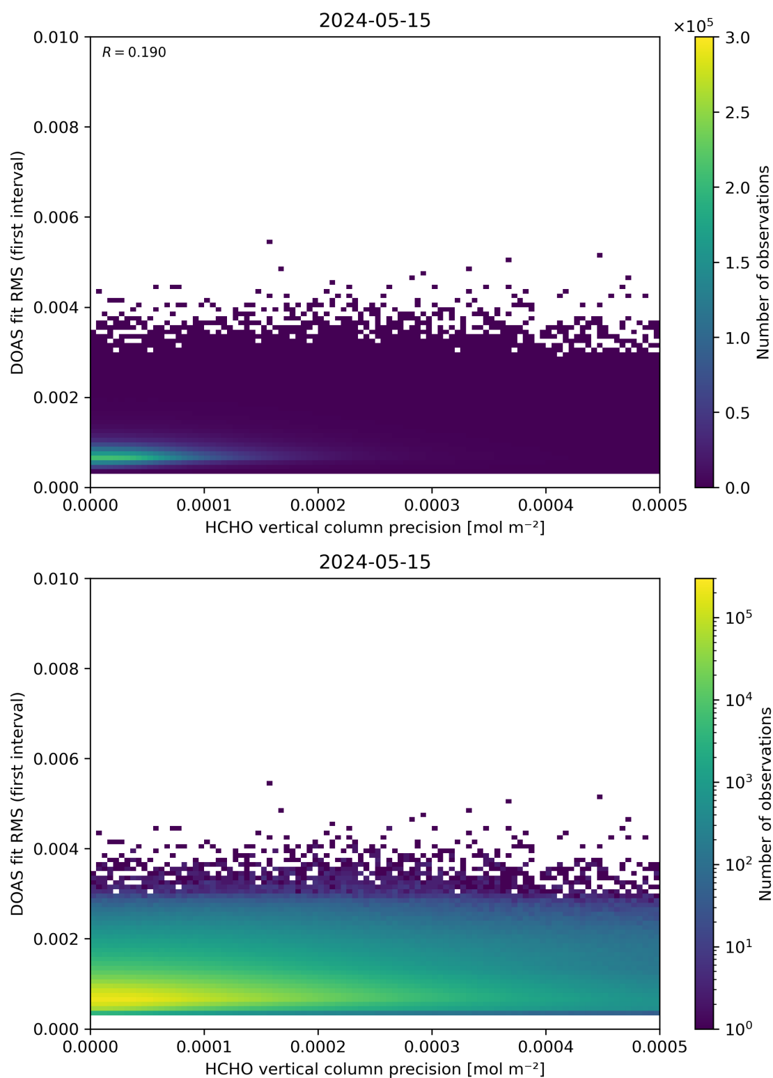
Figure 136: Scatter density plot of “HCHO vertical column precision” against “DOAS fit RMS (first interval)” for 2024-05-14 to 2024-05-16.
