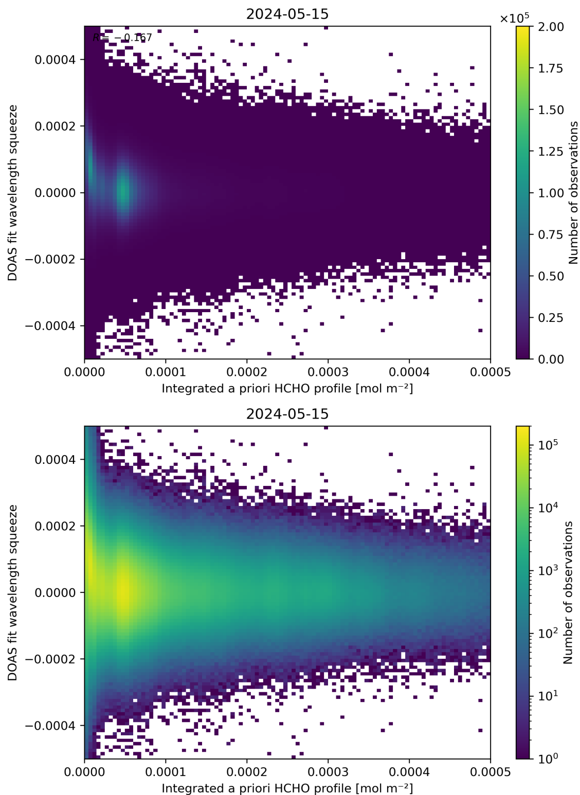
Figure 150: Scatter density plot of “Integrated a priori HCHO profile” against “DOAS fit wavelength squeeze” for 2024-05-14 to 2024-05-16.
