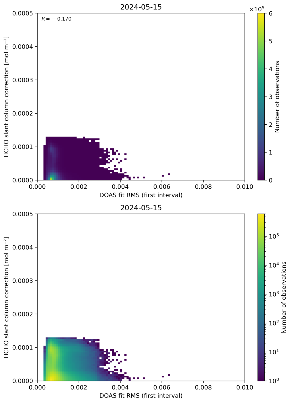
Figure 63: Scatter density plot of “DOAS fit RMS (first interval)” against “HCHO slant column correction” for 2024-05-14 to 2024-05-16.
