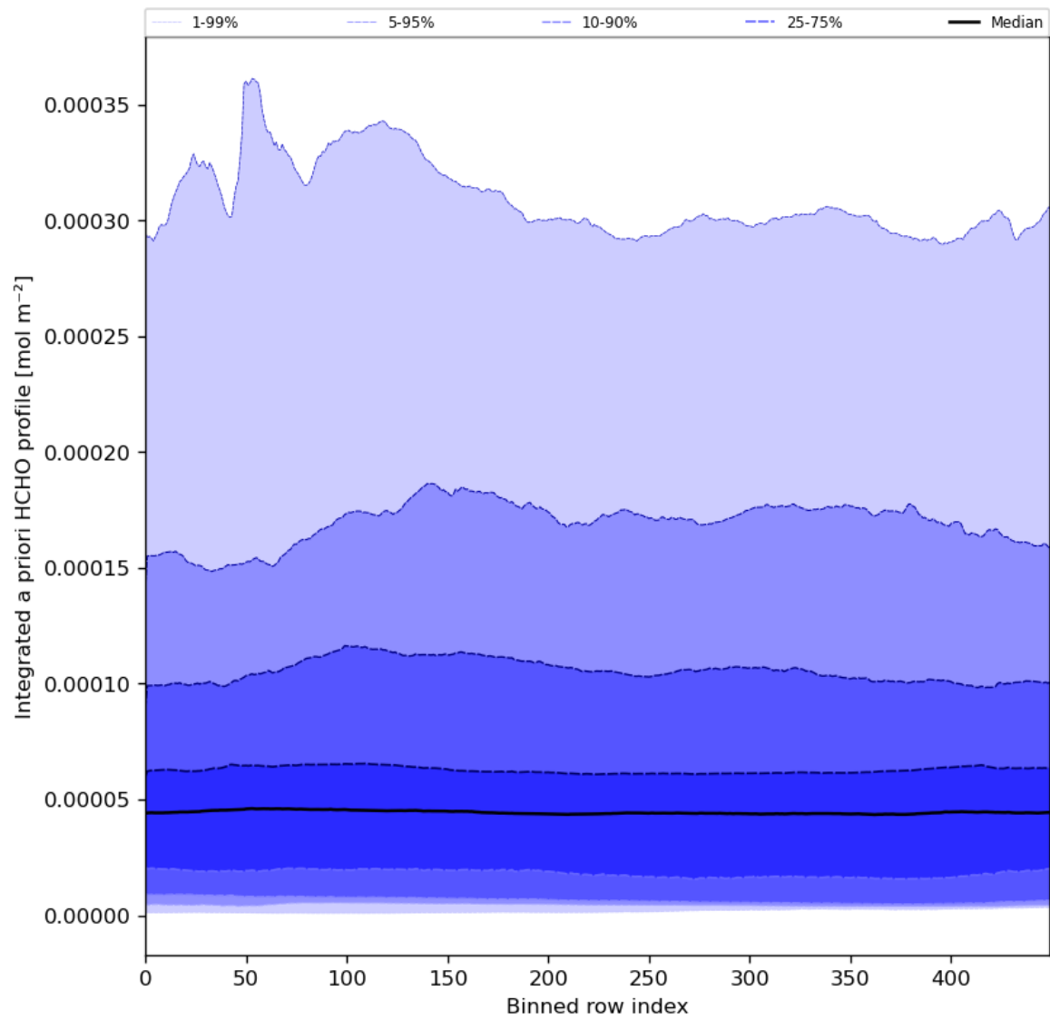
Figure 57: Along track statistics of “Integrated a priori HCHO profile” for 2024-05-14 to 2024-05-16
