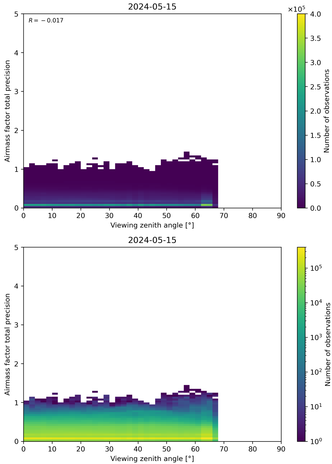
Figure 191: Scatter density plot of “Viewing zenith angle” against “Airmass factor total precision” for 2024-05-14 to 2024-05-16.
