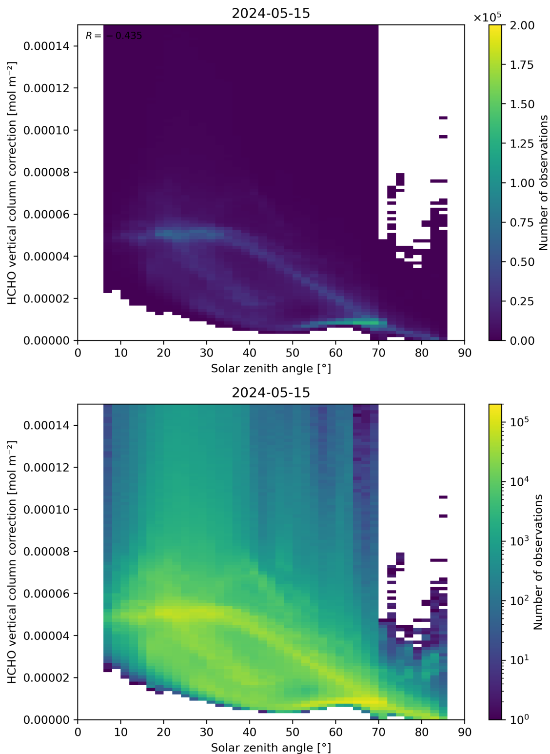
Figure 178: Scatter density plot of “Solar zenith angle” against “HCHO vertical column correction” for 2024-05-14 to 2024-05-16.
