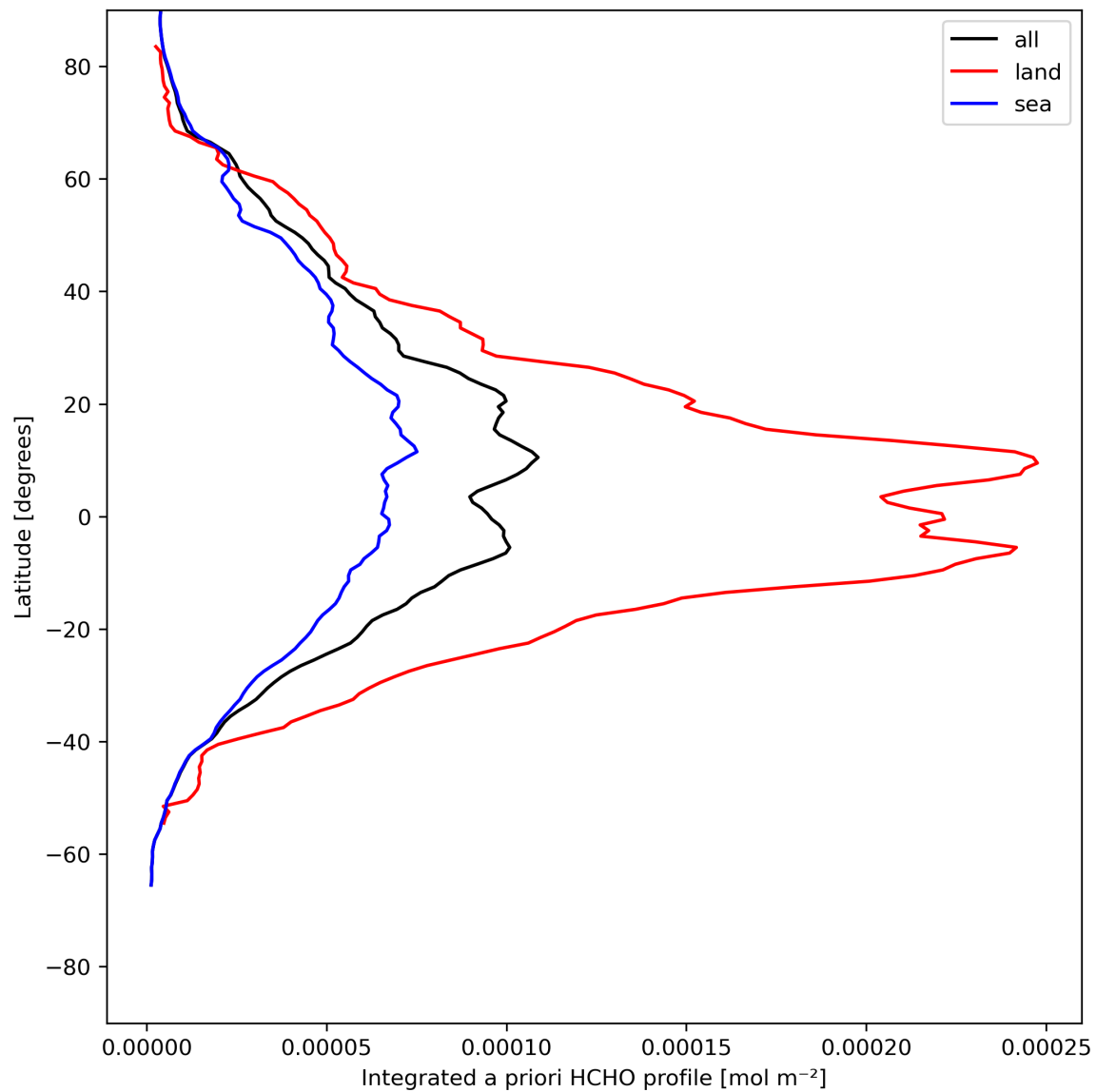
Figure 29: Zonal average of “Integrated a priori HCHO profile” for 2024-05-14 to 2024-05-16.
