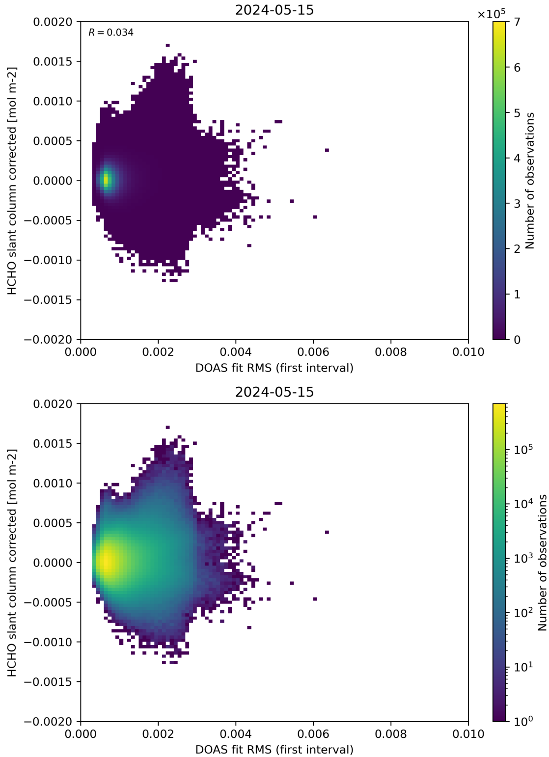
Figure 62: Scatter density plot of “DOAS fit RMS (first interval)” against “HCHO slant column corrected” for 2024-05-14 to 2024-05-16.
