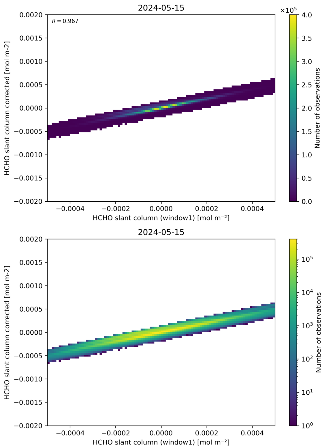
Figure 82: Scatter density plot of “HCHO slant column (window1)” against “HCHO slant column corrected” for 2024-05-14 to 2024-05-16.
