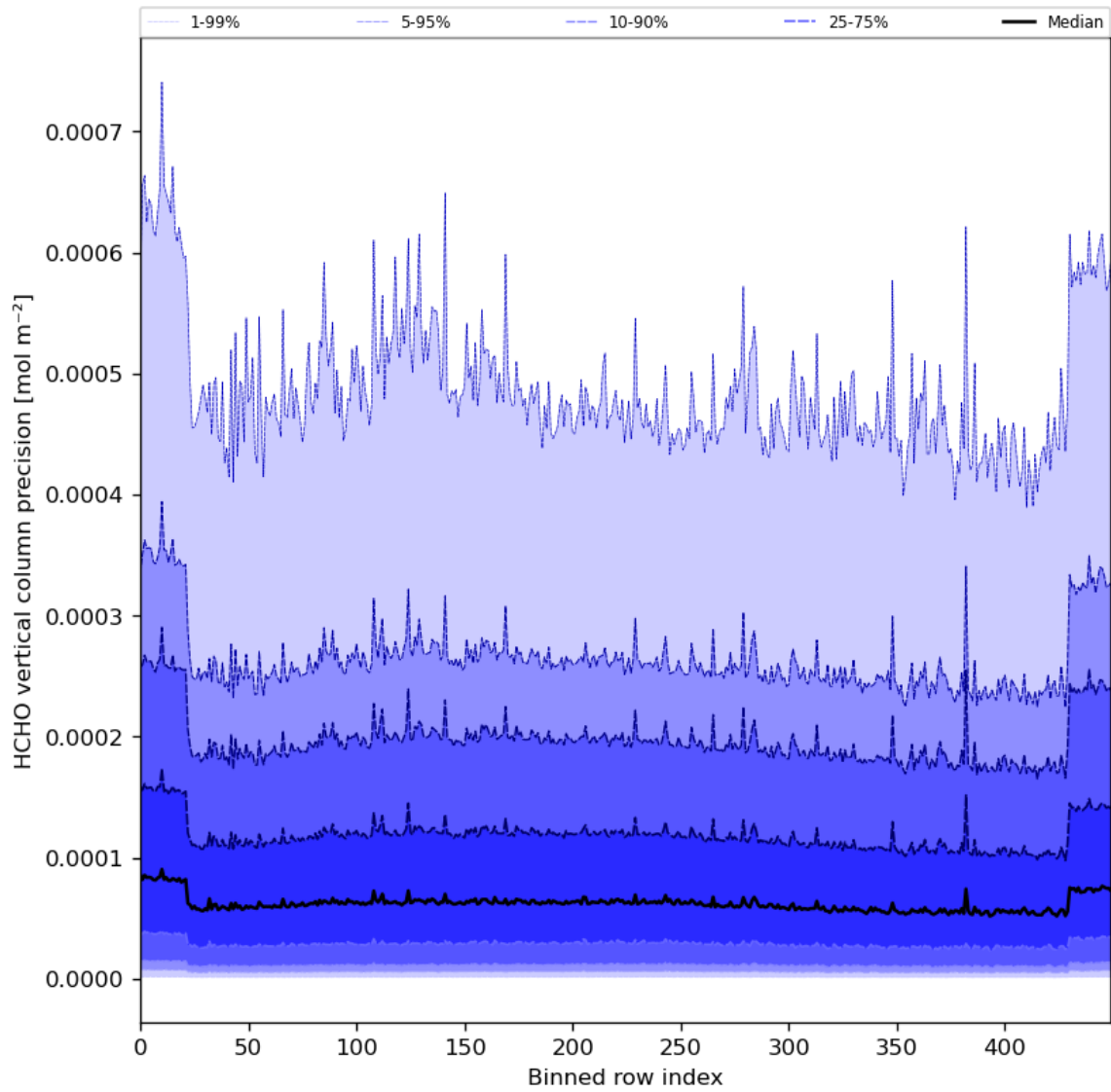
Figure 50: Along track statistics of “HCHO vertical column precision” for 2024-05-14 to 2024-05-16
