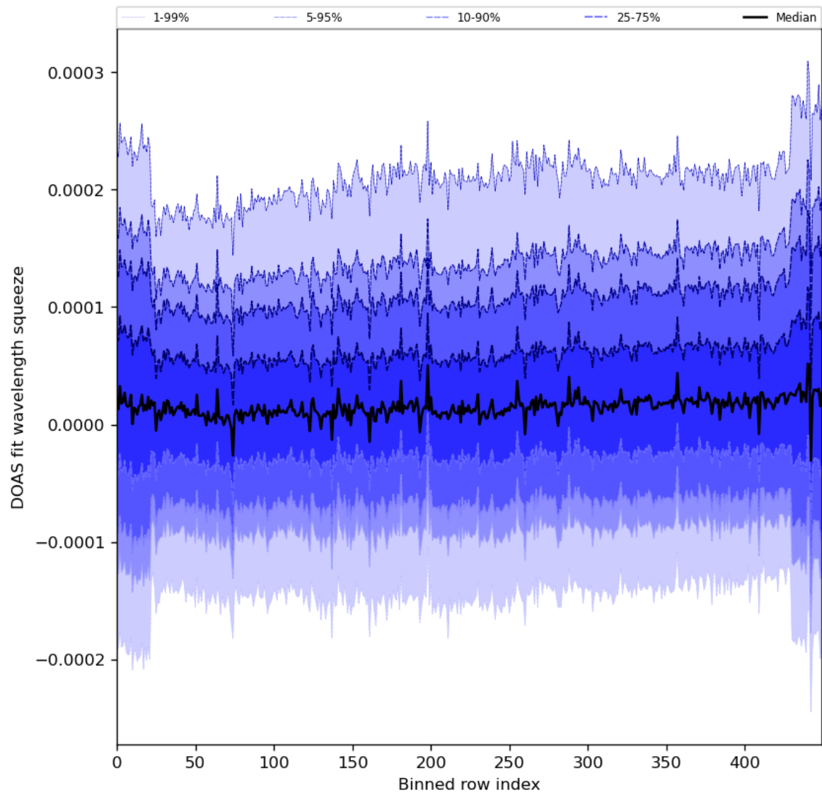
Figure 59: Along track statistics of “DOAS fit wavelength squeeze” for 2024-05-14 to 2024-05-16
