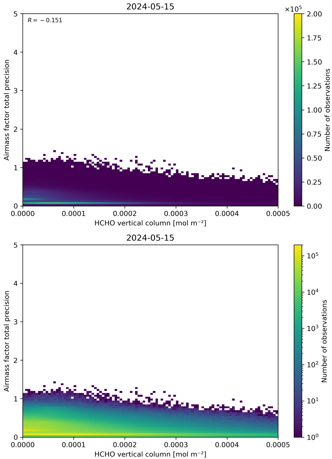
Figure 132: Scatter density plot of “HCHO vertical column” against “Airmass factor total precision” for 2024-05-14 to 2024-05-16.
