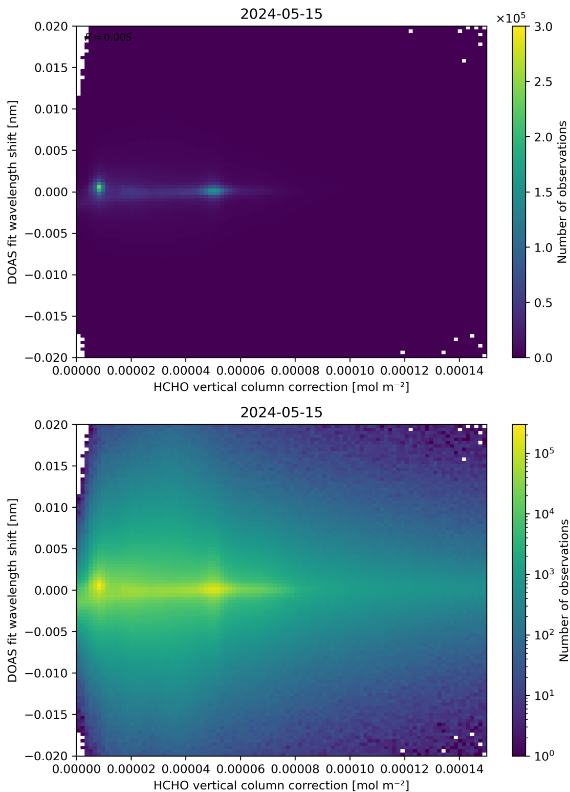
Figure 113: Scatter density plot of “HCHO vertical column correction” against “DOAS fit wavelength shift” for 2024-05-14 to 2024-05-16.
