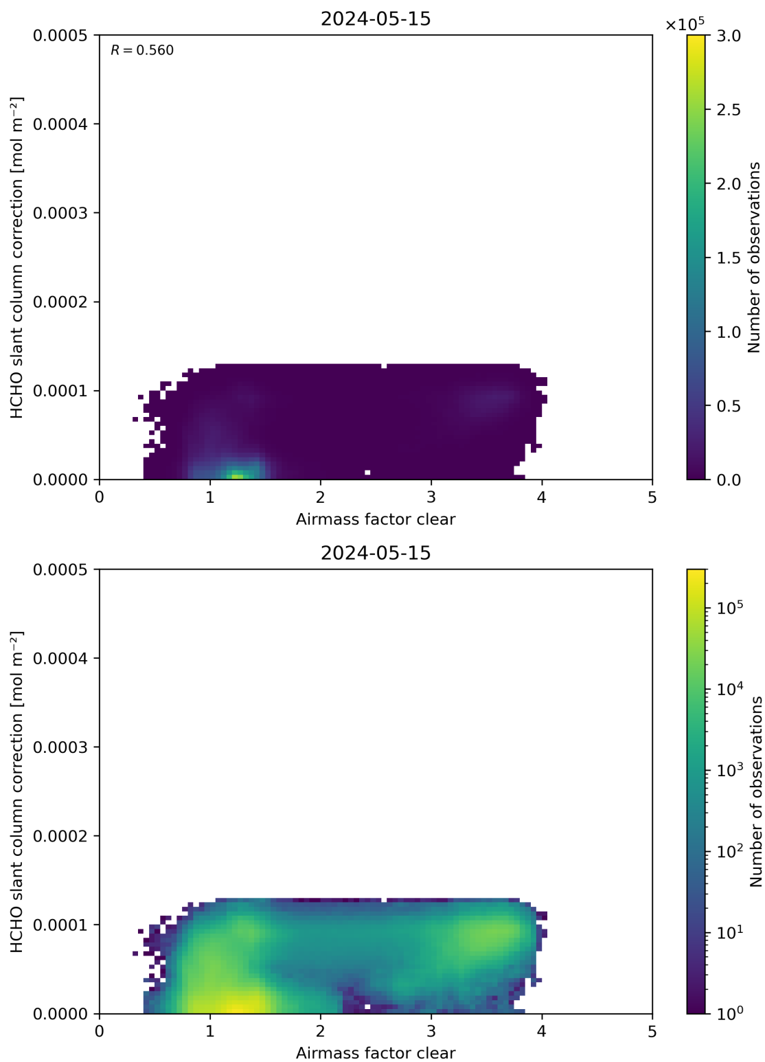
Figure 75: Scatter density plot of “Airmass factor clear” against “HCHO slant column correction” for 2024-05-14 to 2024-05-16.
