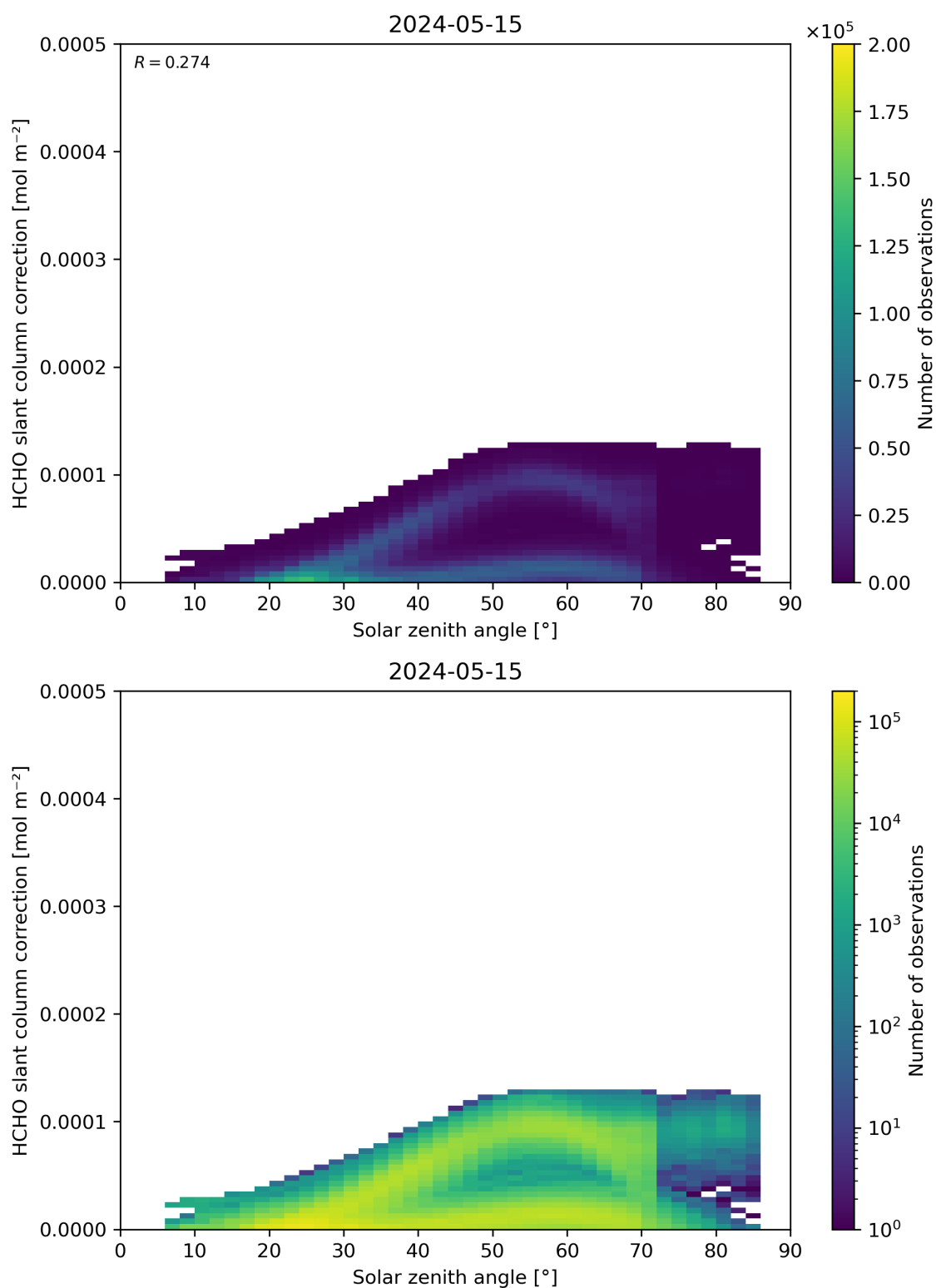
Figure 172: Scatter density plot of “Solar zenith angle” against “HCHO slant column correction” for 2024-05-14 to 2024-05-16.
