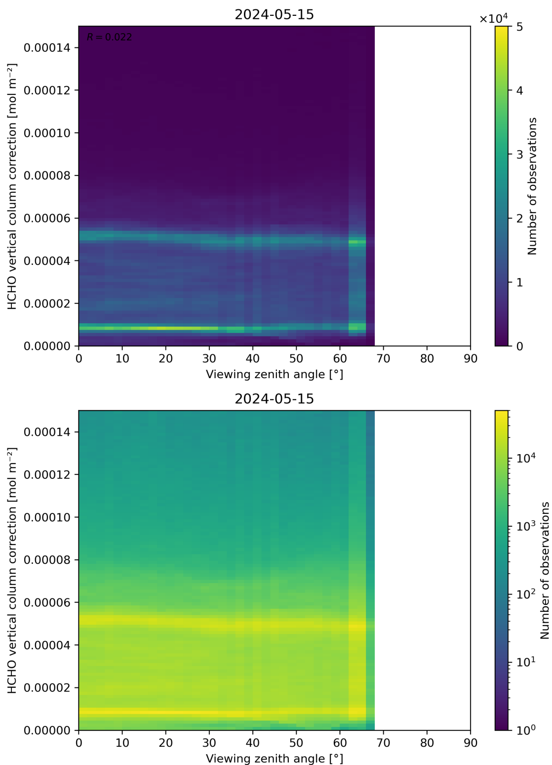
Figure 193: Scatter density plot of “Viewing zenith angle” against “HCHO vertical column correction” for 2024-05-14 to 2024-05-16.
