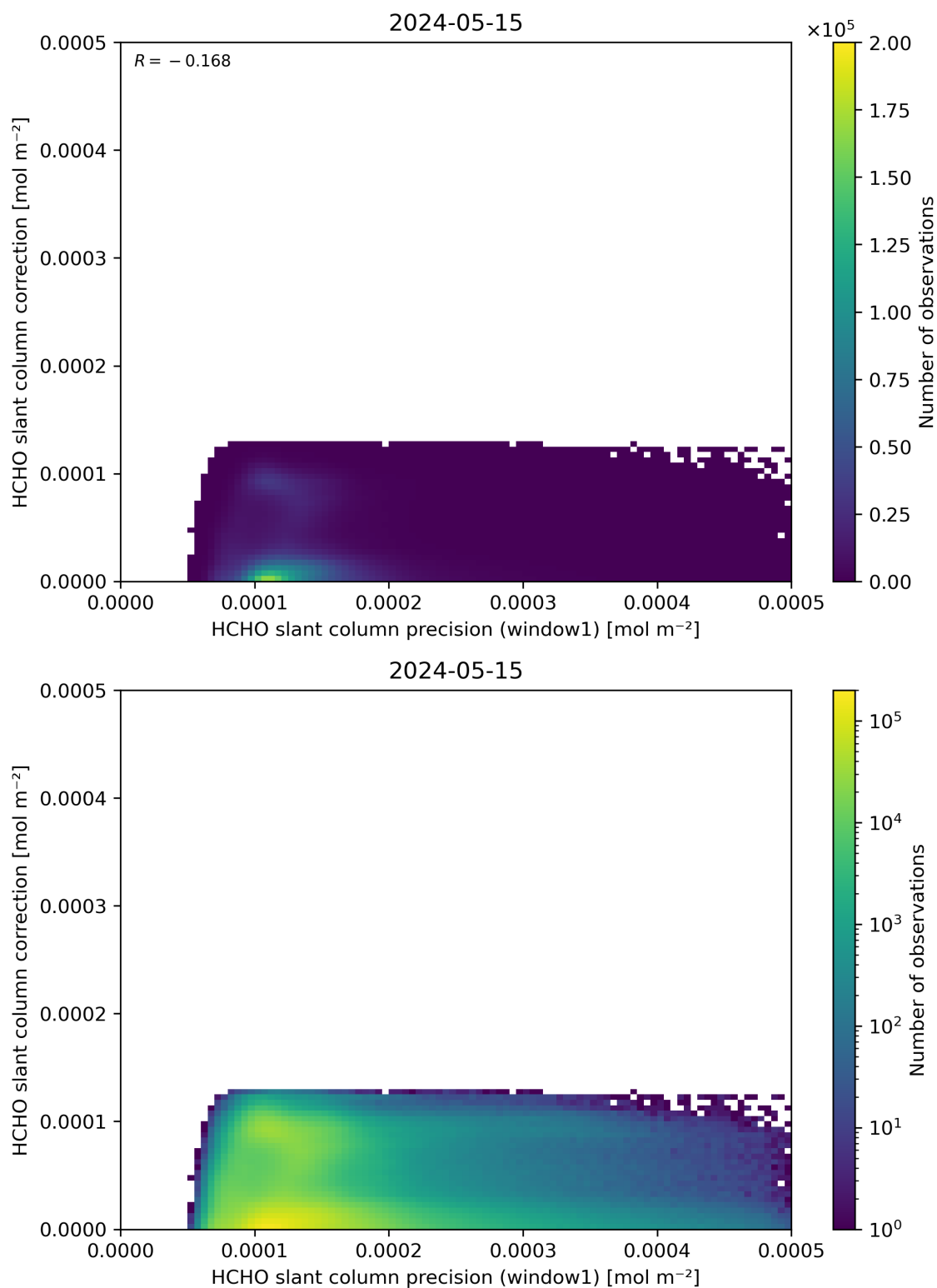
Figure 93: Scatter density plot of “HCHO slant column precision (window1)” against “HCHO slant column correction” for 2024-05-14 to 2024-05-16.
