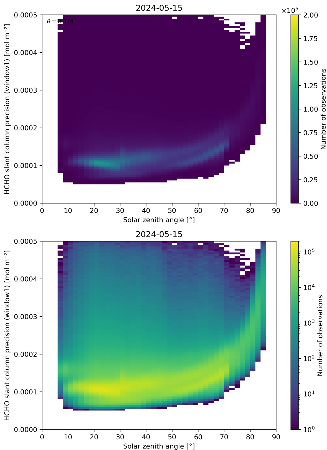
Figure 174: Scatter density plot of “Solar zenith angle” against “HCHO slant column precision (window1)” for 2024-05-14 to 2024-05-16.
