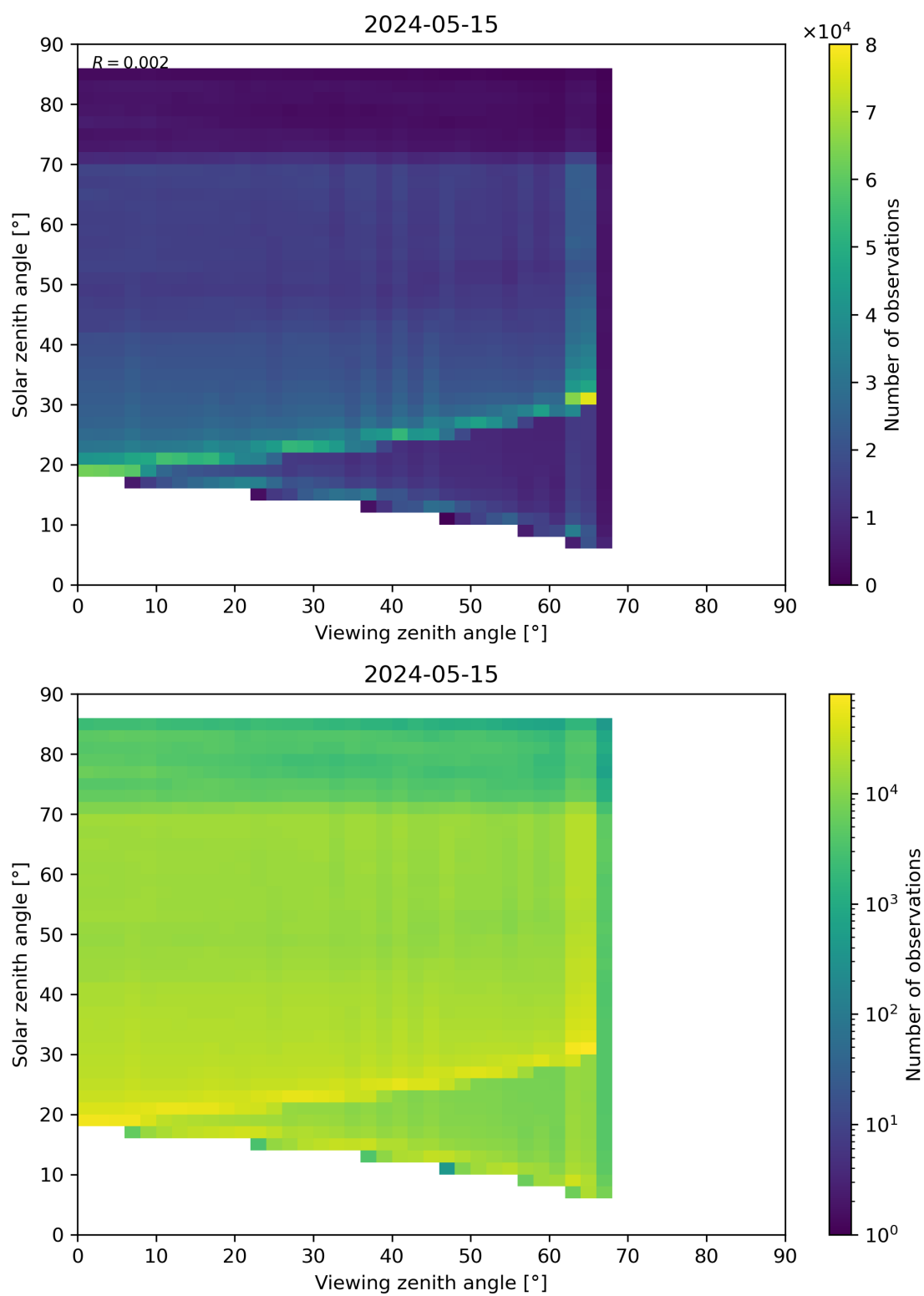
Figure 197: Scatter density plot of “Viewing zenith angle” against “Solar zenith angle” for 2024-05-14 to 2024-05-16.
