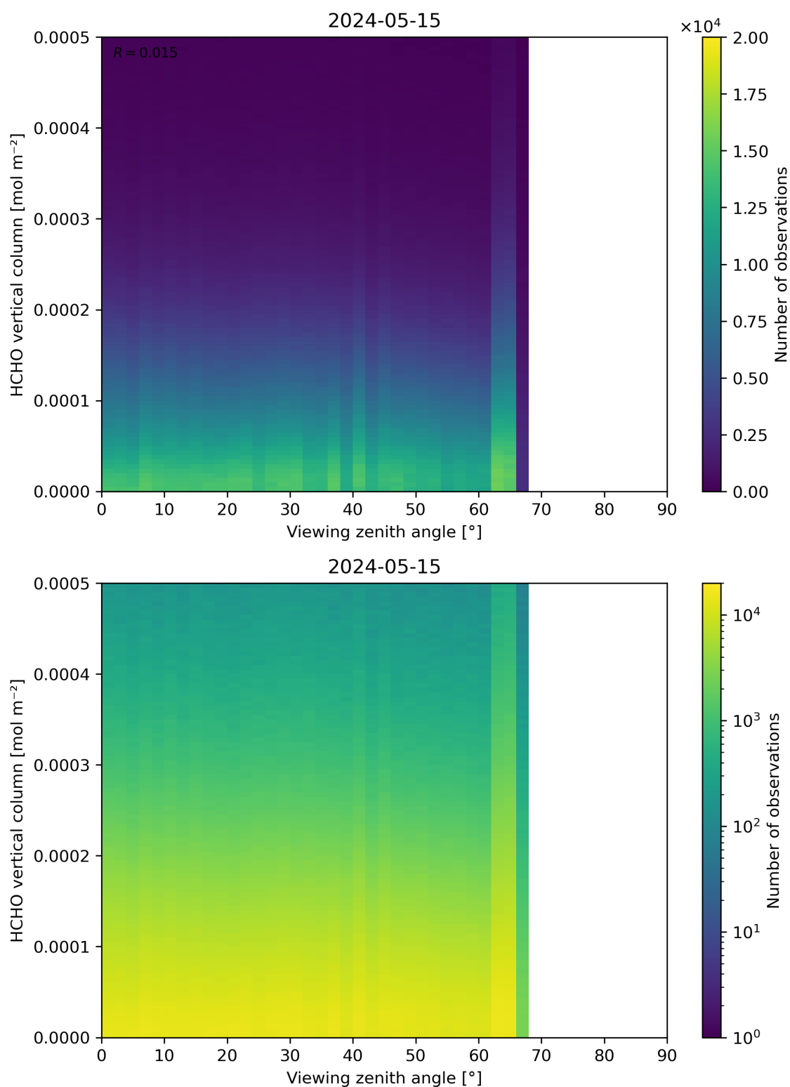
Figure 192: Scatter density plot of “Viewing zenith angle” against “HCHO vertical column” for 2024-05-14 to 2024-05-16.
