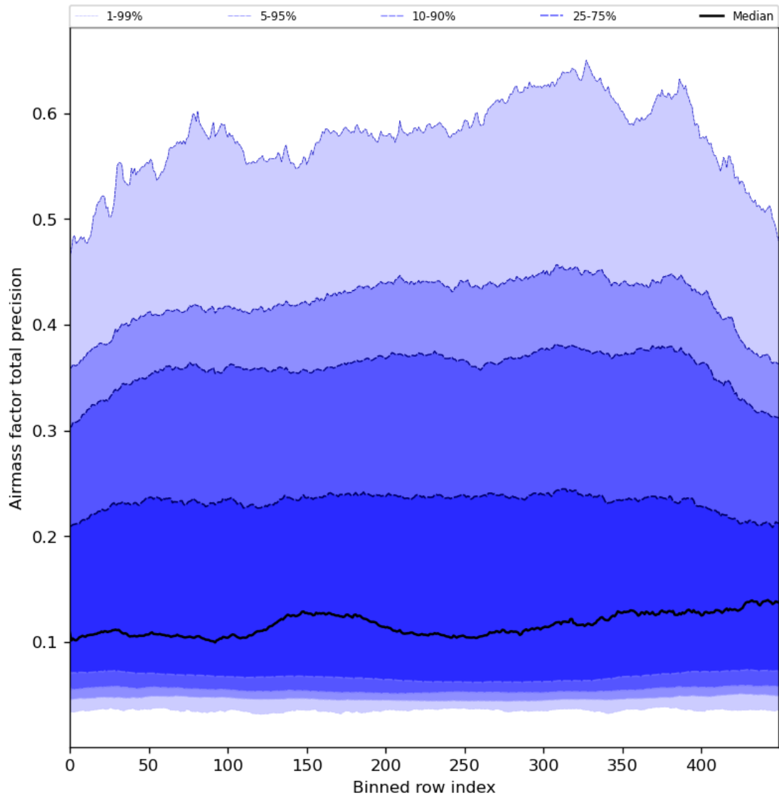
Figure 55: Along track statistics of “Airmass factor total precision” for 2024-05-14 to 2024-05-16
