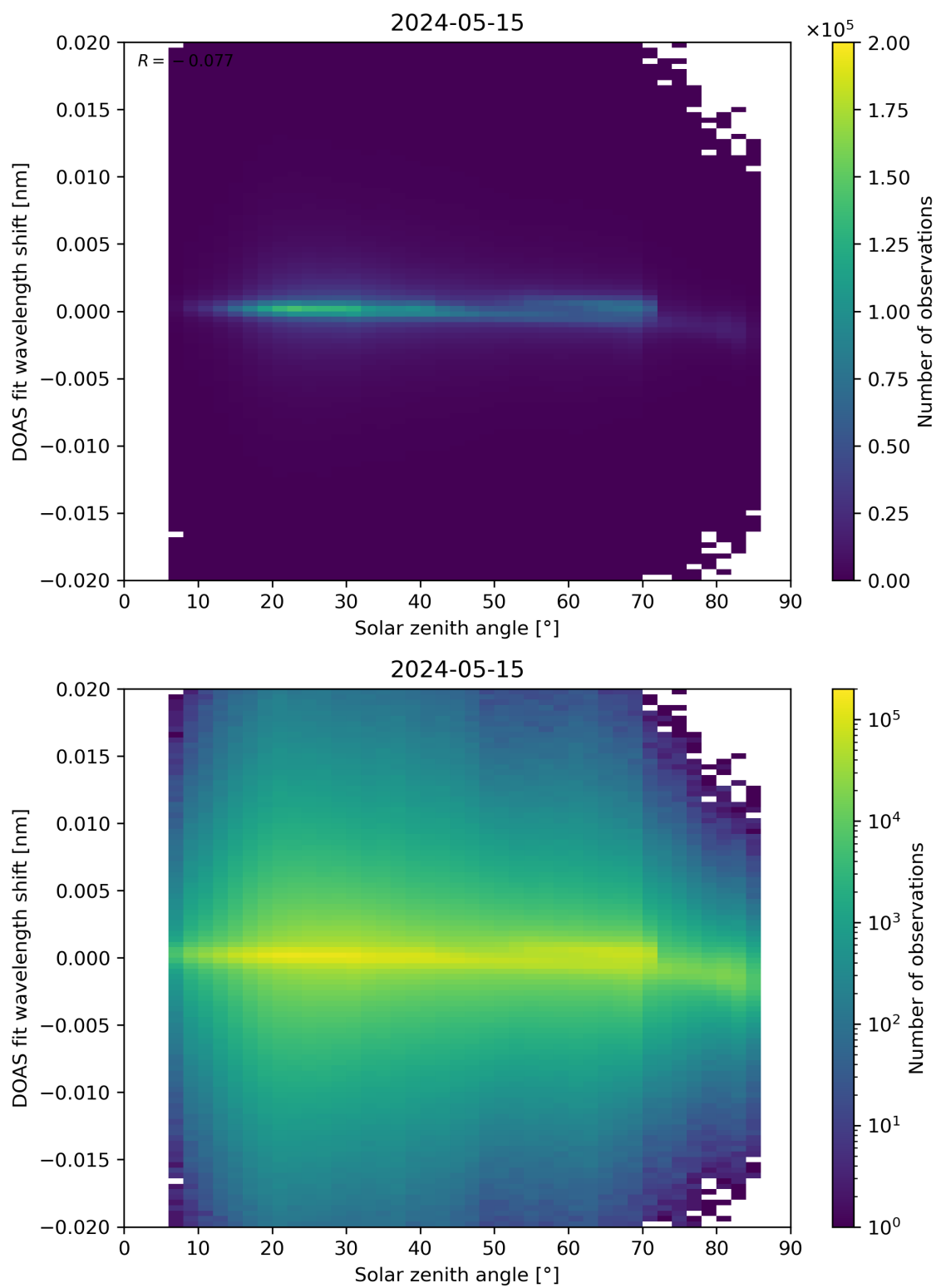
Figure 168: Scatter density plot of “Solar zenith angle” against “DOAS fit wavelength shift” for 2024-05-14 to 2024-05-16.
