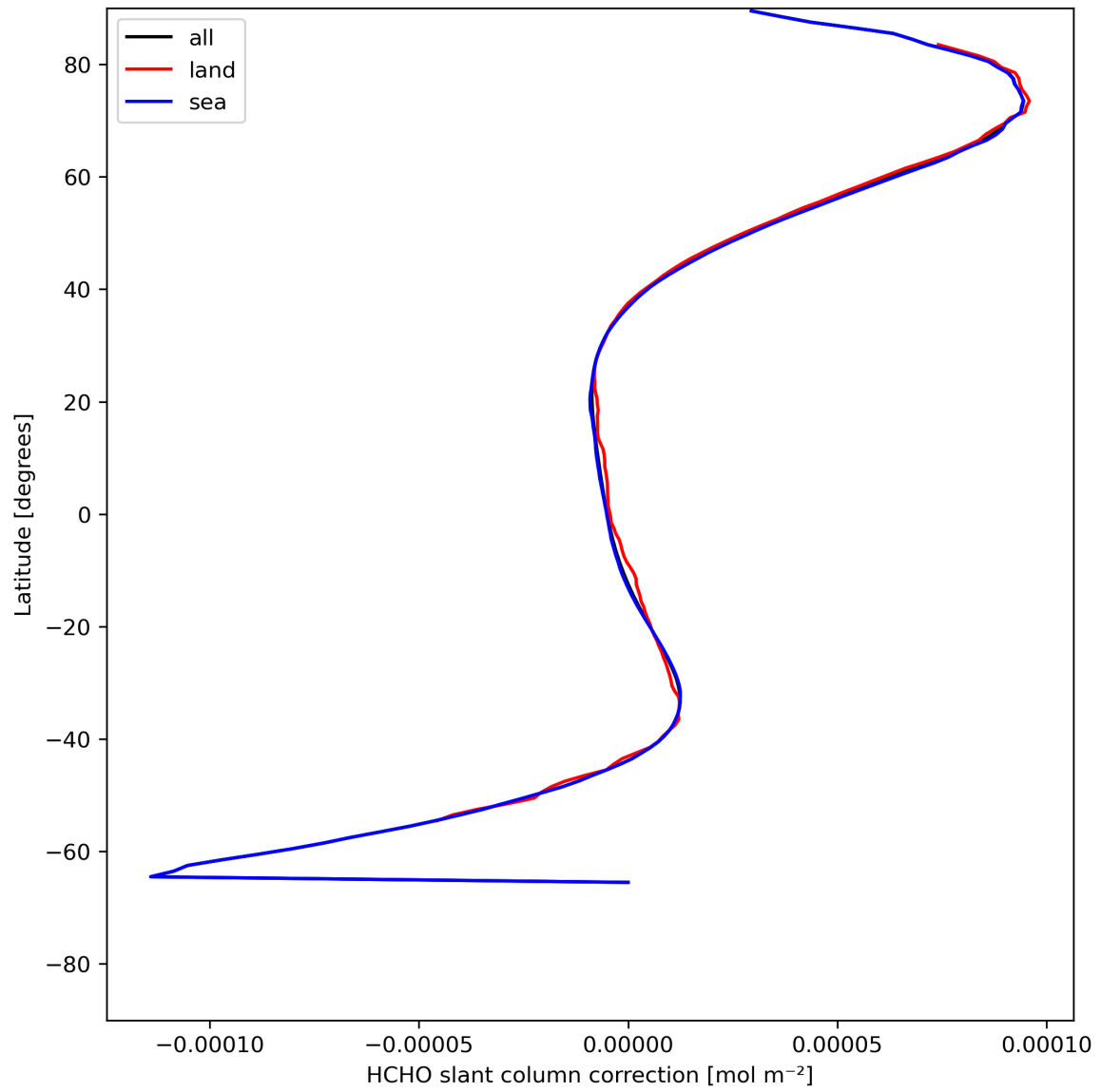
Figure 33: Zonal average of “HCHO slant column correction” for 2024-05-14 to 2024-05-16.
