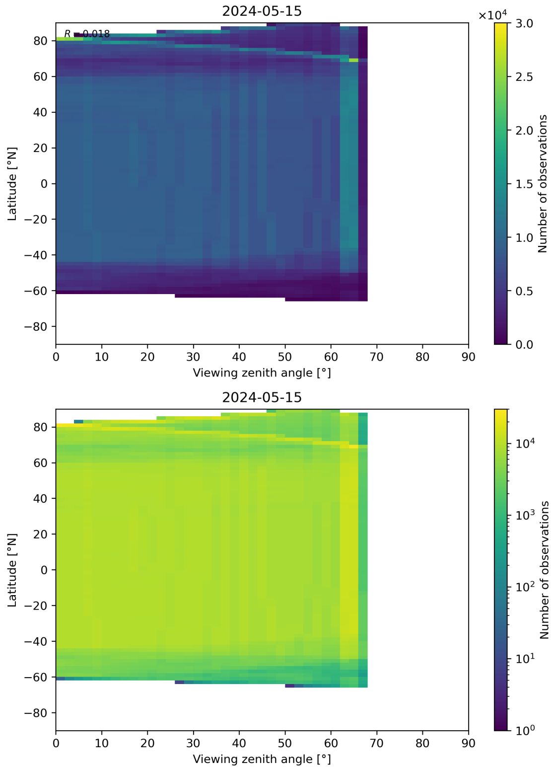
Figure 196: Scatter density plot of “Viewing zenith angle” against “Latitude” for 2024-05-14 to 2024-05-16.
