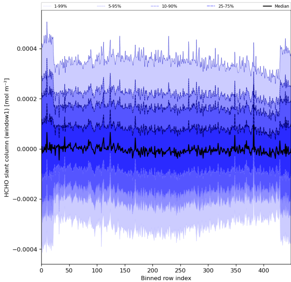
Figure 52: Along track statistics of “HCHO slant column (window1)” for 2024-05-14 to 2024-05-16
