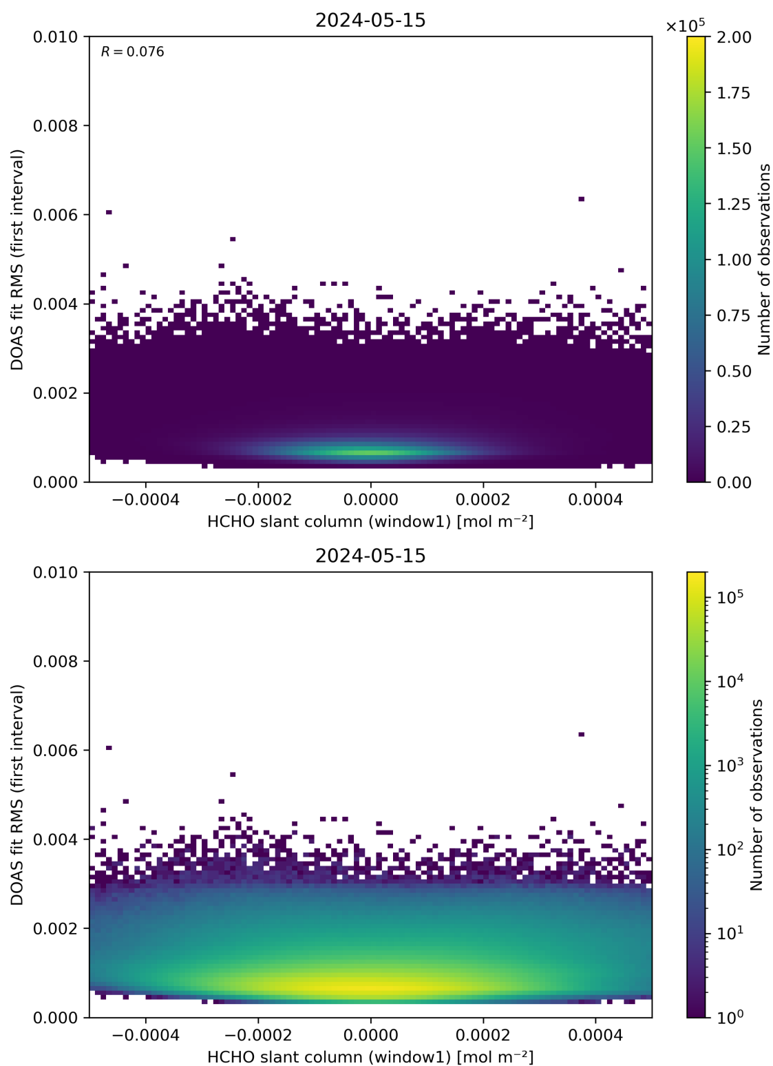
Figure 78: Scatter density plot of “HCHO slant column (window1)” against “DOAS fit RMS (first interval)” for 2024-05-14 to 2024-05-16.
