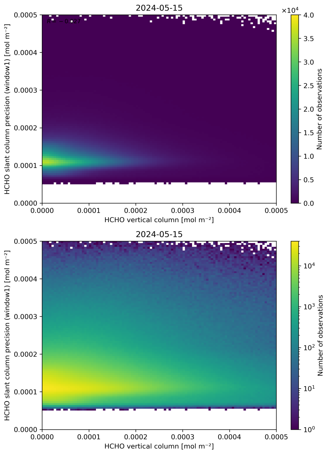
Figure 130: Scatter density plot of “HCHO vertical column” against “HCHO slant column precision (window1)” for 2024-05-14 to 2024-05-16.
