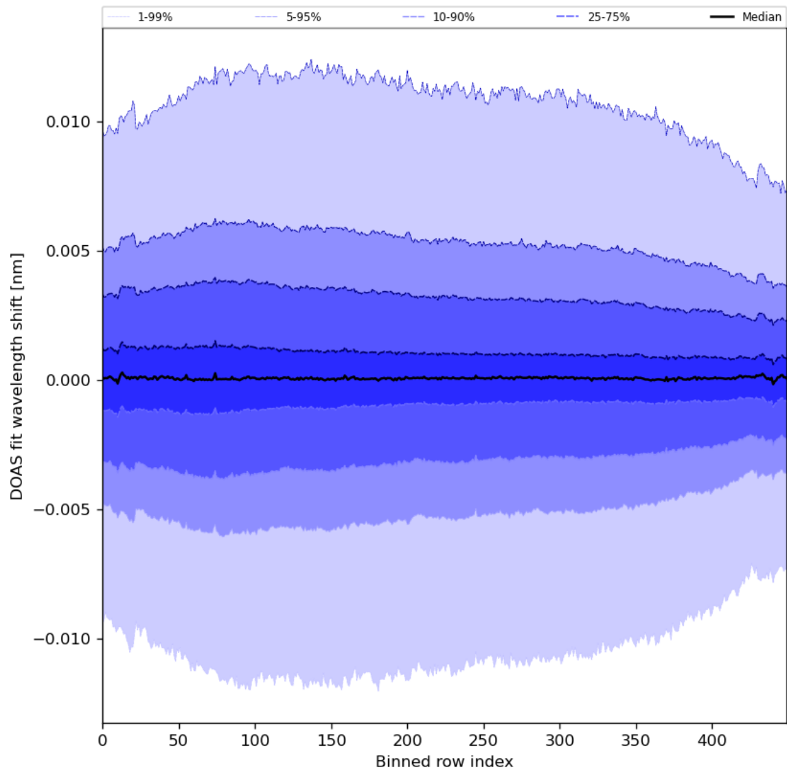
Figure 58: Along track statistics of “DOAS fit wavelength shift” for 2024-05-14 to 2024-05-16
