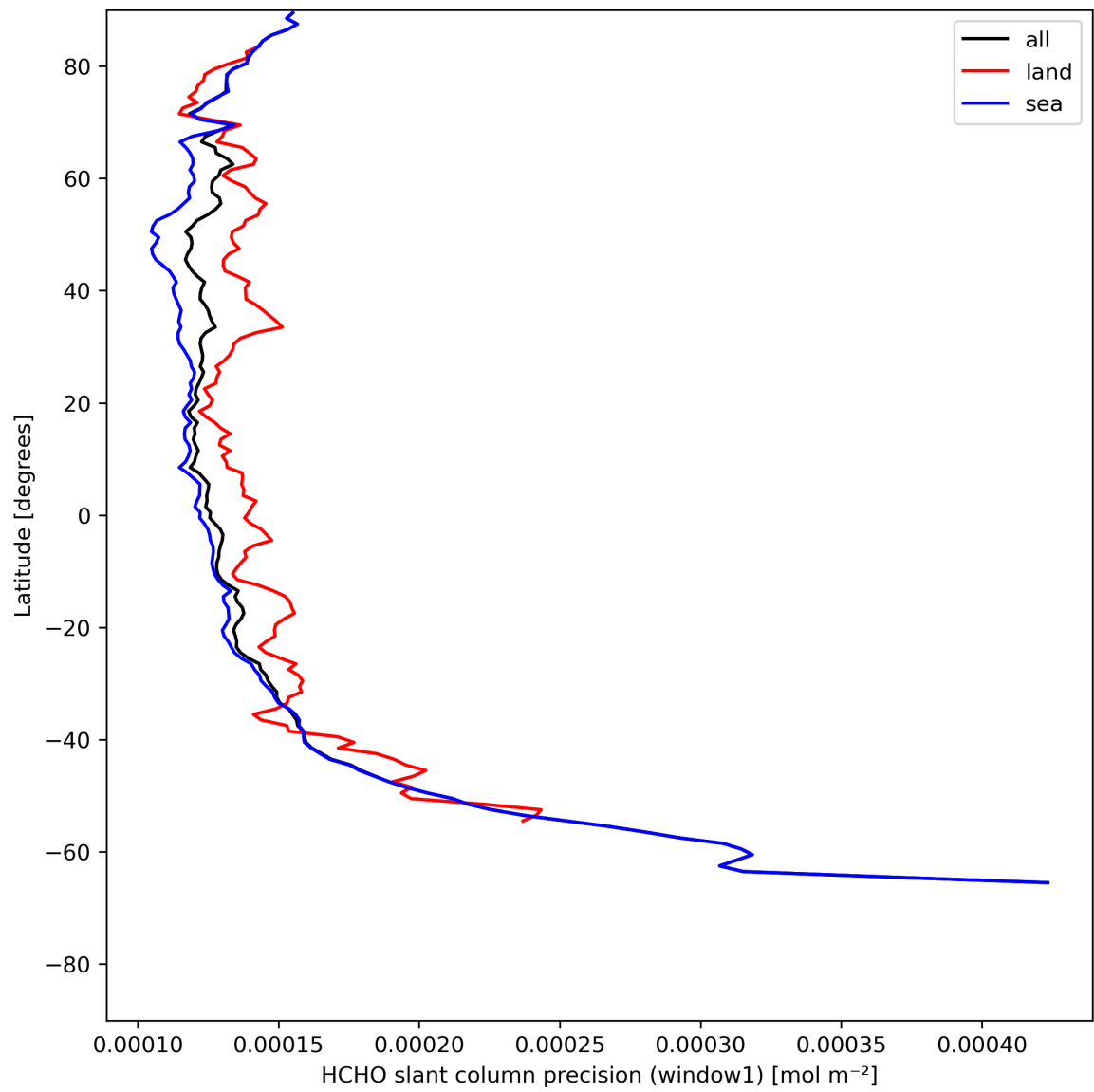
Figure 25: Zonal average of “HCHO slant column precision (window1)” for 2024-05-14 to 2024-05-16.
