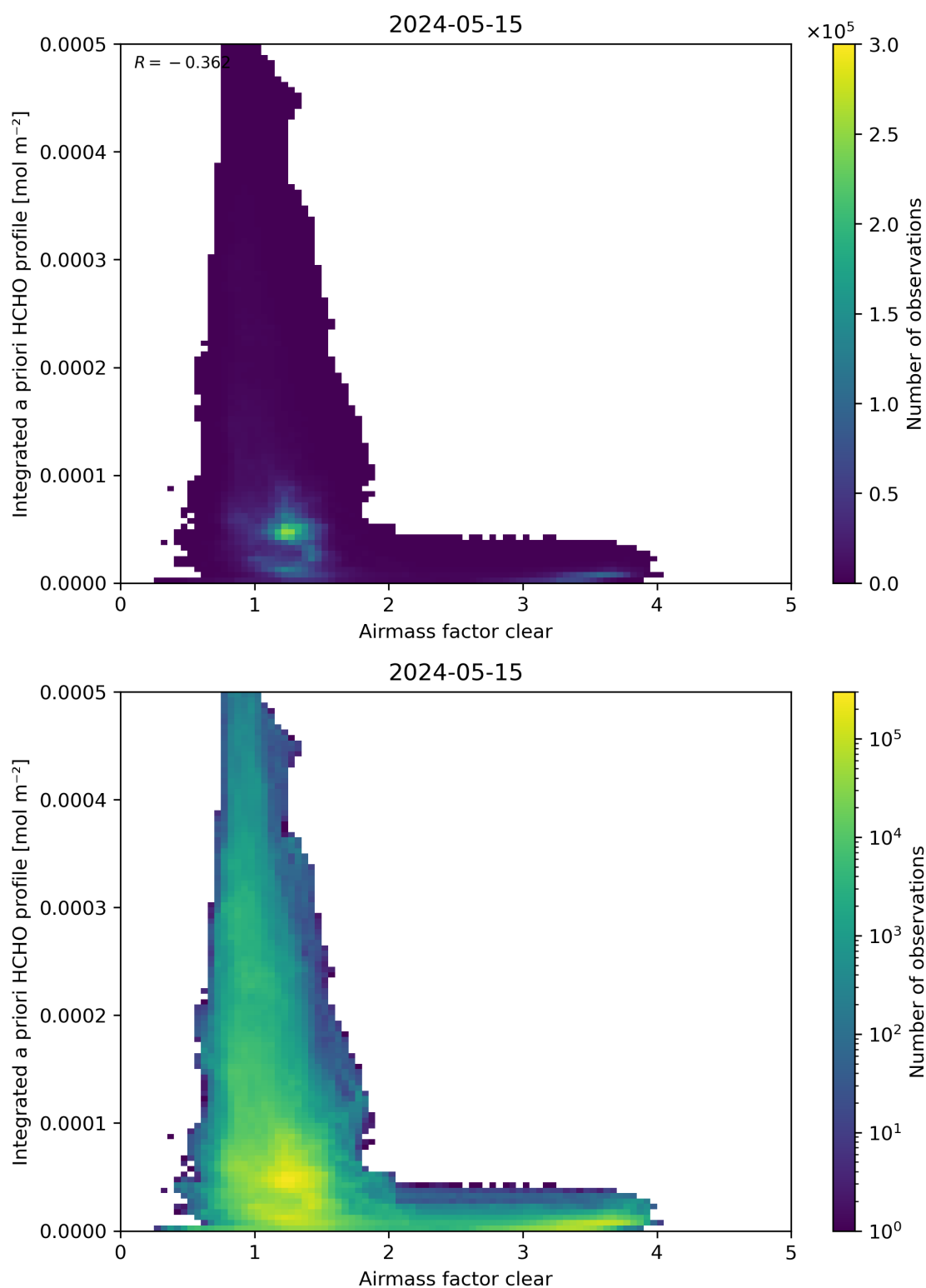
Figure 76: Scatter density plot of “Airmass factor clear” against “Integrated a priori HCHO profile” for 2024-05-14 to 2024-05-16.
