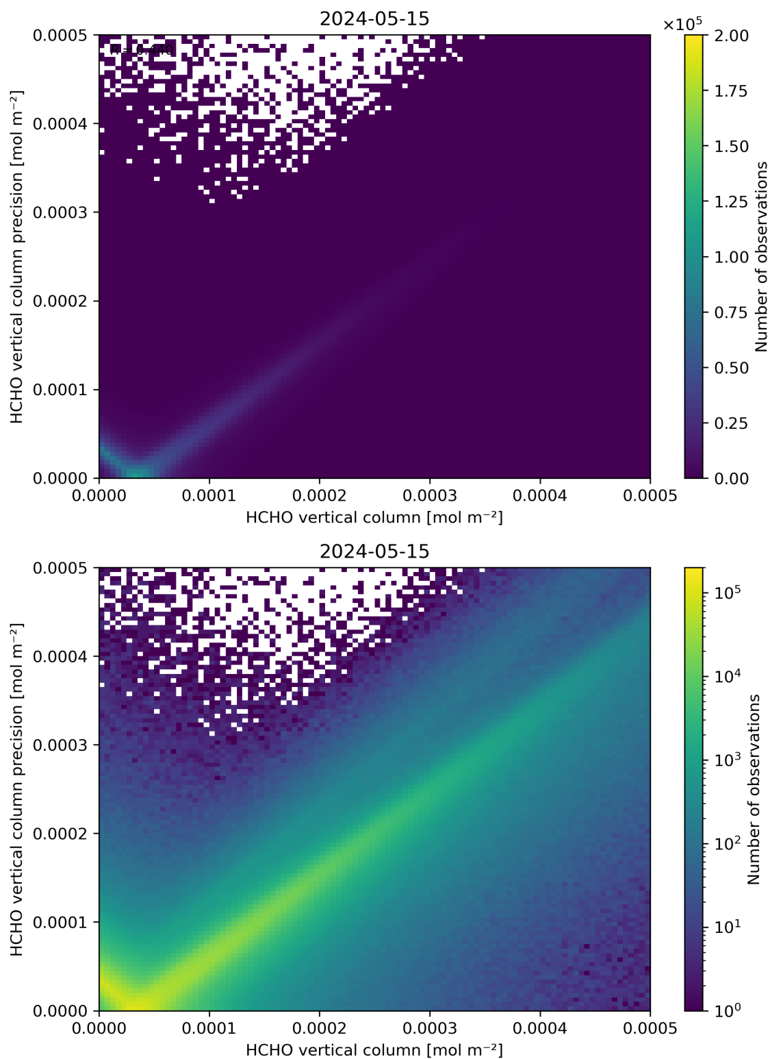
Figure 134: Scatter density plot of “HCHO vertical column” against “HCHO vertical column precision” for 2024-05-14 to 2024-05-16.
