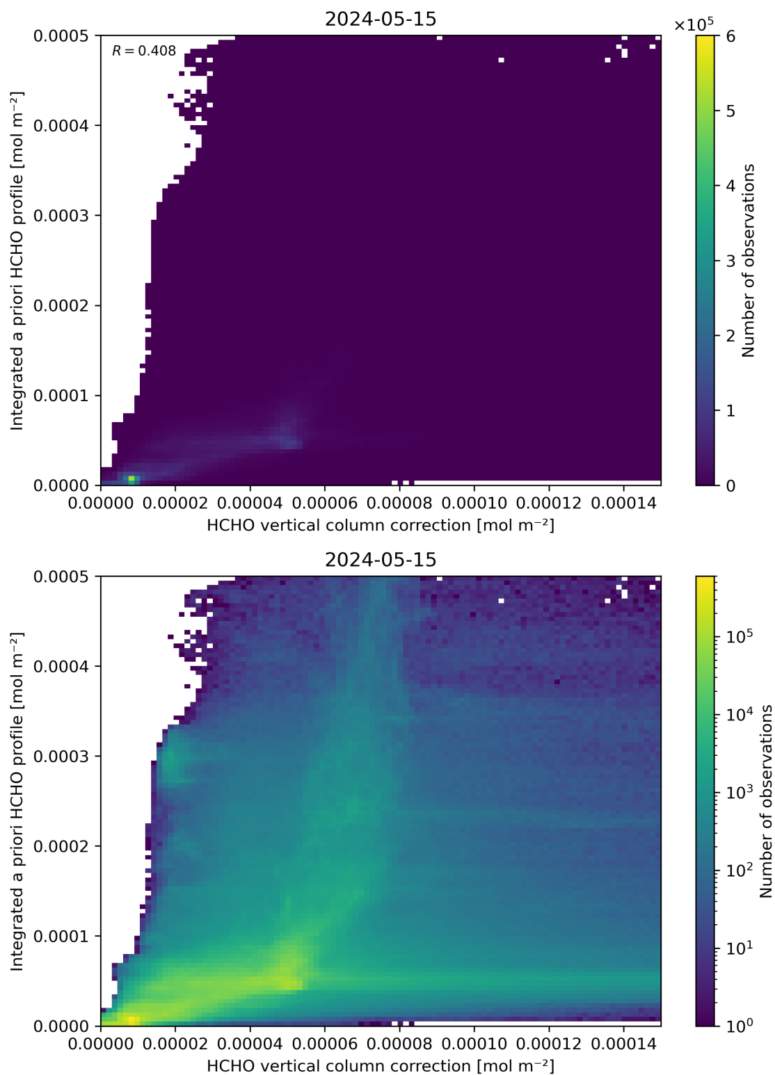
Figure 122: Scatter density plot of “HCHO vertical column correction” against “Integrated a priori HCHO profile” for 2024-05-14 to 2024-05-16.
