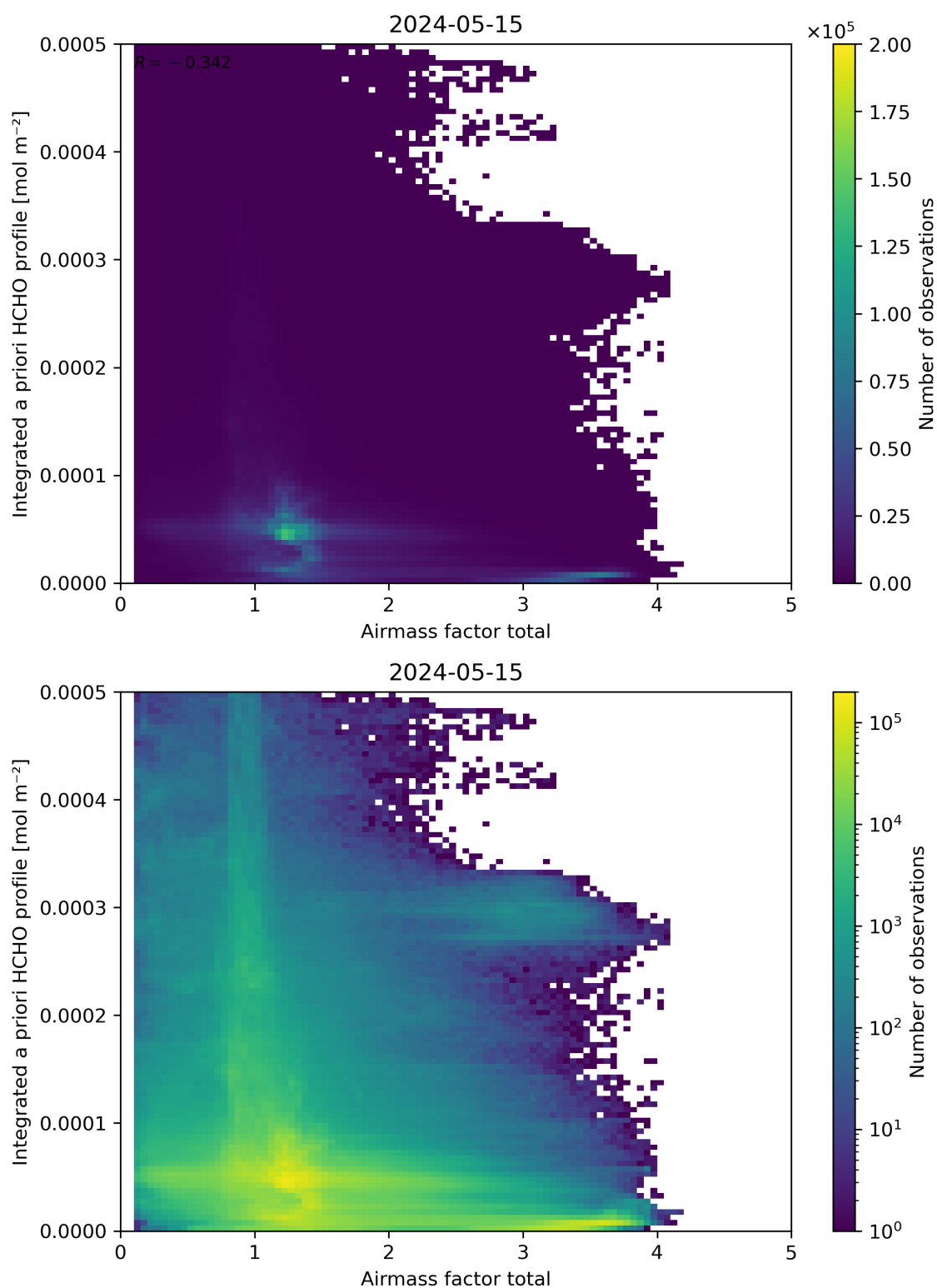
Figure 104: Scatter density plot of “Airmass factor total” against “Integrated a priori HCHO profile” for 2024-05-14 to 2024-05-16.
