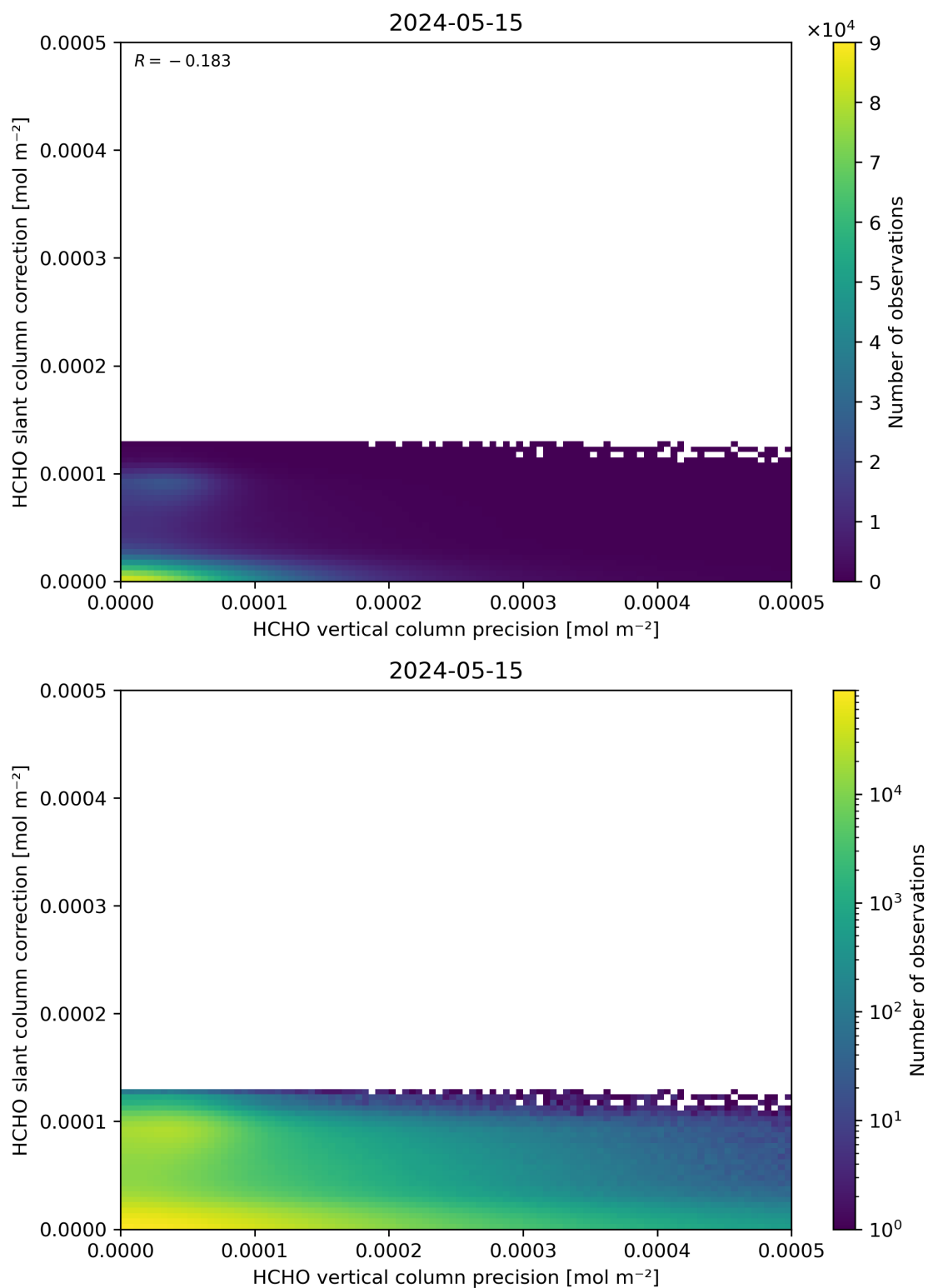
Figure 141: Scatter density plot of “HCHO vertical column precision” against “HCHO slant column correction” for 2024-05-14 to 2024-05-16.
