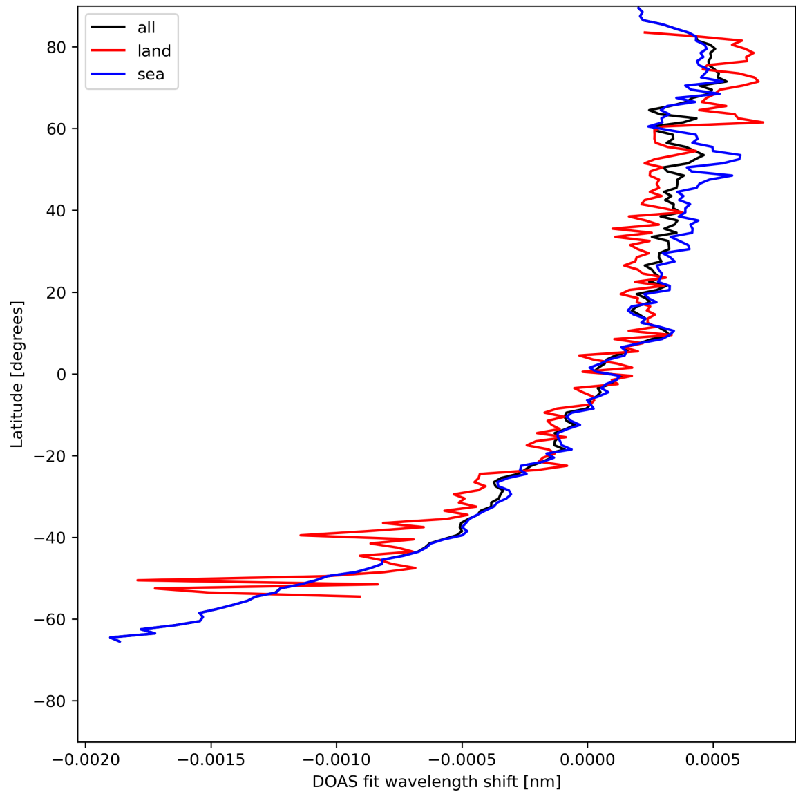
Figure 30: Zonal average of “DOAS fit wavelength shift” for 2024-05-14 to 2024-05-16.
