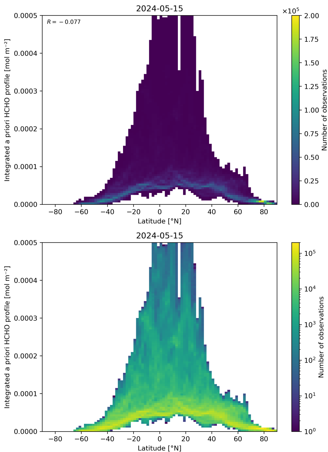
Figure 166: Scatter density plot of “Latitude” against “Integrated a priori HCHO profile” for 2024-05-14 to 2024-05-16.
