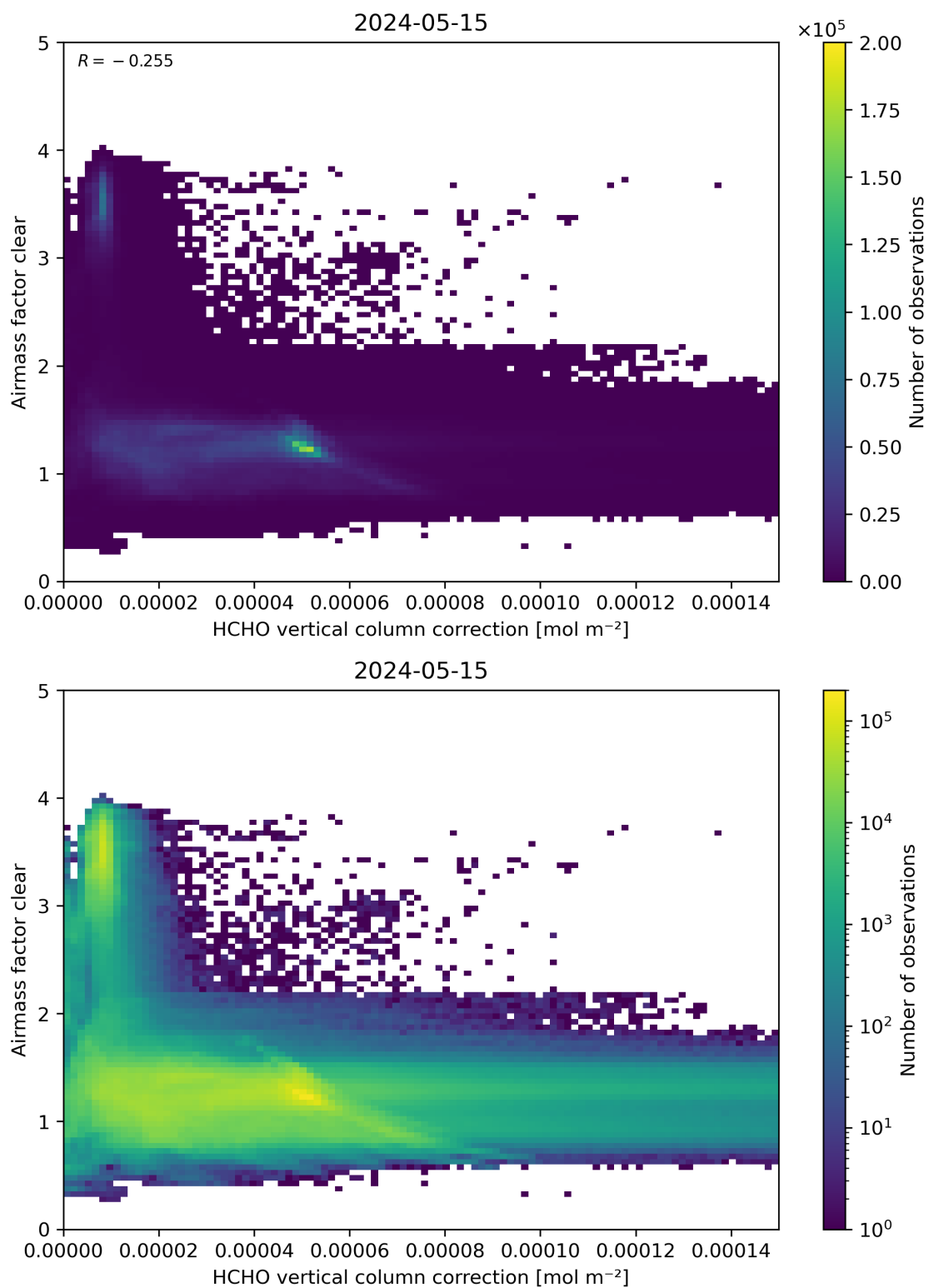
Figure 115: Scatter density plot of “HCHO vertical column correction” against “Airmass factor clear” for 2024-05-14 to 2024-05-16.
