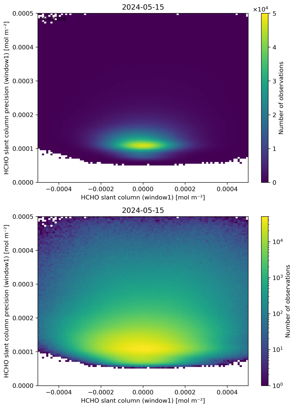
Figure 84: Scatter density plot of “HCHO slant column (window1)” against “HCHO slant column precision (window1)” for 2024-05-14 to 2024-05-16.
