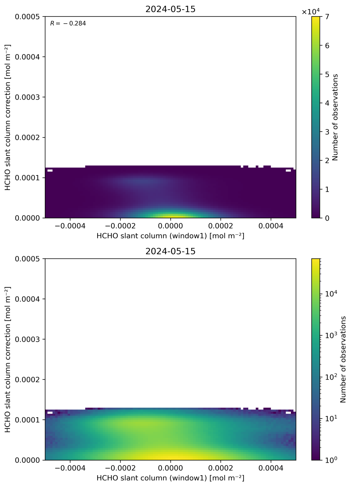
Figure 83: Scatter density plot of “HCHO slant column (window1)” against “HCHO slant column correction” for 2024-05-14 to 2024-05-16.
