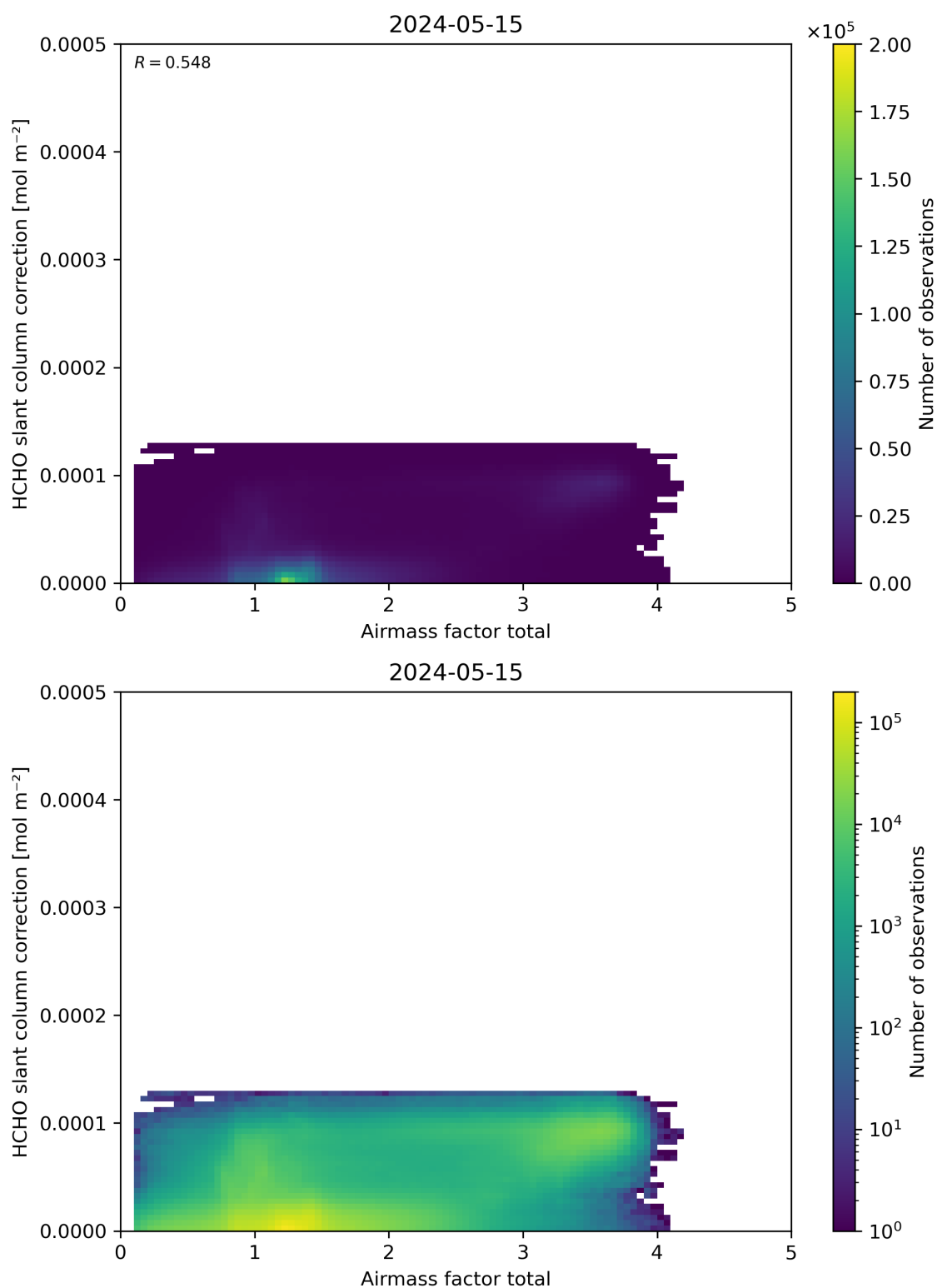
Figure 102: Scatter density plot of “Airmass factor total” against “HCHO slant column correction” for 2024-05-14 to 2024-05-16.
