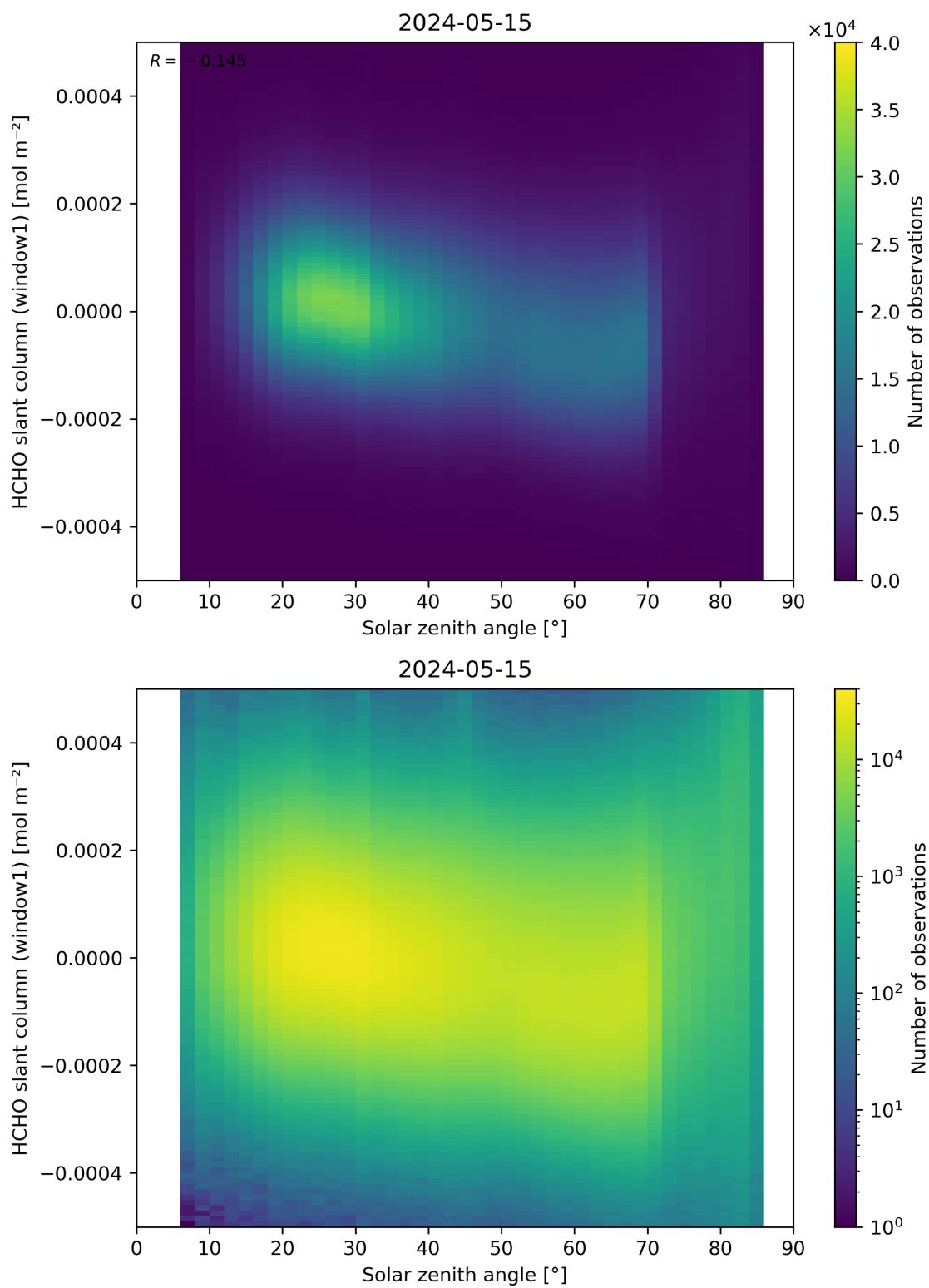
Figure 173: Scatter density plot of “Solar zenith angle” against “HCHO slant column (window1)” for 2024-05-14 to 2024-05-16.
