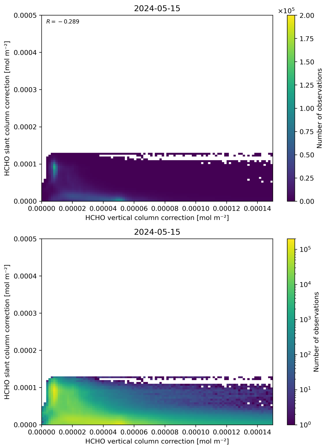
Figure 117: Scatter density plot of “HCHO vertical column correction” against “HCHO slant column correction” for 2024-05-14 to 2024-05-16.
