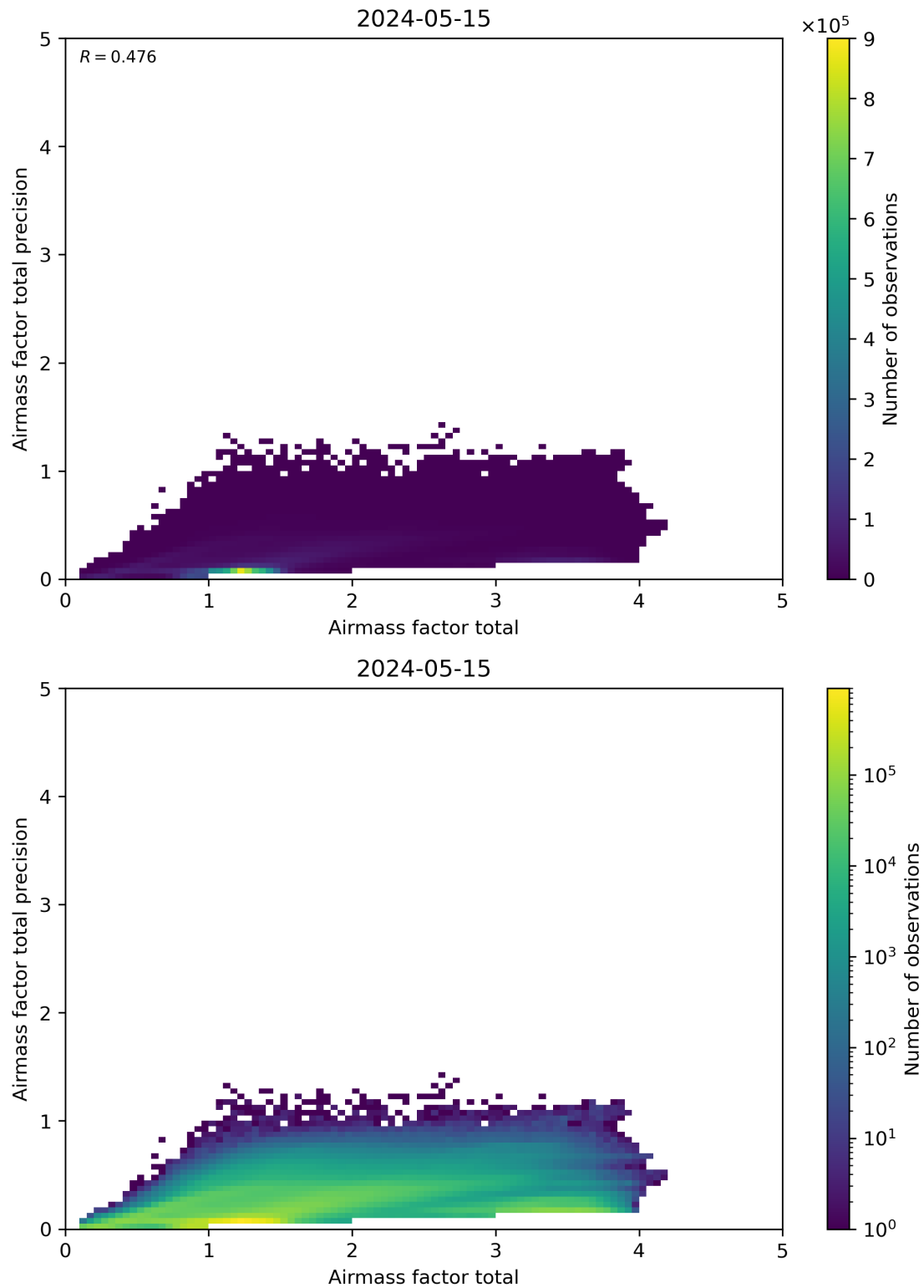
Figure 103: Scatter density plot of “Airmass factor total” against “Airmass factor total precision” for 2024-05-14 to 2024-05-16.
