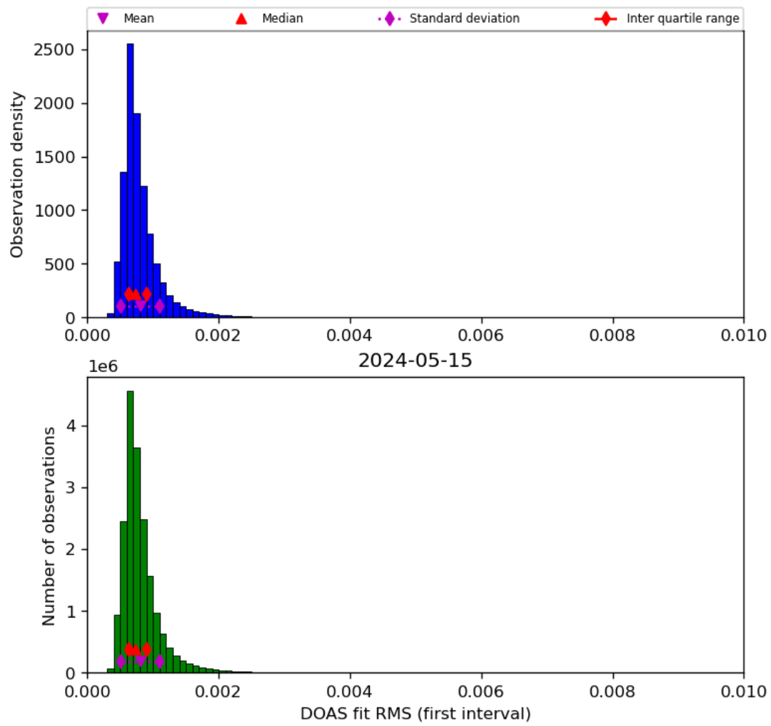
Figure 46: Histogram of “DOAS fit RMS (first interval)” for 2024-05-14 to 2024-05-16
