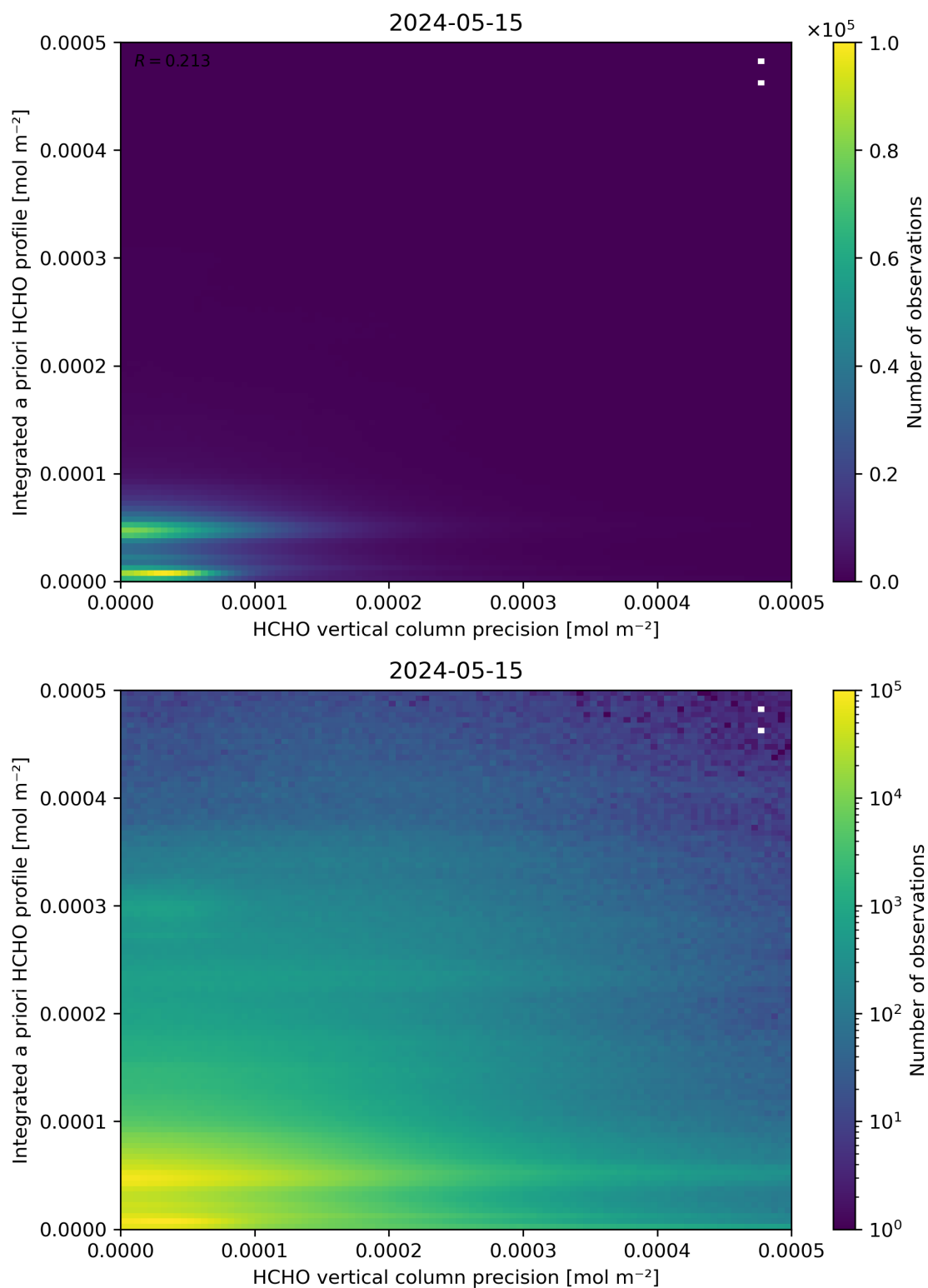
Figure 147: Scatter density plot of “HCHO vertical column precision” against “Integrated a priori HCHO profile” for 2024-05-14 to 2024-05-16.
