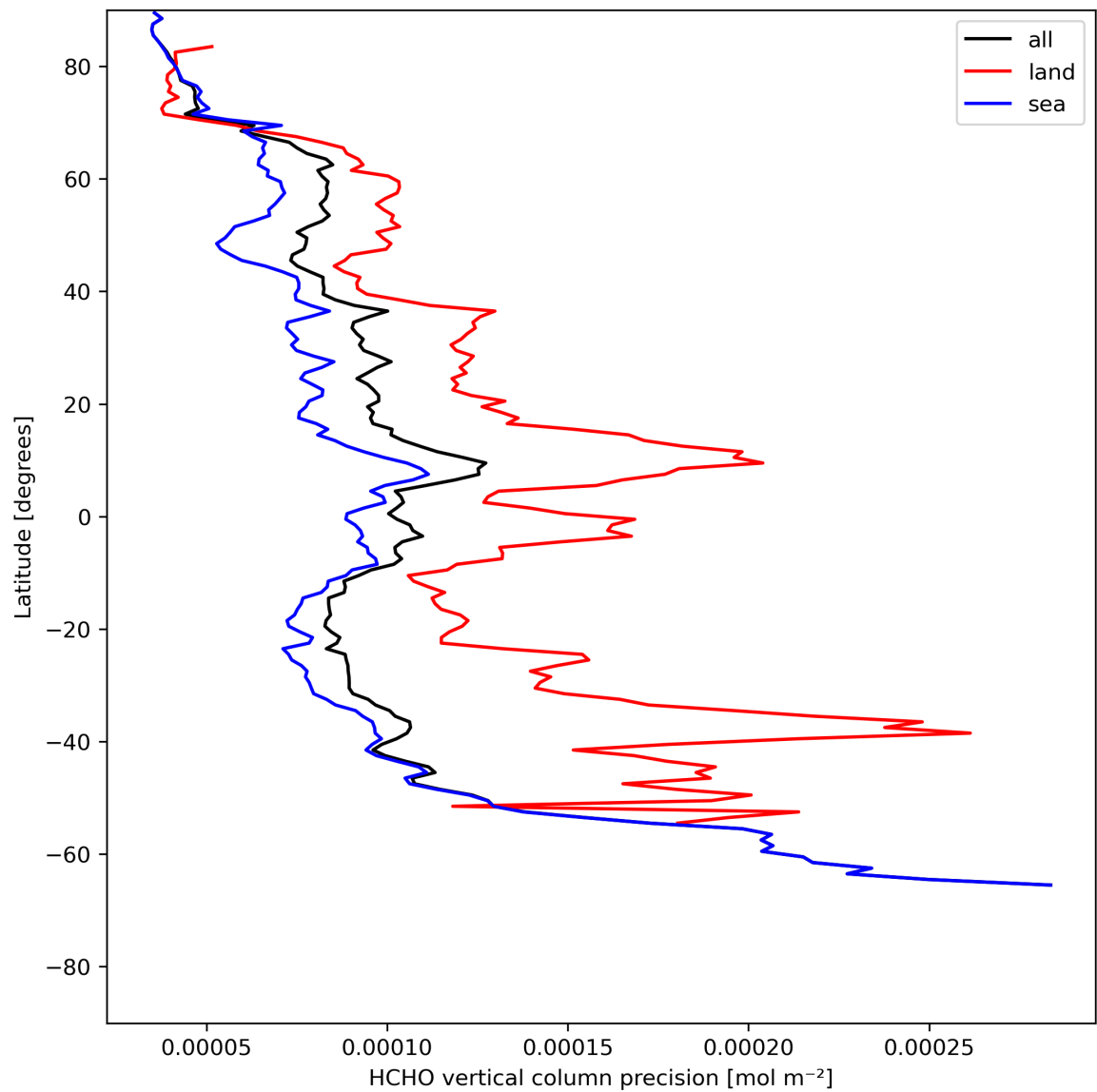
Figure 22: Zonal average of “HCHO vertical column precision” for 2024-05-14 to 2024-05-16.
