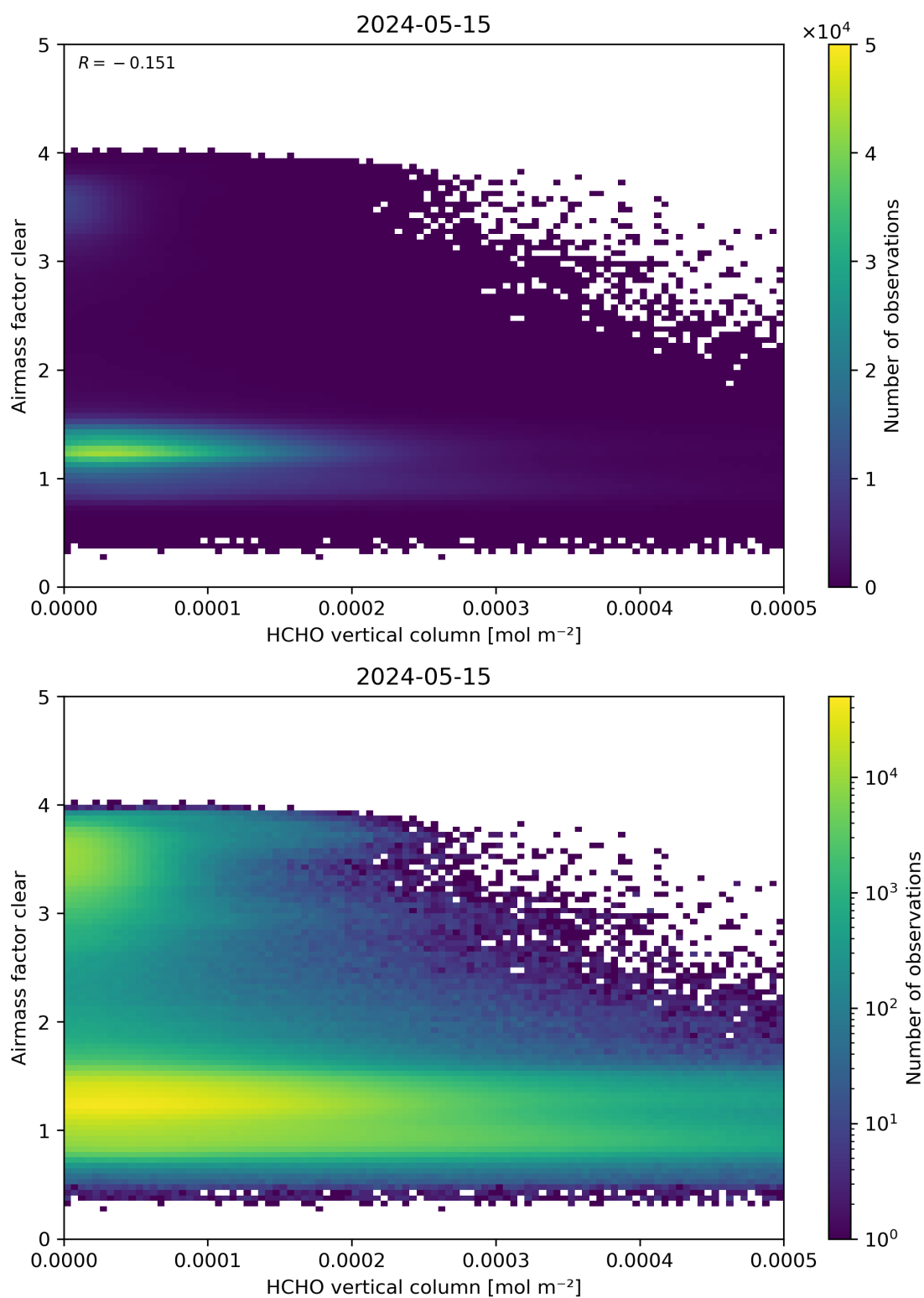
Figure 126: Scatter density plot of “HCHO vertical column” against “Airmass factor clear” for 2024-05-14 to 2024-05-16.
