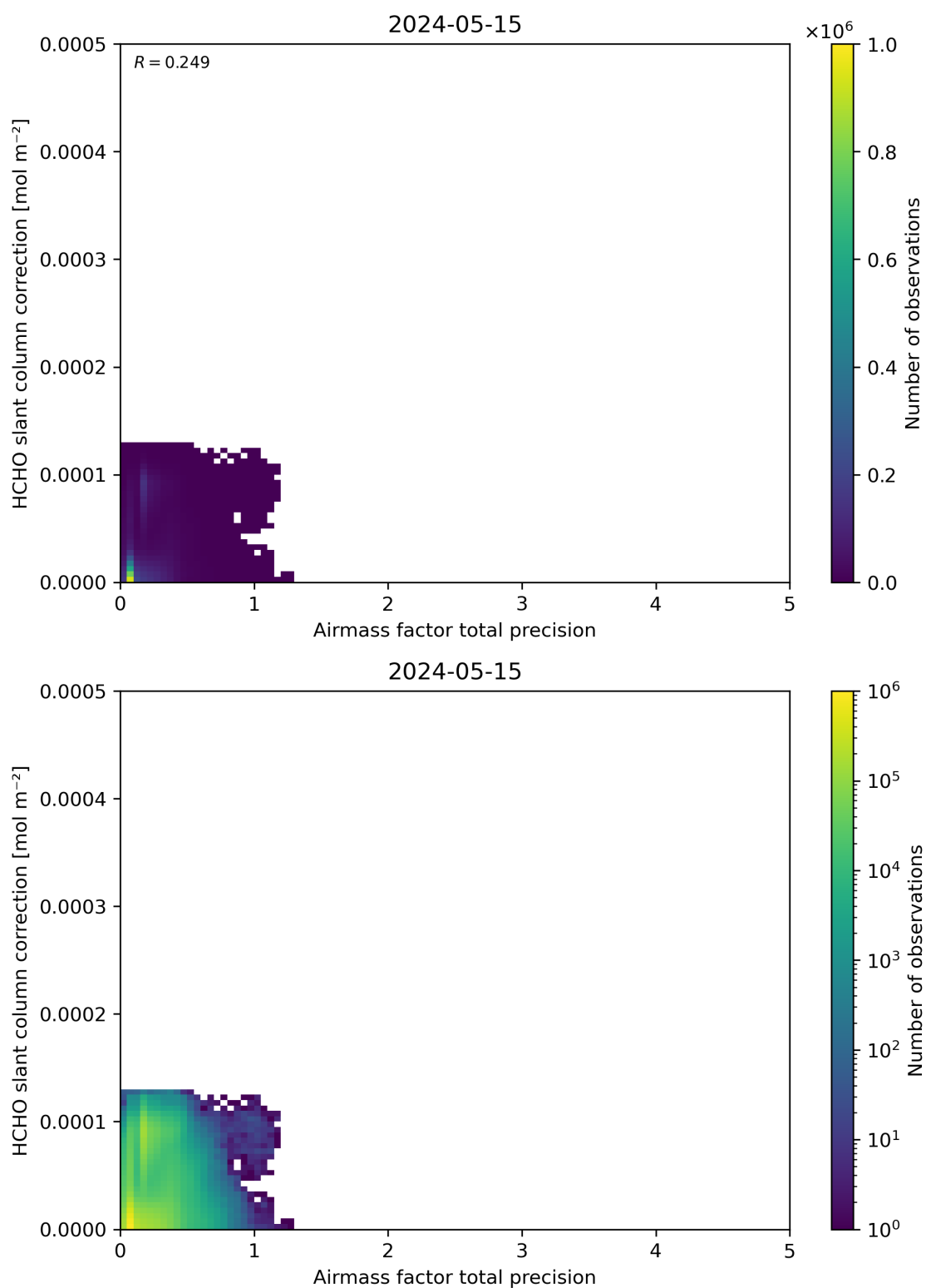
Figure 110: Scatter density plot of “Airmass factor total precision” against “HCHO slant column correction” for 2024-05-14 to 2024-05-16.
