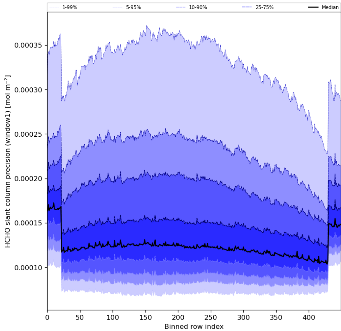
Figure 53: Along track statistics of “HCHO slant column precision (window1)” for 2024-05-14 to 2024-05-16
