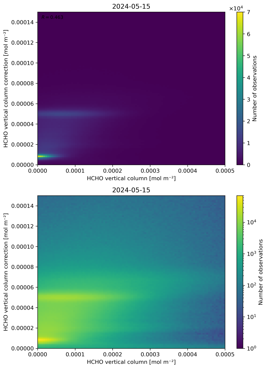
Figure 133: Scatter density plot of “HCHO vertical column” against “HCHO vertical column correction” for 2024-05-14 to 2024-05-16.
