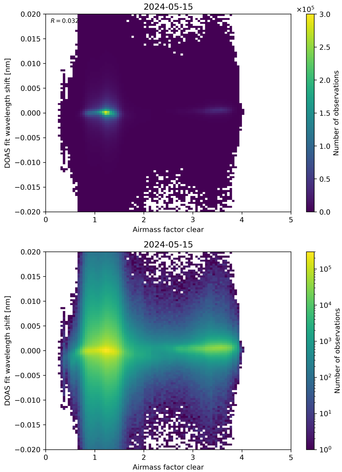
Figure 72: Scatter density plot of “Airmass factor clear” against “DOAS fit wavelength shift” for 2024-05-14 to 2024-05-16.
