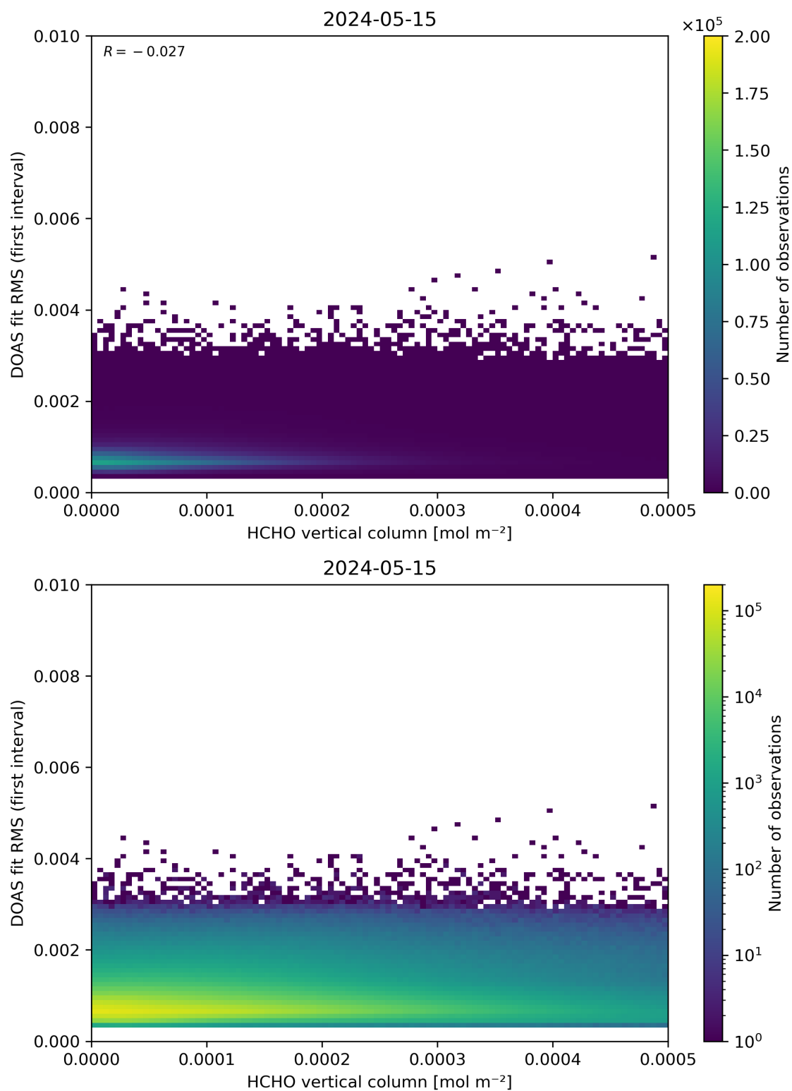
Figure 123: Scatter density plot of “HCHO vertical column” against “DOAS fit RMS (first interval)” for 2024-05-14 to 2024-05-16.
