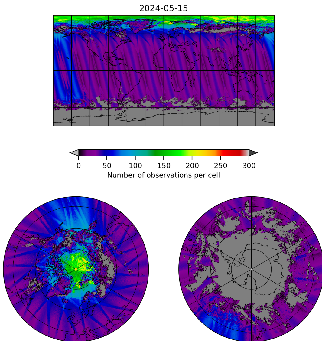
Figure 19: Map of the number of observations for 2024-05-14 to 2024-05-16
