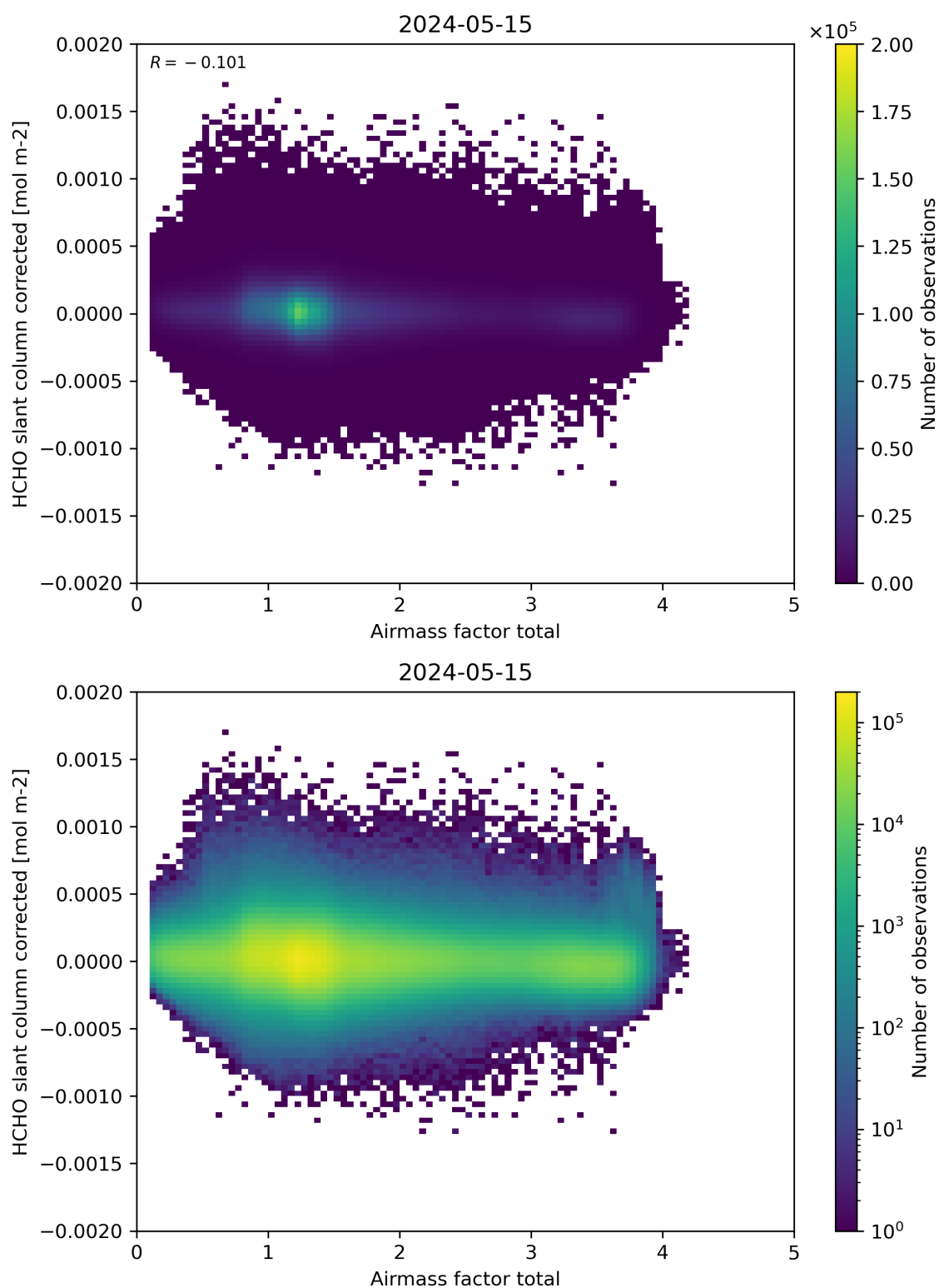
Figure 101: Scatter density plot of “Airmass factor total” against “HCHO slant column corrected” for 2024-05-14 to 2024-05-16.
