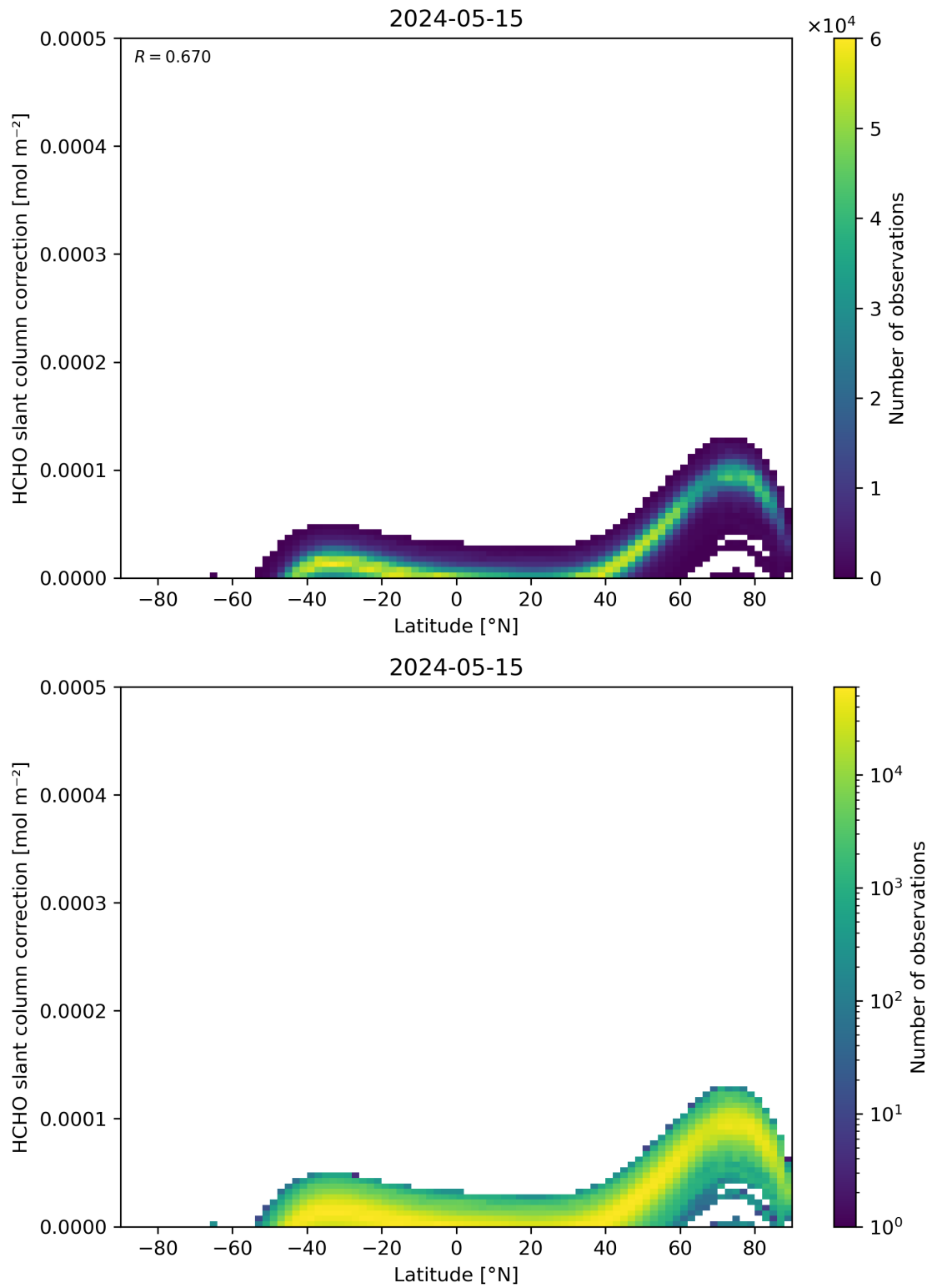
Figure 158: Scatter density plot of “Latitude” against “HCHO slant column correction” for 2024-05-14 to 2024-05-16.
