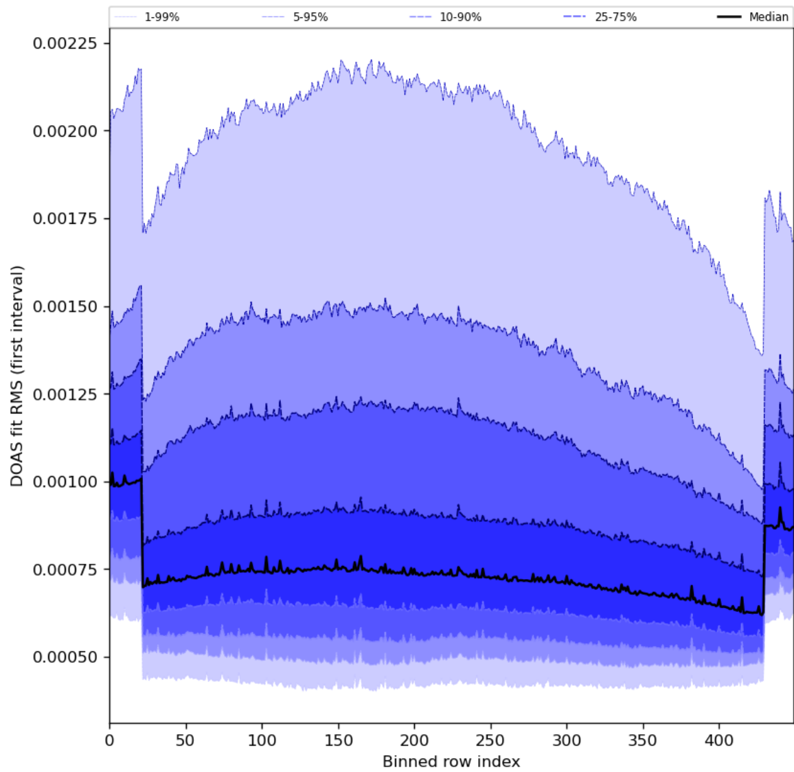
Figure 60: Along track statistics of “DOAS fit RMS (first interval)” for 2024-05-14 to 2024-05-16
