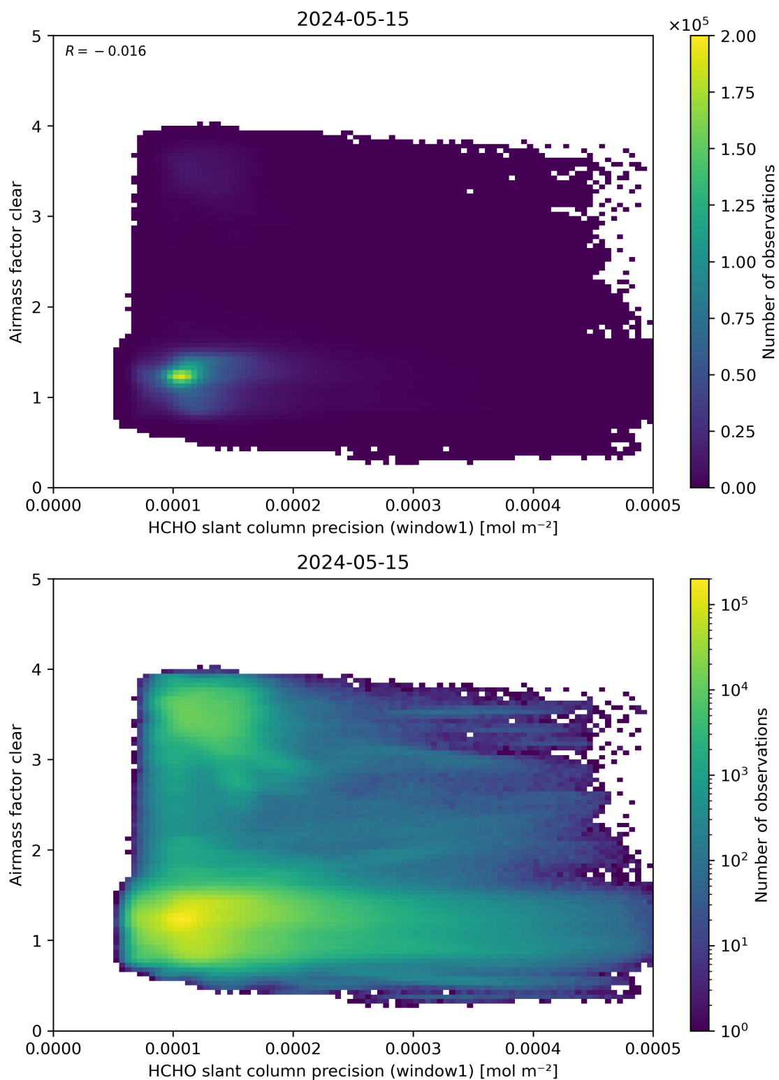
Figure 91: Scatter density plot of “HCHO slant column precision (window1)” against “Airmass factor clear” for 2024-05-14 to 2024-05-16.
