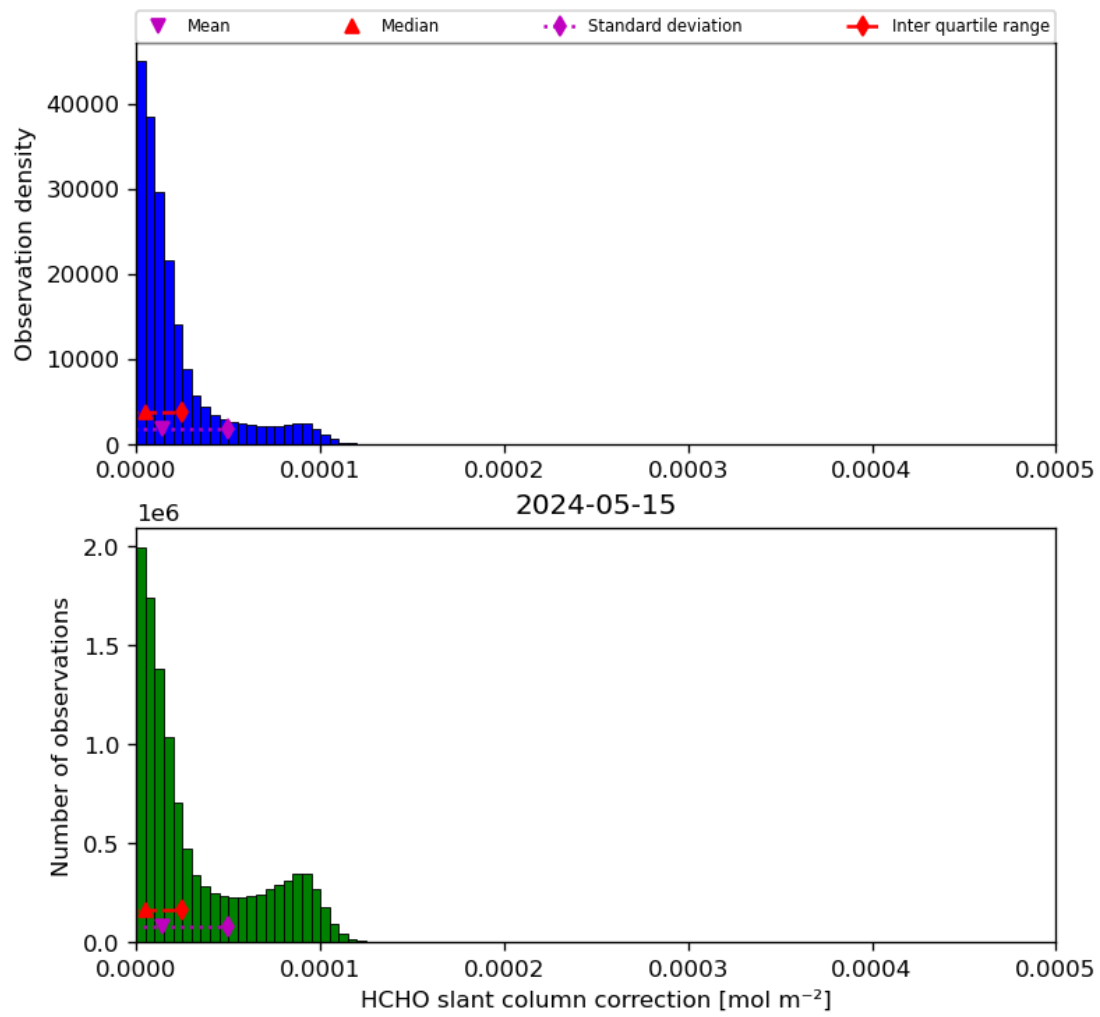
Figure 47: Histogram of “HCHO slant column correction” for 2024-05-14 to 2024-05-16
