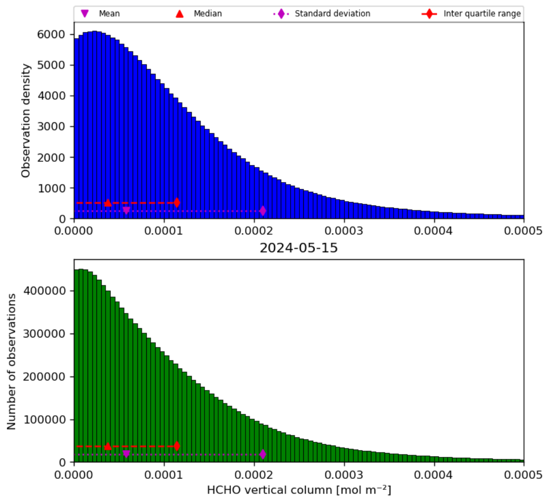
Figure 35: Histogram of “HCHO vertical column” for 2024-05-14 to 2024-05-16
