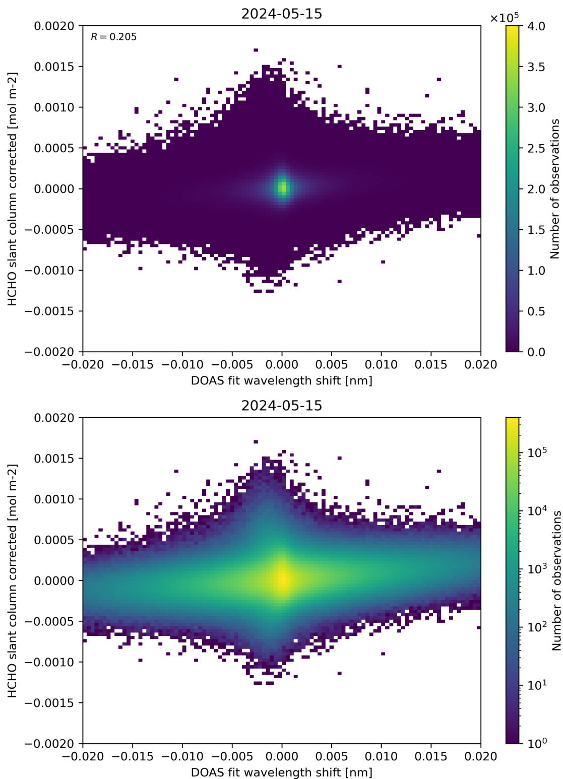
Figure 66: Scatter density plot of “DOAS fit wavelength shift” against “HCHO slant column corrected” for 2024-05-14 to 2024-05-16.
