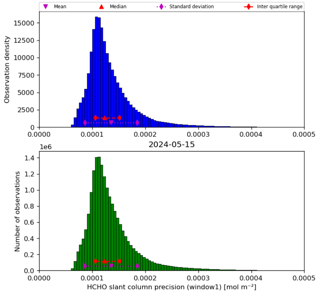
Figure 39: Histogram of “HCHO slant column precision (window1)” for 2024-05-14 to 2024-05-16
