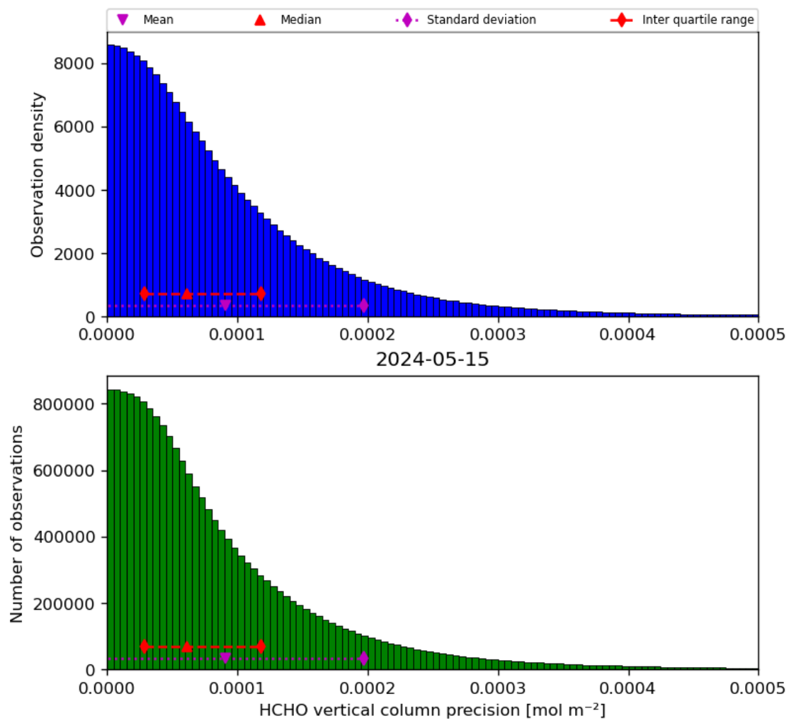
Figure 36: Histogram of “HCHO vertical column precision” for 2024-05-14 to 2024-05-16
