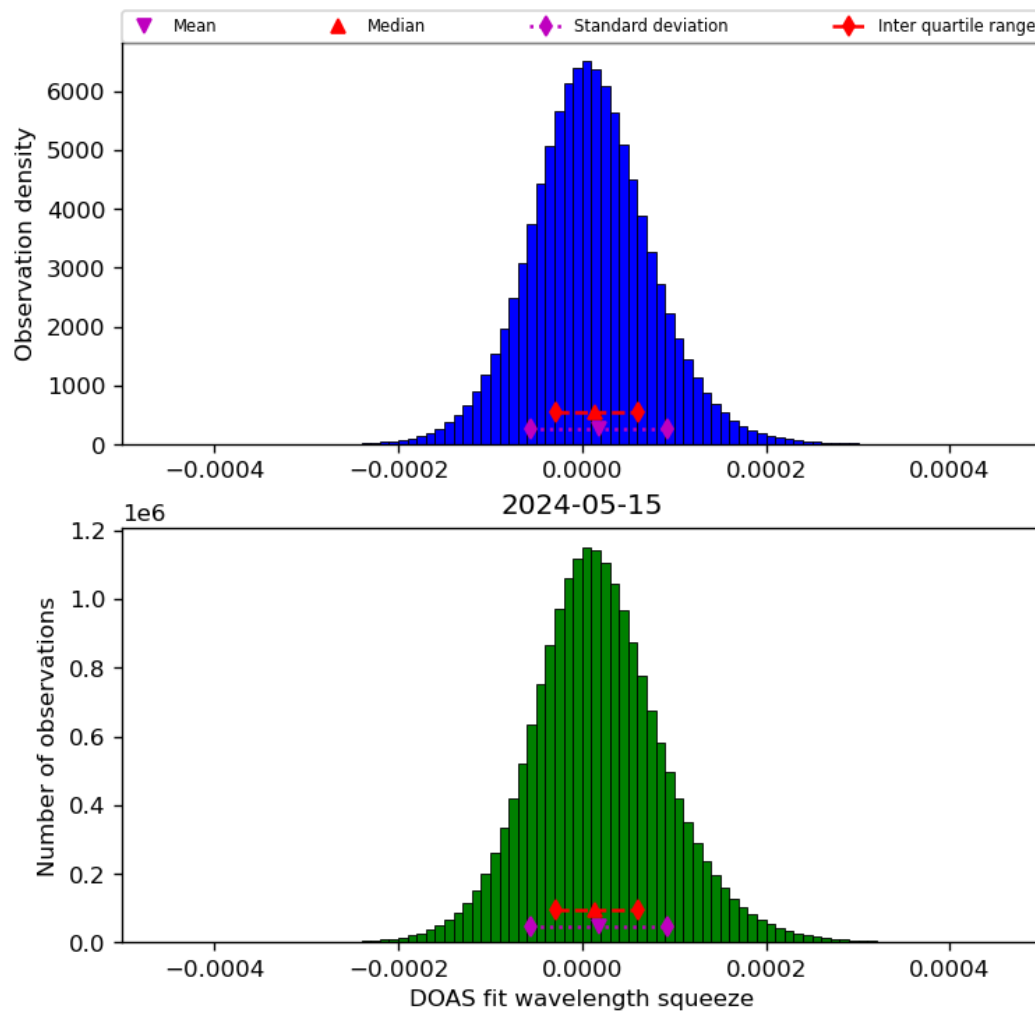
Figure 45: Histogram of “DOAS fit wavelength squeeze” for 2024-05-14 to 2024-05-16
