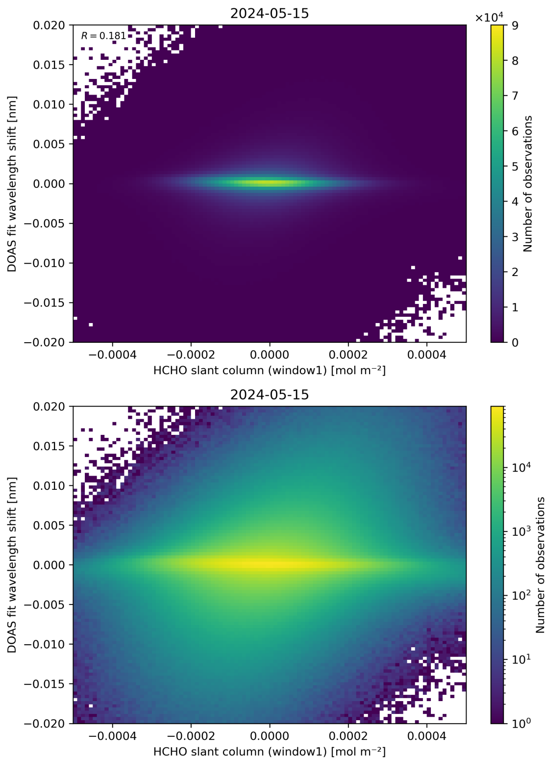
Figure 79: Scatter density plot of “HCHO slant column (window1)” against “DOAS fit wavelength shift” for 2024-05-14 to 2024-05-16.
