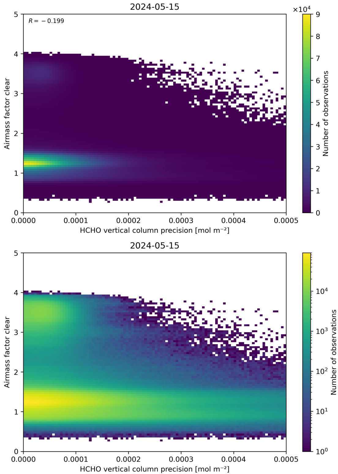
Figure 139: Scatter density plot of “HCHO vertical column precision” against “Airmass factor clear” for 2024-05-14 to 2024-05-16.
