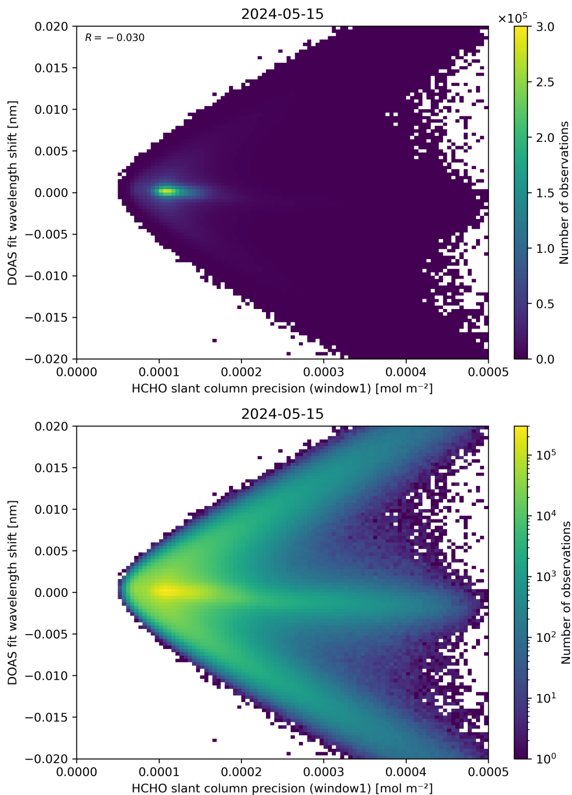
Figure 89: Scatter density plot of “HCHO slant column precision (window1)” against “DOAS fit wavelength shift” for 2024-05-14 to 2024-05-16.
