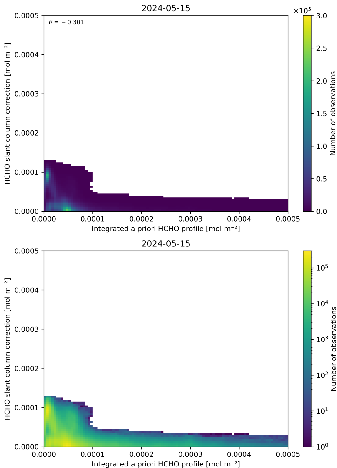
Figure 152: Scatter density plot of “Integrated a priori HCHO profile” against “HCHO slant column correction” for 2024-05-14 to 2024-05-16.
