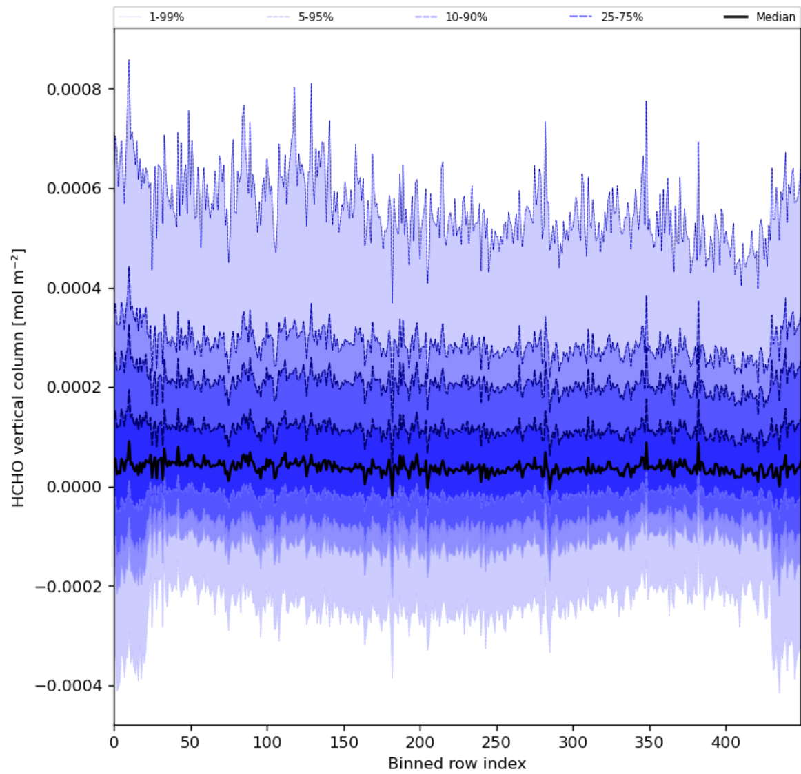
Figure 49: Along track statistics of “HCHO vertical column” for 2024-05-14 to 2024-05-16
