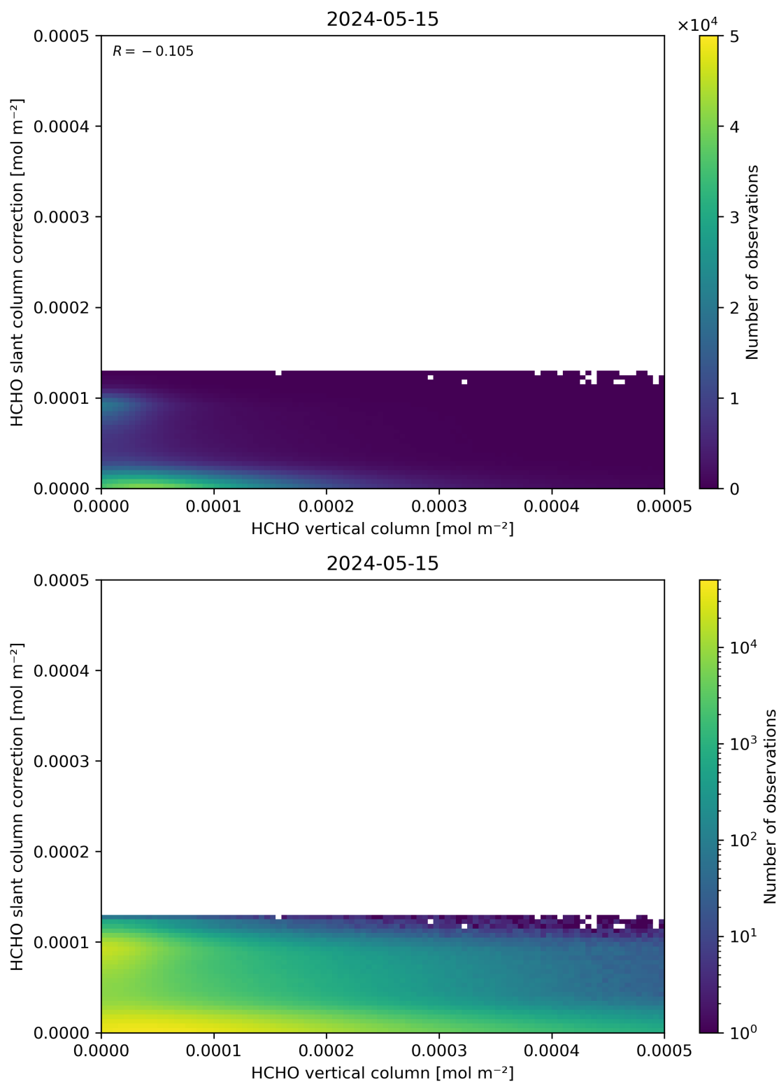
Figure 128: Scatter density plot of “HCHO vertical column” against “HCHO slant column correction” for 2024-05-14 to 2024-05-16.
