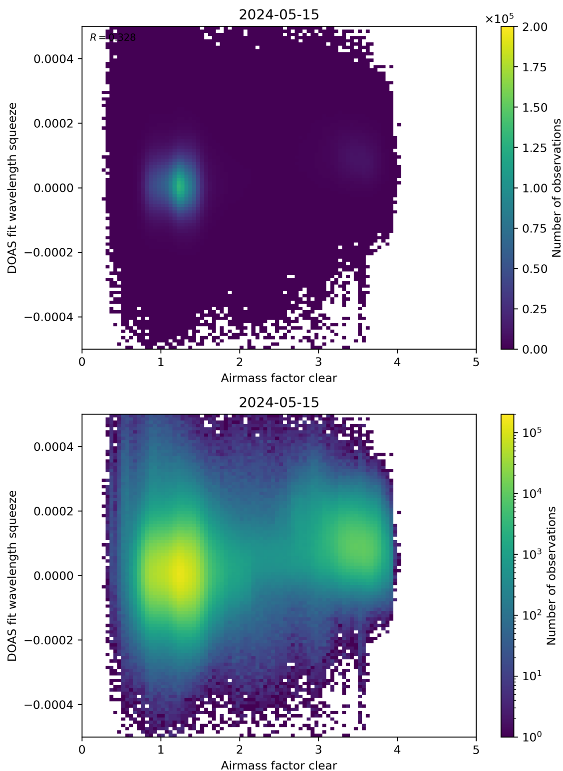
Figure 73: Scatter density plot of “Airmass factor clear” against “DOAS fit wavelength squeeze” for 2024-05-14 to 2024-05-16.
