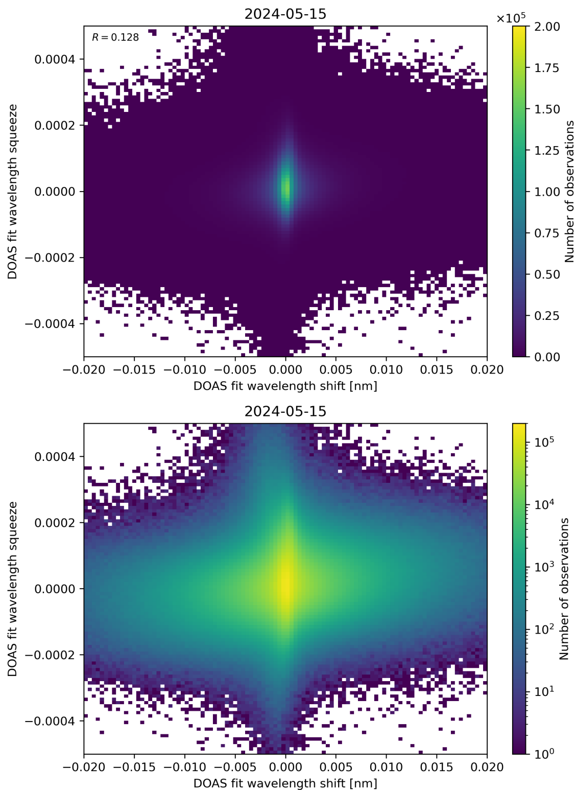
Figure 65: Scatter density plot of “DOAS fit wavelength shift” against “DOAS fit wavelength squeeze” for 2024-05-14 to 2024-05-16.
