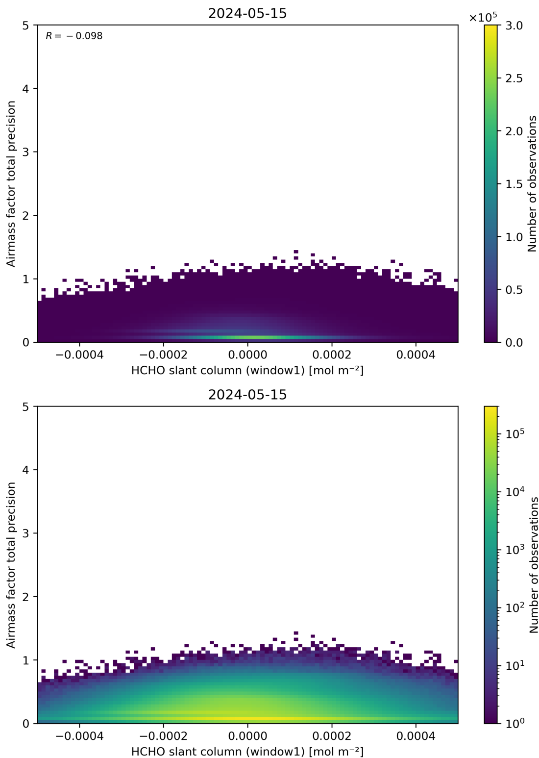
Figure 86: Scatter density plot of “HCHO slant column (window1)” against “Airmass factor total precision” for 2024-05-14 to 2024-05-16.
