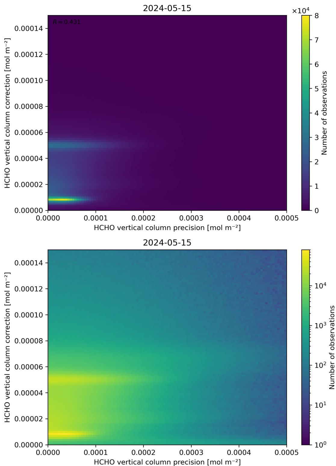
Figure 146: Scatter density plot of “HCHO vertical column precision” against “HCHO vertical column correction” for 2024-05-14 to 2024-05-16.
