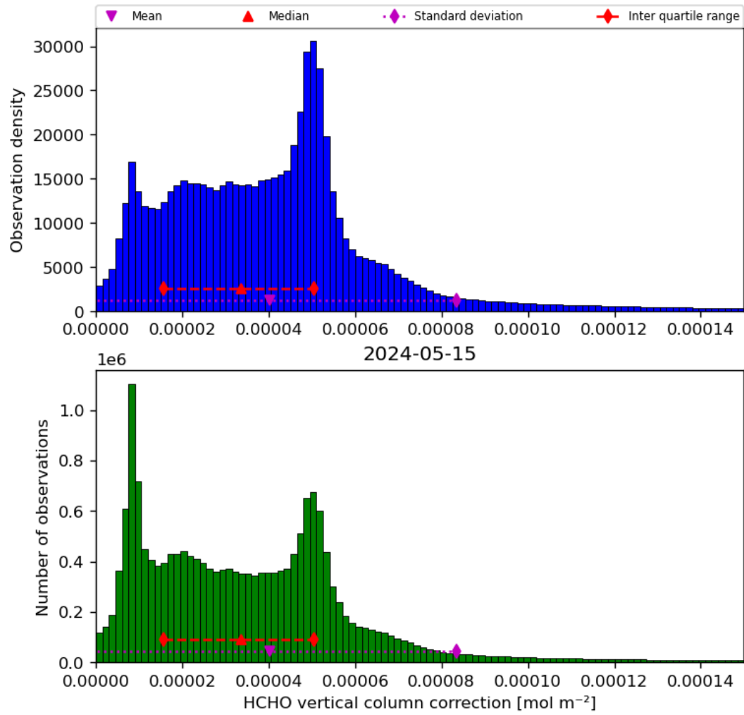
Figure 37: Histogram of “HCHO vertical column correction” for 2024-05-14 to 2024-05-16
