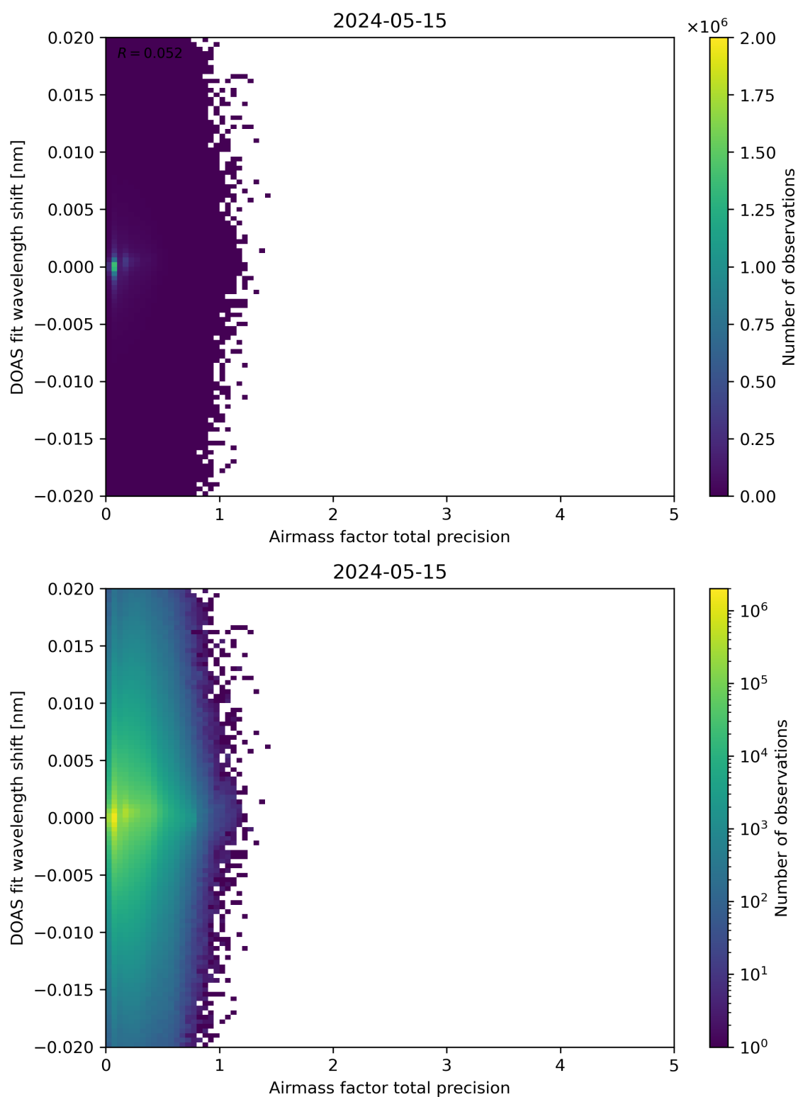
Figure 106: Scatter density plot of “Airmass factor total precision” against “DOAS fit wavelength shift” for 2024-05-14 to 2024-05-16.
