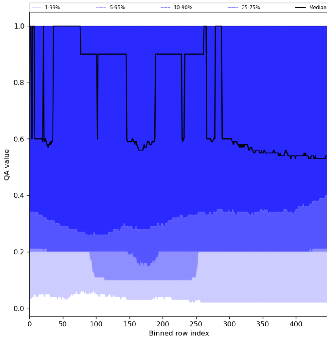
Figure 48: Along track statistics of “QA value” for 2024-05-14 to 2024-05-16
