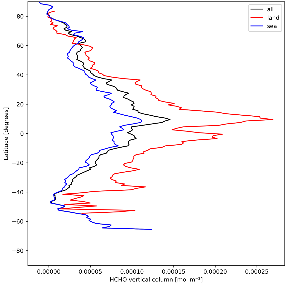
Figure 21: Zonal average of “HCHO vertical column” for 2024-05-14 to 2024-05-16.
