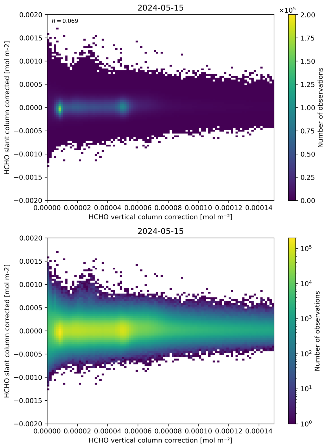
Figure 116: Scatter density plot of “HCHO vertical column correction” against “HCHO slant column corrected” for 2024-05-14 to 2024-05-16.
