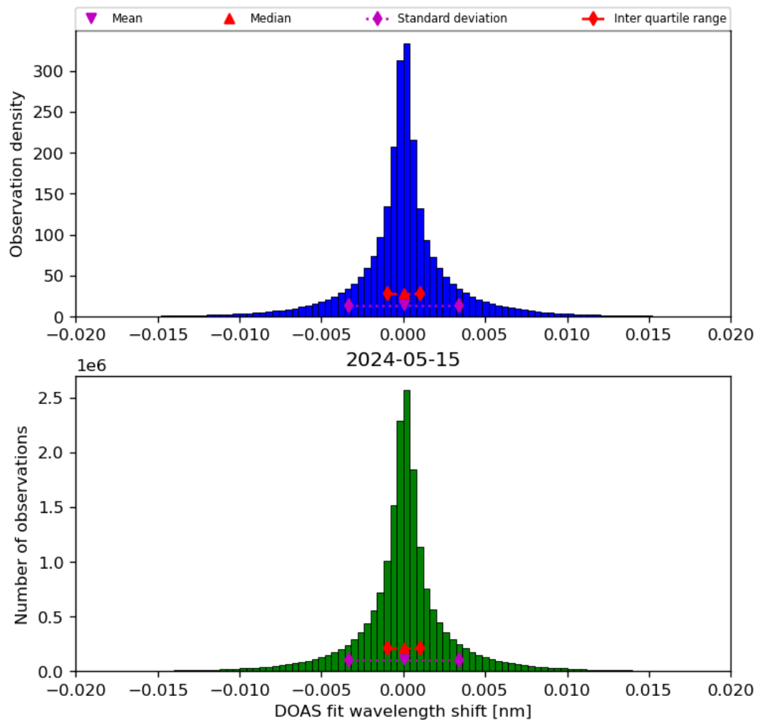
Figure 44: Histogram of “DOAS fit wavelength shift” for 2024-05-14 to 2024-05-16
