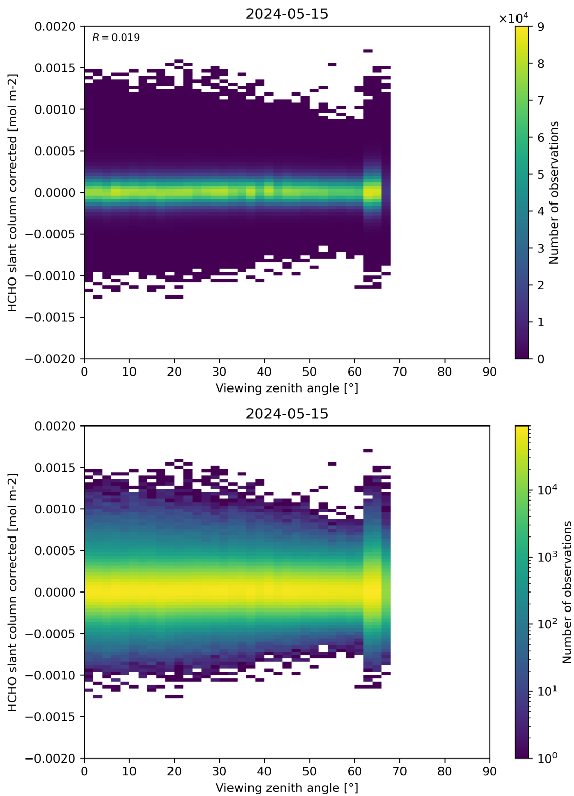
Figure 186: Scatter density plot of “Viewing zenith angle” against “HCHO slant column corrected” for 2024-05-14 to 2024-05-16.
