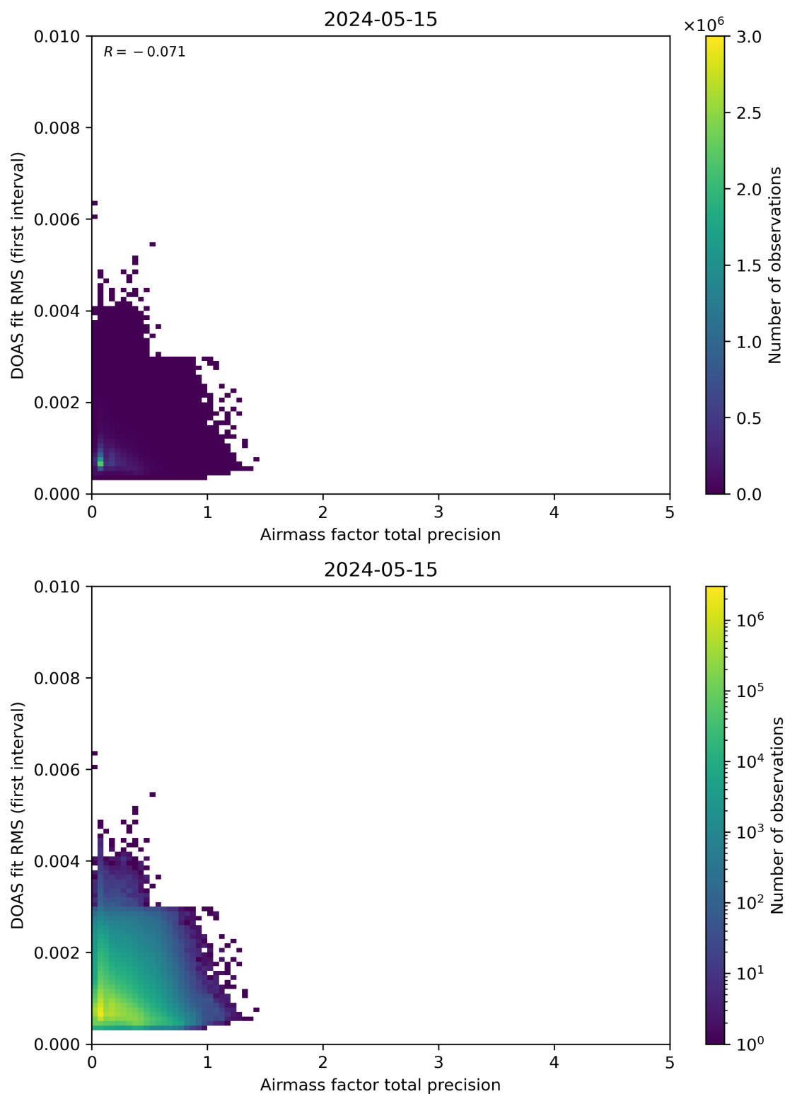
Figure 105: Scatter density plot of “Airmass factor total precision” against “DOAS fit RMS (first interval)” for 2024-05-14 to 2024-05-16.
