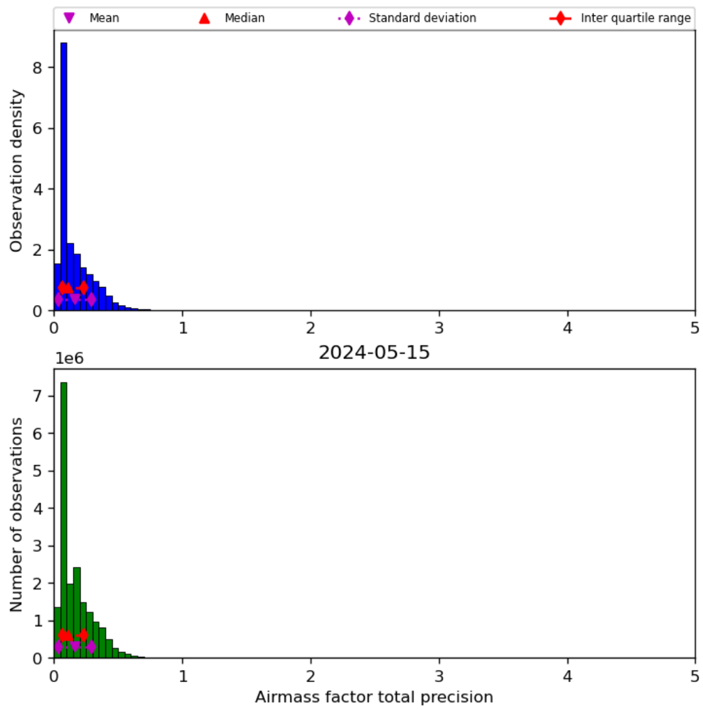
Figure 41: Histogram of “Airmass factor total precision” for 2024-05-14 to 2024-05-16
