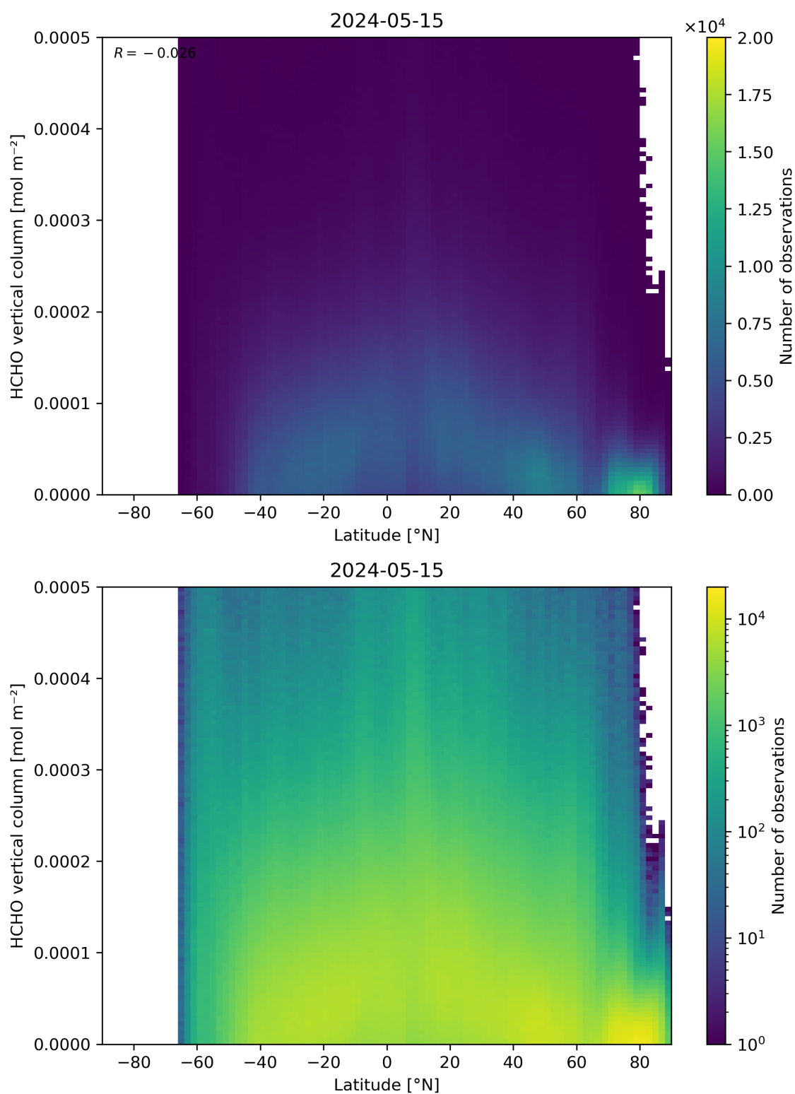
Figure 163: Scatter density plot of “Latitude” against “HCHO vertical column” for 2024-05-14 to 2024-05-16.
