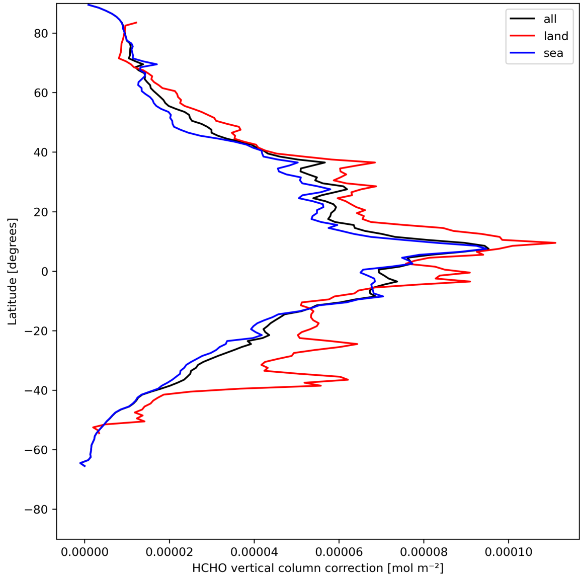
Figure 23: Zonal average of “HCHO vertical column correction” for 2024-05-14 to 2024-05-16.
