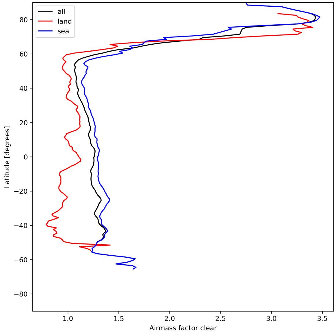
Figure 28: Zonal average of “Airmass factor clear” for 2024-05-14 to 2024-05-16.
