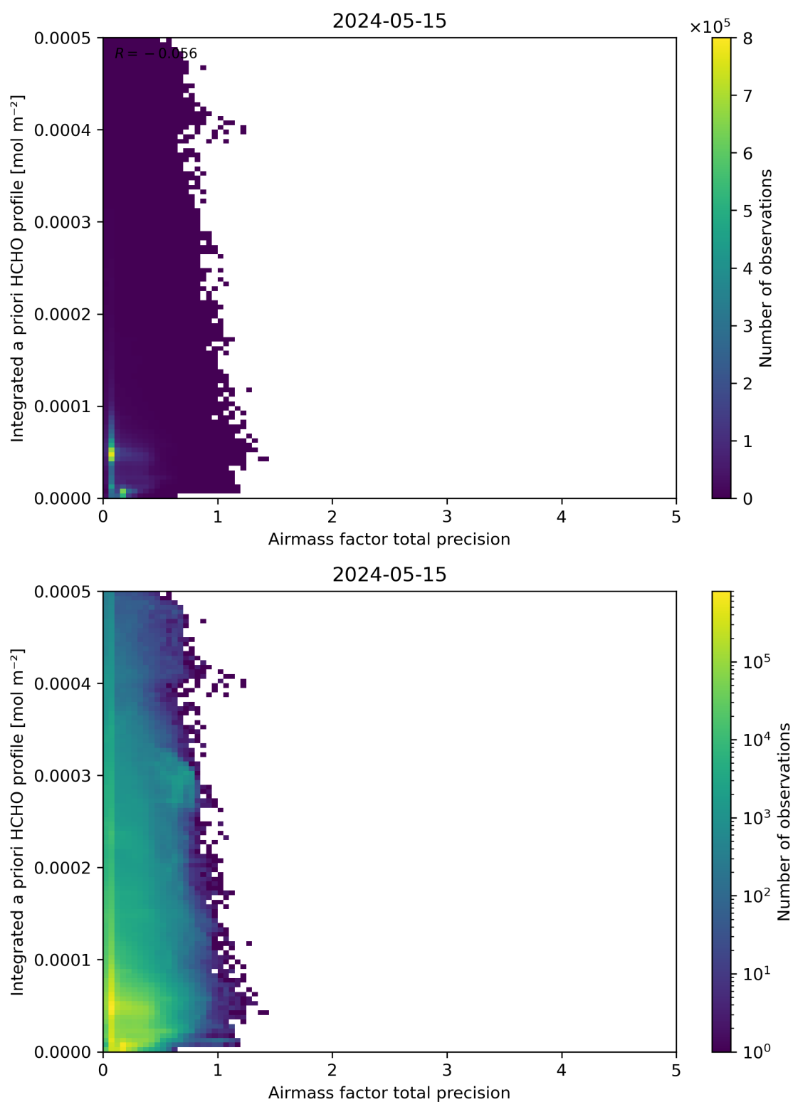
Figure 111: Scatter density plot of “Airmass factor total precision” against “Integrated a priori HCHO profile” for 2024-05-14 to 2024-05-16.
