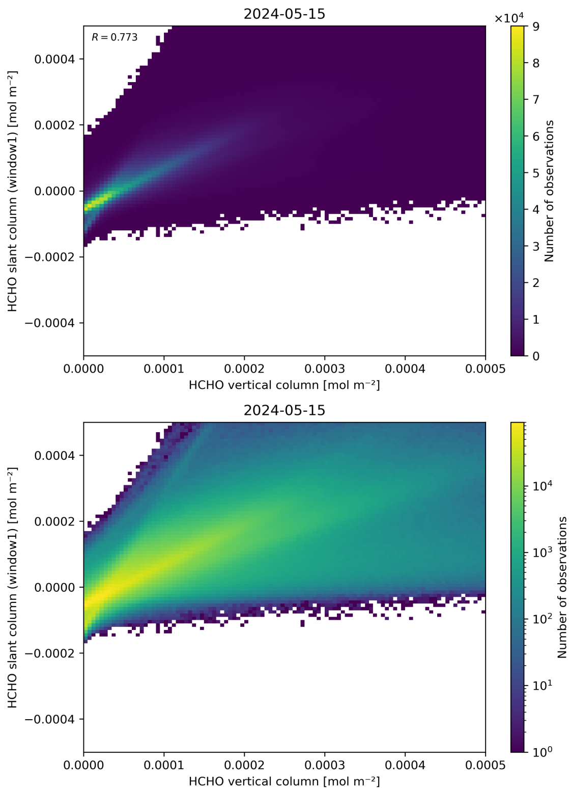
Figure 129: Scatter density plot of “HCHO vertical column” against “HCHO slant column (window1)” for 2024-05-14 to 2024-05-16.
