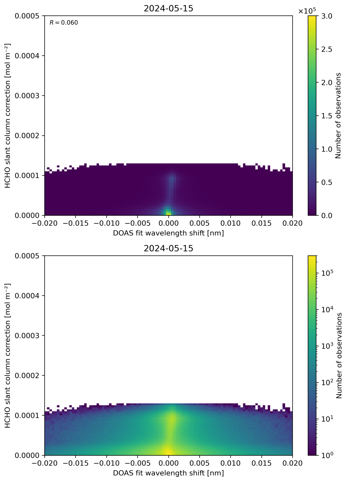
Figure 67: Scatter density plot of “DOAS fit wavelength shift” against “HCHO slant column correction” for 2024-05-14 to 2024-05-16.
