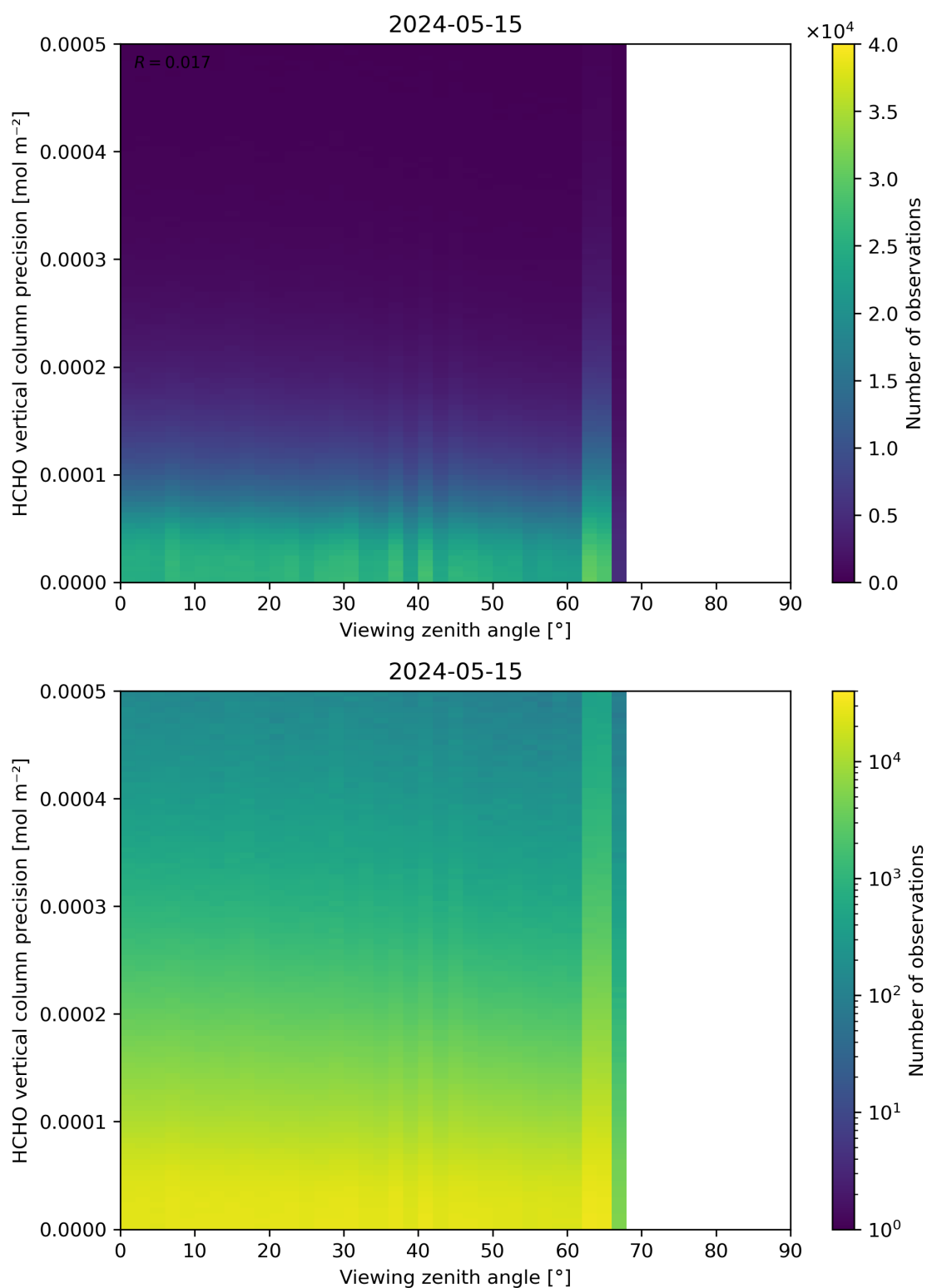
Figure 194: Scatter density plot of “Viewing zenith angle” against “HCHO vertical column precision” for 2024-05-14 to 2024-05-16.
