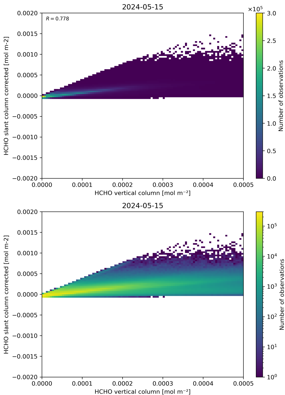
Figure 127: Scatter density plot of “HCHO vertical column” against “HCHO slant column corrected” for 2024-05-14 to 2024-05-16.
