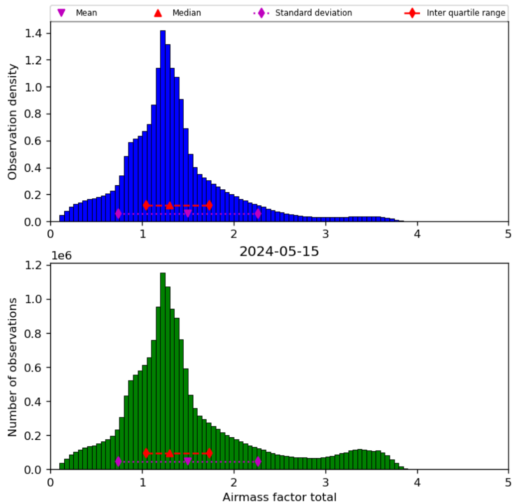
Figure 40: Histogram of “Airmass factor total” for 2024-05-14 to 2024-05-16
