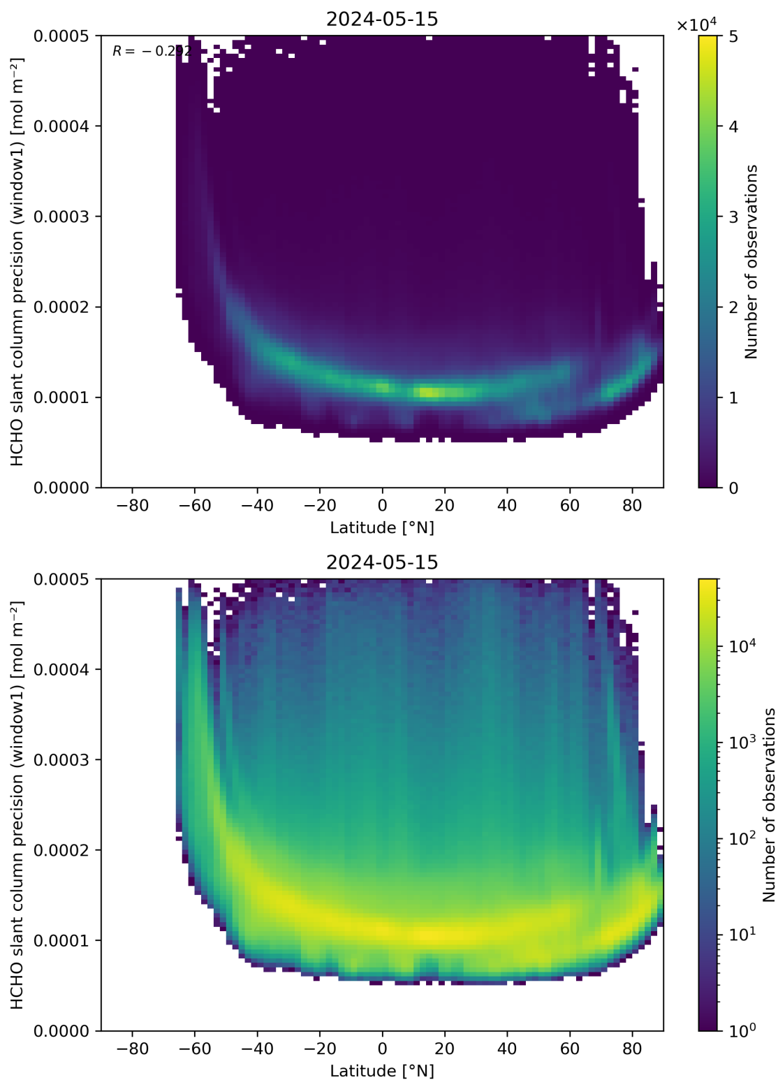
Figure 160: Scatter density plot of “Latitude” against “HCHO slant column precision (window1)” for 2024-05-14 to 2024-05-16.
