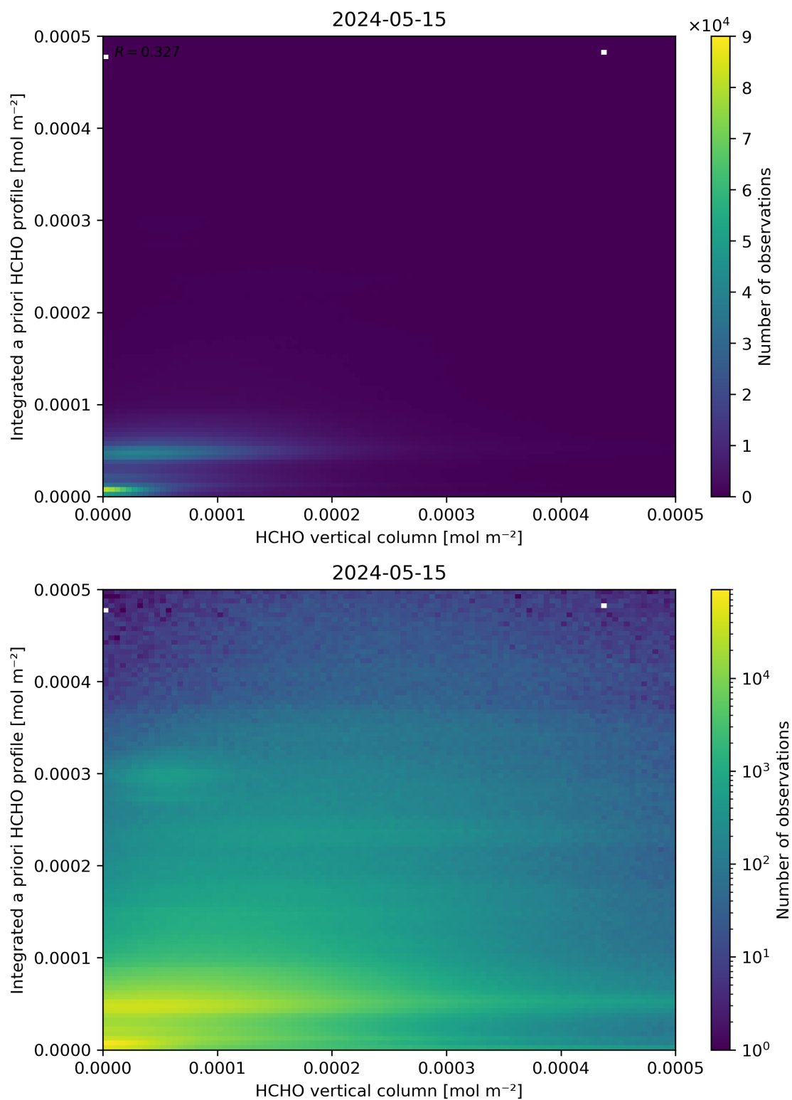
Figure 135: Scatter density plot of “HCHO vertical column” against “Integrated a priori HCHO profile” for 2024-05-14 to 2024-05-16.
