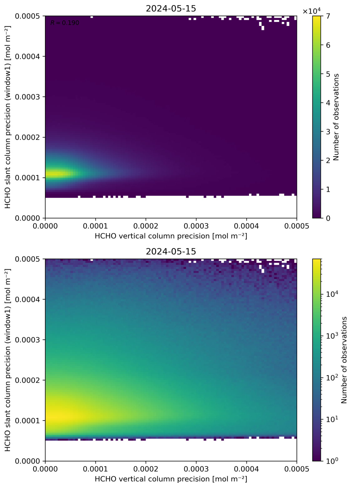
Figure 143: Scatter density plot of “HCHO vertical column precision” against “HCHO slant column precision (window1)” for 2024-05-14 to 2024-05-16.
