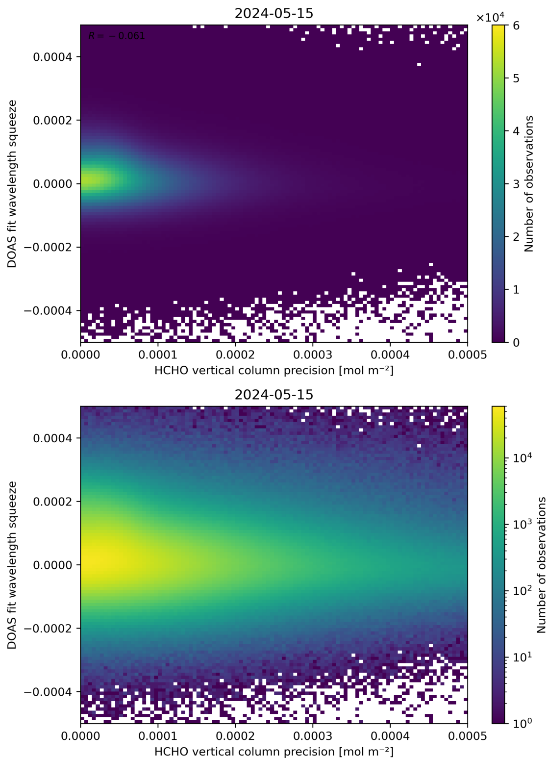
Figure 138: Scatter density plot of “HCHO vertical column precision” against “DOAS fit wavelength squeeze” for 2024-05-14 to 2024-05-16.
