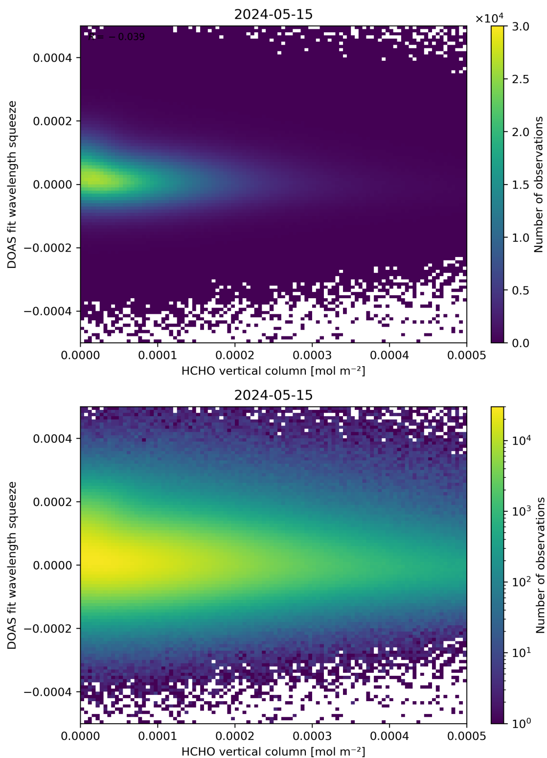
Figure 125: Scatter density plot of “HCHO vertical column” against “DOAS fit wavelength squeeze” for 2024-05-14 to 2024-05-16.
