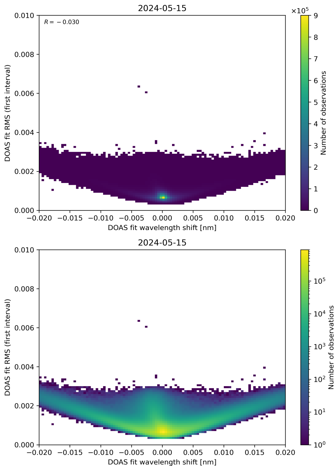
Figure 64: Scatter density plot of “DOAS fit wavelength shift” against “DOAS fit RMS (first interval)” for 2024-05-14 to 2024-05-16.
