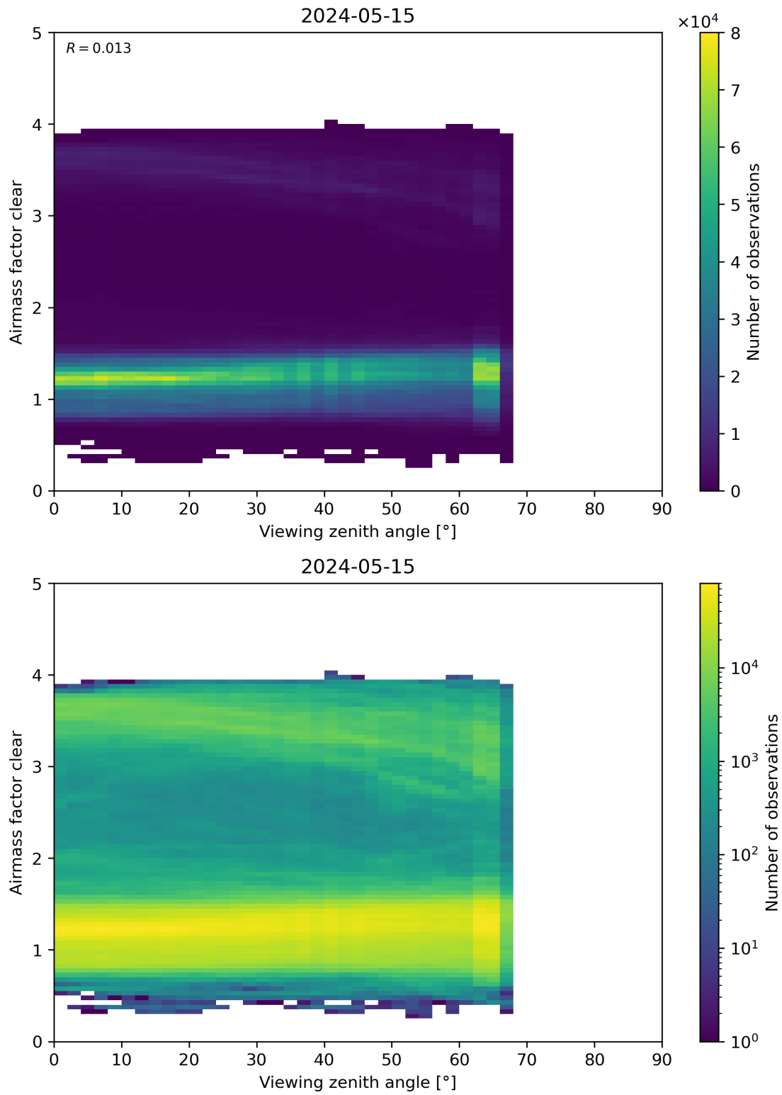
Figure 185: Scatter density plot of “Viewing zenith angle” against “Airmass factor clear” for 2024-05-14 to 2024-05-16.
