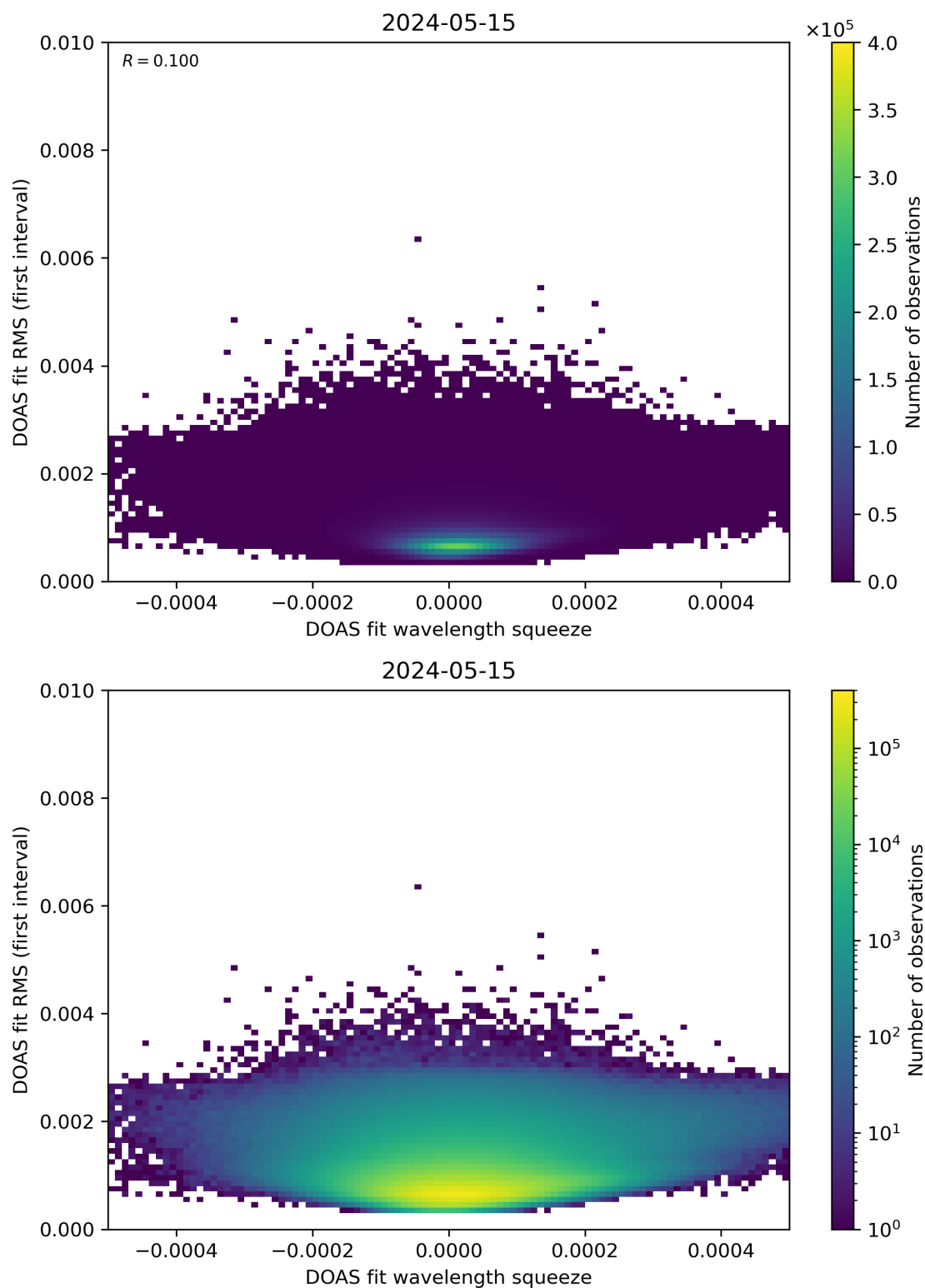
Figure 68: Scatter density plot of “DOAS fit wavelength squeeze” against “DOAS fit RMS (first interval)” for 2024-05-14 to 2024-05-16.
