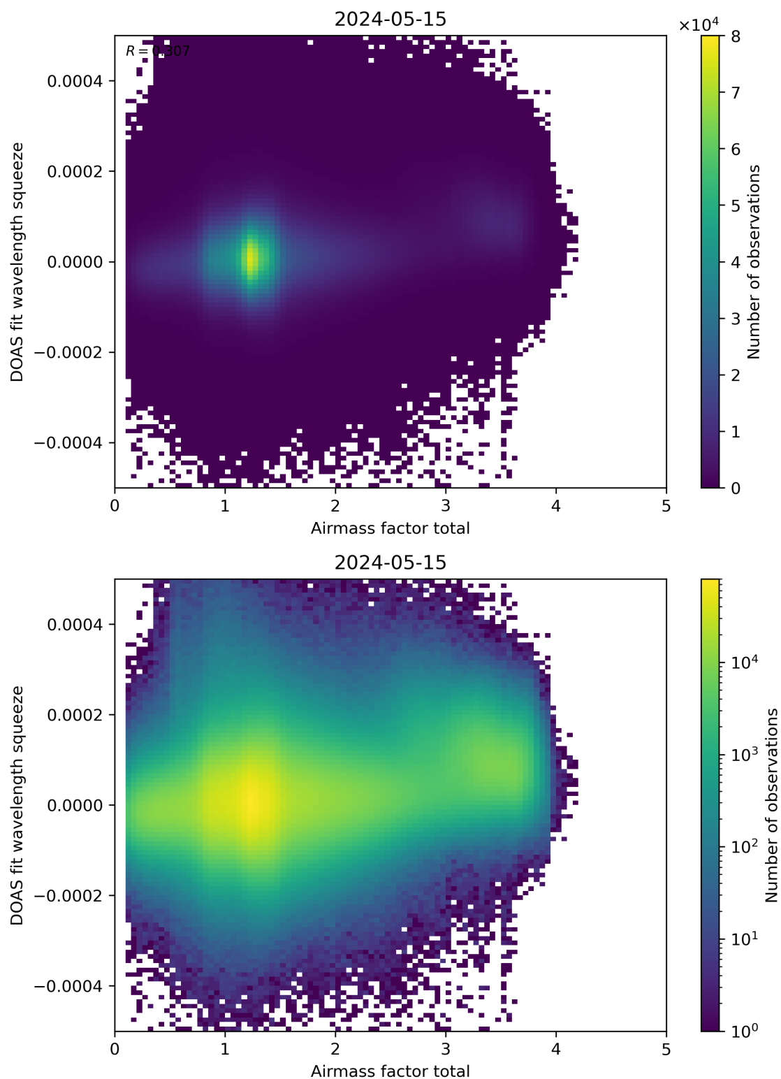
Figure 99: Scatter density plot of “Airmass factor total” against “DOAS fit wavelength squeeze” for 2024-05-14 to 2024-05-16.
