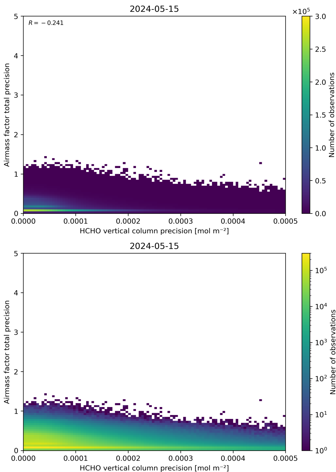
Figure 145: Scatter density plot of “HCHO vertical column precision” against “Airmass factor total precision” for 2024-05-14 to 2024-05-16.
