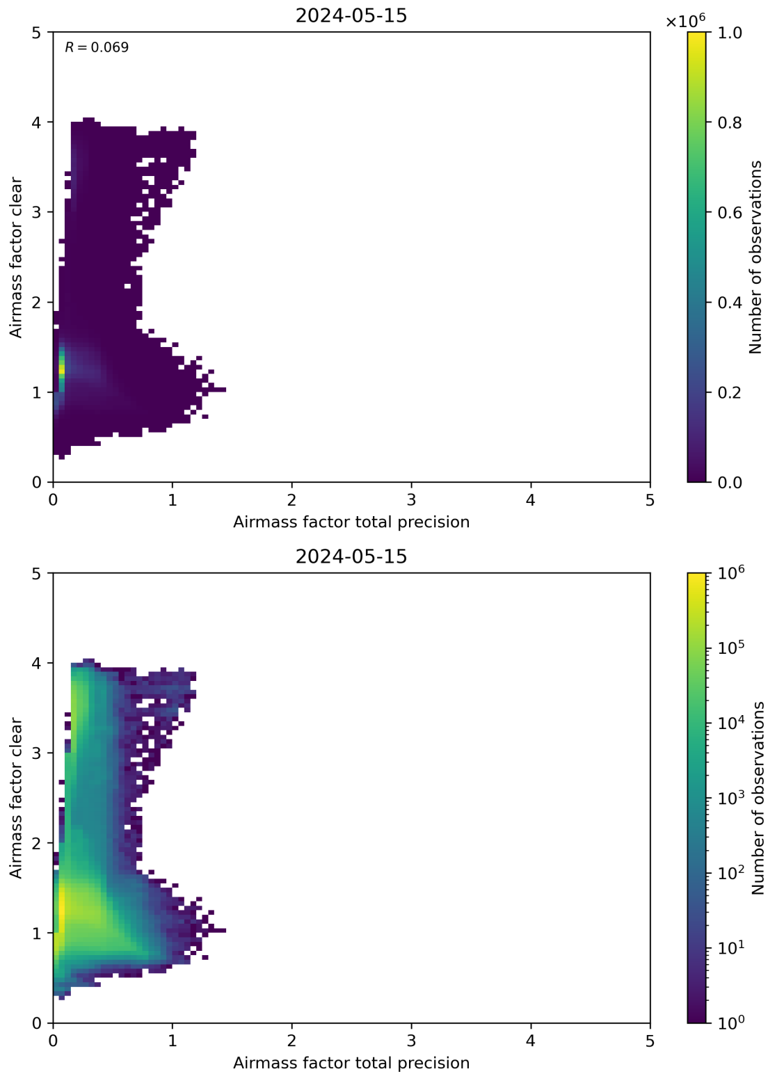
Figure 108: Scatter density plot of “Airmass factor total precision” against “Airmass factor clear” for 2024-05-14 to 2024-05-16.
