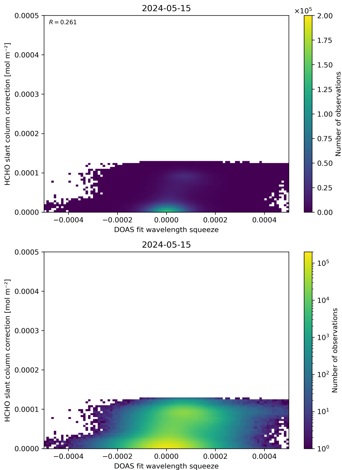
Figure 70: Scatter density plot of “DOAS fit wavelength squeeze” against “HCHO slant column correction” for 2024-05-14 to 2024-05-16.
