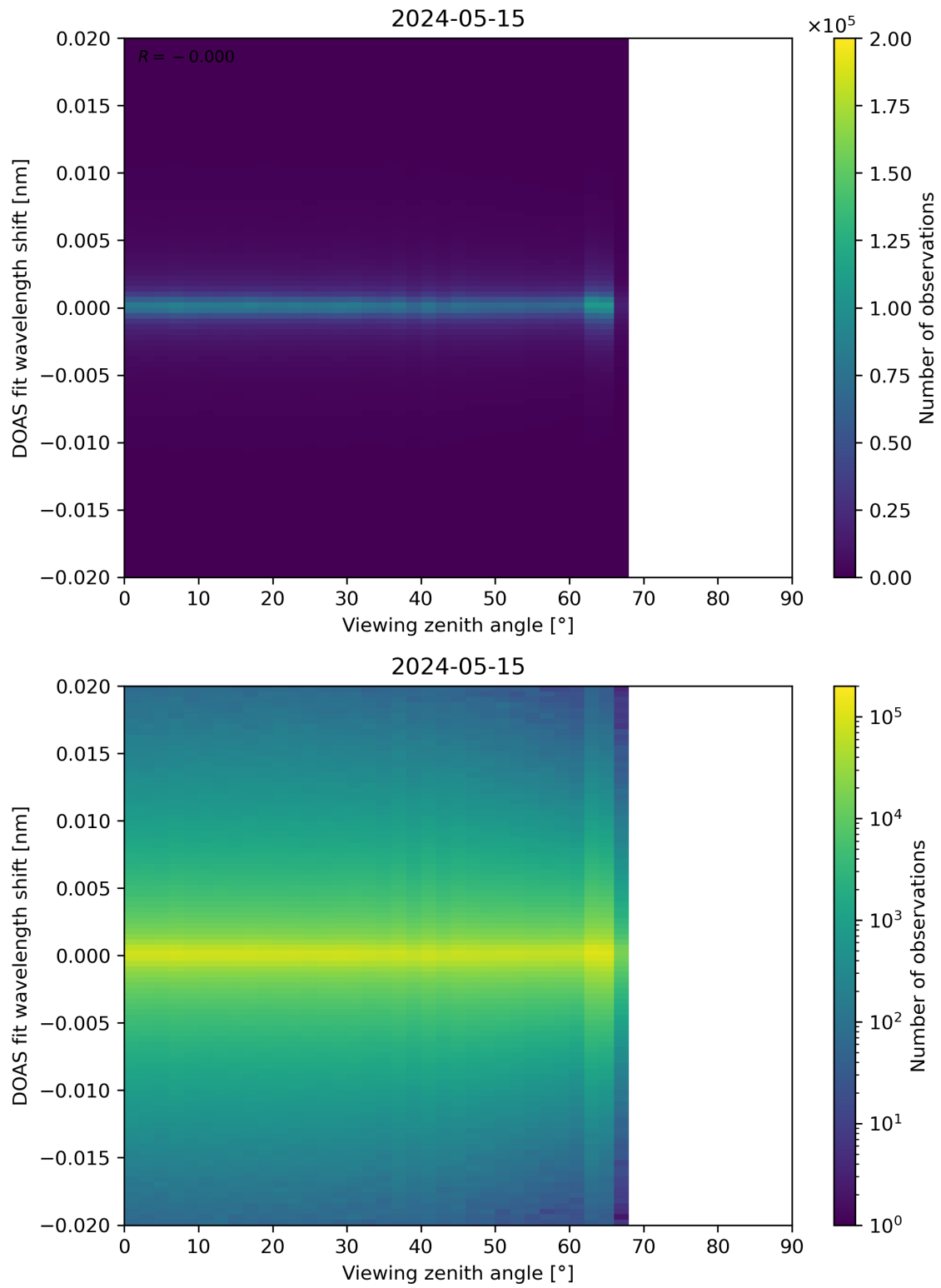
Figure 183: Scatter density plot of “Viewing zenith angle” against “DOAS fit wavelength shift” for 2024-05-14 to 2024-05-16.
