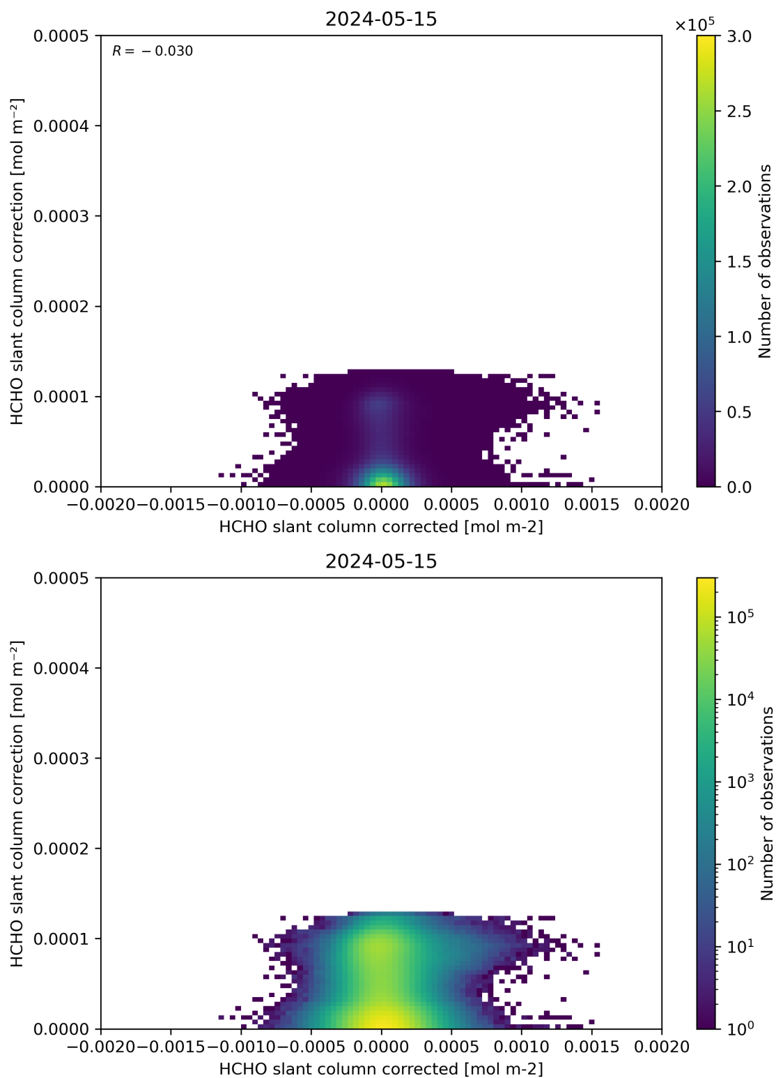
Figure 77: Scatter density plot of “HCHO slant column corrected” against “HCHO slant column correction” for 2024-05-14 to 2024-05-16.
