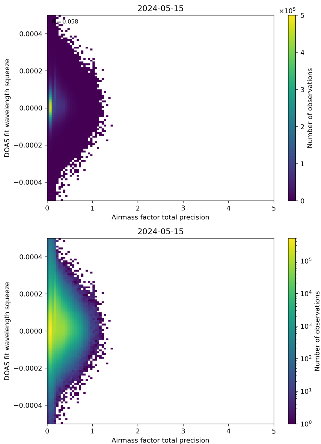
Figure 107: Scatter density plot of “Airmass factor total precision” against “DOAS fit wavelength squeeze” for 2024-05-14 to 2024-05-16.
