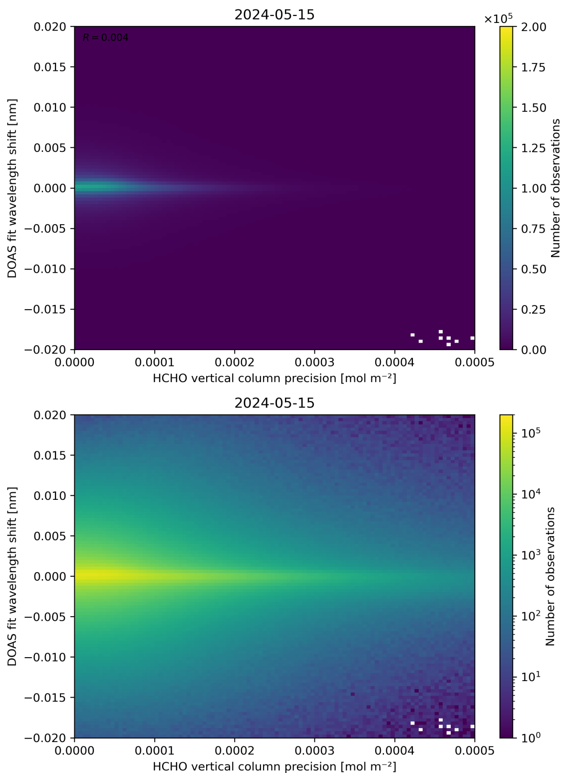
Figure 137: Scatter density plot of “HCHO vertical column precision” against “DOAS fit wavelength shift” for 2024-05-14 to 2024-05-16.
