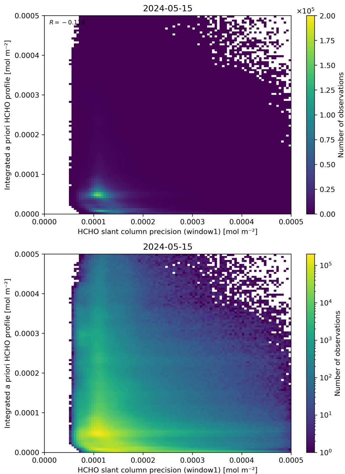
Figure 96: Scatter density plot of “HCHO slant column precision (window1)” against “Integrated a priori HCHO profile” for 2024-05-14 to 2024-05-16.
