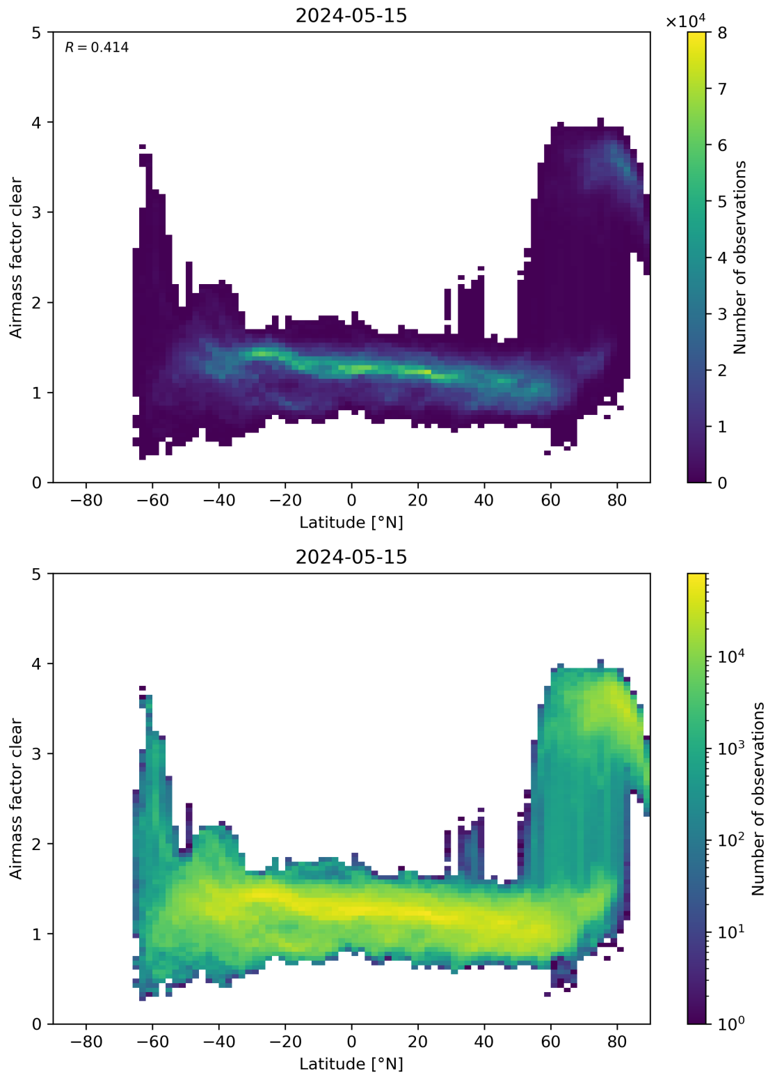
Figure 156: Scatter density plot of “Latitude” against “Airmass factor clear” for 2024-05-14 to 2024-05-16.
