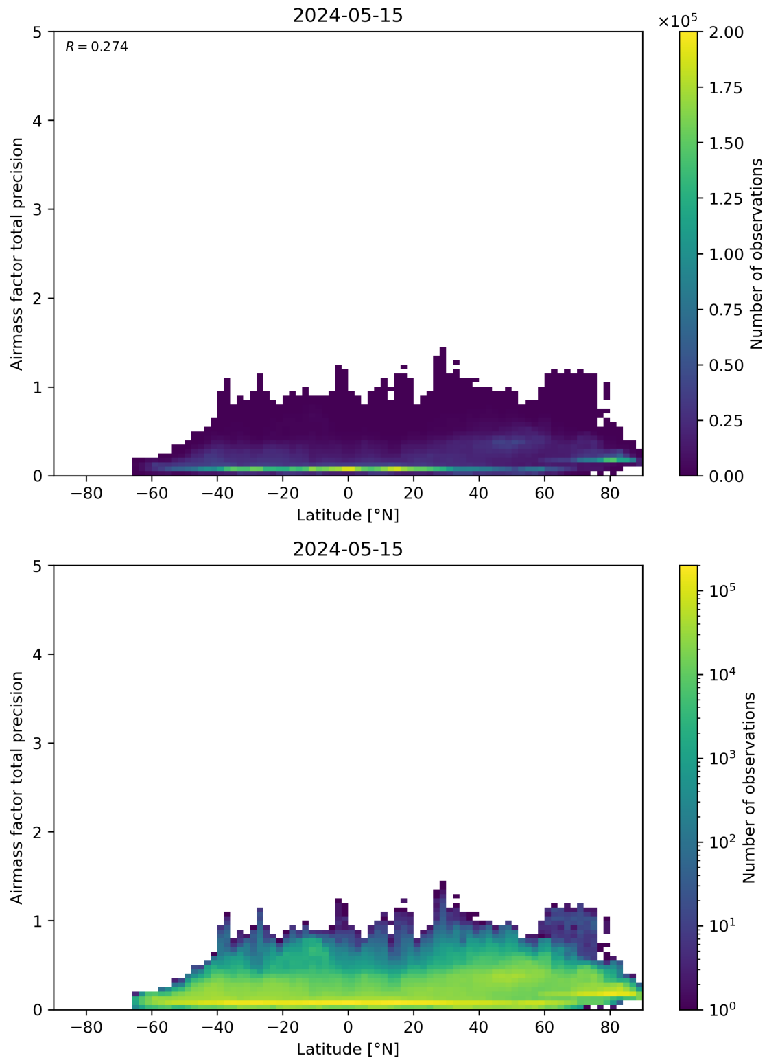
Figure 162: Scatter density plot of “Latitude” against “Airmass factor total precision” for 2024-05-14 to 2024-05-16.
