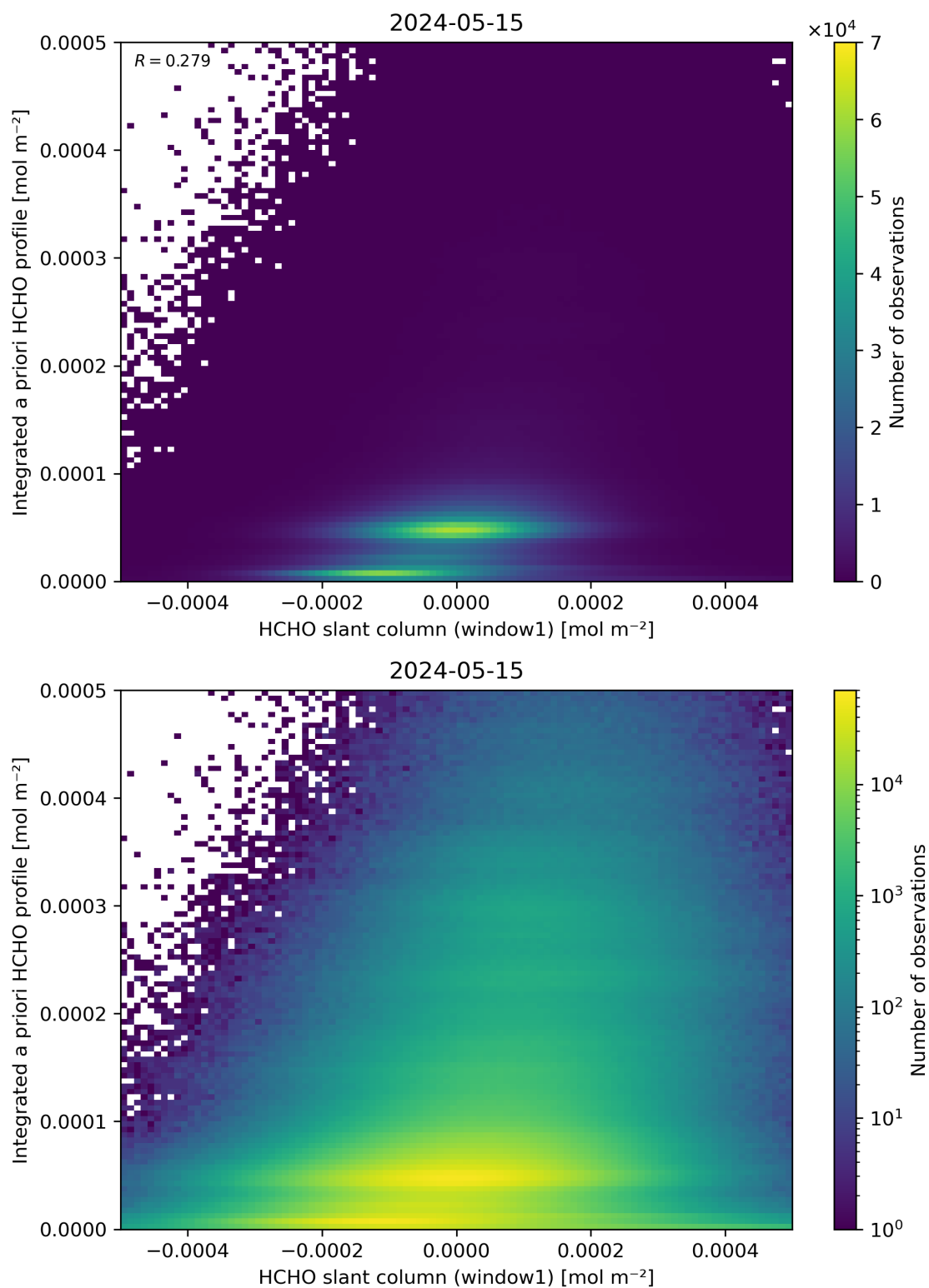
Figure 87: Scatter density plot of “HCHO slant column (window1)” against “Integrated a priori HCHO profile” for 2024-05-14 to 2024-05-16.
