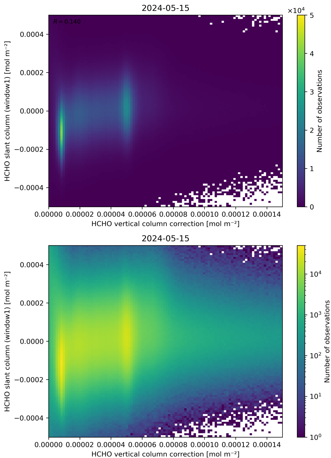
Figure 118: Scatter density plot of “HCHO vertical column correction” against “HCHO slant column (window1)” for 2024-05-14 to 2024-05-16.
