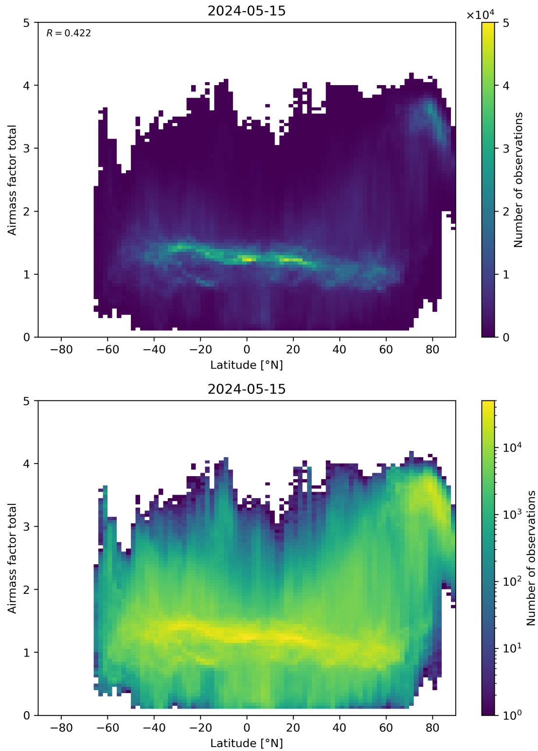
Figure 161: Scatter density plot of “Latitude” against “Airmass factor total” for 2024-05-14 to 2024-05-16.
