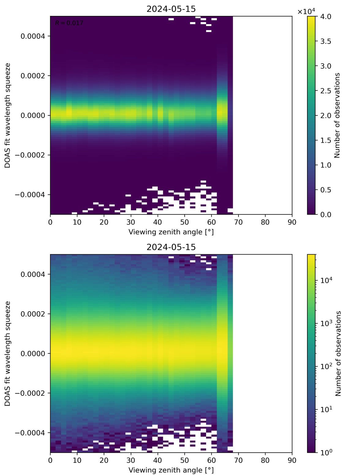
Figure 184: Scatter density plot of “Viewing zenith angle” against “DOAS fit wavelength squeeze” for 2024-05-14 to 2024-05-16.
