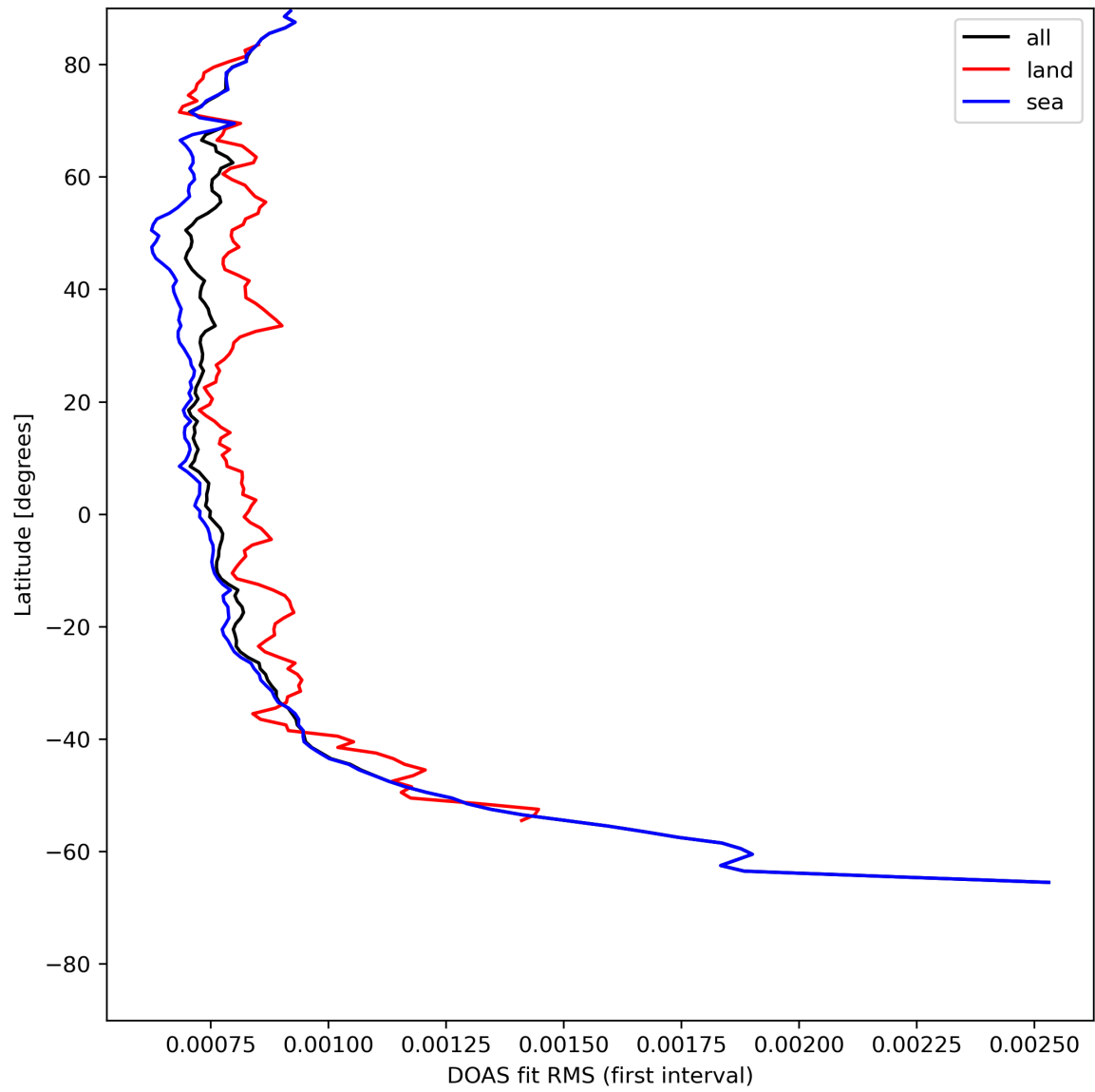
Figure 32: Zonal average of “DOAS fit RMS (first interval)” for 2024-05-14 to 2024-05-16.
