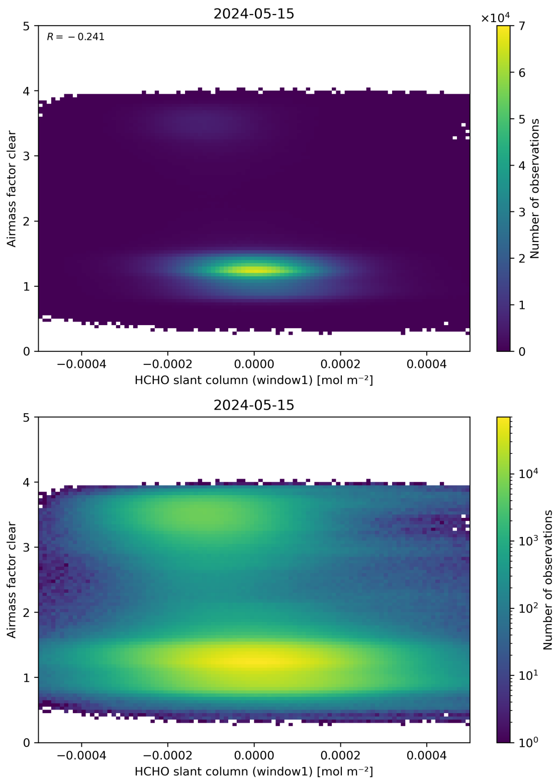
Figure 81: Scatter density plot of “HCHO slant column (window1)” against “Airmass factor clear” for 2024-05-14 to 2024-05-16.
