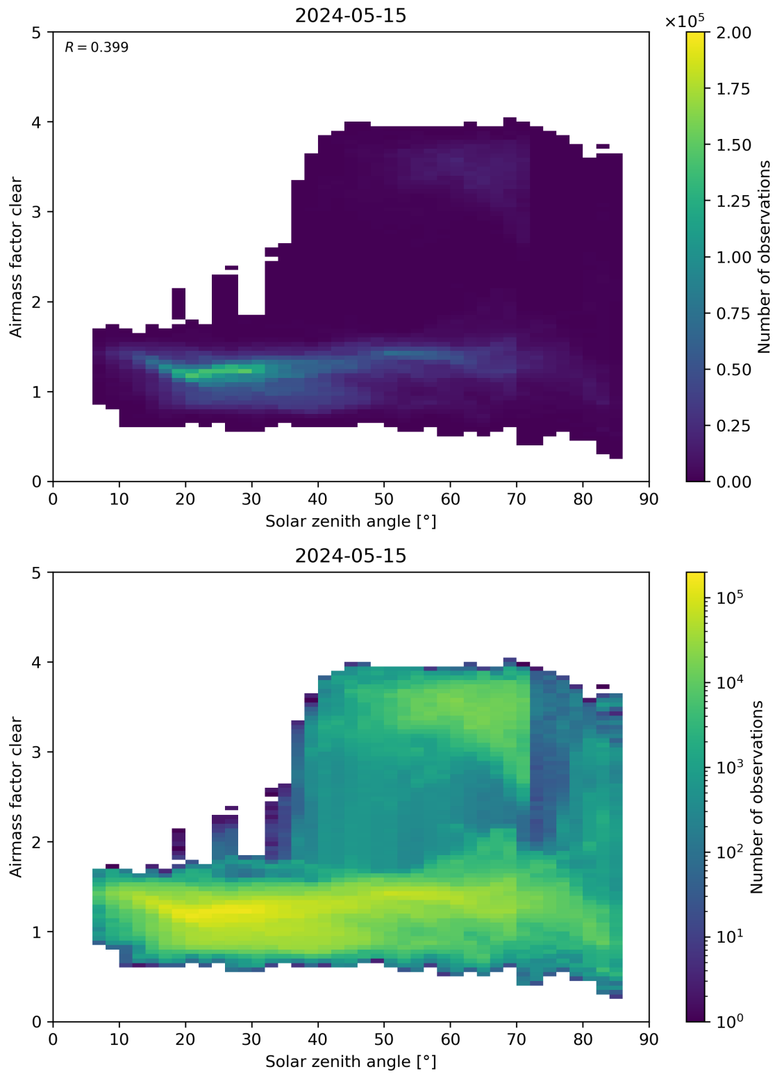
Figure 170: Scatter density plot of “Solar zenith angle” against “Airmass factor clear” for 2024-05-14 to 2024-05-16.
