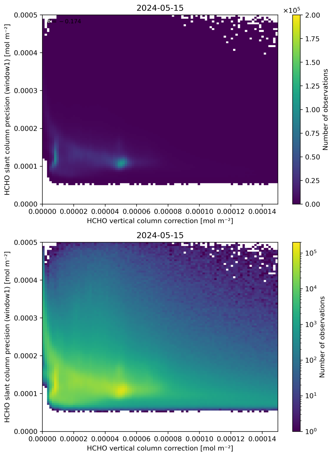
Figure 119: Scatter density plot of “HCHO vertical column correction” against “HCHO slant column precision (window1)” for 2024-05-14 to 2024-05-16.
