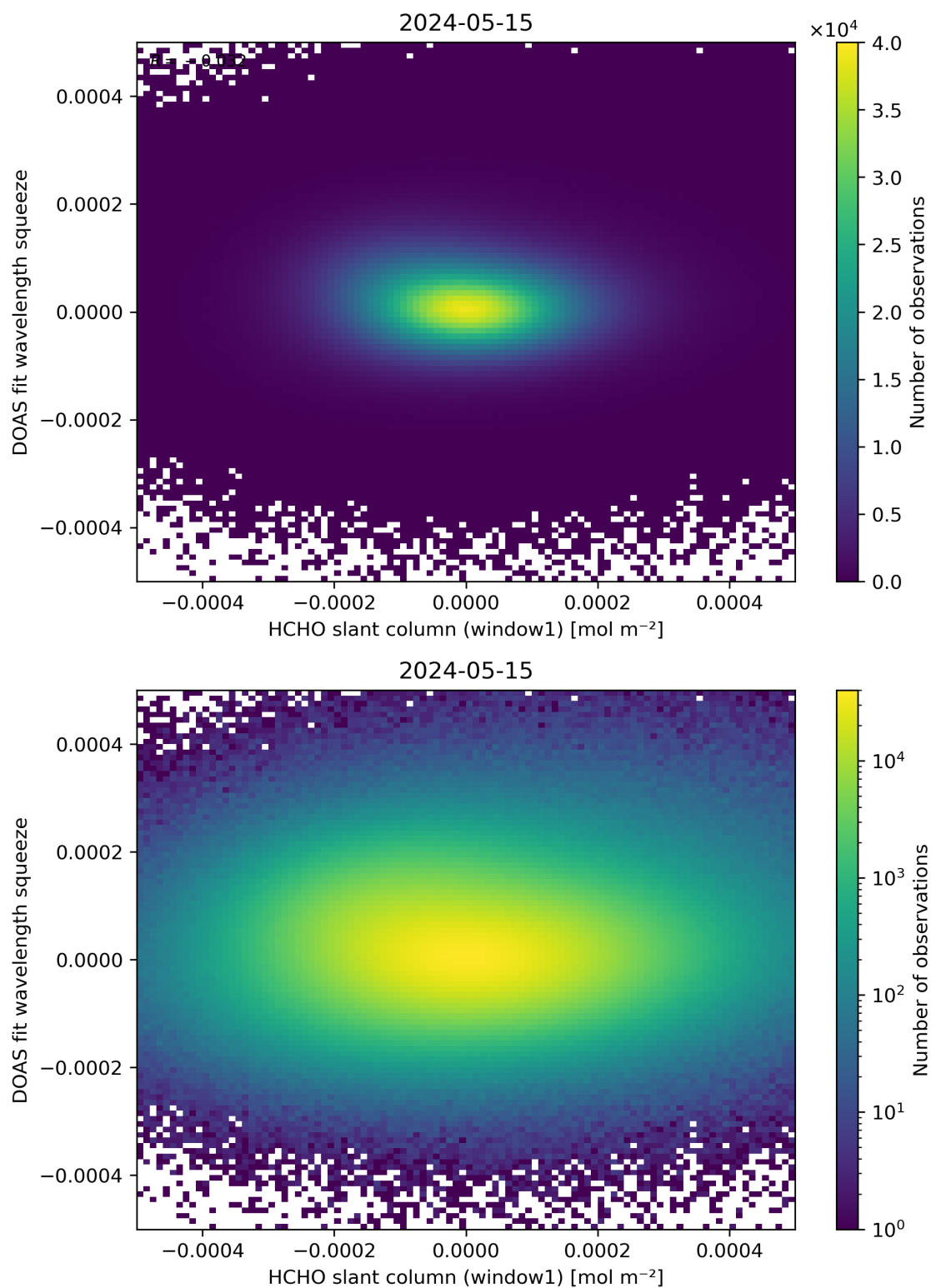
Figure 80: Scatter density plot of “HCHO slant column (window1)” against “DOAS fit wavelength squeeze” for 2024-05-14 to 2024-05-16.
