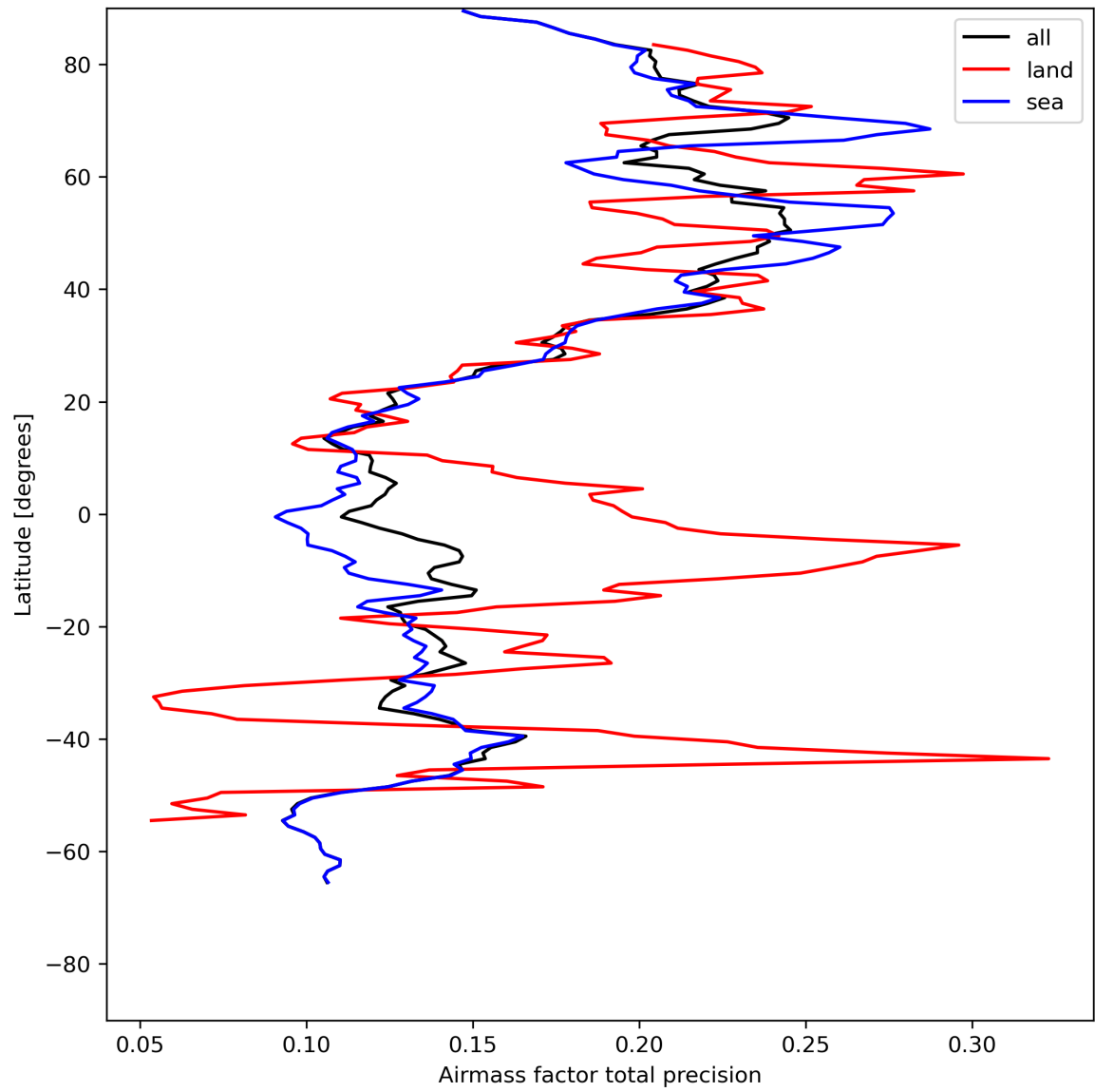
Figure 27: Zonal average of “Airmass factor total precision” for 2024-05-15 to 2024-05-17.
