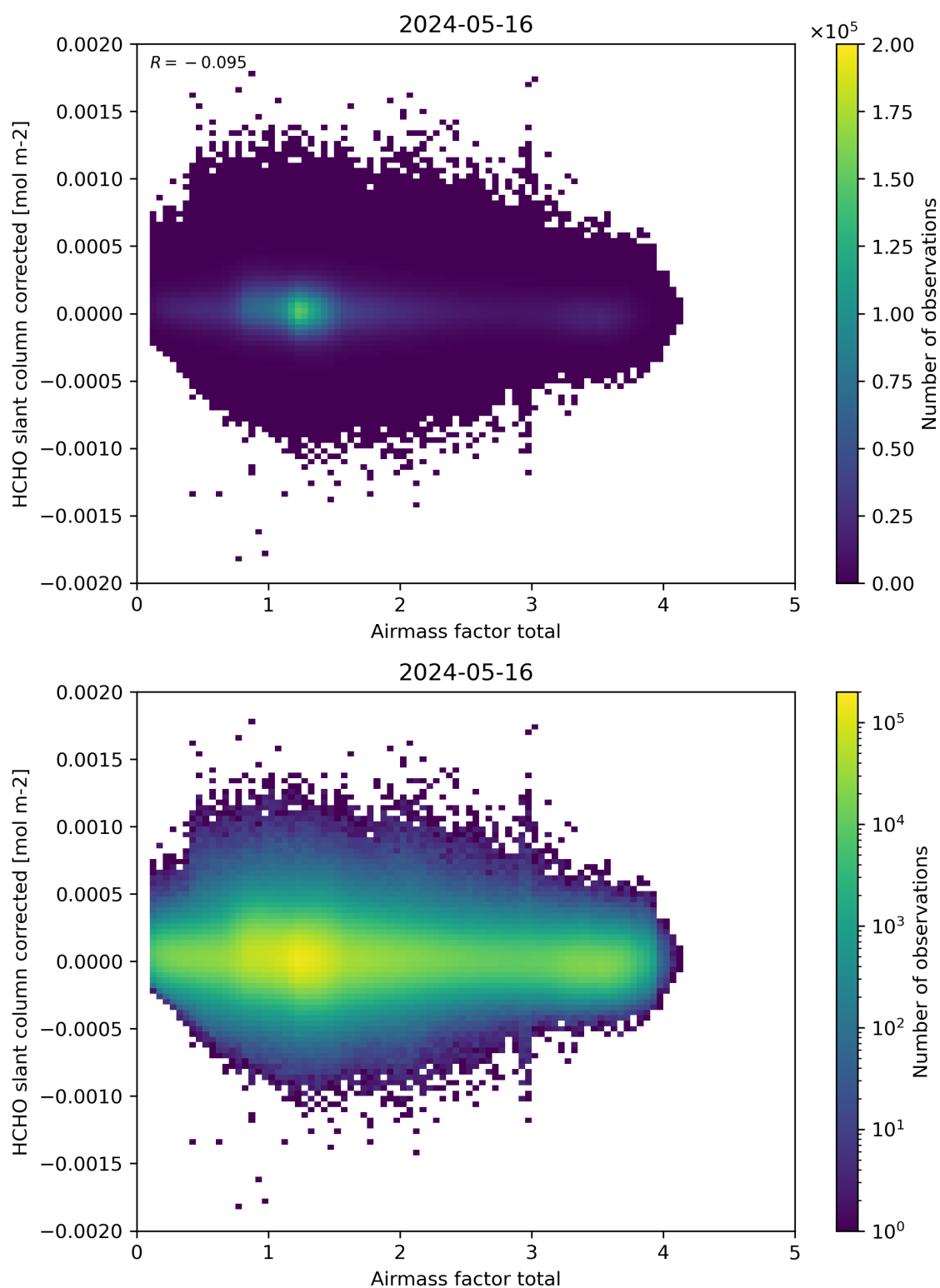
Figure 101: Scatter density plot of “Airmass factor total” against “HCHO slant column corrected” for 2024-05-15 to 2024-05-17.
