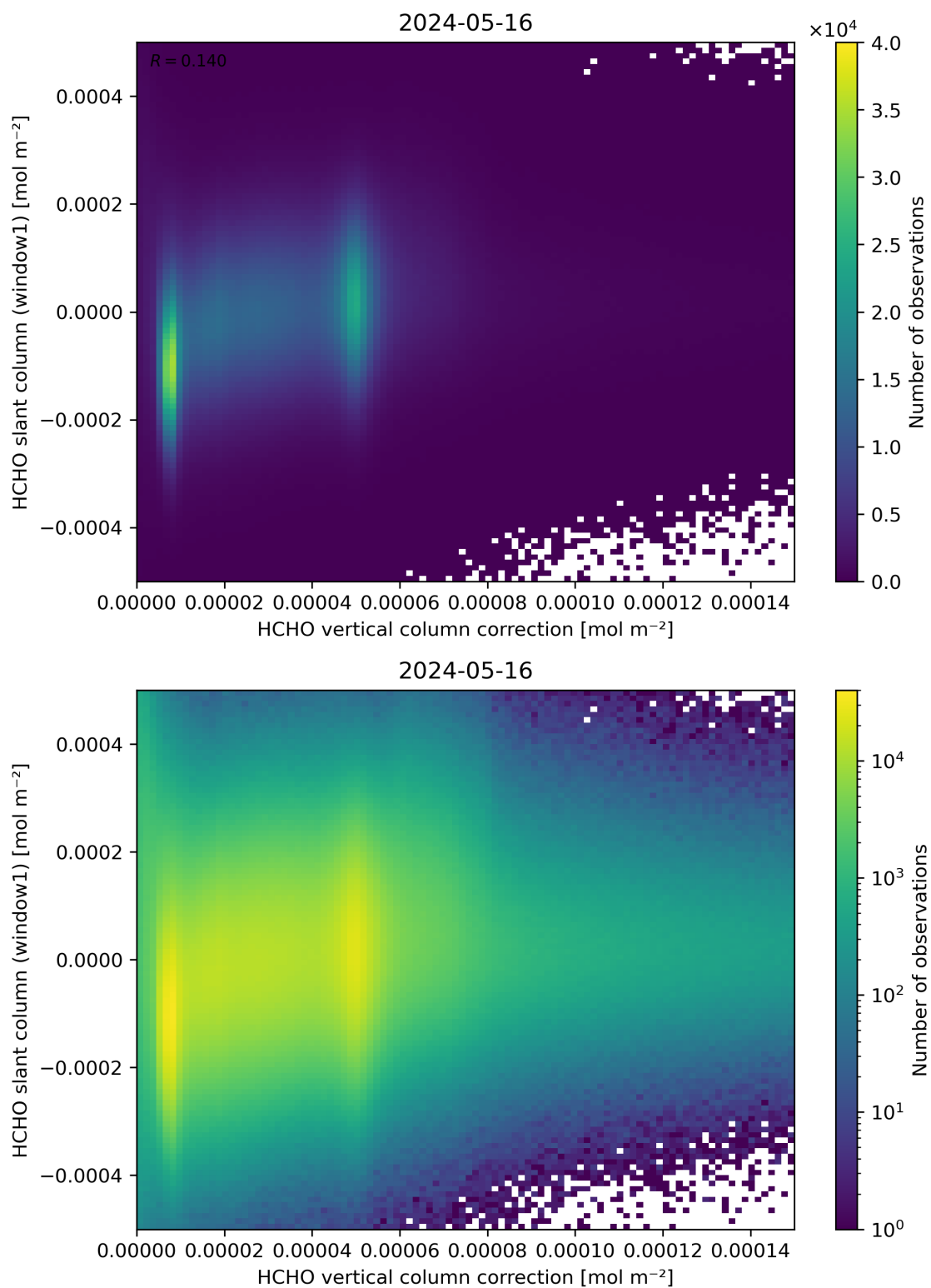
Figure 118: Scatter density plot of “HCHO vertical column correction” against “HCHO slant column (window1)” for 2024-05-15 to 2024-05-17.
