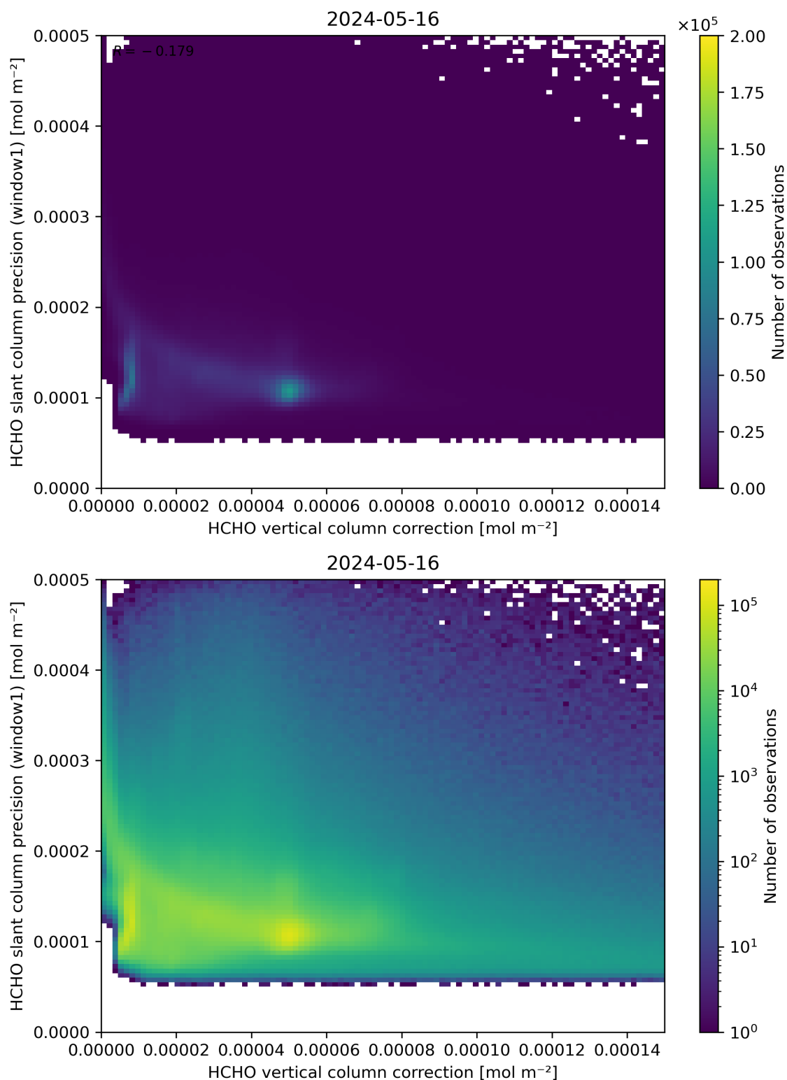
Figure 119: Scatter density plot of “HCHO vertical column correction” against “HCHO slant column precision (window1)” for 2024-05-15 to 2024-05-17.
