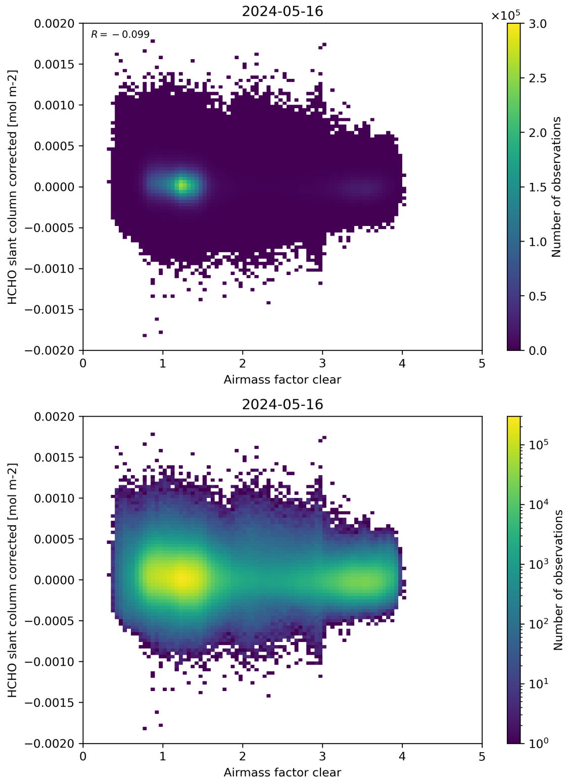
Figure 74: Scatter density plot of “Airmass factor clear” against “HCHO slant column corrected” for 2024-05-15 to 2024-05-17.
