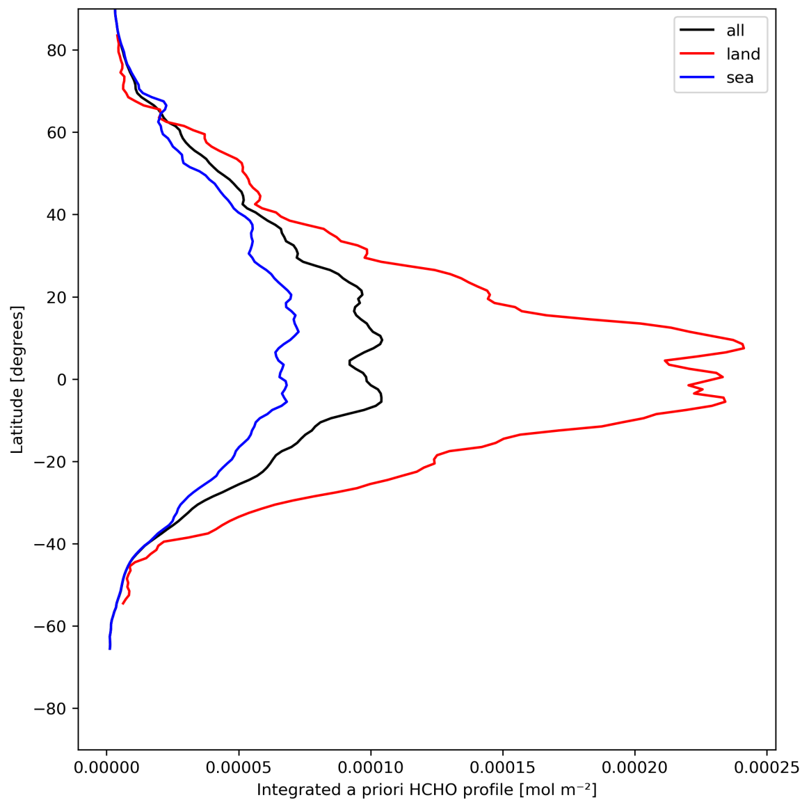
Figure 29: Zonal average of “Integrated a priori HCHO profile” for 2024-05-15 to 2024-05-17.
