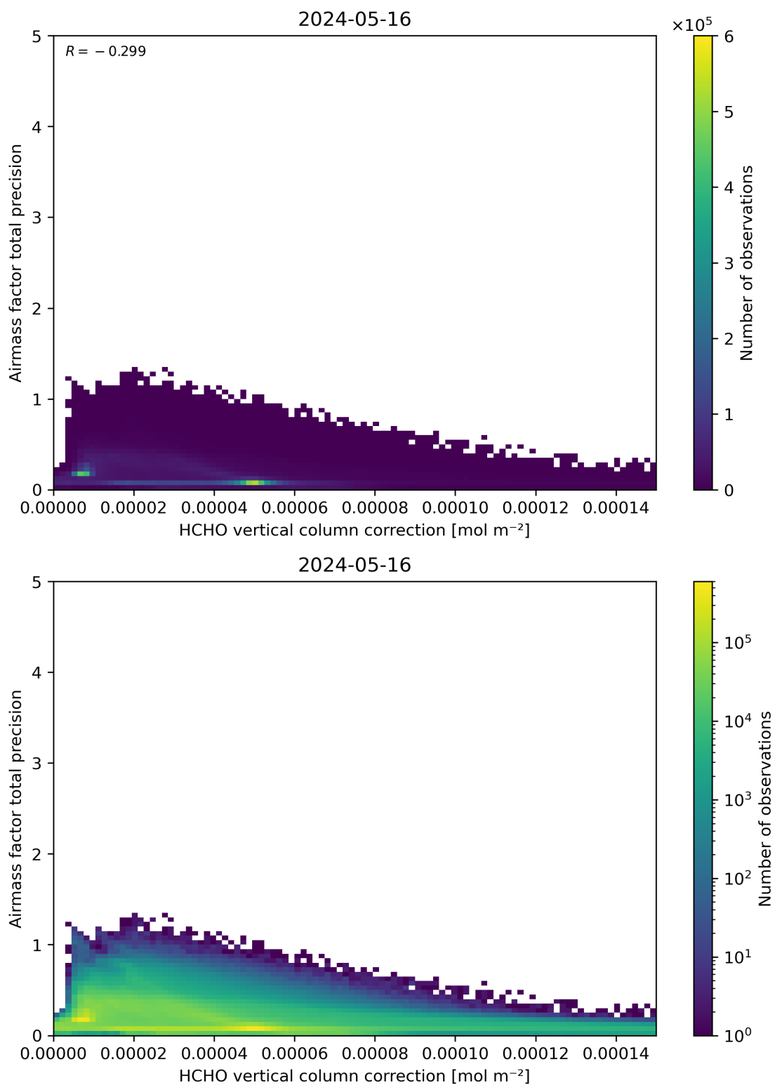
Figure 121: Scatter density plot of “HCHO vertical column correction” against “Airmass factor total precision” for 2024-05-15 to 2024-05-17.
