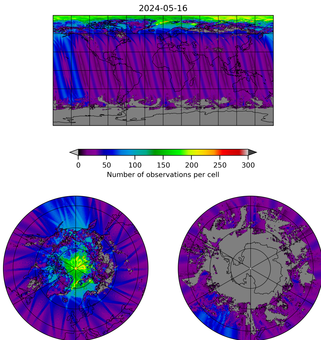
Figure 19: Map of the number of observations for 2024-05-15 to 2024-05-17
