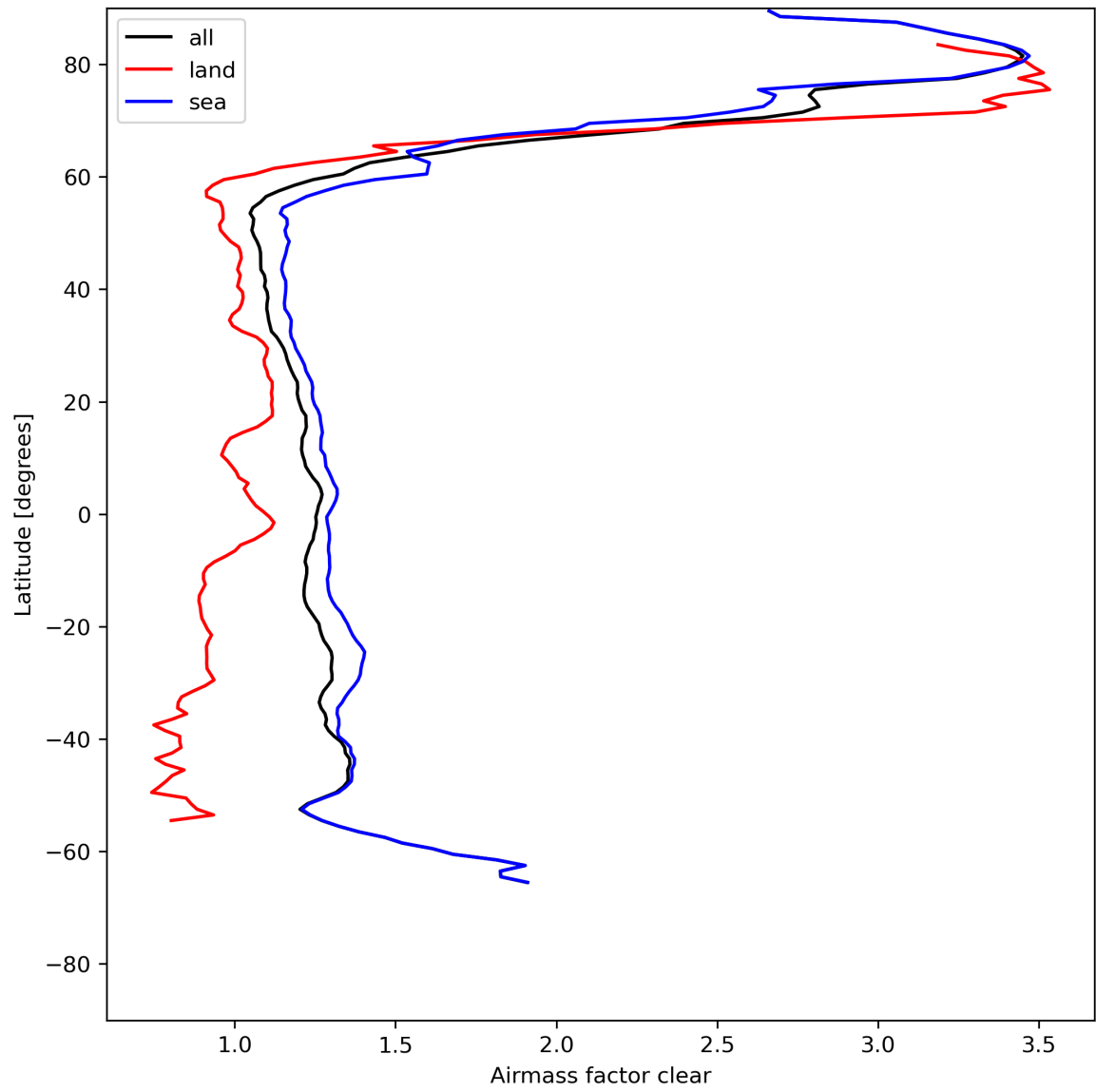
Figure 28: Zonal average of “Airmass factor clear” for 2024-05-15 to 2024-05-17.
