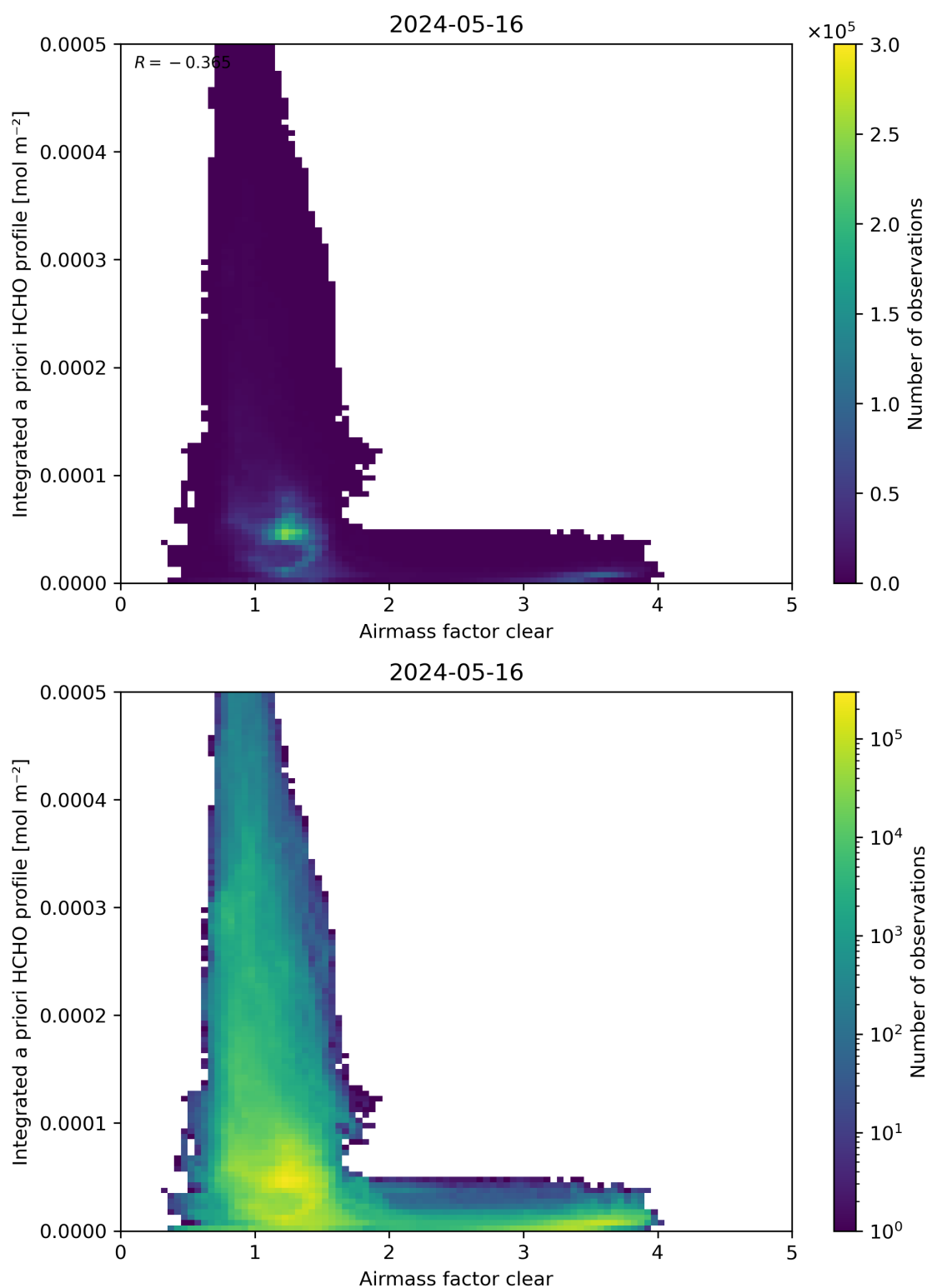
Figure 76: Scatter density plot of “Airmass factor clear” against “Integrated a priori HCHO profile” for 2024-05-15 to 2024-05-17.
