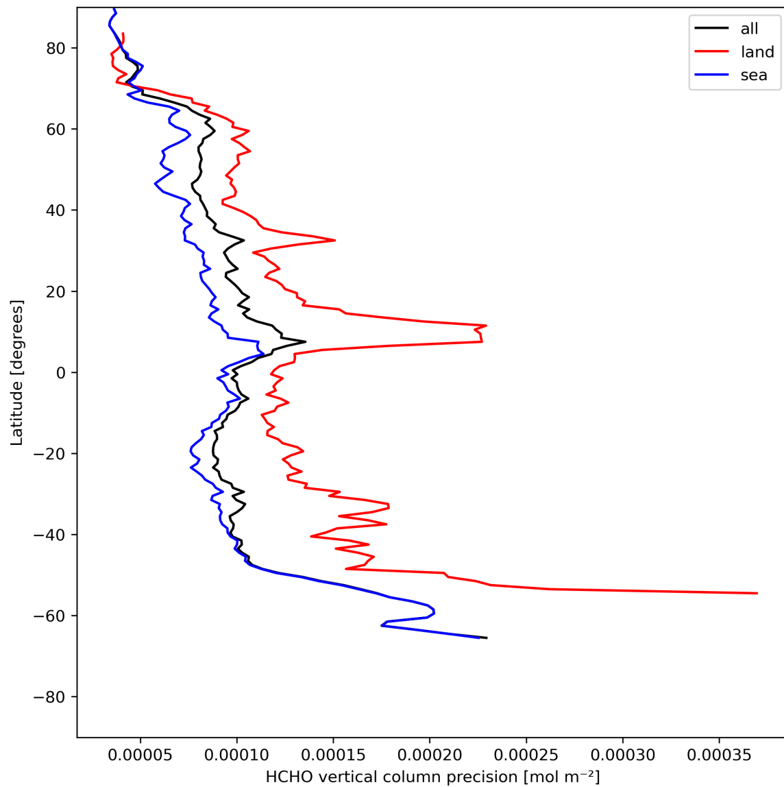
Figure 22: Zonal average of “HCHO vertical column precision” for 2024-05-15 to 2024-05-17.
