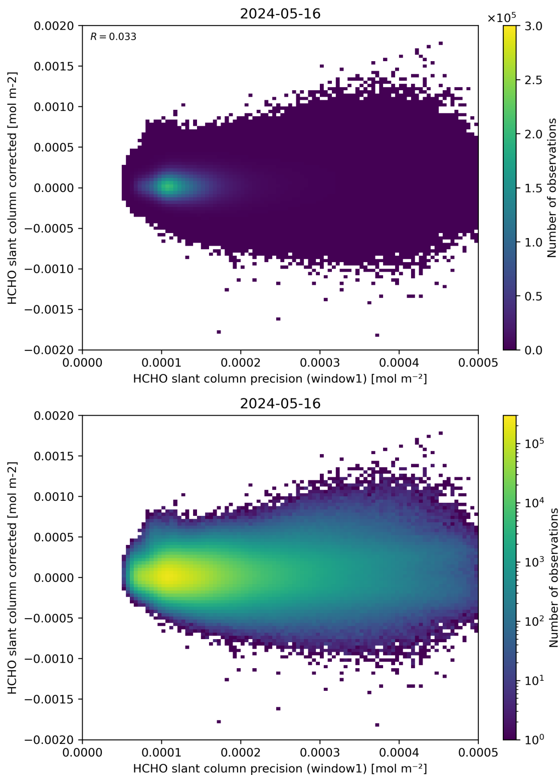
Figure 92: Scatter density plot of “HCHO slant column precision (window1)” against “HCHO slant column corrected” for 2024-05-15 to 2024-05-17.
