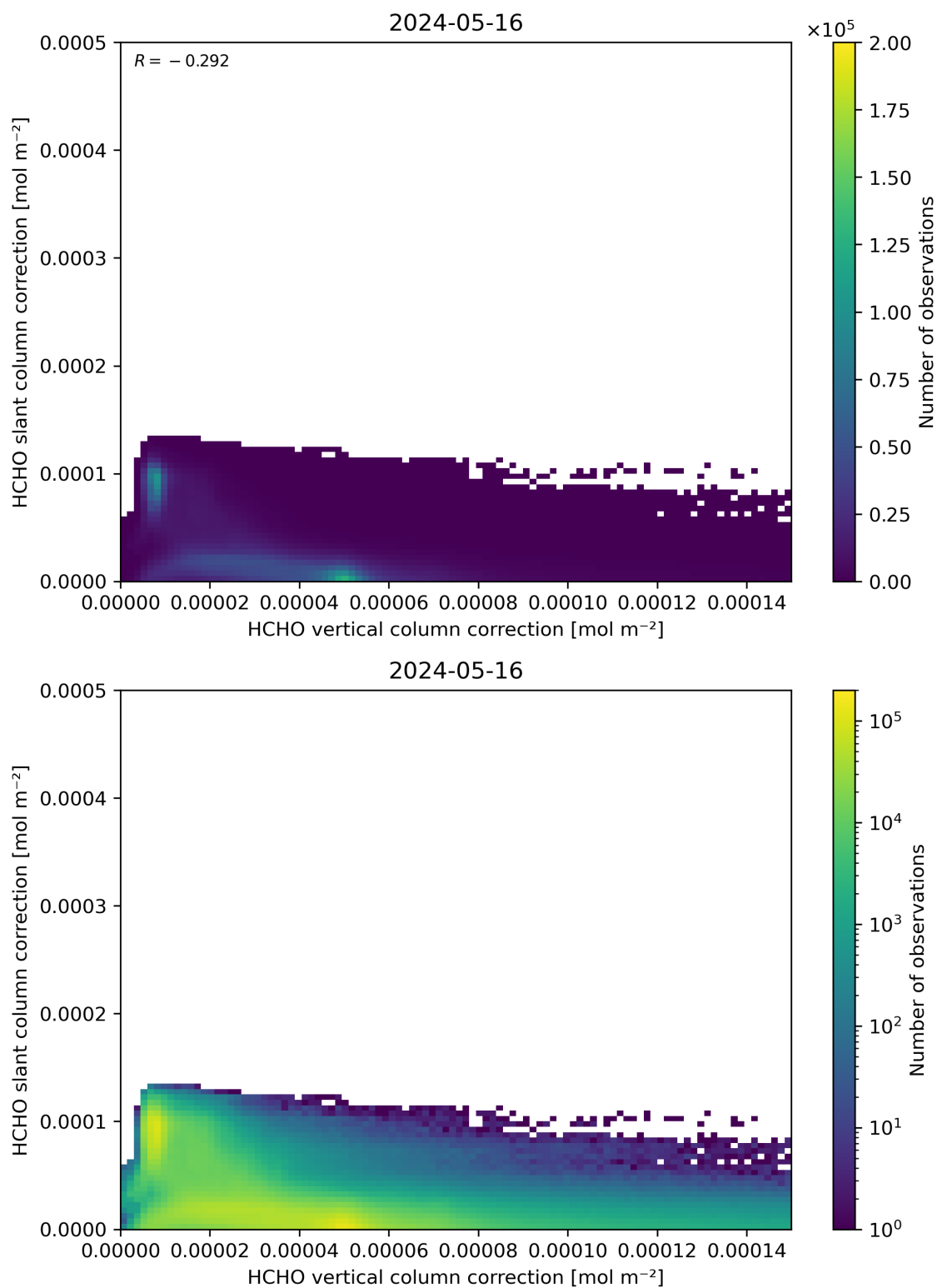
Figure 117: Scatter density plot of “HCHO vertical column correction” against “HCHO slant column correction” for 2024-05-15 to 2024-05-17.
