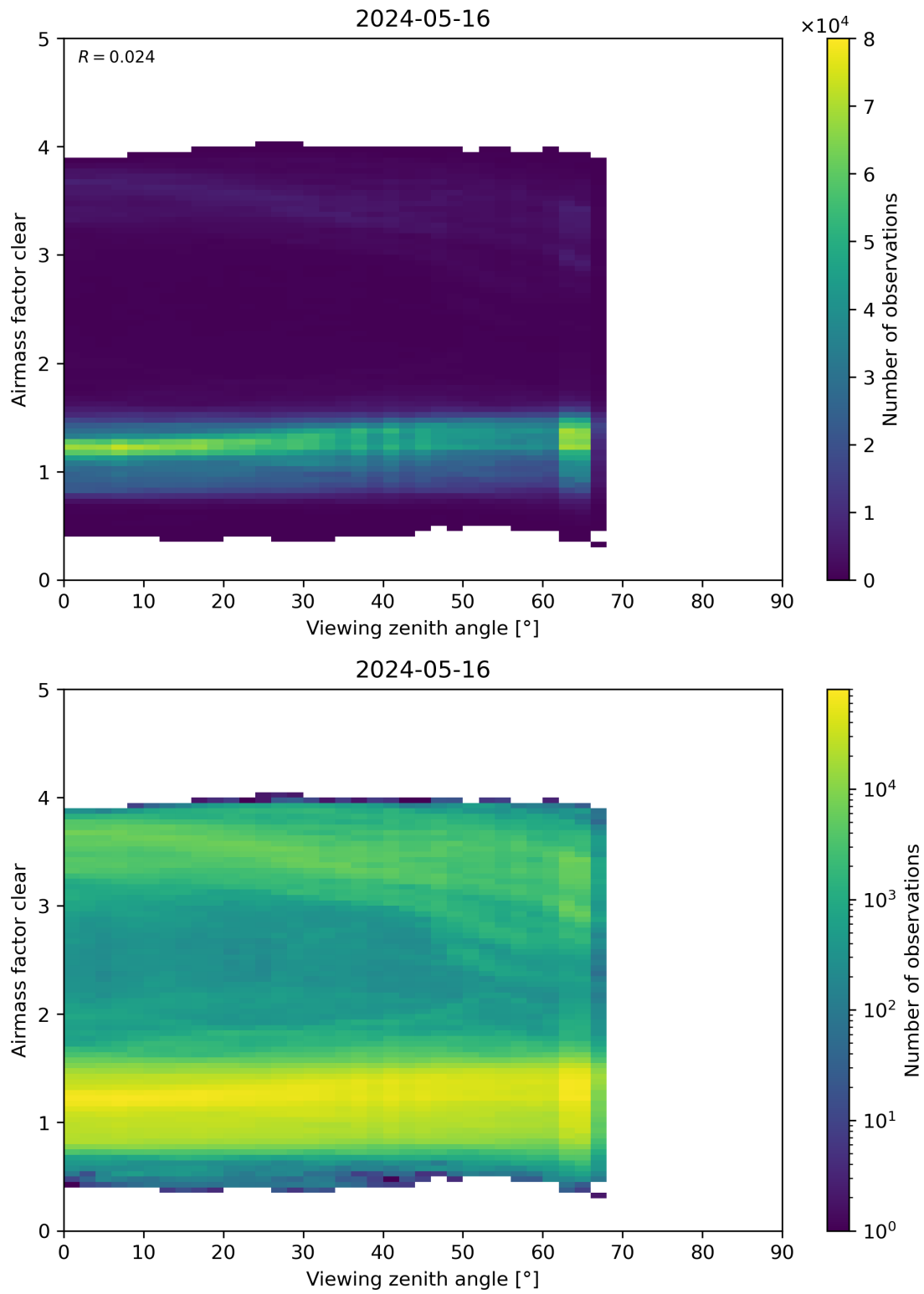
Figure 185: Scatter density plot of “Viewing zenith angle” against “Airmass factor clear” for 2024-05-15 to 2024-05-17.
