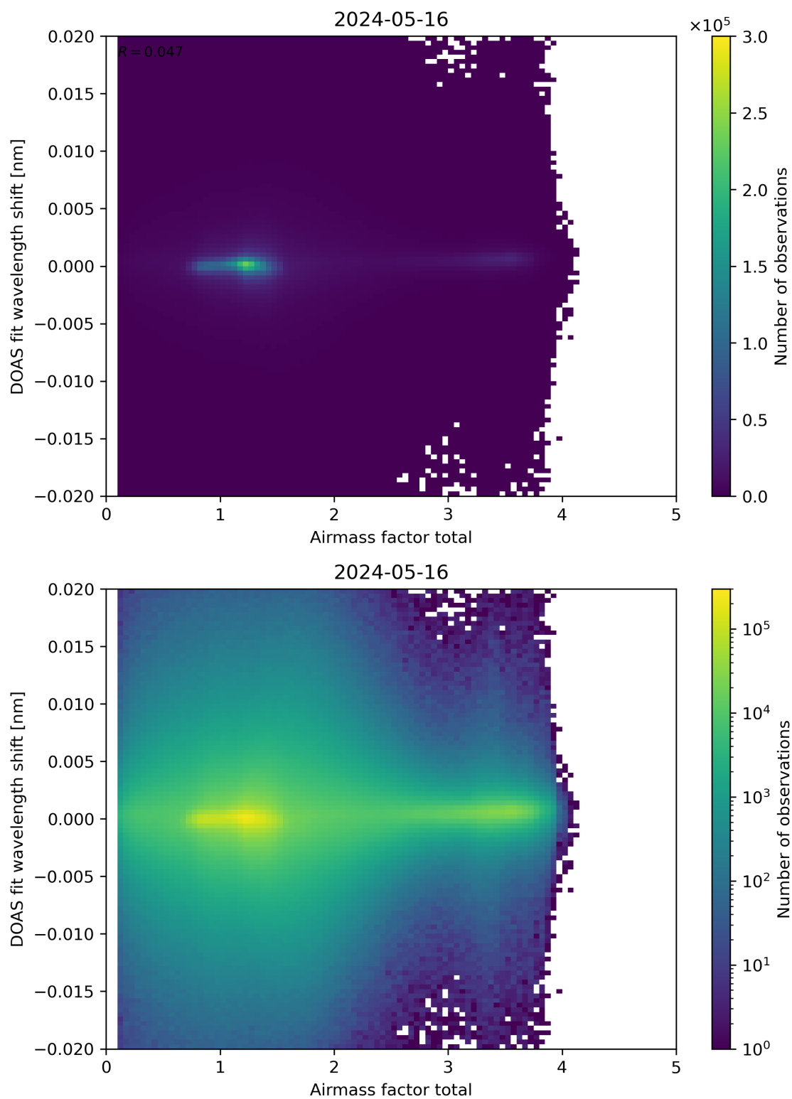
Figure 98: Scatter density plot of “Airmass factor total” against “DOAS fit wavelength shift” for 2024-05-15 to 2024-05-17.
