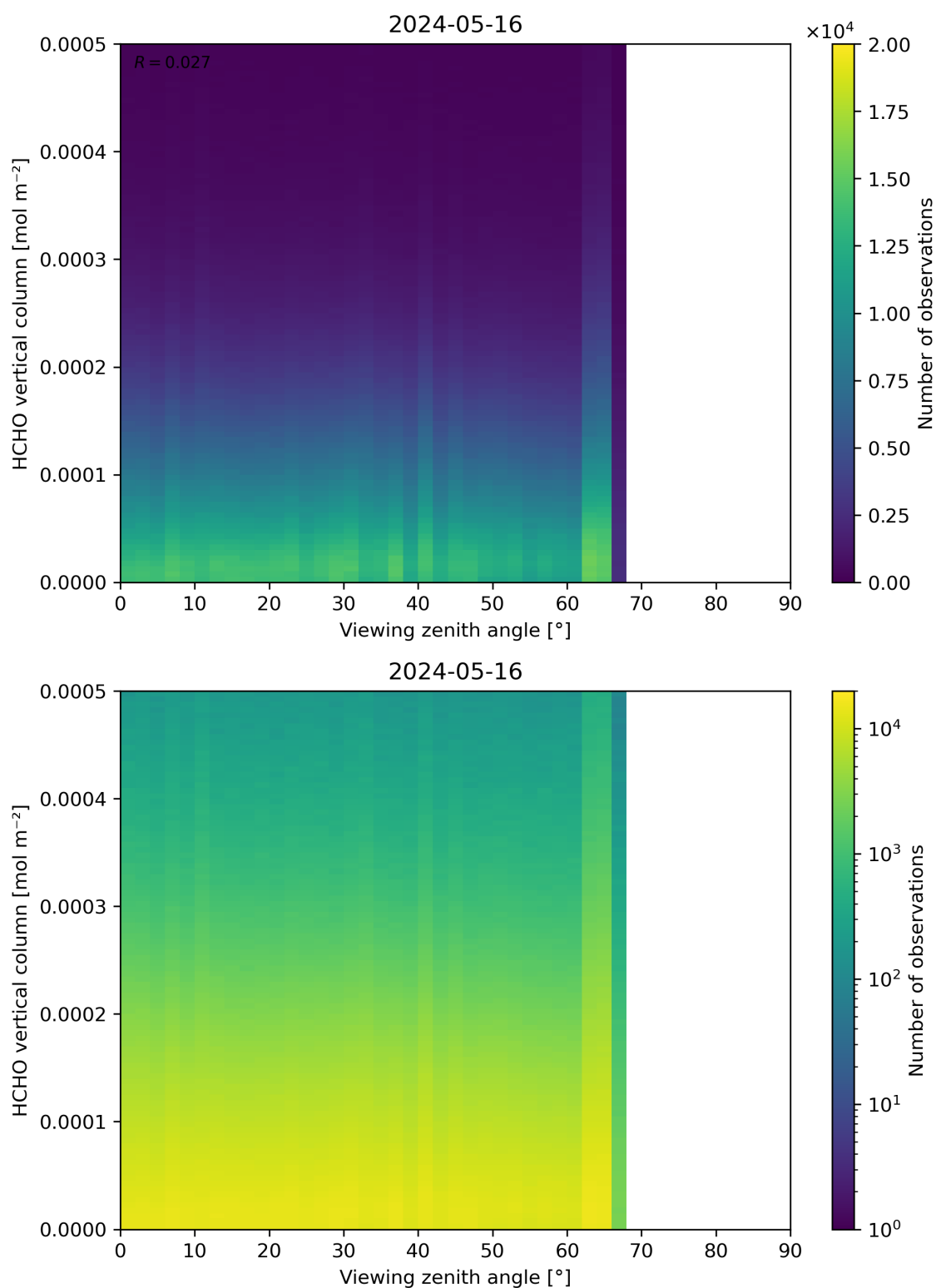
Figure 192: Scatter density plot of “Viewing zenith angle” against “HCHO vertical column” for 2024-05-15 to 2024-05-17.
