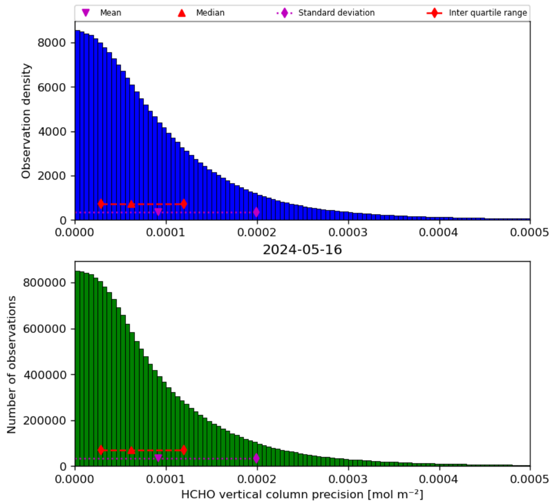
Figure 36: Histogram of “HCHO vertical column precision” for 2024-05-15 to 2024-05-17
