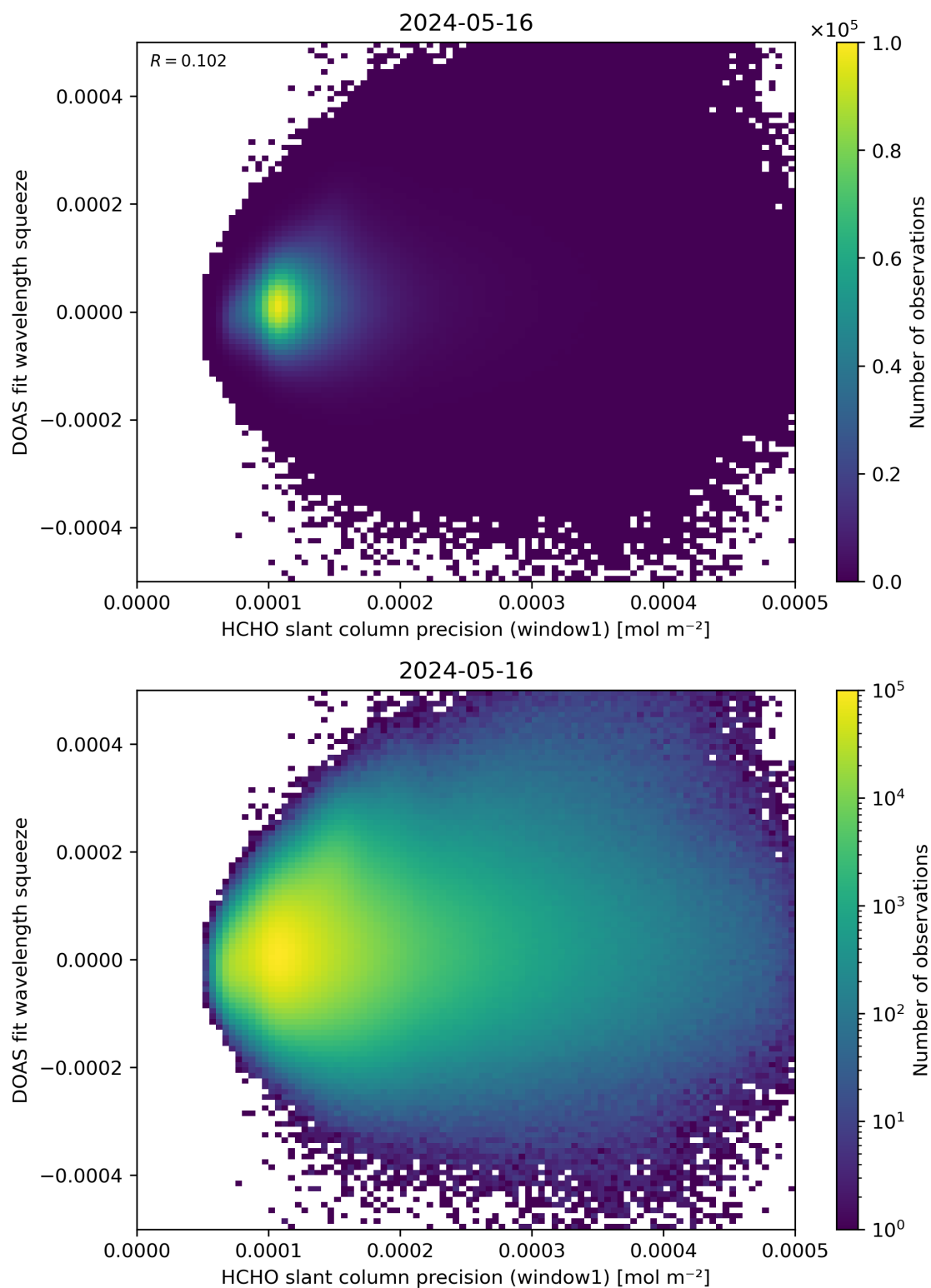
Figure 90: Scatter density plot of “HCHO slant column precision (window1)” against “DOAS fit wavelength squeeze” for 2024-05-15 to 2024-05-17.
