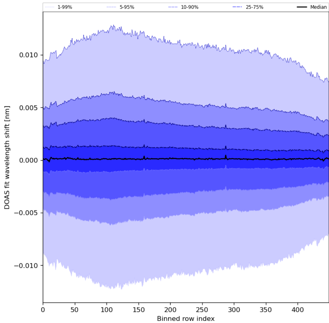
Figure 58: Along track statistics of “DOAS fit wavelength shift” for 2024-05-15 to 2024-05-17
