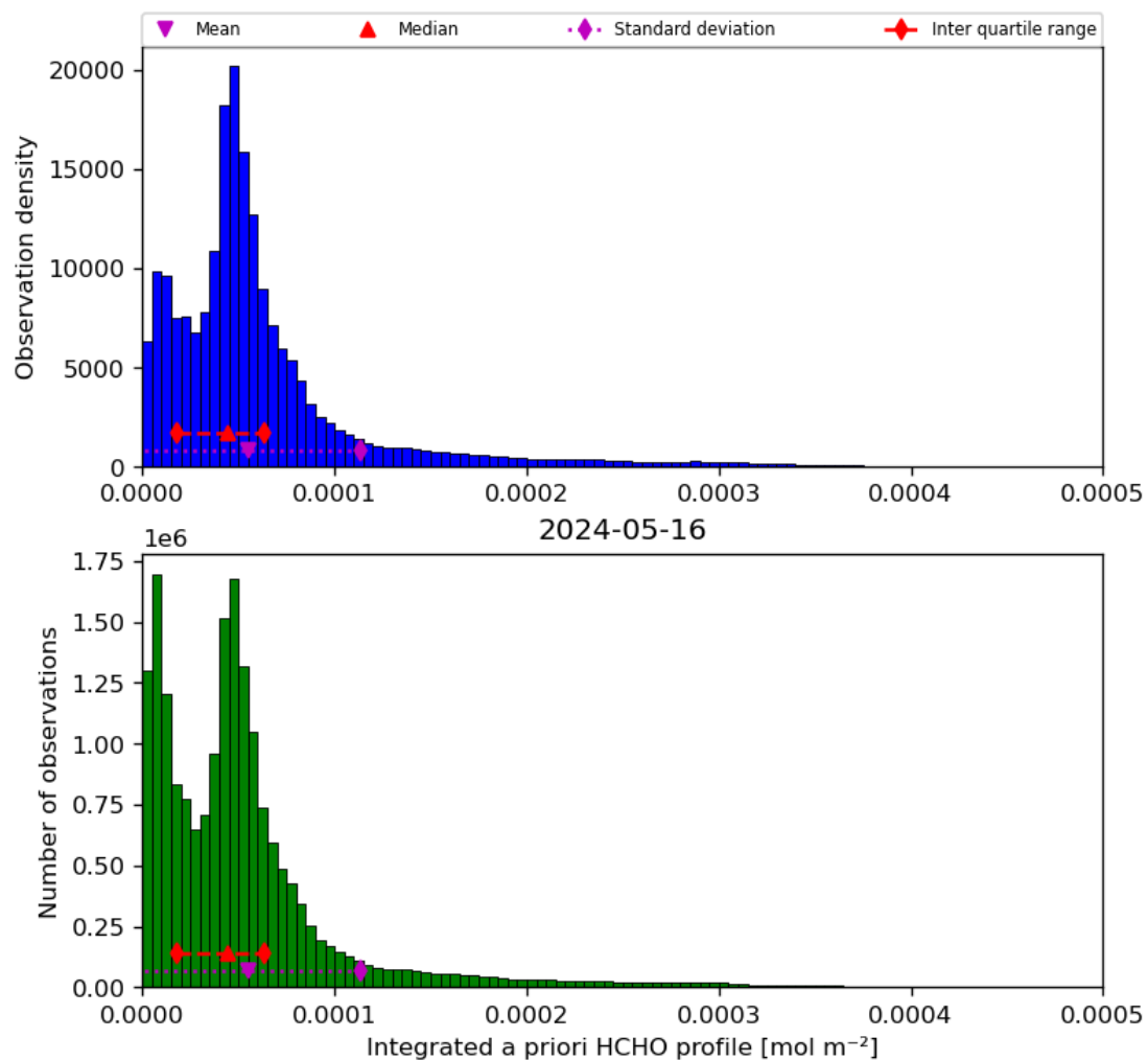
Figure 43: Histogram of “Integrated a priori HCHO profile” for 2024-05-15 to 2024-05-17
