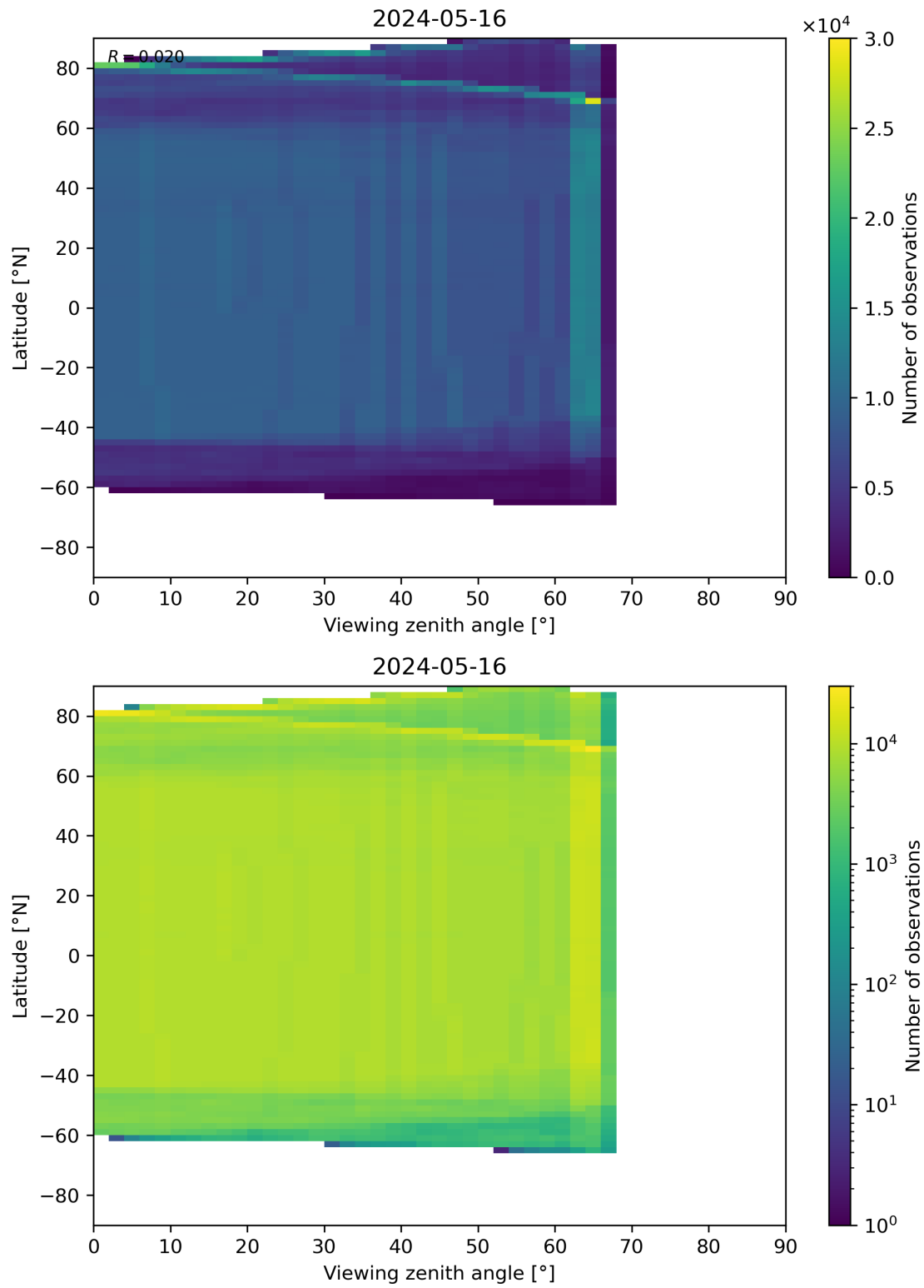
Figure 196: Scatter density plot of “Viewing zenith angle” against “Latitude” for 2024-05-15 to 2024-05-17.
