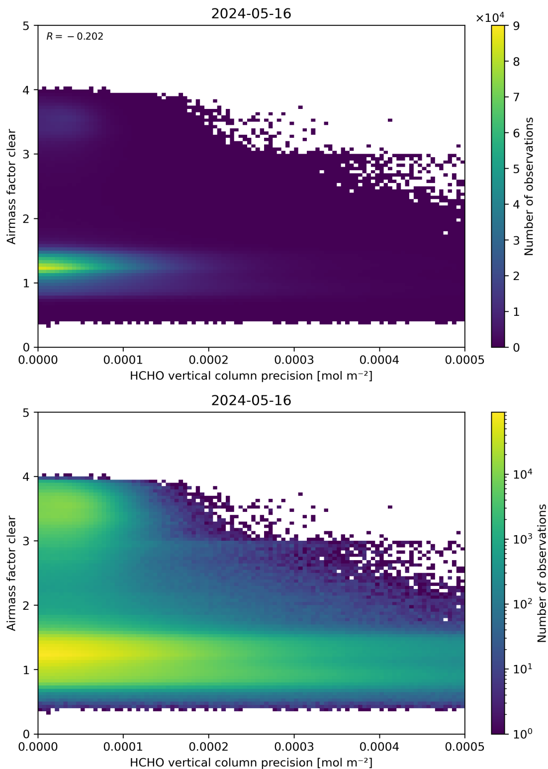
Figure 139: Scatter density plot of “HCHO vertical column precision” against “Airmass factor clear” for 2024-05-15 to 2024-05-17.
