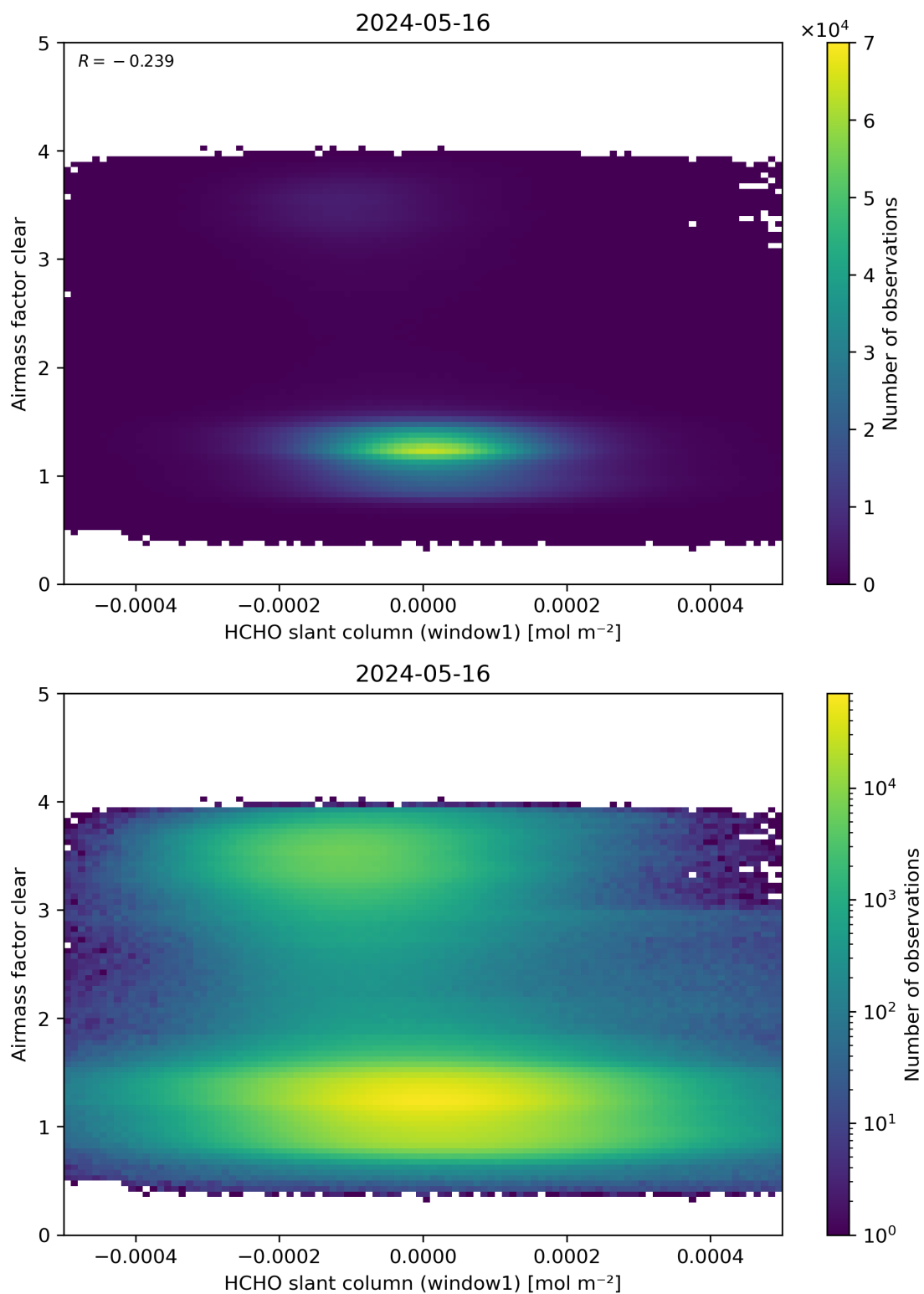
Figure 81: Scatter density plot of “HCHO slant column (window1)” against “Airmass factor clear” for 2024-05-15 to 2024-05-17.
