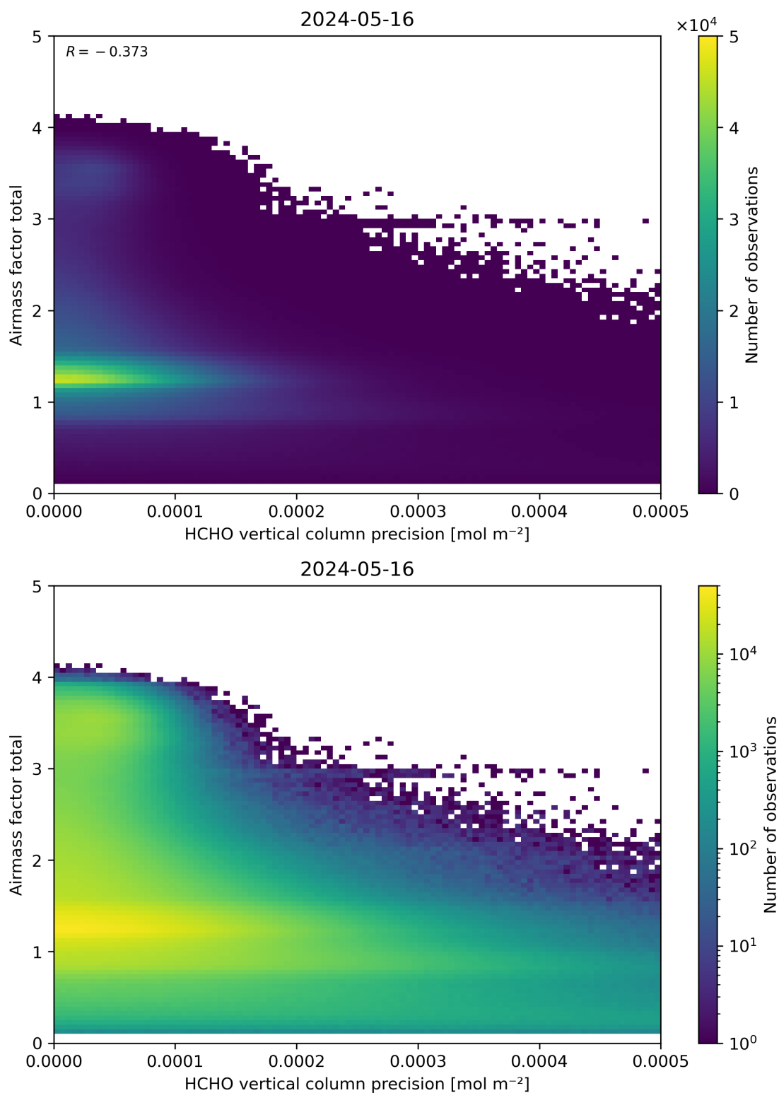
Figure 144: Scatter density plot of “HCHO vertical column precision” against “Airmass factor total” for 2024-05-15 to 2024-05-17.
