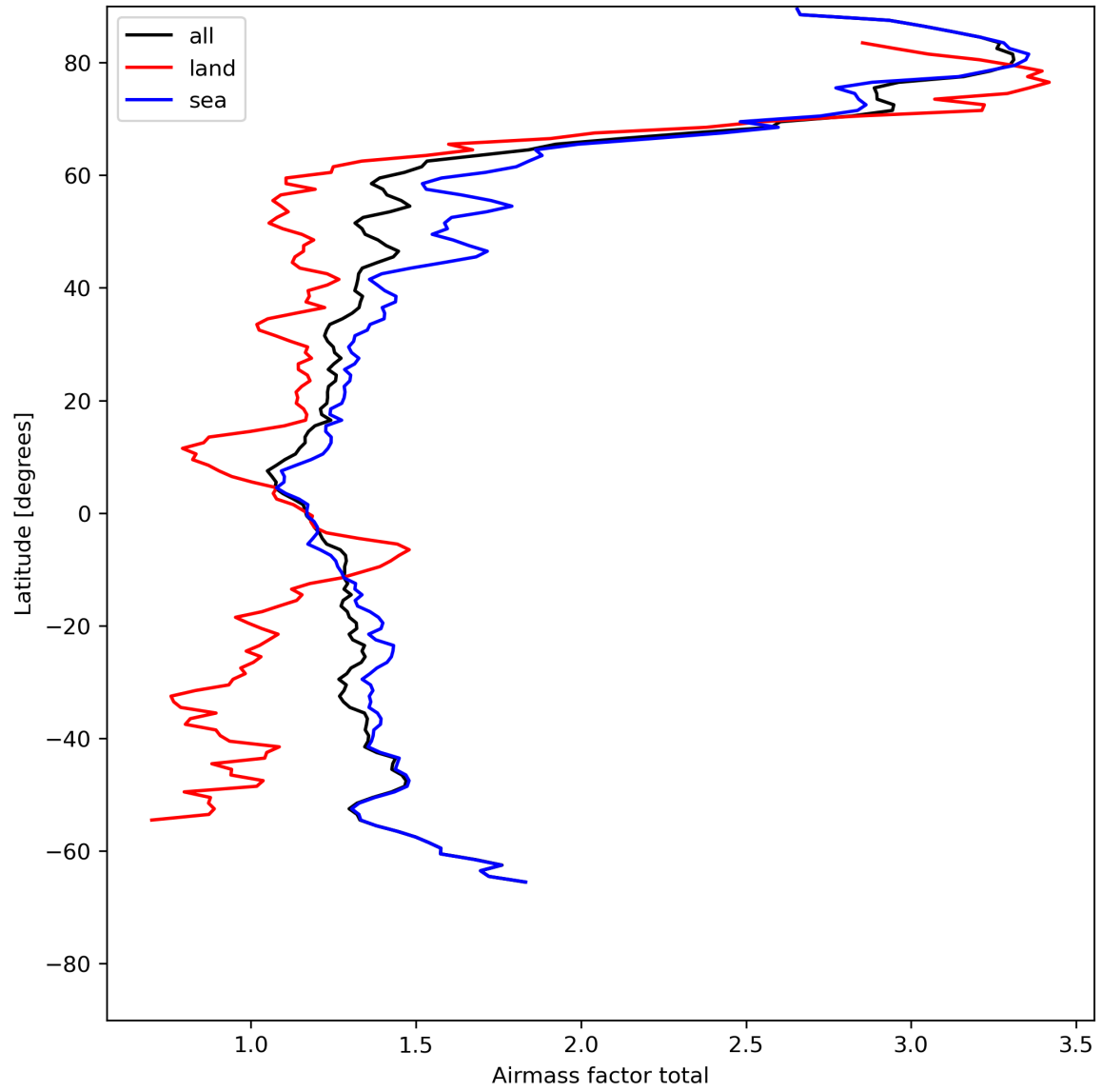
Figure 26: Zonal average of “Airmass factor total” for 2024-05-15 to 2024-05-17.
