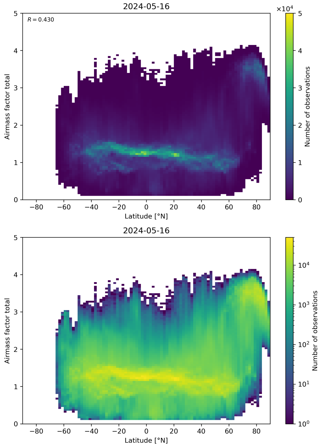
Figure 161: Scatter density plot of “Latitude” against “Airmass factor total” for 2024-05-15 to 2024-05-17.
