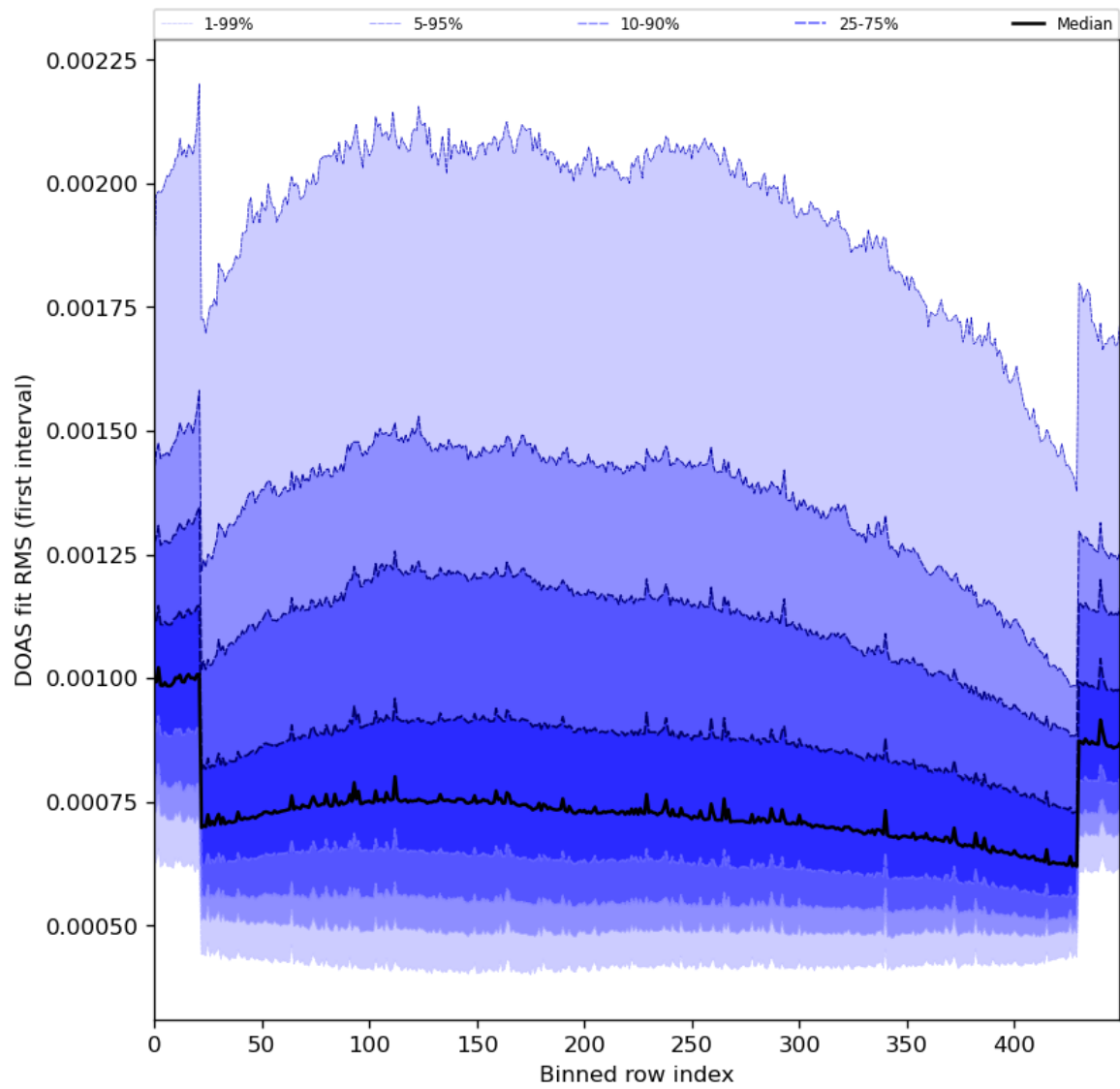
Figure 60: Along track statistics of “DOAS fit RMS (first interval)” for 2024-05-15 to 2024-05-17
