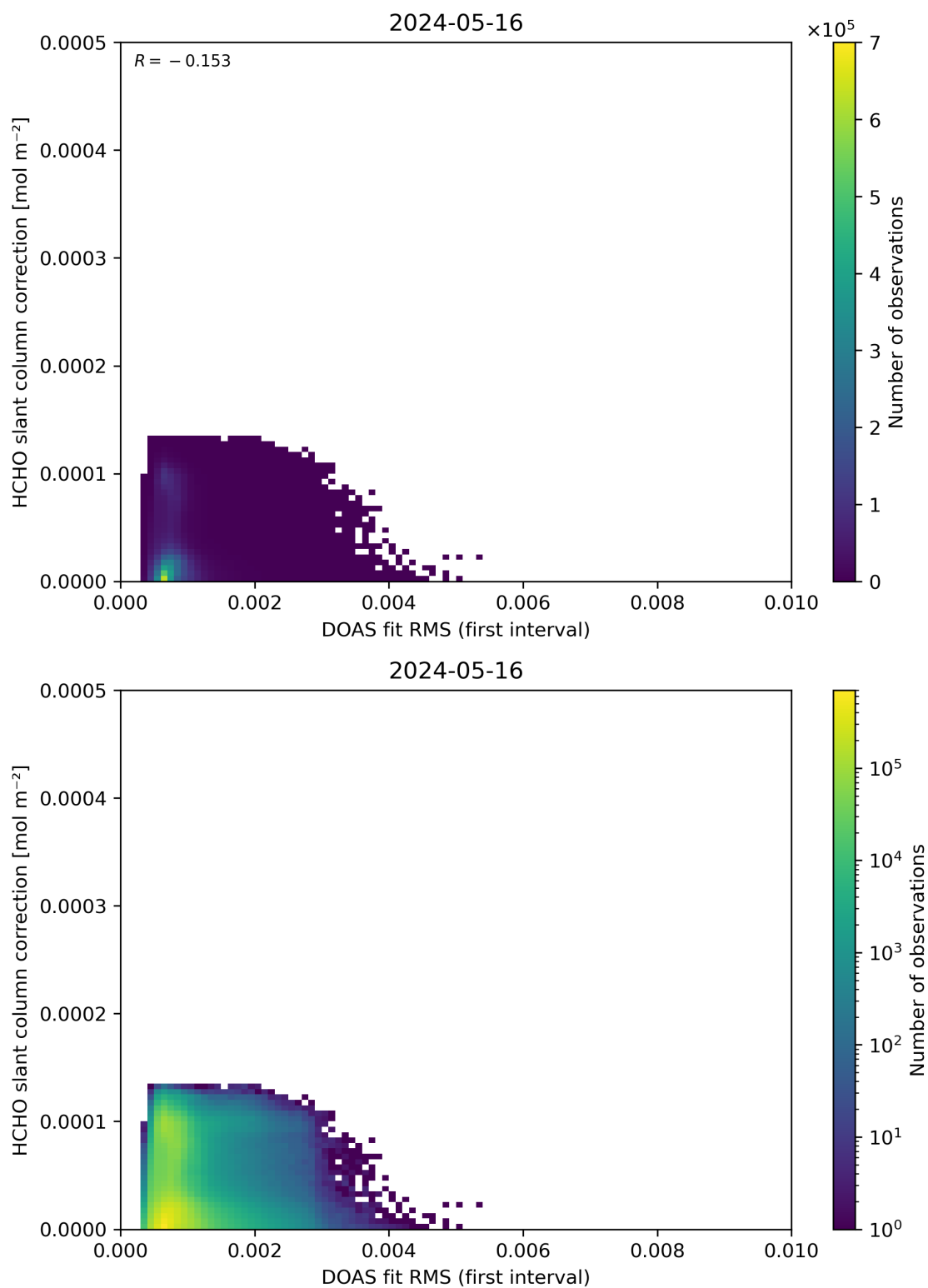
Figure 63: Scatter density plot of “DOAS fit RMS (first interval)” against “HCHO slant column correction” for 2024-05-15 to 2024-05-17.
