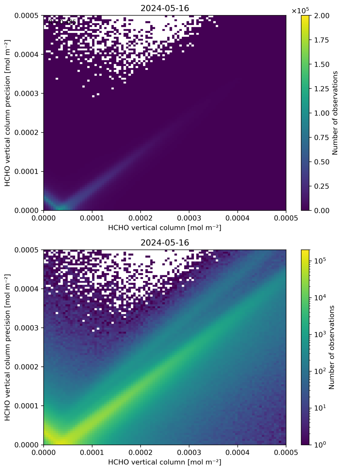
Figure 134: Scatter density plot of “HCHO vertical column” against “HCHO vertical column precision” for 2024-05-15 to 2024-05-17.
