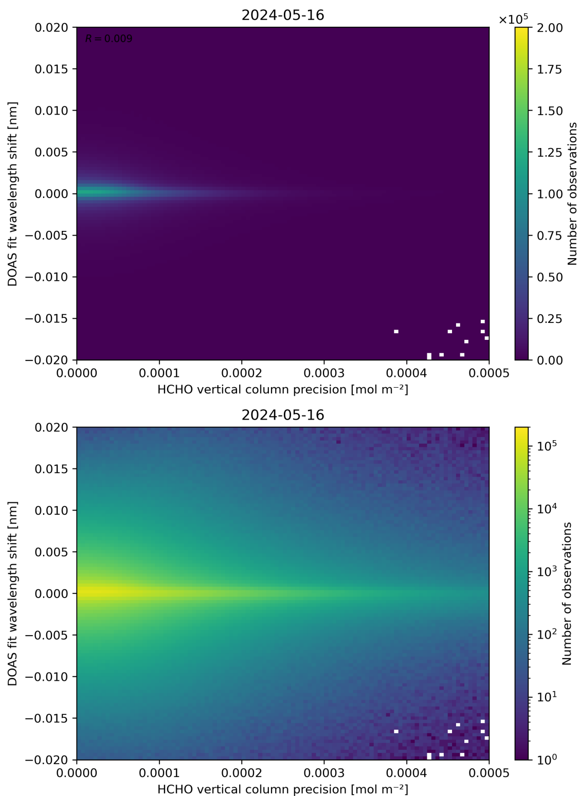
Figure 137: Scatter density plot of “HCHO vertical column precision” against “DOAS fit wavelength shift” for 2024-05-15 to 2024-05-17.
