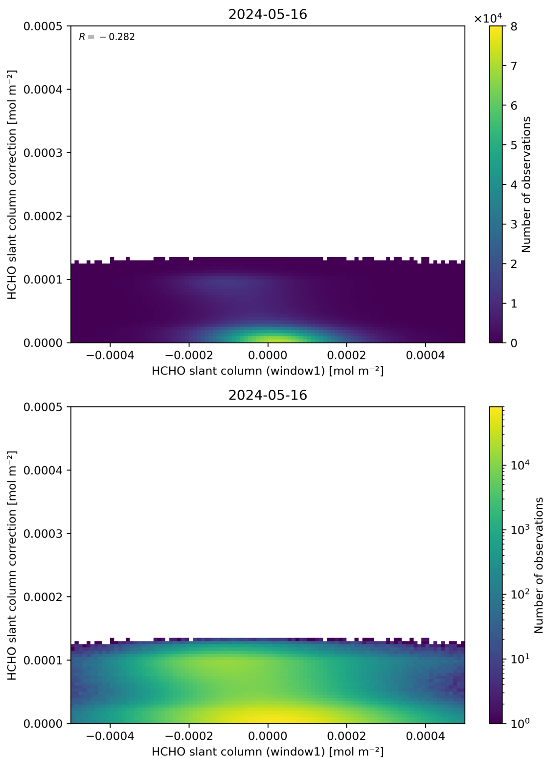
Figure 83: Scatter density plot of “HCHO slant column (window1)” against “HCHO slant column correction” for 2024-05-15 to 2024-05-17.
