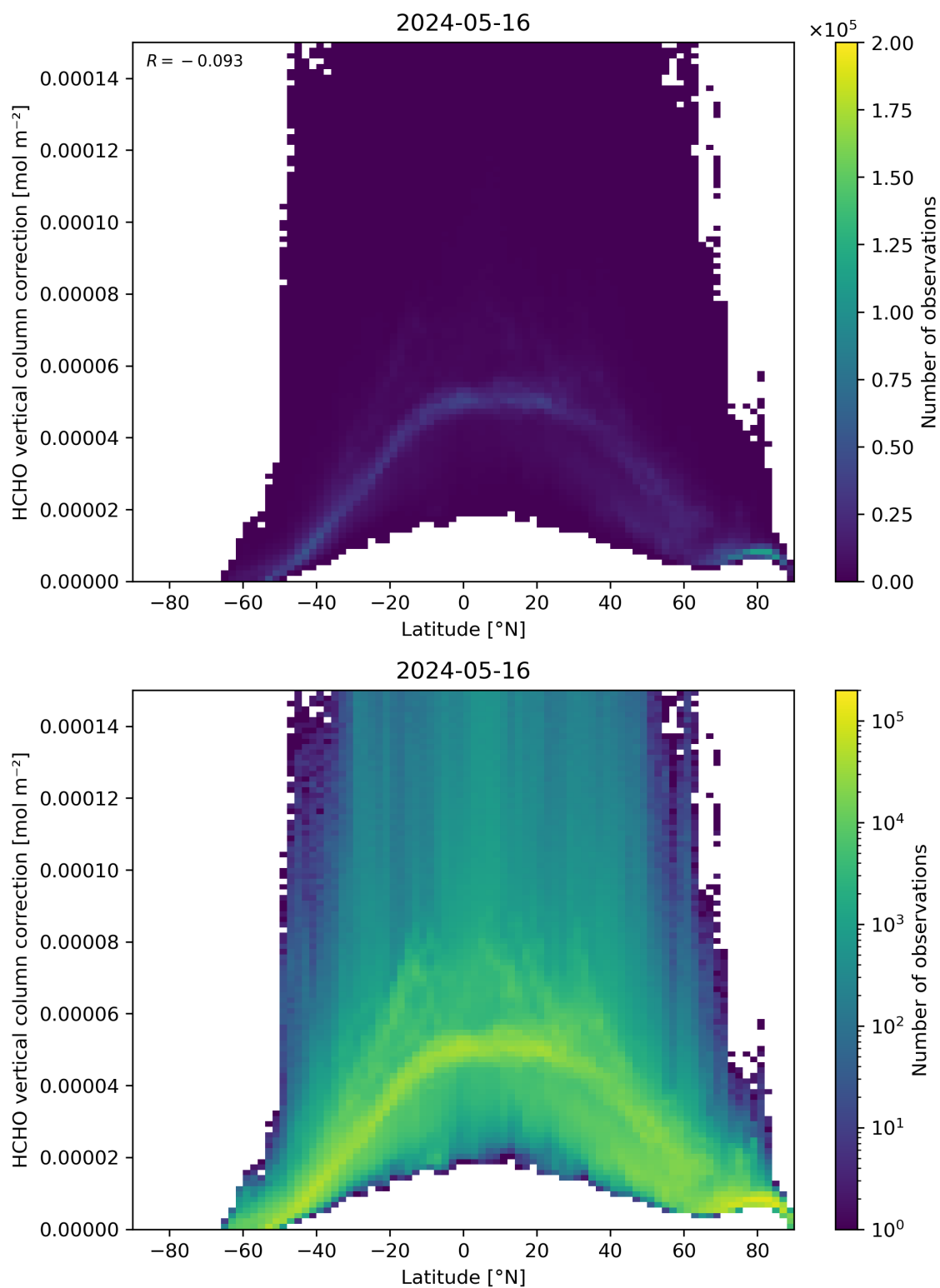
Figure 164: Scatter density plot of “Latitude” against “HCHO vertical column correction” for 2024-05-15 to 2024-05-17.
