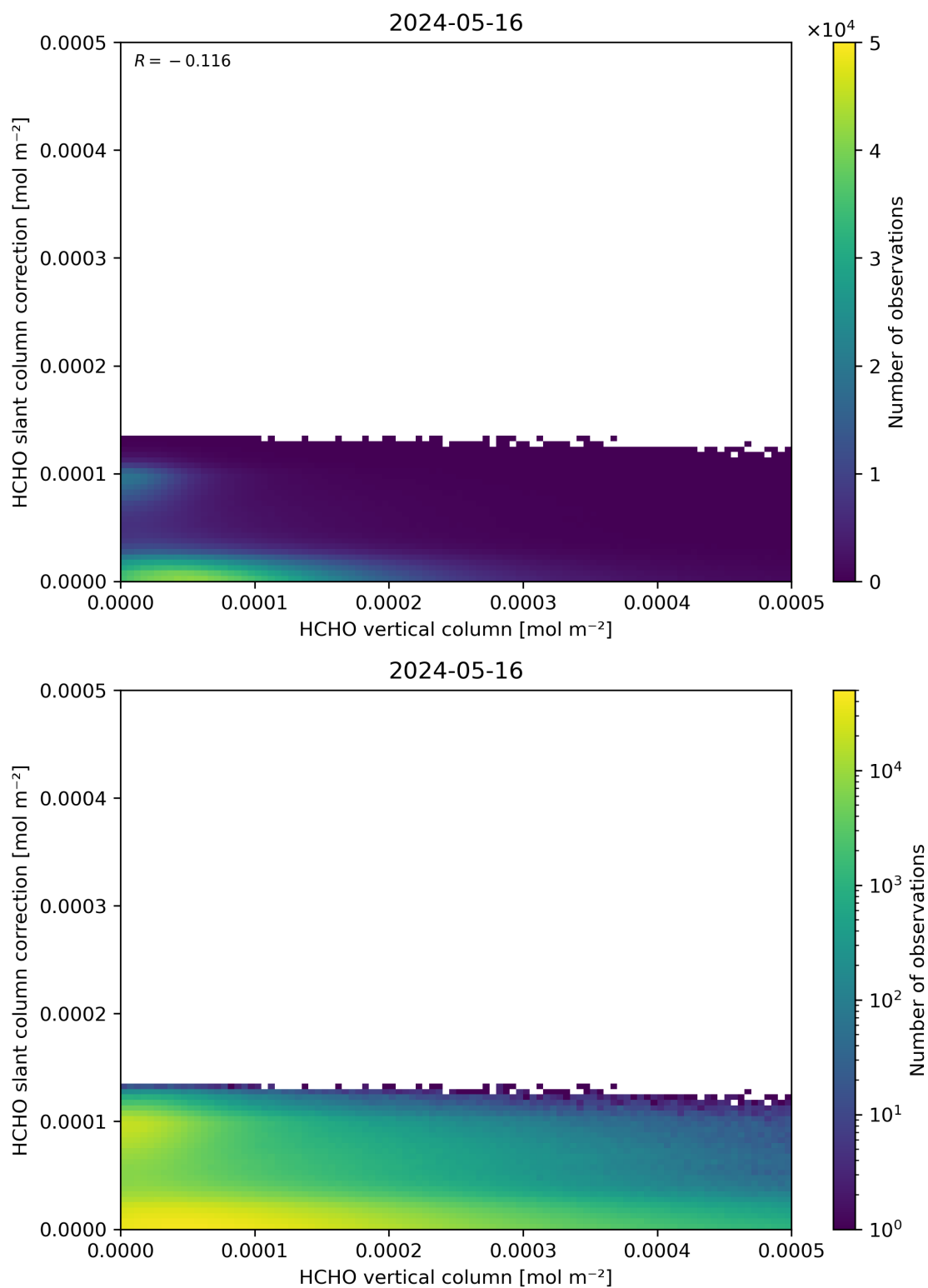
Figure 128: Scatter density plot of “HCHO vertical column” against “HCHO slant column correction” for 2024-05-15 to 2024-05-17.
