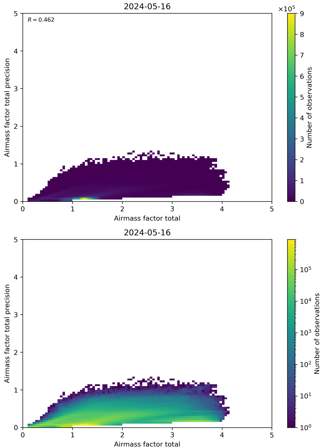
Figure 103: Scatter density plot of “Airmass factor total” against “Airmass factor total precision” for 2024-05-15 to 2024-05-17.
