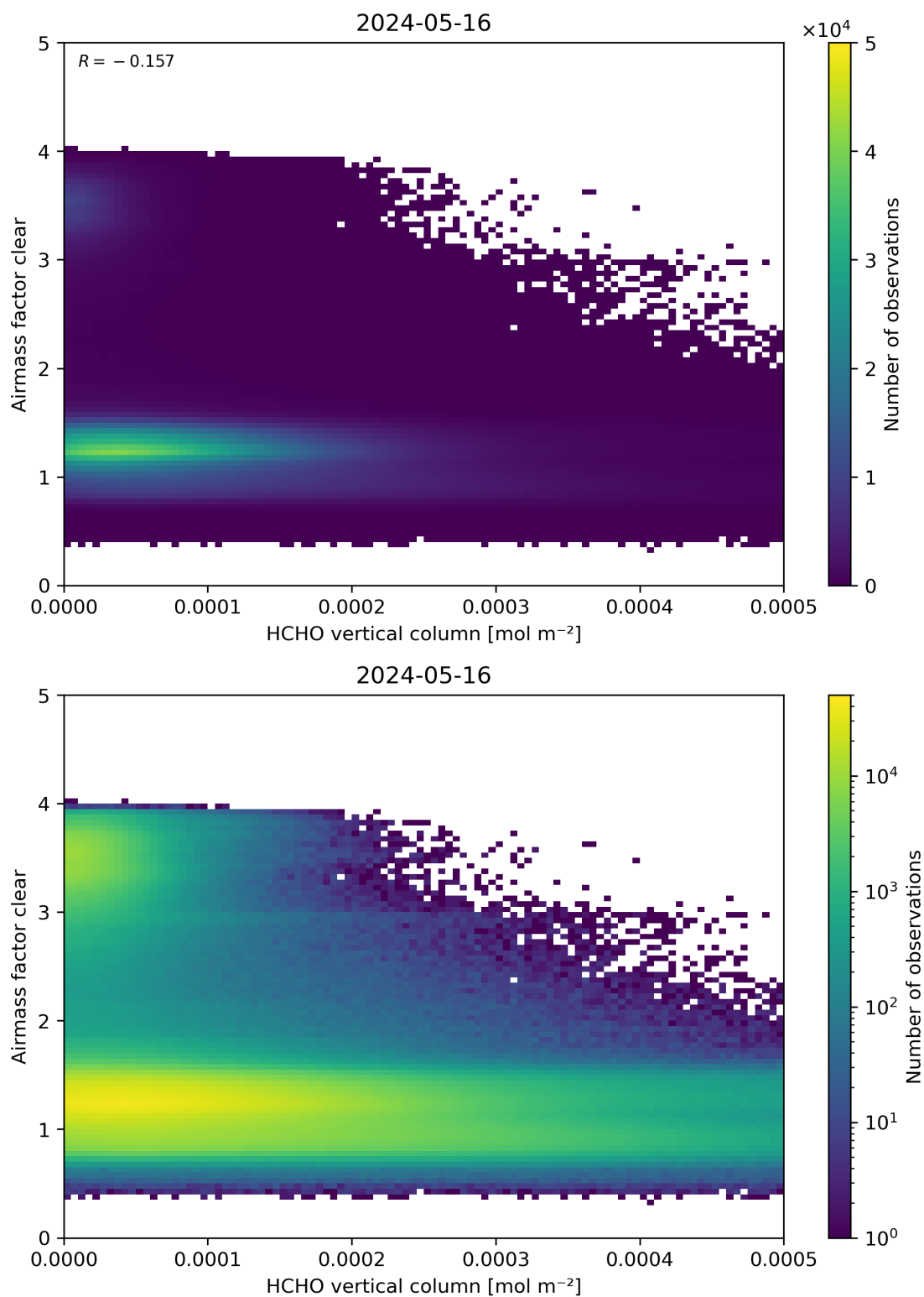
Figure 126: Scatter density plot of “HCHO vertical column” against “Airmass factor clear” for 2024-05-15 to 2024-05-17.
