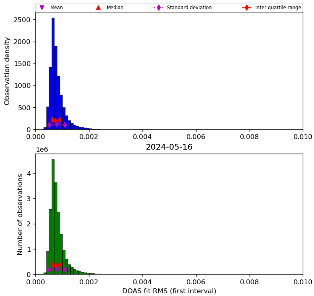
Figure 46: Histogram of “DOAS fit RMS (first interval)” for 2024-05-15 to 2024-05-17
