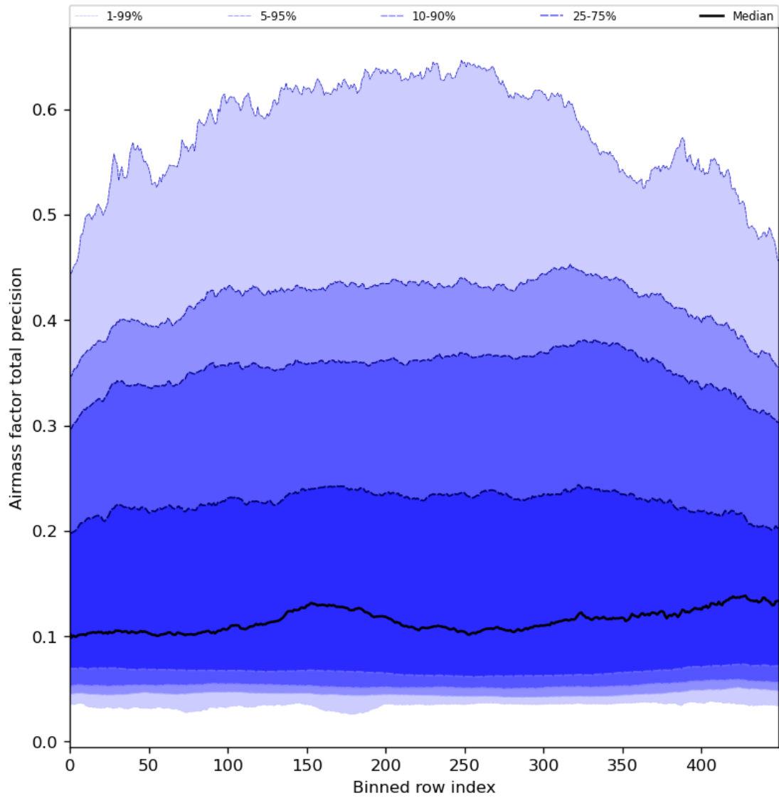
Figure 55: Along track statistics of “Airmass factor total precision” for 2024-05-15 to 2024-05-17
