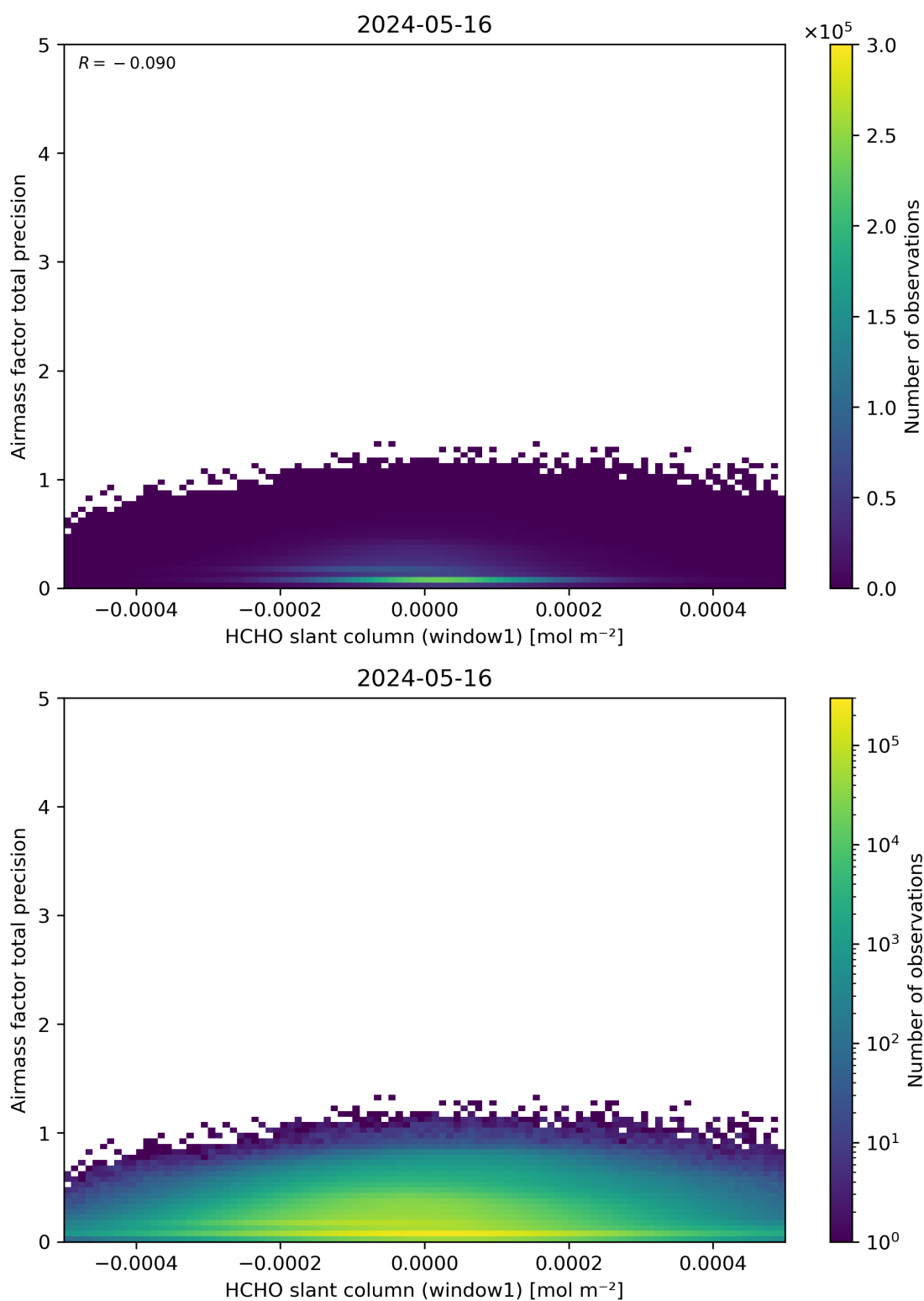
Figure 86: Scatter density plot of “HCHO slant column (window1)” against “Airmass factor total precision” for 2024-05-15 to 2024-05-17.
