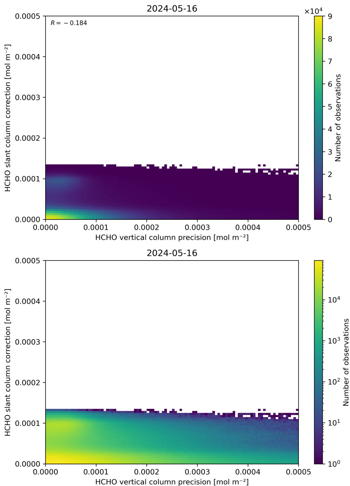
Figure 141: Scatter density plot of “HCHO vertical column precision” against “HCHO slant column correction” for 2024-05-15 to 2024-05-17.
