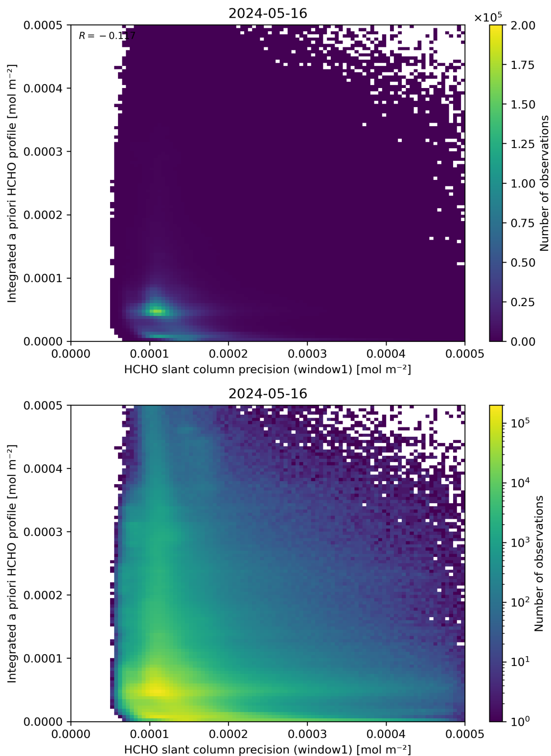
Figure 96: Scatter density plot of “HCHO slant column precision (window1)” against “Integrated a priori HCHO profile” for 2024-05-15 to 2024-05-17.
