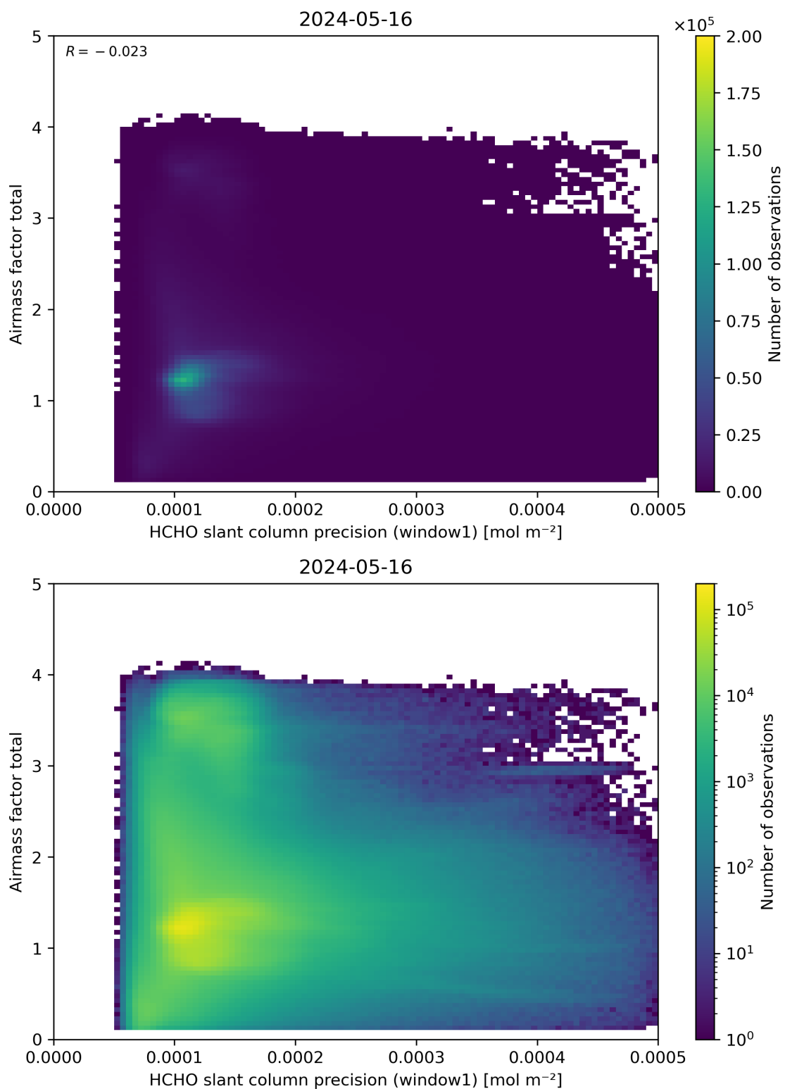
Figure 94: Scatter density plot of “HCHO slant column precision (window1)” against “Airmass factor total” for 2024-05-15 to 2024-05-17.
