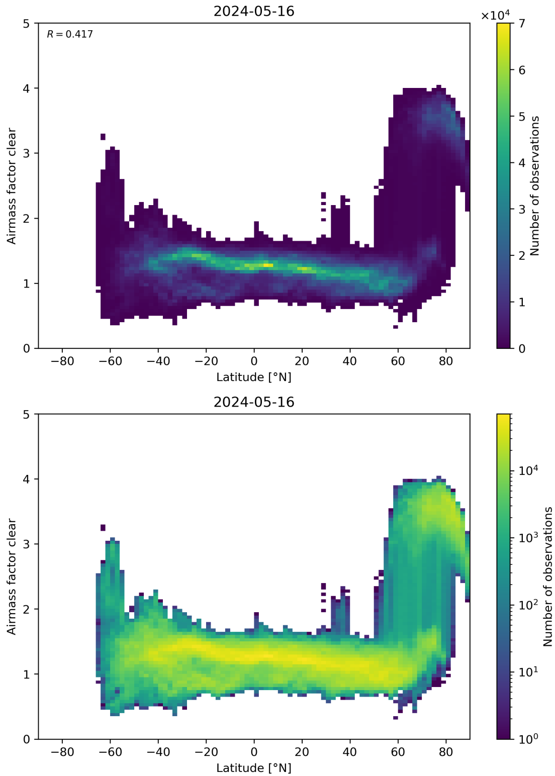
Figure 156: Scatter density plot of “Latitude” against “Airmass factor clear” for 2024-05-15 to 2024-05-17.
