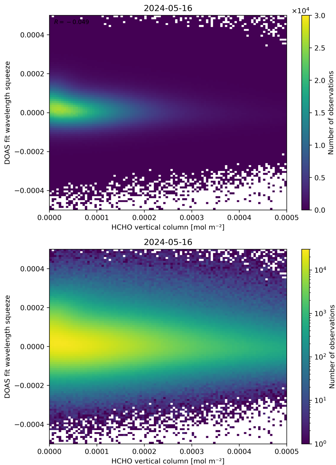
Figure 125: Scatter density plot of “HCHO vertical column” against “DOAS fit wavelength squeeze” for 2024-05-15 to 2024-05-17.
