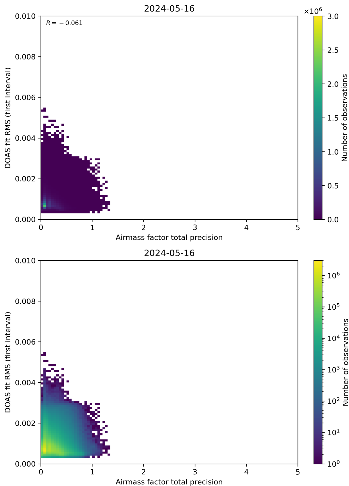
Figure 105: Scatter density plot of “Airmass factor total precision” against “DOAS fit RMS (first interval)” for 2024-05-15 to 2024-05-17.
