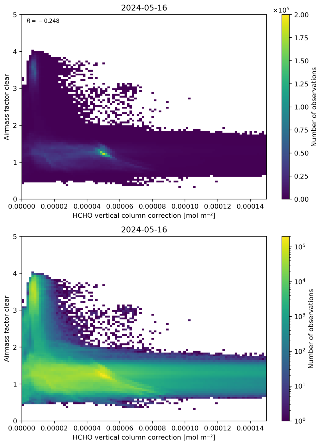
Figure 115: Scatter density plot of “HCHO vertical column correction” against “Airmass factor clear” for 2024-05-15 to 2024-05-17.
