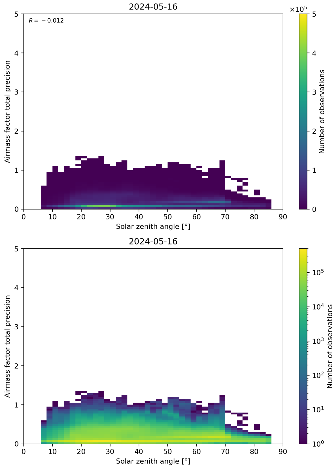
Figure 176: Scatter density plot of “Solar zenith angle” against “Airmass factor total precision” for 2024-05-15 to 2024-05-17.
