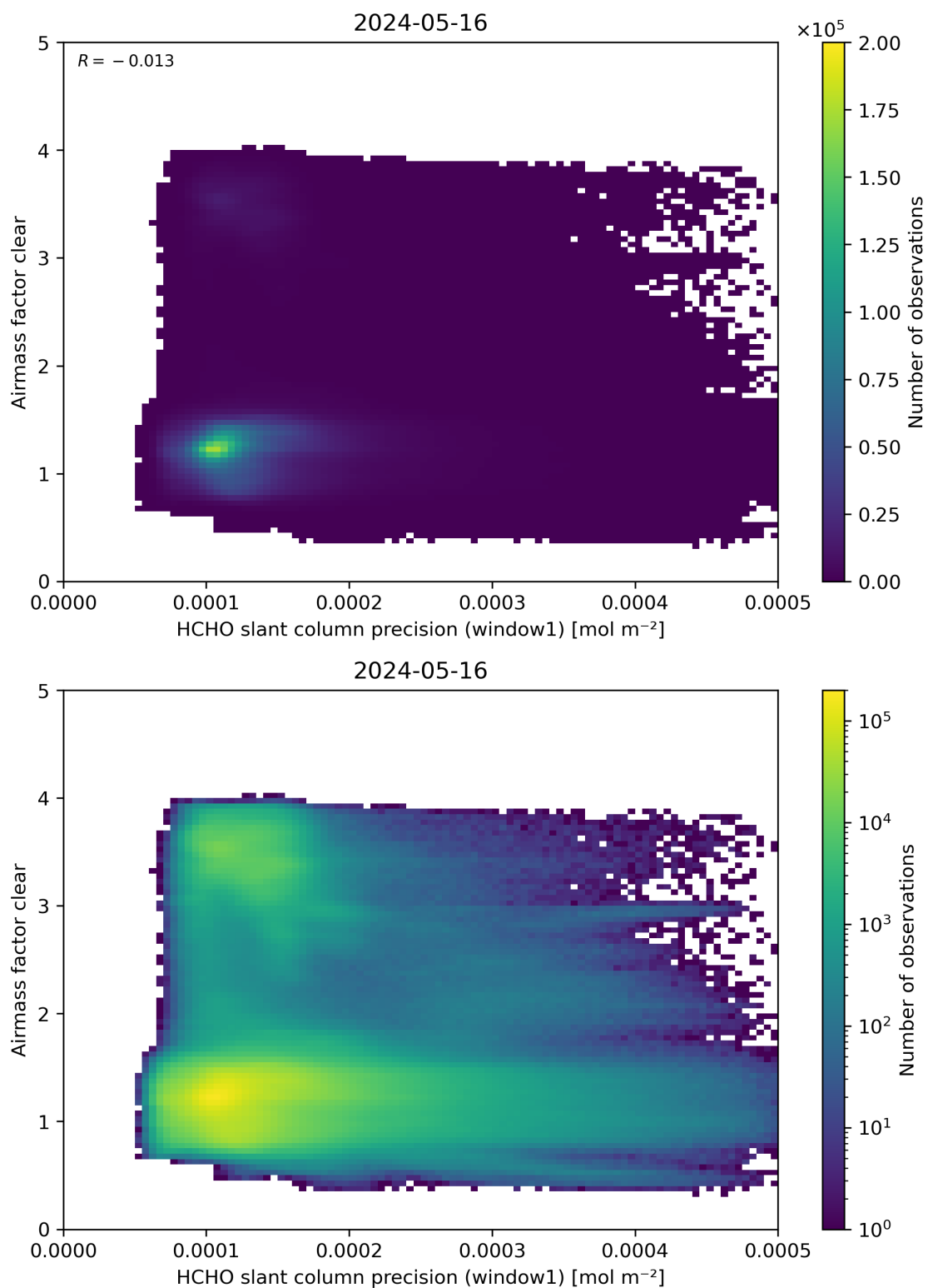
Figure 91: Scatter density plot of “HCHO slant column precision (window1)” against “Airmass factor clear” for 2024-05-15 to 2024-05-17.
