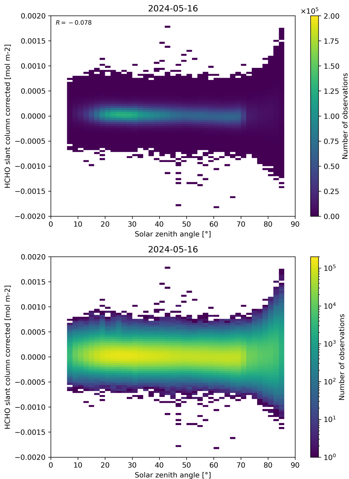
Figure 171: Scatter density plot of “Solar zenith angle” against “HCHO slant column corrected” for 2024-05-15 to 2024-05-17.
