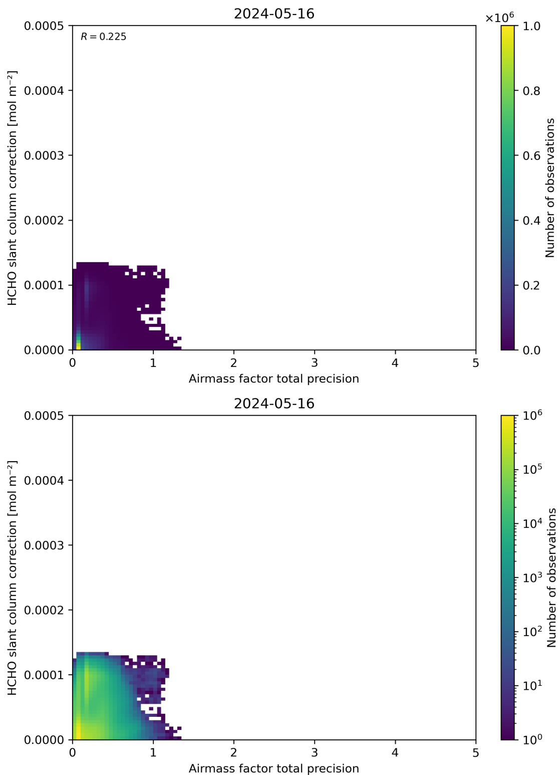
Figure 110: Scatter density plot of “Airmass factor total precision” against “HCHO slant column correction” for 2024-05-15 to 2024-05-17.
