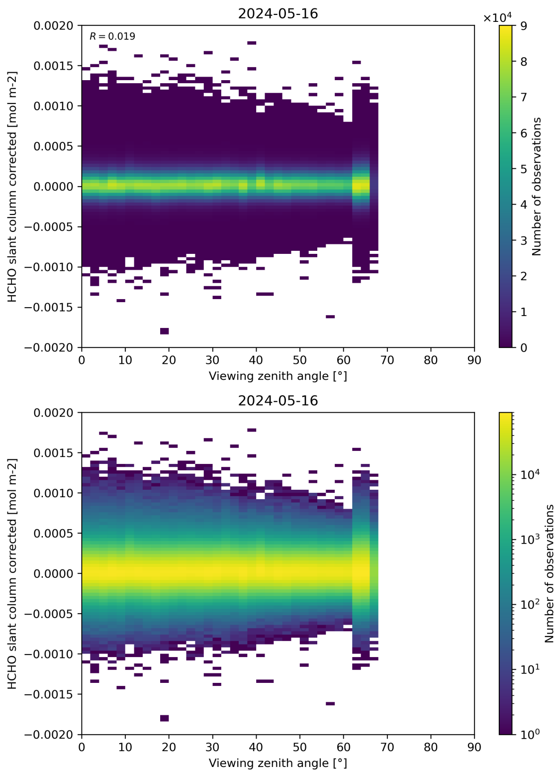
Figure 186: Scatter density plot of “Viewing zenith angle” against “HCHO slant column corrected” for 2024-05-15 to 2024-05-17.
