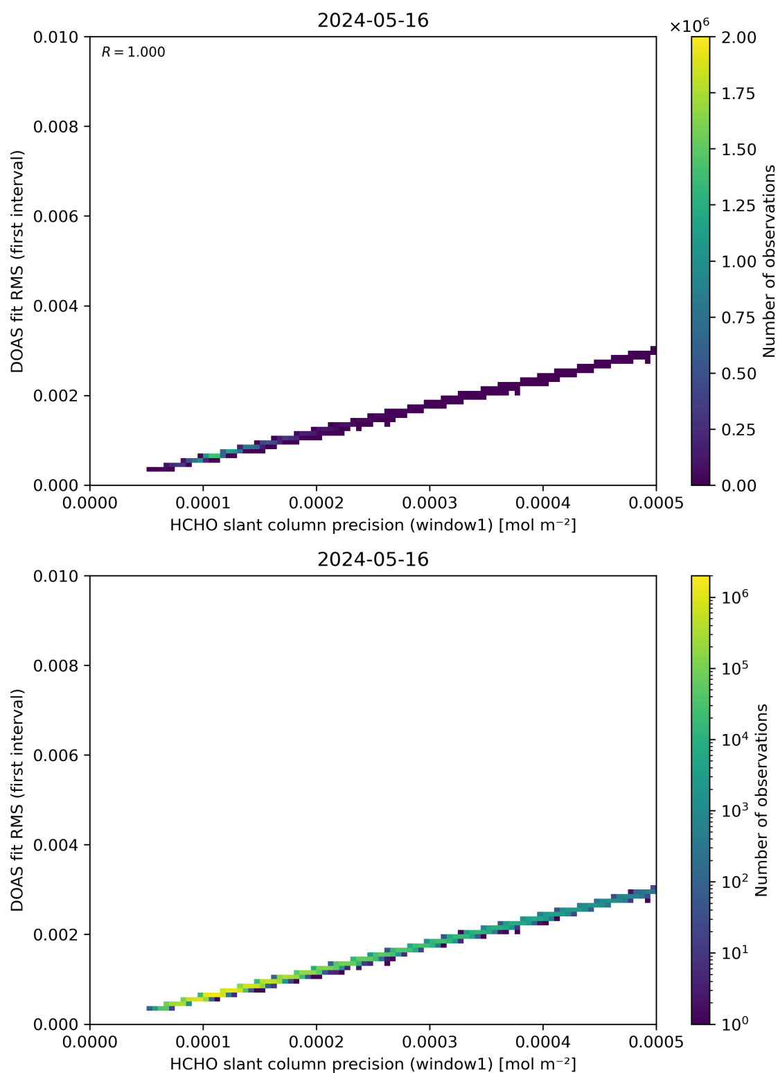
Figure 88: Scatter density plot of “HCHO slant column precision (window1)” against “DOAS fit RMS (first interval)” for 2024-05-15 to 2024-05-17.
