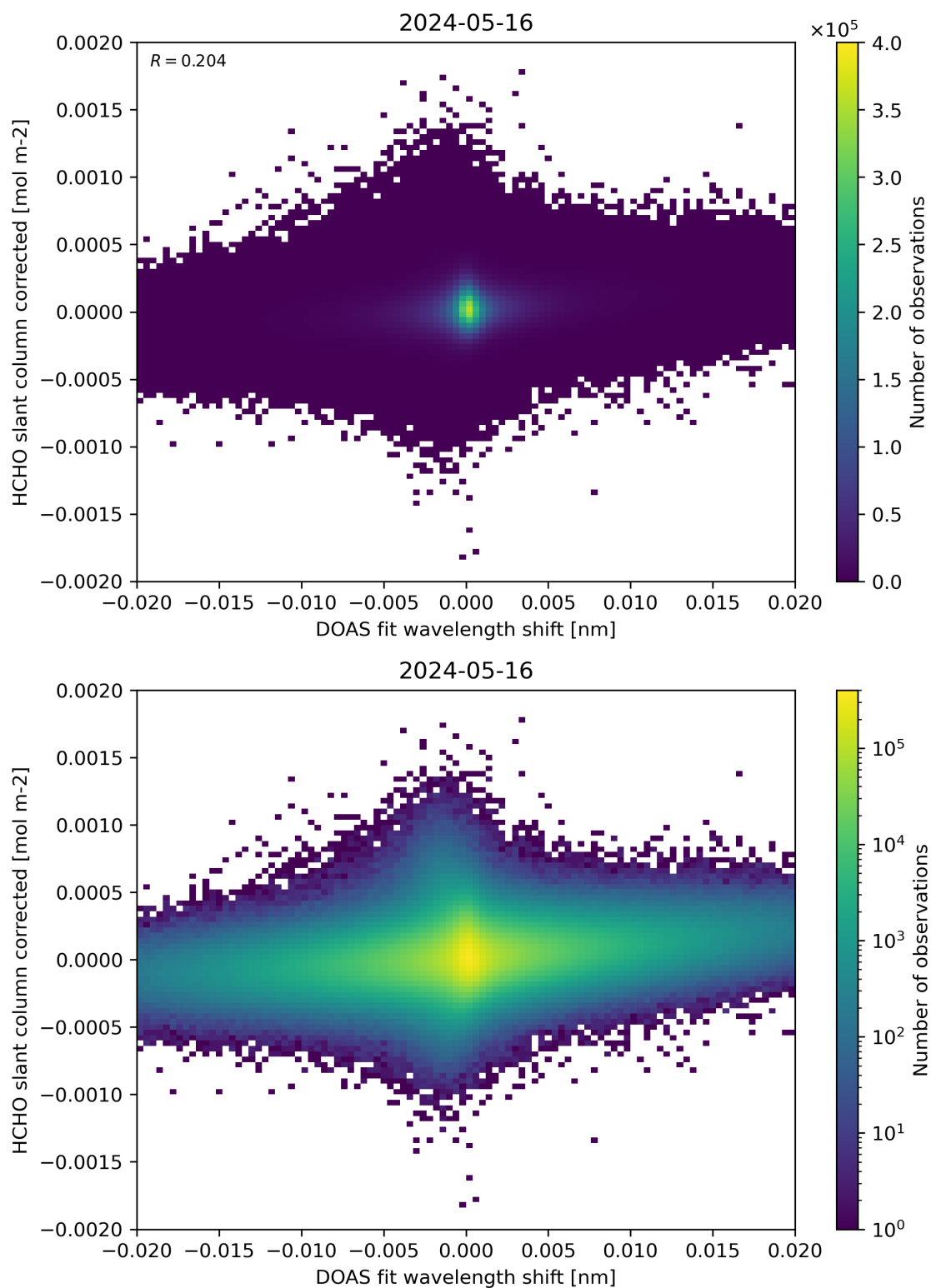
Figure 66: Scatter density plot of “DOAS fit wavelength shift” against “HCHO slant column corrected” for 2024-05-15 to 2024-05-17.
