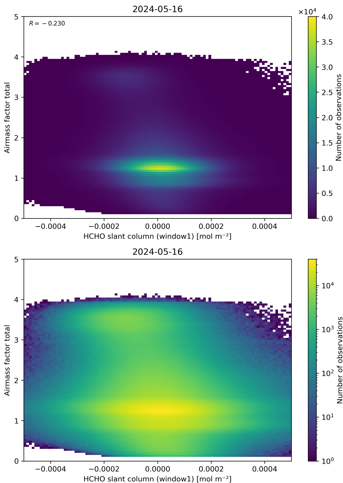
Figure 85: Scatter density plot of “HCHO slant column (window1)” against “Airmass factor total” for 2024-05-15 to 2024-05-17.
