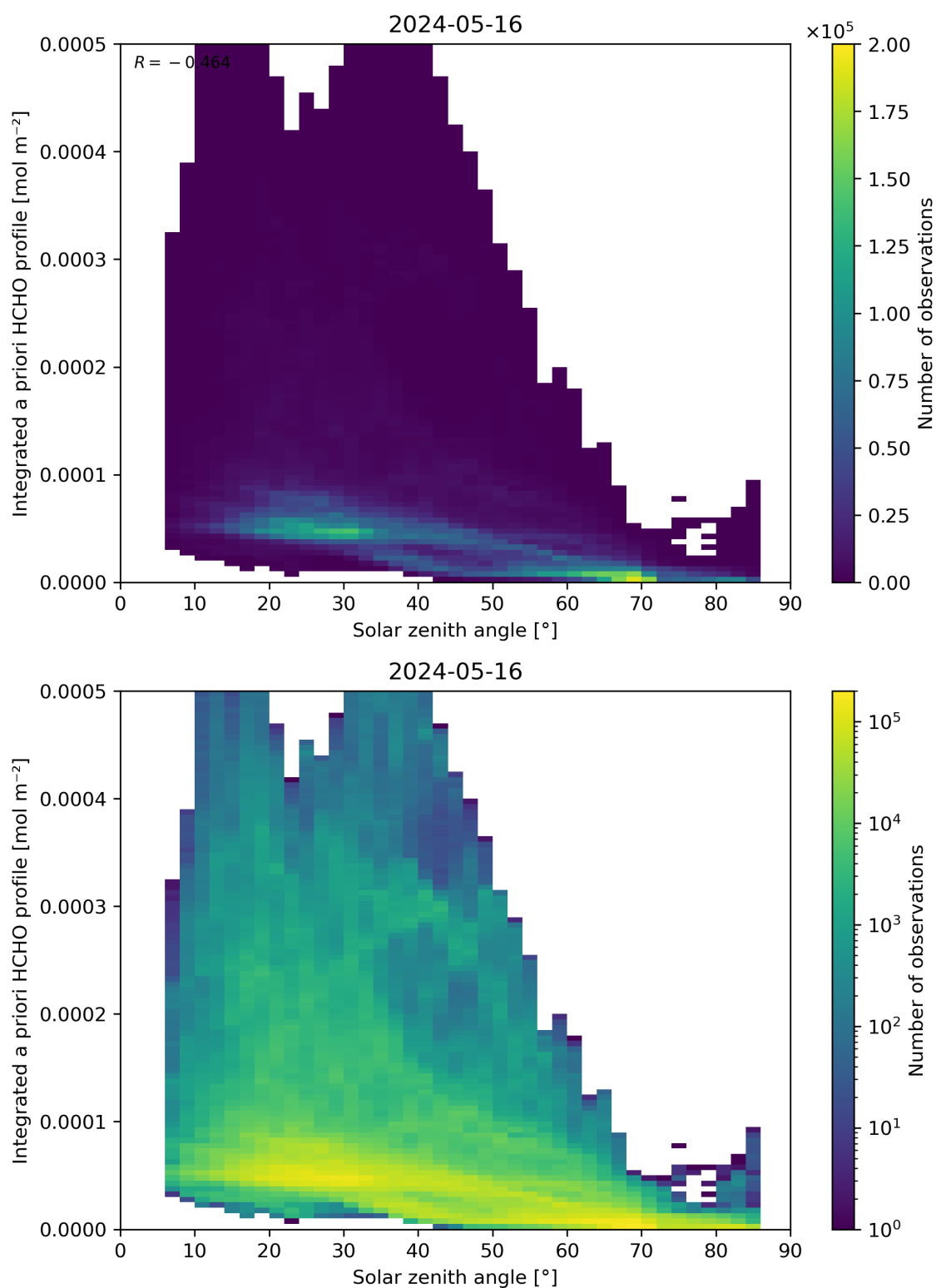
Figure 180: Scatter density plot of “Solar zenith angle” against “Integrated a priori HCHO profile” for 2024-05-15 to 2024-05-17.
