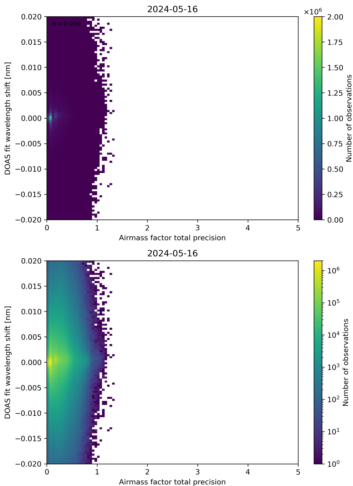
Figure 106: Scatter density plot of “Airmass factor total precision” against “DOAS fit wavelength shift” for 2024-05-15 to 2024-05-17.
