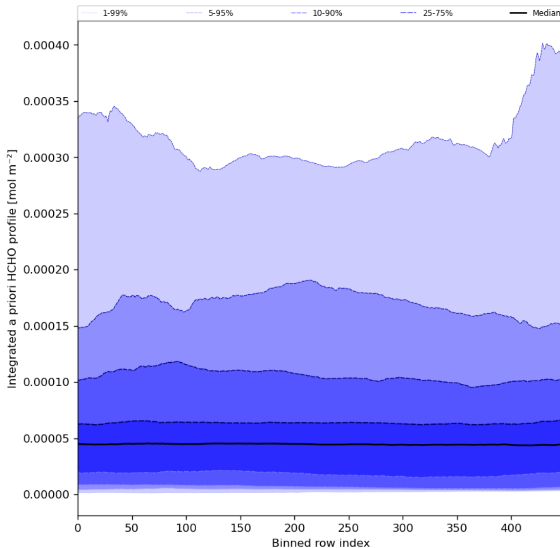
Figure 57: Along track statistics of “Integrated a priori HCHO profile” for 2024-05-15 to 2024-05-17
