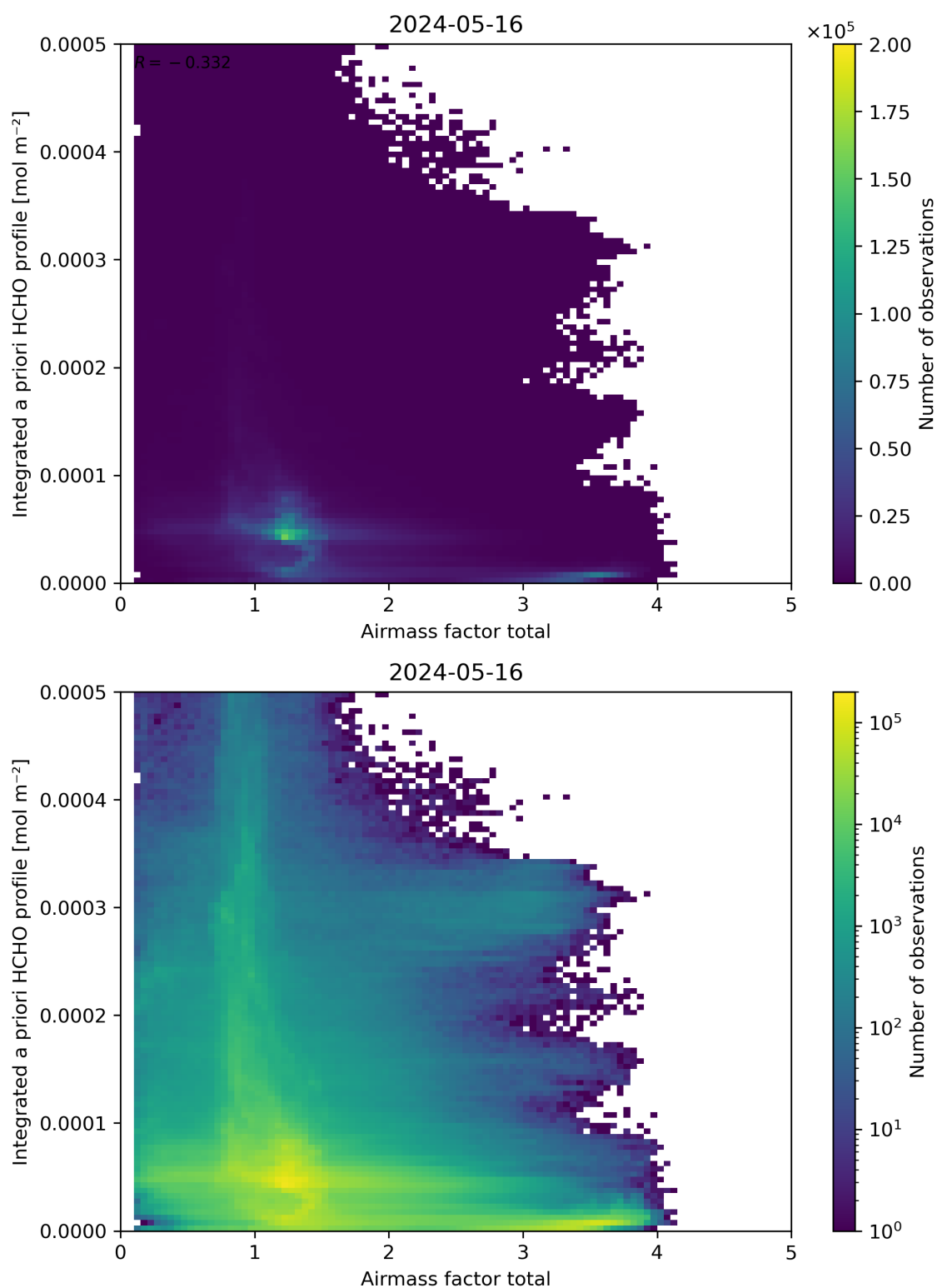
Figure 104: Scatter density plot of “Air mass factor total” against “Integrated a priori HCHO profile” for 2024-05-15 to 2024-05-17.
