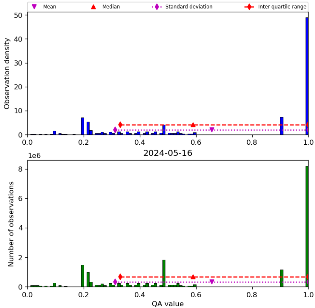
Figure 34: Histogram of “QA value” for 2024-05-15 to 2024-05-17
