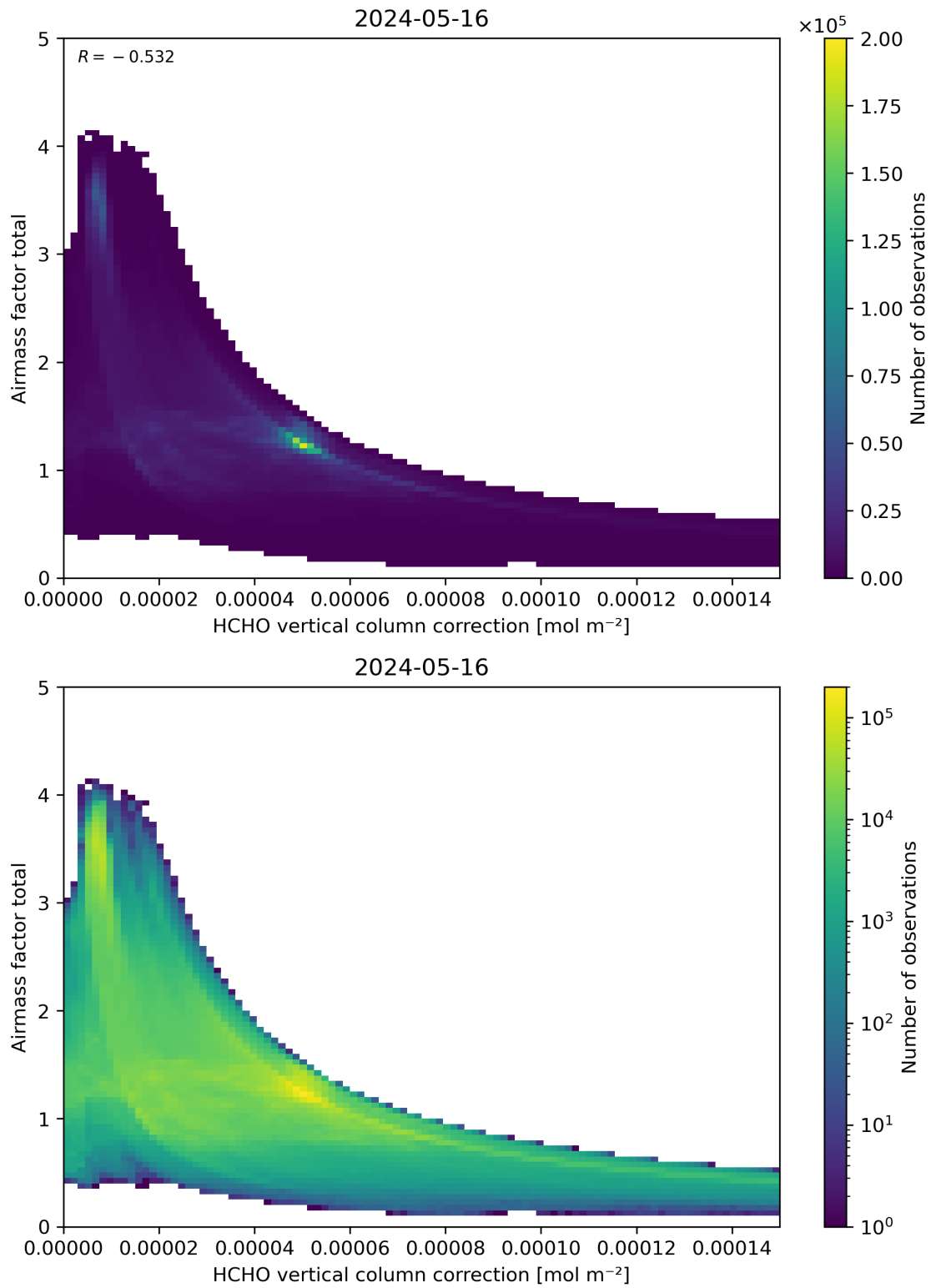
Figure 120: Scatter density plot of “HCHO vertical column correction” against “Airmass factor total” for 2024-05-15 to 2024-05-17.
