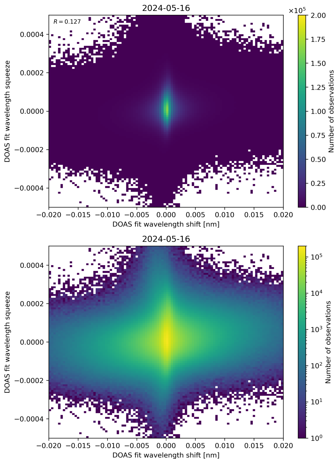
Figure 65: Scatter density plot of “DOAS fit wavelength shift” against “DOAS fit wavelength squeeze” for 2024-05-15 to 2024-05-17.
