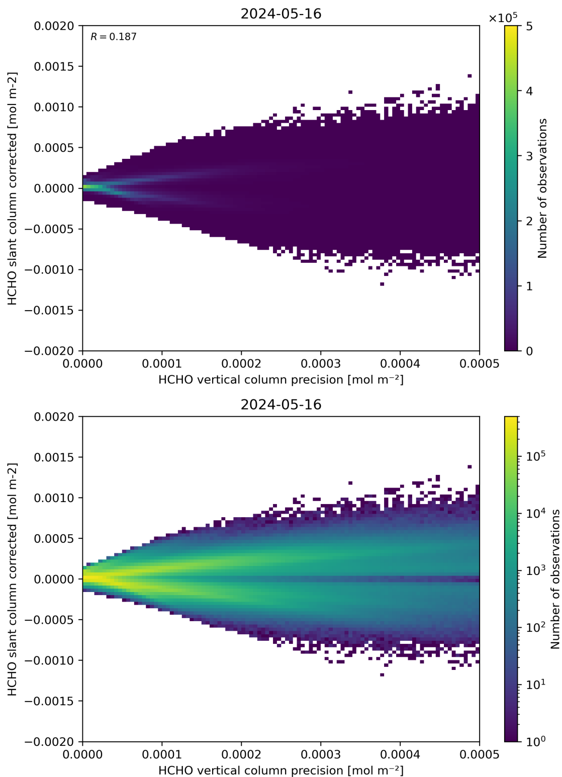
Figure 140: Scatter density plot of “HCHO vertical column precision” against “HCHO slant column corrected” for 2024-05-15 to 2024-05-17.
