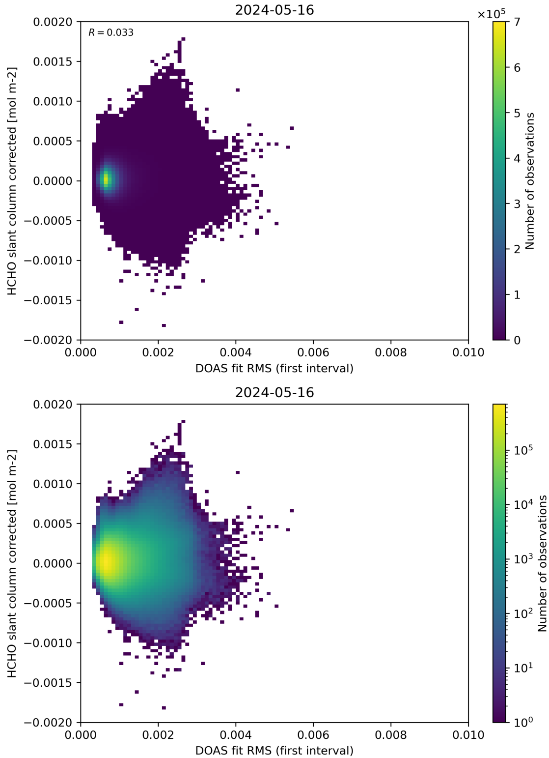
Figure 62: Scatter density plot of “DOAS fit RMS (first interval)” against “HCHO slant column corrected” for 2024-05-15 to 2024-05-17.
