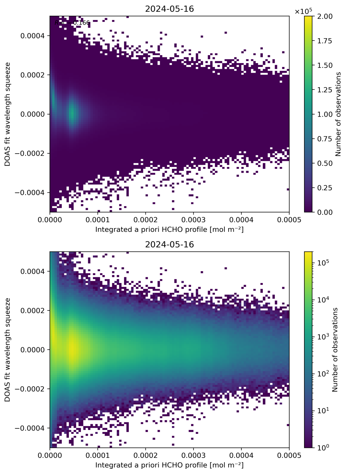
Figure 150: Scatter density plot of “Integrated a priori HCHO profile” against “DOAS fit wavelength squeeze” for 2024-05-15 to 2024-05-17.
