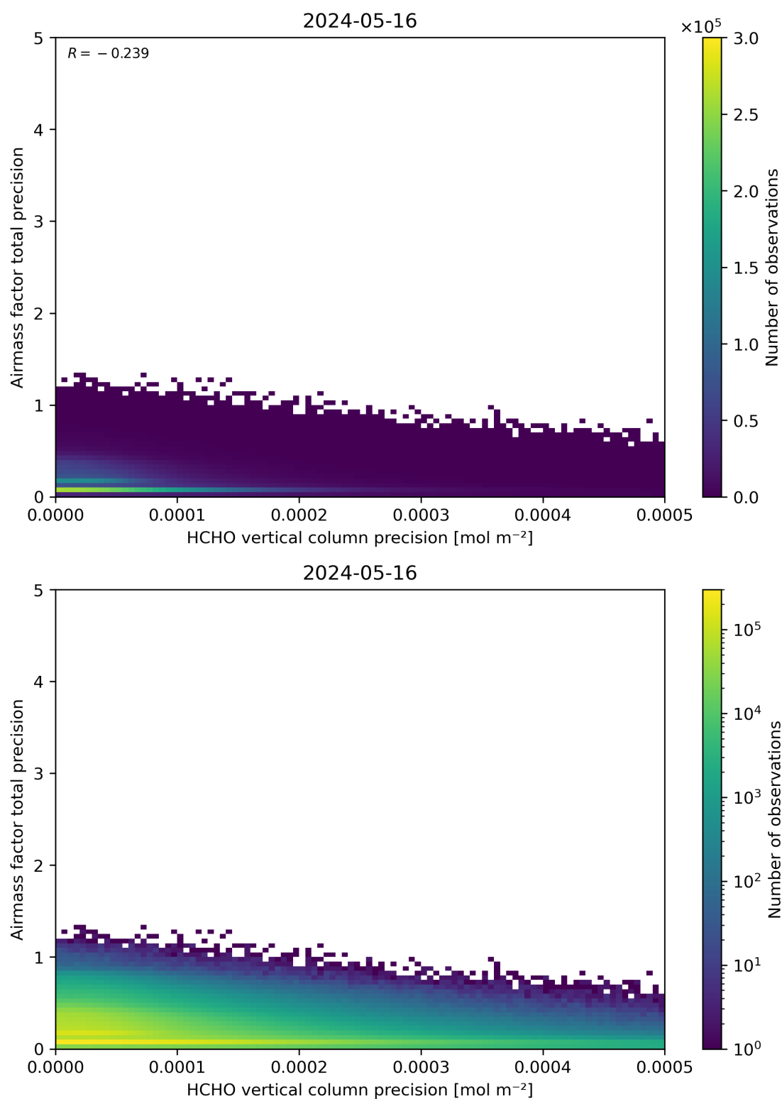
Figure 145: Scatter density plot of “HCHO vertical column precision” against “Airmass factor total precision” for 2024-05-15 to 2024-05-17.
