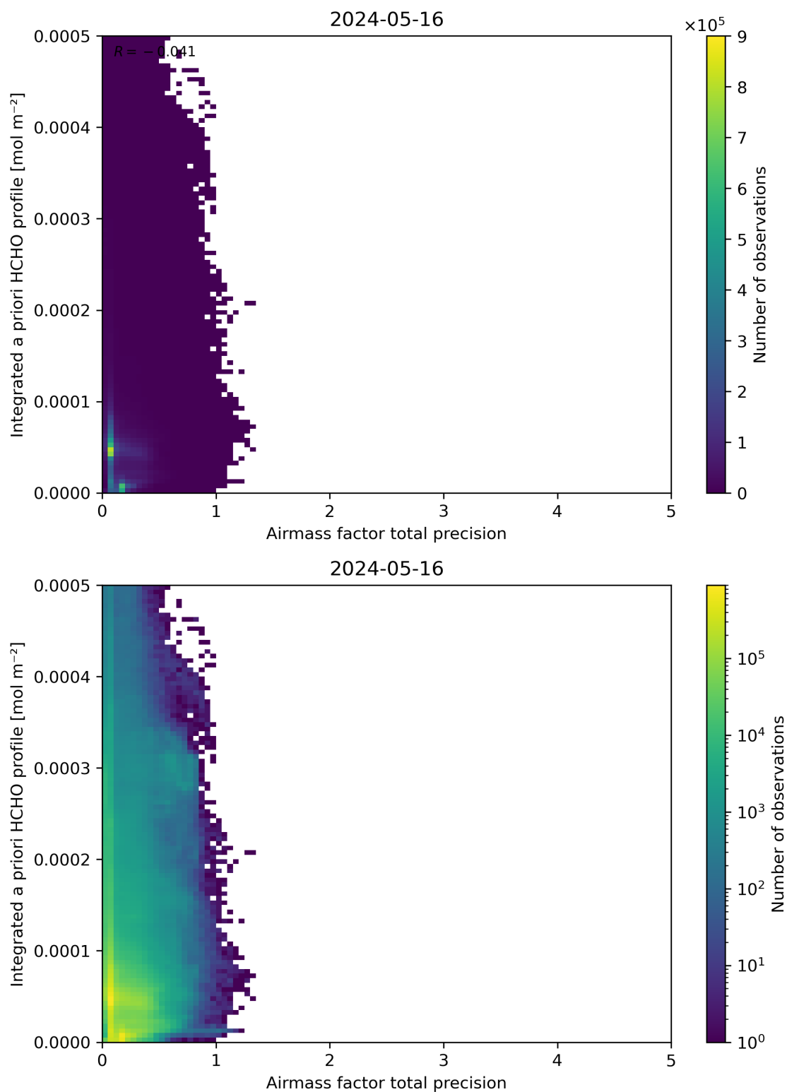
Figure 111: Scatter density plot of “Airmass factor total precision” against “Integrated a priori HCHO profile” for 2024-05-15 to 2024-05-17.
