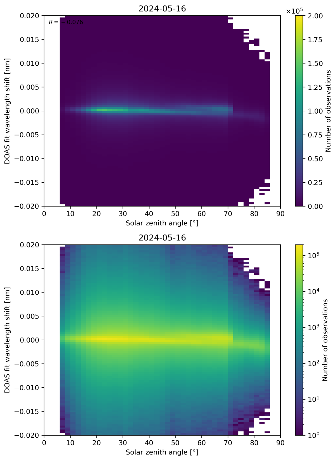
Figure 168: Scatter density plot of “Solar zenith angle” against “DOAS fit wavelength shift” for 2024-05-15 to 2024-05-17.
