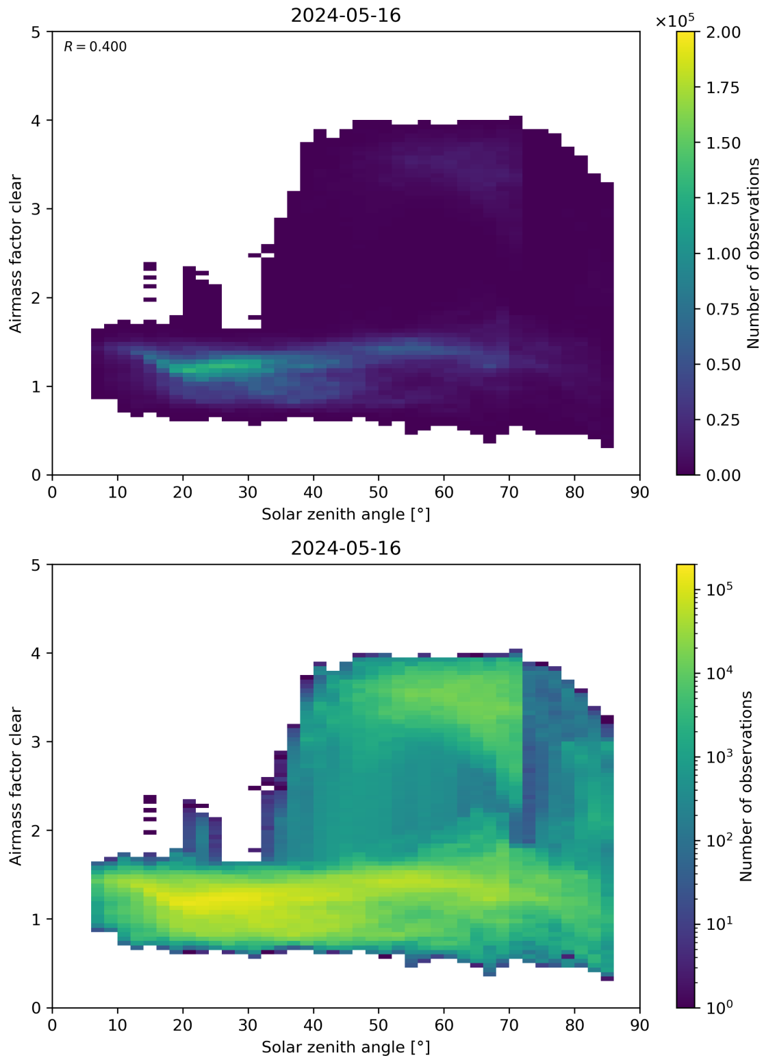
Figure 170: Scatter density plot of “Solar zenith angle” against “Airmass factor clear” for 2024-05-15 to 2024-05-17.
