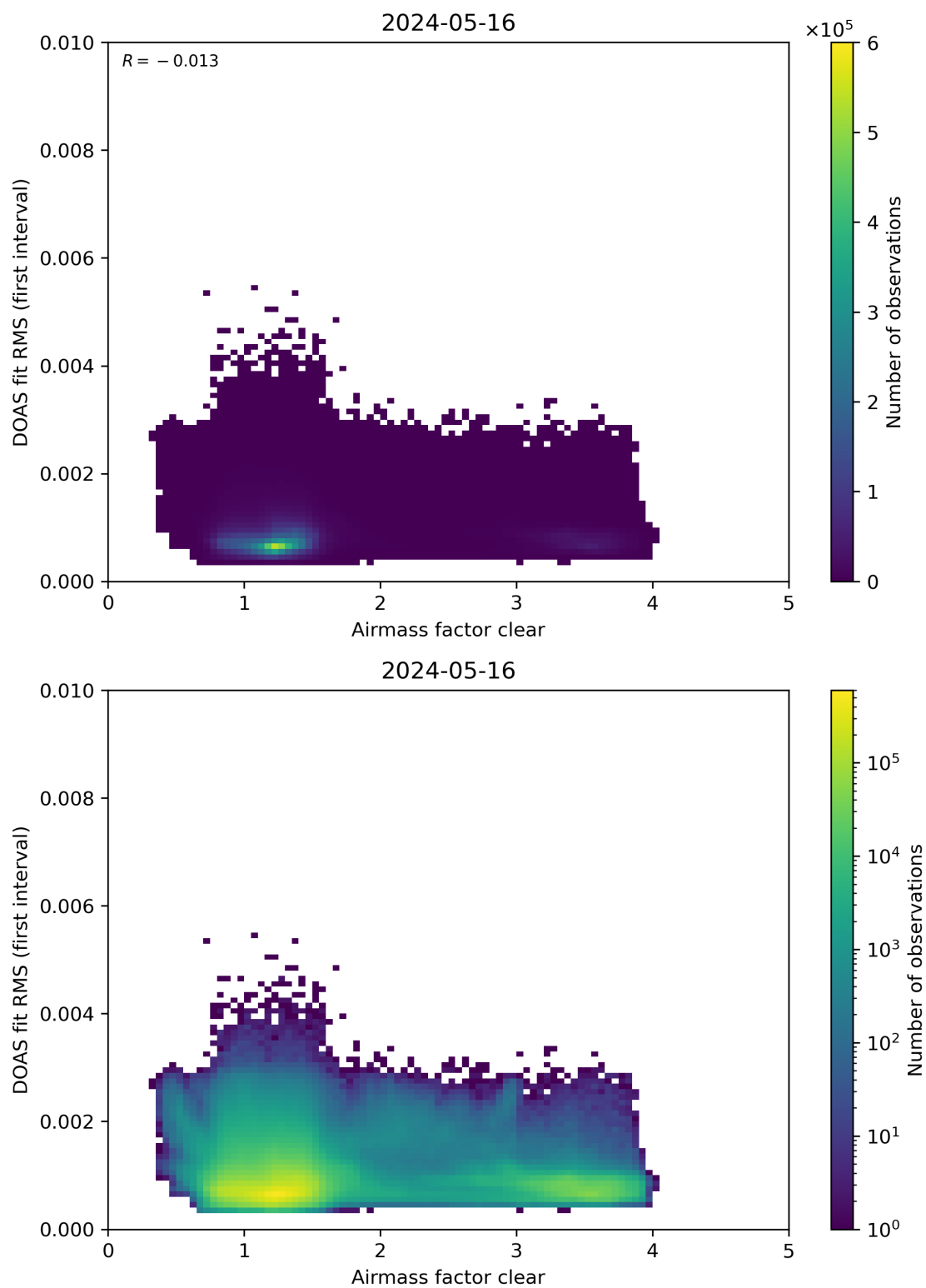
Figure 71: Scatter density plot of “Airmass factor clear” against “DOAS fit RMS (first interval)” for 2024-05-15 to 2024-05-17.
