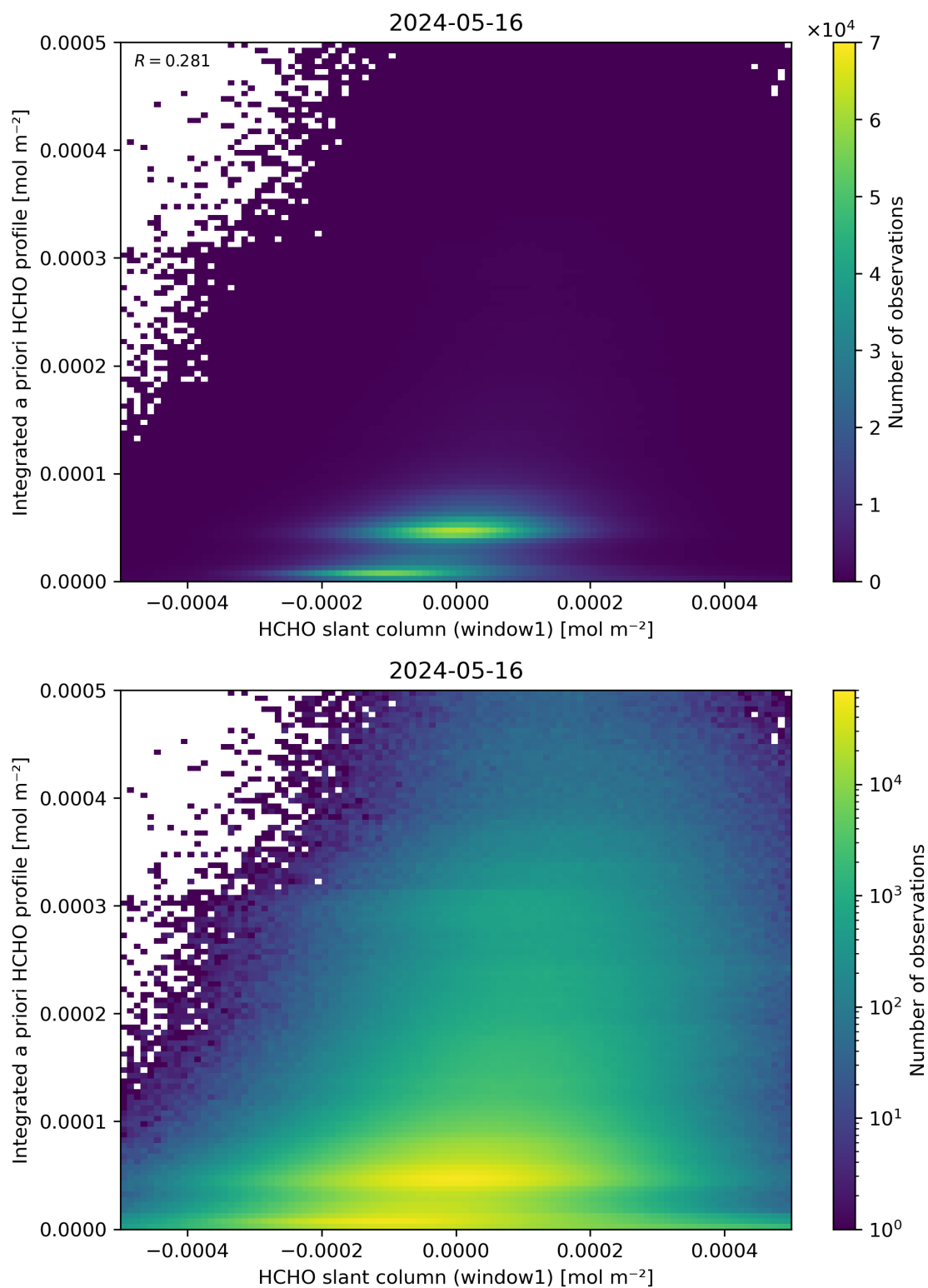
Figure 87: Scatter density plot of “HCHO slant column (window1)” against “Integrated a priori HCHO profile” for 2024-05-15 to 2024-05-17.
