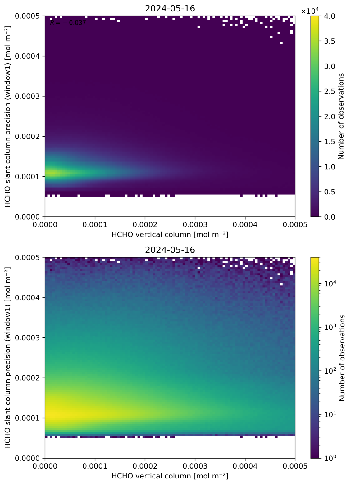
Figure 130: Scatter density plot of “HCHO vertical column” against “HCHO slant column precision (window1)” for 2024-05-15 to 2024-05-17.
