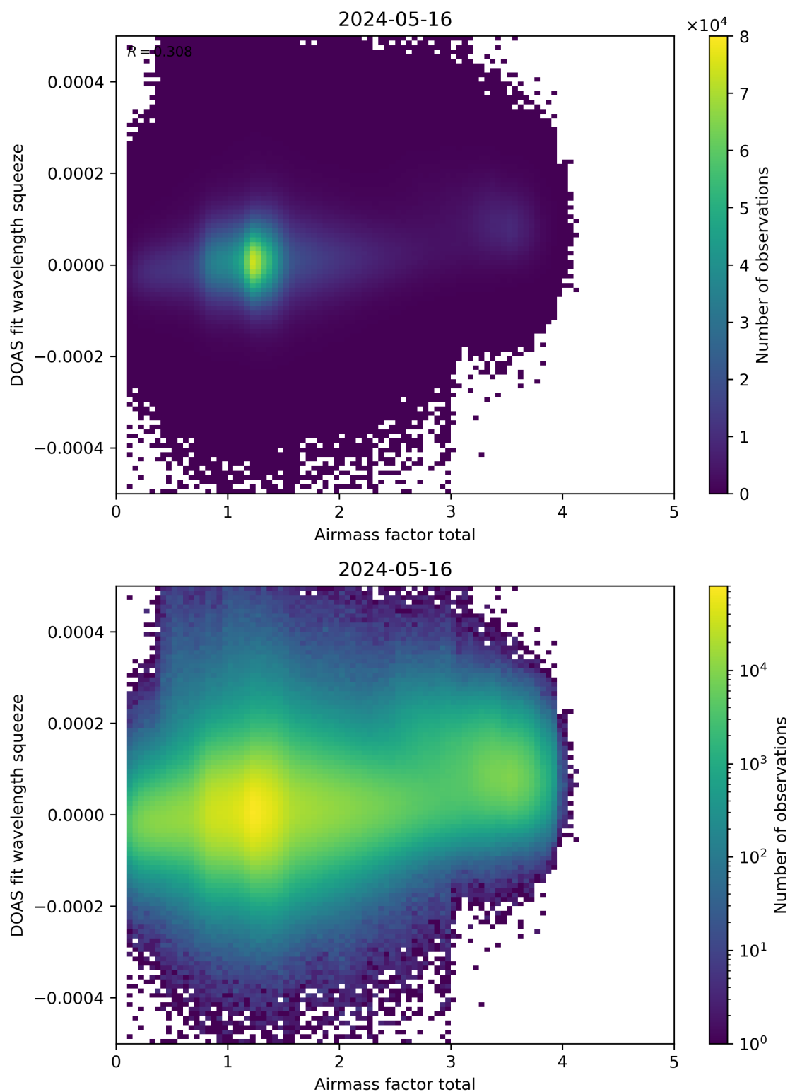
Figure 99: Scatter density plot of “Airmass factor total” against “DOAS fit wavelength squeeze” for 2024-05-15 to 2024-05-17.
