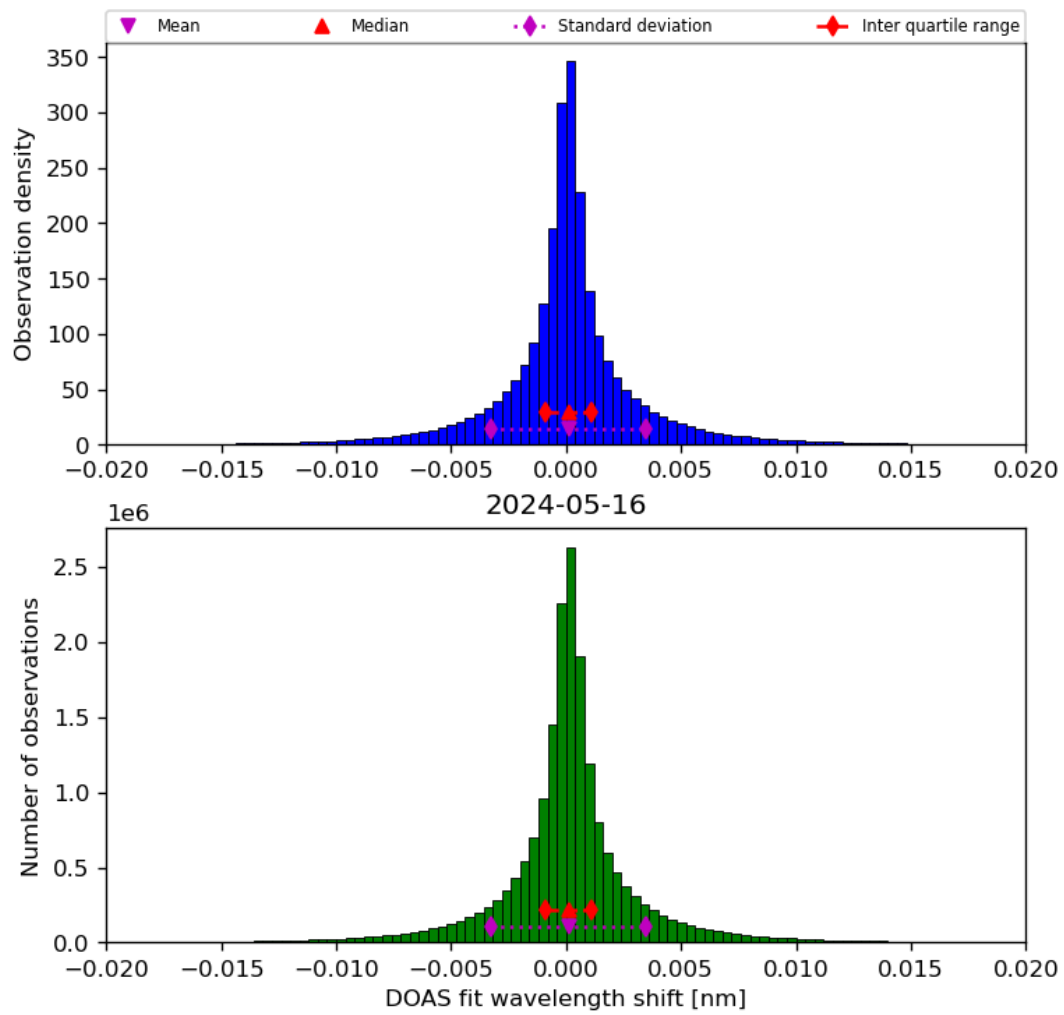
Figure 44: Histogram of “DOAS fit wavelength shift” for 2024-05-15 to 2024-05-17
