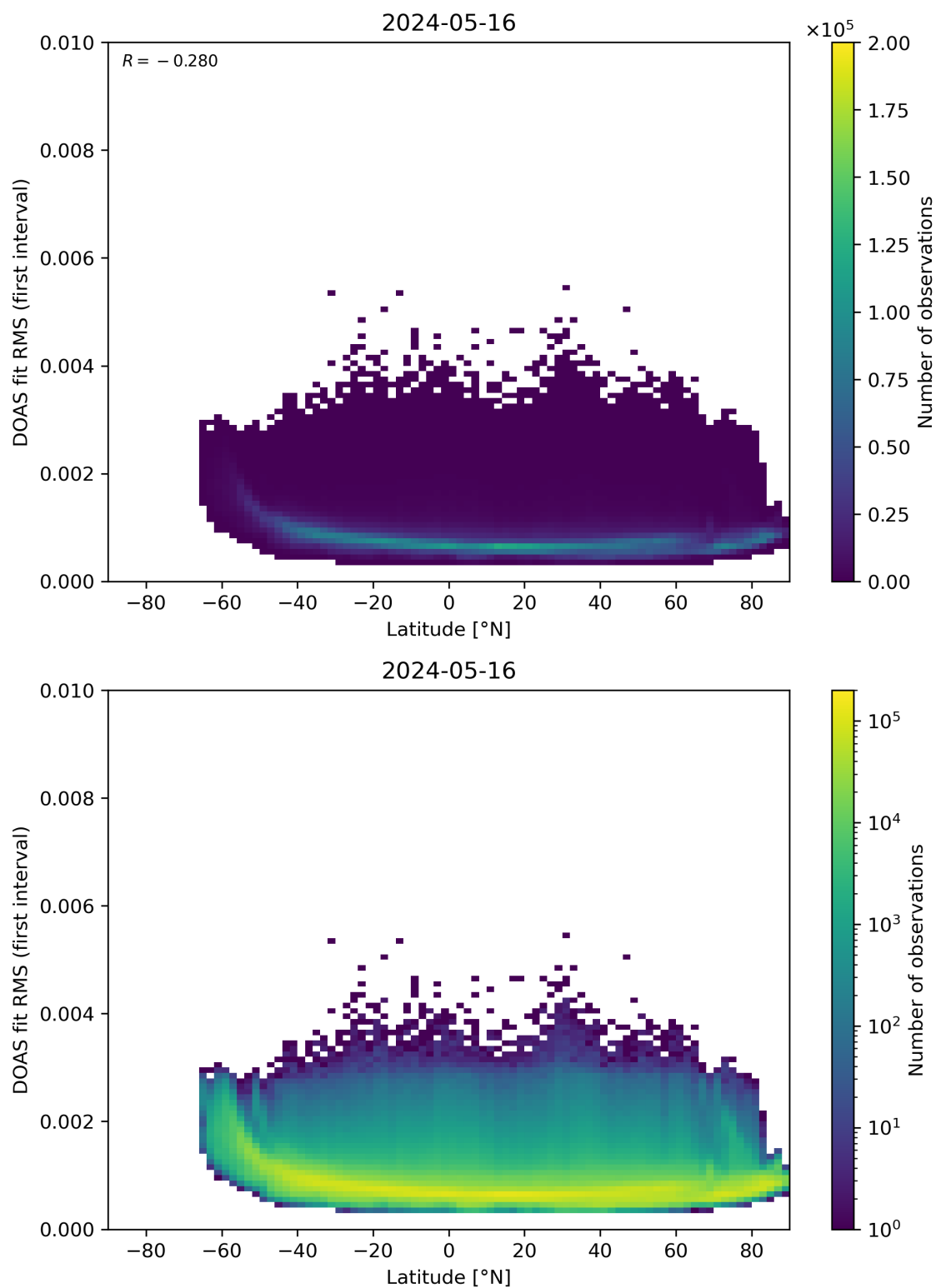
Figure 153: Scatter density plot of “Latitude” against “DOAS fit RMS (first interval)” for 2024-05-15 to 2024-05-17.
