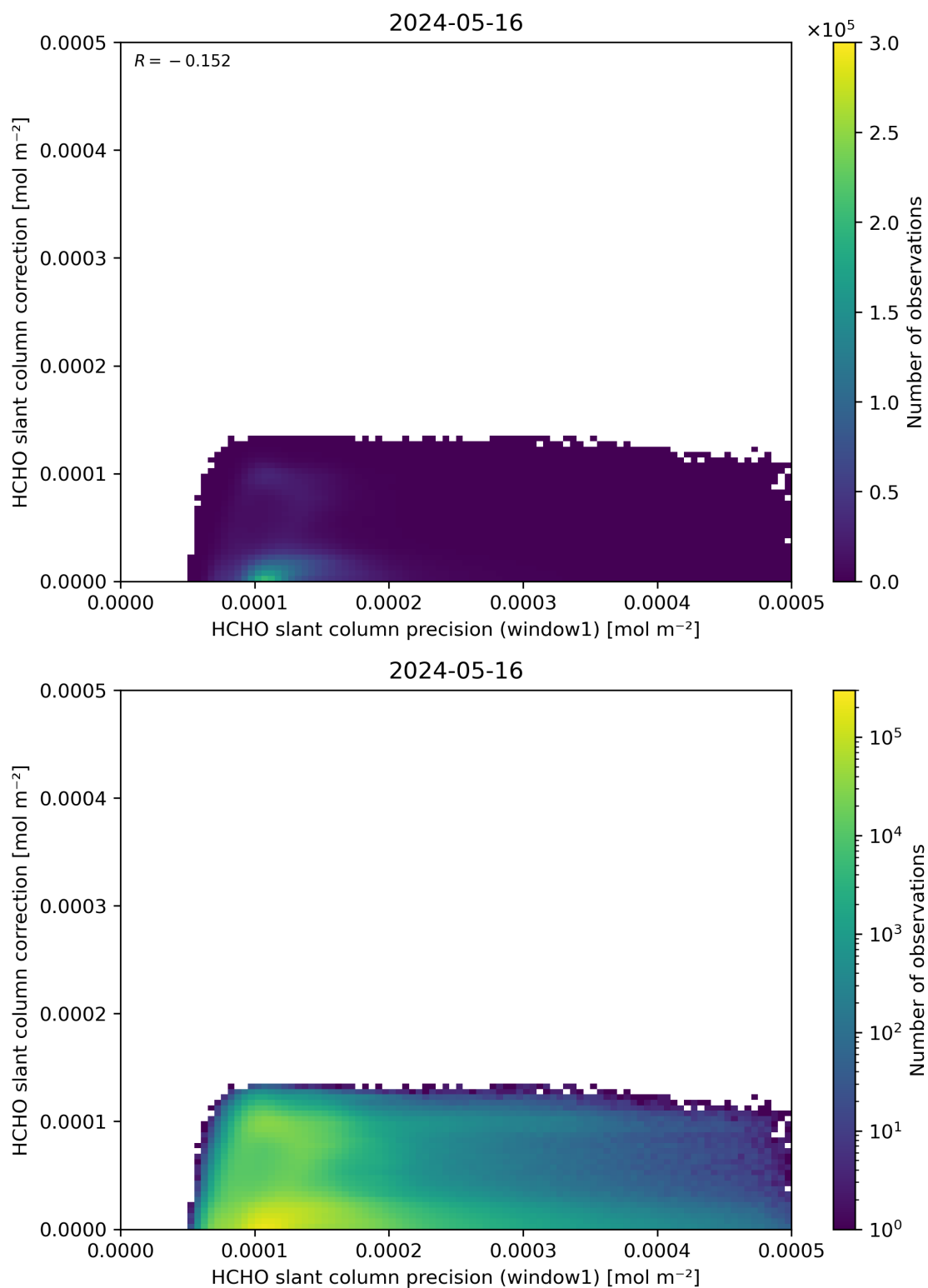
Figure 93: Scatter density plot of “HCHO slant column precision (window1)” against “HCHO slant column correction” for 2024-05-15 to 2024-05-17.
