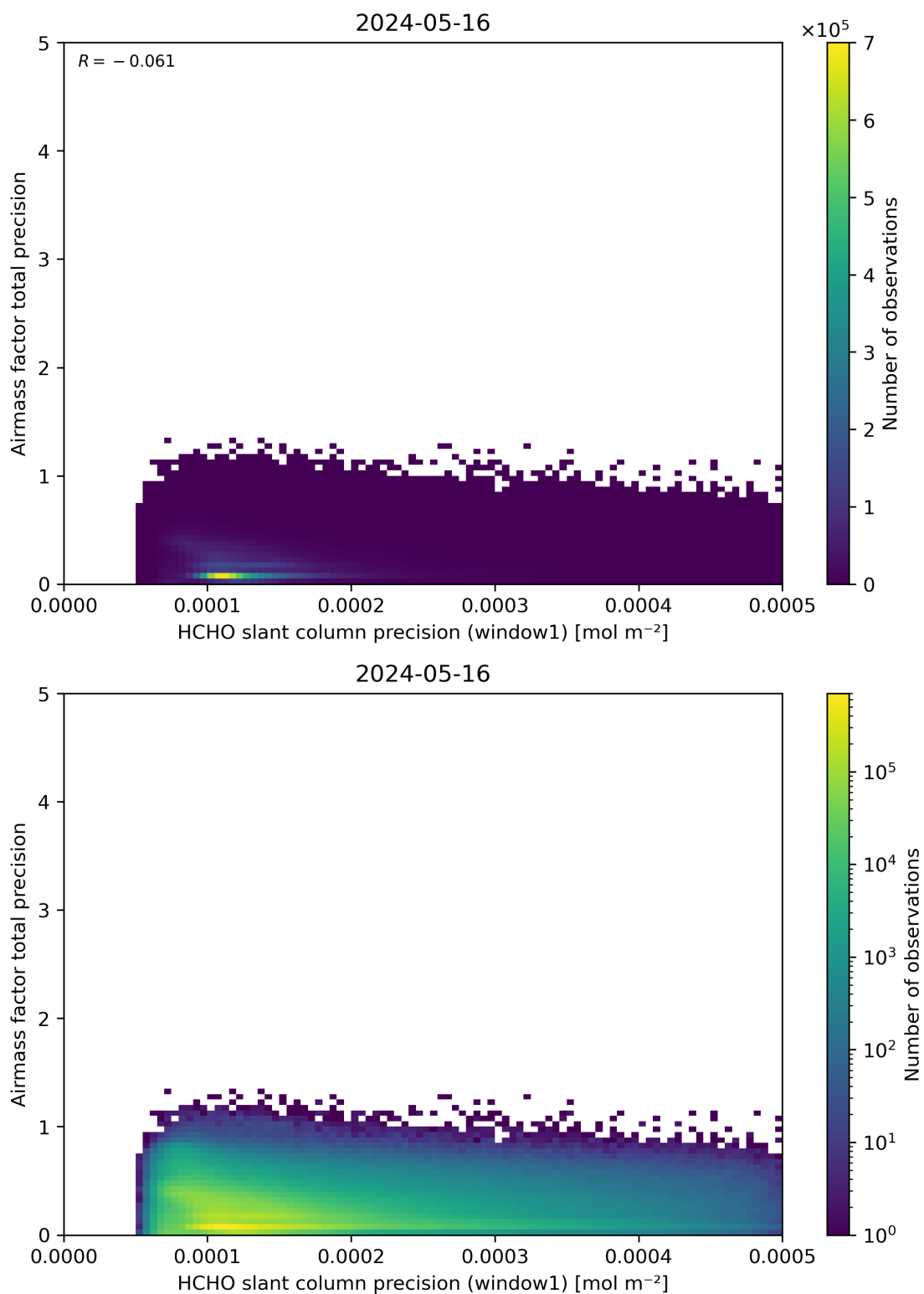
Figure 95: Scatter density plot of “HCHO slant column precision (window1)” against “Airmass factor total precision” for 2024-05-15 to 2024-05-17.
