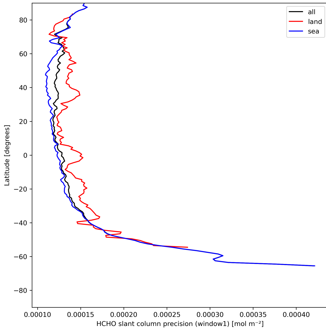
Figure 25: Zonal average of “HCHO slant column precision (window1)” for 2024-05-15 to 2024-05-17.
