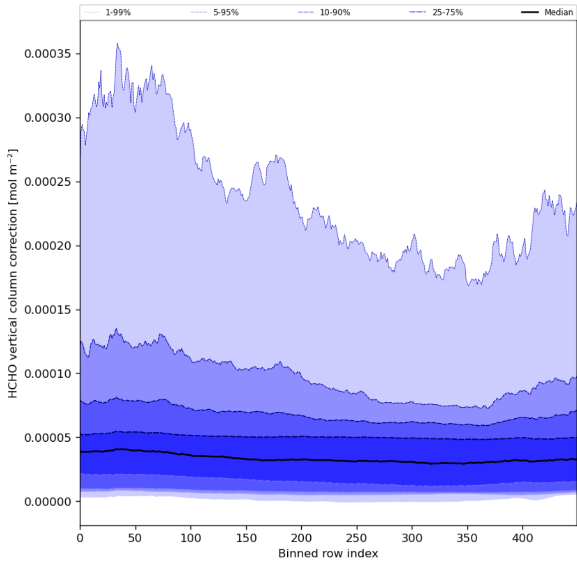
Figure 51: Along track statistics of “HCHO vertical column correction” for 2024-05-15 to 2024-05-17
