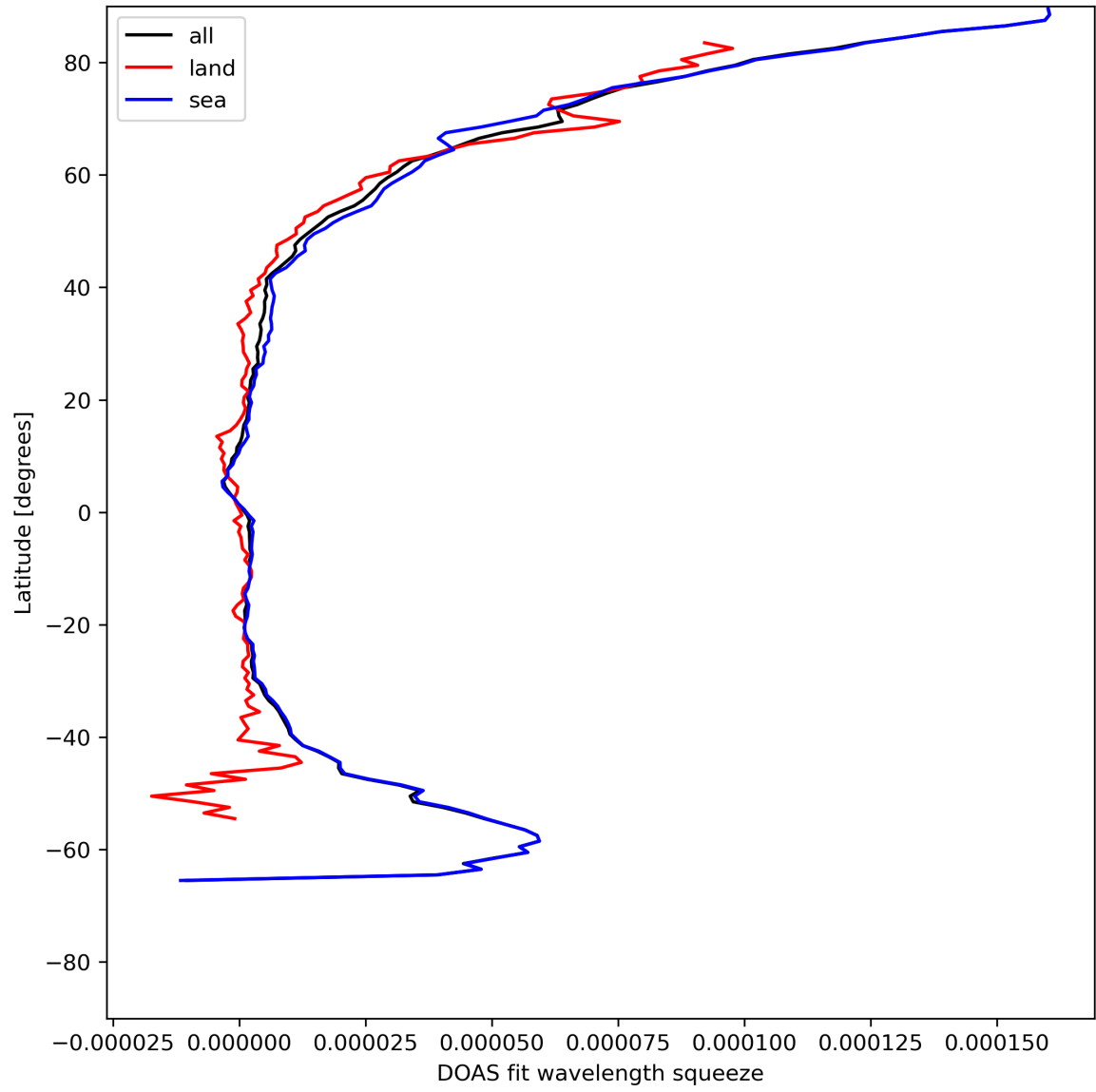
Figure 31: Zonal average of “DOAS fit wavelength squeeze” for 2024-05-15 to 2024-05-17.
