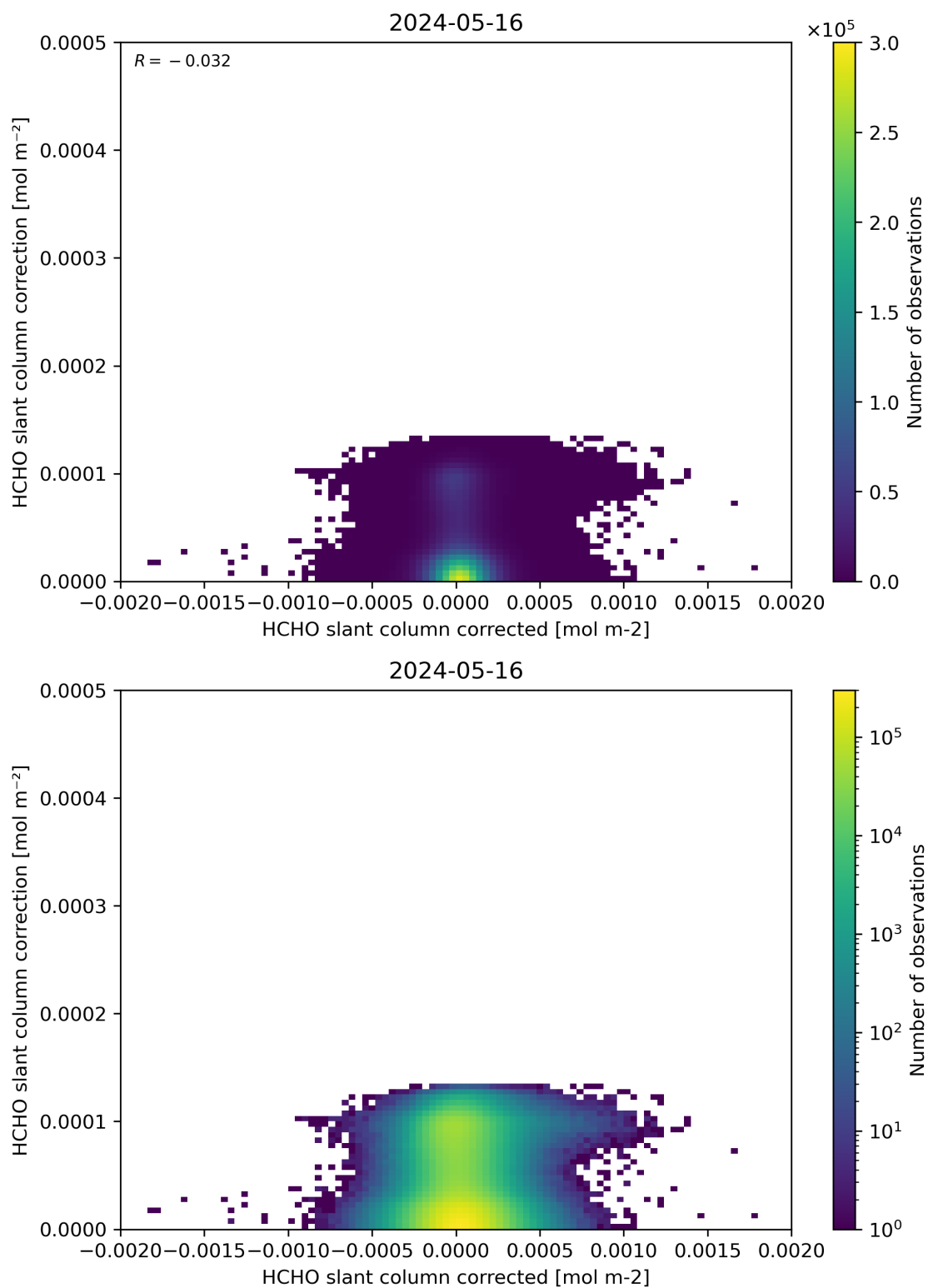
Figure 77: Scatter density plot of “HCHO slant column corrected” against “HCHO slant column correction” for 2024-05-15 to 2024-05-17.
