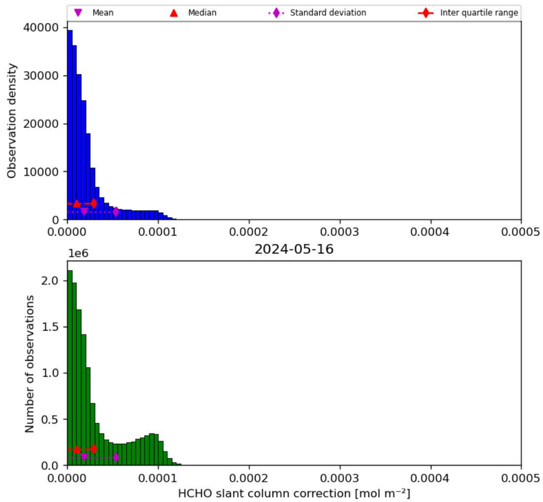
Figure 47: Histogram of “HCHO slant column correction” for 2024-05-15 to 2024-05-17
