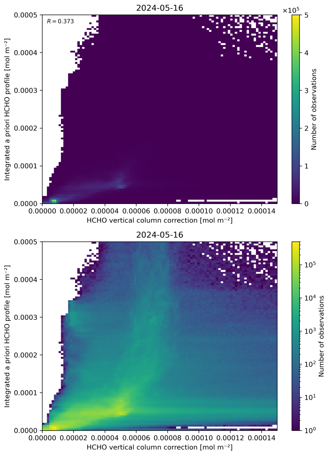
Figure 122: Scatter density plot of “HCHO vertical column correction” against “Integrated a priori HCHO profile” for 2024-05-15 to 2024-05-17.
