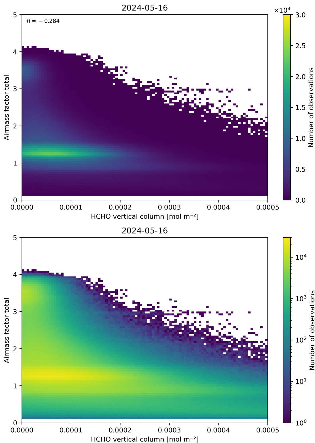
Figure 131: Scatter density plot of “HCHO vertical column” against “Airmass factor total” for 2024-05-15 to 2024-05-17.
