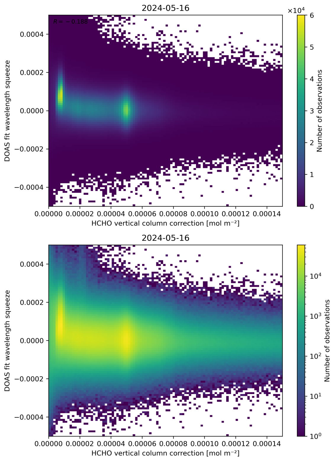
Figure 114: Scatter density plot of “HCHO vertical column correction” against “DOAS fit wavelength squeeze” for 2024-05-15 to 2024-05-17.
