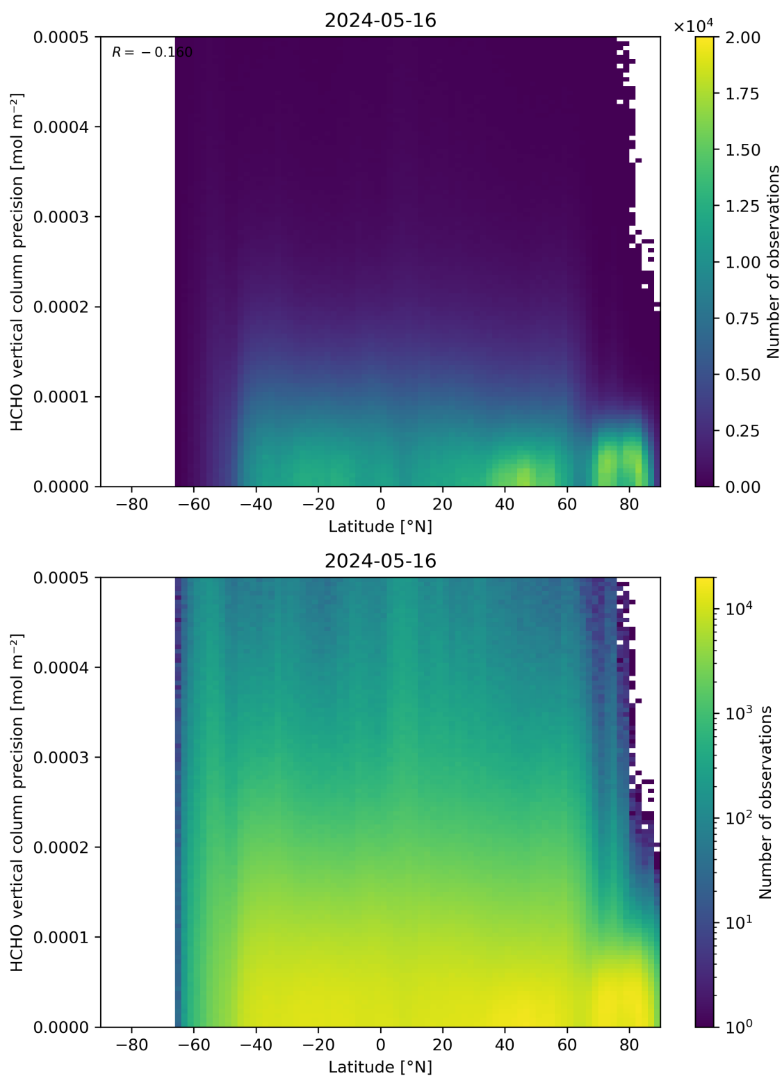
Figure 165: Scatter density plot of “Latitude” against “HCHO vertical column precision” for 2024-05-15 to 2024-05-17.
