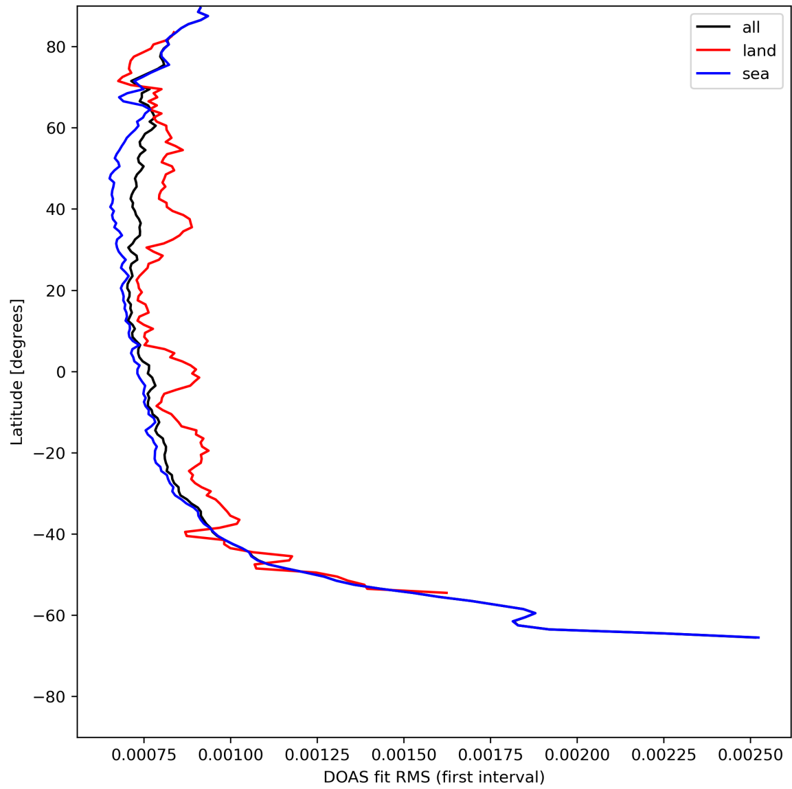
Figure 32: Zonal average of “DOAS fit RMS (first interval)” for 2024-05-15 to 2024-05-17.
