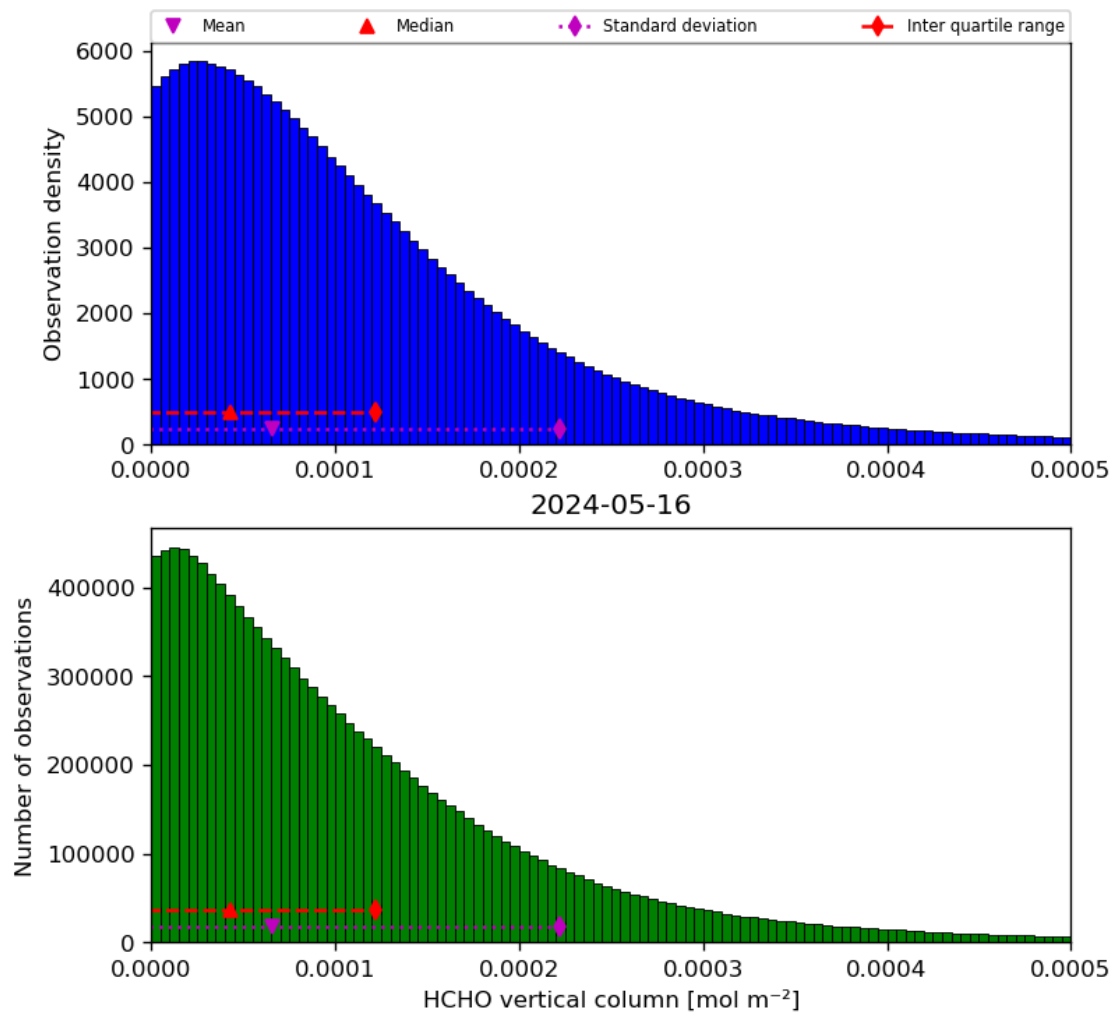
Figure 35: Histogram of “HCHO vertical column” for 2024-05-15 to 2024-05-17
