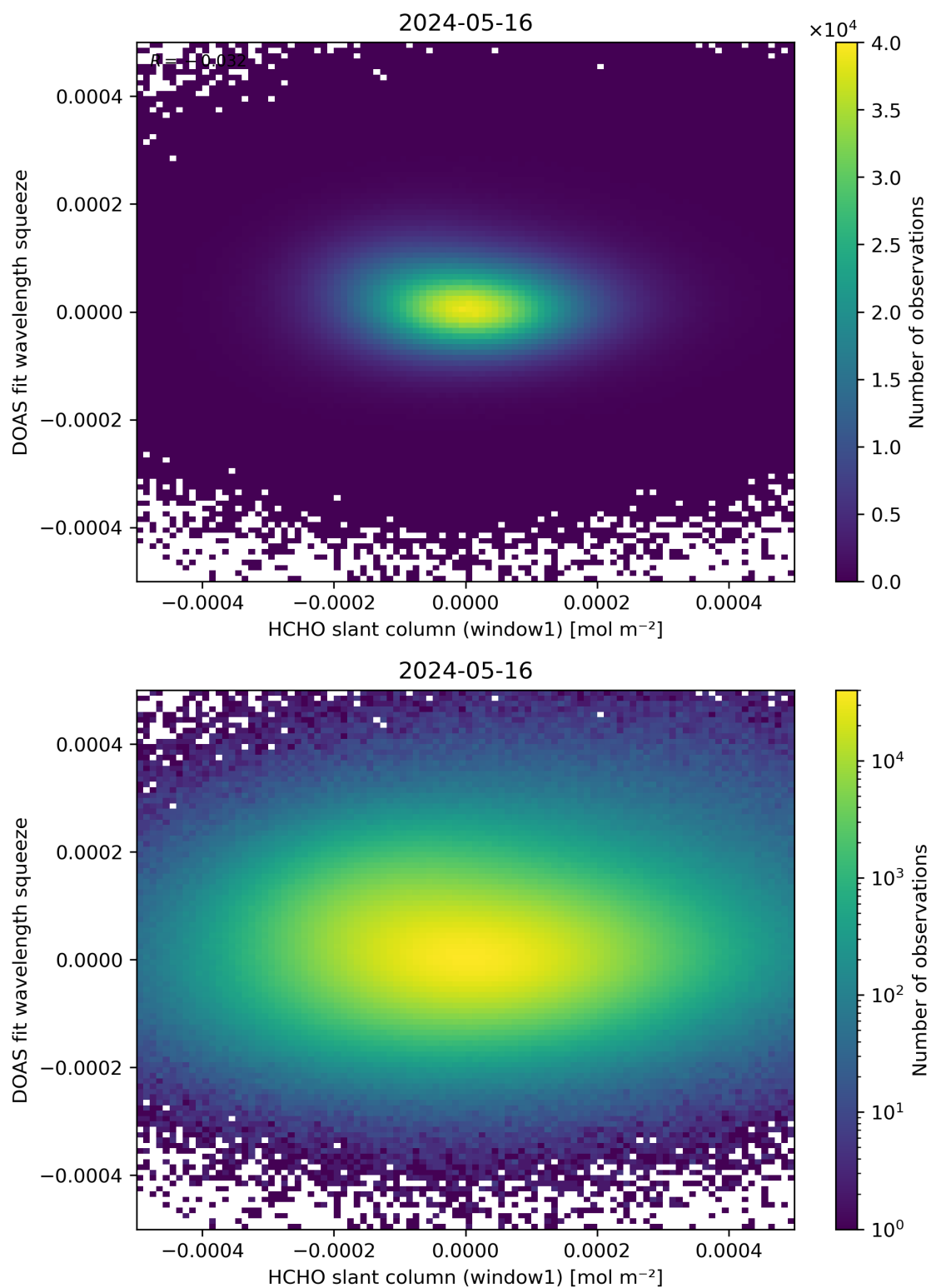
Figure 80: Scatter density plot of “HCHO slant column (window1)” against “DOAS fit wavelength squeeze” for 2024-05-15 to 2024-05-17.
