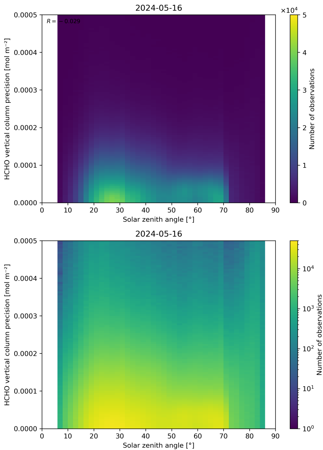
Figure 179: Scatter density plot of “Solar zenith angle” against “HCHO vertical column precision” for 2024-05-15 to 2024-05-17.
