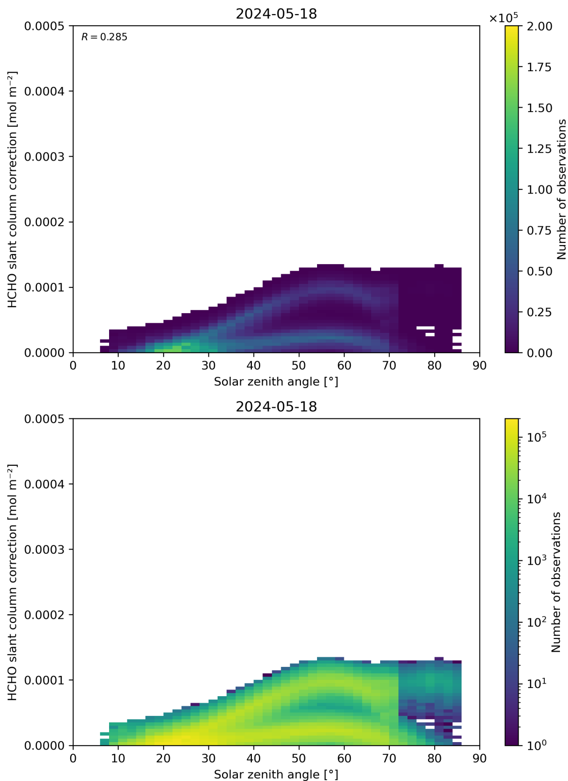
Figure 172: Scatter density plot of “Solar zenith angle” against “HCHO slant column correction” for 2024-05-18 to 2024-05-19.
