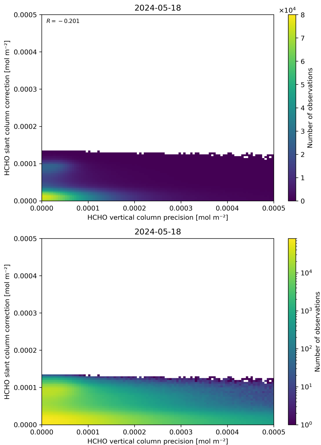
Figure 141: Scatter density plot of “HCHO vertical column precision” against “HCHO slant column correction” for 2024-05-18 to 2024-05-19.
