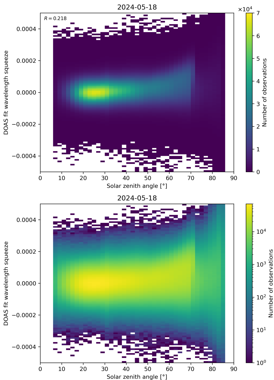
Figure 169: Scatter density plot of “Solar zenith angle” against “DOAS fit wavelength squeeze” for 2024-05-18 to 2024-05-19.
