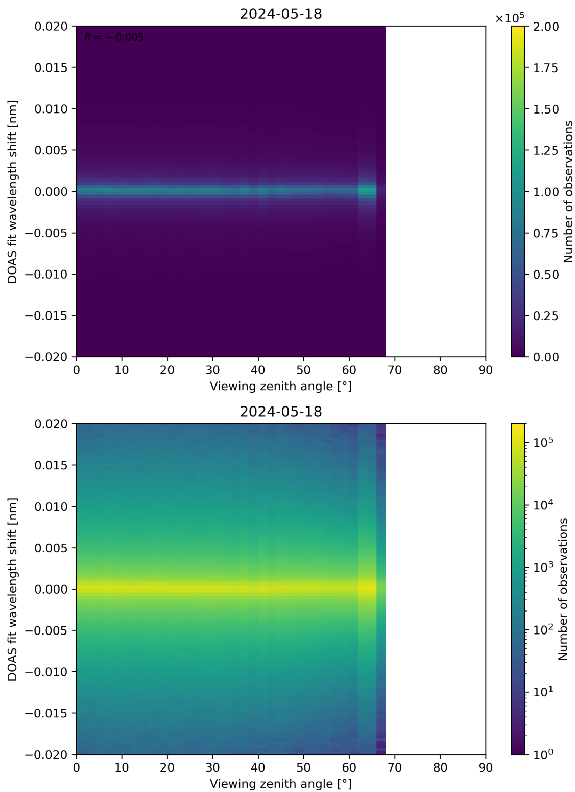
Figure 183: Scatter density plot of “Viewing zenith angle” against “DOAS fit wavelength shift” for 2024-05-18 to 2024-05-19.
