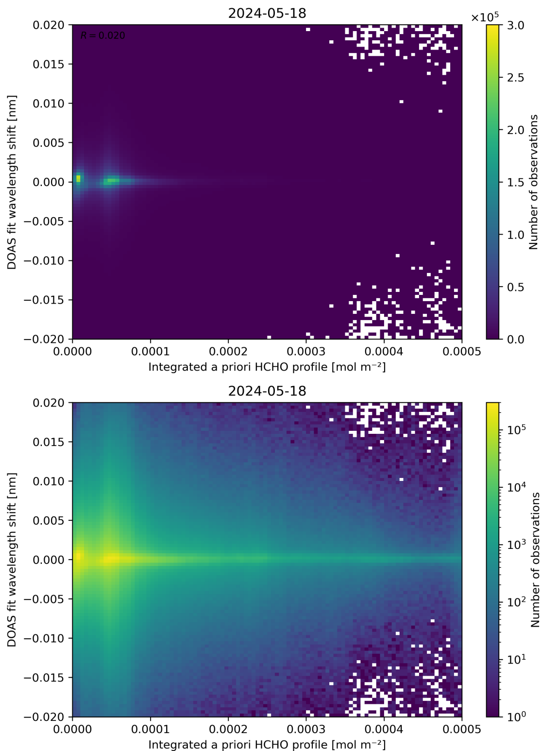
Figure 149: Scatter density plot of “Integrated a priori HCHO profile” against “DOAS fit wavelength shift” for 2024-05-18 to 2024-05-19.
