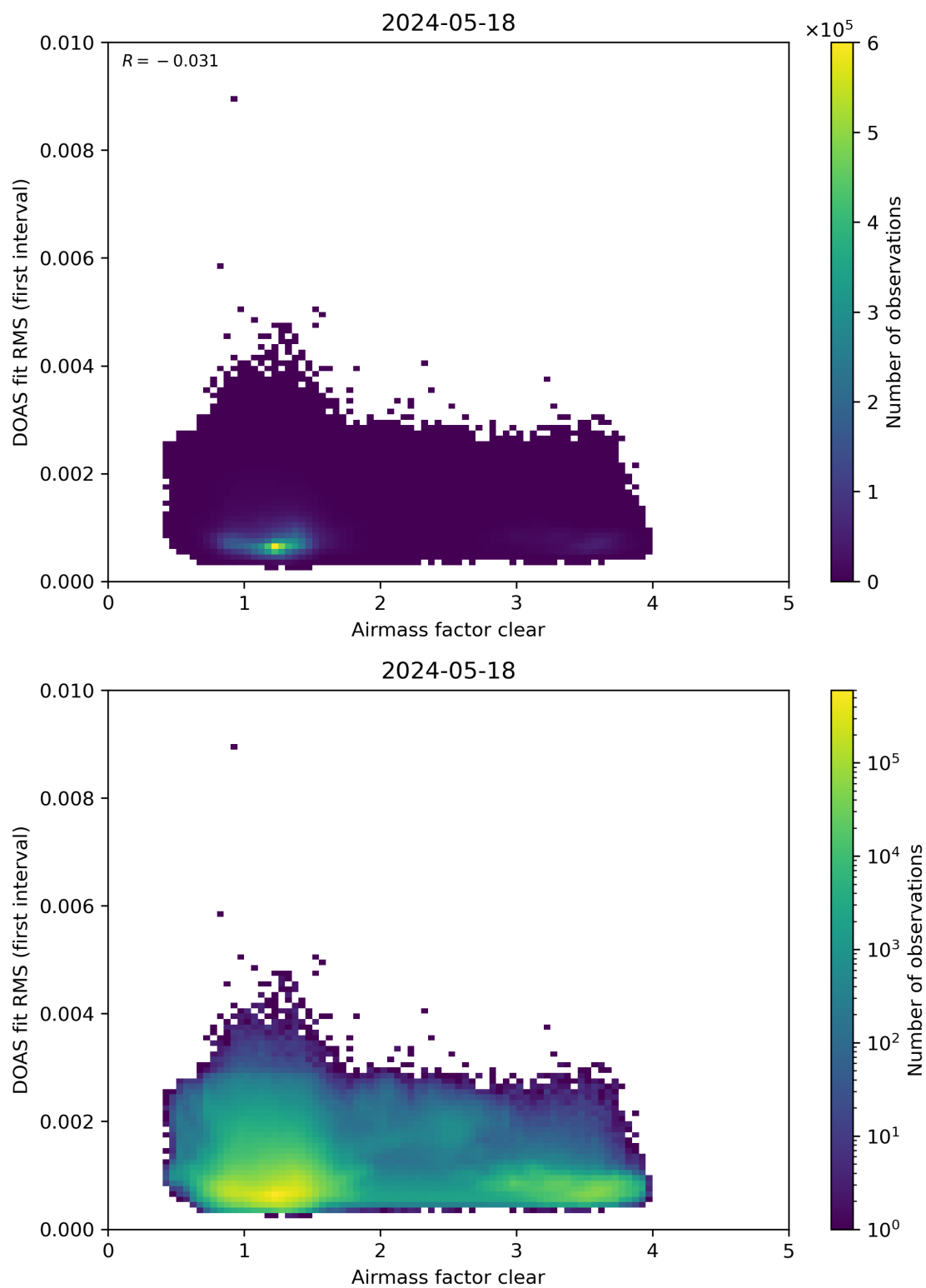
Figure 71: Scatter density plot of “Airmass factor clear” against “DOAS fit RMS (first interval)” for 2024-05-18 to 2024-05-19.
