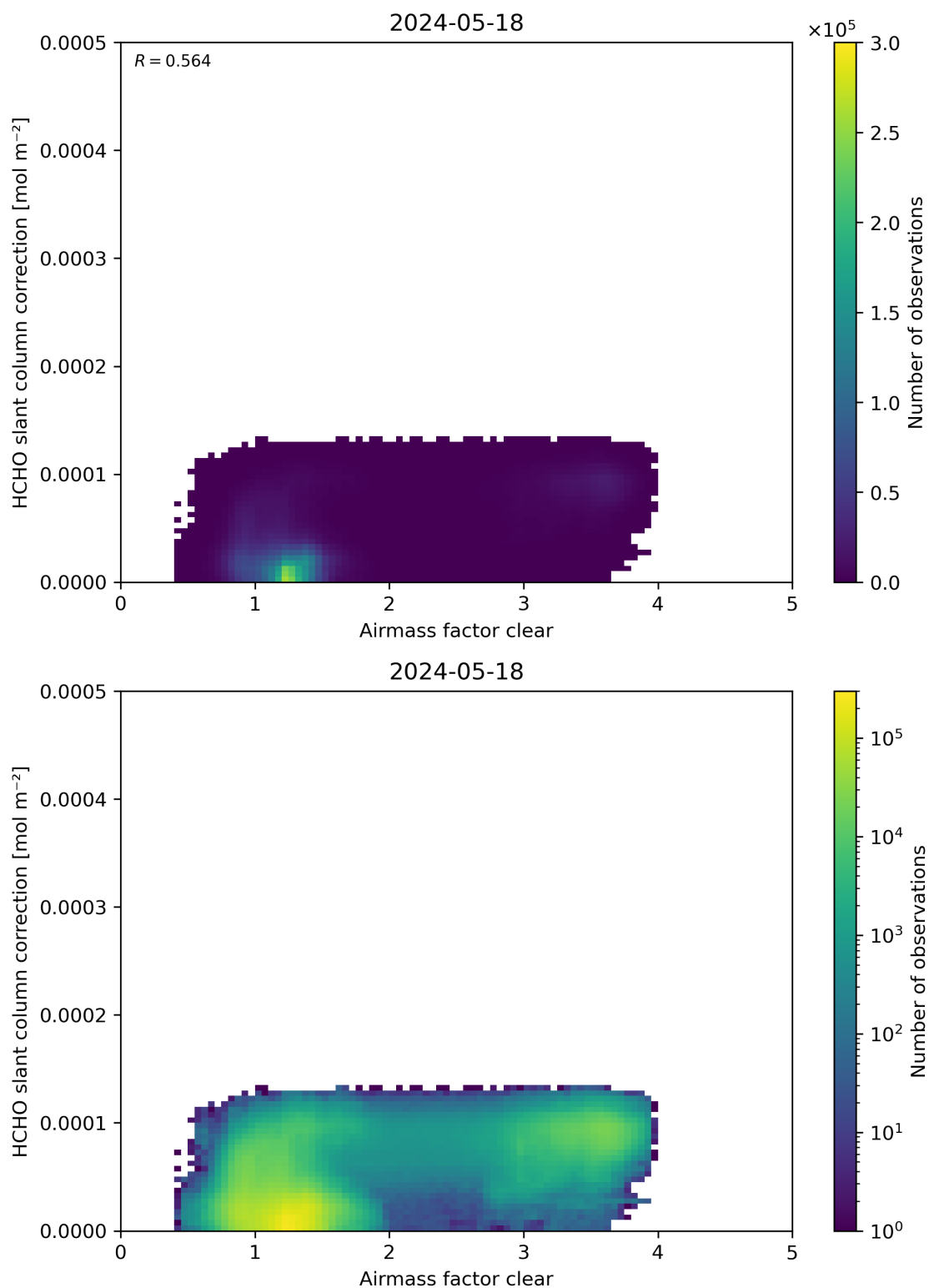
Figure 75: Scatter density plot of “Airmass factor clear” against “HCHO slant column correction” for 2024-05-18 to 2024-05-19.
