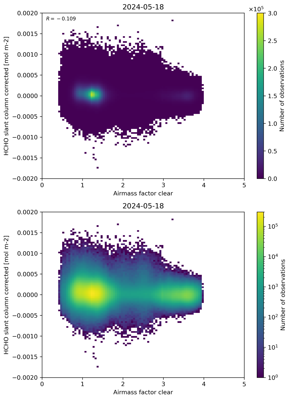
Figure 74: Scatter density plot of “Airmass factor clear” against “HCHO slant column corrected” for 2024-05-18 to 2024-05-19.
