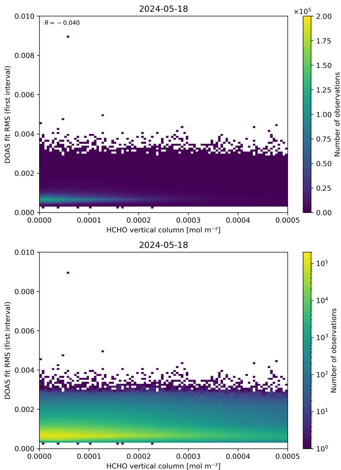
Figure 123: Scatter density plot of “HCHO vertical column” against “DOAS fit RMS (first interval)” for 2024-05-18 to 2024-05-19.
