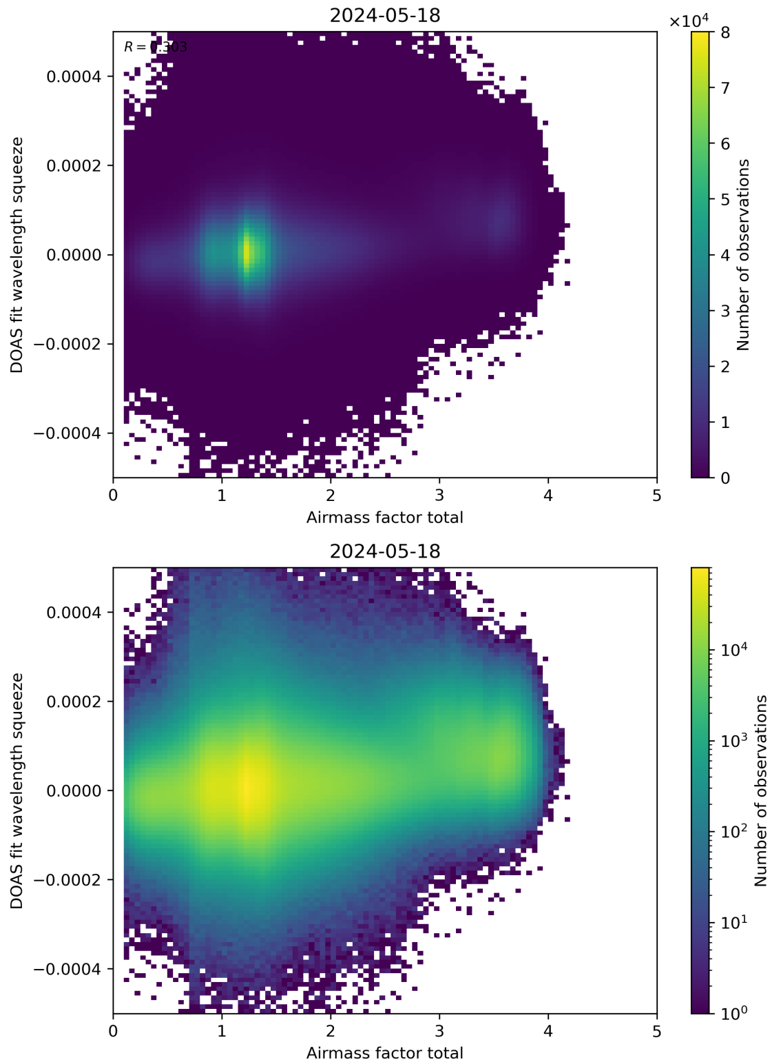
Figure 99: Scatter density plot of “Airmass factor total” against “DOAS fit wavelength squeeze” for 2024-05-18 to 2024-05-19.
