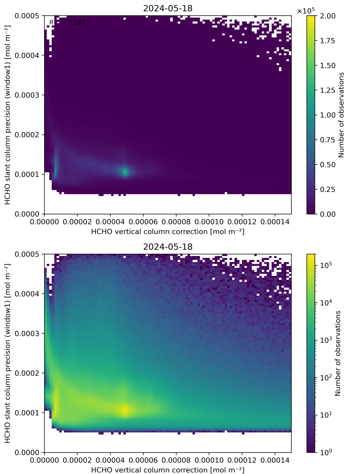
Figure 119: Scatter density plot of “HCHO vertical column correction” against “HCHO slant column precision (window1)” for 2024-05-18 to 2024-05-19.
