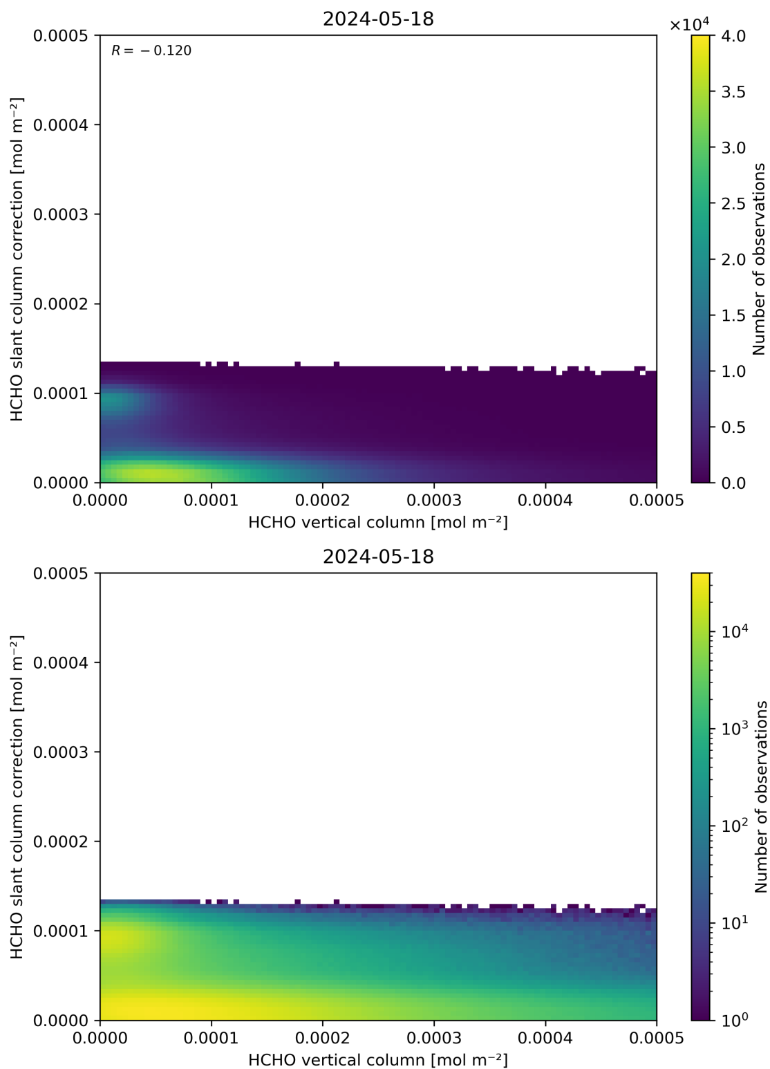
Figure 128: Scatter density plot of “HCHO vertical column” against “HCHO slant column correction” for 2024-05-18 to 2024-05-19.
