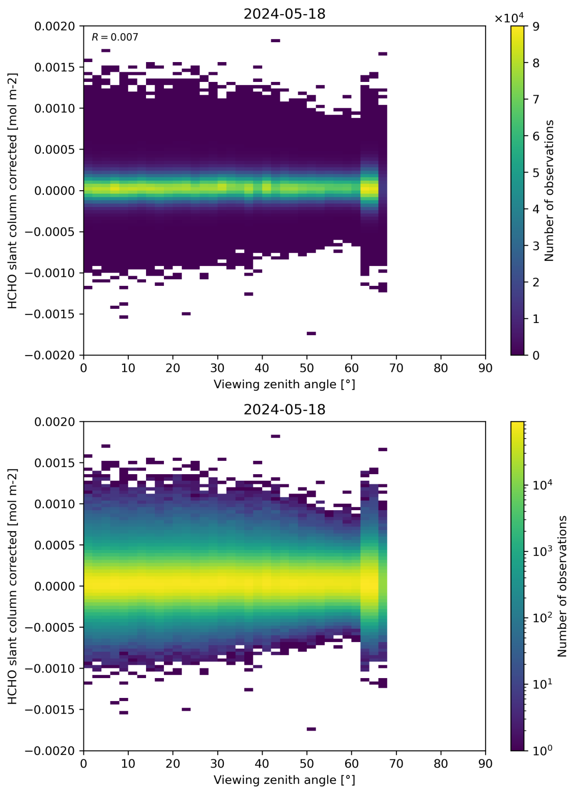
Figure 186: Scatter density plot of “Viewing zenith angle” against “HCHO slant column corrected” for 2024-05-18 to 2024-05-19.
