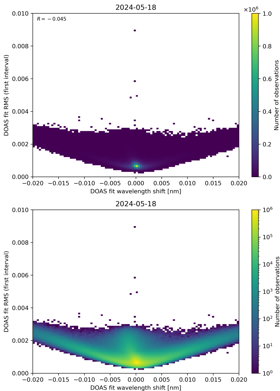
Figure 64: Scatter density plot of “DOAS fit wavelength shift” against “DOAS fit RMS (first interval)” for 2024-05-18 to 2024-05-19.
