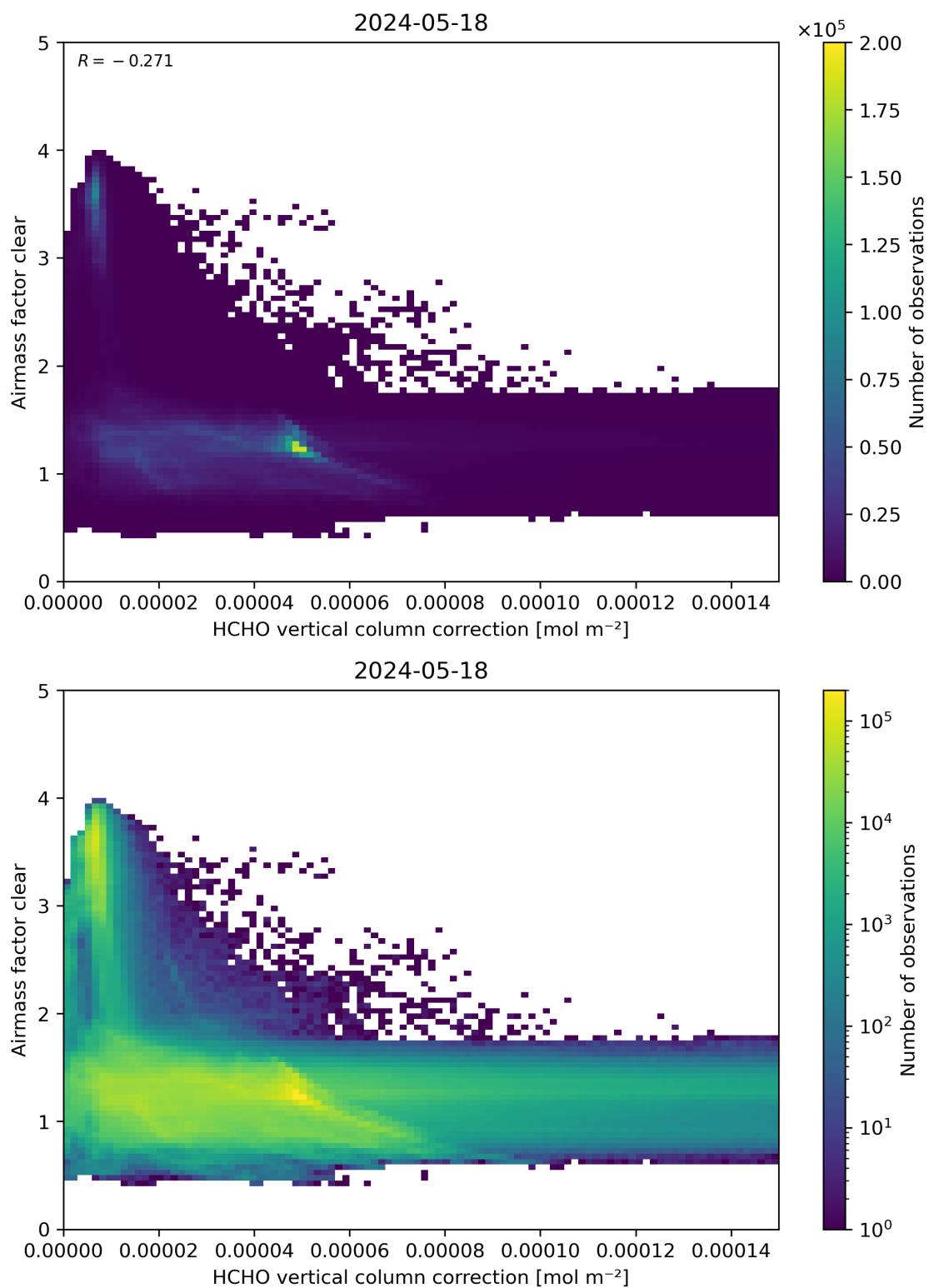
Figure 115: Scatter density plot of “HCHO vertical column correction” against “Airmass factor clear” for 2024-05-18 to 2024-05-19.
