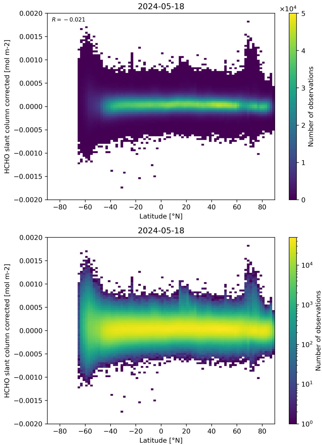
Figure 157: Scatter density plot of “Latitude” against “HCHO slant column corrected” for 2024-05-18 to 2024-05-19.
