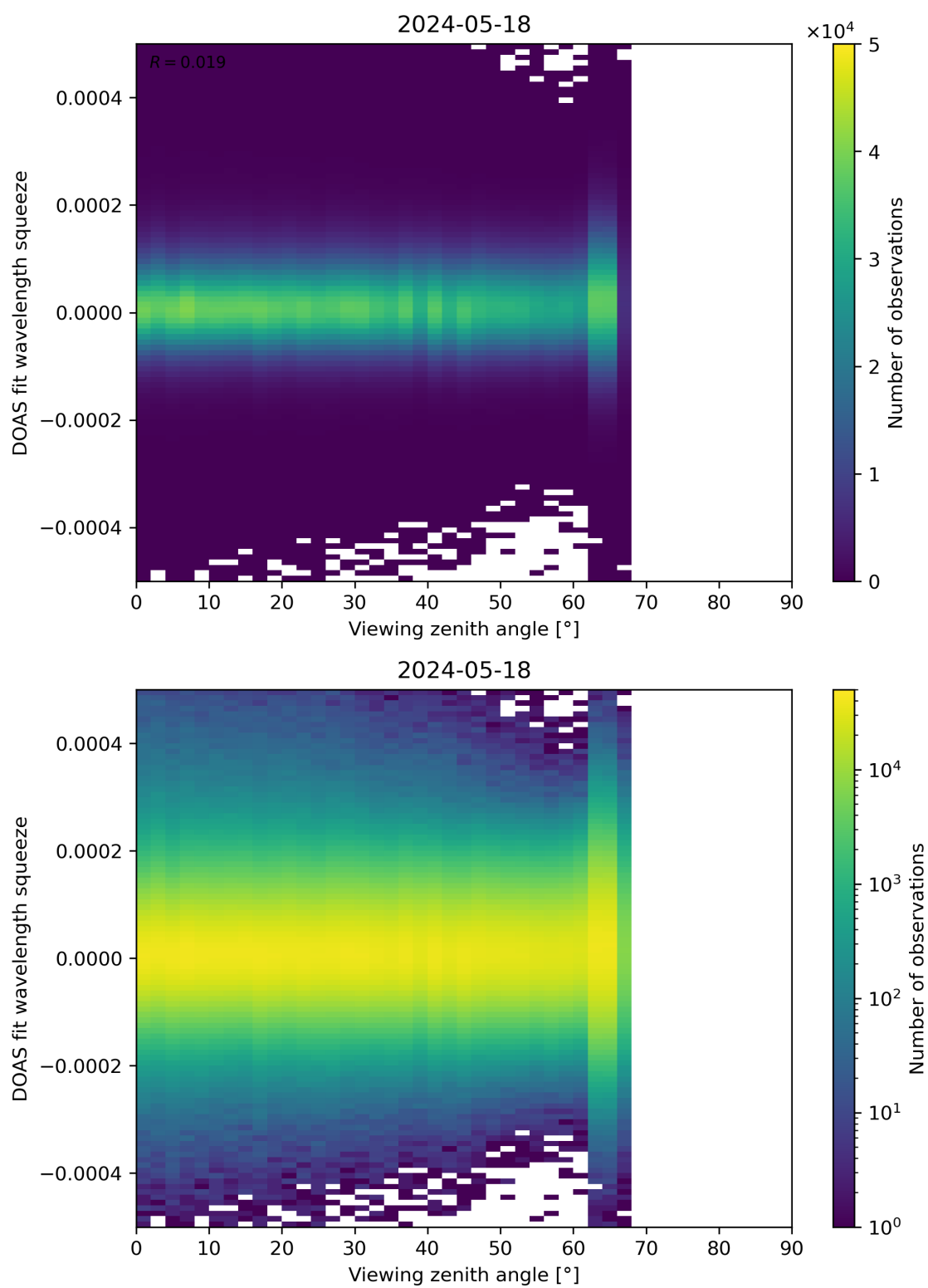
Figure 184: Scatter density plot of “Viewing zenith angle” against “DOAS fit wavelength squeeze” for 2024-05-18 to 2024-05-19.
