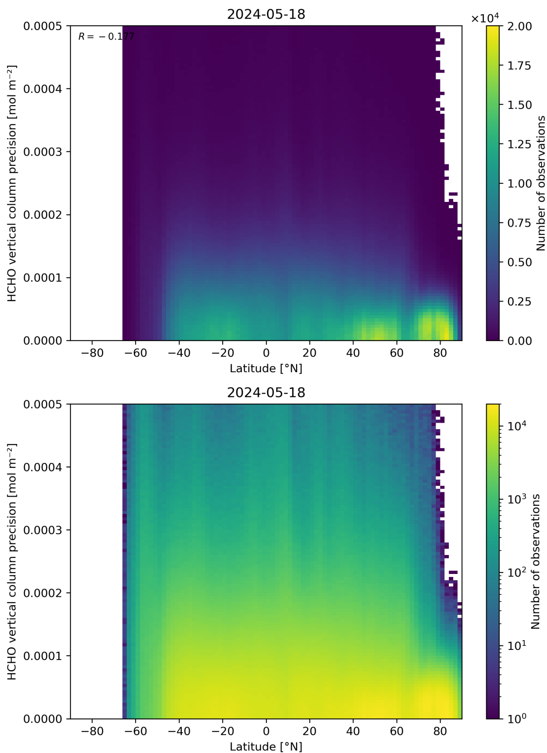
Figure 165: Scatter density plot of “Latitude” against “HCHO vertical column precision” for 2024-05-18 to 2024-05-19.
