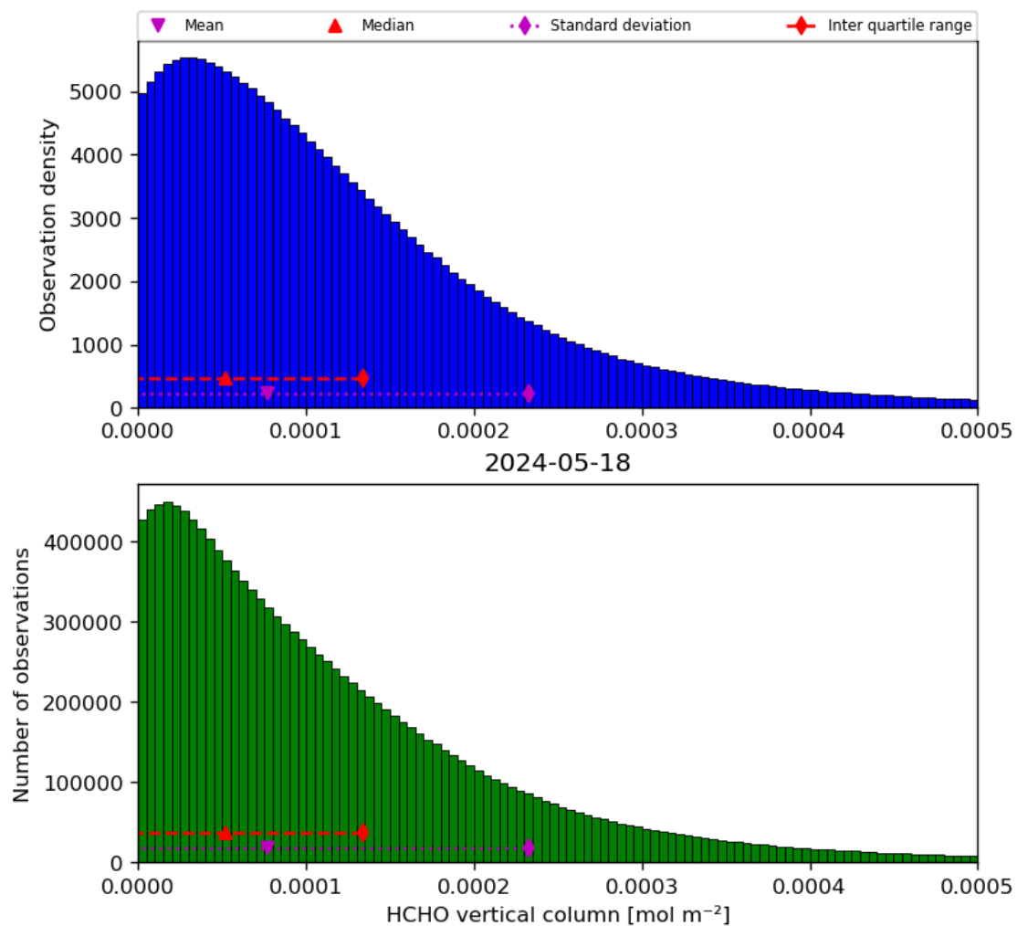
Figure 35: Histogram of “HCHO vertical column” for 2024-05-18 to 2024-05-19
