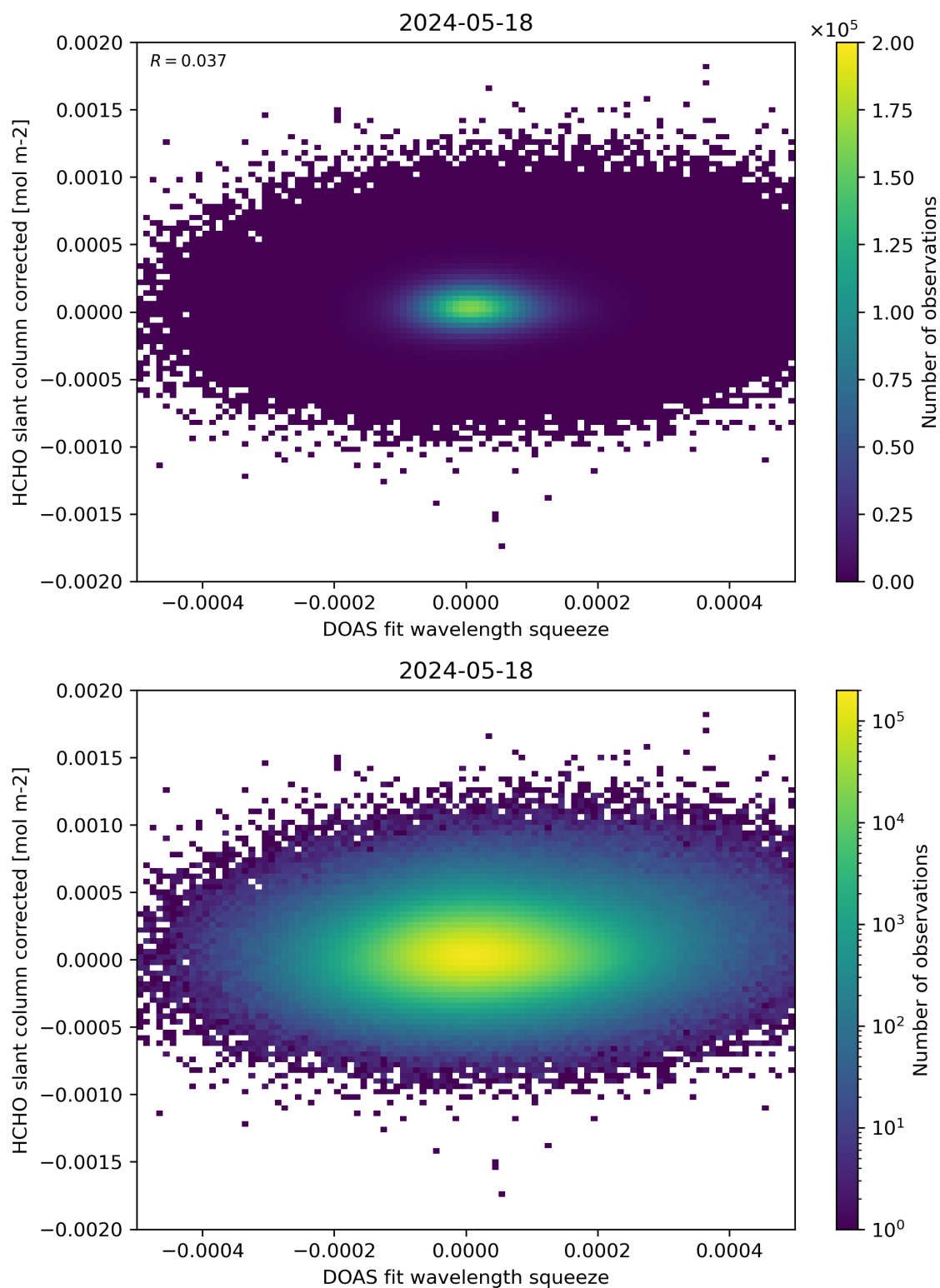
Figure 69: Scatter density plot of “DOAS fit wavelength squeeze” against “HCHO slant column corrected” for 2024-05-18 to 2024-05-19.
