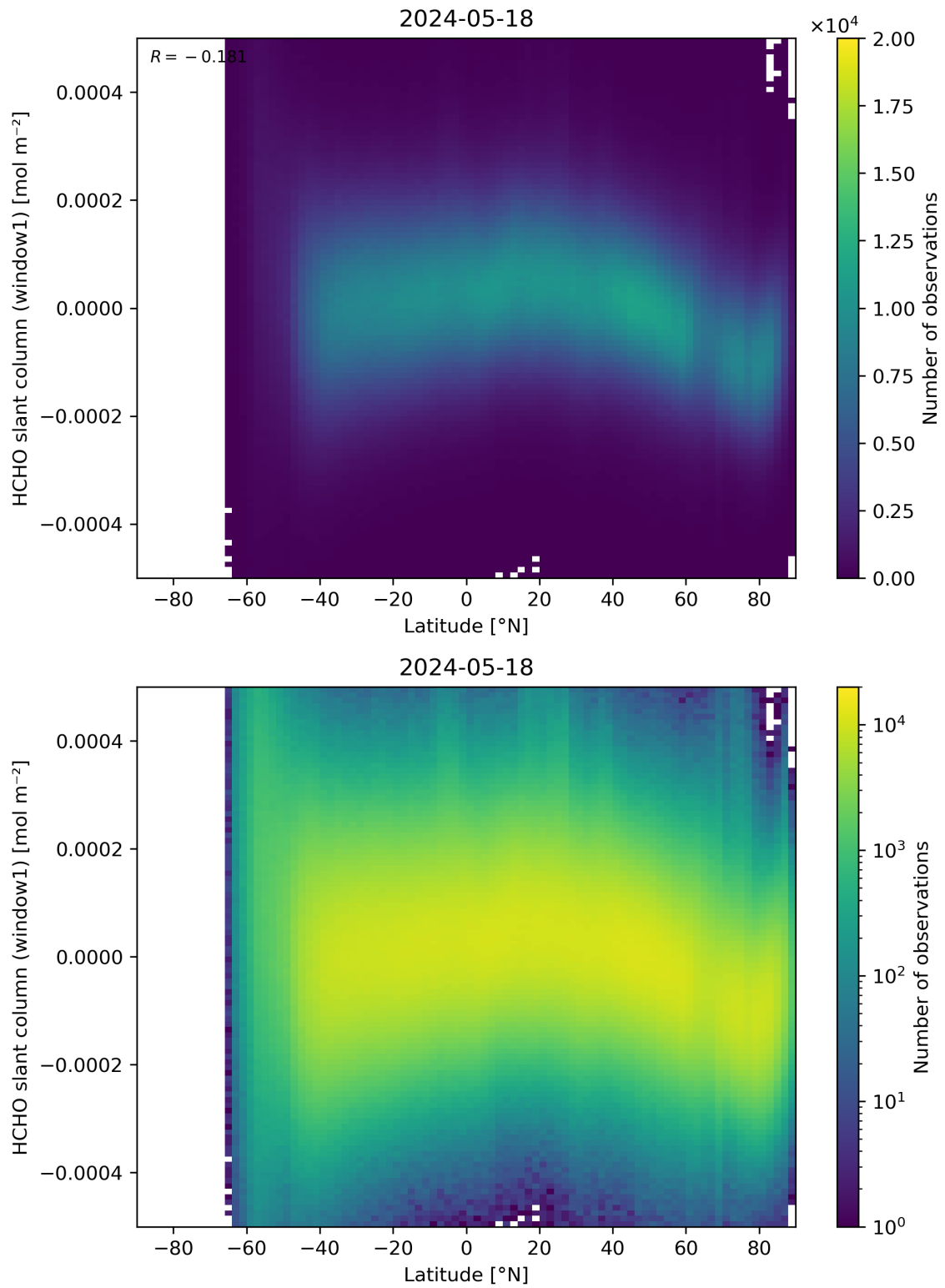
Figure 159: Scatter density plot of “Latitude” against “HCHO slant column (window1)” for 2024-05-18 to 2024-05-19.
