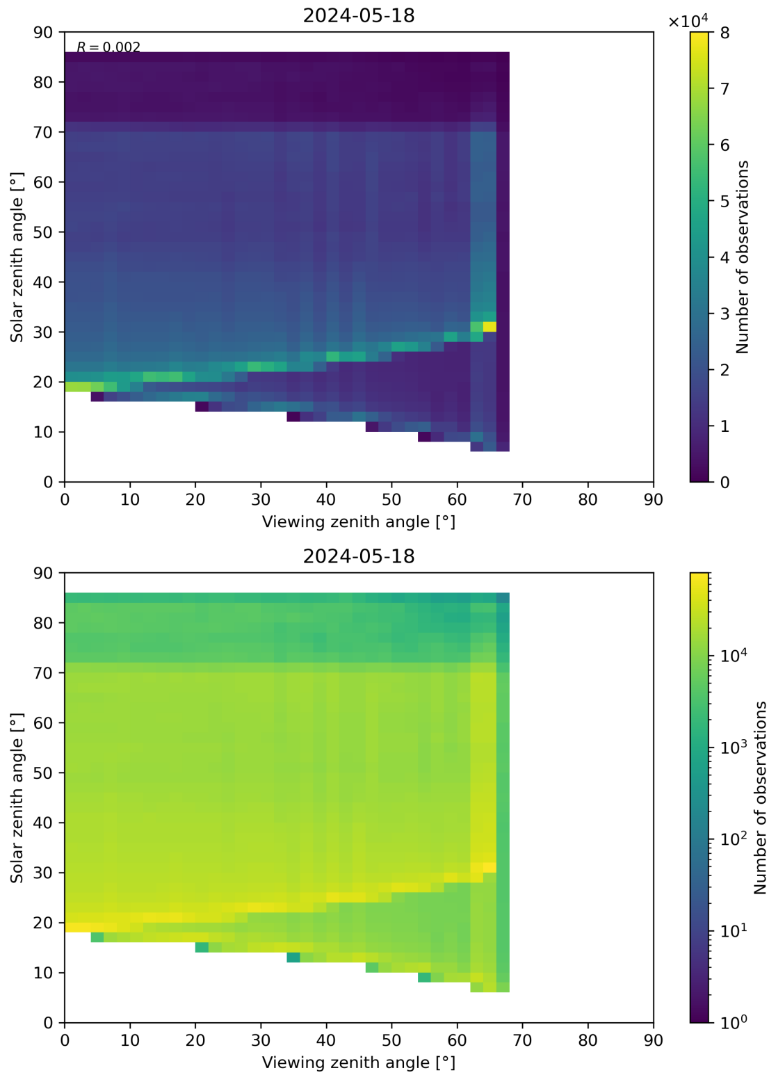
Figure 197: Scatter density plot of “Viewing zenith angle” against “Solar zenith angle” for 2024-05-18 to 2024-05-19.
