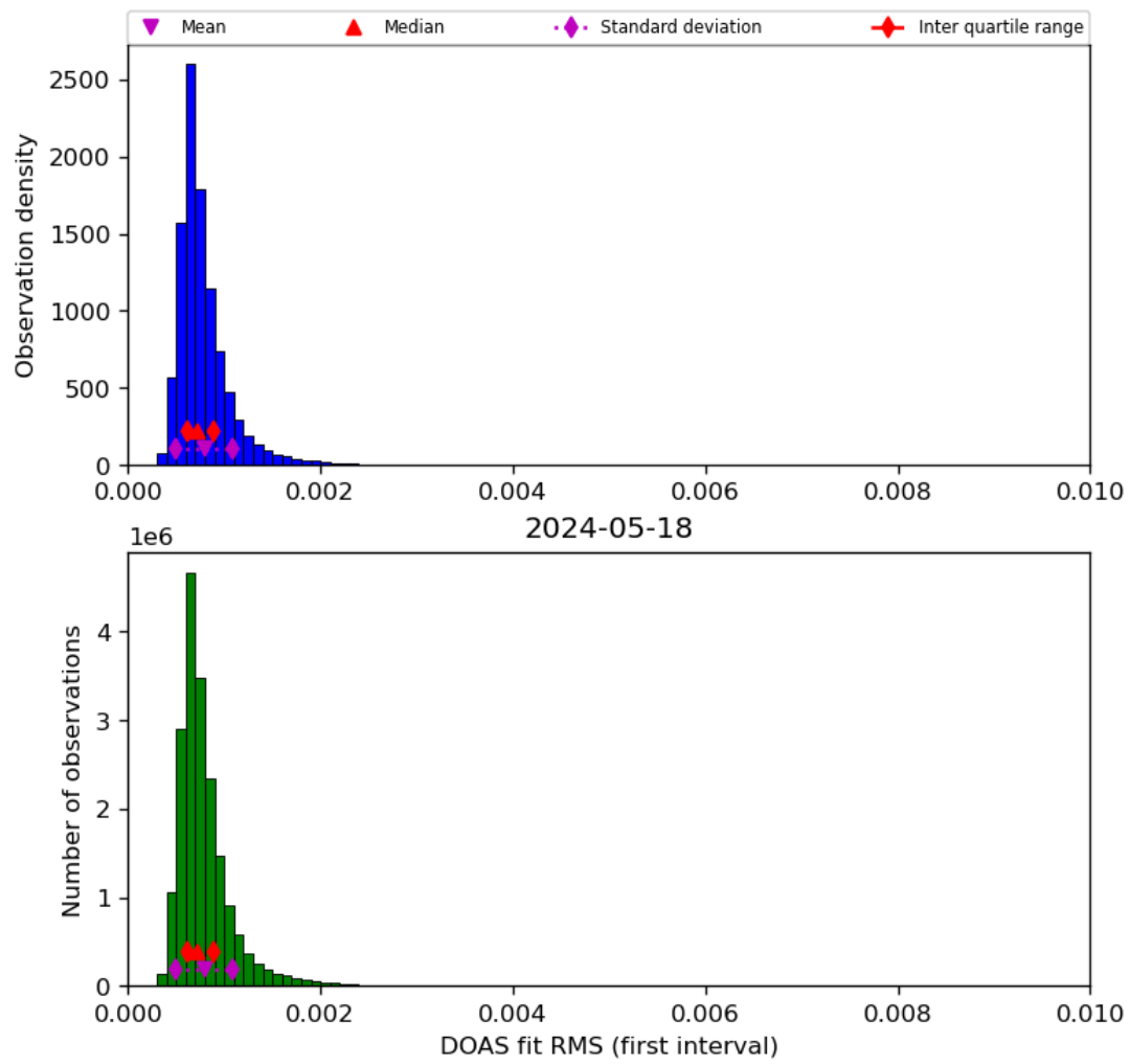
Figure 46: Histogram of “DOAS fit RMS (first interval)” for 2024-05-18 to 2024-05-19
