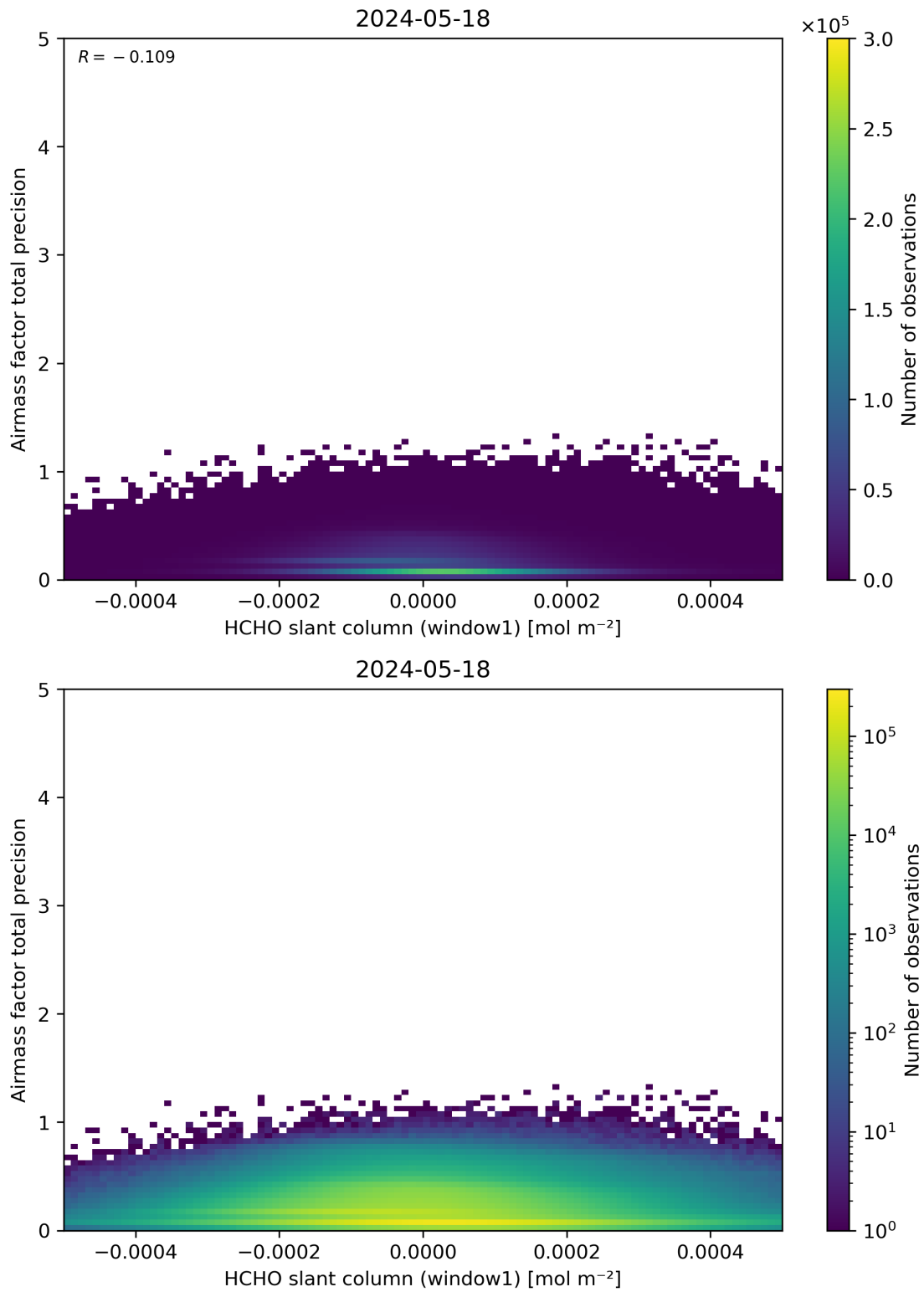
Figure 86: Scatter density plot of “HCHO slant column (window1)” against “Airmass factor total precision” for 2024-05-18 to 2024-05-19.
