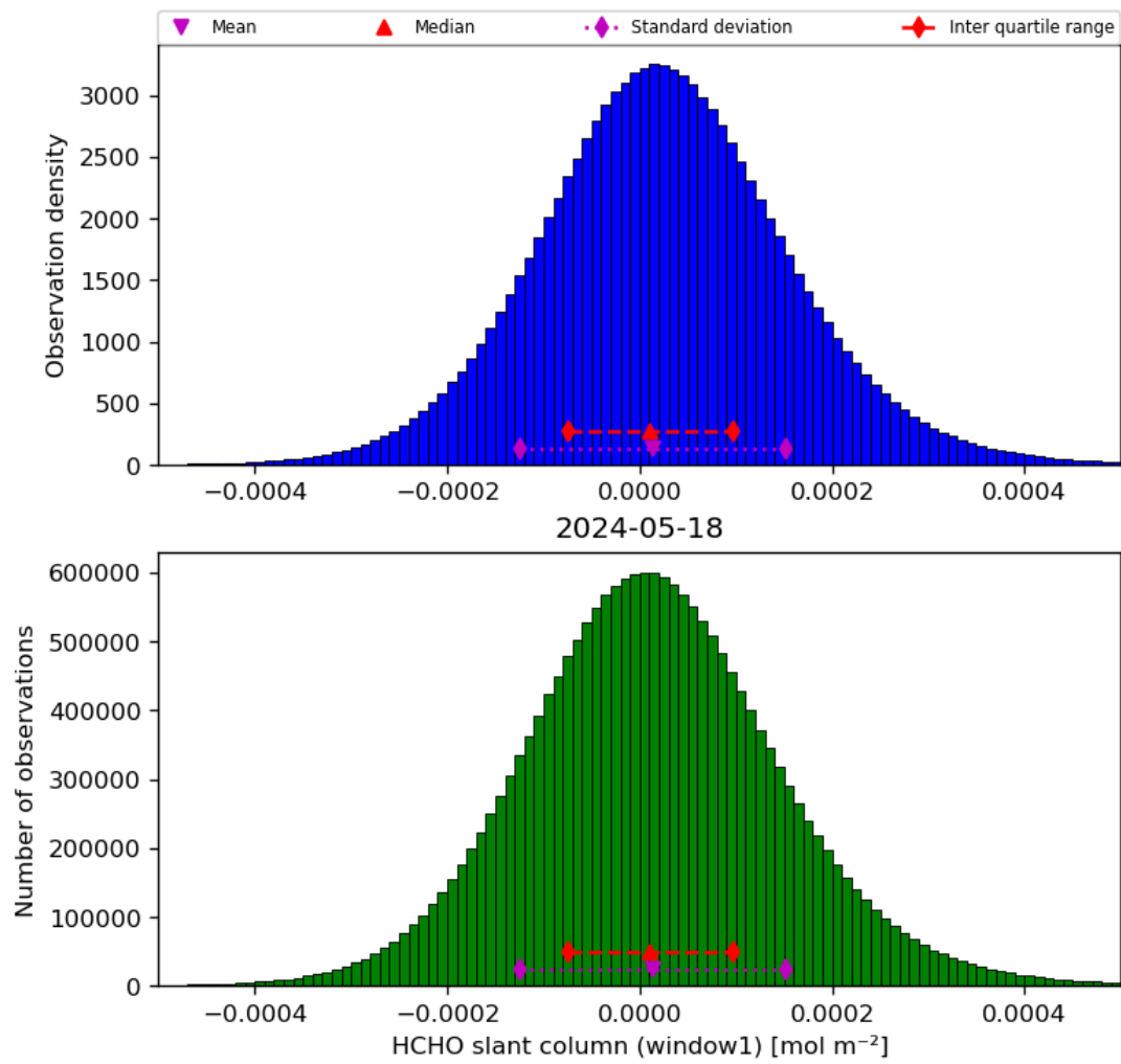
Figure 38: Histogram of “HCHO slant column (window1)” for 2024-05-18 to 2024-05-19
