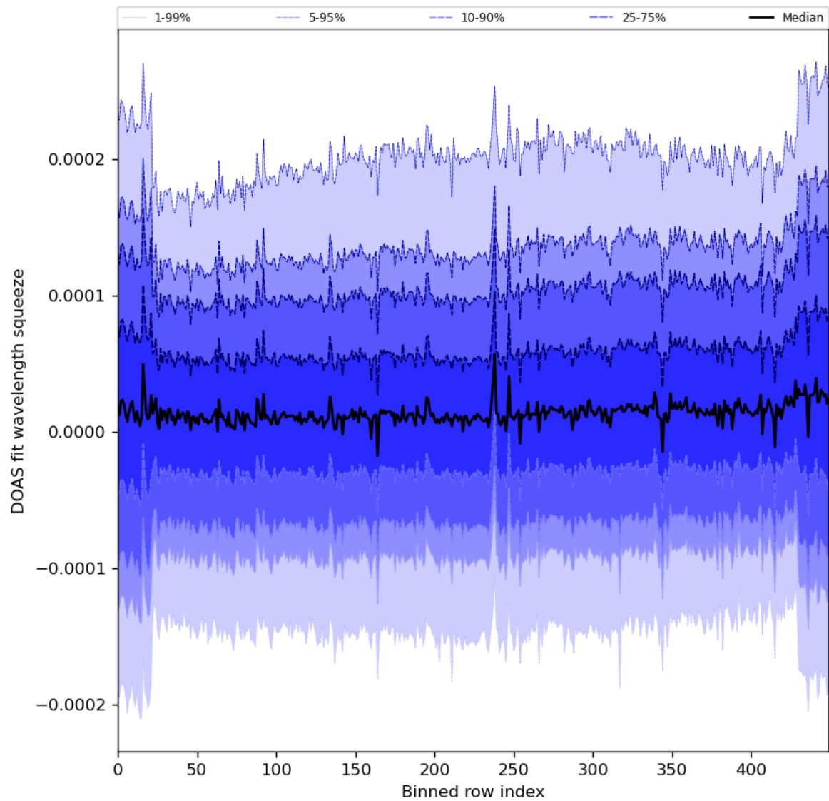
Figure 59: Along track statistics of “DOAS fit wavelength squeeze” for 2024-05-18 to 2024-05-19
