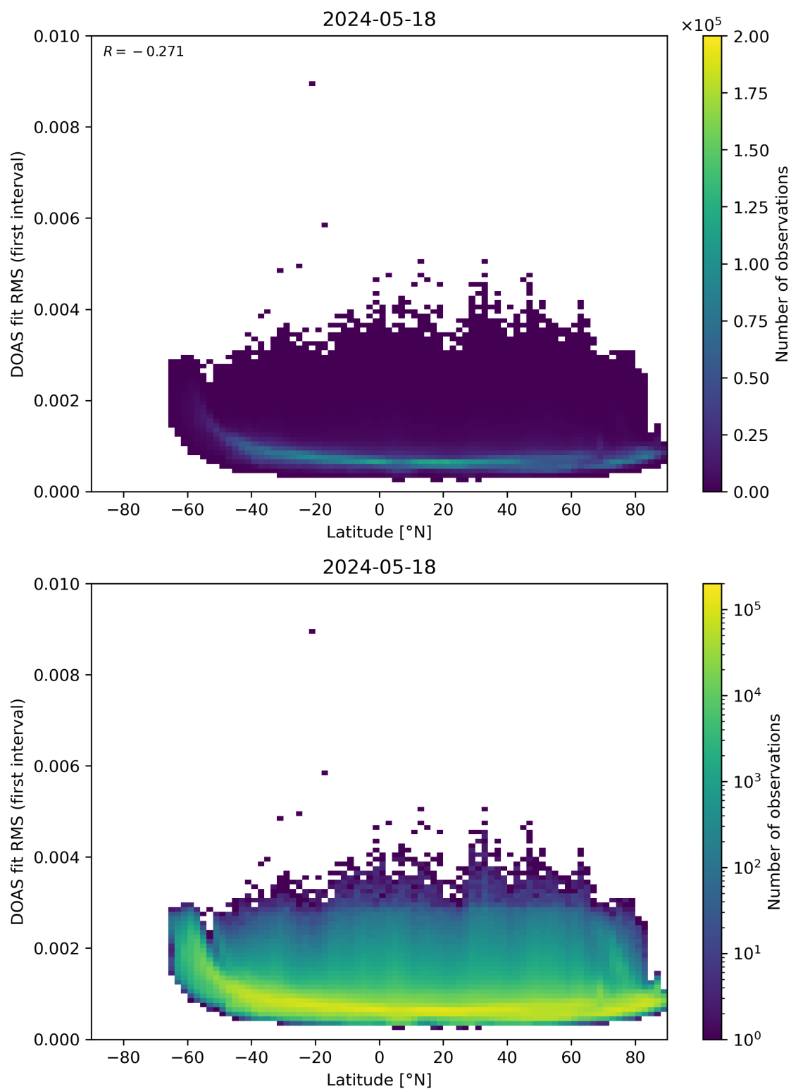
Figure 153: Scatter density plot of “Latitude” against “DOAS fit RMS (first interval)” for 2024-05-18 to 2024-05-19.
