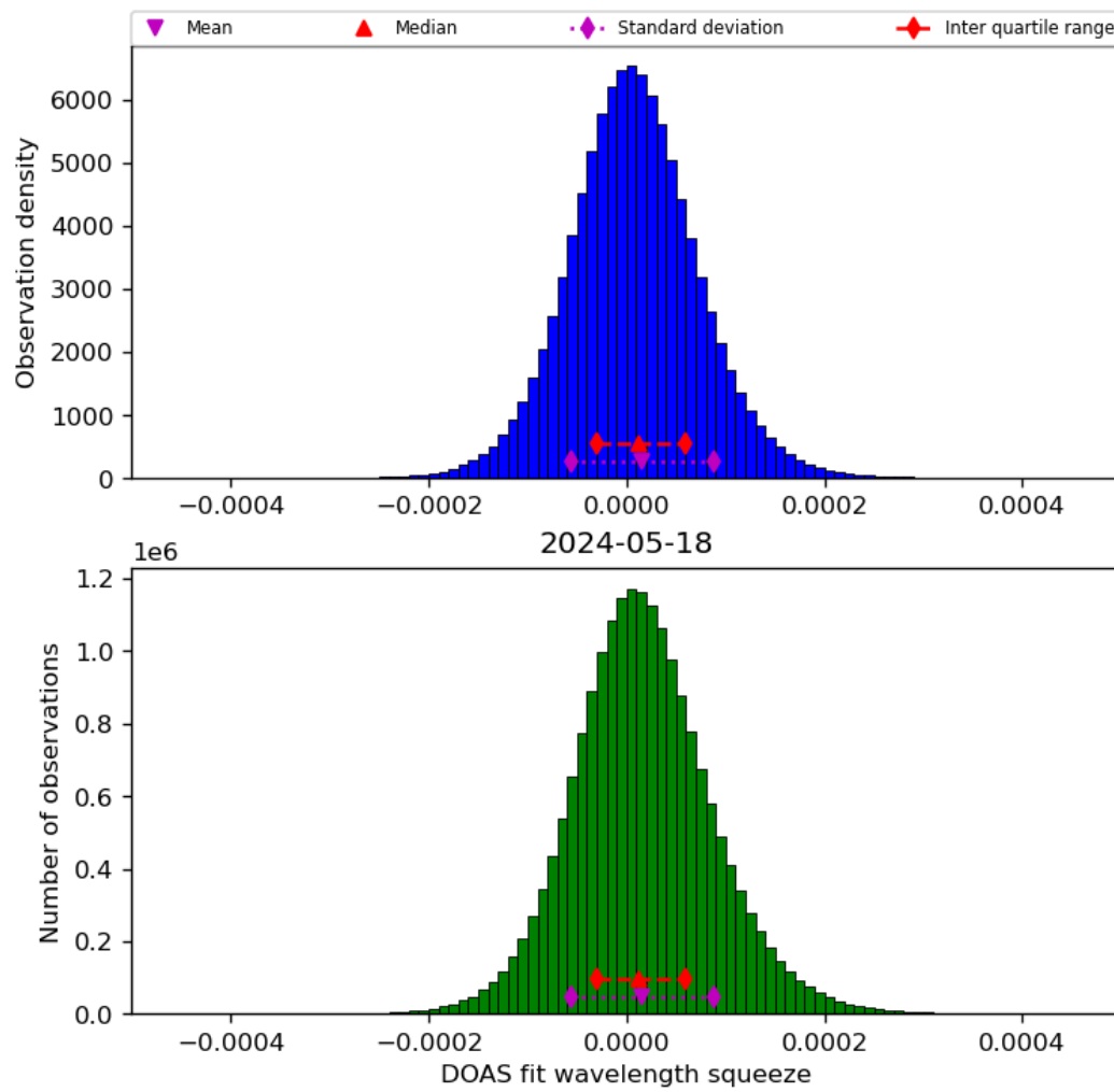
Figure 45: Histogram of “DOAS fit wavelength squeeze” for 2024-05-18 to 2024-05-19
