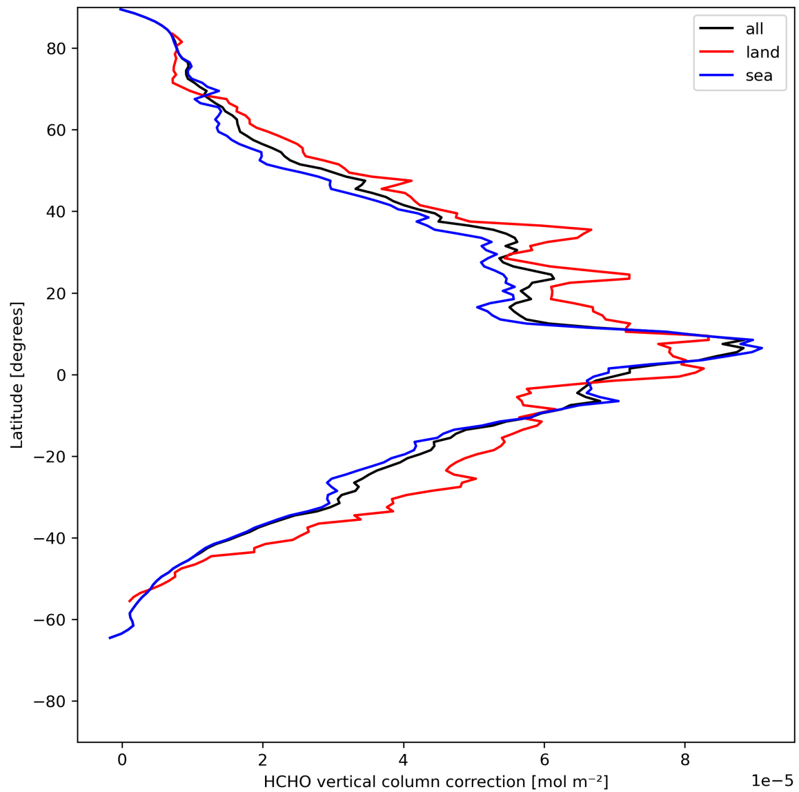
Figure 23: Zonal average of “HCHO vertical column correction” for 2024-05-18 to 2024-05-19.
