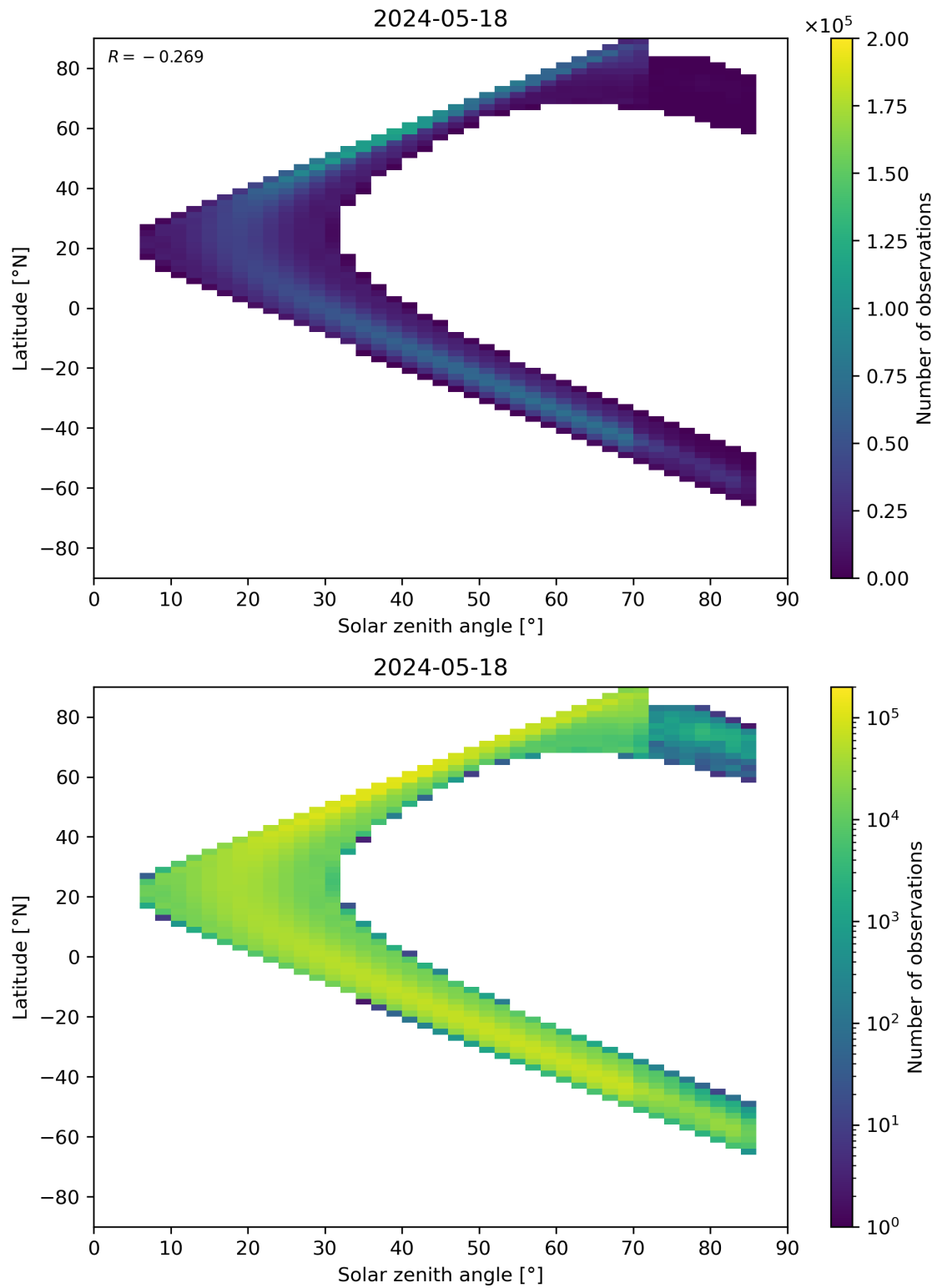
Figure 181: Scatter density plot of “Solar zenith angle” against “Latitude” for 2024-05-18 to 2024-05-19.
