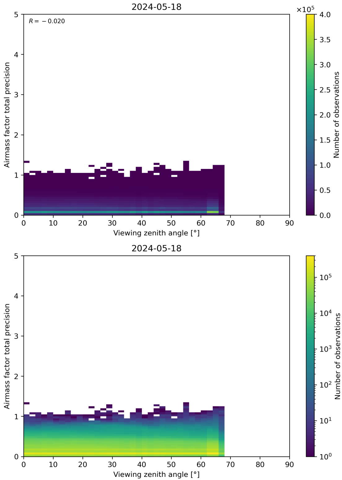
Figure 191: Scatter density plot of “Viewing zenith angle” against “Airmass factor total precision” for 2024-05-18 to 2024-05-19.
