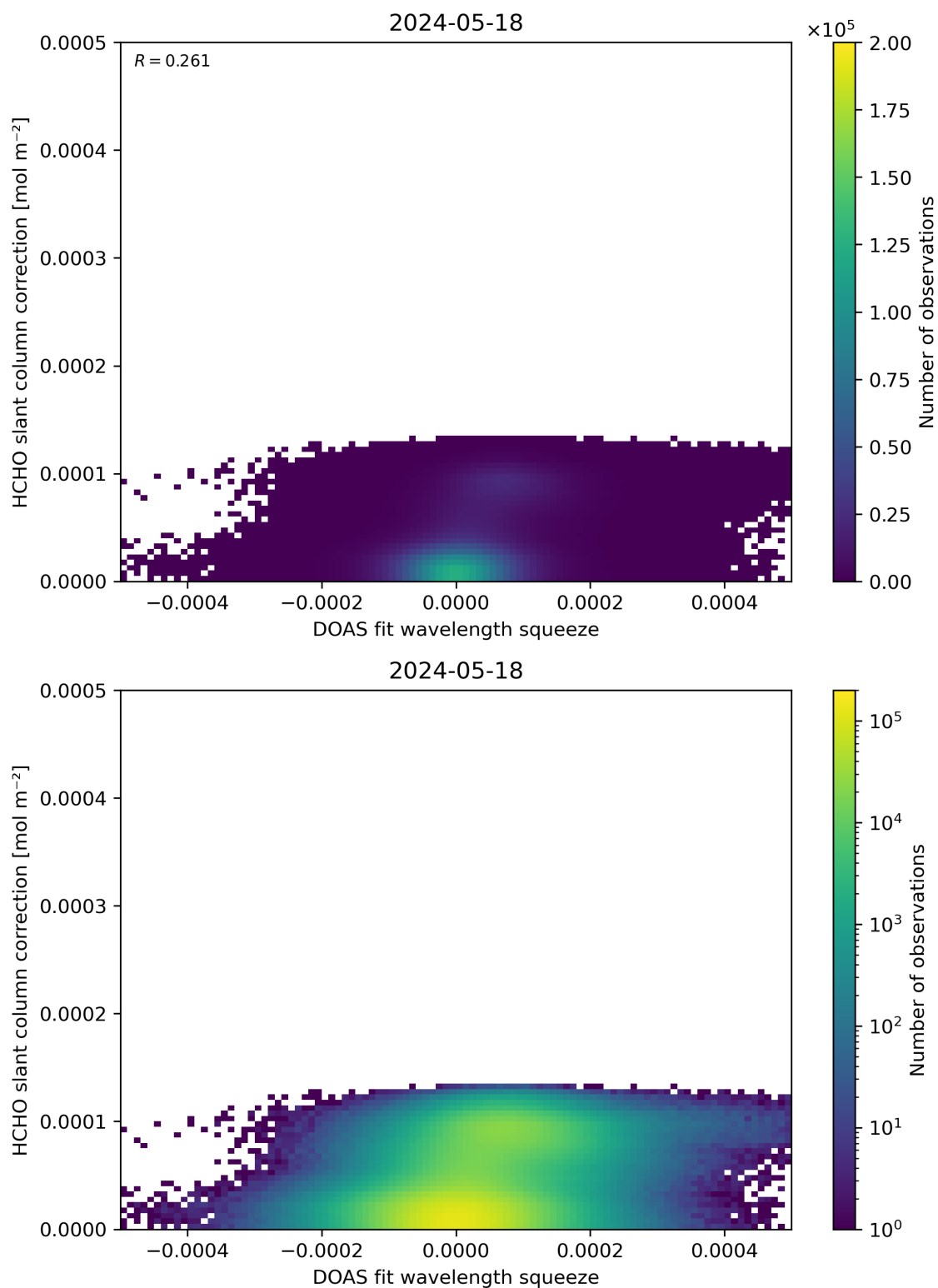
Figure 70: Scatter density plot of “DOAS fit wavelength squeeze” against “HCHO slant column correction” for 2024-05-18 to 2024-05-19.
