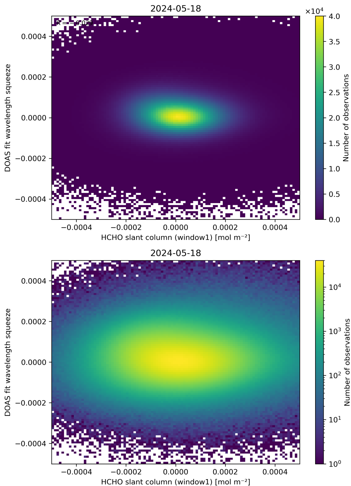
Figure 80: Scatter density plot of “HCHO slant column (window1)” against “DOAS fit wavelength squeeze” for 2024-05-18 to 2024-05-19.
