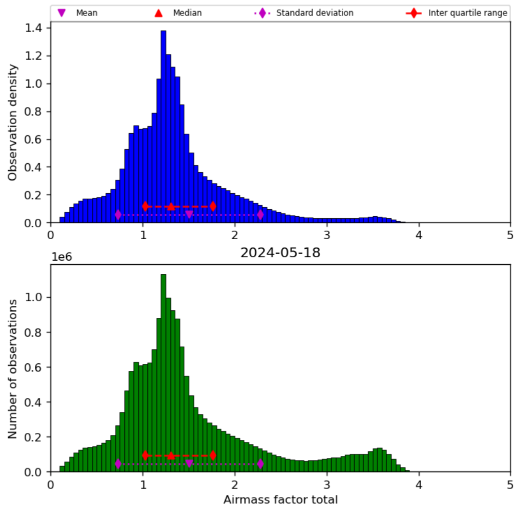
Figure 40: Histogram of “Airmass factor total” for 2024-05-18 to 2024-05-19
