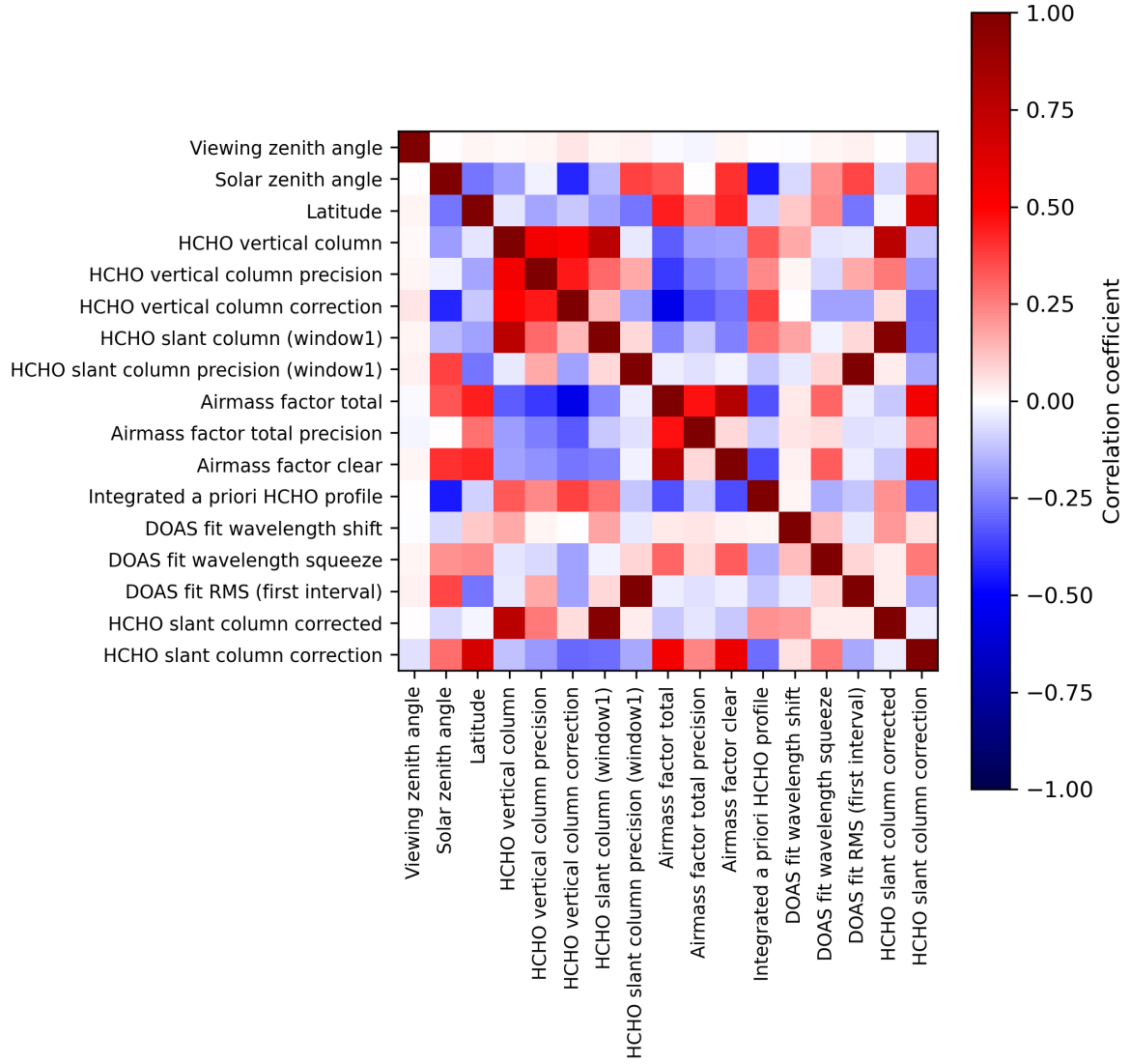
Figure 2: Map of correlation matrix for 2024-05-18 to 2024-05-19.
