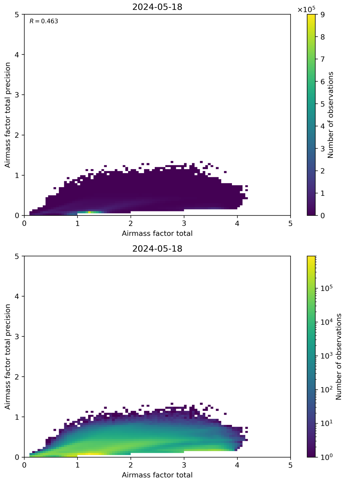
Figure 103: Scatter density plot of “Airmass factor total” against “Airmass factor total precision” for 2024-05-18 to 2024-05-19.
