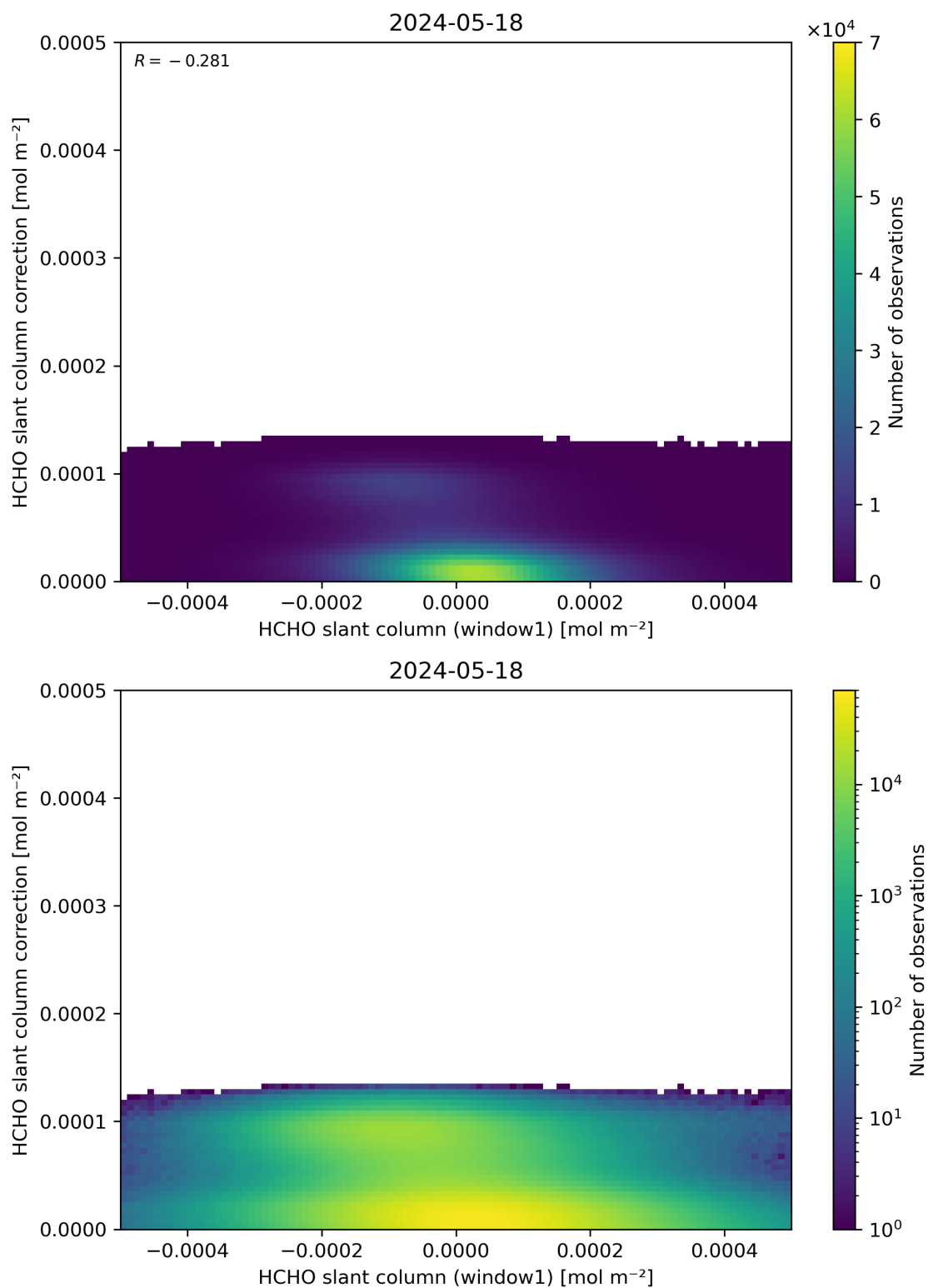
Figure 83: Scatter density plot of “HCHO slant column (window1)” against “HCHO slant column correction” for 2024-05-18 to 2024-05-19.
