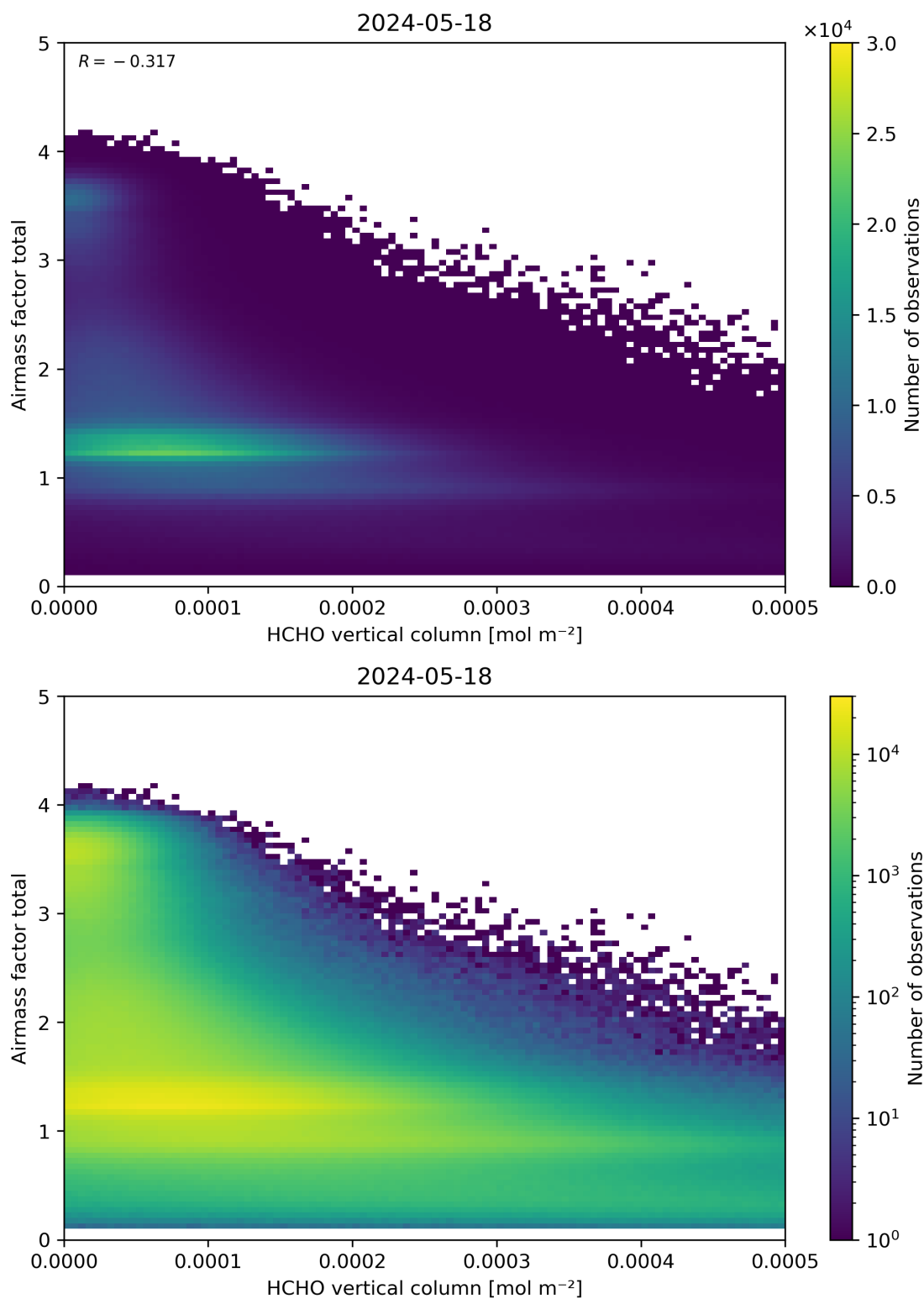
Figure 131: Scatter density plot of “HCHO vertical column” against “Airmass factor total” for 2024-05-18 to 2024-05-19.
