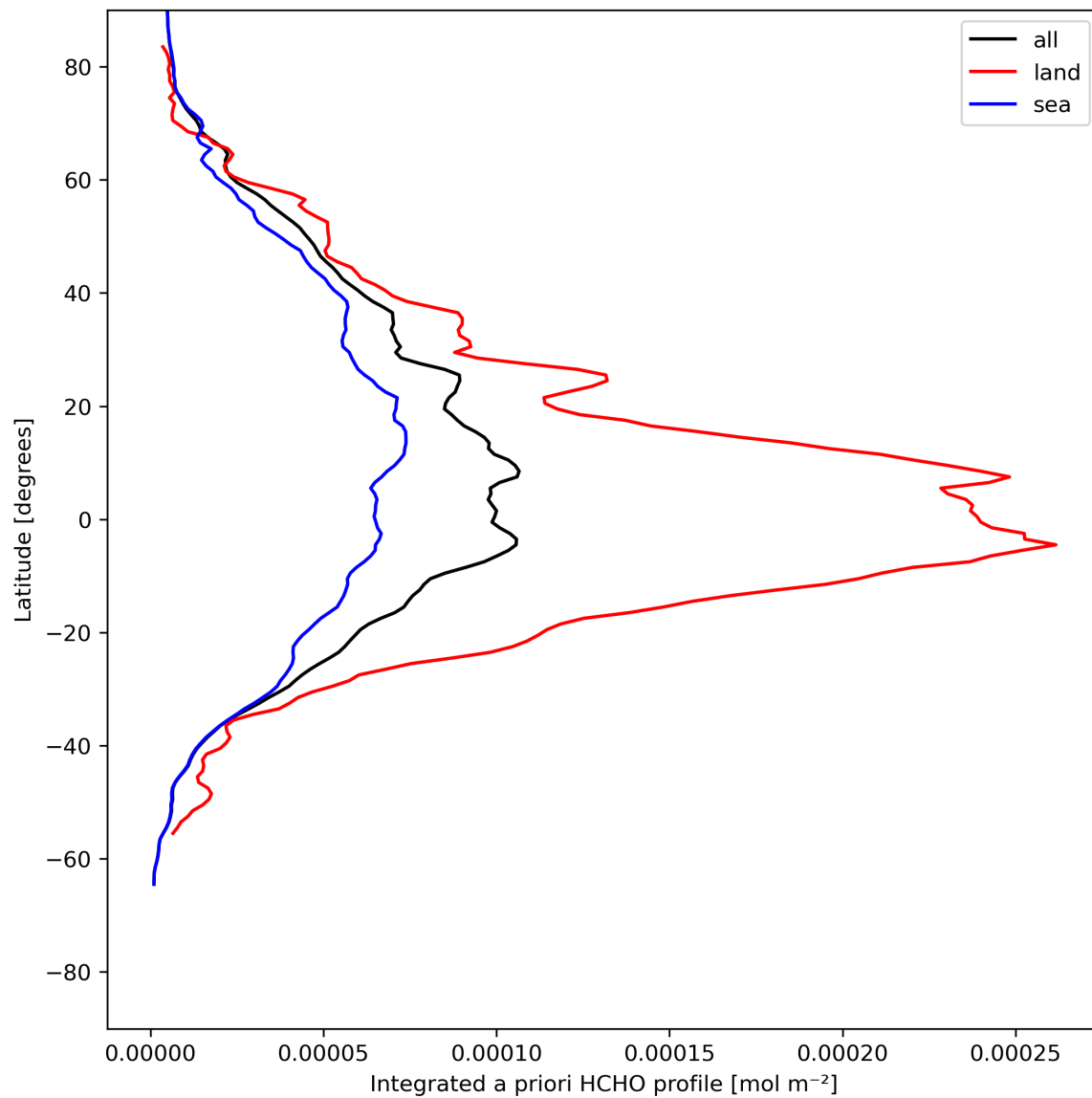
Figure 29: Zonal average of “Integrated a priori HCHO profile” for 2024-05-18 to 2024-05-19.
