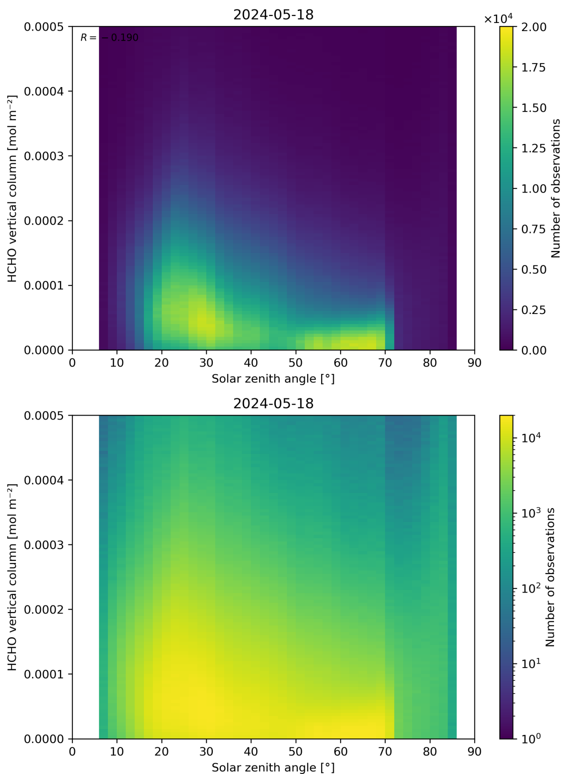
Figure 177: Scatter density plot of “Solar zenith angle” against “HCHO vertical column” for 2024-05-18 to 2024-05-19.
