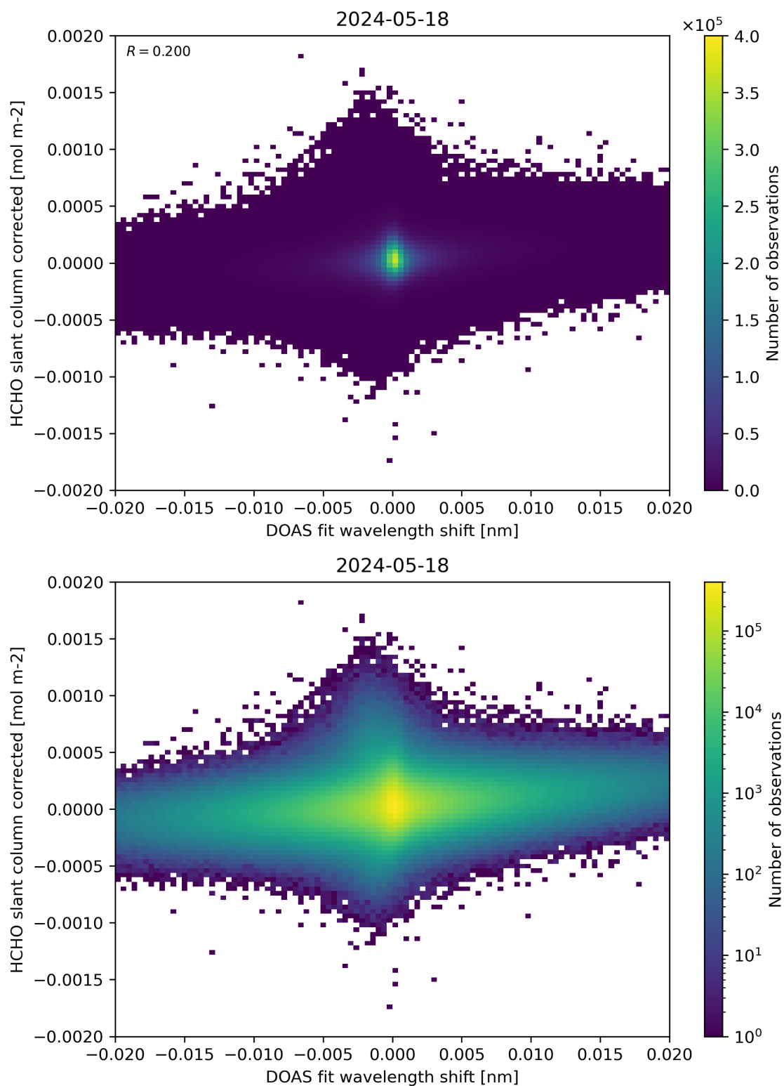
Figure 66: Scatter density plot of “DOAS fit wavelength shift” against “HCHO slant column corrected” for 2024-05-18 to 2024-05-19.
