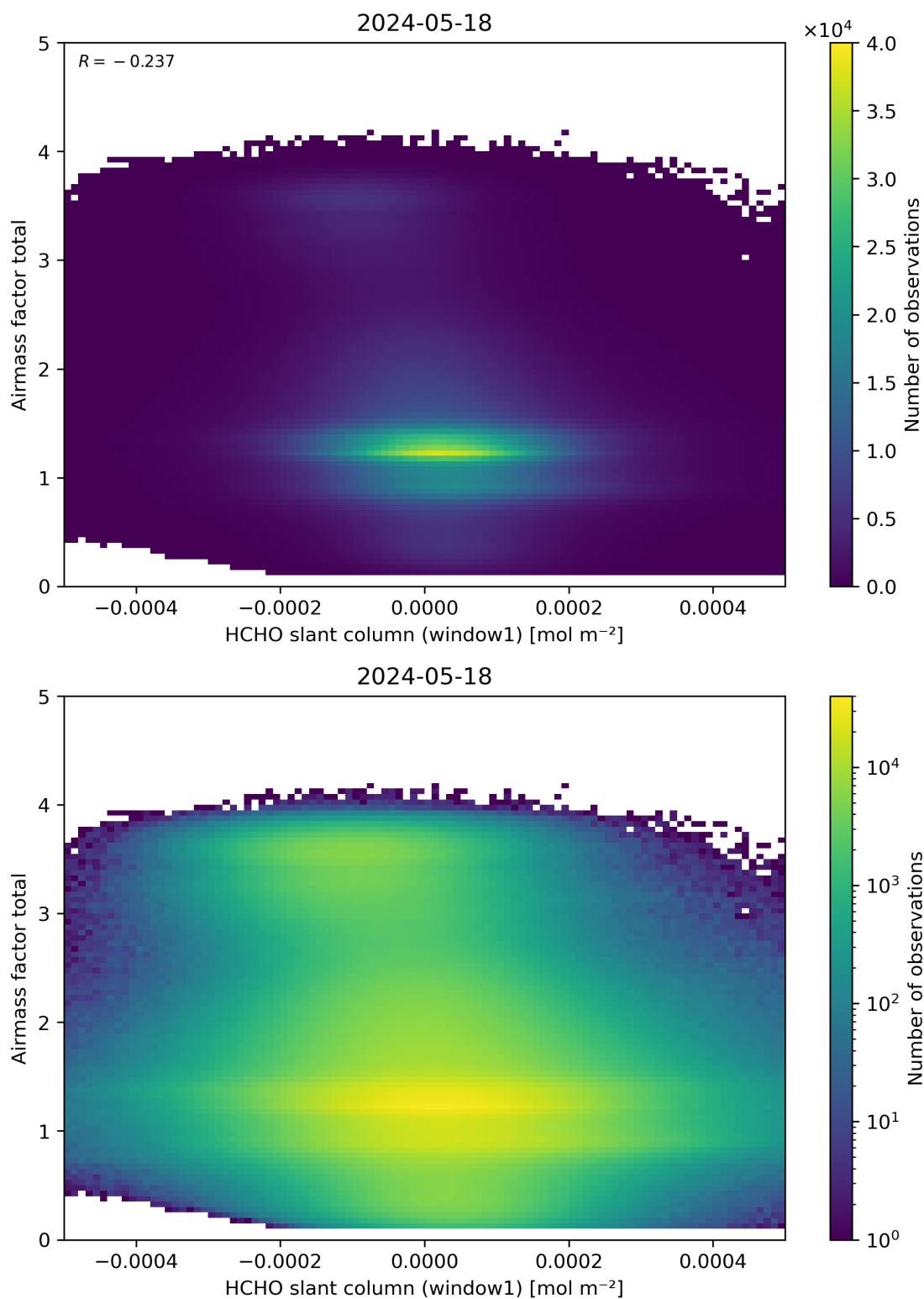
Figure 85: Scatter density plot of “HCHO slant column (window1)” against “Airmass factor total” for 2024-05-18 to 2024-05-19.
