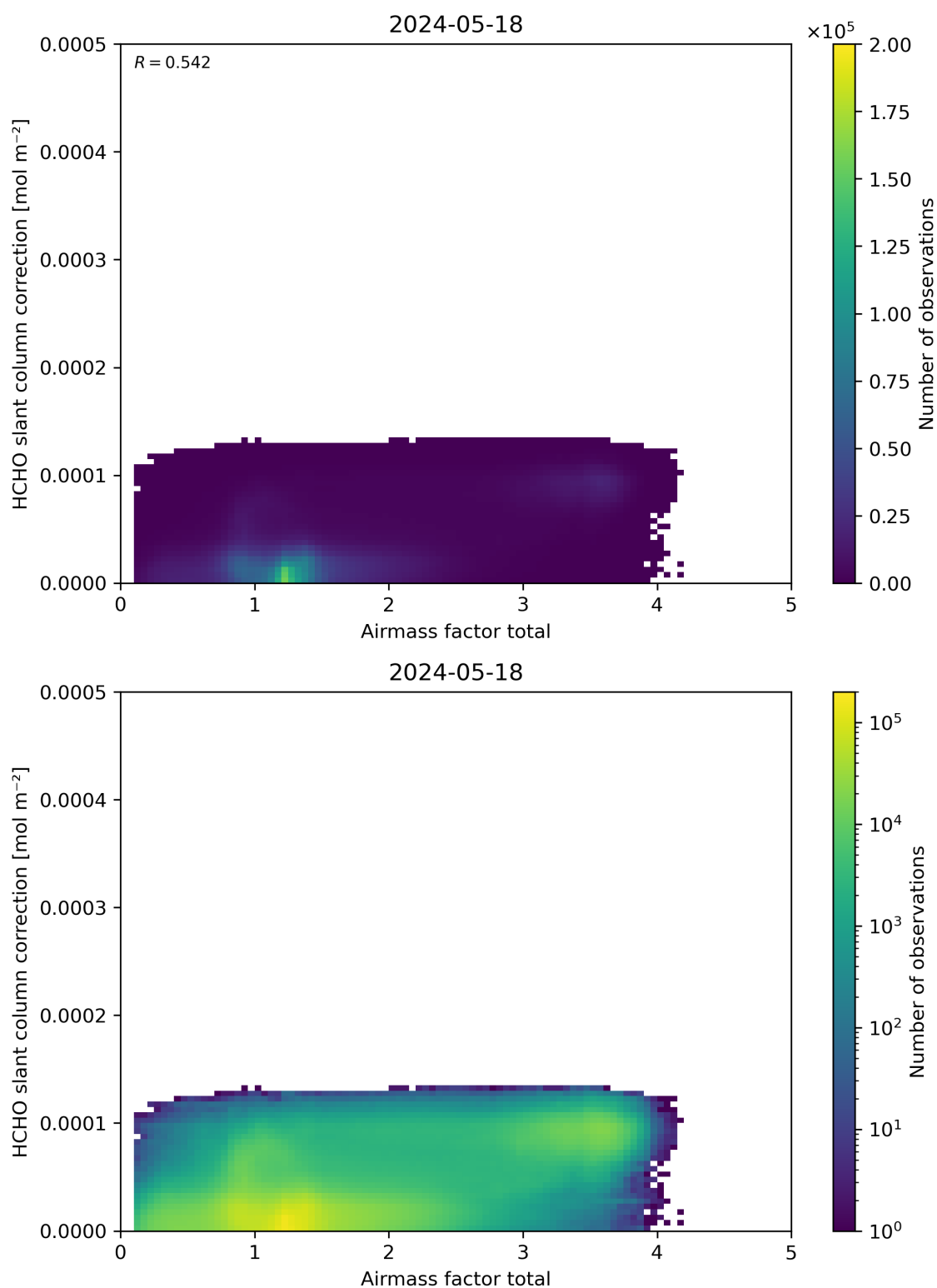
Figure 102: Scatter density plot of “Airmass factor total” against “HCHO slant column correction” for 2024-05-18 to 2024-05-19.
