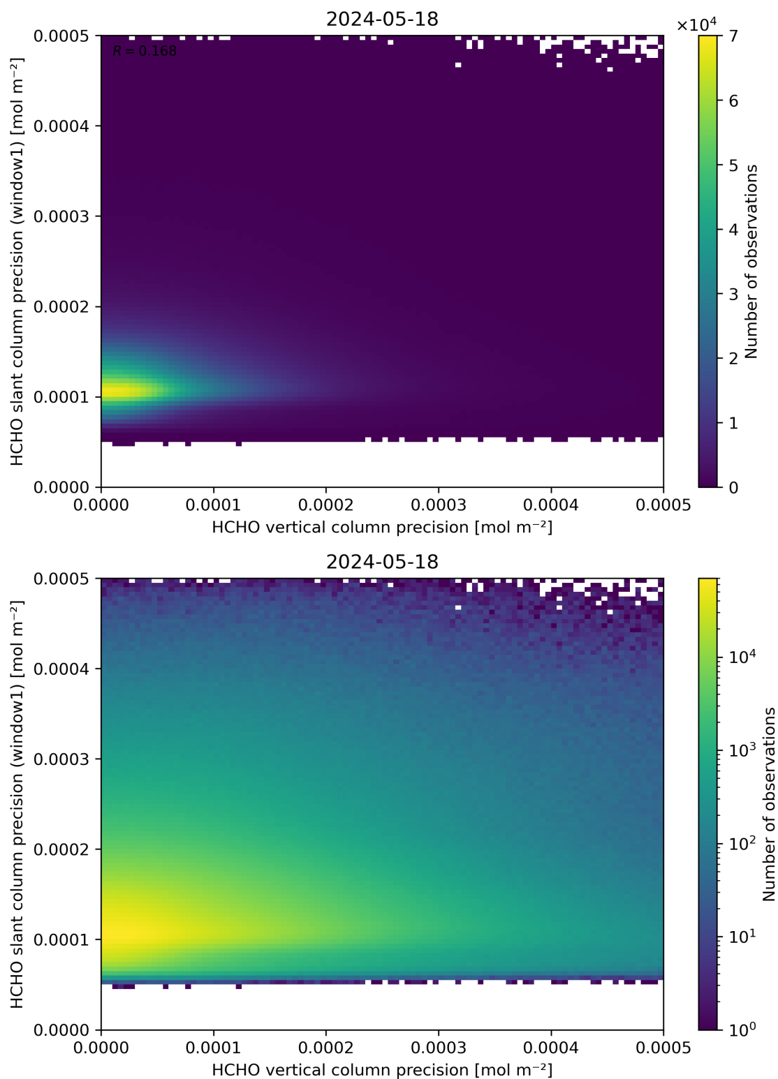
Figure 143: Scatter density plot of “HCHO vertical column precision” against “HCHO slant column precision (window1)” for 2024-05-18 to 2024-05-19.
