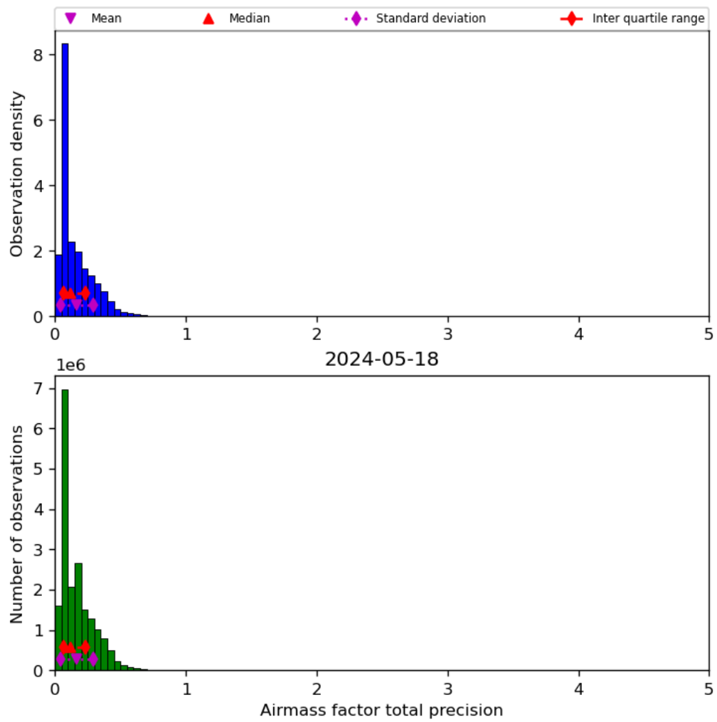
Figure 41: Histogram of “Airmass factor total precision” for 2024-05-18 to 2024-05-19
