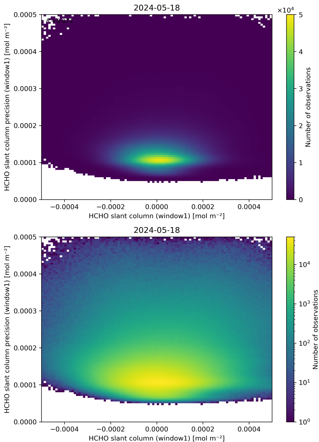
Figure 84: Scatter density plot of “HCHO slant column (window1)” against “HCHO slant column precision (window1)” for 2024-05-18 to 2024-05-19.
