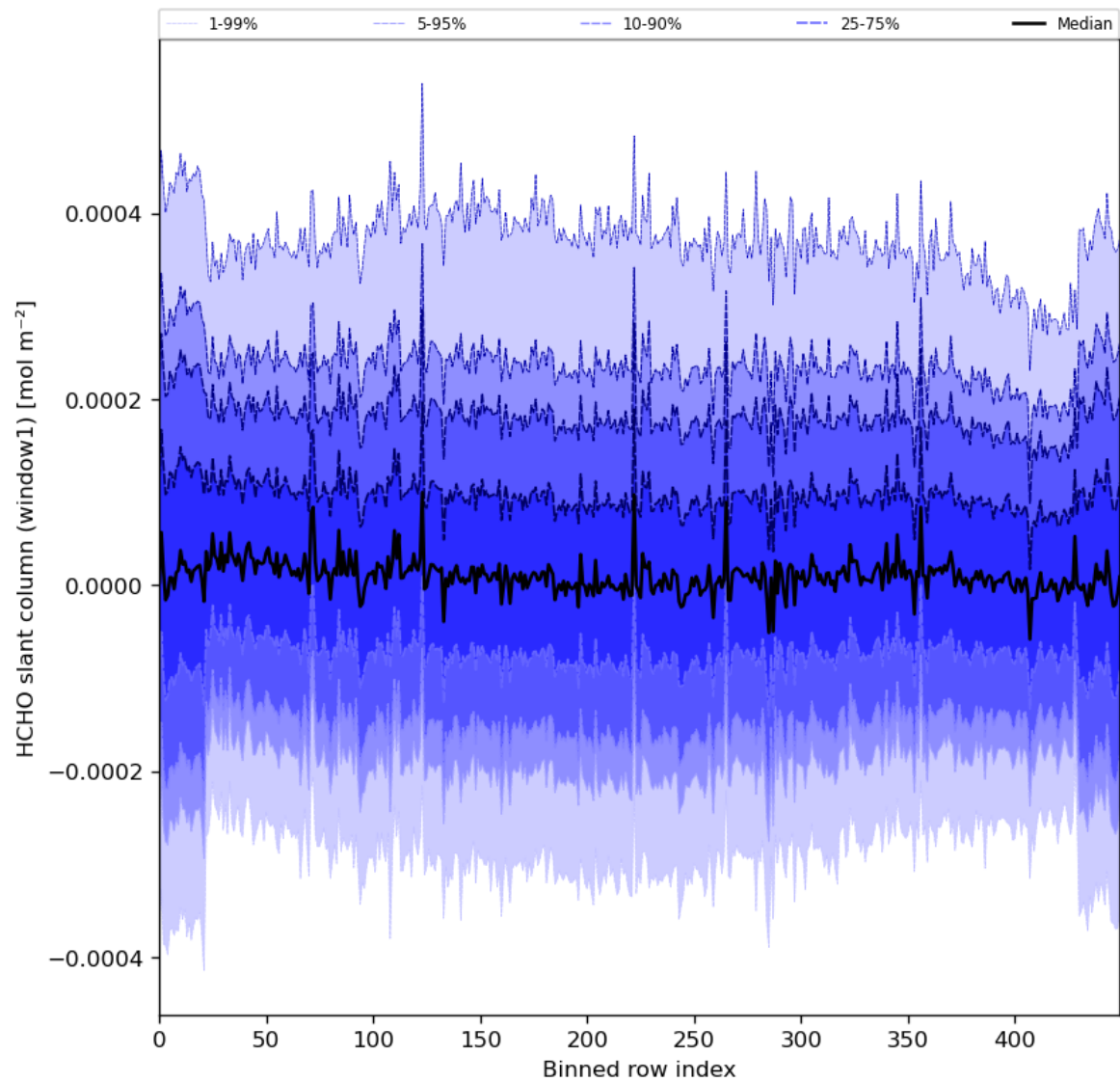
Figure 52: Along track statistics of “HCHO slant column (window1)” for 2024-05-18 to 2024-05-19
