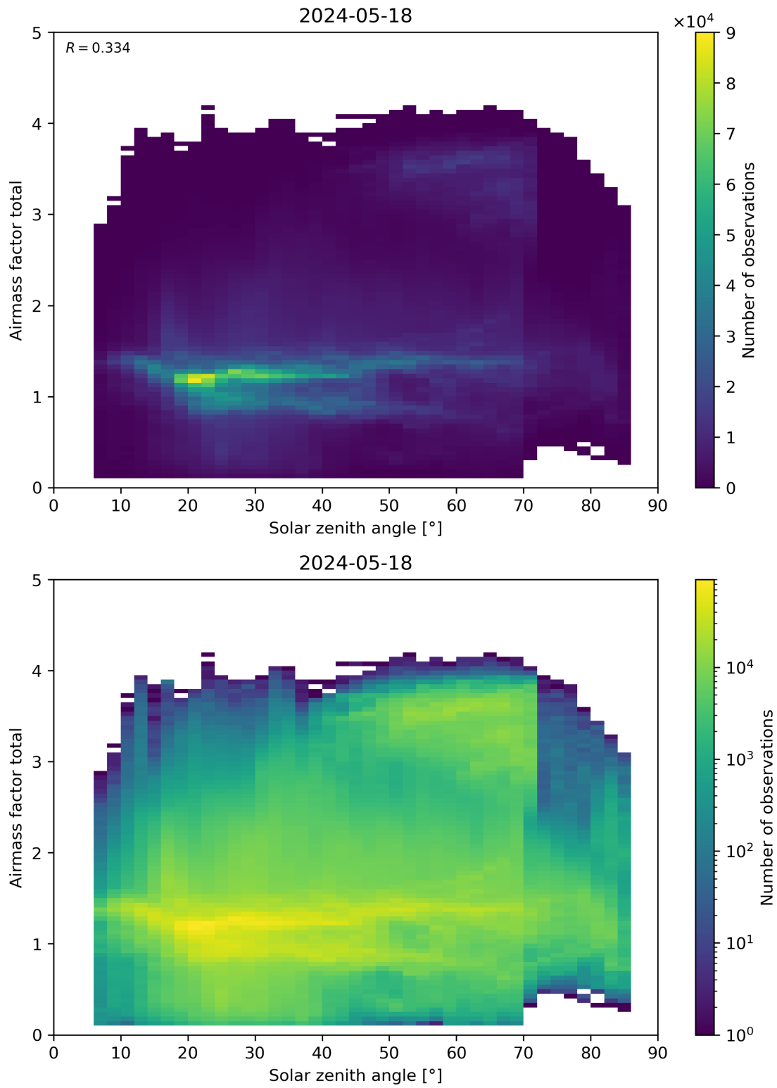
Figure 175: Scatter density plot of “Solar zenith angle” against “Airmass factor total” for 2024-05-18 to 2024-05-19.
