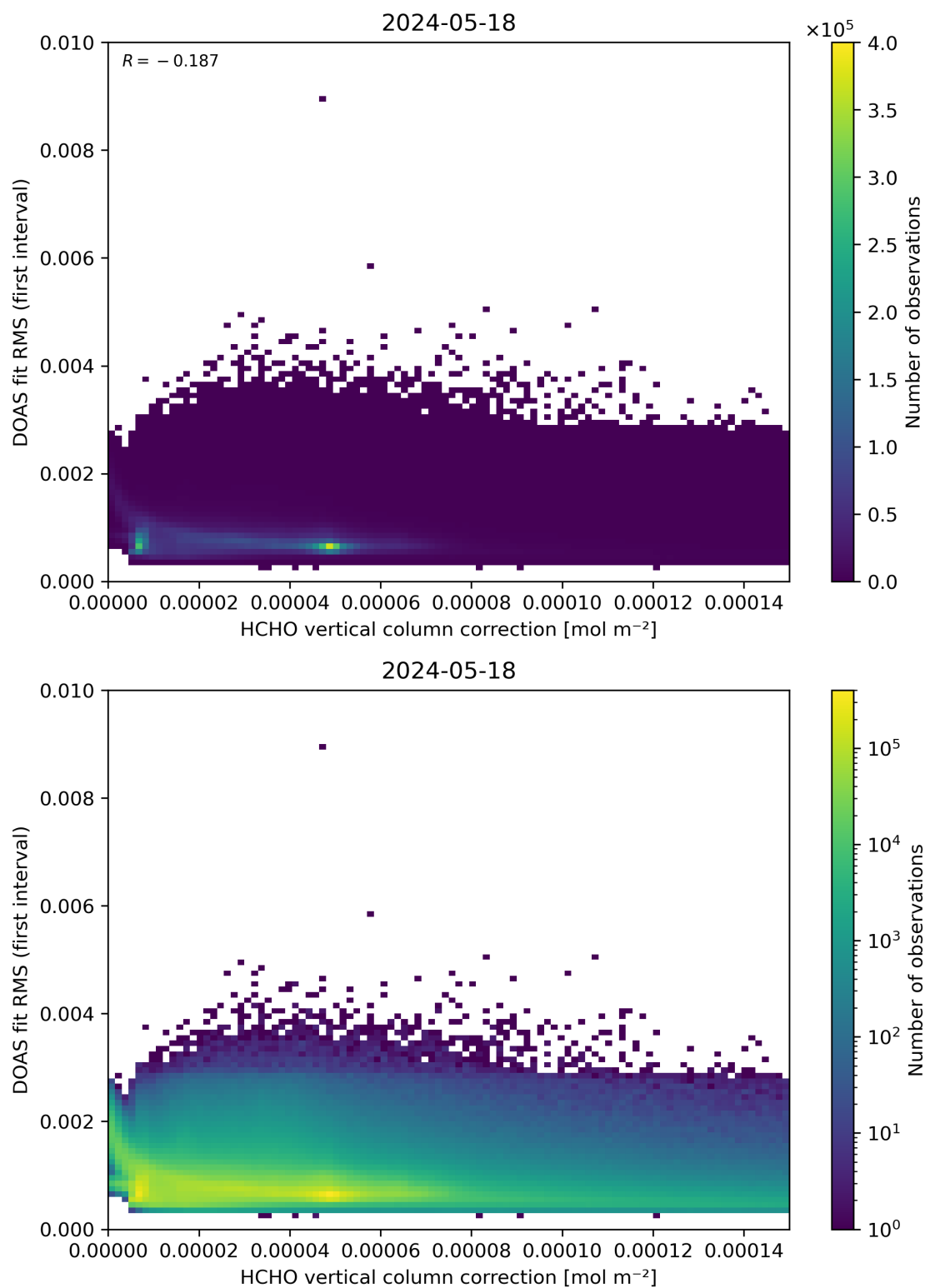
Figure 112: Scatter density plot of “HCHO vertical column correction” against “DOAS fit RMS (first interval)” for 2024-05-18 to 2024-05-19.
