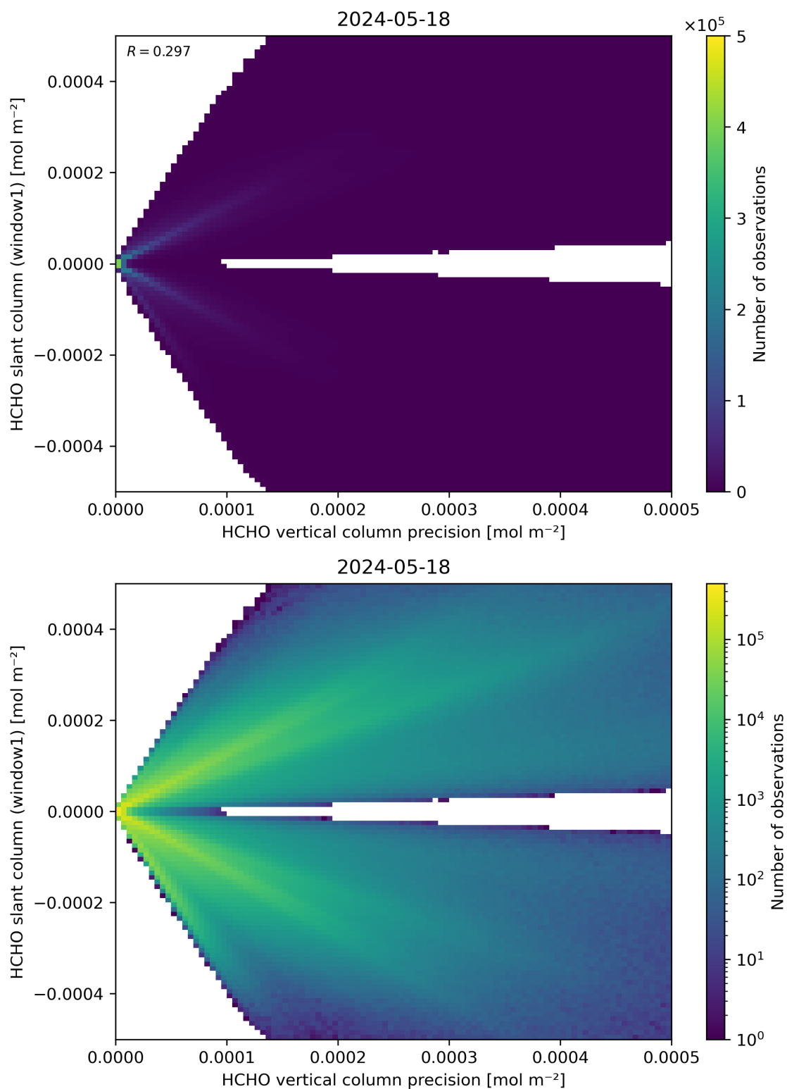
Figure 142: Scatter density plot of “HCHO vertical column precision” against “HCHO slant column (window1)” for 2024-05-18 to 2024-05-19.
