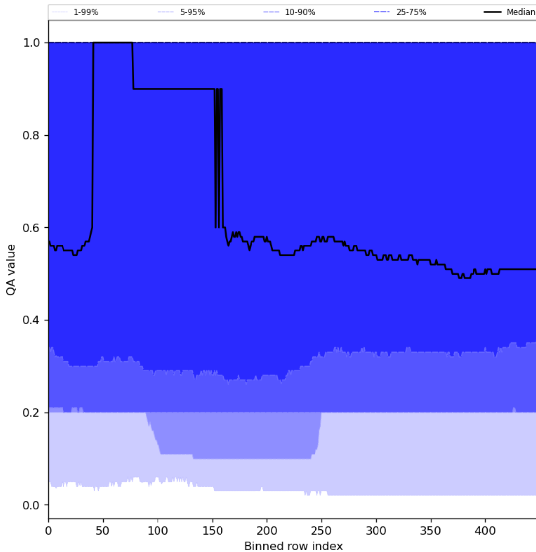
Figure 48: Along track statistics of “QA value” for 2024-05-18 to 2024-05-19
