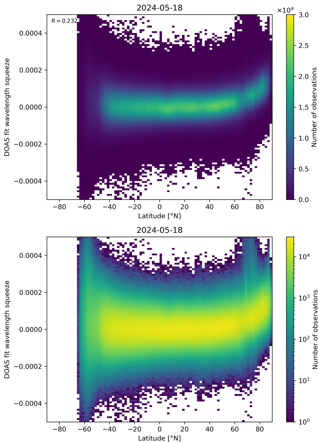
Figure 155: Scatter density plot of “Latitude” against “DOAS fit wavelength squeeze” for 2024-05-18 to 2024-05-19.
