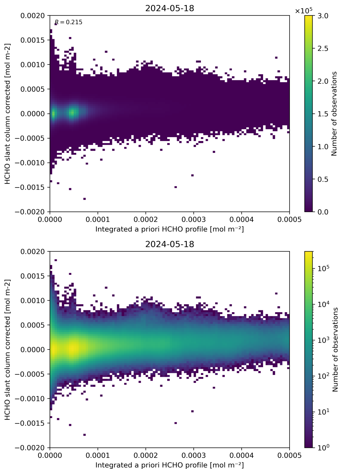
Figure 151: Scatter density plot of “Integrated a priori HCHO profile” against “HCHO slant column corrected” for 2024-05-18 to 2024-05-19.
