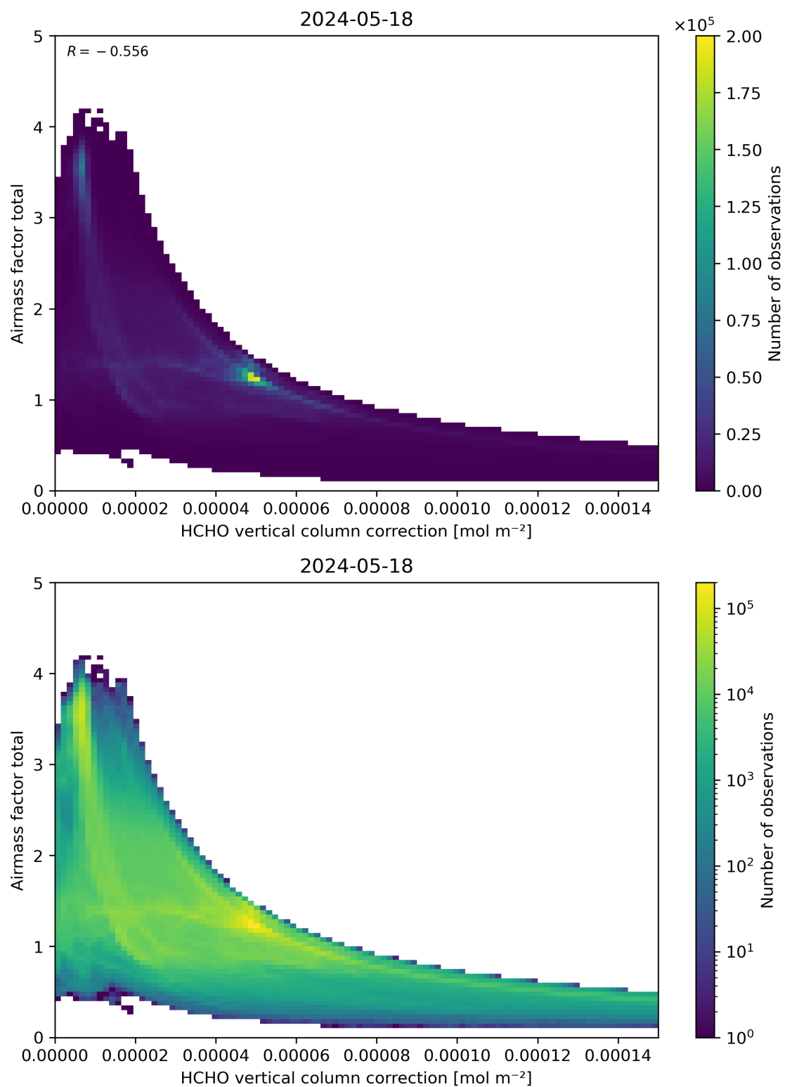
Figure 120: Scatter density plot of “HCHO vertical column correction” against “Airmass factor total” for 2024-05-18 to 2024-05-19.
