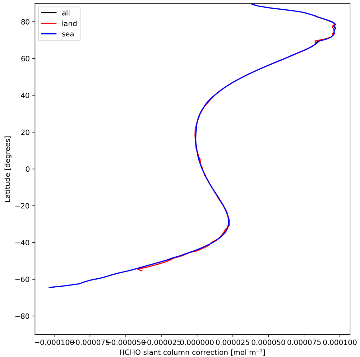
Figure 33: Zonal average of “HCHO slant column correction” for 2024-05-18 to 2024-05-19.
