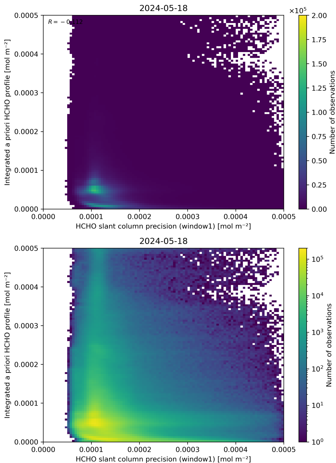
Figure 96: Scatter density plot of “HCHO slant column precision (window1)” against “Integrated a priori HCHO profile” for 2024-05-18 to 2024-05-19.
