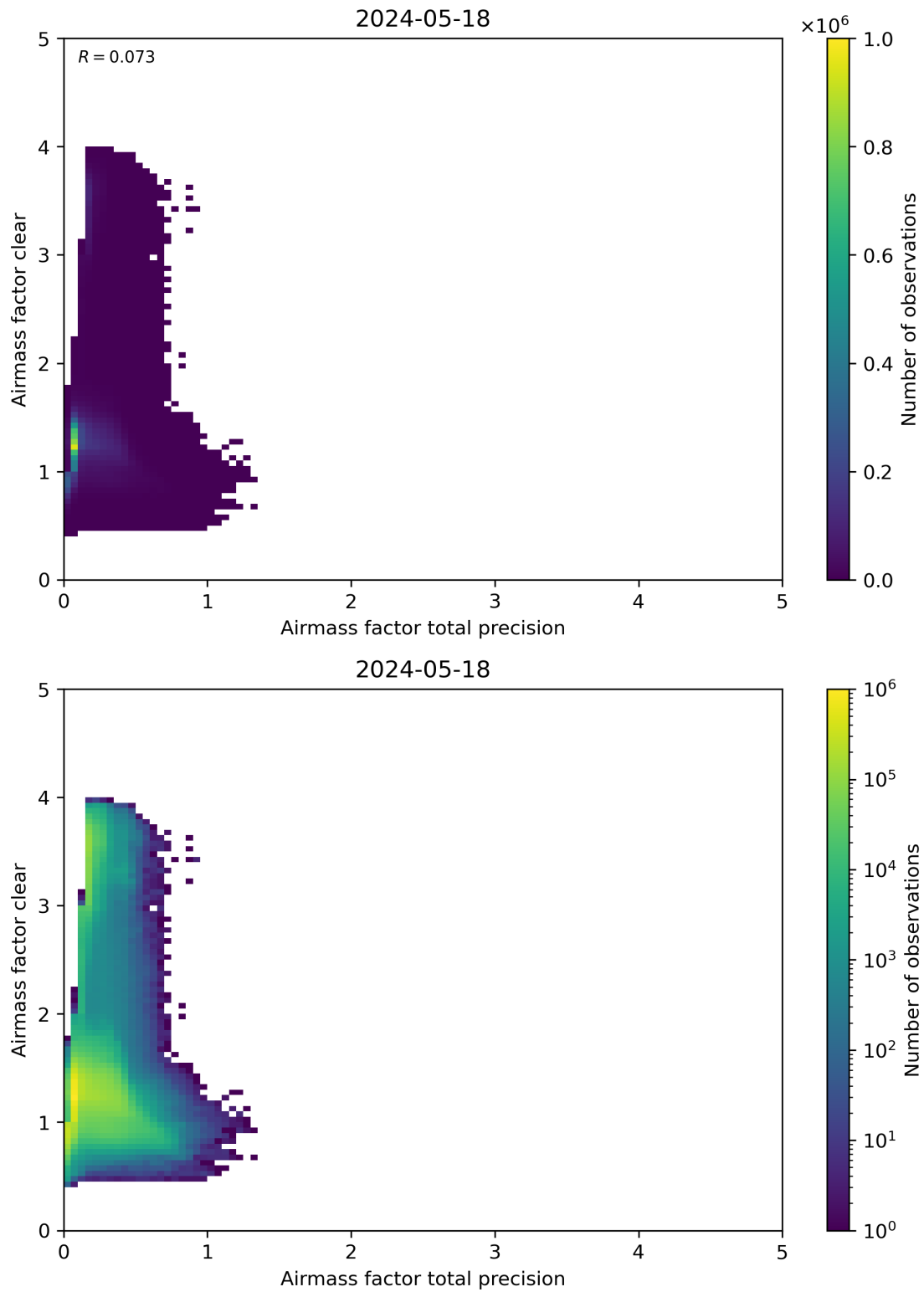
Figure 108: Scatter density plot of “Airmass factor total precision” against “Airmass factor clear” for 2024-05-18 to 2024-05-19.
