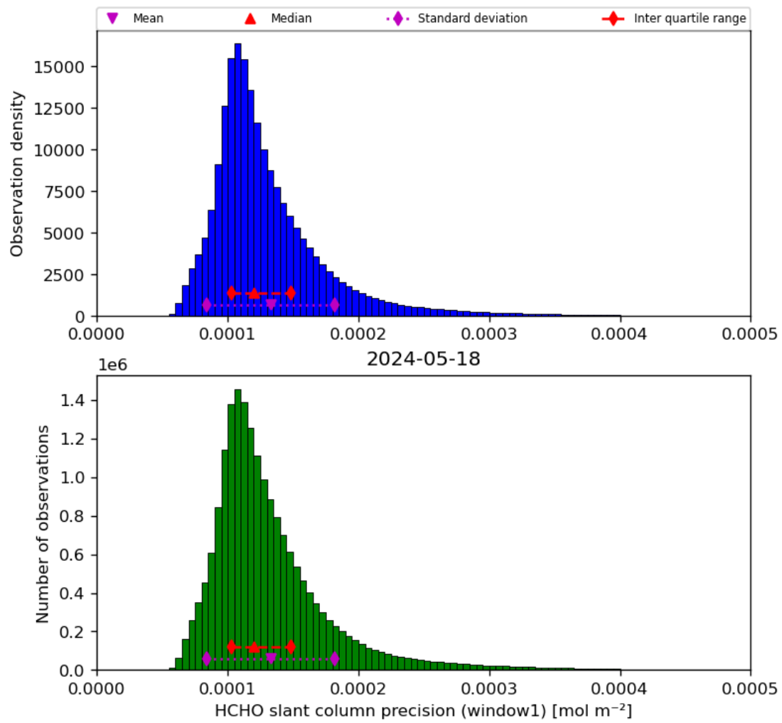
Figure 39: Histogram of “HCHO slant column precision (window1)” for 2024-05-18 to 2024-05-19
