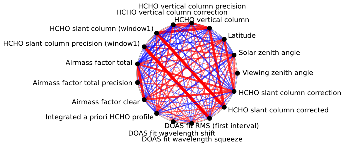
Figure 1: Map of correlation graph for 2024-05-18 to 2024-05-19.
