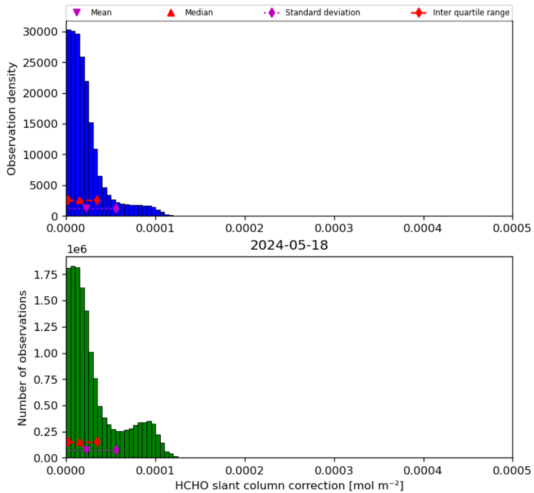
Figure 47: Histogram of “HCHO slant column correction” for 2024-05-18 to 2024-05-19
