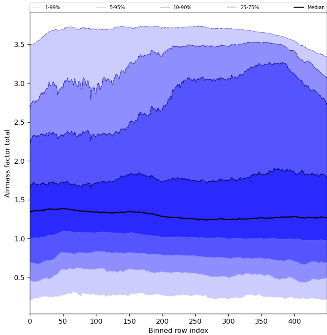
Figure 54: Along track statistics of “Airmass factor total” for 2024-05-18 to 2024-05-19
