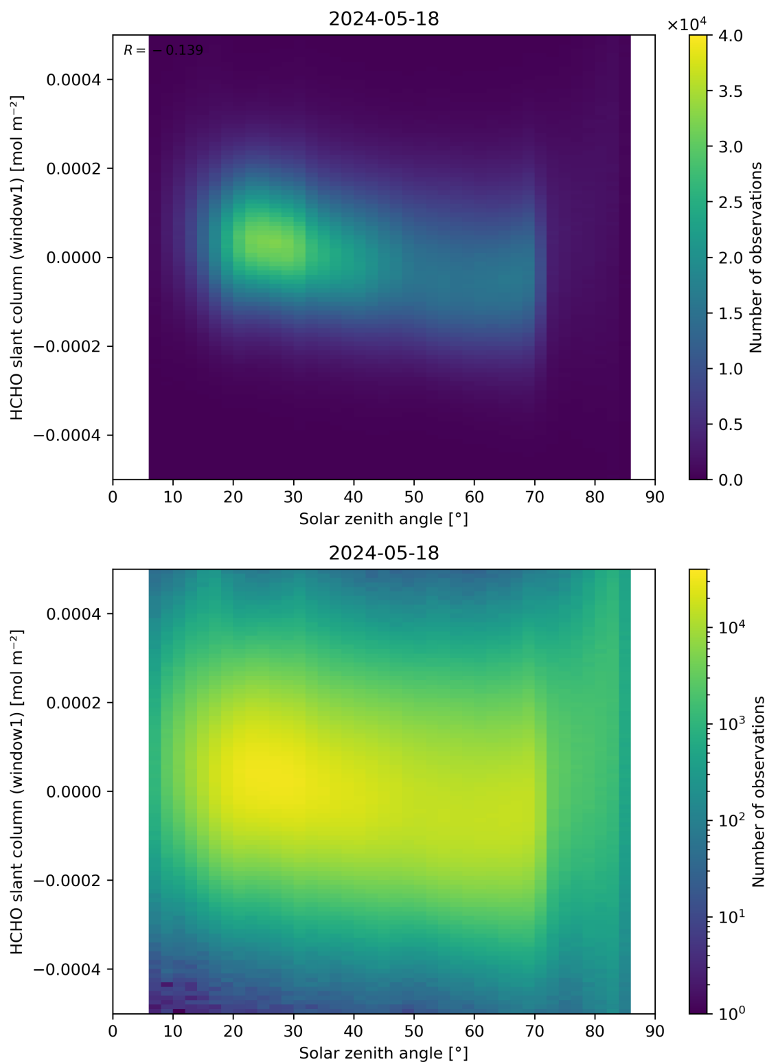
Figure 173: Scatter density plot of “Solar zenith angle” against “HCHO slant column (window1)” for 2024-05-18 to 2024-05-19.
