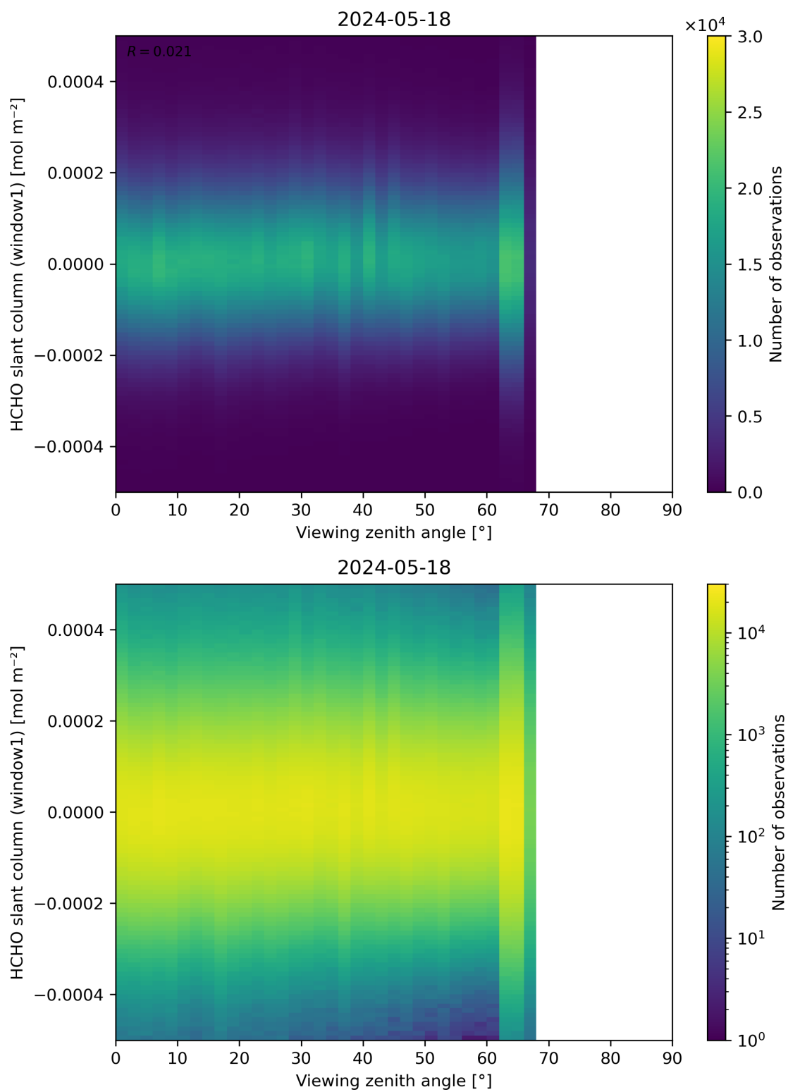
Figure 188: Scatter density plot of “Viewing zenith angle” against “HCHO slant column (window1)” for 2024-05-18 to 2024-05-19.
