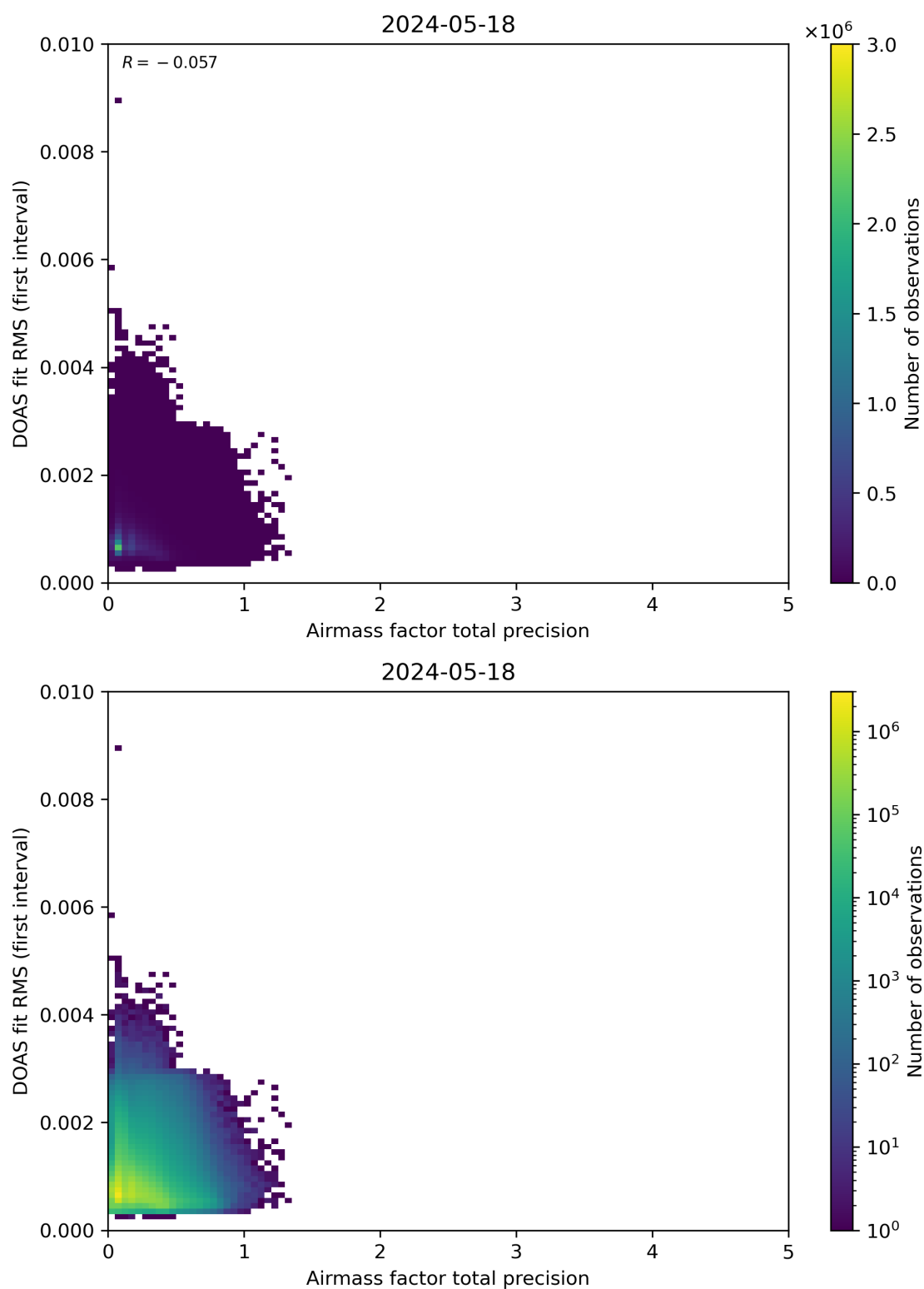
Figure 105: Scatter density plot of “Airmass factor total precision” against “DOAS fit RMS (first interval)” for 2024-05-18 to 2024-05-19.
