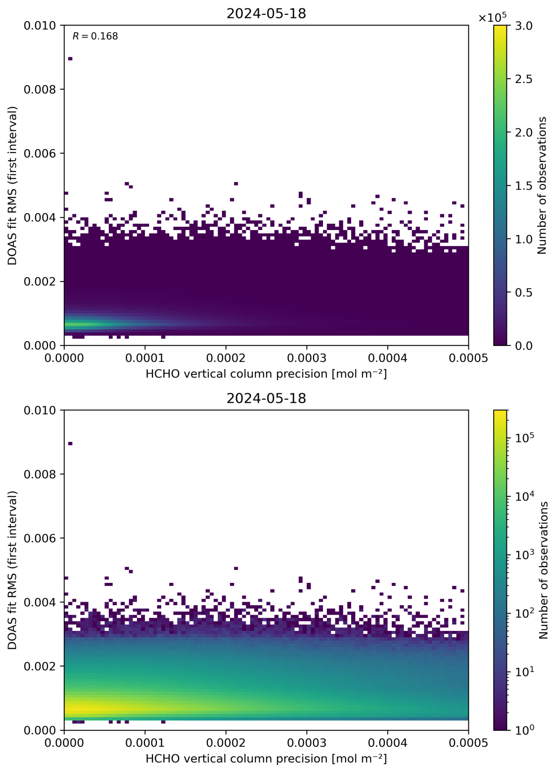
Figure 136: Scatter density plot of “HCHO vertical column precision” against “DOAS fit RMS (first interval)” for 2024-05-18 to 2024-05-19.
