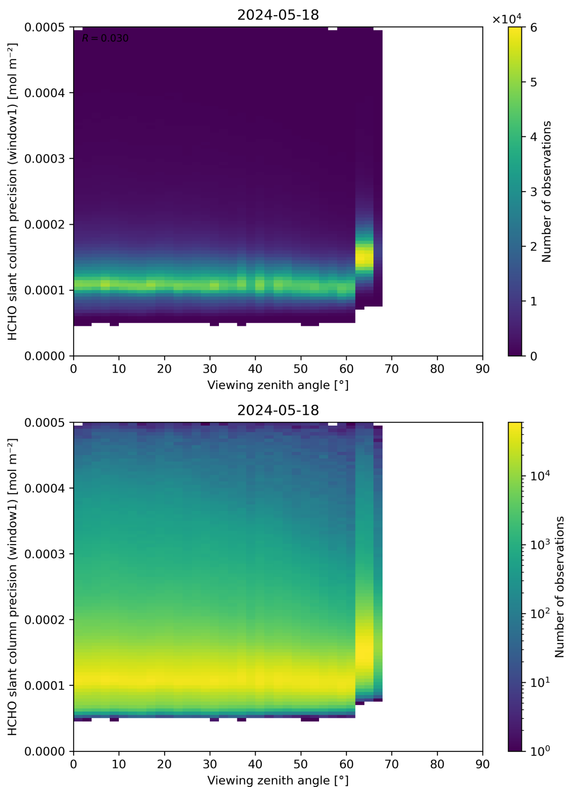
Figure 189: Scatter density plot of “Viewing zenith angle” against “HCHO slant column precision (window1)” for 2024-05-18 to 2024-05-19.
