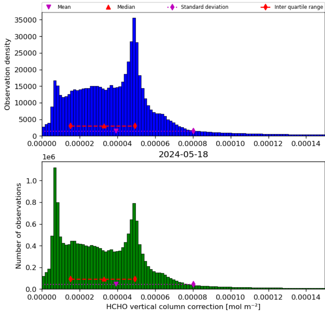
Figure 37: Histogram of “HCHO vertical column correction” for 2024-05-18 to 2024-05-19
