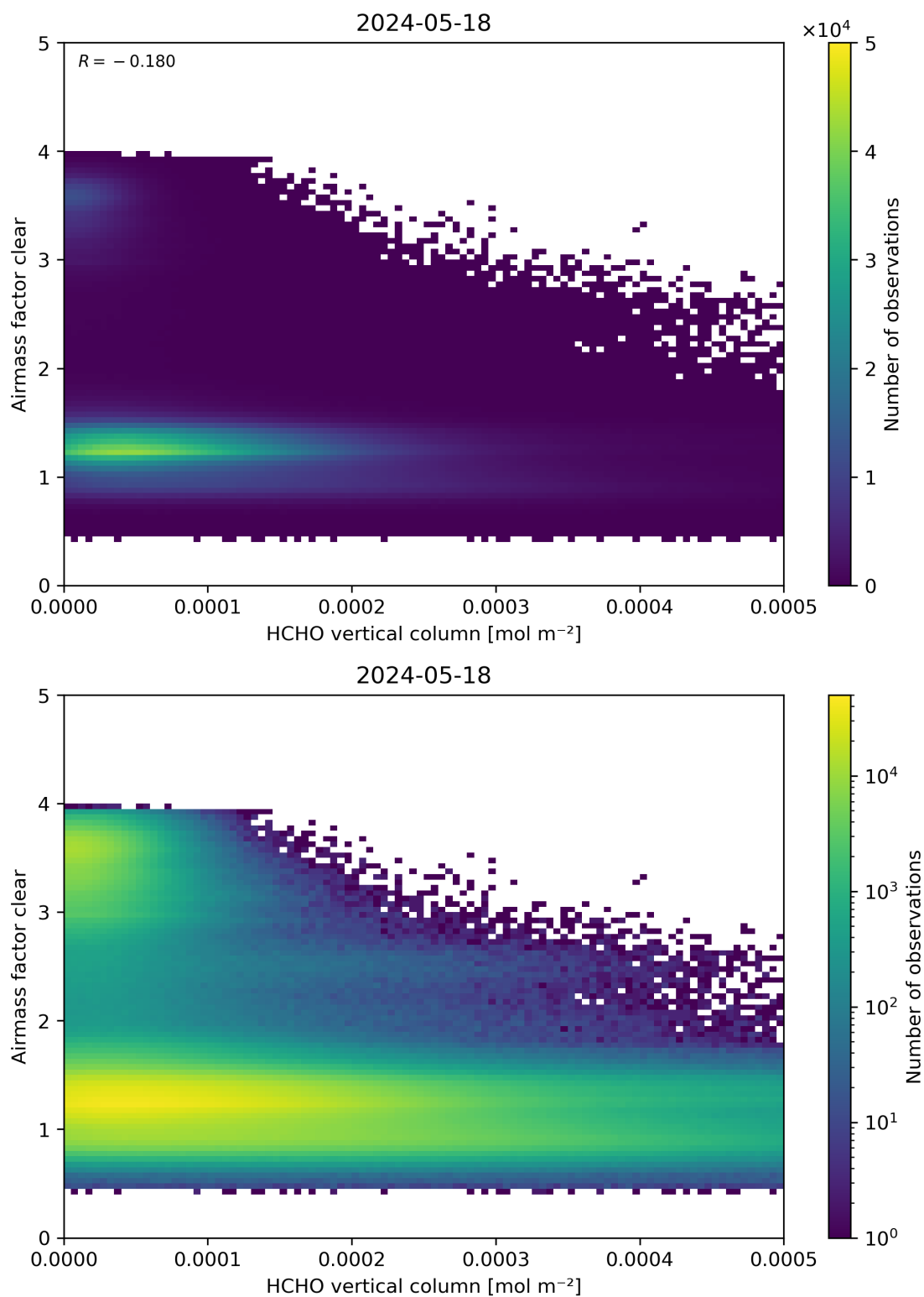
Figure 126: Scatter density plot of “HCHO vertical column” against “Airmass factor clear” for 2024-05-18 to 2024-05-19.
