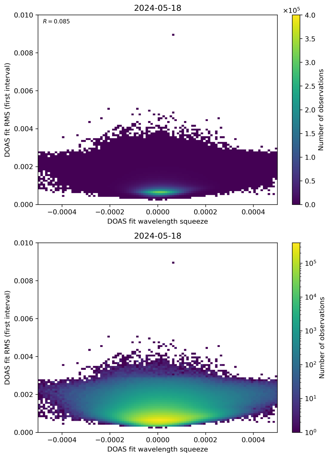
Figure 68: Scatter density plot of “DOAS fit wavelength squeeze” against “DOAS fit RMS (first interval)” for 2024-05-18 to 2024-05-19.
