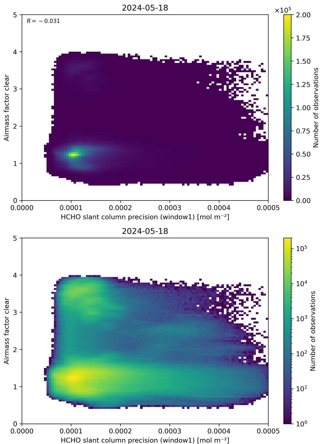
Figure 91: Scatter density plot of “HCHO slant column precision (window1)” against “Airmass factor clear” for 2024-05-18 to 2024-05-19.
