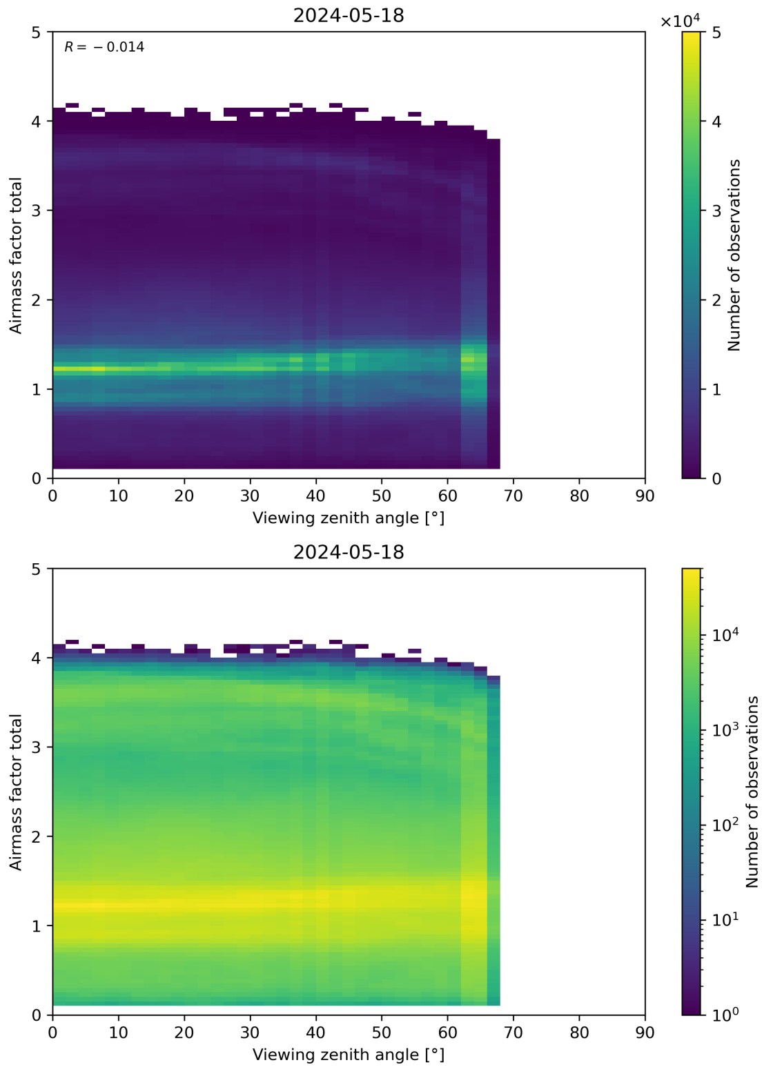
Figure 190: Scatter density plot of “Viewing zenith angle” against “Airmass factor total” for 2024-05-18 to 2024-05-19.
