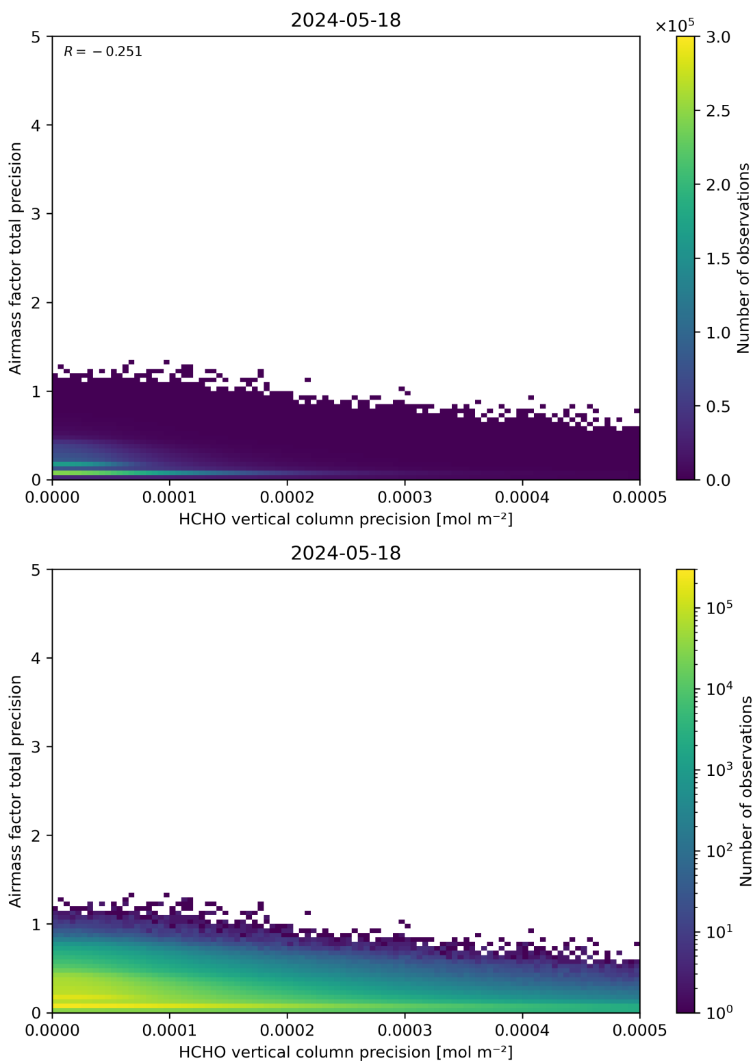
Figure 145: Scatter density plot of “HCHO vertical column precision” against “Airmass factor total precision” for 2024-05-18 to 2024-05-19.
