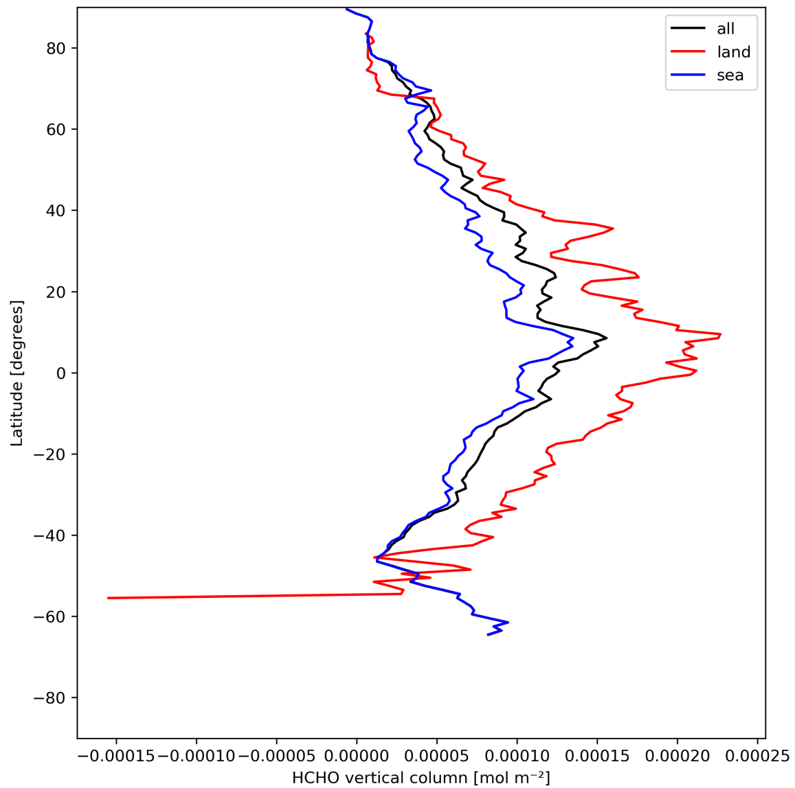
Figure 21: Zonal average of “HCHO vertical column” for 2024-05-18 to 2024-05-19.
