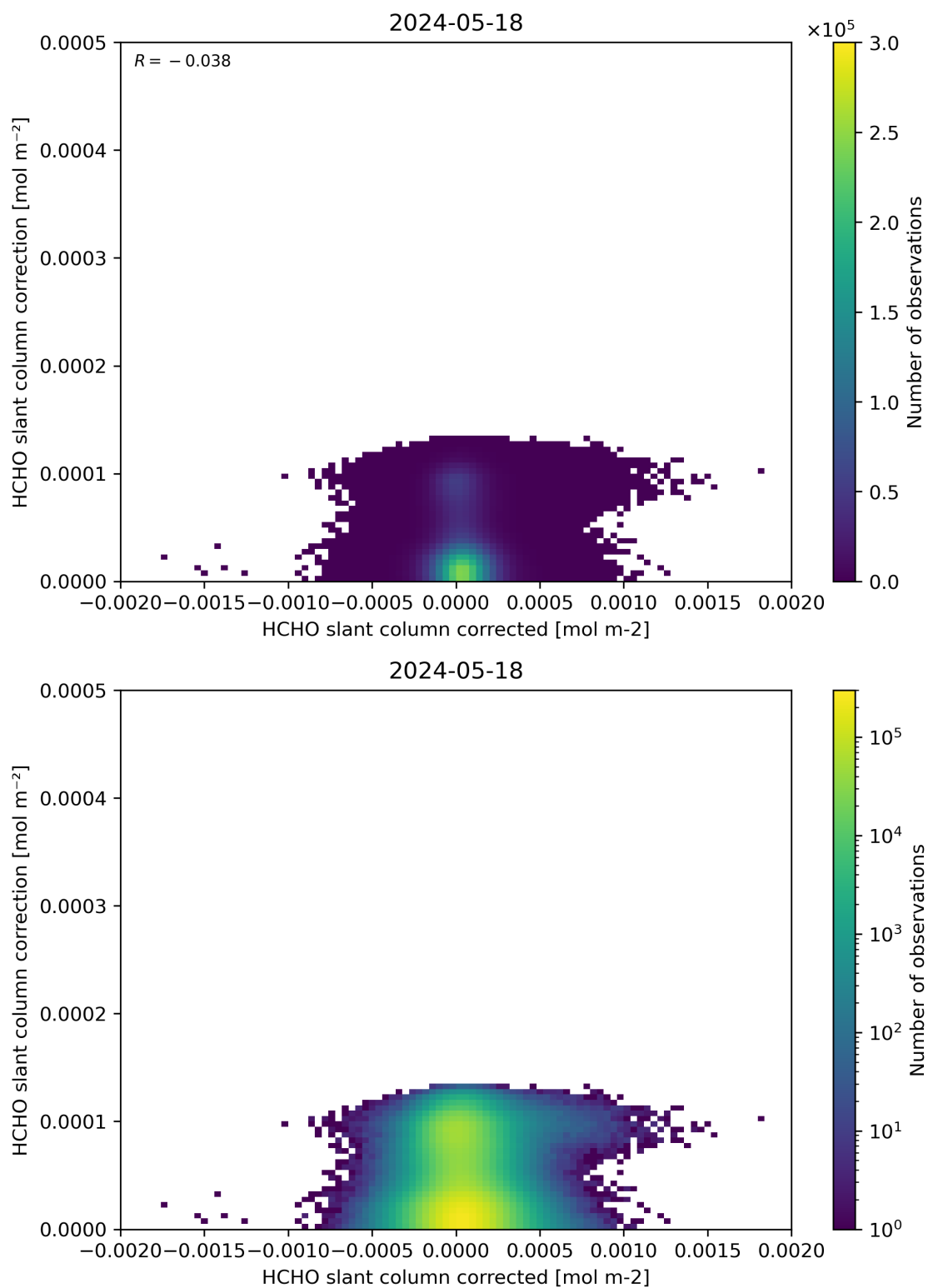
Figure 77: Scatter density plot of “HCHO slant column corrected” against “HCHO slant column correction” for 2024-05-18 to 2024-05-19.
