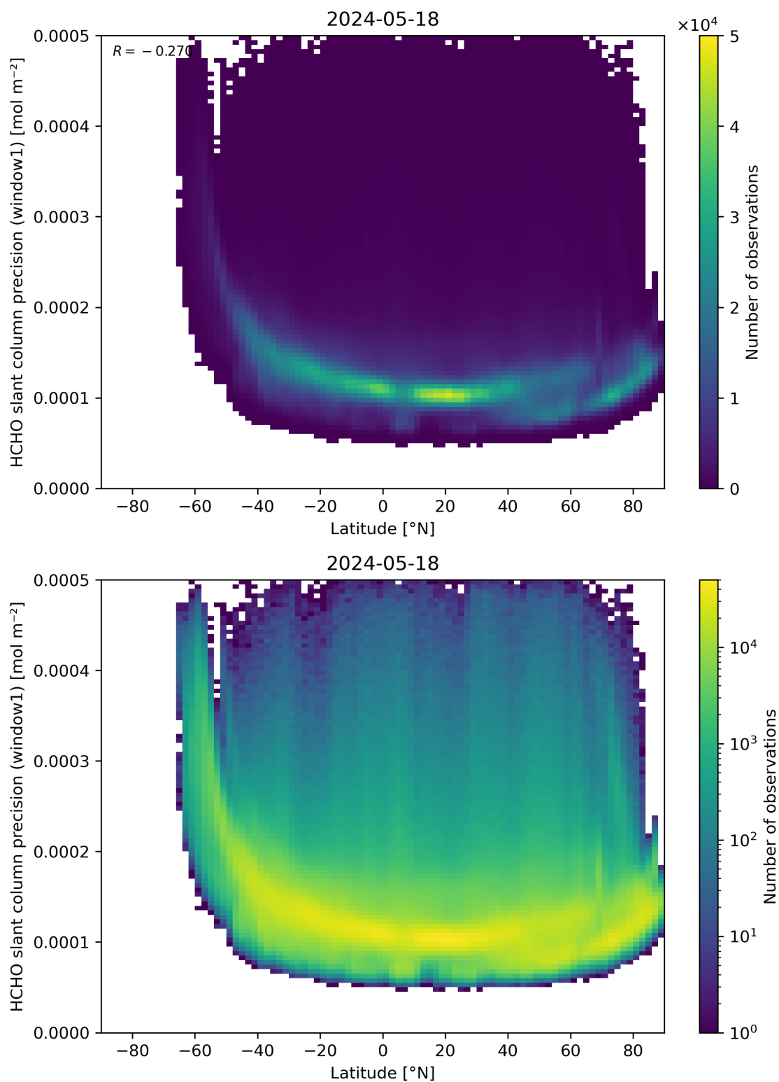
Figure 160: Scatter density plot of “Latitude” against “HCHO slant column precision (window1)” for 2024-05-18 to 2024-05-19.
