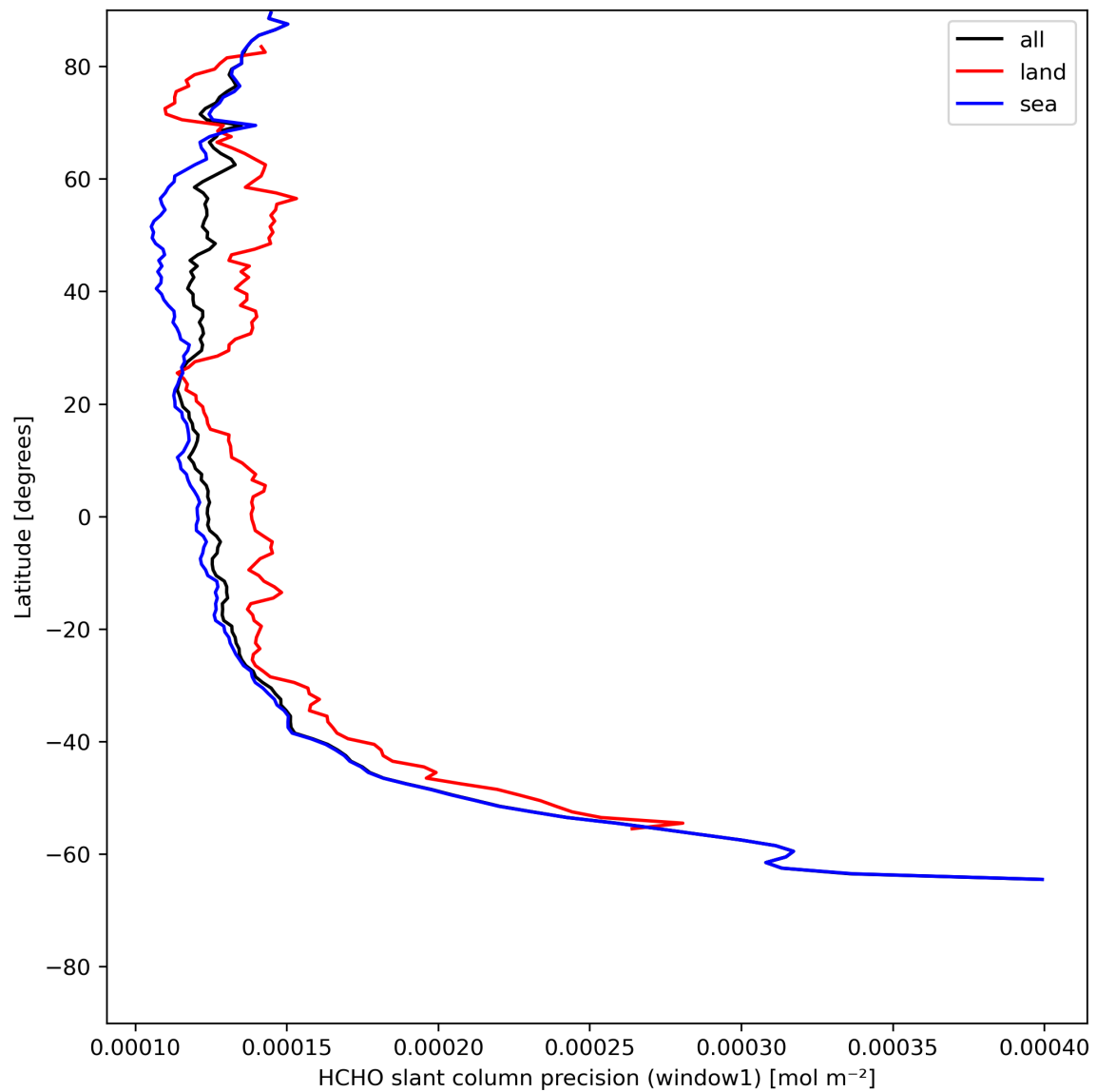
Figure 25: Zonal average of “HCHO slant column precision (window1)” for 2024-05-18 to 2024-05-19.
