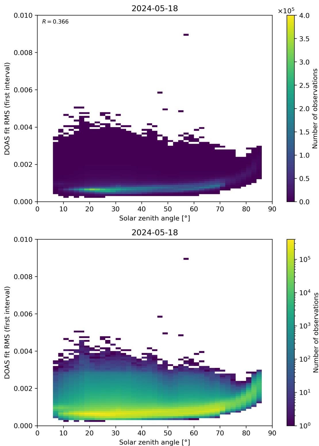
Figure 167: Scatter density plot of “Solar zenith angle” against “DOAS fit RMS (first interval)” for 2024-05-18 to 2024-05-19.
