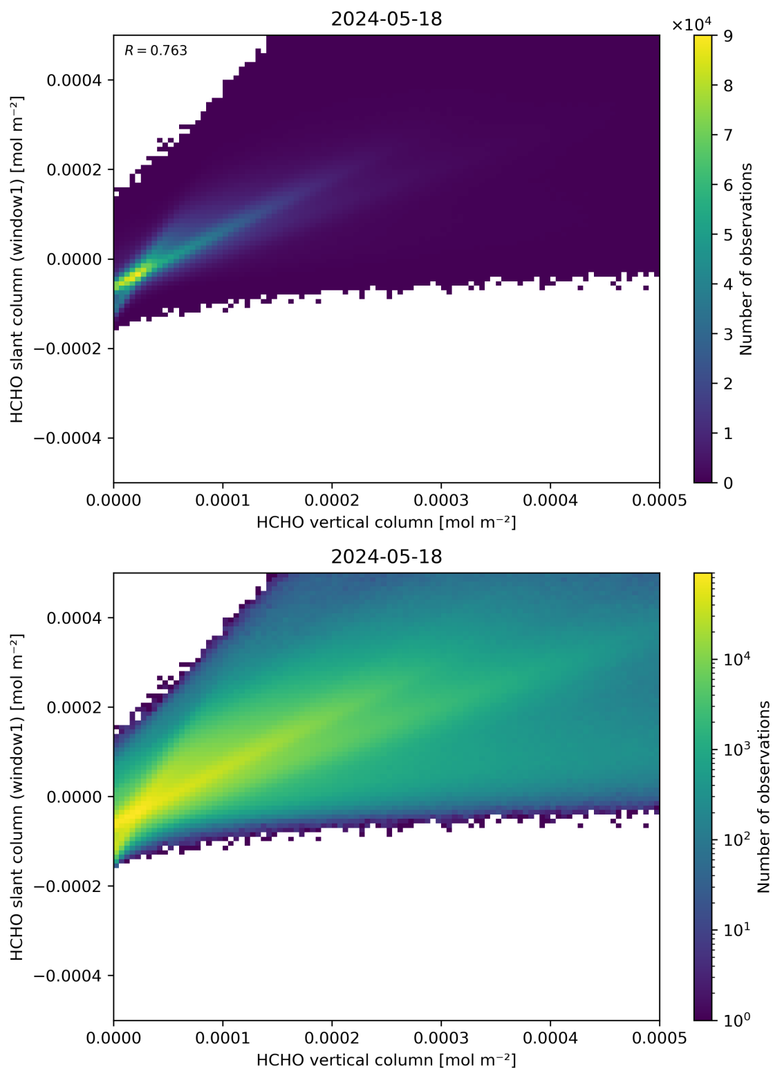
Figure 129: Scatter density plot of “HCHO vertical column” against “HCHO slant column (window1)” for 2024-05-18 to 2024-05-19.
