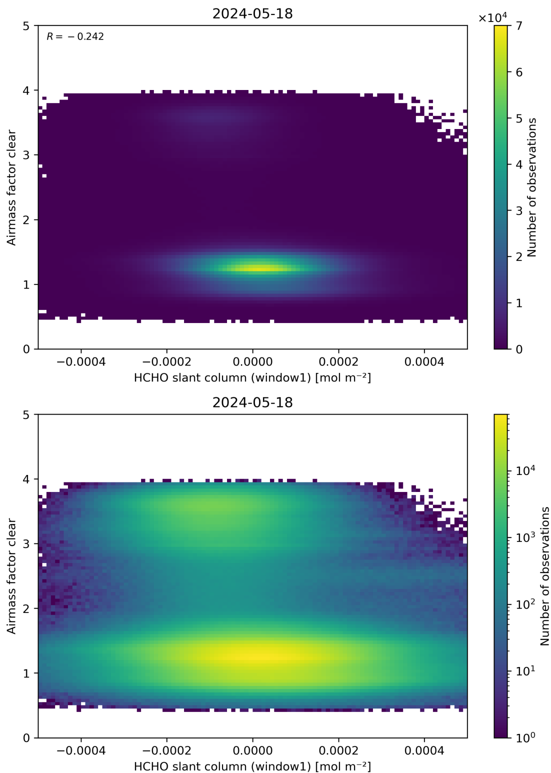
Figure 81: Scatter density plot of “HCHO slant column (window1)” against “Airmass factor clear” for 2024-05-18 to 2024-05-19.
