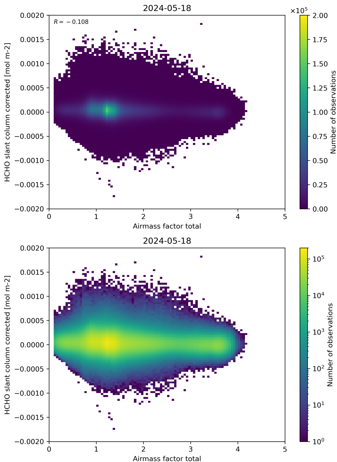
Figure 101: Scatter density plot of “Airmass factor total” against “HCHO slant column corrected” for 2024-05-18 to 2024-05-19.
