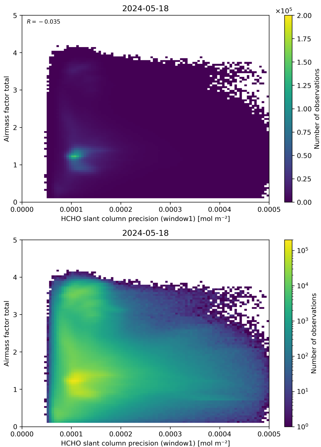
Figure 94: Scatter density plot of “HCHO slant column precision (window1)” against “Airmass factor total” for 2024-05-18 to 2024-05-19.
