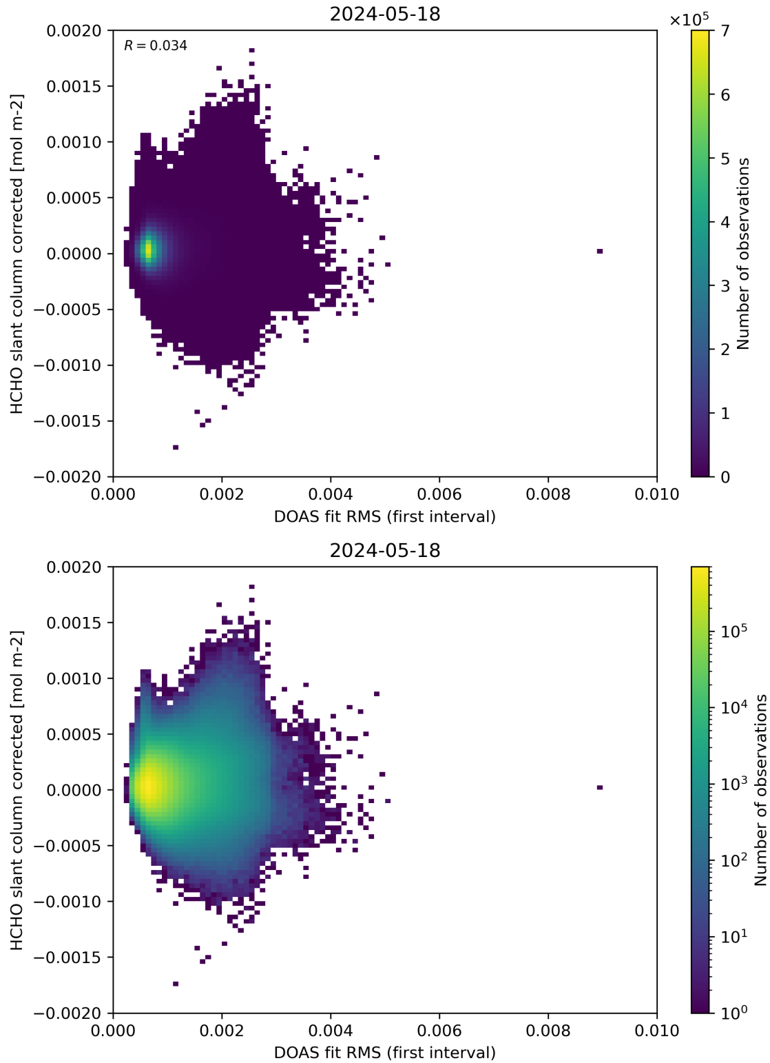
Figure 62: Scatter density plot of “DOAS fit RMS (first interval)” against “HCHO slant column corrected” for 2024-05-18 to 2024-05-19.
