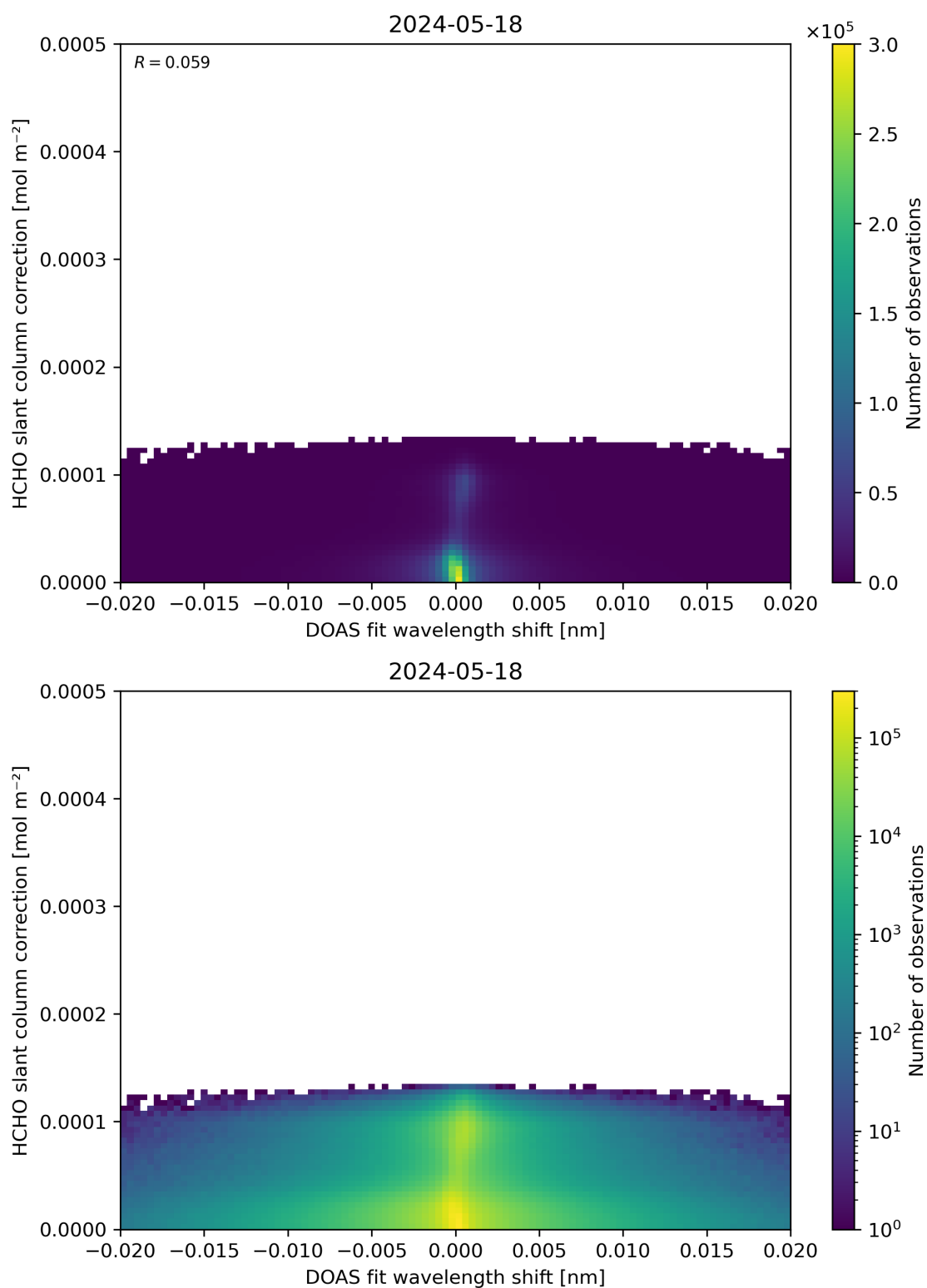
Figure 67: Scatter density plot of “DOAS fit wavelength shift” against “HCHO slant column correction” for 2024-05-18 to 2024-05-19.
