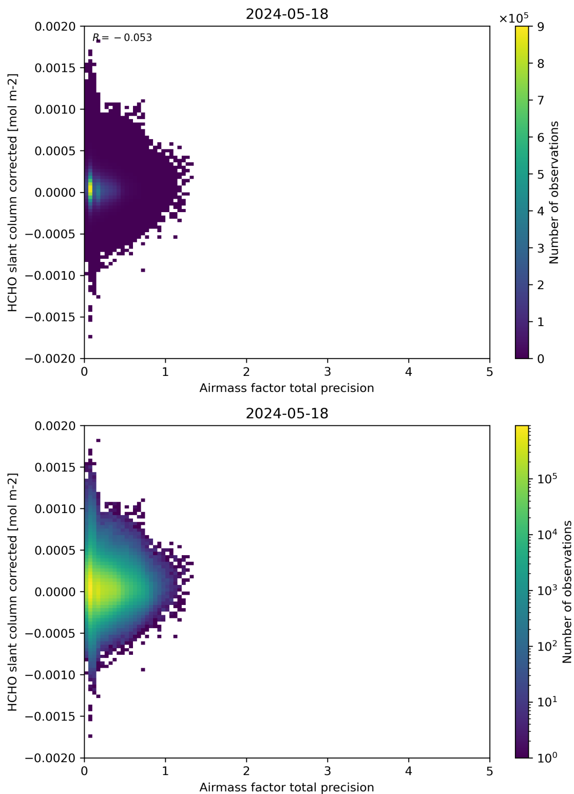
Figure 109: Scatter density plot of “Airmass factor total precision” against “HCHO slant column corrected” for 2024-05-18 to 2024-05-19.
