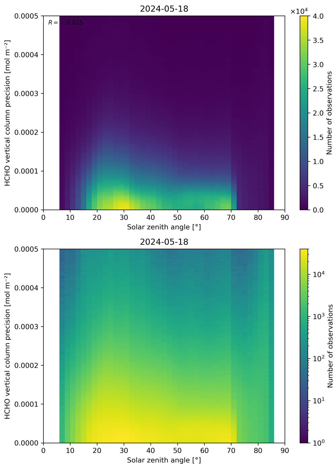
Figure 179: Scatter density plot of “Solar zenith angle” against “HCHO vertical column precision” for 2024-05-18 to 2024-05-19.
