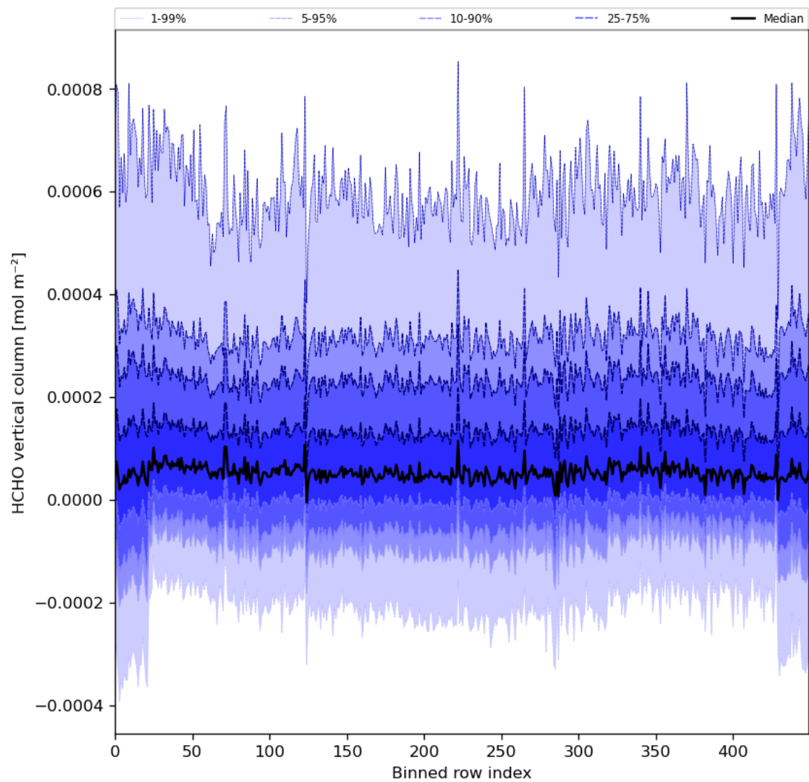
Figure 49: Along track statistics of “HCHO vertical column” for 2024-05-18 to 2024-05-19
