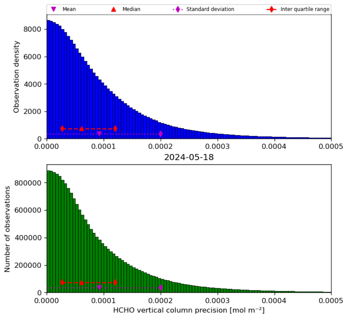
Figure 36: Histogram of “HCHO vertical column precision” for 2024-05-18 to 2024-05-19
