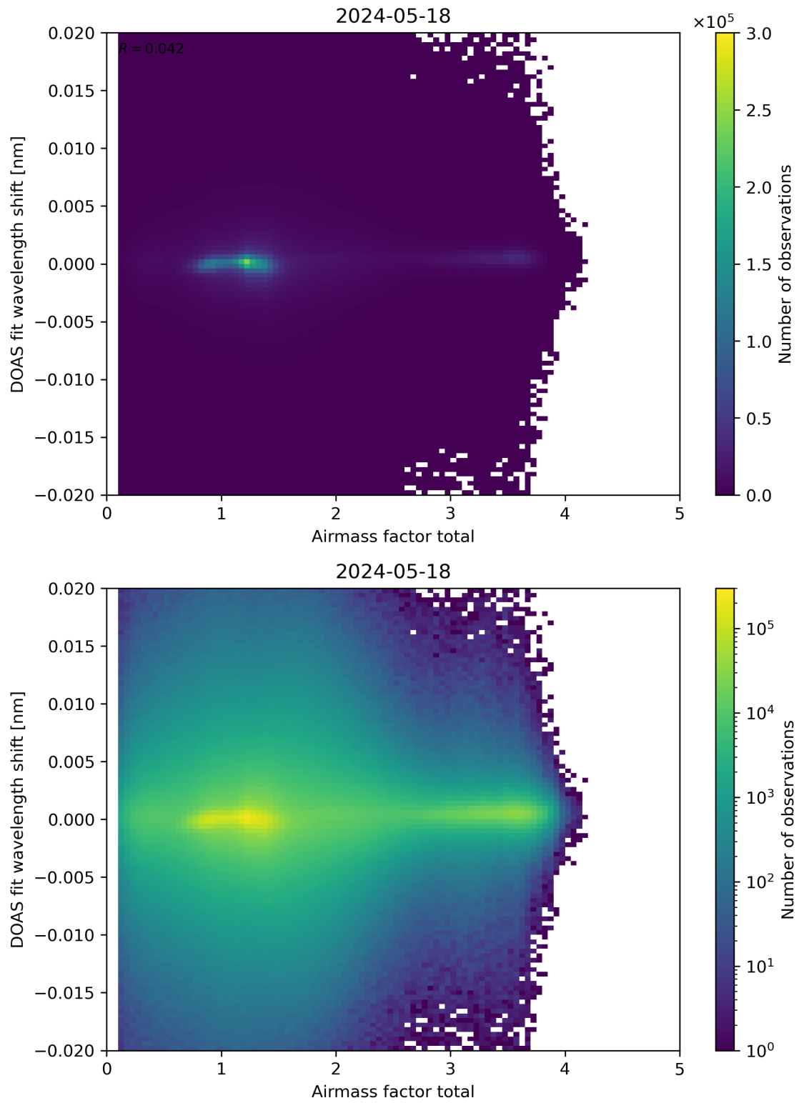
Figure 98: Scatter density plot of “Airmass factor total” against “DOAS fit wavelength shift” for 2024-05-18 to 2024-05-19.
