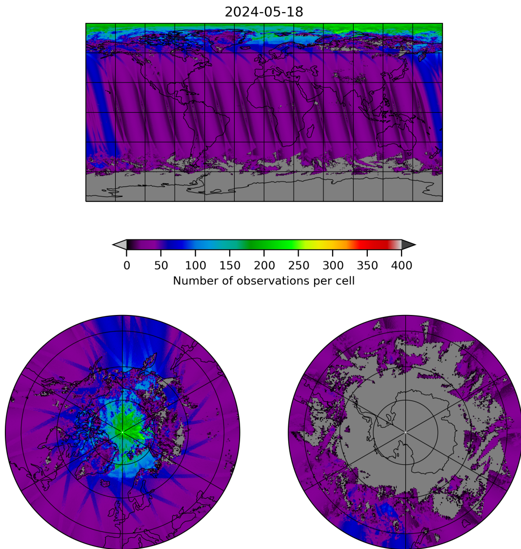
Figure 19: Map of the number of observations for 2024-05-18 to 2024-05-19
