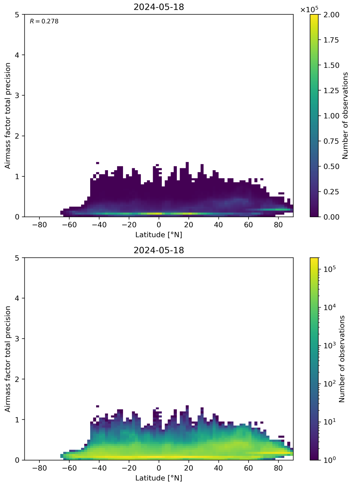
Figure 162: Scatter density plot of “Latitude” against “Airmass factor total precision” for 2024-05-18 to 2024-05-19.
