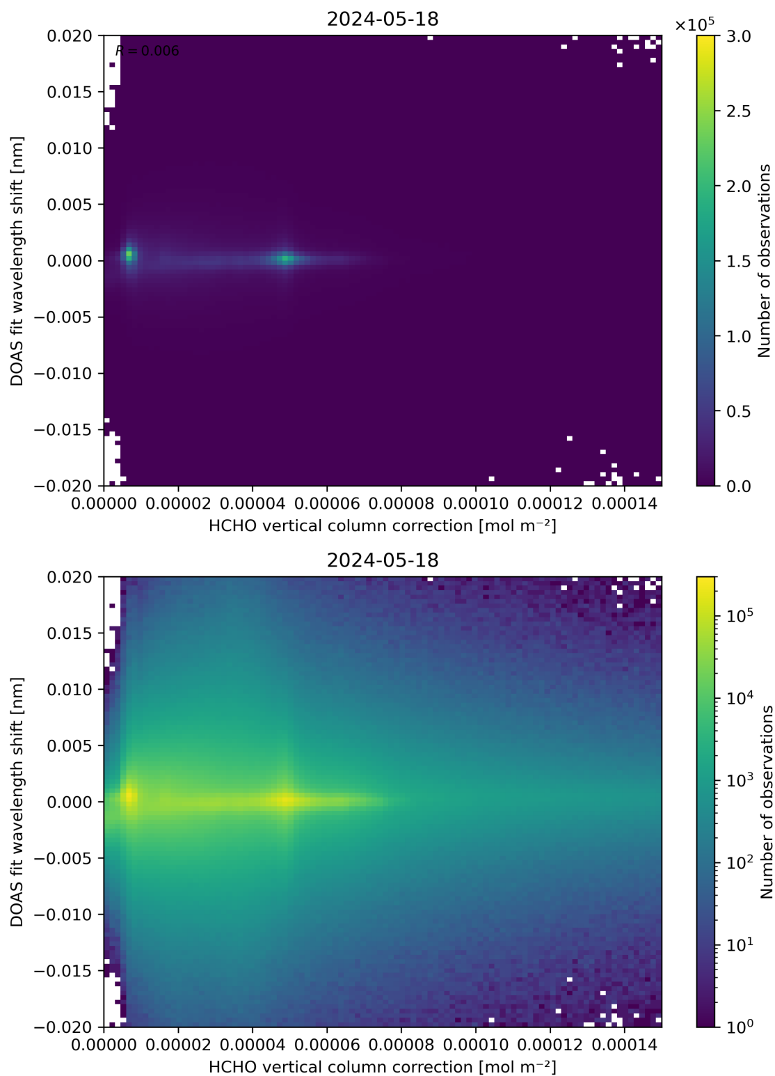
Figure 113: Scatter density plot of “HCHO vertical column correction” against “DOAS fit wavelength shift” for 2024-05-18 to 2024-05-19.
