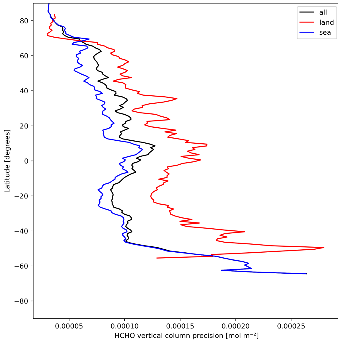
Figure 22: Zonal average of “HCHO vertical column precision” for 2024-05-18 to 2024-05-19.
