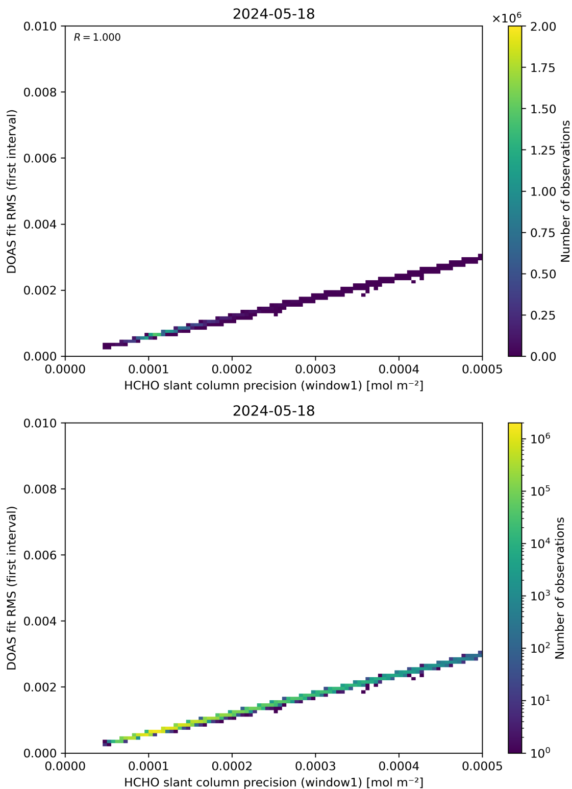
Figure 88: Scatter density plot of “HCHO slant column precision (window1)” against “DOAS fit RMS (first interval)” for 2024-05-18 to 2024-05-19.
