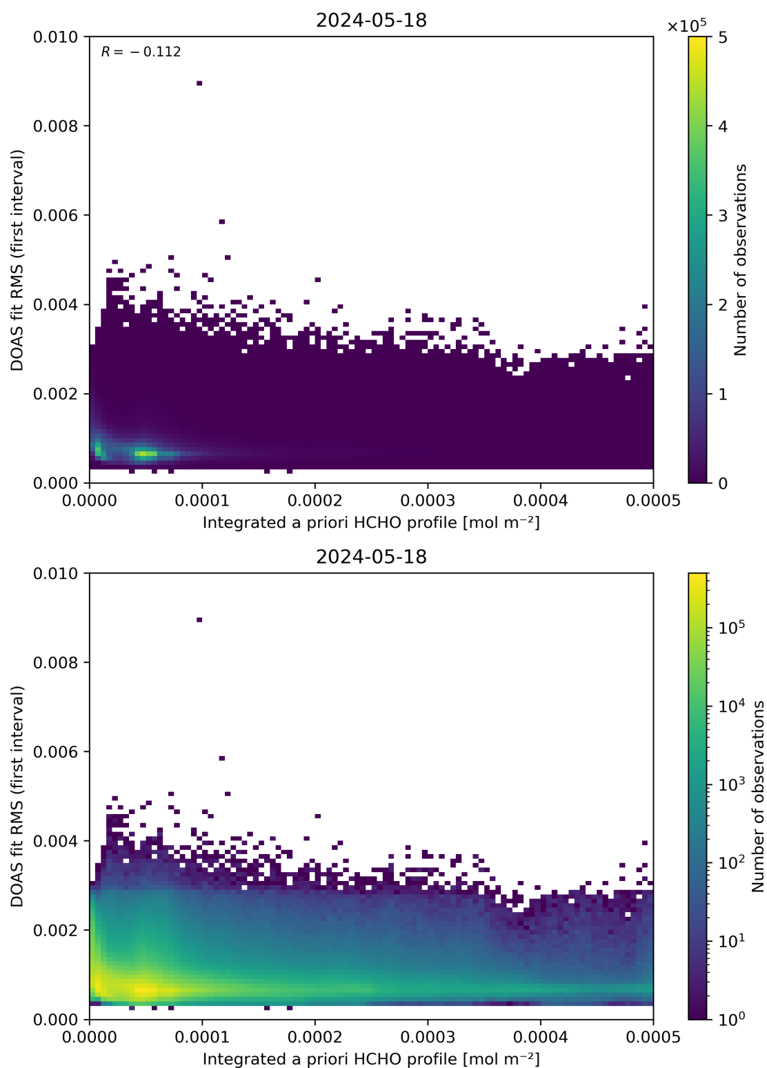
Figure 148: Scatter density plot of “Integrated a priori HCHO profile” against “DOAS fit RMS (first interval)” for 2024-05-18 to 2024-05-19.
