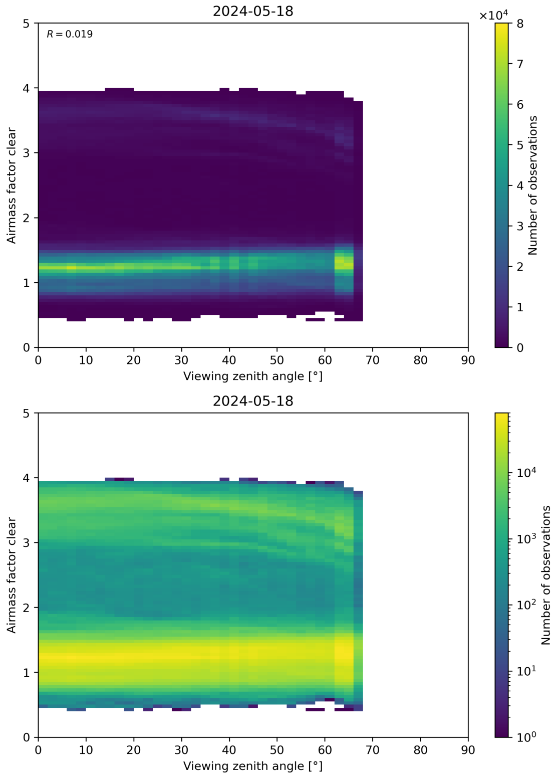
Figure 185: Scatter density plot of “Viewing zenith angle” against “Airmass factor clear” for 2024-05-18 to 2024-05-19.
