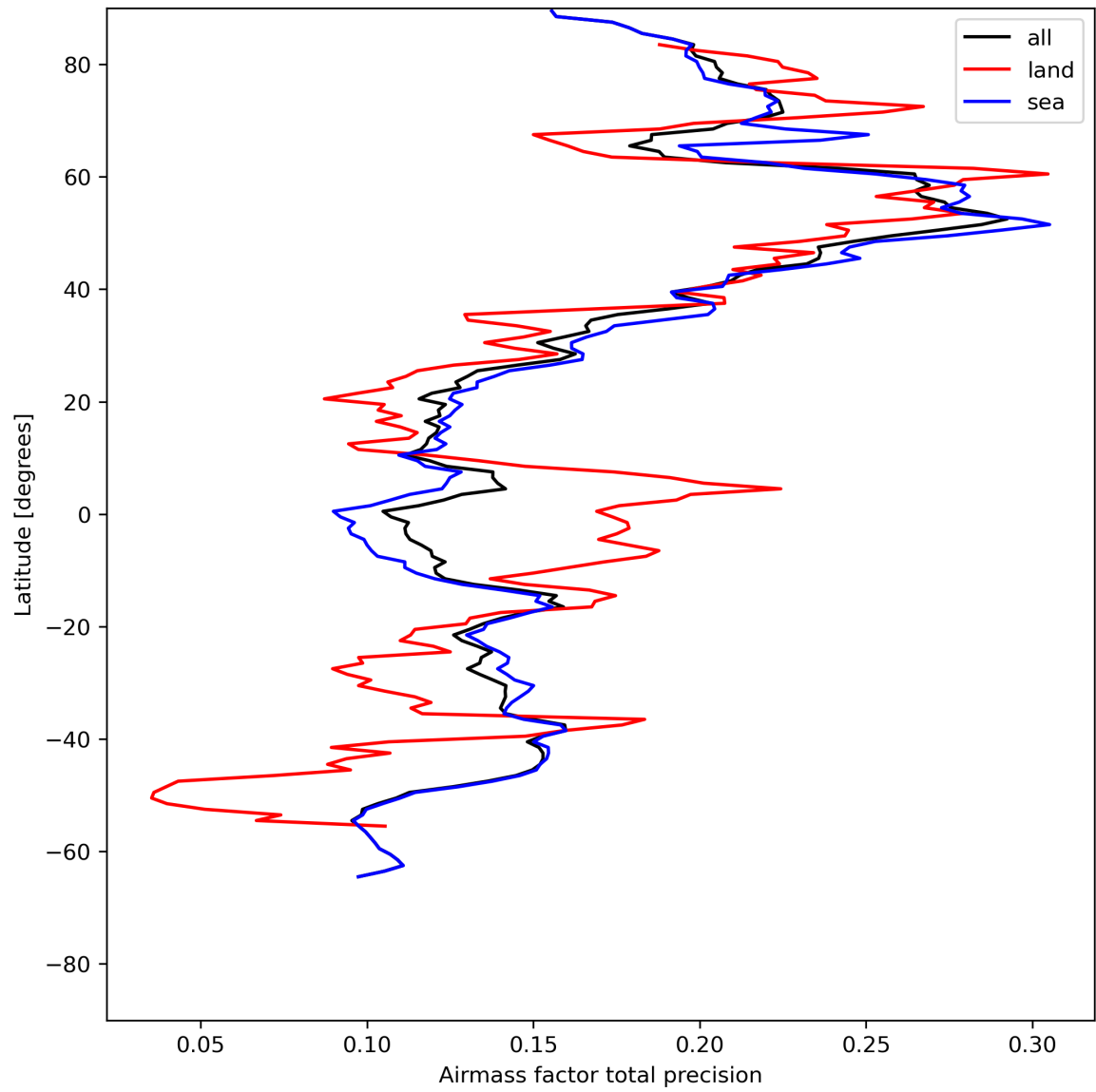
Figure 27: Zonal average of “Airmass factor total precision” for 2024-05-18 to 2024-05-19.
