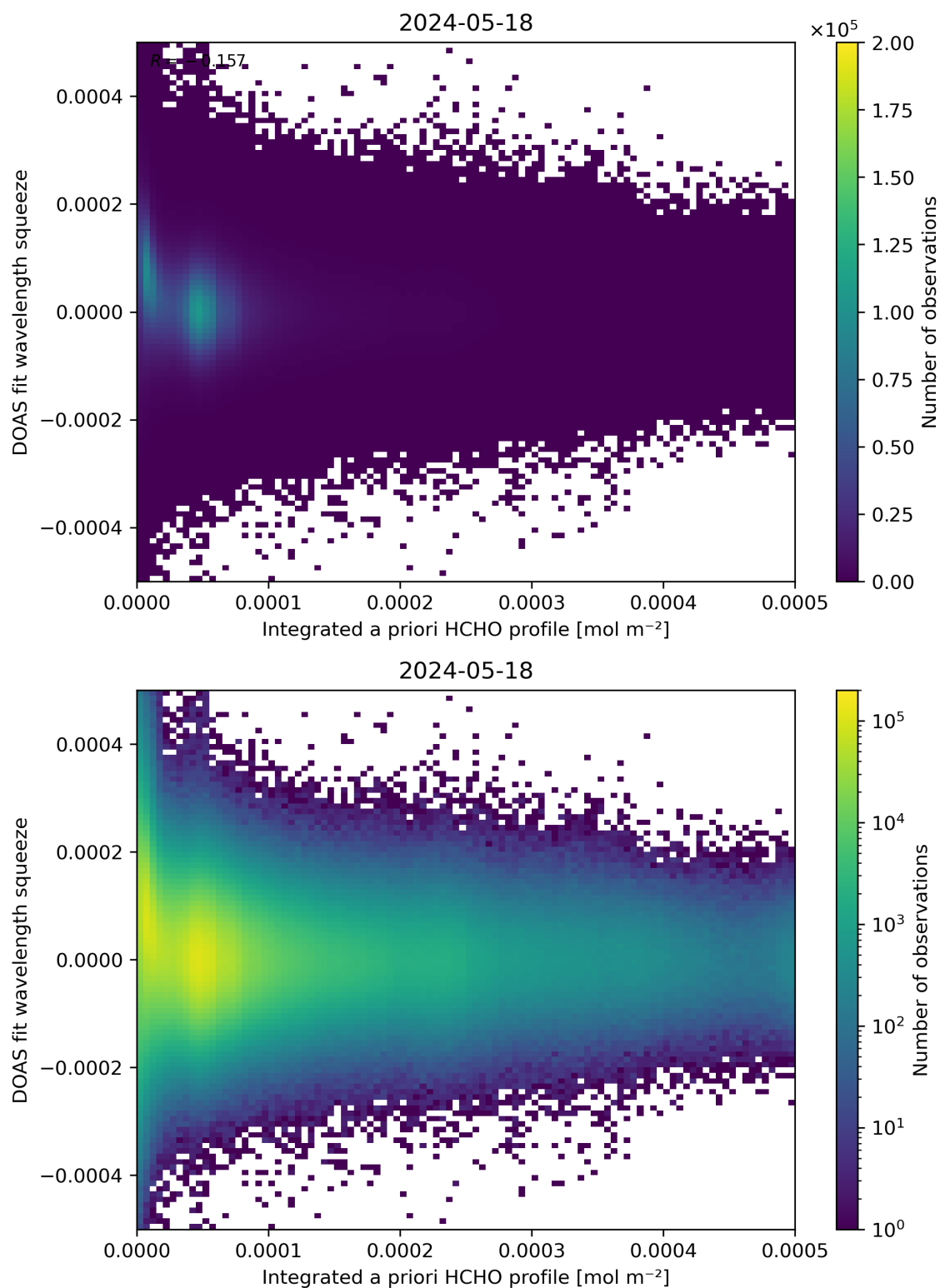
Figure 150: Scatter density plot of “Integrated a priori HCHO profile” against “DOAS fit wavelength squeeze” for 2024-05-18 to 2024-05-19.
