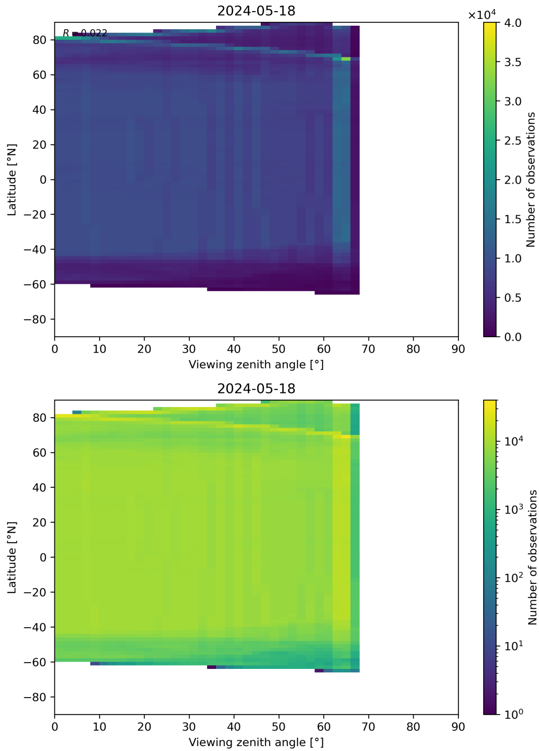
Figure 196: Scatter density plot of “Viewing zenith angle” against “Latitude” for 2024-05-18 to 2024-05-19.
