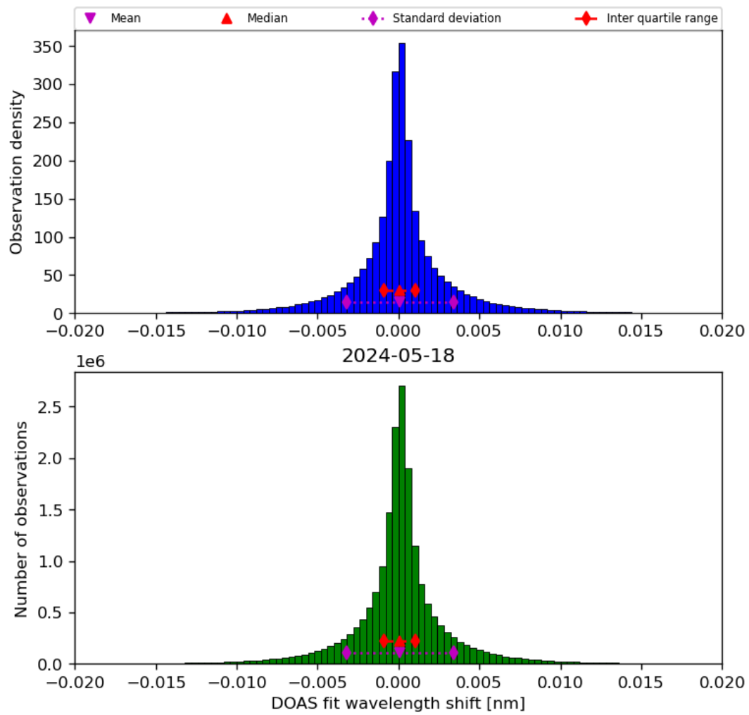
Figure 44: Histogram of “DOAS fit wavelength shift” for 2024-05-18 to 2024-05-19
