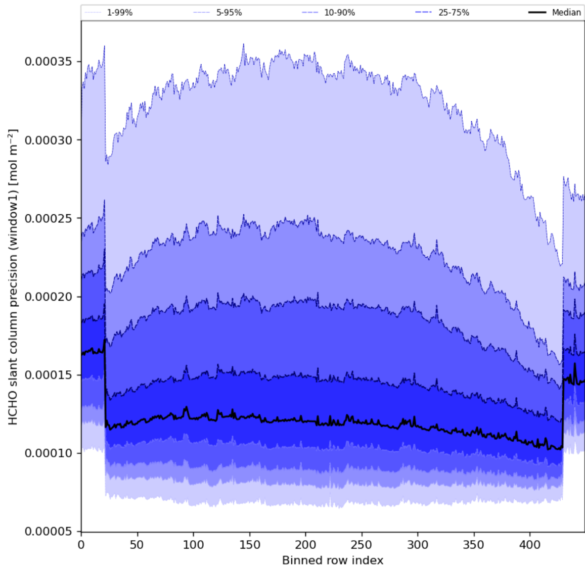
Figure 53: Along track statistics of “HCHO slant column precision (window1)” for 2024-05-18 to 2024-05-19
