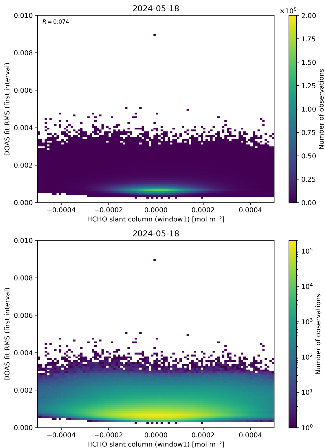
Figure 78: Scatter density plot of “HCHO slant column (window1)” against “DOAS fit RMS (first interval)” for 2024-05-18 to 2024-05-19.
