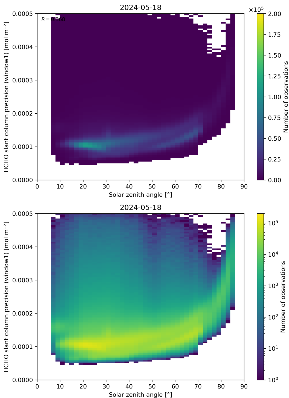
Figure 174: Scatter density plot of “Solar zenith angle” against “HCHO slant column precision (window1)” for 2024-05-18 to 2024-05-19.
