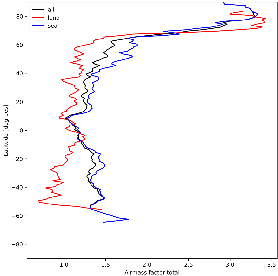
Figure 26: Zonal average of “Airmass factor total” for 2024-05-18 to 2024-05-19.
