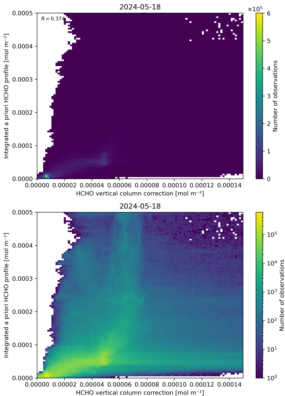
Figure 122: Scatter density plot of “HCHO vertical column correction” against “Integrated a priori HCHO profile” for 2024-05-18 to 2024-05-19.
