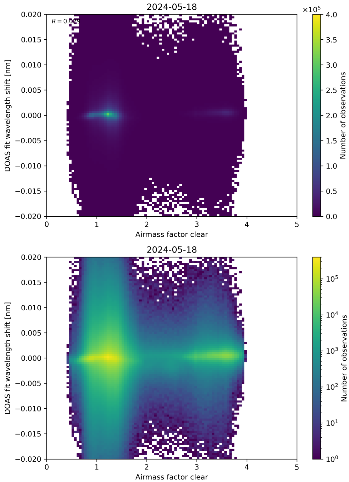
Figure 72: Scatter density plot of “Airmass factor clear” against “DOAS fit wavelength shift” for 2024-05-18 to 2024-05-19.
