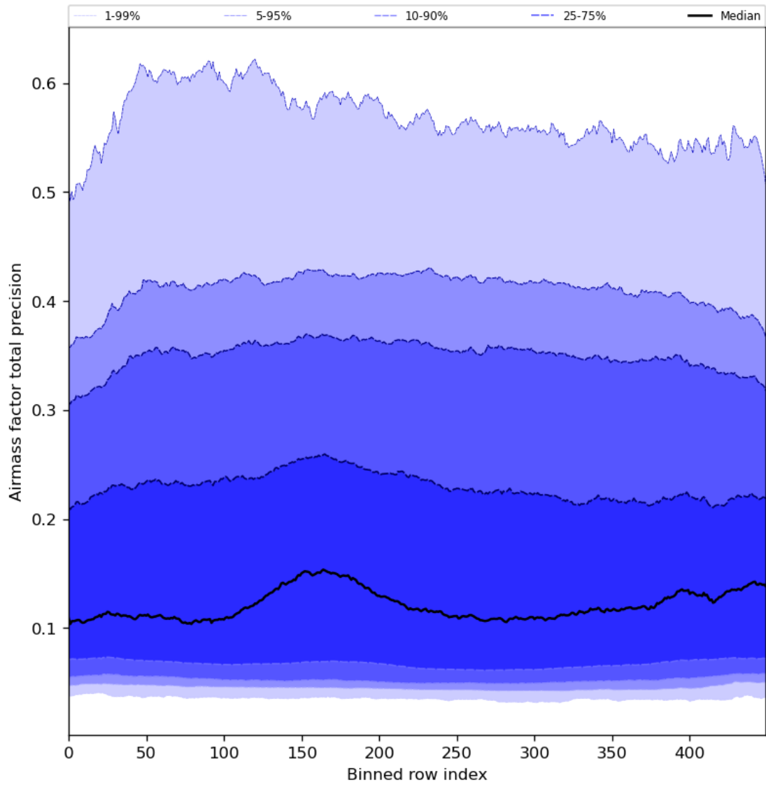
Figure 55: Along track statistics of “Airmass factor total precision” for 2024-05-18 to 2024-05-19
