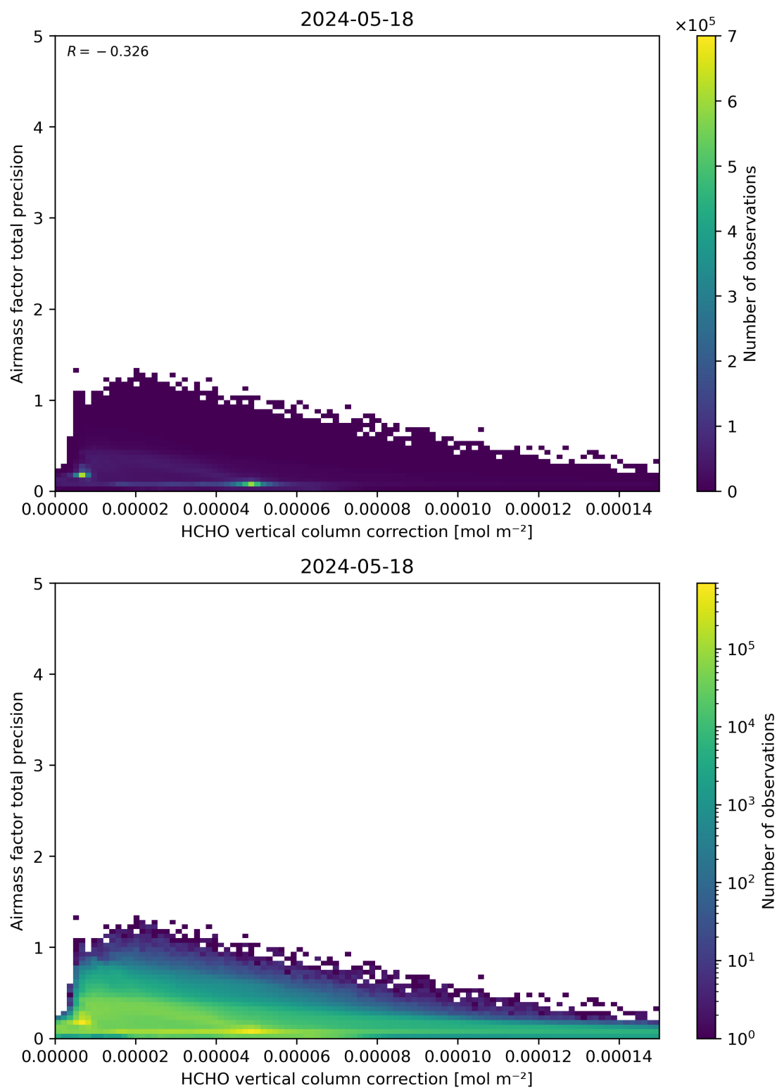
Figure 121: Scatter density plot of “HCHO vertical column correction” against “Airmass factor total precision” for 2024-05-18 to 2024-05-19.
