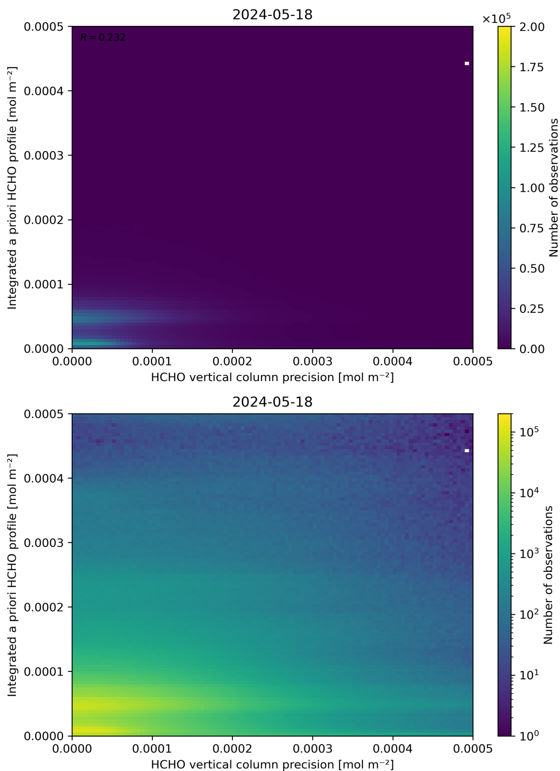
Figure 147: Scatter density plot of “HCHO vertical column precision” against “Integrated a priori HCHO profile” for 2024-05-18 to 2024-05-19.
