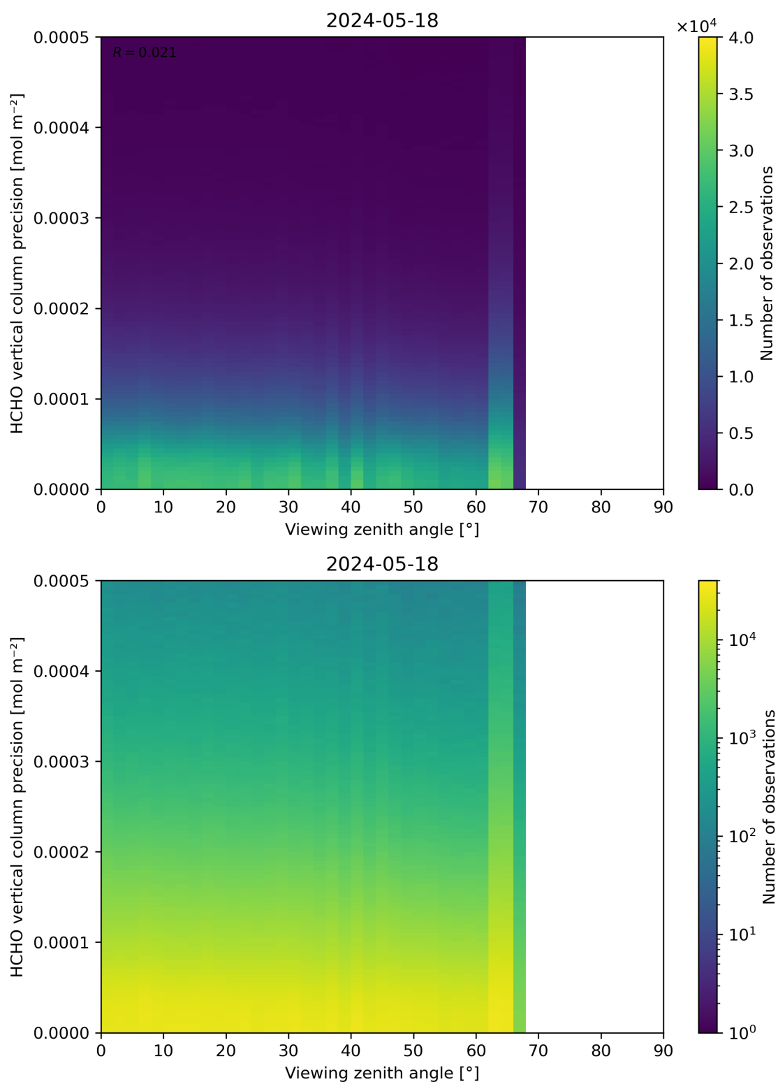
Figure 194: Scatter density plot of “Viewing zenith angle” against “HCHO vertical column precision” for 2024-05-18 to 2024-05-19.
