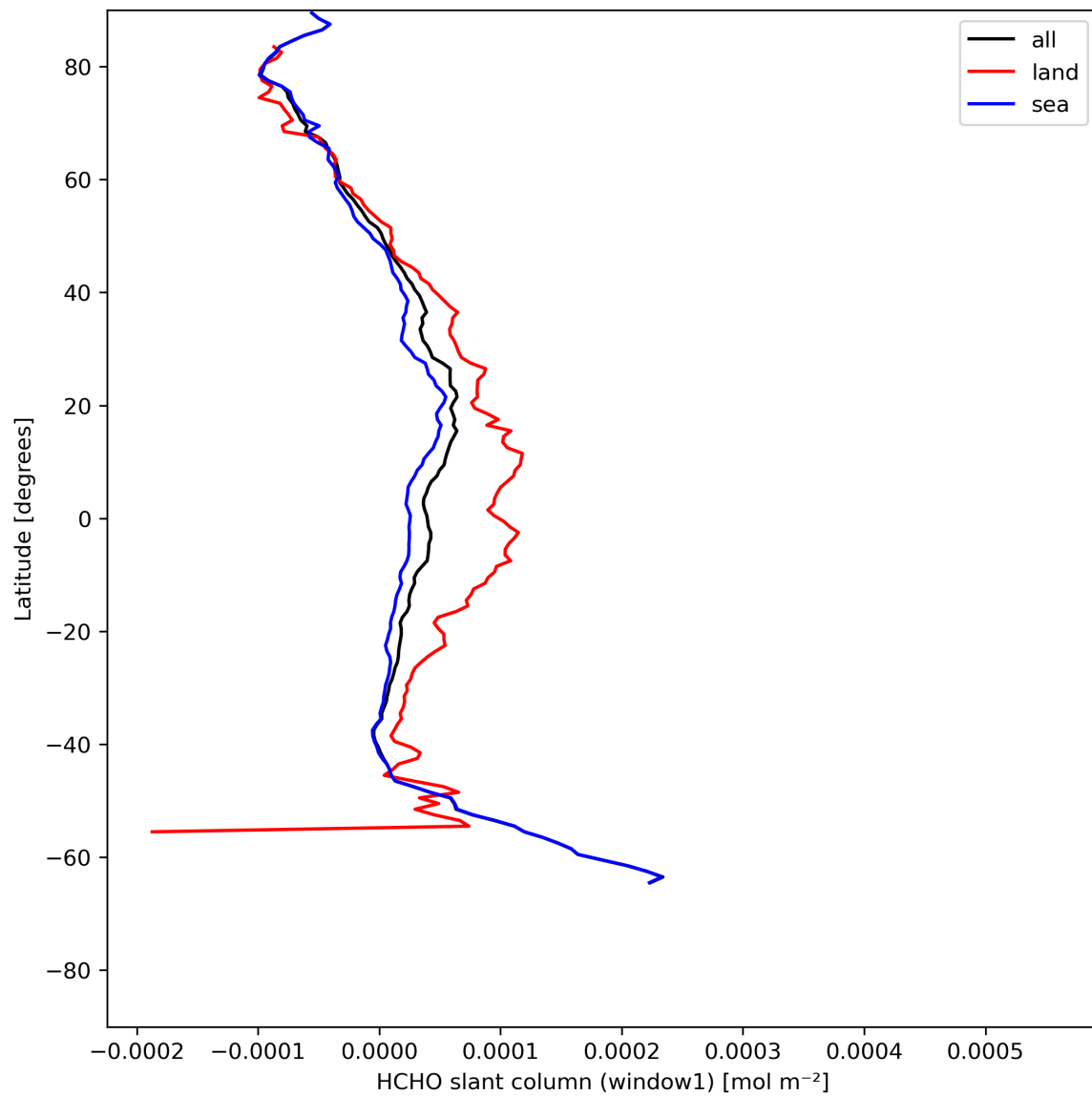
Figure 24: Zonal average of “HCHO slant column (window1)” for 2024-05-18 to 2024-05-19.
