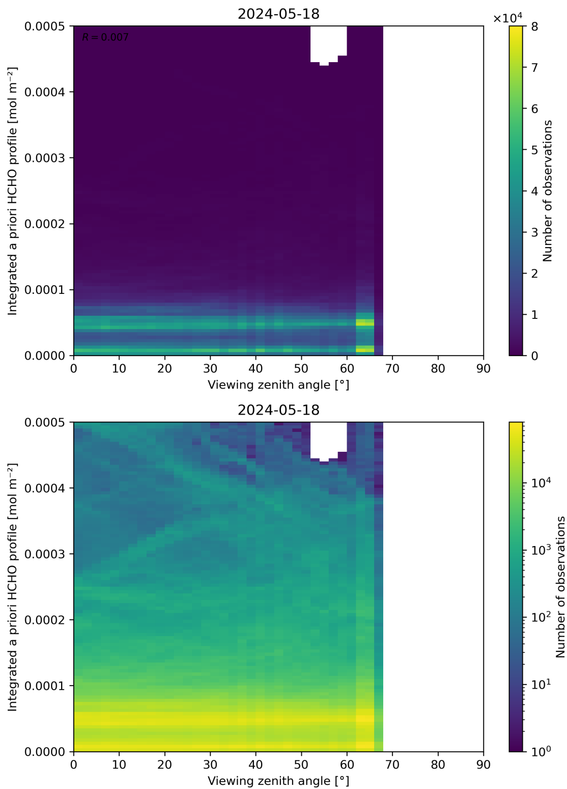
Figure 195: Scatter density plot of “Viewing zenith angle” against “Integrated a priori HCHO profile” for 2024-05-18 to 2024-05-19.
