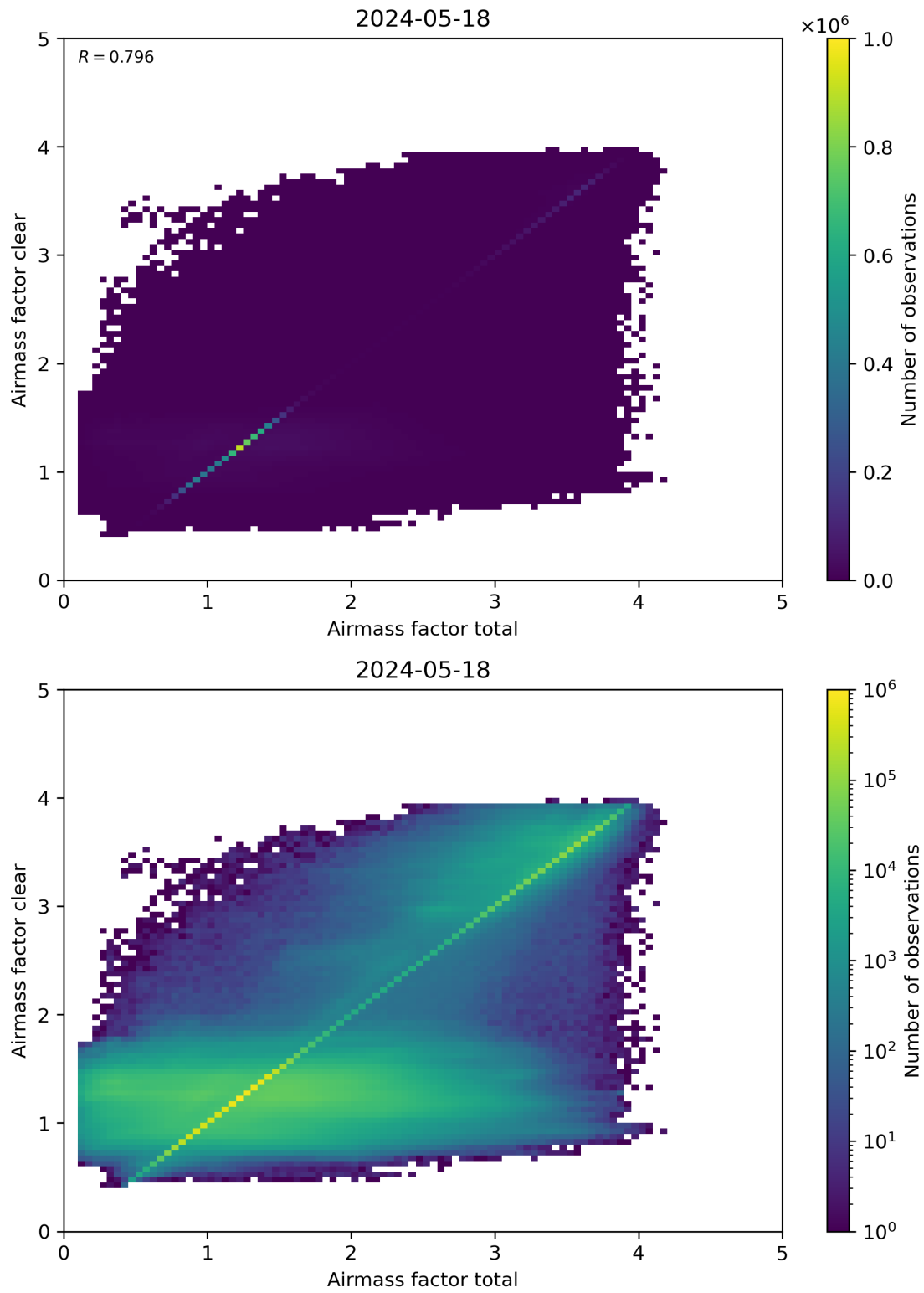
Figure 100: Scatter density plot of “Airmass factor total” against “Airmass factor clear” for 2024-05-18 to 2024-05-19.
