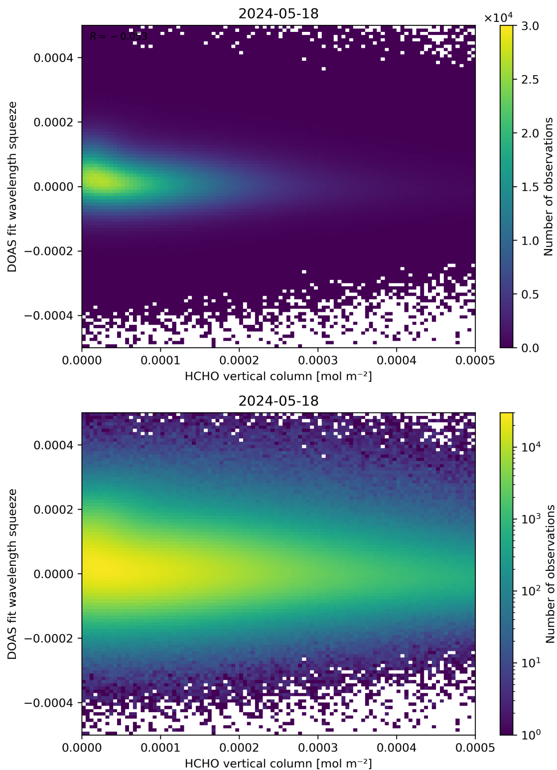
Figure 125: Scatter density plot of “HCHO vertical column” against “DOAS fit wavelength squeeze” for 2024-05-18 to 2024-05-19.
