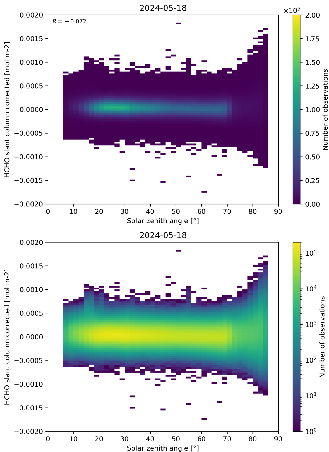
Figure 171: Scatter density plot of “Solar zenith angle” against “HCHO slant column corrected” for 2024-05-18 to 2024-05-19.
