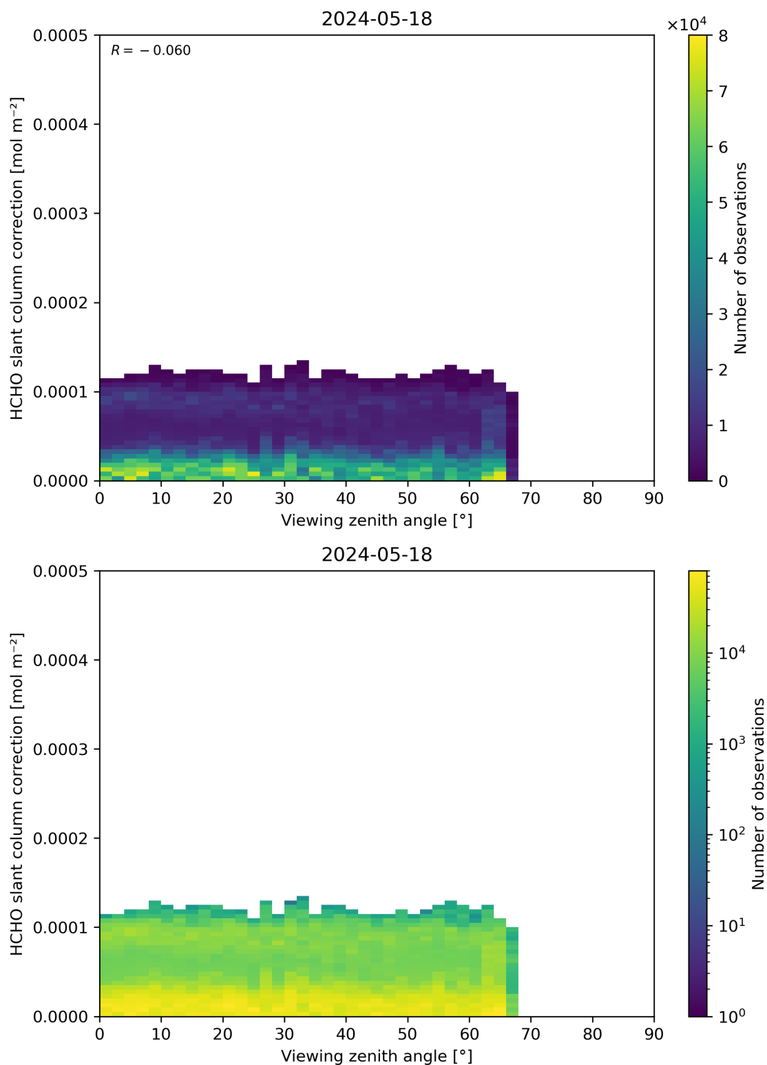
Figure 187: Scatter density plot of “Viewing zenith angle” against “HCHO slant column correction” for 2024-05-18 to 2024-05-19.
