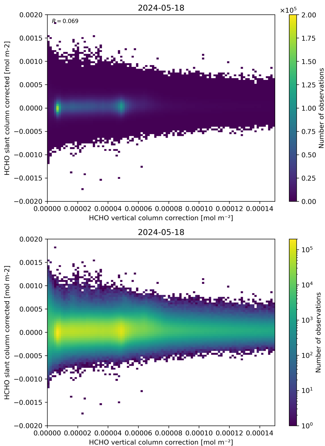
Figure 116: Scatter density plot of “HCHO vertical column correction” against “HCHO slant column corrected” for 2024-05-18 to 2024-05-19.
