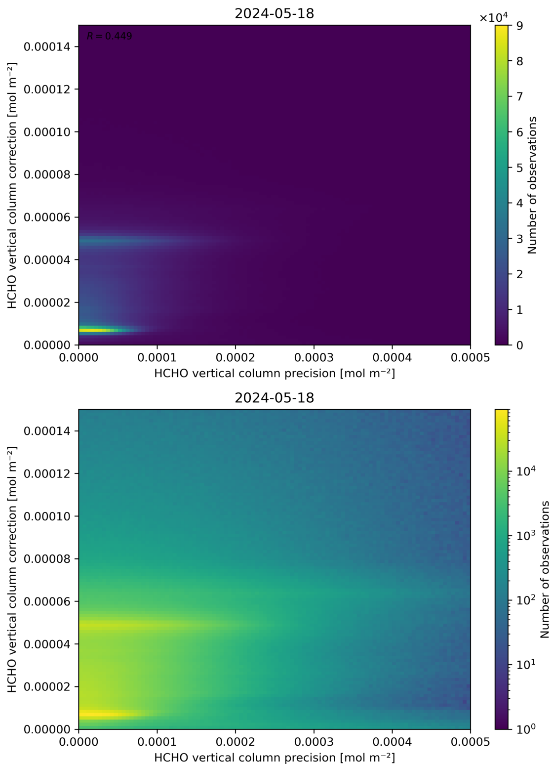
Figure 146: Scatter density plot of “HCHO vertical column precision” against “HCHO vertical column correction” for 2024-05-18 to 2024-05-19.
