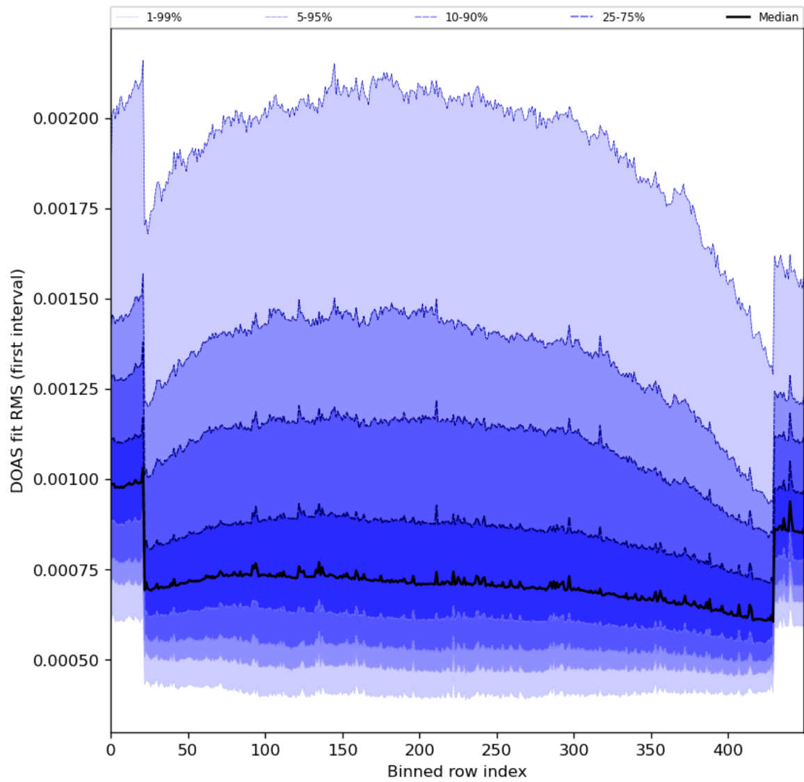
Figure 60: Along track statistics of “DOAS fit RMS (first interval)” for 2024-05-18 to 2024-05-19
