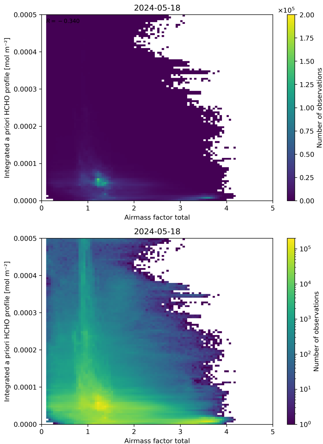
Figure 104: Scatter density plot of “Airmass factor total” against “Integrated a priori HCHO profile” for 2024-05-18 to 2024-05-19.
