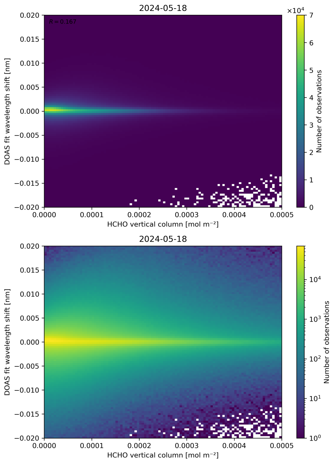
Figure 124: Scatter density plot of “HCHO vertical column” against “DOAS fit wavelength shift” for 2024-05-18 to 2024-05-19.
