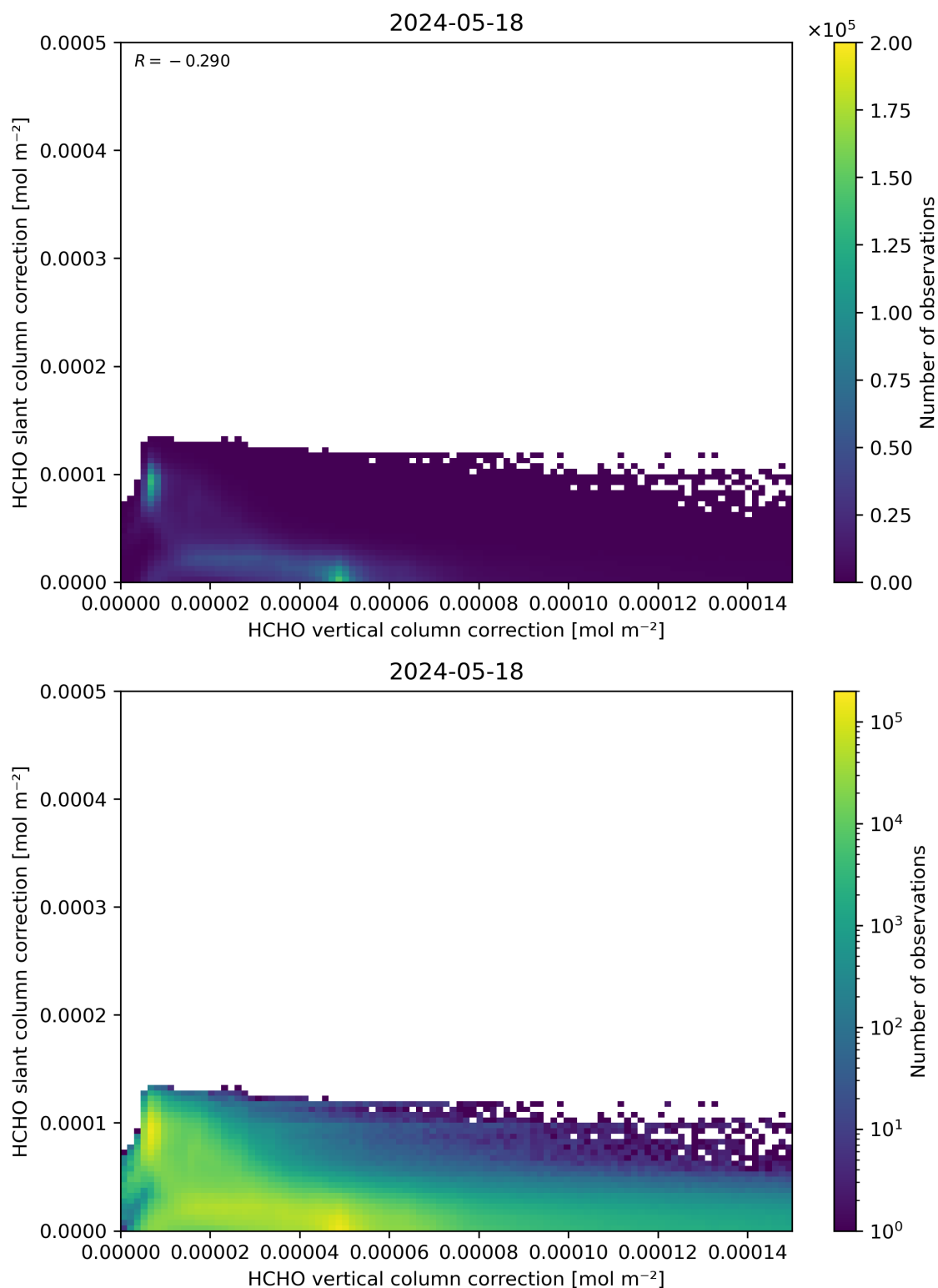
Figure 117: Scatter density plot of “HCHO vertical column correction” against “HCHO slant column correction” for 2024-05-18 to 2024-05-19.
