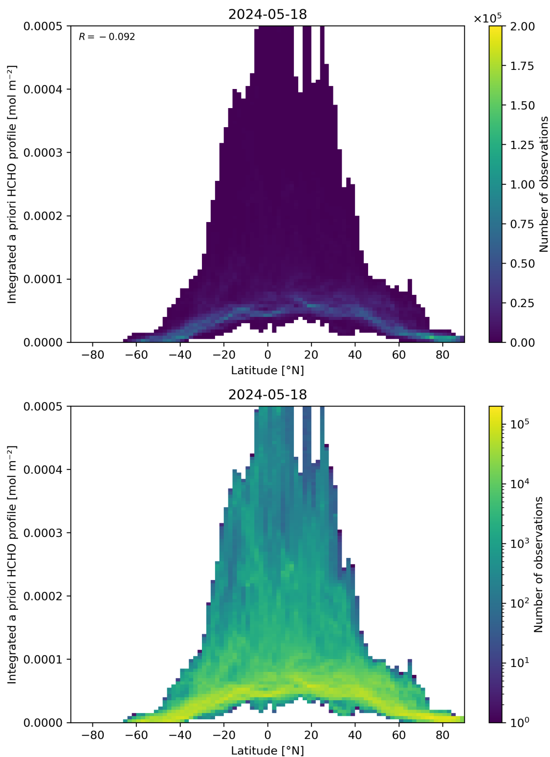
Figure 166: Scatter density plot of “Latitude” against “Integrated a priori HCHO profile” for 2024-05-18 to 2024-05-19.
