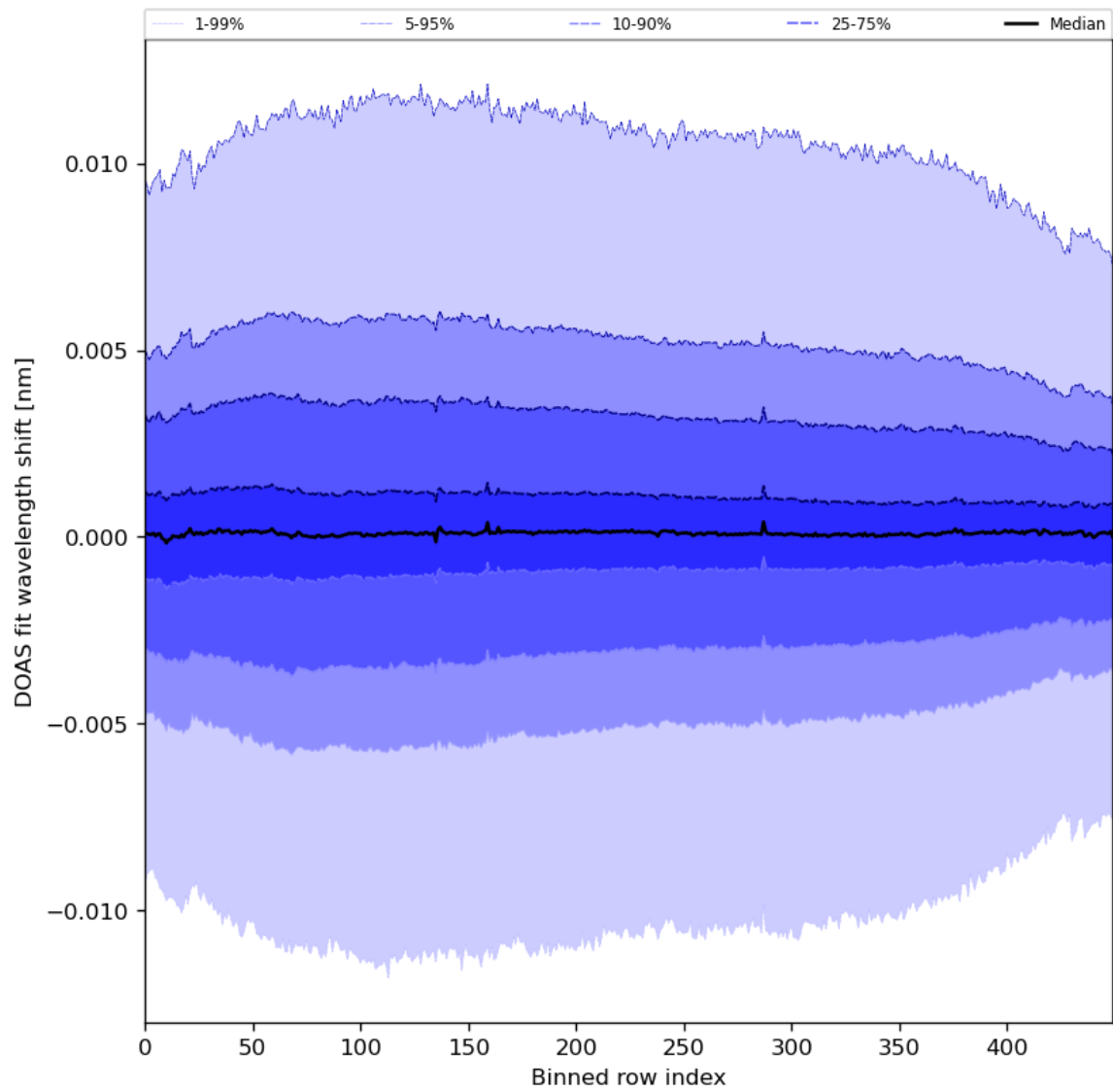
Figure 58: Along track statistics of “DOAS fit wavelength shift” for 2024-05-18 to 2024-05-19
