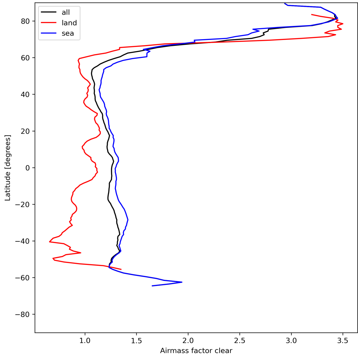
Figure 28: Zonal average of “Airmass factor clear” for 2024-05-18 to 2024-05-19.
