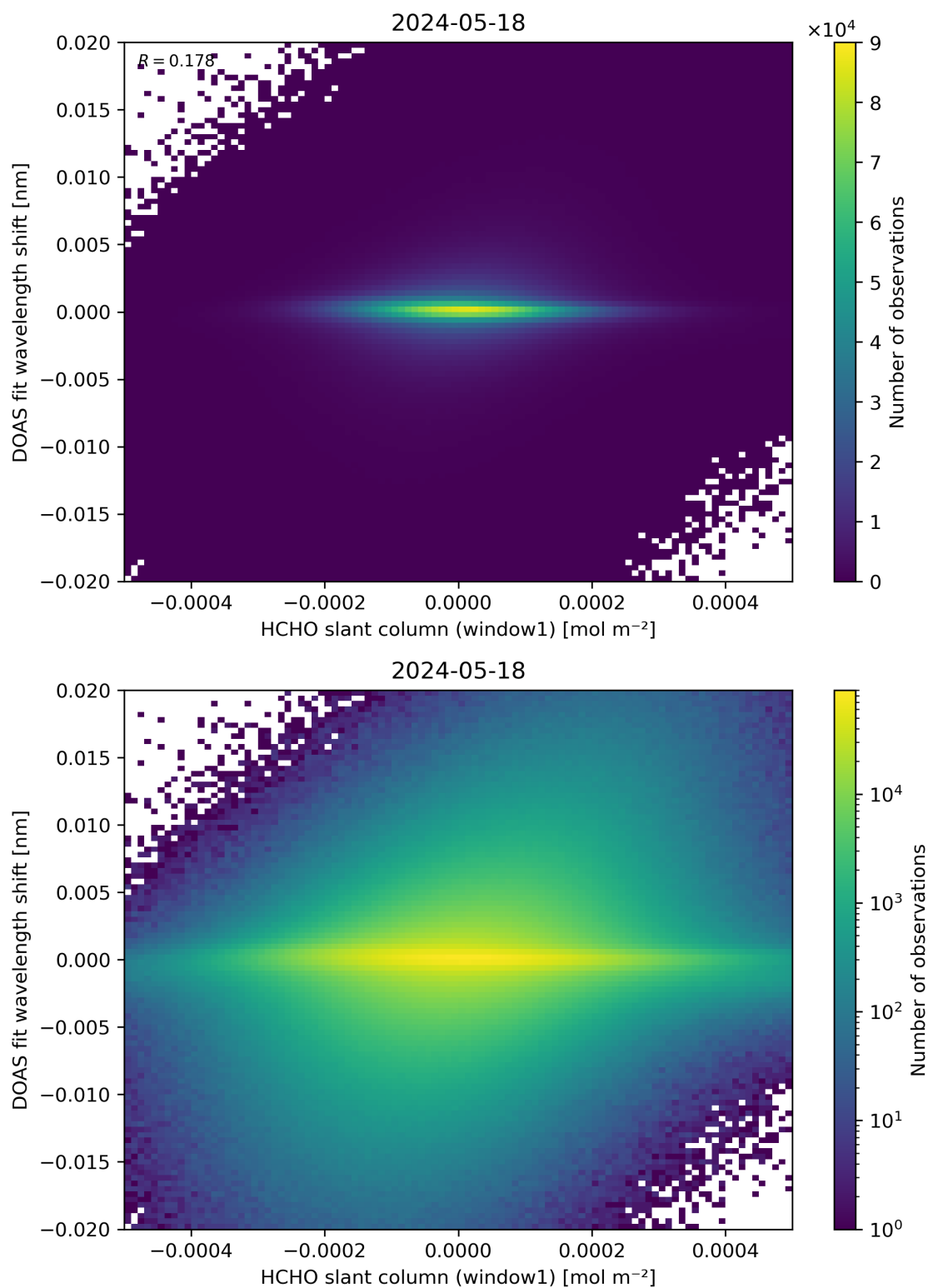
Figure 79: Scatter density plot of “HCHO slant column (window1)” against “DOAS fit wavelength shift” for 2024-05-18 to 2024-05-19.
