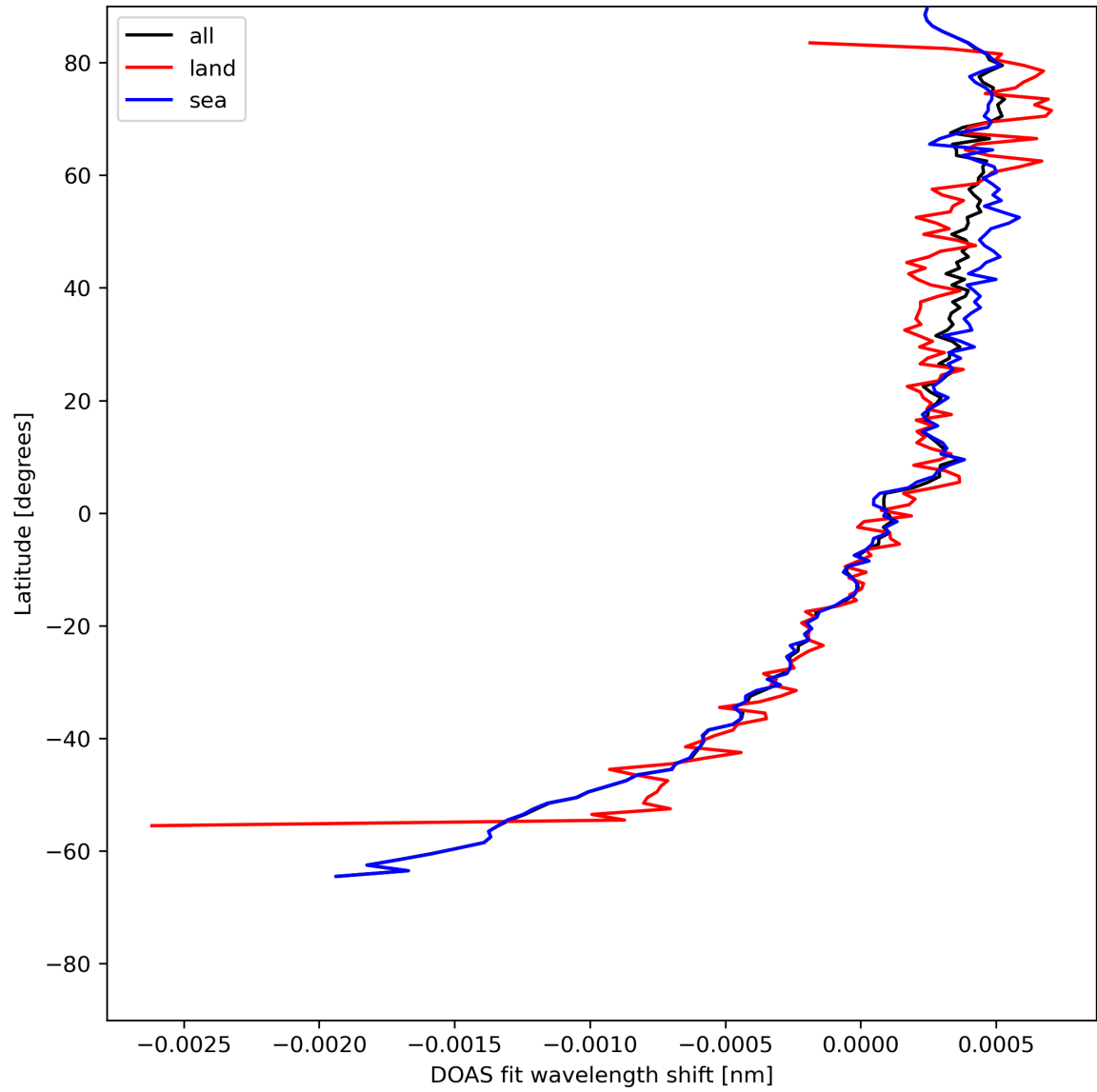
Figure 30: Zonal average of “DOAS fit wavelength shift” for 2024-05-18 to 2024-05-19.
