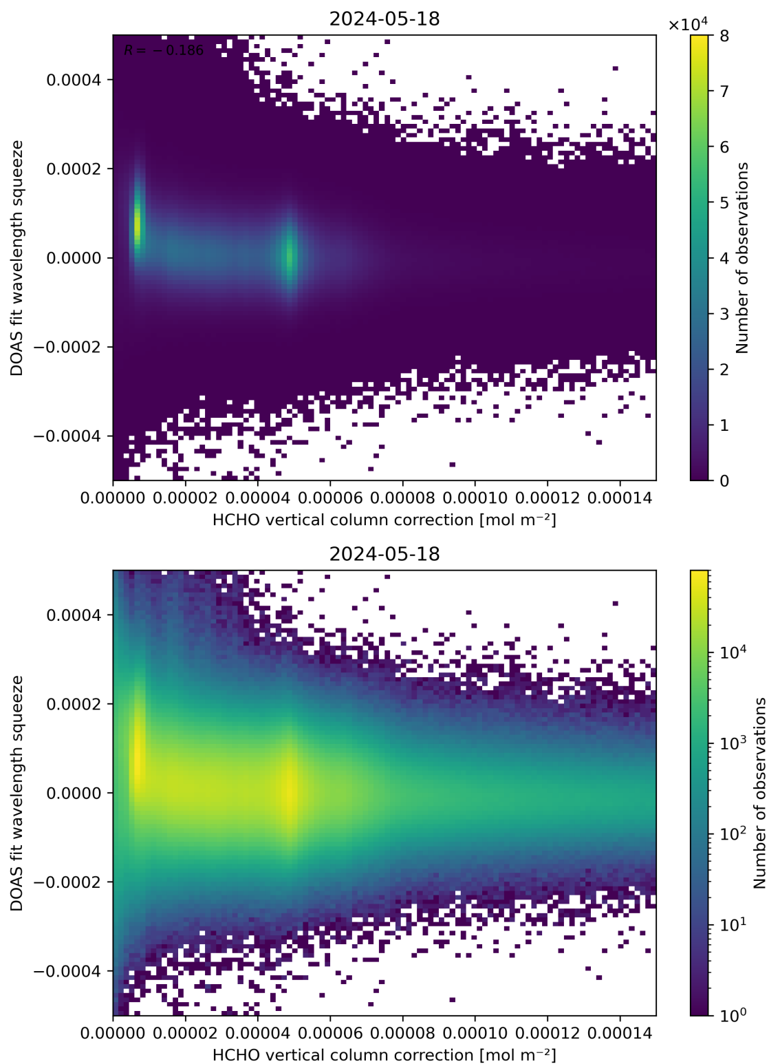
Figure 114: Scatter density plot of “HCHO vertical column correction” against “DOAS fit wavelength squeeze” for 2024-05-18 to 2024-05-19.
