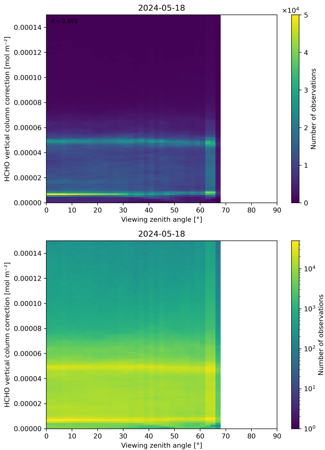
Figure 193: Scatter density plot of “Viewing zenith angle” against “HCHO vertical column correction” for 2024-05-18 to 2024-05-19.
