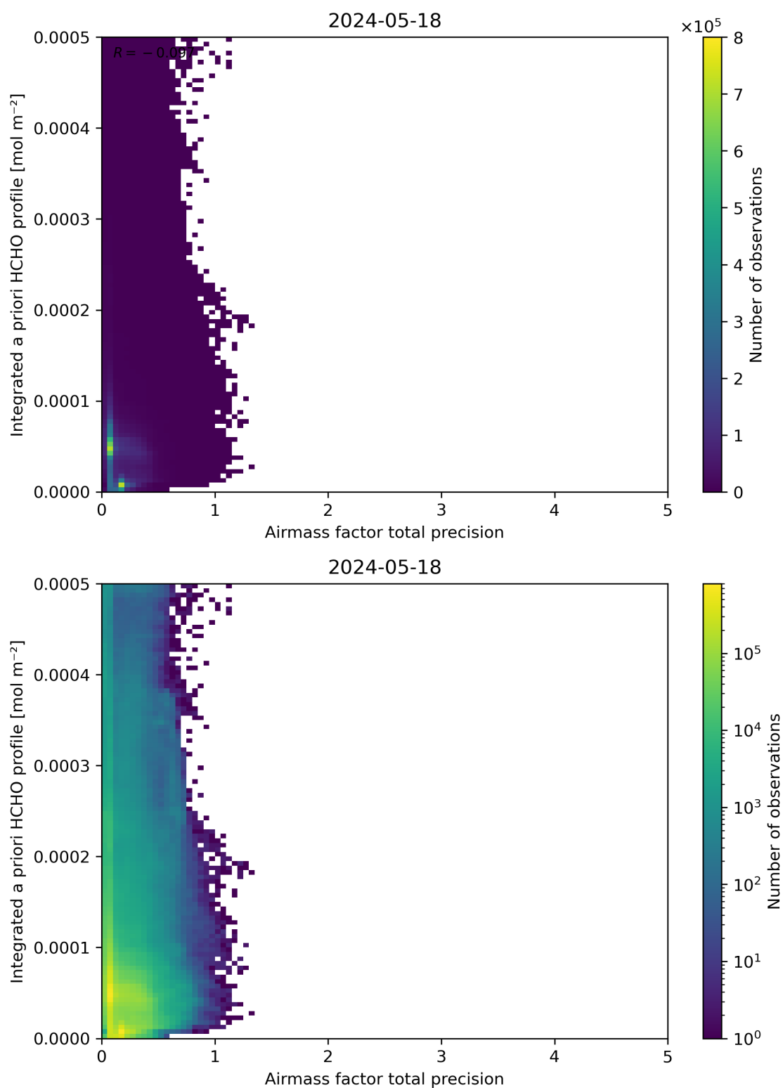
Figure 111: Scatter density plot of “Airmass factor total precision” against “Integrated a priori HCHO profile” for 2024-05-18 to 2024-05-19.
