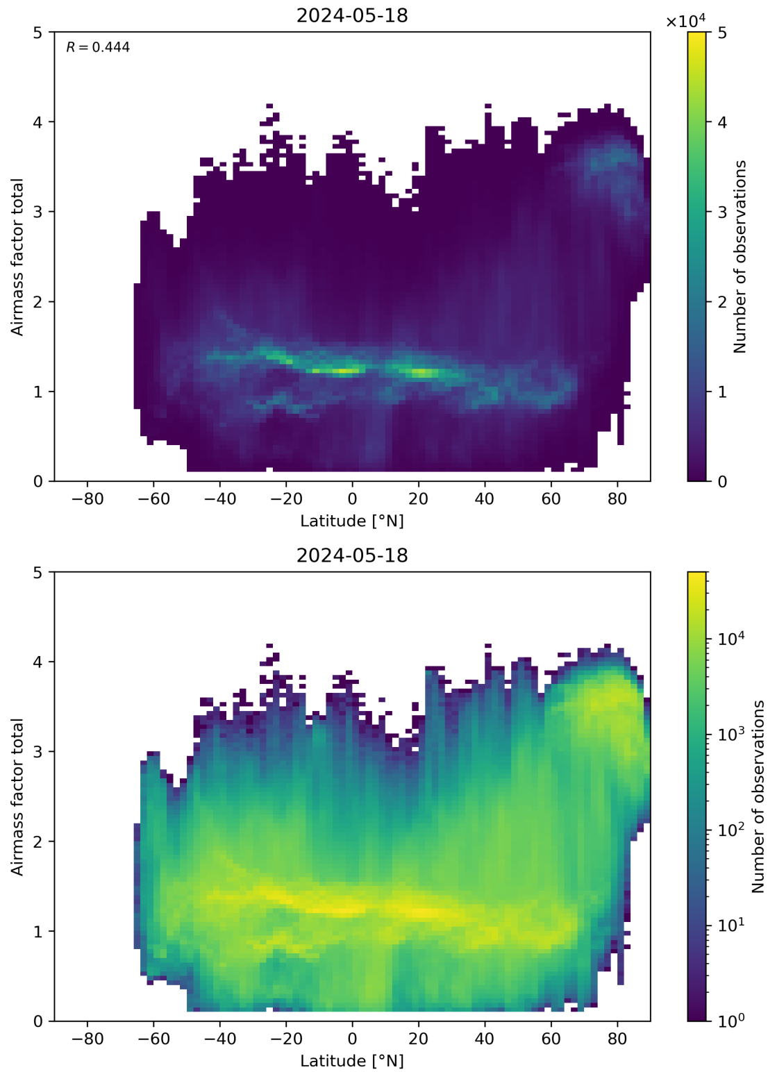
Figure 161: Scatter density plot of “Latitude” against “Airmass factor total” for 2024-05-18 to 2024-05-19.
