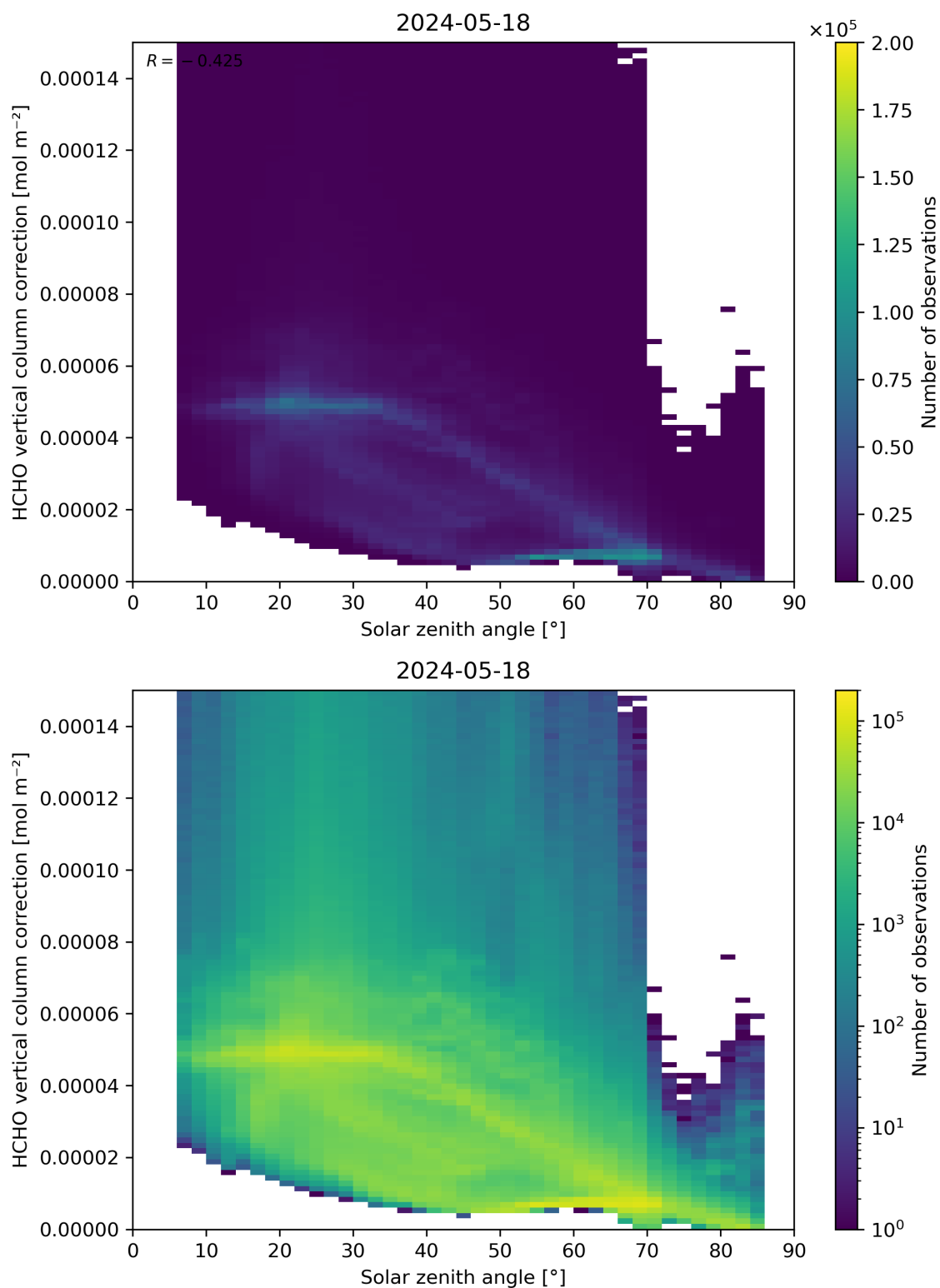
Figure 178: Scatter density plot of “Solar zenith angle” against “HCHO vertical column correction” for 2024-05-18 to 2024-05-19.
