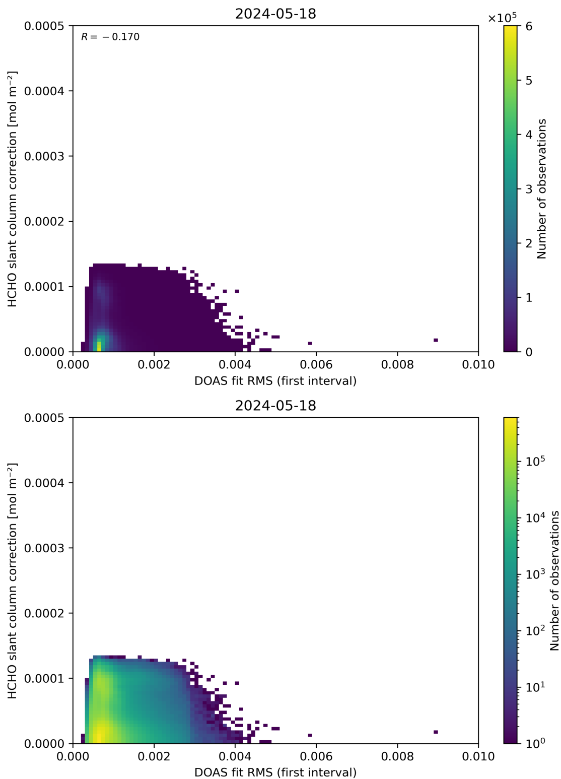
Figure 63: Scatter density plot of “DOAS fit RMS (first interval)” against “HCHO slant column correction” for 2024-05-18 to 2024-05-19.
