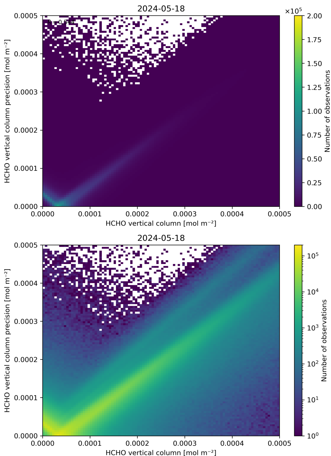
Figure 134: Scatter density plot of “HCHO vertical column” against “HCHO vertical column precision” for 2024-05-18 to 2024-05-19.
