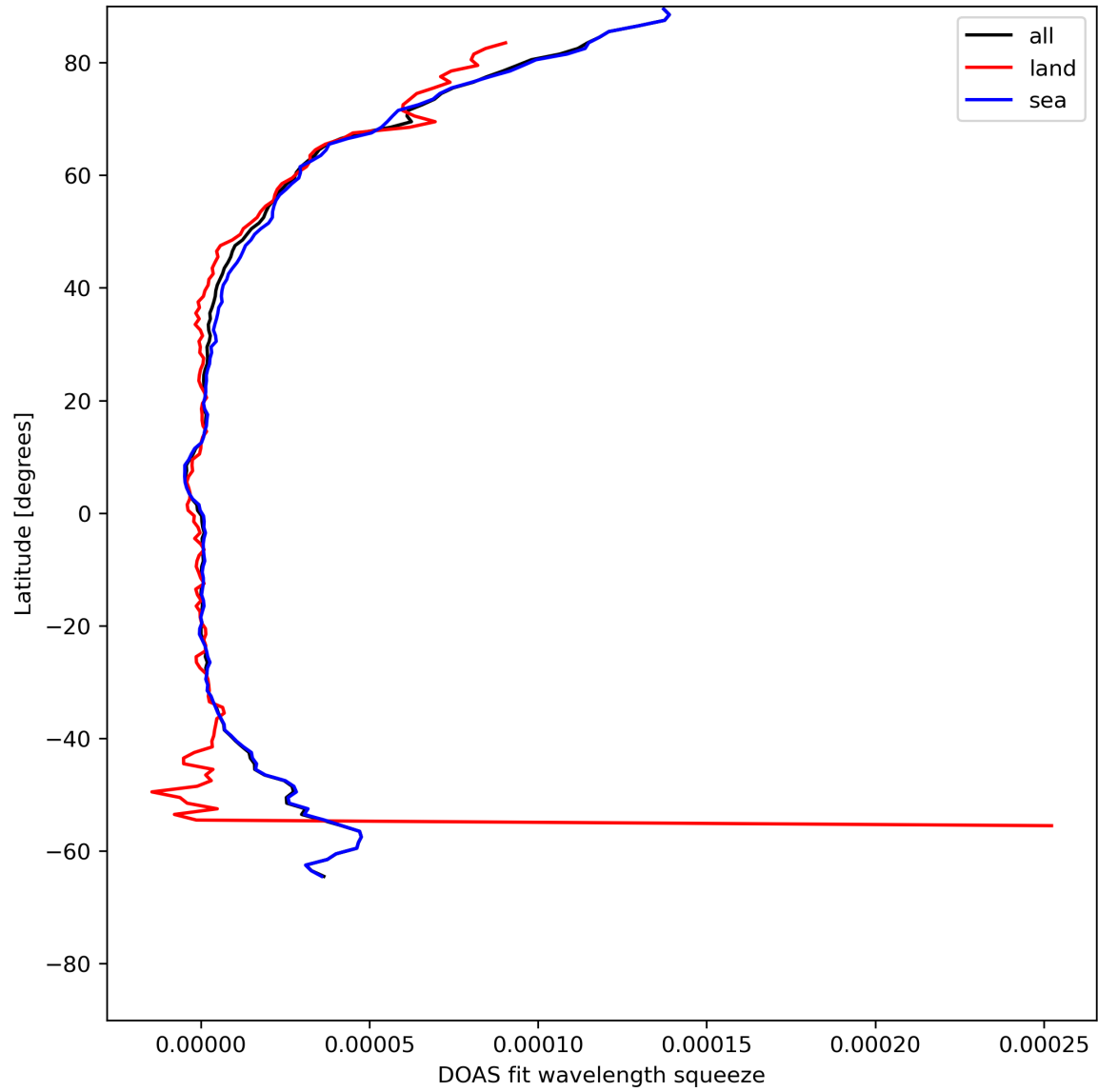
Figure 31: Zonal average of “DOAS fit wavelength squeeze” for 2024-05-18 to 2024-05-19.
