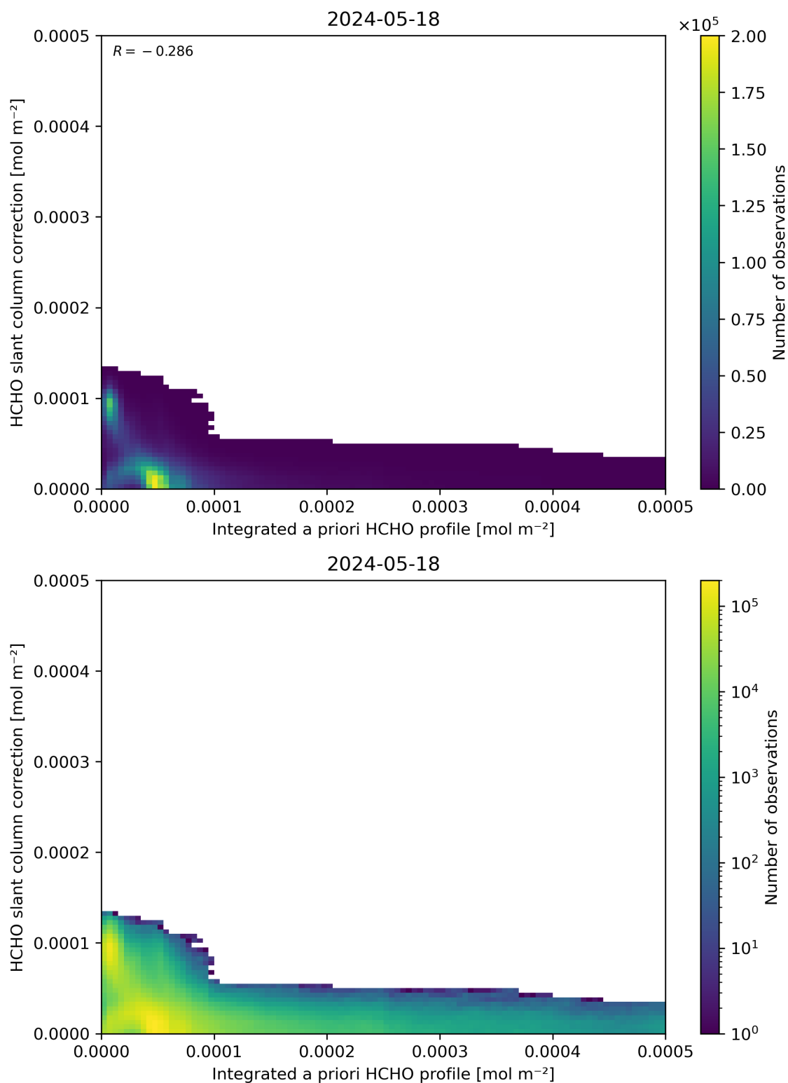
Figure 152: Scatter density plot of “Integrated a priori HCHO profile” against “HCHO slant column correction” for 2024-05-18 to 2024-05-19.
