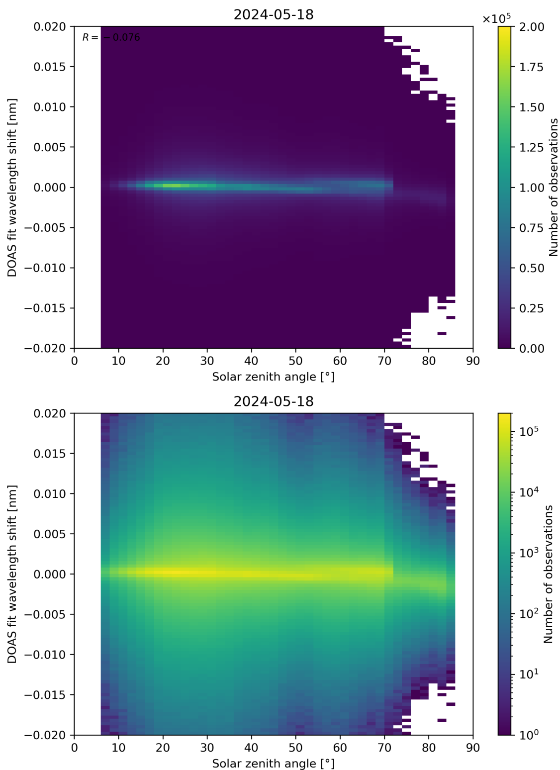
Figure 168: Scatter density plot of “Solar zenith angle” against “DOAS fit wavelength shift” for 2024-05-18 to 2024-05-19.
