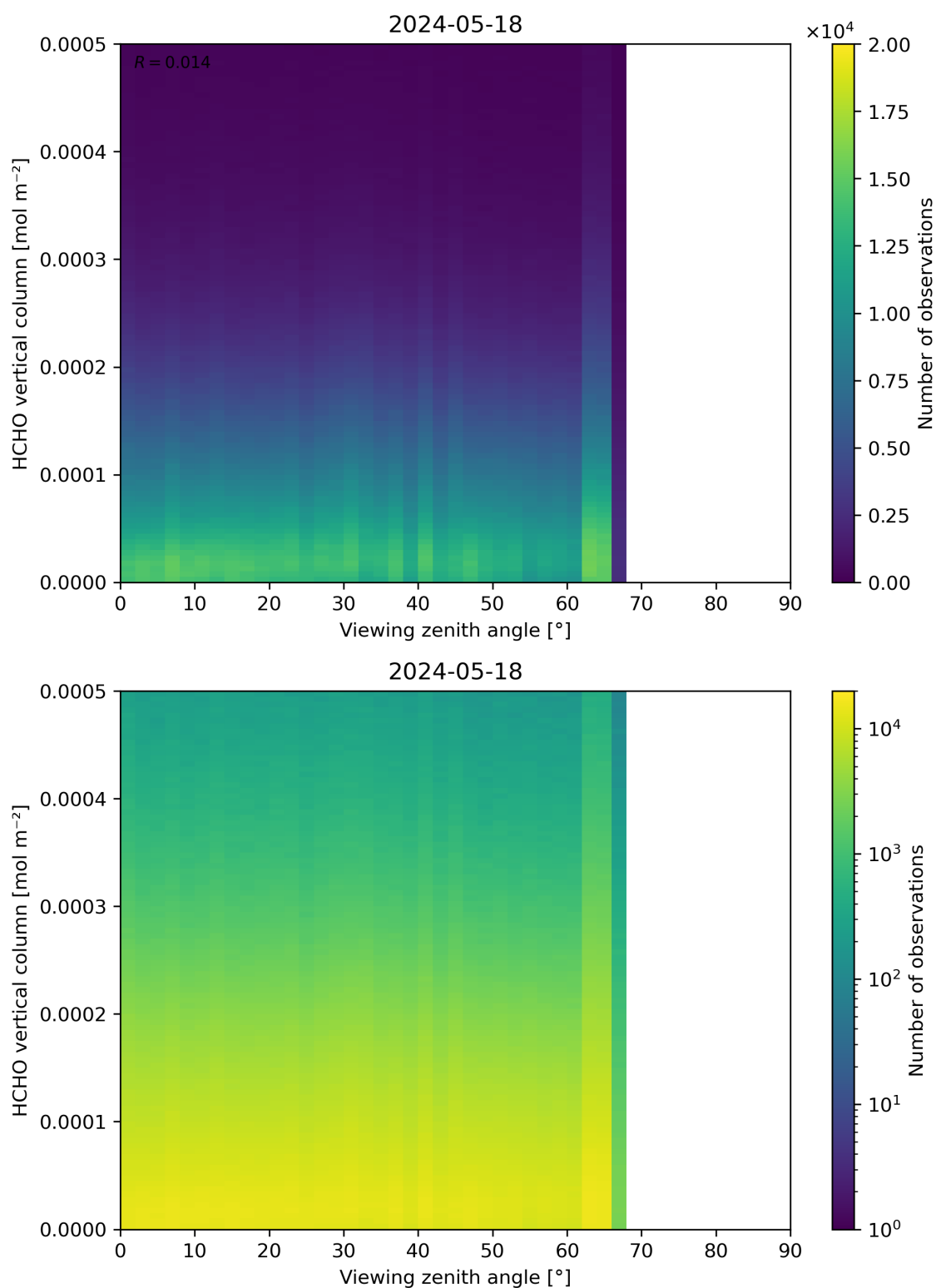
Figure 192: Scatter density plot of “Viewing zenith angle” against “HCHO vertical column” for 2024-05-18 to 2024-05-19.
