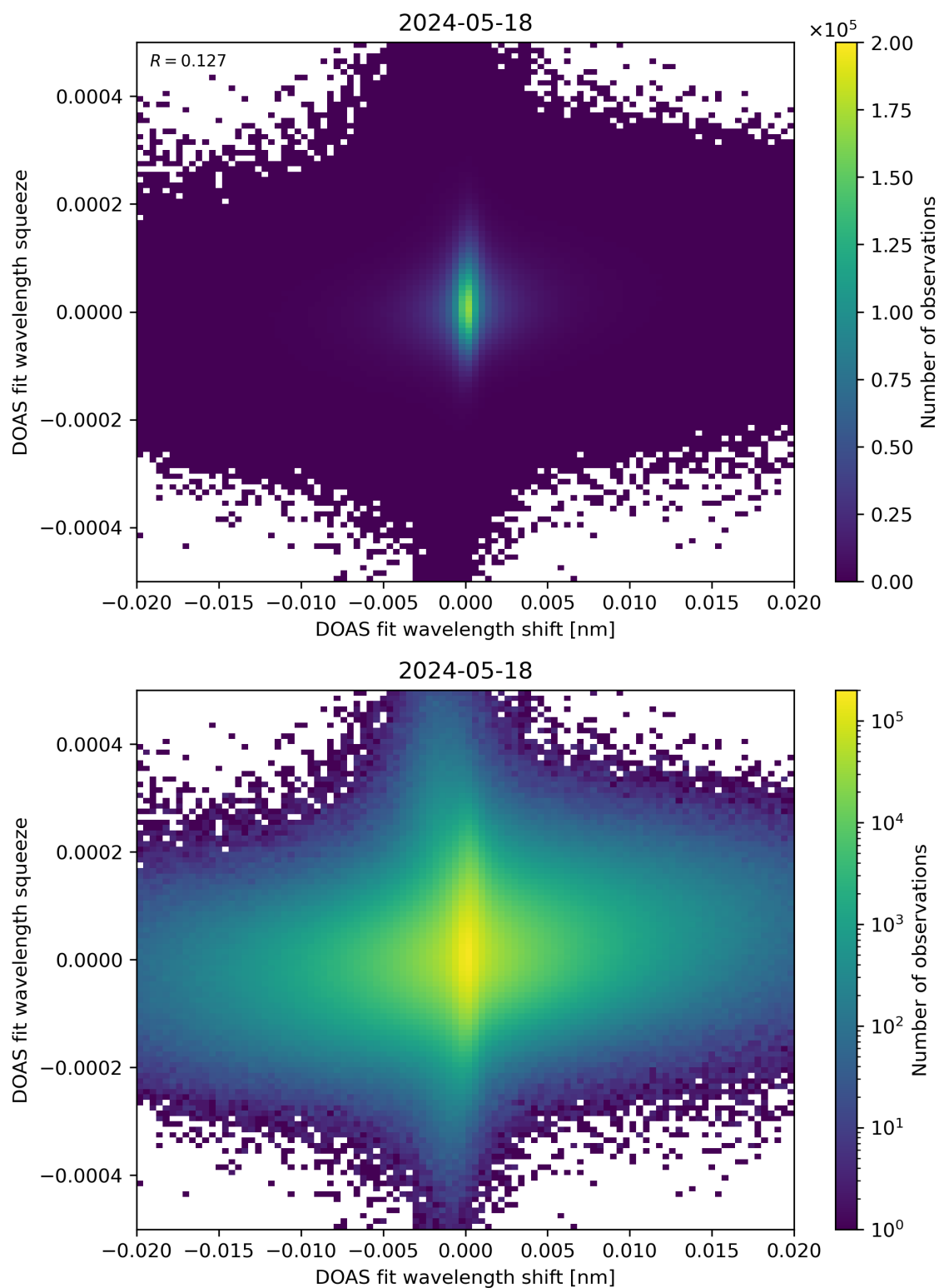
Figure 65: Scatter density plot of “DOAS fit wavelength shift” against “DOAS fit wavelength squeeze” for 2024-05-18 to 2024-05-19.
