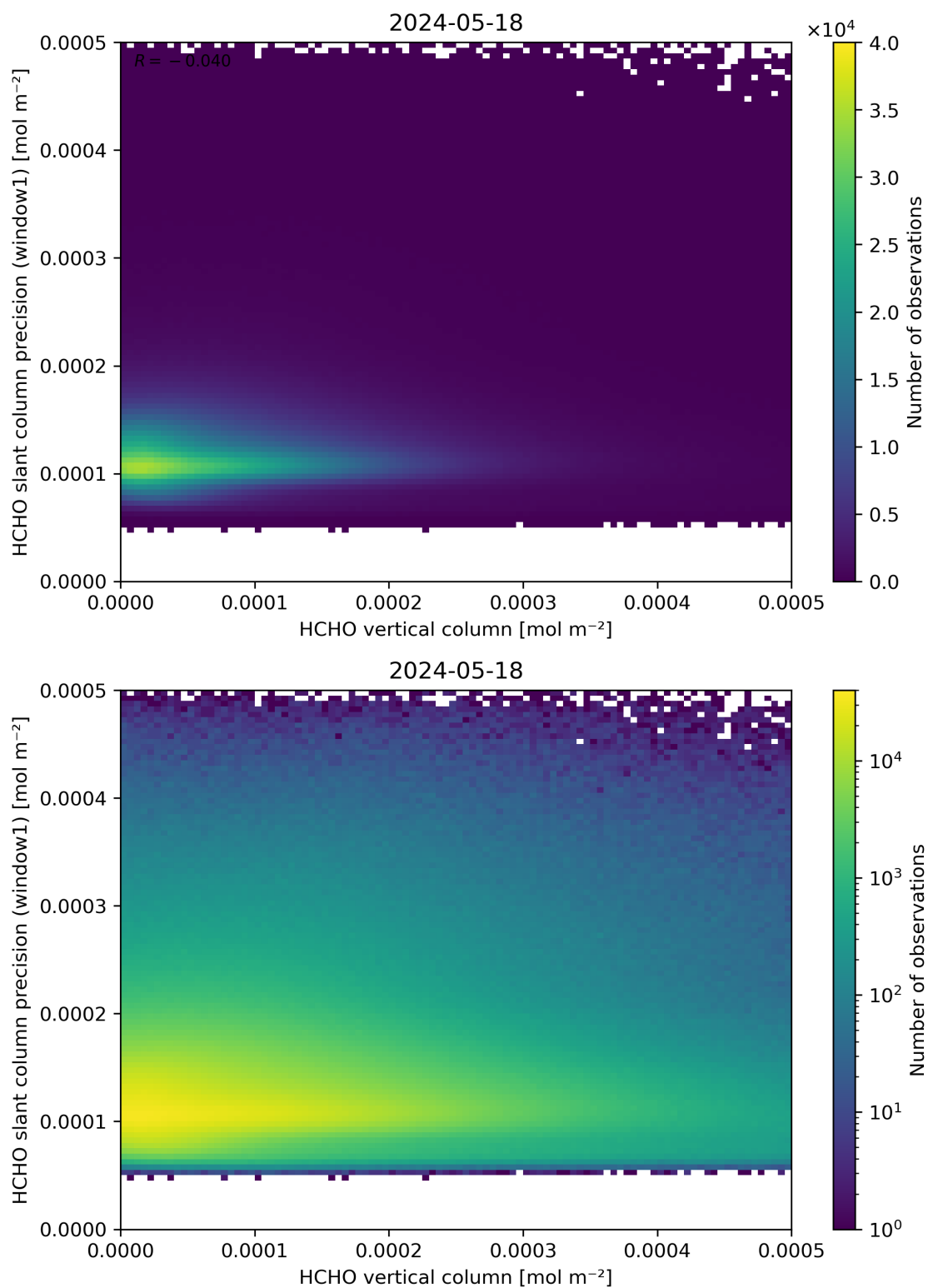
Figure 130: Scatter density plot of “HCHO vertical column” against “HCHO slant column precision (window1)” for 2024-05-18 to 2024-05-19.
