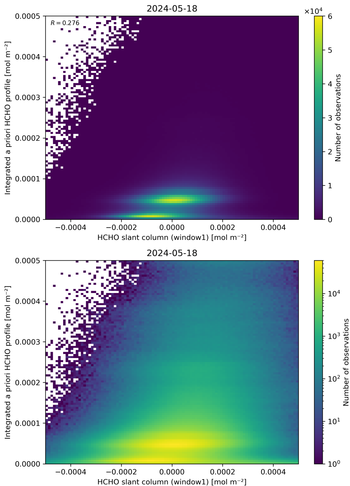
Figure 87: Scatter density plot of “HCHO slant column (window1)” against “Integrated a priori HCHO profile” for 2024-05-18 to 2024-05-19.
