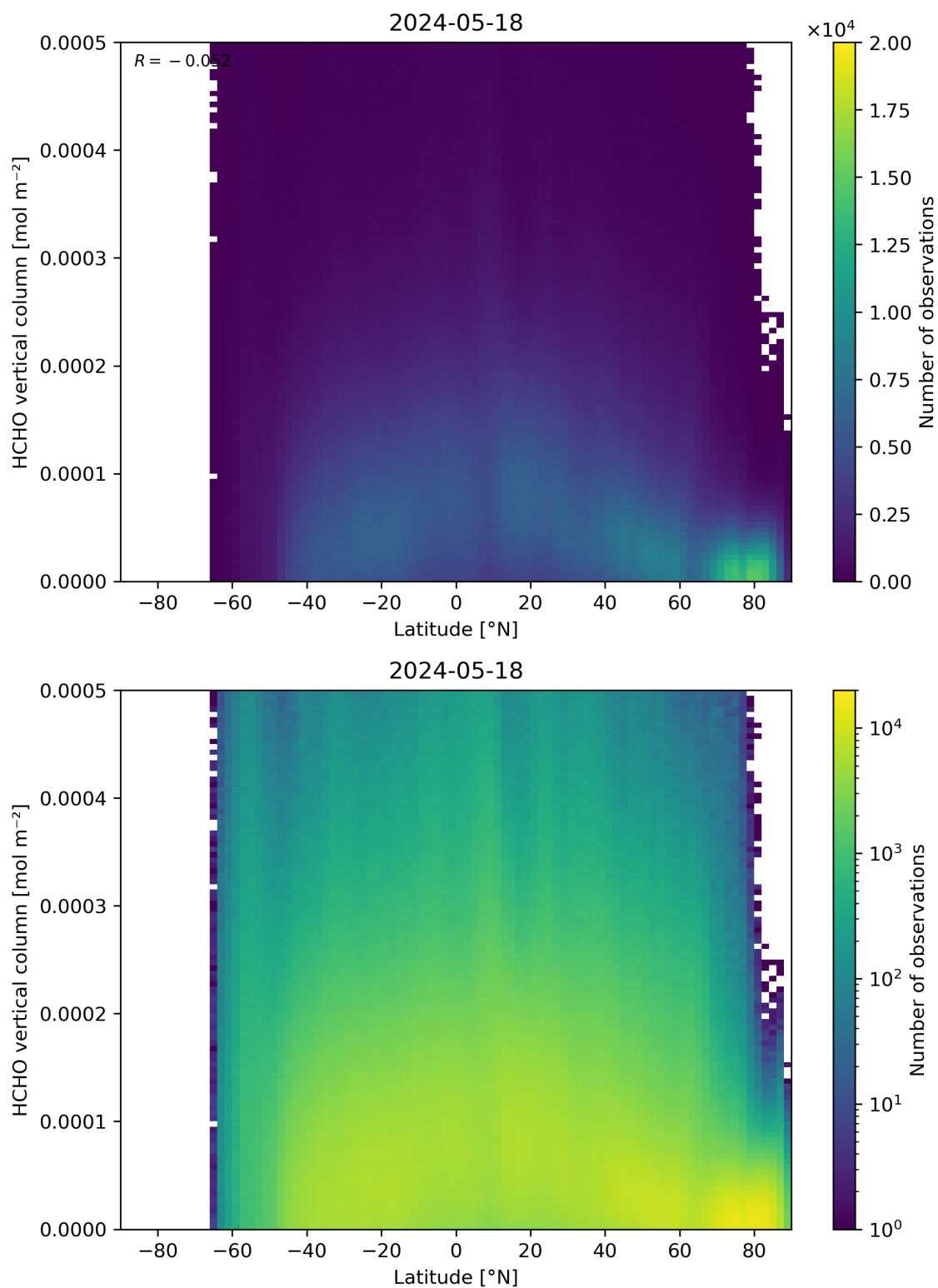
Figure 163: Scatter density plot of “Latitude” against “HCHO vertical column” for 2024-05-18 to 2024-05-19.
