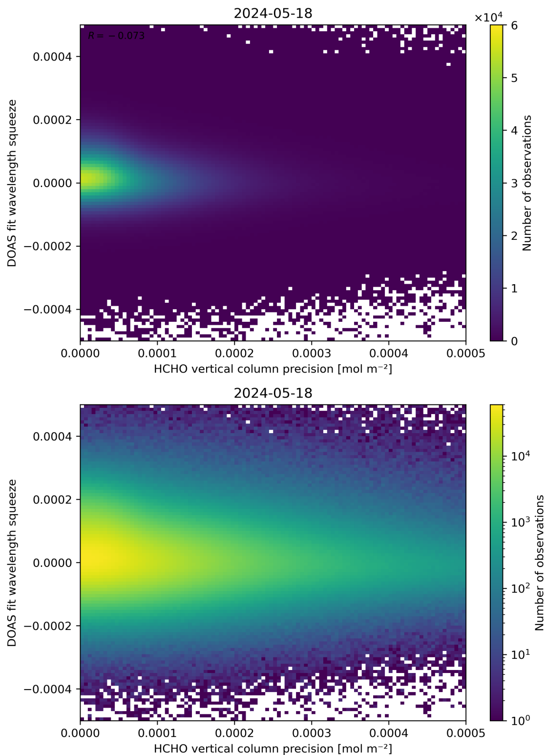
Figure 138: Scatter density plot of “HCHO vertical column precision” against “DOAS fit wavelength squeeze” for 2024-05-18 to 2024-05-19.
