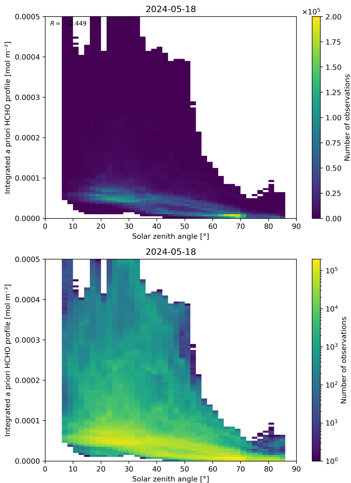
Figure 180: Scatter density plot of “Solar zenith angle” against “Integrated a priori HCHO profile” for 2024-05-18 to 2024-05-19.
