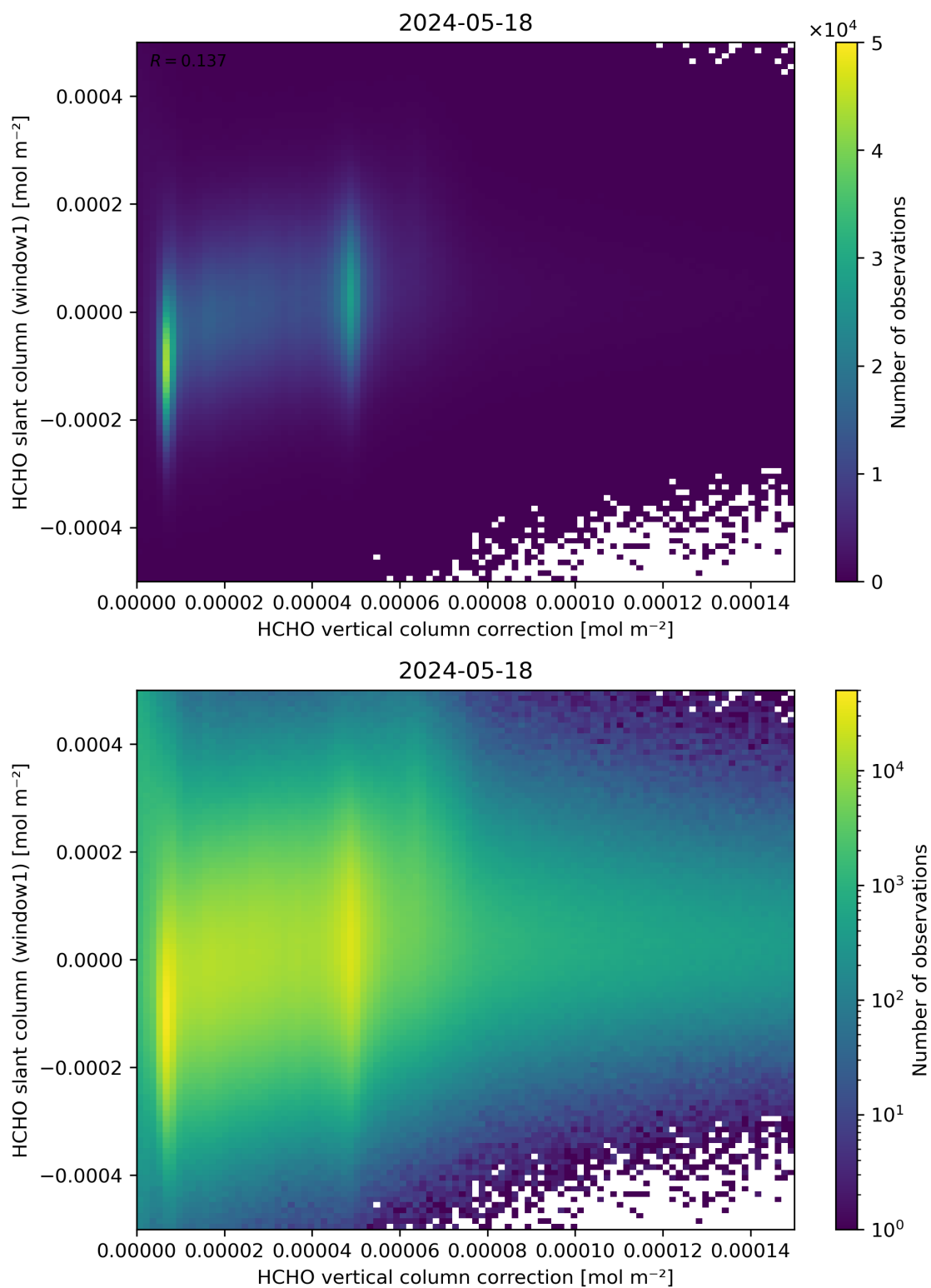
Figure 118: Scatter density plot of “HCHO vertical column correction” against “HCHO slant column (window1)” for 2024-05-18 to 2024-05-19.
