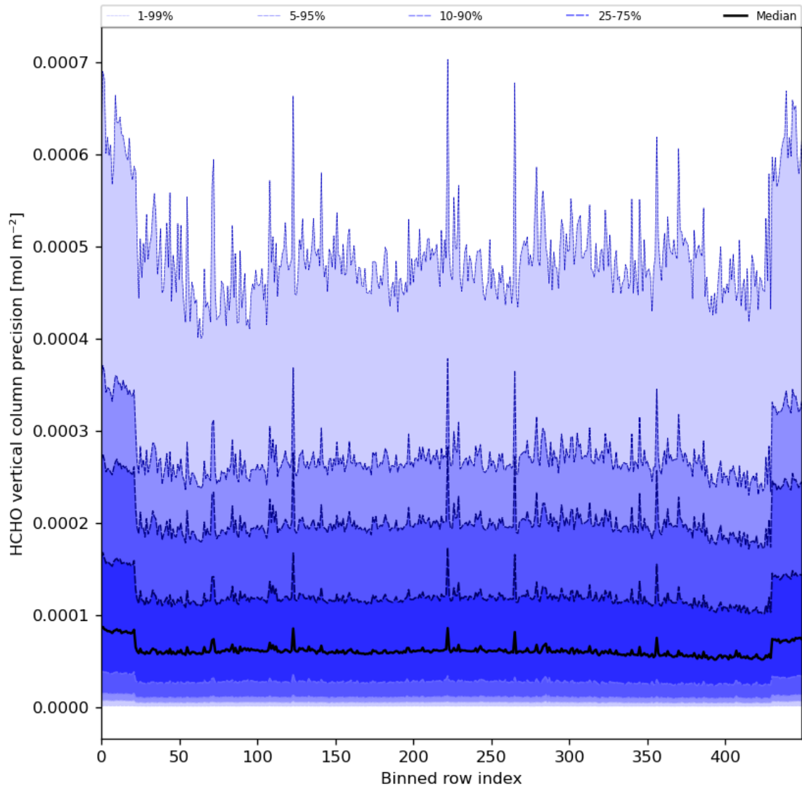
Figure 50: Along track statistics of “HCHO vertical column precision” for 2024-05-18 to 2024-05-19
