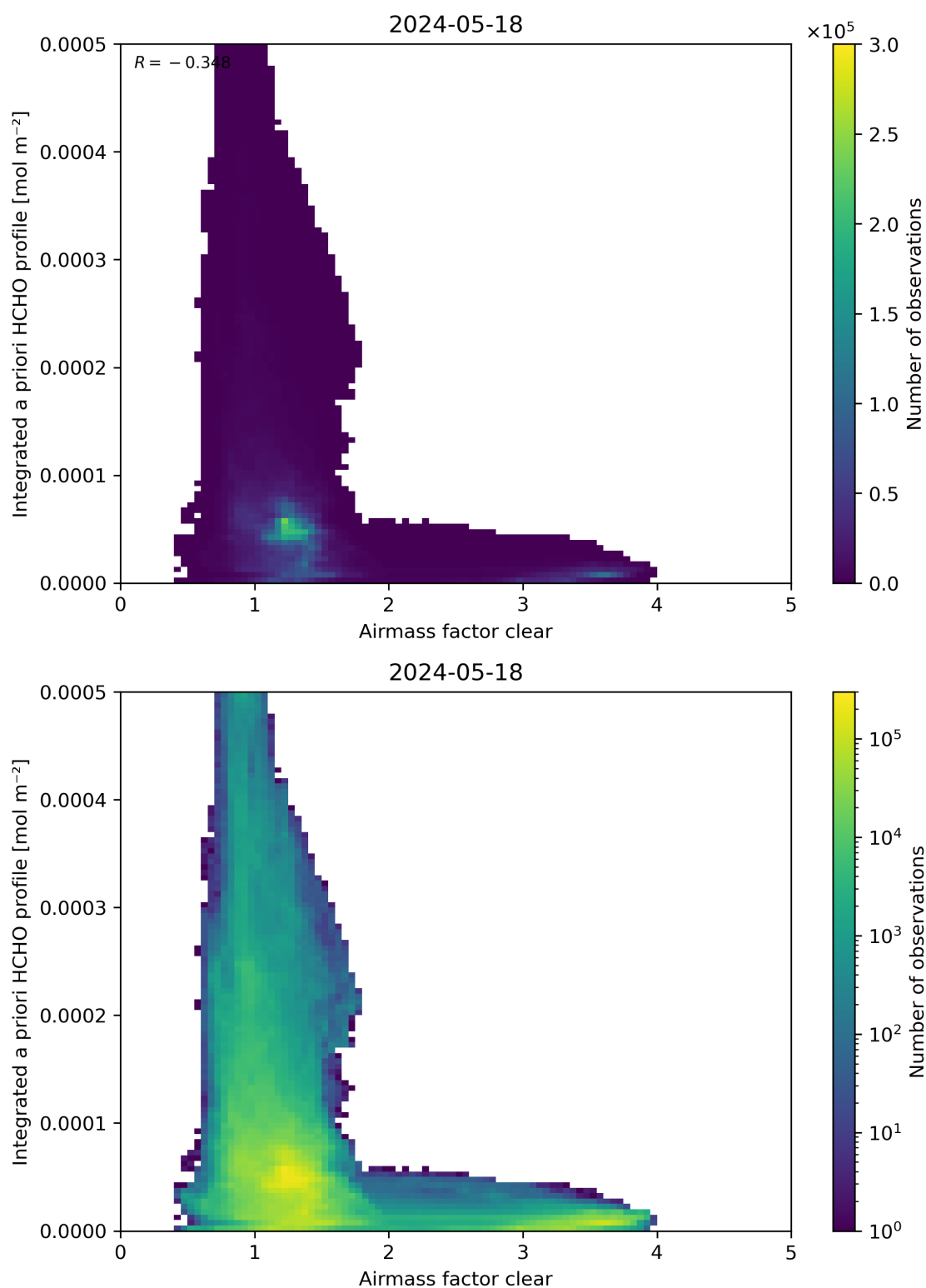
Figure 76: Scatter density plot of “Airmass factor clear” against “Integrated a priori HCHO profile” for 2024-05-18 to 2024-05-19.
