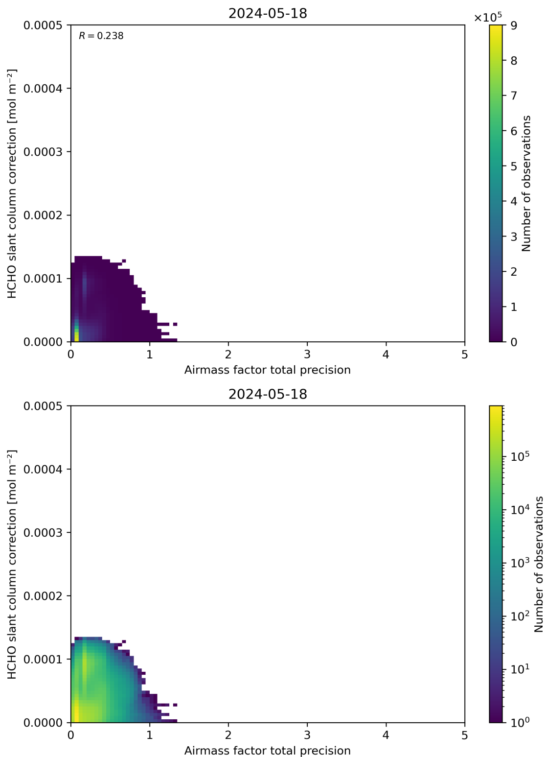
Figure 110: Scatter density plot of “Airmass factor total precision” against “HCHO slant column correction” for 2024-05-18 to 2024-05-19.
