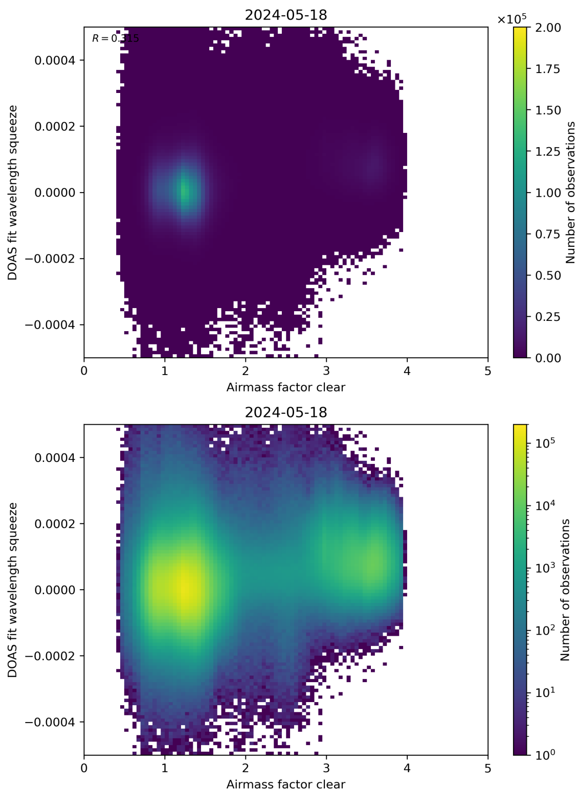
Figure 73: Scatter density plot of “Airmass factor clear” against “DOAS fit wavelength squeeze” for 2024-05-18 to 2024-05-19.
