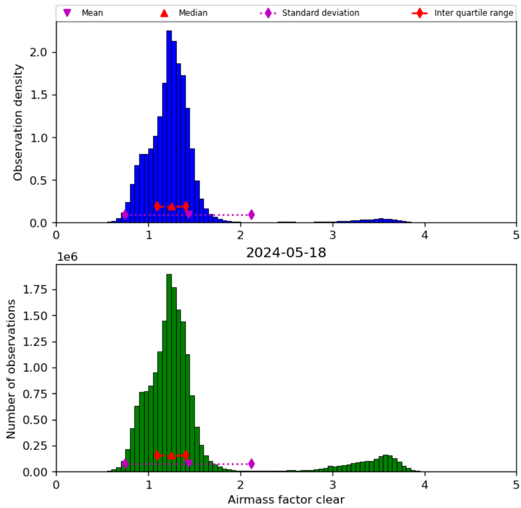
Figure 42: Histogram of “Airmass factor clear” for 2024-05-18 to 2024-05-19
