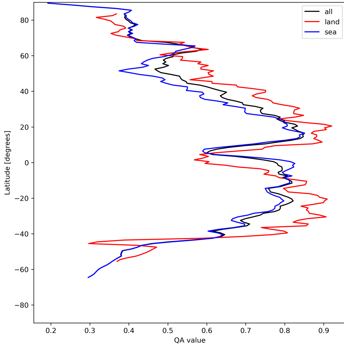
Figure 20: Zonal average of “QA value” for 2024-05-18 to 2024-05-19.
