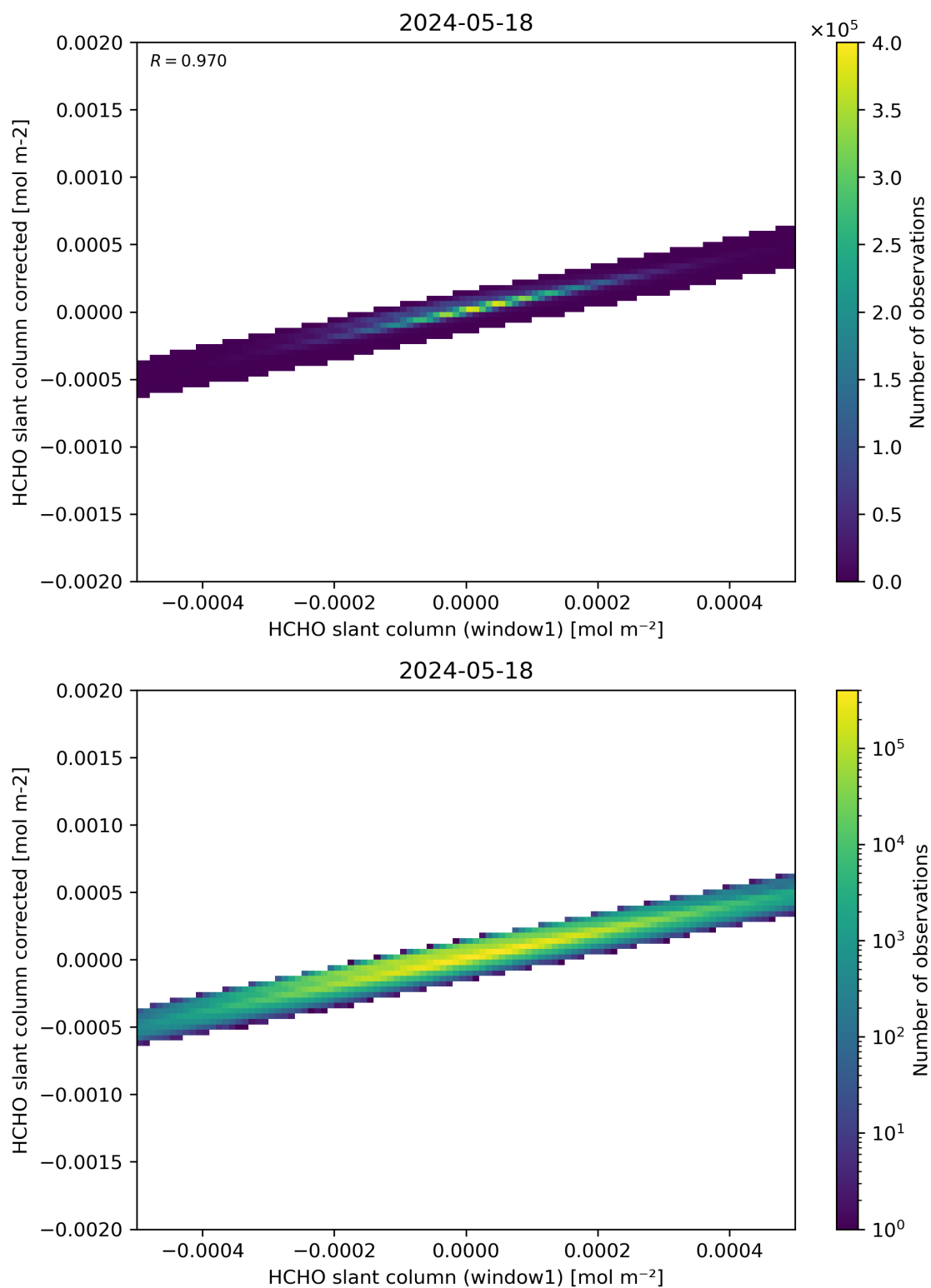
Figure 82: Scatter density plot of “HCHO slant column (window1)” against “HCHO slant column corrected” for 2024-05-18 to 2024-05-19.
