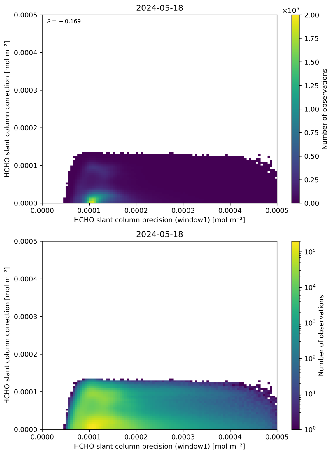
Figure 93: Scatter density plot of “HCHO slant column precision (window1)” against “HCHO slant column correction” for 2024-05-18 to 2024-05-19.
