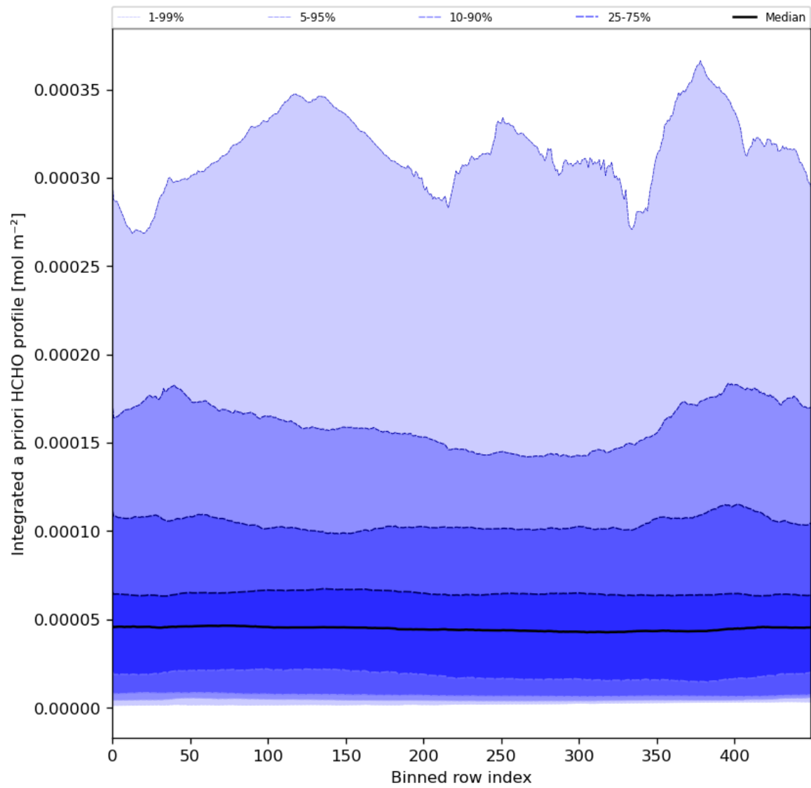
Figure 57: Along track statistics of “Integrated a priori HCHO profile” for 2024-05-18 to 2024-05-19
