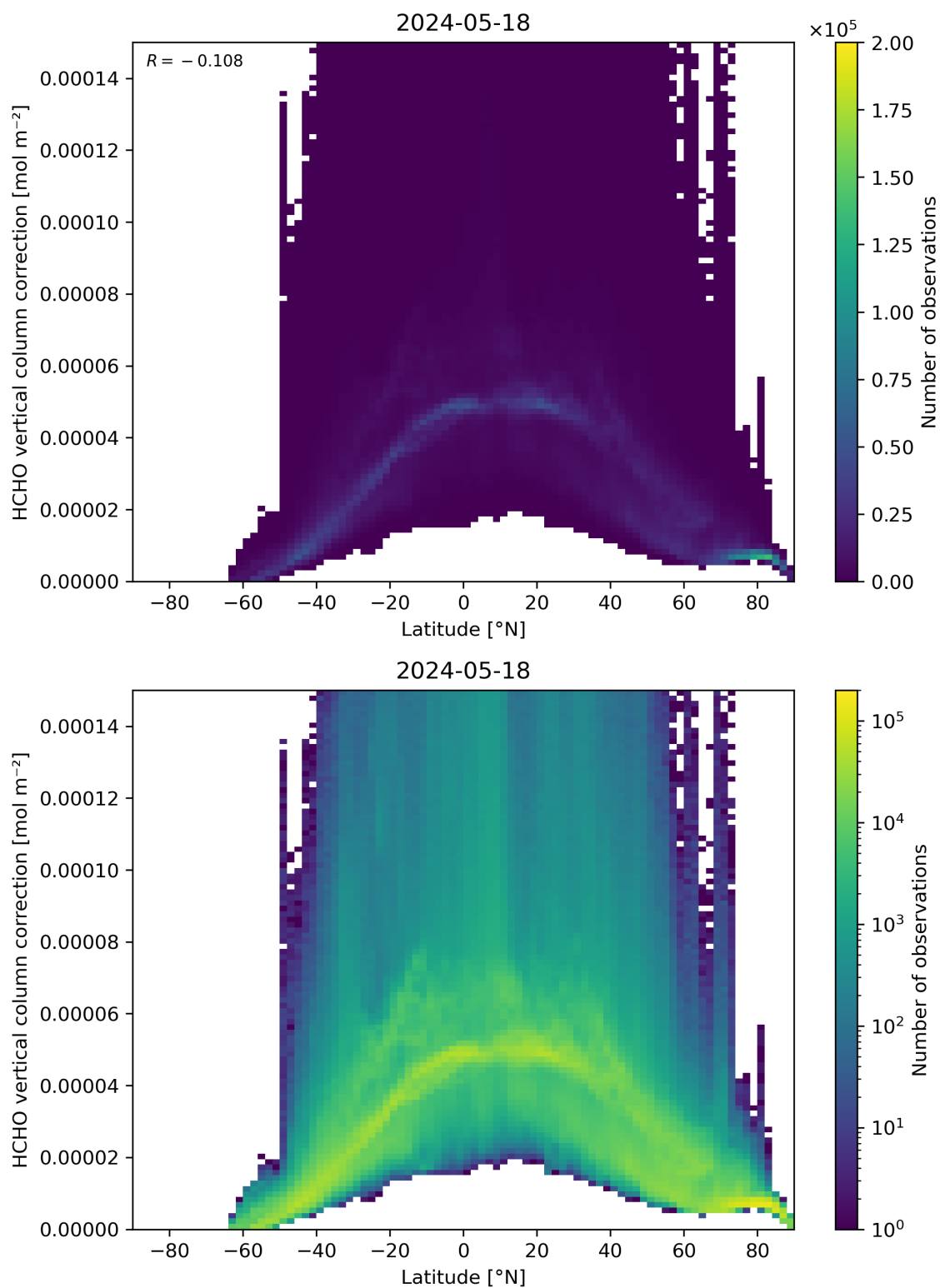
Figure 164: Scatter density plot of “Latitude” against “HCHO vertical column correction” for 2024-05-18 to 2024-05-19.
