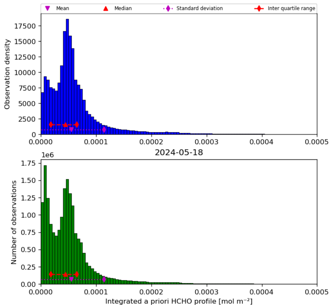
Figure 43: Histogram of “Integrated a priori HCHO profile” for 2024-05-18 to 2024-05-19
