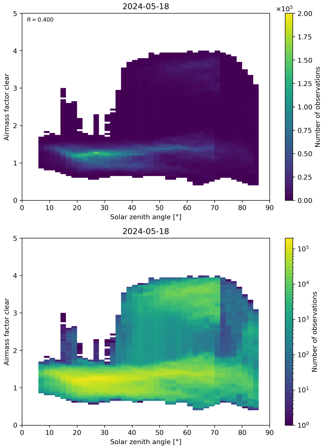
Figure 170: Scatter density plot of “Solar zenith angle” against “Airmass factor clear” for 2024-05-18 to 2024-05-19.
