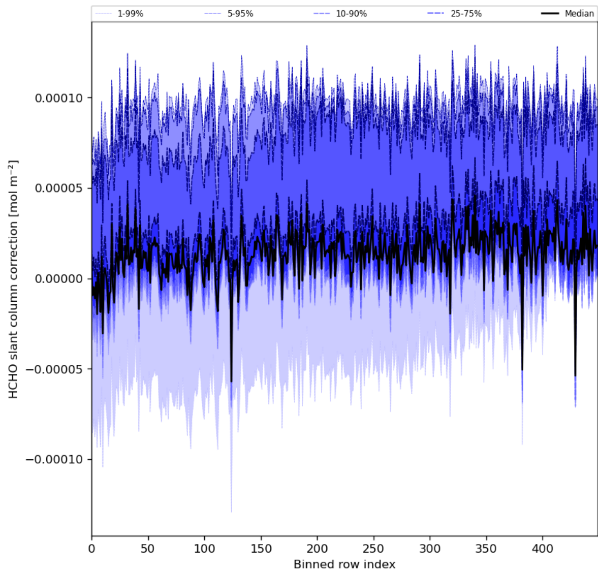
Figure 61: Along track statistics of “HCHO slant column correction” for 2024-05-18 to 2024-05-19
