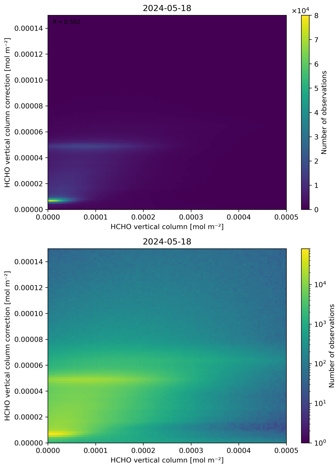
Figure 133: Scatter density plot of “HCHO vertical column” against “HCHO vertical column correction” for 2024-05-18 to 2024-05-19.
