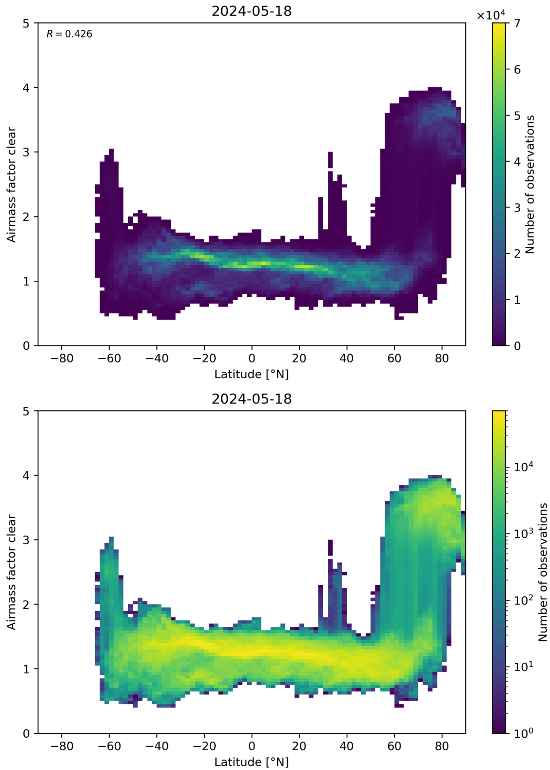
Figure 156: Scatter density plot of “Latitude” against “Airmass factor clear” for 2024-05-18 to 2024-05-19.
