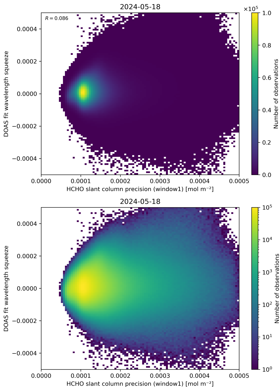
Figure 90: Scatter density plot of “HCHO slant column precision (window1)” against “DOAS fit wavelength squeeze” for 2024-05-18 to 2024-05-19.
