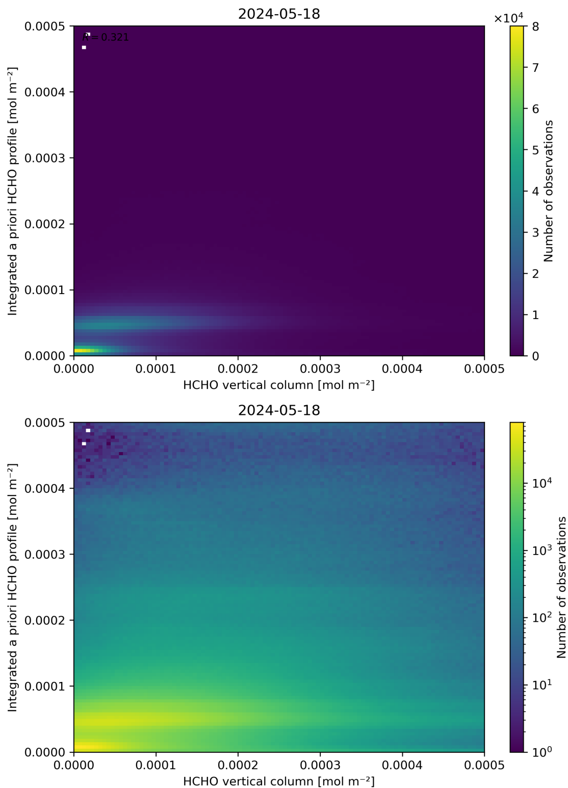
Figure 135: Scatter density plot of “HCHO vertical column” against “Integrated a priori HCHO profile” for 2024-05-18 to 2024-05-19.
