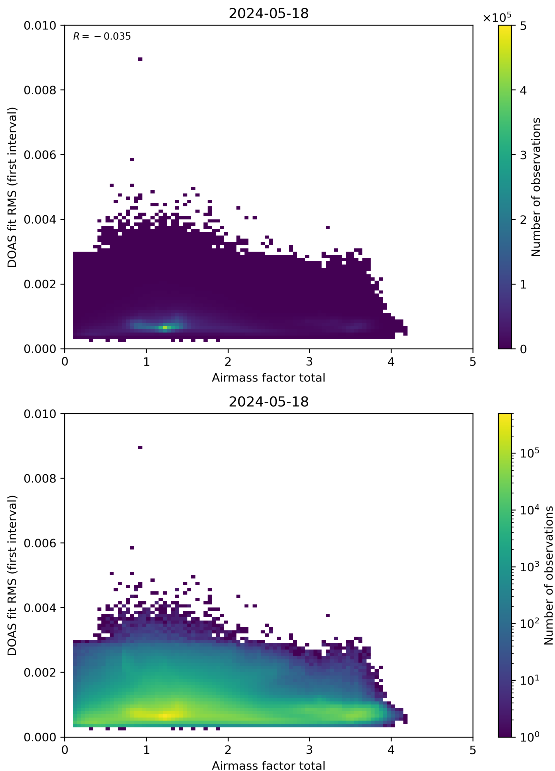
Figure 97: Scatter density plot of “Airmass factor total” against “DOAS fit RMS (first interval)” for 2024-05-18 to 2024-05-19.
