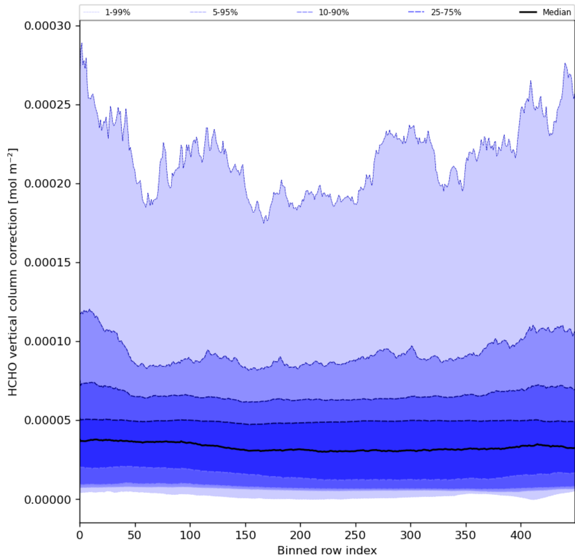
Figure 51: Along track statistics of “HCHO vertical column correction” for 2024-05-18 to 2024-05-19
