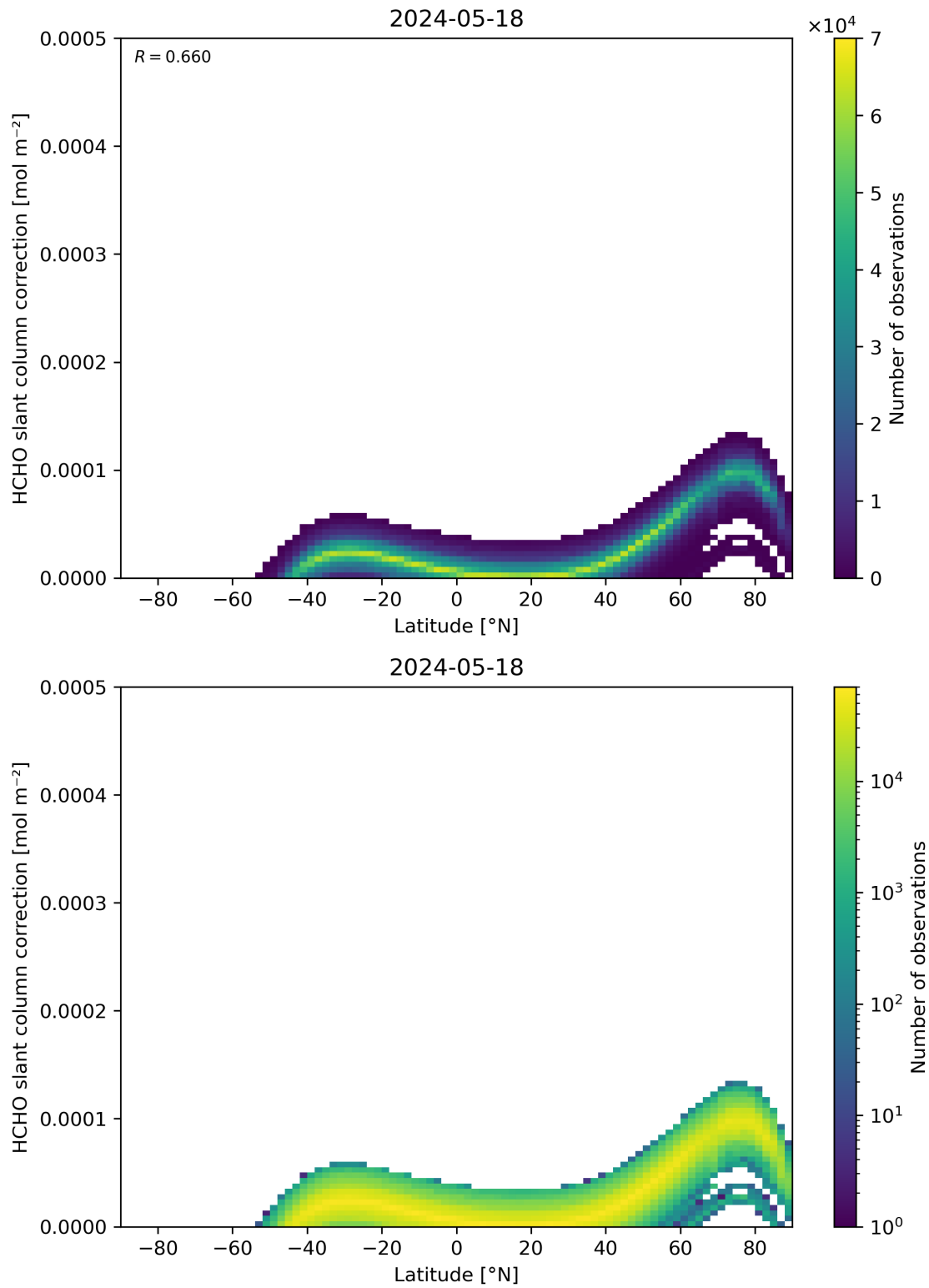
Figure 158: Scatter density plot of “Latitude” against “HCHO slant column correction” for 2024-05-18 to 2024-05-19.
