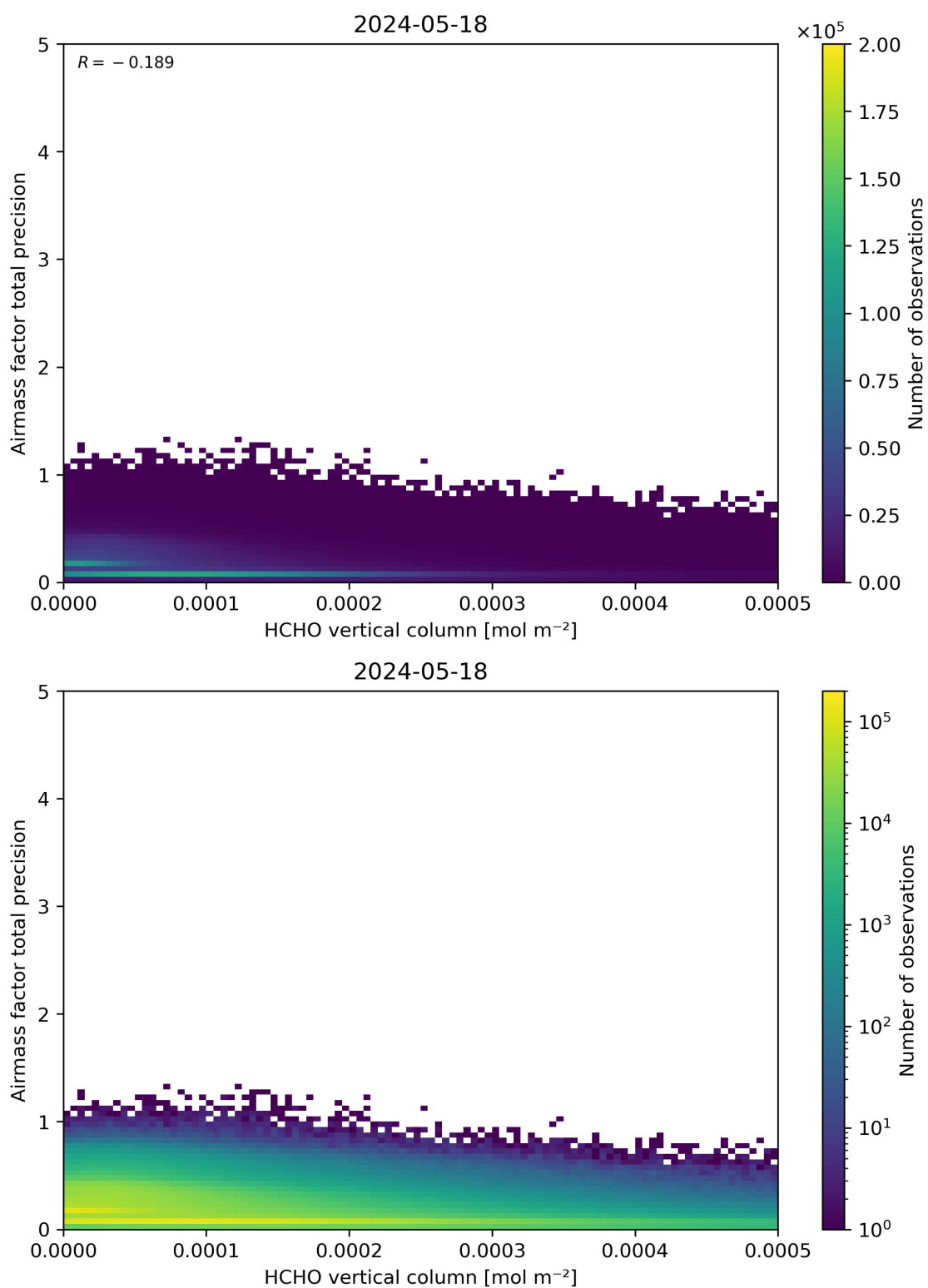
Figure 132: Scatter density plot of “HCHO vertical column” against “Airmass factor total precision” for 2024-05-18 to 2024-05-19.
