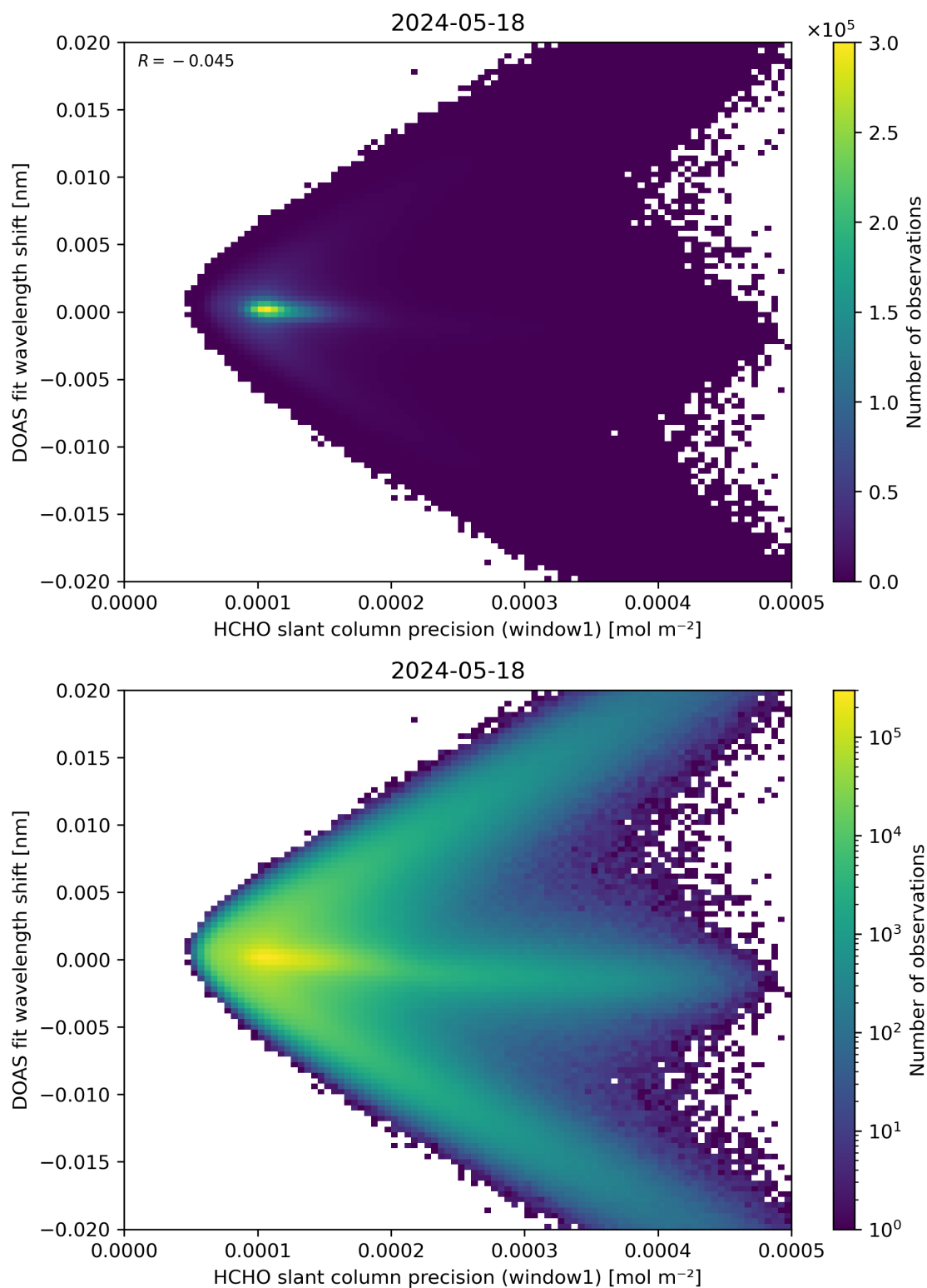
Figure 89: Scatter density plot of “HCHO slant column precision (window1)” against “DOAS fit wavelength shift” for 2024-05-18 to 2024-05-19.
