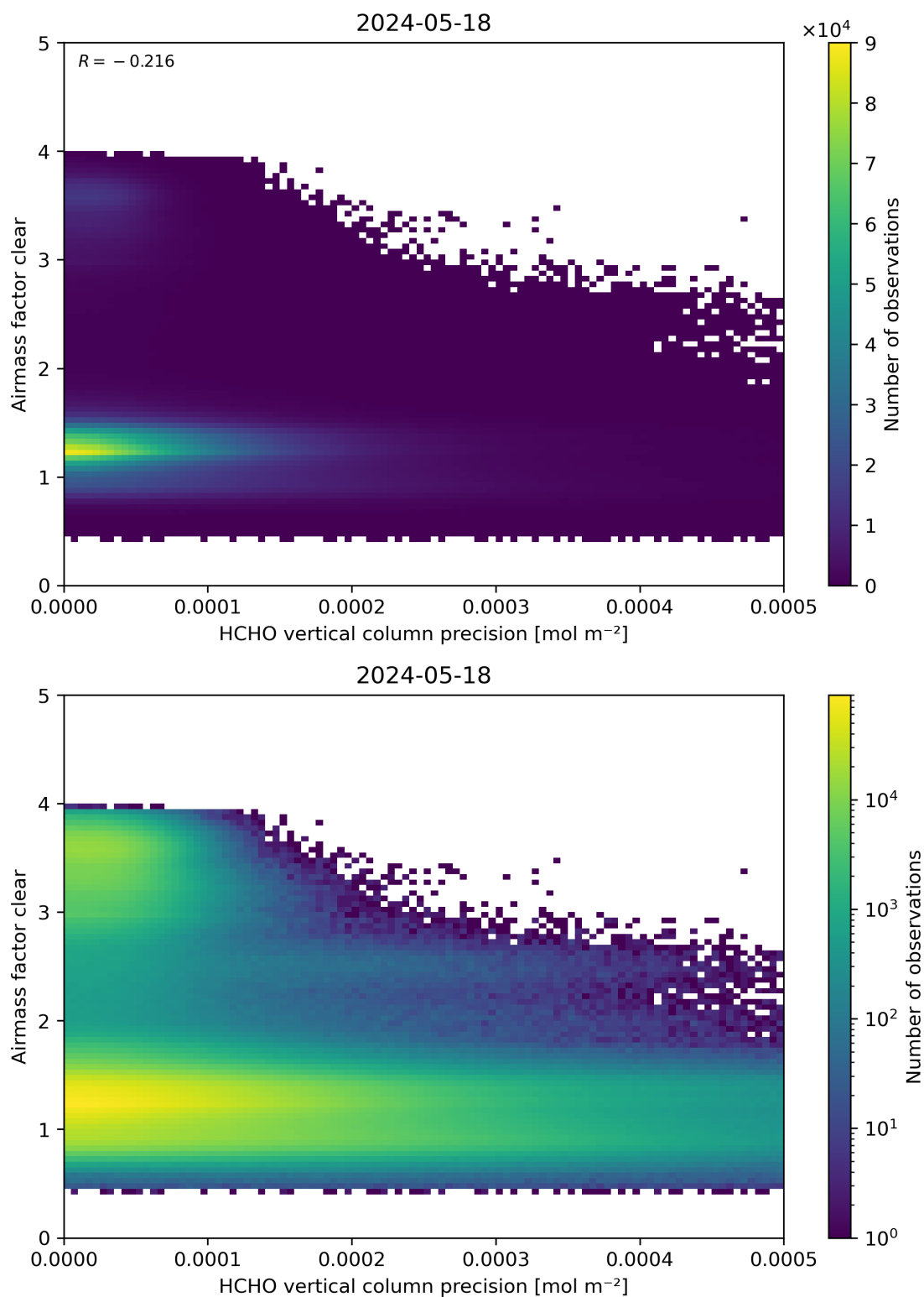
Figure 139: Scatter density plot of “HCHO vertical column precision” against “Airmass factor clear” for 2024-05-18 to 2024-05-19.
