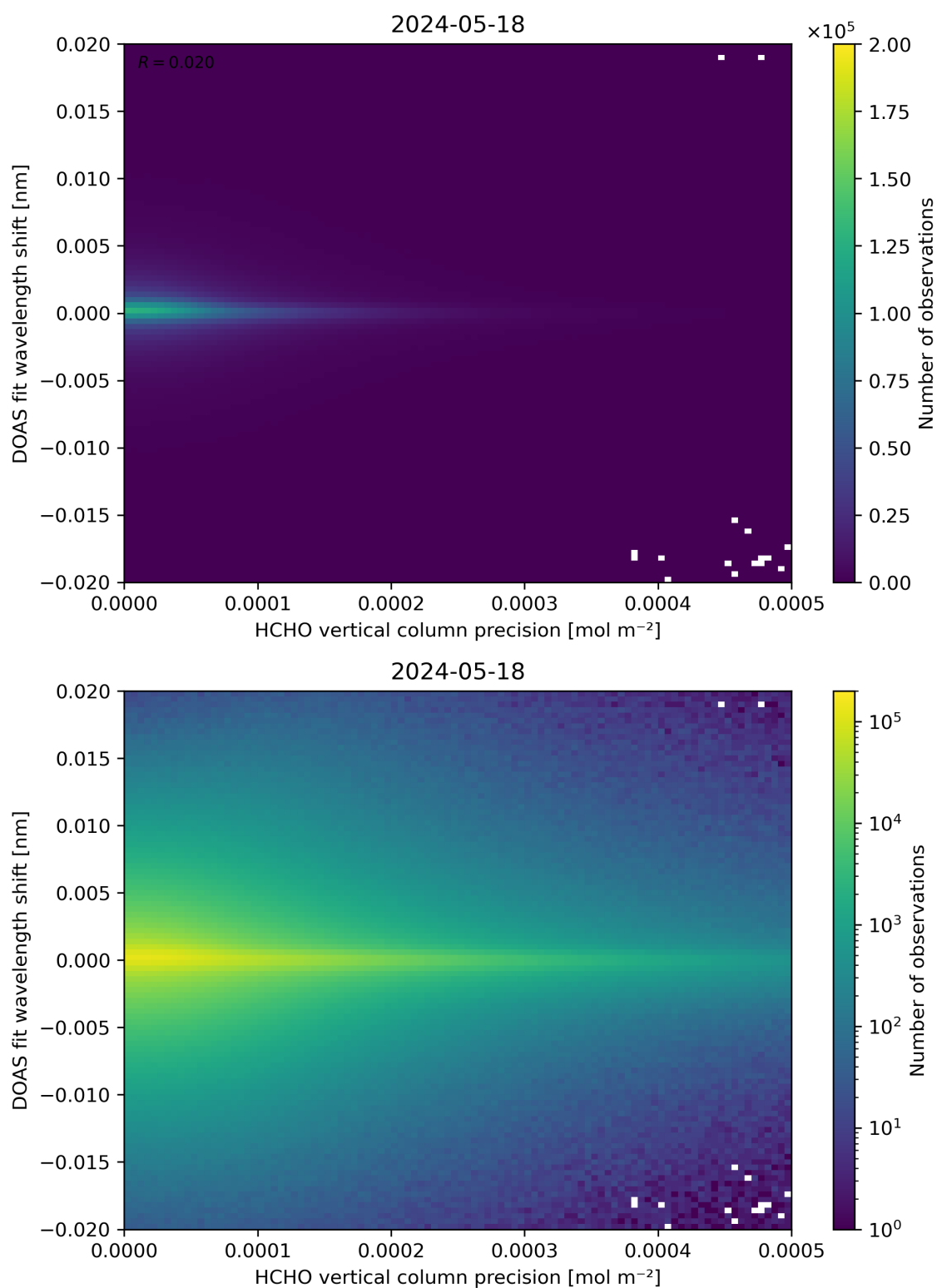
Figure 137: Scatter density plot of “HCHO vertical column precision” against “DOAS fit wavelength shift” for 2024-05-18 to 2024-05-19.
