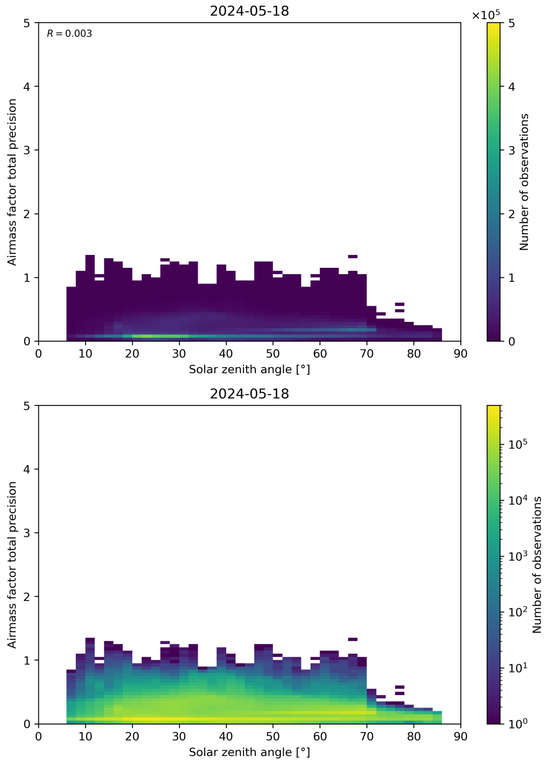
Figure 176: Scatter density plot of “Solar zenith angle” against “Airmass factor total precision” for 2024-05-18 to 2024-05-19.
