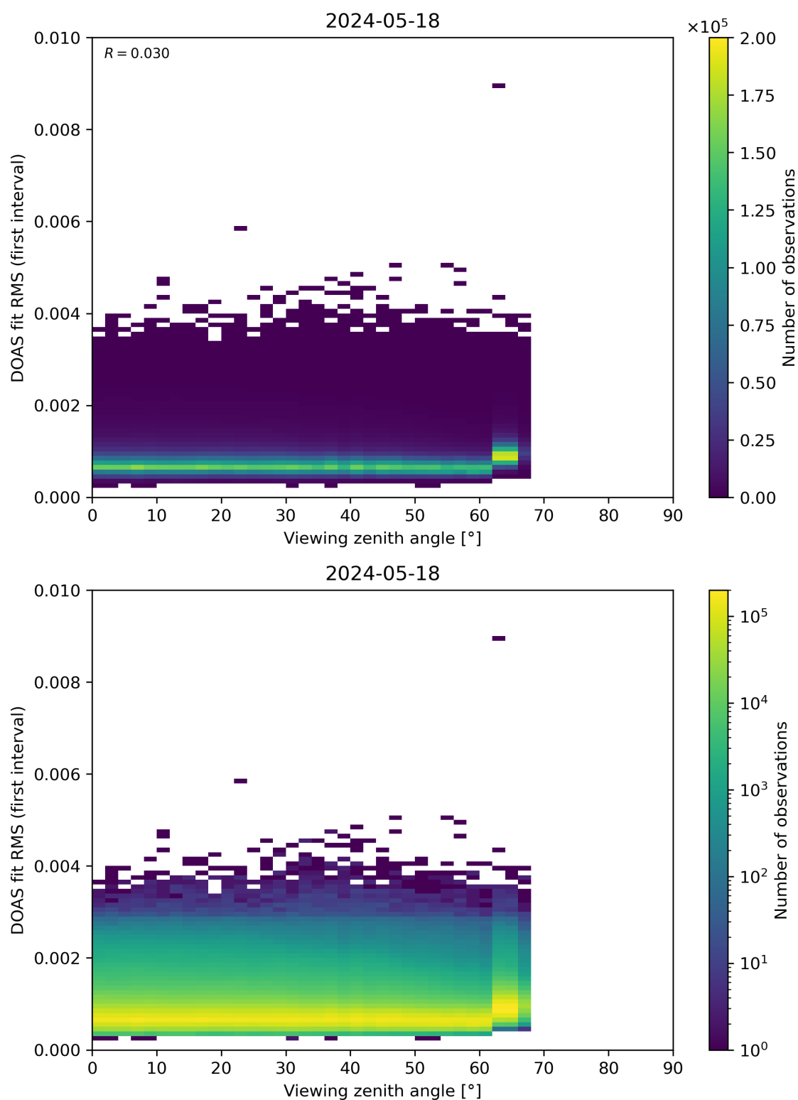
Figure 182: Scatter density plot of “Viewing zenith angle” against “DOAS fit RMS (first interval)” for 2024-05-18 to 2024-05-19.
