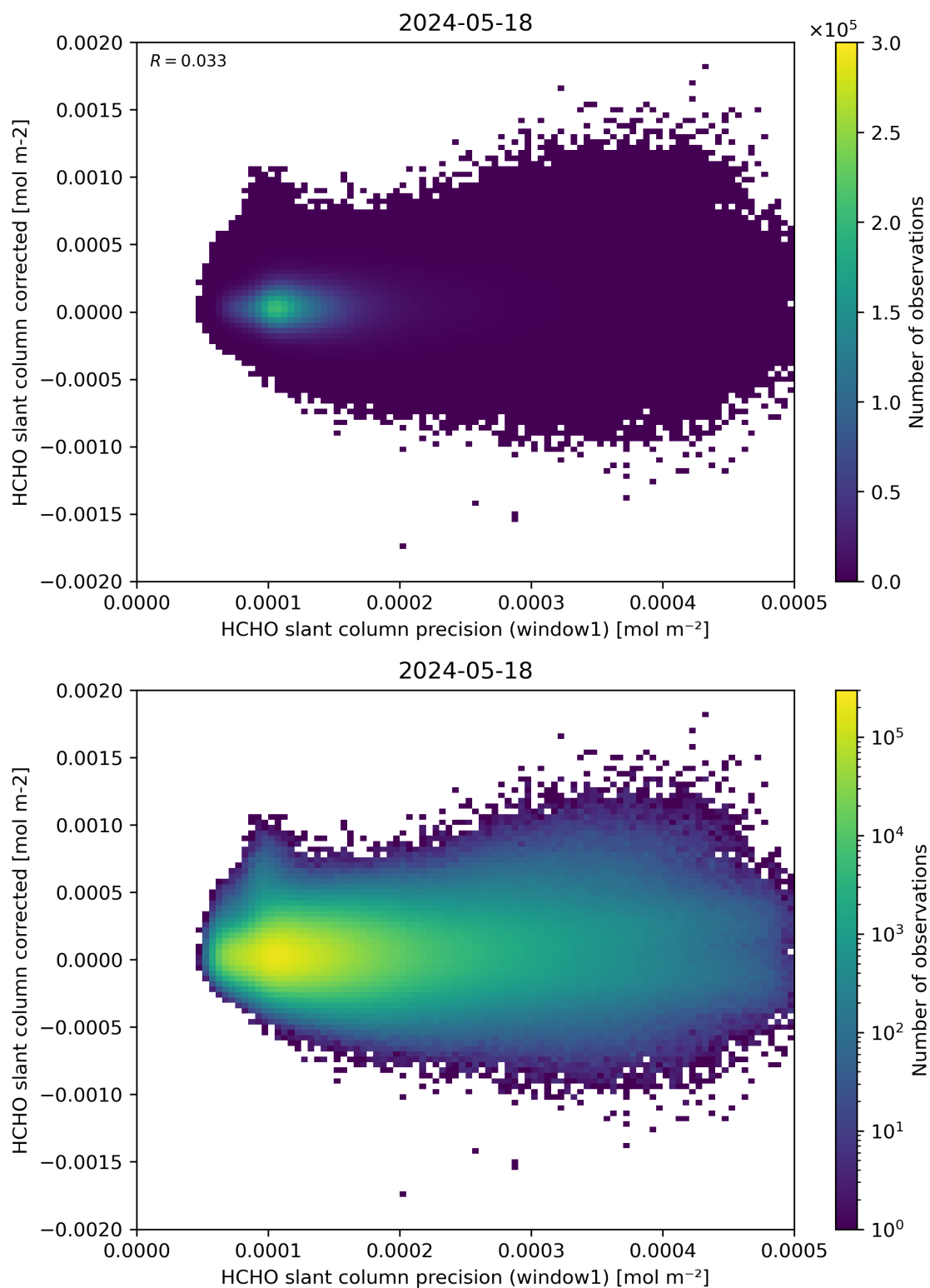
Figure 92: Scatter density plot of “HCHO slant column precision (window1)” against “HCHO slant column corrected” for 2024-05-18 to 2024-05-19.
