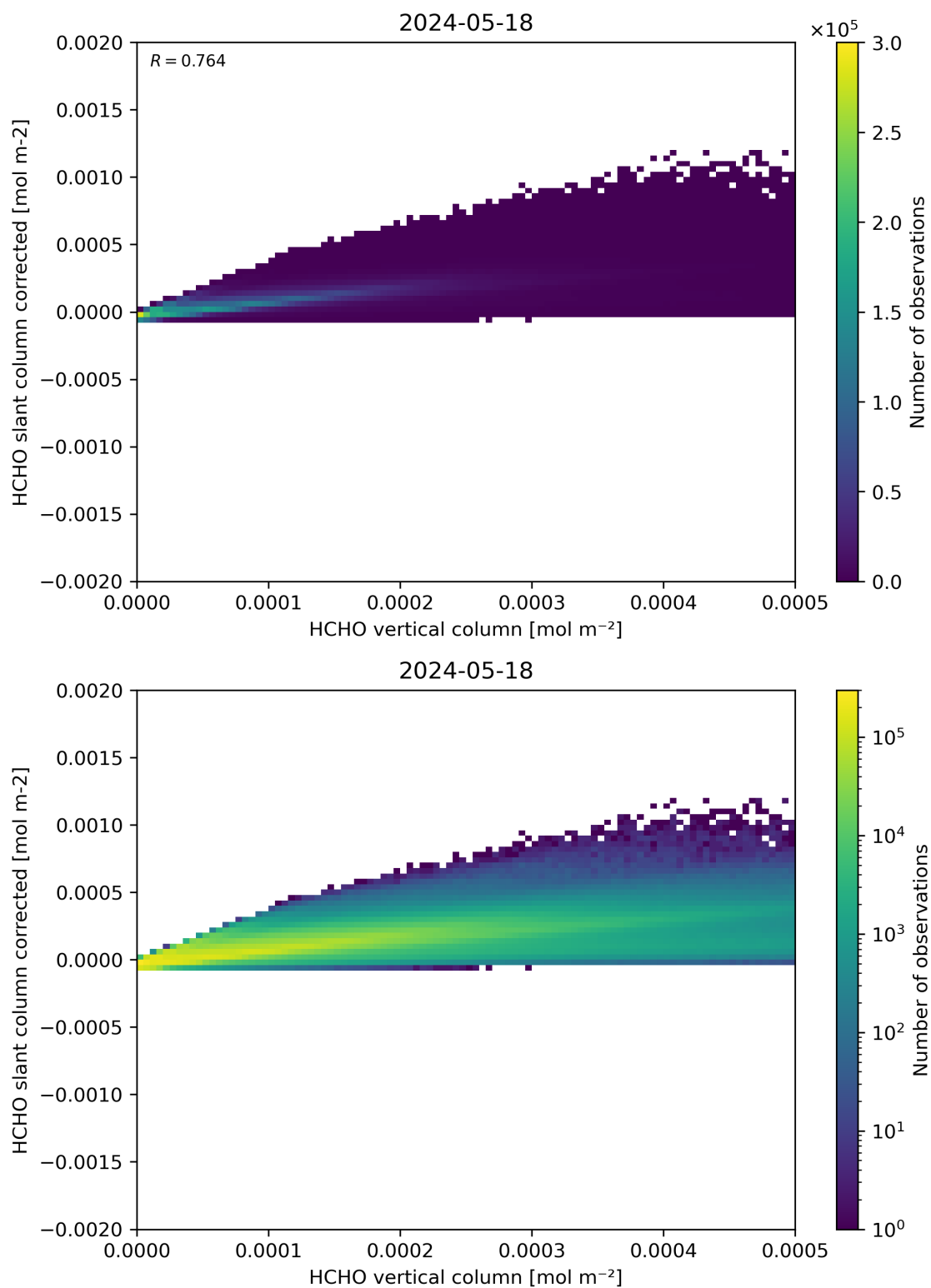
Figure 127: Scatter density plot of “HCHO vertical column” against “HCHO slant column corrected” for 2024-05-18 to 2024-05-19.
