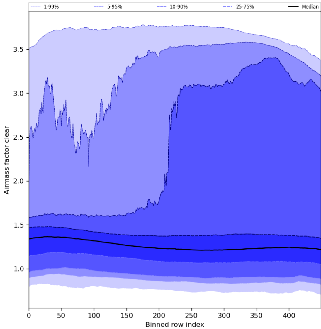
Figure 56: Along track statistics of “Airmass factor clear” for 2024-05-18 to 2024-05-19
