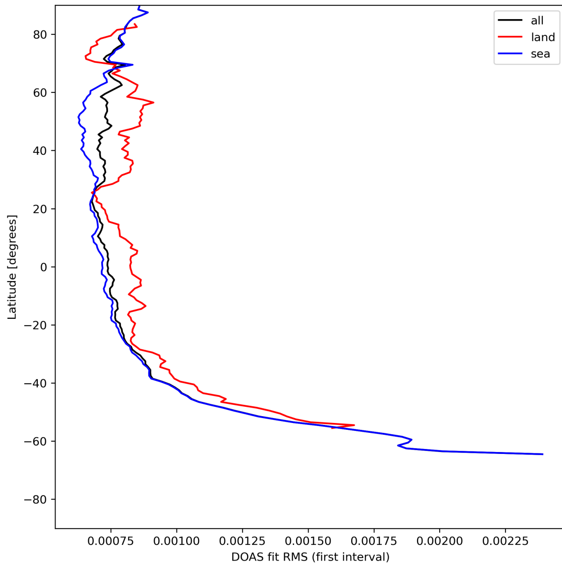
Figure 32: Zonal average of “DOAS fit RMS (first interval)” for 2024-05-18 to 2024-05-19.
