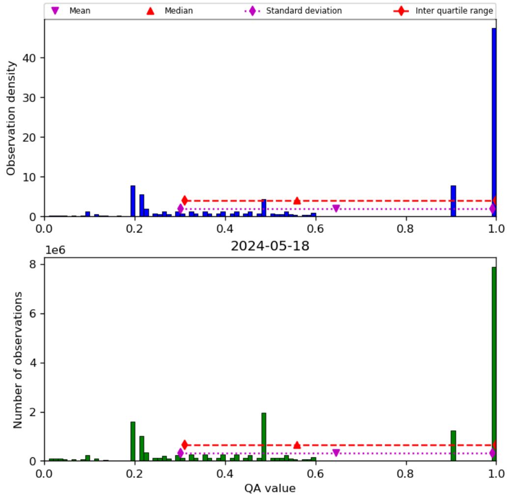
Figure 34: Histogram of “QA value” for 2024-05-18 to 2024-05-19
