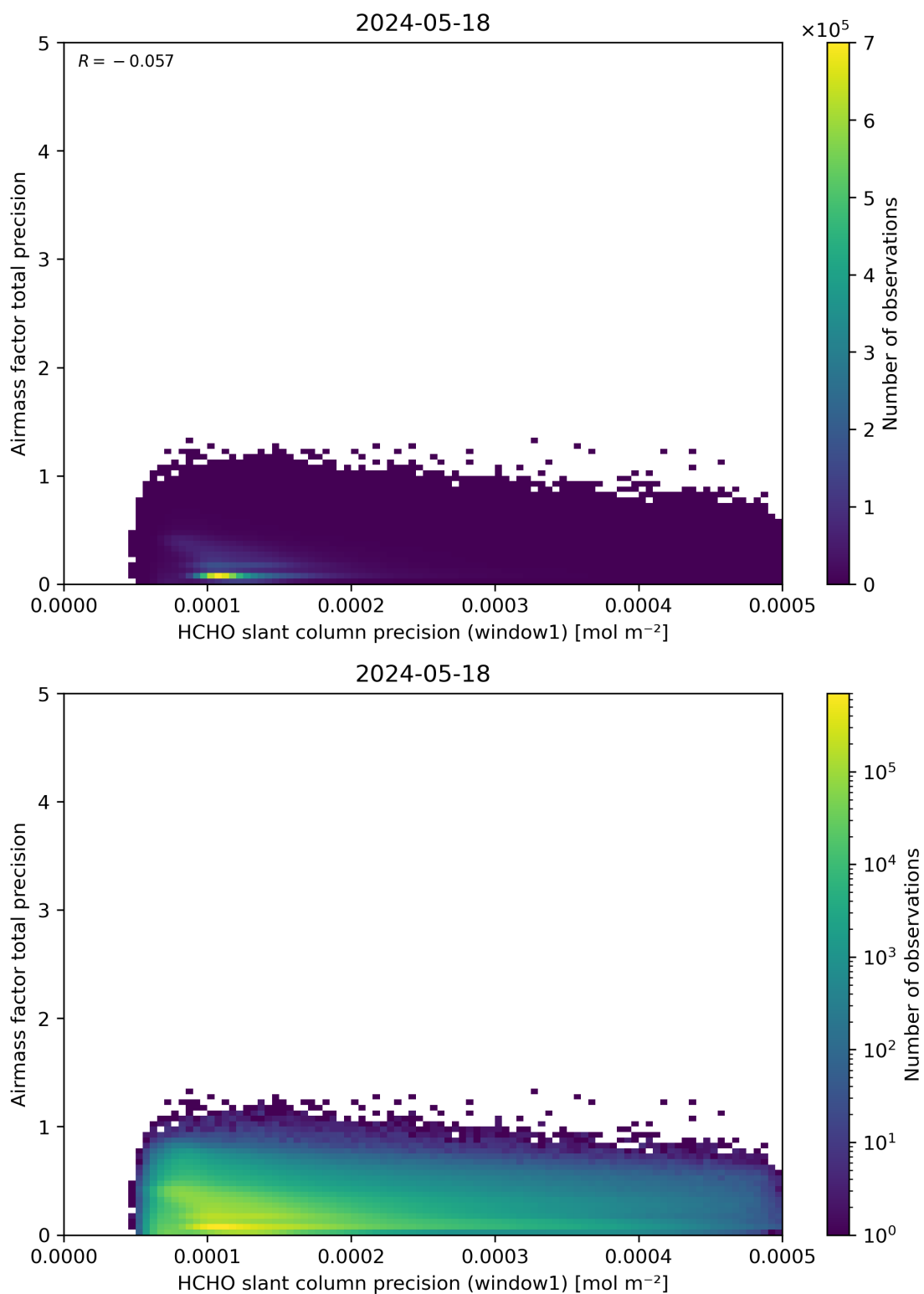
Figure 95: Scatter density plot of “HCHO slant column precision (window1)” against “Airmass factor total precision” for 2024-05-18 to 2024-05-19.
