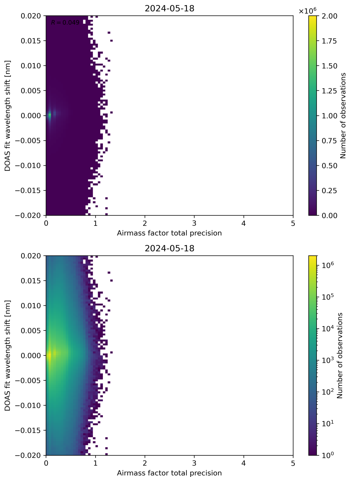
Figure 106: Scatter density plot of “Airmass factor total precision” against “DOAS fit wavelength shift” for 2024-05-18 to 2024-05-19.
