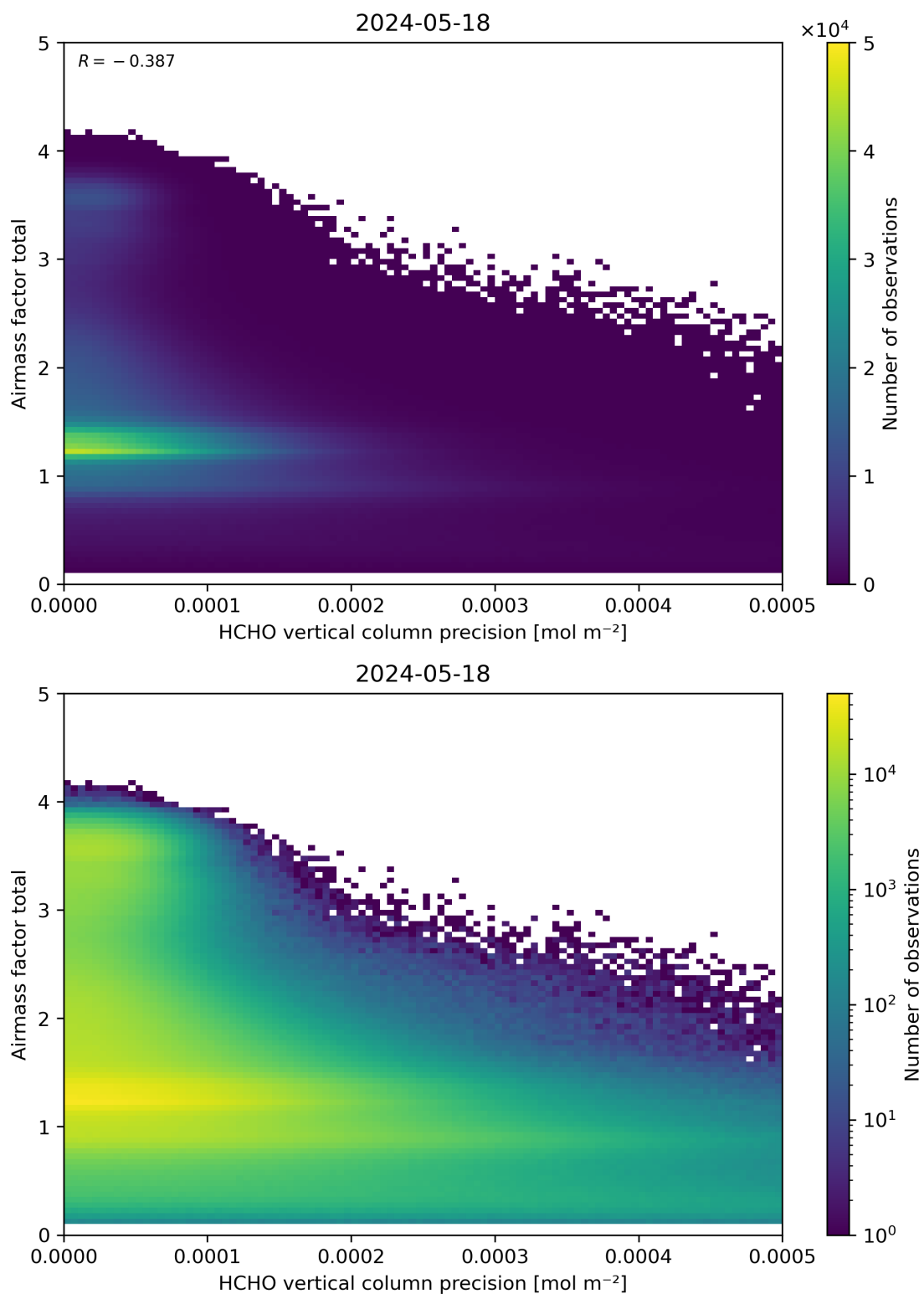
Figure 144: Scatter density plot of “HCHO vertical column precision” against “Airmass factor total” for 2024-05-18 to 2024-05-19.
