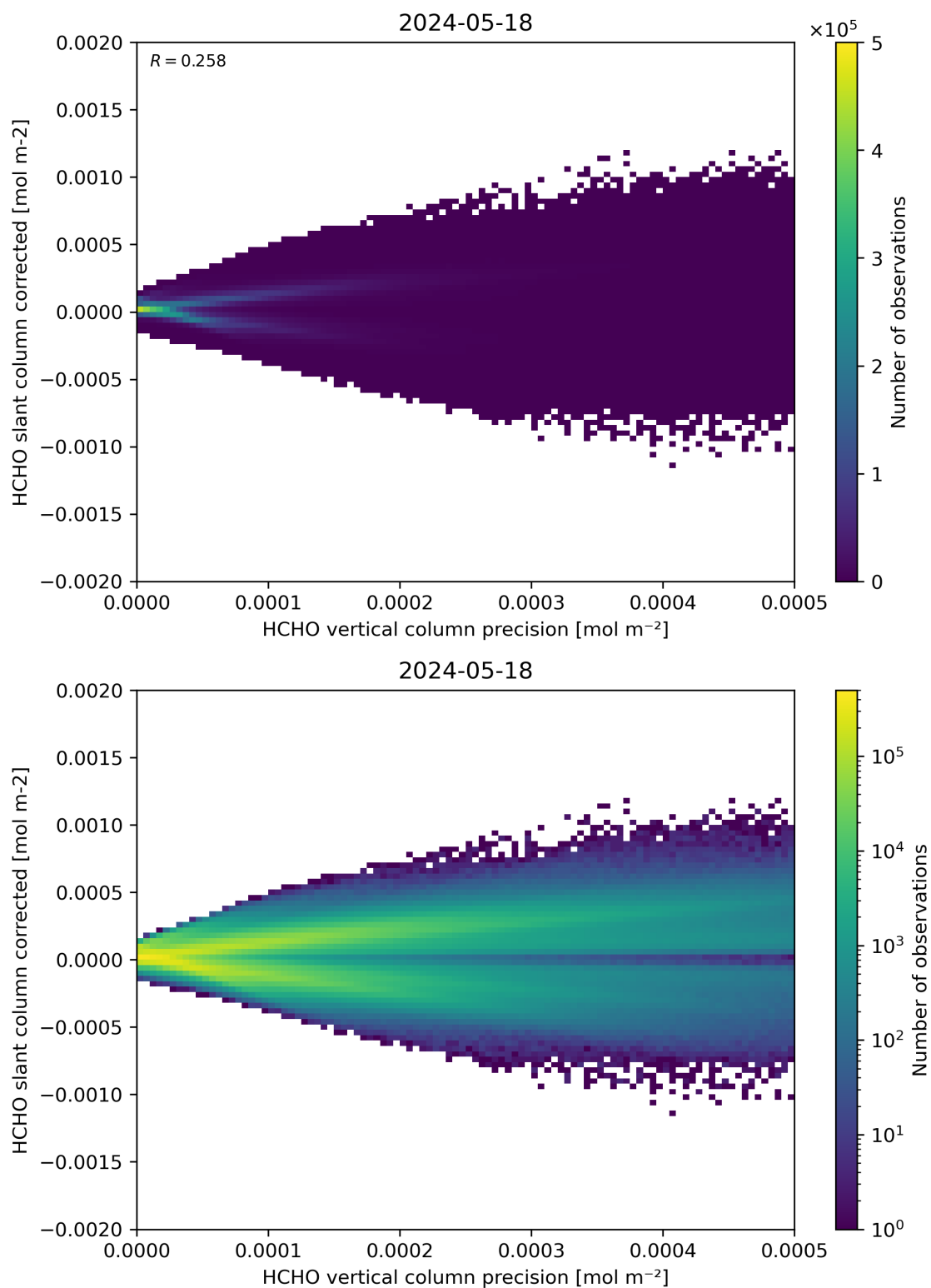
Figure 140: Scatter density plot of “HCHO vertical column precision” against “HCHO slant column corrected” for 2024-05-18 to 2024-05-19.
