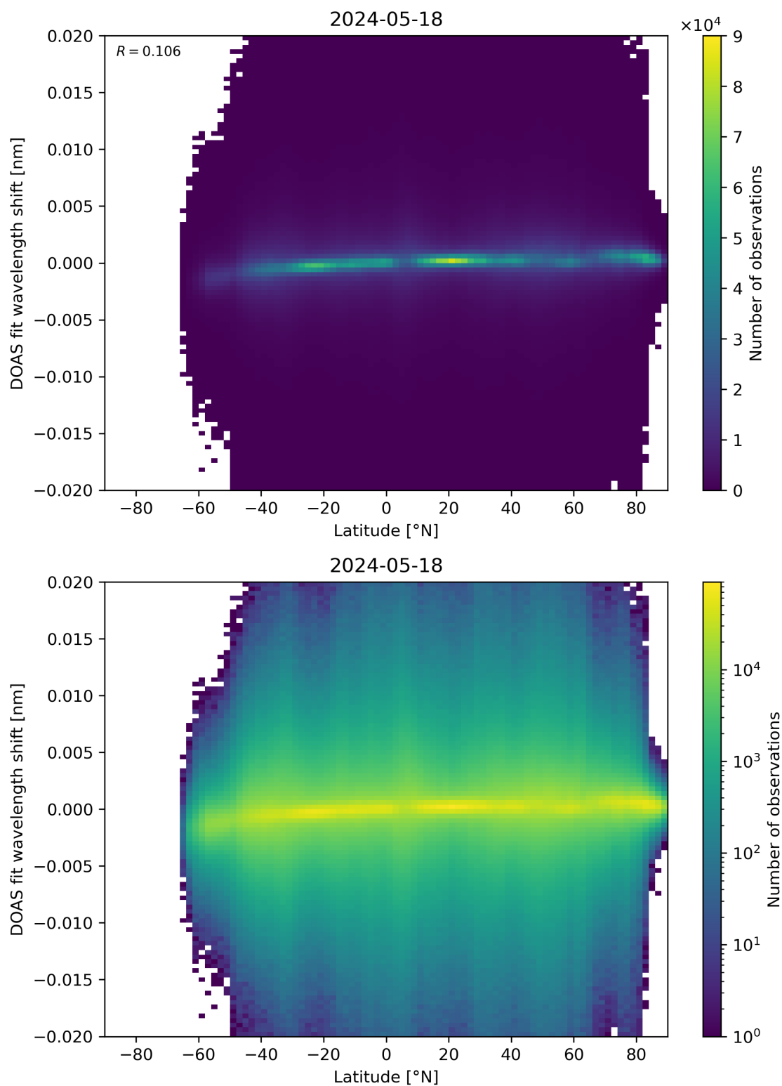
Figure 154: Scatter density plot of “Latitude” against “DOAS fit wavelength shift” for 2024-05-18 to 2024-05-19.
