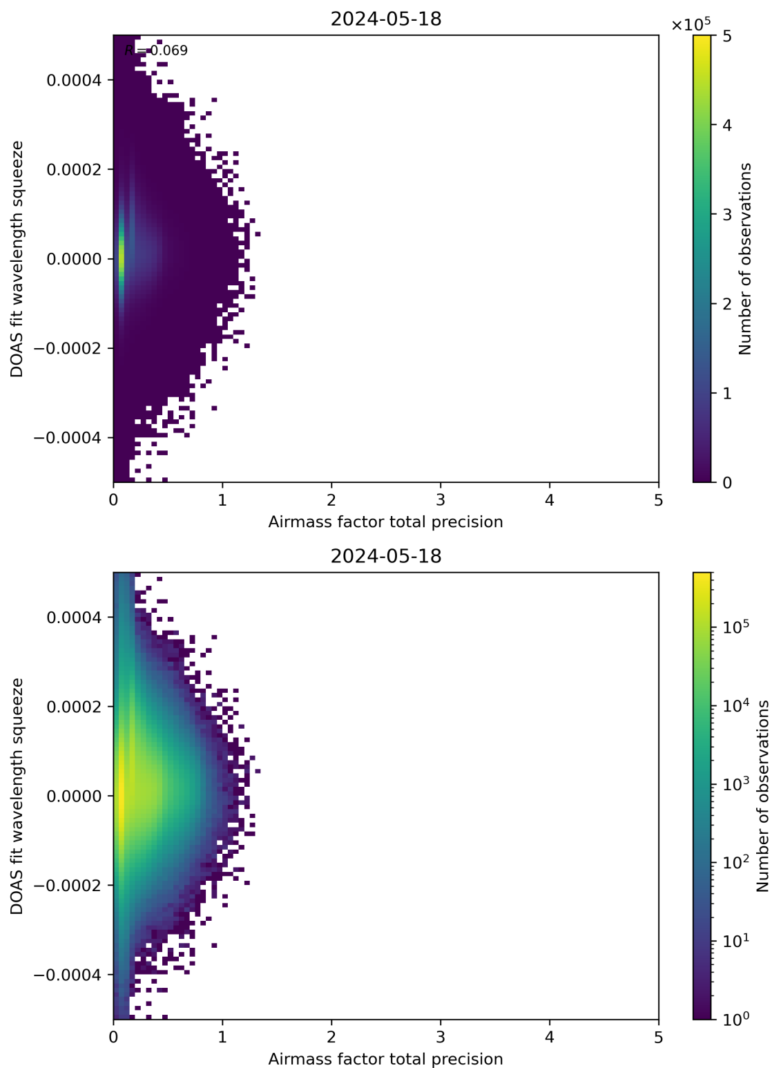
Figure 107: Scatter density plot of “Airmass factor total precision” against “DOAS fit wavelength squeeze” for 2024-05-18 to 2024-05-19.
