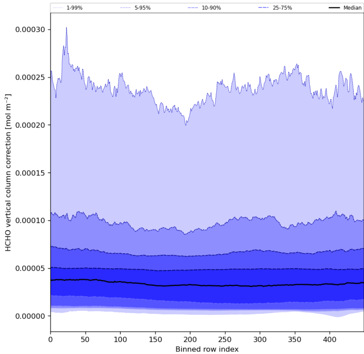
Figure 51: Along track statistics of “HCHO vertical column correction” for 2024-05-18 to 2024-05-20
