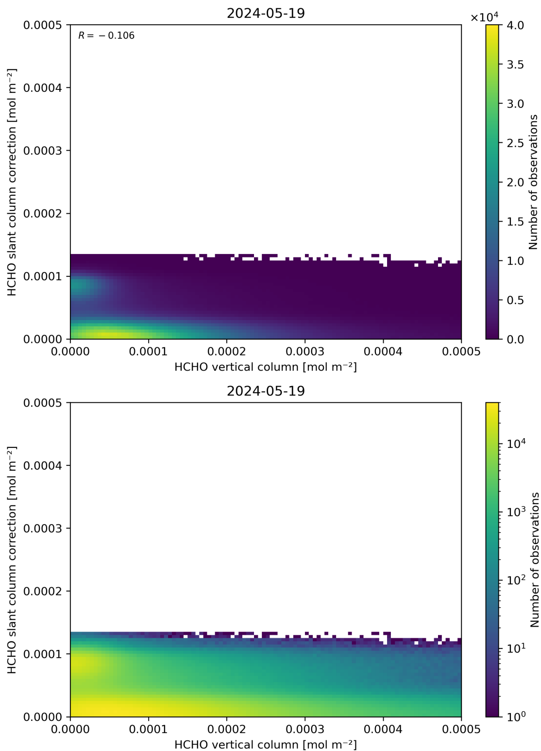
Figure 128: Scatter density plot of “HCHO vertical column” against “HCHO slant column correction” for 2024-05-18 to 2024-05-20.
