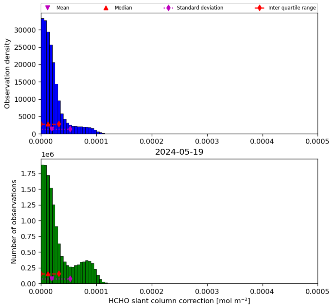
Figure 47: Histogram of “HCHO slant column correction” for 2024-05-18 to 2024-05-20
