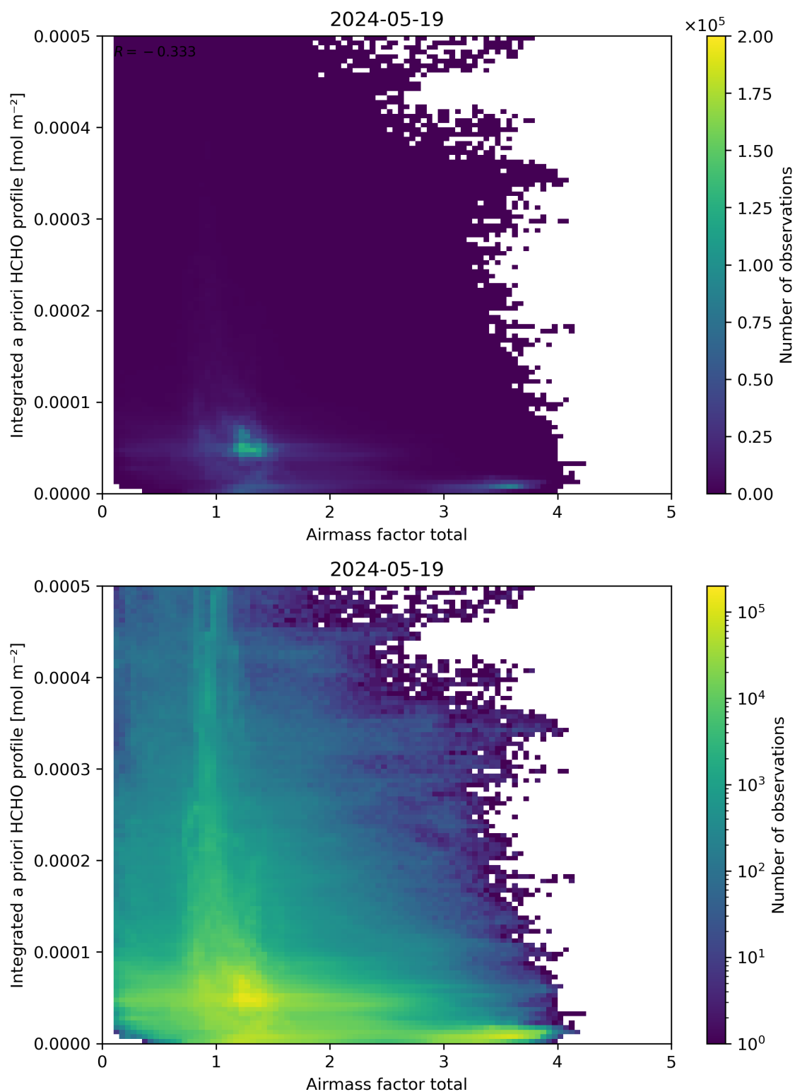
Figure 104: Scatter density plot of “Airmass factor total” against “Integrated a priori HCHO profile” for 2024-05-18 to 2024-05-20.
