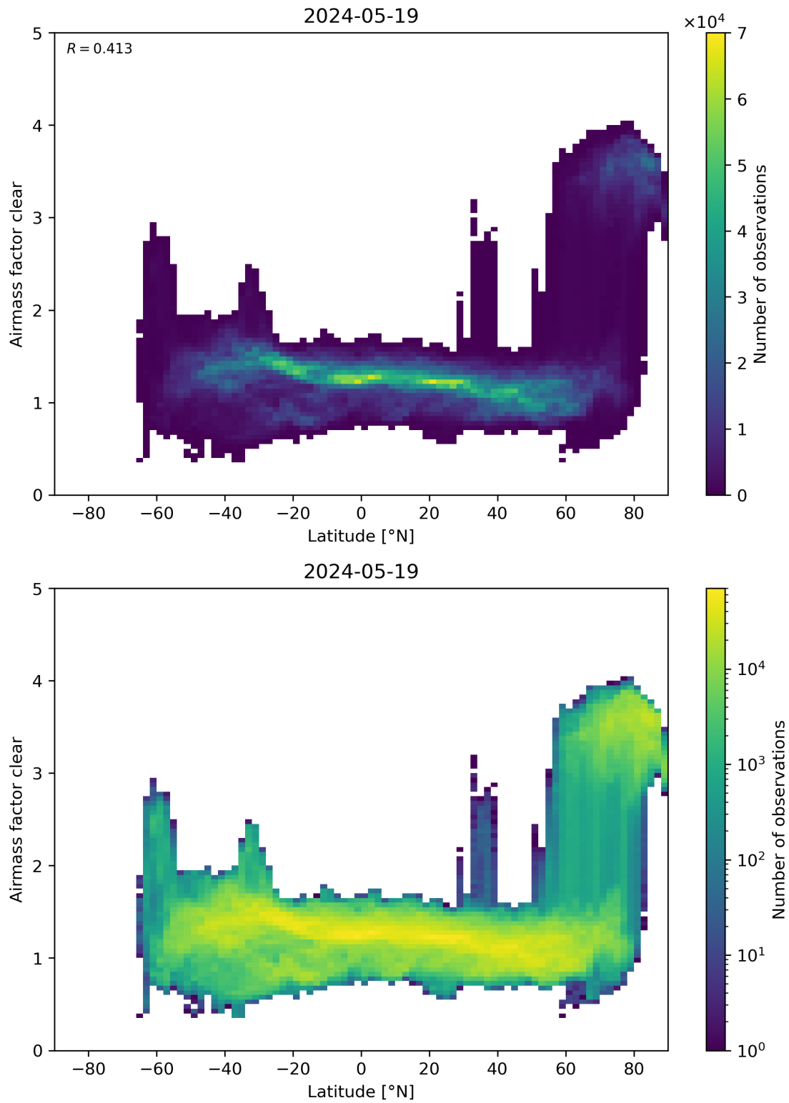
Figure 156: Scatter density plot of “Latitude” against “Airmass factor clear” for 2024-05-18 to 2024-05-20.
