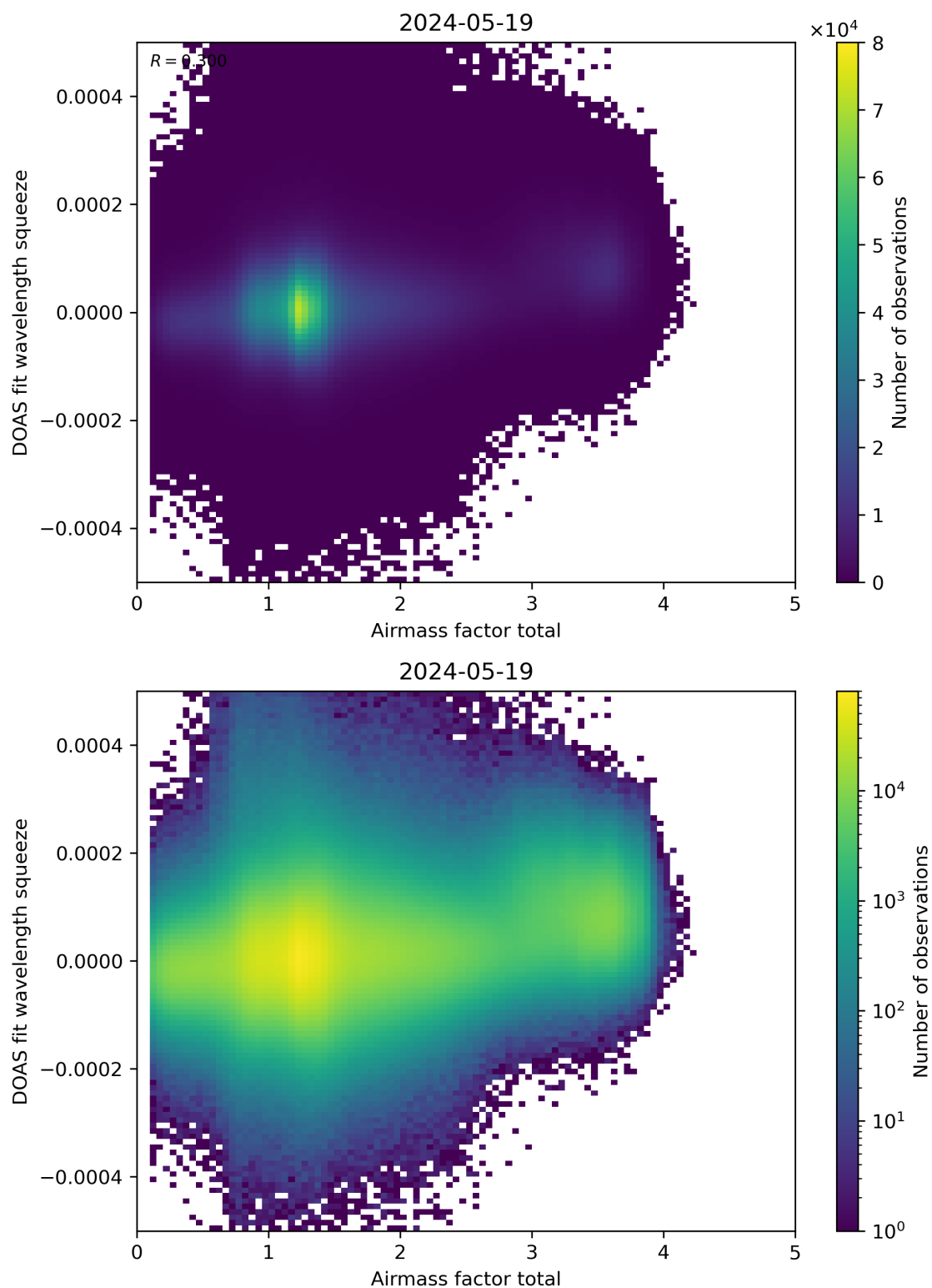
Figure 99: Scatter density plot of “Airmass factor total” against “DOAS fit wavelength squeeze” for 2024-05-18 to 2024-05-20.
