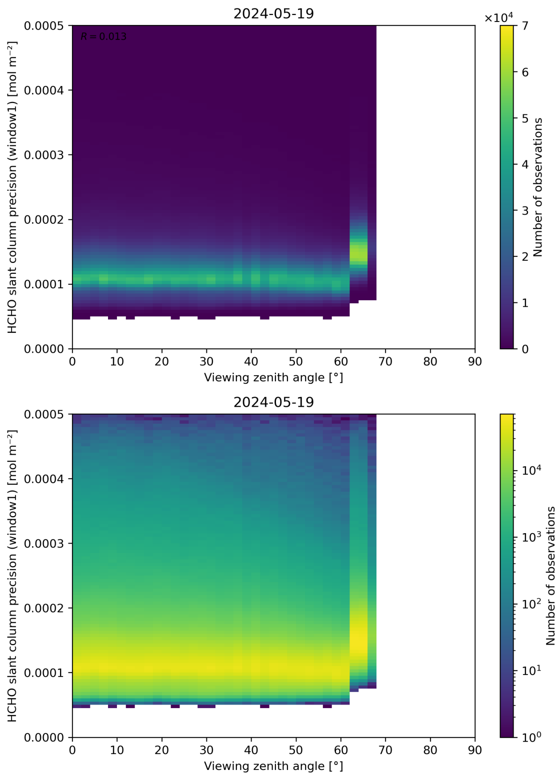
Figure 189: Scatter density plot of “Viewing zenith angle” against “HCHO slant column precision (window1)” for 2024-05-18 to 2024-05-20.
