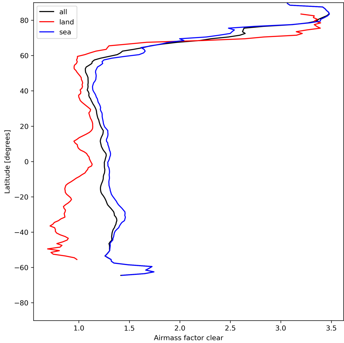
Figure 28: Zonal average of “Airmass factor clear” for 2024-05-18 to 2024-05-20.
