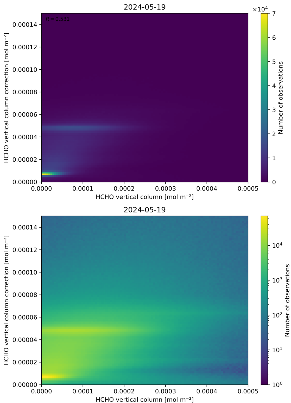
Figure 133: Scatter density plot of “HCHO vertical column” against “HCHO vertical column correction” for 2024-05-18 to 2024-05-20.
