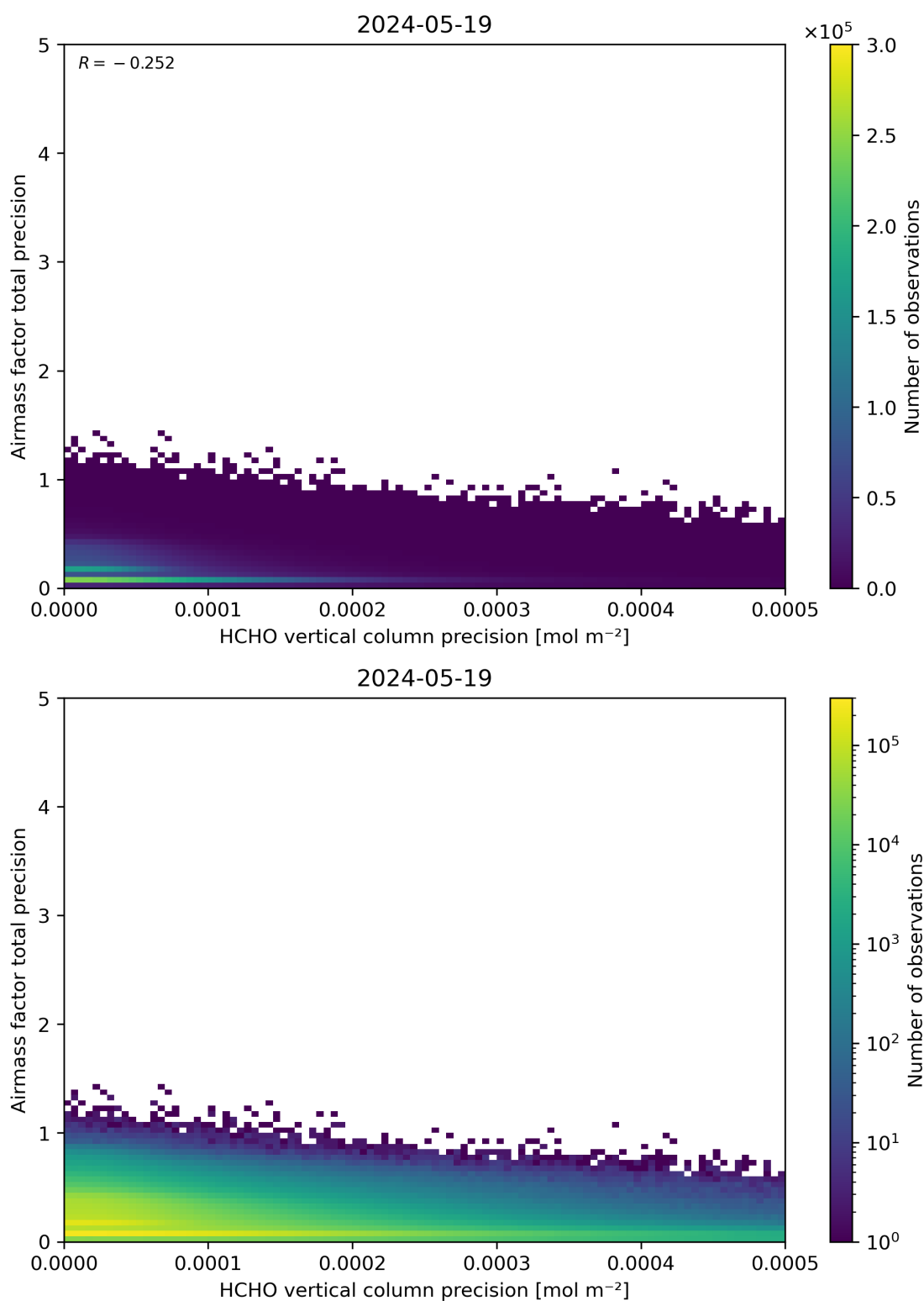
Figure 145: Scatter density plot of “HCHO vertical column precision” against “Airmass factor total precision” for 2024-05-18 to 2024-05-20.
