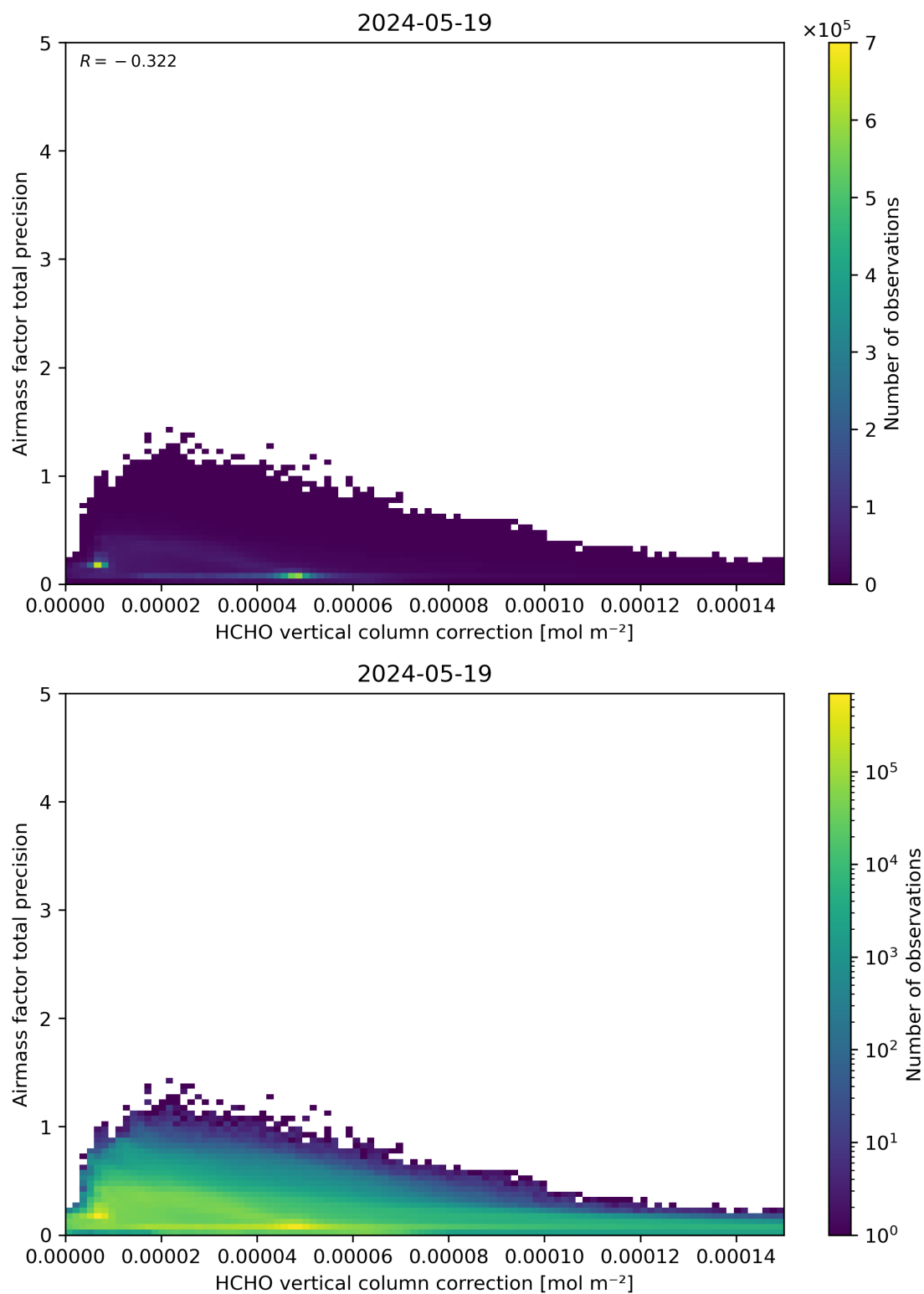
Figure 121: Scatter density plot of “HCHO vertical column correction” against “Airmass factor total precision” for 2024-05-18 to 2024-05-20.
