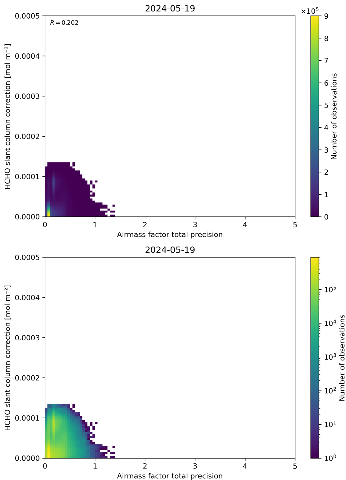
Figure 110: Scatter density plot of “Airmass factor total precision” against “HCHO slant column correction” for 2024-05-18 to 2024-05-20.
