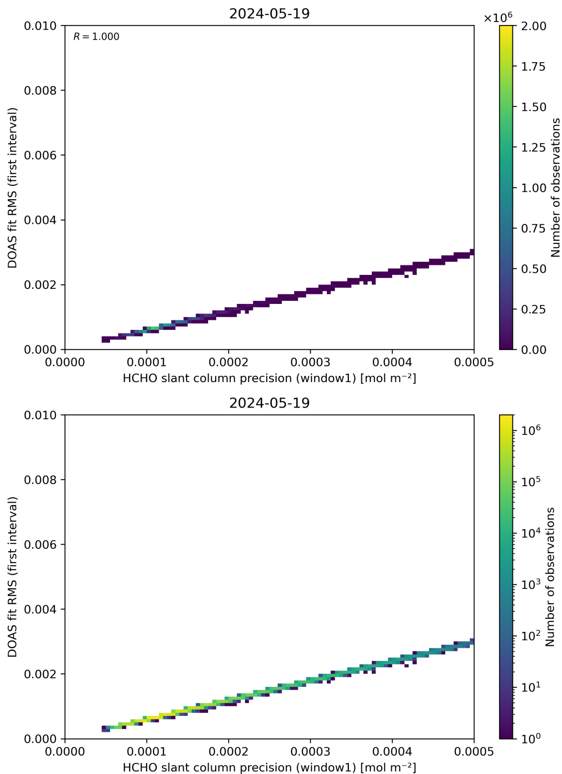
Figure 88: Scatter density plot of “HCHO slant column precision (window1)” against “DOAS fit RMS (first interval)” for 2024-05-18 to 2024-05-20.
