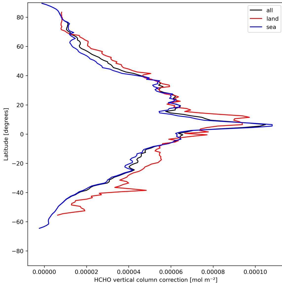
Figure 23: Zonal average of “HCHO vertical column correction” for 2024-05-18 to 2024-05-20.
