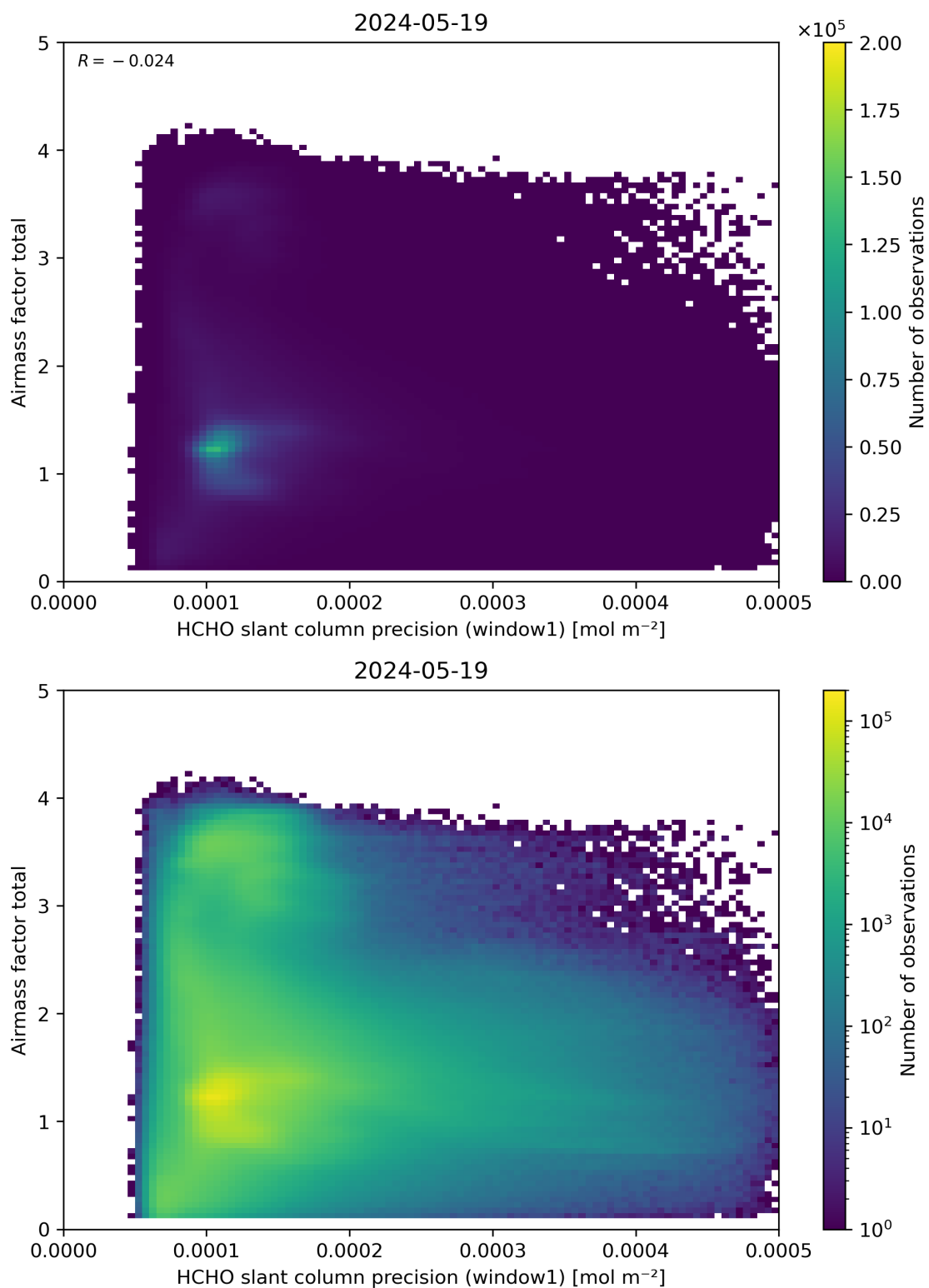
Figure 94: Scatter density plot of “HCHO slant column precision (window1)” against “Airmass factor total” for 2024-05-18 to 2024-05-20.
