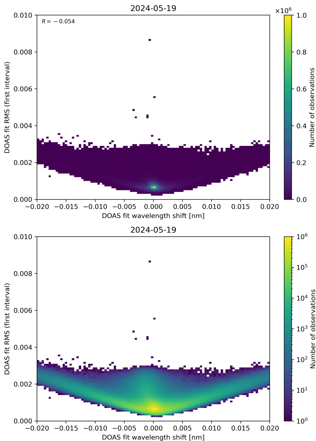
Figure 64: Scatter density plot of “DOAS fit wavelength shift” against “DOAS fit RMS (first interval)” for 2024-05-18 to 2024-05-20.
