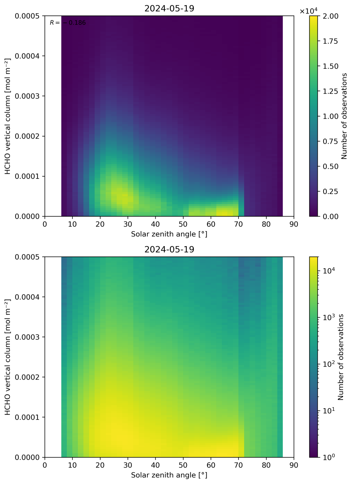
Figure 177: Scatter density plot of “Solar zenith angle” against “HCHO vertical column” for 2024-05-18 to 2024-05-20.
