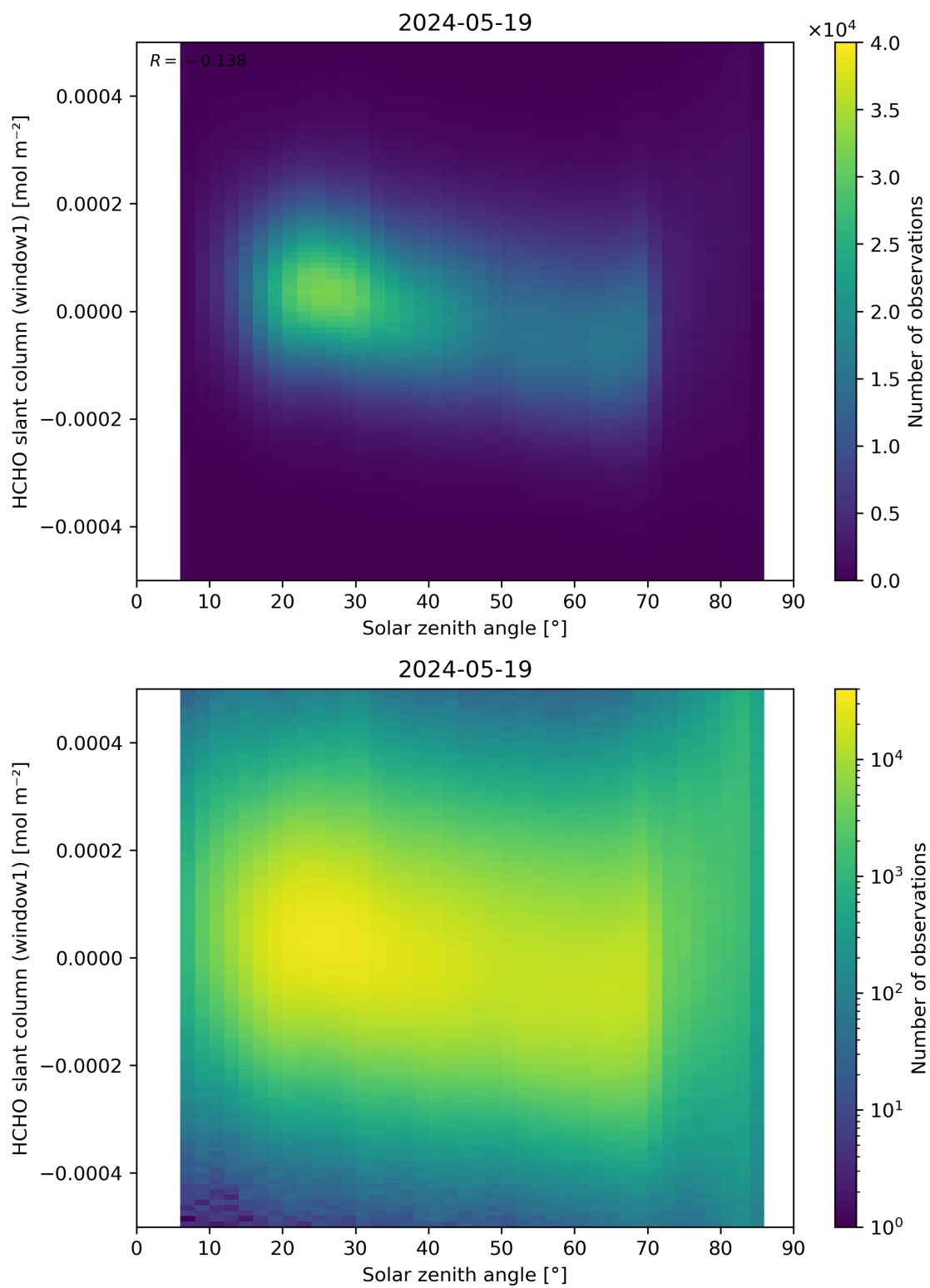
Figure 173: Scatter density plot of “Solar zenith angle” against “HCHO slant column (window1)” for 2024-05-18 to 2024-05-20.
