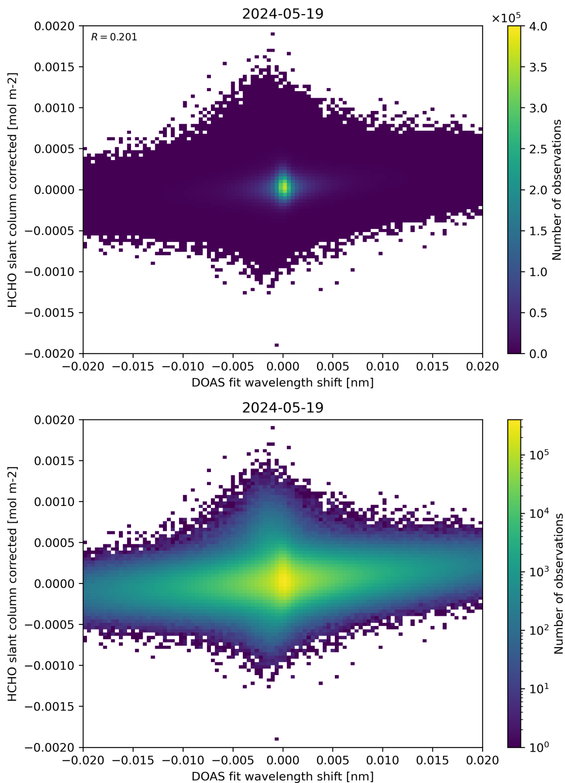
Figure 66: Scatter density plot of “DOAS fit wavelength shift” against “HCHO slant column corrected” for 2024-05-18 to 2024-05-20.
