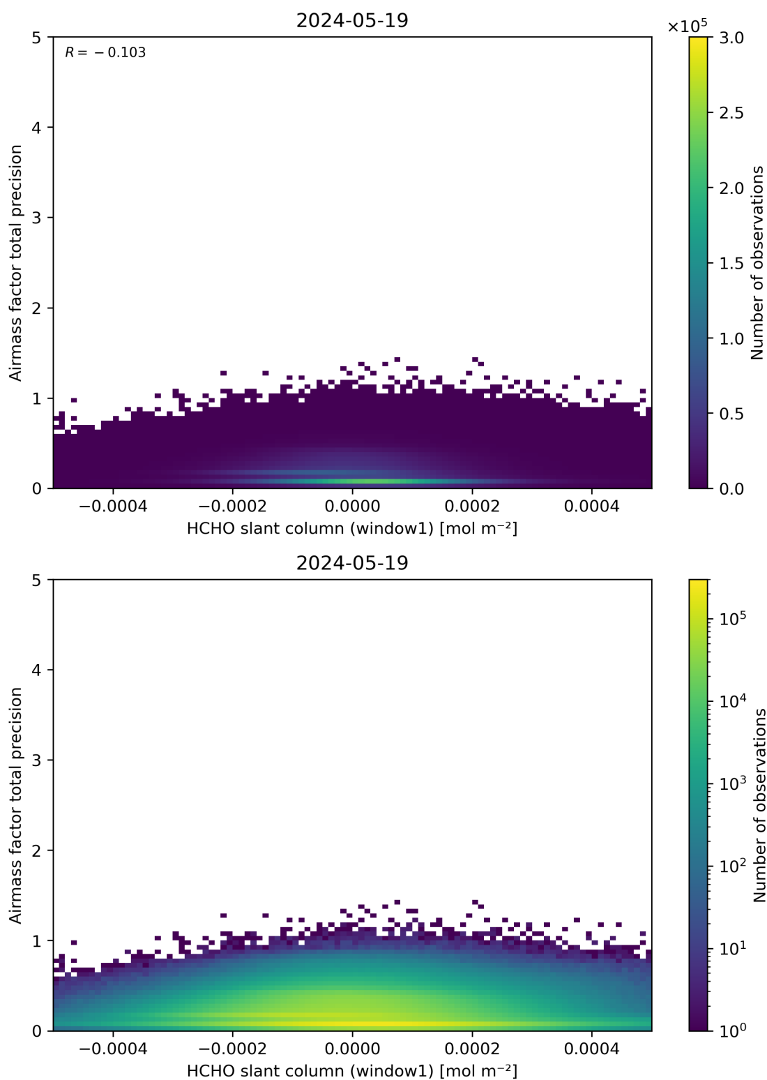
Figure 86: Scatter density plot of “HCHO slant column (window1)” against “Airmass factor total precision” for 2024-05-18 to 2024-05-20.
