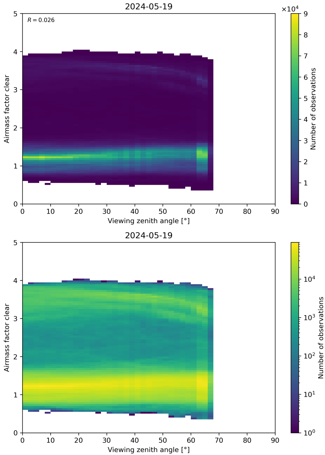
Figure 185: Scatter density plot of “Viewing zenith angle” against “Airmass factor clear” for 2024-05-18 to 2024-05-20.
