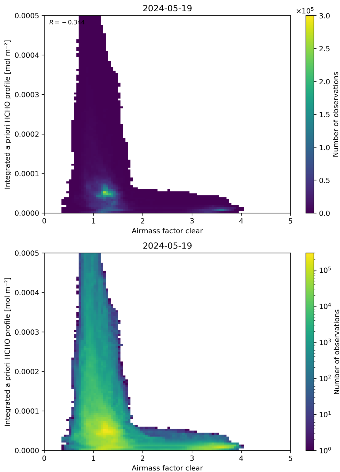
Figure 76: Scatter density plot of “Airmass factor clear” against “Integrated a priori HCHO profile” for 2024-05-18 to 2024-05-20.
