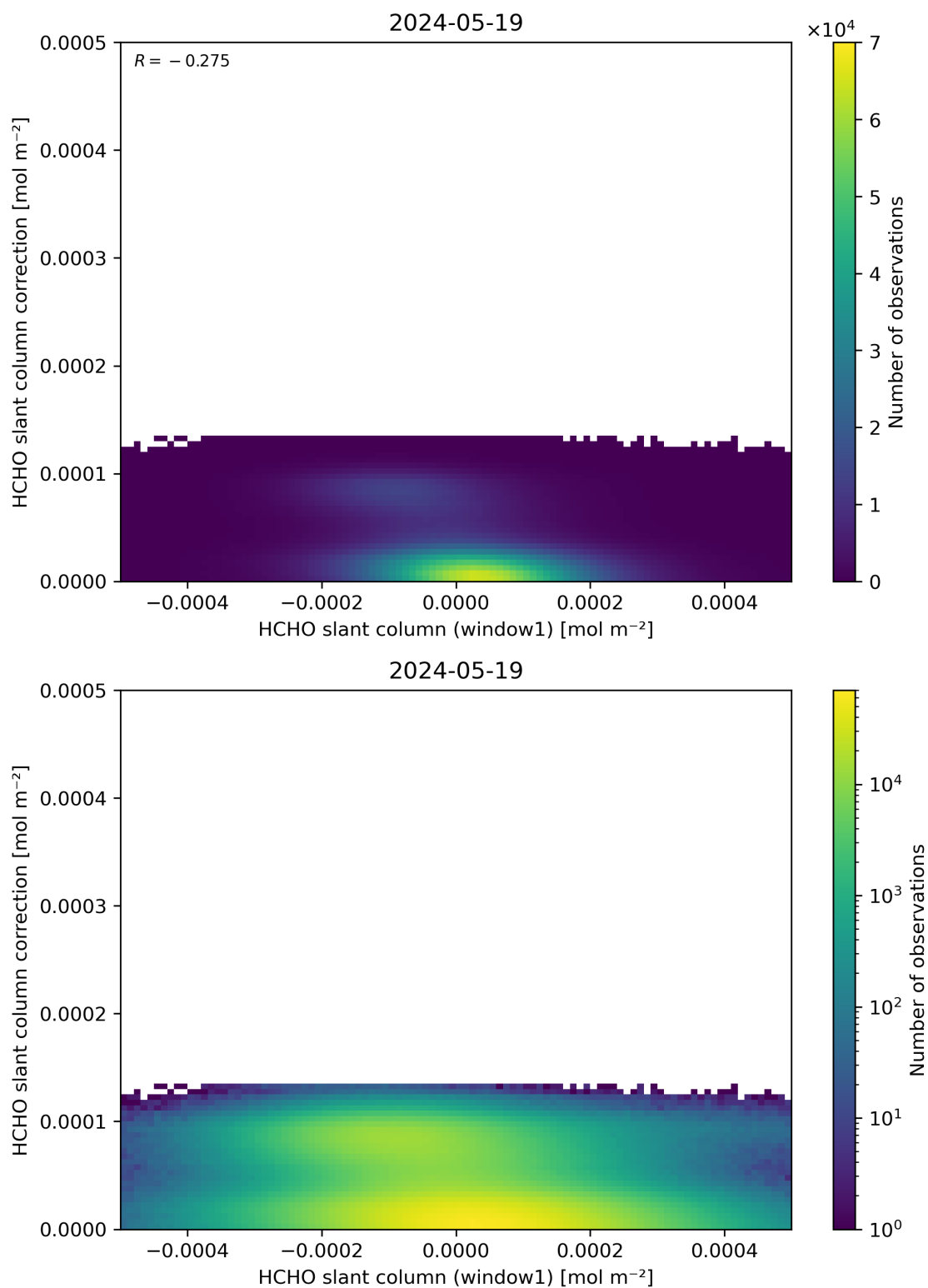
Figure 83: Scatter density plot of “HCHO slant column (window1)” against “HCHO slant column correction” for 2024-05-18 to 2024-05-20.
