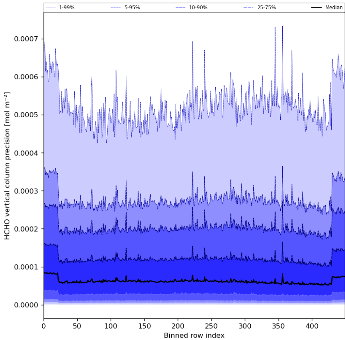
Figure 50: Along track statistics of “HCHO vertical column precision” for 2024-05-18 to 2024-05-20
