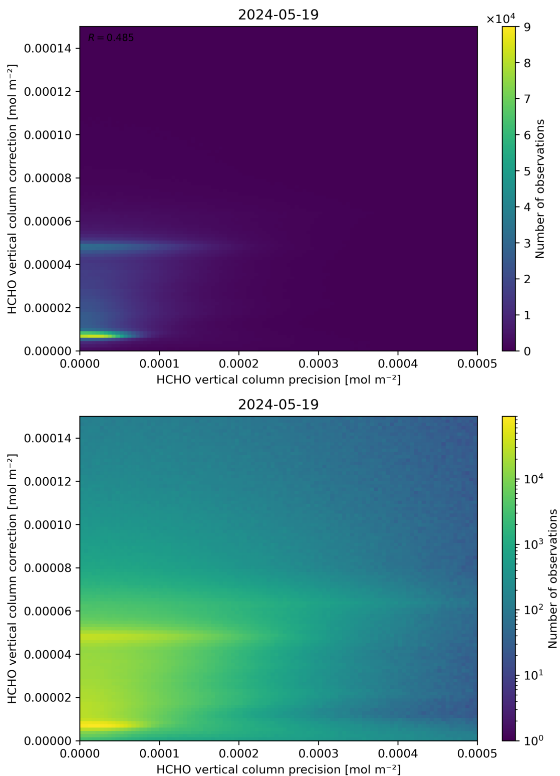
Figure 146: Scatter density plot of “HCHO vertical column precision” against “HCHO vertical column correction” for 2024-05-18 to 2024-05-20.
