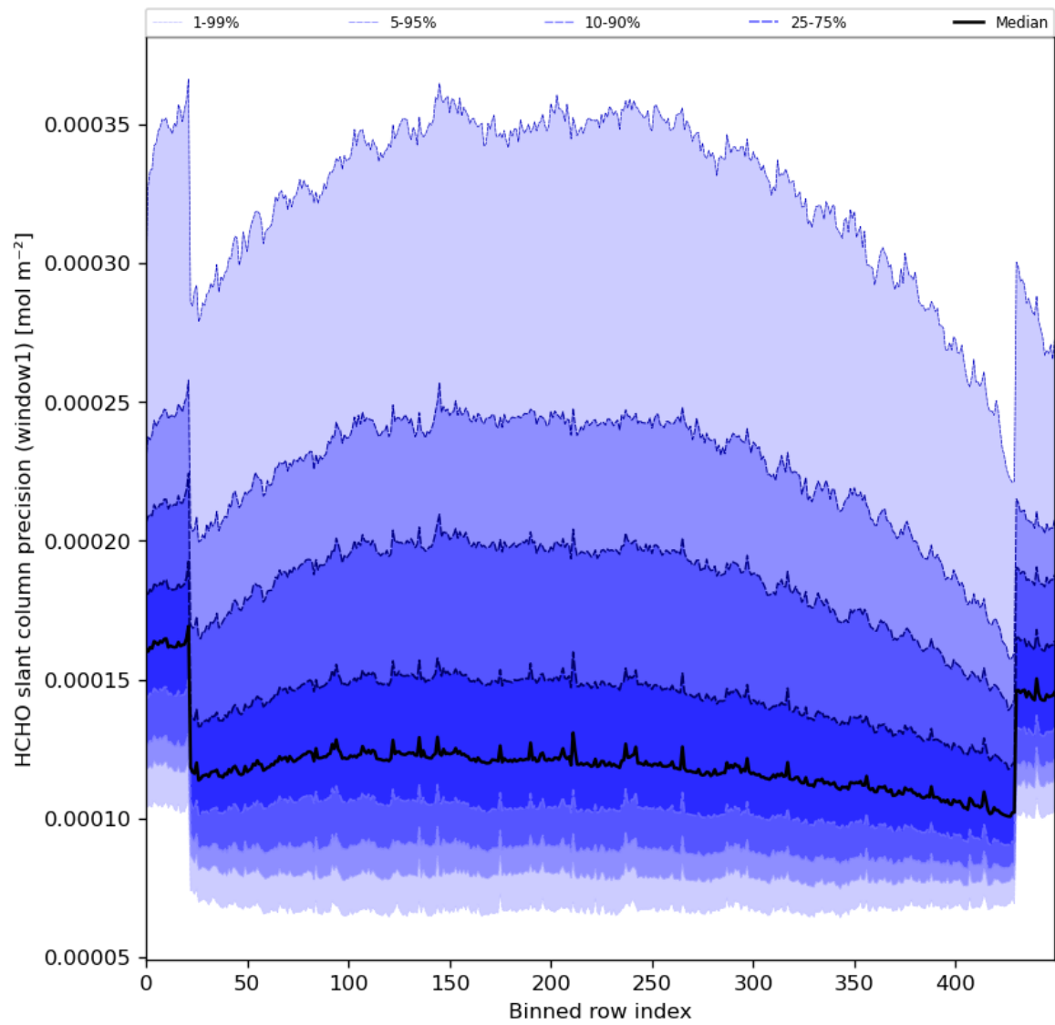
Figure 53: Along track statistics of “HCHO slant column precision (window1)” for 2024-05-18 to 2024-05-20
