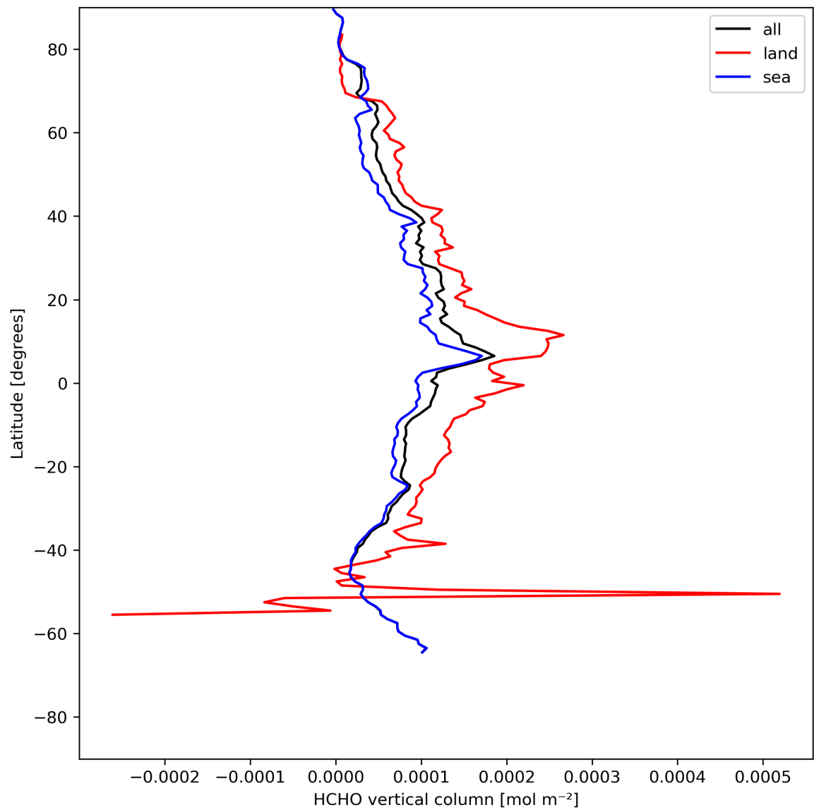
Figure 21: Zonal average of “HCHO vertical column” for 2024-05-18 to 2024-05-20.
