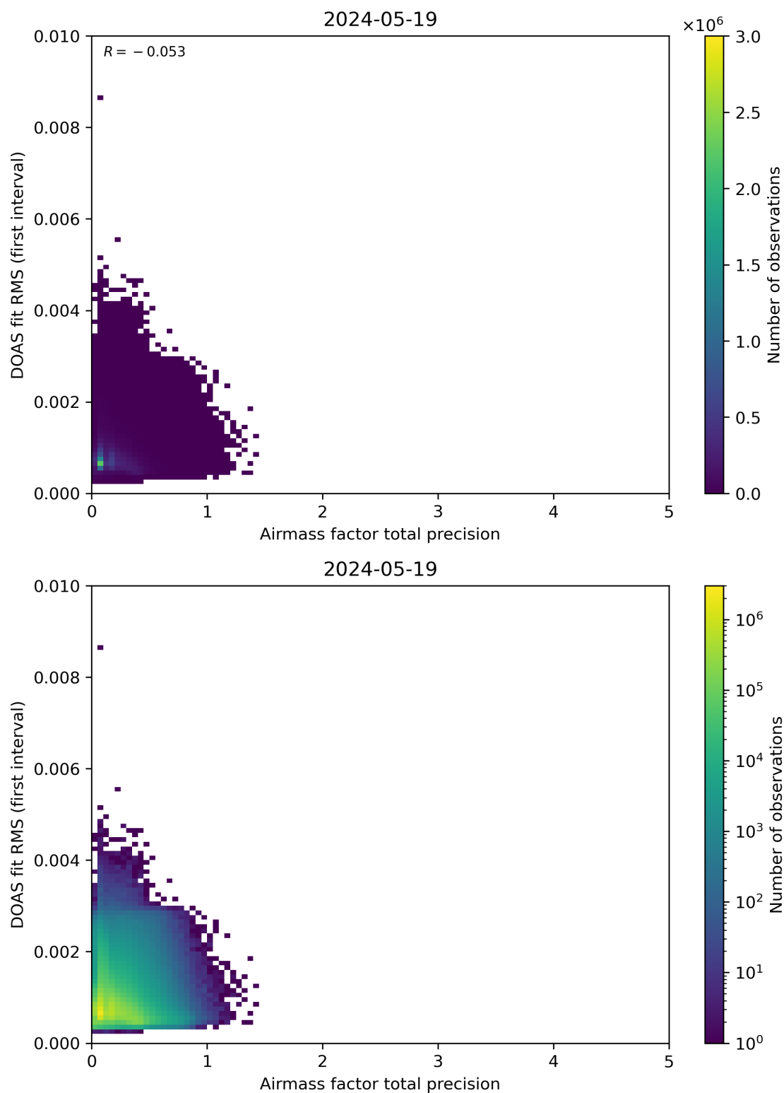
Figure 105: Scatter density plot of “Airmass factor total precision” against “DOAS fit RMS (first interval)” for 2024-05-18 to 2024-05-20.
