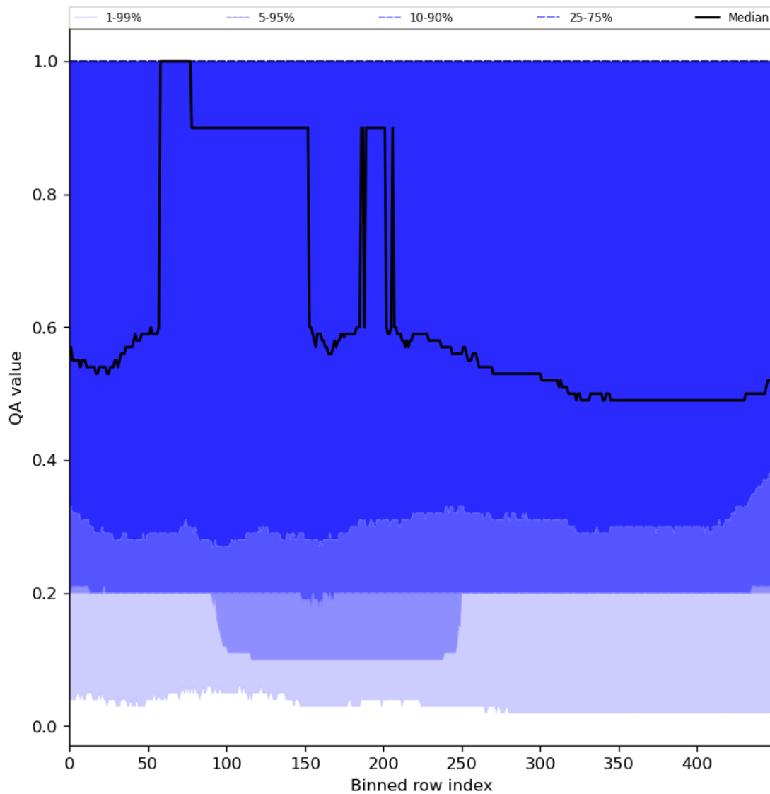
Figure 48: Along track statistics of “QA value” for 2024-05-18 to 2024-05-20
