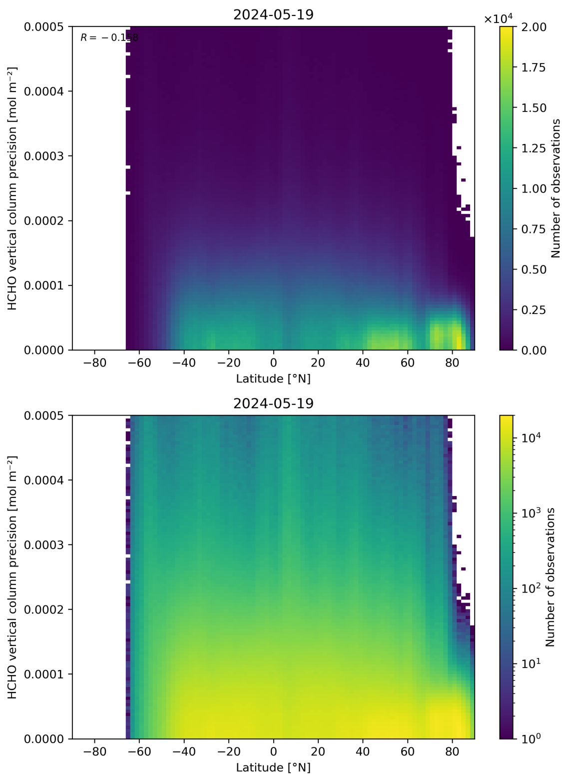
Figure 165: Scatter density plot of “Latitude” against “HCHO vertical column precision” for 2024-05-18 to 2024-05-20.
