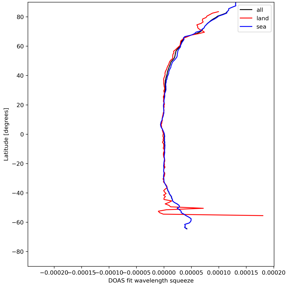
Figure 31: Zonal average of “DOAS fit wavelength squeeze” for 2024-05-18 to 2024-05-20.
