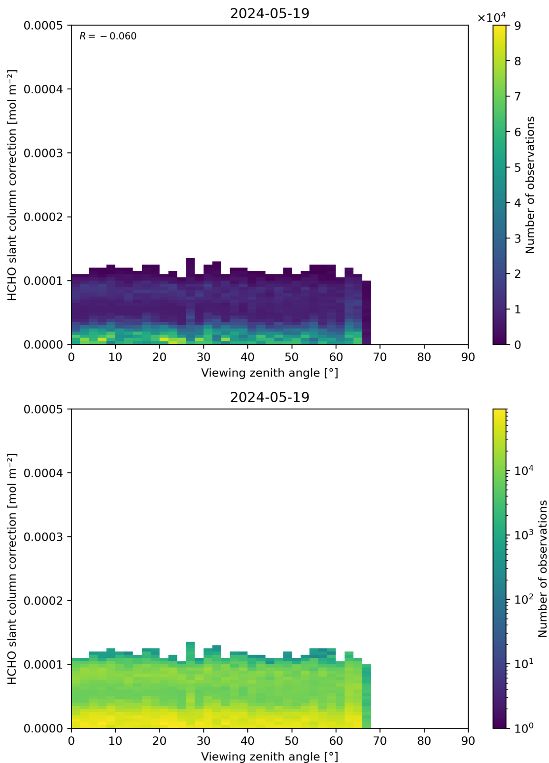
Figure 187: Scatter density plot of “Viewing zenith angle” against “HCHO slant column correction” for 2024-05-18 to 2024-05-20.
