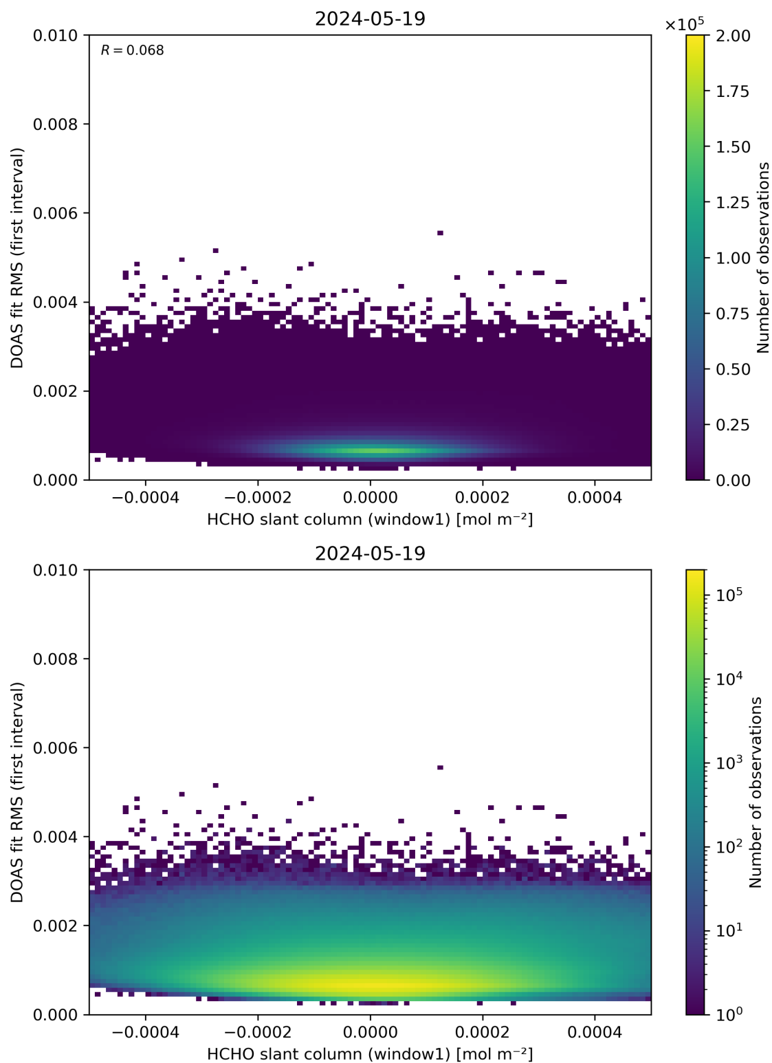
Figure 78: Scatter density plot of “HCHO slant column (window1)” against “DOAS fit RMS (first interval)” for 2024-05-18 to 2024-05-20.
