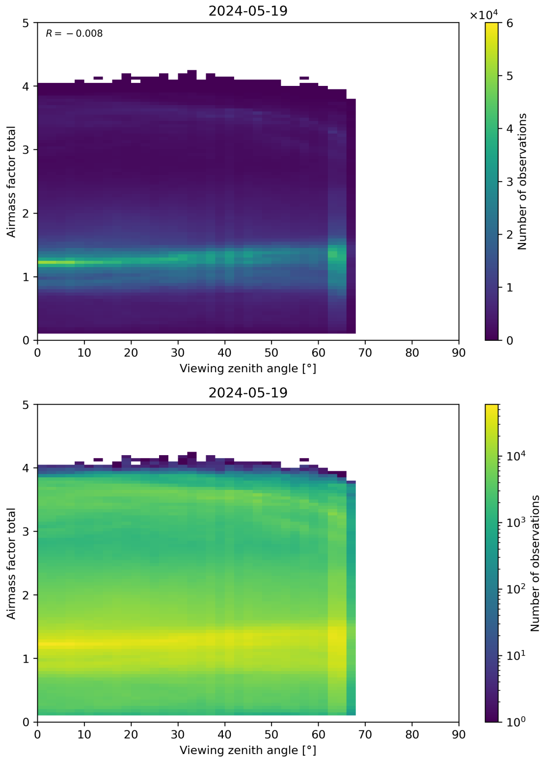
Figure 190: Scatter density plot of “Viewing zenith angle” against “Airmass factor total” for 2024-05-18 to 2024-05-20.
