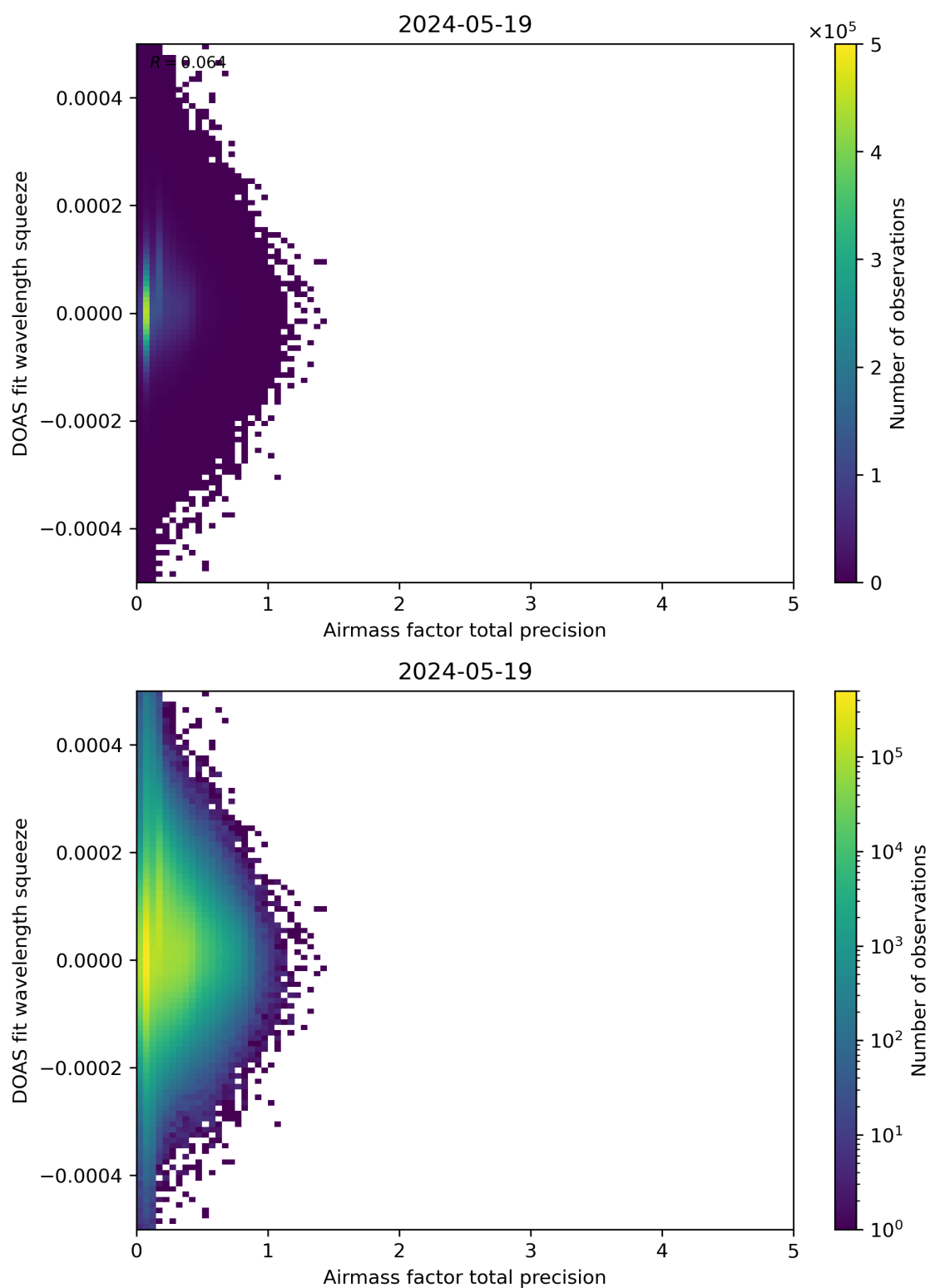
Figure 107: Scatter density plot of “Airmass factor total precision” against “DOAS fit wavelength squeeze” for 2024-05-18 to 2024-05-20.
