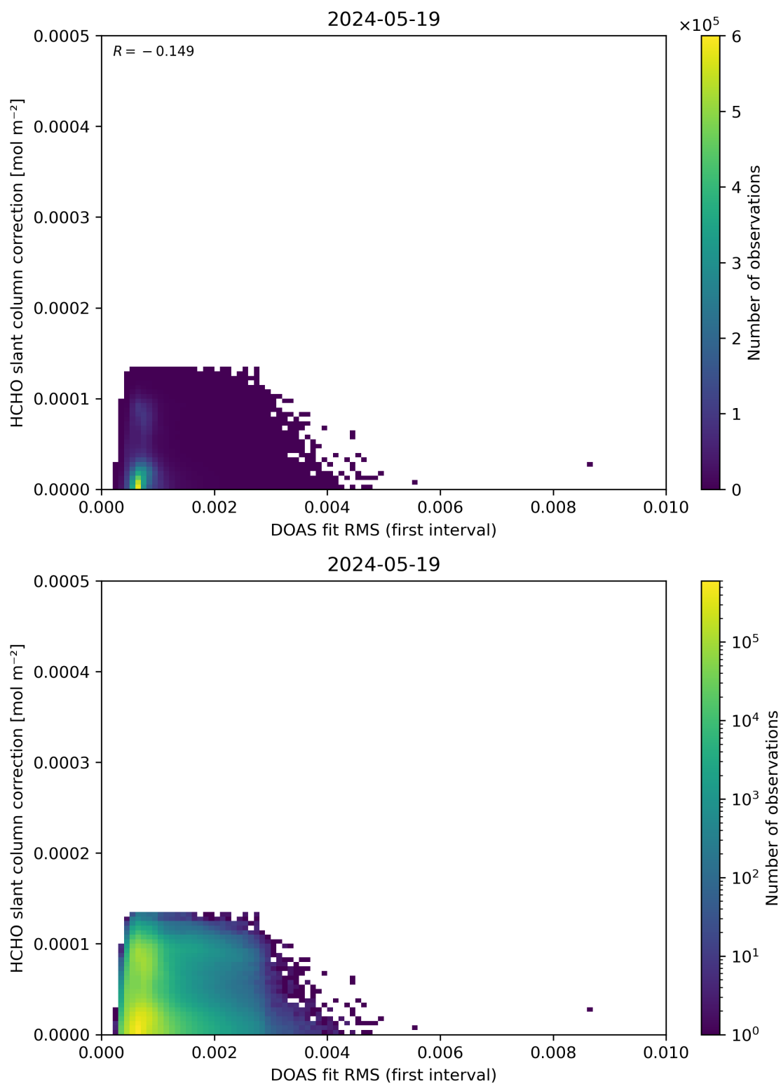
Figure 63: Scatter density plot of “DOAS fit RMS (first interval)” against “HCHO slant column correction” for 2024-05-18 to 2024-05-20.
