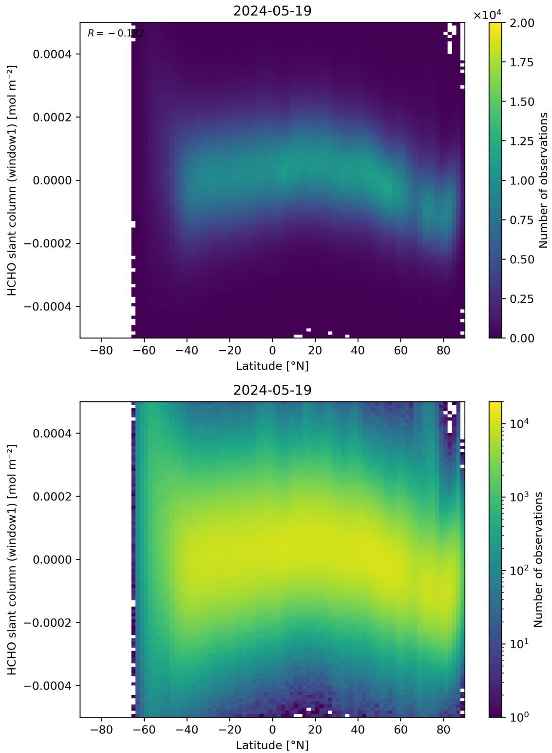
Figure 159: Scatter density plot of “Latitude” against “HCHO slant column (window1)” for 2024-05-18 to 2024-05-20.
