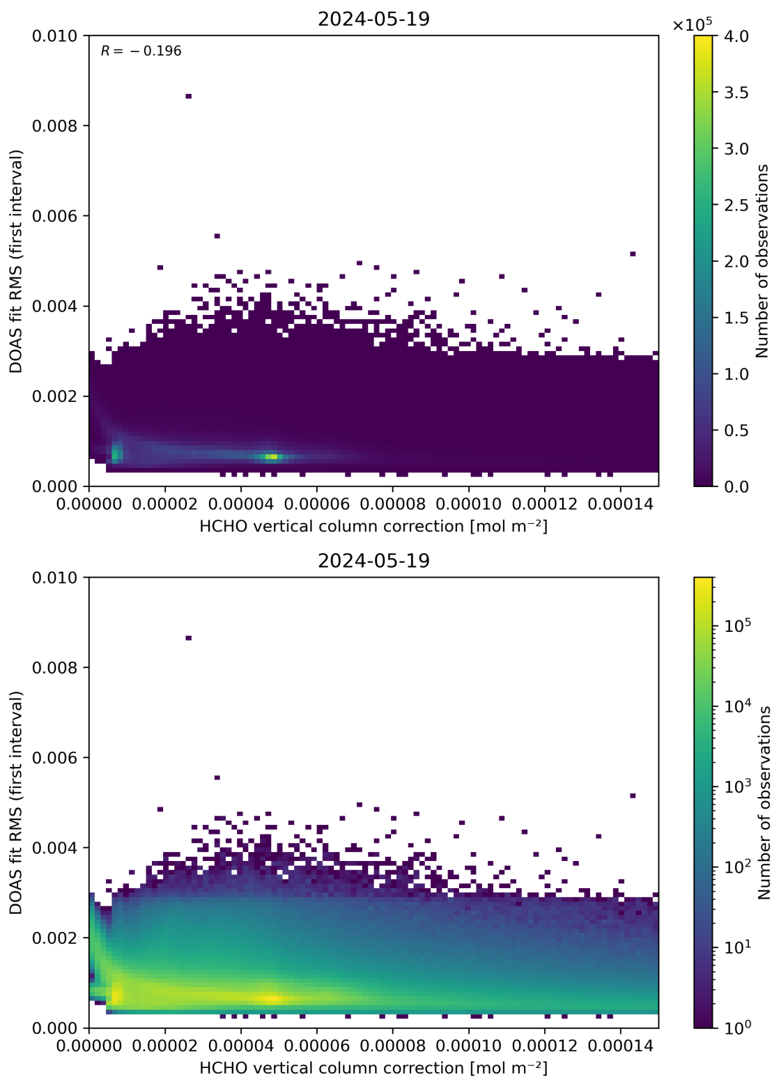
Figure 112: Scatter density plot of “HCHO vertical column correction” against “DOAS fit RMS (first interval)” for 2024-05-18 to 2024-05-20.
