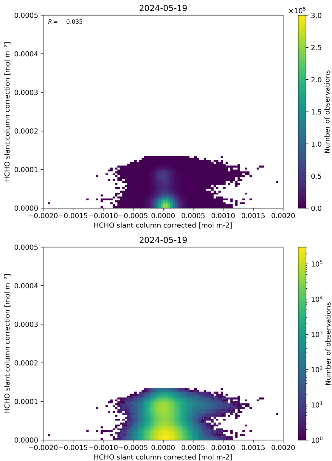
Figure 77: Scatter density plot of “HCHO slant column corrected” against “HCHO slant column correction” for 2024-05-18 to 2024-05-20.
