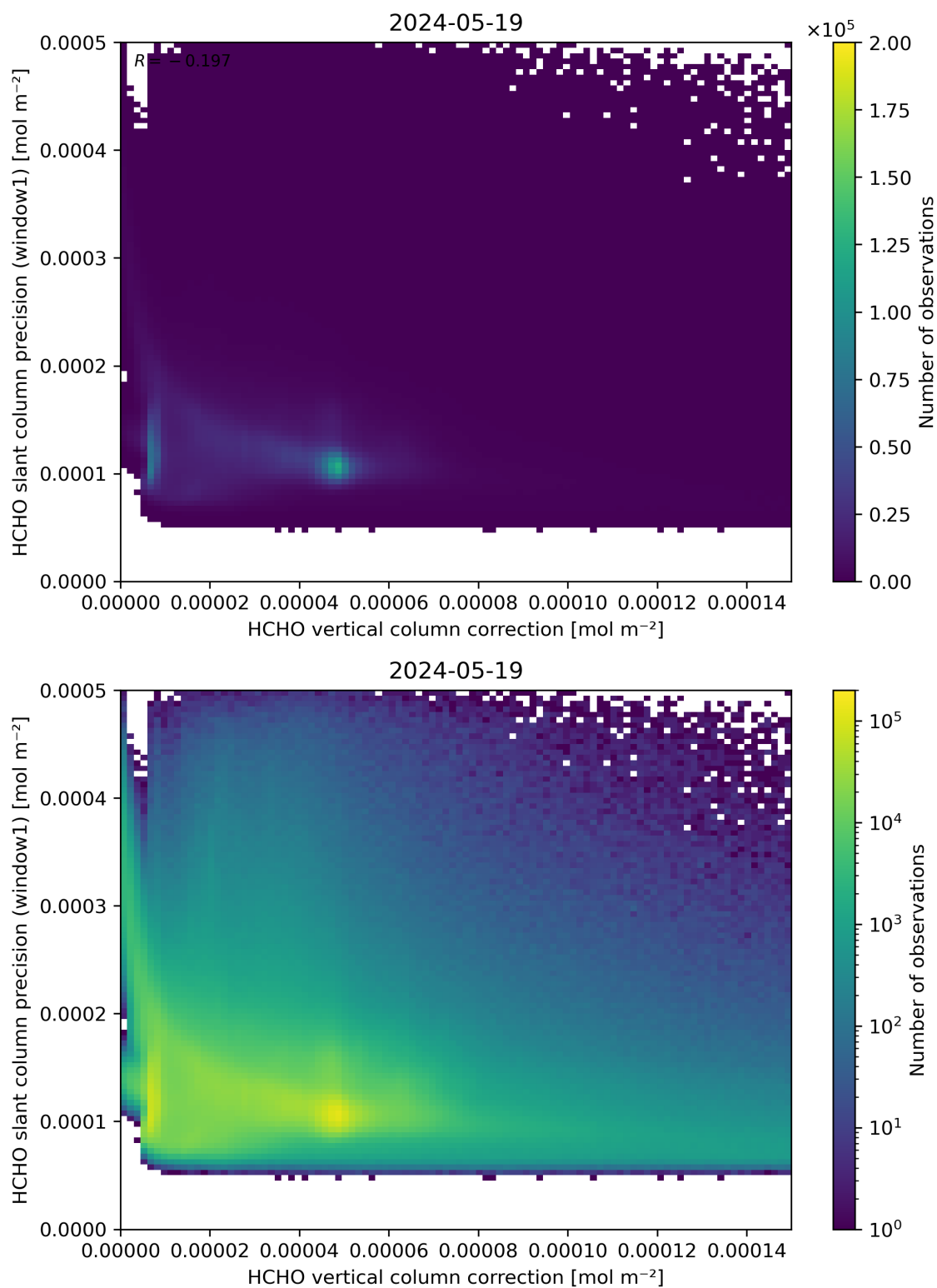
Figure 119: Scatter density plot of “HCHO vertical column correction” against “HCHO slant column precision (window1)” for 2024-05-18 to 2024-05-20.
