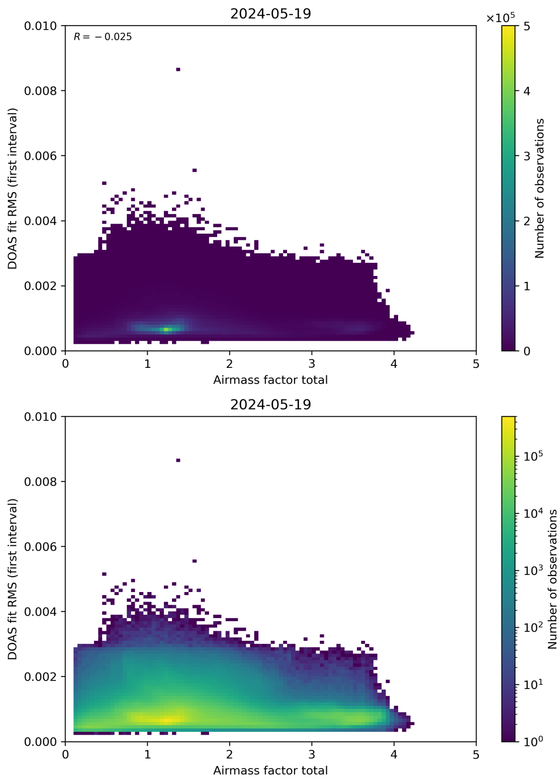
Figure 97: Scatter density plot of “Airmass factor total” against “DOAS fit RMS (first interval)” for 2024-05-18 to 2024-05-20.
