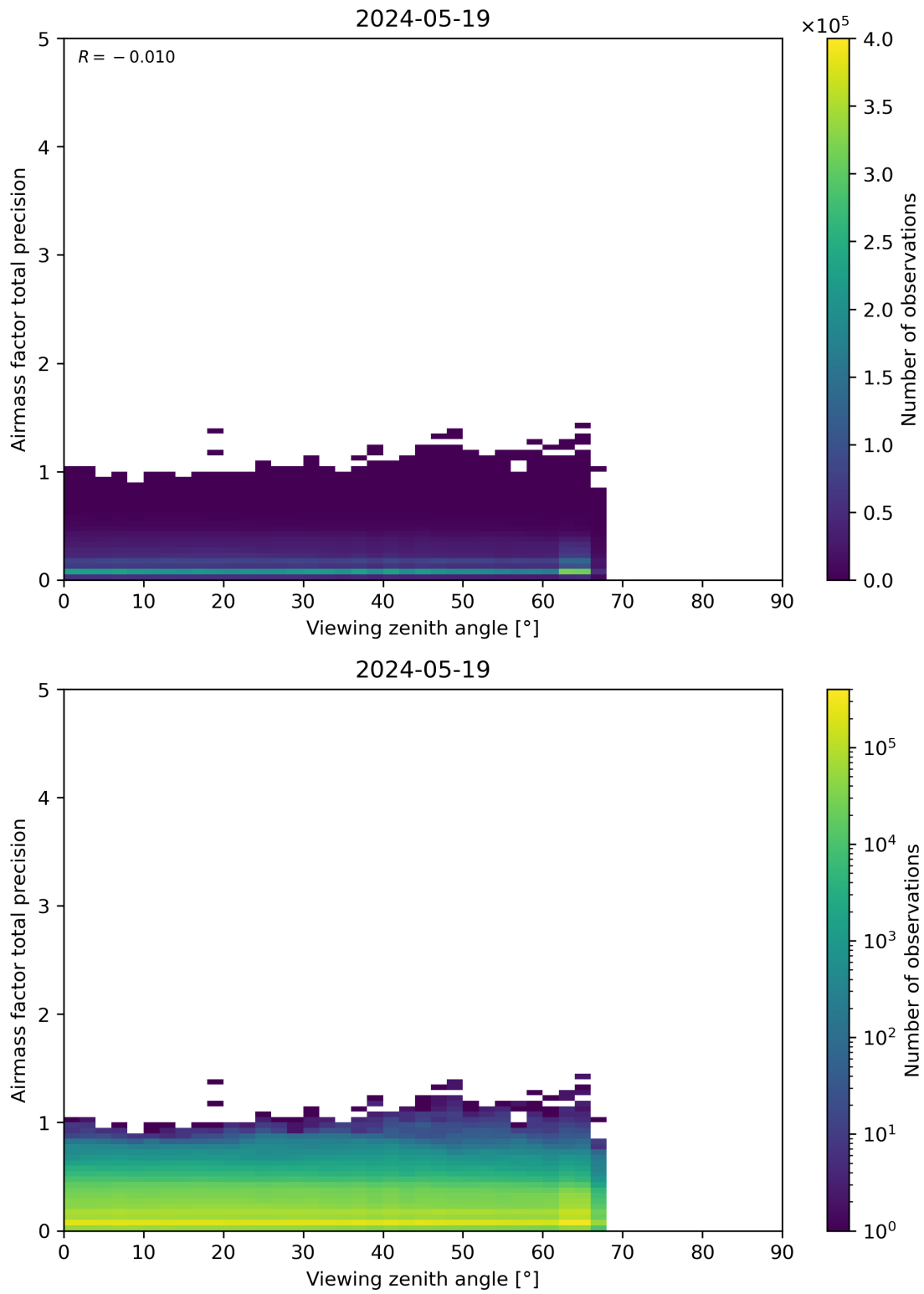
Figure 191: Scatter density plot of “Viewing zenith angle” against “Airmass factor total precision” for 2024-05-18 to 2024-05-20.
