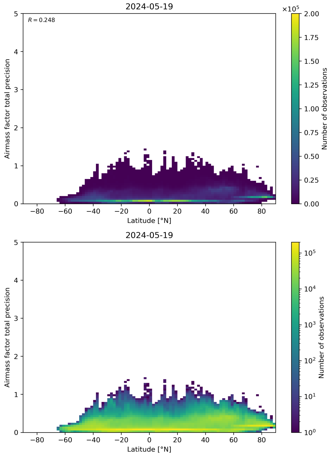
Figure 162: Scatter density plot of “Latitude” against “Airmass factor total precision” for 2024-05-18 to 2024-05-20.
