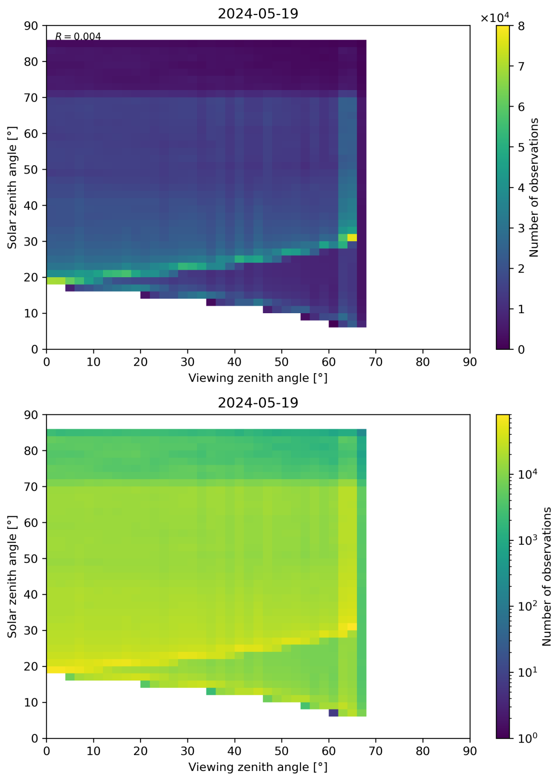
Figure 197: Scatter density plot of “Viewing zenith angle” against “Solar zenith angle” for 2024-05-18 to 2024-05-20.
