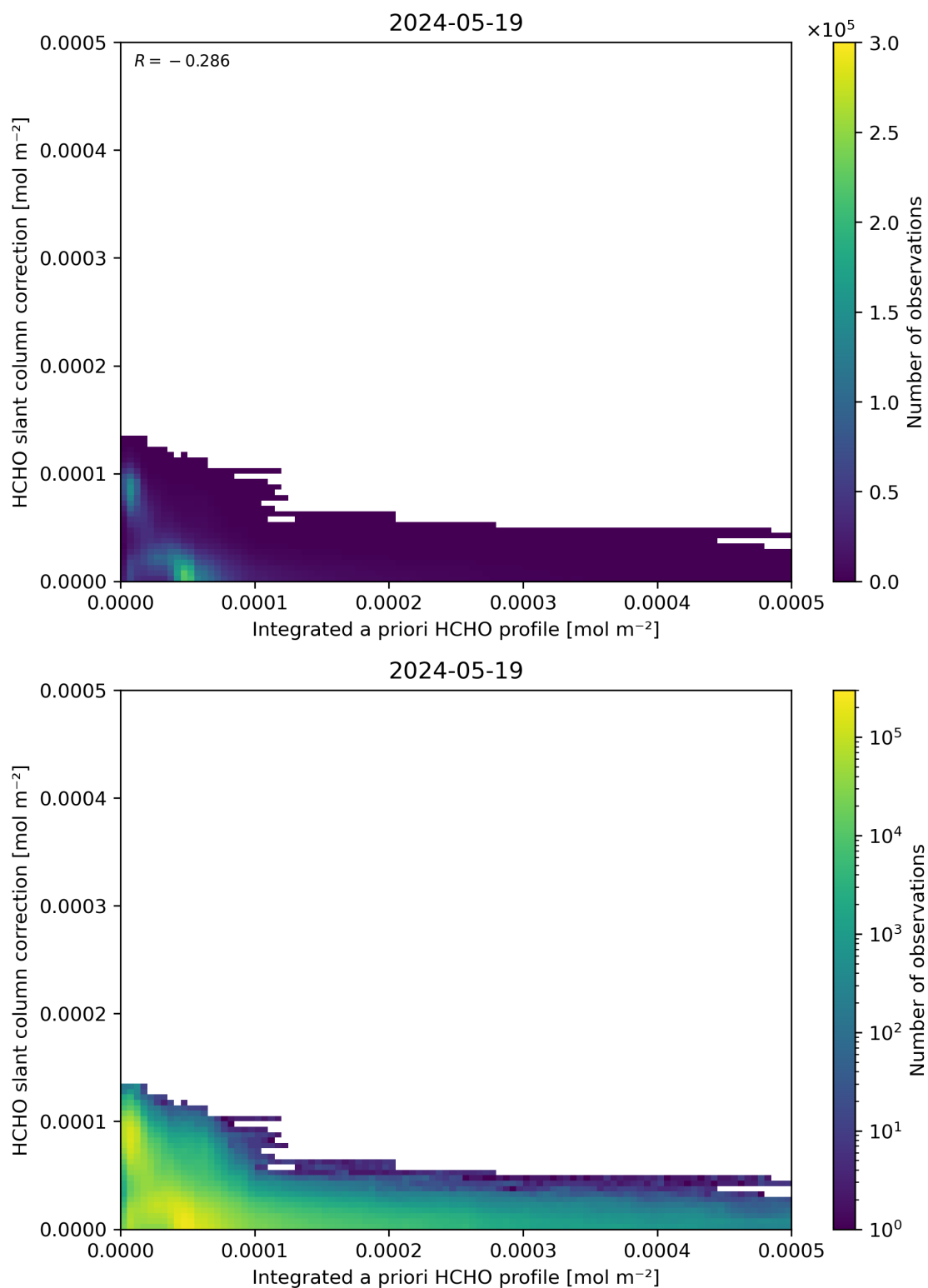
Figure 152: Scatter density plot of “Integrated a priori HCHO profile” against “HCHO slant column correction” for 2024-05-18 to 2024-05-20.
