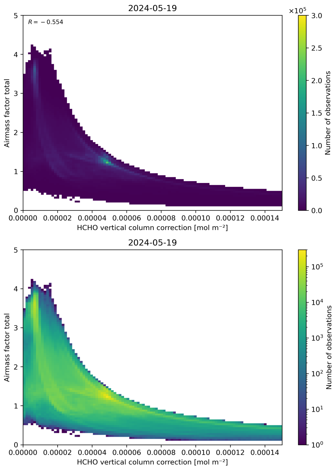
Figure 120: Scatter density plot of “HCHO vertical column correction” against “Airmass factor total” for 2024-05-18 to 2024-05-20.
