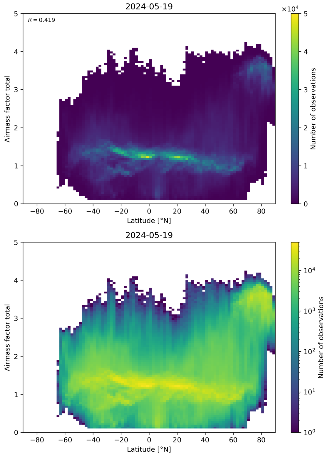
Figure 161: Scatter density plot of “Latitude” against “Airmass factor total” for 2024-05-18 to 2024-05-20.
