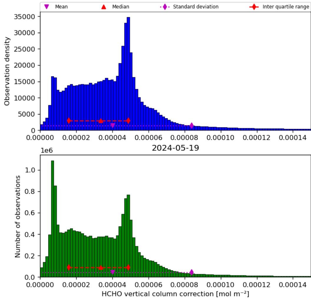
Figure 37: Histogram of “HCHO vertical column correction” for 2024-05-18 to 2024-05-20
