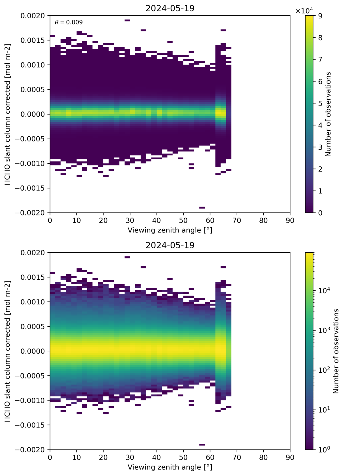
Figure 186: Scatter density plot of “Viewing zenith angle” against “HCHO slant column corrected” for 2024-05-18 to 2024-05-20.
