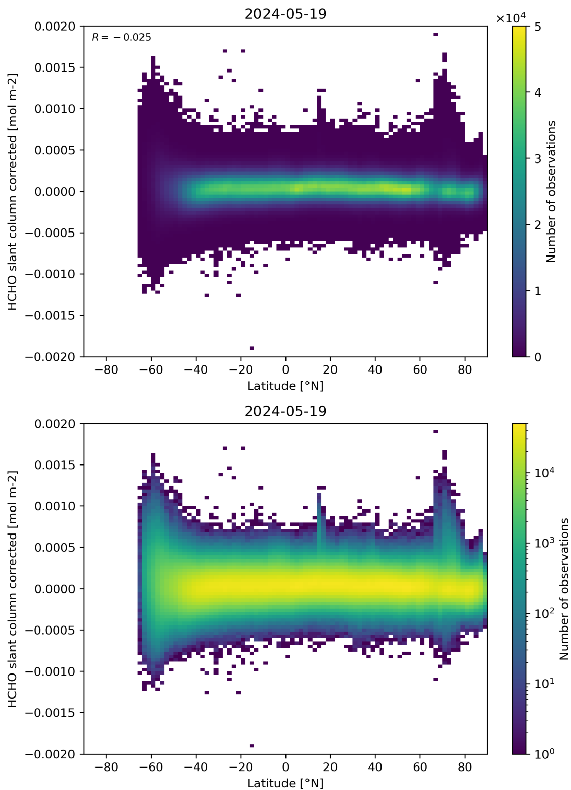
Figure 157: Scatter density plot of “Latitude” against “HCHO slant column corrected” for 2024-05-18 to 2024-05-20.
