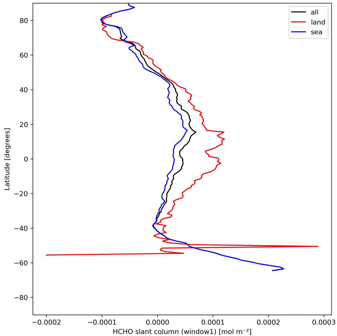
Figure 24: Zonal average of “HCHO slant column (window1)” for 2024-05-18 to 2024-05-20.
