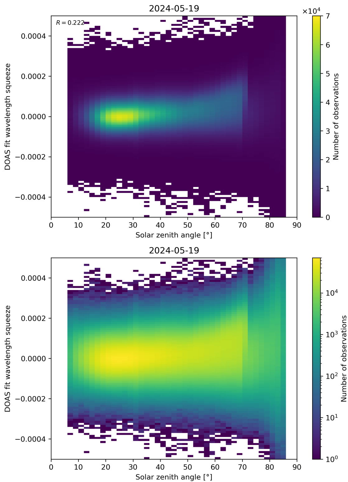
Figure 169: Scatter density plot of “Solar zenith angle” against “DOAS fit wavelength squeeze” for 2024-05-18 to 2024-05-20.
