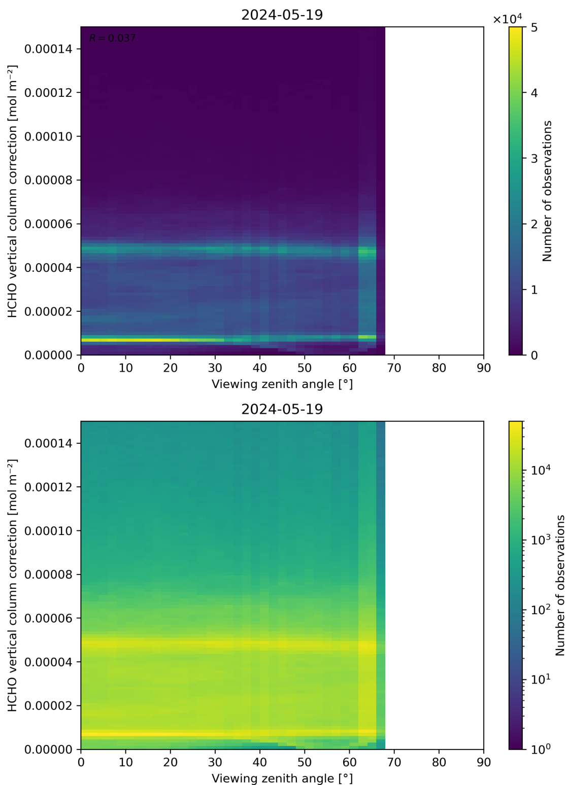
Figure 193: Scatter density plot of “Viewing zenith angle” against “HCHO vertical column correction” for 2024-05-18 to 2024-05-20.
