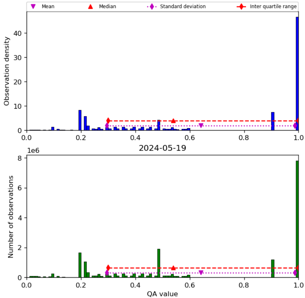
Figure 34: Histogram of “QA value” for 2024-05-18 to 2024-05-20
