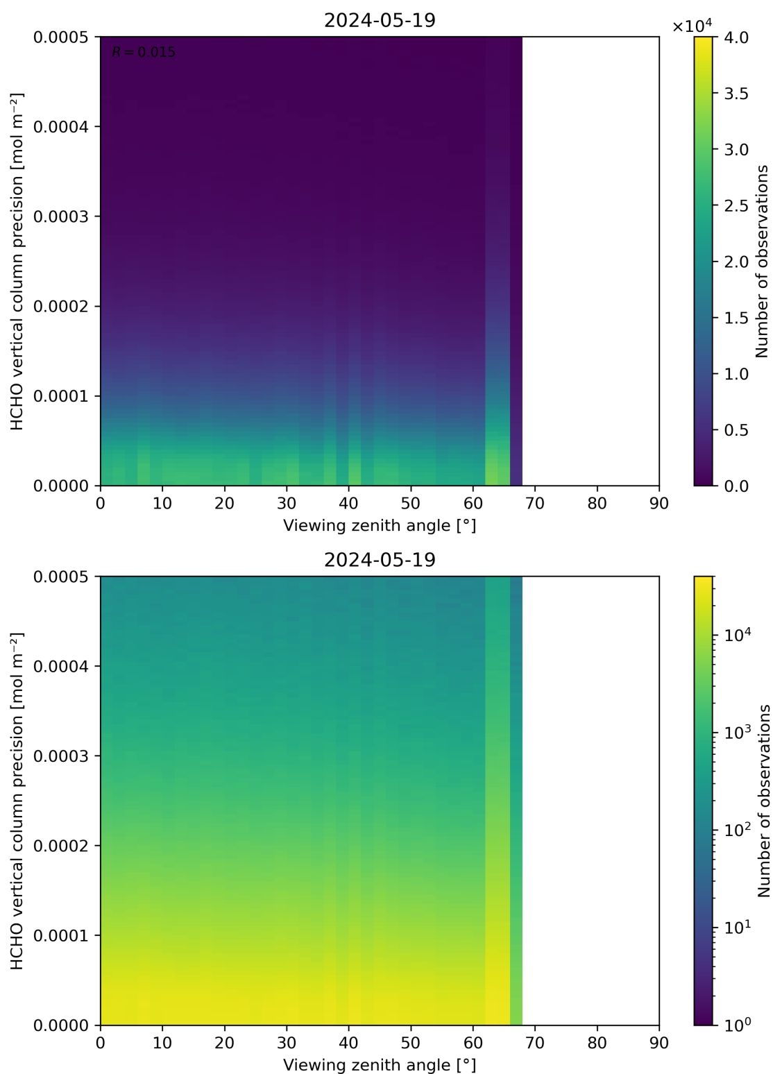
Figure 194: Scatter density plot of “Viewing zenith angle” against “HCHO vertical column precision” for 2024-05-18 to 2024-05-20.
