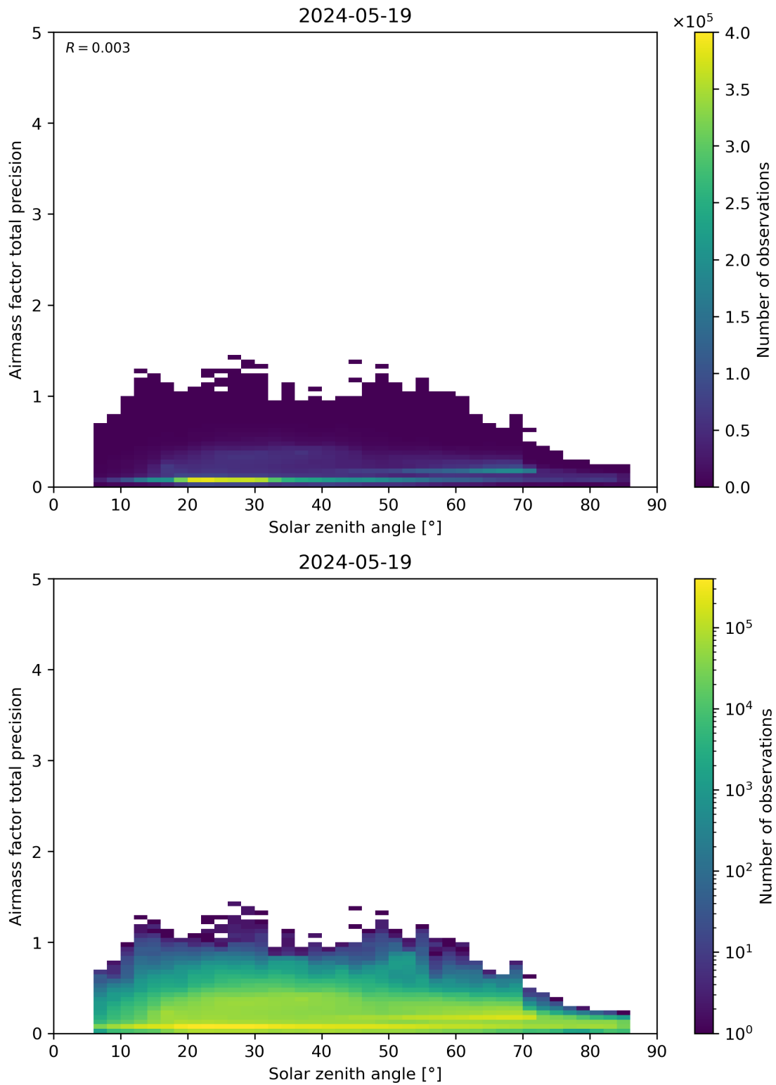
Figure 176: Scatter density plot of “Solar zenith angle” against “Airmass factor total precision” for 2024-05-18 to 2024-05-20.
