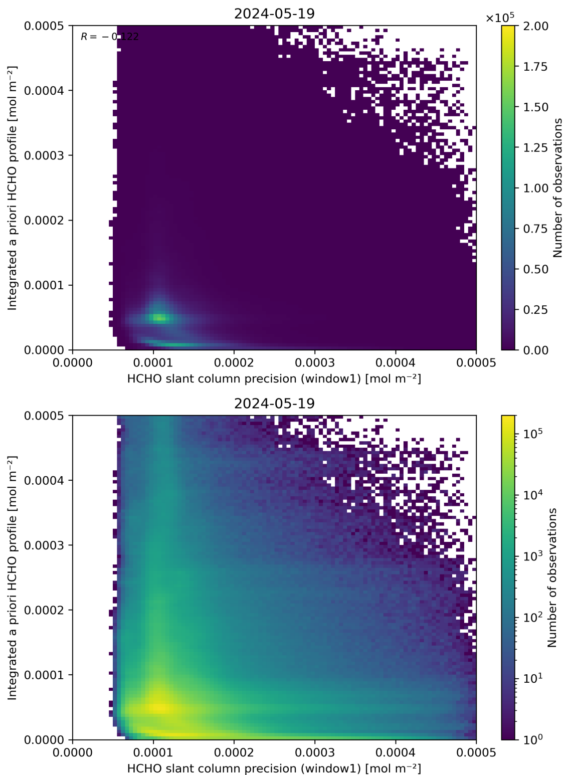
Figure 96: Scatter density plot of “HCHO slant column precision (window1)” against “Integrated a priori HCHO profile” for 2024-05-18 to 2024-05-20.
