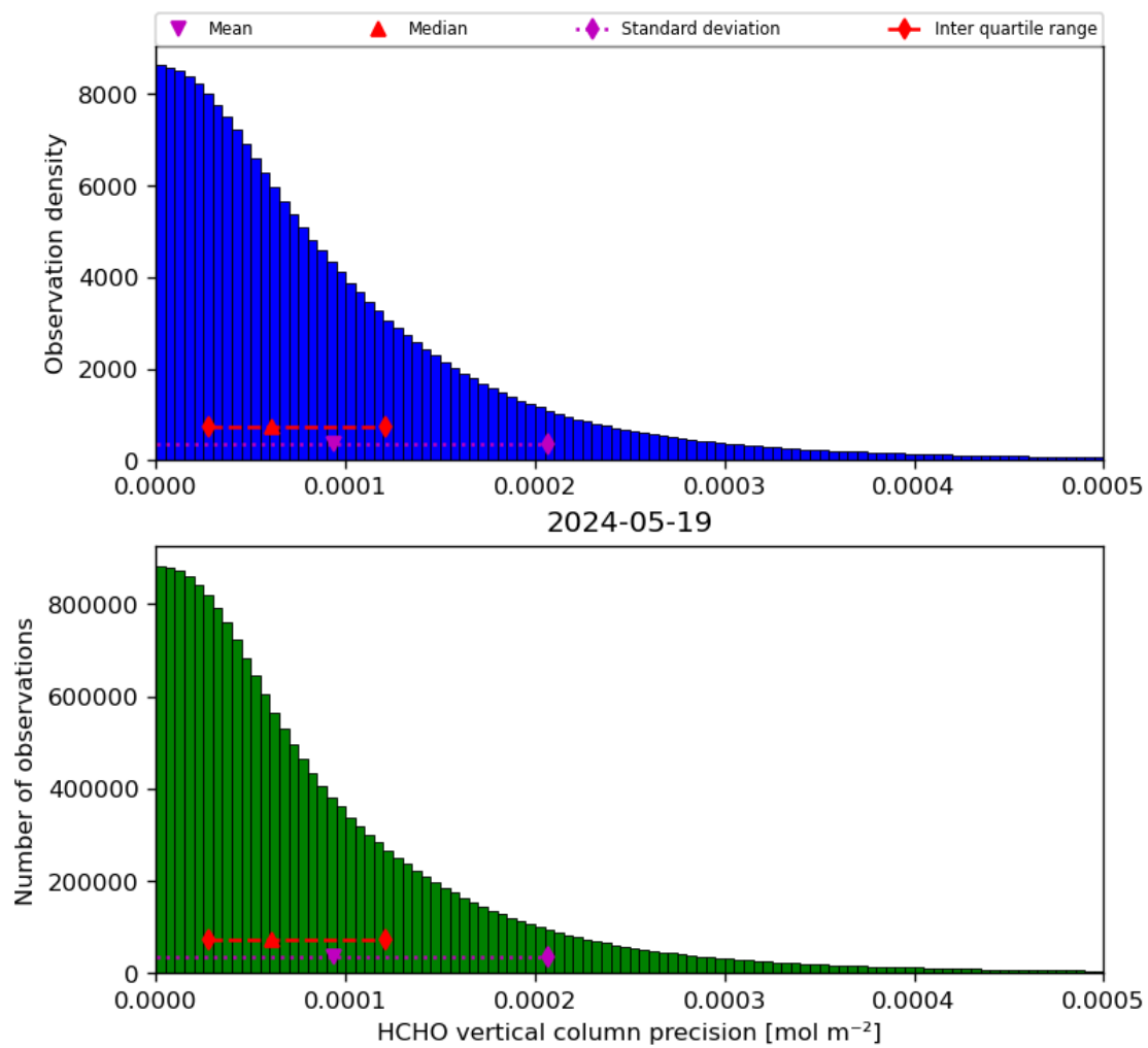
Figure 36: Histogram of “HCHO vertical column precision” for 2024-05-18 to 2024-05-20
