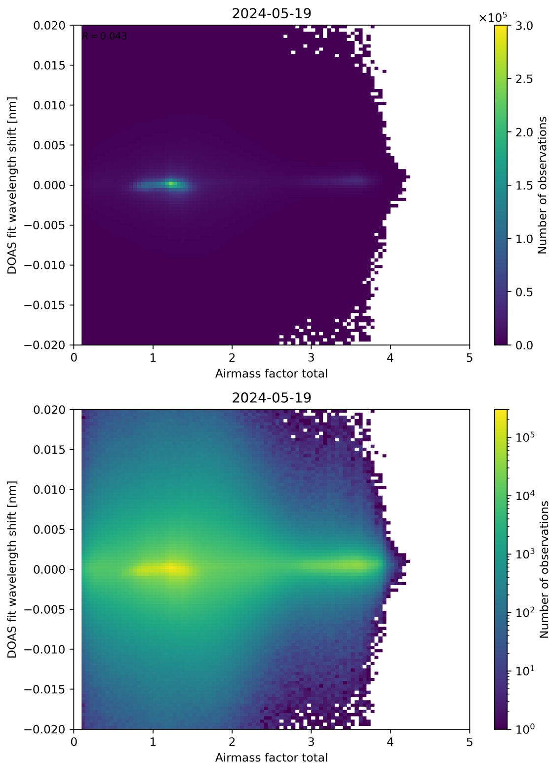
Figure 98: Scatter density plot of “Airmass factor total” against “DOAS fit wavelength shift” for 2024-05-18 to 2024-05-20.
