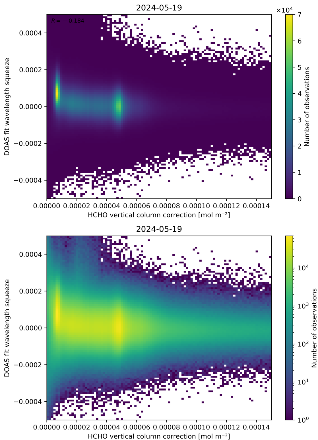
Figure 114: Scatter density plot of “HCHO vertical column correction” against “DOAS fit wavelength squeeze” for 2024-05-18 to 2024-05-20.
