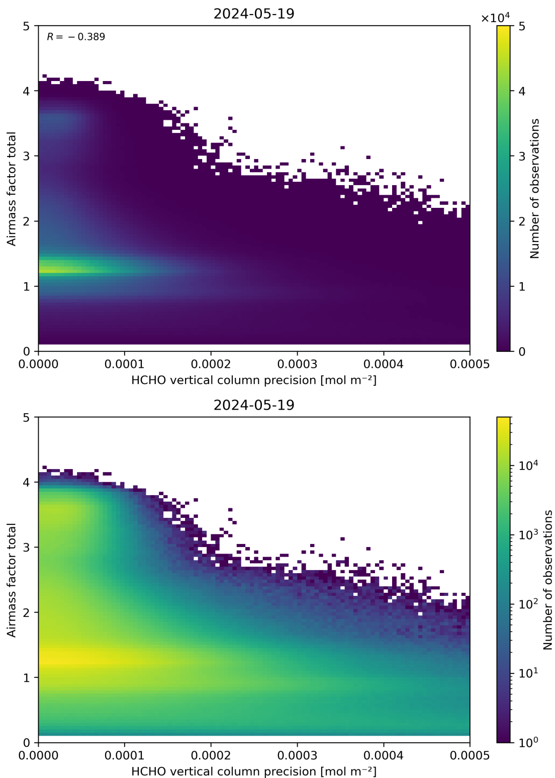
Figure 144: Scatter density plot of “HCHO vertical column precision” against “Airmass factor total” for 2024-05-18 to 2024-05-20.
