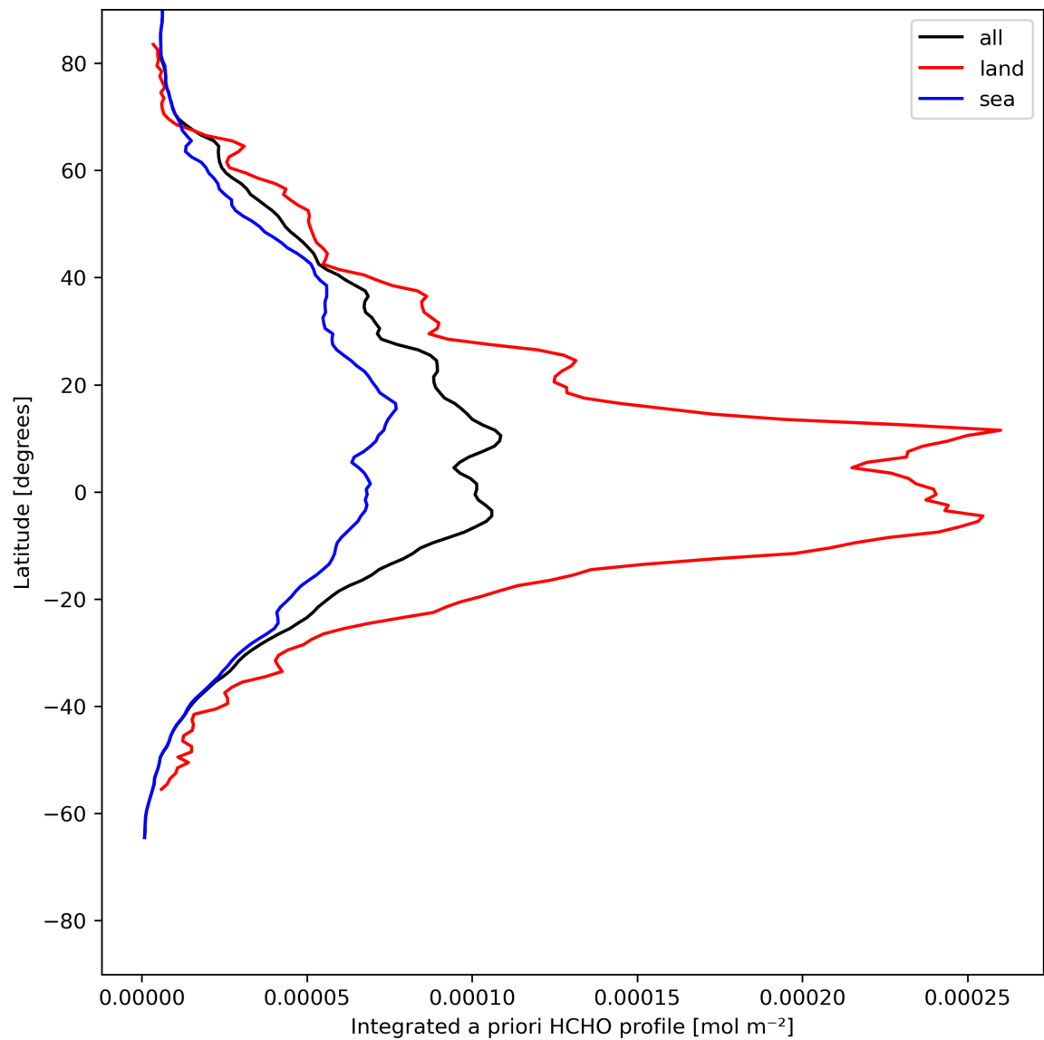
Figure 29: Zonal average of “Integrated a priori HCHO profile” for 2024-05-18 to 2024-05-20.
