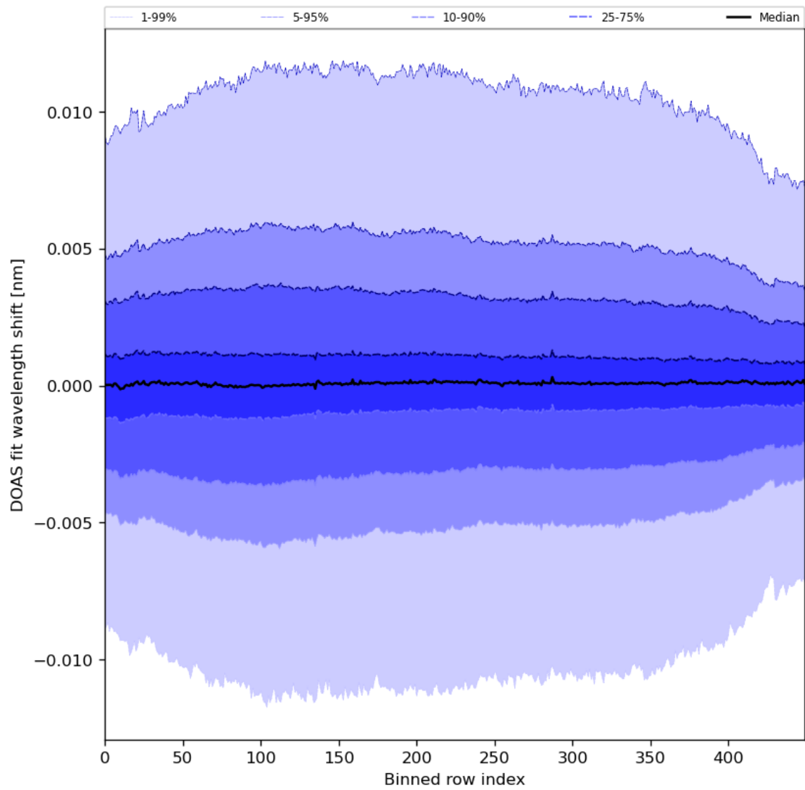
Figure 58: Along track statistics of “DOAS fit wavelength shift” for 2024-05-18 to 2024-05-20
