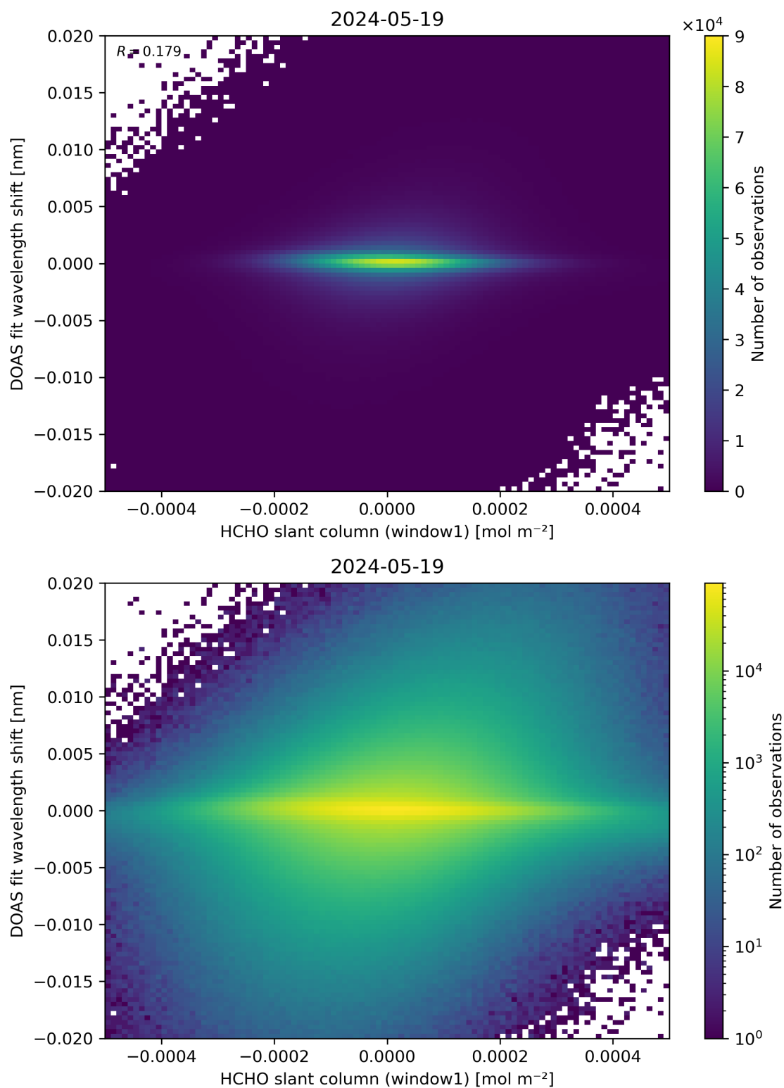
Figure 79: Scatter density plot of “HCHO slant column (window1)” against “DOAS fit wavelength shift” for 2024-05-18 to 2024-05-20.
