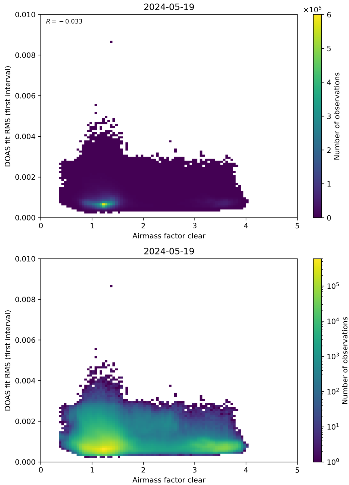
Figure 71: Scatter density plot of “Airmass factor clear” against “DOAS fit RMS (first interval)” for 2024-05-18 to 2024-05-20.
