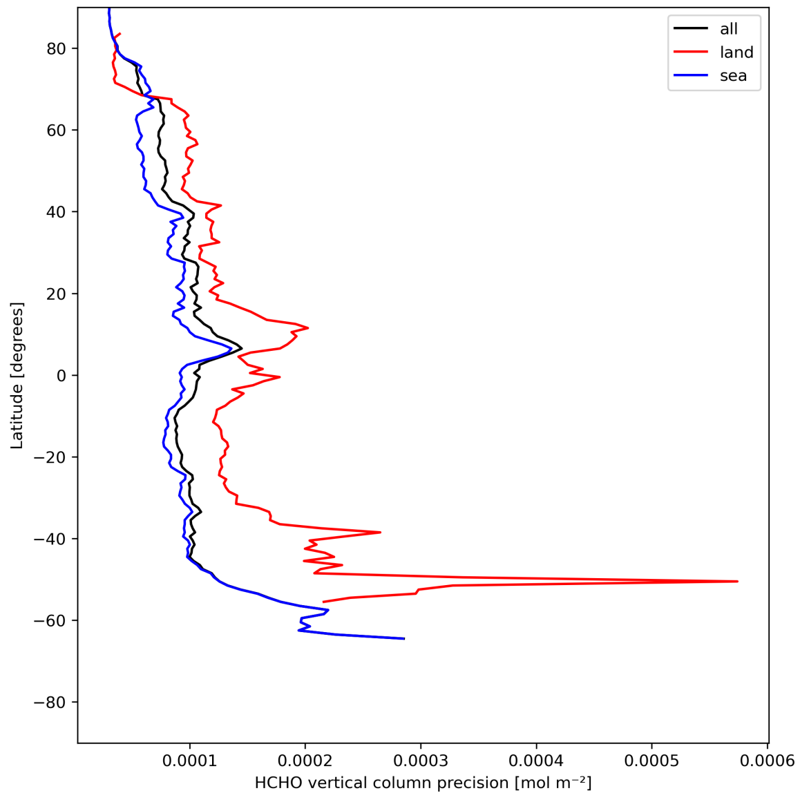
Figure 22: Zonal average of “HCHO vertical column precision” for 2024-05-18 to 2024-05-20.
