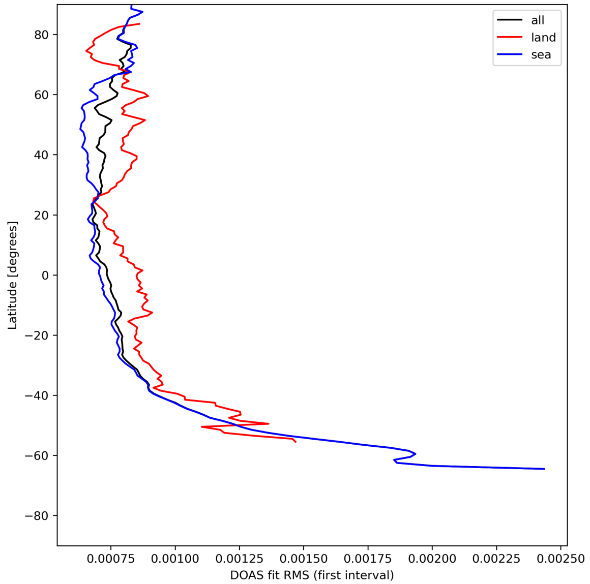
Figure 32: Zonal average of “DOAS fit RMS (first interval)” for 2024-05-18 to 2024-05-20.
