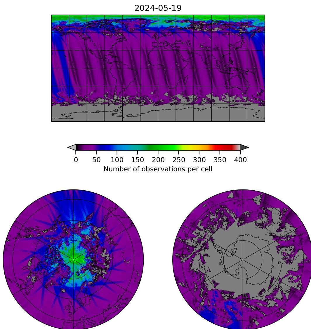
Figure 19: Map of the number of observations for 2024-05-18 to 2024-05-20
