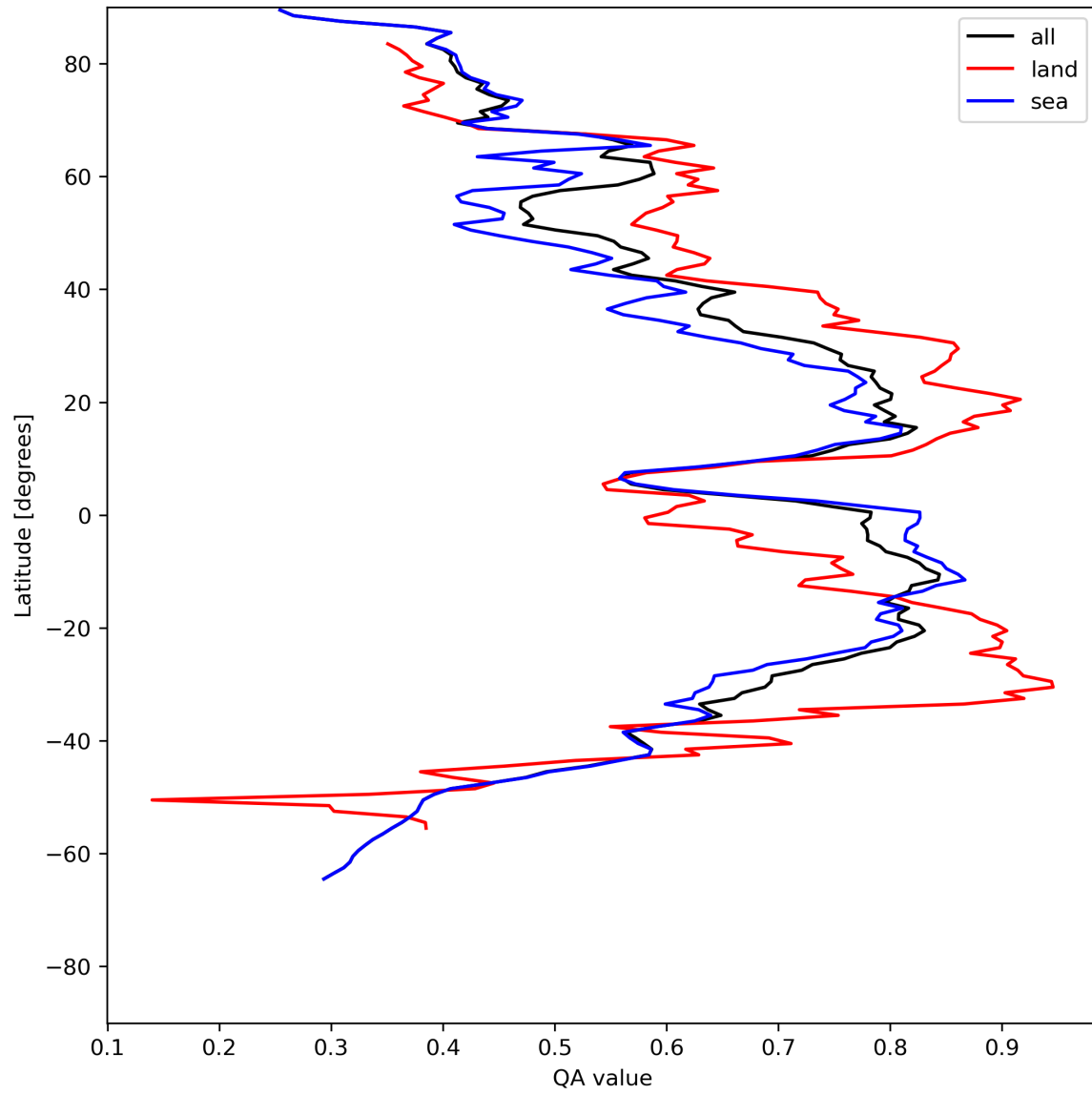
Figure 20: Zonal average of “QA value” for 2024-05-18 to 2024-05-20.
