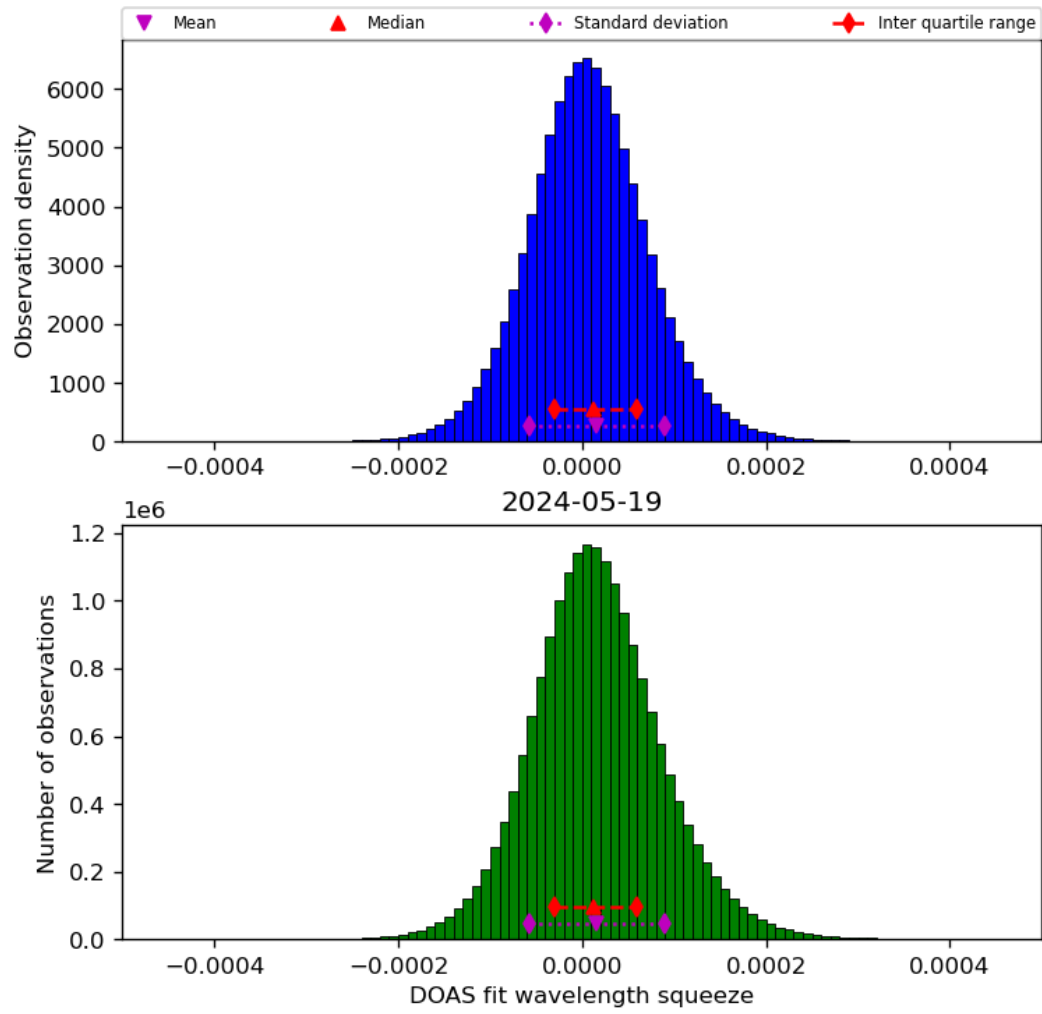
Figure 45: Histogram of “DOAS fit wavelength squeeze” for 2024-05-18 to 2024-05-20
