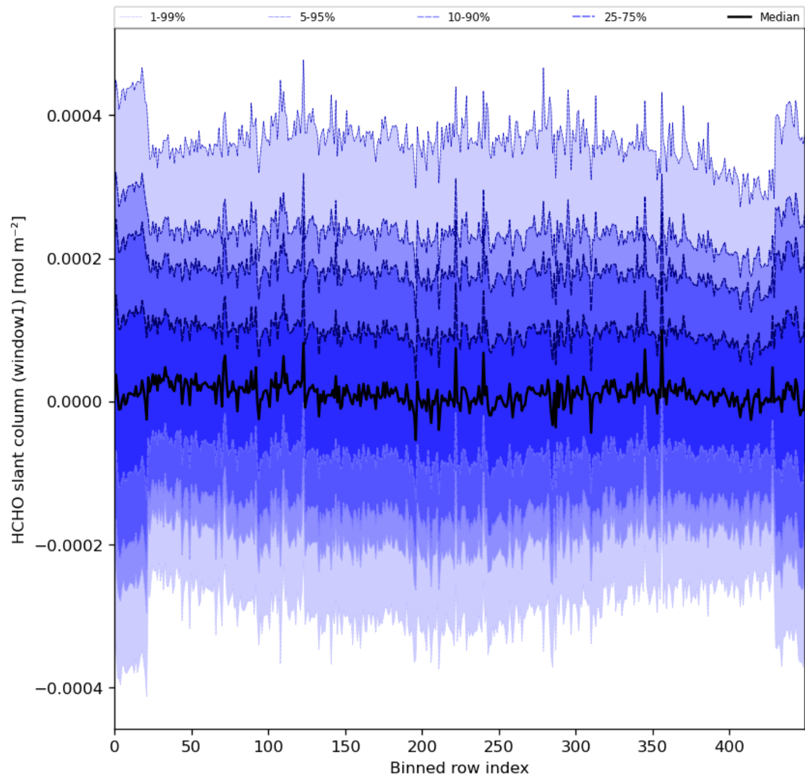
Figure 52: Along track statistics of “HCHO slant column (window1)” for 2024-05-18 to 2024-05-20
