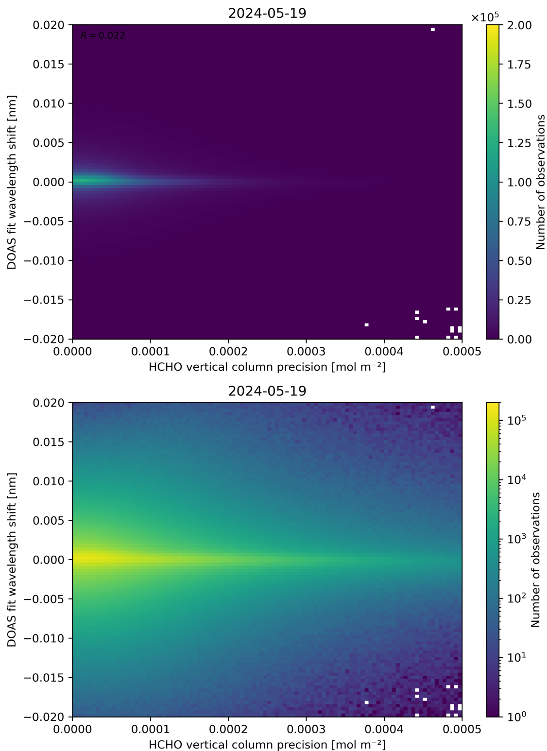
Figure 137: Scatter density plot of “HCHO vertical column precision” against “DOAS fit wavelength shift” for 2024-05-18 to 2024-05-20.
