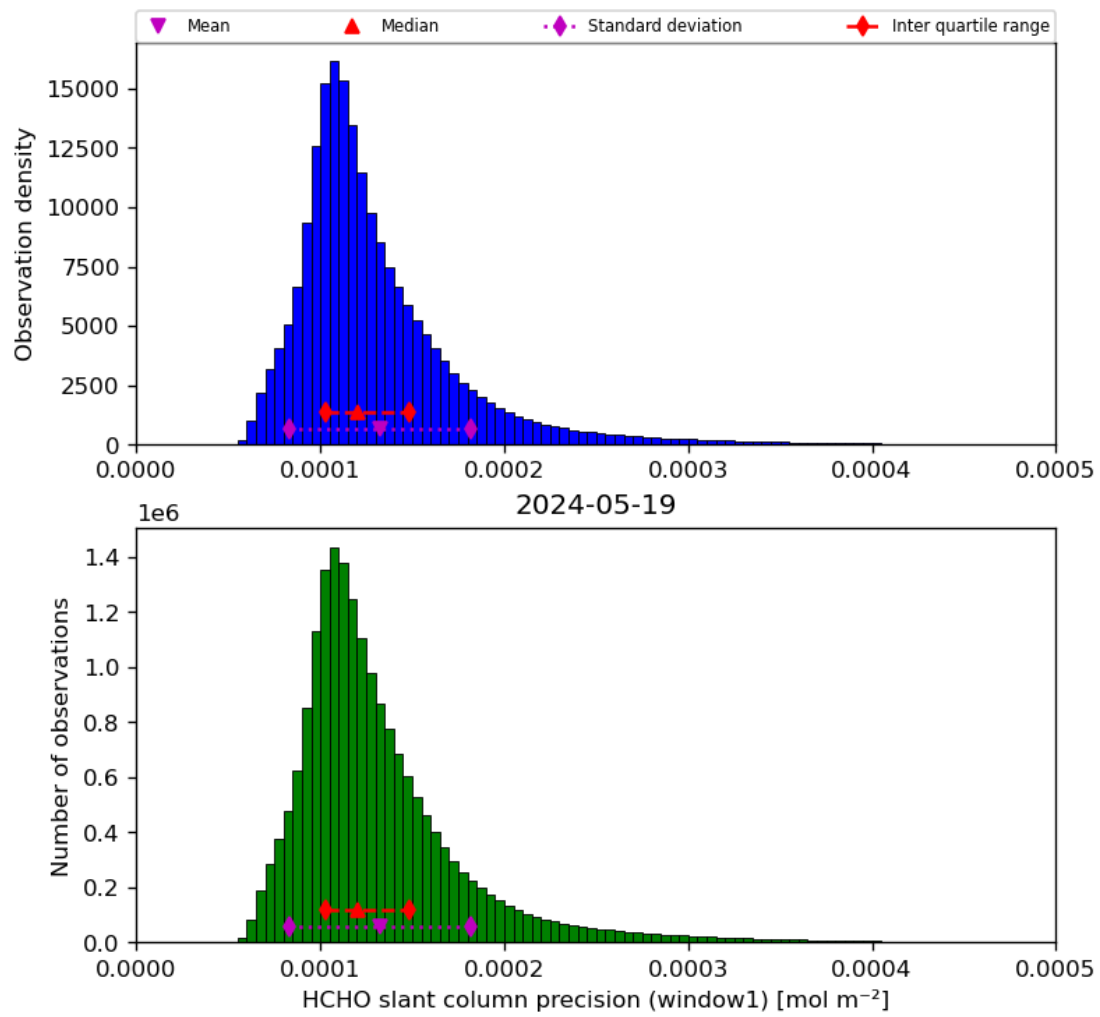
Figure 39: Histogram of “HCHO slant column precision (window1)” for 2024-05-18 to 2024-05-20
