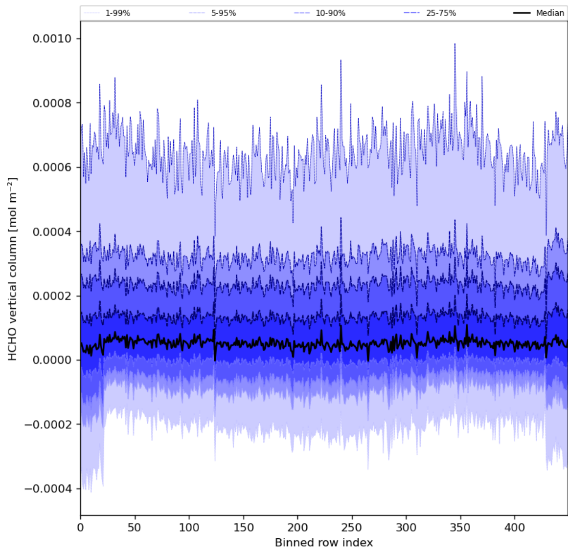
Figure 49: Along track statistics of “HCHO vertical column” for 2024-05-18 to 2024-05-20
