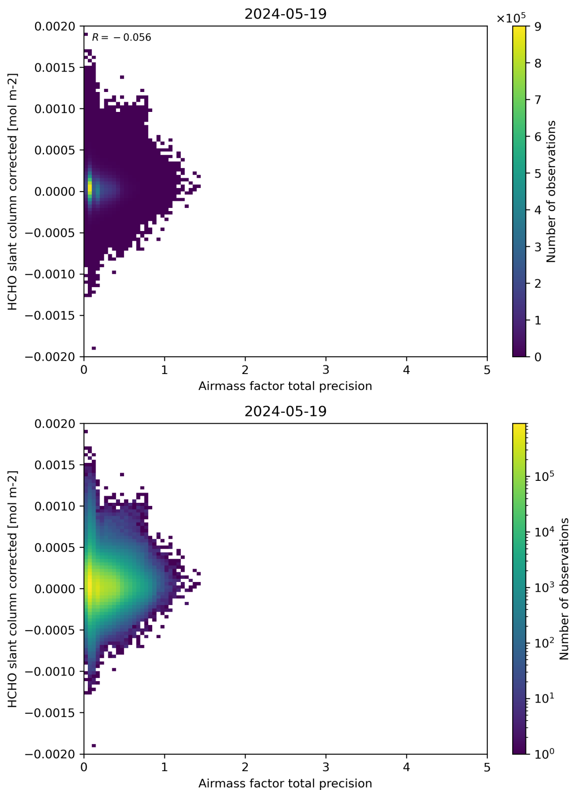
Figure 109: Scatter density plot of “Airmass factor total precision” against “HCHO slant column corrected” for 2024-05-18 to 2024-05-20.
