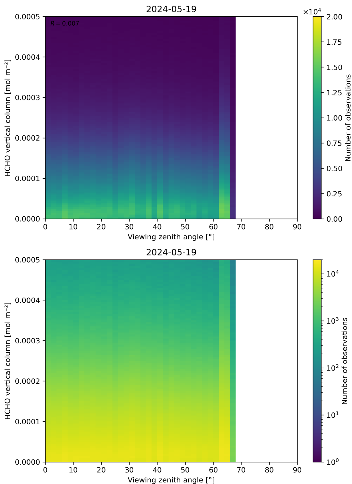
Figure 192: Scatter density plot of “Viewing zenith angle” against “HCHO vertical column” for 2024-05-18 to 2024-05-20.
