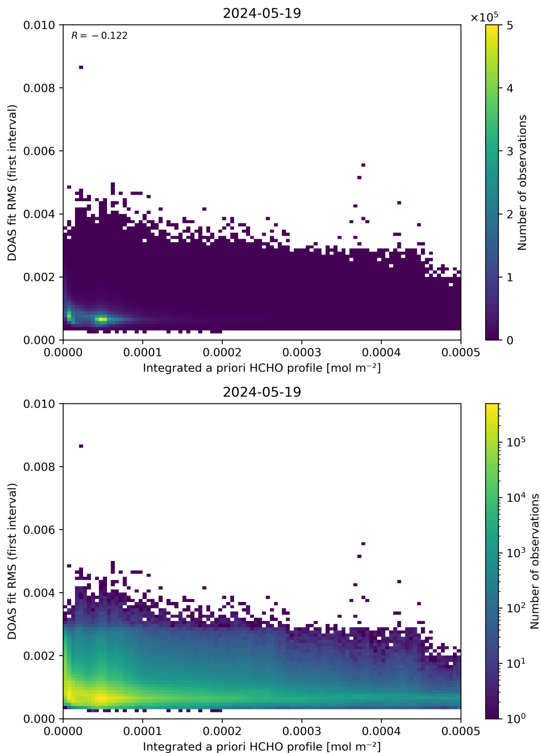
Figure 148: Scatter density plot of “Integrated a priori HCHO profile” against “DOAS fit RMS (first interval)” for 2024-05-18 to 2024-05-20.
