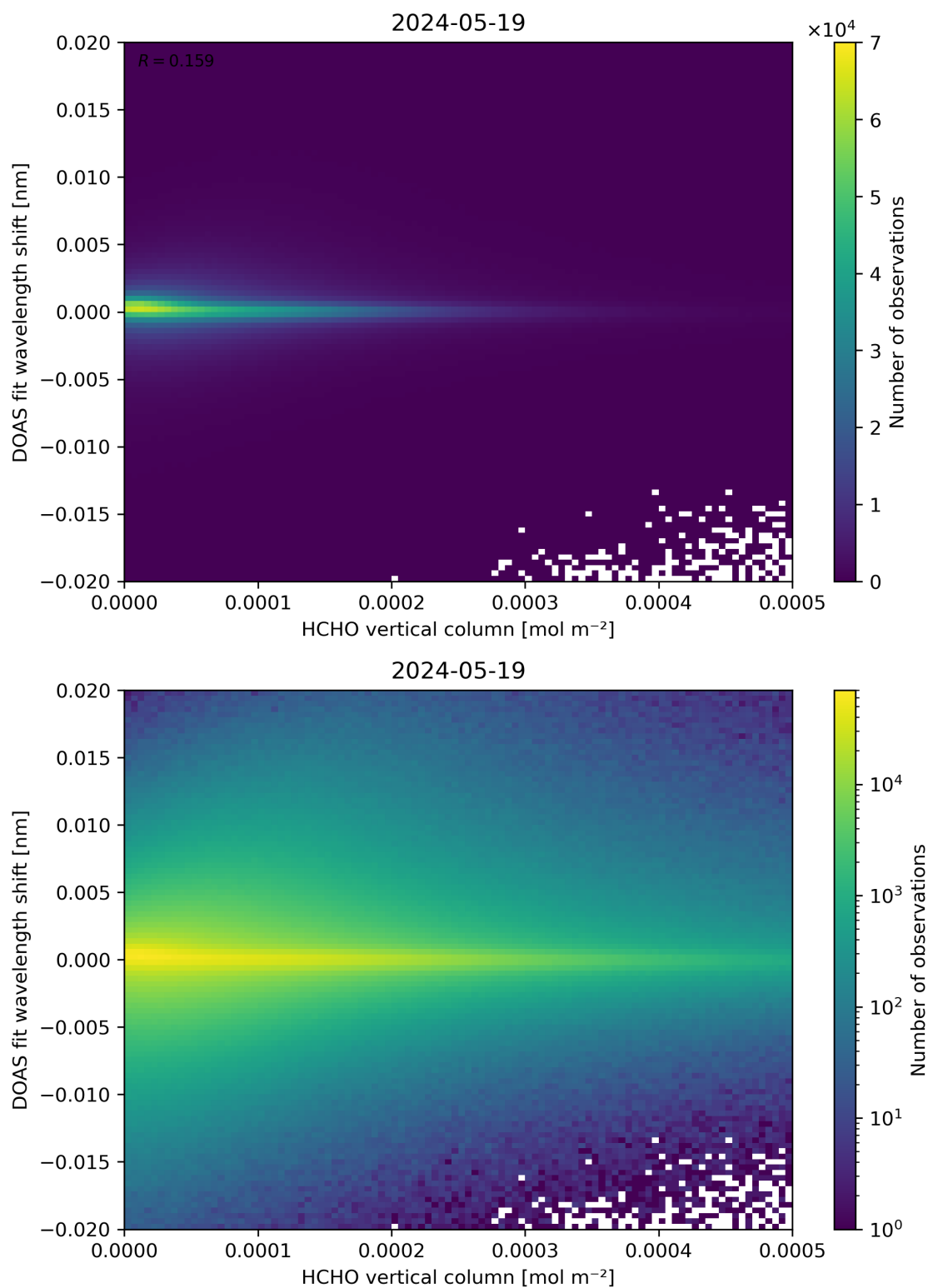
Figure 124: Scatter density plot of “HCHO vertical column” against “DOAS fit wavelength shift” for 2024-05-18 to 2024-05-20.
