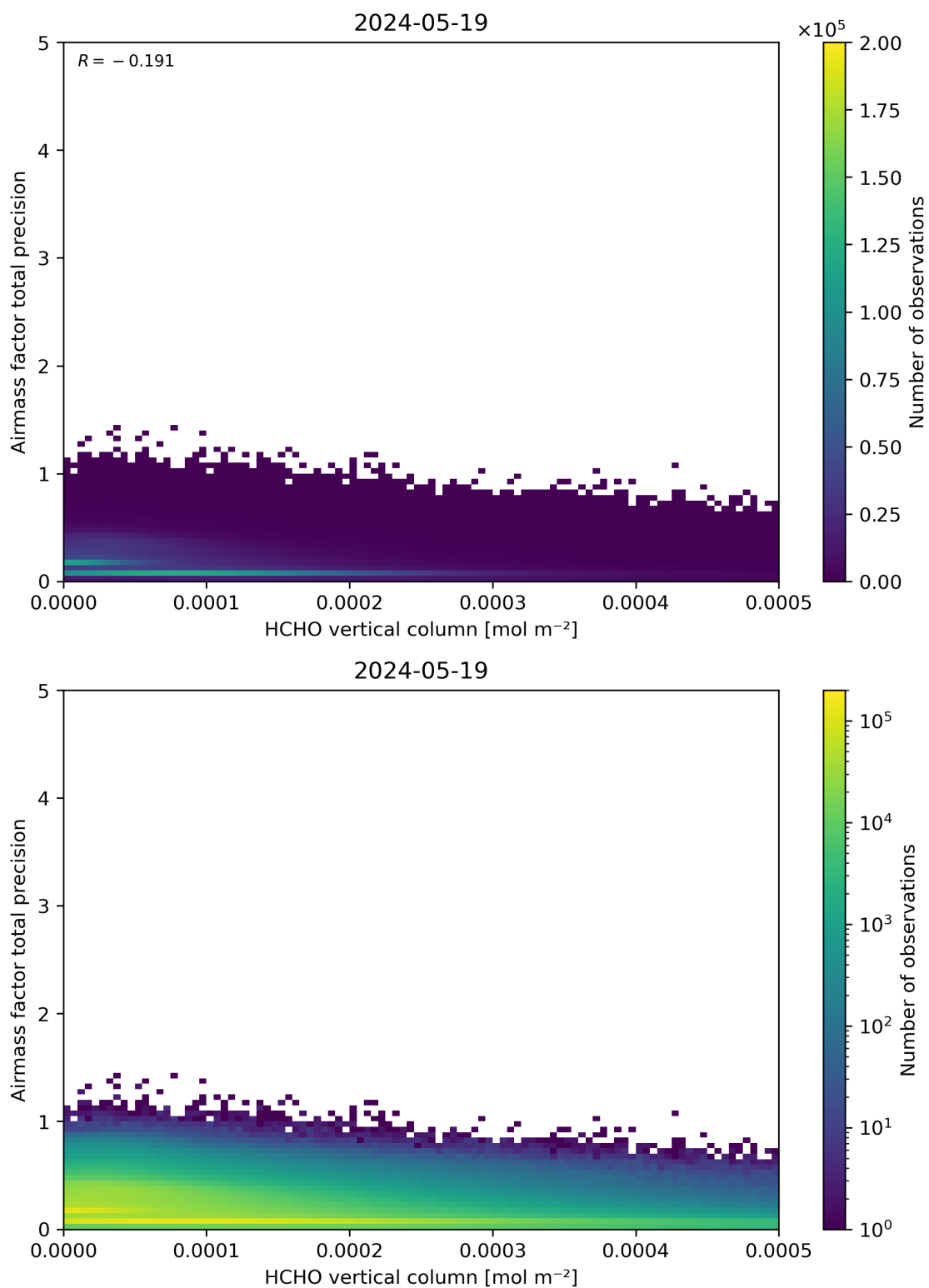
Figure 132: Scatter density plot of “HCHO vertical column” against “Airmass factor total precision” for 2024-05-18 to 2024-05-20.
