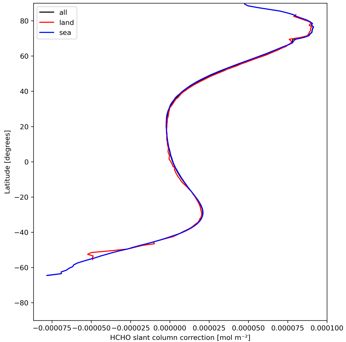
Figure 33: Zonal average of “HCHO slant column correction” for 2024-05-18 to 2024-05-20.
