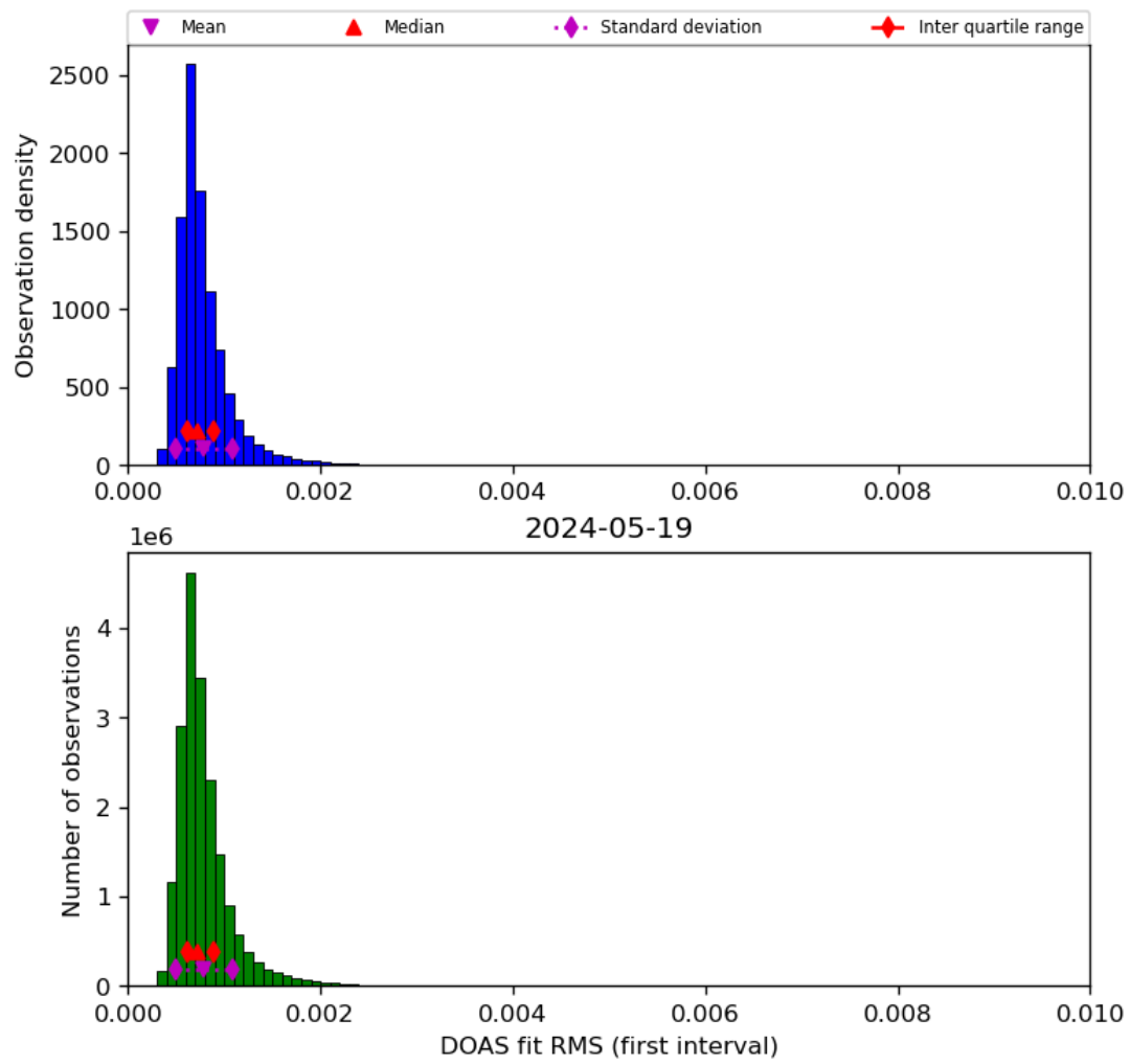
Figure 46: Histogram of “DOAS fit RMS (first interval)” for 2024-05-18 to 2024-05-20
