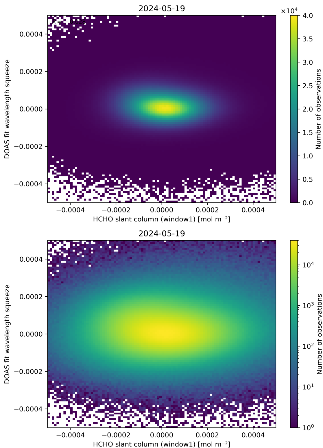
Figure 80: Scatter density plot of “HCHO slant column (window1)” against “DOAS fit wavelength squeeze” for 2024-05-18 to 2024-05-20.
