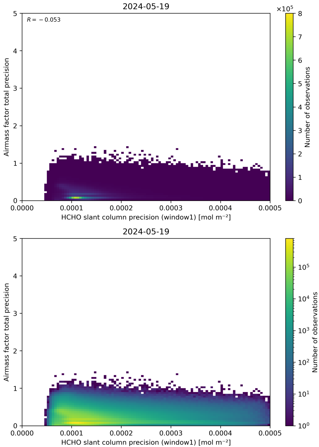
Figure 95: Scatter density plot of “HCHO slant column precision (window1)” against “Airmass factor total precision” for 2024-05-18 to 2024-05-20.
