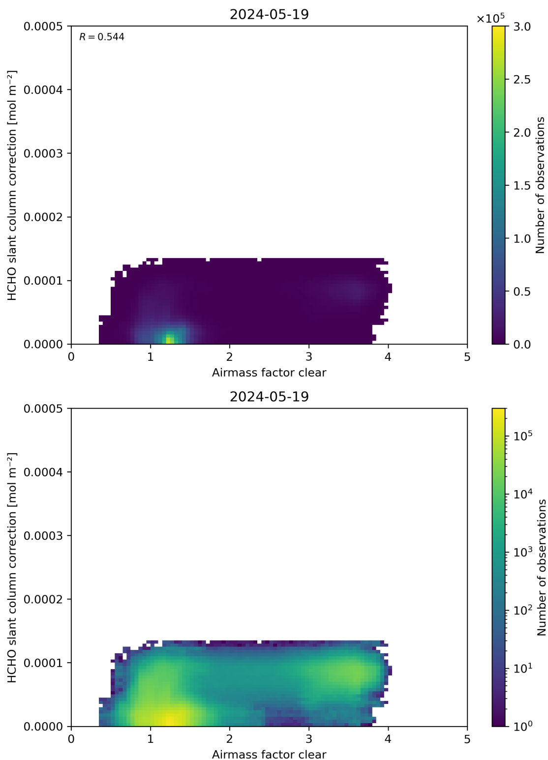
Figure 75: Scatter density plot of “Airmass factor clear” against “HCHO slant column correction” for 2024-05-18 to 2024-05-20.
