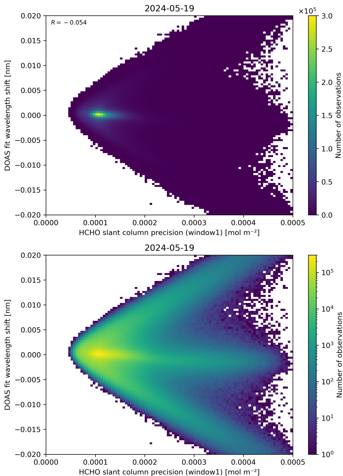
Figure 89: Scatter density plot of “HCHO slant column precision (window1)” against “DOAS fit wavelength shift” for 2024-05-18 to 2024-05-20.
