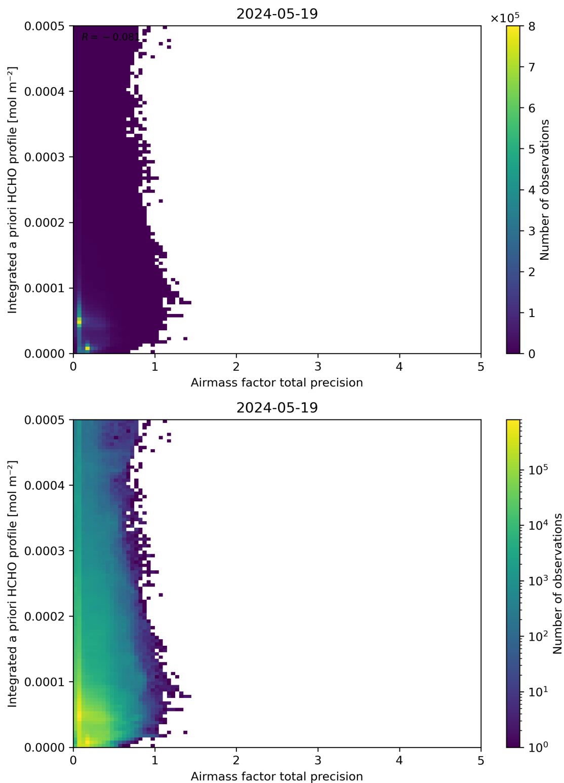
Figure 111: Scatter density plot of “Airmass factor total precision” against “Integrated a priori HCHO profile” for 2024-05-18 to 2024-05-20.
