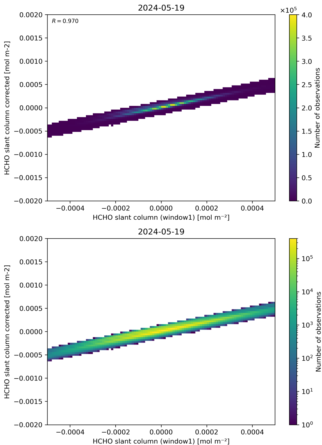
Figure 82: Scatter density plot of “HCHO slant column (window1)” against “HCHO slant column corrected” for 2024-05-18 to 2024-05-20.
