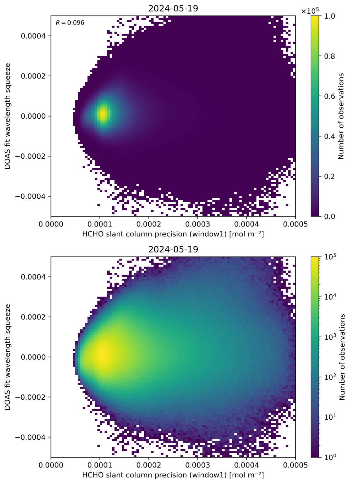
Figure 90: Scatter density plot of “HCHO slant column precision (window1)” against “DOAS fit wavelength squeeze” for 2024-05-18 to 2024-05-20.
