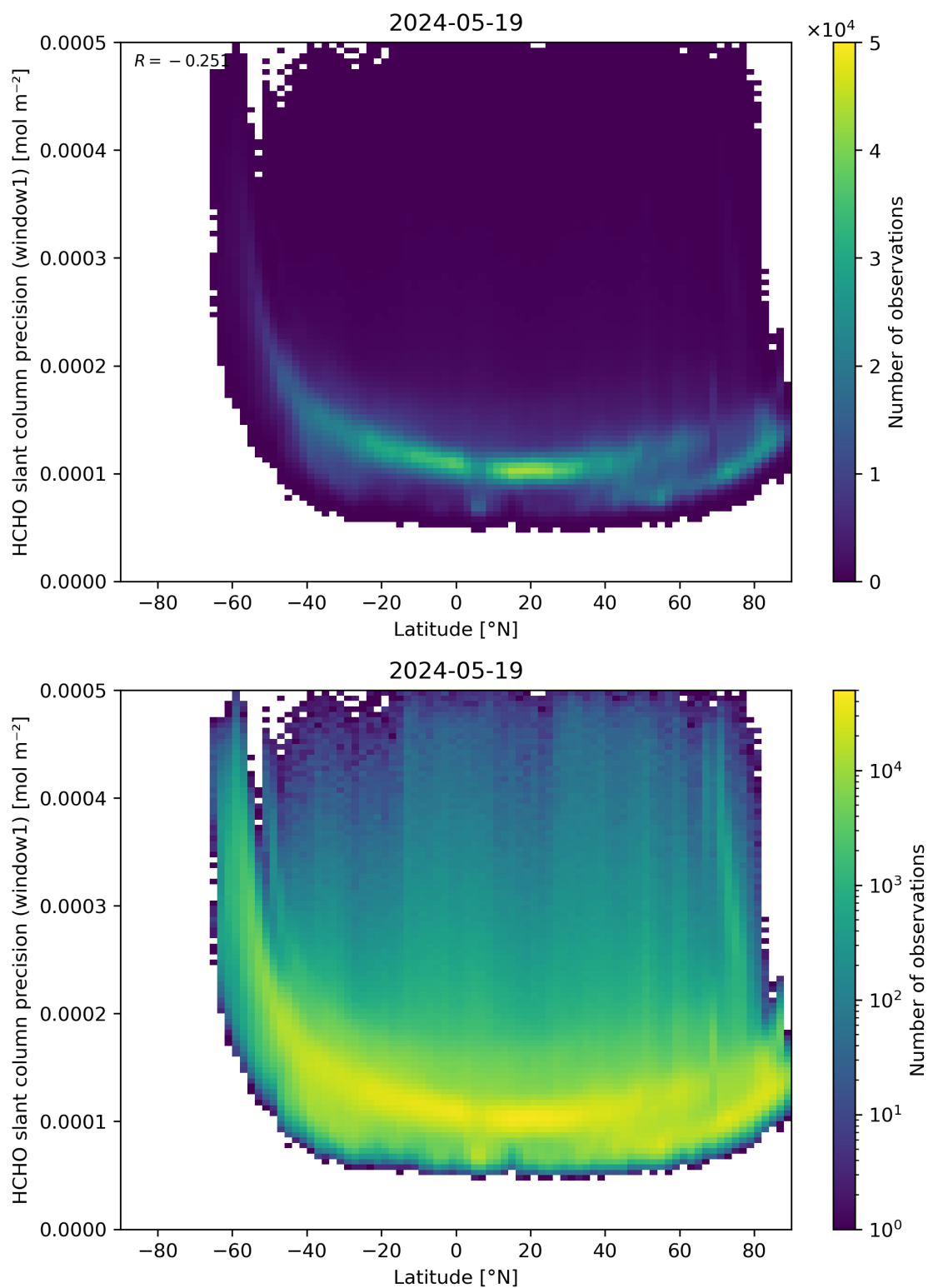
Figure 160: Scatter density plot of “Latitude” against “HCHO slant column precision (window1)” for 2024-05-18 to 2024-05-20.
