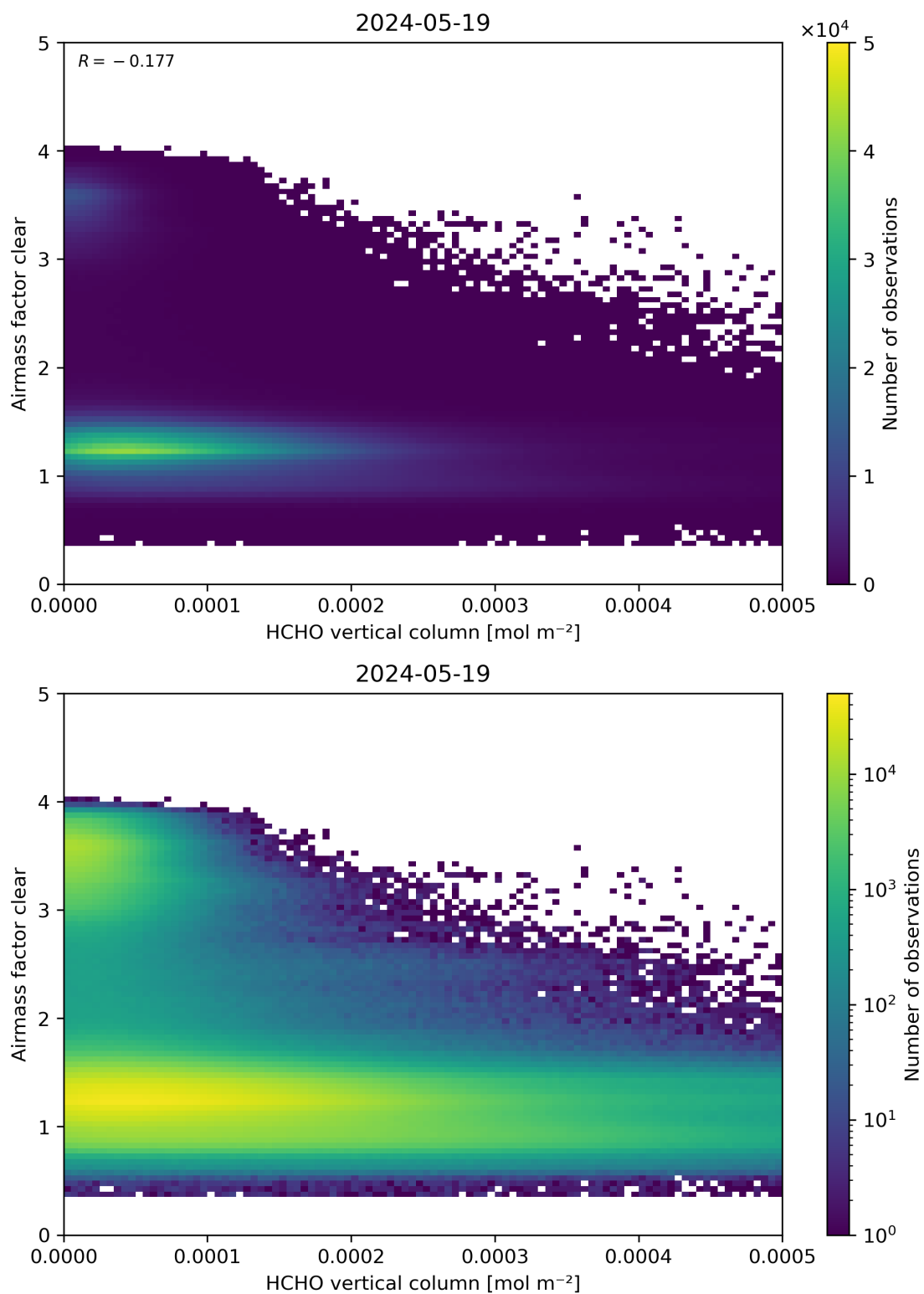
Figure 126: Scatter density plot of “HCHO vertical column” against “Airmass factor clear” for 2024-05-18 to 2024-05-20.
