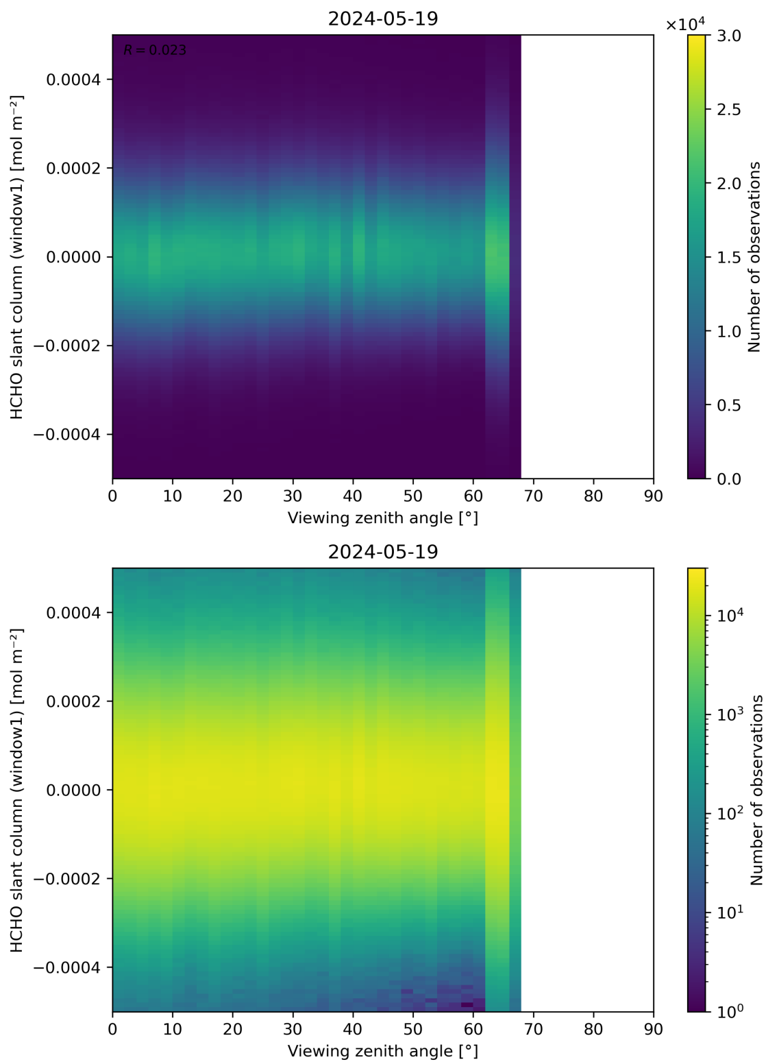
Figure 188: Scatter density plot of “Viewing zenith angle” against “HCHO slant column (window1)” for 2024-05-18 to 2024-05-20.
