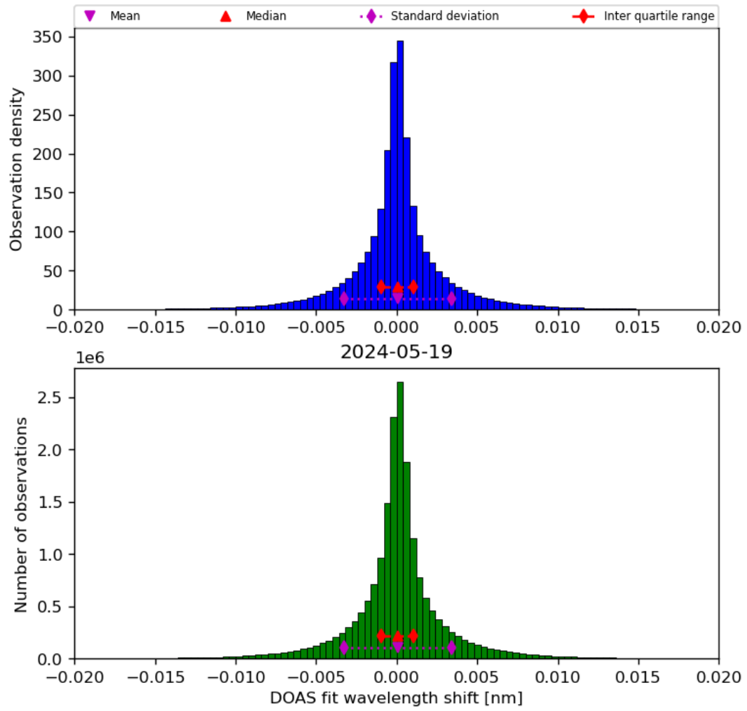
Figure 44: Histogram of “DOAS fit wavelength shift” for 2024-05-18 to 2024-05-20
