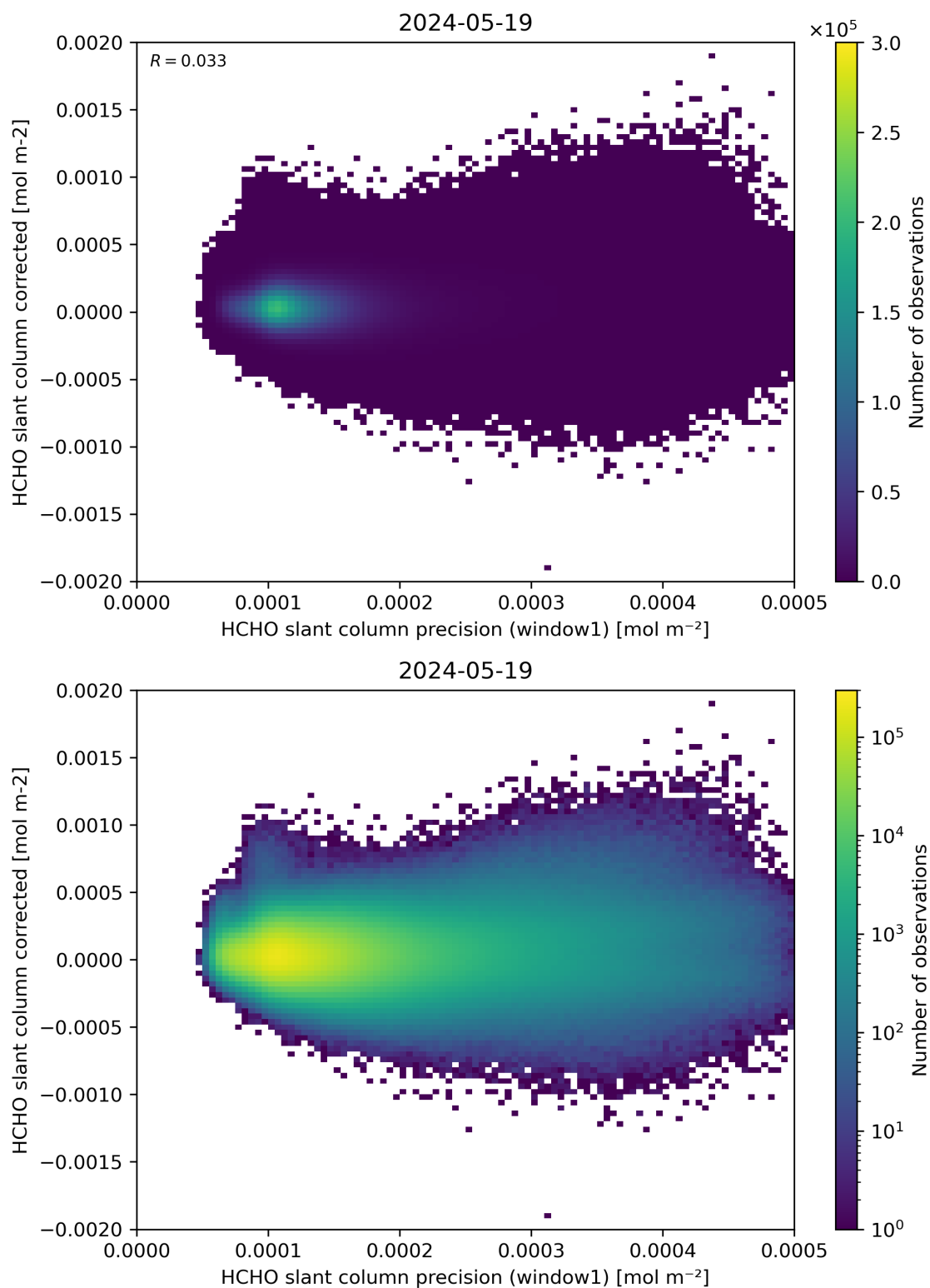
Figure 92: Scatter density plot of “HCHO slant column precision (window1)” against “HCHO slant column corrected” for 2024-05-18 to 2024-05-20.
