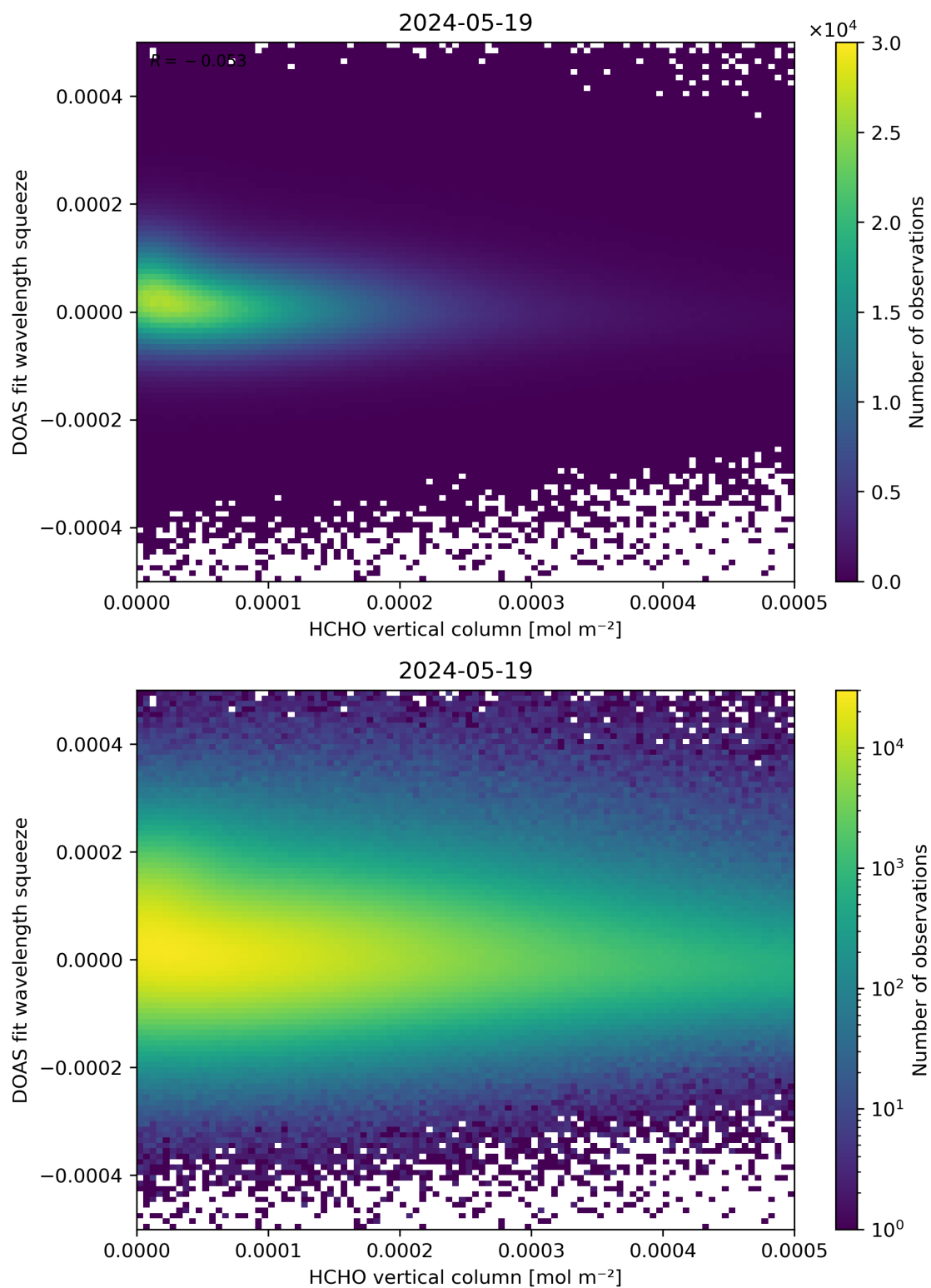
Figure 125: Scatter density plot of “HCHO vertical column” against “DOAS fit wavelength squeeze” for 2024-05-18 to 2024-05-20.
