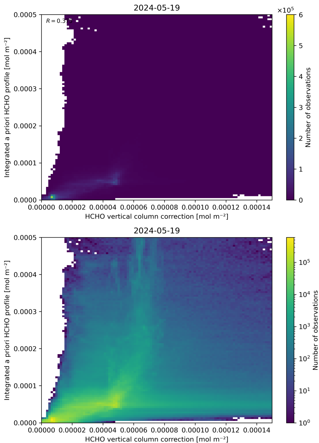
Figure 122: Scatter density plot of “HCHO vertical column correction” against “Integrated a priori HCHO profile” for 2024-05-18 to 2024-05-20.
