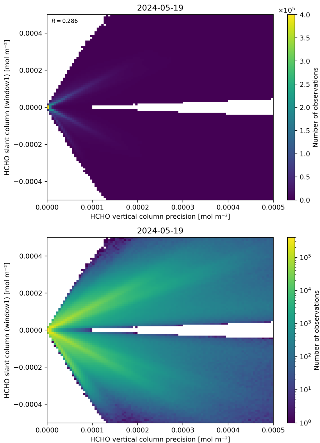
Figure 142: Scatter density plot of “HCHO vertical column precision” against “HCHO slant column (window1)” for 2024-05-18 to 2024-05-20.
