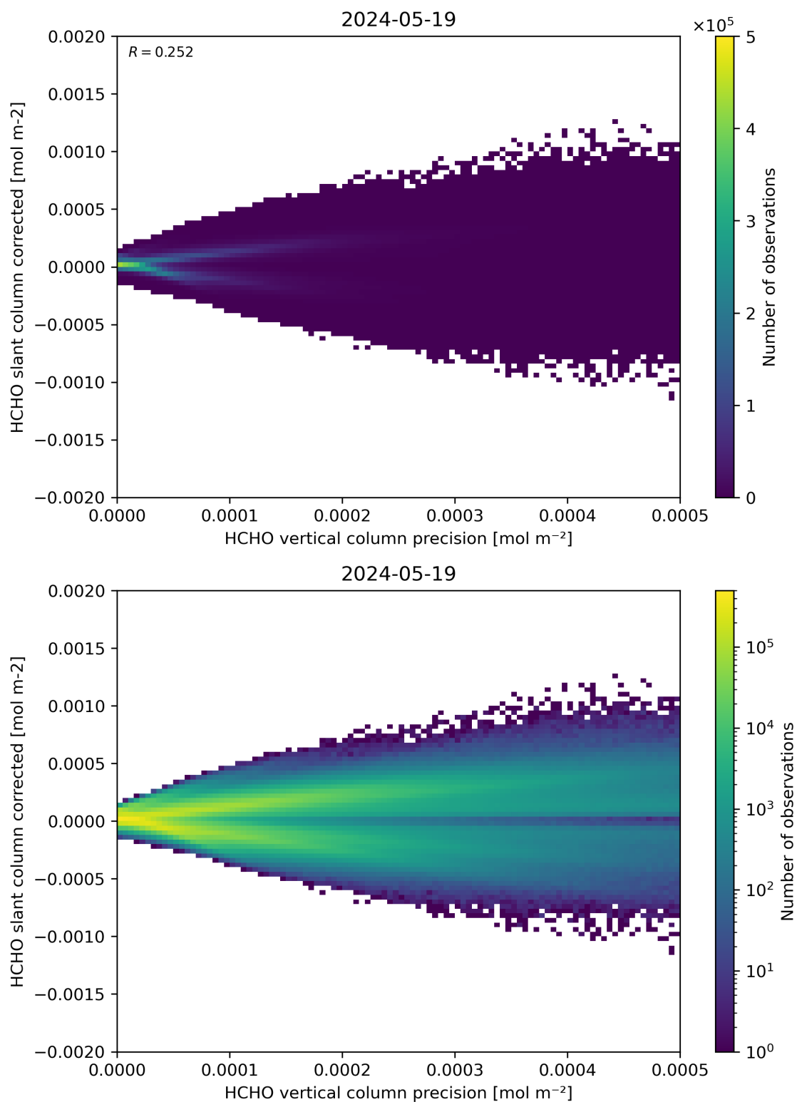
Figure 140: Scatter density plot of “HCHO vertical column precision” against “HCHO slant column corrected” for 2024-05-18 to 2024-05-20.
