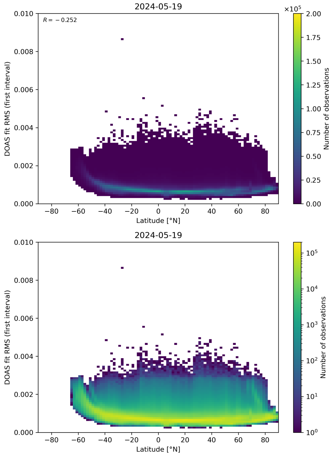
Figure 153: Scatter density plot of “Latitude” against “DOAS fit RMS (first interval)” for 2024-05-18 to 2024-05-20.
