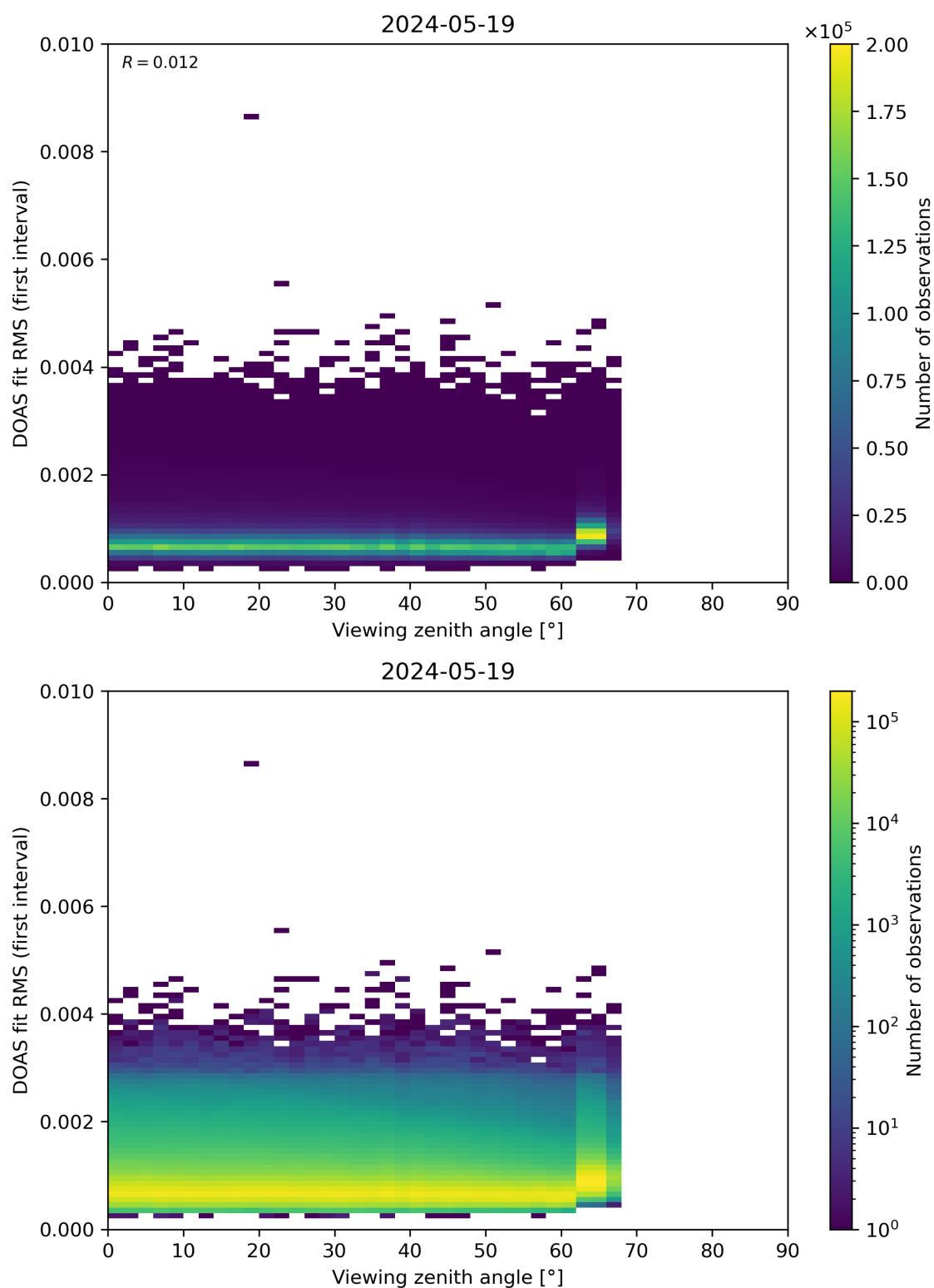
Figure 182: Scatter density plot of “Viewing zenith angle” against “DOAS fit RMS (first interval)” for 2024-05-18 to 2024-05-20.
