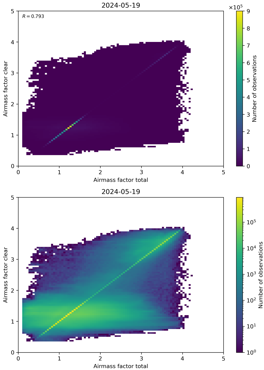
Figure 100: Scatter density plot of “Airmass factor total” against “Airmass factor clear” for 2024-05-18 to 2024-05-20.
