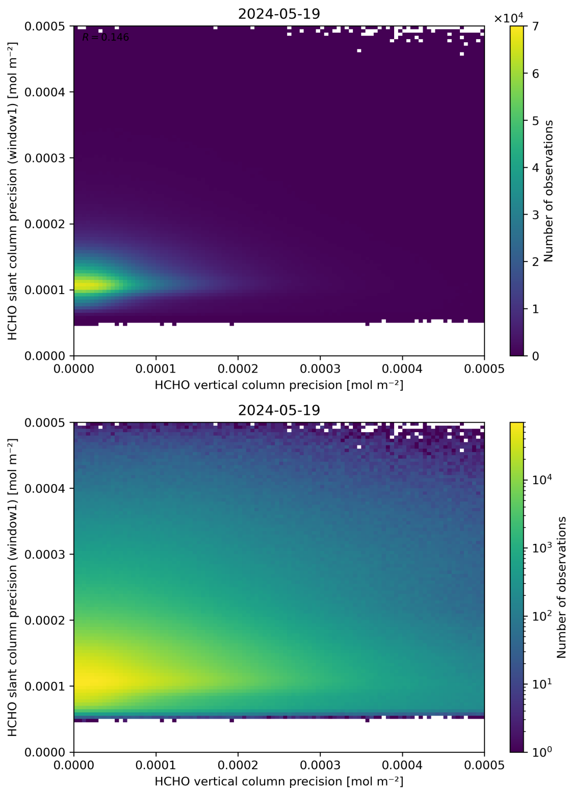
Figure 143: Scatter density plot of “HCHO vertical column precision” against “HCHO slant column precision (window1)” for 2024-05-18 to 2024-05-20.
