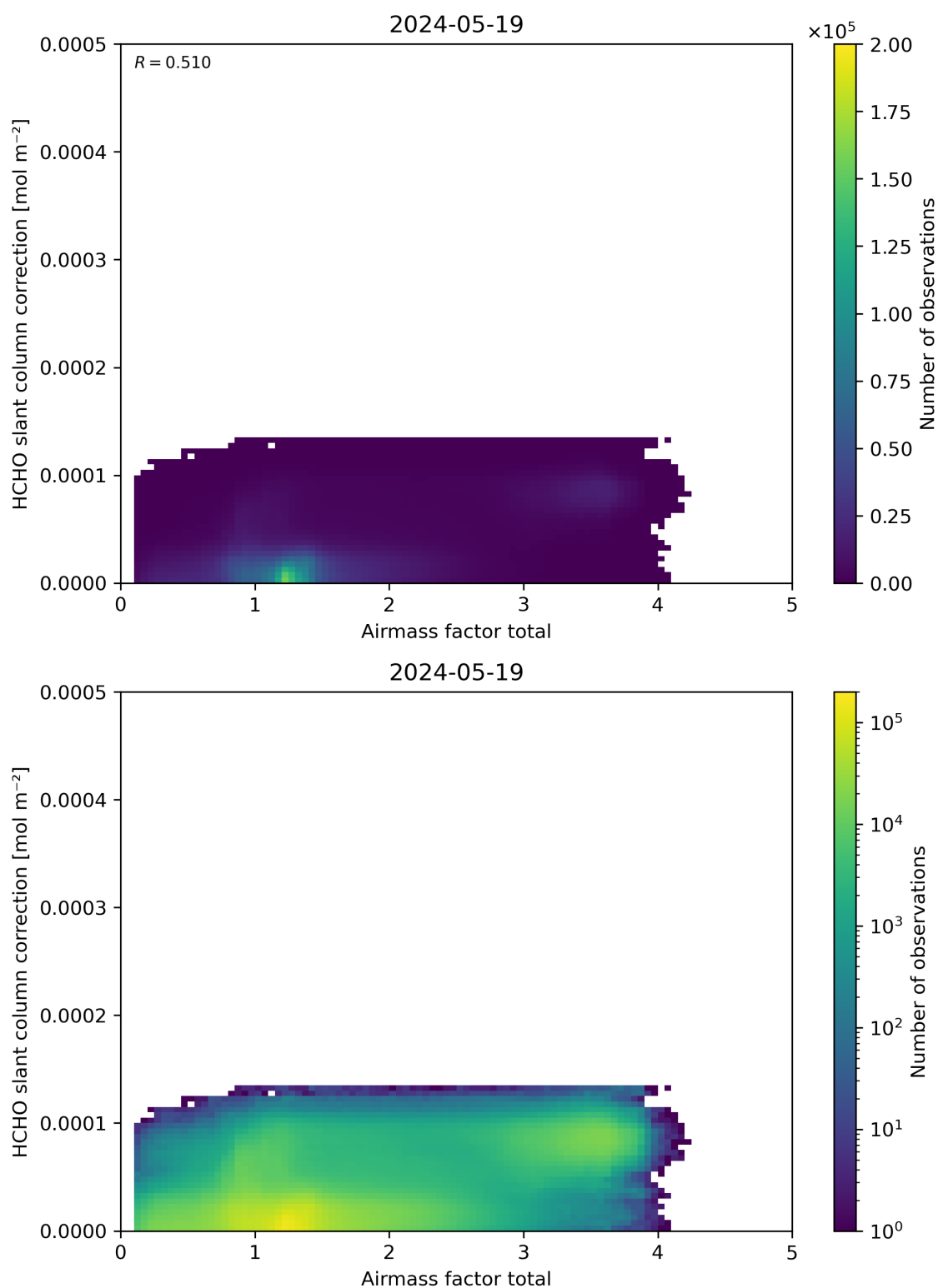
Figure 102: Scatter density plot of “Airmass factor total” against “HCHO slant column correction” for 2024-05-18 to 2024-05-20.
