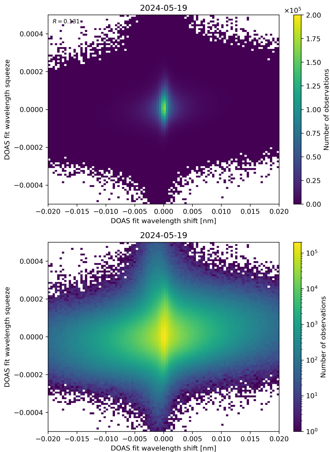
Figure 65: Scatter density plot of “DOAS fit wavelength shift” against “DOAS fit wavelength squeeze” for 2024-05-18 to 2024-05-20.
