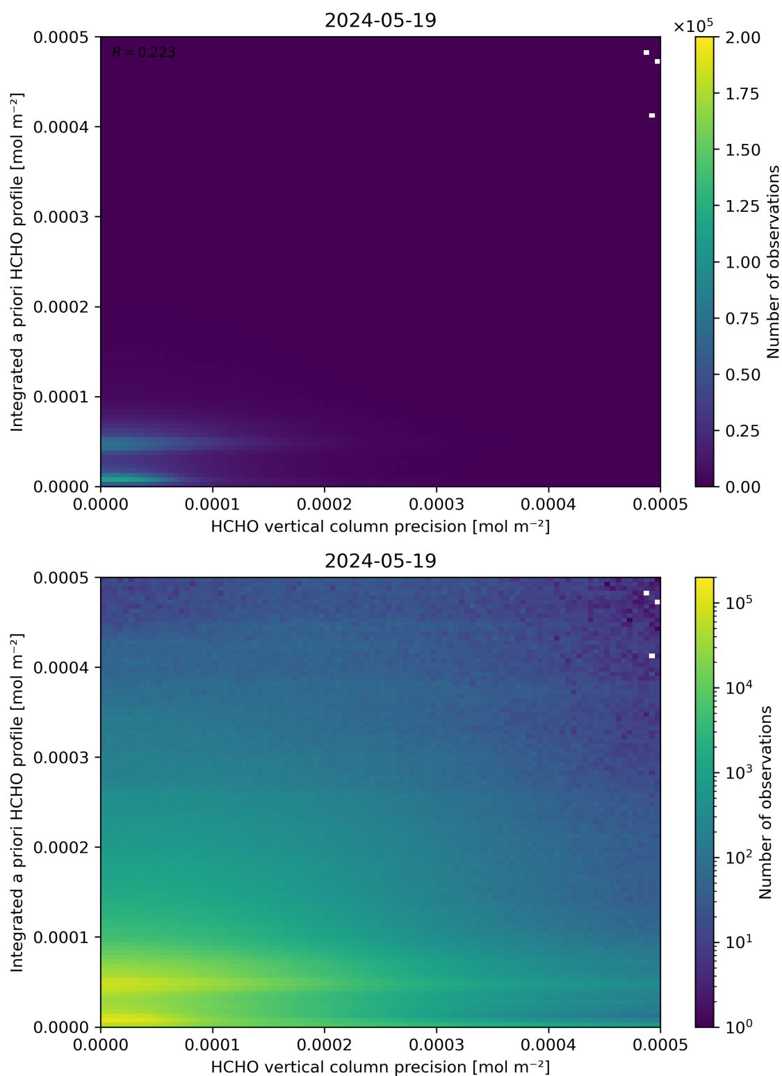
Figure 147: Scatter density plot of “HCHO vertical column precision” against “Integrated a priori HCHO profile” for 2024-05-18 to 2024-05-20.
