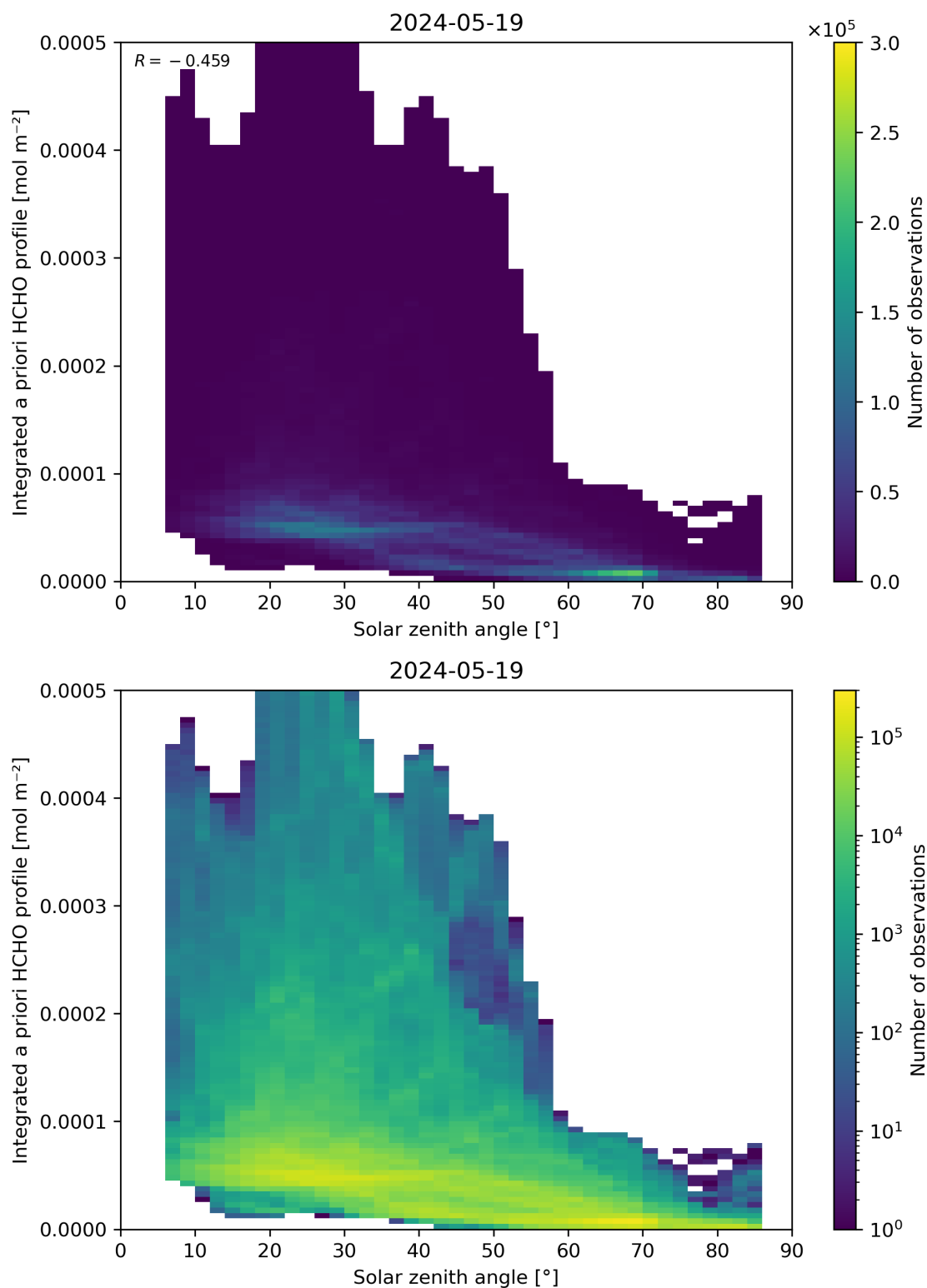
Figure 180: Scatter density plot of “Solar zenith angle” against “Integrated a priori HCHO profile” for 2024-05-18 to 2024-05-20.
