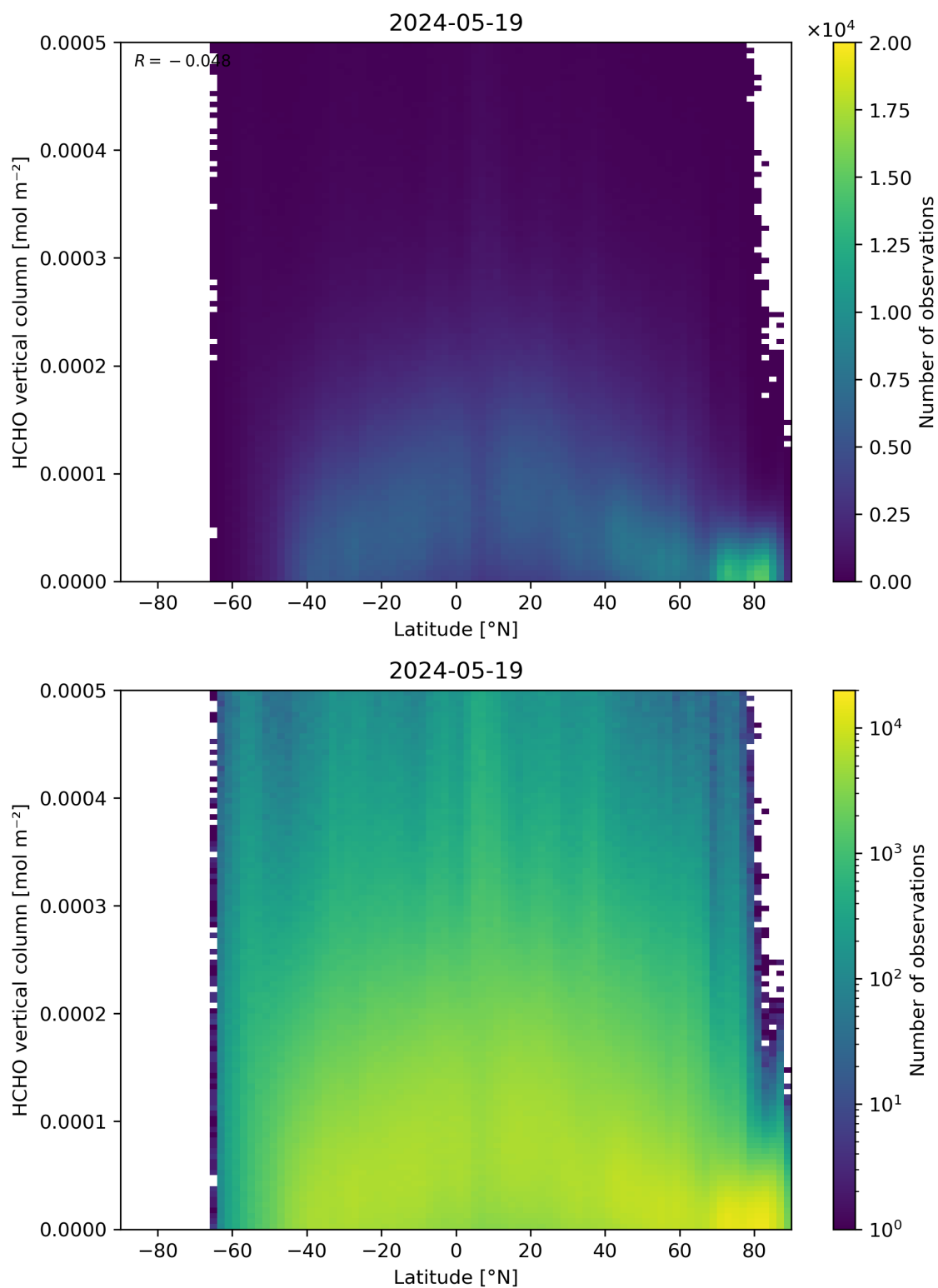
Figure 163: Scatter density plot of “Latitude” against “HCHO vertical column” for 2024-05-18 to 2024-05-20.
