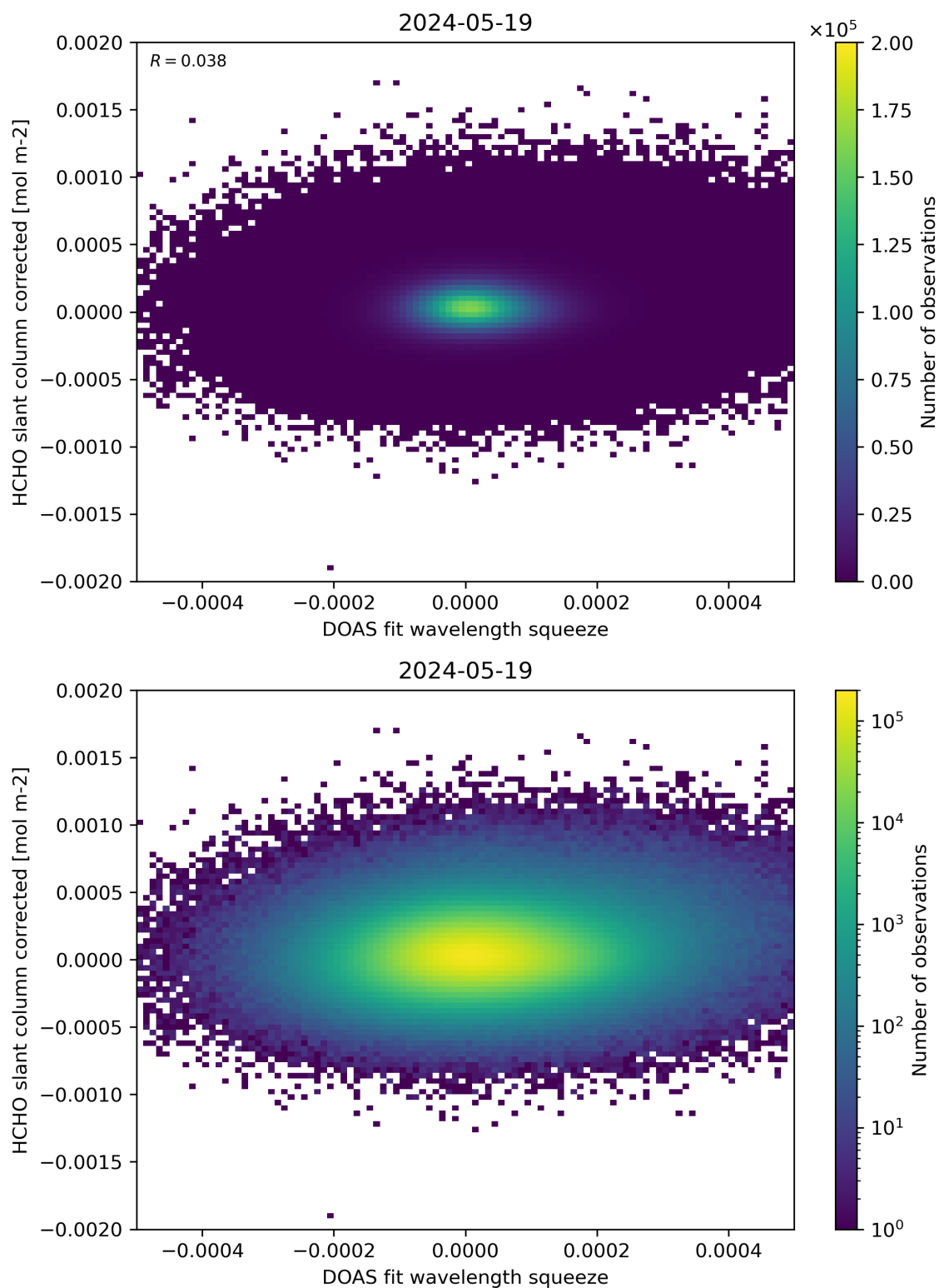
Figure 69: Scatter density plot of “DOAS fit wavelength squeeze” against “HCHO slant column corrected” for 2024-05-18 to 2024-05-20.
