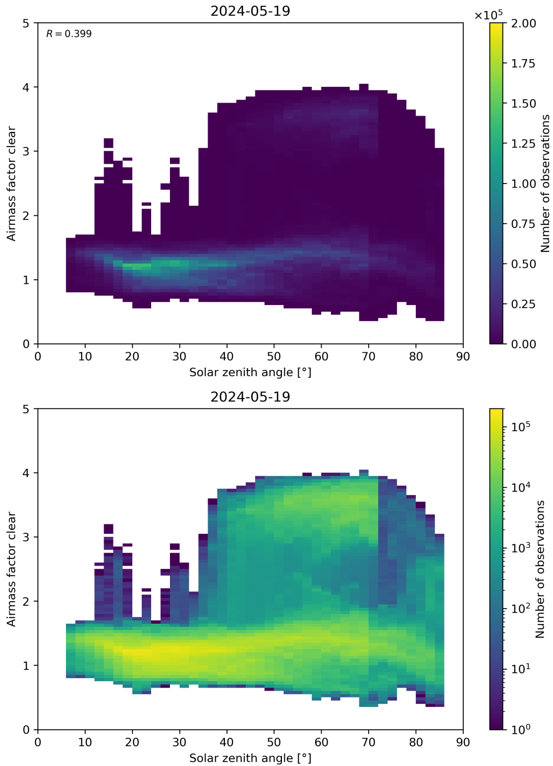
Figure 170: Scatter density plot of “Solar zenith angle” against “Airmass factor clear” for 2024-05-18 to 2024-05-20.
