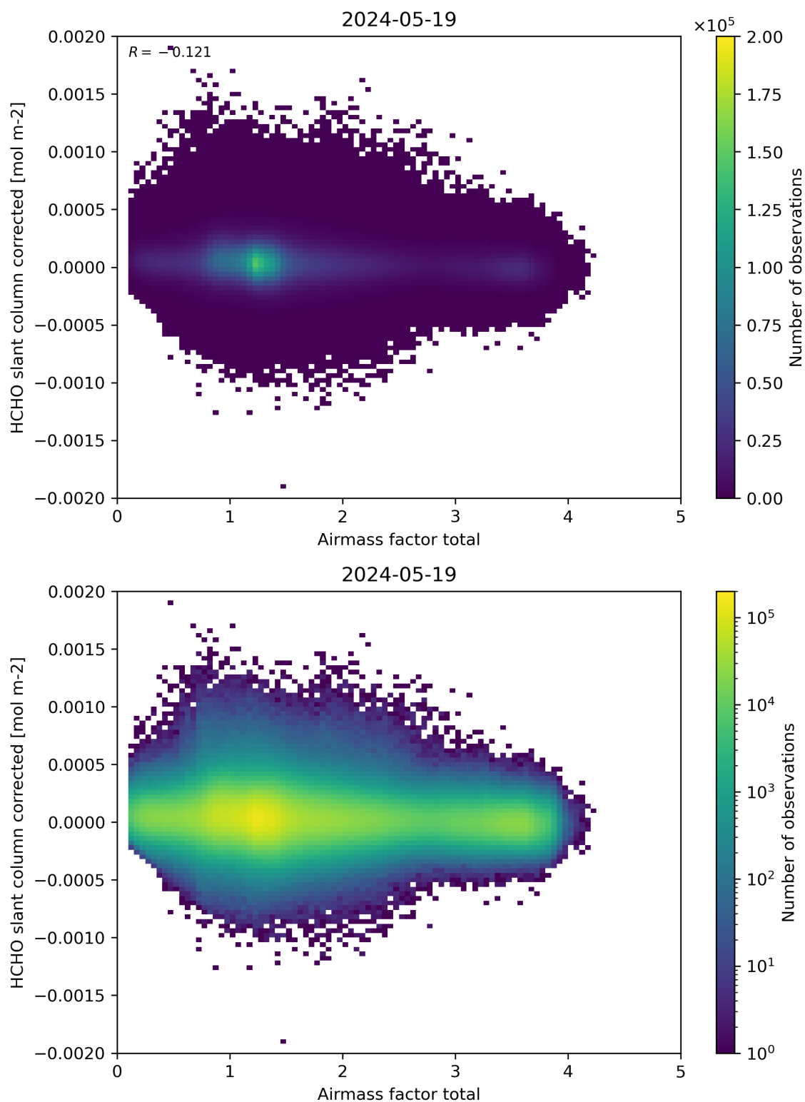
Figure 101: Scatter density plot of “Airmass factor total” against “HCHO slant column corrected” for 2024-05-18 to 2024-05-20.
