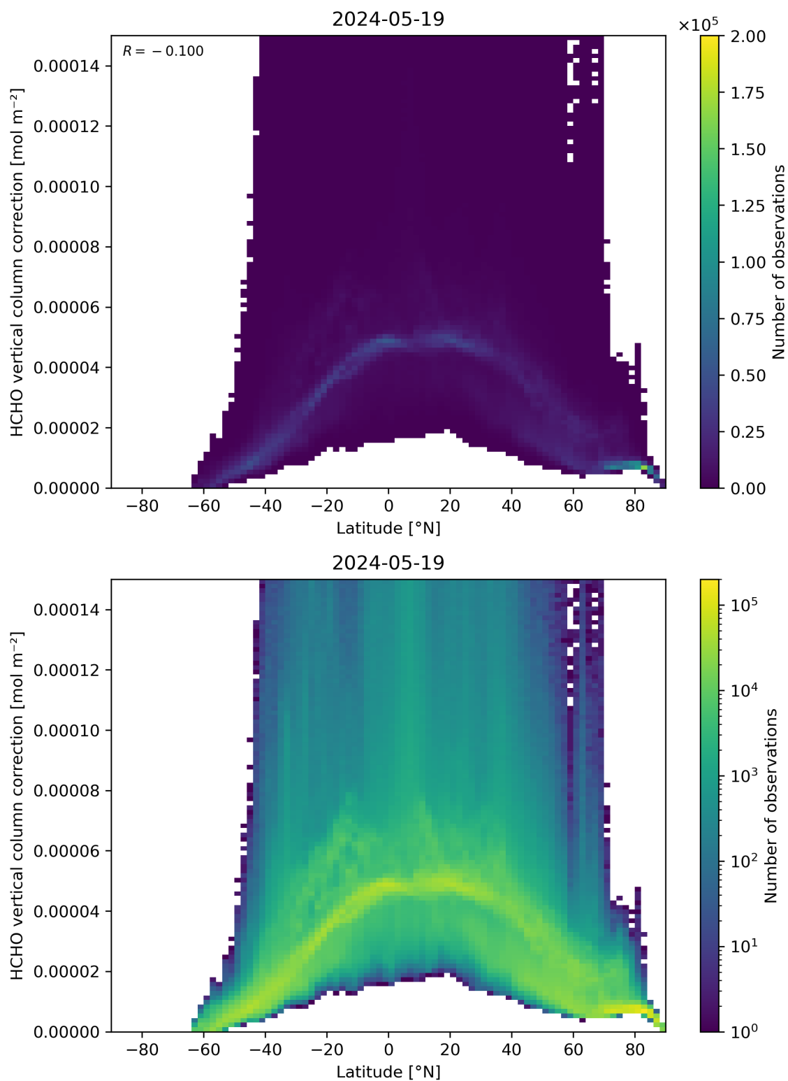
Figure 164: Scatter density plot of “Latitude” against “HCHO vertical column correction” for 2024-05-18 to 2024-05-20.
