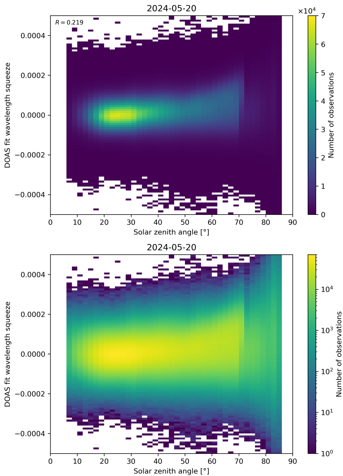
Figure 169: Scatter density plot of “Solar zenith angle” against “DOAS fit wavelength squeeze” for 2024-05-19 to 2024-05-21.
