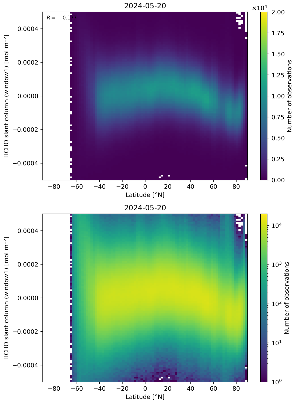
Figure 159: Scatter density plot of “Latitude” against “HCHO slant column (window1)” for 2024-05-19 to 2024-05-21.
