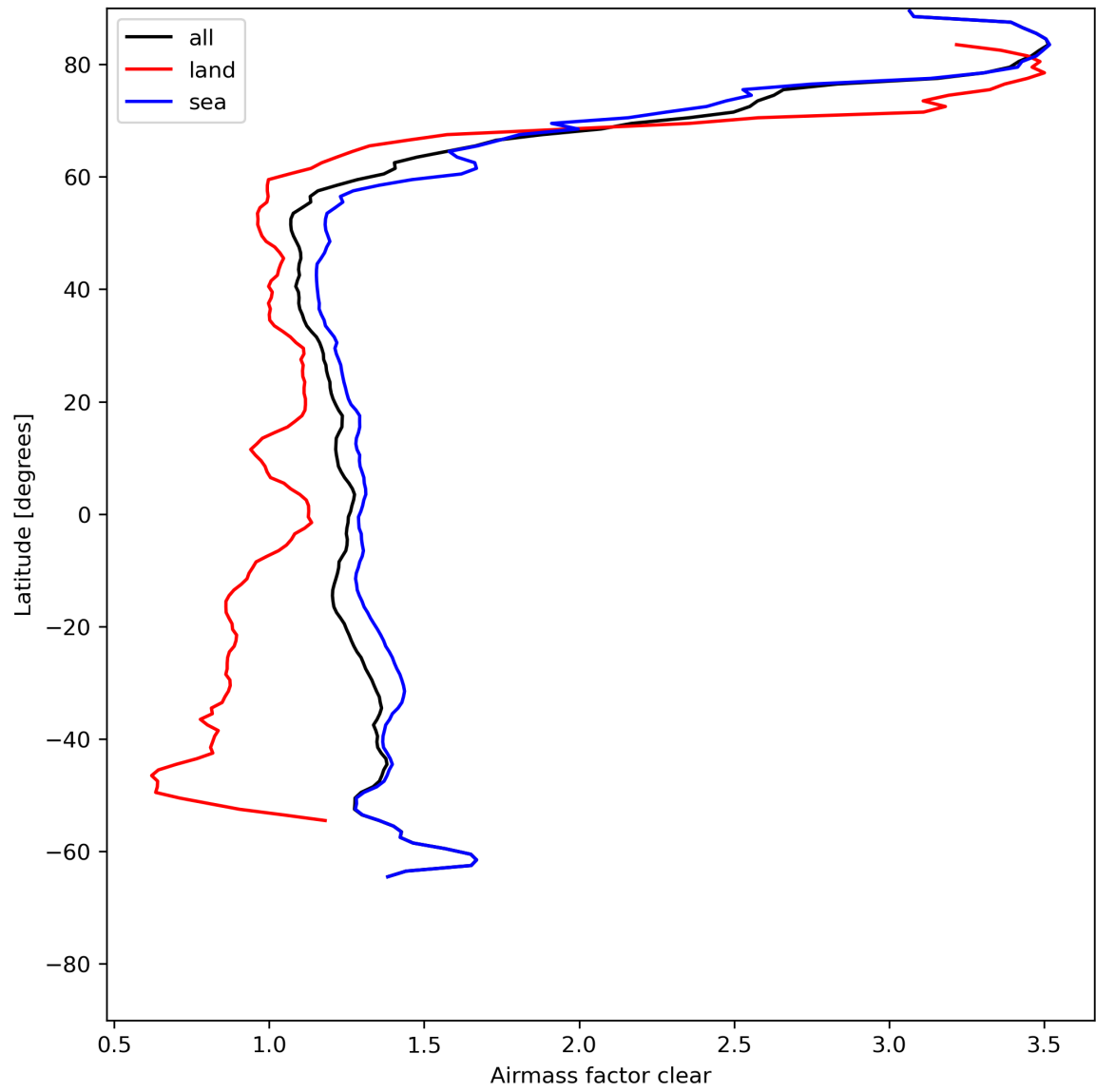
Figure 28: Zonal average of “Airmass factor clear” for 2024-05-19 to 2024-05-21.
