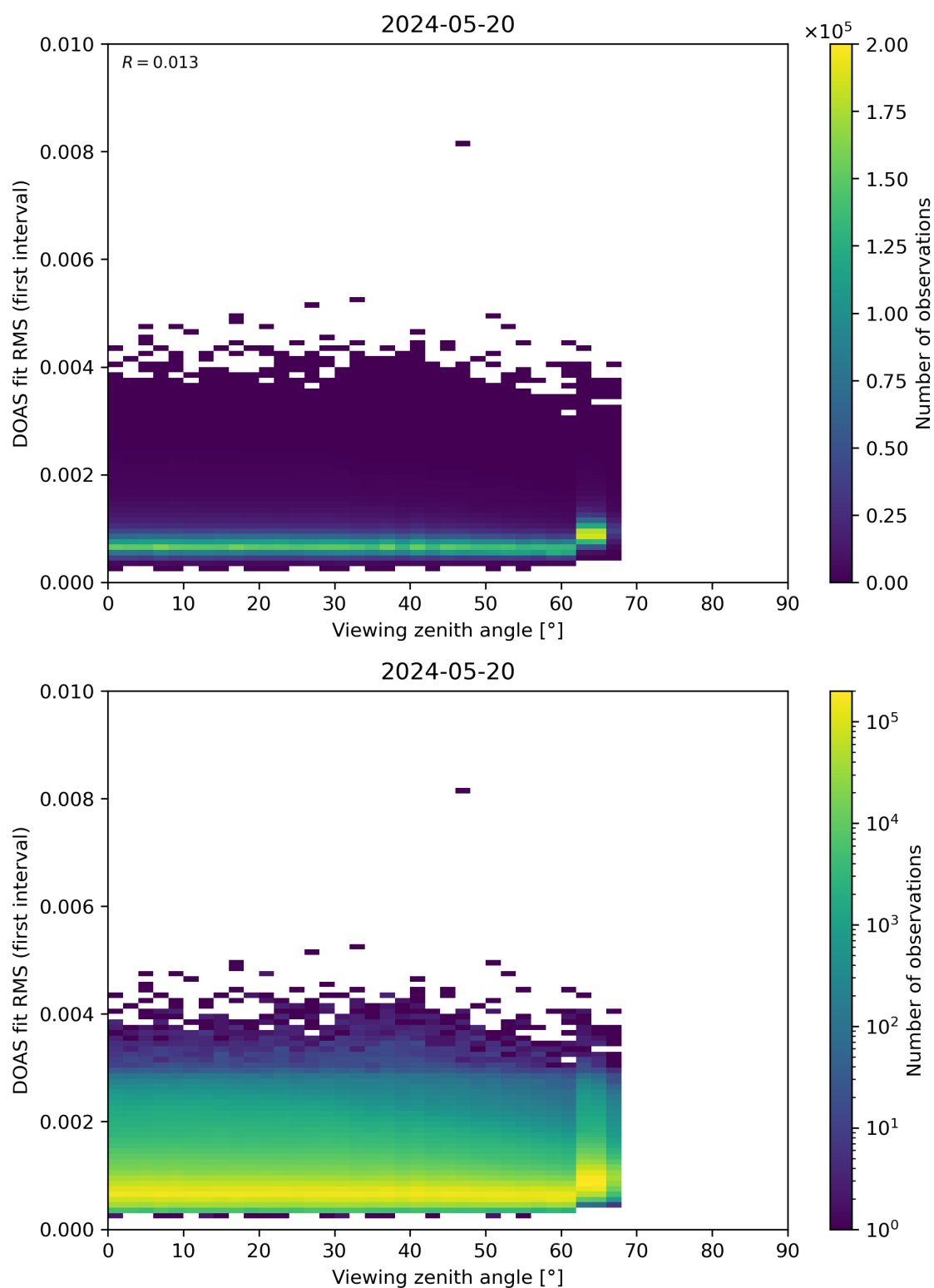
Figure 182: Scatter density plot of “Viewing zenith angle” against “DOAS fit RMS (first interval)” for 2024-05-19 to 2024-05-21.
