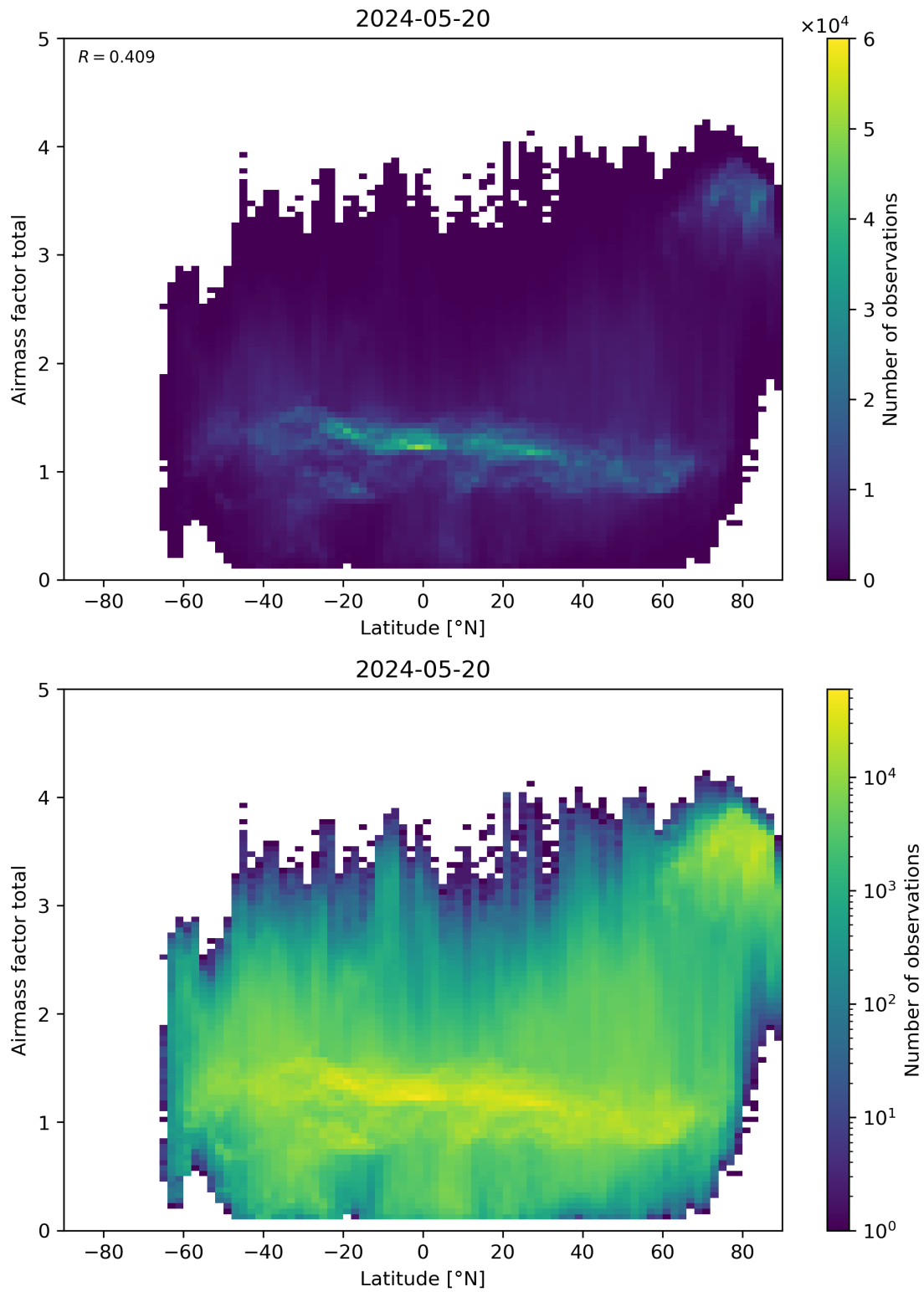
Figure 161: Scatter density plot of “Latitude” against “Airmass factor total” for 2024-05-19 to 2024-05-21.
