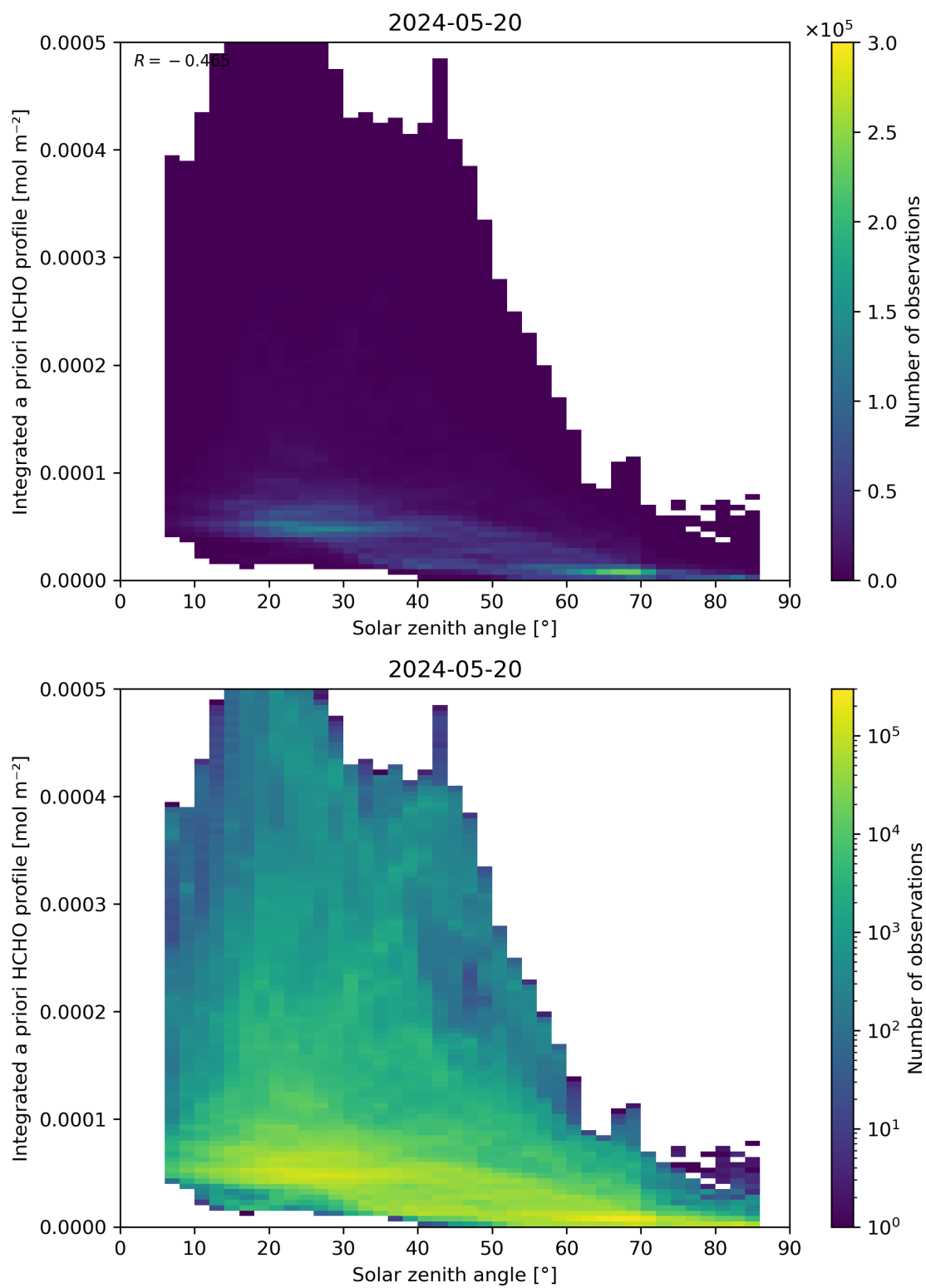
Figure 180: Scatter density plot of “Solar zenith angle” against “Integrated a priori HCHO profile” for 2024-05-19 to 2024-05-21.
