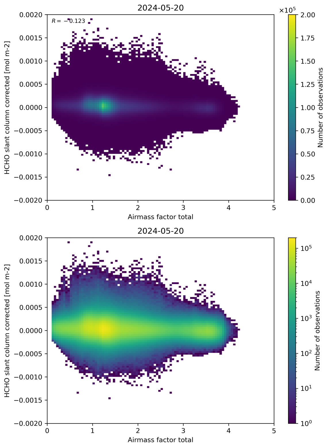
Figure 101: Scatter density plot of “Airmass factor total” against “HCHO slant column corrected” for 2024-05-19 to 2024-05-21.
