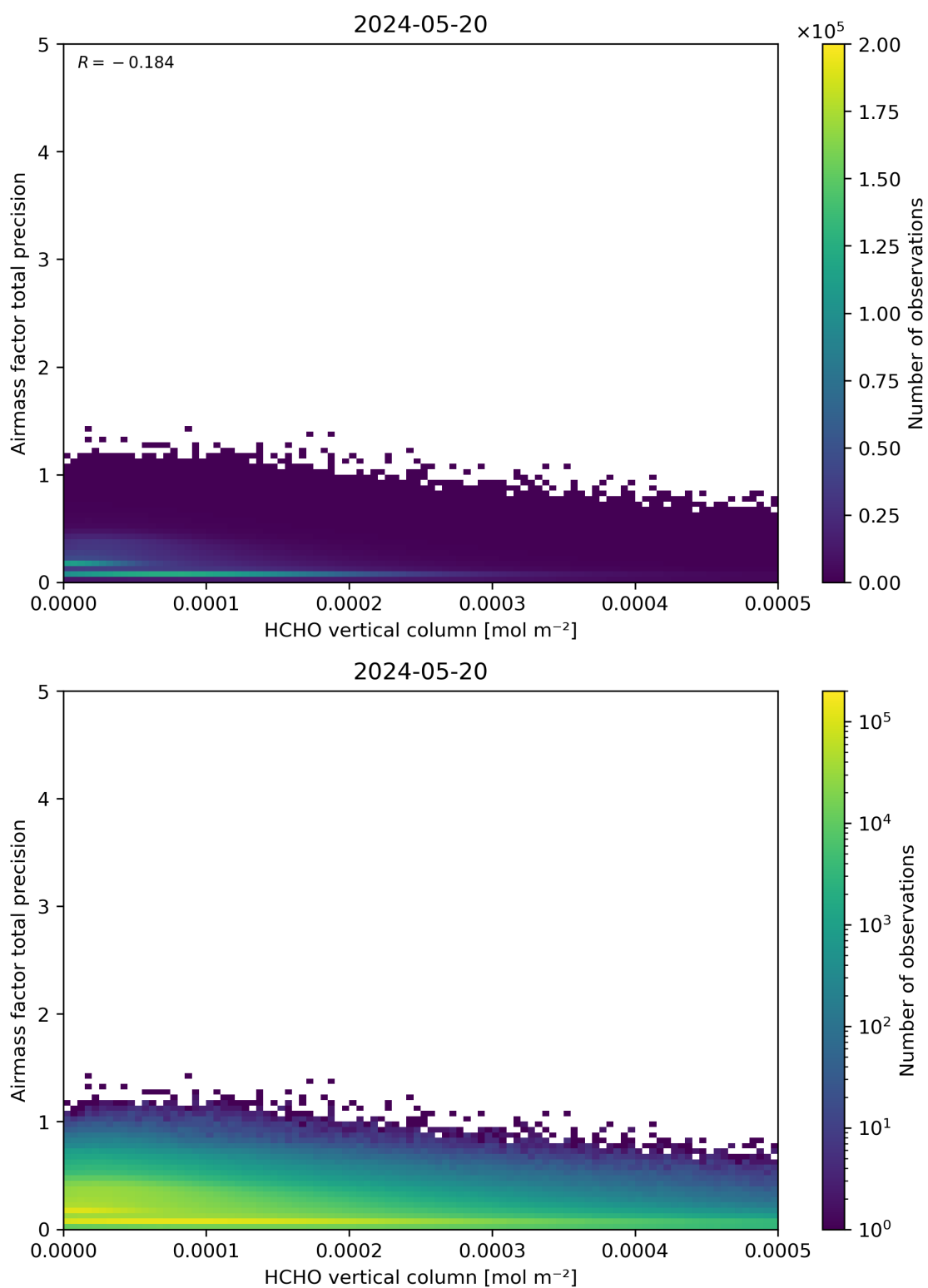
Figure 132: Scatter density plot of “HCHO vertical column” against “Airmass factor total precision” for 2024-05-19 to 2024-05-21.
