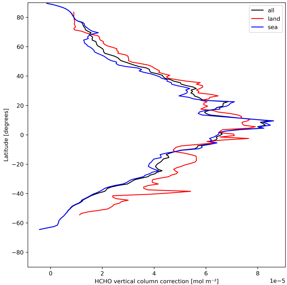
Figure 23: Zonal average of “HCHO vertical column correction” for 2024-05-19 to 2024-05-21.
