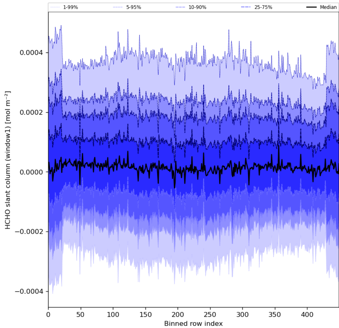
Figure 52: Along track statistics of “HCHO slant column (window1)” for 2024-05-19 to 2024-05-21
