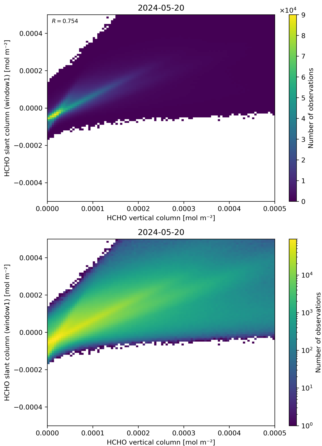
Figure 129: Scatter density plot of “HCHO vertical column” against “HCHO slant column (window1)” for 2024-05-19 to 2024-05-21.
