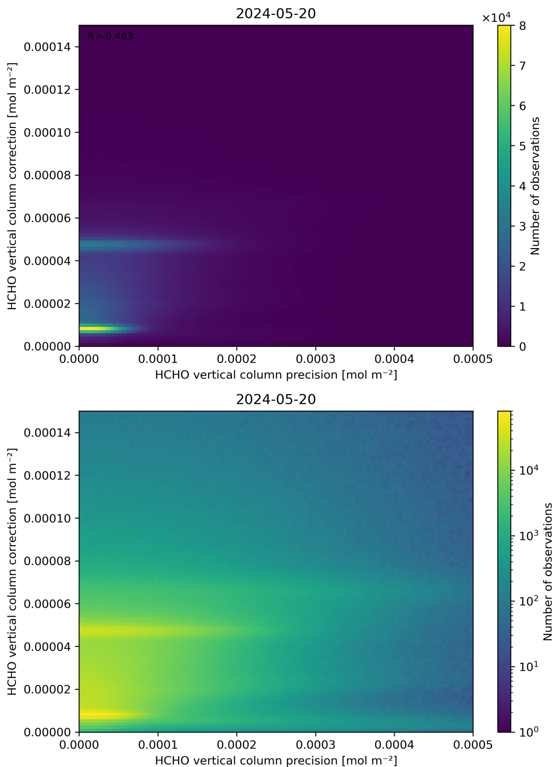
Figure 146: Scatter density plot of “HCHO vertical column precision” against “HCHO vertical column correction” for 2024-05-19 to 2024-05-21.
