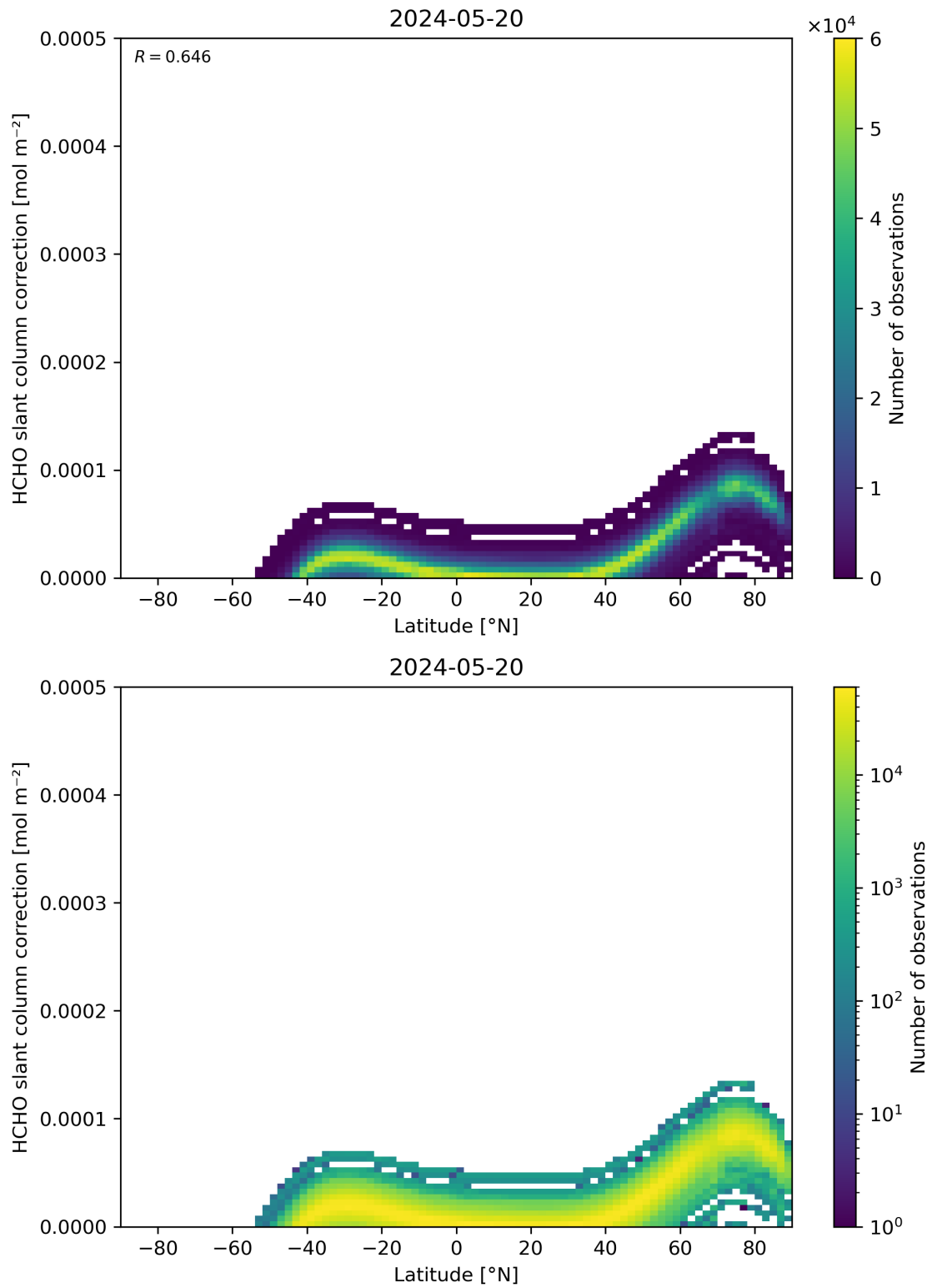
Figure 158: Scatter density plot of “Latitude” against “HCHO slant column correction” for 2024-05-19 to 2024-05-21.
