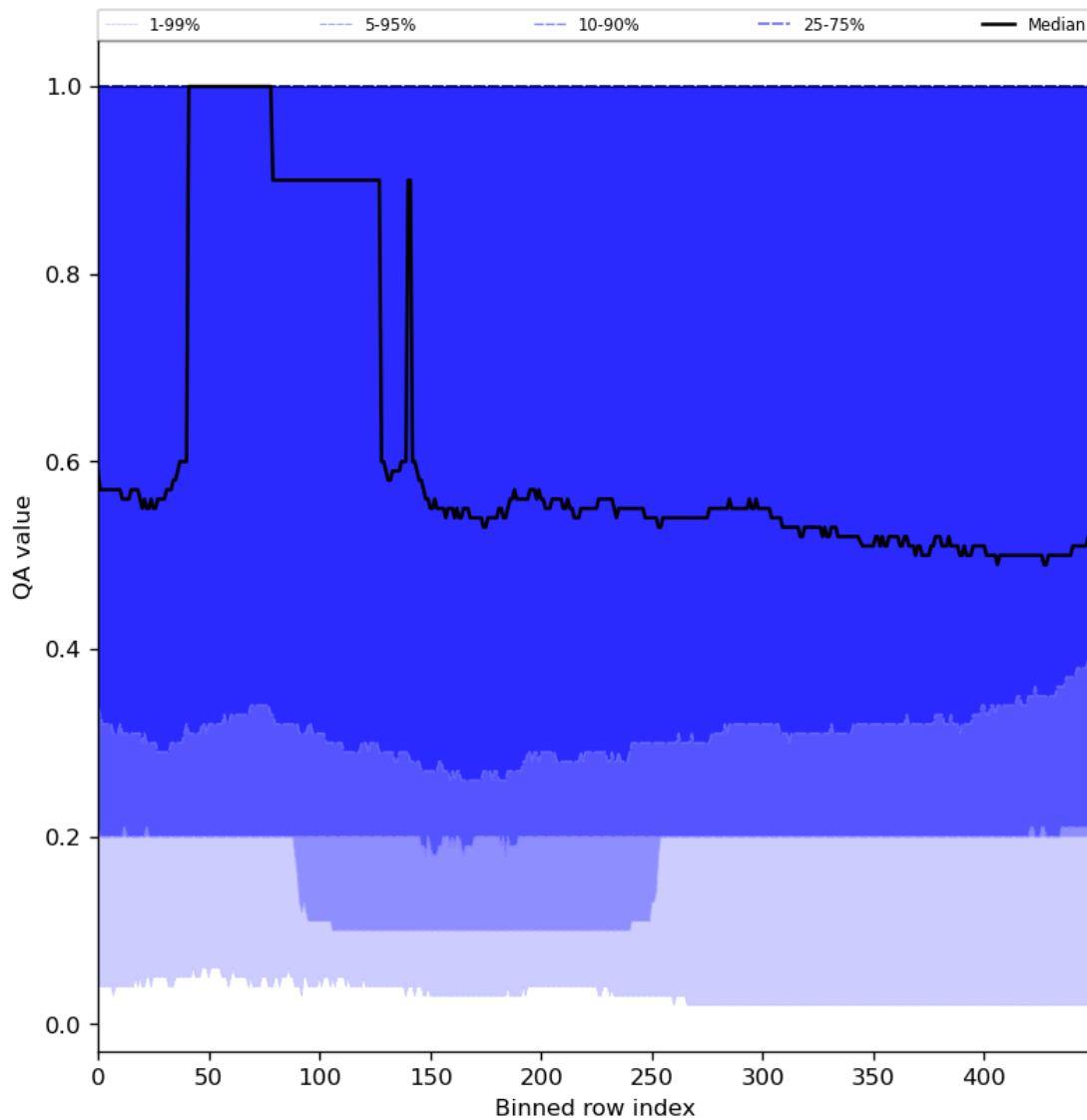
Figure 48: Along track statistics of “QA value” for 2024-05-19 to 2024-05-21
