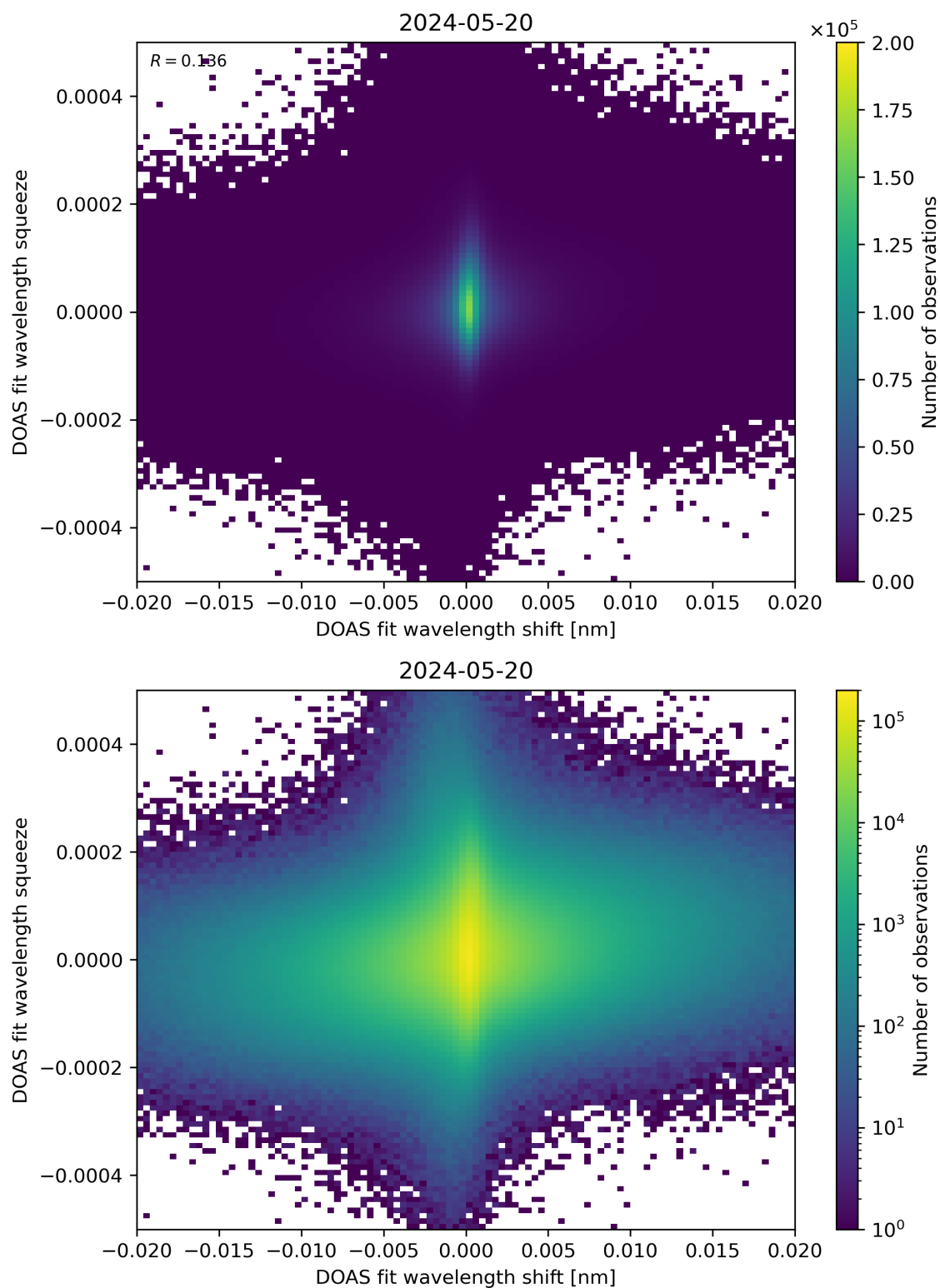
Figure 65: Scatter density plot of “DOAS fit wavelength shift” against “DOAS fit wavelength squeeze” for 2024-05-19 to 2024-05-21.
