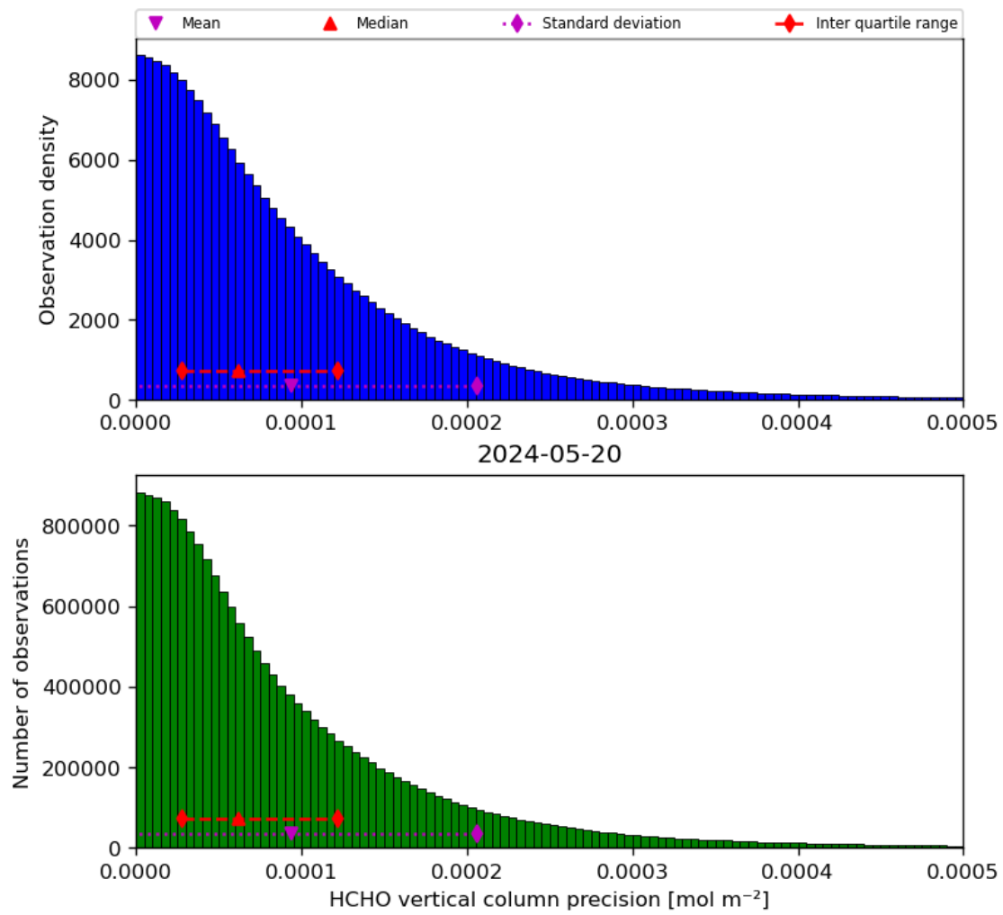
Figure 36: Histogram of “HCHO vertical column precision” for 2024-05-19 to 2024-05-21
