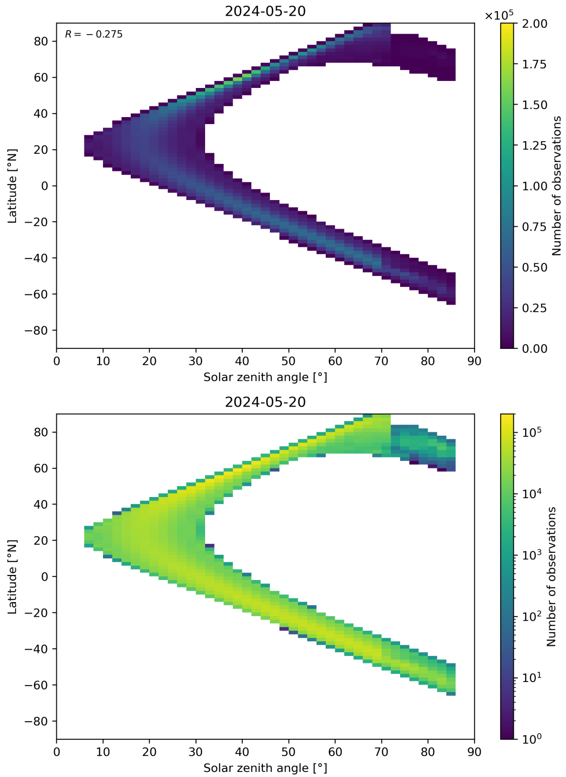
Figure 181: Scatter density plot of “Solar zenith angle” against “Latitude” for 2024-05-19 to 2024-05-21.
