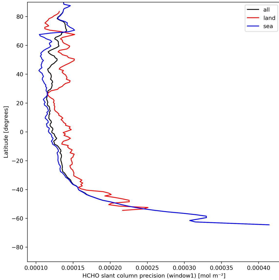
Figure 25: Zonal average of “HCHO slant column precision (window1)” for 2024-05-19 to 2024-05-21.
