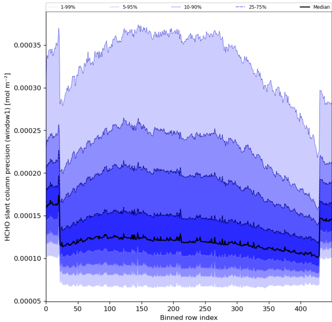
Figure 53: Along track statistics of “HCHO slant column precision (window1)” for 2024-05-19 to 2024-05-21
