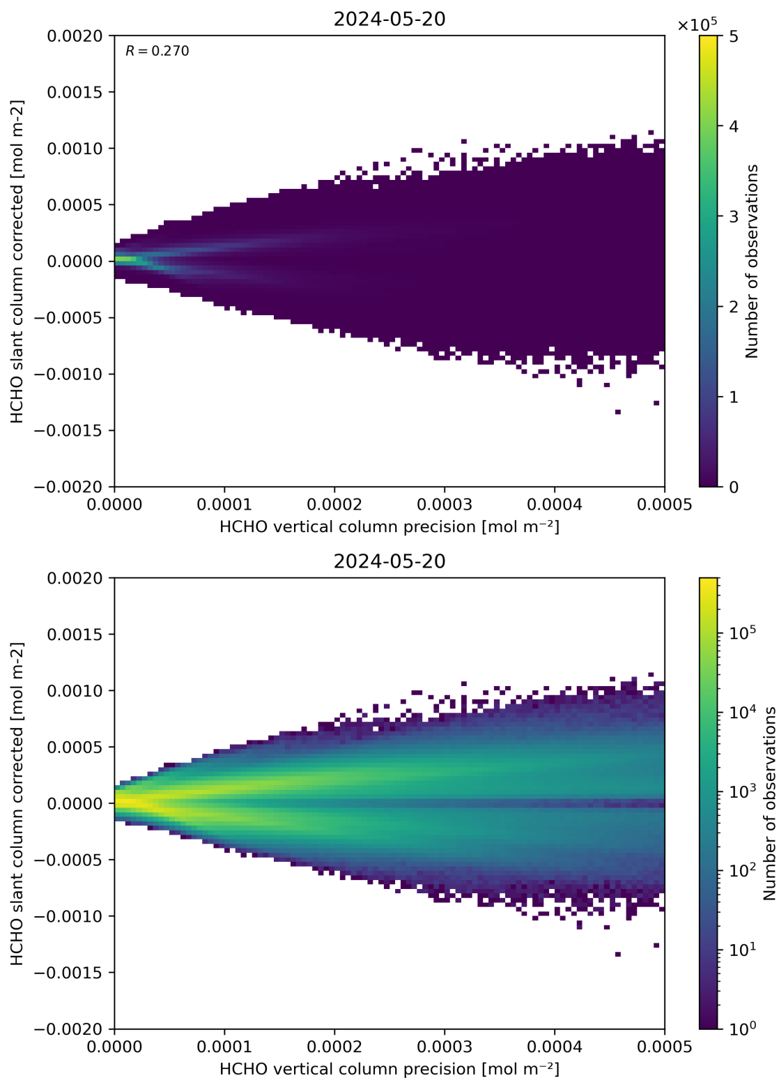
Figure 140: Scatter density plot of “HCHO vertical column precision” against “HCHO slant column corrected” for 2024-05-19 to 2024-05-21.
