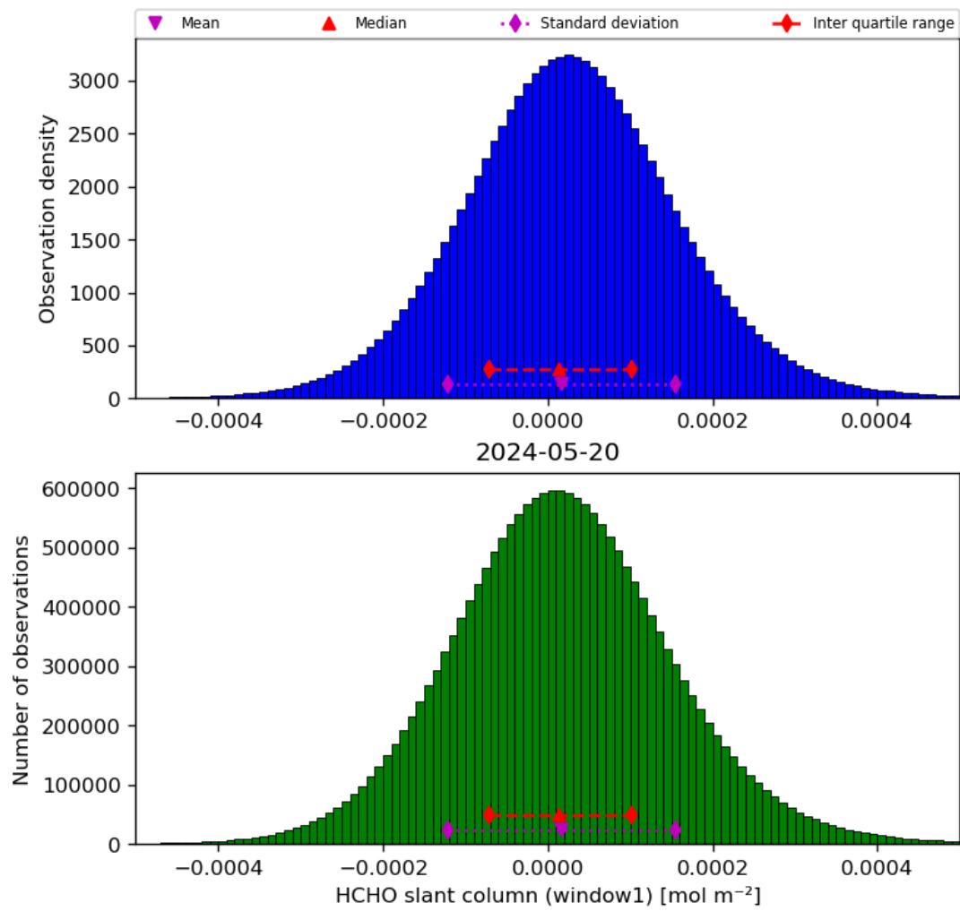
Figure 38: Histogram of “HCHO slant column (window1)” for 2024-05-19 to 2024-05-21
