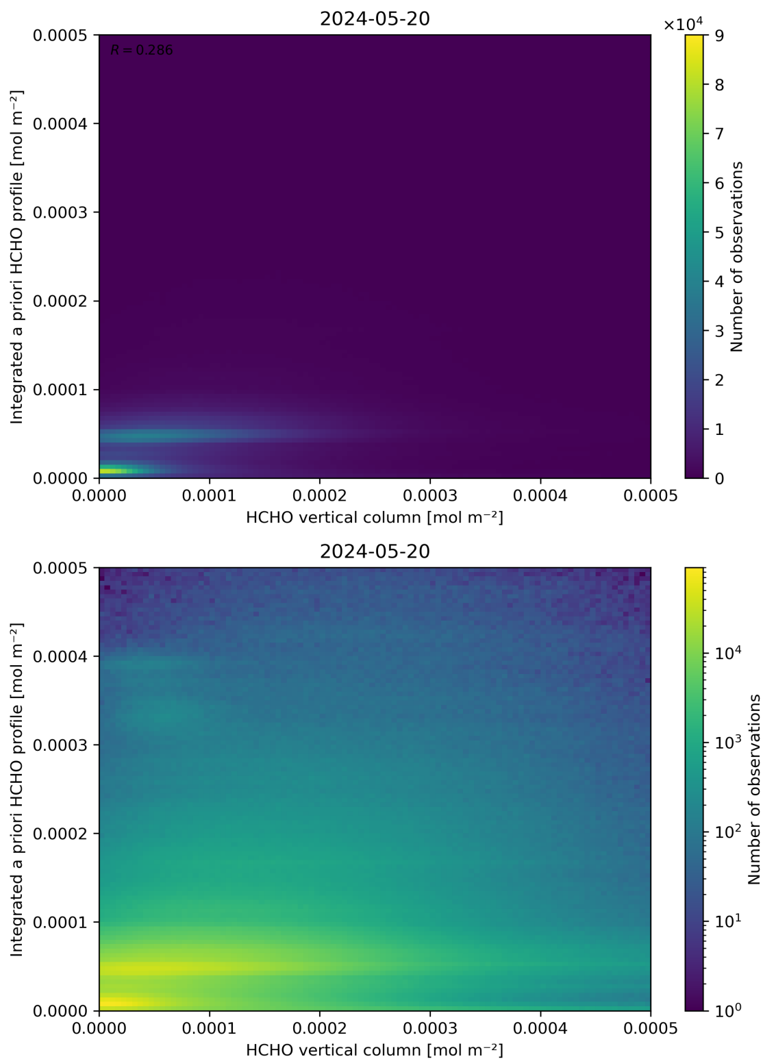
Figure 135: Scatter density plot of “HCHO vertical column” against “Integrated a priori HCHO profile” for 2024-05-19 to 2024-05-21.
