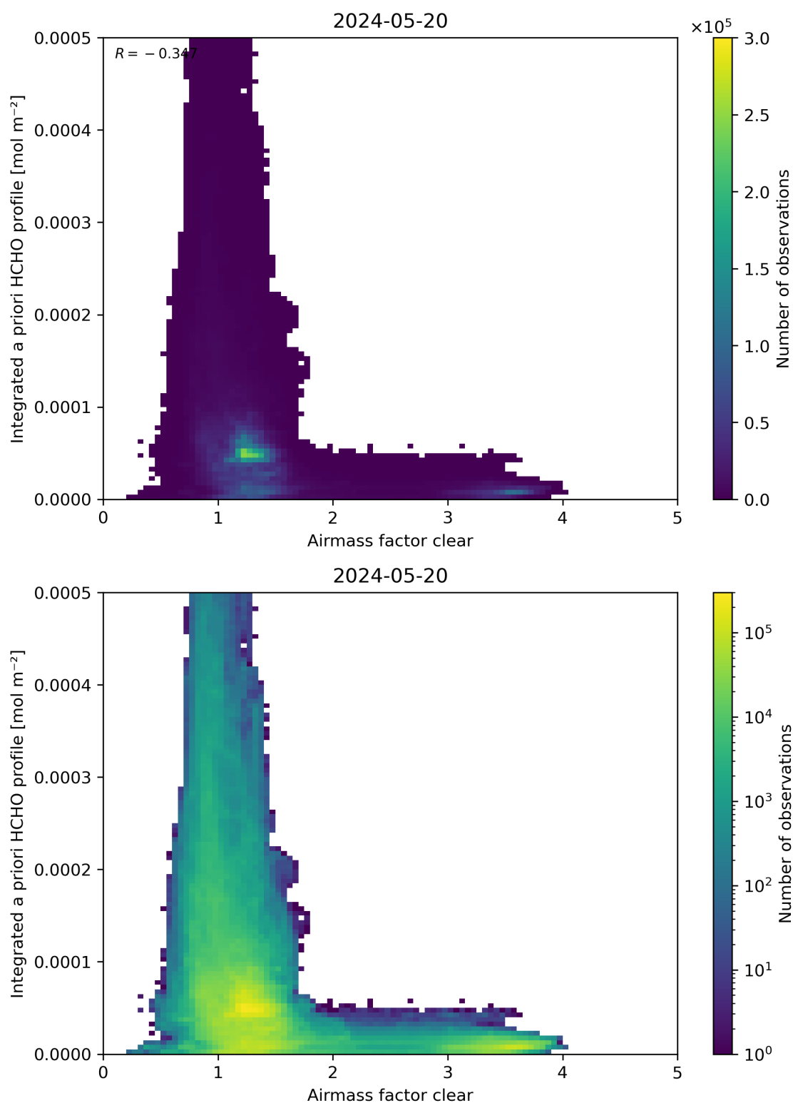
Figure 76: Scatter density plot of “Airmass factor clear” against “Integrated a priori HCHO profile” for 2024-05-19 to 2024-05-21.
