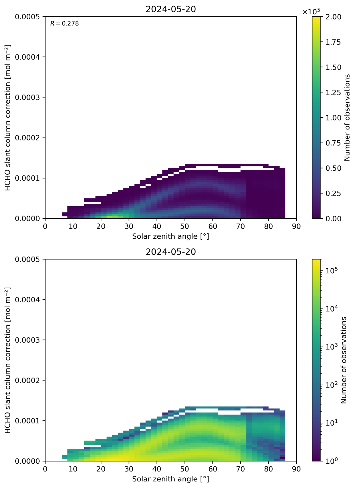
Figure 172: Scatter density plot of “Solar zenith angle” against “HCHO slant column correction” for 2024-05-19 to 2024-05-21.
