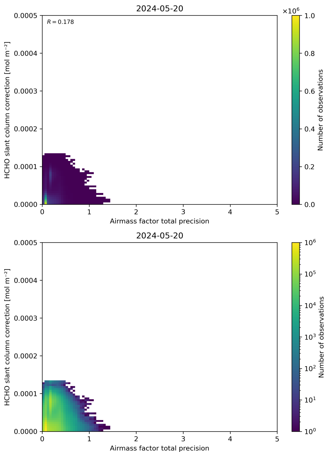
Figure 110: Scatter density plot of “Airmass factor total precision” against “HCHO slant column correction” for 2024-05-19 to 2024-05-21.
