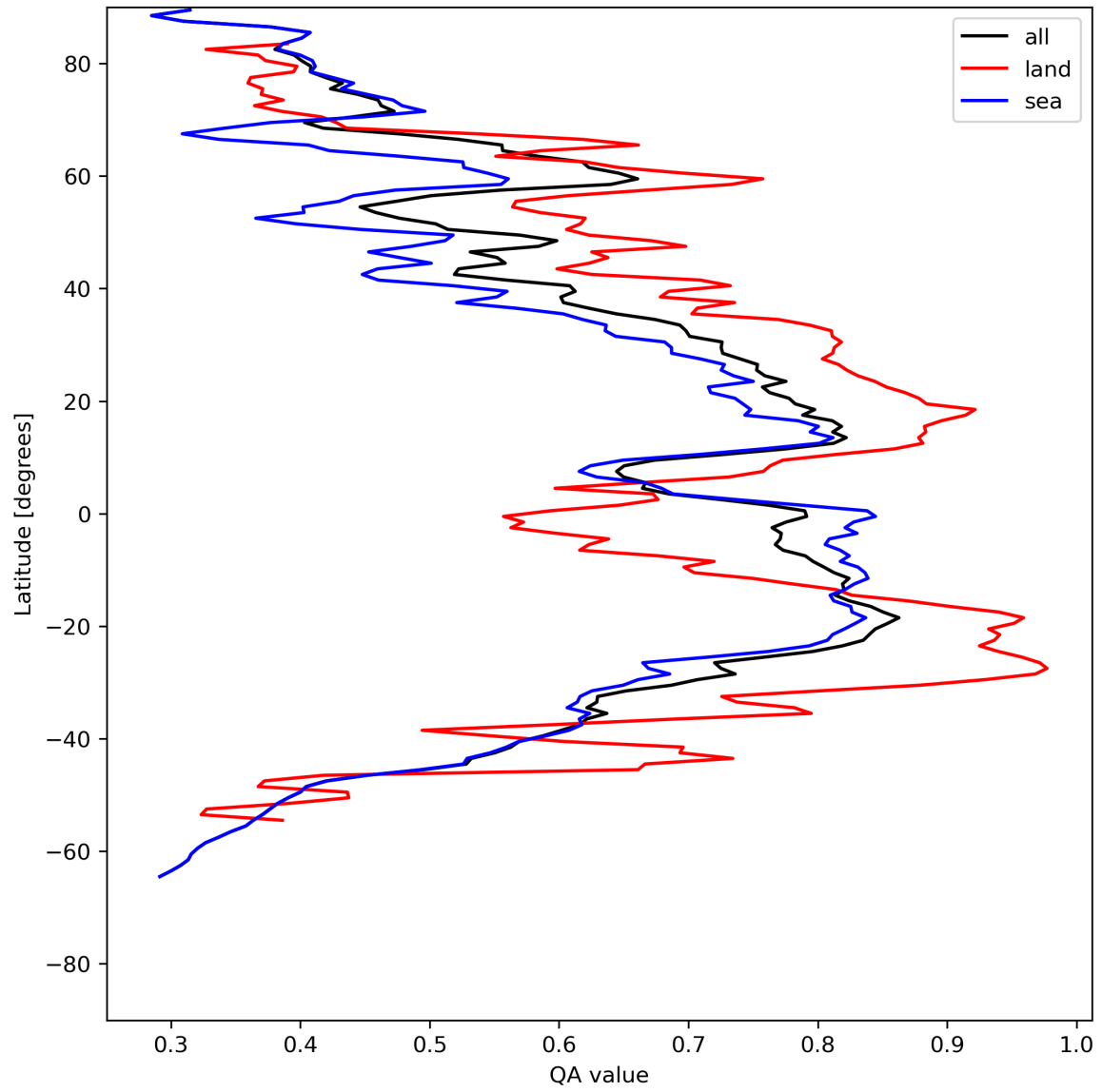
Figure 20: Zonal average of “QA value” for 2024-05-19 to 2024-05-21.
