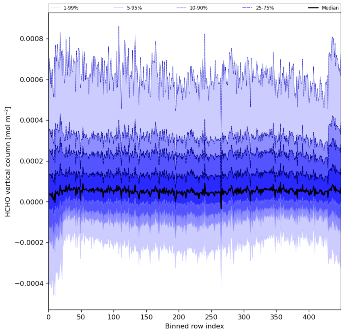
Figure 49: Along track statistics of “HCHO vertical column” for 2024-05-19 to 2024-05-21
