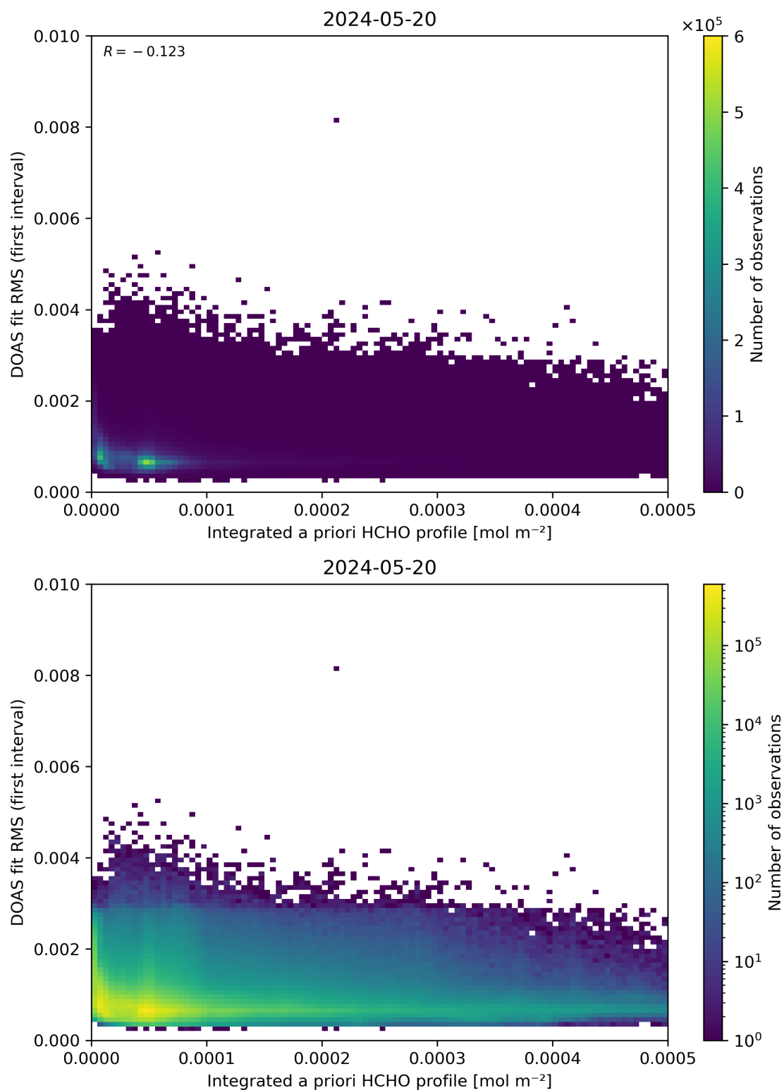
Figure 148: Scatter density plot of “Integrated a priori HCHO profile” against “DOAS fit RMS (first interval)” for 2024-05-19 to 2024-05-21.
