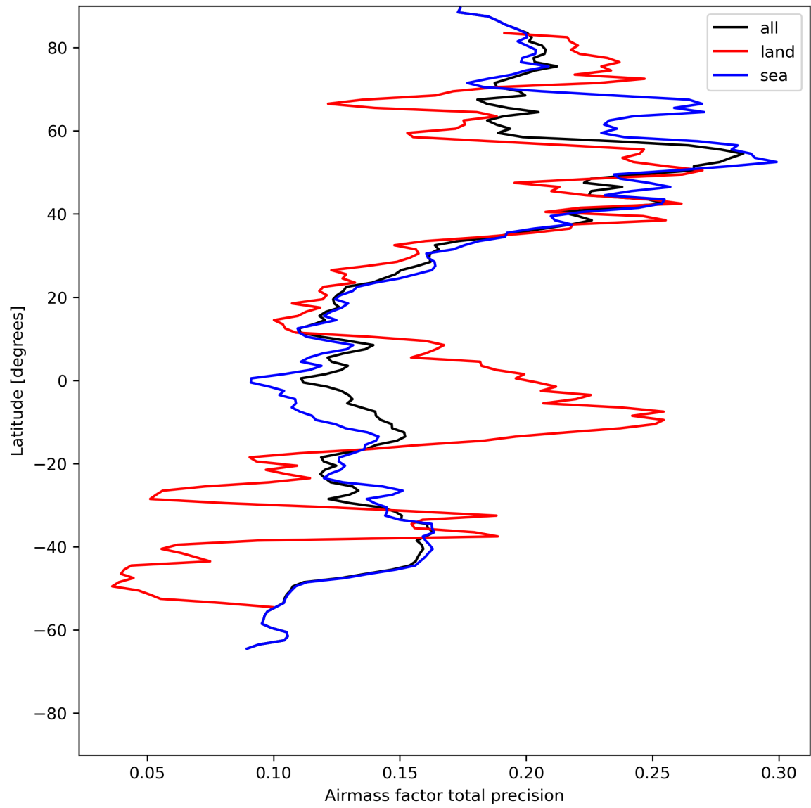
Figure 27: Zonal average of “Airmass factor total precision” for 2024-05-19 to 2024-05-21.
