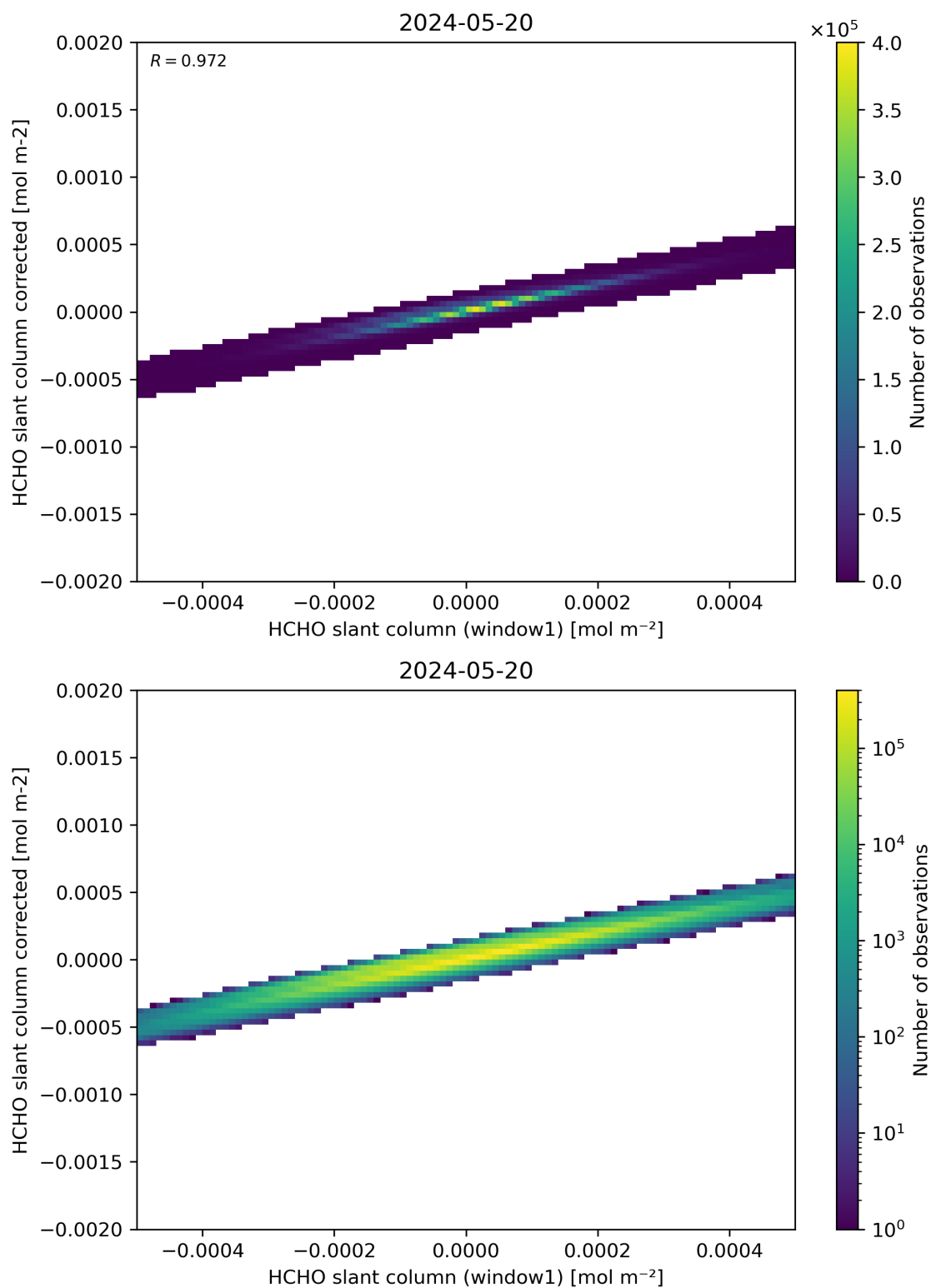
Figure 82: Scatter density plot of “HCHO slant column (window1)” against “HCHO slant column corrected” for 2024-05-19 to 2024-05-21.
