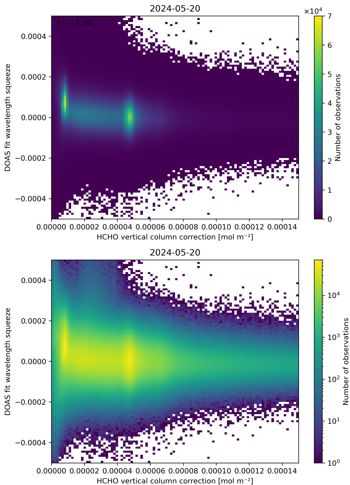
Figure 114: Scatter density plot of “HCHO vertical column correction” against “DOAS fit wavelength squeeze” for 2024-05-19 to 2024-05-21.
