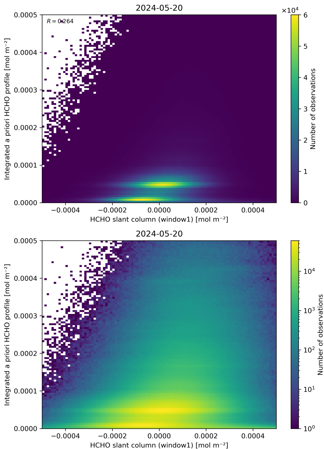
Figure 87: Scatter density plot of “HCHO slant column (window1)” against “Integrated a priori HCHO profile” for 2024-05-19 to 2024-05-21.
