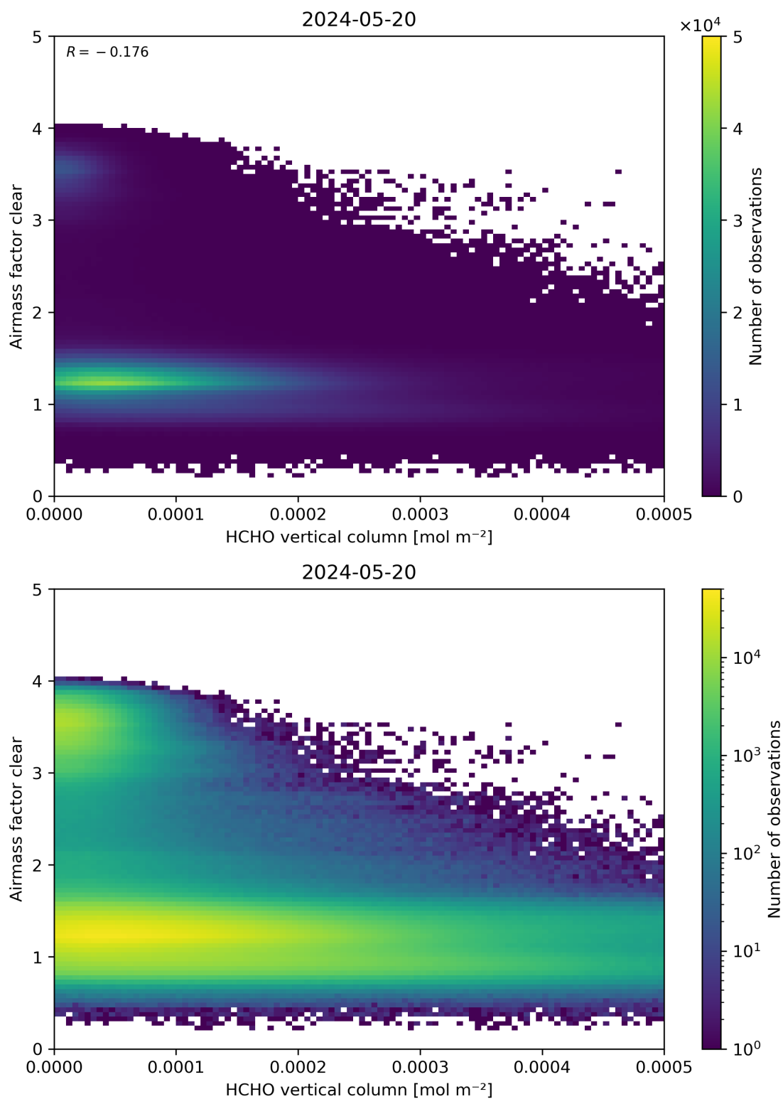
Figure 126: Scatter density plot of “HCHO vertical column” against “Airmass factor clear” for 2024-05-19 to 2024-05-21.
