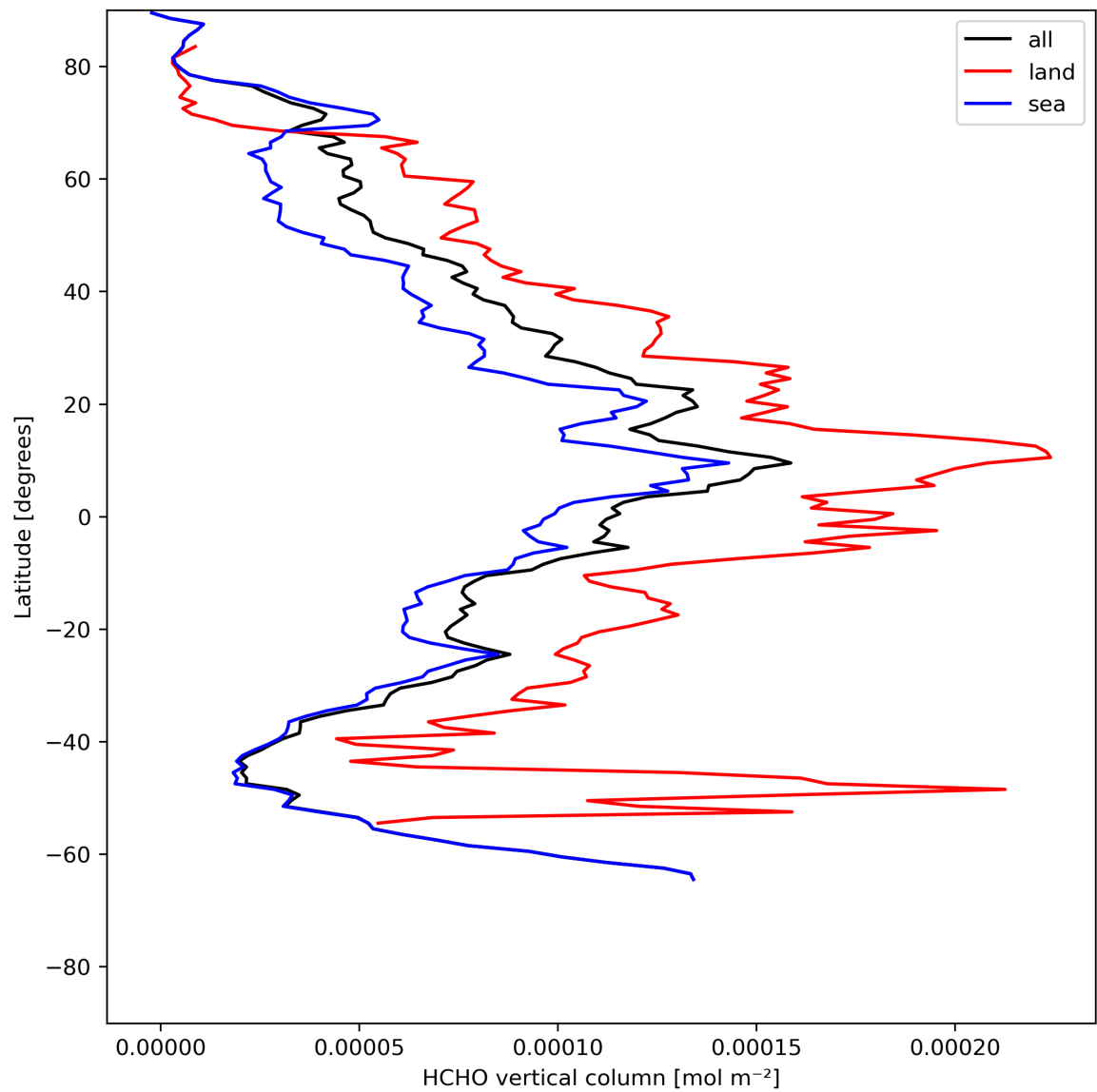
Figure 21: Zonal average of “HCHO vertical column” for 2024-05-19 to 2024-05-21.
