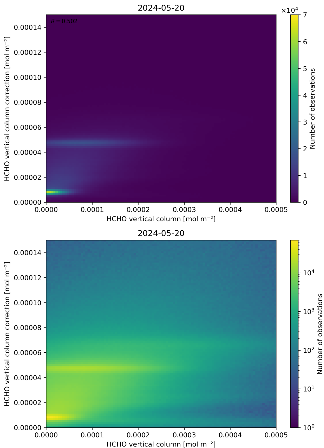
Figure 133: Scatter density plot of “HCHO vertical column” against “HCHO vertical column correction” for 2024-05-19 to 2024-05-21.
