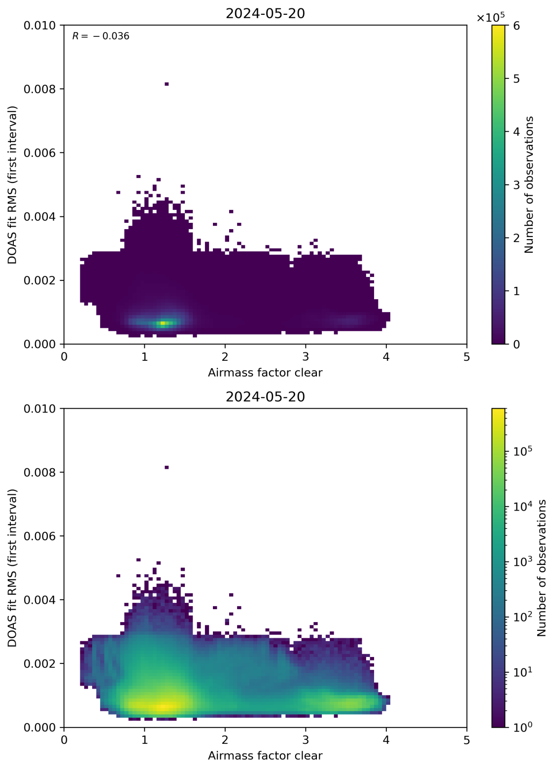
Figure 71: Scatter density plot of “Airmass factor clear” against “DOAS fit RMS (first interval)” for 2024-05-19 to 2024-05-21.
