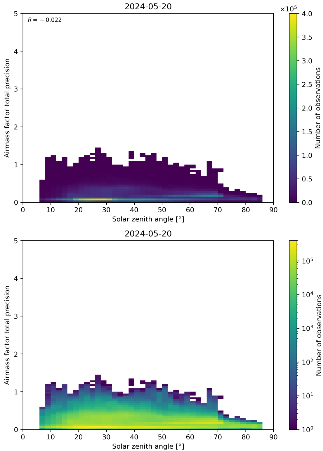
Figure 176: Scatter density plot of “Solar zenith angle” against “Airmass factor total precision” for 2024-05-19 to 2024-05-21.
