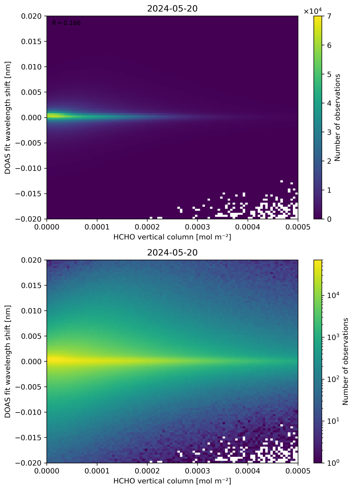
Figure 124: Scatter density plot of “HCHO vertical column” against “DOAS fit wavelength shift” for 2024-05-19 to 2024-05-21.
