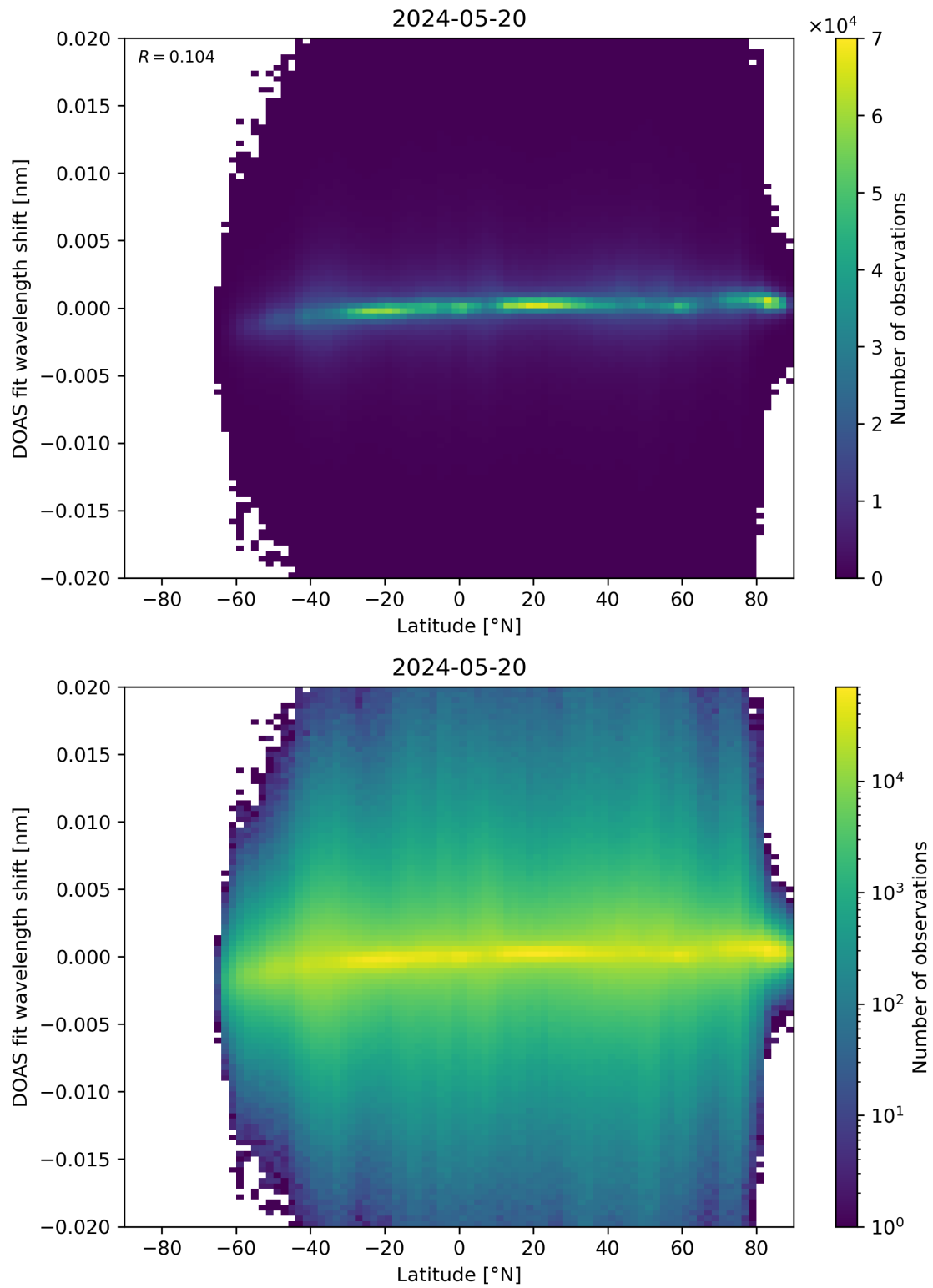
Figure 154: Scatter density plot of “Latitude” against “DOAS fit wavelength shift” for 2024-05-19 to 2024-05-21.
