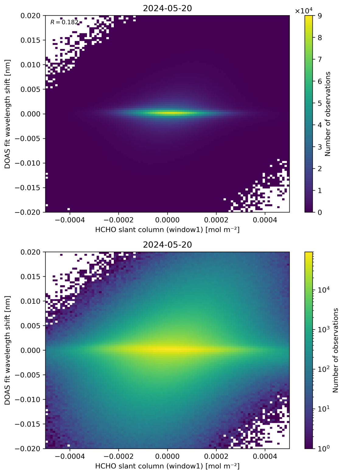
Figure 79: Scatter density plot of “HCHO slant column (window1)” against “DOAS fit wavelength shift” for 2024-05-19 to 2024-05-21.
