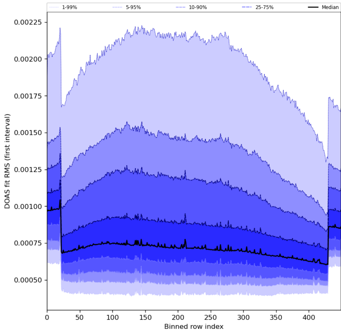
Figure 60: Along track statistics of “DOAS fit RMS (first interval)” for 2024-05-19 to 2024-05-21
