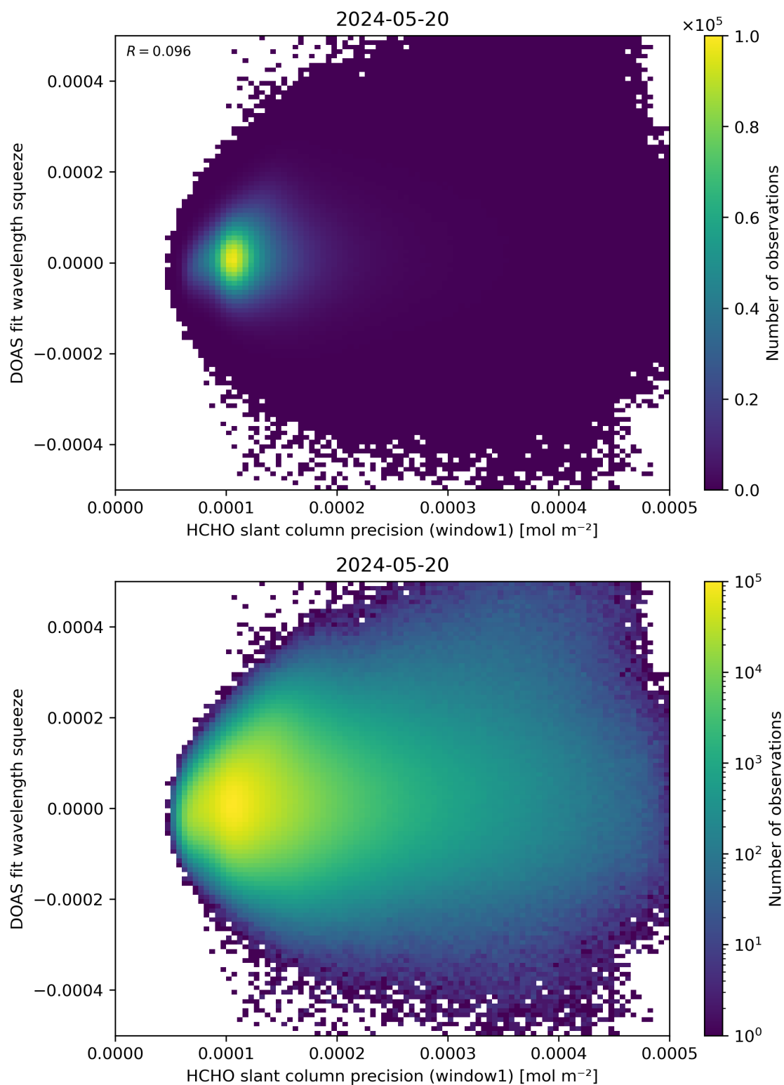
Figure 90: Scatter density plot of “HCHO slant column precision (window1)” against “DOAS fit wavelength squeeze” for 2024-05-19 to 2024-05-21.
