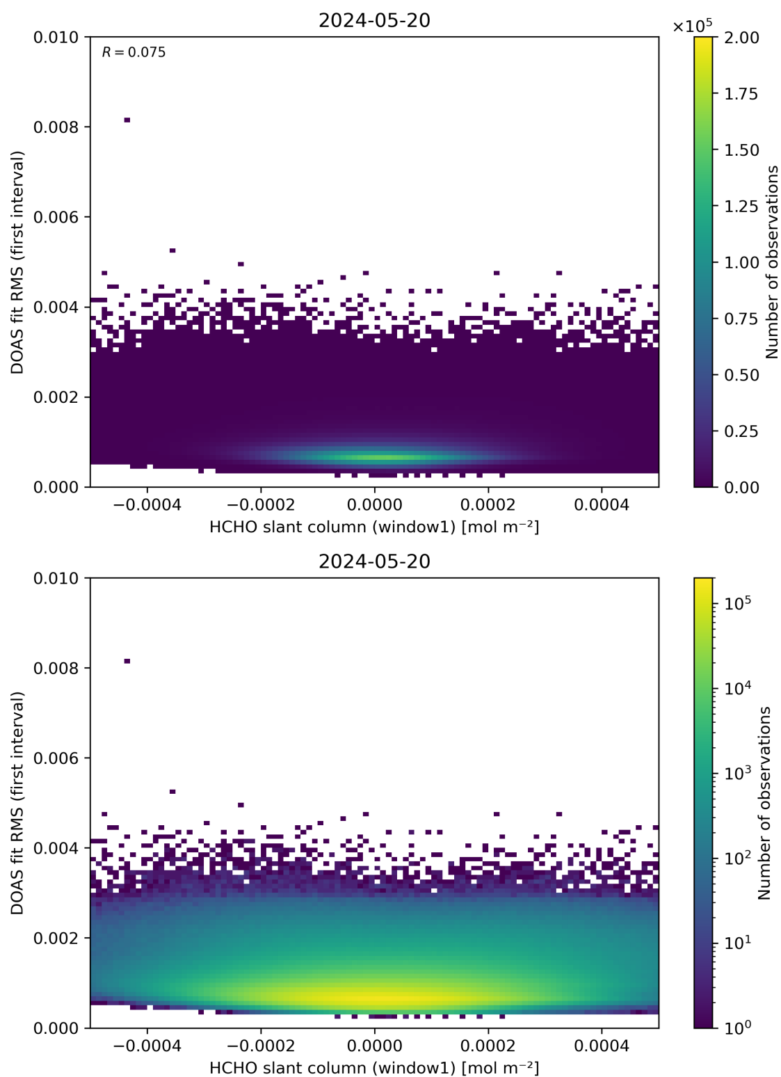
Figure 78: Scatter density plot of “HCHO slant column (window1)” against “DOAS fit RMS (first interval)” for 2024-05-19 to 2024-05-21.
