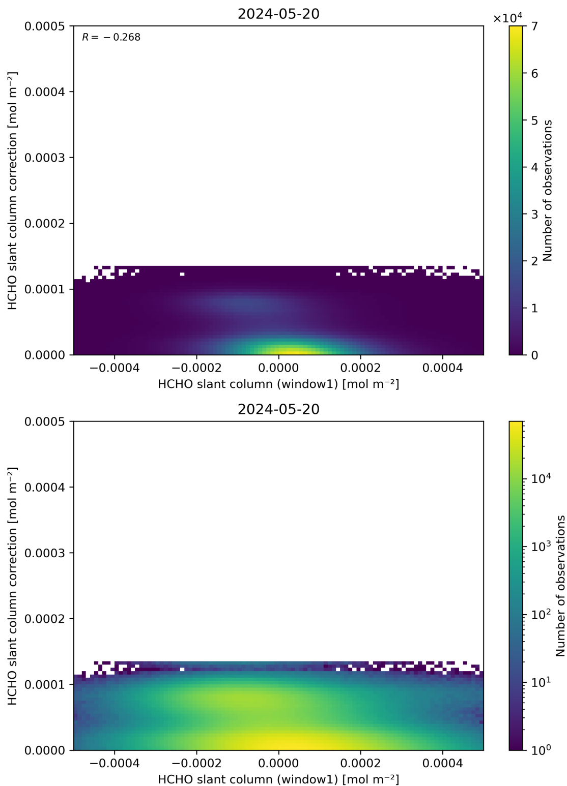
Figure 83: Scatter density plot of “HCHO slant column (window1)” against “HCHO slant column correction” for 2024-05-19 to 2024-05-21.
