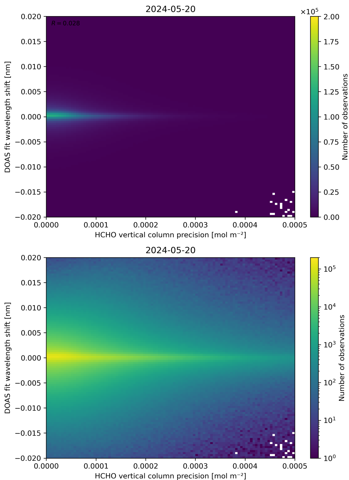
Figure 137: Scatter density plot of “HCHO vertical column precision” against “DOAS fit wavelength shift” for 2024-05-19 to 2024-05-21.
