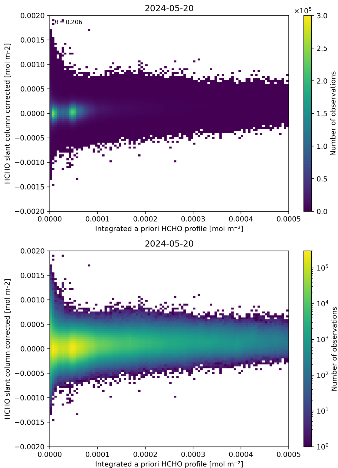
Figure 151: Scatter density plot of “Integrated a priori HCHO profile” against “HCHO slant column corrected” for 2024-05-19 to 2024-05-21.
