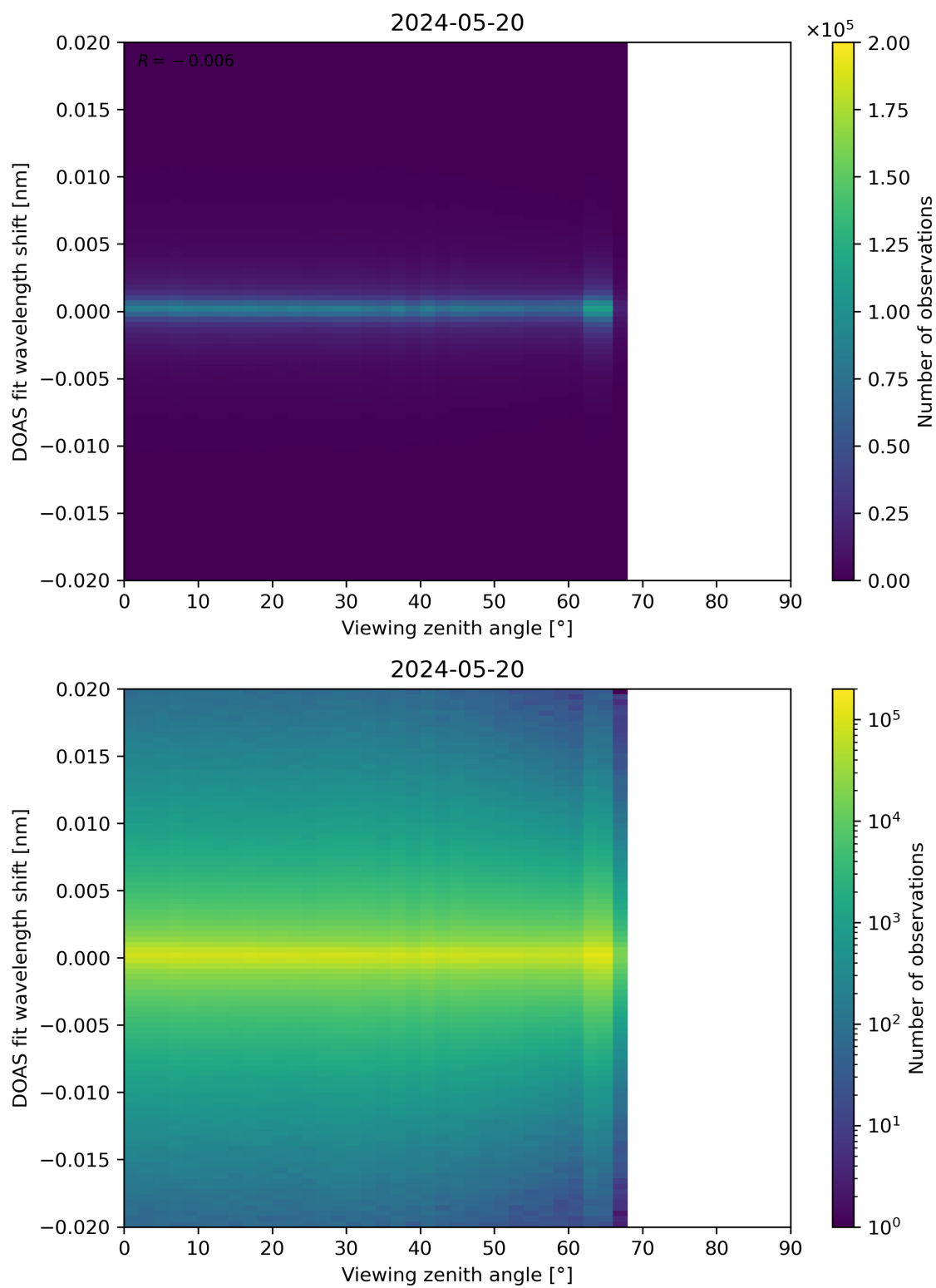
Figure 183: Scatter density plot of “Viewing zenith angle” against “DOAS fit wavelength shift” for 2024-05-19 to 2024-05-21.
