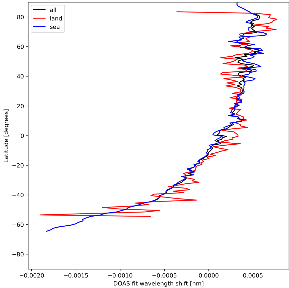
Figure 30: Zonal average of “DOAS fit wavelength shift” for 2024-05-19 to 2024-05-21.
