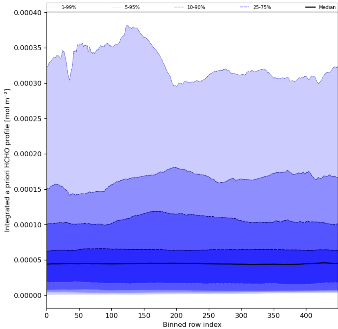
Figure 57: Along track statistics of “Integrated a priori HCHO profile” for 2024-05-19 to 2024-05-21
