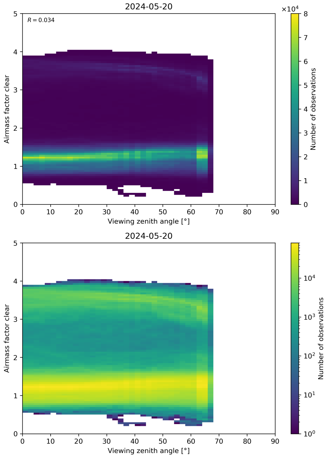
Figure 185: Scatter density plot of “Viewing zenith angle” against “Airmass factor clear” for 2024-05-19 to 2024-05-21.
