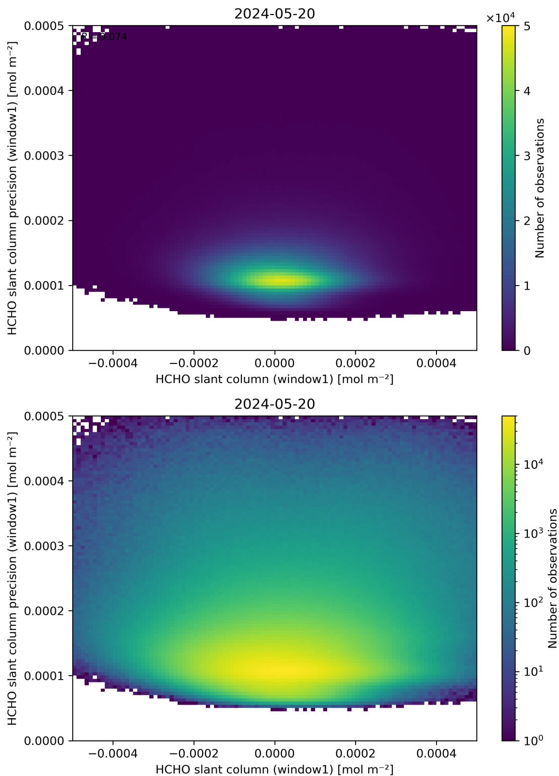
Figure 84: Scatter density plot of “HCHO slant column (window1)” against “HCHO slant column precision (window1)” for 2024-05-19 to 2024-05-21.
