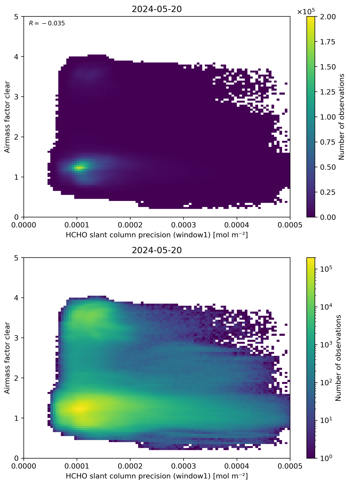
Figure 91: Scatter density plot of “HCHO slant column precision (window1)” against “Airmass factor clear” for 2024-05-19 to 2024-05-21.
