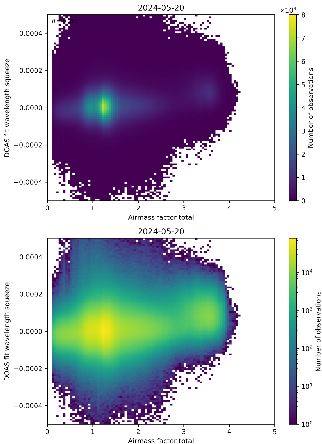
Figure 99: Scatter density plot of “Airmass factor total” against “DOAS fit wavelength squeeze” for 2024-05-19 to 2024-05-21.
