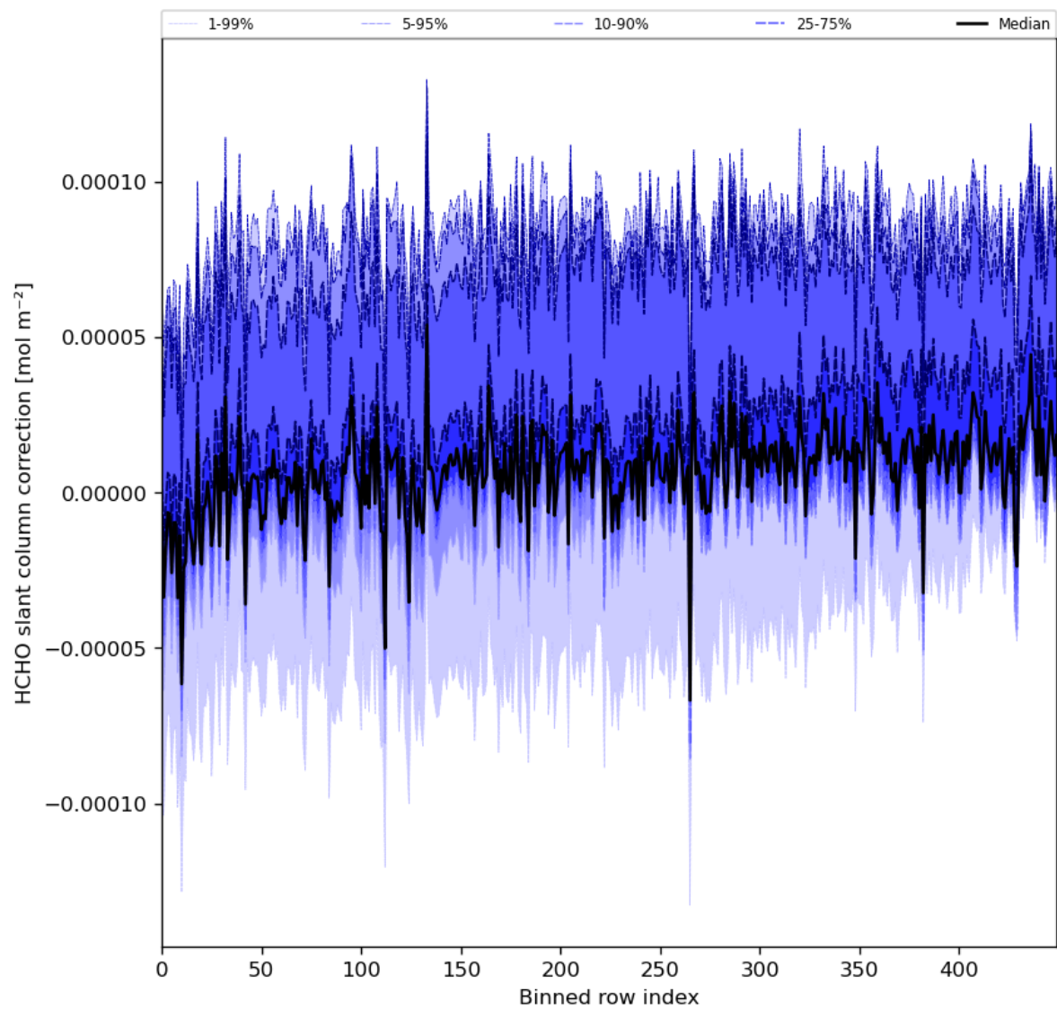
Figure 61: Along track statistics of “HCHO slant column correction” for 2024-05-19 to 2024-05-21
