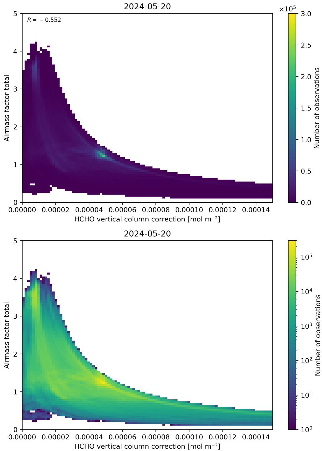
Figure 120: Scatter density plot of “HCHO vertical column correction” against “Airmass factor total” for 2024-05-19 to 2024-05-21.
