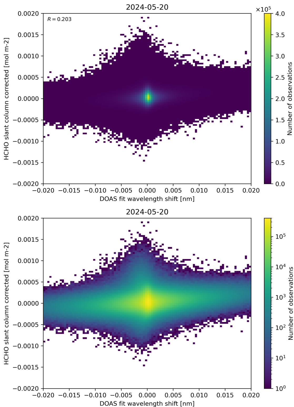
Figure 66: Scatter density plot of “DOAS fit wavelength shift” against “HCHO slant column corrected” for 2024-05-19 to 2024-05-21.
