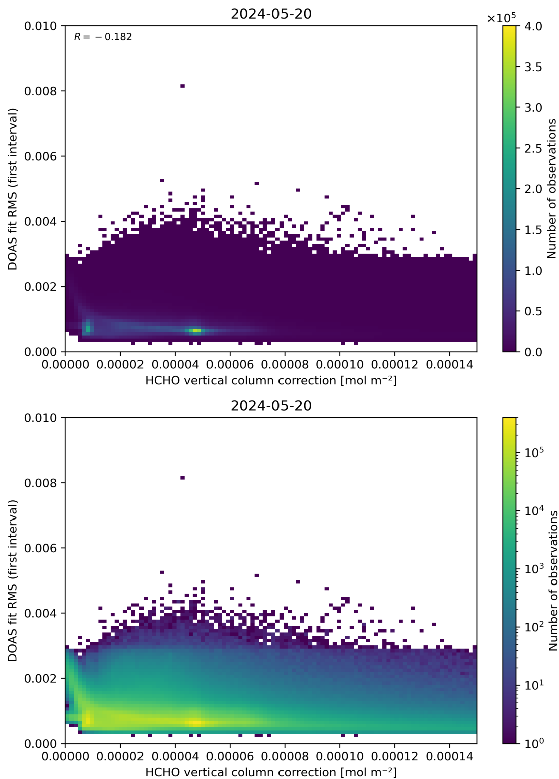
Figure 112: Scatter density plot of “HCHO vertical column correction” against “DOAS fit RMS (first interval)” for 2024-05-19 to 2024-05-21.
