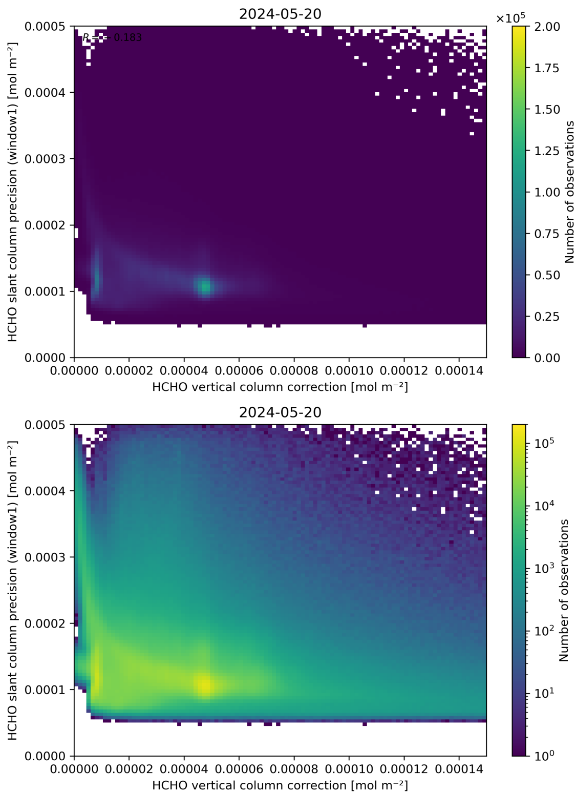
Figure 119: Scatter density plot of “HCHO vertical column correction” against “HCHO slant column precision (window1)” for 2024-05-19 to 2024-05-21.
