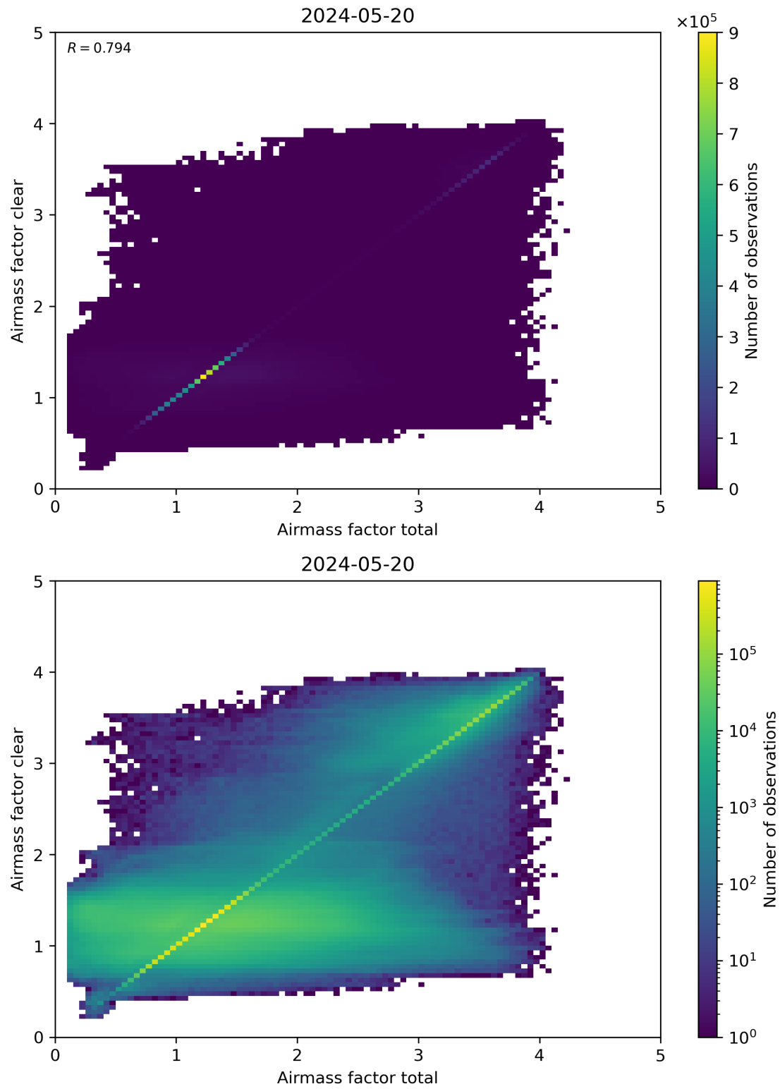
Figure 100: Scatter density plot of “Airmass factor total” against “Airmass factor clear” for 2024-05-19 to 2024-05-21.
