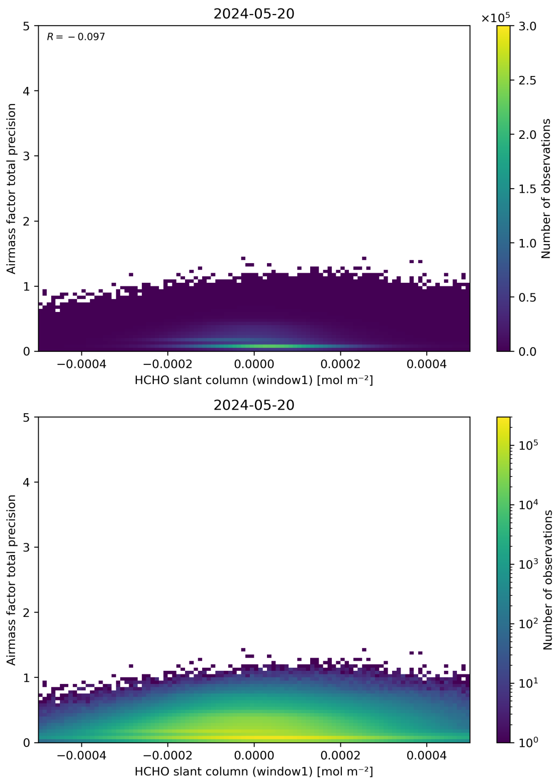
Figure 86: Scatter density plot of “HCHO slant column (window1)” against “Airmass factor total precision” for 2024-05-19 to 2024-05-21.
