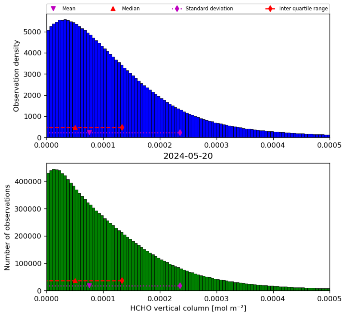
Figure 35: Histogram of “HCHO vertical column” for 2024-05-19 to 2024-05-21
