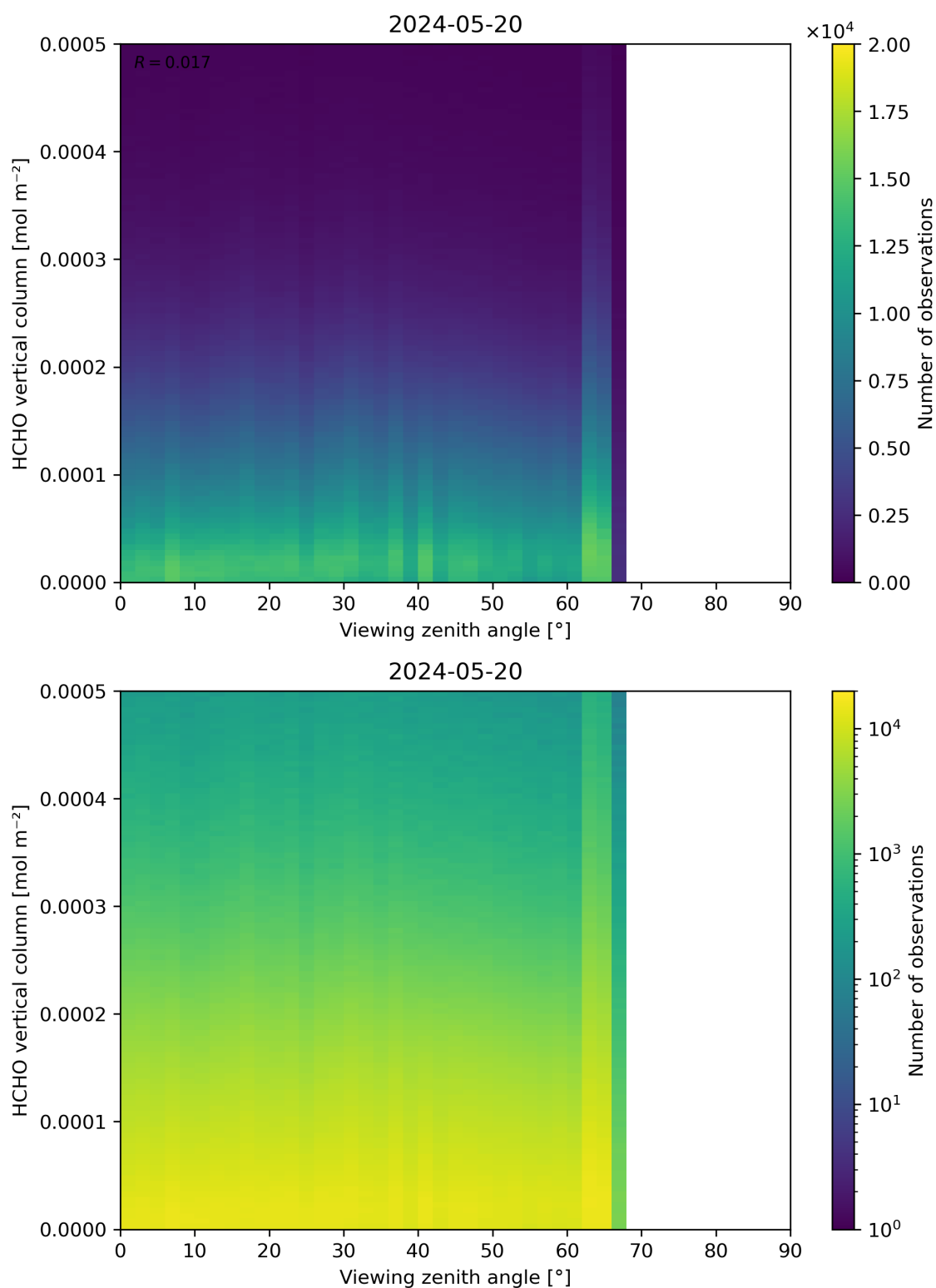
Figure 192: Scatter density plot of “Viewing zenith angle” against “HCHO vertical column” for 2024-05-19 to 2024-05-21.
