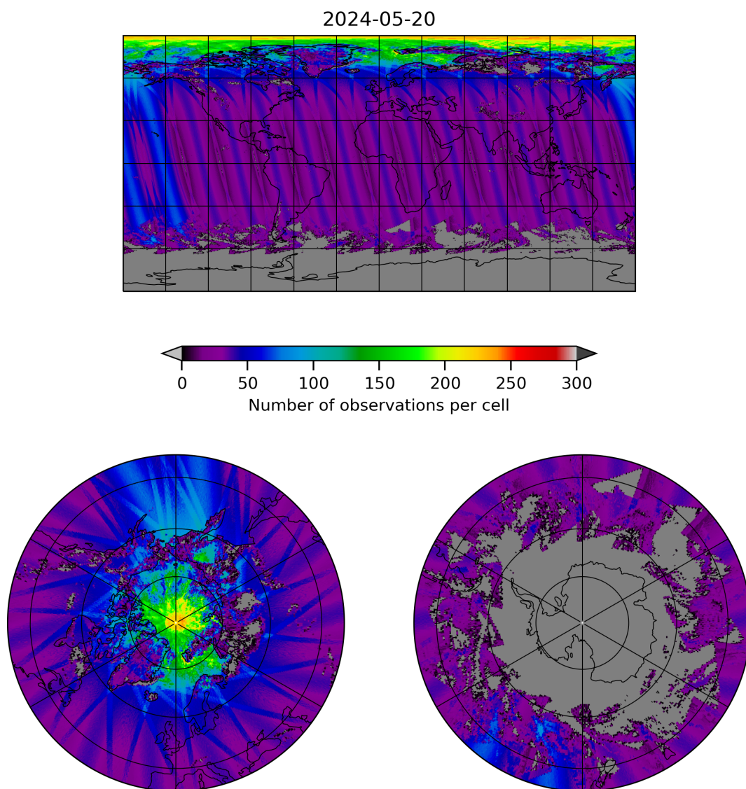
Figure 19: Map of the number of observations for 2024-05-19 to 2024-05-21
