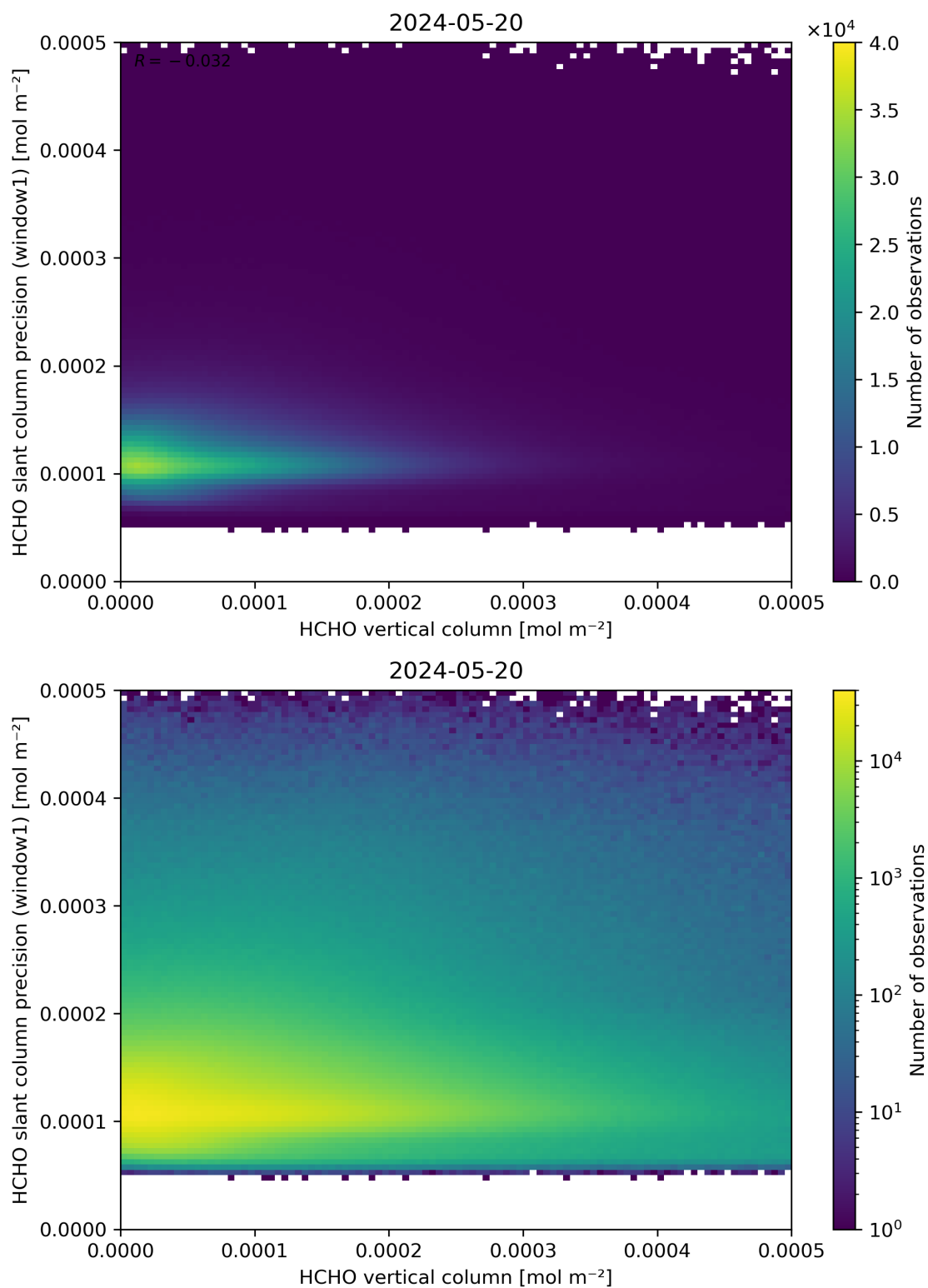
Figure 130: Scatter density plot of “HCHO vertical column” against “HCHO slant column precision (window1)” for 2024-05-19 to 2024-05-21.
