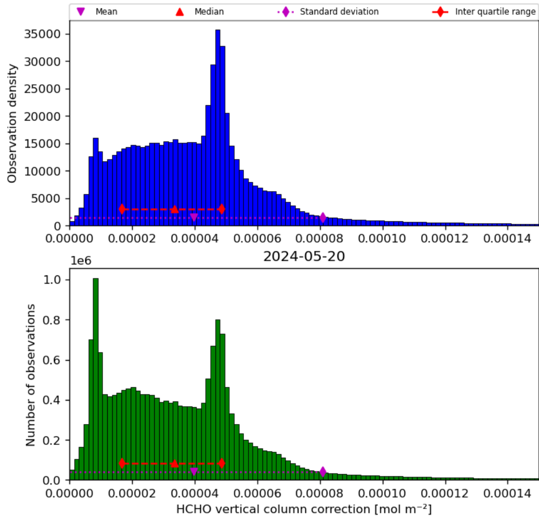
Figure 37: Histogram of “HCHO vertical column correction” for 2024-05-19 to 2024-05-21
