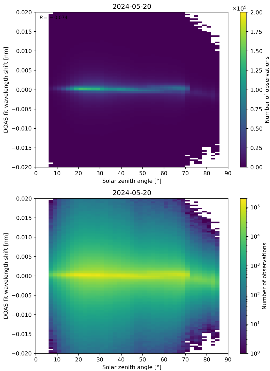
Figure 168: Scatter density plot of “Solar zenith angle” against “DOAS fit wavelength shift” for 2024-05-19 to 2024-05-21.
