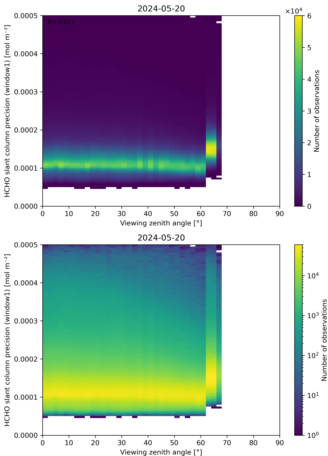
Figure 189: Scatter density plot of “Viewing zenith angle” against “HCHO slant column precision (window1)” for 2024-05-19 to 2024-05-21.
