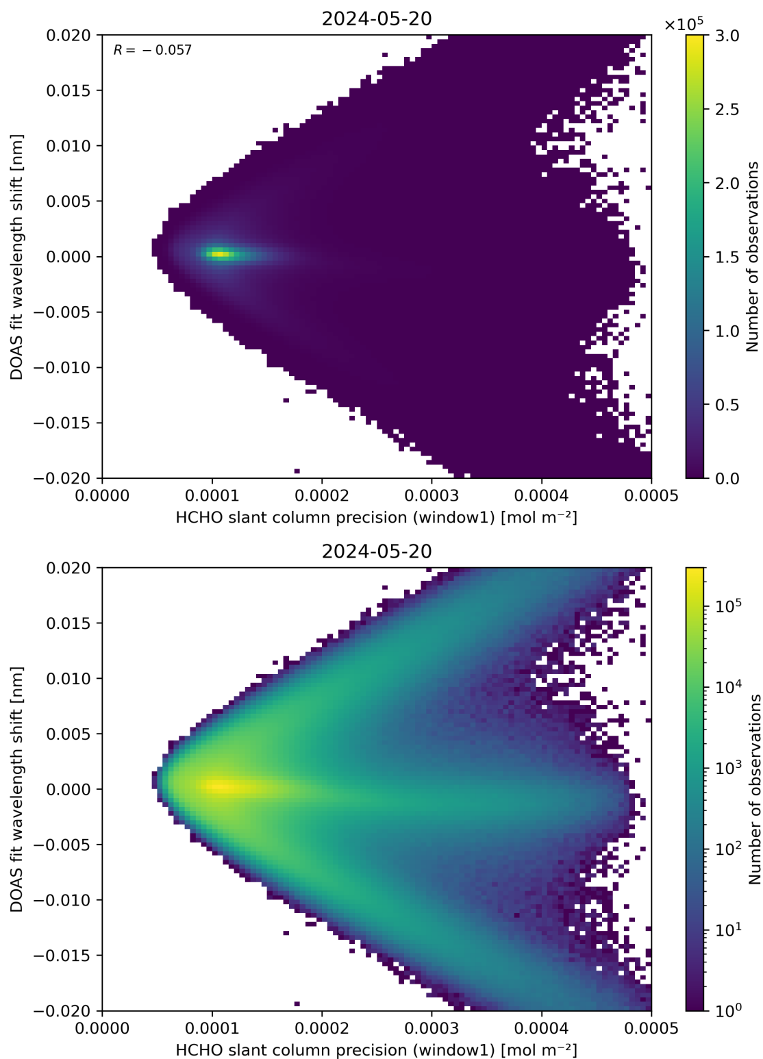
Figure 89: Scatter density plot of “HCHO slant column precision (window1)” against “DOAS fit wavelength shift” for 2024-05-19 to 2024-05-21.
