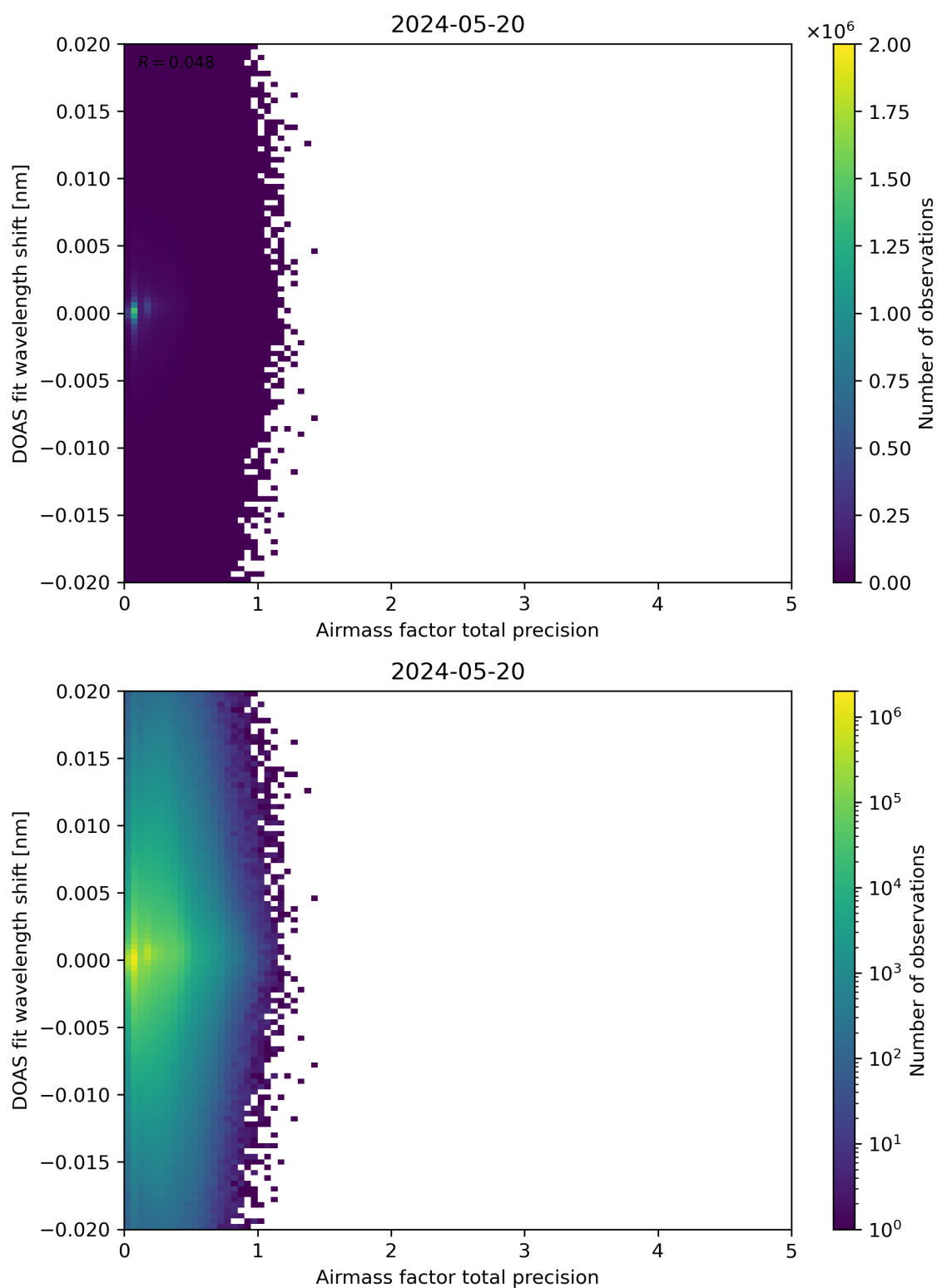
Figure 106: Scatter density plot of “Airmass factor total precision” against “DOAS fit wavelength shift” for 2024-05-19 to 2024-05-21.
