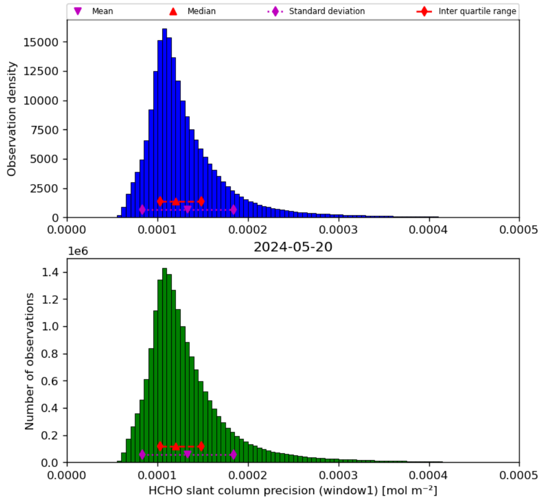
Figure 39: Histogram of “HCHO slant column precision (window1)” for 2024-05-19 to 2024-05-21
