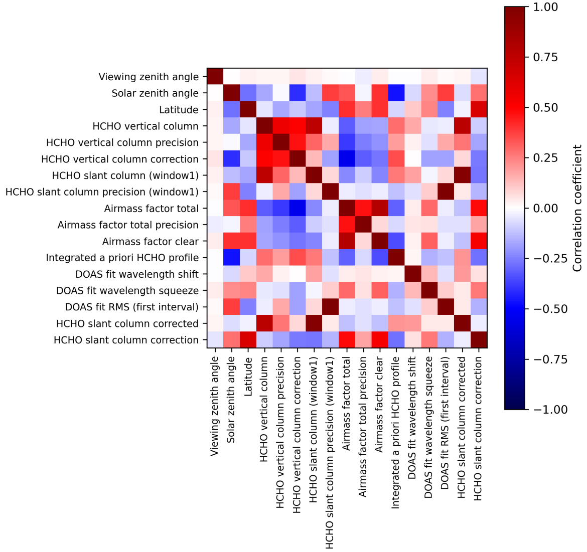
Figure 2: Map of correlation matrix for 2024-05-19 to 2024-05-21.
