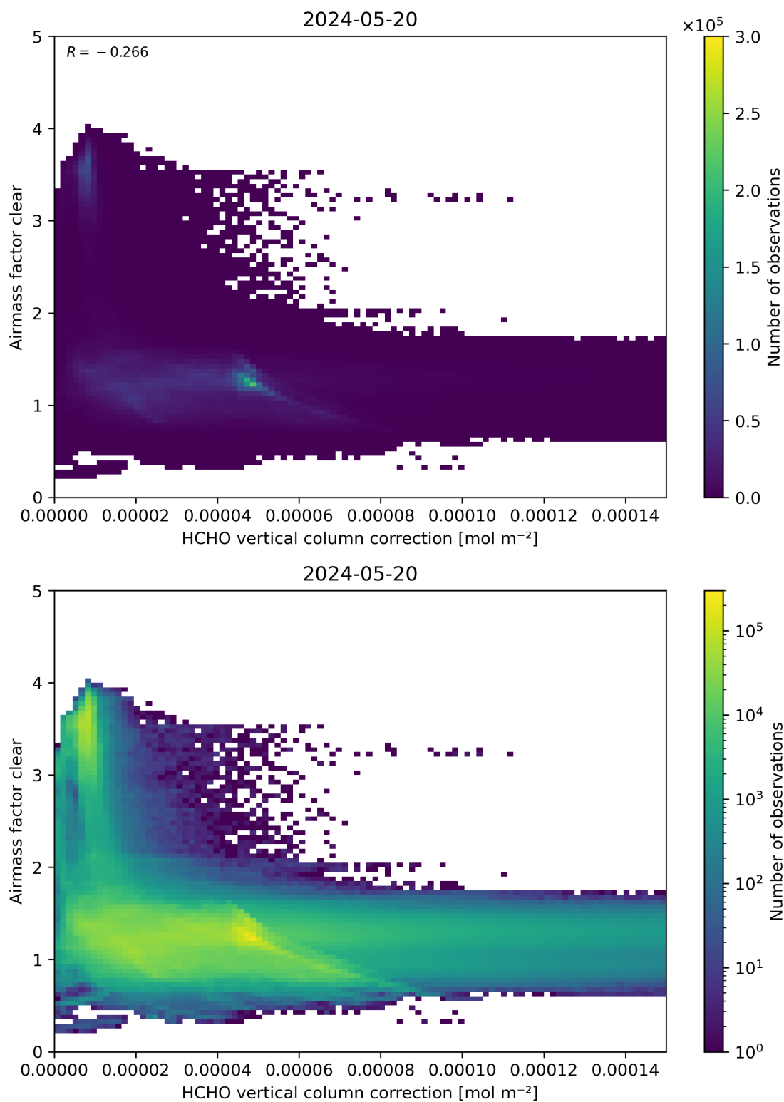
Figure 115: Scatter density plot of “HCHO vertical column correction” against “Airmass factor clear” for 2024-05-19 to 2024-05-21.
