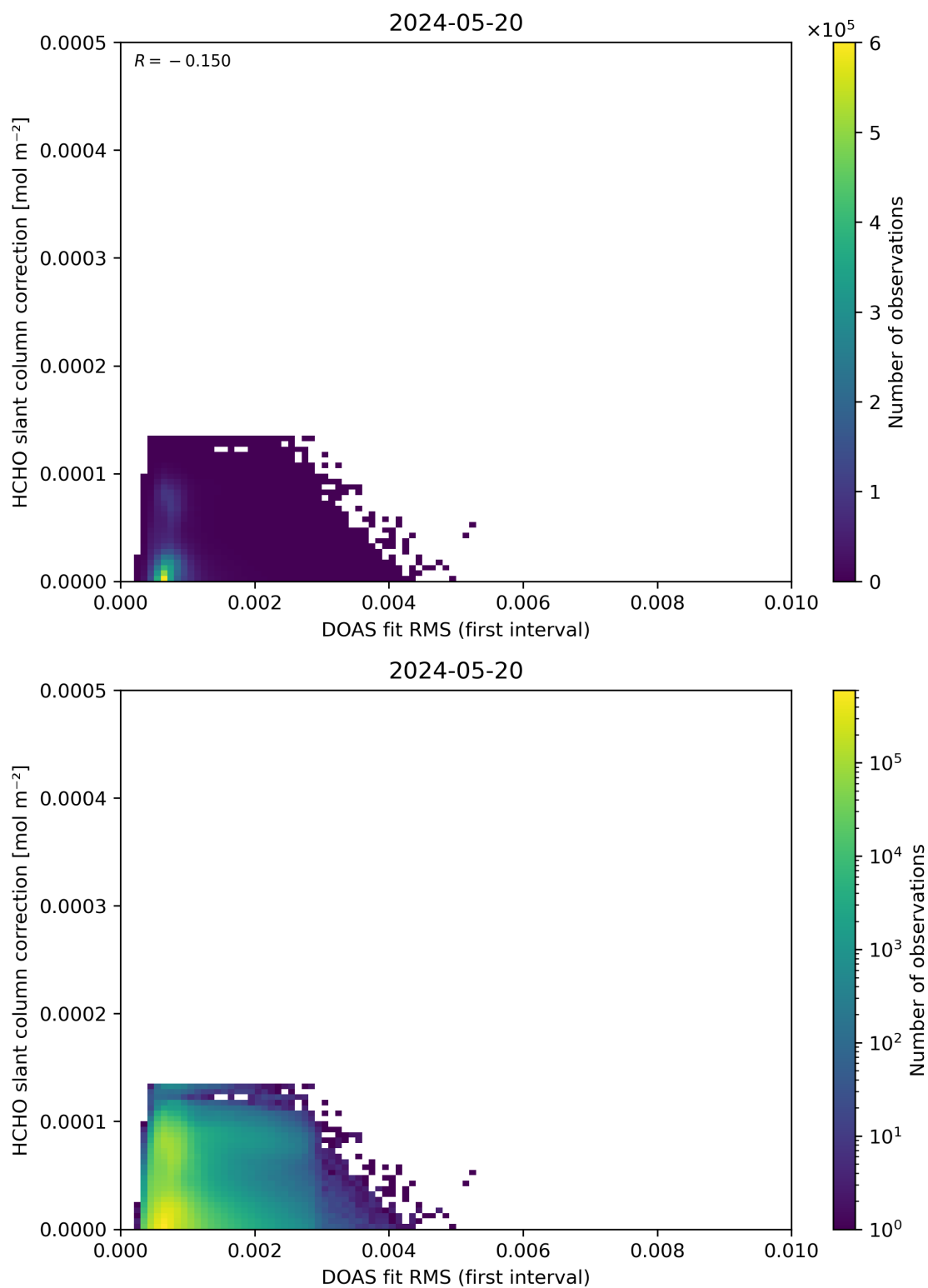
Figure 63: Scatter density plot of “DOAS fit RMS (first interval)” against “HCHO slant column correction” for 2024-05-19 to 2024-05-21.
