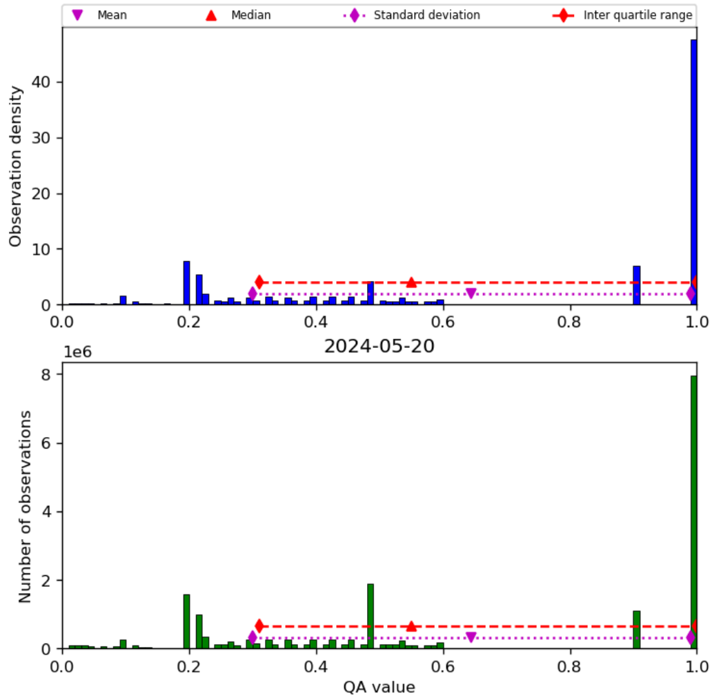
Figure 34: Histogram of “QA value” for 2024-05-19 to 2024-05-21
