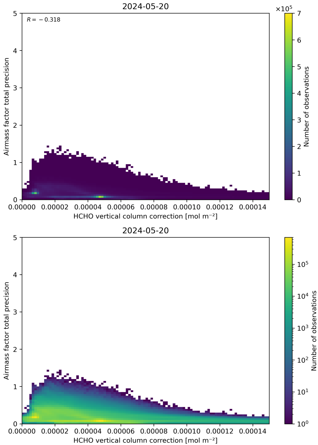
Figure 121: Scatter density plot of “HCHO vertical column correction” against “Airmass factor total precision” for 2024-05-19 to 2024-05-21.
