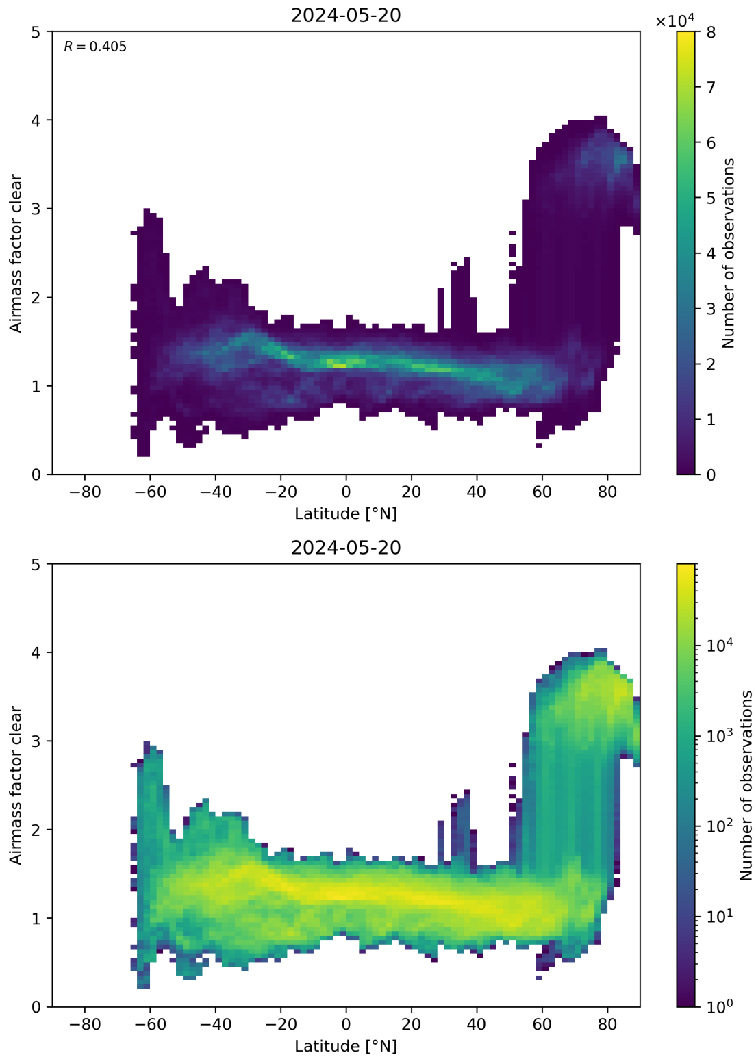
Figure 156: Scatter density plot of “Latitude” against “Airmass factor clear” for 2024-05-19 to 2024-05-21.
