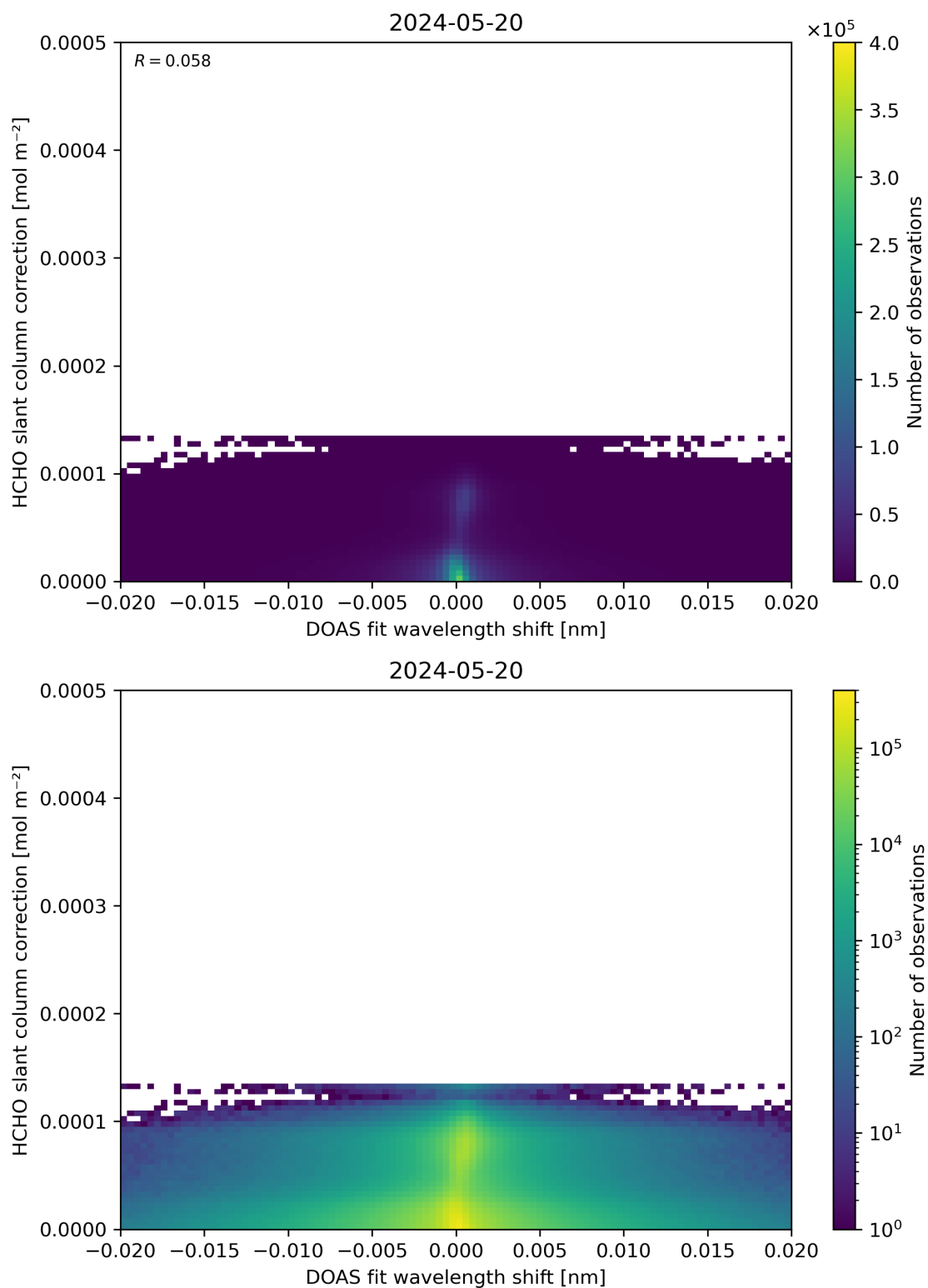
Figure 67: Scatter density plot of “DOAS fit wavelength shift” against “HCHO slant column correction” for 2024-05-19 to 2024-05-21.
