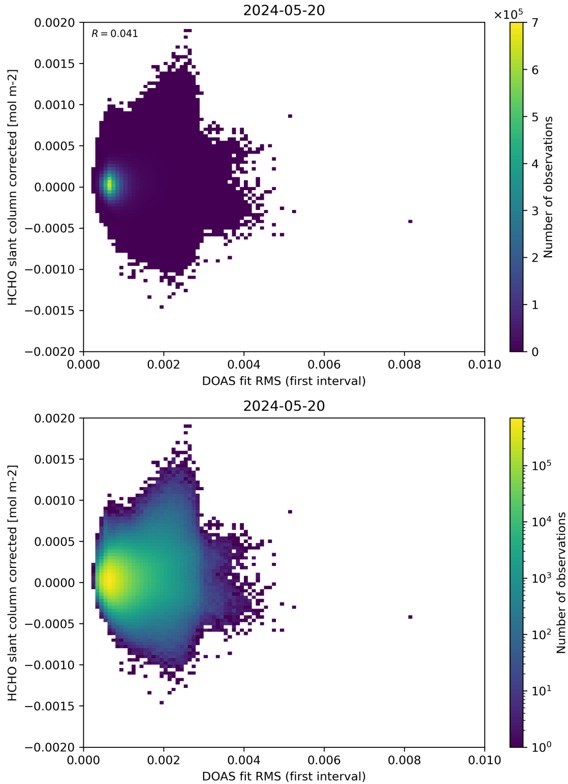
Figure 62: Scatter density plot of “DOAS fit RMS (first interval)” against “HCHO slant column corrected” for 2024-05-19 to 2024-05-21.
