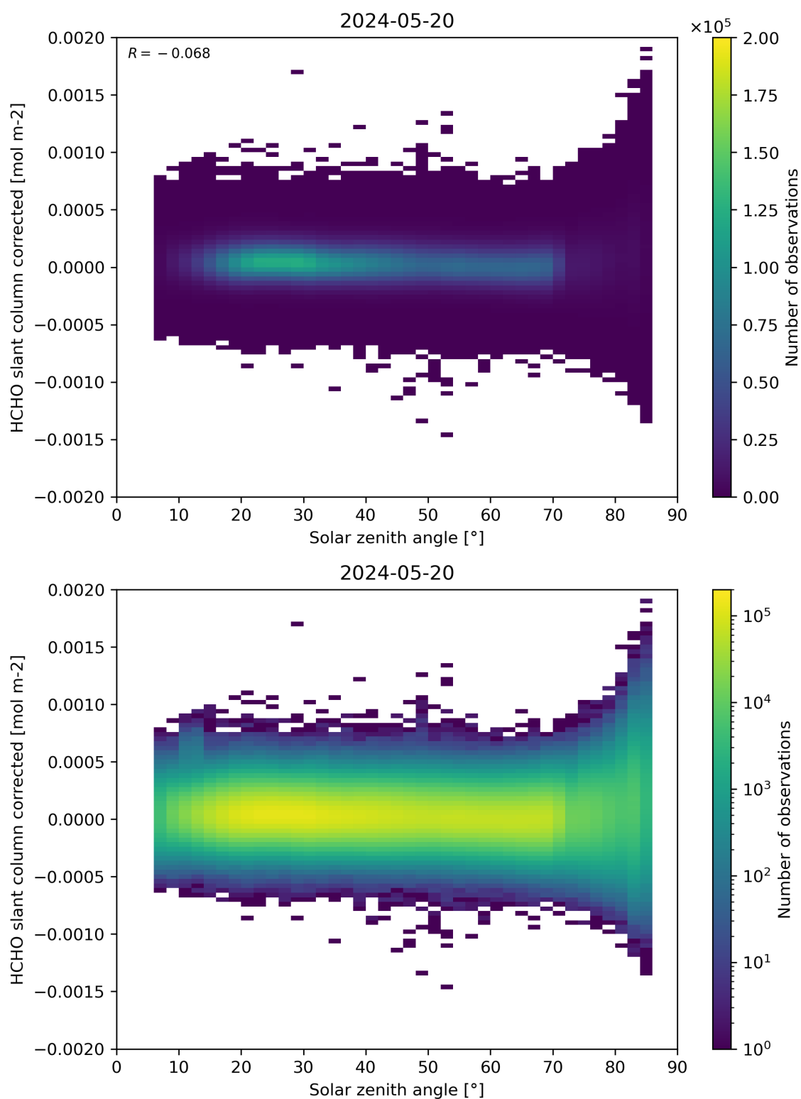
Figure 171: Scatter density plot of “Solar zenith angle” against “HCHO slant column corrected” for 2024-05-19 to 2024-05-21.
