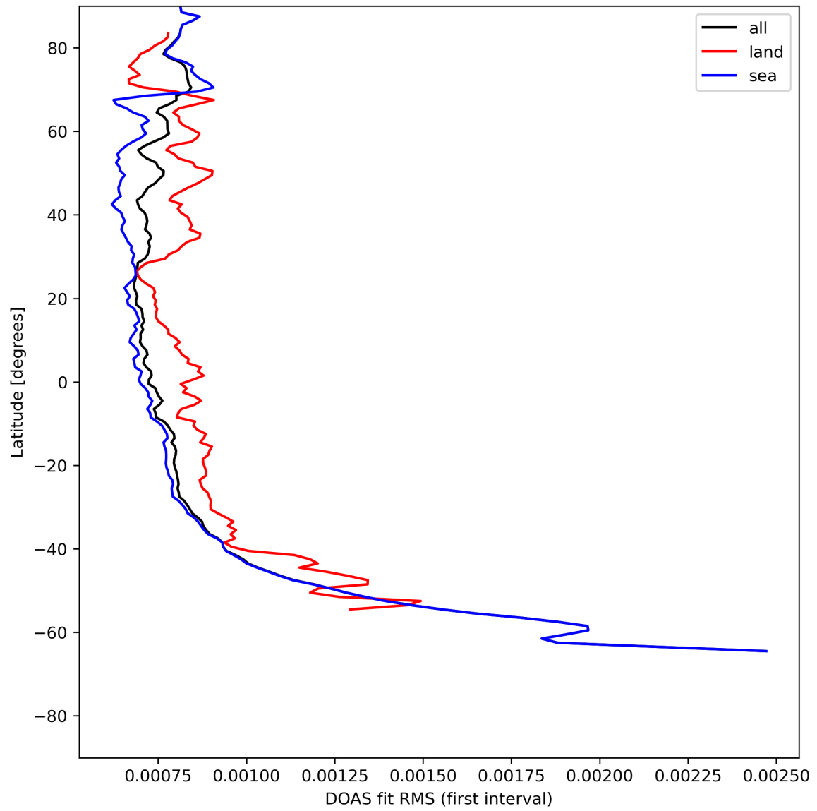
Figure 32: Zonal average of “DOAS fit RMS (first interval)” for 2024-05-19 to 2024-05-21.
