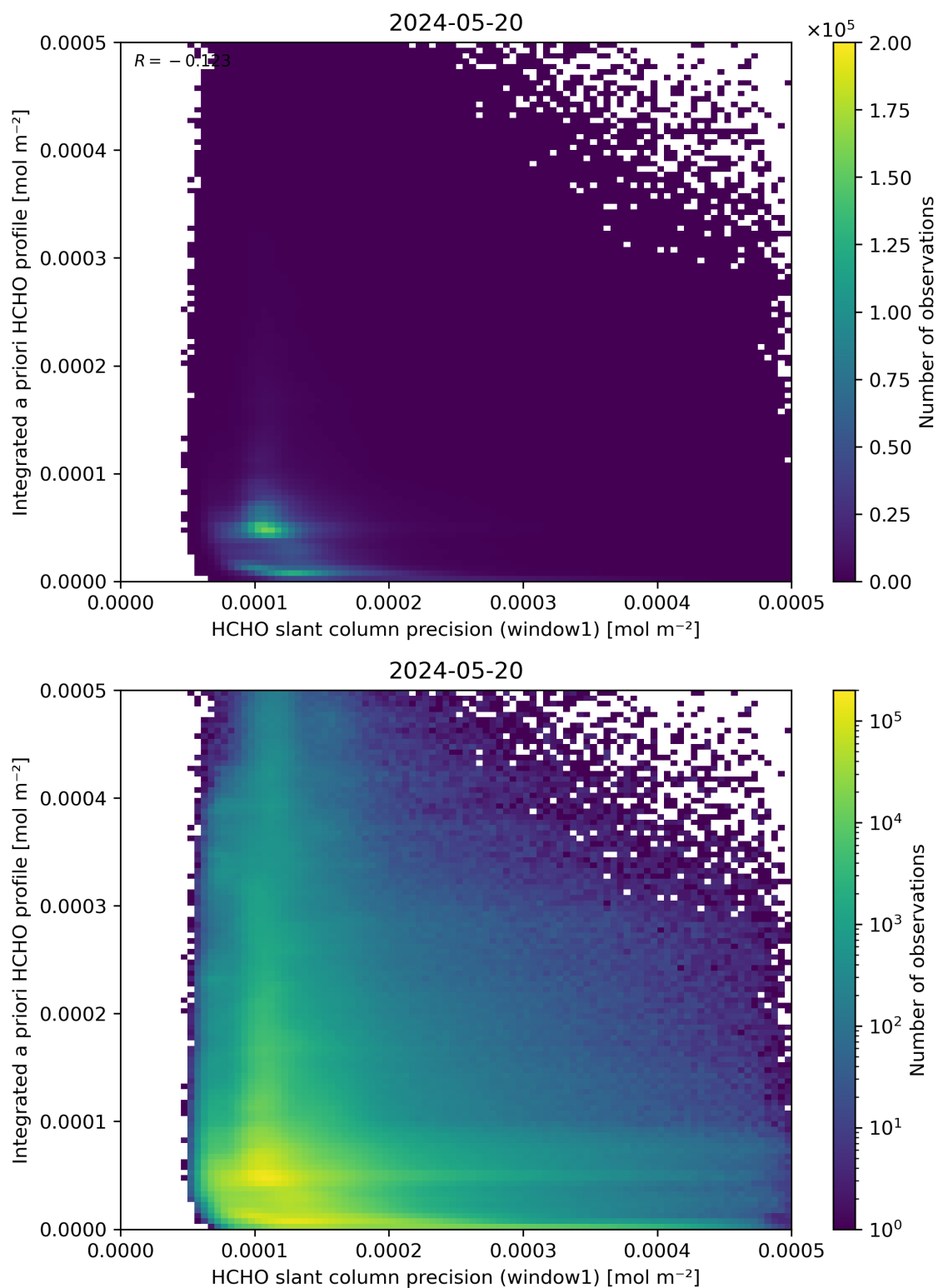
Figure 96: Scatter density plot of “HCHO slant column precision (window1)” against “Integrated a priori HCHO profile” for 2024-05-19 to 2024-05-21.
