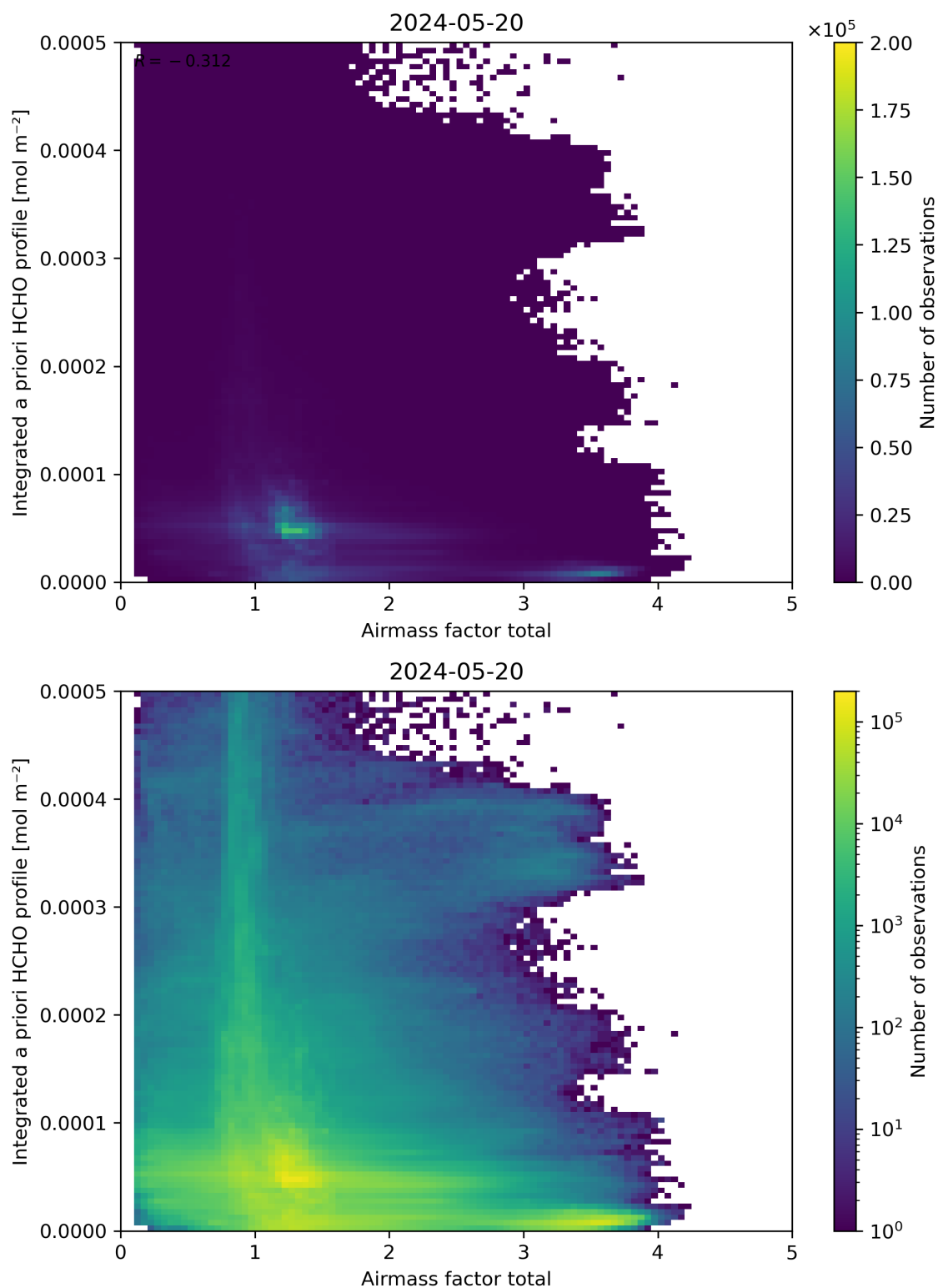
Figure 104: Scatter density plot of “Airmass factor total” against “Integrated a priori HCHO profile” for 2024-05-19 to 2024-05-21.
