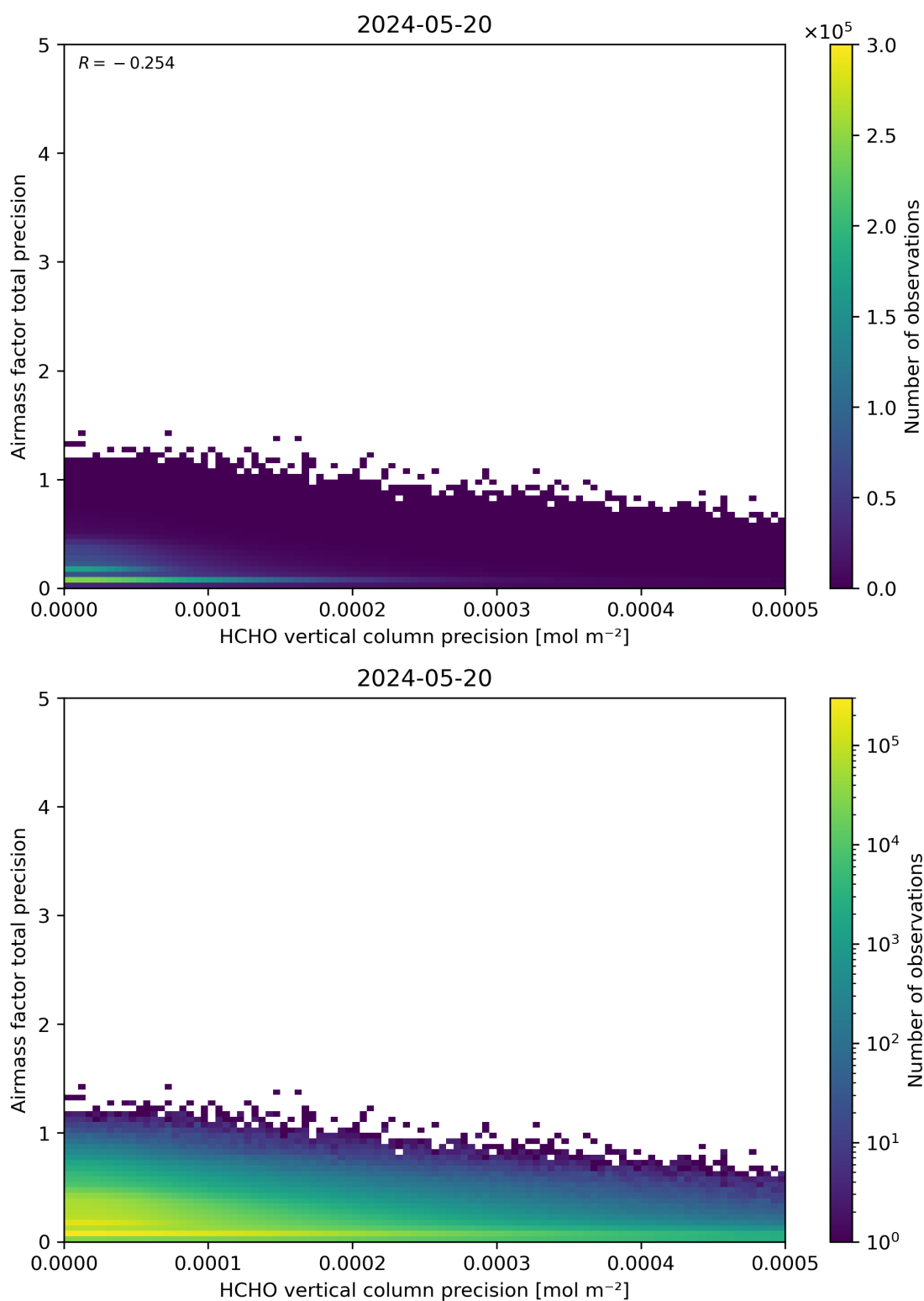
Figure 145: Scatter density plot of “HCHO vertical column precision” against “Airmass factor total precision” for 2024-05-19 to 2024-05-21.
