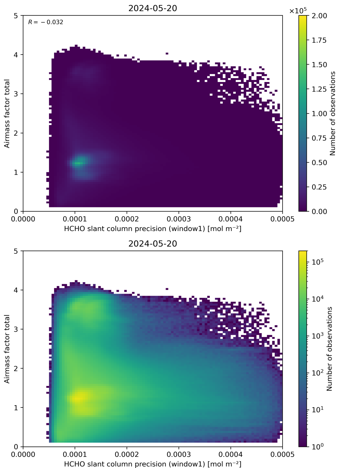
Figure 94: Scatter density plot of “HCHO slant column precision (window1)” against “Airmass factor total” for 2024-05-19 to 2024-05-21.
