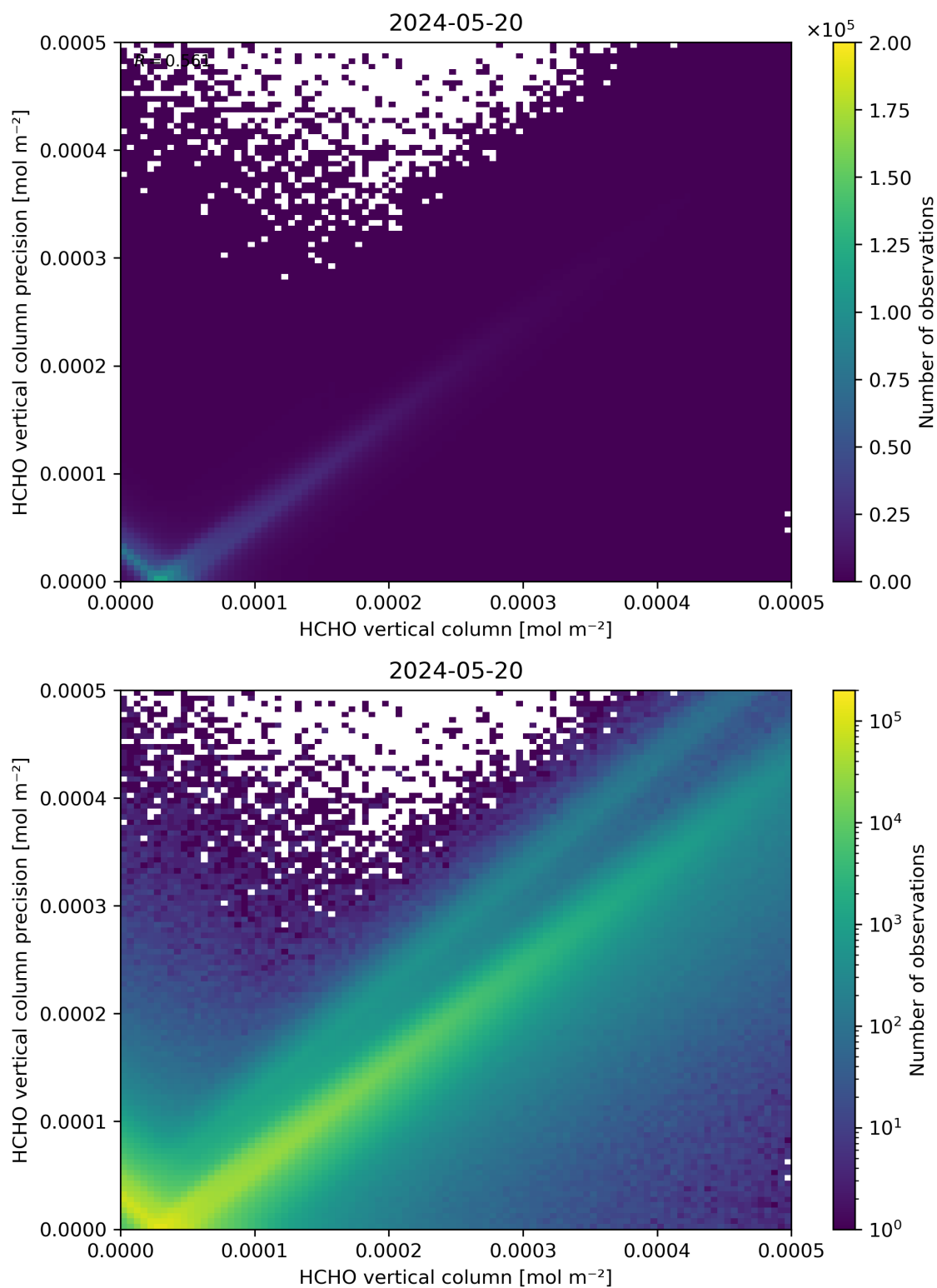
Figure 134: Scatter density plot of “HCHO vertical column” against “HCHO vertical column precision” for 2024-05-19 to 2024-05-21.
