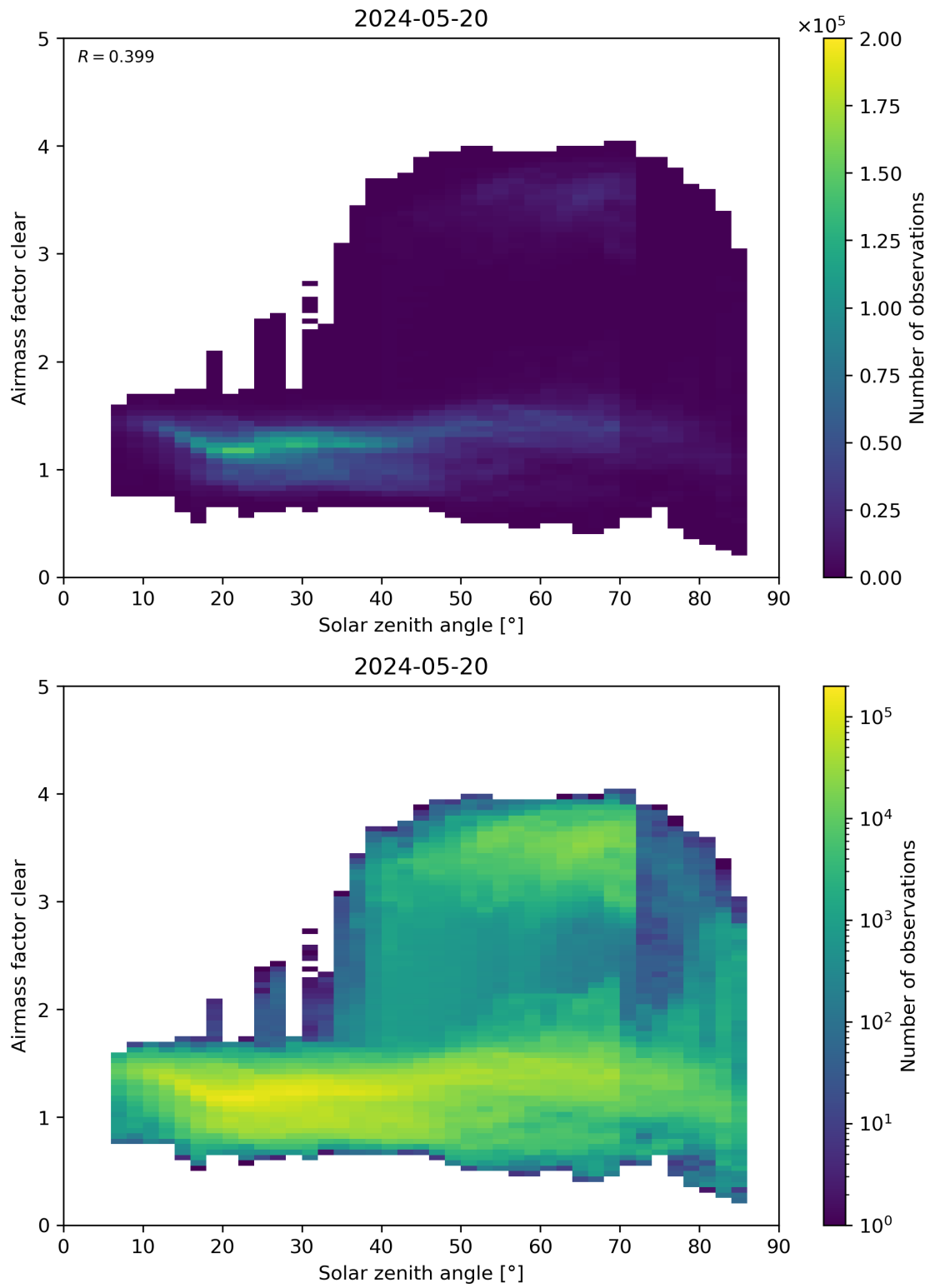
Figure 170: Scatter density plot of “Solar zenith angle” against “Airmass factor clear” for 2024-05-19 to 2024-05-21.
