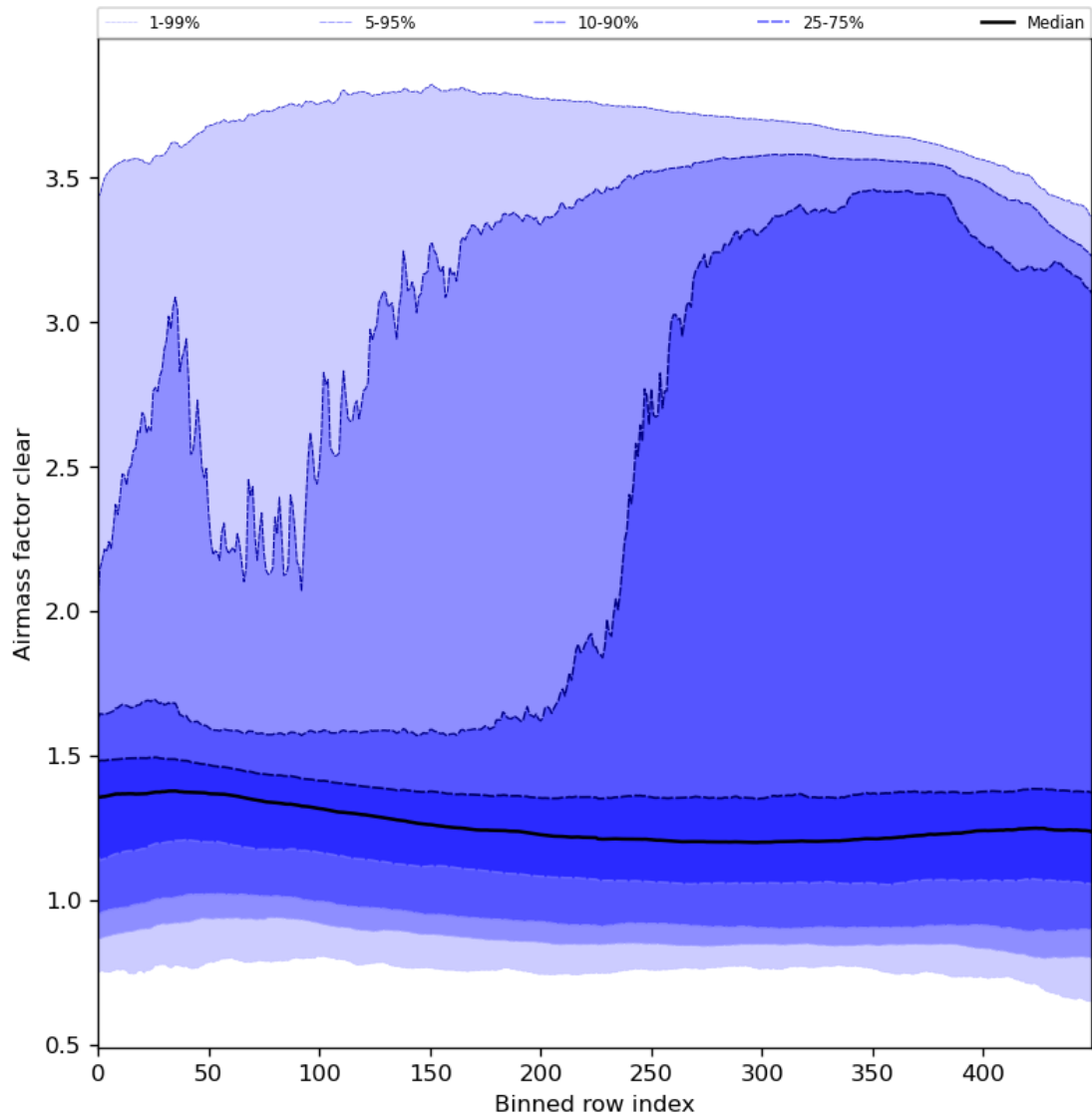
Figure 56: Along track statistics of “Airmass factor clear” for 2024-05-19 to 2024-05-21
