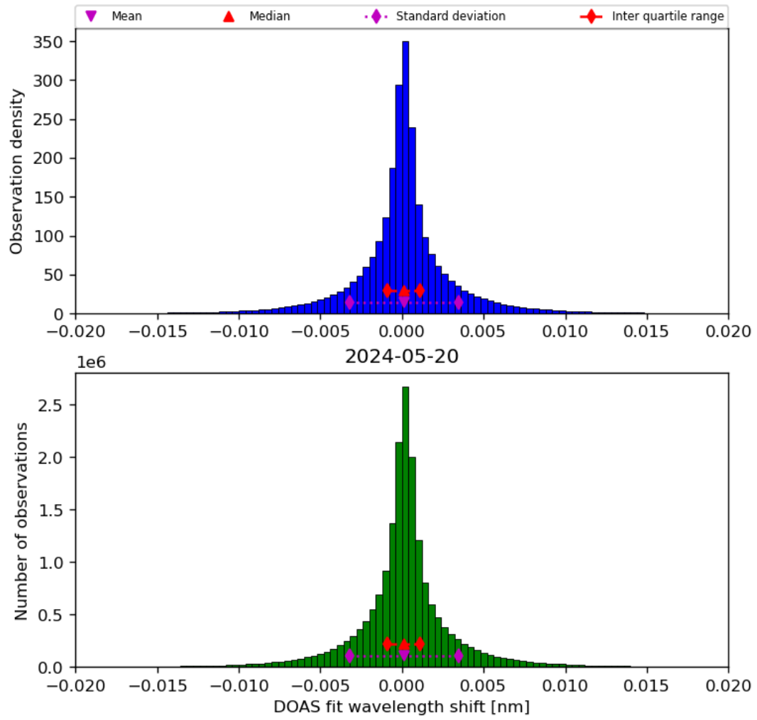
Figure 44: Histogram of “DOAS fit wavelength shift” for 2024-05-19 to 2024-05-21
