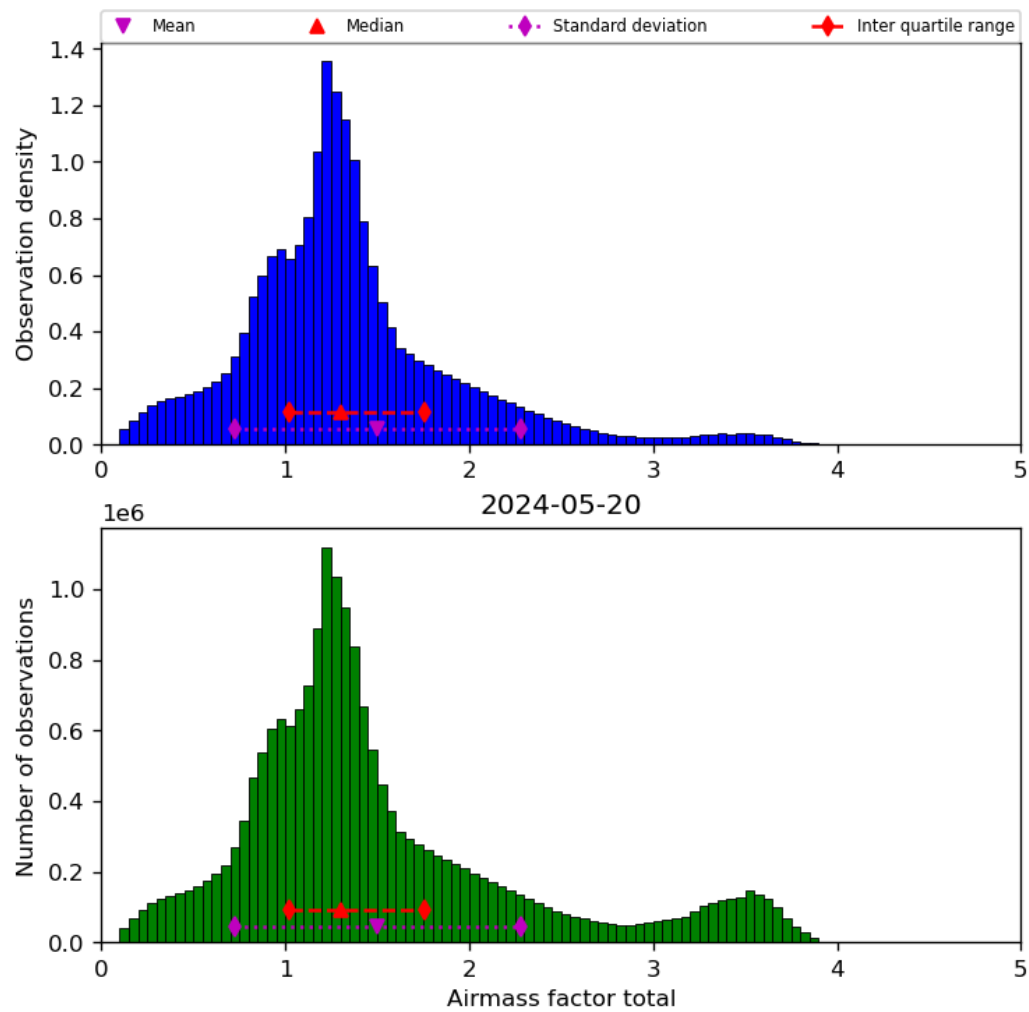
Figure 40: Histogram of “Airmass factor total” for 2024-05-19 to 2024-05-21
