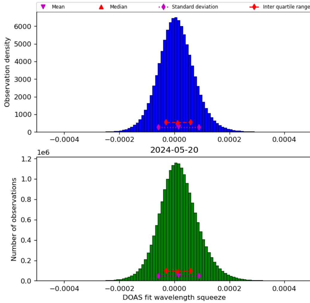
Figure 45: Histogram of “DOAS fit wavelength squeeze” for 2024-05-19 to 2024-05-21
