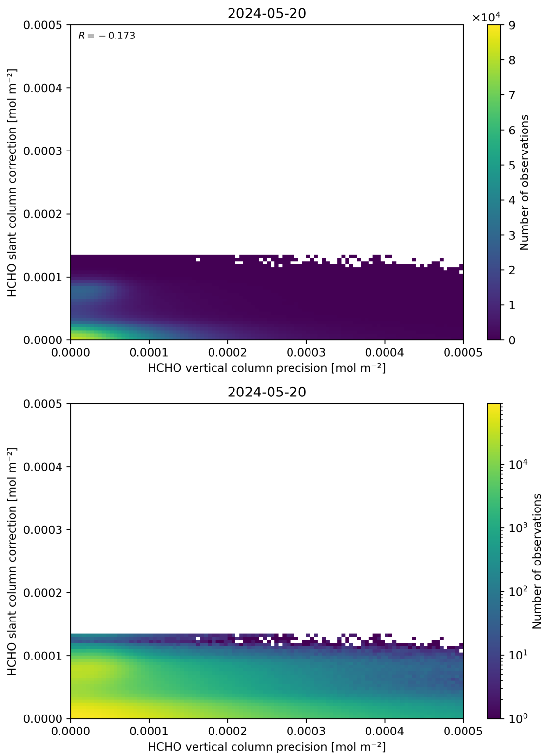
Figure 141: Scatter density plot of “HCHO vertical column precision” against “HCHO slant column correction” for 2024-05-19 to 2024-05-21.
