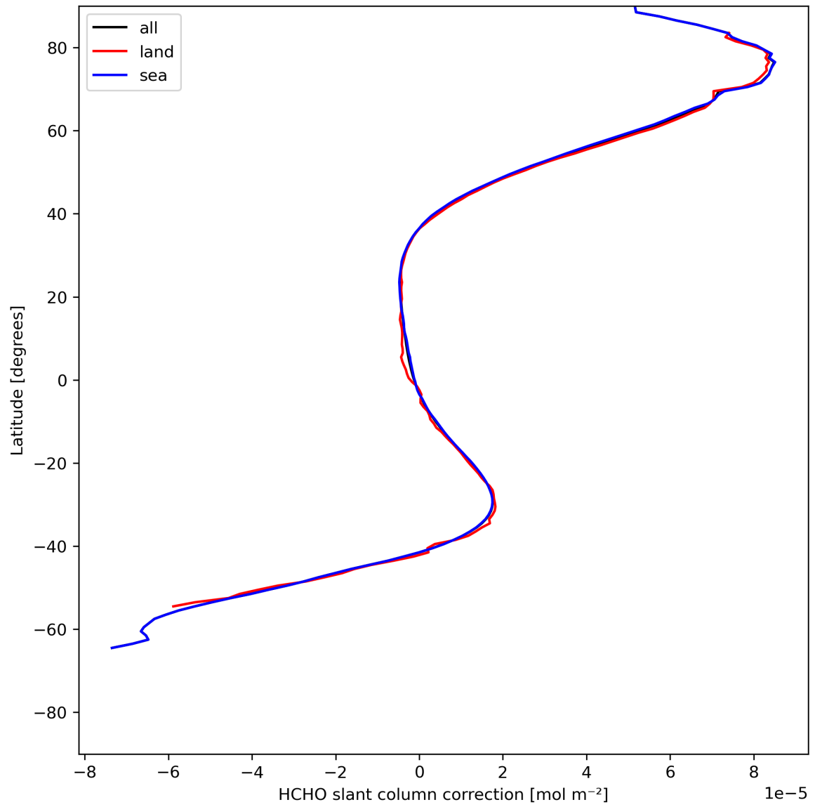
Figure 33: Zonal average of “HCHO slant column correction” for 2024-05-19 to 2024-05-21.
