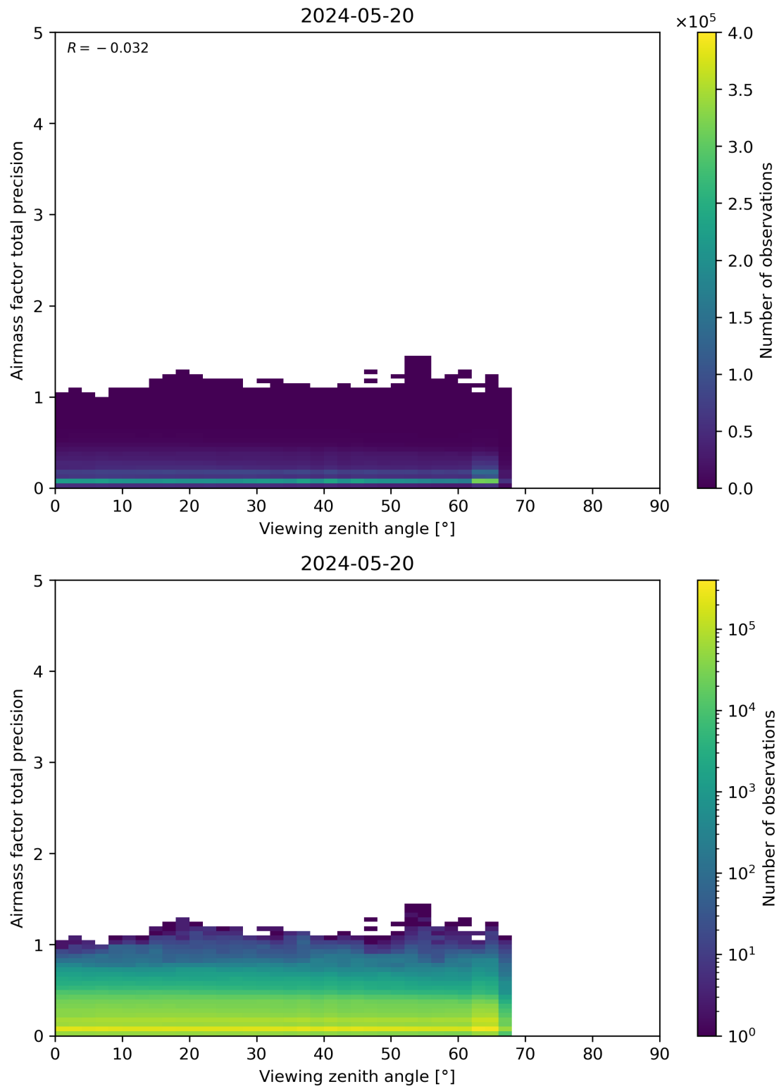
Figure 191: Scatter density plot of “Viewing zenith angle” against “Airmass factor total precision” for 2024-05-19 to 2024-05-21.
