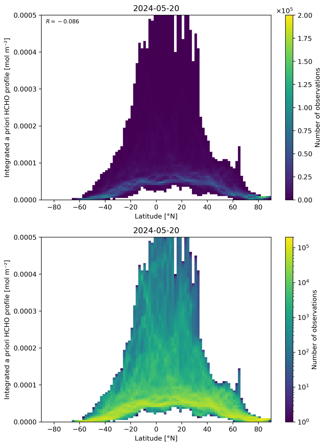
Figure 166: Scatter density plot of “Latitude” against “Integrated a priori HCHO profile” for 2024-05-19 to 2024-05-21.
