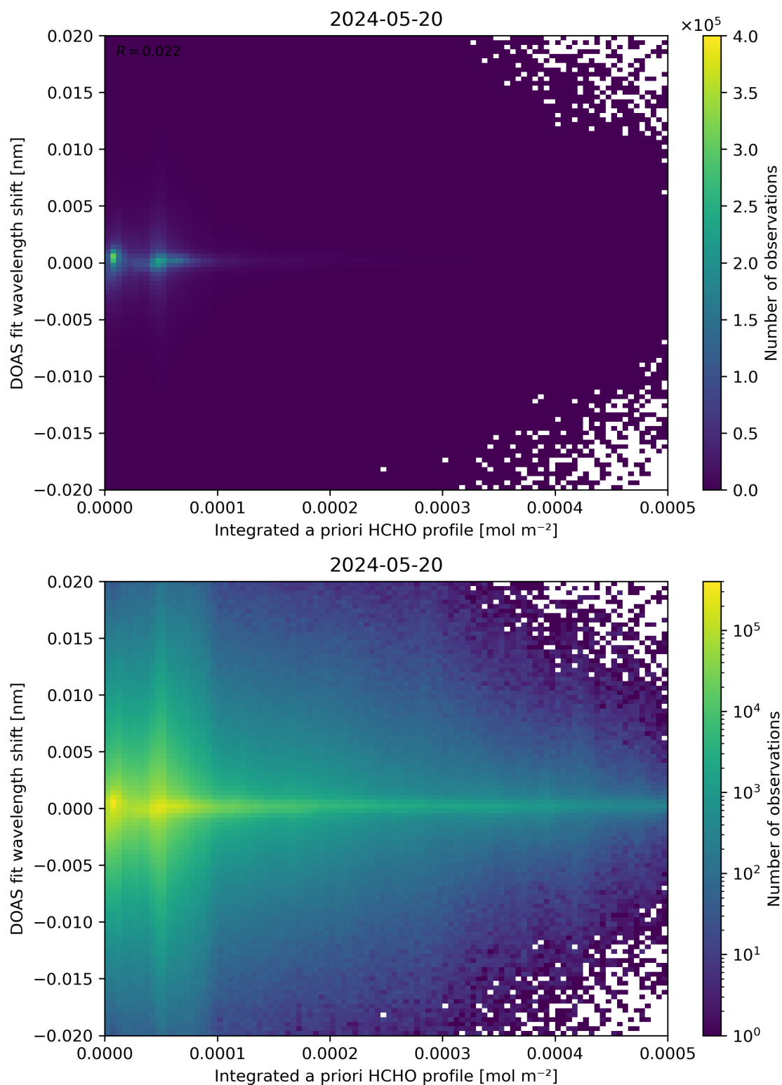
Figure 149: Scatter density plot of “Integrated a priori HCHO profile” against “DOAS fit wavelength shift” for 2024-05-19 to 2024-05-21.
