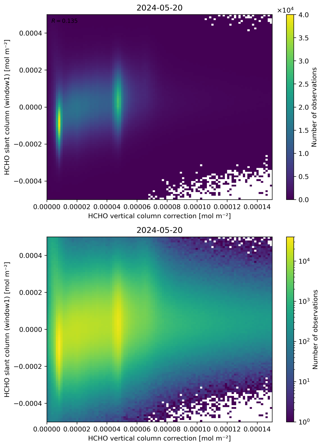
Figure 118: Scatter density plot of “HCHO vertical column correction” against “HCHO slant column (window1)” for 2024-05-19 to 2024-05-21.
