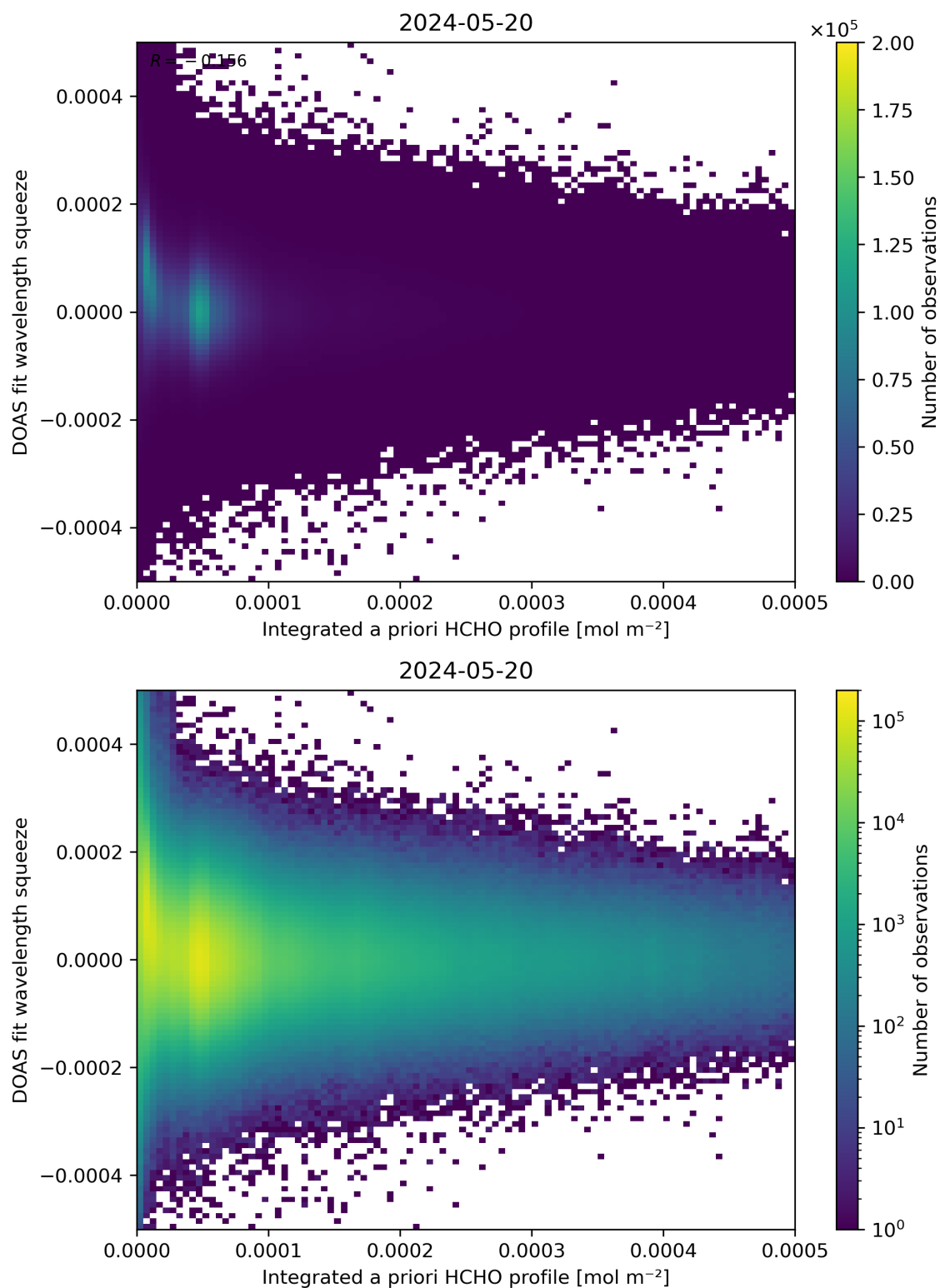
Figure 150: Scatter density plot of “Integrated a priori HCHO profile” against “DOAS fit wavelength squeeze” for 2024-05-19 to 2024-05-21.
