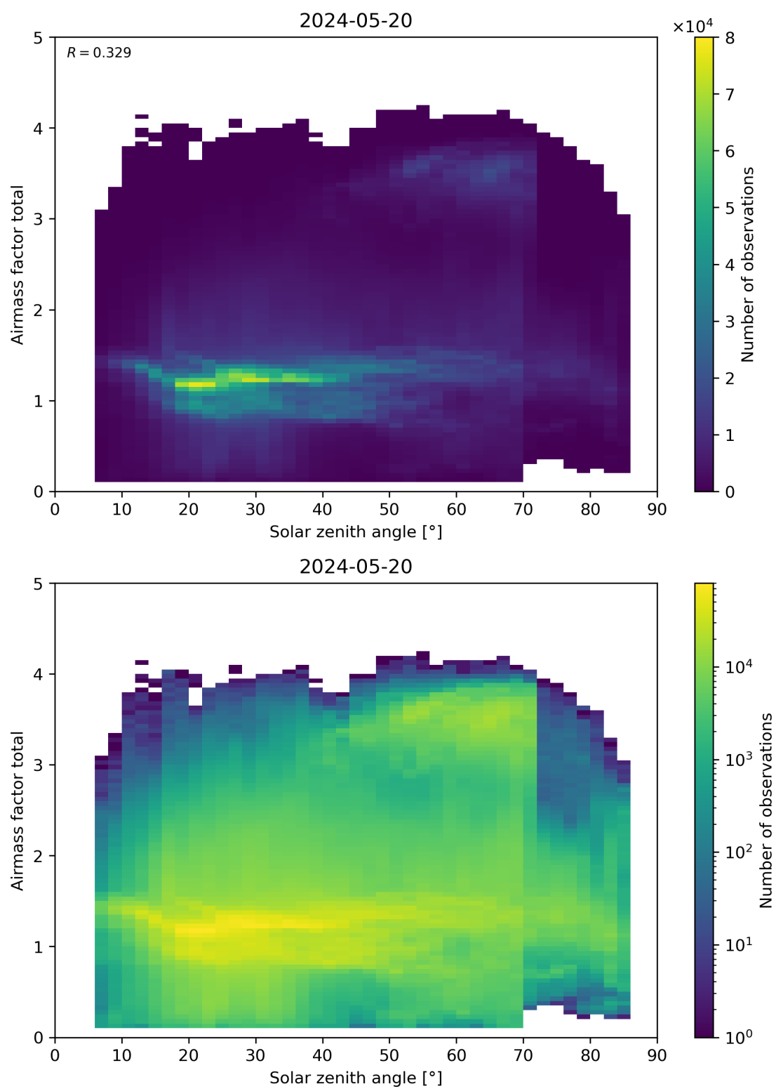
Figure 175: Scatter density plot of “Solar zenith angle” against “Airmass factor total” for 2024-05-19 to 2024-05-21.
