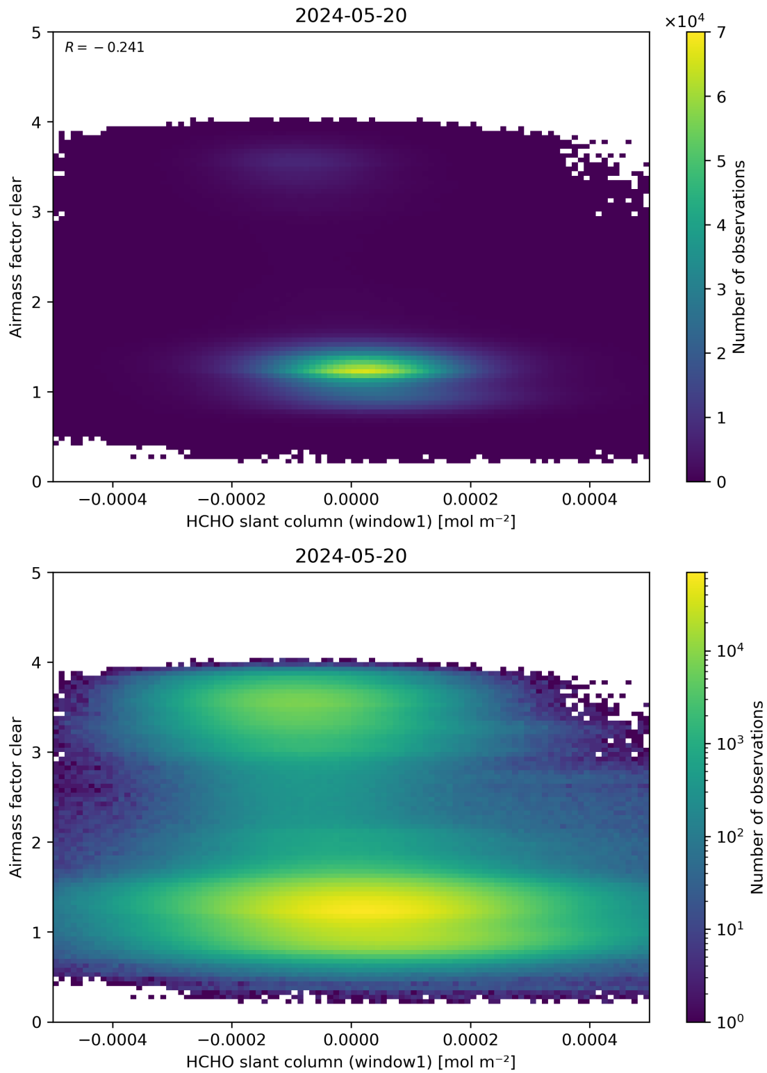
Figure 81: Scatter density plot of “HCHO slant column (window1)” against “Airmass factor clear” for 2024-05-19 to 2024-05-21.
