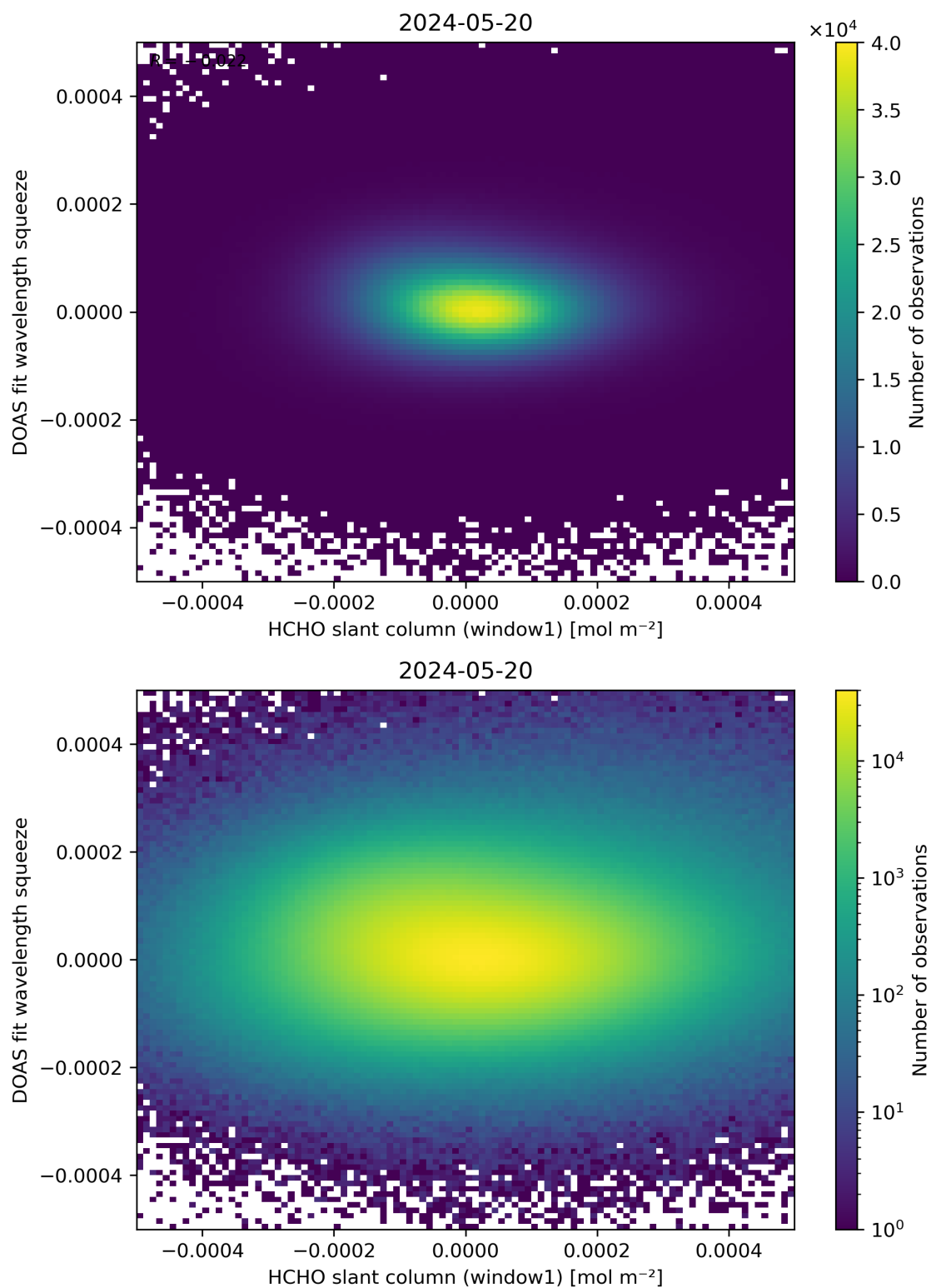
Figure 80: Scatter density plot of “HCHO slant column (window1)” against “DOAS fit wavelength squeeze” for 2024-05-19 to 2024-05-21.
