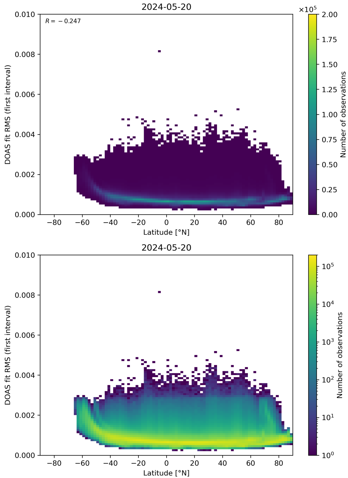
Figure 153: Scatter density plot of “Latitude” against “DOAS fit RMS (first interval)” for 2024-05-19 to 2024-05-21.
