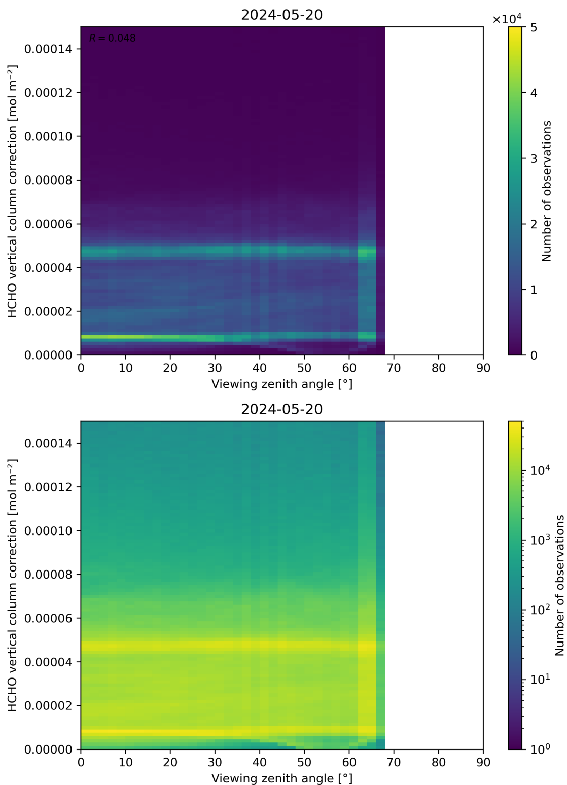
Figure 193: Scatter density plot of “Viewing zenith angle” against “HCHO vertical column correction” for 2024-05-19 to 2024-05-21.
