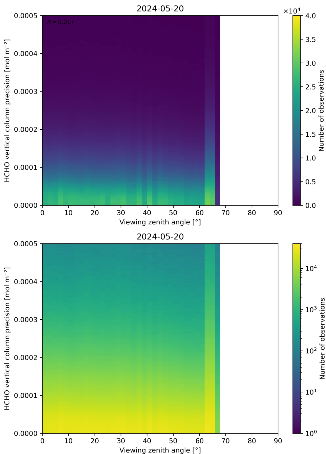
Figure 194: Scatter density plot of “Viewing zenith angle” against “HCHO vertical column precision” for 2024-05-19 to 2024-05-21.
