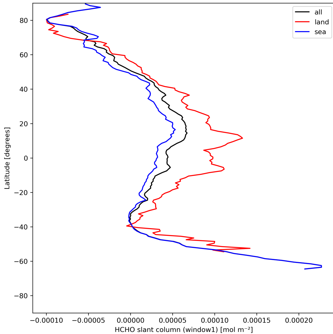
Figure 24: Zonal average of “HCHO slant column (window1)” for 2024-05-19 to 2024-05-21.
