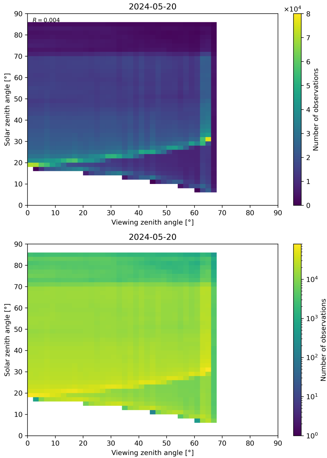
Figure 197: Scatter density plot of “Viewing zenith angle” against “Solar zenith angle” for 2024-05-19 to 2024-05-21.
