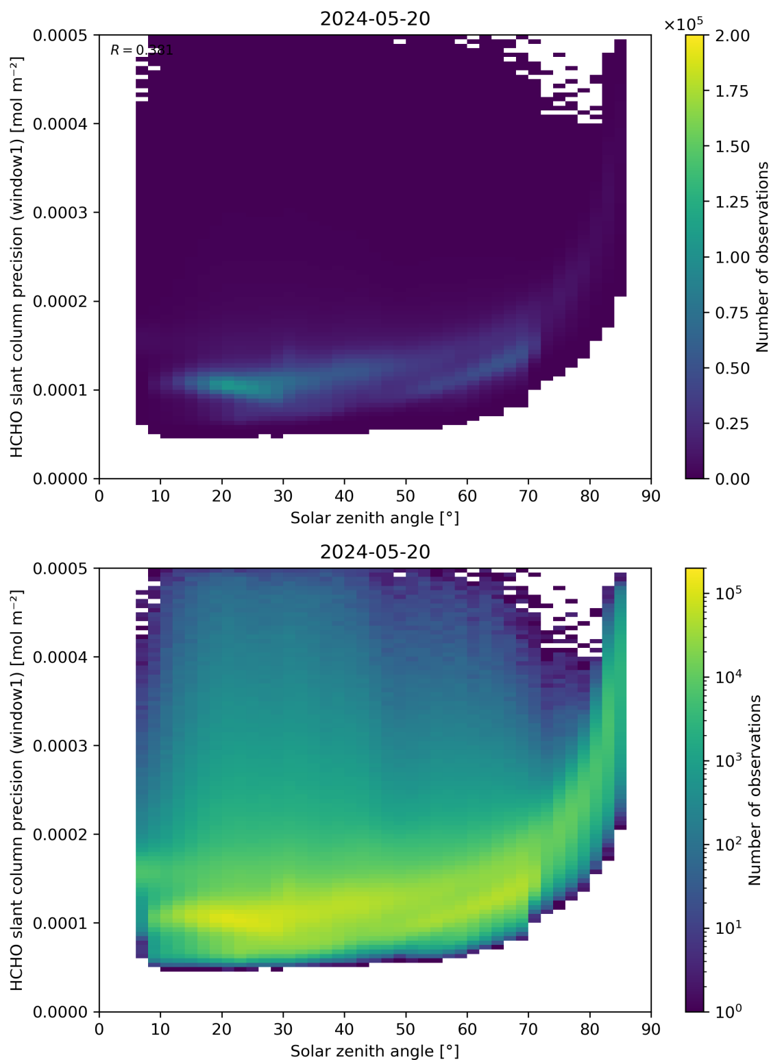
Figure 174: Scatter density plot of “Solar zenith angle” against “HCHO slant column precision (window1)” for 2024-05-19 to 2024-05-21.
