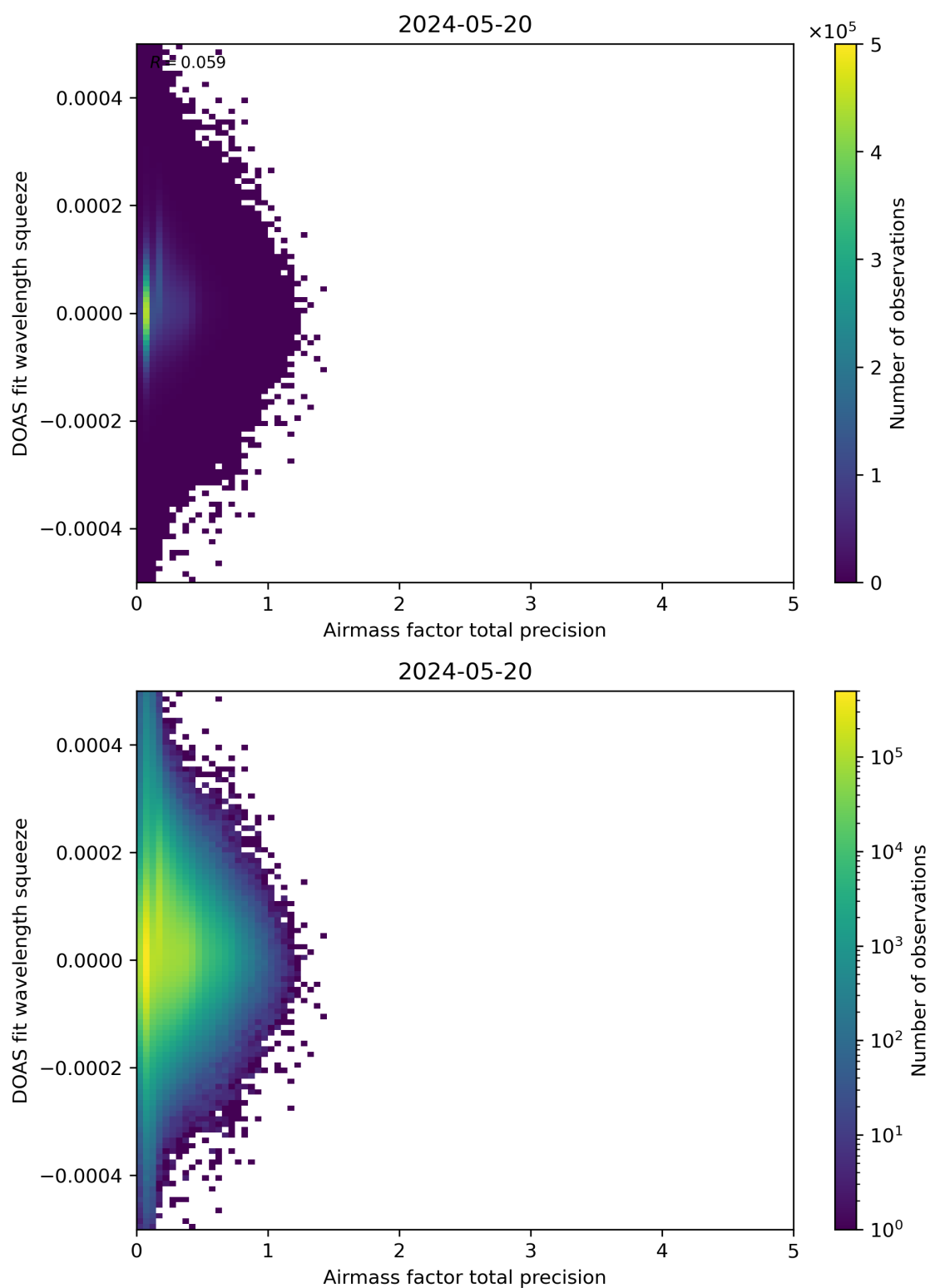
Figure 107: Scatter density plot of “Airmass factor total precision” against “DOAS fit wavelength squeeze” for 2024-05-19 to 2024-05-21.
