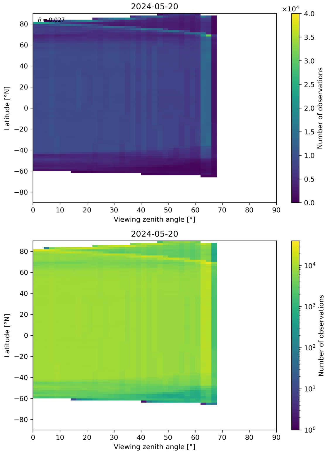
Figure 196: Scatter density plot of “Viewing zenith angle” against “Latitude” for 2024-05-19 to 2024-05-21.
