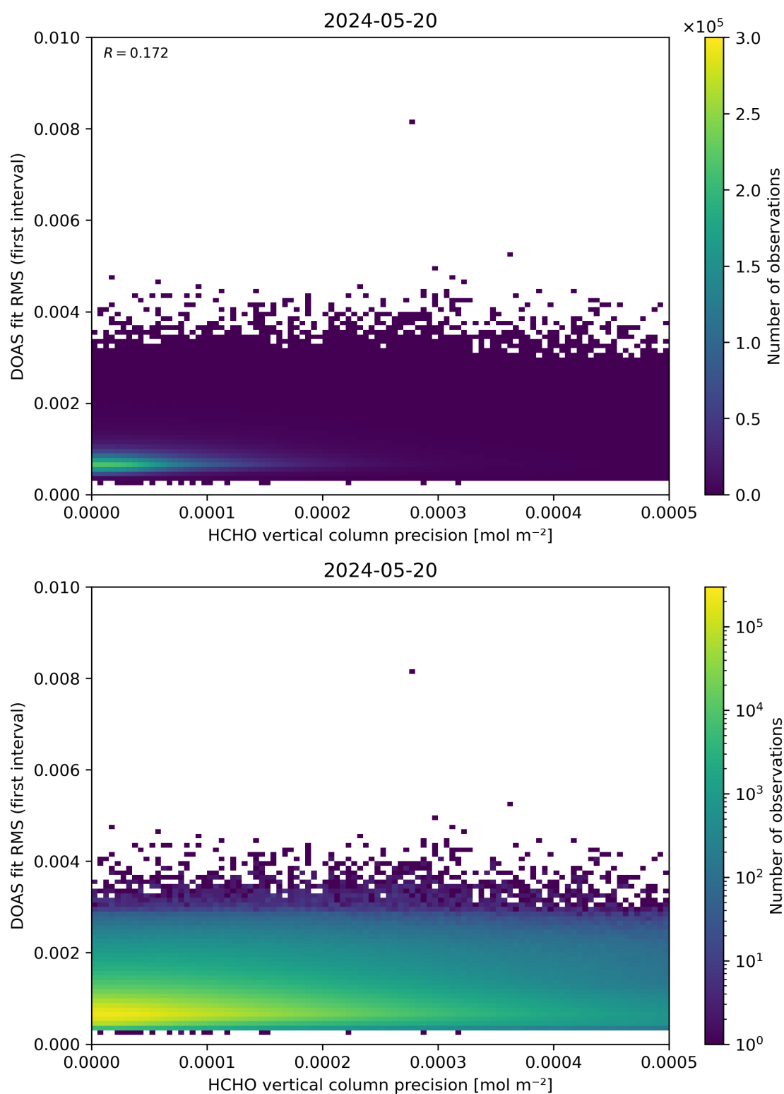
Figure 136: Scatter density plot of “HCHO vertical column precision” against “DOAS fit RMS (first interval)” for 2024-05-19 to 2024-05-21.
