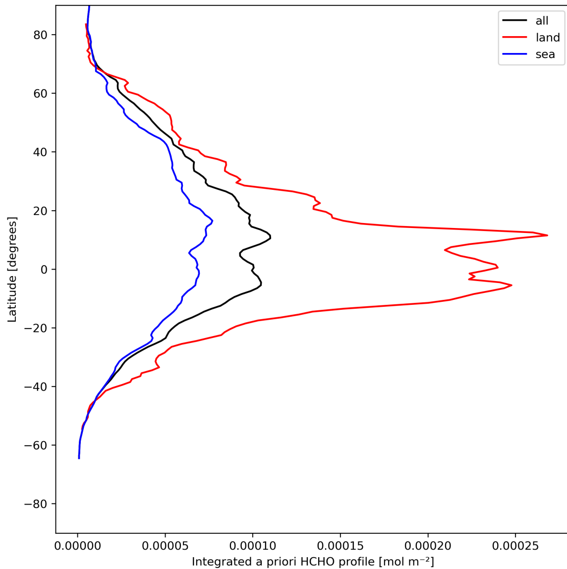
Figure 29: Zonal average of “Integrated a priori HCHO profile” for 2024-05-19 to 2024-05-21.
