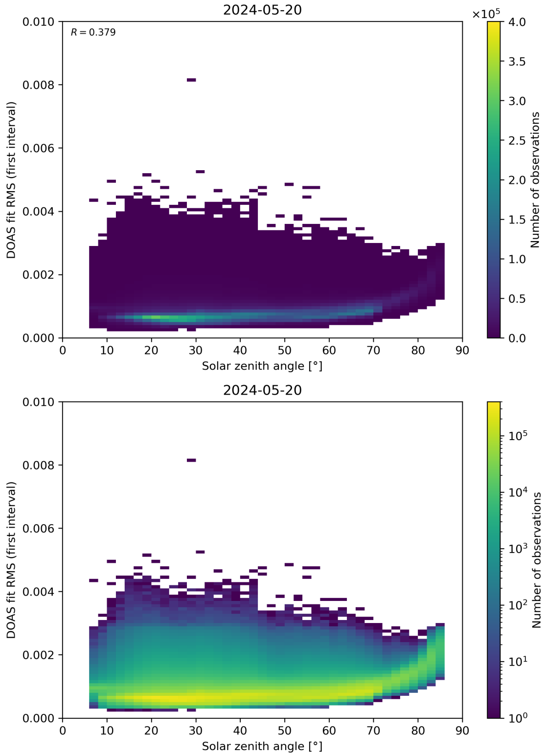
Figure 167: Scatter density plot of “Solar zenith angle” against “DOAS fit RMS (first interval)” for 2024-05-19 to 2024-05-21.
