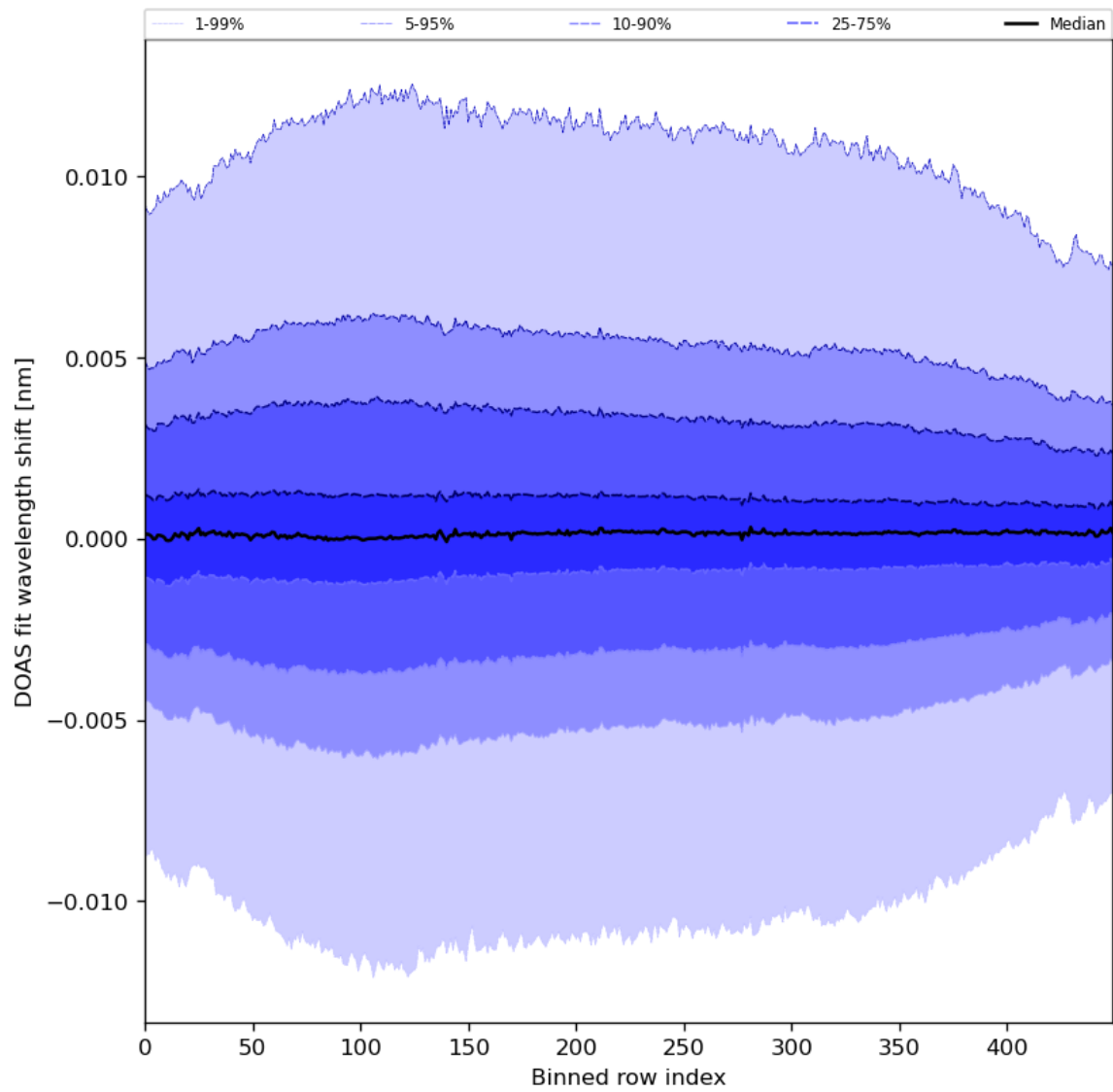
Figure 58: Along track statistics of “DOAS fit wavelength shift” for 2024-05-19 to 2024-05-21
