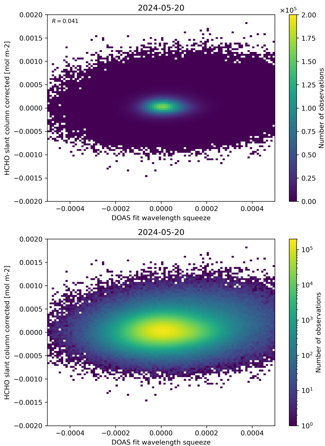
Figure 69: Scatter density plot of “DOAS fit wavelength squeeze” against “HCHO slant column corrected” for 2024-05-19 to 2024-05-21.
