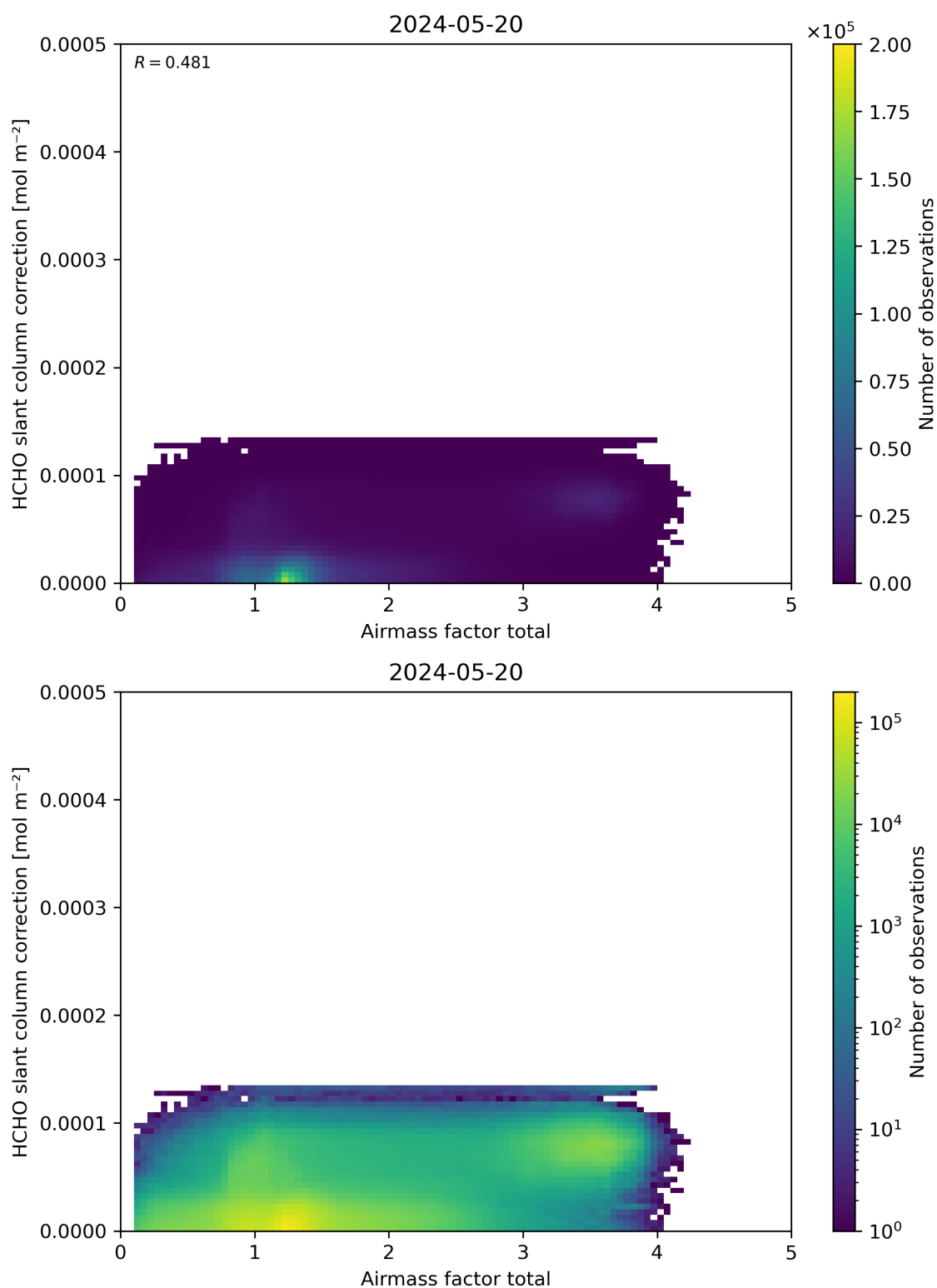
Figure 102: Scatter density plot of “Airmass factor total” against “HCHO slant column correction” for 2024-05-19 to 2024-05-21.
