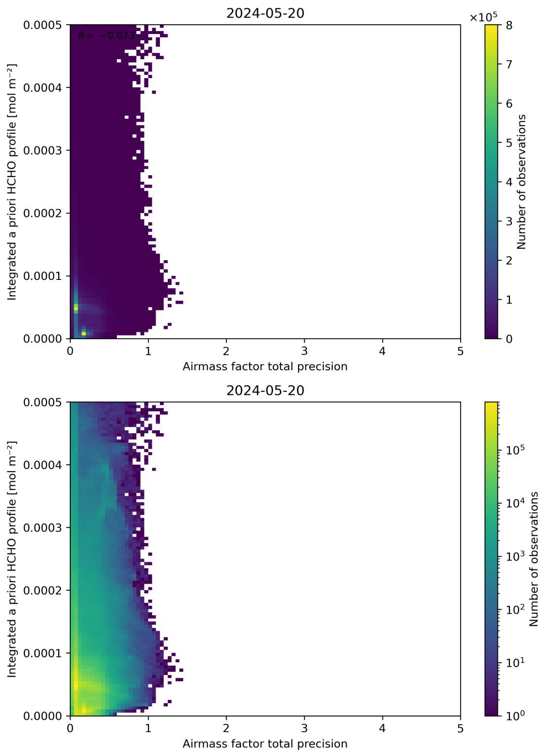
Figure 111: Scatter density plot of “Airmass factor total precision” against “Integrated a priori HCHO profile” for 2024-05-19 to 2024-05-21.
