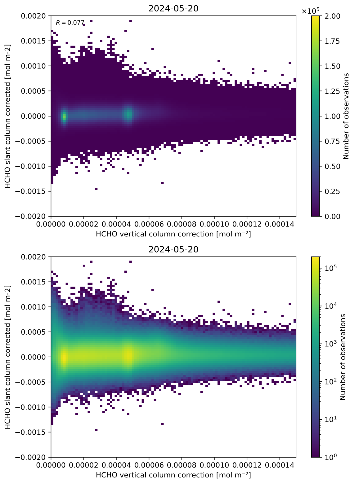
Figure 116: Scatter density plot of “HCHO vertical column correction” against “HCHO slant column corrected” for 2024-05-19 to 2024-05-21.
