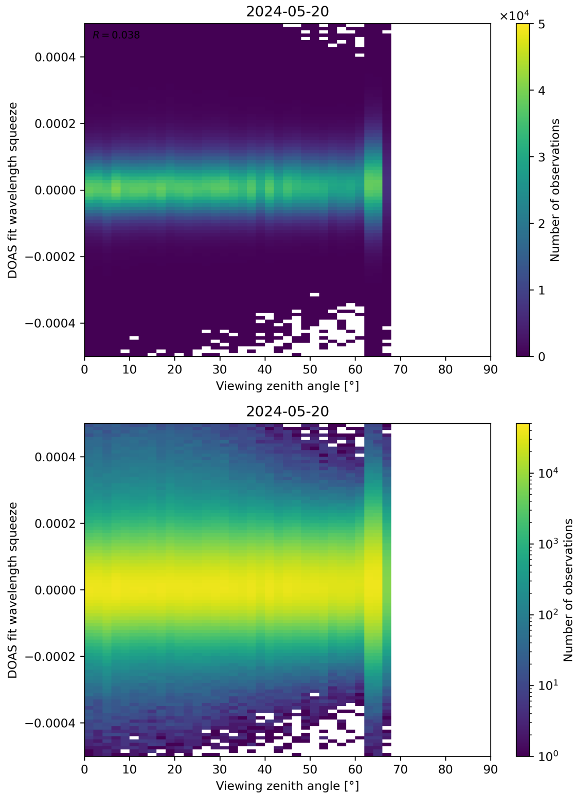
Figure 184: Scatter density plot of “Viewing zenith angle” against “DOAS fit wavelength squeeze” for 2024-05-19 to 2024-05-21.
