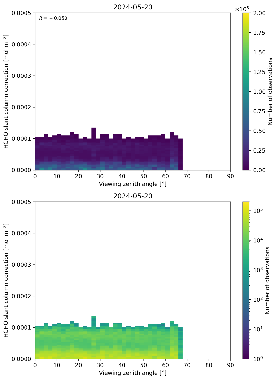
Figure 187: Scatter density plot of “Viewing zenith angle” against “HCHO slant column correction” for 2024-05-19 to 2024-05-21.
