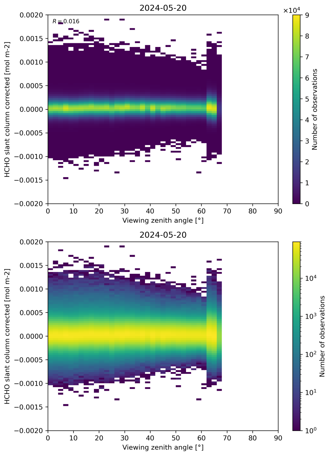
Figure 186: Scatter density plot of “Viewing zenith angle” against “HCHO slant column corrected” for 2024-05-19 to 2024-05-21.
