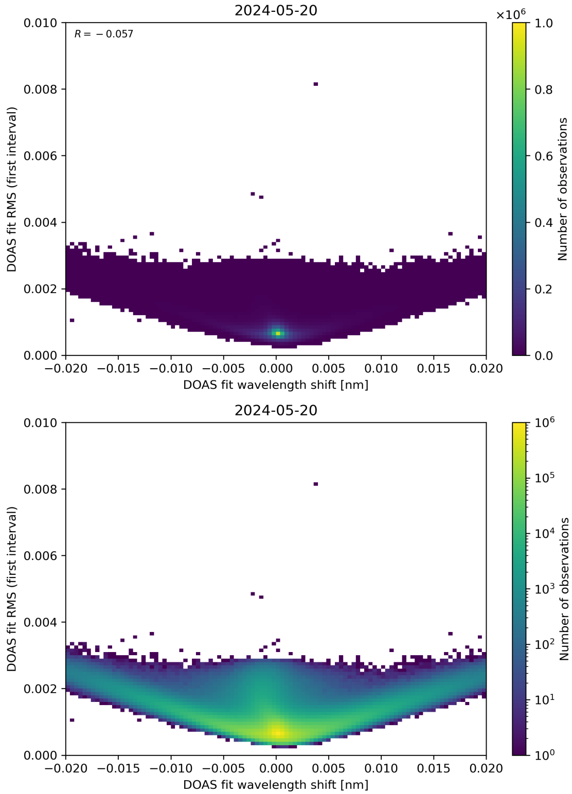
Figure 64: Scatter density plot of “DOAS fit wavelength shift” against “DOAS fit RMS (first interval)” for 2024-05-19 to 2024-05-21.
