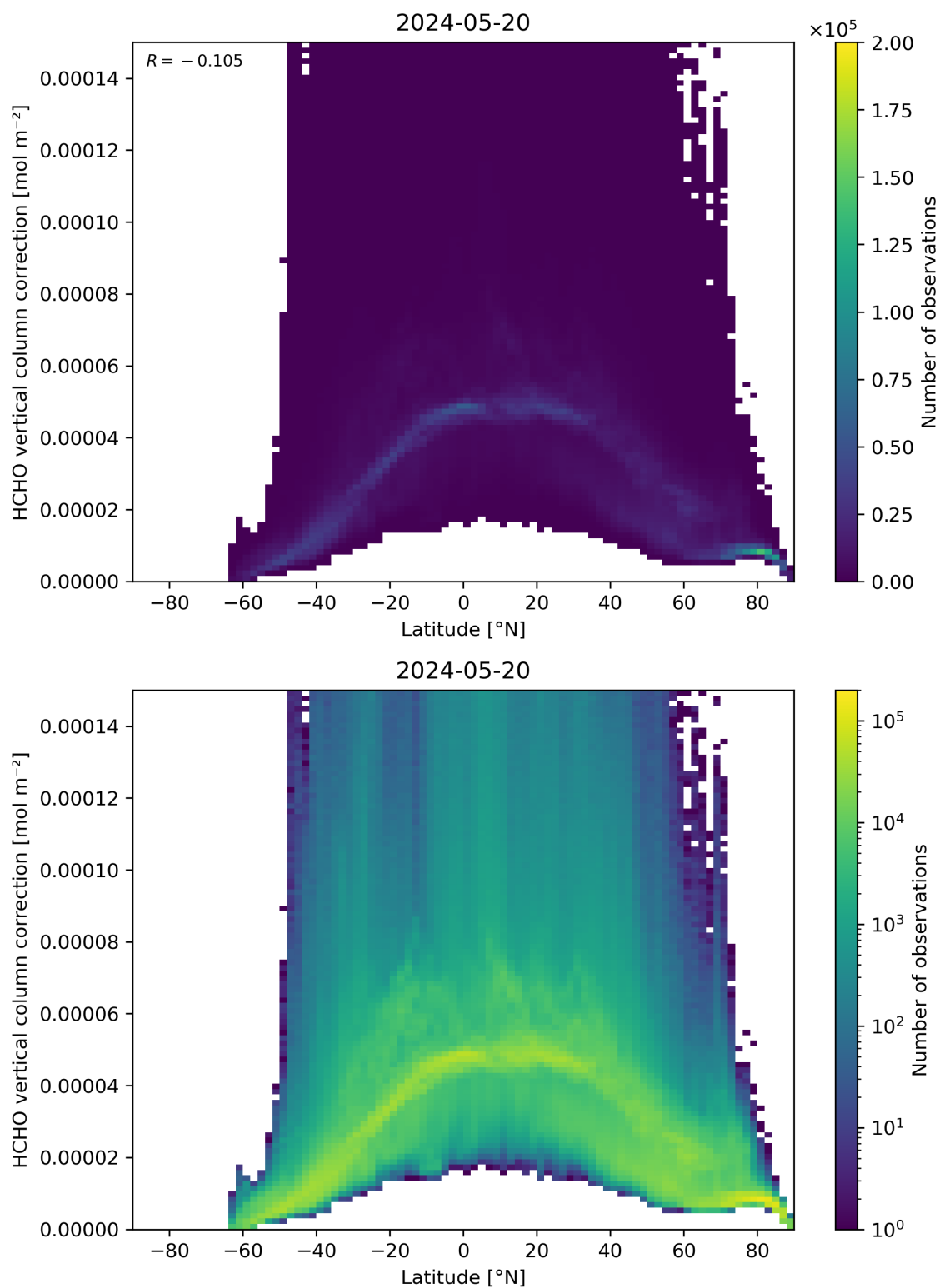
Figure 164: Scatter density plot of “Latitude” against “HCHO vertical column correction” for 2024-05-19 to 2024-05-21.
