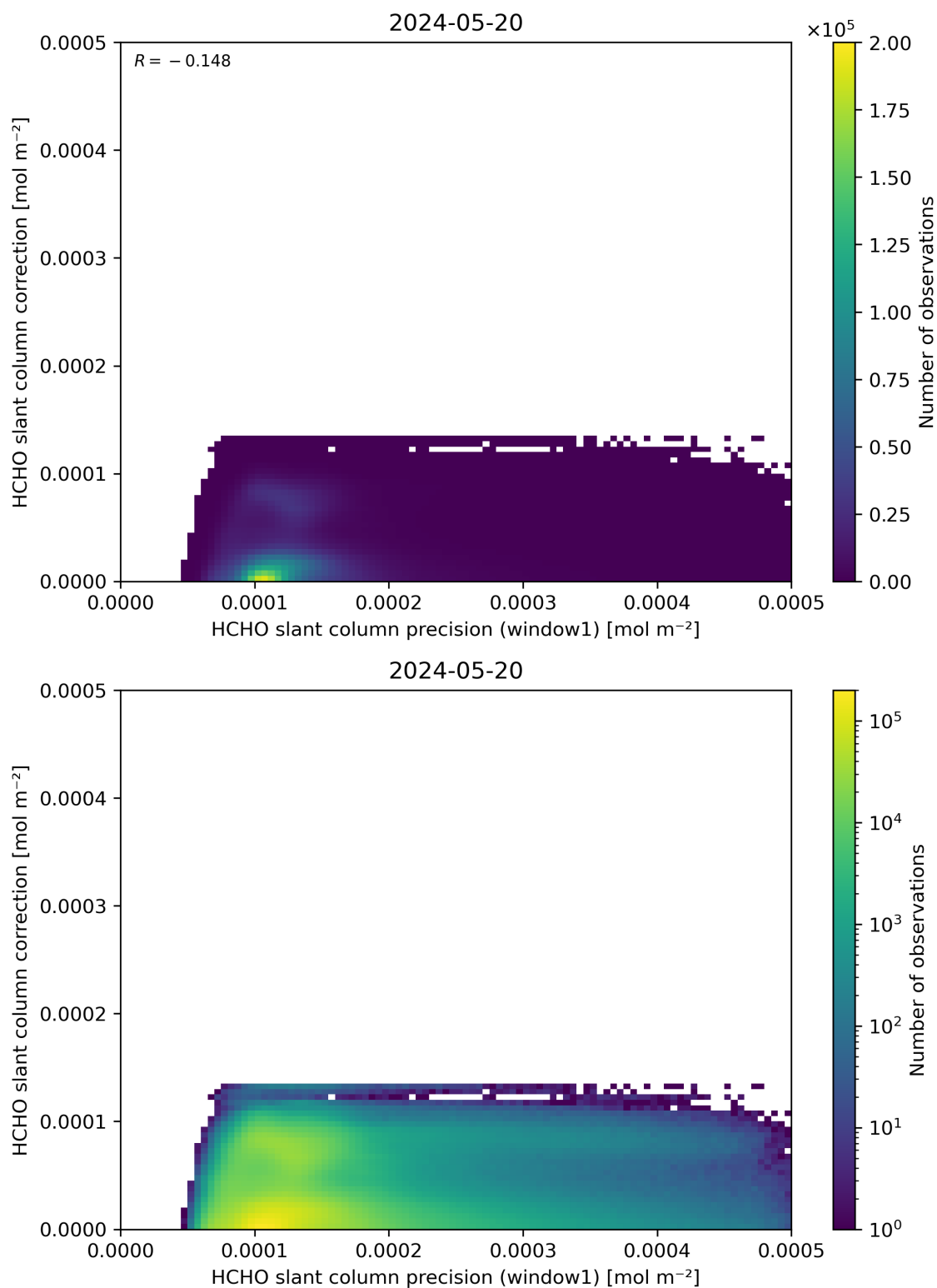
Figure 93: Scatter density plot of “HCHO slant column precision (window1)” against “HCHO slant column correction” for 2024-05-19 to 2024-05-21.
