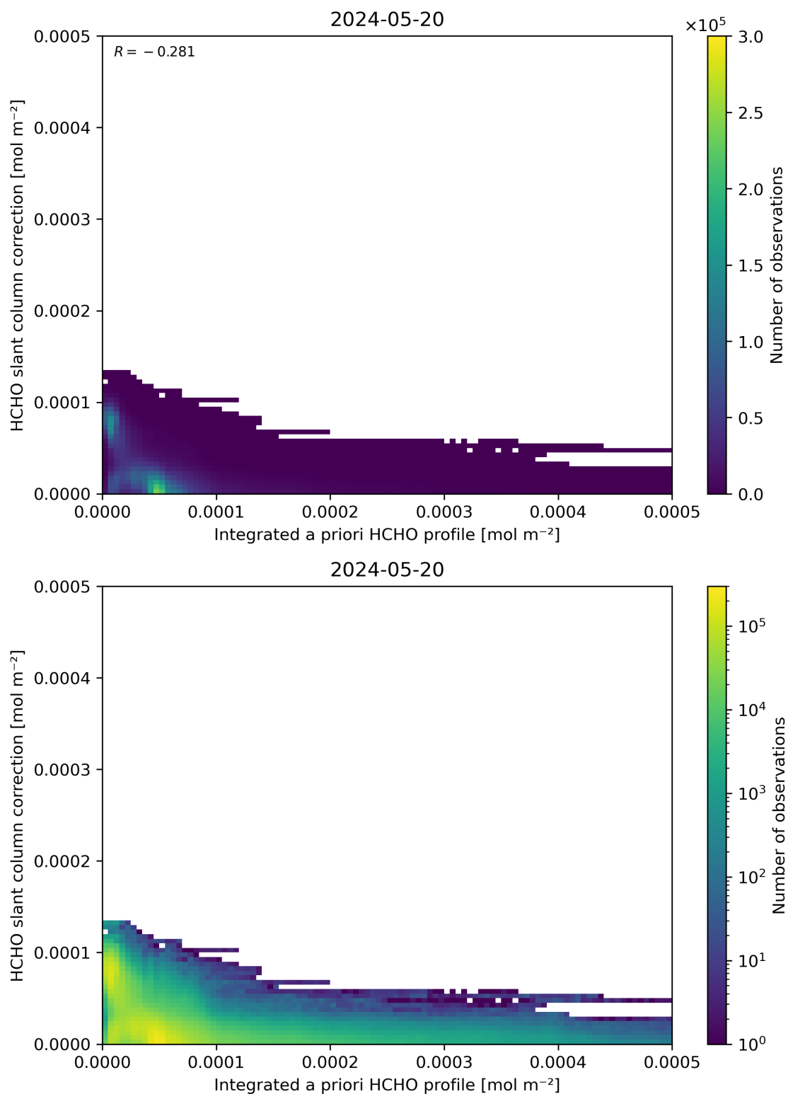
Figure 152: Scatter density plot of “Integrated a priori HCHO profile” against “HCHO slant column correction” for 2024-05-19 to 2024-05-21.
