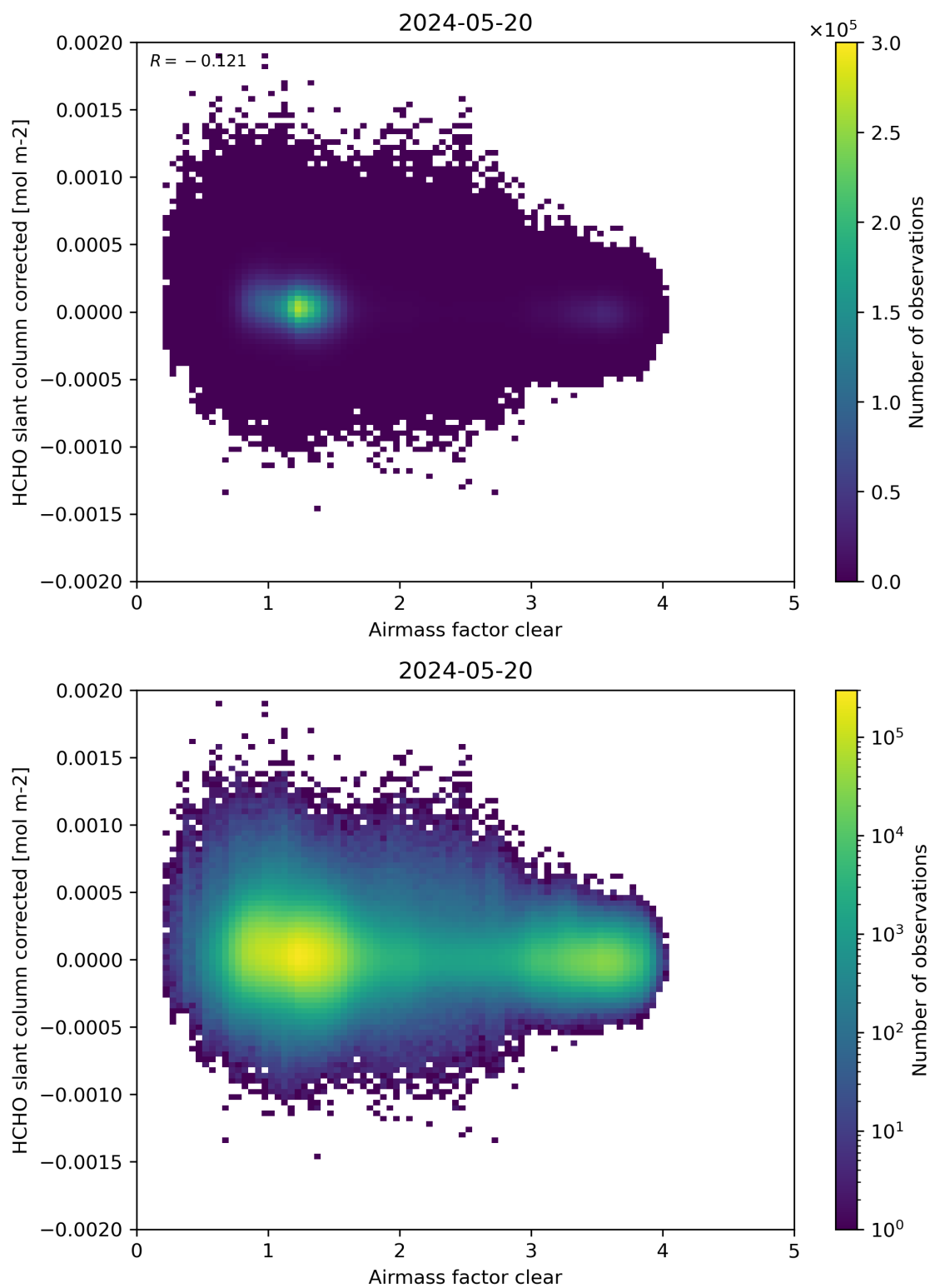
Figure 74: Scatter density plot of “Airmass factor clear” against “HCHO slant column corrected” for 2024-05-19 to 2024-05-21.
