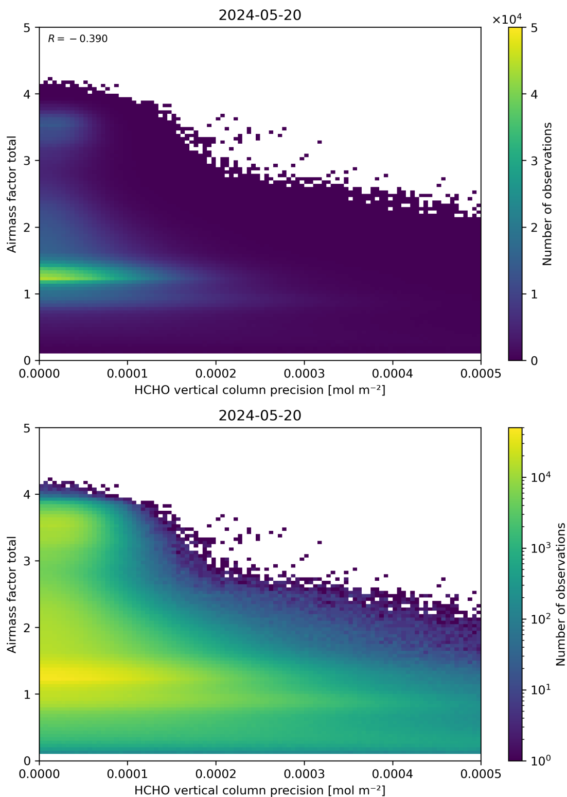
Figure 144: Scatter density plot of “HCHO vertical column precision” against “Airmass factor total” for 2024-05-19 to 2024-05-21.
