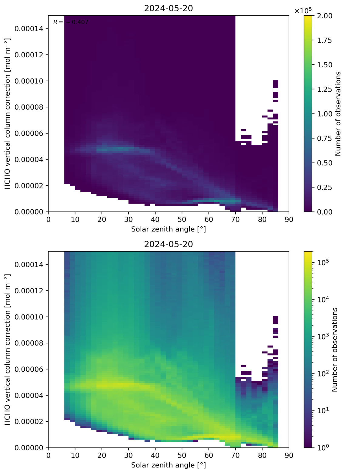
Figure 178: Scatter density plot of “Solar zenith angle” against “HCHO vertical column correction” for 2024-05-19 to 2024-05-21.
