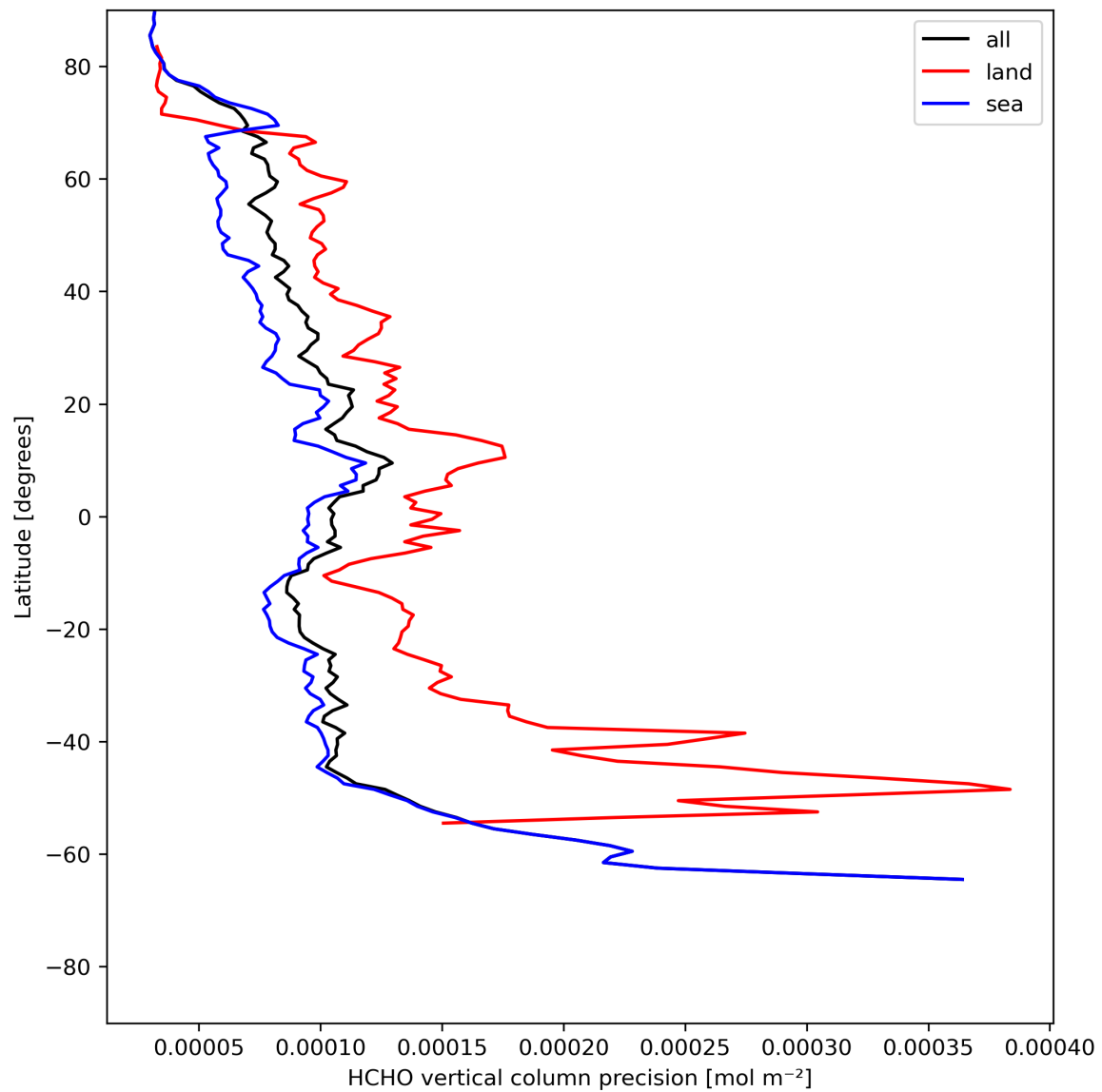
Figure 22: Zonal average of “HCHO vertical column precision” for 2024-05-19 to 2024-05-21.
