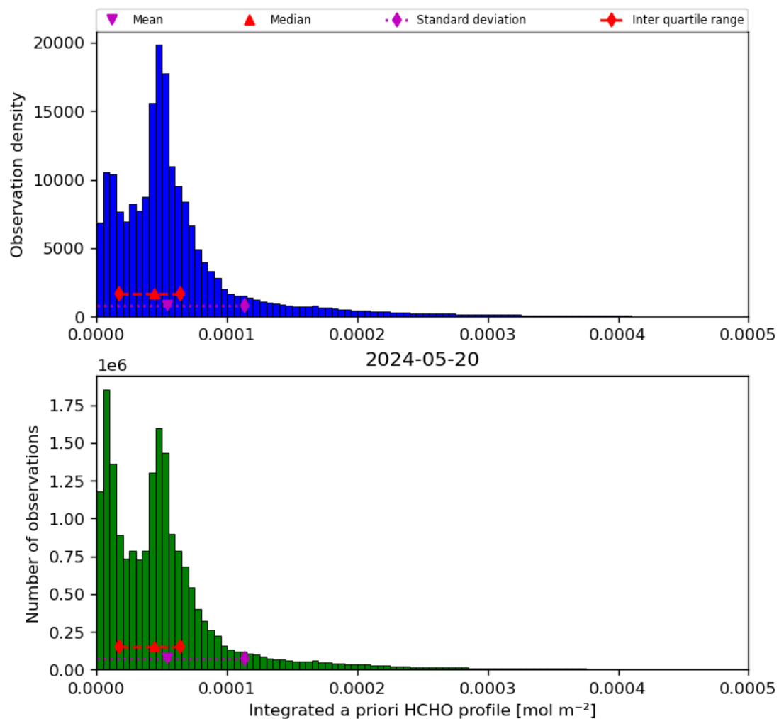
Figure 43: Histogram of “Integrated a priori HCHO profile” for 2024-05-19 to 2024-05-21
