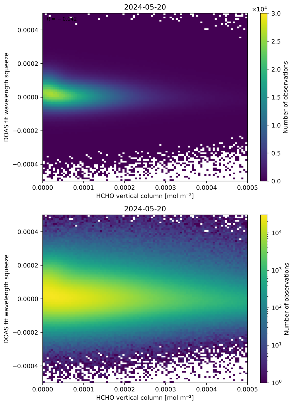
Figure 125: Scatter density plot of “HCHO vertical column” against “DOAS fit wavelength squeeze” for 2024-05-19 to 2024-05-21.
