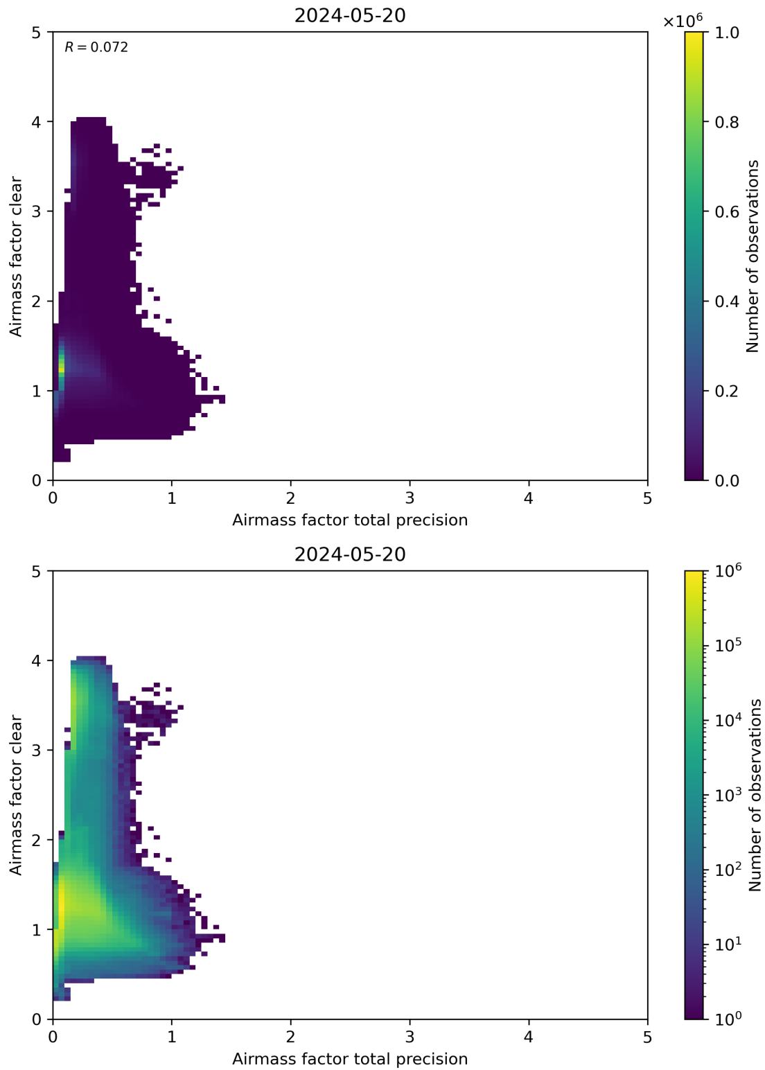
Figure 108: Scatter density plot of “Airmass factor total precision” against “Airmass factor clear” for 2024-05-19 to 2024-05-21.
