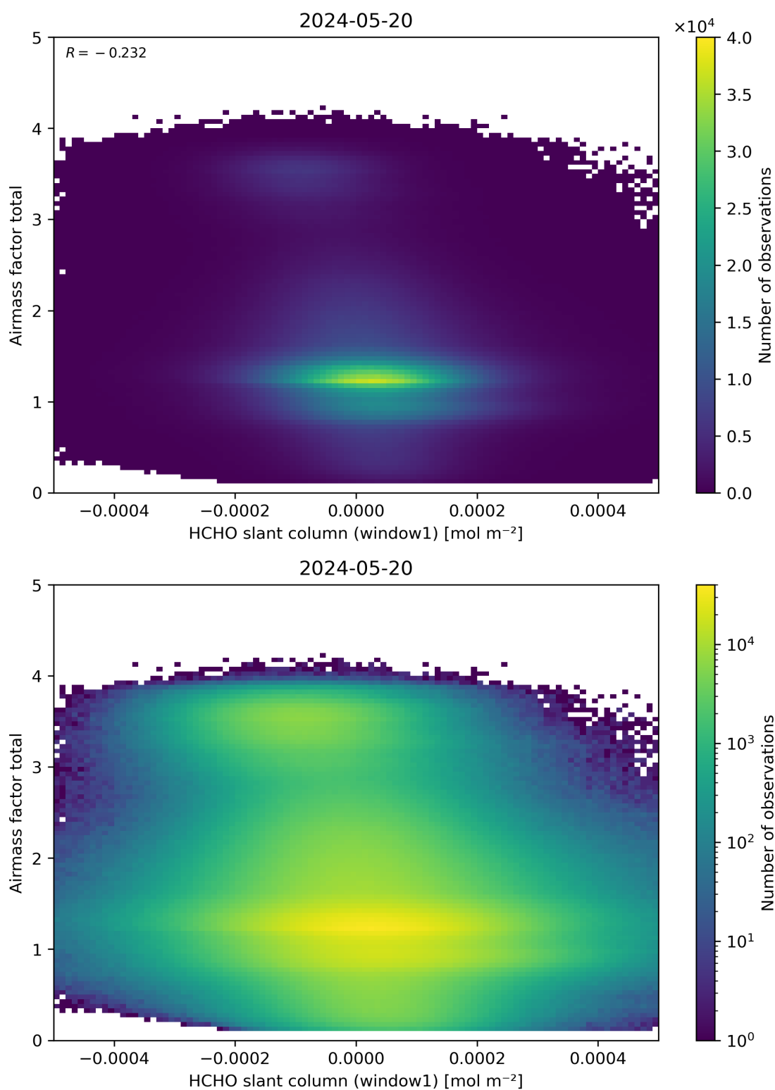
Figure 85: Scatter density plot of “HCHO slant column (window1)” against “Airmass factor total” for 2024-05-19 to 2024-05-21.
