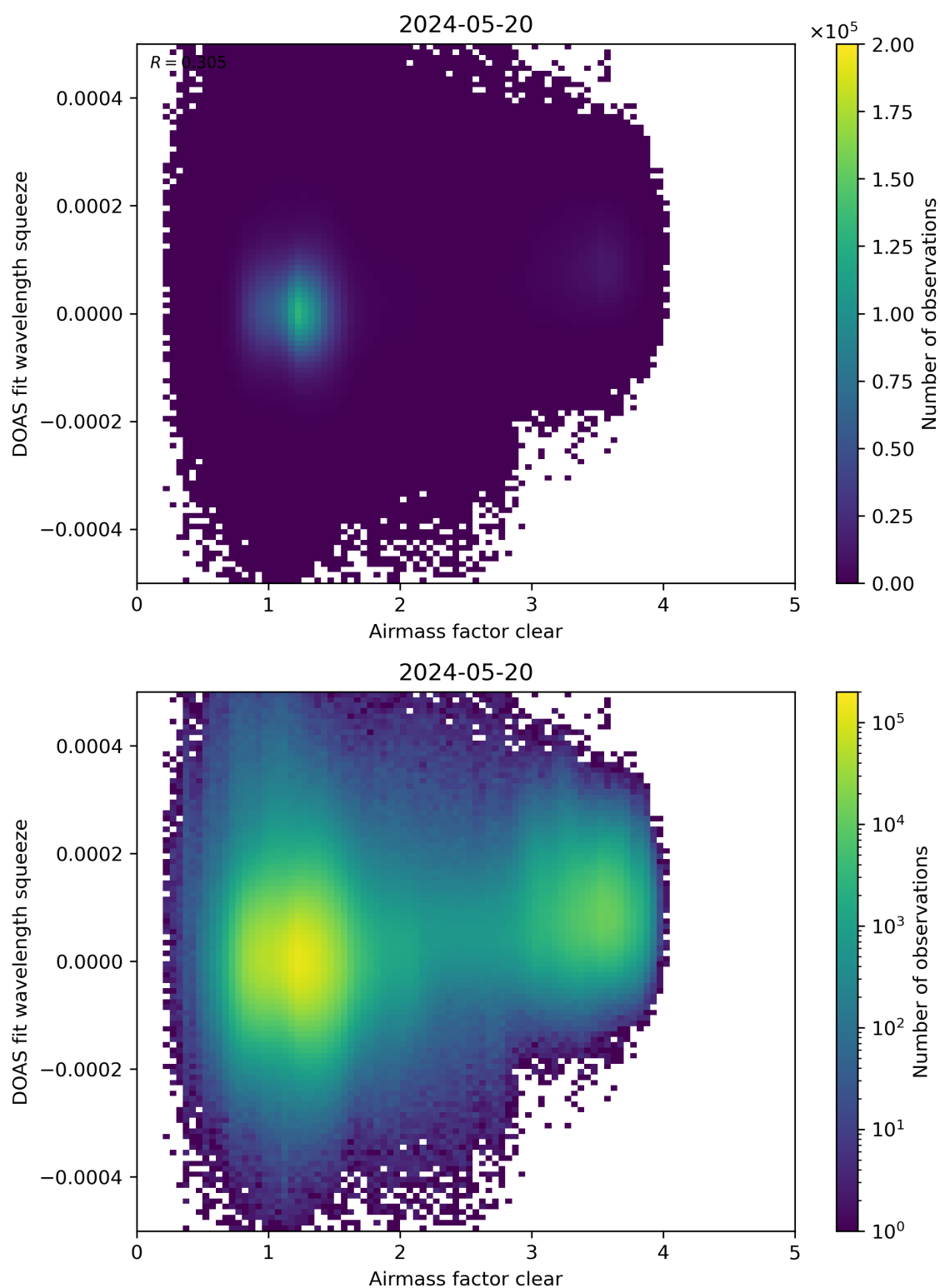
Figure 73: Scatter density plot of “Airmass factor clear” against “DOAS fit wavelength squeeze” for 2024-05-19 to 2024-05-21.
