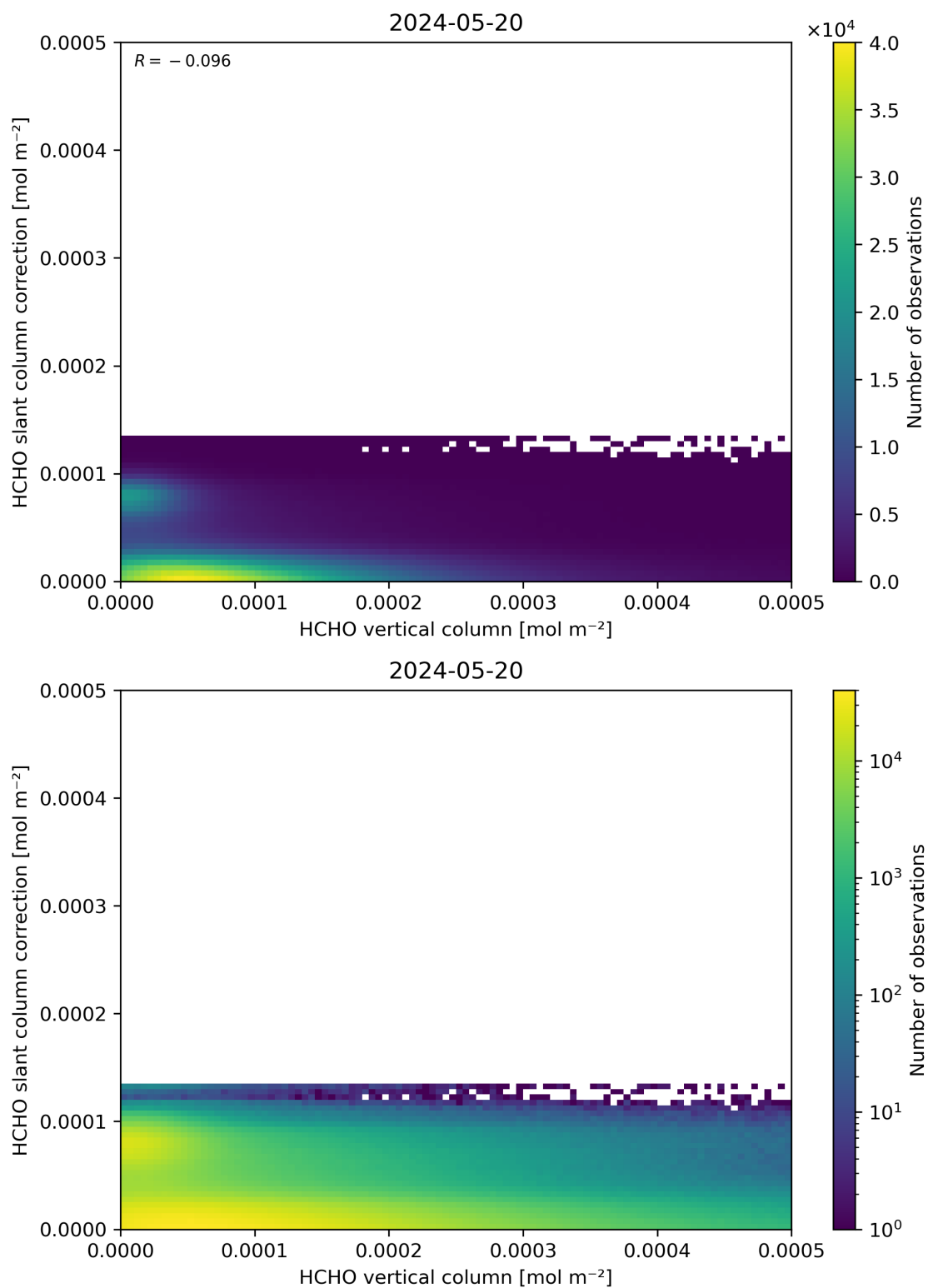
Figure 128: Scatter density plot of “HCHO vertical column” against “HCHO slant column correction” for 2024-05-19 to 2024-05-21.
