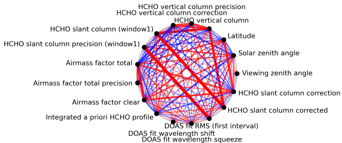
Figure 1: Map of correlation graph for 2024-05-19 to 2024-05-21.
