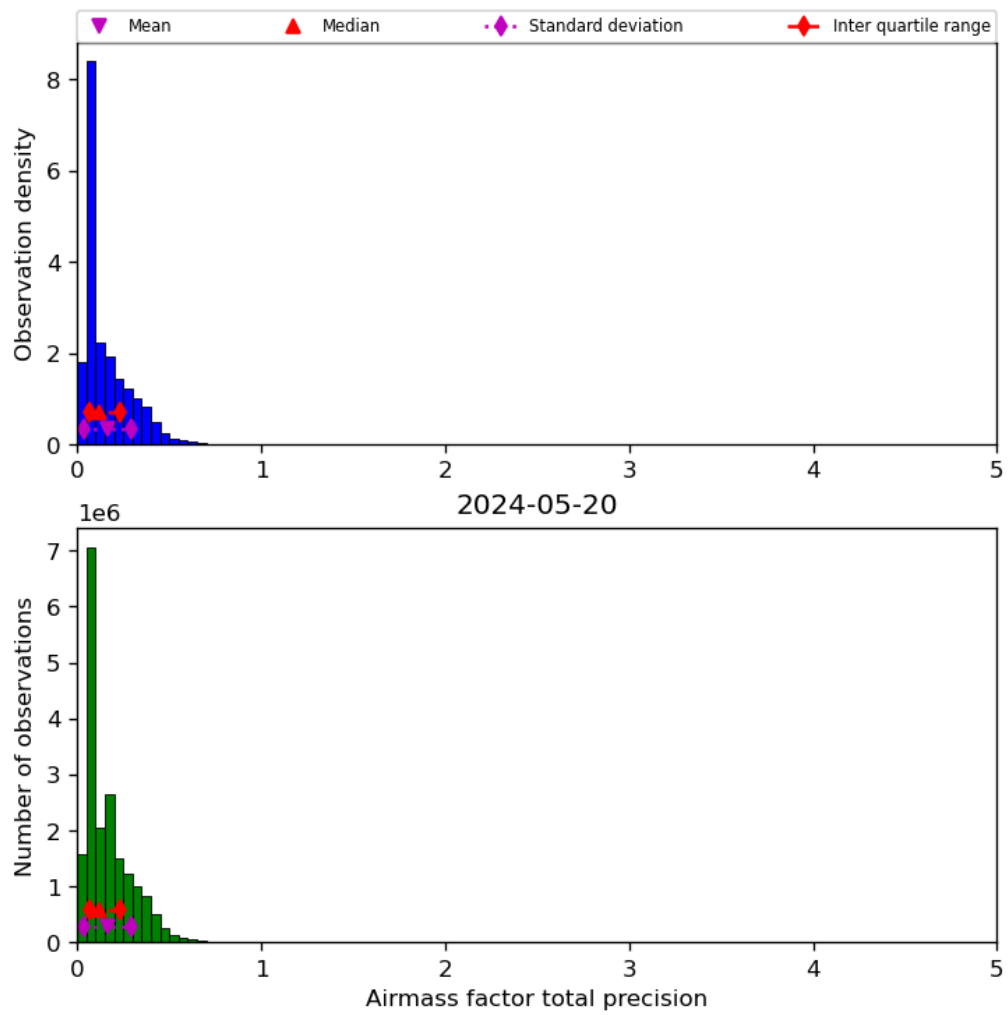
Figure 41: Histogram of “Airmass factor total precision” for 2024-05-19 to 2024-05-21
