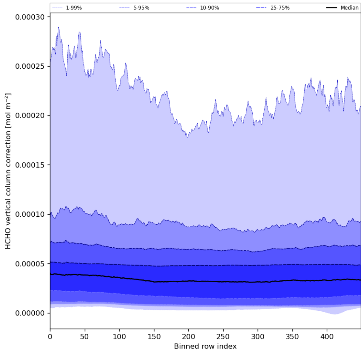
Figure 51: Along track statistics of “HCHO vertical column correction” for 2024-05-19 to 2024-05-21
