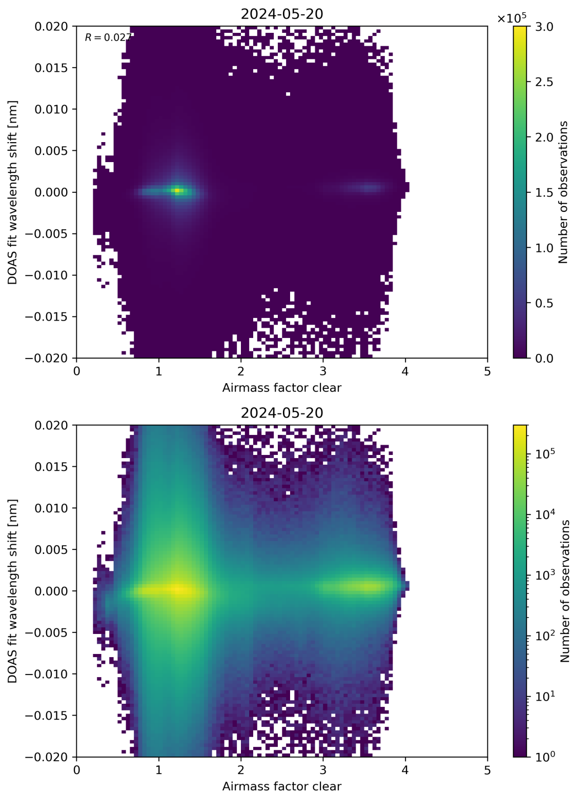
Figure 72: Scatter density plot of “Airmass factor clear” against “DOAS fit wavelength shift” for 2024-05-19 to 2024-05-21.
