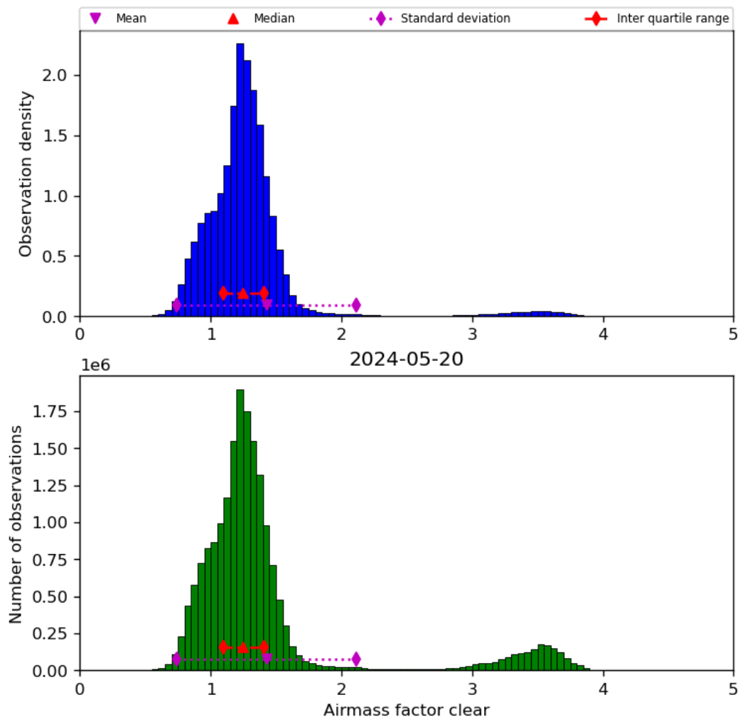
Figure 42: Histogram of “Airmass factor clear” for 2024-05-19 to 2024-05-21
