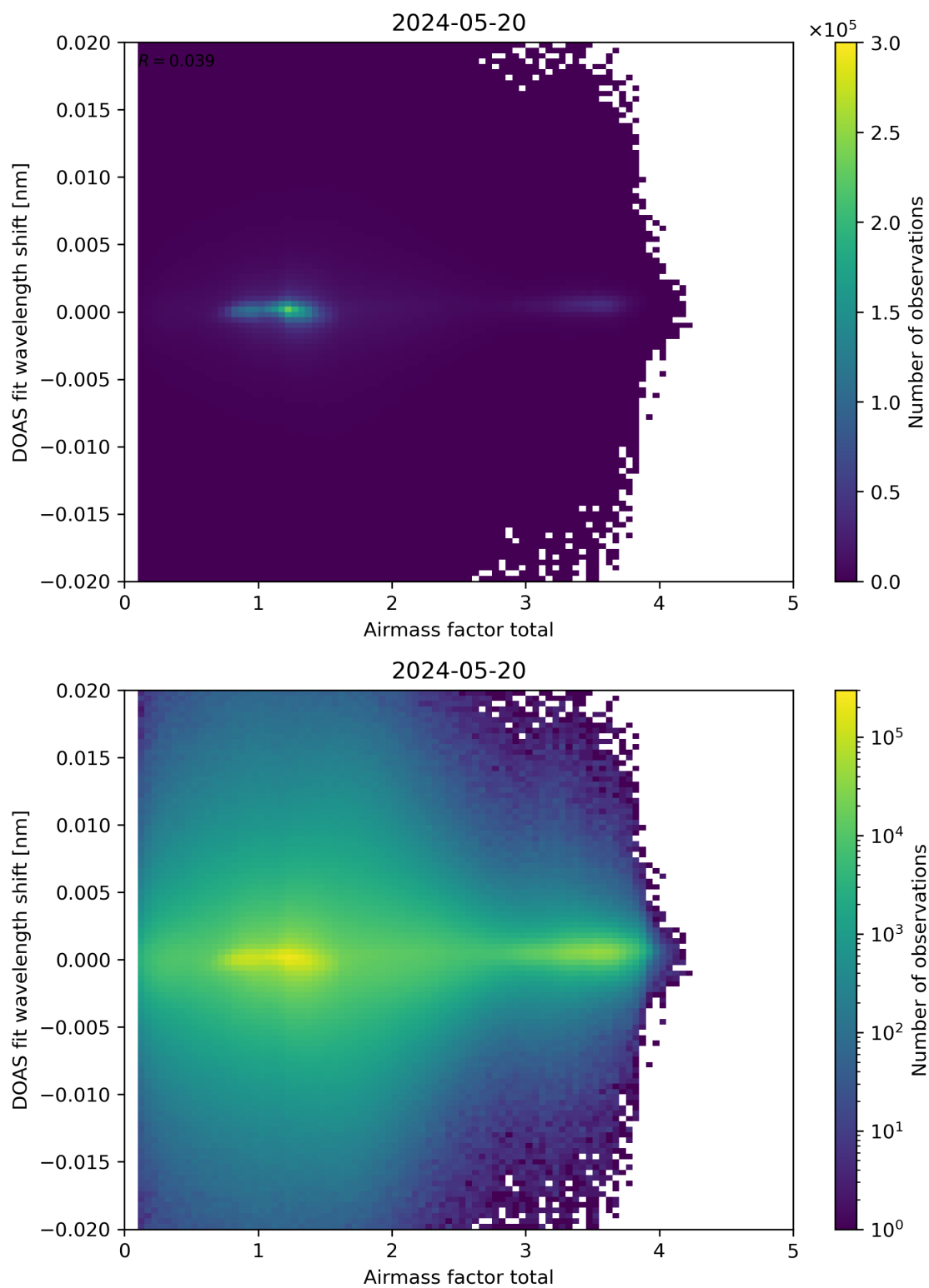
Figure 98: Scatter density plot of “Airmass factor total” against “DOAS fit wavelength shift” for 2024-05-19 to 2024-05-21.
