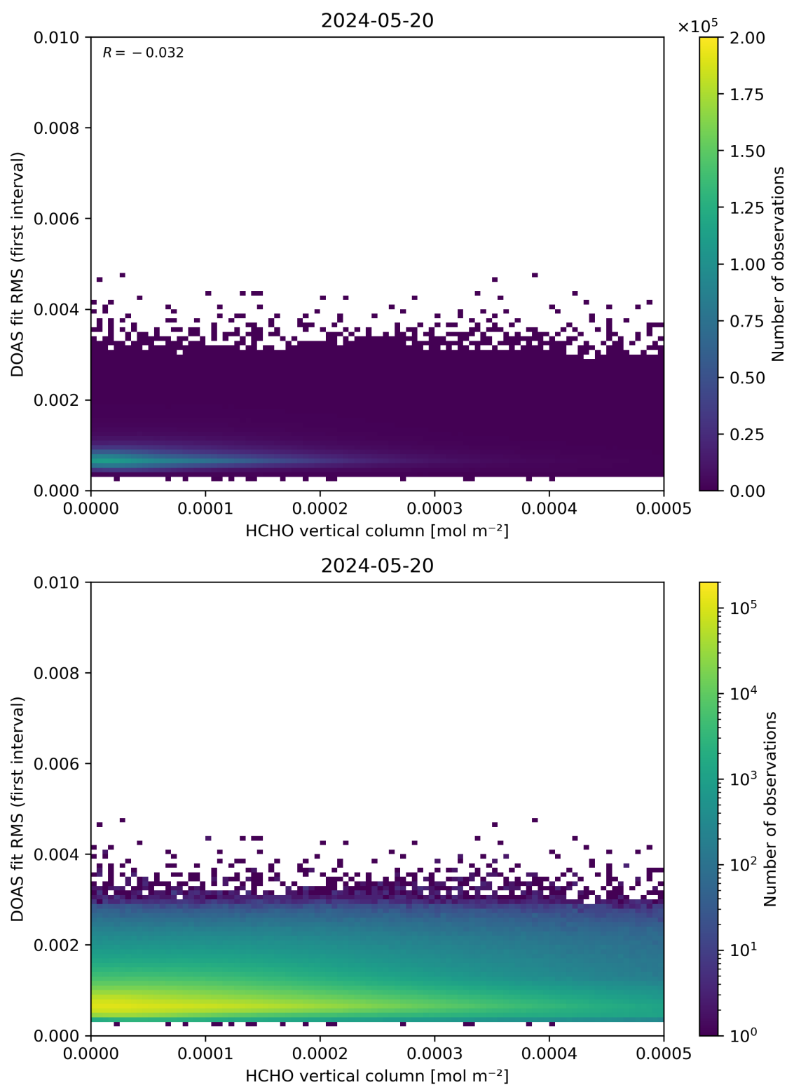
Figure 123: Scatter density plot of “HCHO vertical column” against “DOAS fit RMS (first interval)” for 2024-05-19 to 2024-05-21.
