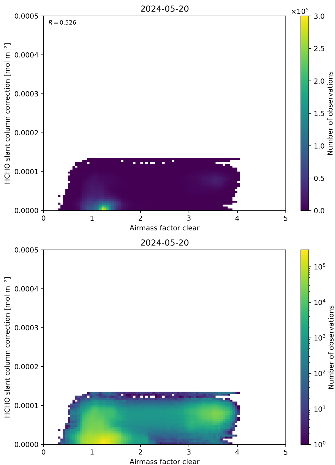
Figure 75: Scatter density plot of “Airmass factor clear” against “HCHO slant column correction” for 2024-05-19 to 2024-05-21.
