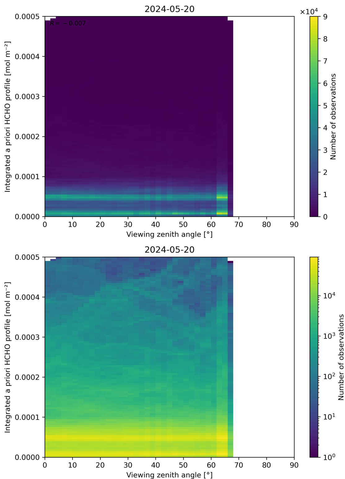
Figure 195: Scatter density plot of “Viewing zenith angle” against “Integrated a priori HCHO profile” for 2024-05-19 to 2024-05-21.
