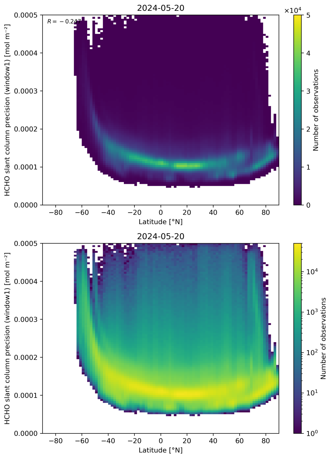
Figure 160: Scatter density plot of “Latitude” against “HCHO slant column precision (window1)” for 2024-05-19 to 2024-05-21.
