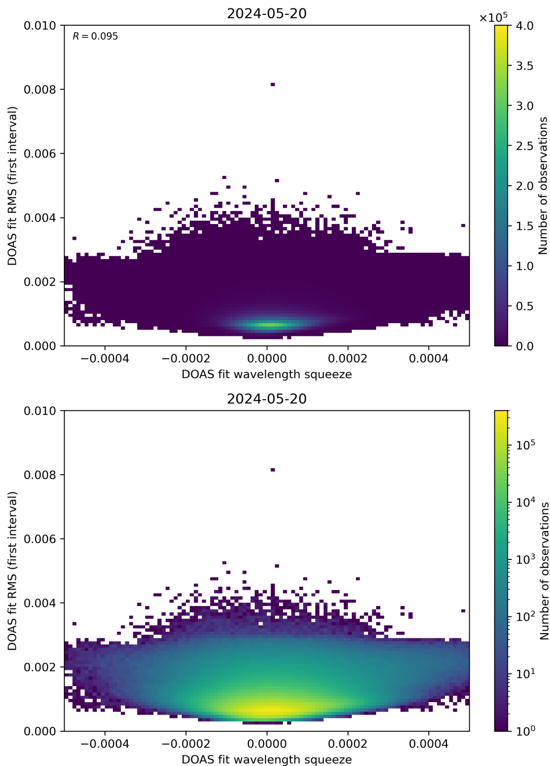
Figure 68: Scatter density plot of “DOAS fit wavelength squeeze” against “DOAS fit RMS (first interval)” for 2024-05-19 to 2024-05-21.
