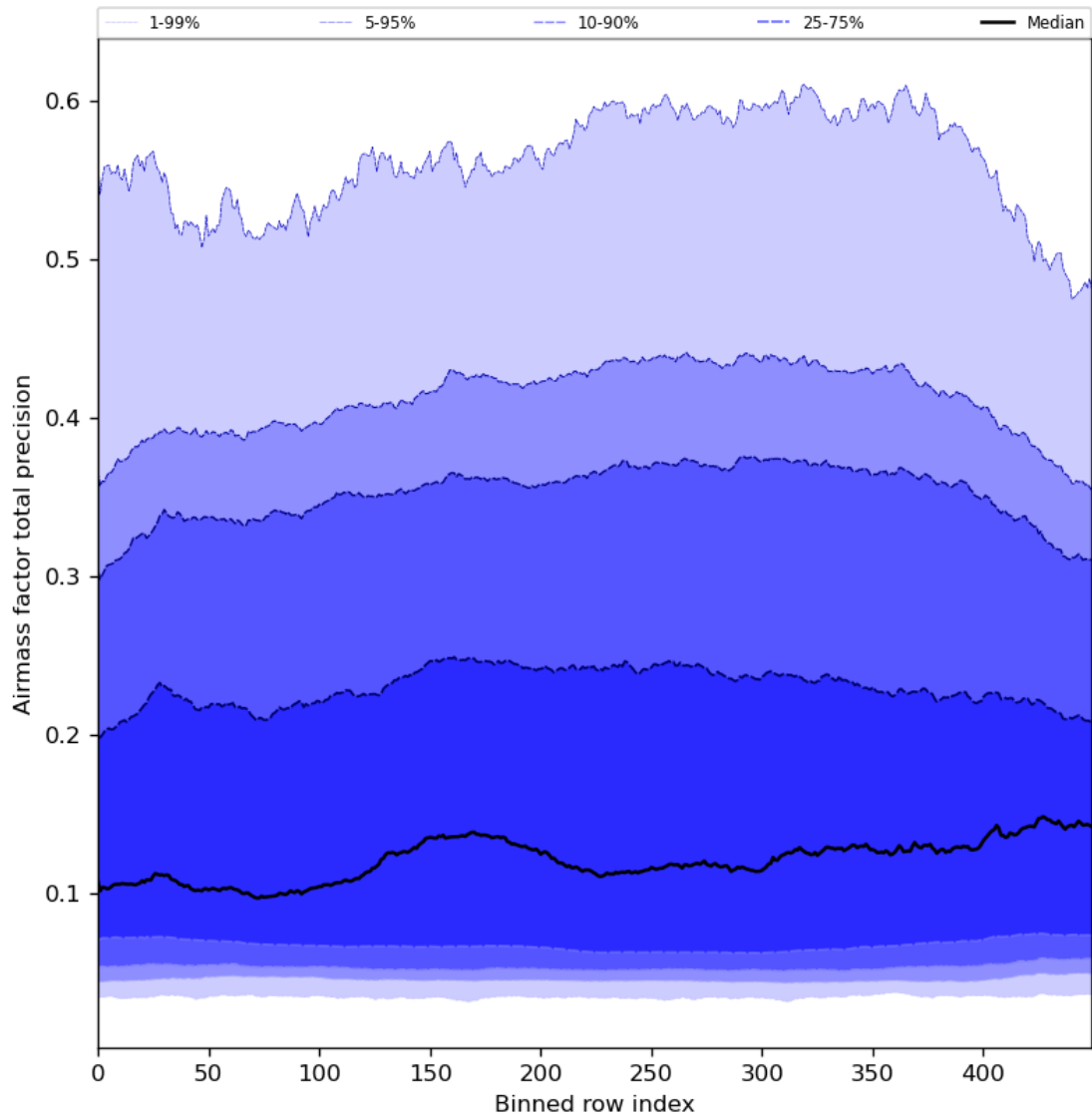
Figure 55: Along track statistics of “Airmass factor total precision” for 2024-05-19 to 2024-05-21
