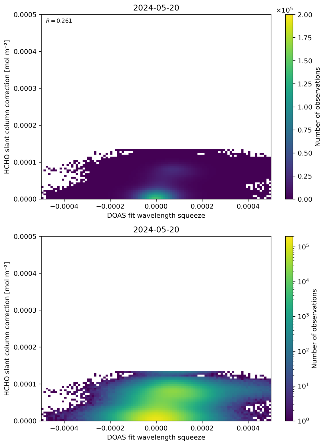
Figure 70: Scatter density plot of “DOAS fit wavelength squeeze” against “HCHO slant column correction” for 2024-05-19 to 2024-05-21.
