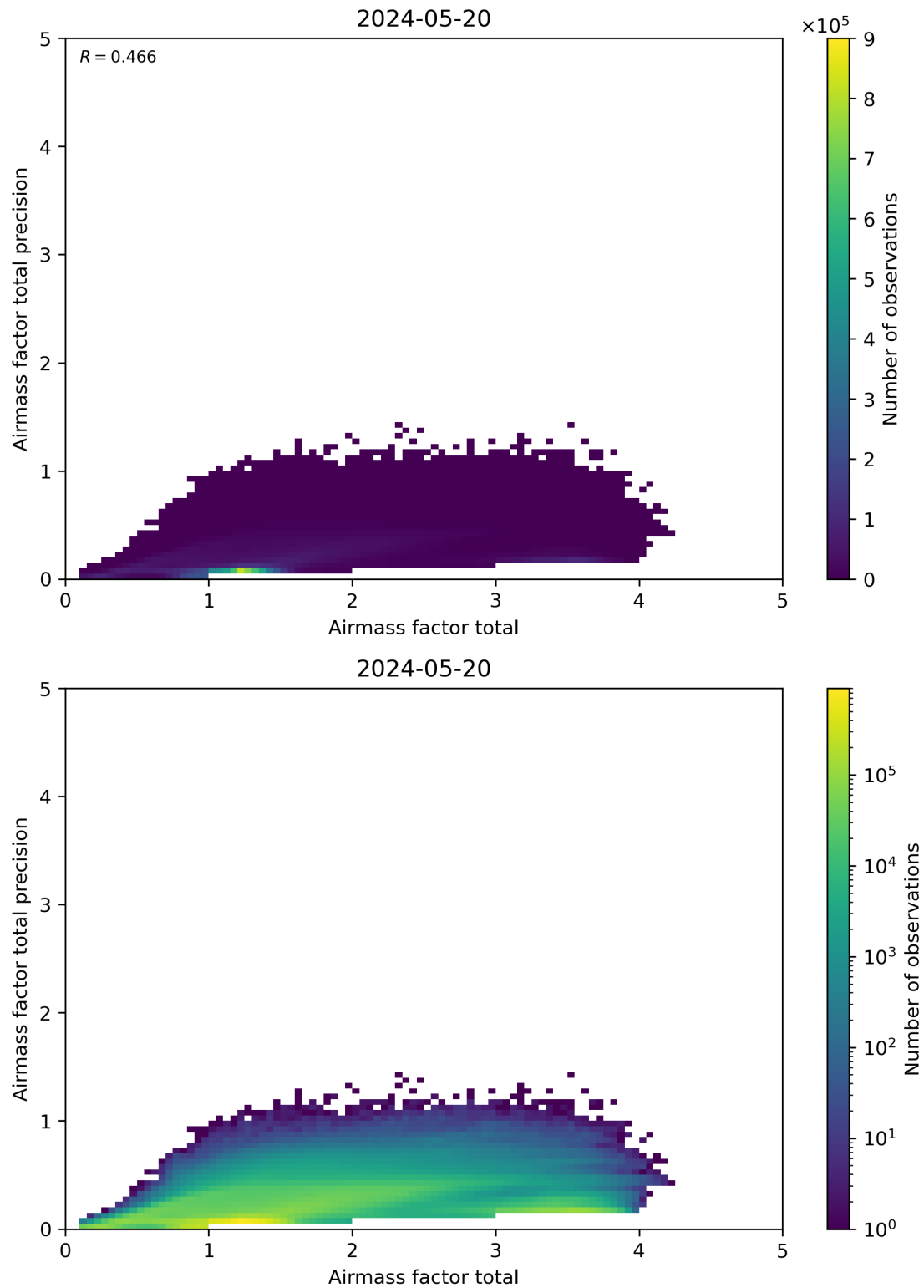
Figure 103: Scatter density plot of “Airmass factor total” against “Airmass factor total precision” for 2024-05-19 to 2024-05-21.
