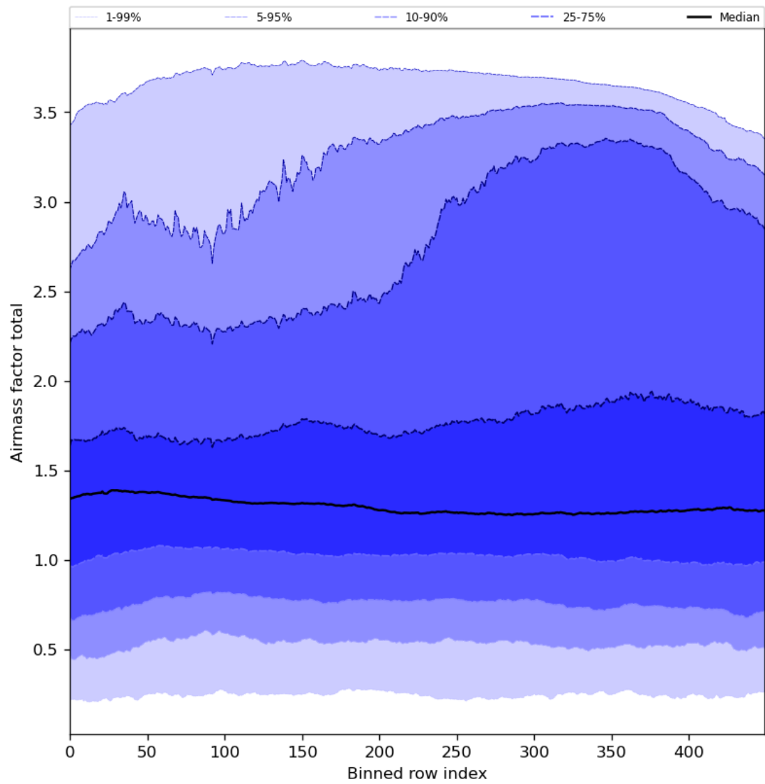
Figure 54: Along track statistics of “Airmass factor total” for 2024-05-19 to 2024-05-21
