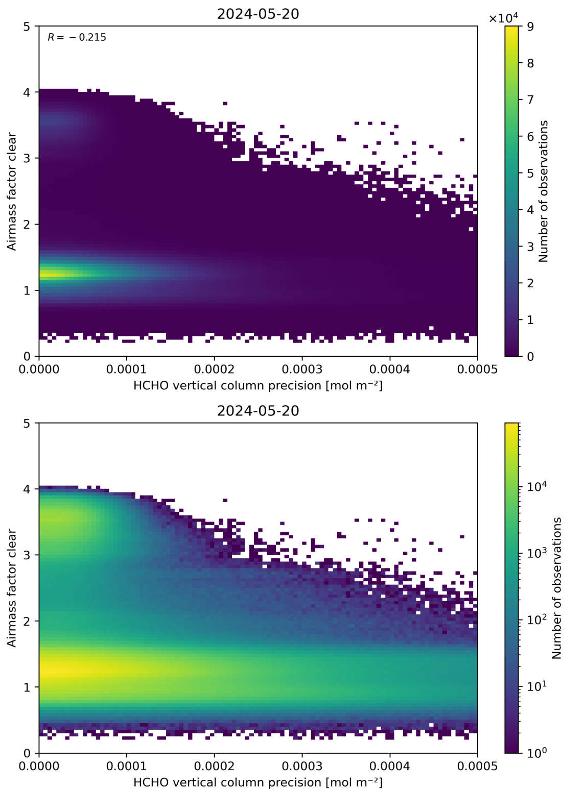
Figure 139: Scatter density plot of “HCHO vertical column precision” against “Airmass factor clear” for 2024-05-19 to 2024-05-21.
