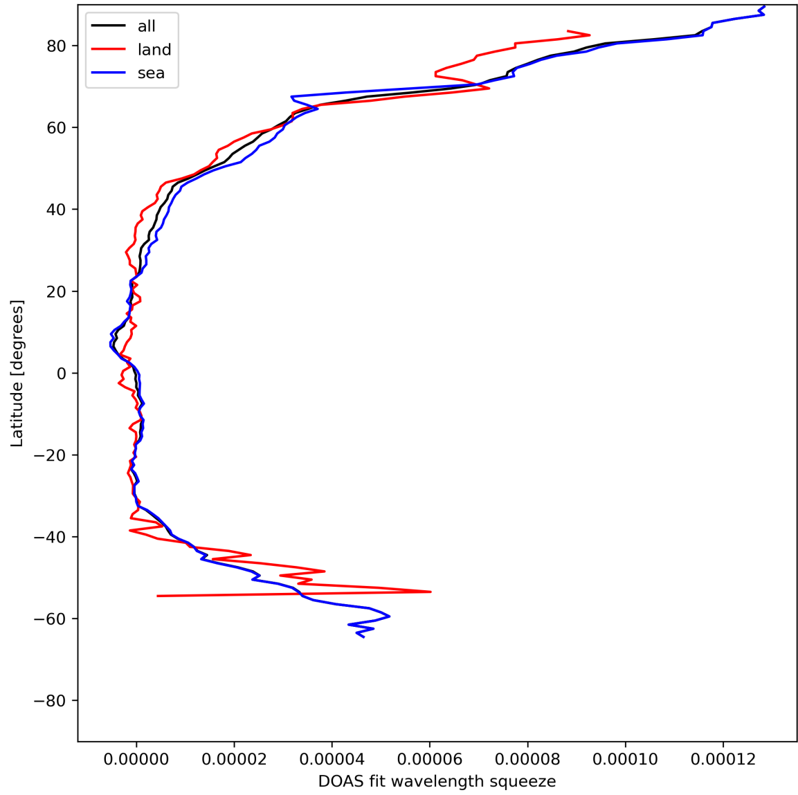
Figure 31: Zonal average of “DOAS fit wavelength squeeze” for 2024-05-19 to 2024-05-21.
