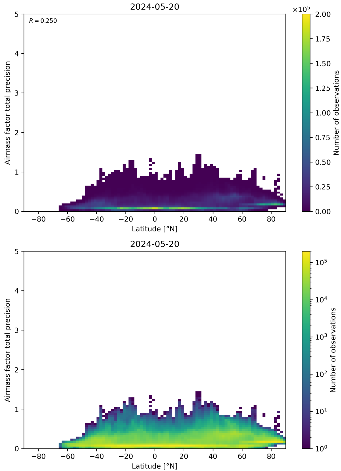
Figure 162: Scatter density plot of “Latitude” against “Airmass factor total precision” for 2024-05-19 to 2024-05-21.
