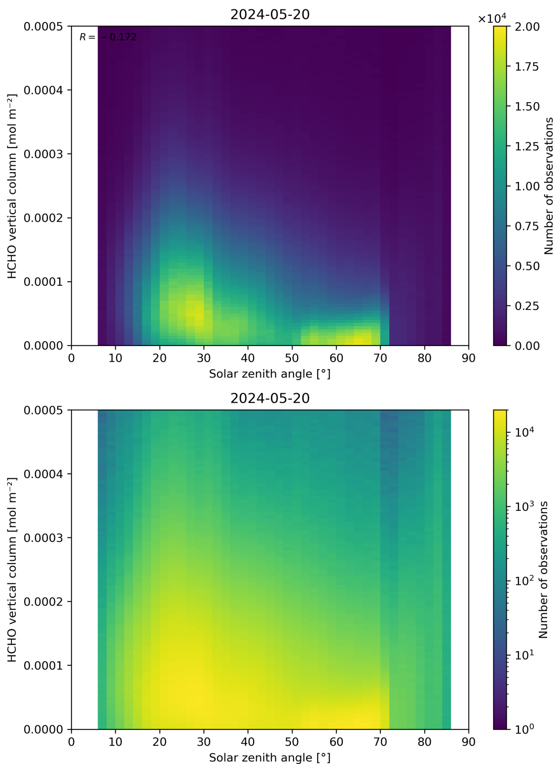
Figure 177: Scatter density plot of “Solar zenith angle” against “HCHO vertical column” for 2024-05-19 to 2024-05-21.
