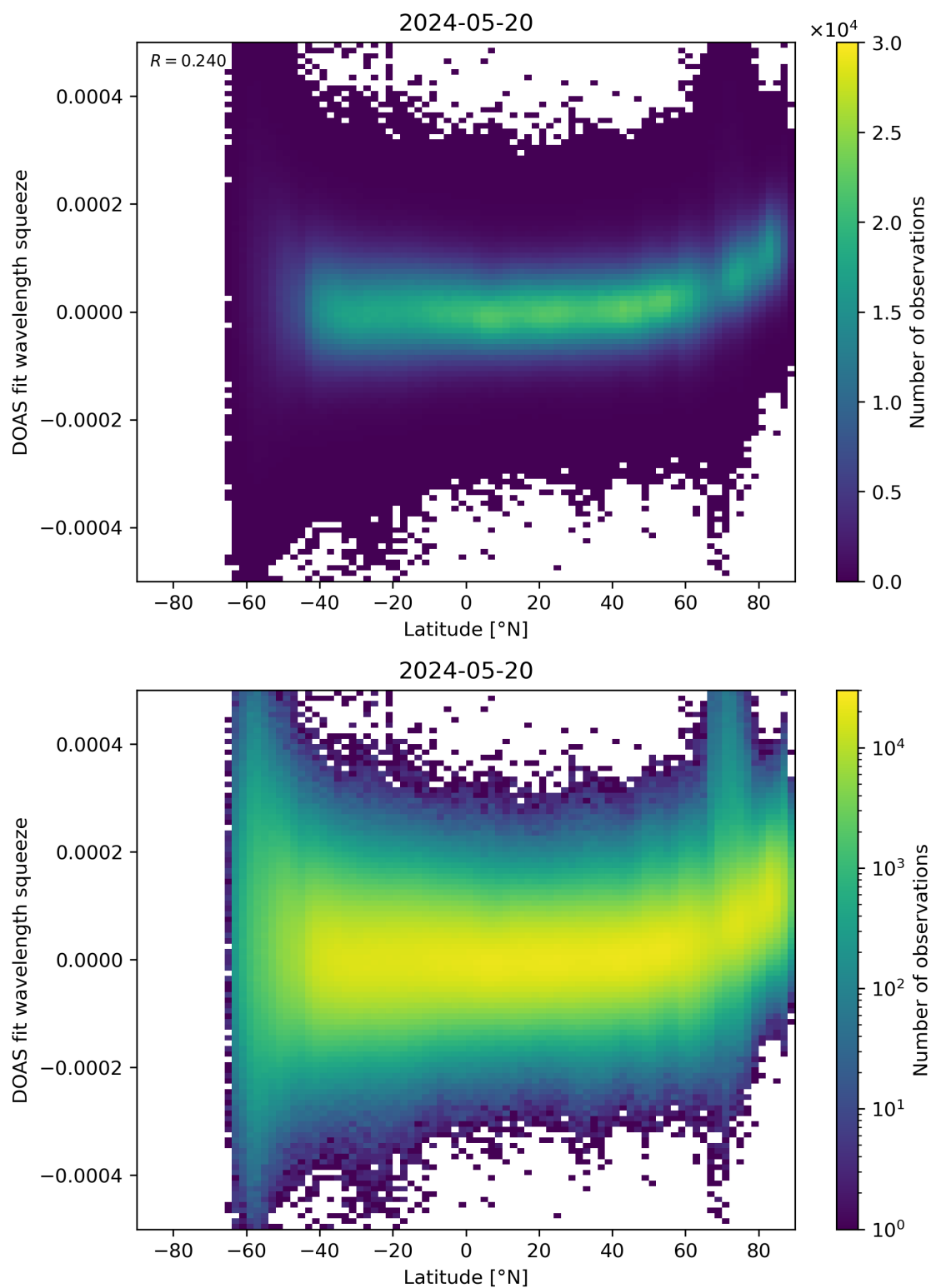
Figure 155: Scatter density plot of “Latitude” against “DOAS fit wavelength squeeze” for 2024-05-19 to 2024-05-21.
