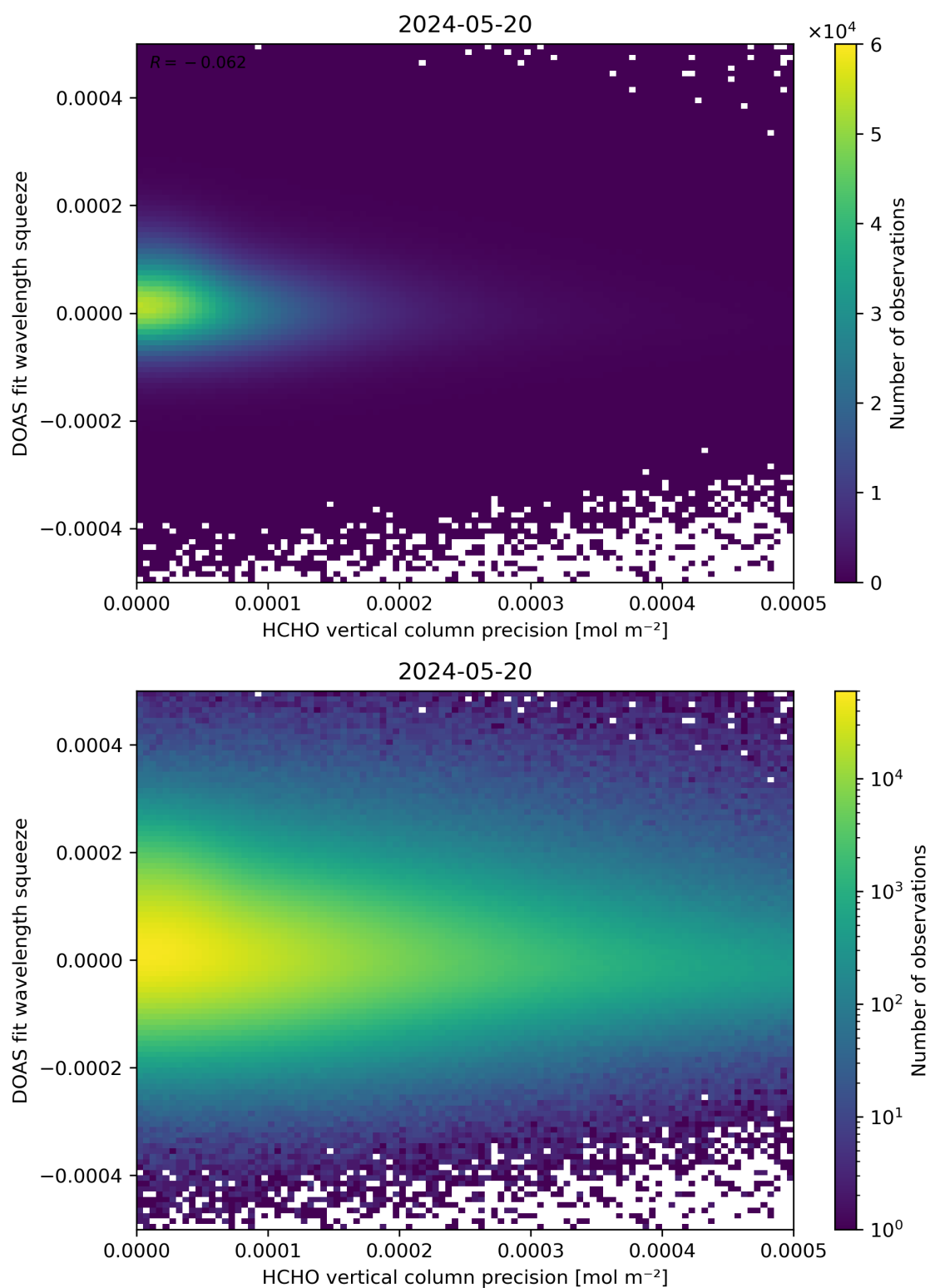
Figure 138: Scatter density plot of “HCHO vertical column precision” against “DOAS fit wavelength squeeze” for 2024-05-19 to 2024-05-21.
