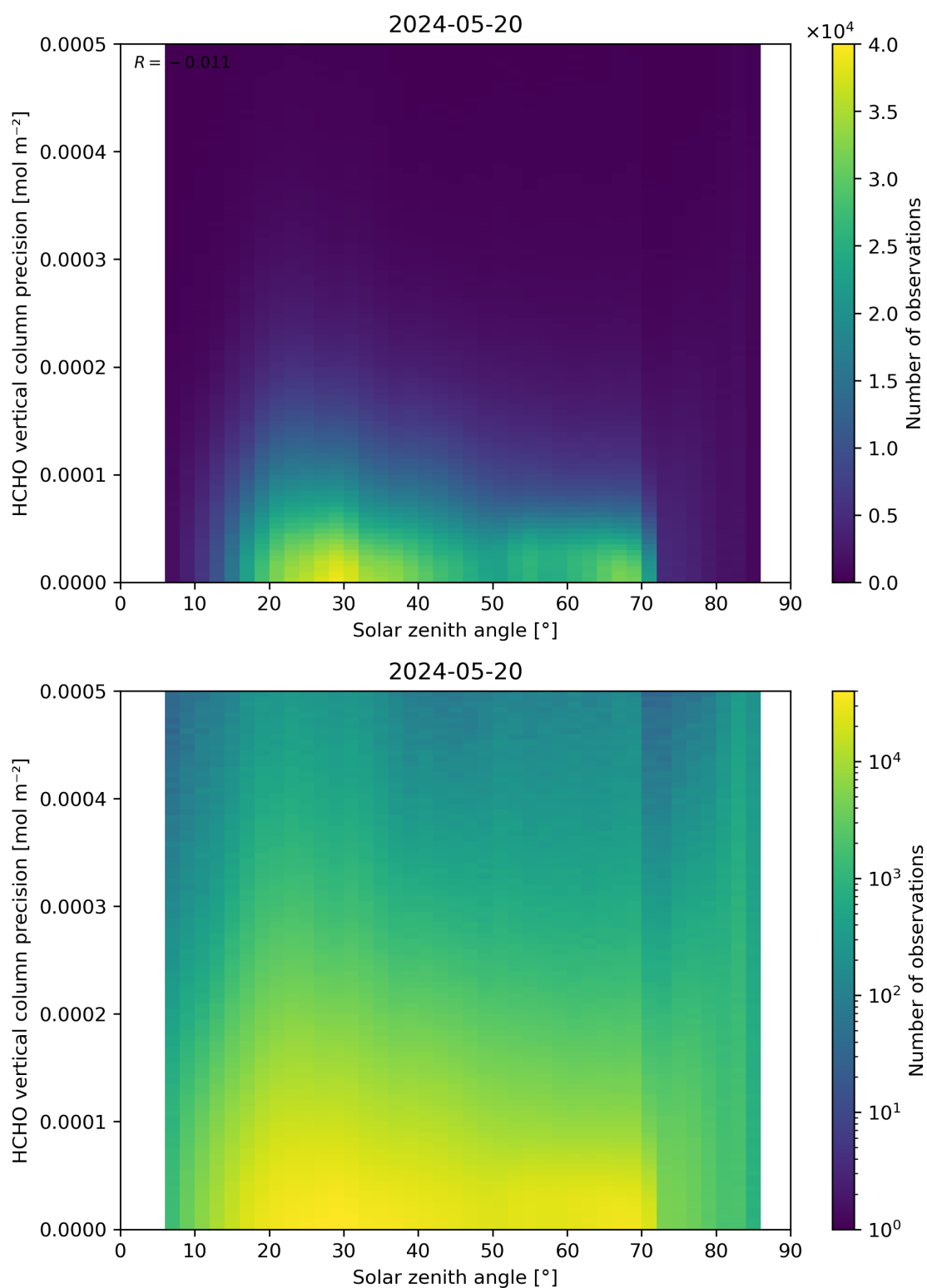
Figure 179: Scatter density plot of “Solar zenith angle” against “HCHO vertical column precision” for 2024-05-19 to 2024-05-21.
