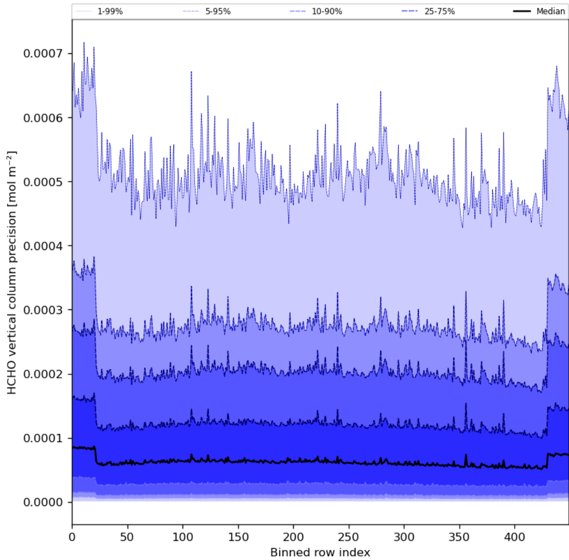
Figure 50: Along track statistics of “HCHO vertical column precision” for 2024-05-19 to 2024-05-21
