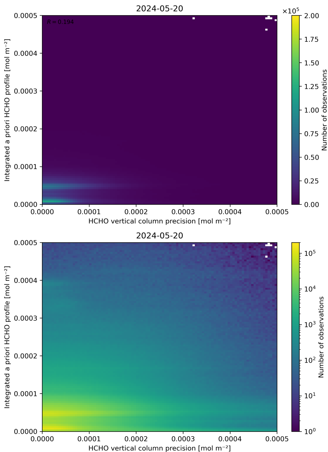
Figure 147: Scatter density plot of “HCHO vertical column precision” against “Integrated a priori HCHO profile” for 2024-05-19 to 2024-05-21.
