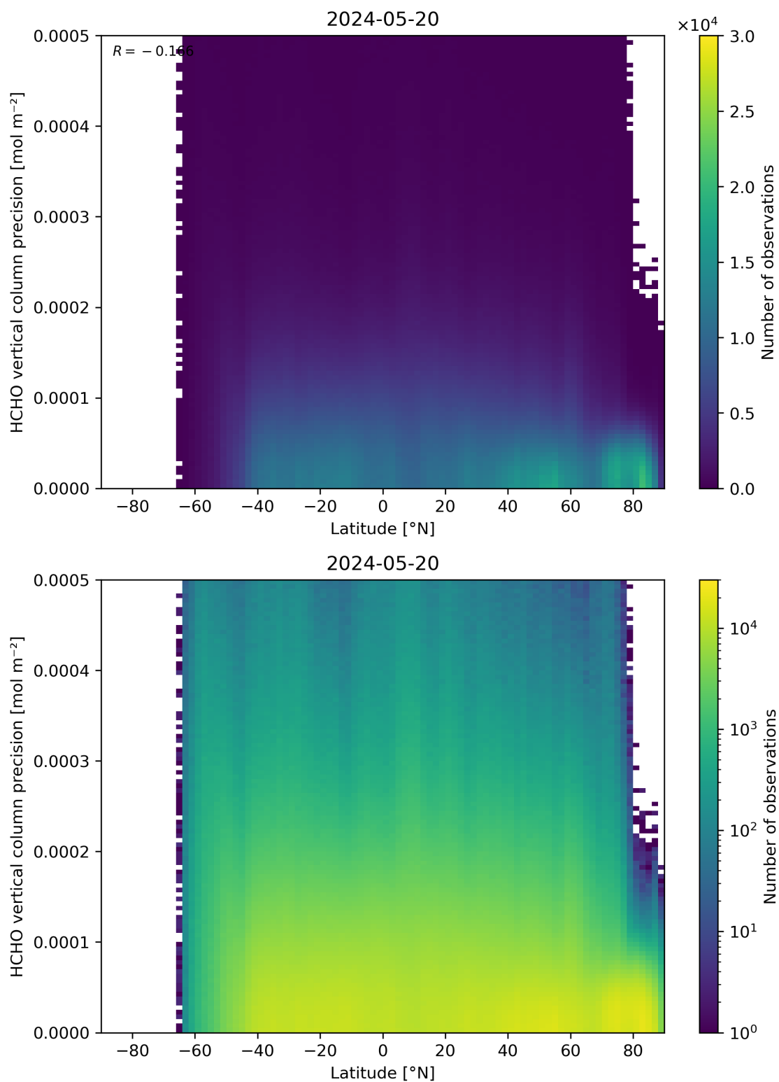
Figure 165: Scatter density plot of “Latitude” against “HCHO vertical column precision” for 2024-05-19 to 2024-05-21.
