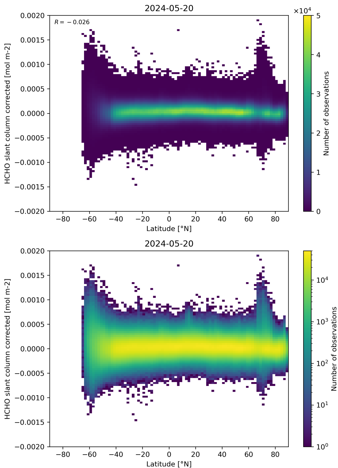
Figure 157: Scatter density plot of “Latitude” against “HCHO slant column corrected” for 2024-05-19 to 2024-05-21.
