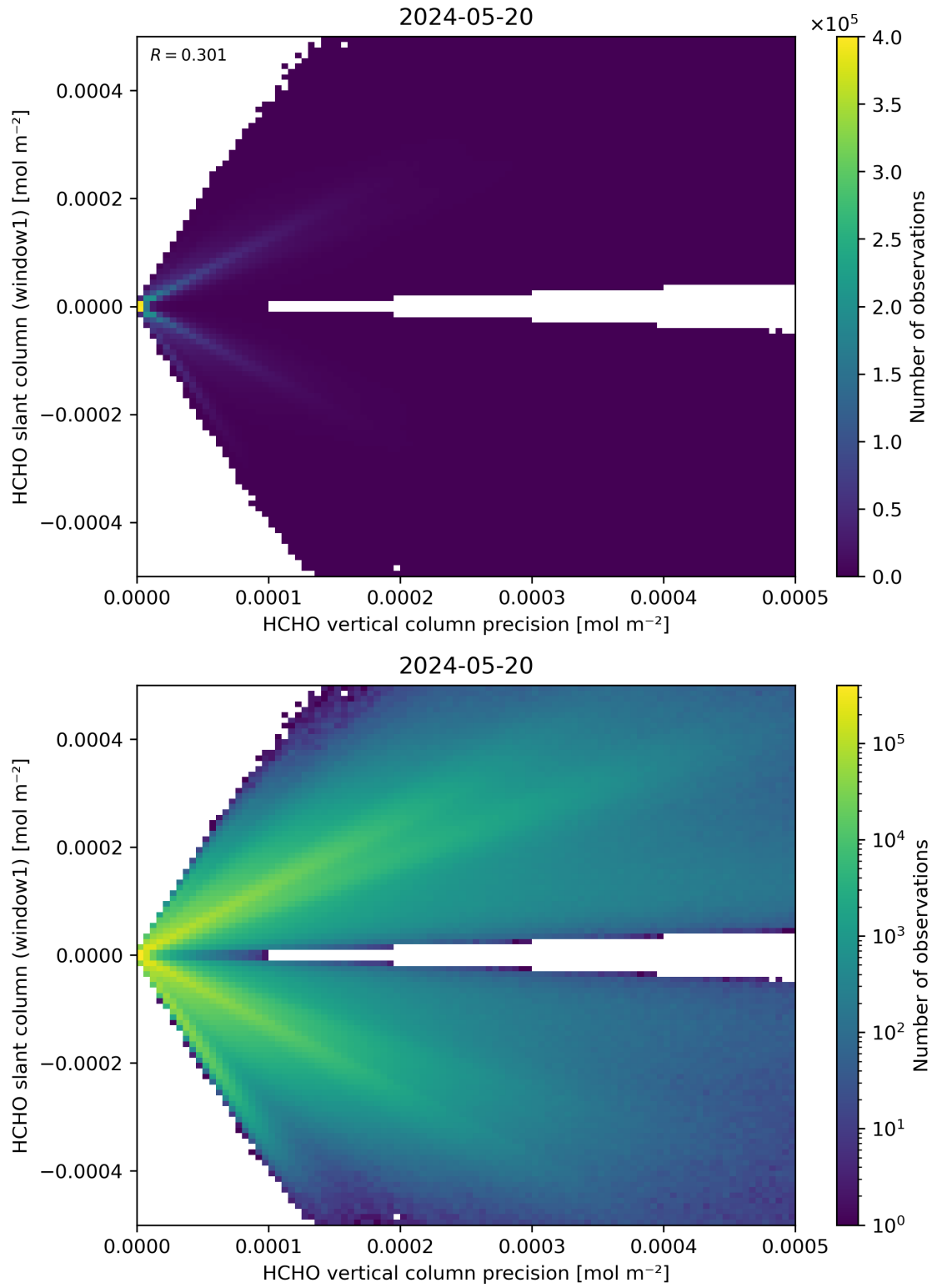
Figure 142: Scatter density plot of “HCHO vertical column precision” against “HCHO slant column (window1)” for 2024-05-19 to 2024-05-21.
