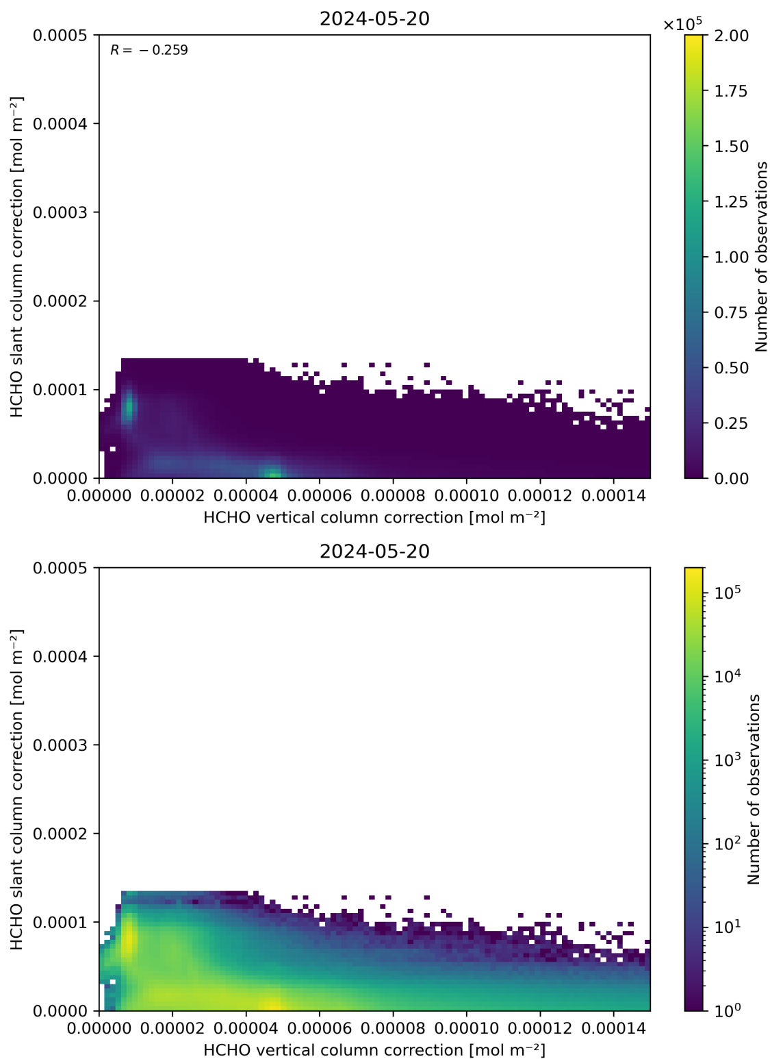
Figure 117: Scatter density plot of “HCHO vertical column correction” against “HCHO slant column correction” for 2024-05-19 to 2024-05-21.
