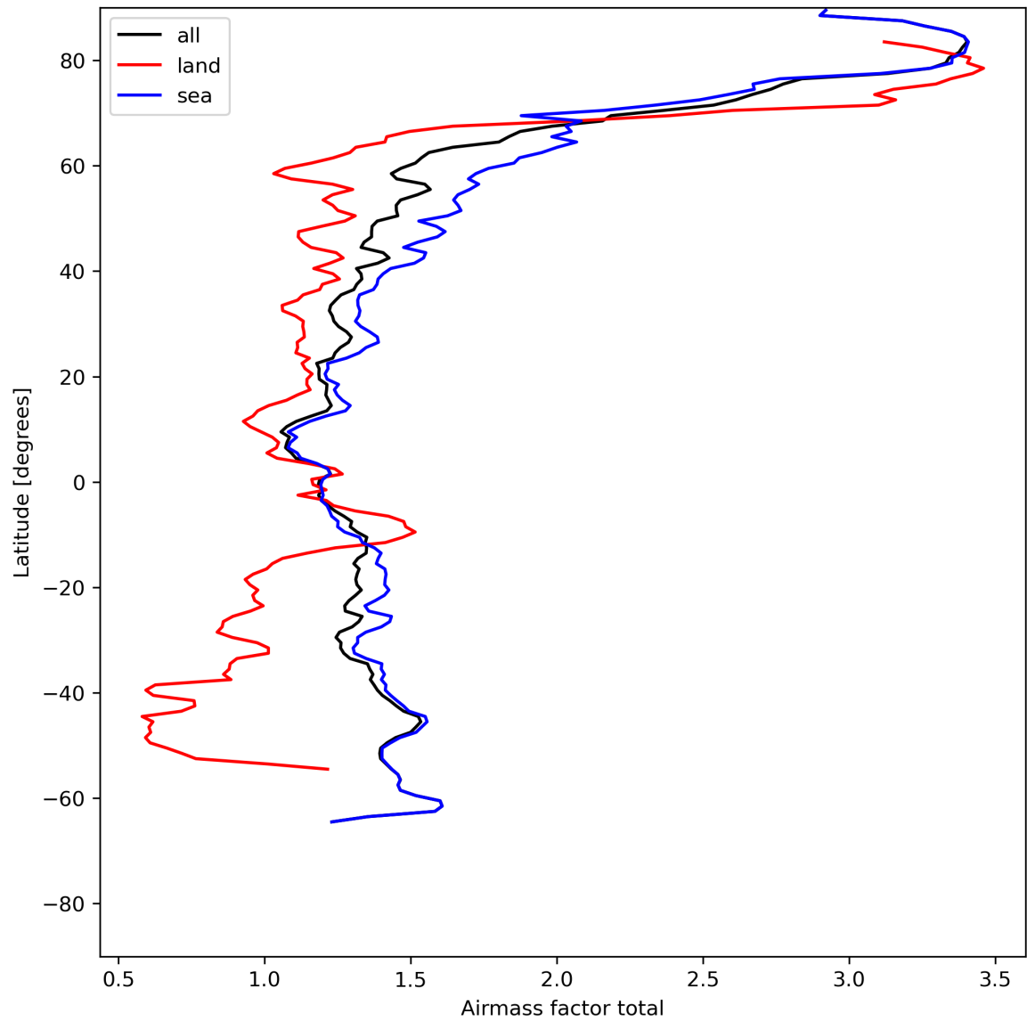
Figure 26: Zonal average of “Airmass factor total” for 2024-05-19 to 2024-05-21.
