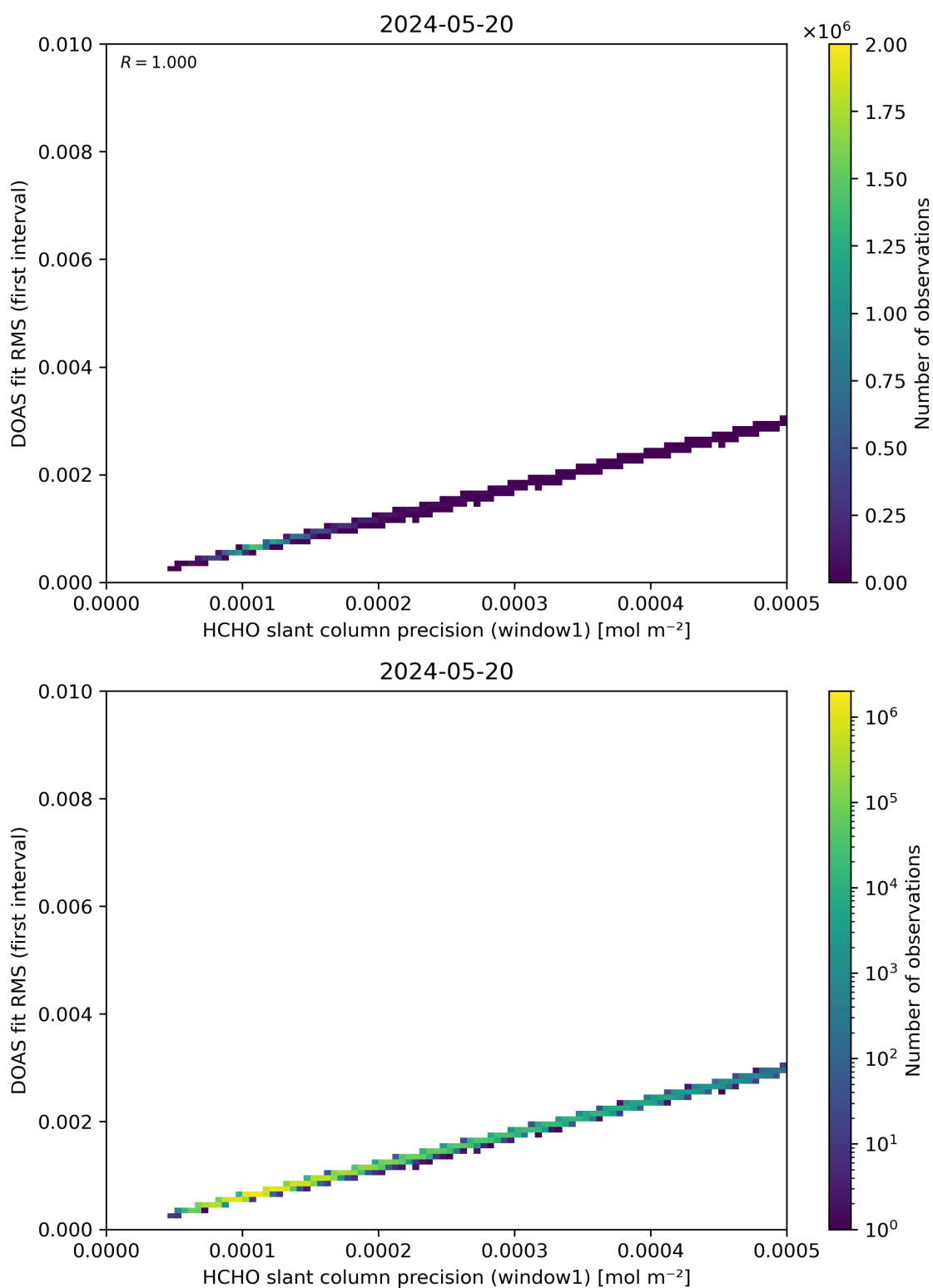
Figure 88: Scatter density plot of “HCHO slant column precision (window1)” against “DOAS fit RMS (first interval)” for 2024-05-19 to 2024-05-21.
