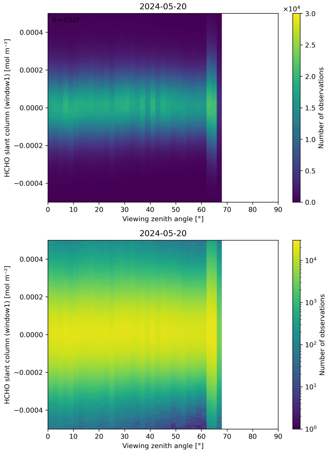
Figure 188: Scatter density plot of “Viewing zenith angle” against “HCHO slant column (window1)” for 2024-05-19 to 2024-05-21.
