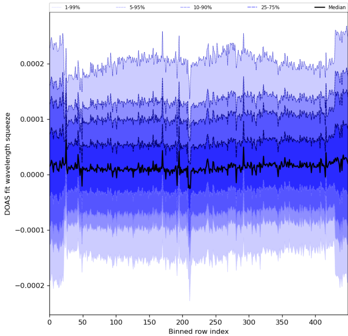
Figure 59: Along track statistics of “DOAS fit wavelength squeeze” for 2024-05-19 to 2024-05-21
