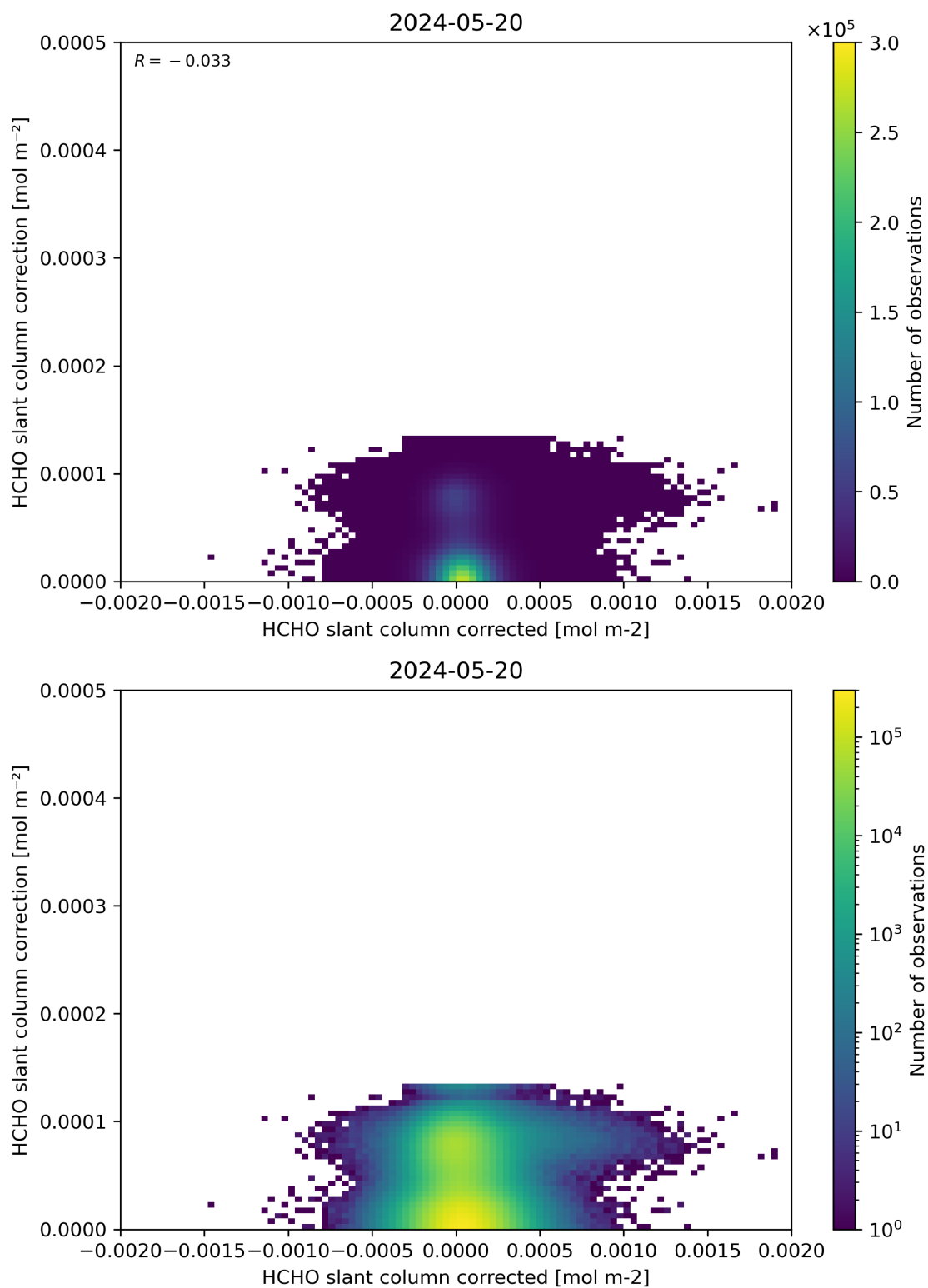
Figure 77: Scatter density plot of “HCHO slant column corrected” against “HCHO slant column correction” for 2024-05-19 to 2024-05-21.
