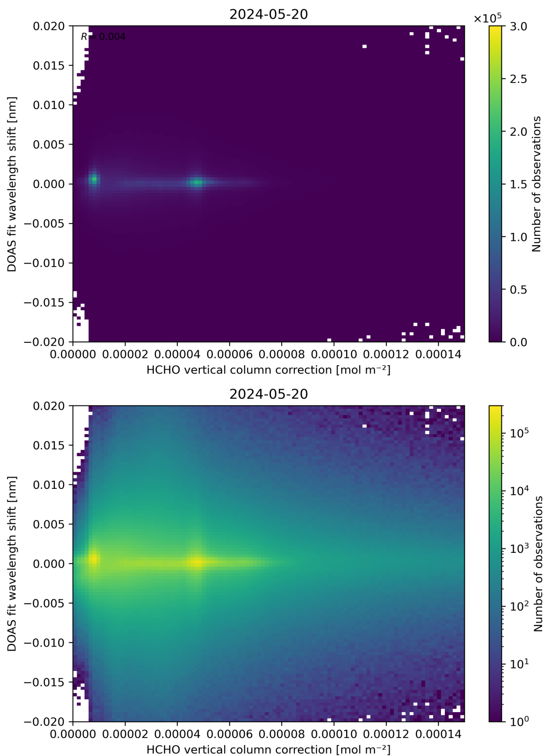
Figure 113: Scatter density plot of “HCHO vertical column correction” against “DOAS fit wavelength shift” for 2024-05-19 to 2024-05-21.
