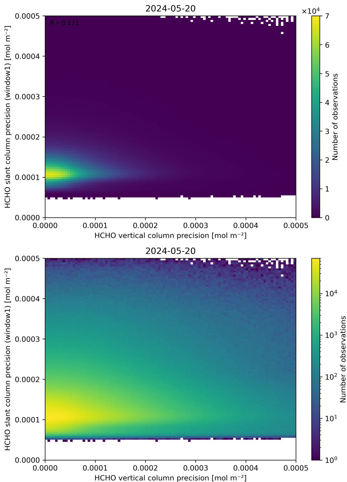
Figure 143: Scatter density plot of “HCHO vertical column precision” against “HCHO slant column precision (window1)” for 2024-05-19 to 2024-05-21.
