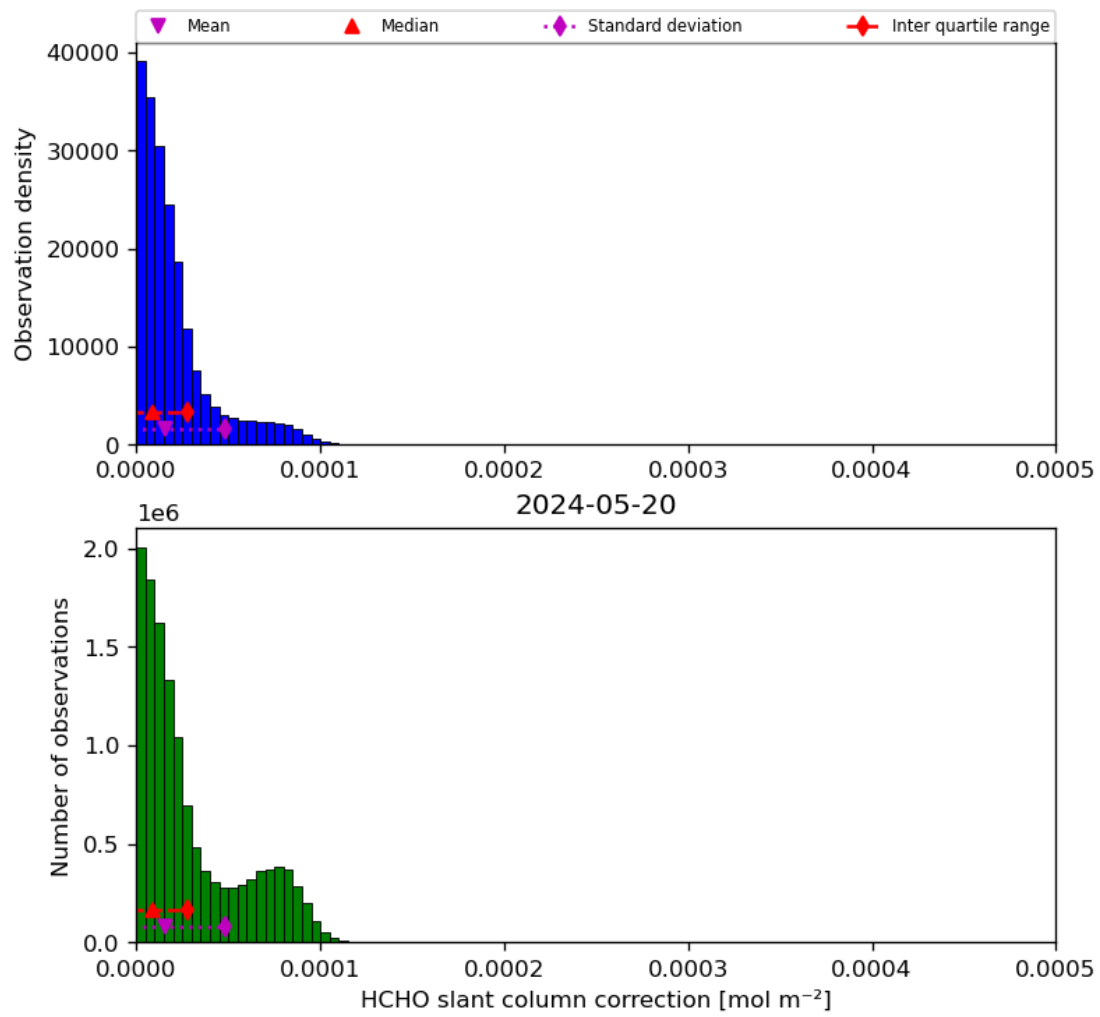
Figure 47: Histogram of “HCHO slant column correction” for 2024-05-19 to 2024-05-21
