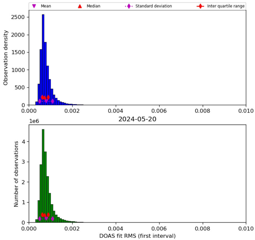
Figure 46: Histogram of “DOAS fit RMS (first interval)” for 2024-05-19 to 2024-05-21
