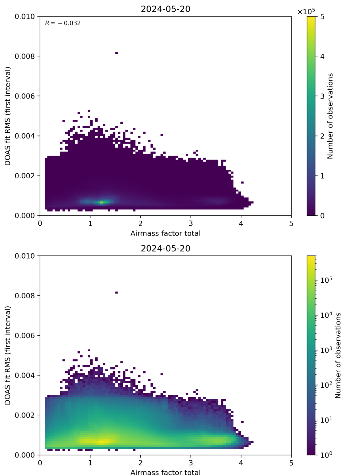
Figure 97: Scatter density plot of “Airmass factor total” against “DOAS fit RMS (first interval)” for 2024-05-19 to 2024-05-21.
