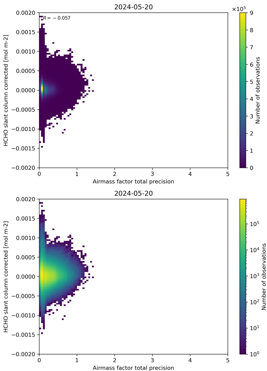
Figure 109: Scatter density plot of “Airmass factor total precision” against “HCHO slant column corrected” for 2024-05-19 to 2024-05-21.
