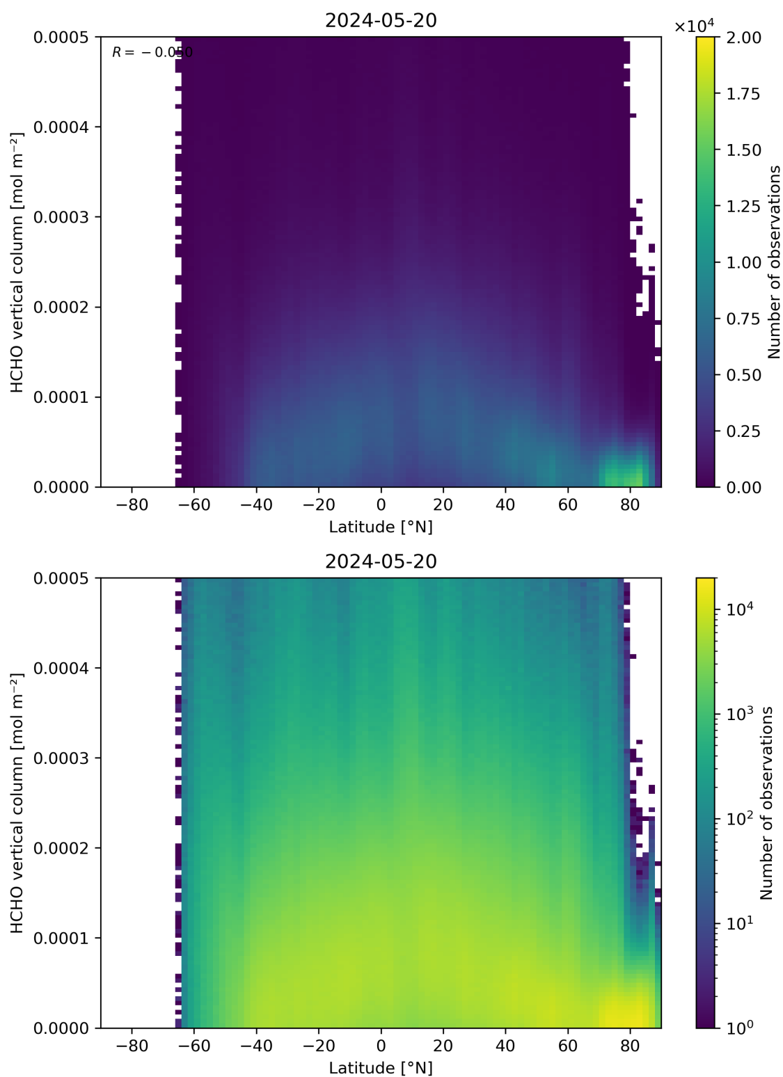
Figure 163: Scatter density plot of “Latitude” against “HCHO vertical column” for 2024-05-19 to 2024-05-21.
