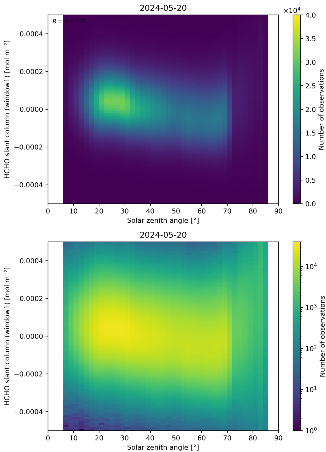
Figure 173: Scatter density plot of “Solar zenith angle” against “HCHO slant column (window1)” for 2024-05-19 to 2024-05-21.
