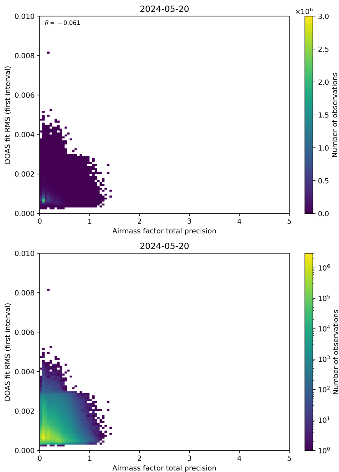
Figure 105: Scatter density plot of “Airmass factor total precision” against “DOAS fit RMS (first interval)” for 2024-05-19 to 2024-05-21.
