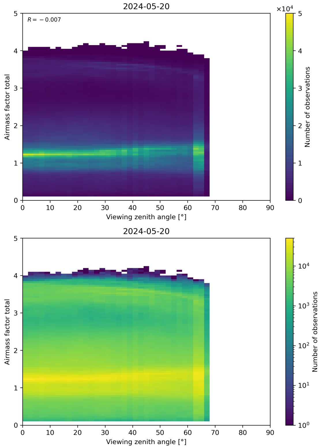
Figure 190: Scatter density plot of “Viewing zenith angle” against “Airmass factor total” for 2024-05-19 to 2024-05-21.
