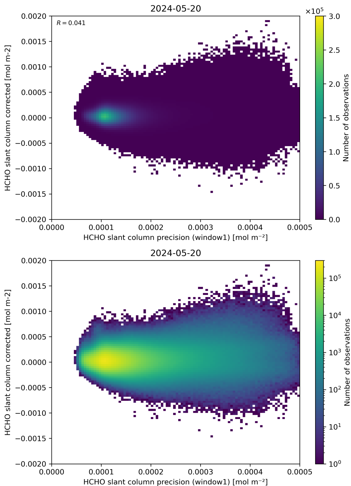
Figure 92: Scatter density plot of “HCHO slant column precision (window1)” against “HCHO slant column corrected” for 2024-05-19 to 2024-05-21.
