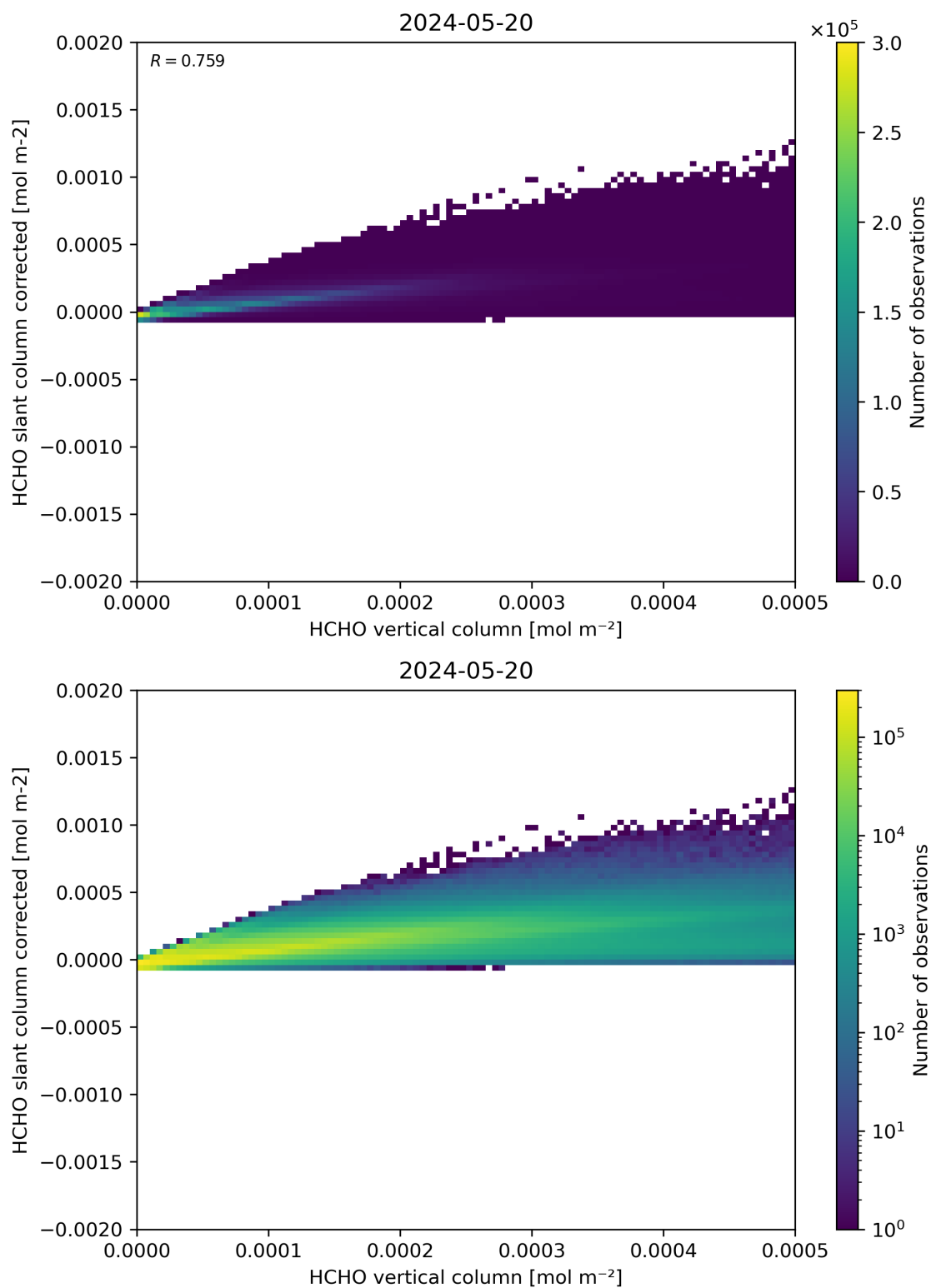
Figure 127: Scatter density plot of “HCHO vertical column” against “HCHO slant column corrected” for 2024-05-19 to 2024-05-21.
