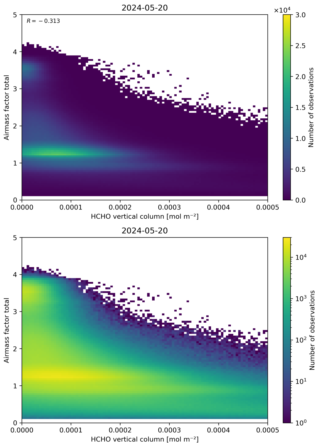
Figure 131: Scatter density plot of “HCHO vertical column” against “Airmass factor total” for 2024-05-19 to 2024-05-21.
