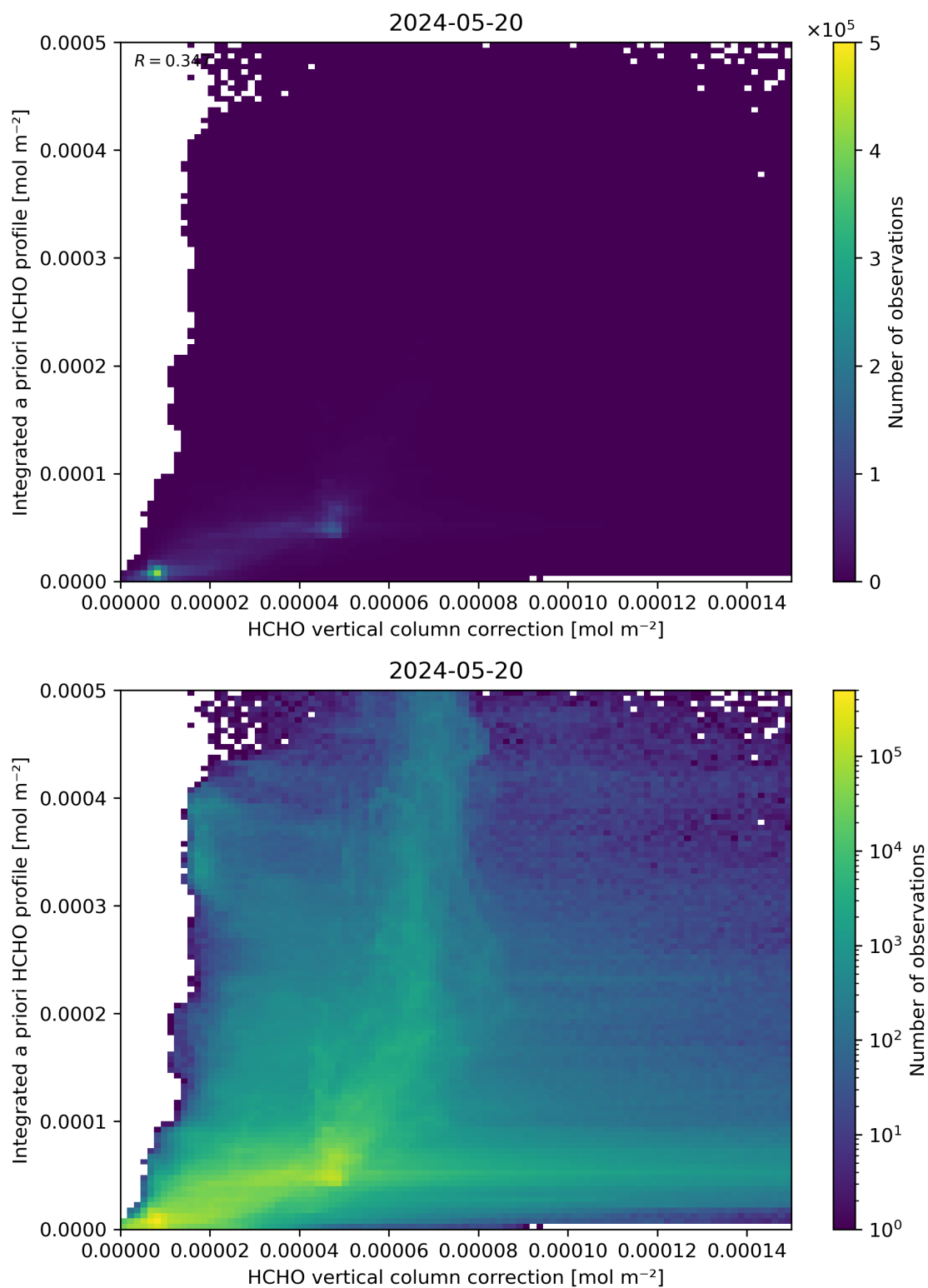
Figure 122: Scatter density plot of “HCHO vertical column correction” against “Integrated a priori HCHO profile” for 2024-05-19 to 2024-05-21.
