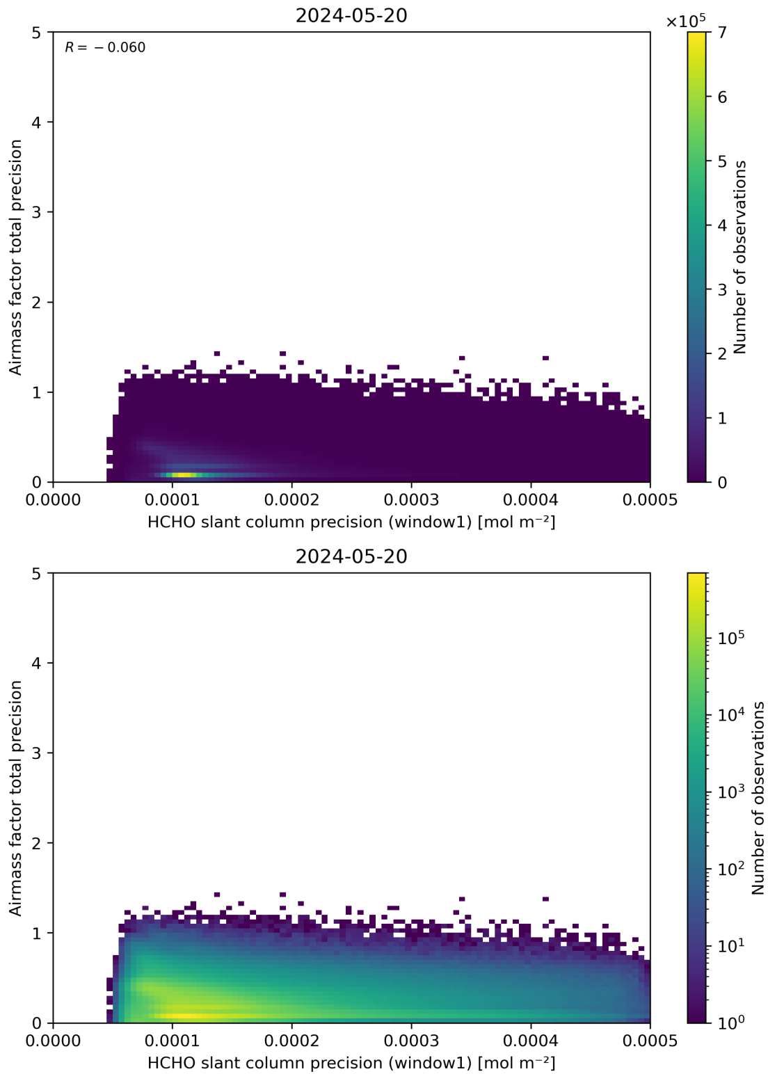
Figure 95: Scatter density plot of “HCHO slant column precision (window1)” against “Airmass factor total precision” for 2024-05-19 to 2024-05-21.
