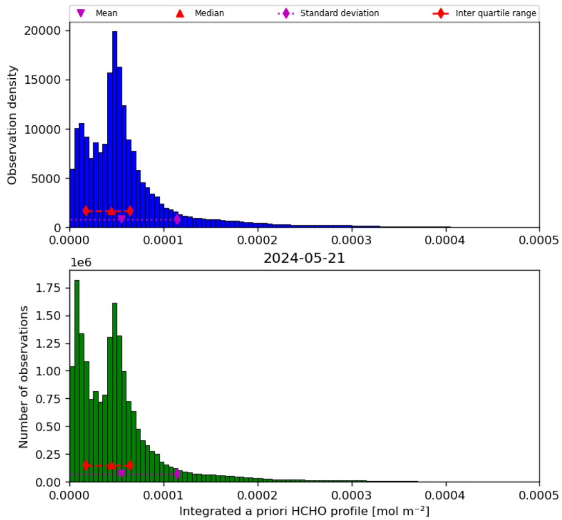
Figure 43: Histogram of “Integrated a priori HCHO profile” for 2024-05-20 to 2024-05-22
