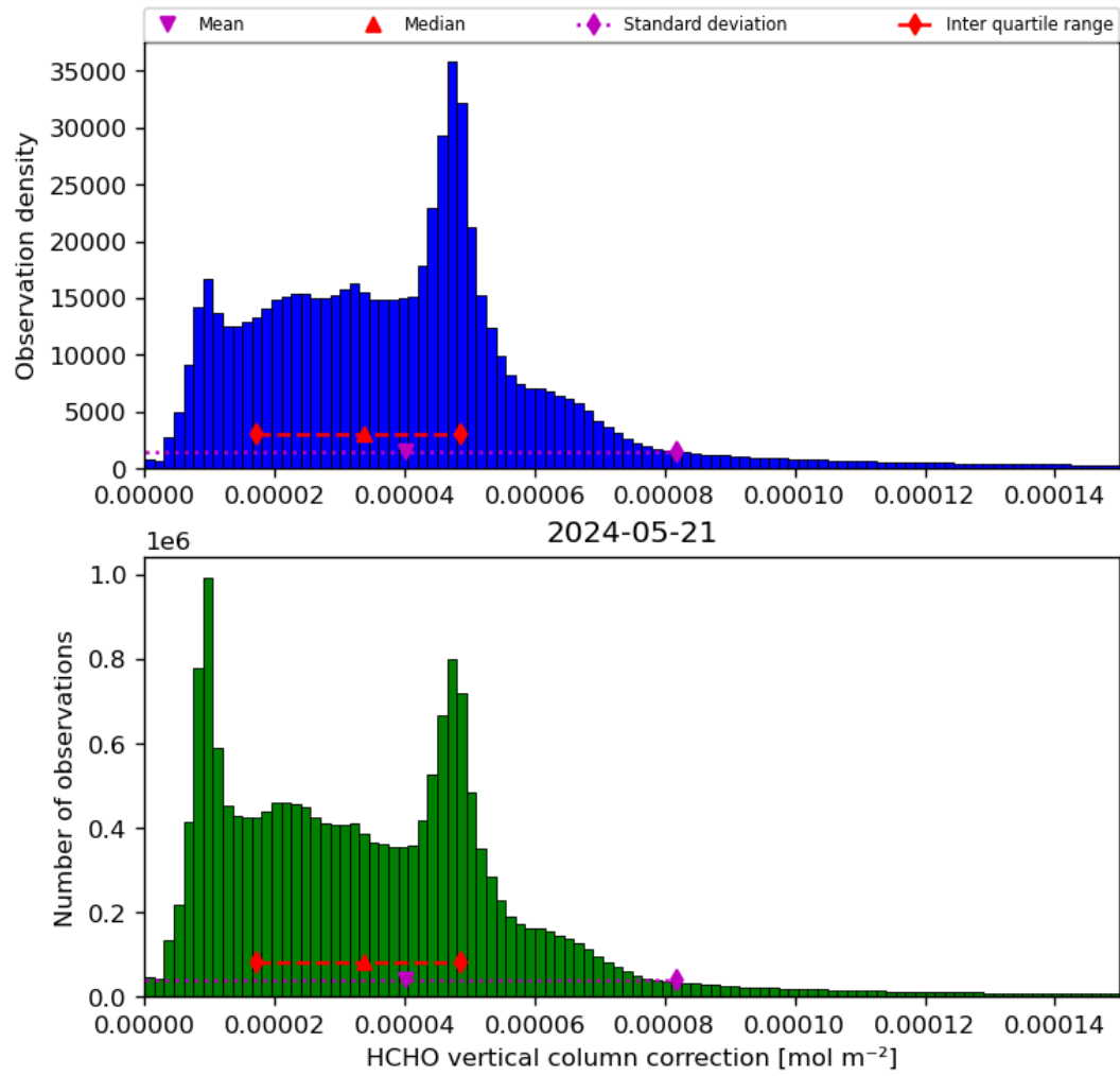
Figure 37: Histogram of “HCHO vertical column correction” for 2024-05-20 to 2024-05-22
