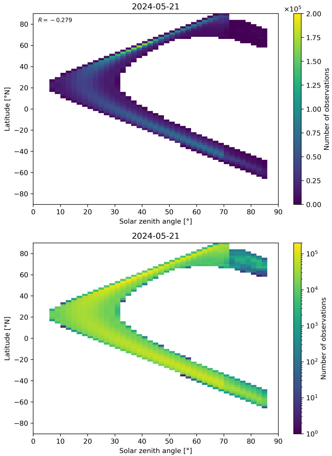
Figure 181: Scatter density plot of “Solar zenith angle” against “Latitude” for 2024-05-20 to 2024-05-22.
