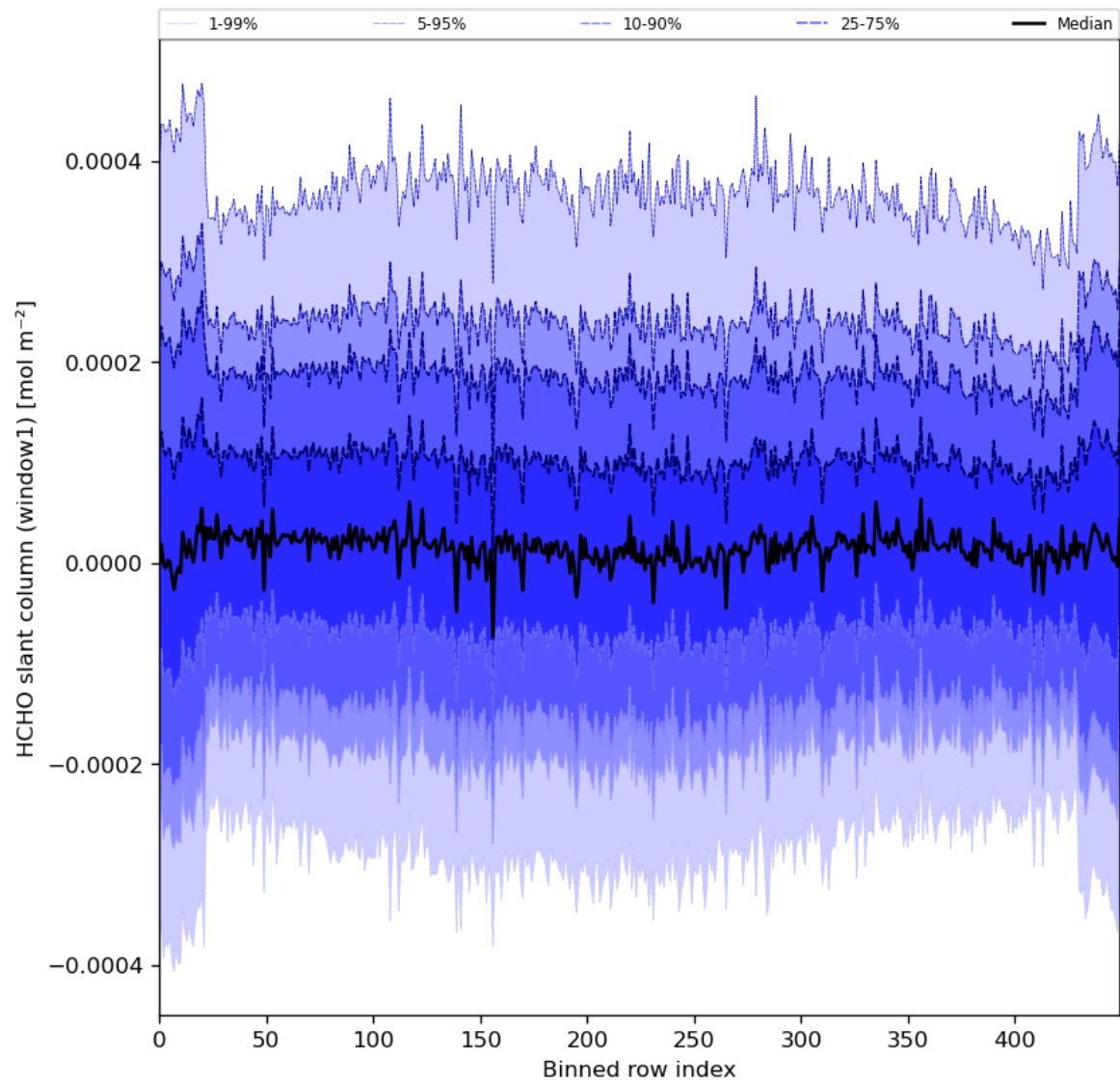
Figure 52: Along track statistics of “HCHO slant column (window1)” for 2024-05-20 to 2024-05-22
