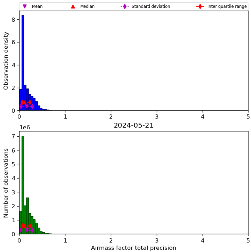
Figure 41: Histogram of “Airmass factor total precision” for 2024-05-20 to 2024-05-22
