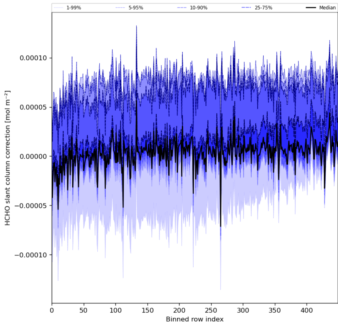
Figure 61: Along track statistics of “HCHO slant column correction” for 2024-05-20 to 2024-05-22
