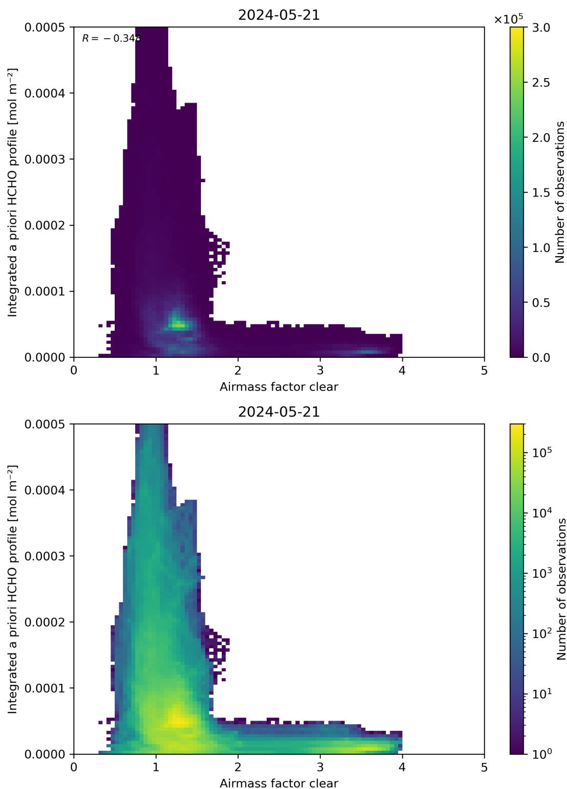
Figure 76: Scatter density plot of “Airmass factor clear” against “Integrated a priori HCHO profile” for 2024-05-20 to 2024-05-22.
