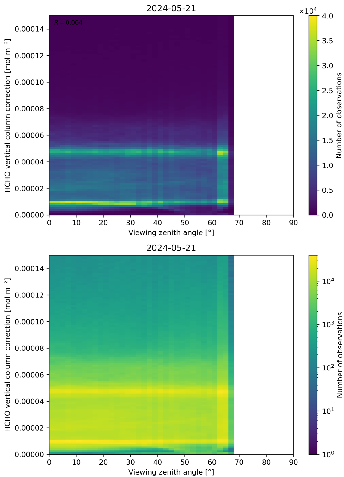
Figure 193: Scatter density plot of “Viewing zenith angle” against “HCHO vertical column correction” for 2024-05-20 to 2024-05-22.
