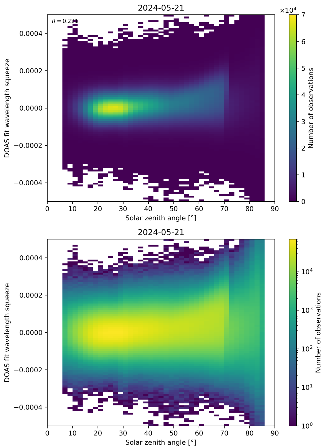
Figure 169: Scatter density plot of “Solar zenith angle” against “DOAS fit wavelength squeeze” for 2024-05-20 to 2024-05-22.
