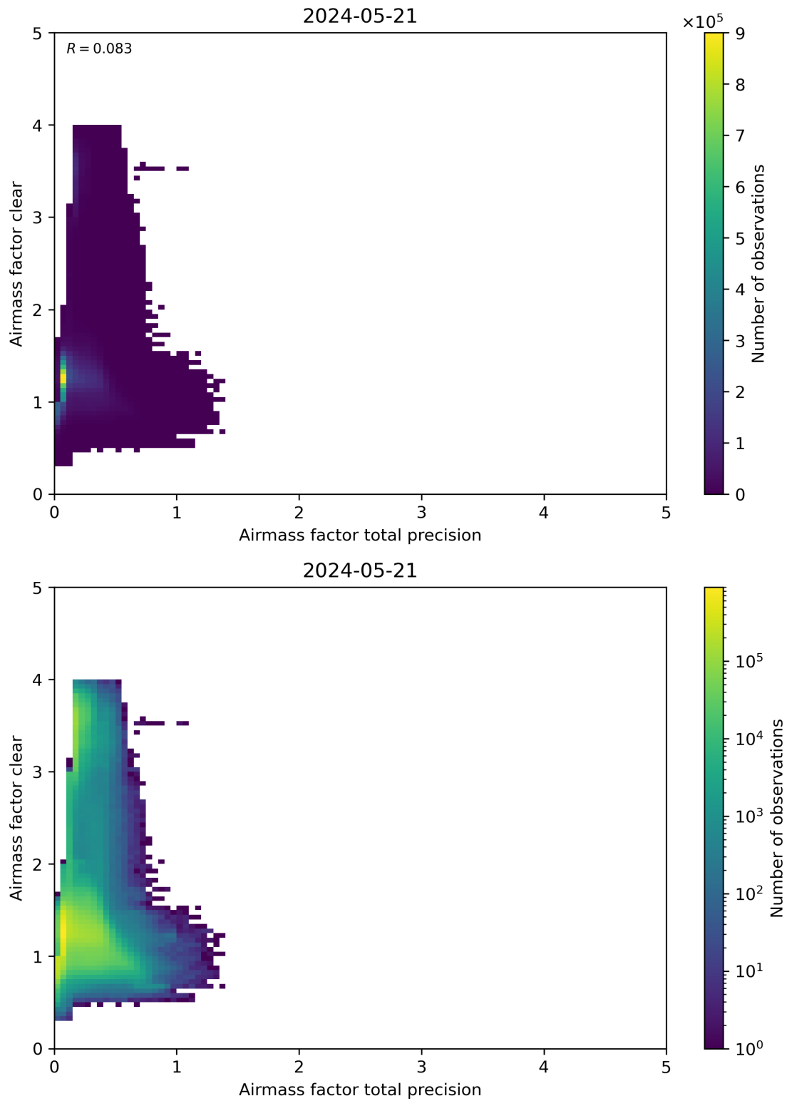
Figure 108: Scatter density plot of “Airmass factor total precision” against “Airmass factor clear” for 2024-05-20 to 2024-05-22.
