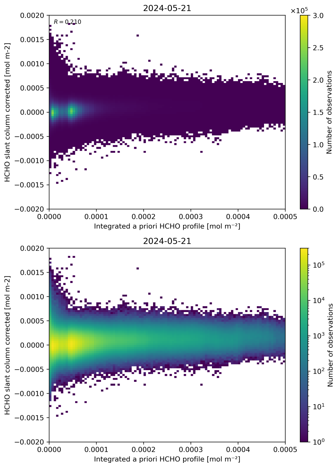
Figure 151: Scatter density plot of “Integrated a priori HCHO profile” against “HCHO slant column corrected” for 2024-05-20 to 2024-05-22.
