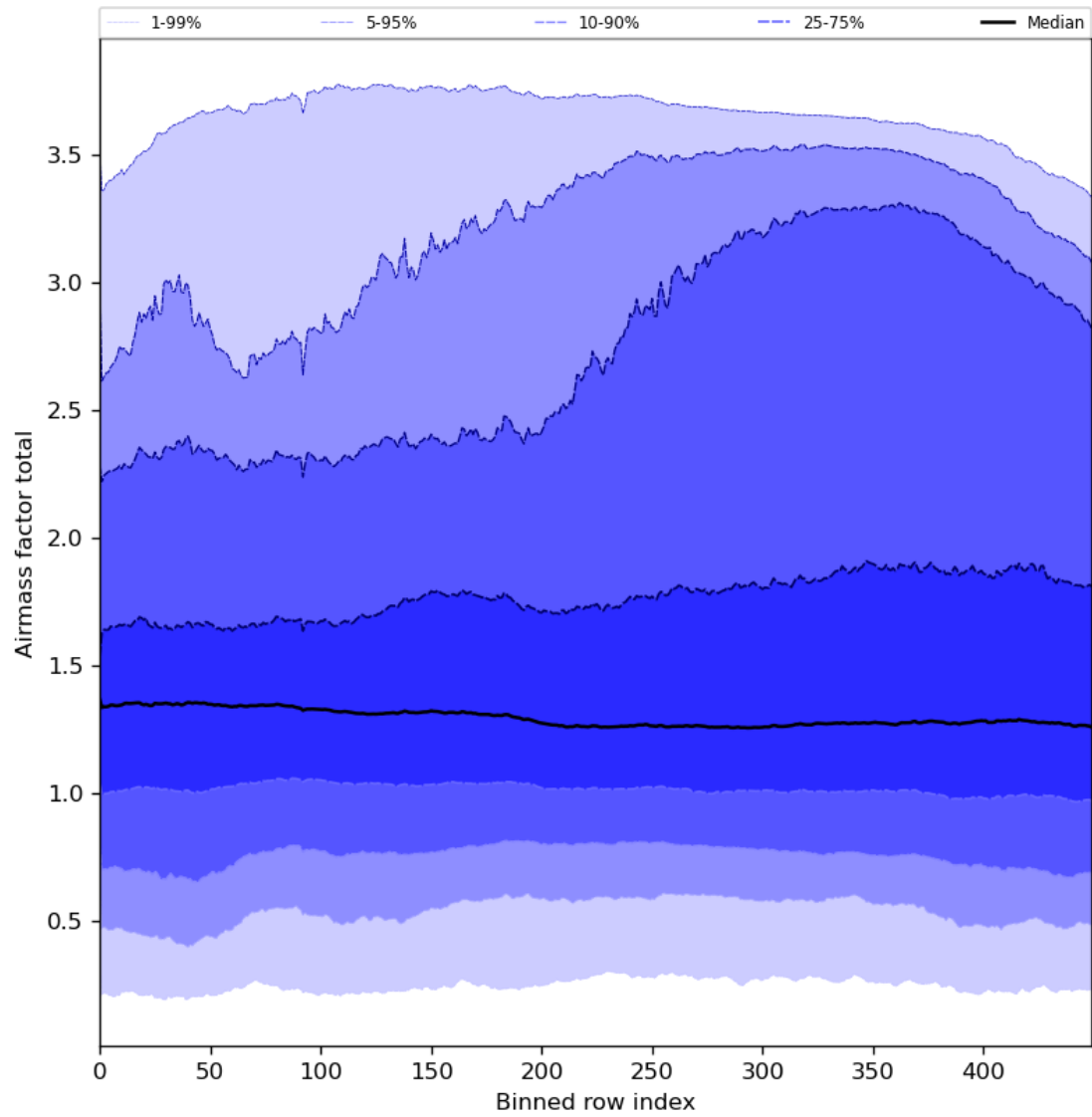
Figure 54: Along track statistics of “Airmass factor total” for 2024-05-20 to 2024-05-22
