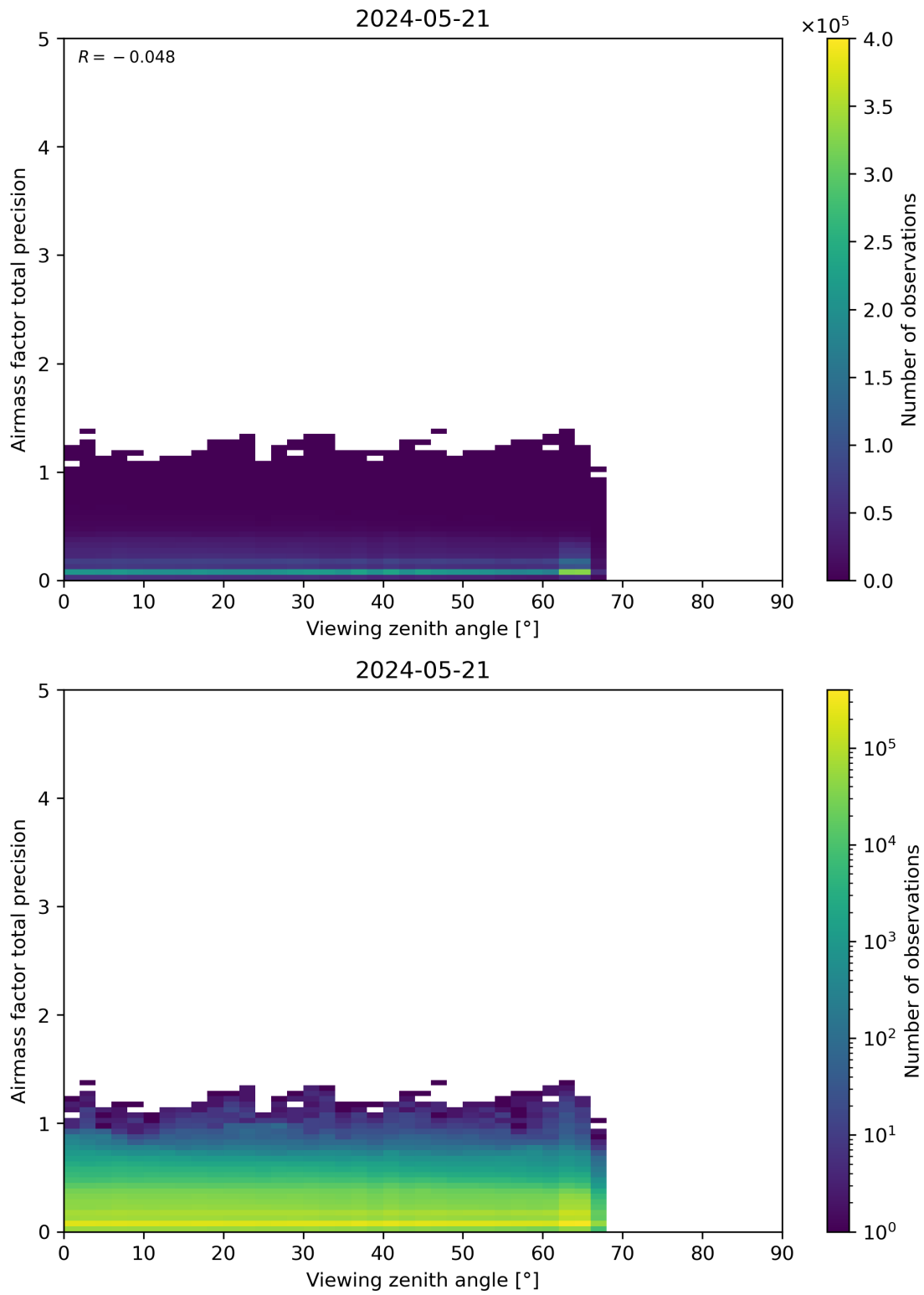
Figure 191: Scatter density plot of “Viewing zenith angle” against “Airmass factor total precision” for 2024-05-20 to 2024-05-22.
