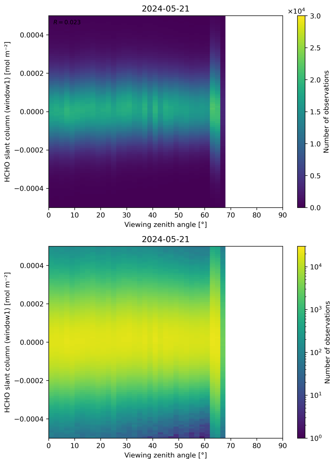
Figure 188: Scatter density plot of “Viewing zenith angle” against “HCHO slant column (window1)” for 2024-05-20 to 2024-05-22.
