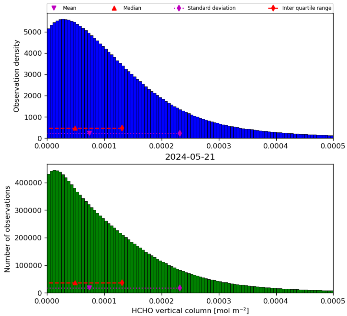
Figure 35: Histogram of “HCHO vertical column” for 2024-05-20 to 2024-05-22
