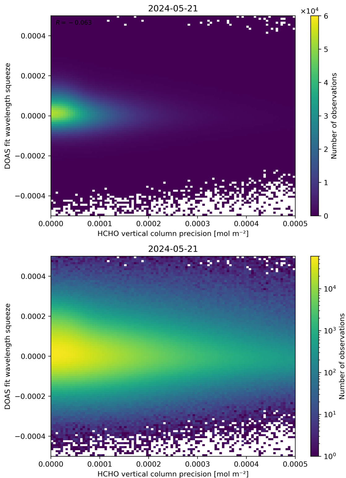
Figure 138: Scatter density plot of “HCHO vertical column precision” against “DOAS fit wavelength squeeze” for 2024-05-20 to 2024-05-22.
