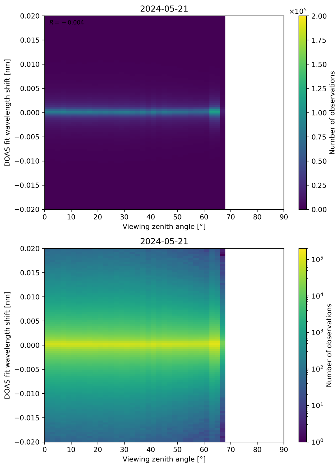
Figure 183: Scatter density plot of “Viewing zenith angle” against “DOAS fit wavelength shift” for 2024-05-20 to 2024-05-22.
