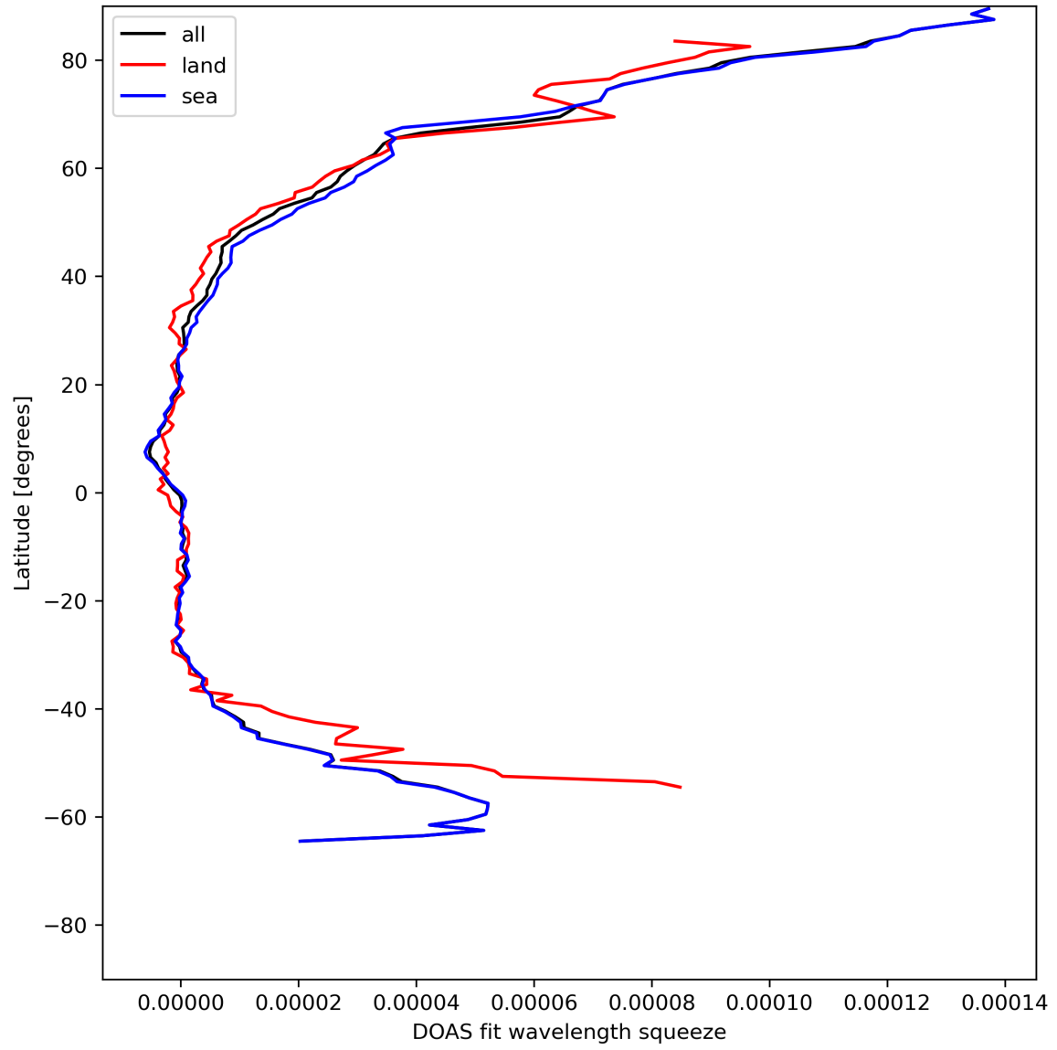
Figure 31: Zonal average of “DOAS fit wavelength squeeze” for 2024-05-20 to 2024-05-22.
