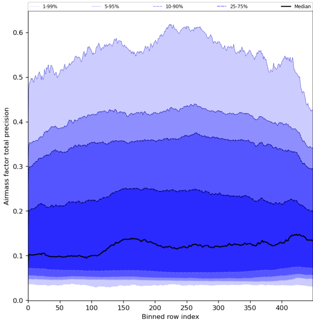
Figure 55: Along track statistics of “Airmass factor total precision” for 2024-05-20 to 2024-05-22
