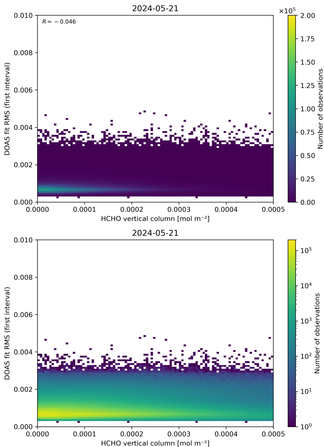
Figure 123: Scatter density plot of “HCHO vertical column” against “DOAS fit RMS (first interval)” for 2024-05-20 to 2024-05-22.
