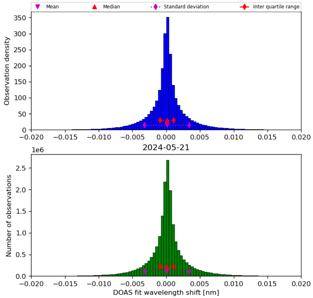
Figure 44: Histogram of “DOAS fit wavelength shift” for 2024-05-20 to 2024-05-22
