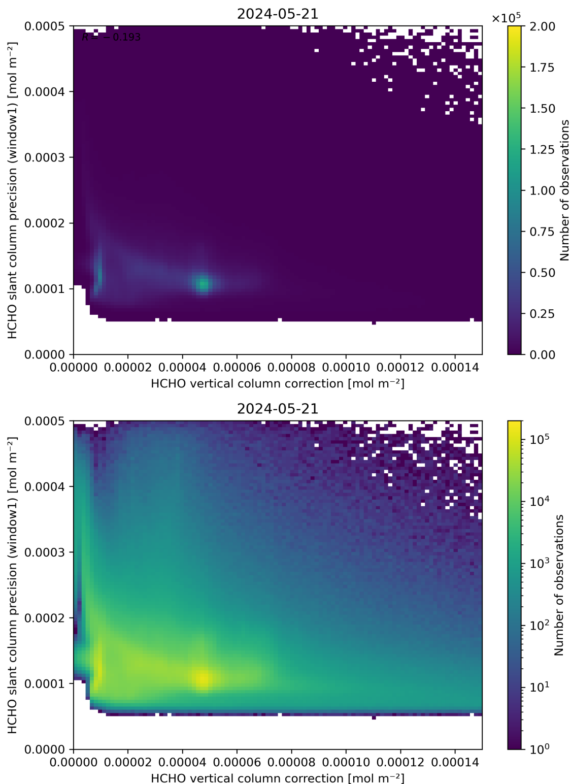
Figure 119: Scatter density plot of “HCHO vertical column correction” against “HCHO slant column precision (window1)” for 2024-05-20 to 2024-05-22.
