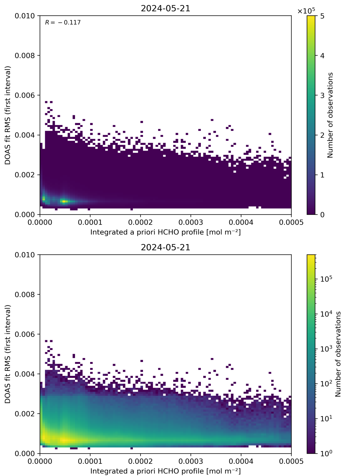
Figure 148: Scatter density plot of “Integrated a priori HCHO profile” against “DOAS fit RMS (first interval)” for 2024-05-20 to 2024-05-22.
