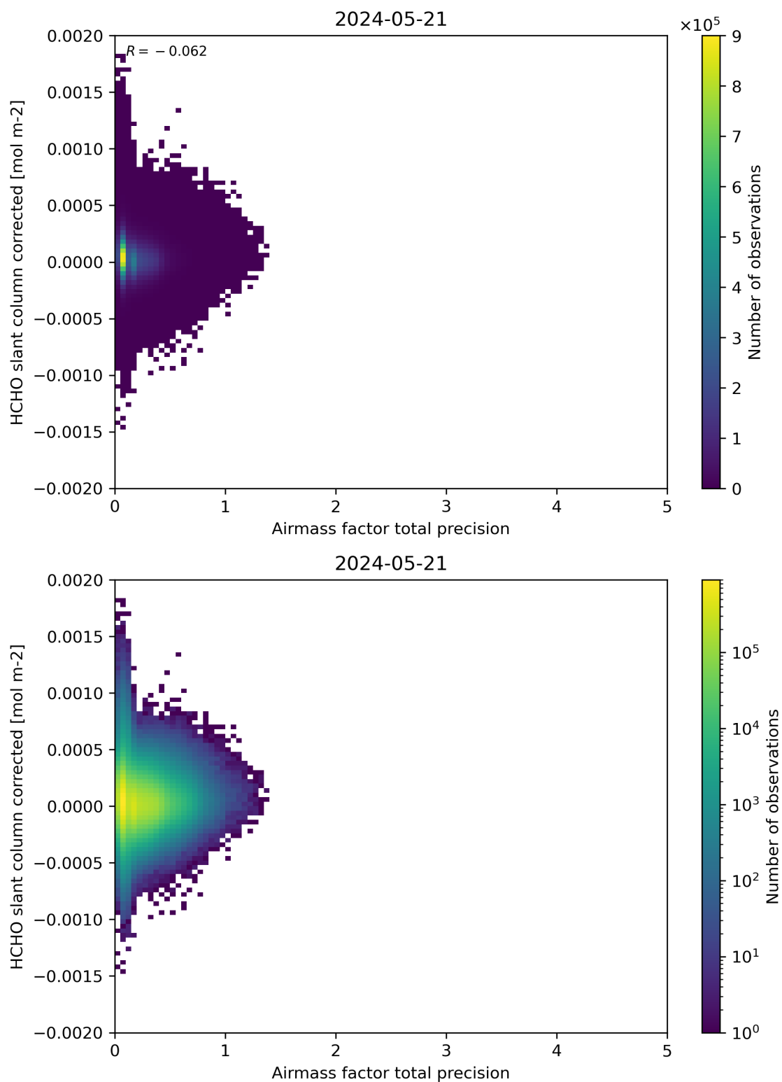
Figure 109: Scatter density plot of “Airmass factor total precision” against “HCHO slant column corrected” for 2024-05-20 to 2024-05-22.
