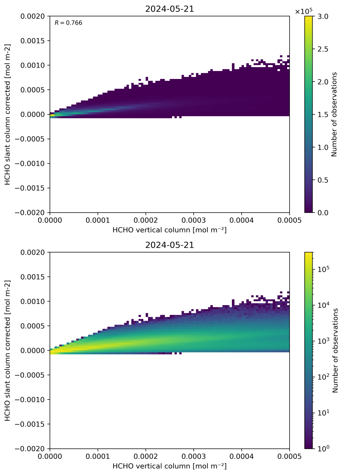
Figure 127: Scatter density plot of “HCHO vertical column” against “HCHO slant column corrected” for 2024-05-20 to 2024-05-22.
