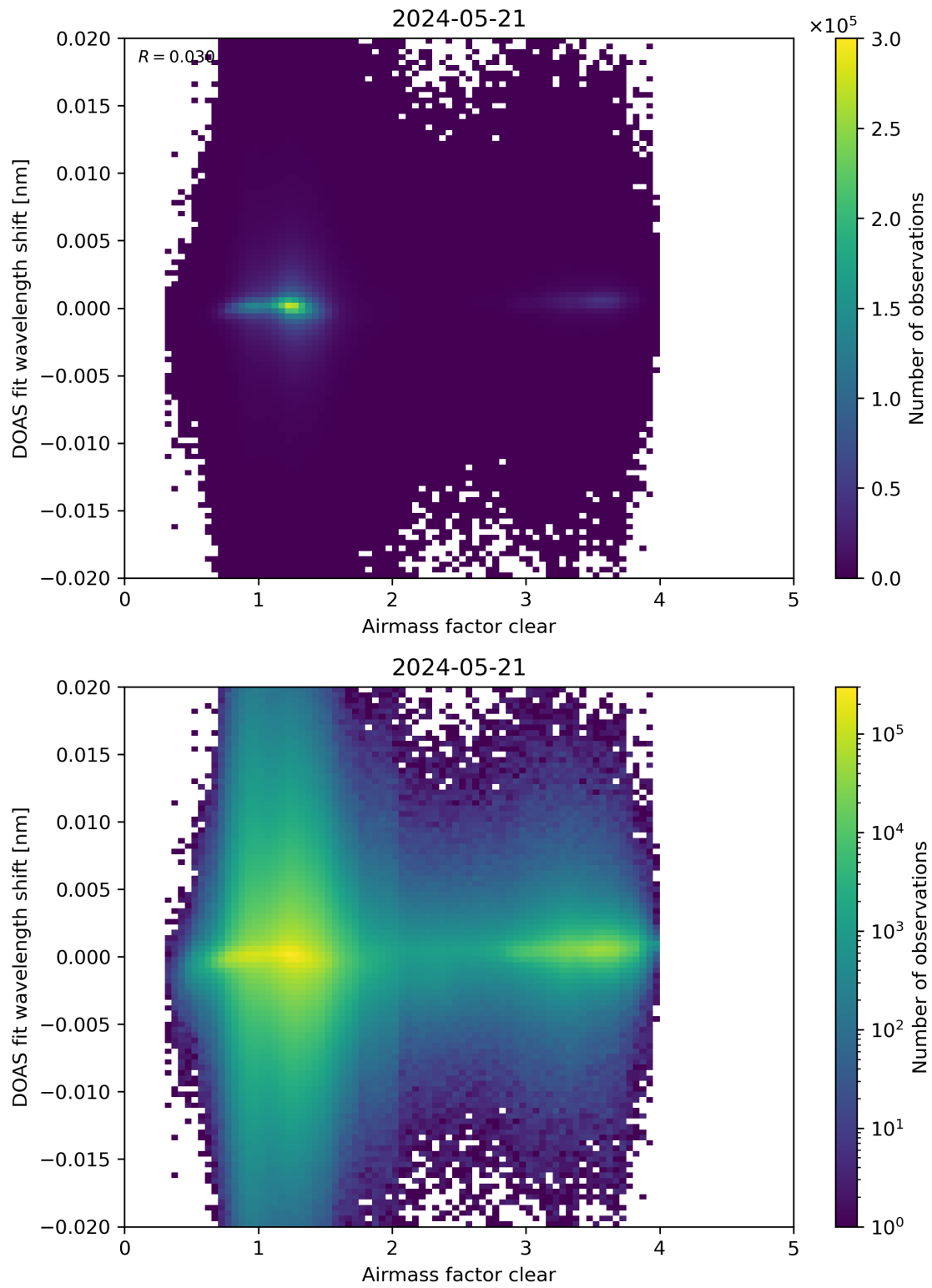
Figure 72: Scatter density plot of “Airmass factor clear” against “DOAS fit wavelength shift” for 2024-05-20 to 2024-05-22.
