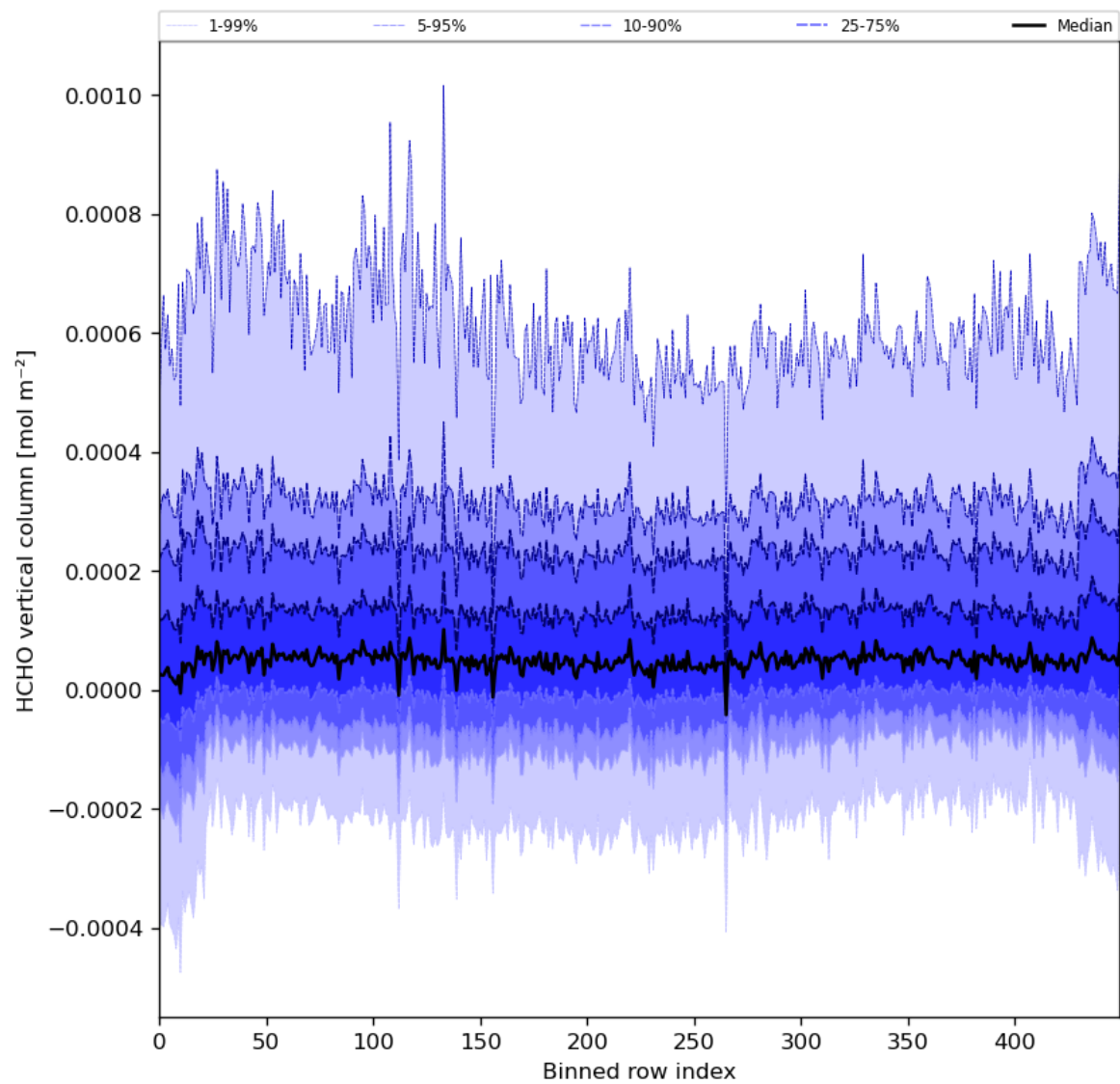
Figure 49: Along track statistics of “HCHO vertical column” for 2024-05-20 to 2024-05-22
