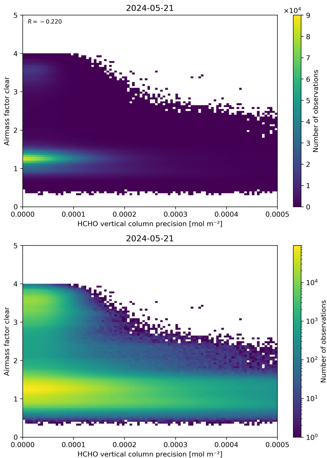
Figure 139: Scatter density plot of “HCHO vertical column precision” against “Airmass factor clear” for 2024-05-20 to 2024-05-22.
