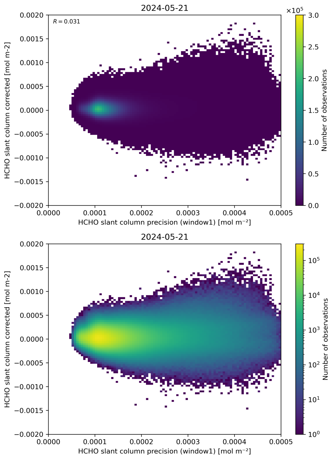
Figure 92: Scatter density plot of “HCHO slant column precision (window1)” against “HCHO slant column corrected” for 2024-05-20 to 2024-05-22.
