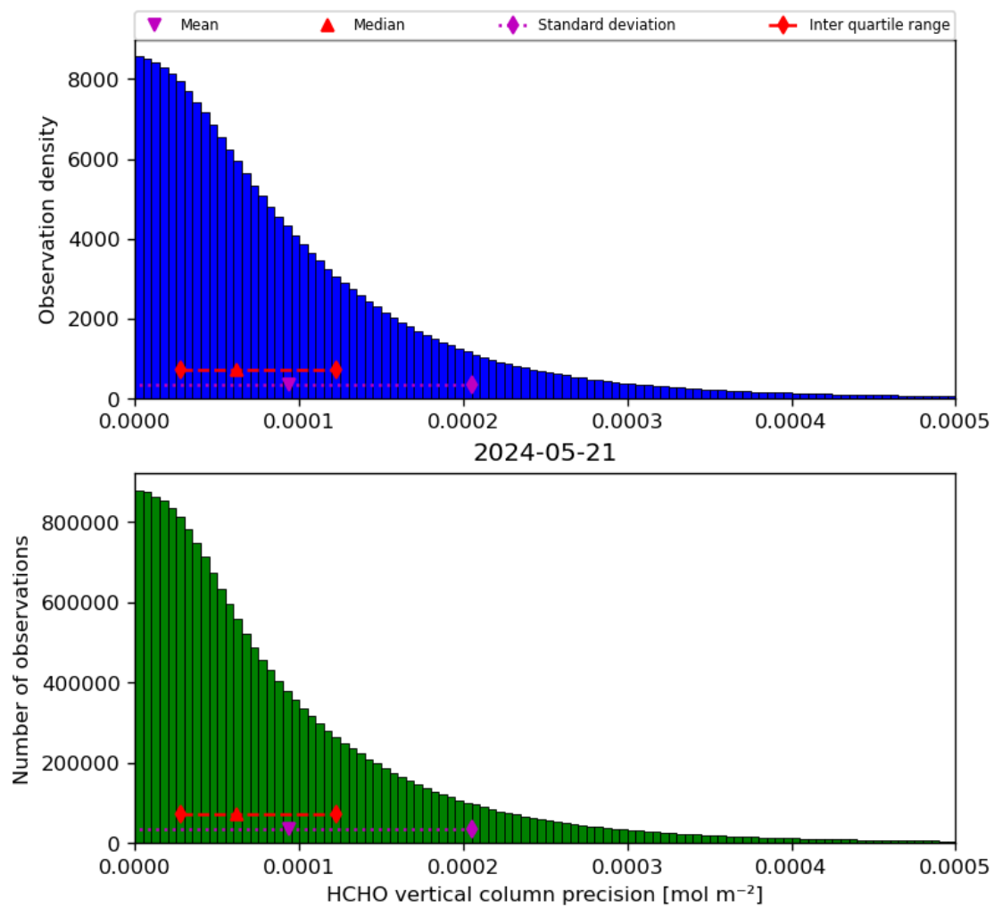
Figure 36: Histogram of “HCHO vertical column precision” for 2024-05-20 to 2024-05-22
