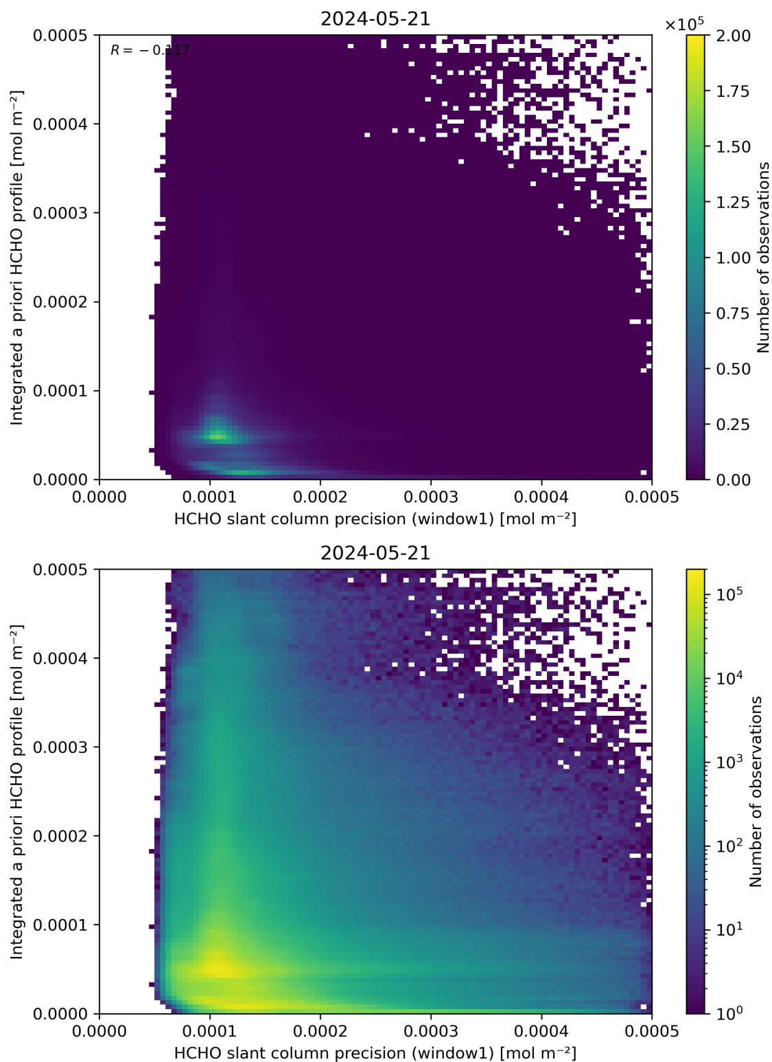
Figure 96: Scatter density plot of “HCHO slant column precision (window1)” against “Integrated a priori HCHO profile” for 2024-05-20 to 2024-05-22.
