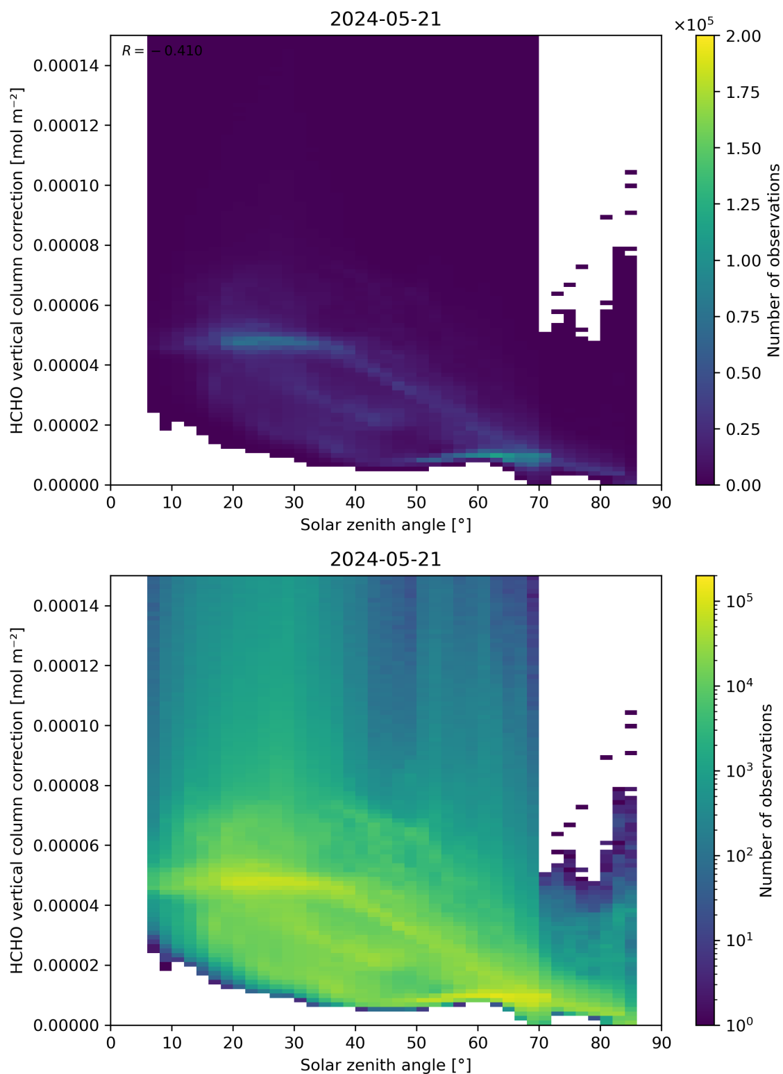
Figure 178: Scatter density plot of “Solar zenith angle” against “HCHO vertical column correction” for 2024-05-20 to 2024-05-22.
