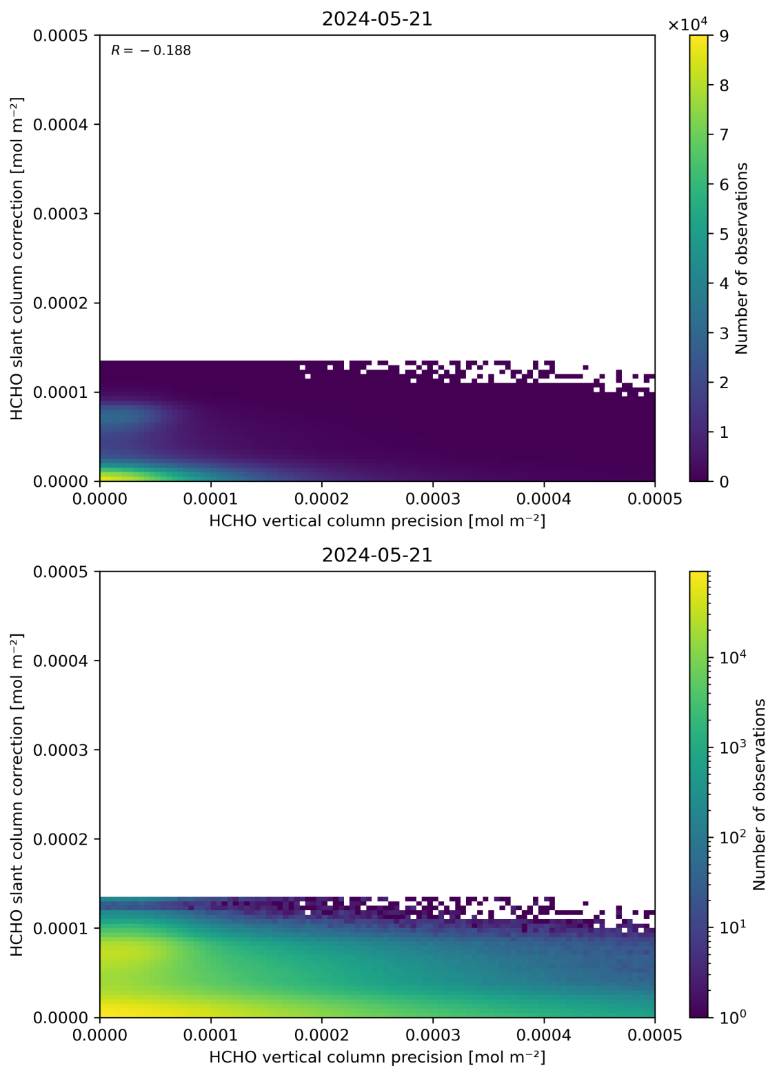
Figure 141: Scatter density plot of “HCHO vertical column precision” against “HCHO slant column correction” for 2024-05-20 to 2024-05-22.
