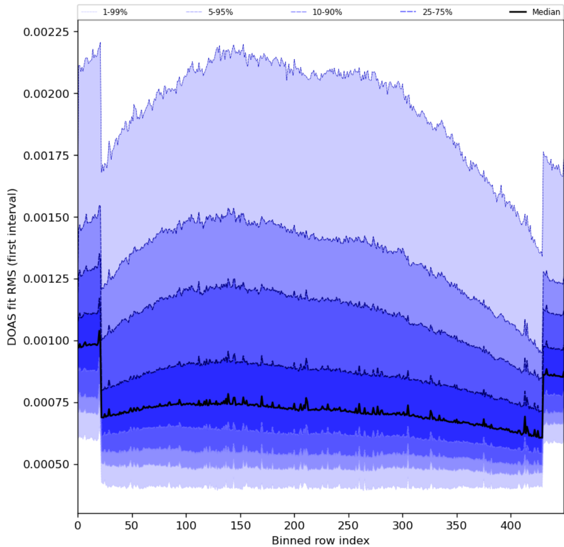
Figure 60: Along track statistics of “DOAS fit RMS (first interval)” for 2024-05-20 to 2024-05-22
