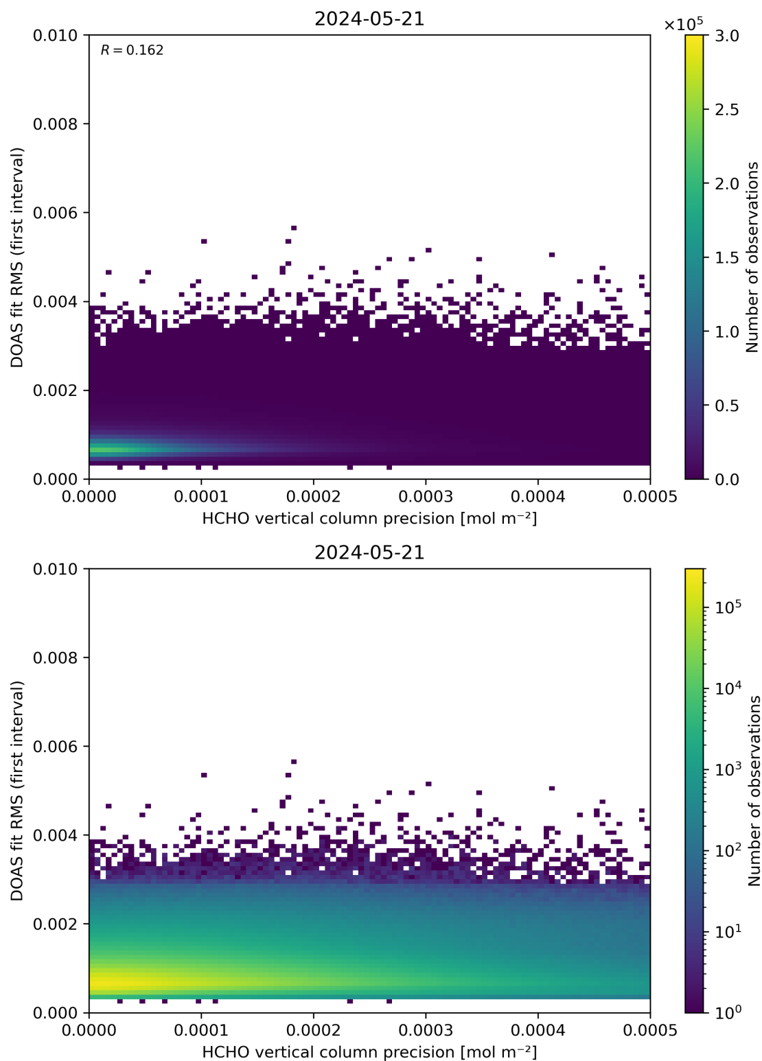
Figure 136: Scatter density plot of “HCHO vertical column precision” against “DOAS fit RMS (first interval)” for 2024-05-20 to 2024-05-22.
