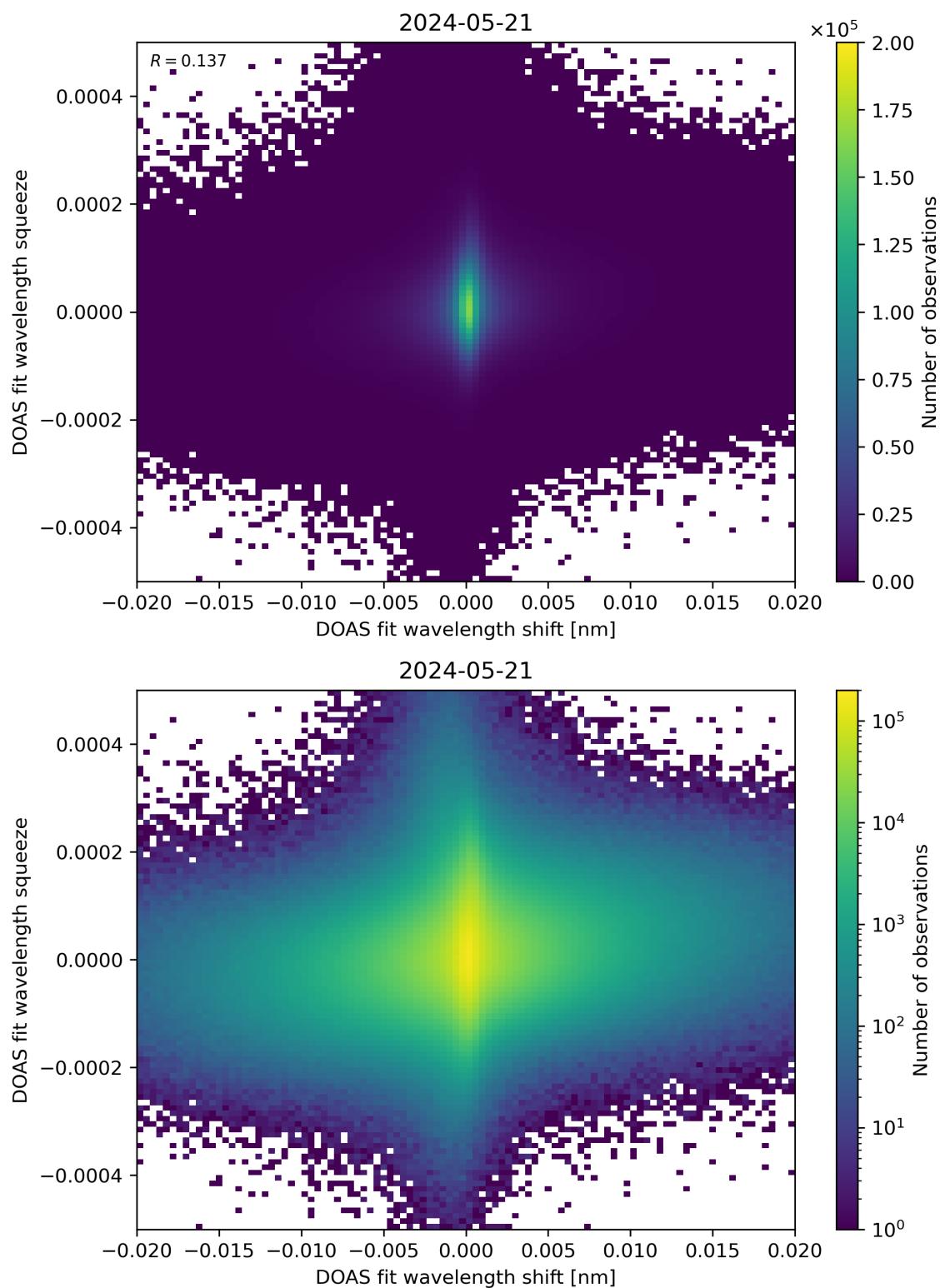
Figure 65: Scatter density plot of “DOAS fit wavelength shift” against “DOAS fit wavelength squeeze” for 2024-05-20 to 2024-05-22.
