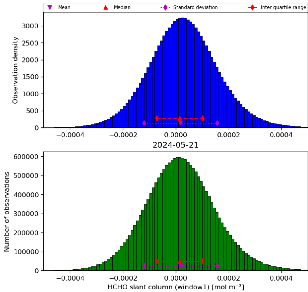
Figure 38: Histogram of “HCHO slant column (window1)” for 2024-05-20 to 2024-05-22
