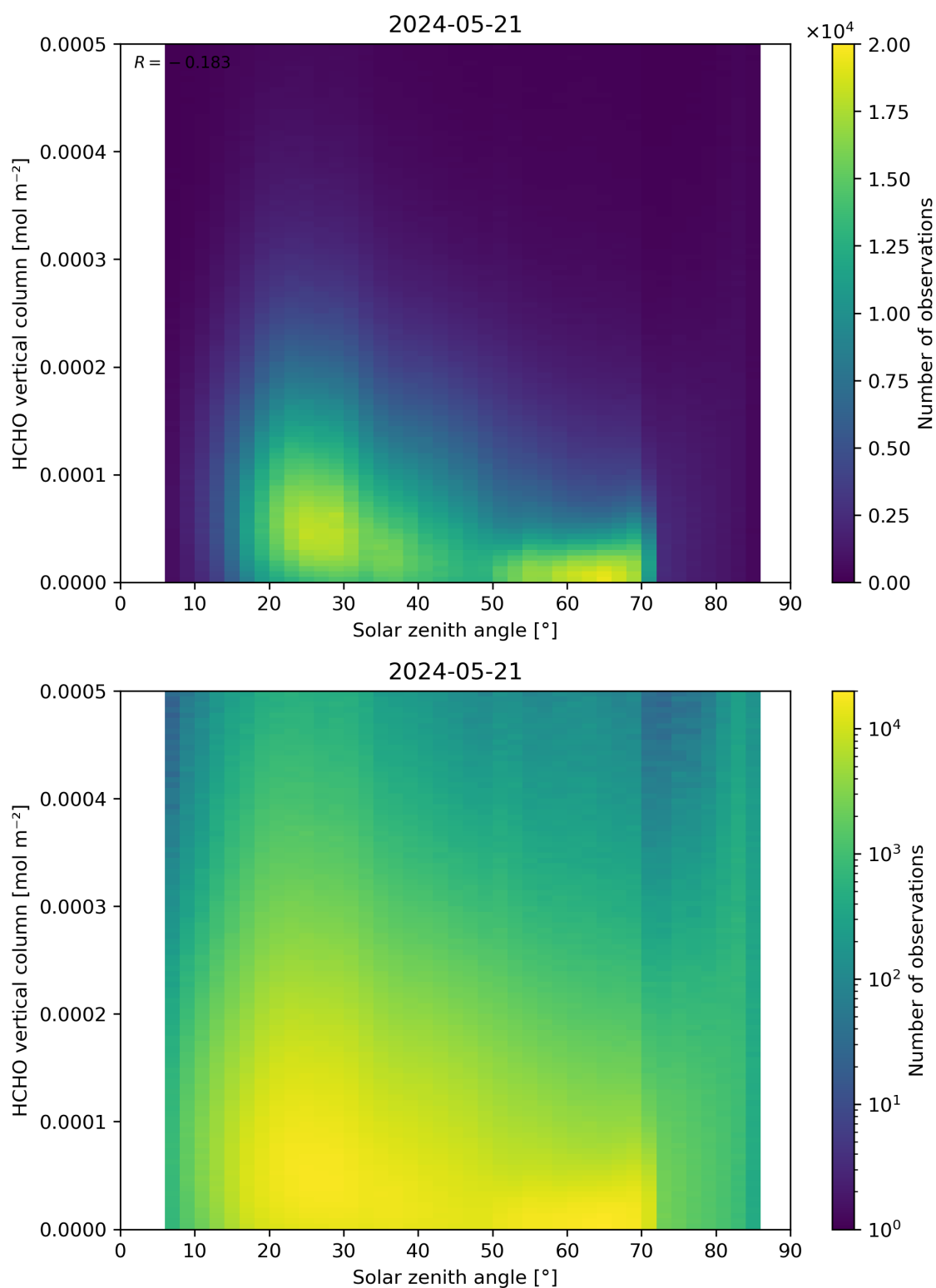
Figure 177: Scatter density plot of “Solar zenith angle” against “HCHO vertical column” for 2024-05-20 to 2024-05-22.
