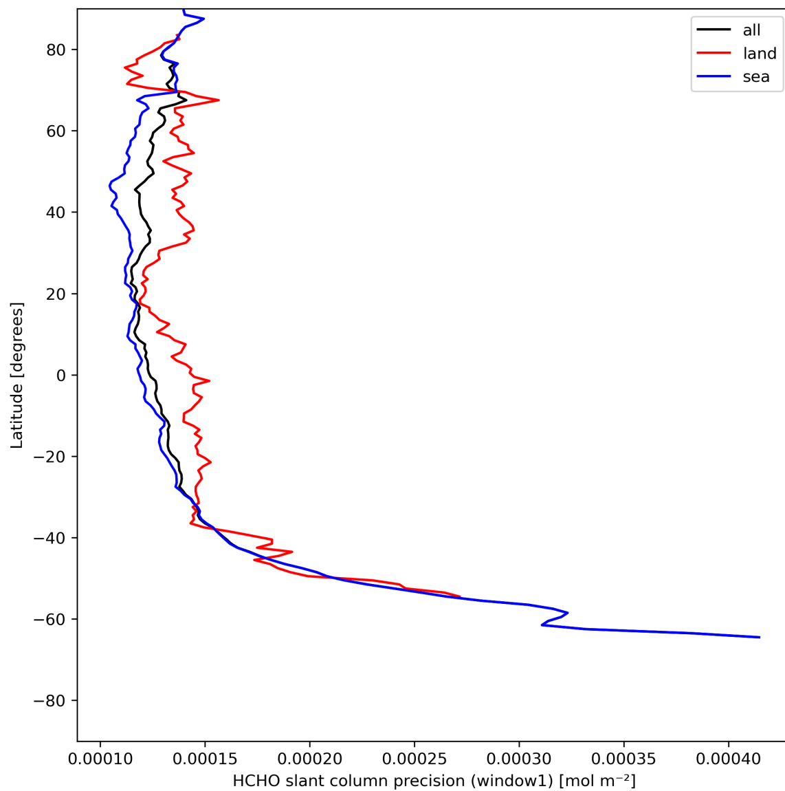
Figure 25: Zonal average of “HCHO slant column precision (window1)” for 2024-05-20 to 2024-05-22.
