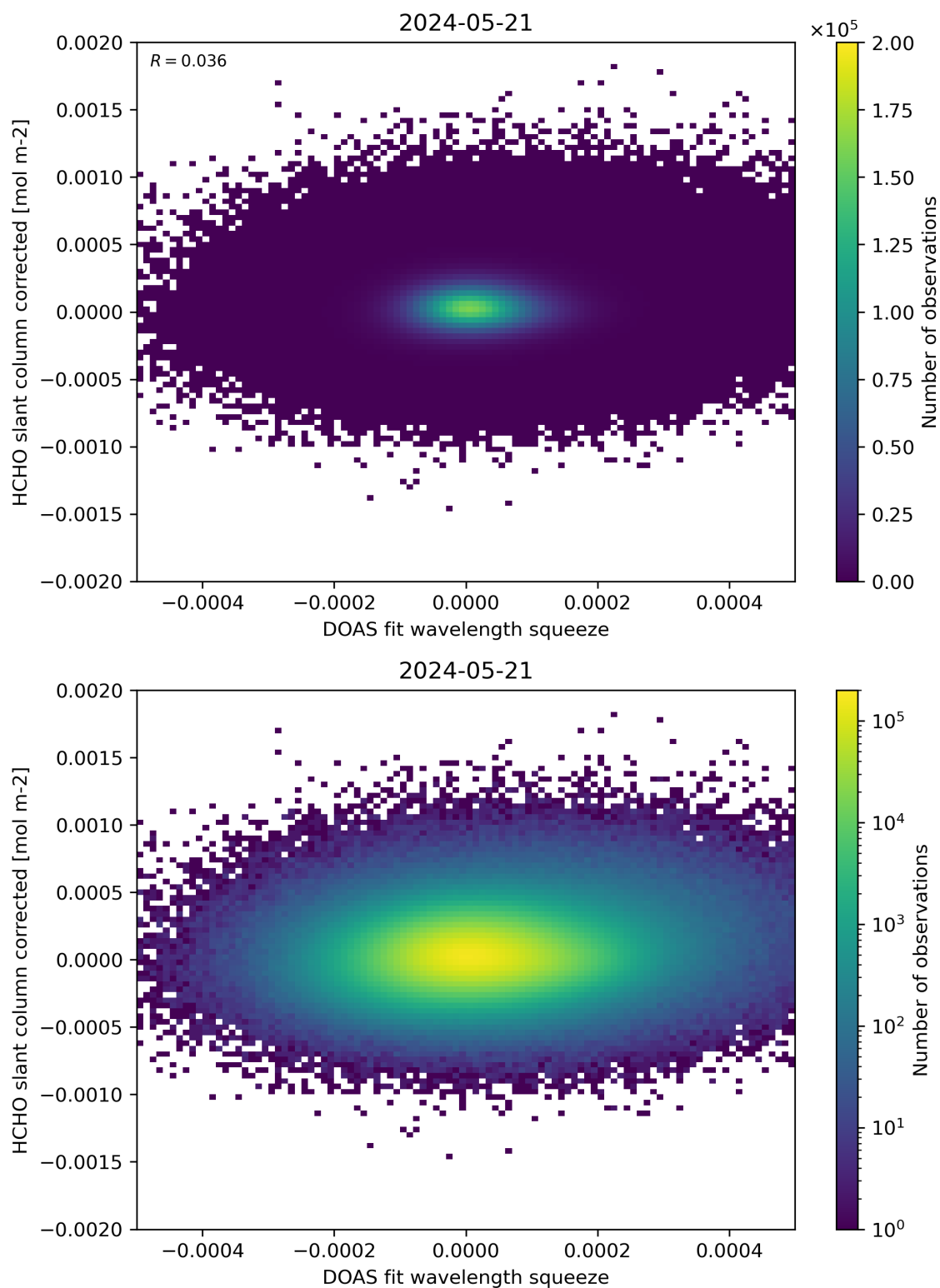
Figure 69: Scatter density plot of “DOAS fit wavelength squeeze” against “HCHO slant column corrected” for 2024-05-20 to 2024-05-22.
