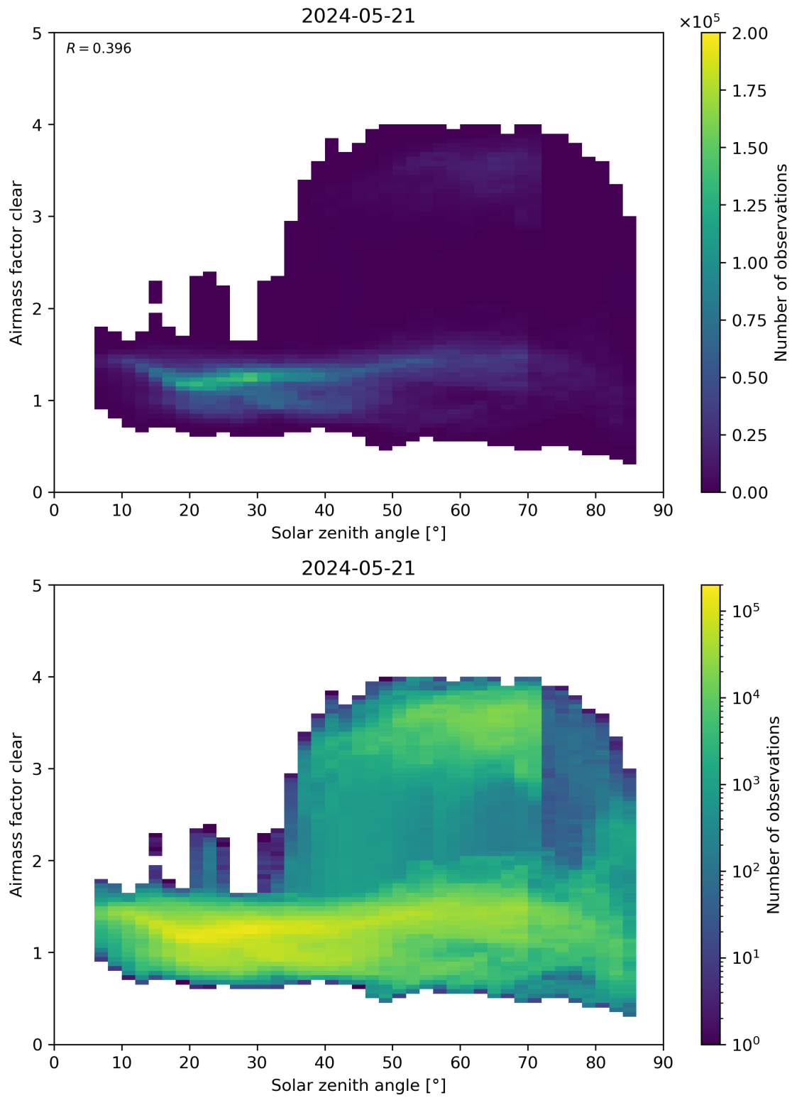
Figure 170: Scatter density plot of “Solar zenith angle” against “Airmass factor clear” for 2024-05-20 to 2024-05-22.
