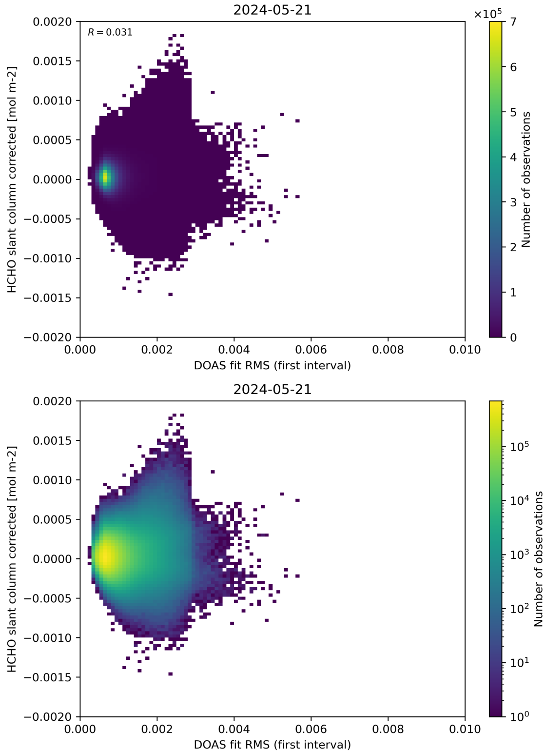
Figure 62: Scatter density plot of “DOAS fit RMS (first interval)” against “HCHO slant column corrected” for 2024-05-20 to 2024-05-22.
