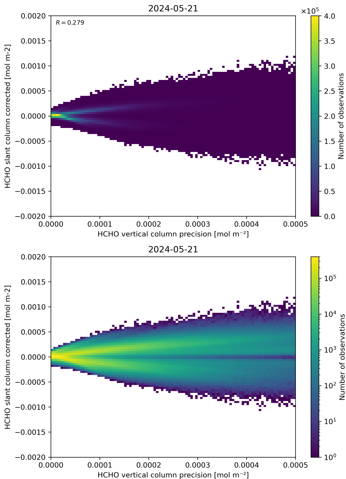
Figure 140: Scatter density plot of “HCHO vertical column precision” against “HCHO slant column corrected” for 2024-05-20 to 2024-05-22.
