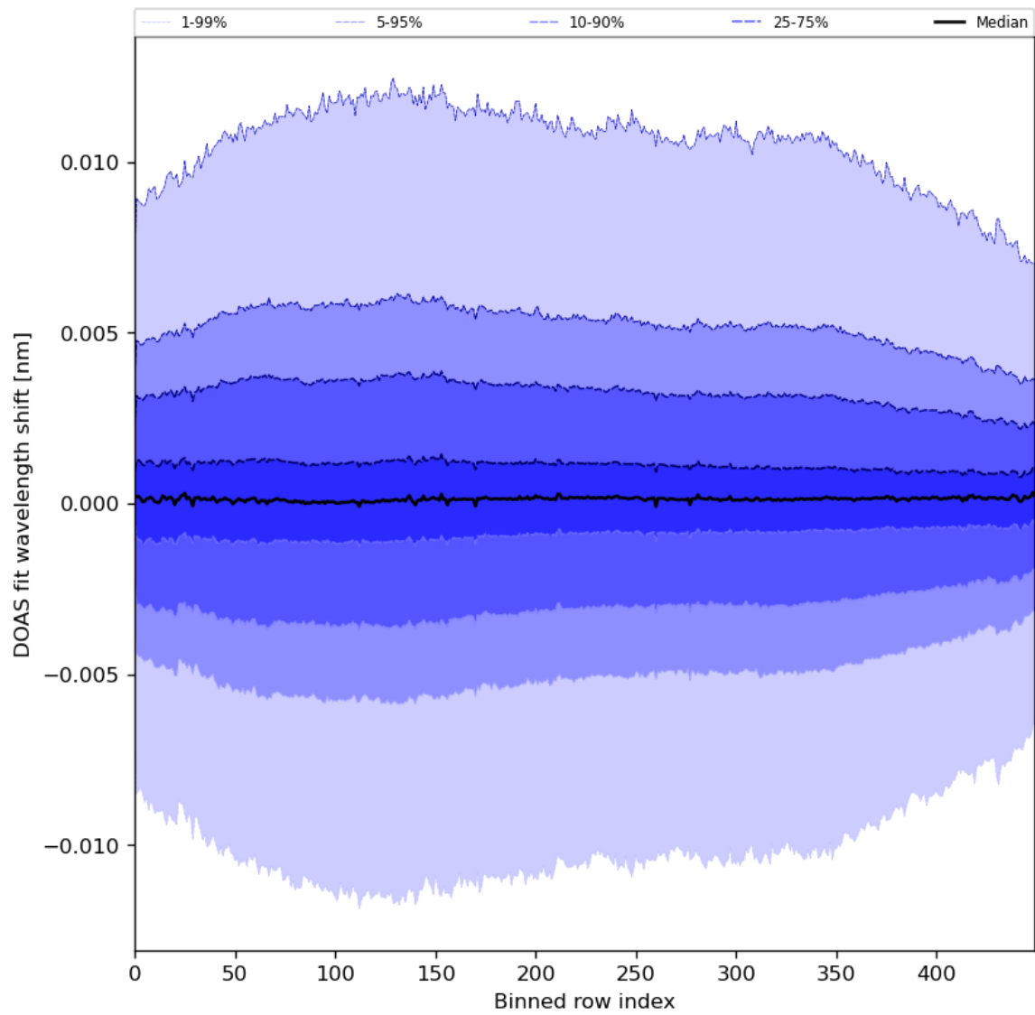
Figure 58: Along track statistics of “DOAS fit wavelength shift” for 2024-05-20 to 2024-05-22
