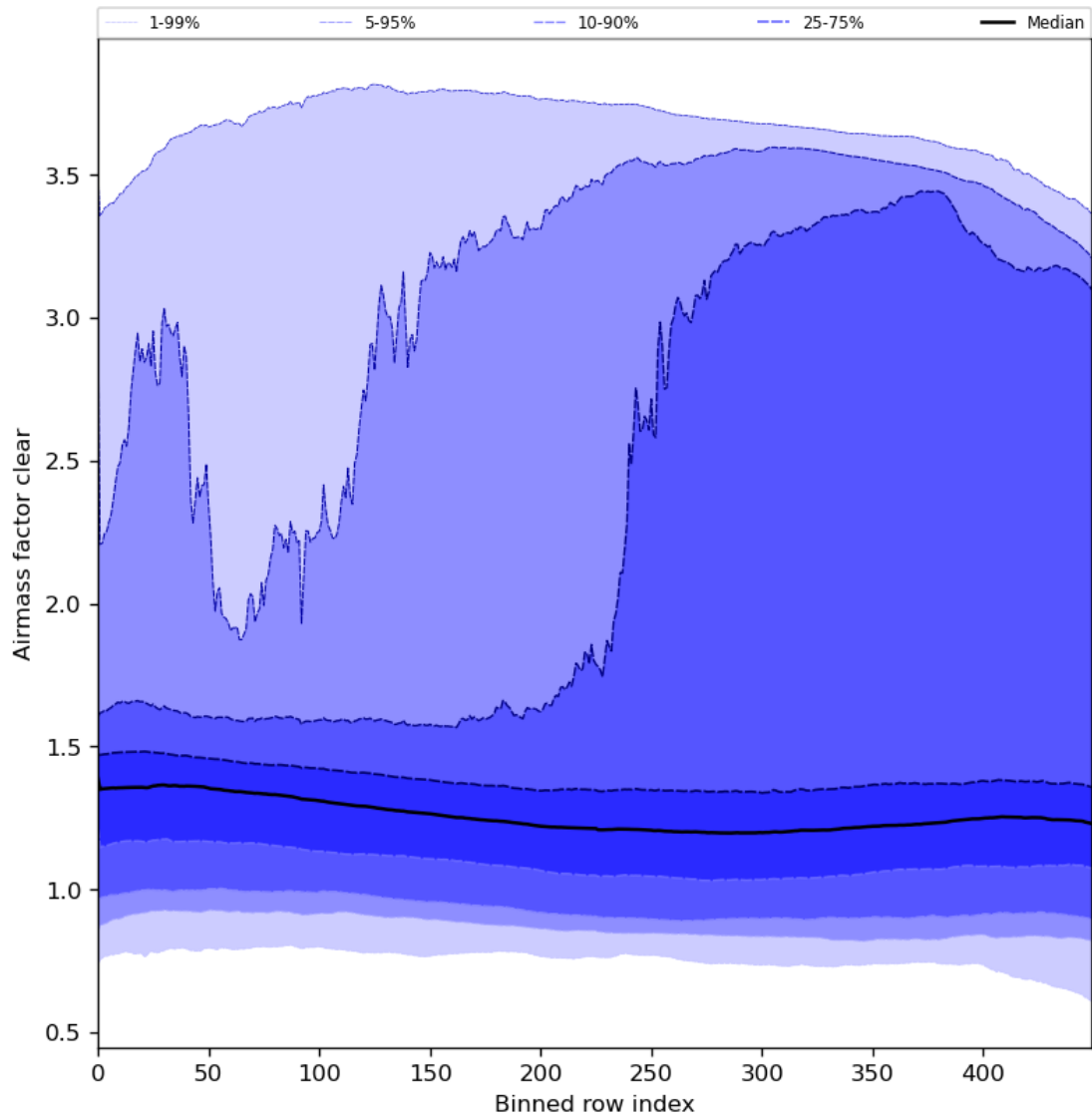
Figure 56: Along track statistics of “Airmass factor clear” for 2024-05-20 to 2024-05-22
