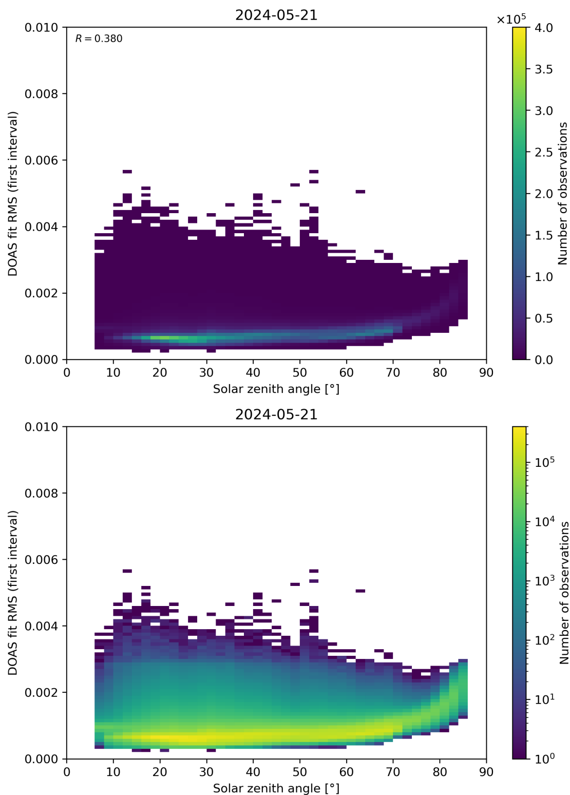
Figure 167: Scatter density plot of “Solar zenith angle” against “DOAS fit RMS (first interval)” for 2024-05-20 to 2024-05-22.
