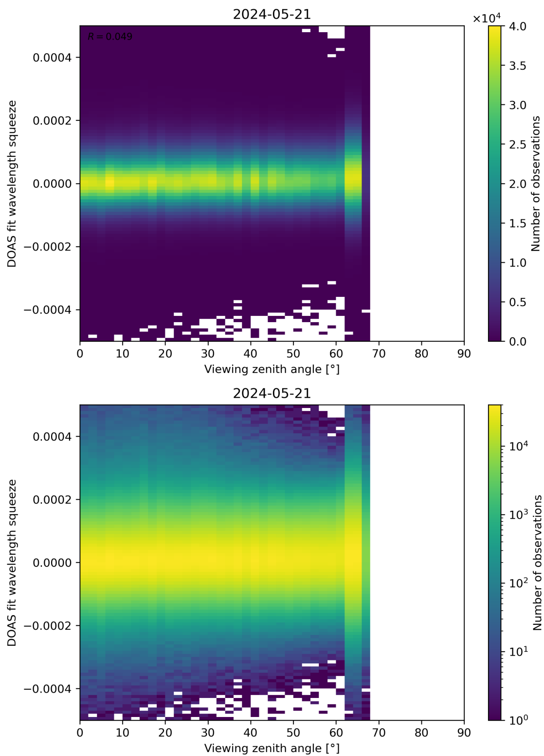
Figure 184: Scatter density plot of “Viewing zenith angle” against “DOAS fit wavelength squeeze” for 2024-05-20 to 2024-05-22.
