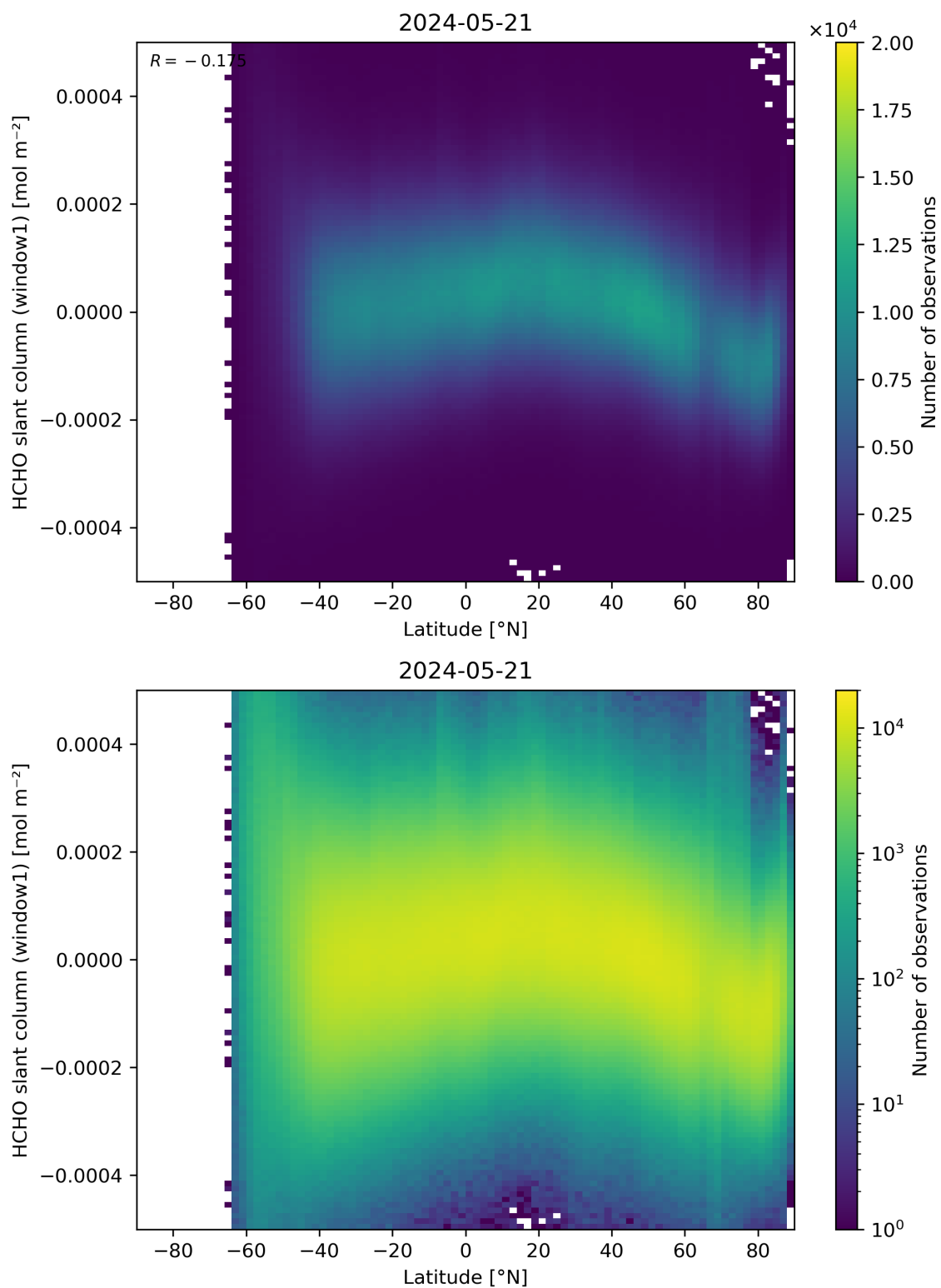
Figure 159: Scatter density plot of “Latitude” against “HCHO slant column (window1)” for 2024-05-20 to 2024-05-22.
