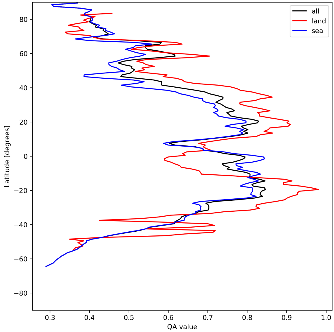
Figure 20: Zonal average of “QA value” for 2024-05-20 to 2024-05-22.
