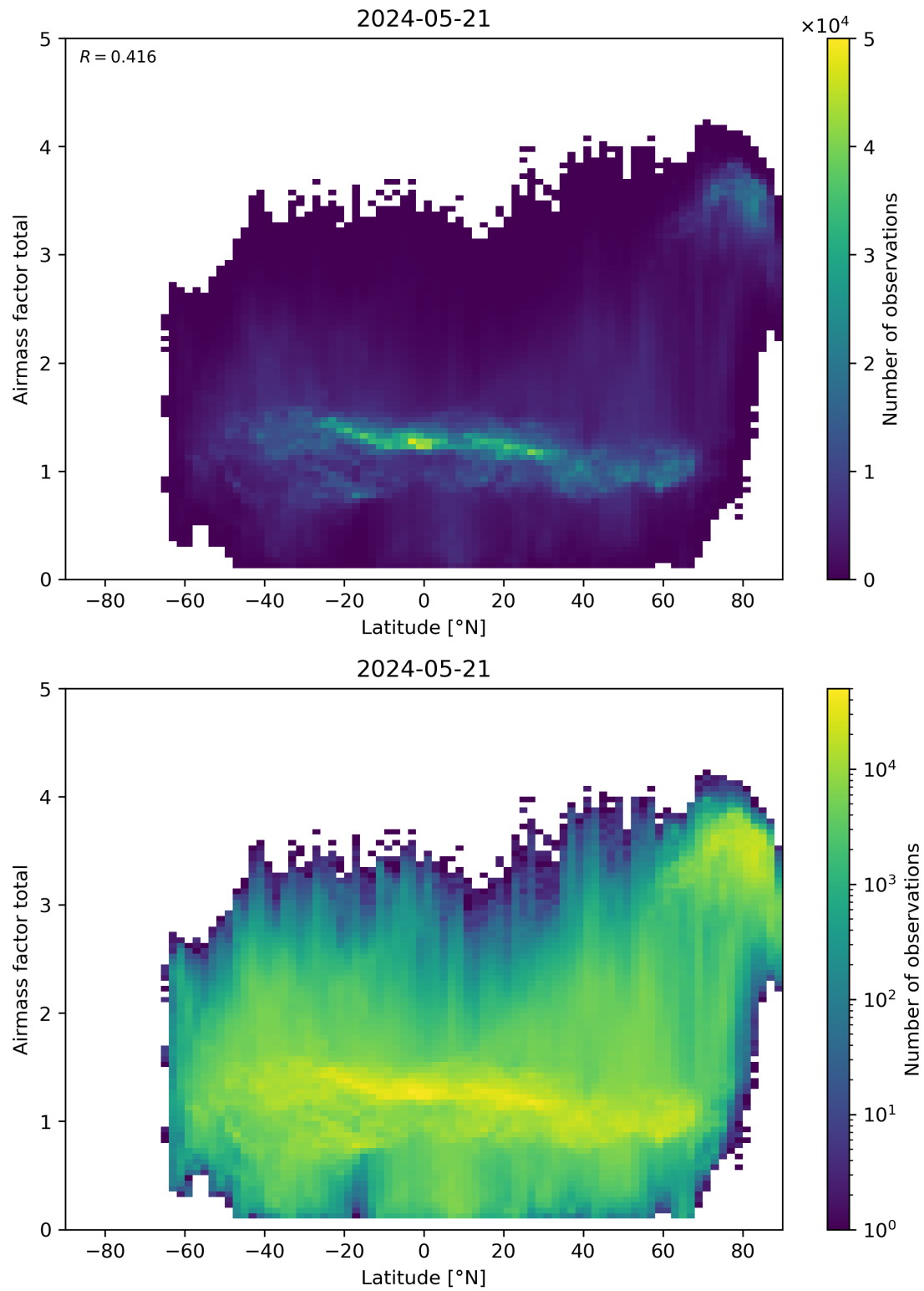
Figure 161: Scatter density plot of “Latitude” against “Airmass factor total” for 2024-05-20 to 2024-05-22.
