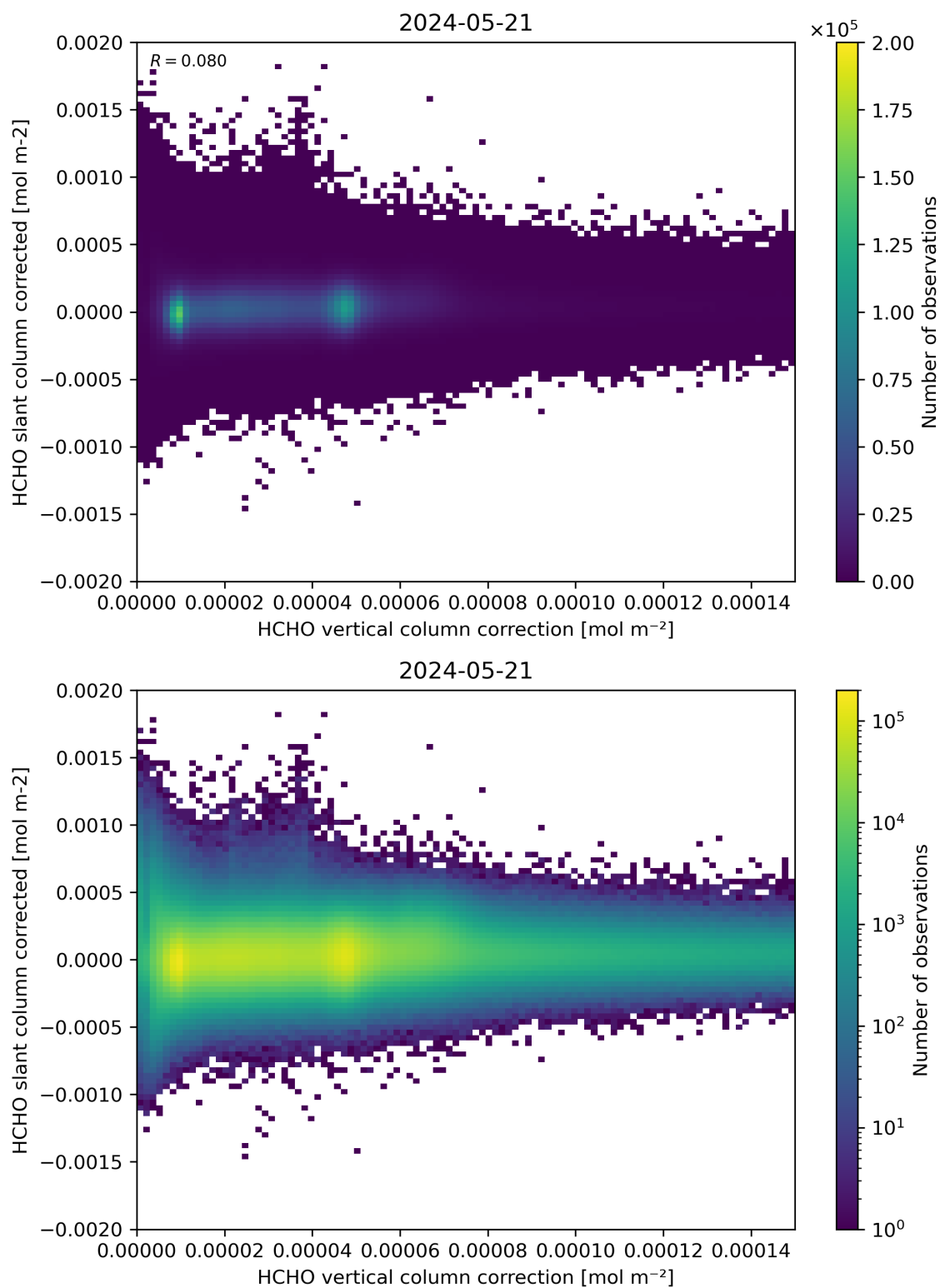
Figure 116: Scatter density plot of “HCHO vertical column correction” against “HCHO slant column corrected” for 2024-05-20 to 2024-05-22.
