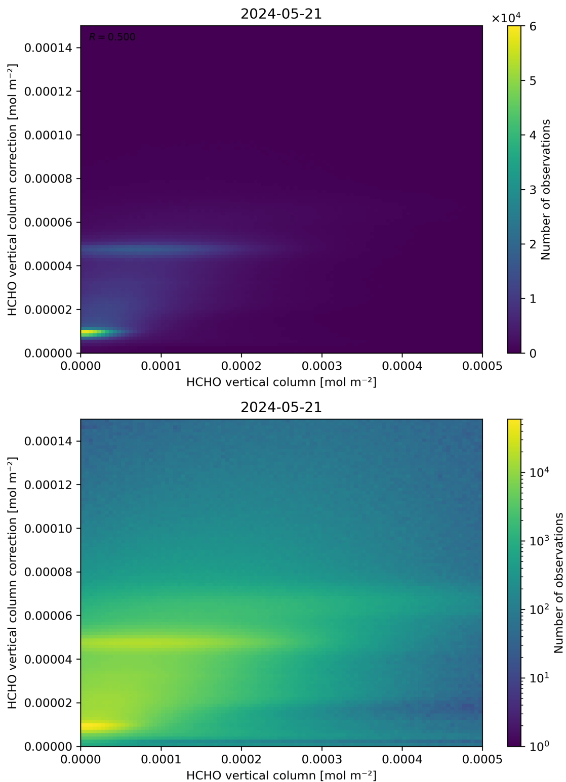
Figure 133: Scatter density plot of “HCHO vertical column” against “HCHO vertical column correction” for 2024-05-20 to 2024-05-22.
