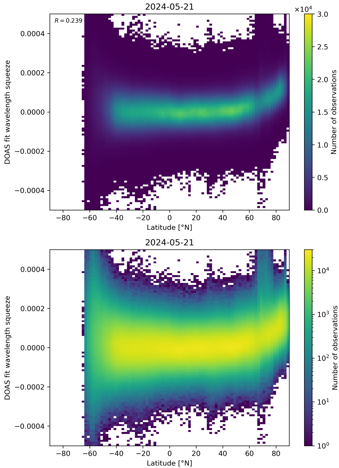
Figure 155: Scatter density plot of “Latitude” against “DOAS fit wavelength squeeze” for 2024-05-20 to 2024-05-22.
