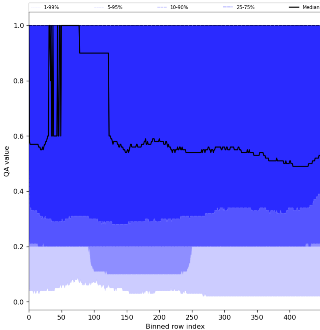
Figure 48: Along track statistics of “QA value” for 2024-05-20 to 2024-05-22
