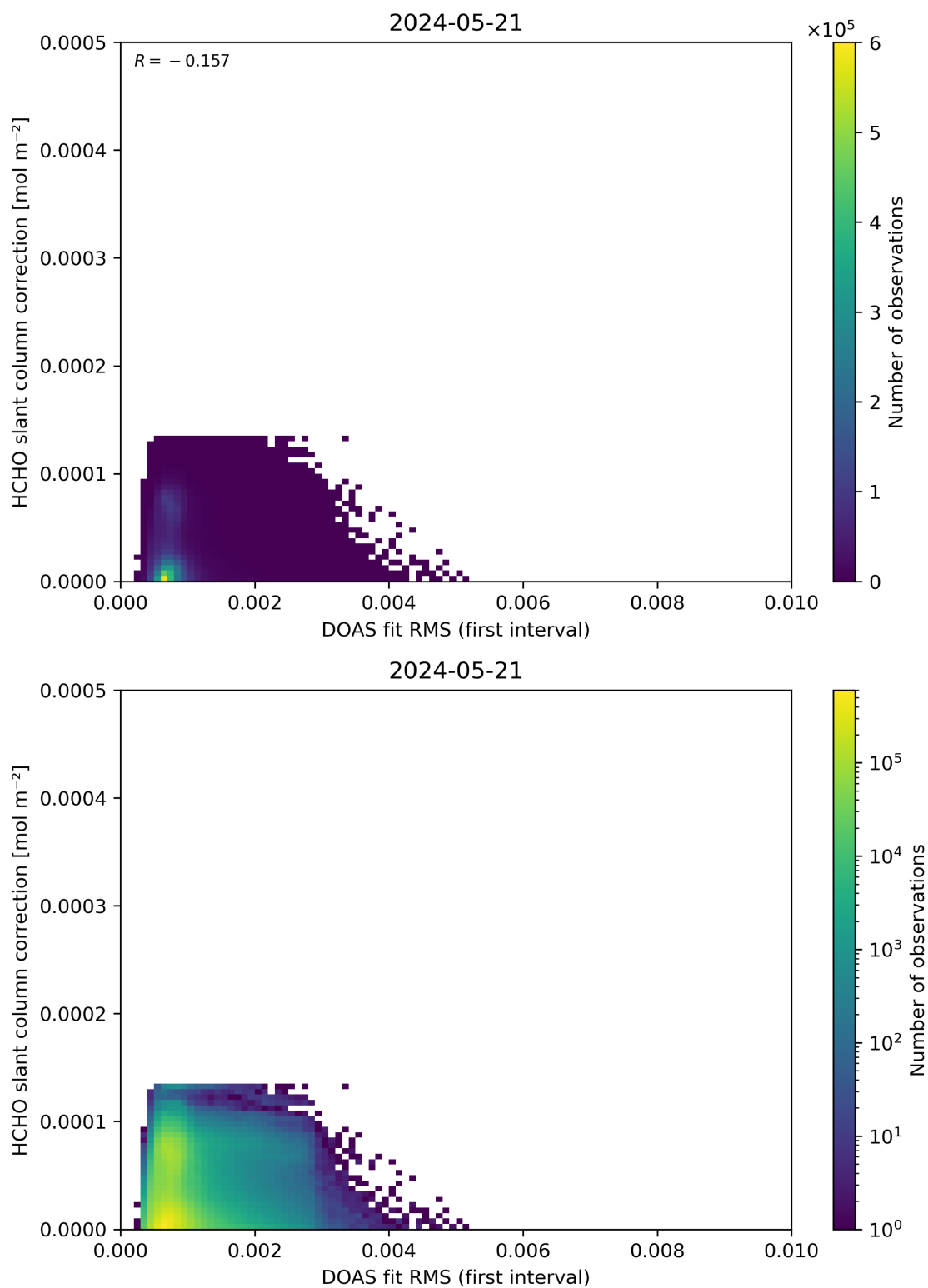
Figure 63: Scatter density plot of “DOAS fit RMS (first interval)” against “HCHO slant column correction” for 2024-05-20 to 2024-05-22.
