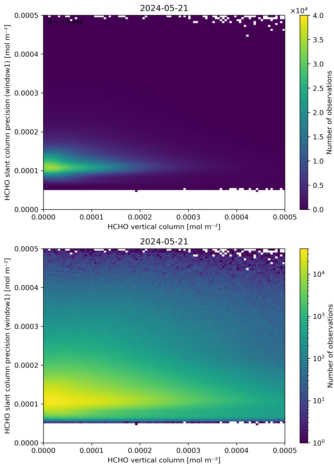
Figure 130: Scatter density plot of “HCHO vertical column” against “HCHO slant column precision (window1)” for 2024-05-20 to 2024-05-22.
