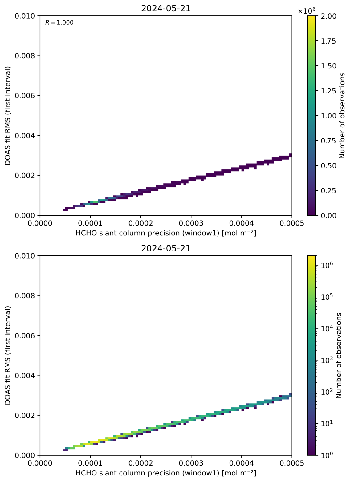
Figure 88: Scatter density plot of “HCHO slant column precision (window1)” against “DOAS fit RMS (first interval)” for 2024-05-20 to 2024-05-22.
