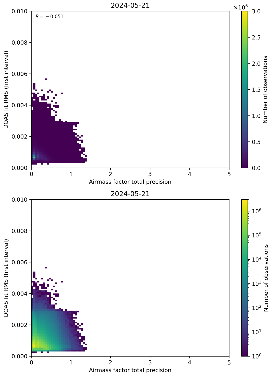
Figure 105: Scatter density plot of “Airmass factor total precision” against “DOAS fit RMS (first interval)” for 2024-05-20 to 2024-05-22.
