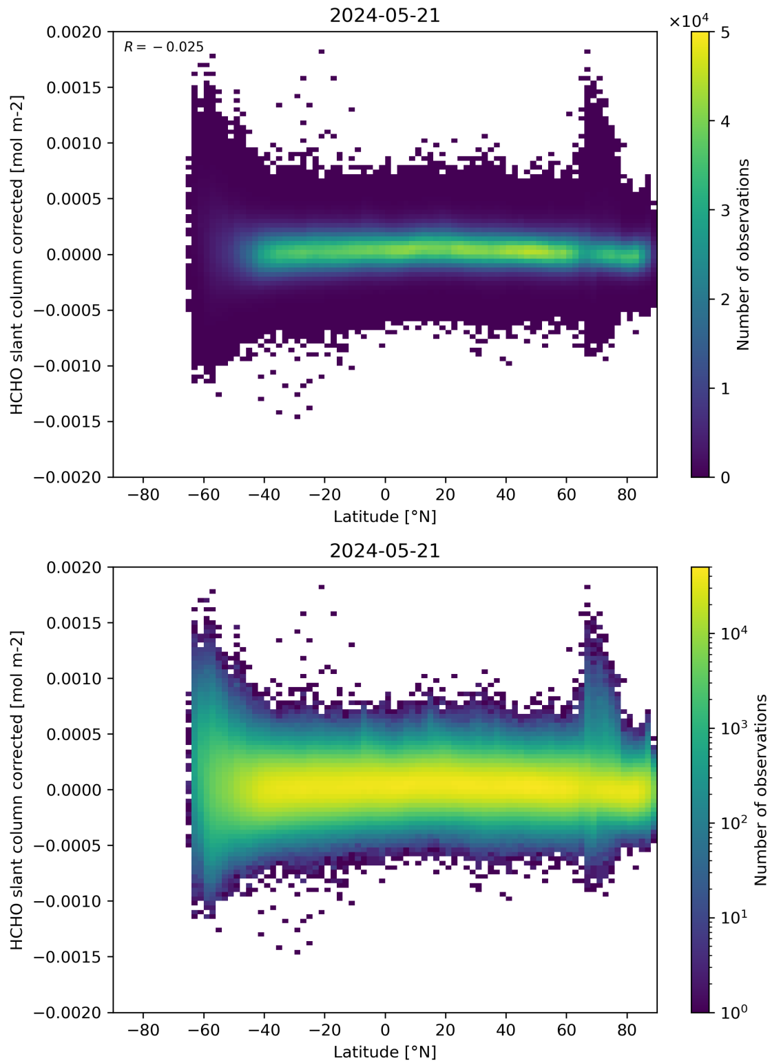
Figure 157: Scatter density plot of “Latitude” against “HCHO slant column corrected” for 2024-05-20 to 2024-05-22.
