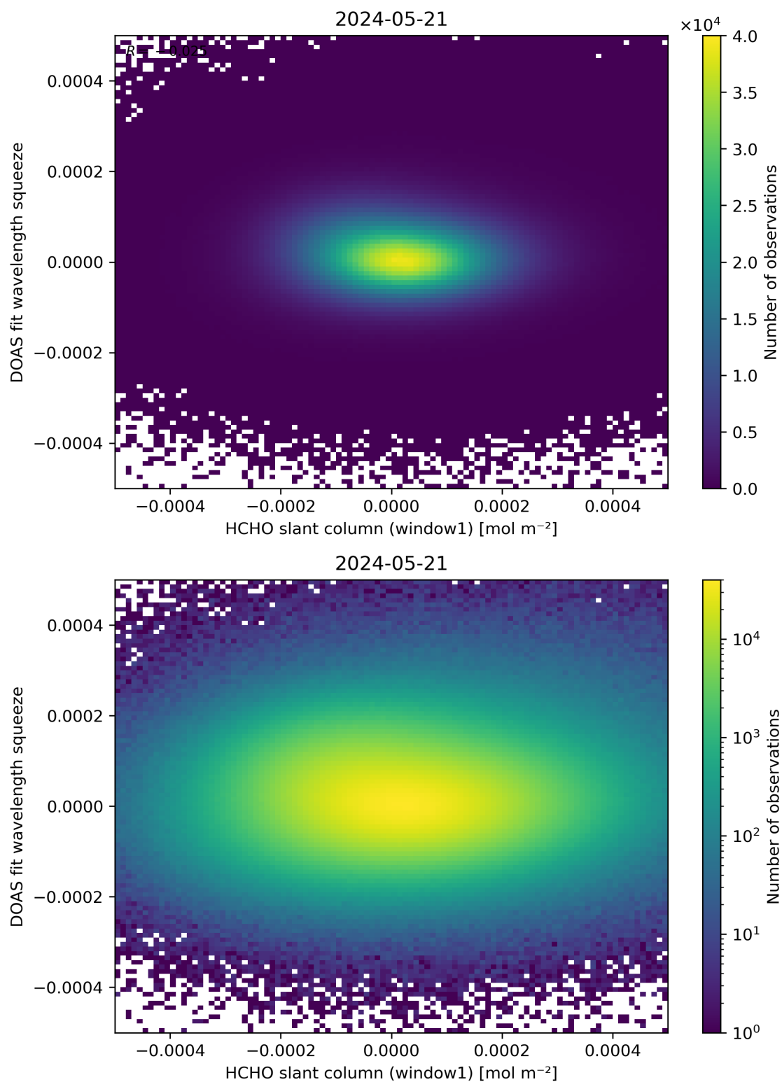
Figure 80: Scatter density plot of “HCHO slant column (window1)” against “DOAS fit wavelength squeeze” for 2024-05-20 to 2024-05-22.
