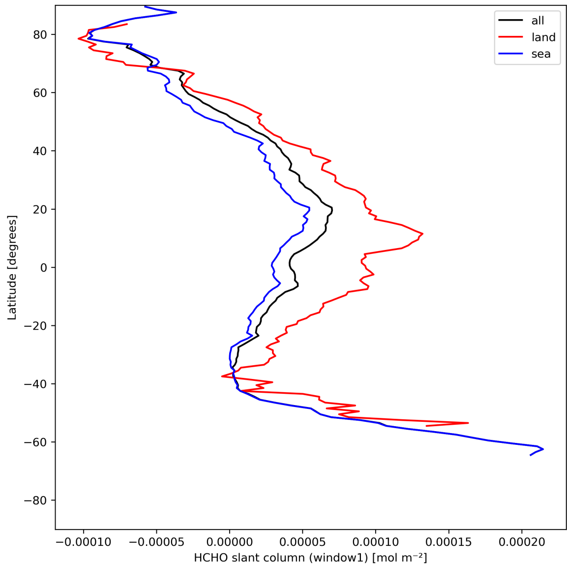
Figure 24: Zonal average of “HCHO slant column (window1)” for 2024-05-20 to 2024-05-22.
