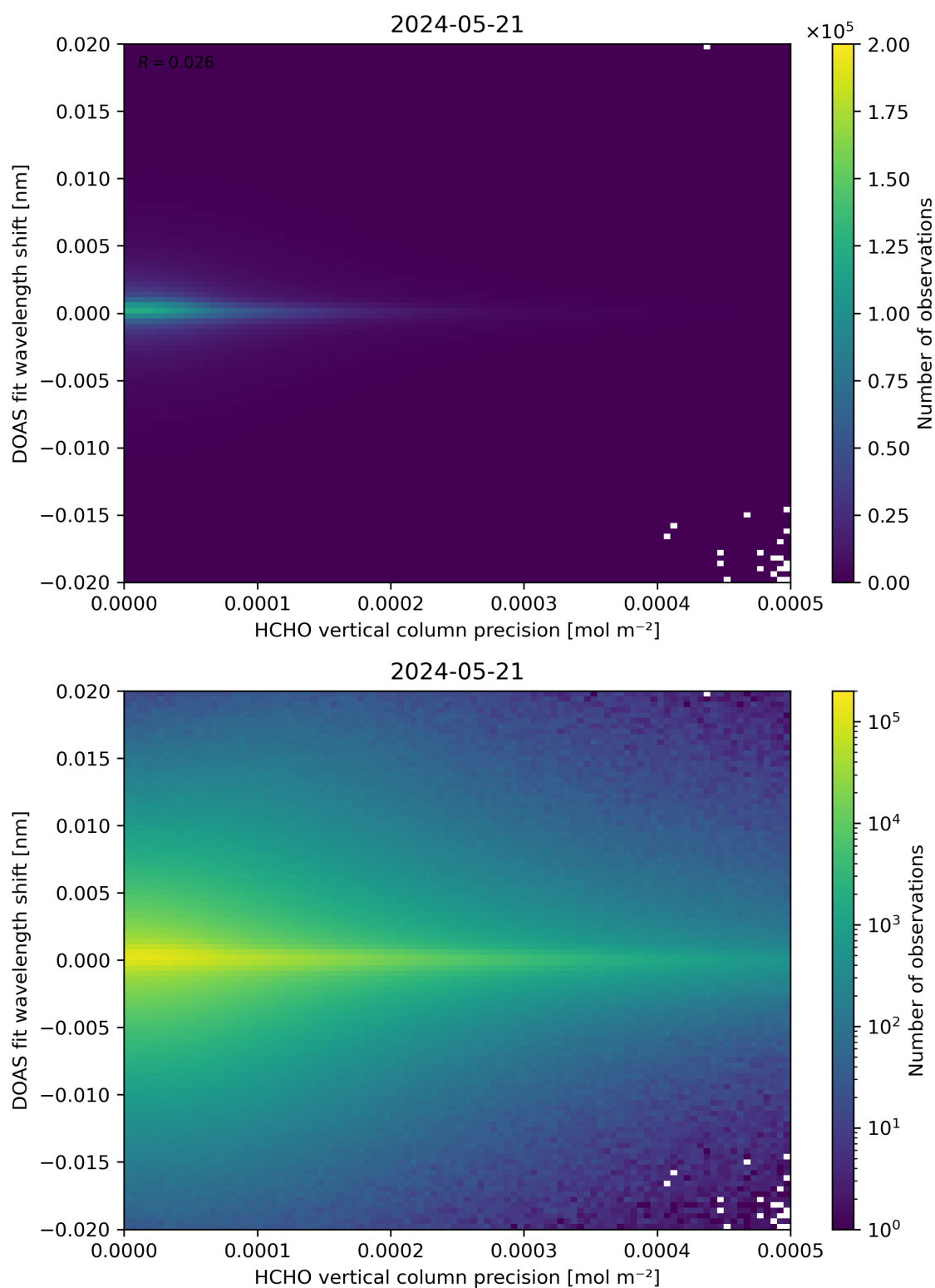
Figure 137: Scatter density plot of “HCHO vertical column precision” against “DOAS fit wavelength shift” for 2024-05-20 to 2024-05-22.
