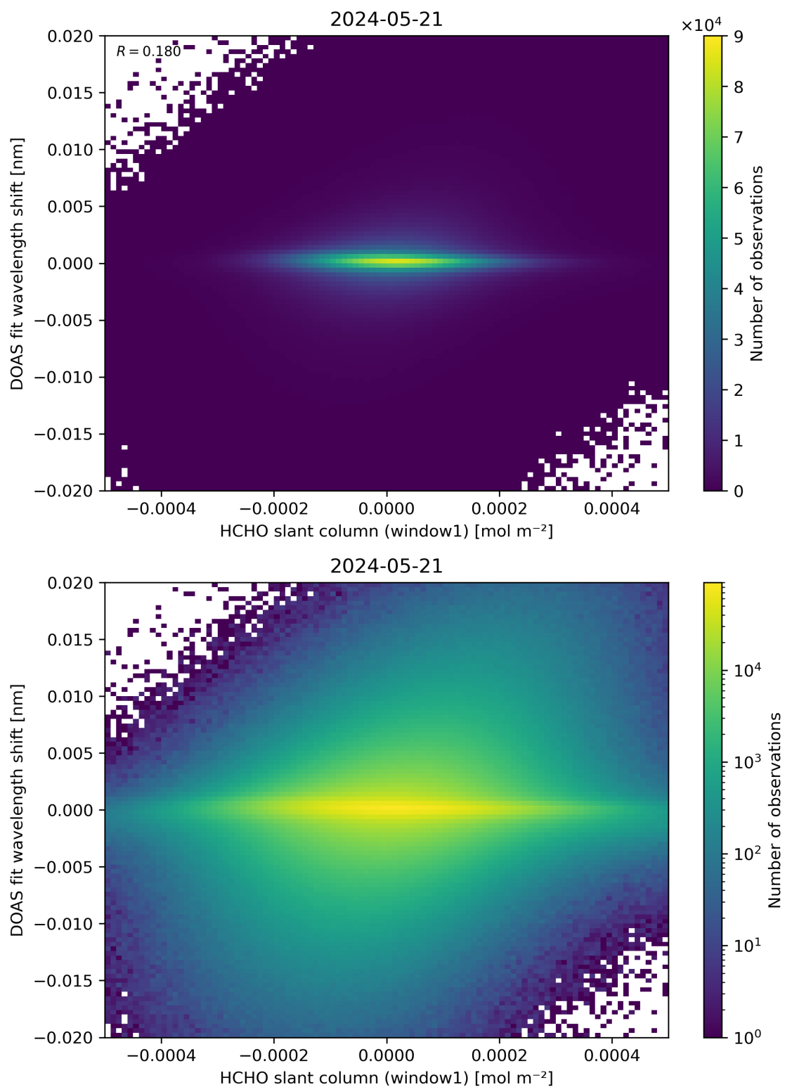
Figure 79: Scatter density plot of “HCHO slant column (window1)” against “DOAS fit wavelength shift” for 2024-05-20 to 2024-05-22.
