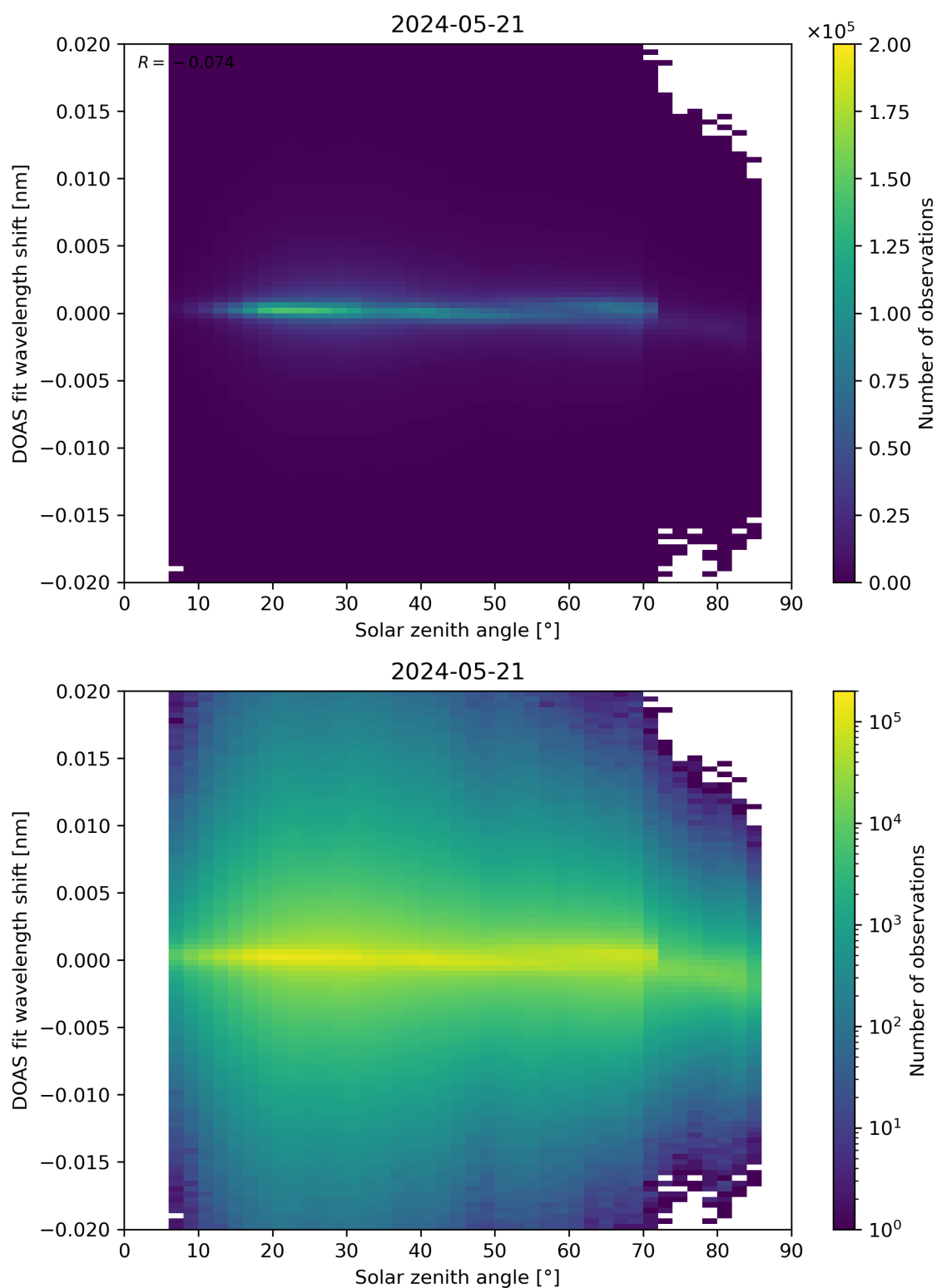
Figure 168: Scatter density plot of “Solar zenith angle” against “DOAS fit wavelength shift” for 2024-05-20 to 2024-05-22.
