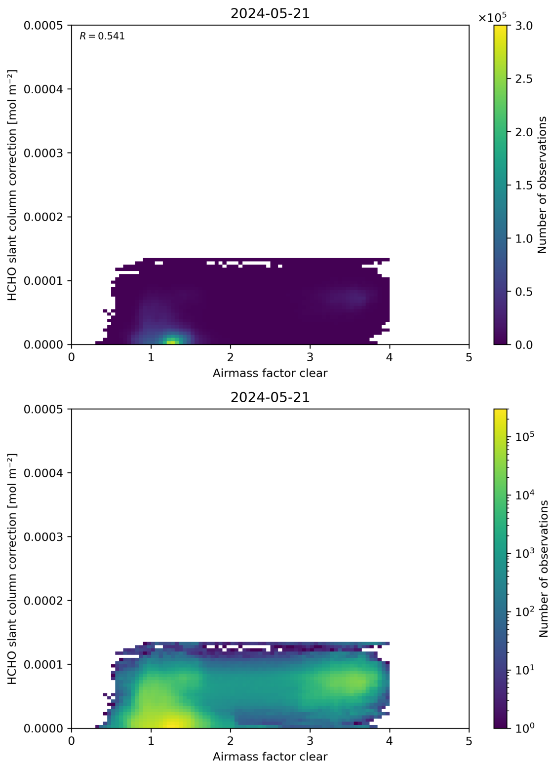
Figure 75: Scatter density plot of “Airmass factor clear” against “HCHO slant column correction” for 2024-05-20 to 2024-05-22.
