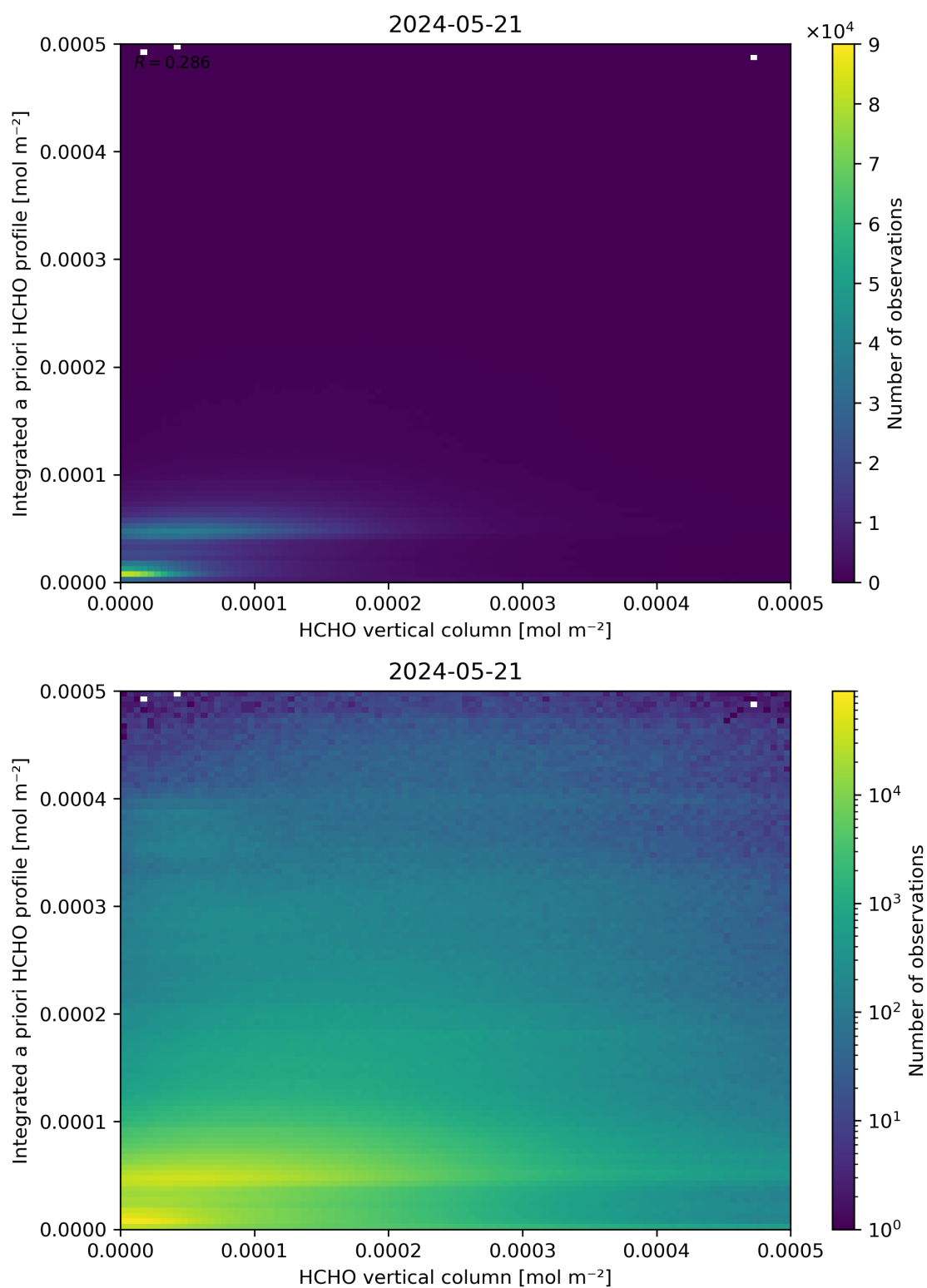
Figure 135: Scatter density plot of “HCHO vertical column” against “Integrated a priori HCHO profile” for 2024-05-20 to 2024-05-22.
