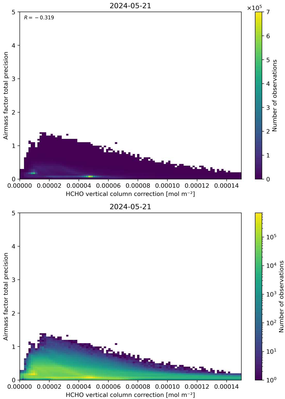
Figure 121: Scatter density plot of “HCHO vertical column correction” against “Airmass factor total precision” for 2024-05-20 to 2024-05-22.
