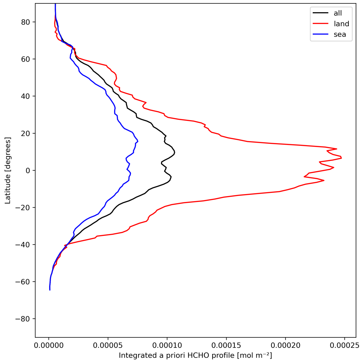
Figure 29: Zonal average of “Integrated a priori HCHO profile” for 2024-05-20 to 2024-05-22.
