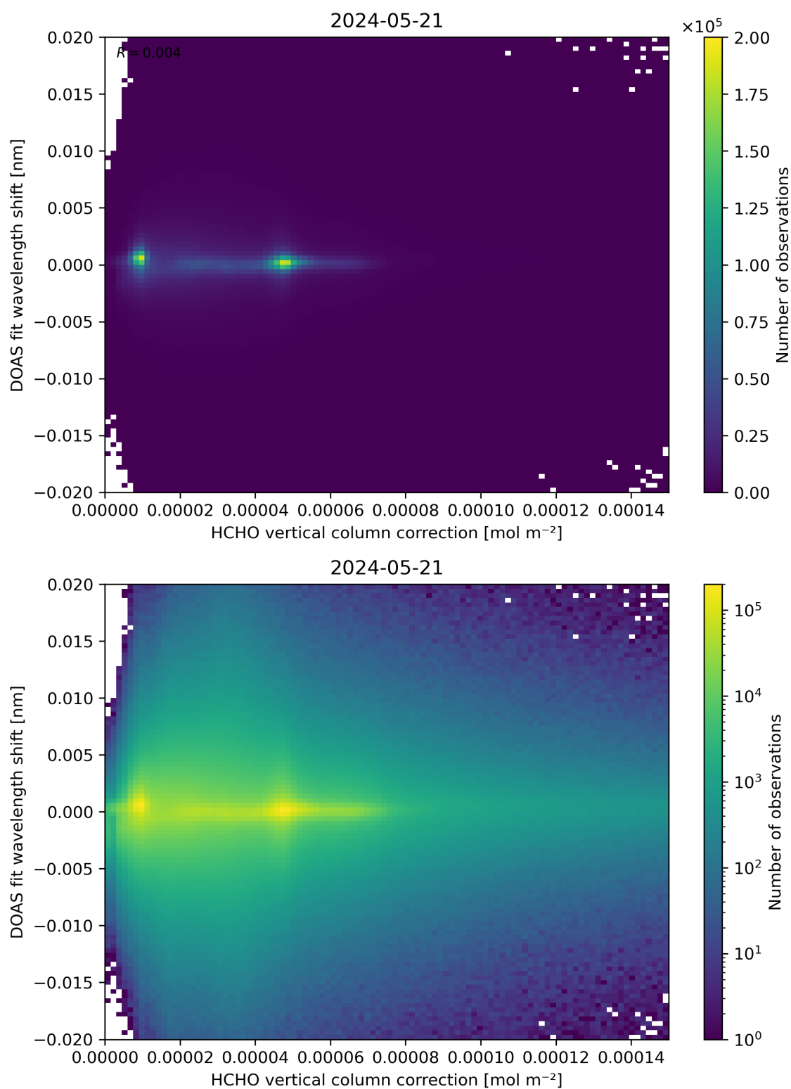
Figure 113: Scatter density plot of “HCHO vertical column correction” against “DOAS fit wavelength shift” for 2024-05-20 to 2024-05-22.
