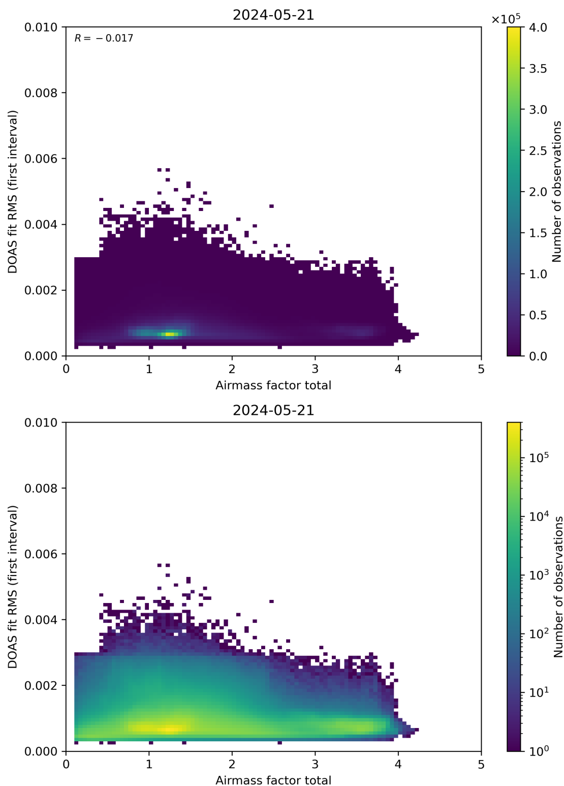
Figure 97: Scatter density plot of “Airmass factor total” against “DOAS fit RMS (first interval)” for 2024-05-20 to 2024-05-22.
