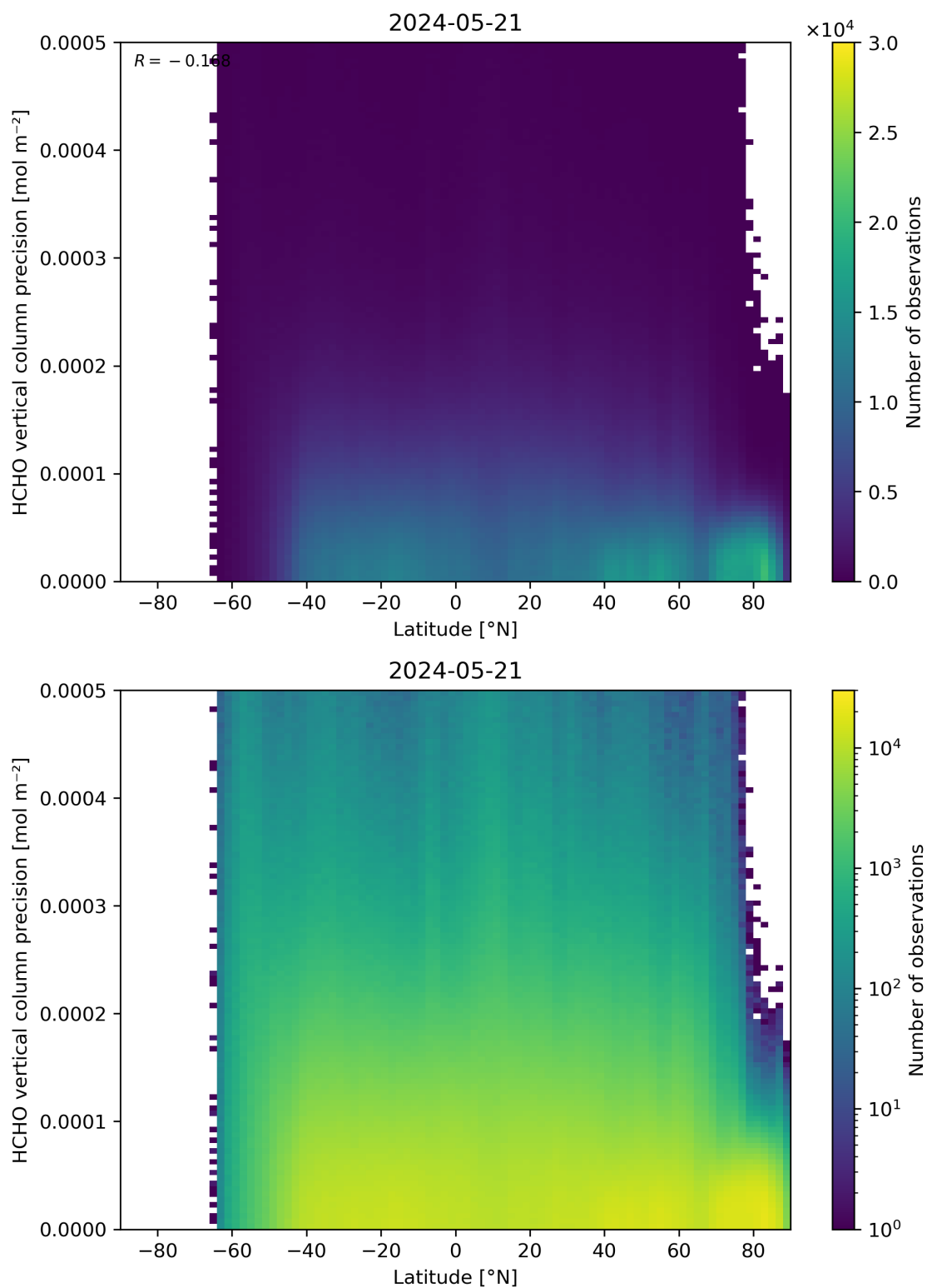
Figure 165: Scatter density plot of “Latitude” against “HCHO vertical column precision” for 2024-05-20 to 2024-05-22.
