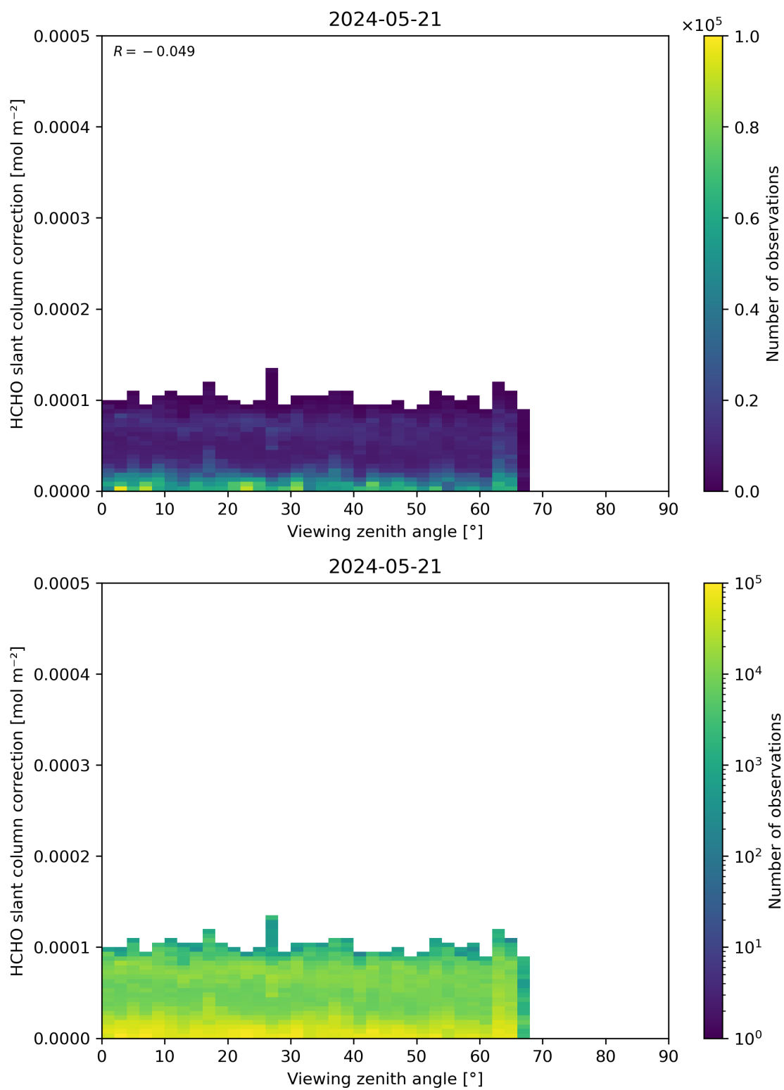
Figure 187: Scatter density plot of “Viewing zenith angle” against “HCHO slant column correction” for 2024-05-20 to 2024-05-22.
