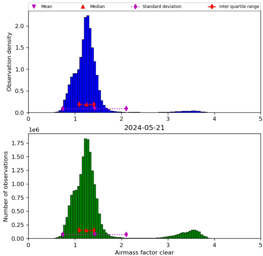
Figure 42: Histogram of “Airmass factor clear” for 2024-05-20 to 2024-05-22
