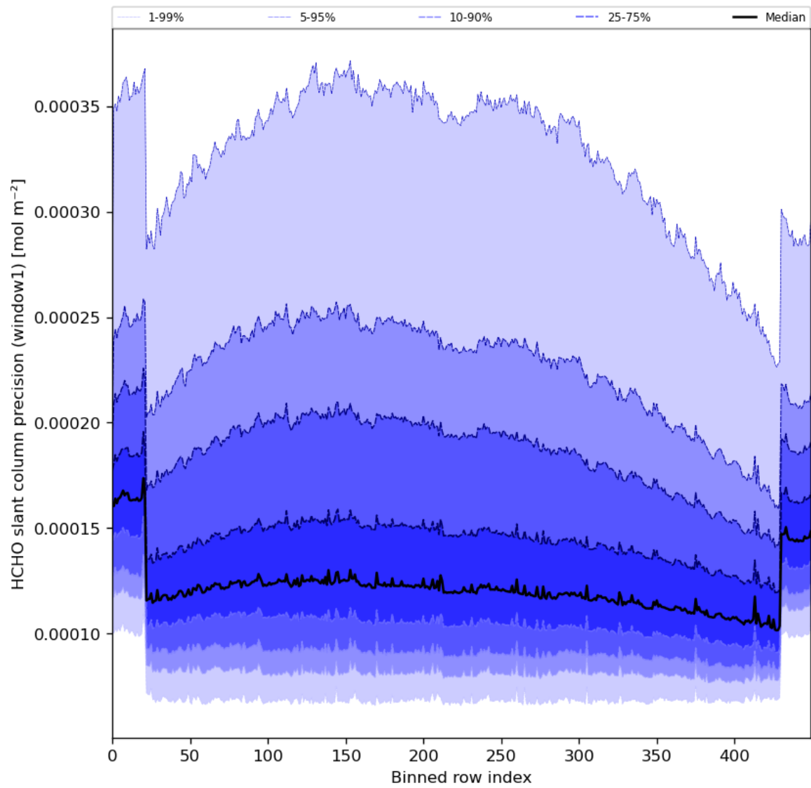
Figure 53: Along track statistics of “HCHO slant column precision (window1)” for 2024-05-20 to 2024-05-22
