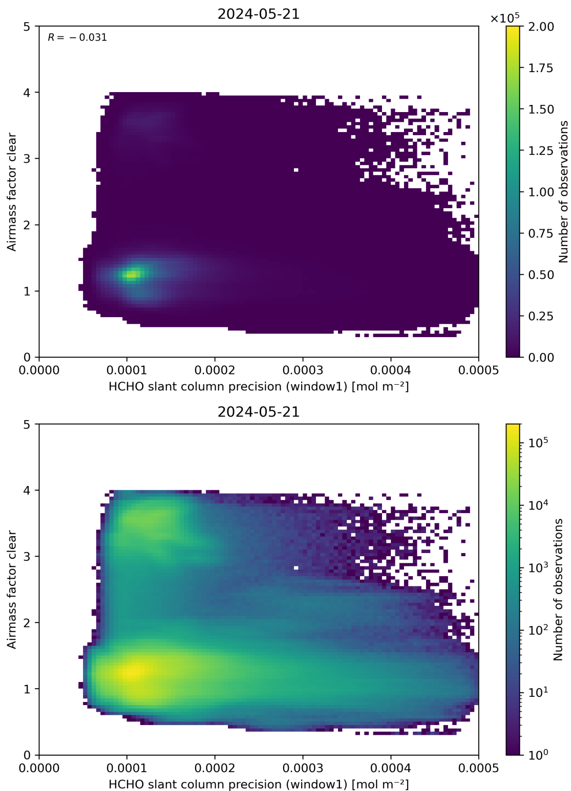
Figure 91: Scatter density plot of “HCHO slant column precision (window1)” against “Airmass factor clear” for 2024-05-20 to 2024-05-22.
