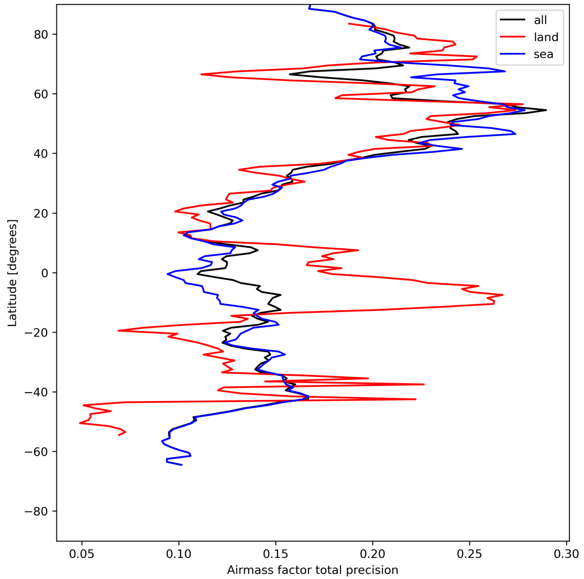
Figure 27: Zonal average of “Airmass factor total precision” for 2024-05-20 to 2024-05-22.
