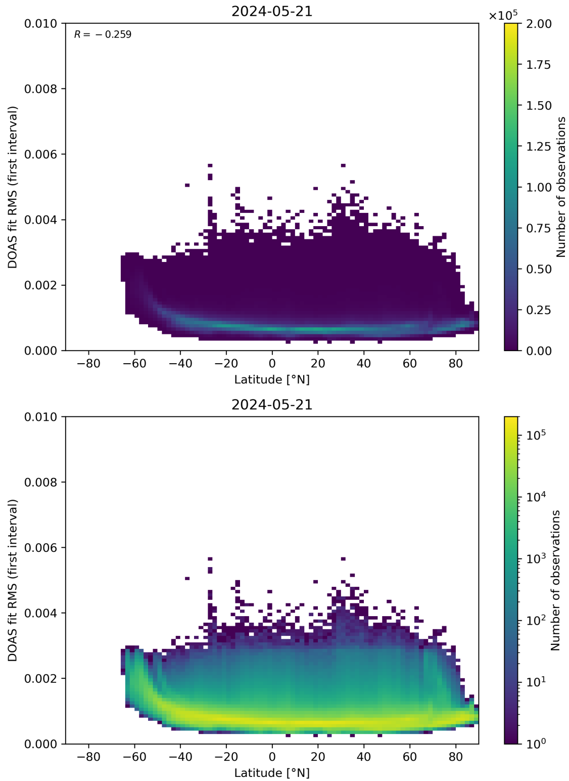
Figure 153: Scatter density plot of “Latitude” against “DOAS fit RMS (first interval)” for 2024-05-20 to 2024-05-22.
