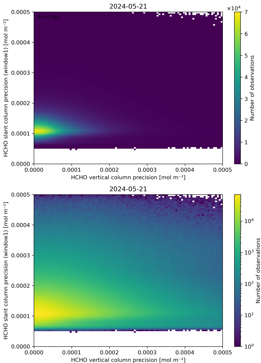
Figure 143: Scatter density plot of “HCHO vertical column precision” against “HCHO slant column precision (window1)” for 2024-05-20 to 2024-05-22.
