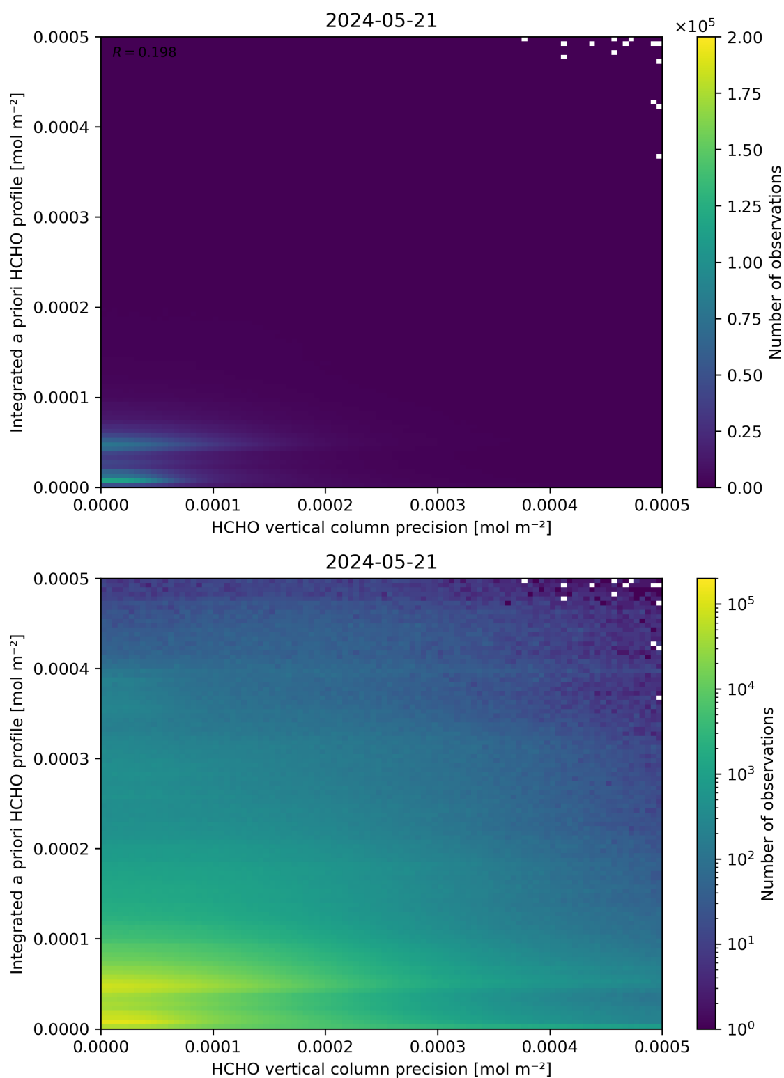
Figure 147: Scatter density plot of “HCHO vertical column precision” against “Integrated a priori HCHO profile” for 2024-05-20 to 2024-05-22.
