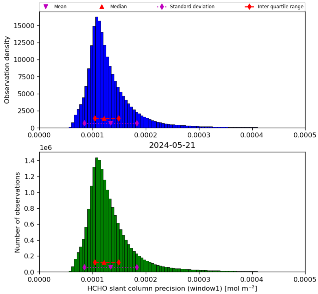
Figure 39: Histogram of “HCHO slant column precision (window1)” for 2024-05-20 to 2024-05-22
