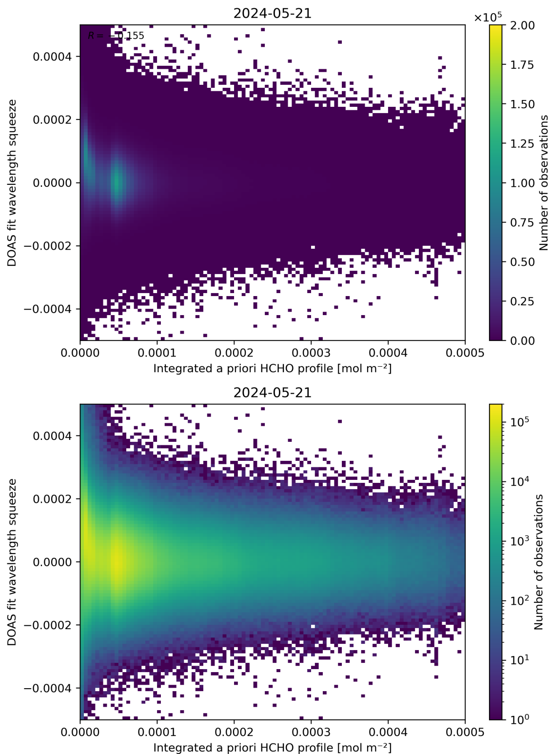
Figure 150: Scatter density plot of “Integrated a priori HCHO profile” against “DOAS fit wavelength squeeze” for 2024-05-20 to 2024-05-22.
