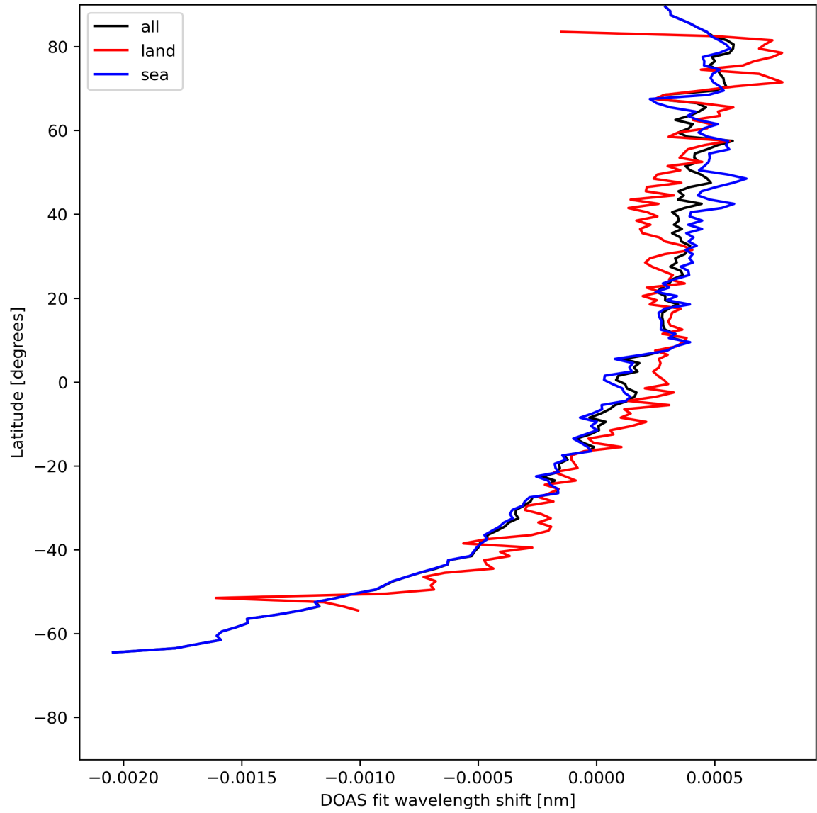
Figure 30: Zonal average of “DOAS fit wavelength shift” for 2024-05-20 to 2024-05-22.
