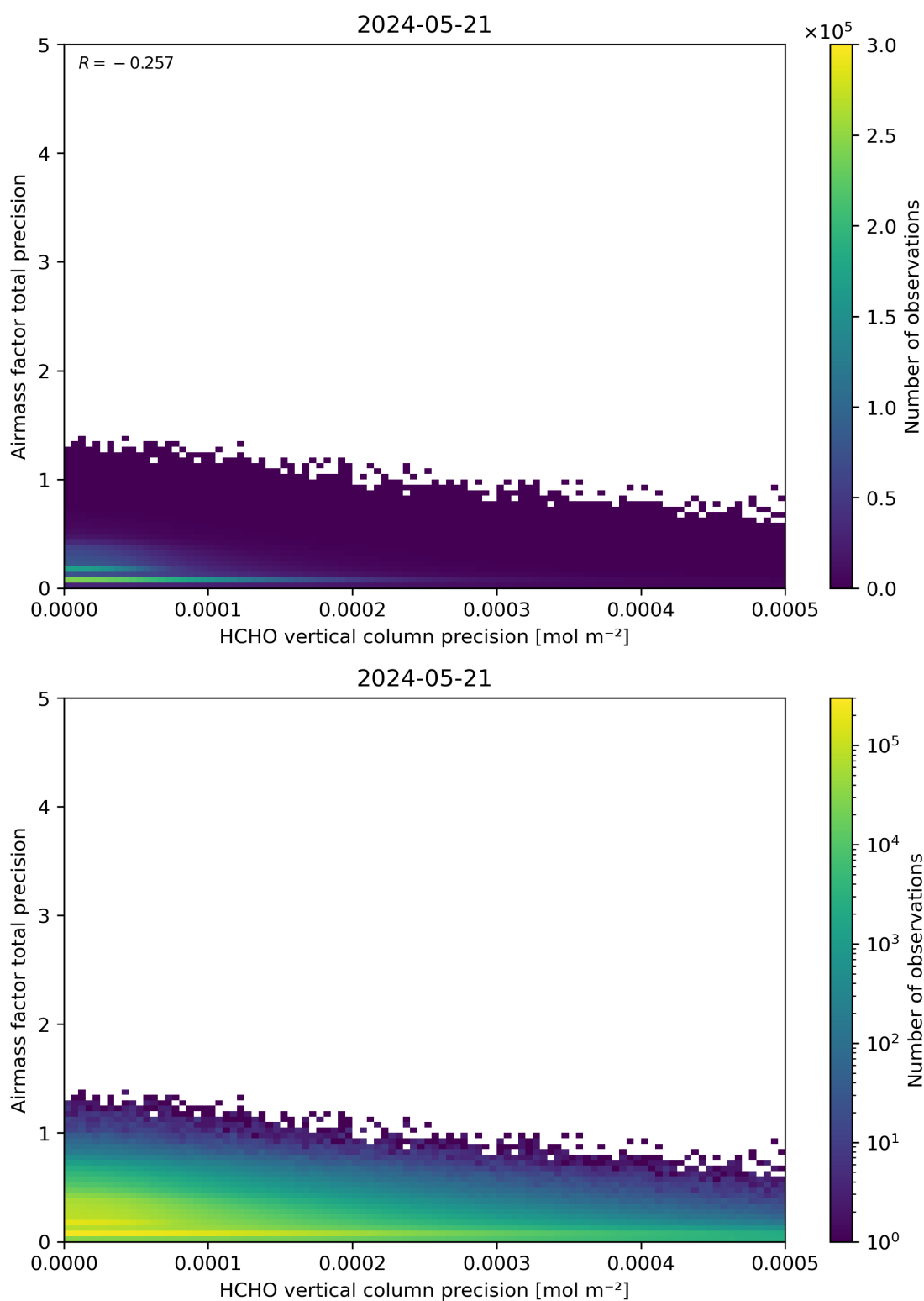
Figure 145: Scatter density plot of “HCHO vertical column precision” against “Airmass factor total precision” for 2024-05-20 to 2024-05-22.
