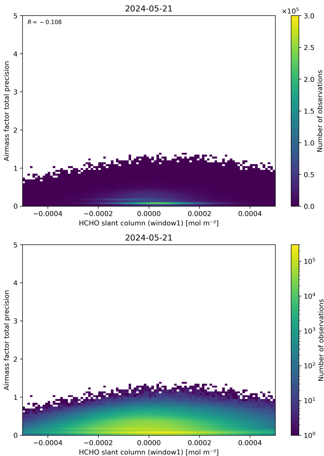
Figure 86: Scatter density plot of “HCHO slant column (window1)” against “Airmass factor total precision” for 2024-05-20 to 2024-05-22.
