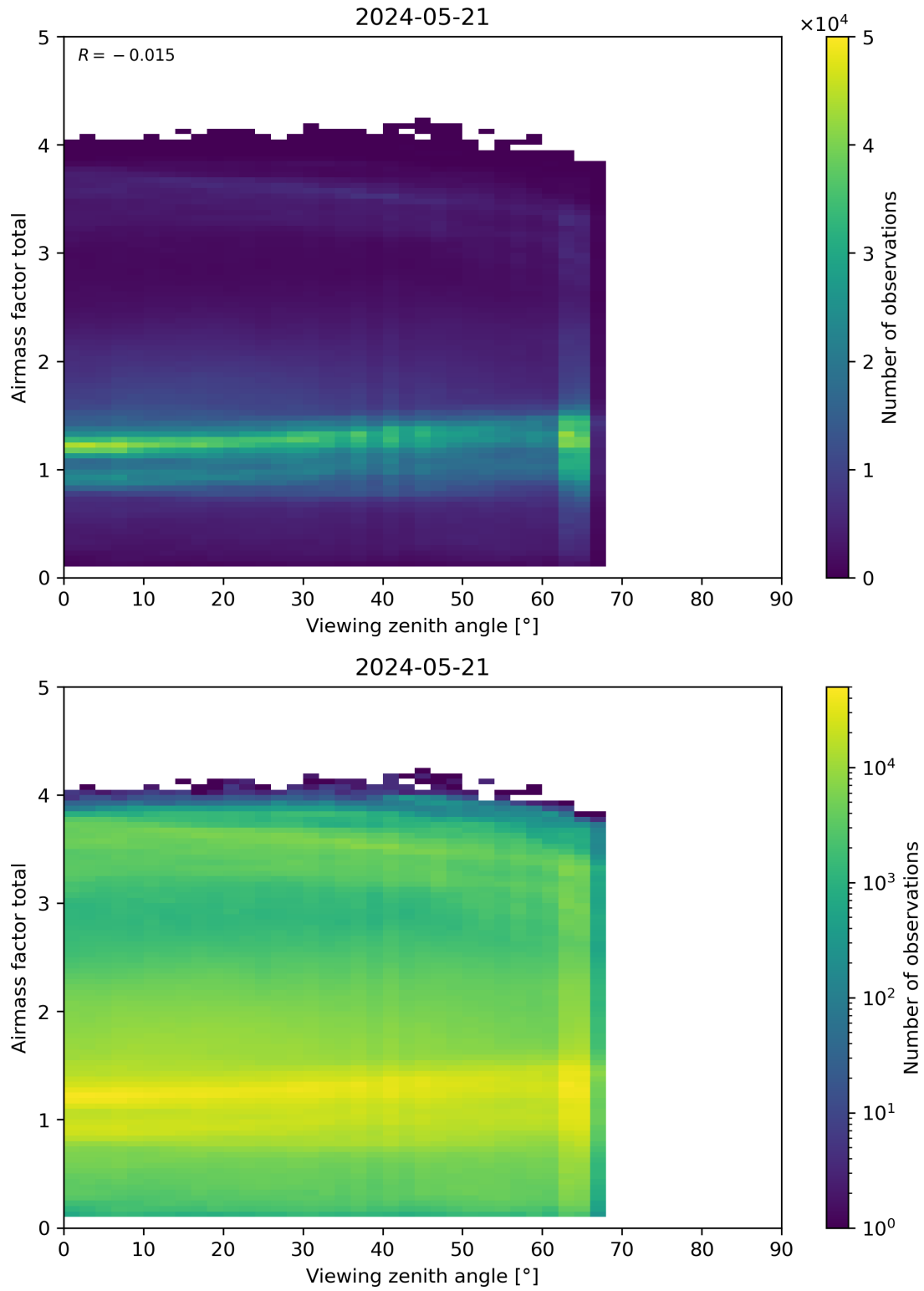
Figure 190: Scatter density plot of “Viewing zenith angle” against “Airmass factor total” for 2024-05-20 to 2024-05-22.
