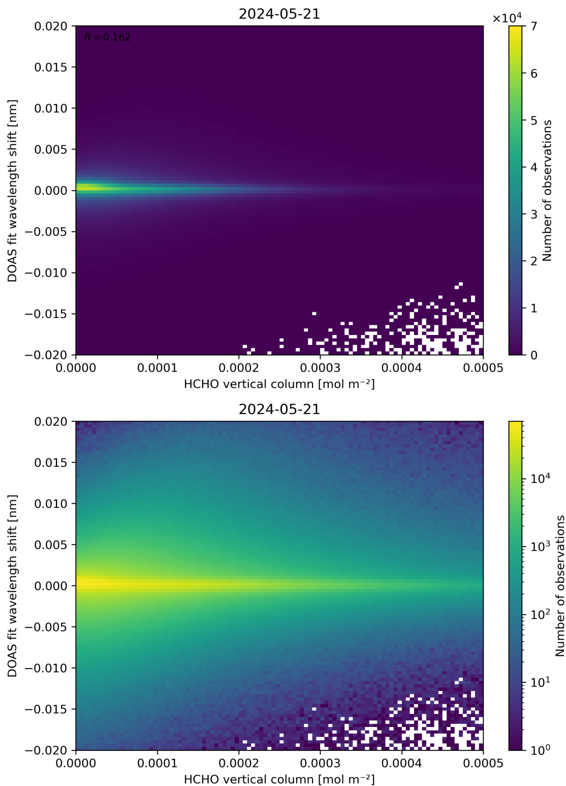
Figure 124: Scatter density plot of “HCHO vertical column” against “DOAS fit wavelength shift” for 2024-05-20 to 2024-05-22.
