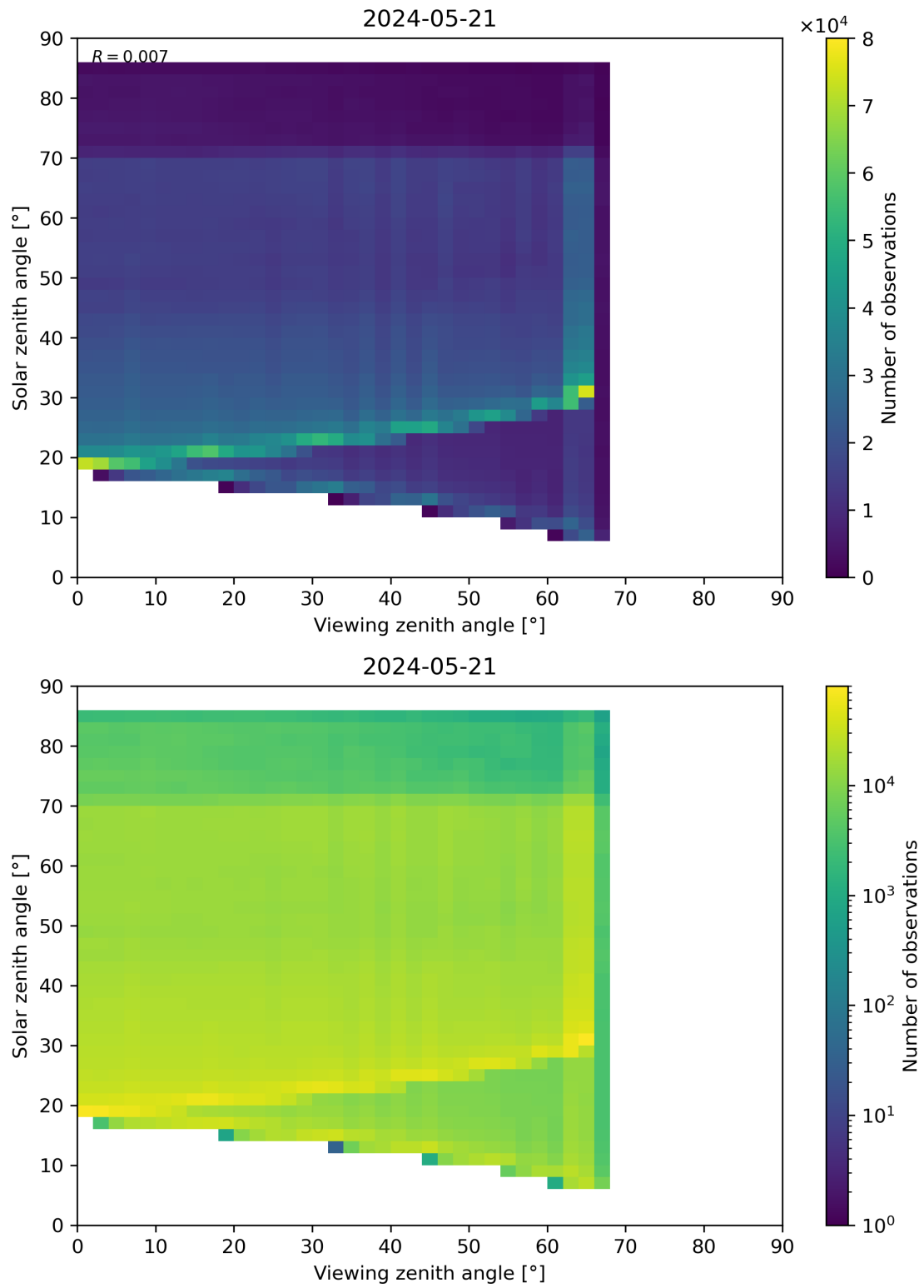
Figure 197: Scatter density plot of “Viewing zenith angle” against “Solar zenith angle” for 2024-05-20 to 2024-05-22.
