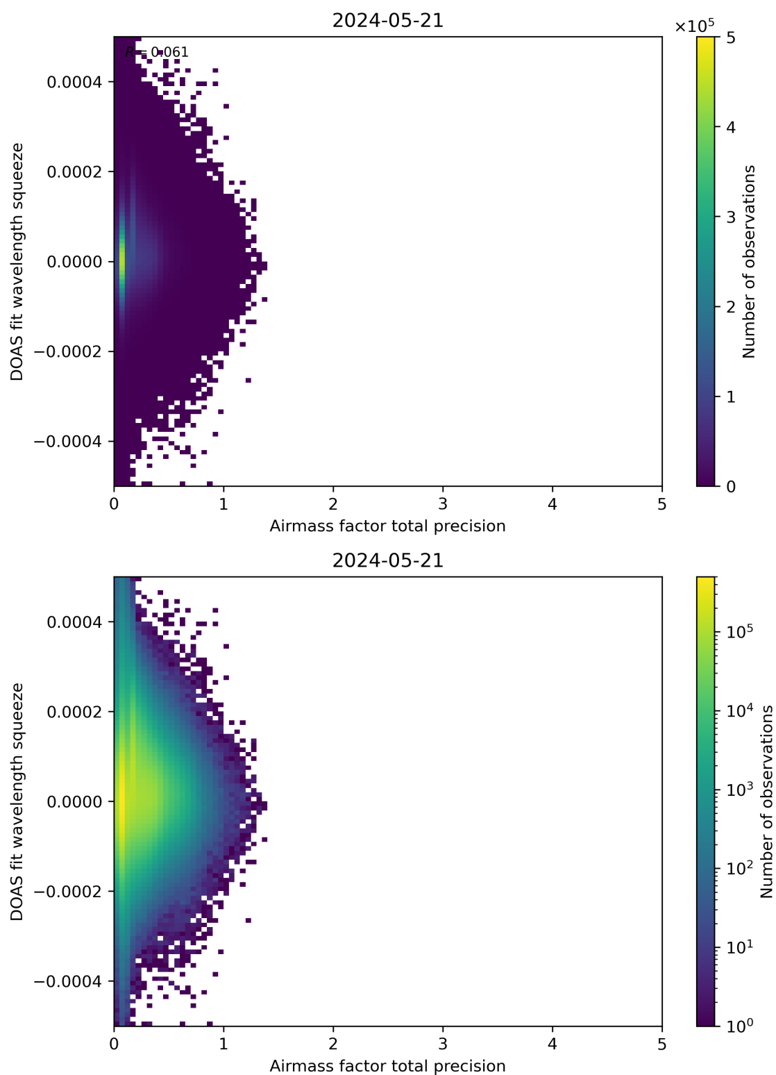
Figure 107: Scatter density plot of “Airmass factor total precision” against “DOAS fit wavelength squeeze” for 2024-05-20 to 2024-05-22.
