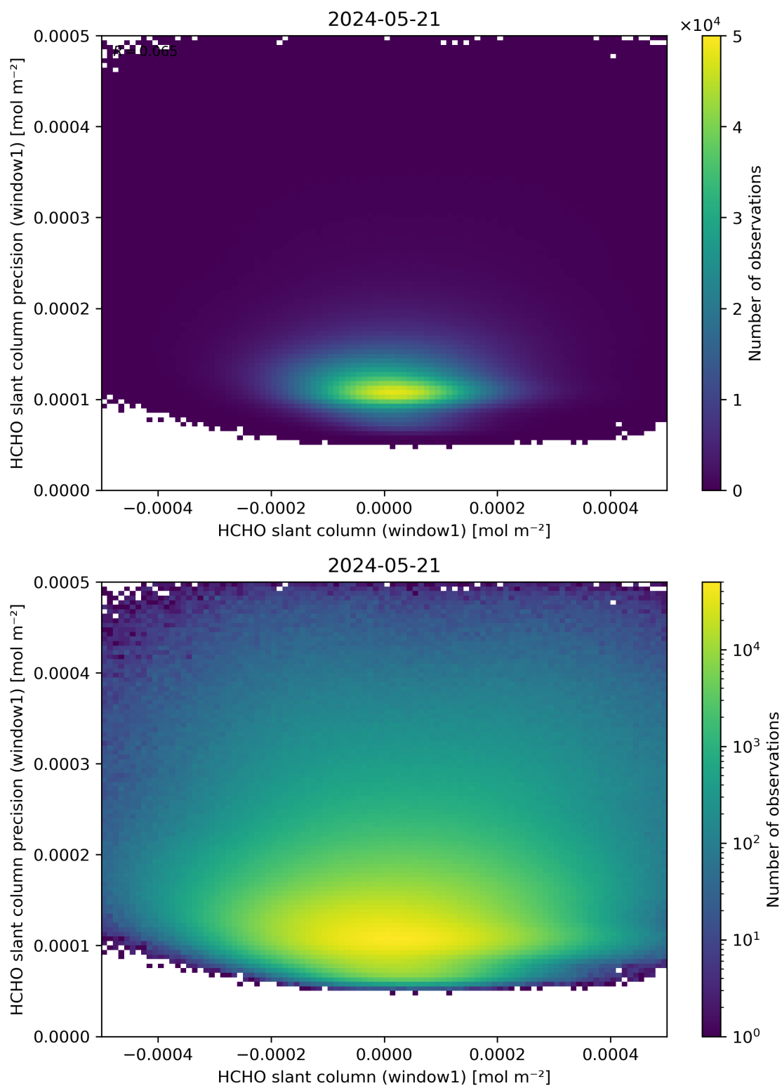
Figure 84: Scatter density plot of “HCHO slant column (window1)” against “HCHO slant column precision (window1)” for 2024-05-20 to 2024-05-22.
