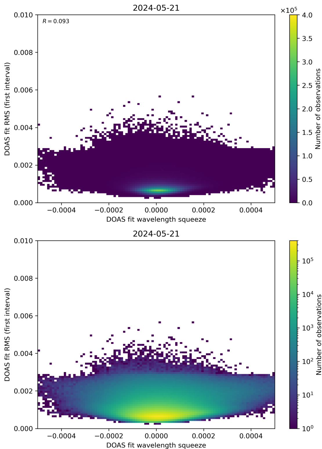
Figure 68: Scatter density plot of “DOAS fit wavelength squeeze” against “DOAS fit RMS (first interval)” for 2024-05-20 to 2024-05-22.
