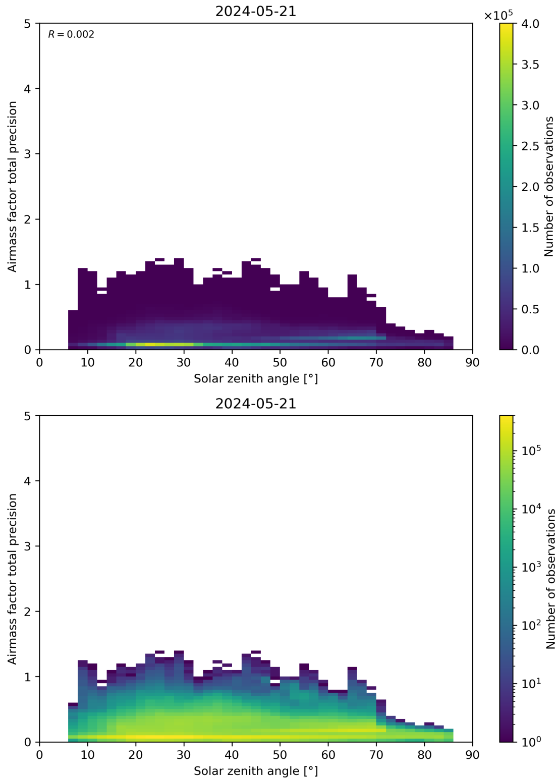
Figure 176: Scatter density plot of “Solar zenith angle” against “Airmass factor total precision” for 2024-05-20 to 2024-05-22.
