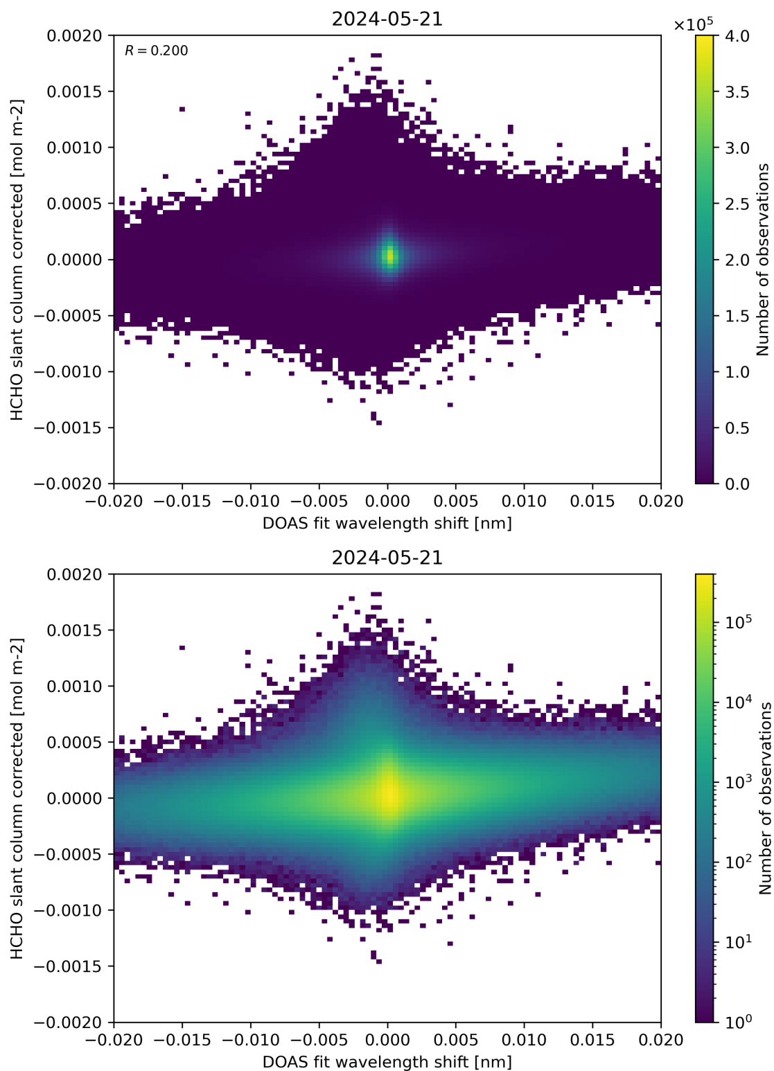
Figure 66: Scatter density plot of “DOAS fit wavelength shift” against “HCHO slant column corrected” for 2024-05-20 to 2024-05-22.
