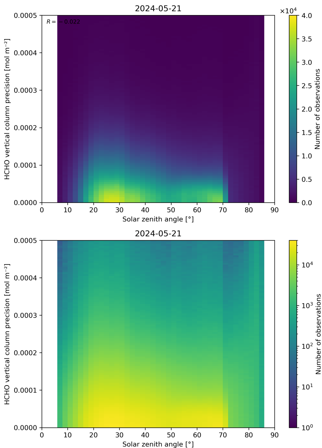
Figure 179: Scatter density plot of “Solar zenith angle” against “HCHO vertical column precision” for 2024-05-20 to 2024-05-22.
