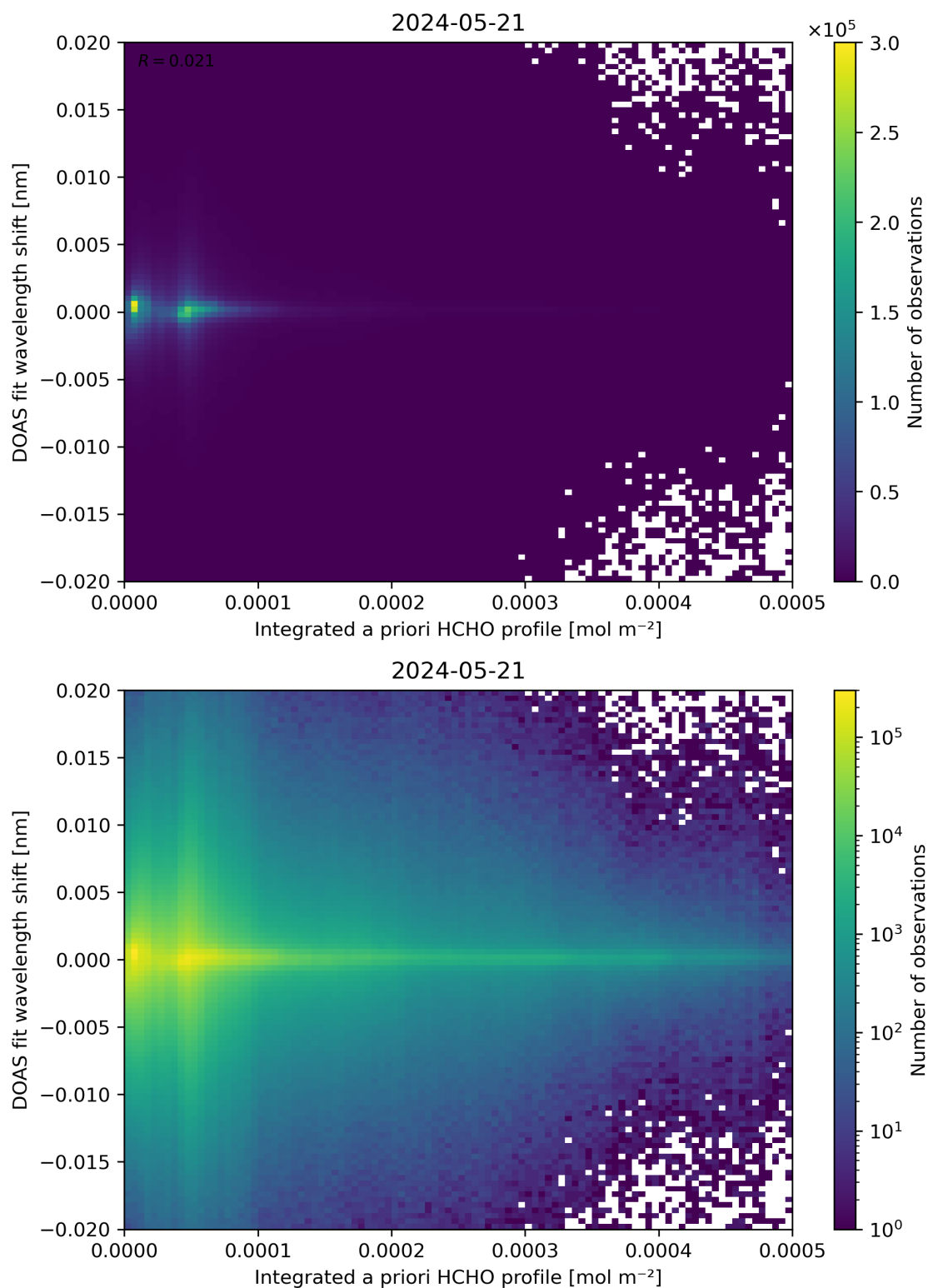
Figure 149: Scatter density plot of “Integrated a priori HCHO profile” against “DOAS fit wavelength shift” for 2024-05-20 to 2024-05-22.
