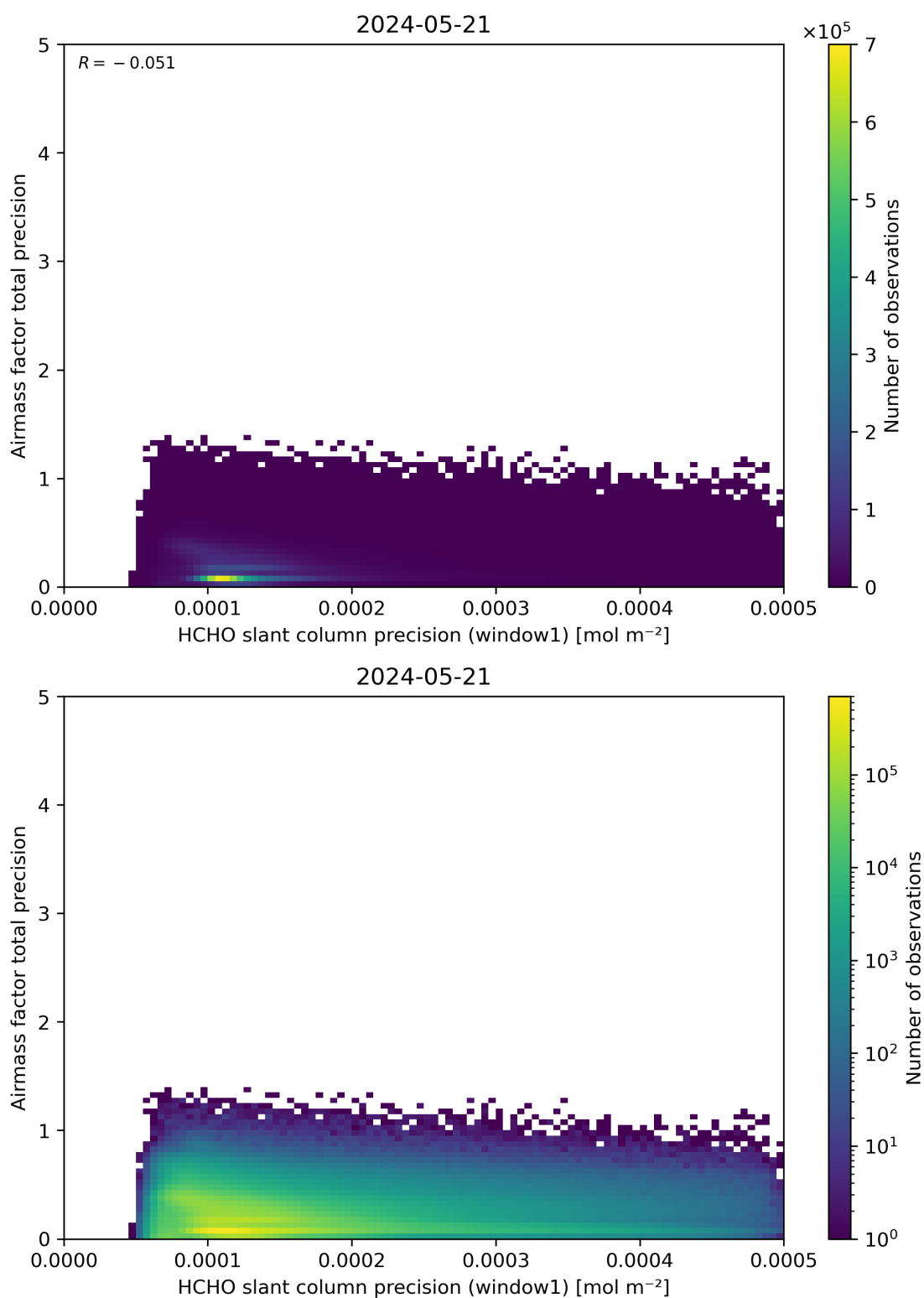
Figure 95: Scatter density plot of “HCHO slant column precision (window1)” against “Airmass factor total precision” for 2024-05-20 to 2024-05-22.
