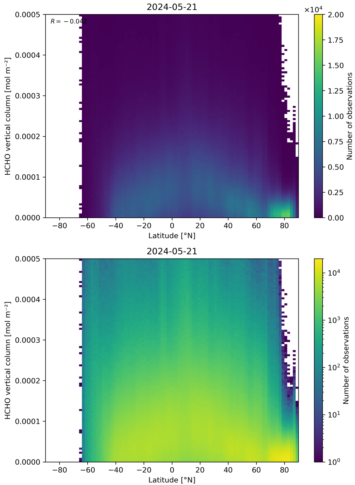
Figure 163: Scatter density plot of “Latitude” against “HCHO vertical column” for 2024-05-20 to 2024-05-22.
