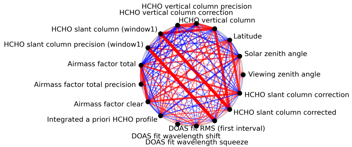
Figure 1: Map of correlation graph for 2024-05-20 to 2024-05-22.
