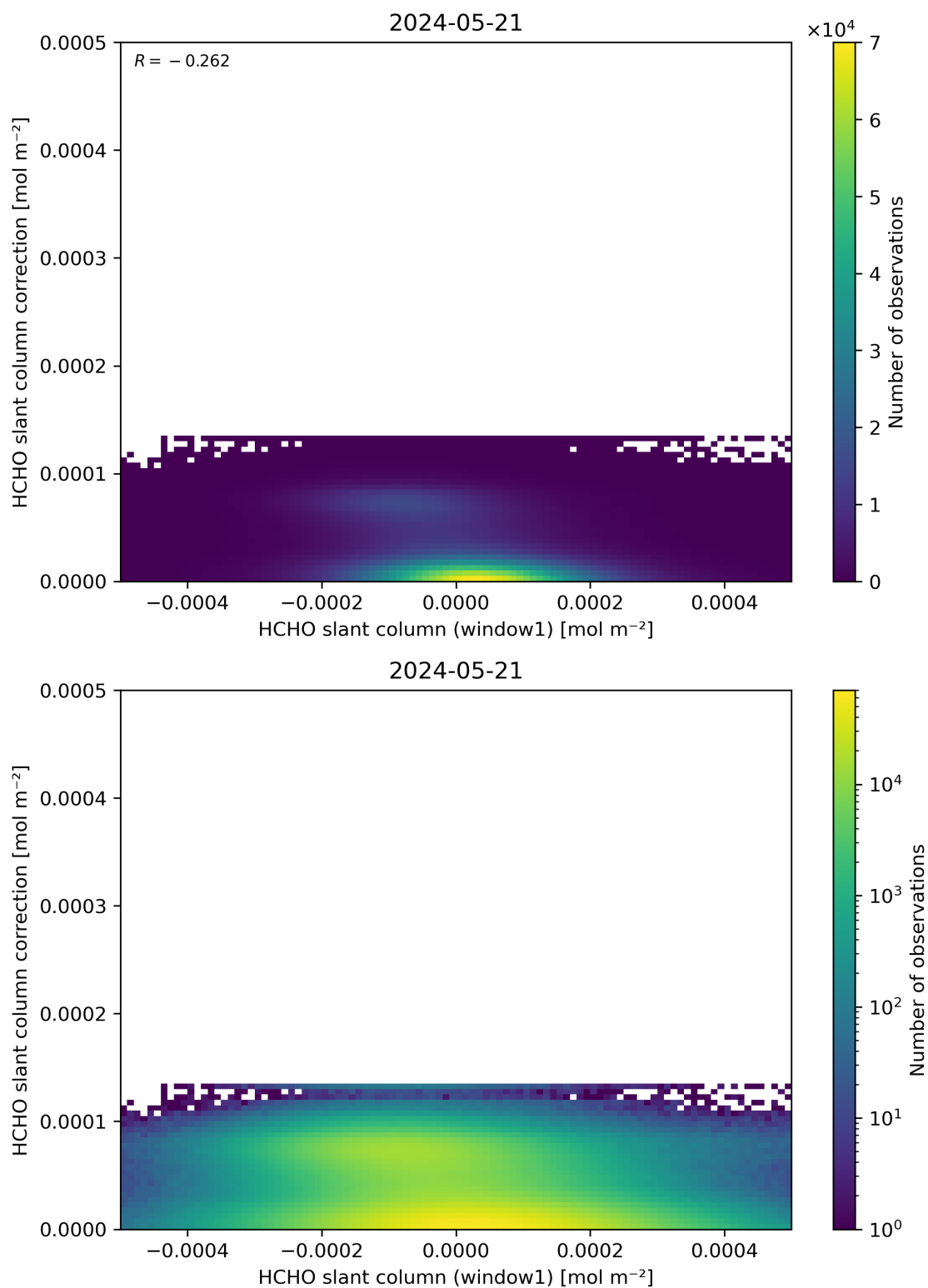
Figure 83: Scatter density plot of “HCHO slant column (window1)” against “HCHO slant column correction” for 2024-05-20 to 2024-05-22.
