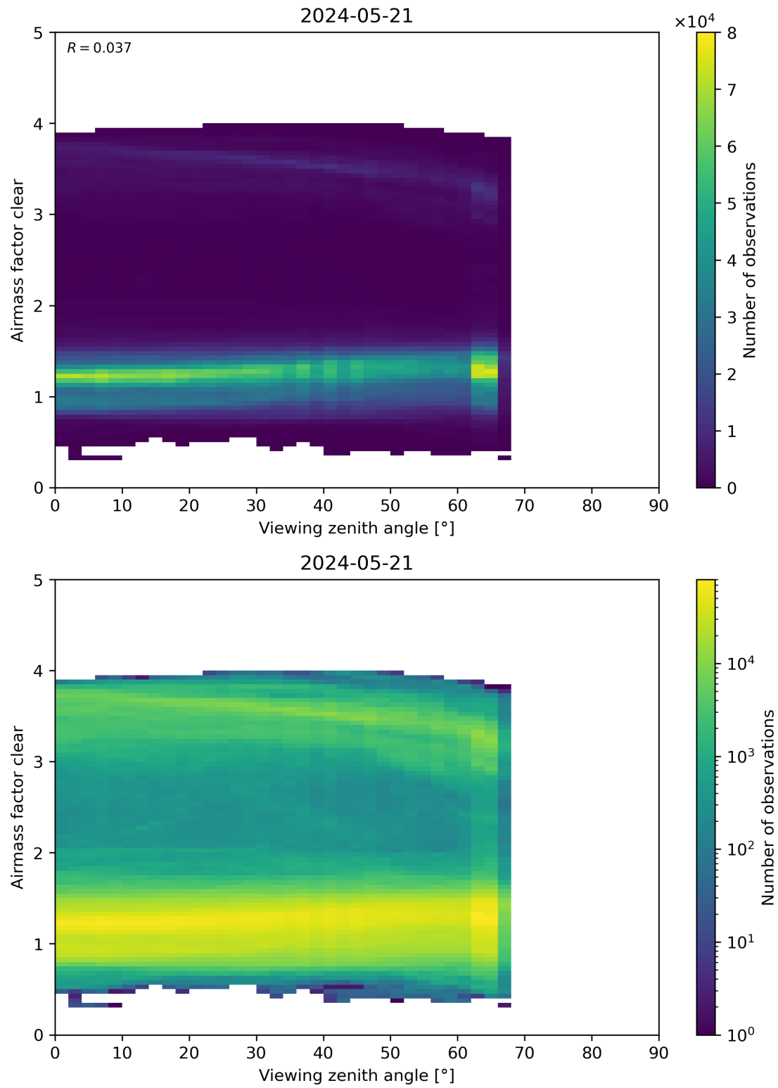
Figure 185: Scatter density plot of “Viewing zenith angle” against “Airmass factor clear” for 2024-05-20 to 2024-05-22.
