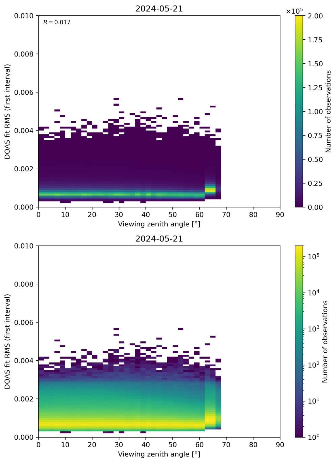
Figure 182: Scatter density plot of “Viewing zenith angle” against “DOAS fit RMS (first interval)” for 2024-05-20 to 2024-05-22.
