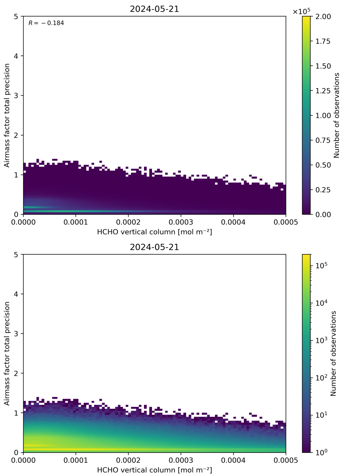
Figure 132: Scatter density plot of “HCHO vertical column” against “Airmass factor total precision” for 2024-05-20 to 2024-05-22.
