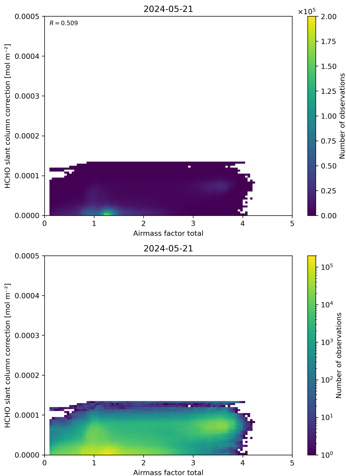
Figure 102: Scatter density plot of “Airmass factor total” against “HCHO slant column correction” for 2024-05-20 to 2024-05-22.
