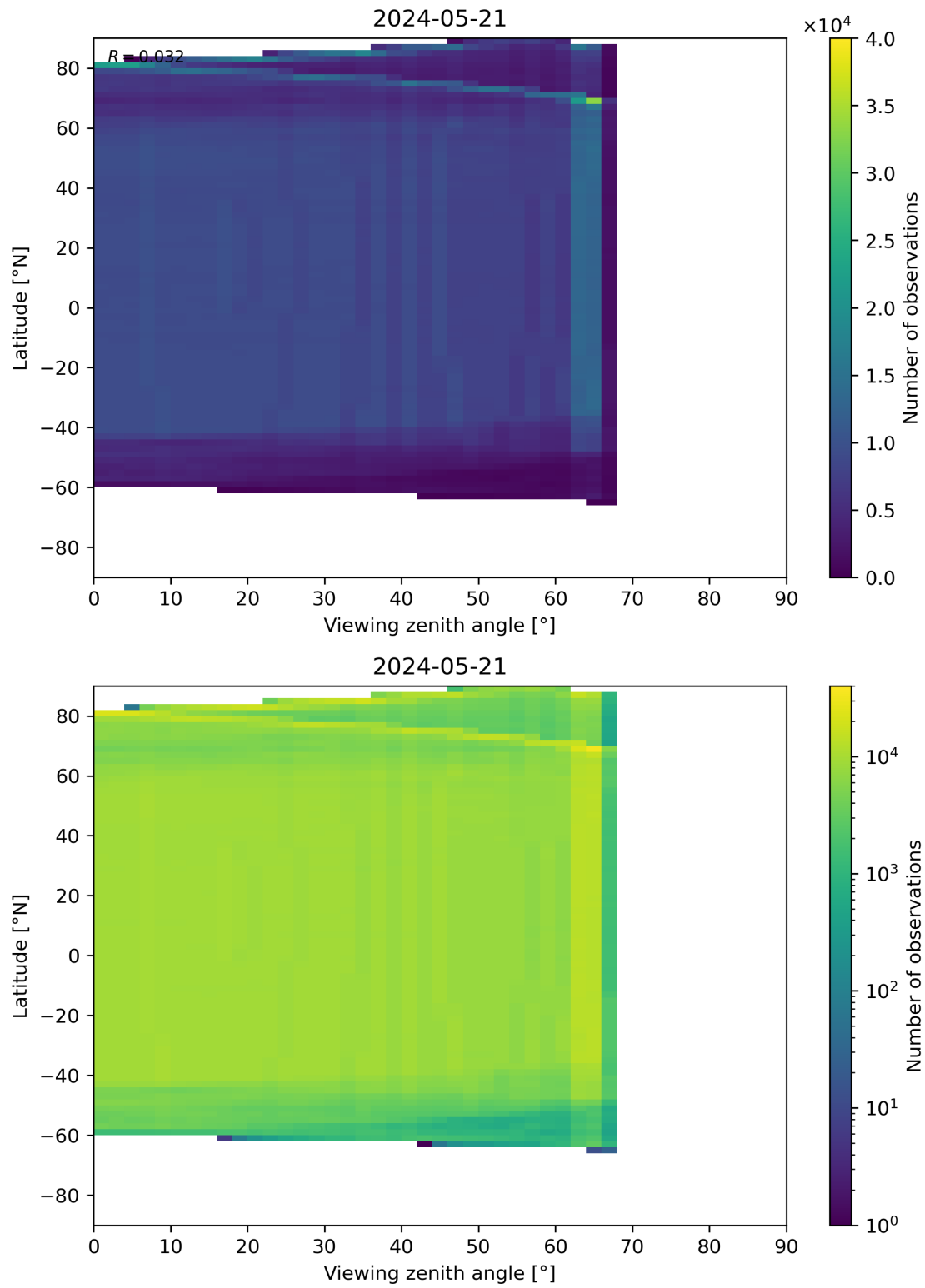
Figure 196: Scatter density plot of “Viewing zenith angle” against “Latitude” for 2024-05-20 to 2024-05-22.
