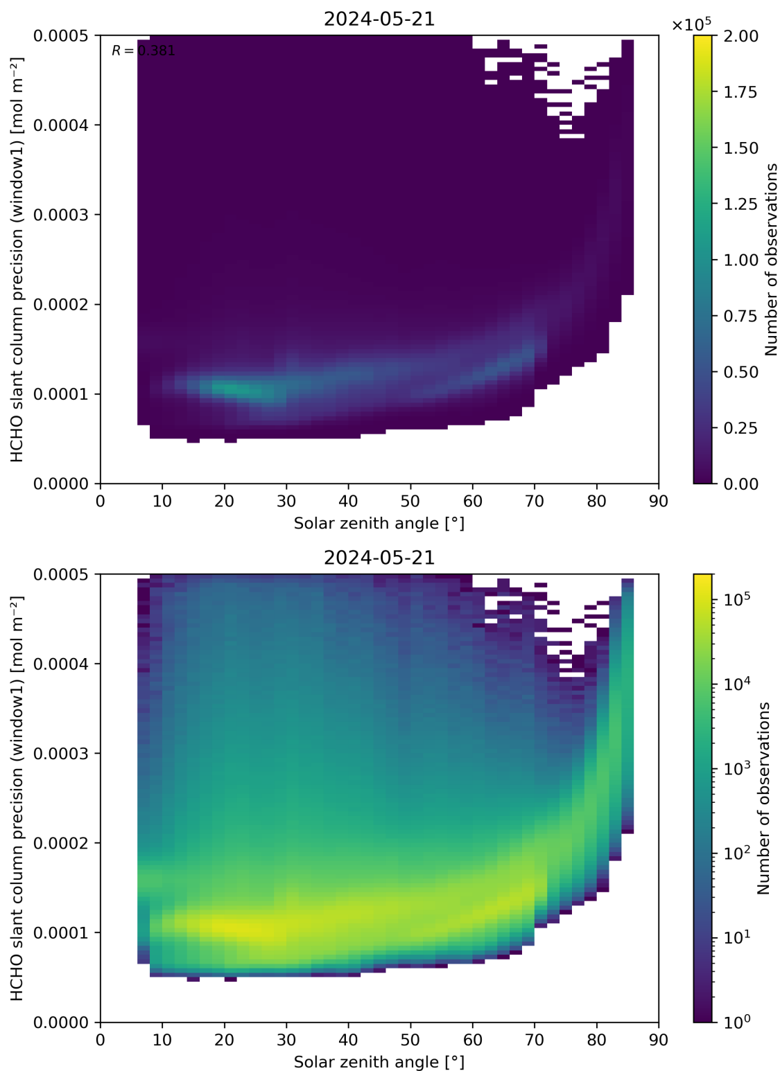
Figure 174: Scatter density plot of “Solar zenith angle” against “HCHO slant column precision (window1)” for 2024-05-20 to 2024-05-22.
