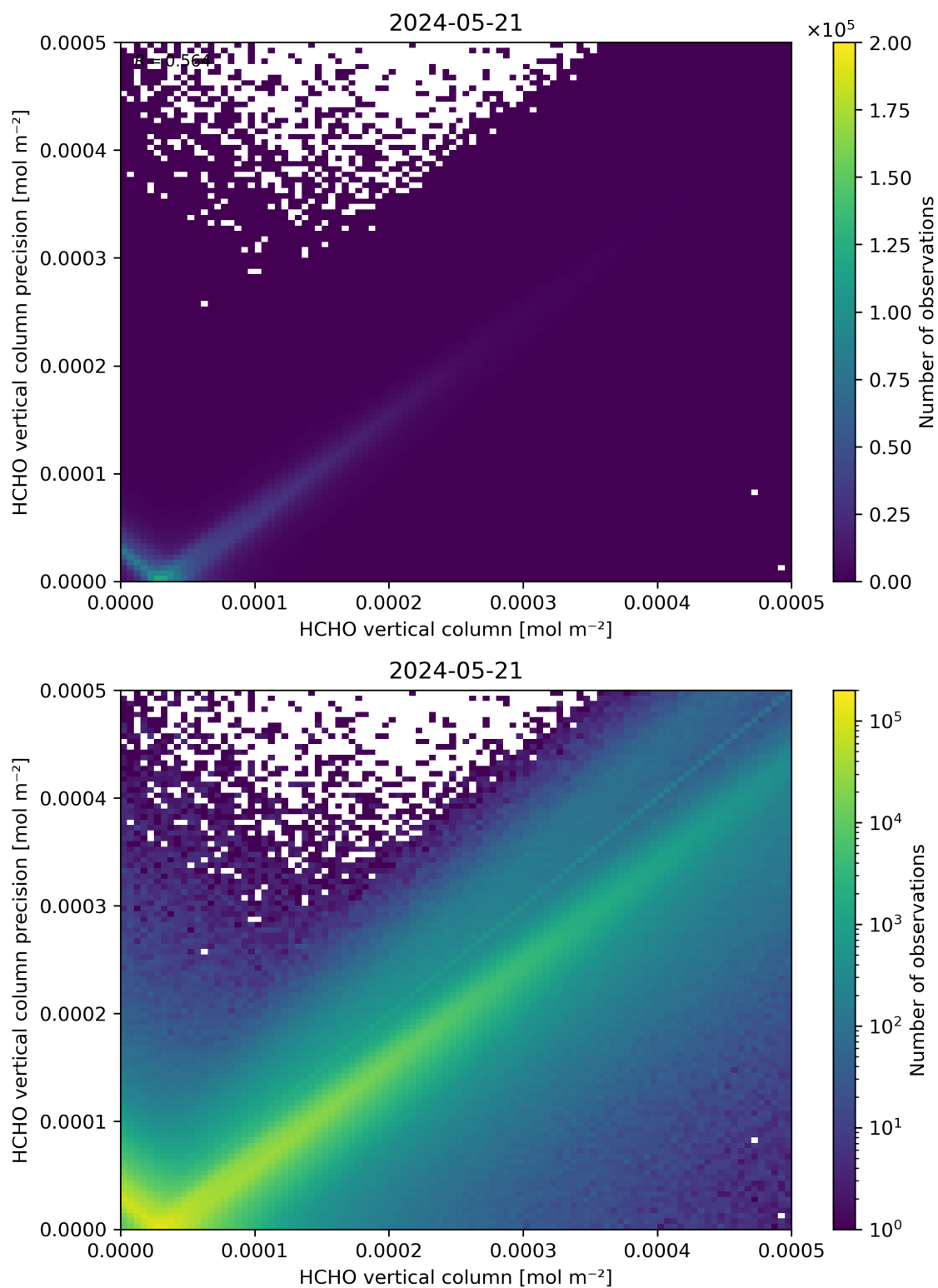
Figure 134: Scatter density plot of “HCHO vertical column” against “HCHO vertical column precision” for 2024-05-20 to 2024-05-22.
