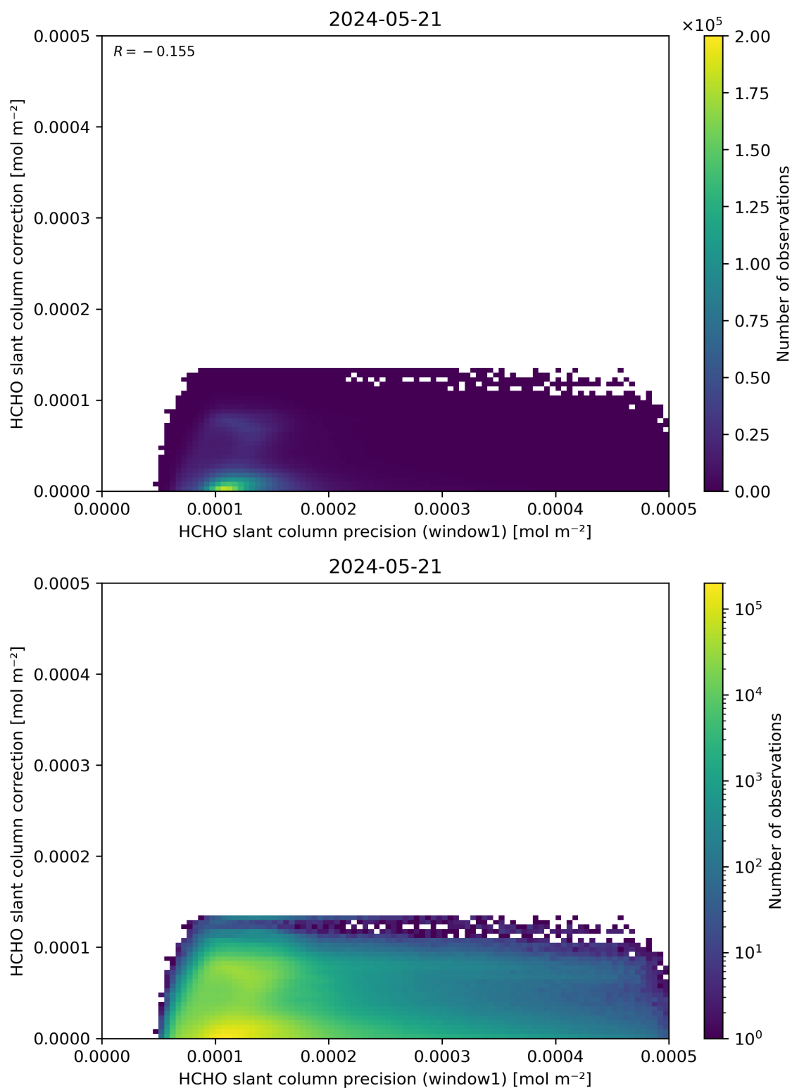
Figure 93: Scatter density plot of “HCHO slant column precision (window1)” against “HCHO slant column correction” for 2024-05-20 to 2024-05-22.
