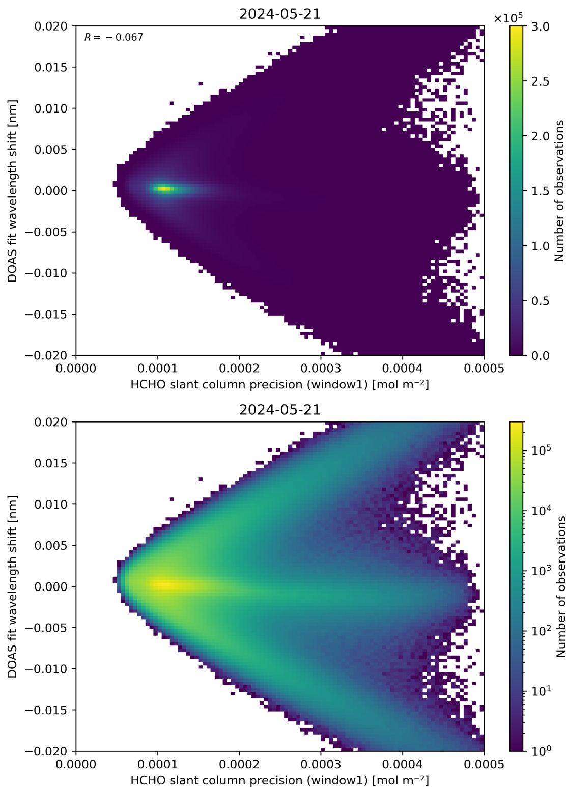
Figure 89: Scatter density plot of “HCHO slant column precision (window1)” against “DOAS fit wavelength shift” for 2024-05-20 to 2024-05-22.
