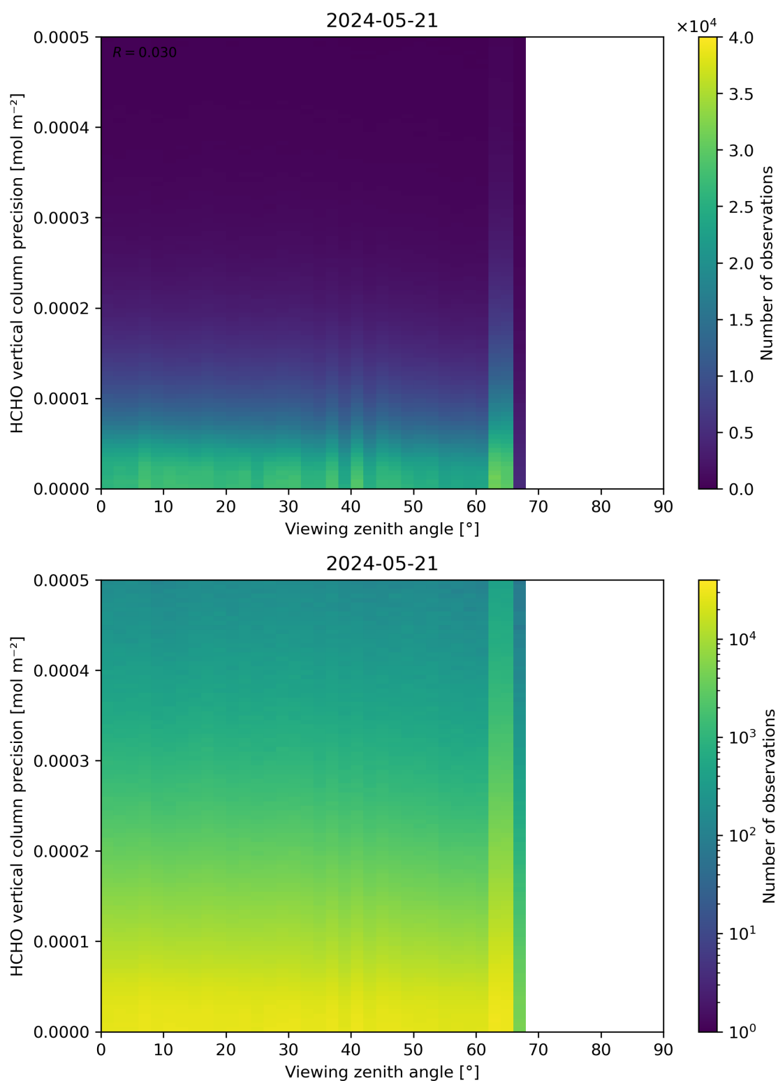
Figure 194: Scatter density plot of “Viewing zenith angle” against “HCHO vertical column precision” for 2024-05-20 to 2024-05-22.
