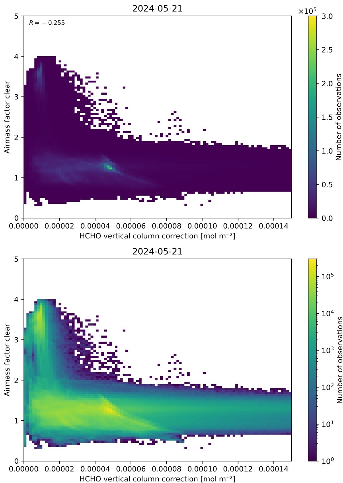
Figure 115: Scatter density plot of “HCHO vertical column correction” against “Airmass factor clear” for 2024-05-20 to 2024-05-22.
