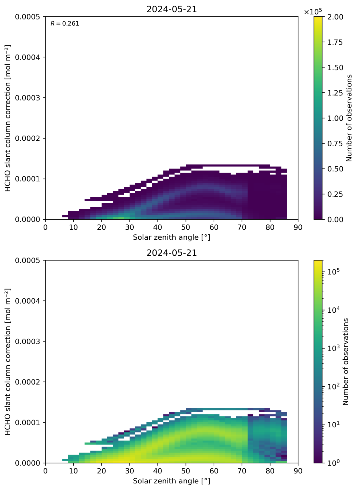
Figure 172: Scatter density plot of “Solar zenith angle” against “HCHO slant column correction” for 2024-05-20 to 2024-05-22.
