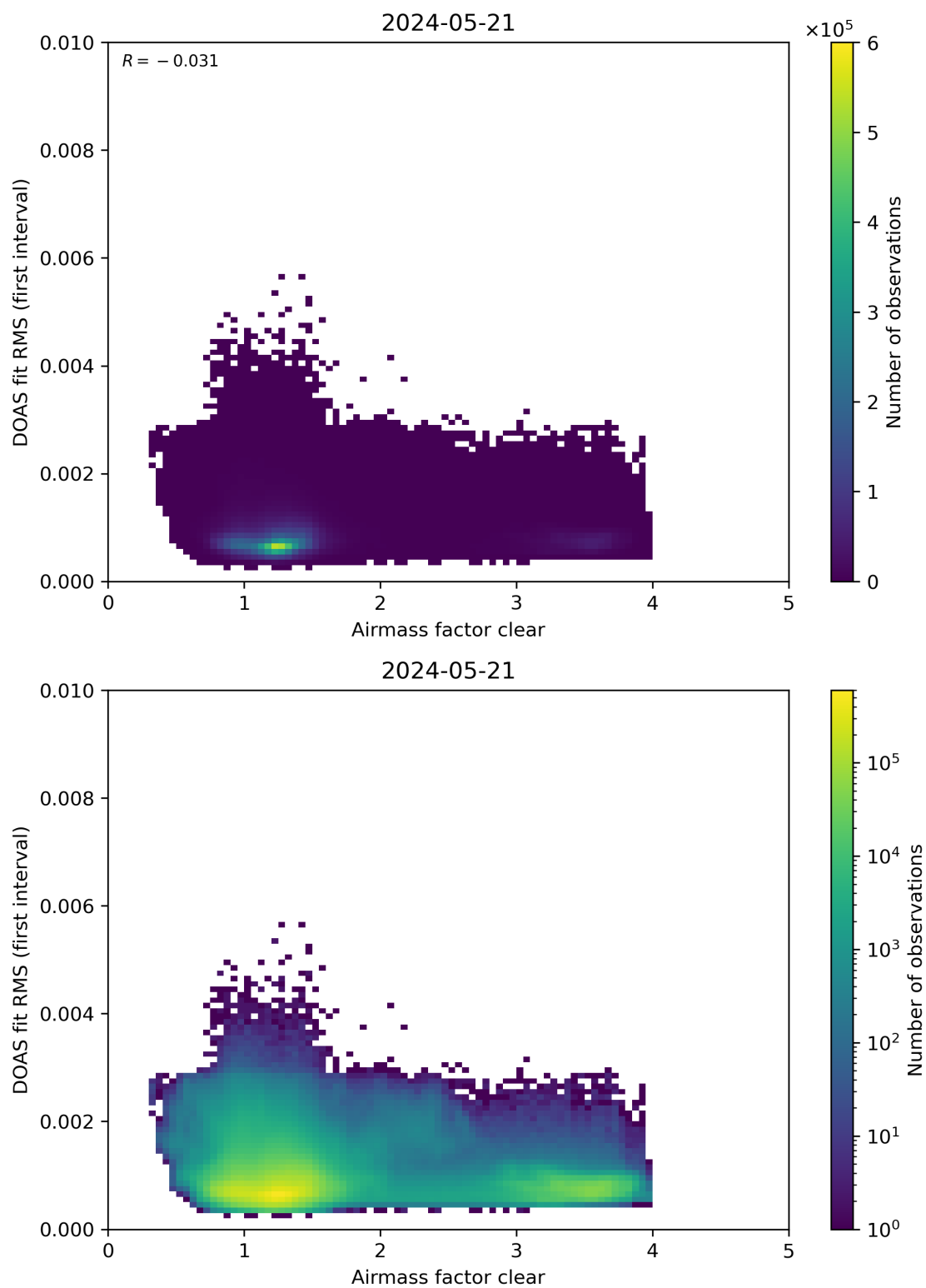
Figure 71: Scatter density plot of “Airmass factor clear” against “DOAS fit RMS (first interval)” for 2024-05-20 to 2024-05-22.
