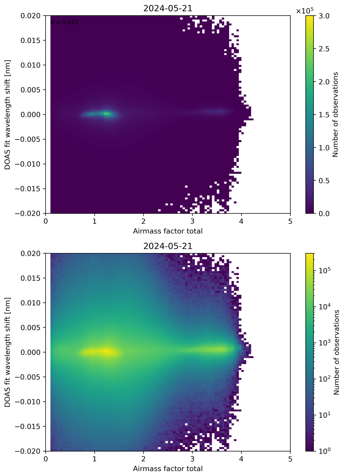
Figure 98: Scatter density plot of “Airmass factor total” against “DOAS fit wavelength shift” for 2024-05-20 to 2024-05-22.
