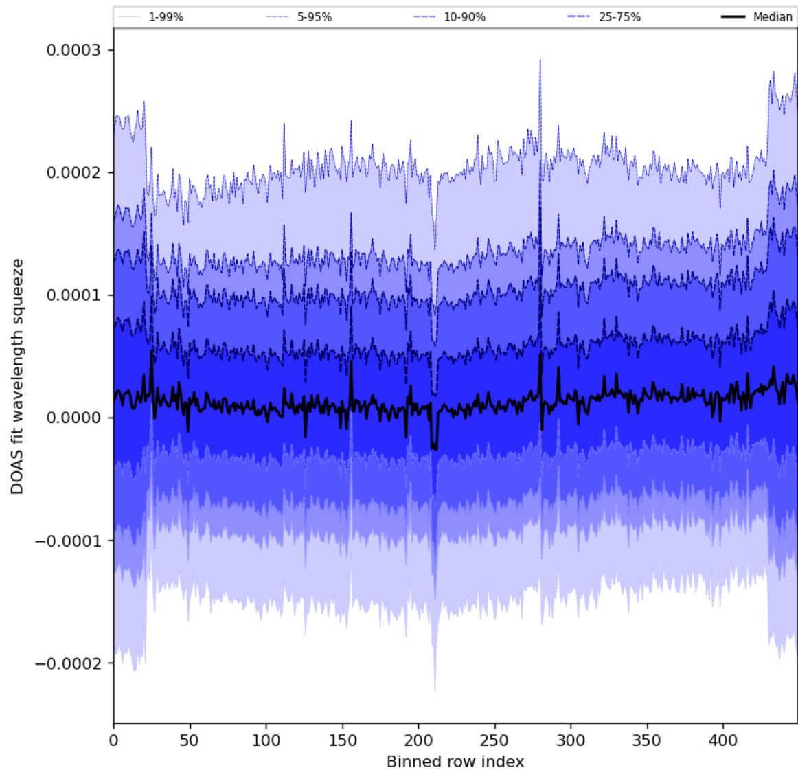
Figure 59: Along track statistics of “DOAS fit wavelength squeeze” for 2024-05-20 to 2024-05-22
