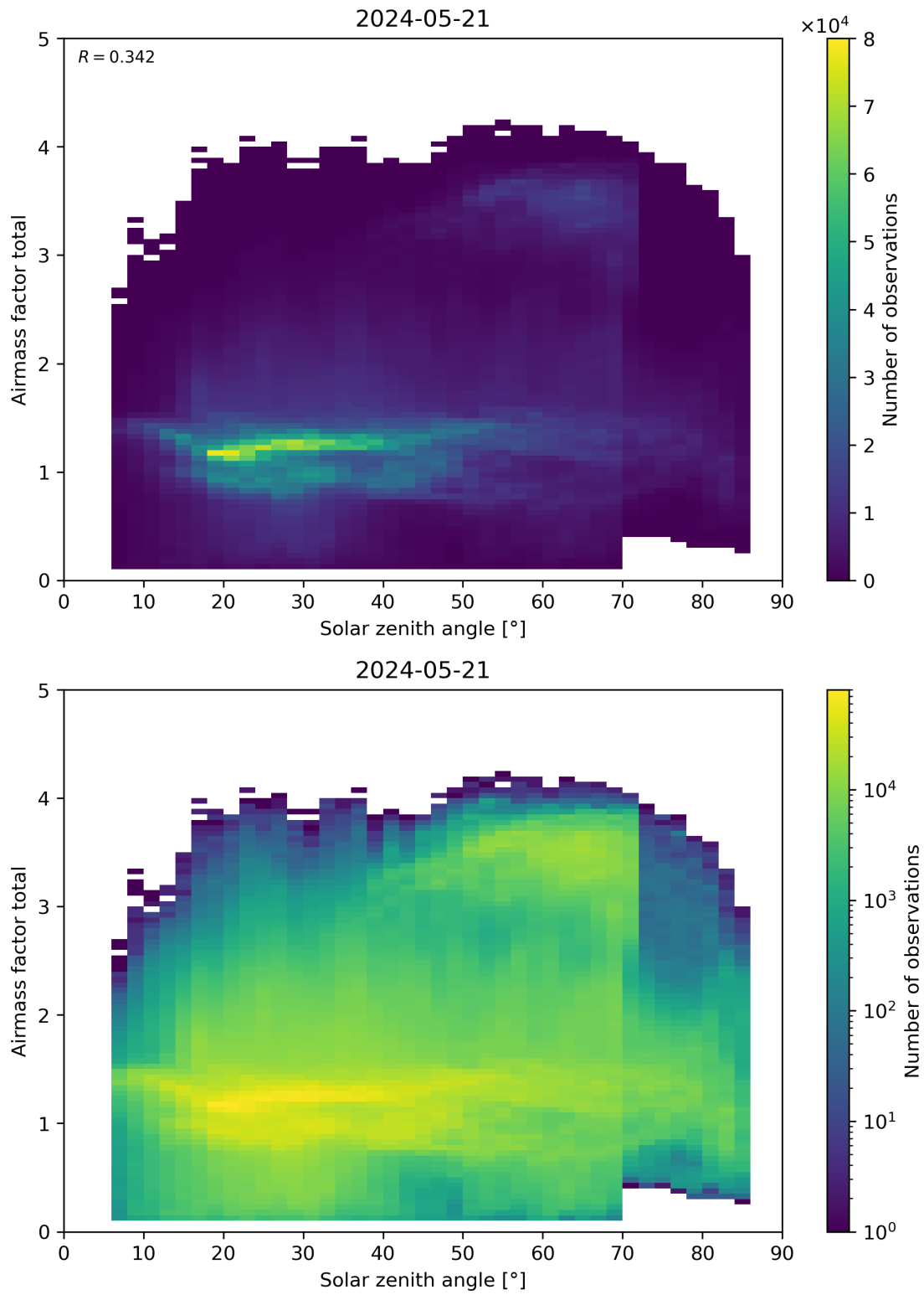
Figure 175: Scatter density plot of “Solar zenith angle” against “Airmass factor total” for 2024-05-20 to 2024-05-22.
