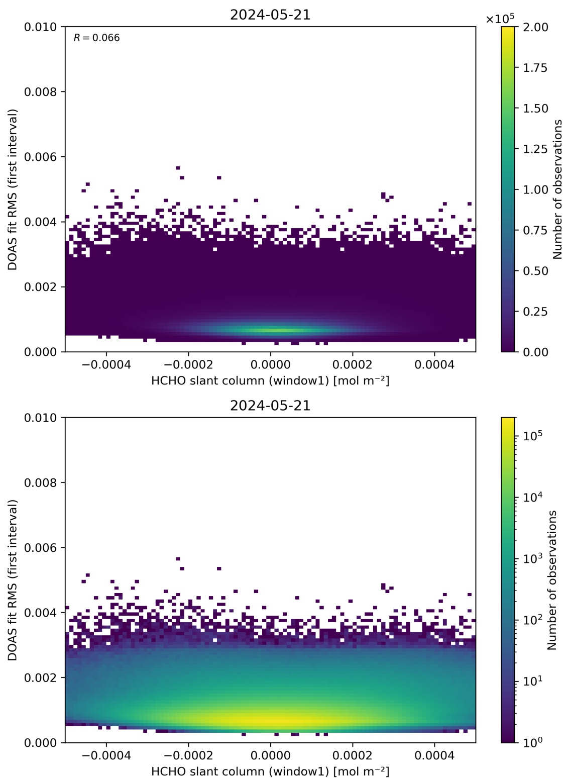
Figure 78: Scatter density plot of “HCHO slant column (window1)” against “DOAS fit RMS (first interval)” for 2024-05-20 to 2024-05-22.
