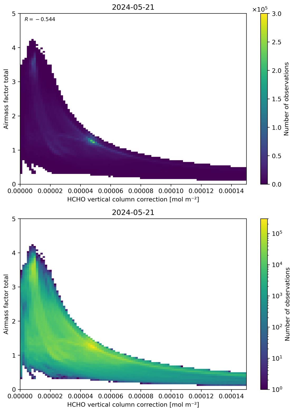
Figure 120: Scatter density plot of “HCHO vertical column correction” against “Airmass factor total” for 2024-05-20 to 2024-05-22.
