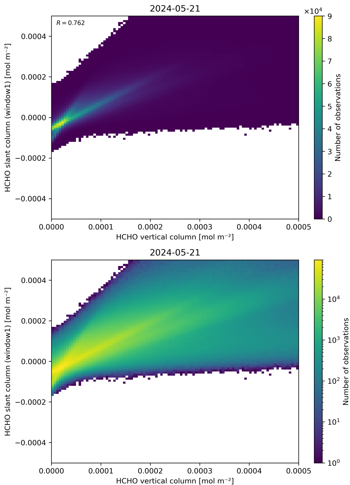
Figure 129: Scatter density plot of “HCHO vertical column” against “HCHO slant column (window1)” for 2024-05-20 to 2024-05-22.
