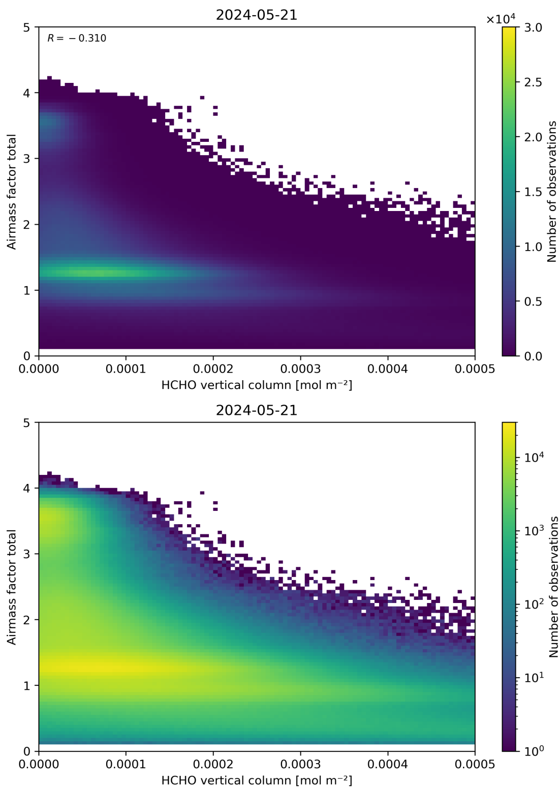
Figure 131: Scatter density plot of “HCHO vertical column” against “Airmass factor total” for 2024-05-20 to 2024-05-22.
