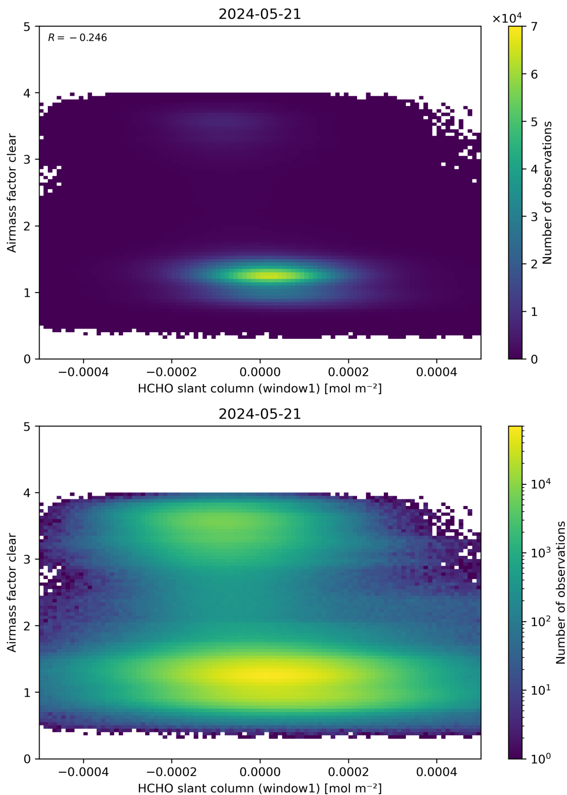
Figure 81: Scatter density plot of “HCHO slant column (window1)” against “Airmass factor clear” for 2024-05-20 to 2024-05-22.
