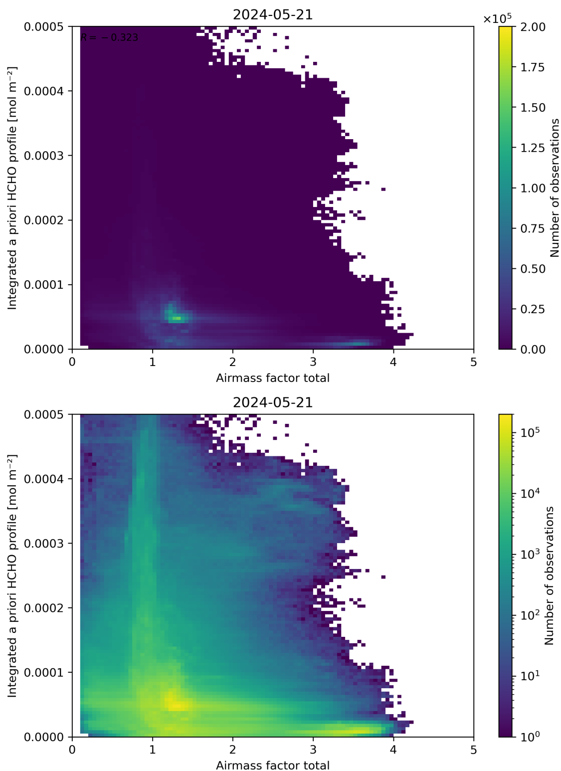
Figure 104: Scatter density plot of “Airmass factor total” against “Integrated a priori HCHO profile” for 2024-05-20 to 2024-05-22.
