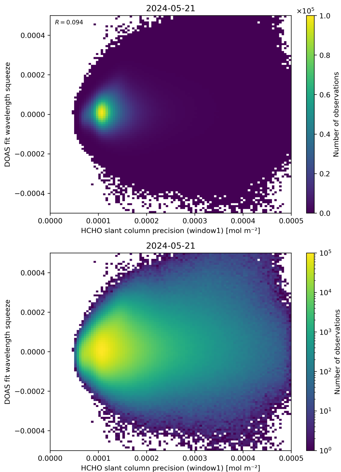
Figure 90: Scatter density plot of “HCHO slant column precision (window1)” against “DOAS fit wavelength squeeze” for 2024-05-20 to 2024-05-22.
