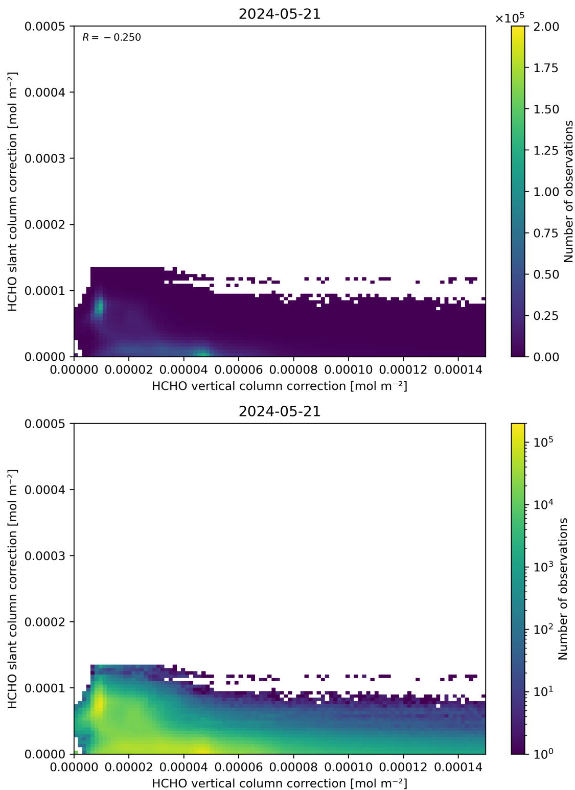
Figure 117: Scatter density plot of “HCHO vertical column correction” against “HCHO slant column correction” for 2024-05-20 to 2024-05-22.
