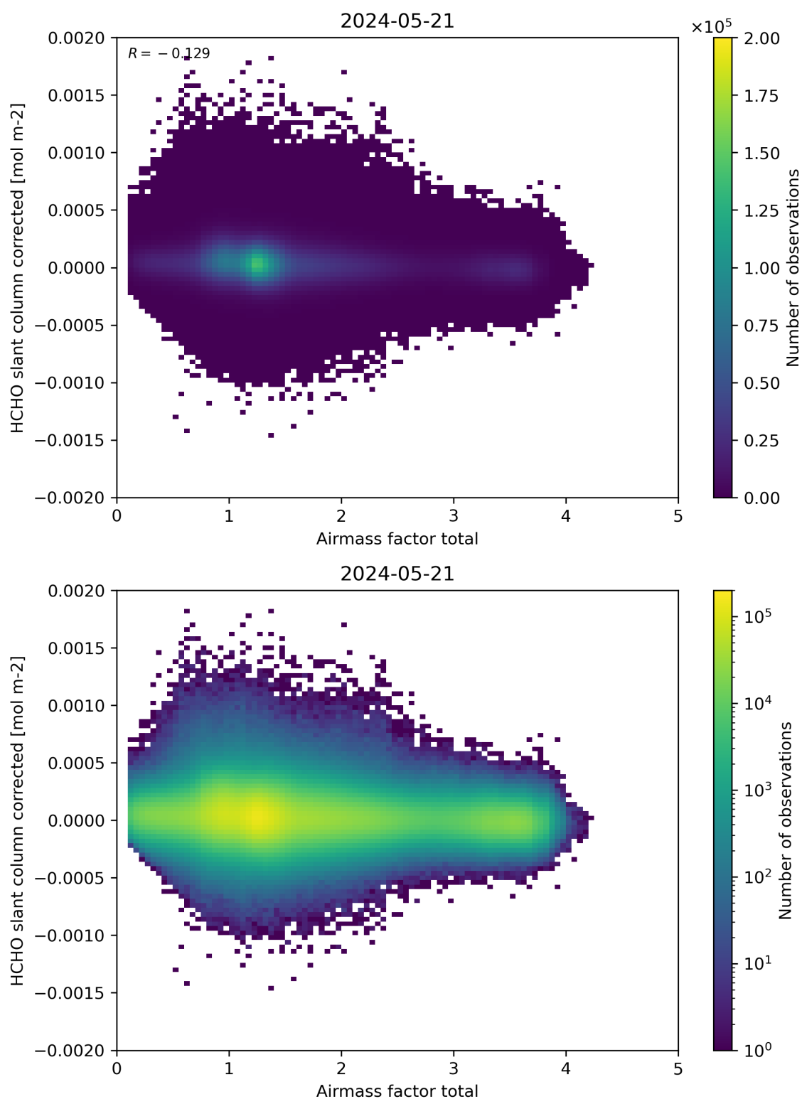
Figure 101: Scatter density plot of “Airmass factor total” against “HCHO slant column corrected” for 2024-05-20 to 2024-05-22.
