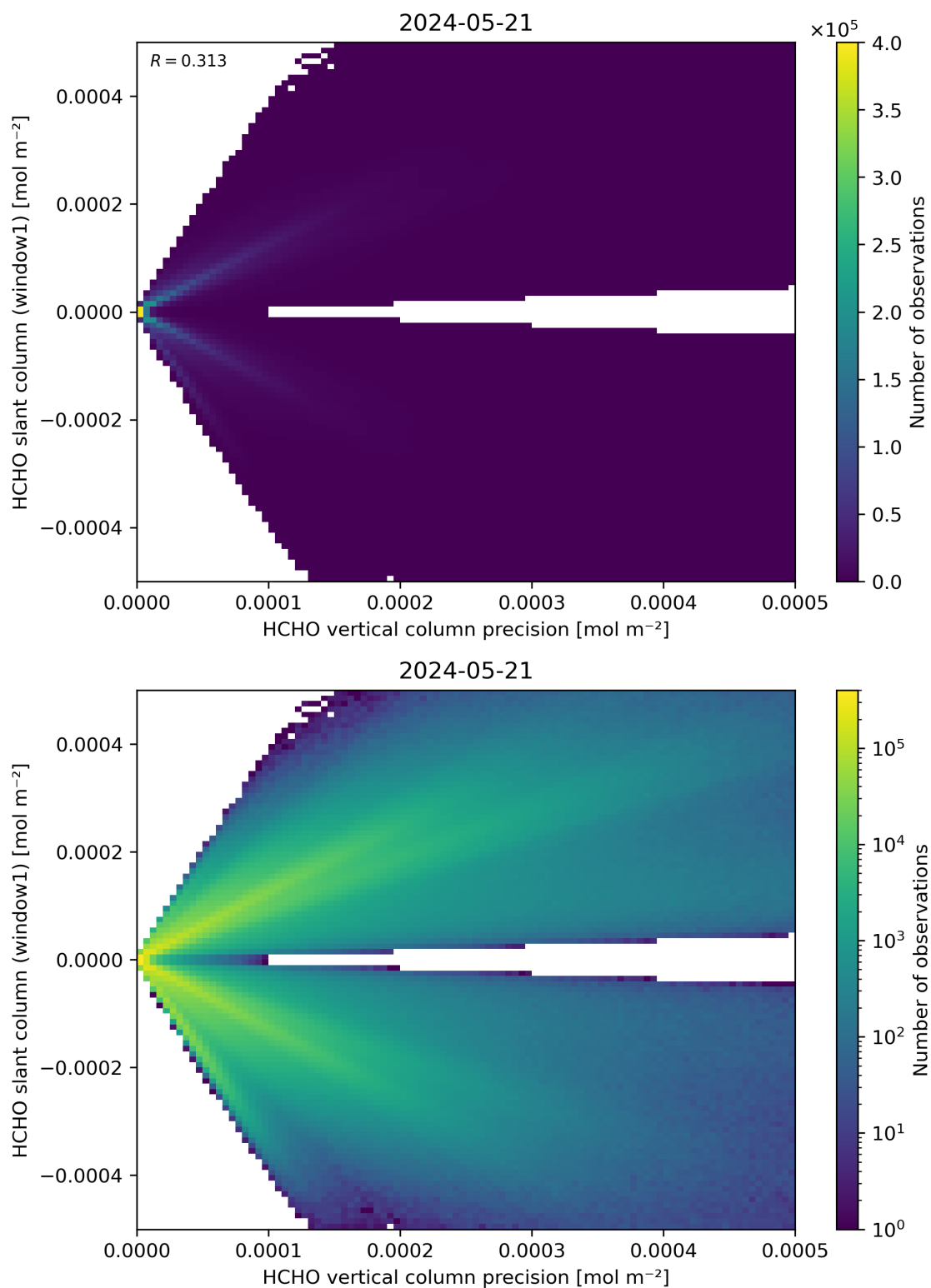
Figure 142: Scatter density plot of “HCHO vertical column precision” against “HCHO slant column (window1)” for 2024-05-20 to 2024-05-22.
