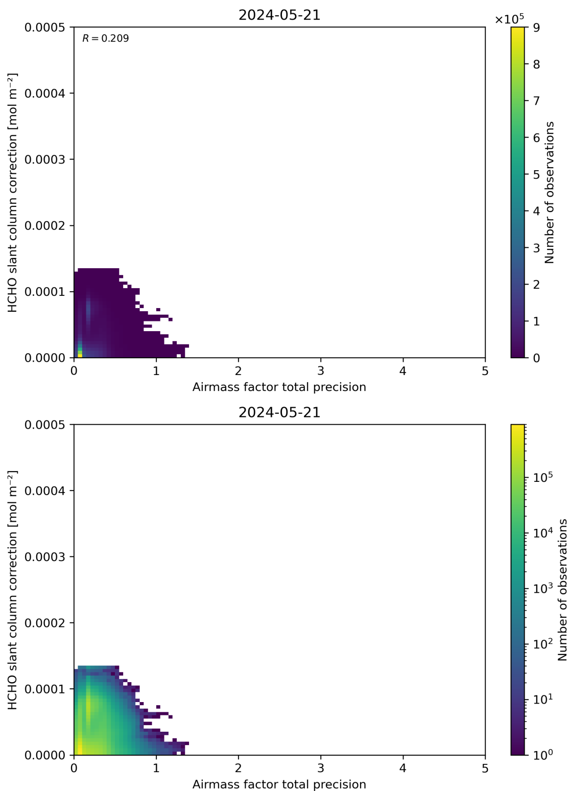
Figure 110: Scatter density plot of “Airmass factor total precision” against “HCHO slant column correction” for 2024-05-20 to 2024-05-22.
