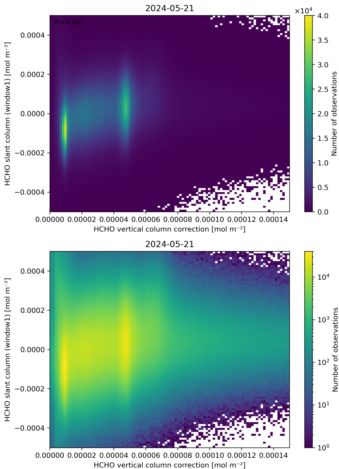
Figure 118: Scatter density plot of “HCHO vertical column correction” against “HCHO slant column (window1)” for 2024-05-20 to 2024-05-22.
