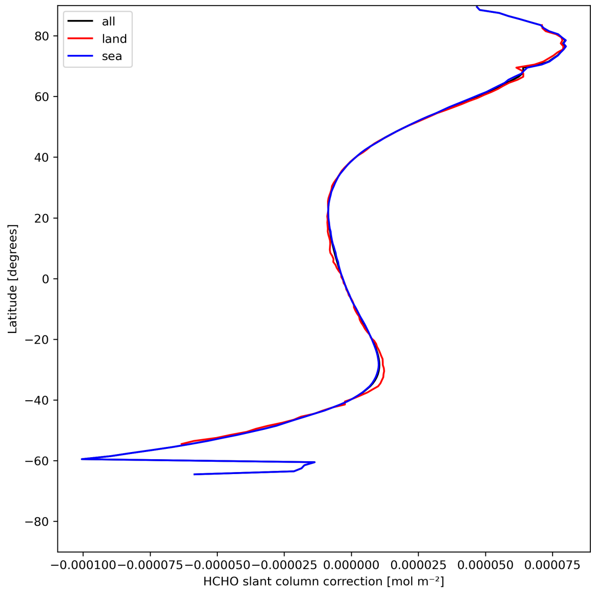
Figure 33: Zonal average of “HCHO slant column correction” for 2024-05-20 to 2024-05-22.
