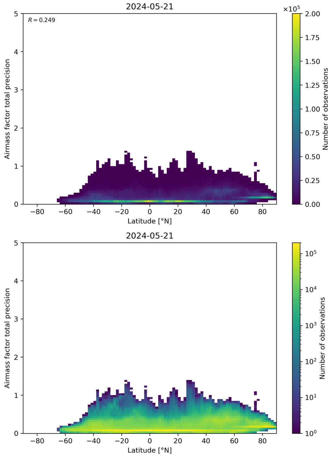
Figure 162: Scatter density plot of “Latitude” against “Airmass factor total precision” for 2024-05-20 to 2024-05-22.
