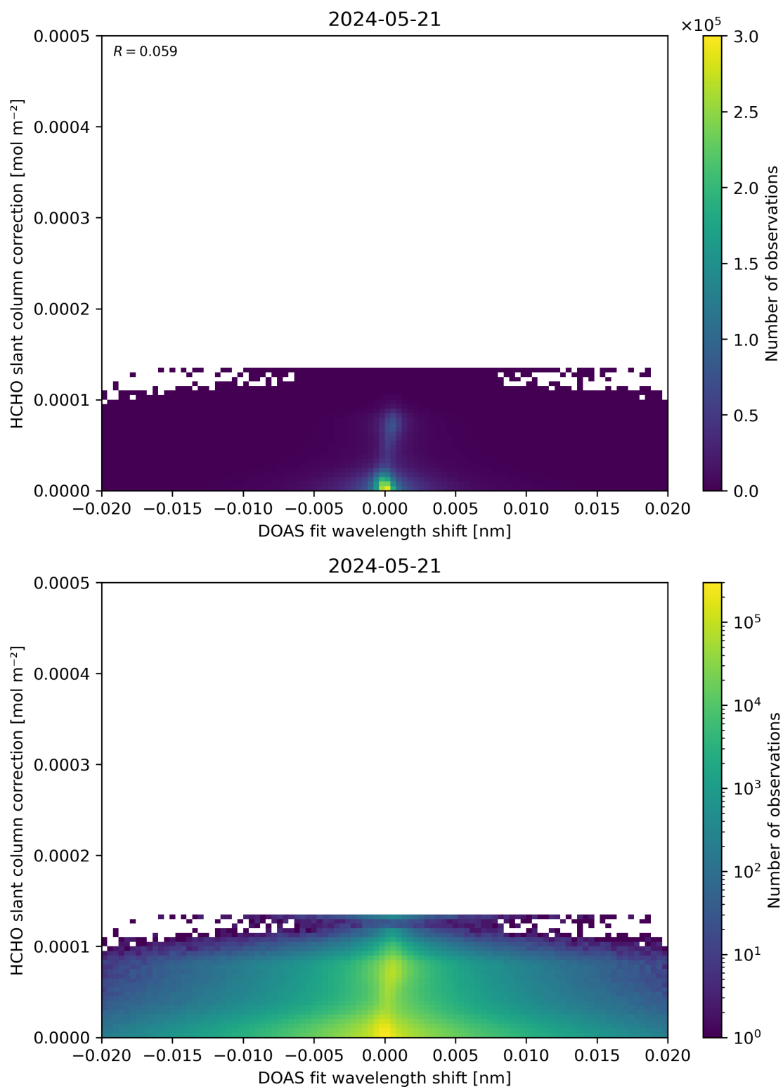
Figure 67: Scatter density plot of “DOAS fit wavelength shift” against “HCHO slant column correction” for 2024-05-20 to 2024-05-22.
