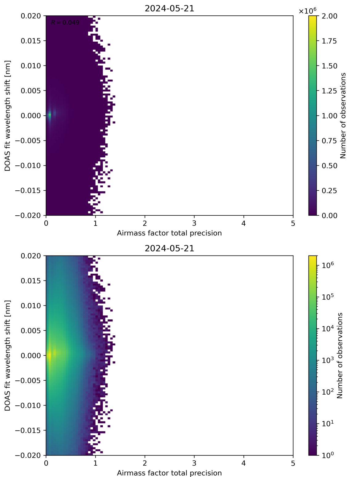
Figure 106: Scatter density plot of “Airmass factor total precision” against “DOAS fit wavelength shift” for 2024-05-20 to 2024-05-22.
