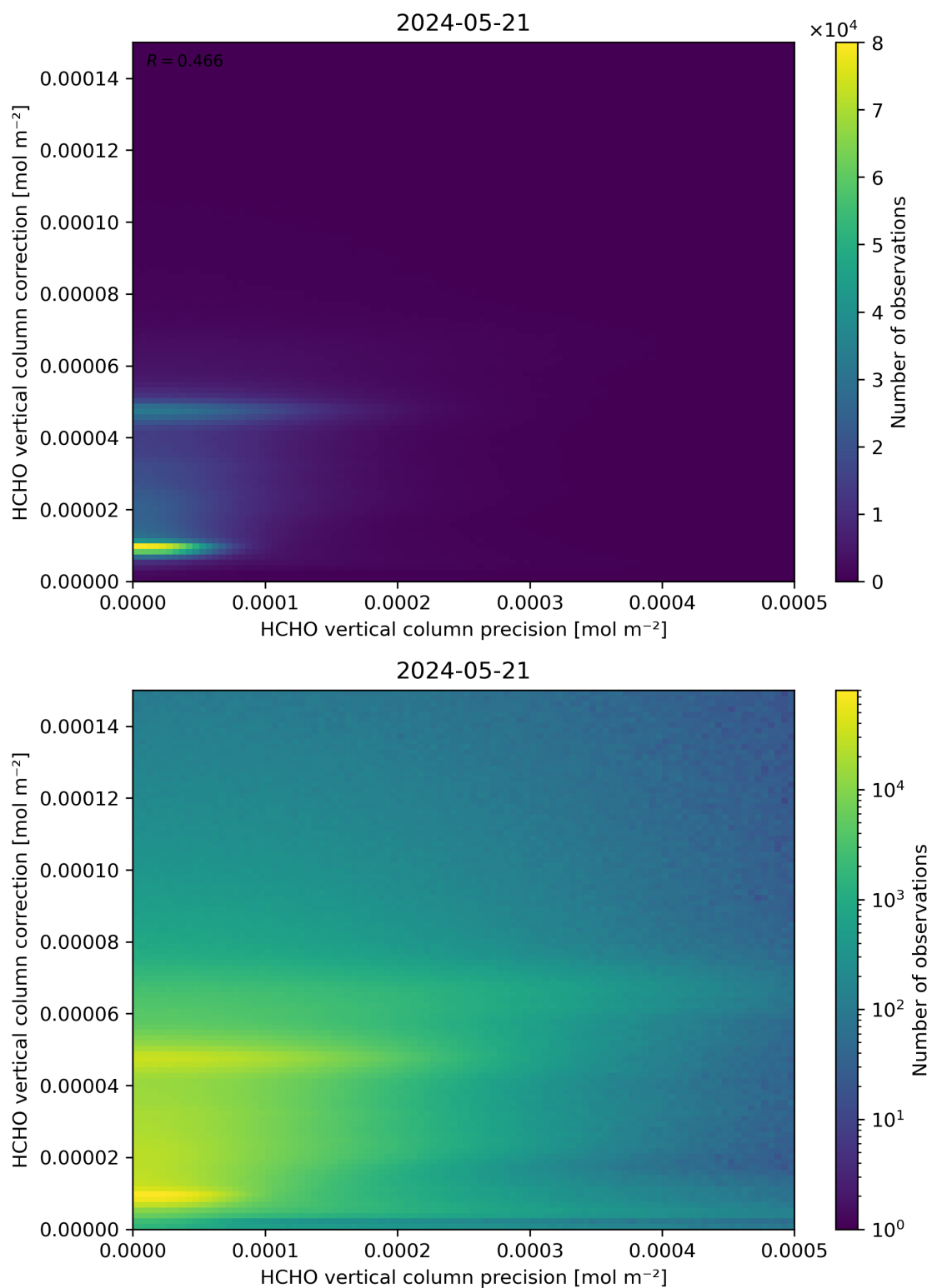
Figure 146: Scatter density plot of “HCHO vertical column precision” against “HCHO vertical column correction” for 2024-05-20 to 2024-05-22.
