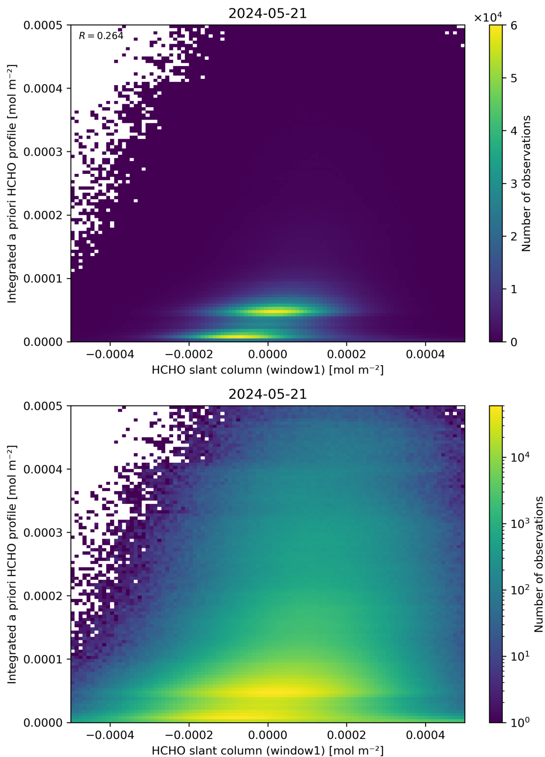
Figure 87: Scatter density plot of “HCHO slant column (window1)” against “Integrated a priori HCHO profile” for 2024-05-20 to 2024-05-22.
