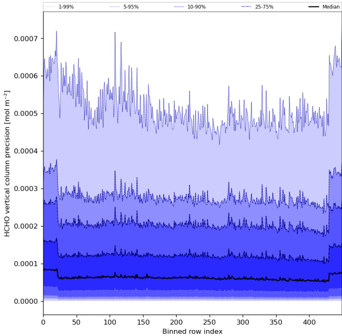
Figure 50: Along track statistics of “HCHO vertical column precision” for 2024-05-20 to 2024-05-22
