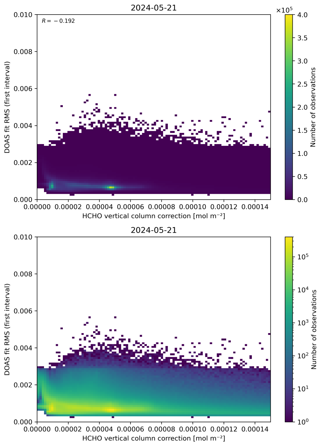
Figure 112: Scatter density plot of “HCHO vertical column correction” against “DOAS fit RMS (first interval)” for 2024-05-20 to 2024-05-22.
