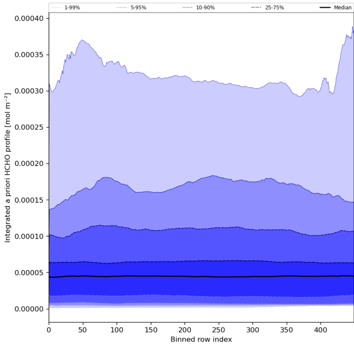
Figure 57: Along track statistics of “Integrated a priori HCHO profile” for 2024-05-20 to 2024-05-22
