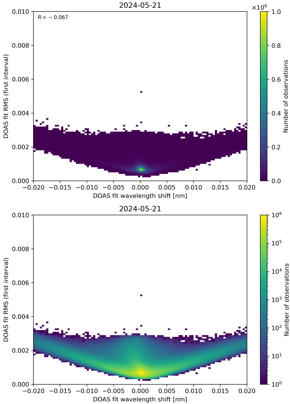
Figure 64: Scatter density plot of “DOAS fit wavelength shift” against “DOAS fit RMS (first interval)” for 2024-05-20 to 2024-05-22.
