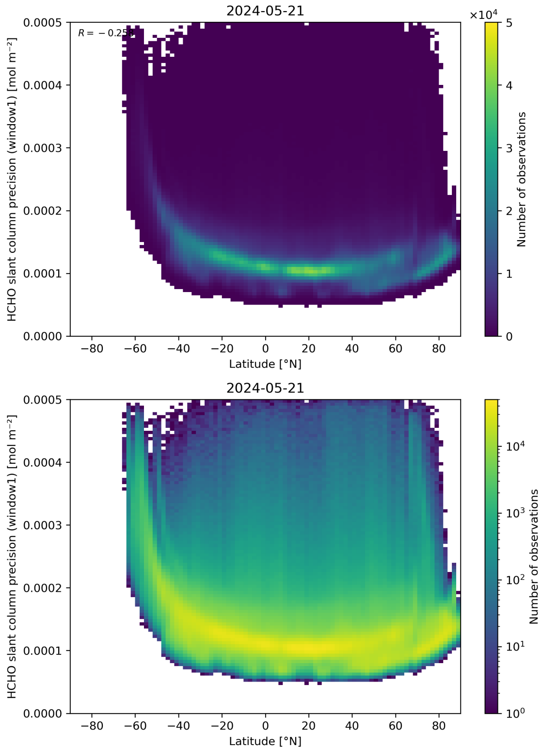
Figure 160: Scatter density plot of “Latitude” against “HCHO slant column precision (window1)” for 2024-05-20 to 2024-05-22.
