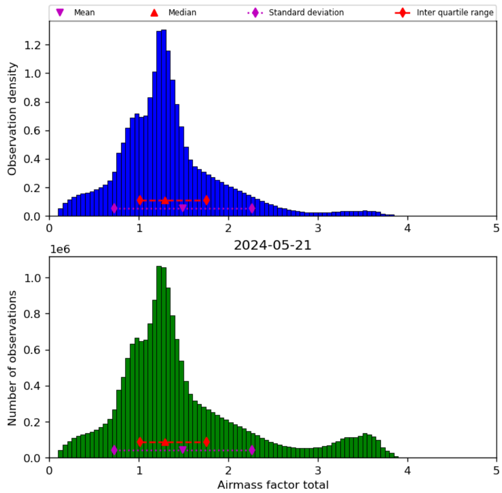
Figure 40: Histogram of “Airmass factor total” for 2024-05-20 to 2024-05-22
