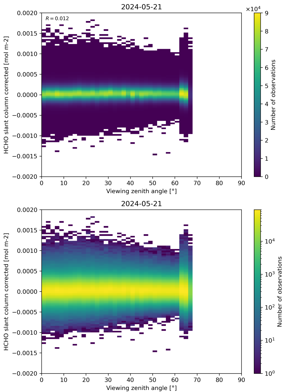
Figure 186: Scatter density plot of “Viewing zenith angle” against “HCHO slant column corrected” for 2024-05-20 to 2024-05-22.
