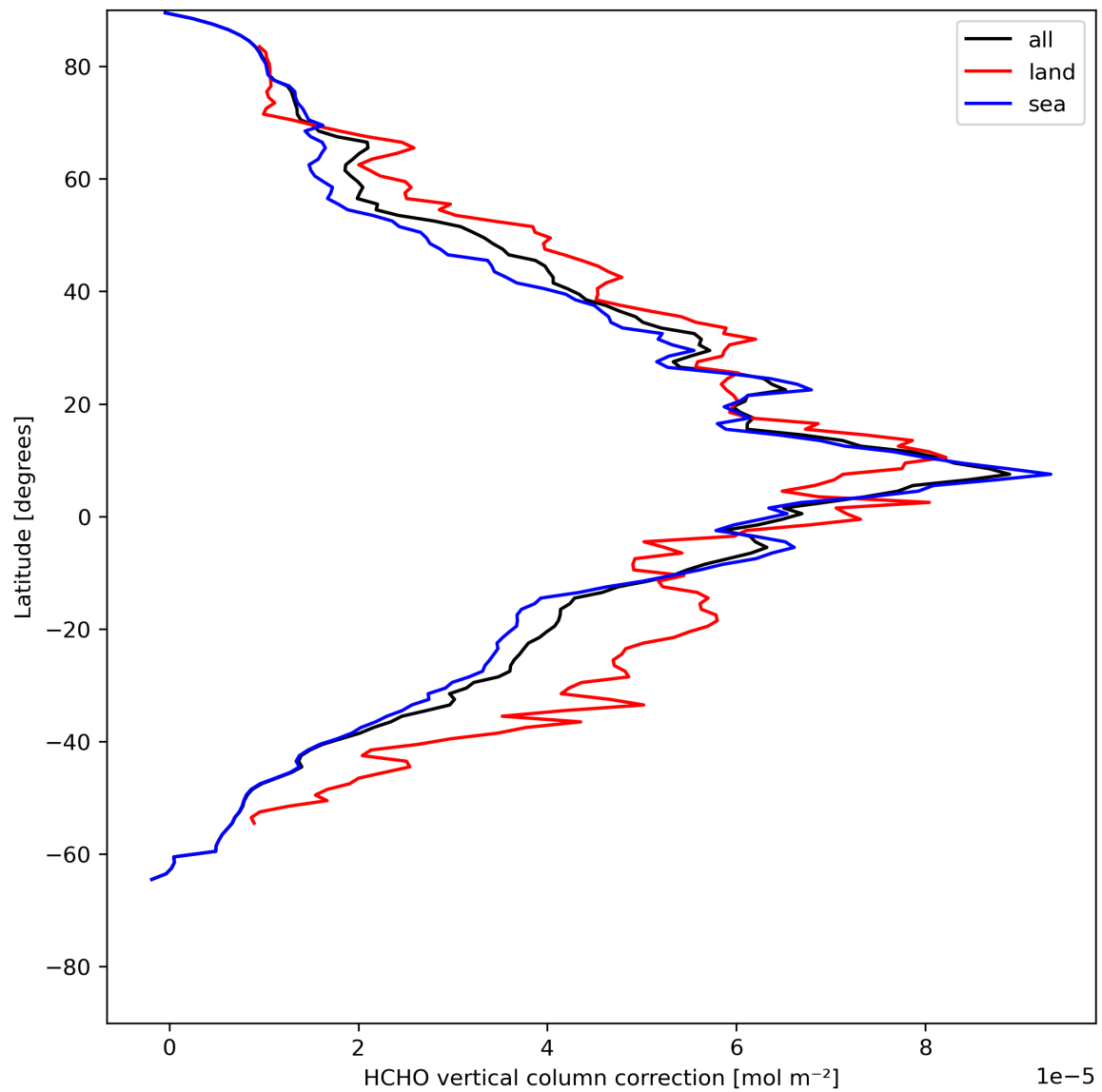
Figure 23: Zonal average of “HCHO vertical column correction” for 2024-05-20 to 2024-05-22.
