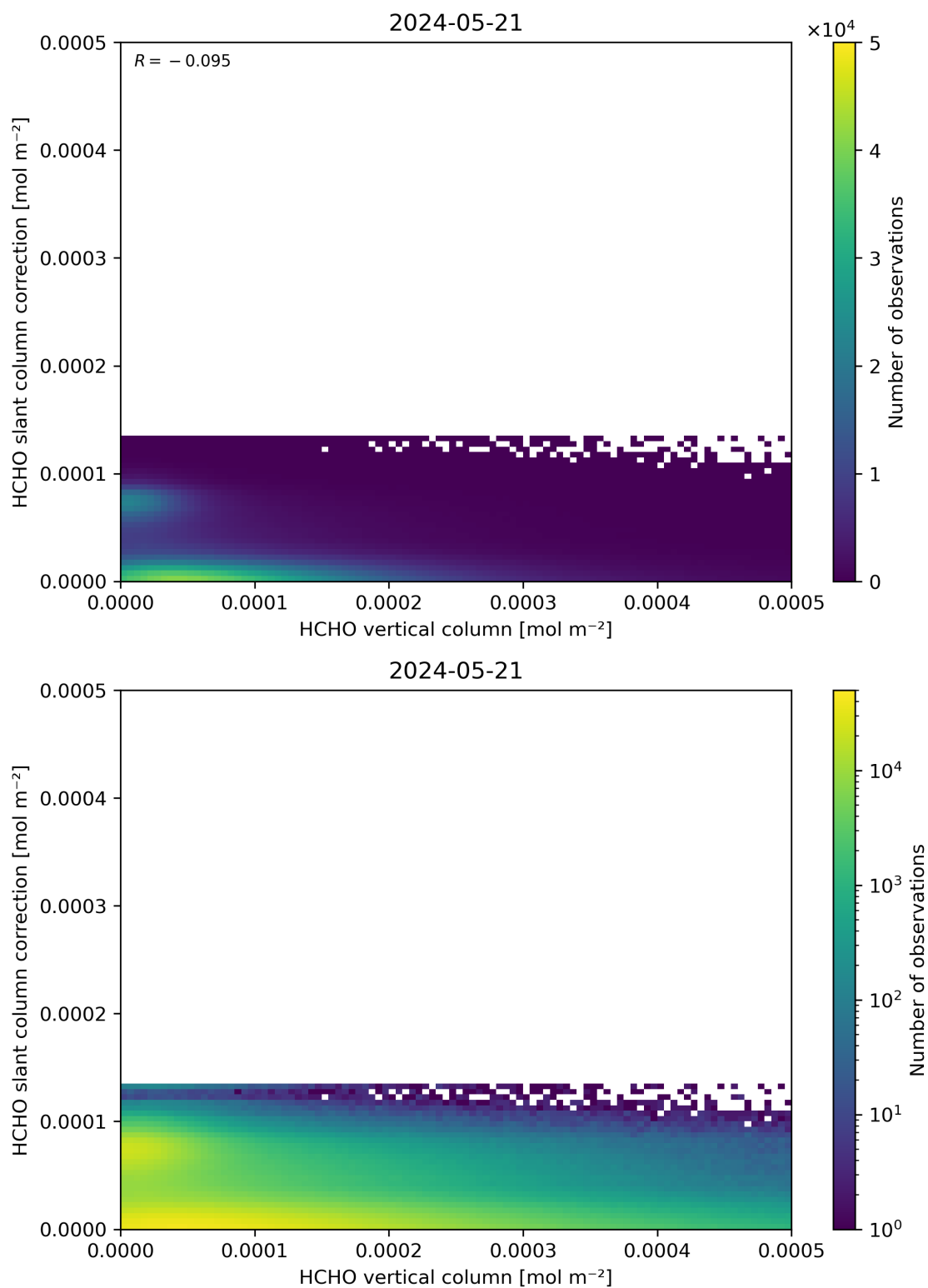
Figure 128: Scatter density plot of “HCHO vertical column” against “HCHO slant column correction” for 2024-05-20 to 2024-05-22.
