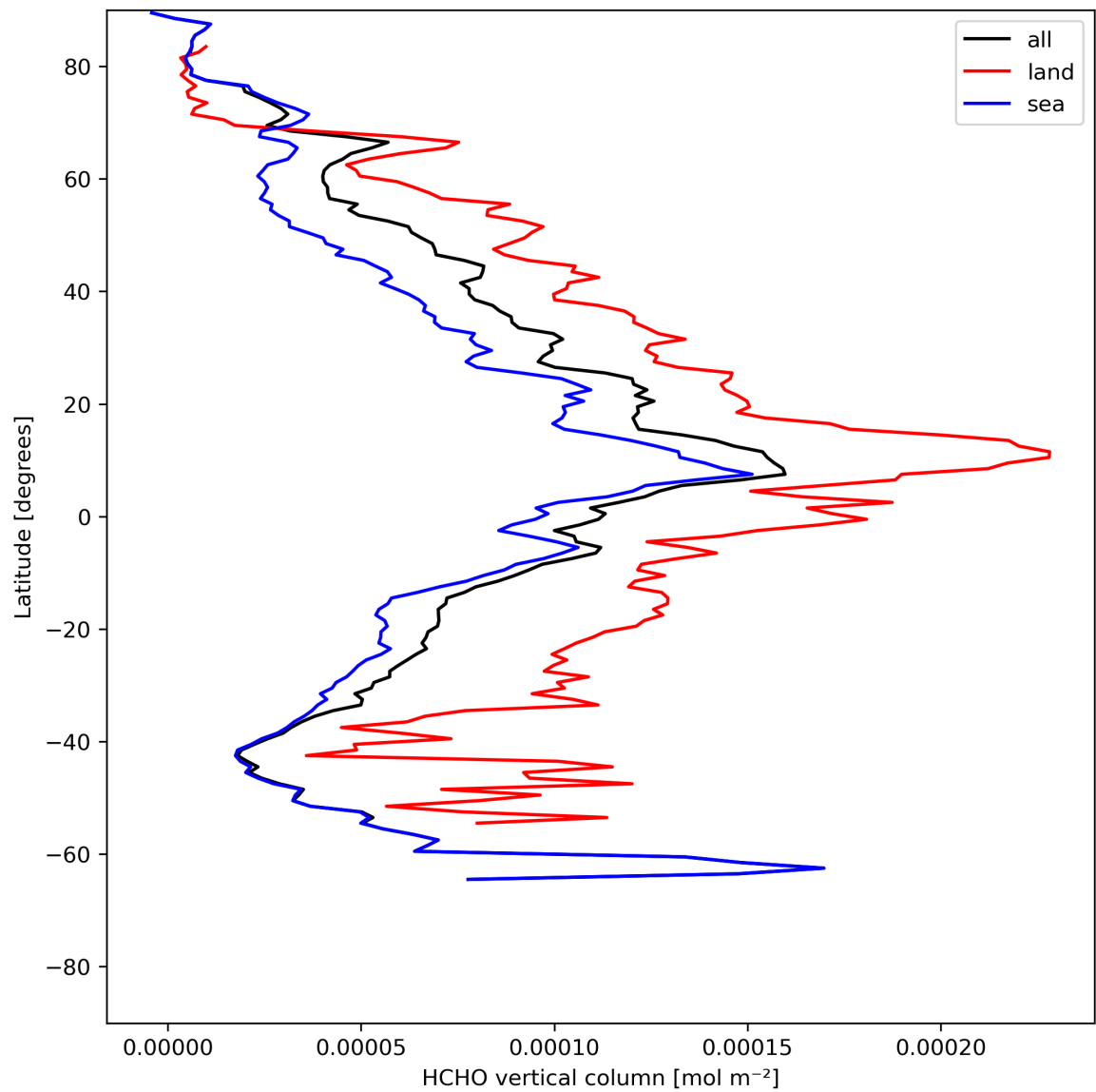
Figure 21: Zonal average of “HCHO vertical column” for 2024-05-20 to 2024-05-22.
