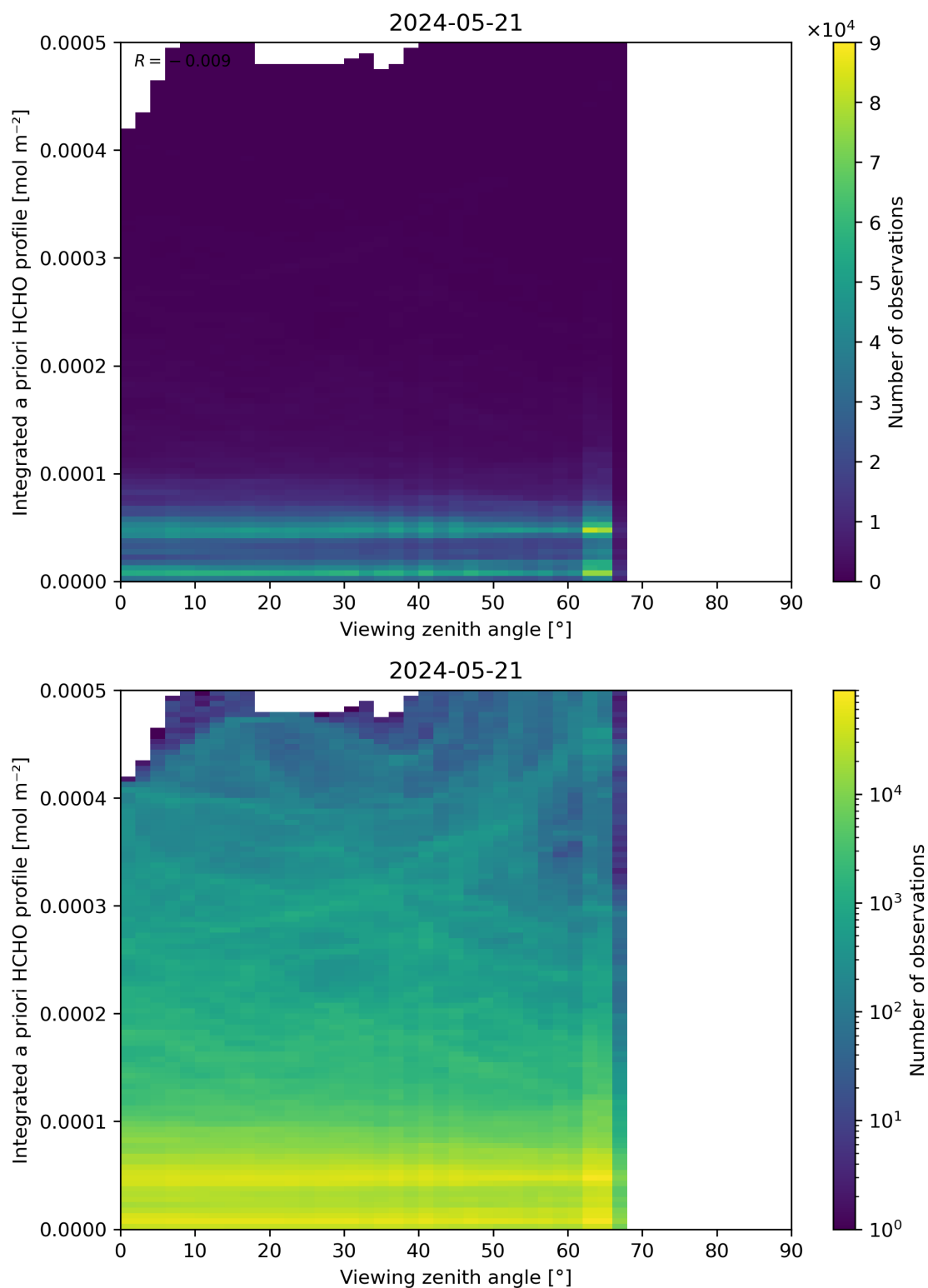
Figure 195: Scatter density plot of “Viewing zenith angle” against “Integrated a priori HCHO profile” for 2024-05-20 to 2024-05-22.
