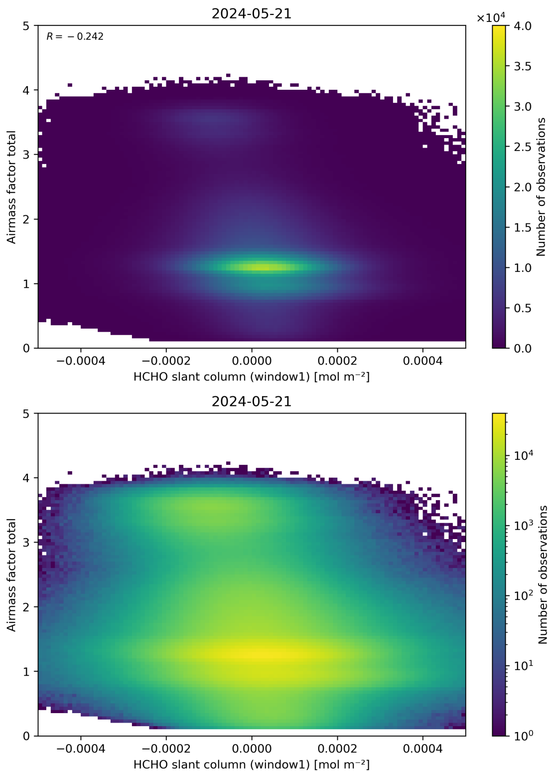
Figure 85: Scatter density plot of “HCHO slant column (window1)” against “Airmass factor total” for 2024-05-20 to 2024-05-22.
