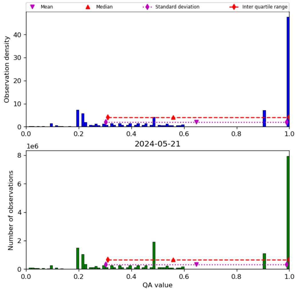
Figure 34: Histogram of “QA value” for 2024-05-20 to 2024-05-22
