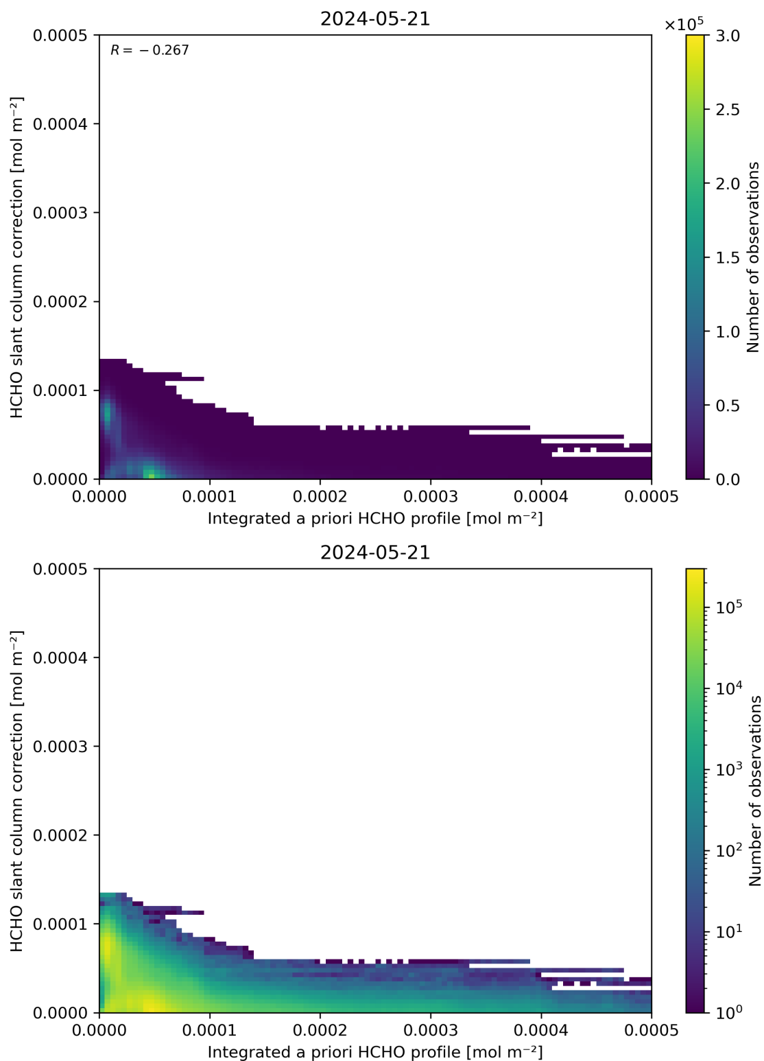
Figure 152: Scatter density plot of “Integrated a priori HCHO profile” against “HCHO slant column correction” for 2024-05-20 to 2024-05-22.
