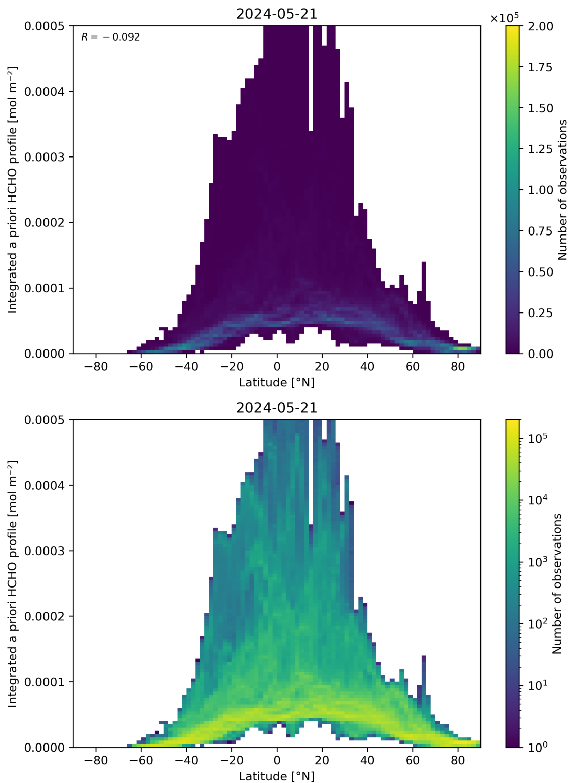
Figure 166: Scatter density plot of “Latitude” against “Integrated a priori HCHO profile” for 2024-05-20 to 2024-05-22.
