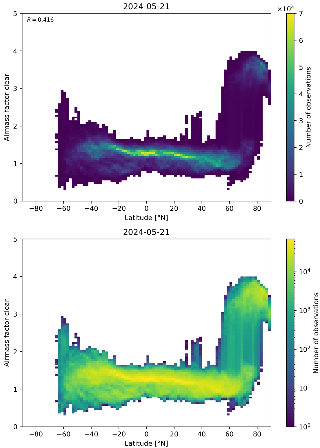
Figure 156: Scatter density plot of “Latitude” against “Airmass factor clear” for 2024-05-20 to 2024-05-22.
