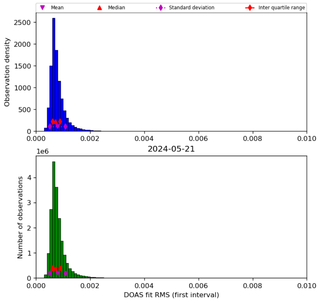
Figure 46: Histogram of “DOAS fit RMS (first interval)” for 2024-05-20 to 2024-05-22
