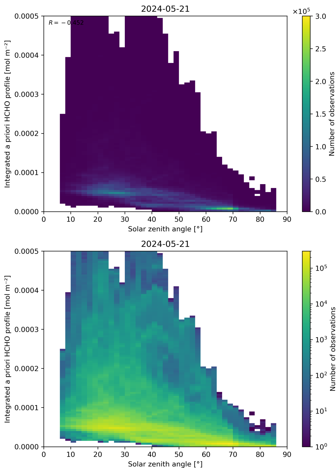
Figure 180: Scatter density plot of “Solar zenith angle” against “Integrated a priori HCHO profile” for 2024-05-20 to 2024-05-22.
