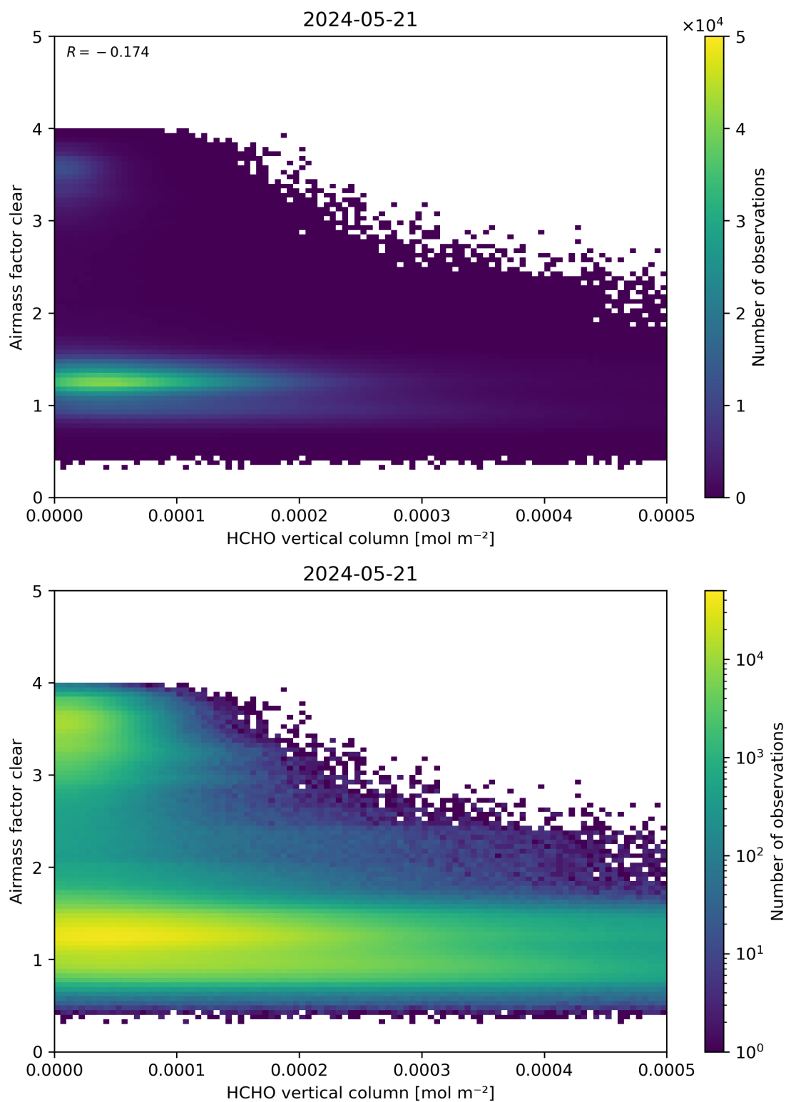
Figure 126: Scatter density plot of “HCHO vertical column” against “Airmass factor clear” for 2024-05-20 to 2024-05-22.
