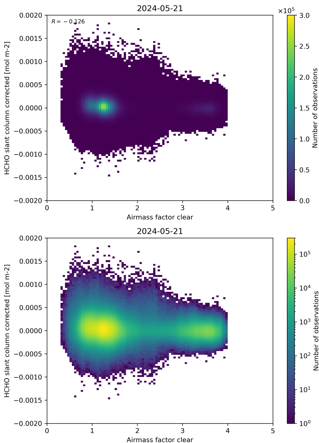
Figure 74: Scatter density plot of “Airmass factor clear” against “HCHO slant column corrected” for 2024-05-20 to 2024-05-22.
