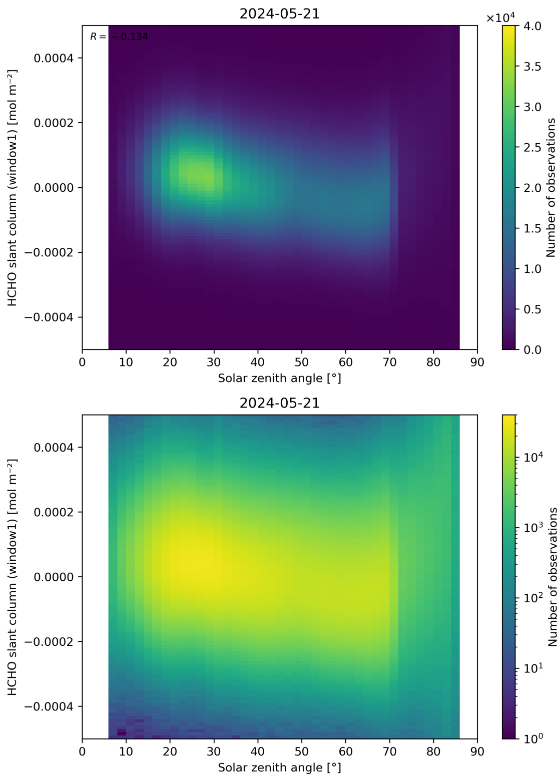
Figure 173: Scatter density plot of “Solar zenith angle” against “HCHO slant column (window1)” for 2024-05-20 to 2024-05-22.
