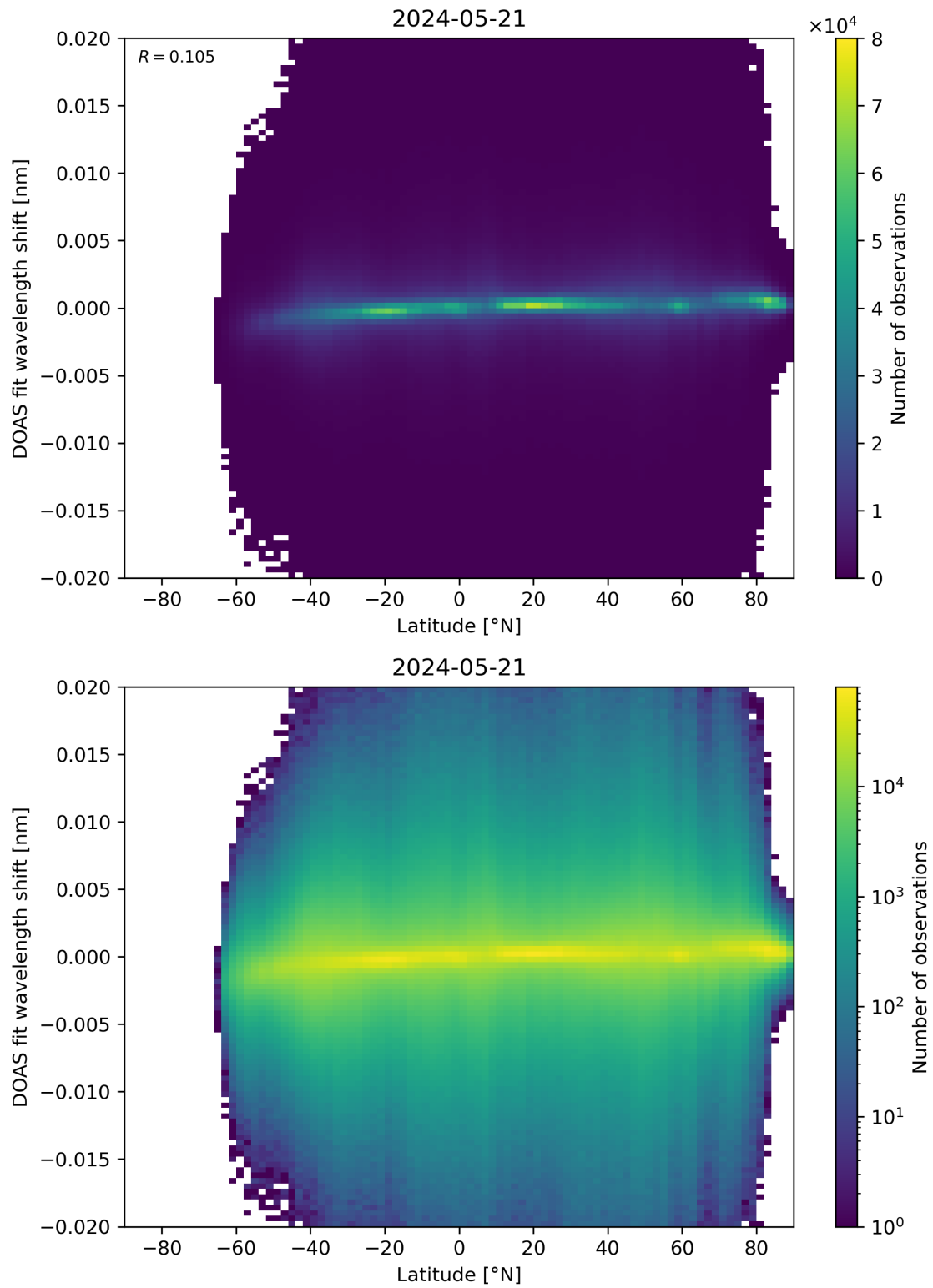
Figure 154: Scatter density plot of “Latitude” against “DOAS fit wavelength shift” for 2024-05-20 to 2024-05-22.
