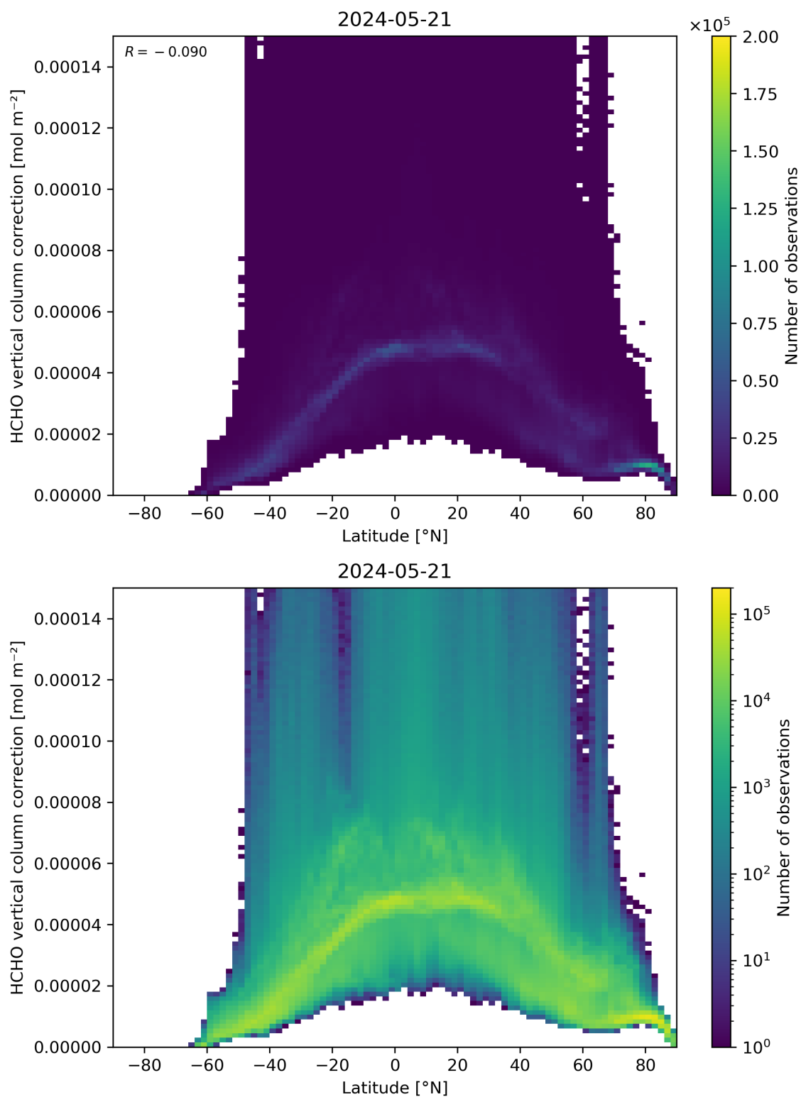
Figure 164: Scatter density plot of “Latitude” against “HCHO vertical column correction” for 2024-05-20 to 2024-05-22.
