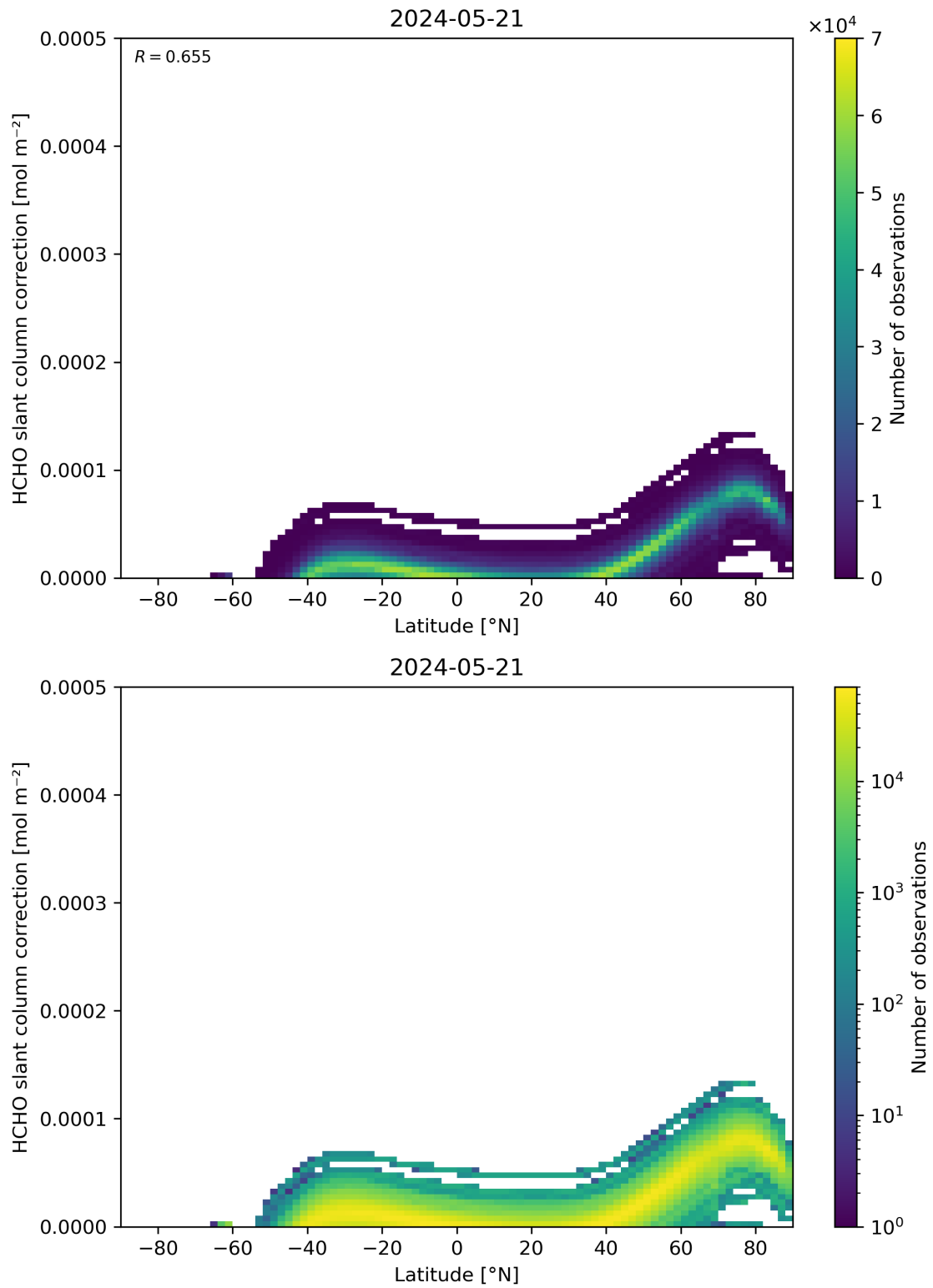
Figure 158: Scatter density plot of “Latitude” against “HCHO slant column correction” for 2024-05-20 to 2024-05-22.
