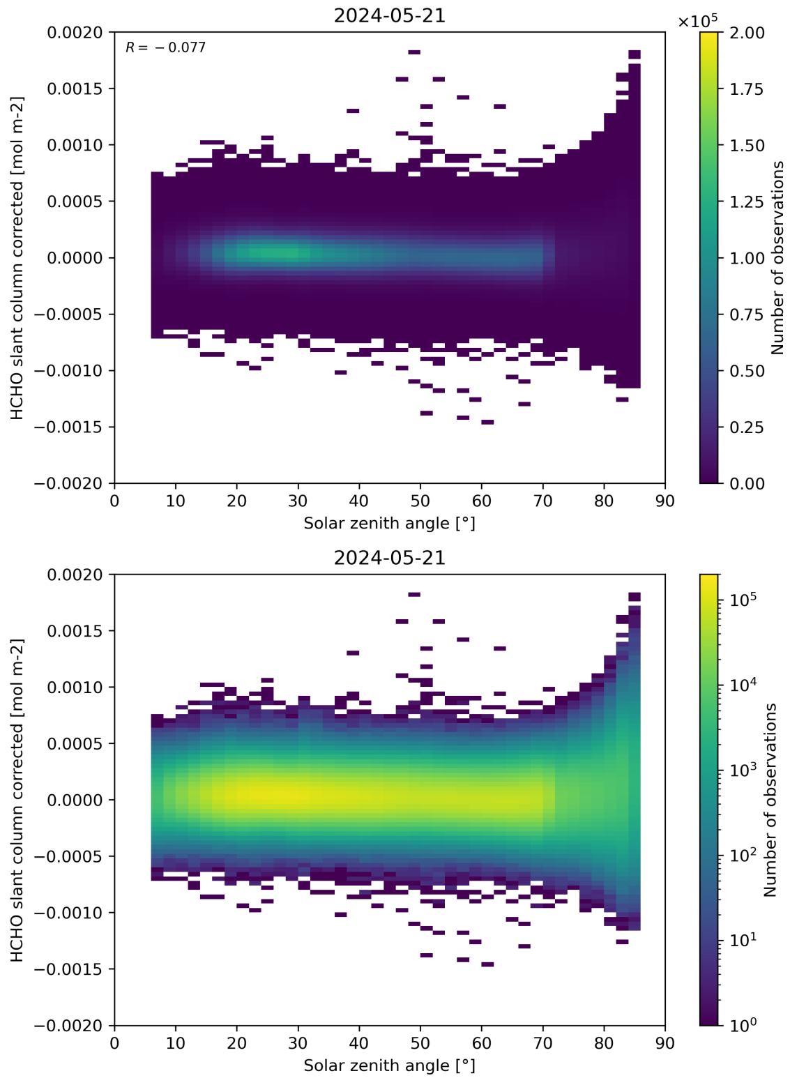
Figure 171: Scatter density plot of “Solar zenith angle” against “HCHO slant column corrected” for 2024-05-20 to 2024-05-22.
