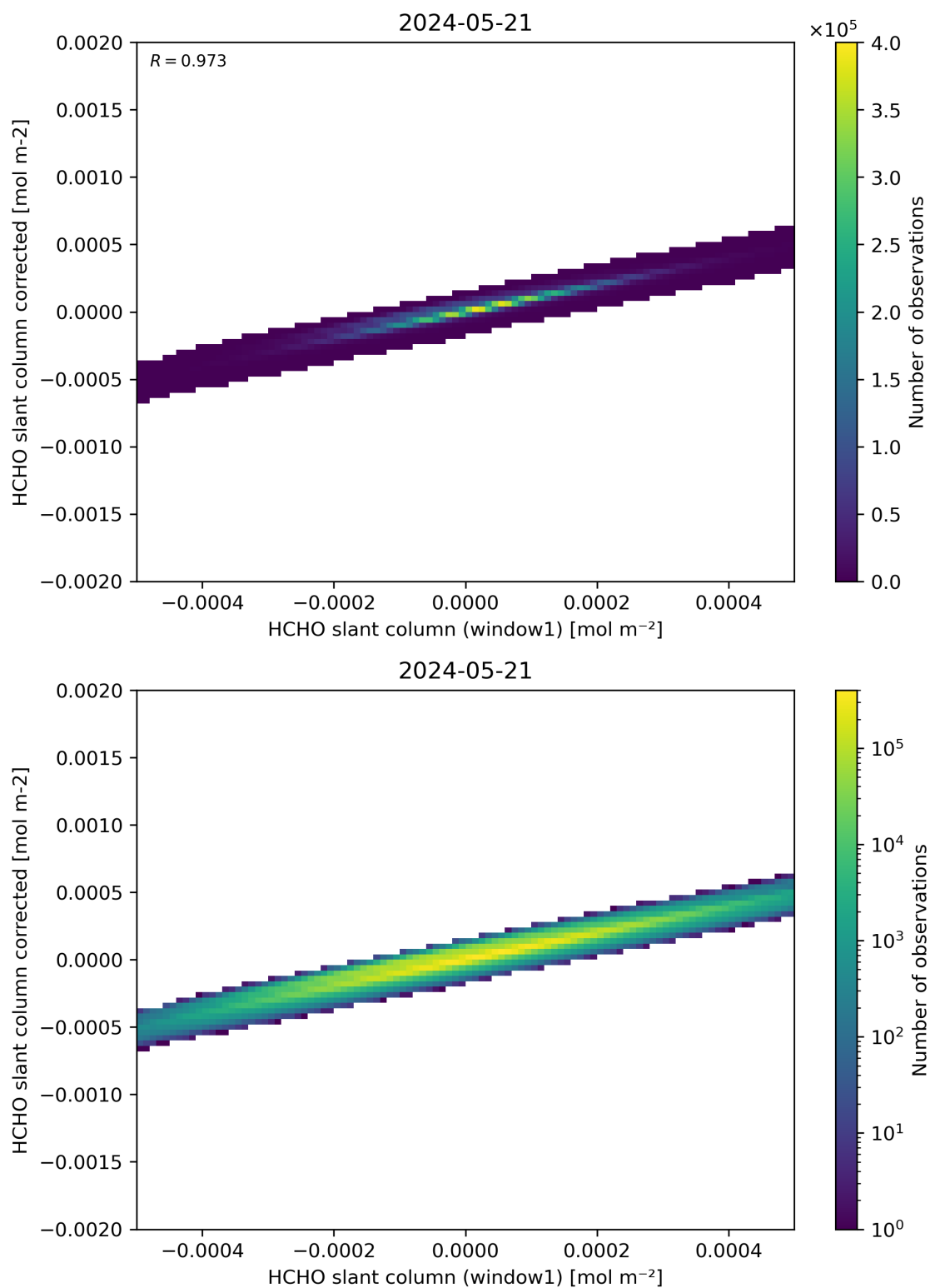
Figure 82: Scatter density plot of “HCHO slant column (window1)” against “HCHO slant column corrected” for 2024-05-20 to 2024-05-22.
