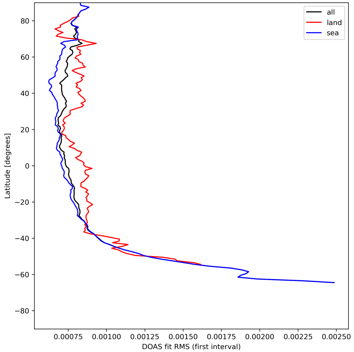
Figure 32: Zonal average of “DOAS fit RMS (first interval)” for 2024-05-20 to 2024-05-22.
