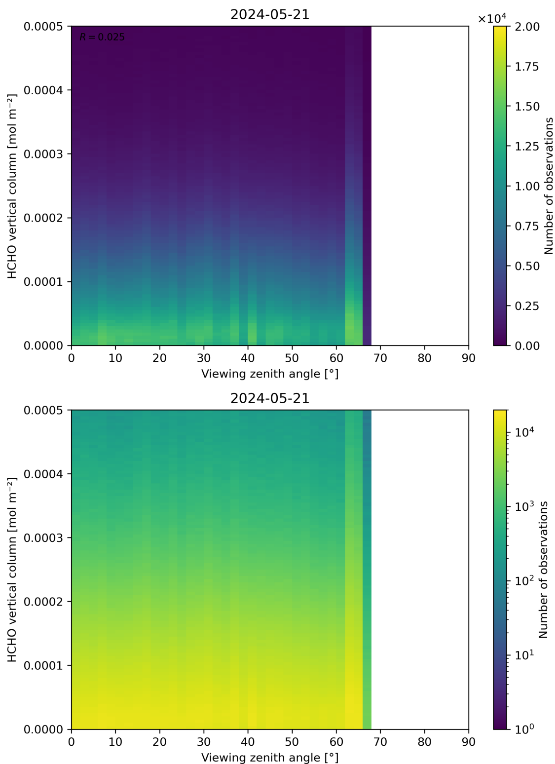
Figure 192: Scatter density plot of “Viewing zenith angle” against “HCHO vertical column” for 2024-05-20 to 2024-05-22.
