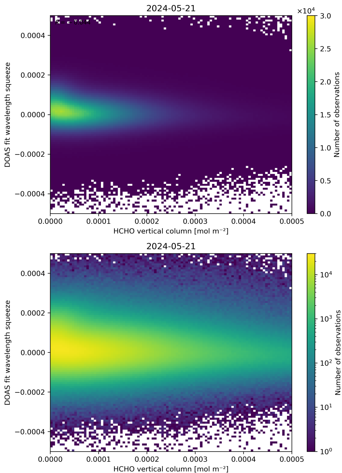
Figure 125: Scatter density plot of “HCHO vertical column” against “DOAS fit wavelength squeeze” for 2024-05-20 to 2024-05-22.
