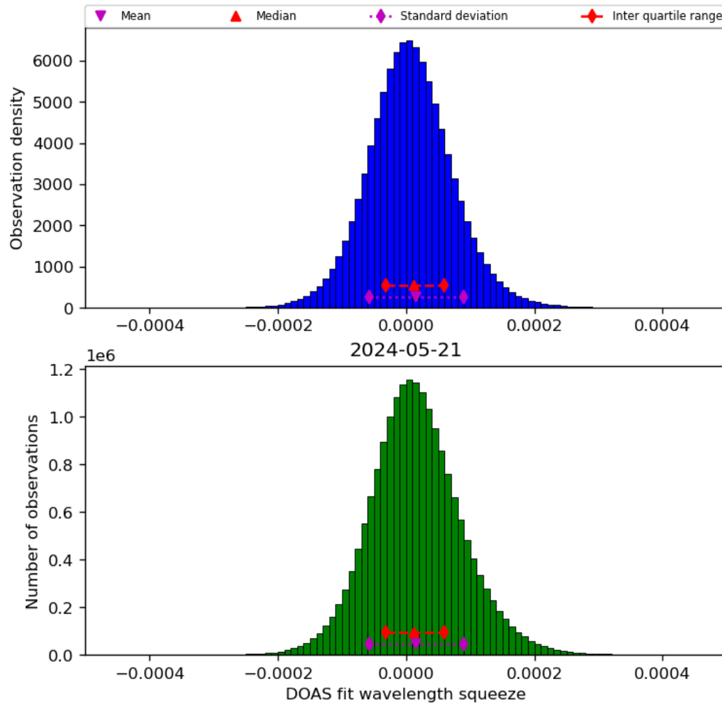
Figure 45: Histogram of “DOAS fit wavelength squeeze” for 2024-05-20 to 2024-05-22
