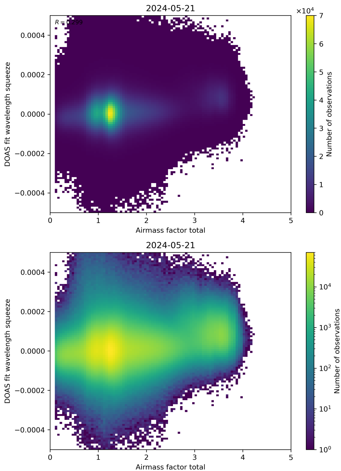
Figure 99: Scatter density plot of “Airmass factor total” against “DOAS fit wavelength squeeze” for 2024-05-20 to 2024-05-22.
