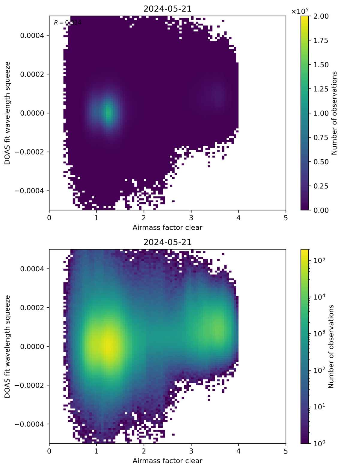
Figure 73: Scatter density plot of “Airmass factor clear” against “DOAS fit wavelength squeeze” for 2024-05-20 to 2024-05-22.
