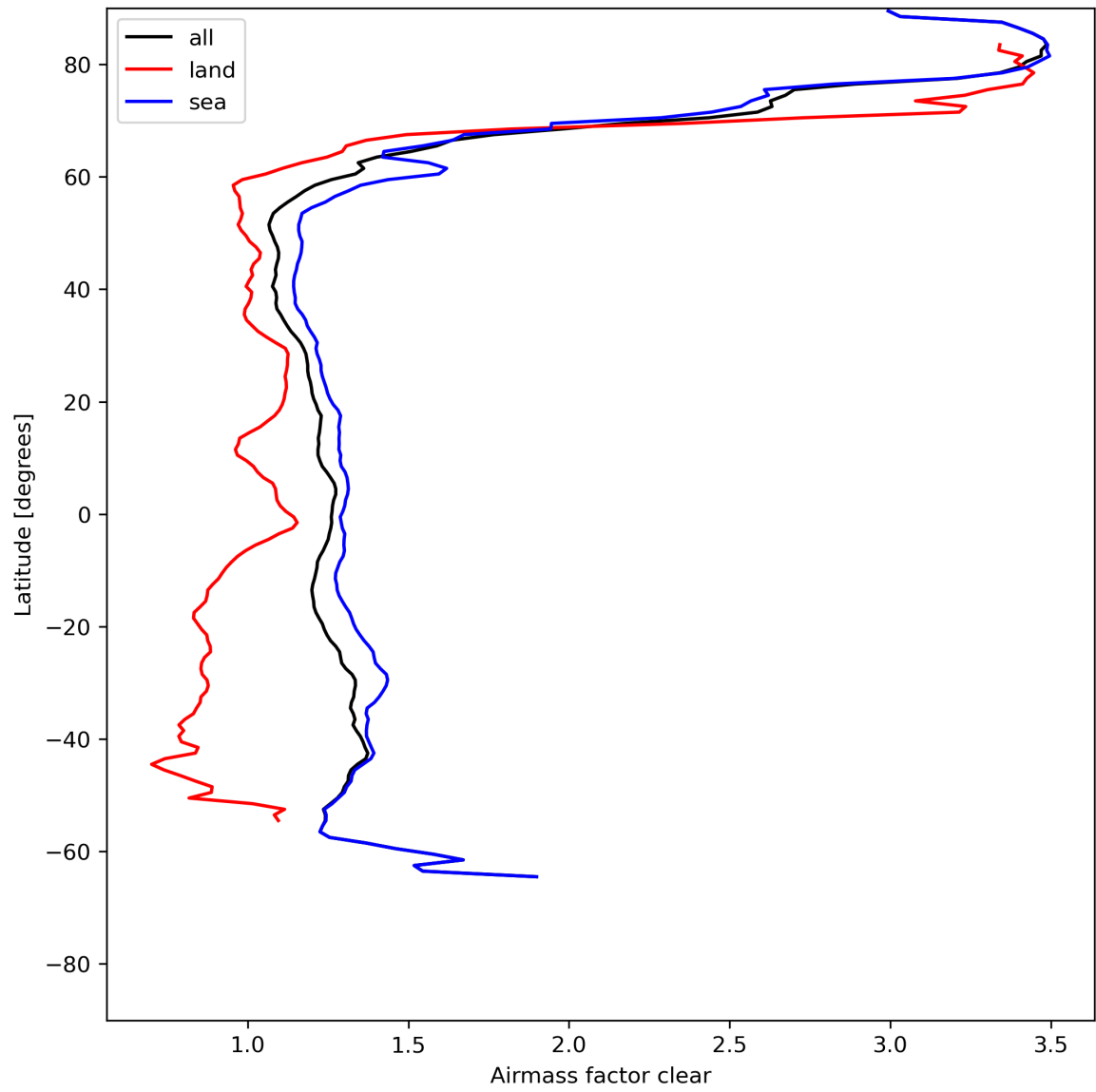
Figure 28: Zonal average of “Airmass factor clear” for 2024-05-20 to 2024-05-22.
