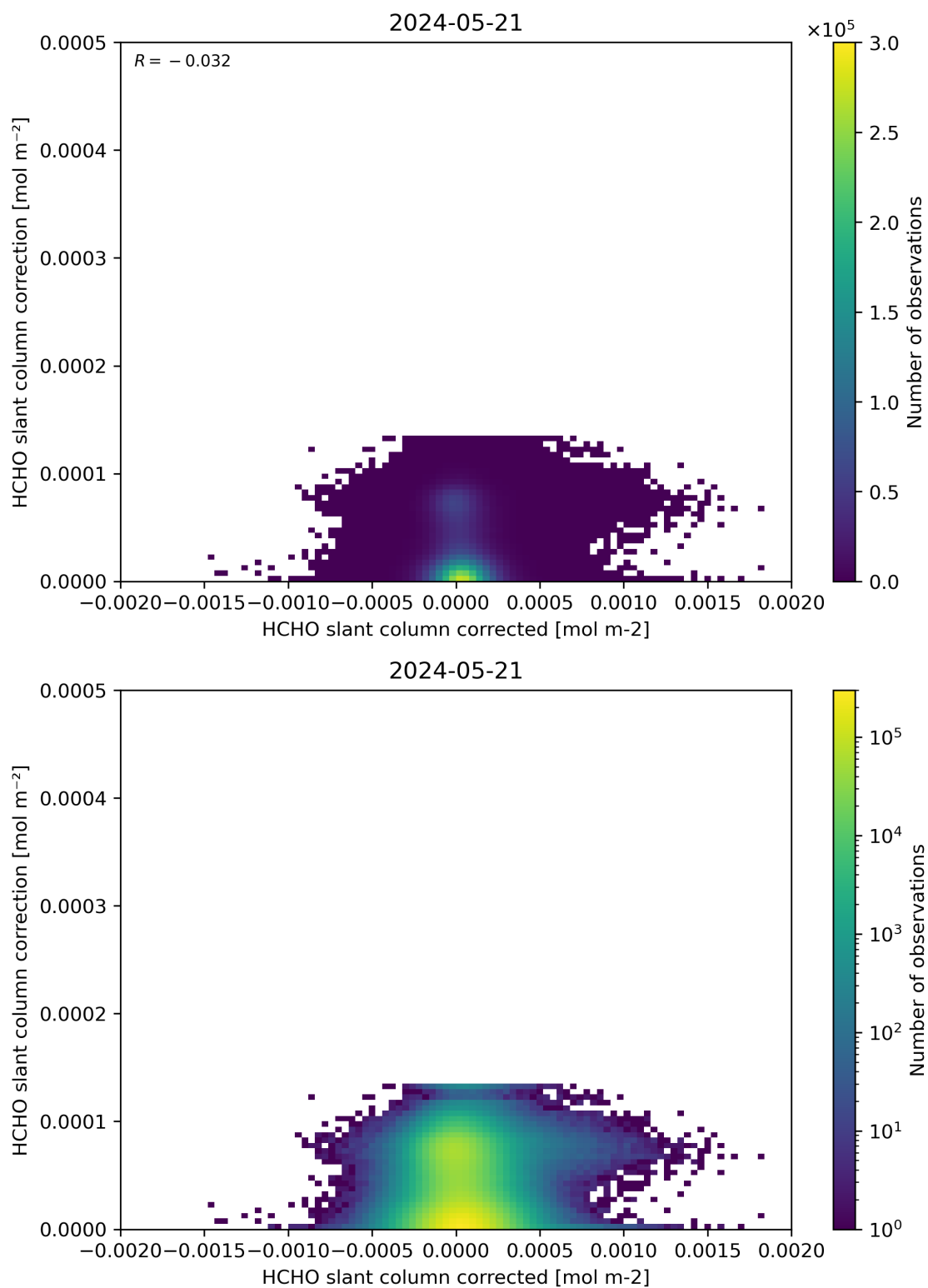
Figure 77: Scatter density plot of “HCHO slant column corrected” against “HCHO slant column correction” for 2024-05-20 to 2024-05-22.
