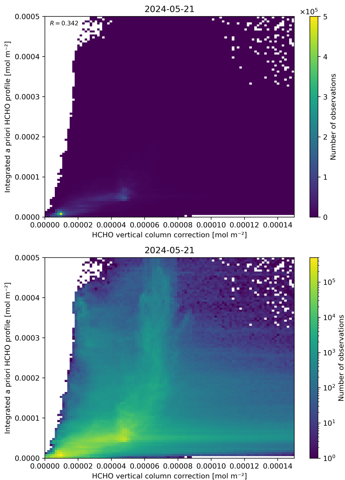
Figure 122: Scatter density plot of “HCHO vertical column correction” against “Integrated a priori HCHO profile” for 2024-05-20 to 2024-05-22.
