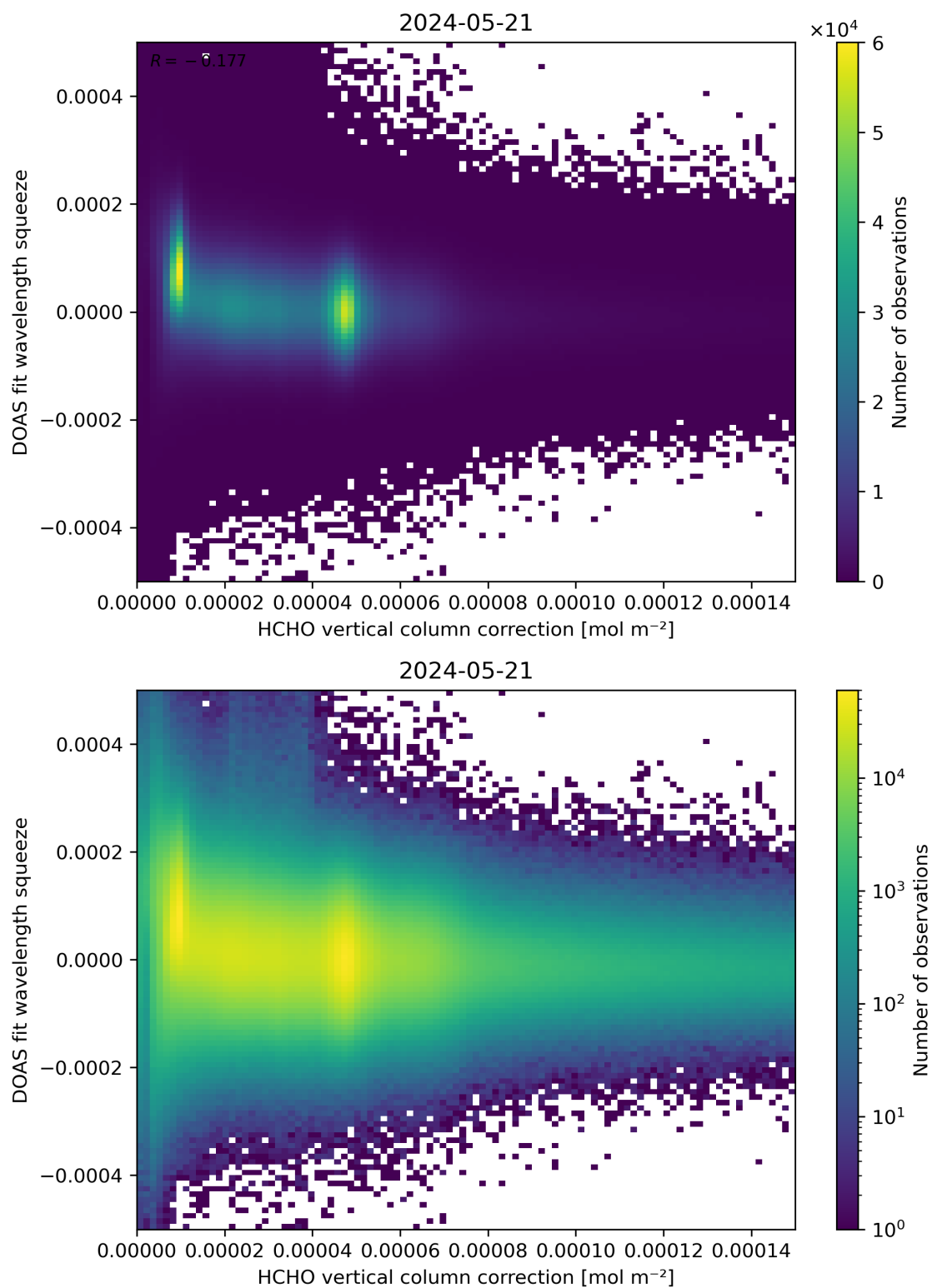
Figure 114: Scatter density plot of “HCHO vertical column correction” against “DOAS fit wavelength squeeze” for 2024-05-20 to 2024-05-22.
