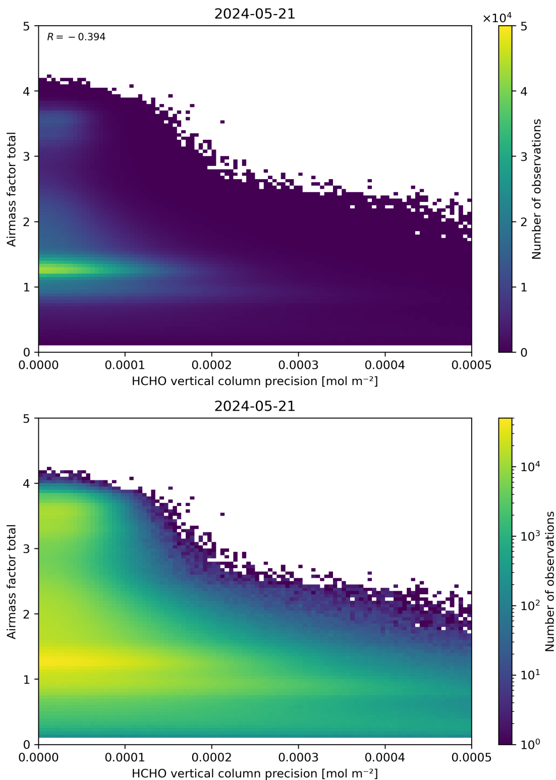
Figure 144: Scatter density plot of “HCHO vertical column precision” against “Airmass factor total” for 2024-05-20 to 2024-05-22.
