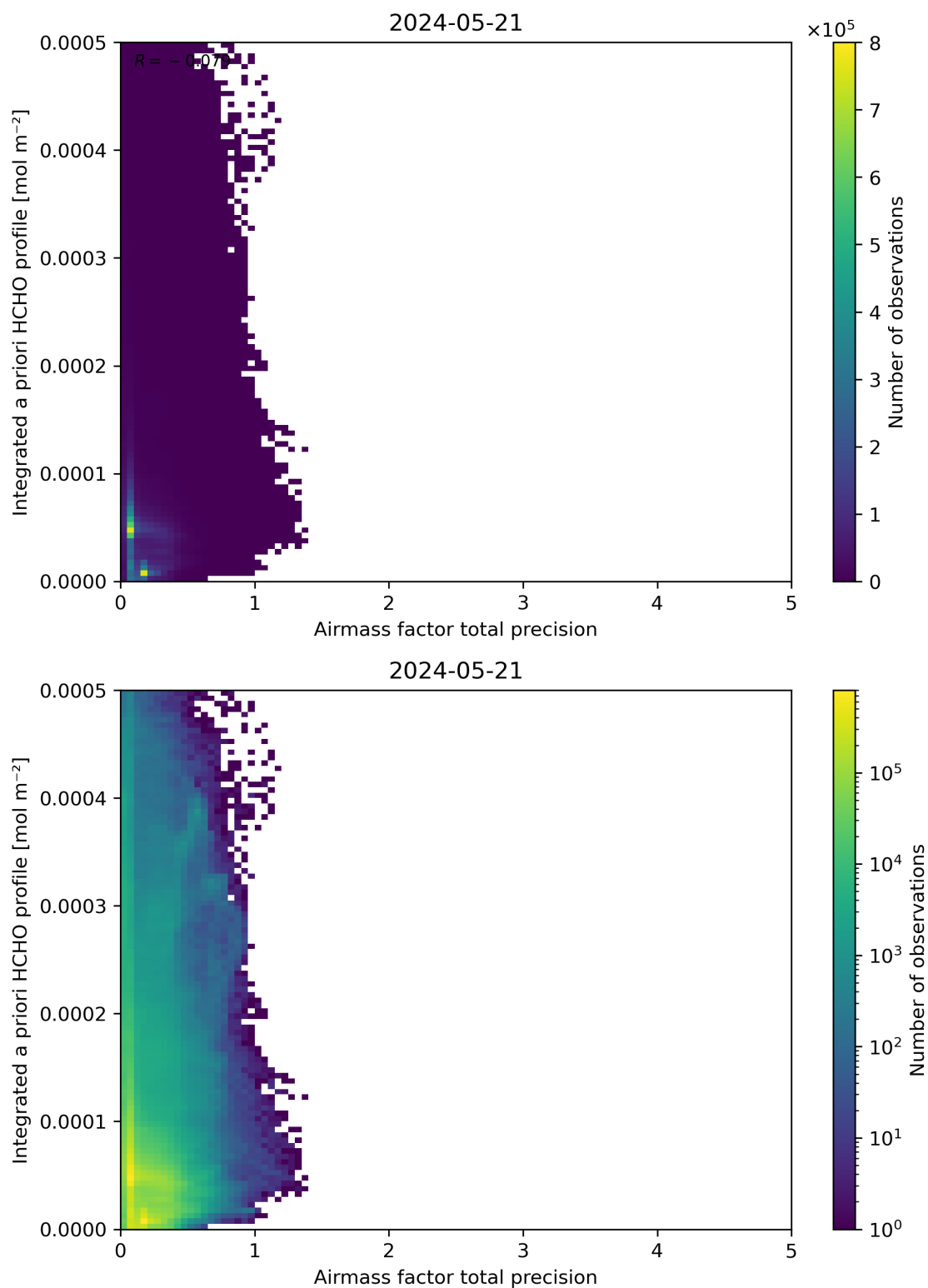
Figure 111: Scatter density plot of “Airmass factor total precision” against “Integrated a priori HCHO profile” for 2024-05-20 to 2024-05-22.
