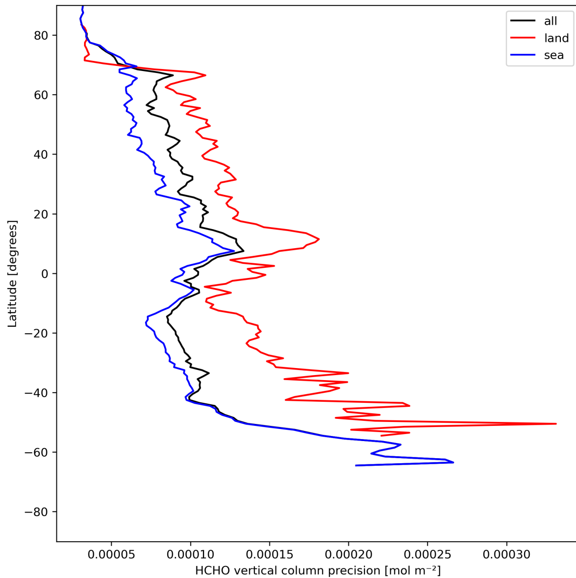
Figure 22: Zonal average of “HCHO vertical column precision” for 2024-05-20 to 2024-05-22.
