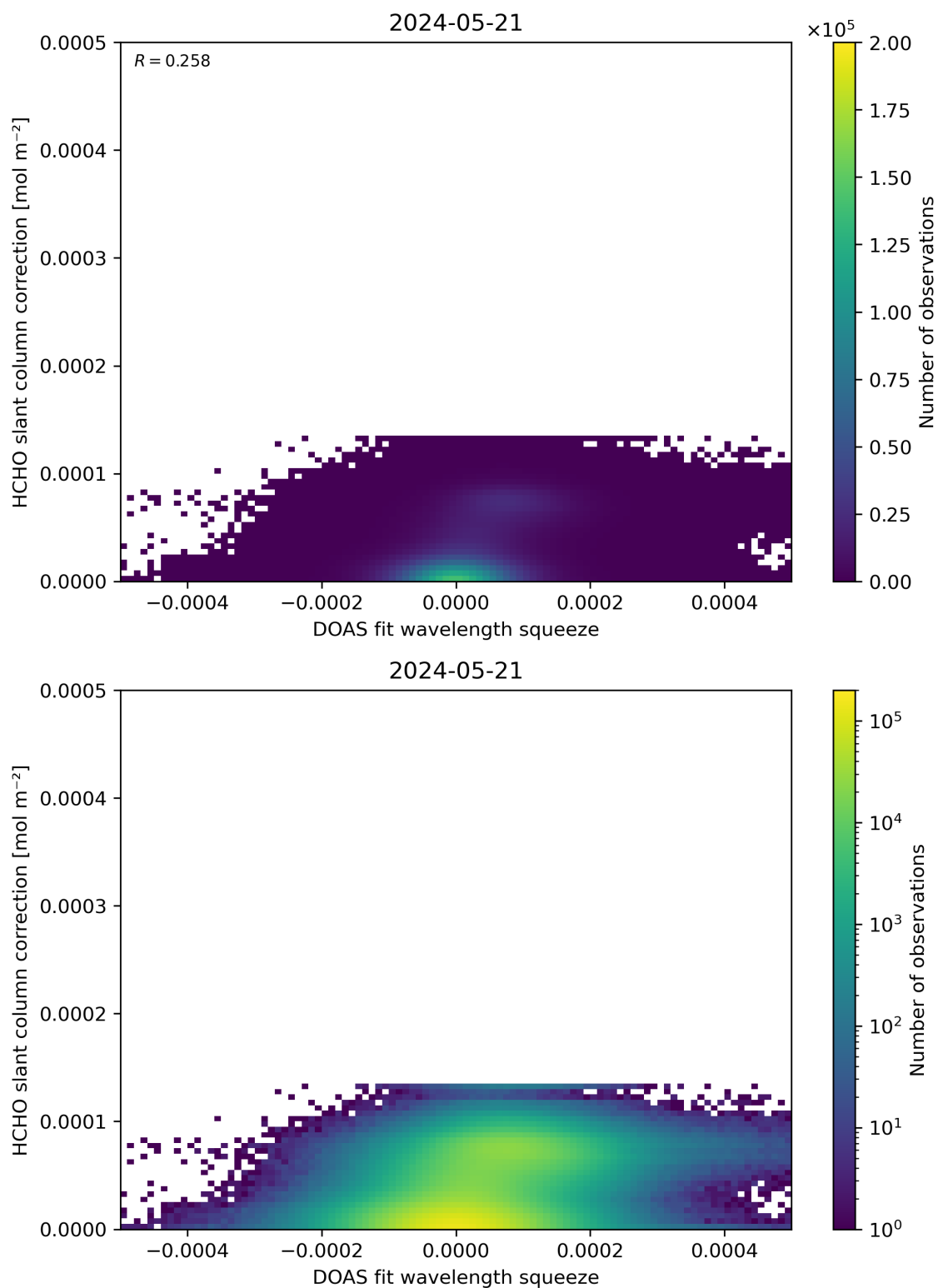
Figure 70: Scatter density plot of “DOAS fit wavelength squeeze” against “HCHO slant column correction” for 2024-05-20 to 2024-05-22.
