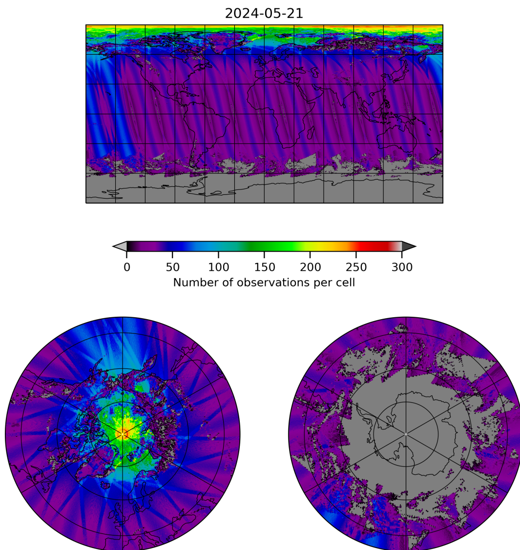
Figure 19: Map of the number of observations for 2024-05-20 to 2024-05-22
