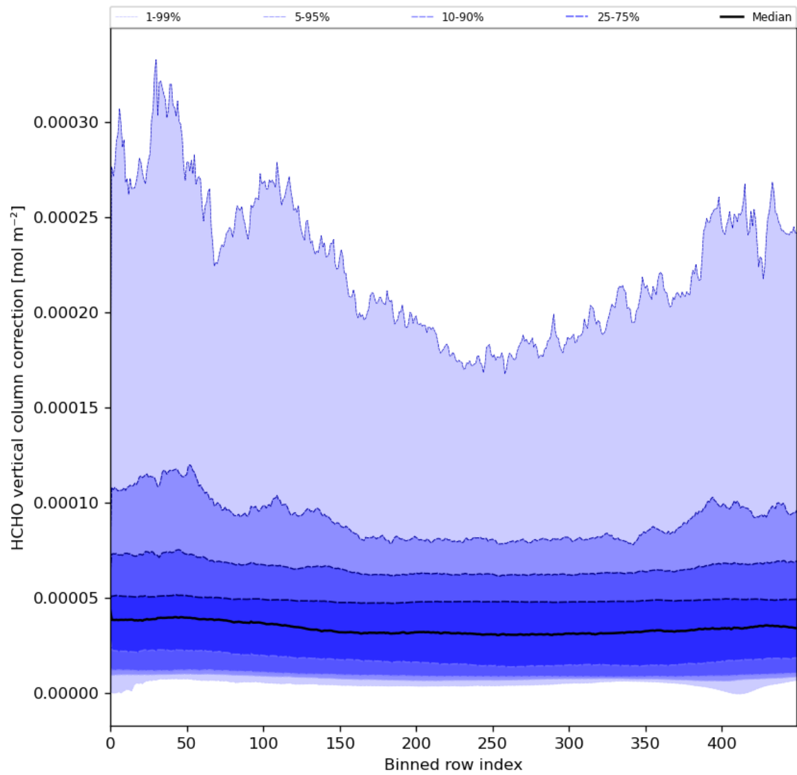
Figure 51: Along track statistics of “HCHO vertical column correction” for 2024-05-20 to 2024-05-22
