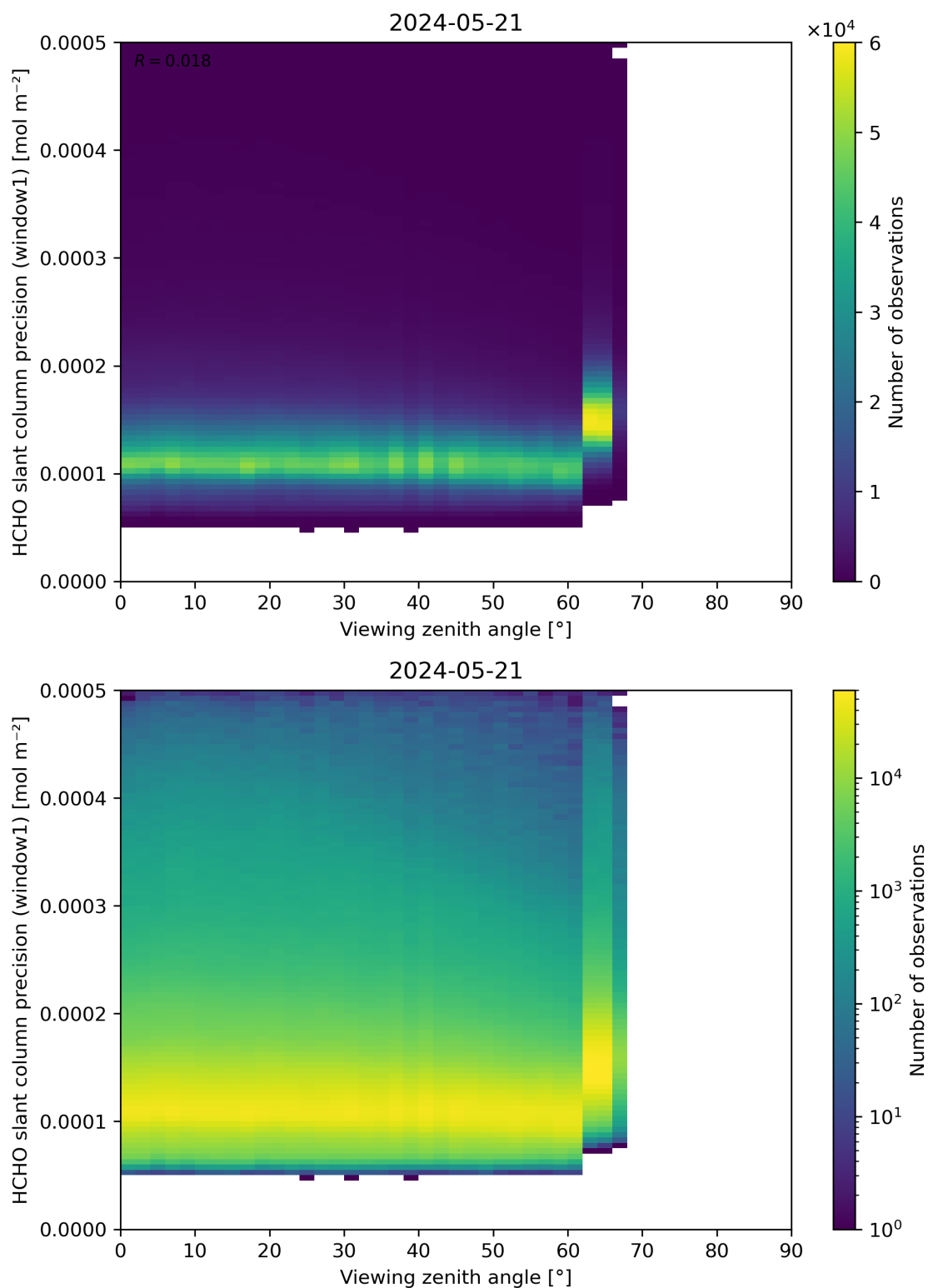
Figure 189: Scatter density plot of “Viewing zenith angle” against “HCHO slant column precision (window1)” for 2024-05-20 to 2024-05-22.
