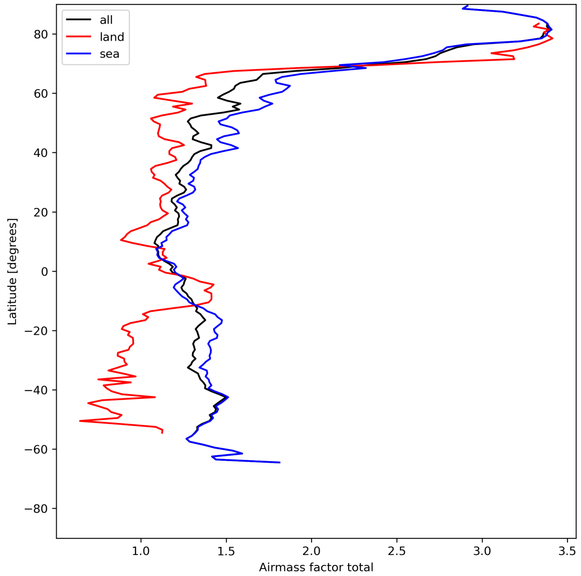
Figure 26: Zonal average of “Airmass factor total” for 2024-05-20 to 2024-05-22.
