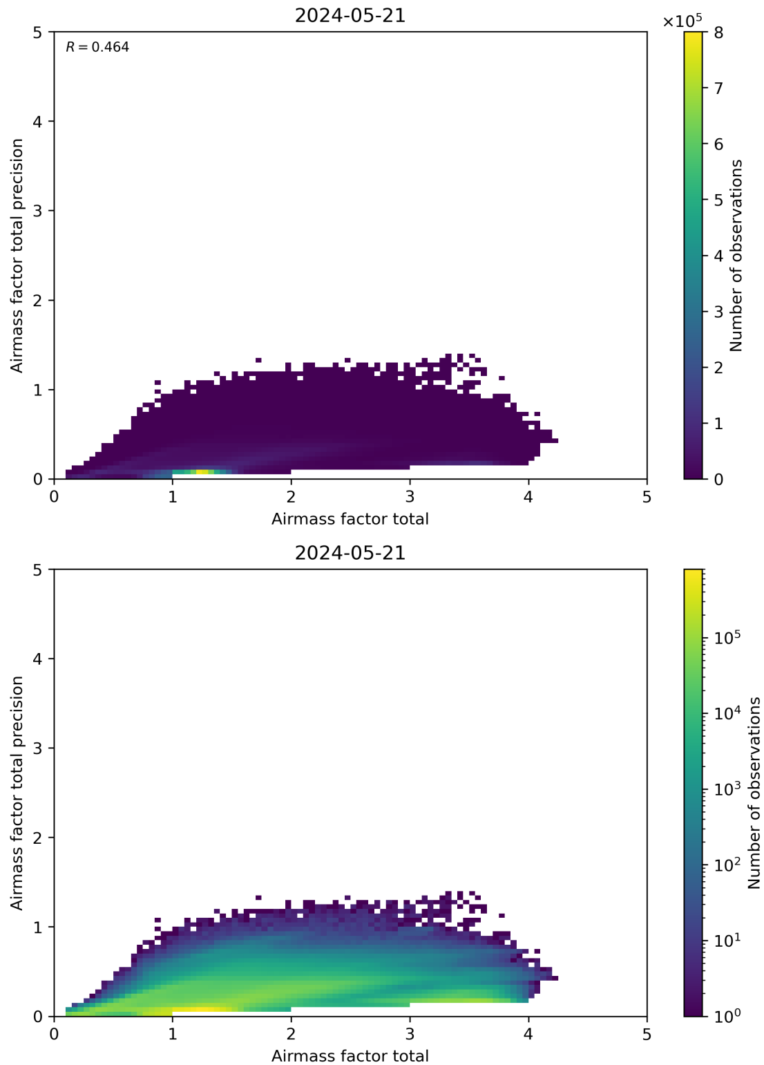
Figure 103: Scatter density plot of “Airmass factor total” against “Airmass factor total precision” for 2024-05-20 to 2024-05-22.
