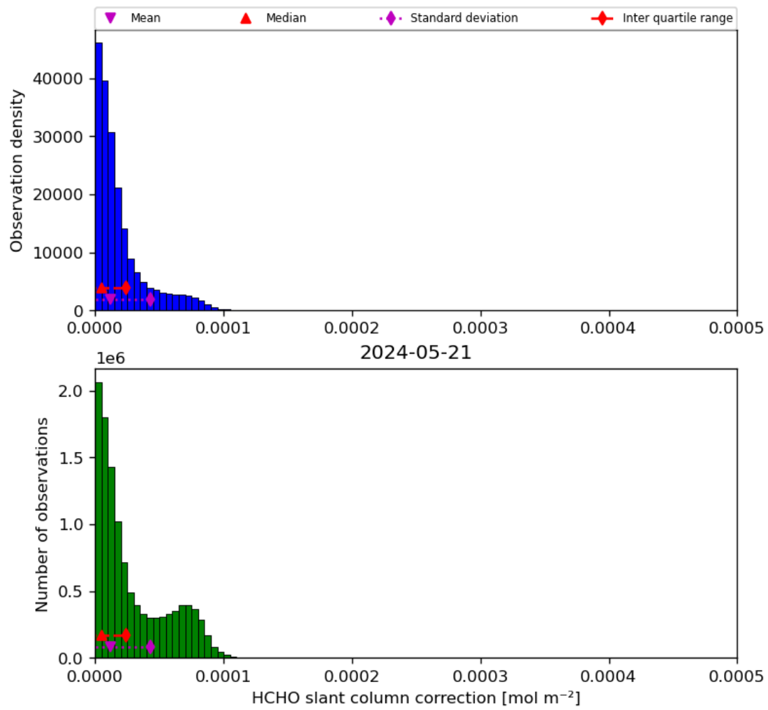
Figure 47: Histogram of “HCHO slant column correction” for 2024-05-20 to 2024-05-22
