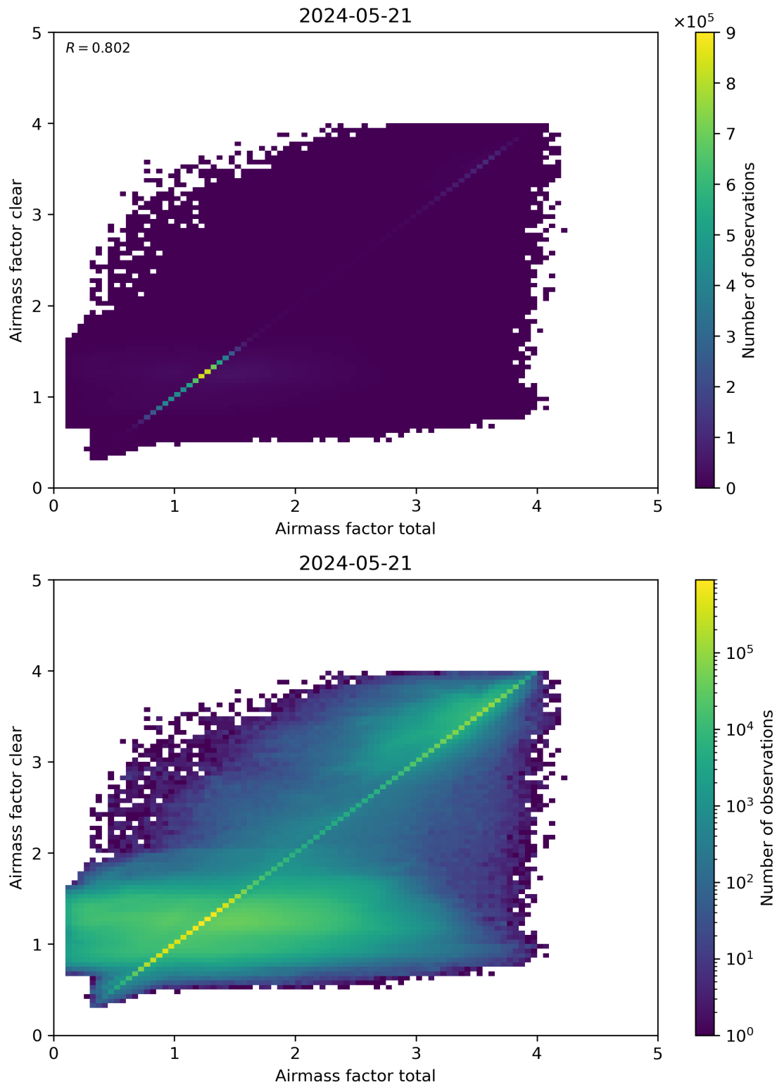
Figure 100: Scatter density plot of “Airmass factor total” against “Airmass factor clear” for 2024-05-20 to 2024-05-22.
