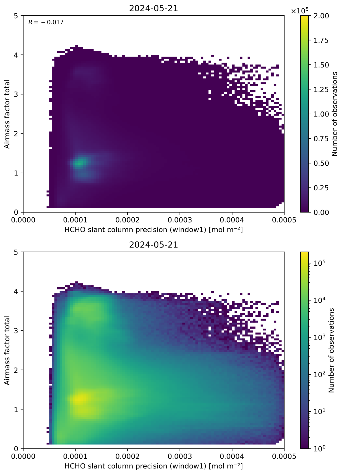
Figure 94: Scatter density plot of “HCHO slant column precision (window1)” against “Airmass factor total” for 2024-05-20 to 2024-05-22.
