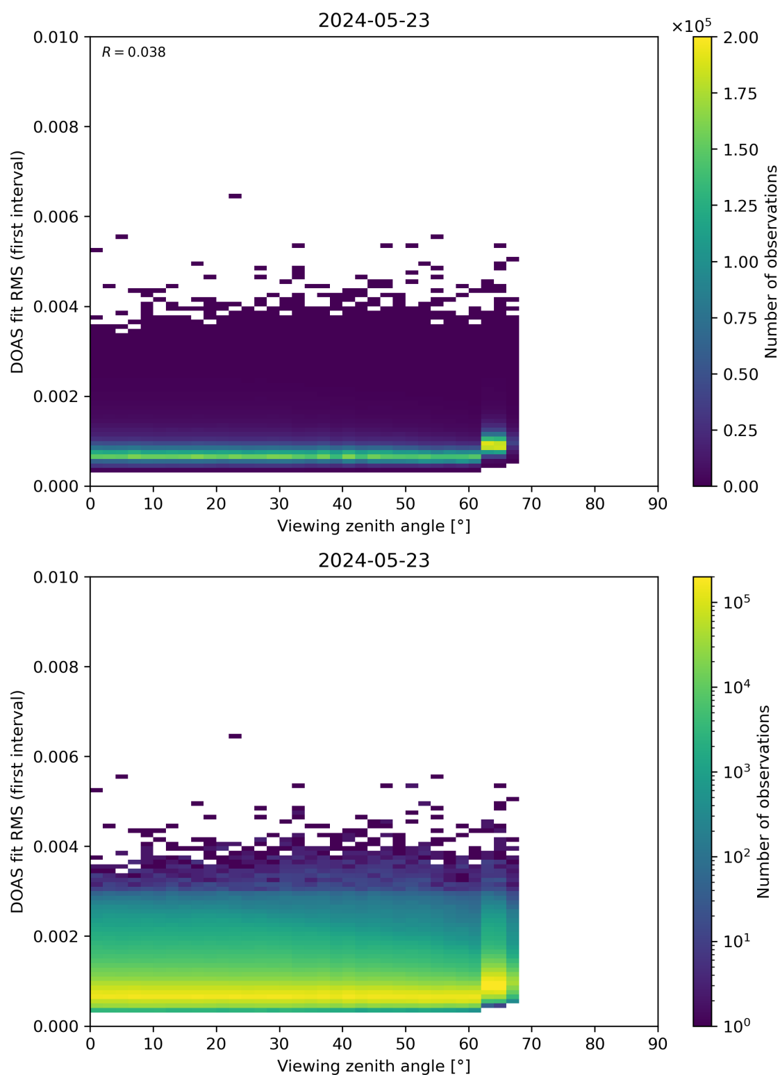
Figure 182: Scatter density plot of “Viewing zenith angle” against “DOAS fit RMS (first interval)” for 2024-05-23 to 2024-05-24.
