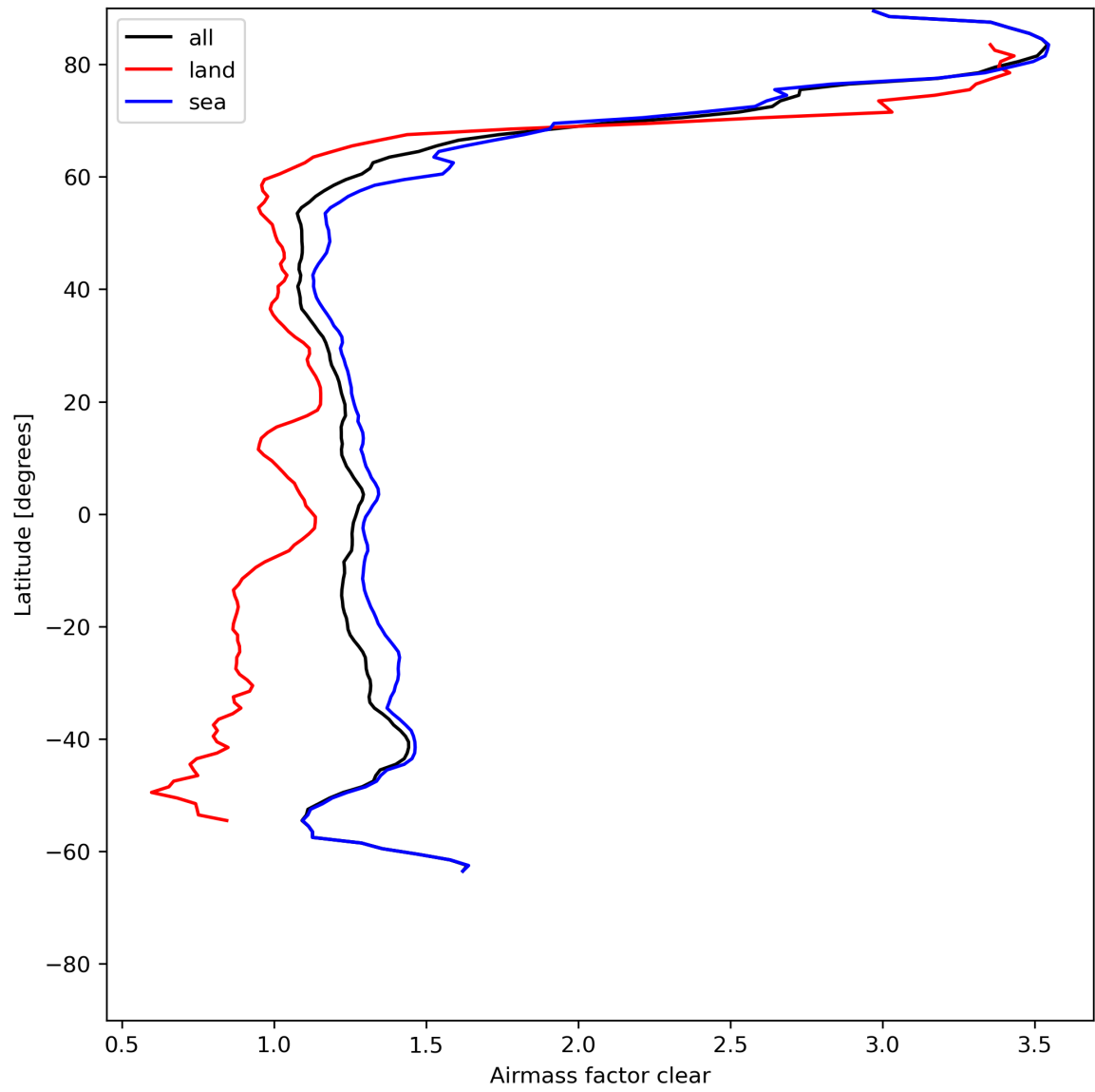
Figure 28: Zonal average of “Airmass factor clear” for 2024-05-23 to 2024-05-24.
