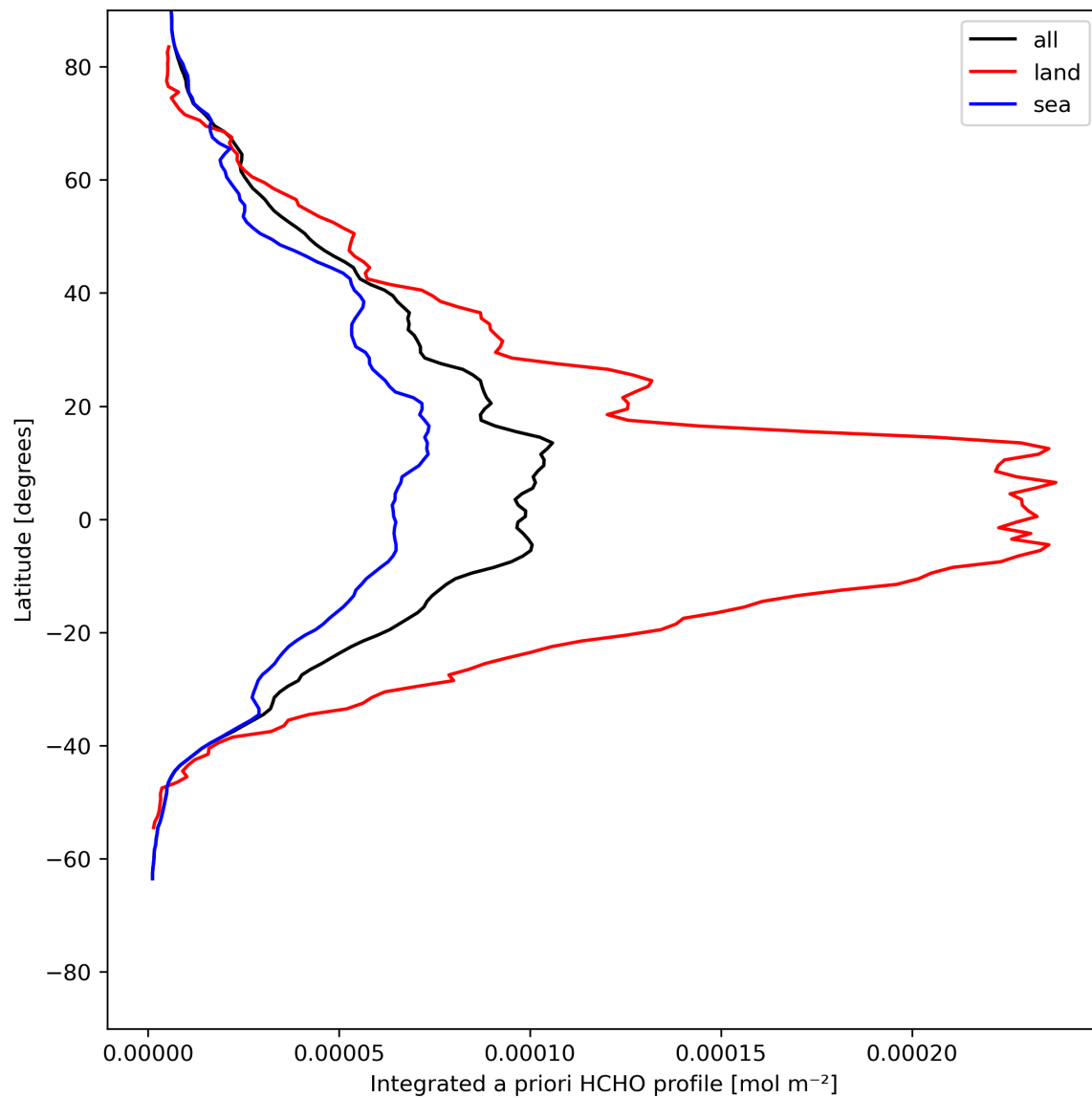
Figure 29: Zonal average of “Integrated a priori HCHO profile” for 2024-05-23 to 2024-05-24.
