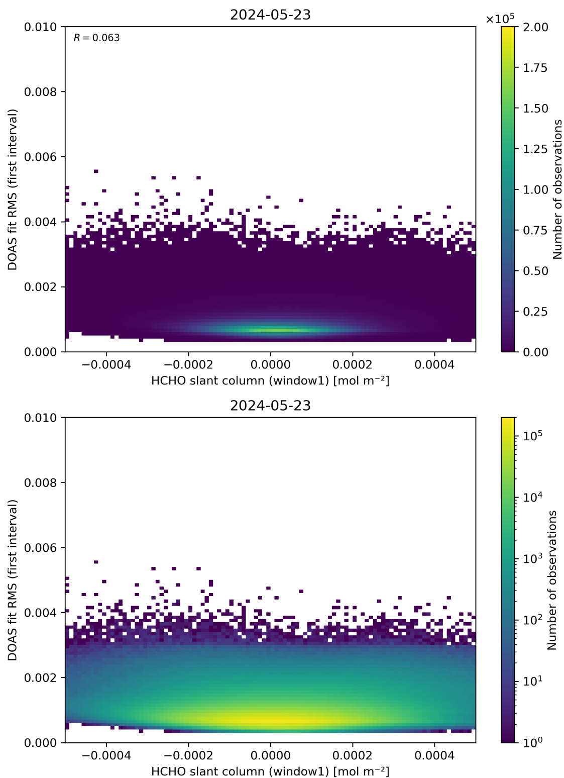
Figure 78: Scatter density plot of “HCHO slant column (window1)” against “DOAS fit RMS (first interval)” for 2024-05-23 to 2024-05-24.
