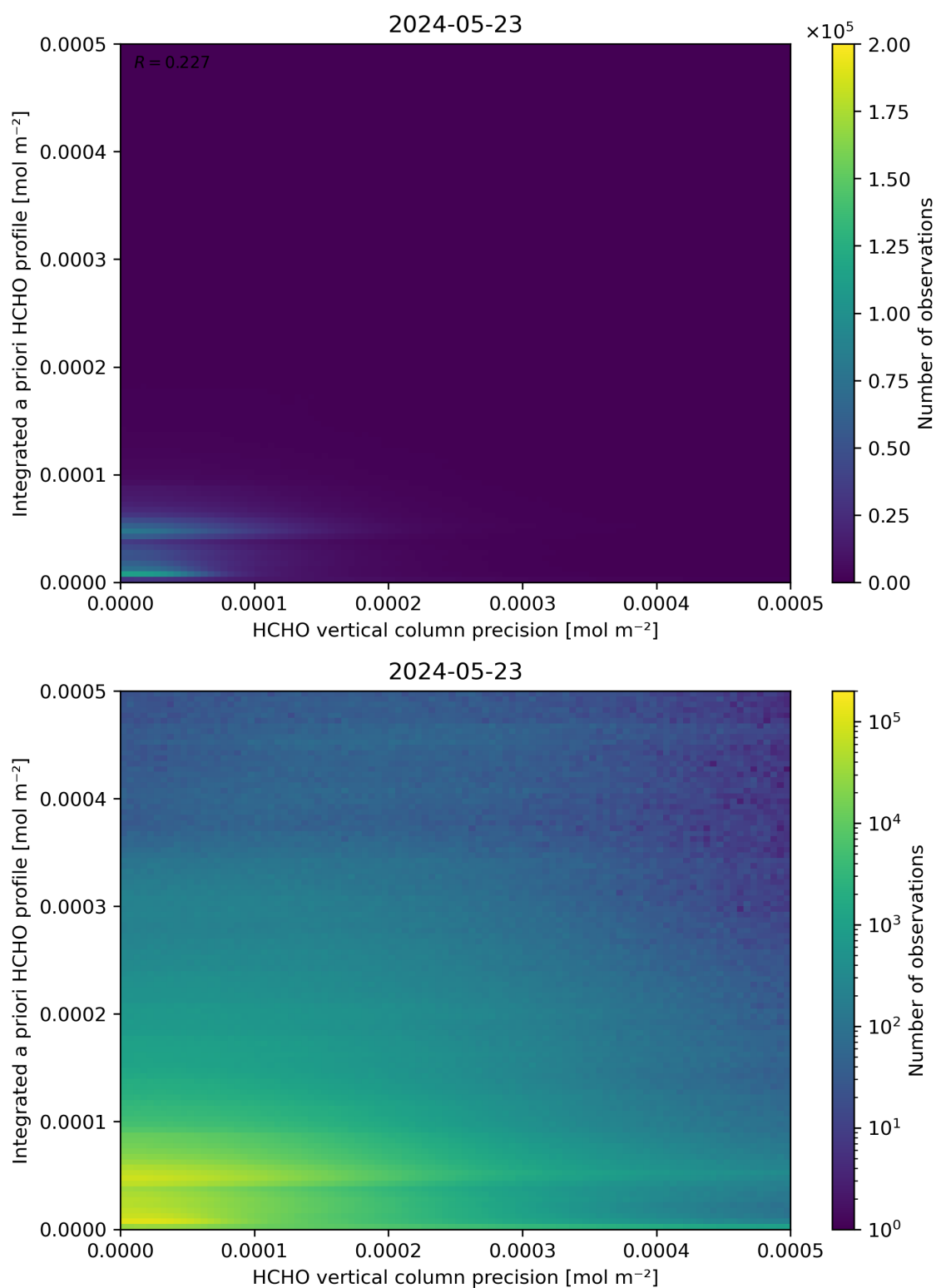
Figure 147: Scatter density plot of “HCHO vertical column precision” against “Integrated a priori HCHO profile” for 2024-05-23 to 2024-05-24.
