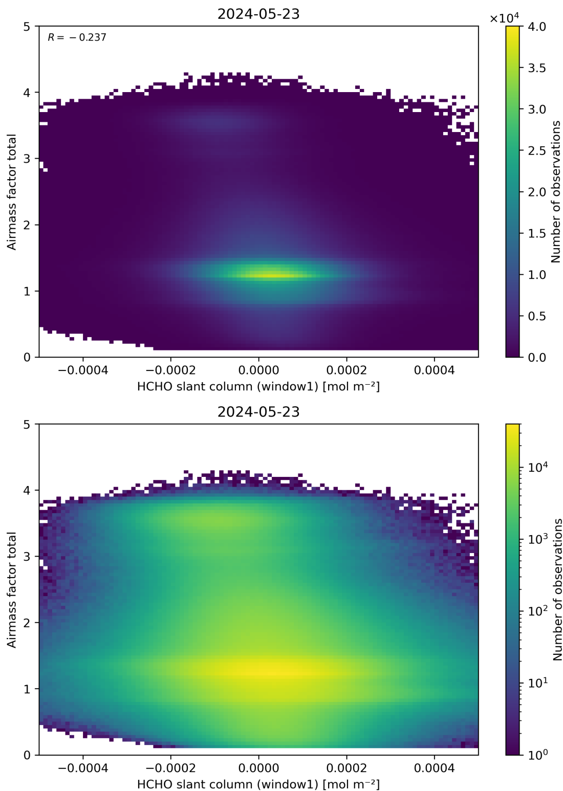
Figure 85: Scatter density plot of “HCHO slant column (window1)” against “Airmass factor total” for 2024-05-23 to 2024-05-24.
