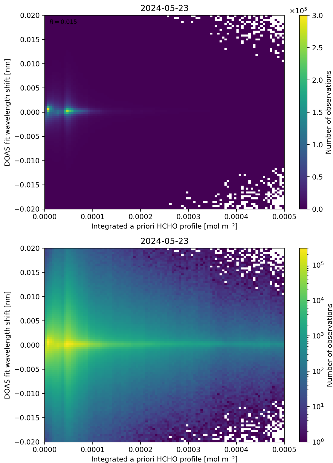
Figure 149: Scatter density plot of “Integrated a priori HCHO profile” against “DOAS fit wavelength shift” for 2024-05-23 to 2024-05-24.
