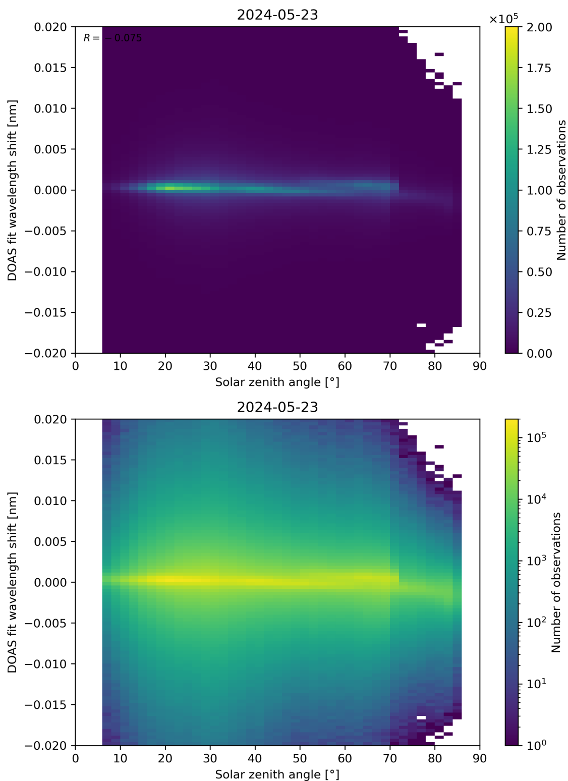
Figure 168: Scatter density plot of “Solar zenith angle” against “DOAS fit wavelength shift” for 2024-05-23 to 2024-05-24.
