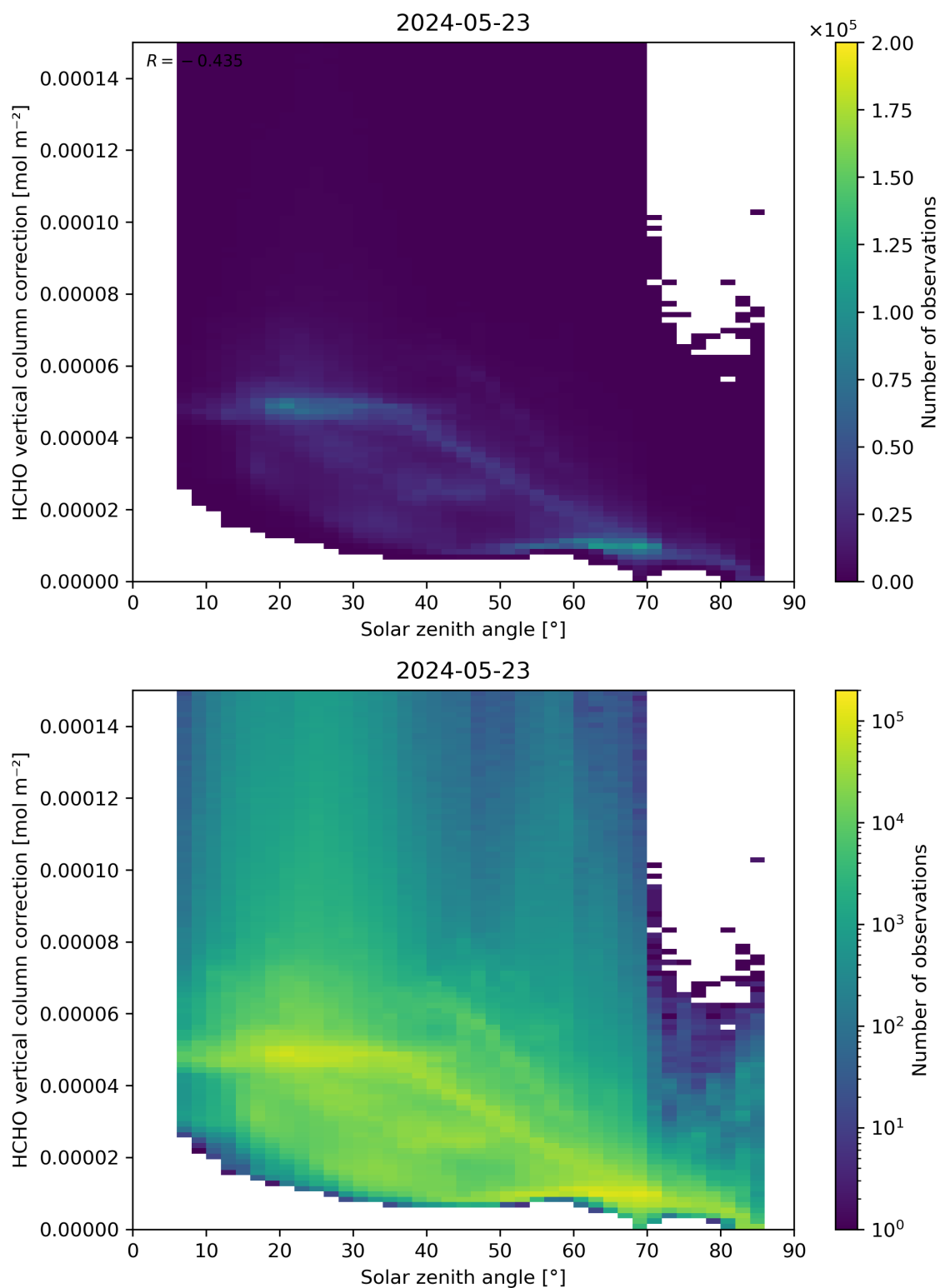
Figure 178: Scatter density plot of “Solar zenith angle” against “HCHO vertical column correction” for 2024-05-23 to 2024-05-24.
