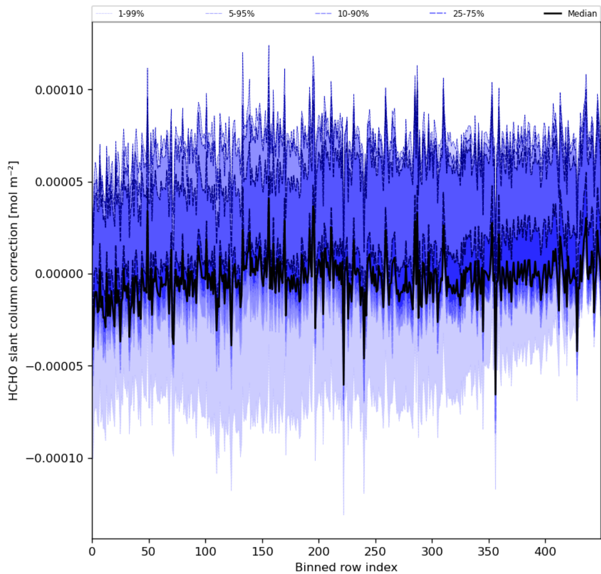
Figure 61: Along track statistics of “HCHO slant column correction” for 2024-05-23 to 2024-05-24
