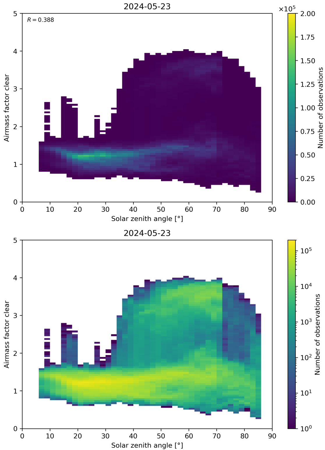
Figure 170: Scatter density plot of “Solar zenith angle” against “Airmass factor clear” for 2024-05-23 to 2024-05-24.
