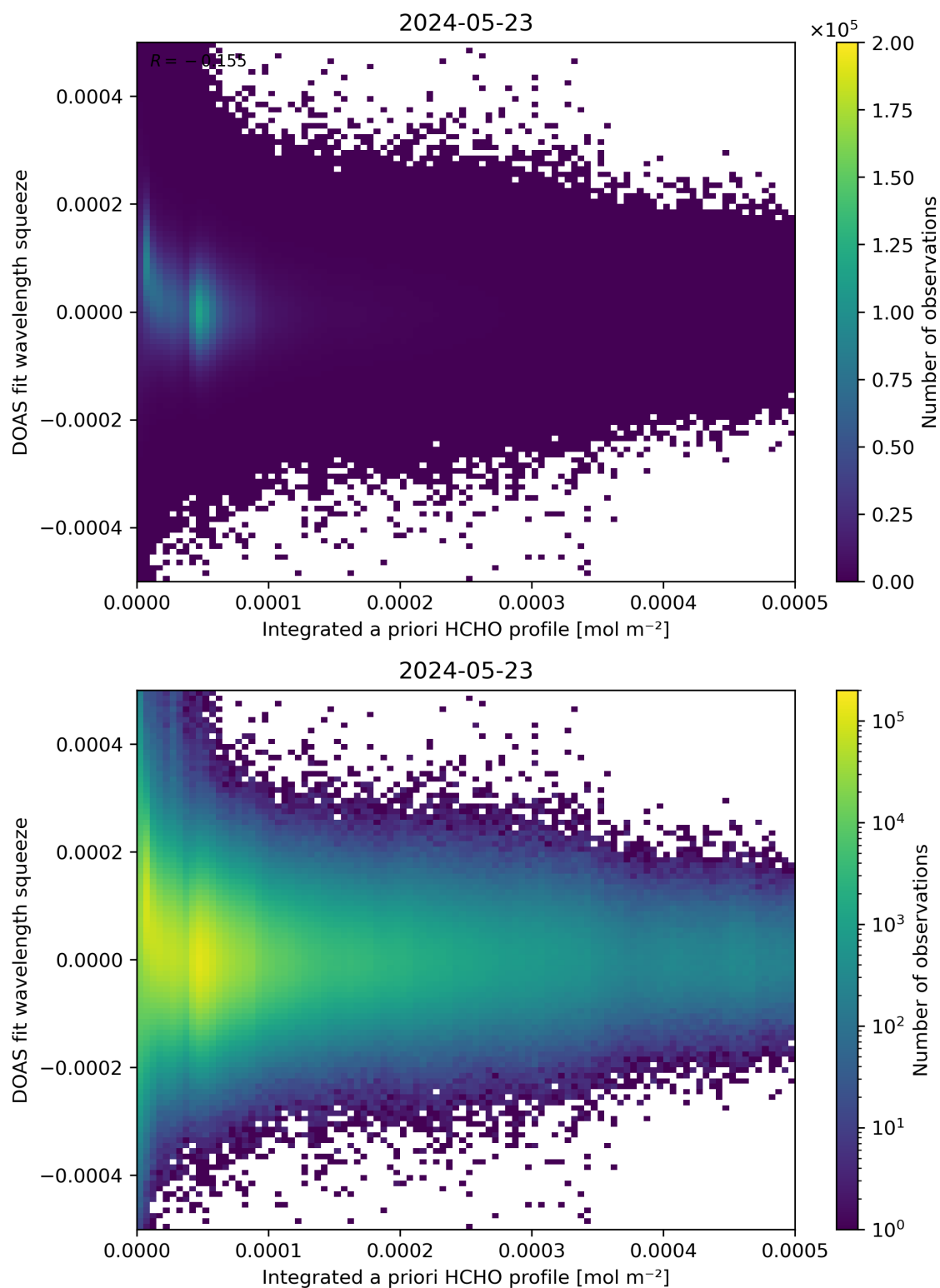
Figure 150: Scatter density plot of “Integrated a priori HCHO profile” against “DOAS fit wavelength squeeze” for 2024-05-23 to 2024-05-24.
