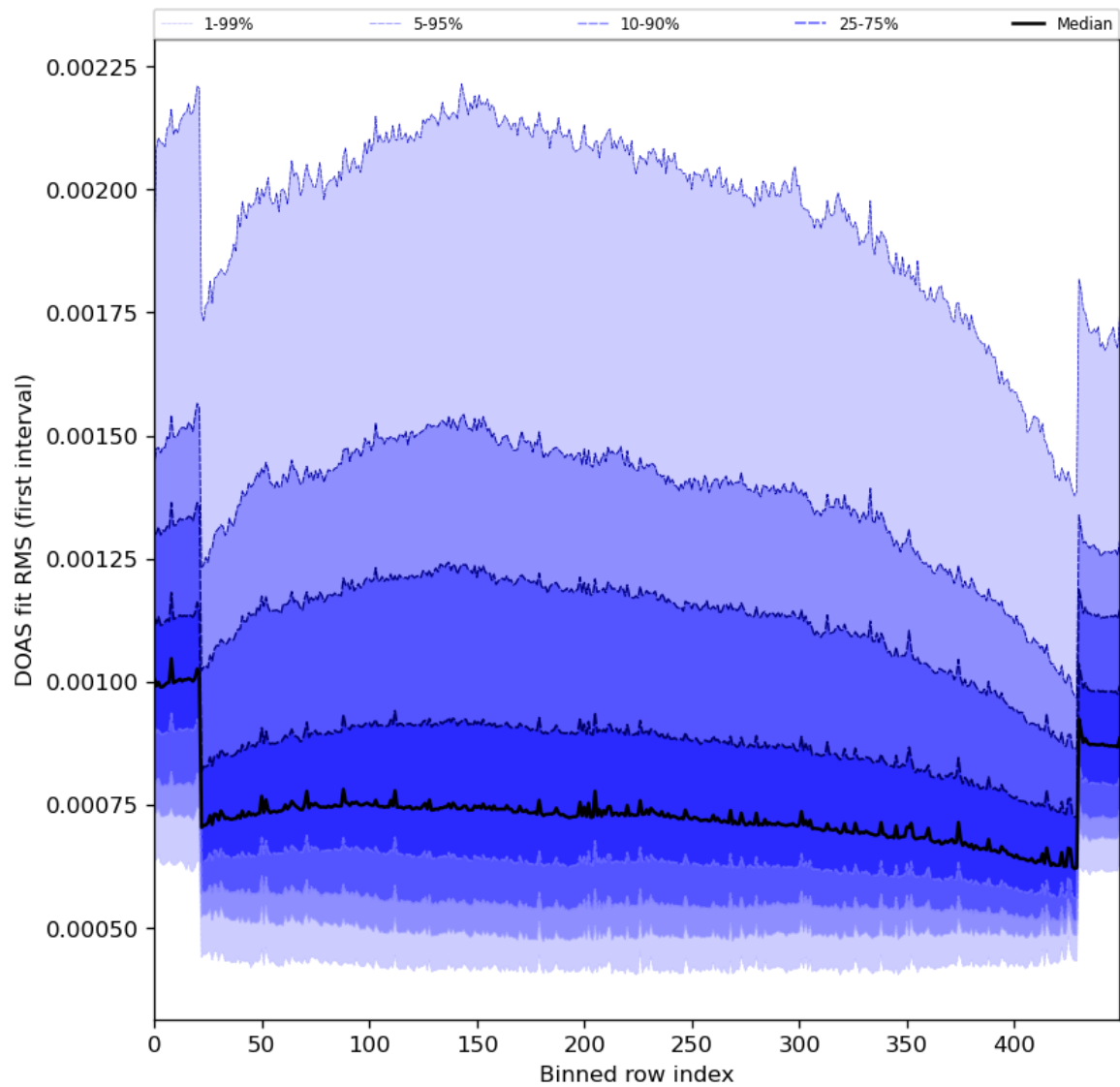
Figure 60: Along track statistics of “DOAS fit RMS (first interval)” for 2024-05-23 to 2024-05-24
