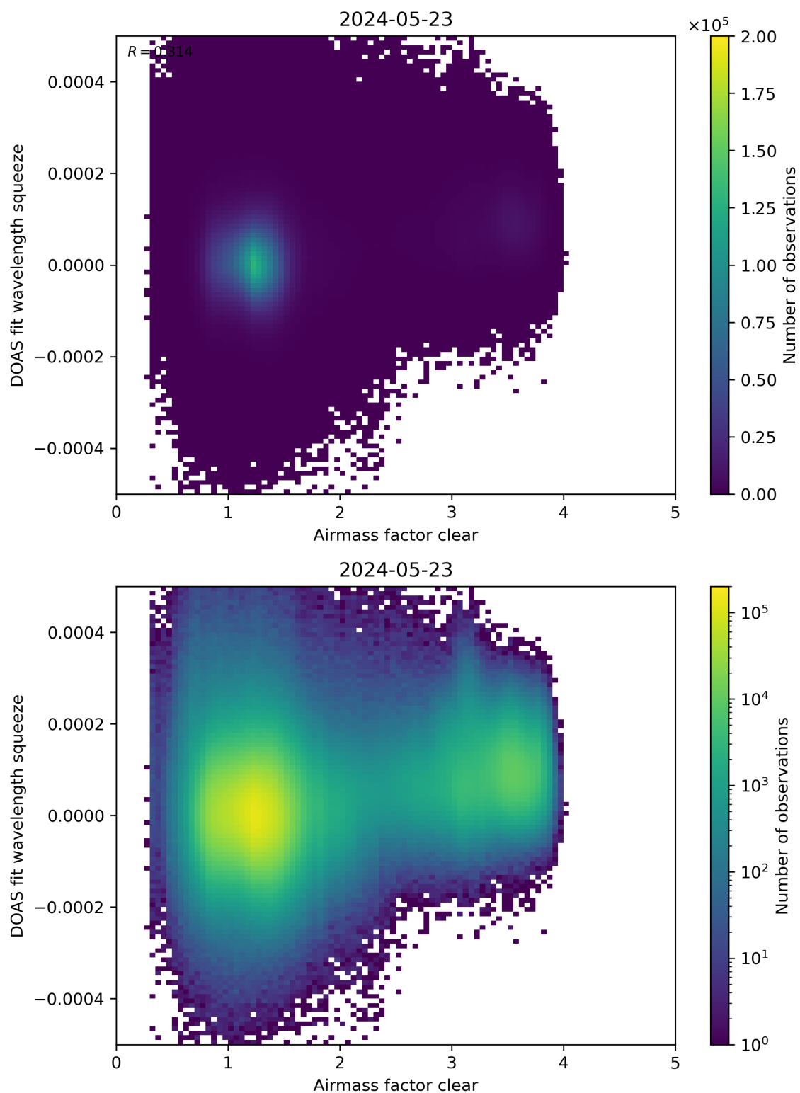
Figure 73: Scatter density plot of “Airmass factor clear” against “DOAS fit wavelength squeeze” for 2024-05-23 to 2024-05-24.
