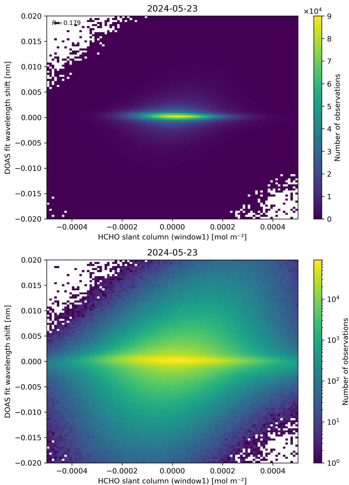
Figure 79: Scatter density plot of “HCHO slant column (window1)” against “DOAS fit wavelength shift” for 2024-05-23 to 2024-05-24.
