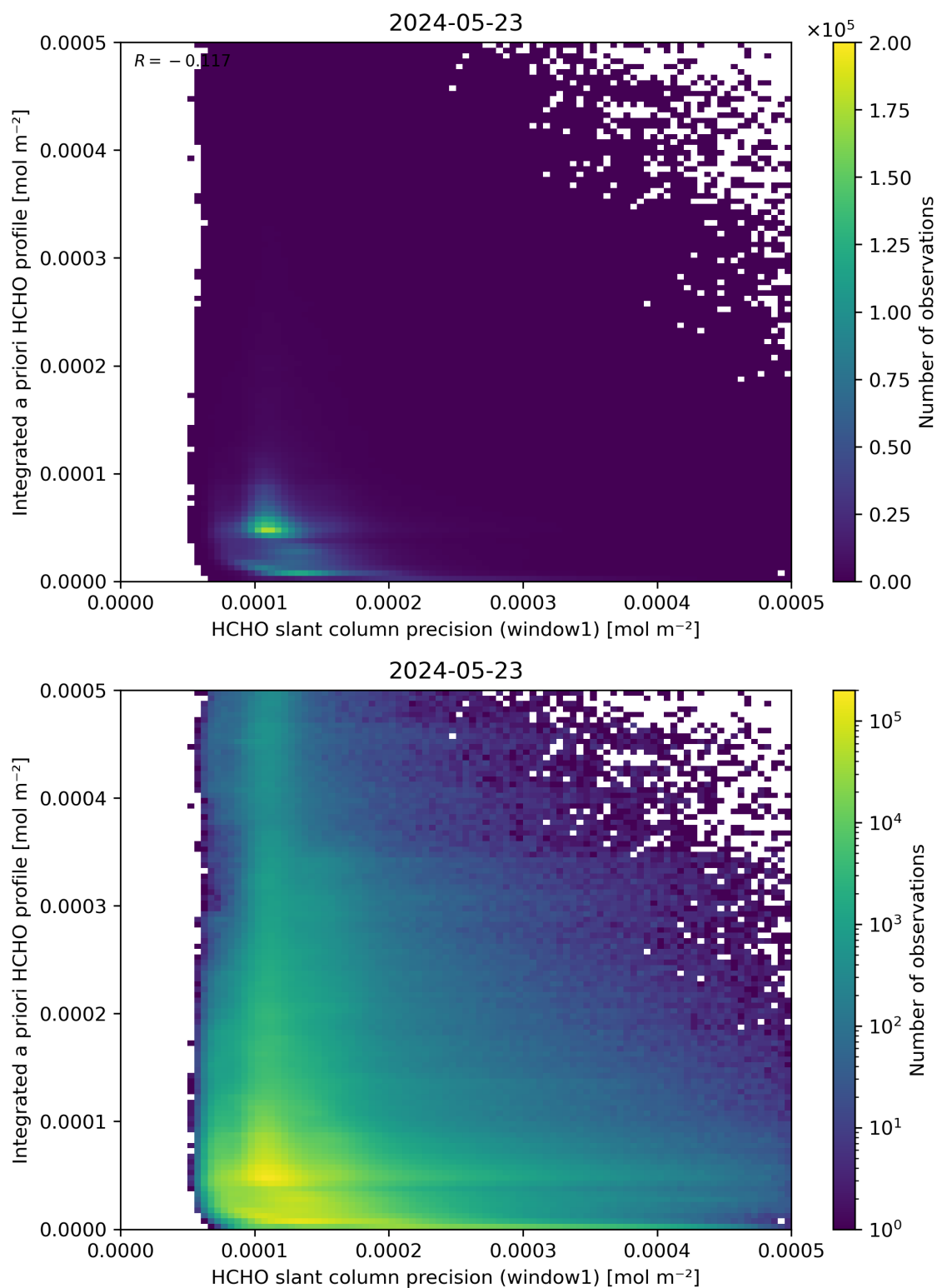
Figure 96: Scatter density plot of “HCHO slant column precision (window1)” against “Integrated a priori HCHO profile” for 2024-05-23 to 2024-05-24.
