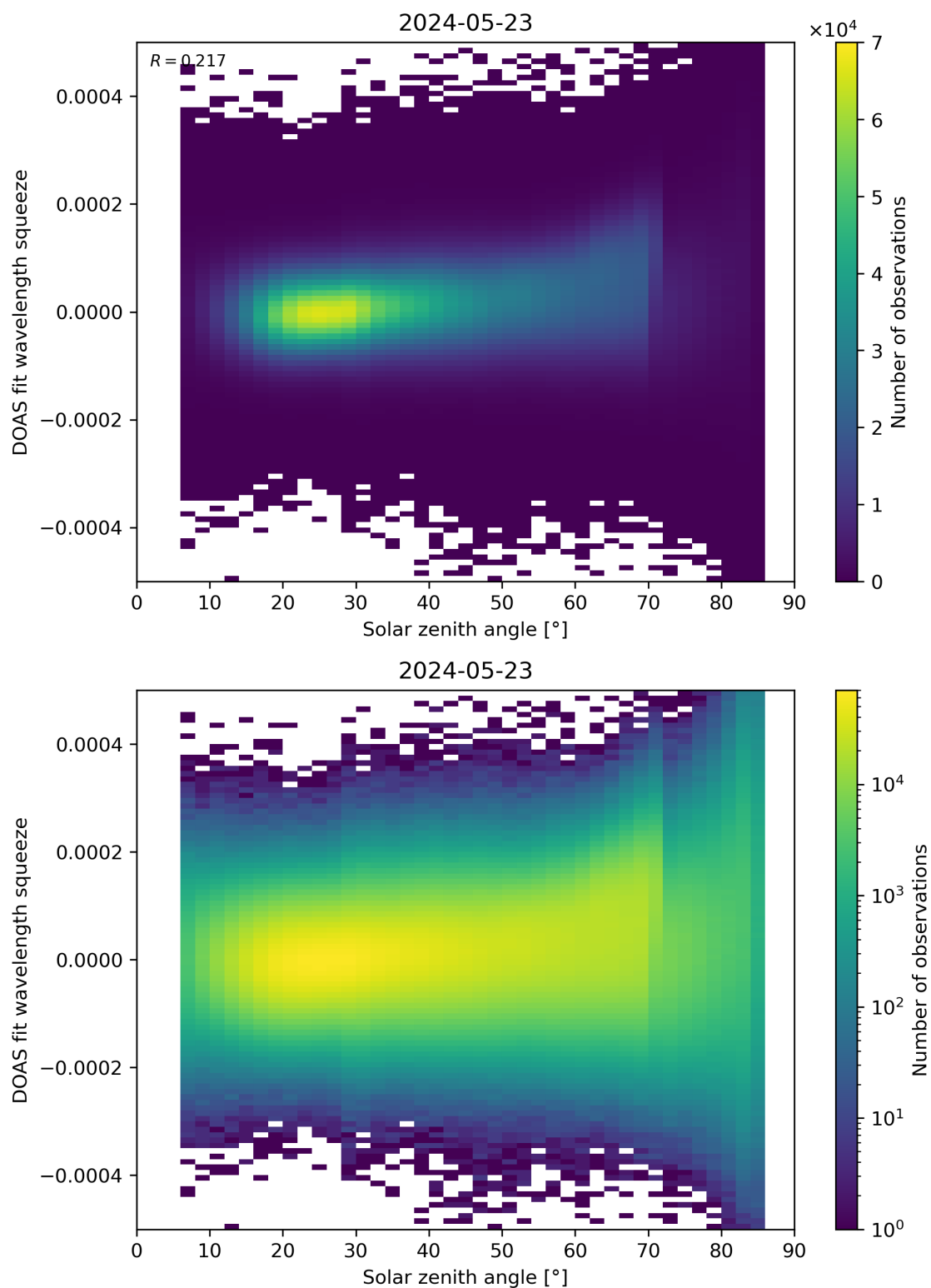
Figure 169: Scatter density plot of “Solar zenith angle” against “DOAS fit wavelength squeeze” for 2024-05-23 to 2024-05-24.
