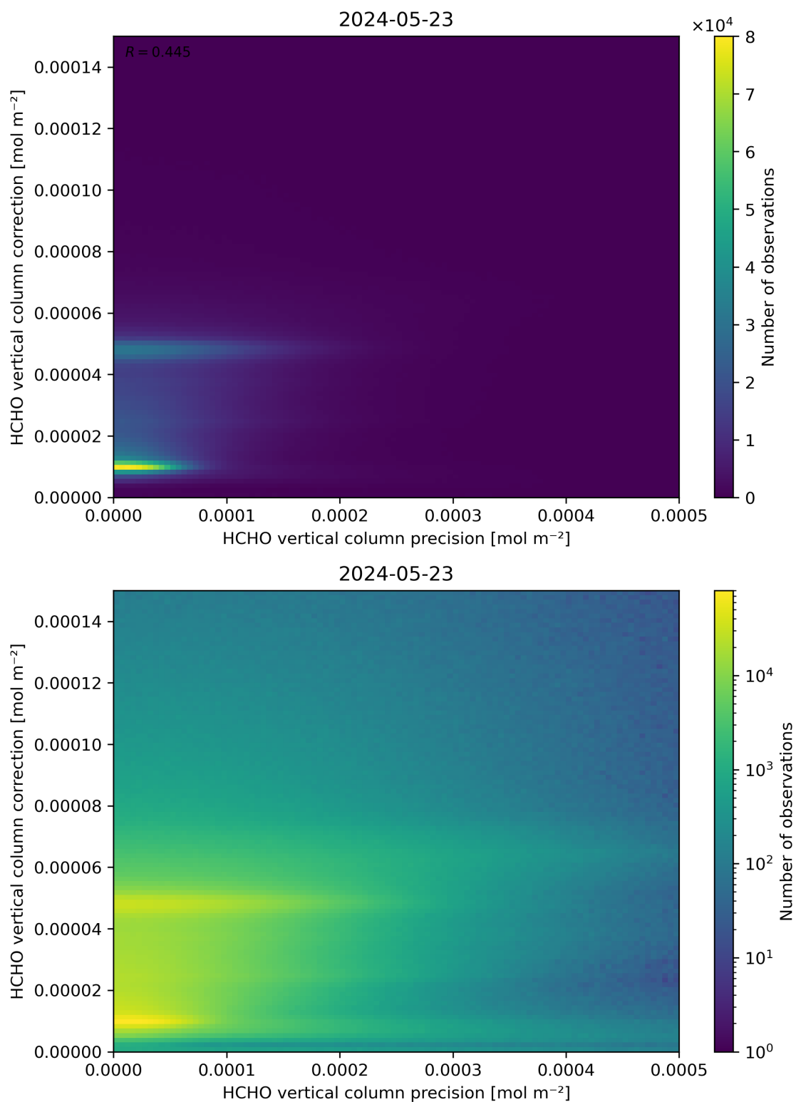
Figure 146: Scatter density plot of “HCHO vertical column precision” against “HCHO vertical column correction” for 2024-05-23 to 2024-05-24.
