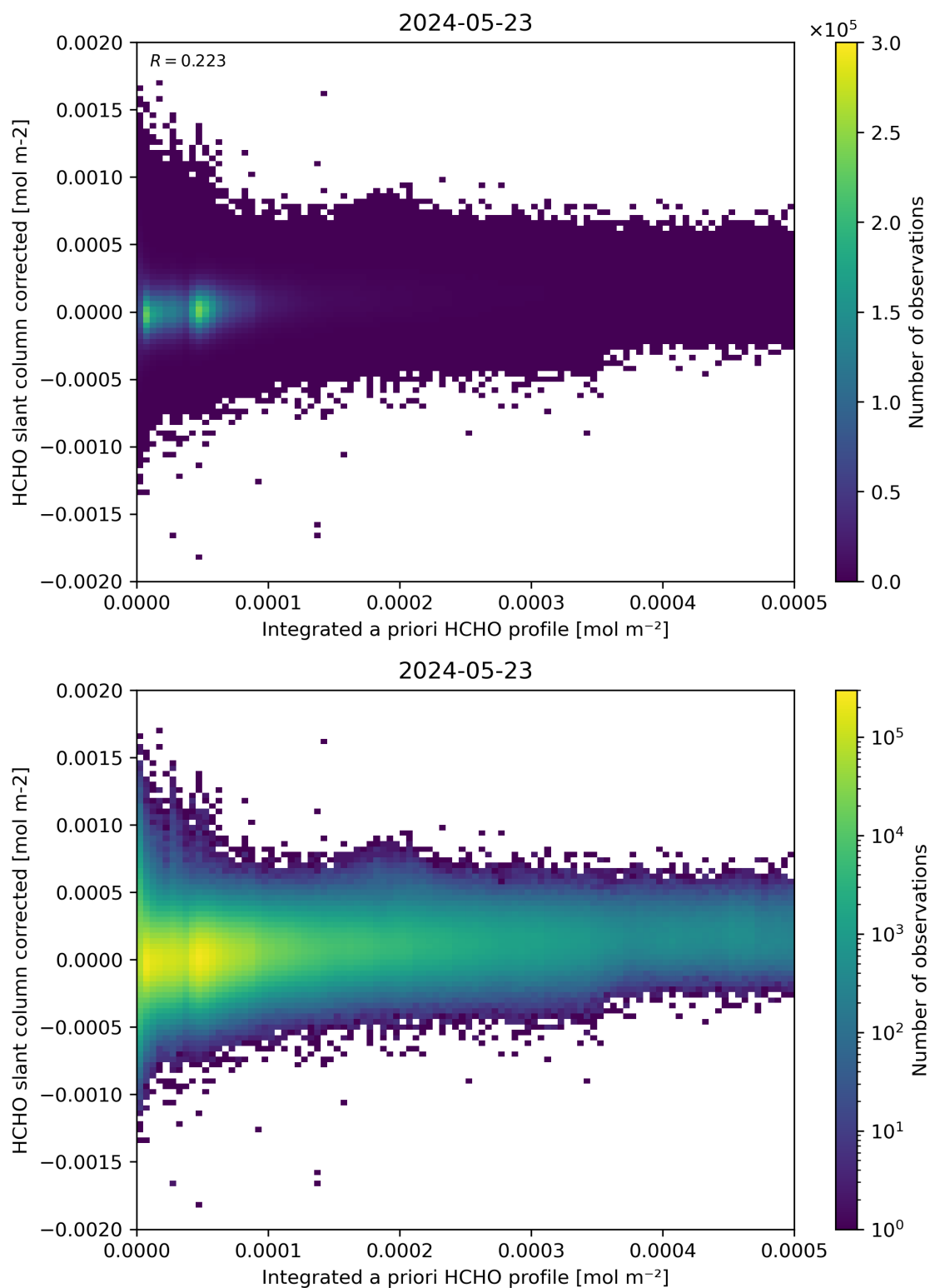
Figure 151: Scatter density plot of “Integrated a priori HCHO profile” against “HCHO slant column corrected” for 2024-05-23 to 2024-05-24.
