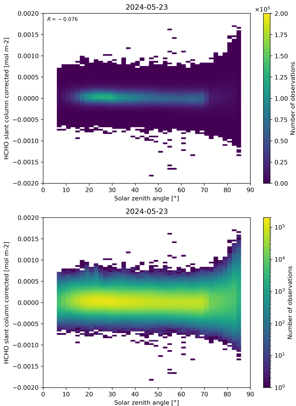
Figure 171: Scatter density plot of “Solar zenith angle” against “HCHO slant column corrected” for 2024-05-23 to 2024-05-24.
