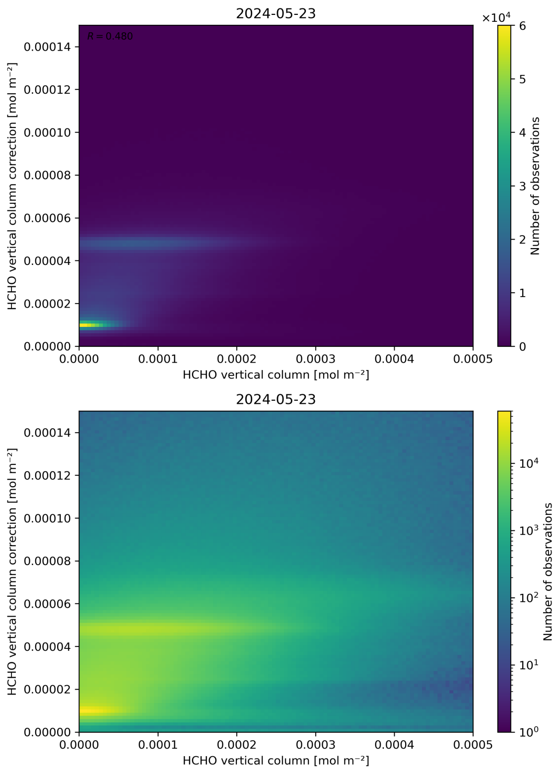
Figure 133: Scatter density plot of “HCHO vertical column” against “HCHO vertical column correction” for 2024-05-23 to 2024-05-24.
