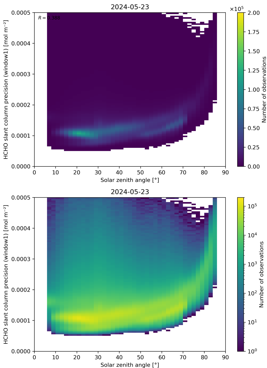
Figure 174: Scatter density plot of “Solar zenith angle” against “HCHO slant column precision (window1)” for 2024-05-23 to 2024-05-24.
