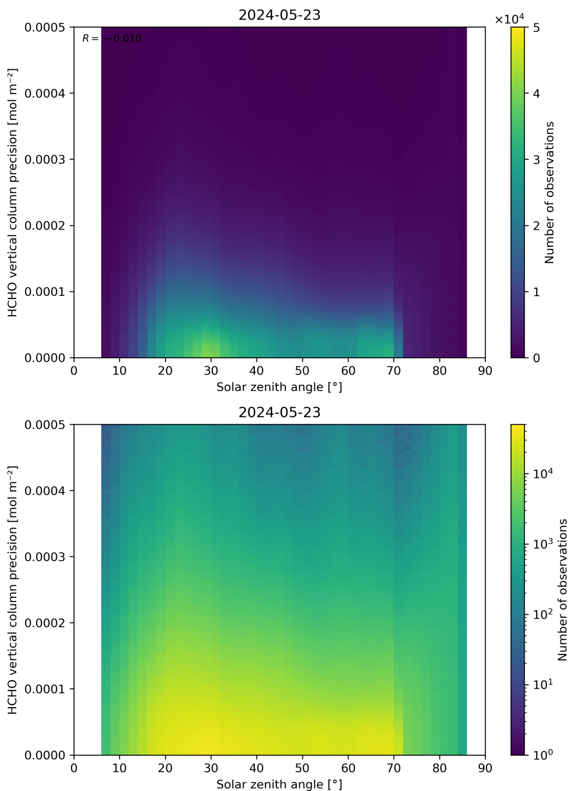
Figure 179: Scatter density plot of “Solar zenith angle” against “HCHO vertical column precision” for 2024-05-23 to 2024-05-24.
