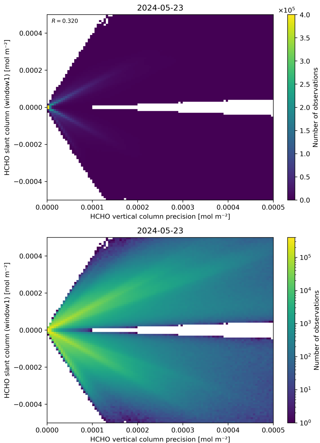
Figure 142: Scatter density plot of “HCHO vertical column precision” against “HCHO slant column (window1)” for 2024-05-23 to 2024-05-24.
