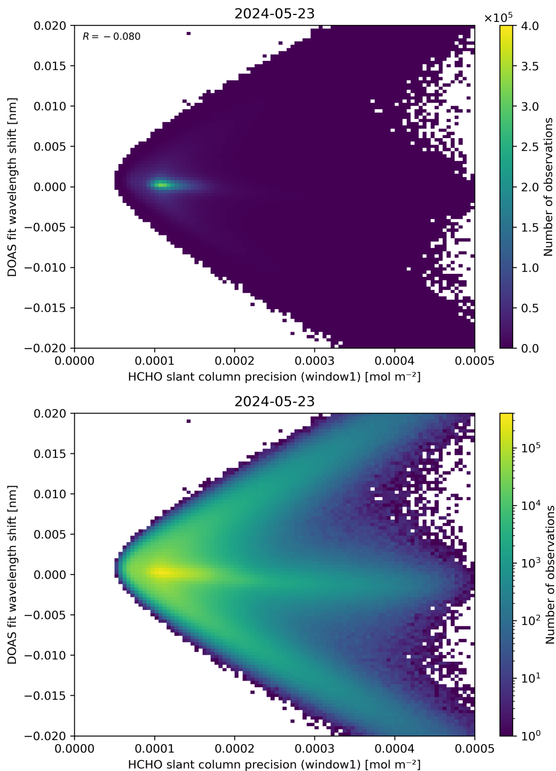
Figure 89: Scatter density plot of “HCHO slant column precision (window1)” against “DOAS fit wavelength shift” for 2024-05-23 to 2024-05-24.
