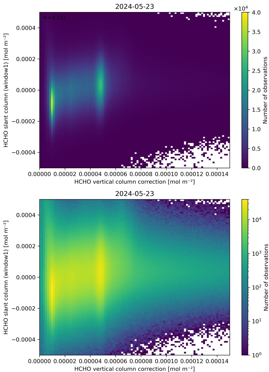
Figure 118: Scatter density plot of “HCHO vertical column correction” against “HCHO slant column (window1)” for 2024-05-23 to 2024-05-24.
