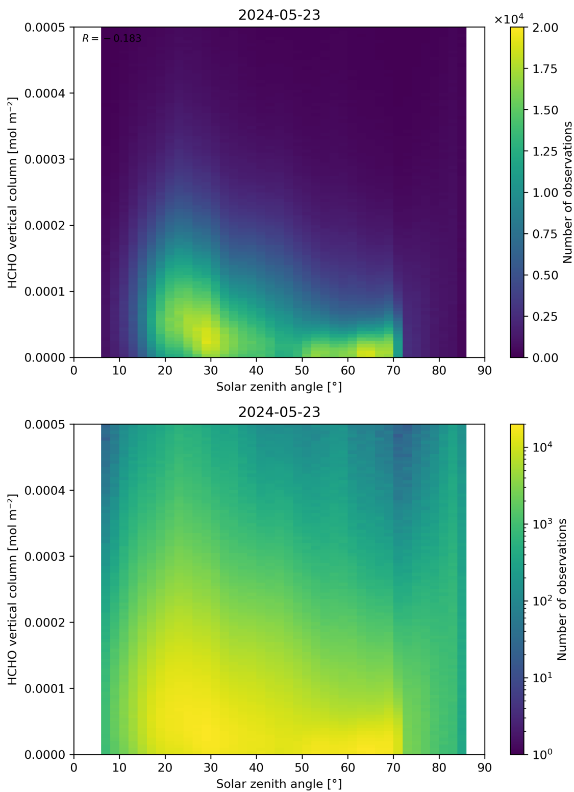
Figure 177: Scatter density plot of “Solar zenith angle” against “HCHO vertical column” for 2024-05-23 to 2024-05-24.
