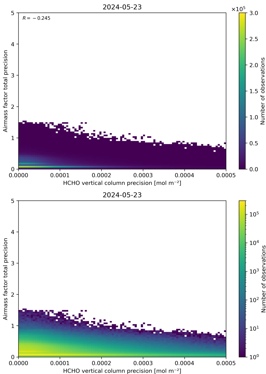
Figure 145: Scatter density plot of “HCHO vertical column precision” against “Airmass factor total precision” for 2024-05-23 to 2024-05-24.
