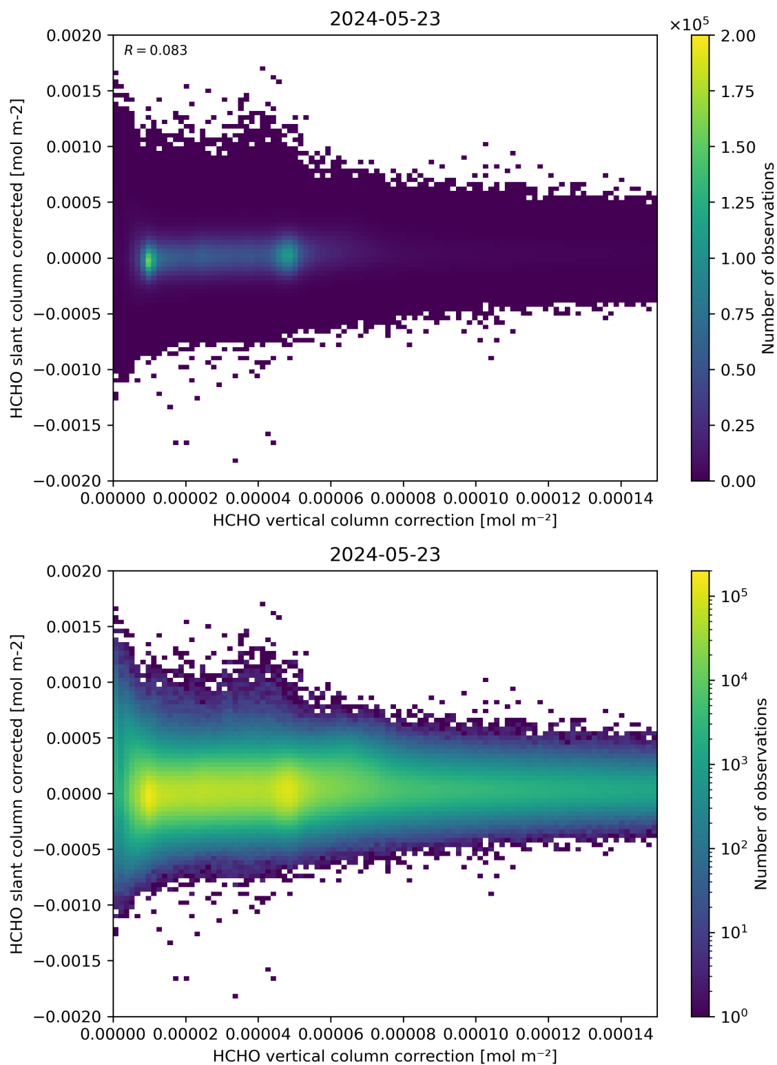
Figure 116: Scatter density plot of “HCHO vertical column correction” against “HCHO slant column corrected” for 2024-05-23 to 2024-05-24.
