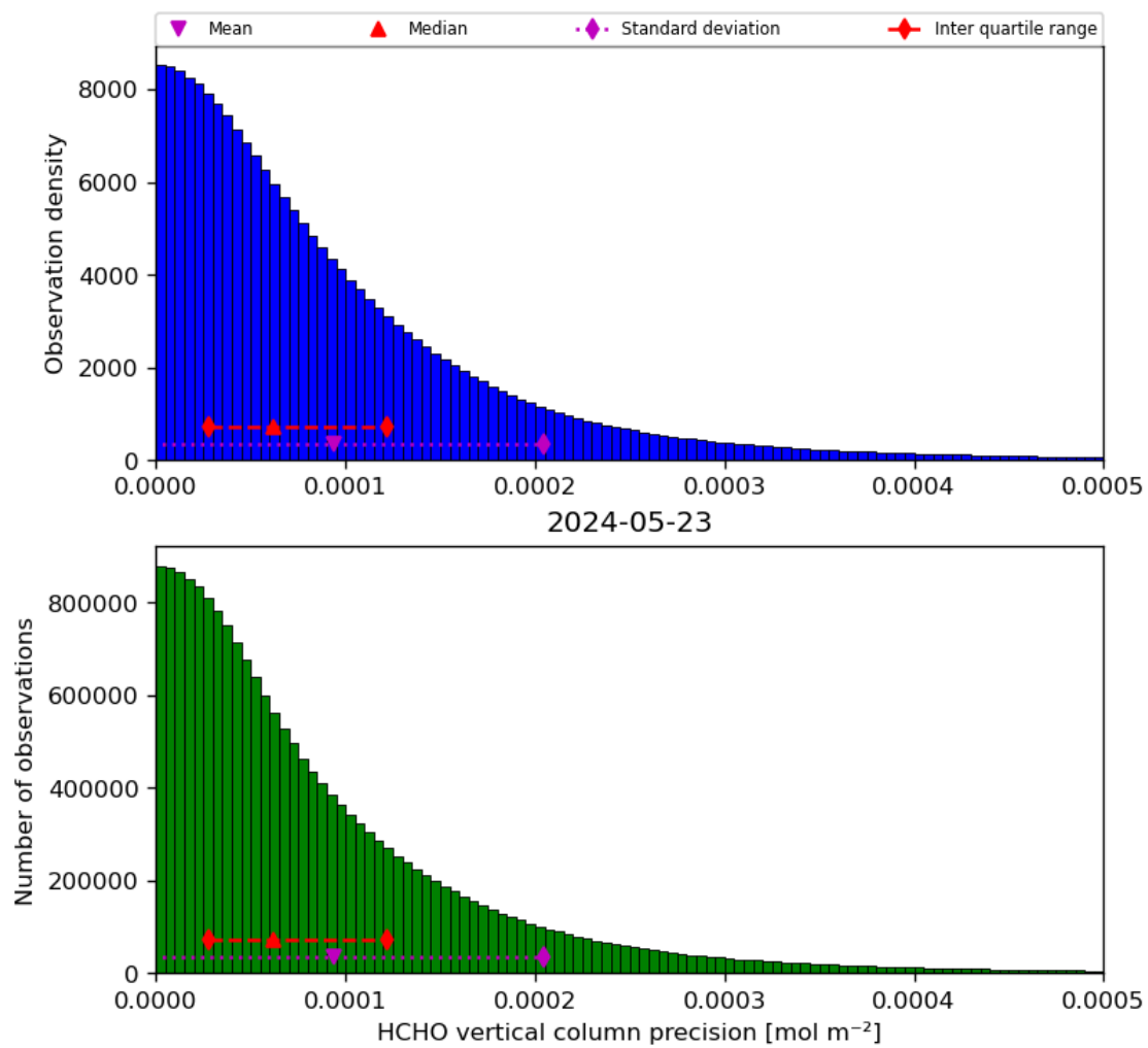
Figure 36: Histogram of “HCHO vertical column precision” for 2024-05-23 to 2024-05-24
