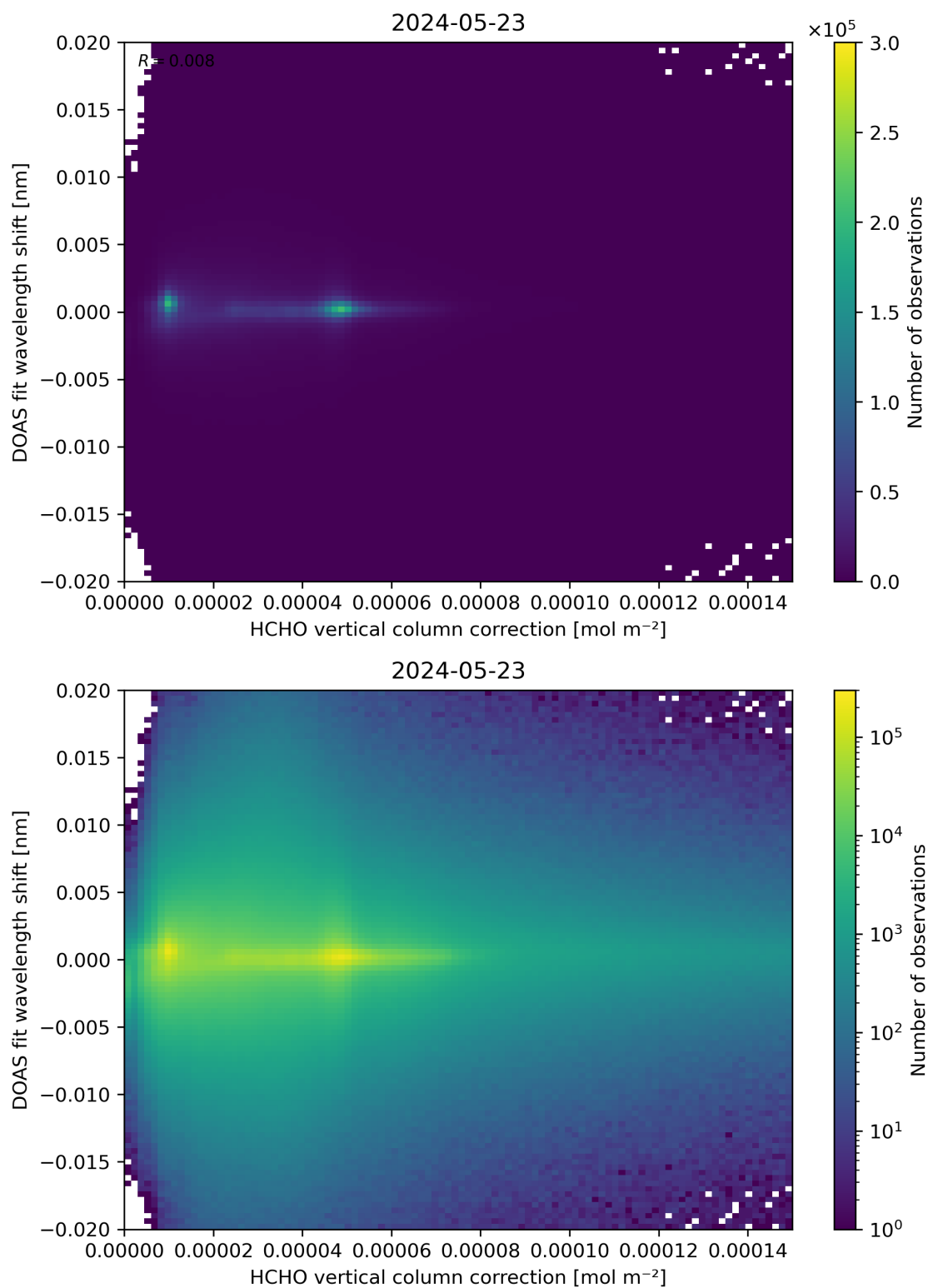
Figure 113: Scatter density plot of “HCHO vertical column correction” against “DOAS fit wavelength shift” for 2024-05-23 to 2024-05-24.
