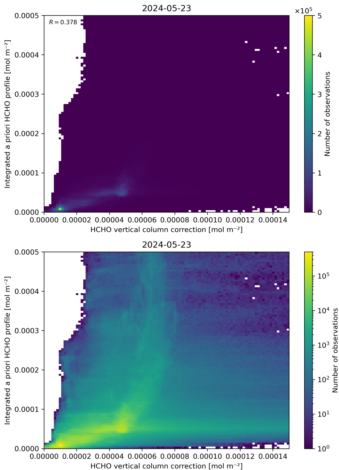
Figure 122: Scatter density plot of “HCHO vertical column correction” against “Integrated a priori HCHO profile” for 2024-05-23 to 2024-05-24.
