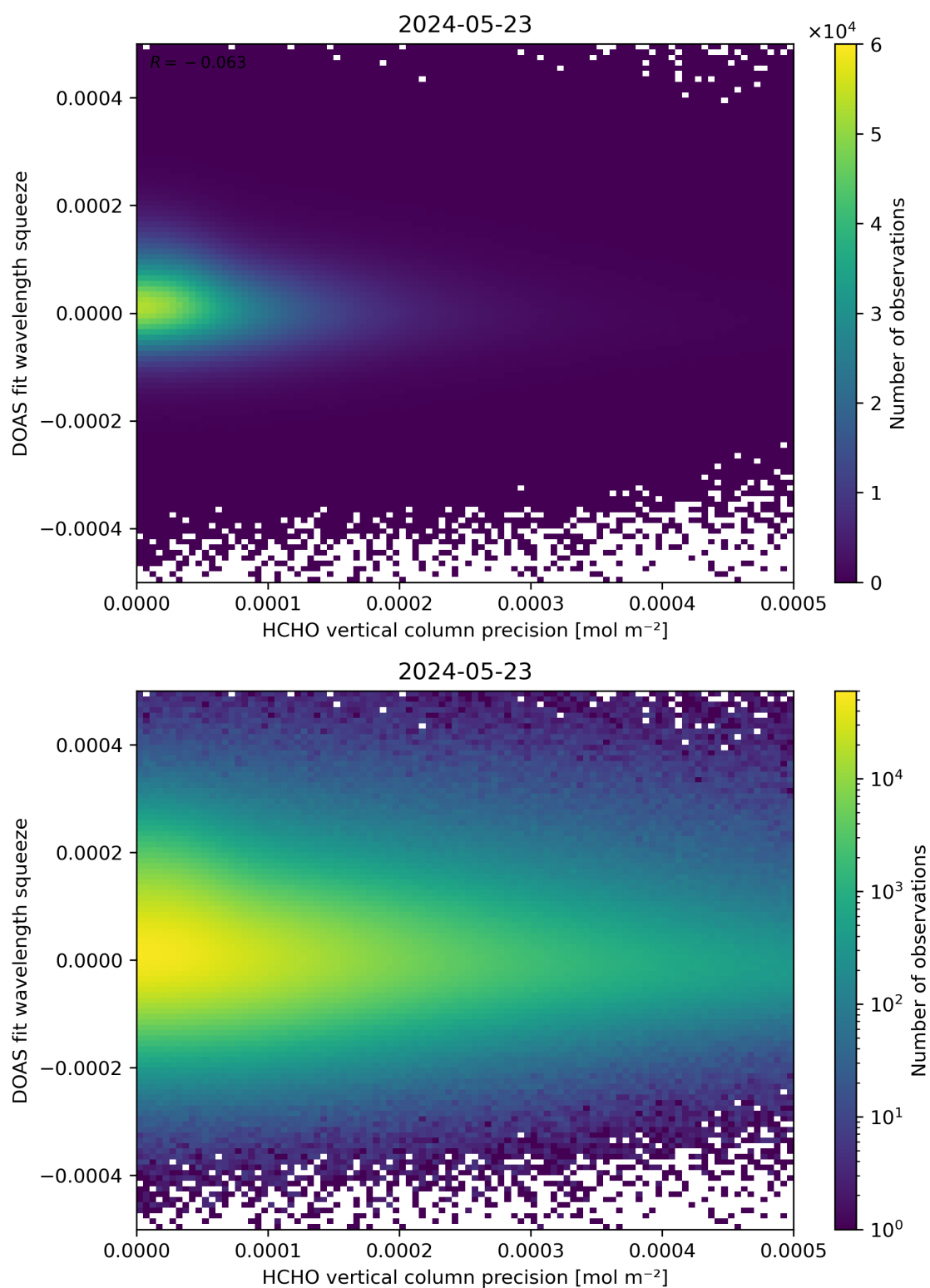
Figure 138: Scatter density plot of “HCHO vertical column precision” against “DOAS fit wavelength squeeze” for 2024-05-23 to 2024-05-24.
