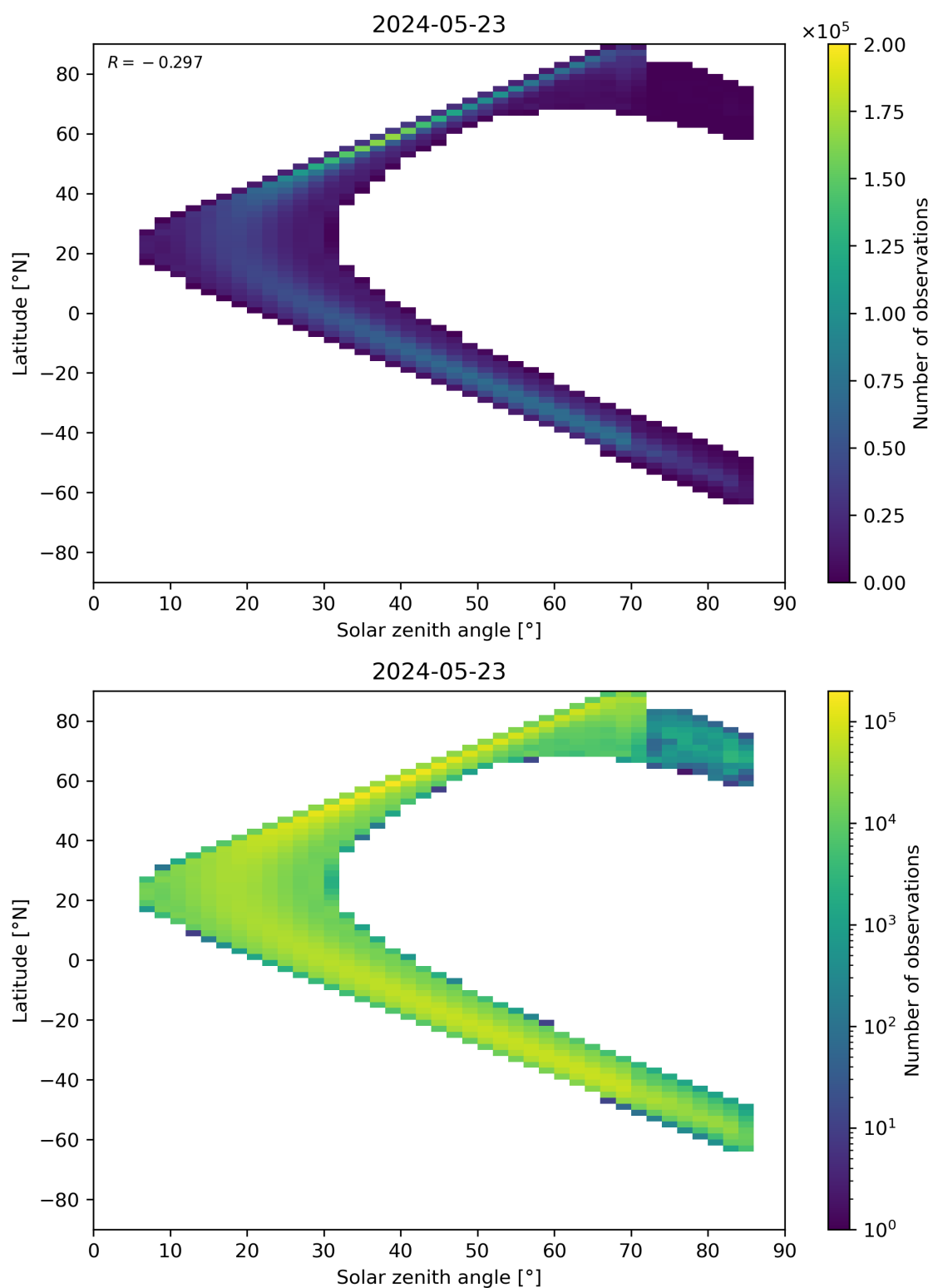
Figure 181: Scatter density plot of “Solar zenith angle” against “Latitude” for 2024-05-23 to 2024-05-24.
