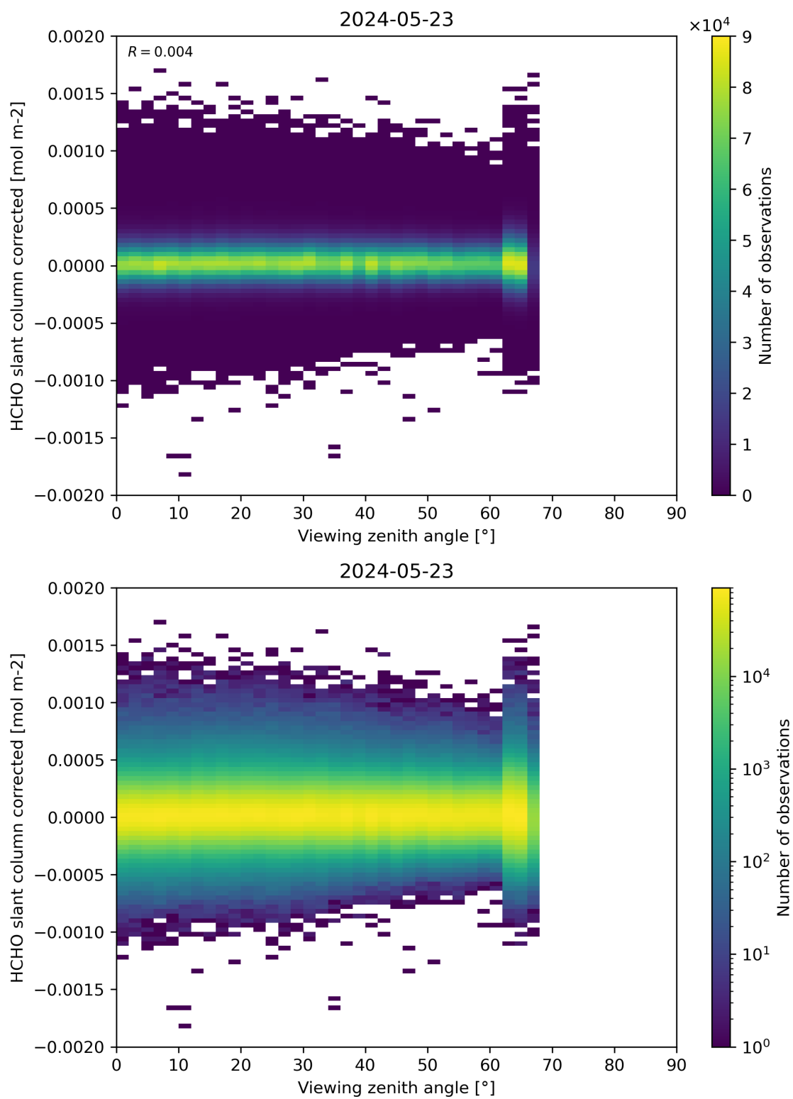
Figure 186: Scatter density plot of “Viewing zenith angle” against “HCHO slant column corrected” for 2024-05-23 to 2024-05-24.
