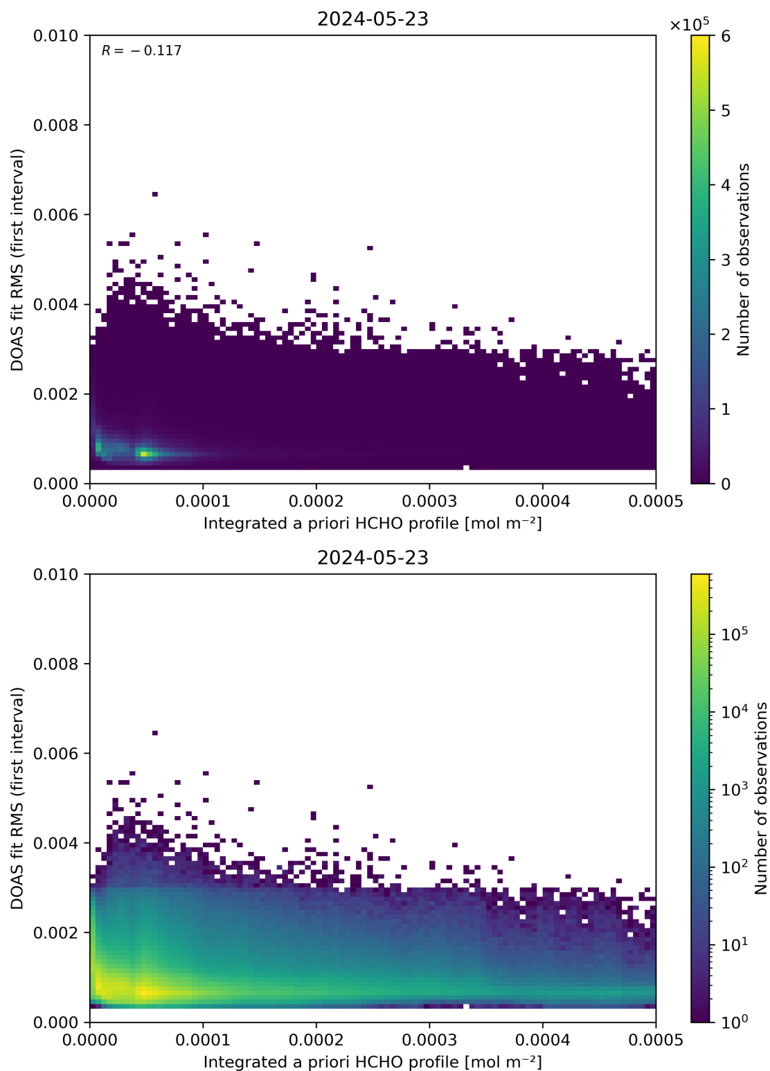
Figure 148: Scatter density plot of “Integrated a priori HCHO profile” against “DOAS fit RMS (first interval)” for 2024-05-23 to 2024-05-24.
