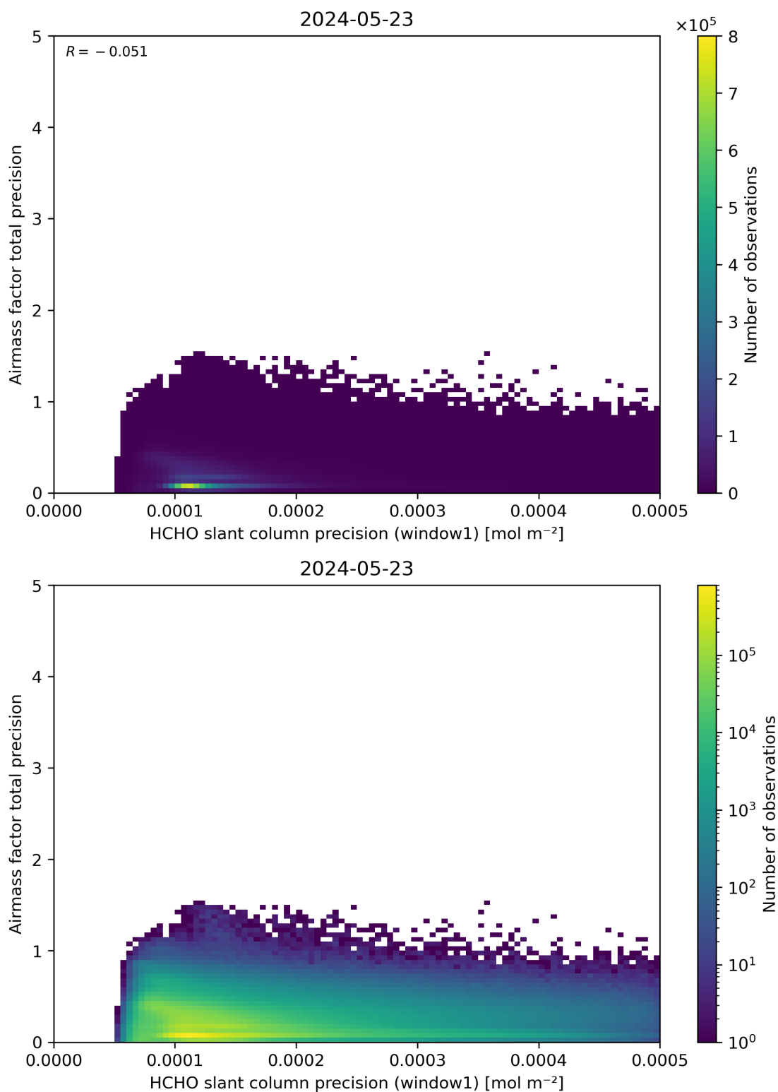
Figure 95: Scatter density plot of “HCHO slant column precision (window1)” against “Airmass factor total precision” for 2024-05-23 to 2024-05-24.
