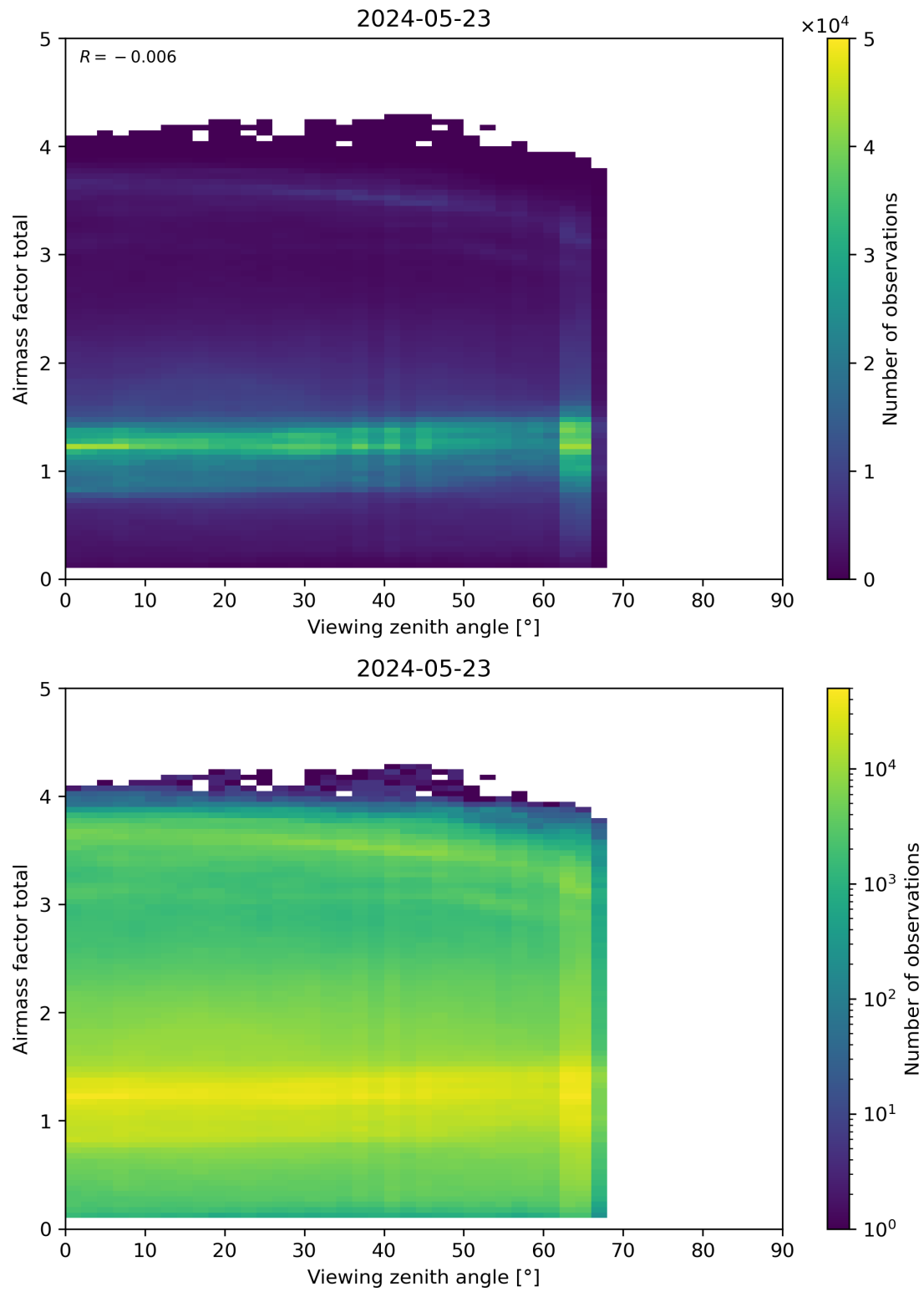
Figure 190: Scatter density plot of “Viewing zenith angle” against “Airmass factor total” for 2024-05-23 to 2024-05-24.
