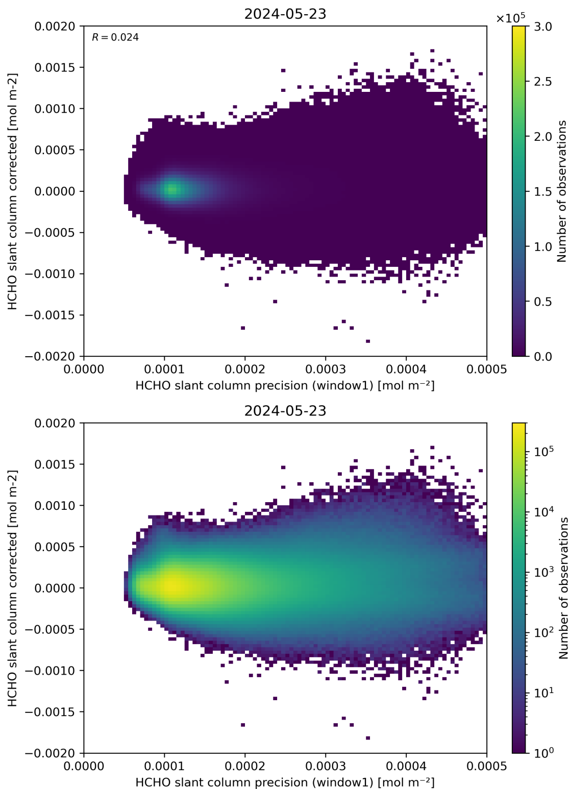
Figure 92: Scatter density plot of “HCHO slant column precision (window1)” against “HCHO slant column corrected” for 2024-05-23 to 2024-05-24.
