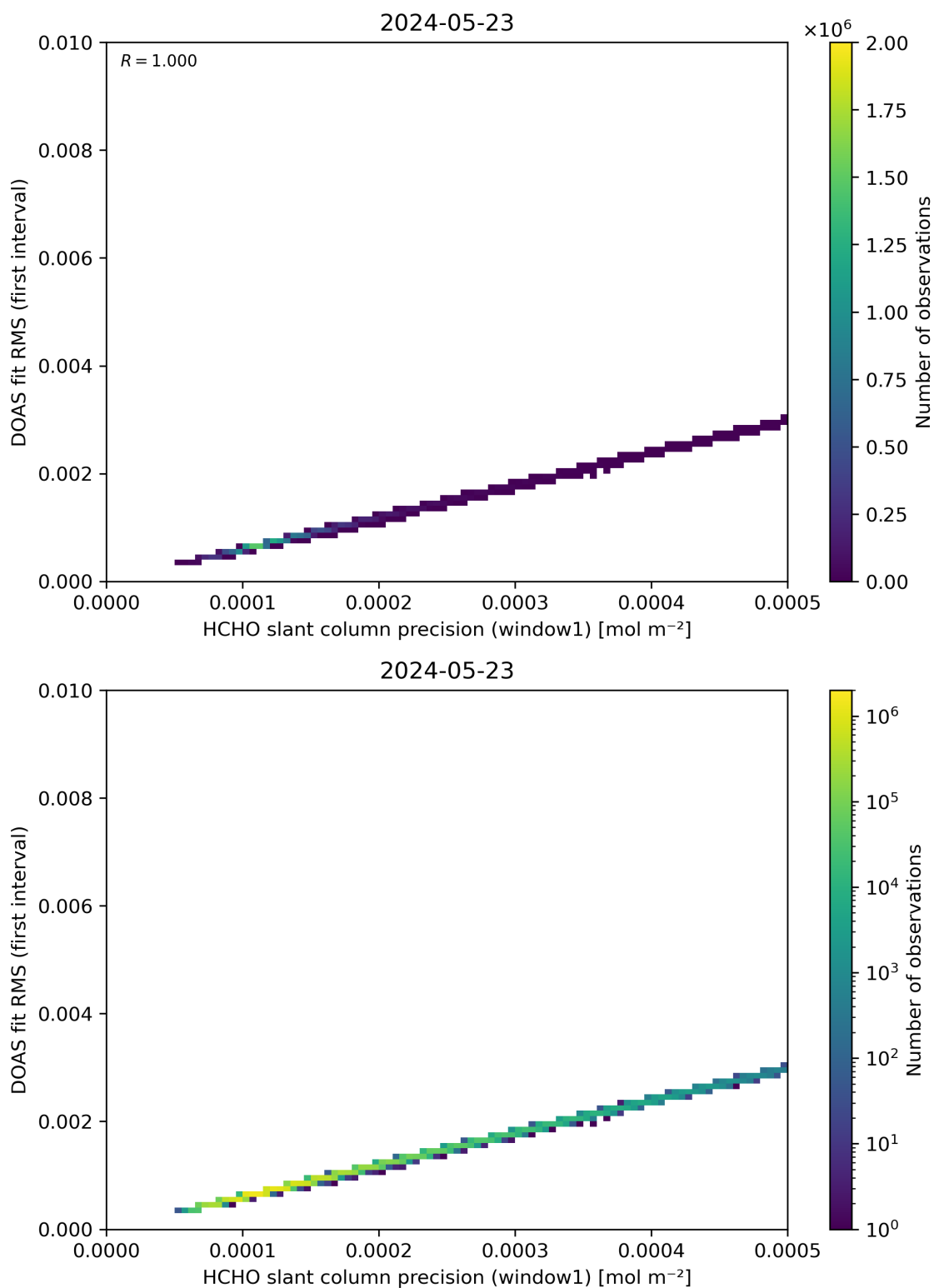
Figure 88: Scatter density plot of “HCHO slant column precision (window1)” against “DOAS fit RMS (first interval)” for 2024-05-23 to 2024-05-24.
