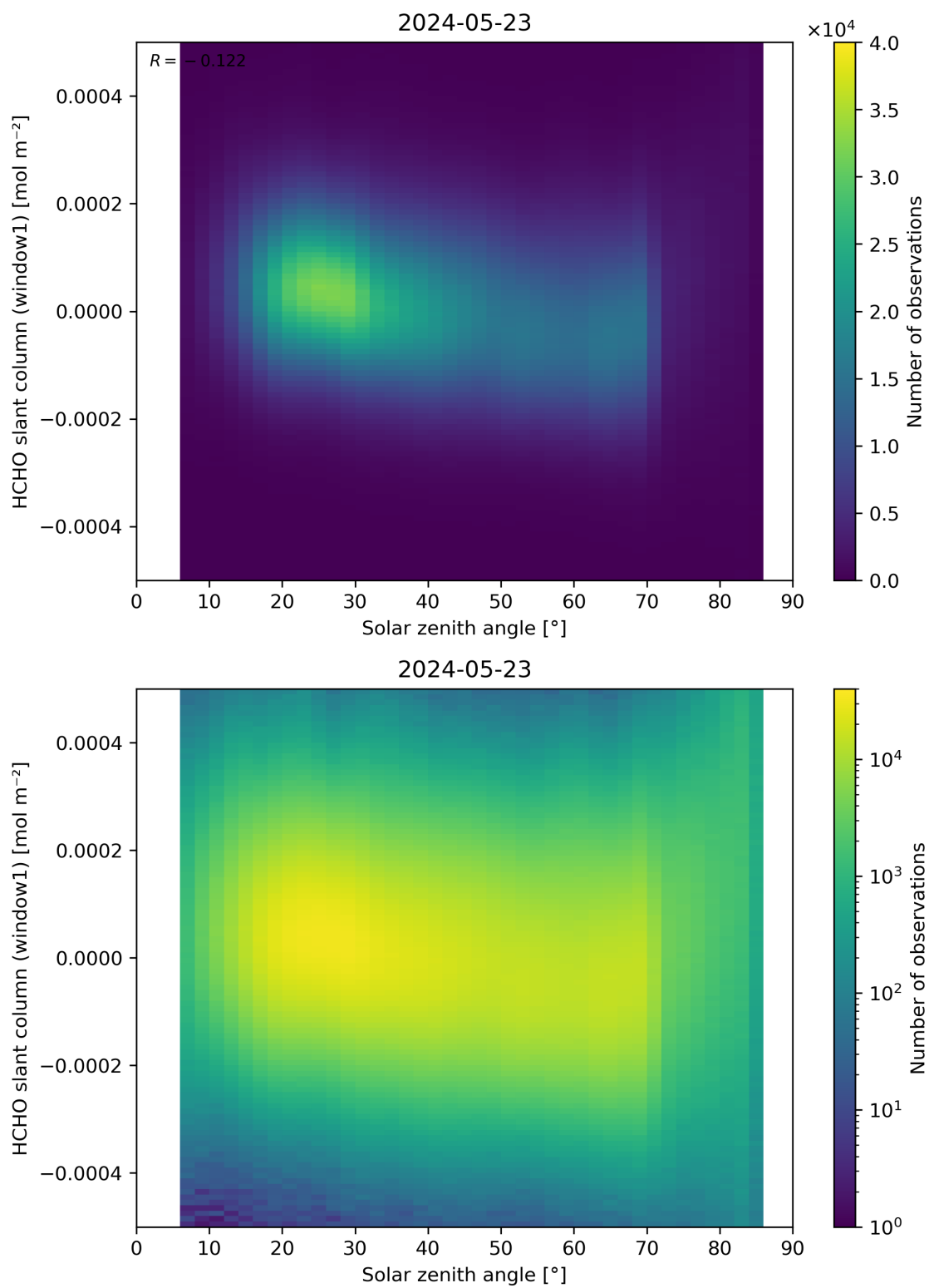
Figure 173: Scatter density plot of “Solar zenith angle” against “HCHO slant column (window1)” for 2024-05-23 to 2024-05-24.
