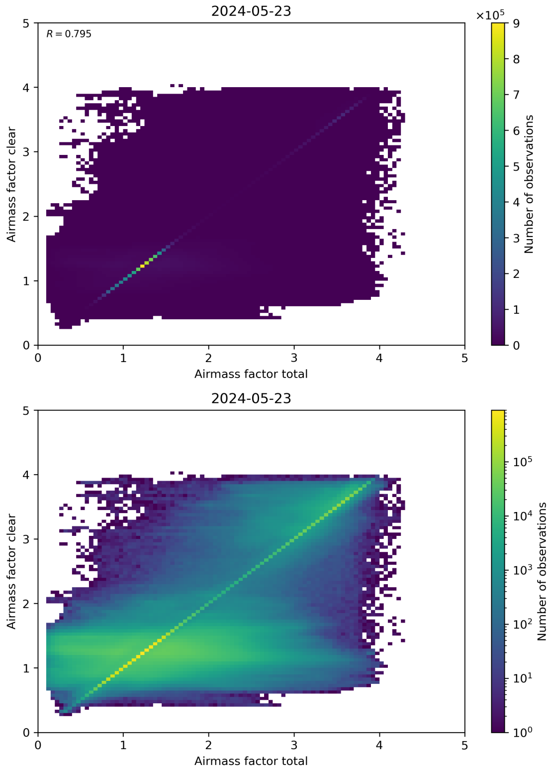
Figure 100: Scatter density plot of “Airmass factor total” against “Airmass factor clear” for 2024-05-23 to 2024-05-24.
