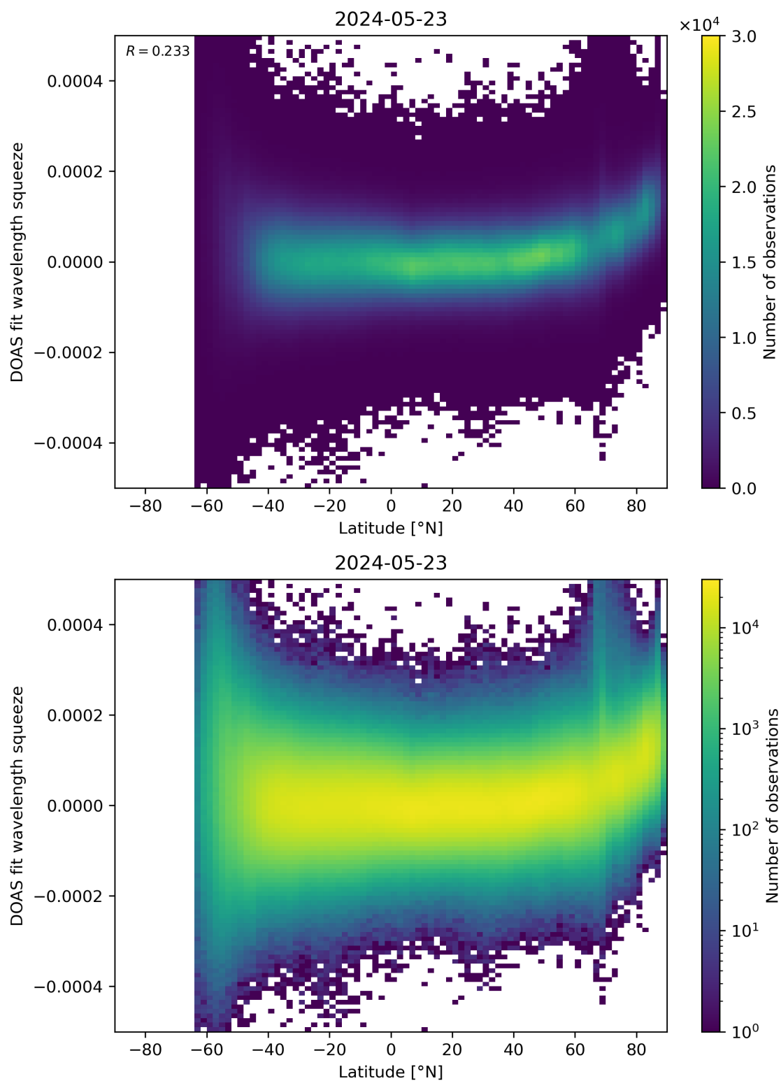
Figure 155: Scatter density plot of “Latitude” against “DOAS fit wavelength squeeze” for 2024-05-23 to 2024-05-24.
