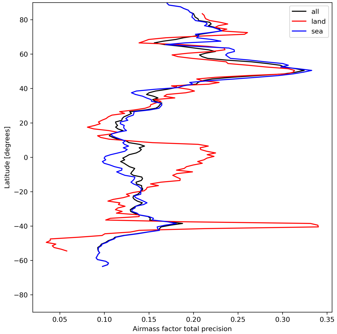
Figure 27: Zonal average of “Airmass factor total precision” for 2024-05-23 to 2024-05-24.
