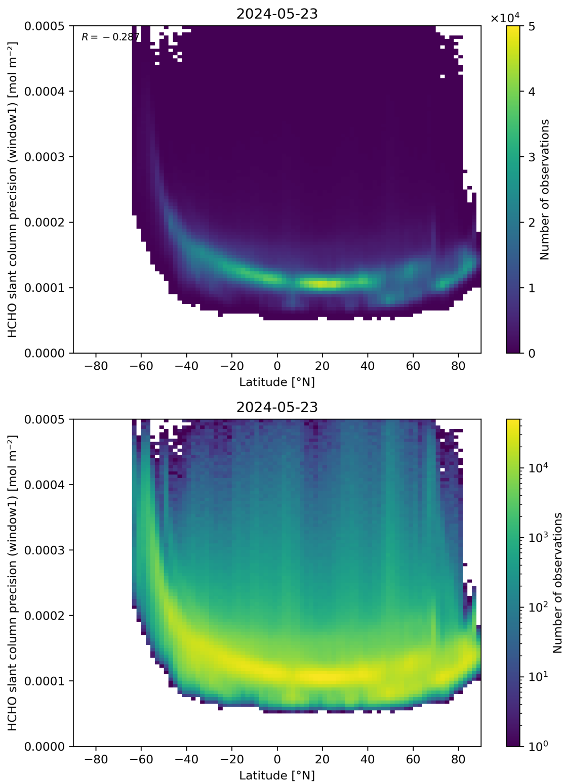
Figure 160: Scatter density plot of “Latitude” against “HCHO slant column precision (window1)” for 2024-05-23 to 2024-05-24.
