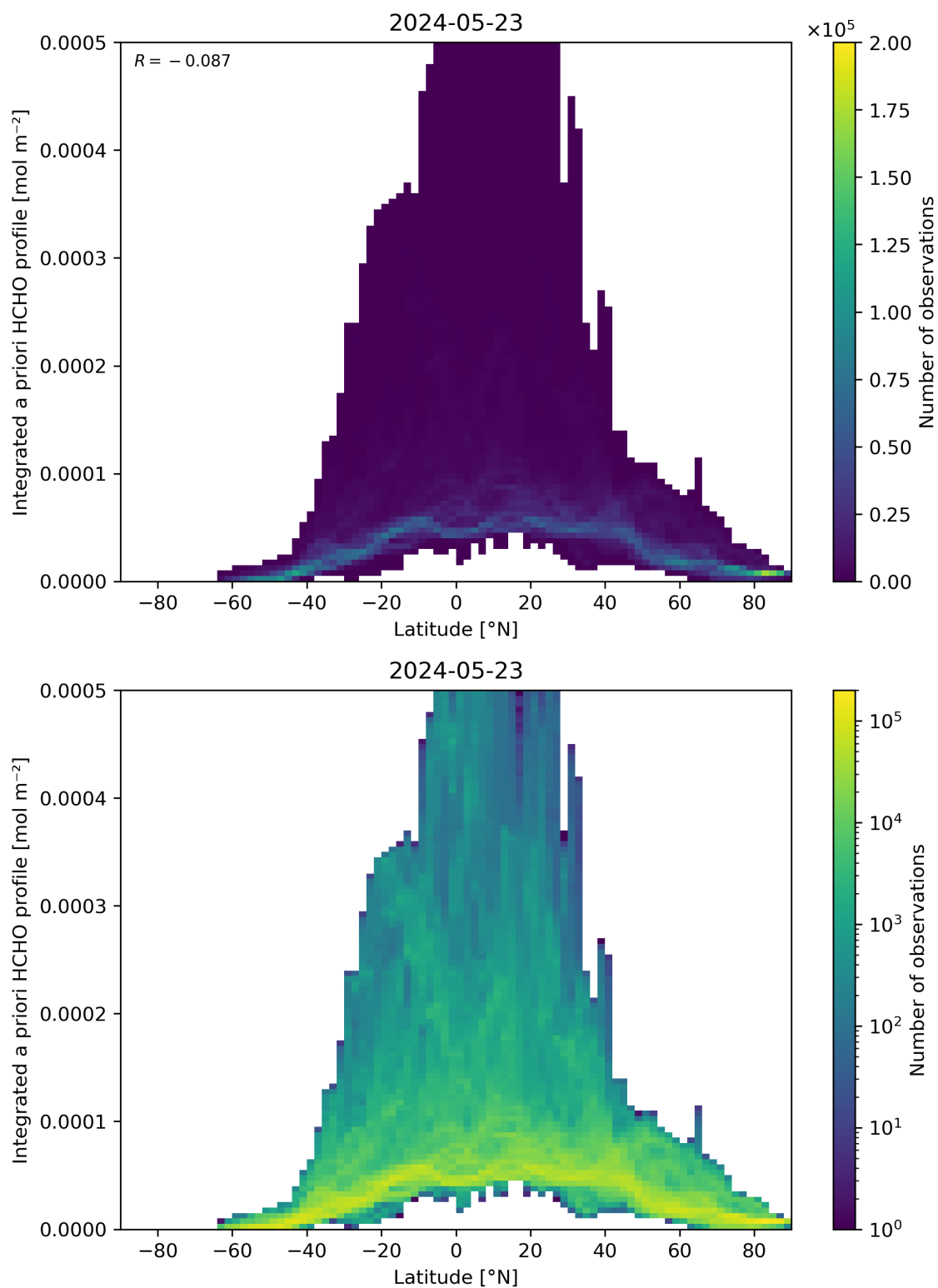
Figure 166: Scatter density plot of “Latitude” against “Integrated a priori HCHO profile” for 2024-05-23 to 2024-05-24.
