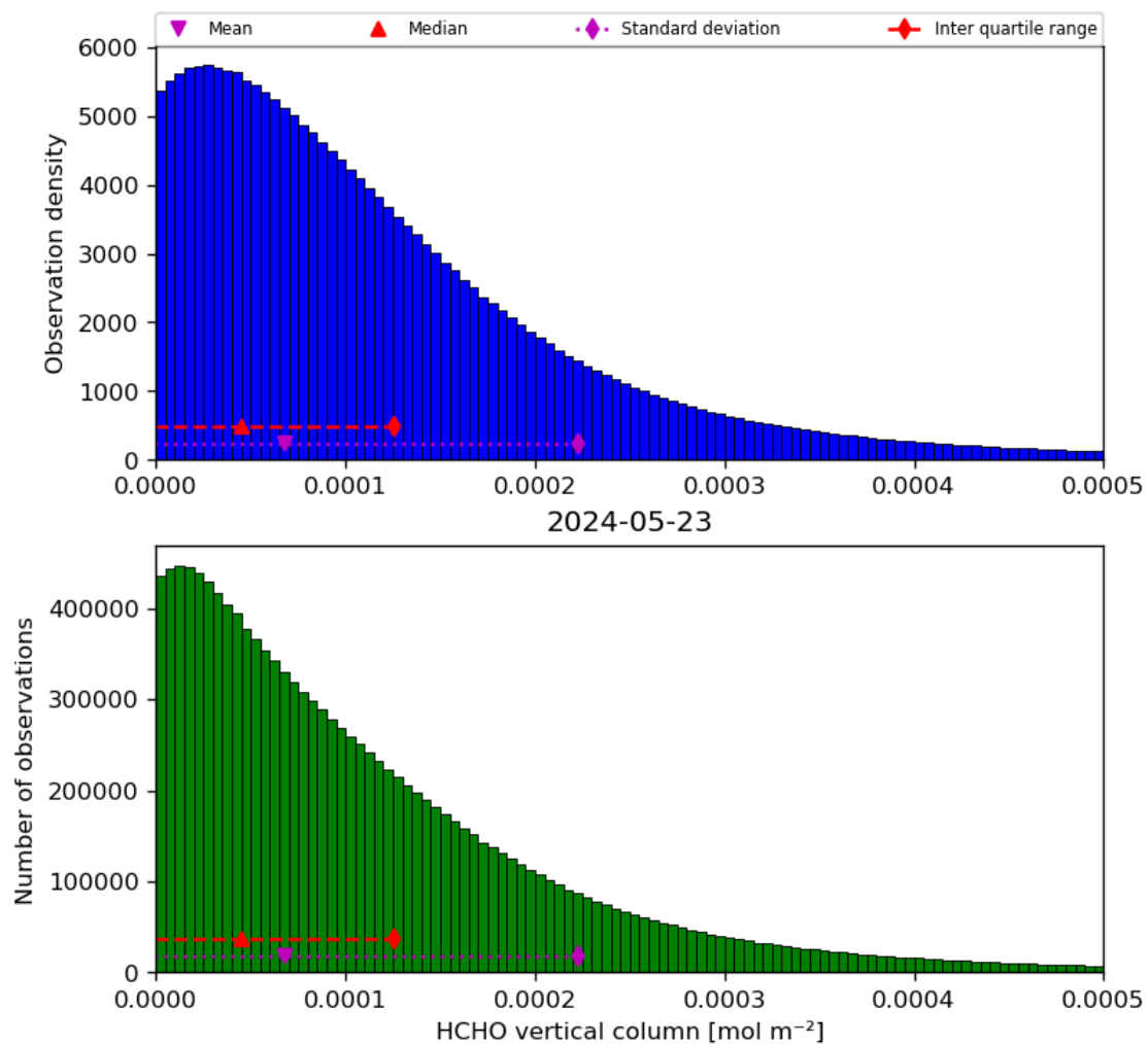
Figure 35: Histogram of “HCHO vertical column” for 2024-05-23 to 2024-05-24
