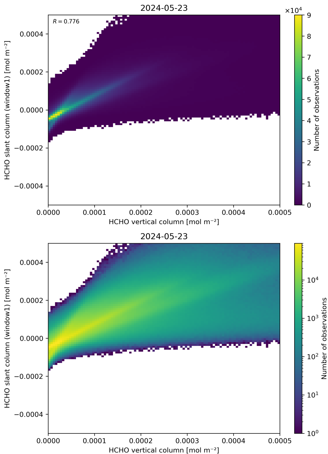
Figure 129: Scatter density plot of “HCHO vertical column” against “HCHO slant column (window1)” for 2024-05-23 to 2024-05-24.
