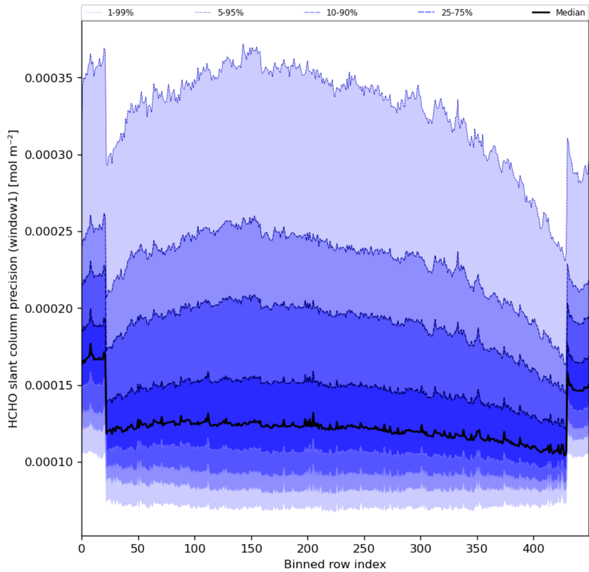
Figure 53: Along track statistics of “HCHO slant column precision (window1)” for 2024-05-23 to 2024-05-24
