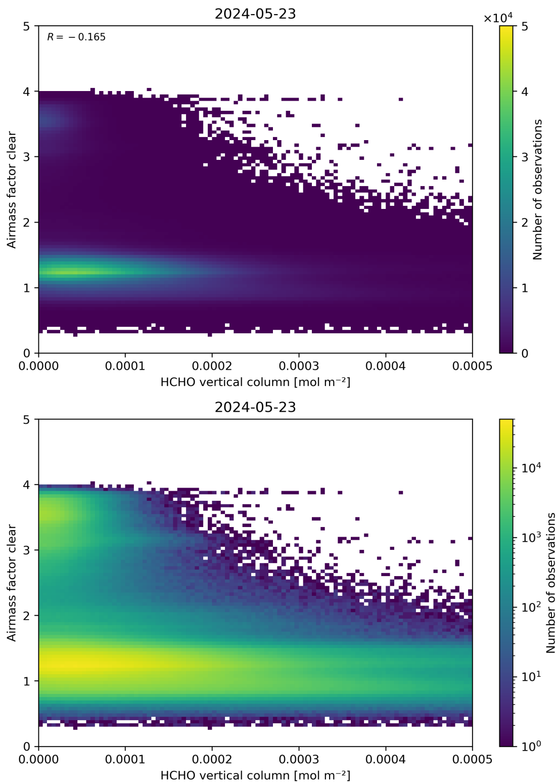
Figure 126: Scatter density plot of “HCHO vertical column” against “Airmass factor clear” for 2024-05-23 to 2024-05-24.
