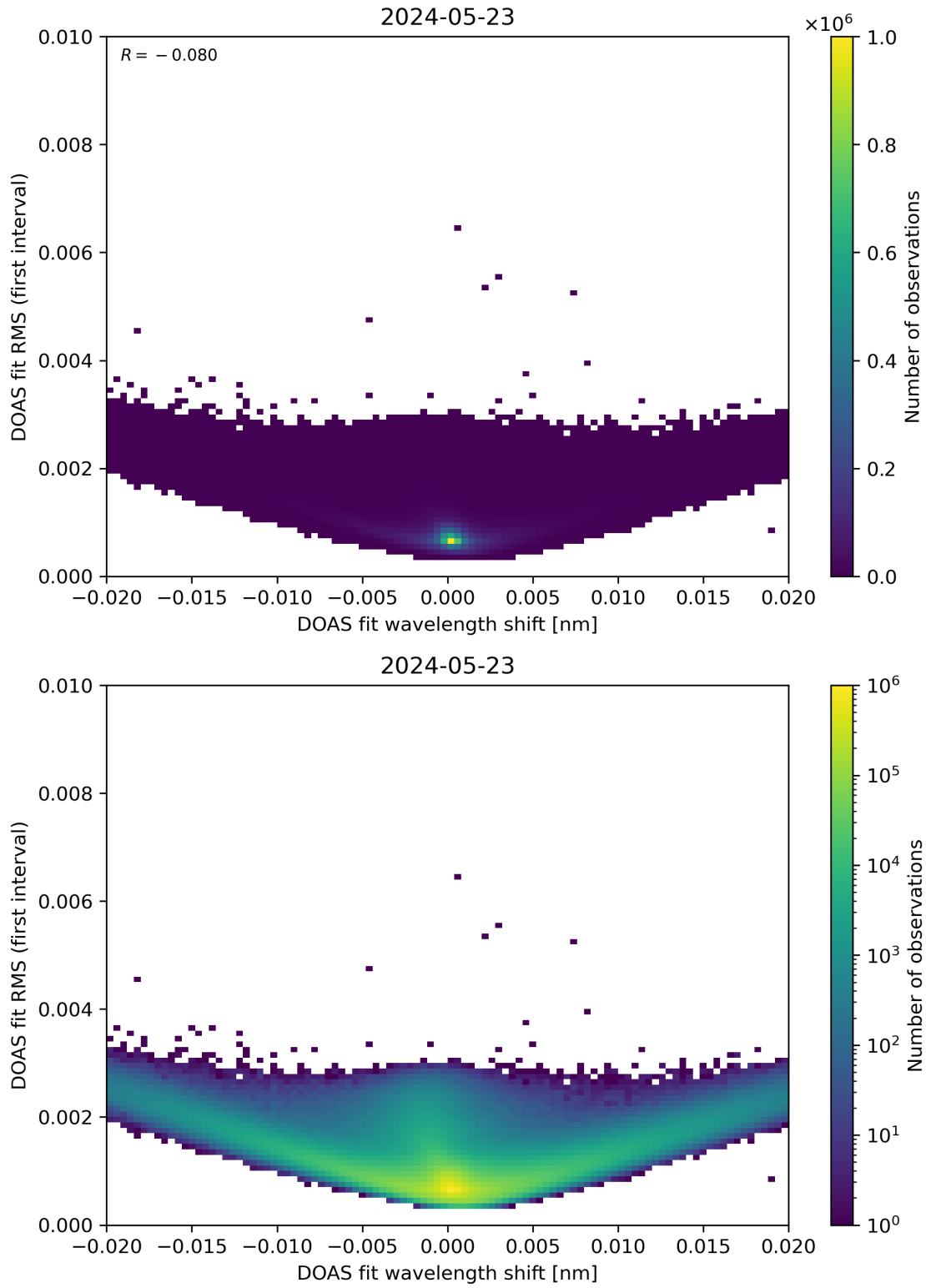
Figure 64: Scatter density plot of “DOAS fit wavelength shift” against “DOAS fit RMS (first interval)” for 2024-05-23 to 2024-05-24.
