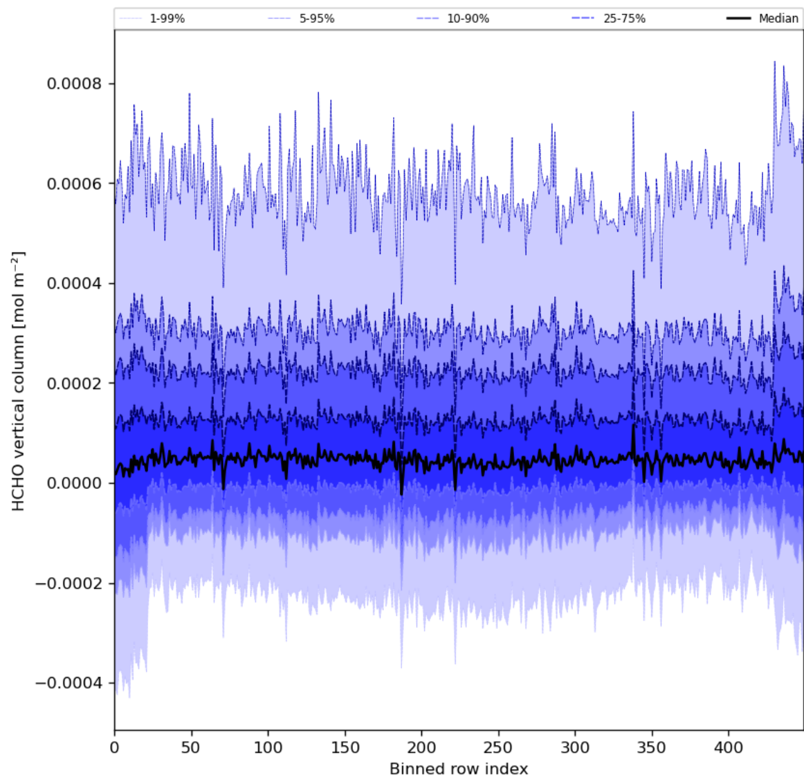
Figure 49: Along track statistics of “HCHO vertical column” for 2024-05-23 to 2024-05-24
