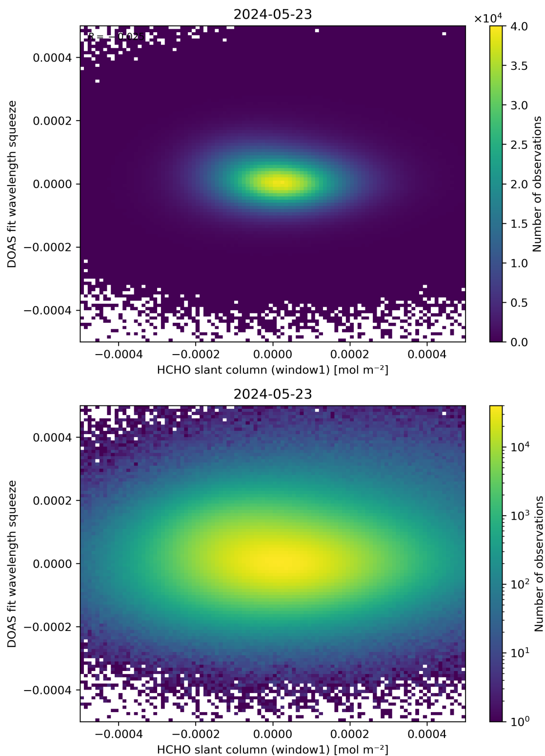
Figure 80: Scatter density plot of “HCHO slant column (window1)” against “DOAS fit wavelength squeeze” for 2024-05-23 to 2024-05-24.
