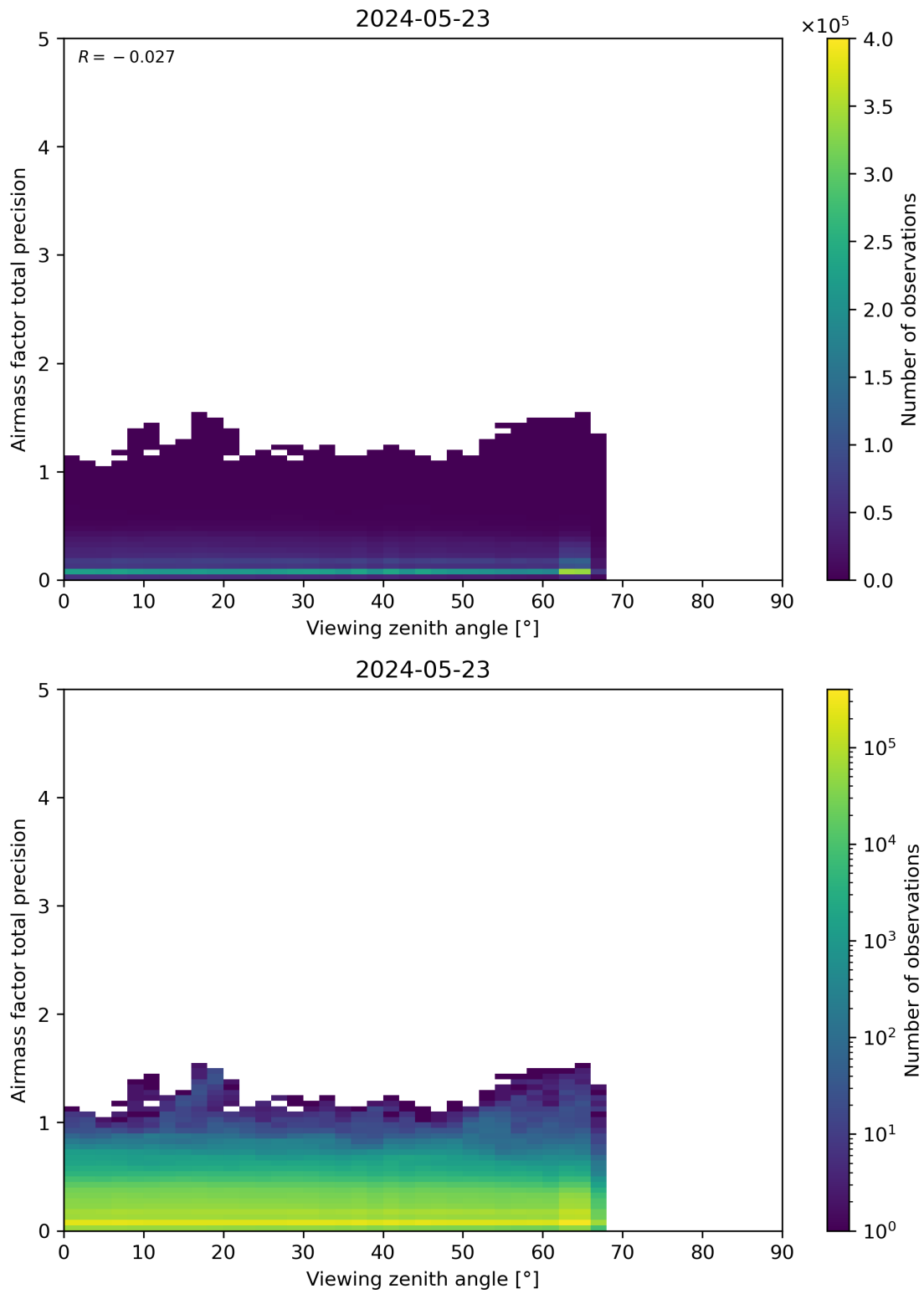
Figure 191: Scatter density plot of “Viewing zenith angle” against “Airmass factor total precision” for 2024-05-23 to 2024-05-24.
