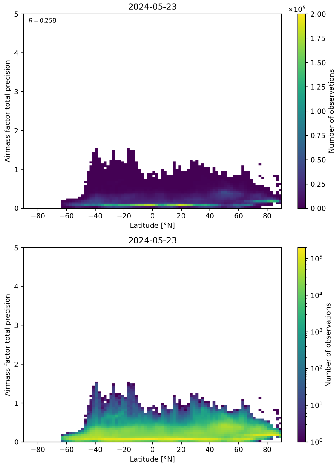
Figure 162: Scatter density plot of “Latitude” against “Airmass factor total precision” for 2024-05-23 to 2024-05-24.
