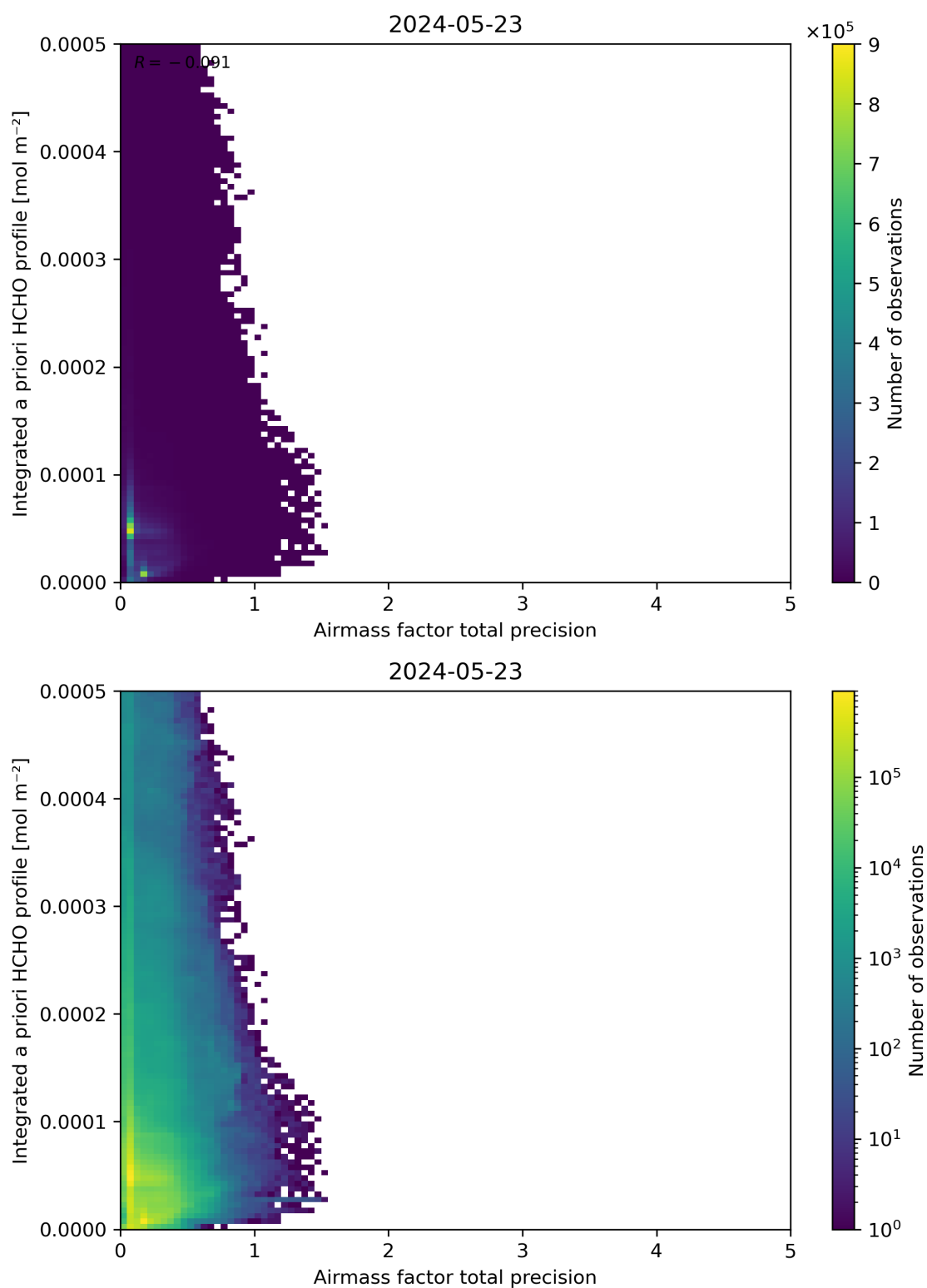
Figure 111: Scatter density plot of “Airmass factor total precision” against “Integrated a priori HCHO profile” for 2024-05-23 to 2024-05-24.
