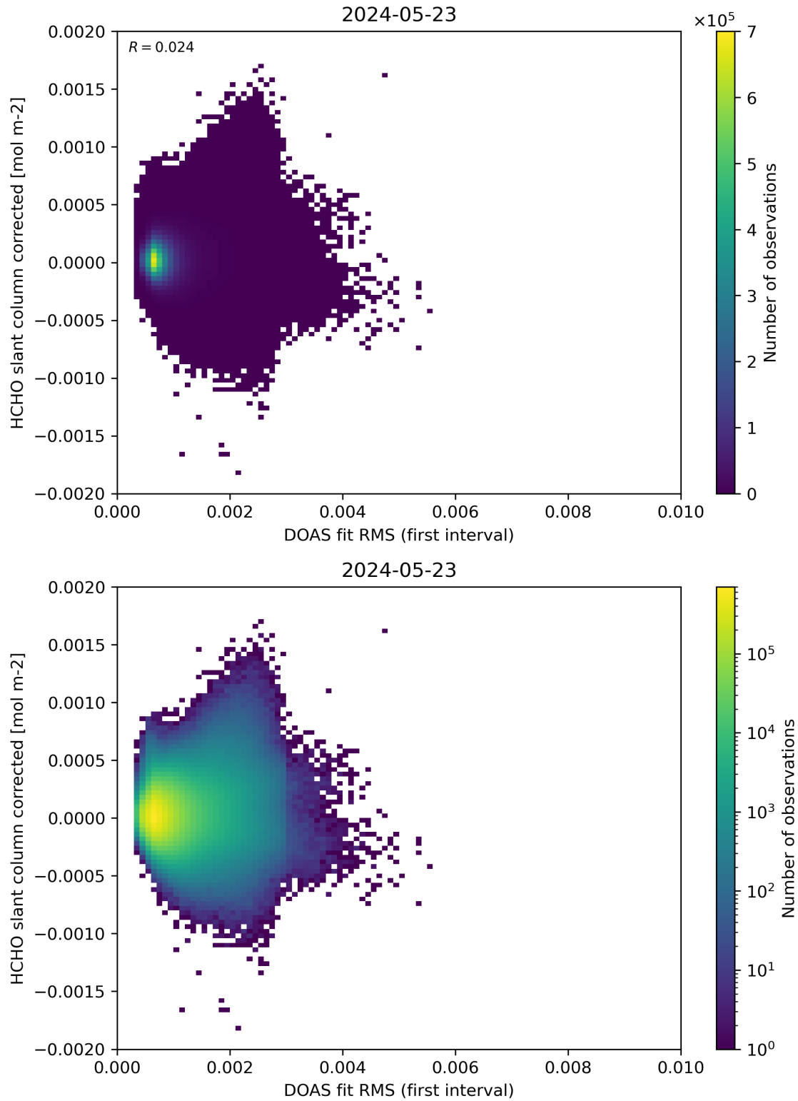
Figure 62: Scatter density plot of “DOAS fit RMS (first interval)” against “HCHO slant column corrected” for 2024-05-23 to 2024-05-24.
