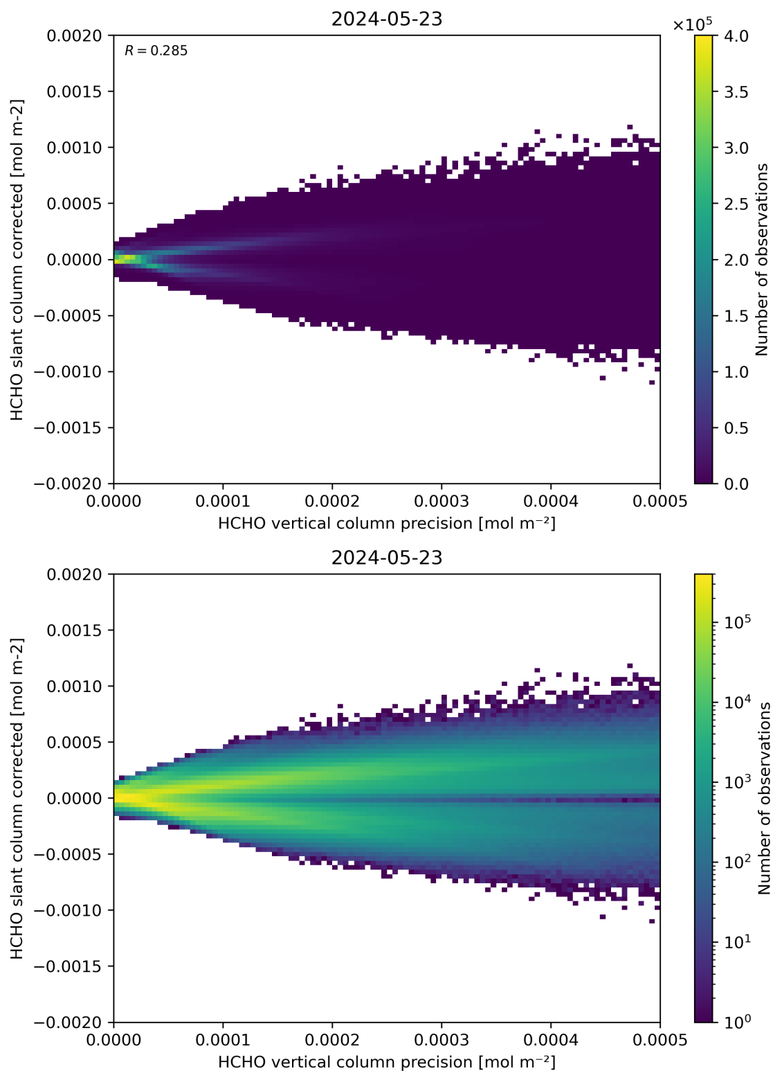
Figure 140: Scatter density plot of “HCHO vertical column precision” against “HCHO slant column corrected” for 2024-05-23 to 2024-05-24.
