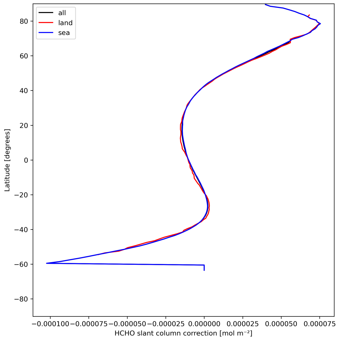
Figure 33: Zonal average of “HCHO slant column correction” for 2024-05-23 to 2024-05-24.
