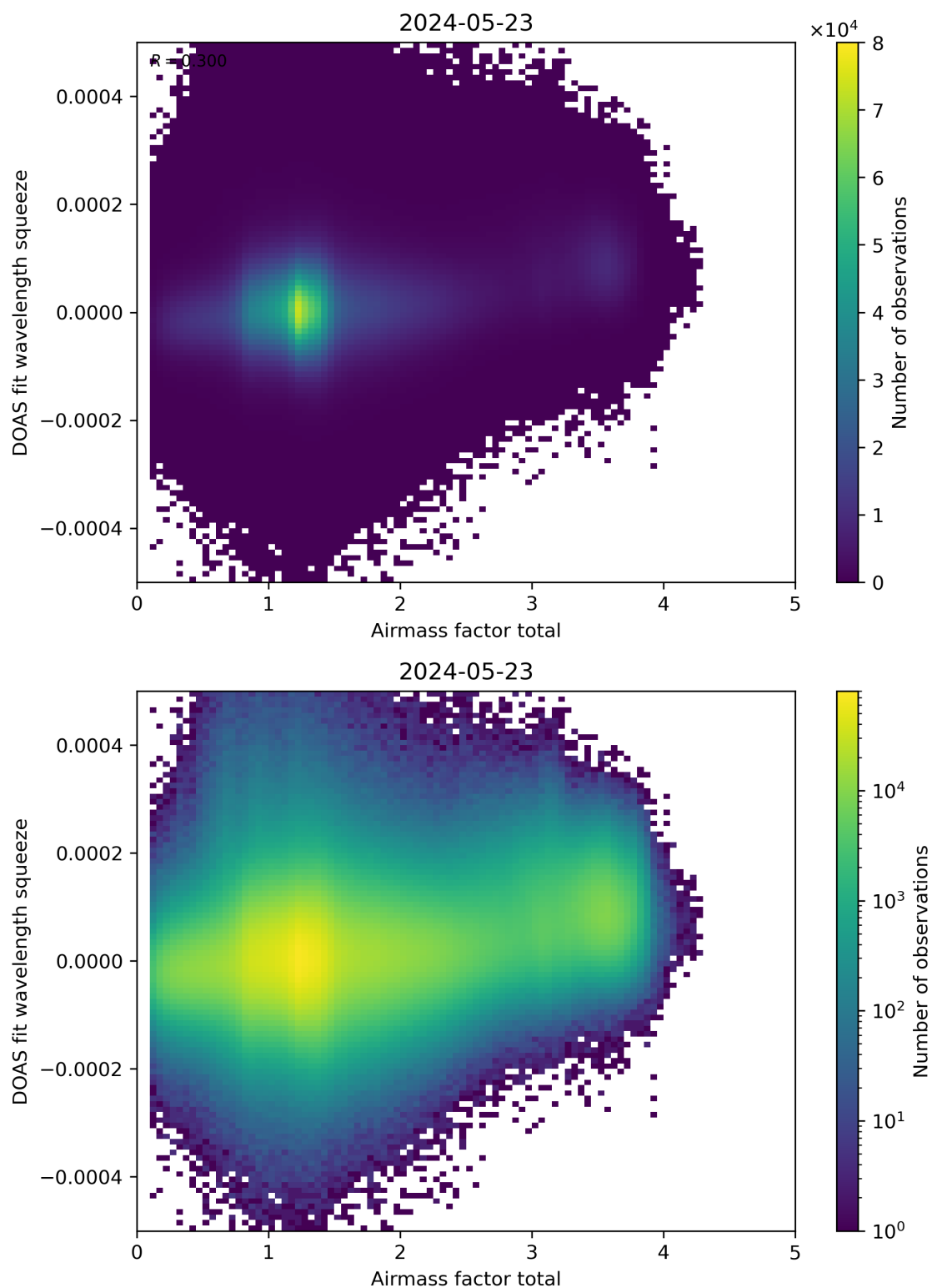
Figure 99: Scatter density plot of “Airmass factor total” against “DOAS fit wavelength squeeze” for 2024-05-23 to 2024-05-24.
