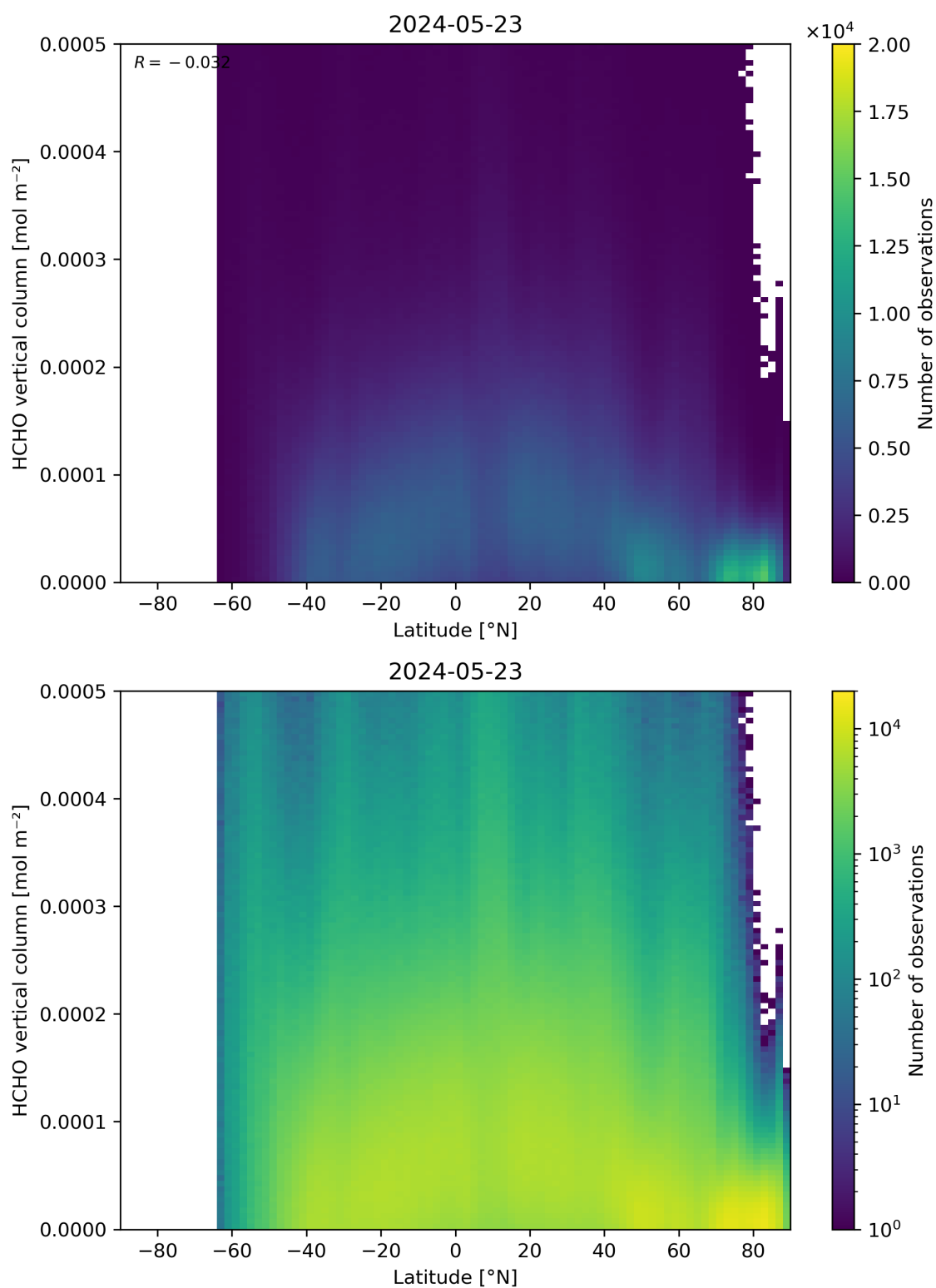
Figure 163: Scatter density plot of “Latitude” against “HCHO vertical column” for 2024-05-23 to 2024-05-24.
