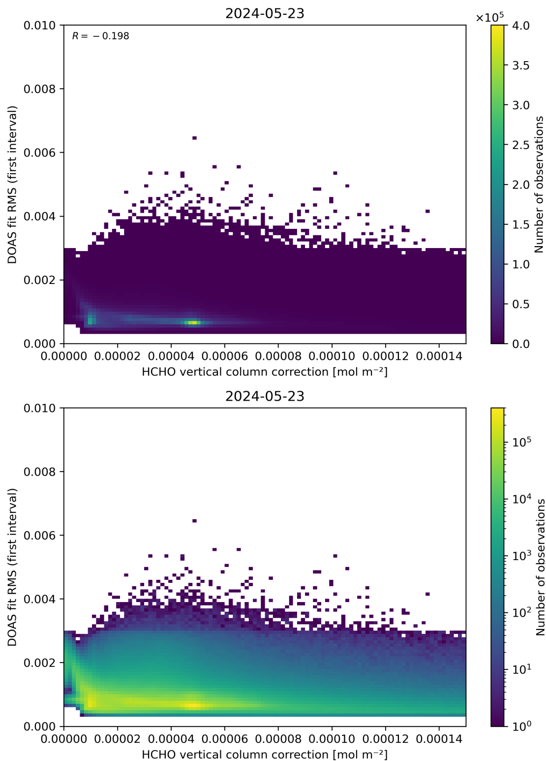
Figure 112: Scatter density plot of “HCHO vertical column correction” against “DOAS fit RMS (first interval)” for 2024-05-23 to 2024-05-24.
