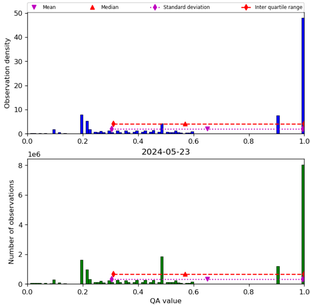
Figure 34: Histogram of “QA value” for 2024-05-23 to 2024-05-24
