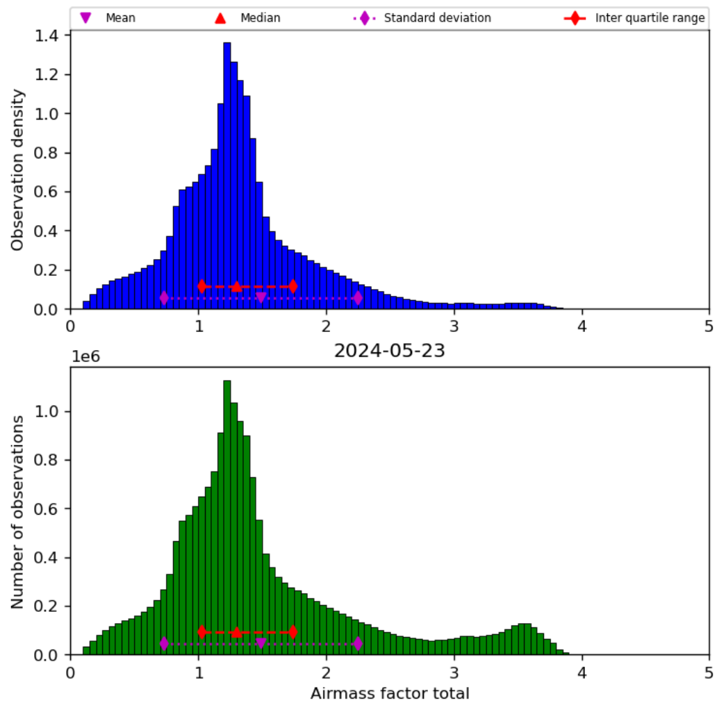
Figure 40: Histogram of “Airmass factor total” for 2024-05-23 to 2024-05-24
