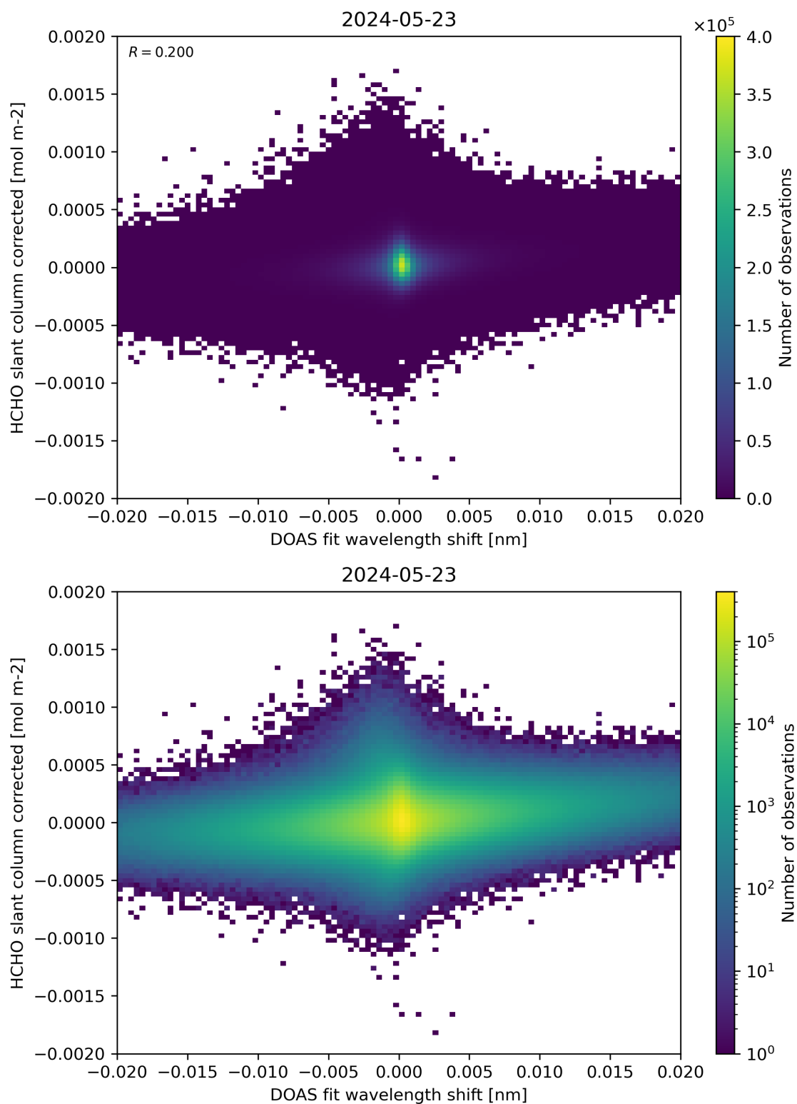
Figure 66: Scatter density plot of “DOAS fit wavelength shift” against “HCHO slant column corrected” for 2024-05-23 to 2024-05-24.
