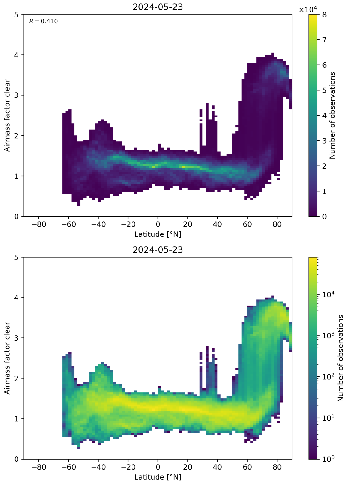
Figure 156: Scatter density plot of “Latitude” against “Airmass factor clear” for 2024-05-23 to 2024-05-24.
