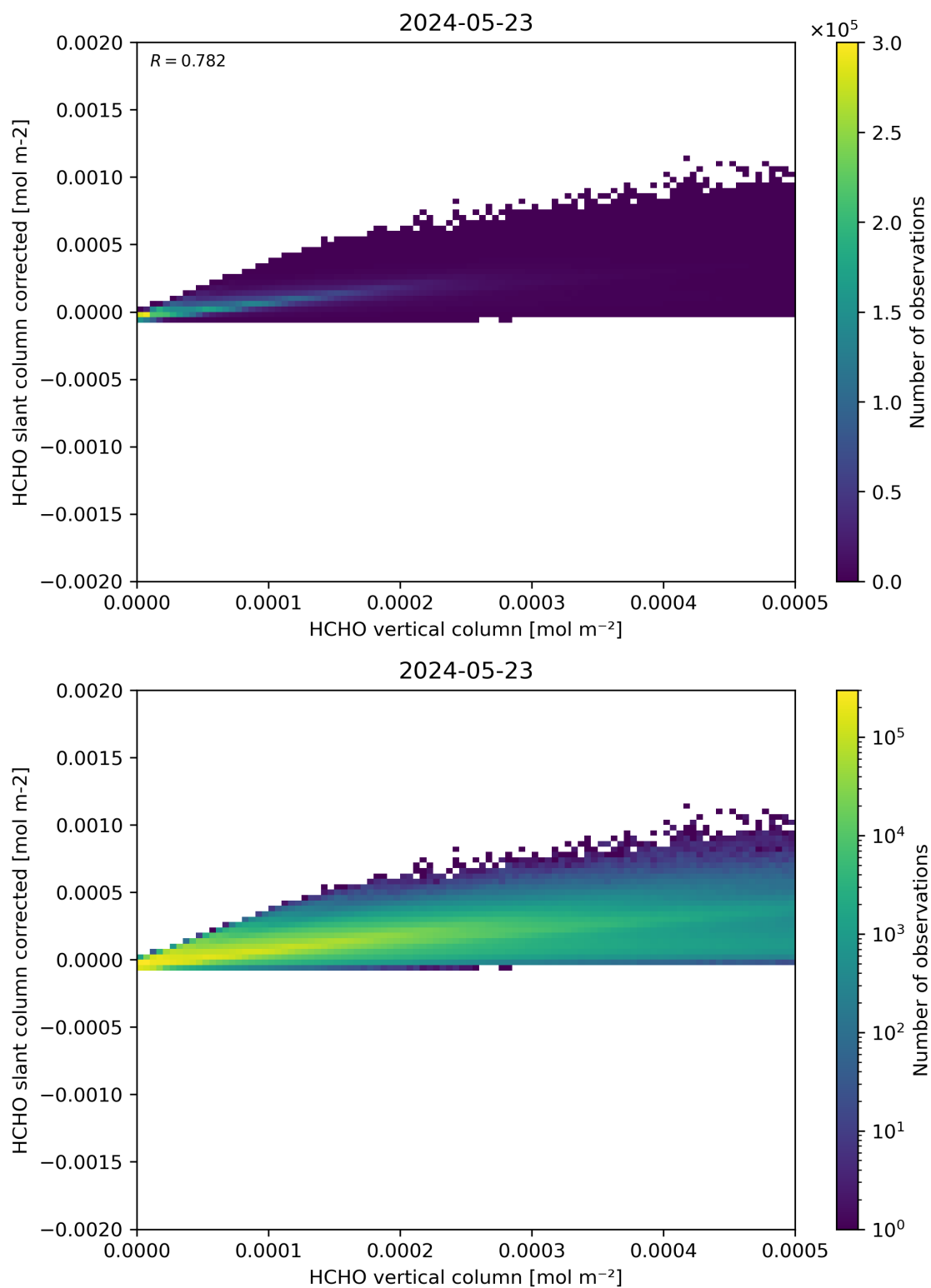
Figure 127: Scatter density plot of “HCHO vertical column” against “HCHO slant column corrected” for 2024-05-23 to 2024-05-24.
