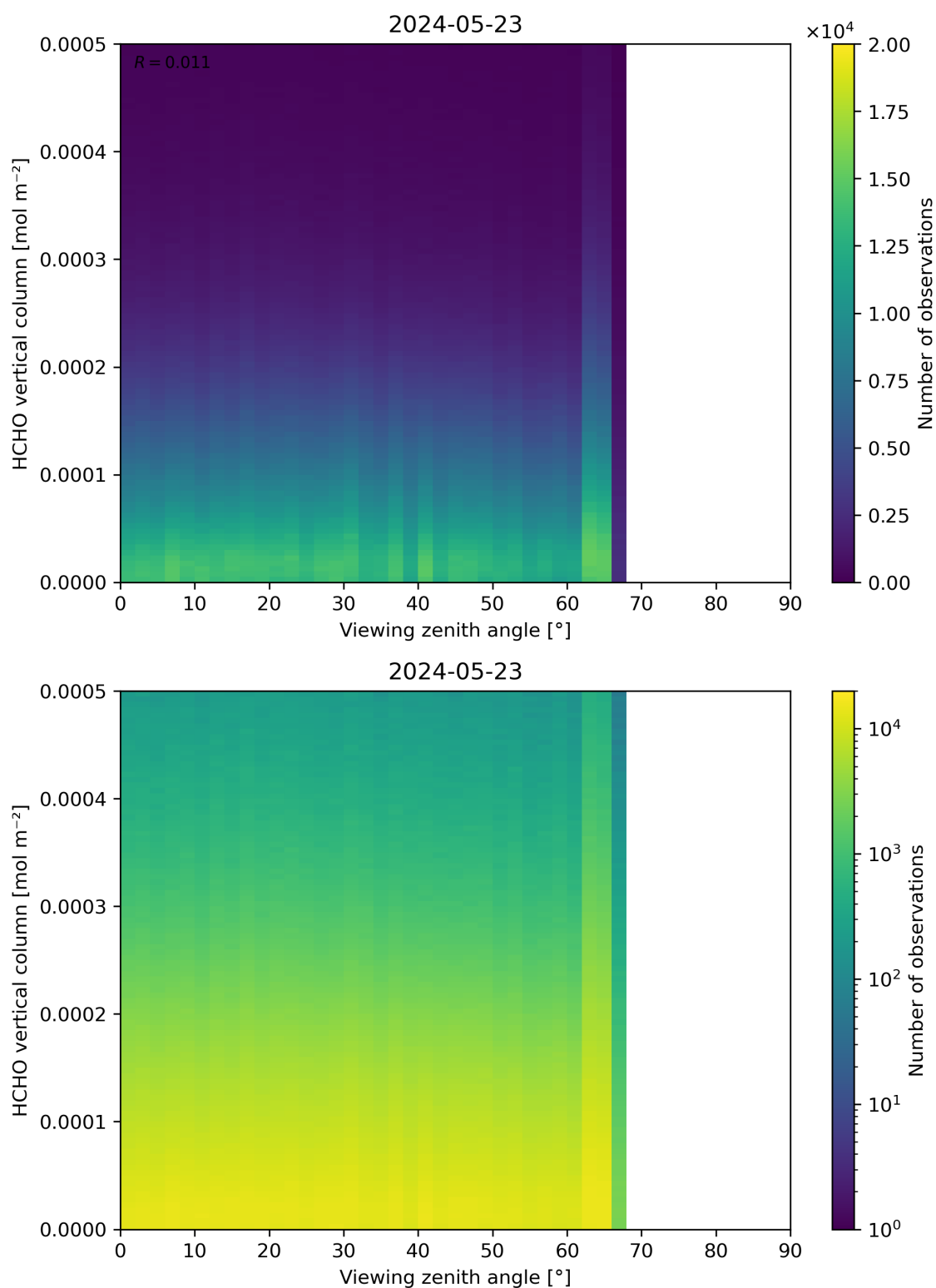
Figure 192: Scatter density plot of “Viewing zenith angle” against “HCHO vertical column” for 2024-05-23 to 2024-05-24.
