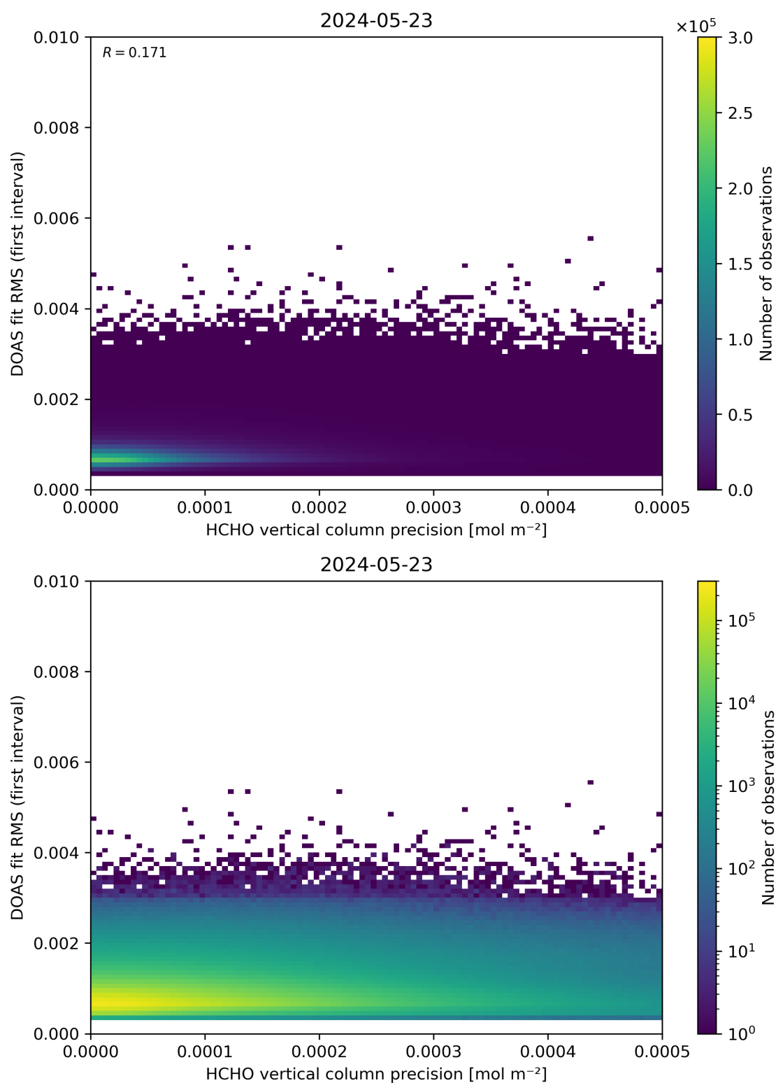
Figure 136: Scatter density plot of “HCHO vertical column precision” against “DOAS fit RMS (first interval)” for 2024-05-23 to 2024-05-24.
