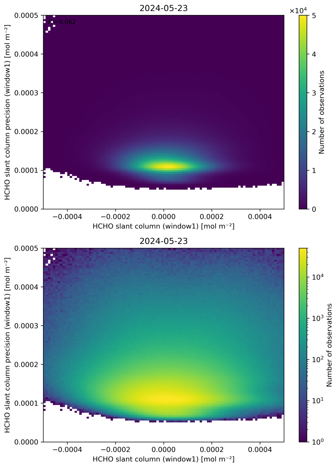
Figure 84: Scatter density plot of “HCHO slant column (window1)” against “HCHO slant column precision (window1)” for 2024-05-23 to 2024-05-24.
