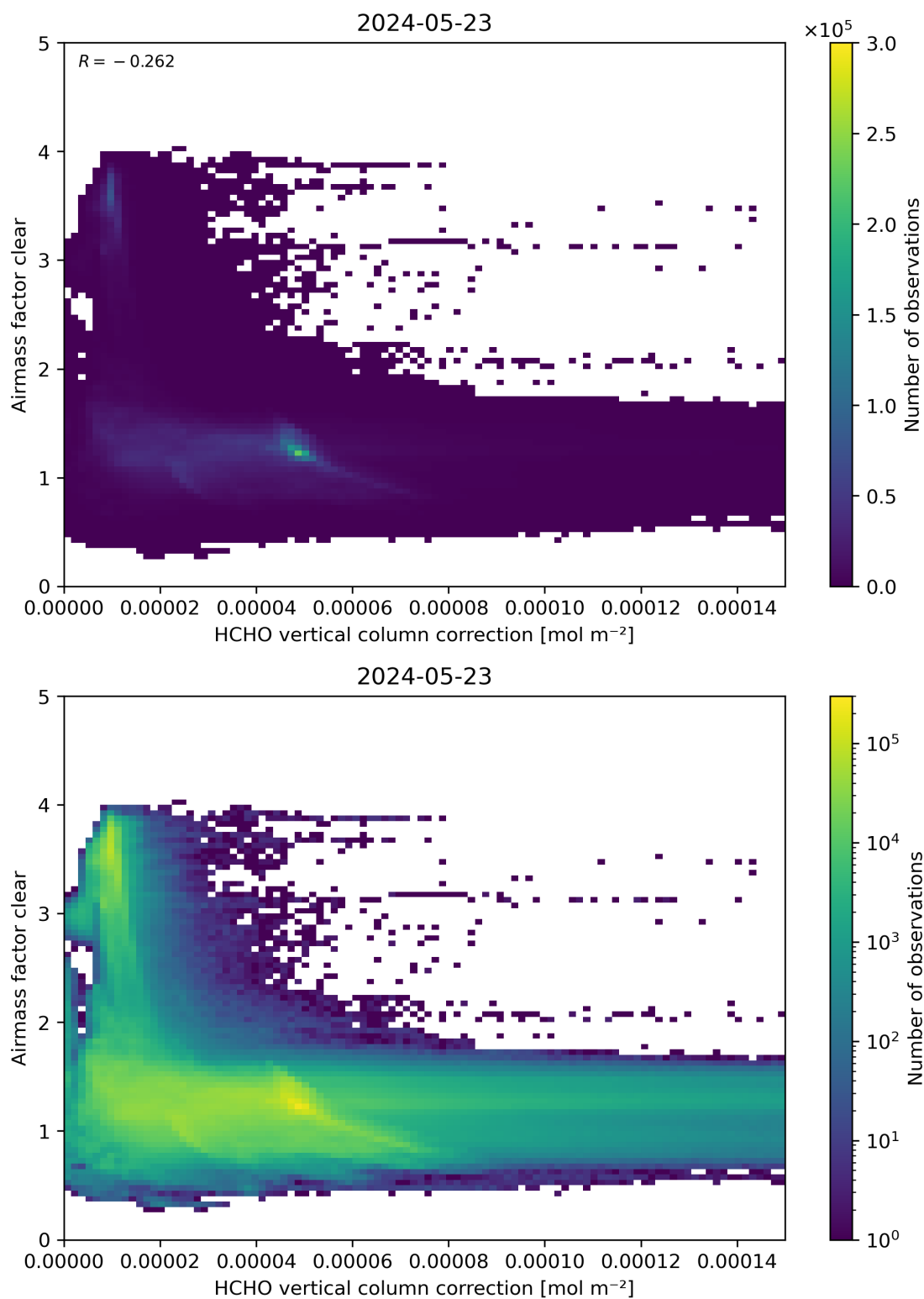
Figure 115: Scatter density plot of “HCHO vertical column correction” against “Airmass factor clear” for 2024-05-23 to 2024-05-24.
