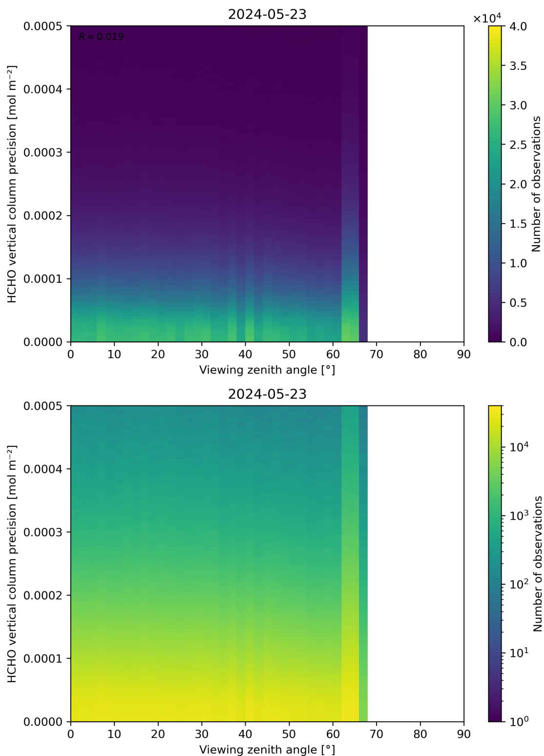
Figure 194: Scatter density plot of “Viewing zenith angle” against “HCHO vertical column precision” for 2024-05-23 to 2024-05-24.
