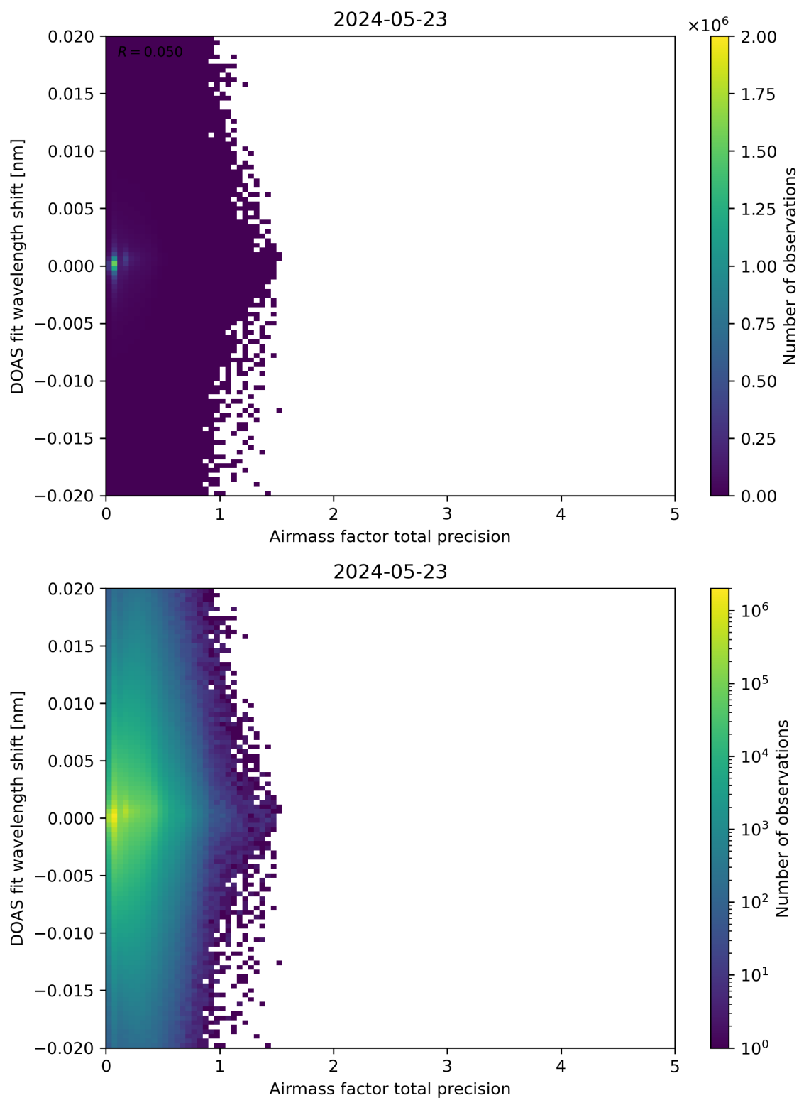
Figure 106: Scatter density plot of “Airmass factor total precision” against “DOAS fit wavelength shift” for 2024-05-23 to 2024-05-24.
