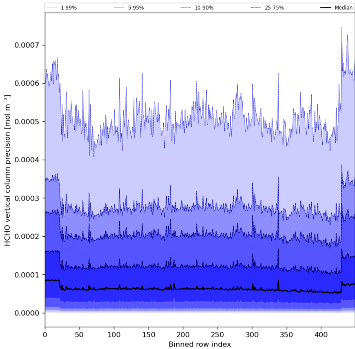
Figure 50: Along track statistics of “HCHO vertical column precision” for 2024-05-23 to 2024-05-24
