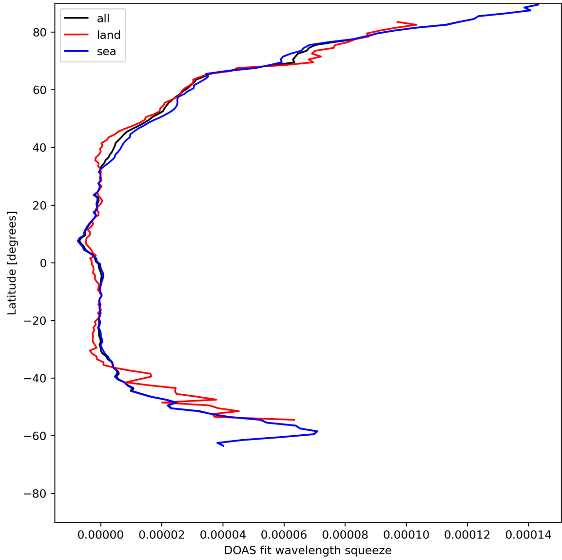
Figure 31: Zonal average of “DOAS fit wavelength squeeze” for 2024-05-23 to 2024-05-24.
