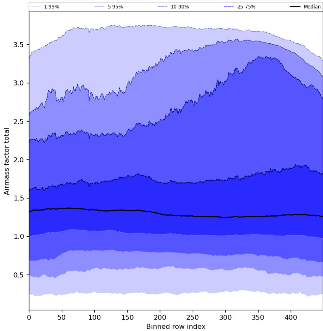
Figure 54: Along track statistics of “Airmass factor total” for 2024-05-23 to 2024-05-24
