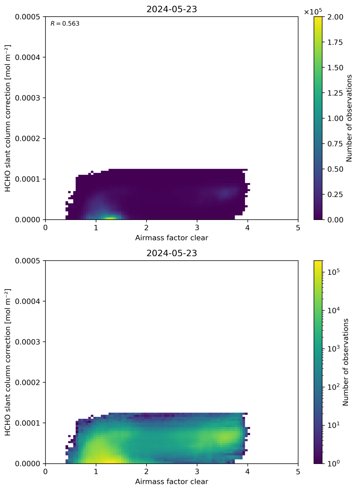
Figure 75: Scatter density plot of “Airmass factor clear” against “HCHO slant column correction” for 2024-05-23 to 2024-05-24.
