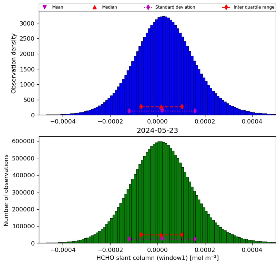
Figure 38: Histogram of “HCHO slant column (window1)” for 2024-05-23 to 2024-05-24
