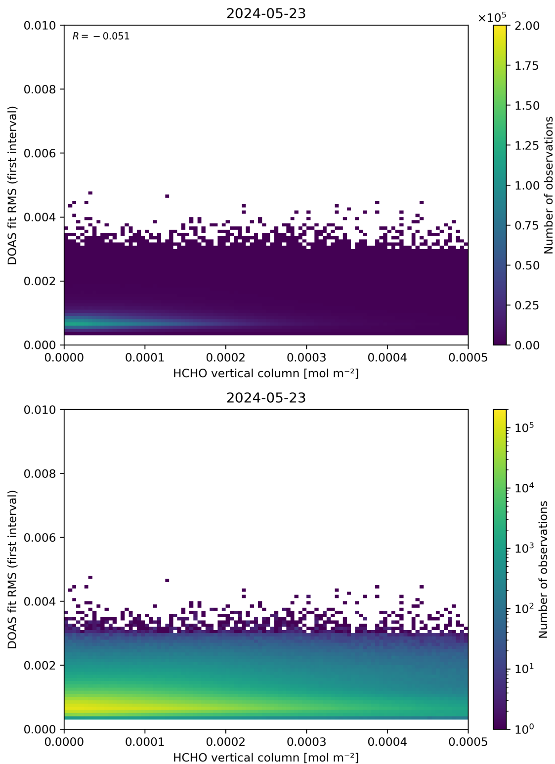
Figure 123: Scatter density plot of “HCHO vertical column” against “DOAS fit RMS (first interval)” for 2024-05-23 to 2024-05-24.
