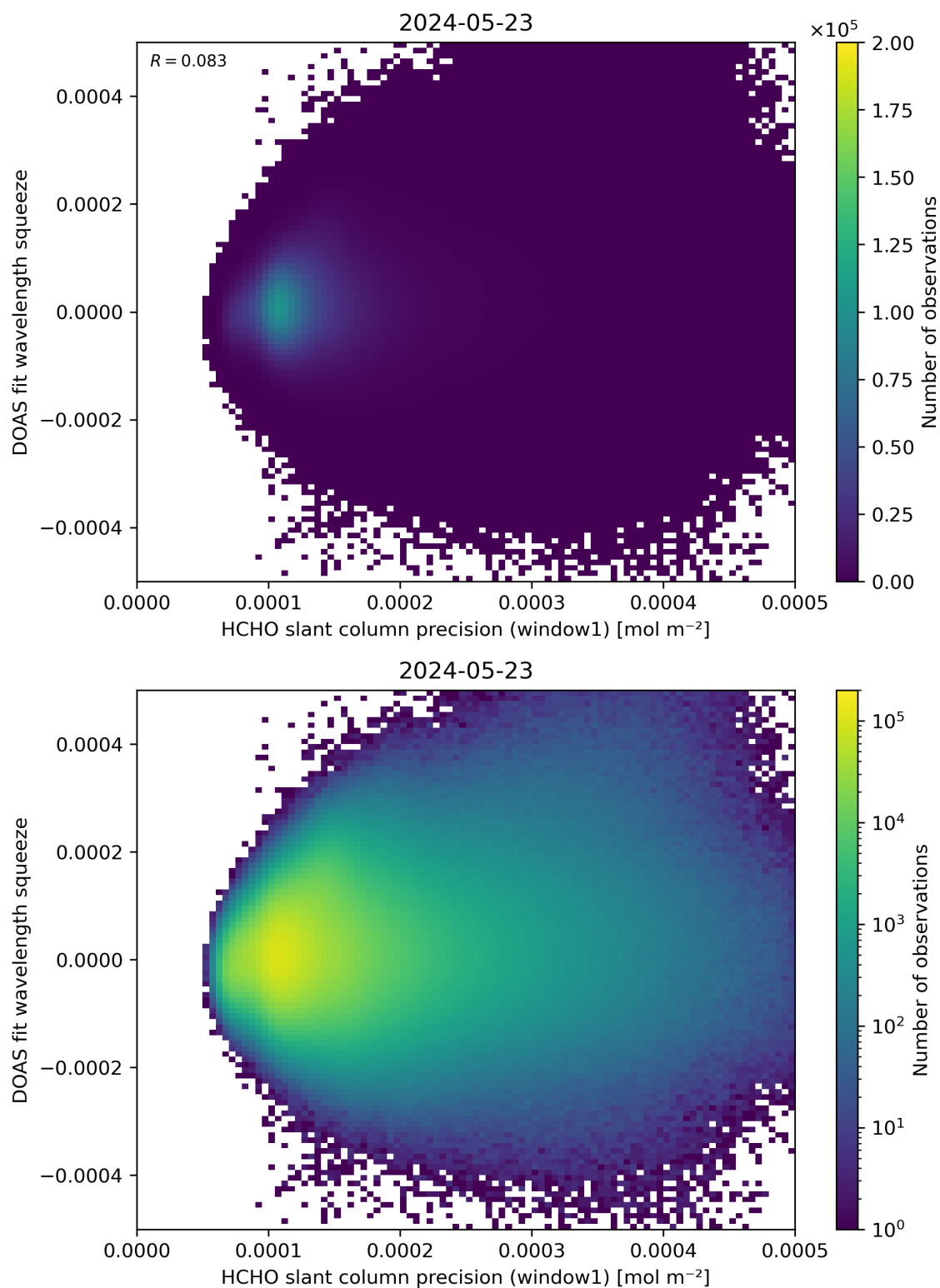
Figure 90: Scatter density plot of “HCHO slant column precision (window1)” against “DOAS fit wavelength squeeze” for 2024-05-23 to 2024-05-24.
