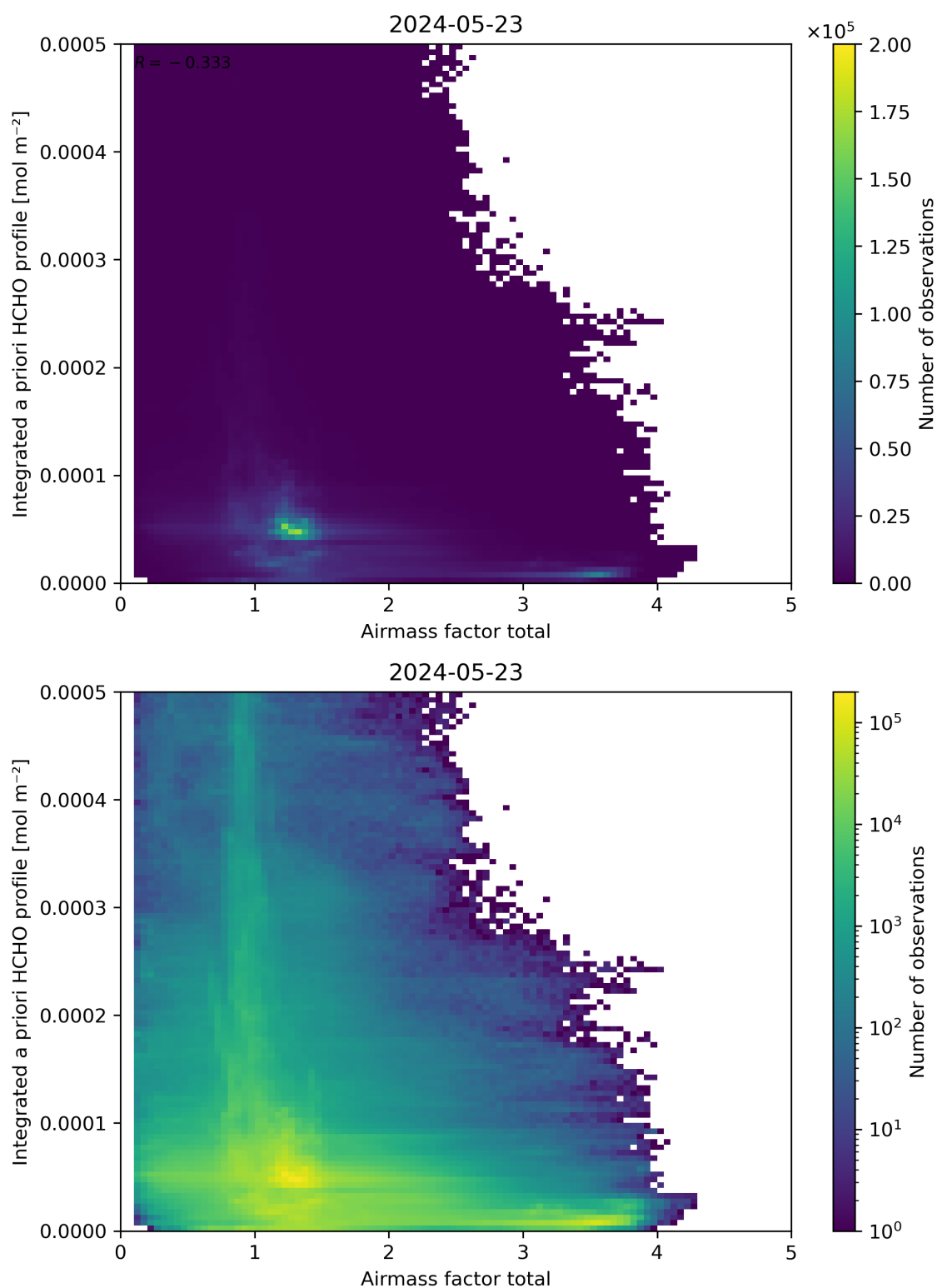
Figure 104: Scatter density plot of “Airmass factor total” against “Integrated a priori HCHO profile” for 2024-05-23 to 2024-05-24.
