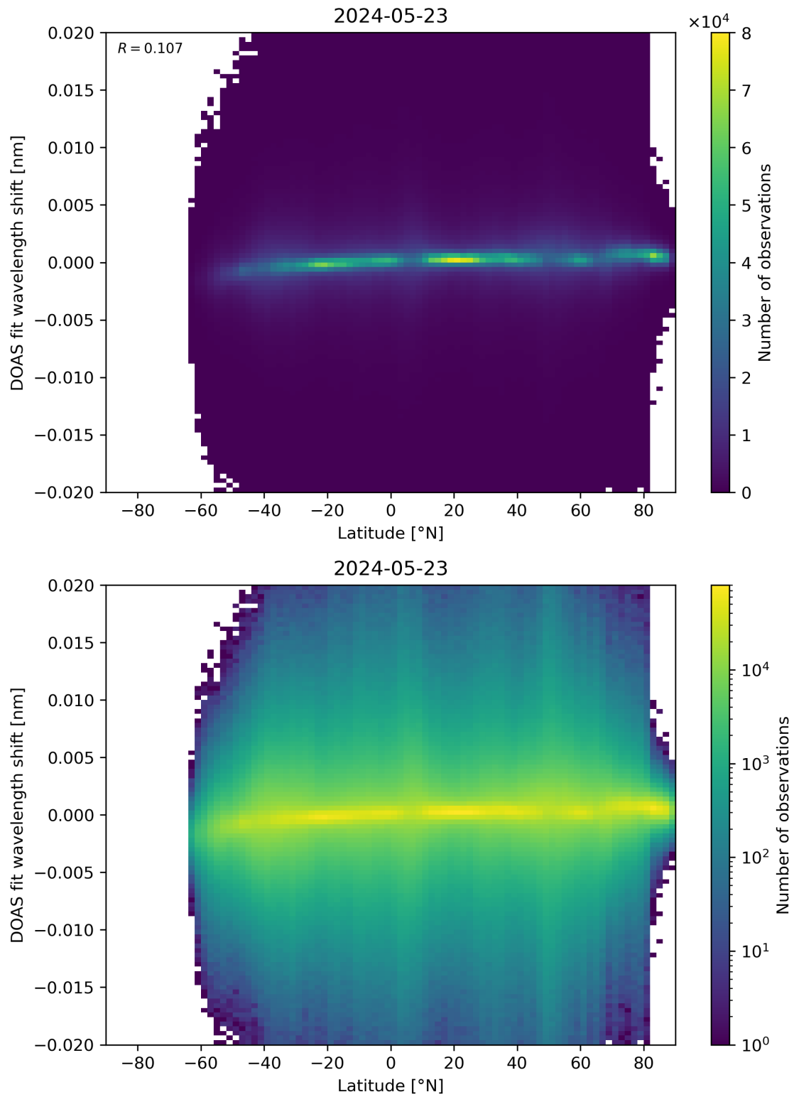
Figure 154: Scatter density plot of “Latitude” against “DOAS fit wavelength shift” for 2024-05-23 to 2024-05-24.
