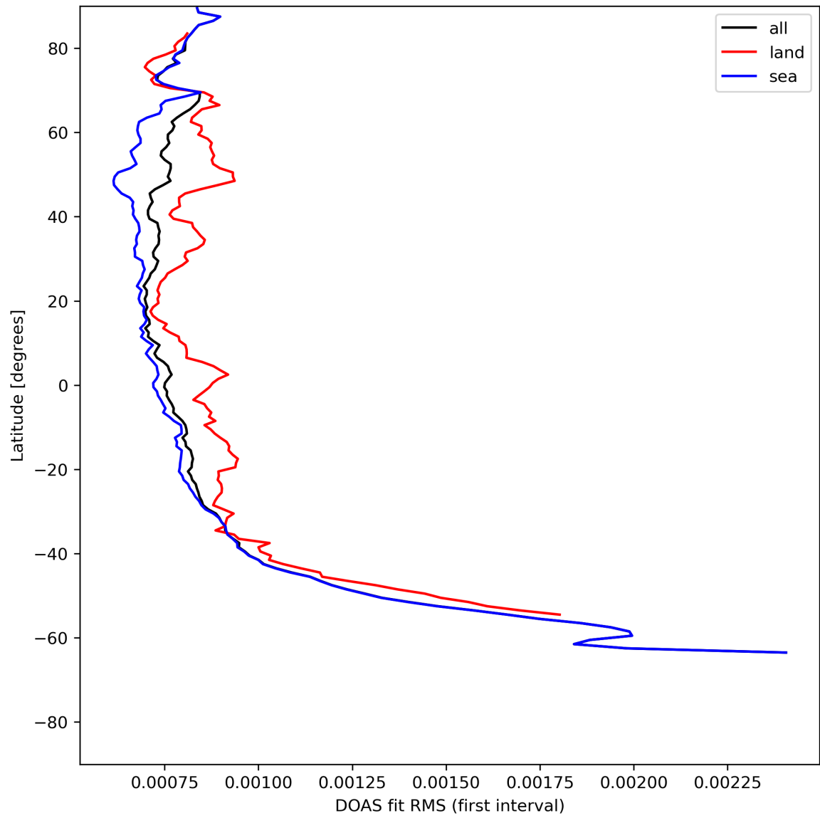
Figure 32: Zonal average of “DOAS fit RMS (first interval)” for 2024-05-23 to 2024-05-24.
