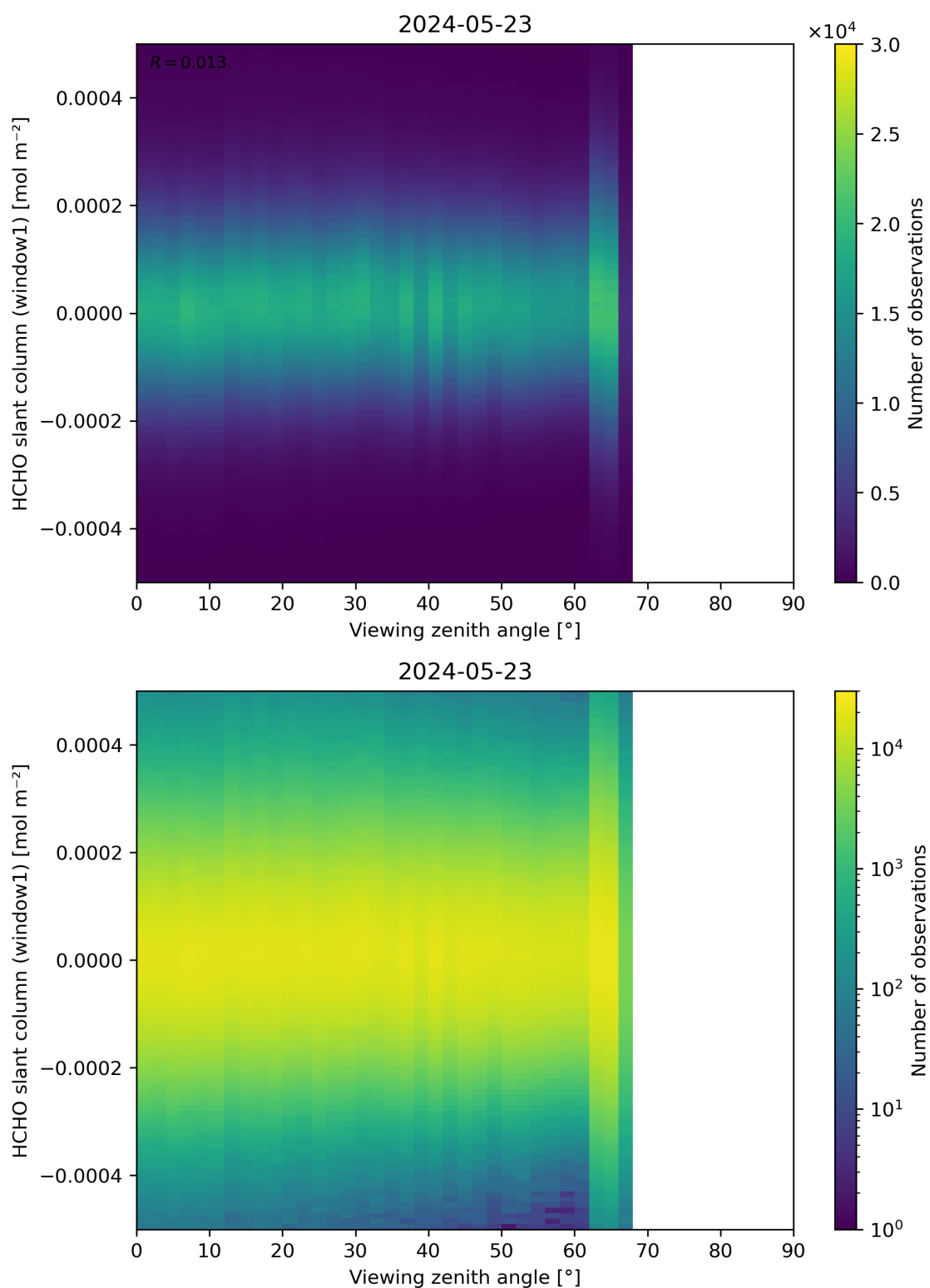
Figure 188: Scatter density plot of “Viewing zenith angle” against “HCHO slant column (window1)” for 2024-05-23 to 2024-05-24.
