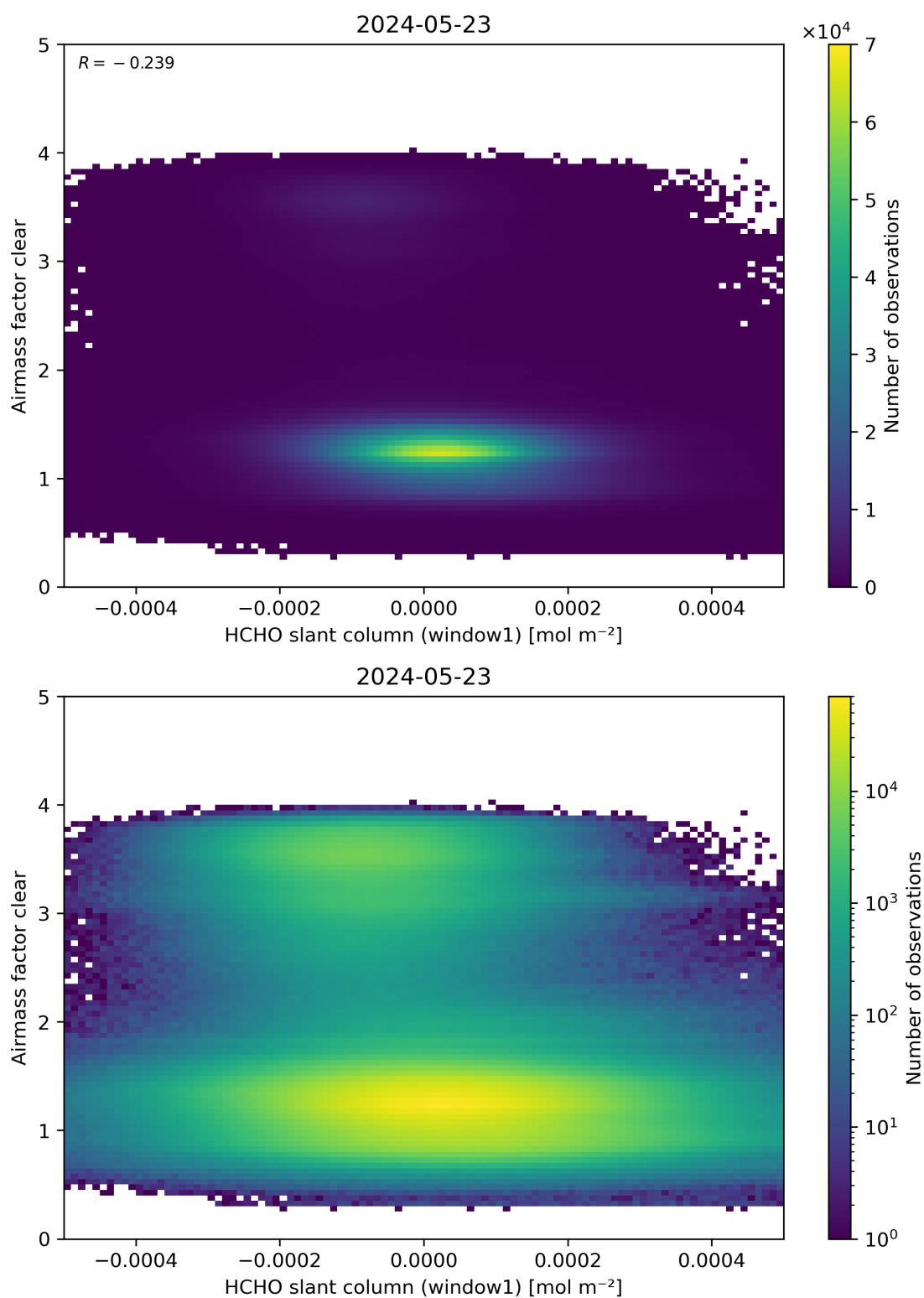
Figure 81: Scatter density plot of “HCHO slant column (window1)” against “Airmass factor clear” for 2024-05-23 to 2024-05-24.
