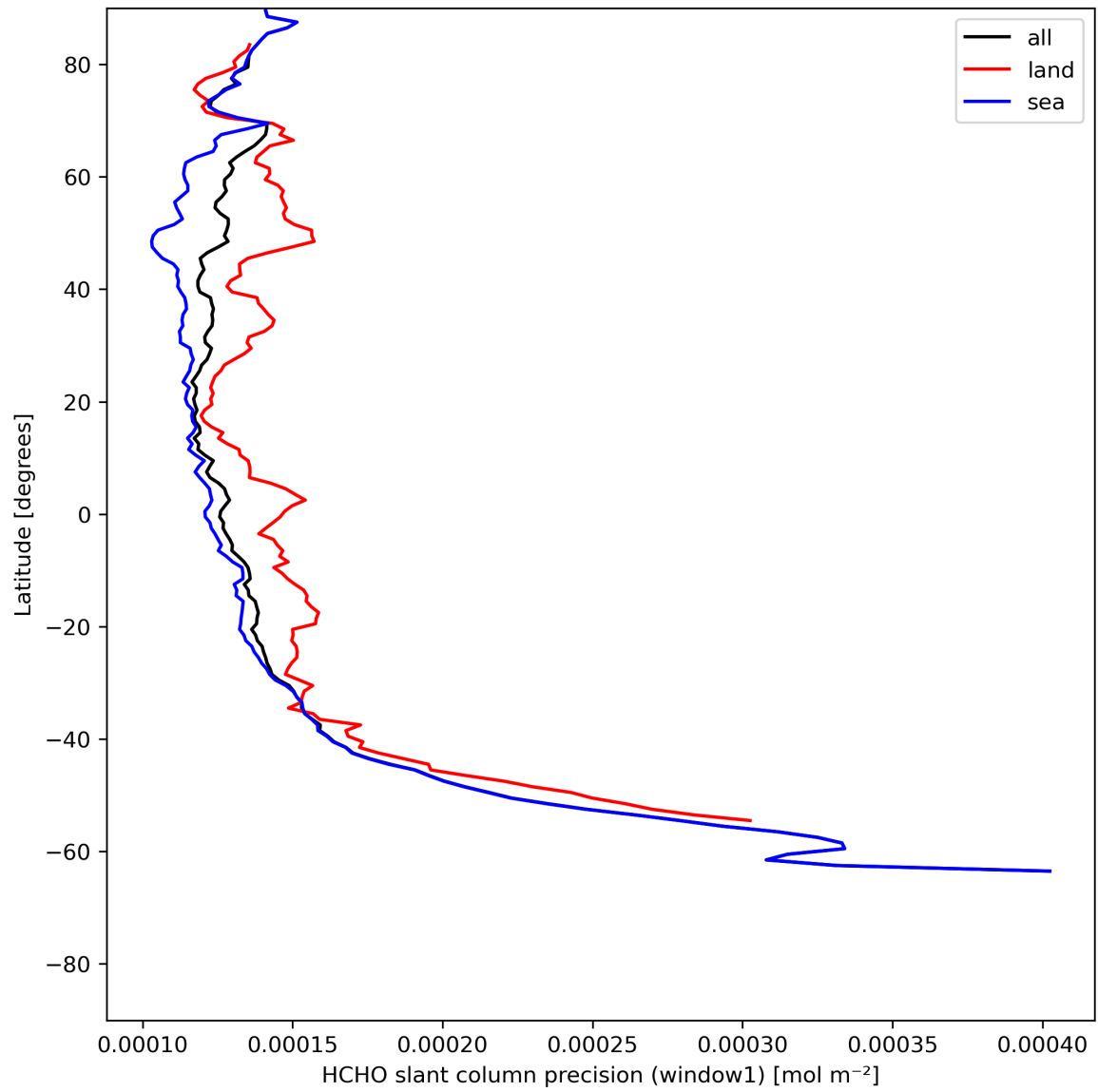
Figure 25: Zonal average of “HCHO slant column precision (window1)” for 2024-05-23 to 2024-05-24.
