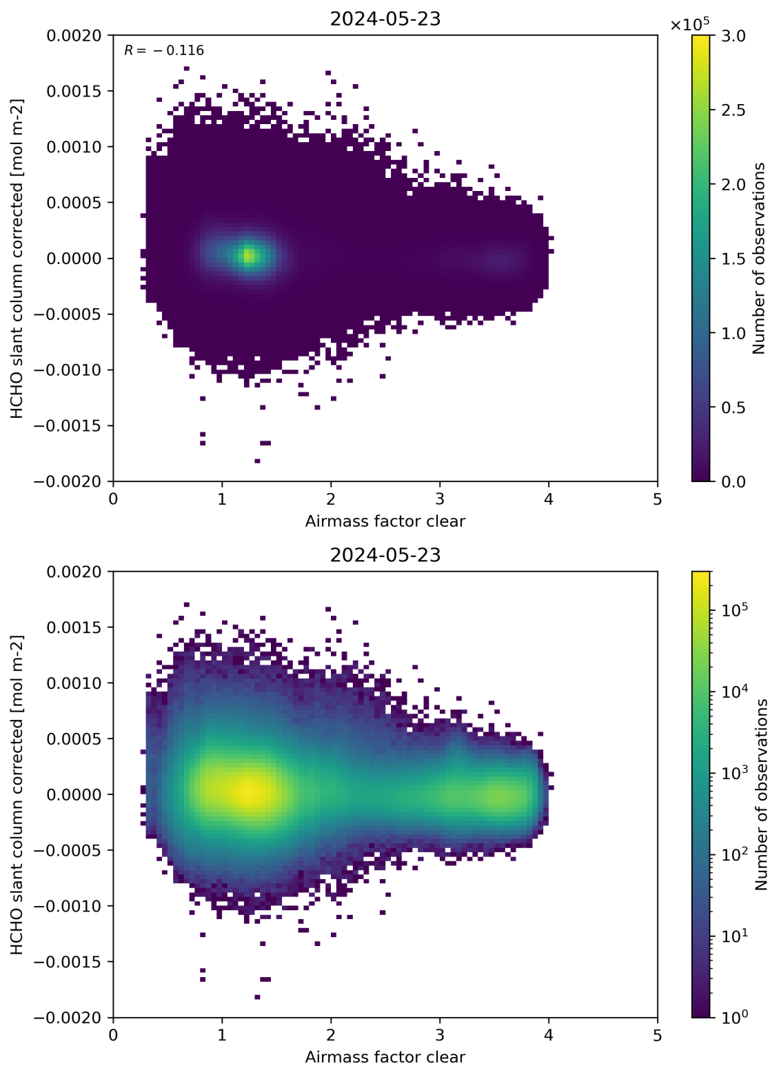
Figure 74: Scatter density plot of “Airmass factor clear” against “HCHO slant column corrected” for 2024-05-23 to 2024-05-24.
