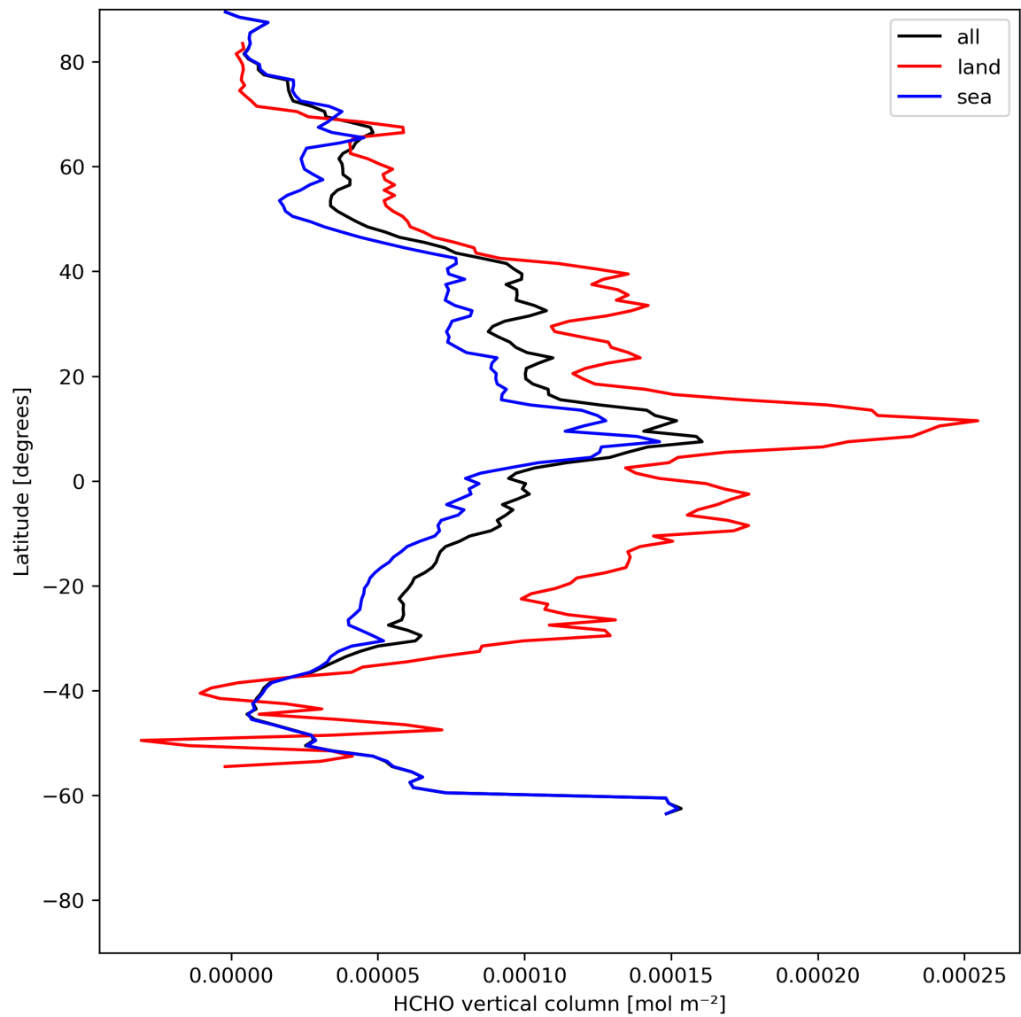
Figure 21: Zonal average of “HCHO vertical column” for 2024-05-23 to 2024-05-24.
