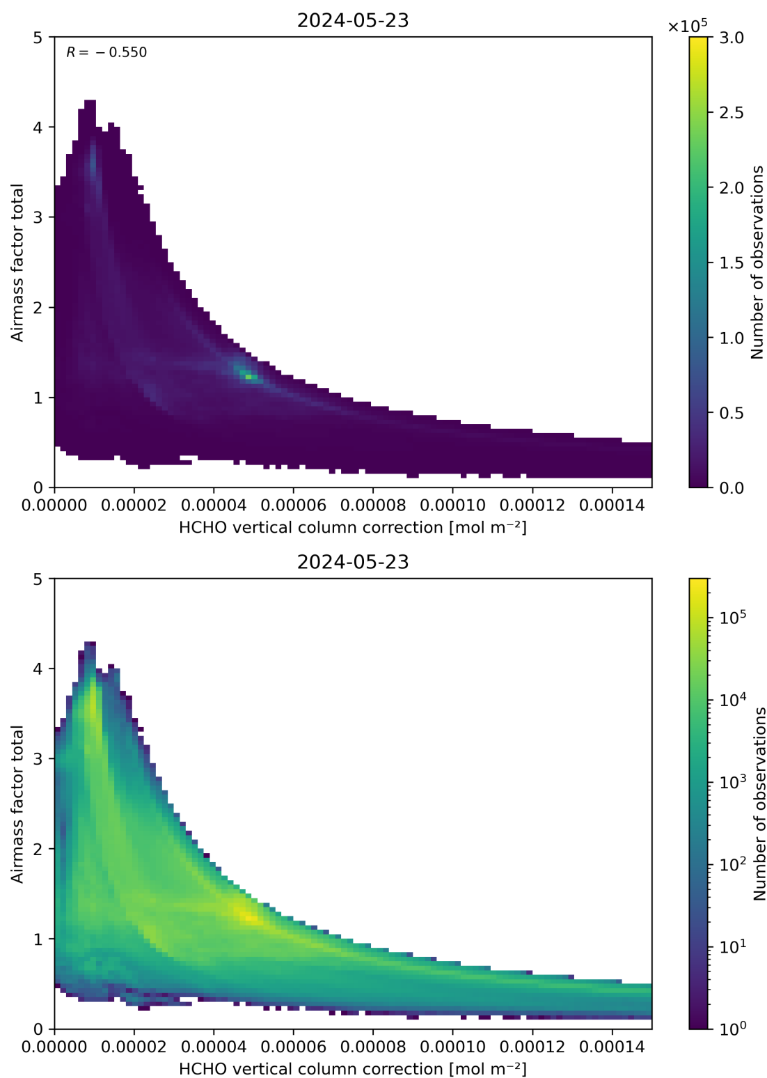
Figure 120: Scatter density plot of “HCHO vertical column correction” against “Airmass factor total” for 2024-05-23 to 2024-05-24.
