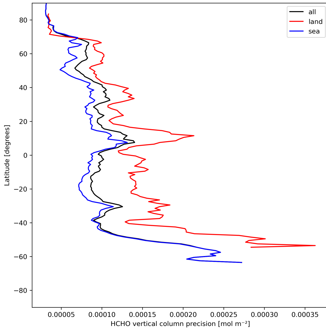
Figure 22: Zonal average of “HCHO vertical column precision” for 2024-05-23 to 2024-05-24.
