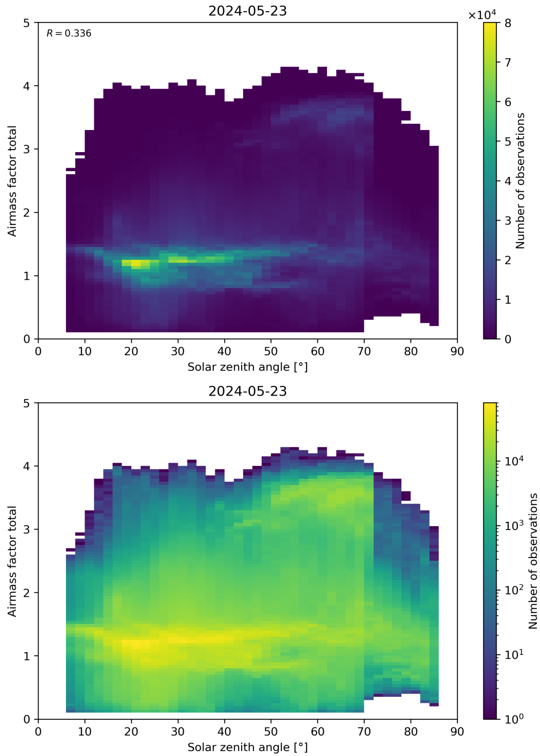
Figure 175: Scatter density plot of “Solar zenith angle” against “Airmass factor total” for 2024-05-23 to 2024-05-24.
