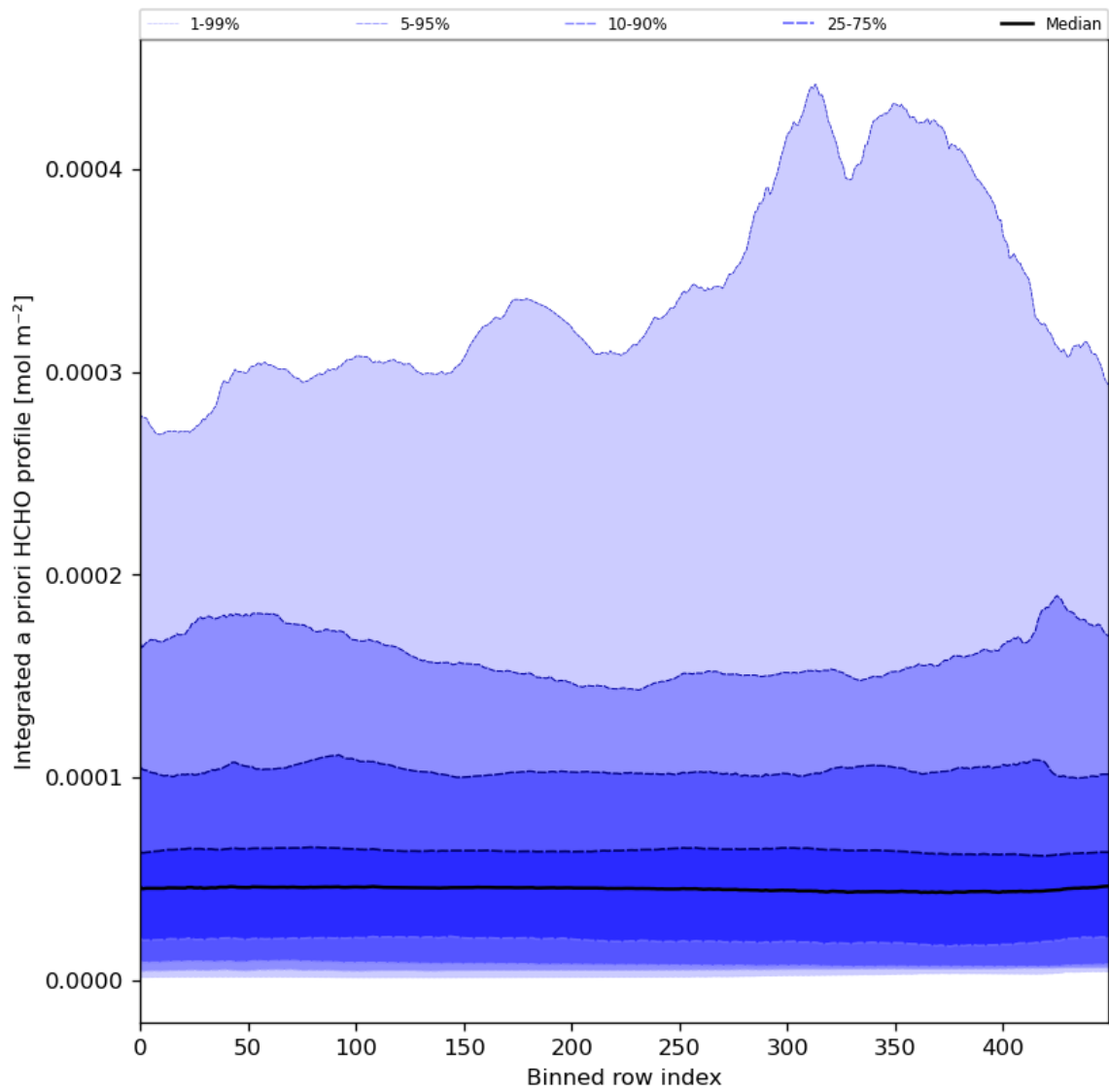
Figure 57: Along track statistics of “Integrated a priori HCHO profile” for 2024-05-23 to 2024-05-24
