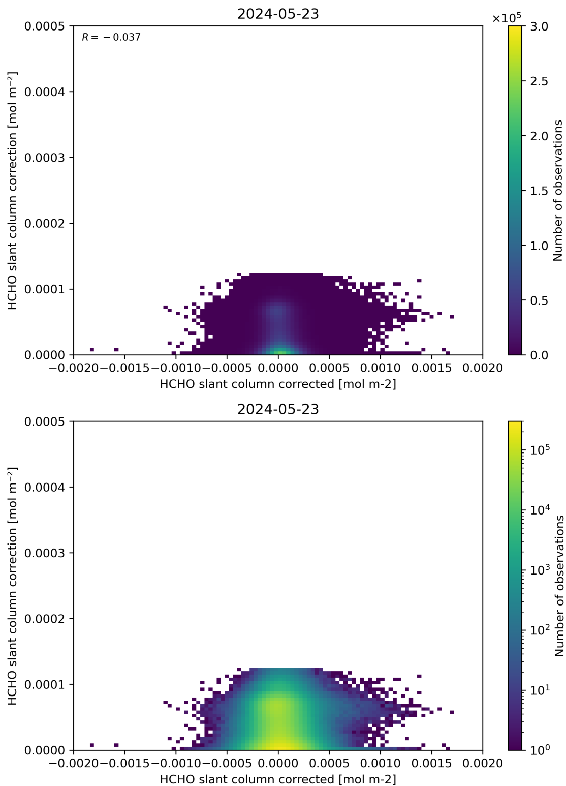
Figure 77: Scatter density plot of “HCHO slant column corrected” against “HCHO slant column correction” for 2024-05-23 to 2024-05-24.
