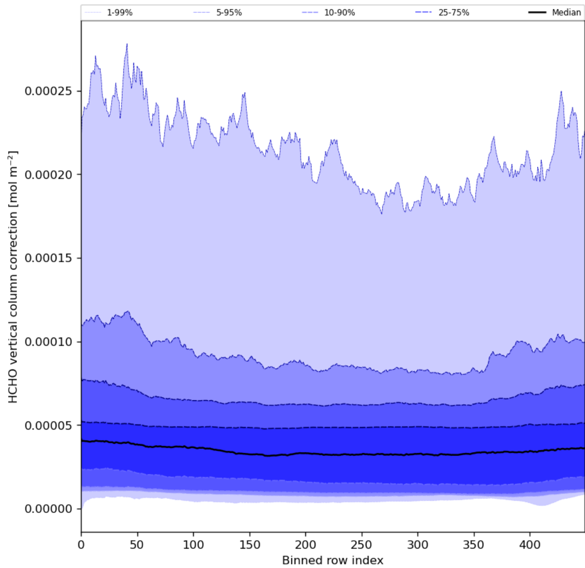
Figure 51: Along track statistics of “HCHO vertical column correction” for 2024-05-23 to 2024-05-24
