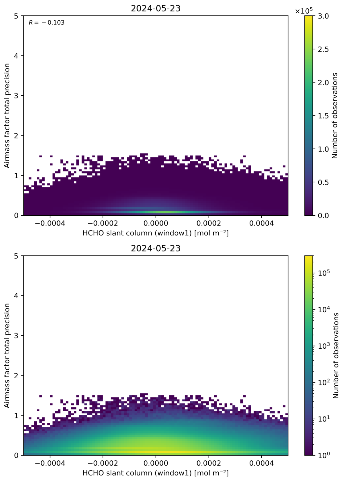
Figure 86: Scatter density plot of “HCHO slant column (window1)” against “Airmass factor total precision” for 2024-05-23 to 2024-05-24.
