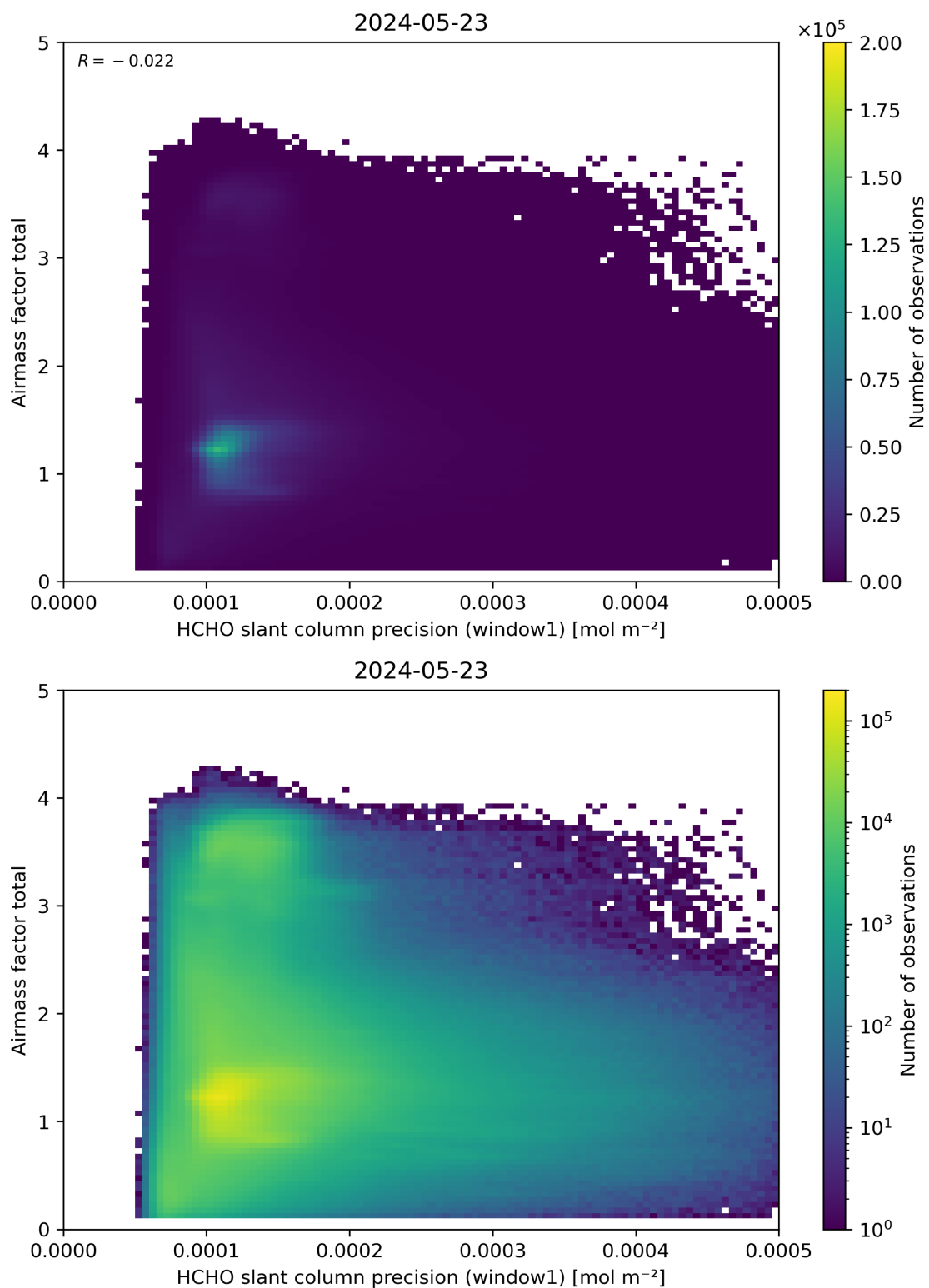
Figure 94: Scatter density plot of “HCHO slant column precision (window1)” against “Airmass factor total” for 2024-05-23 to 2024-05-24.
