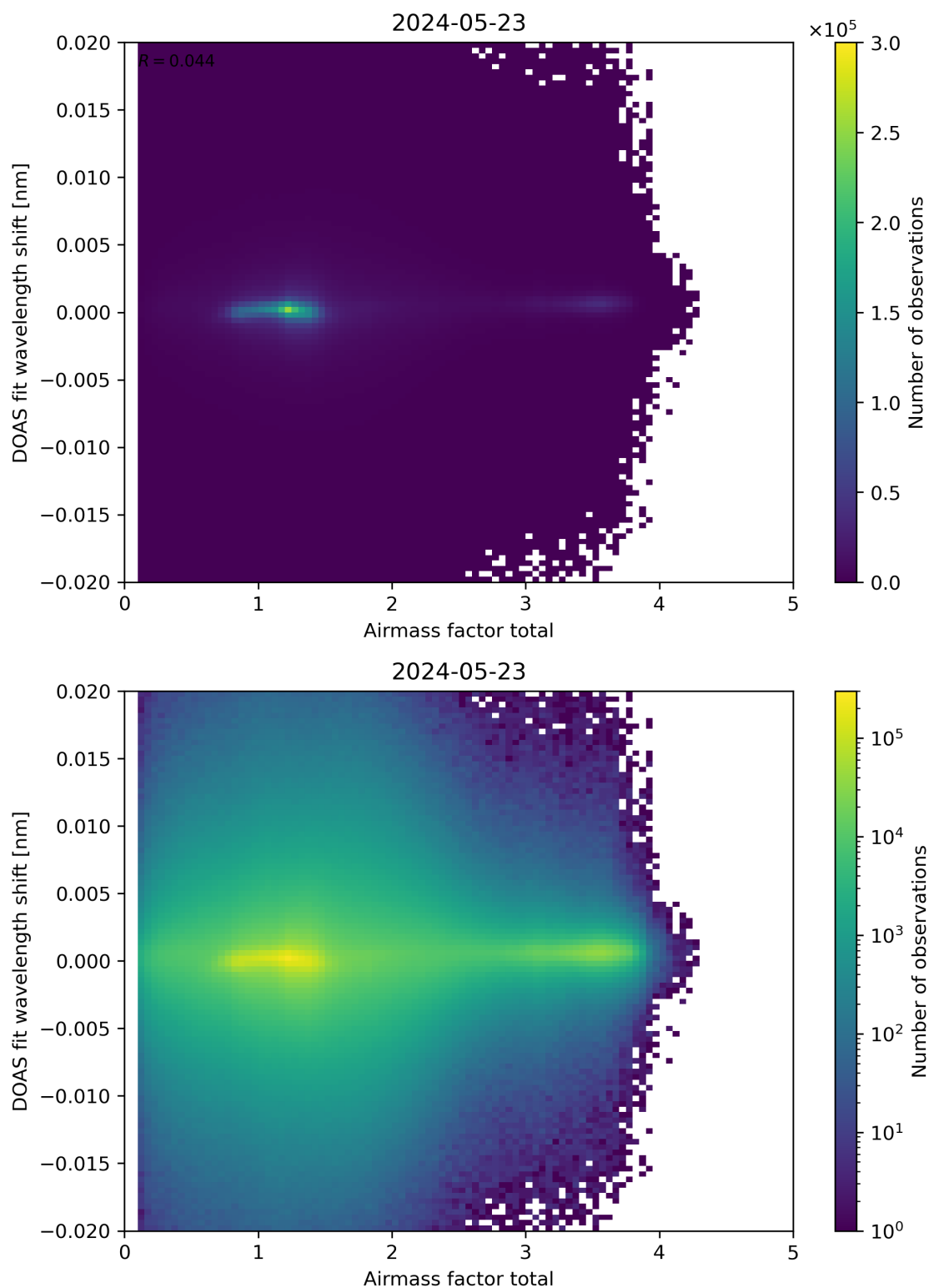
Figure 98: Scatter density plot of “Airmass factor total” against “DOAS fit wavelength shift” for 2024-05-23 to 2024-05-24.
