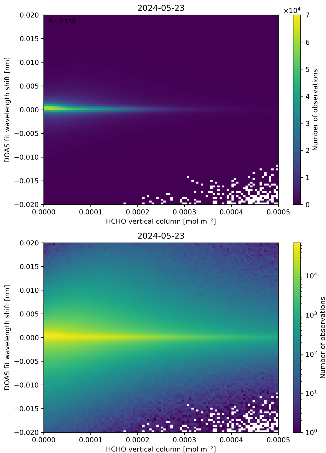
Figure 124: Scatter density plot of “HCHO vertical column” against “DOAS fit wavelength shift” for 2024-05-23 to 2024-05-24.
