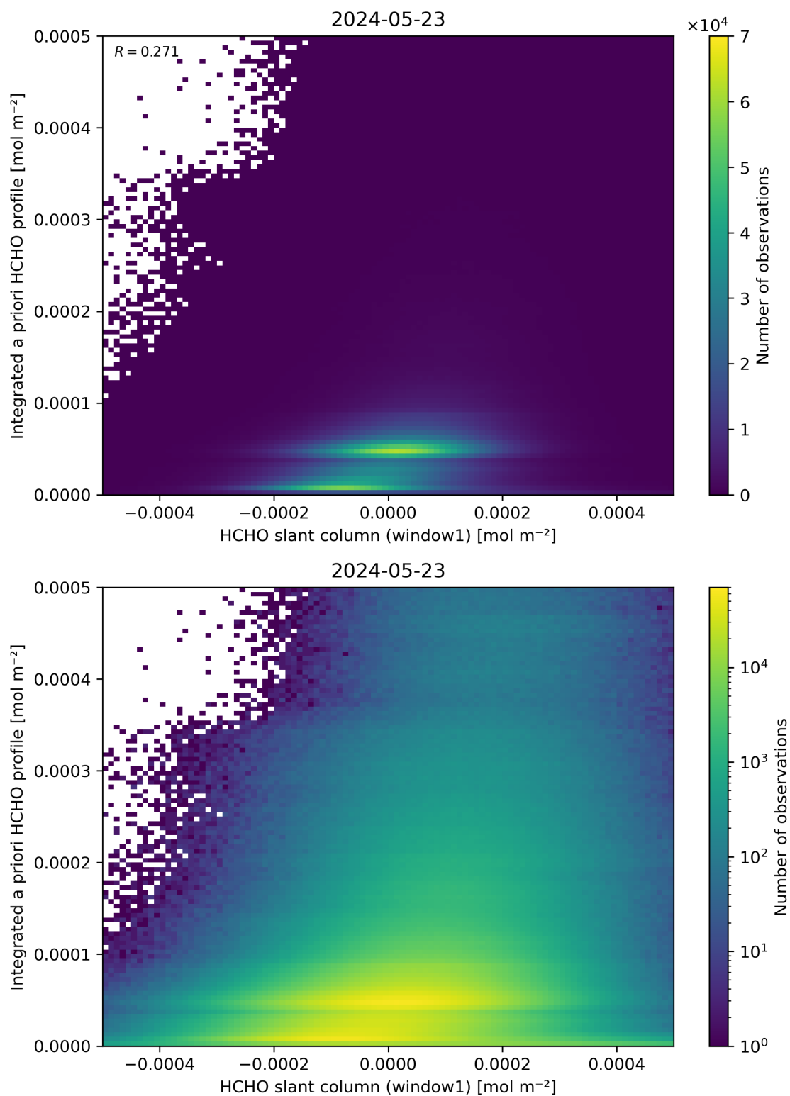
Figure 87: Scatter density plot of “HCHO slant column (window1)” against “Integrated a priori HCHO profile” for 2024-05-23 to 2024-05-24.
