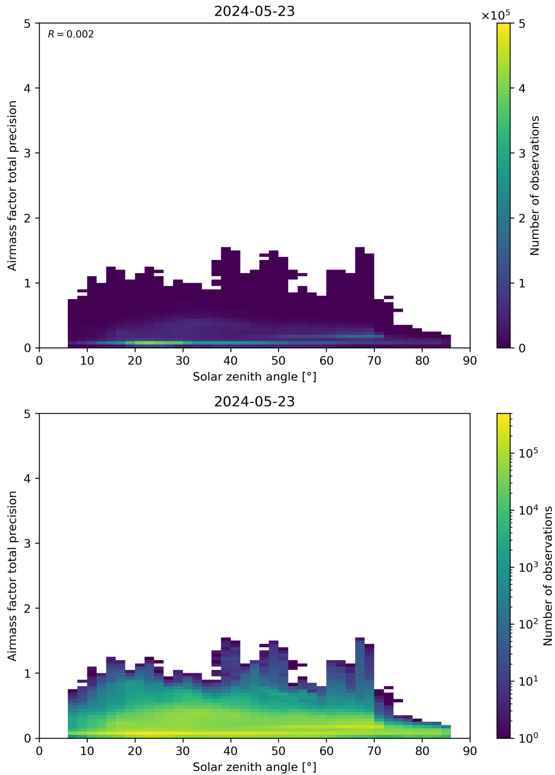
Figure 176: Scatter density plot of “Solar zenith angle” against “Airmass factor total precision” for 2024-05-23 to 2024-05-24.
