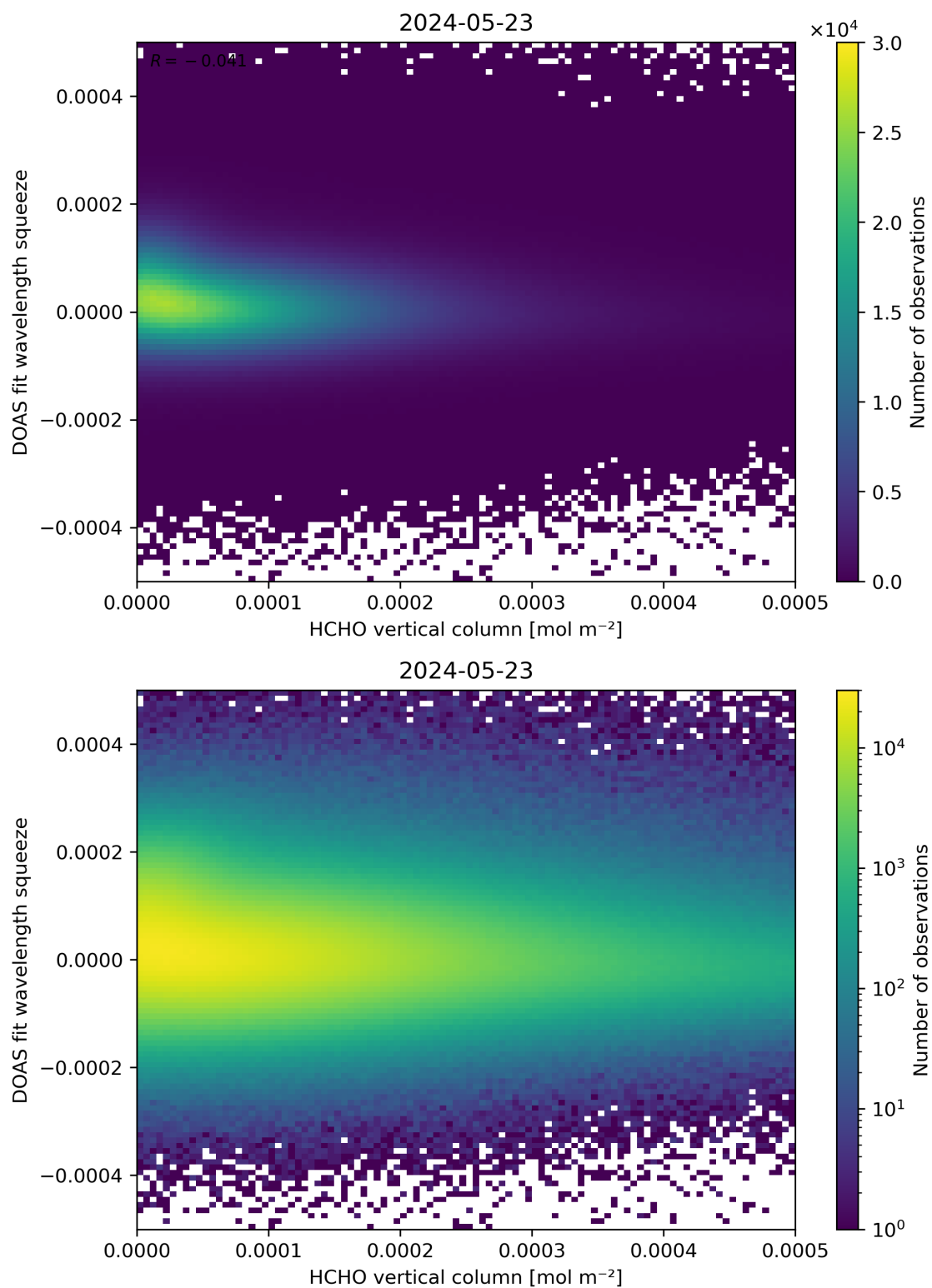
Figure 125: Scatter density plot of “HCHO vertical column” against “DOAS fit wavelength squeeze” for 2024-05-23 to 2024-05-24.
