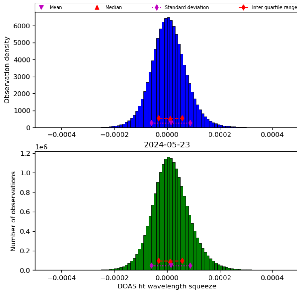
Figure 45: Histogram of “DOAS fit wavelength squeeze” for 2024-05-23 to 2024-05-24
