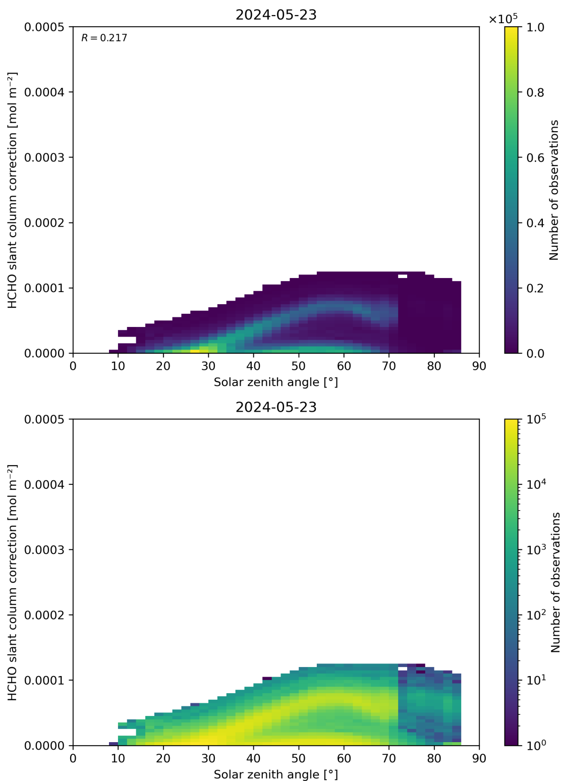
Figure 172: Scatter density plot of “Solar zenith angle” against “HCHO slant column correction” for 2024-05-23 to 2024-05-24.
