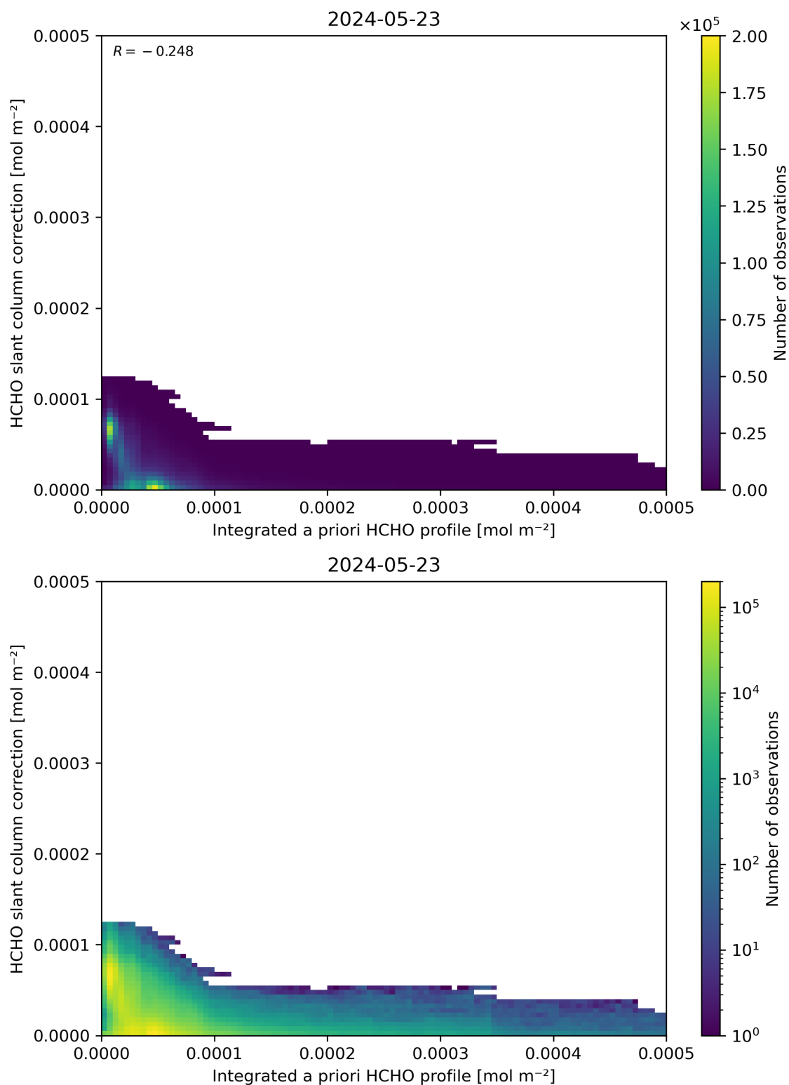
Figure 152: Scatter density plot of “Integrated a priori HCHO profile” against “HCHO slant column correction” for 2024-05-23 to 2024-05-24.
