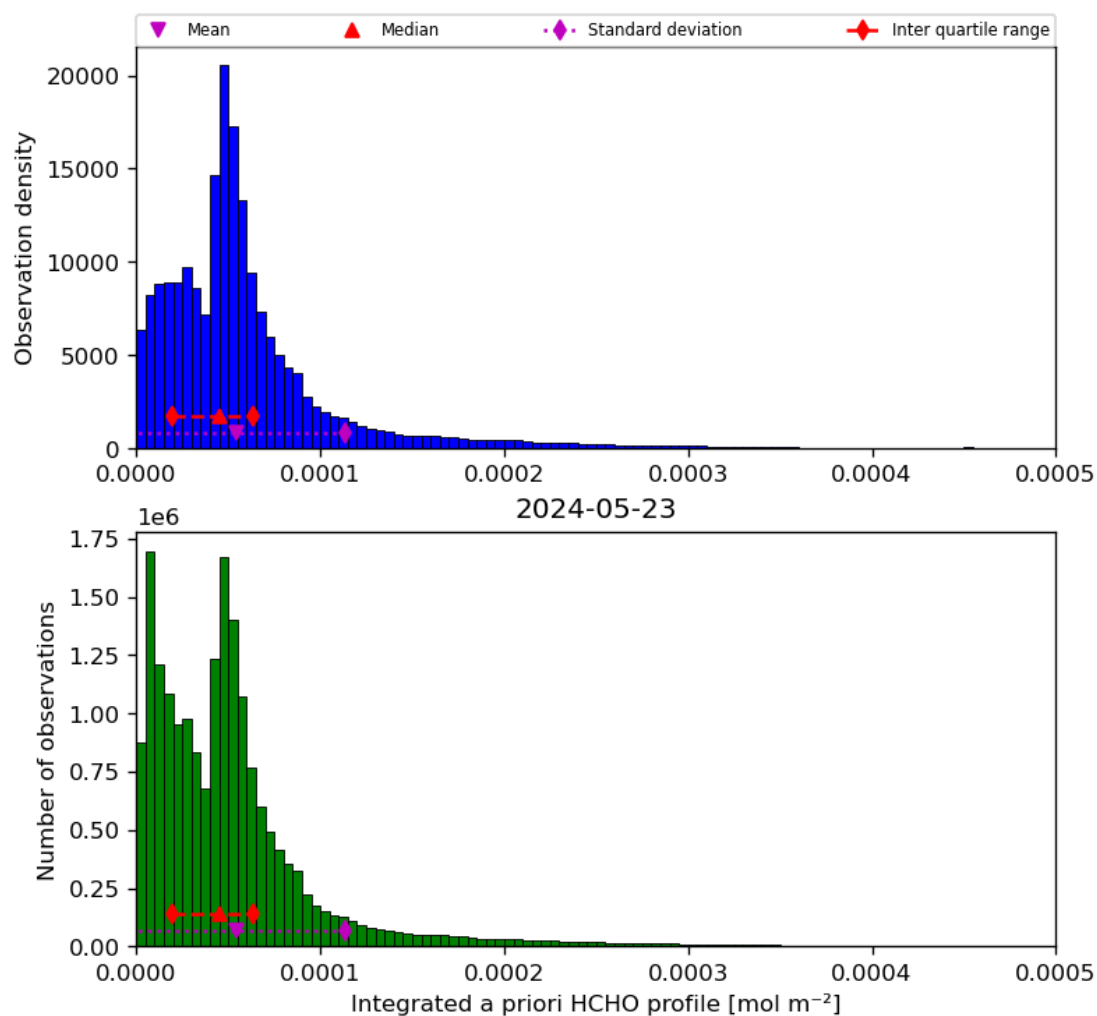
Figure 43: Histogram of “Integrated a priori HCHO profile” for 2024-05-23 to 2024-05-24
