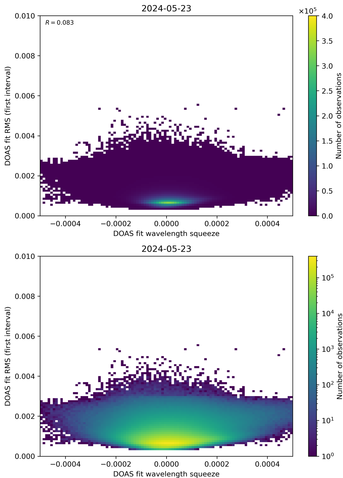
Figure 68: Scatter density plot of “DOAS fit wavelength squeeze” against “DOAS fit RMS (first interval)” for 2024-05-23 to 2024-05-24.
