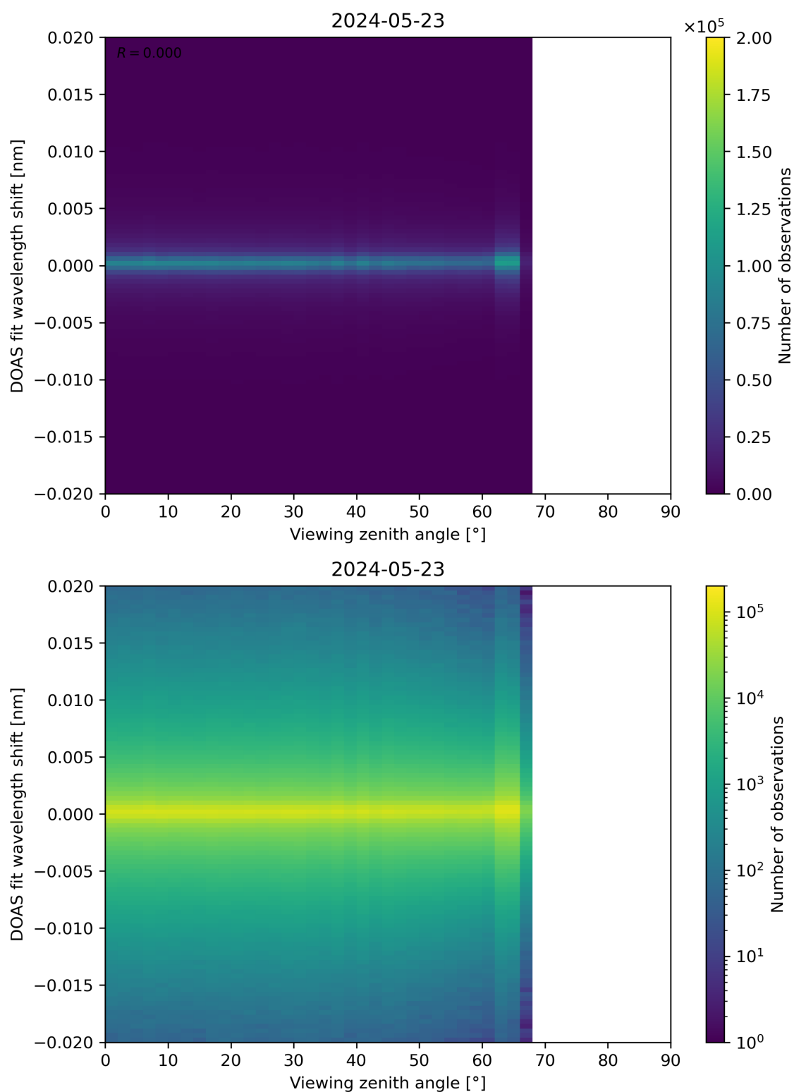
Figure 183: Scatter density plot of “Viewing zenith angle” against “DOAS fit wavelength shift” for 2024-05-23 to 2024-05-24.
