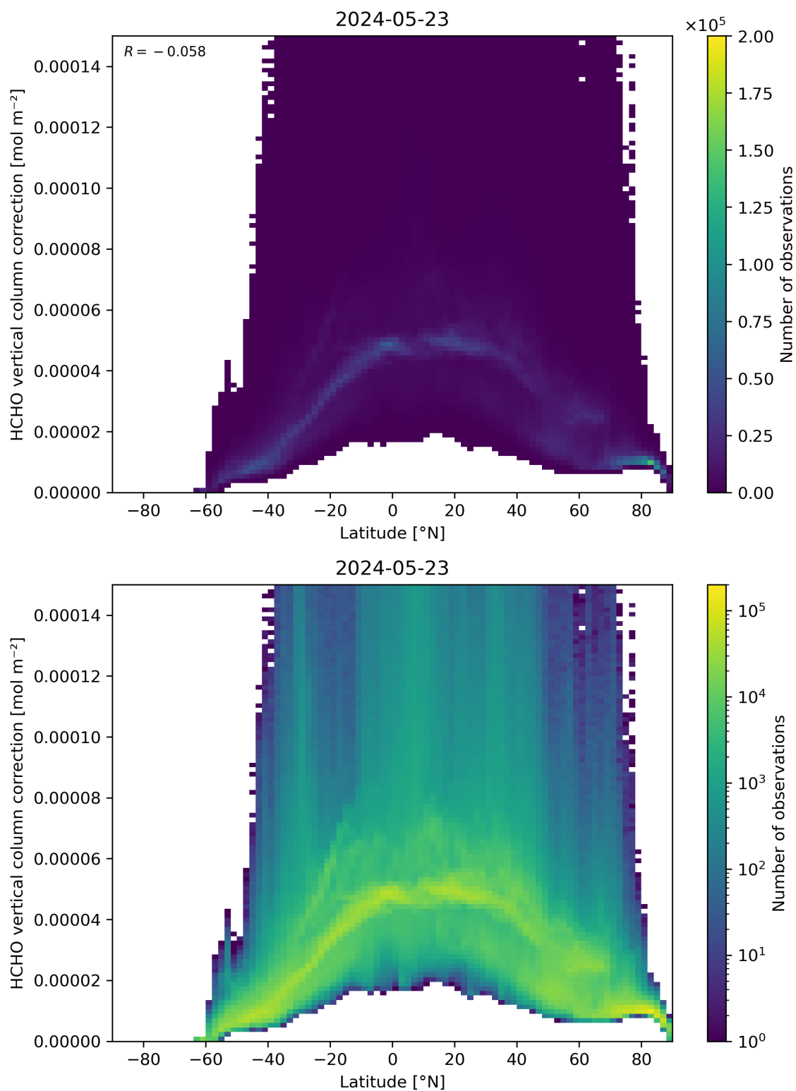
Figure 164: Scatter density plot of “Latitude” against “HCHO vertical column correction” for 2024-05-23 to 2024-05-24.
