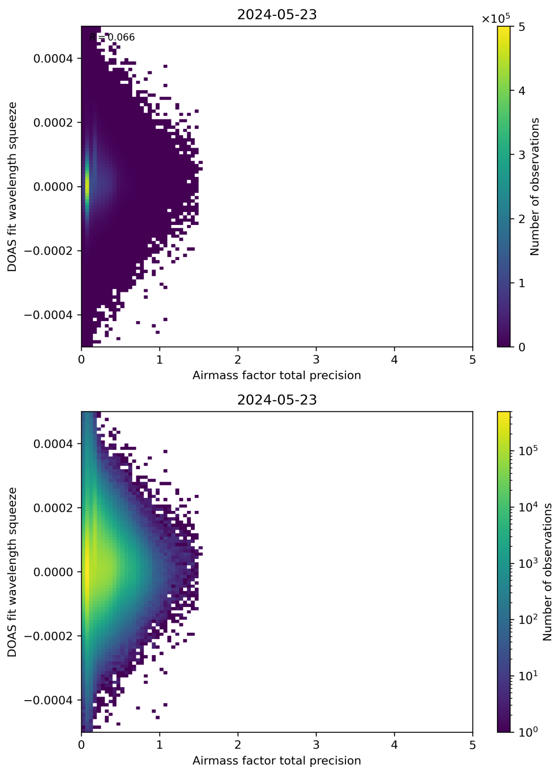
Figure 107: Scatter density plot of “Airmass factor total precision” against “DOAS fit wavelength squeeze” for 2024-05-23 to 2024-05-24.
