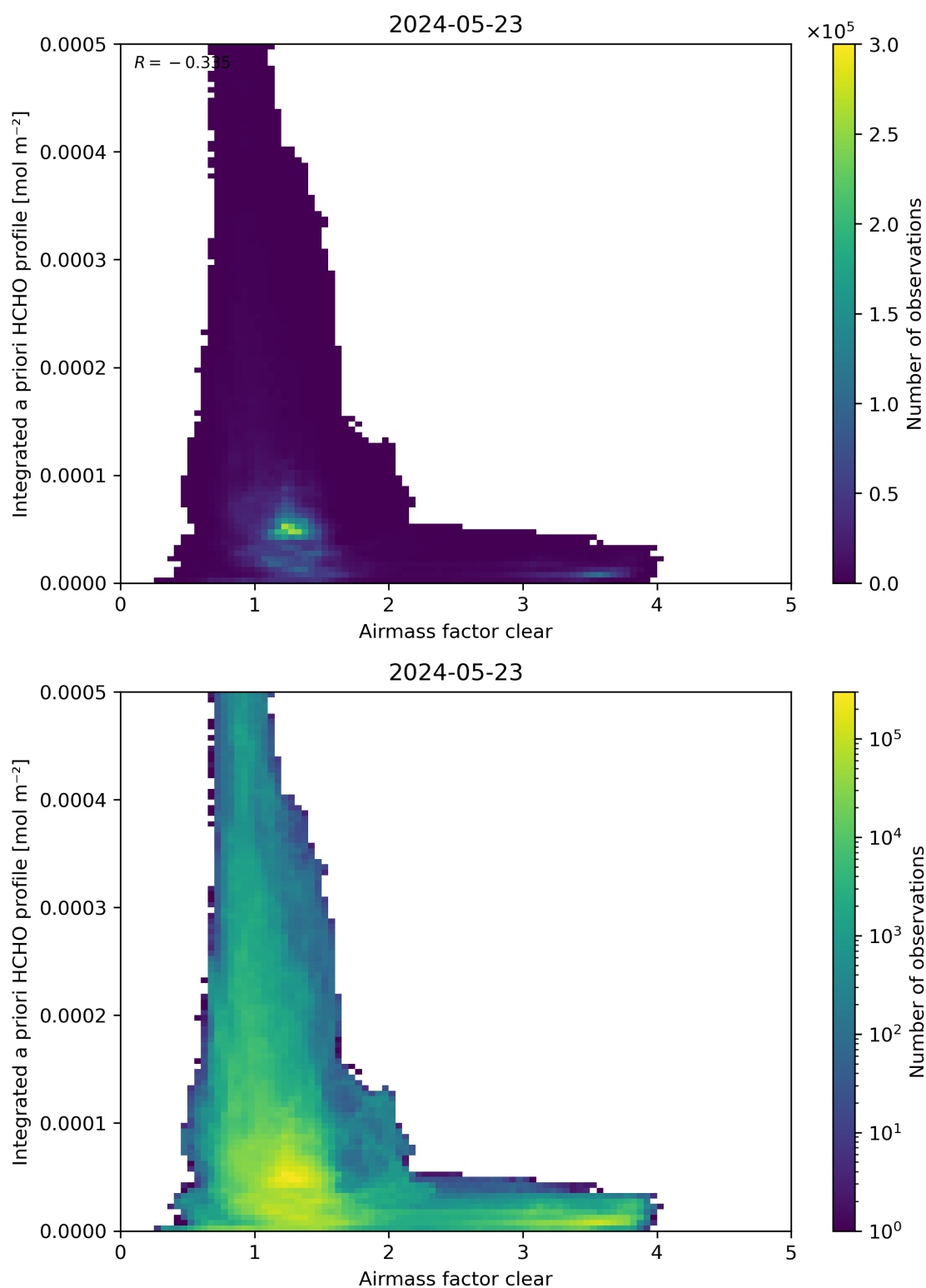
Figure 76: Scatter density plot of “Airmass factor clear” against “Integrated a priori HCHO profile” for 2024-05-23 to 2024-05-24.
