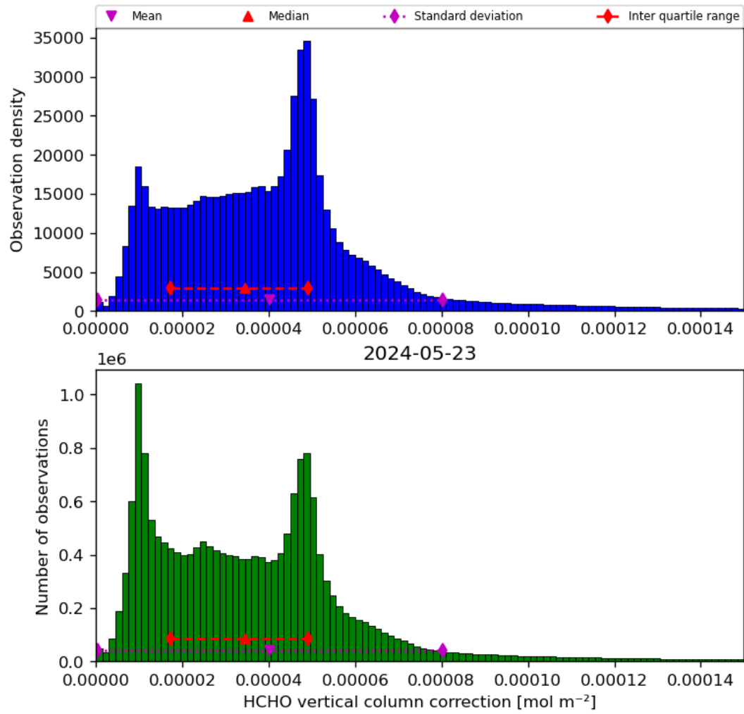
Figure 37: Histogram of “HCHO vertical column correction” for 2024-05-23 to 2024-05-24
