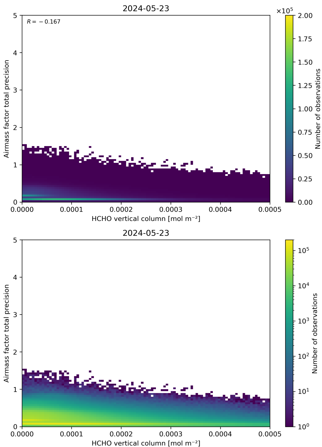
Figure 132: Scatter density plot of “HCHO vertical column” against “Airmass factor total precision” for 2024-05-23 to 2024-05-24.
