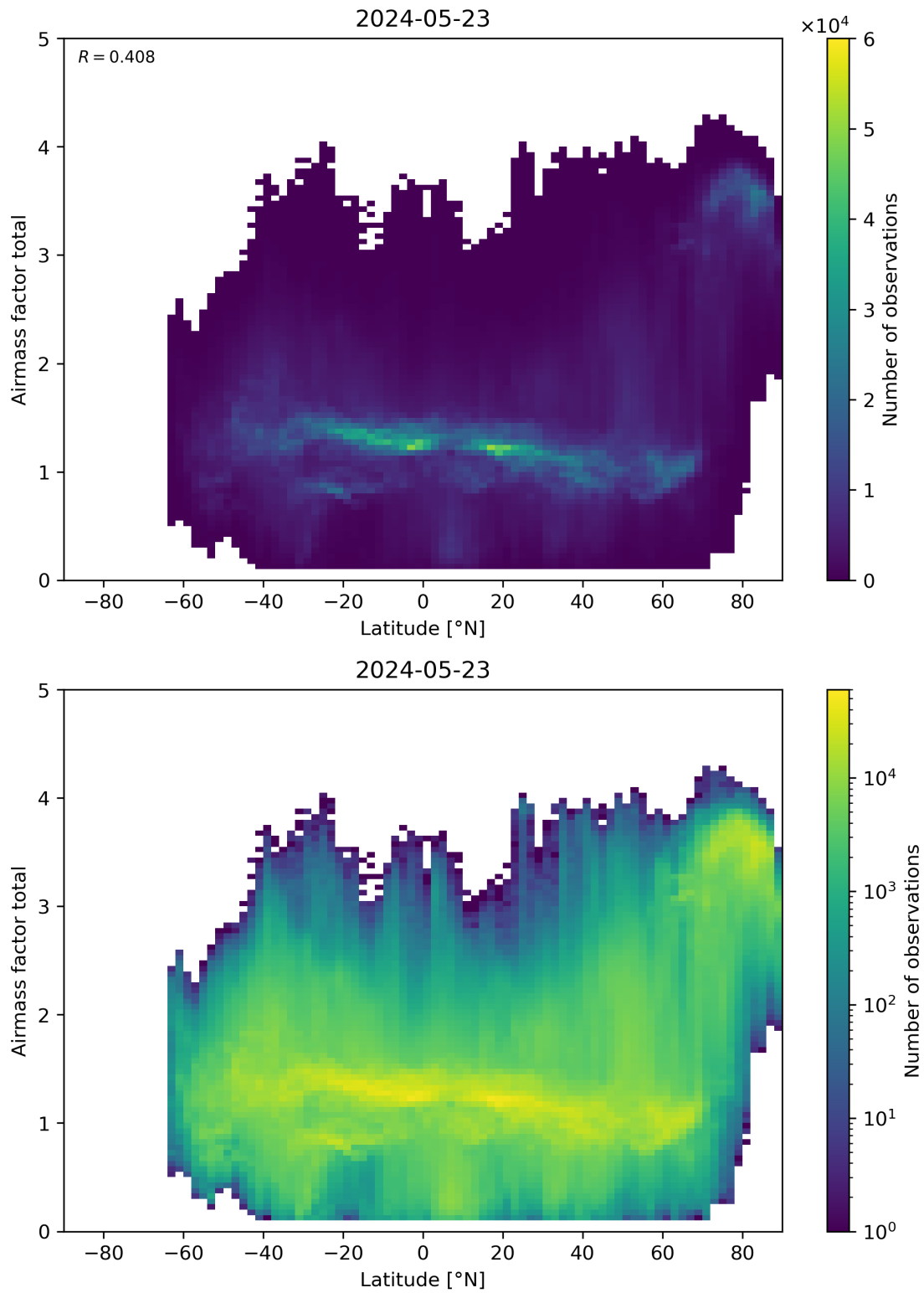
Figure 161: Scatter density plot of “Latitude” against “Airmass factor total” for 2024-05-23 to 2024-05-24.
