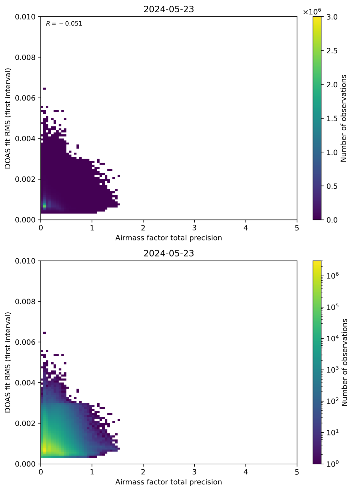
Figure 105: Scatter density plot of “Airmass factor total precision” against “DOAS fit RMS (first interval)” for 2024-05-23 to 2024-05-24.
