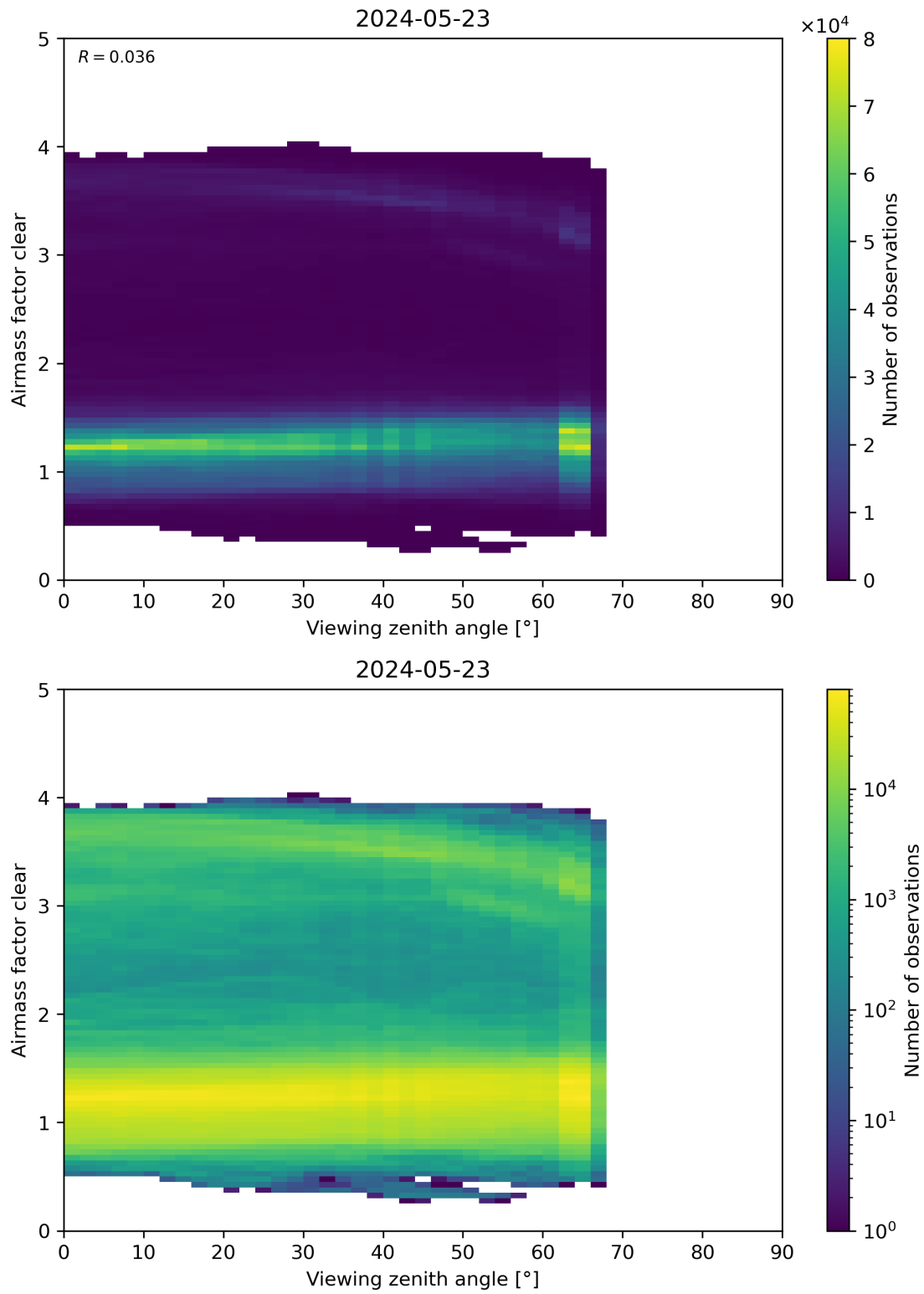
Figure 185: Scatter density plot of “Viewing zenith angle” against “Airmass factor clear” for 2024-05-23 to 2024-05-24.
