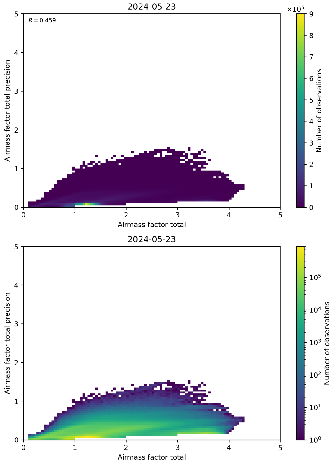
Figure 103: Scatter density plot of “Airmass factor total” against “Airmass factor total precision” for 2024-05-23 to 2024-05-24.
