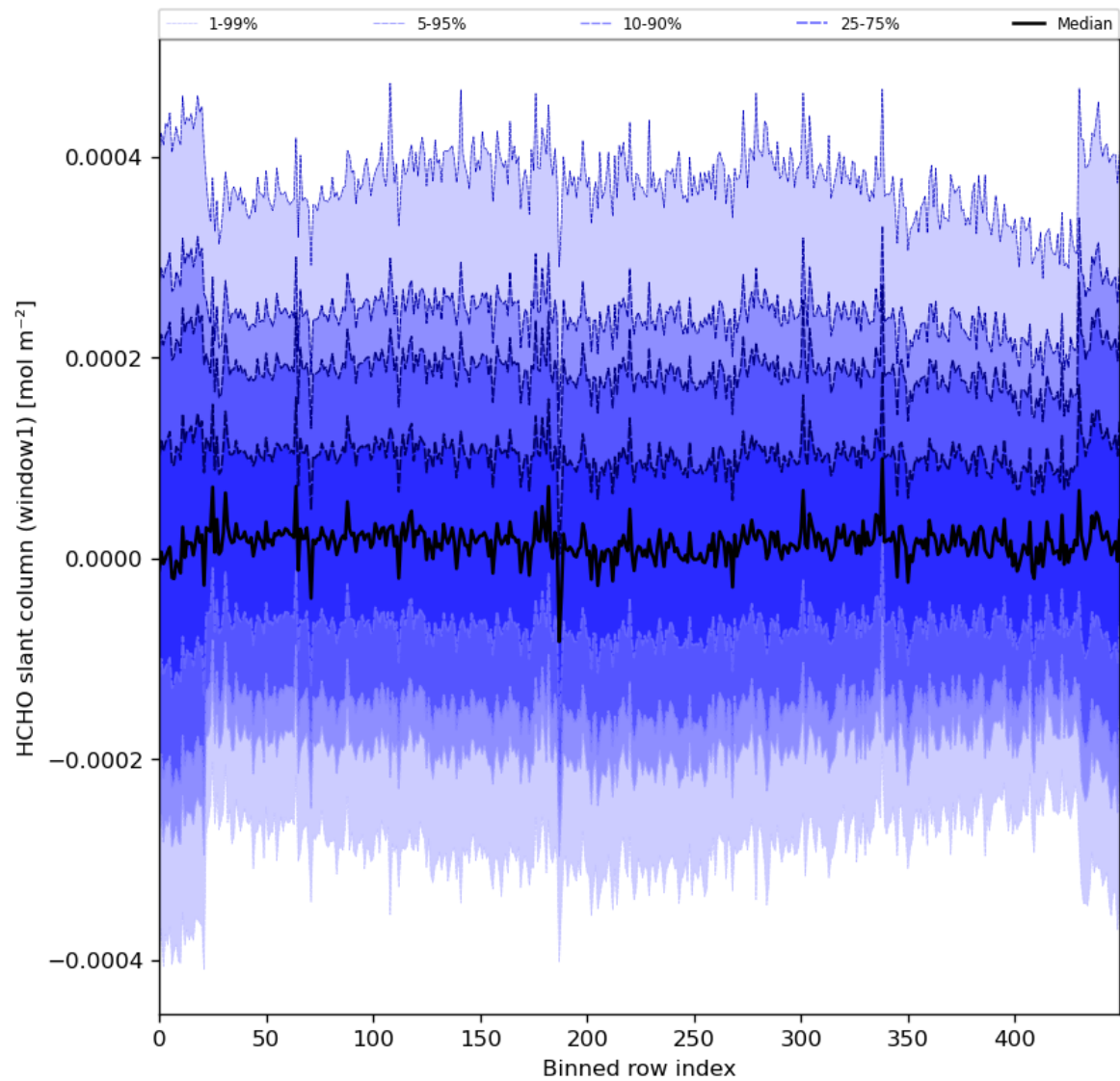
Figure 52: Along track statistics of “HCHO slant column (window1)” for 2024-05-23 to 2024-05-24
