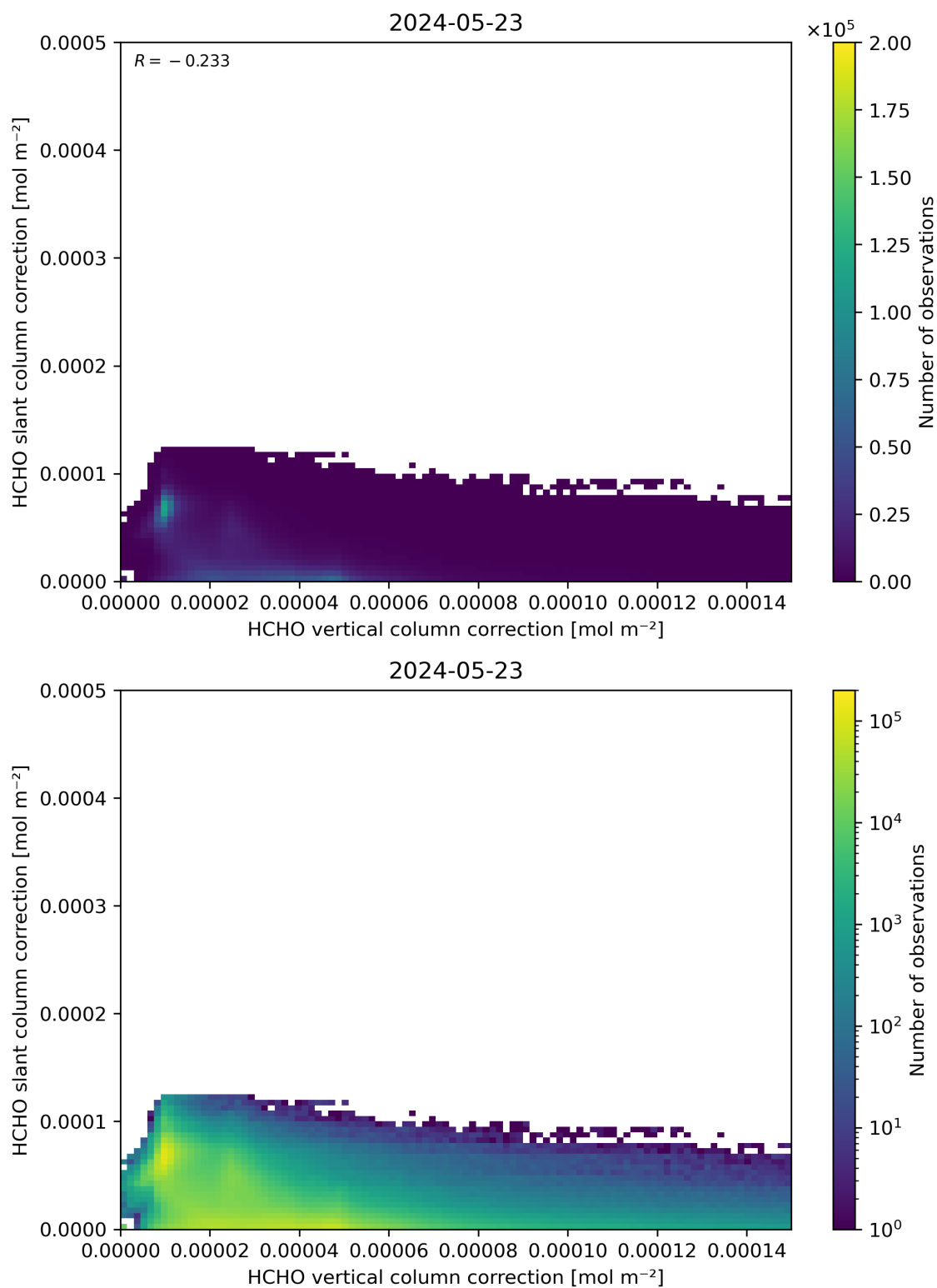
Figure 117: Scatter density plot of “HCHO vertical column correction” against “HCHO slant column correction” for 2024-05-23 to 2024-05-24.
