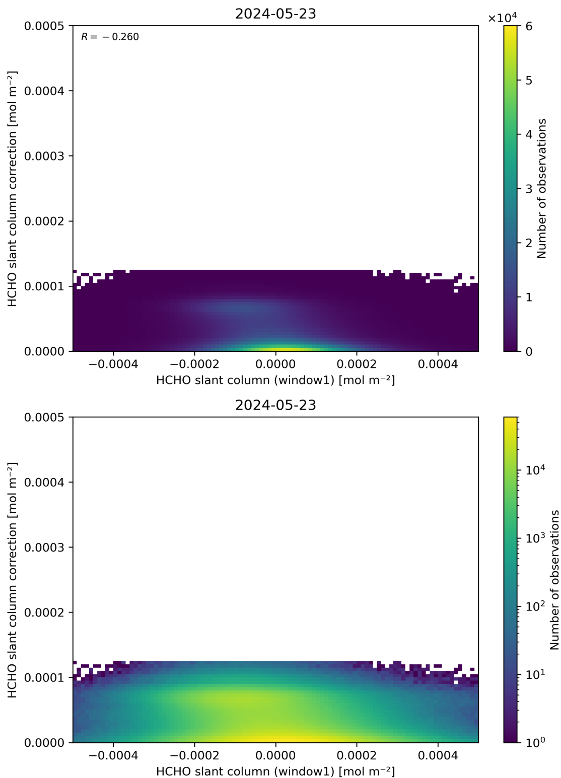
Figure 83: Scatter density plot of “HCHO slant column (window1)” against “HCHO slant column correction” for 2024-05-23 to 2024-05-24.
