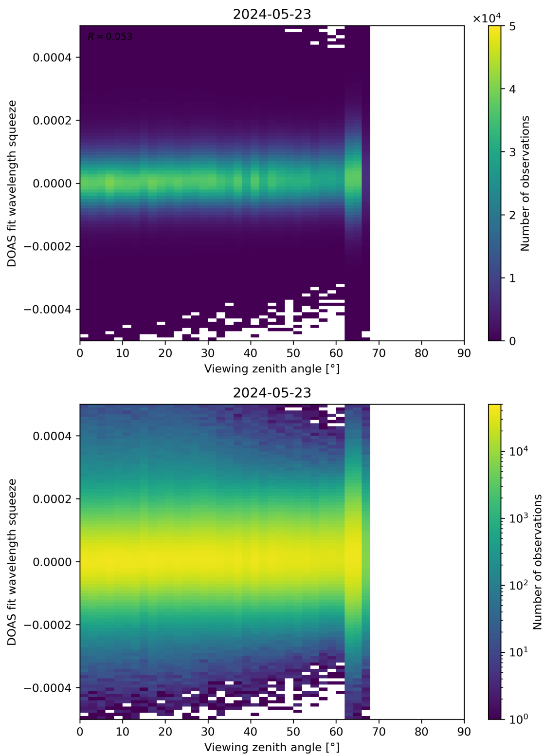
Figure 184: Scatter density plot of “Viewing zenith angle” against “DOAS fit wavelength squeeze” for 2024-05-23 to 2024-05-24.
