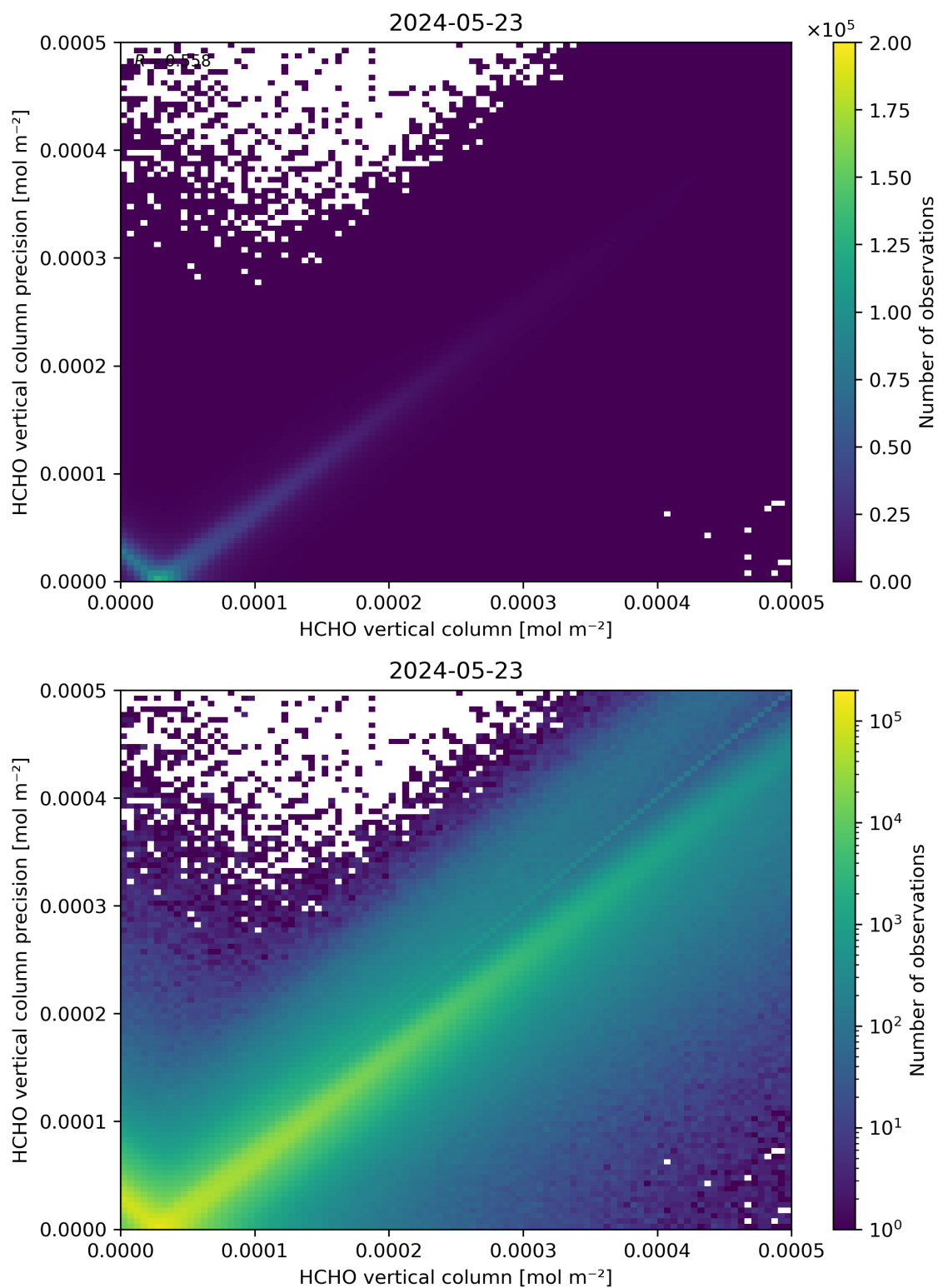
Figure 134: Scatter density plot of “HCHO vertical column” against “HCHO vertical column precision” for 2024-05-23 to 2024-05-24.
