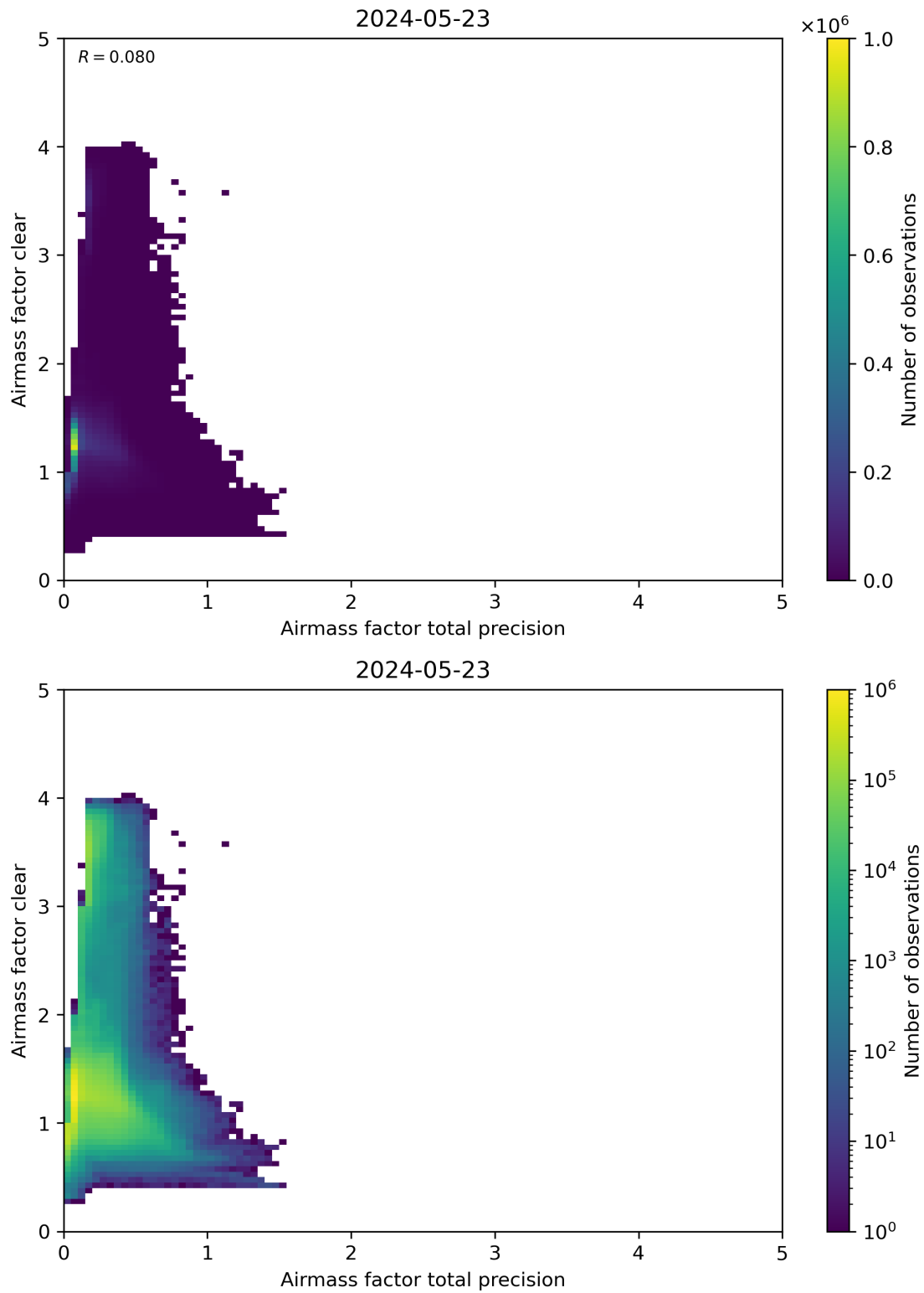
Figure 108: Scatter density plot of “Airmass factor total precision” against “Airmass factor clear” for 2024-05-23 to 2024-05-24.
