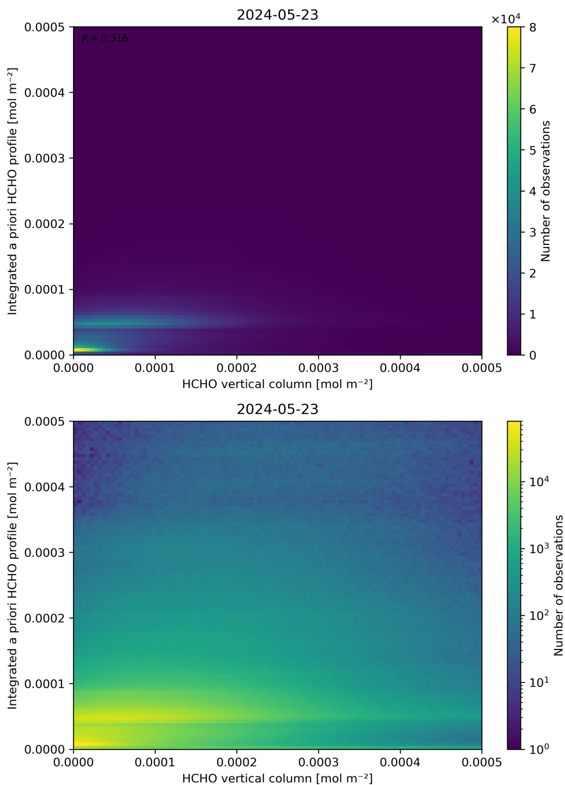
Figure 135: Scatter density plot of “HCHO vertical column” against “Integrated a priori HCHO profile” for 2024-05-23 to 2024-05-24.
