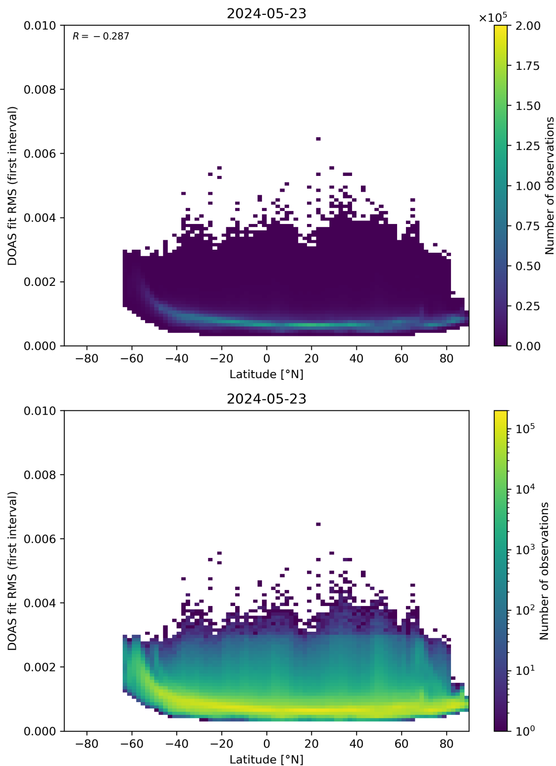
Figure 153: Scatter density plot of “Latitude” against “DOAS fit RMS (first interval)” for 2024-05-23 to 2024-05-24.
