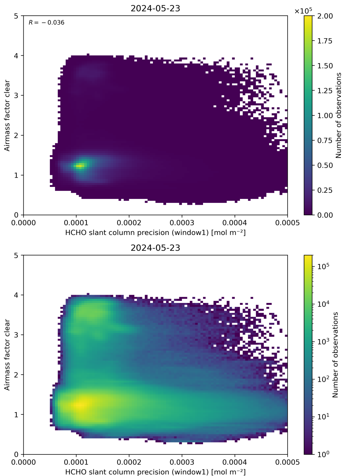
Figure 91: Scatter density plot of “HCHO slant column precision (window1)” against “Airmass factor clear” for 2024-05-23 to 2024-05-24.
