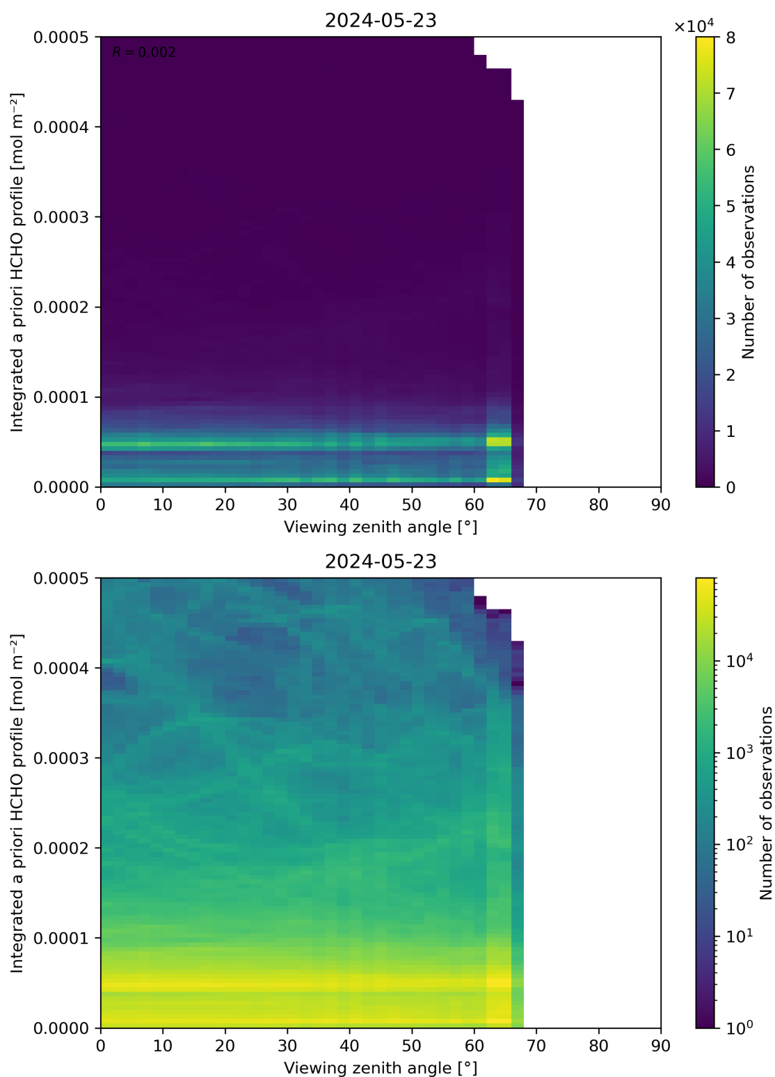
Figure 195: Scatter density plot of “Viewing zenith angle” against “Integrated a priori HCHO profile” for 2024-05-23 to 2024-05-24.
