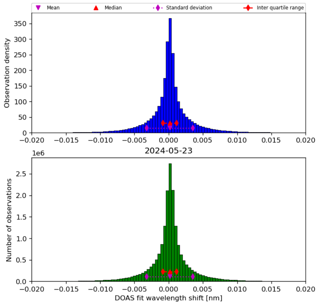
Figure 44: Histogram of “DOAS fit wavelength shift” for 2024-05-23 to 2024-05-24
