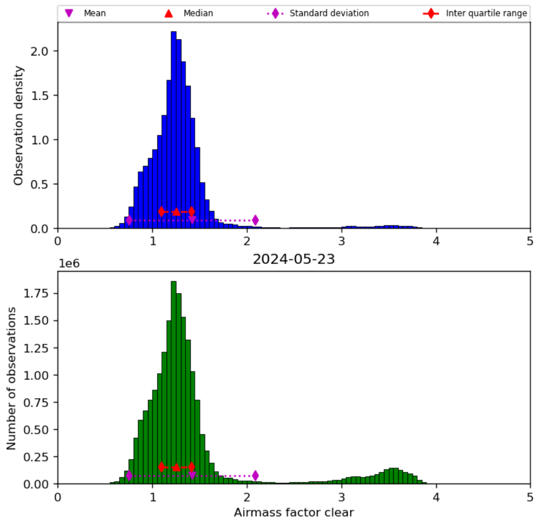
Figure 42: Histogram of “Airmass factor clear” for 2024-05-23 to 2024-05-24
