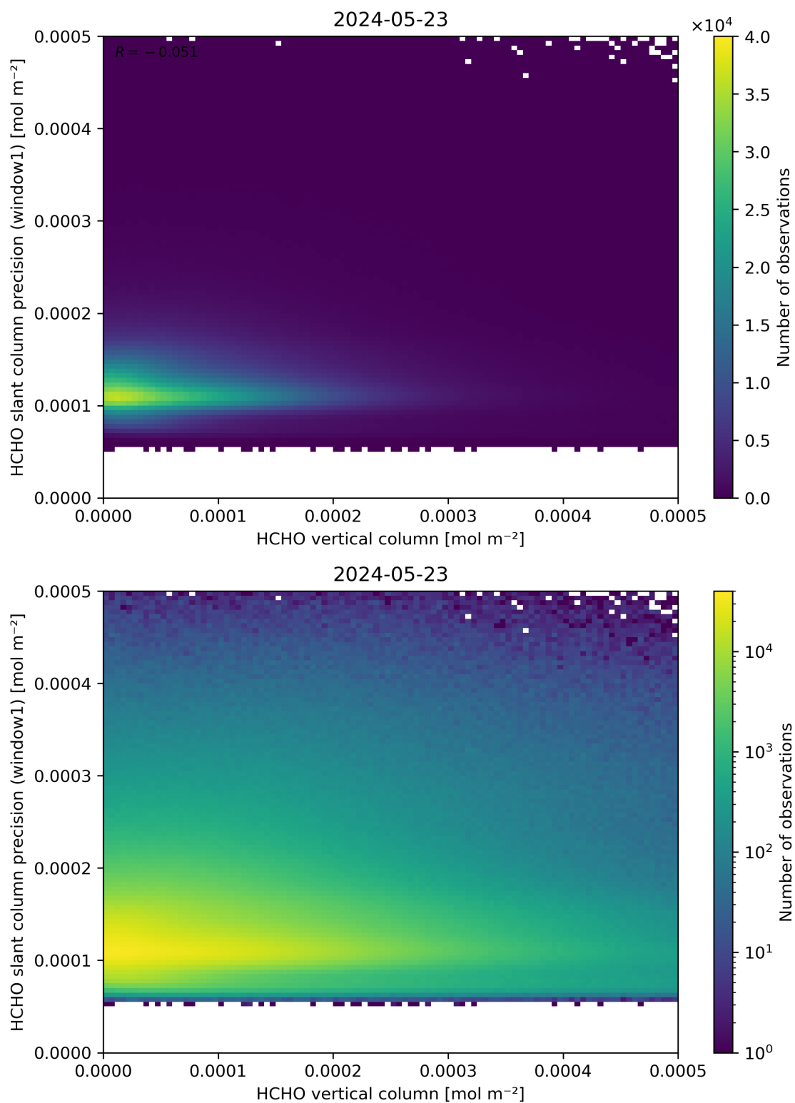
Figure 130: Scatter density plot of “HCHO vertical column” against “HCHO slant column precision (window1)” for 2024-05-23 to 2024-05-24.
