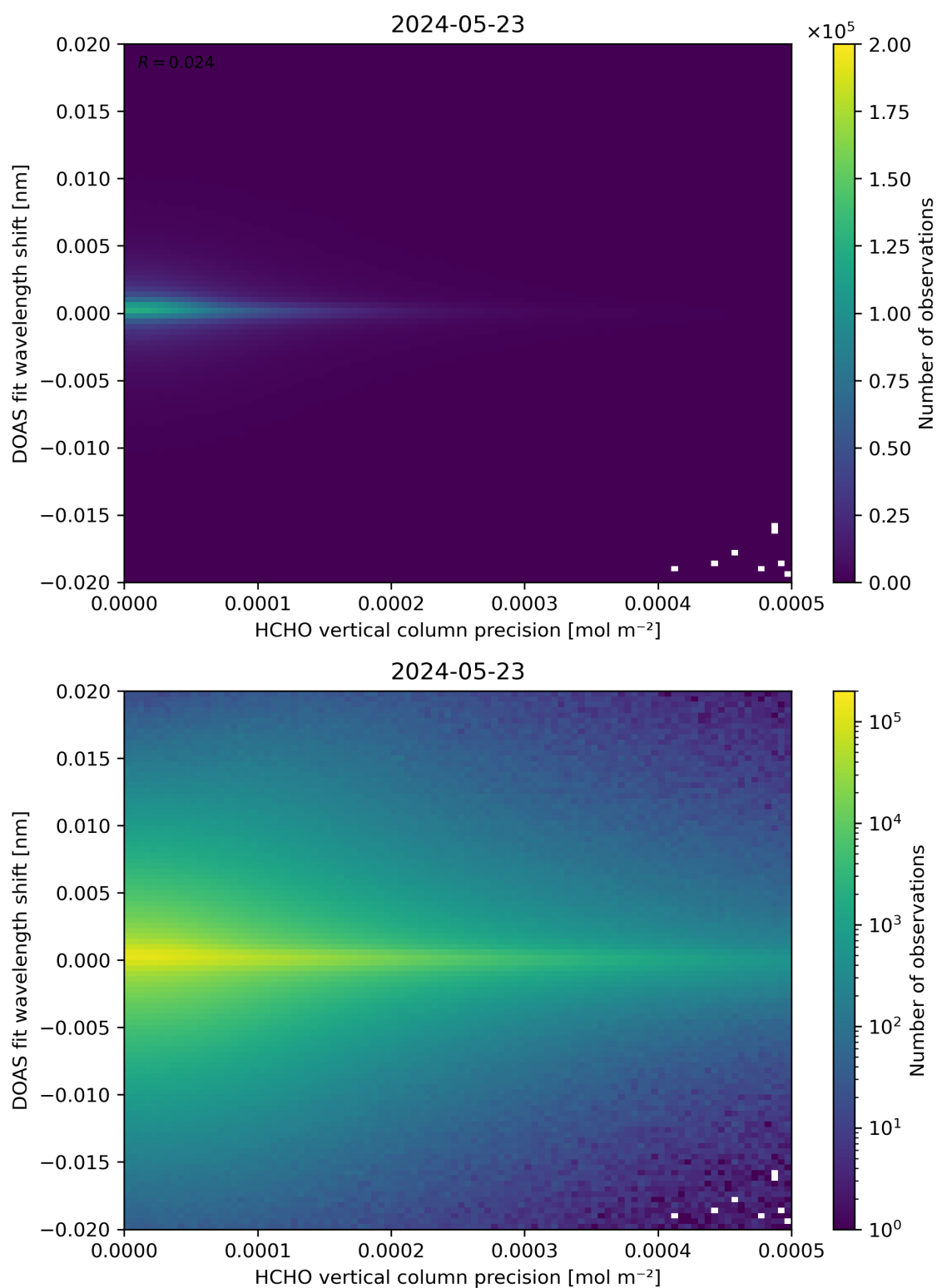
Figure 137: Scatter density plot of “HCHO vertical column precision” against “DOAS fit wavelength shift” for 2024-05-23 to 2024-05-24.
