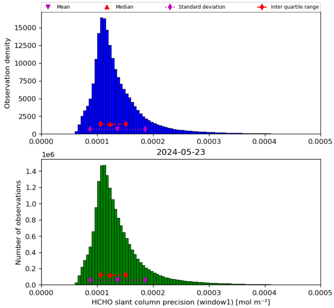
Figure 39: Histogram of “HCHO slant column precision (window1)” for 2024-05-23 to 2024-05-24
