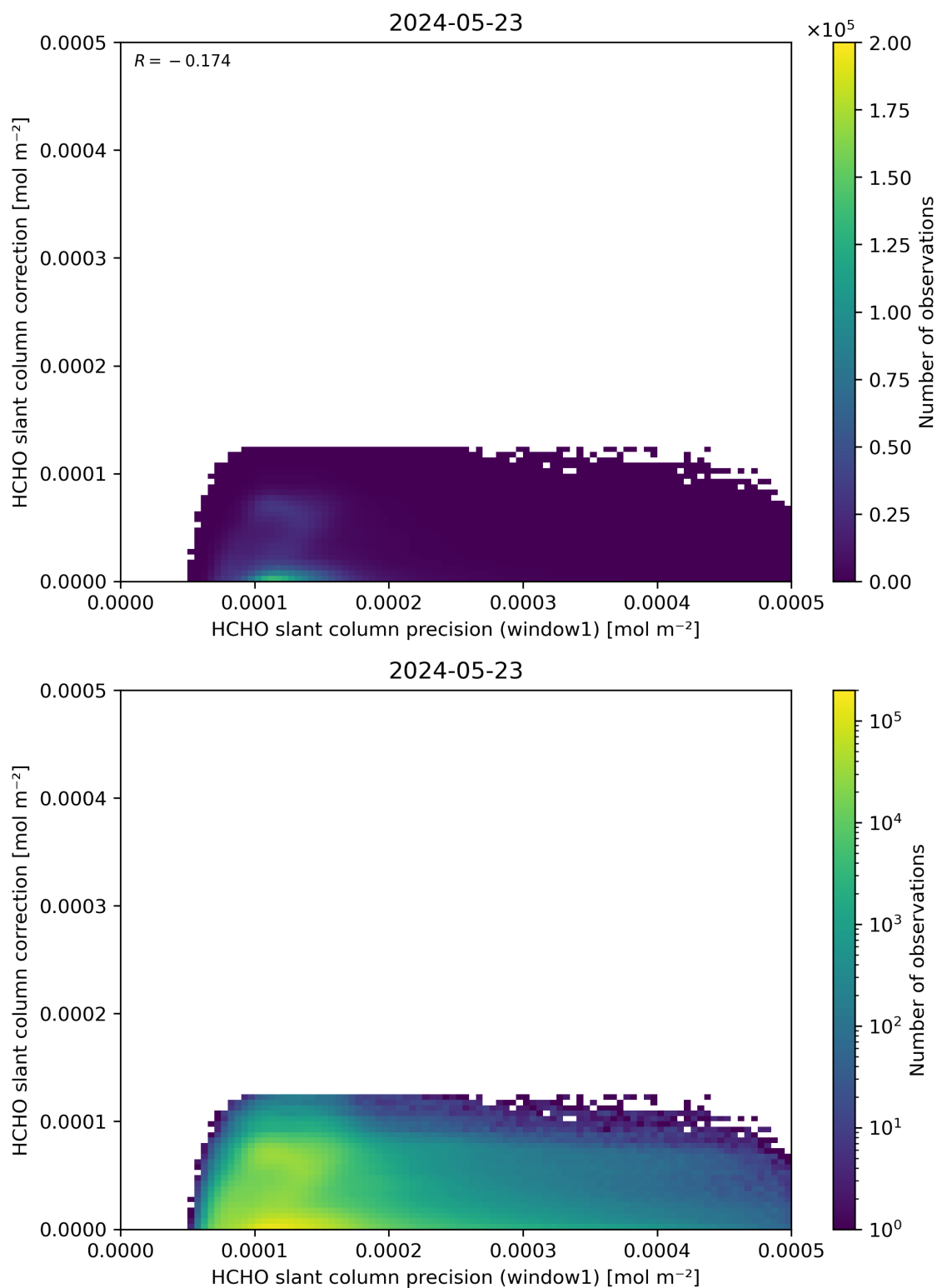
Figure 93: Scatter density plot of “HCHO slant column precision (window1)” against “HCHO slant column correction” for 2024-05-23 to 2024-05-24.
