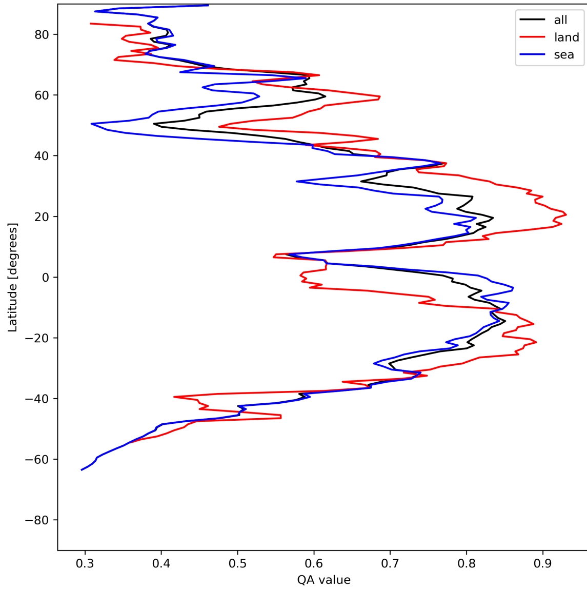
Figure 20: Zonal average of “QA value” for 2024-05-23 to 2024-05-24.
