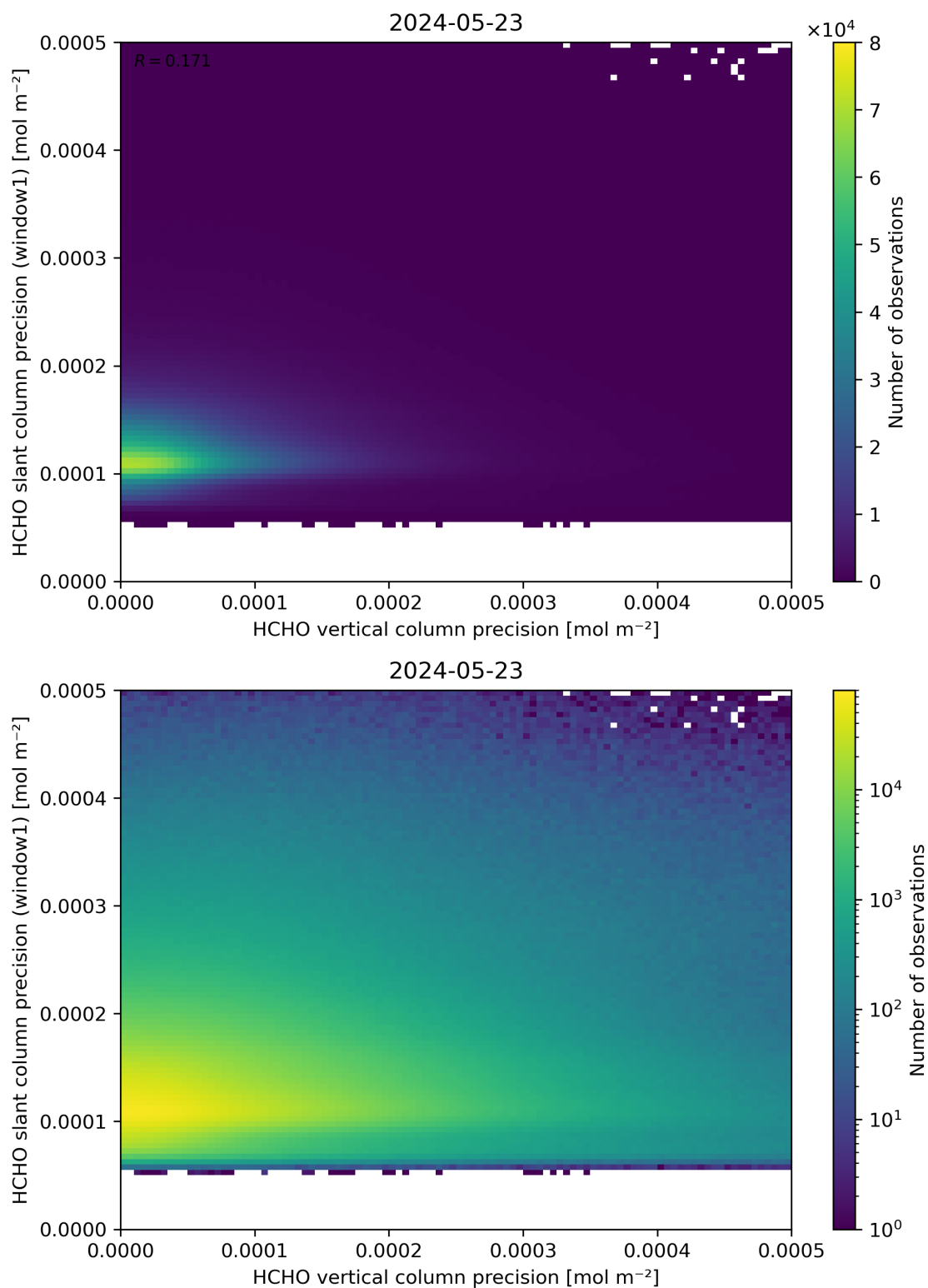
Figure 143: Scatter density plot of “HCHO vertical column precision” against “HCHO slant column precision (window1)” for 2024-05-23 to 2024-05-24.
