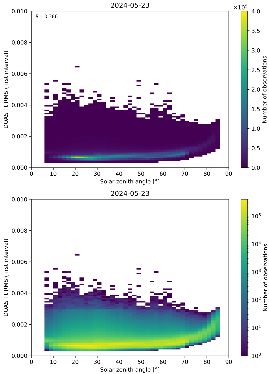
Figure 167: Scatter density plot of “Solar zenith angle” against “DOAS fit RMS (first interval)” for 2024-05-23 to 2024-05-24.
