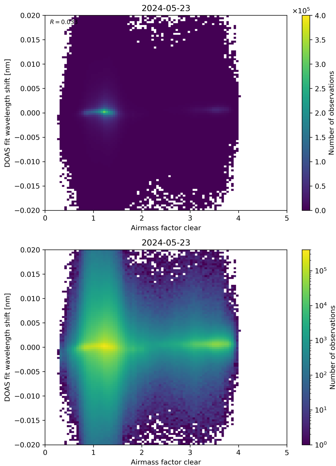
Figure 72: Scatter density plot of “Airmass factor clear” against “DOAS fit wavelength shift” for 2024-05-23 to 2024-05-24.
