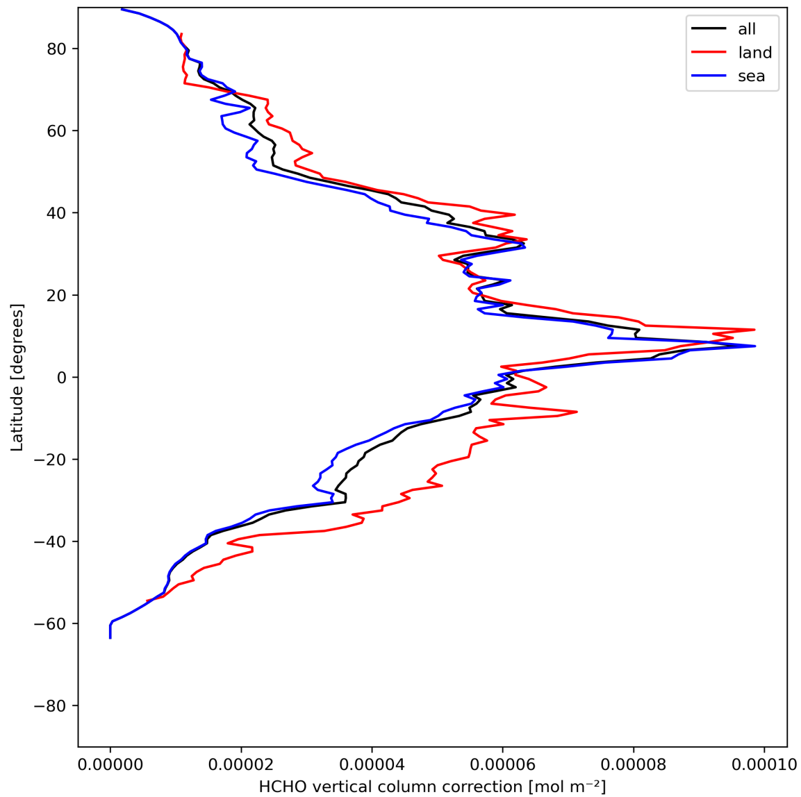
Figure 23: Zonal average of “HCHO vertical column correction” for 2024-05-23 to 2024-05-24.
