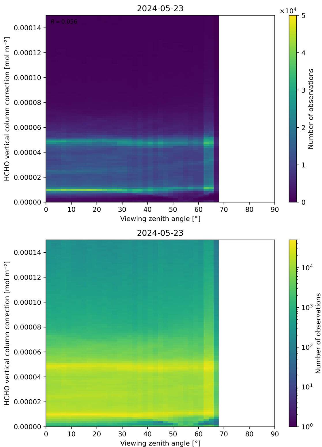
Figure 193: Scatter density plot of “Viewing zenith angle” against “HCHO vertical column correction” for 2024-05-23 to 2024-05-24.
