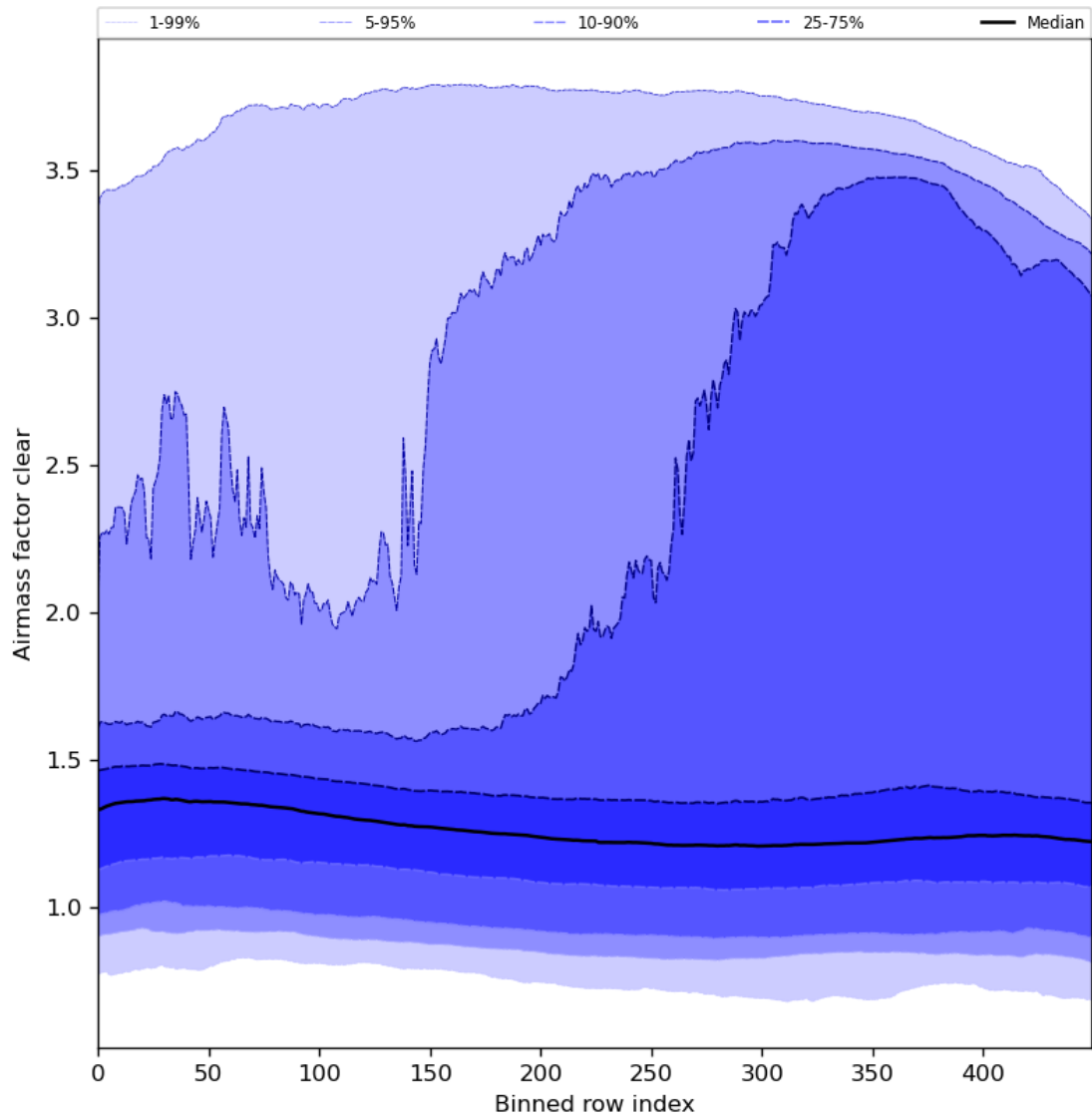
Figure 56: Along track statistics of “Airmass factor clear” for 2024-05-23 to 2024-05-24
