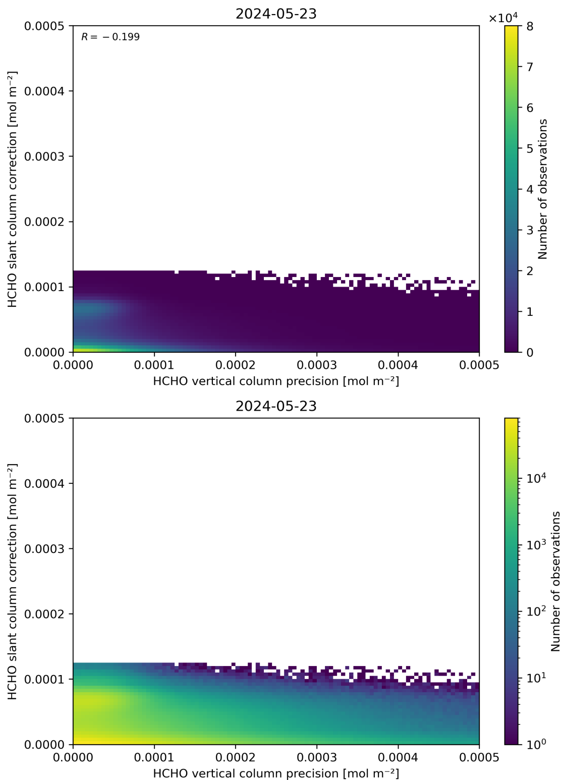
Figure 141: Scatter density plot of “HCHO vertical column precision” against “HCHO slant column correction” for 2024-05-23 to 2024-05-24.
