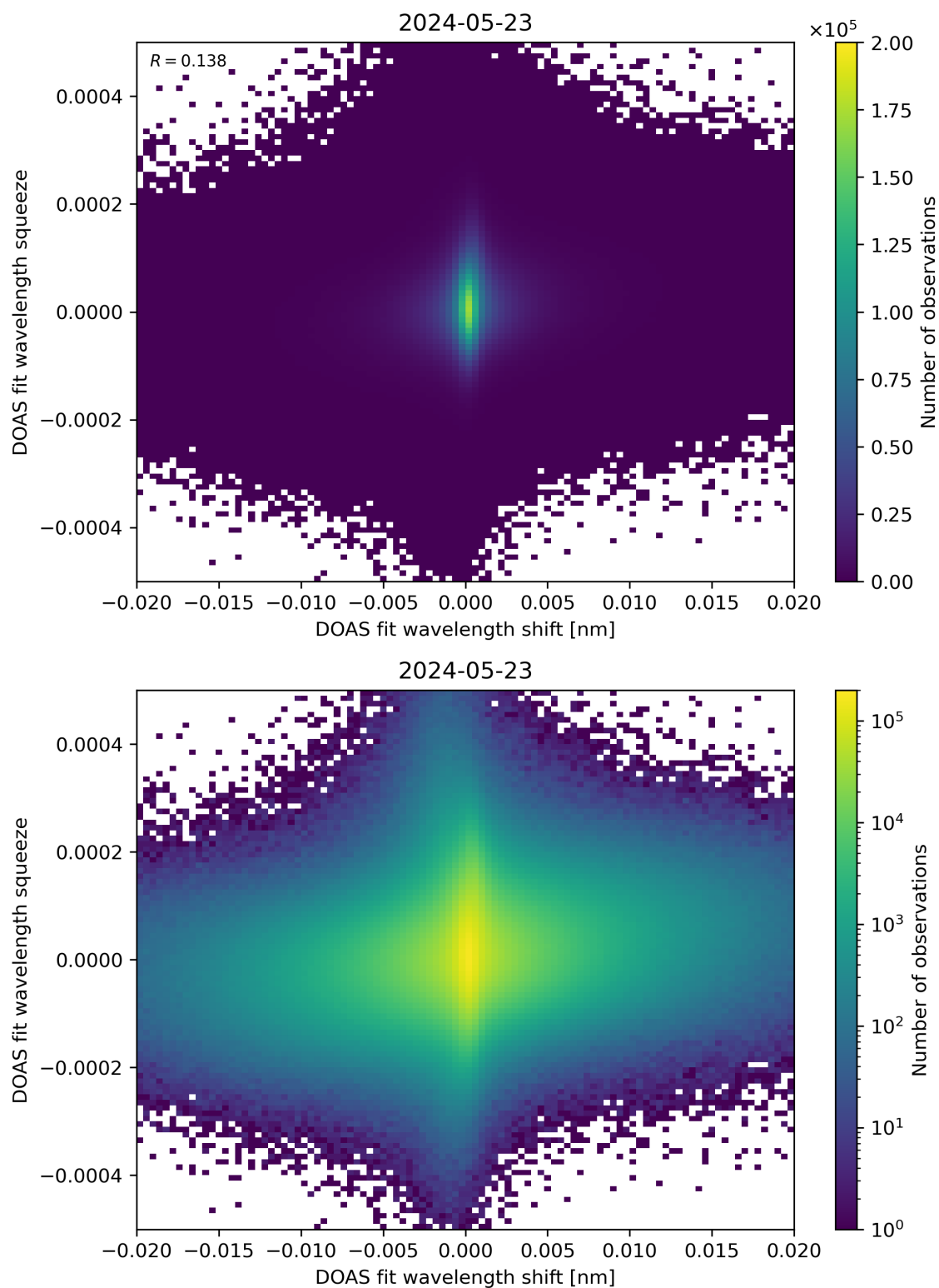
Figure 65: Scatter density plot of “DOAS fit wavelength shift” against “DOAS fit wavelength squeeze” for 2024-05-23 to 2024-05-24.
