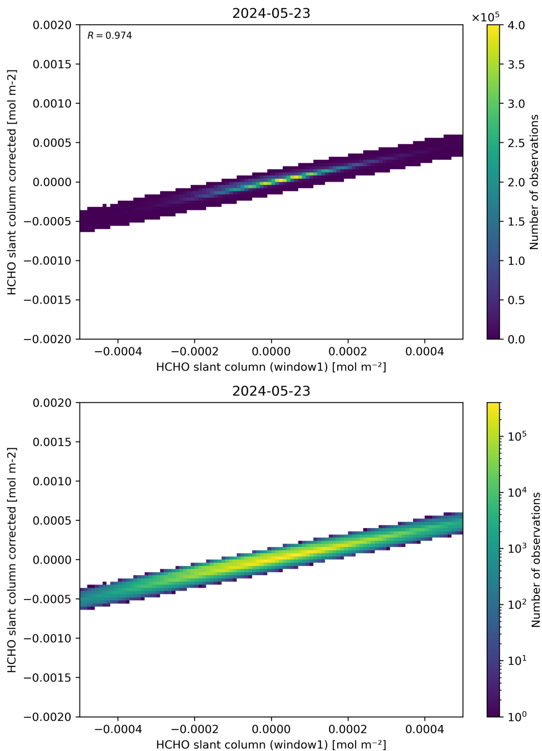
Figure 82: Scatter density plot of “HCHO slant column (window1)” against “HCHO slant column corrected” for 2024-05-23 to 2024-05-24.
