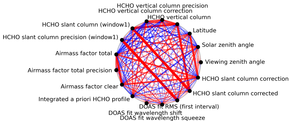
Figure 1: Map of correlation graph for 2024-05-23 to 2024-05-24.
