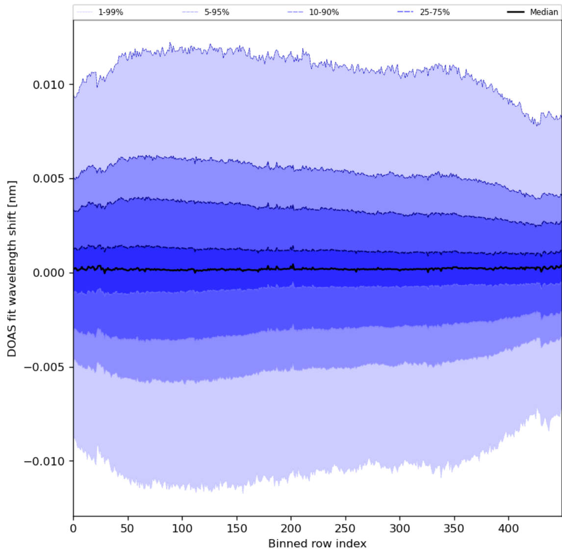
Figure 58: Along track statistics of “DOAS fit wavelength shift” for 2024-05-23 to 2024-05-24
