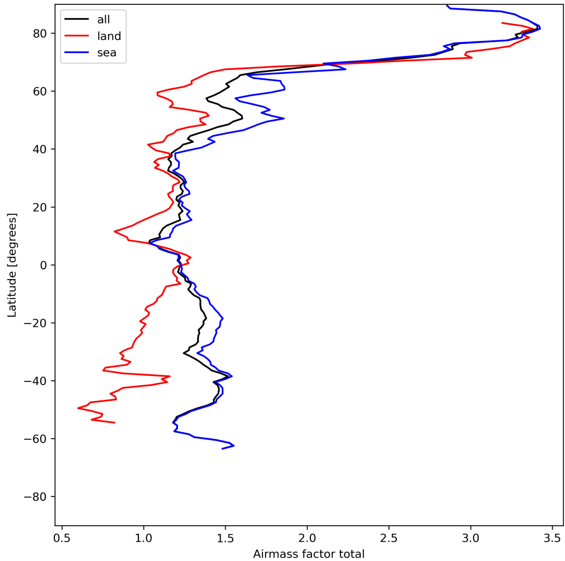
Figure 26: Zonal average of “Airmass factor total” for 2024-05-23 to 2024-05-24.
