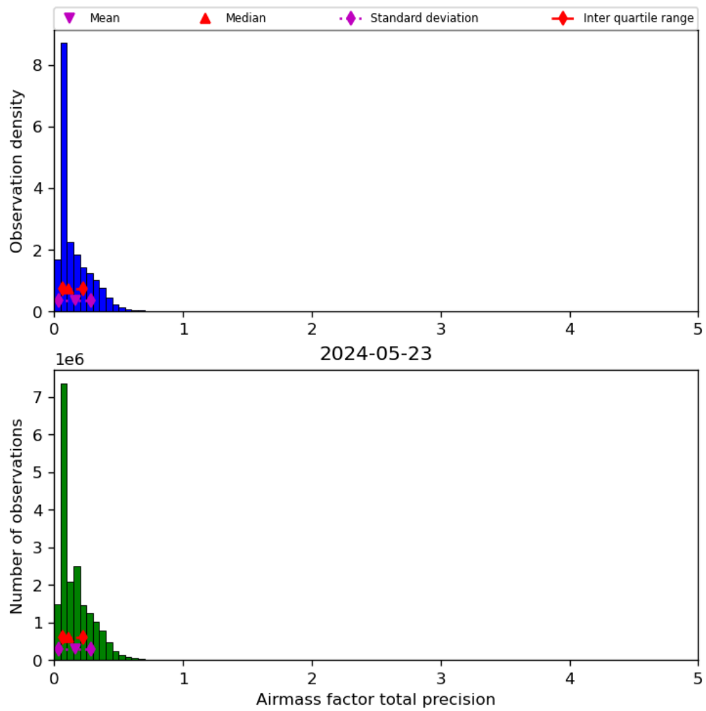
Figure 41: Histogram of “Airmass factor total precision” for 2024-05-23 to 2024-05-24
