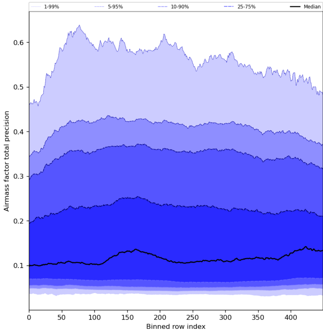
Figure 55: Along track statistics of “Airmass factor total precision” for 2024-05-23 to 2024-05-24
