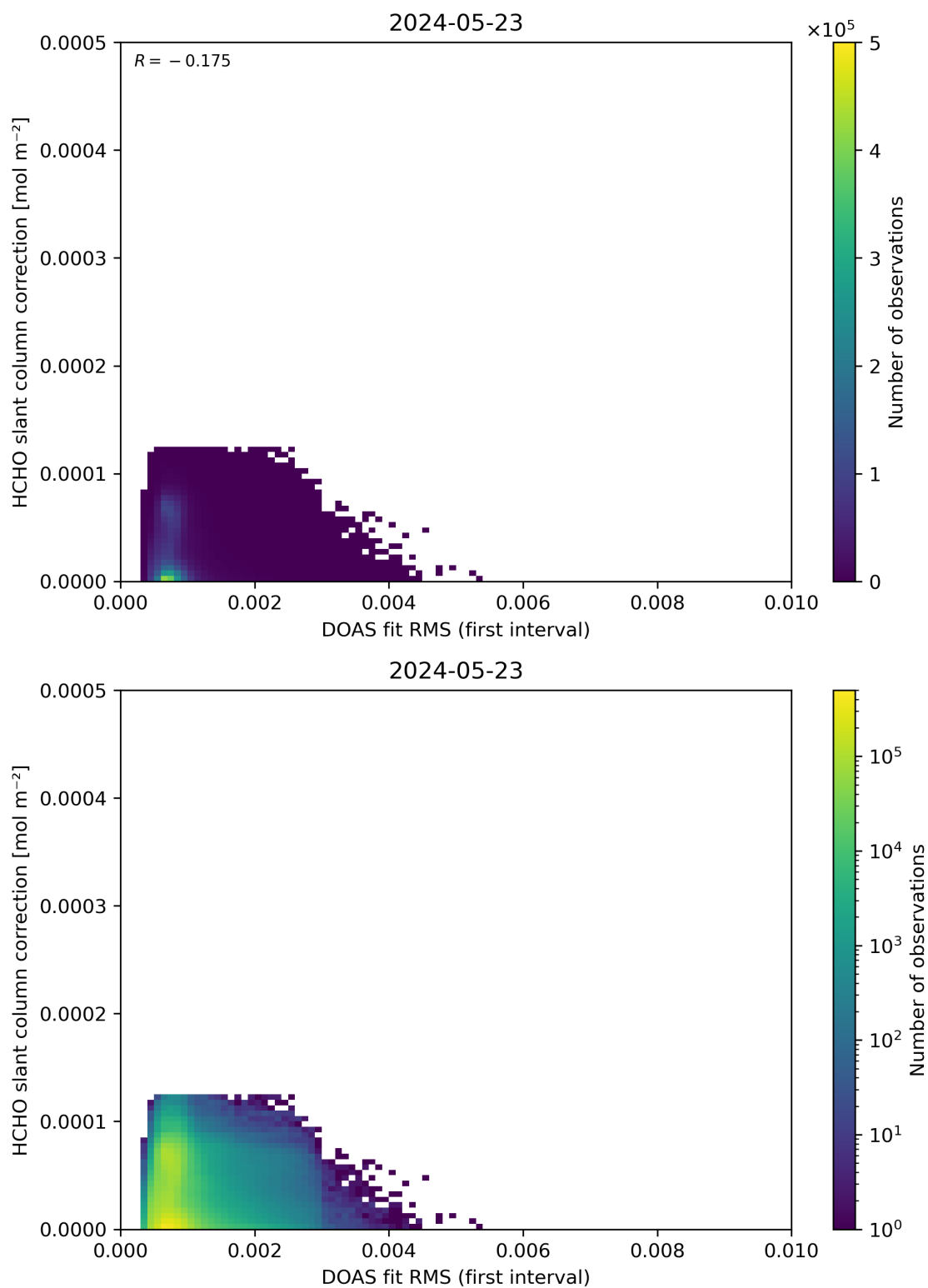
Figure 63: Scatter density plot of “DOAS fit RMS (first interval)” against “HCHO slant column correction” for 2024-05-23 to 2024-05-24.
