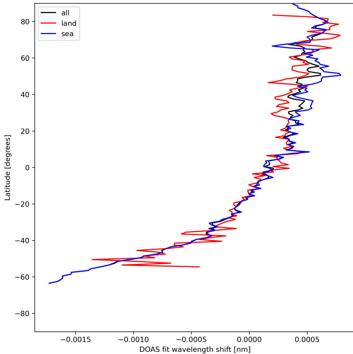
Figure 30: Zonal average of “DOAS fit wavelength shift” for 2024-05-23 to 2024-05-24.
