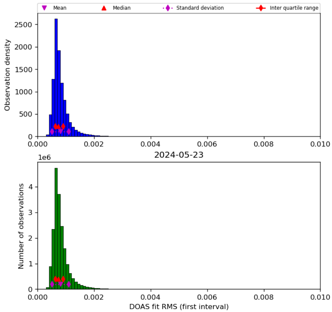
Figure 46: Histogram of “DOAS fit RMS (first interval)” for 2024-05-23 to 2024-05-24
