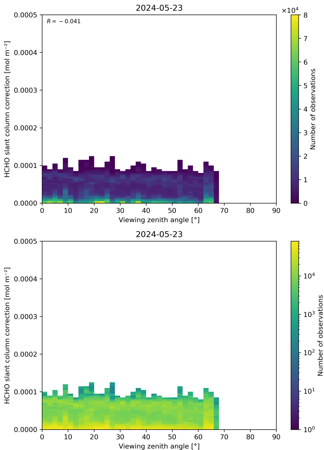
Figure 187: Scatter density plot of “Viewing zenith angle” against “HCHO slant column correction” for 2024-05-23 to 2024-05-24.
