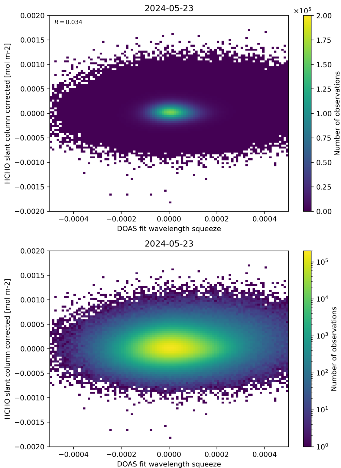
Figure 69: Scatter density plot of “DOAS fit wavelength squeeze” against “HCHO slant column corrected” for 2024-05-23 to 2024-05-24.
