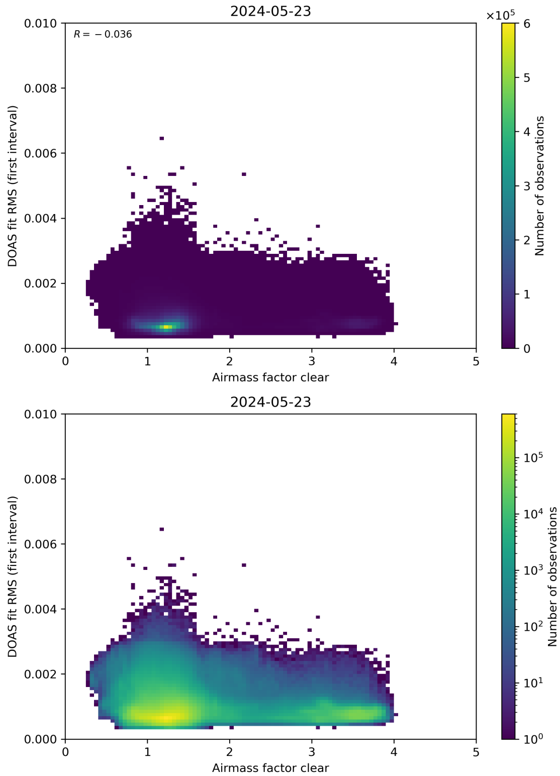
Figure 71: Scatter density plot of “Airmass factor clear” against “DOAS fit RMS (first interval)” for 2024-05-23 to 2024-05-24.
