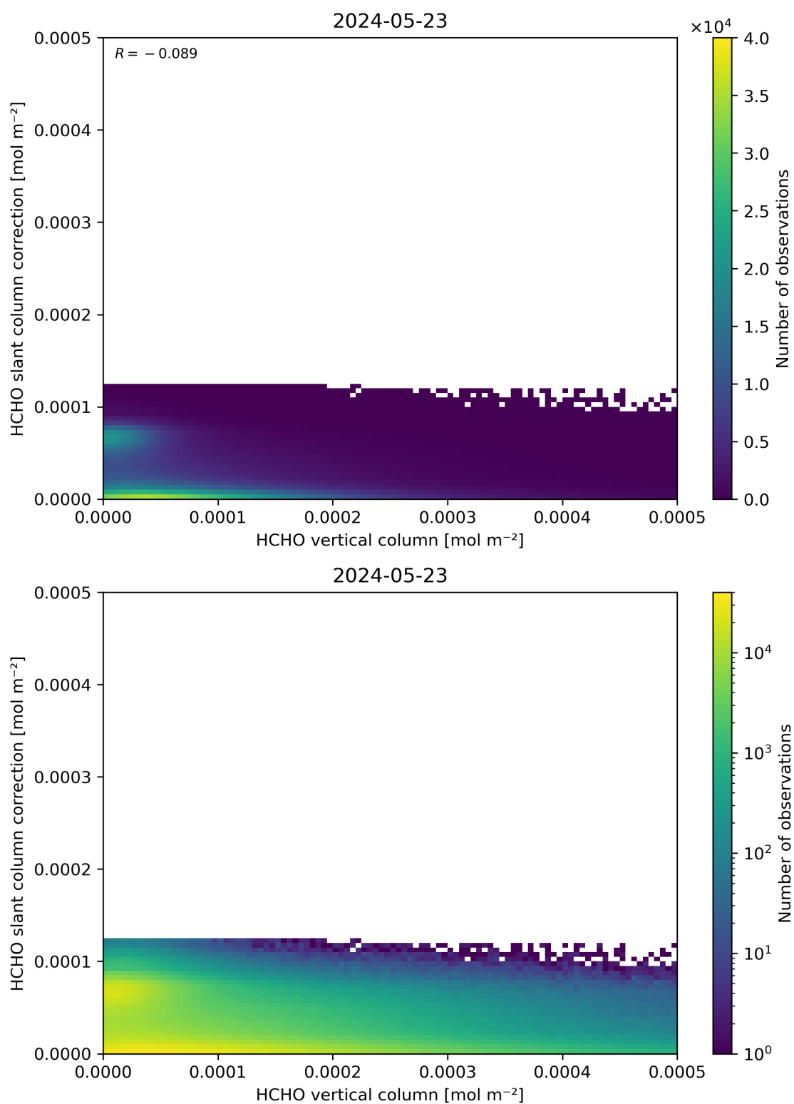
Figure 128: Scatter density plot of “HCHO vertical column” against “HCHO slant column correction” for 2024-05-23 to 2024-05-24.
