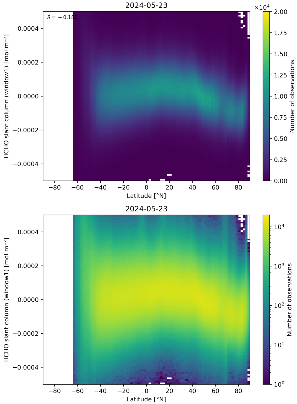
Figure 159: Scatter density plot of “Latitude” against “HCHO slant column (window1)” for 2024-05-23 to 2024-05-24.
