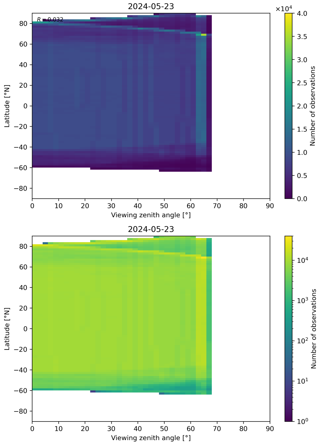
Figure 196: Scatter density plot of “Viewing zenith angle” against “Latitude” for 2024-05-23 to 2024-05-24.
