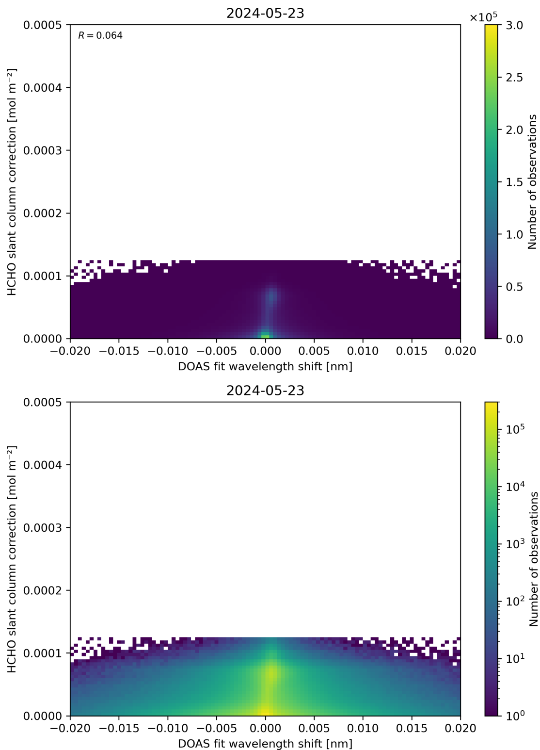
Figure 67: Scatter density plot of “DOAS fit wavelength shift” against “HCHO slant column correction” for 2024-05-23 to 2024-05-24.
