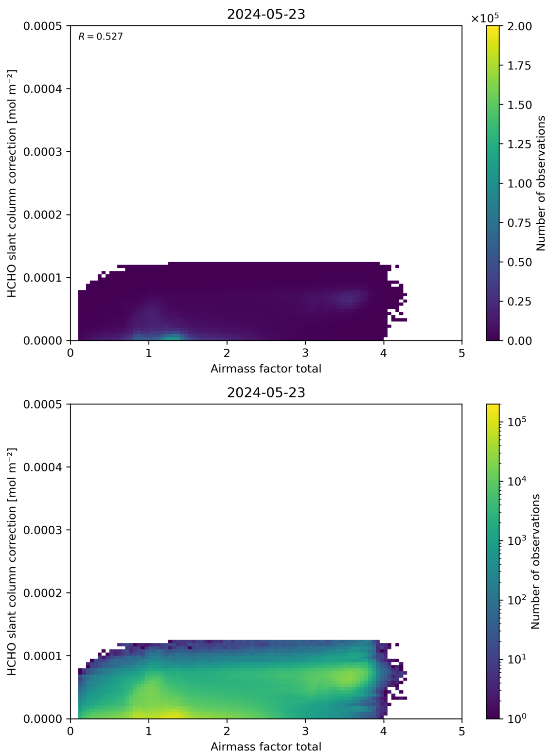
Figure 102: Scatter density plot of “Airmass factor total” against “HCHO slant column correction” for 2024-05-23 to 2024-05-24.
