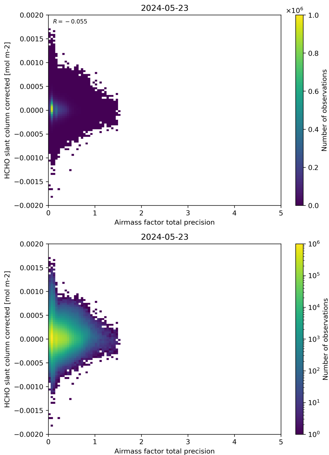
Figure 109: Scatter density plot of “Airmass factor total precision” against “HCHO slant column corrected” for 2024-05-23 to 2024-05-24.
