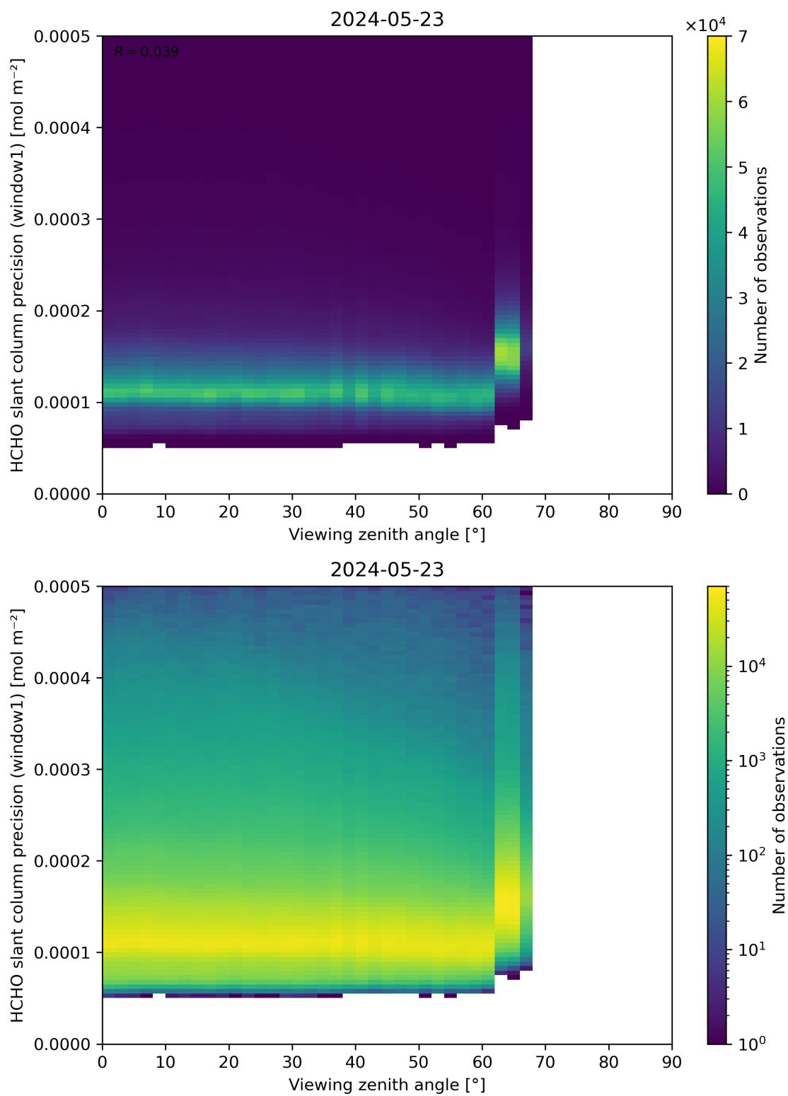
Figure 189: Scatter density plot of “Viewing zenith angle” against “HCHO slant column precision (window1)” for 2024-05-23 to 2024-05-24.
