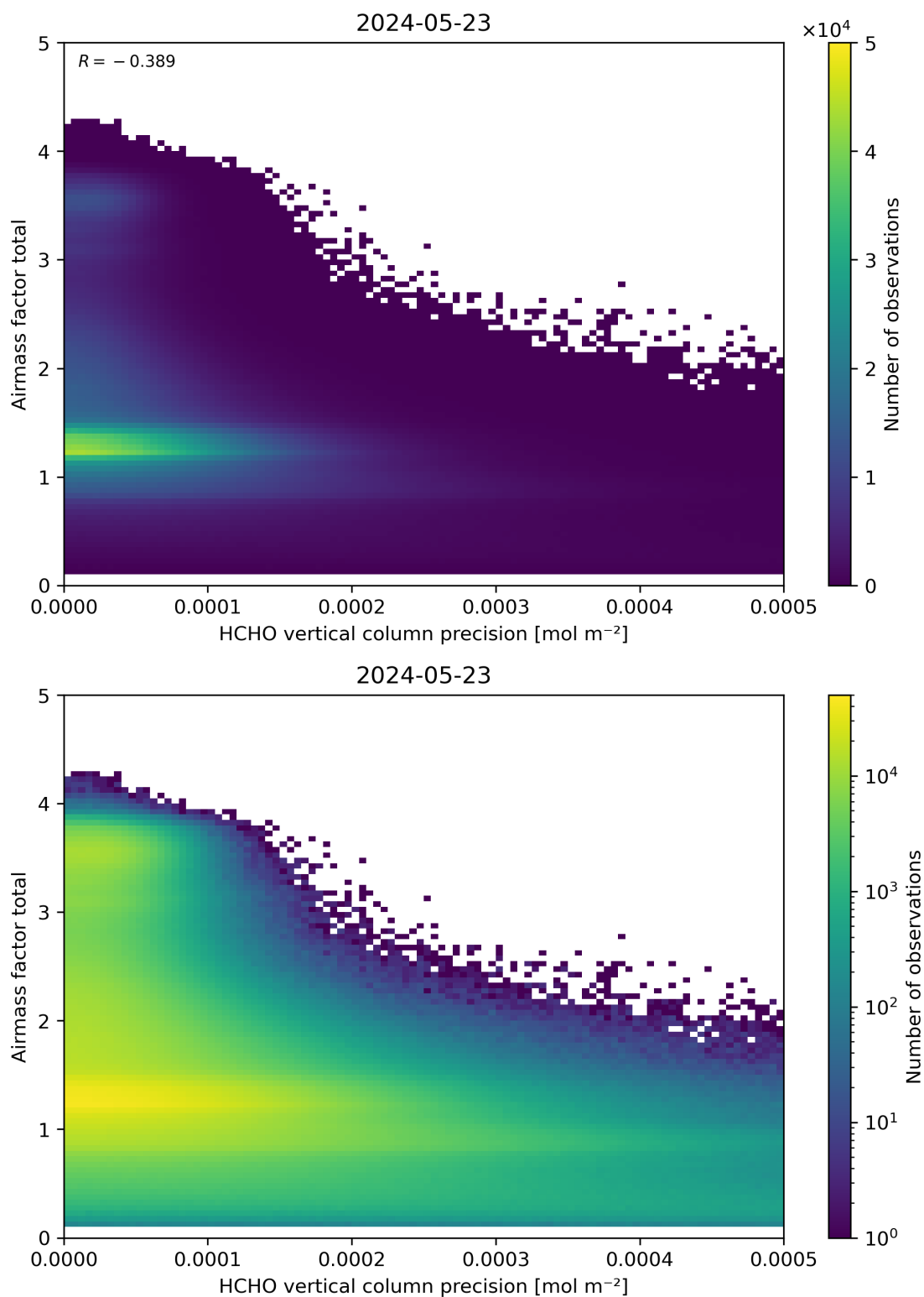
Figure 144: Scatter density plot of “HCHO vertical column precision” against “Airmass factor total” for 2024-05-23 to 2024-05-24.
