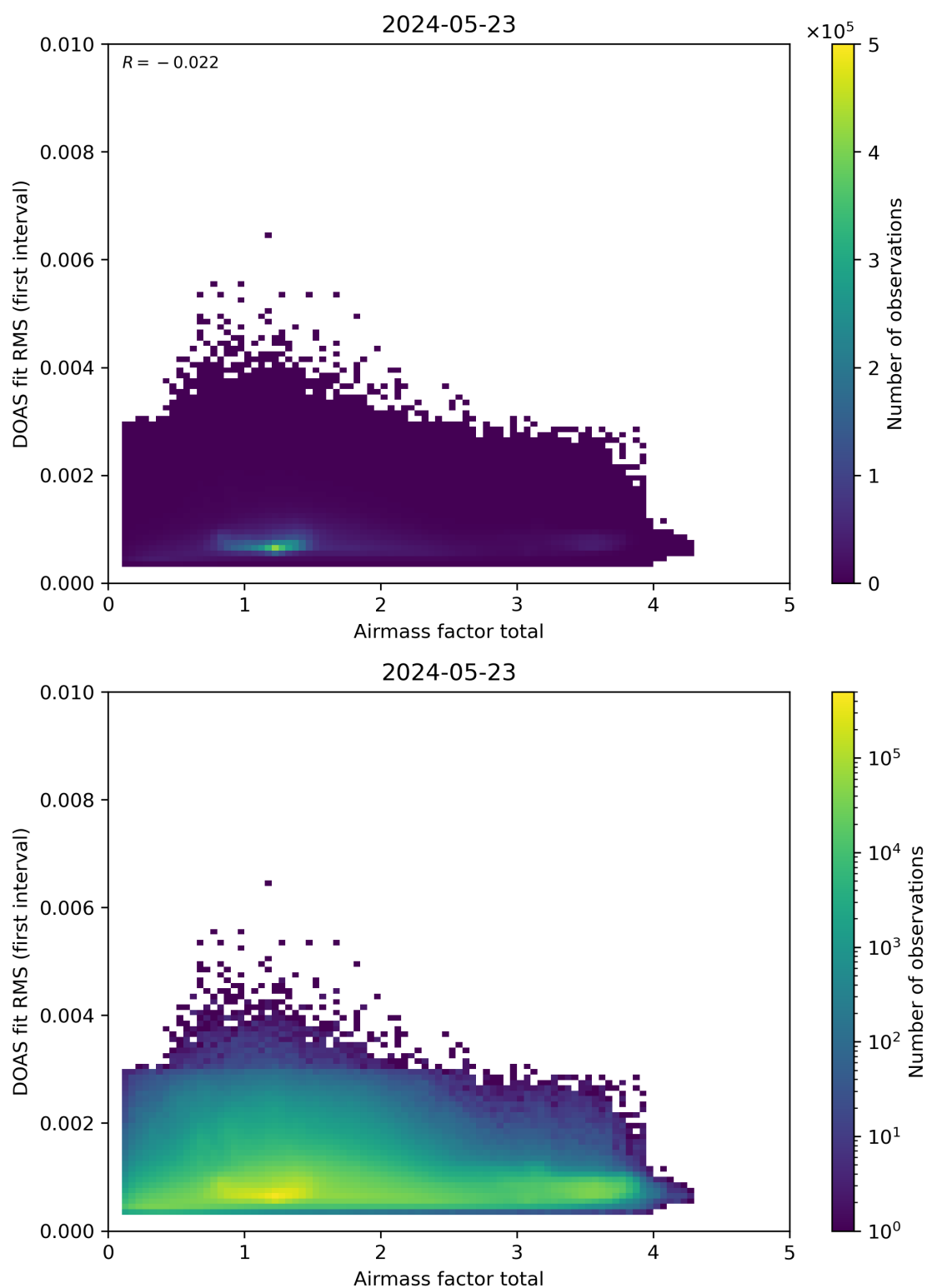
Figure 97: Scatter density plot of “Airmass factor total” against “DOAS fit RMS (first interval)” for 2024-05-23 to 2024-05-24.
