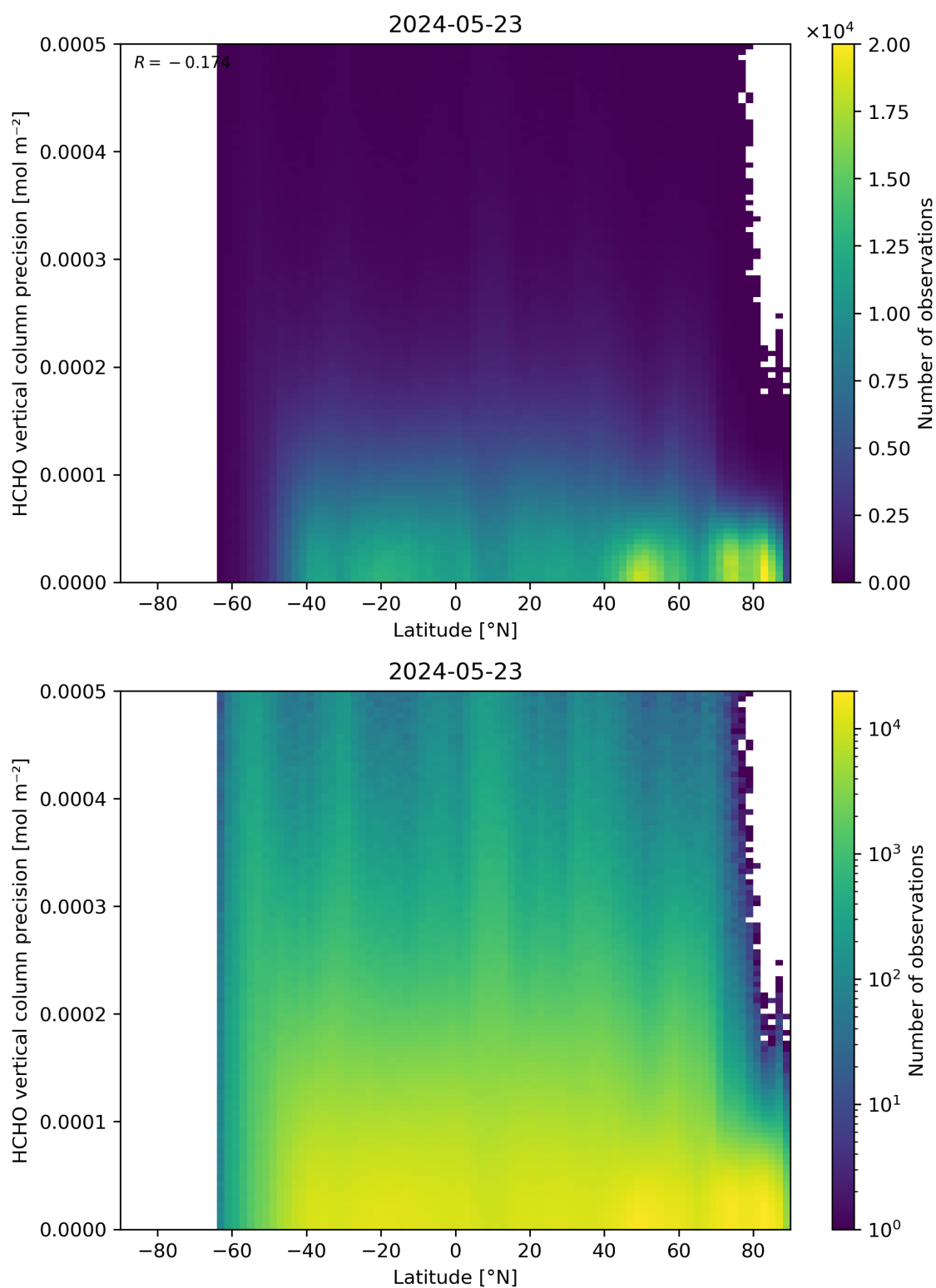
Figure 165: Scatter density plot of “Latitude” against “HCHO vertical column precision” for 2024-05-23 to 2024-05-24.
