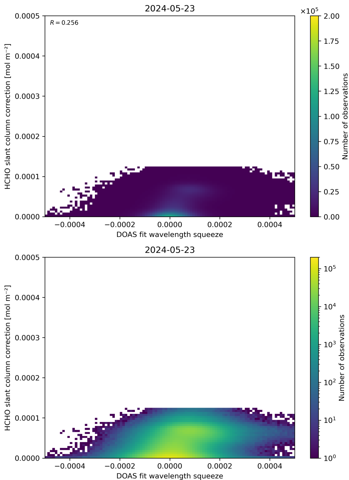
Figure 70: Scatter density plot of “DOAS fit wavelength squeeze” against “HCHO slant column correction” for 2024-05-23 to 2024-05-24.
