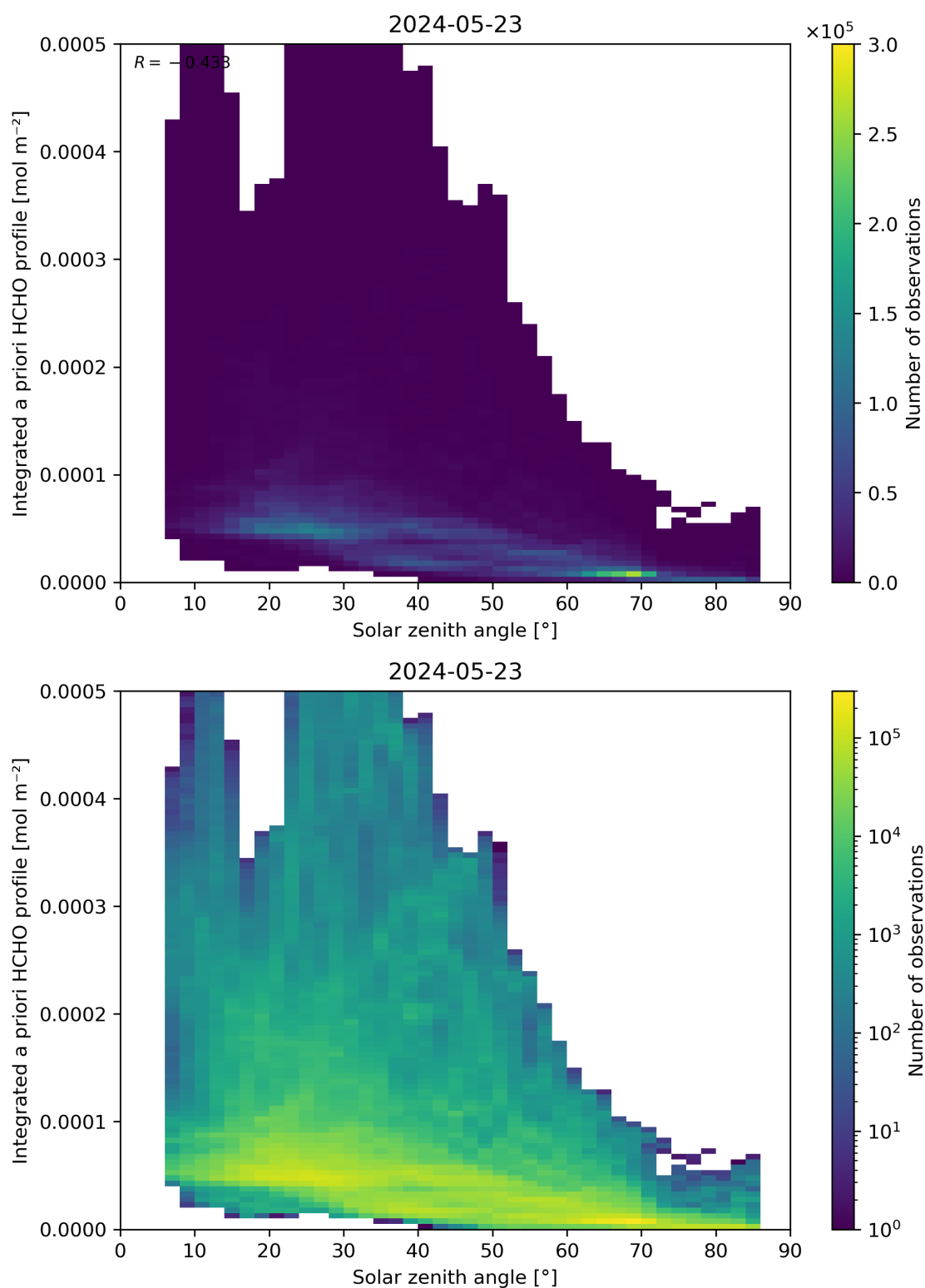
Figure 180: Scatter density plot of “Solar zenith angle” against “Integrated a priori HCHO profile” for 2024-05-23 to 2024-05-24.
