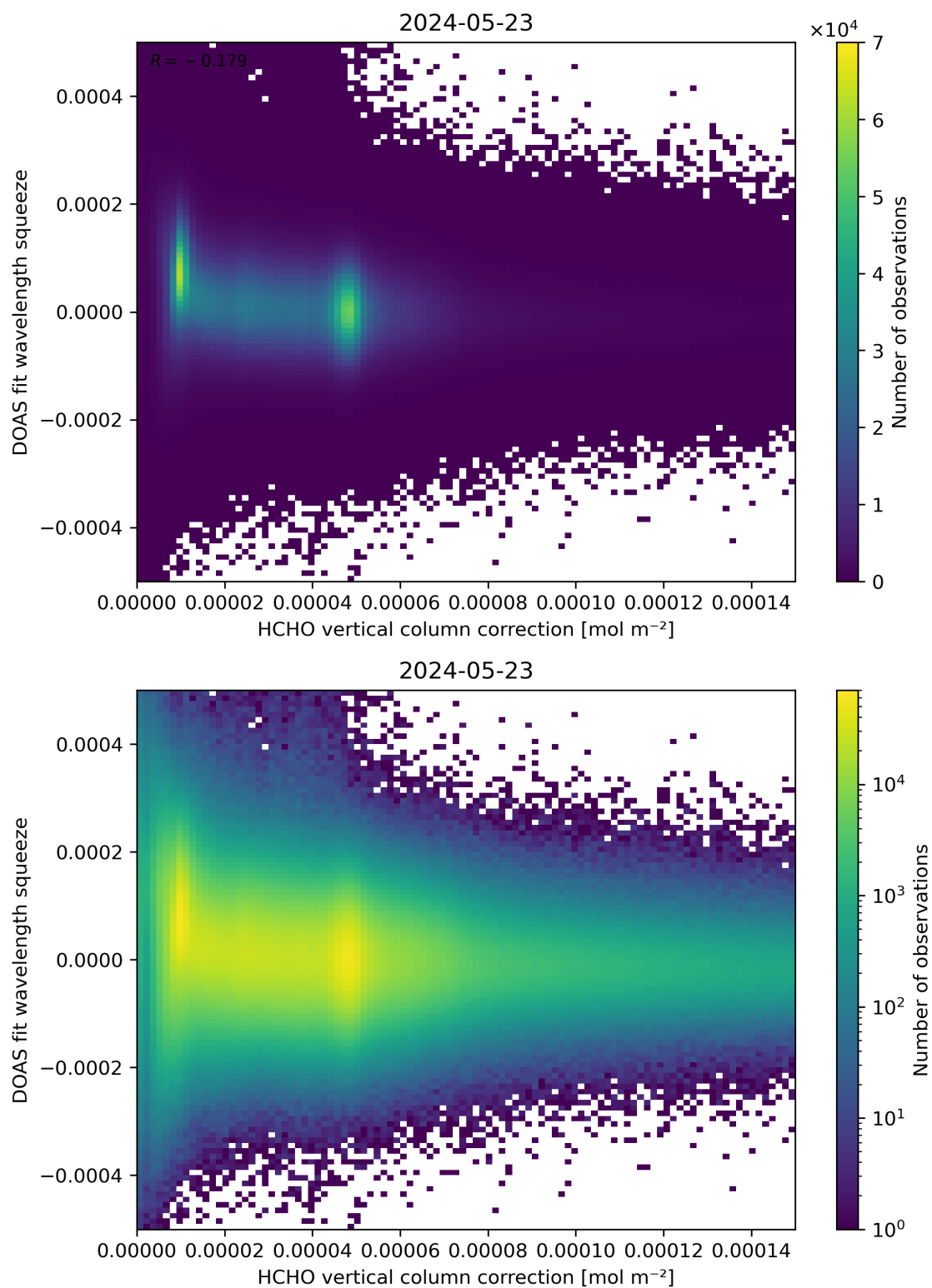
Figure 114: Scatter density plot of “HCHO vertical column correction” against “DOAS fit wavelength squeeze” for 2024-05-23 to 2024-05-24.
