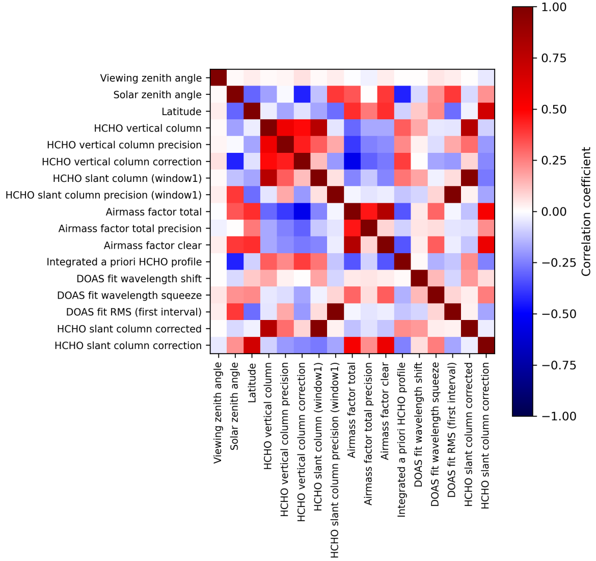
Figure 2: Map of correlation matrix for 2024-05-23 to 2024-05-24.
