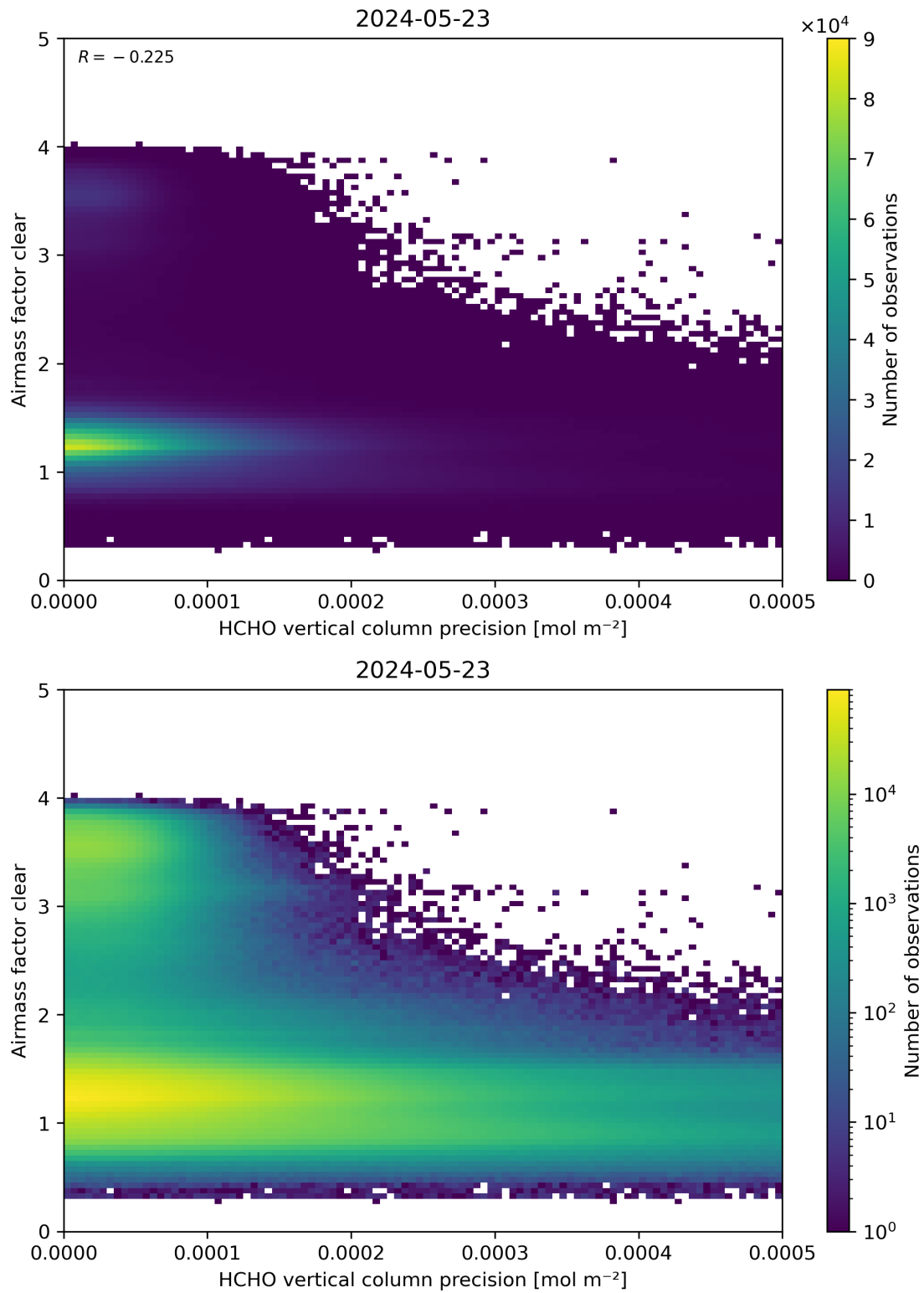
Figure 139: Scatter density plot of “HCHO vertical column precision” against “Airmass factor clear” for 2024-05-23 to 2024-05-24.
