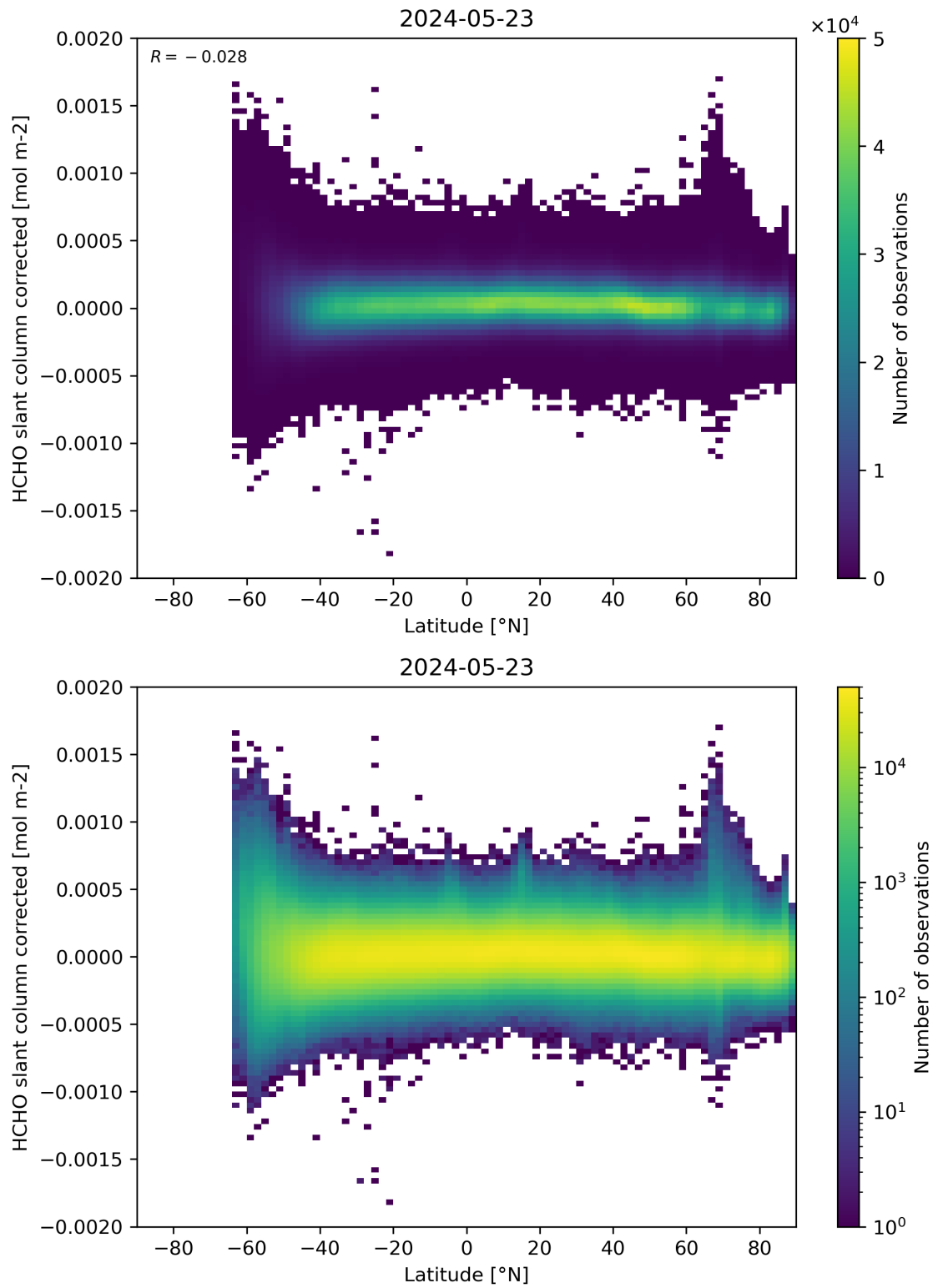
Figure 157: Scatter density plot of “Latitude” against “HCHO slant column corrected” for 2024-05-23 to 2024-05-24.
