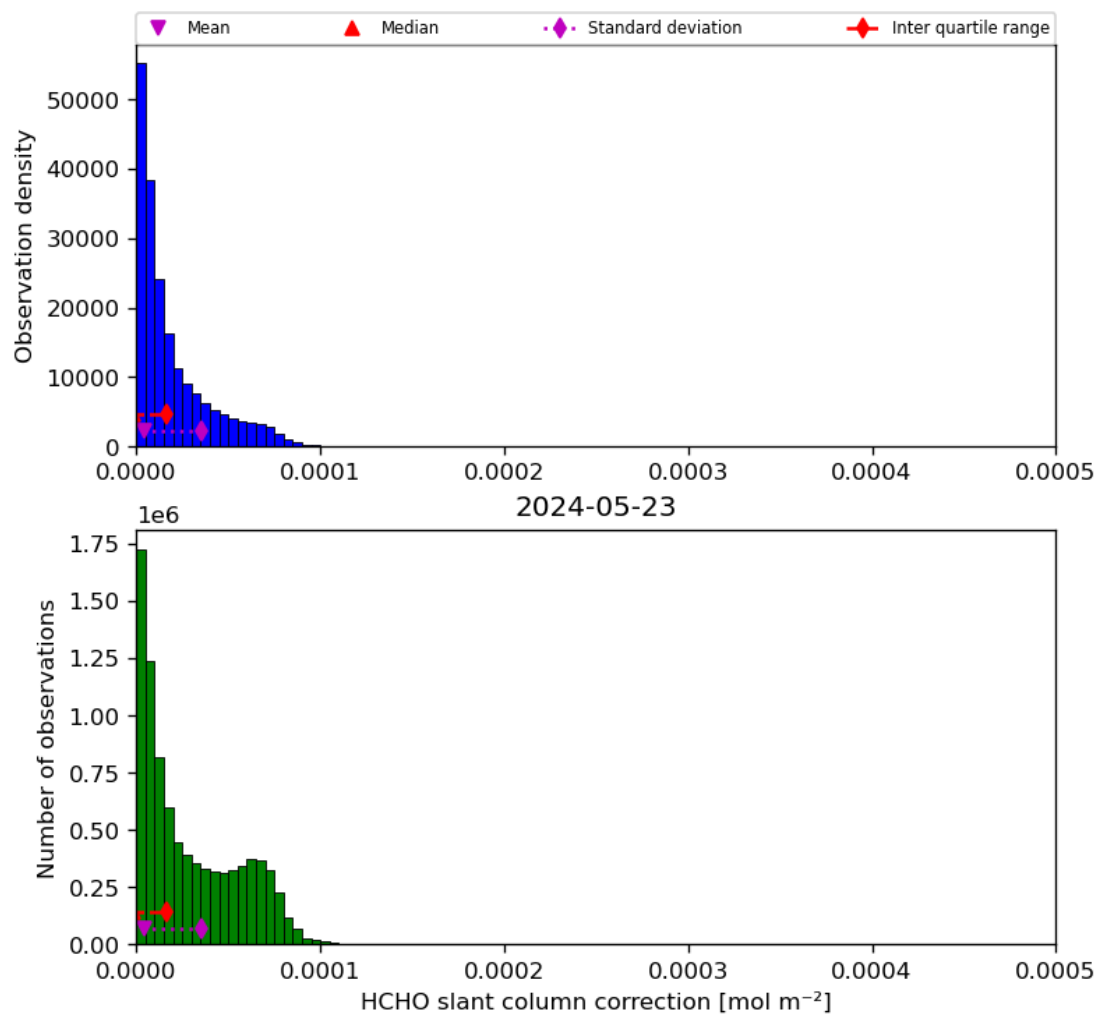
Figure 47: Histogram of “HCHO slant column correction” for 2024-05-23 to 2024-05-24
