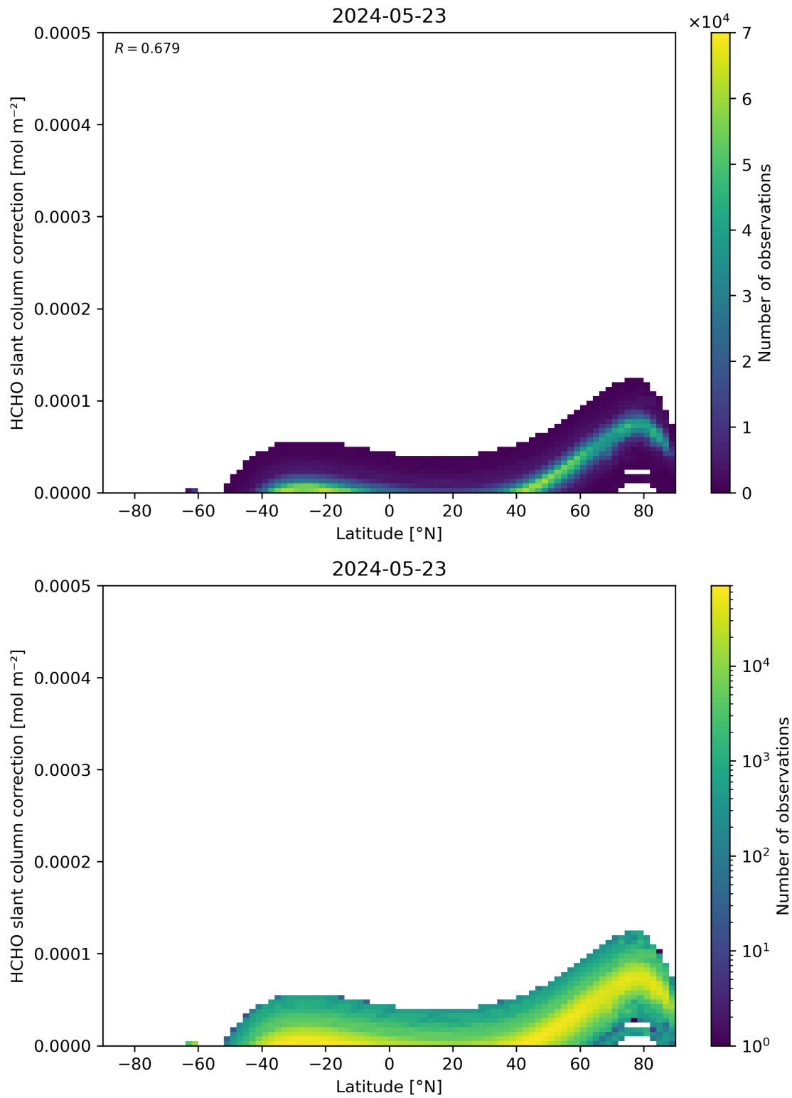
Figure 158: Scatter density plot of “Latitude” against “HCHO slant column correction” for 2024-05-23 to 2024-05-24.
