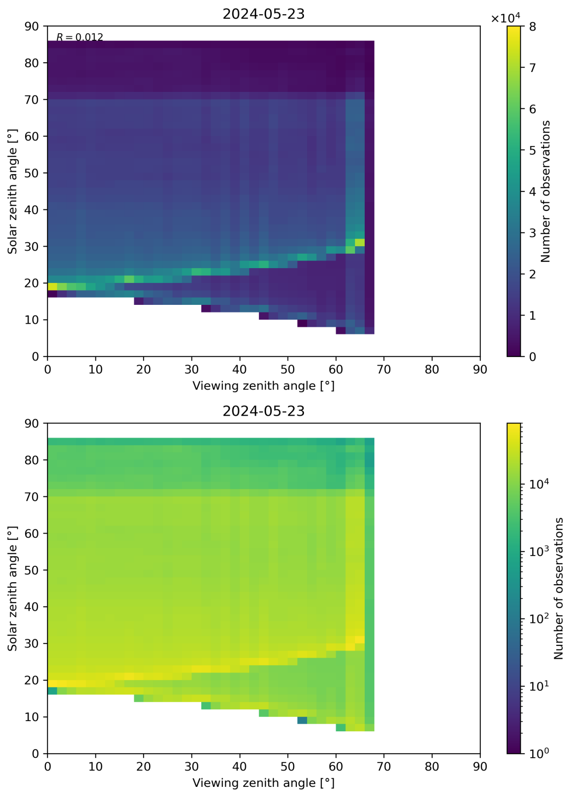
Figure 197: Scatter density plot of “Viewing zenith angle” against “Solar zenith angle” for 2024-05-23 to 2024-05-24.
