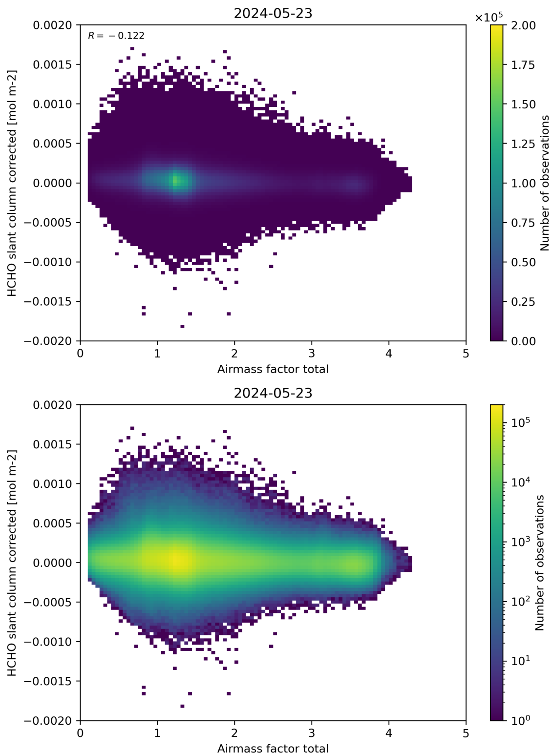
Figure 101: Scatter density plot of “Airmass factor total” against “HCHO slant column corrected” for 2024-05-23 to 2024-05-24.
