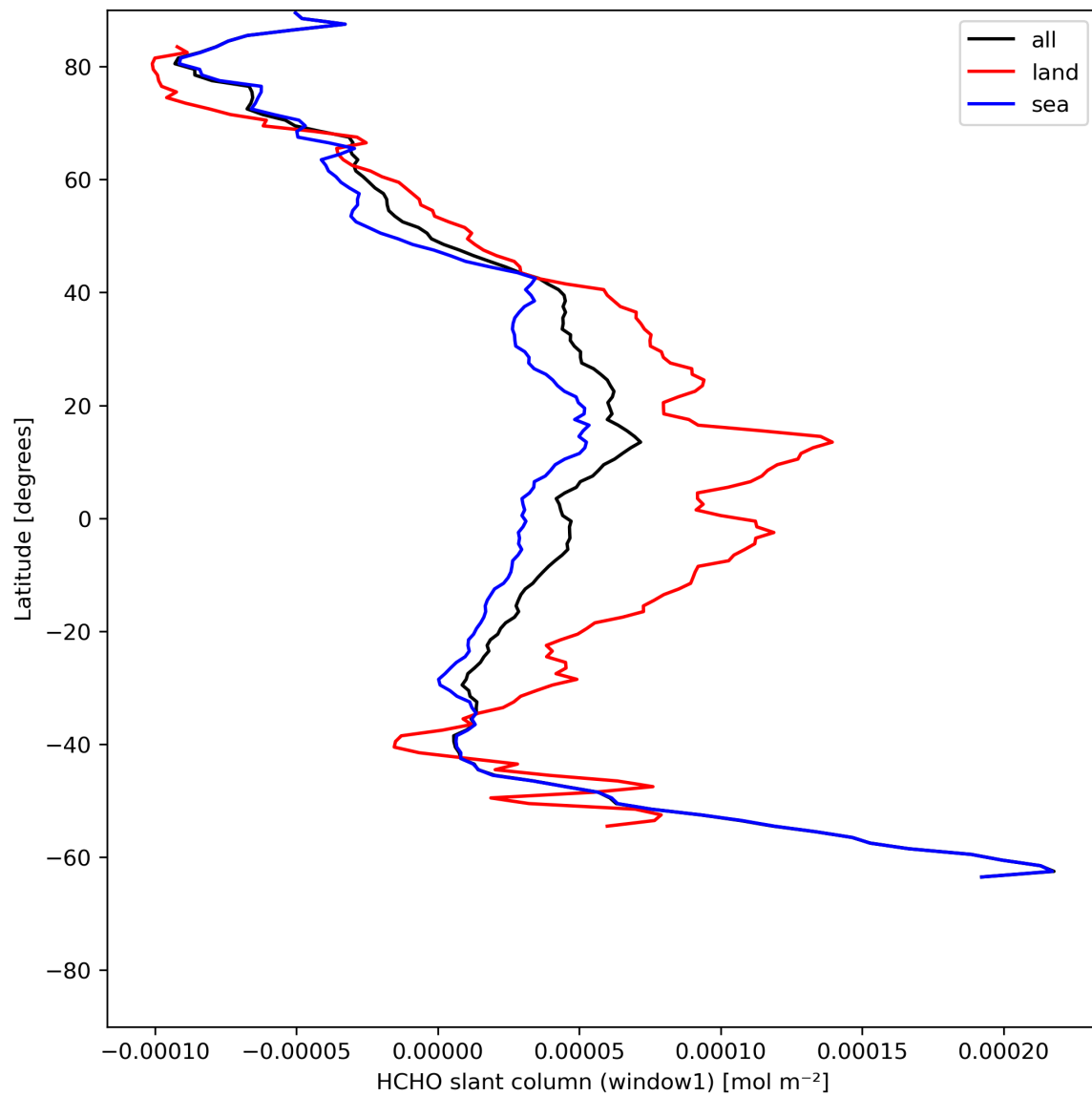
Figure 24: Zonal average of “HCHO slant column (window1)” for 2024-05-23 to 2024-05-24.
