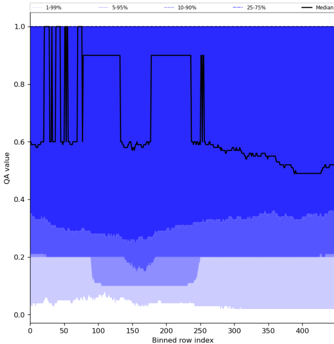
Figure 48: Along track statistics of “QA value” for 2024-05-23 to 2024-05-24
