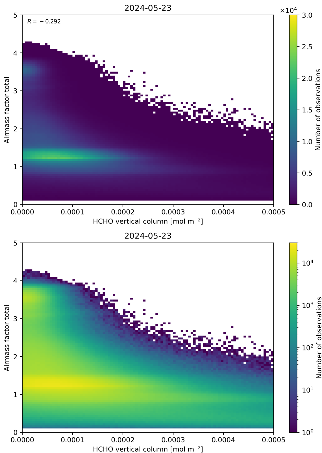
Figure 131: Scatter density plot of “HCHO vertical column” against “Airmass factor total” for 2024-05-23 to 2024-05-24.
