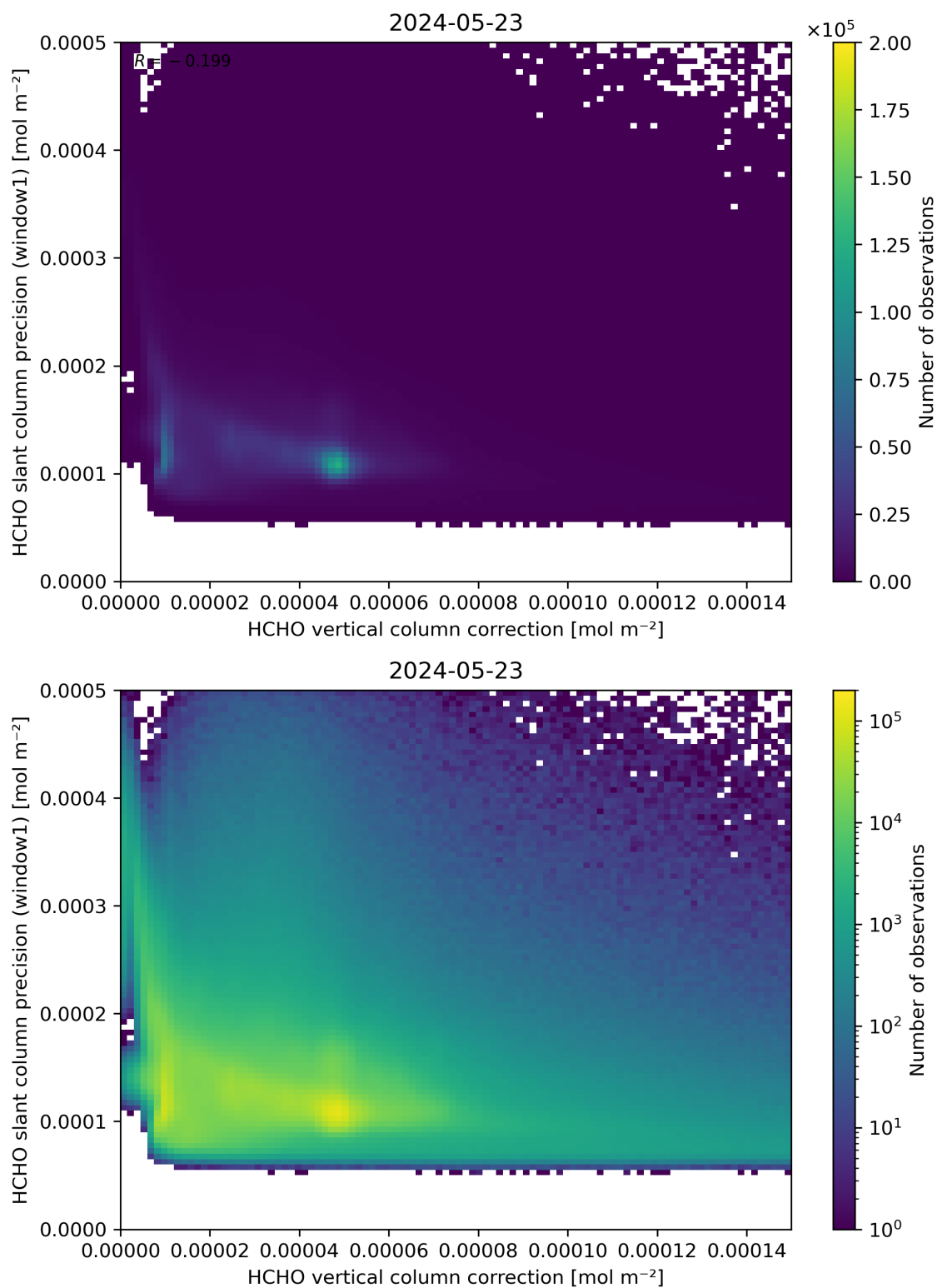
Figure 119: Scatter density plot of “HCHO vertical column correction” against “HCHO slant column precision (window1)” for 2024-05-23 to 2024-05-24.
