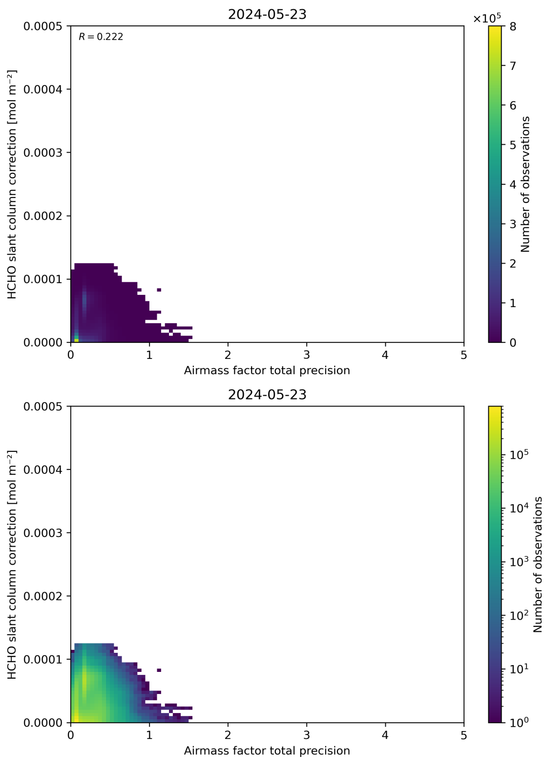
Figure 110: Scatter density plot of “Airmass factor total precision” against “HCHO slant column correction” for 2024-05-23 to 2024-05-24.
