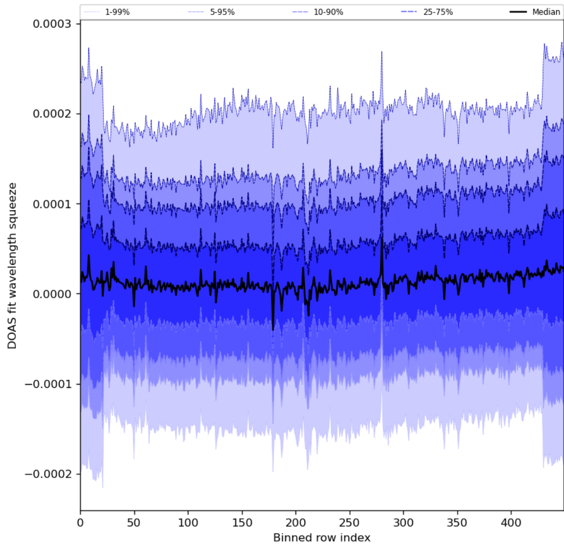
Figure 59: Along track statistics of “DOAS fit wavelength squeeze” for 2024-05-23 to 2024-05-24
