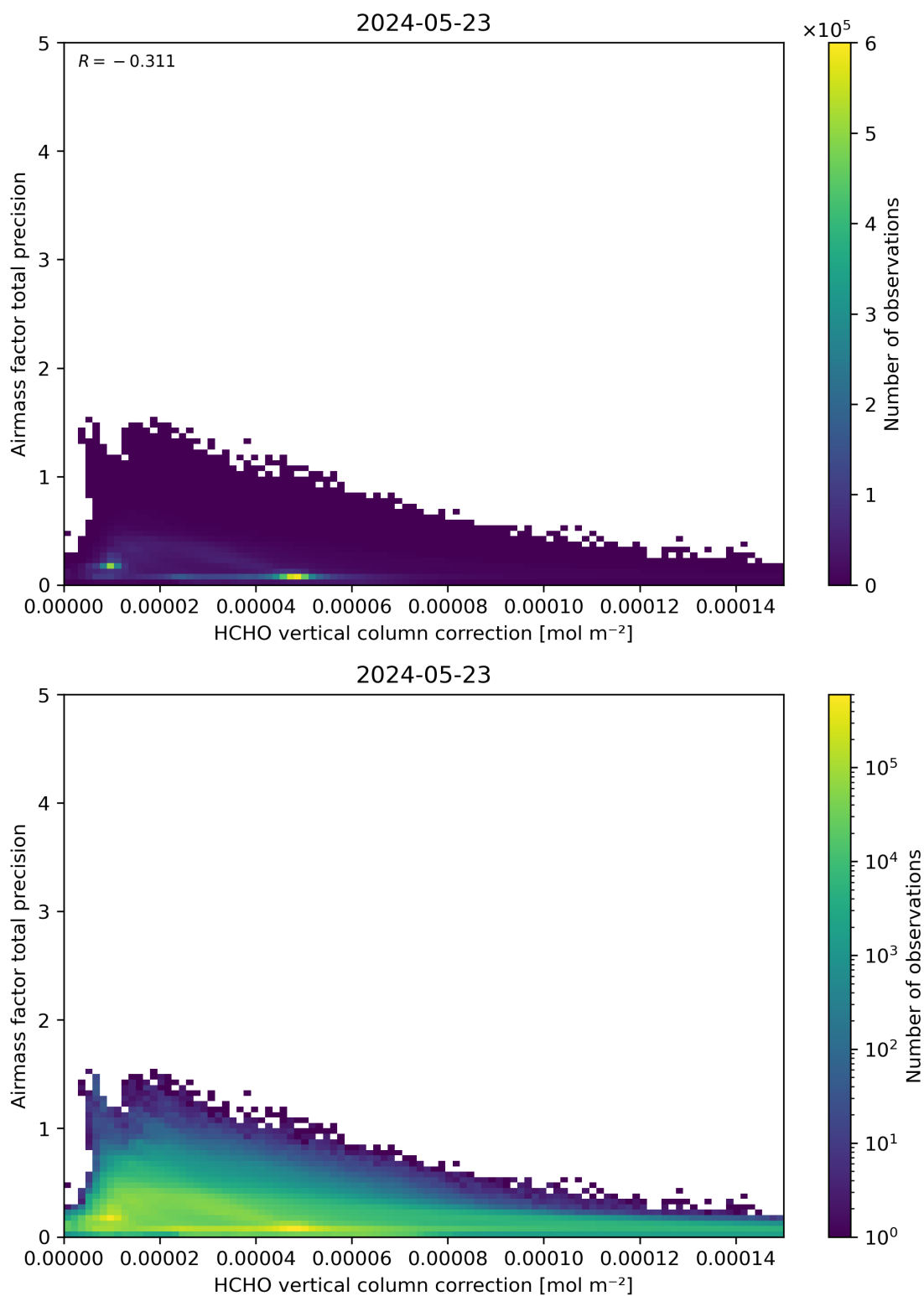
Figure 121: Scatter density plot of “HCHO vertical column correction” against “Airmass factor total precision” for 2024-05-23 to 2024-05-24.
