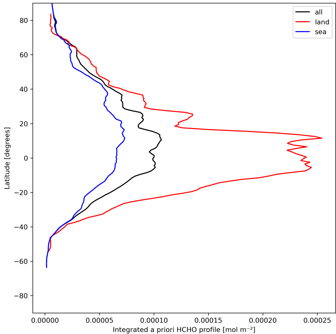
Figure 29: Zonal average of “Integrated a priori HCHO profile” for 2024-05-23 to 2024-05-25.
