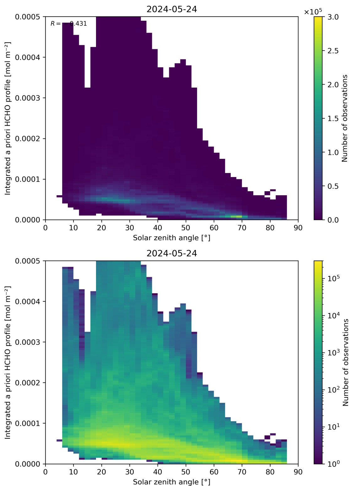
Figure 180: Scatter density plot of “Solar zenith angle” against “Integrated a priori HCHO profile” for 2024-05-23 to 2024-05-25.
