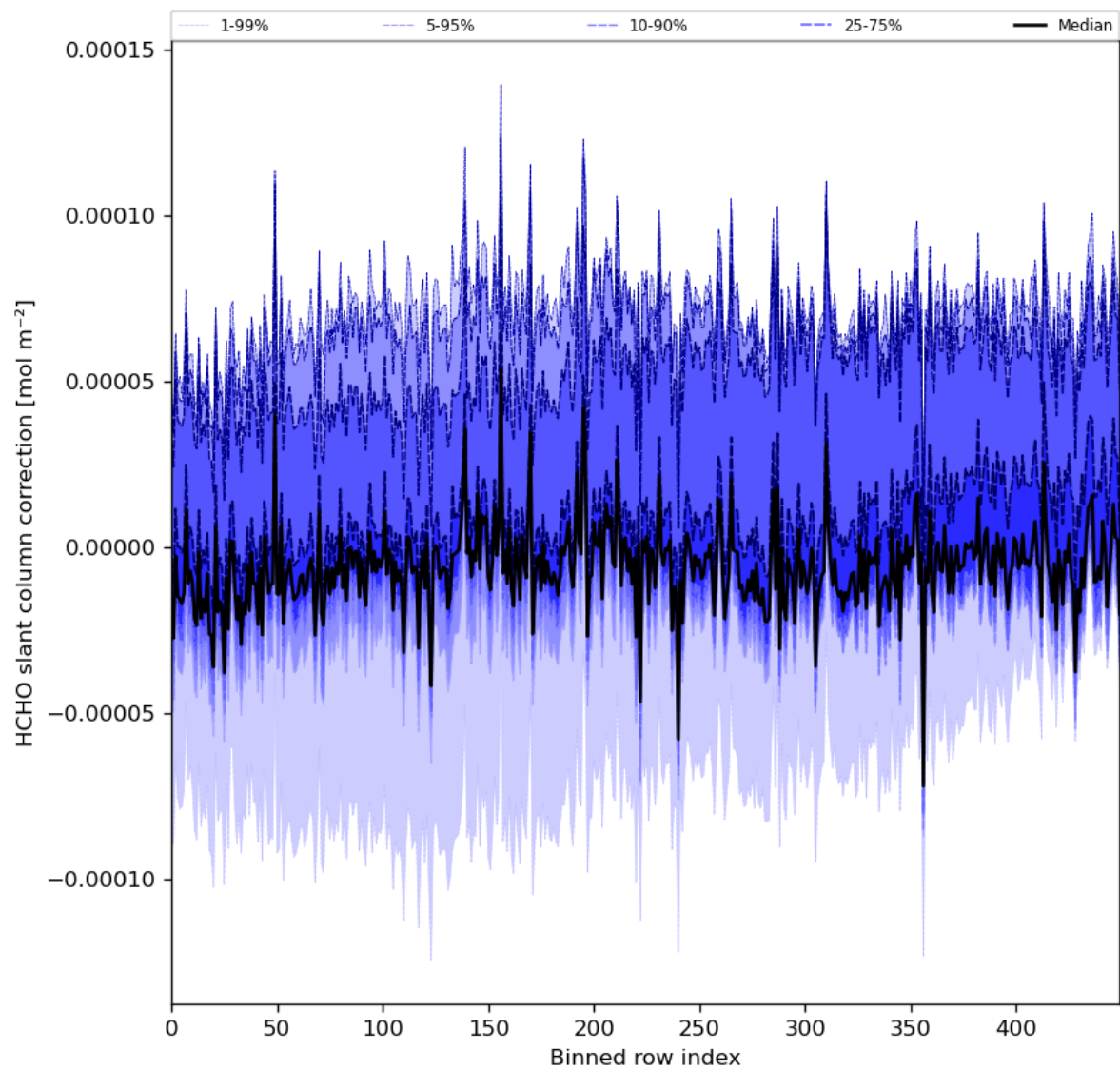
Figure 61: Along track statistics of “HCHO slant column correction” for 2024-05-23 to 2024-05-25
