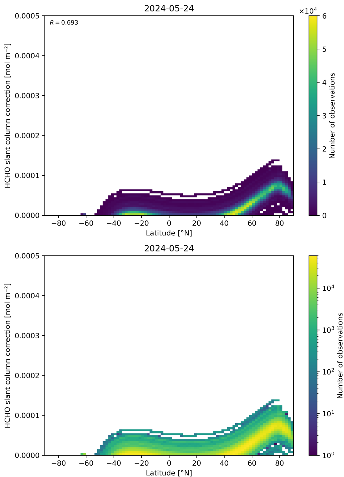
Figure 158: Scatter density plot of “Latitude” against “HCHO slant column correction” for 2024-05-23 to 2024-05-25.
