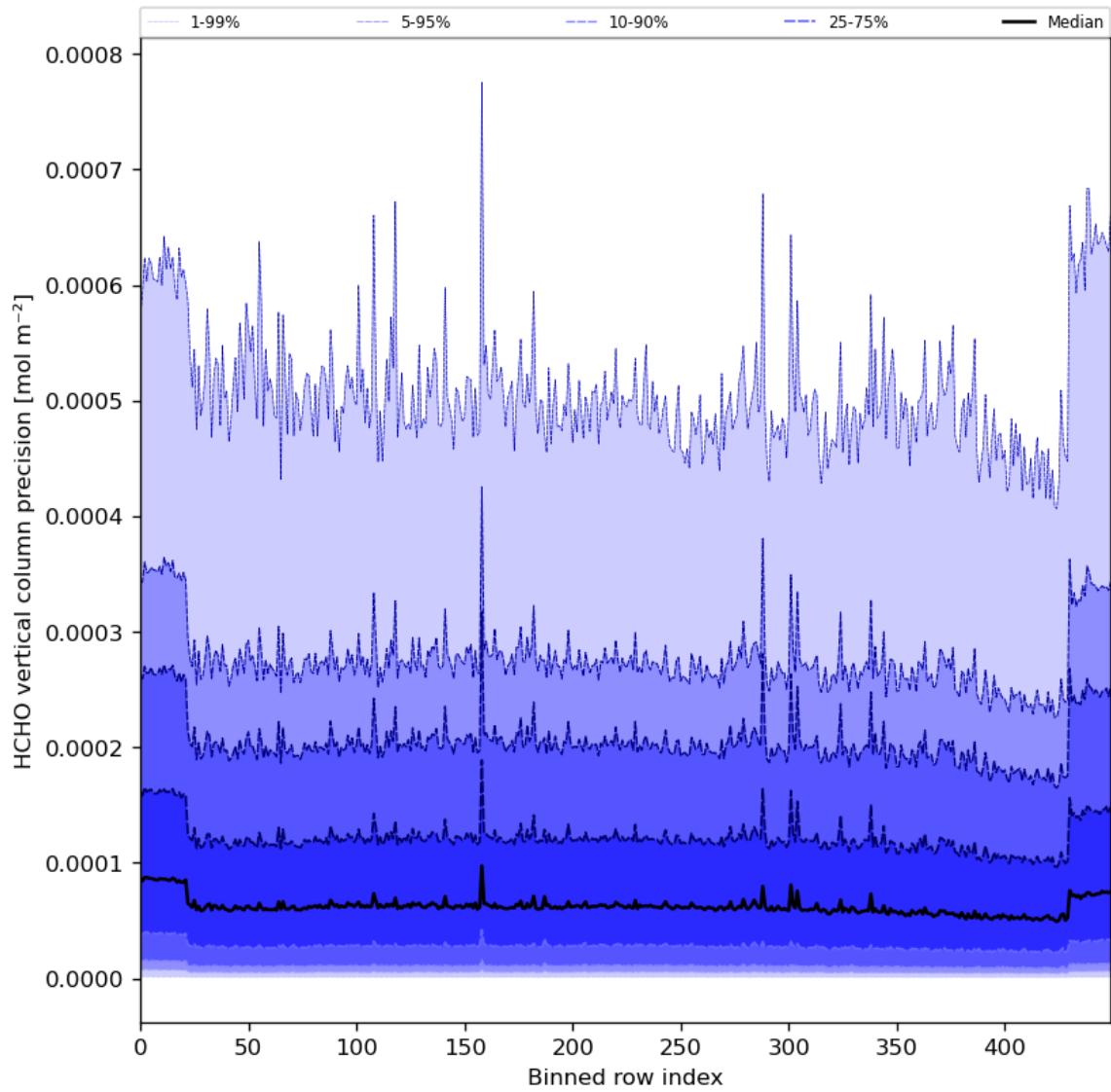
Figure 50: Along track statistics of “HCHO vertical column precision” for 2024-05-23 to 2024-05-25
