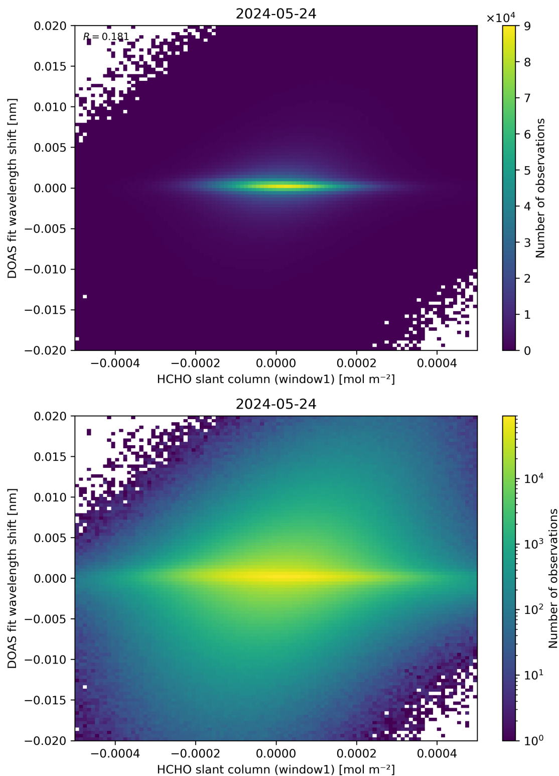
Figure 79: Scatter density plot of “HCHO slant column (window1)” against “DOAS fit wavelength shift” for 2024-05-23 to 2024-05-25.
