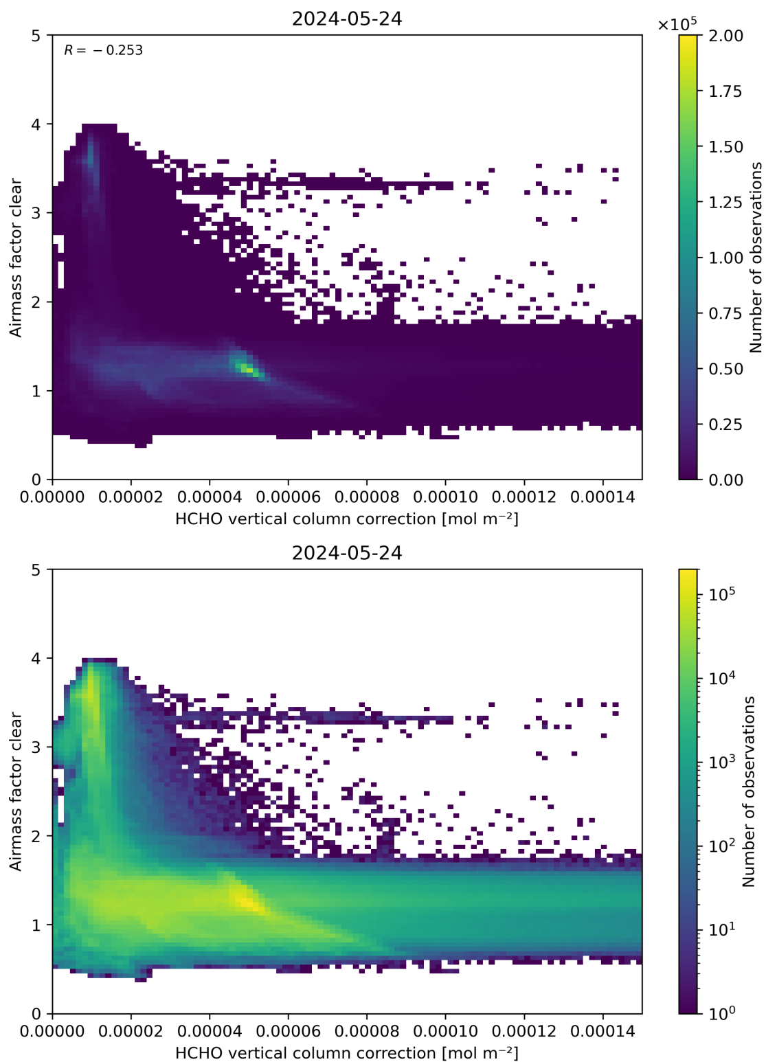
Figure 115: Scatter density plot of “HCHO vertical column correction” against “Airmass factor clear” for 2024-05-23 to 2024-05-25.
