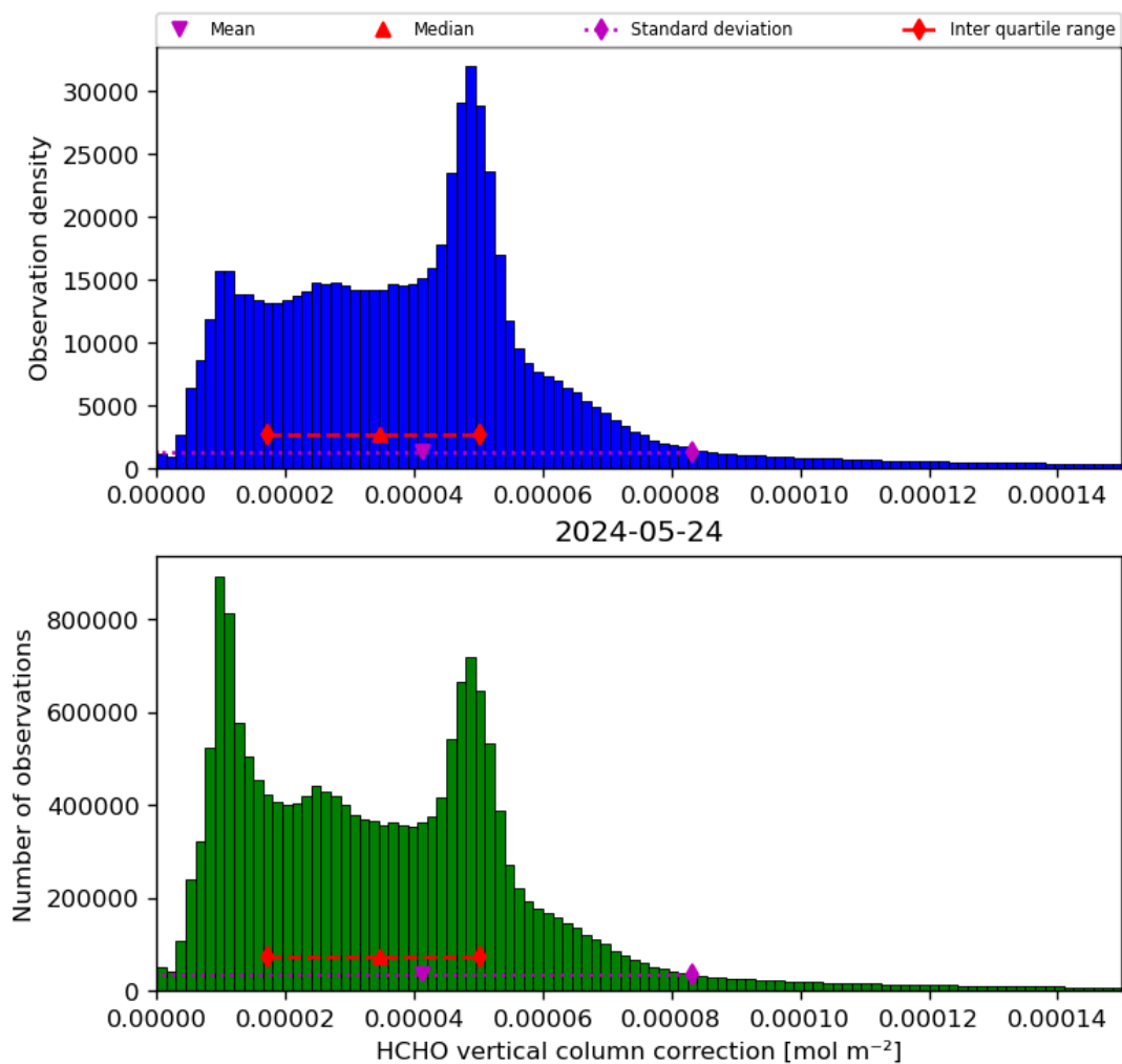
Figure 37: Histogram of “HCHO vertical column correction” for 2024-05-23 to 2024-05-25
