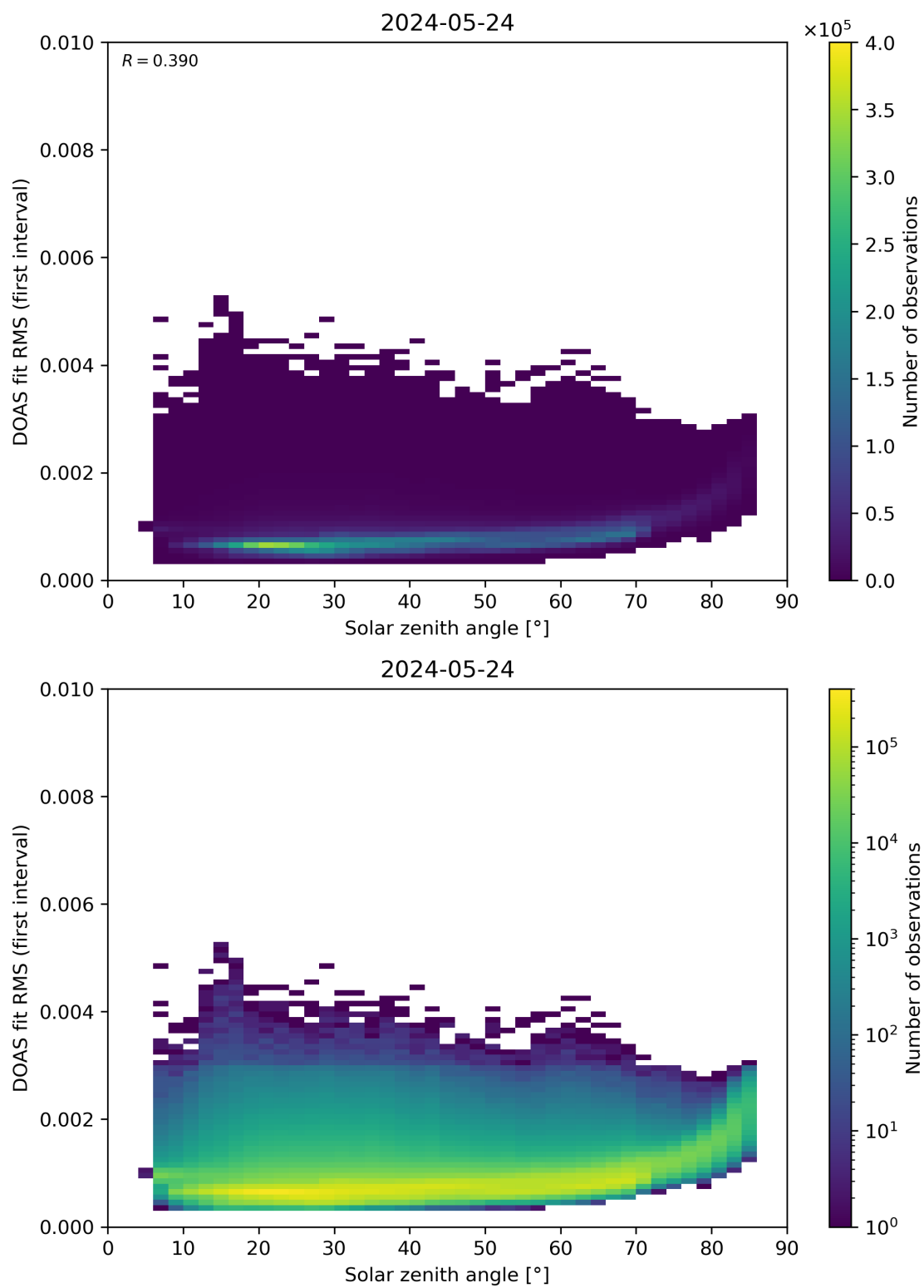
Figure 167: Scatter density plot of “Solar zenith angle” against “DOAS fit RMS (first interval)” for 2024-05-23 to 2024-05-25.
