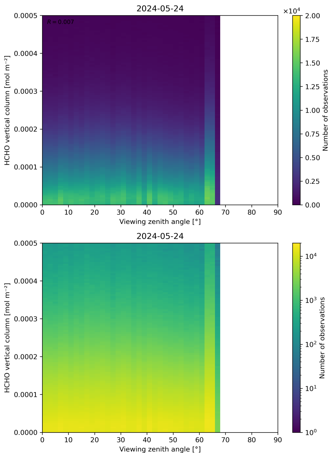
Figure 192: Scatter density plot of “Viewing zenith angle” against “HCHO vertical column” for 2024-05-23 to 2024-05-25.
