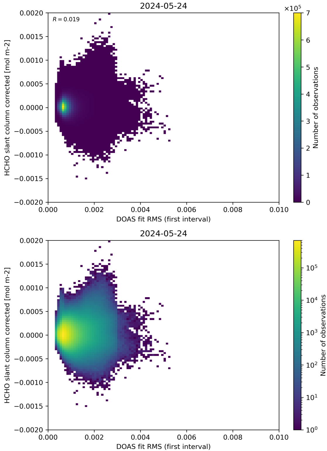
Figure 62: Scatter density plot of “DOAS fit RMS (first interval)” against “HCHO slant column corrected” for 2024-05-23 to 2024-05-25.
