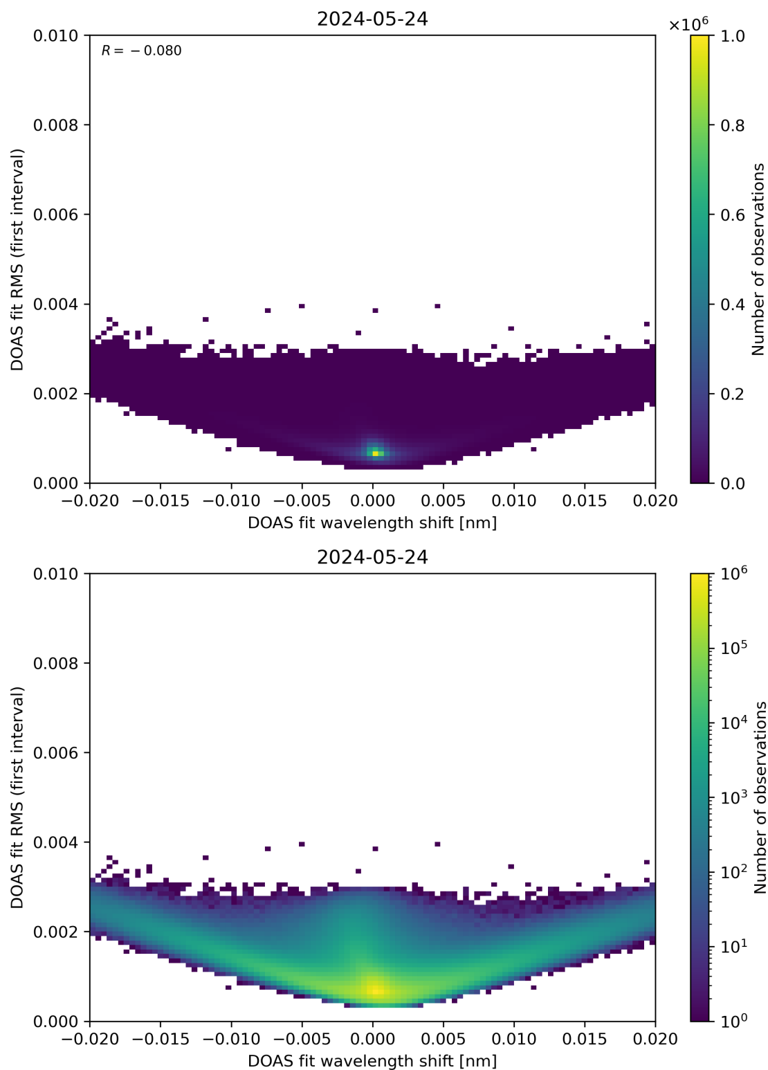
Figure 64: Scatter density plot of “DOAS fit wavelength shift” against “DOAS fit RMS (first interval)” for 2024-05-23 to 2024-05-25.
