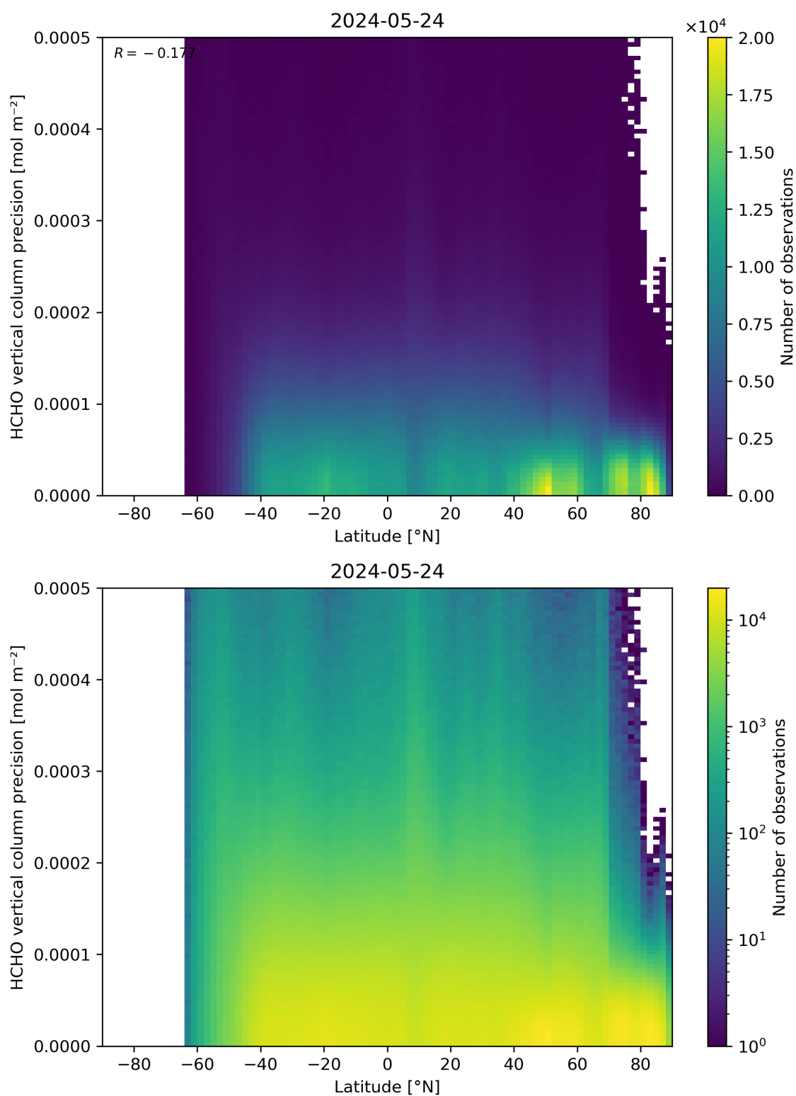
Figure 165: Scatter density plot of “Latitude” against “HCHO vertical column precision” for 2024-05-23 to 2024-05-25.
