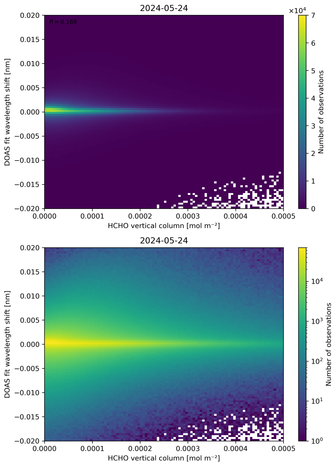
Figure 124: Scatter density plot of “HCHO vertical column” against “DOAS fit wavelength shift” for 2024-05-23 to 2024-05-25.
