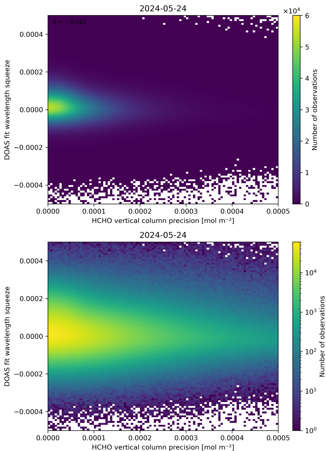
Figure 138: Scatter density plot of “HCHO vertical column precision” against “DOAS fit wavelength squeeze” for 2024-05-23 to 2024-05-25.
