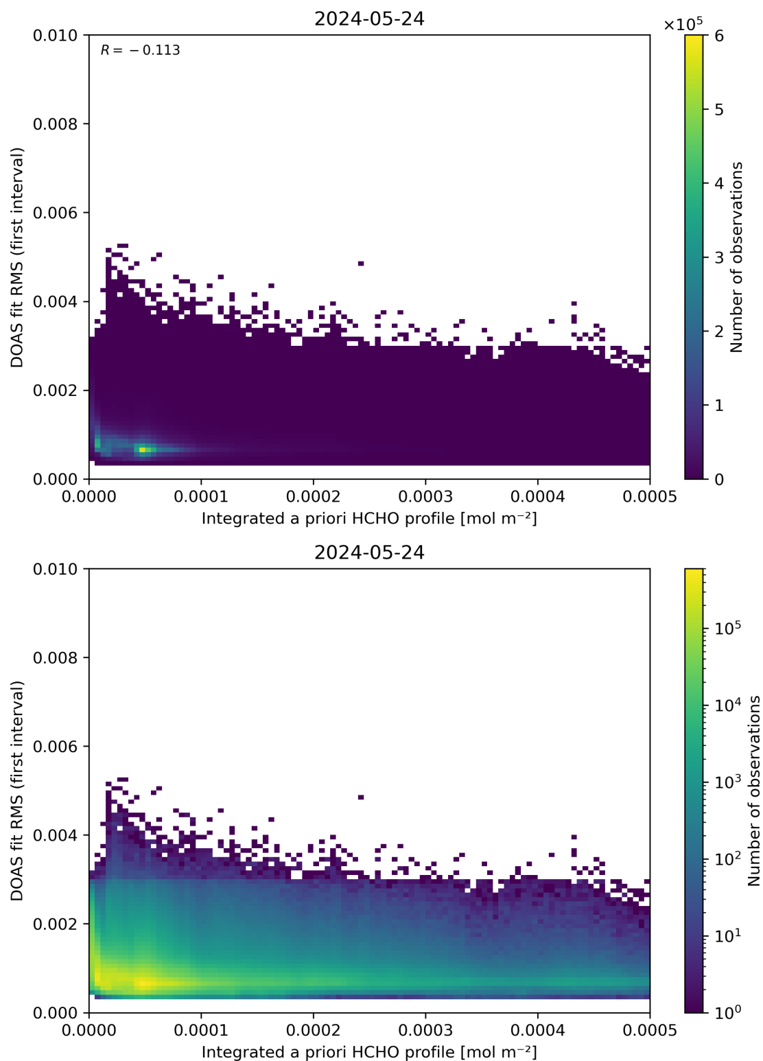
Figure 148: Scatter density plot of “Integrated a priori HCHO profile” against “DOAS fit RMS (first interval)” for 2024-05-23 to 2024-05-25.
