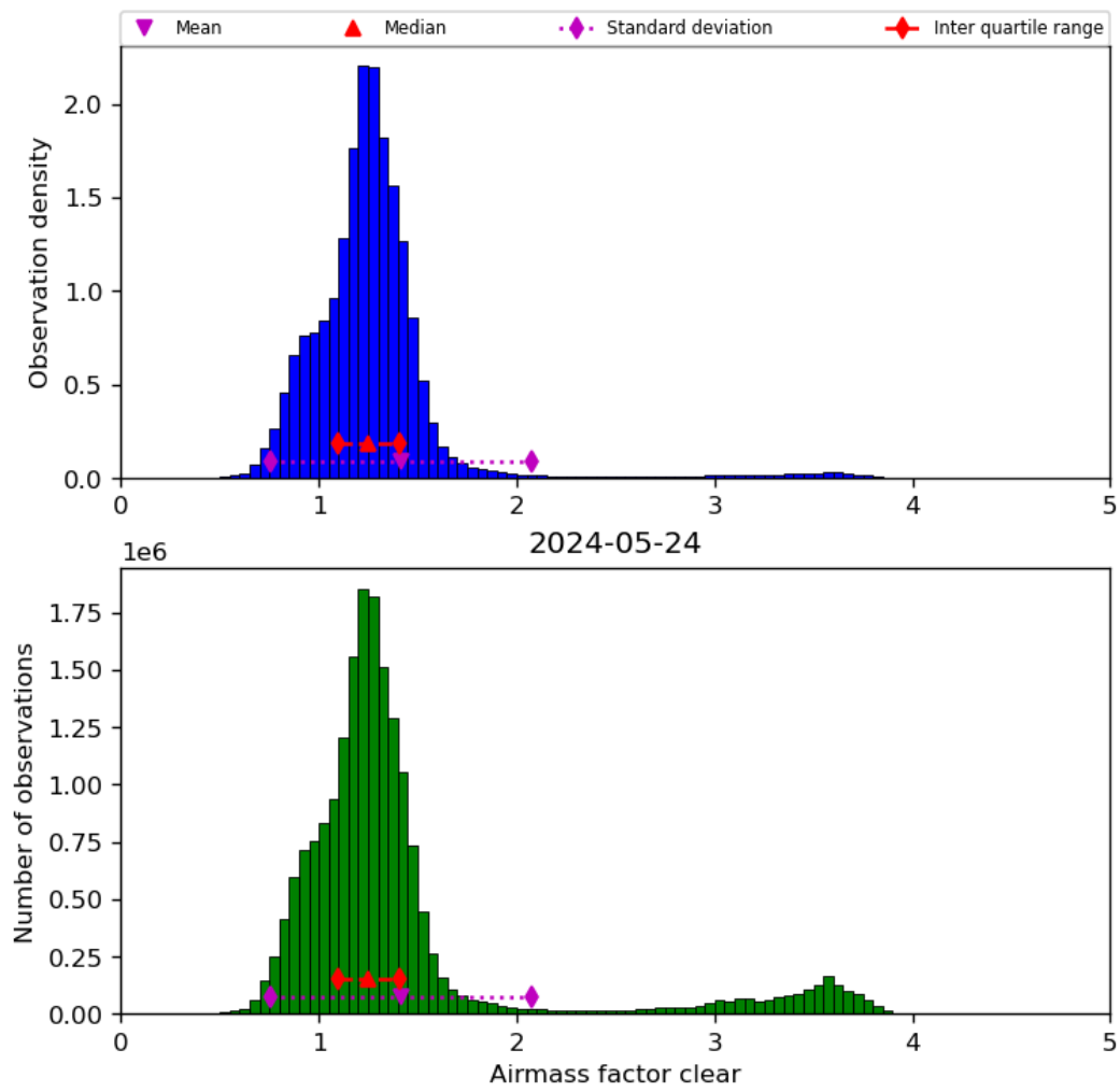
Figure 42: Histogram of “Airmass factor clear” for 2024-05-23 to 2024-05-25
