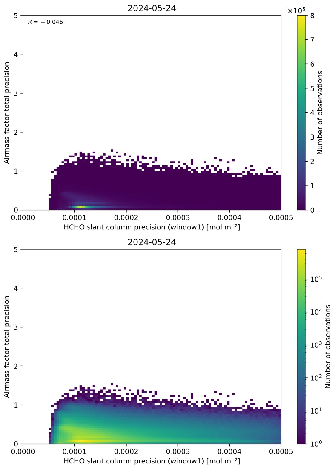
Figure 95: Scatter density plot of “HCHO slant column precision (window1)” against “Airmass factor total precision” for 2024-05-23 to 2024-05-25.
