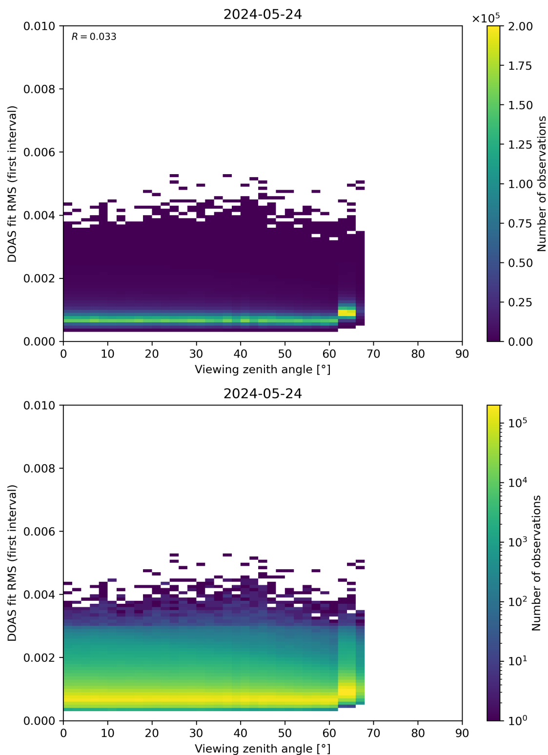
Figure 182: Scatter density plot of “Viewing zenith angle” against “DOAS fit RMS (first interval)” for 2024-05-23 to 2024-05-25.
