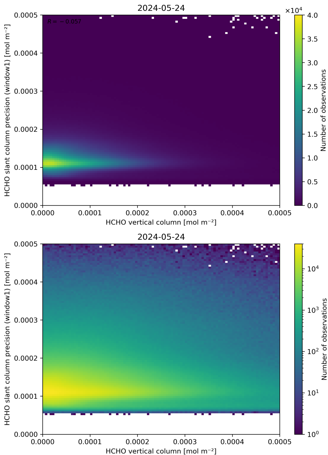
Figure 130: Scatter density plot of “HCHO vertical column” against “HCHO slant column precision (window1)” for 2024-05-23 to 2024-05-25.
