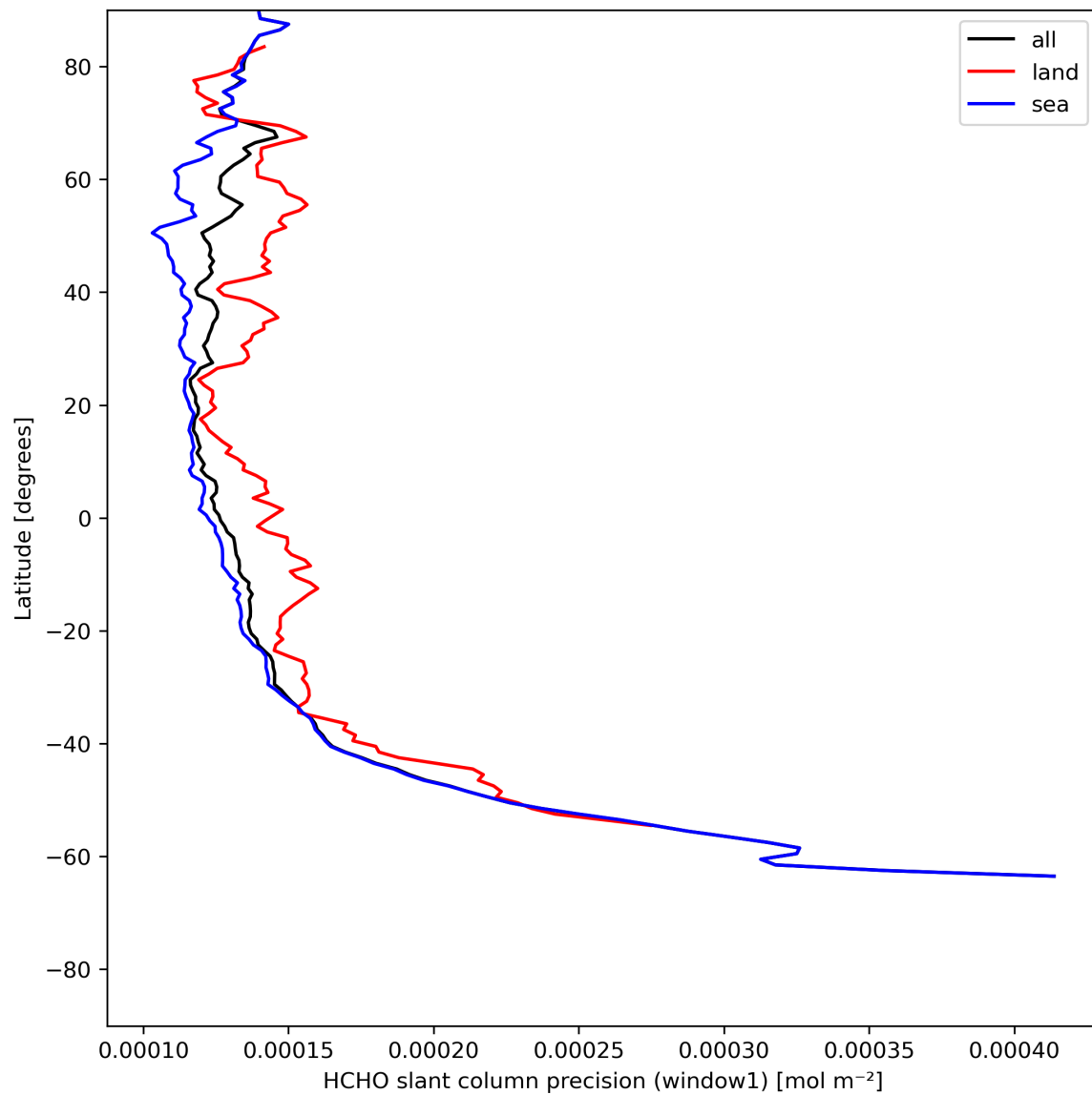
Figure 25: Zonal average of “HCHO slant column precision (window1)” for 2024-05-23 to 2024-05-25.
