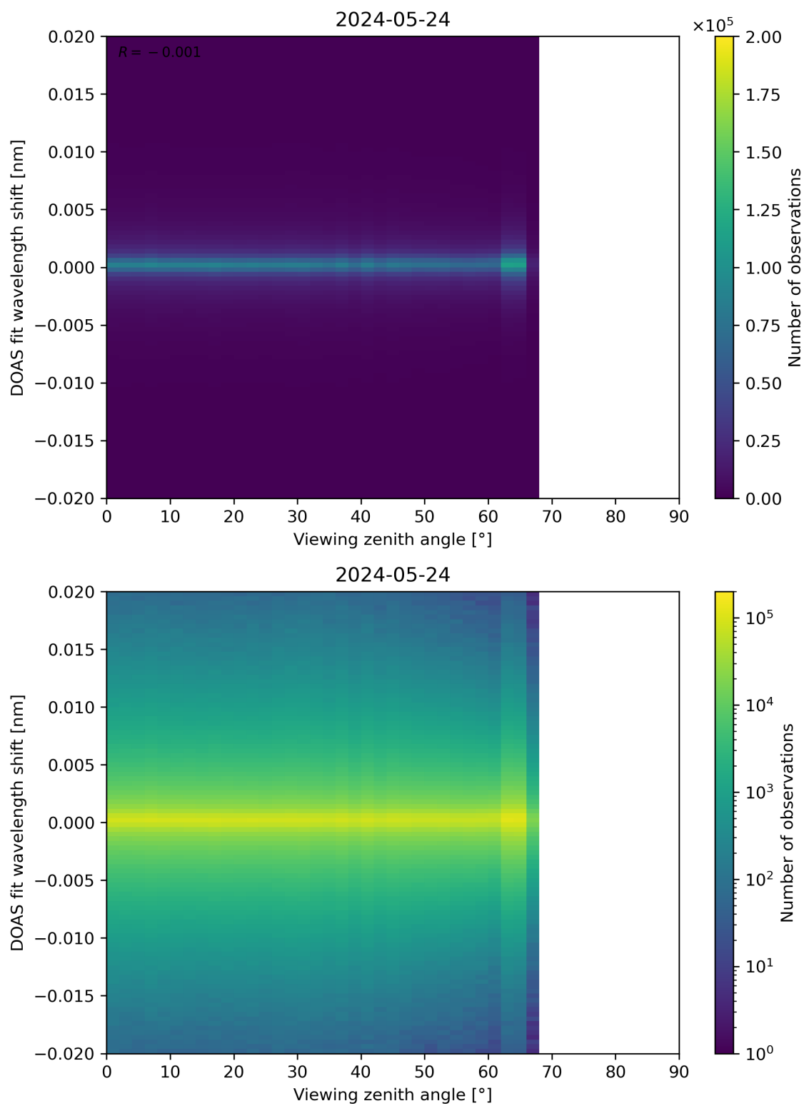
Figure 183: Scatter density plot of “Viewing zenith angle” against “DOAS fit wavelength shift” for 2024-05-23 to 2024-05-25.
