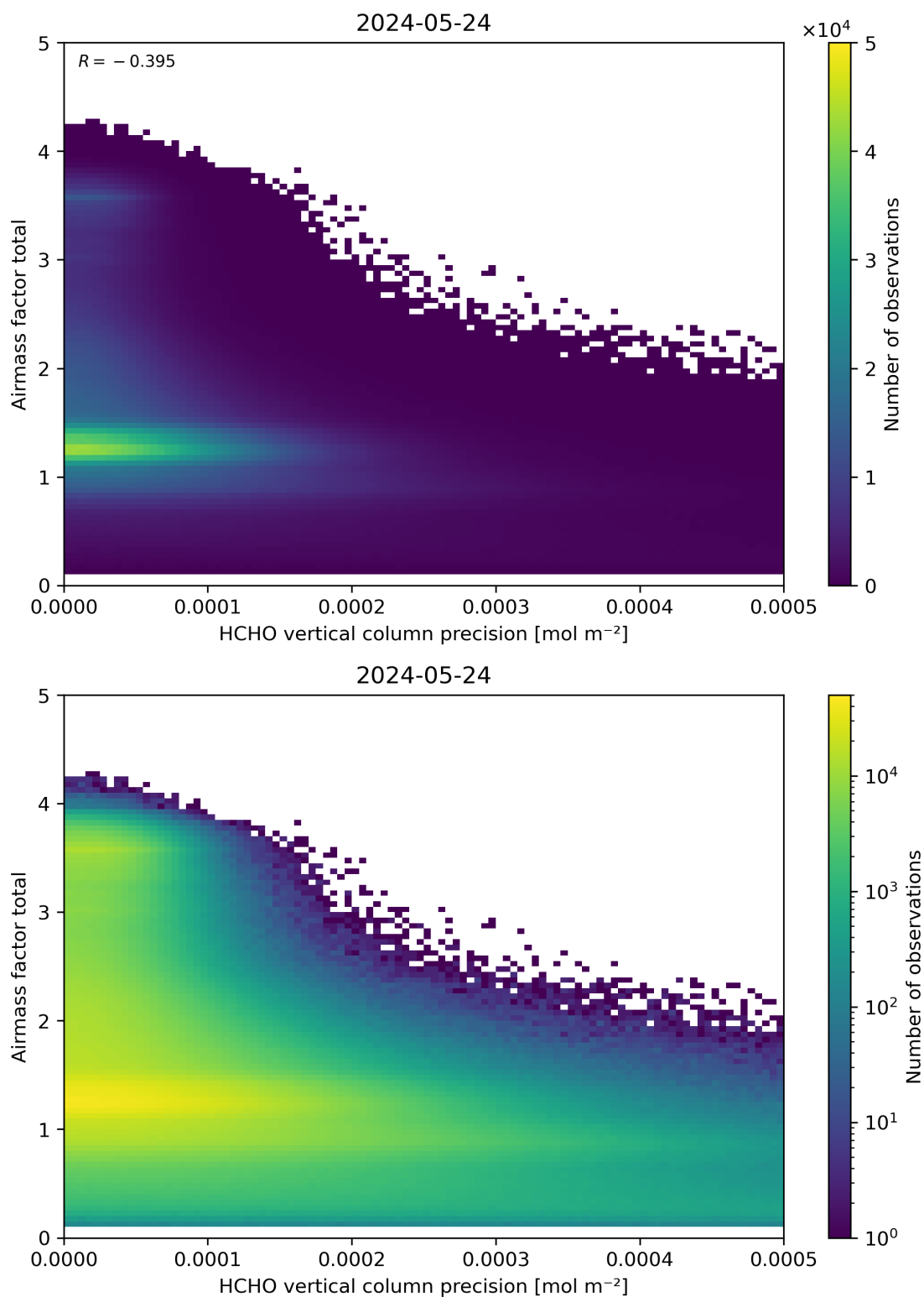
Figure 144: Scatter density plot of “HCHO vertical column precision” against “Airmass factor total” for 2024-05-23 to 2024-05-25.
