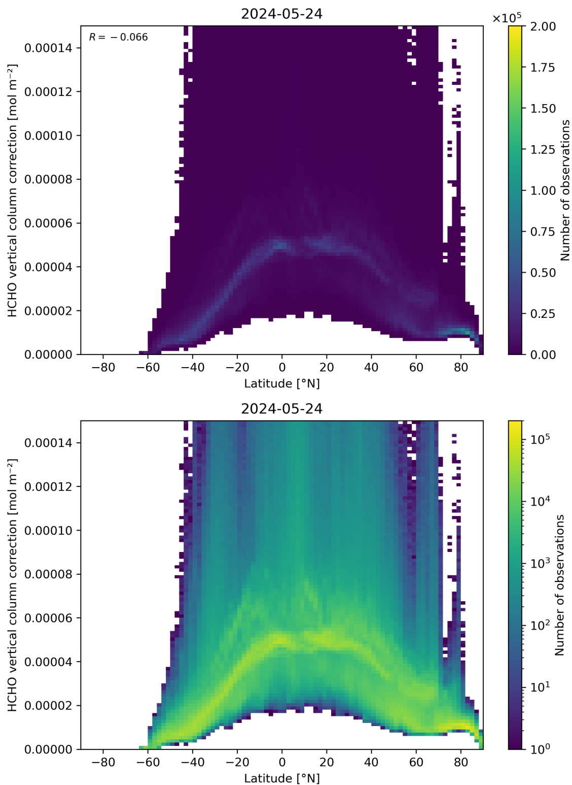
Figure 164: Scatter density plot of “Latitude” against “HCHO vertical column correction” for 2024-05-23 to 2024-05-25.
