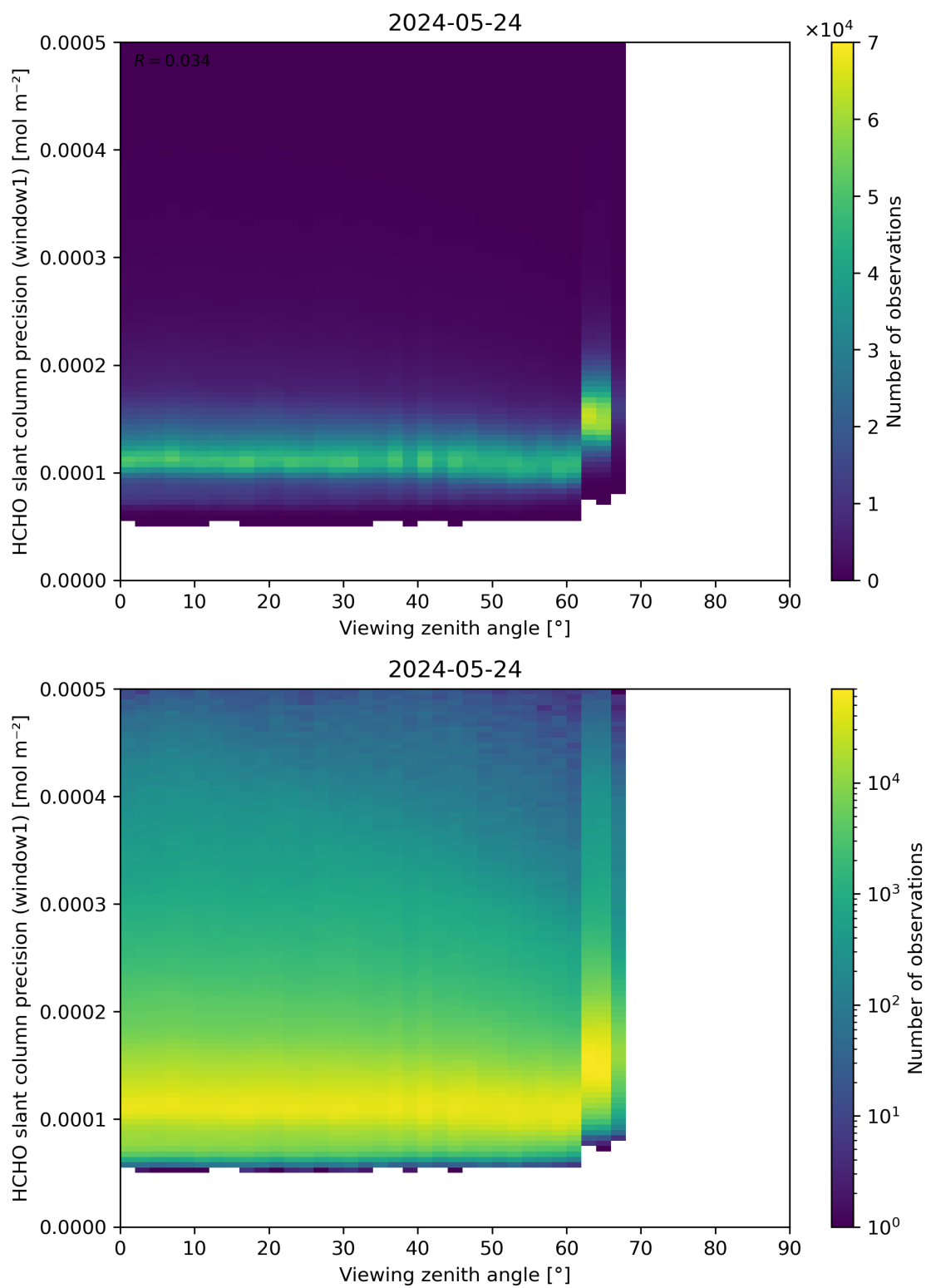
Figure 189: Scatter density plot of “Viewing zenith angle” against “HCHO slant column precision (window1)” for 2024-05-23 to 2024-05-25.
