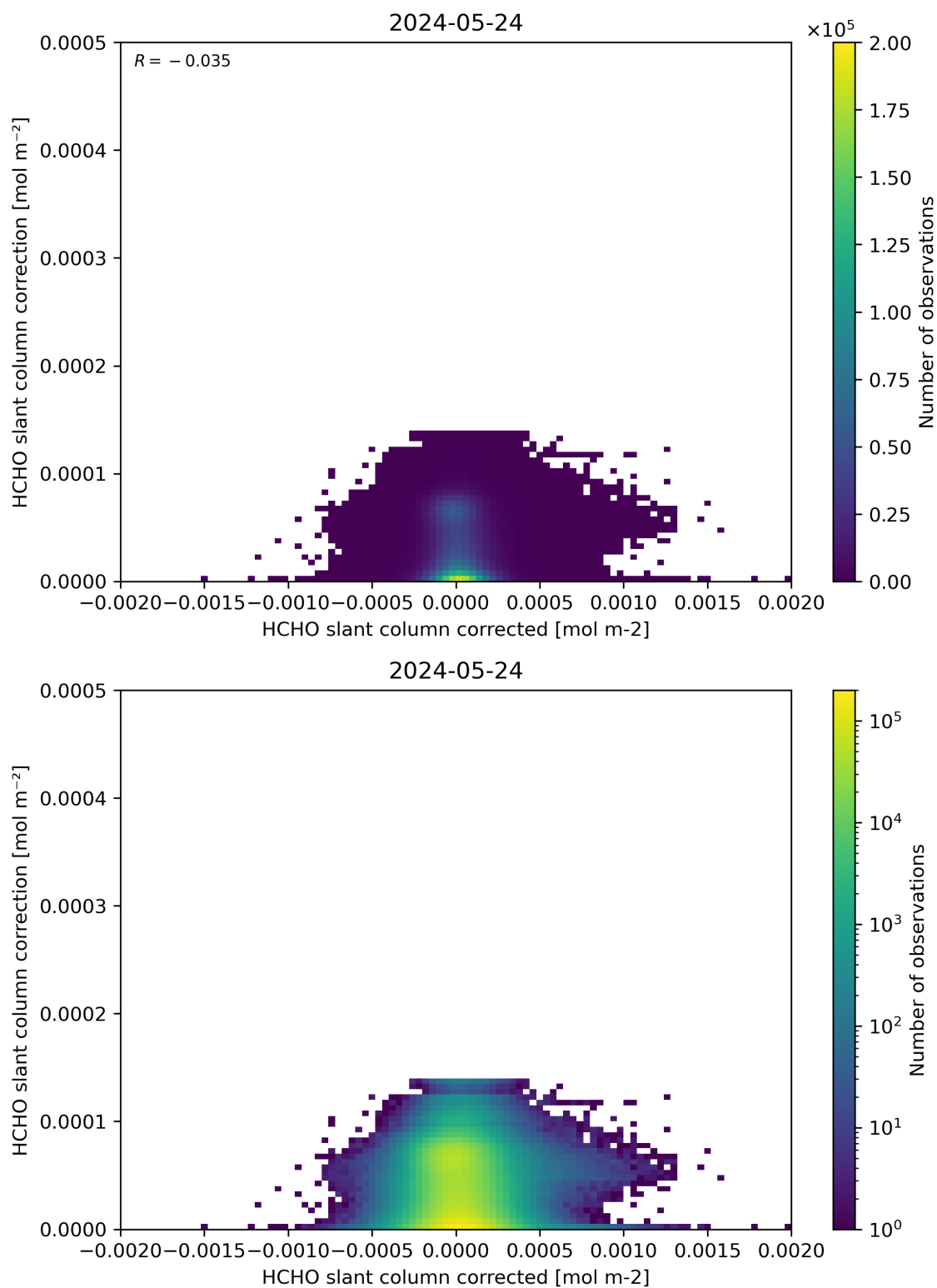
Figure 77: Scatter density plot of “HCHO slant column corrected” against “HCHO slant column correction” for 2024-05-23 to 2024-05-25.
