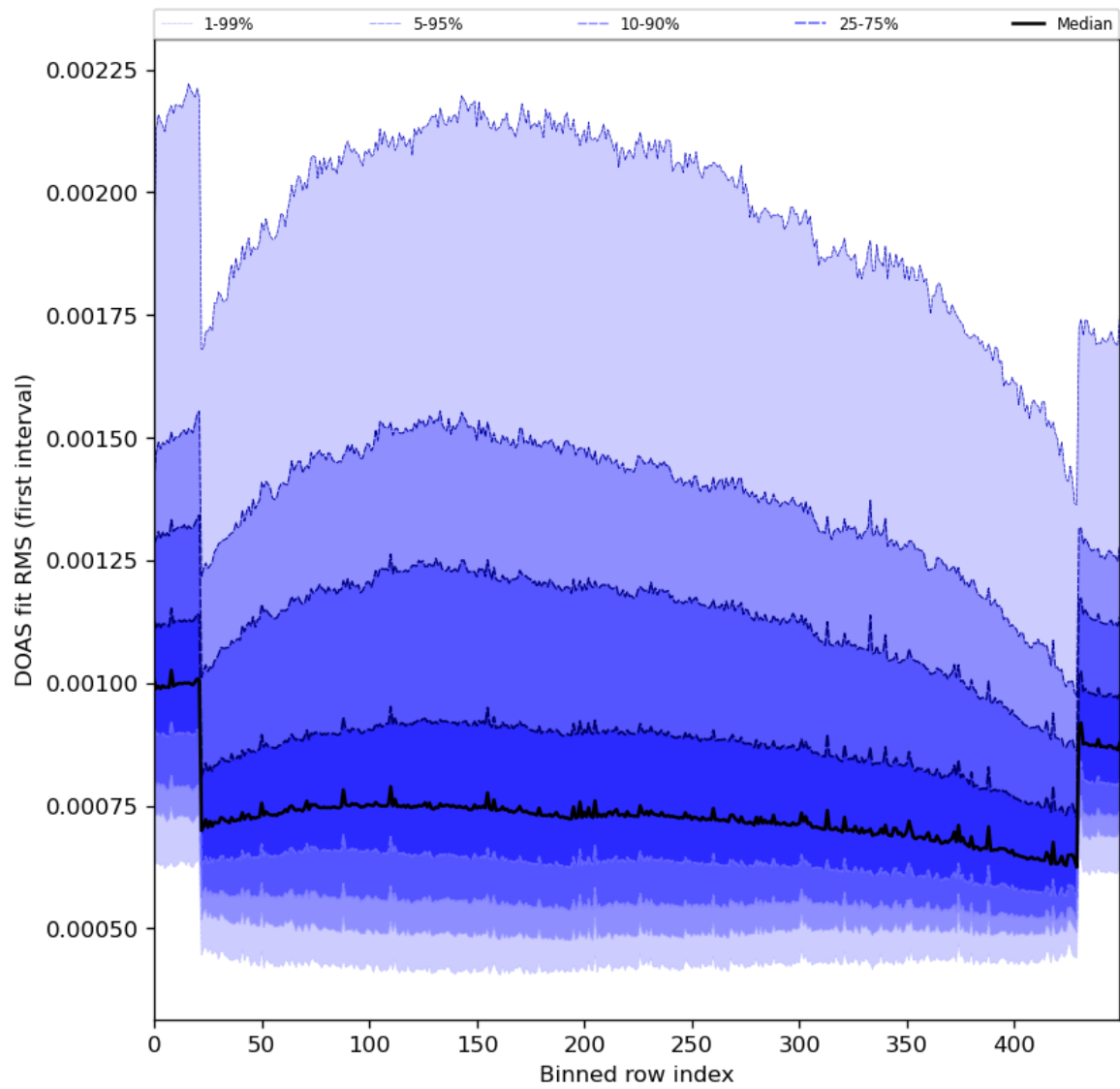
Figure 60: Along track statistics of “DOAS fit RMS (first interval)” for 2024-05-23 to 2024-05-25
