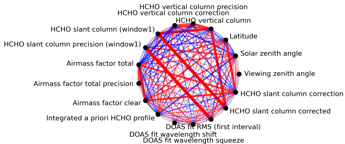
Figure 1: Map of correlation graph for 2024-05-23 to 2024-05-25.
