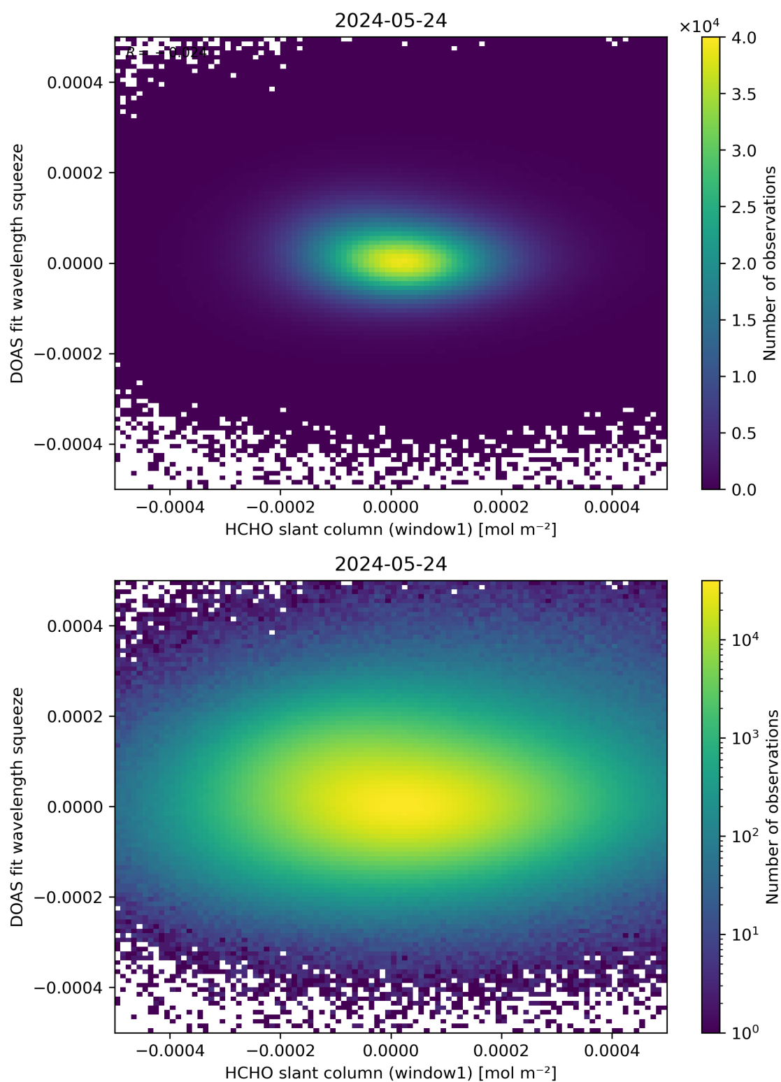
Figure 80: Scatter density plot of “HCHO slant column (window1)” against “DOAS fit wavelength squeeze” for 2024-05-23 to 2024-05-25.
