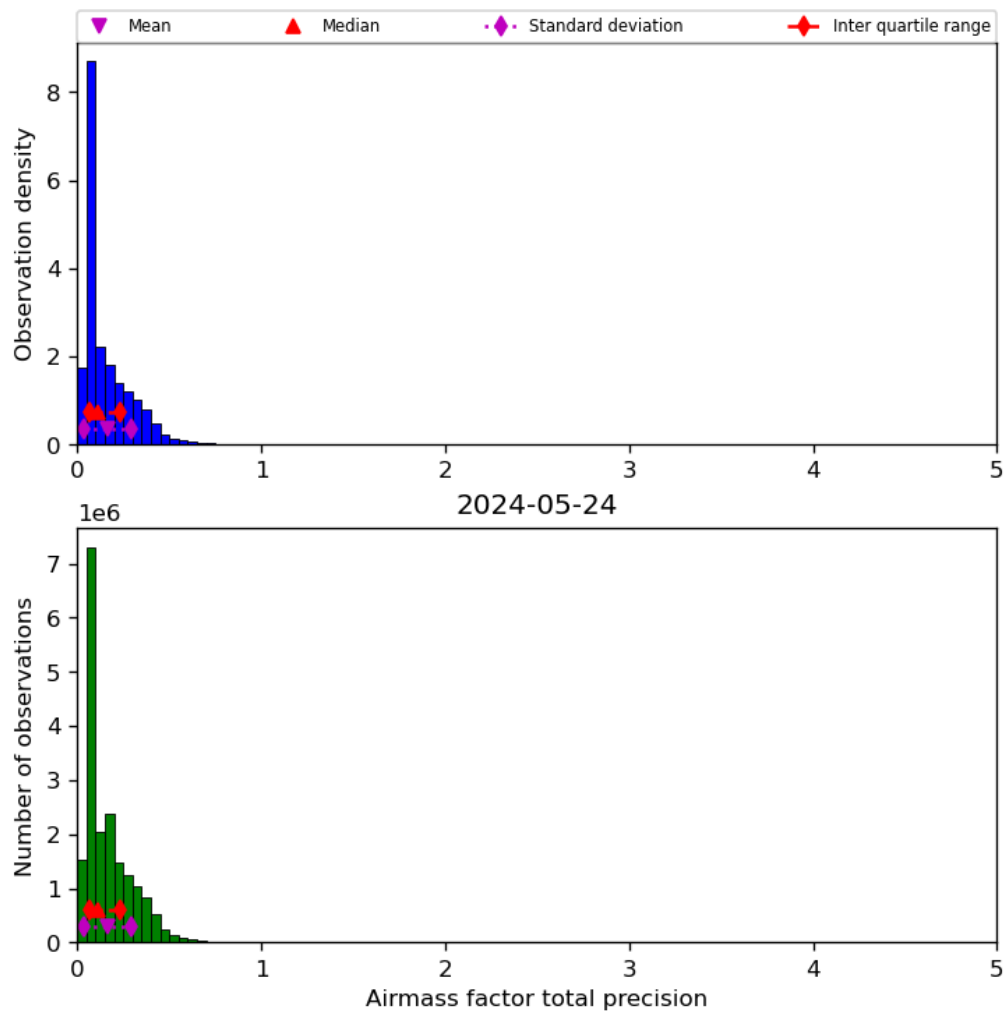
Figure 41: Histogram of "Airmass factor total precision" for 2024-05-23 to 2024-05-25
