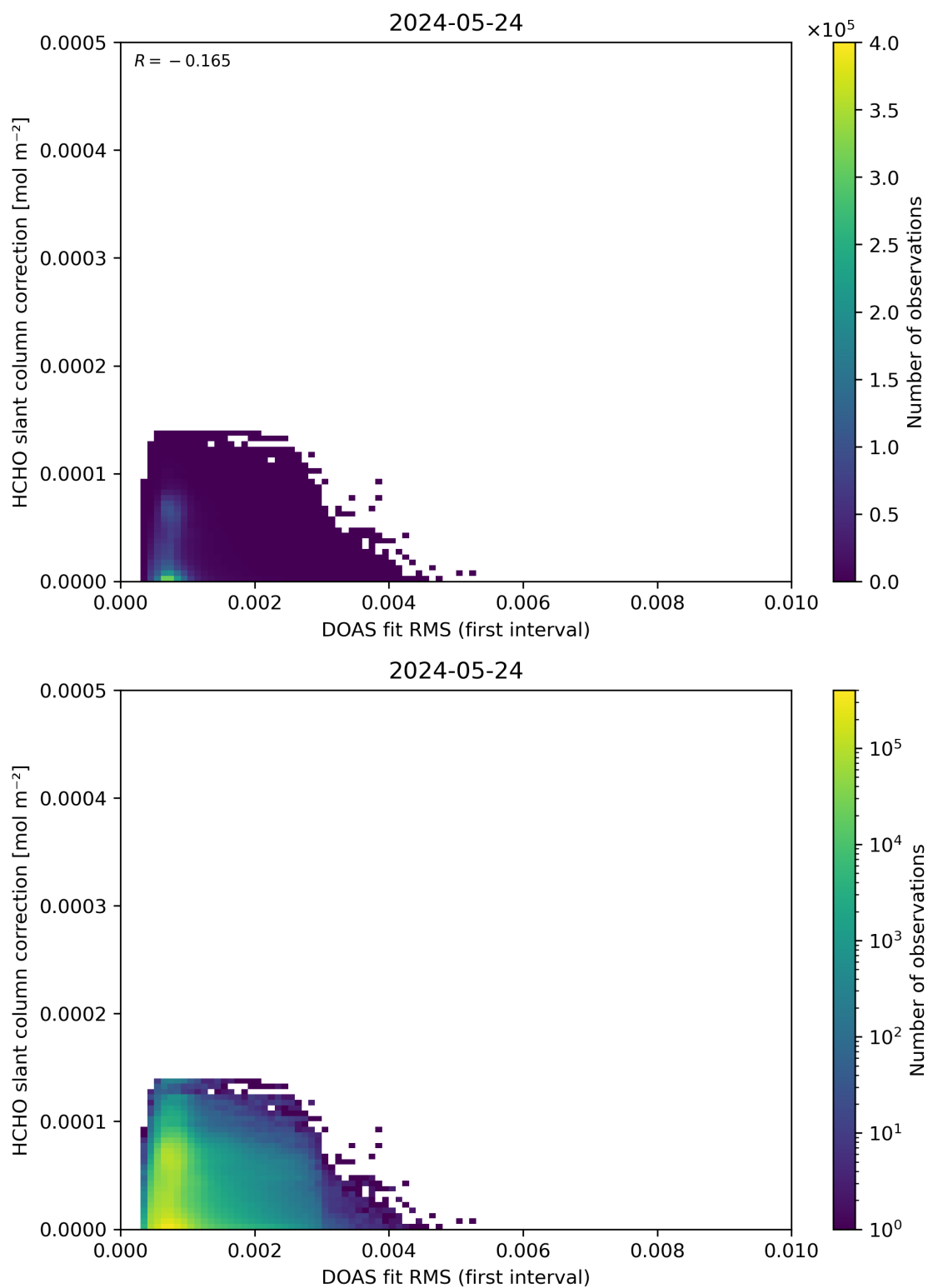
Figure 63: Scatter density plot of “DOAS fit RMS (first interval)” against “HCHO slant column correction” for 2024-05-23 to 2024-05-25.
