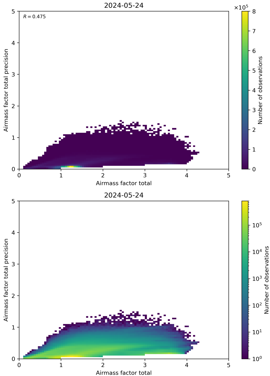
Figure 103: Scatter density plot of “Airmass factor total” against “Airmass factor total precision” for 2024-05-23 to 2024-05-25.
