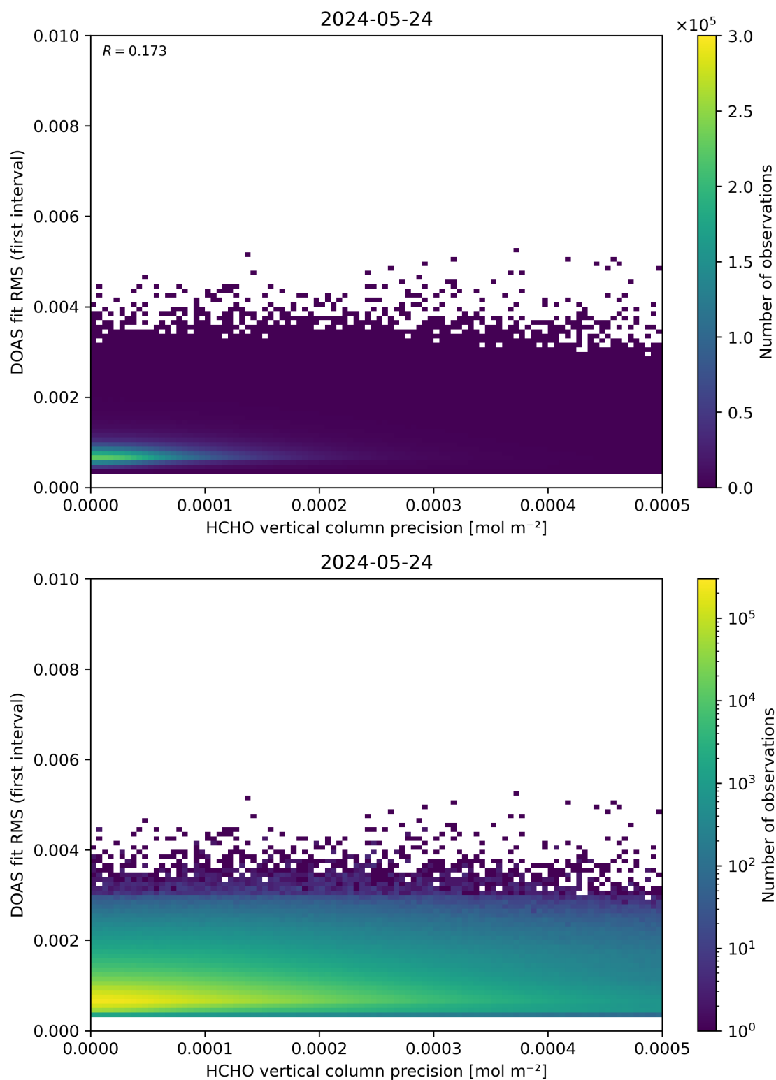
Figure 136: Scatter density plot of “HCHO vertical column precision” against “DOAS fit RMS (first interval)” for 2024-05-23 to 2024-05-25.
