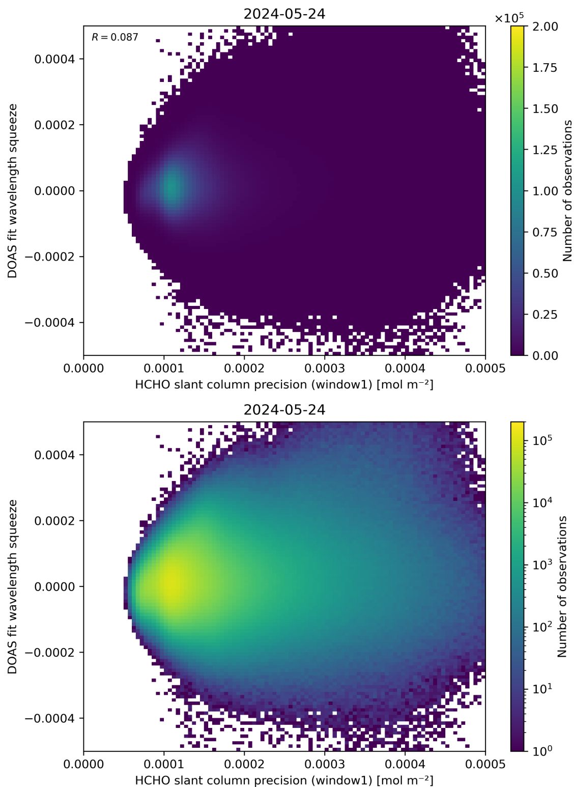
Figure 90: Scatter density plot of “HCHO slant column precision (window1)” against “DOAS fit wavelength squeeze” for 2024-05-23 to 2024-05-25.
