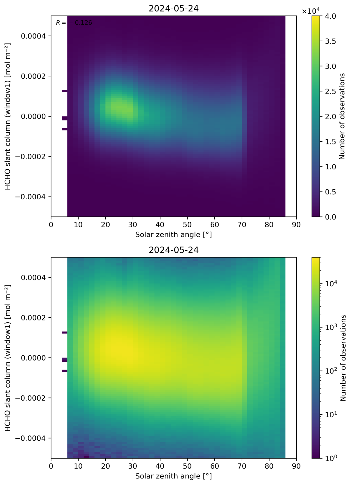
Figure 173: Scatter density plot of “Solar zenith angle” against “HCHO slant column (window1)” for 2024-05-23 to 2024-05-25.
