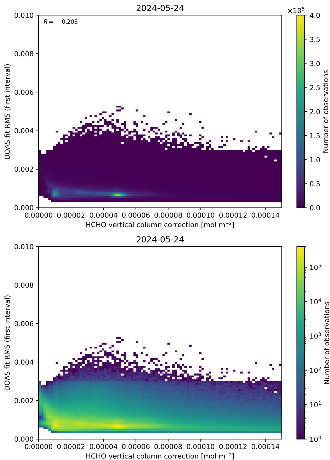
Figure 112: Scatter density plot of “HCHO vertical column correction” against “DOAS fit RMS (first interval)” for 2024-05-23 to 2024-05-25.
