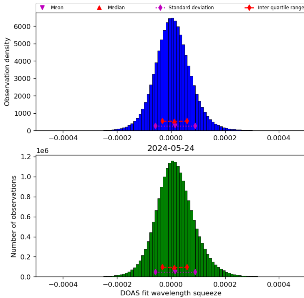
Figure 45: Histogram of “DOAS fit wavelength squeeze” for 2024-05-23 to 2024-05-25
