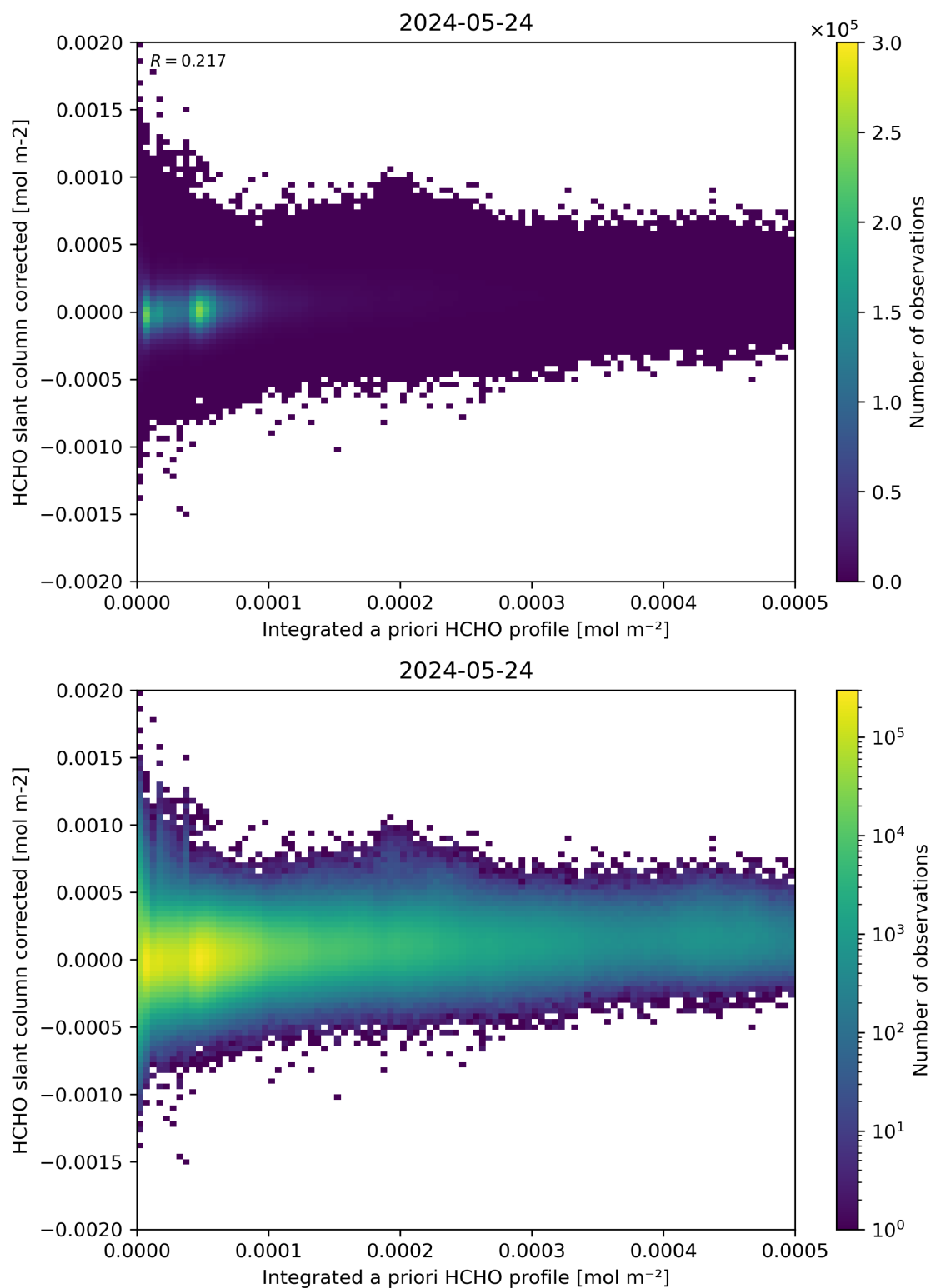
Figure 151: Scatter density plot of “Integrated a priori HCHO profile” against “HCHO slant column corrected” for 2024-05-23 to 2024-05-25.
