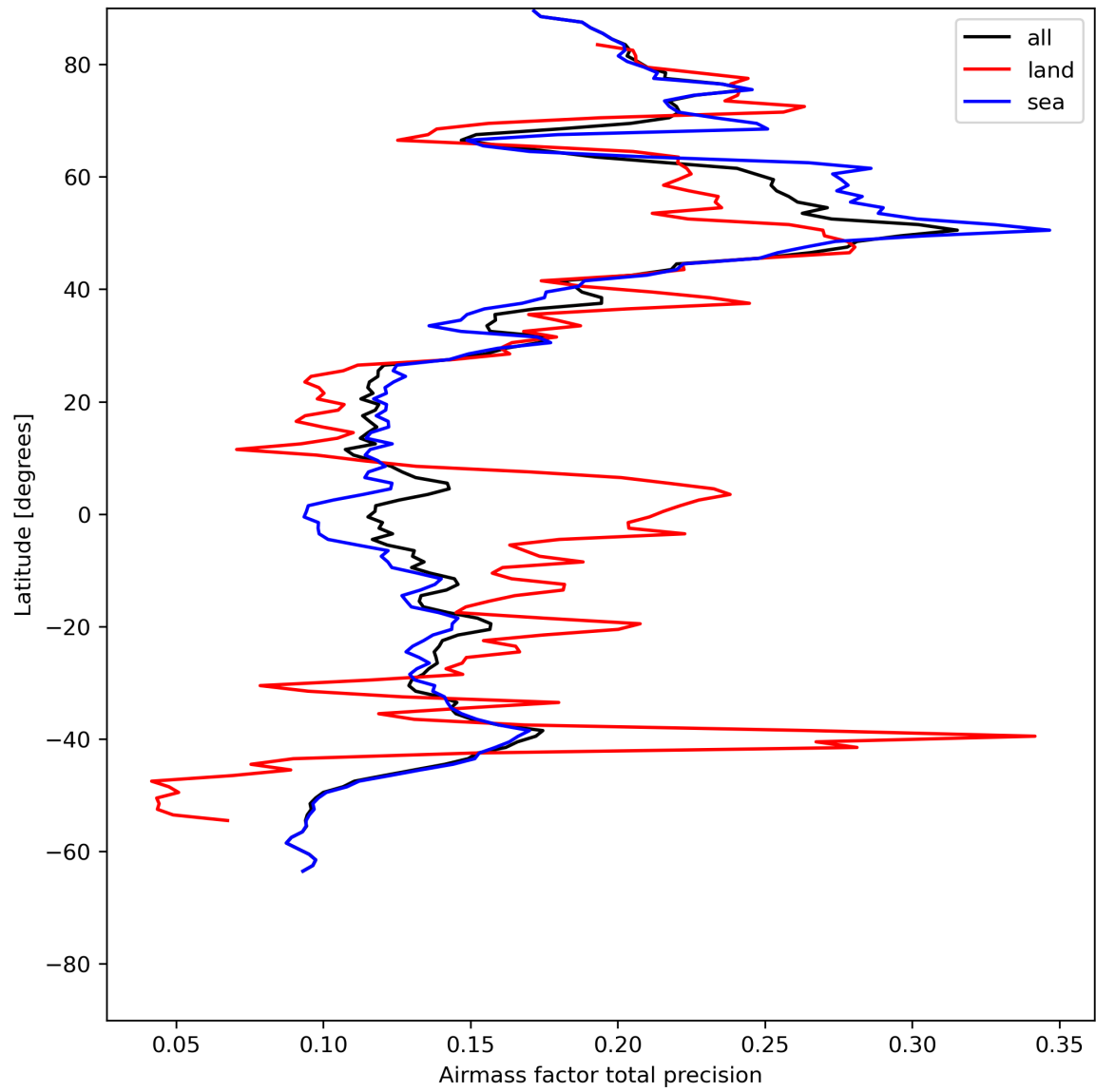
Figure 27: Zonal average of “Airmass factor total precision” for 2024-05-23 to 2024-05-25.
