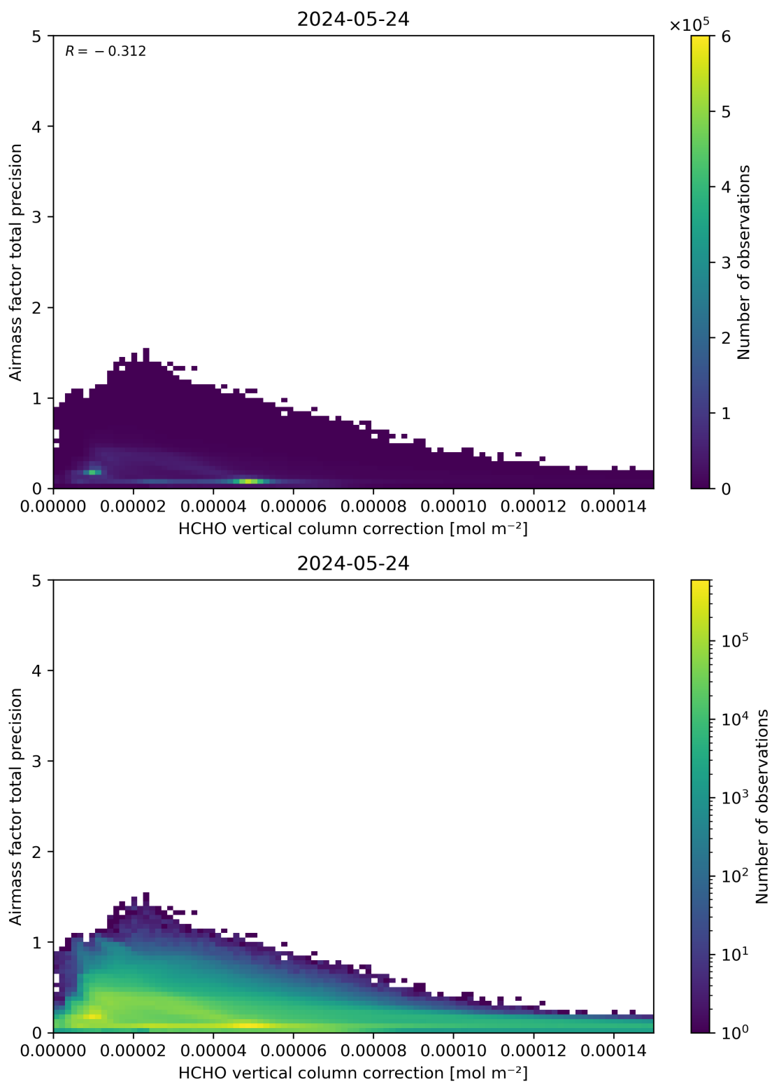
Figure 121: Scatter density plot of “HCHO vertical column correction” against “Airmass factor total precision” for 2024-05-23 to 2024-05-25.
