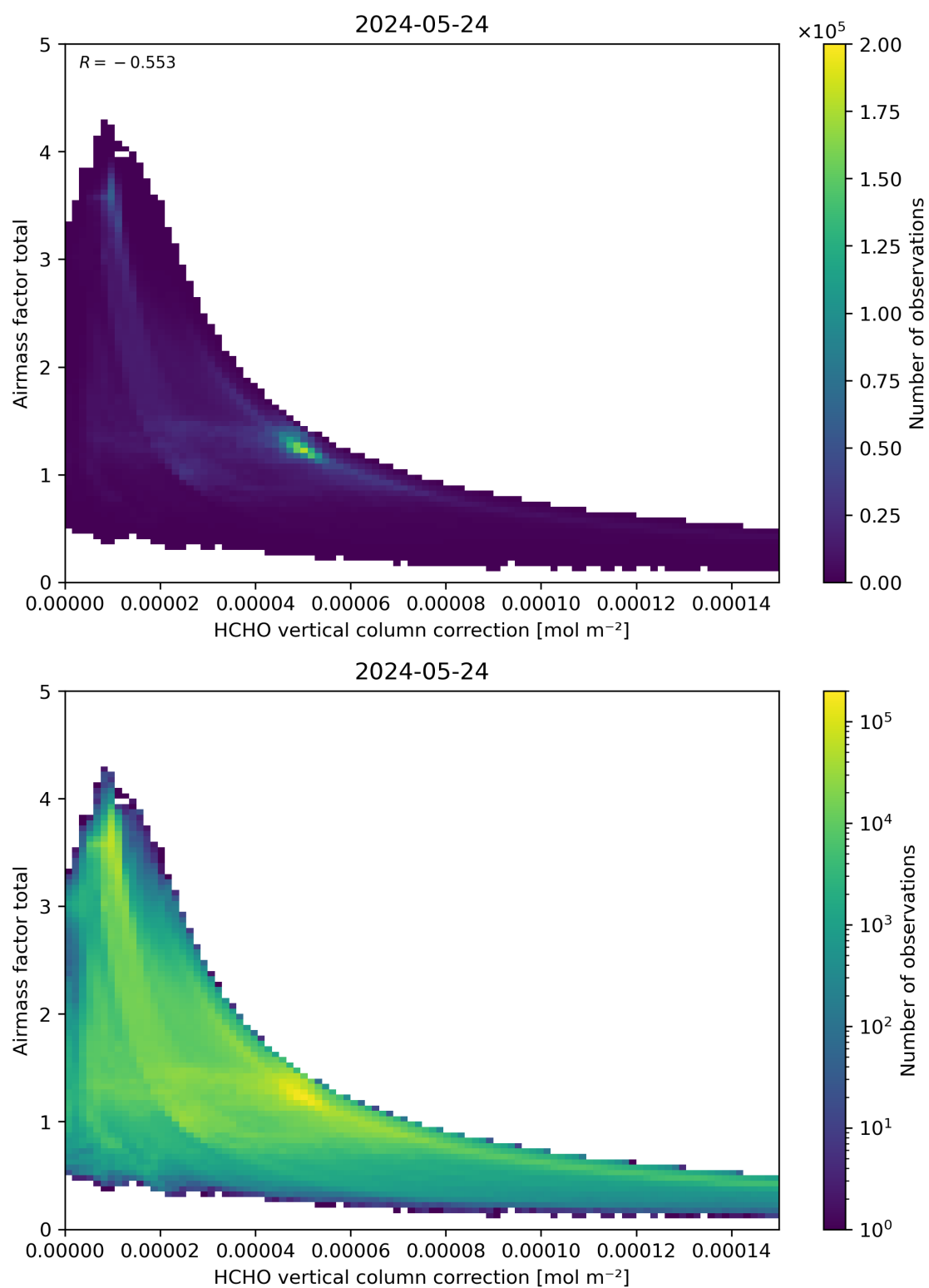
Figure 120: Scatter density plot of “HCHO vertical column correction” against “Airmass factor total” for 2024-05-23 to 2024-05-25.
