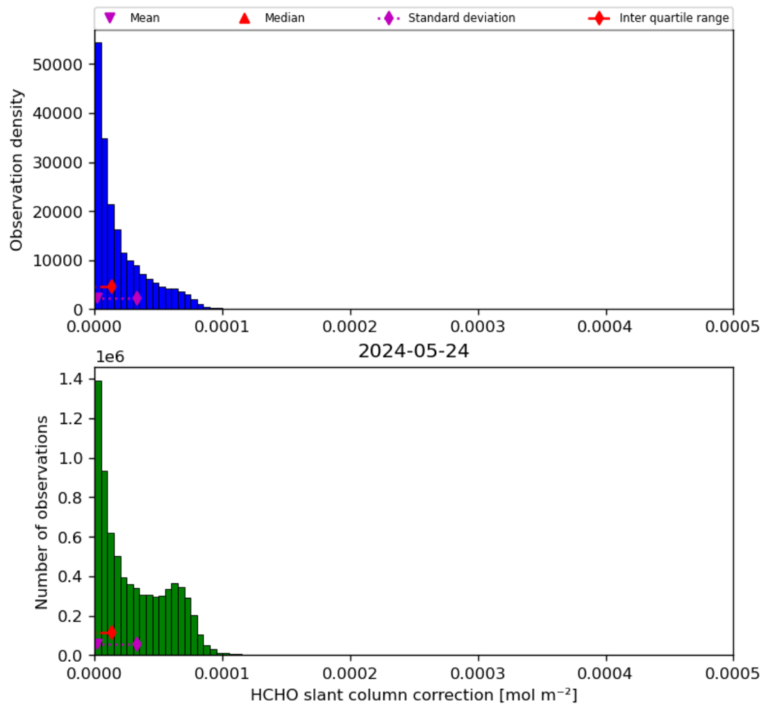
Figure 47: Histogram of “HCHO slant column correction” for 2024-05-23 to 2024-05-25
