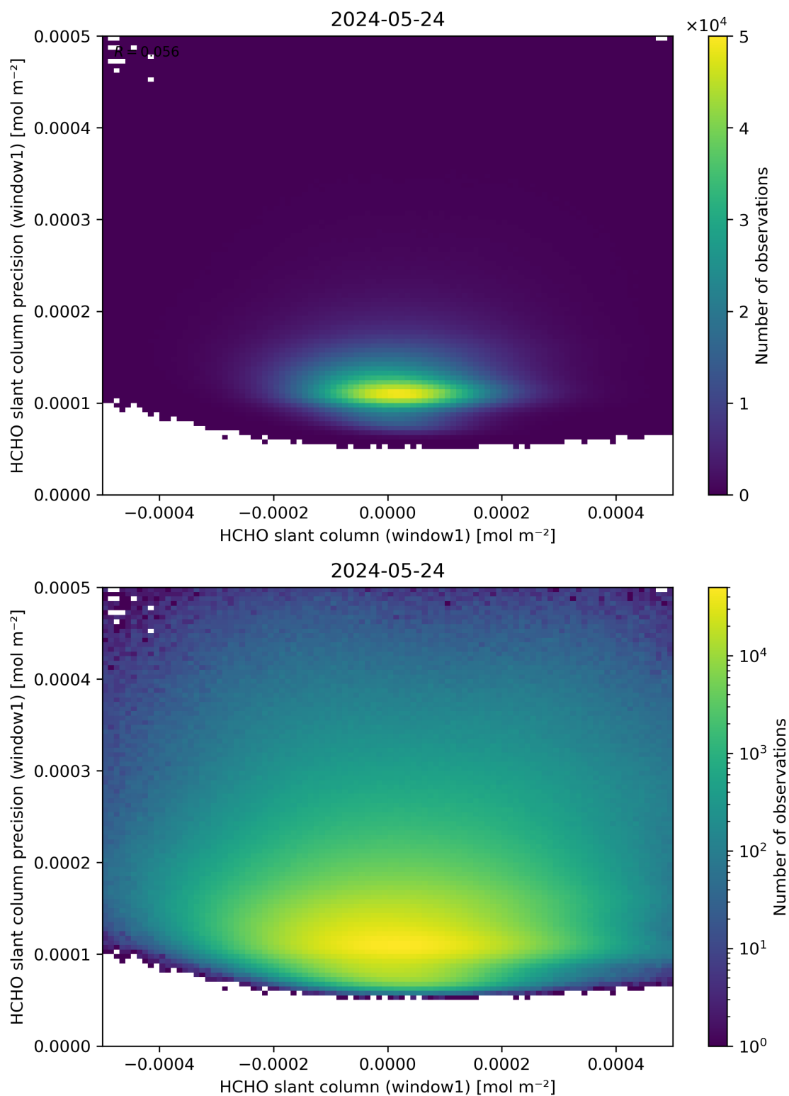
Figure 84: Scatter density plot of “HCHO slant column (window1)” against “HCHO slant column precision (window1)” for 2024-05-23 to 2024-05-25.
