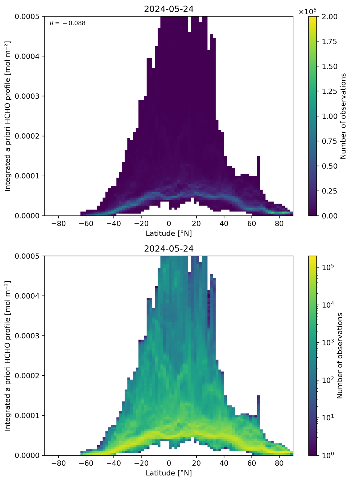
Figure 166: Scatter density plot of “Latitude” against “Integrated a priori HCHO profile” for 2024-05-23 to 2024-05-25.
