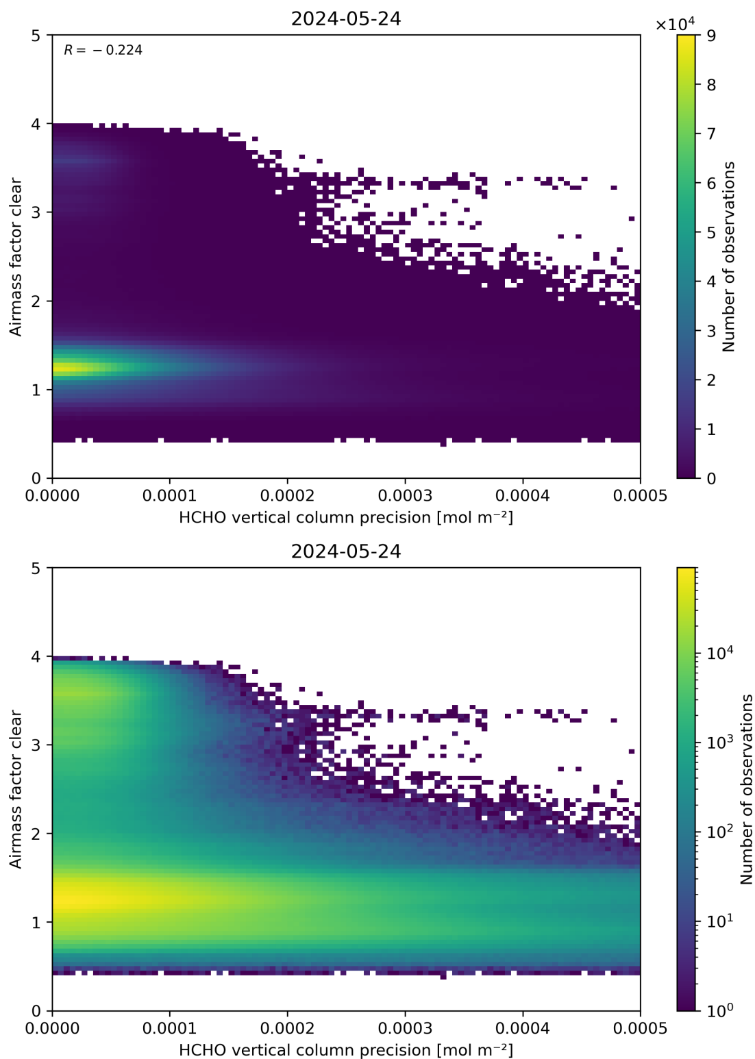
Figure 139: Scatter density plot of “HCHO vertical column precision” against “Airmass factor clear” for 2024-05-23 to 2024-05-25.
