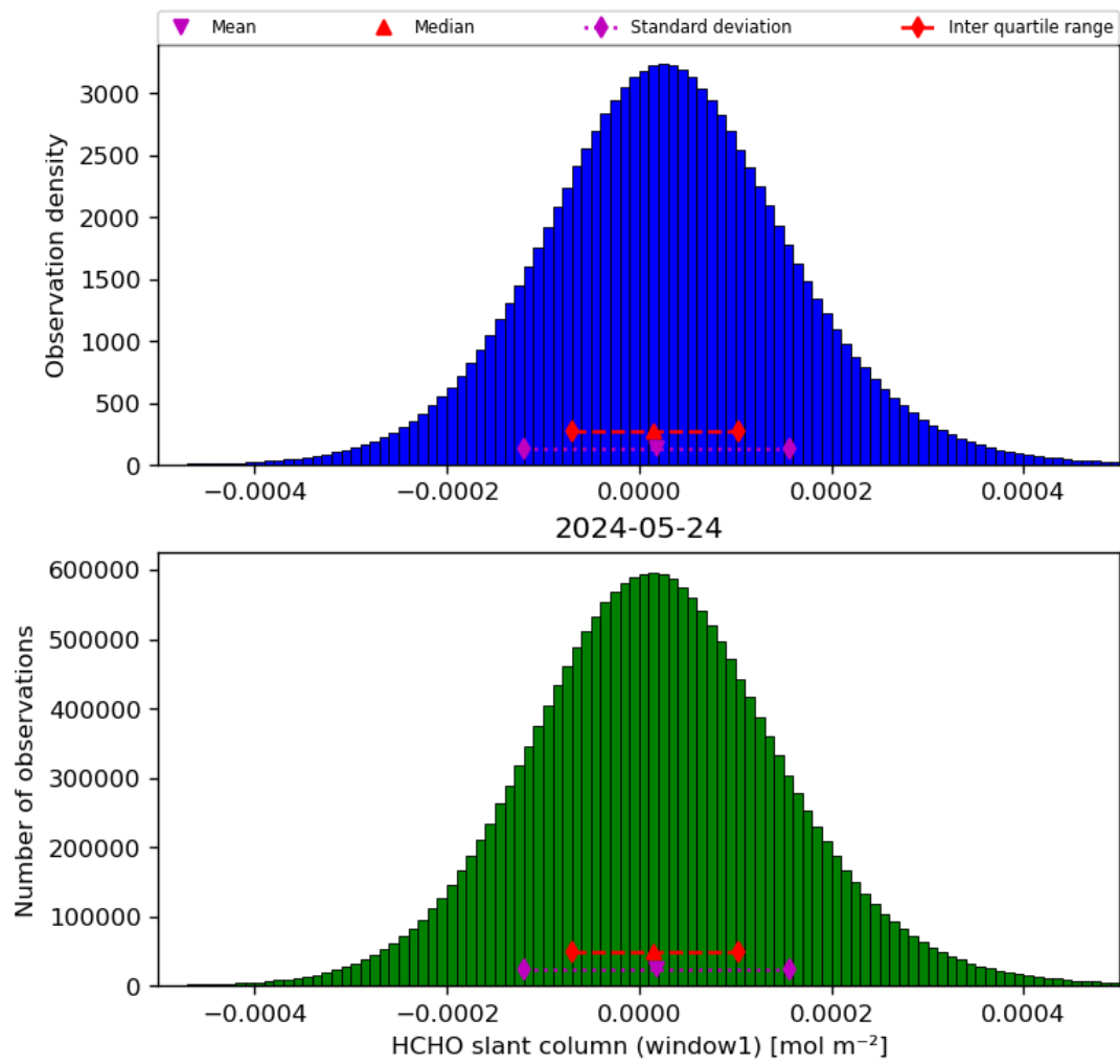
Figure 38: Histogram of “HCHO slant column (window1)” for 2024-05-23 to 2024-05-25
