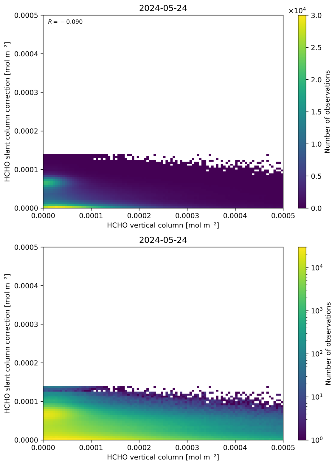
Figure 128: Scatter density plot of “HCHO vertical column” against “HCHO slant column correction” for 2024-05-23 to 2024-05-25.
