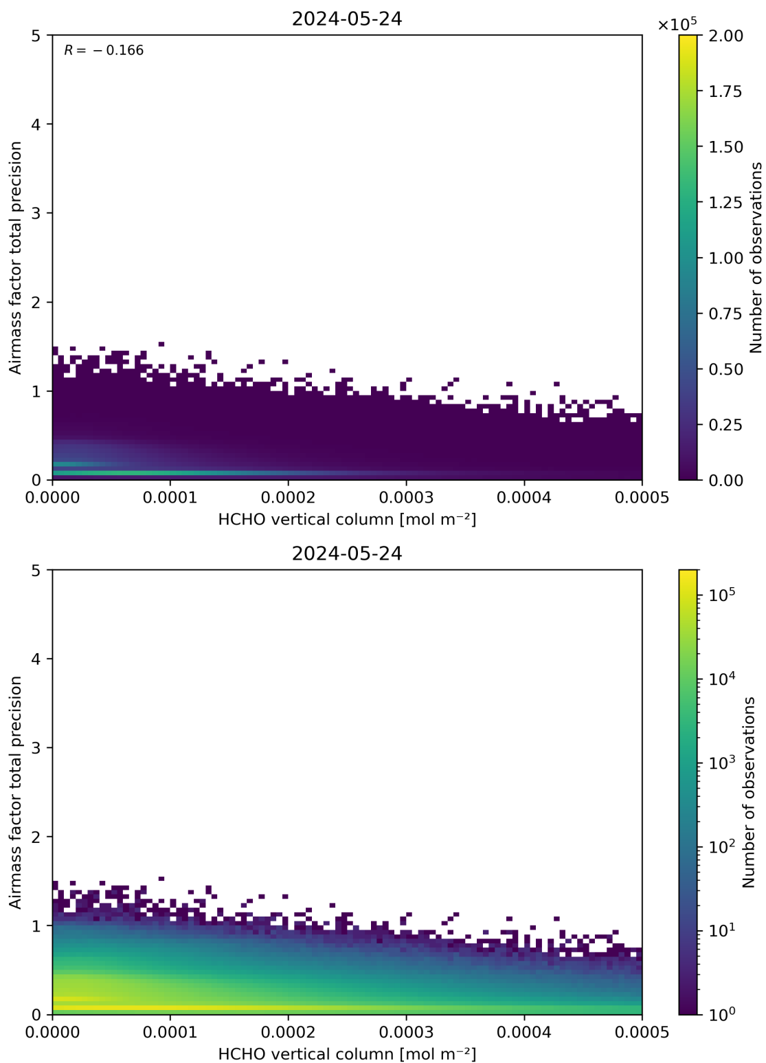
Figure 132: Scatter density plot of “HCHO vertical column” against “Airmass factor total precision” for 2024-05-23 to 2024-05-25.
