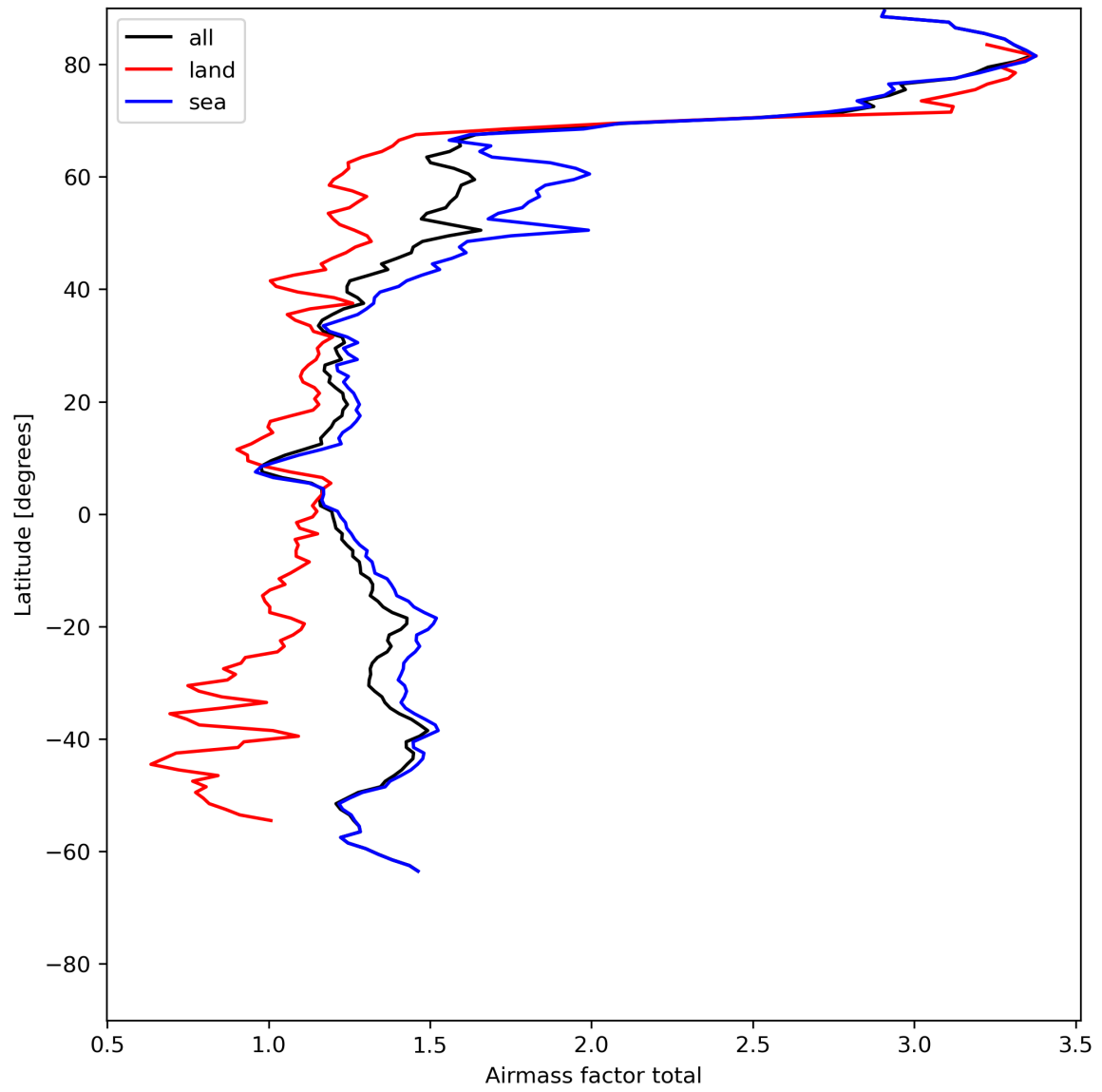
Figure 26: Zonal average of “Airmass factor total” for 2024-05-23 to 2024-05-25.
