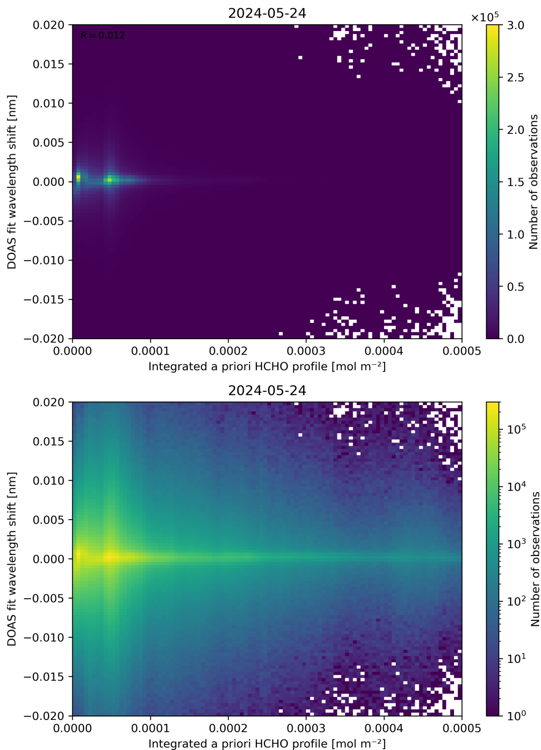
Figure 149: Scatter density plot of “Integrated a priori HCHO profile” against “DOAS fit wavelength shift” for 2024-05-23 to 2024-05-25.
