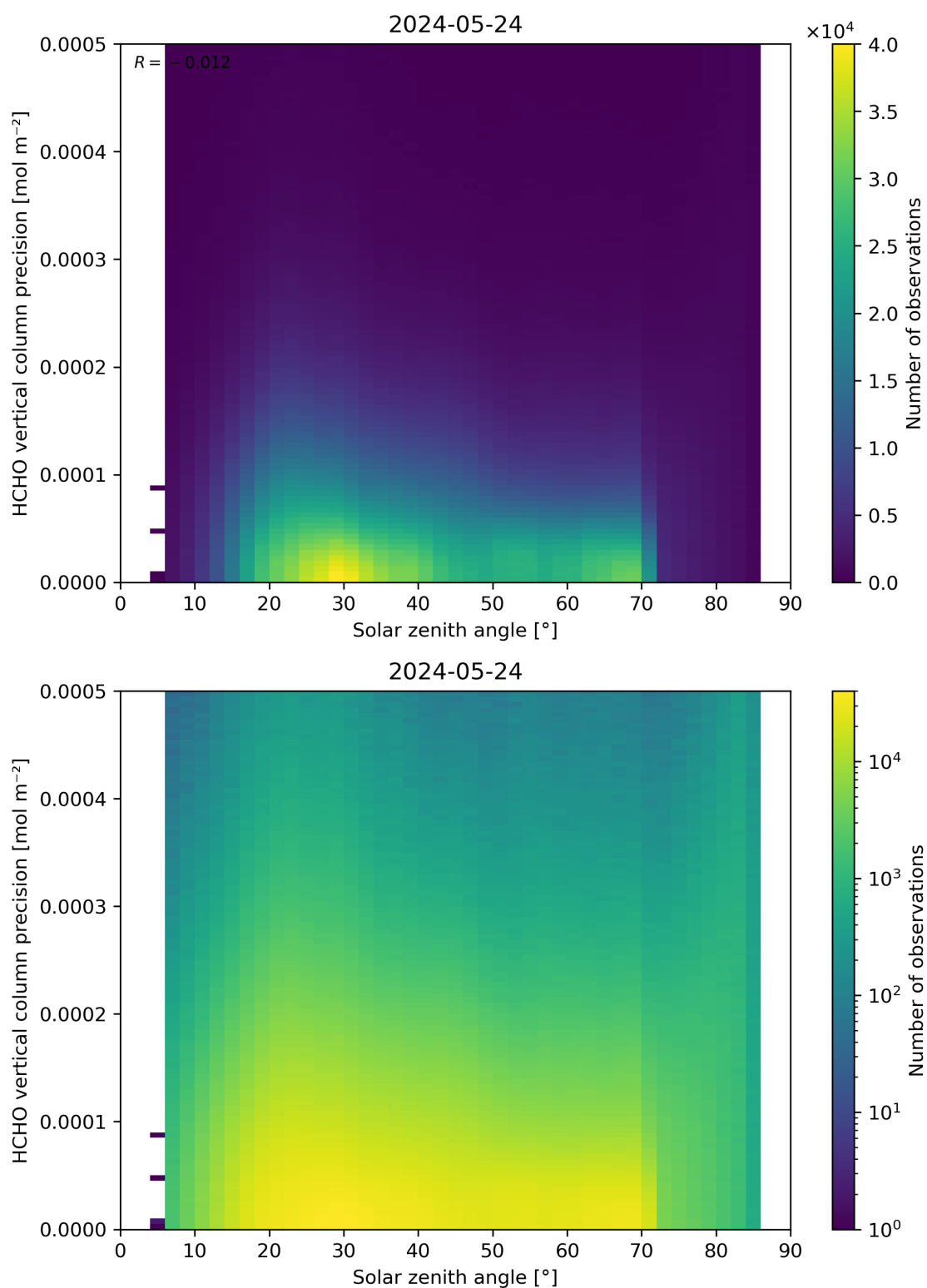
Figure 179: Scatter density plot of “Solar zenith angle” against “HCHO vertical column precision” for 2024-05-23 to 2024-05-25.
