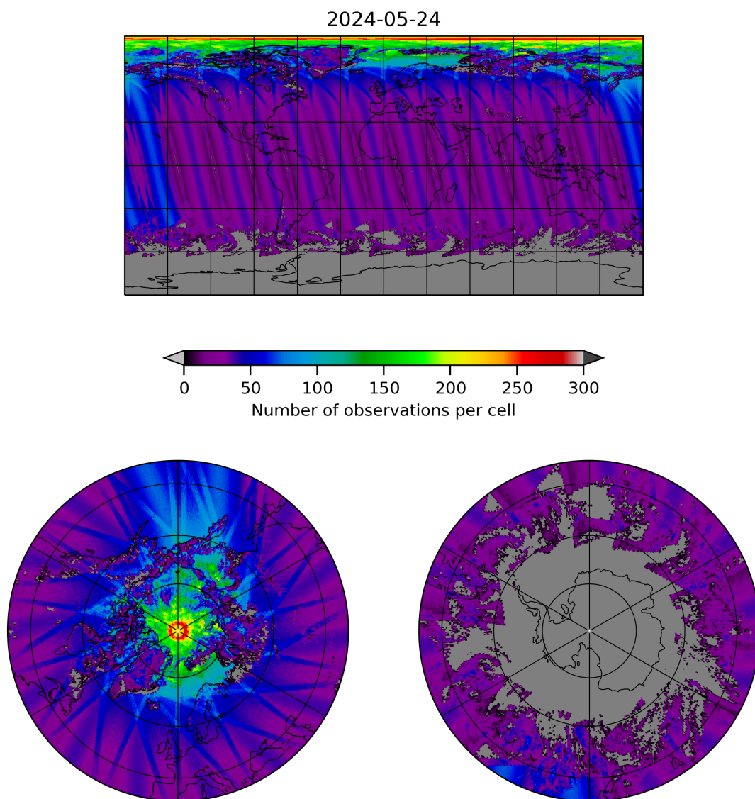
Figure 19: Map of the number of observations for 2024-05-23 to 2024-05-25
