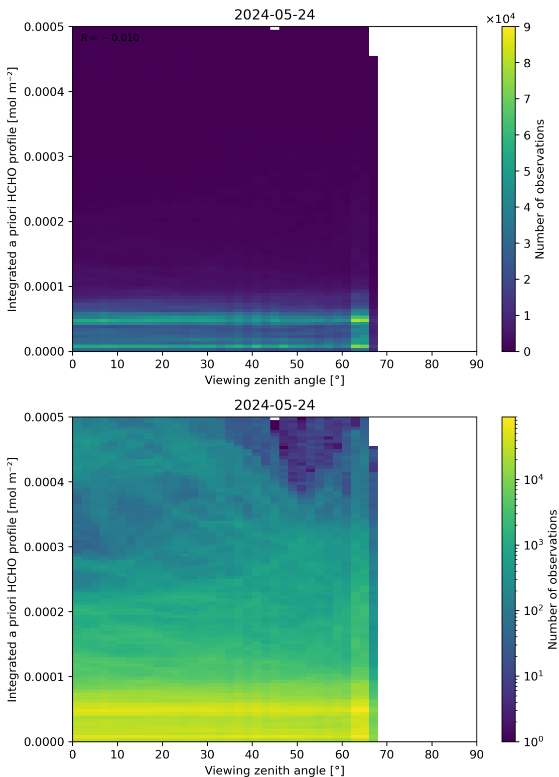
Figure 195: Scatter density plot of “Viewing zenith angle” against “Integrated a priori HCHO profile” for 2024-05-23 to 2024-05-25.
