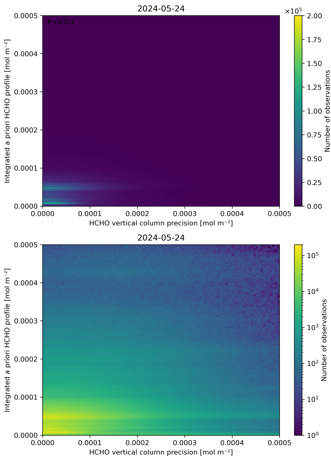
Figure 147: Scatter density plot of “HCHO vertical column precision” against “Integrated a priori HCHO profile” for 2024-05-23 to 2024-05-25.
