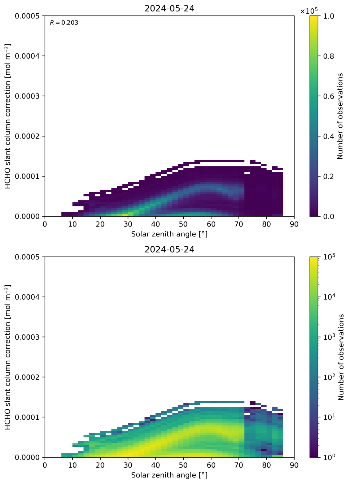
Figure 172: Scatter density plot of “Solar zenith angle” against “HCHO slant column correction” for 2024-05-23 to 2024-05-25.
