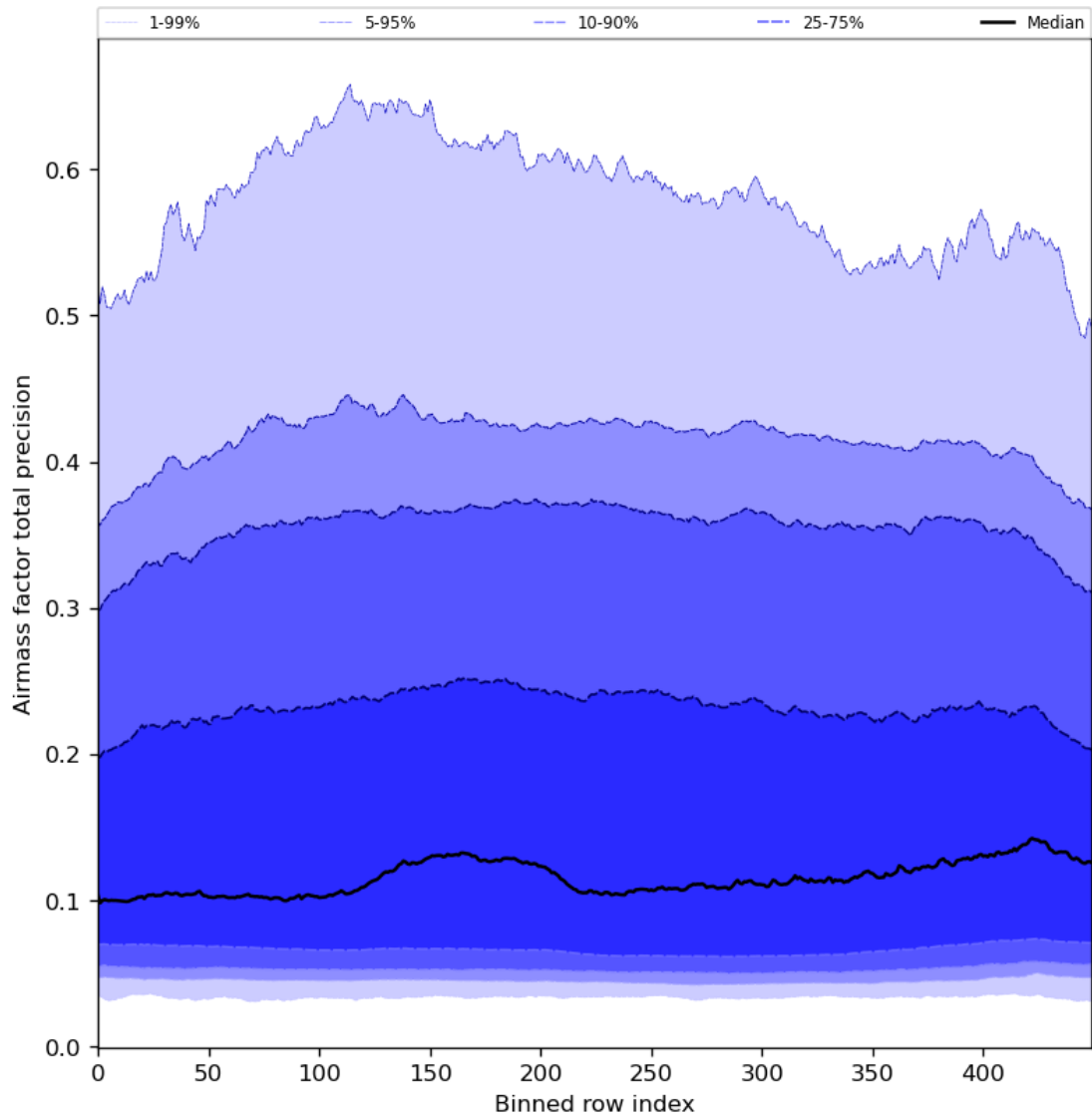
Figure 55: Along track statistics of “Airmass factor total precision” for 2024-05-23 to 2024-05-25
