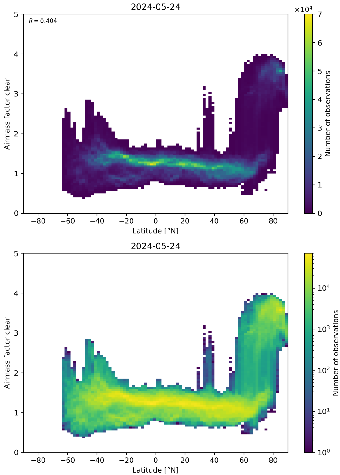
Figure 156: Scatter density plot of “Latitude” against “Airmass factor clear” for 2024-05-23 to 2024-05-25.
