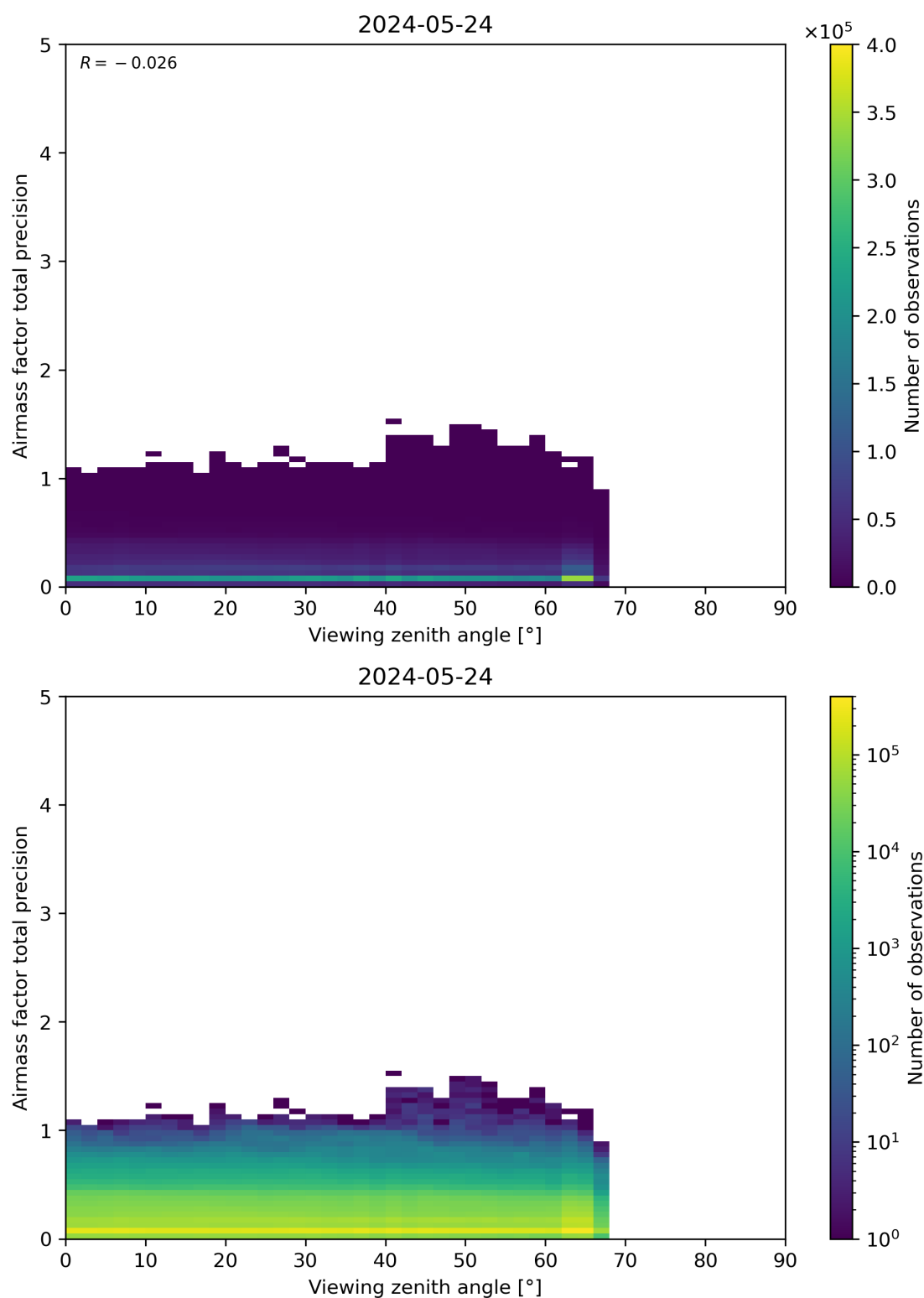
Figure 191: Scatter density plot of “Viewing zenith angle” against “Airmass factor total precision” for 2024-05-23 to 2024-05-25.
