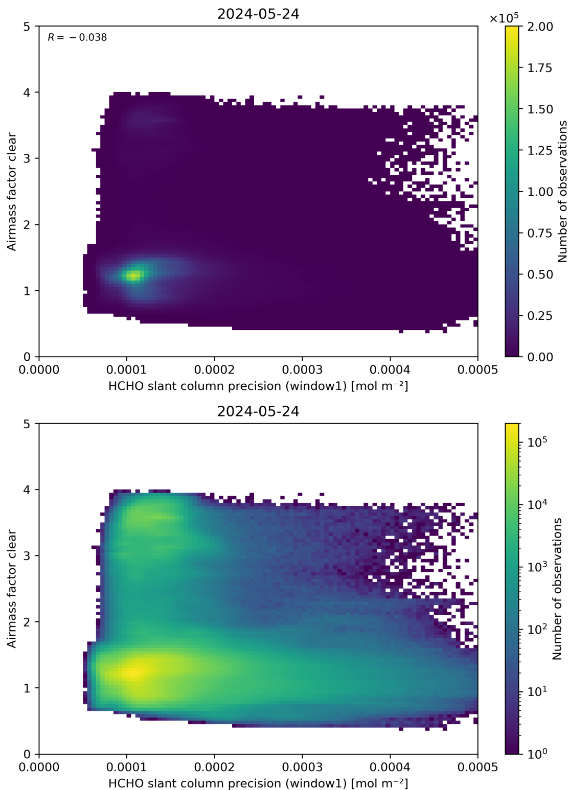
Figure 91: Scatter density plot of “HCHO slant column precision (window1)” against “Airmass factor clear” for 2024-05-23 to 2024-05-25.
