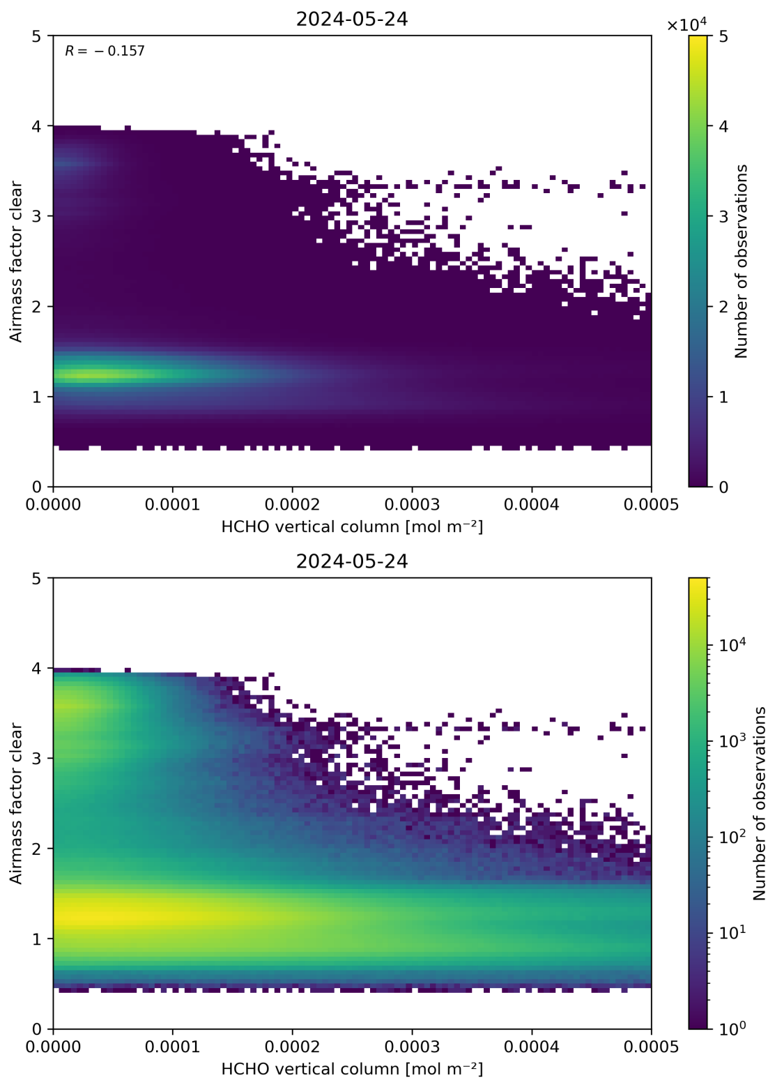
Figure 126: Scatter density plot of “HCHO vertical column” against “Airmass factor clear” for 2024-05-23 to 2024-05-25.
