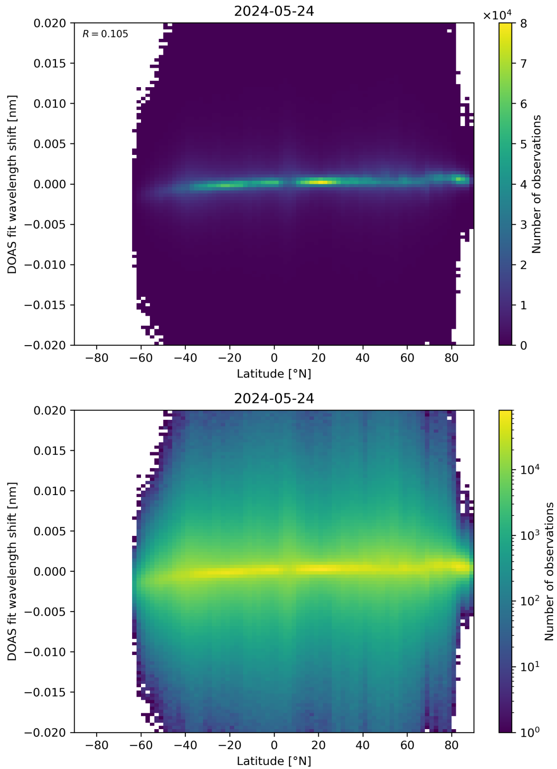
Figure 154: Scatter density plot of “Latitude” against “DOAS fit wavelength shift” for 2024-05-23 to 2024-05-25.
