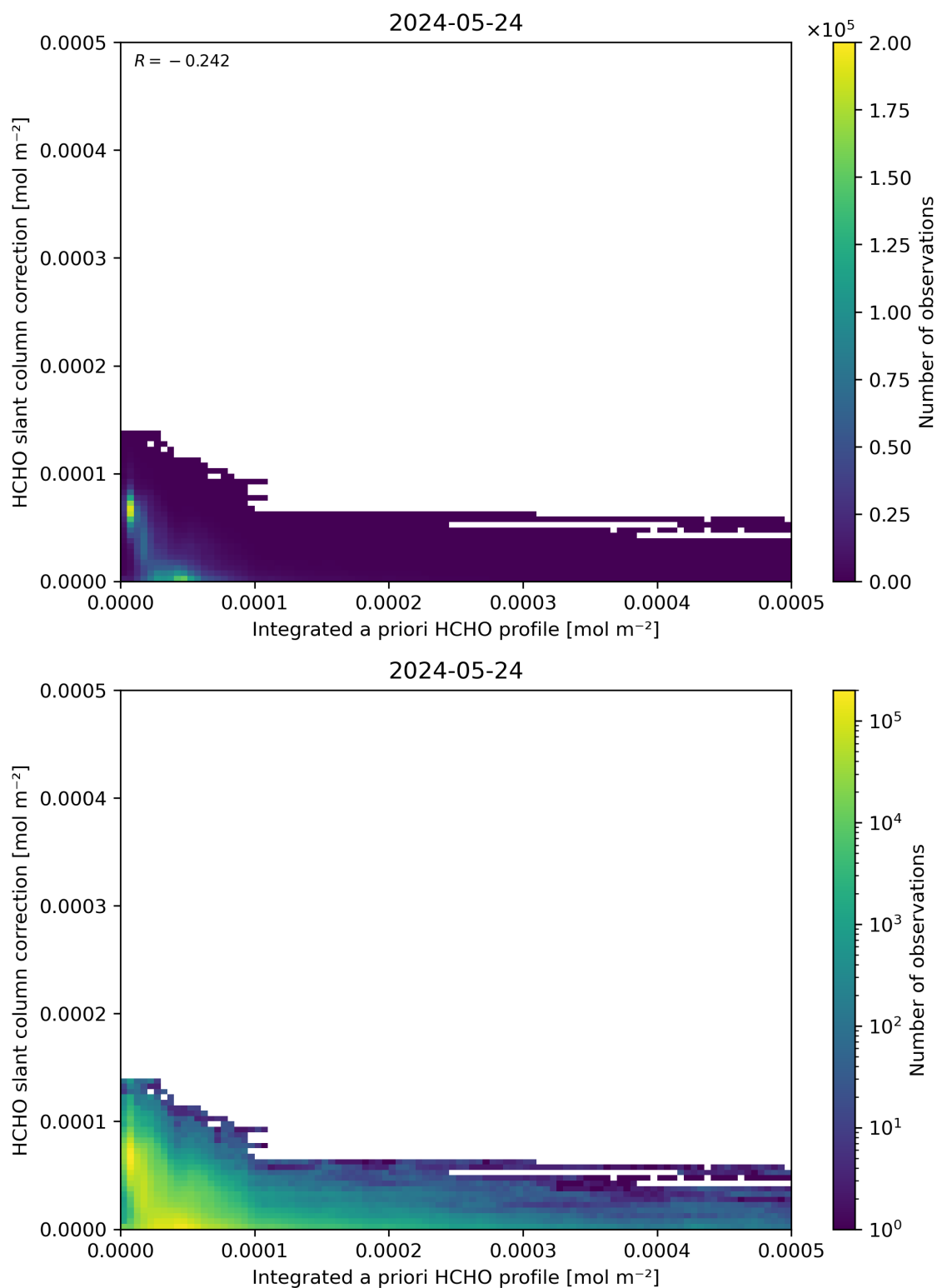
Figure 152: Scatter density plot of “Integrated a priori HCHO profile” against “HCHO slant column correction” for 2024-05-23 to 2024-05-25.
