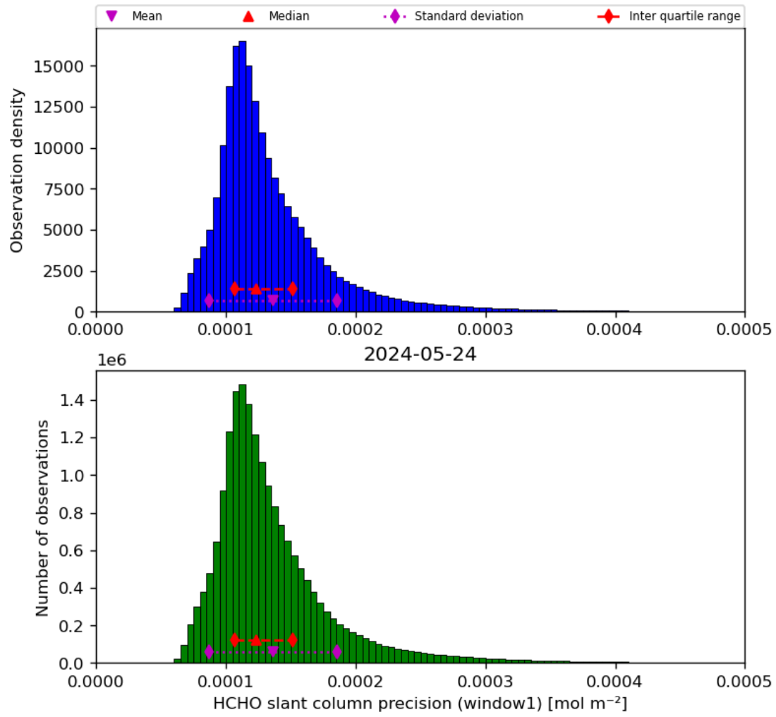
Figure 39: Histogram of “HCHO slant column precision (window1)” for 2024-05-23 to 2024-05-25
