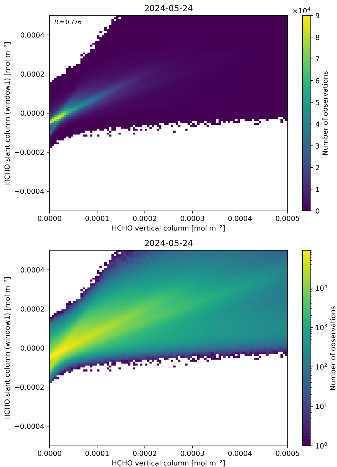
Figure 129: Scatter density plot of “HCHO vertical column” against “HCHO slant column (window1)” for 2024-05-23 to 2024-05-25.
