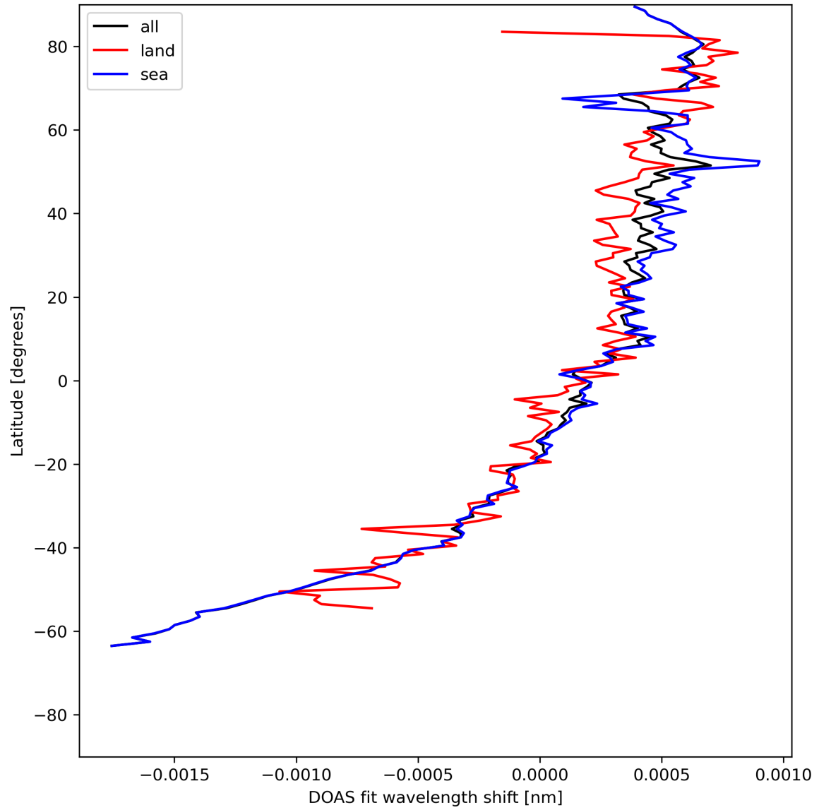
Figure 30: Zonal average of "DOAS fit wavelength shift" for 2024-05-23 to 2024-05-25.
