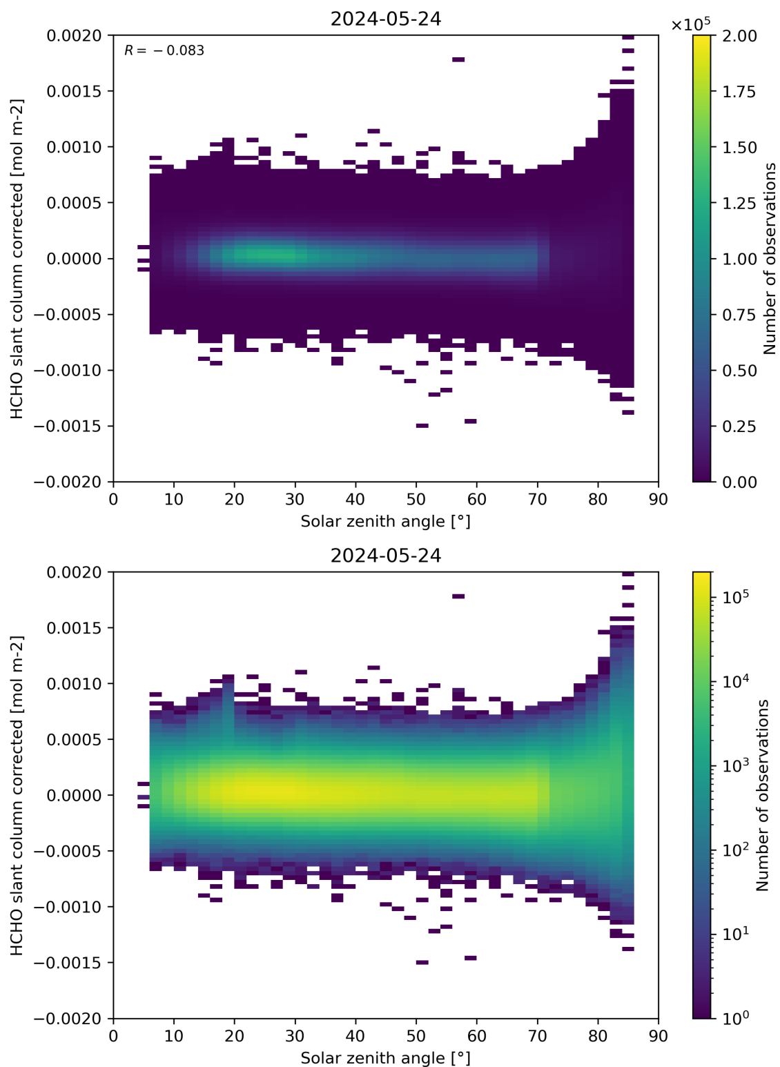
Figure 171: Scatter density plot of “Solar zenith angle” against “HCHO slant column corrected” for 2024-05-23 to 2024-05-25.
