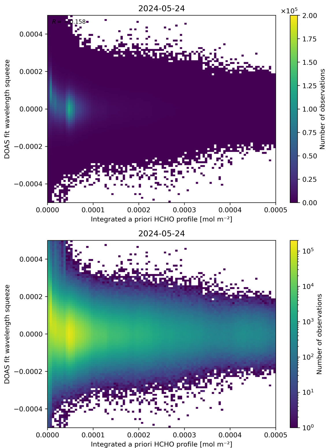
Figure 150: Scatter density plot of “Integrated a priori HCHO profile” against “DOAS fit wavelength squeeze” for 2024-05-23 to 2024-05-25.
