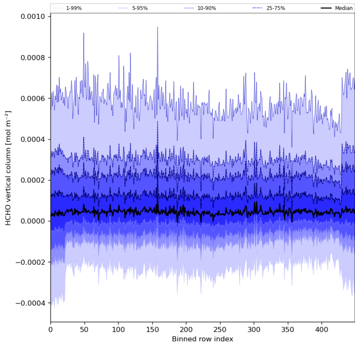
Figure 49: Along track statistics of “HCHO vertical column” for 2024-05-23 to 2024-05-25
