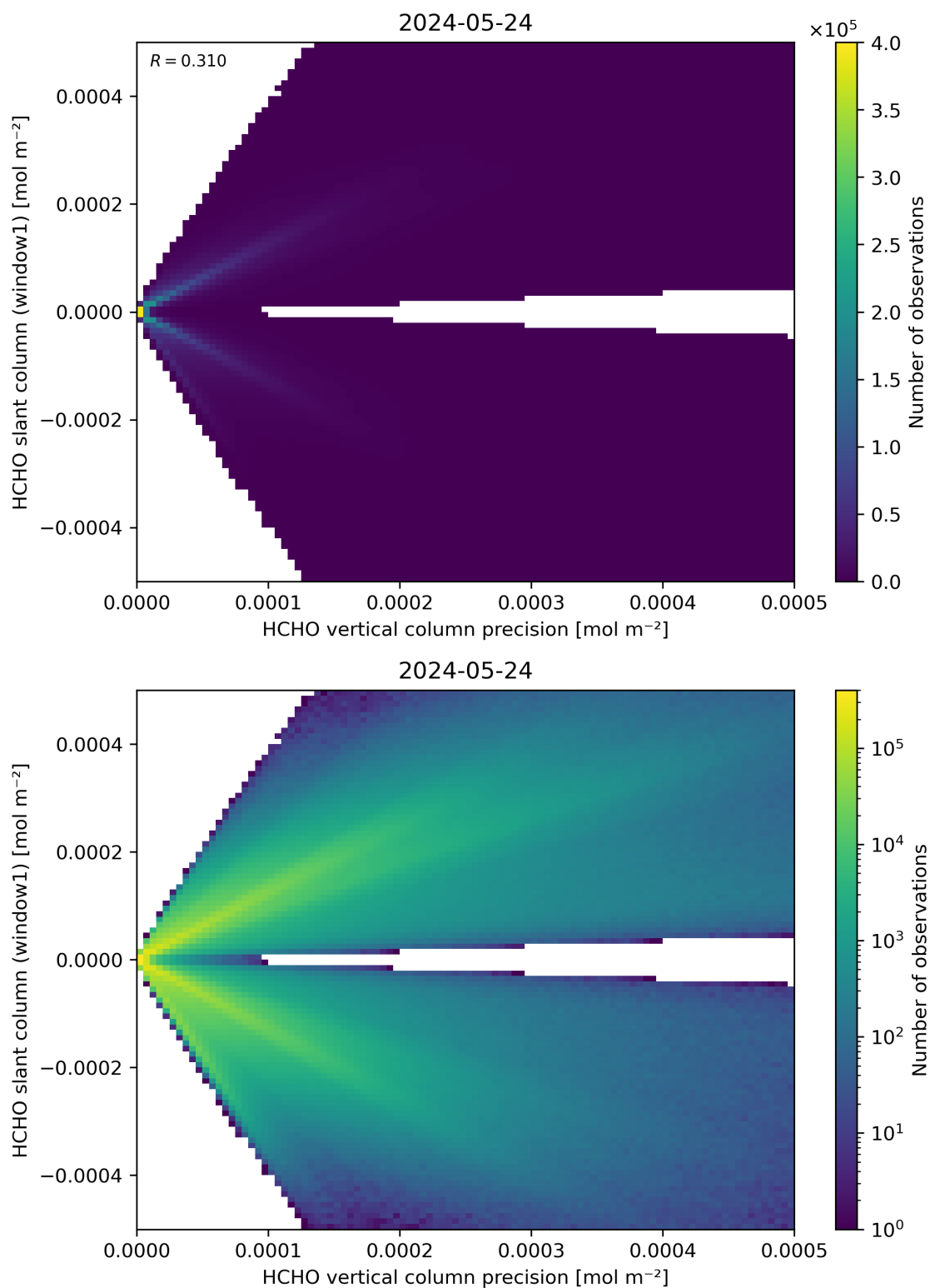
Figure 142: Scatter density plot of “HCHO vertical column precision” against “HCHO slant column (window1)” for 2024-05-23 to 2024-05-25.
