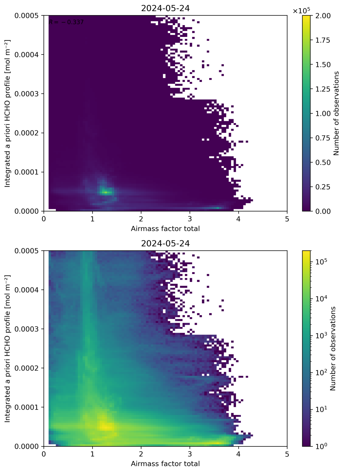
Figure 104: Scatter density plot of “Airmass factor total” against “Integrated a priori HCHO profile” for 2024-05-23 to 2024-05-25.
