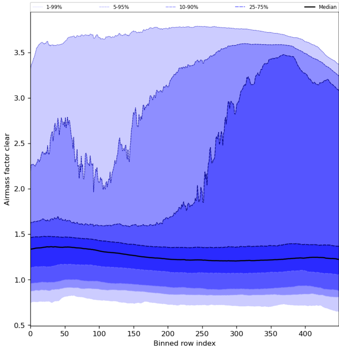
Figure 56: Along track statistics of “Airmass factor clear” for 2024-05-23 to 2024-05-25
