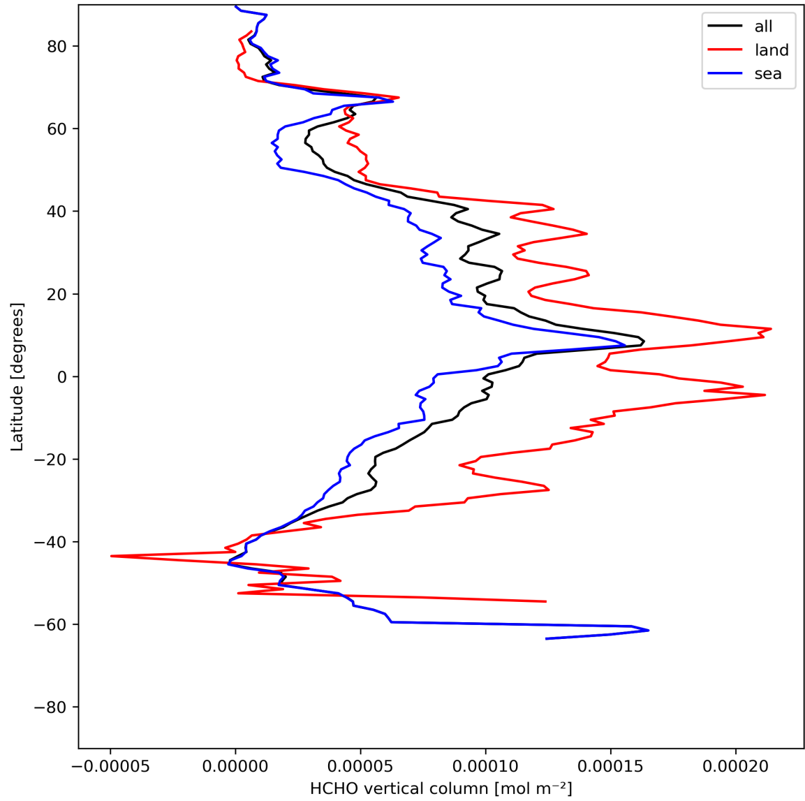
Figure 21: Zonal average of “HCHO vertical column” for 2024-05-23 to 2024-05-25.
