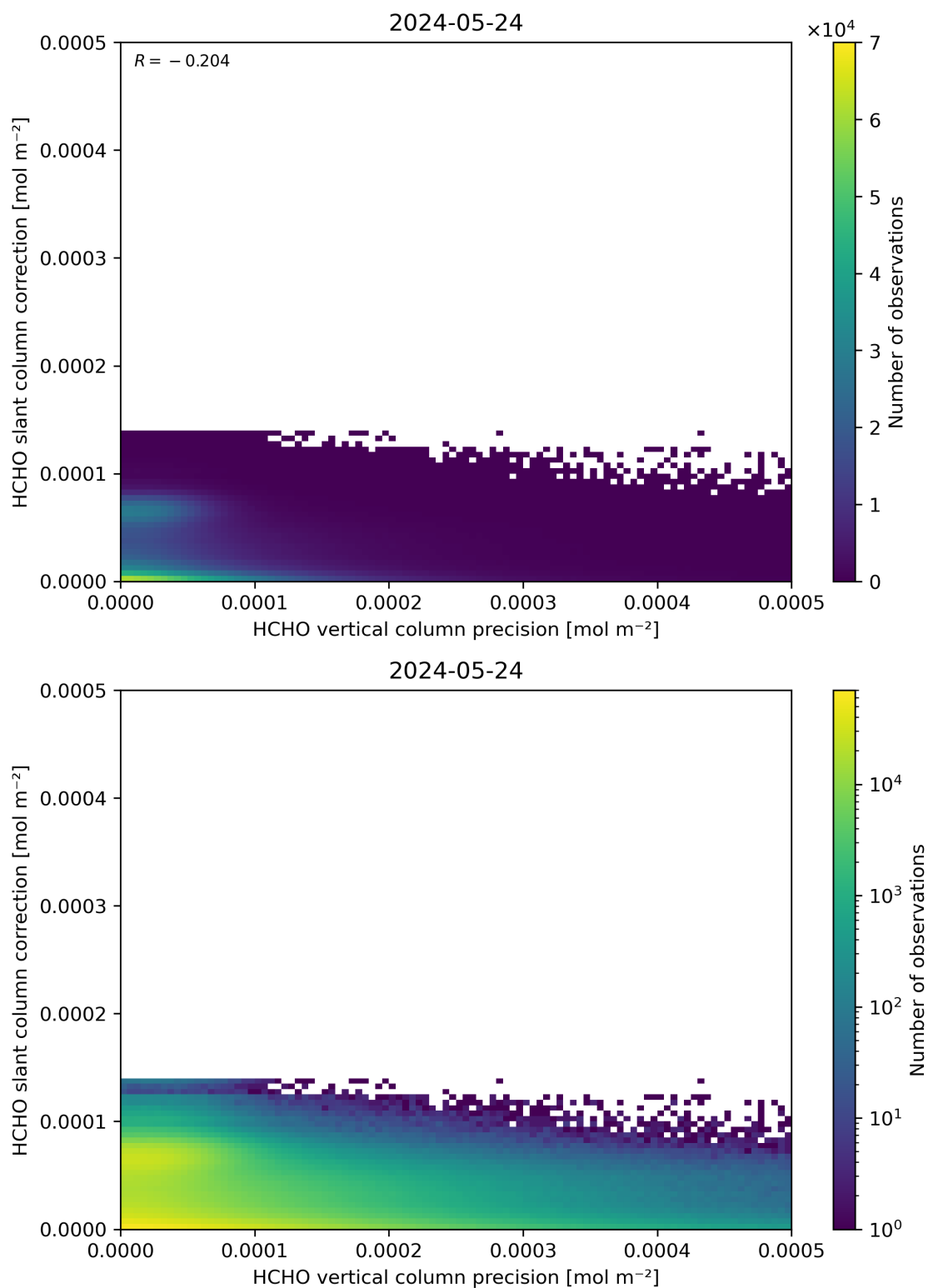
Figure 141: Scatter density plot of “HCHO vertical column precision” against “HCHO slant column correction” for 2024-05-23 to 2024-05-25.
