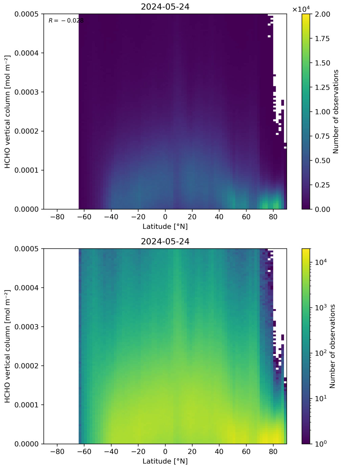
Figure 163: Scatter density plot of “Latitude” against “HCHO vertical column” for 2024-05-23 to 2024-05-25.
