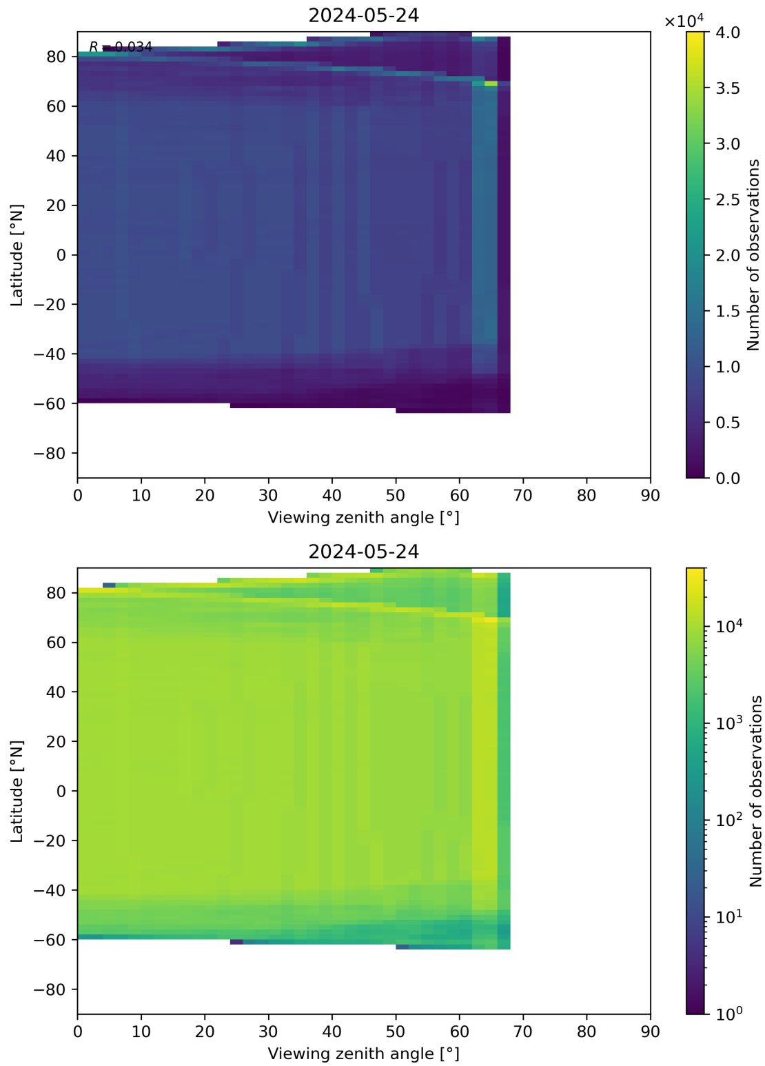
Figure 196: Scatter density plot of “Viewing zenith angle” against “Latitude” for 2024-05-23 to 2024-05-25.
