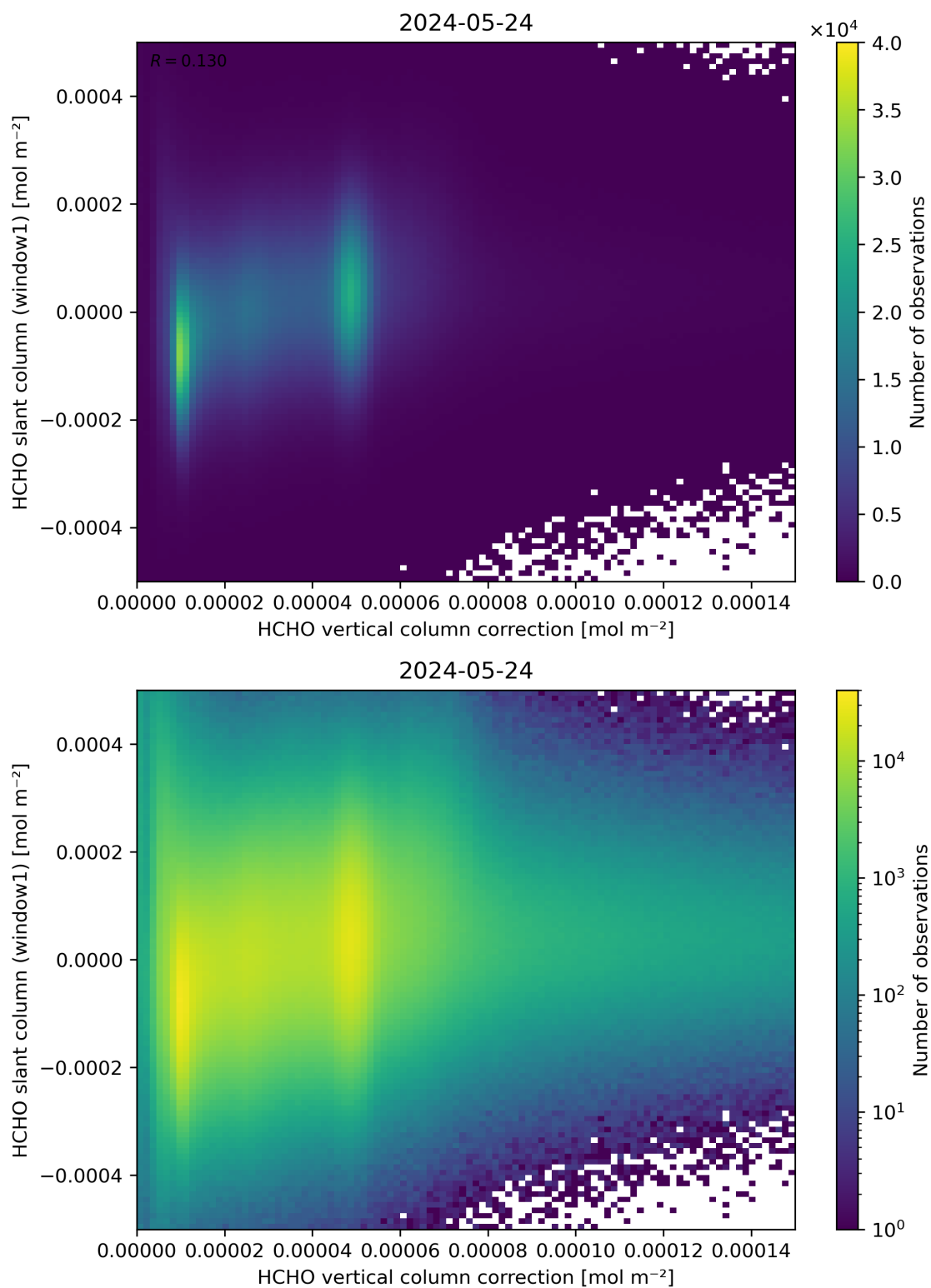
Figure 118: Scatter density plot of “HCHO vertical column correction” against “HCHO slant column (window1)” for 2024-05-23 to 2024-05-25.
