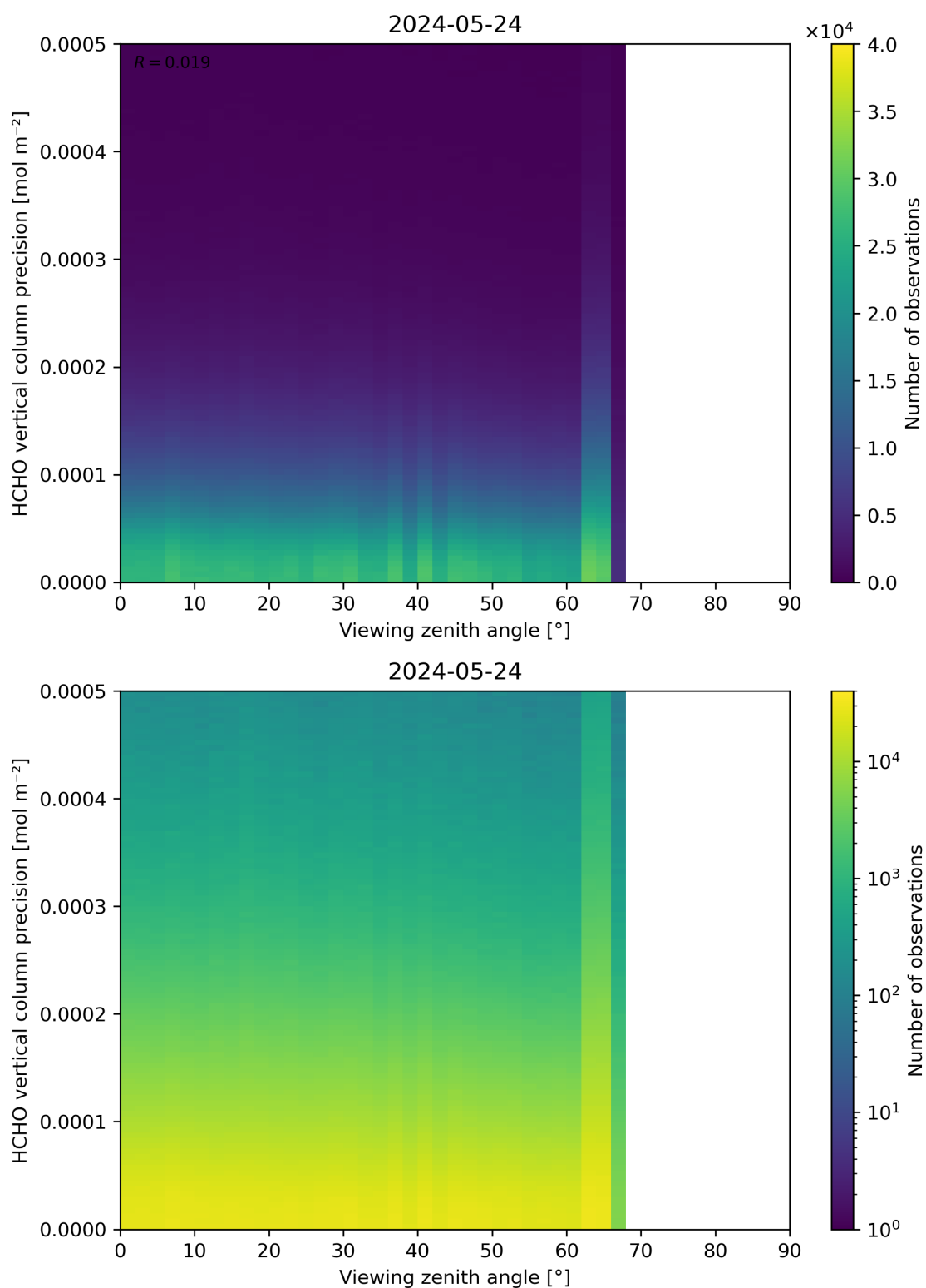
Figure 194: Scatter density plot of “Viewing zenith angle” against “HCHO vertical column precision” for 2024-05-23 to 2024-05-25.
