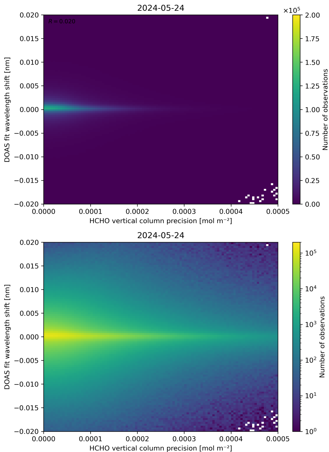
Figure 137: Scatter density plot of “HCHO vertical column precision” against “DOAS fit wavelength shift” for 2024-05-23 to 2024-05-25.
