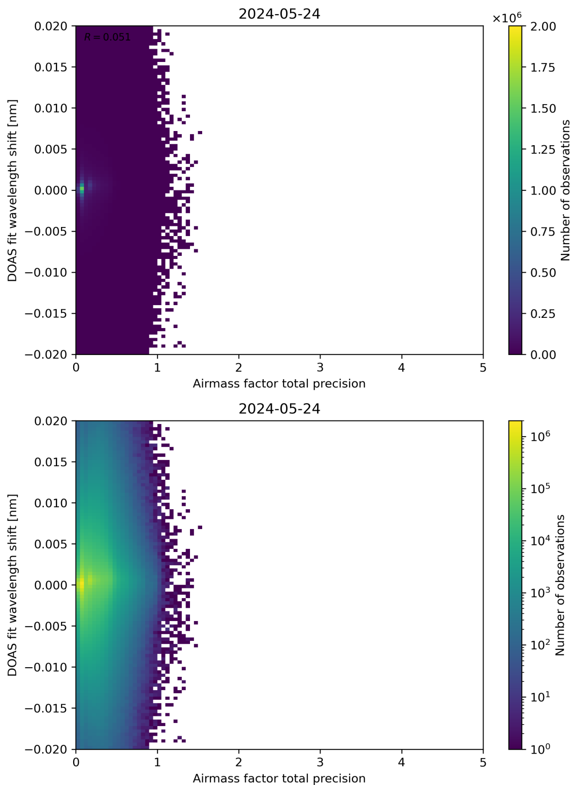
Figure 106: Scatter density plot of “Airmass factor total precision” against “DOAS fit wavelength shift” for 2024-05-23 to 2024-05-25.
