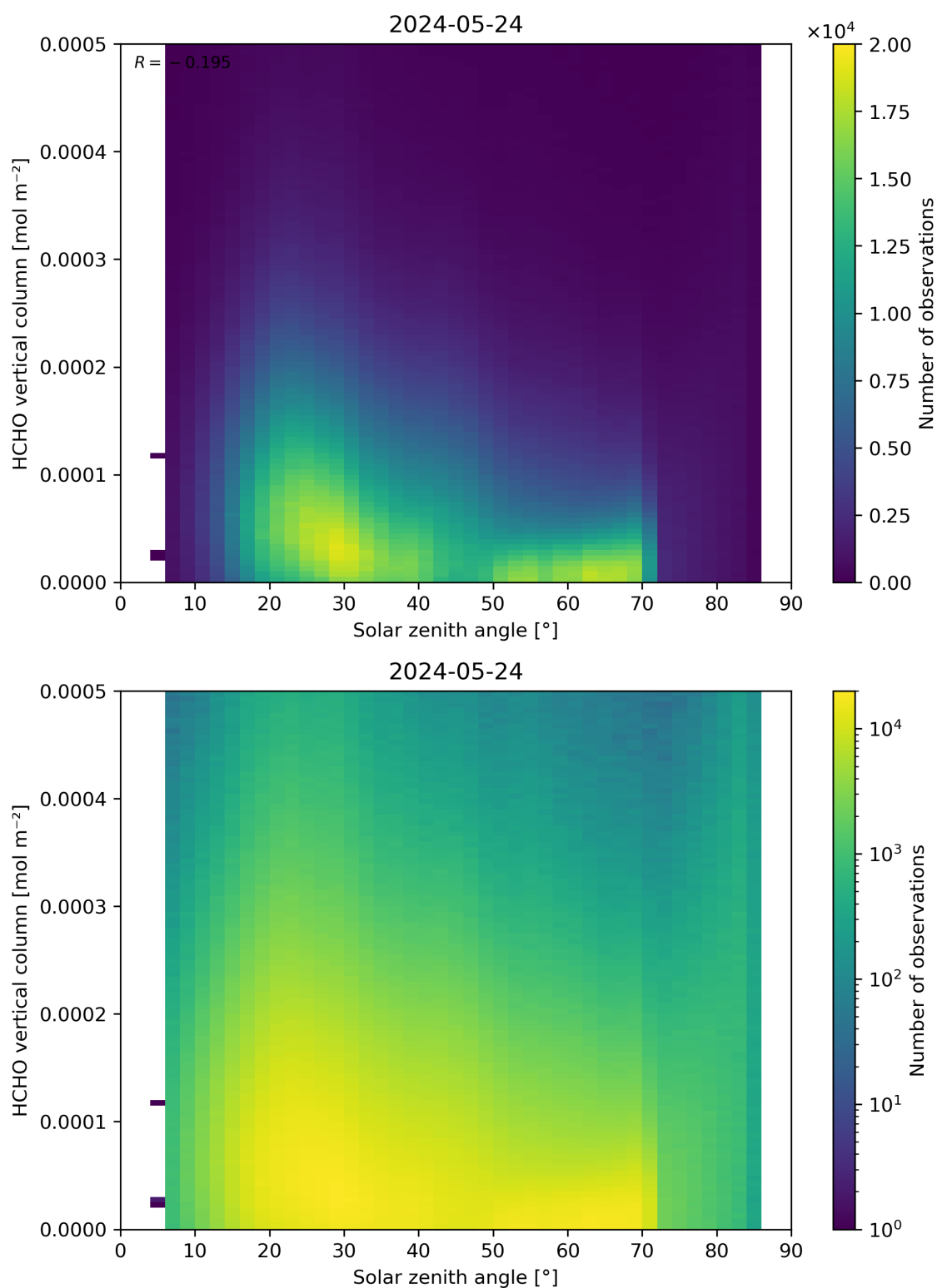
Figure 177: Scatter density plot of “Solar zenith angle” against “HCHO vertical column” for 2024-05-23 to 2024-05-25.
