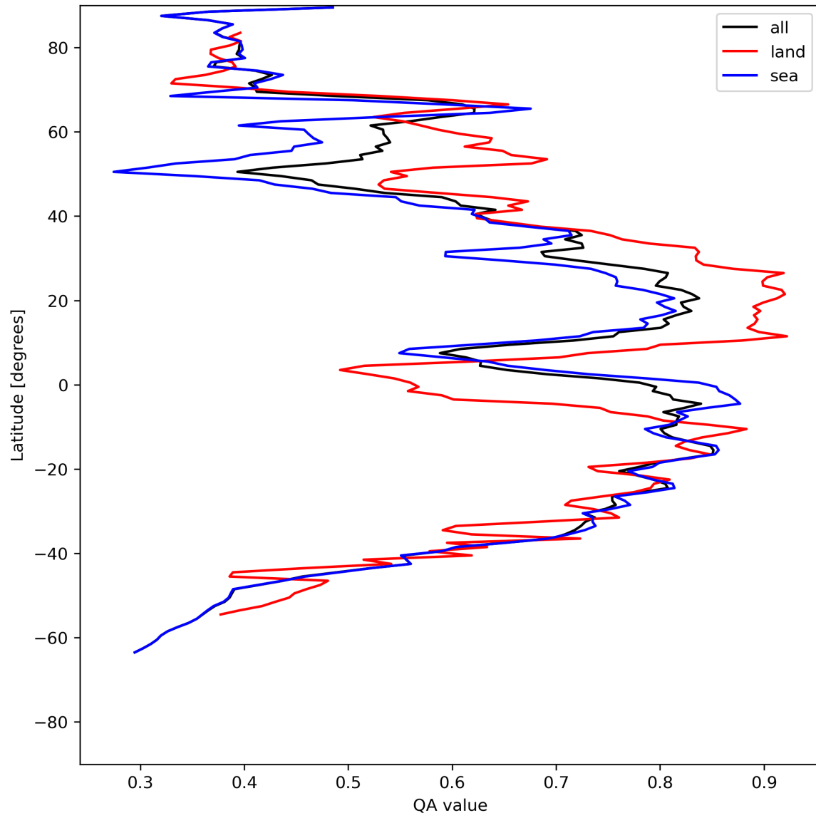
Figure 20: Zonal average of “QA value” for 2024-05-23 to 2024-05-25.
