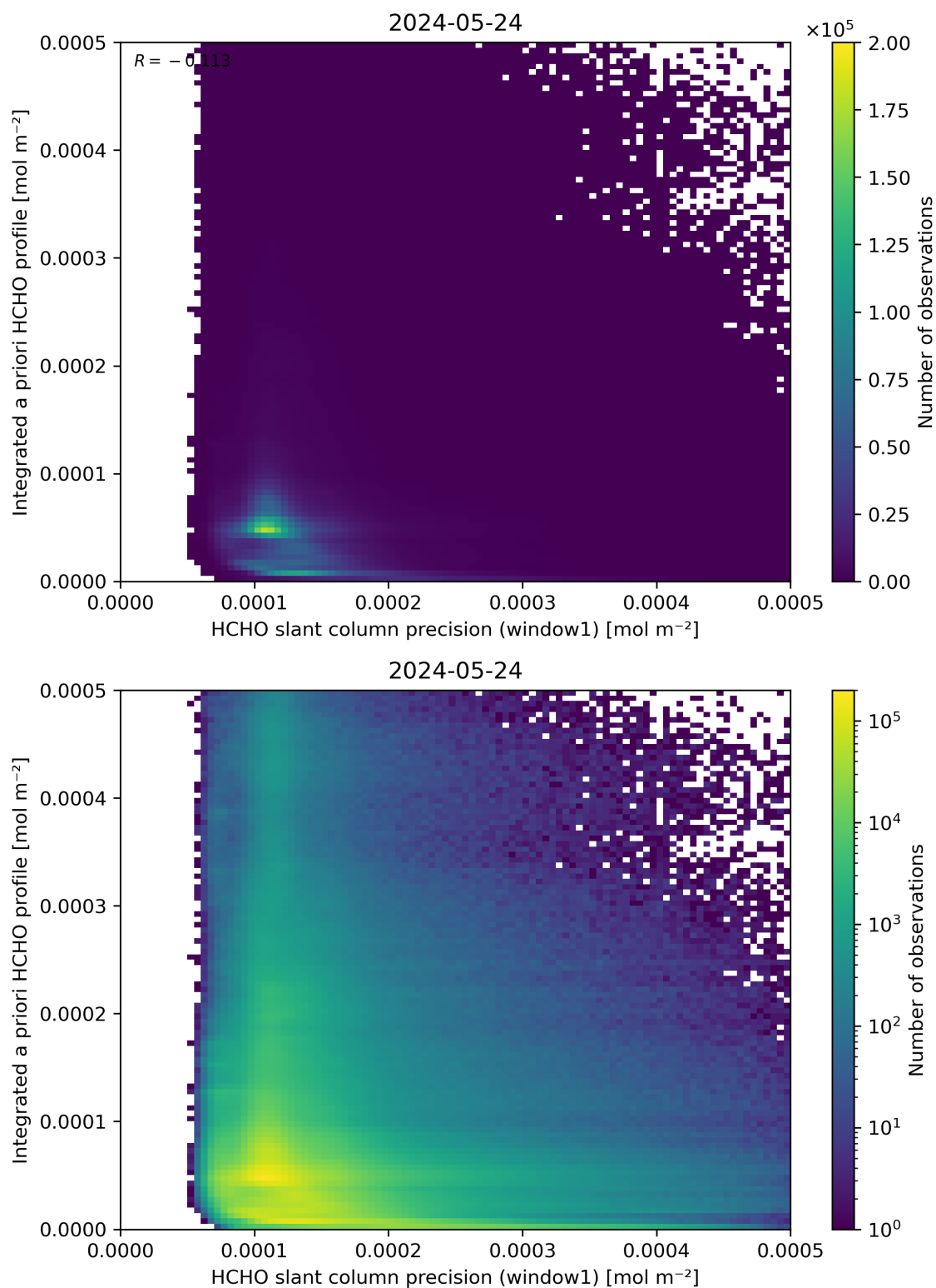
Figure 96: Scatter density plot of “HCHO slant column precision (window1)” against “Integrated a priori HCHO profile” for 2024-05-23 to 2024-05-25.
