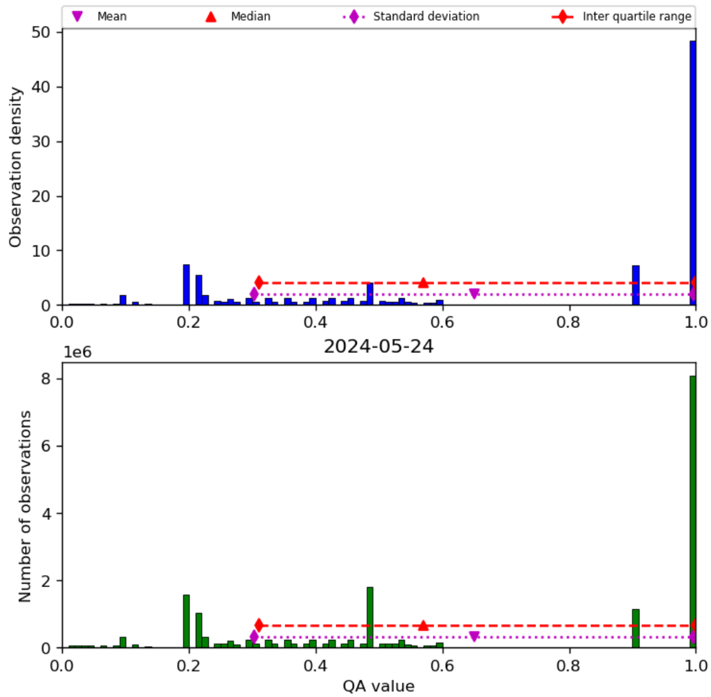
Figure 34: Histogram of “QA value” for 2024-05-23 to 2024-05-25
