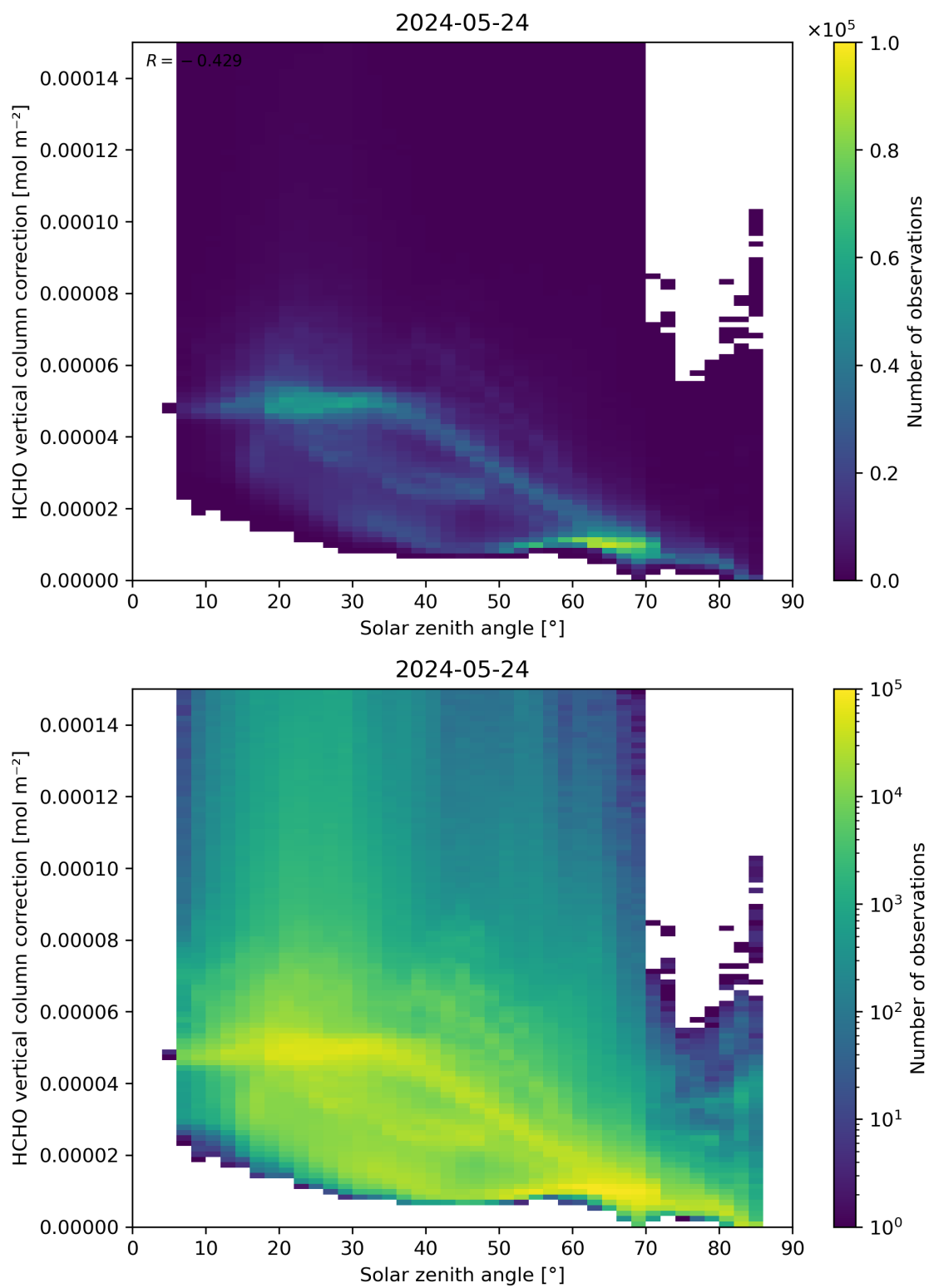
Figure 178: Scatter density plot of “Solar zenith angle” against “HCHO vertical column correction” for 2024-05-23 to 2024-05-25.
