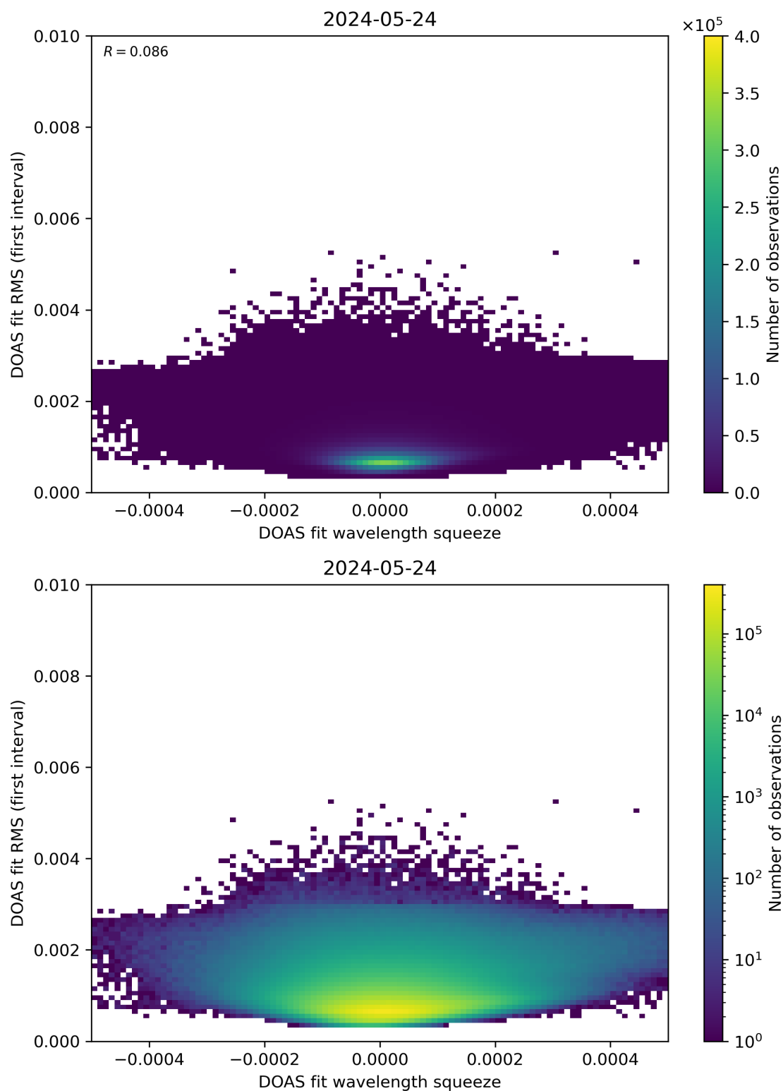
Figure 68: Scatter density plot of “DOAS fit wavelength squeeze” against “DOAS fit RMS (first interval)” for 2024-05-23 to 2024-05-25.
