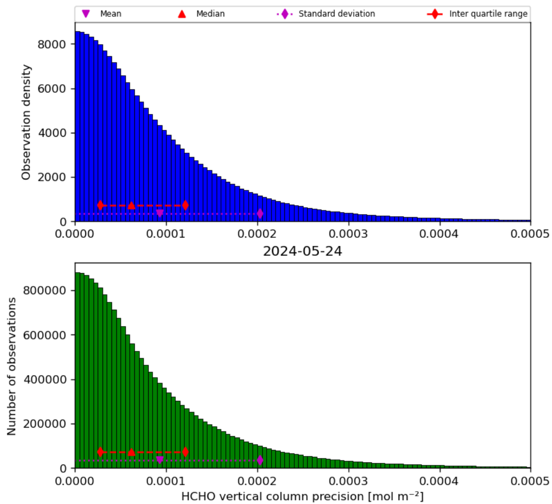
Figure 36: Histogram of “HCHO vertical column precision” for 2024-05-23 to 2024-05-25
