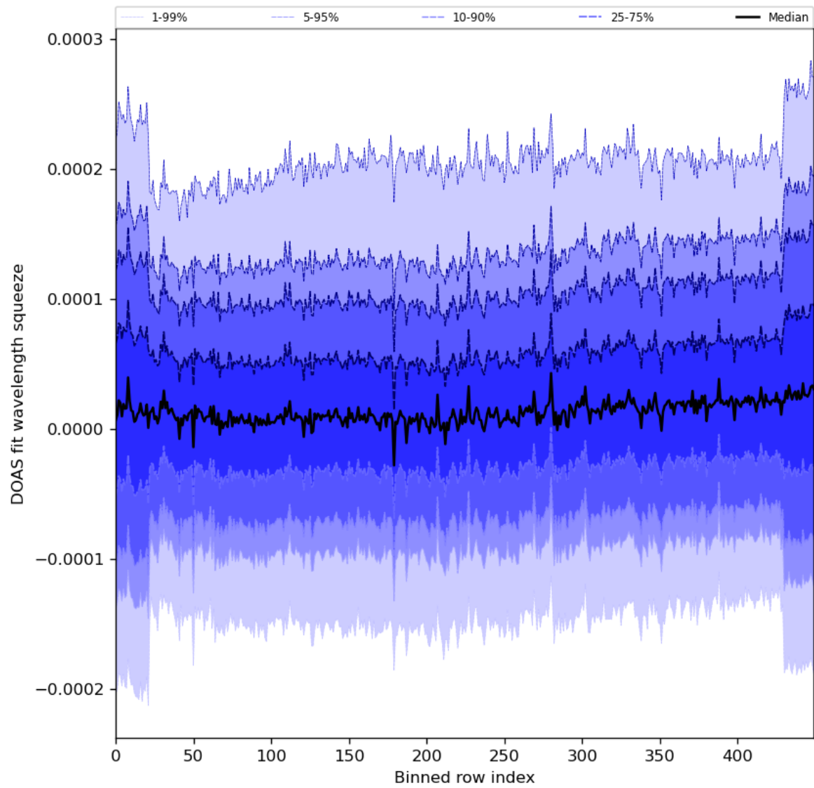
Figure 59: Along track statistics of “DOAS fit wavelength squeeze” for 2024-05-23 to 2024-05-25
