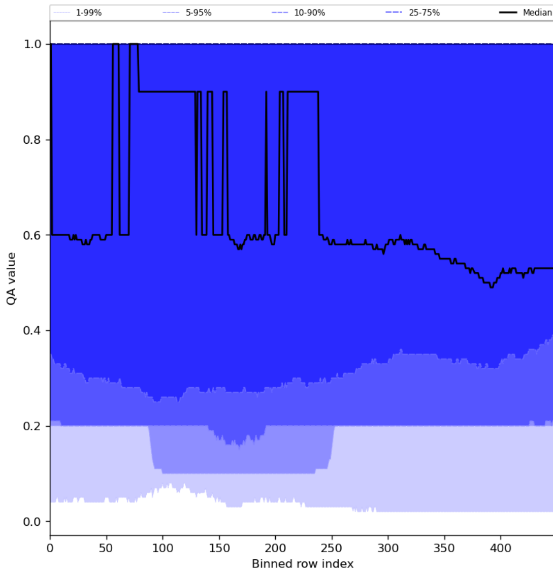
Figure 48: Along track statistics of “QA value” for 2024-05-23 to 2024-05-25
