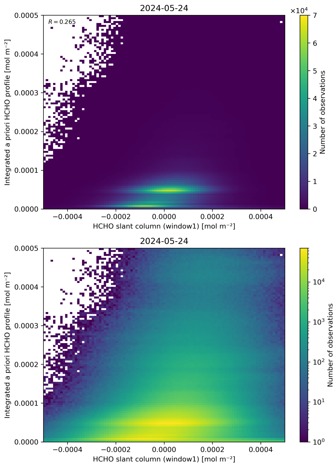
Figure 87: Scatter density plot of “HCHO slant column (window1)” against “Integrated a priori HCHO profile” for 2024-05-23 to 2024-05-25.
