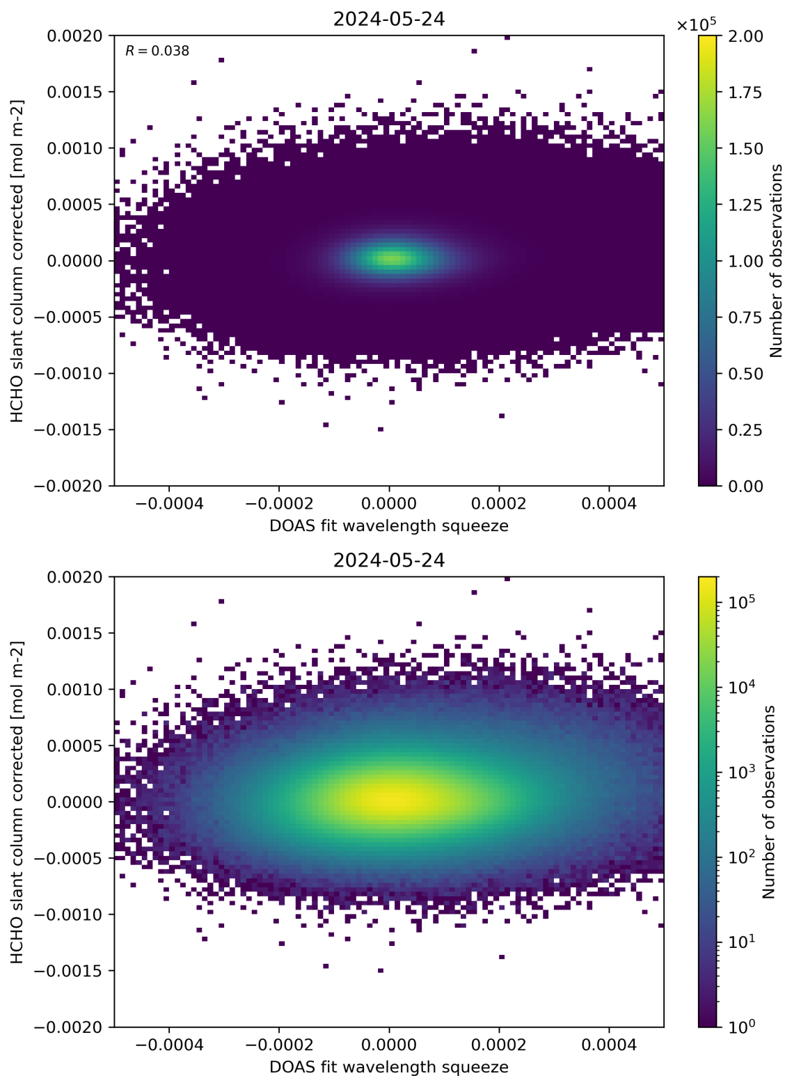
Figure 69: Scatter density plot of “DOAS fit wavelength squeeze” against “HCHO slant column corrected” for 2024-05-23 to 2024-05-25.
