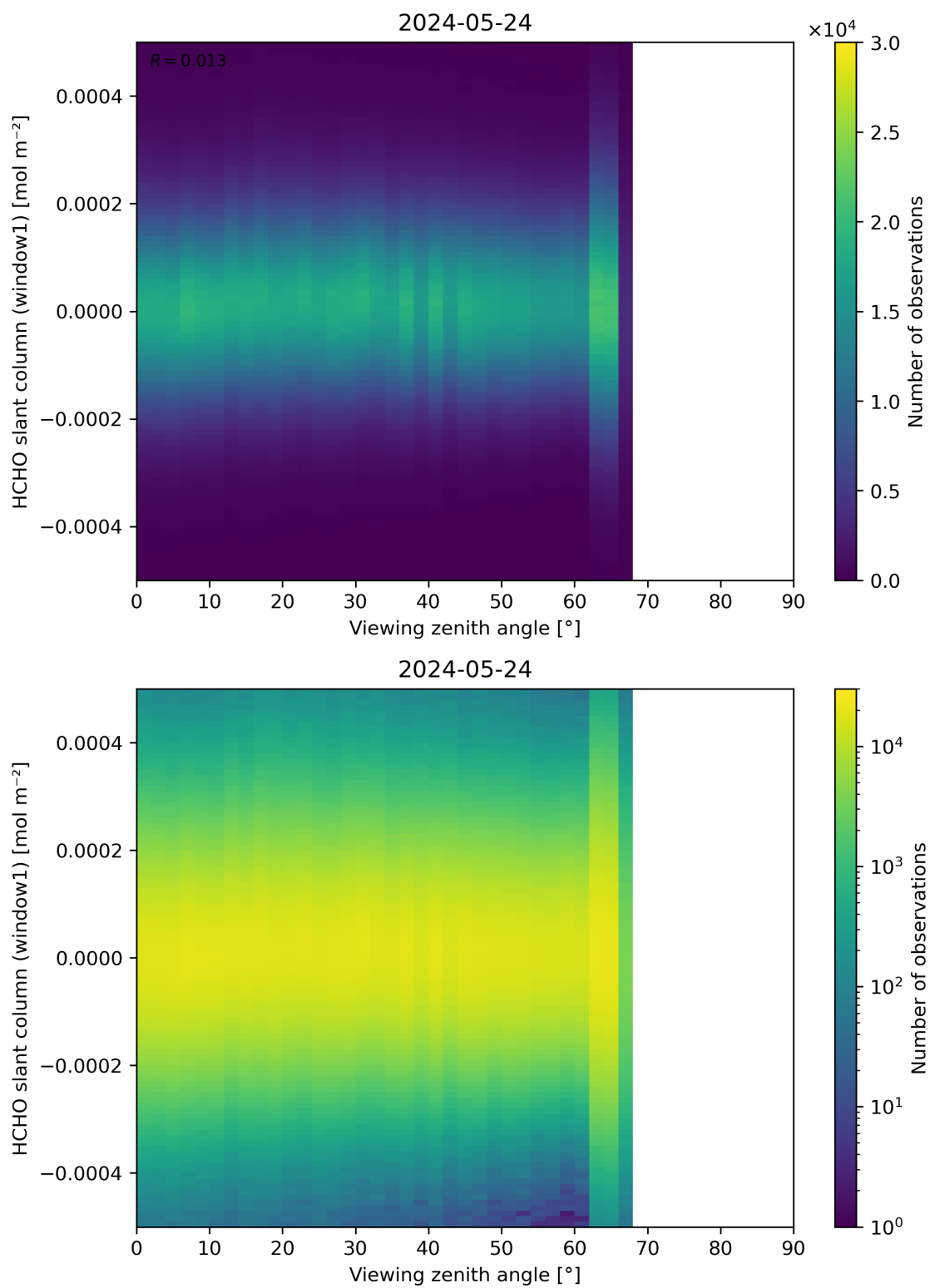
Figure 188: Scatter density plot of “Viewing zenith angle” against “HCHO slant column (window1)” for 2024-05-23 to 2024-05-25.
