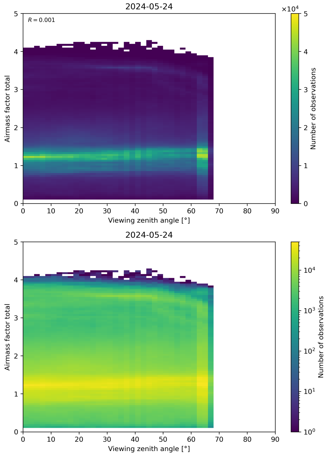
Figure 190: Scatter density plot of “Viewing zenith angle” against “Airmass factor total” for 2024-05-23 to 2024-05-25.
