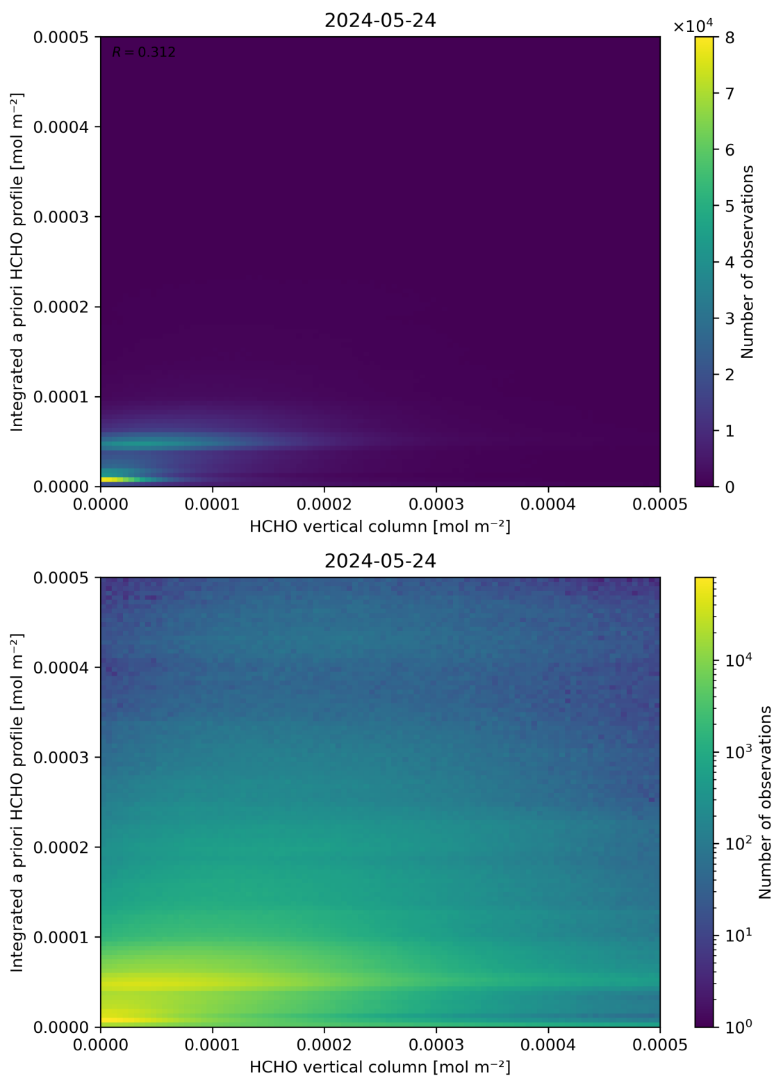
Figure 135: Scatter density plot of “HCHO vertical column” against “Integrated a priori HCHO profile” for 2024-05-23 to 2024-05-25.
