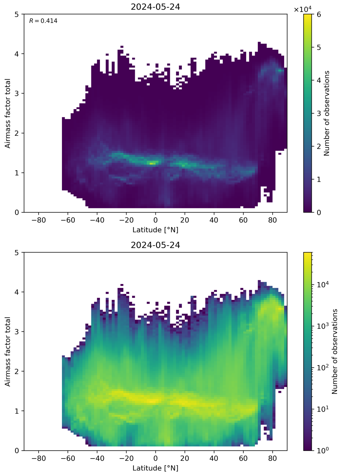
Figure 161: Scatter density plot of “Latitude” against “Airmass factor total” for 2024-05-23 to 2024-05-25.
