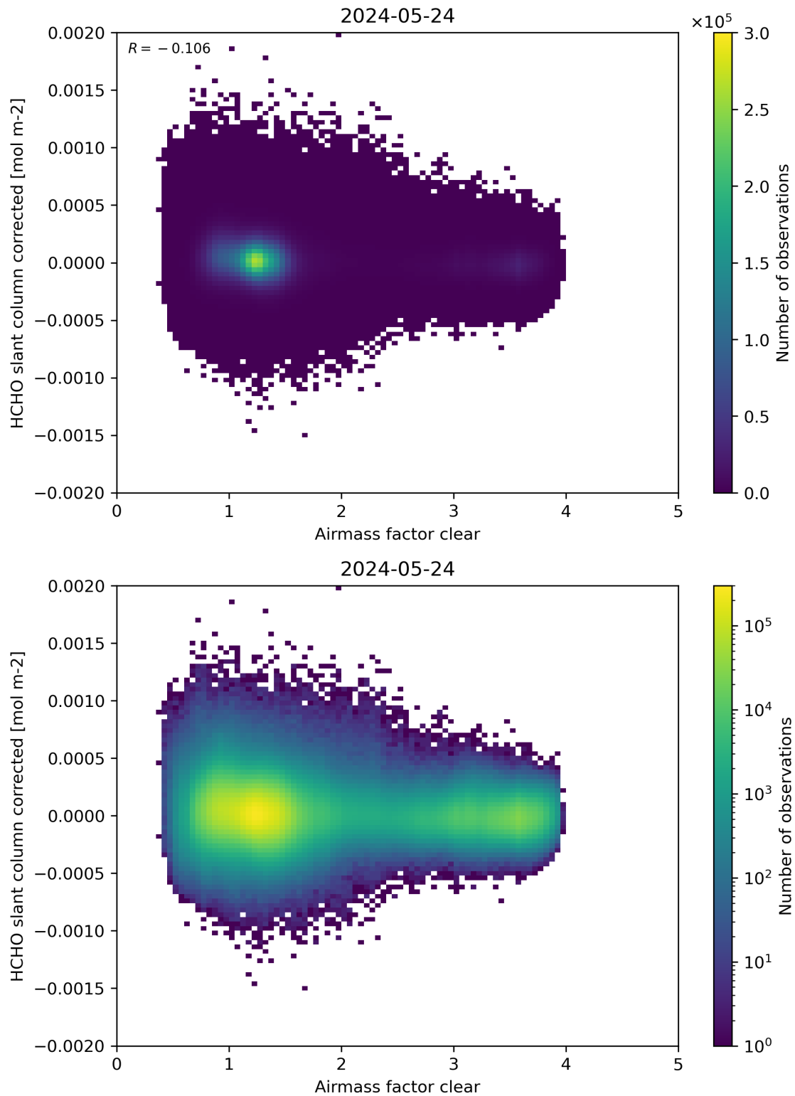
Figure 74: Scatter density plot of “Airmass factor clear” against “HCHO slant column corrected” for 2024-05-23 to 2024-05-25.
