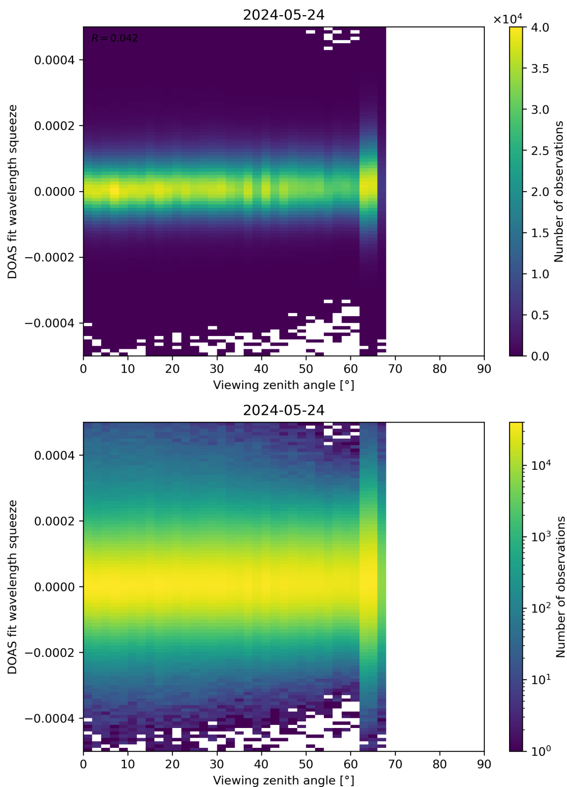
Figure 184: Scatter density plot of “Viewing zenith angle” against “DOAS fit wavelength squeeze” for 2024-05-23 to 2024-05-25.
