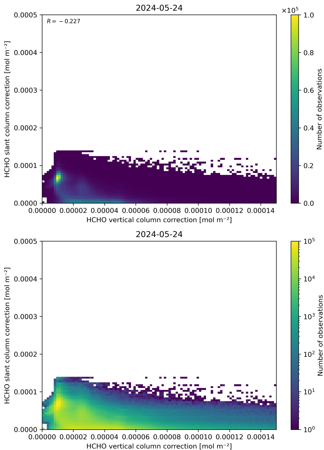
Figure 117: Scatter density plot of “HCHO vertical column correction” against “HCHO slant column correction” for 2024-05-23 to 2024-05-25.
