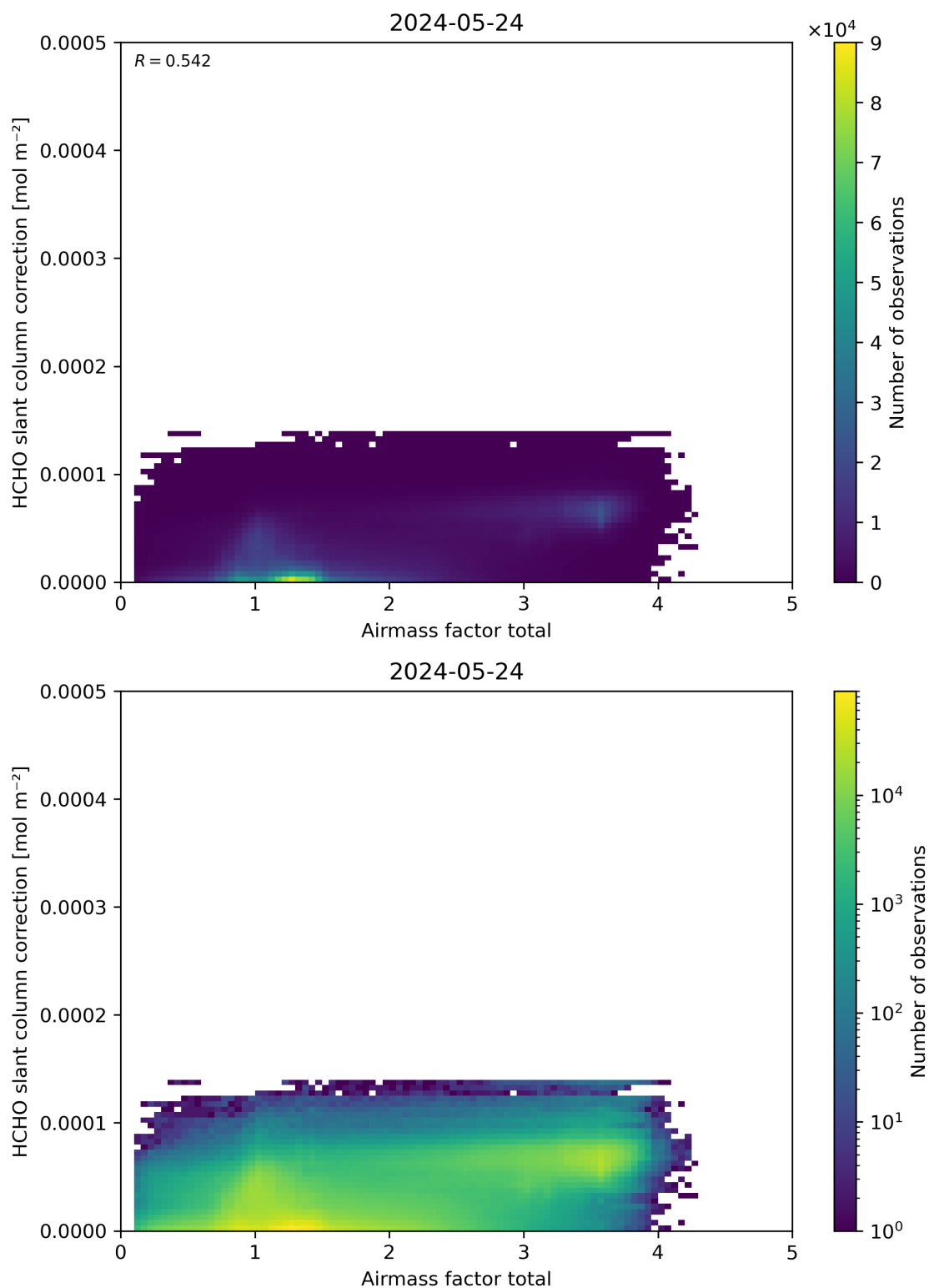
Figure 102: Scatter density plot of “Airmass factor total” against “HCHO slant column correction” for 2024-05-23 to 2024-05-25.
