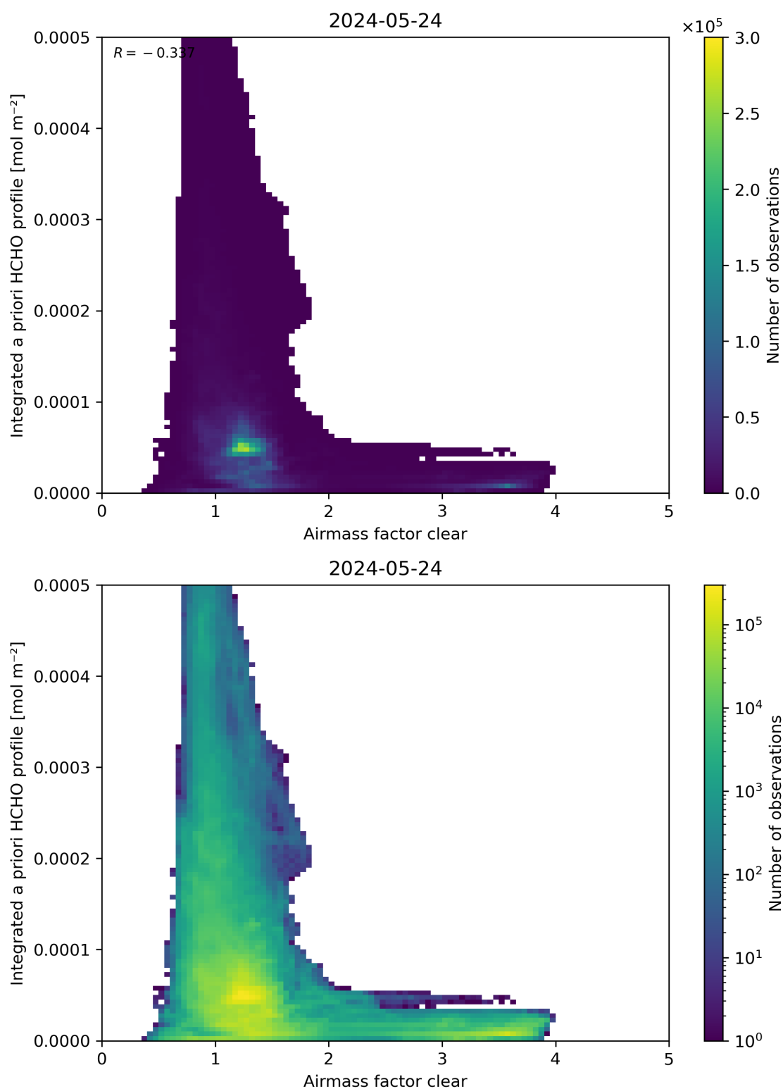
Figure 76: Scatter density plot of “Airmass factor clear” against “Integrated a priori HCHO profile” for 2024-05-23 to 2024-05-25.
