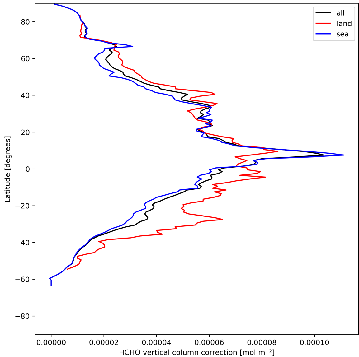
Figure 23: Zonal average of “HCHO vertical column correction” for 2024-05-23 to 2024-05-25.
