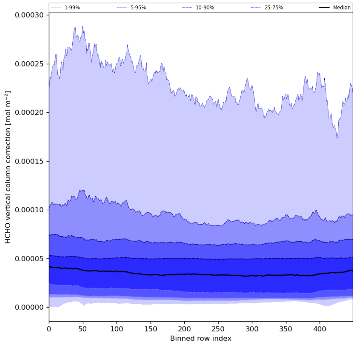
Figure 51: Along track statistics of “HCHO vertical column correction” for 2024-05-23 to 2024-05-25
