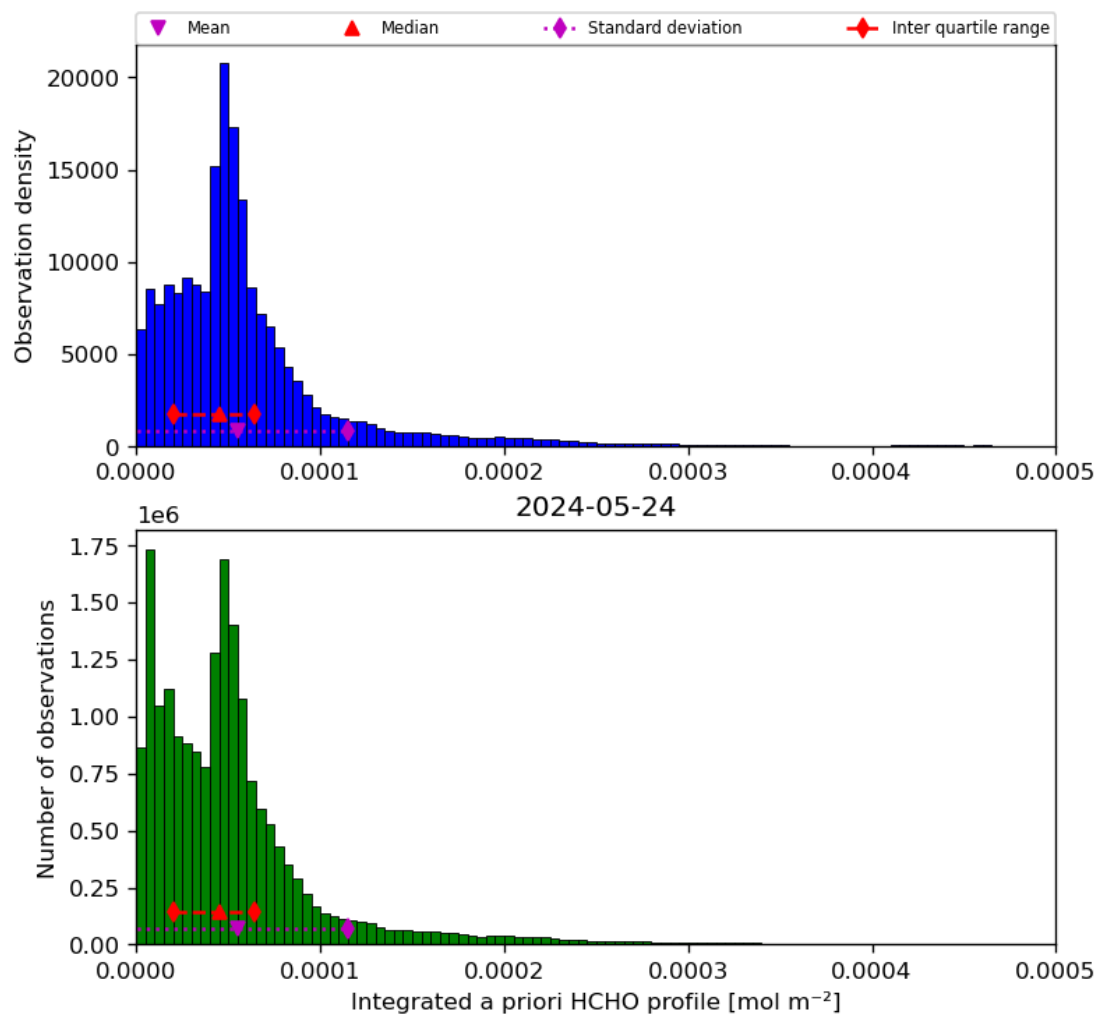
Figure 43: Histogram of “Integrated a priori HCHO profile” for 2024-05-23 to 2024-05-25
