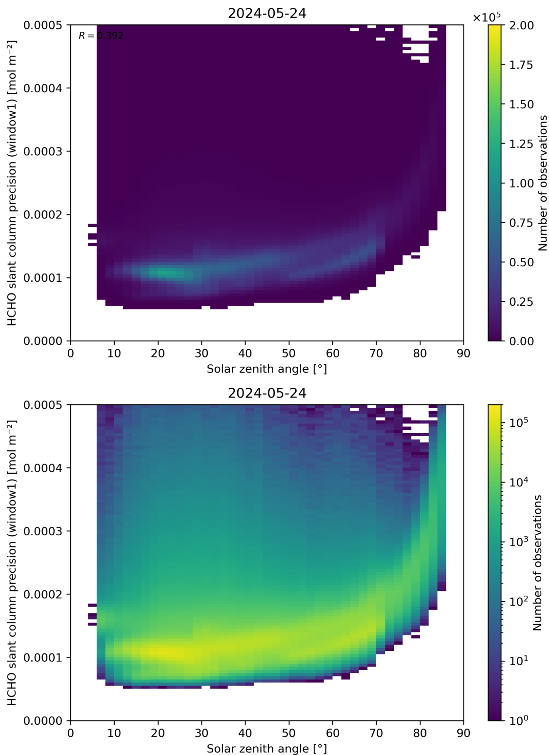
Figure 174: Scatter density plot of “Solar zenith angle” against “HCHO slant column precision (window1)” for 2024-05-23 to 2024-05-25.
