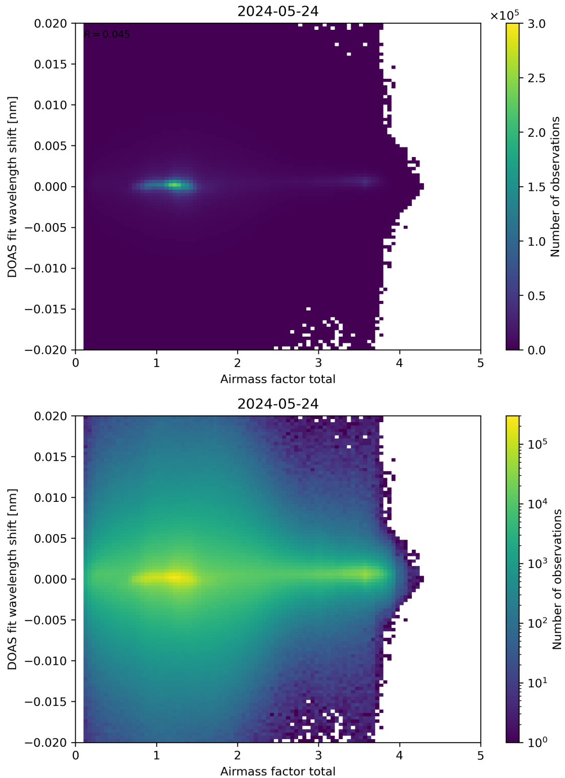
Figure 98: Scatter density plot of “Airmass factor total” against “DOAS fit wavelength shift” for 2024-05-23 to 2024-05-25.
