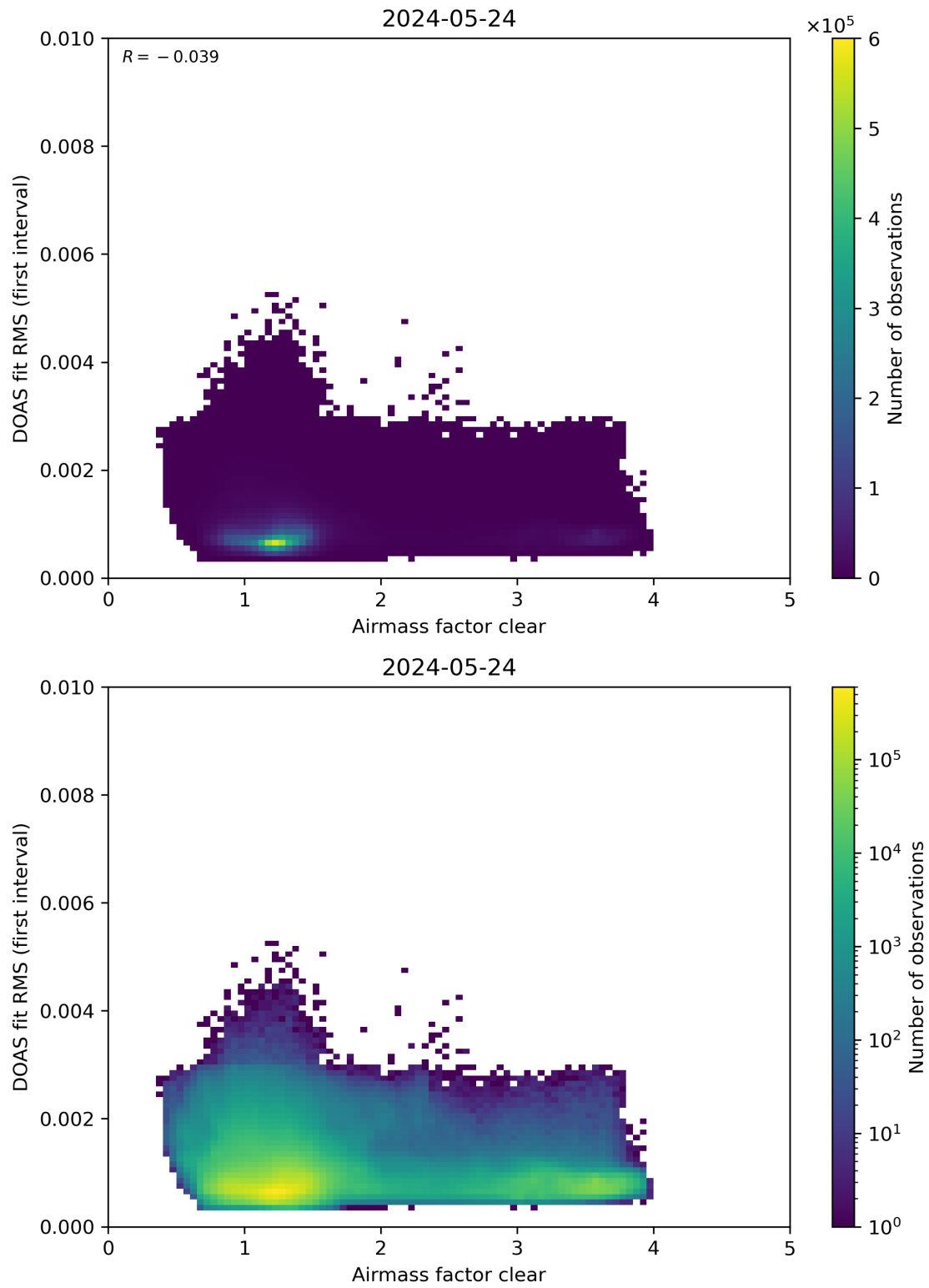
Figure 71: Scatter density plot of “Airmass factor clear” against “DOAS fit RMS (first interval)” for 2024-05-23 to 2024-05-25.
