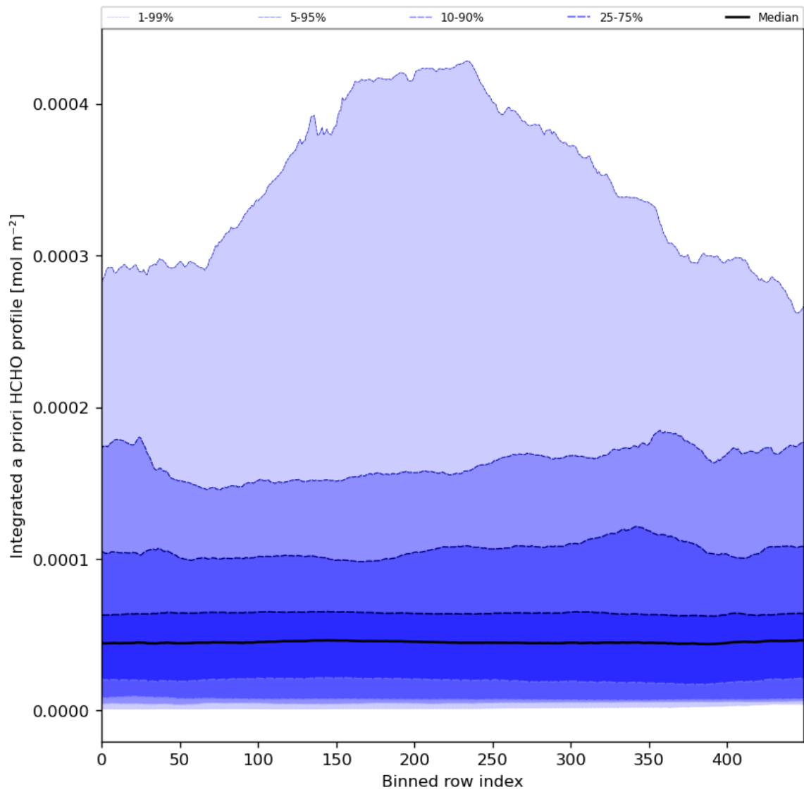
Figure 57: Along track statistics of “Integrated a priori HCHO profile” for 2024-05-23 to 2024-05-25
