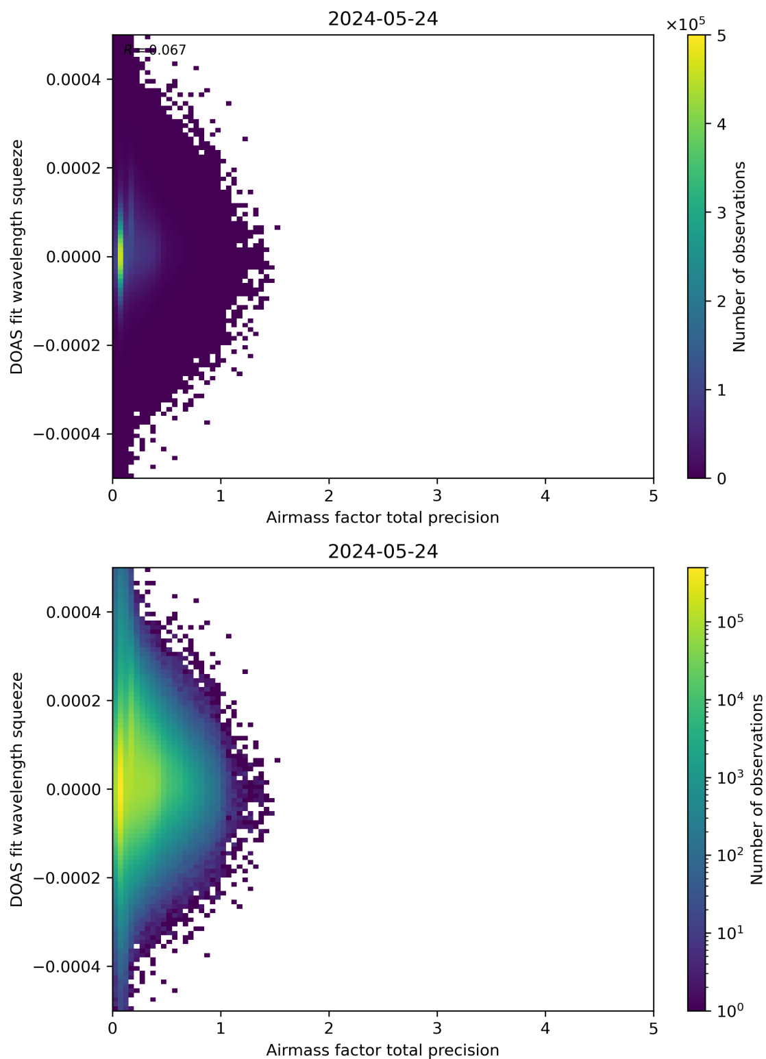
Figure 107: Scatter density plot of “Airmass factor total precision” against “DOAS fit wavelength squeeze” for 2024-05-23 to 2024-05-25.
