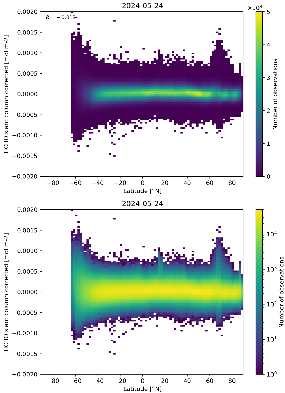
Figure 157: Scatter density plot of “Latitude” against “HCHO slant column corrected” for 2024-05-23 to 2024-05-25.
