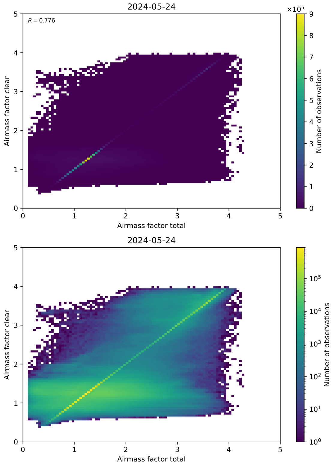
Figure 100: Scatter density plot of “Airmass factor total” against “Airmass factor clear” for 2024-05-23 to 2024-05-25.
