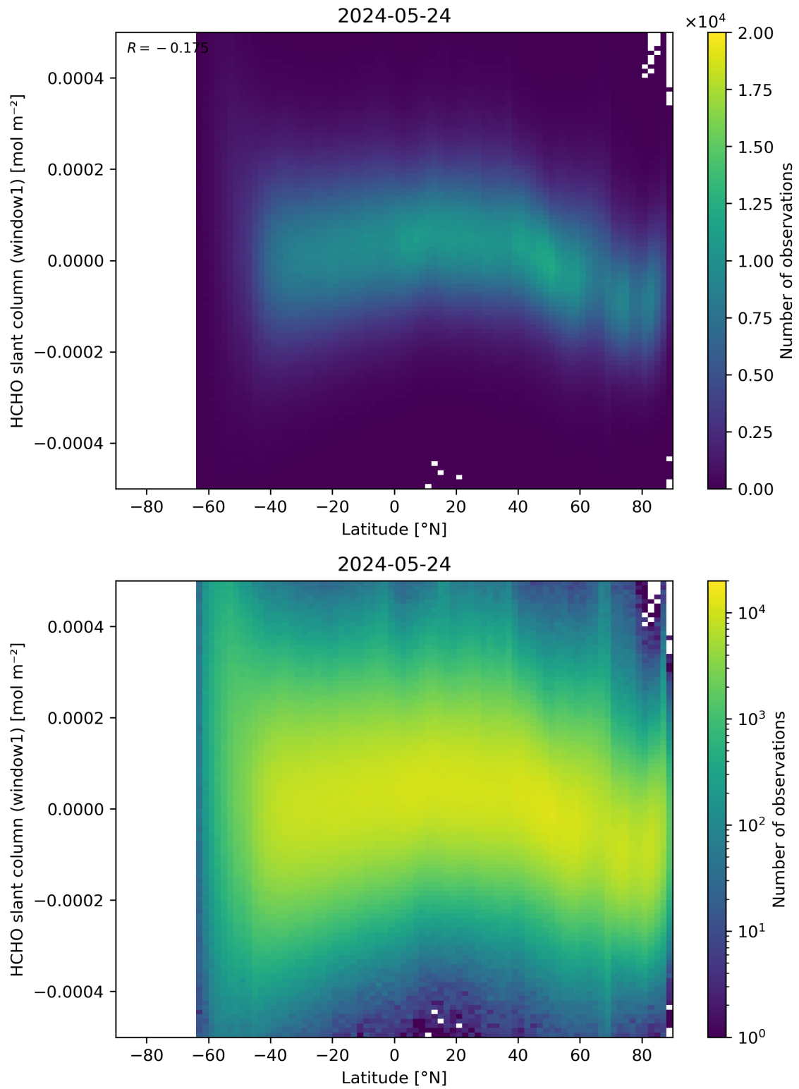
Figure 159: Scatter density plot of “Latitude” against “HCHO slant column (window1)” for 2024-05-23 to 2024-05-25.
