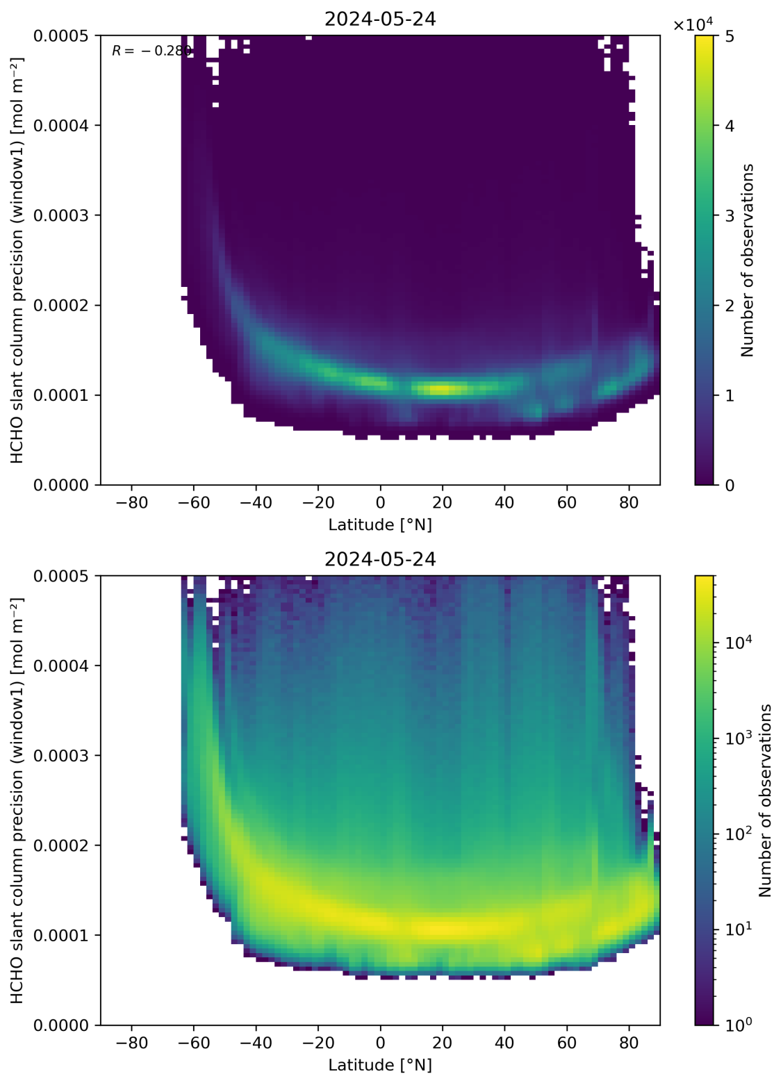
Figure 160: Scatter density plot of “Latitude” against “HCHO slant column precision (window1)” for 2024-05-23 to 2024-05-25.
