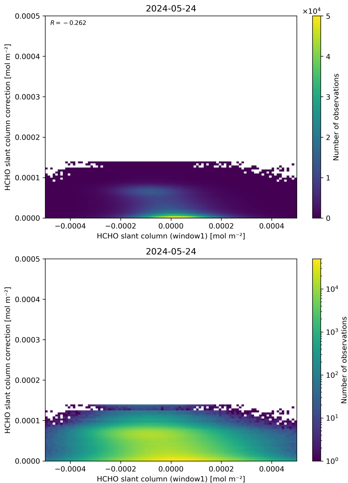
Figure 83: Scatter density plot of “HCHO slant column (window1)” against “HCHO slant column correction” for 2024-05-23 to 2024-05-25.
