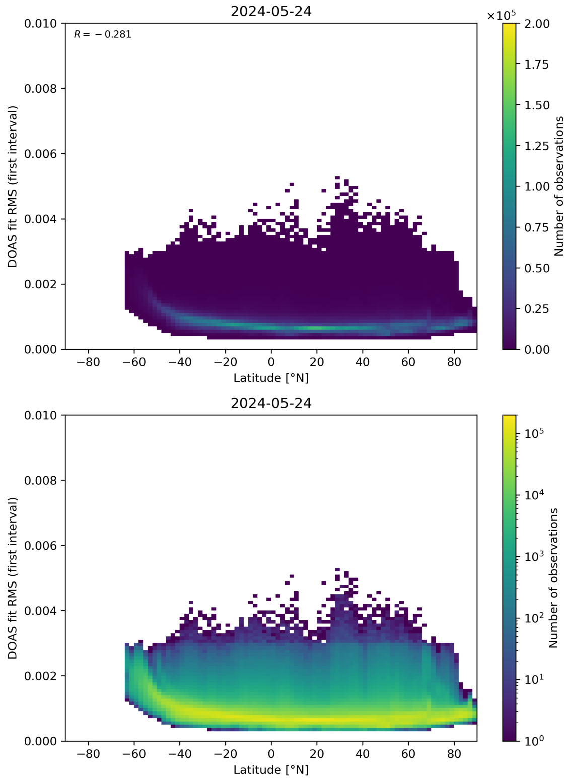
Figure 153: Scatter density plot of “Latitude” against “DOAS fit RMS (first interval)” for 2024-05-23 to 2024-05-25.
