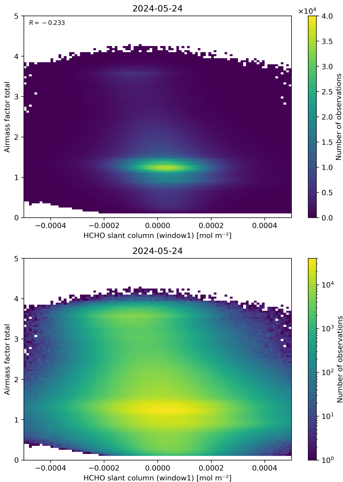
Figure 85: Scatter density plot of “HCHO slant column (window1)” against “Airmass factor total” for 2024-05-23 to 2024-05-25.
