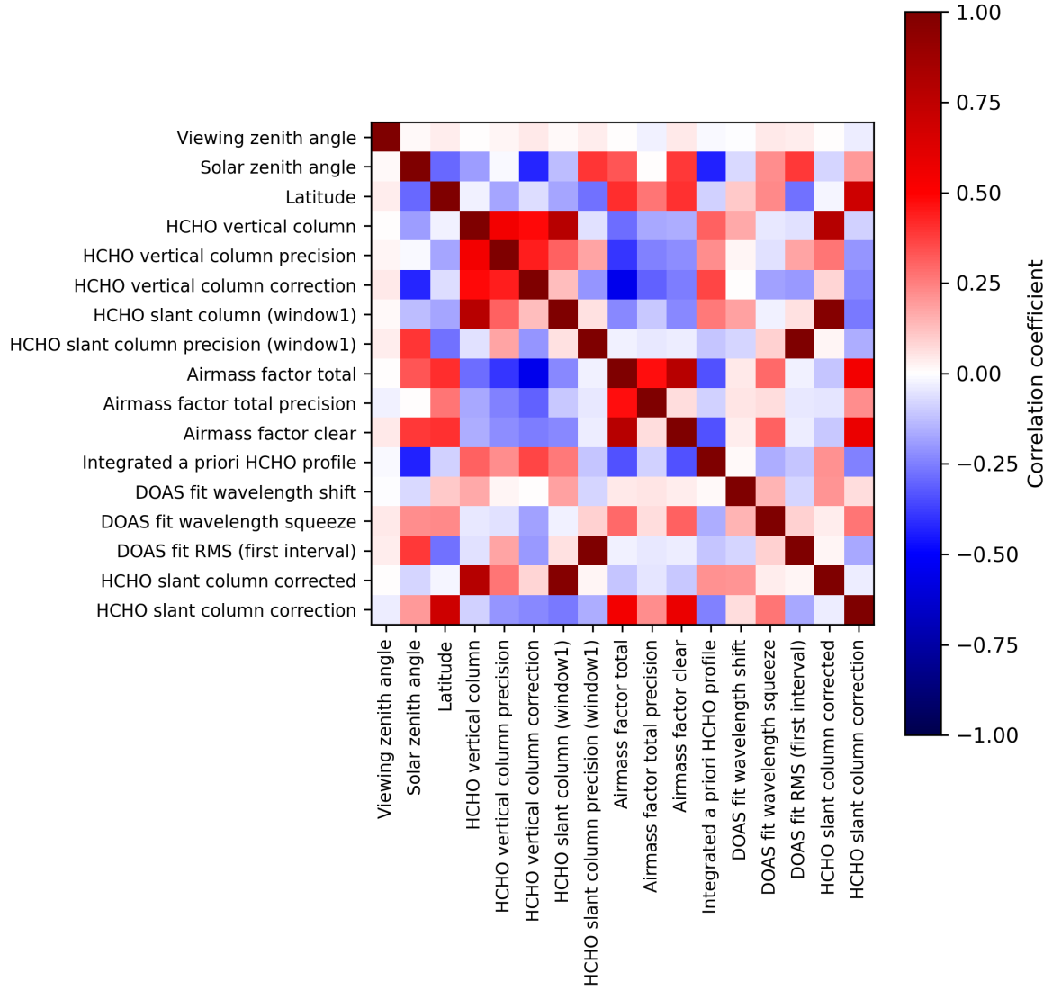
Figure 2: Map of correlation matrix for 2024-05-23 to 2024-05-25.
