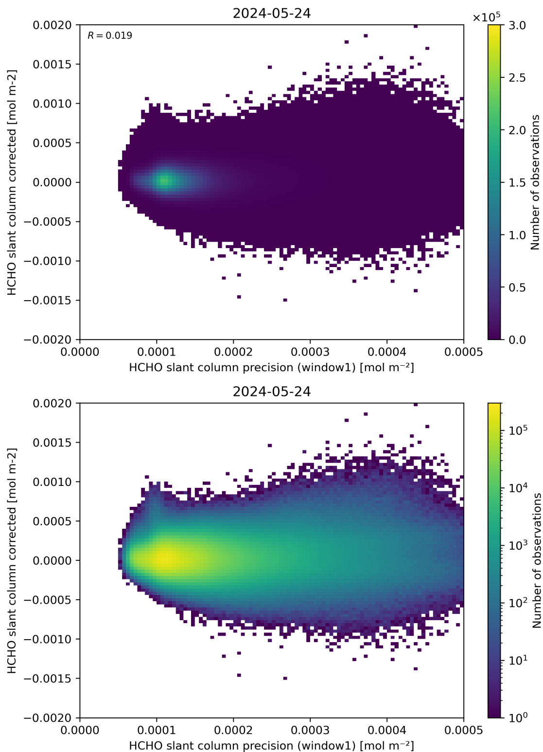
Figure 92: Scatter density plot of “HCHO slant column precision (window1)” against “HCHO slant column corrected” for 2024-05-23 to 2024-05-25.
