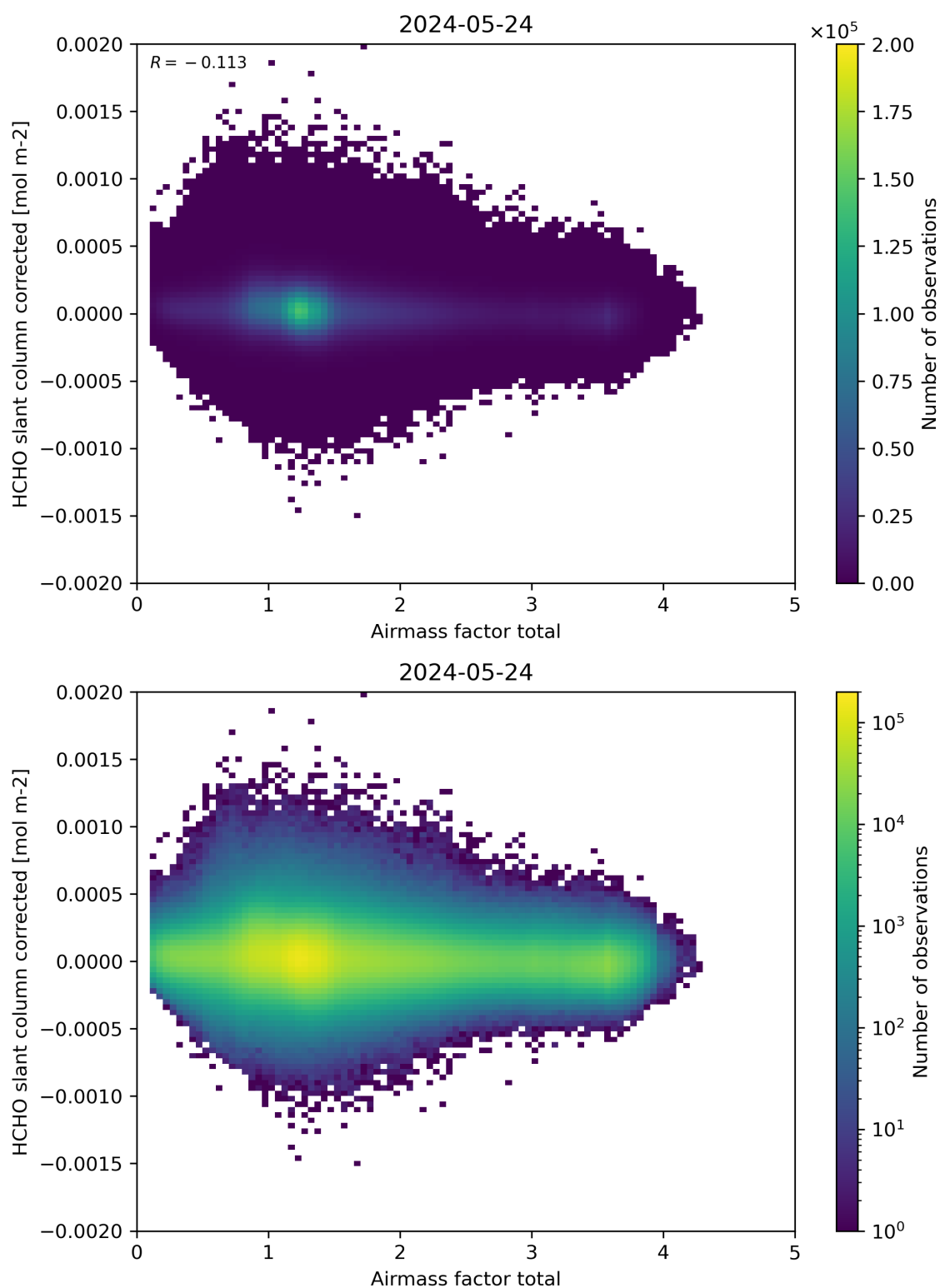
Figure 101: Scatter density plot of “Airmass factor total” against “HCHO slant column corrected” for 2024-05-23 to 2024-05-25.
