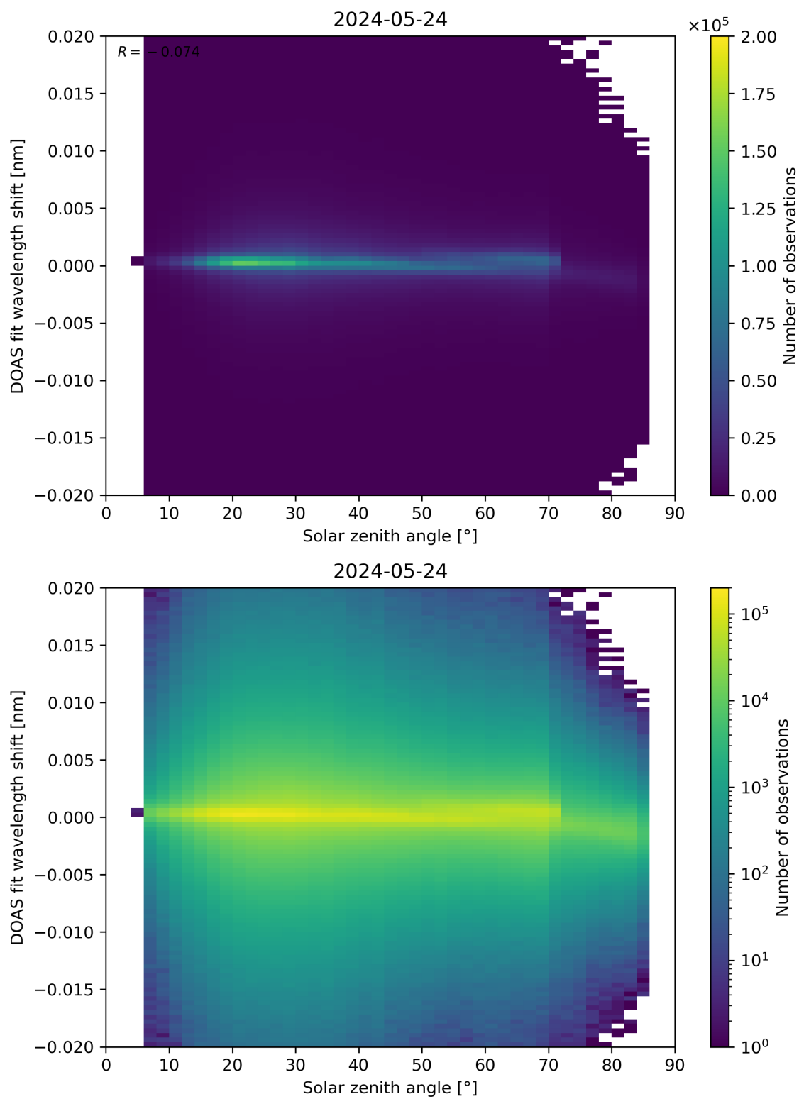
Figure 168: Scatter density plot of “Solar zenith angle” against “DOAS fit wavelength shift” for 2024-05-23 to 2024-05-25.
