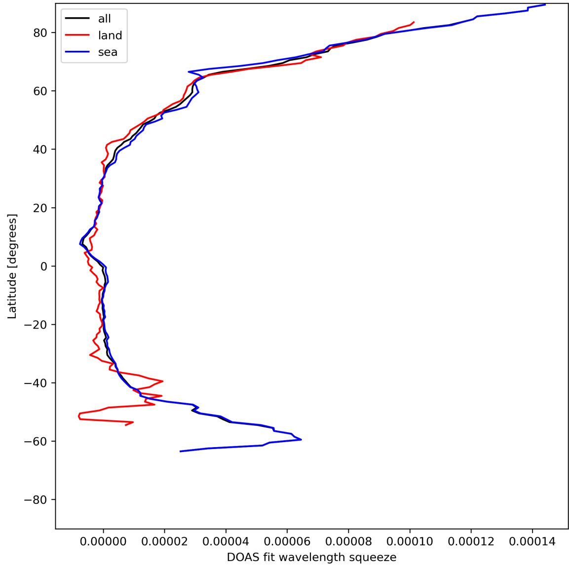
Figure 31: Zonal average of “DOAS fit wavelength squeeze” for 2024-05-23 to 2024-05-25.
