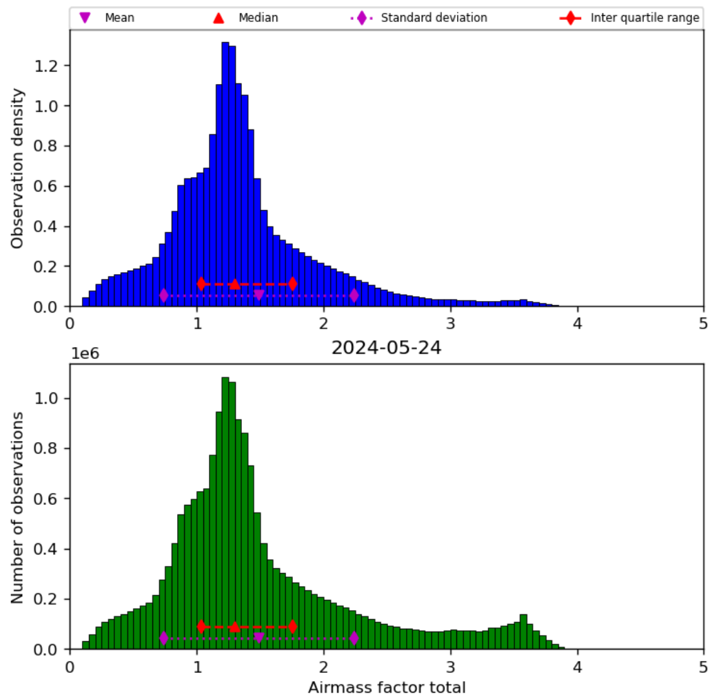
Figure 40: Histogram of “Airmass factor total” for 2024-05-23 to 2024-05-25
