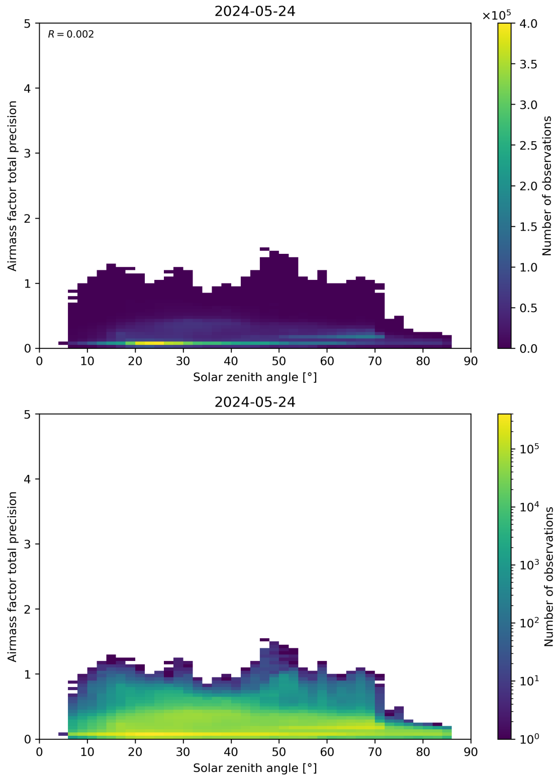
Figure 176: Scatter density plot of “Solar zenith angle” against “Airmass factor total precision” for 2024-05-23 to 2024-05-25.
