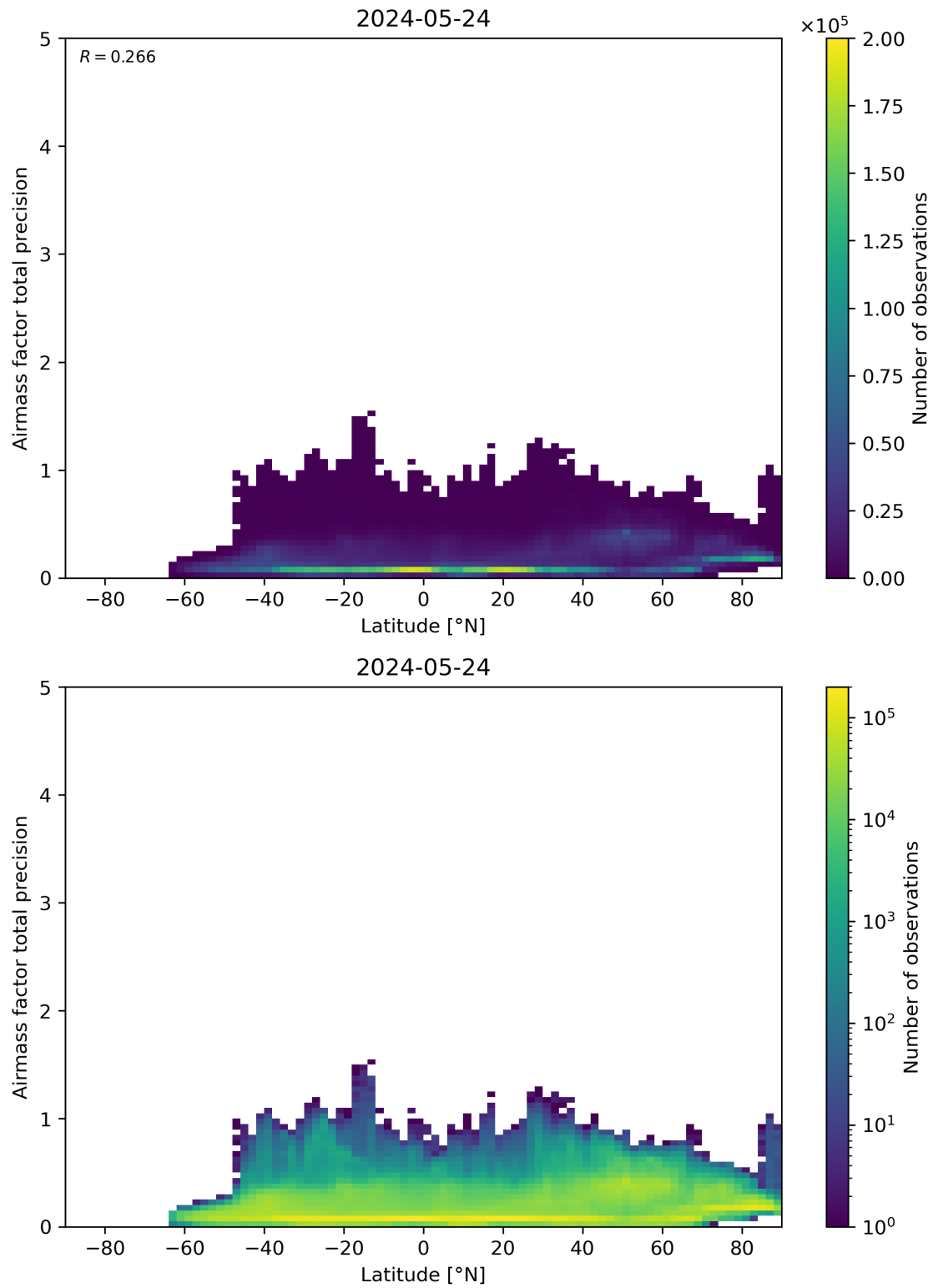
Figure 162: Scatter density plot of “Latitude” against “Airmass factor total precision” for 2024-05-23 to 2024-05-25.
