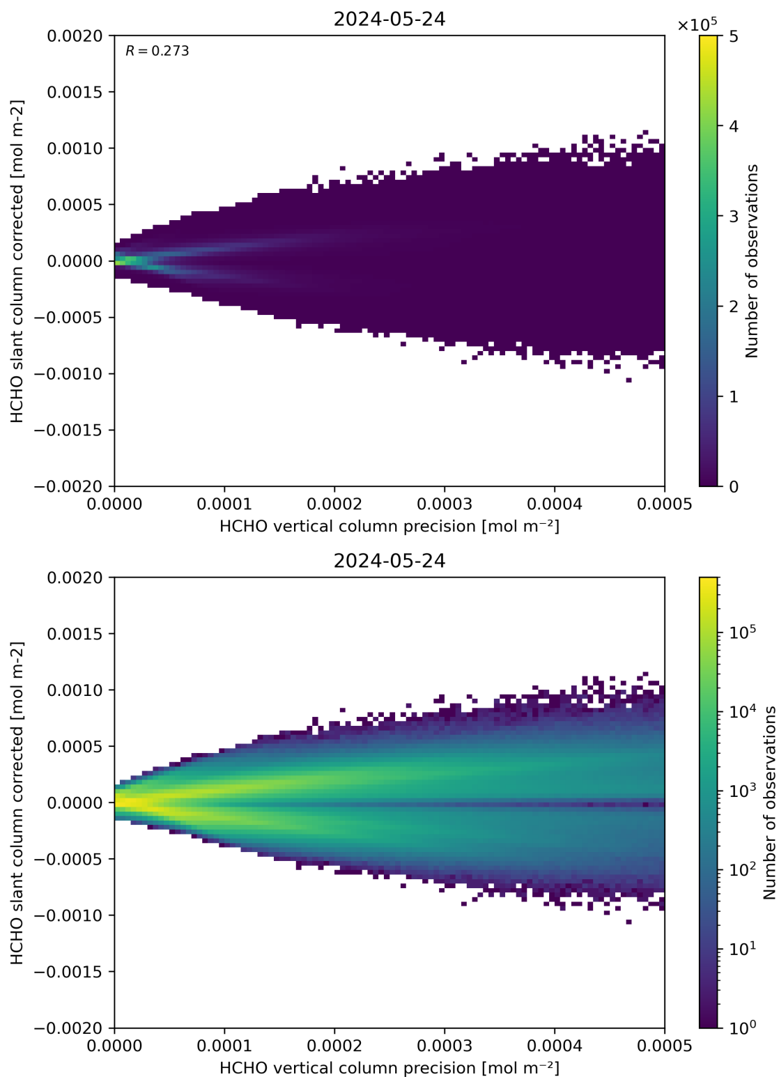
Figure 140: Scatter density plot of “HCHO vertical column precision” against “HCHO slant column corrected” for 2024-05-23 to 2024-05-25.
