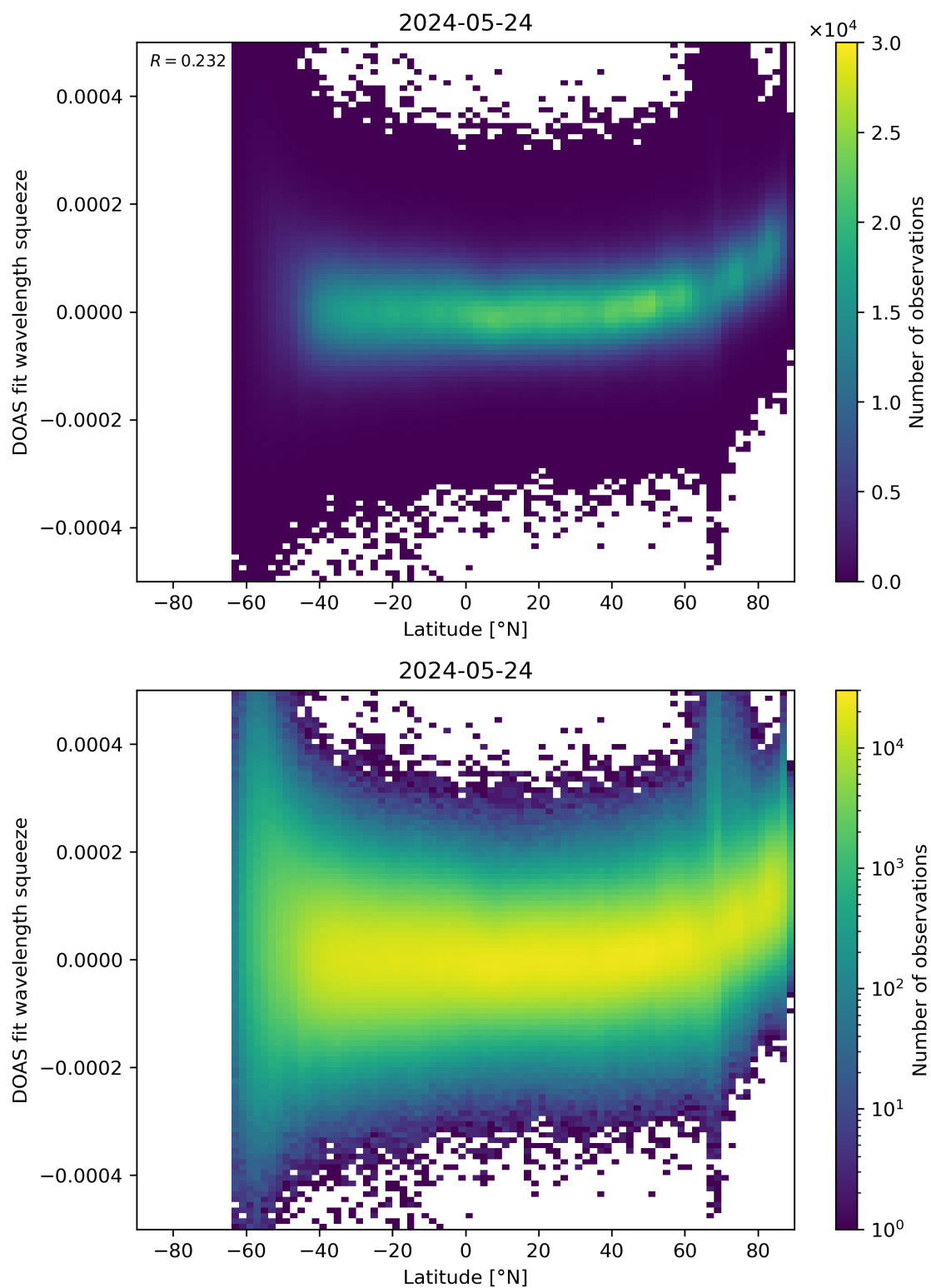
Figure 155: Scatter density plot of “Latitude” against “DOAS fit wavelength squeeze” for 2024-05-23 to 2024-05-25.
