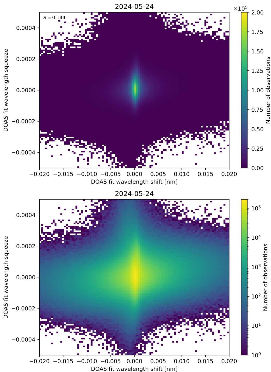
Figure 65: Scatter density plot of “DOAS fit wavelength shift” against “DOAS fit wavelength squeeze” for 2024-05-23 to 2024-05-25.
