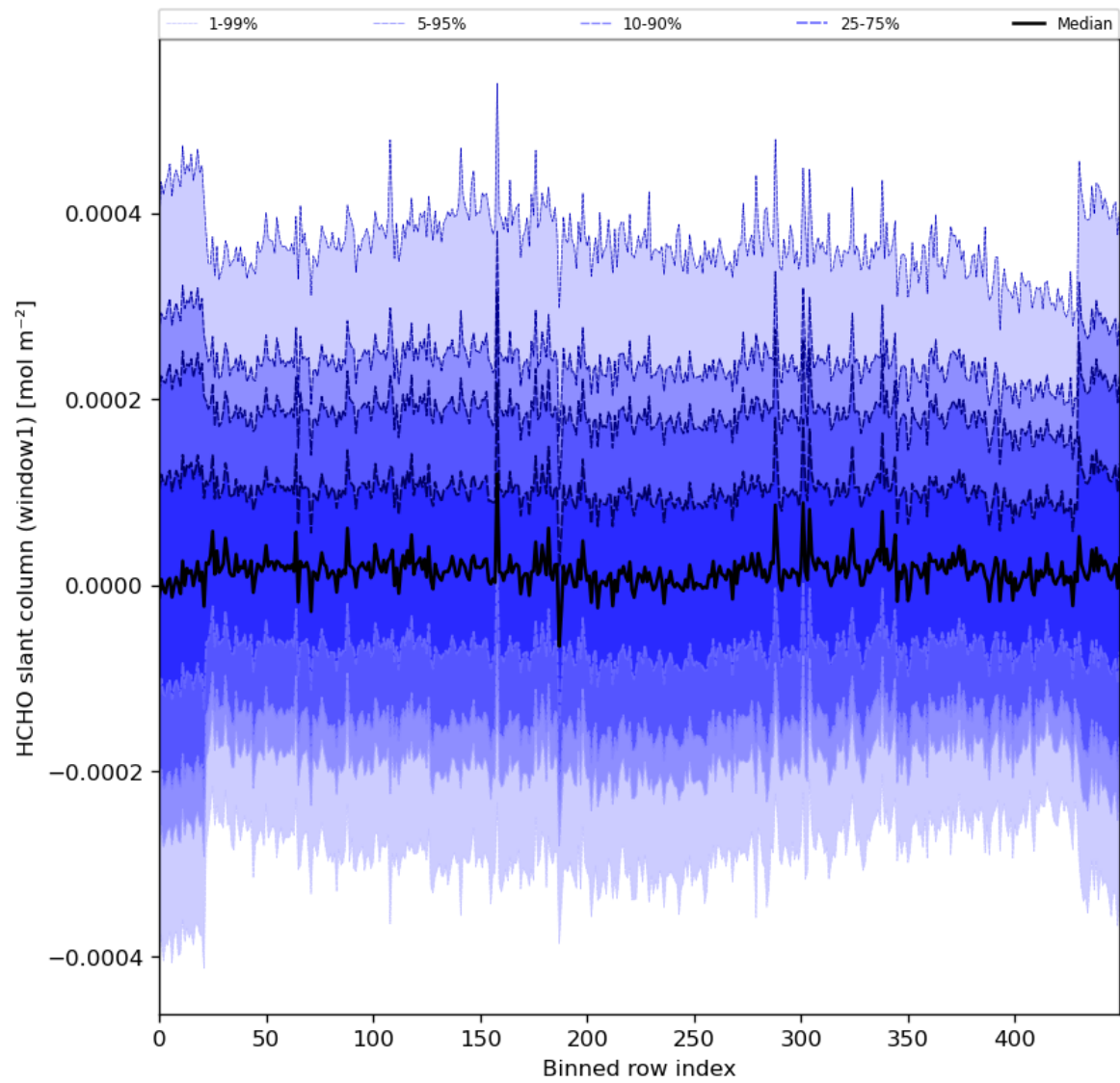
Figure 52: Along track statistics of “HCHO slant column (window1)” for 2024-05-23 to 2024-05-25
