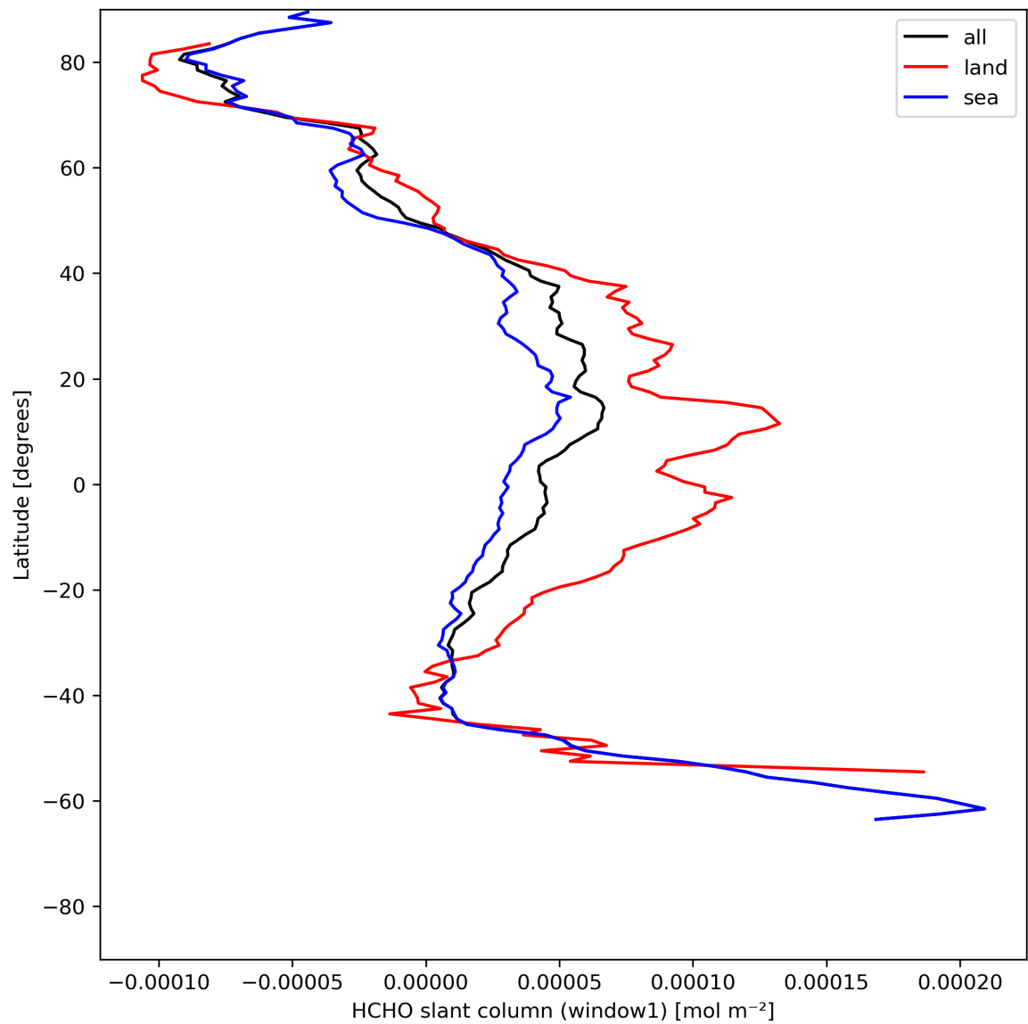
Figure 24: Zonal average of “HCHO slant column (window1)” for 2024-05-23 to 2024-05-25.
