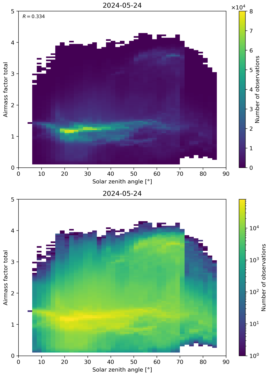
Figure 175: Scatter density plot of “Solar zenith angle” against “Airmass factor total” for 2024-05-23 to 2024-05-25.
