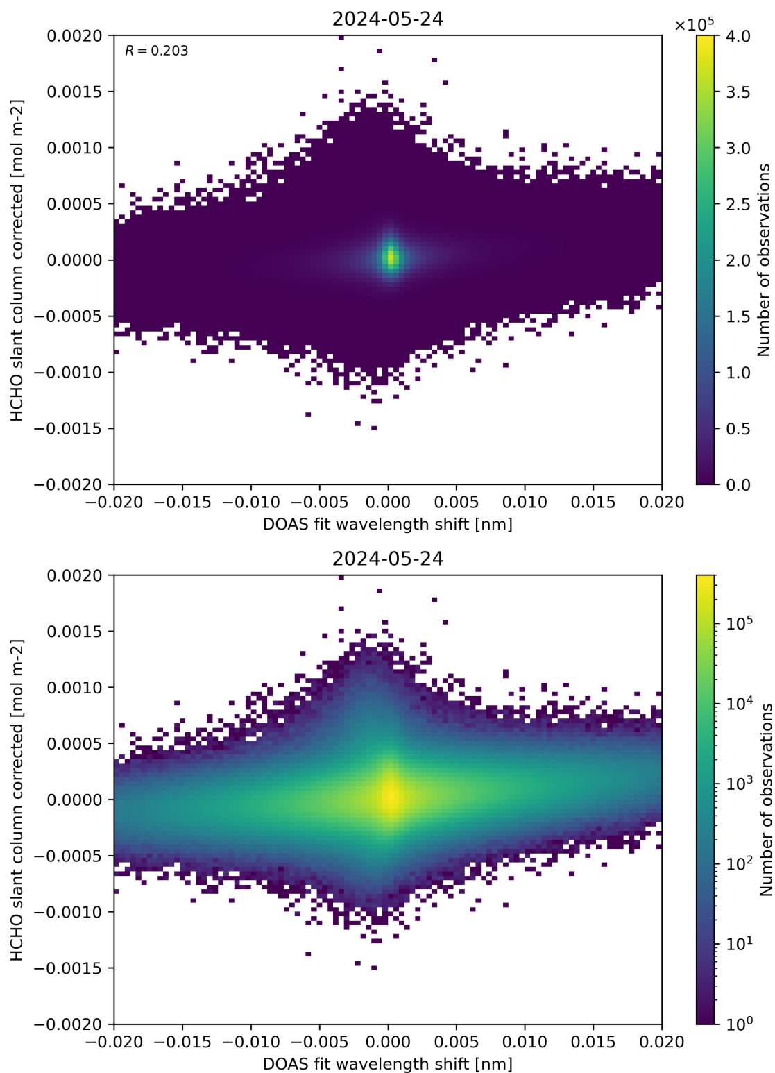
Figure 66: Scatter density plot of “DOAS fit wavelength shift” against “HCHO slant column corrected” for 2024-05-23 to 2024-05-25.
