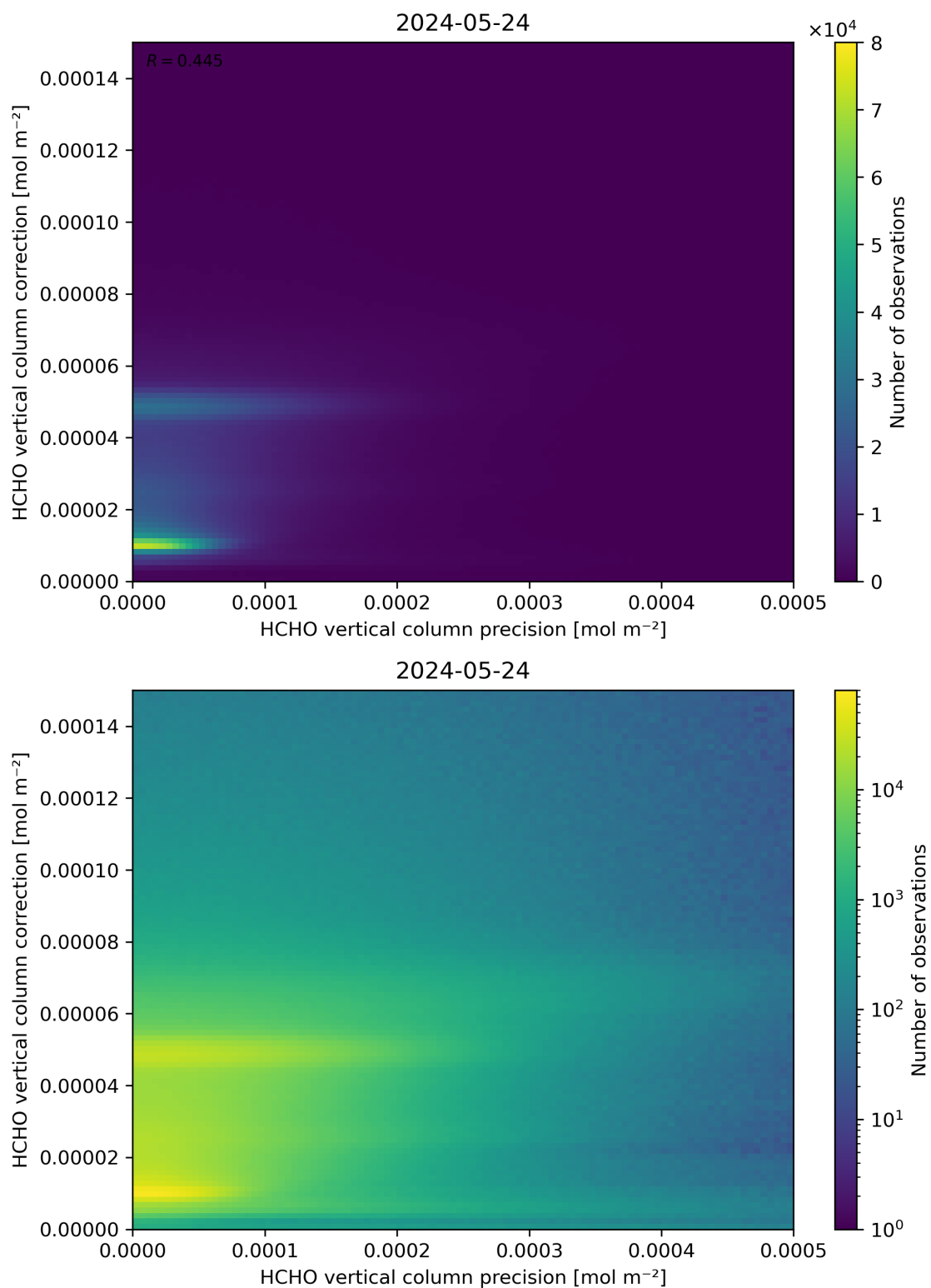
Figure 146: Scatter density plot of “HCHO vertical column precision” against “HCHO vertical column correction” for 2024-05-23 to 2024-05-25.
