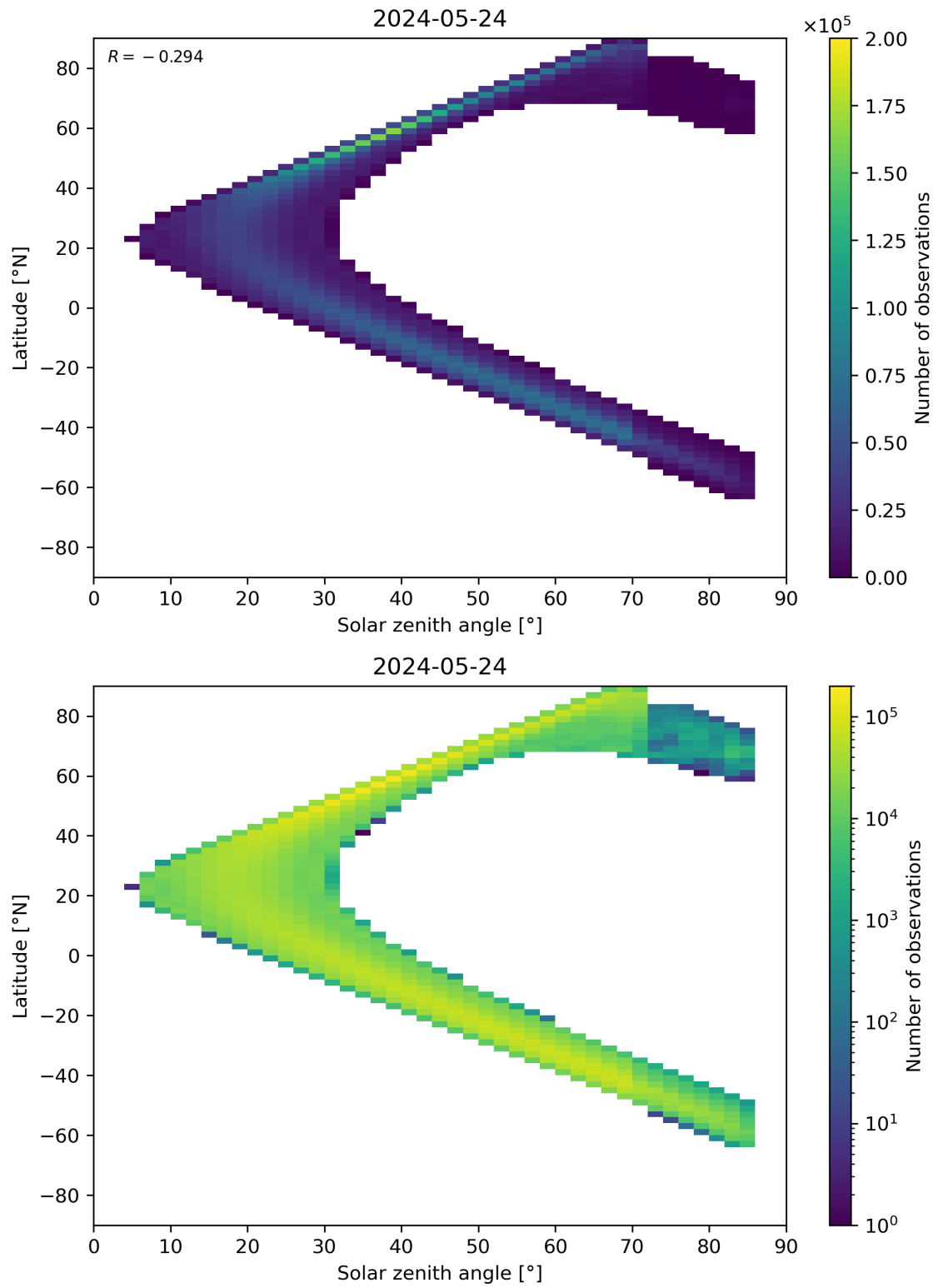
Figure 181: Scatter density plot of “Solar zenith angle” against “Latitude” for 2024-05-23 to 2024-05-25.
