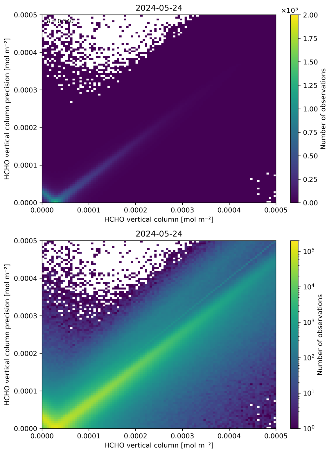
Figure 134: Scatter density plot of “HCHO vertical column” against “HCHO vertical column precision” for 2024-05-23 to 2024-05-25.
