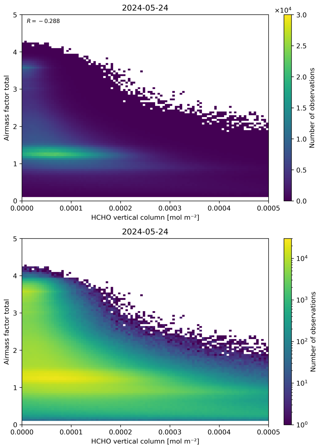
Figure 131: Scatter density plot of “HCHO vertical column” against “Airmass factor total” for 2024-05-23 to 2024-05-25.
