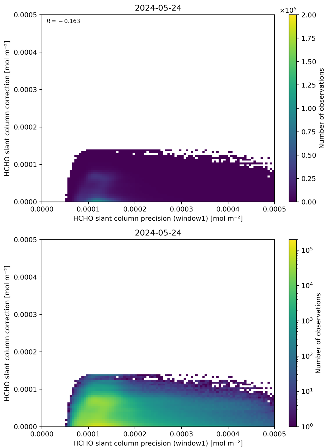
Figure 93: Scatter density plot of “HCHO slant column precision (window1)” against “HCHO slant column correction” for 2024-05-23 to 2024-05-25.
