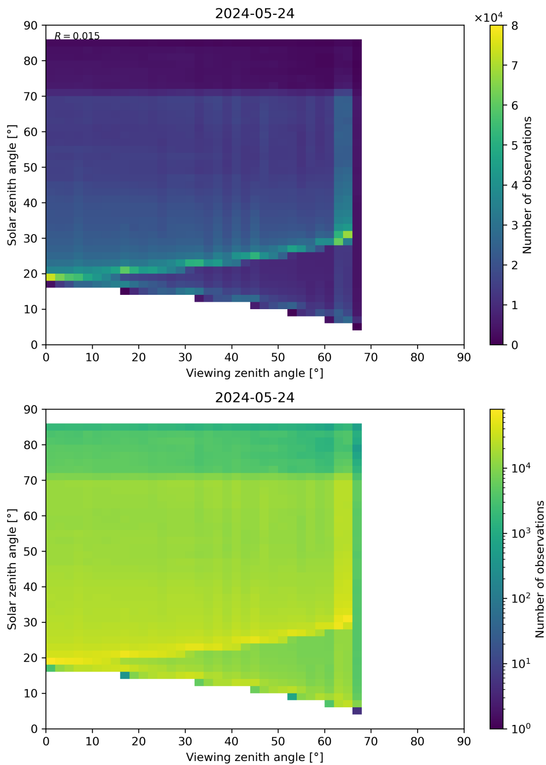
Figure 197: Scatter density plot of “Viewing zenith angle” against “Solar zenith angle” for 2024-05-23 to 2024-05-25.
