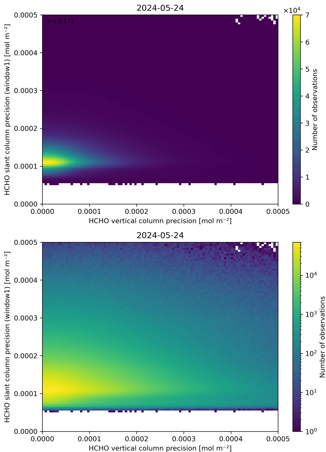
Figure 143: Scatter density plot of “HCHO vertical column precision” against “HCHO slant column precision (window1)” for 2024-05-23 to 2024-05-25.
