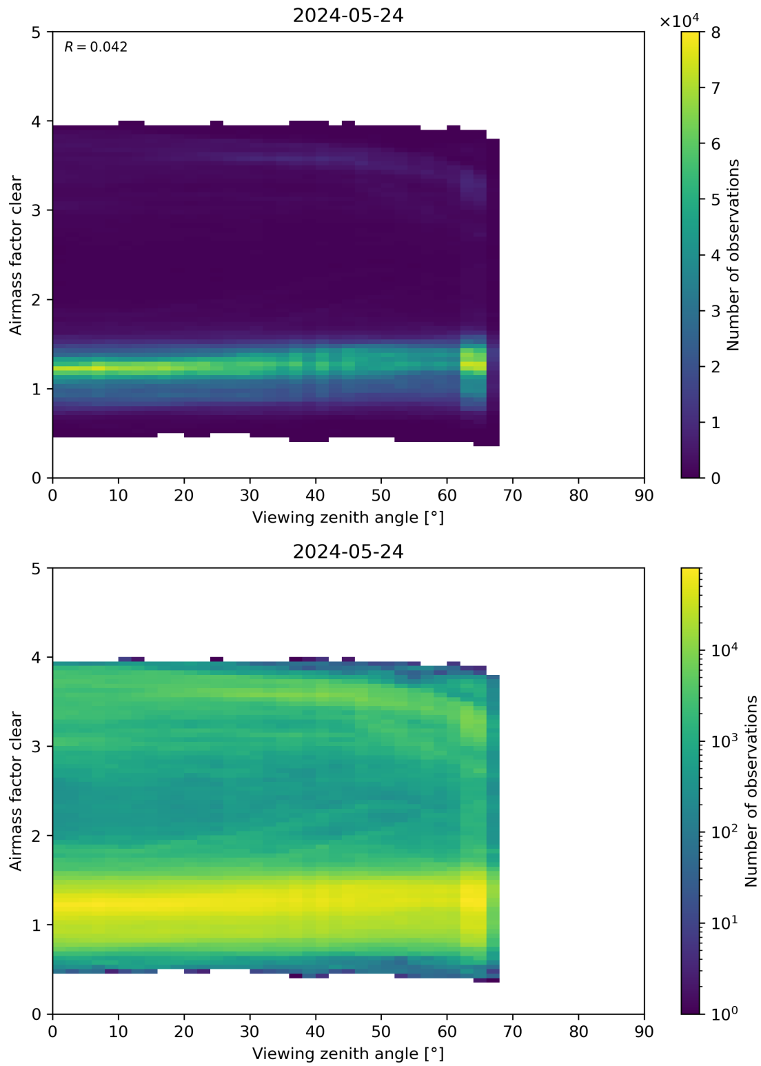
Figure 185: Scatter density plot of “Viewing zenith angle” against “Airmass factor clear” for 2024-05-23 to 2024-05-25.
