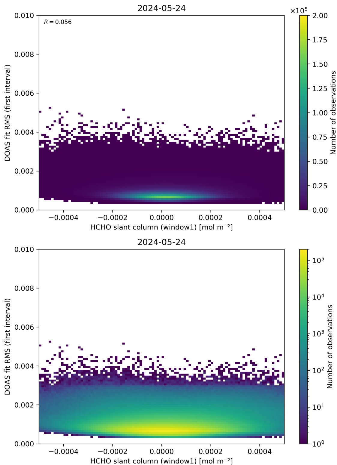
Figure 78: Scatter density plot of “HCHO slant column (window1)” against “DOAS fit RMS (first interval)” for 2024-05-23 to 2024-05-25.
