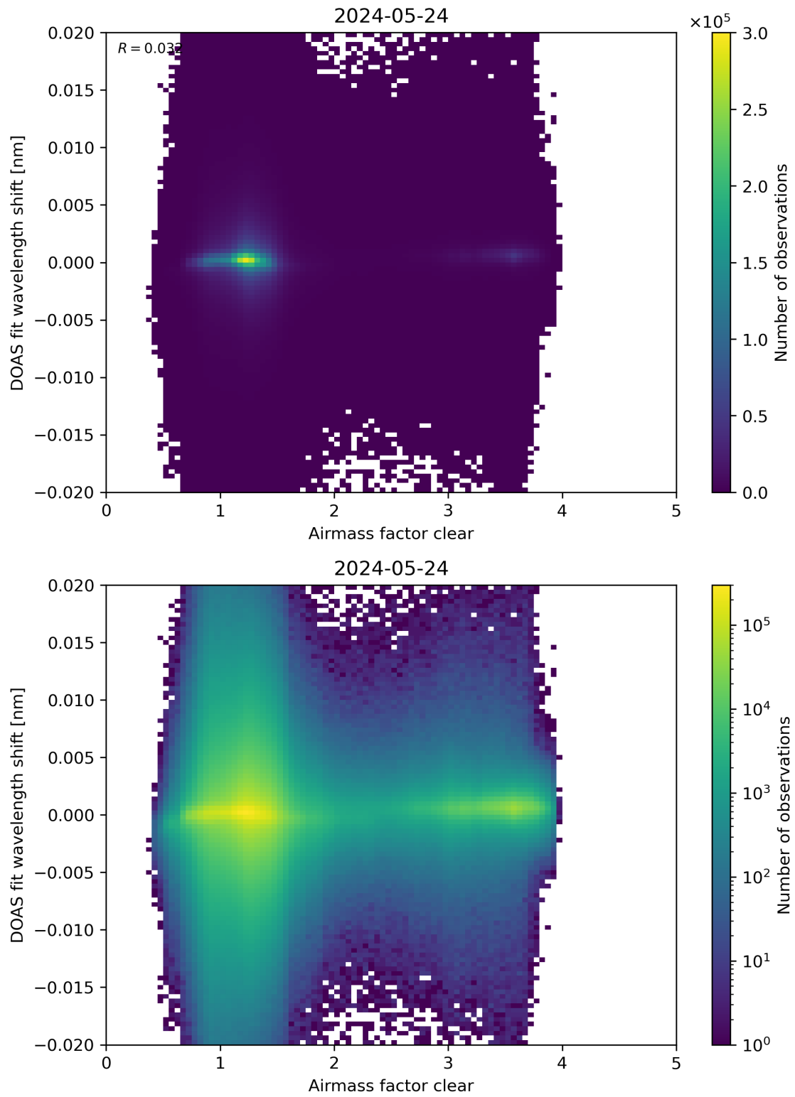
Figure 72: Scatter density plot of “Airmass factor clear” against “DOAS fit wavelength shift” for 2024-05-23 to 2024-05-25.
