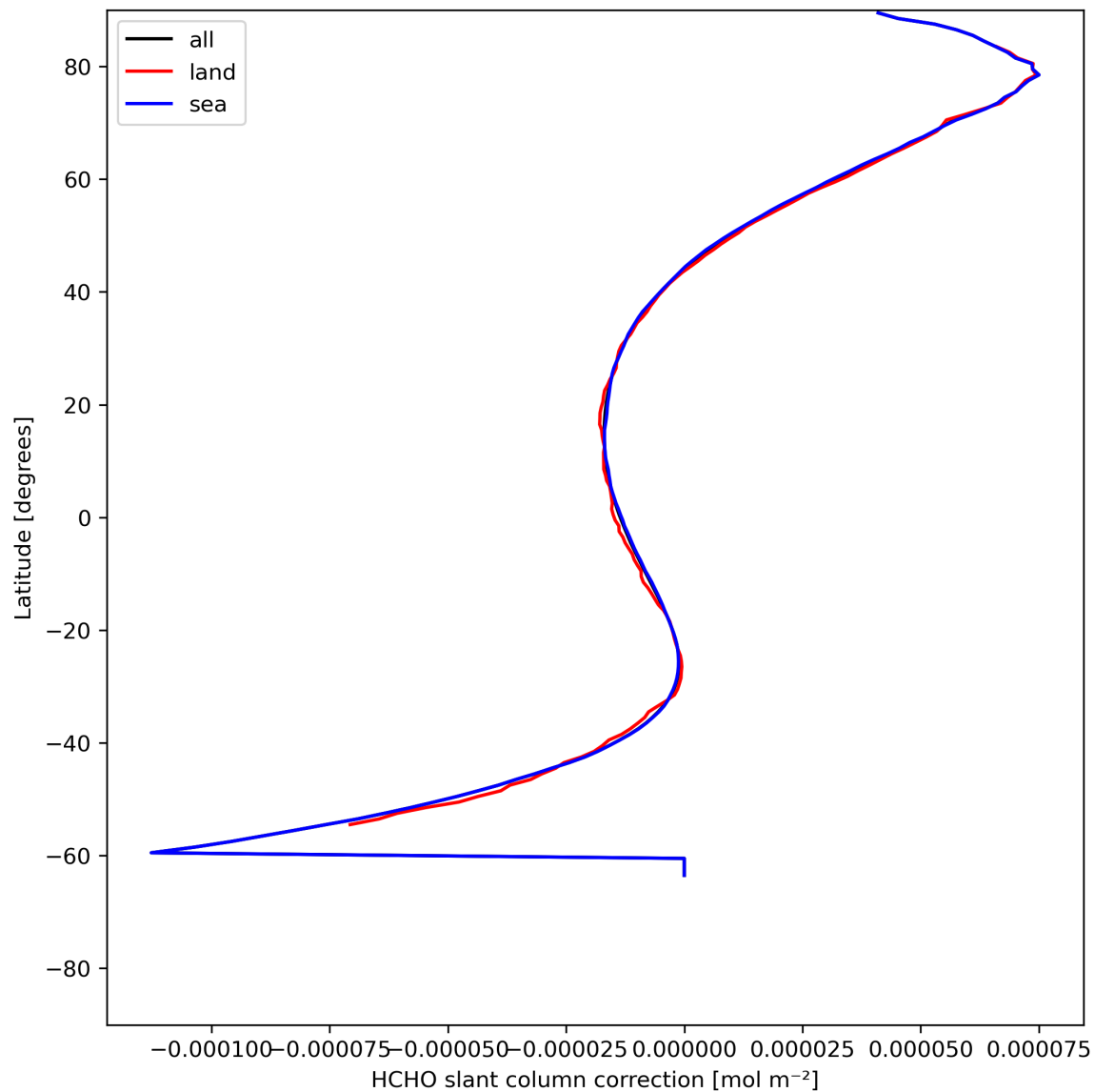
Figure 33: Zonal average of “HCHO slant column correction” for 2024-05-23 to 2024-05-25.
