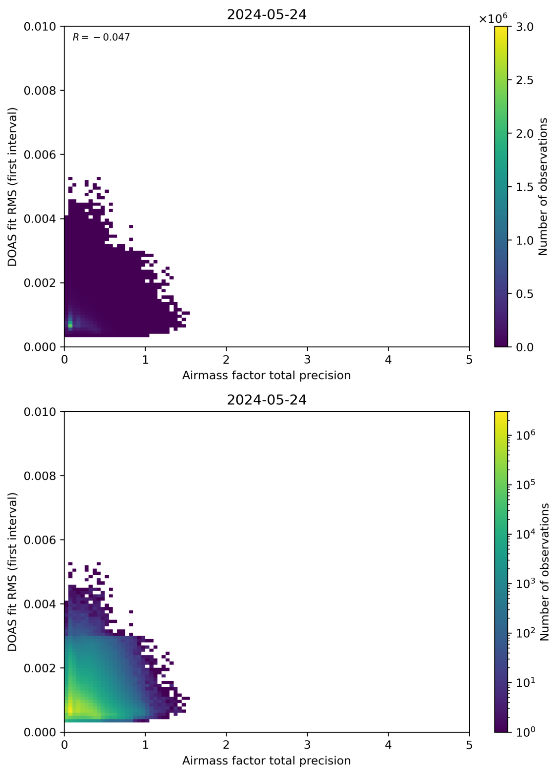
Figure 105: Scatter density plot of “Airmass factor total precision” against “DOAS fit RMS (first interval)” for 2024-05-23 to 2024-05-25.
