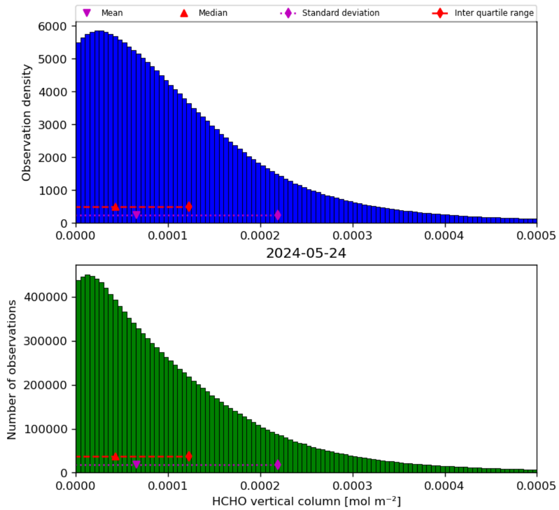
Figure 35: Histogram of “HCHO vertical column” for 2024-05-23 to 2024-05-25
