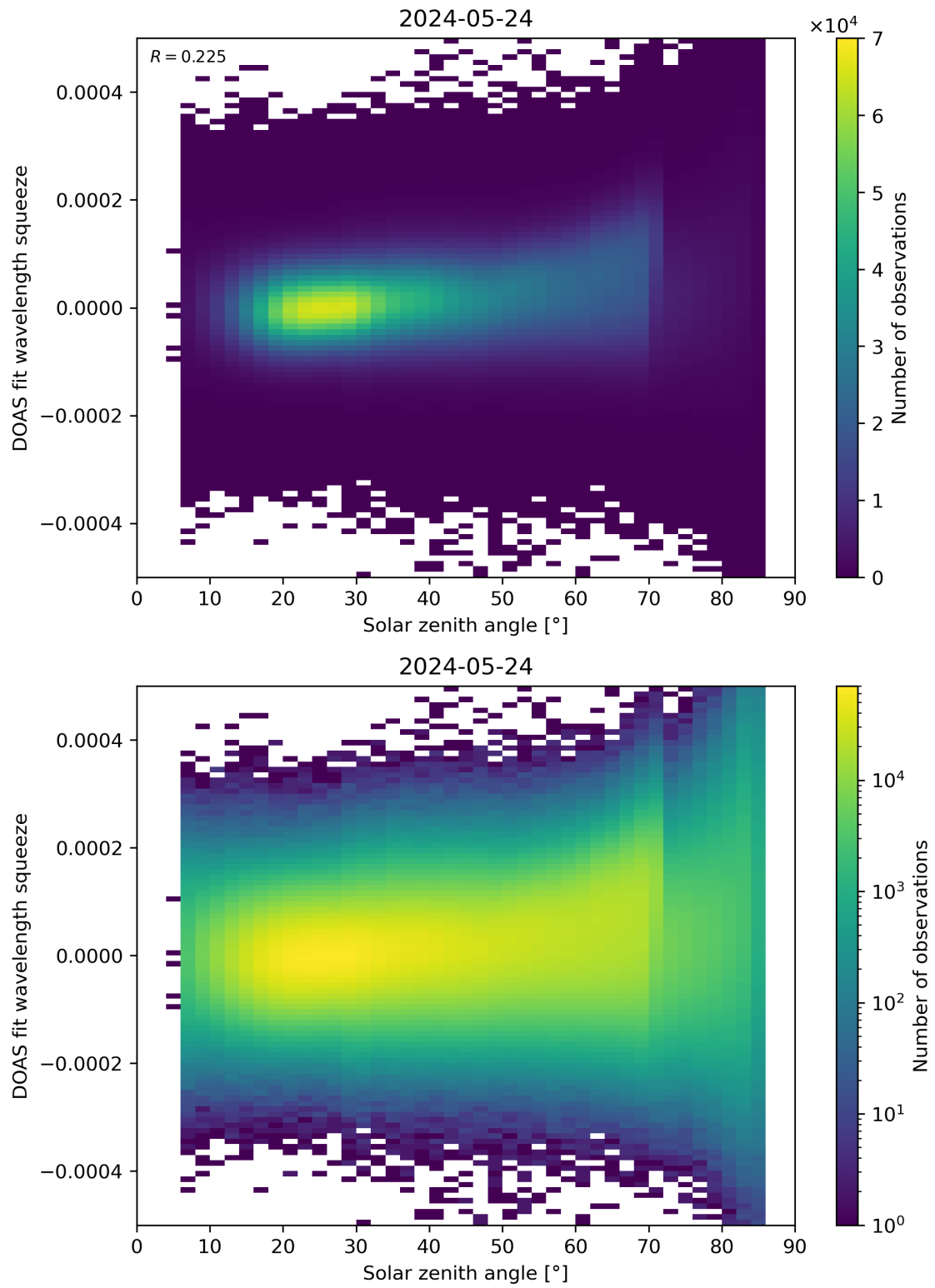
Figure 169: Scatter density plot of “Solar zenith angle” against “DOAS fit wavelength squeeze” for 2024-05-23 to 2024-05-25.
