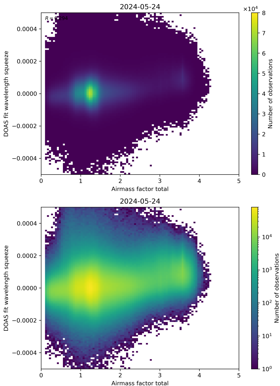
Figure 99: Scatter density plot of “Airmass factor total” against “DOAS fit wavelength squeeze” for 2024-05-23 to 2024-05-25.
