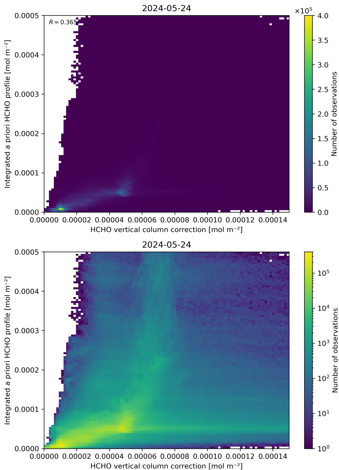
Figure 122: Scatter density plot of “HCHO vertical column correction” against “Integrated a priori HCHO profile” for 2024-05-23 to 2024-05-25.
