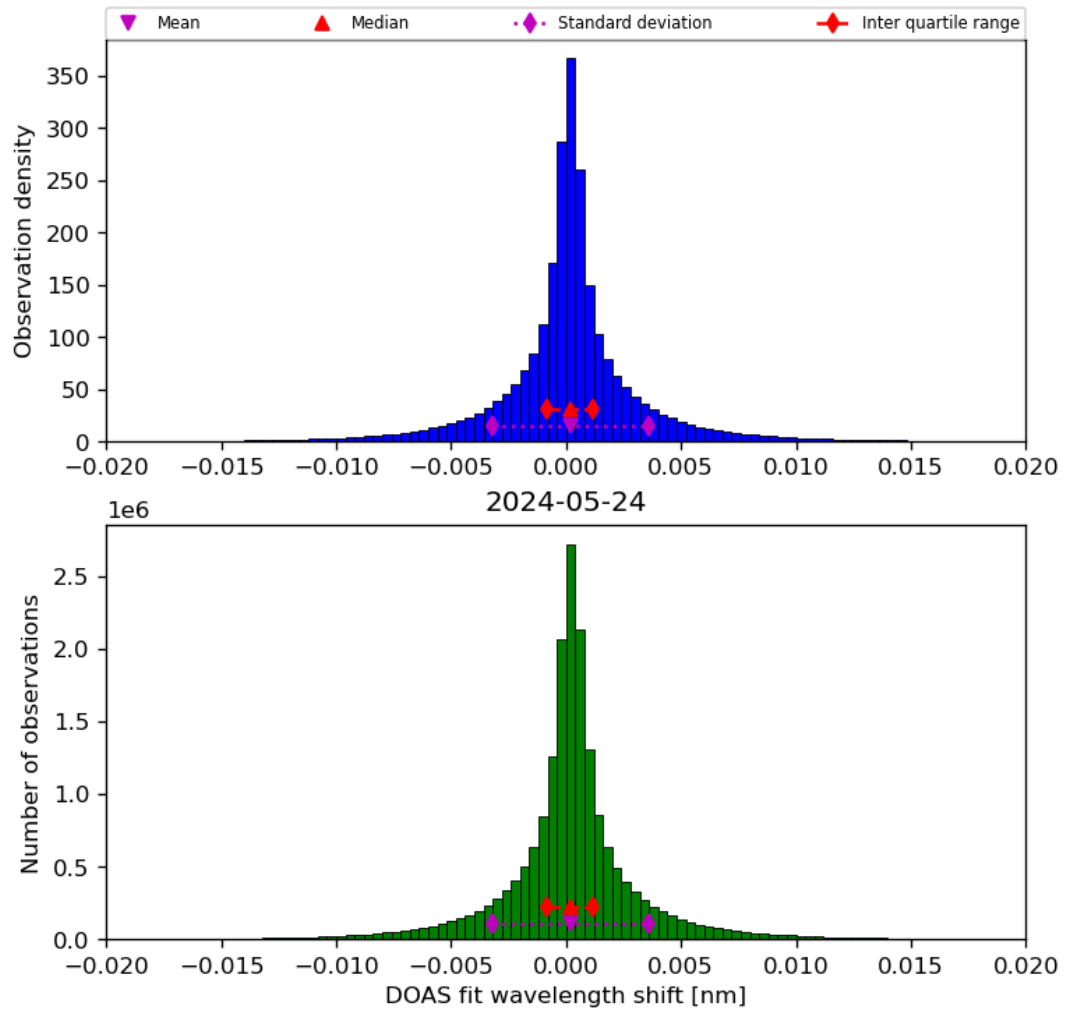
Figure 44: Histogram of “DOAS fit wavelength shift” for 2024-05-23 to 2024-05-25
