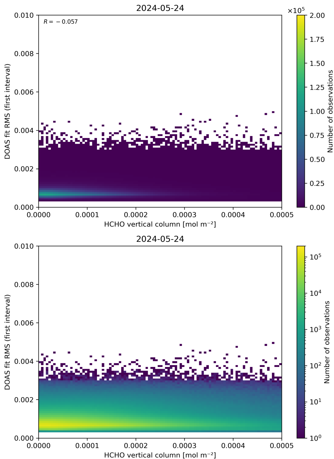
Figure 123: Scatter density plot of “HCHO vertical column” against “DOAS fit RMS (first interval)” for 2024-05-23 to 2024-05-25.
