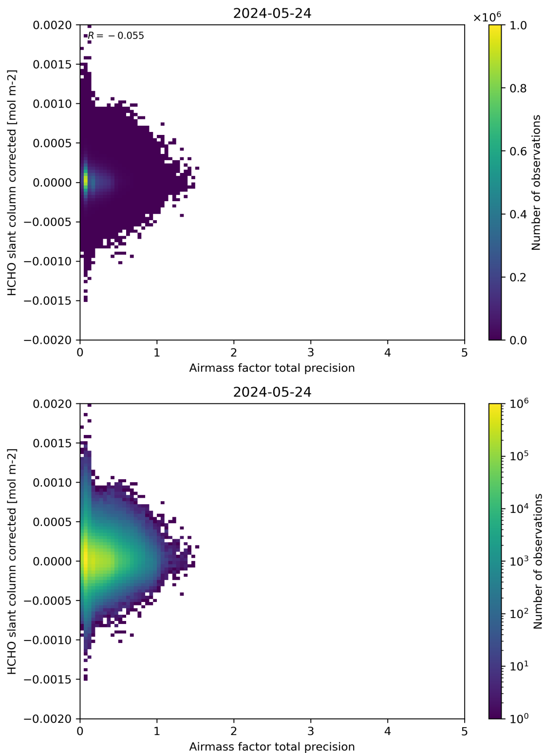
Figure 109: Scatter density plot of “Airmass factor total precision” against “HCHO slant column corrected” for 2024-05-23 to 2024-05-25.
