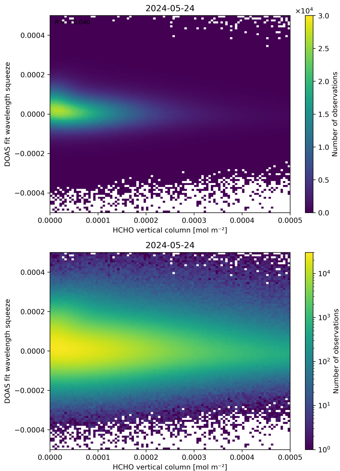
Figure 125: Scatter density plot of “HCHO vertical column” against “DOAS fit wavelength squeeze” for 2024-05-23 to 2024-05-25.
