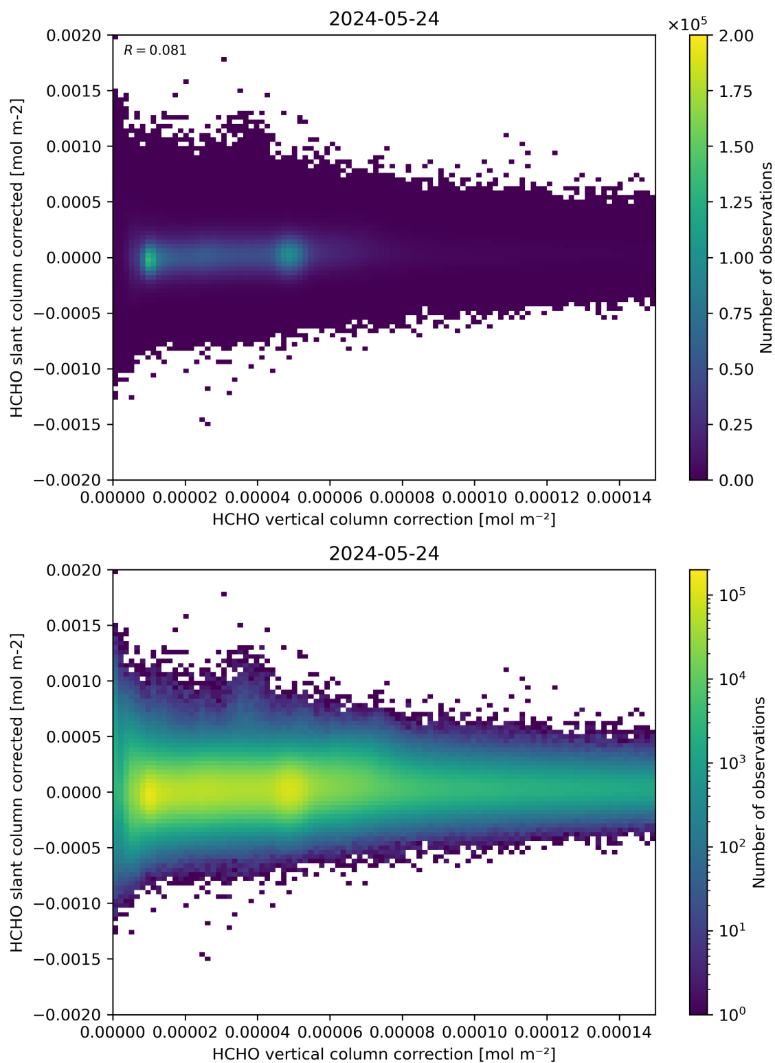
Figure 116: Scatter density plot of “HCHO vertical column correction” against “HCHO slant column corrected” for 2024-05-23 to 2024-05-25.
