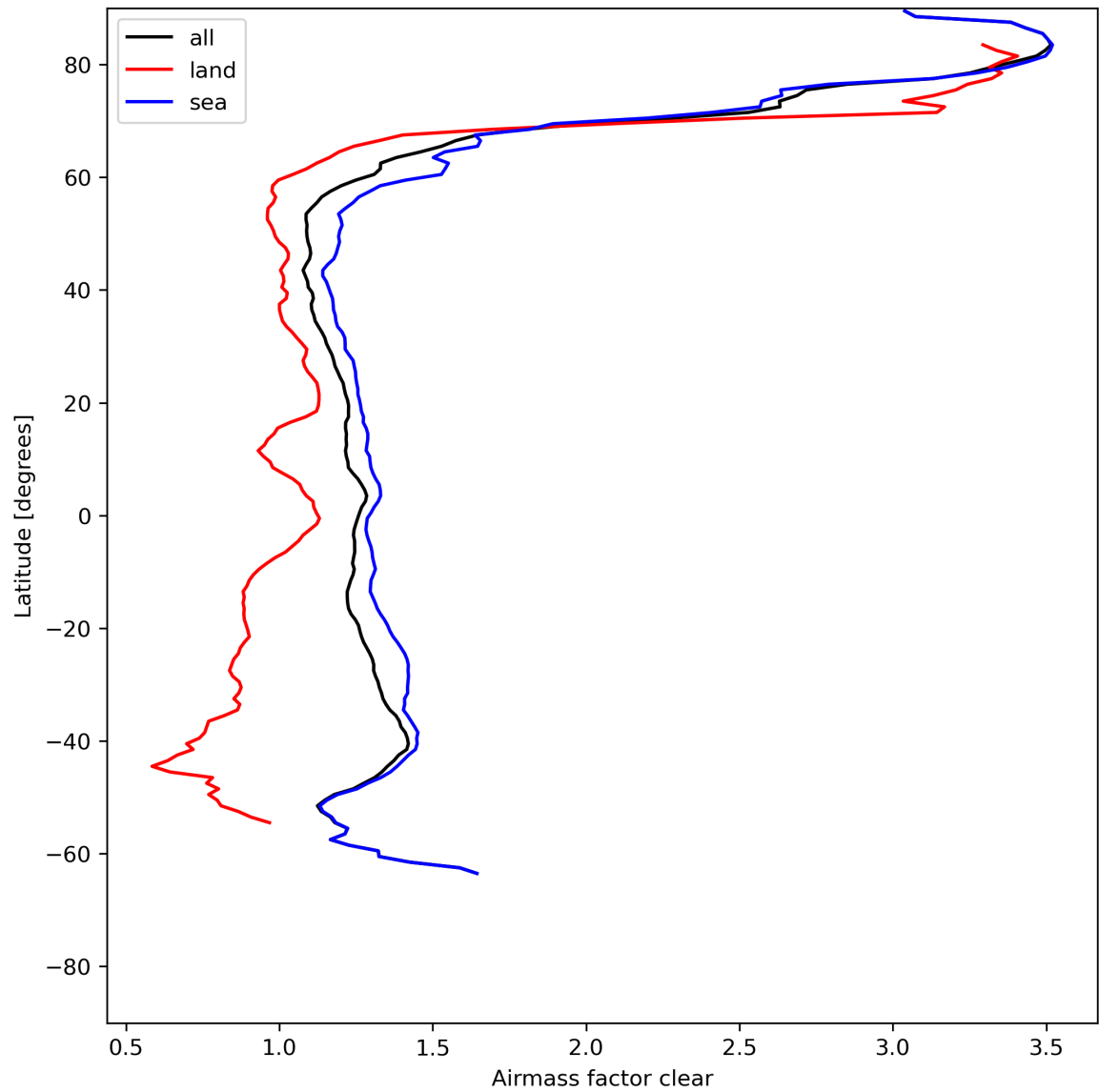
Figure 28: Zonal average of “Airmass factor clear” for 2024-05-23 to 2024-05-25.
