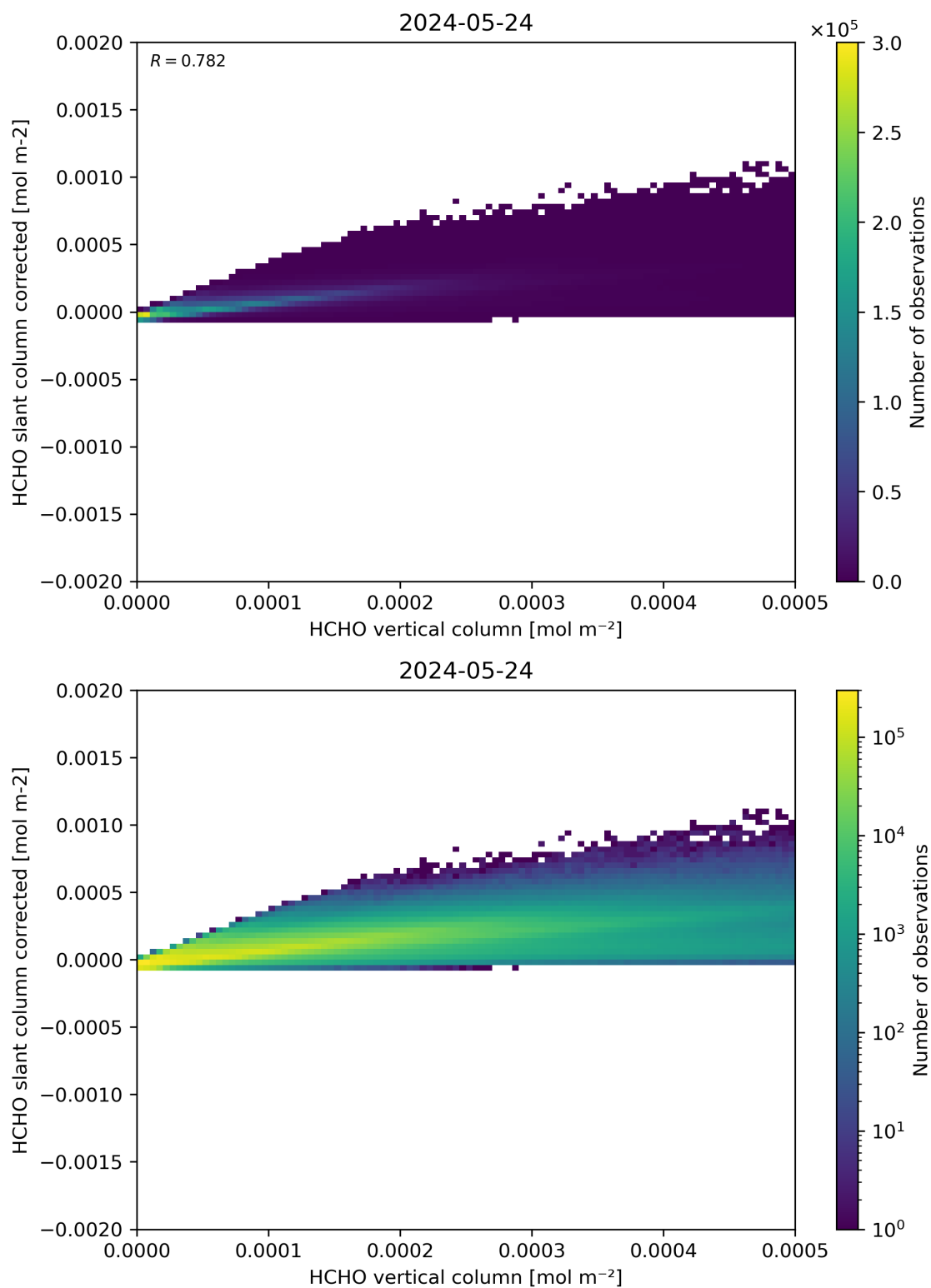
Figure 127: Scatter density plot of “HCHO vertical column” against “HCHO slant column corrected” for 2024-05-23 to 2024-05-25.
