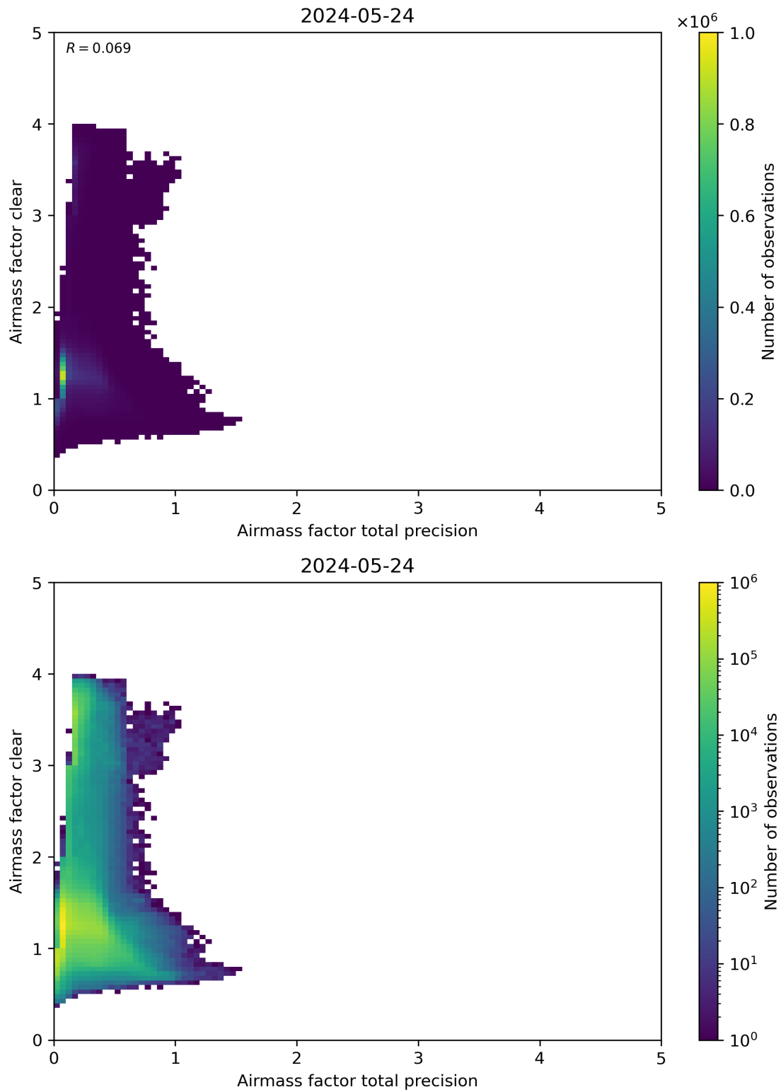
Figure 108: Scatter density plot of “Airmass factor total precision” against “Airmass factor clear” for 2024-05-23 to 2024-05-25.
