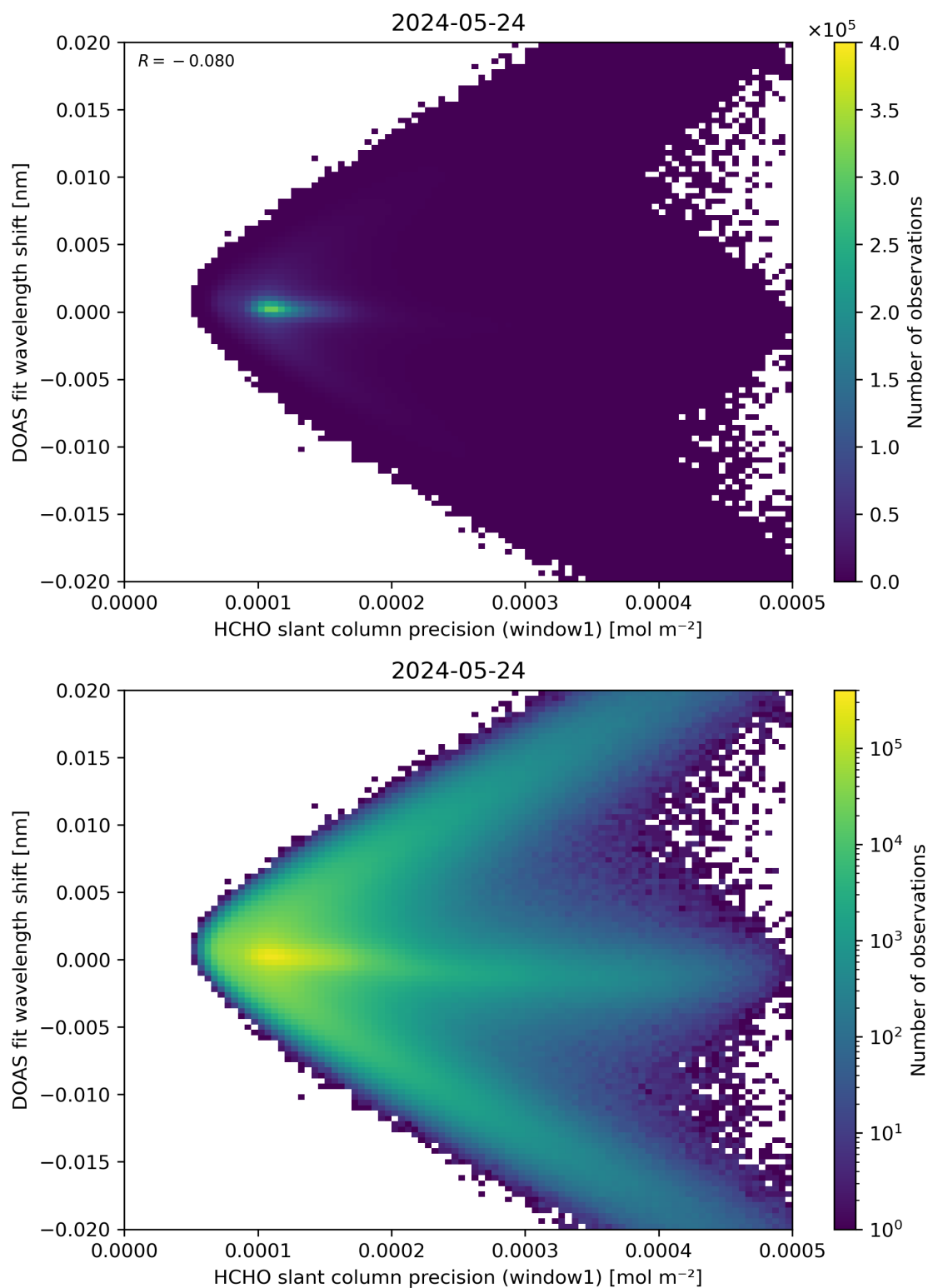
Figure 89: Scatter density plot of “HCHO slant column precision (window1)” against “DOAS fit wavelength shift” for 2024-05-23 to 2024-05-25.
