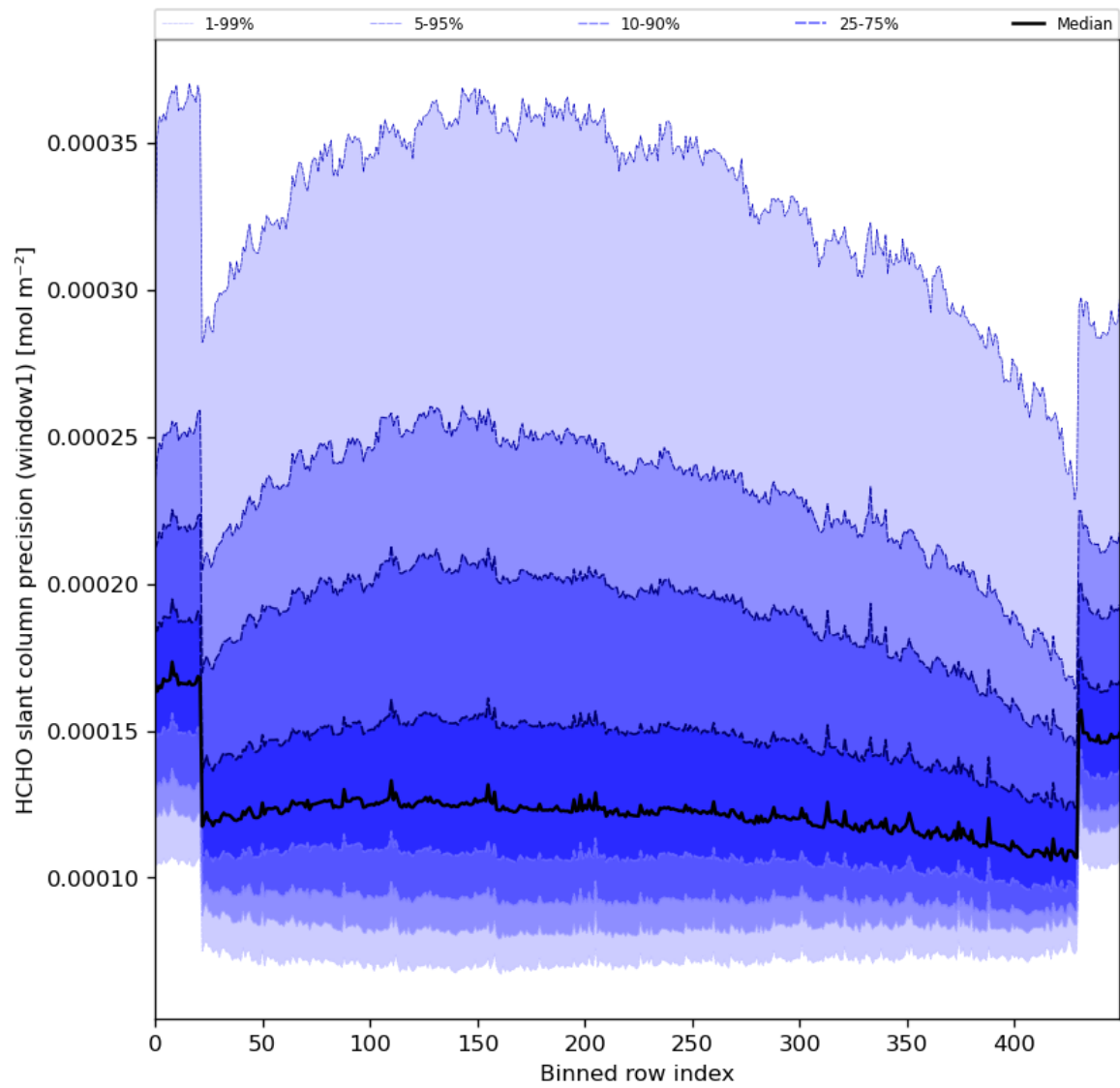
Figure 53: Along track statistics of “HCHO slant column precision (window1)” for 2024-05-23 to 2024-05-25
