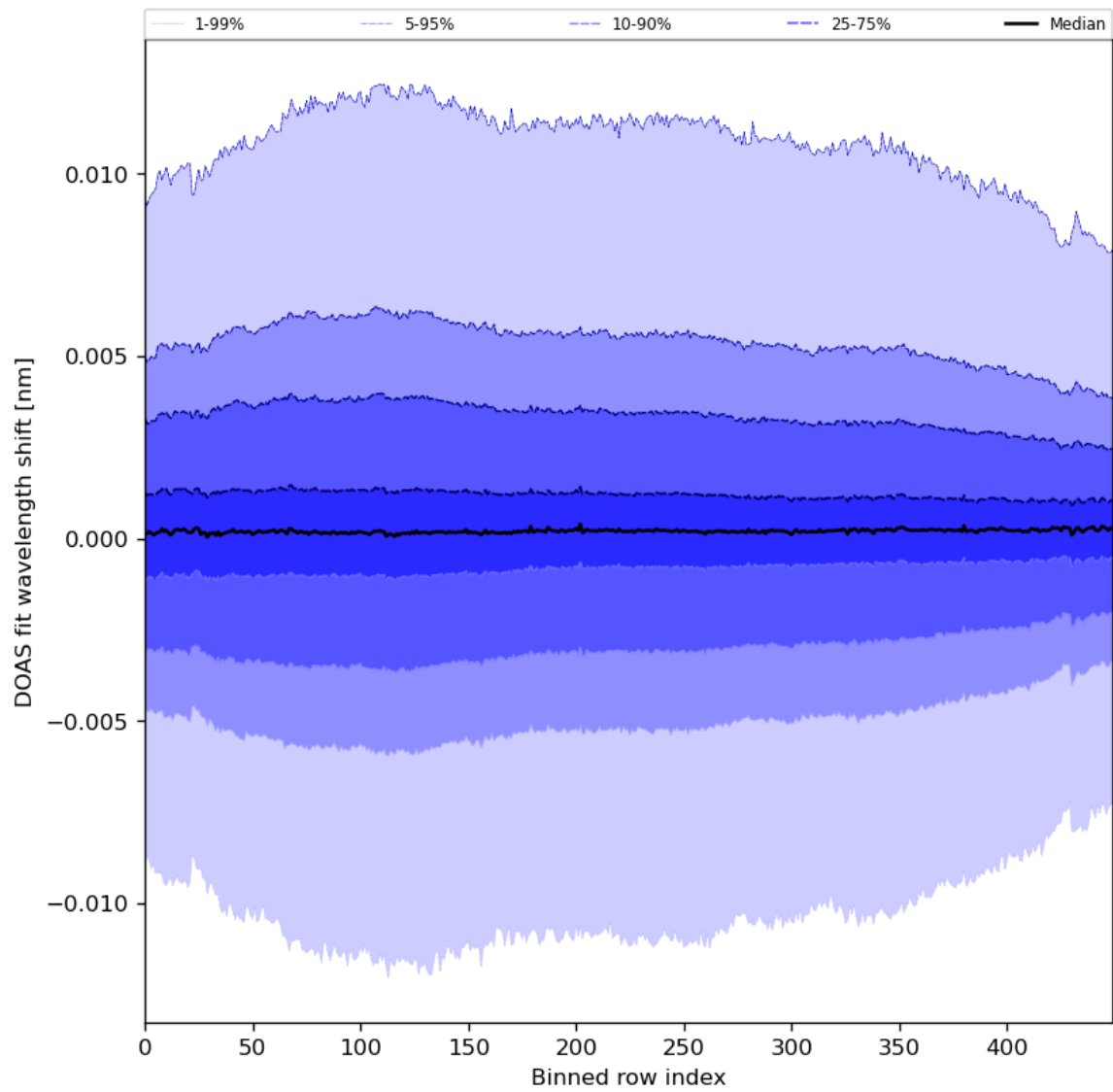
Figure 58: Along track statistics of “DOAS fit wavelength shift” for 2024-05-23 to 2024-05-25
