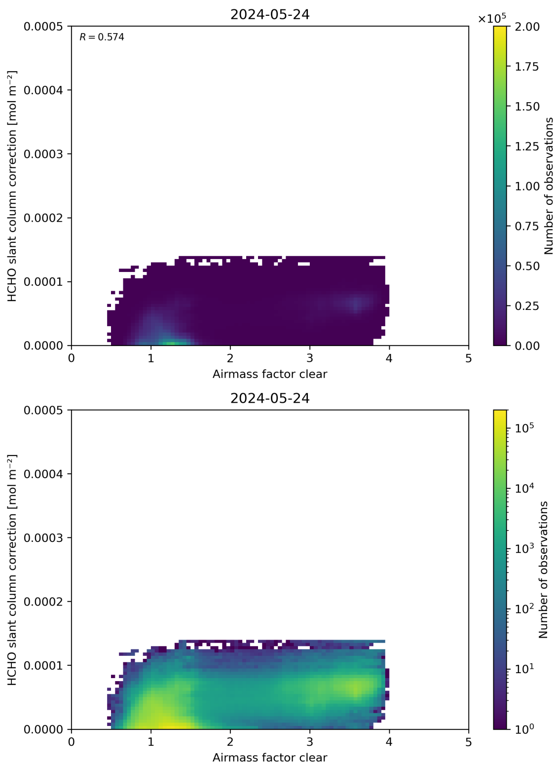
Figure 75: Scatter density plot of “Airmass factor clear” against “HCHO slant column correction” for 2024-05-23 to 2024-05-25.
