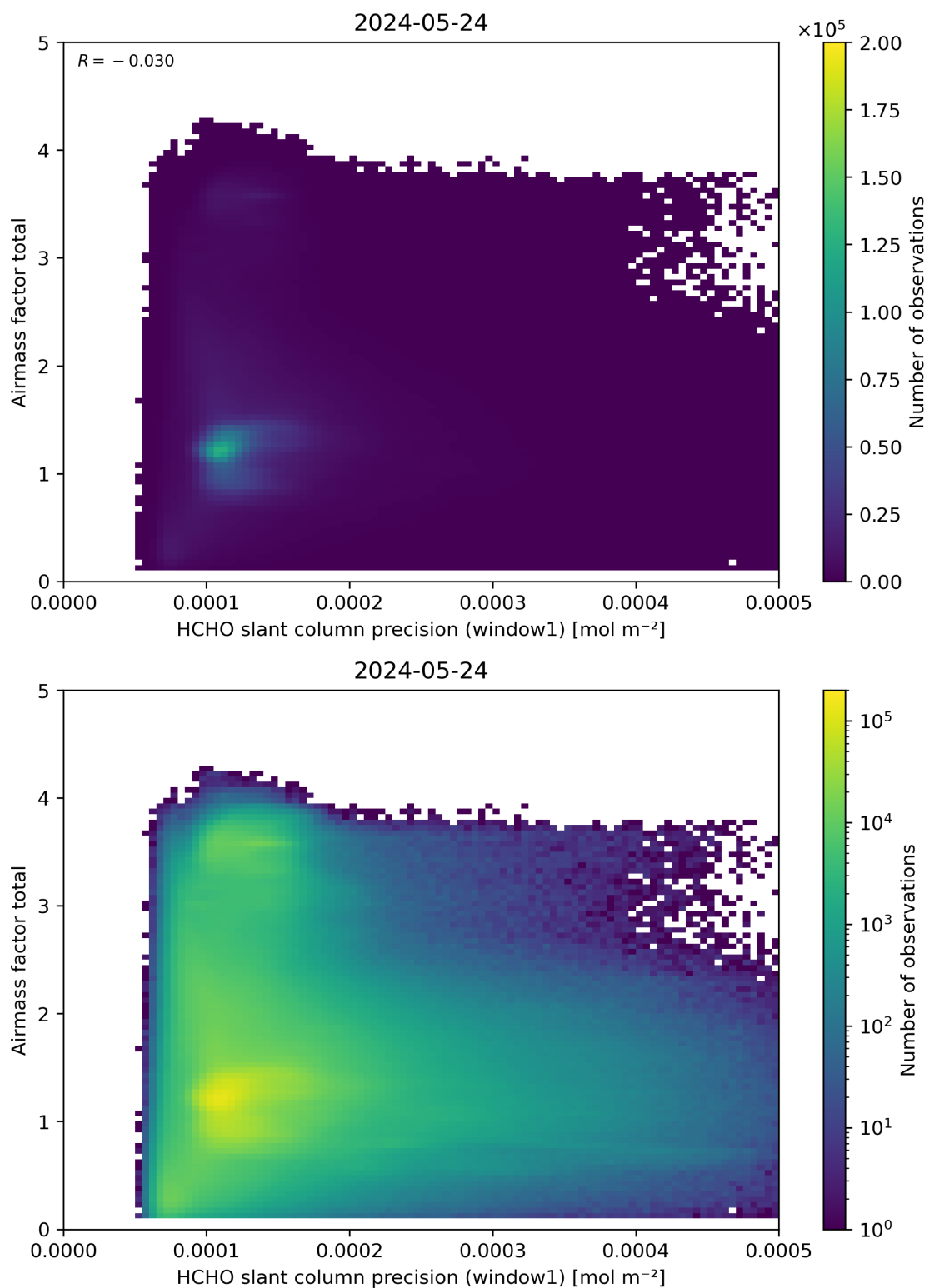
Figure 94: Scatter density plot of “HCHO slant column precision (window1)” against “Airmass factor total” for 2024-05-23 to 2024-05-25.
