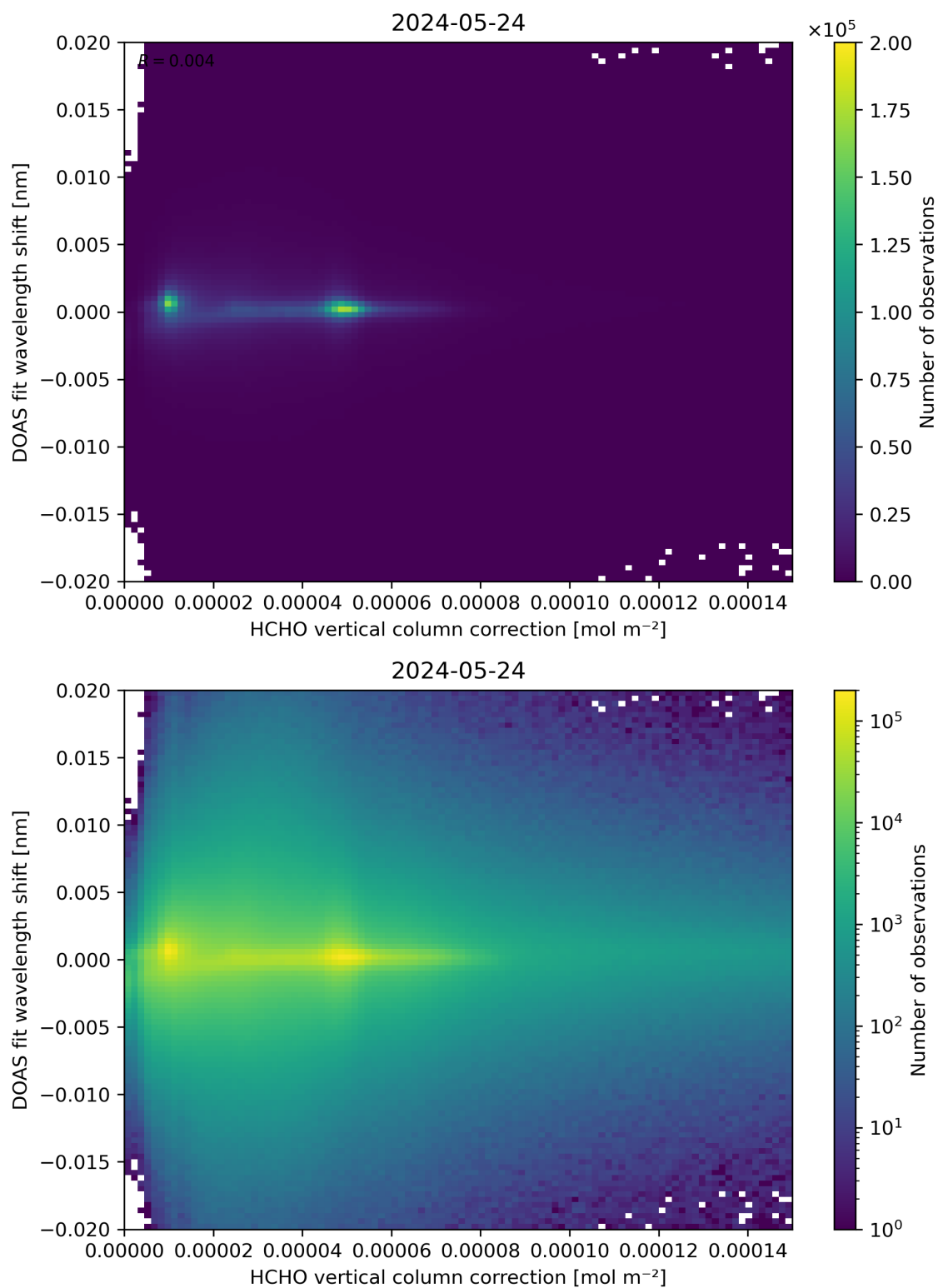
Figure 113: Scatter density plot of “HCHO vertical column correction” against “DOAS fit wavelength shift” for 2024-05-23 to 2024-05-25.
