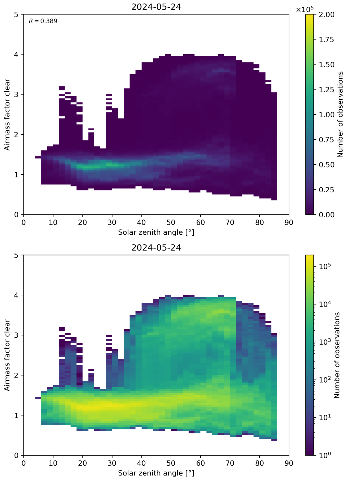
Figure 170: Scatter density plot of “Solar zenith angle” against “Airmass factor clear” for 2024-05-23 to 2024-05-25.
