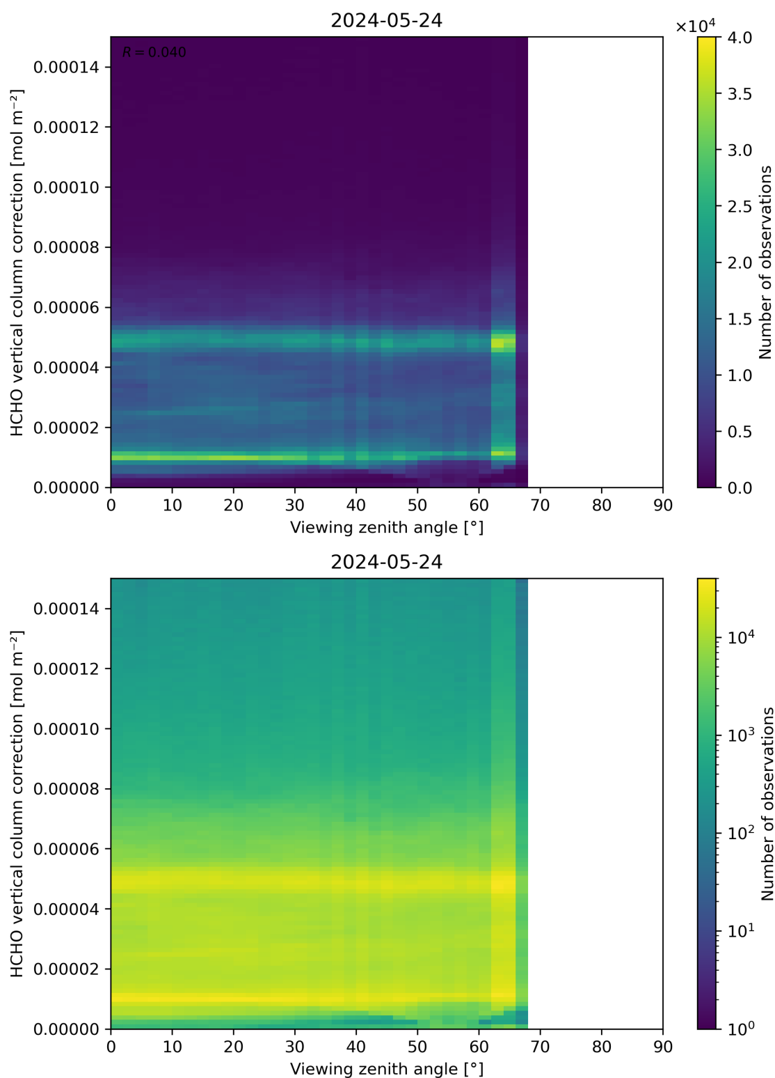
Figure 193: Scatter density plot of “Viewing zenith angle” against “HCHO vertical column correction” for 2024-05-23 to 2024-05-25.
