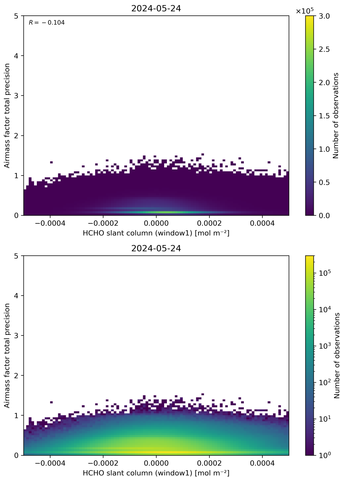
Figure 86: Scatter density plot of “HCHO slant column (window1)” against “Airmass factor total precision” for 2024-05-23 to 2024-05-25.
