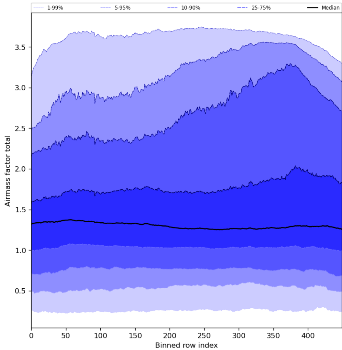
Figure 54: Along track statistics of “Airmass factor total” for 2024-05-23 to 2024-05-25
