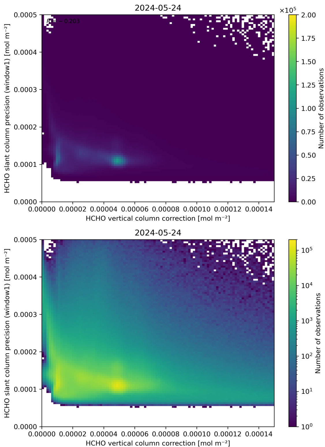
Figure 119: Scatter density plot of “HCHO vertical column correction” against “HCHO slant column precision (window1)” for 2024-05-23 to 2024-05-25.
