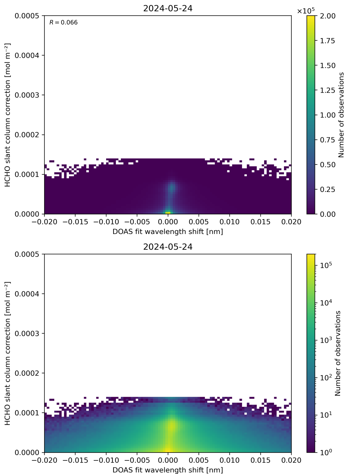
Figure 67: Scatter density plot of “DOAS fit wavelength shift” against “HCHO slant column correction” for 2024-05-23 to 2024-05-25.
