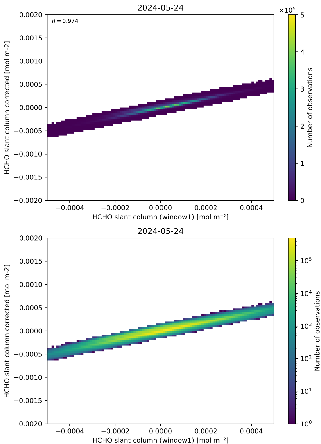
Figure 82: Scatter density plot of “HCHO slant column (window1)” against “HCHO slant column corrected” for 2024-05-23 to 2024-05-25.
