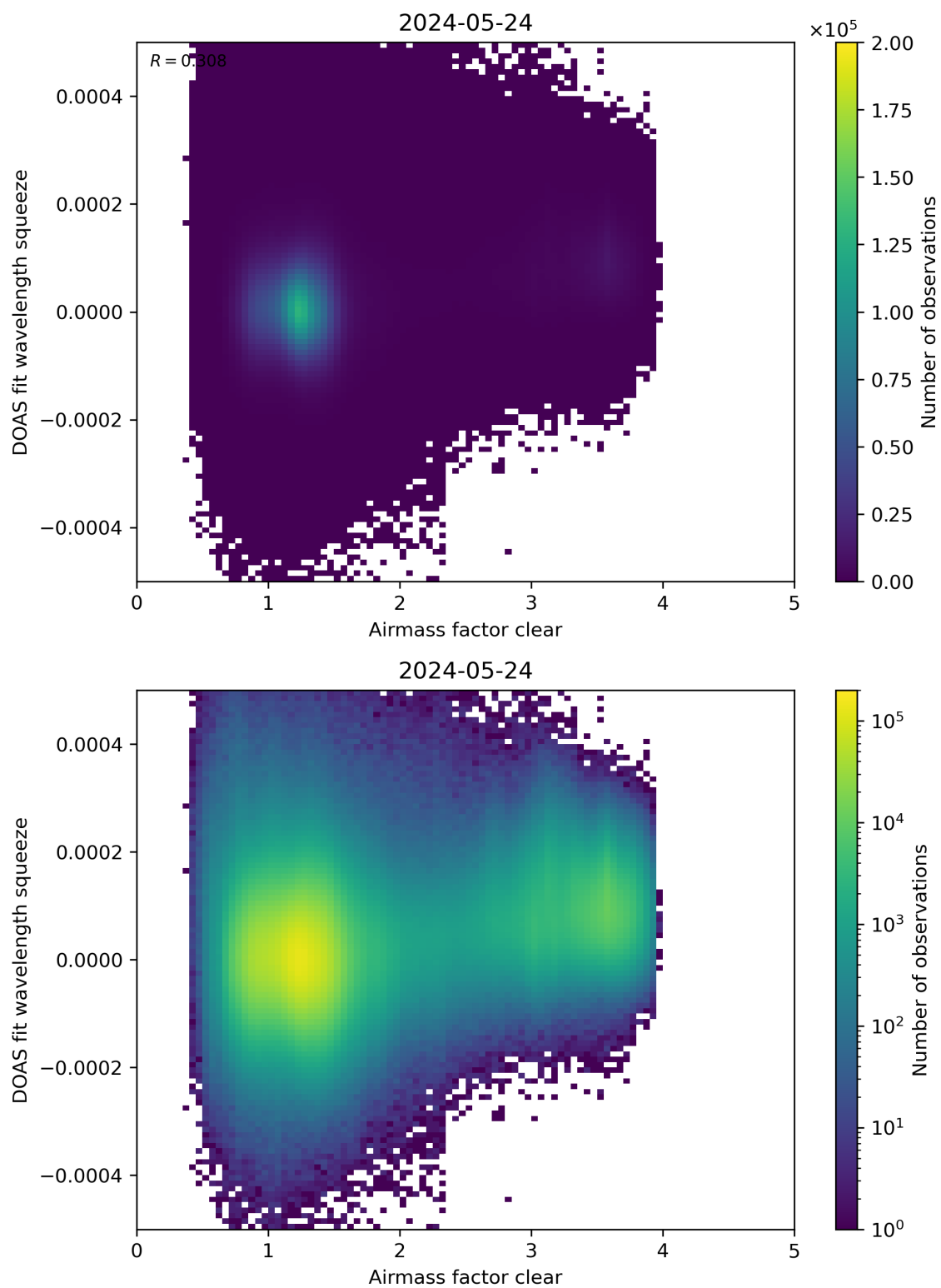
Figure 73: Scatter density plot of “Airmass factor clear” against “DOAS fit wavelength squeeze” for 2024-05-23 to 2024-05-25.
