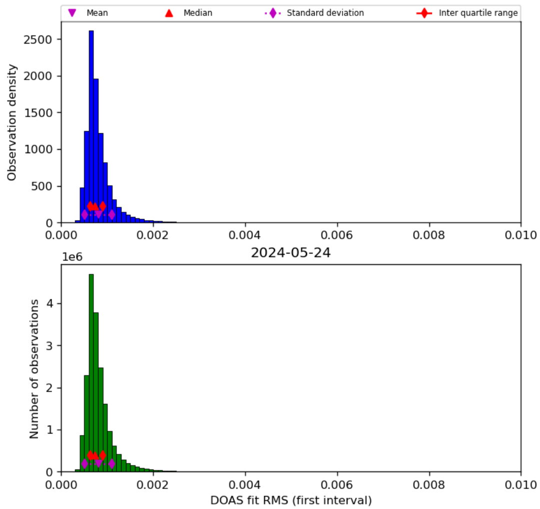
Figure 46: Histogram of “DOAS fit RMS (first interval)” for 2024-05-23 to 2024-05-25
