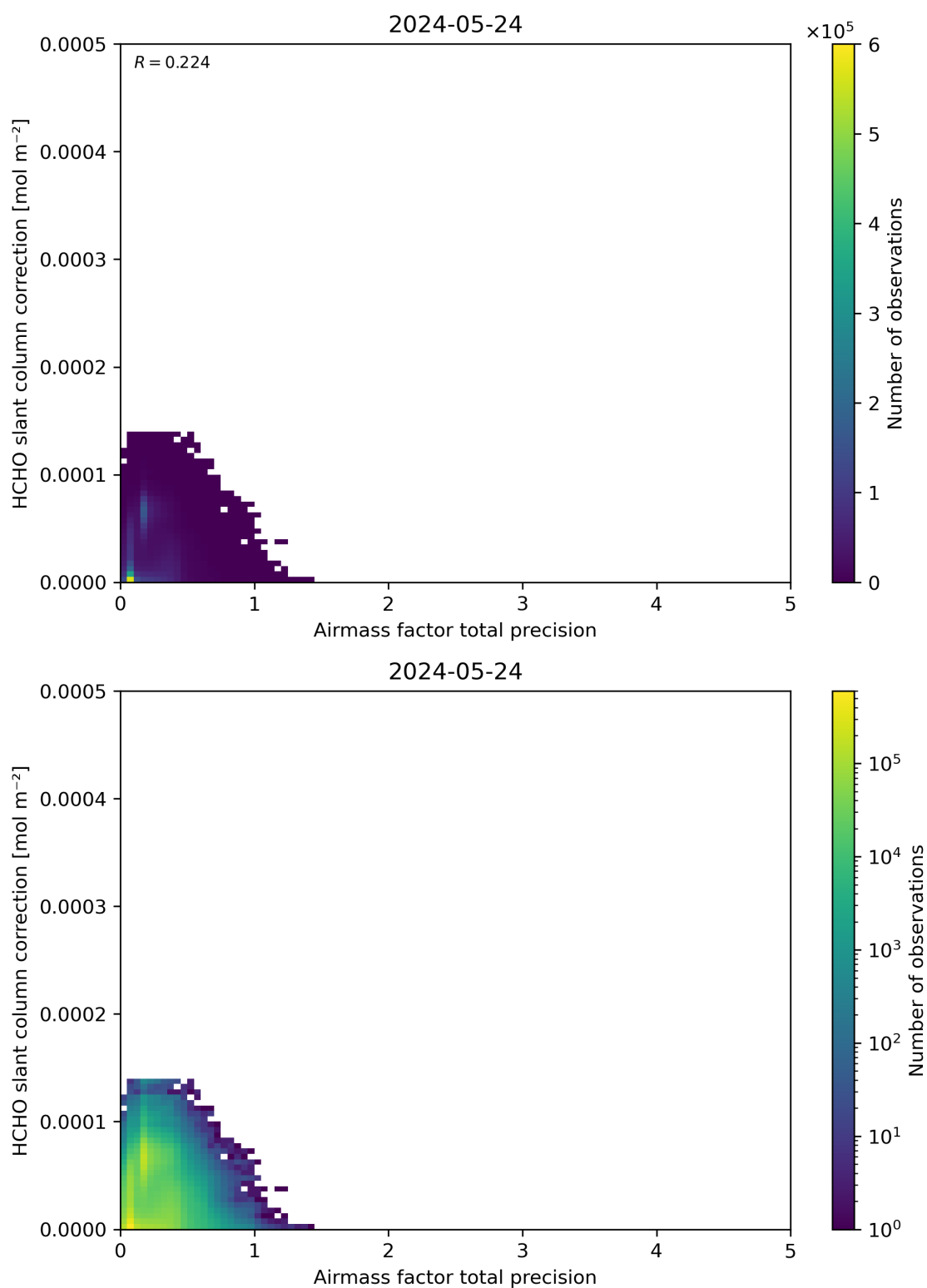
Figure 110: Scatter density plot of “Airmass factor total precision” against “HCHO slant column correction” for 2024-05-23 to 2024-05-25.
