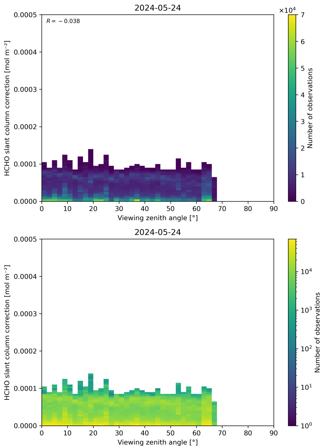
Figure 187: Scatter density plot of “Viewing zenith angle” against “HCHO slant column correction” for 2024-05-23 to 2024-05-25.
