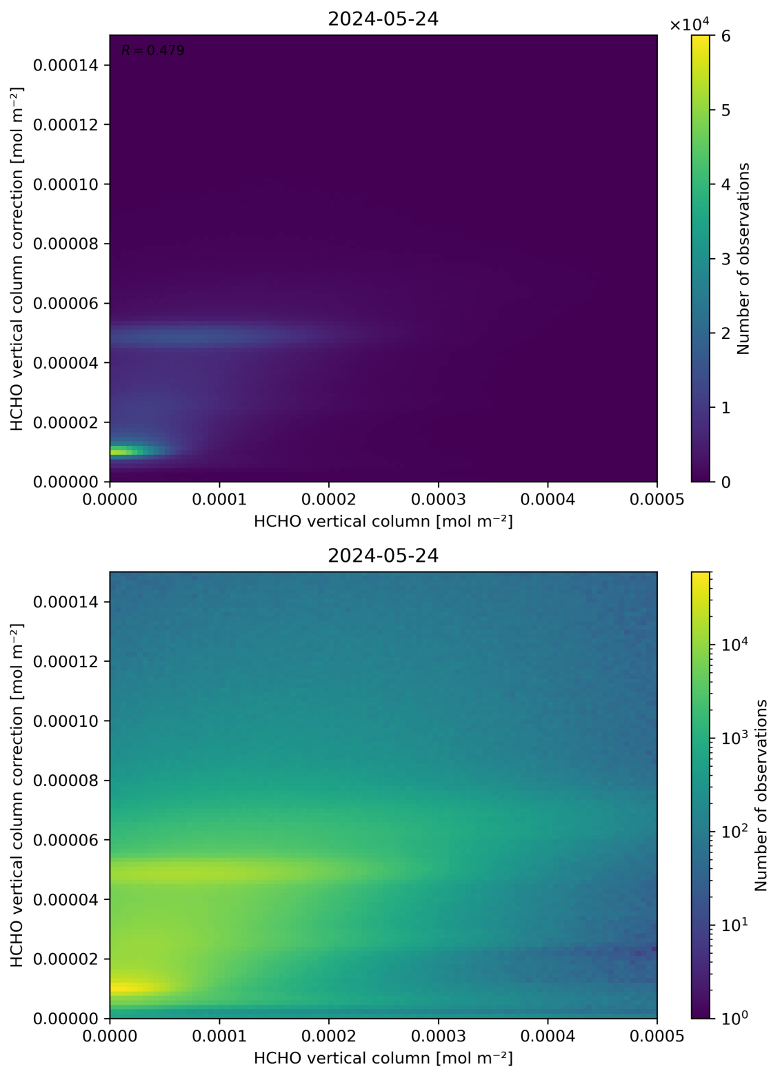
Figure 133: Scatter density plot of “HCHO vertical column” against “HCHO vertical column correction” for 2024-05-23 to 2024-05-25.
