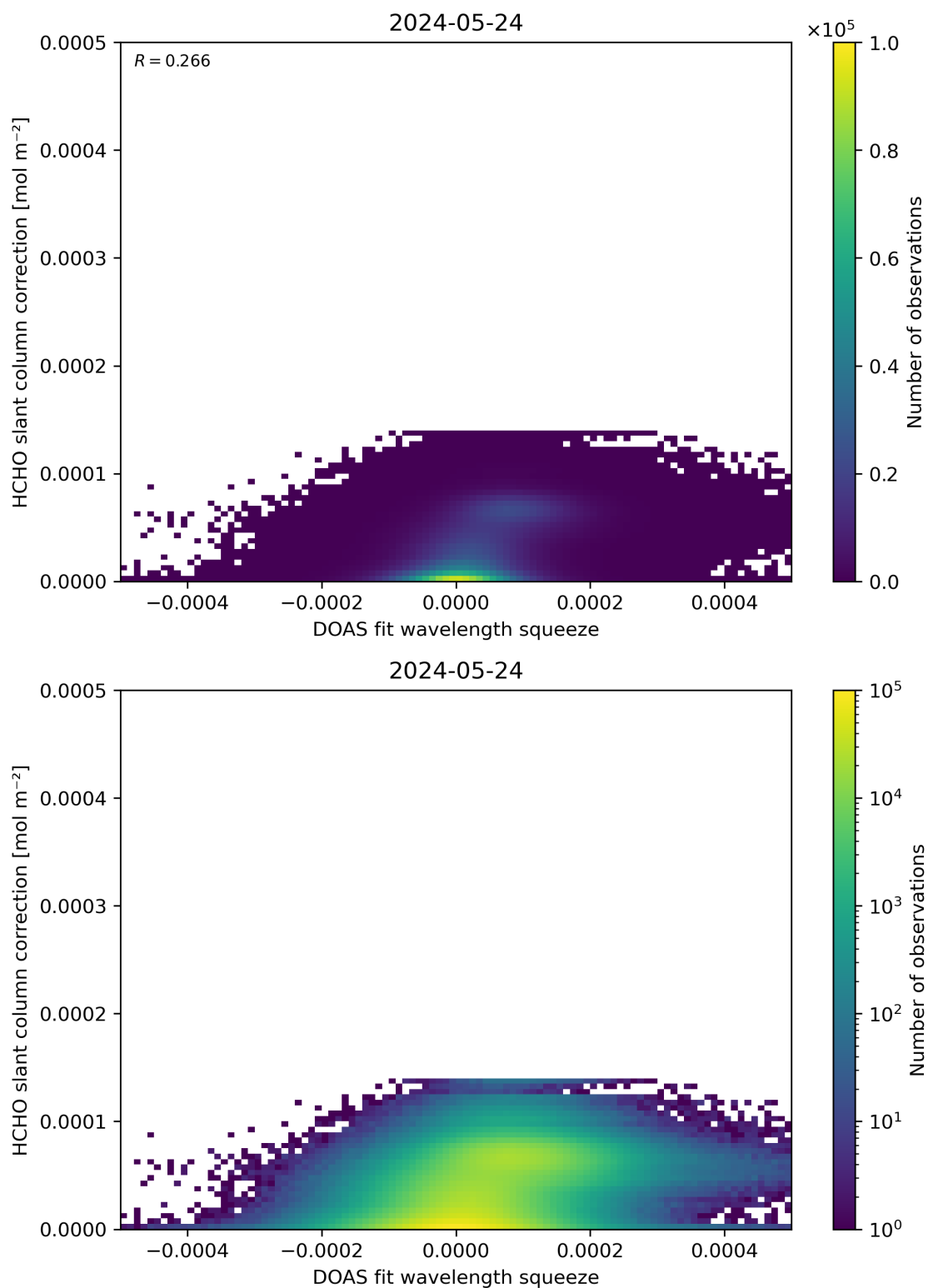
Figure 70: Scatter density plot of “DOAS fit wavelength squeeze” against “HCHO slant column correction” for 2024-05-23 to 2024-05-25.
