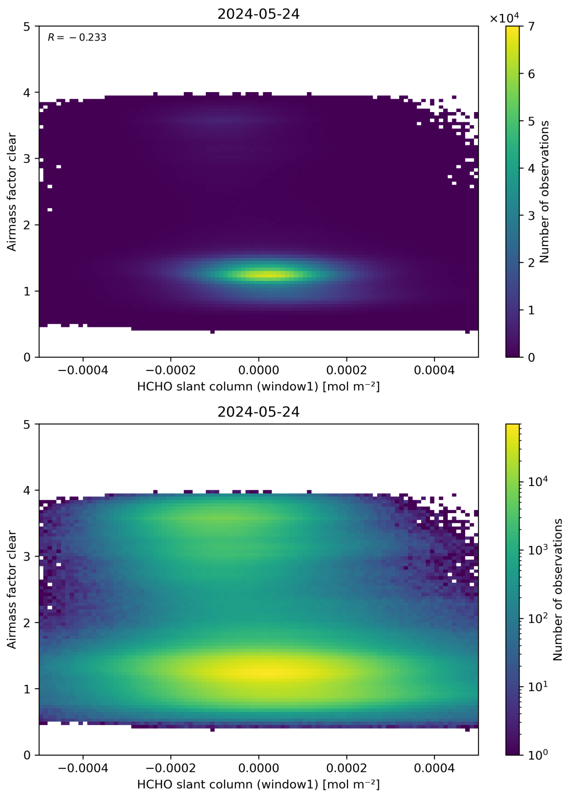
Figure 81: Scatter density plot of “HCHO slant column (window1)” against “Airmass factor clear” for 2024-05-23 to 2024-05-25.
