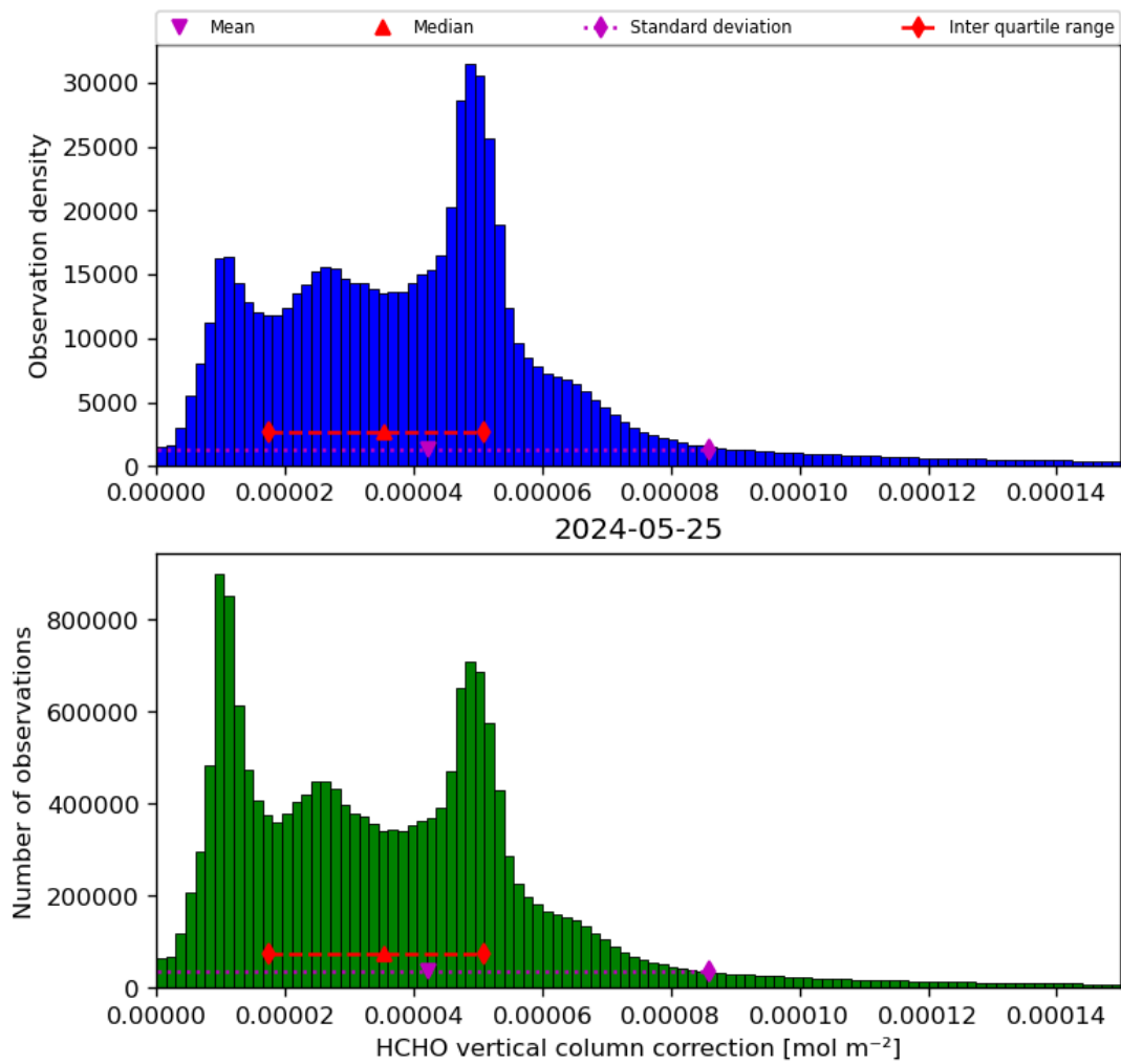
Figure 37: Histogram of “HCHO vertical column correction” for 2024-05-24 to 2024-05-26
