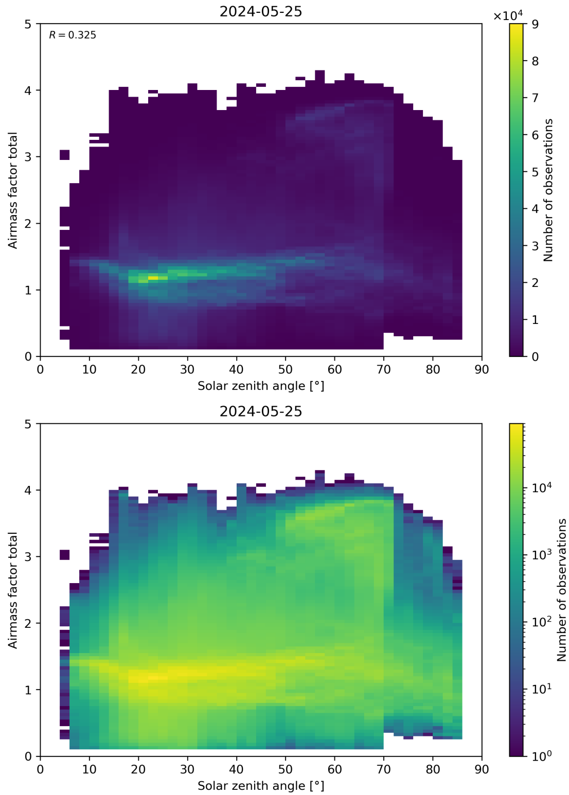
Figure 175: Scatter density plot of “Solar zenith angle” against “Airmass factor total” for 2024-05-24 to 2024-05-26.
