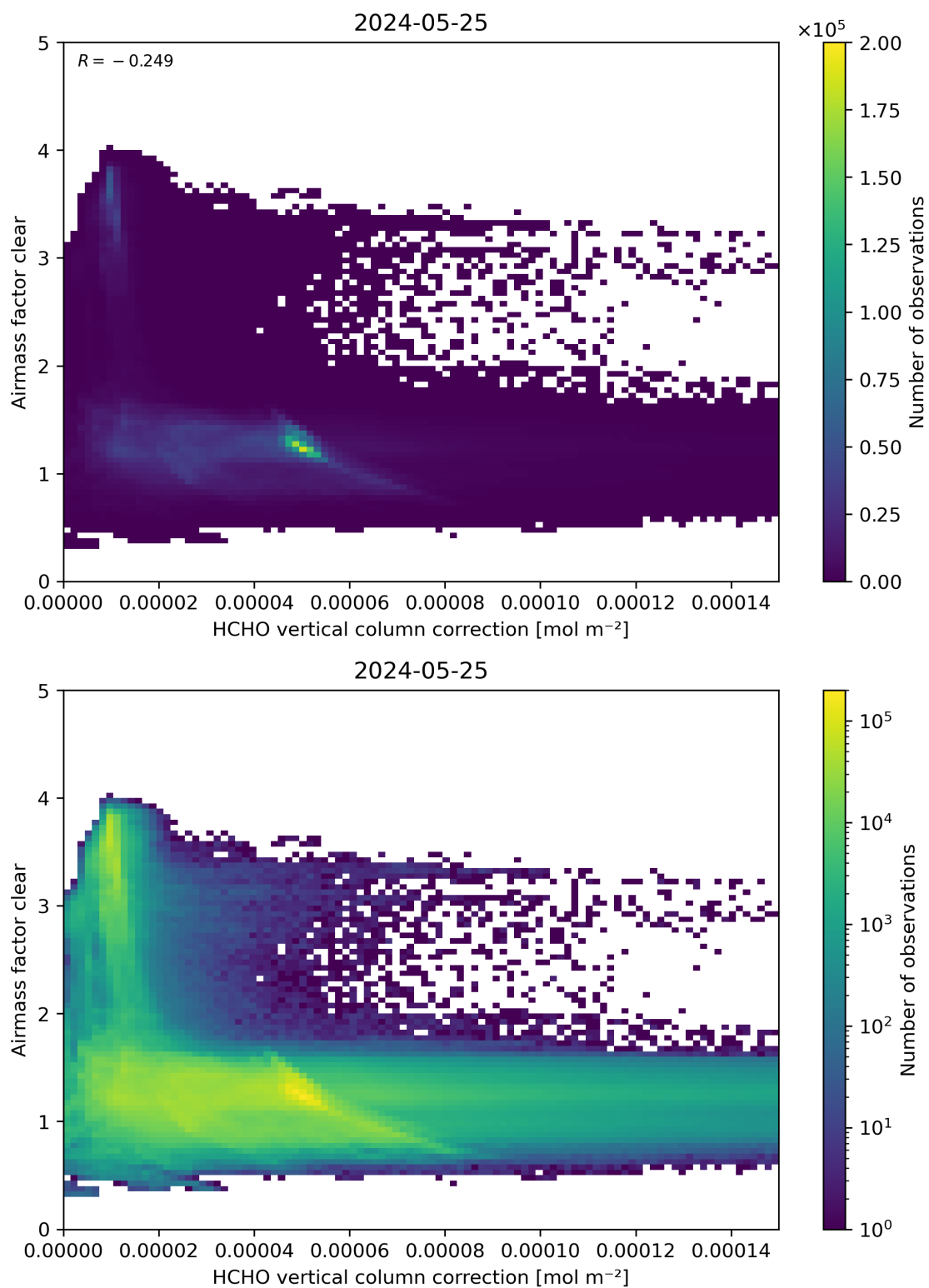
Figure 115: Scatter density plot of “HCHO vertical column correction” against “Airmass factor clear” for 2024-05-24 to 2024-05-26.
