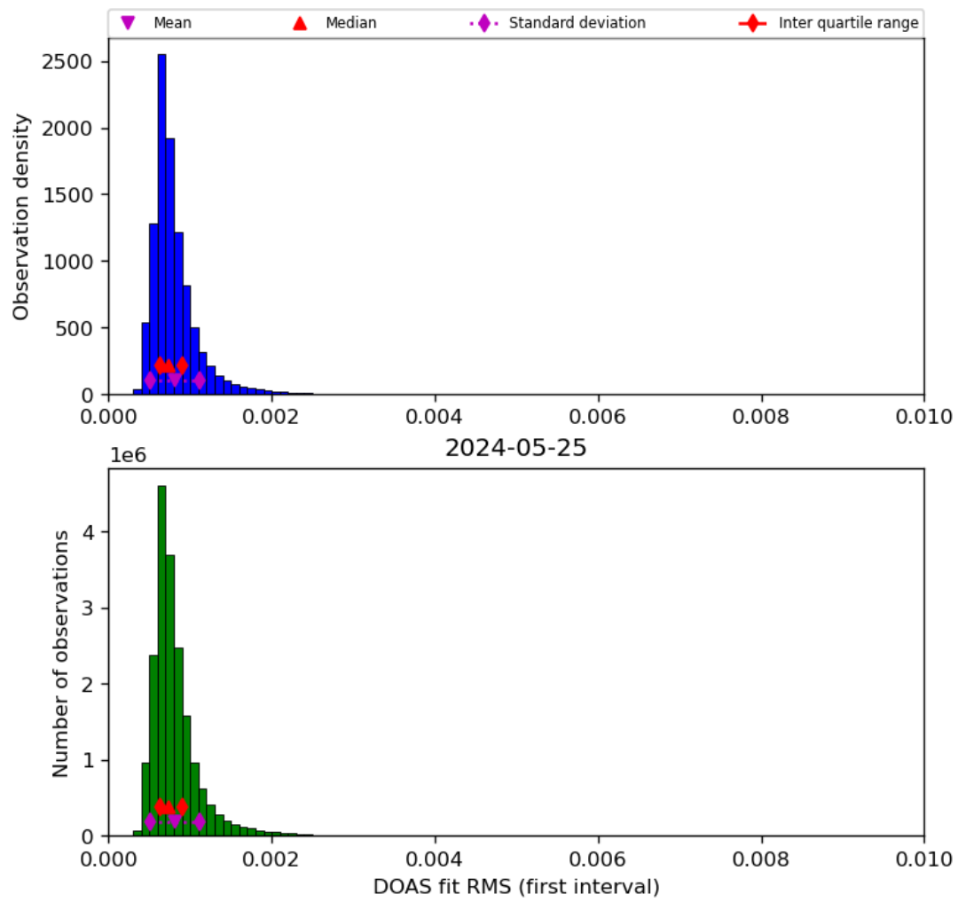
Figure 46: Histogram of “DOAS fit RMS (first interval)” for 2024-05-24 to 2024-05-26
