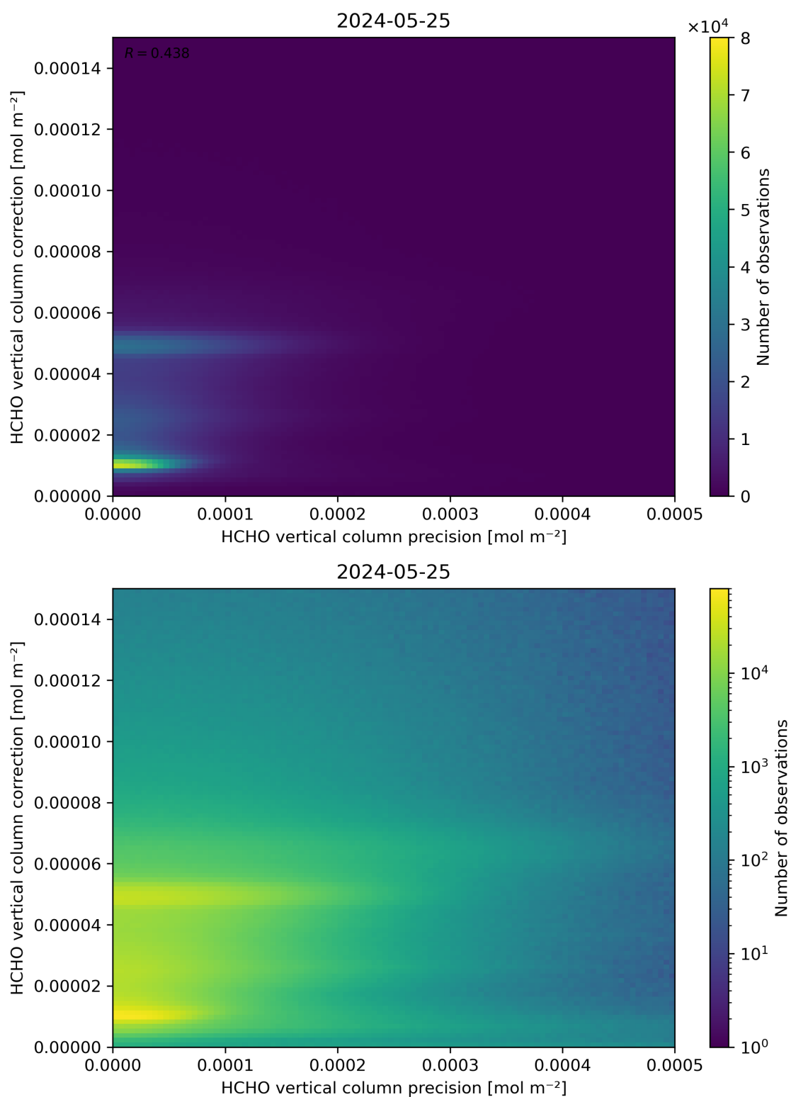
Figure 146: Scatter density plot of “HCHO vertical column precision” against “HCHO vertical column correction” for 2024-05-24 to 2024-05-26.
