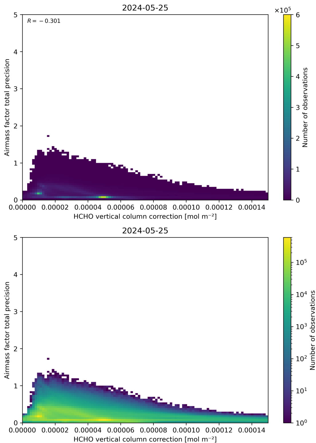
Figure 121: Scatter density plot of “HCHO vertical column correction” against “Airmass factor total precision” for 2024-05-24 to 2024-05-26.
