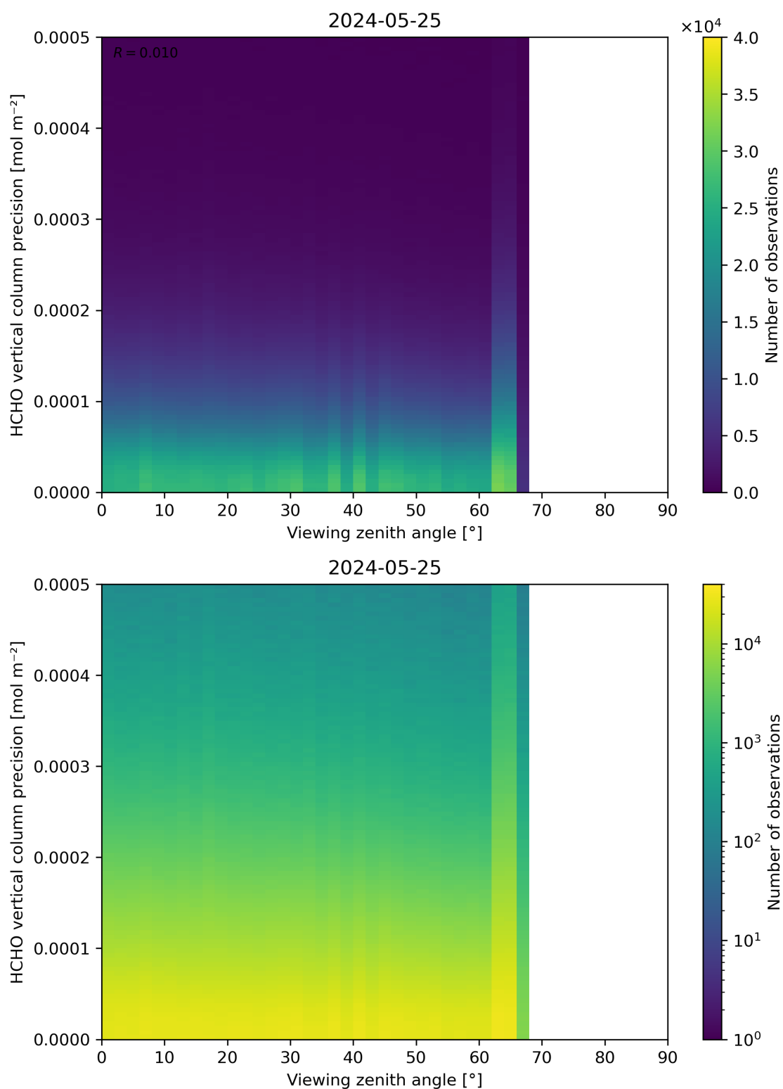
Figure 194: Scatter density plot of “Viewing zenith angle” against “HCHO vertical column precision” for 2024-05-24 to 2024-05-26.
