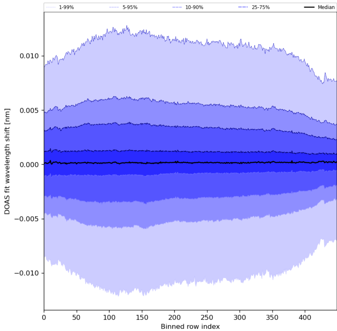
Figure 58: Along track statistics of “DOAS fit wavelength shift” for 2024-05-24 to 2024-05-26
