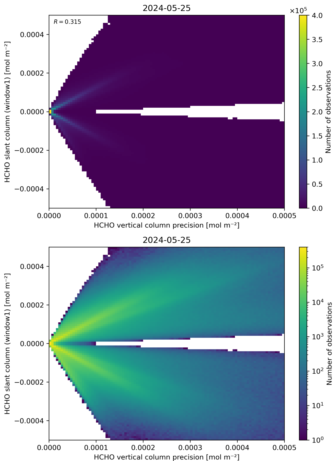
Figure 142: Scatter density plot of “HCHO vertical column precision” against “HCHO slant column (window1)” for 2024-05-24 to 2024-05-26.
