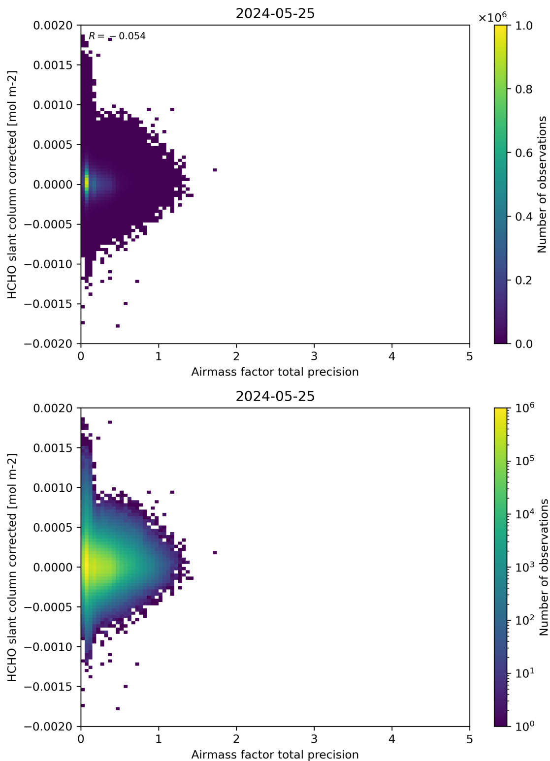
Figure 109: Scatter density plot of “Airmass factor total precision” against “HCHO slant column corrected” for 2024-05-24 to 2024-05-26.
