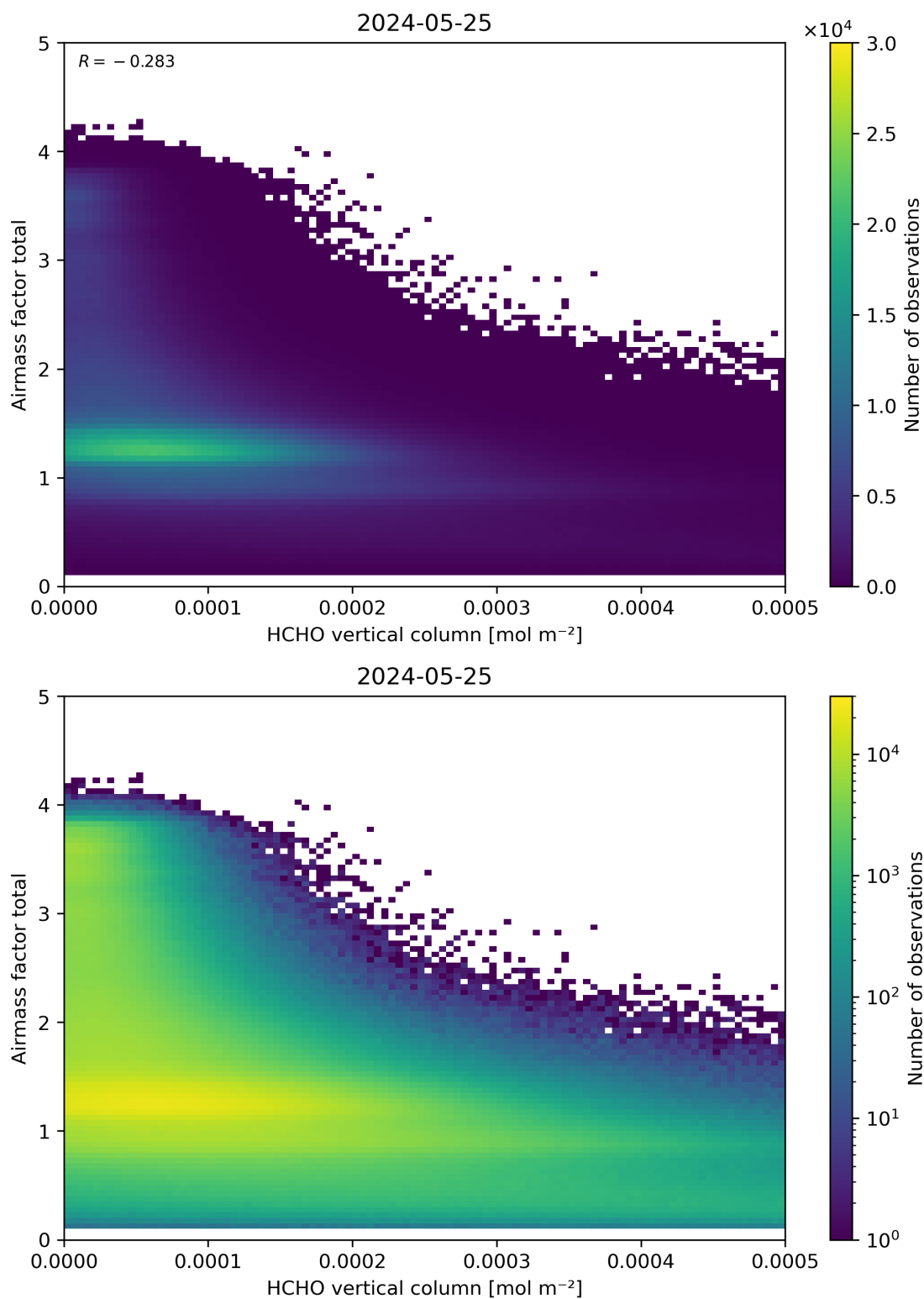
Figure 131: Scatter density plot of “HCHO vertical column” against “Airmass factor total” for 2024-05-24 to 2024-05-26.
