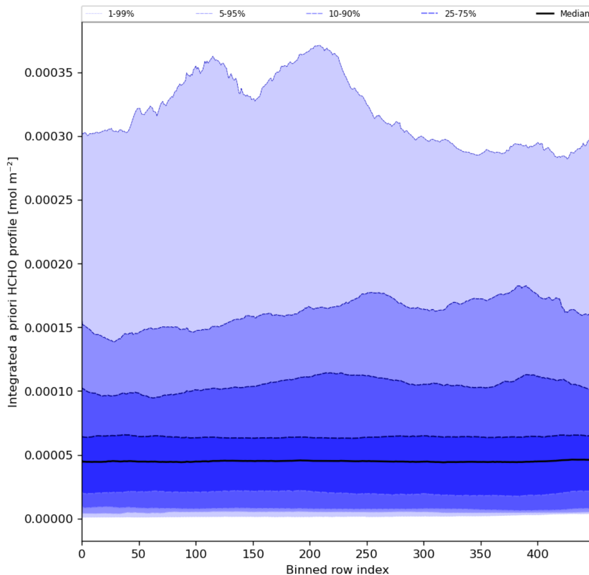
Figure 57: Along track statistics of "Integrated a priori HCHO profile" for 2024-05-24 to 2024-05-26
