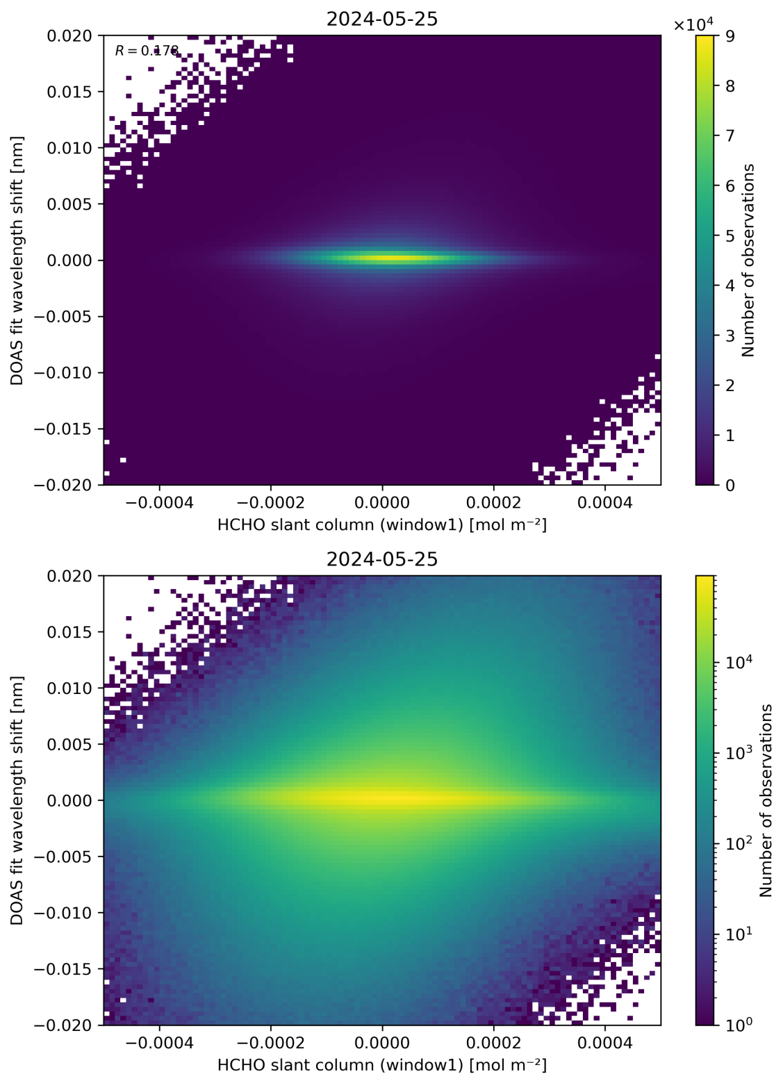
Figure 79: Scatter density plot of “HCHO slant column (window1)” against “DOAS fit wavelength shift” for 2024-05-24 to 2024-05-26.
