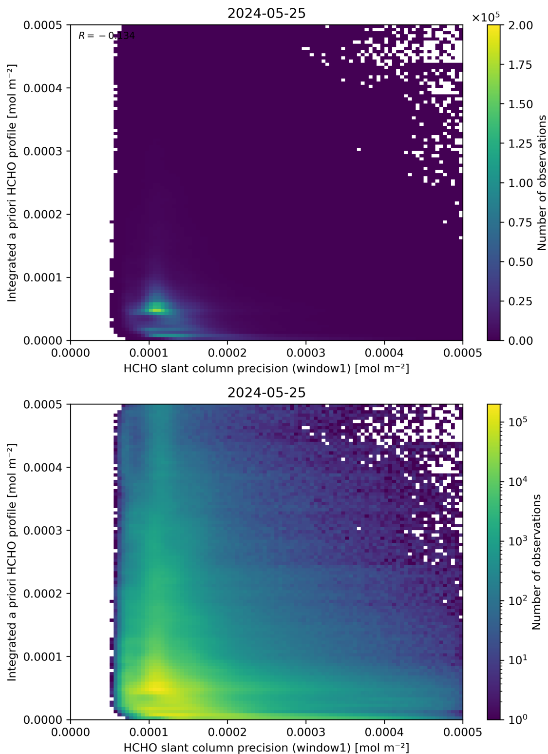
Figure 96: Scatter density plot of “HCHO slant column precision (window1)” against “Integrated a priori HCHO profile” for 2024-05-24 to 2024-05-26.
