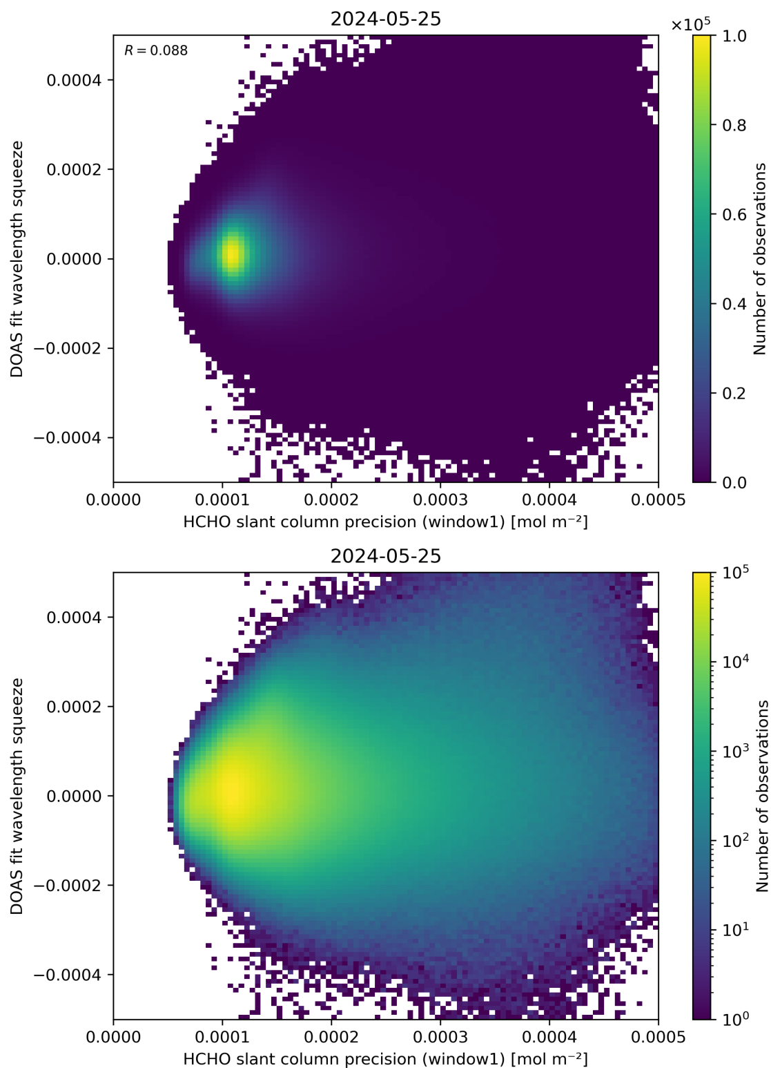
Figure 90: Scatter density plot of “HCHO slant column precision (window1)” against “DOAS fit wavelength squeeze” for 2024-05-24 to 2024-05-26.
