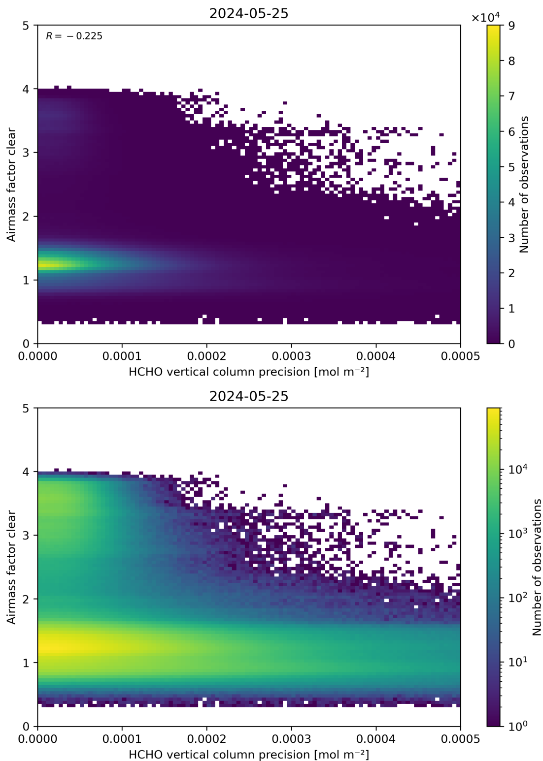
Figure 139: Scatter density plot of “HCHO vertical column precision” against “Airmass factor clear” for 2024-05-24 to 2024-05-26.
