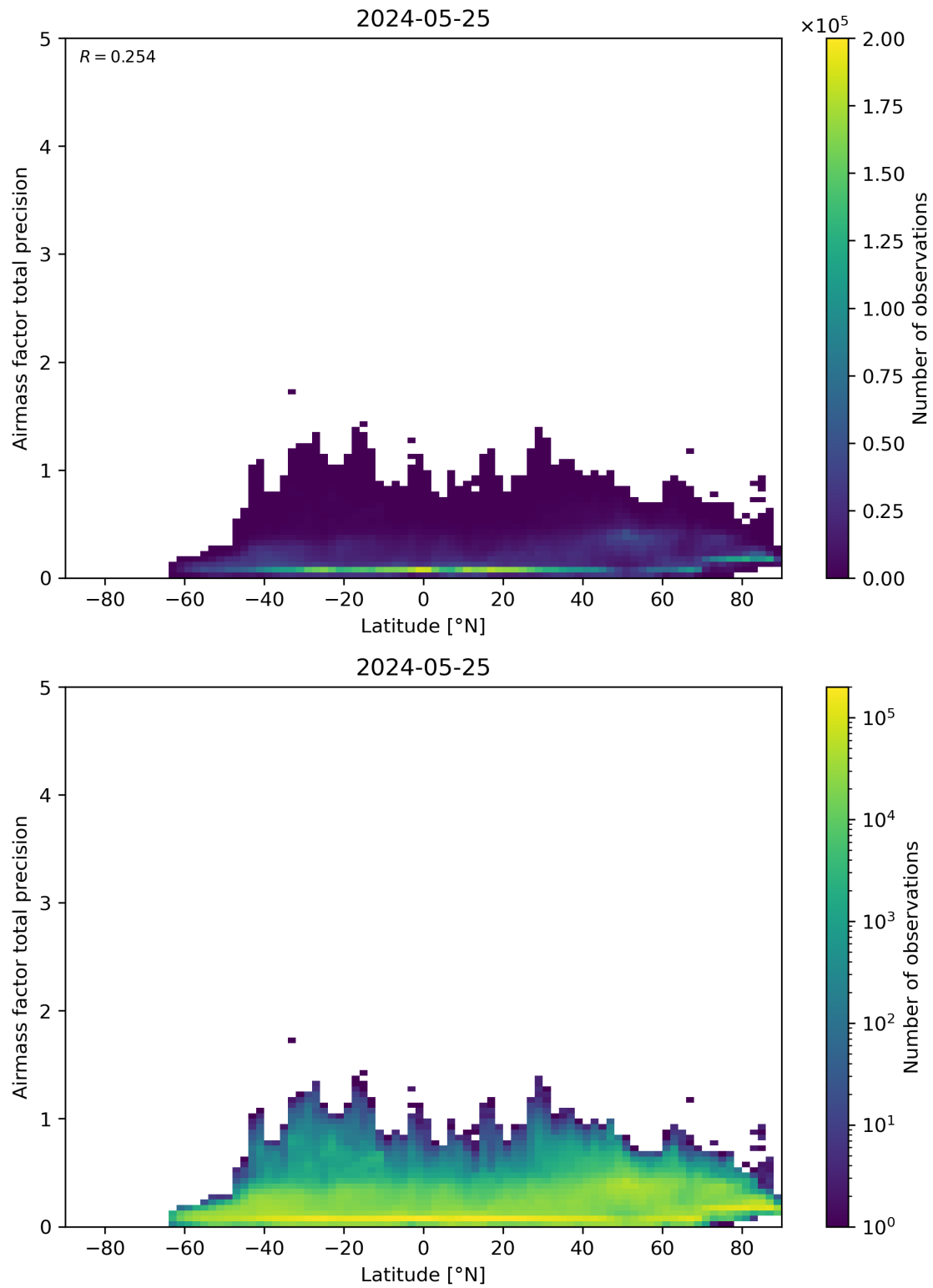
Figure 162: Scatter density plot of “Latitude” against “Airmass factor total precision” for 2024-05-24 to 2024-05-26.
