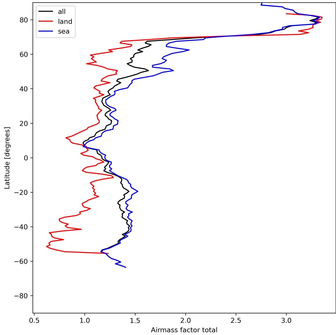
Figure 26: Zonal average of “Airmass factor total” for 2024-05-24 to 2024-05-26.
