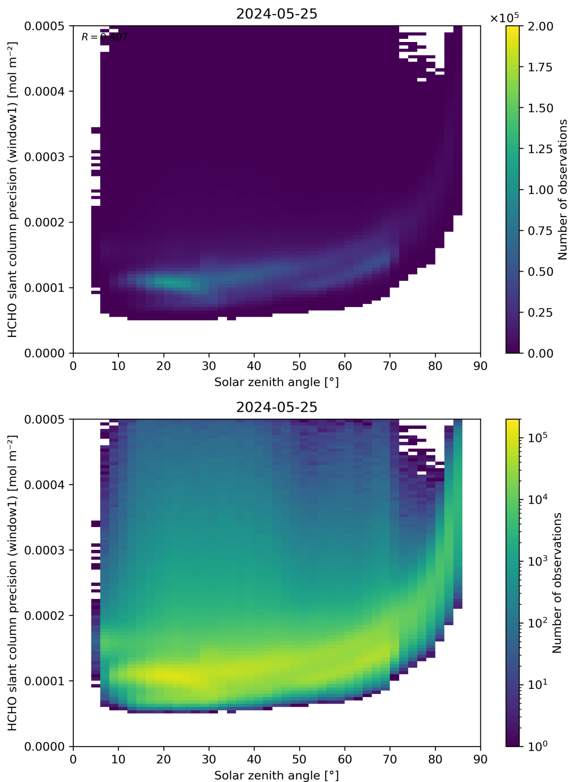
Figure 174: Scatter density plot of “Solar zenith angle” against “HCHO slant column precision (window1)” for 2024-05-24 to 2024-05-26.
