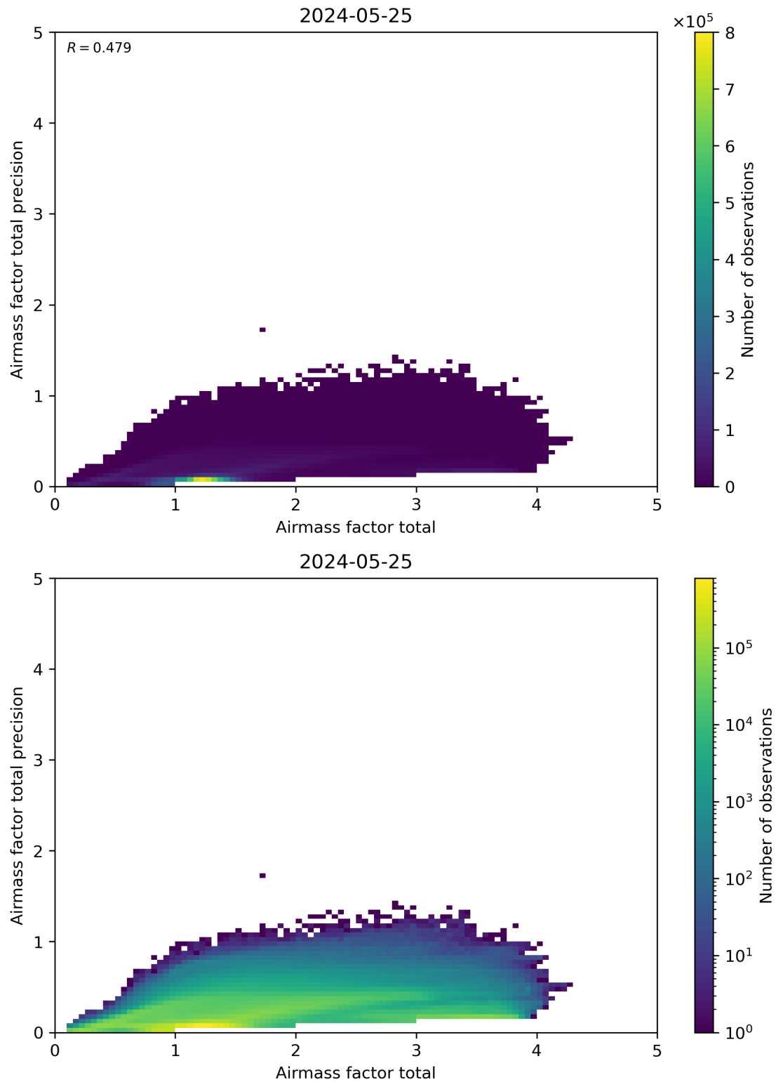
Figure 103: Scatter density plot of “Airmass factor total” against “Airmass factor total precision” for 2024-05-24 to 2024-05-26.
