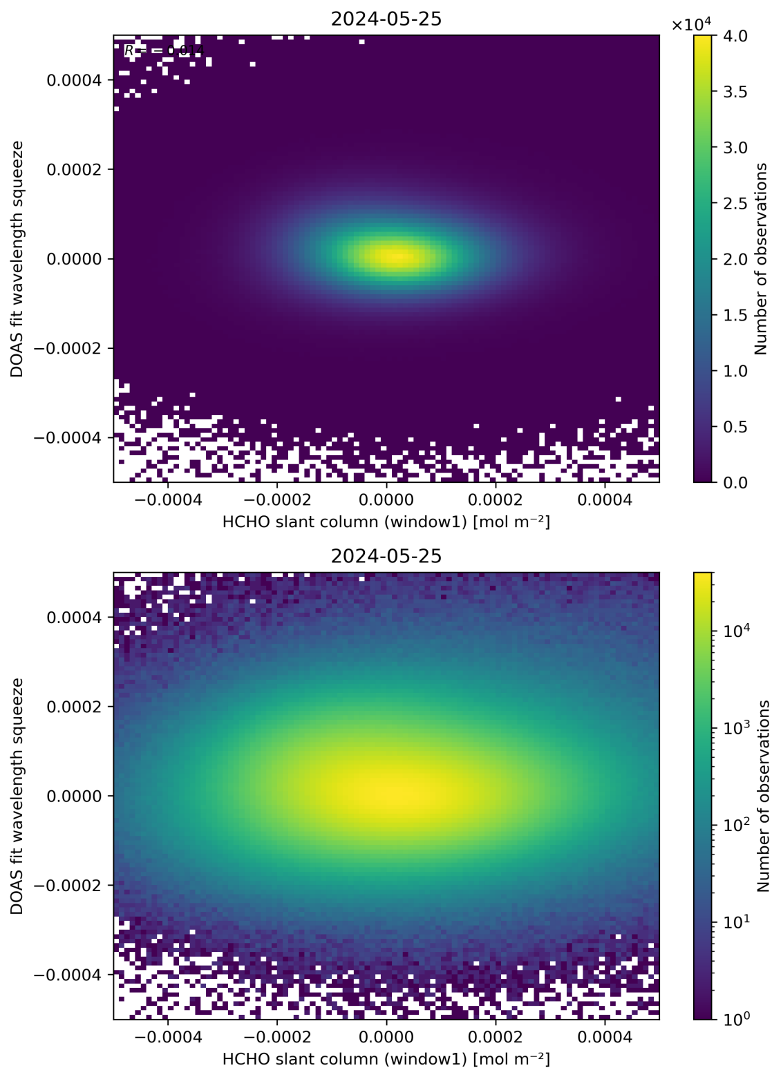
Figure 80: Scatter density plot of “HCHO slant column (window1)” against “DOAS fit wavelength squeeze” for 2024-05-24 to 2024-05-26.
