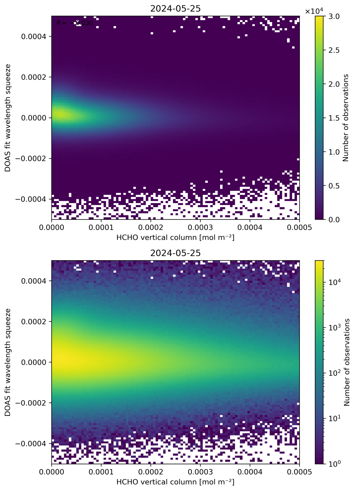
Figure 125: Scatter density plot of “HCHO vertical column” against “DOAS fit wavelength squeeze” for 2024-05-24 to 2024-05-26.
