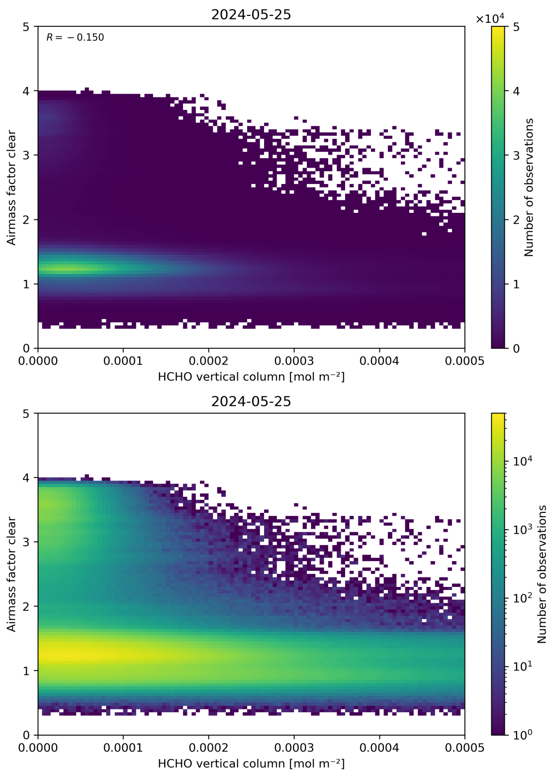
Figure 126: Scatter density plot of “HCHO vertical column” against “Airmass factor clear” for 2024-05-24 to 2024-05-26.
