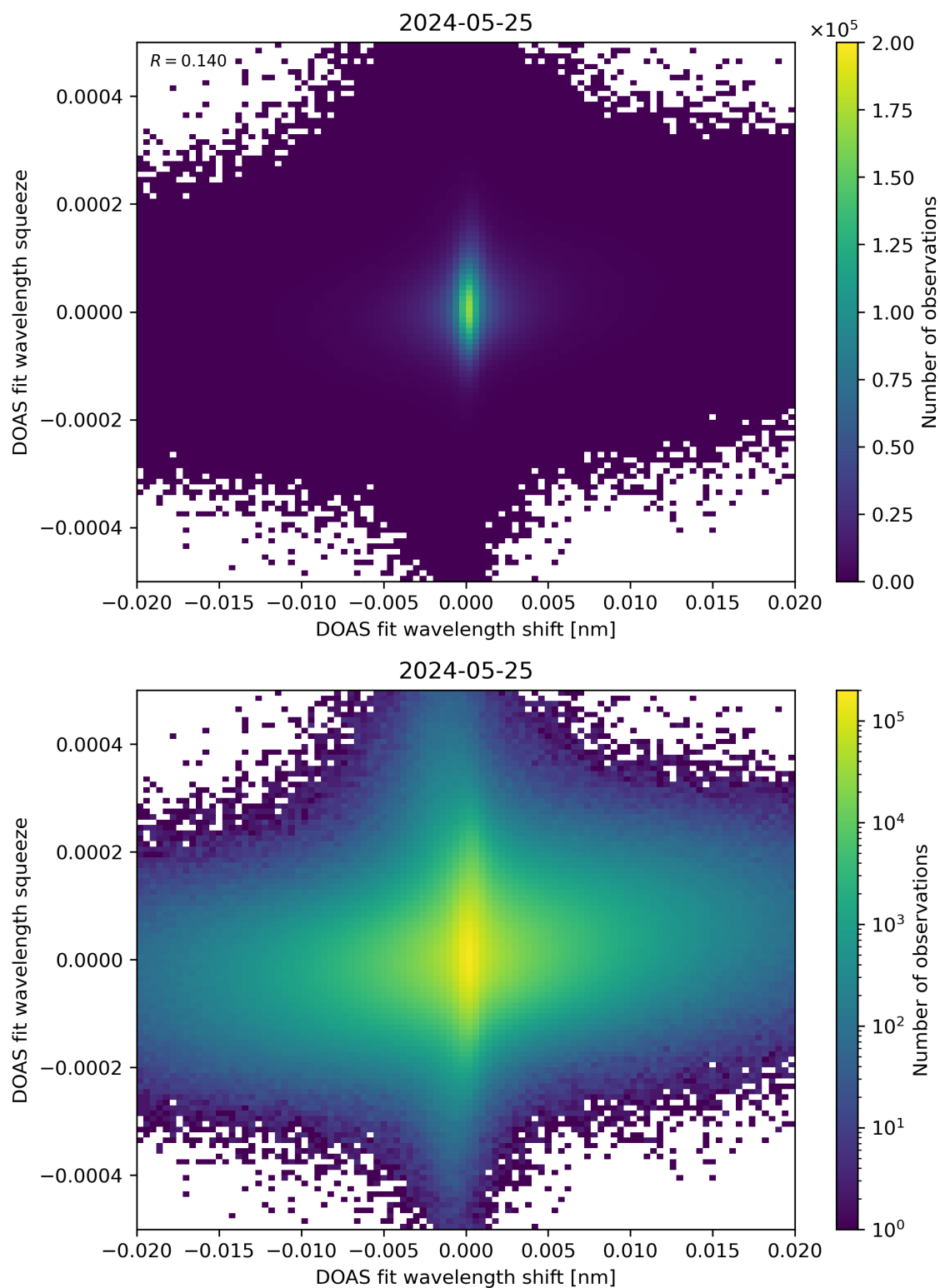
Figure 65: Scatter density plot of “DOAS fit wavelength shift” against “DOAS fit wavelength squeeze” for 2024-05-24 to 2024-05-26.
