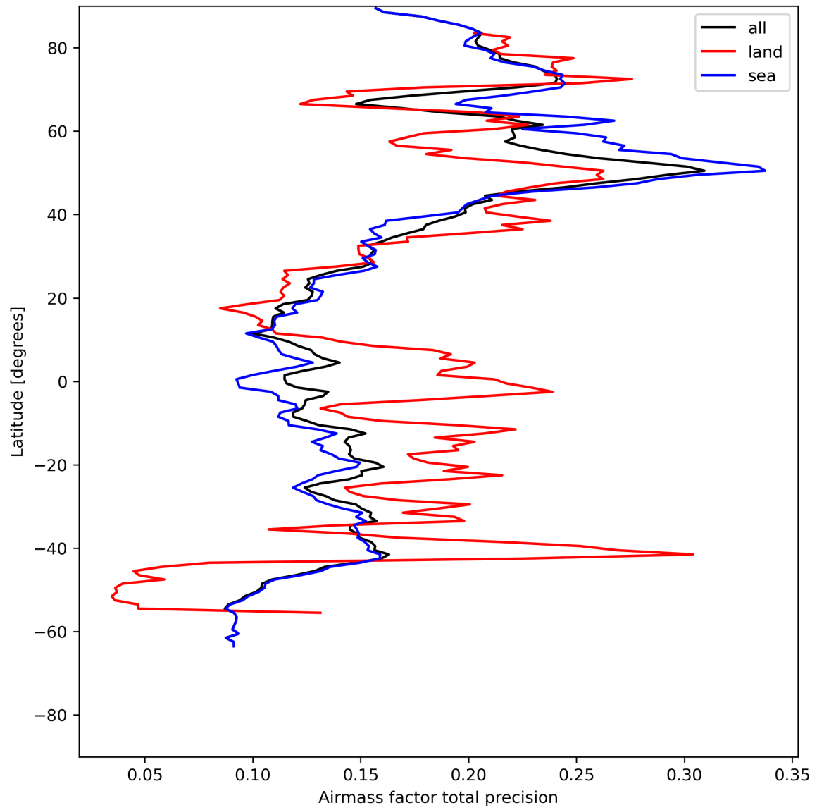
Figure 27: Zonal average of “Airmass factor total precision” for 2024-05-24 to 2024-05-26.
