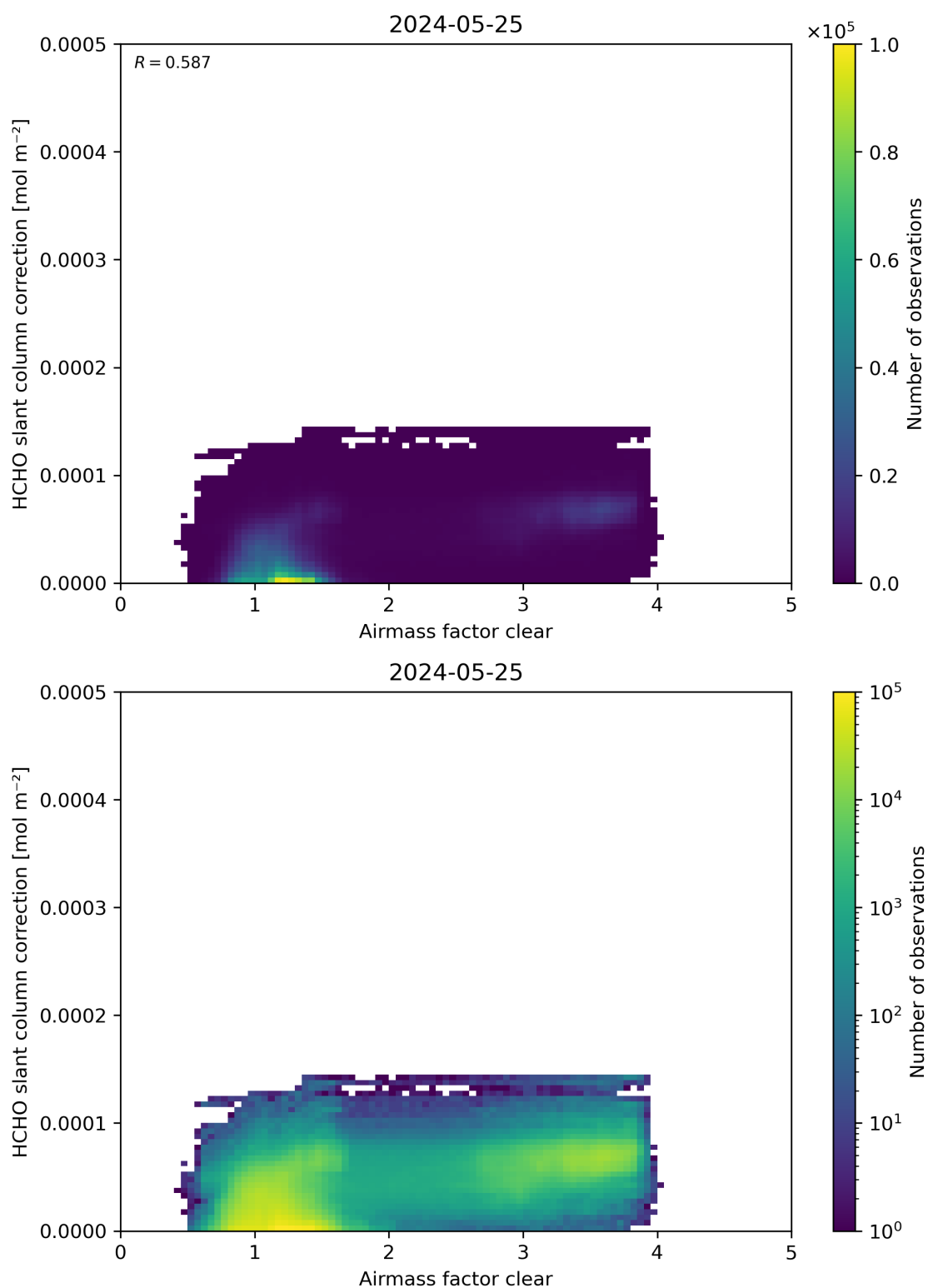
Figure 75: Scatter density plot of “Airmass factor clear” against “HCHO slant column correction” for 2024-05-24 to 2024-05-26.
