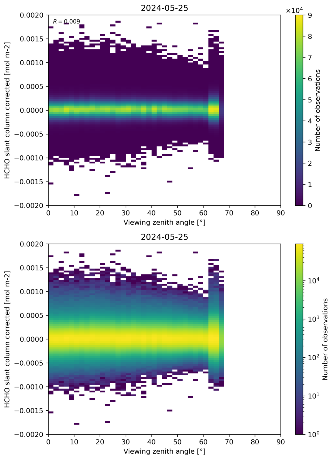
Figure 186: Scatter density plot of “Viewing zenith angle” against “HCHO slant column corrected” for 2024-05-24 to 2024-05-26.
