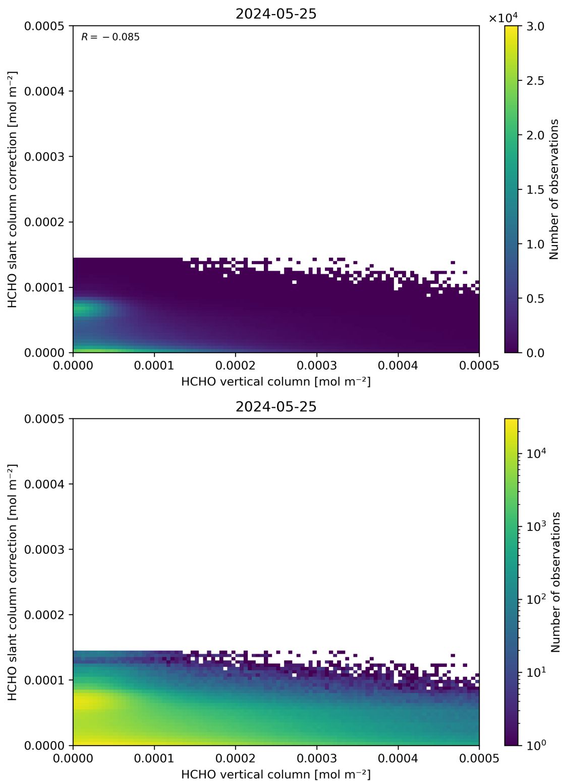
Figure 128: Scatter density plot of “HCHO vertical column” against “HCHO slant column correction” for 2024-05-24 to 2024-05-26.
