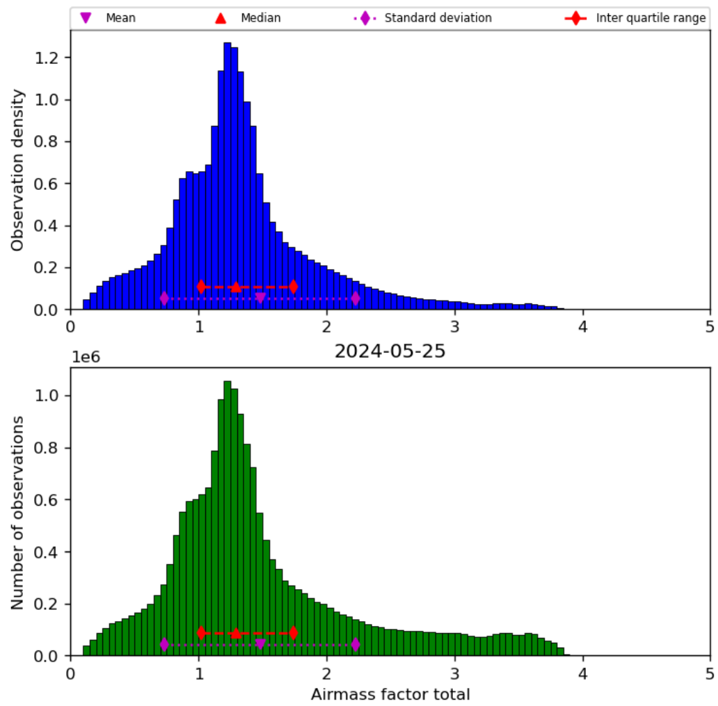
Figure 40: Histogram of “Airmass factor total” for 2024-05-24 to 2024-05-26
