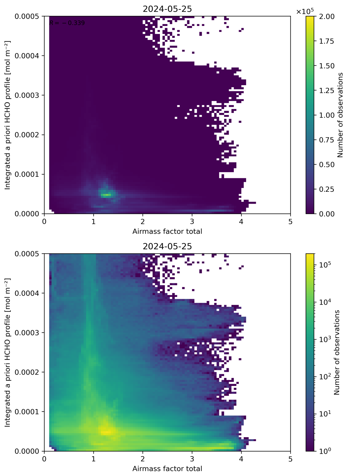
Figure 104: Scatter density plot of “Airmass factor total” against “Integrated a priori HCHO profile” for 2024-05-24 to 2024-05-26.
