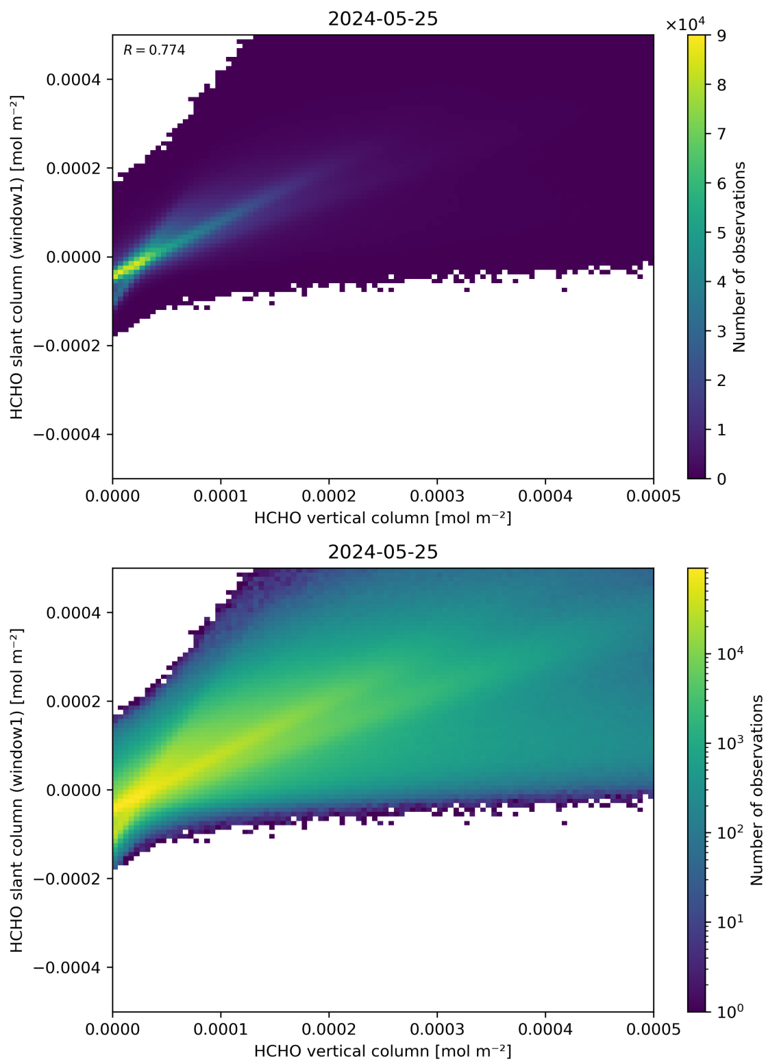
Figure 129: Scatter density plot of “HCHO vertical column” against “HCHO slant column (window1)” for 2024-05-24 to 2024-05-26.
