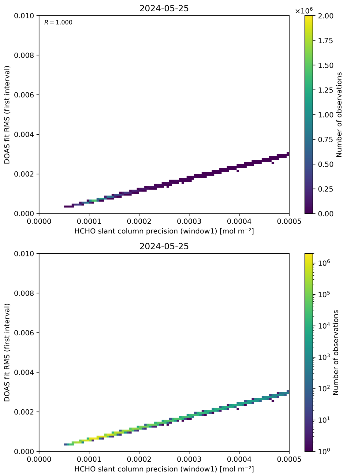
Figure 88: Scatter density plot of “HCHO slant column precision (window1)” against “DOAS fit RMS (first interval)” for 2024-05-24 to 2024-05-26.
