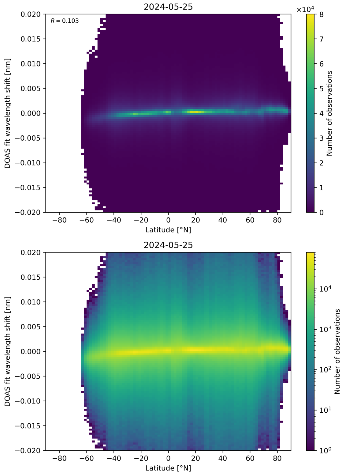
Figure 154: Scatter density plot of “Latitude” against “DOAS fit wavelength shift” for 2024-05-24 to 2024-05-26.
