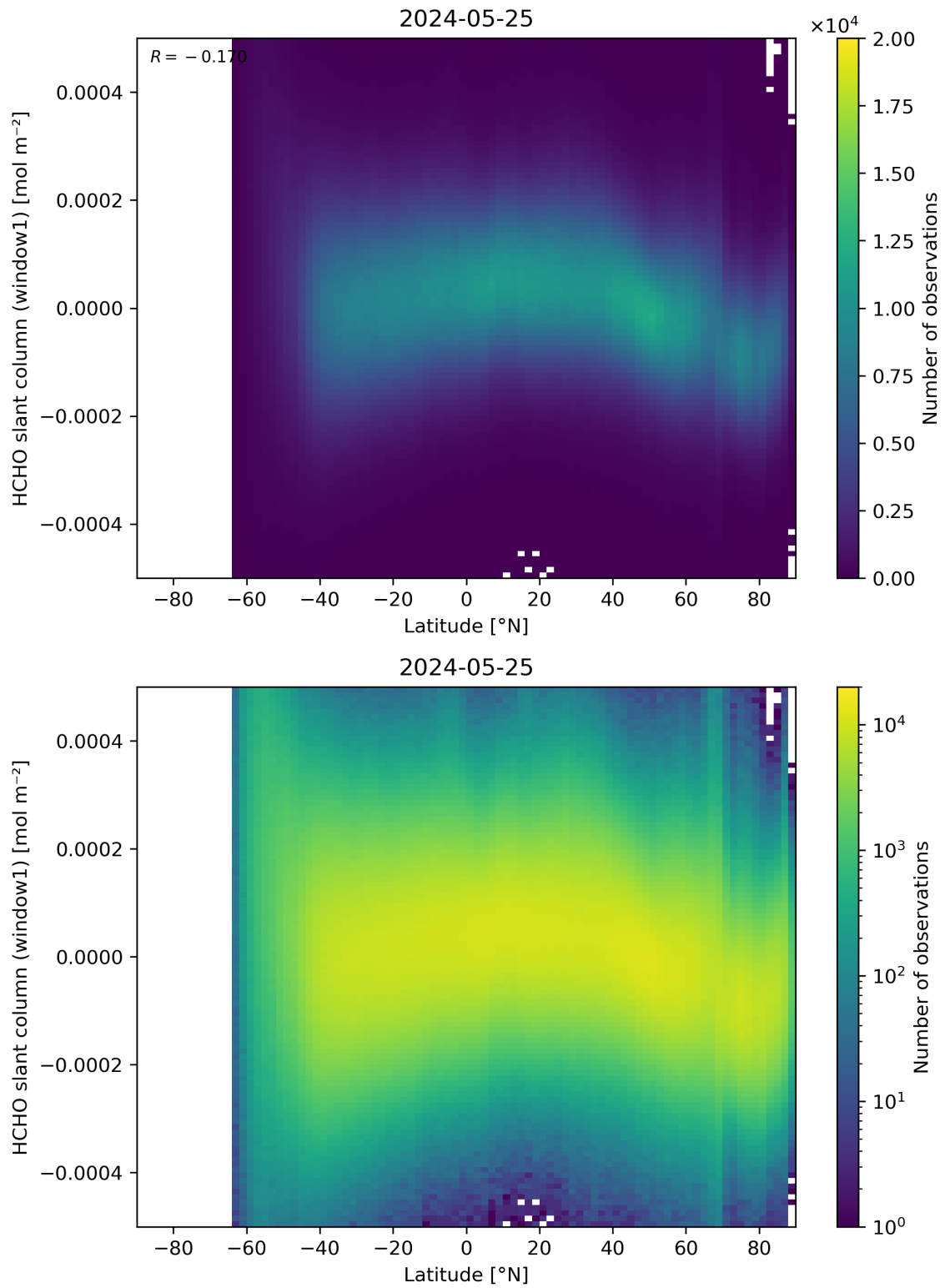
Figure 159: Scatter density plot of “Latitude” against “HCHO slant column (window1)” for 2024-05-24 to 2024-05-26.
