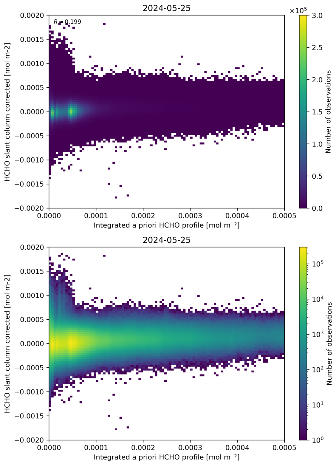
Figure 151: Scatter density plot of “Integrated a priori HCHO profile” against “HCHO slant column corrected” for 2024-05-24 to 2024-05-26.
