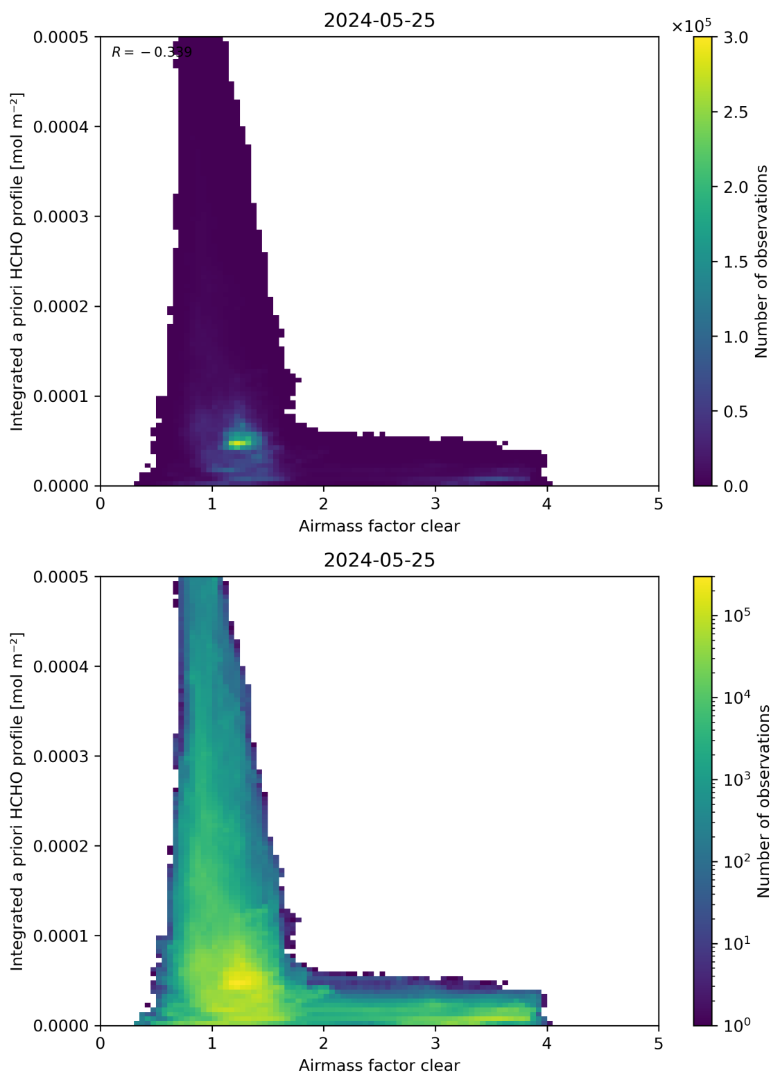
Figure 76: Scatter density plot of “Airmass factor clear” against “Integrated a priori HCHO profile” for 2024-05-24 to 2024-05-26.
