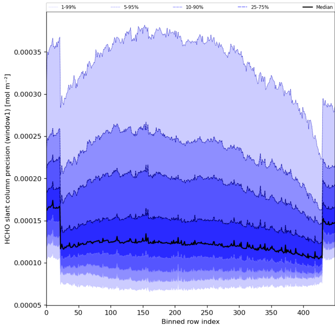
Figure 53: Along track statistics of “HCHO slant column precision (window1)” for 2024-05-24 to 2024-05-26
