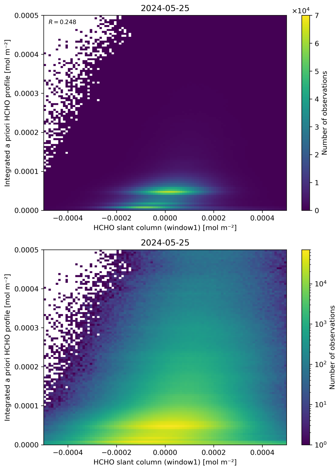
Figure 87: Scatter density plot of “HCHO slant column (window1)” against “Integrated a priori HCHO profile” for 2024-05-24 to 2024-05-26.
