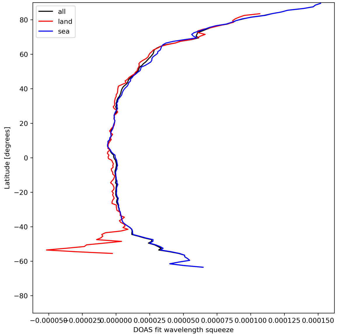
Figure 31: Zonal average of “DOAS fit wavelength squeeze” for 2024-05-24 to 2024-05-26.
