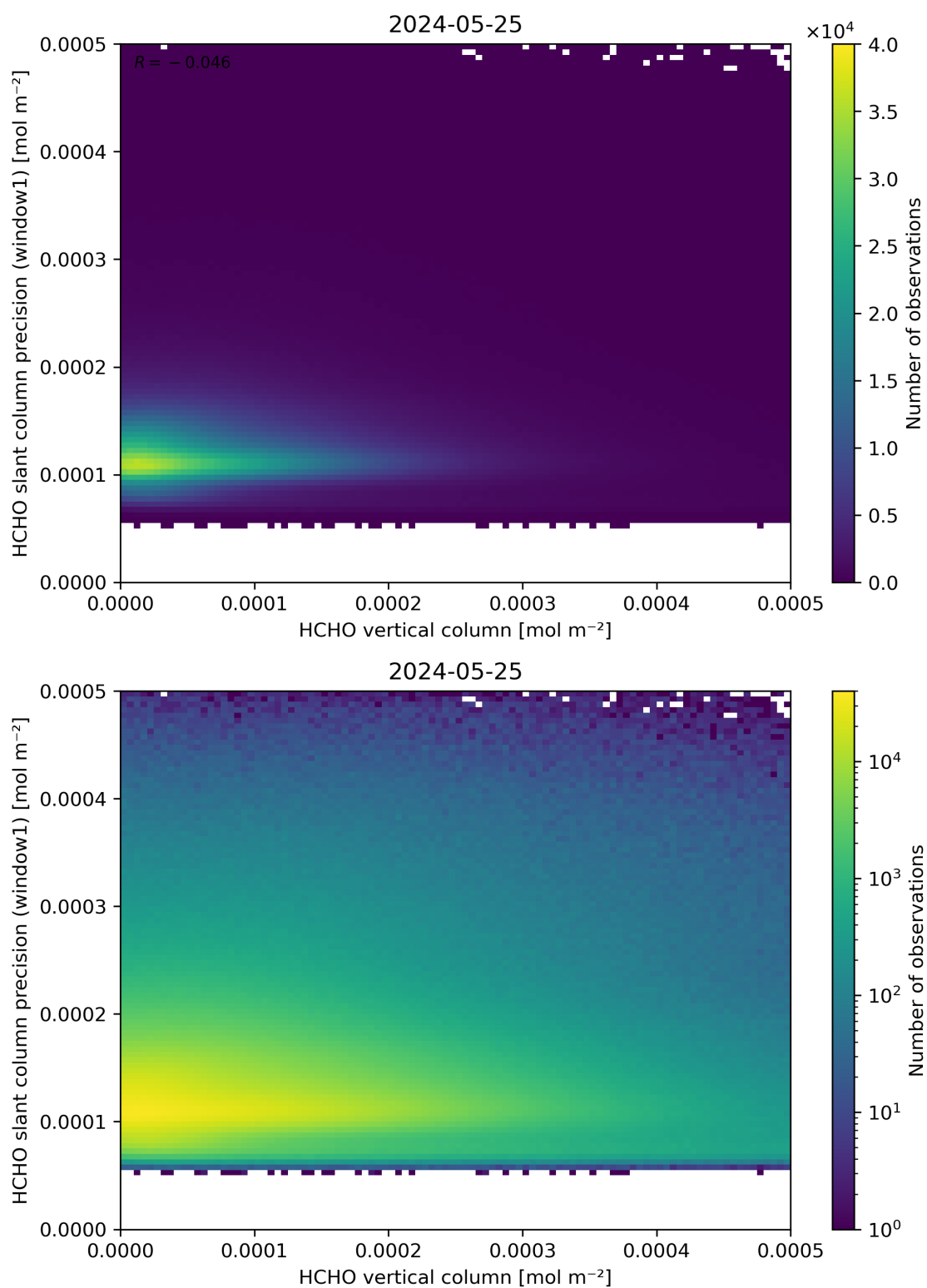
Figure 130: Scatter density plot of “HCHO vertical column” against “HCHO slant column precision (window1)” for 2024-05-24 to 2024-05-26.
