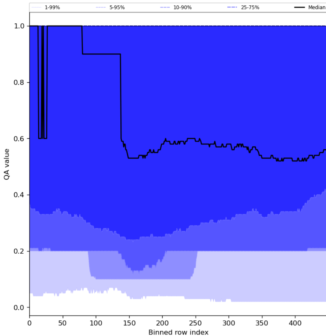
Figure 48: Along track statistics of “QA value” for 2024-05-24 to 2024-05-26
