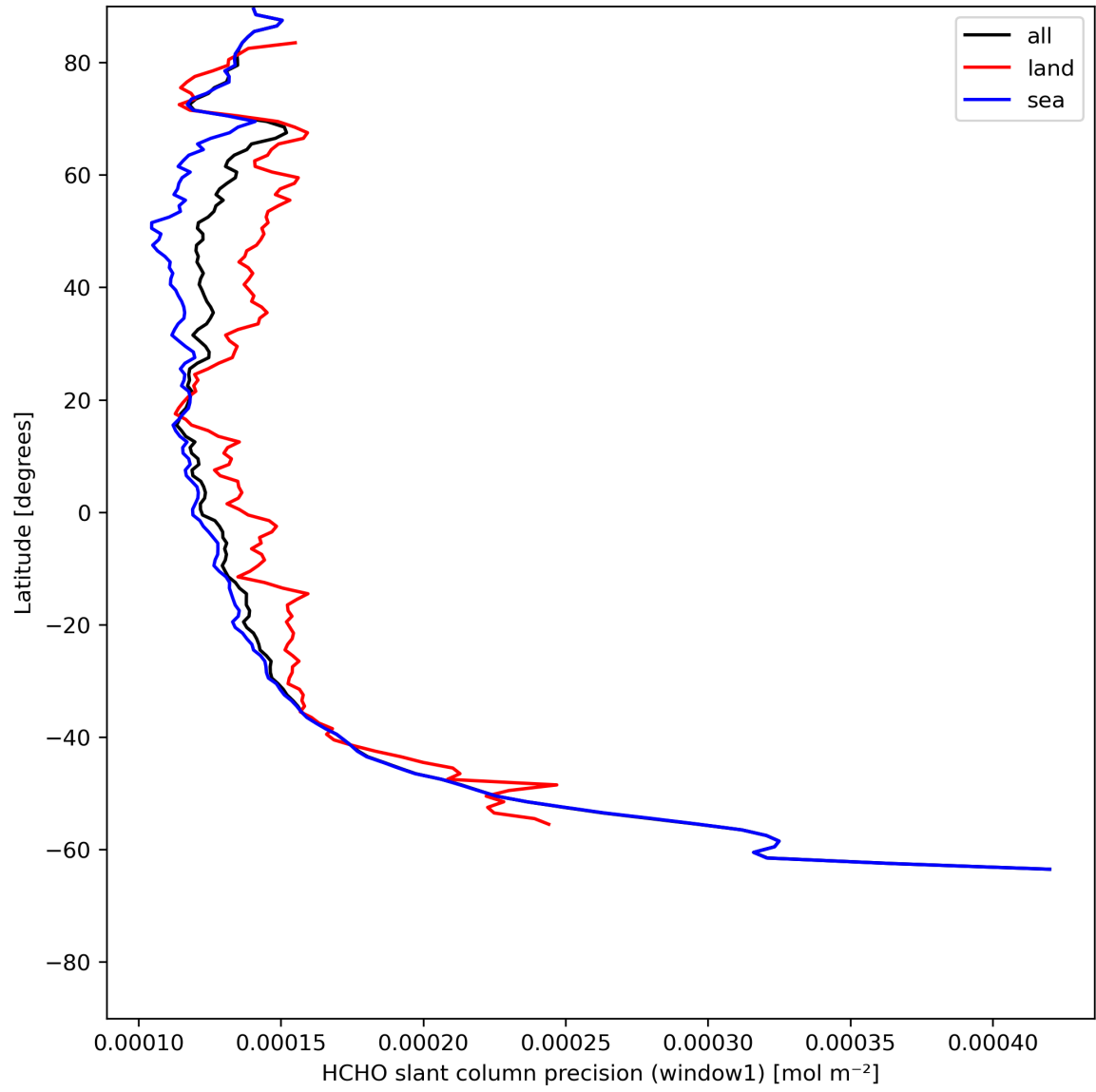
Figure 25: Zonal average of “HCHO slant column precision (window1)” for 2024-05-24 to 2024-05-26.
