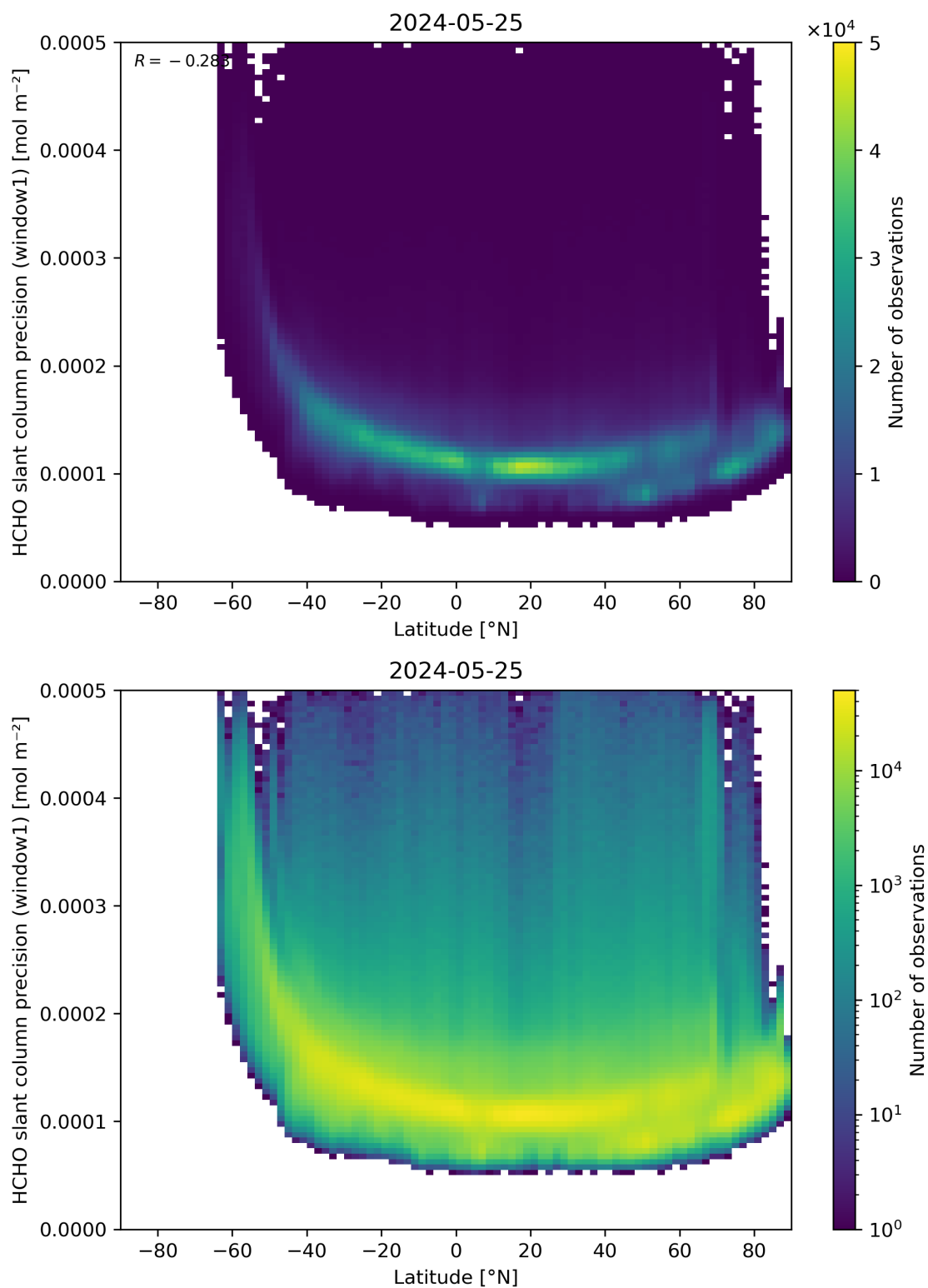
Figure 160: Scatter density plot of “Latitude” against “HCHO slant column precision (window1)” for 2024-05-24 to 2024-05-26.
