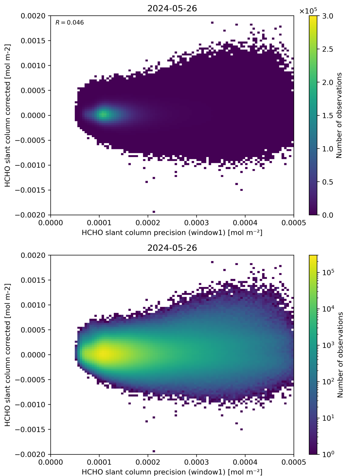
Figure 92: Scatter density plot of “HCHO slant column precision (window1)” against “HCHO slant column corrected” for 2024-05-25 to 2024-05-27.
