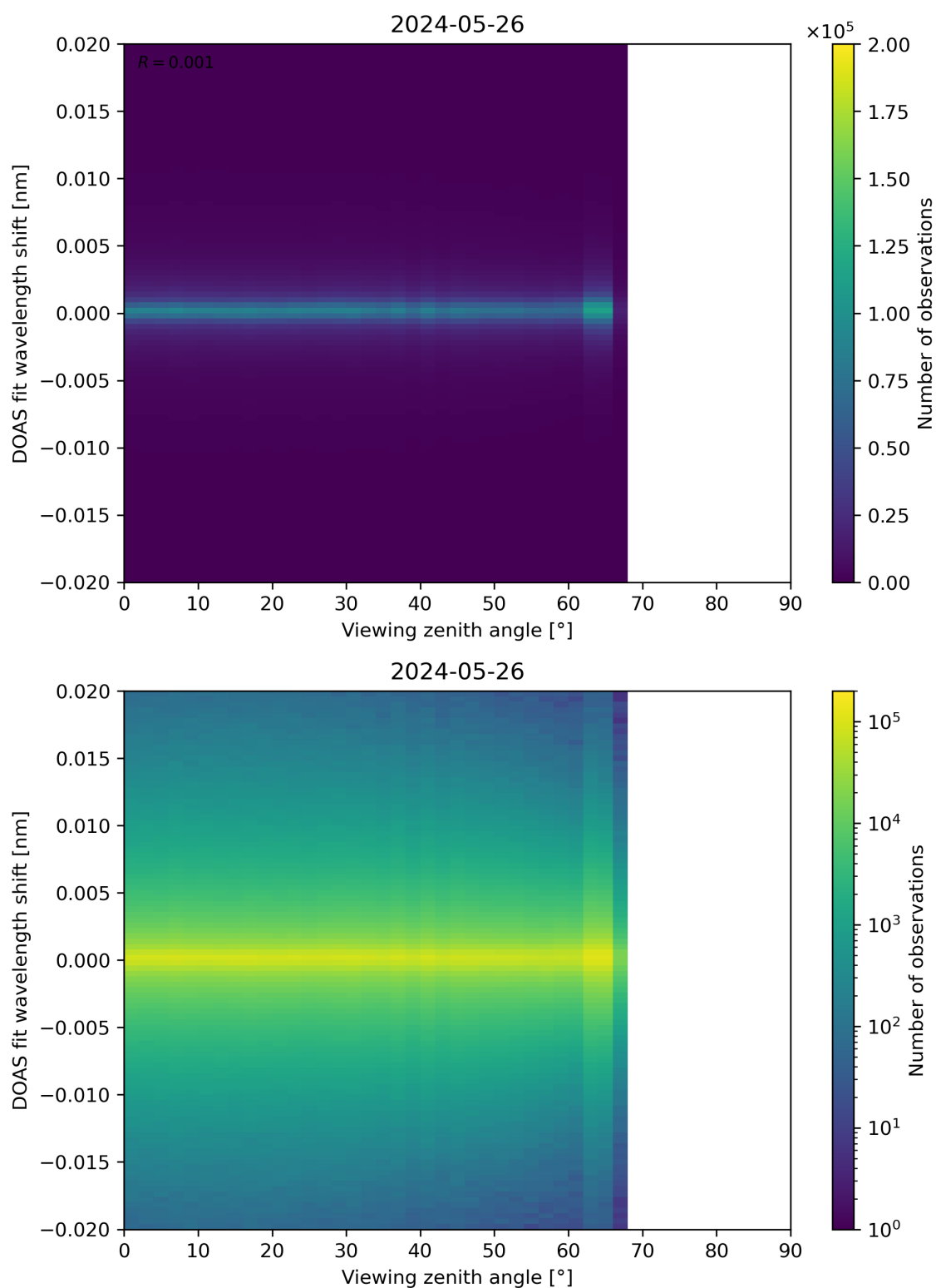
Figure 183: Scatter density plot of “Viewing zenith angle” against “DOAS fit wavelength shift” for 2024-05-25 to 2024-05-27.
