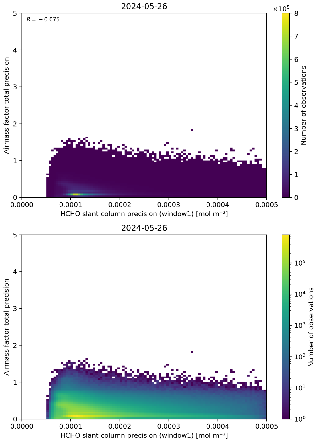
Figure 95: Scatter density plot of “HCHO slant column precision (window1)” against “Airmass factor total precision” for 2024-05-25 to 2024-05-27.
