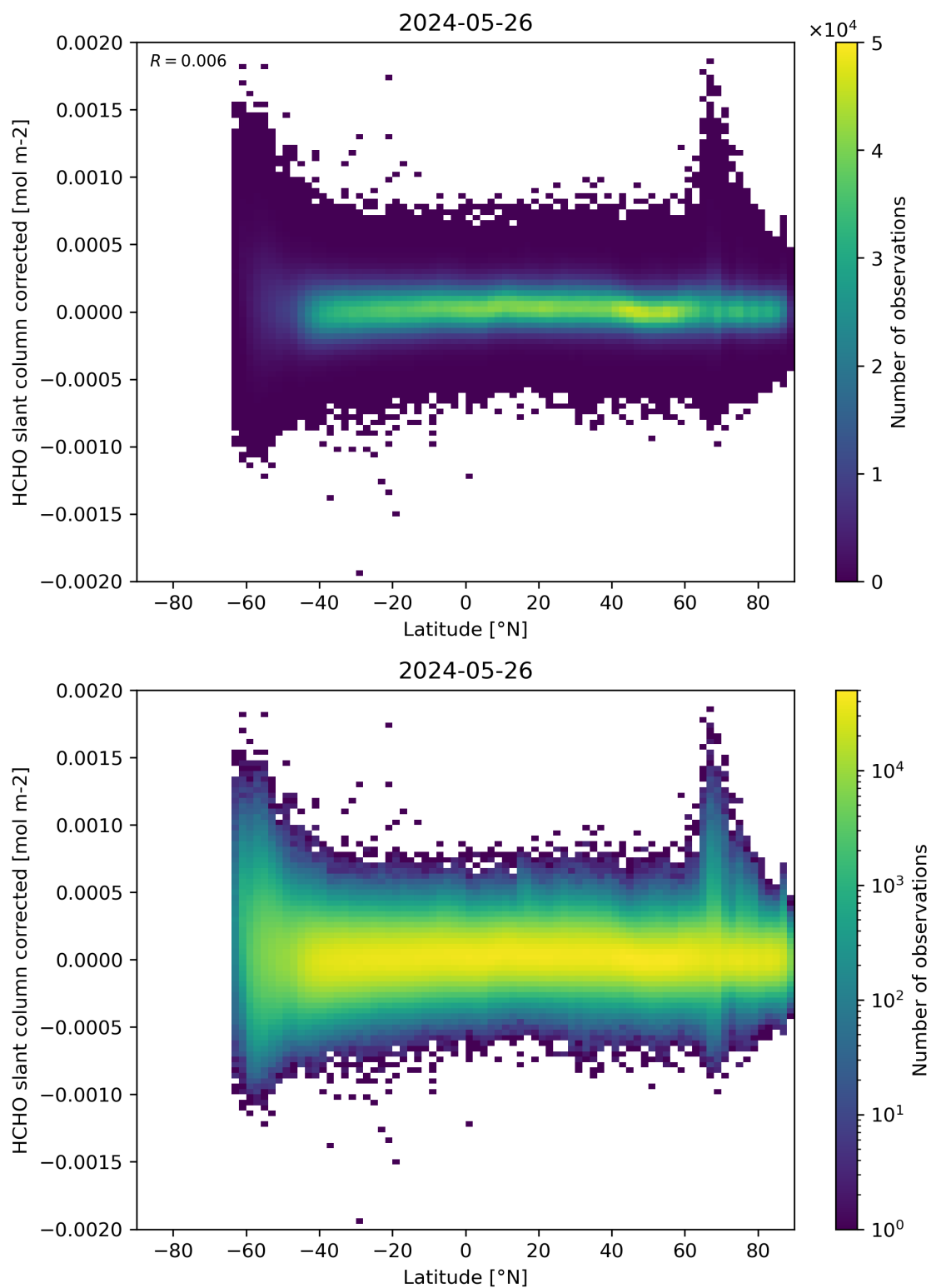
Figure 157: Scatter density plot of “Latitude” against “HCHO slant column corrected” for 2024-05-25 to 2024-05-27.
