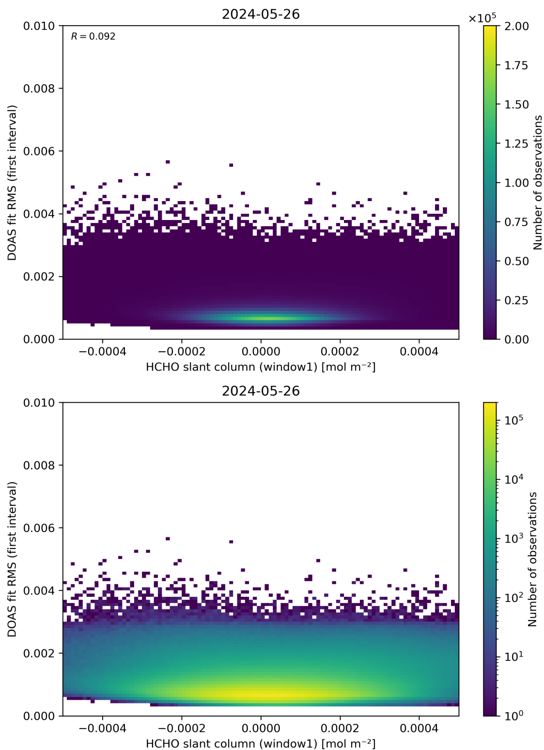
Figure 78: Scatter density plot of “HCHO slant column (window1)” against “DOAS fit RMS (first interval)” for 2024-05-25 to 2024-05-27.
