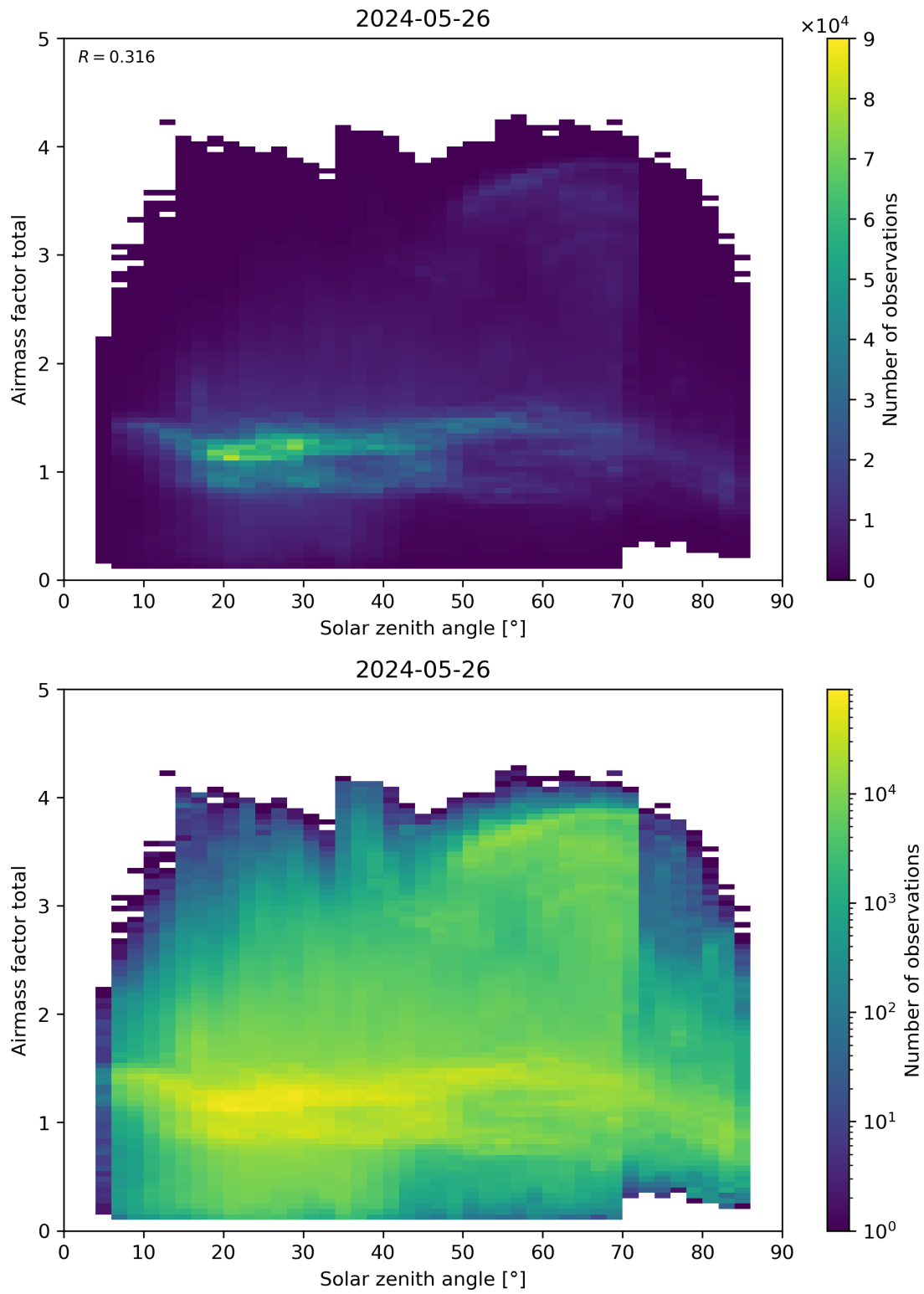
Figure 175: Scatter density plot of “Solar zenith angle” against “Airmass factor total” for 2024-05-25 to 2024-05-27.
