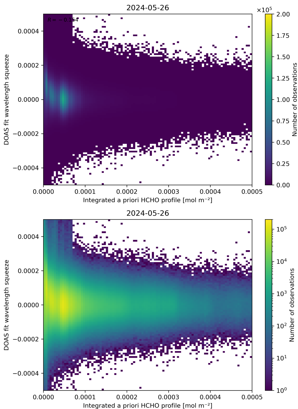
Figure 150: Scatter density plot of “Integrated a priori HCHO profile” against “DOAS fit wavelength squeeze” for 2024-05-25 to 2024-05-27.
