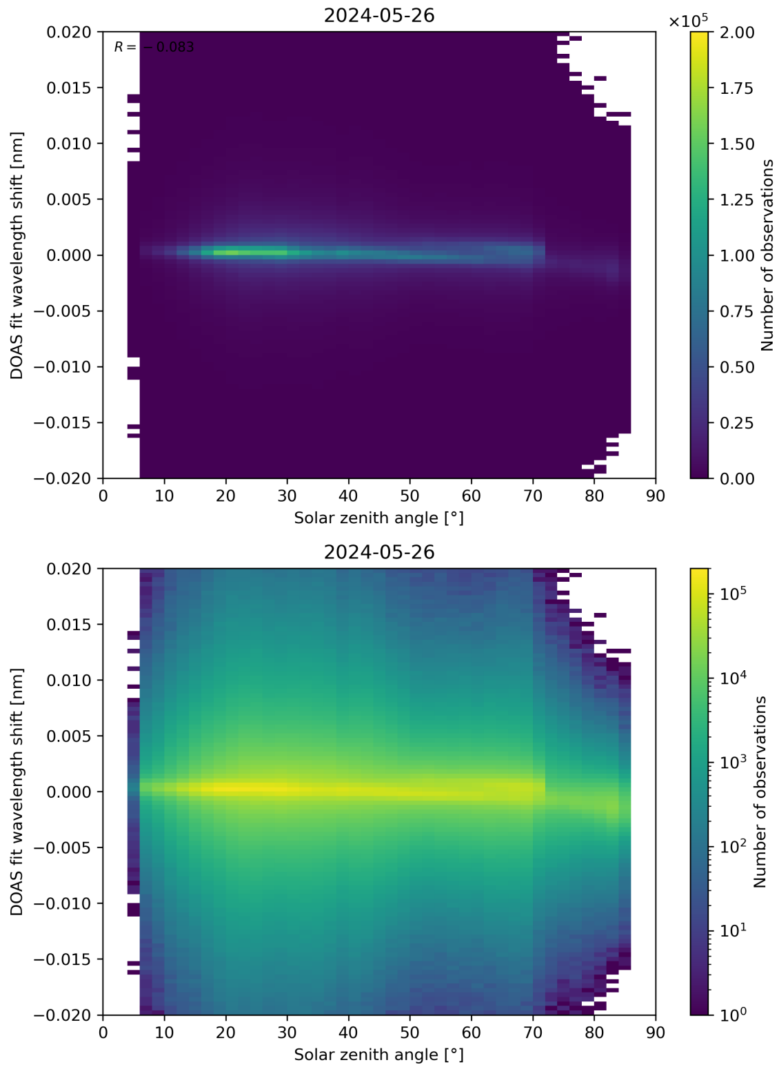
Figure 168: Scatter density plot of “Solar zenith angle” against “DOAS fit wavelength shift” for 2024-05-25 to 2024-05-27.
