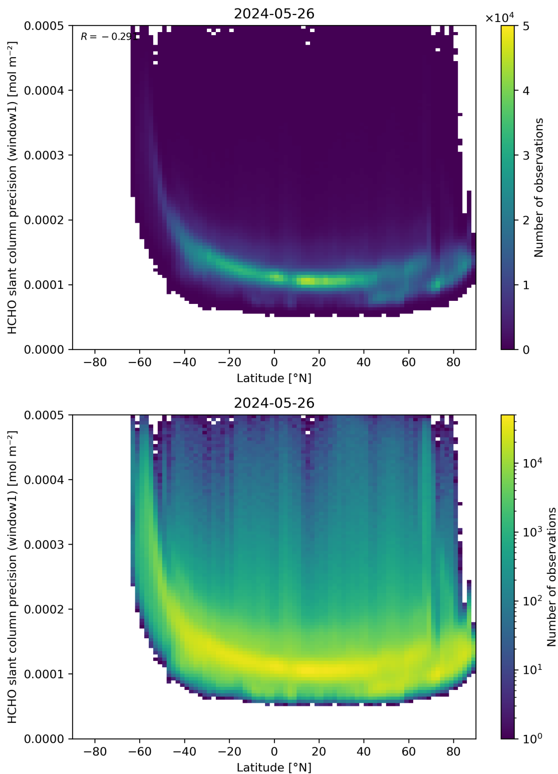
Figure 160: Scatter density plot of “Latitude” against “HCHO slant column precision (window1)” for 2024-05-25 to 2024-05-27.
