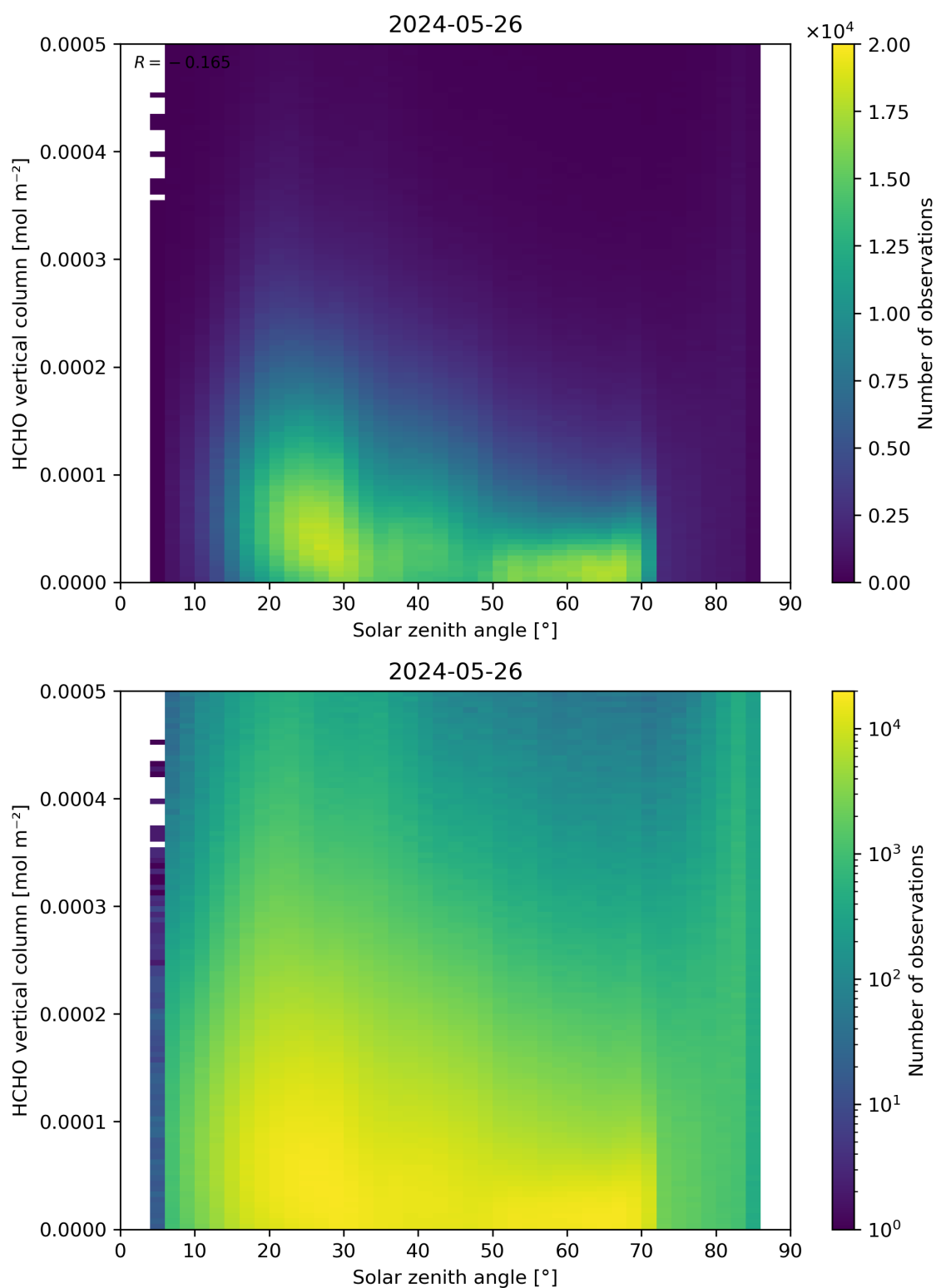
Figure 177: Scatter density plot of “Solar zenith angle” against “HCHO vertical column” for 2024-05-25 to 2024-05-27.
