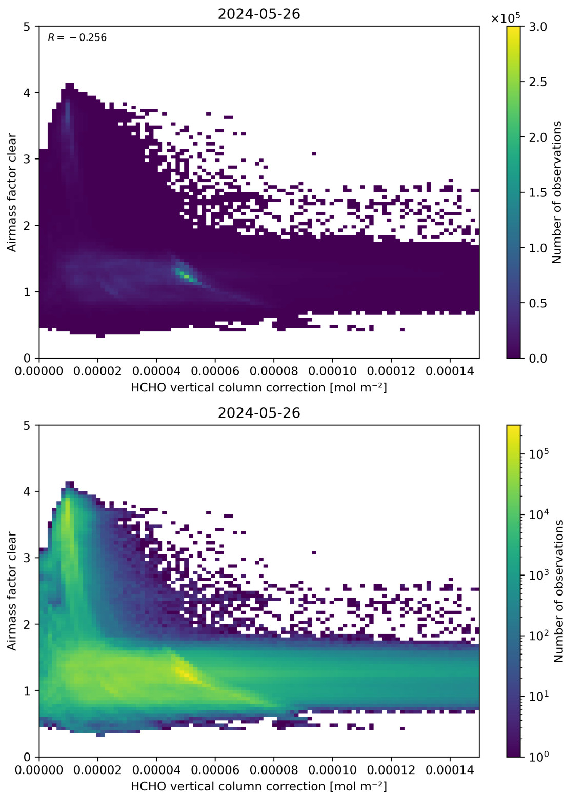
Figure 115: Scatter density plot of “HCHO vertical column correction” against “Airmass factor clear” for 2024-05-25 to 2024-05-27.
