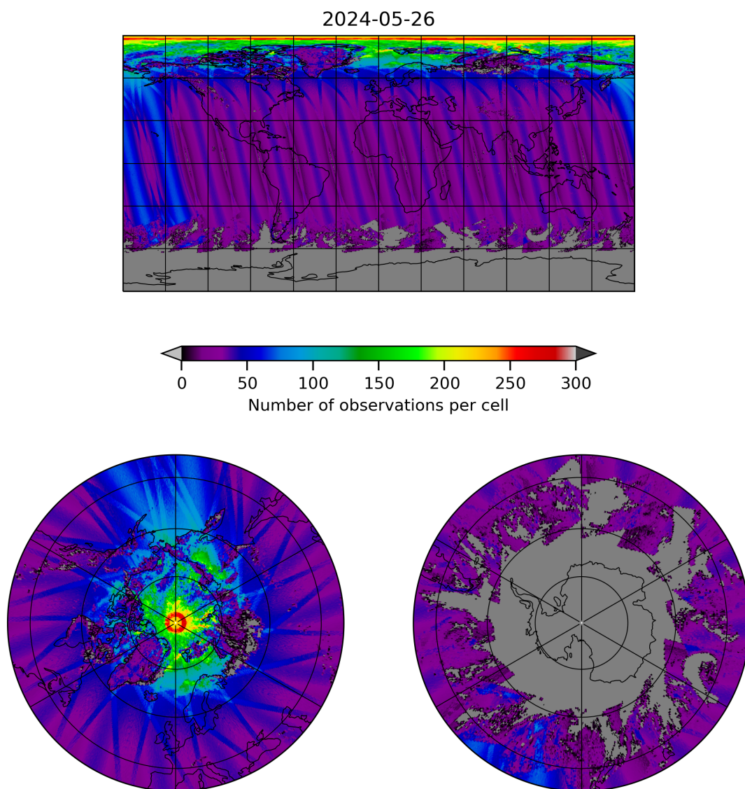
Figure 19: Map of the number of observations for 2024-05-25 to 2024-05-27
