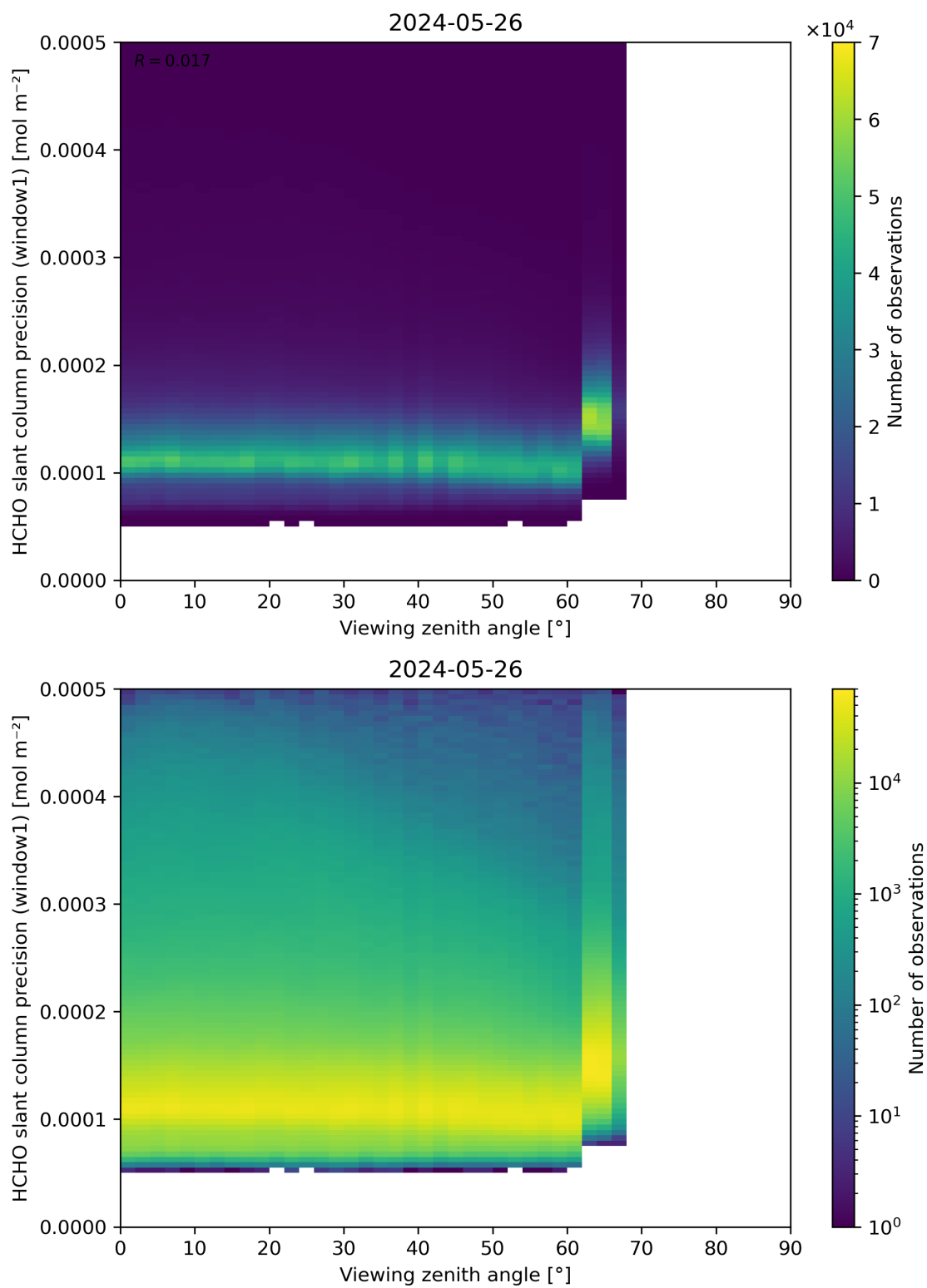
Figure 189: Scatter density plot of “Viewing zenith angle” against “HCHO slant column precision (window1)” for 2024-05-25 to 2024-05-27.
