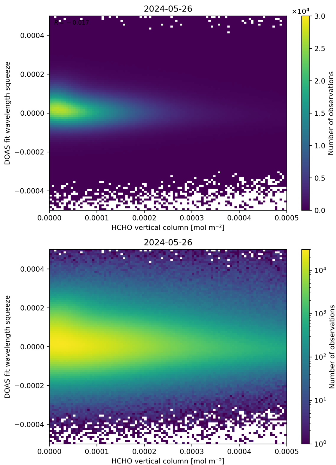
Figure 125: Scatter density plot of “HCHO vertical column” against “DOAS fit wavelength squeeze” for 2024-05-25 to 2024-05-27.
