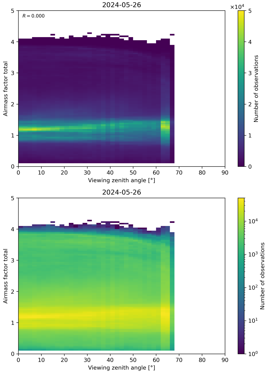
Figure 190: Scatter density plot of “Viewing zenith angle” against “Airmass factor total” for 2024-05-25 to 2024-05-27.
