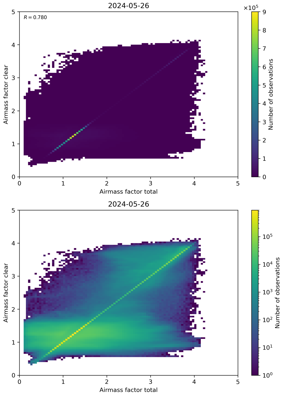
Figure 100: Scatter density plot of “Airmass factor total” against “Airmass factor clear” for 2024-05-25 to 2024-05-27.
