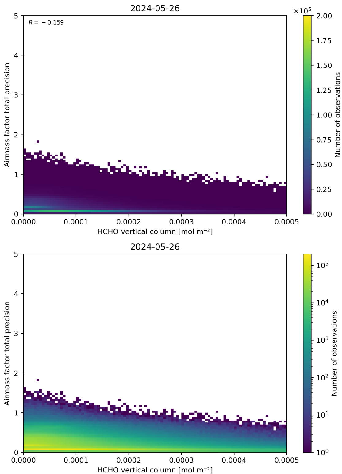
Figure 132: Scatter density plot of “HCHO vertical column” against “Airmass factor total precision” for 2024-05-25 to 2024-05-27.
