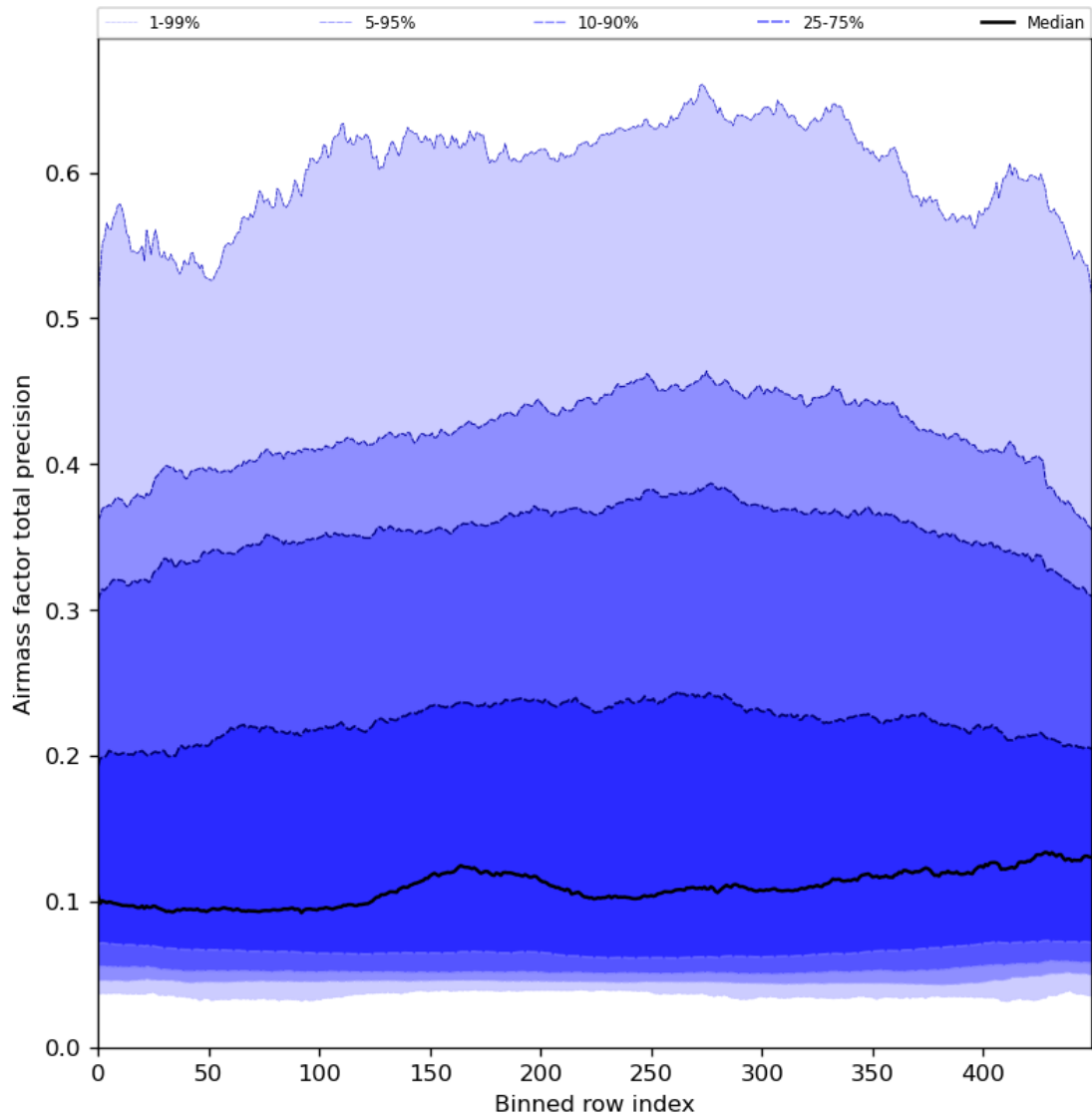
Figure 55: Along track statistics of “Airmass factor total precision” for 2024-05-25 to 2024-05-27
