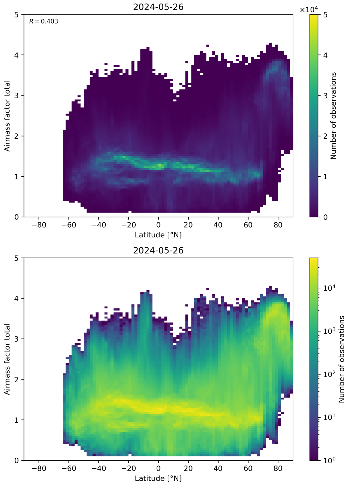
Figure 161: Scatter density plot of “Latitude” against “Airmass factor total” for 2024-05-25 to 2024-05-27.
