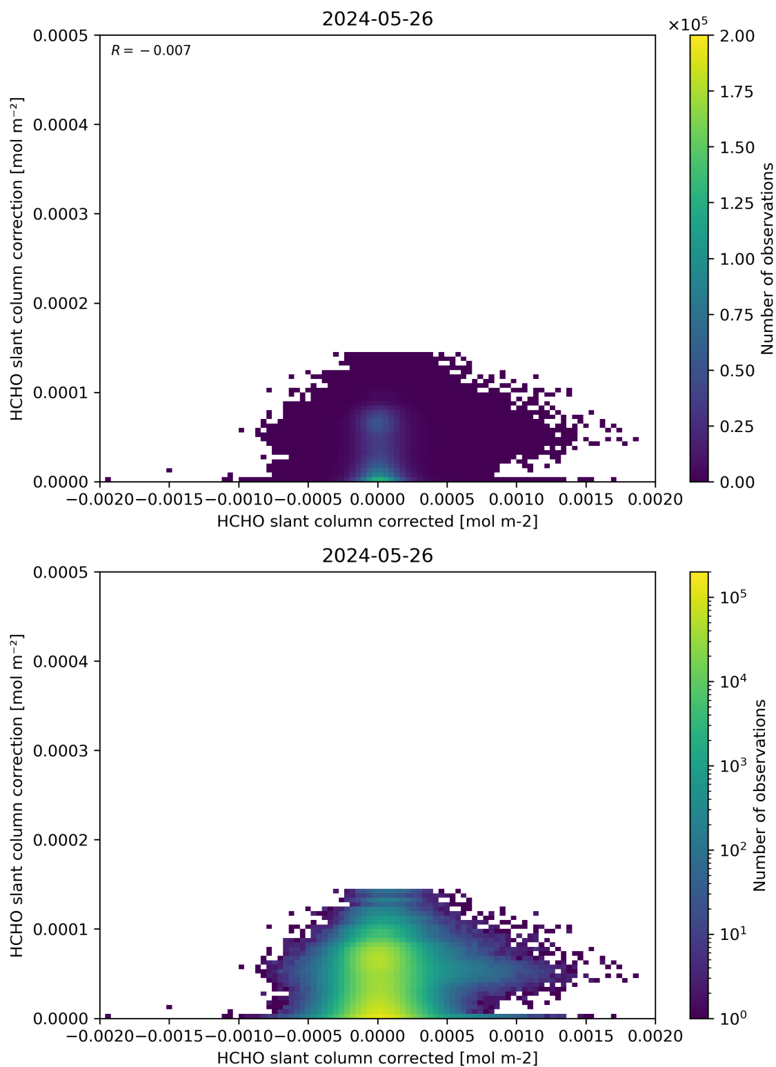
Figure 77: Scatter density plot of “HCHO slant column corrected” against “HCHO slant column correction” for 2024-05-25 to 2024-05-27.
