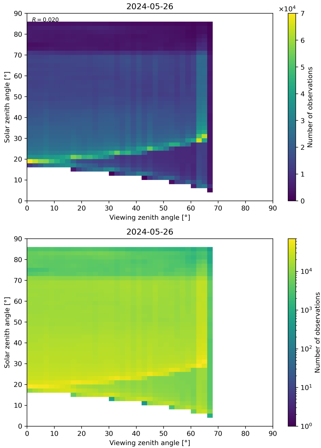
Figure 197: Scatter density plot of “Viewing zenith angle” against “Solar zenith angle” for 2024-05-25 to 2024-05-27.
