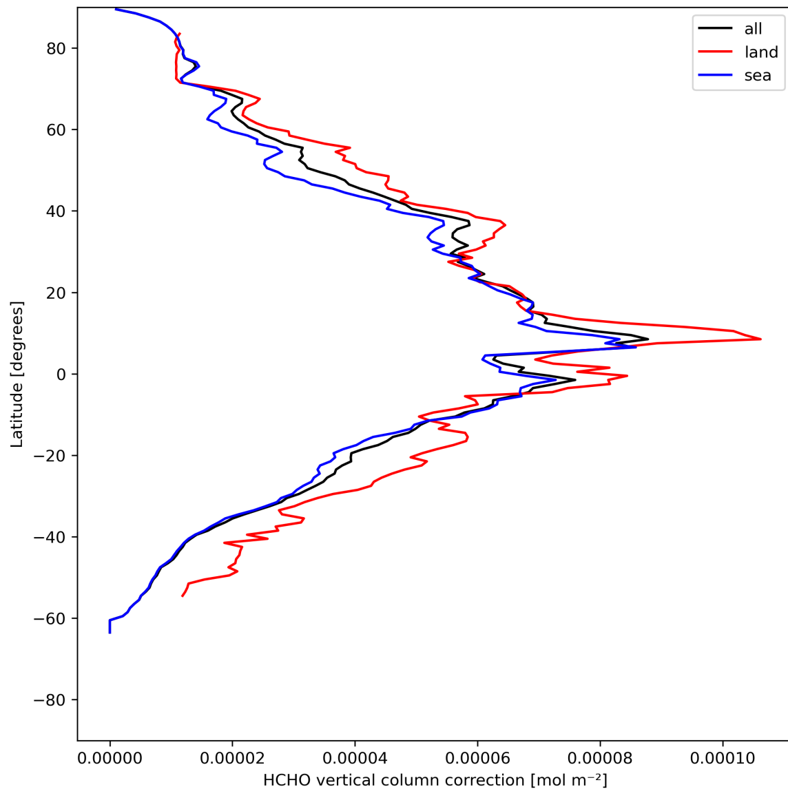
Figure 23: Zonal average of “HCHO vertical column correction” for 2024-05-25 to 2024-05-27.
