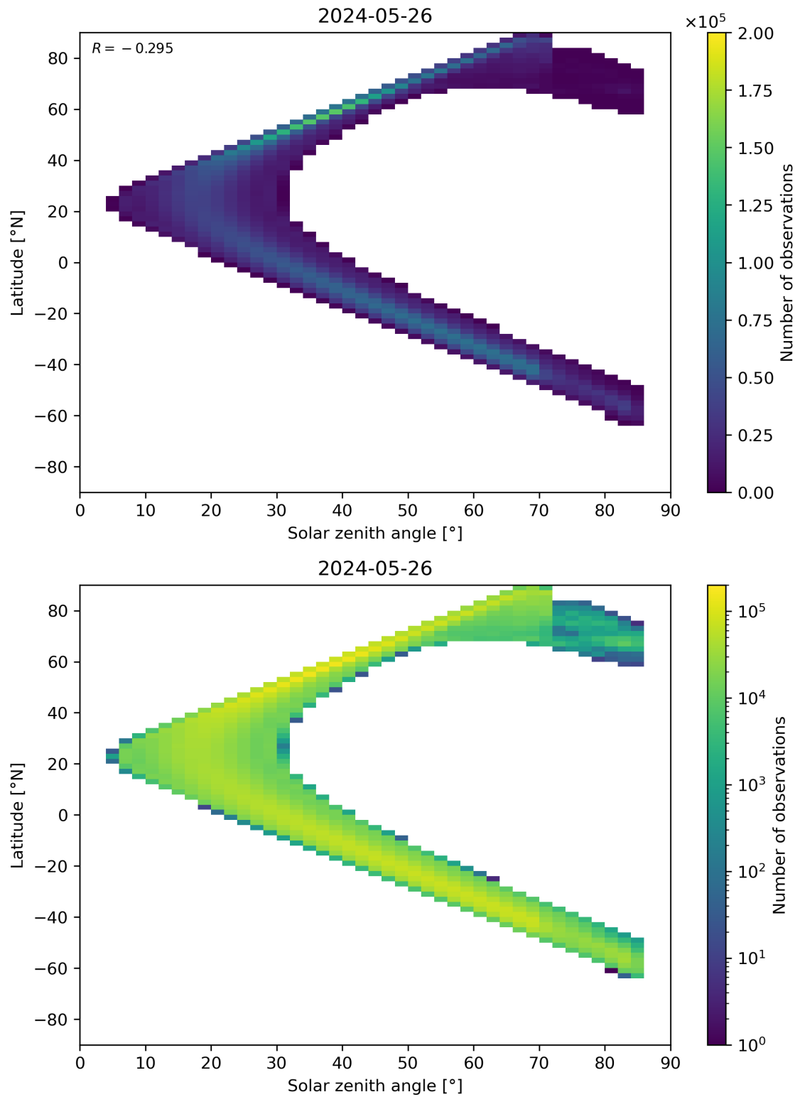
Figure 181: Scatter density plot of “Solar zenith angle” against “Latitude” for 2024-05-25 to 2024-05-27.
