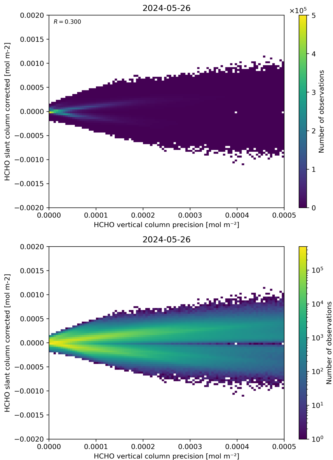
Figure 140: Scatter density plot of “HCHO vertical column precision” against “HCHO slant column corrected” for 2024-05-25 to 2024-05-27.
