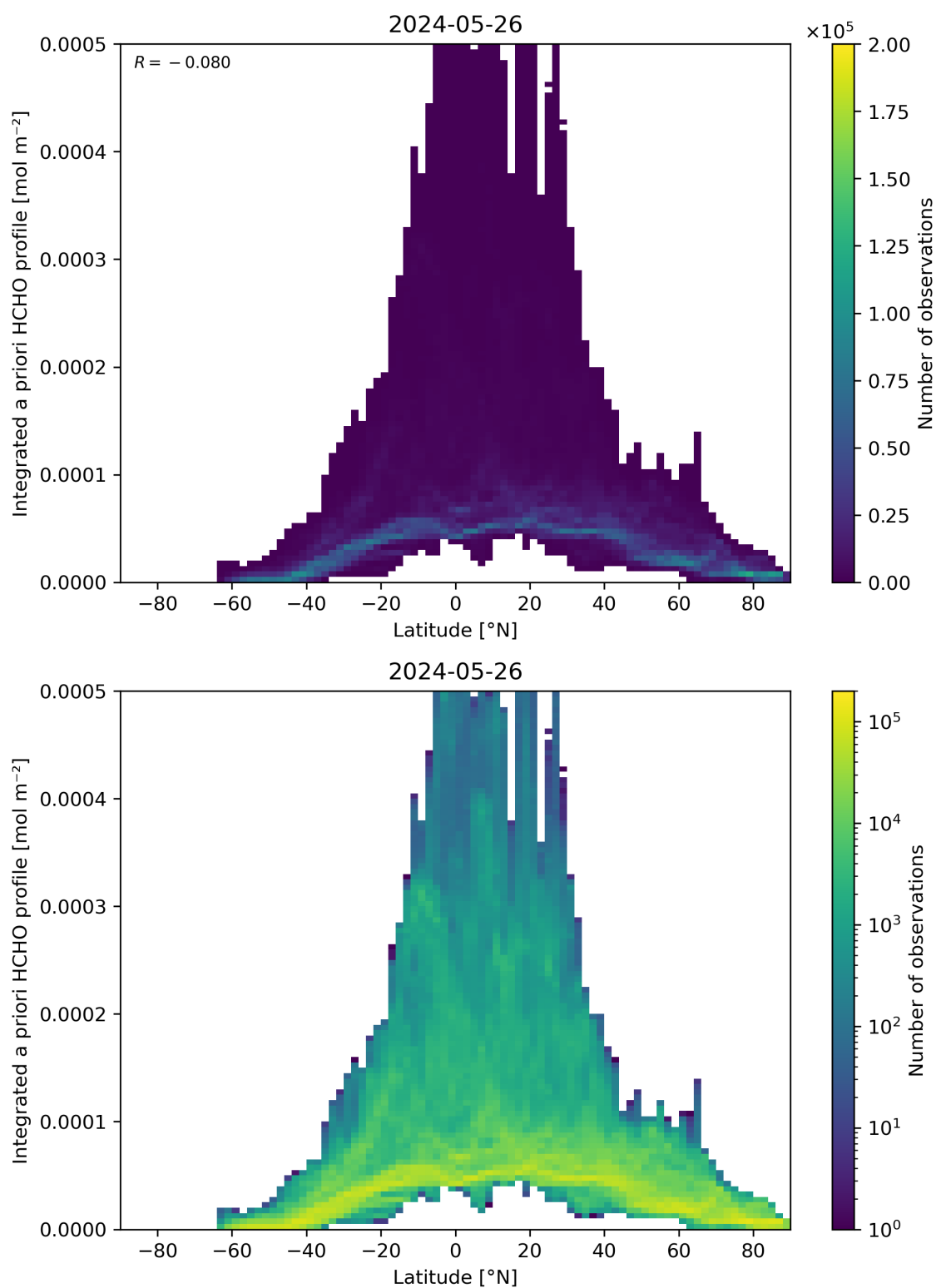
Figure 166: Scatter density plot of “Latitude” against “Integrated a priori HCHO profile” for 2024-05-25 to 2024-05-27.
