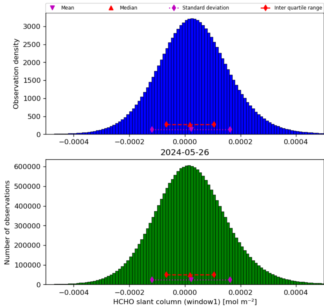
Figure 38: Histogram of “HCHO slant column (window1)” for 2024-05-25 to 2024-05-27
