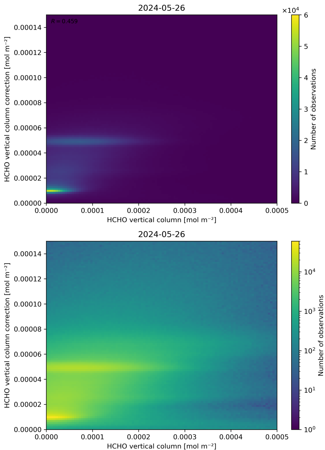
Figure 133: Scatter density plot of “HCHO vertical column” against “HCHO vertical column correction” for 2024-05-25 to 2024-05-27.
