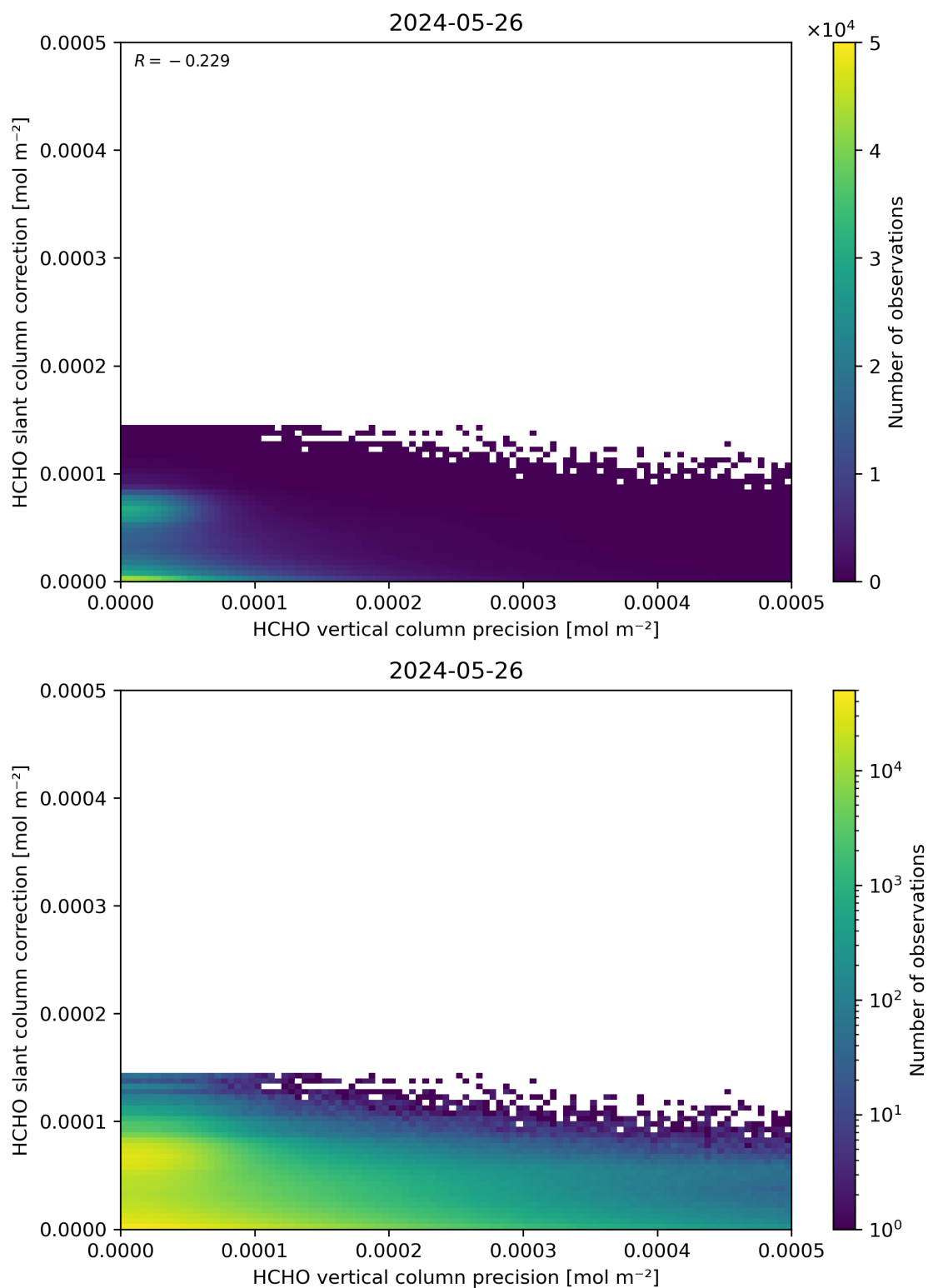
Figure 141: Scatter density plot of “HCHO vertical column precision” against “HCHO slant column correction” for 2024-05-25 to 2024-05-27.
