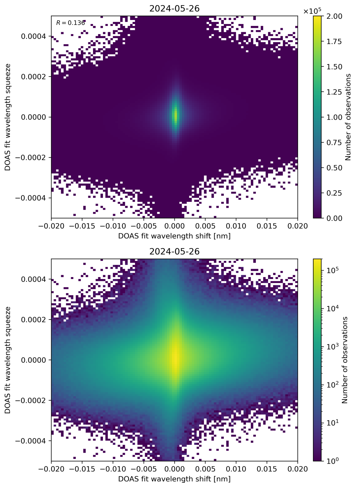
Figure 65: Scatter density plot of “DOAS fit wavelength shift” against “DOAS fit wavelength squeeze” for 2024-05-25 to 2024-05-27.
