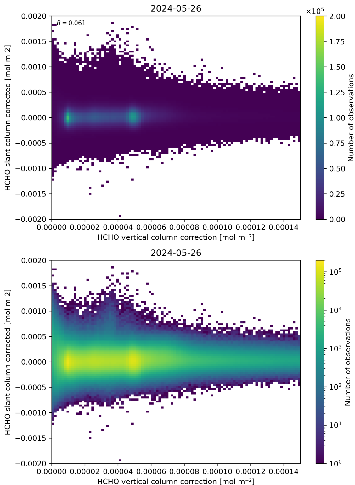
Figure 116: Scatter density plot of “HCHO vertical column correction” against “HCHO slant column corrected” for 2024-05-25 to 2024-05-27.
