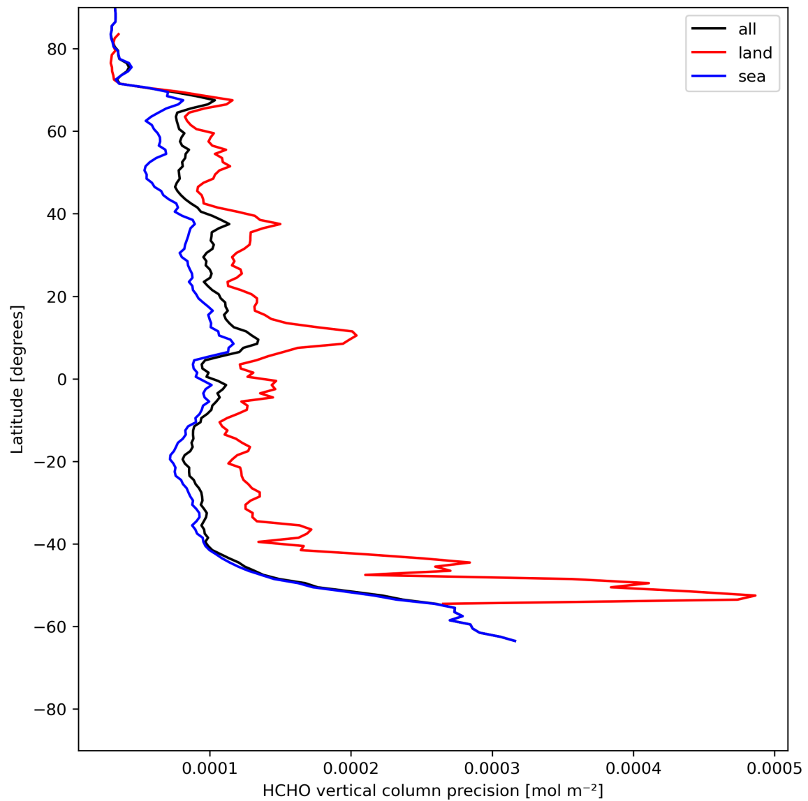
Figure 22: Zonal average of “HCHO vertical column precision” for 2024-05-25 to 2024-05-27.
