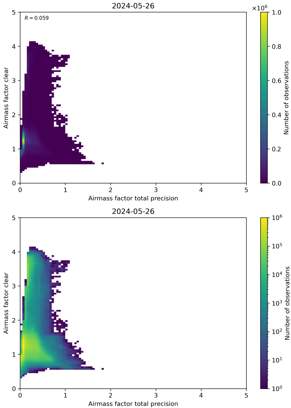
Figure 108: Scatter density plot of “Airmass factor total precision” against “Airmass factor clear” for 2024-05-25 to 2024-05-27.
