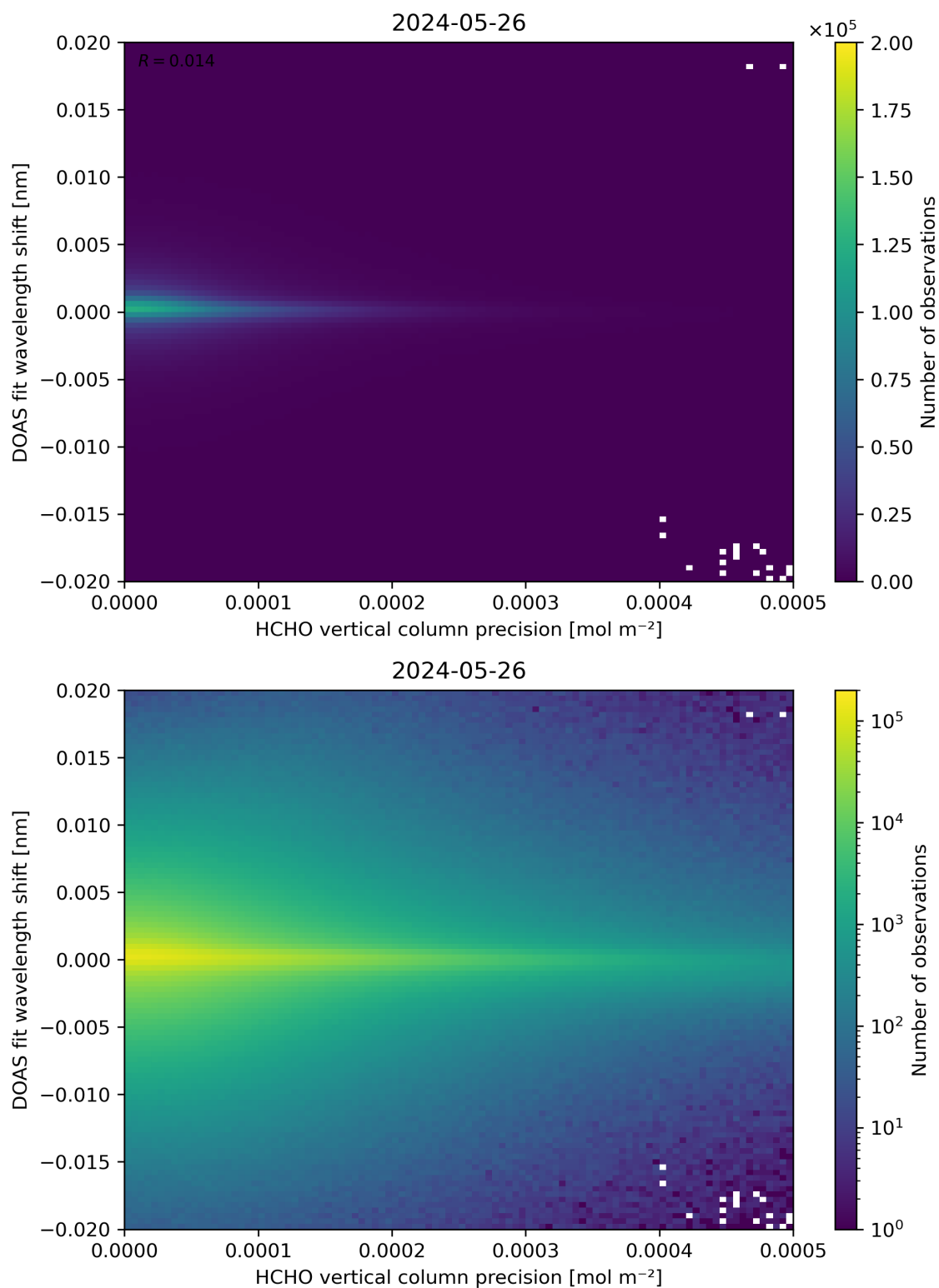
Figure 137: Scatter density plot of “HCHO vertical column precision” against “DOAS fit wavelength shift” for 2024-05-25 to 2024-05-27.
