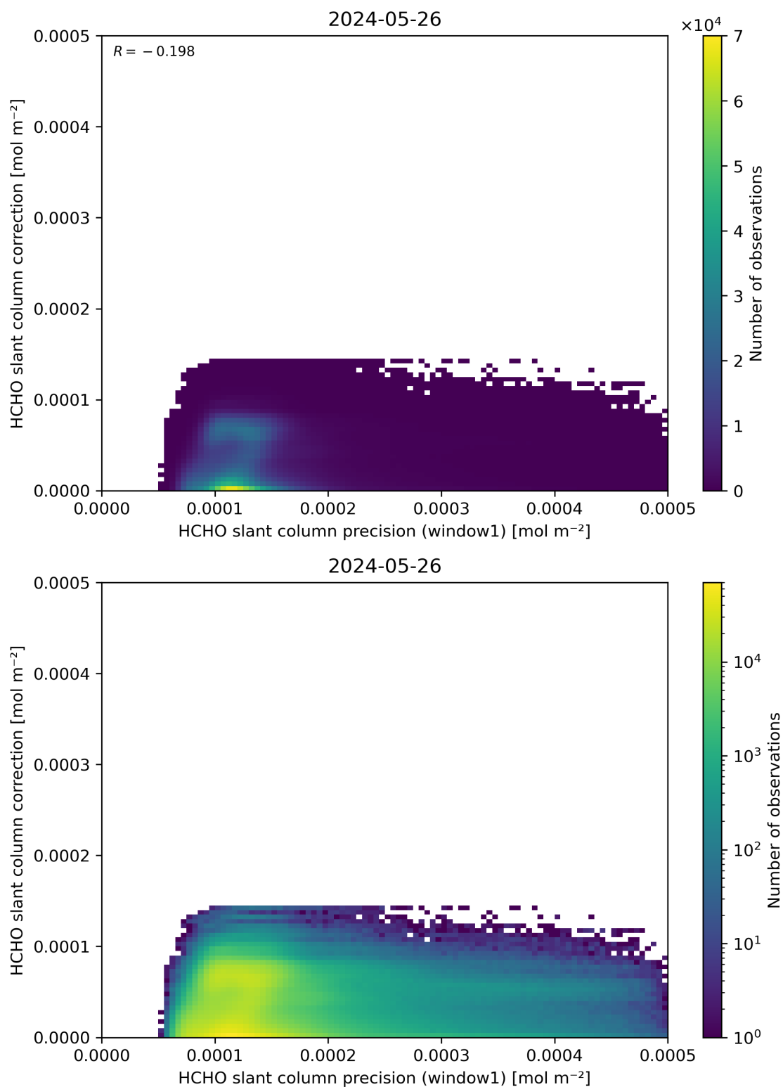
Figure 93: Scatter density plot of “HCHO slant column precision (window1)” against “HCHO slant column correction” for 2024-05-25 to 2024-05-27.
