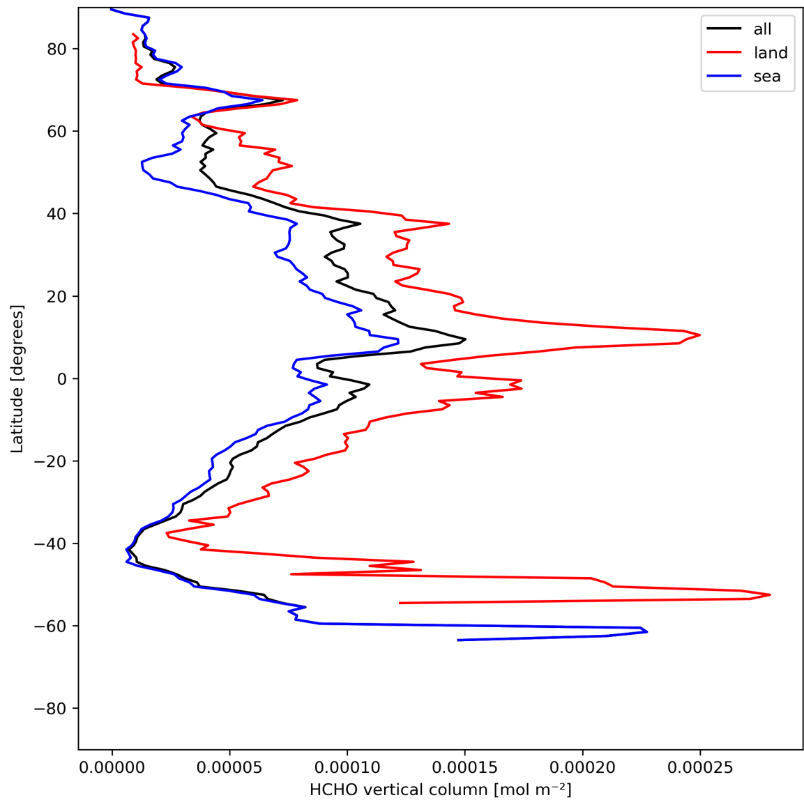
Figure 21: Zonal average of “HCHO vertical column” for 2024-05-25 to 2024-05-27.
