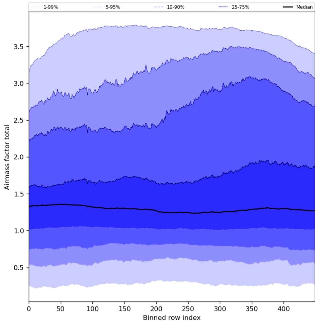
Figure 54: Along track statistics of “Airmass factor total” for 2024-05-25 to 2024-05-27
