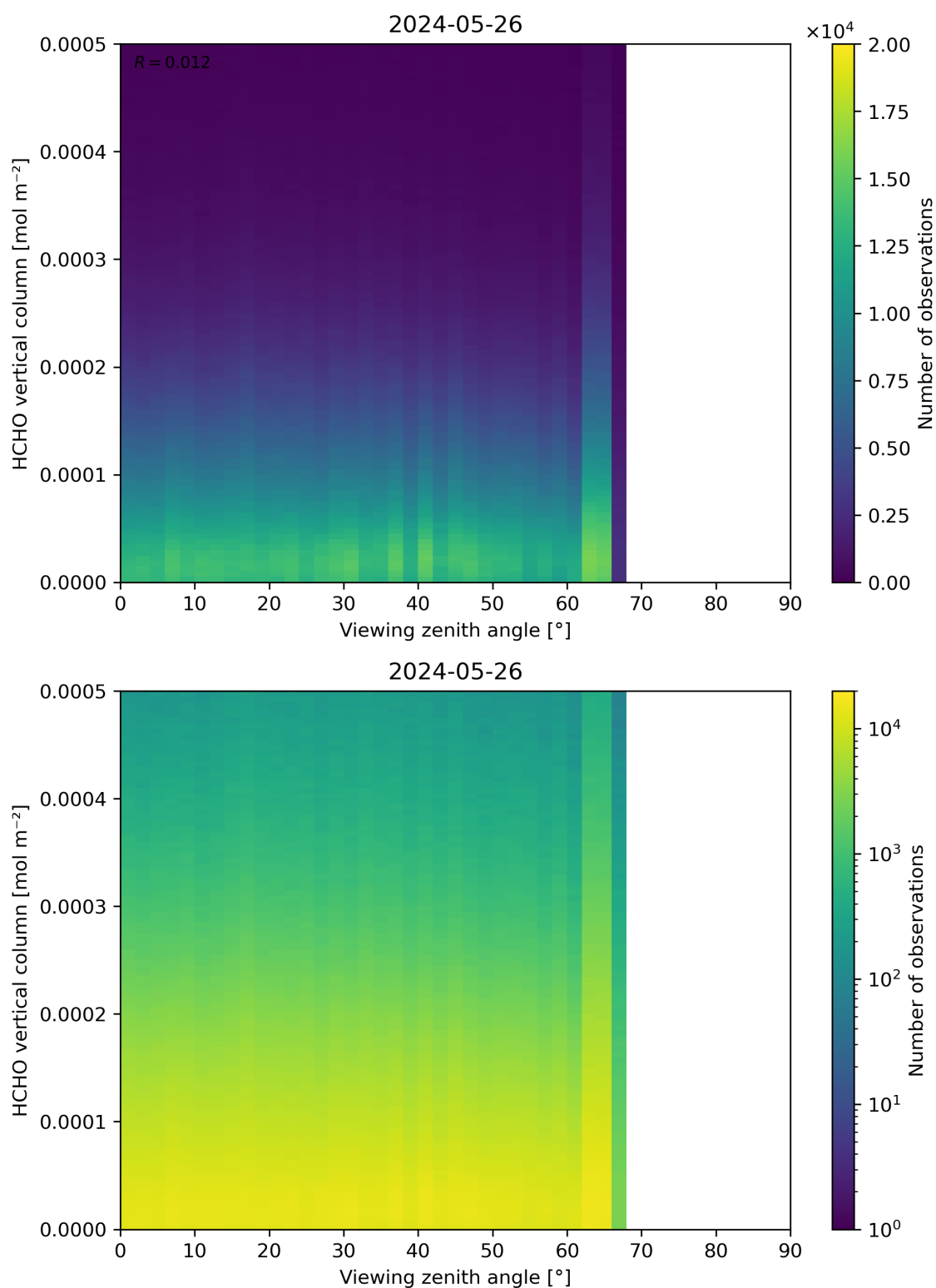
Figure 192: Scatter density plot of “Viewing zenith angle” against “HCHO vertical column” for 2024-05-25 to 2024-05-27.
