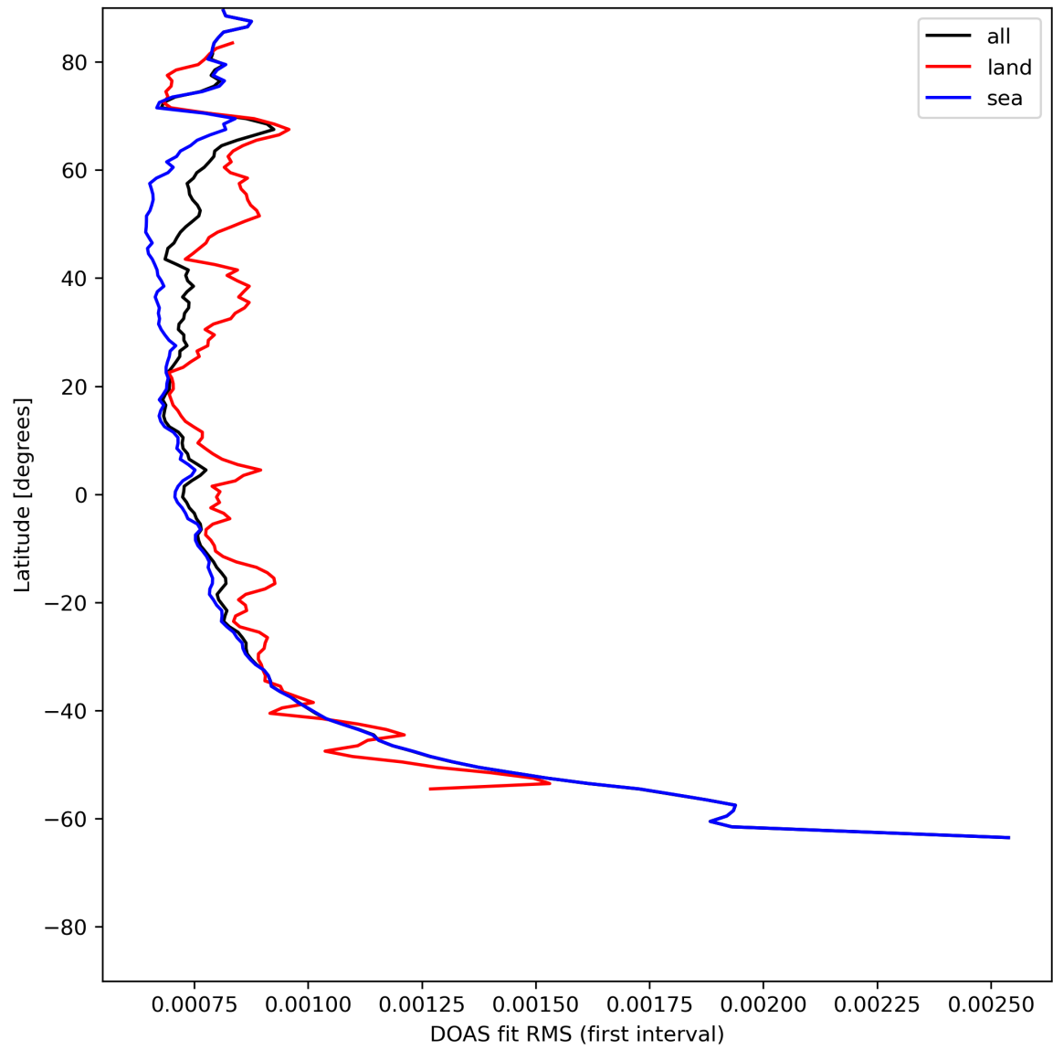
Figure 32: Zonal average of “DOAS fit RMS (first interval)” for 2024-05-25 to 2024-05-27.
