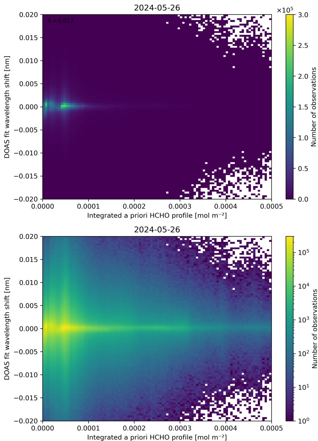
Figure 149: Scatter density plot of “Integrated a priori HCHO profile” against “DOAS fit wavelength shift” for 2024-05-25 to 2024-05-27.
