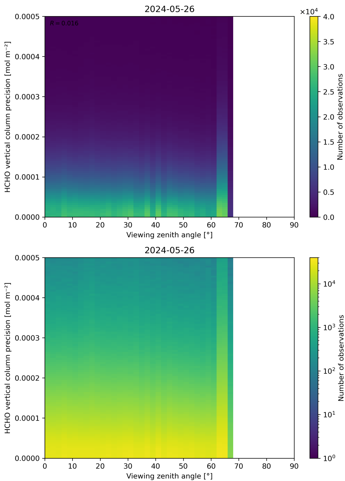
Figure 194: Scatter density plot of “Viewing zenith angle” against “HCHO vertical column precision” for 2024-05-25 to 2024-05-27.
