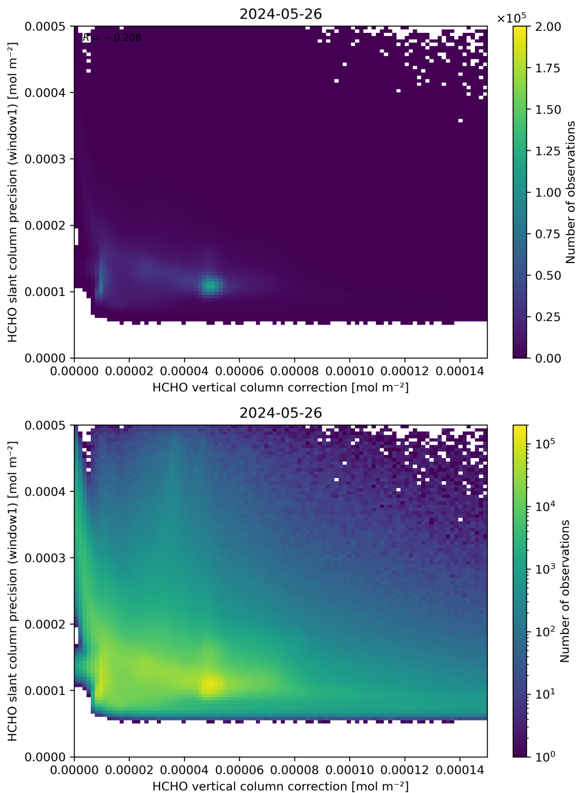
Figure 119: Scatter density plot of “HCHO vertical column correction” against “HCHO slant column precision (window1)” for 2024-05-25 to 2024-05-27.
