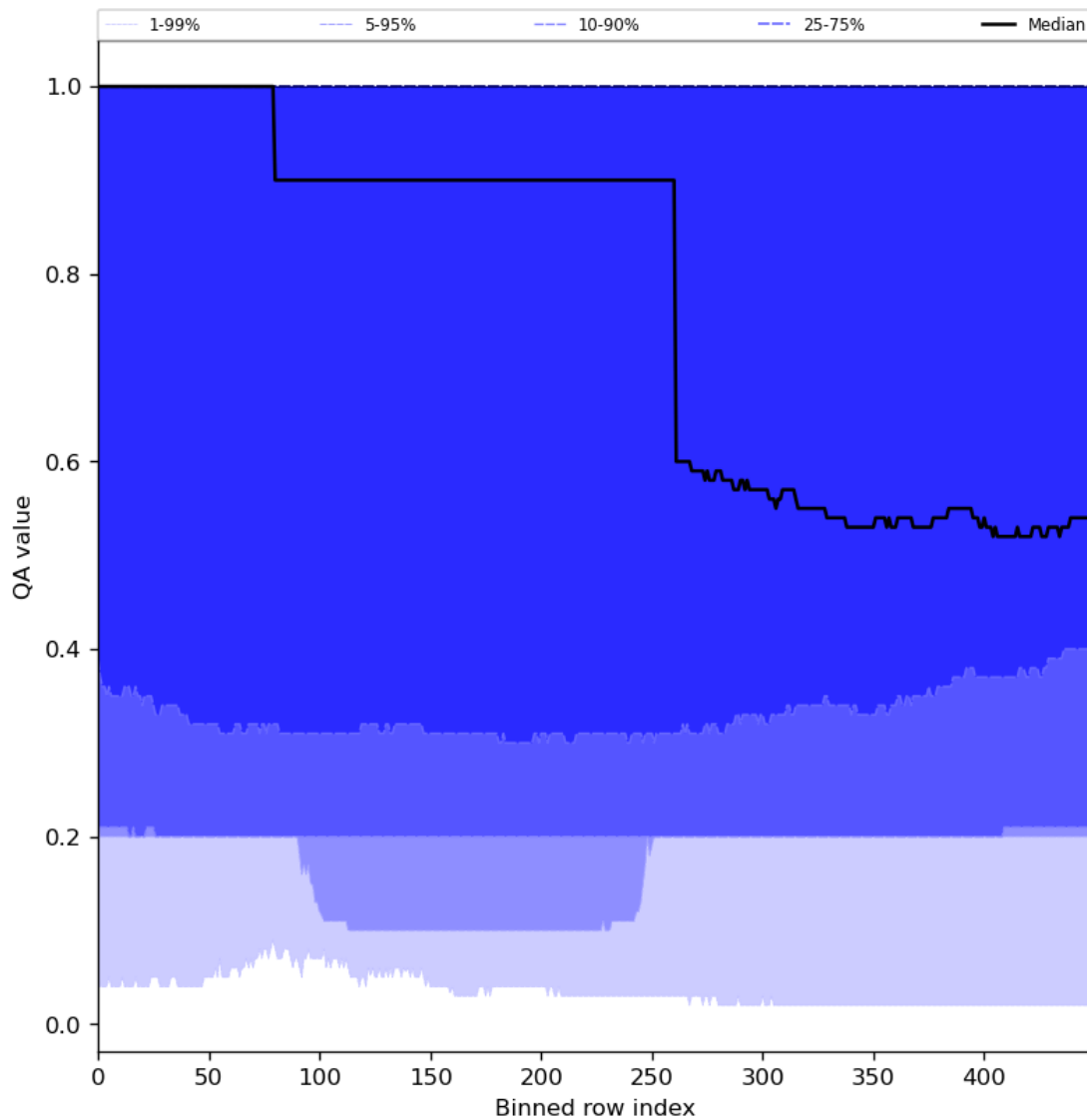
Figure 48: Along track statistics of “QA value” for 2024-05-25 to 2024-05-27
