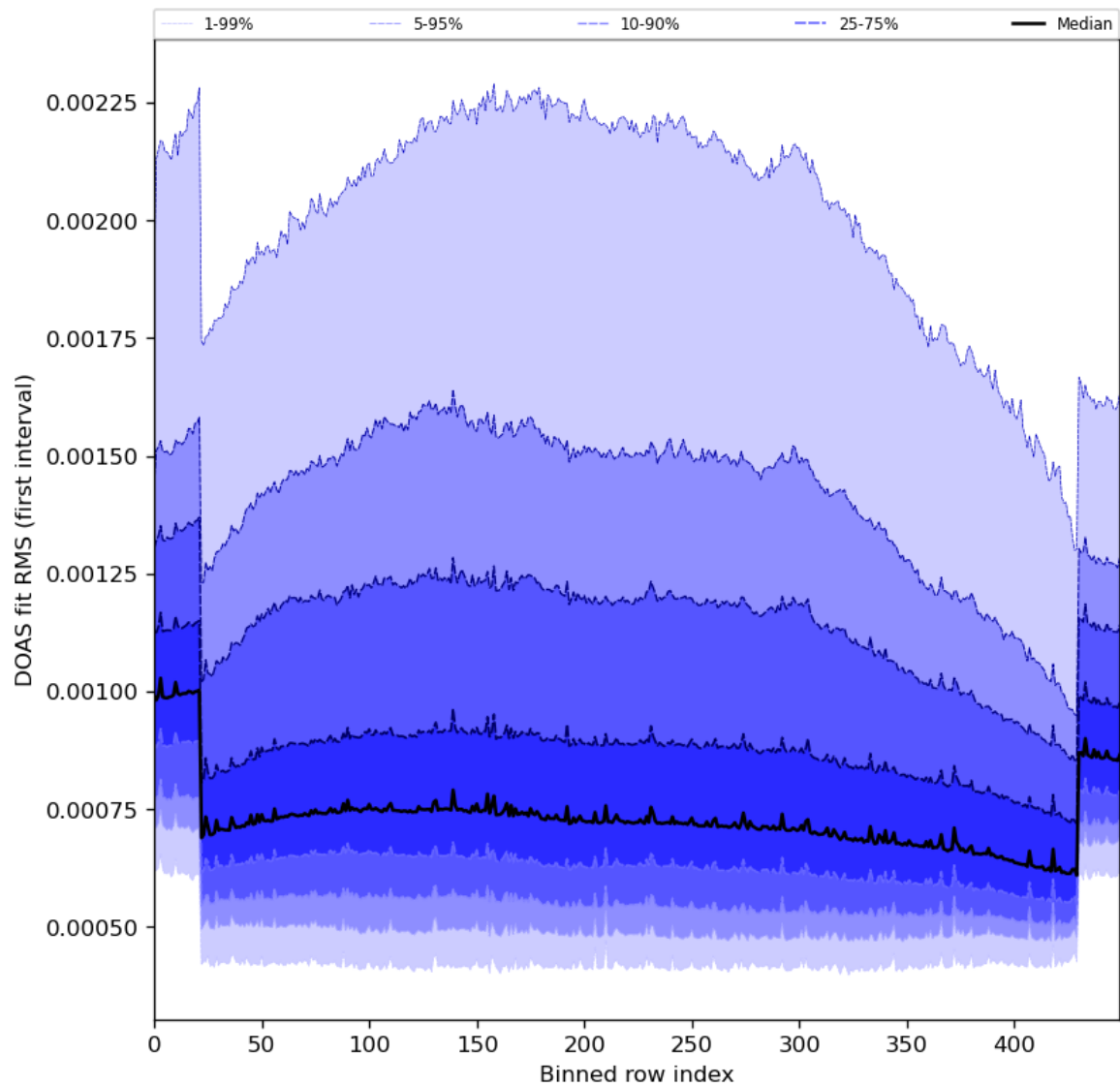
Figure 60: Along track statistics of “DOAS fit RMS (first interval)” for 2024-05-25 to 2024-05-27
