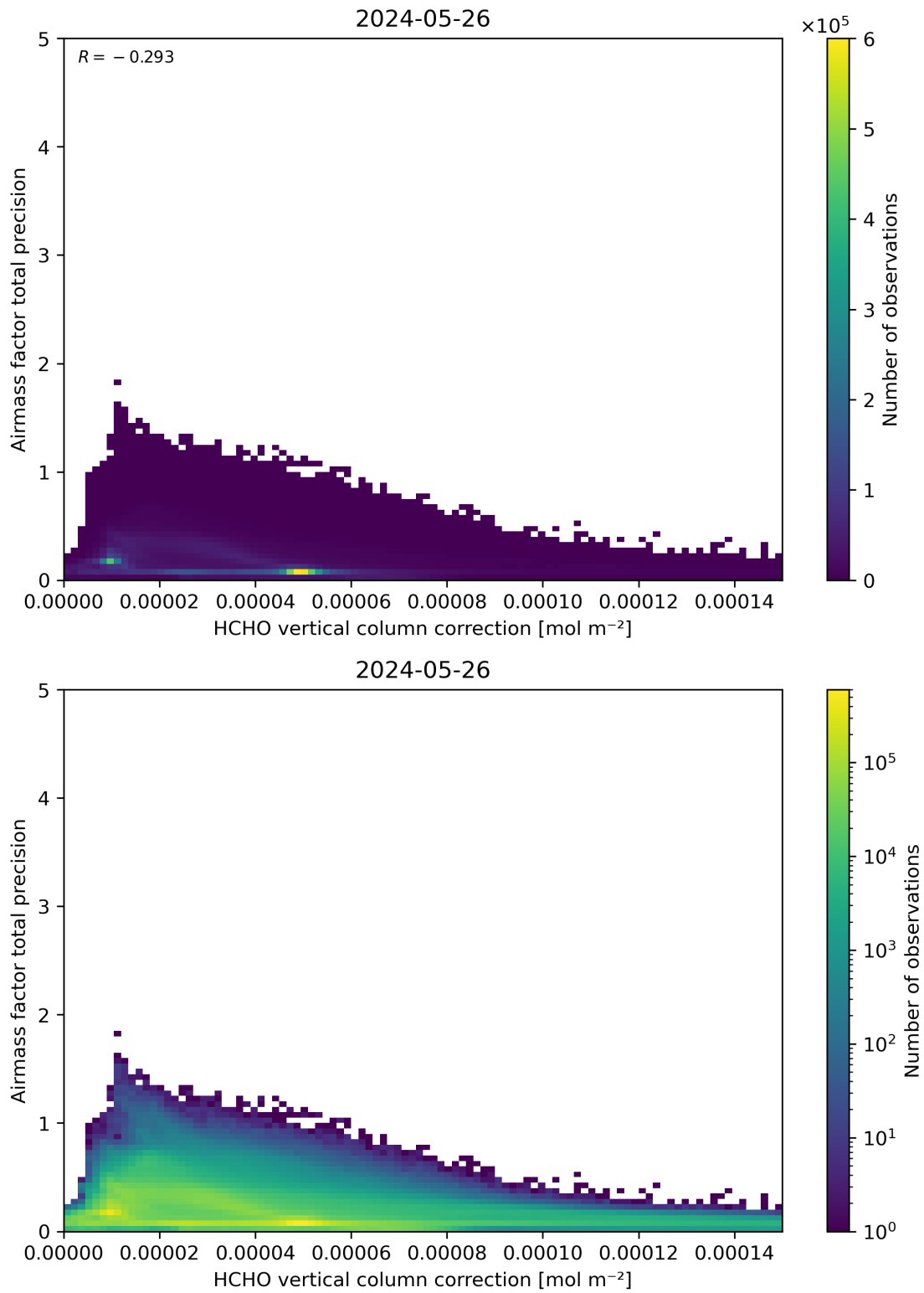
Figure 121: Scatter density plot of “HCHO vertical column correction” against “Airmass factor total precision” for 2024-05-25 to 2024-05-27.
