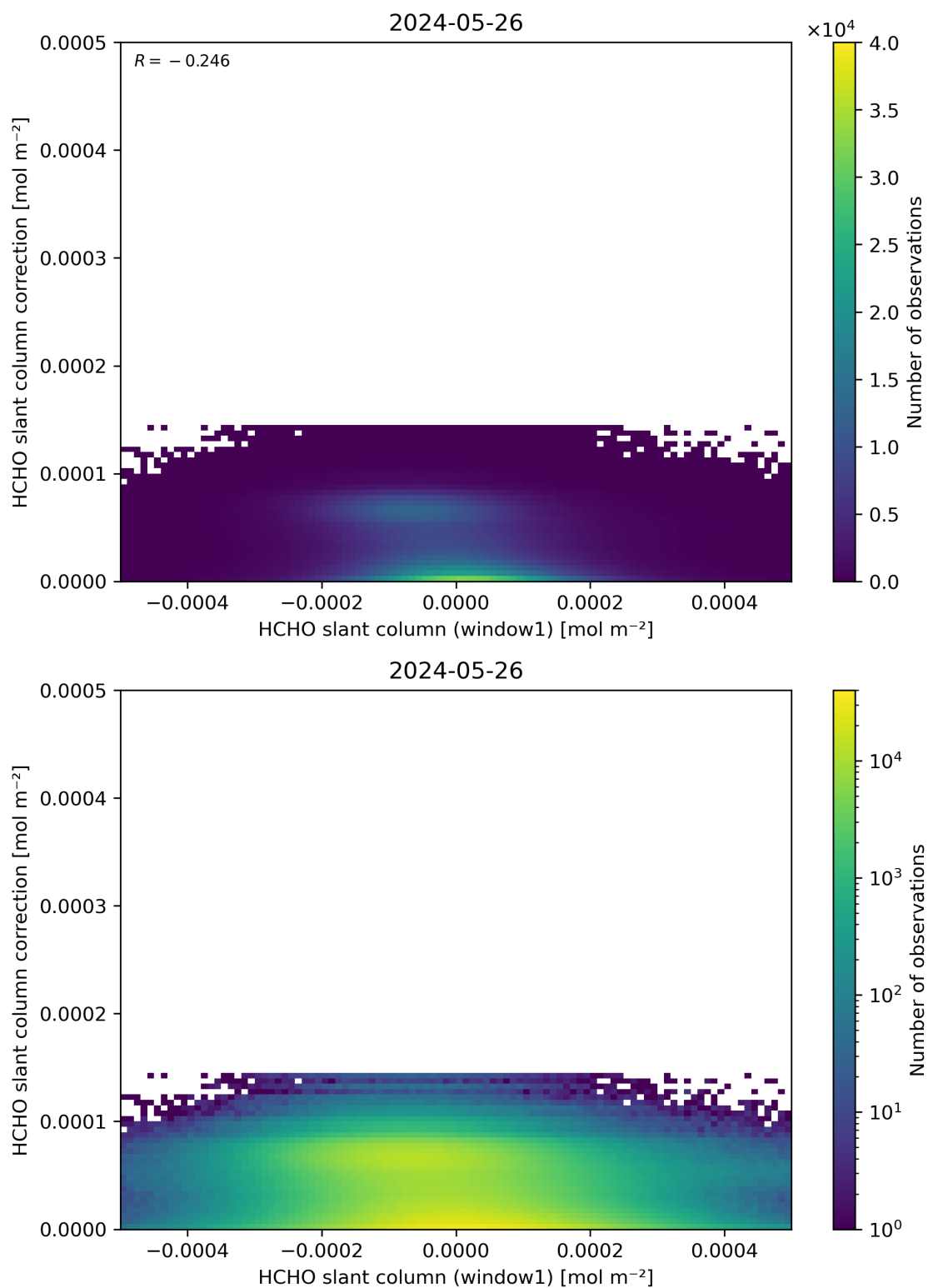
Figure 83: Scatter density plot of “HCHO slant column (window1)” against “HCHO slant column correction” for 2024-05-25 to 2024-05-27.
