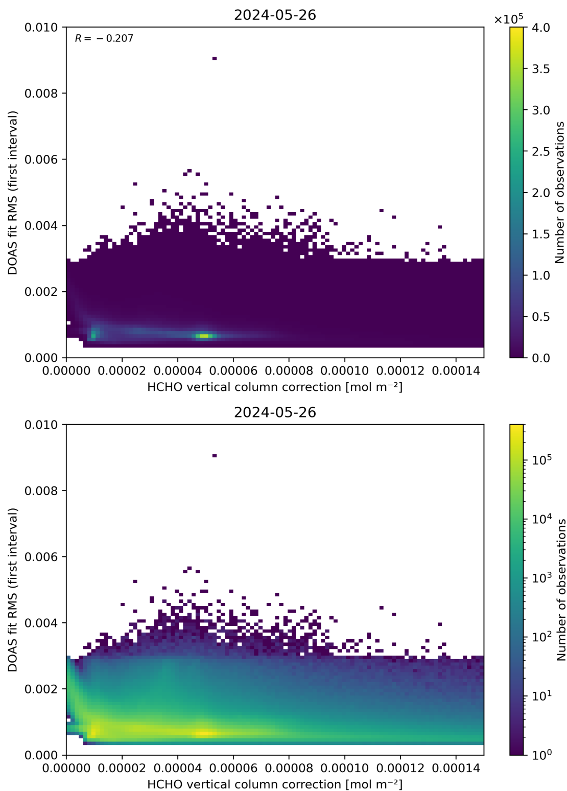
Figure 112: Scatter density plot of “HCHO vertical column correction” against “DOAS fit RMS (first interval)” for 2024-05-25 to 2024-05-27.
