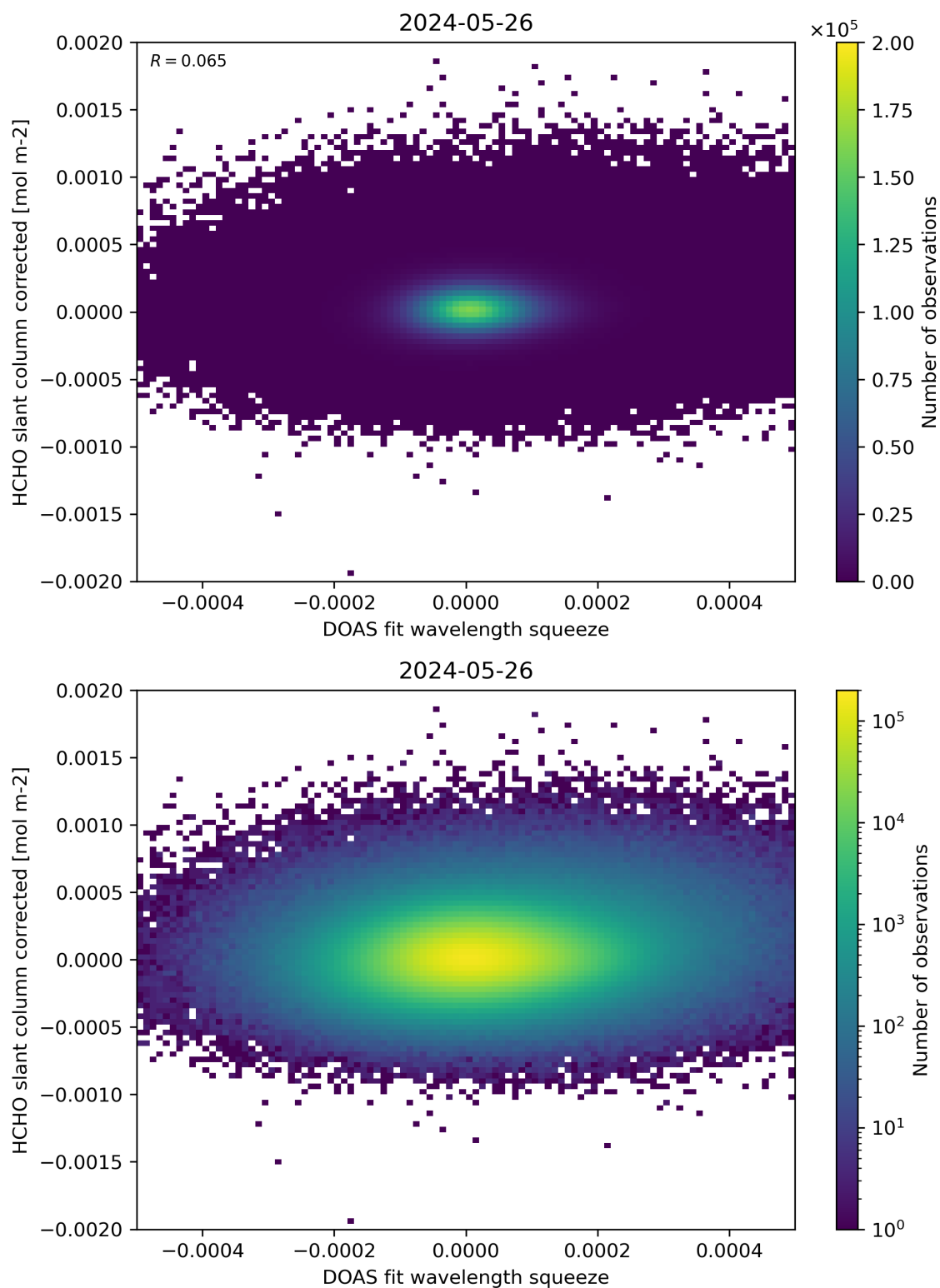
Figure 69: Scatter density plot of “DOAS fit wavelength squeeze” against “HCHO slant column corrected” for 2024-05-25 to 2024-05-27.
