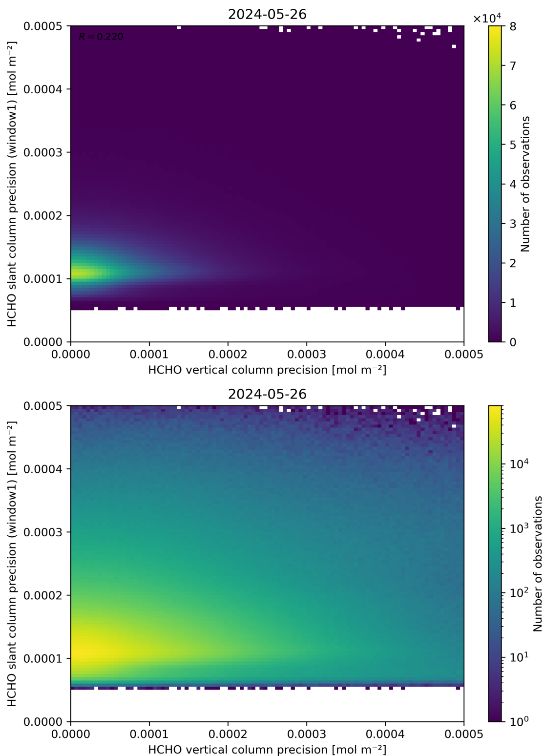
Figure 143: Scatter density plot of “HCHO vertical column precision” against “HCHO slant column precision (window1)” for 2024-05-25 to 2024-05-27.
