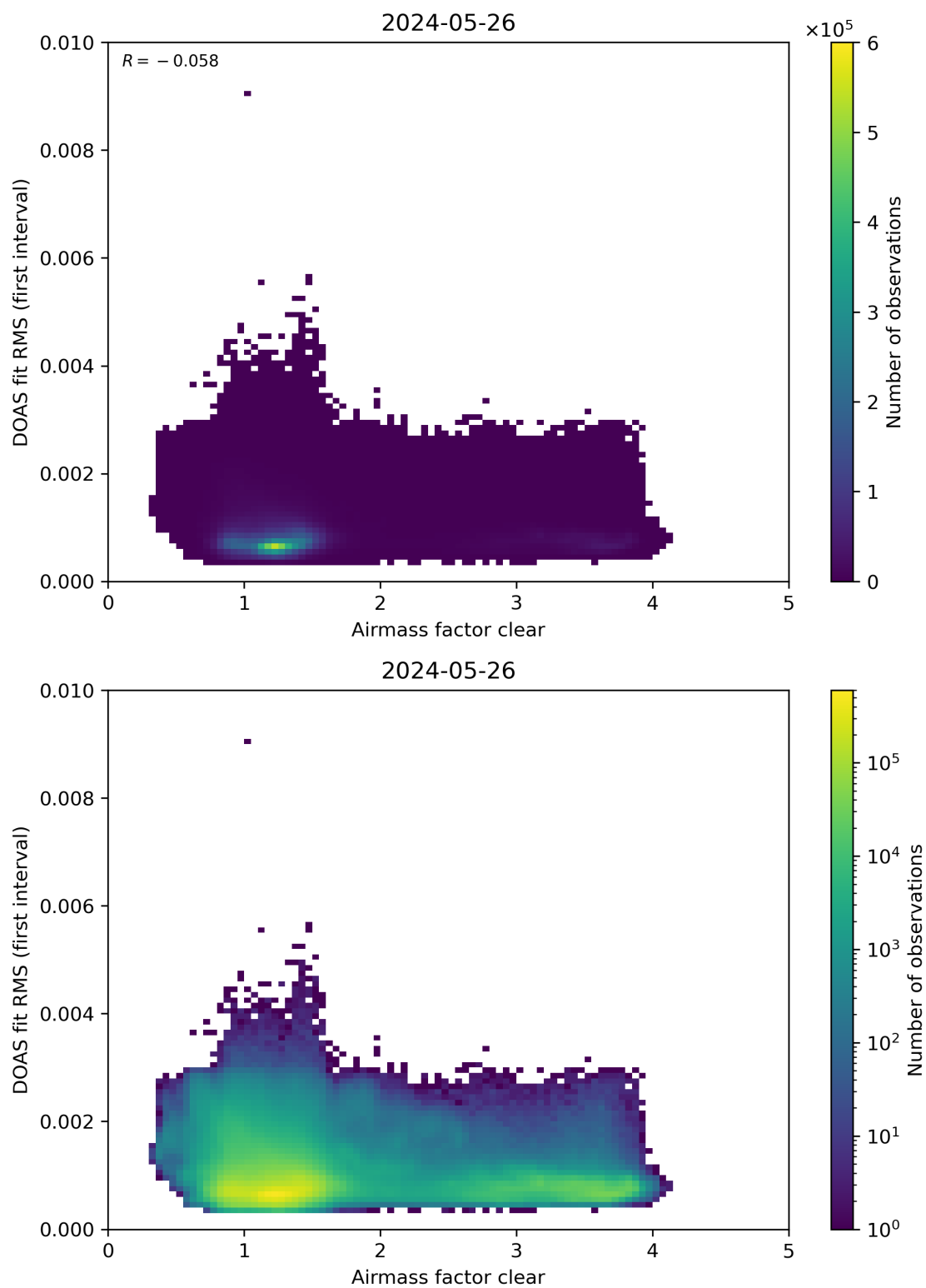
Figure 71: Scatter density plot of “Airmass factor clear” against “DOAS fit RMS (first interval)” for 2024-05-25 to 2024-05-27.
