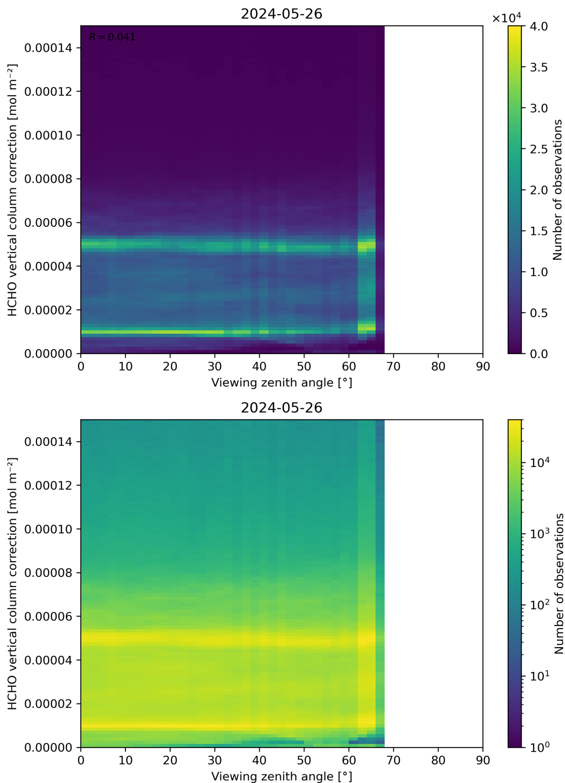
Figure 193: Scatter density plot of “Viewing zenith angle” against “HCHO vertical column correction” for 2024-05-25 to 2024-05-27.
