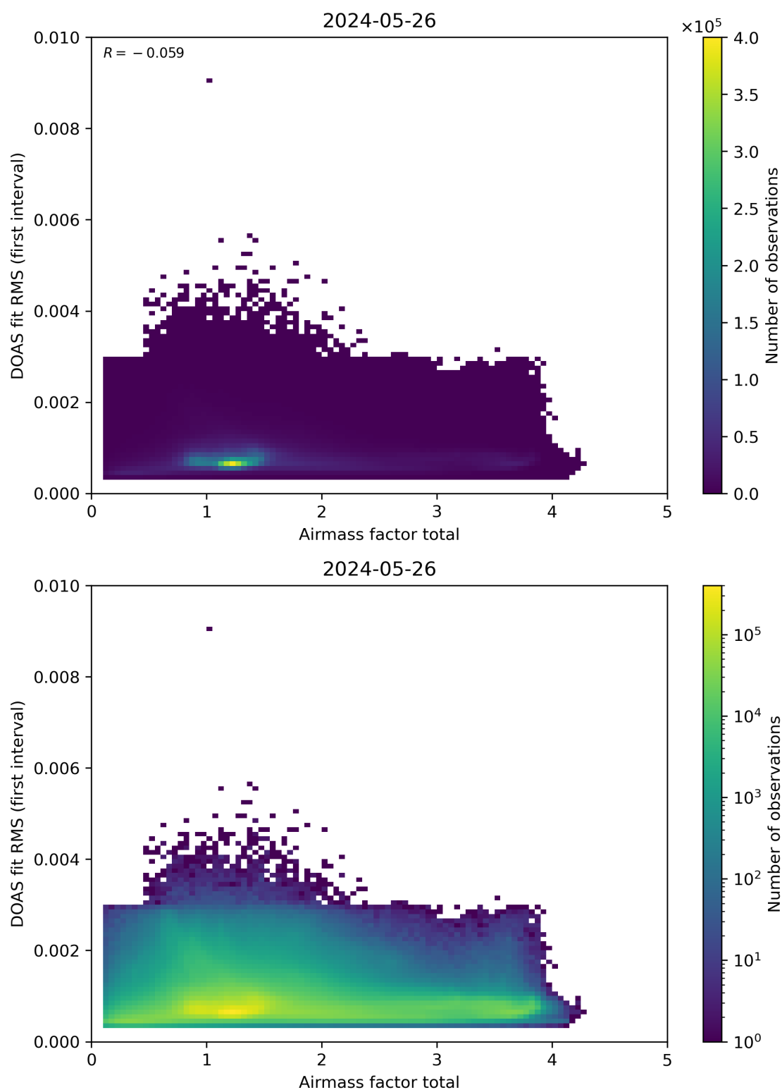
Figure 97: Scatter density plot of “Airmass factor total” against “DOAS fit RMS (first interval)” for 2024-05-25 to 2024-05-27.
