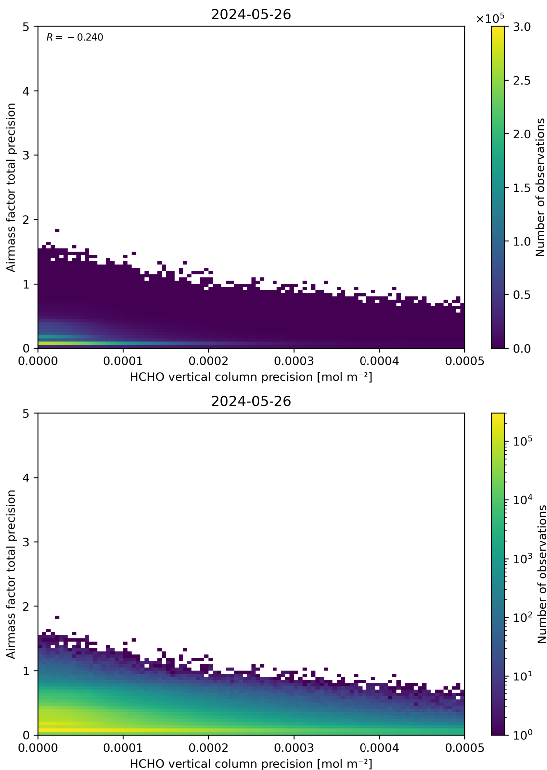
Figure 145: Scatter density plot of “HCHO vertical column precision” against “Airmass factor total precision” for 2024-05-25 to 2024-05-27.
