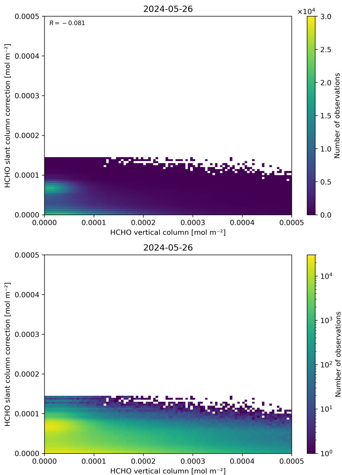
Figure 128: Scatter density plot of “HCHO vertical column” against “HCHO slant column correction” for 2024-05-25 to 2024-05-27.
