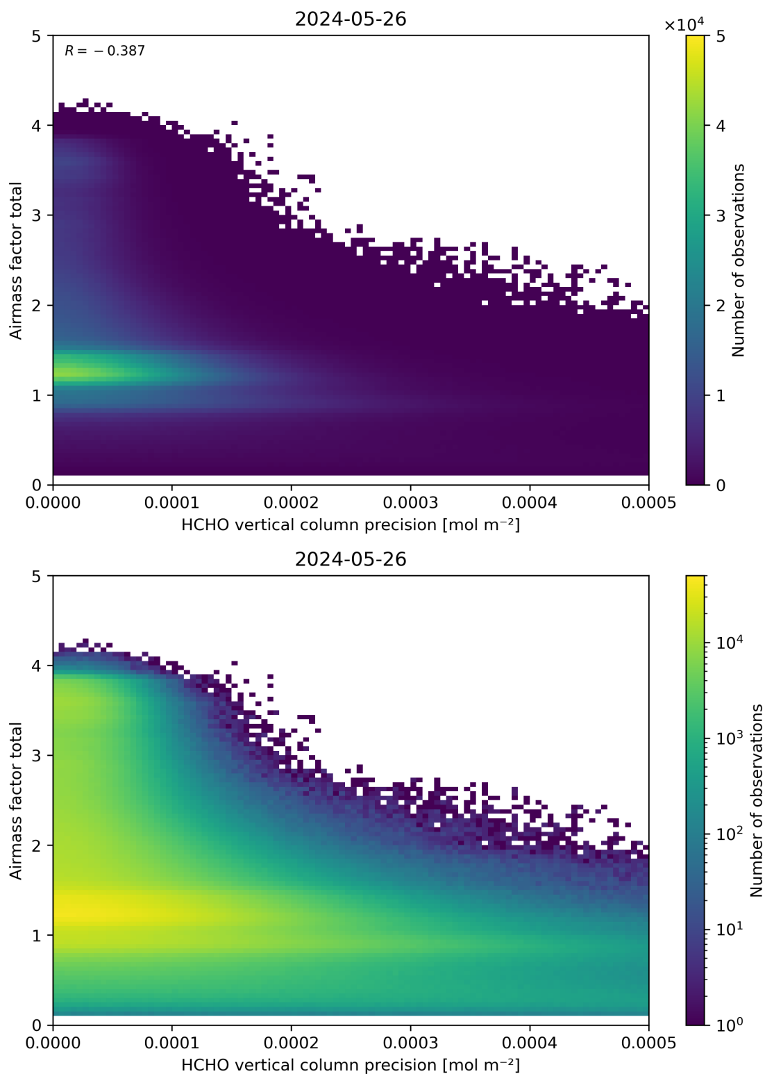
Figure 144: Scatter density plot of “HCHO vertical column precision” against “Airmass factor total” for 2024-05-25 to 2024-05-27.
