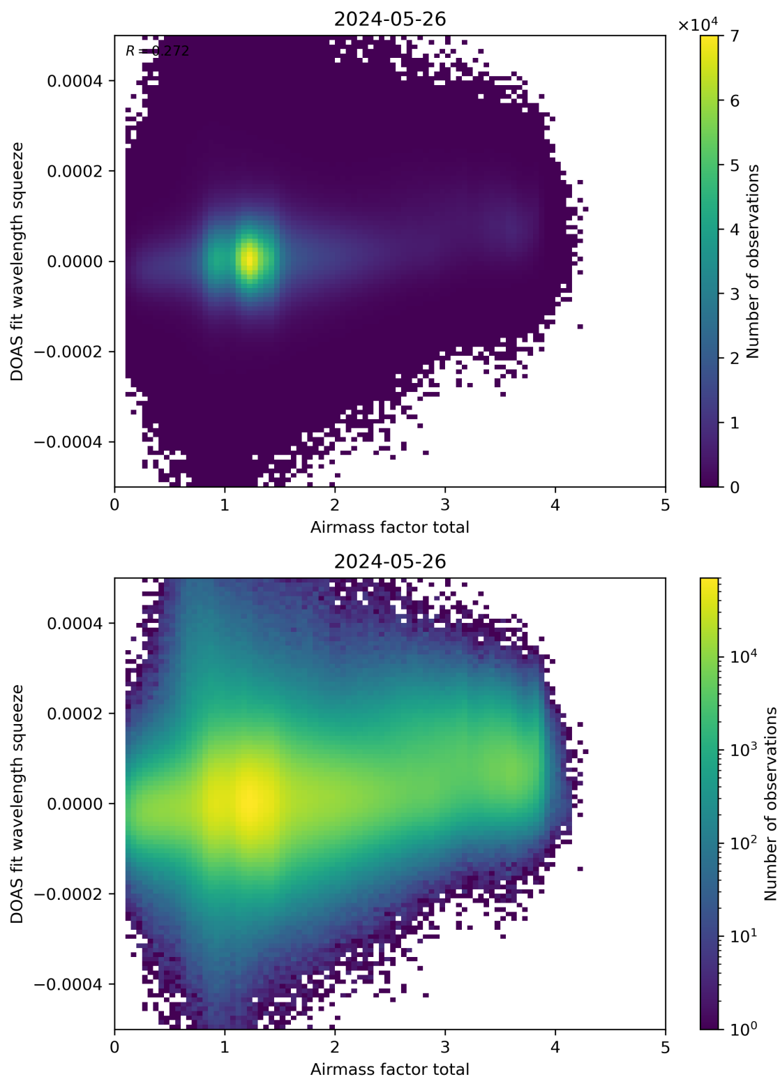
Figure 99: Scatter density plot of “Airmass factor total” against “DOAS fit wavelength squeeze” for 2024-05-25 to 2024-05-27.
