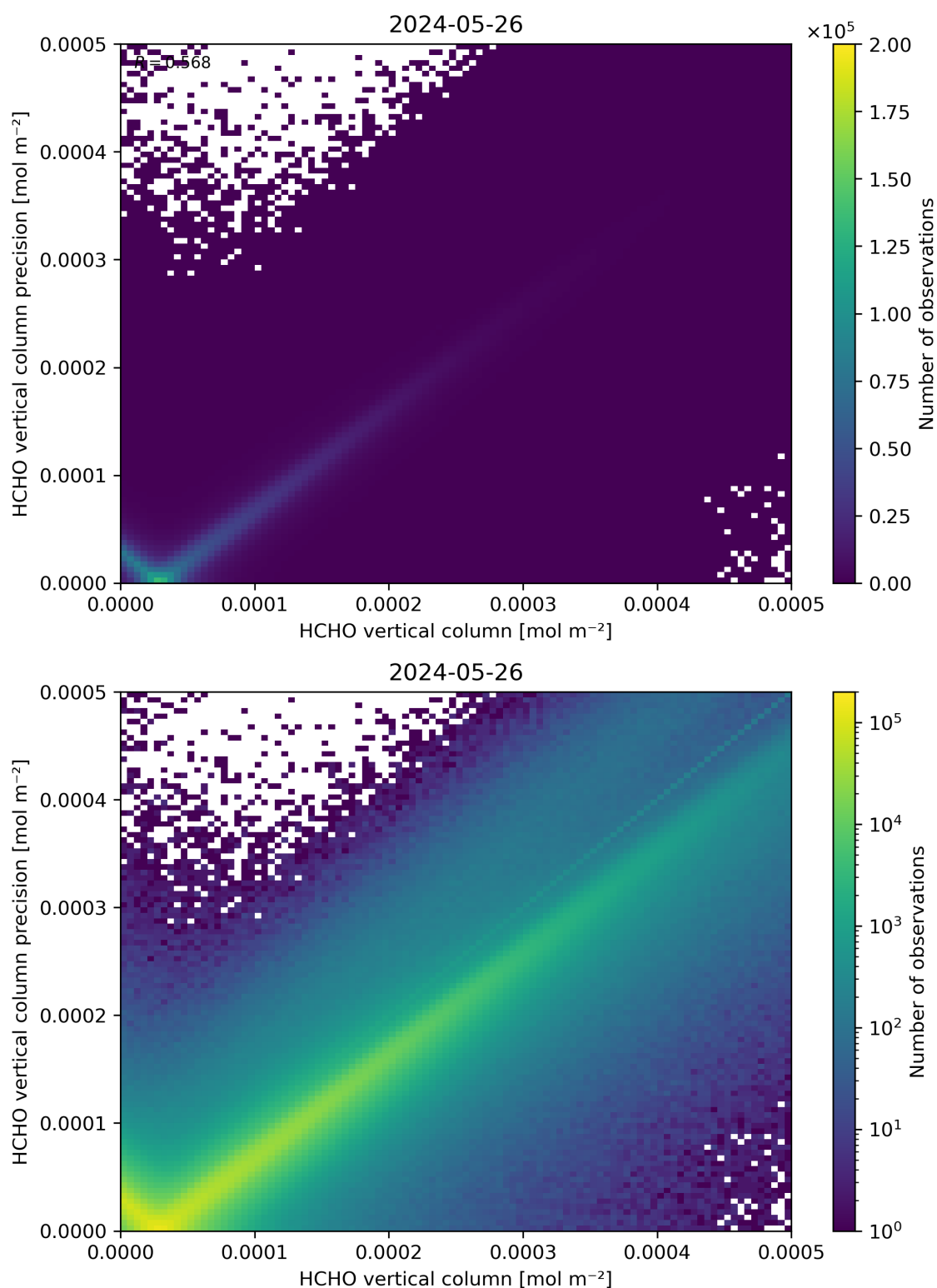
Figure 134: Scatter density plot of “HCHO vertical column” against “HCHO vertical column precision” for 2024-05-25 to 2024-05-27.
