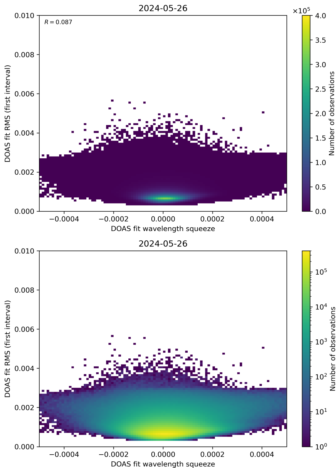
Figure 68: Scatter density plot of “DOAS fit wavelength squeeze” against “DOAS fit RMS (first interval)” for 2024-05-25 to 2024-05-27.
