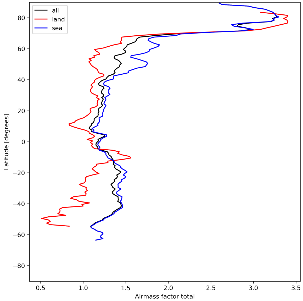
Figure 26: Zonal average of “Airmass factor total” for 2024-05-25 to 2024-05-27.
