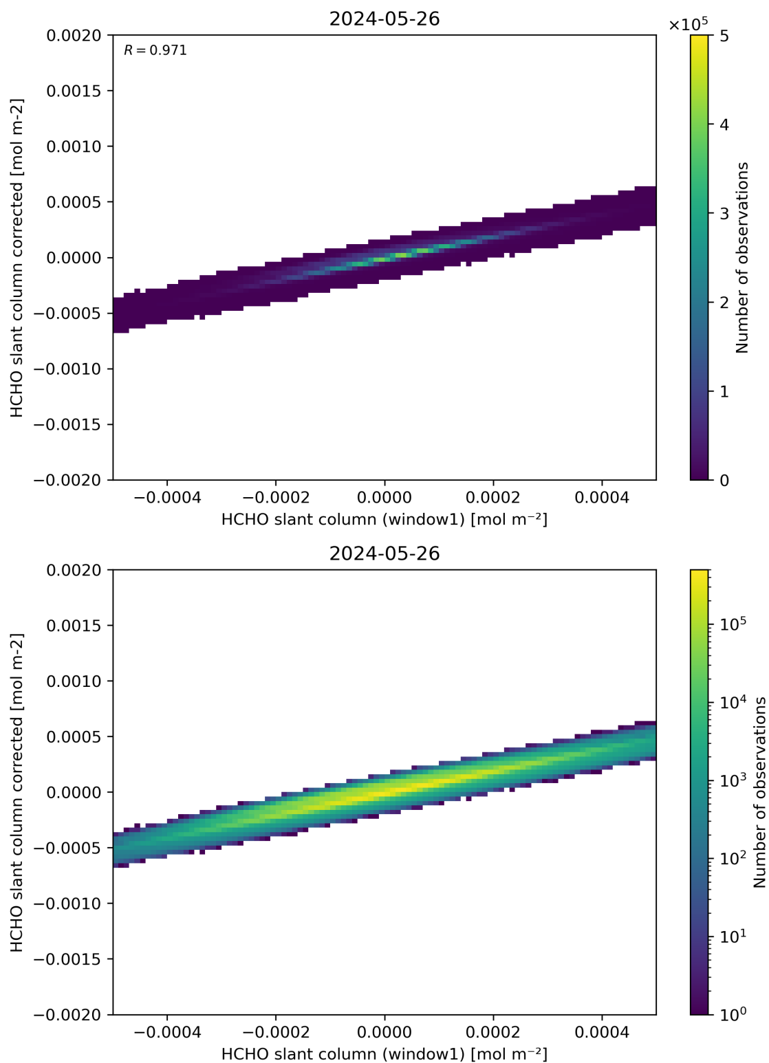
Figure 82: Scatter density plot of “HCHO slant column (window1)” against “HCHO slant column corrected” for 2024-05-25 to 2024-05-27.
