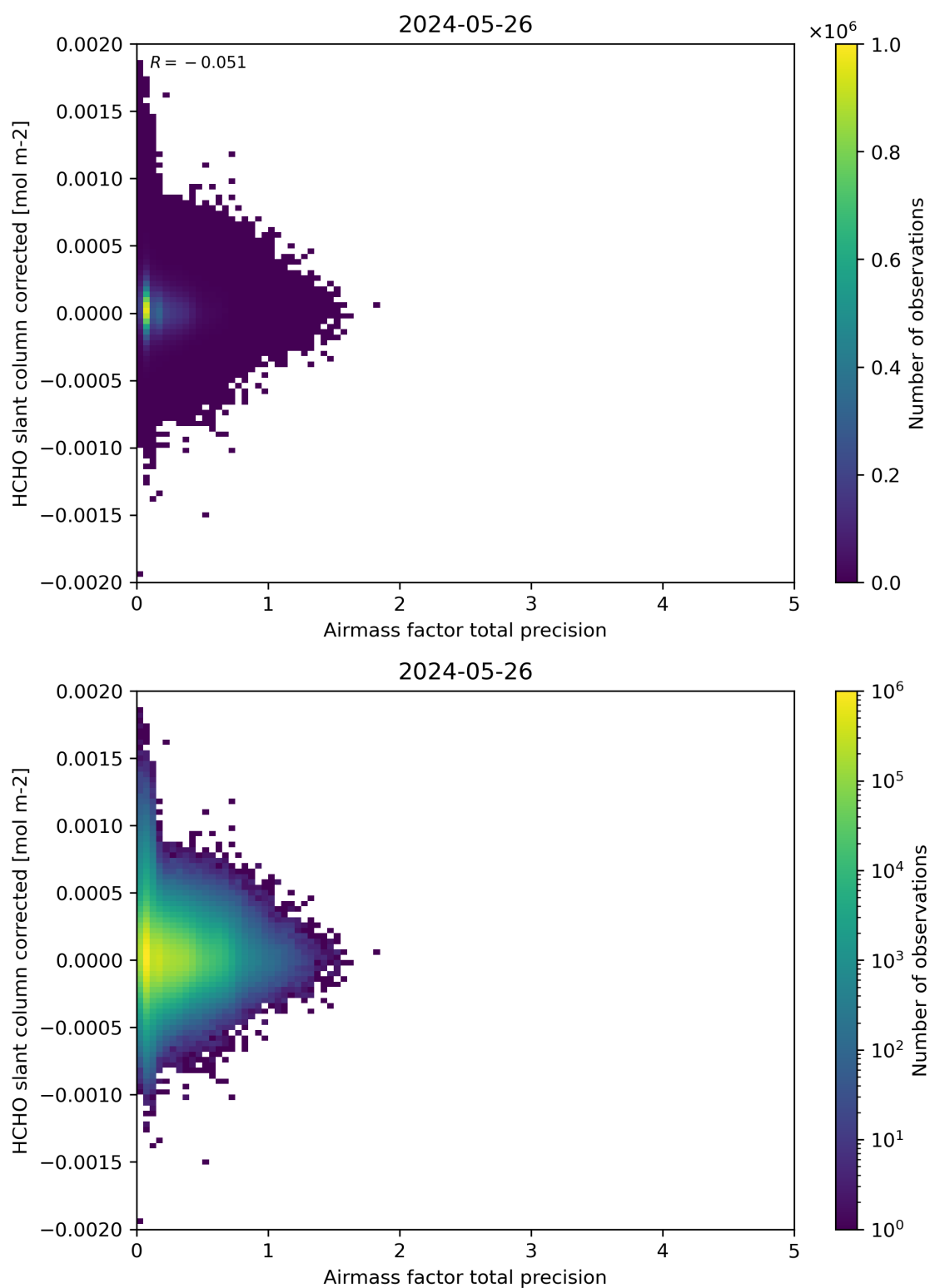
Figure 109: Scatter density plot of “Airmass factor total precision” against “HCHO slant column corrected” for 2024-05-25 to 2024-05-27.
