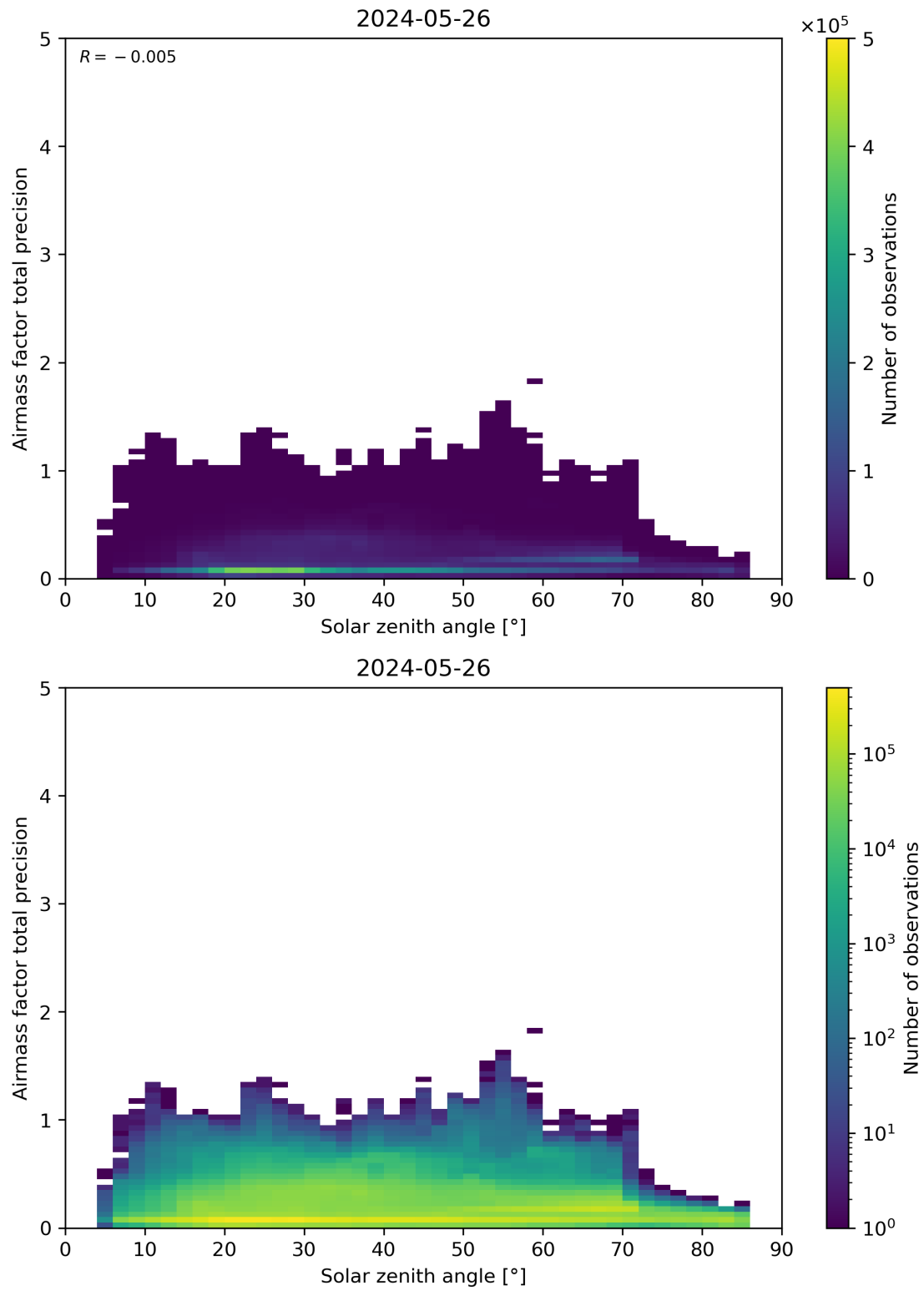
Figure 176: Scatter density plot of “Solar zenith angle” against “Airmass factor total precision” for 2024-05-25 to 2024-05-27.
