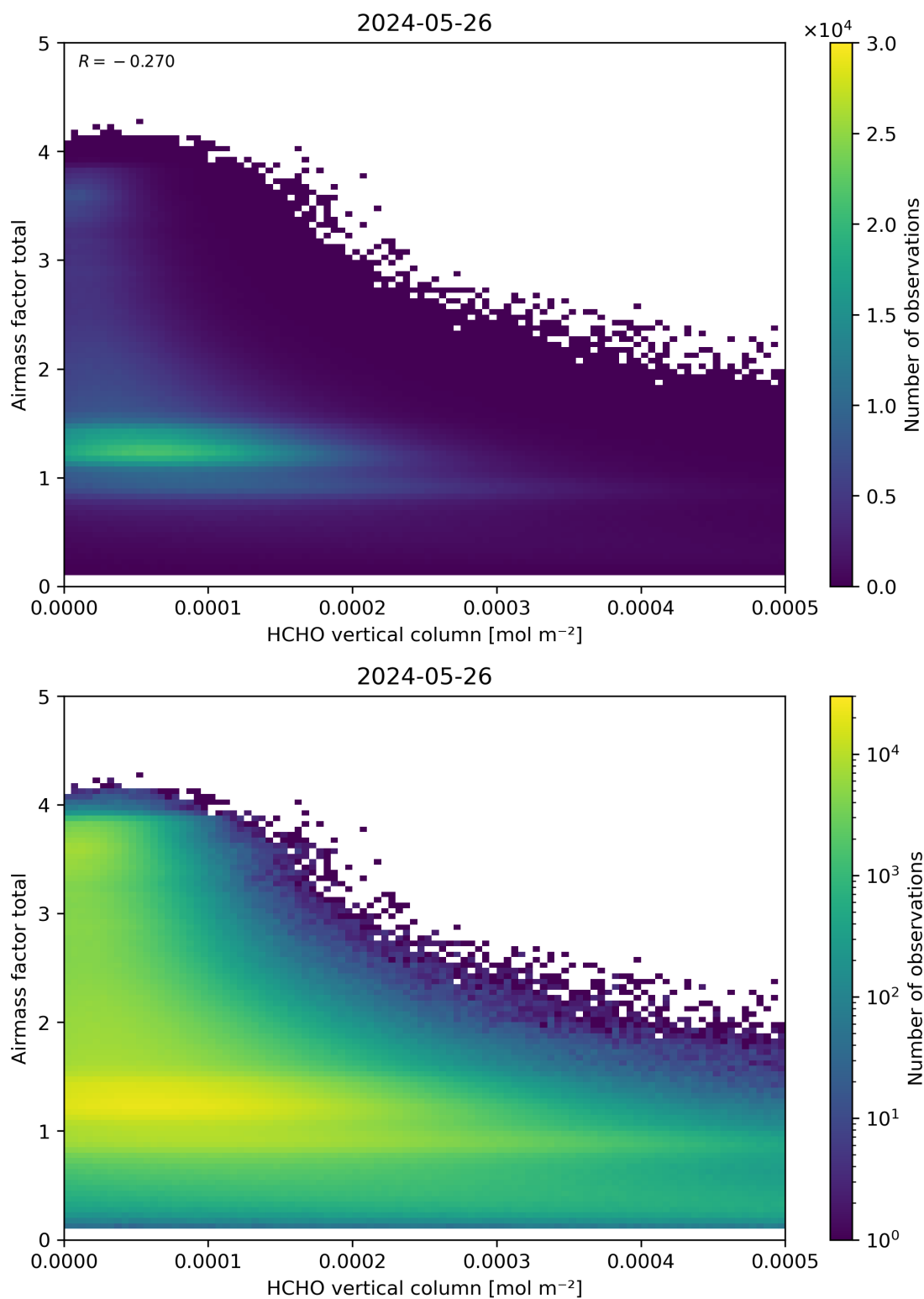
Figure 131: Scatter density plot of “HCHO vertical column” against “Airmass factor total” for 2024-05-25 to 2024-05-27.
