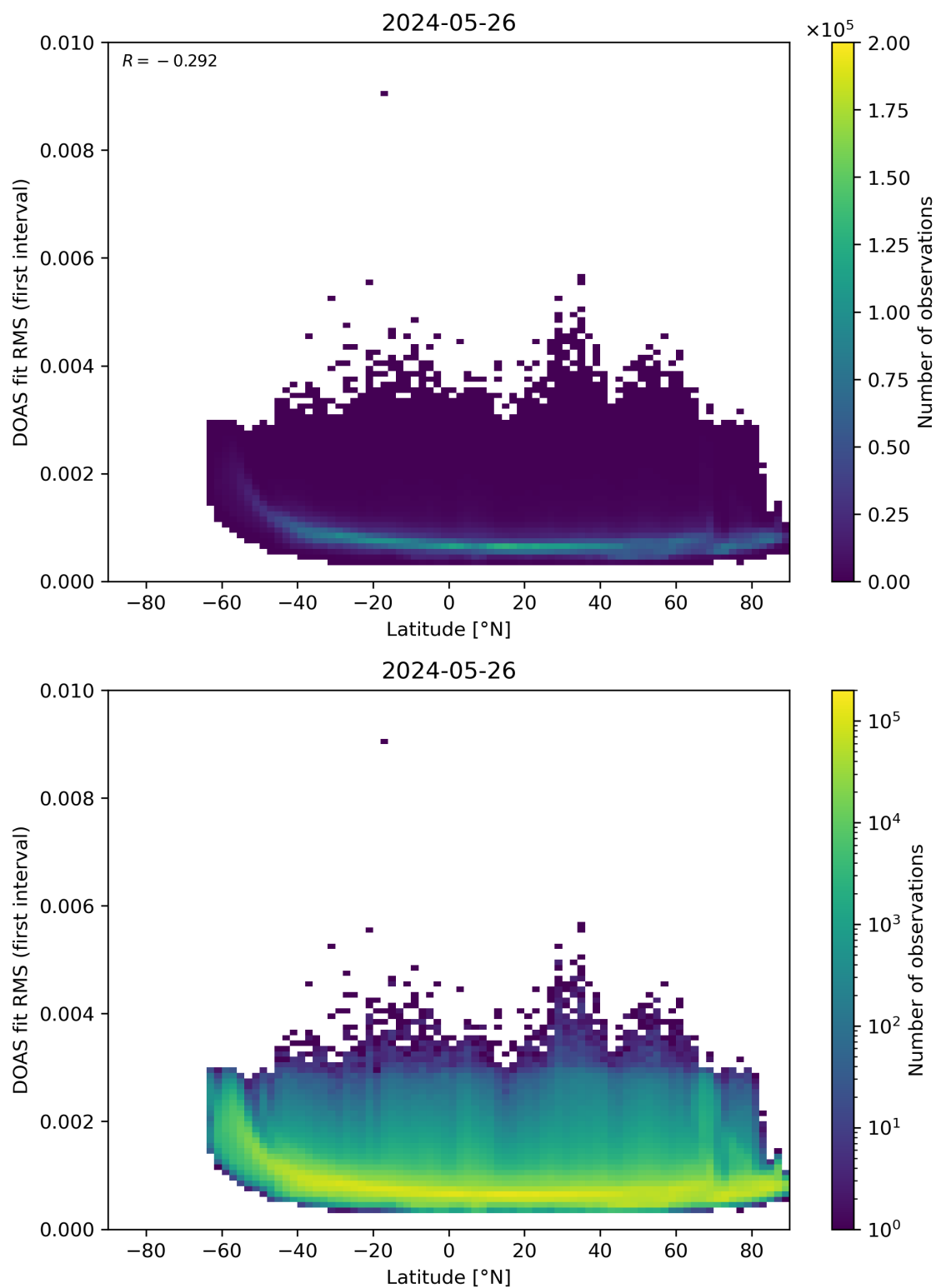
Figure 153: Scatter density plot of “Latitude” against “DOAS fit RMS (first interval)” for 2024-05-25 to 2024-05-27.
