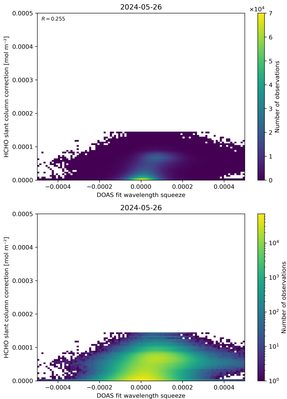
Figure 70: Scatter density plot of “DOAS fit wavelength squeeze” against “HCHO slant column correction” for 2024-05-25 to 2024-05-27.
