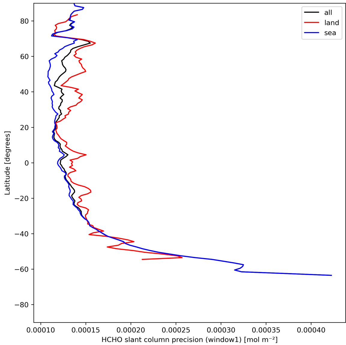
Figure 25: Zonal average of “HCHO slant column precision (window1)” for 2024-05-25 to 2024-05-27.
