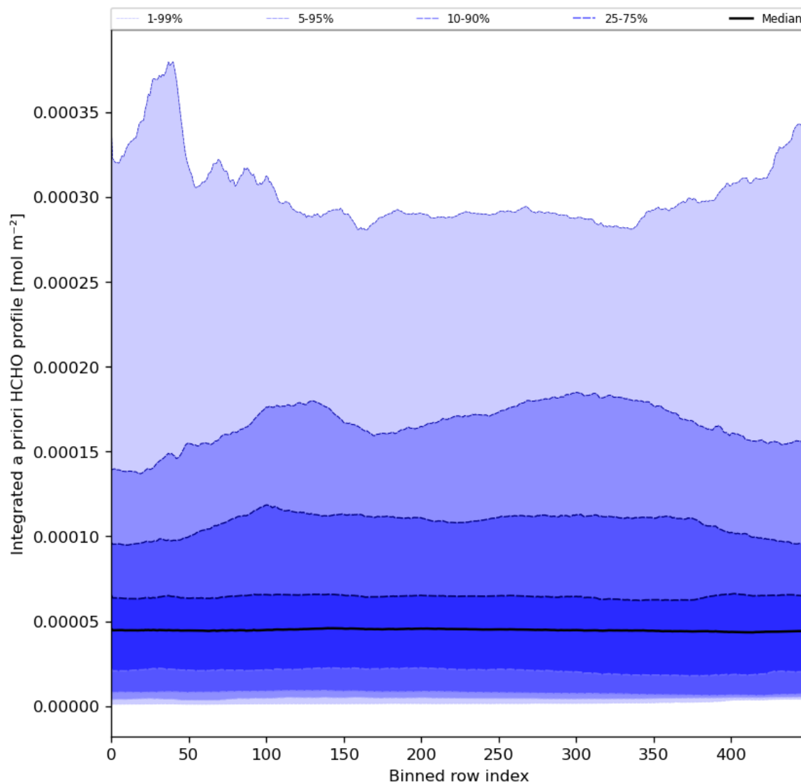
Figure 57: Along track statistics of “Integrated a priori HCHO profile” for 2024-05-25 to 2024-05-27
