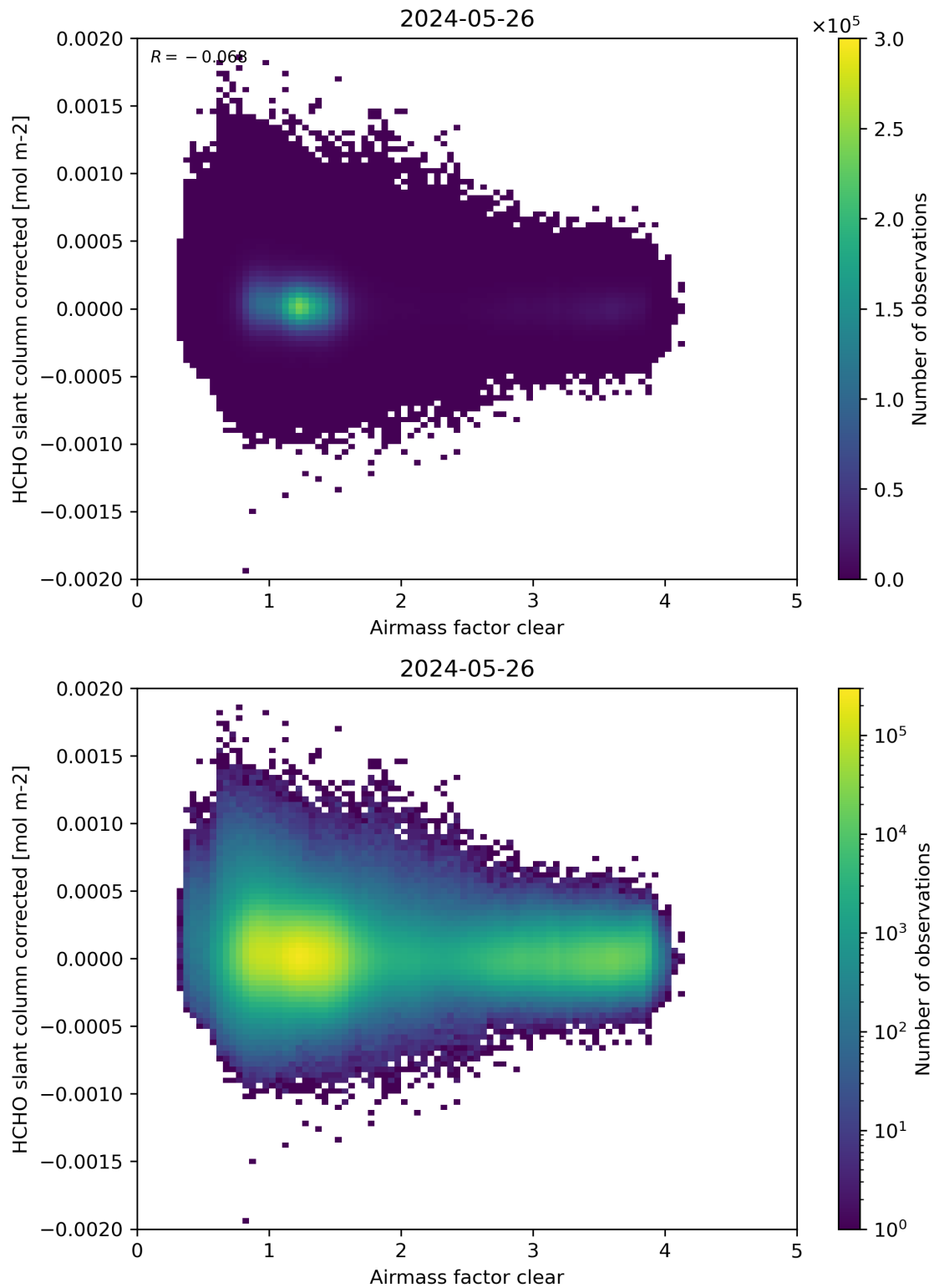
Figure 74: Scatter density plot of “Airmass factor clear” against “HCHO slant column corrected” for 2024-05-25 to 2024-05-27.
