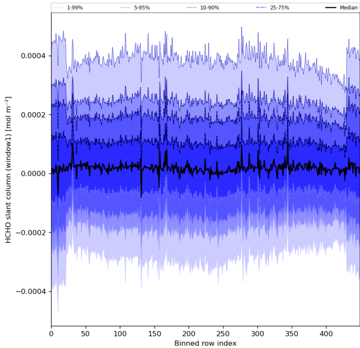
Figure 52: Along track statistics of “HCHO slant column (window1)” for 2024-05-25 to 2024-05-27
