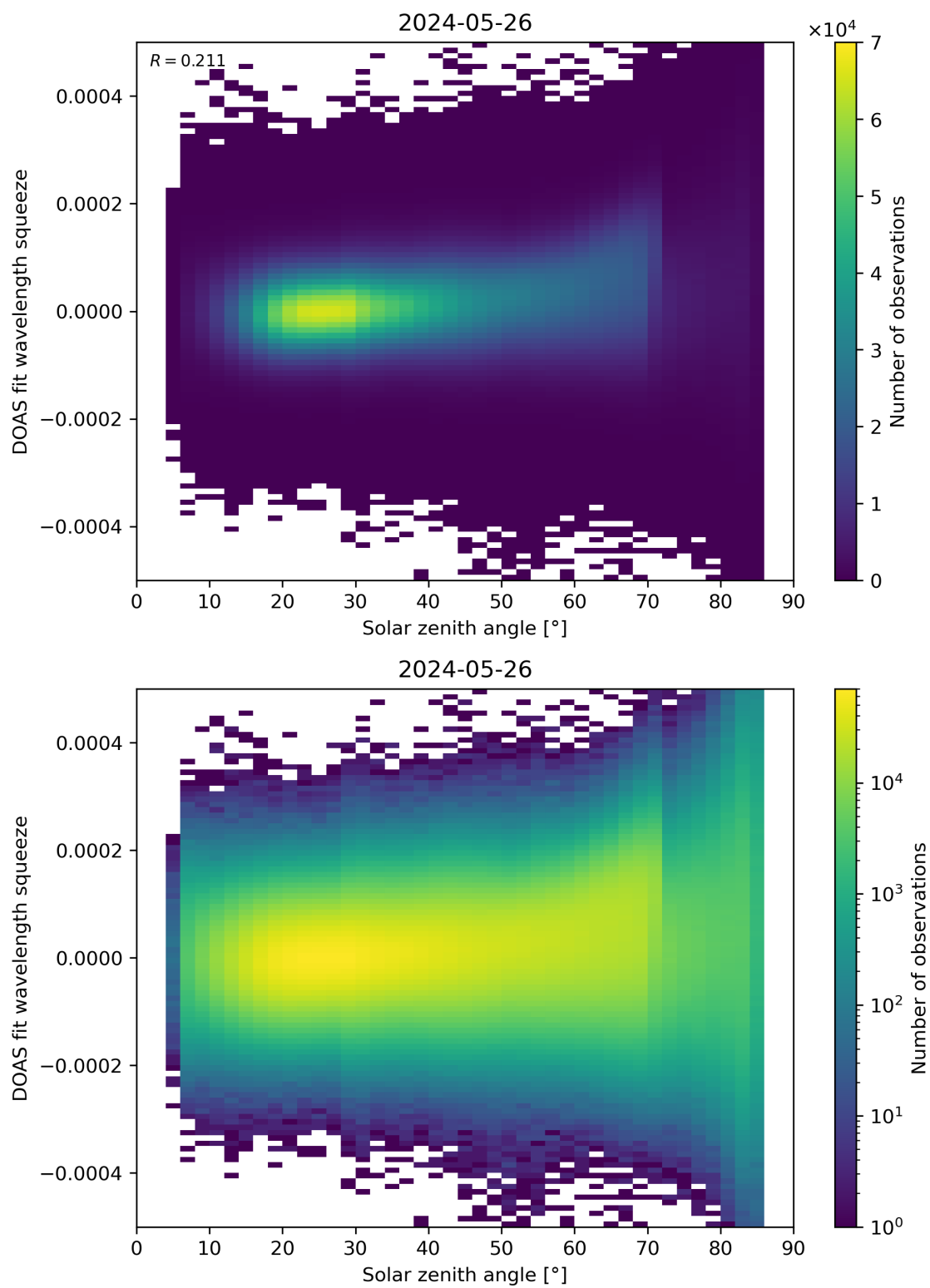
Figure 169: Scatter density plot of “Solar zenith angle” against “DOAS fit wavelength squeeze” for 2024-05-25 to 2024-05-27.
