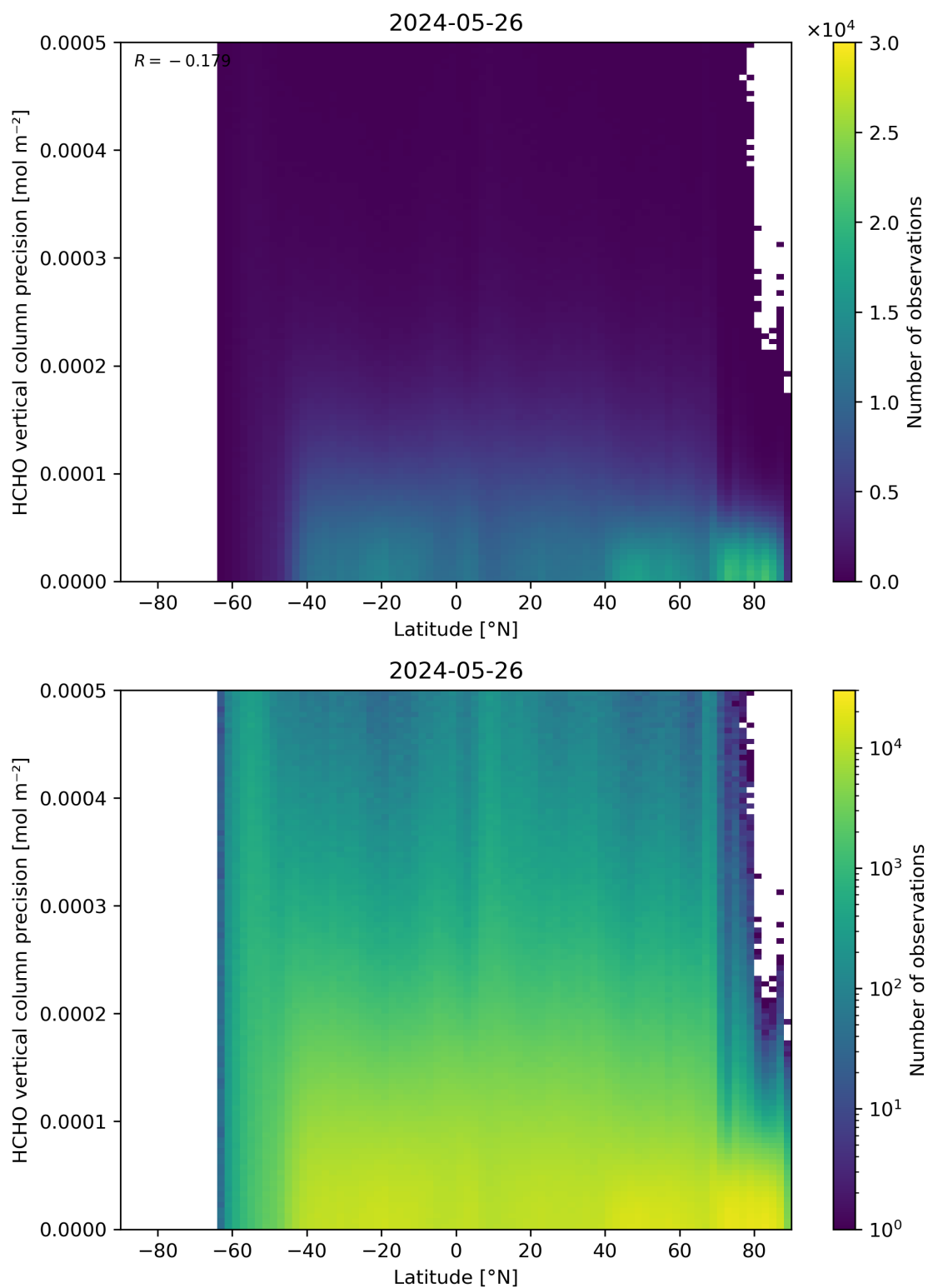
Figure 165: Scatter density plot of “Latitude” against “HCHO vertical column precision” for 2024-05-25 to 2024-05-27.
