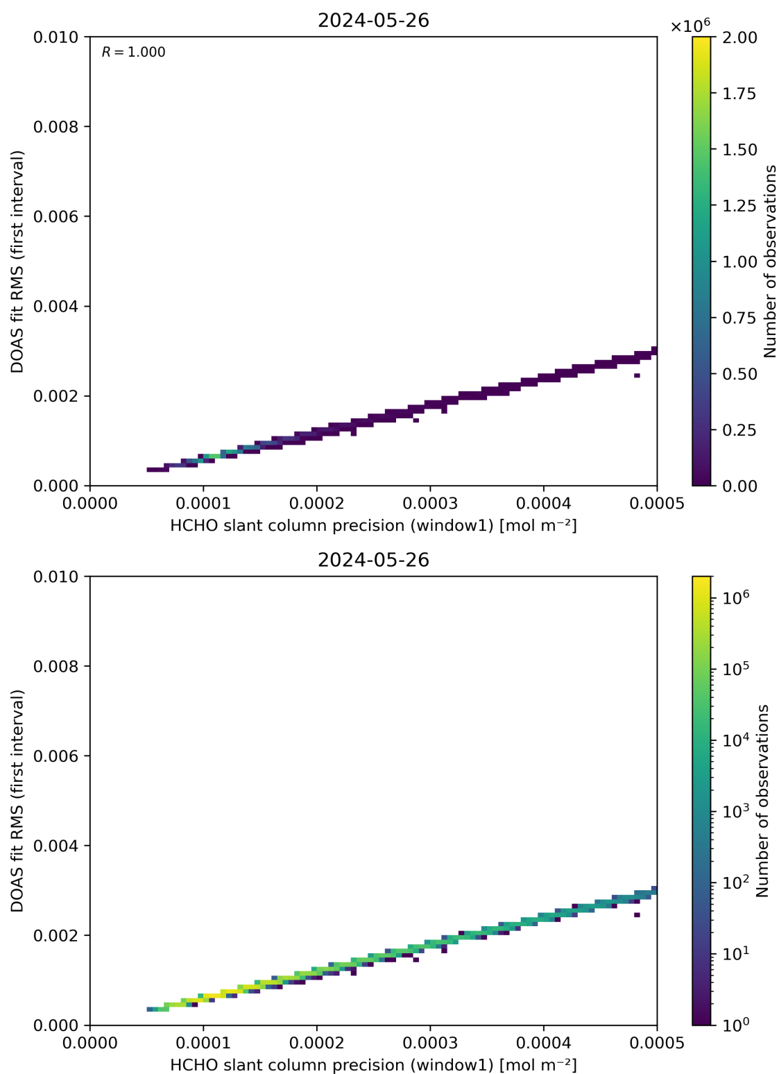
Figure 88: Scatter density plot of “HCHO slant column precision (window1)” against “DOAS fit RMS (first interval)” for 2024-05-25 to 2024-05-27.
