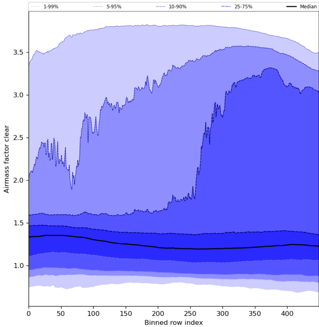
Figure 56: Along track statistics of “Airmass factor clear” for 2024-05-25 to 2024-05-27
