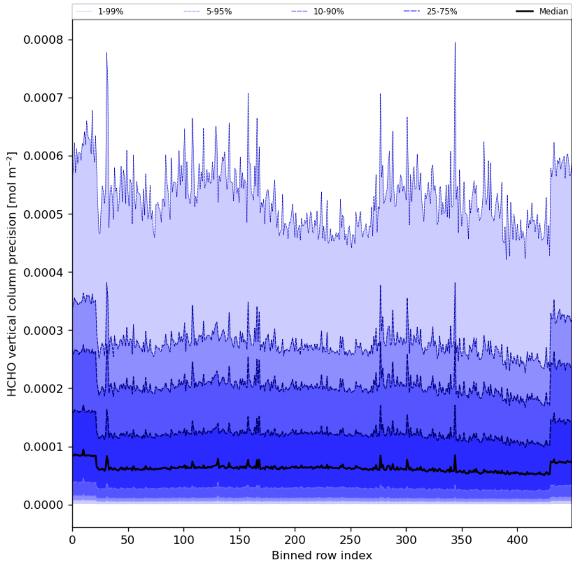
Figure 50: Along track statistics of “HCHO vertical column precision” for 2024-05-25 to 2024-05-27
