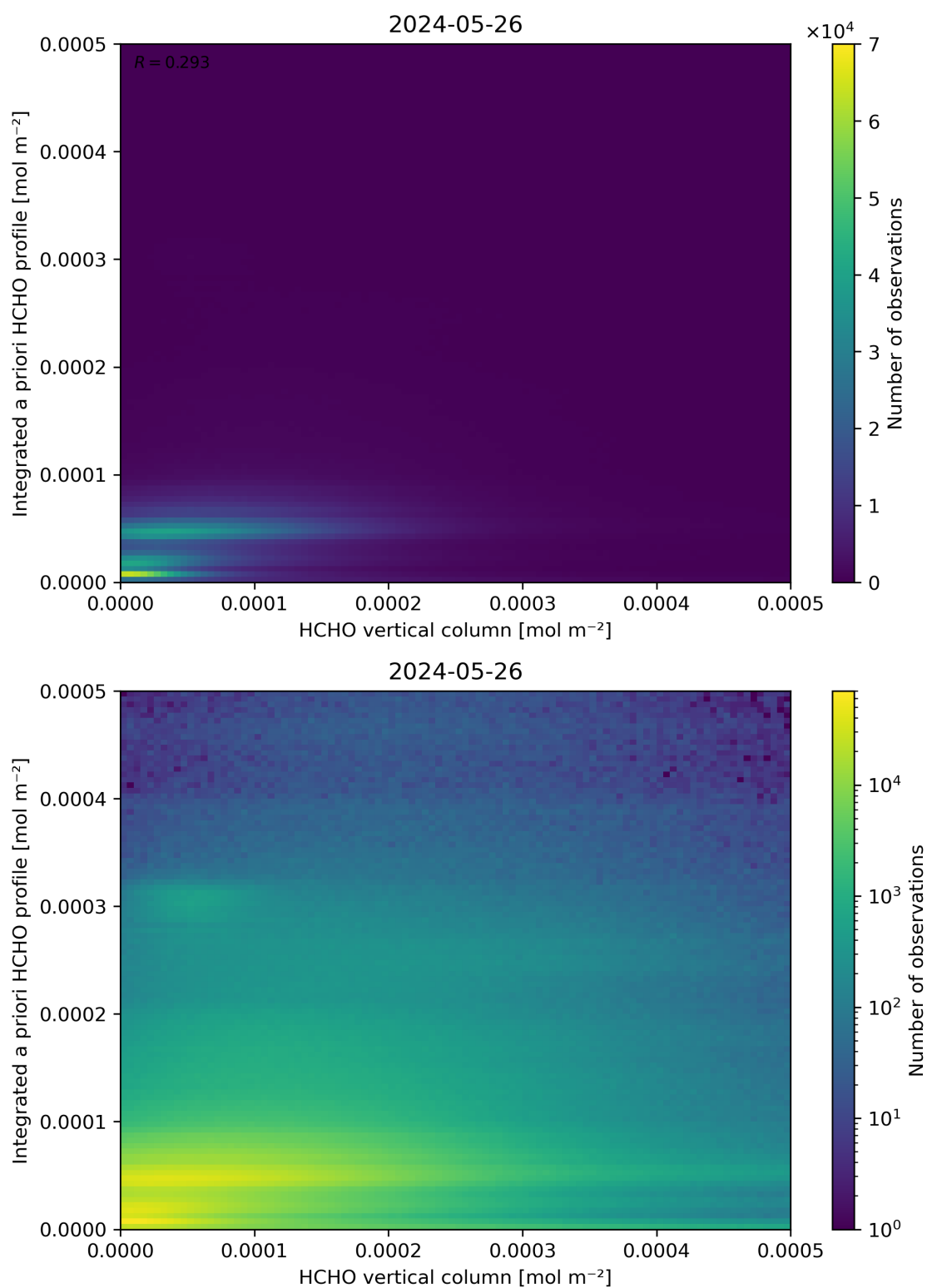
Figure 135: Scatter density plot of “HCHO vertical column” against “Integrated a priori HCHO profile” for 2024-05-25 to 2024-05-27.
