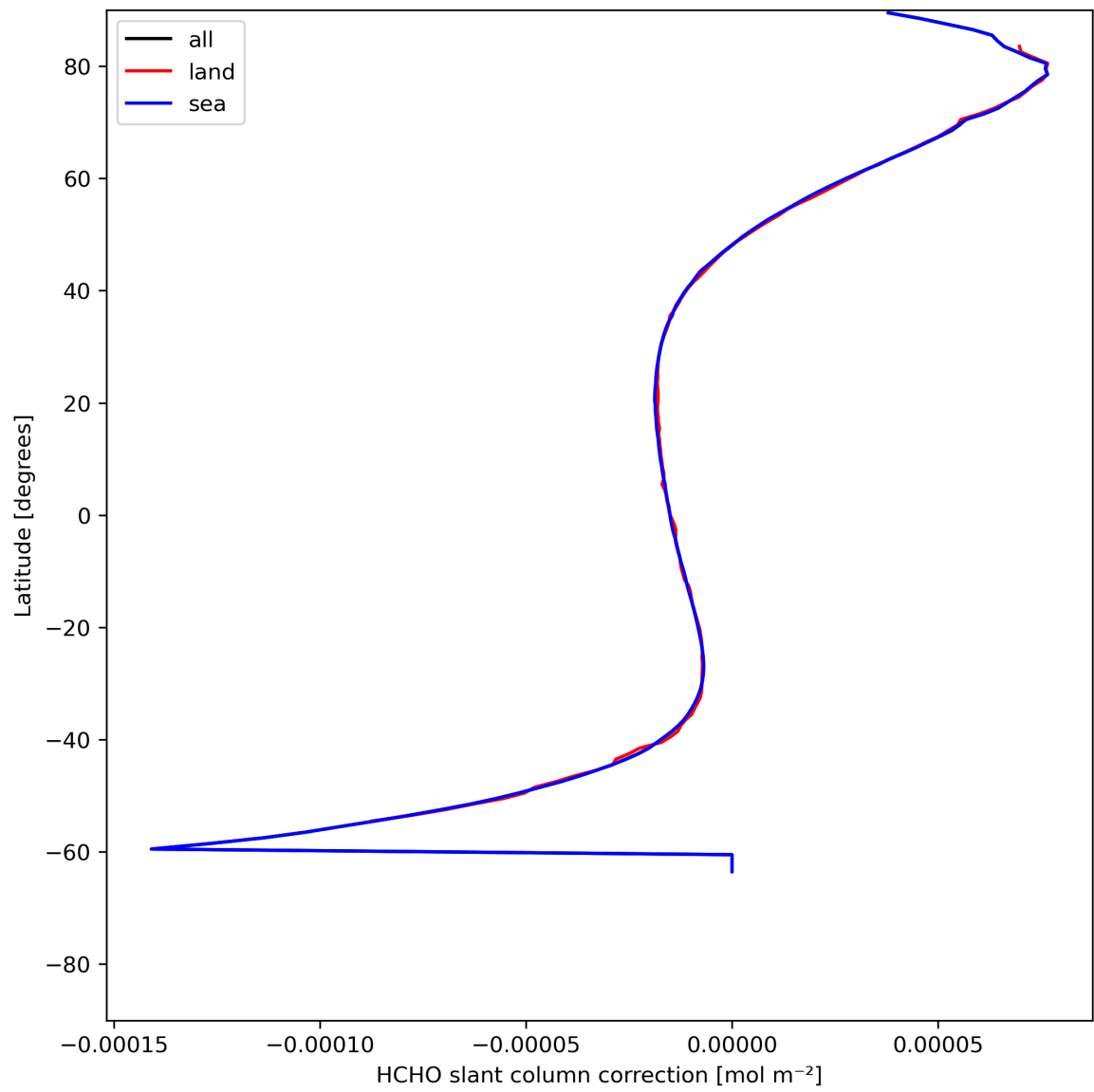
Figure 33: Zonal average of “HCHO slant column correction” for 2024-05-25 to 2024-05-27.
