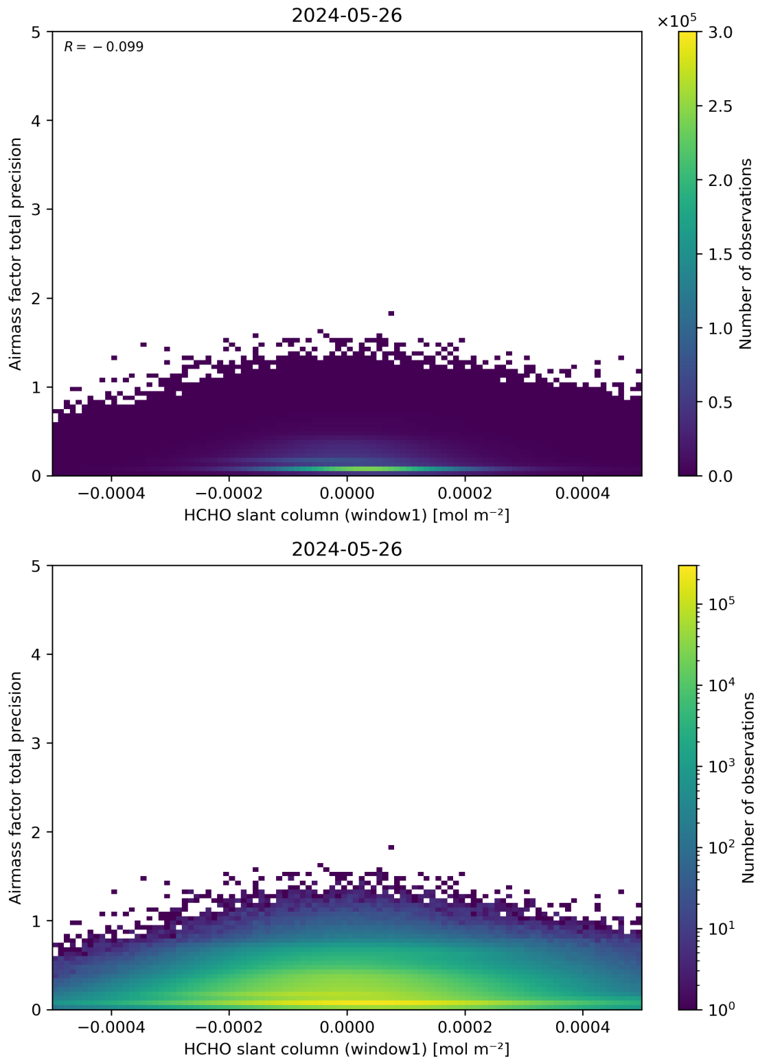
Figure 86: Scatter density plot of “HCHO slant column (window1)” against “Airmass factor total precision” for 2024-05-25 to 2024-05-27.
