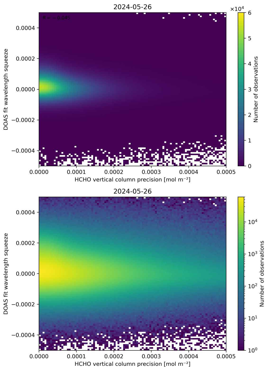
Figure 138: Scatter density plot of “HCHO vertical column precision” against “DOAS fit wavelength squeeze” for 2024-05-25 to 2024-05-27.
