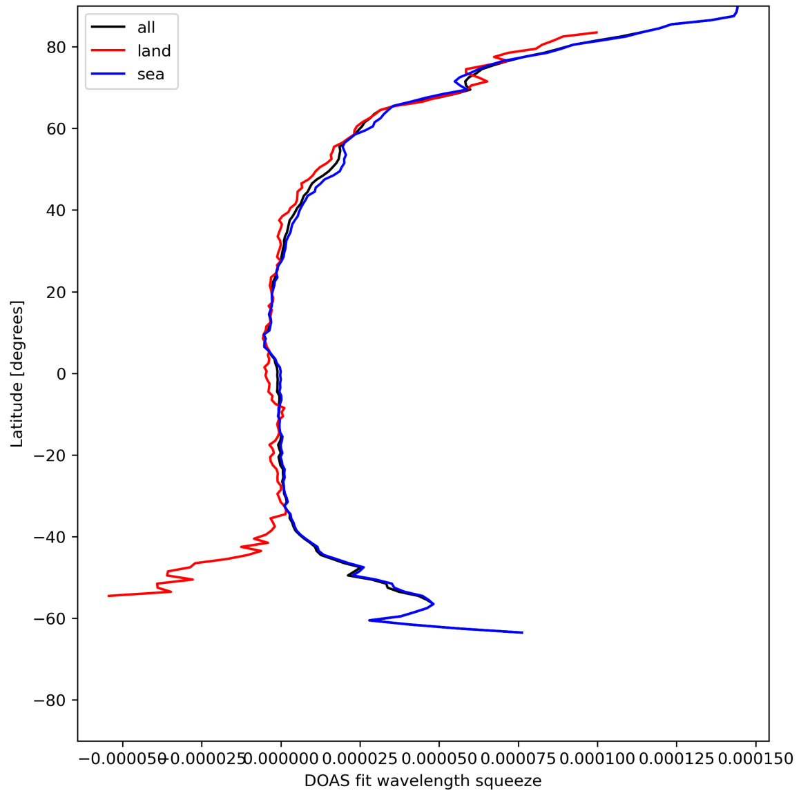
Figure 31: Zonal average of “DOAS fit wavelength squeeze” for 2024-05-25 to 2024-05-27.
