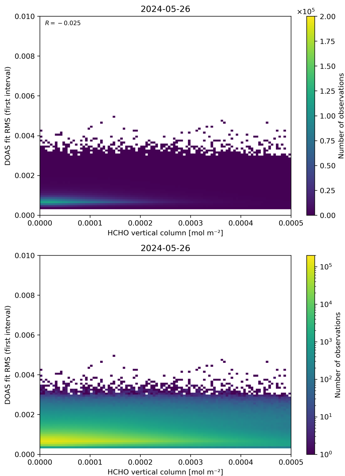
Figure 123: Scatter density plot of “HCHO vertical column” against “DOAS fit RMS (first interval)” for 2024-05-25 to 2024-05-27.
