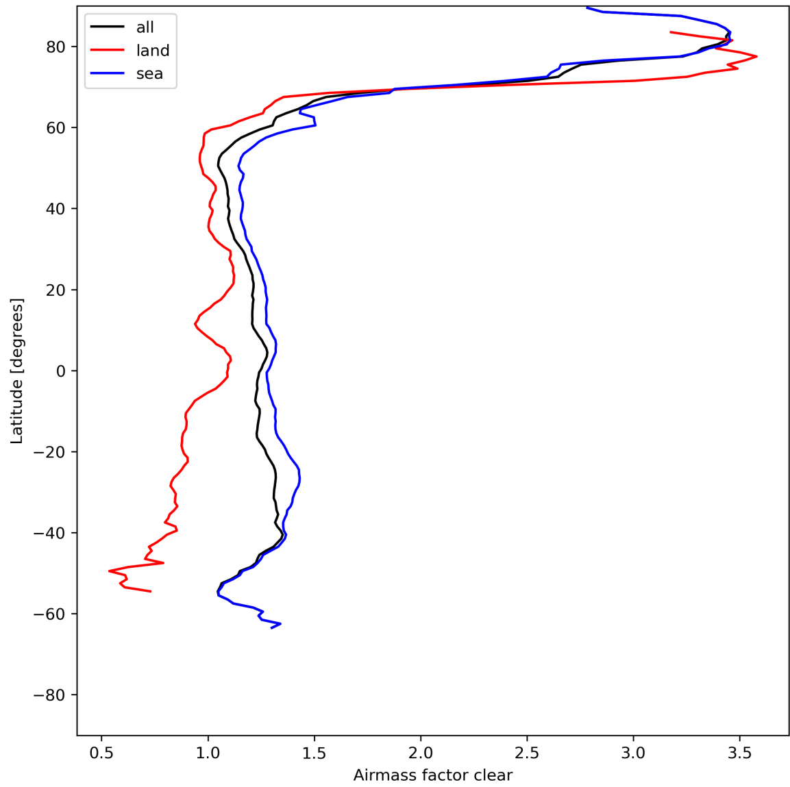
Figure 28: Zonal average of “Airmass factor clear” for 2024-05-25 to 2024-05-27.
