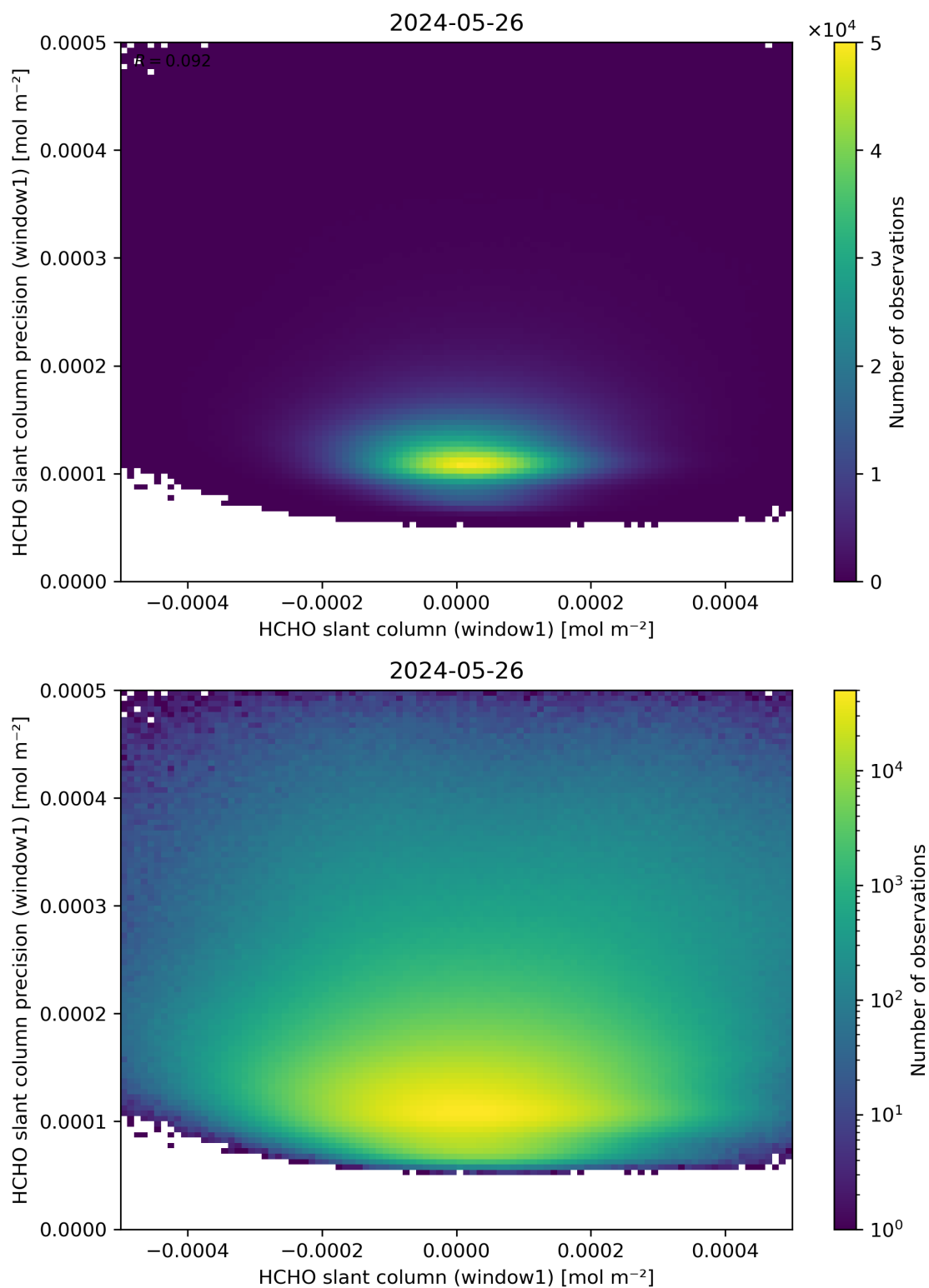
Figure 84: Scatter density plot of “HCHO slant column (window1)” against “HCHO slant column precision (window1)” for 2024-05-25 to 2024-05-27.
