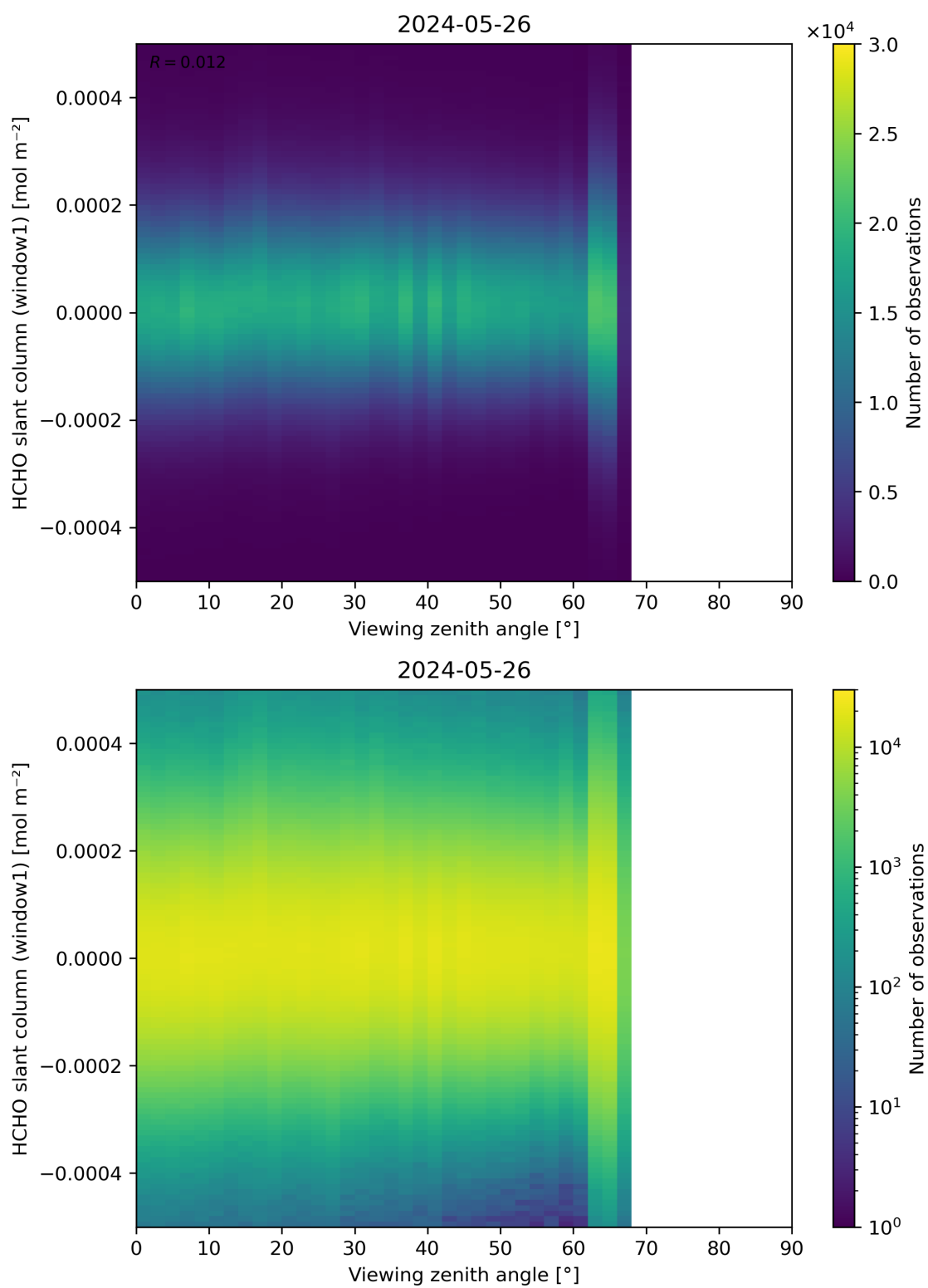
Figure 188: Scatter density plot of “Viewing zenith angle” against “HCHO slant column (window1)” for 2024-05-25 to 2024-05-27.
