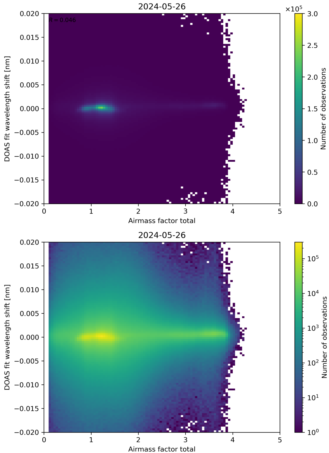
Figure 98: Scatter density plot of “Airmass factor total” against “DOAS fit wavelength shift” for 2024-05-25 to 2024-05-27.
