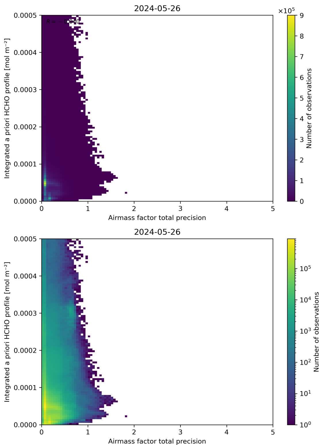
Figure 111: Scatter density plot of “Airmass factor total precision” against “Integrated a priori HCHO profile” for 2024-05-25 to 2024-05-27.
