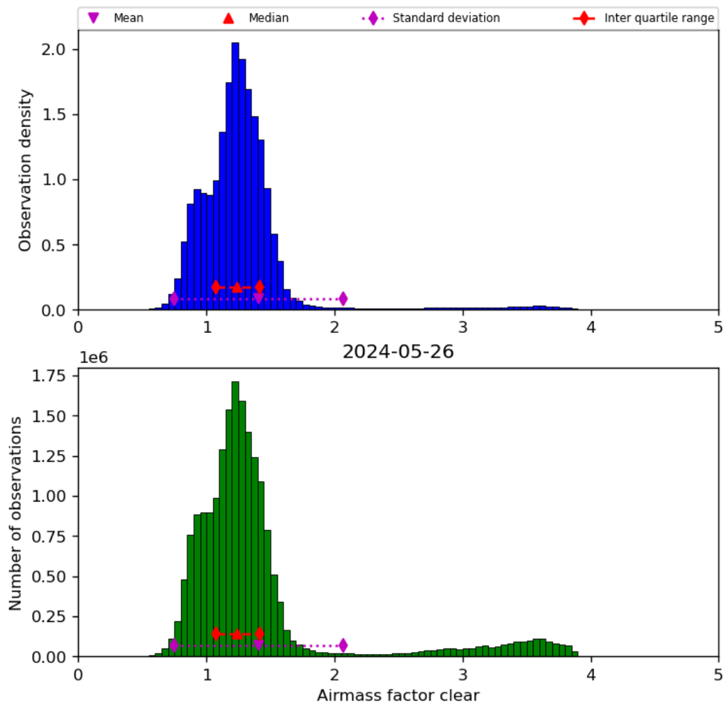
Figure 42: Histogram of “Airmass factor clear” for 2024-05-25 to 2024-05-27
