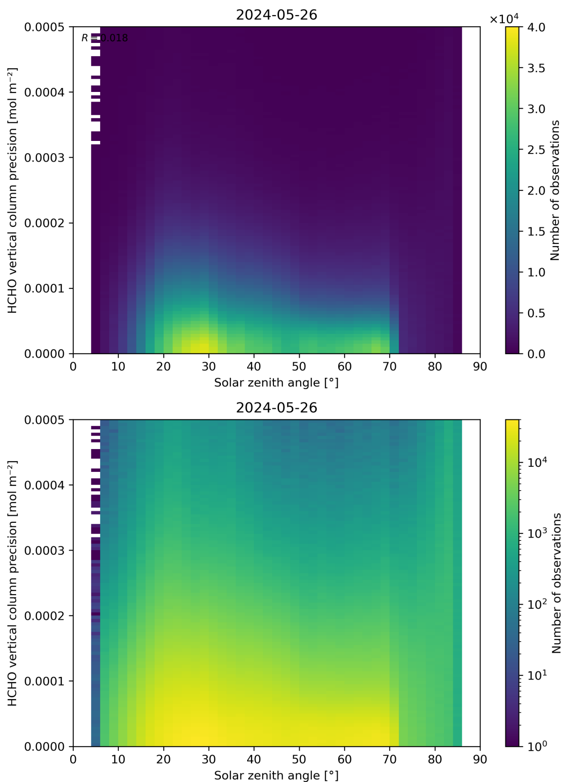
Figure 179: Scatter density plot of “Solar zenith angle” against “HCHO vertical column precision” for 2024-05-25 to 2024-05-27.
