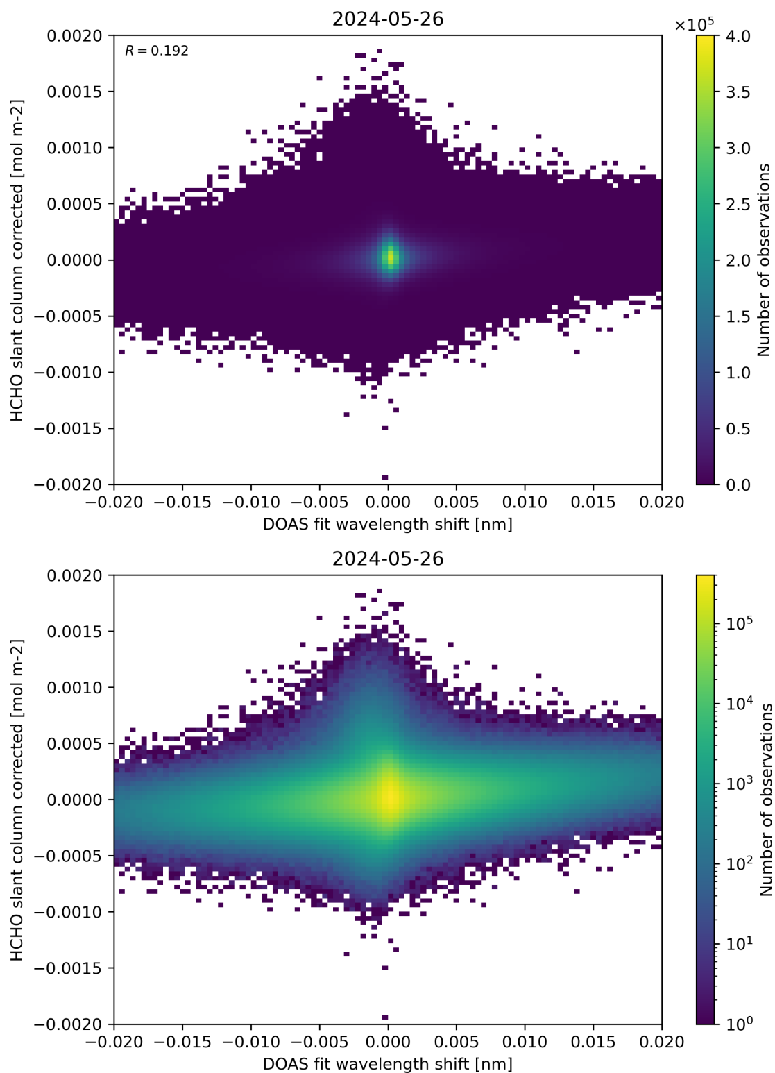
Figure 66: Scatter density plot of “DOAS fit wavelength shift” against “HCHO slant column corrected” for 2024-05-25 to 2024-05-27.
