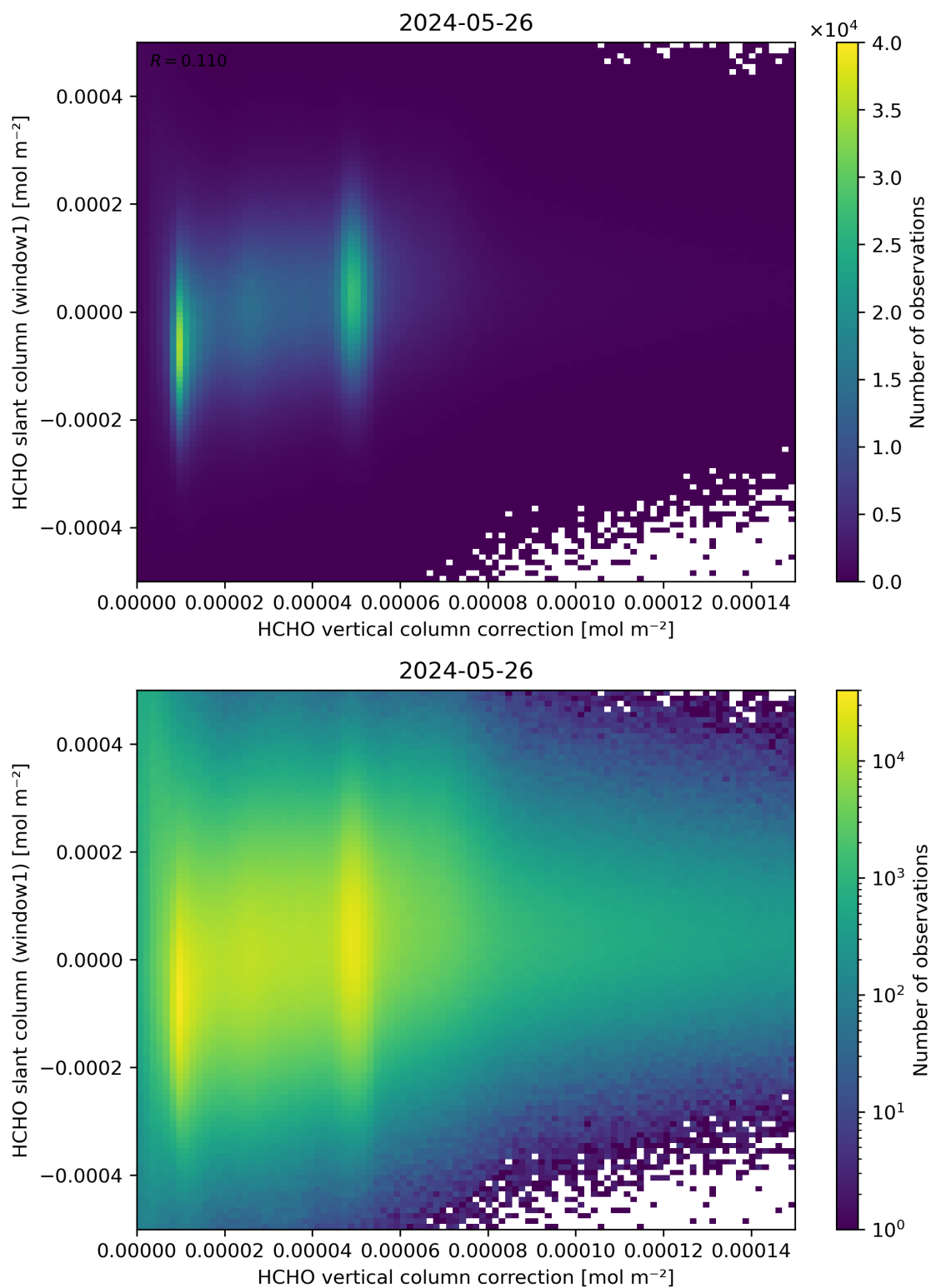
Figure 118: Scatter density plot of “HCHO vertical column correction” against “HCHO slant column (window1)” for 2024-05-25 to 2024-05-27.
