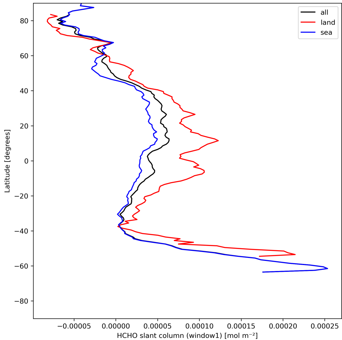
Figure 24: Zonal average of “HCHO slant column (window1)” for 2024-05-25 to 2024-05-27.
