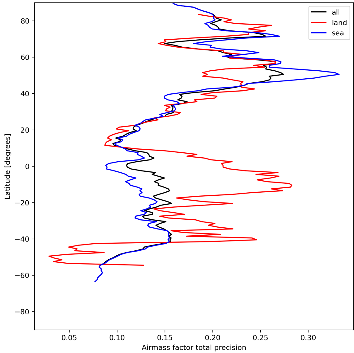
Figure 27: Zonal average of “Airmass factor total precision” for 2024-05-25 to 2024-05-27.
