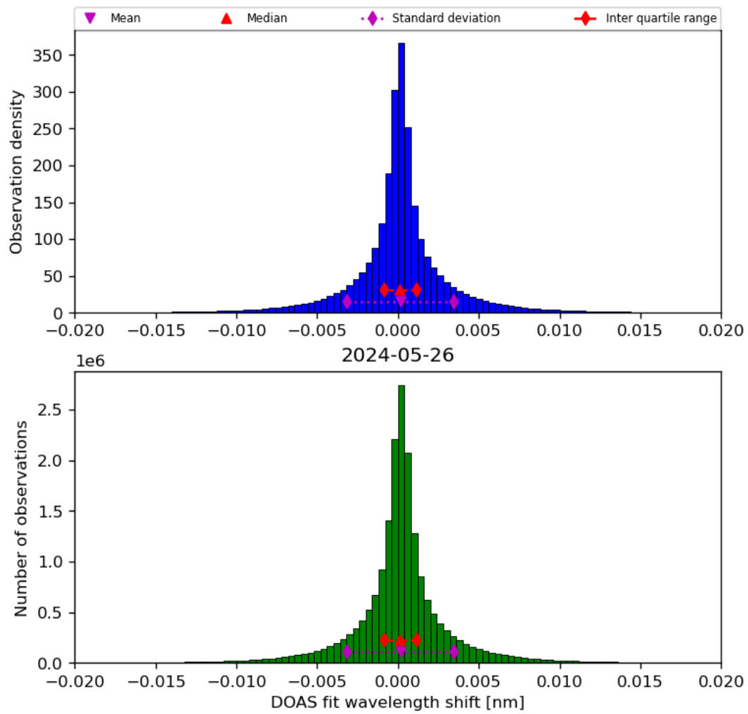
Figure 44: Histogram of “DOAS fit wavelength shift” for 2024-05-25 to 2024-05-27
