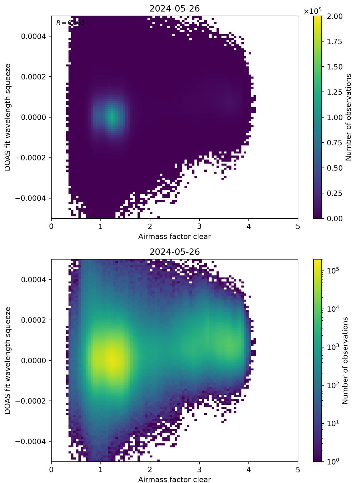
Figure 73: Scatter density plot of “Airmass factor clear” against “DOAS fit wavelength squeeze” for 2024-05-25 to 2024-05-27.
