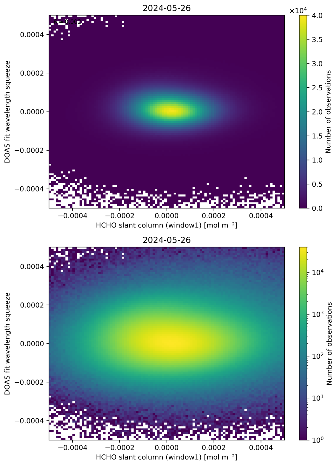
Figure 80: Scatter density plot of “HCHO slant column (window1)” against “DOAS fit wavelength squeeze” for 2024-05-25 to 2024-05-27.
