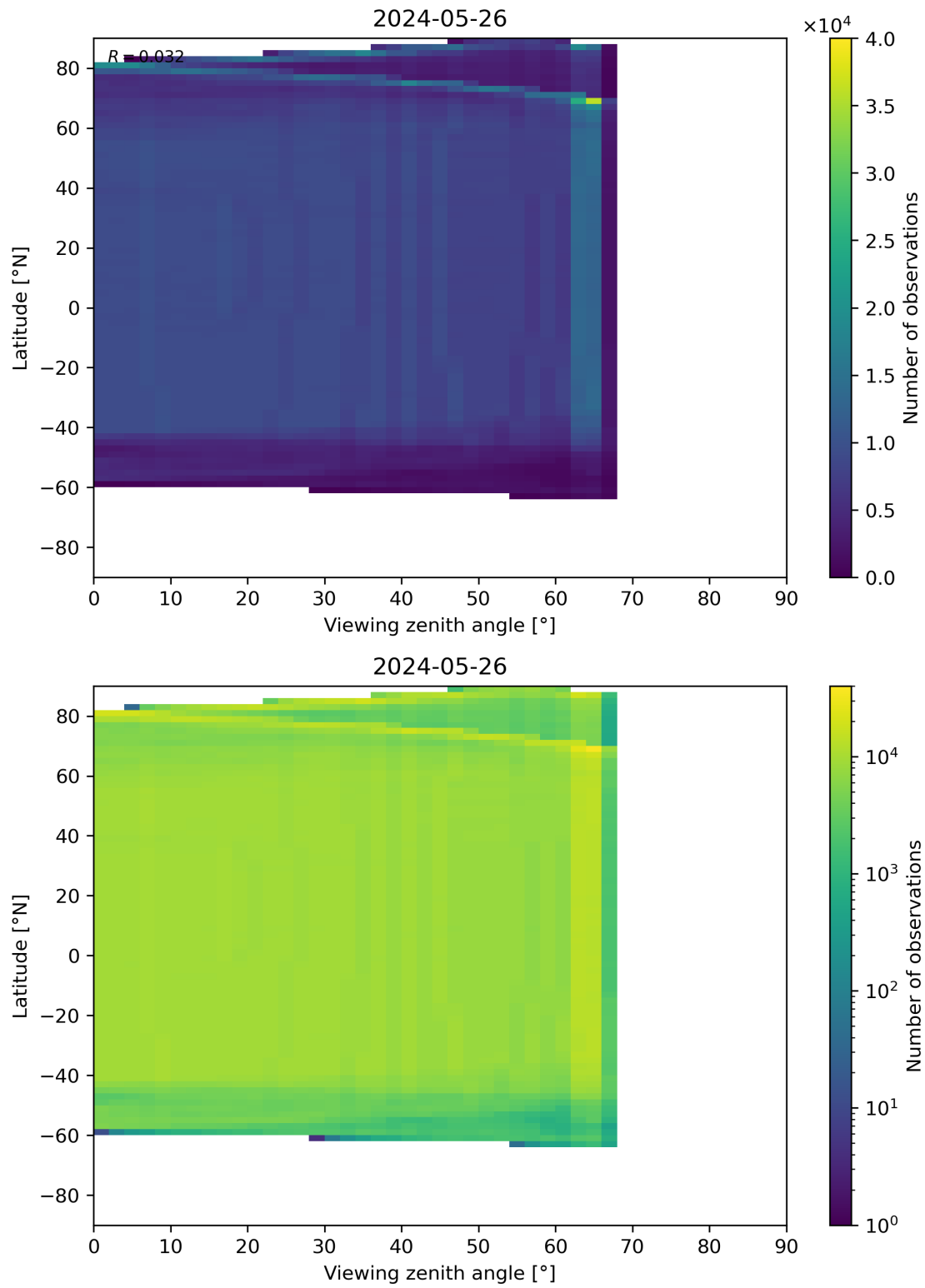
Figure 196: Scatter density plot of “Viewing zenith angle” against “Latitude” for 2024-05-25 to 2024-05-27.
