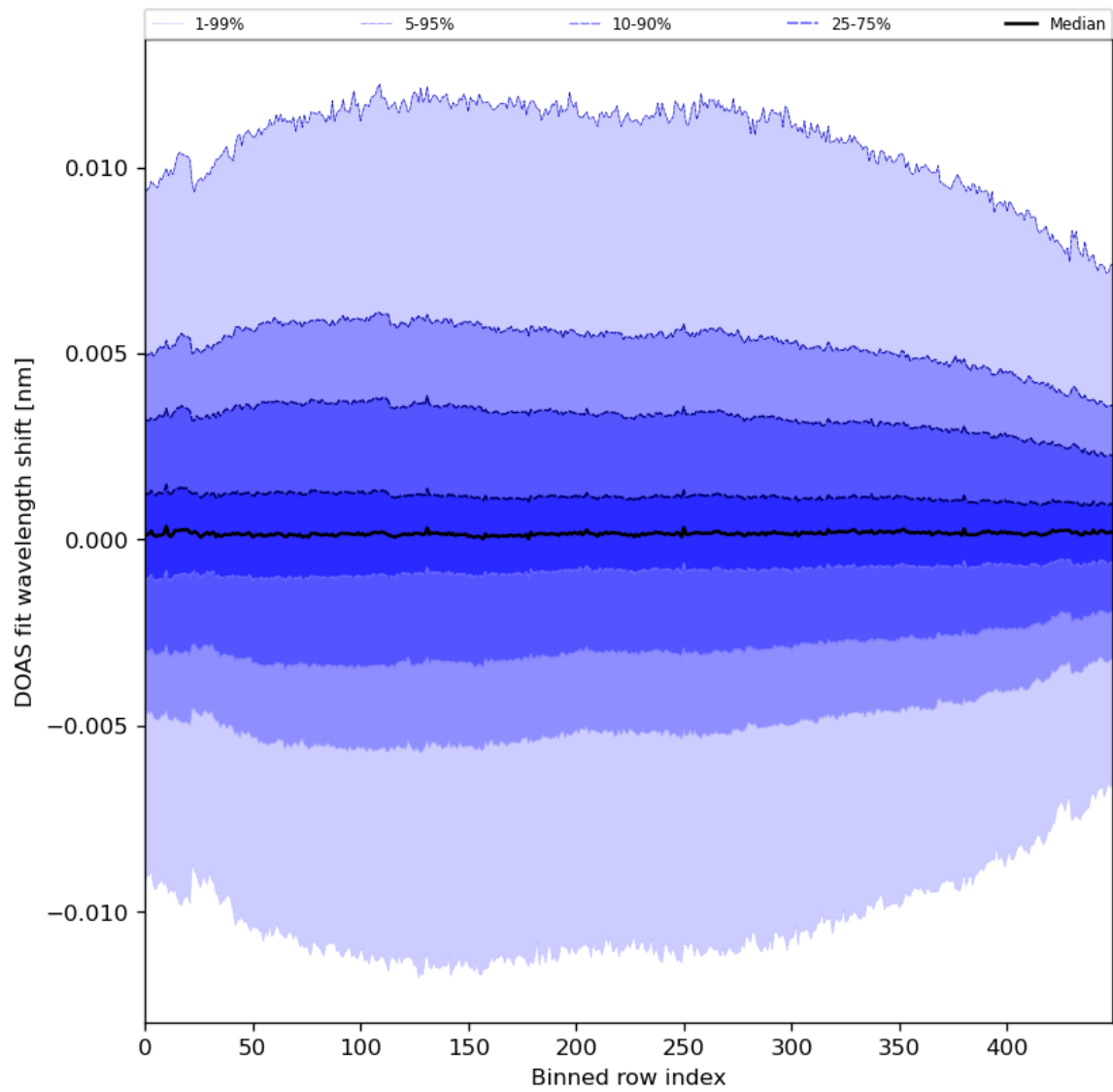
Figure 58: Along track statistics of “DOAS fit wavelength shift” for 2024-05-25 to 2024-05-27
