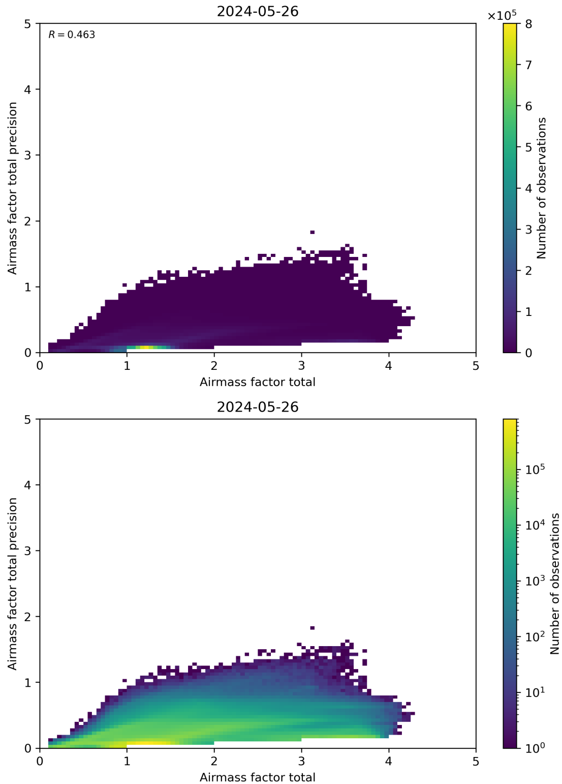
Figure 103: Scatter density plot of “Airmass factor total” against “Airmass factor total precision” for 2024-05-25 to 2024-05-27.
