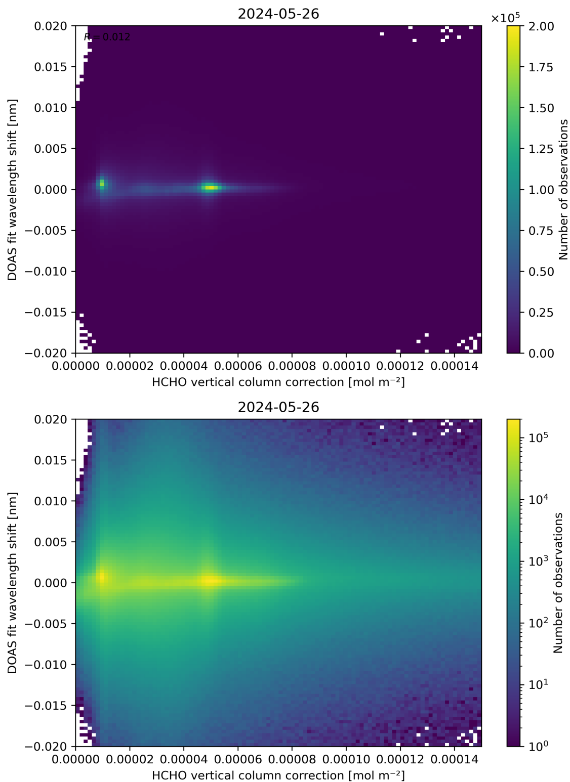
Figure 113: Scatter density plot of “HCHO vertical column correction” against “DOAS fit wavelength shift” for 2024-05-25 to 2024-05-27.
