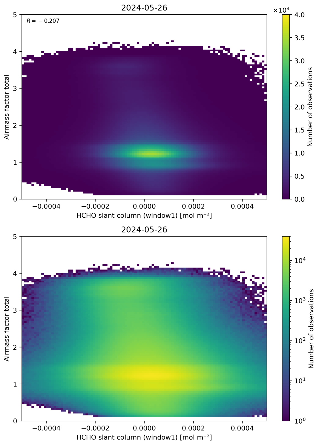
Figure 85: Scatter density plot of “HCHO slant column (window1)” against “Airmass factor total” for 2024-05-25 to 2024-05-27.
