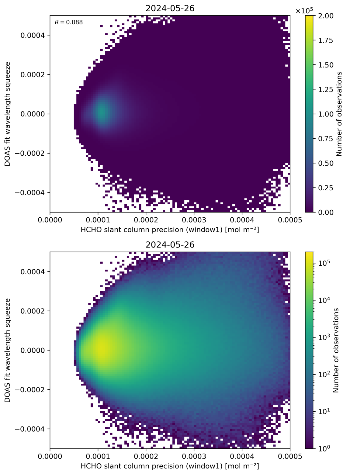
Figure 90: Scatter density plot of “HCHO slant column precision (window1)” against “DOAS fit wavelength squeeze” for 2024-05-25 to 2024-05-27.
