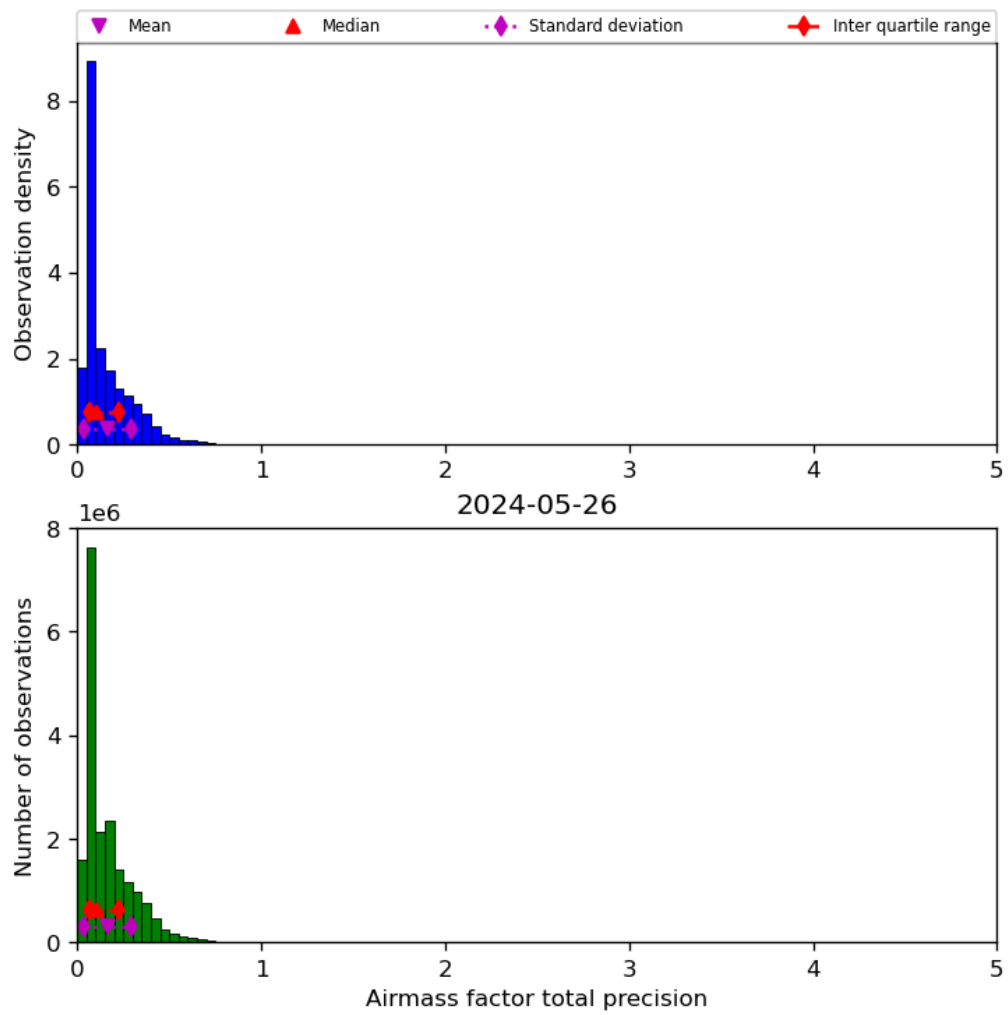
Figure 41: Histogram of “Airmass factor total precision” for 2024-05-25 to 2024-05-27
