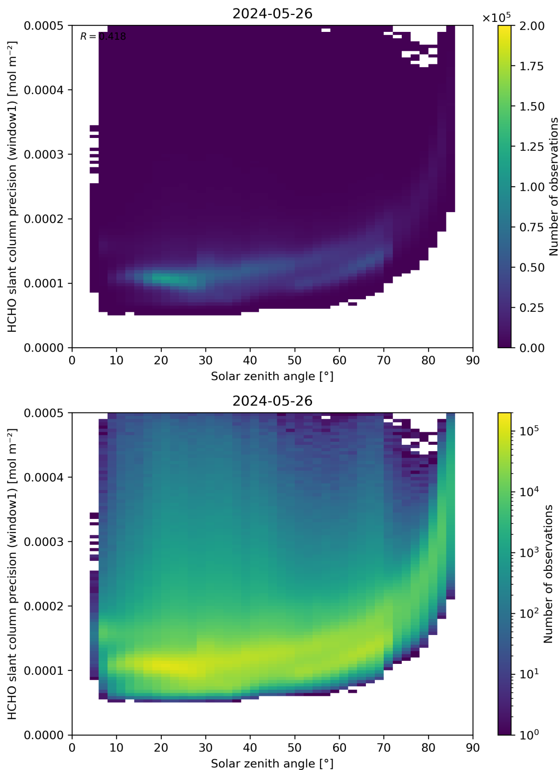
Figure 174: Scatter density plot of “Solar zenith angle” against “HCHO slant column precision (window1)” for 2024-05-25 to 2024-05-27.
