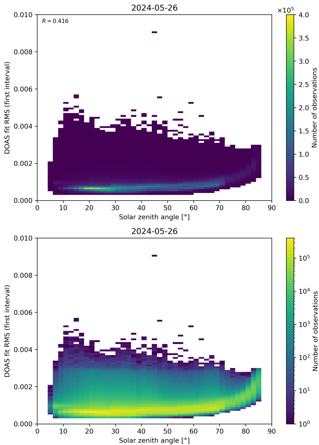
Figure 167: Scatter density plot of “Solar zenith angle” against “DOAS fit RMS (first interval)” for 2024-05-25 to 2024-05-27.
