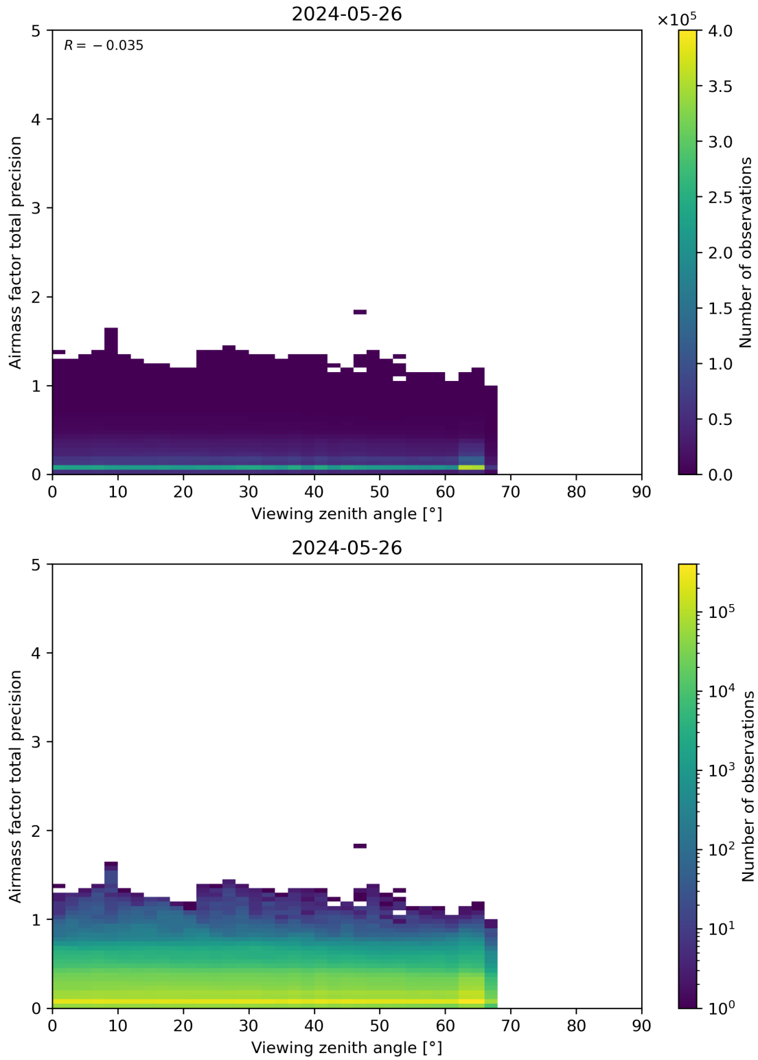
Figure 191: Scatter density plot of “Viewing zenith angle” against “Airmass factor total precision” for 2024-05-25 to 2024-05-27.
