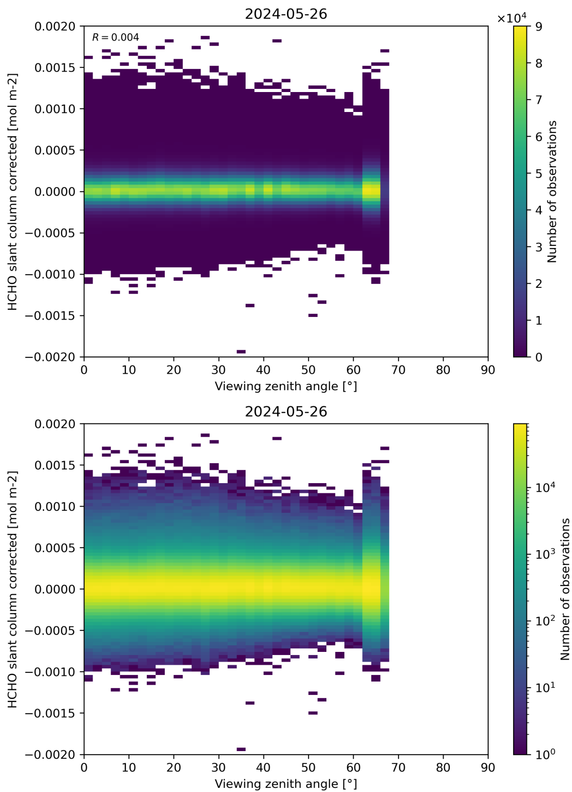
Figure 186: Scatter density plot of “Viewing zenith angle” against “HCHO slant column corrected” for 2024-05-25 to 2024-05-27.
