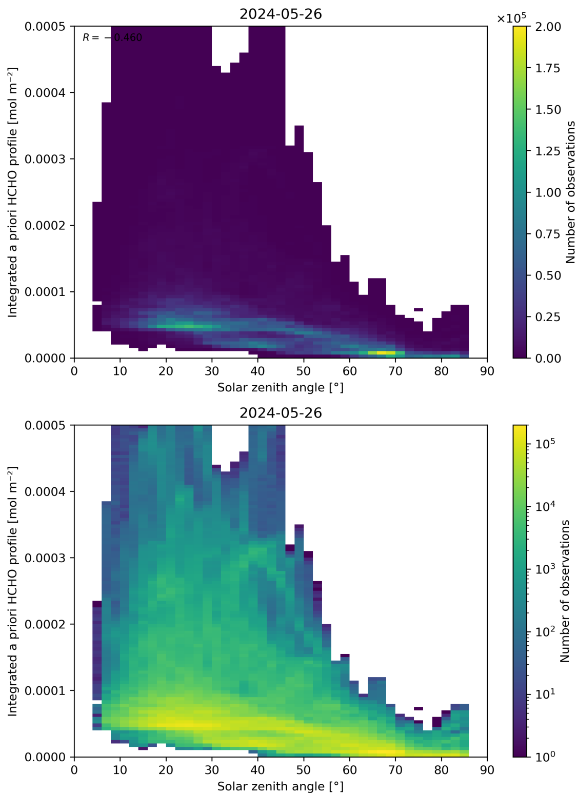
Figure 180: Scatter density plot of “Solar zenith angle” against “Integrated a priori HCHO profile” for 2024-05-25 to 2024-05-27.
