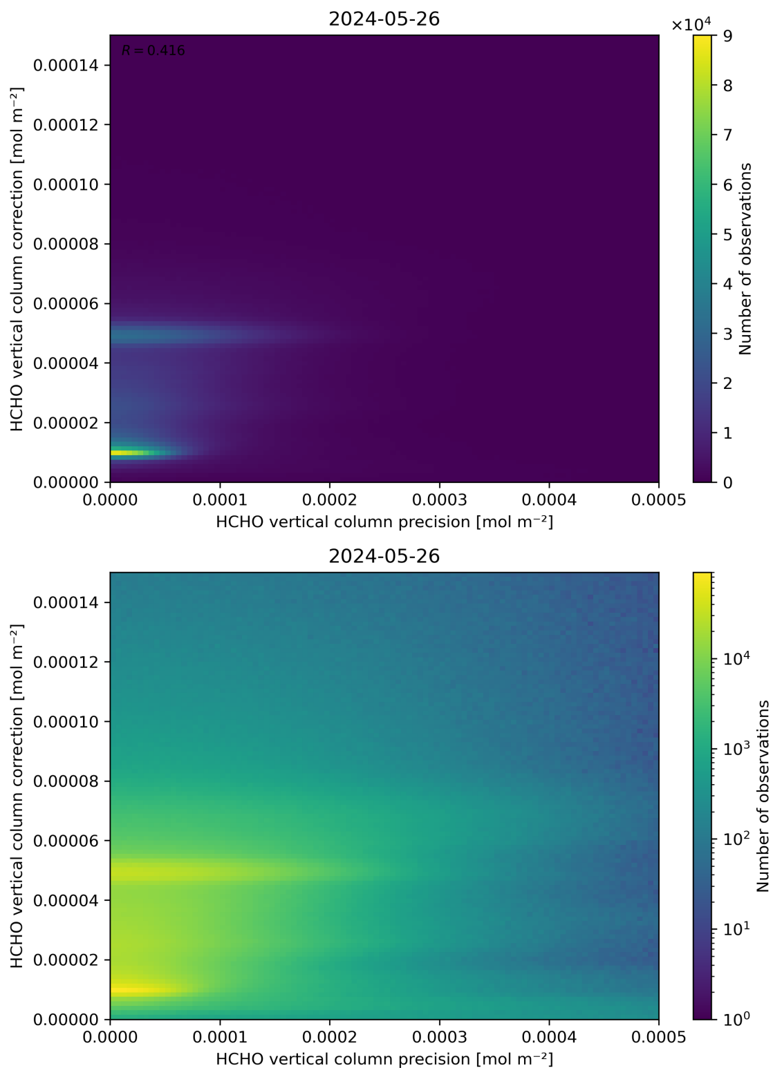
Figure 146: Scatter density plot of “HCHO vertical column precision” against “HCHO vertical column correction” for 2024-05-25 to 2024-05-27.
