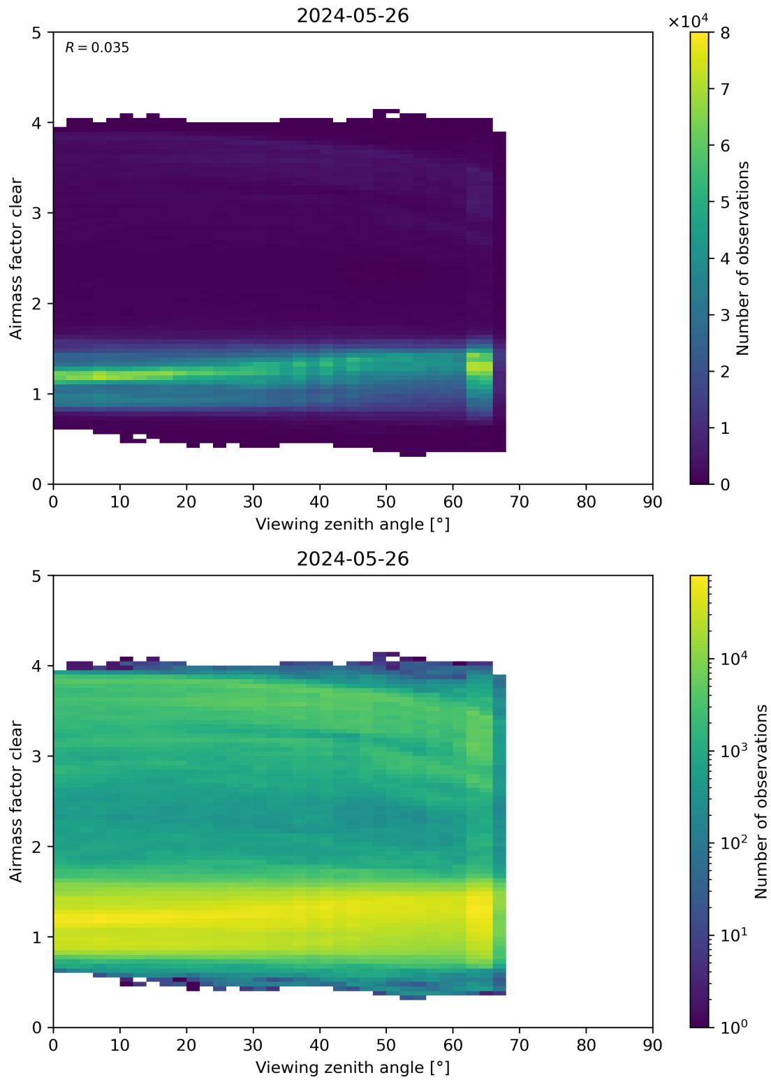
Figure 185: Scatter density plot of “Viewing zenith angle” against “Airmass factor clear” for 2024-05-25 to 2024-05-27.
