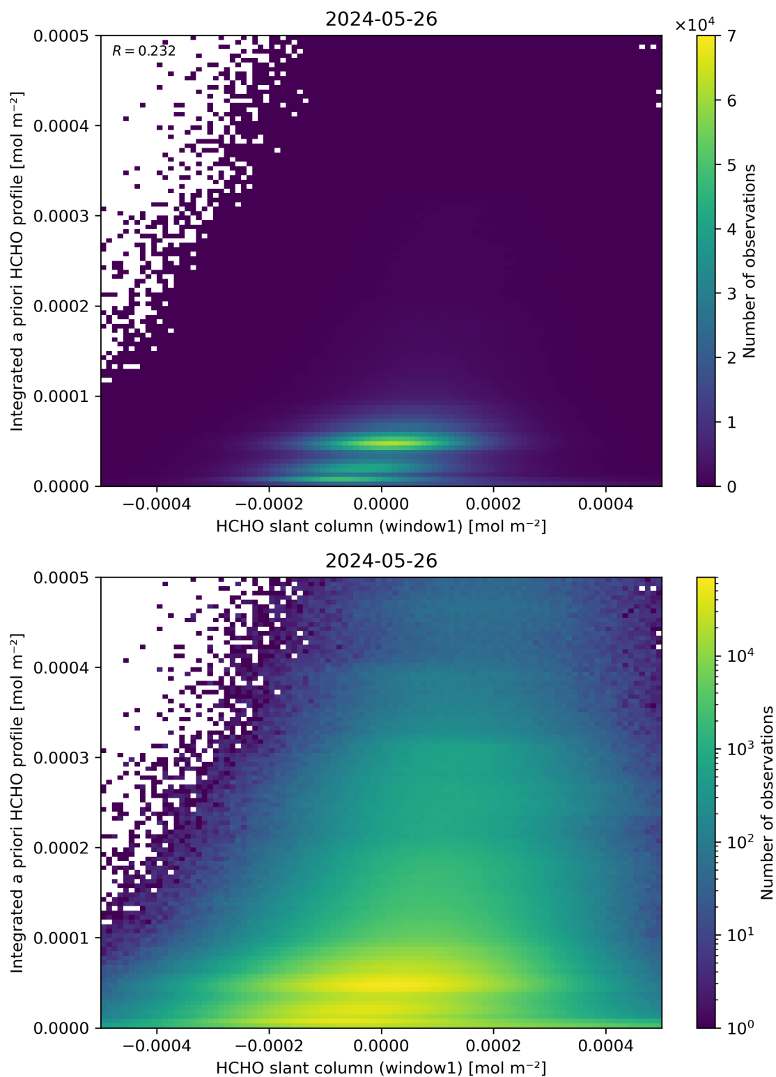
Figure 87: Scatter density plot of “HCHO slant column (window1)” against “Integrated a priori HCHO profile” for 2024-05-25 to 2024-05-27.
