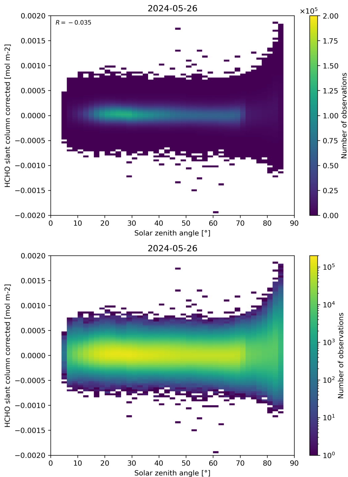
Figure 171: Scatter density plot of “Solar zenith angle” against “HCHO slant column corrected” for 2024-05-25 to 2024-05-27.
