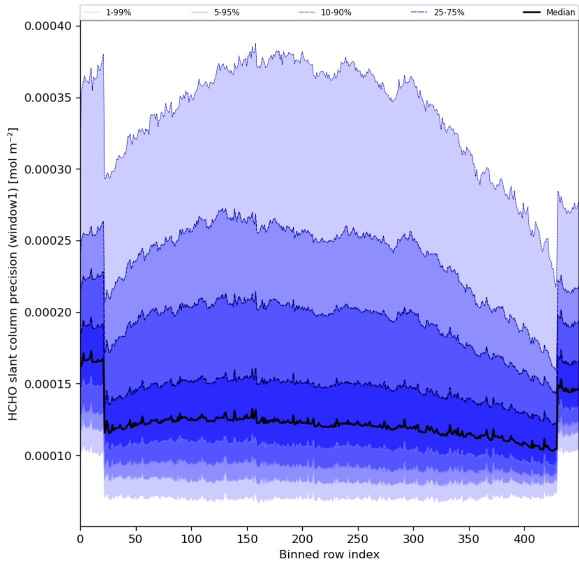
Figure 53: Along track statistics of “HCHO slant column precision (window1)” for 2024-05-25 to 2024-05-27
