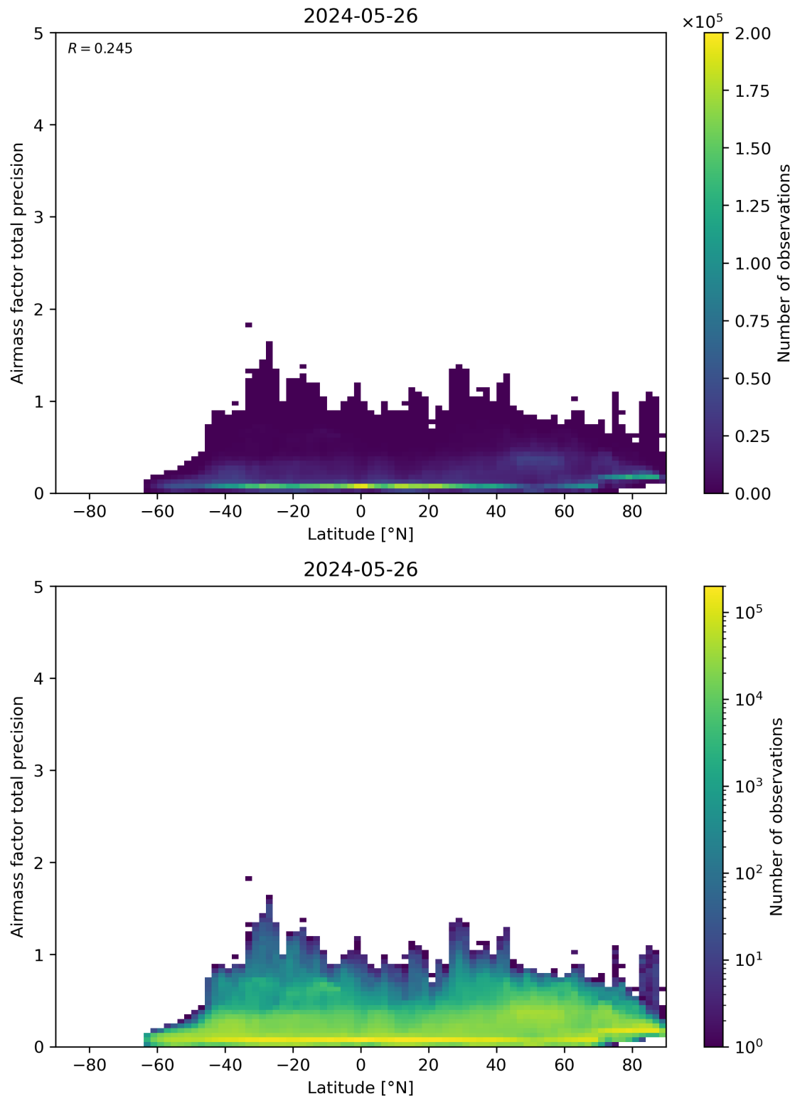
Figure 162: Scatter density plot of “Latitude” against “Airmass factor total precision” for 2024-05-25 to 2024-05-27.
