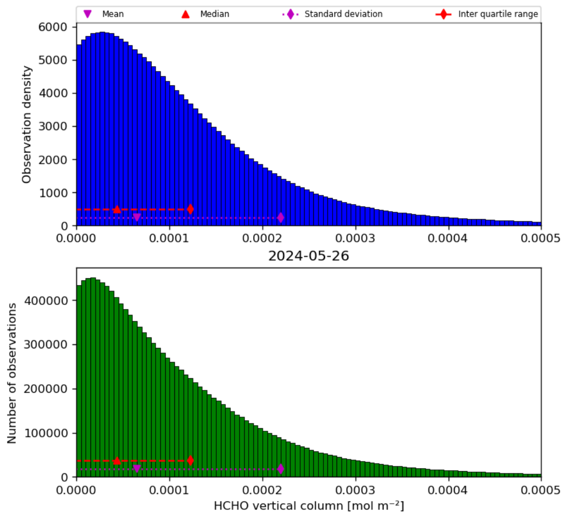
Figure 35: Histogram of “HCHO vertical column” for 2024-05-25 to 2024-05-27
