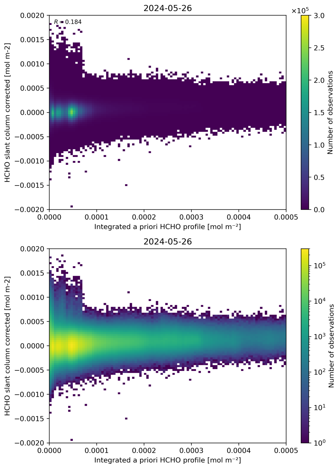
Figure 151: Scatter density plot of “Integrated a priori HCHO profile” against “HCHO slant column corrected” for 2024-05-25 to 2024-05-27.
