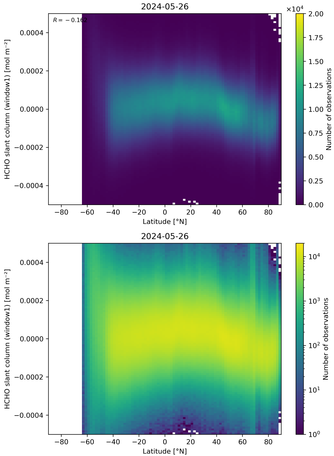
Figure 159: Scatter density plot of “Latitude” against “HCHO slant column (window1)” for 2024-05-25 to 2024-05-27.
