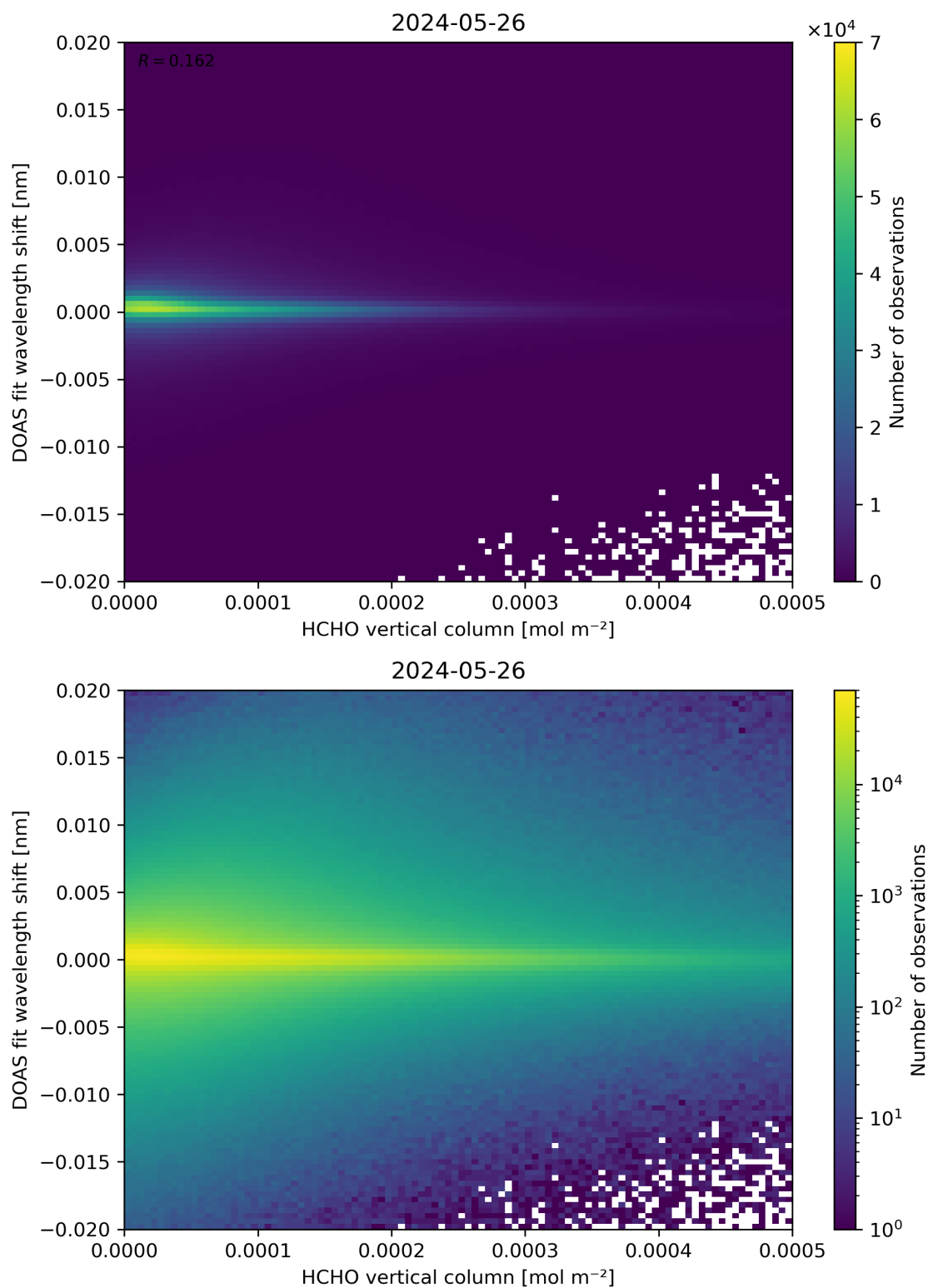
Figure 124: Scatter density plot of “HCHO vertical column” against “DOAS fit wavelength shift” for 2024-05-25 to 2024-05-27.
