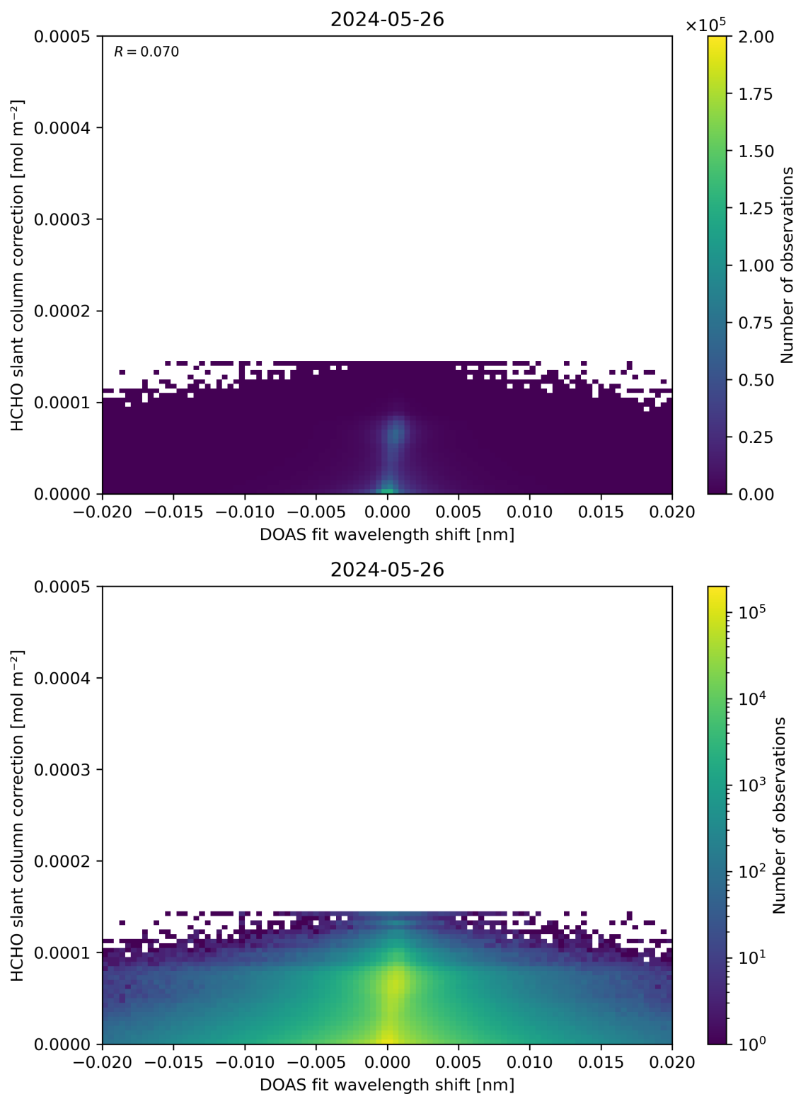
Figure 67: Scatter density plot of “DOAS fit wavelength shift” against “HCHO slant column correction” for 2024-05-25 to 2024-05-27.
