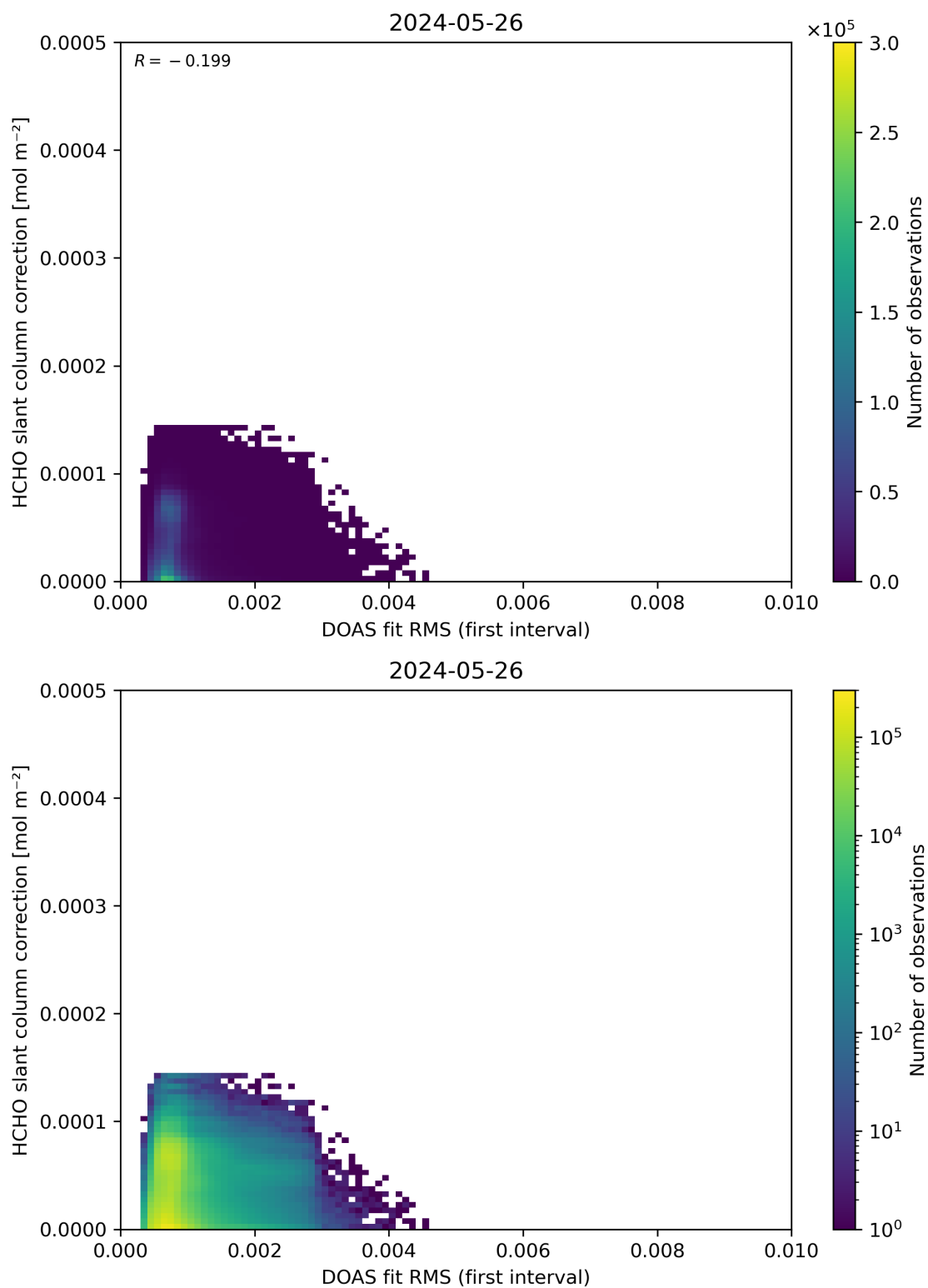
Figure 63: Scatter density plot of “DOAS fit RMS (first interval)” against “HCHO slant column correction” for 2024-05-25 to 2024-05-27.
