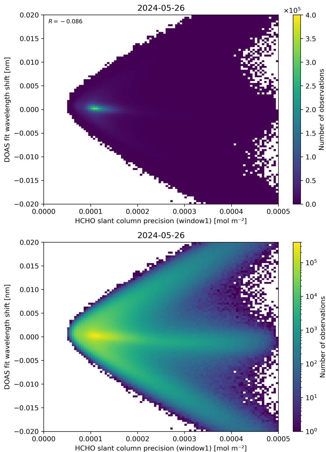
Figure 89: Scatter density plot of “HCHO slant column precision (window1)” against “DOAS fit wavelength shift” for 2024-05-25 to 2024-05-27.
