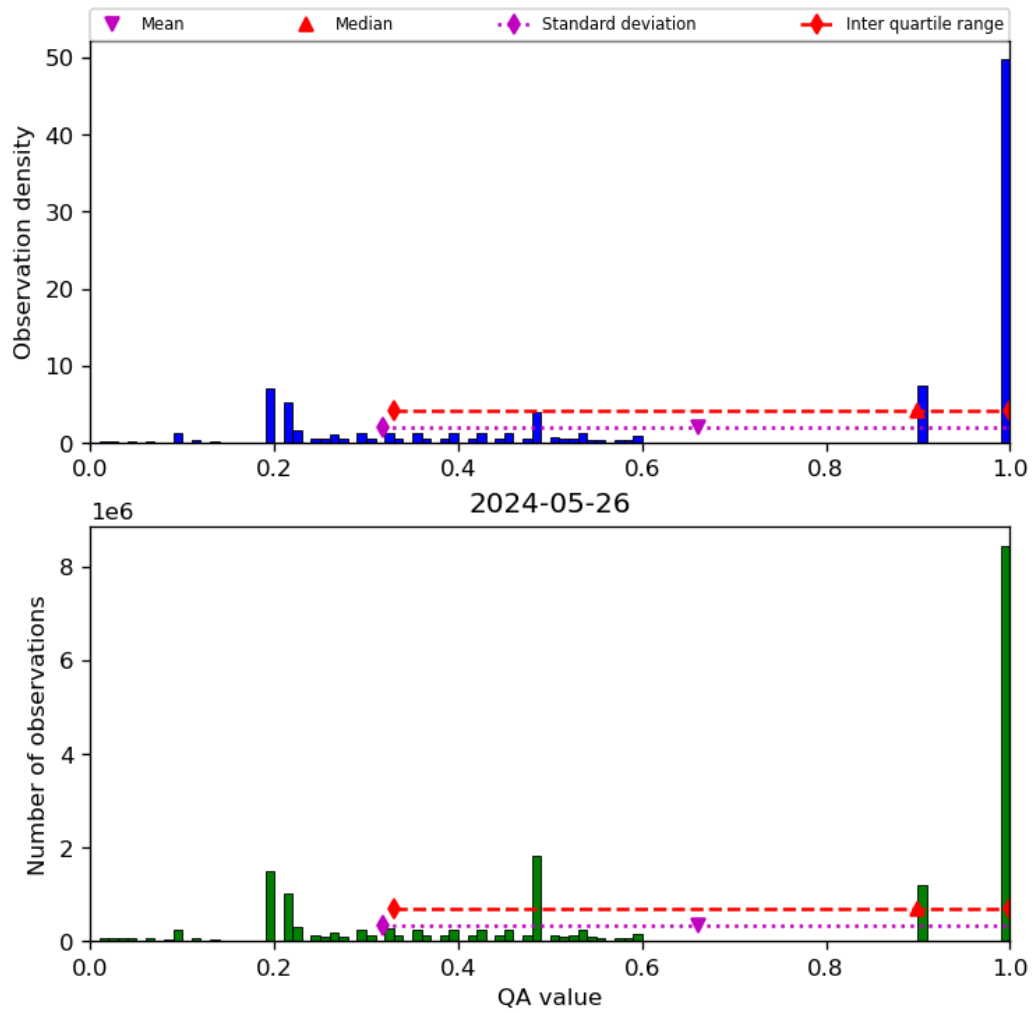
Figure 34: Histogram of “QA value” for 2024-05-25 to 2024-05-27
