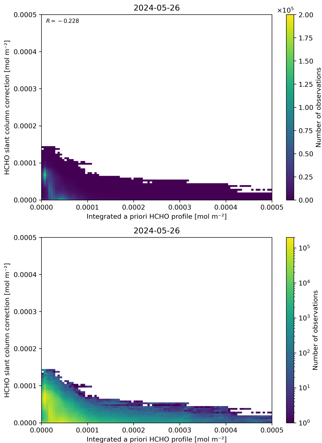
Figure 152: Scatter density plot of “Integrated a priori HCHO profile” against “HCHO slant column correction” for 2024-05-25 to 2024-05-27.
