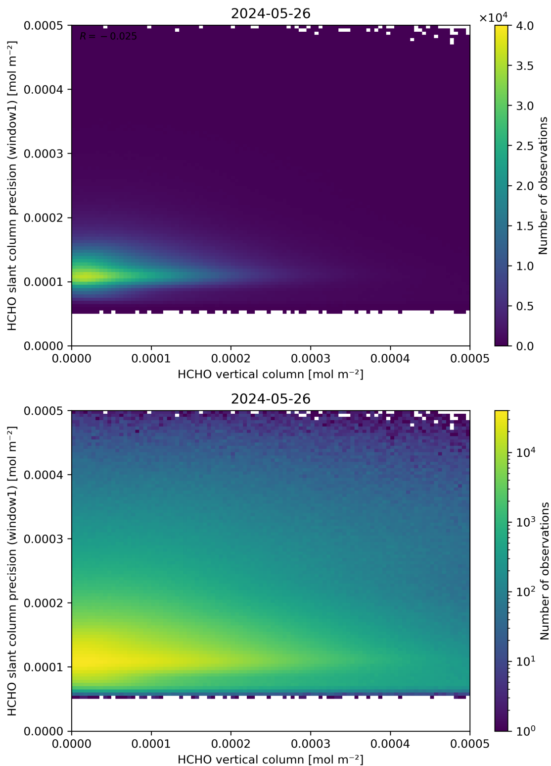
Figure 130: Scatter density plot of “HCHO vertical column” against “HCHO slant column precision (window1)” for 2024-05-25 to 2024-05-27.
