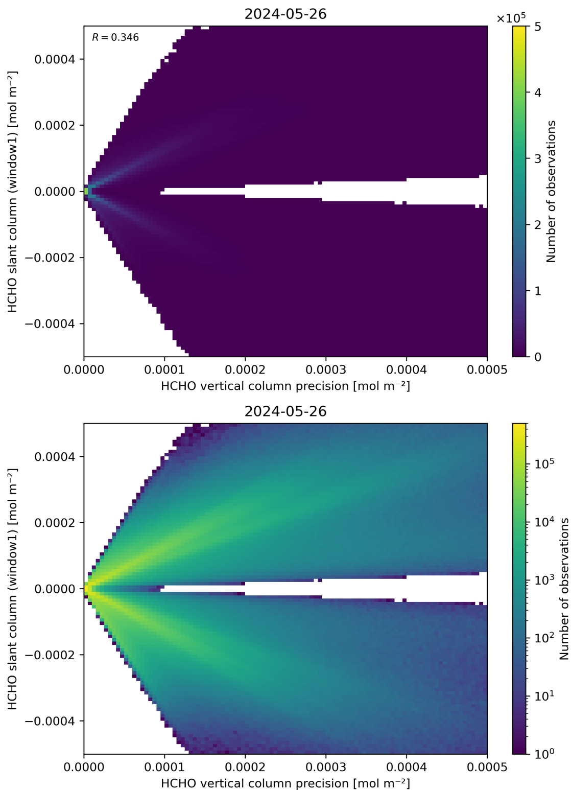
Figure 142: Scatter density plot of “HCHO vertical column precision” against “HCHO slant column (window1)” for 2024-05-25 to 2024-05-27.
