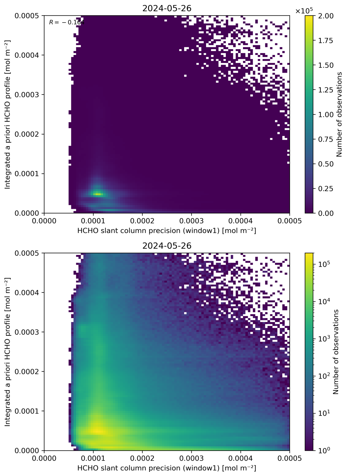
Figure 96: Scatter density plot of “HCHO slant column precision (window1)” against “Integrated a priori HCHO profile” for 2024-05-25 to 2024-05-27.
