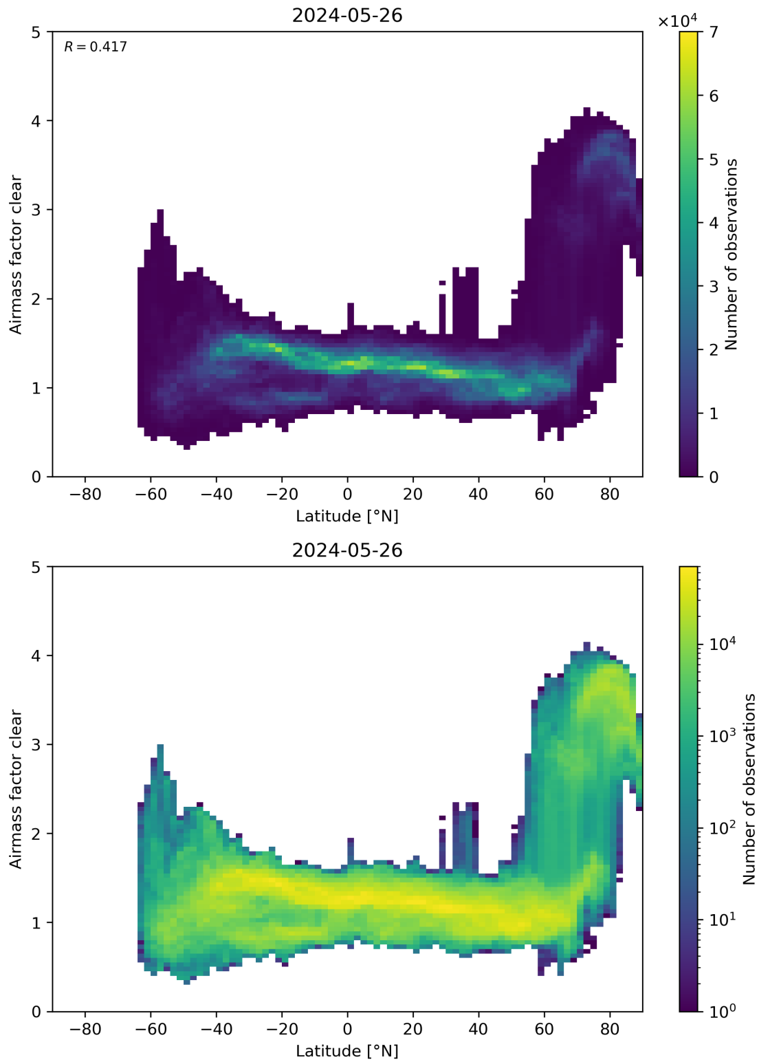
Figure 156: Scatter density plot of “Latitude” against “Airmass factor clear” for 2024-05-25 to 2024-05-27.
