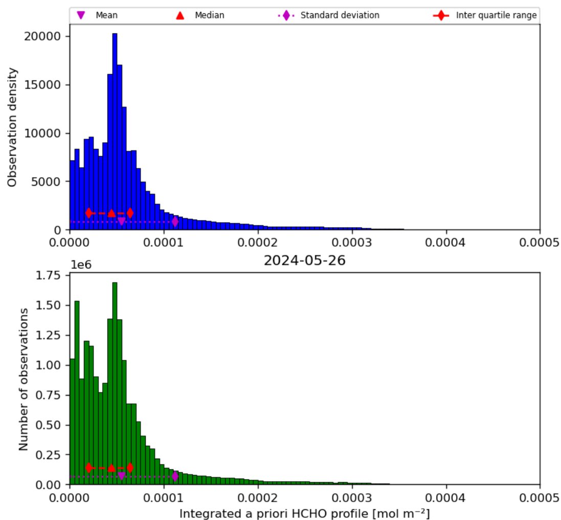
Figure 43: Histogram of “Integrated a priori HCHO profile” for 2024-05-25 to 2024-05-27
