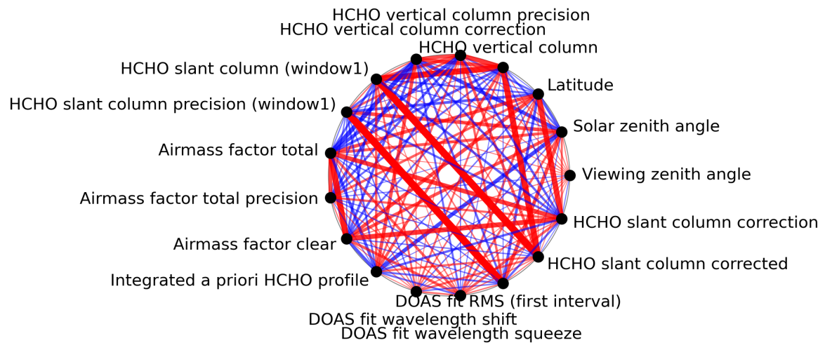
Figure 1: Map of correlation graph for 2024-05-25 to 2024-05-27.
