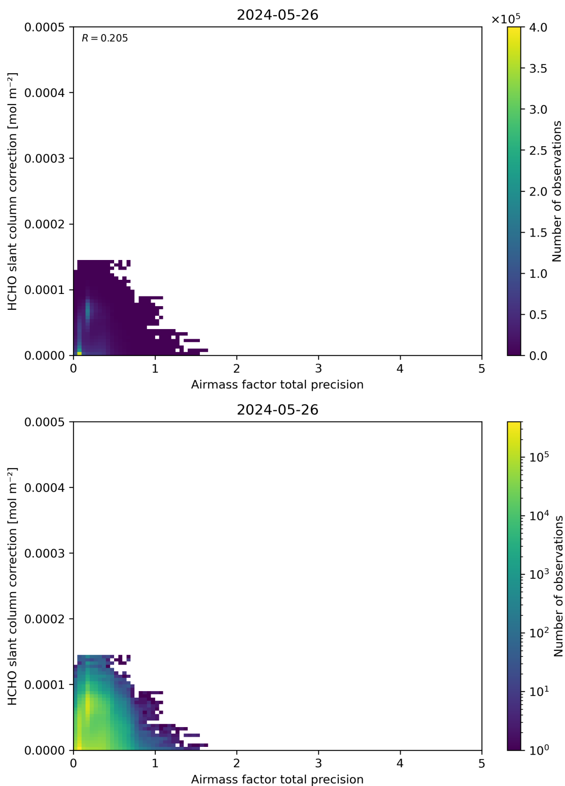
Figure 110: Scatter density plot of “Airmass factor total precision” against “HCHO slant column correction” for 2024-05-25 to 2024-05-27.
