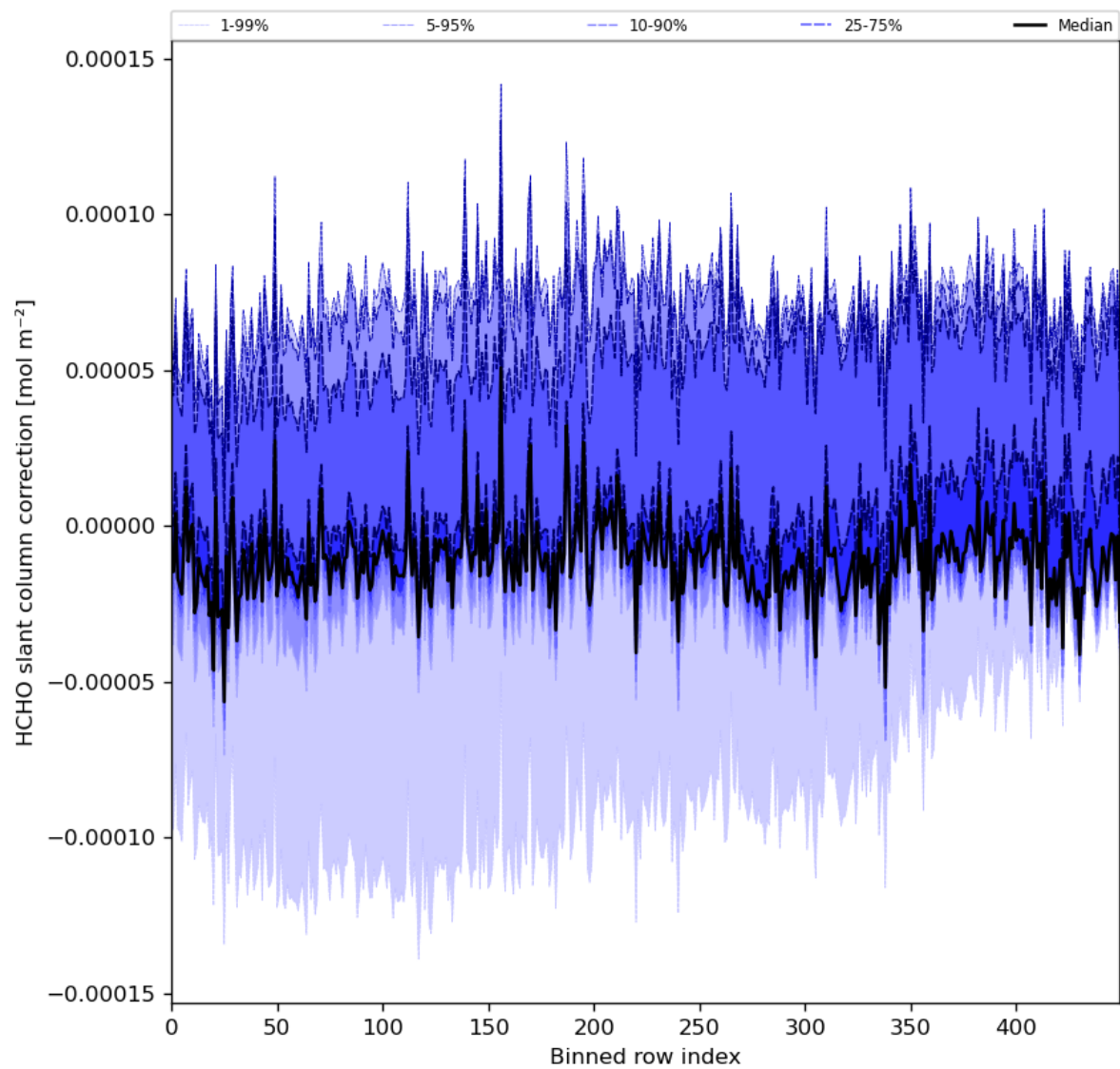
Figure 61: Along track statistics of “HCHO slant column correction” for 2024-05-25 to 2024-05-27
