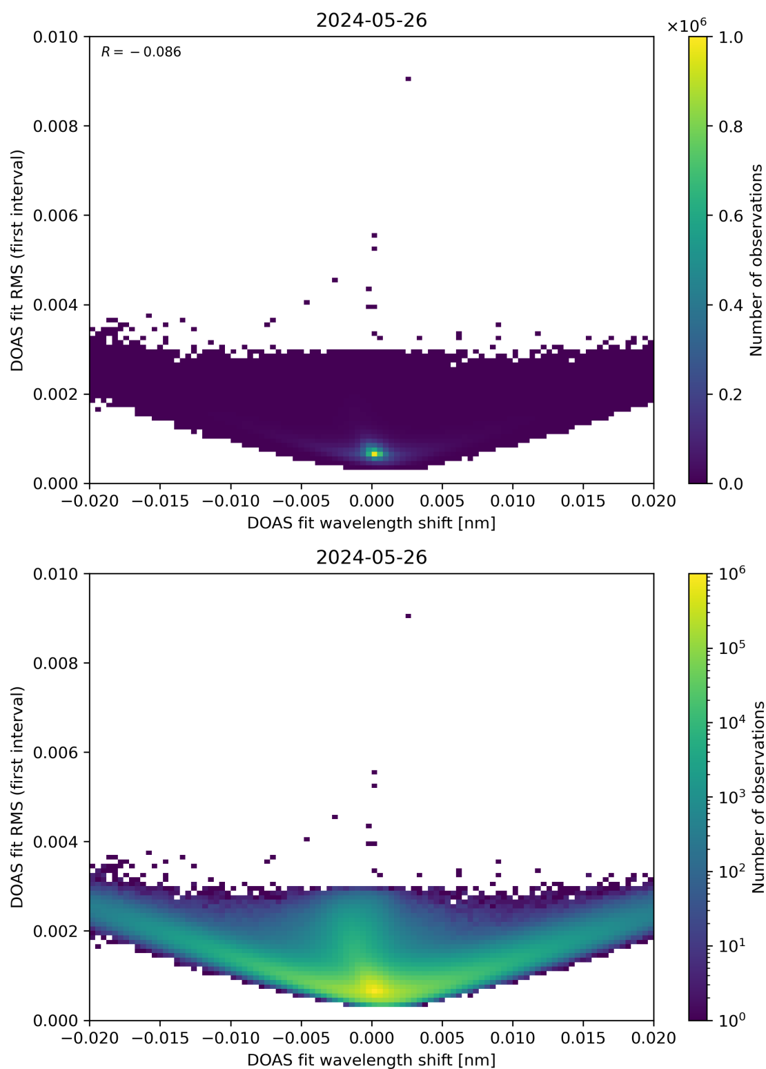
Figure 64: Scatter density plot of “DOAS fit wavelength shift” against “DOAS fit RMS (first interval)” for 2024-05-25 to 2024-05-27.
