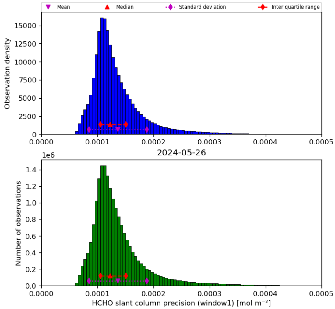
Figure 39: Histogram of “HCHO slant column precision (window1)” for 2024-05-25 to 2024-05-27
