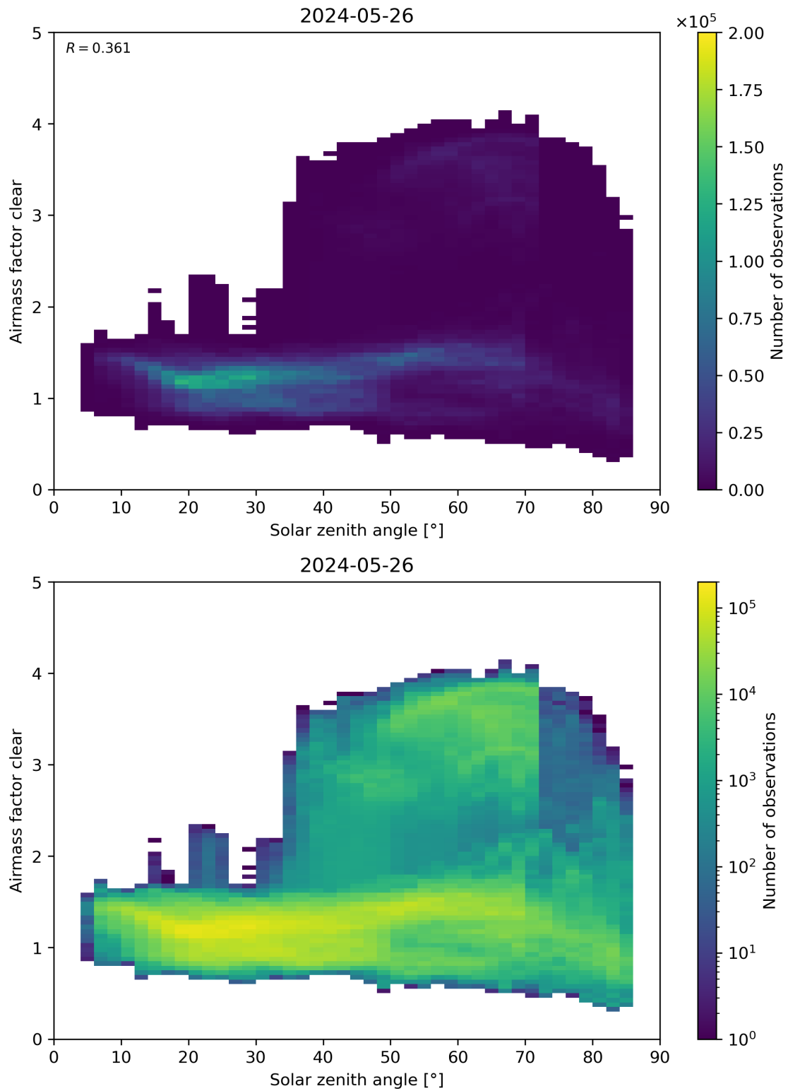
Figure 170: Scatter density plot of “Solar zenith angle” against “Airmass factor clear” for 2024-05-25 to 2024-05-27.
