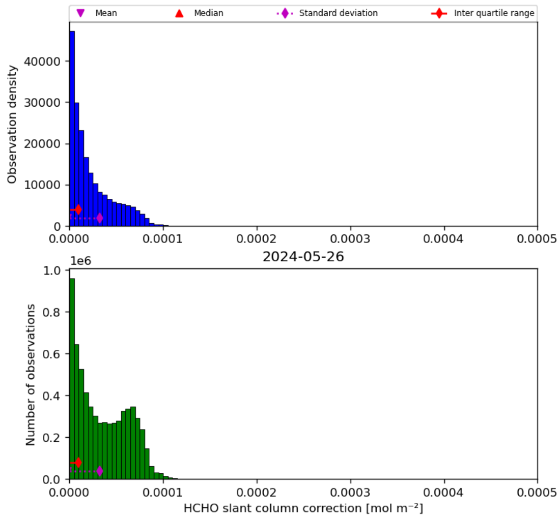
Figure 47: Histogram of “HCHO slant column correction” for 2024-05-25 to 2024-05-27
