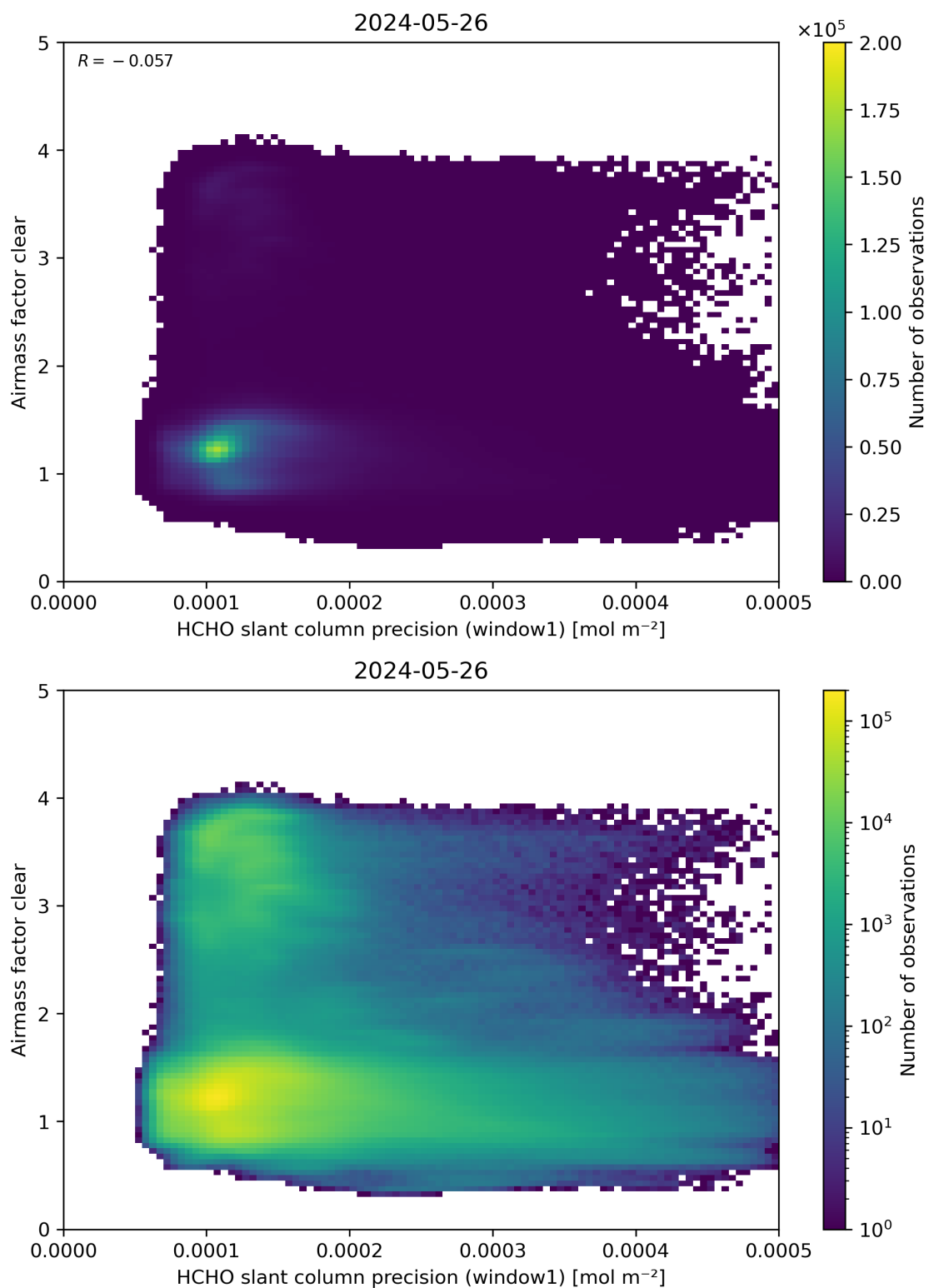
Figure 91: Scatter density plot of “HCHO slant column precision (window1)” against “Airmass factor clear” for 2024-05-25 to 2024-05-27.
