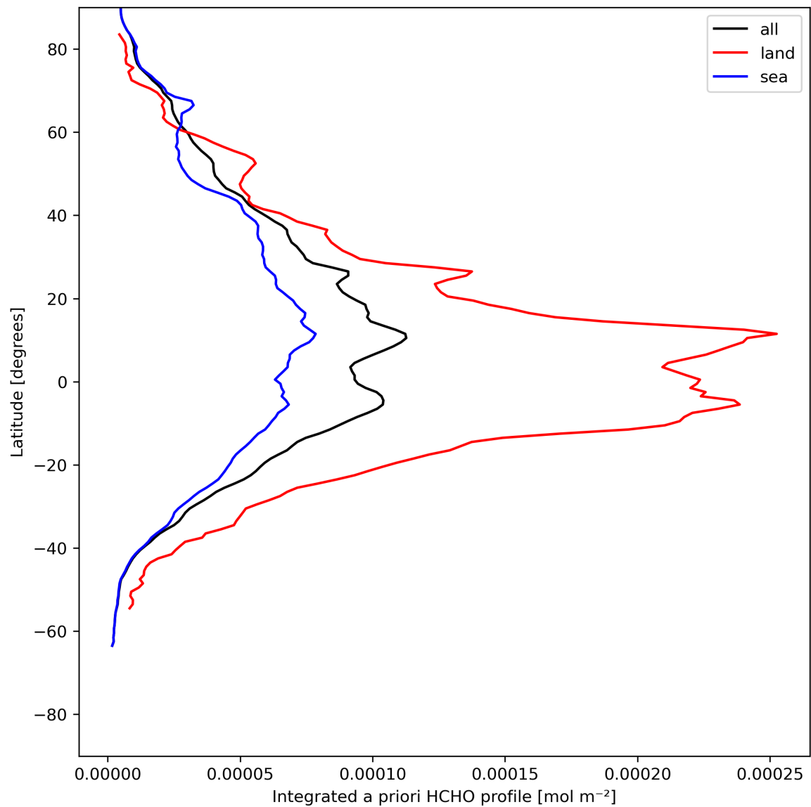
Figure 29: Zonal average of “Integrated a priori HCHO profile” for 2024-05-25 to 2024-05-27.
