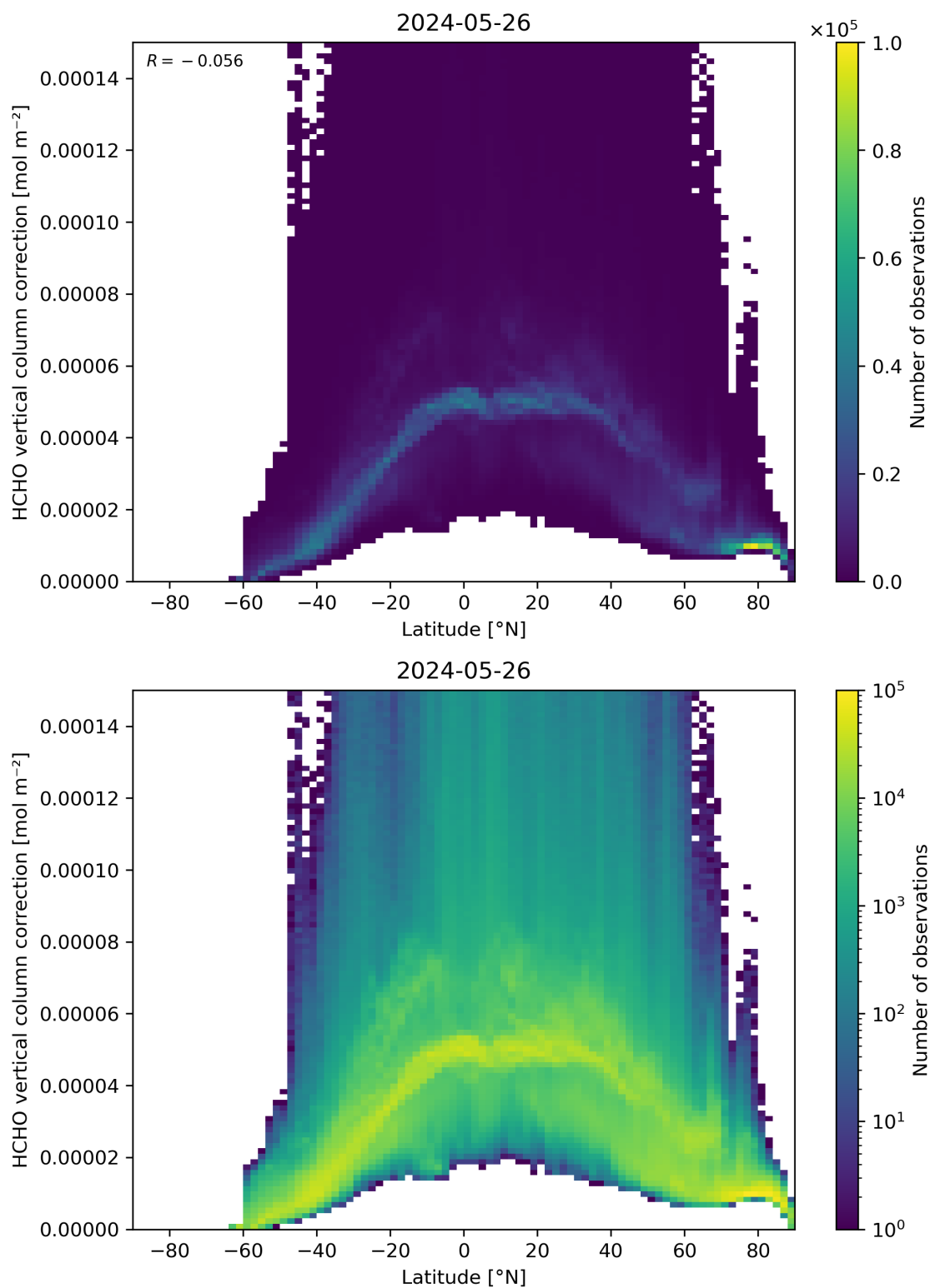
Figure 164: Scatter density plot of “Latitude” against “HCHO vertical column correction” for 2024-05-25 to 2024-05-27.
