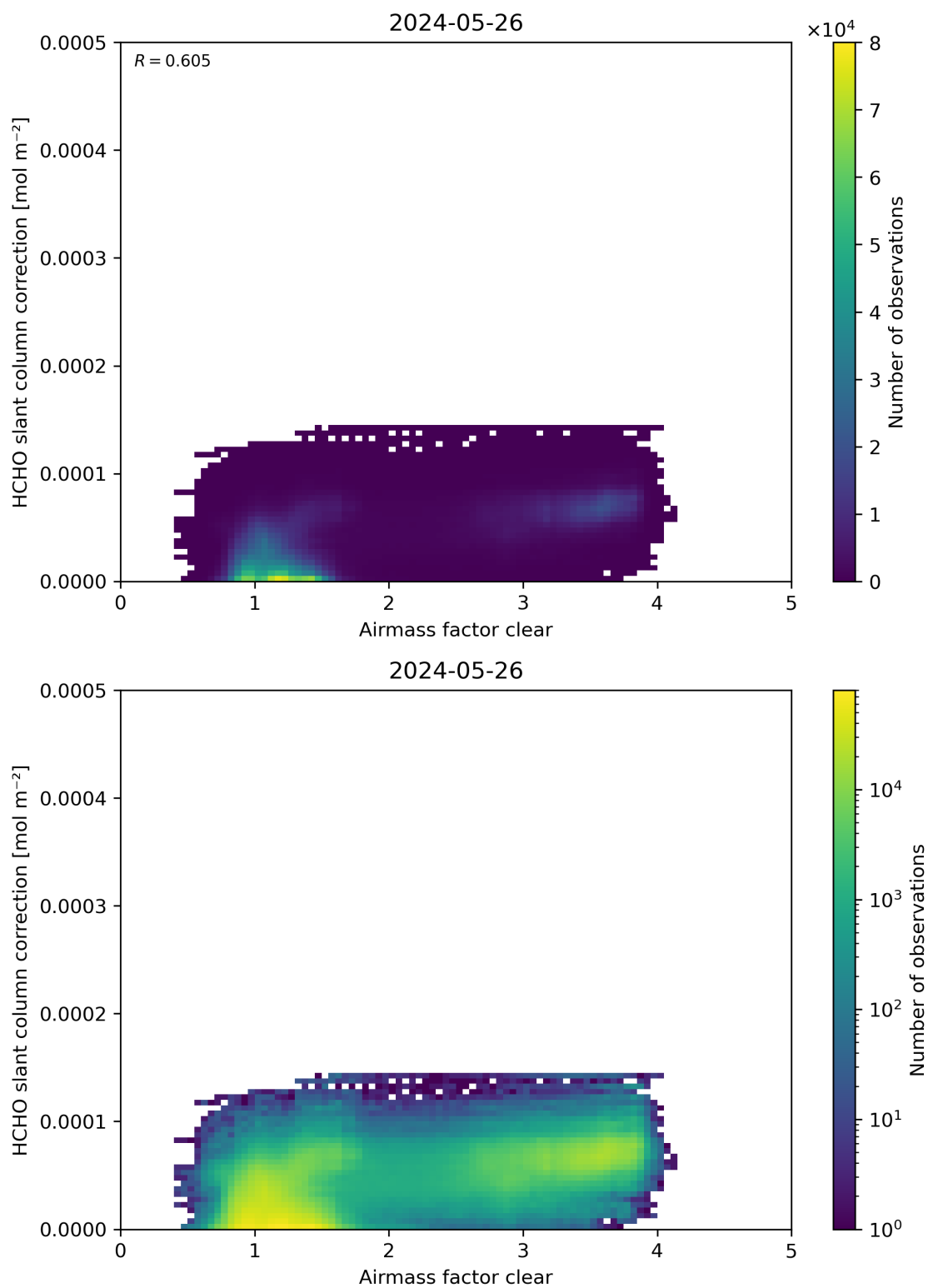
Figure 75: Scatter density plot of “Airmass factor clear” against “HCHO slant column correction” for 2024-05-25 to 2024-05-27.
