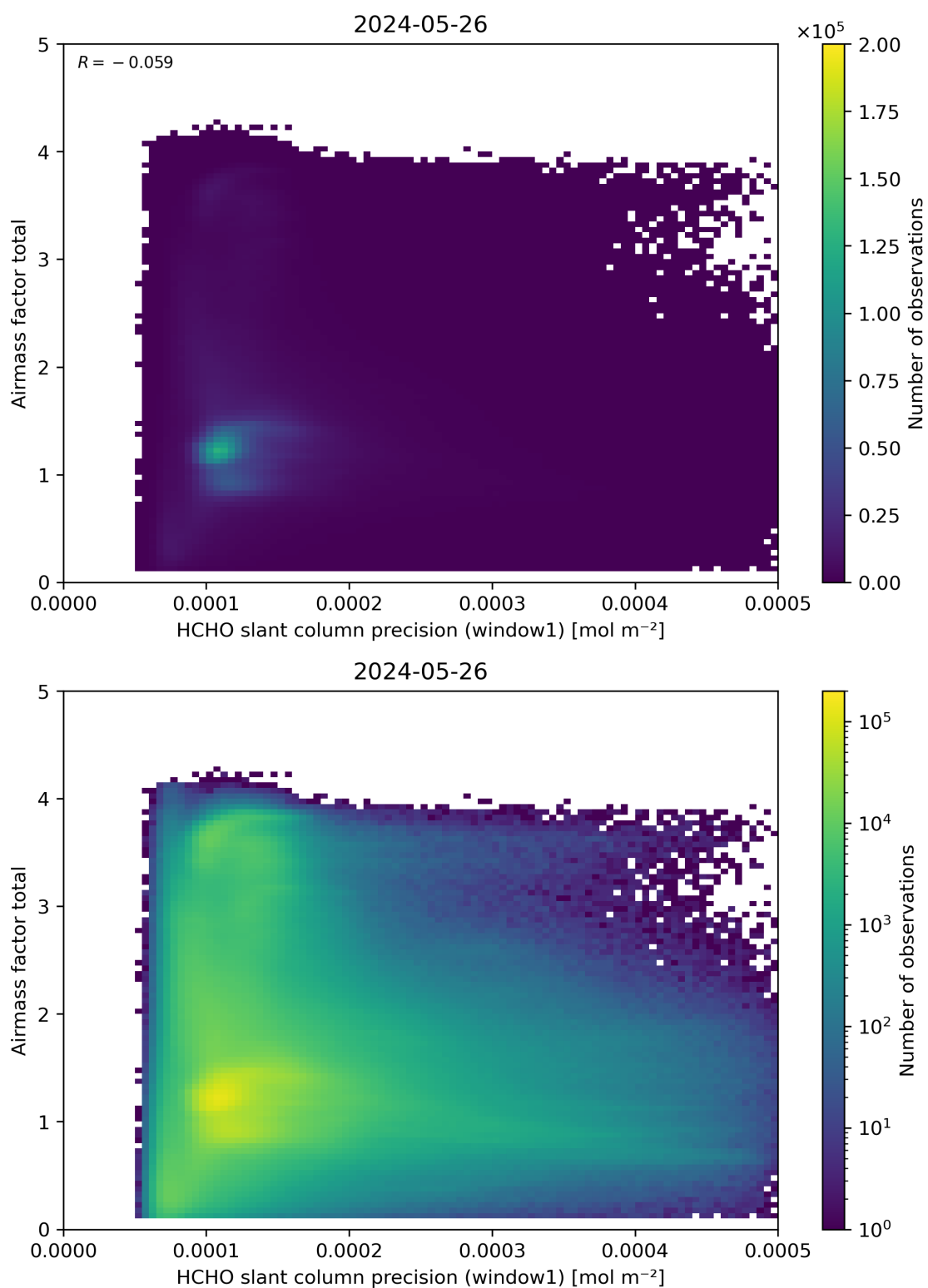
Figure 94: Scatter density plot of “HCHO slant column precision (window1)” against “Airmass factor total” for 2024-05-25 to 2024-05-27.
