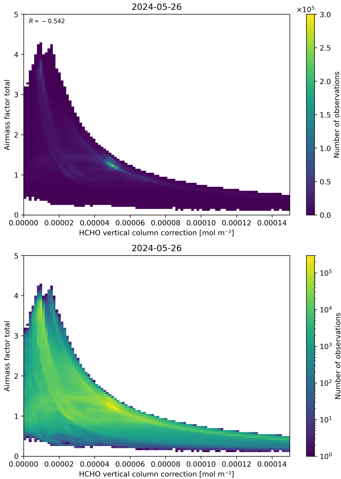
Figure 120: Scatter density plot of “HCHO vertical column correction” against “Airmass factor total” for 2024-05-25 to 2024-05-27.
