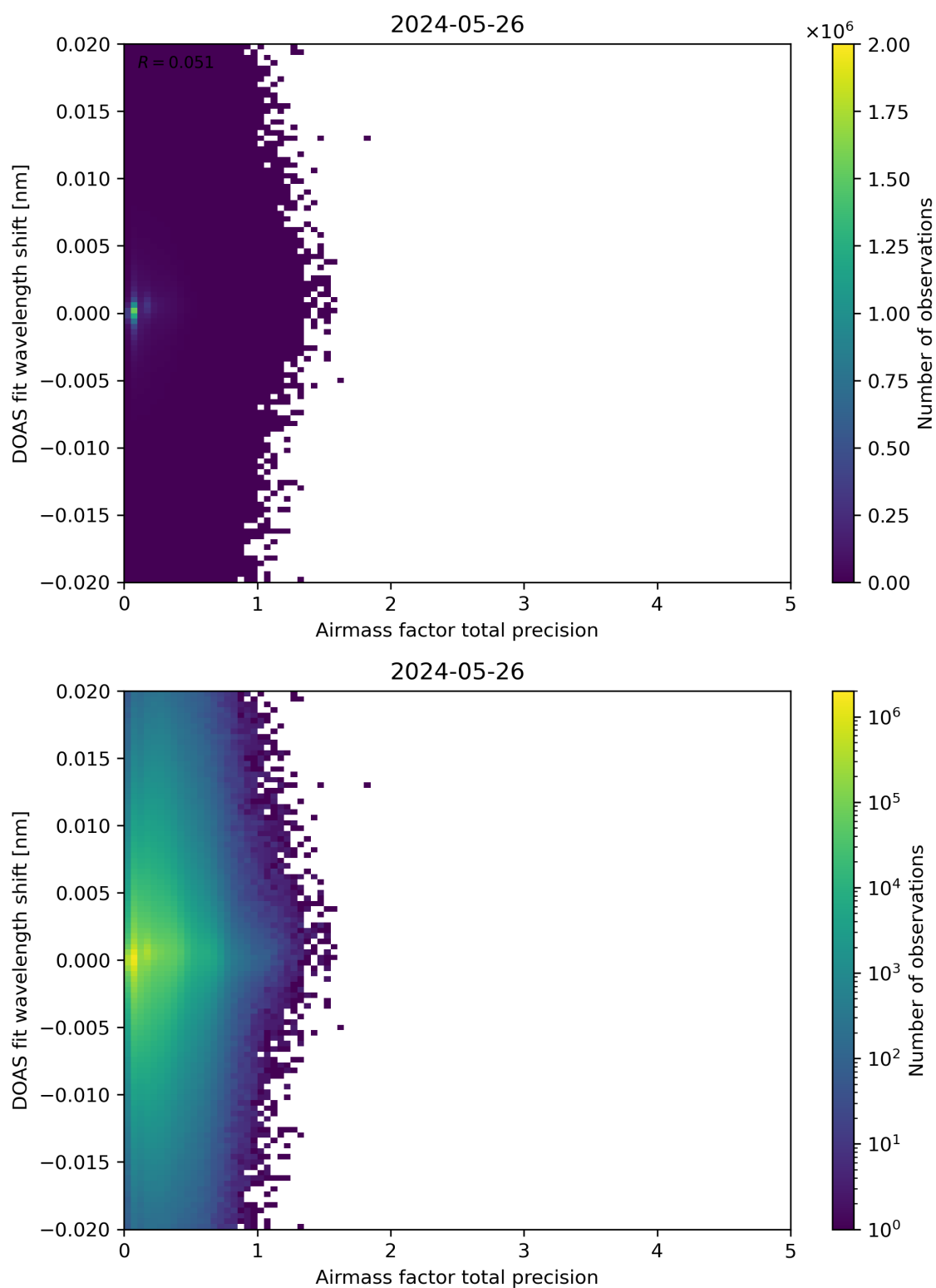
Figure 106: Scatter density plot of “Airmass factor total precision” against “DOAS fit wavelength shift” for 2024-05-25 to 2024-05-27.
