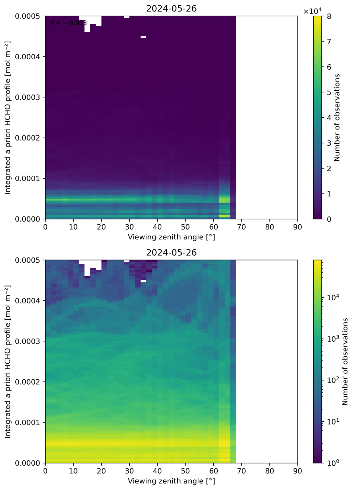
Figure 195: Scatter density plot of “Viewing zenith angle” against “Integrated a priori HCHO profile” for 2024-05-25 to 2024-05-27.
