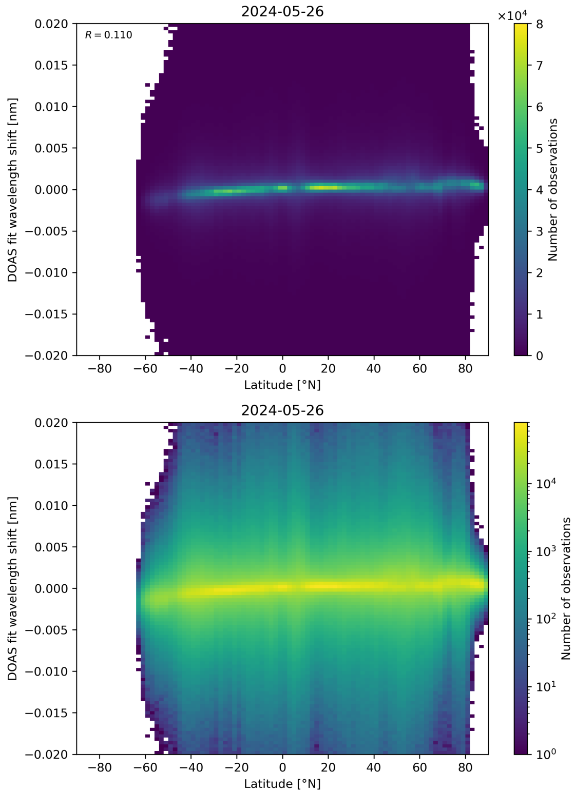
Figure 154: Scatter density plot of “Latitude” against “DOAS fit wavelength shift” for 2024-05-25 to 2024-05-27.
