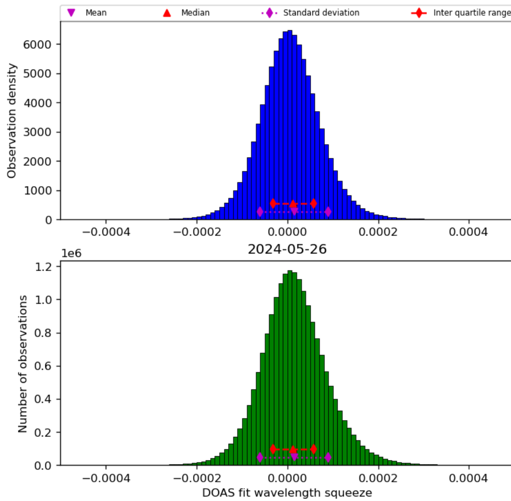
Figure 45: Histogram of “DOAS fit wavelength squeeze” for 2024-05-25 to 2024-05-27
