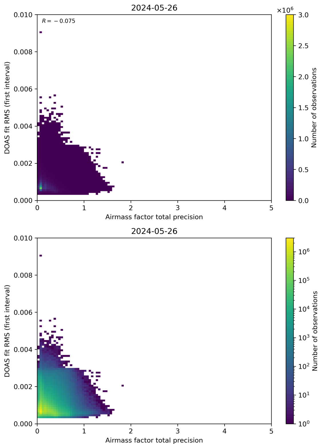
Figure 105: Scatter density plot of “Airmass factor total precision” against “DOAS fit RMS (first interval)” for 2024-05-25 to 2024-05-27.
