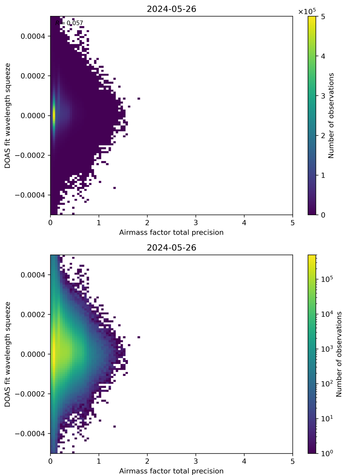
Figure 107: Scatter density plot of “Airmass factor total precision” against “DOAS fit wavelength squeeze” for 2024-05-25 to 2024-05-27.
