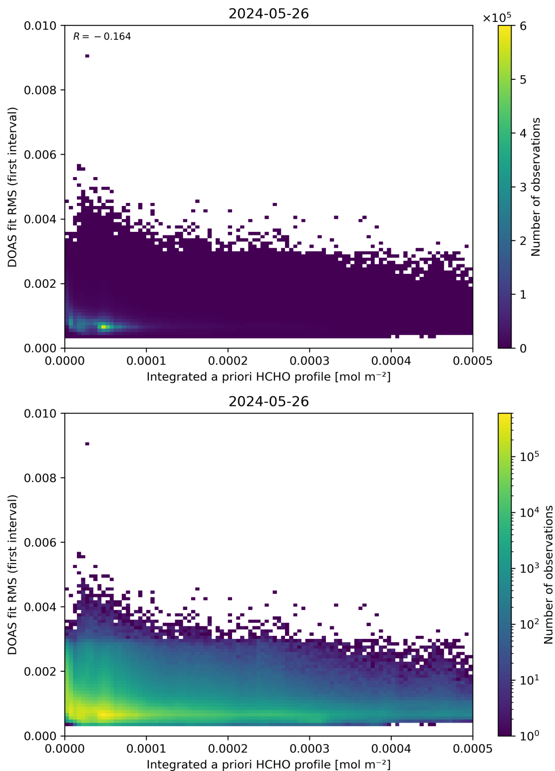
Figure 148: Scatter density plot of “Integrated a priori HCHO profile” against “DOAS fit RMS (first interval)” for 2024-05-25 to 2024-05-27.
