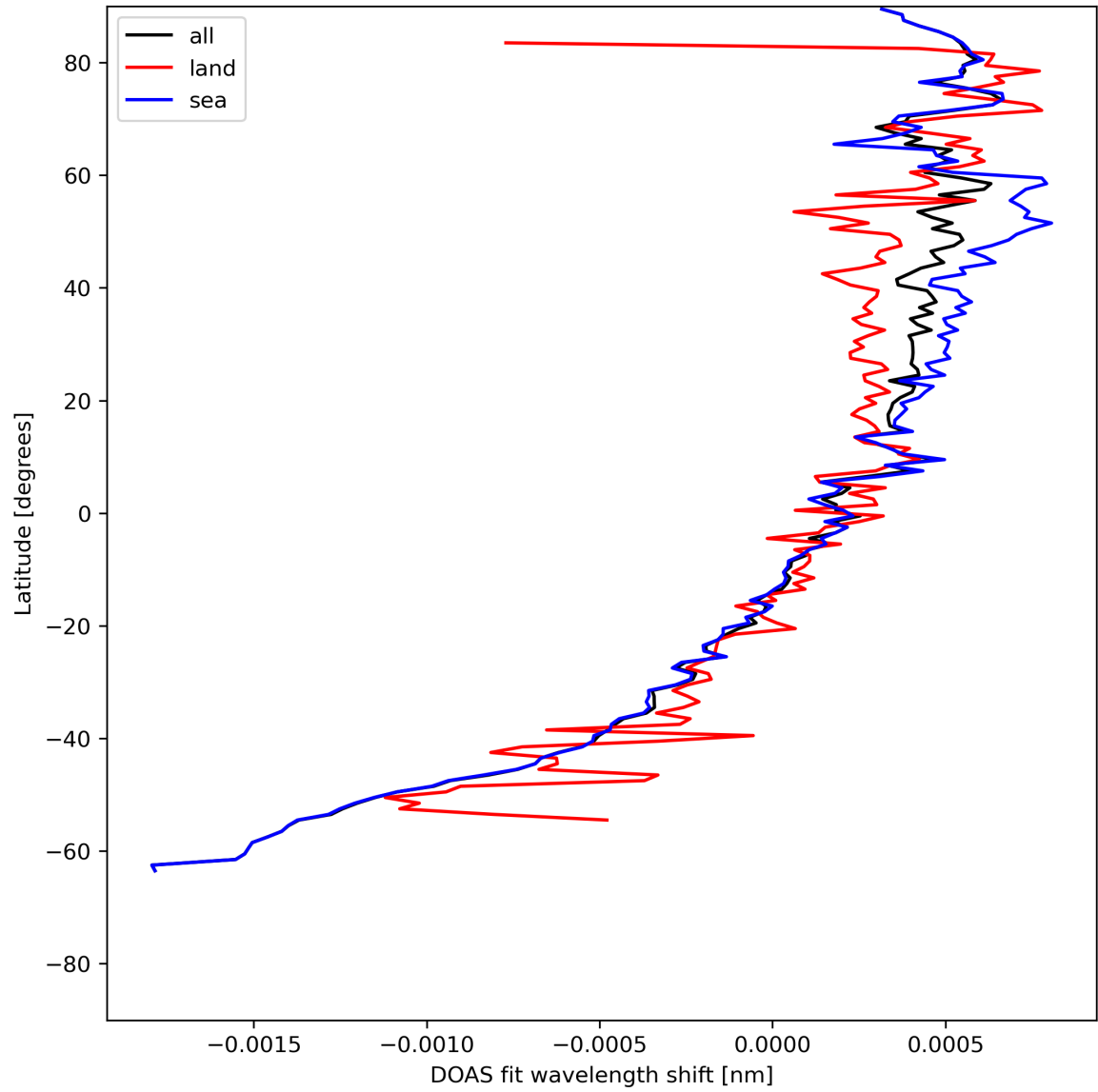
Figure 30: Zonal average of "DOAS fit wavelength shift" for 2024-05-25 to 2024-05-27.
