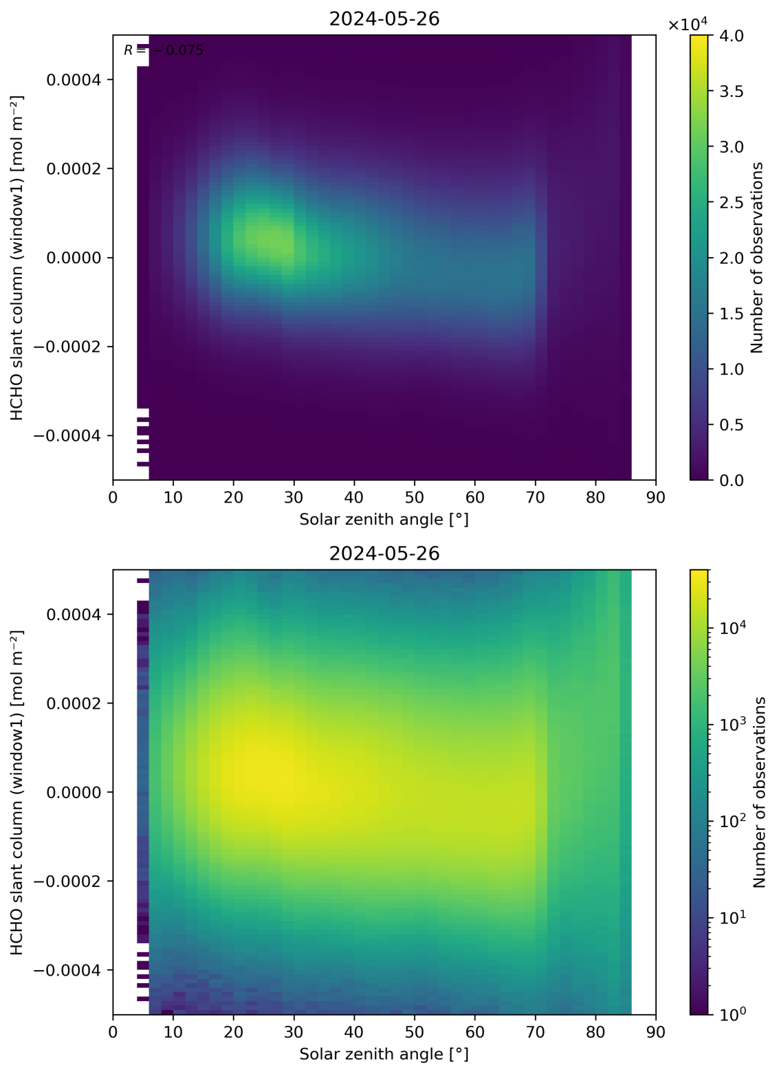
Figure 173: Scatter density plot of “Solar zenith angle” against “HCHO slant column (window1)” for 2024-05-25 to 2024-05-27.
