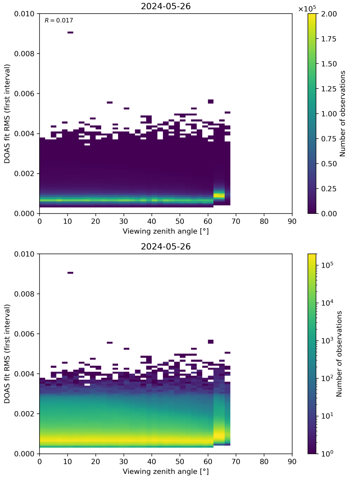
Figure 182: Scatter density plot of “Viewing zenith angle” against “DOAS fit RMS (first interval)” for 2024-05-25 to 2024-05-27.
