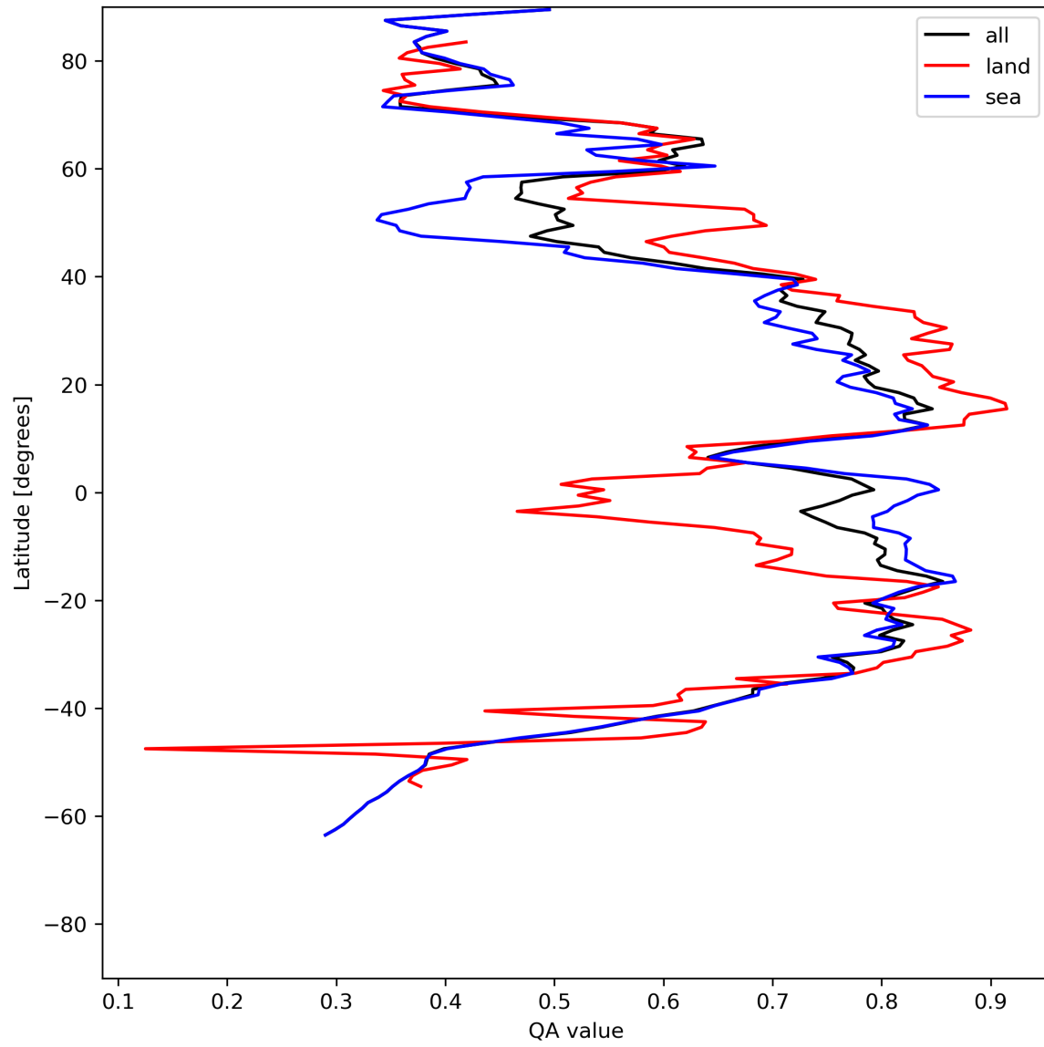
Figure 20: Zonal average of “QA value” for 2024-05-25 to 2024-05-27.
