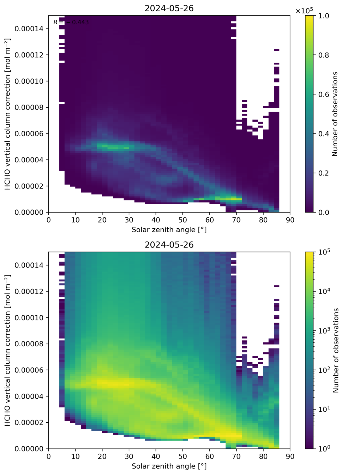
Figure 178: Scatter density plot of “Solar zenith angle” against “HCHO vertical column correction” for 2024-05-25 to 2024-05-27.
