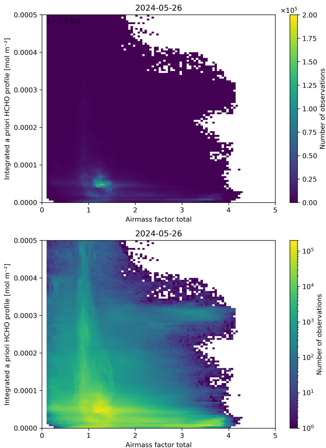
Figure 104: Scatter density plot of “Airmass factor total” against “Integrated a priori HCHO profile” for 2024-05-25 to 2024-05-27.
