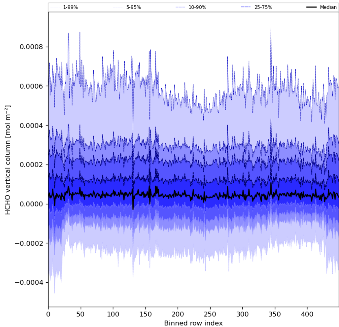
Figure 49: Along track statistics of “HCHO vertical column” for 2024-05-25 to 2024-05-27
