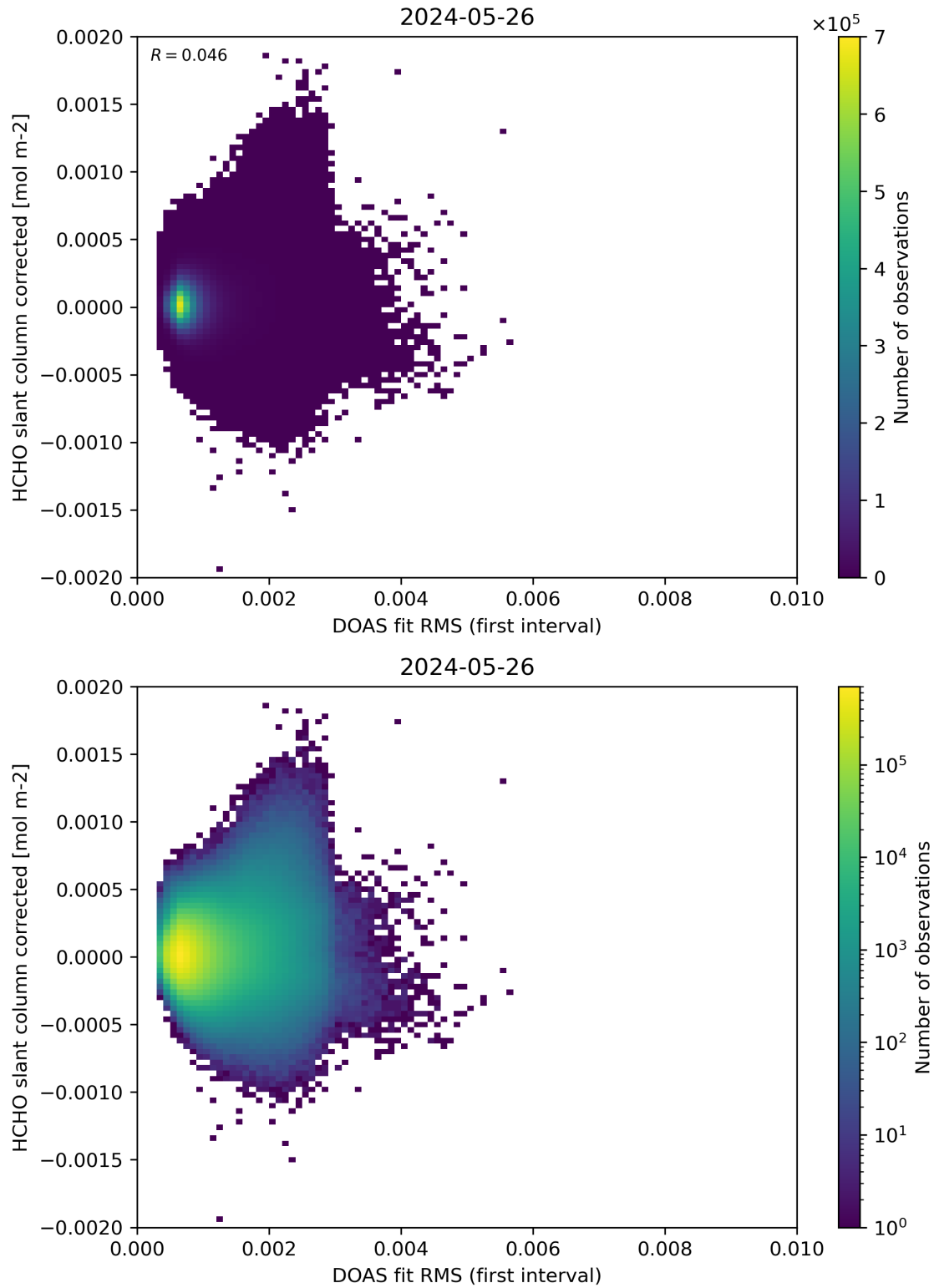
Figure 62: Scatter density plot of “DOAS fit RMS (first interval)” against “HCHO slant column corrected” for 2024-05-25 to 2024-05-27.
