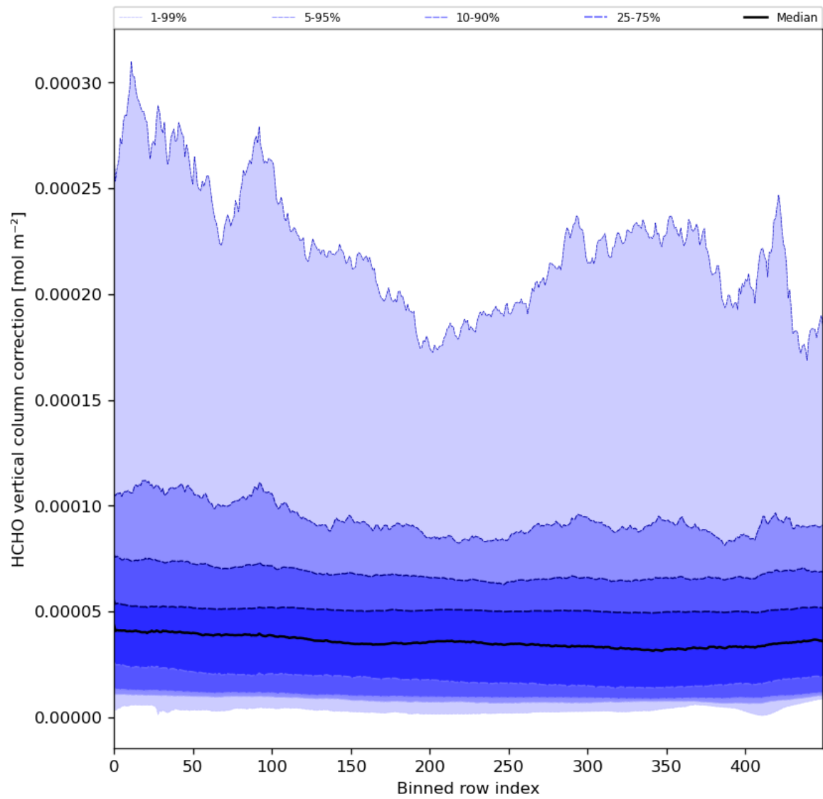
Figure 51: Along track statistics of “HCHO vertical column correction” for 2024-05-25 to 2024-05-27
