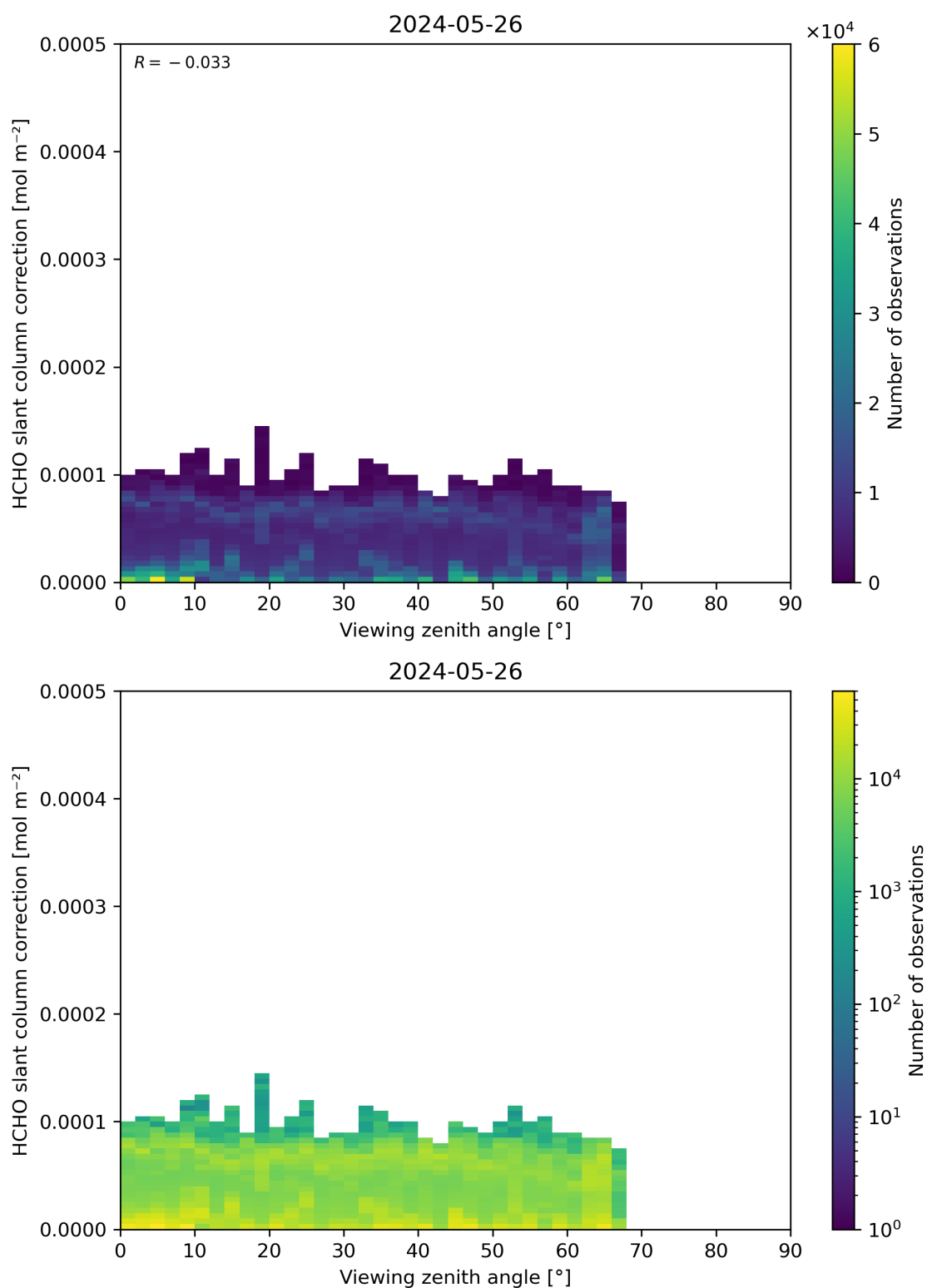
Figure 187: Scatter density plot of “Viewing zenith angle” against “HCHO slant column correction” for 2024-05-25 to 2024-05-27.
