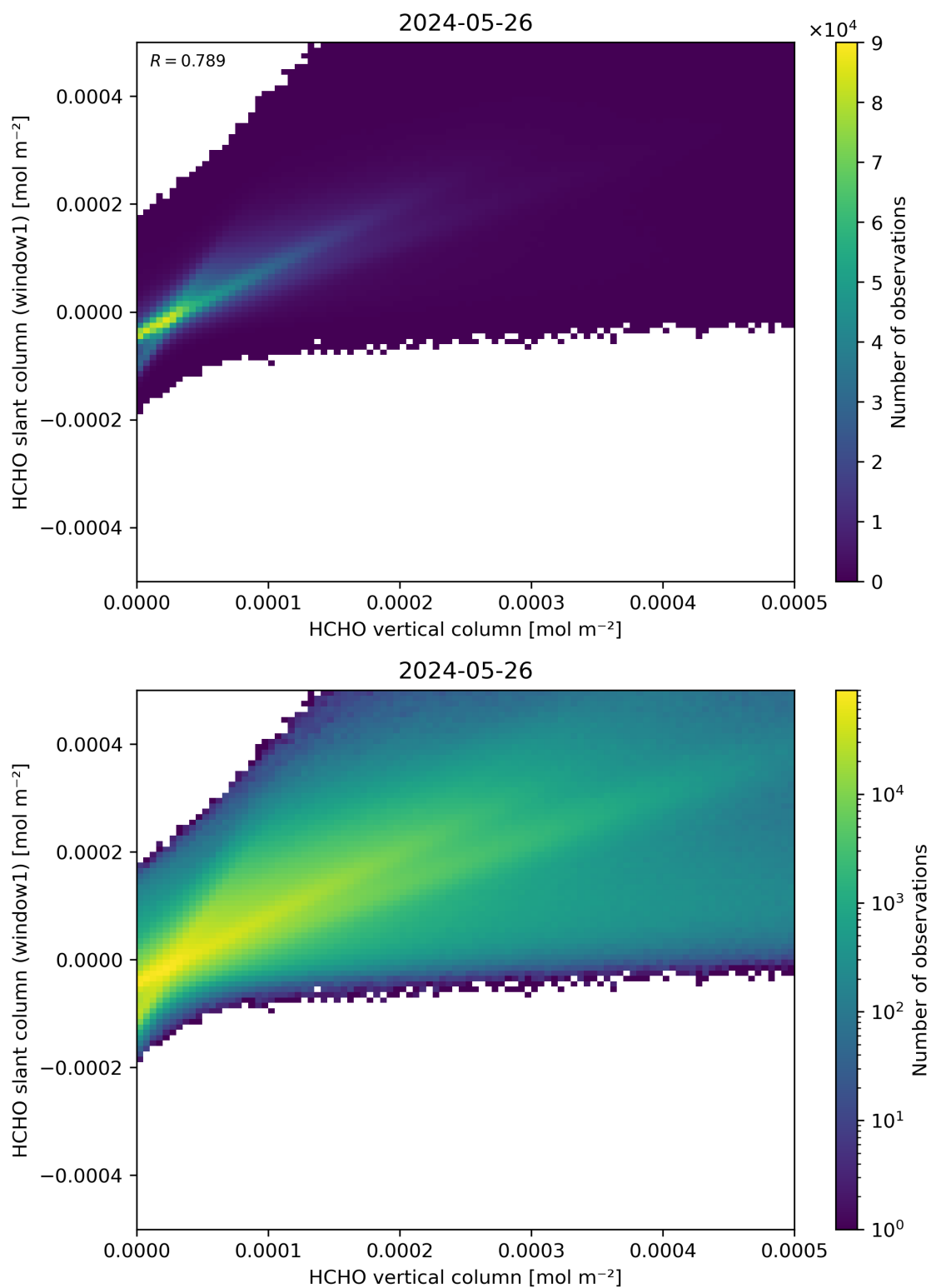
Figure 129: Scatter density plot of “HCHO vertical column” against “HCHO slant column (window1)” for 2024-05-25 to 2024-05-27.
