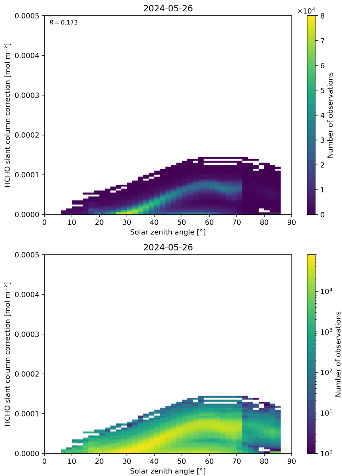
Figure 172: Scatter density plot of “Solar zenith angle” against “HCHO slant column correction” for 2024-05-25 to 2024-05-27.
