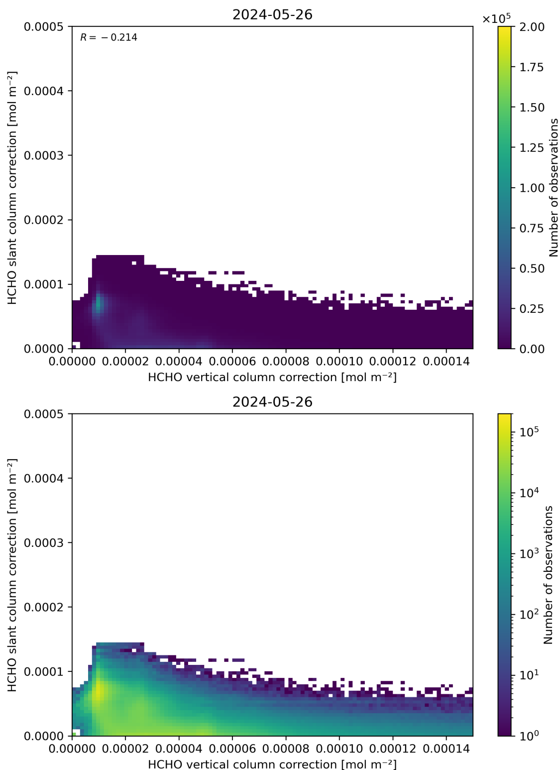
Figure 117: Scatter density plot of “HCHO vertical column correction” against “HCHO slant column correction” for 2024-05-25 to 2024-05-27.
