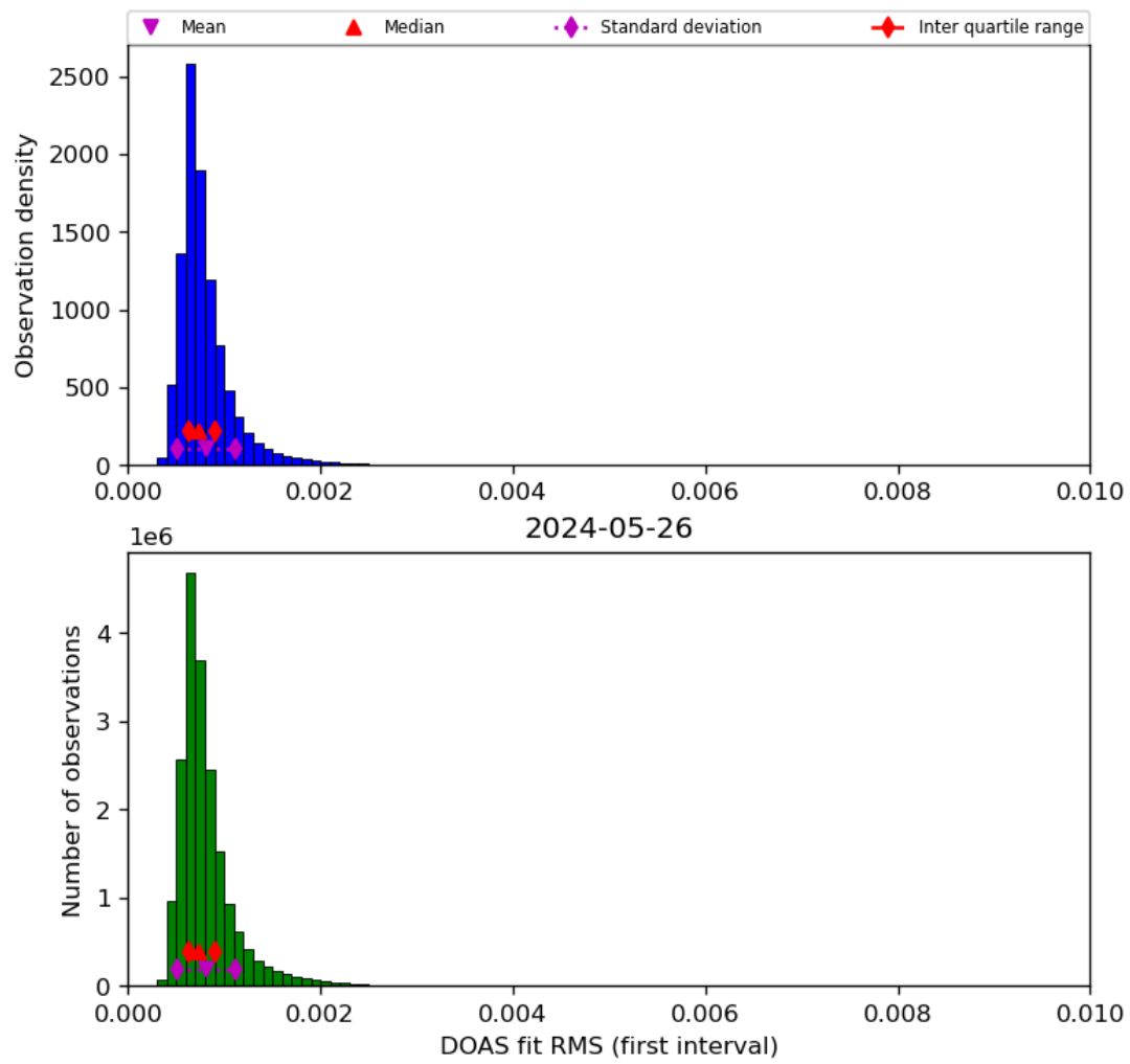
Figure 46: Histogram of “DOAS fit RMS (first interval)” for 2024-05-25 to 2024-05-27
