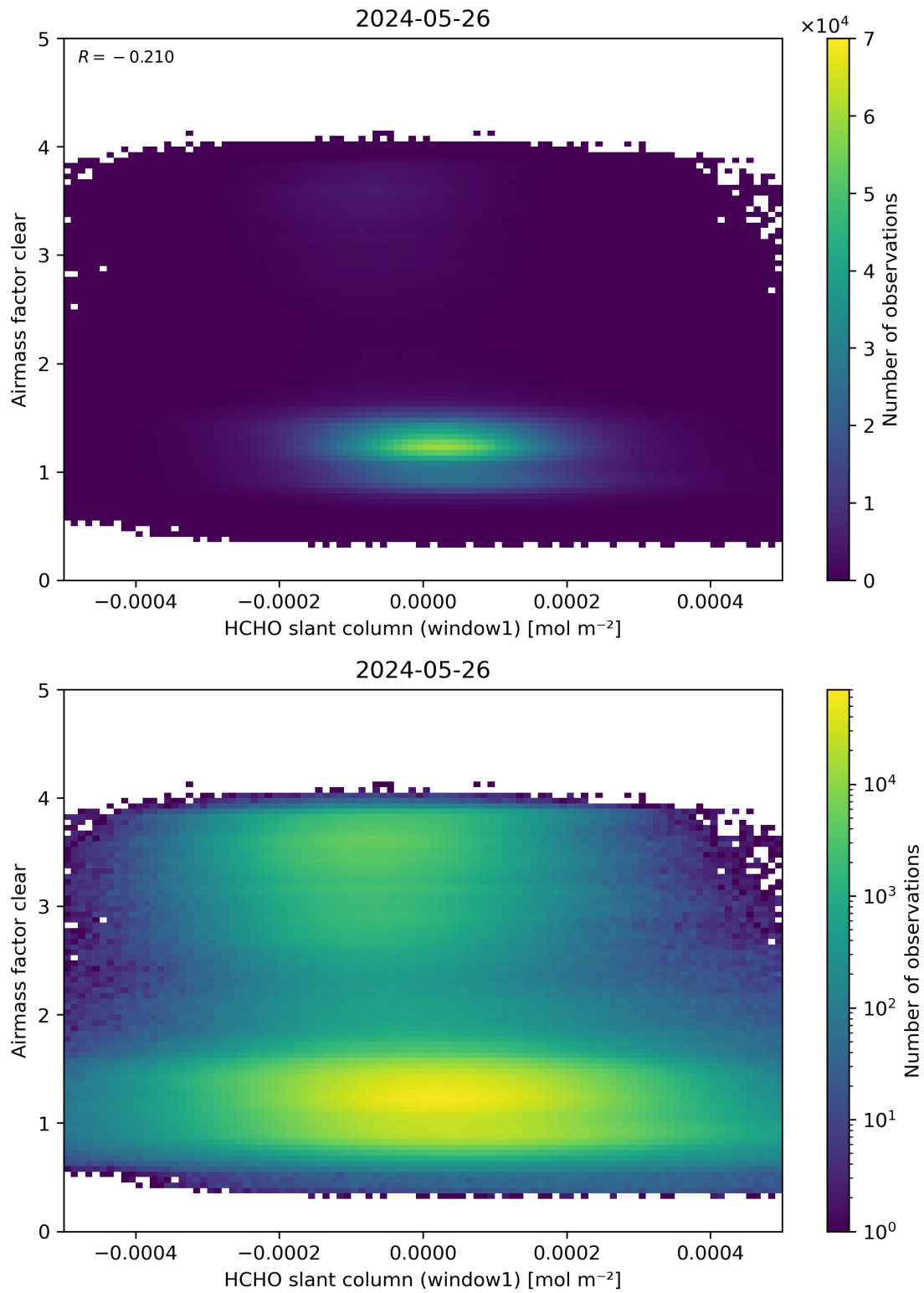
Figure 81: Scatter density plot of “HCHO slant column (window1)” against “Airmass factor clear” for 2024-05-25 to 2024-05-27.
