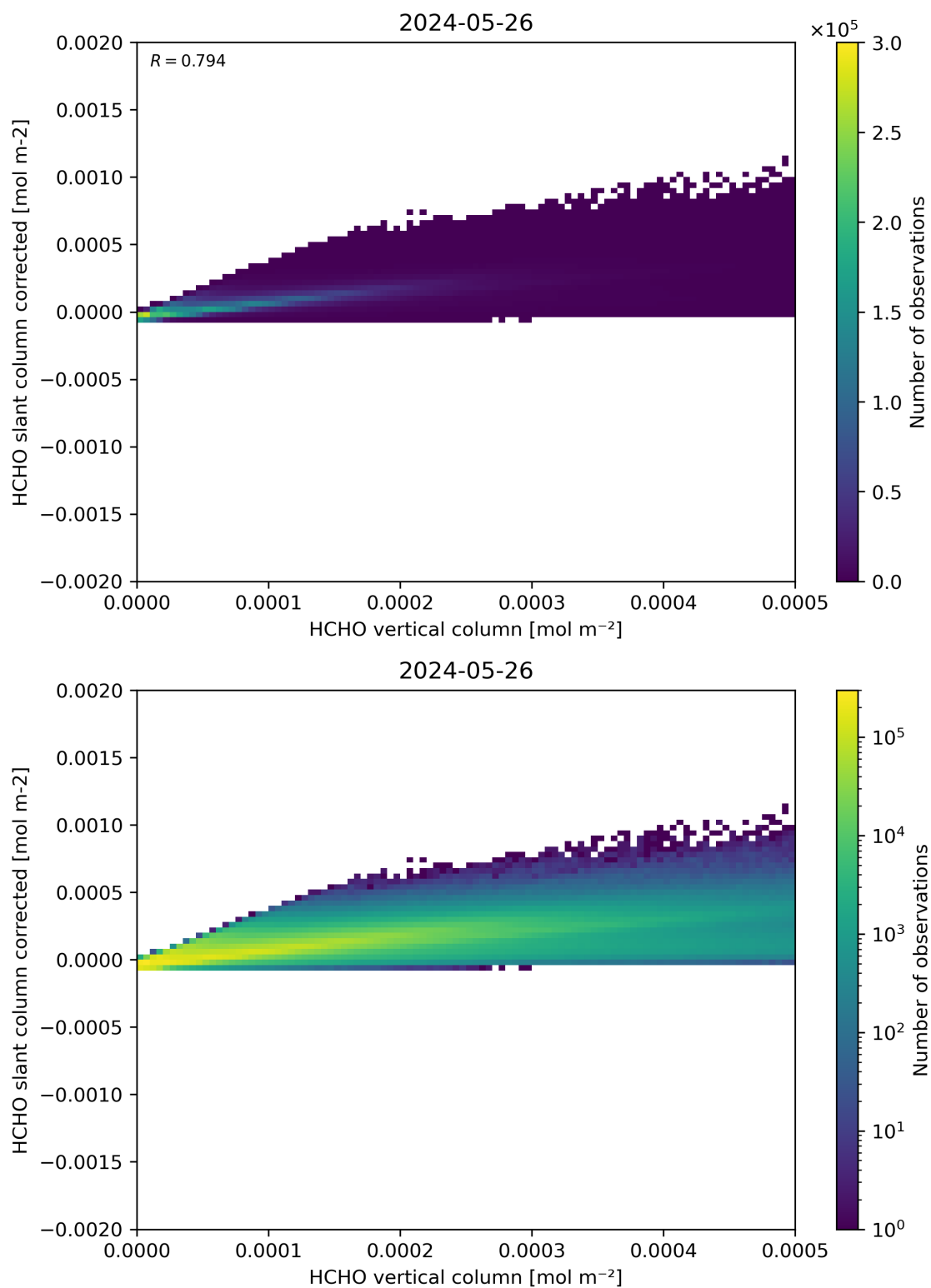
Figure 127: Scatter density plot of “HCHO vertical column” against “HCHO slant column corrected” for 2024-05-25 to 2024-05-27.
