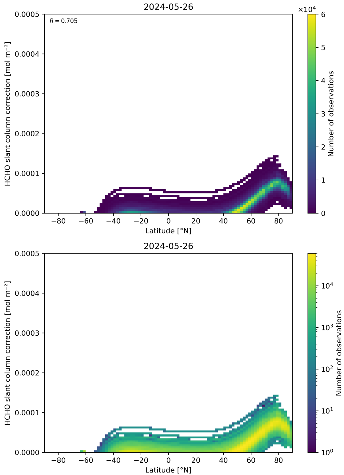
Figure 158: Scatter density plot of “Latitude” against “HCHO slant column correction” for 2024-05-25 to 2024-05-27.
