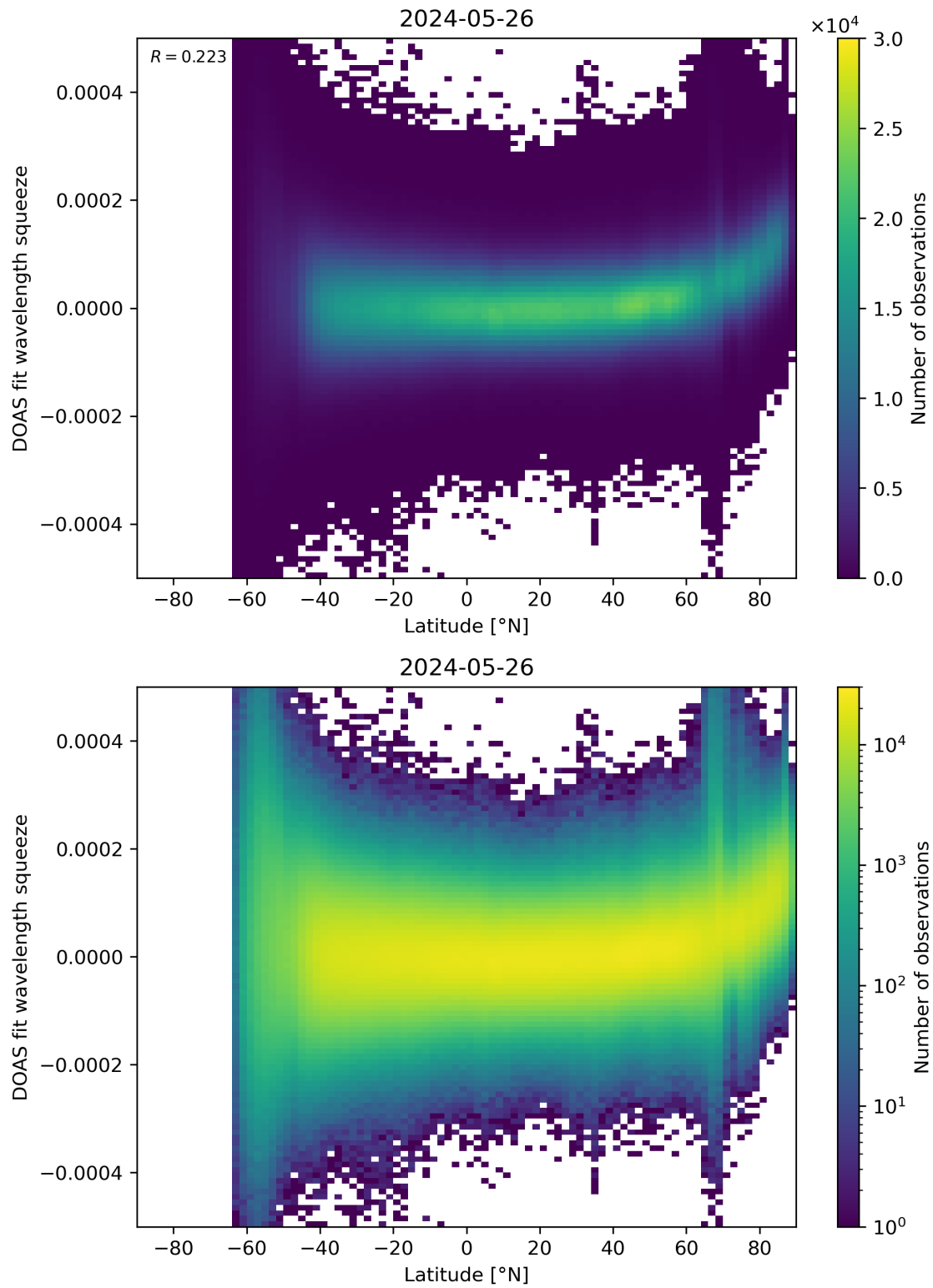
Figure 155: Scatter density plot of “Latitude” against “DOAS fit wavelength squeeze” for 2024-05-25 to 2024-05-27.
