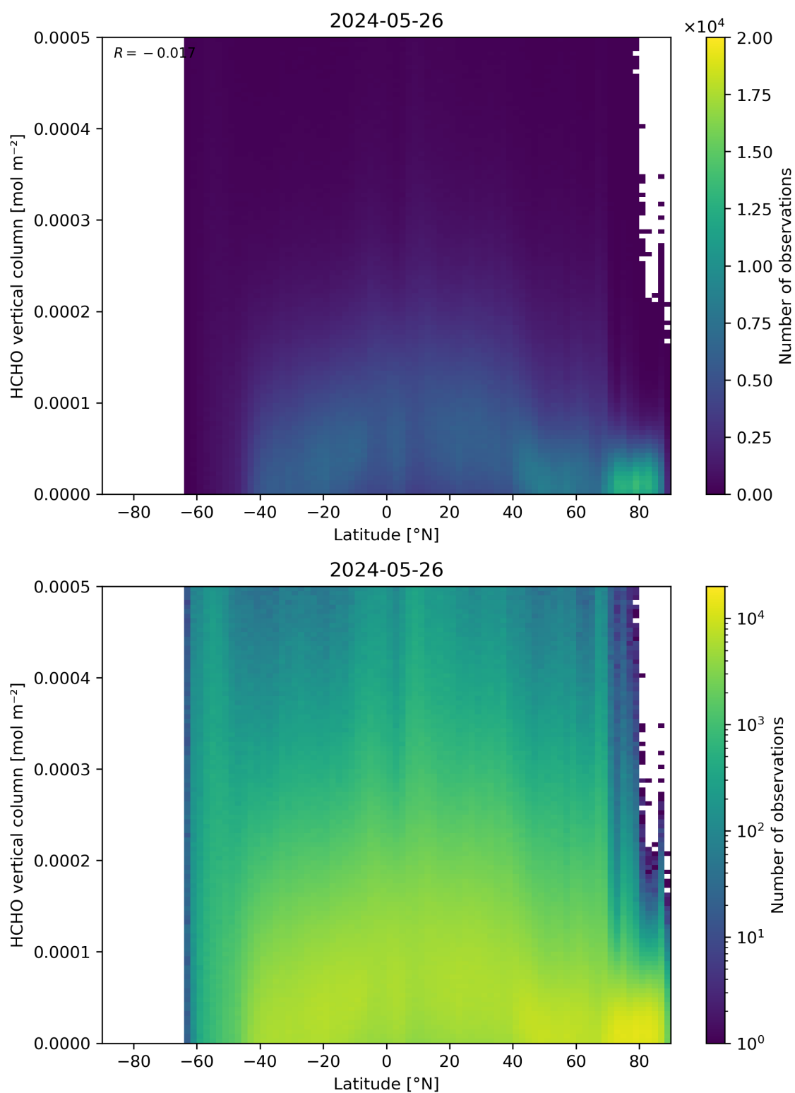
Figure 163: Scatter density plot of “Latitude” against “HCHO vertical column” for 2024-05-25 to 2024-05-27.
