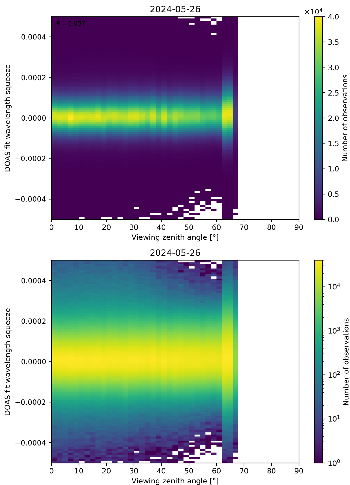
Figure 184: Scatter density plot of “Viewing zenith angle” against “DOAS fit wavelength squeeze” for 2024-05-25 to 2024-05-27.
