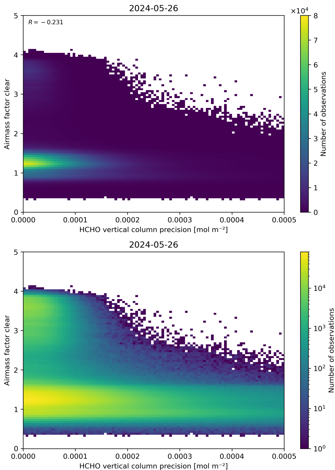
Figure 139: Scatter density plot of “HCHO vertical column precision” against “Airmass factor clear” for 2024-05-25 to 2024-05-27.
