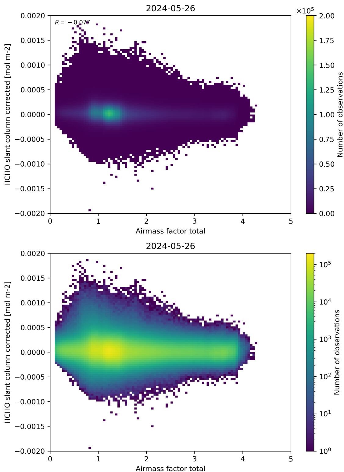
Figure 101: Scatter density plot of “Airmass factor total” against “HCHO slant column corrected” for 2024-05-25 to 2024-05-27.
