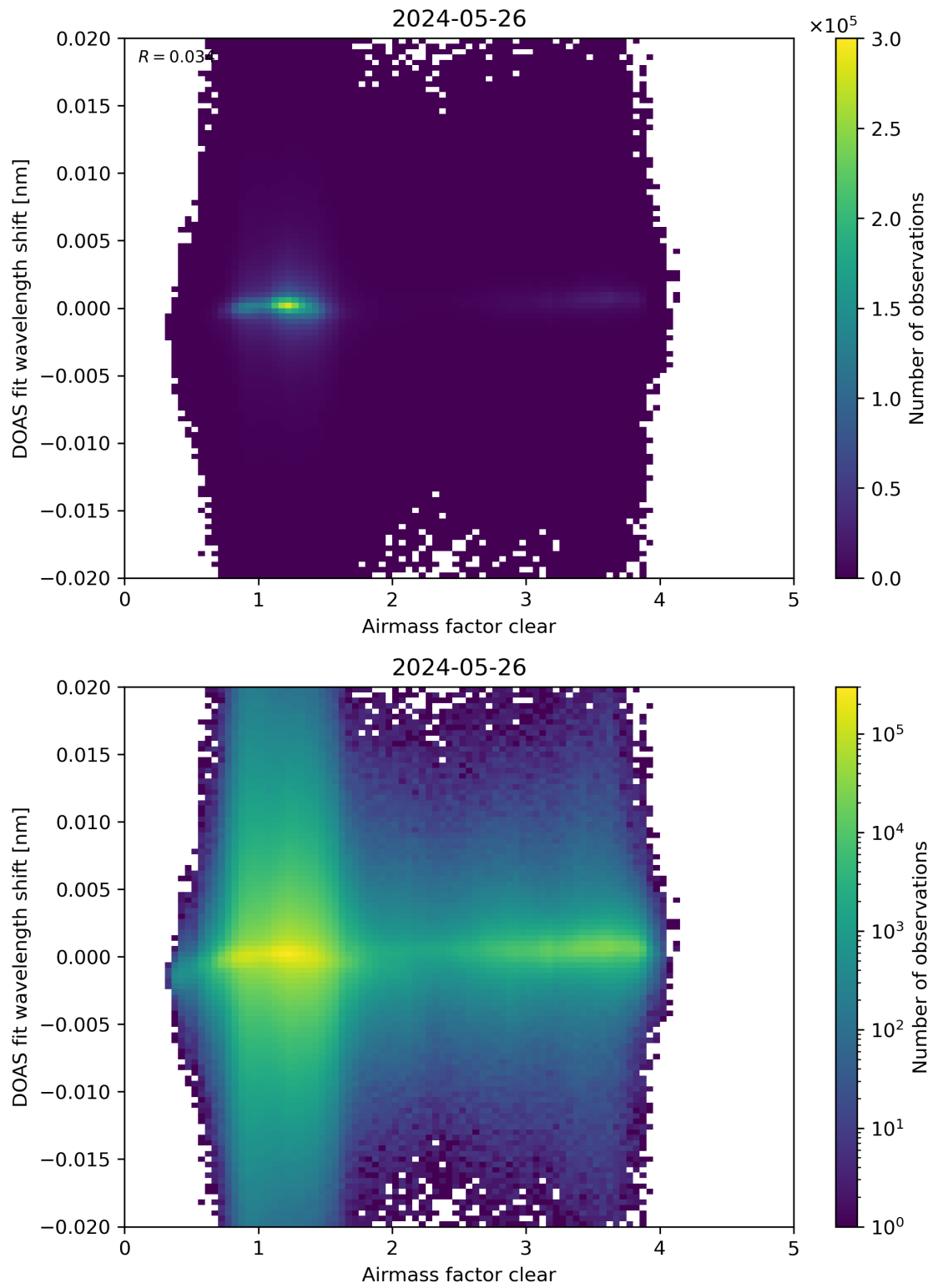
Figure 72: Scatter density plot of “Airmass factor clear” against “DOAS fit wavelength shift” for 2024-05-25 to 2024-05-27.
