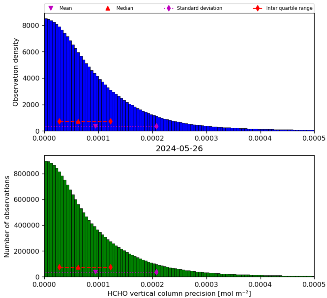
Figure 36: Histogram of “HCHO vertical column precision” for 2024-05-25 to 2024-05-27
