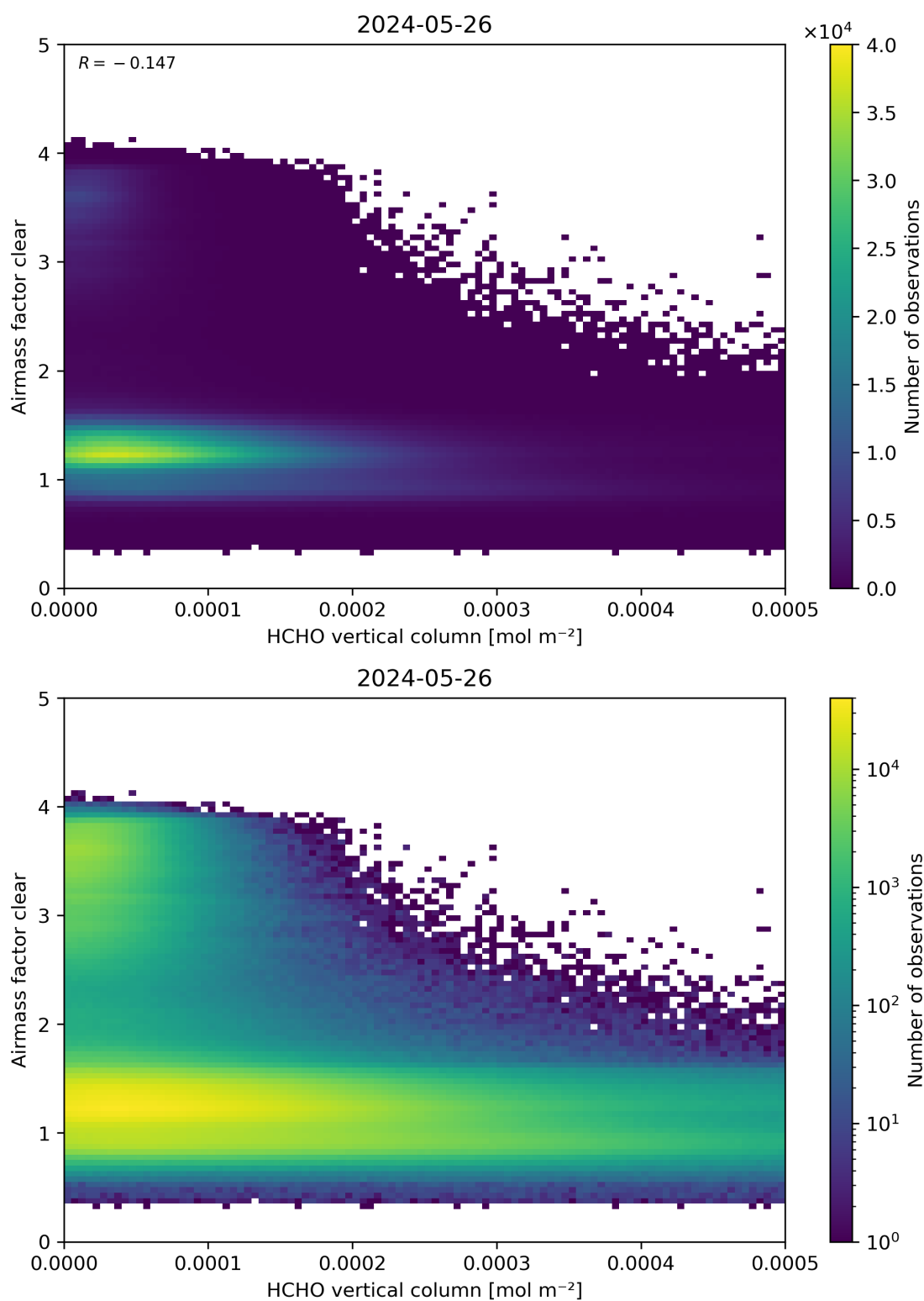
Figure 126: Scatter density plot of “HCHO vertical column” against “Airmass factor clear” for 2024-05-25 to 2024-05-27.
