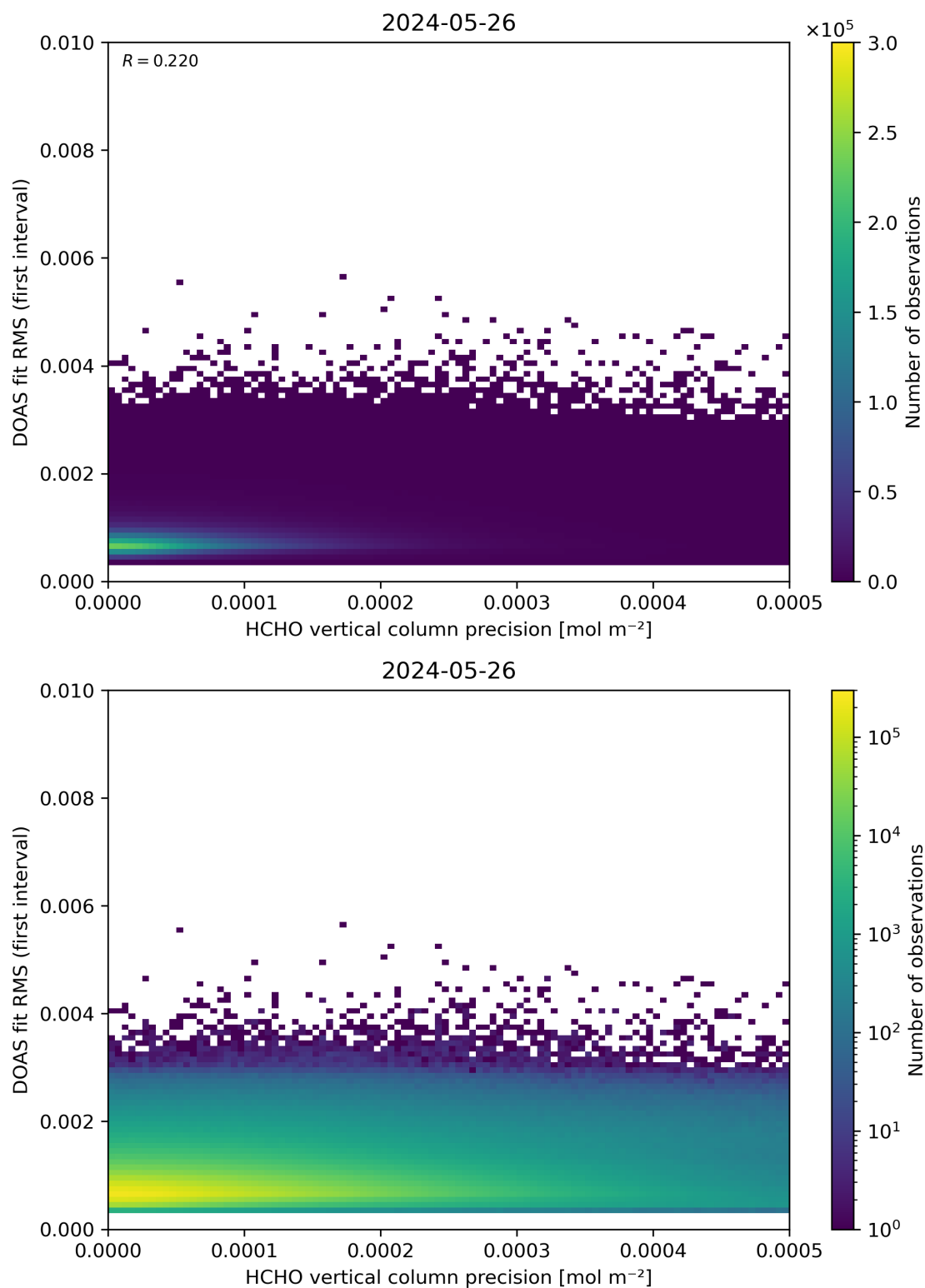
Figure 136: Scatter density plot of “HCHO vertical column precision” against “DOAS fit RMS (first interval)” for 2024-05-25 to 2024-05-27.
