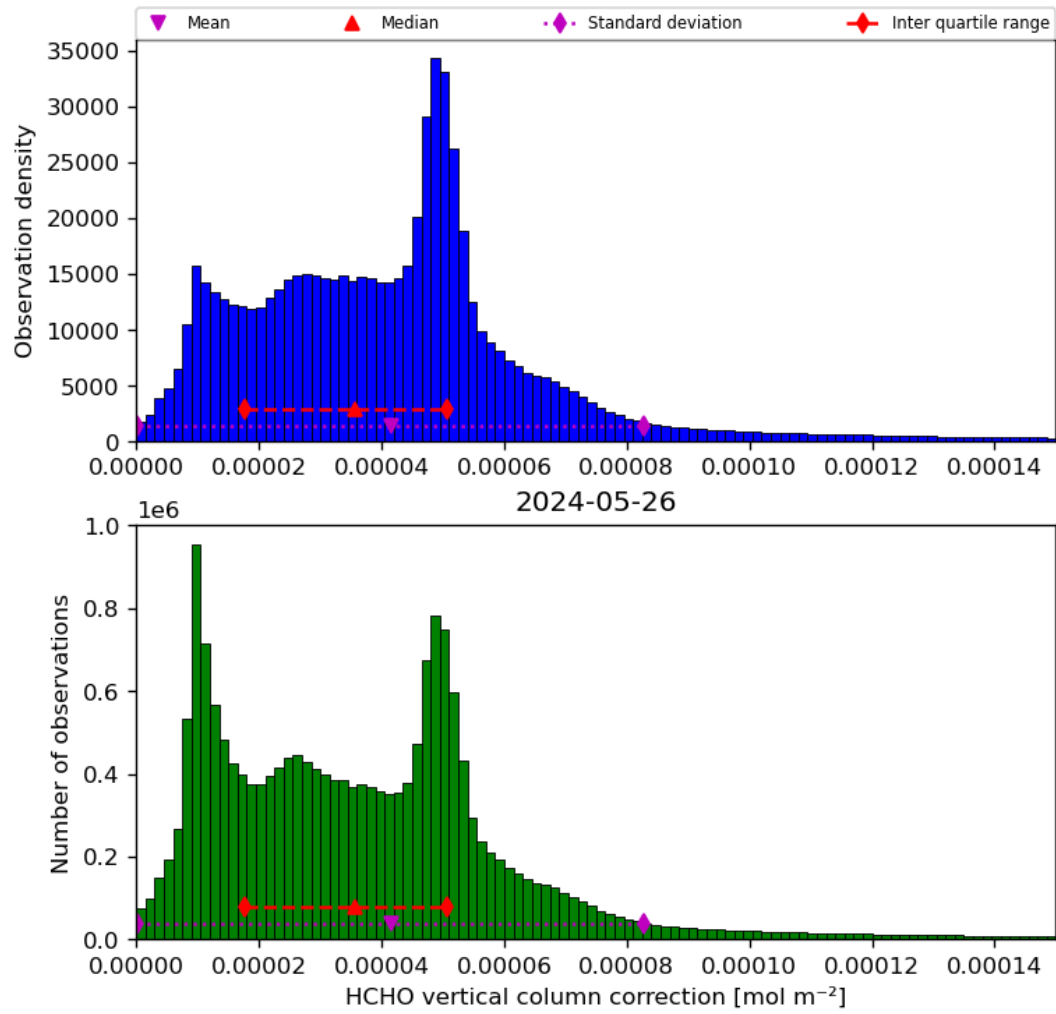
Figure 37: Histogram of “HCHO vertical column correction” for 2024-05-25 to 2024-05-27
