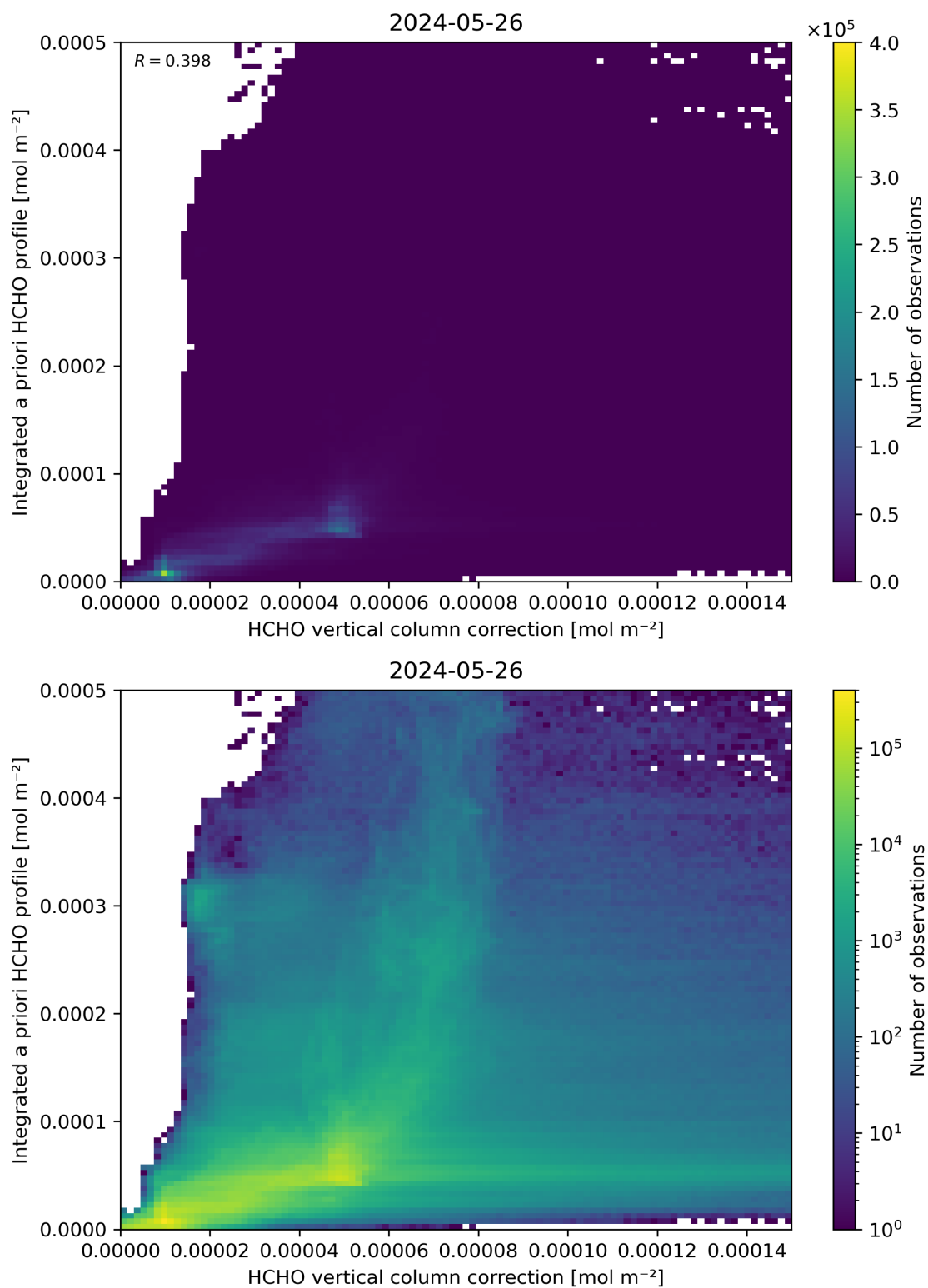
Figure 122: Scatter density plot of “HCHO vertical column correction” against “Integrated a priori HCHO profile” for 2024-05-25 to 2024-05-27.
