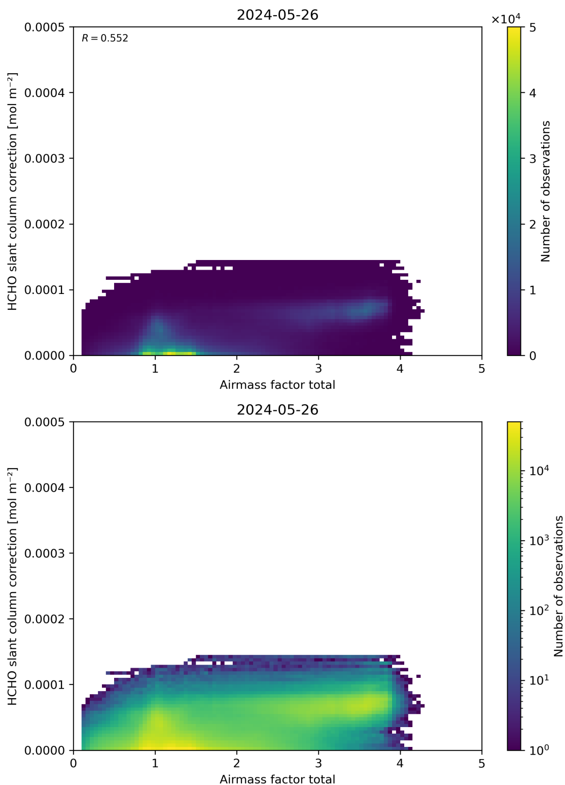
Figure 102: Scatter density plot of “Airmass factor total” against “HCHO slant column correction” for 2024-05-25 to 2024-05-27.
