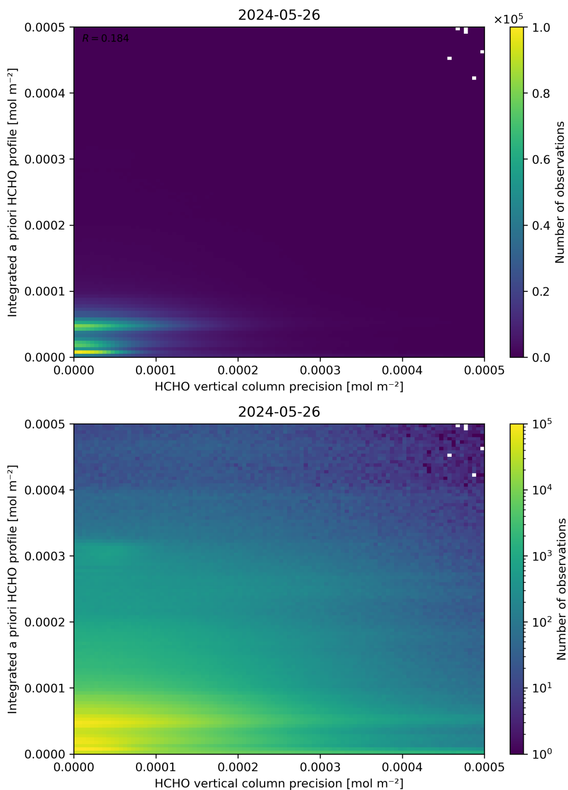
Figure 147: Scatter density plot of “HCHO vertical column precision” against “Integrated a priori HCHO profile” for 2024-05-25 to 2024-05-27.
