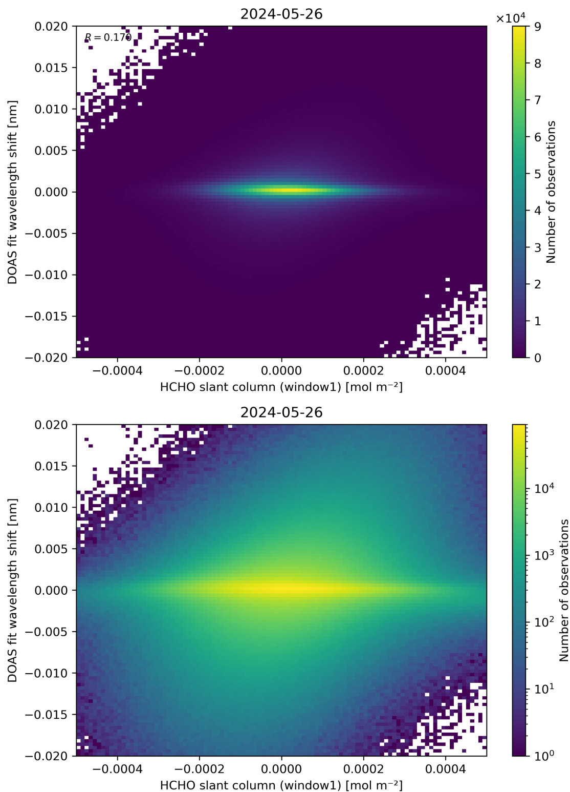
Figure 79: Scatter density plot of “HCHO slant column (window1)” against “DOAS fit wavelength shift” for 2024-05-25 to 2024-05-27.
