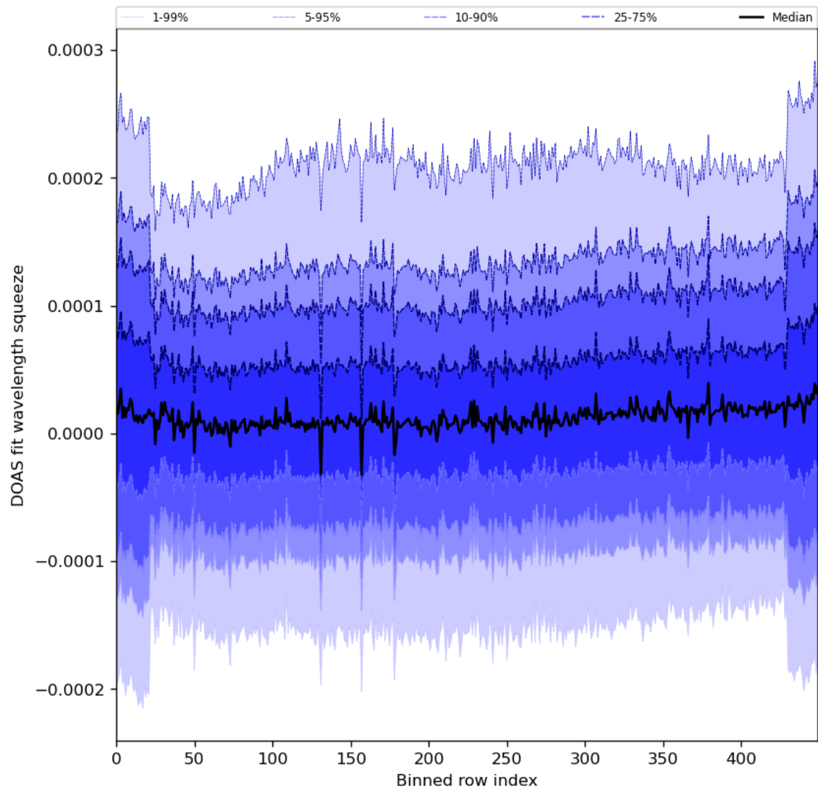
Figure 59: Along track statistics of “DOAS fit wavelength squeeze” for 2024-05-25 to 2024-05-27
