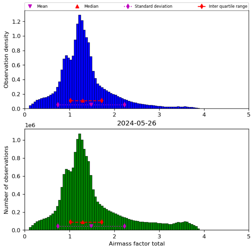
Figure 40: Histogram of “Airmass factor total” for 2024-05-25 to 2024-05-27
