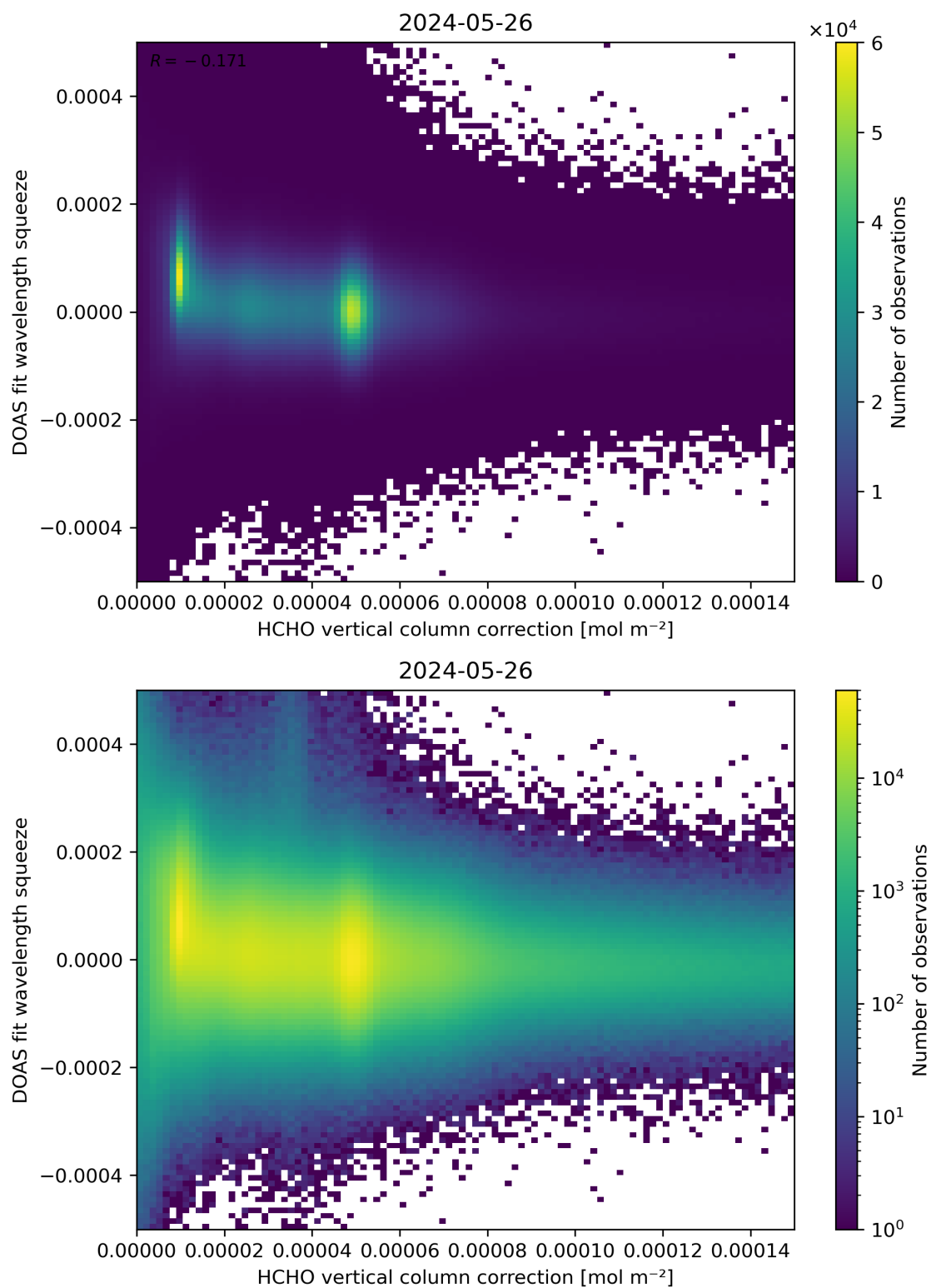
Figure 114: Scatter density plot of “HCHO vertical column correction” against “DOAS fit wavelength squeeze” for 2024-05-25 to 2024-05-27.
