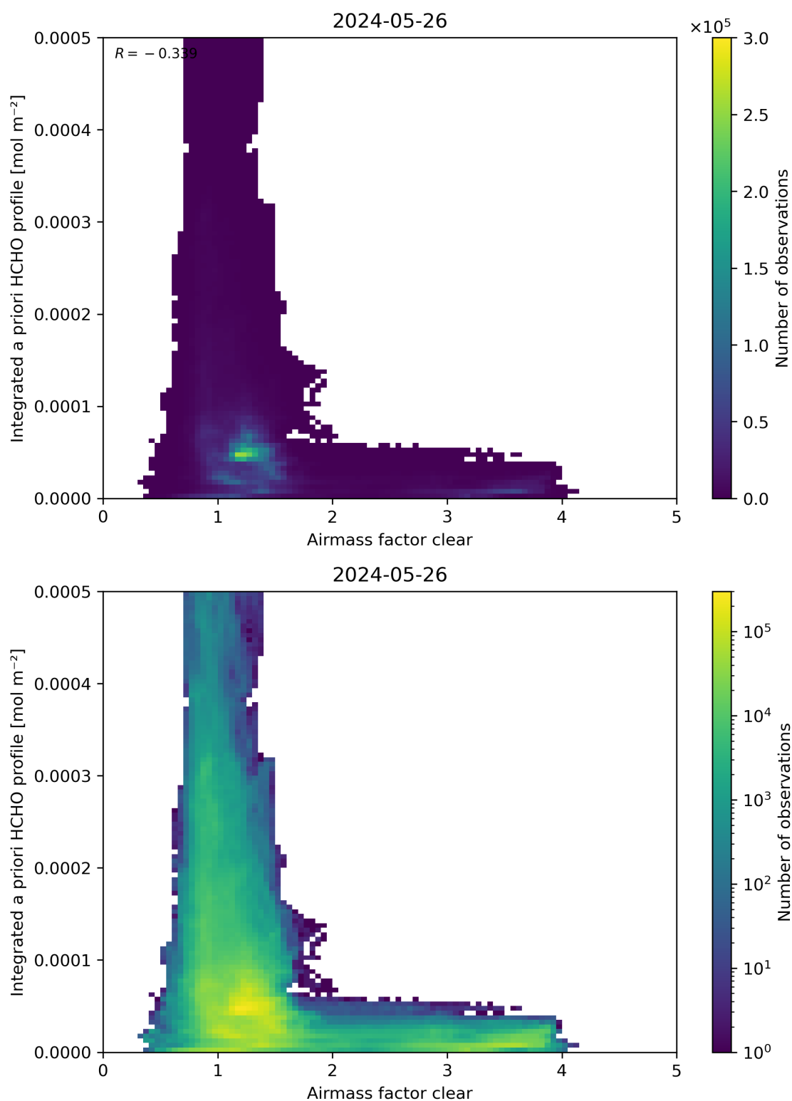
Figure 76: Scatter density plot of “Airmass factor clear” against “Integrated a priori HCHO profile” for 2024-05-25 to 2024-05-27.
