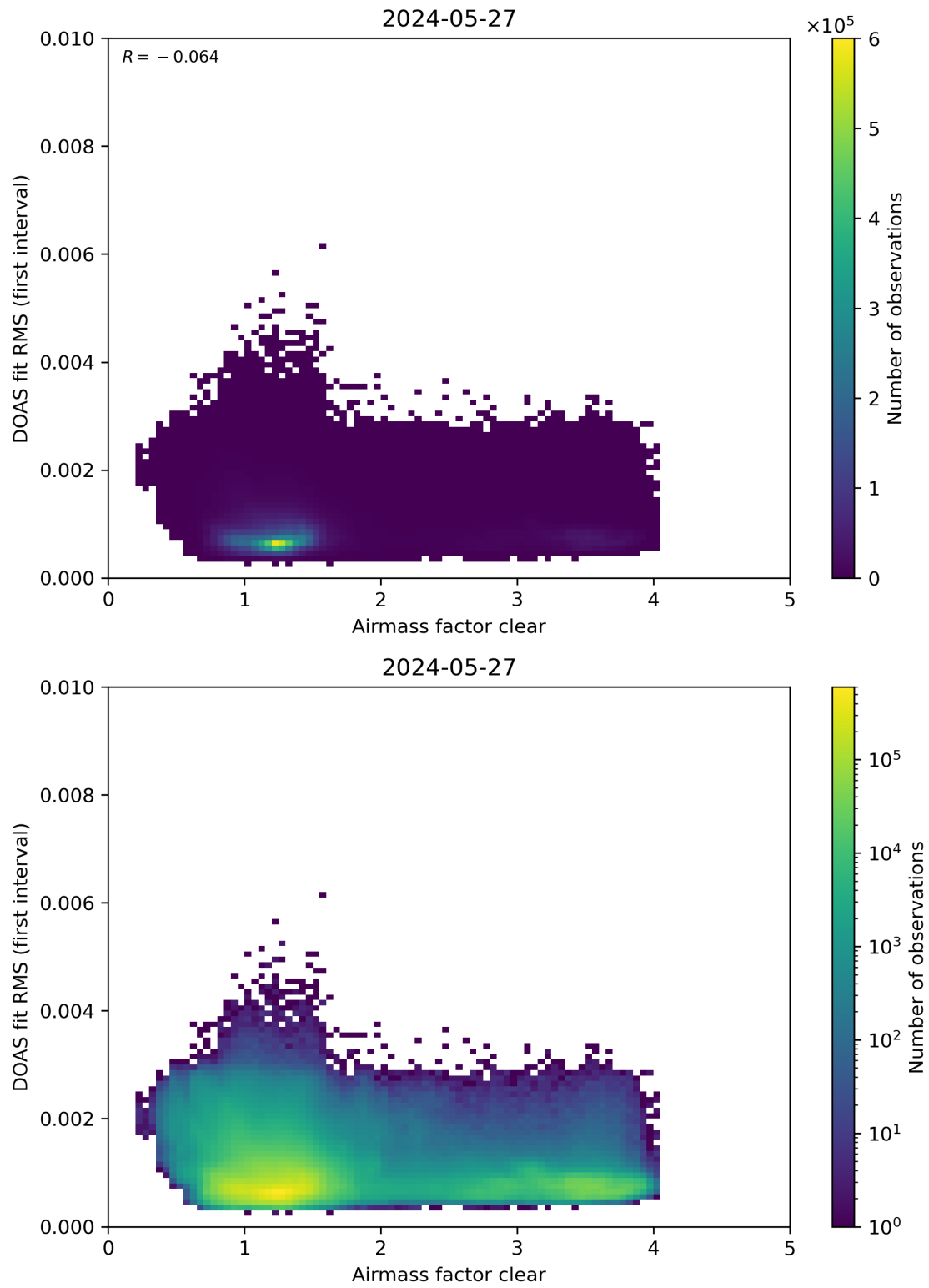
Figure 71: Scatter density plot of “Airmass factor clear” against “DOAS fit RMS (first interval)” for 2024-05-26 to 2024-05-28.
