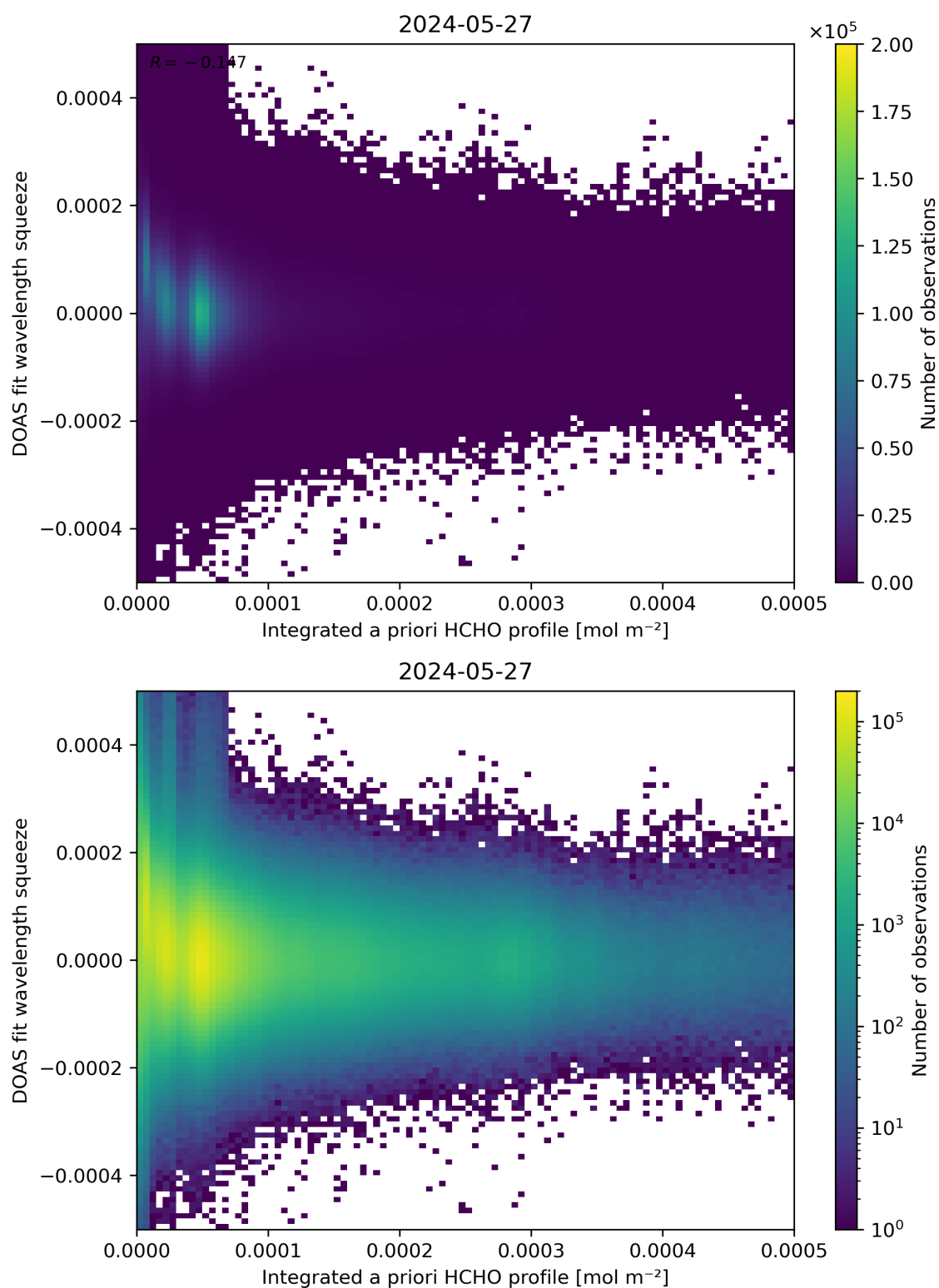
Figure 150: Scatter density plot of “Integrated a priori HCHO profile” against “DOAS fit wavelength squeeze” for 2024-05-26 to 2024-05-28.
