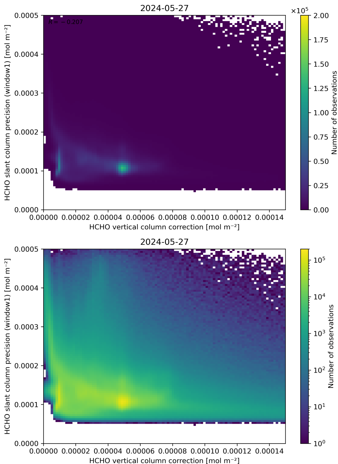
Figure 119: Scatter density plot of “HCHO vertical column correction” against “HCHO slant column precision (window1)” for 2024-05-26 to 2024-05-28.
