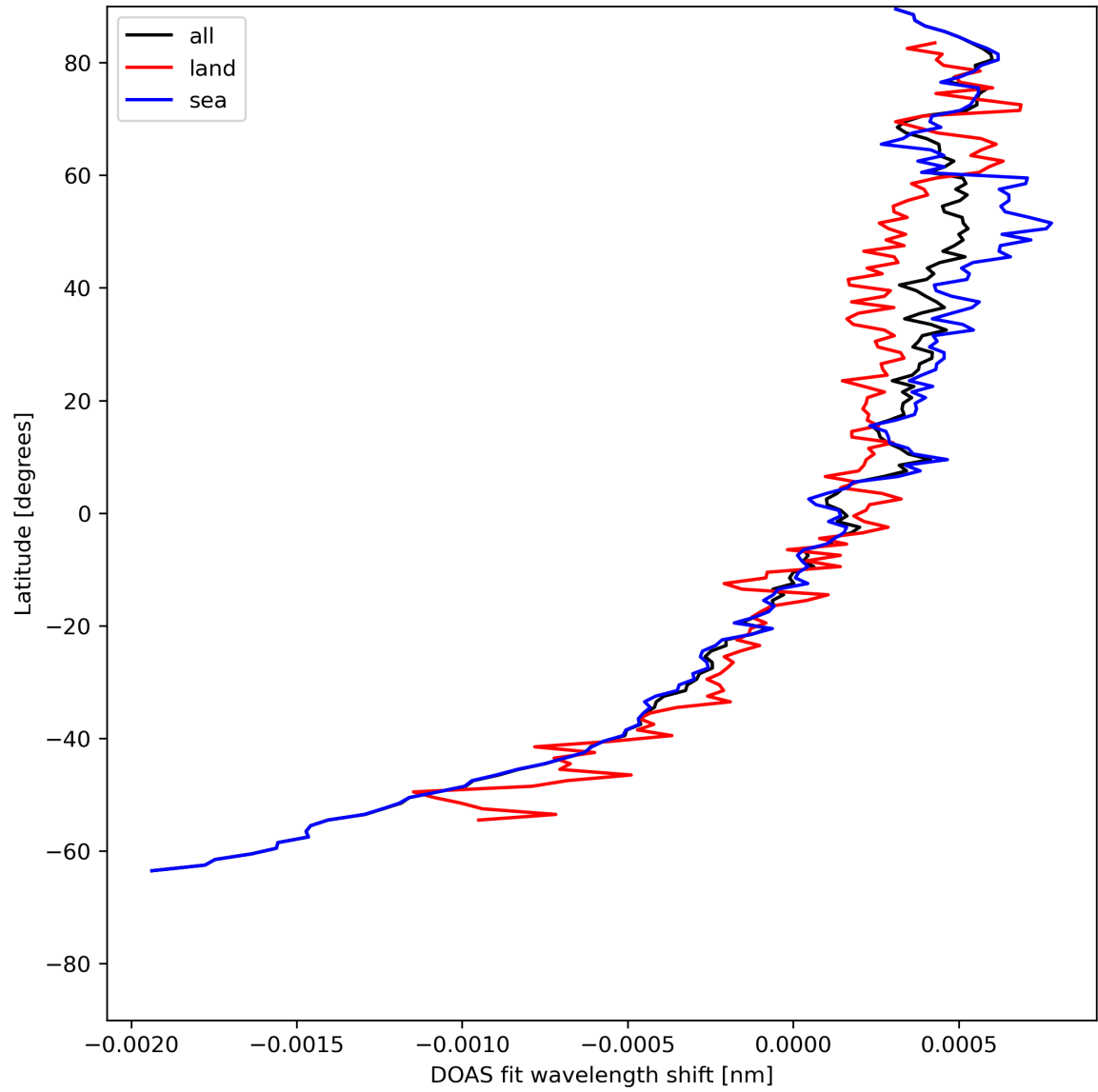
Figure 30: Zonal average of “DOAS fit wavelength shift” for 2024-05-26 to 2024-05-28.
