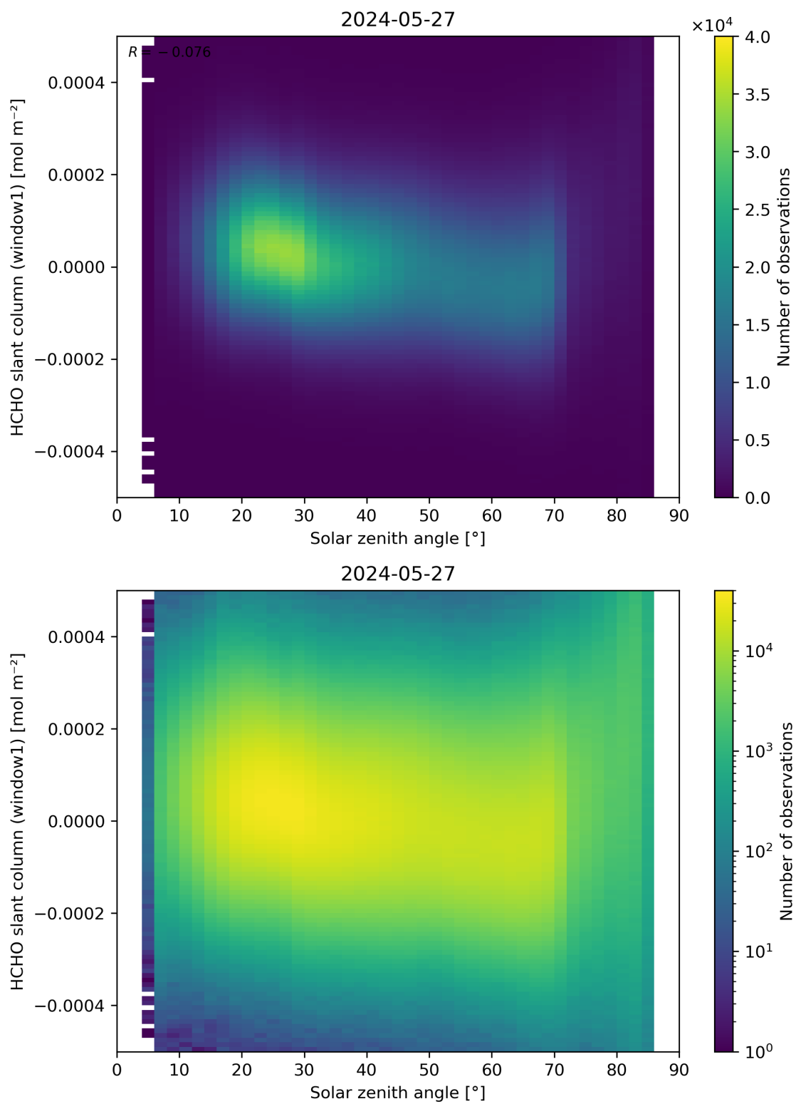
Figure 173: Scatter density plot of “Solar zenith angle” against “HCHO slant column (window1)” for 2024-05-26 to 2024-05-28.
