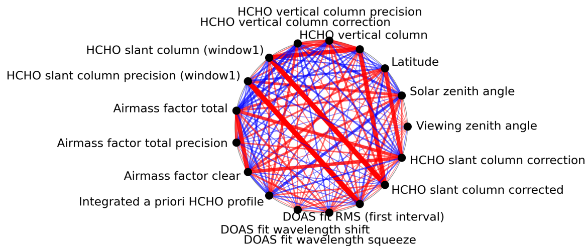
Figure 1: Map of correlation graph for 2024-05-26 to 2024-05-28.
