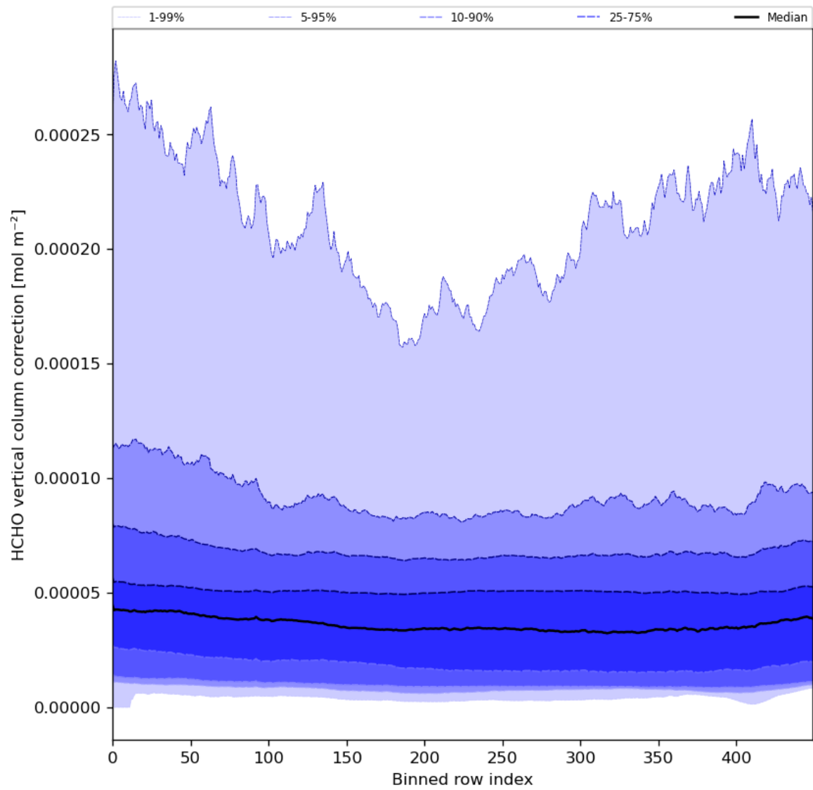
Figure 51: Along track statistics of “HCHO vertical column correction” for 2024-05-26 to 2024-05-28
