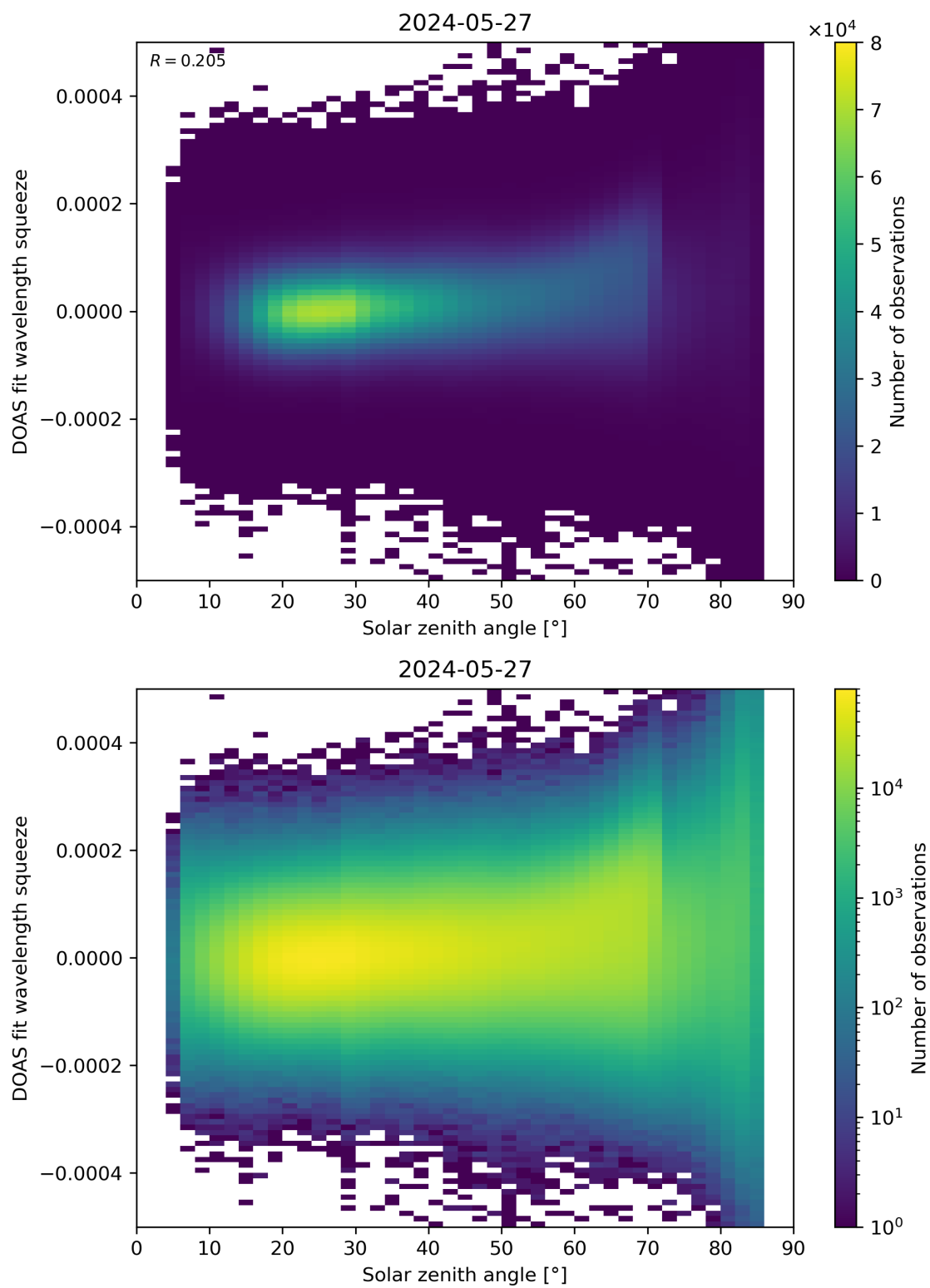
Figure 169: Scatter density plot of “Solar zenith angle” against “DOAS fit wavelength squeeze” for 2024-05-26 to 2024-05-28.
