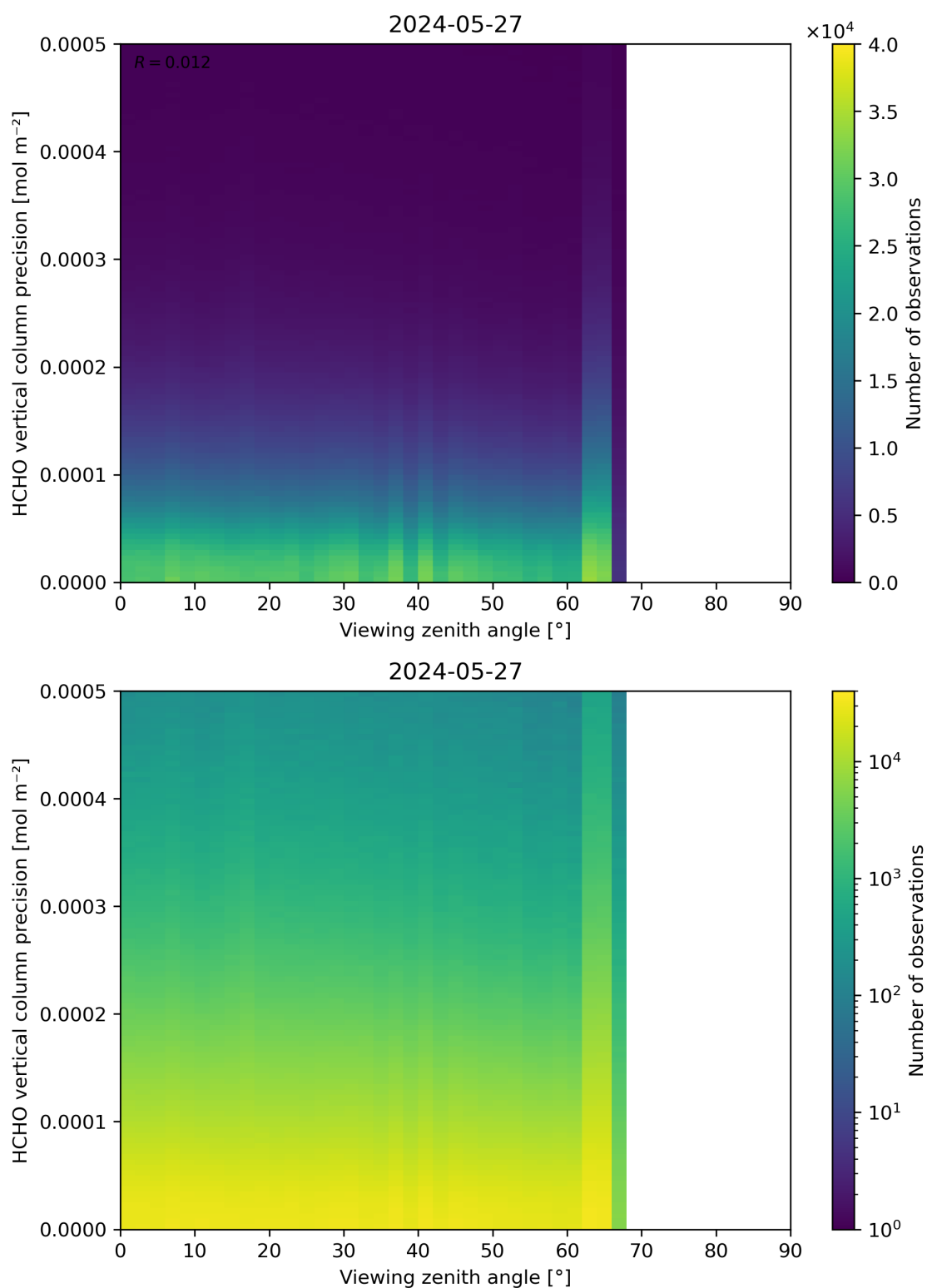
Figure 194: Scatter density plot of “Viewing zenith angle” against “HCHO vertical column precision” for 2024-05-26 to 2024-05-28.
