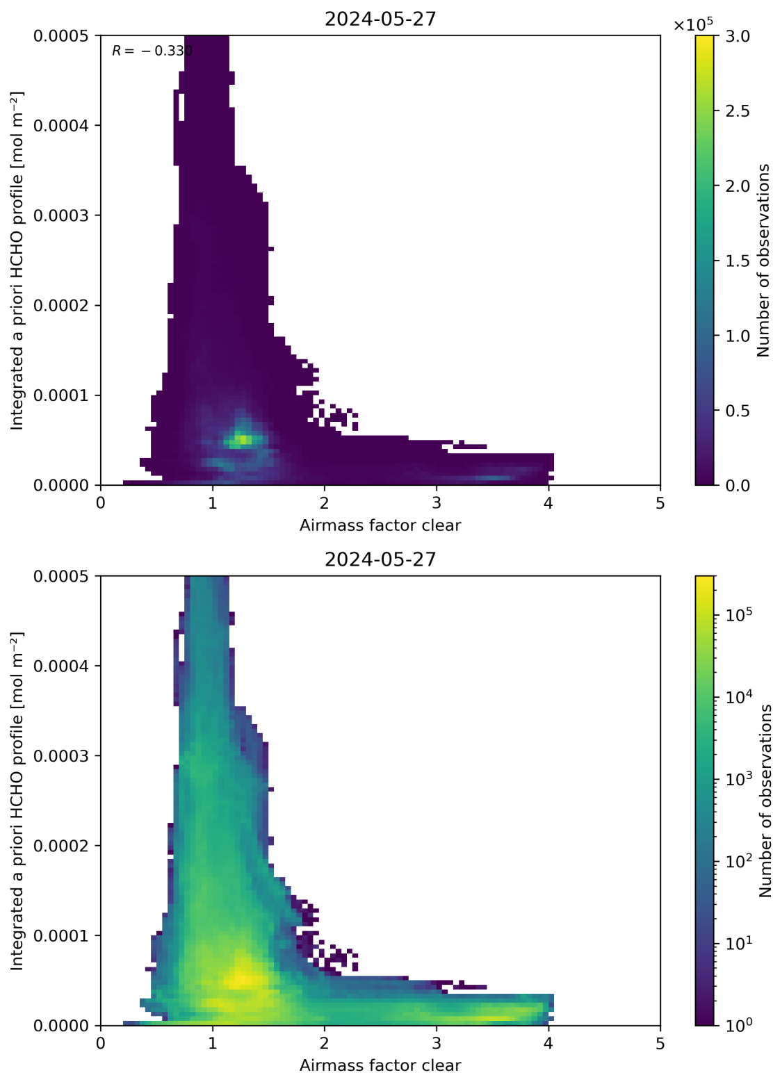
Figure 76: Scatter density plot of “Airmass factor clear” against “Integrated a priori HCHO profile” for 2024-05-26 to 2024-05-28.
