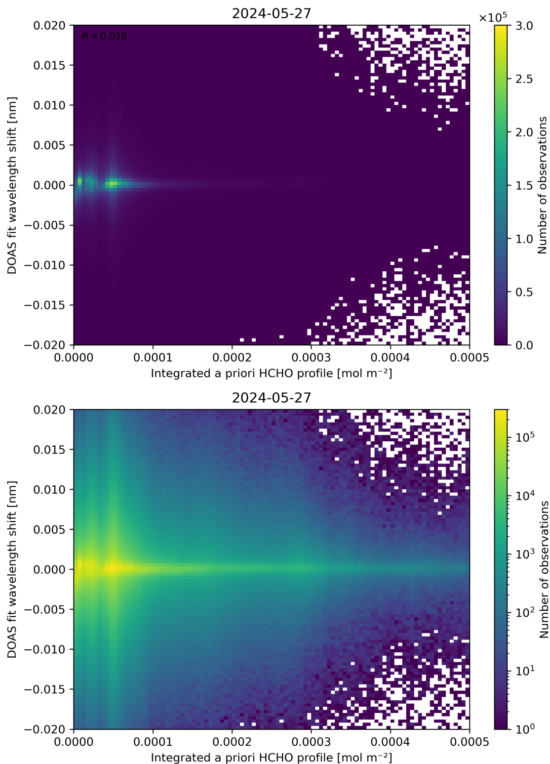
Figure 149: Scatter density plot of “Integrated a priori HCHO profile” against “DOAS fit wavelength shift” for 2024-05-26 to 2024-05-28.
