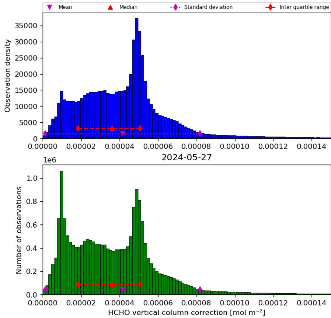
Figure 37: Histogram of “HCHO vertical column correction” for 2024-05-26 to 2024-05-28
