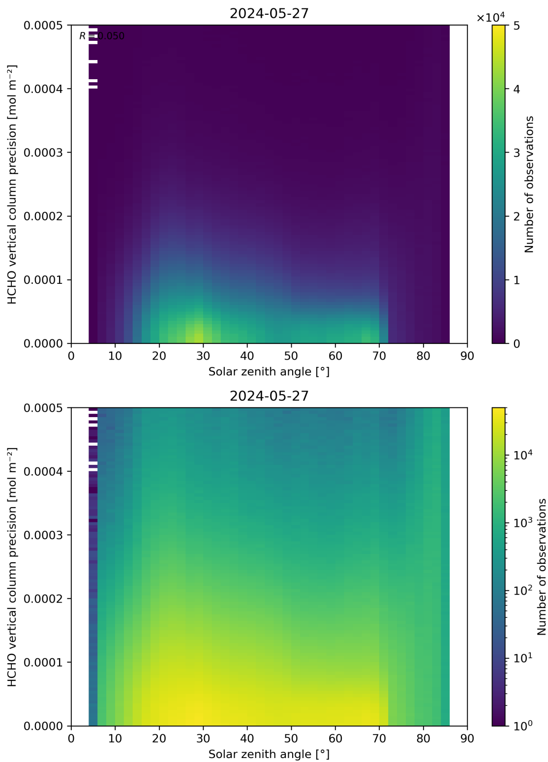
Figure 179: Scatter density plot of “Solar zenith angle” against “HCHO vertical column precision” for 2024-05-26 to 2024-05-28.
