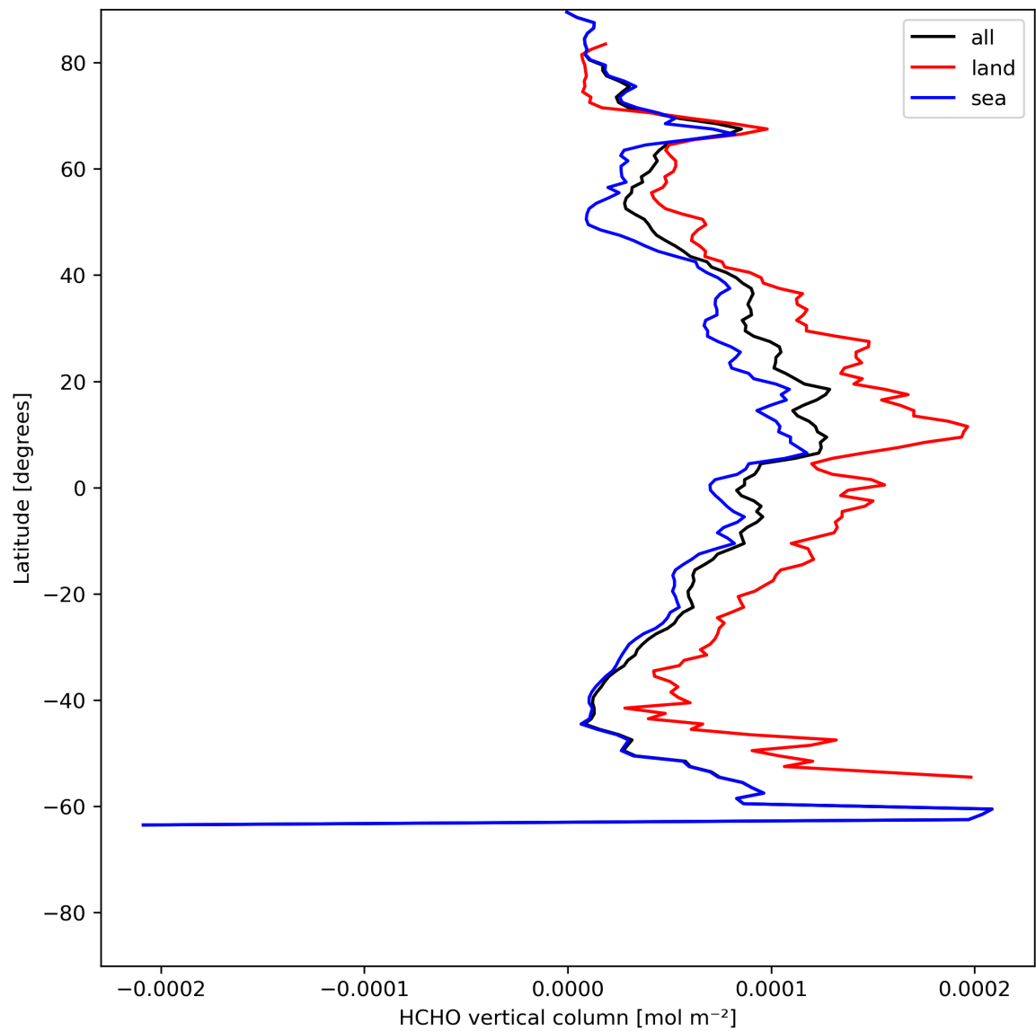
Figure 21: Zonal average of “HCHO vertical column” for 2024-05-26 to 2024-05-28.
