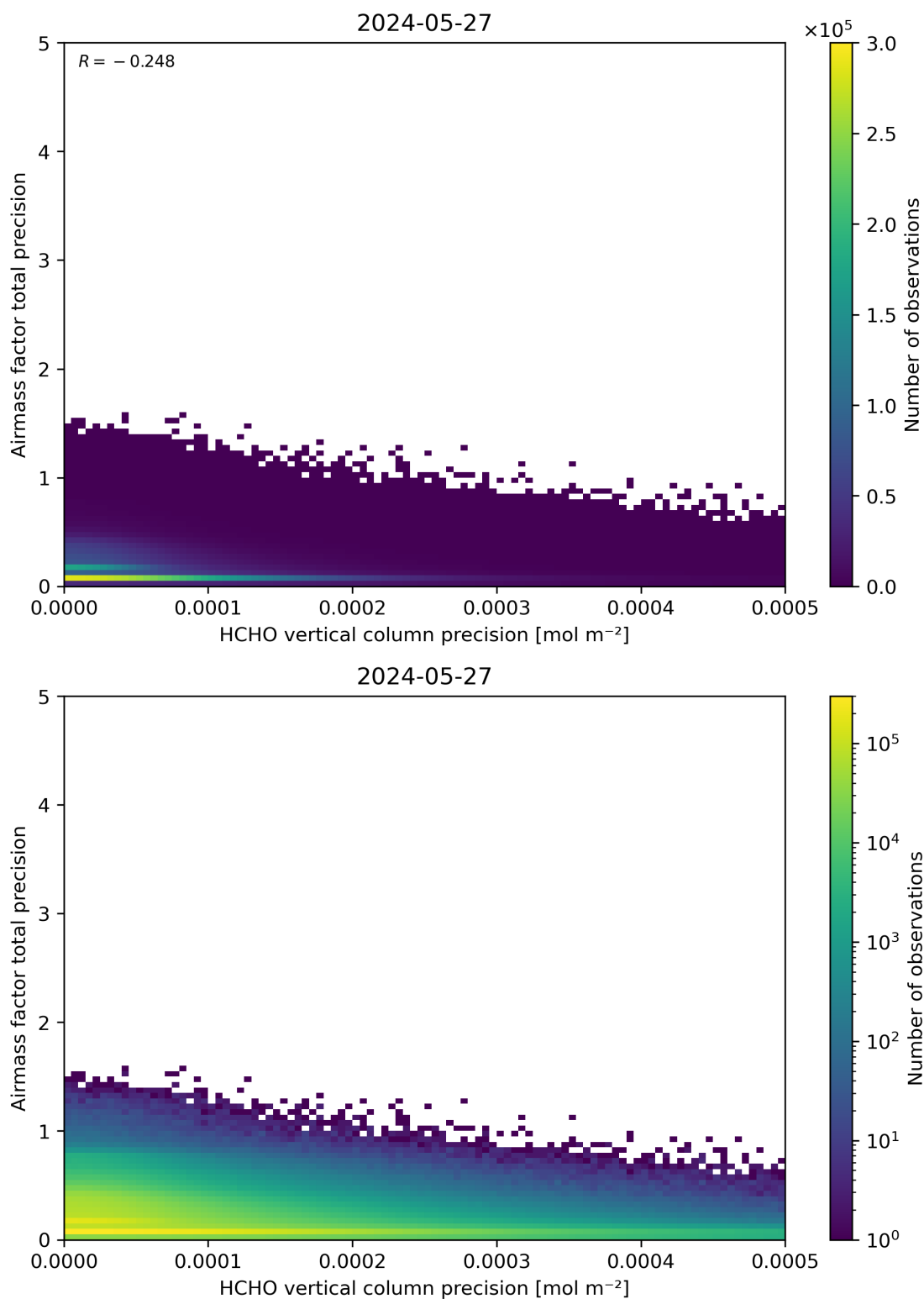
Figure 145: Scatter density plot of “HCHO vertical column precision” against “Airmass factor total precision” for 2024-05-26 to 2024-05-28.
