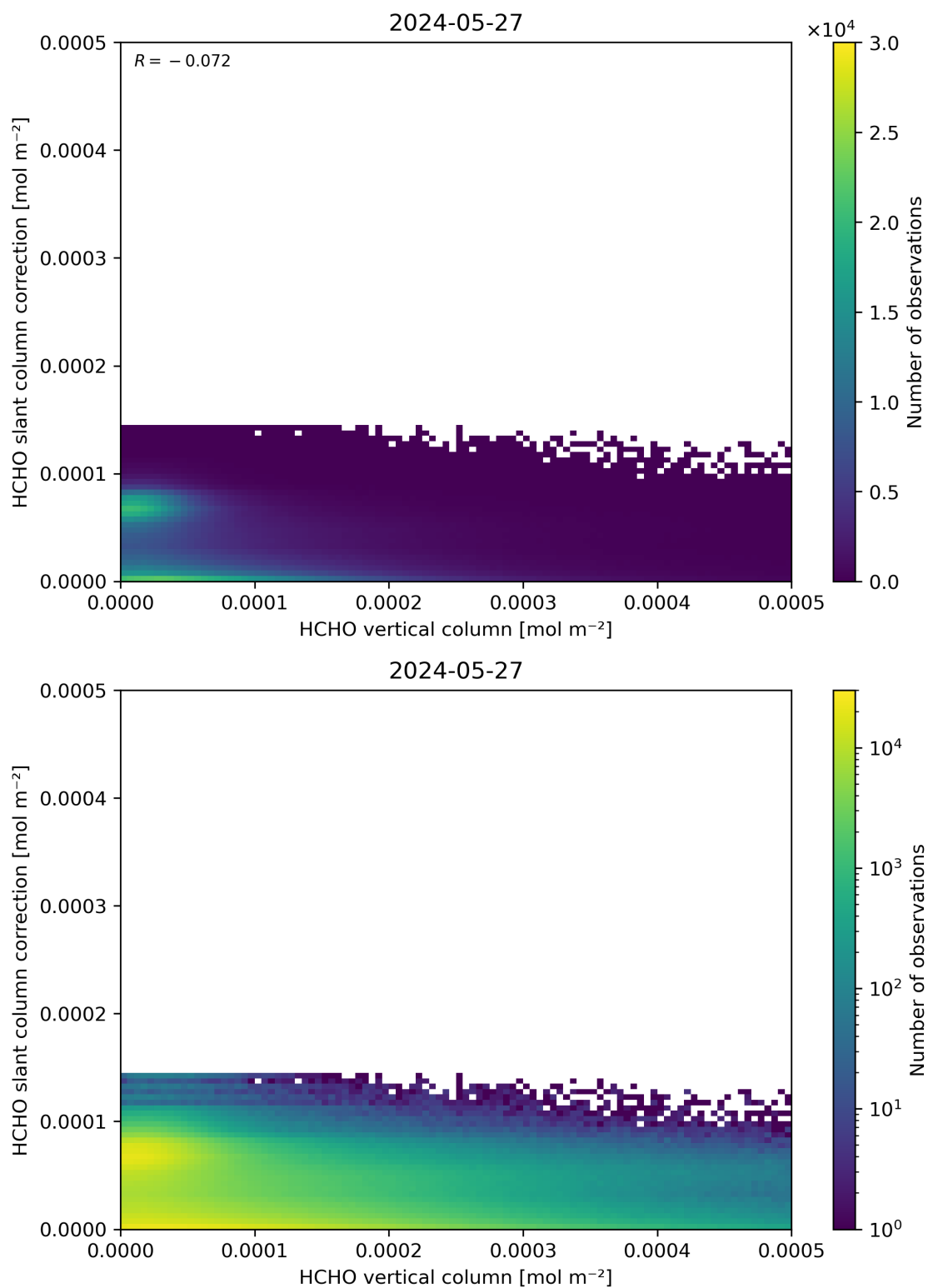
Figure 128: Scatter density plot of “HCHO vertical column” against “HCHO slant column correction” for 2024-05-26 to 2024-05-28.
