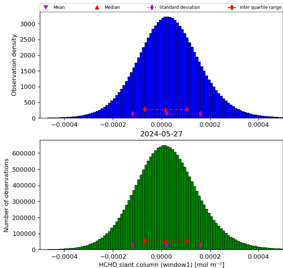
Figure 38: Histogram of “HCHO slant column (window1)” for 2024-05-26 to 2024-05-28
