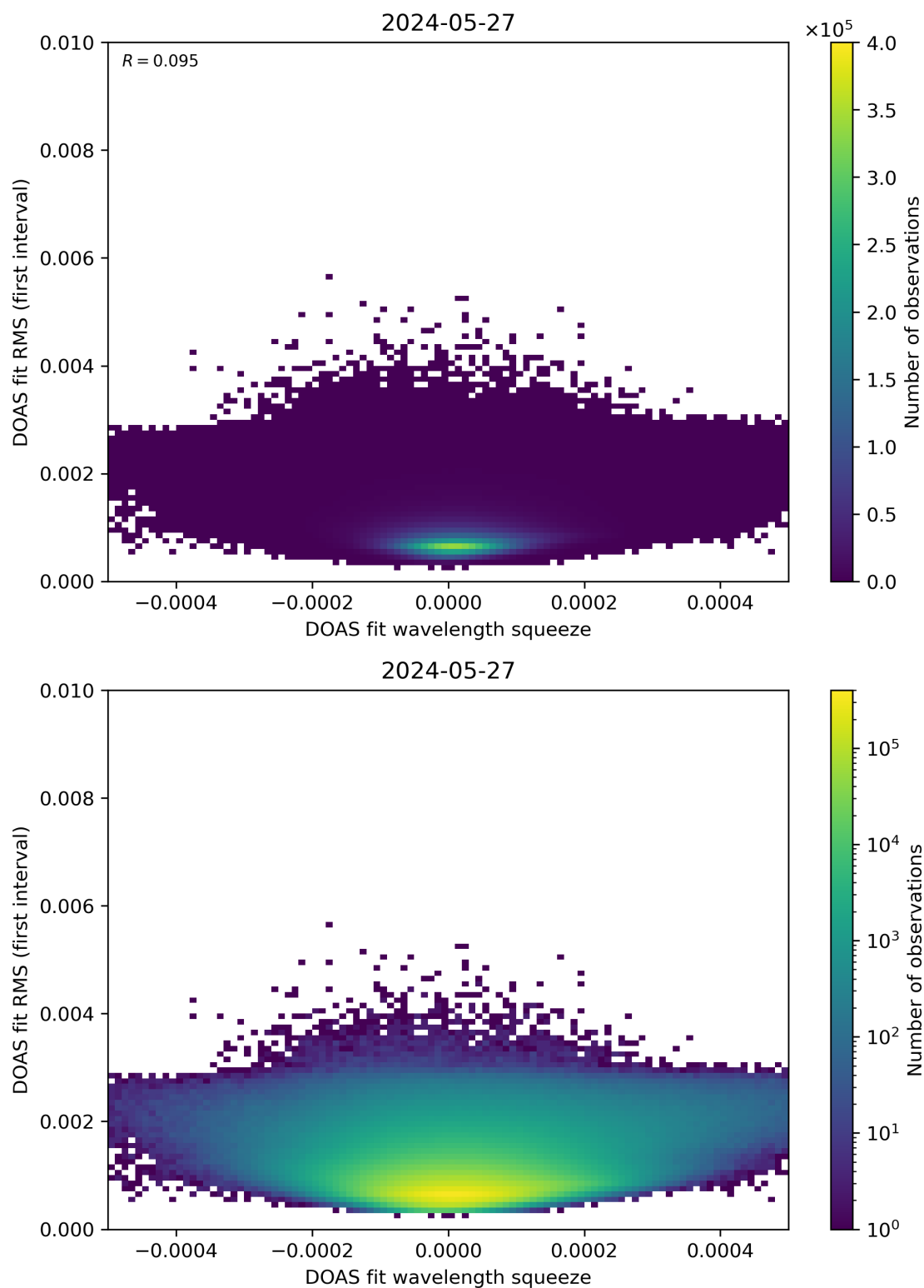
Figure 68: Scatter density plot of “DOAS fit wavelength squeeze” against “DOAS fit RMS (first interval)” for 2024-05-26 to 2024-05-28.
