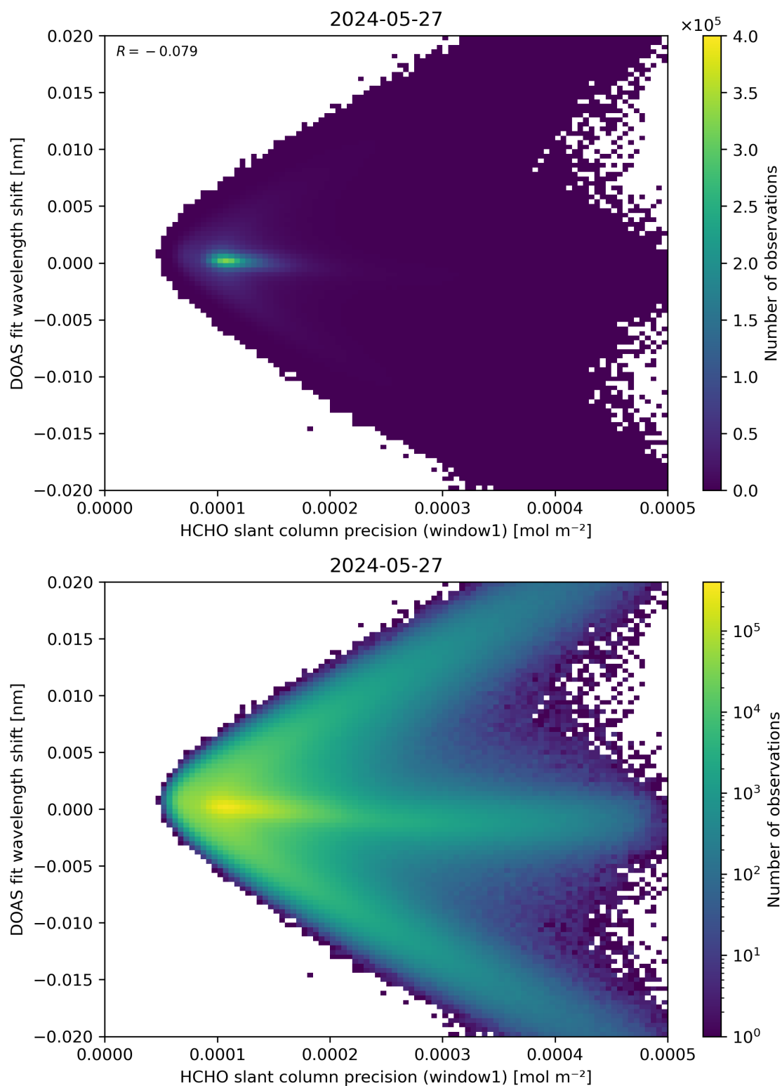
Figure 89: Scatter density plot of “HCHO slant column precision (window1)” against “DOAS fit wavelength shift” for 2024-05-26 to 2024-05-28.
