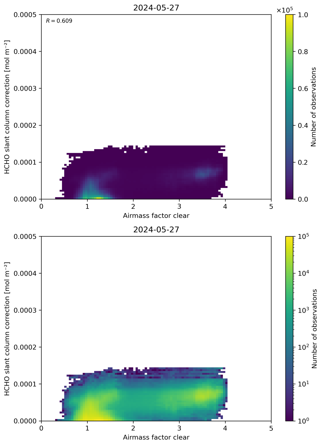
Figure 75: Scatter density plot of “Airmass factor clear” against “HCHO slant column correction” for 2024-05-26 to 2024-05-28.
