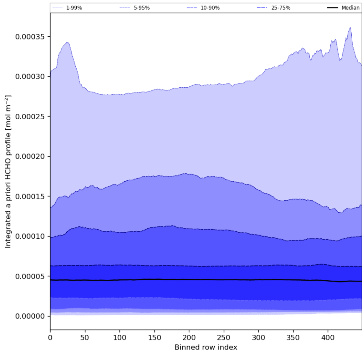
Figure 57: Along track statistics of "Integrated a priori HCHO profile" for 2024-05-26 to 2024-05-28
