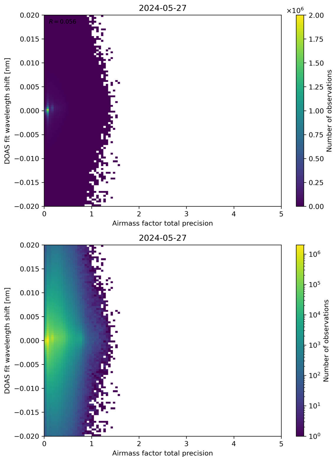
Figure 106: Scatter density plot of “Airmass factor total precision” against “DOAS fit wavelength shift” for 2024-05-26 to 2024-05-28.
