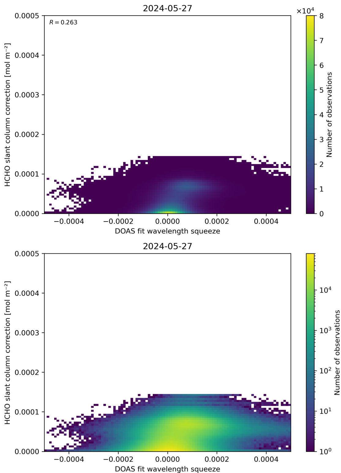
Figure 70: Scatter density plot of “DOAS fit wavelength squeeze” against “HCHO slant column correction” for 2024-05-26 to 2024-05-28.
