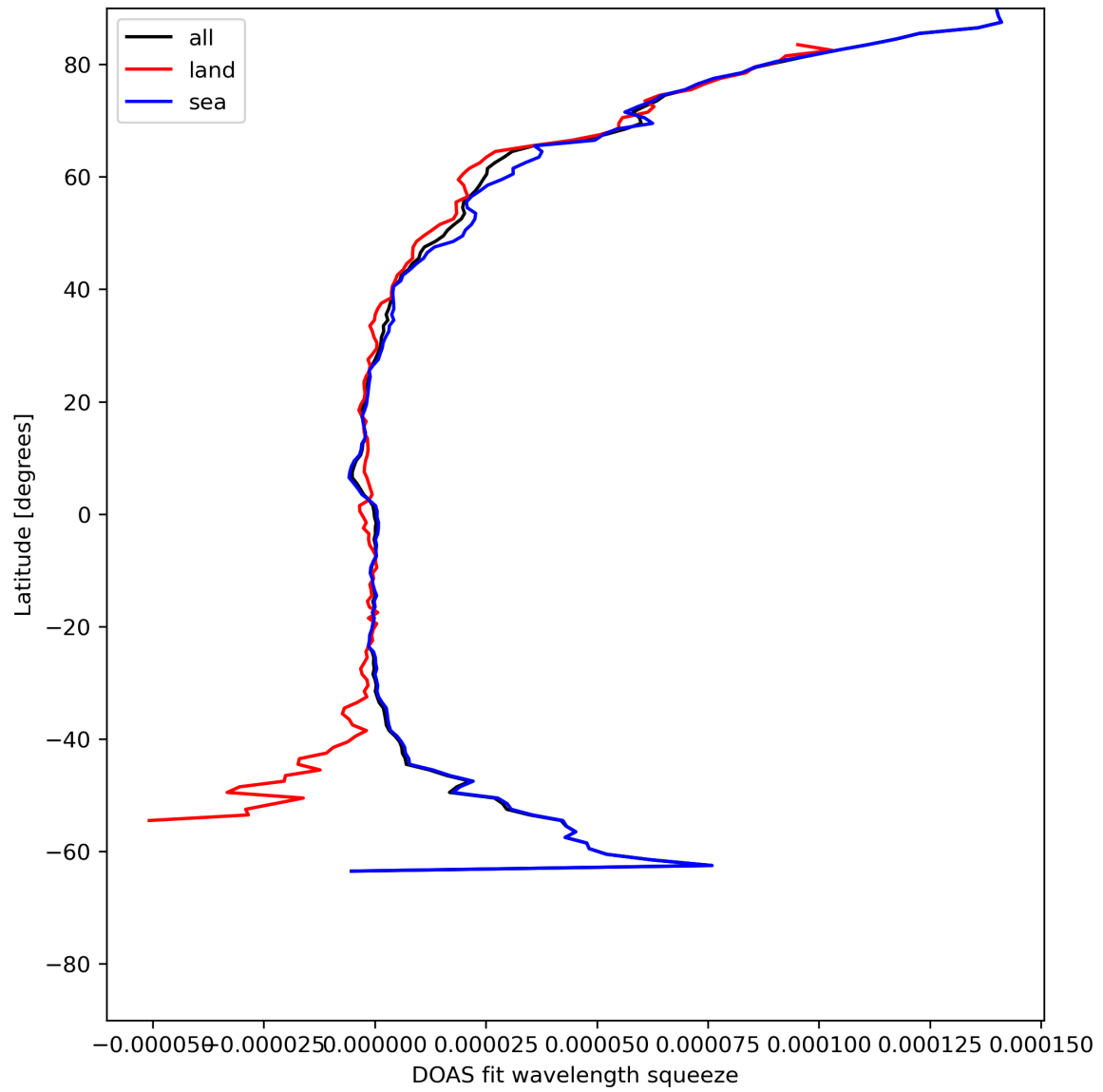
Figure 31: Zonal average of “DOAS fit wavelength squeeze” for 2024-05-26 to 2024-05-28.
