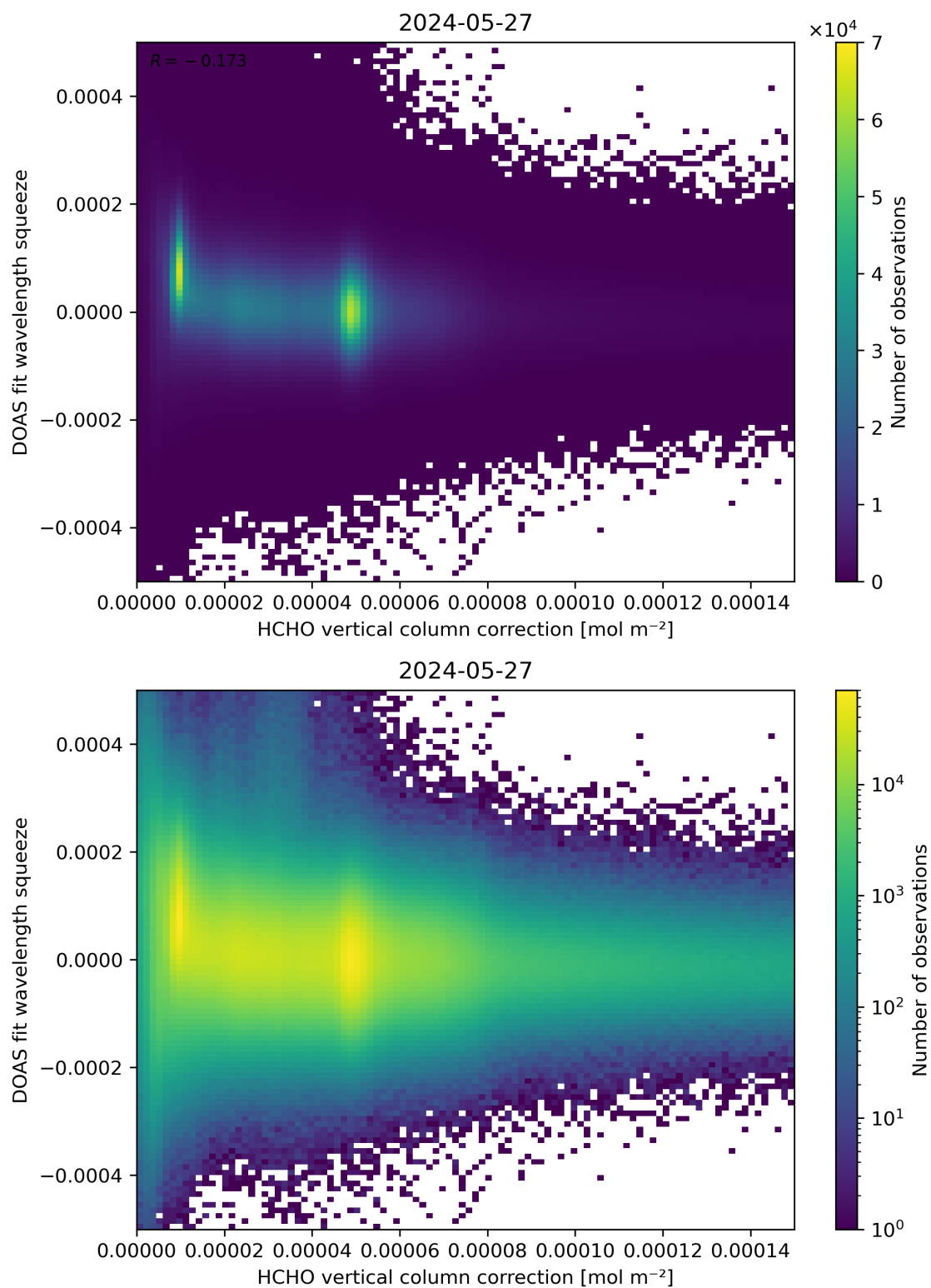
Figure 114: Scatter density plot of “HCHO vertical column correction” against “DOAS fit wavelength squeeze” for 2024-05-26 to 2024-05-28.
