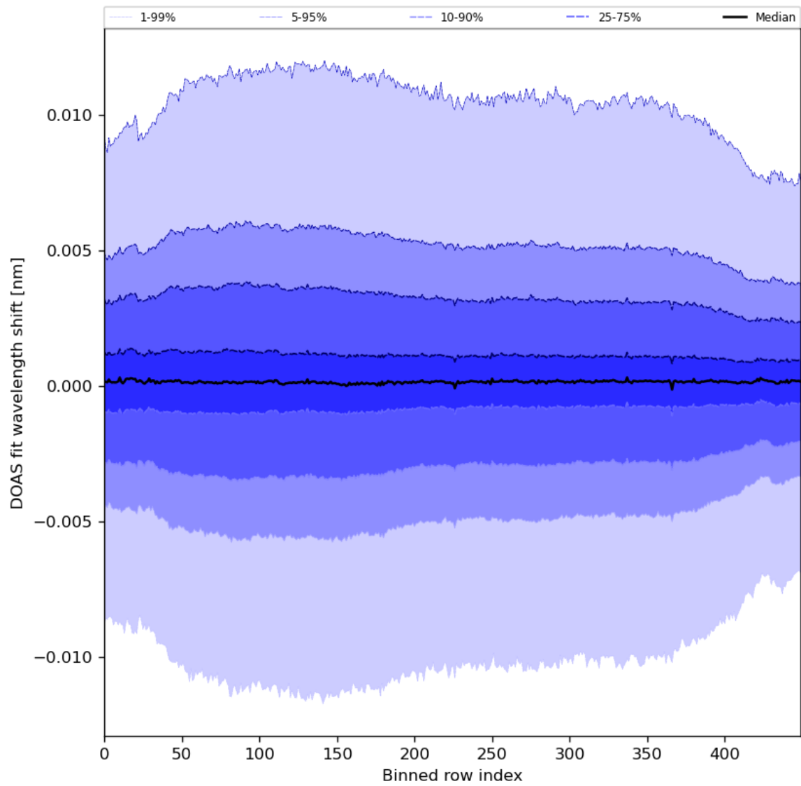
Figure 58: Along track statistics of “DOAS fit wavelength shift” for 2024-05-26 to 2024-05-28
