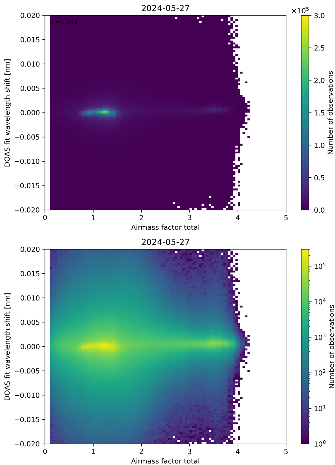
Figure 98: Scatter density plot of “Airmass factor total” against “DOAS fit wavelength shift” for 2024-05-26 to 2024-05-28.
