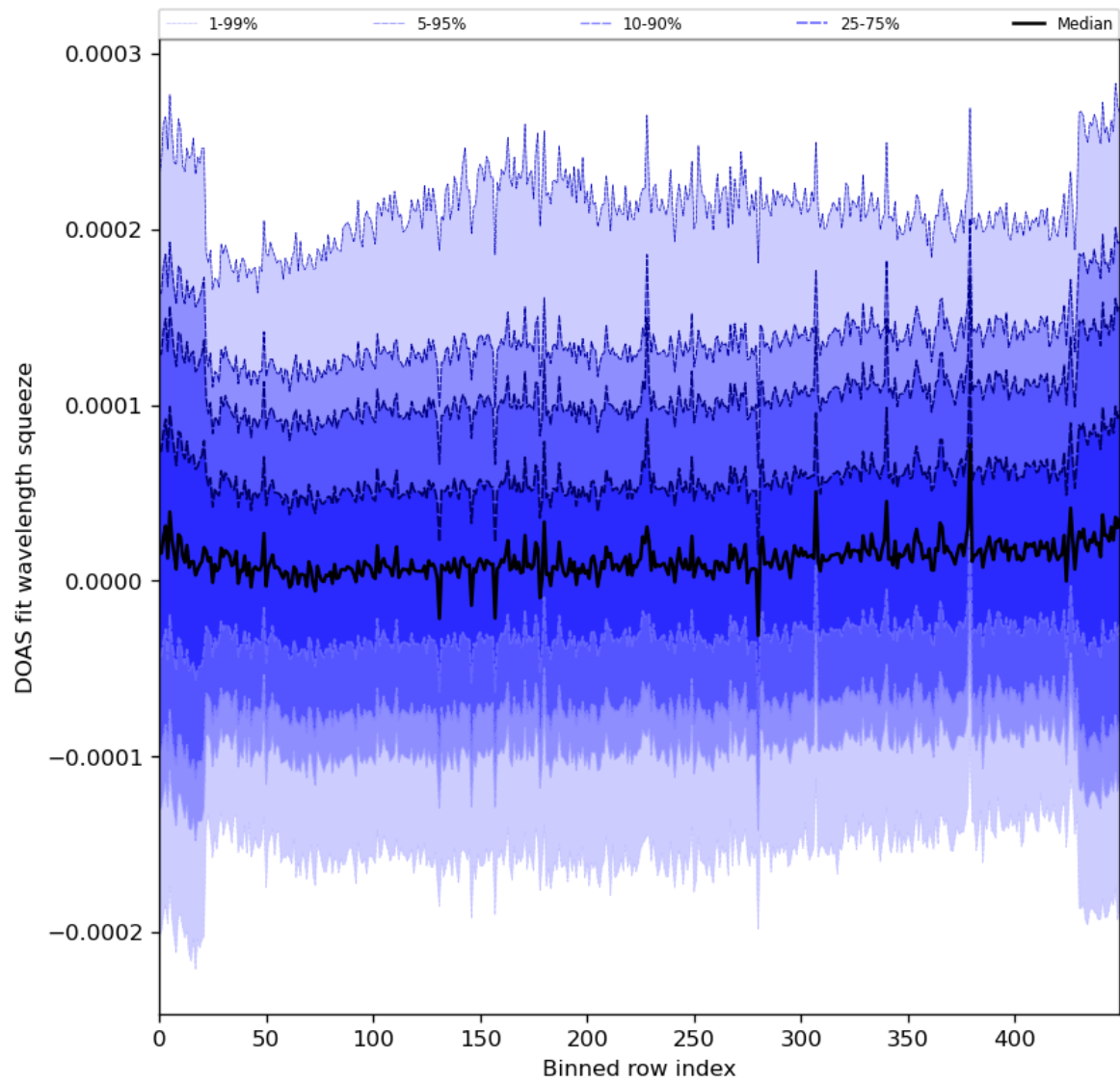
Figure 59: Along track statistics of “DOAS fit wavelength squeeze” for 2024-05-26 to 2024-05-28
