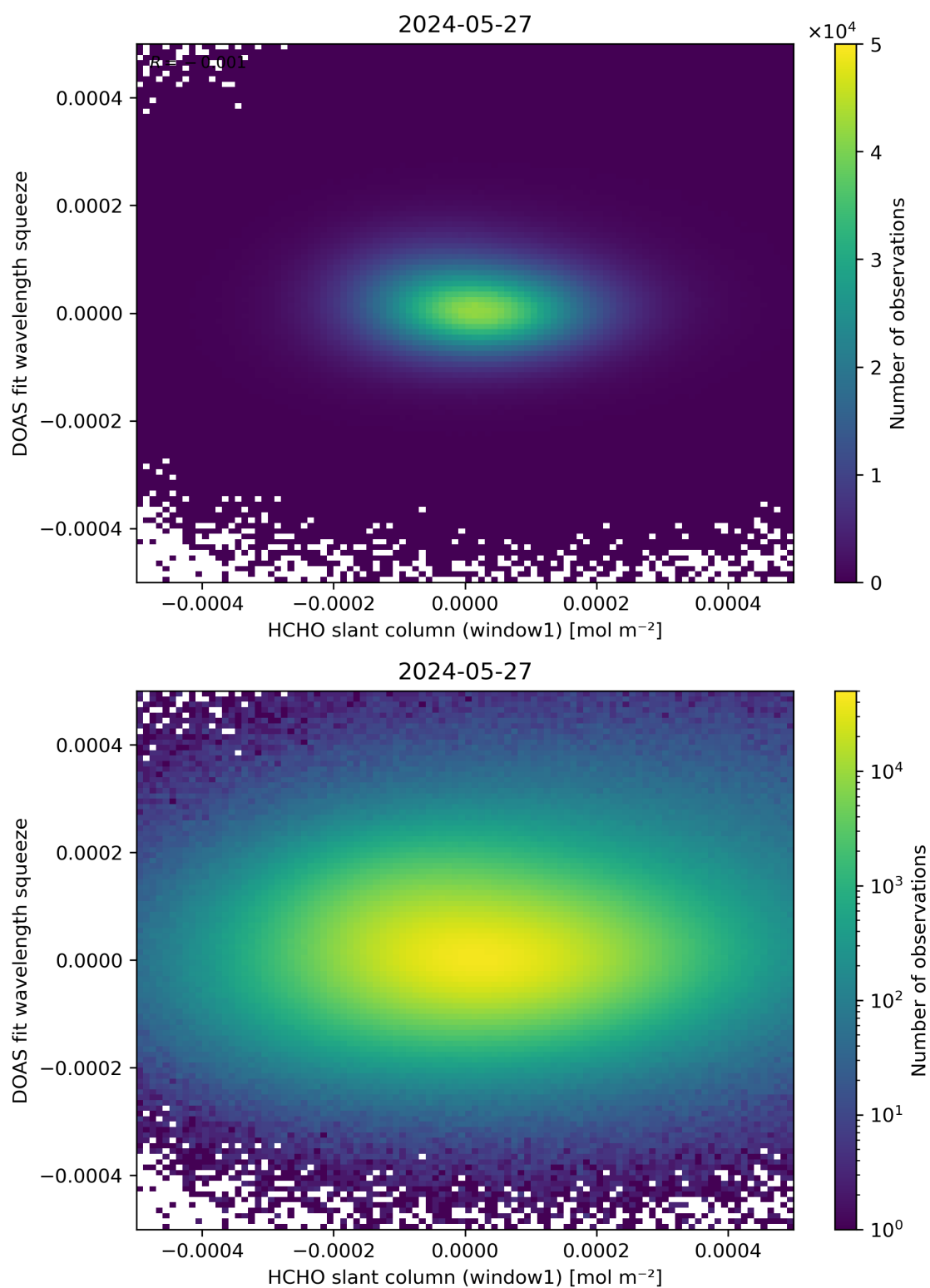
Figure 80: Scatter density plot of “HCHO slant column (window1)” against “DOAS fit wavelength squeeze” for 2024-05-26 to 2024-05-28.
