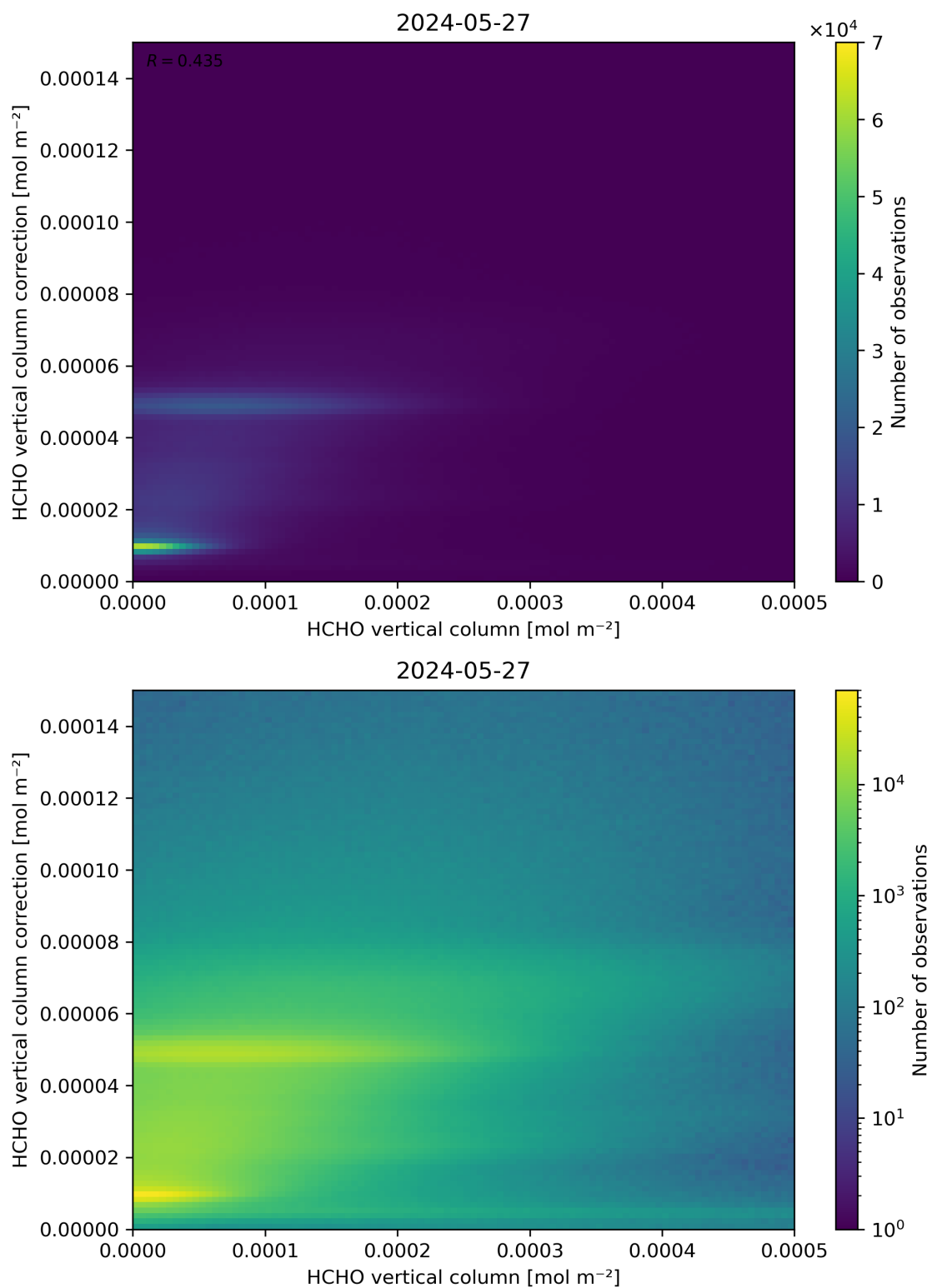
Figure 133: Scatter density plot of “HCHO vertical column” against “HCHO vertical column correction” for 2024-05-26 to 2024-05-28.
