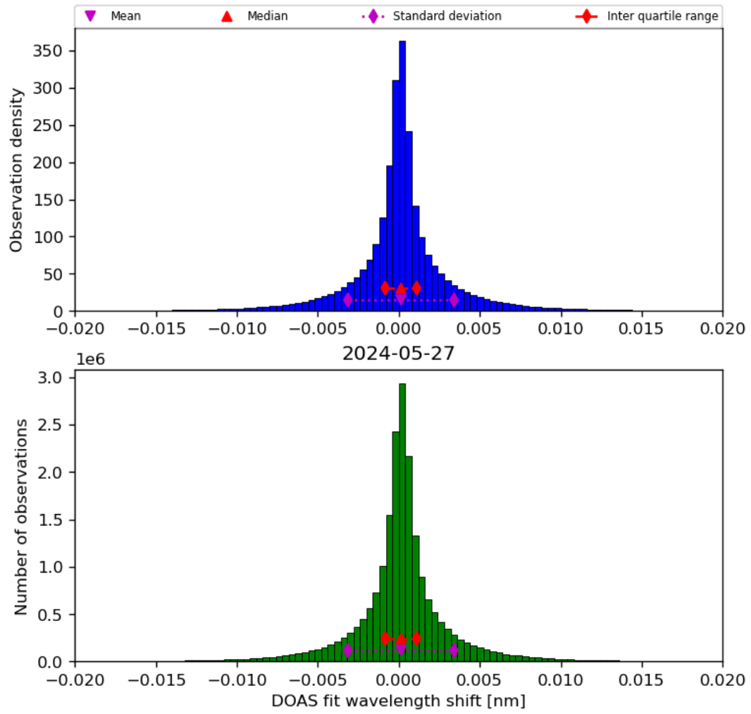
Figure 44: Histogram of “DOAS fit wavelength shift” for 2024-05-26 to 2024-05-28
