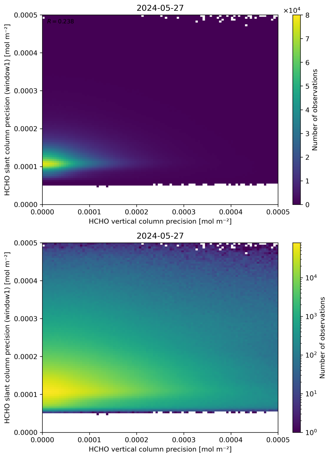
Figure 143: Scatter density plot of “HCHO vertical column precision” against “HCHO slant column precision (window1)” for 2024-05-26 to 2024-05-28.
