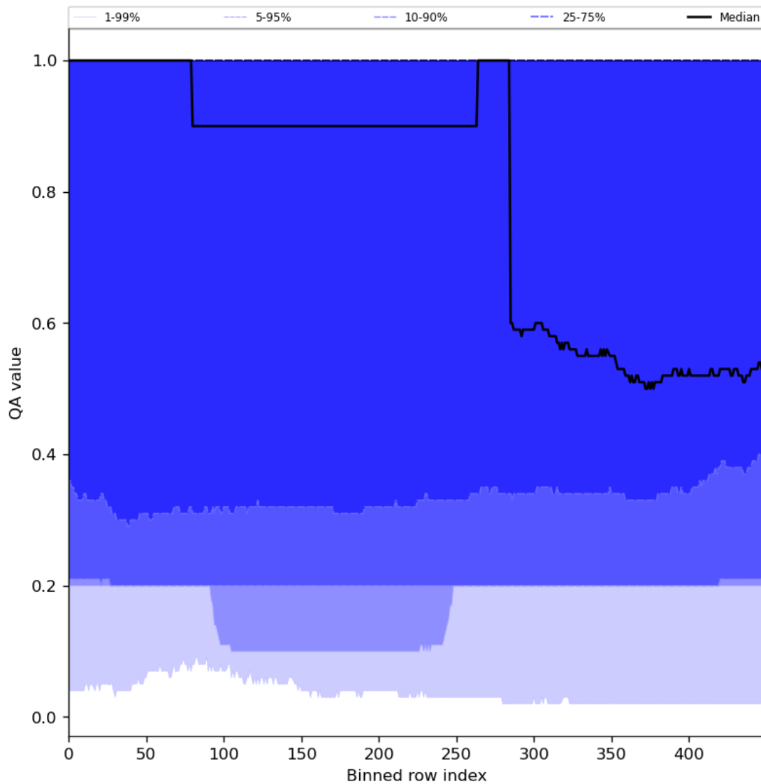
Figure 48: Along track statistics of “QA value” for 2024-05-26 to 2024-05-28
