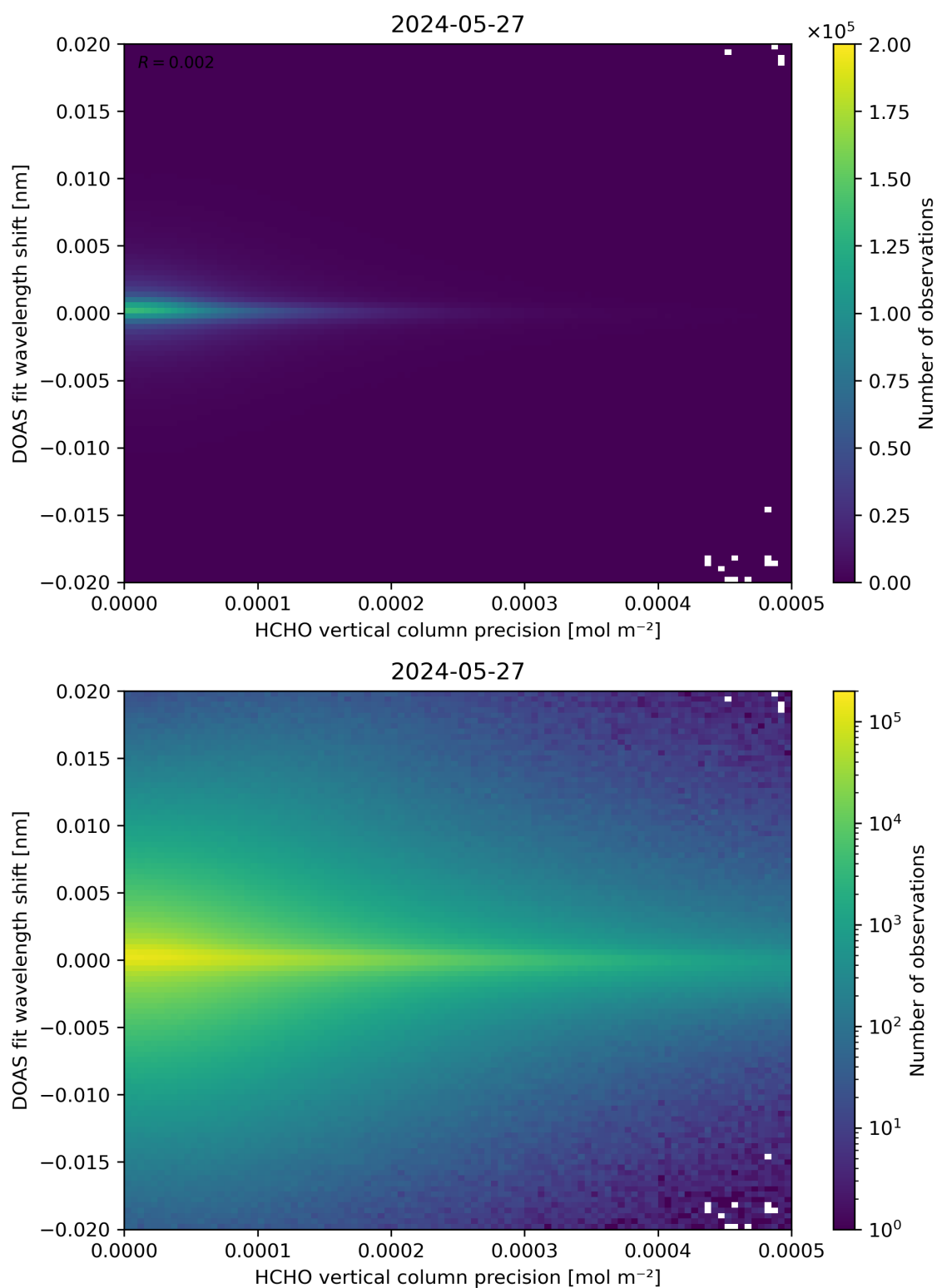
Figure 137: Scatter density plot of “HCHO vertical column precision” against “DOAS fit wavelength shift” for 2024-05-26 to 2024-05-28.
