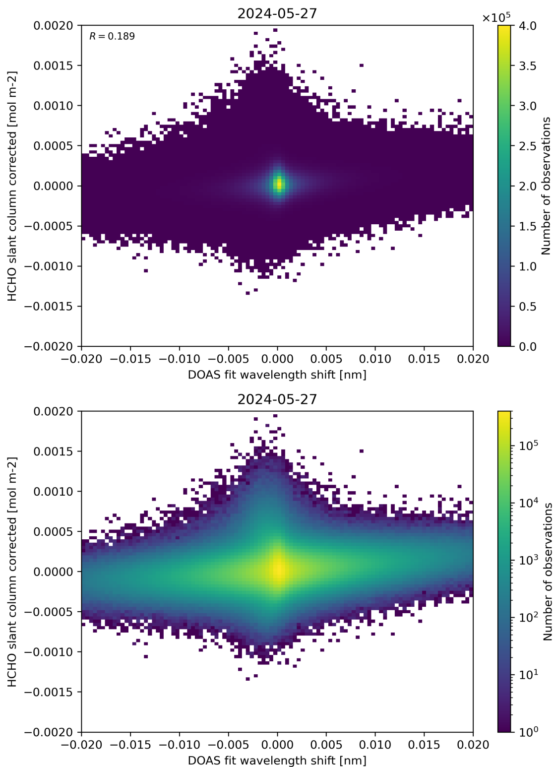
Figure 66: Scatter density plot of “DOAS fit wavelength shift” against “HCHO slant column corrected” for 2024-05-26 to 2024-05-28.
