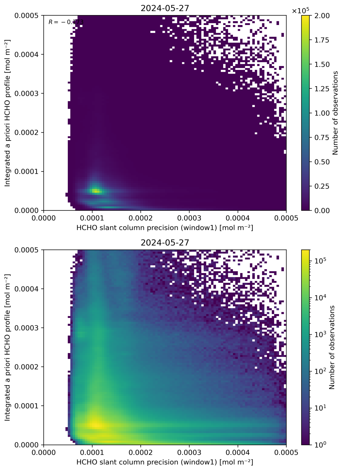
Figure 96: Scatter density plot of “HCHO slant column precision (window1)” against “Integrated a priori HCHO profile” for 2024-05-26 to 2024-05-28.
