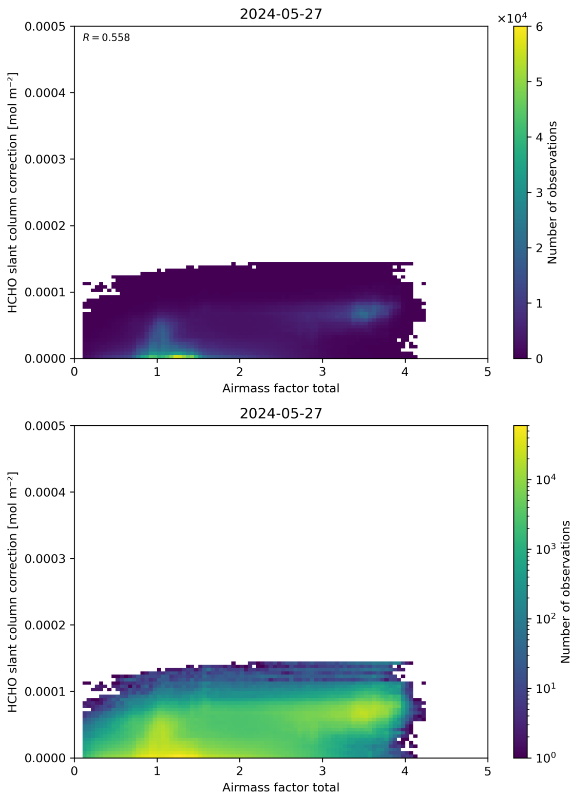
Figure 102: Scatter density plot of “Airmass factor total” against “HCHO slant column correction” for 2024-05-26 to 2024-05-28.
