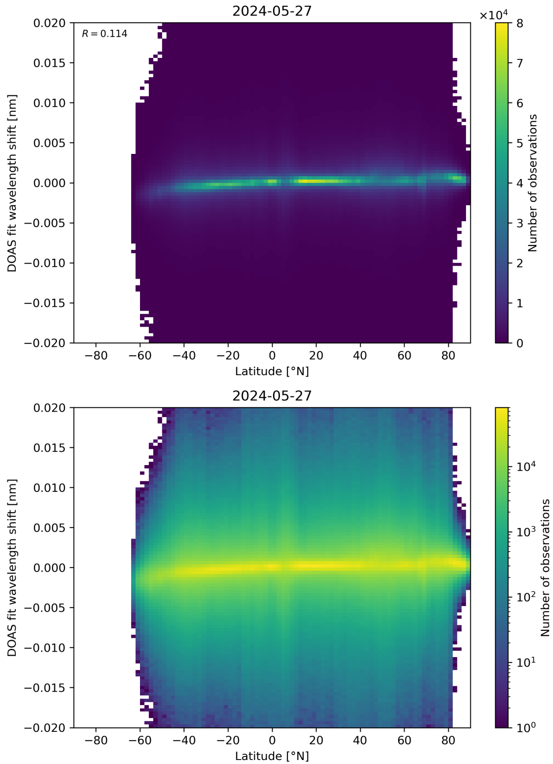
Figure 154: Scatter density plot of “Latitude” against “DOAS fit wavelength shift” for 2024-05-26 to 2024-05-28.
