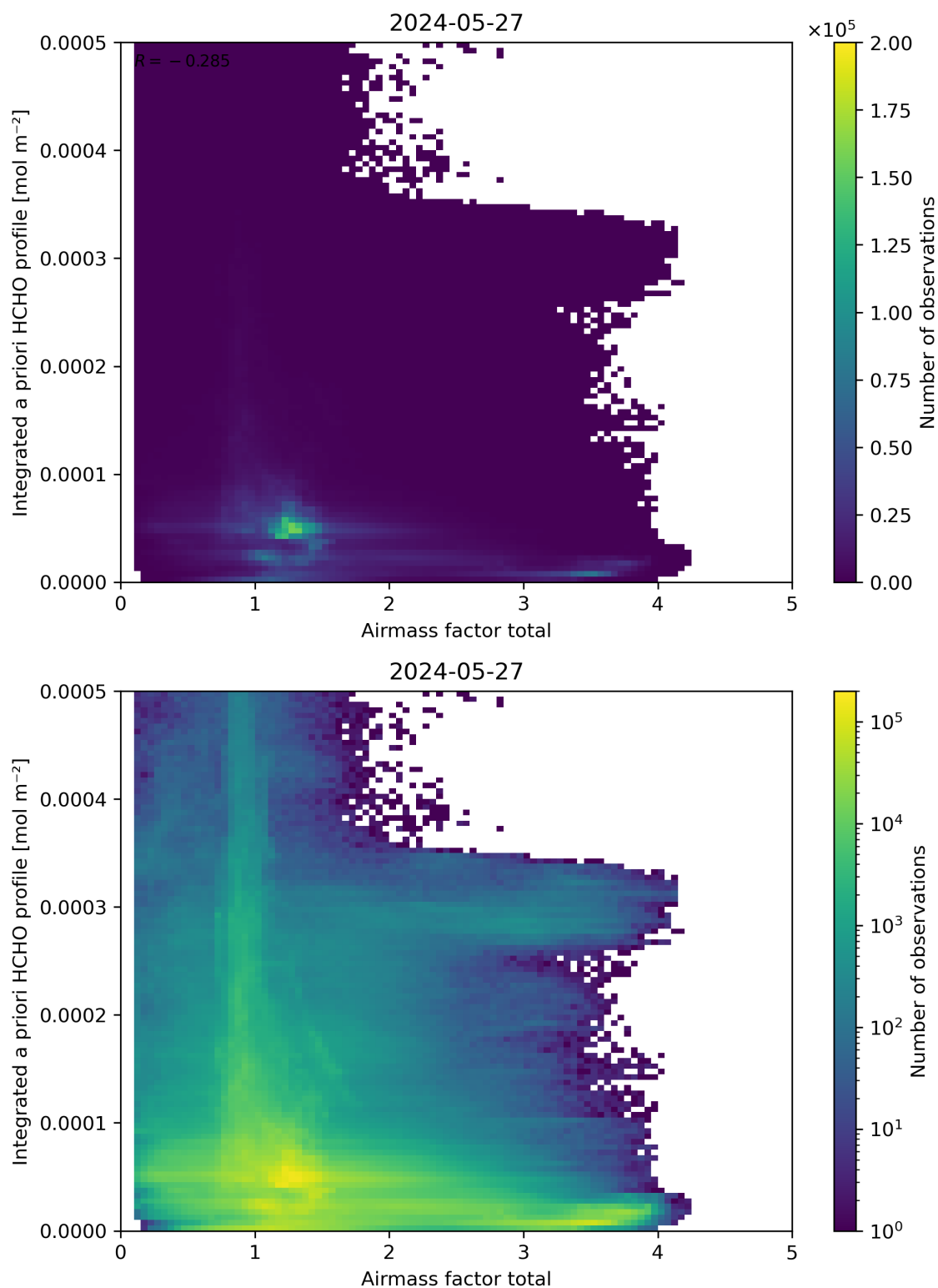
Figure 104: Scatter density plot of “Airmass factor total” against “Integrated a priori HCHO profile” for 2024-05-26 to 2024-05-28.
