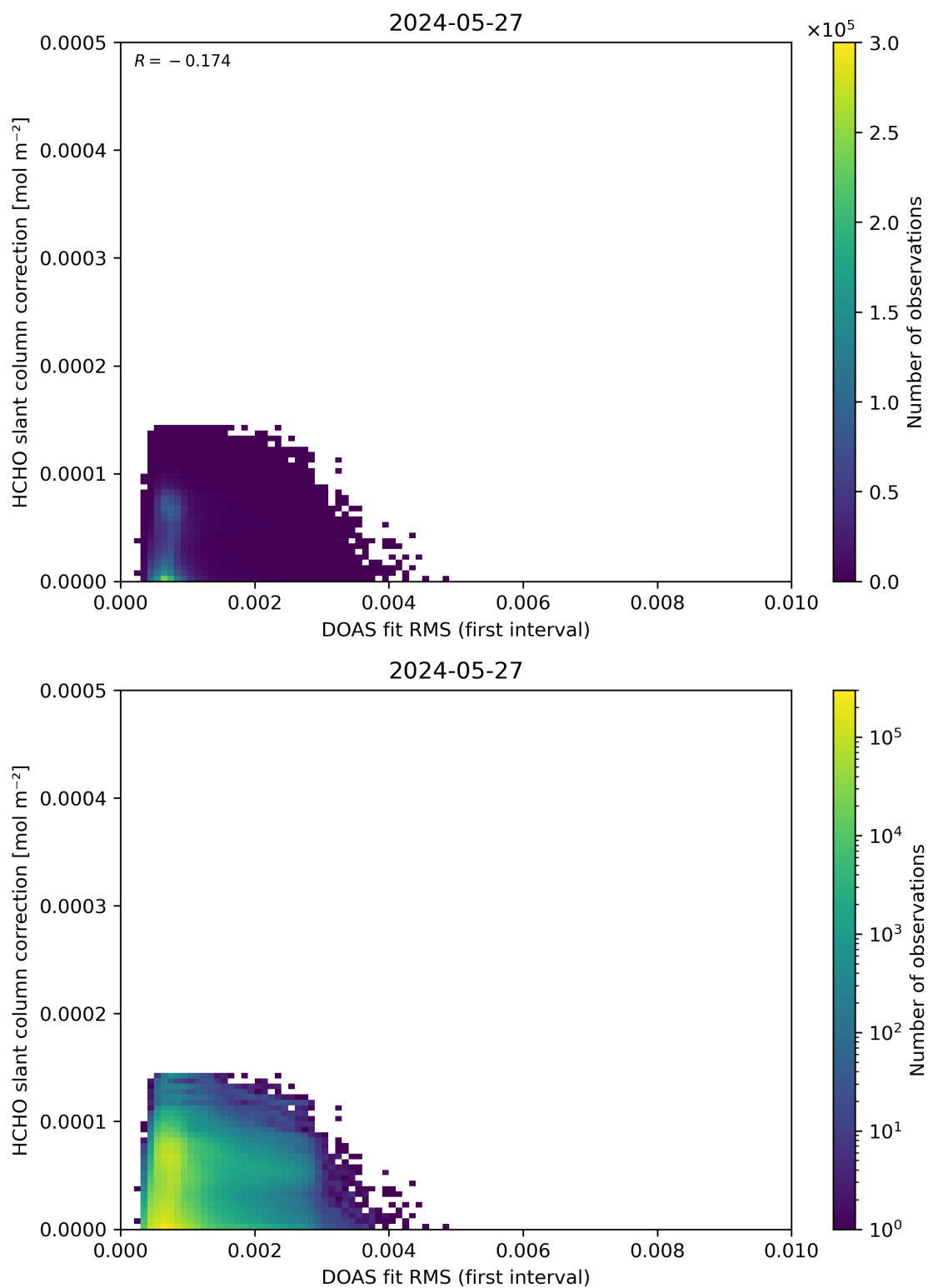
Figure 63: Scatter density plot of “DOAS fit RMS (first interval)” against “HCHO slant column correction” for 2024-05-26 to 2024-05-28.
