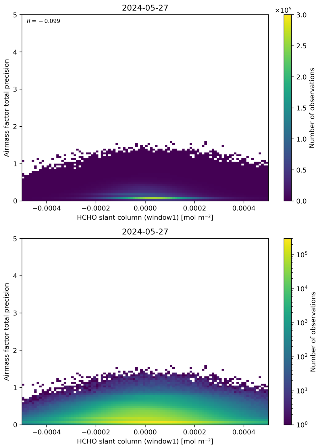
Figure 86: Scatter density plot of “HCHO slant column (window1)” against “Airmass factor total precision” for 2024-05-26 to 2024-05-28.
