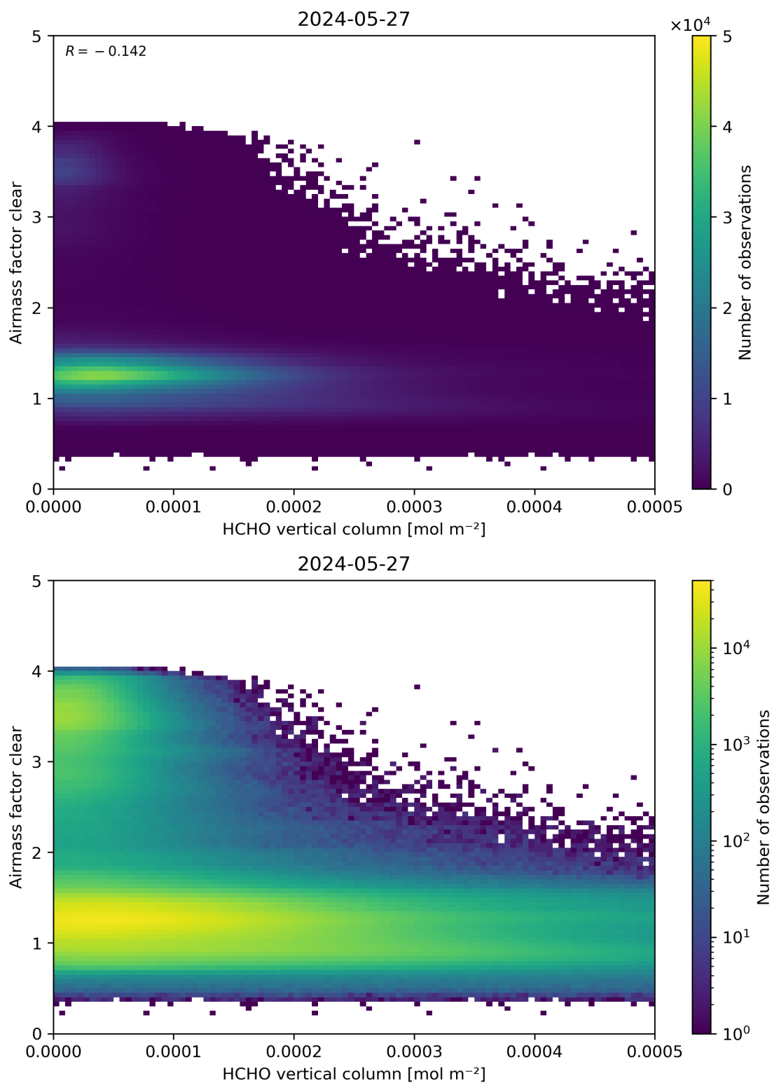
Figure 126: Scatter density plot of “HCHO vertical column” against “Airmass factor clear” for 2024-05-26 to 2024-05-28.
