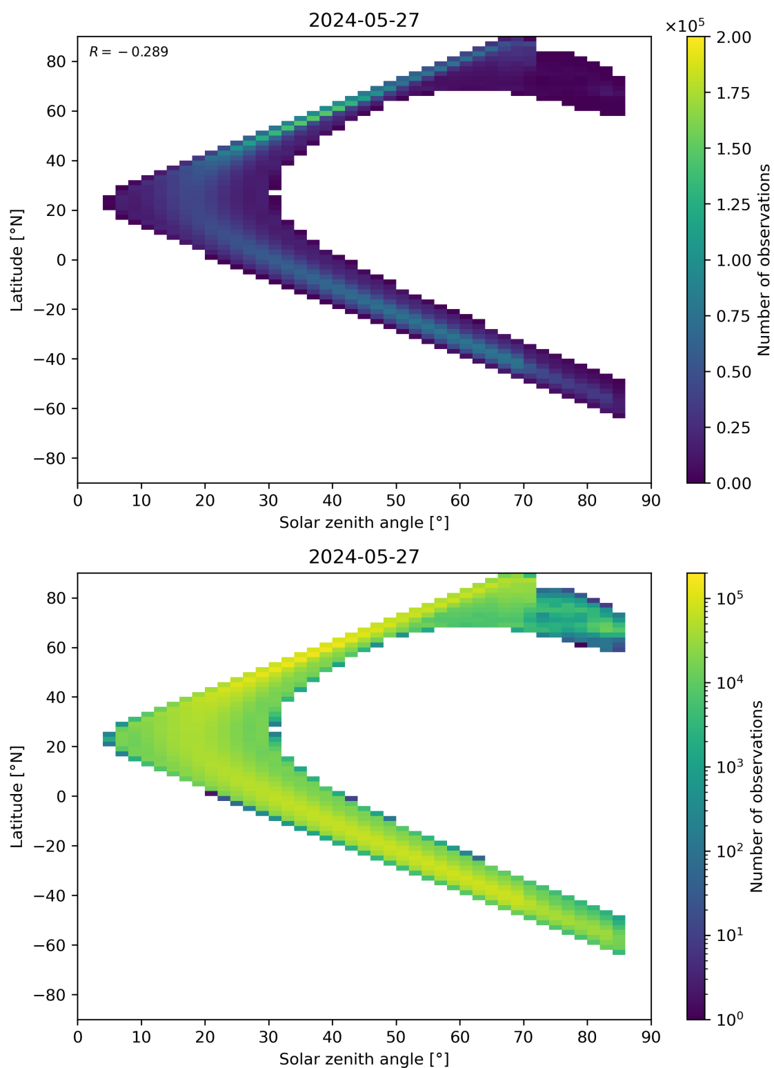
Figure 181: Scatter density plot of “Solar zenith angle” against “Latitude” for 2024-05-26 to 2024-05-28.
