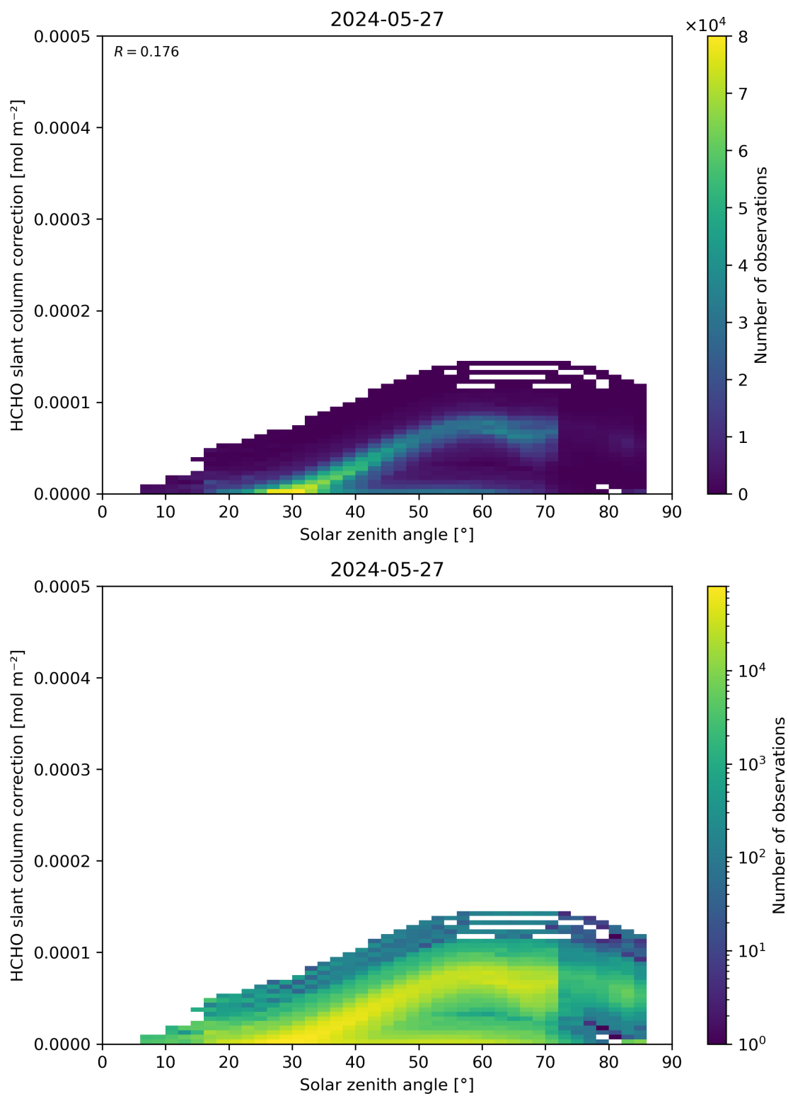
Figure 172: Scatter density plot of “Solar zenith angle” against “HCHO slant column correction” for 2024-05-26 to 2024-05-28.
