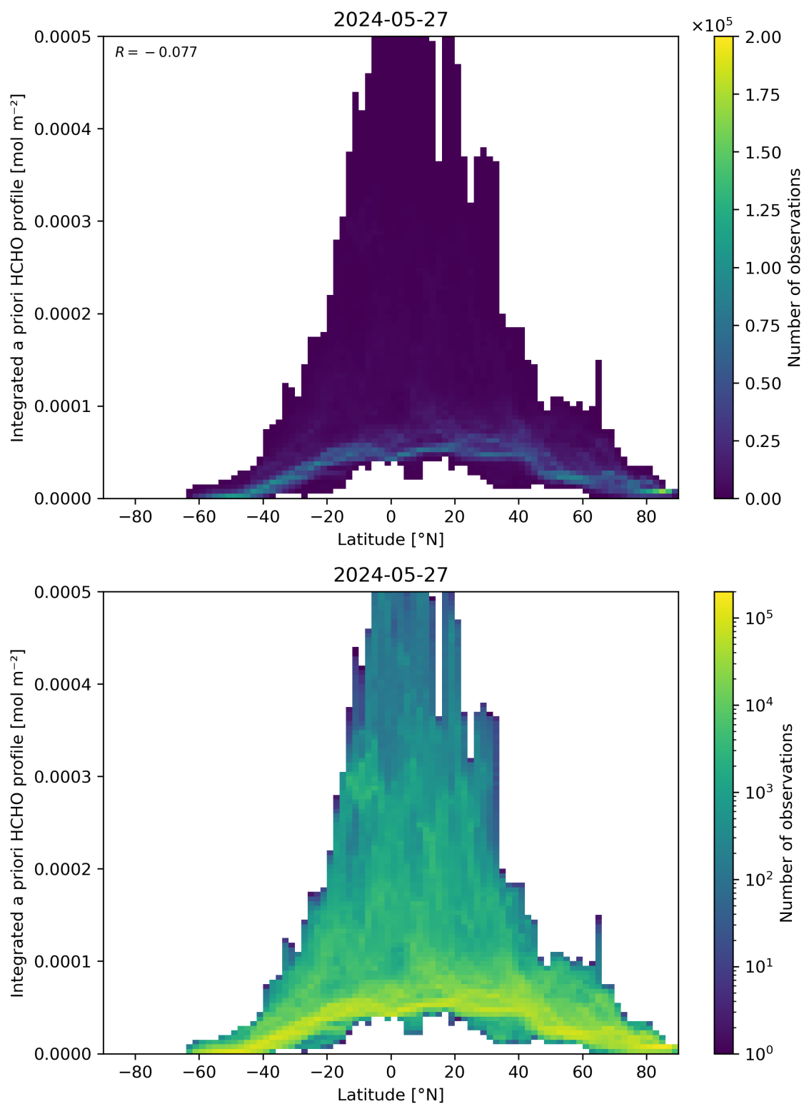
Figure 166: Scatter density plot of “Latitude” against “Integrated a priori HCHO profile” for 2024-05-26 to 2024-05-28.
