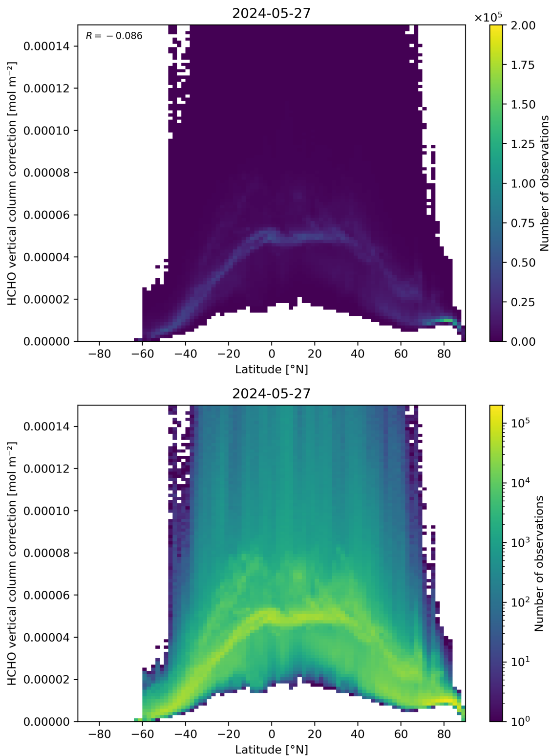
Figure 164: Scatter density plot of “Latitude” against “HCHO vertical column correction” for 2024-05-26 to 2024-05-28.
