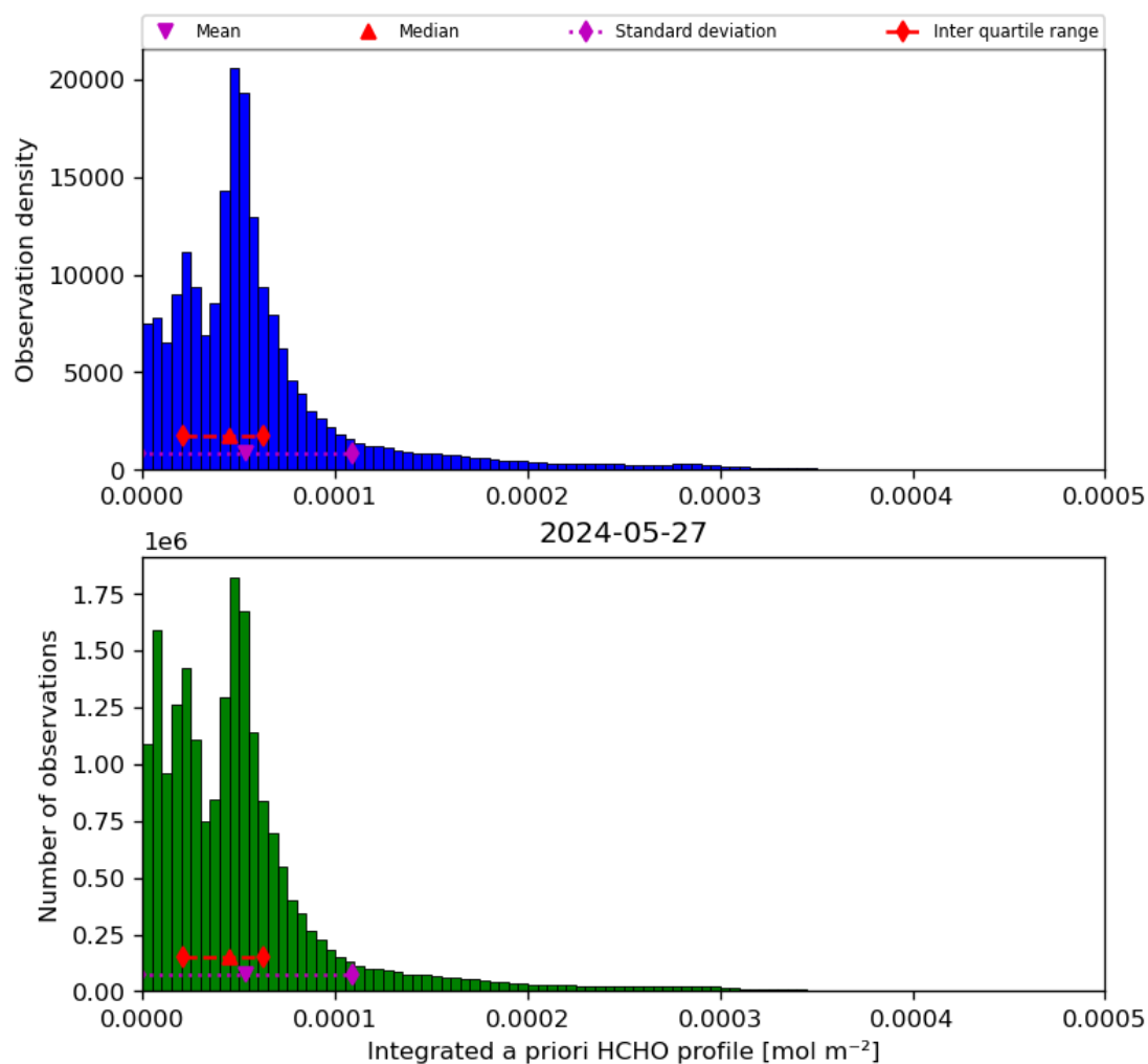
Figure 43: Histogram of “Integrated a priori HCHO profile” for 2024-05-26 to 2024-05-28
