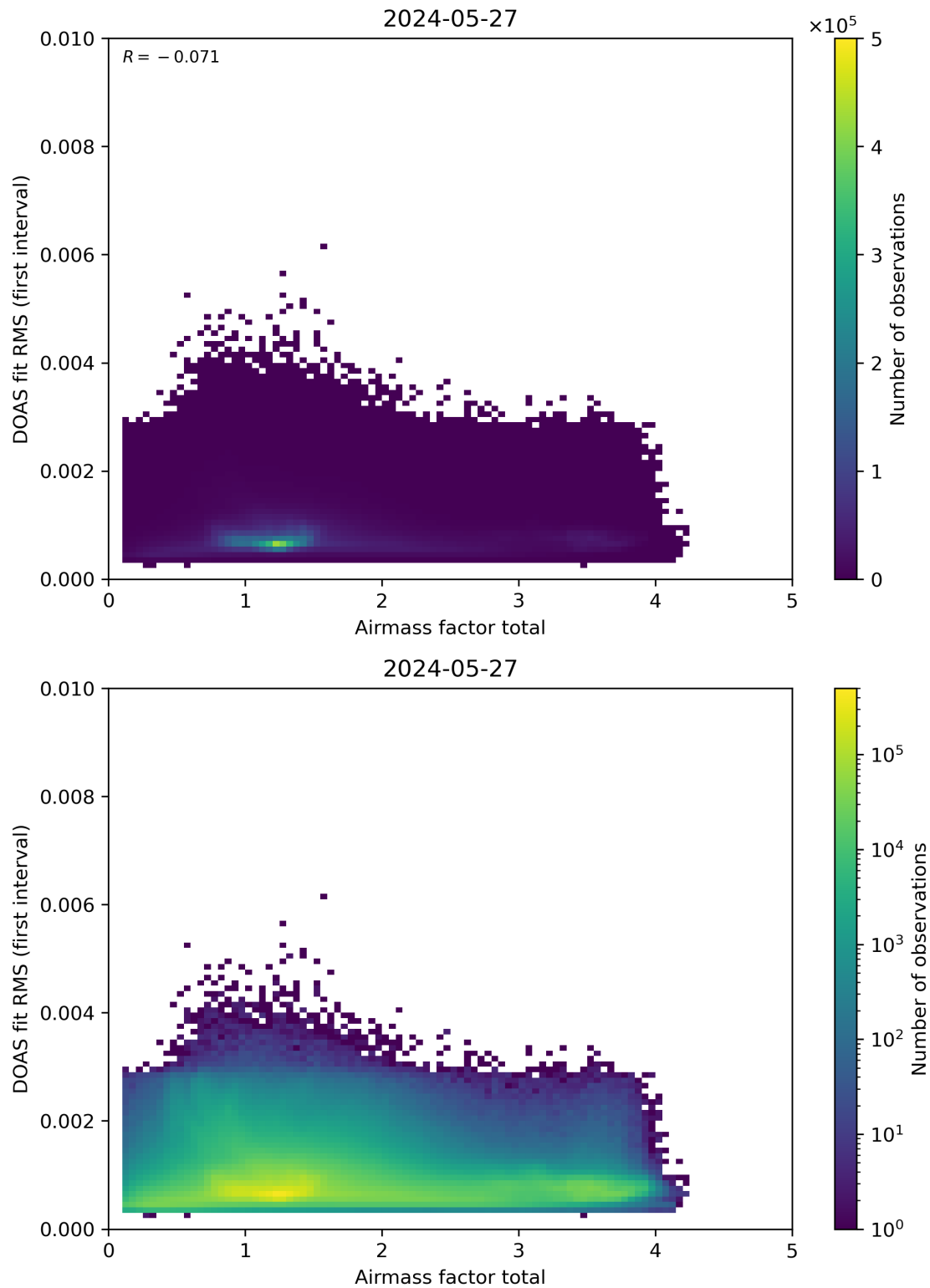
Figure 97: Scatter density plot of “Airmass factor total” against “DOAS fit RMS (first interval)” for 2024-05-26 to 2024-05-28.
