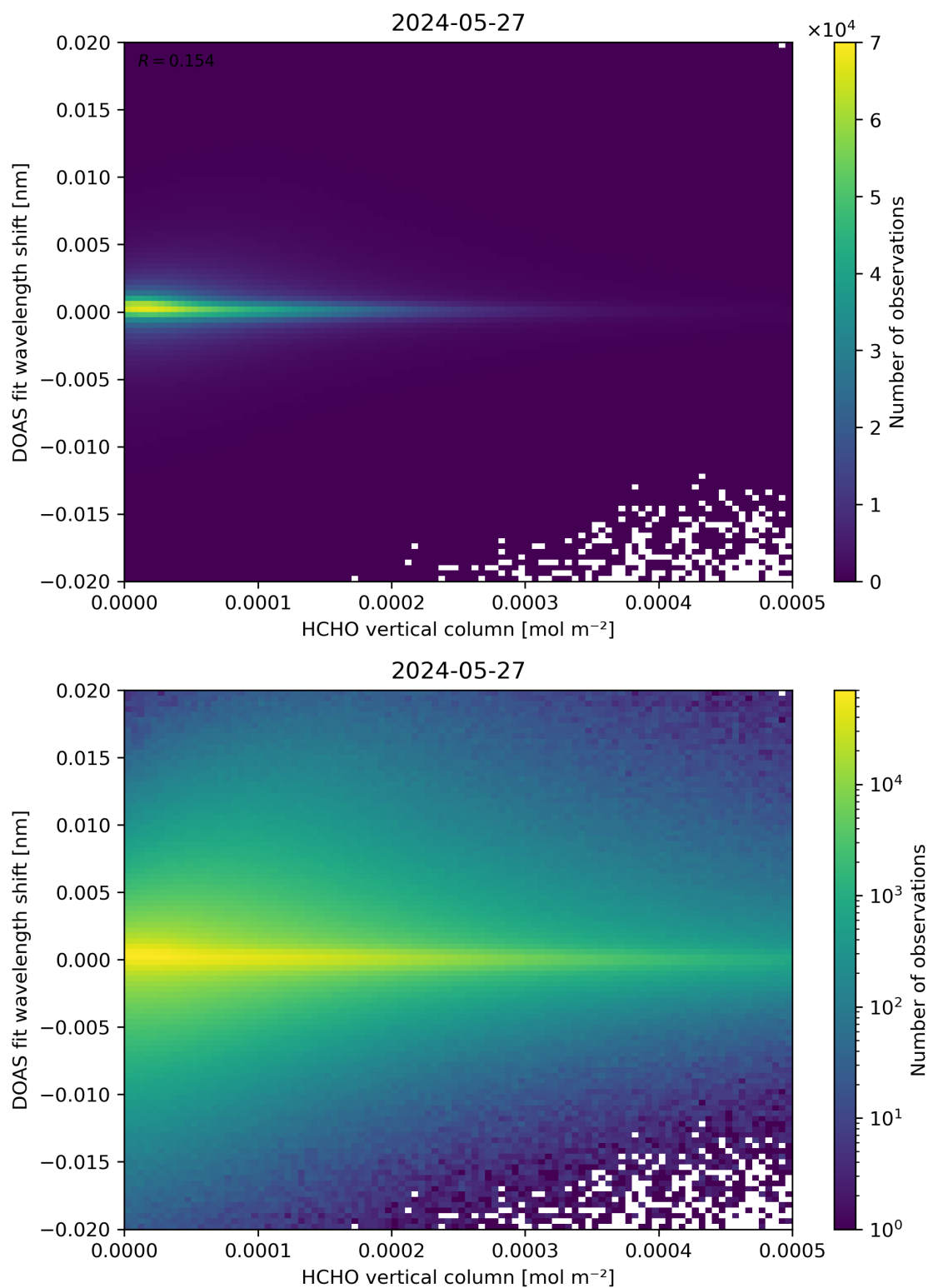
Figure 124: Scatter density plot of “HCHO vertical column” against “DOAS fit wavelength shift” for 2024-05-26 to 2024-05-28.
