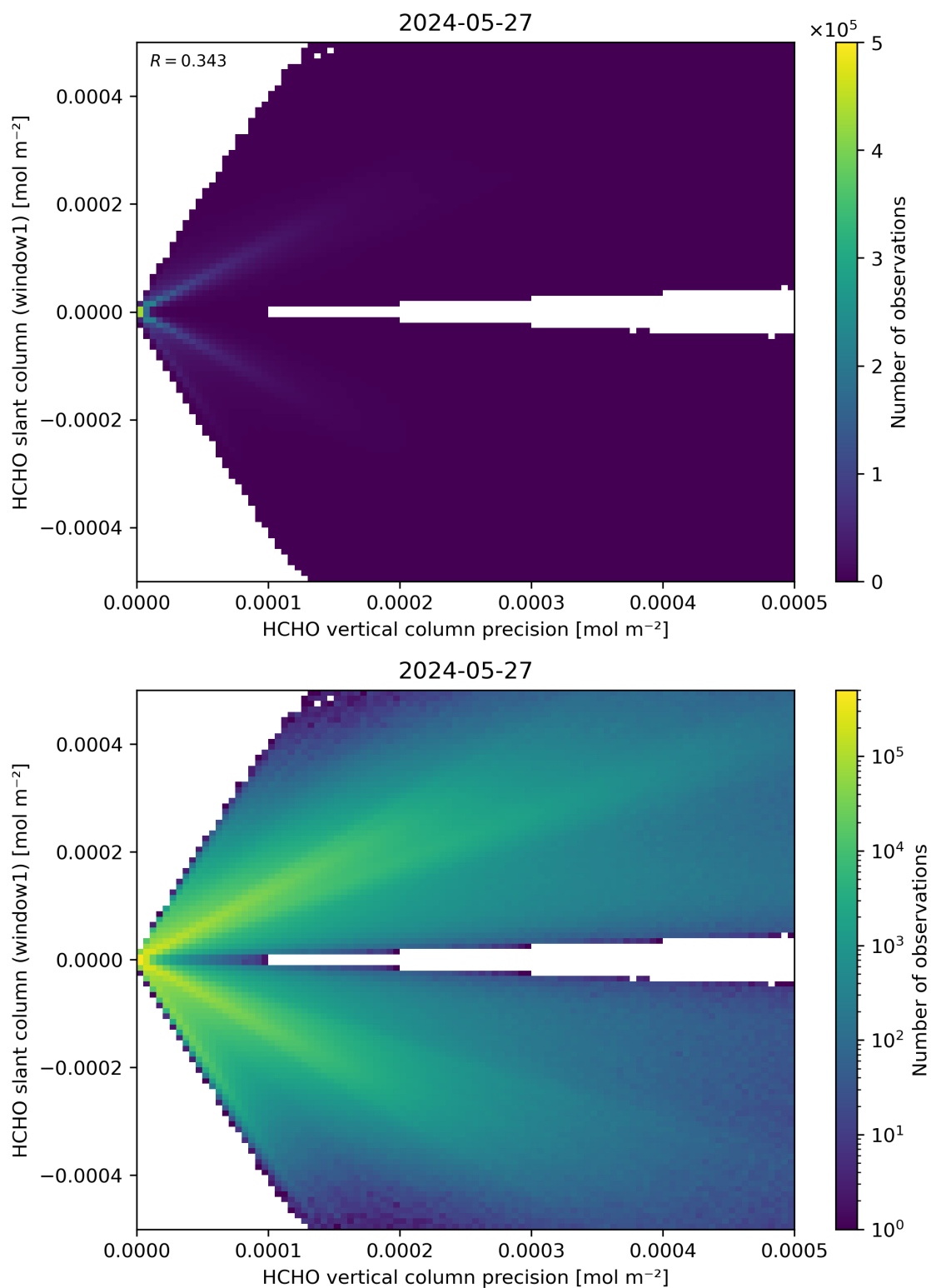
Figure 142: Scatter density plot of “HCHO vertical column precision” against “HCHO slant column (window1)” for 2024-05-26 to 2024-05-28.
