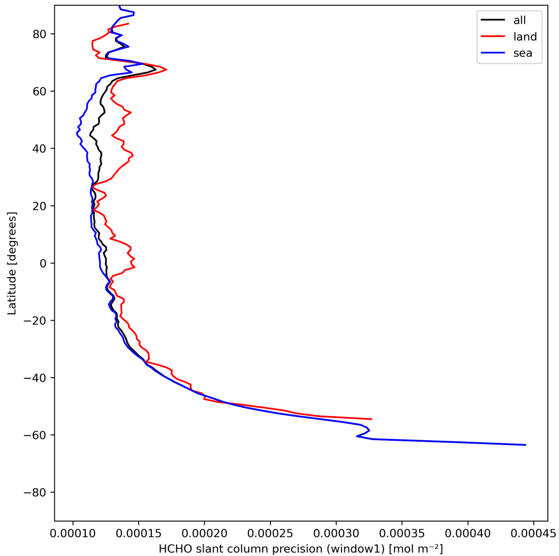
Figure 25: Zonal average of “HCHO slant column precision (window1)” for 2024-05-26 to 2024-05-28.
