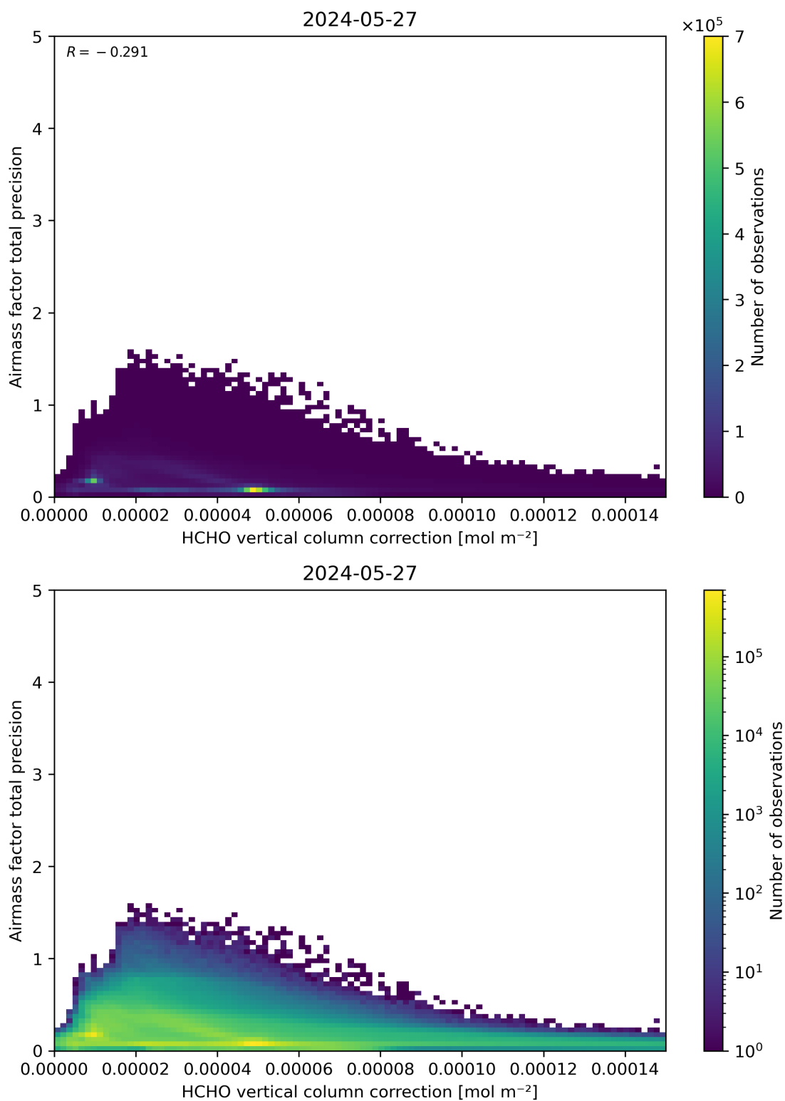
Figure 121: Scatter density plot of “HCHO vertical column correction” against “Airmass factor total precision” for 2024-05-26 to 2024-05-28.
