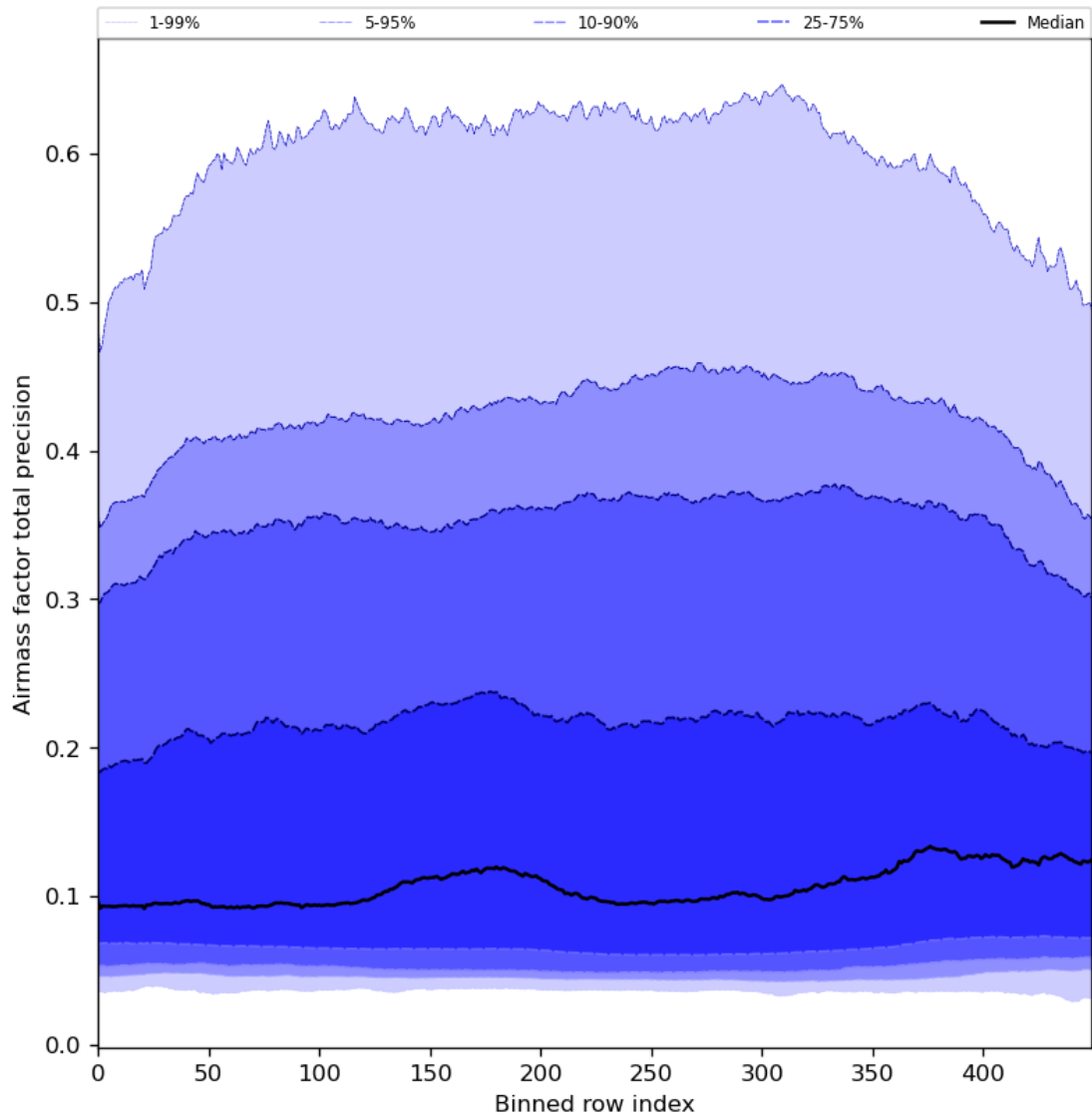
Figure 55: Along track statistics of “Airmass factor total precision” for 2024-05-26 to 2024-05-28
