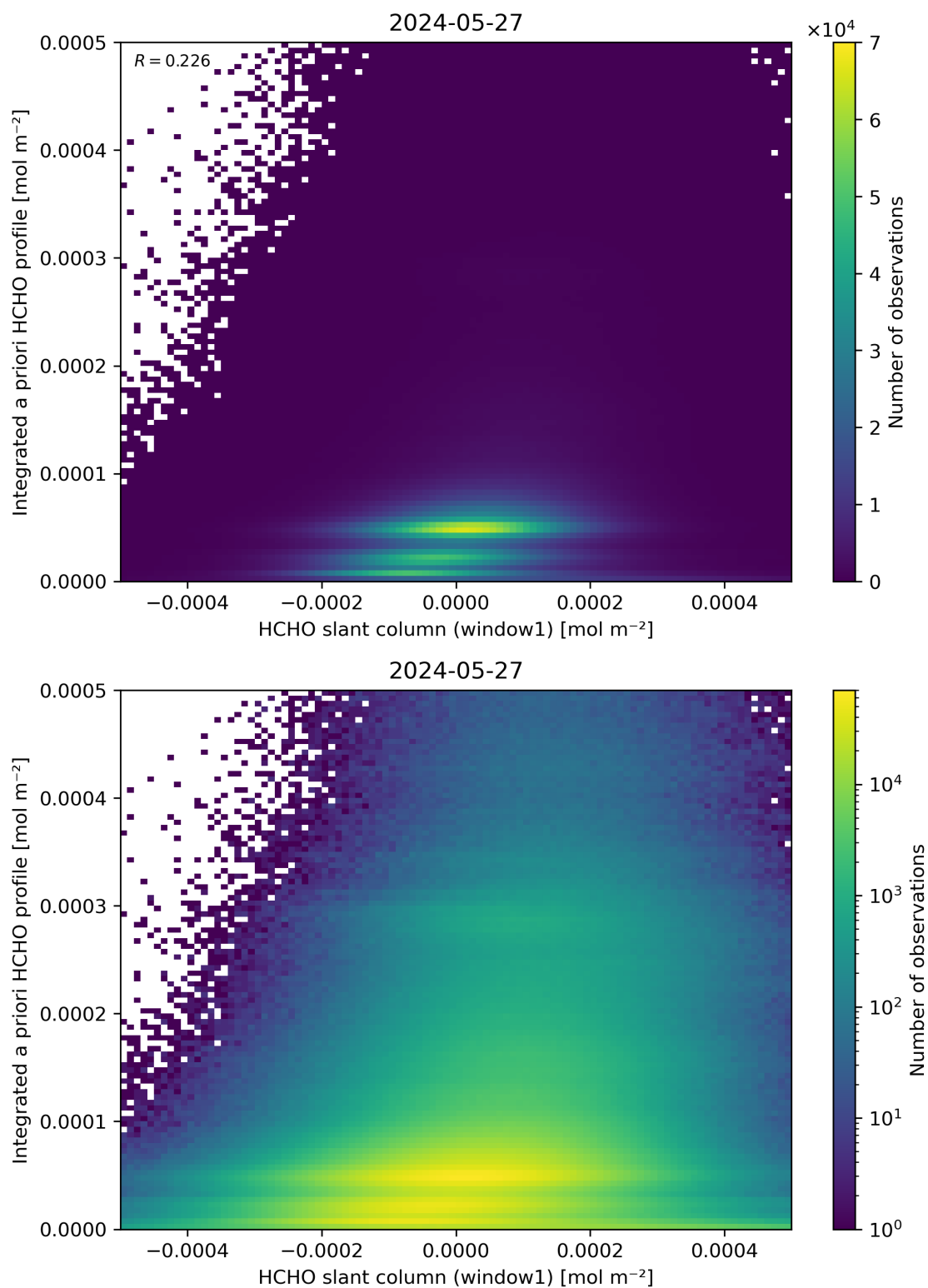
Figure 87: Scatter density plot of “HCHO slant column (window1)” against “Integrated a priori HCHO profile” for 2024-05-26 to 2024-05-28.
