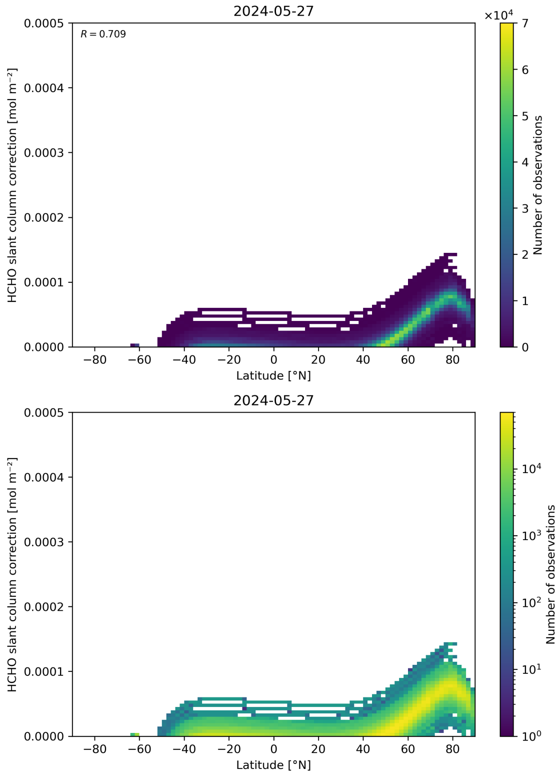
Figure 158: Scatter density plot of “Latitude” against “HCHO slant column correction” for 2024-05-26 to 2024-05-28.
