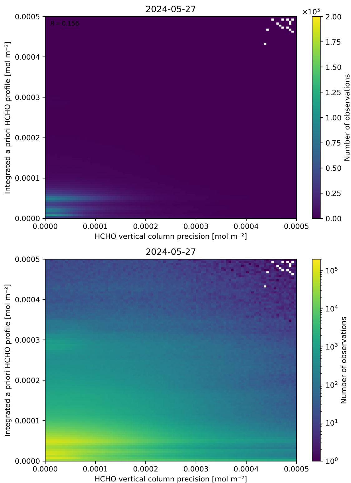
Figure 147: Scatter density plot of “HCHO vertical column precision” against “Integrated a priori HCHO profile” for 2024-05-26 to 2024-05-28.
