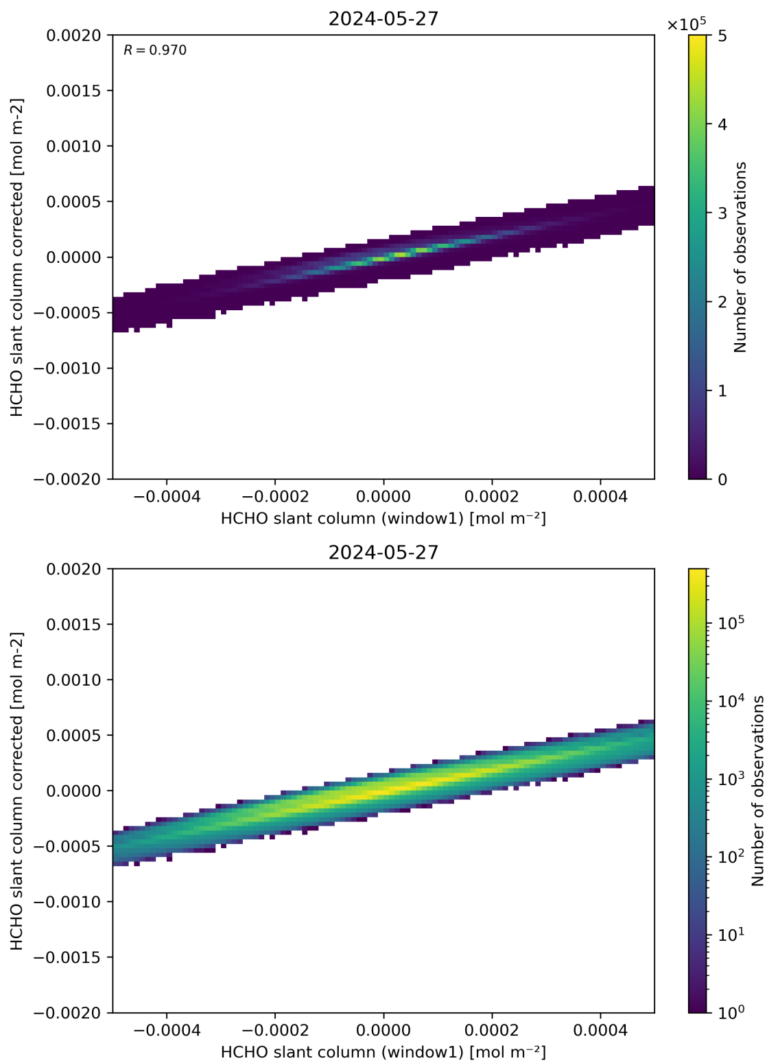
Figure 82: Scatter density plot of “HCHO slant column (window1)” against “HCHO slant column corrected” for 2024-05-26 to 2024-05-28.
