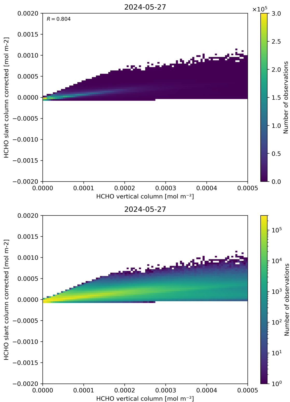
Figure 127: Scatter density plot of “HCHO vertical column” against “HCHO slant column corrected” for 2024-05-26 to 2024-05-28.
