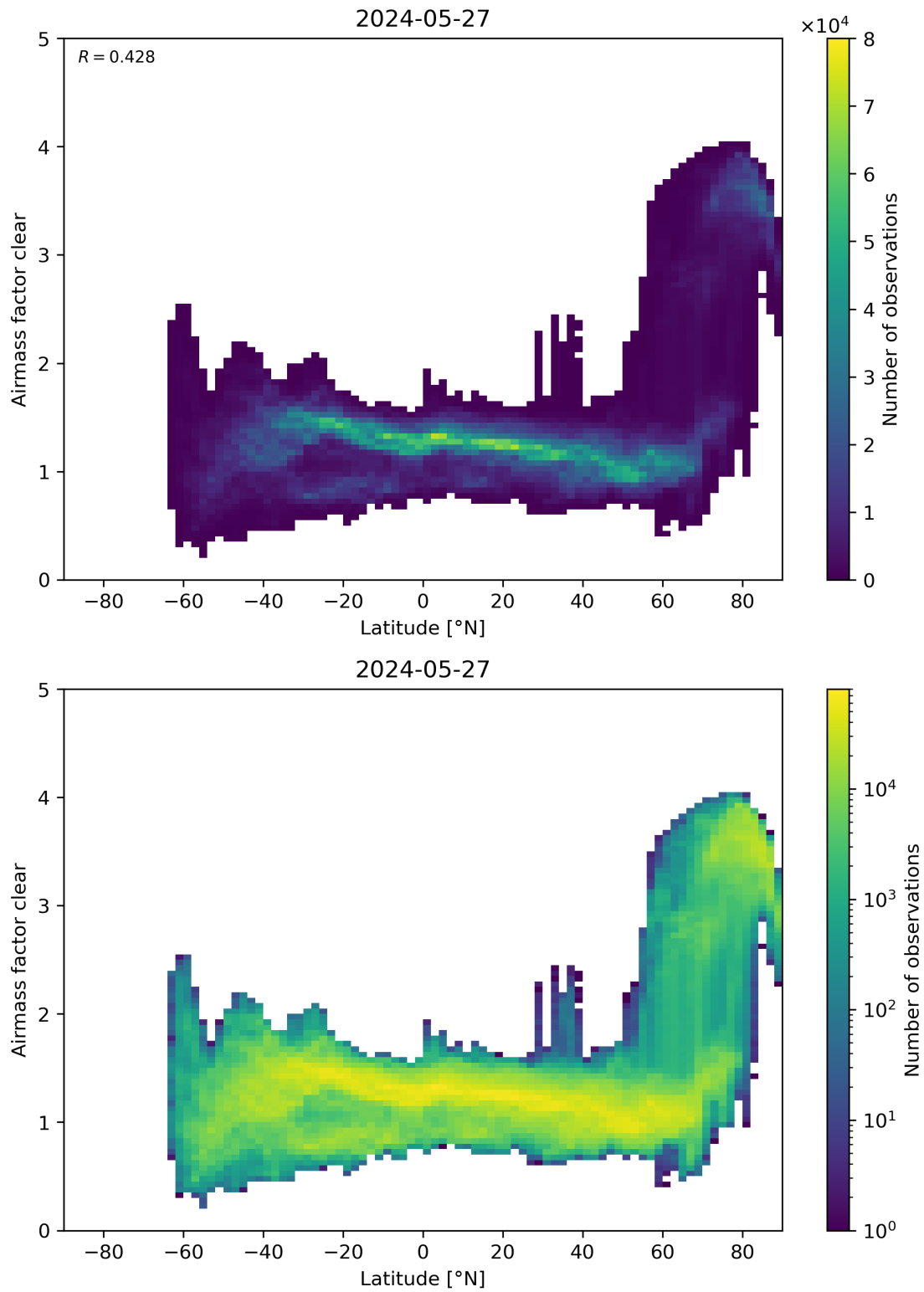
Figure 156: Scatter density plot of “Latitude” against “Airmass factor clear” for 2024-05-26 to 2024-05-28.
