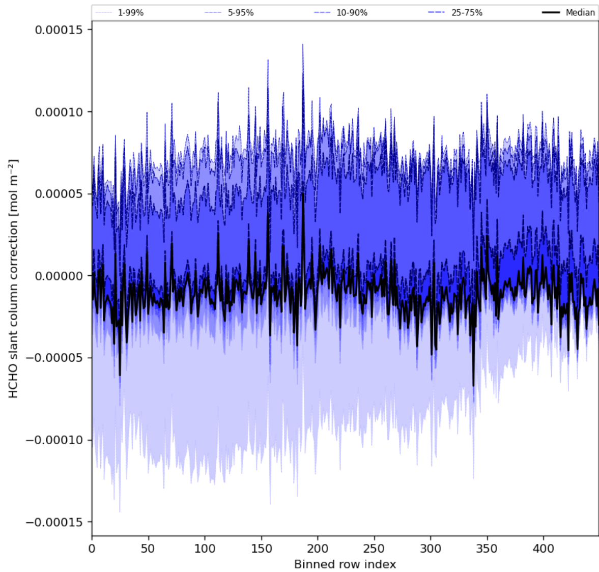
Figure 61: Along track statistics of “HCHO slant column correction” for 2024-05-26 to 2024-05-28
