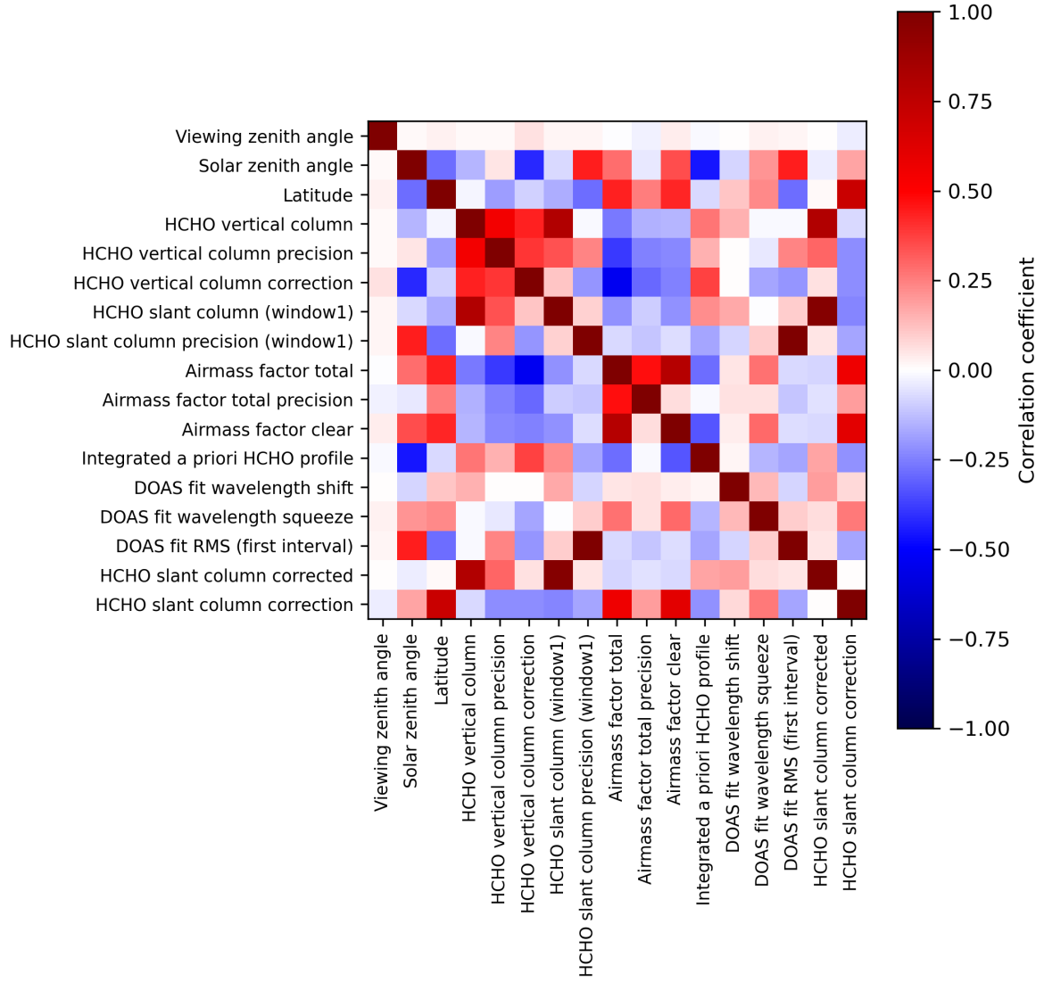
Figure 2: Map of correlation matrix for 2024-05-26 to 2024-05-28.
