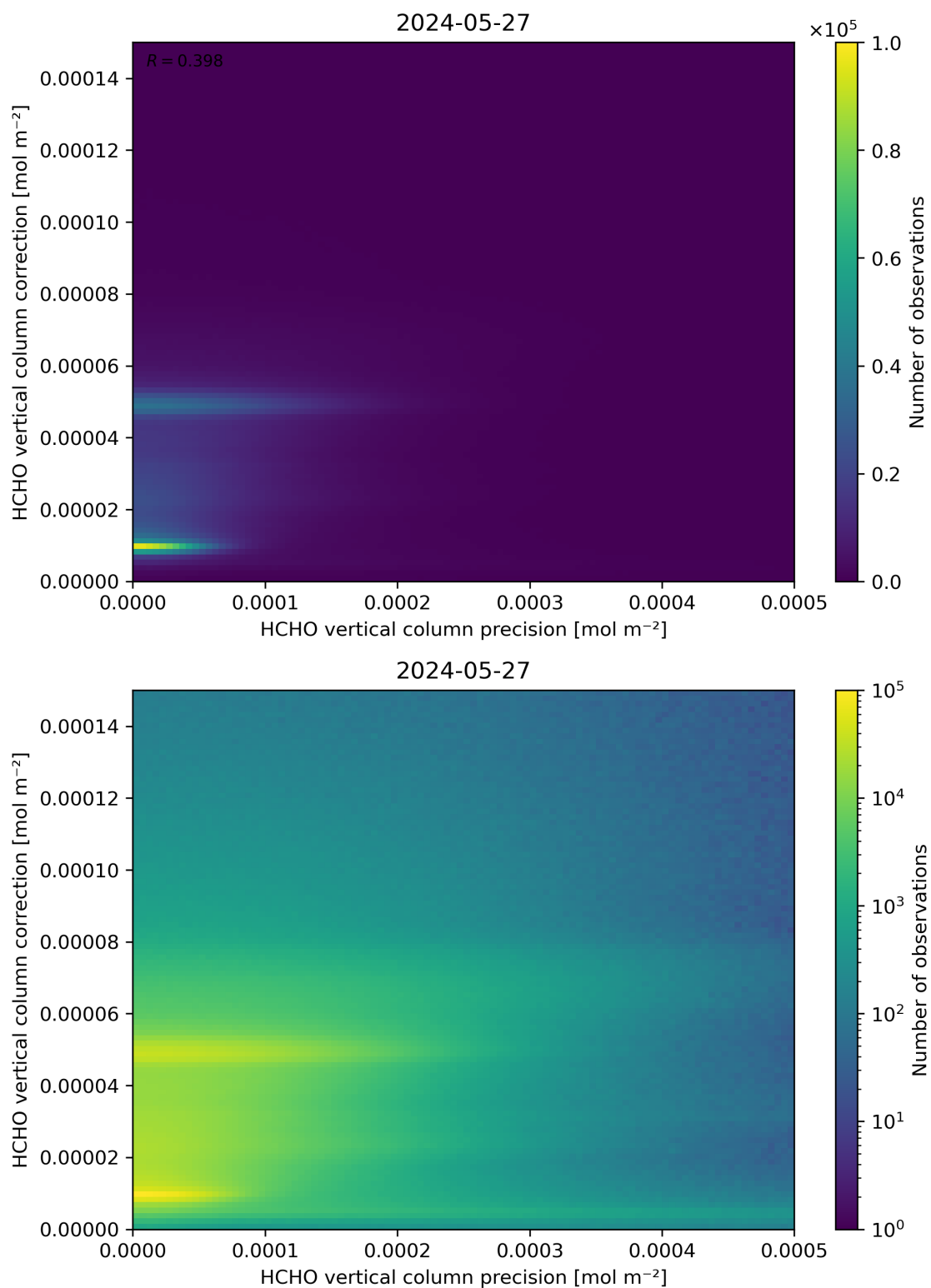
Figure 146: Scatter density plot of “HCHO vertical column precision” against “HCHO vertical column correction” for 2024-05-26 to 2024-05-28.
