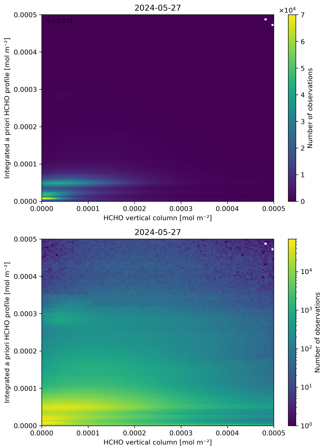
Figure 135: Scatter density plot of “HCHO vertical column” against “Integrated a priori HCHO profile” for 2024-05-26 to 2024-05-28.
