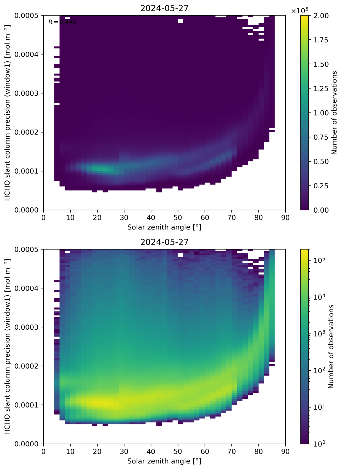
Figure 174: Scatter density plot of “Solar zenith angle” against “HCHO slant column precision (window1)” for 2024-05-26 to 2024-05-28.
