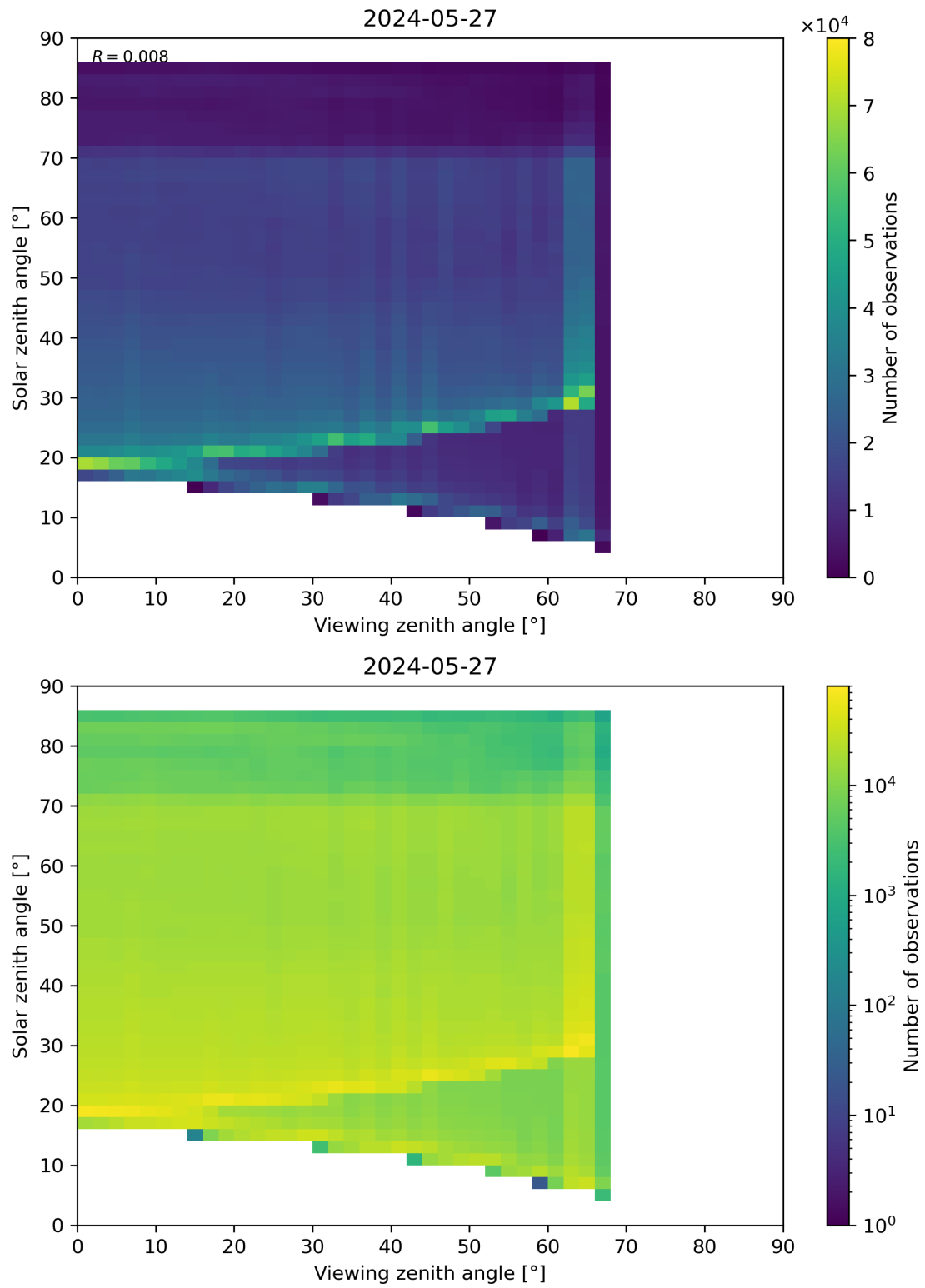
Figure 197: Scatter density plot of “Viewing zenith angle” against “Solar zenith angle” for 2024-05-26 to 2024-05-28.
