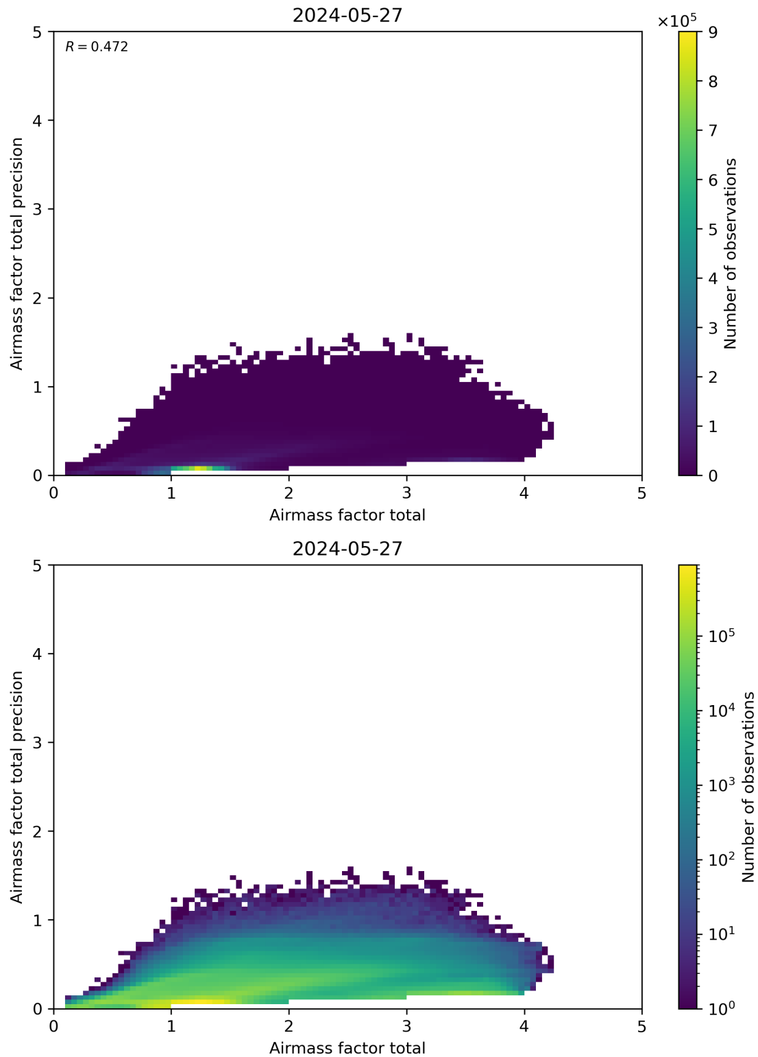
Figure 103: Scatter density plot of “Airmass factor total” against “Airmass factor total precision” for 2024-05-26 to 2024-05-28.
