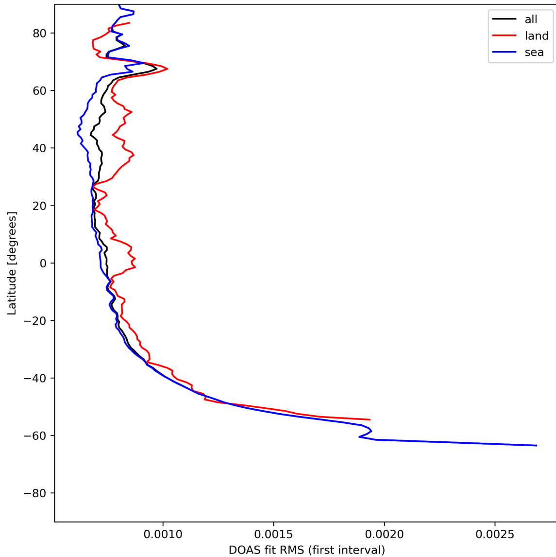
Figure 32: Zonal average of “DOAS fit RMS (first interval)” for 2024-05-26 to 2024-05-28.
