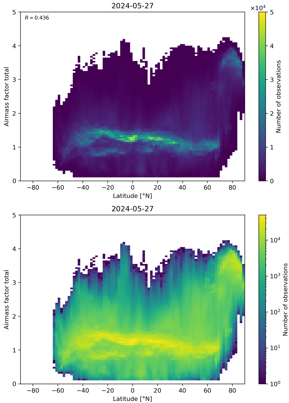
Figure 161: Scatter density plot of “Latitude” against “Airmass factor total” for 2024-05-26 to 2024-05-28.
