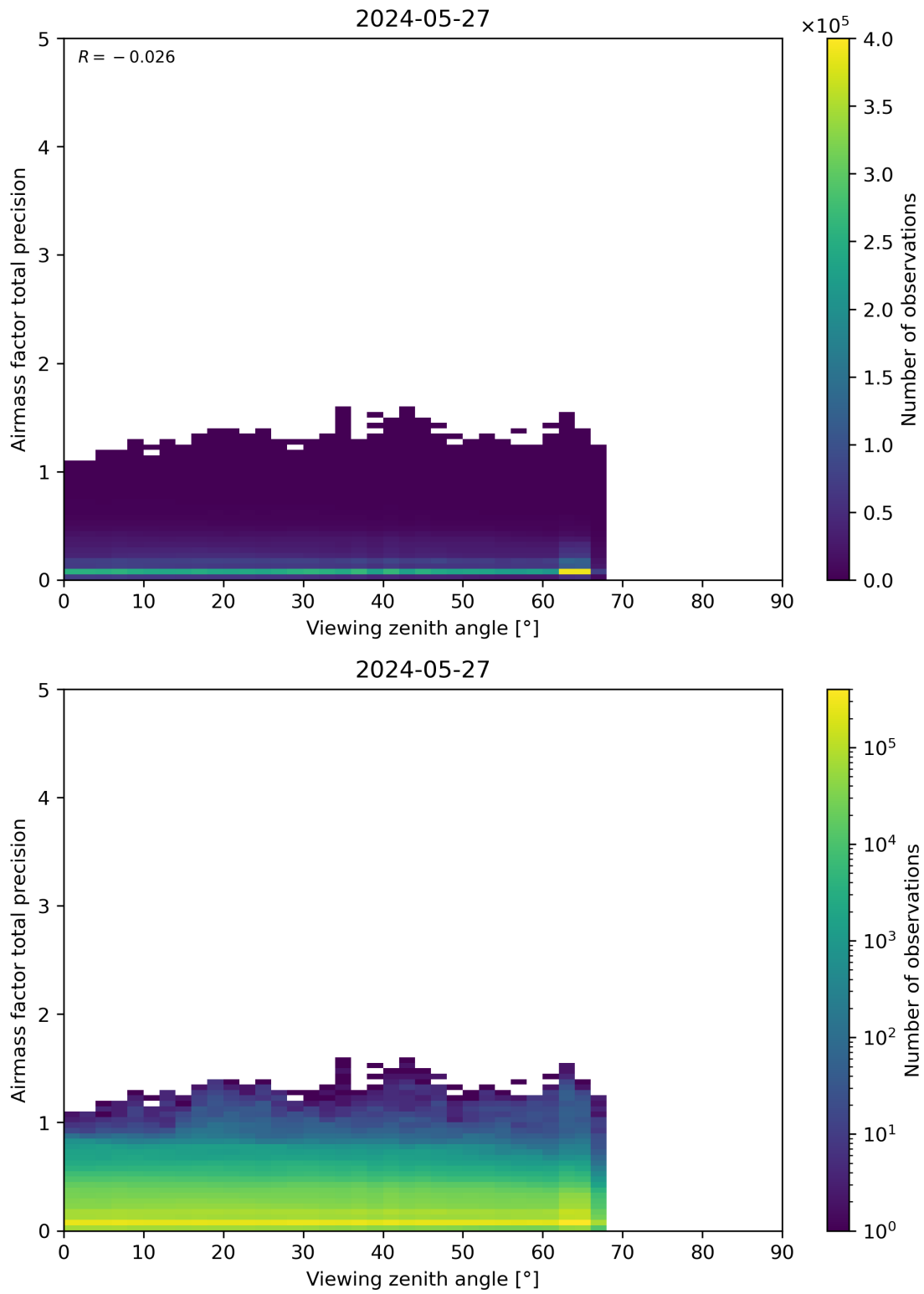
Figure 191: Scatter density plot of “Viewing zenith angle” against “Airmass factor total precision” for 2024-05-26 to 2024-05-28.
