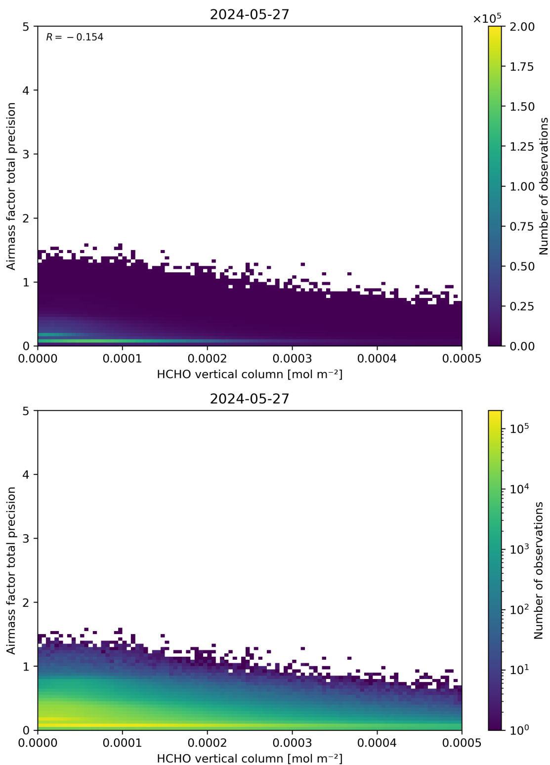
Figure 132: Scatter density plot of “HCHO vertical column” against “Airmass factor total precision” for 2024-05-26 to 2024-05-28.
