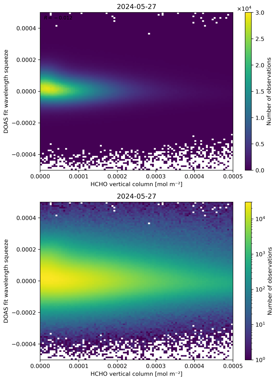
Figure 125: Scatter density plot of “HCHO vertical column” against “DOAS fit wavelength squeeze” for 2024-05-26 to 2024-05-28.
