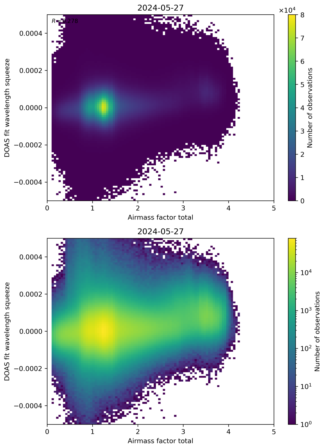
Figure 99: Scatter density plot of “Airmass factor total” against “DOAS fit wavelength squeeze” for 2024-05-26 to 2024-05-28.
