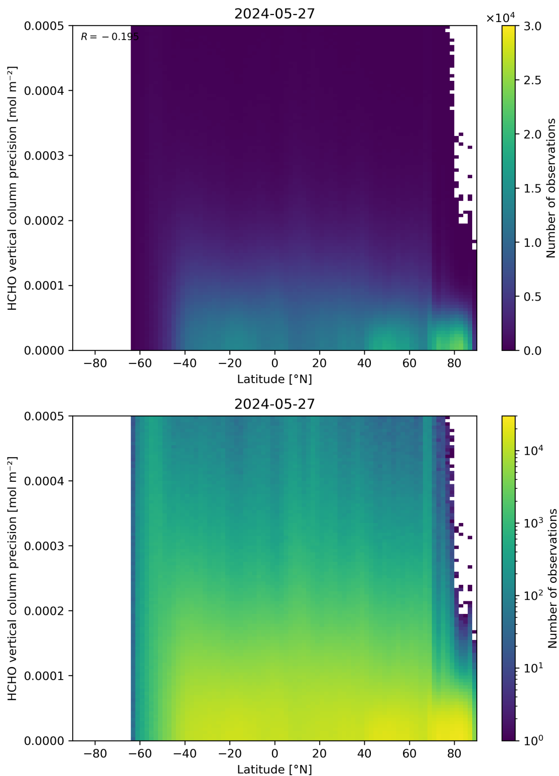
Figure 165: Scatter density plot of “Latitude” against “HCHO vertical column precision” for 2024-05-26 to 2024-05-28.
