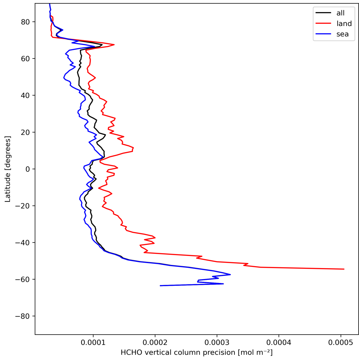
Figure 22: Zonal average of “HCHO vertical column precision” for 2024-05-26 to 2024-05-28.
