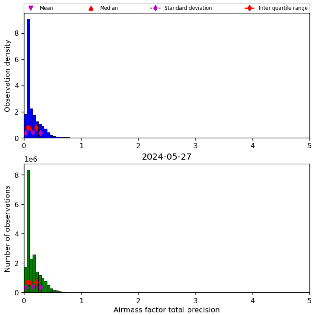
Figure 41: Histogram of “Airmass factor total precision” for 2024-05-26 to 2024-05-28
