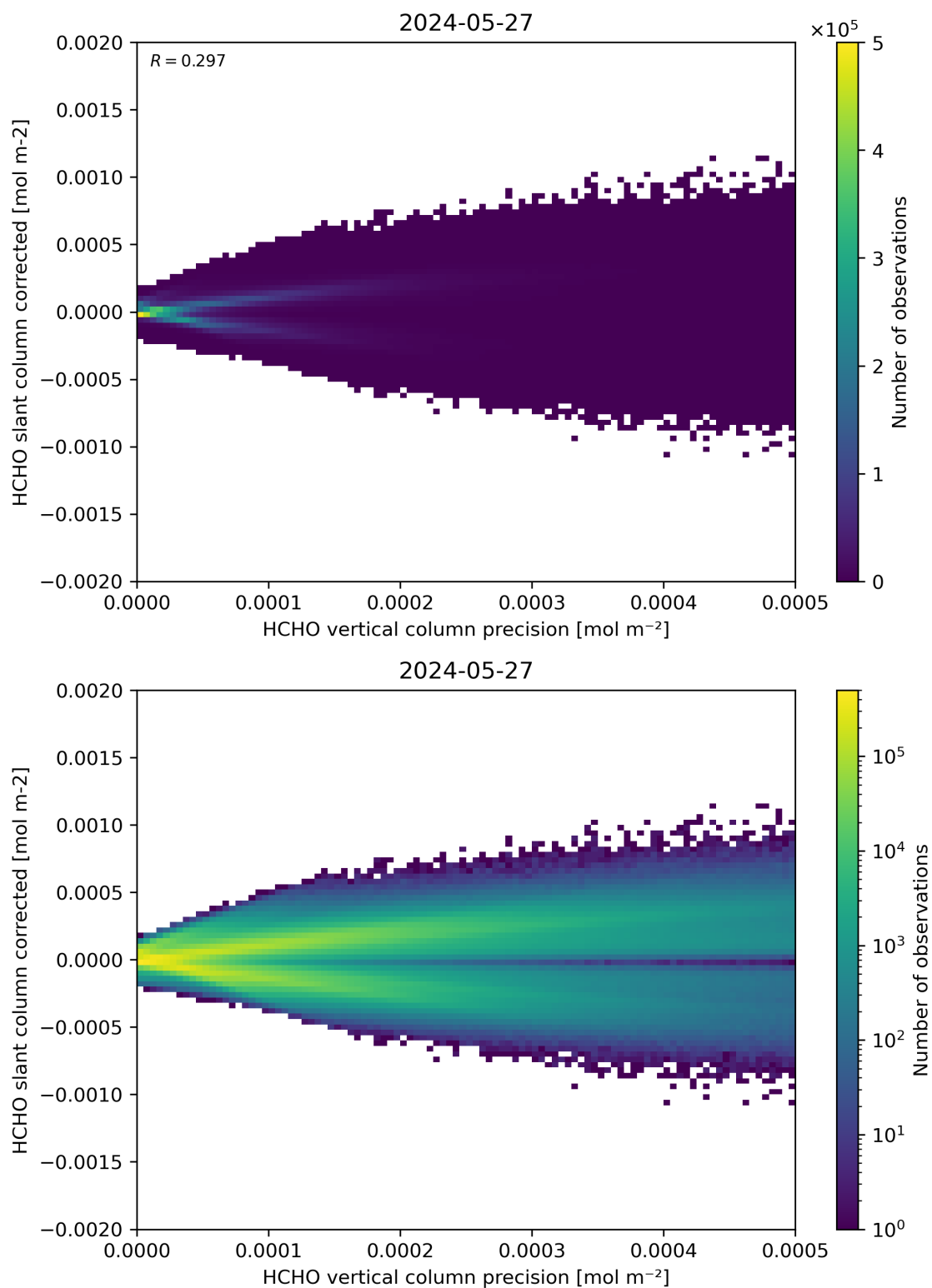
Figure 140: Scatter density plot of “HCHO vertical column precision” against “HCHO slant column corrected” for 2024-05-26 to 2024-05-28.
