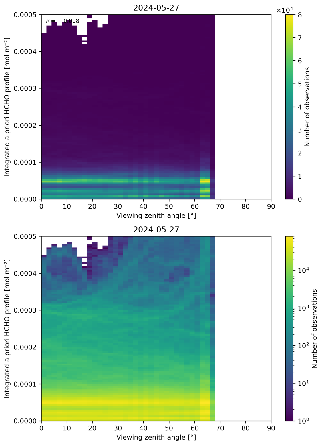
Figure 195: Scatter density plot of “Viewing zenith angle” against “Integrated a priori HCHO profile” for 2024-05-26 to 2024-05-28.
