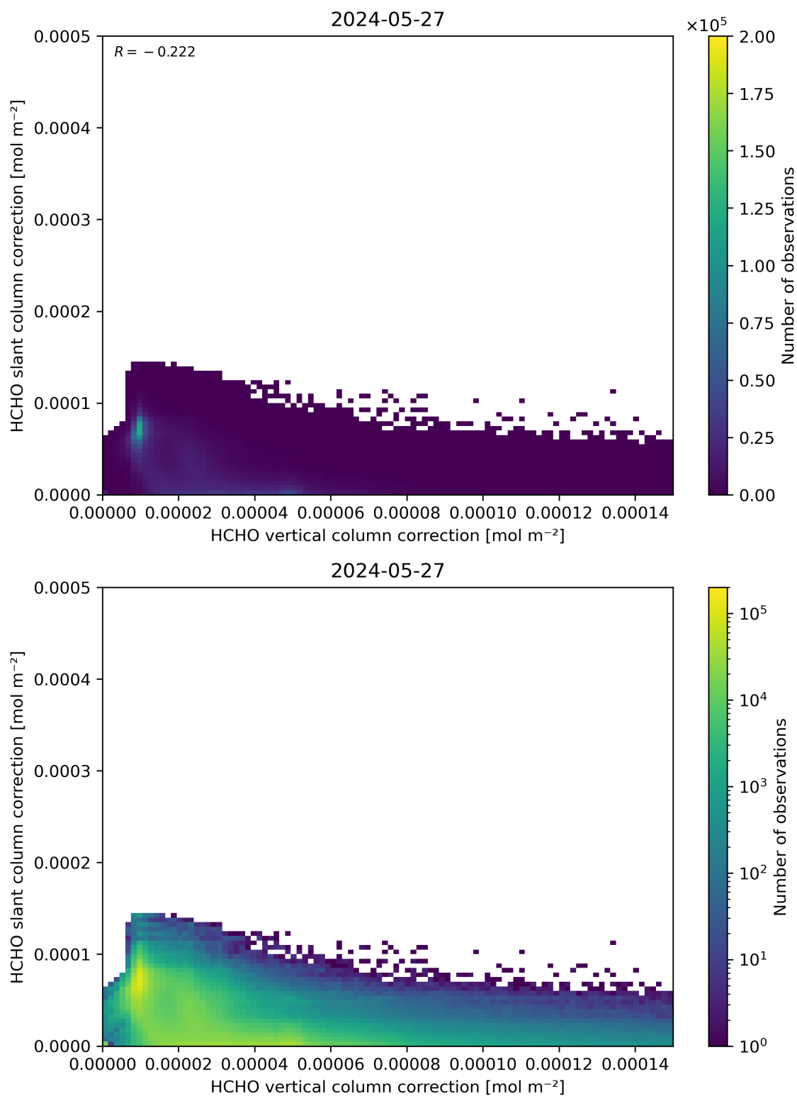
Figure 117: Scatter density plot of “HCHO vertical column correction” against “HCHO slant column correction” for 2024-05-26 to 2024-05-28.
