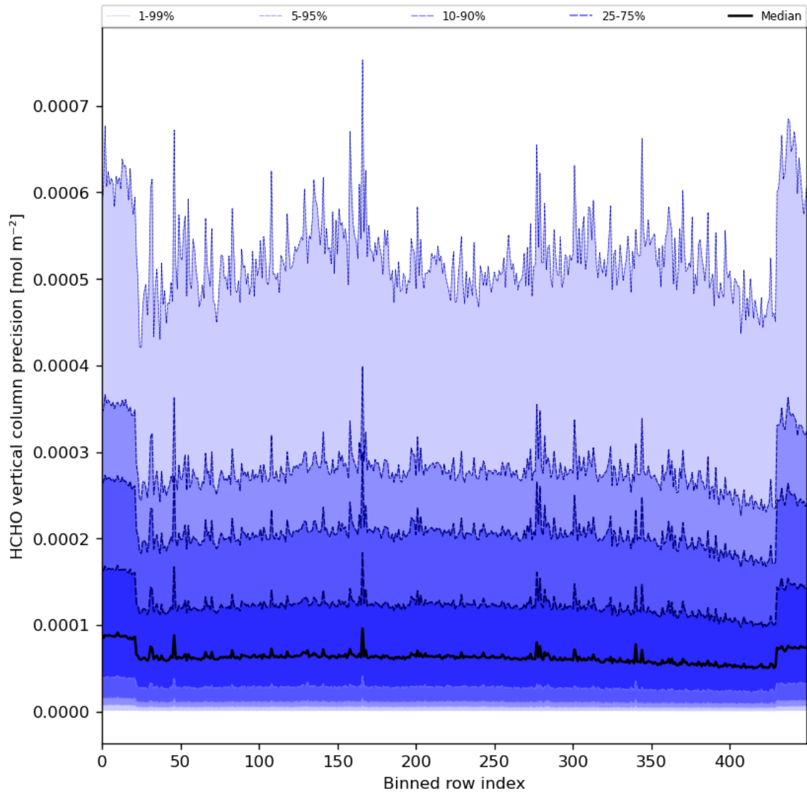
Figure 50: Along track statistics of “HCHO vertical column precision” for 2024-05-26 to 2024-05-28
