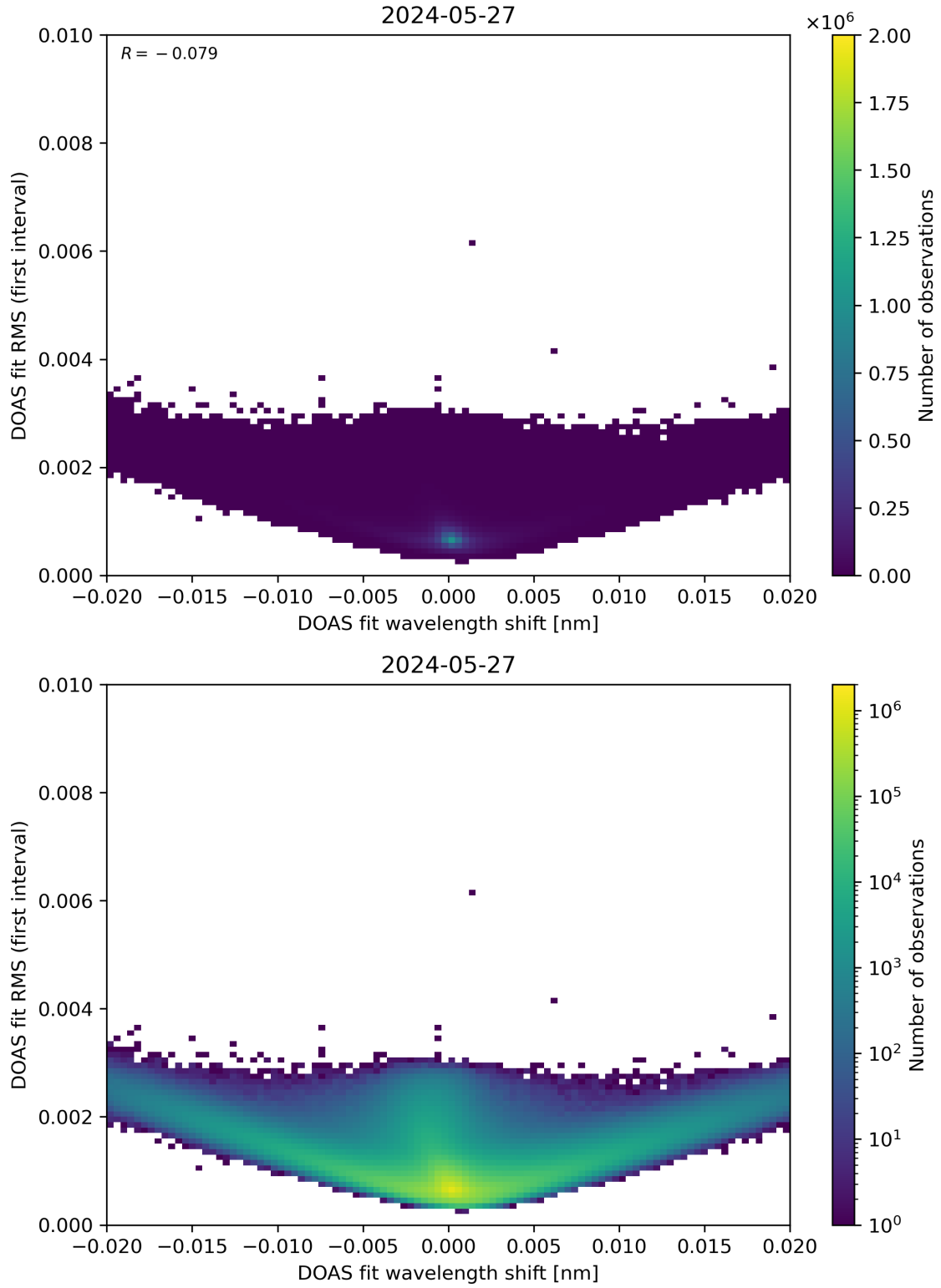
Figure 64: Scatter density plot of “DOAS fit wavelength shift” against “DOAS fit RMS (first interval)” for 2024-05-26 to 2024-05-28.
