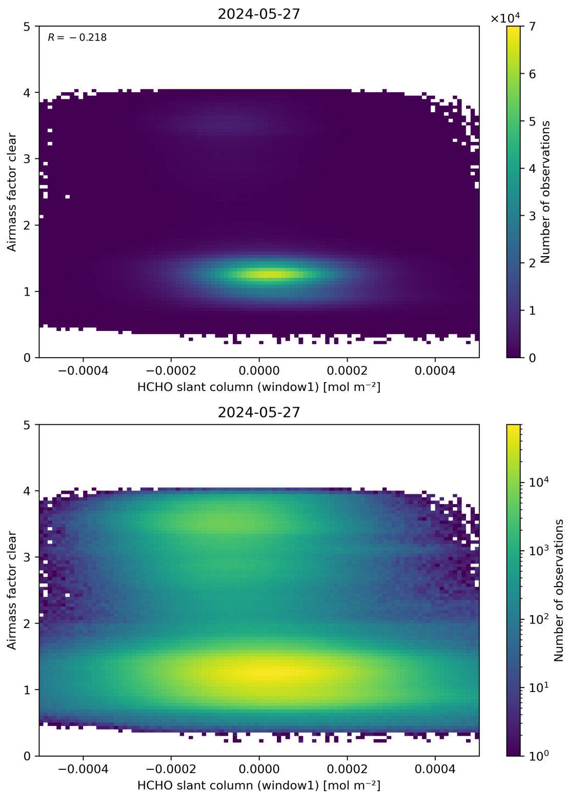
Figure 81: Scatter density plot of “HCHO slant column (window1)” against “Airmass factor clear” for 2024-05-26 to 2024-05-28.
