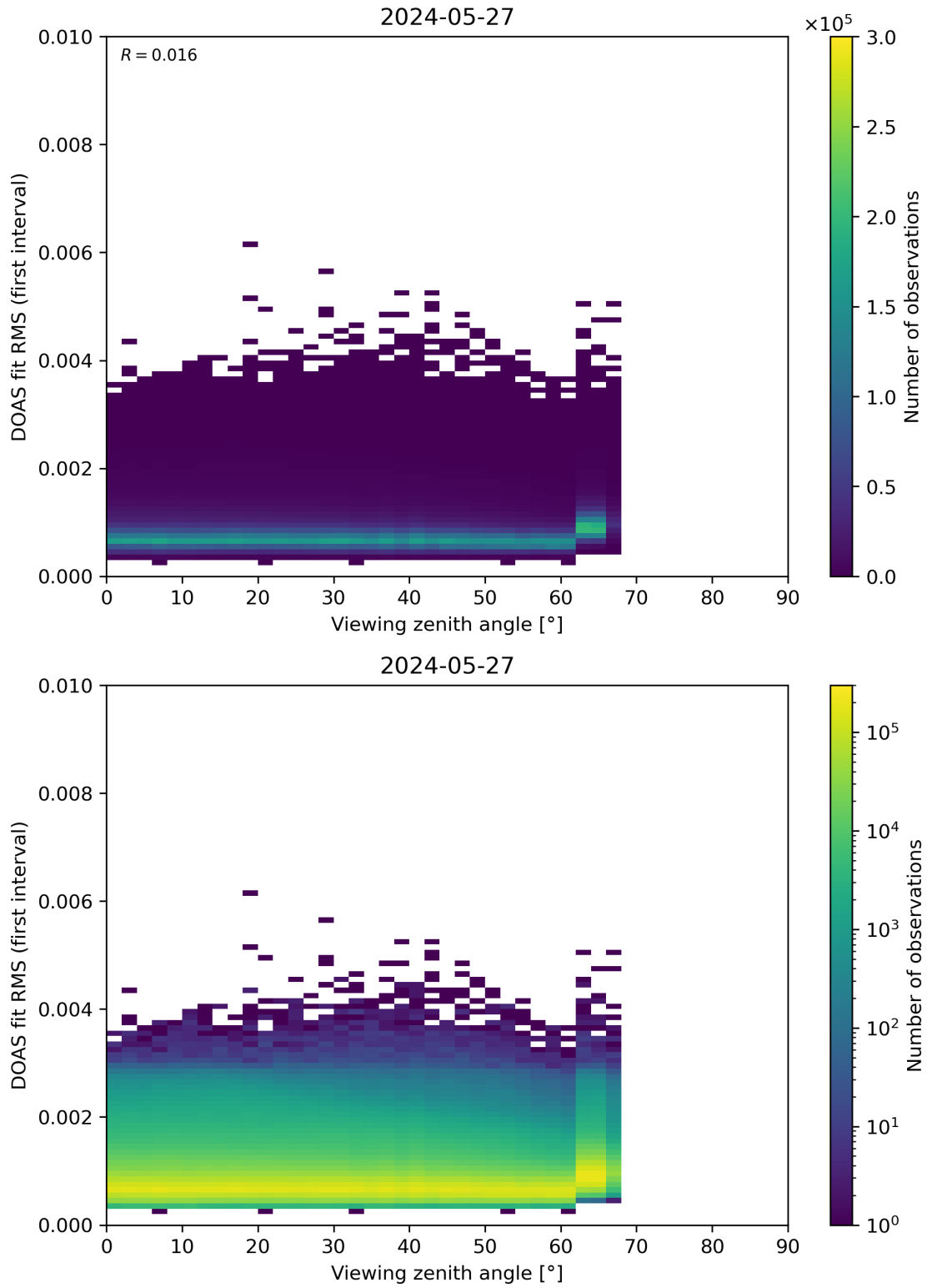
Figure 182: Scatter density plot of “Viewing zenith angle” against “DOAS fit RMS (first interval)” for 2024-05-26 to 2024-05-28.
