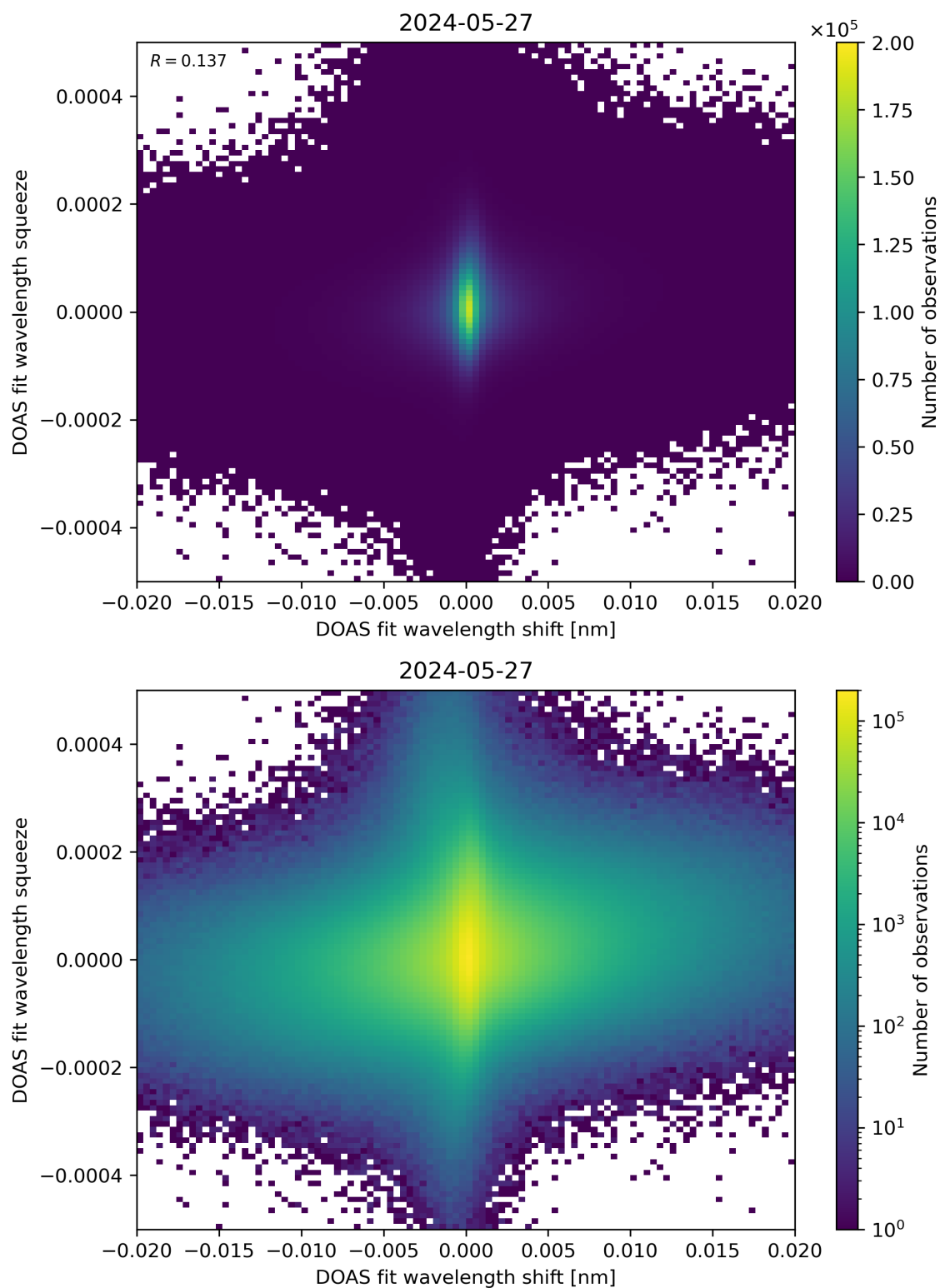
Figure 65: Scatter density plot of “DOAS fit wavelength shift” against “DOAS fit wavelength squeeze” for 2024-05-26 to 2024-05-28.
