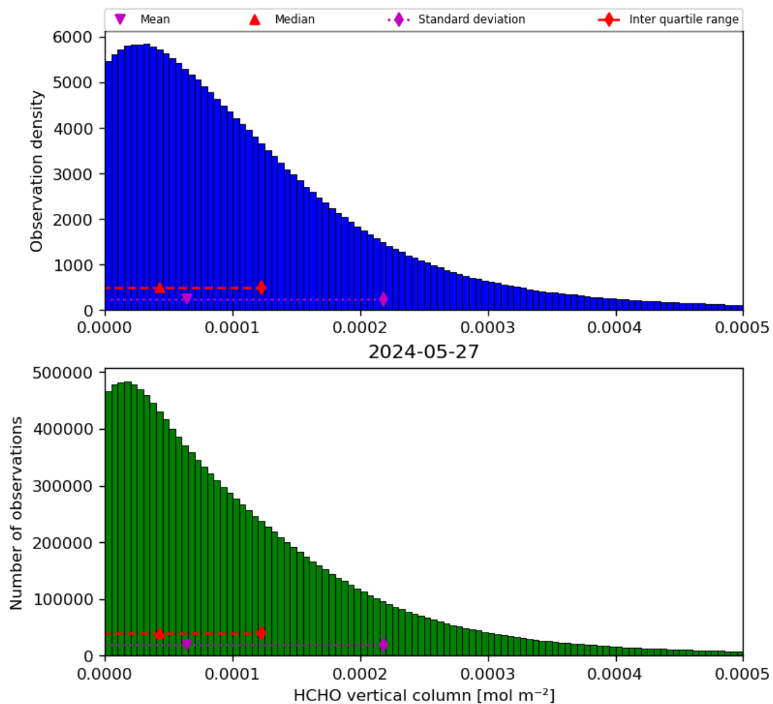
Figure 35: Histogram of “HCHO vertical column” for 2024-05-26 to 2024-05-28
