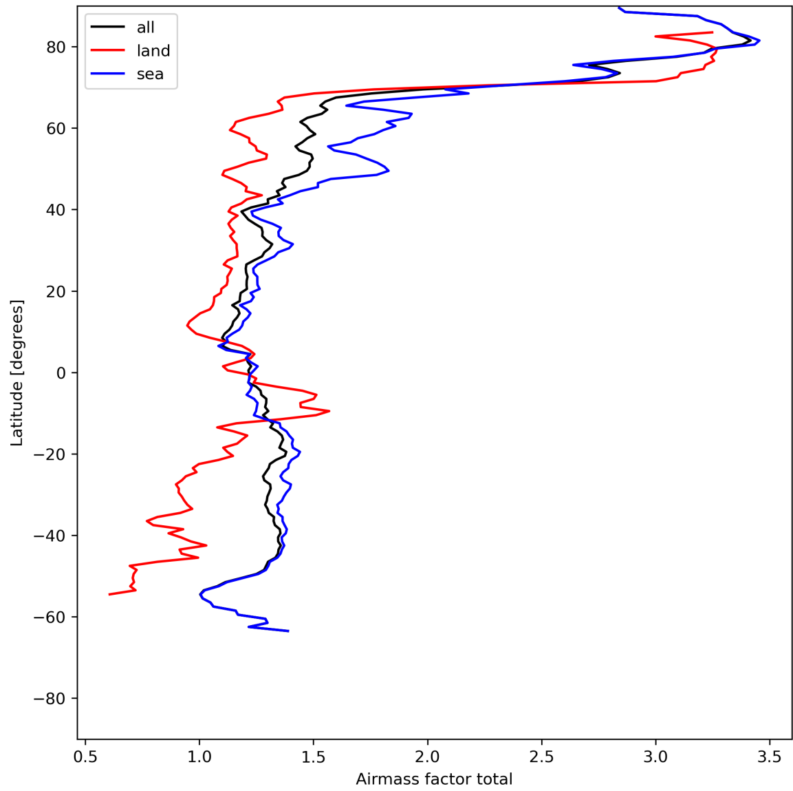
Figure 26: Zonal average of “Airmass factor total” for 2024-05-26 to 2024-05-28.
