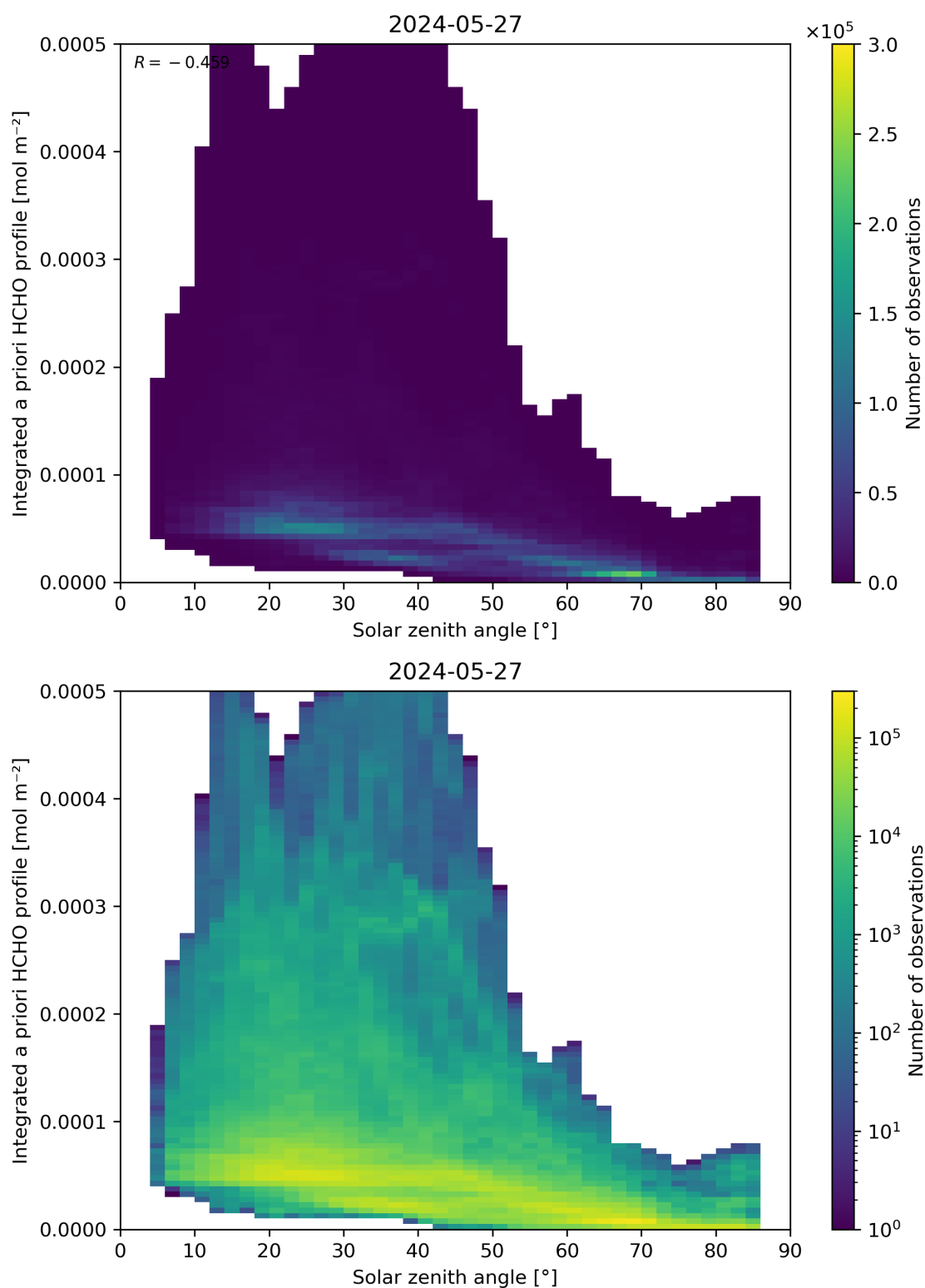
Figure 180: Scatter density plot of “Solar zenith angle” against “Integrated a priori HCHO profile” for 2024-05-26 to 2024-05-28.
