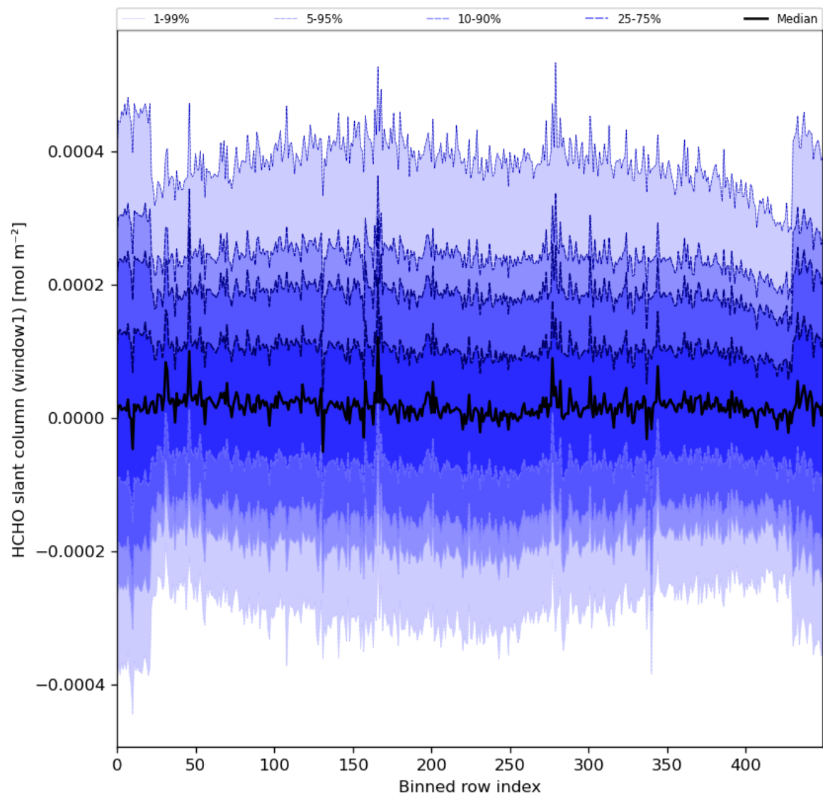
Figure 52: Along track statistics of “HCHO slant column (window1)” for 2024-05-26 to 2024-05-28
