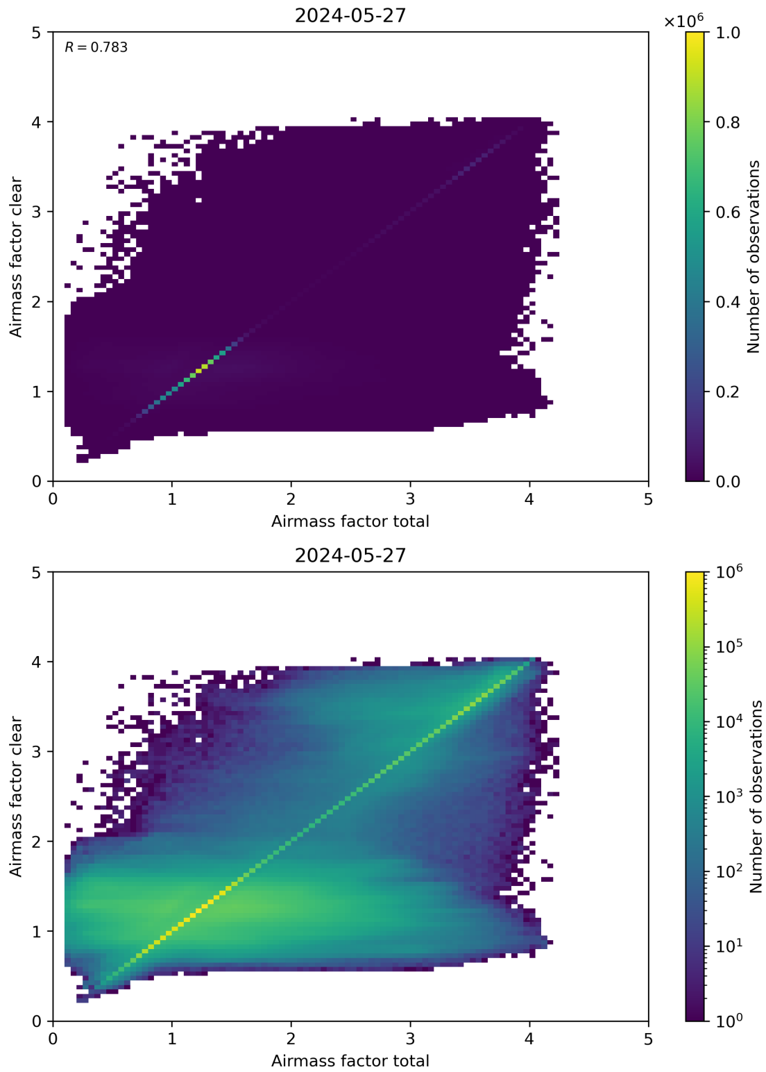
Figure 100: Scatter density plot of “Airmass factor total” against “Airmass factor clear” for 2024-05-26 to 2024-05-28.
