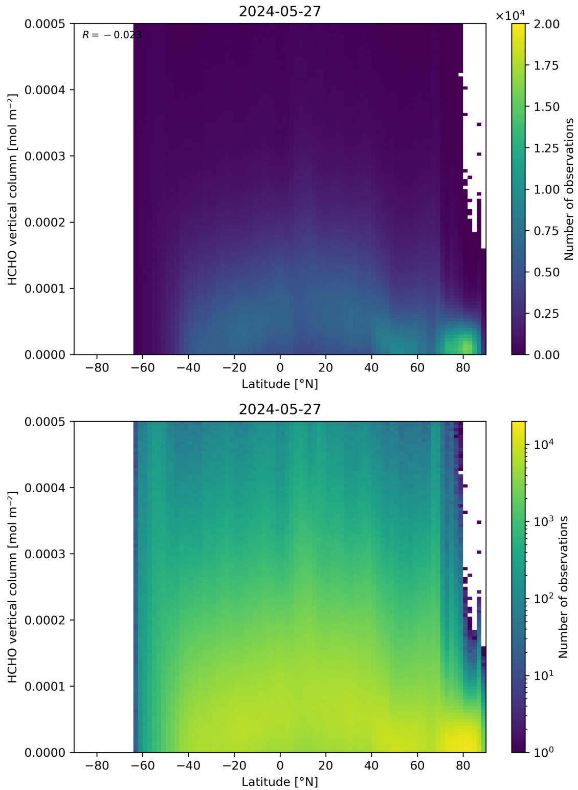
Figure 163: Scatter density plot of “Latitude” against “HCHO vertical column” for 2024-05-26 to 2024-05-28.
