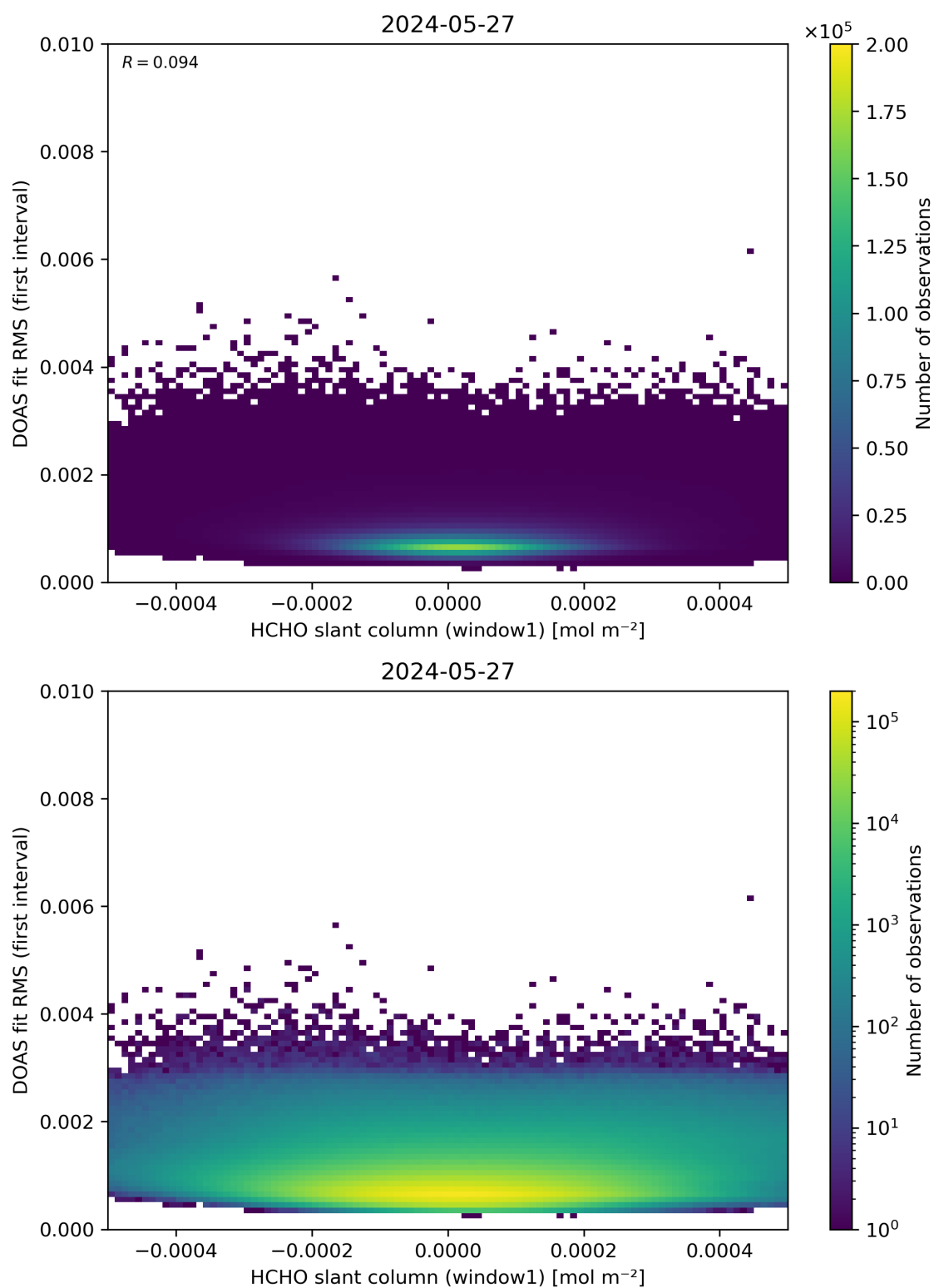
Figure 78: Scatter density plot of “HCHO slant column (window1)” against “DOAS fit RMS (first interval)” for 2024-05-26 to 2024-05-28.
