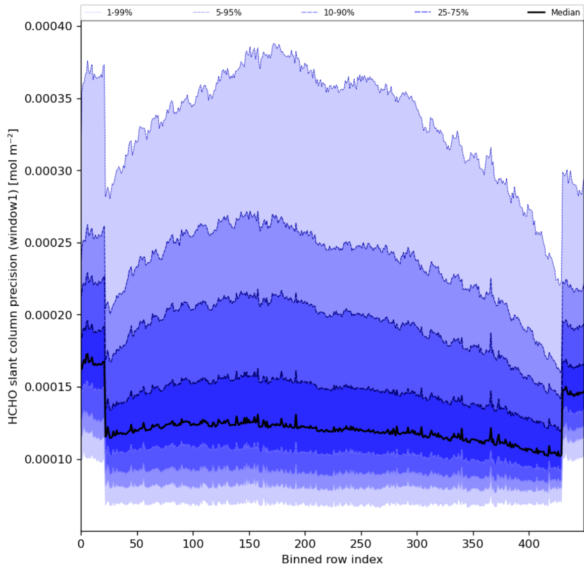
Figure 53: Along track statistics of “HCHO slant column precision (window1)” for 2024-05-26 to 2024-05-28
