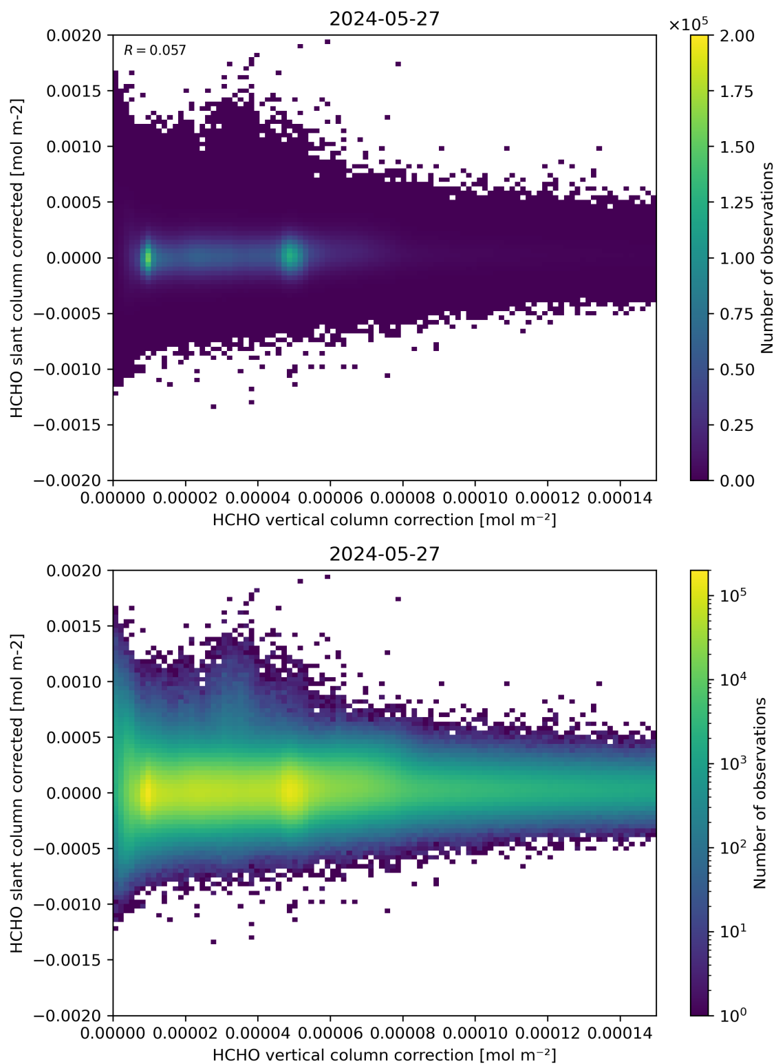
Figure 116: Scatter density plot of “HCHO vertical column correction” against “HCHO slant column corrected” for 2024-05-26 to 2024-05-28.
