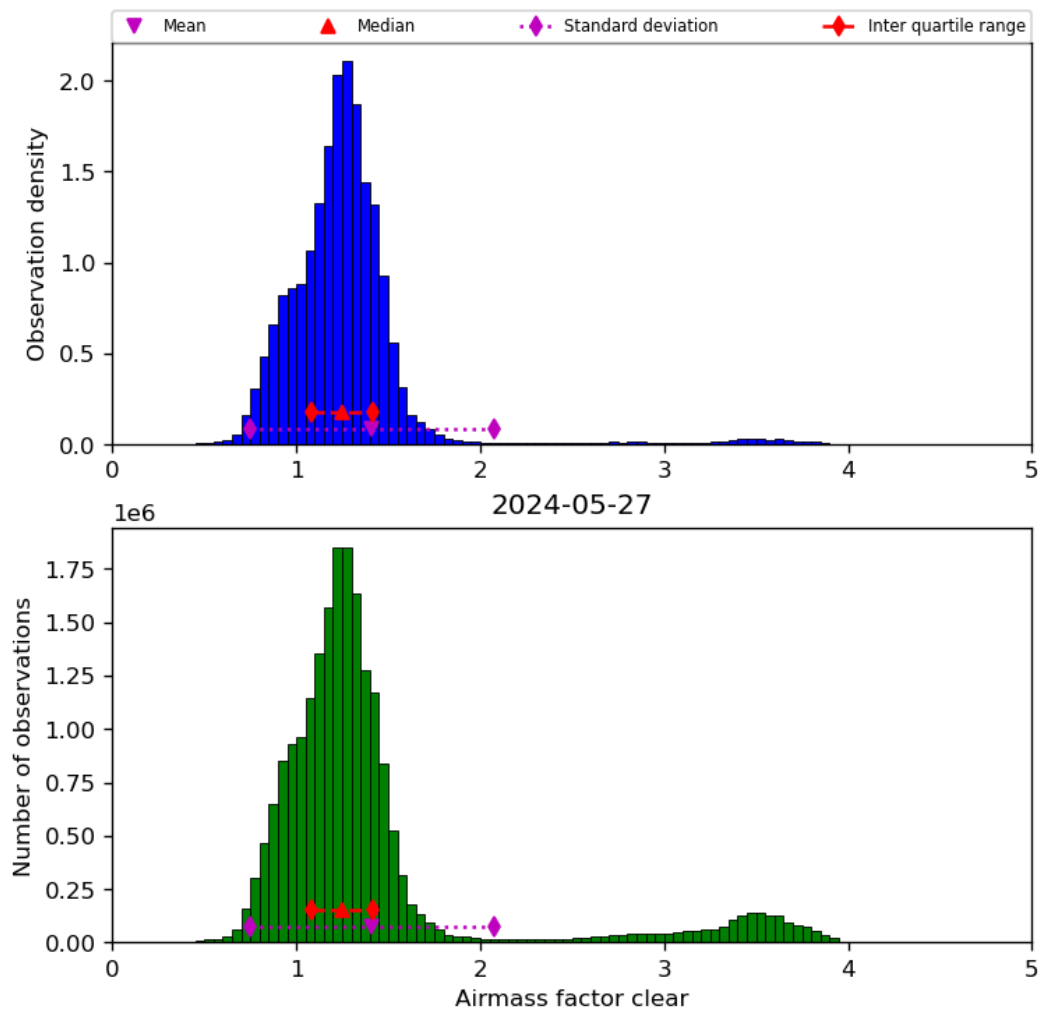
Figure 42: Histogram of “Airmass factor clear” for 2024-05-26 to 2024-05-28
