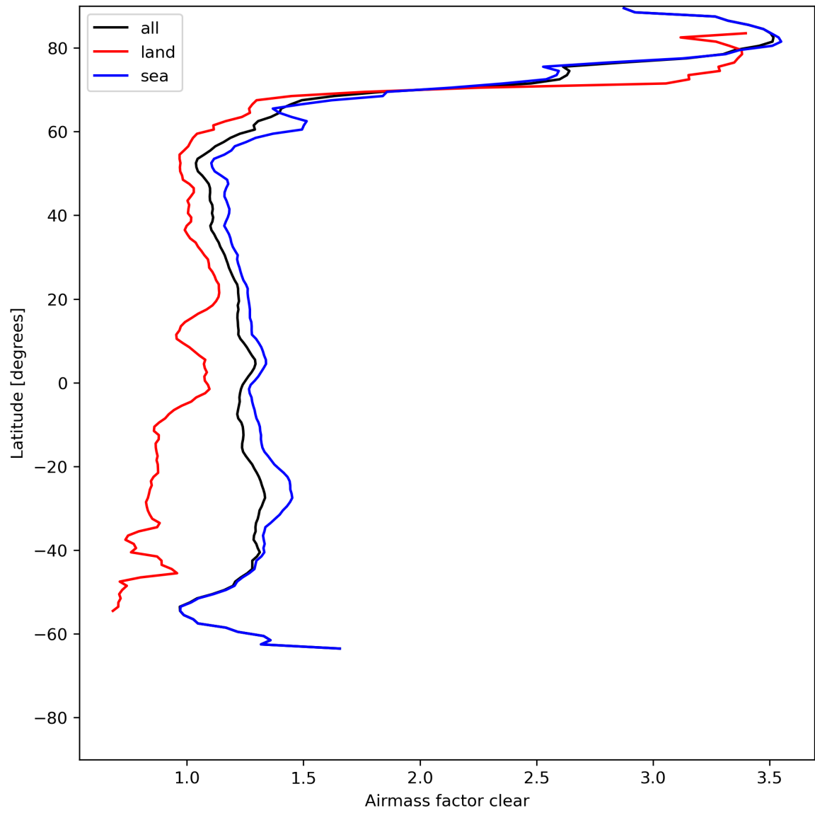
Figure 28: Zonal average of “Airmass factor clear” for 2024-05-26 to 2024-05-28.
