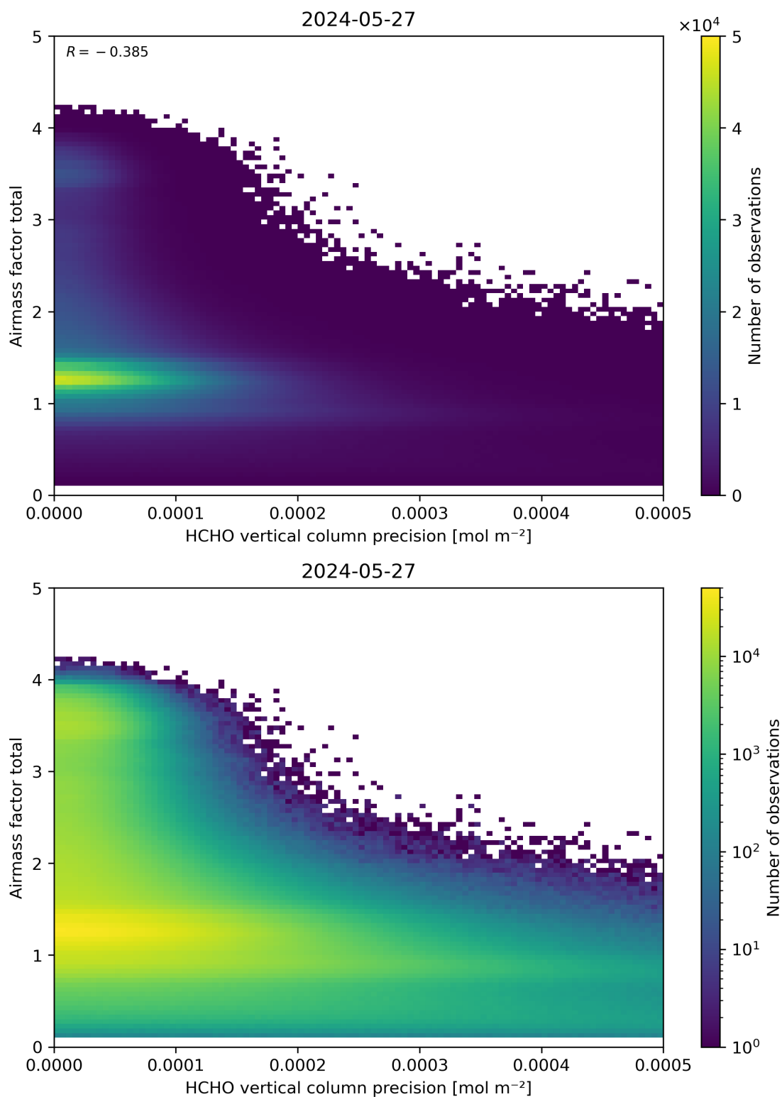
Figure 144: Scatter density plot of “HCHO vertical column precision” against “Airmass factor total” for 2024-05-26 to 2024-05-28.
