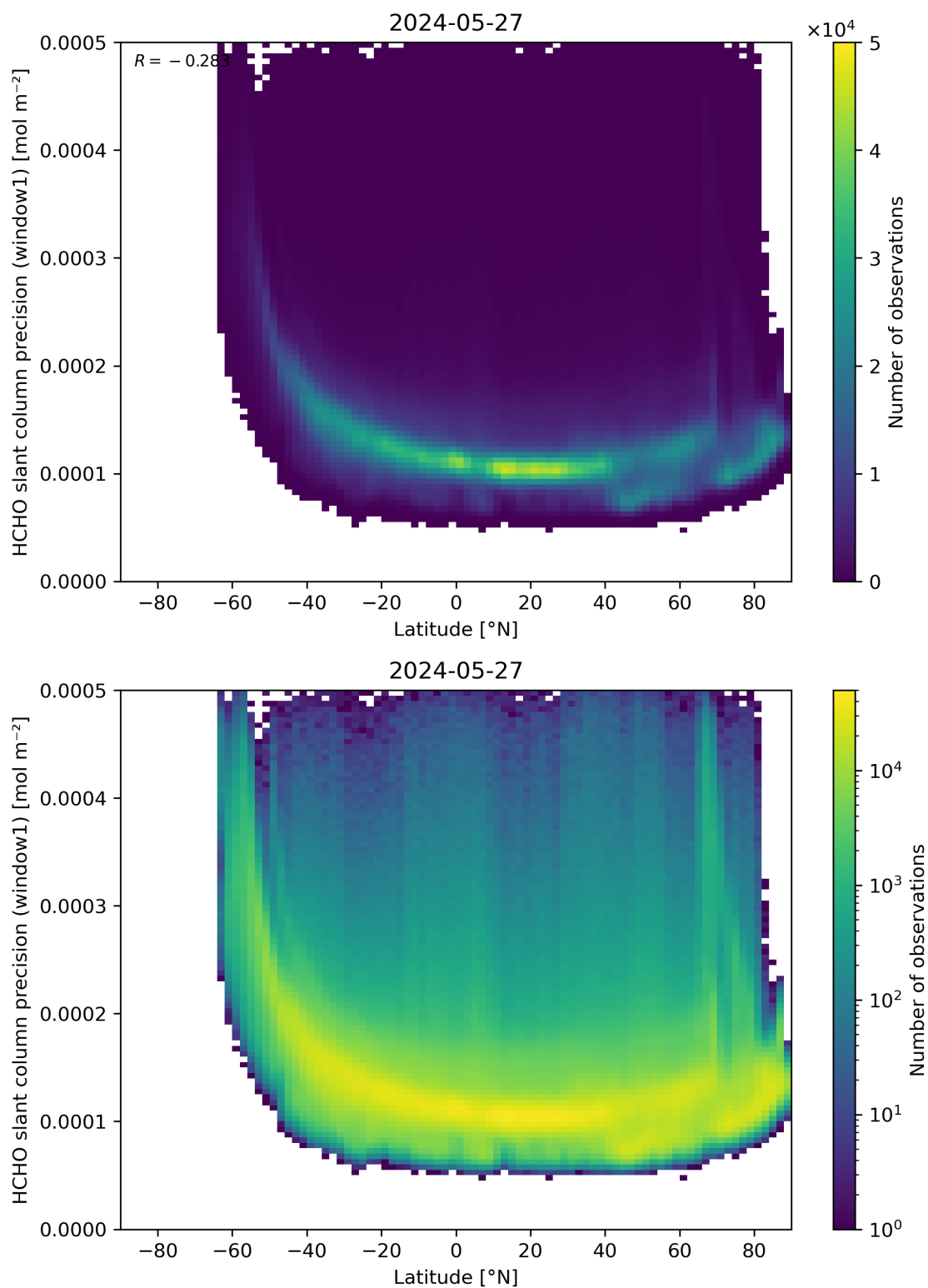
Figure 160: Scatter density plot of “Latitude” against “HCHO slant column precision (window1)” for 2024-05-26 to 2024-05-28.
