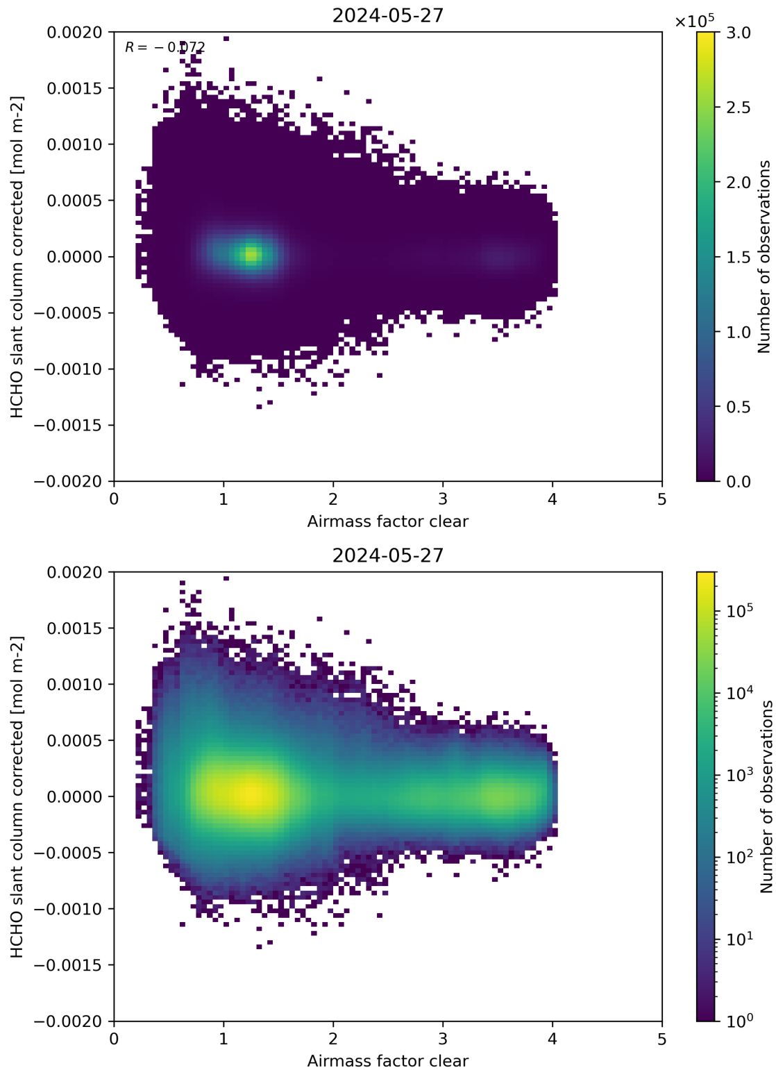
Figure 74: Scatter density plot of “Airmass factor clear” against “HCHO slant column corrected” for 2024-05-26 to 2024-05-28.
