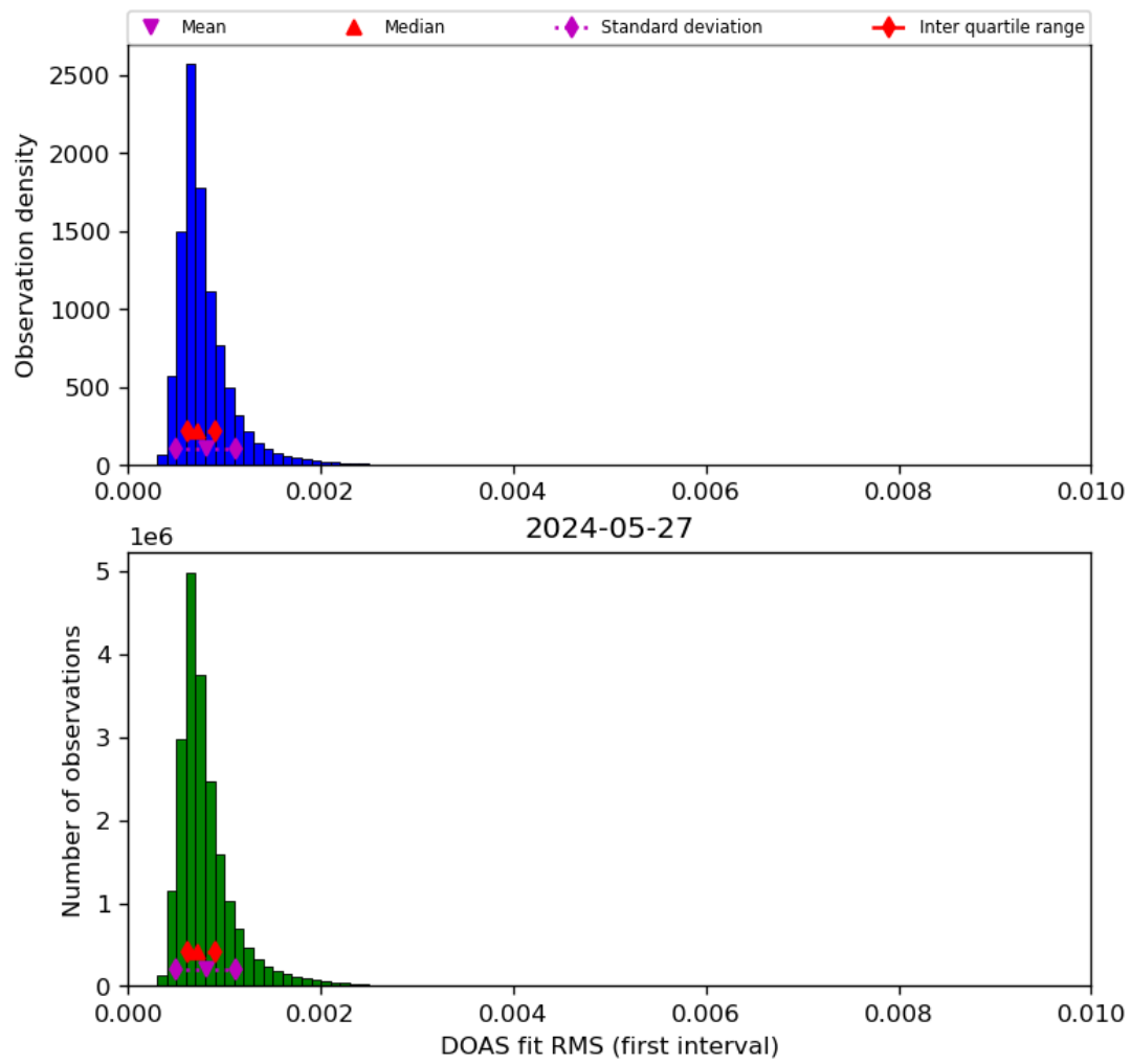
Figure 46: Histogram of “DOAS fit RMS (first interval)” for 2024-05-26 to 2024-05-28
