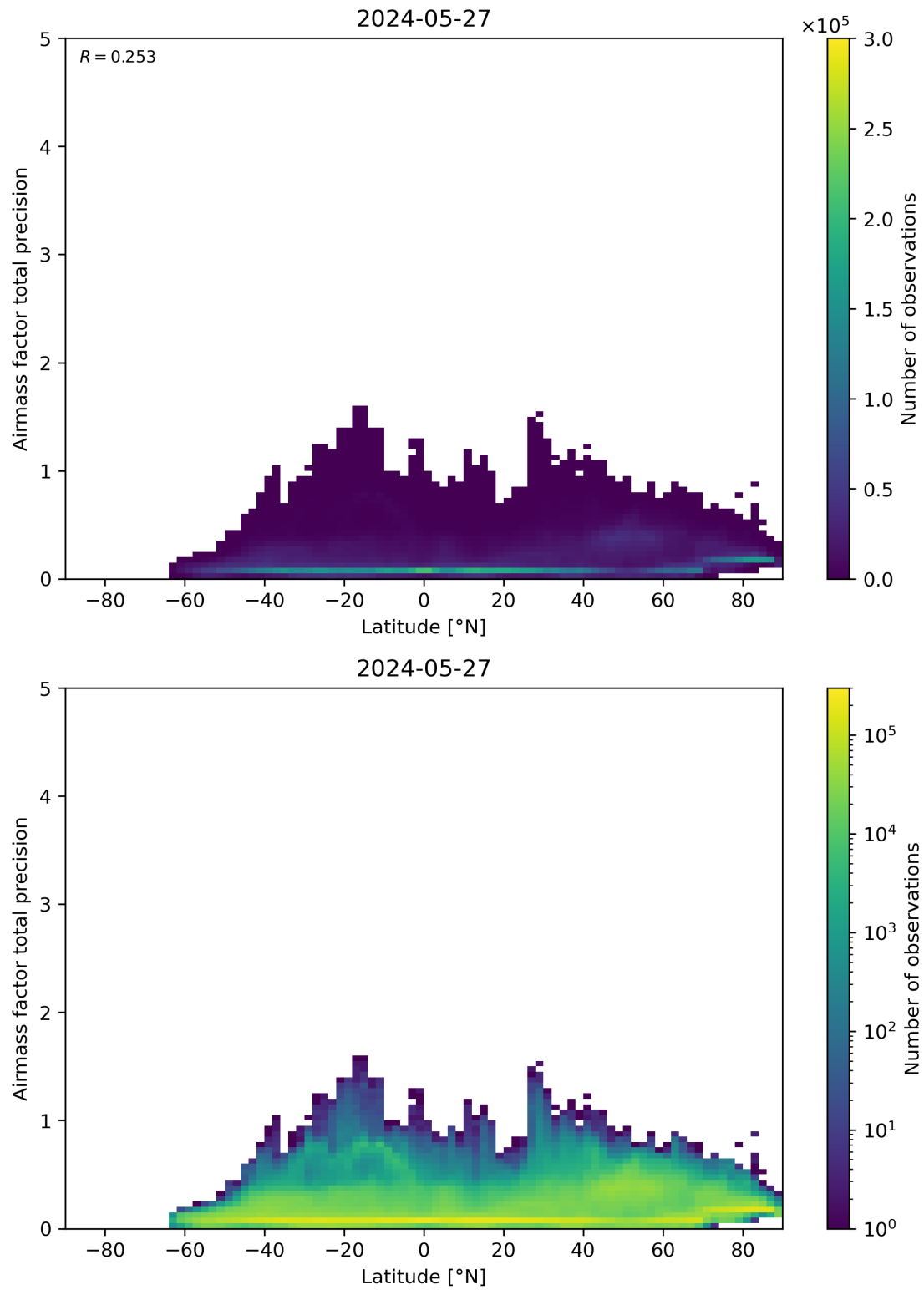
Figure 162: Scatter density plot of “Latitude” against “Airmass factor total precision” for 2024-05-26 to 2024-05-28.
