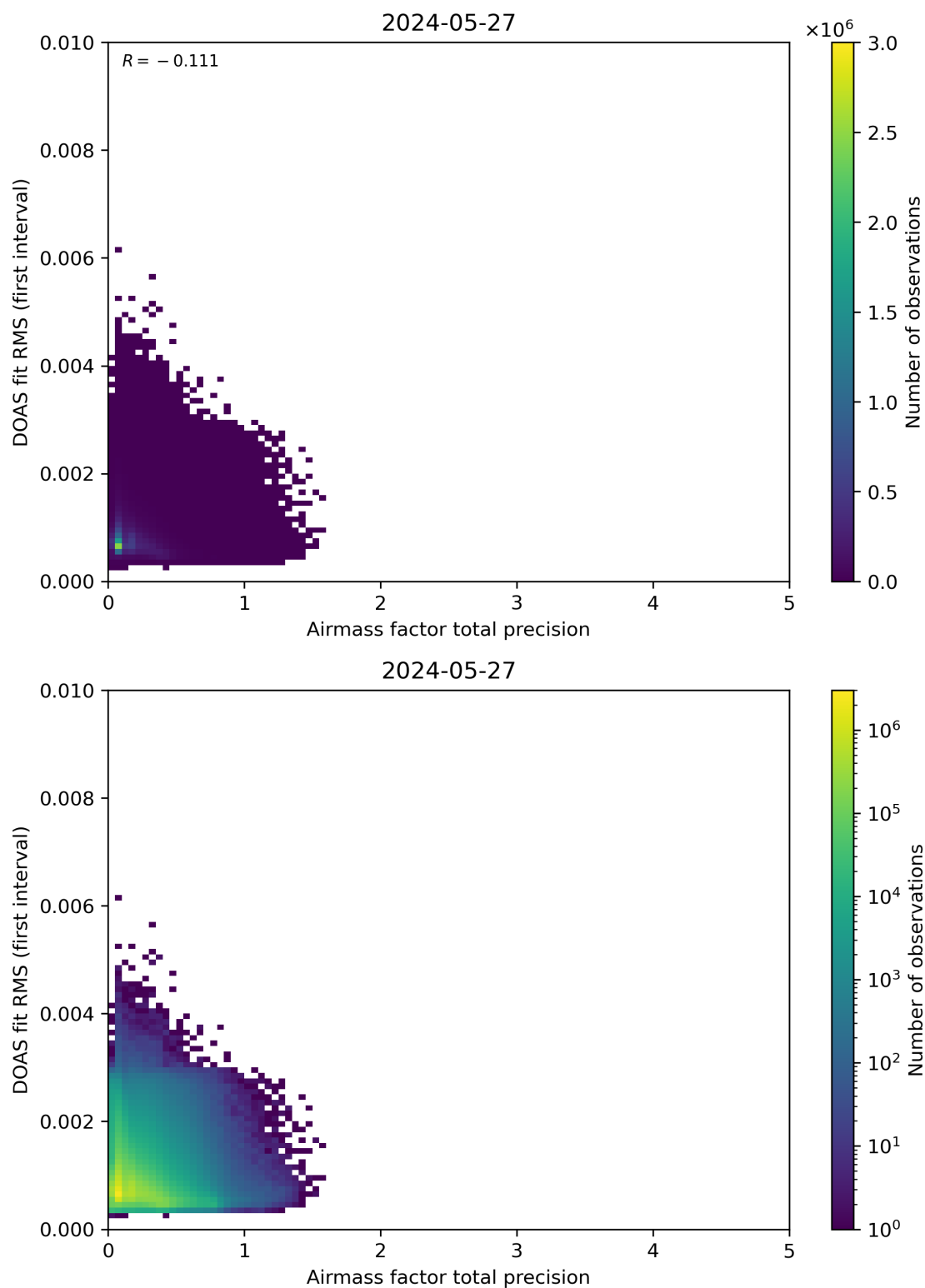
Figure 105: Scatter density plot of “Airmass factor total precision” against “DOAS fit RMS (first interval)” for 2024-05-26 to 2024-05-28.
