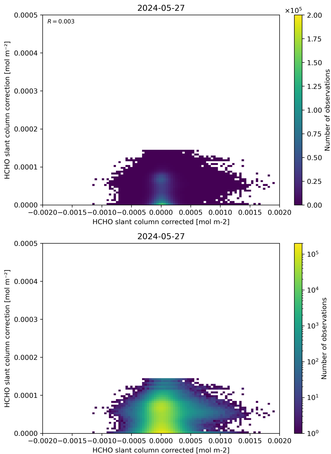
Figure 77: Scatter density plot of “HCHO slant column corrected” against “HCHO slant column correction” for 2024-05-26 to 2024-05-28.
