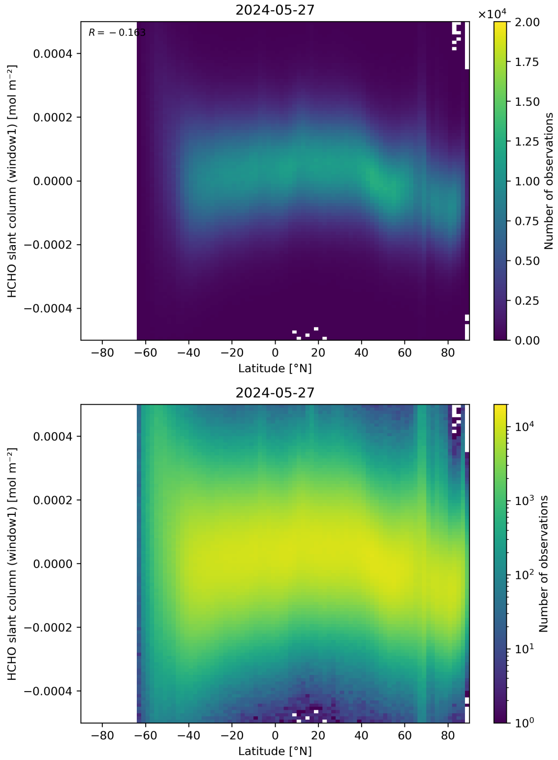
Figure 159: Scatter density plot of “Latitude” against “HCHO slant column (window1)” for 2024-05-26 to 2024-05-28.
