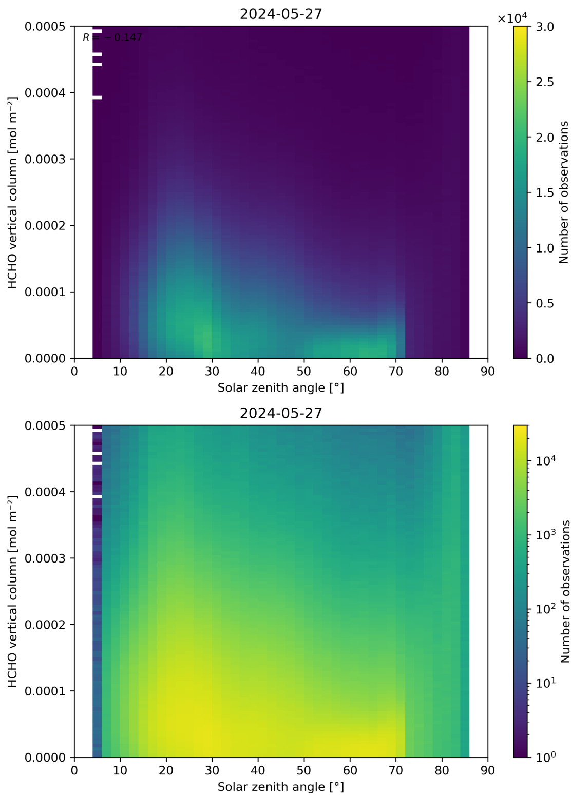
Figure 177: Scatter density plot of “Solar zenith angle” against “HCHO vertical column” for 2024-05-26 to 2024-05-28.
