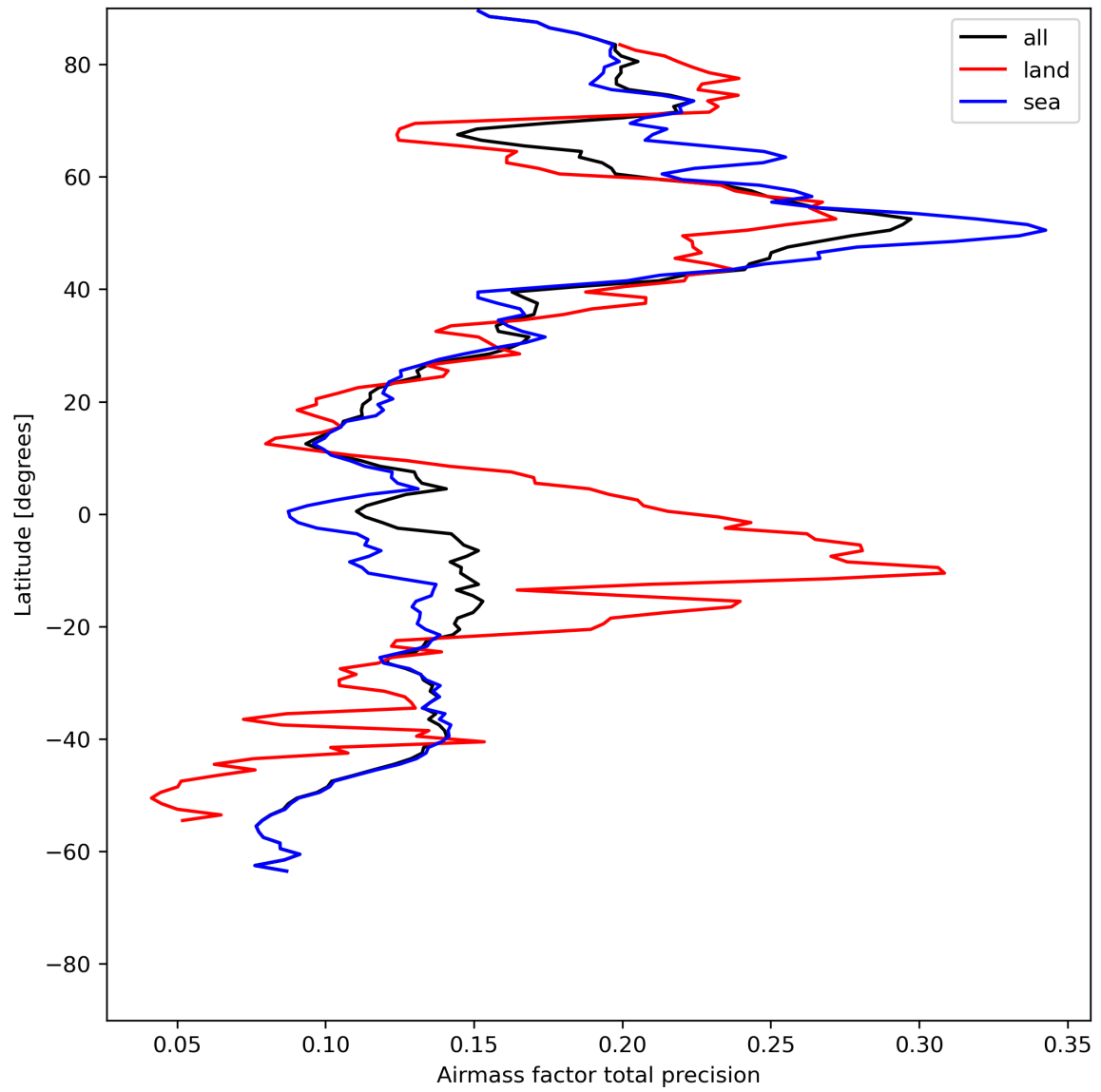
Figure 27: Zonal average of “Airmass factor total precision” for 2024-05-26 to 2024-05-28.
