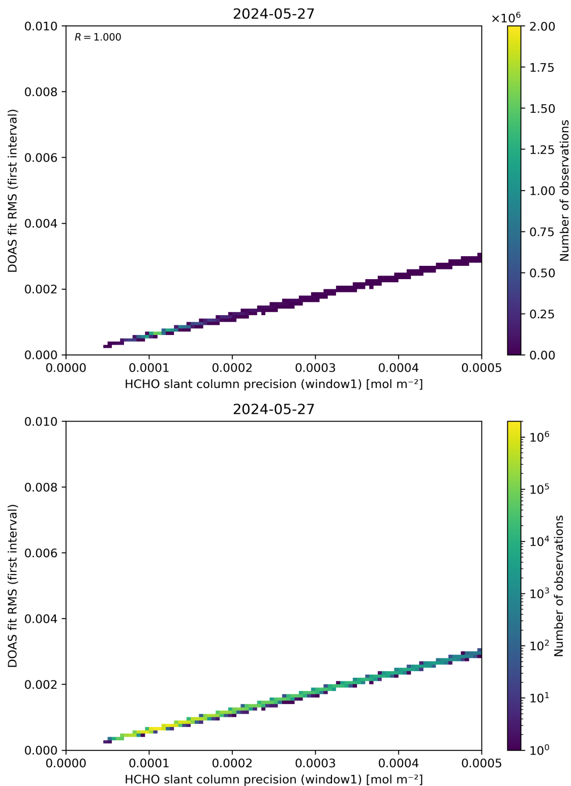
Figure 88: Scatter density plot of “HCHO slant column precision (window1)” against “DOAS fit RMS (first interval)” for 2024-05-26 to 2024-05-28.
