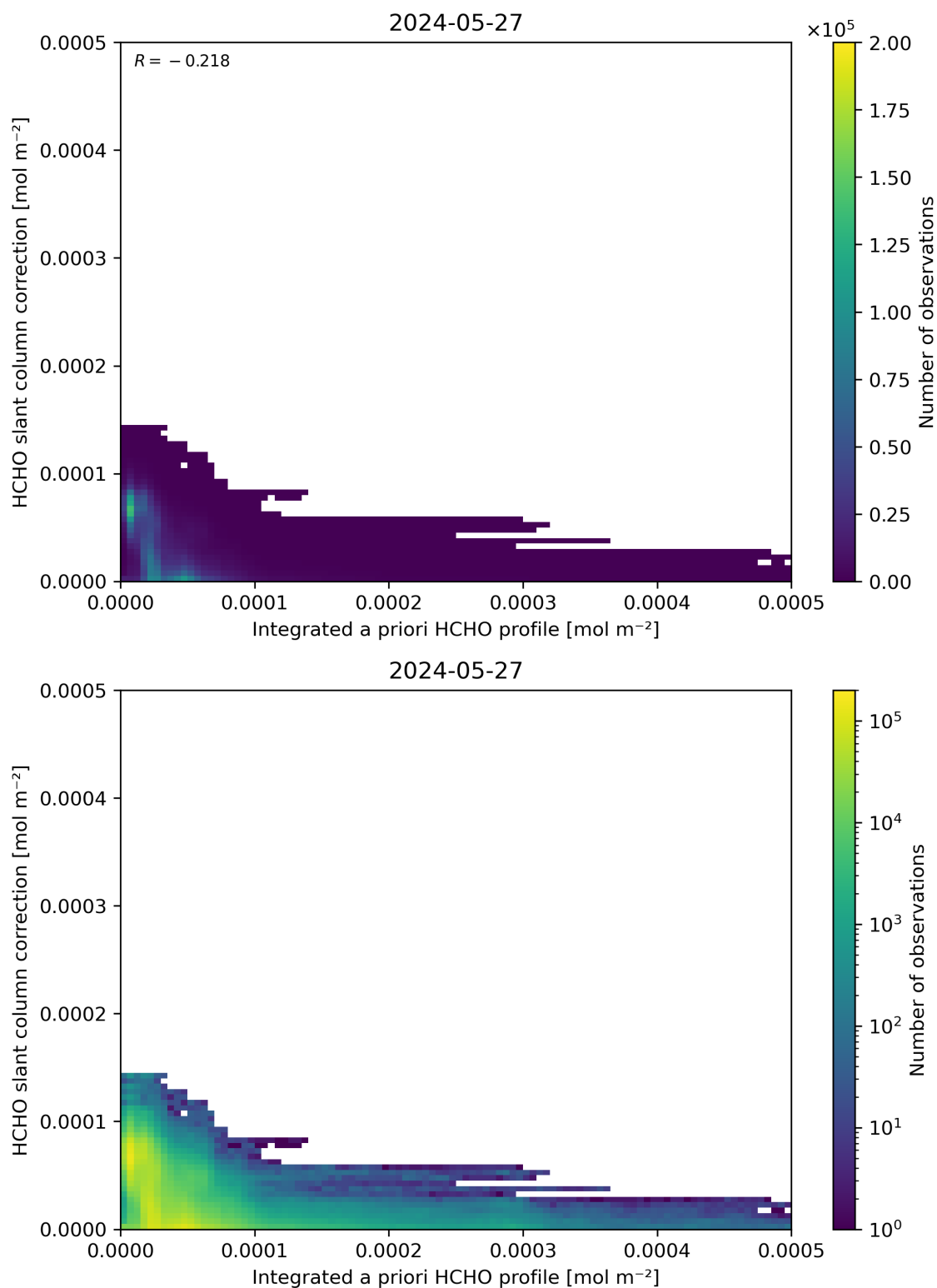
Figure 152: Scatter density plot of “Integrated a priori HCHO profile” against “HCHO slant column correction” for 2024-05-26 to 2024-05-28.
