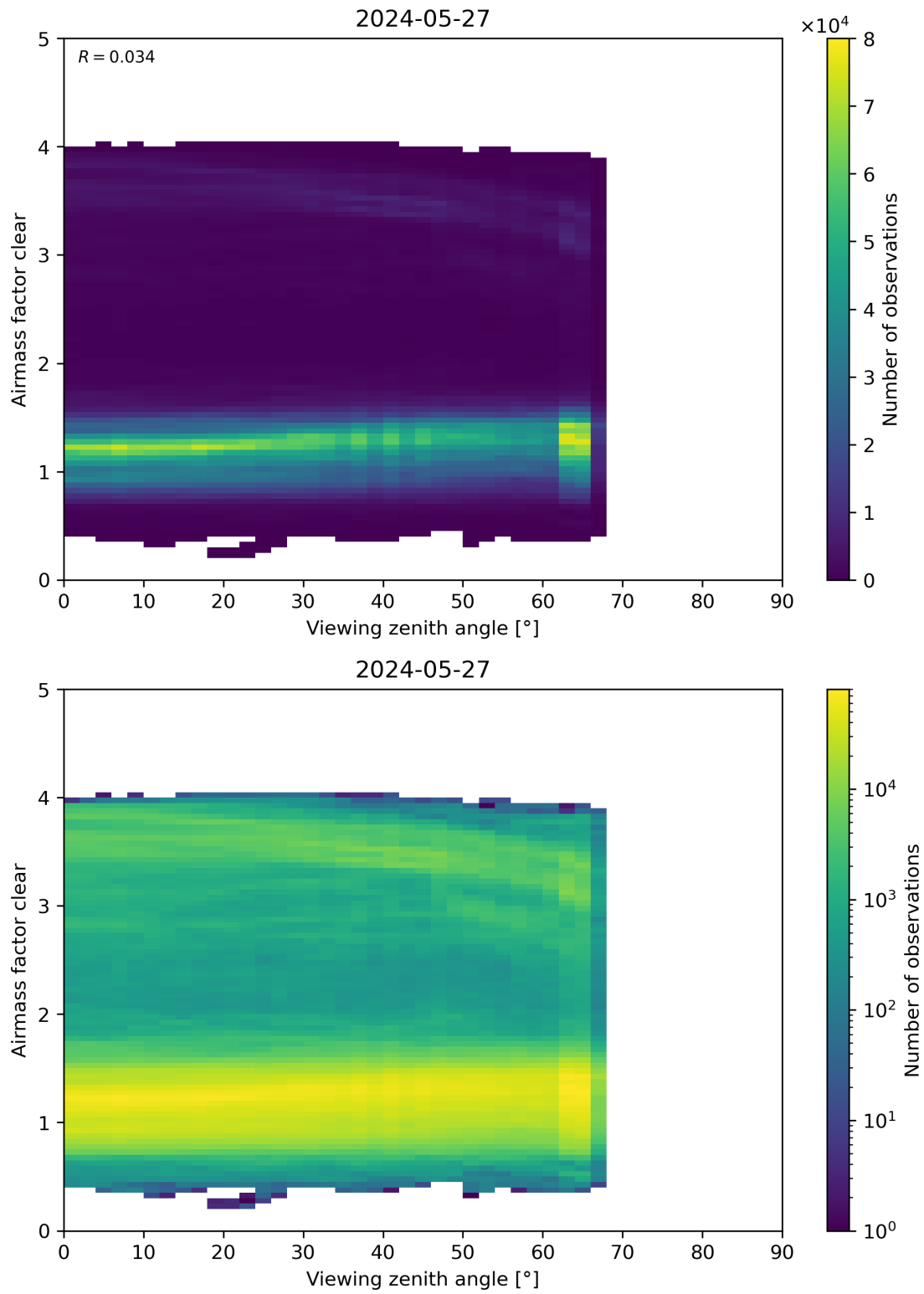
Figure 185: Scatter density plot of “Viewing zenith angle” against “Airmass factor clear” for 2024-05-26 to 2024-05-28.
