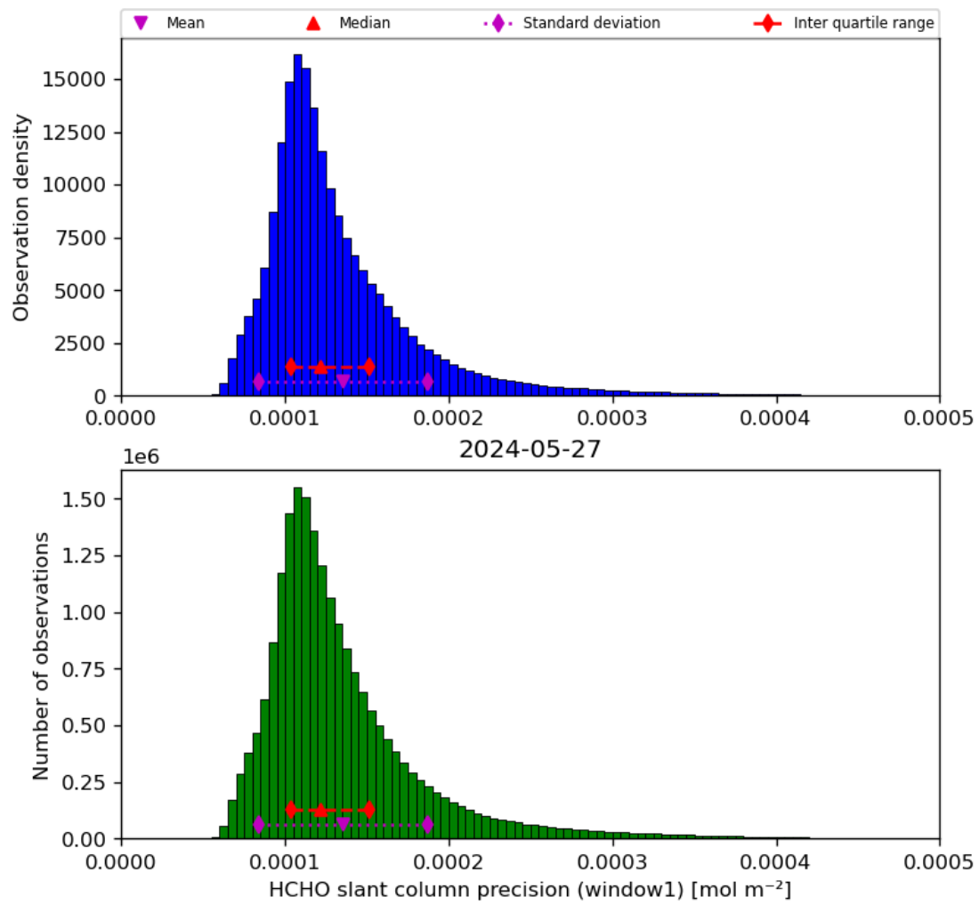
Figure 39: Histogram of “HCHO slant column precision (window1)” for 2024-05-26 to 2024-05-28
