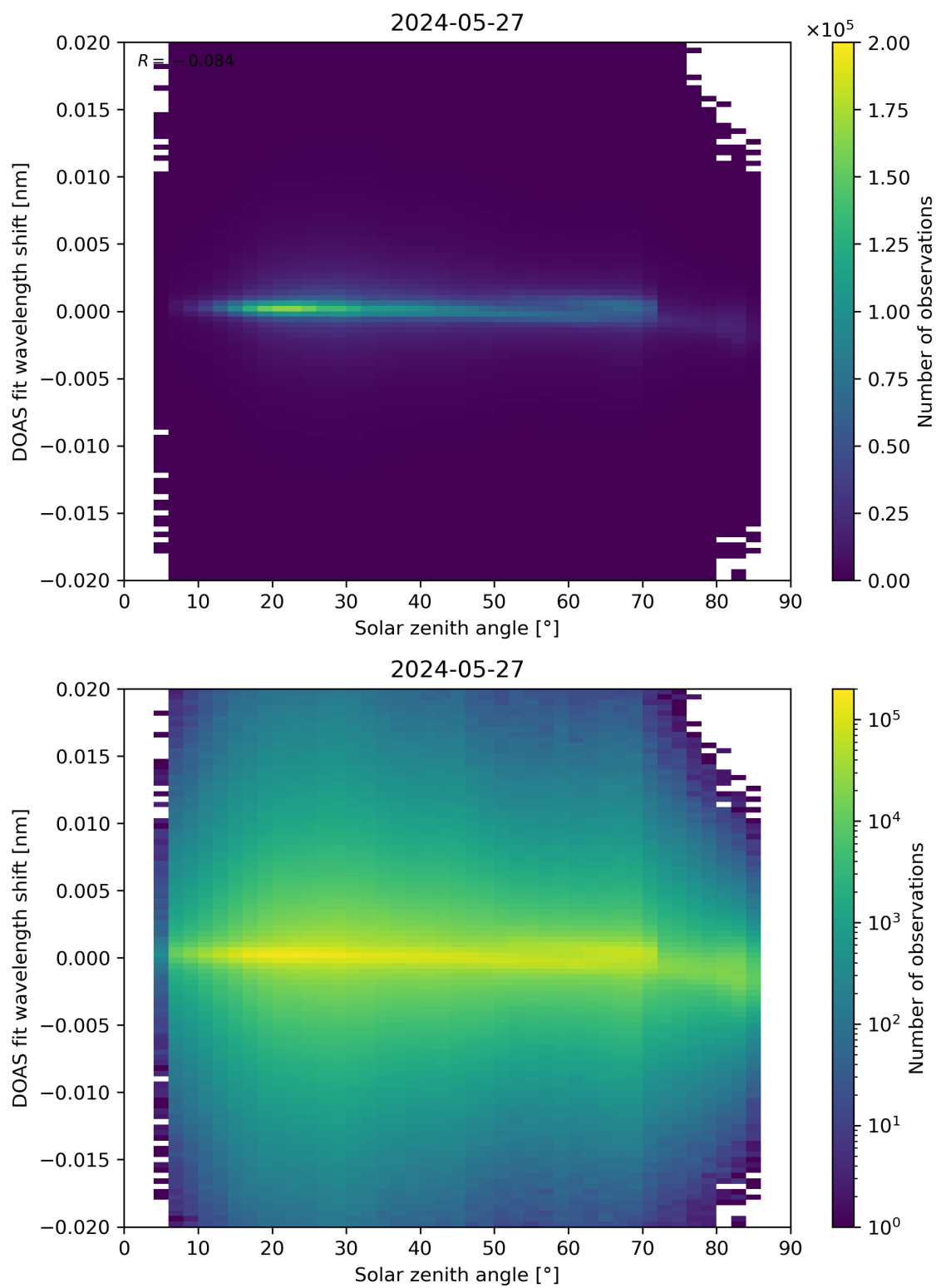
Figure 168: Scatter density plot of “Solar zenith angle” against “DOAS fit wavelength shift” for 2024-05-26 to 2024-05-28.
