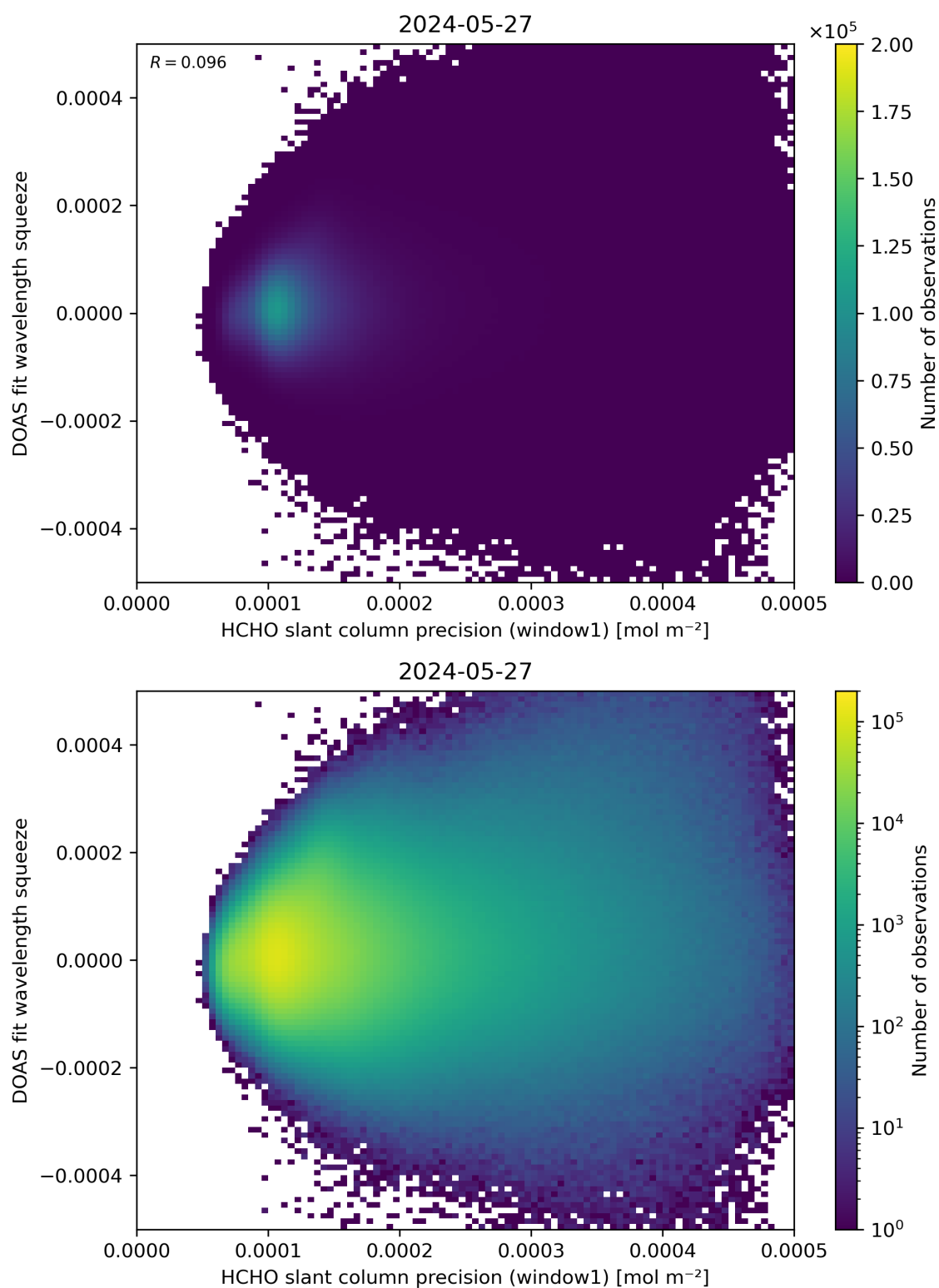
Figure 90: Scatter density plot of “HCHO slant column precision (window1)” against “DOAS fit wavelength squeeze” for 2024-05-26 to 2024-05-28.
