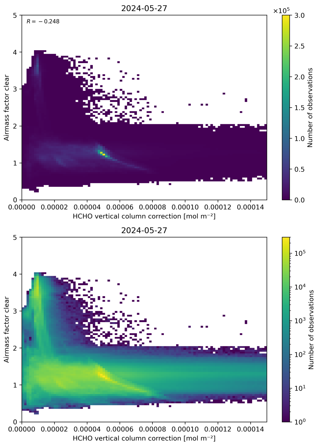
Figure 115: Scatter density plot of “HCHO vertical column correction” against “Airmass factor clear” for 2024-05-26 to 2024-05-28.
