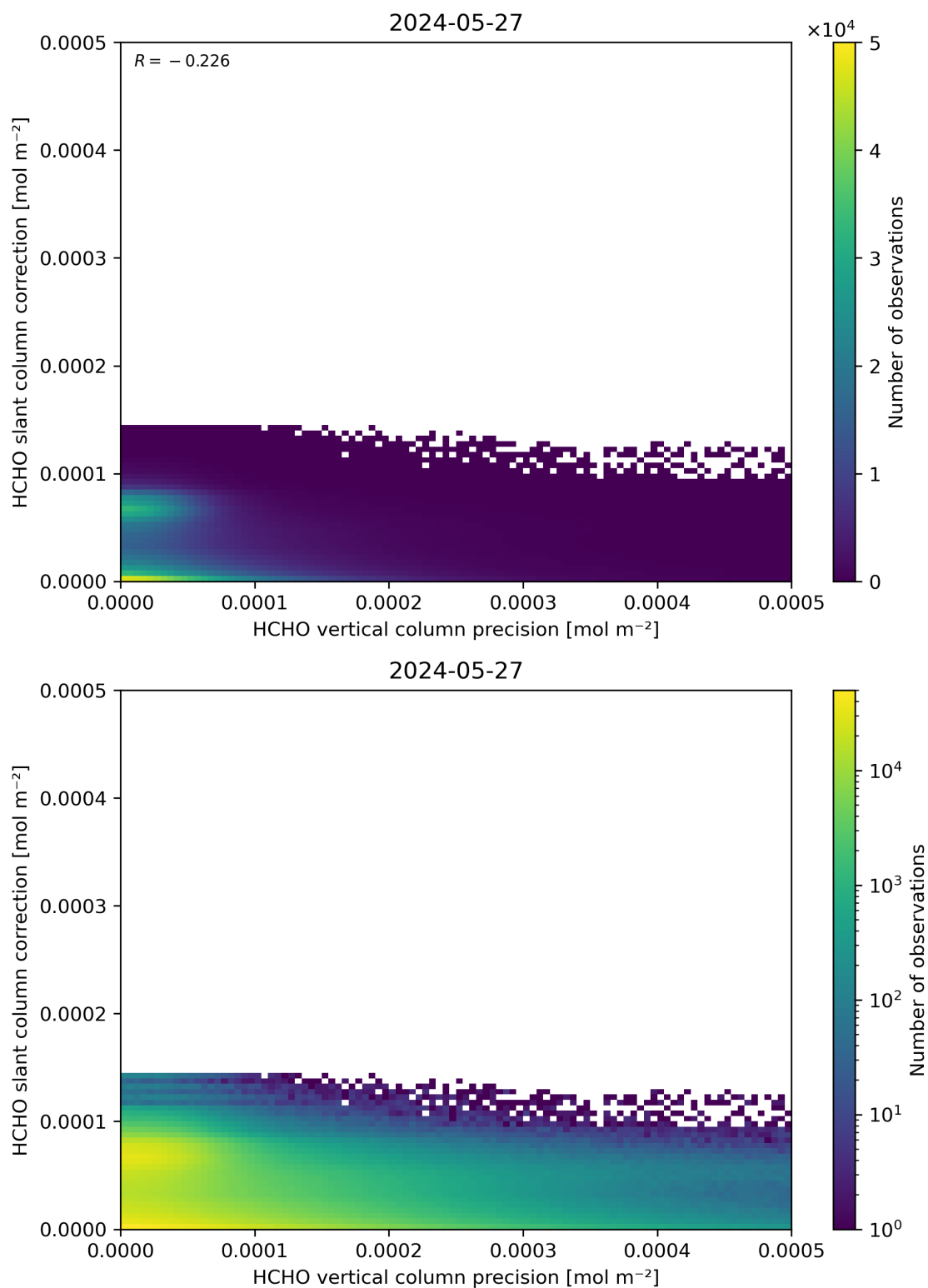
Figure 141: Scatter density plot of “HCHO vertical column precision” against “HCHO slant column correction” for 2024-05-26 to 2024-05-28.
