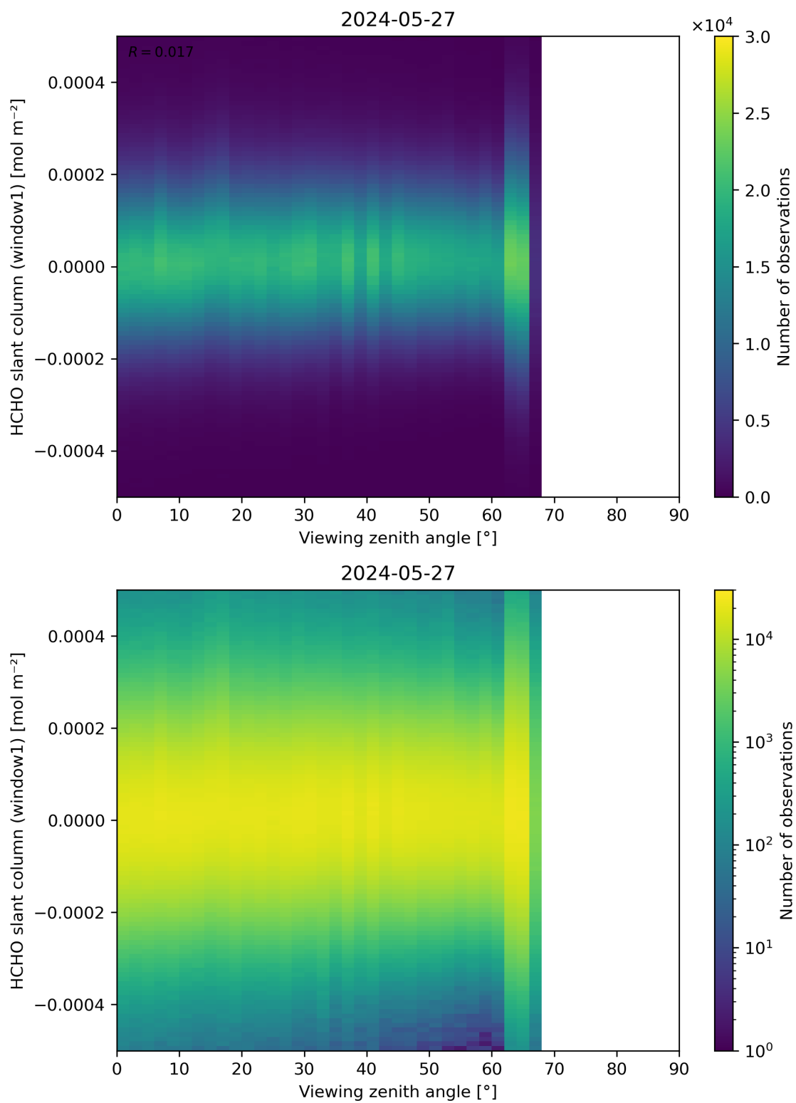
Figure 188: Scatter density plot of “Viewing zenith angle” against “HCHO slant column (window1)” for 2024-05-26 to 2024-05-28.
