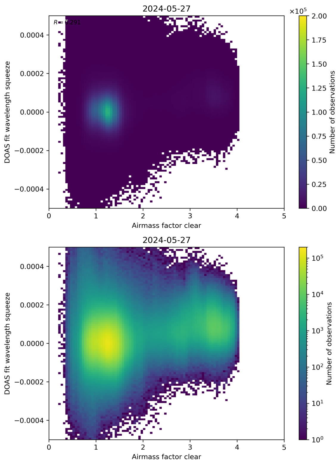
Figure 73: Scatter density plot of “Airmass factor clear” against “DOAS fit wavelength squeeze” for 2024-05-26 to 2024-05-28.
