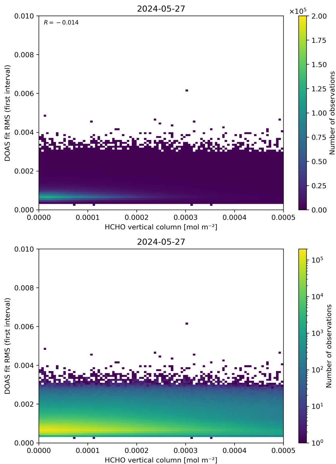
Figure 123: Scatter density plot of “HCHO vertical column” against “DOAS fit RMS (first interval)” for 2024-05-26 to 2024-05-28.
