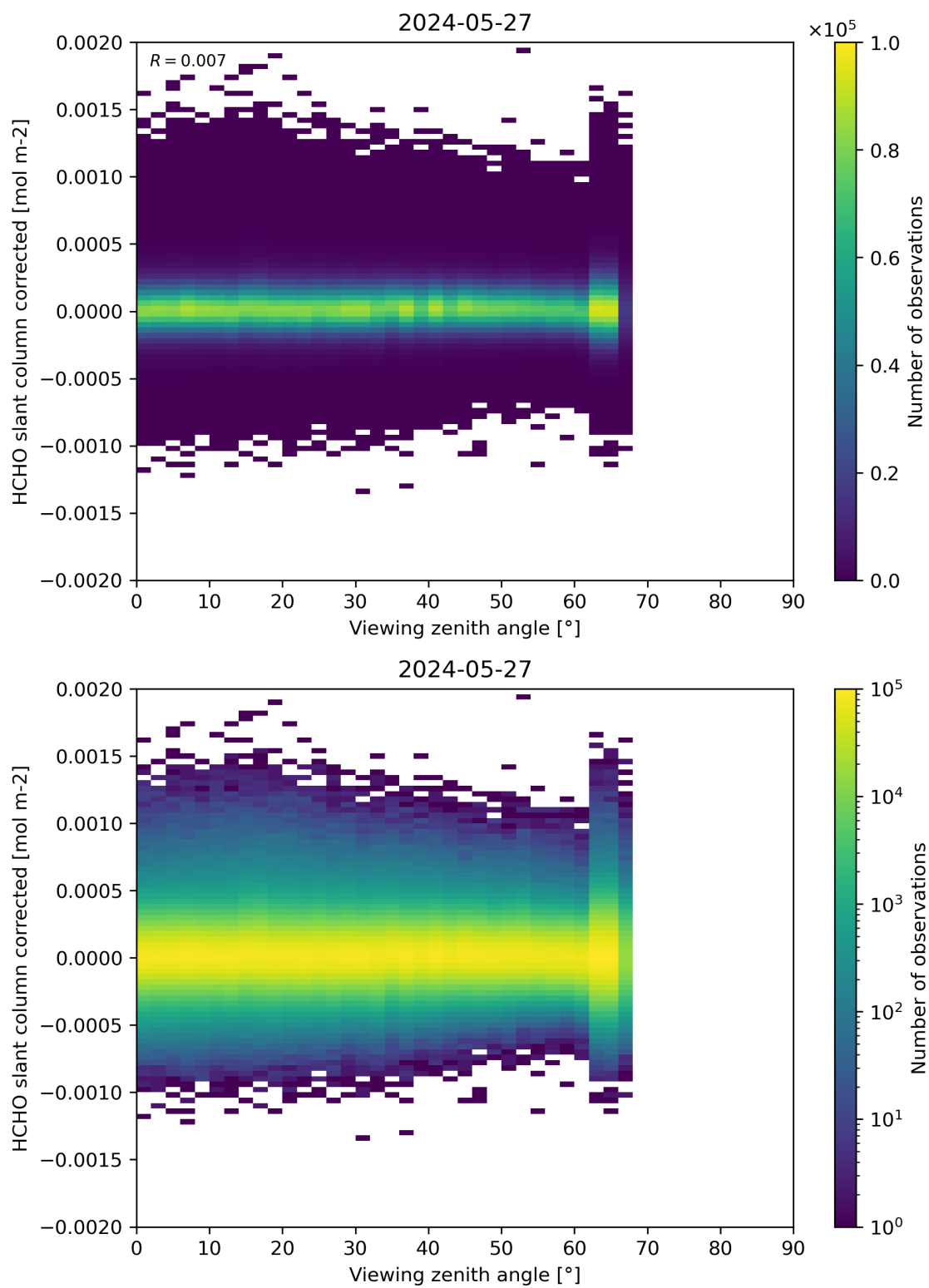
Figure 186: Scatter density plot of “Viewing zenith angle” against “HCHO slant column corrected” for 2024-05-26 to 2024-05-28.
