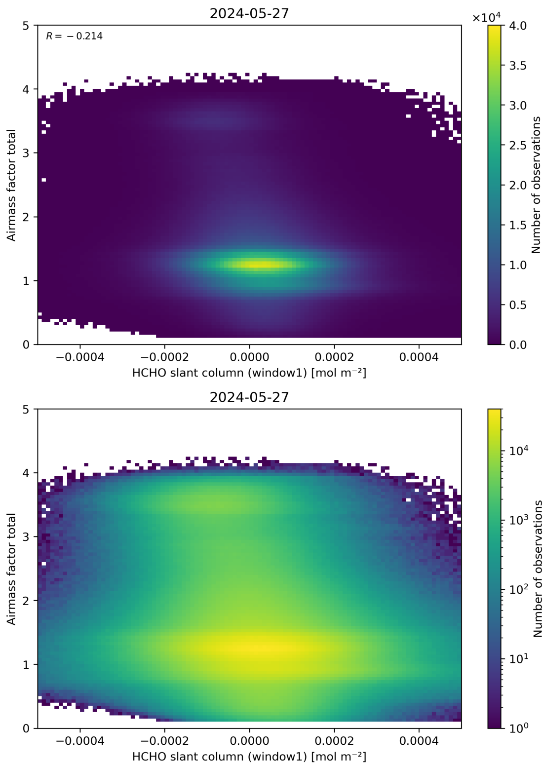
Figure 85: Scatter density plot of “HCHO slant column (window1)” against “Airmass factor total” for 2024-05-26 to 2024-05-28.
