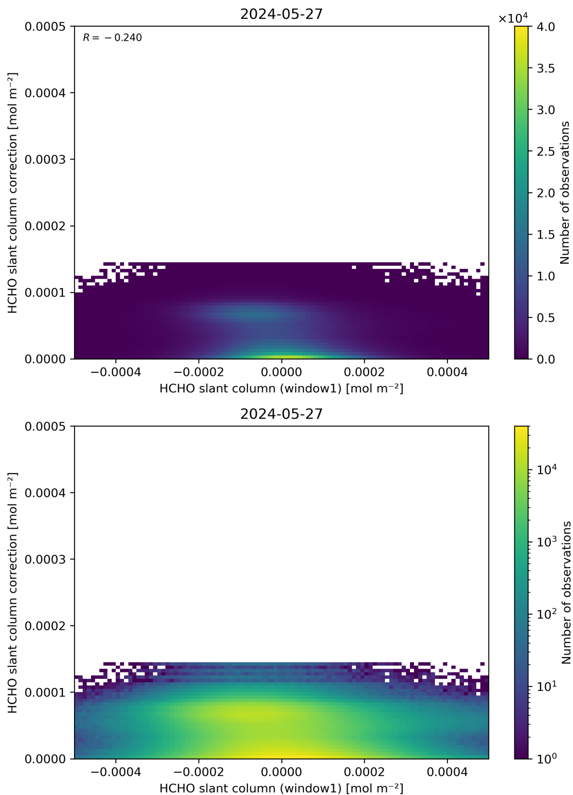
Figure 83: Scatter density plot of “HCHO slant column (window1)” against “HCHO slant column correction” for 2024-05-26 to 2024-05-28.
