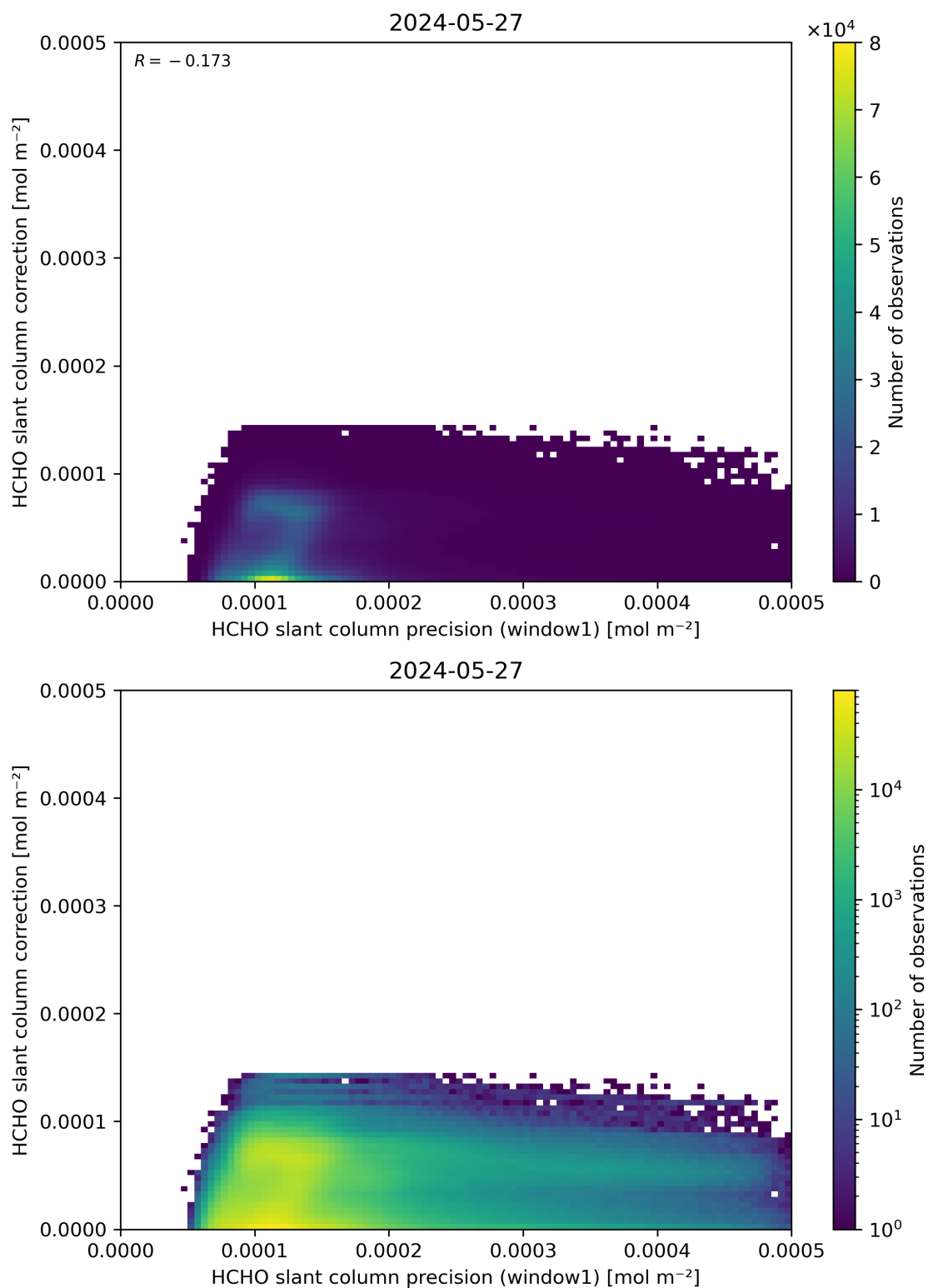
Figure 93: Scatter density plot of “HCHO slant column precision (window1)” against “HCHO slant column correction” for 2024-05-26 to 2024-05-28.
