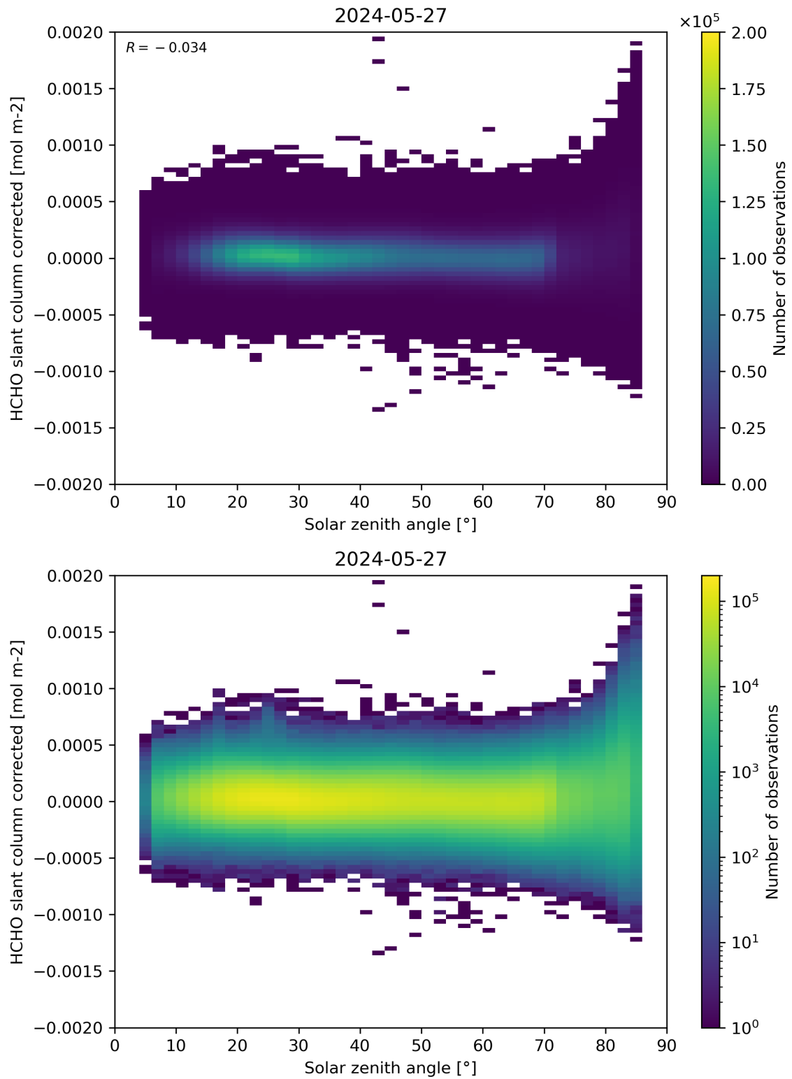
Figure 171: Scatter density plot of “Solar zenith angle” against “HCHO slant column corrected” for 2024-05-26 to 2024-05-28.
