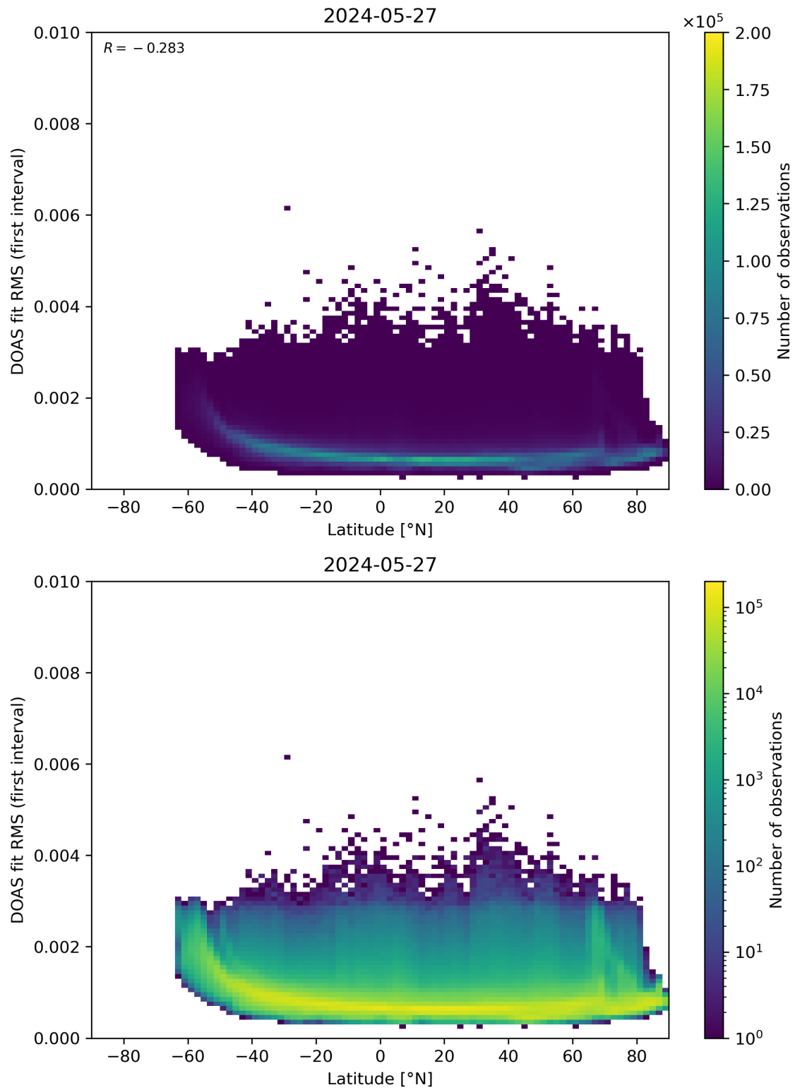
Figure 153: Scatter density plot of “Latitude” against “DOAS fit RMS (first interval)” for 2024-05-26 to 2024-05-28.
