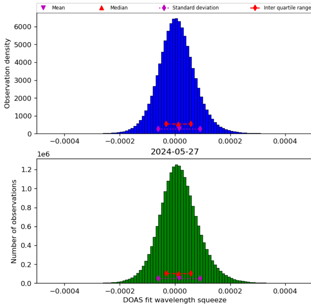
Figure 45: Histogram of “DOAS fit wavelength squeeze” for 2024-05-26 to 2024-05-28
