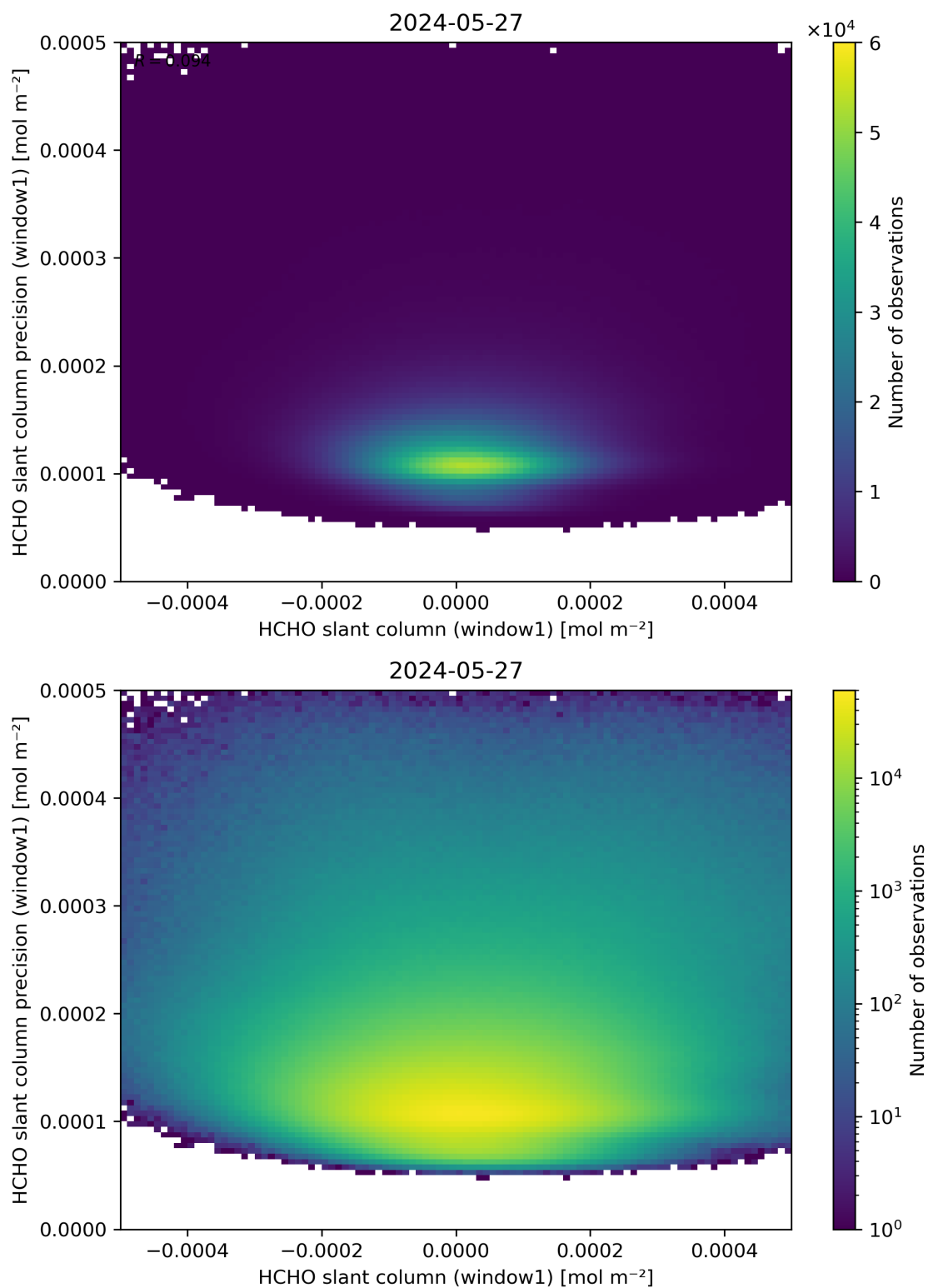
Figure 84: Scatter density plot of “HCHO slant column (window1)” against “HCHO slant column precision (window1)” for 2024-05-26 to 2024-05-28.
