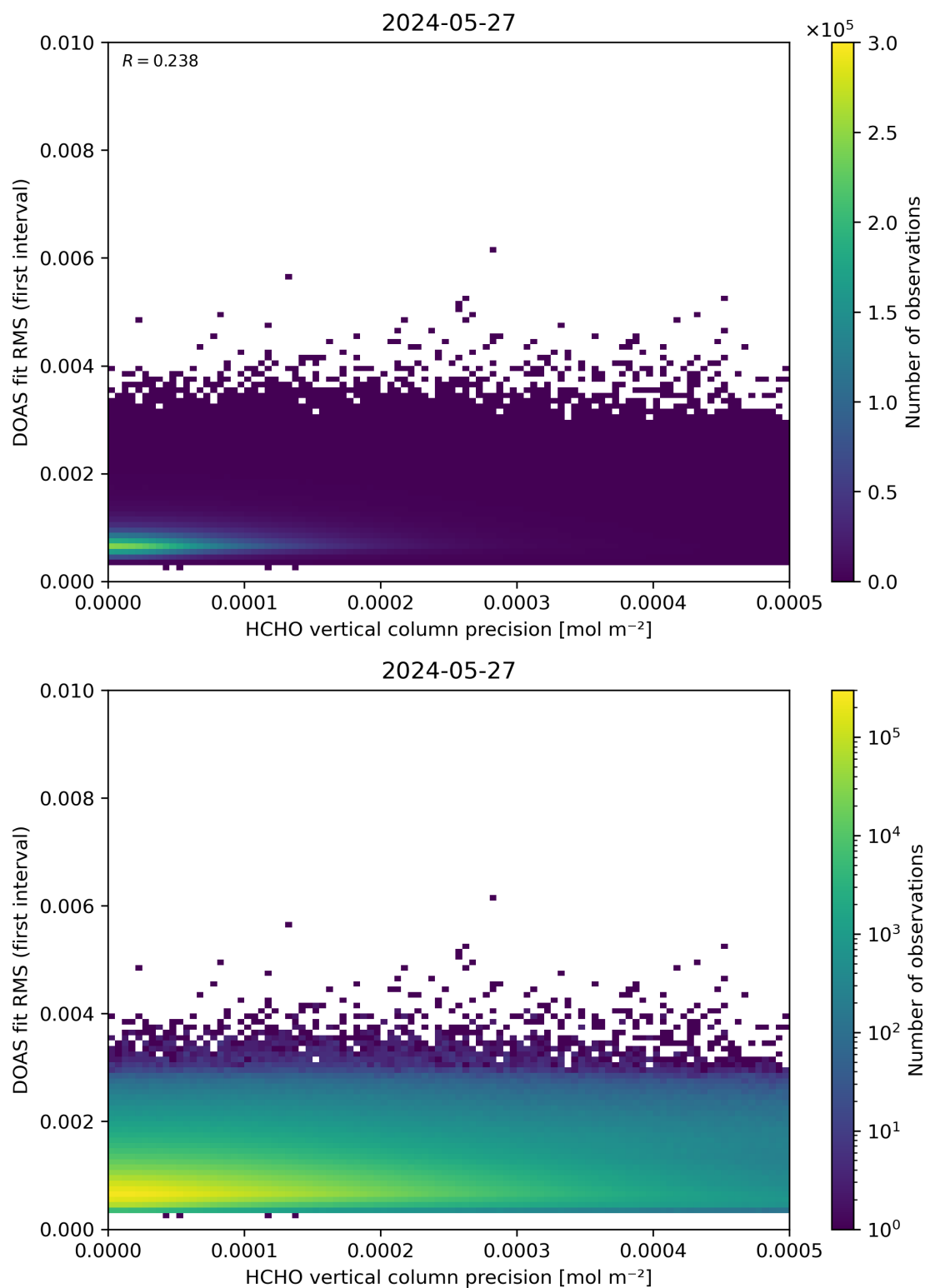
Figure 136: Scatter density plot of “HCHO vertical column precision” against “DOAS fit RMS (first interval)” for 2024-05-26 to 2024-05-28.
