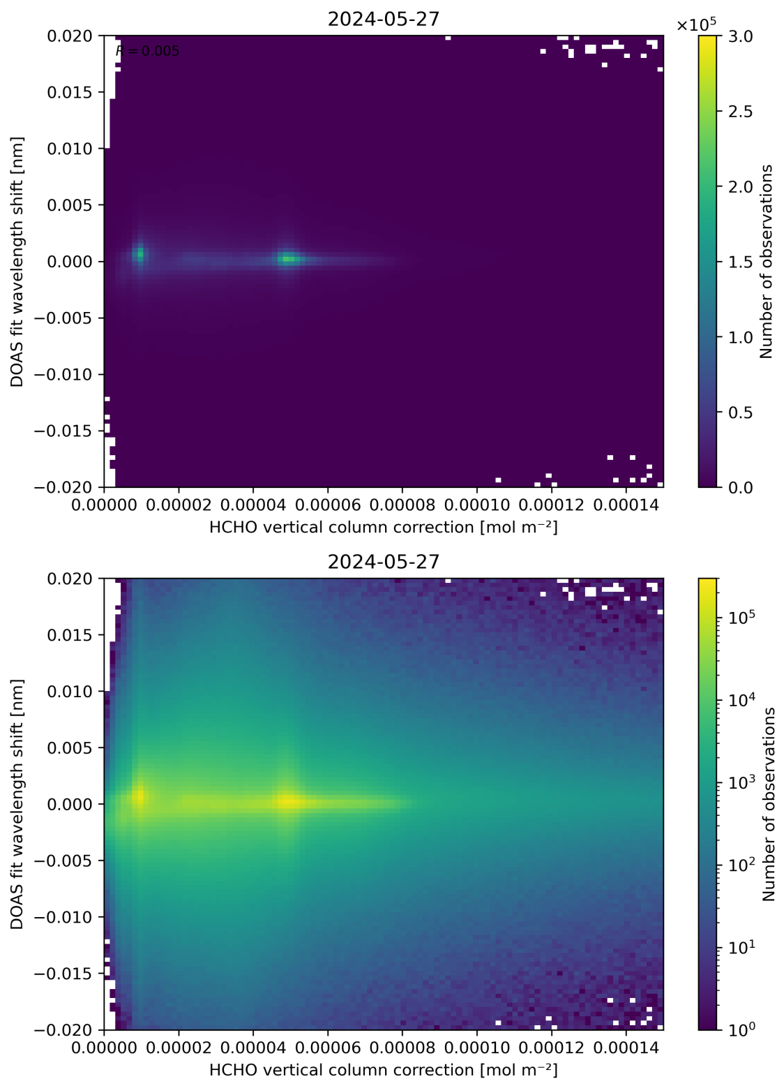
Figure 113: Scatter density plot of “HCHO vertical column correction” against “DOAS fit wavelength shift” for 2024-05-26 to 2024-05-28.
