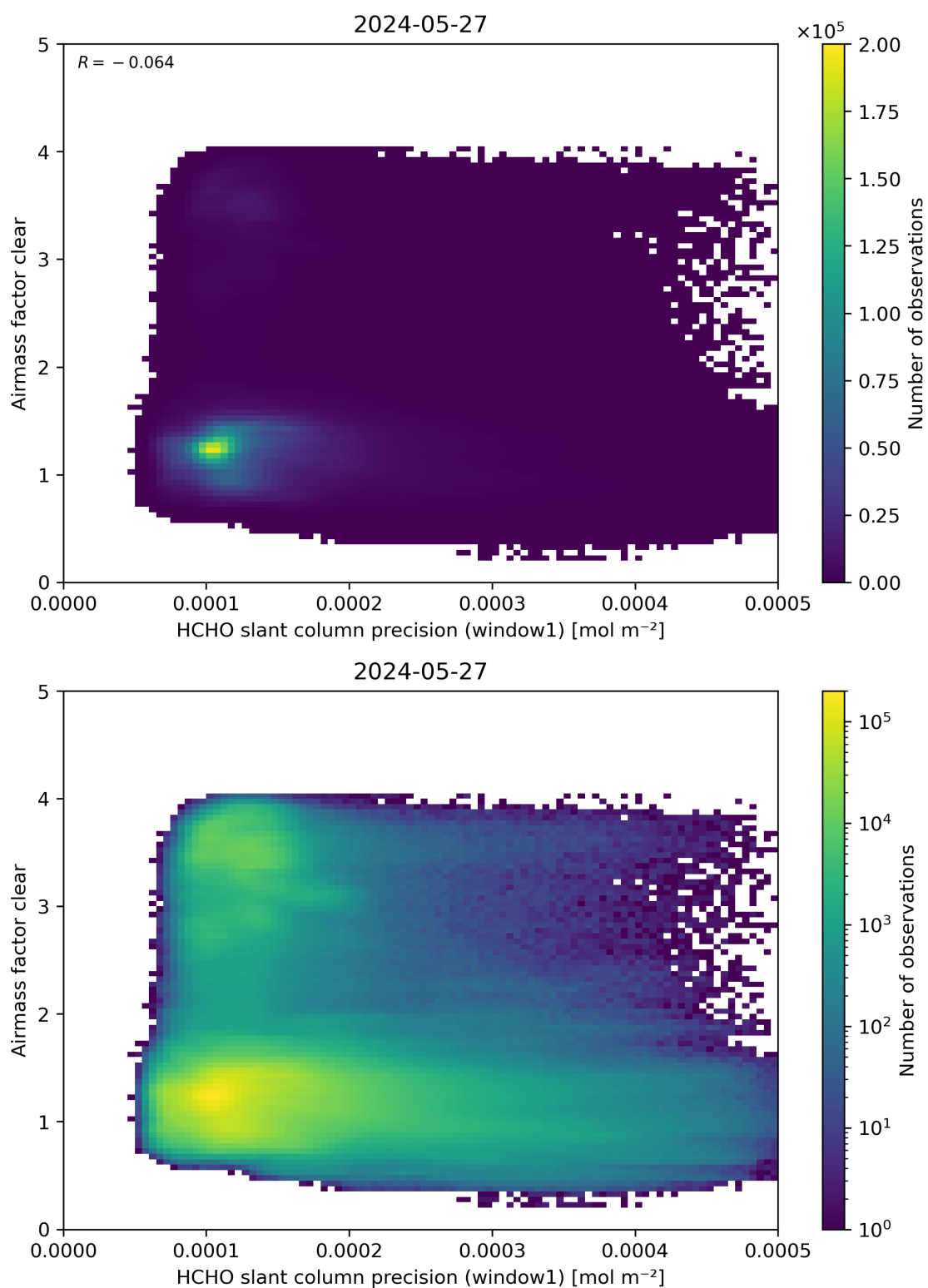
Figure 91: Scatter density plot of “HCHO slant column precision (window1)” against “Airmass factor clear” for 2024-05-26 to 2024-05-28.
