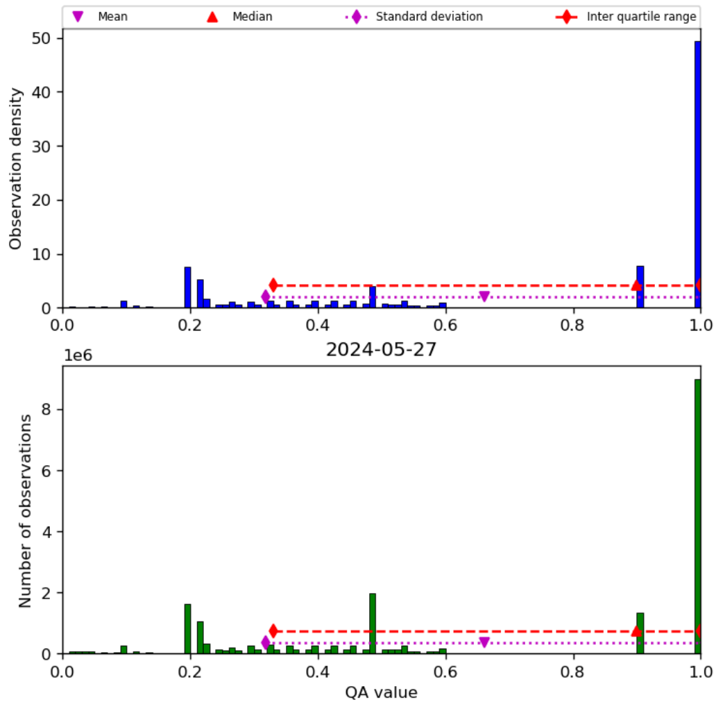
Figure 34: Histogram of “QA value” for 2024-05-26 to 2024-05-28
