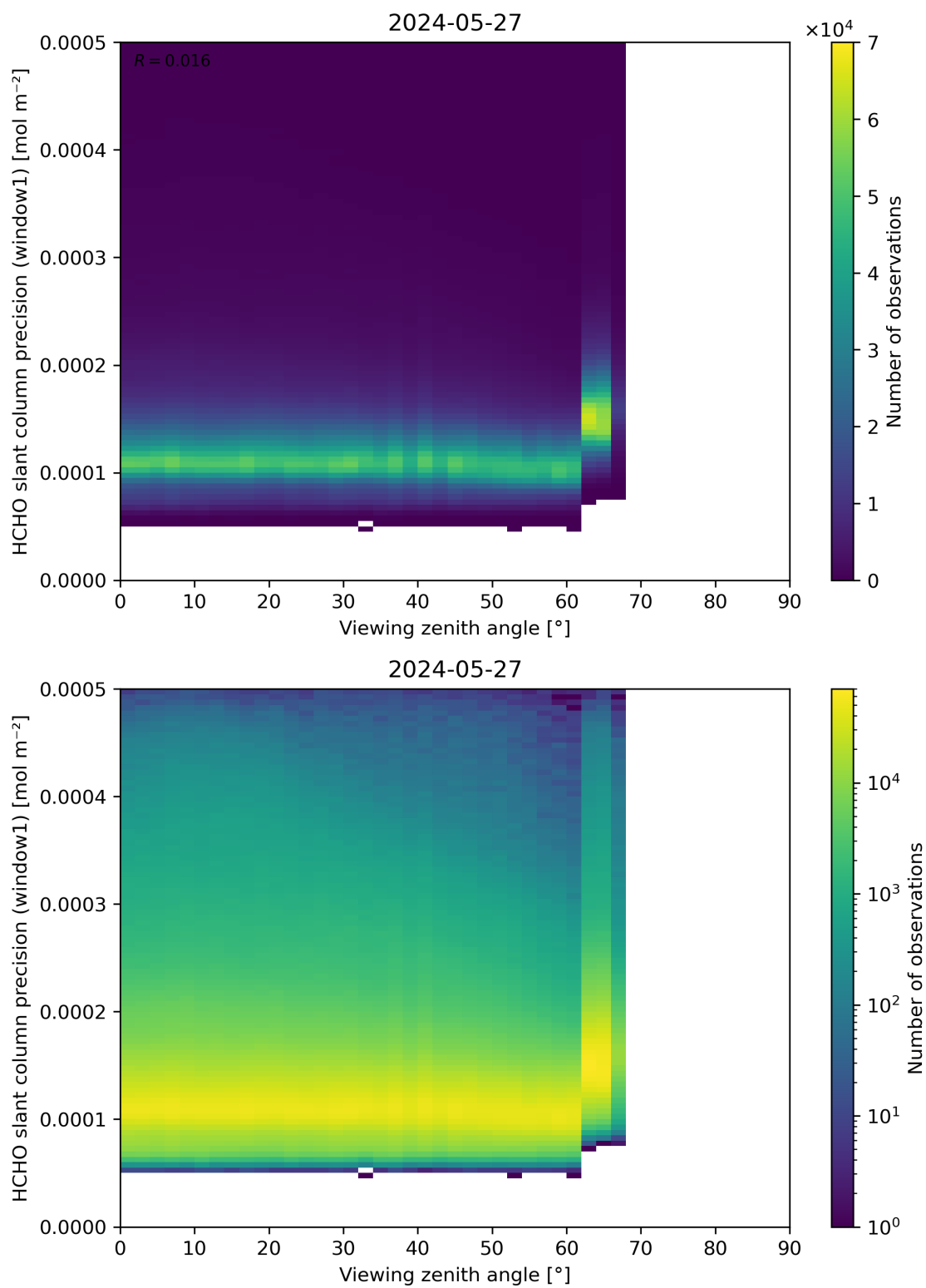
Figure 189: Scatter density plot of “Viewing zenith angle” against “HCHO slant column precision (window1)” for 2024-05-26 to 2024-05-28.
