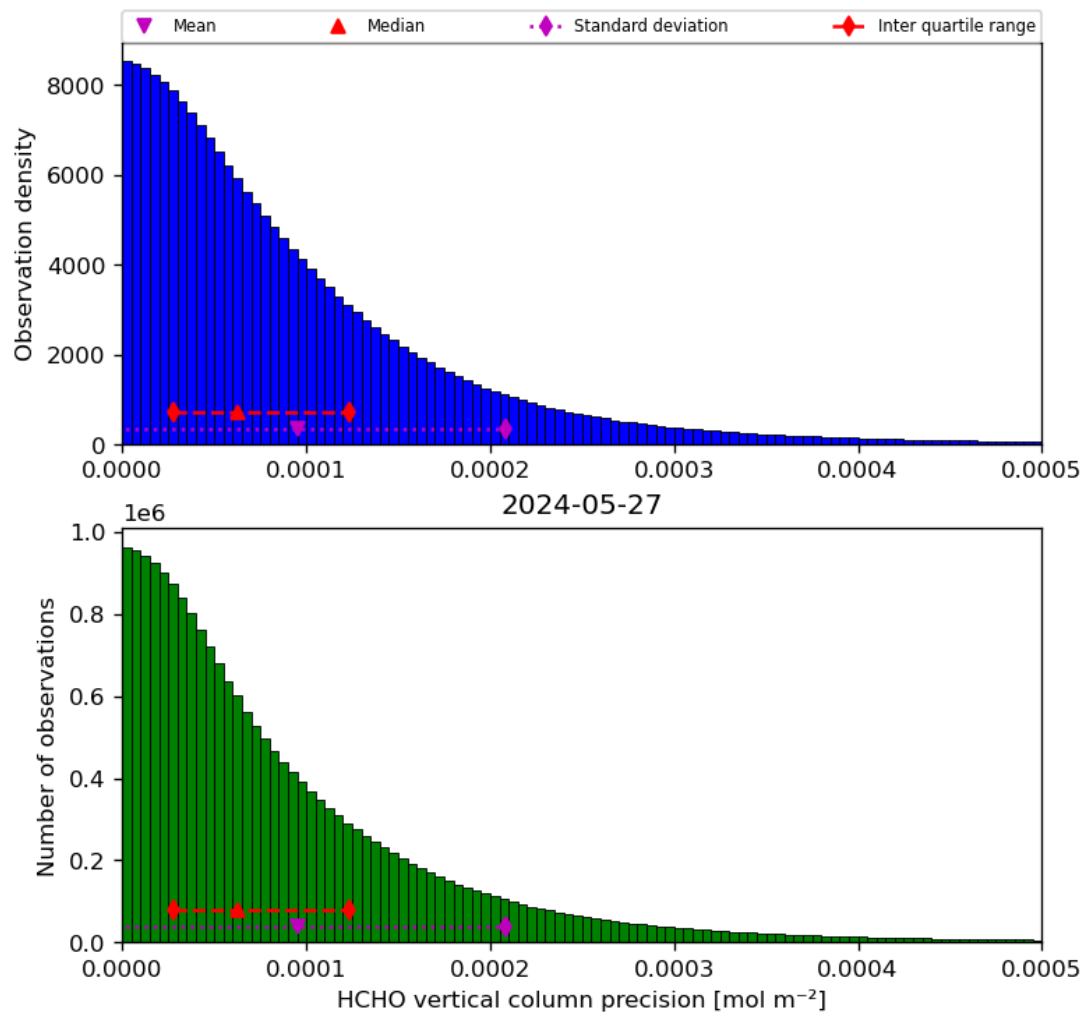
Figure 36: Histogram of “HCHO vertical column precision” for 2024-05-26 to 2024-05-28
