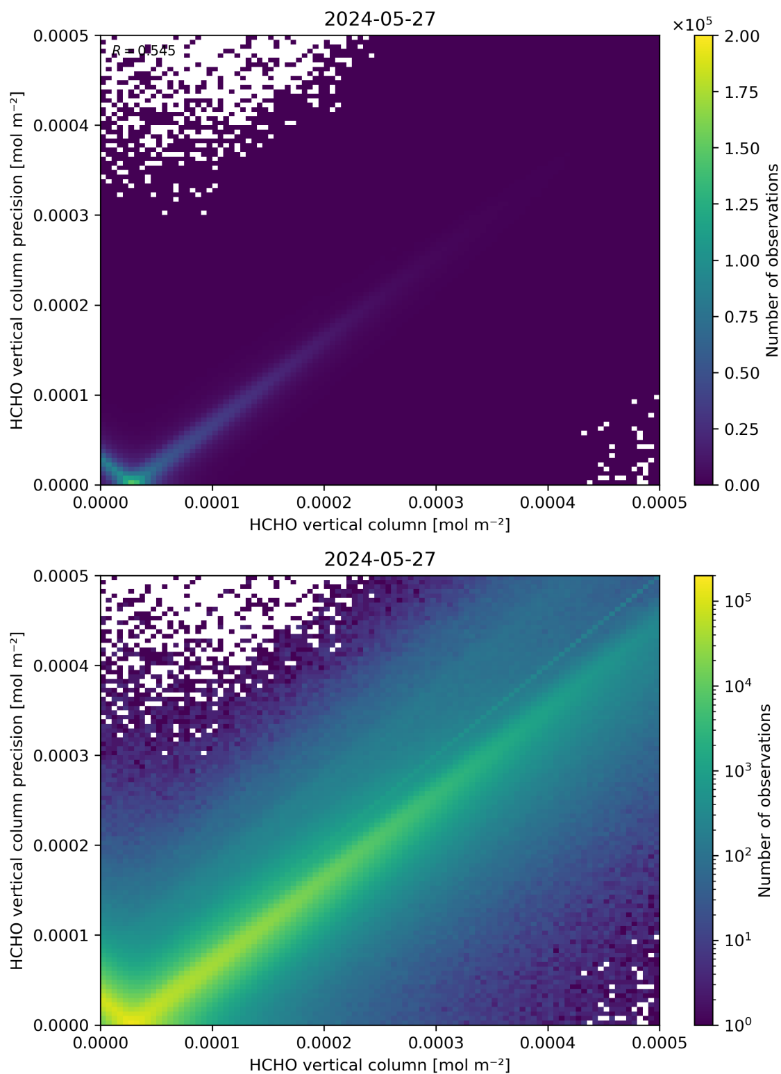
Figure 134: Scatter density plot of “HCHO vertical column” against “HCHO vertical column precision” for 2024-05-26 to 2024-05-28.
