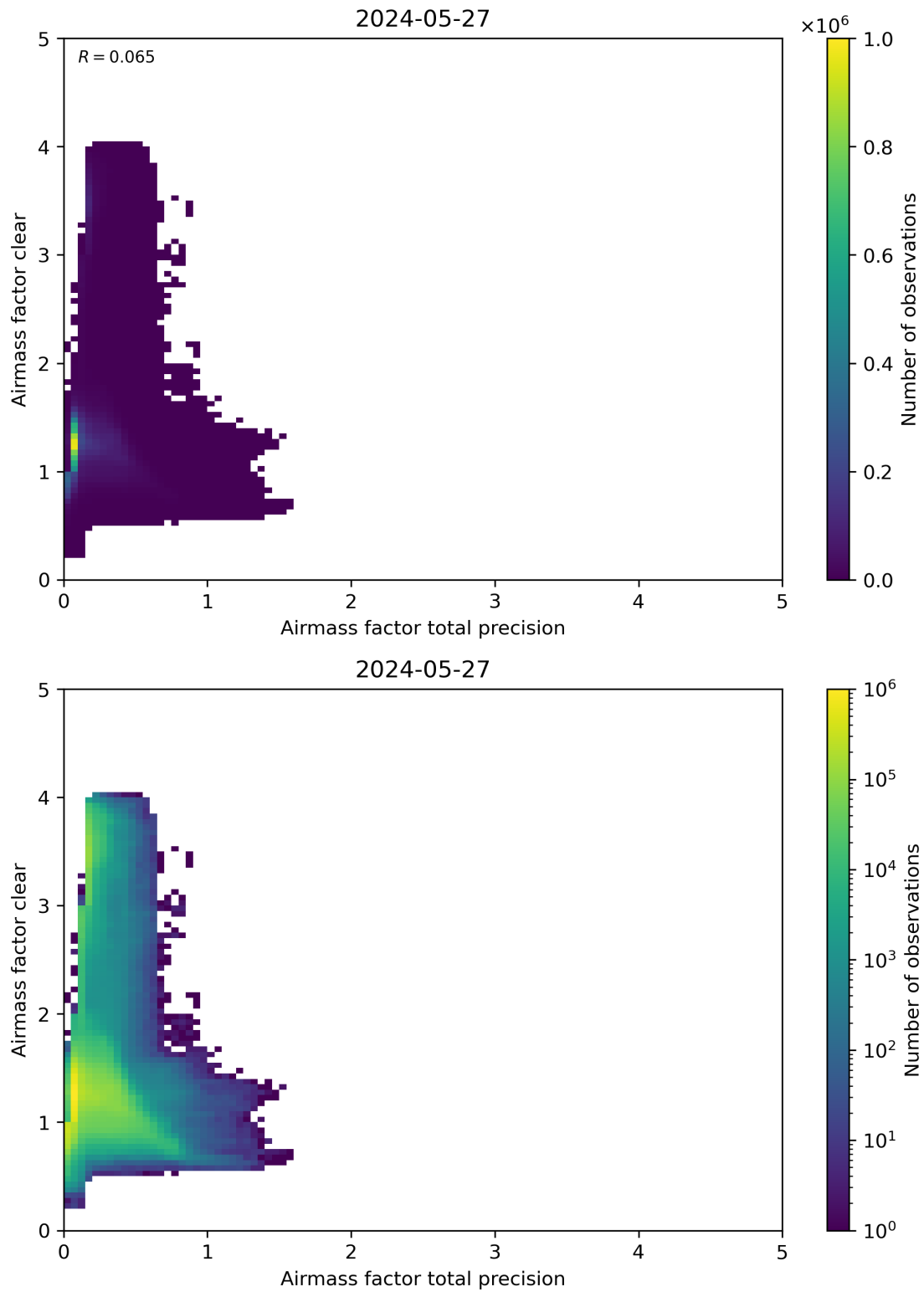
Figure 108: Scatter density plot of “Airmass factor total precision” against “Airmass factor clear” for 2024-05-26 to 2024-05-28.
