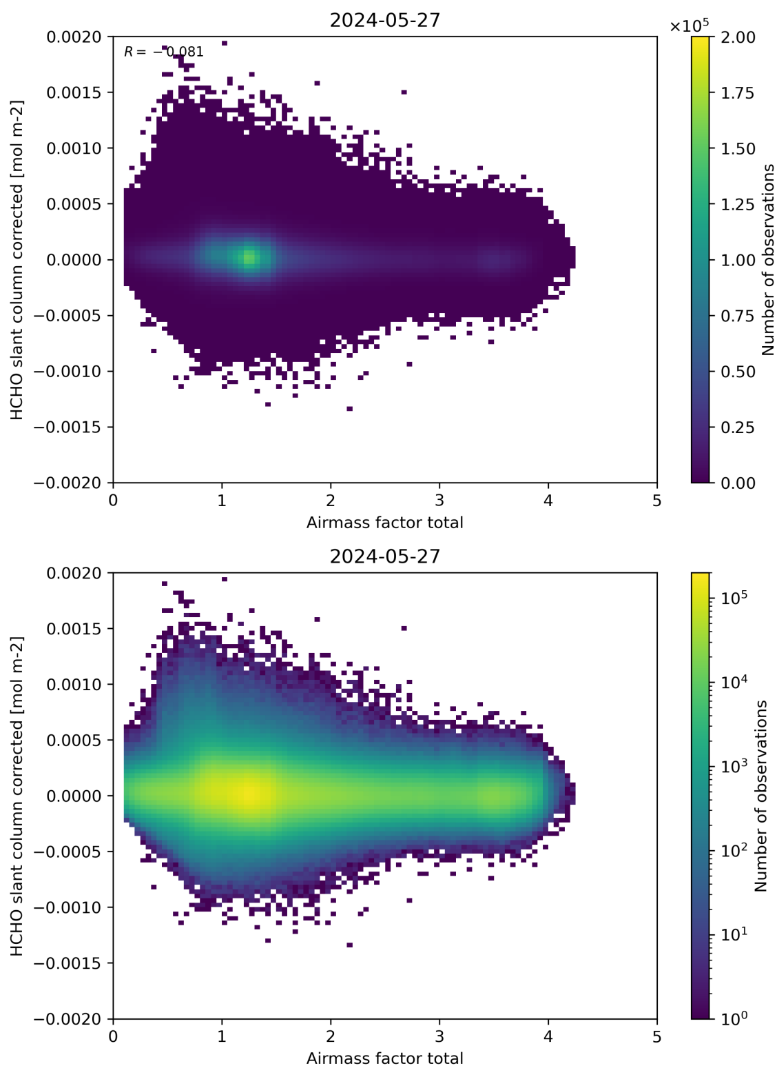
Figure 101: Scatter density plot of “Airmass factor total” against “HCHO slant column corrected” for 2024-05-26 to 2024-05-28.
