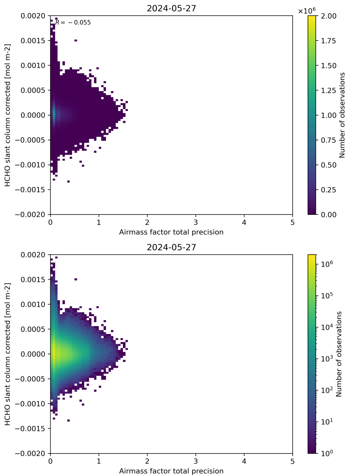
Figure 109: Scatter density plot of “Airmass factor total precision” against “HCHO slant column corrected” for 2024-05-26 to 2024-05-28.
