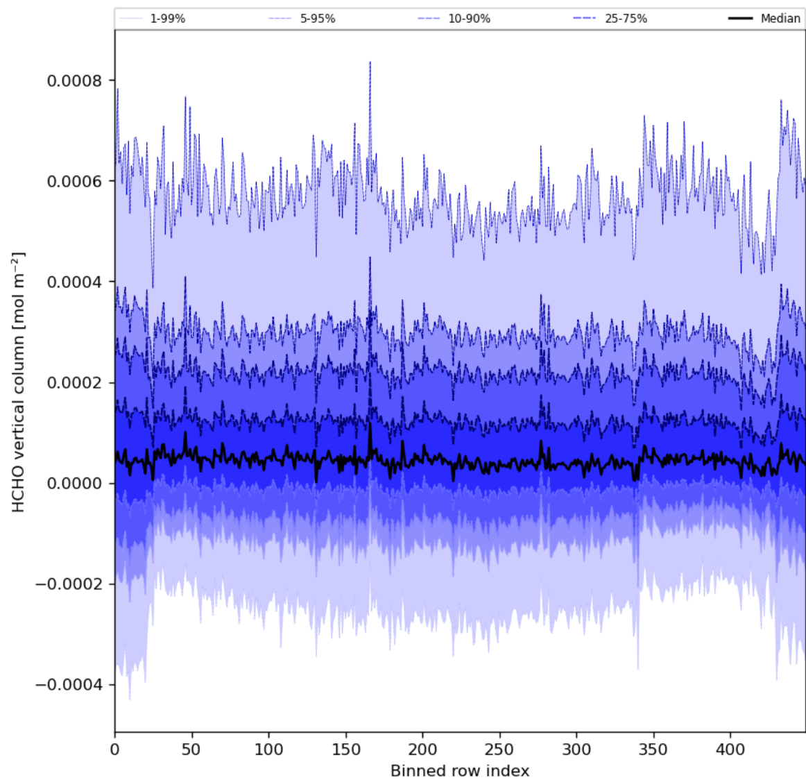
Figure 49: Along track statistics of “HCHO vertical column” for 2024-05-26 to 2024-05-28
