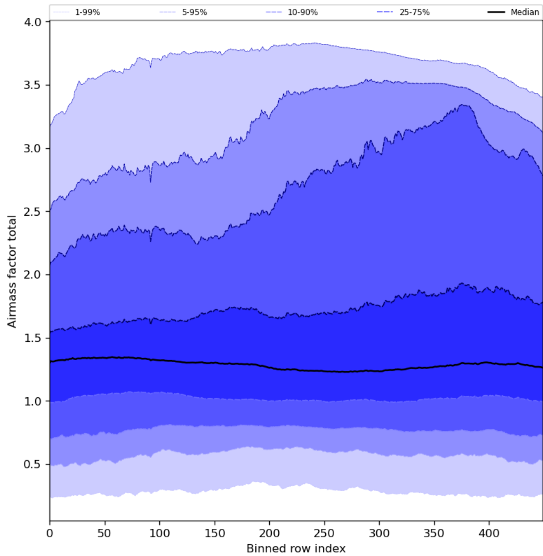
Figure 54: Along track statistics of “Airmass factor total” for 2024-05-26 to 2024-05-28
