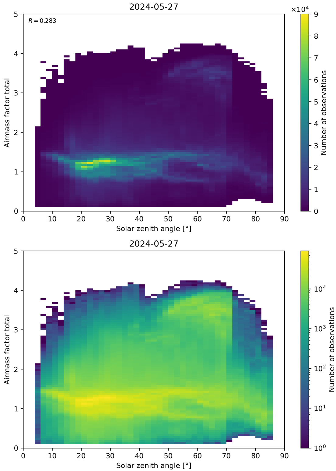
Figure 175: Scatter density plot of “Solar zenith angle” against “Airmass factor total” for 2024-05-26 to 2024-05-28.
