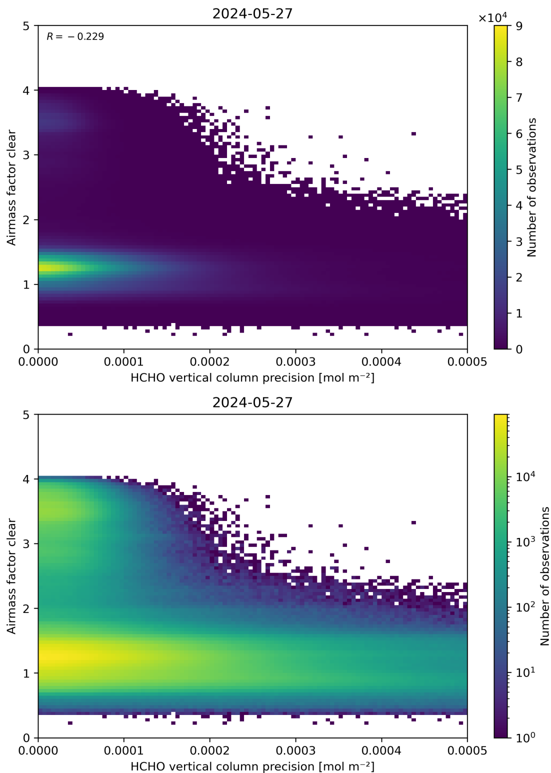
Figure 139: Scatter density plot of “HCHO vertical column precision” against “Airmass factor clear” for 2024-05-26 to 2024-05-28.
