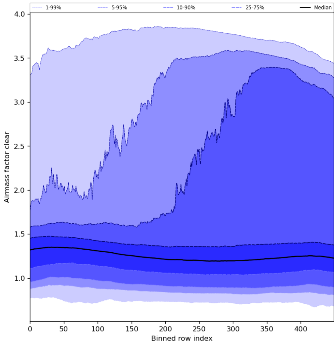
Figure 56: Along track statistics of “Airmass factor clear” for 2024-05-26 to 2024-05-28
