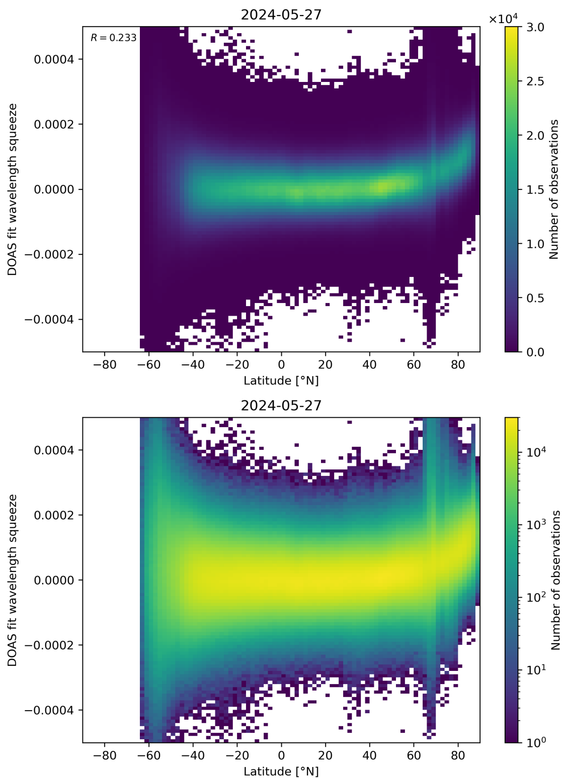
Figure 155: Scatter density plot of “Latitude” against “DOAS fit wavelength squeeze” for 2024-05-26 to 2024-05-28.
