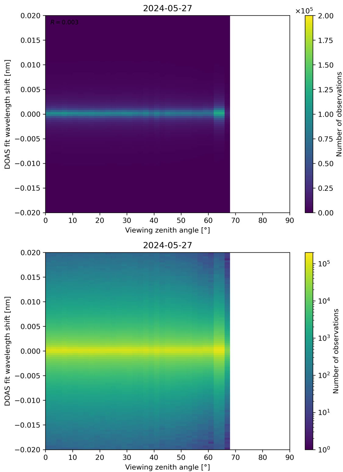
Figure 183: Scatter density plot of “Viewing zenith angle” against “DOAS fit wavelength shift” for 2024-05-26 to 2024-05-28.
