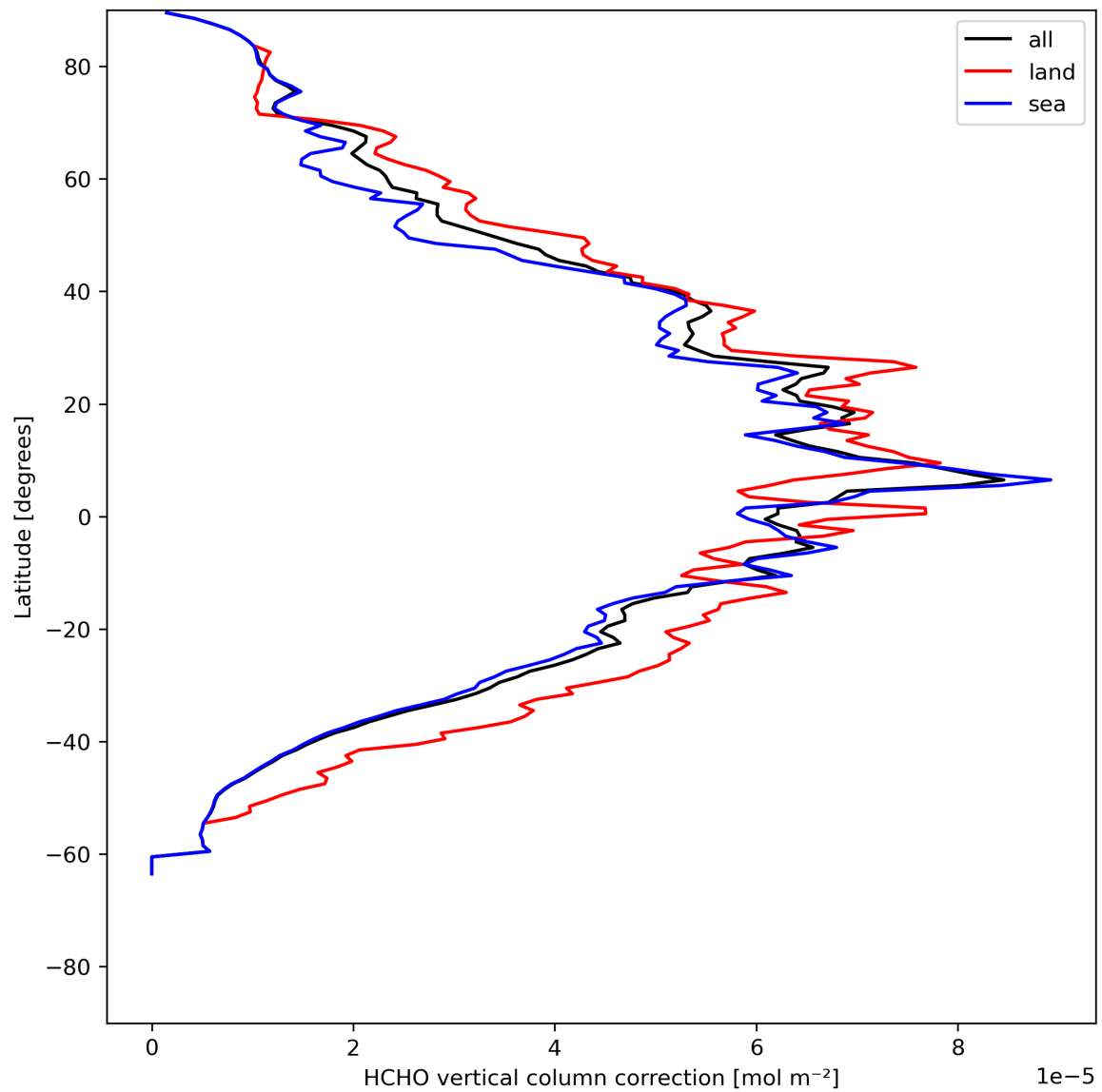
Figure 23: Zonal average of “HCHO vertical column correction” for 2024-05-26 to 2024-05-28.
