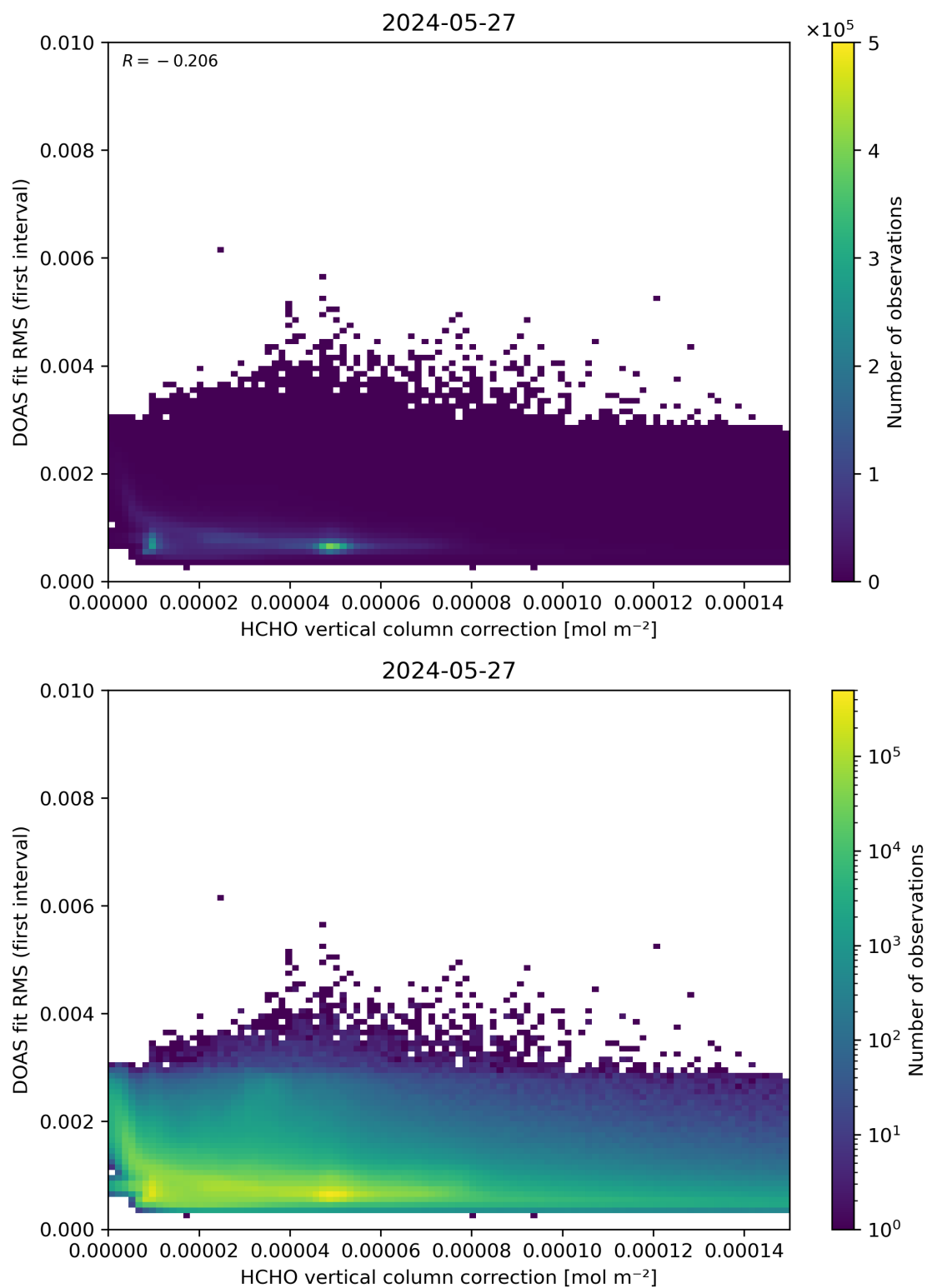
Figure 112: Scatter density plot of “HCHO vertical column correction” against “DOAS fit RMS (first interval)” for 2024-05-26 to 2024-05-28.
