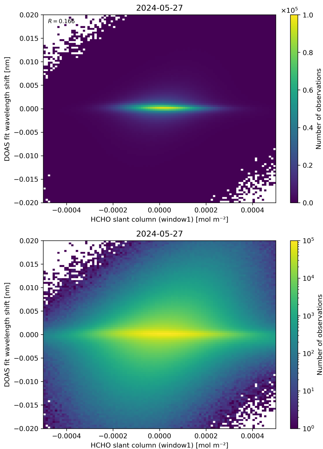
Figure 79: Scatter density plot of “HCHO slant column (window1)” against “DOAS fit wavelength shift” for 2024-05-26 to 2024-05-28.
