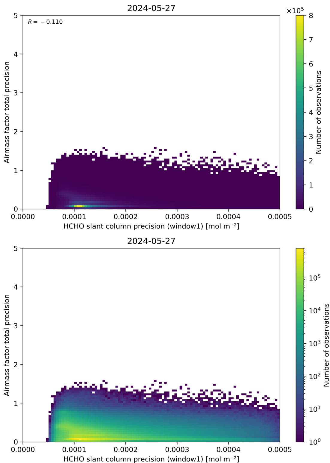
Figure 95: Scatter density plot of “HCHO slant column precision (window1)” against “Airmass factor total precision” for 2024-05-26 to 2024-05-28.
