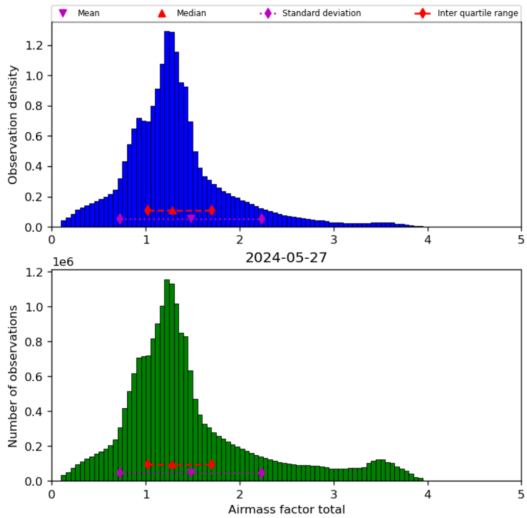
Figure 40: Histogram of “Airmass factor total” for 2024-05-26 to 2024-05-28
