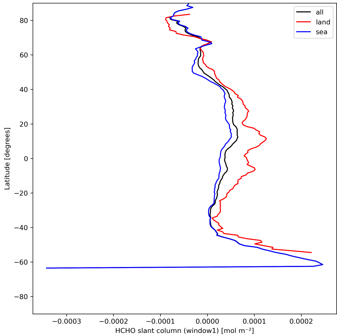
Figure 24: Zonal average of “HCHO slant column (window1)” for 2024-05-26 to 2024-05-28.
