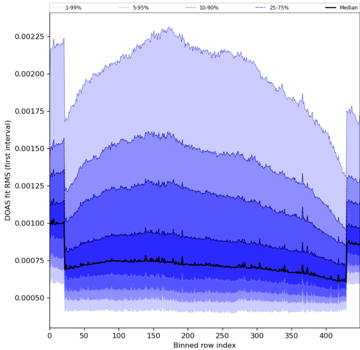
Figure 60: Along track statistics of “DOAS fit RMS (first interval)” for 2024-05-26 to 2024-05-28
