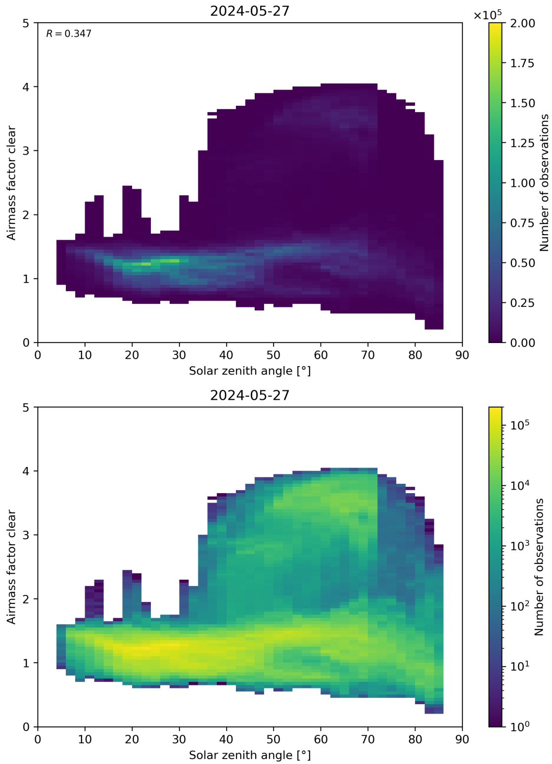
Figure 170: Scatter density plot of “Solar zenith angle” against “Airmass factor clear” for 2024-05-26 to 2024-05-28.
