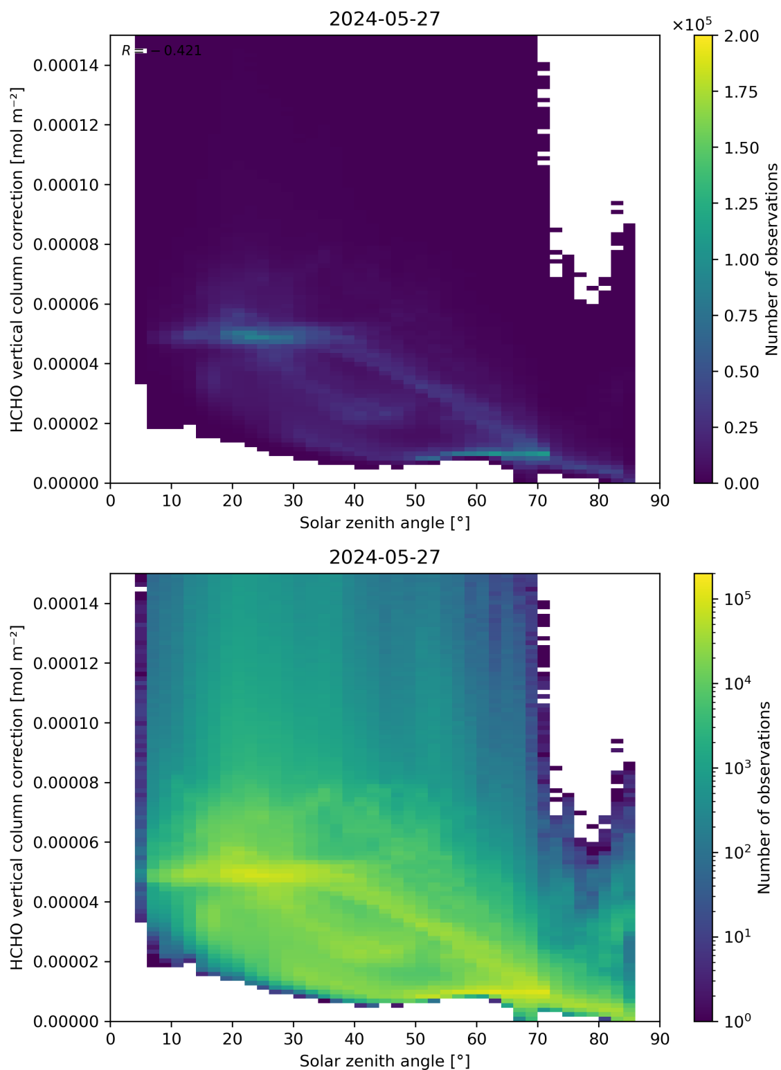
Figure 178: Scatter density plot of “Solar zenith angle” against “HCHO vertical column correction” for 2024-05-26 to 2024-05-28.
