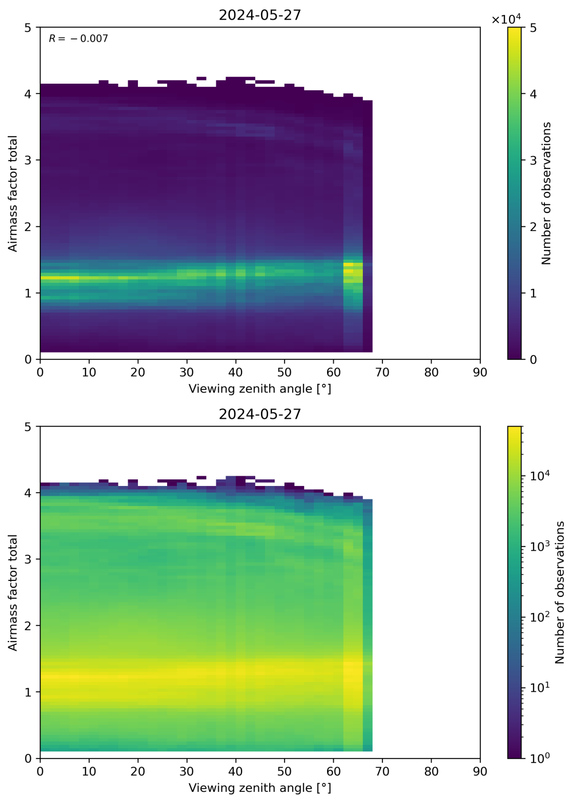
Figure 190: Scatter density plot of “Viewing zenith angle” against “Airmass factor total” for 2024-05-26 to 2024-05-28.
