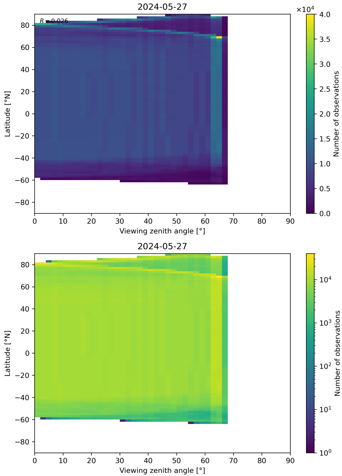
Figure 196: Scatter density plot of “Viewing zenith angle” against “Latitude” for 2024-05-26 to 2024-05-28.
