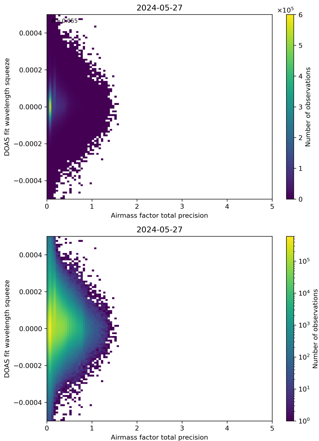
Figure 107: Scatter density plot of “Airmass factor total precision” against “DOAS fit wavelength squeeze” for 2024-05-26 to 2024-05-28.
