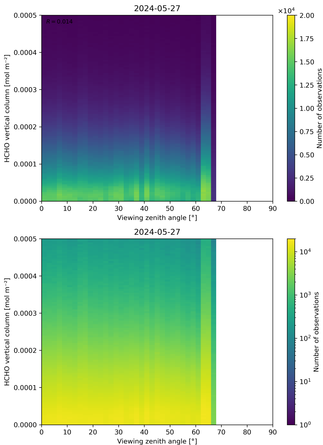
Figure 192: Scatter density plot of “Viewing zenith angle” against “HCHO vertical column” for 2024-05-26 to 2024-05-28.
