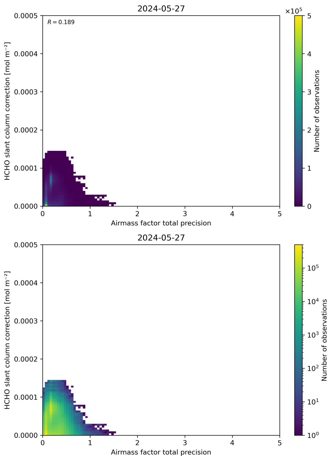
Figure 110: Scatter density plot of “Airmass factor total precision” against “HCHO slant column correction” for 2024-05-26 to 2024-05-28.
