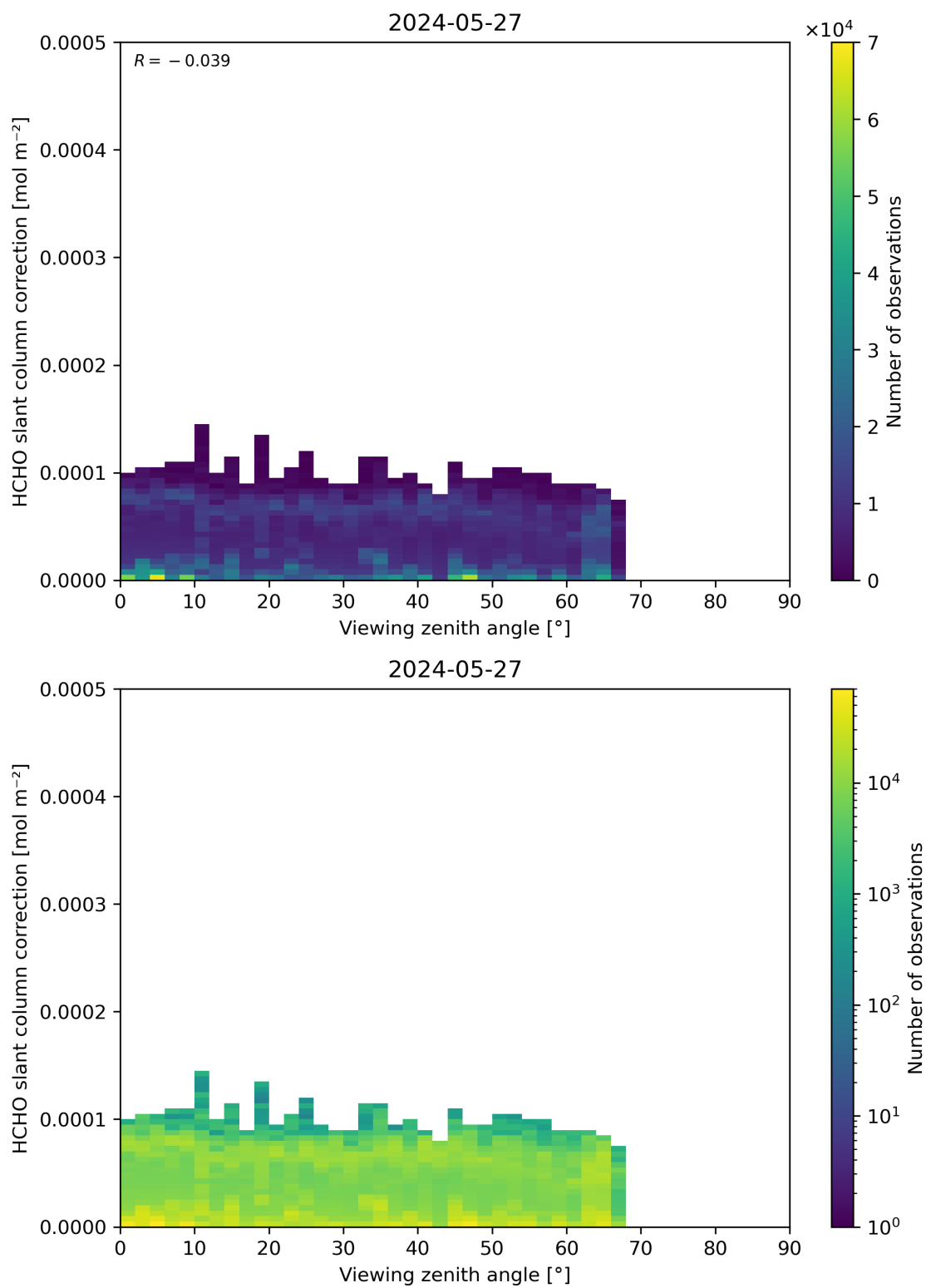
Figure 187: Scatter density plot of “Viewing zenith angle” against “HCHO slant column correction” for 2024-05-26 to 2024-05-28.
