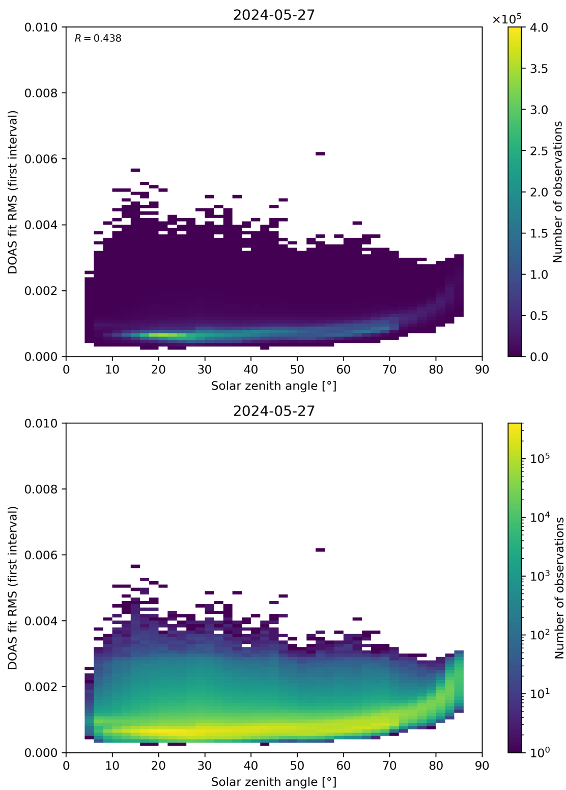
Figure 167: Scatter density plot of “Solar zenith angle” against “DOAS fit RMS (first interval)” for 2024-05-26 to 2024-05-28.
