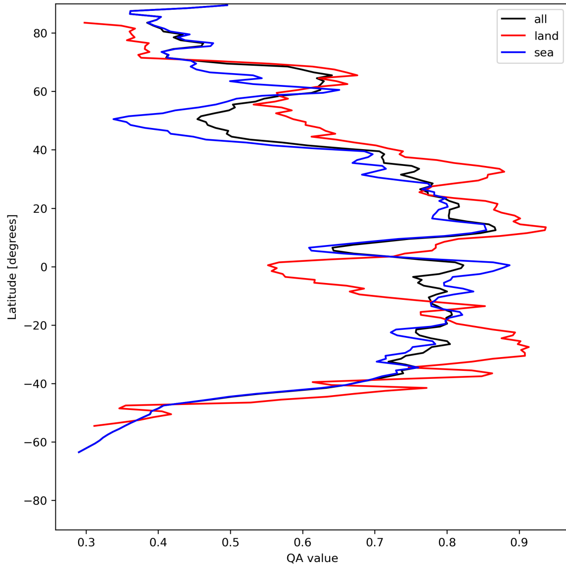
Figure 20: Zonal average of “QA value” for 2024-05-26 to 2024-05-28.
