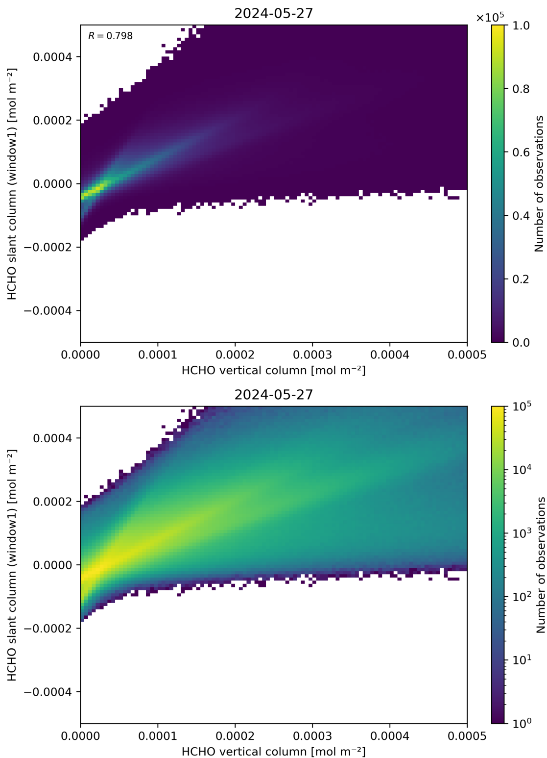
Figure 129: Scatter density plot of “HCHO vertical column” against “HCHO slant column (window1)” for 2024-05-26 to 2024-05-28.
