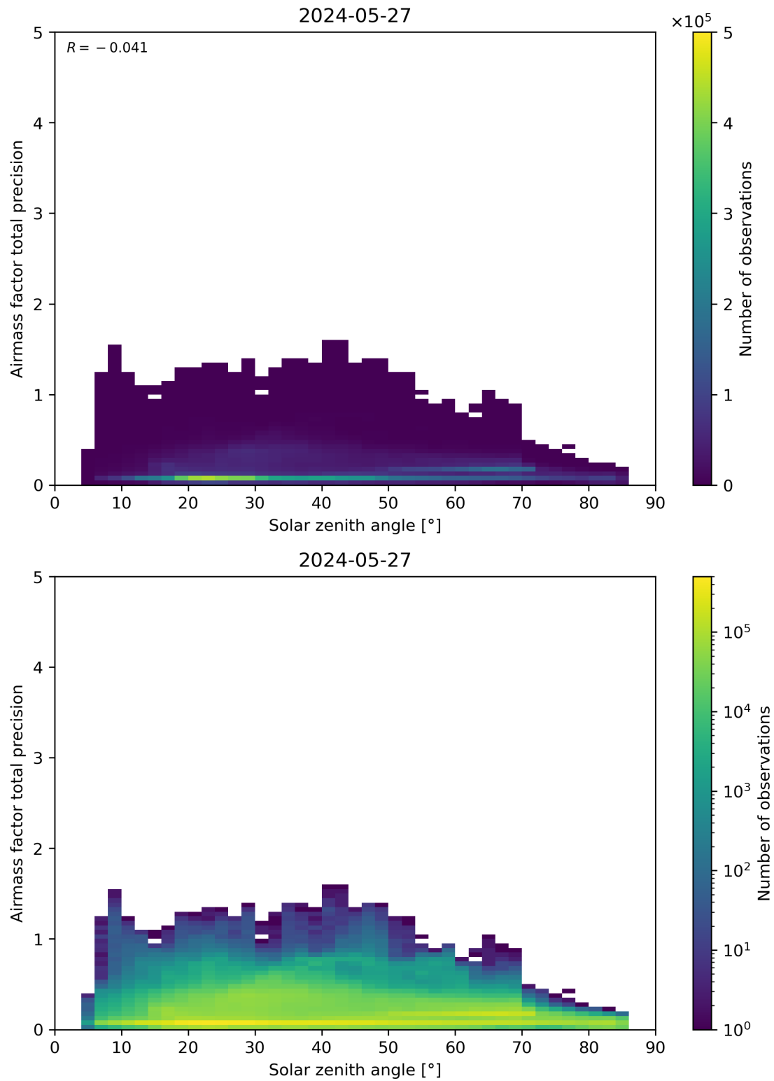
Figure 176: Scatter density plot of “Solar zenith angle” against “Airmass factor total precision” for 2024-05-26 to 2024-05-28.
