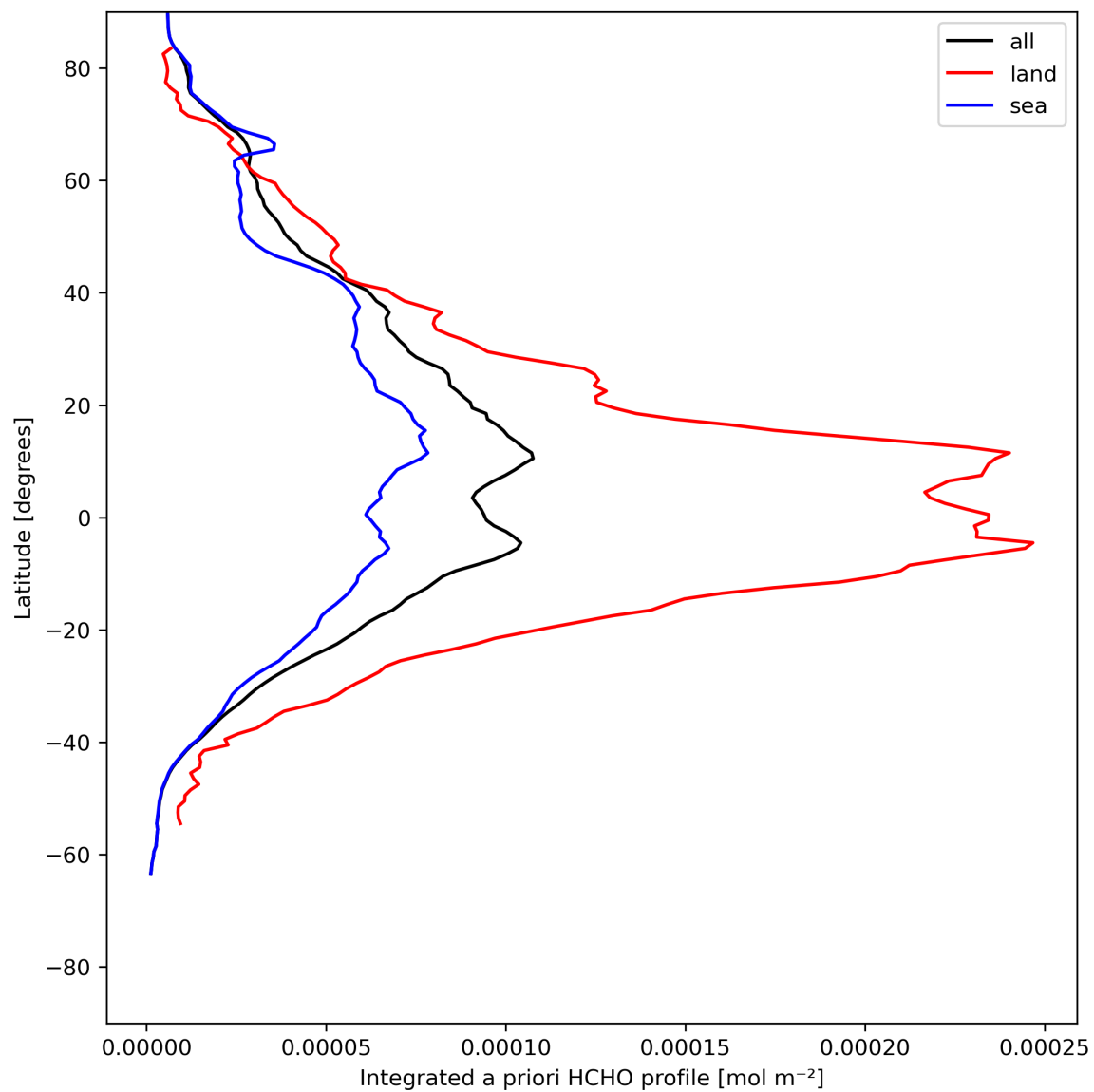
Figure 29: Zonal average of “Integrated a priori HCHO profile” for 2024-05-26 to 2024-05-28.
