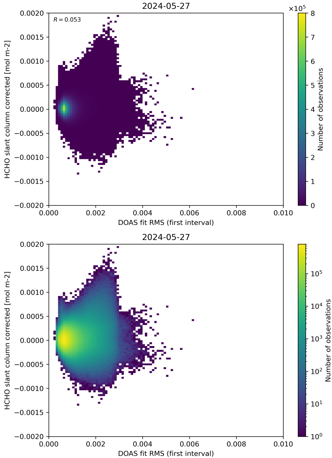
Figure 62: Scatter density plot of “DOAS fit RMS (first interval)” against “HCHO slant column corrected” for 2024-05-26 to 2024-05-28.
