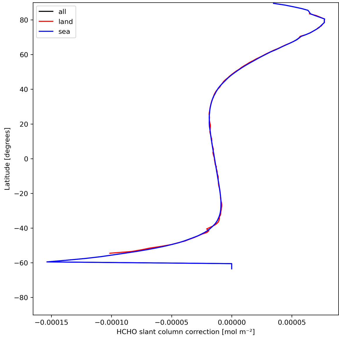
Figure 33: Zonal average of “HCHO slant column correction” for 2024-05-26 to 2024-05-28.
