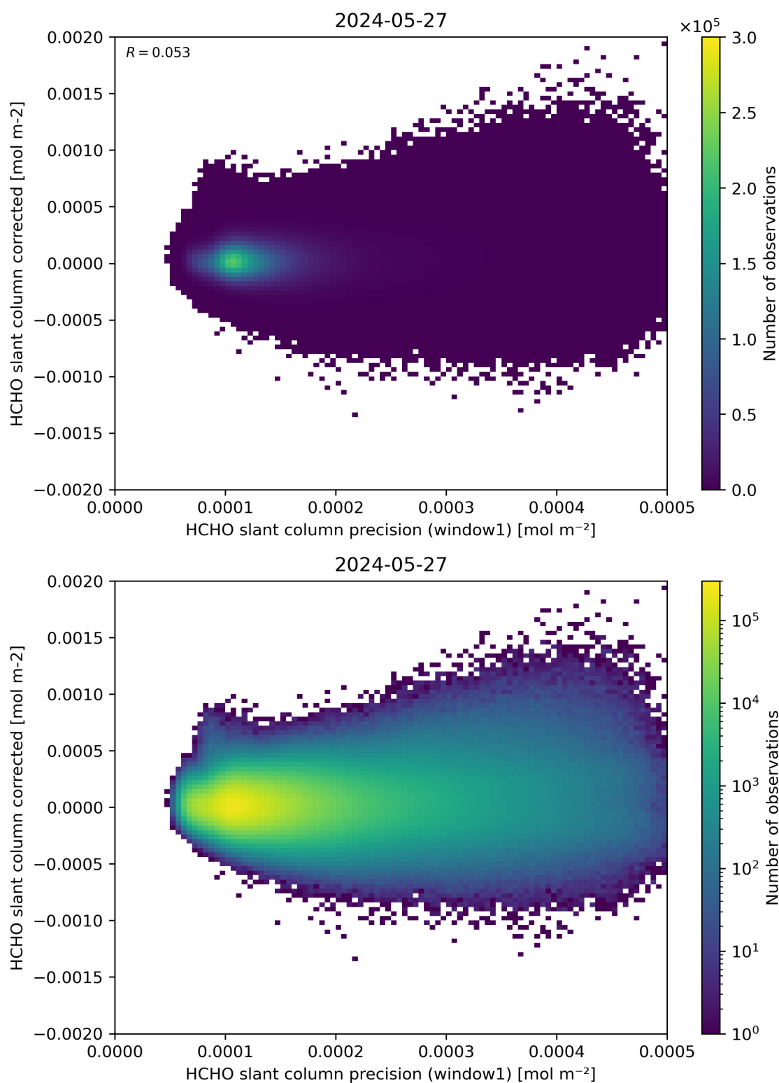
Figure 92: Scatter density plot of “HCHO slant column precision (window1)” against “HCHO slant column corrected” for 2024-05-26 to 2024-05-28.
