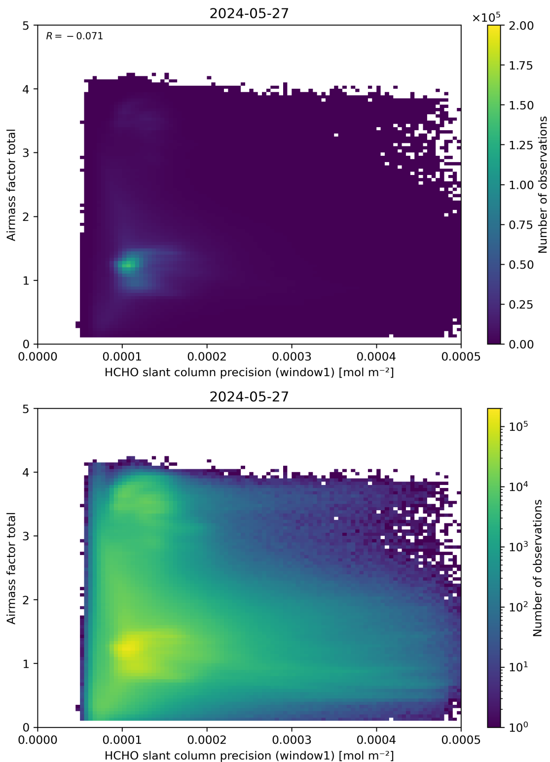
Figure 94: Scatter density plot of “HCHO slant column precision (window1)” against “Airmass factor total” for 2024-05-26 to 2024-05-28.
