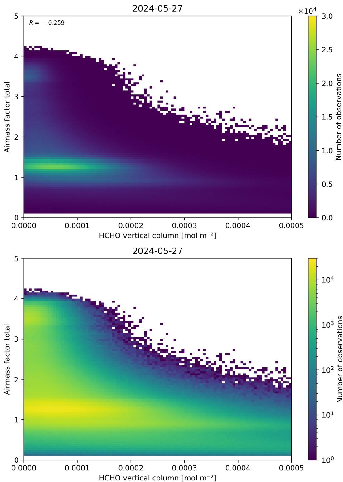
Figure 131: Scatter density plot of “HCHO vertical column” against “Airmass factor total” for 2024-05-26 to 2024-05-28.
