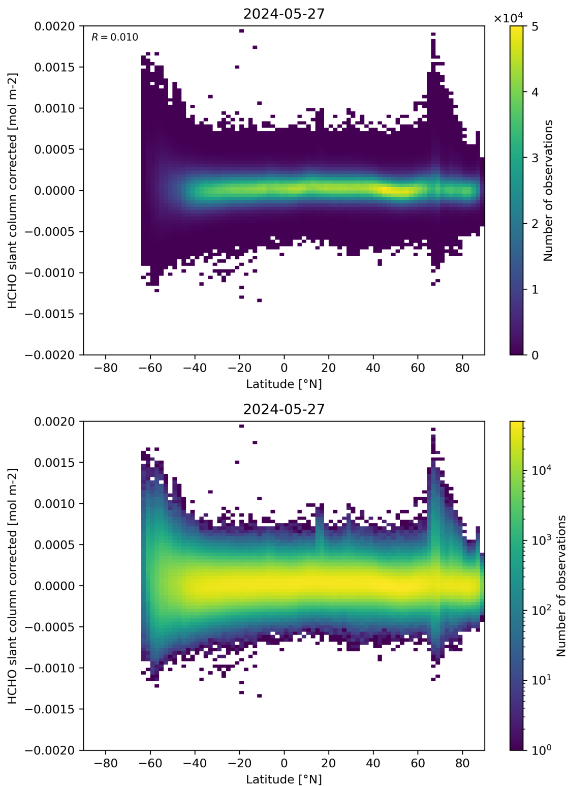
Figure 157: Scatter density plot of “Latitude” against “HCHO slant column corrected” for 2024-05-26 to 2024-05-28.
