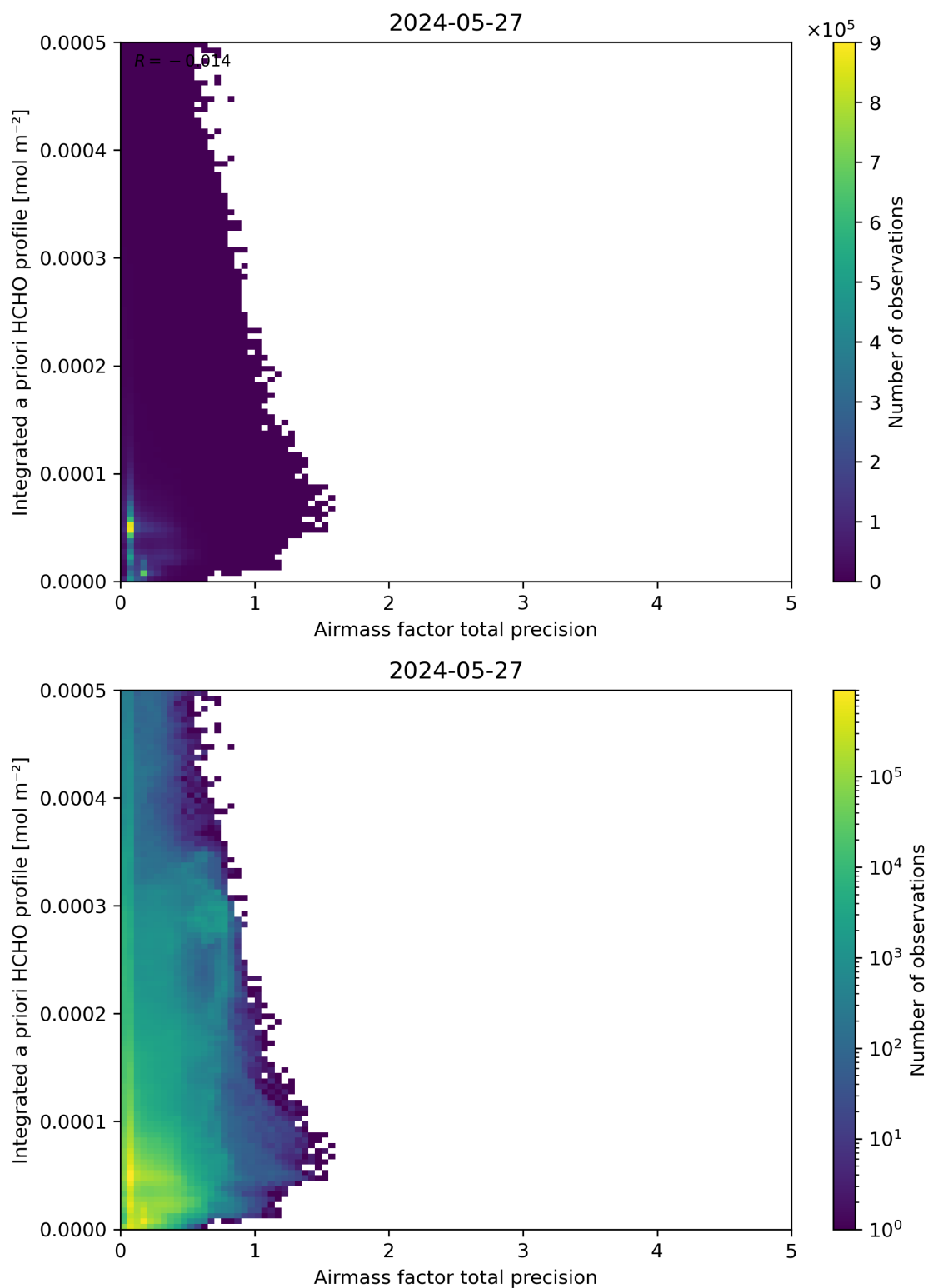
Figure 111: Scatter density plot of “Airmass factor total precision” against “Integrated a priori HCHO profile” for 2024-05-26 to 2024-05-28.
