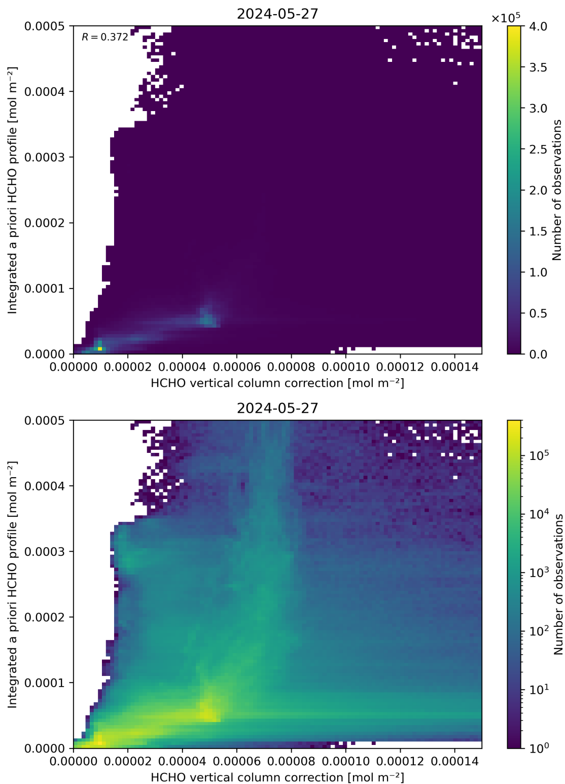
Figure 122: Scatter density plot of “HCHO vertical column correction” against “Integrated a priori HCHO profile” for 2024-05-26 to 2024-05-28.
