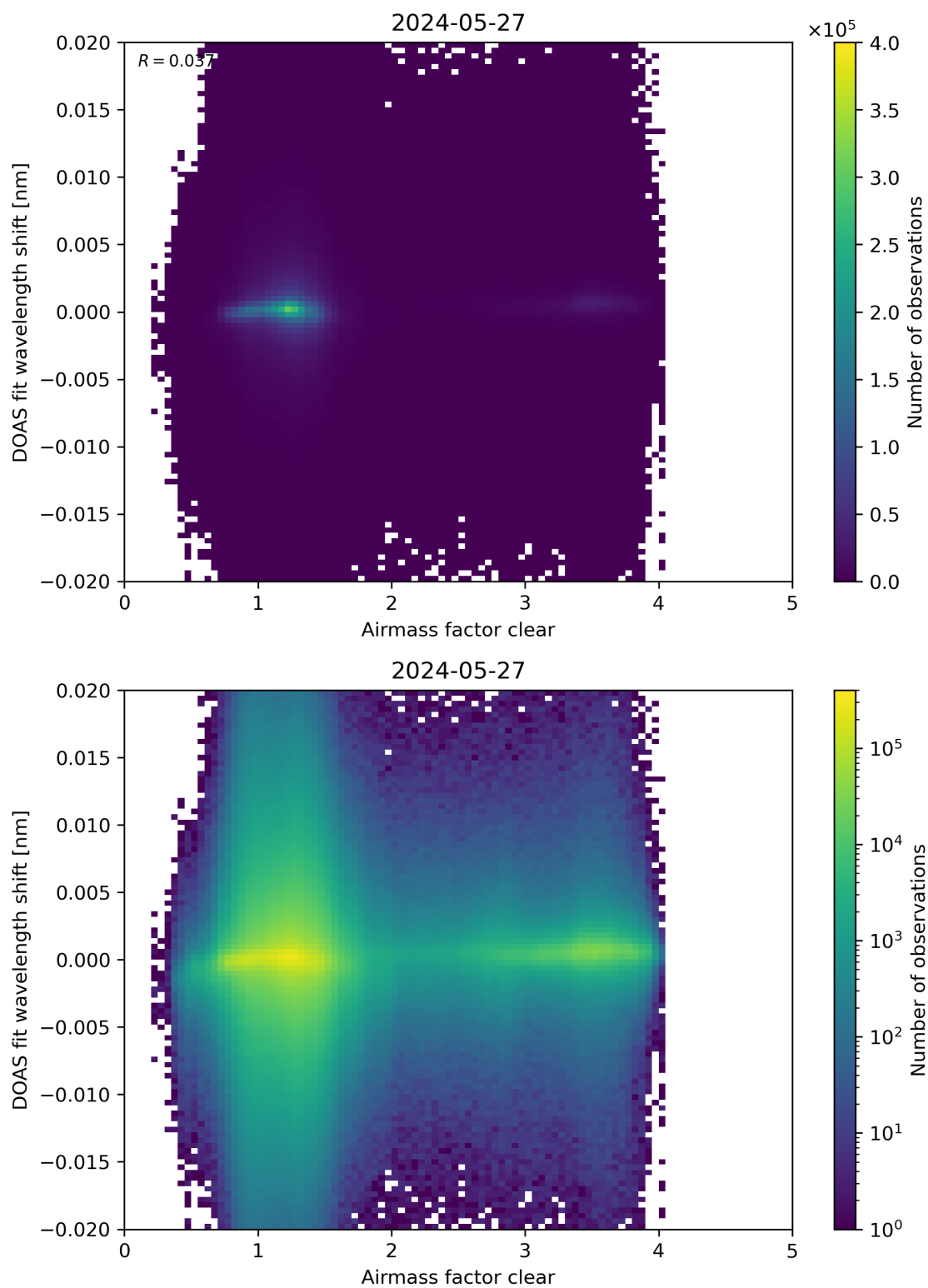
Figure 72: Scatter density plot of “Airmass factor clear” against “DOAS fit wavelength shift” for 2024-05-26 to 2024-05-28.
