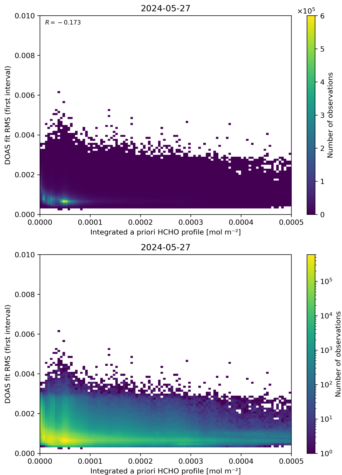
Figure 148: Scatter density plot of “Integrated a priori HCHO profile” against “DOAS fit RMS (first interval)” for 2024-05-26 to 2024-05-28.
