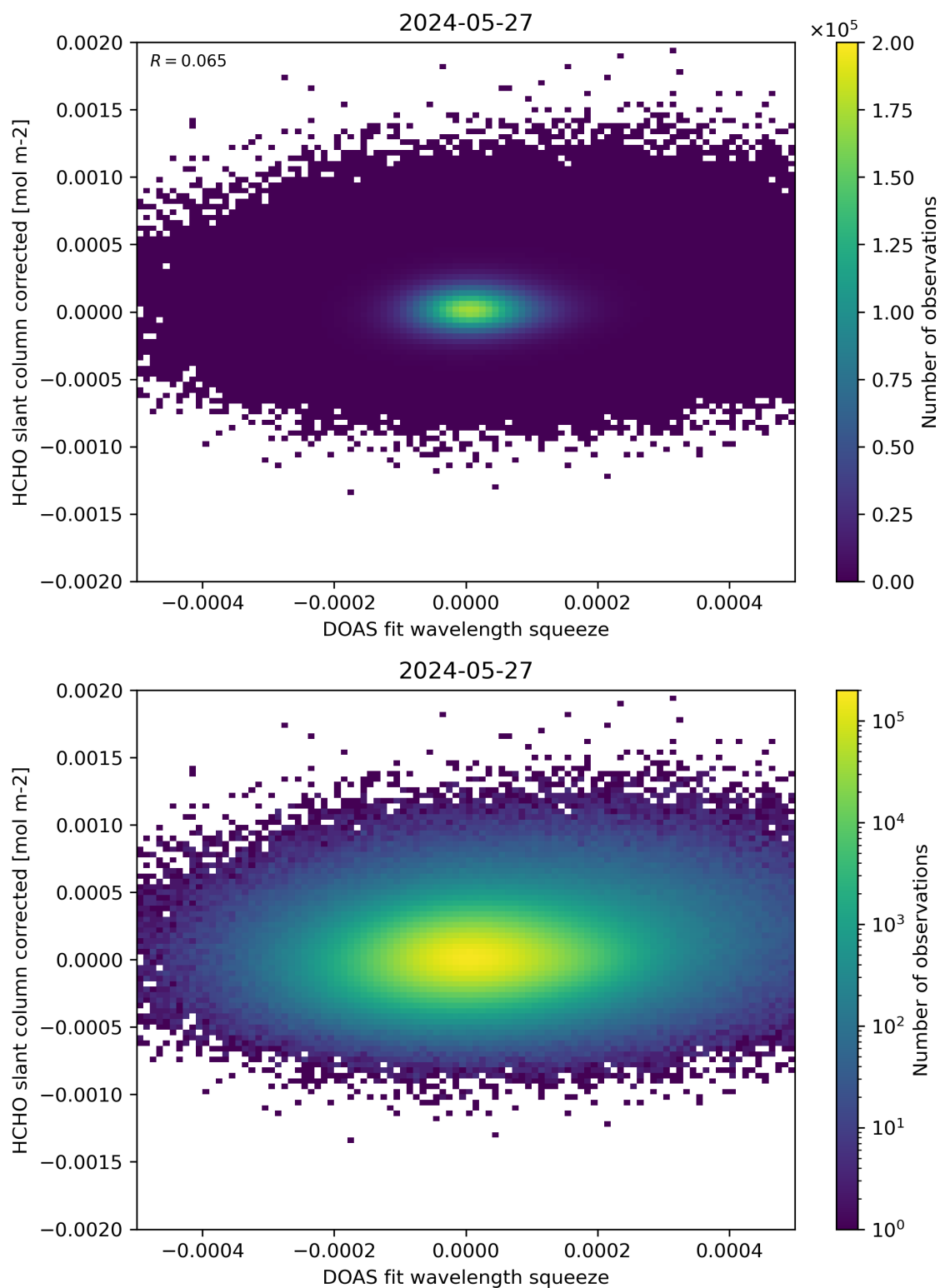
Figure 69: Scatter density plot of “DOAS fit wavelength squeeze” against “HCHO slant column corrected” for 2024-05-26 to 2024-05-28.
