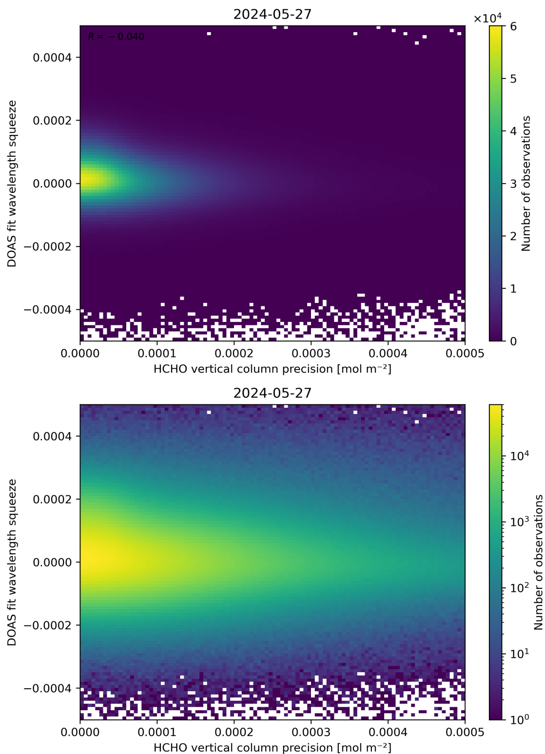
Figure 138: Scatter density plot of “HCHO vertical column precision” against “DOAS fit wavelength squeeze” for 2024-05-26 to 2024-05-28.
