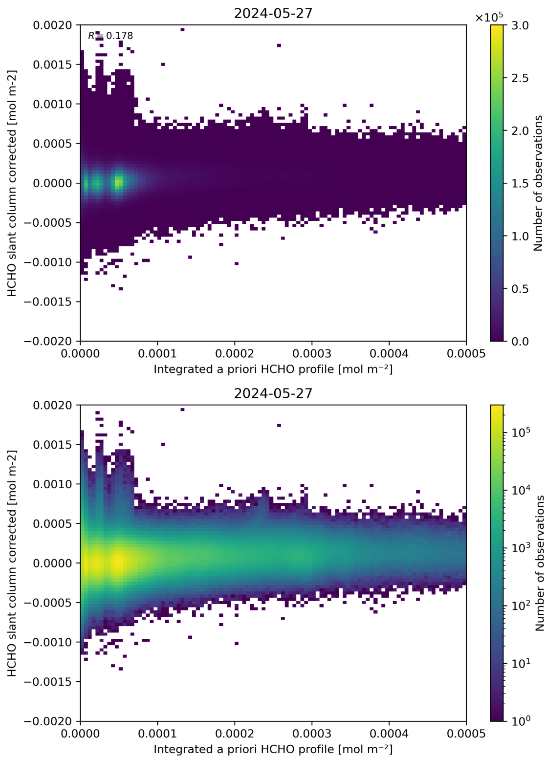
Figure 151: Scatter density plot of “Integrated a priori HCHO profile” against “HCHO slant column corrected” for 2024-05-26 to 2024-05-28.
