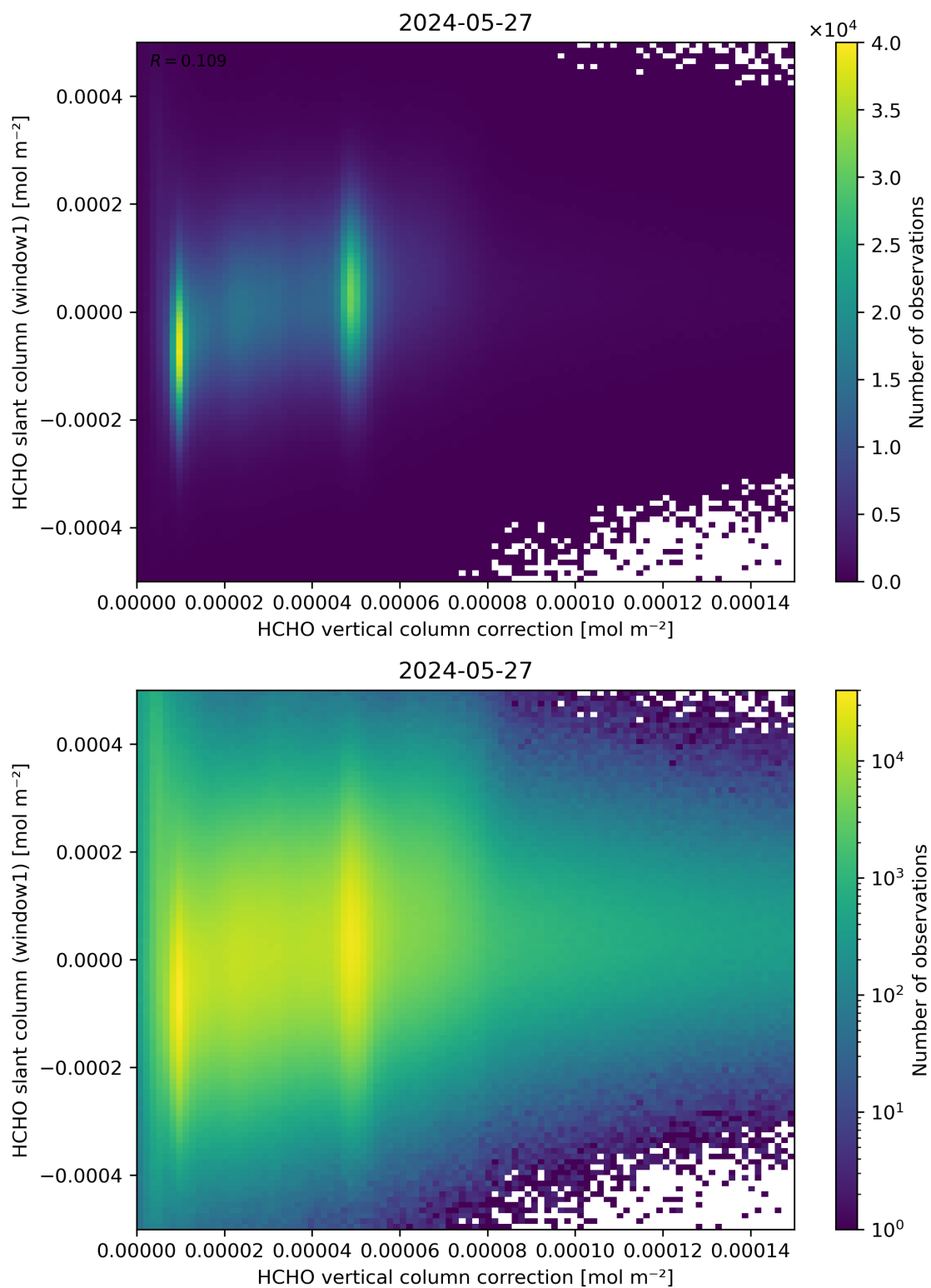
Figure 118: Scatter density plot of “HCHO vertical column correction” against “HCHO slant column (window1)” for 2024-05-26 to 2024-05-28.
