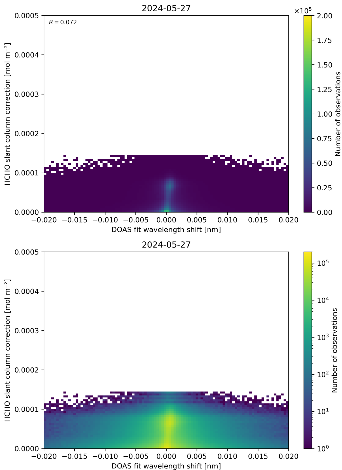
Figure 67: Scatter density plot of “DOAS fit wavelength shift” against “HCHO slant column correction” for 2024-05-26 to 2024-05-28.
