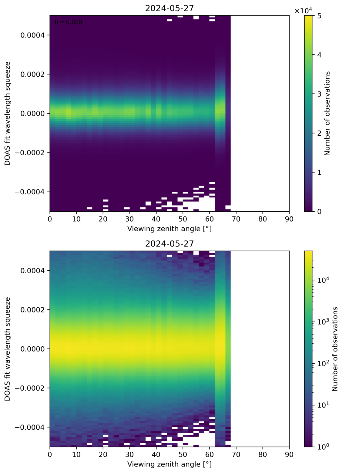
Figure 184: Scatter density plot of “Viewing zenith angle” against “DOAS fit wavelength squeeze” for 2024-05-26 to 2024-05-28.
