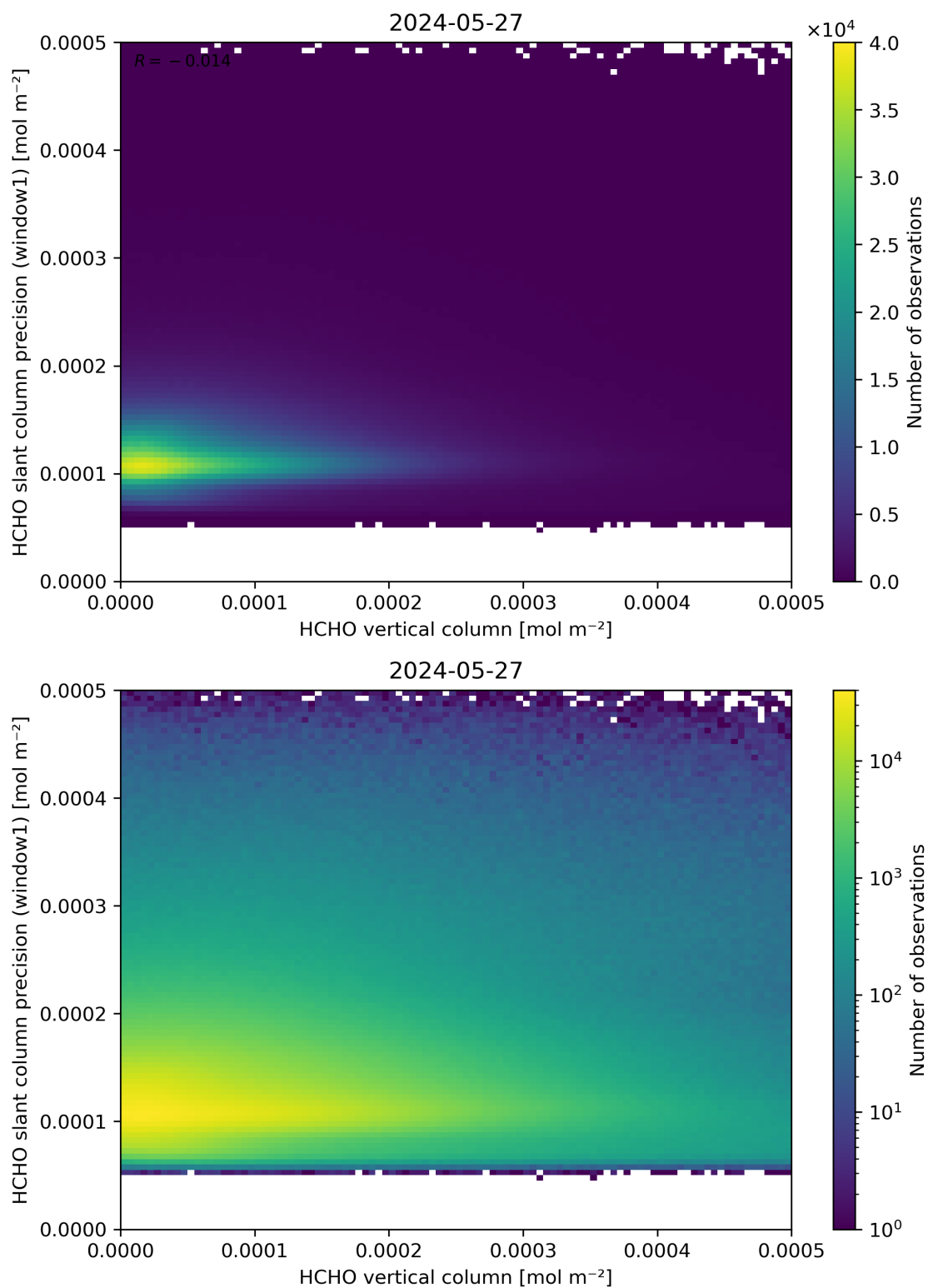
Figure 130: Scatter density plot of “HCHO vertical column” against “HCHO slant column precision (window1)” for 2024-05-26 to 2024-05-28.
