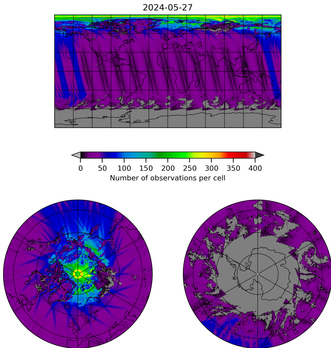
Figure 19: Map of the number of observations for 2024-05-26 to 2024-05-28
