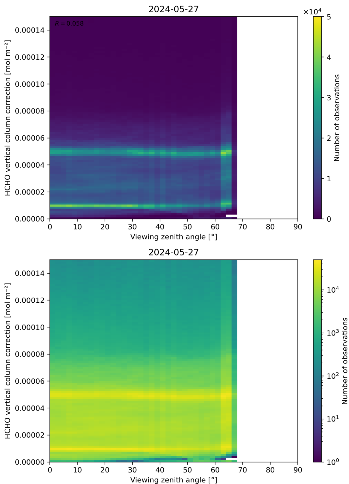
Figure 193: Scatter density plot of “Viewing zenith angle” against “HCHO vertical column correction” for 2024-05-26 to 2024-05-28.
