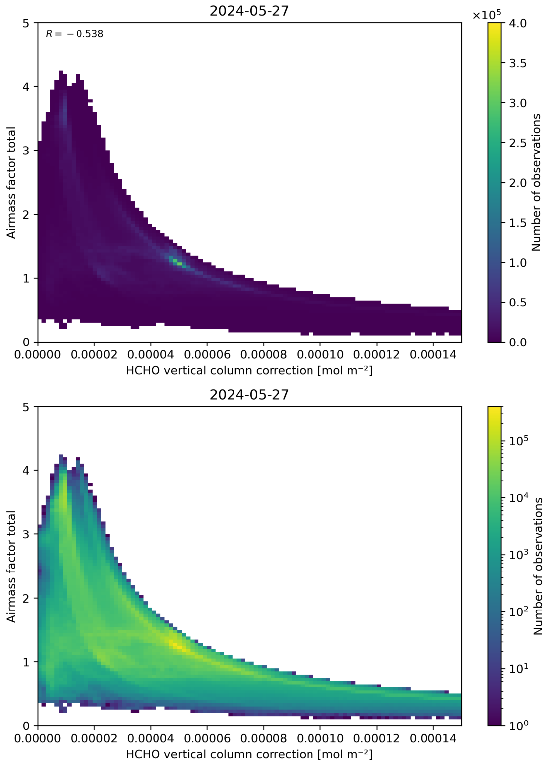
Figure 120: Scatter density plot of “HCHO vertical column correction” against “Airmass factor total” for 2024-05-26 to 2024-05-28.
