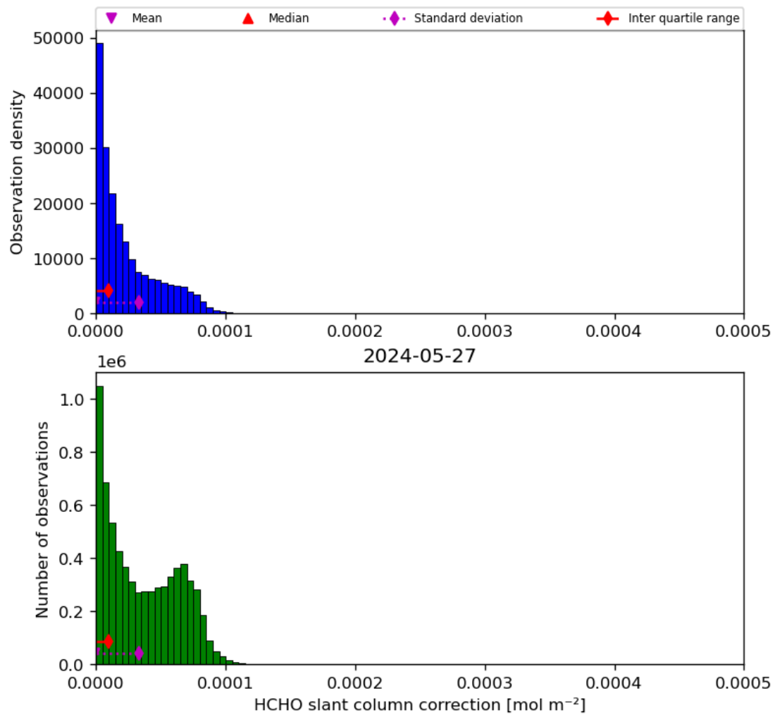
Figure 47: Histogram of “HCHO slant column correction” for 2024-05-26 to 2024-05-28
