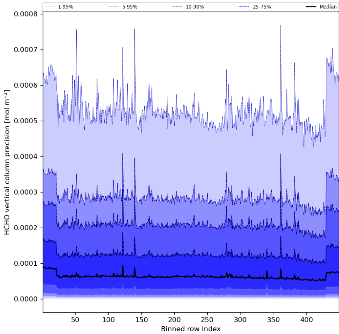
Figure 50: Along track statistics of “HCHO vertical column precision” for 2024-05-28 to 2024-05-30
