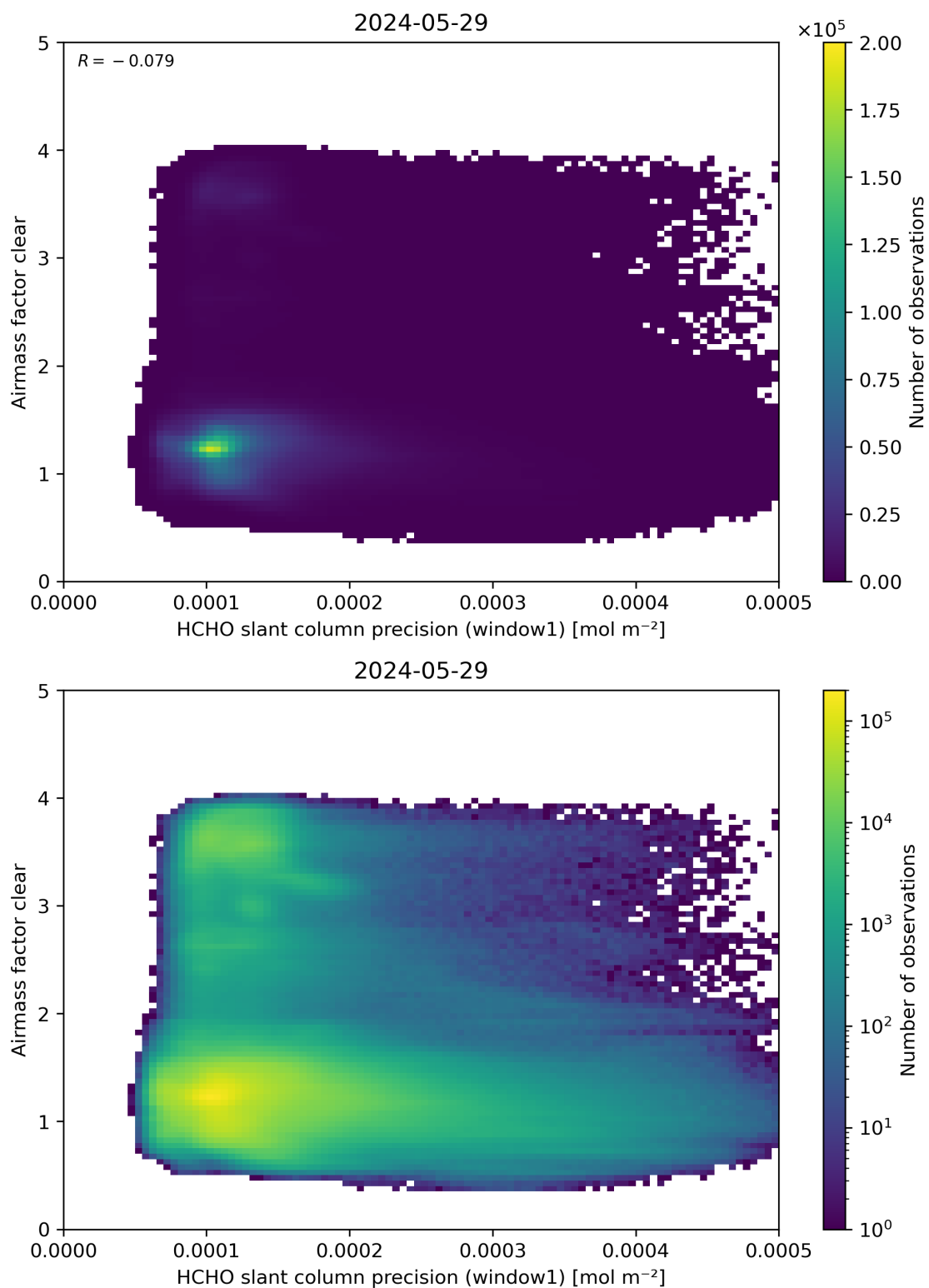
Figure 91: Scatter density plot of “HCHO slant column precision (window1)” against “Airmass factor clear” for 2024-05-28 to 2024-05-30.
