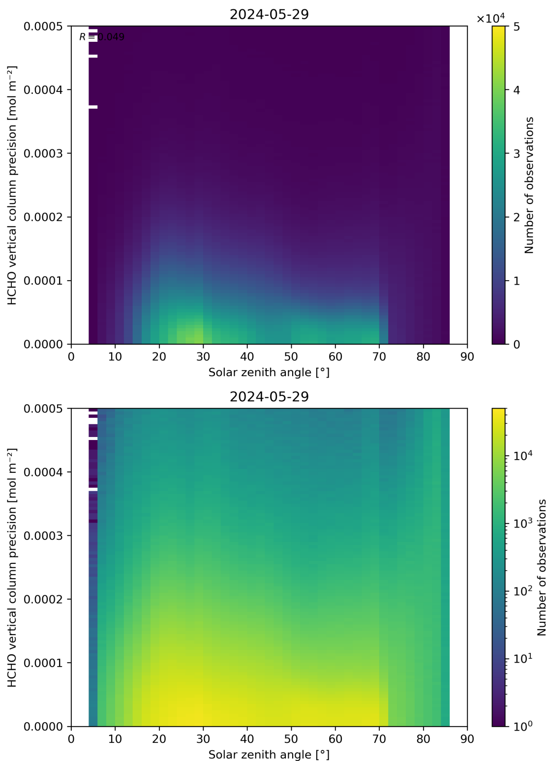
Figure 179: Scatter density plot of “Solar zenith angle” against “HCHO vertical column precision” for 2024-05-28 to 2024-05-30.
