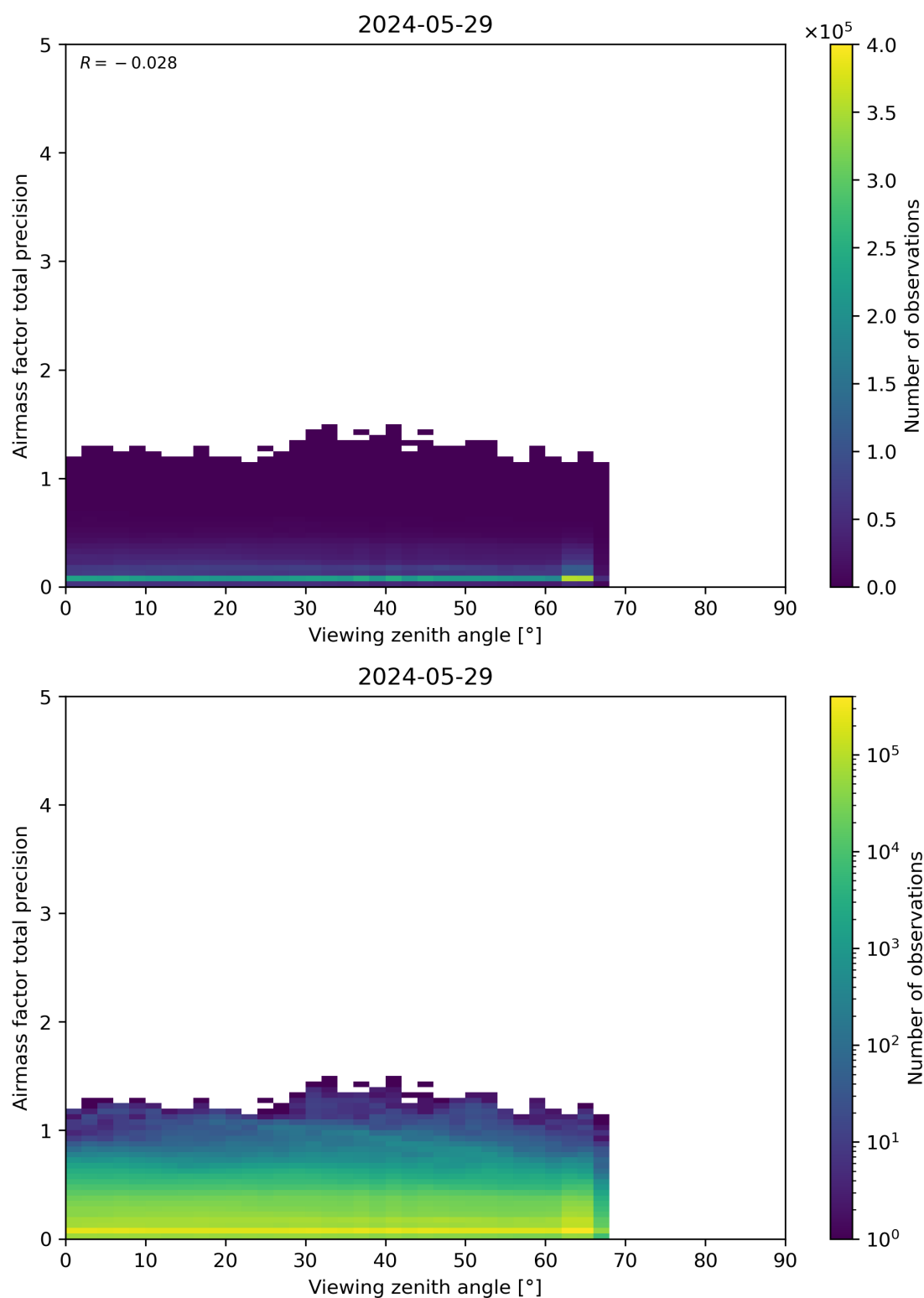
Figure 191: Scatter density plot of “Viewing zenith angle” against “Airmass factor total precision” for 2024-05-28 to 2024-05-30.
