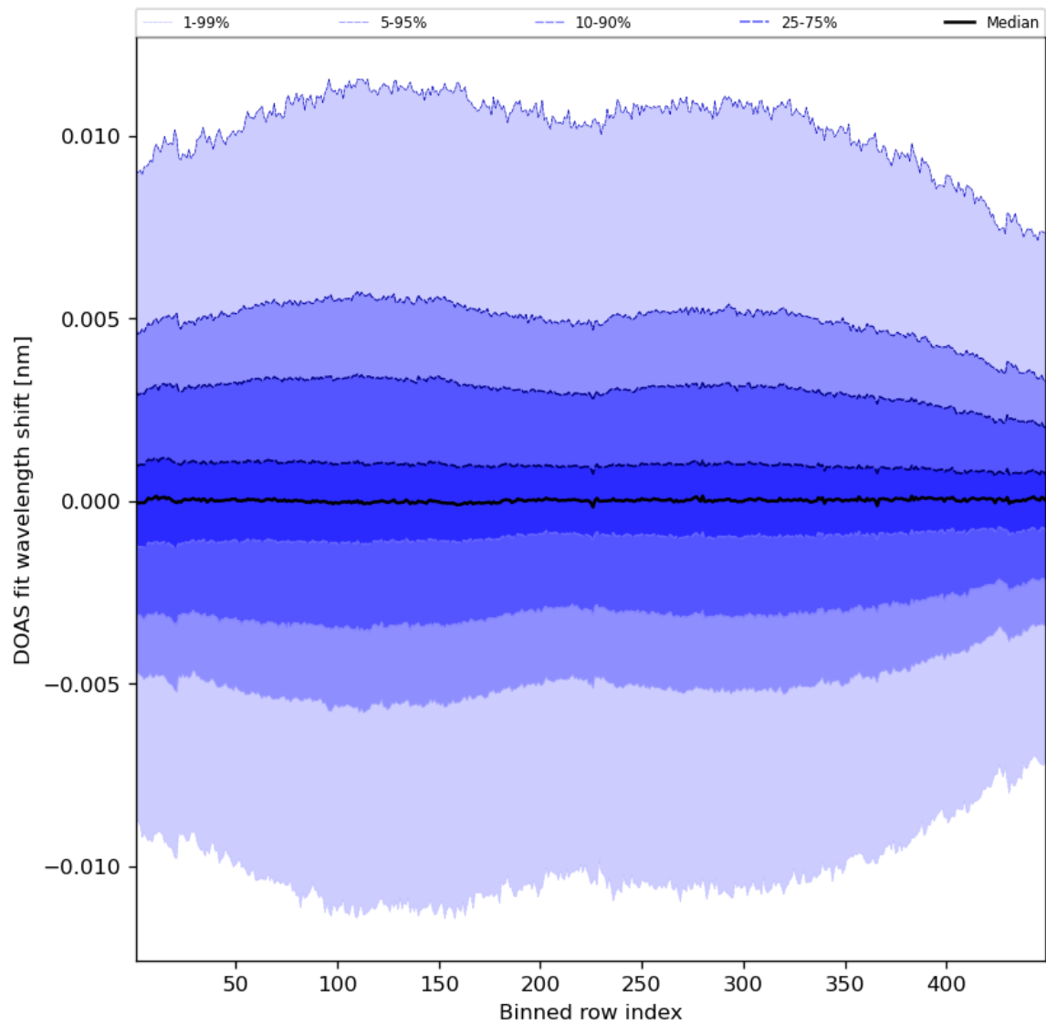
Figure 58: Along track statistics of “DOAS fit wavelength shift” for 2024-05-28 to 2024-05-30
