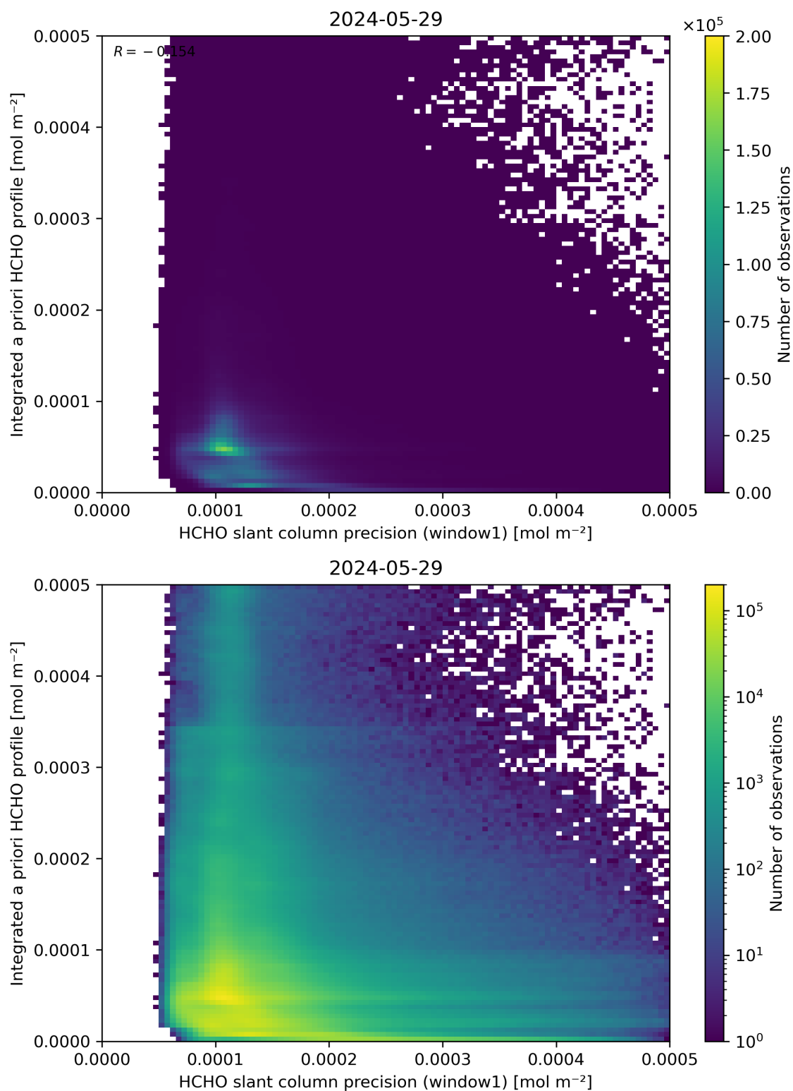
Figure 96: Scatter density plot of “HCHO slant column precision (window1)” against “Integrated a priori HCHO profile” for 2024-05-28 to 2024-05-30.
