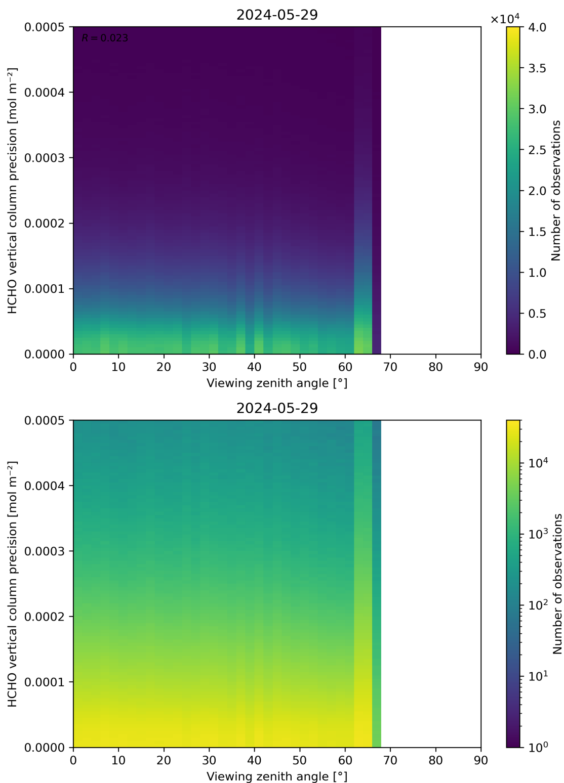
Figure 194: Scatter density plot of “Viewing zenith angle” against “HCHO vertical column precision” for 2024-05-28 to 2024-05-30.
