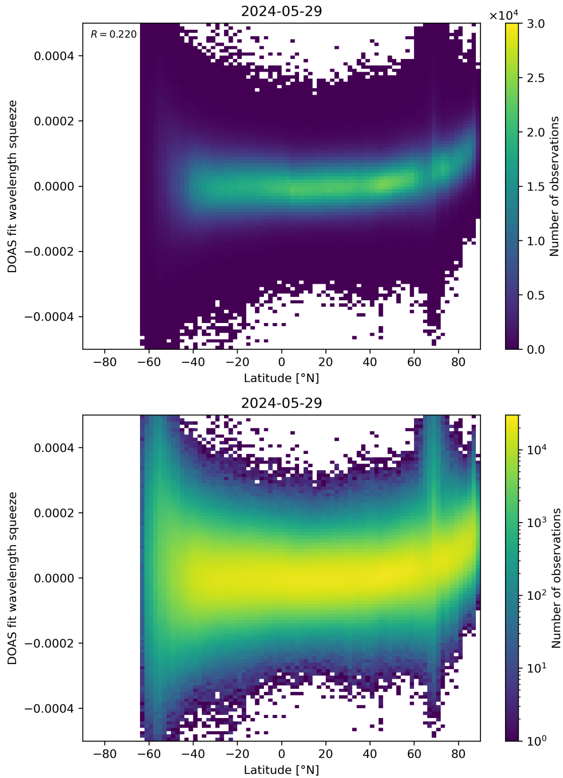
Figure 155: Scatter density plot of “Latitude” against “DOAS fit wavelength squeeze” for 2024-05-28 to 2024-05-30.
