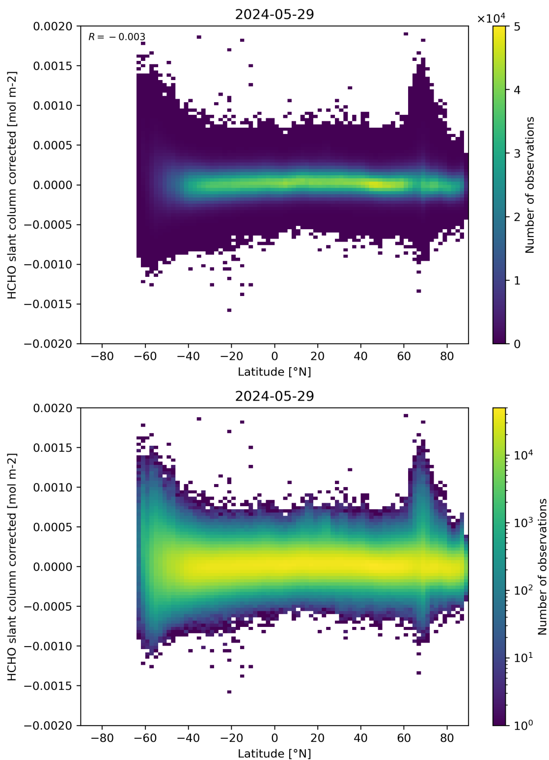
Figure 157: Scatter density plot of “Latitude” against “HCHO slant column corrected” for 2024-05-28 to 2024-05-30.
