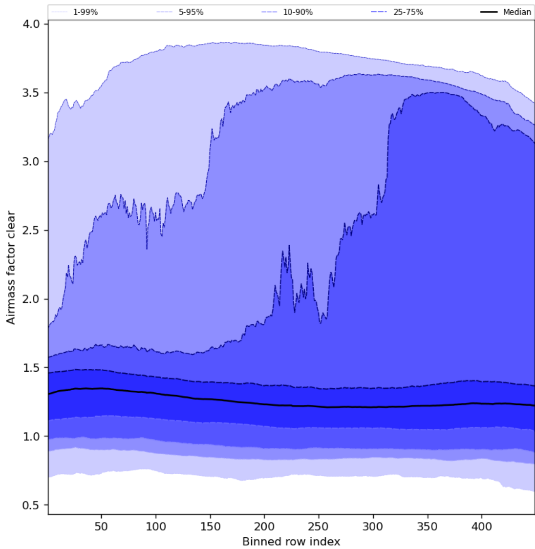
Figure 56: Along track statistics of “Airmass factor clear” for 2024-05-28 to 2024-05-30
