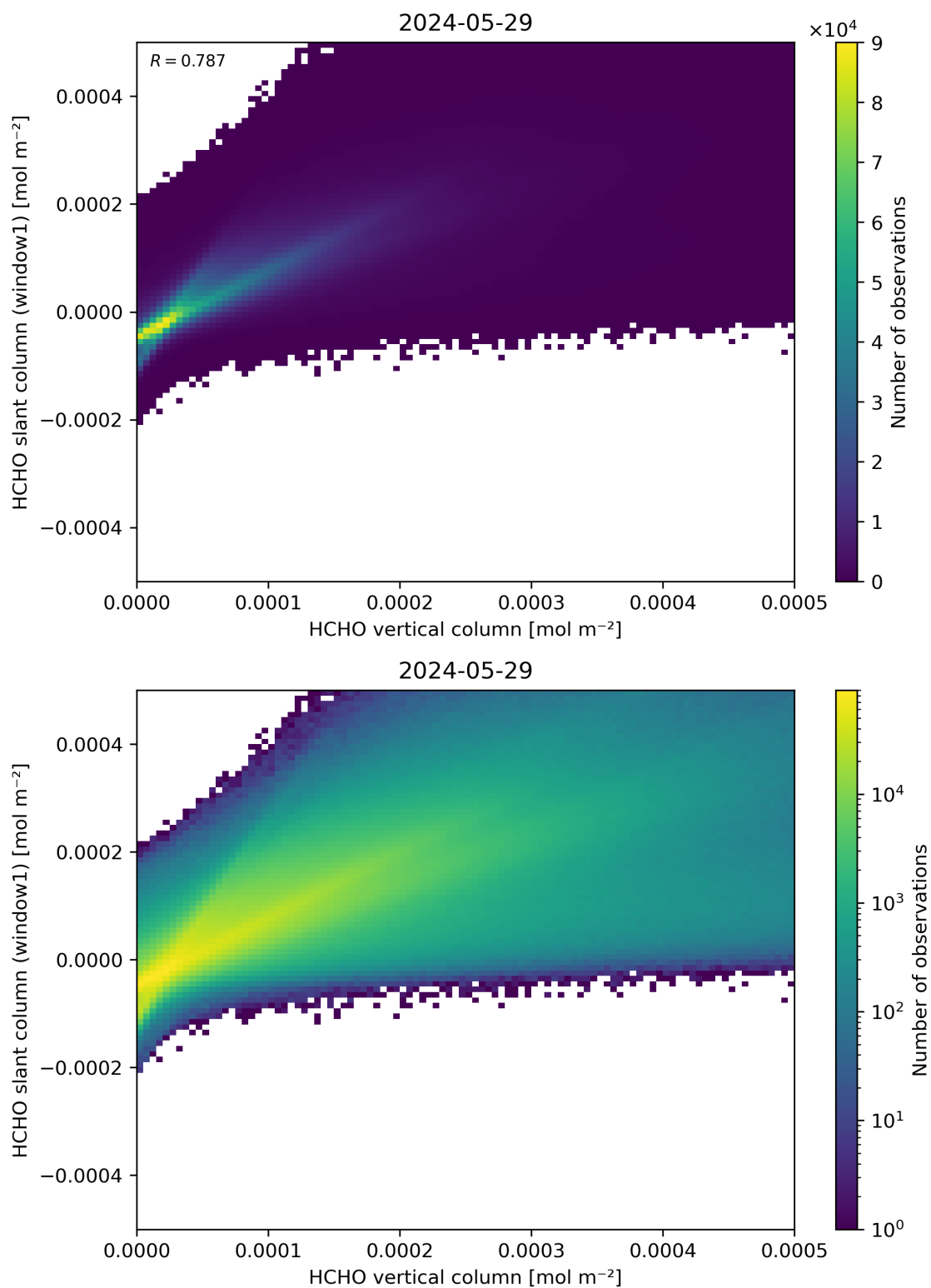
Figure 129: Scatter density plot of “HCHO vertical column” against “HCHO slant column (window1)” for 2024-05-28 to 2024-05-30.
