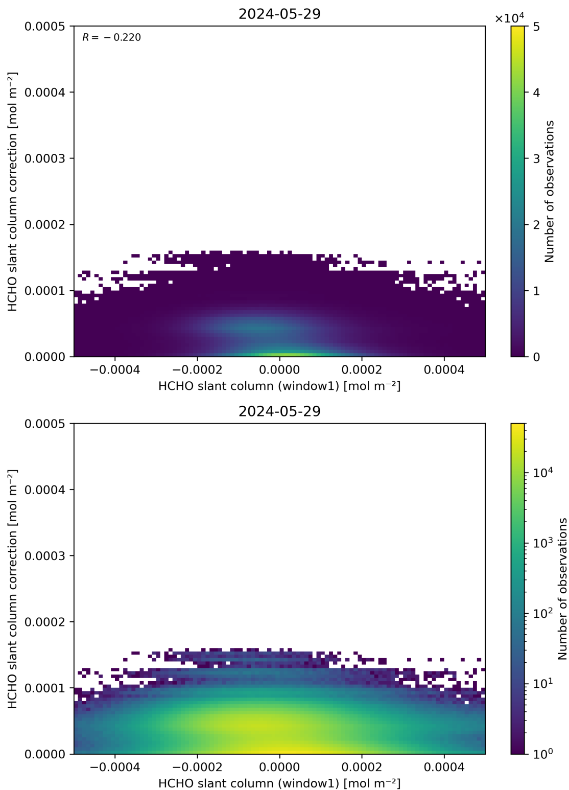
Figure 83: Scatter density plot of “HCHO slant column (window1)” against “HCHO slant column correction” for 2024-05-28 to 2024-05-30.
