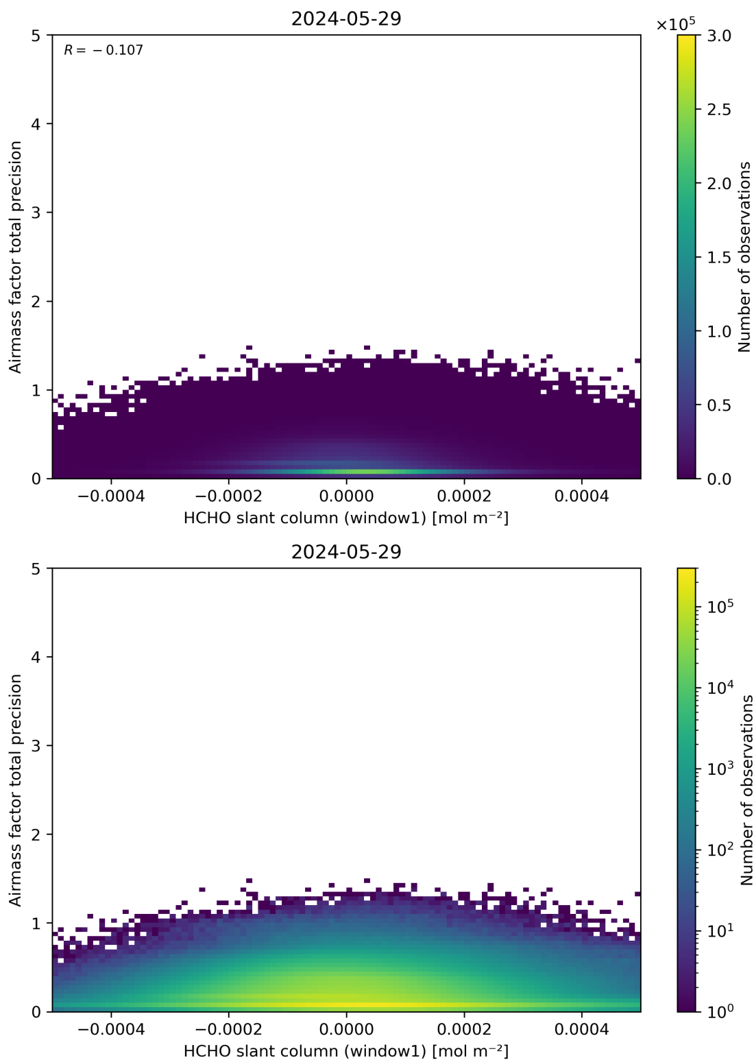
Figure 86: Scatter density plot of “HCHO slant column (window1)” against “Airmass factor total precision” for 2024-05-28 to 2024-05-30.
