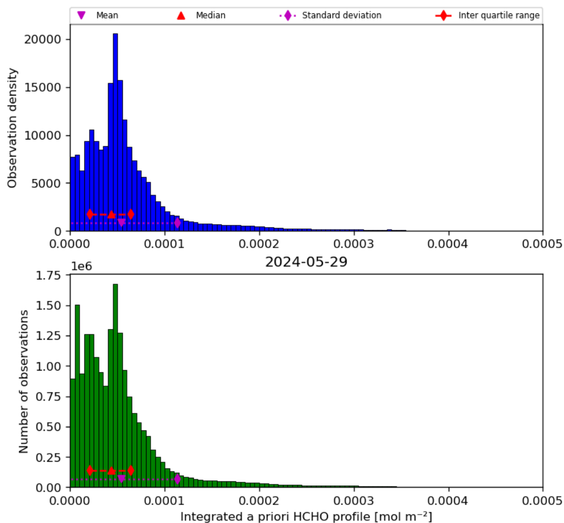
Figure 43: Histogram of “Integrated a priori HCHO profile” for 2024-05-28 to 2024-05-30
