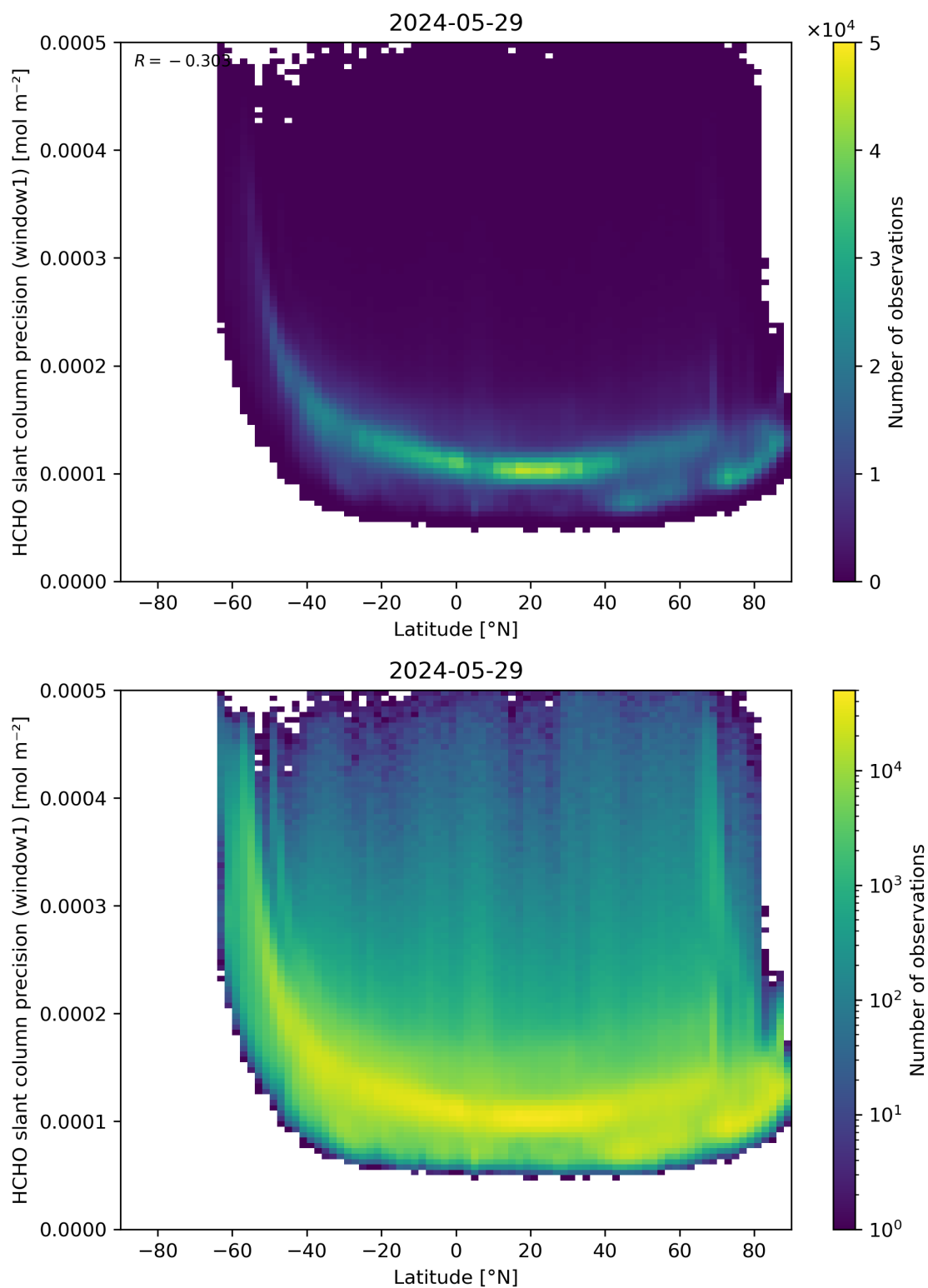
Figure 160: Scatter density plot of “Latitude” against “HCHO slant column precision (window1)” for 2024-05-28 to 2024-05-30.
