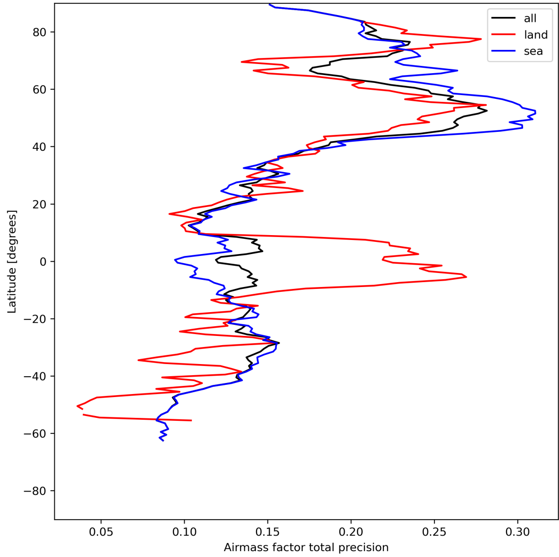
Figure 27: Zonal average of “Airmass factor total precision” for 2024-05-28 to 2024-05-30.
