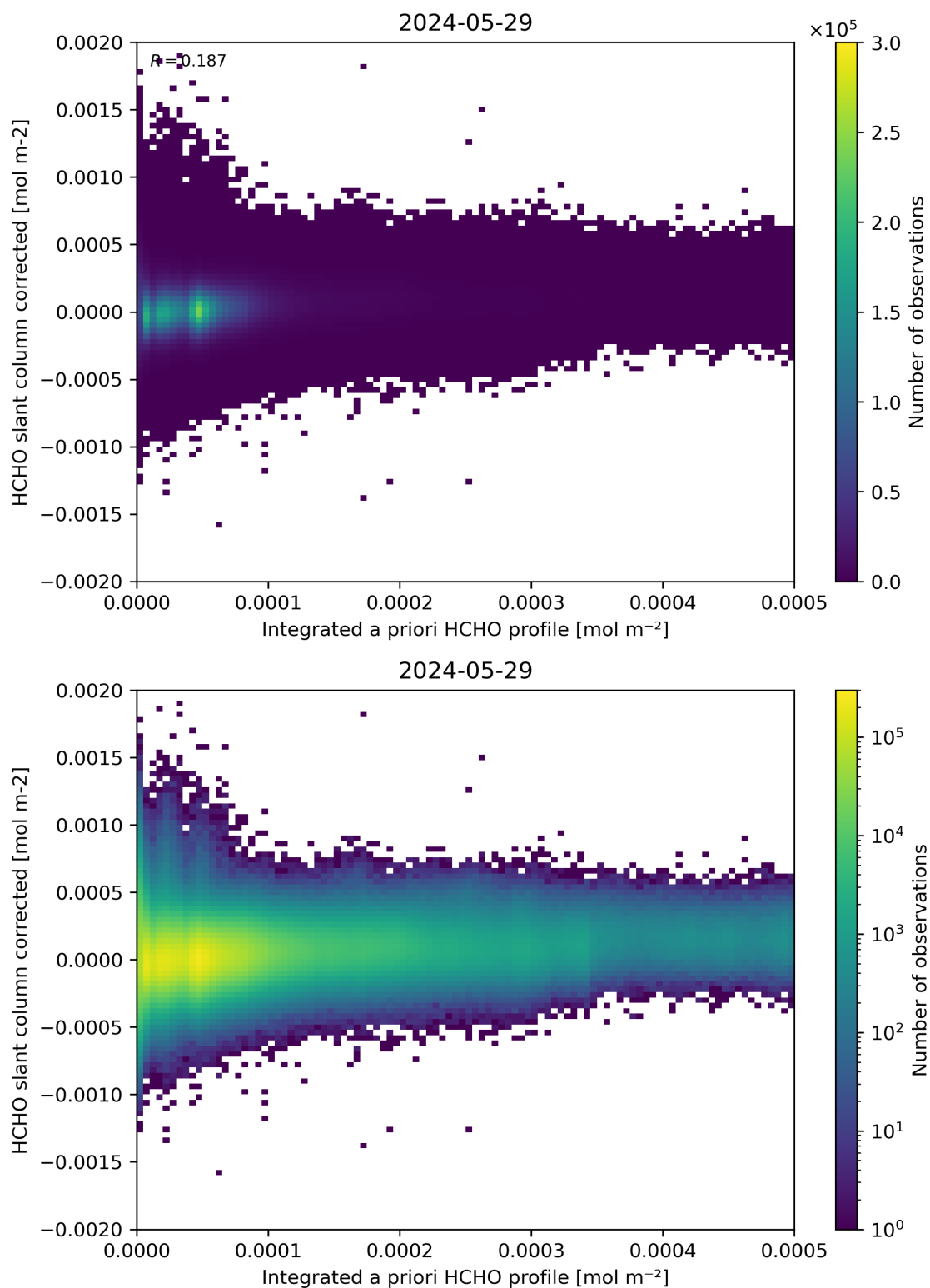
Figure 151: Scatter density plot of “Integrated a priori HCHO profile” against “HCHO slant column corrected” for 2024-05-28 to 2024-05-30.
