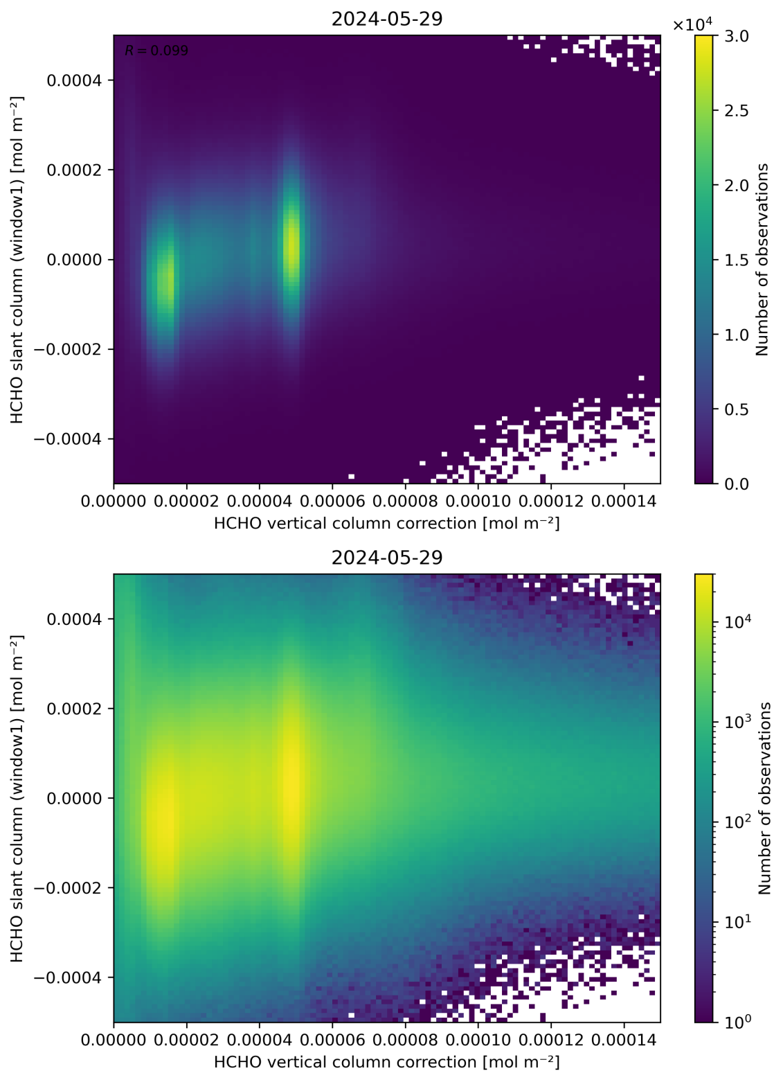
Figure 118: Scatter density plot of “HCHO vertical column correction” against “HCHO slant column (window1)” for 2024-05-28 to 2024-05-30.
