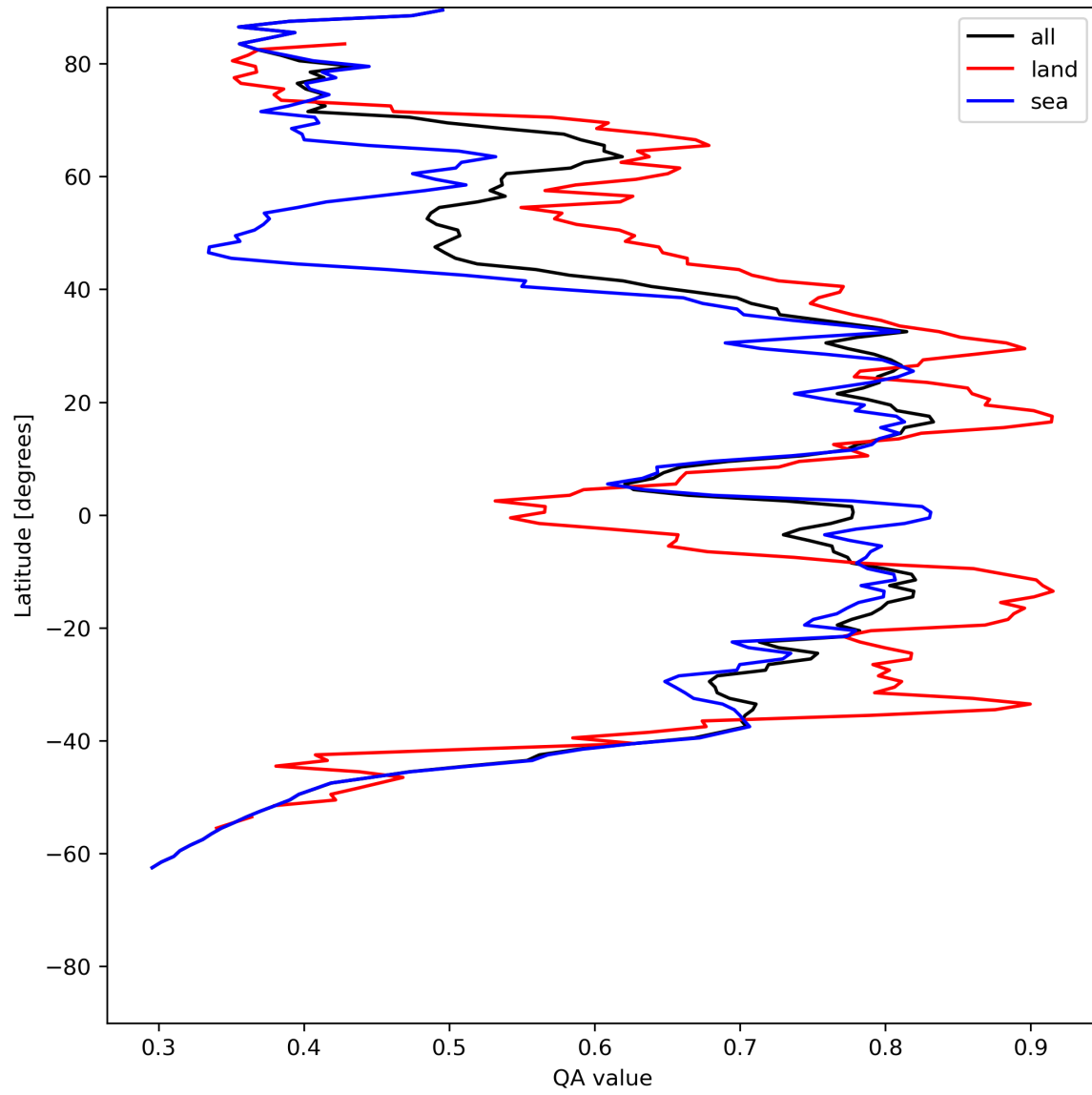
Figure 20: Zonal average of “QA value” for 2024-05-28 to 2024-05-30.
