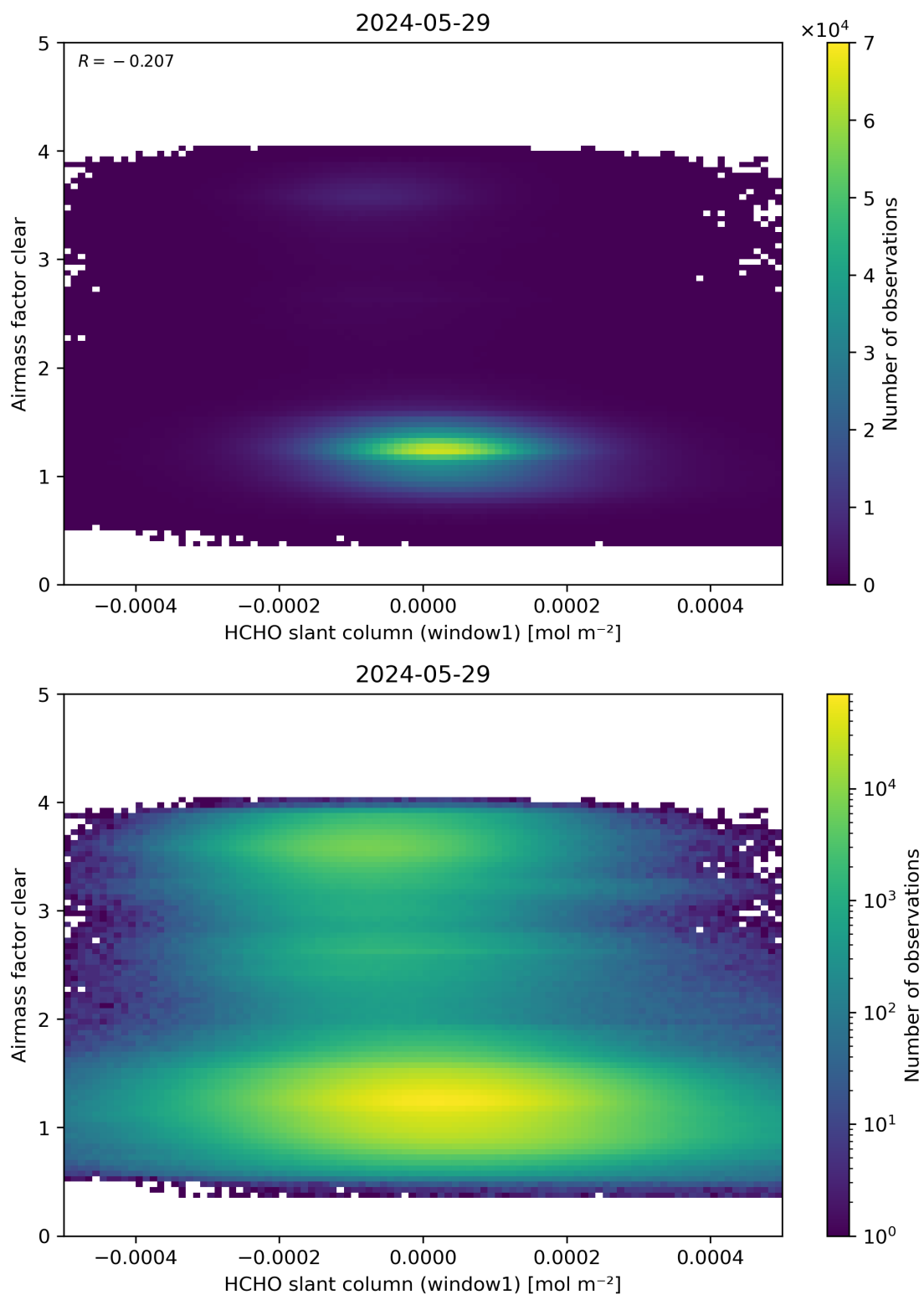
Figure 81: Scatter density plot of “HCHO slant column (window1)” against “Airmass factor clear” for 2024-05-28 to 2024-05-30.
