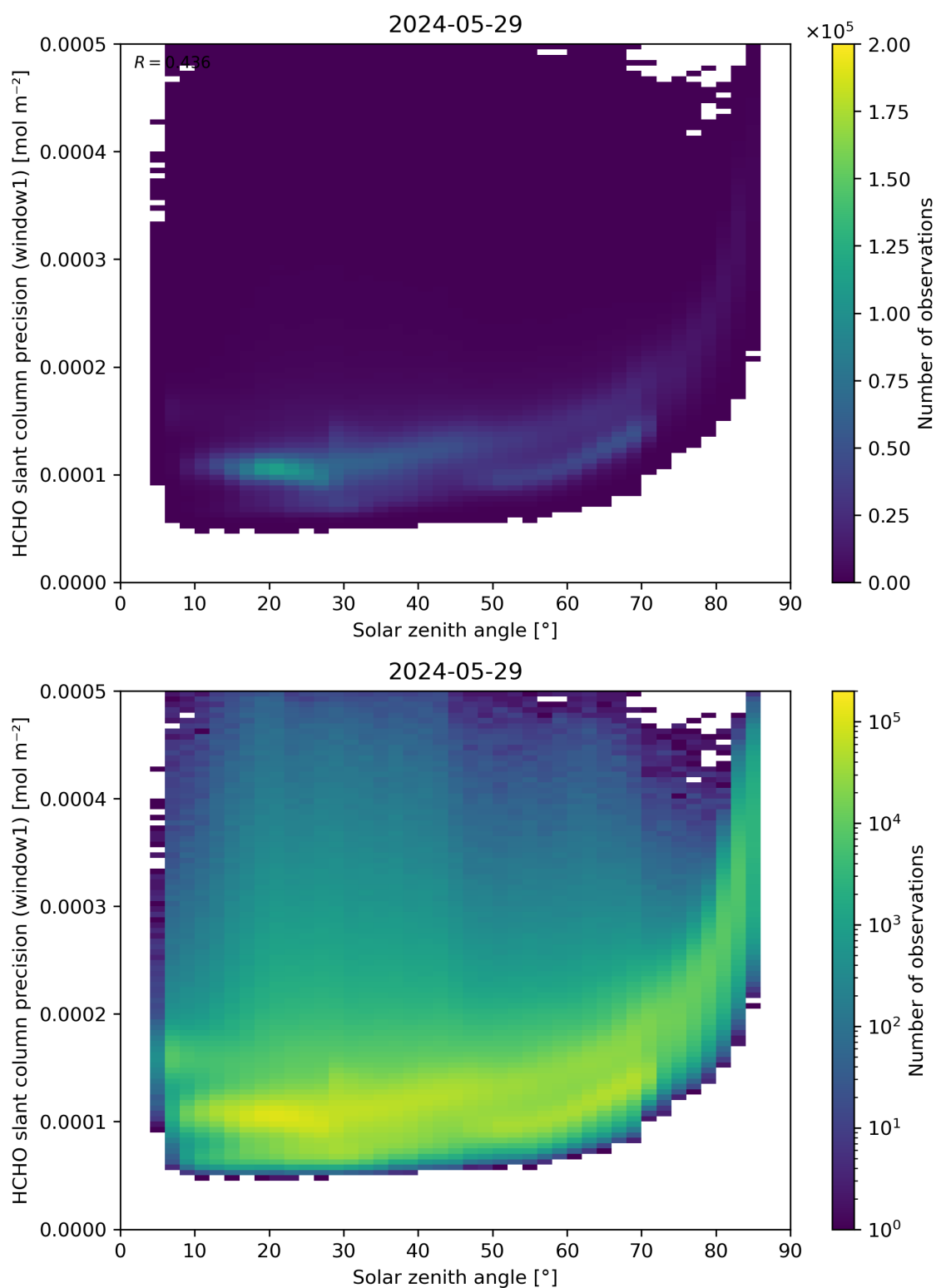
Figure 174: Scatter density plot of “Solar zenith angle” against “HCHO slant column precision (window1)” for 2024-05-28 to 2024-05-30.
