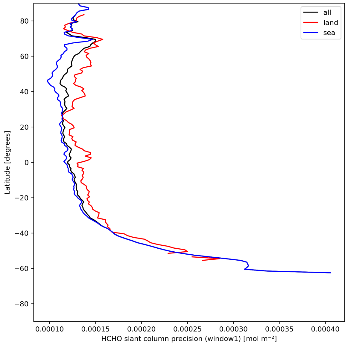
Figure 25: Zonal average of “HCHO slant column precision (window1)” for 2024-05-28 to 2024-05-30.
