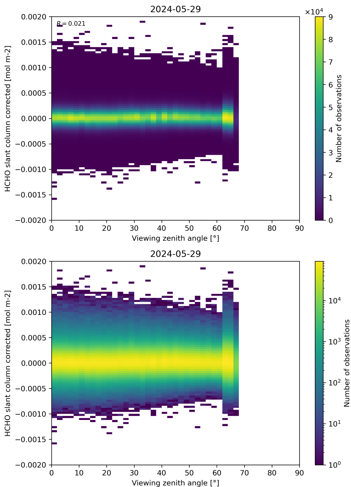
Figure 186: Scatter density plot of “Viewing zenith angle” against “HCHO slant column corrected” for 2024-05-28 to 2024-05-30.
