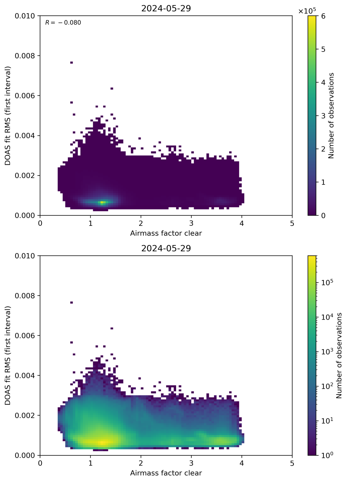
Figure 71: Scatter density plot of “Airmass factor clear” against “DOAS fit RMS (first interval)” for 2024-05-28 to 2024-05-30.
