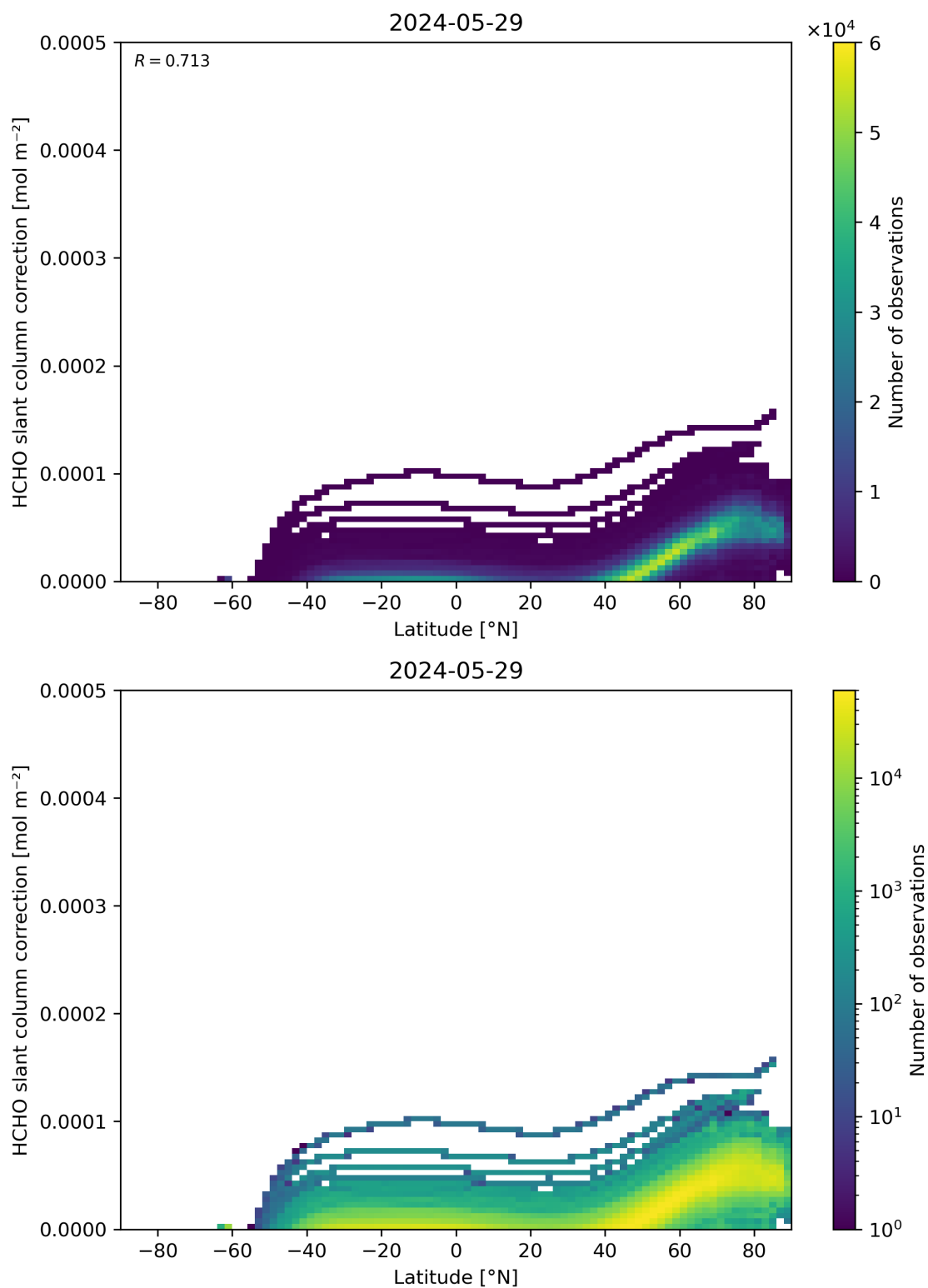
Figure 158: Scatter density plot of “Latitude” against “HCHO slant column correction” for 2024-05-28 to 2024-05-30.
