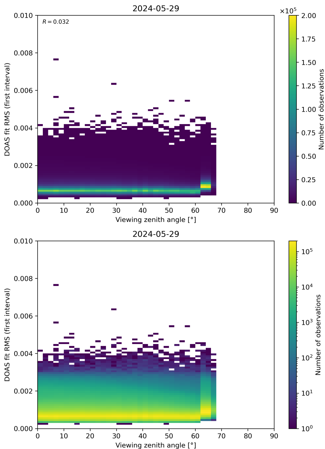
Figure 182: Scatter density plot of “Viewing zenith angle” against “DOAS fit RMS (first interval)” for 2024-05-28 to 2024-05-30.
