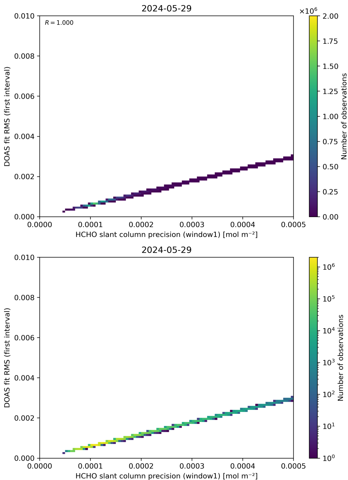
Figure 88: Scatter density plot of “HCHO slant column precision (window1)” against “DOAS fit RMS (first interval)” for 2024-05-28 to 2024-05-30.
