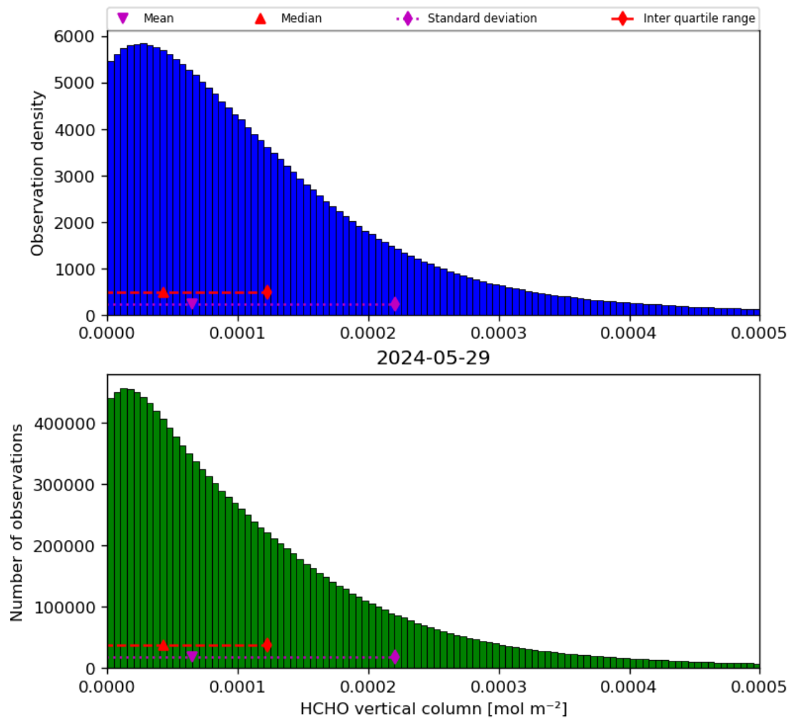
Figure 35: Histogram of “HCHO vertical column” for 2024-05-28 to 2024-05-30
