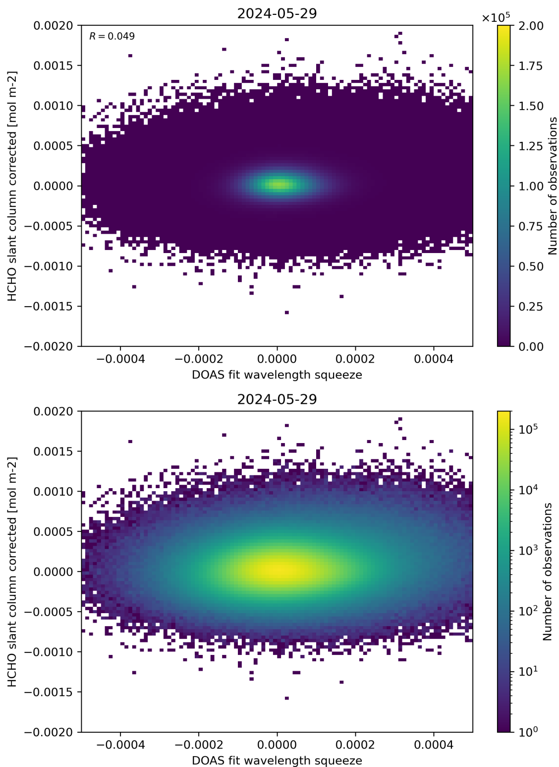
Figure 69: Scatter density plot of “DOAS fit wavelength squeeze” against “HCHO slant column corrected” for 2024-05-28 to 2024-05-30.
