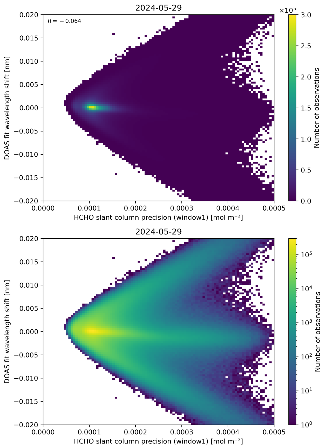
Figure 89: Scatter density plot of “HCHO slant column precision (window1)” against “DOAS fit wavelength shift” for 2024-05-28 to 2024-05-30.
