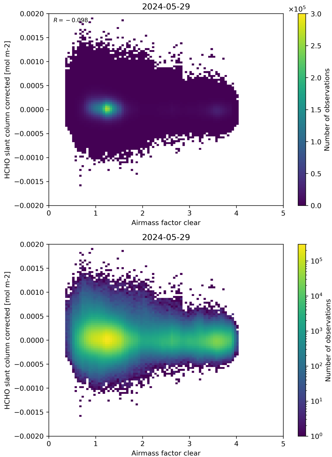
Figure 74: Scatter density plot of “Airmass factor clear” against “HCHO slant column corrected” for 2024-05-28 to 2024-05-30.
