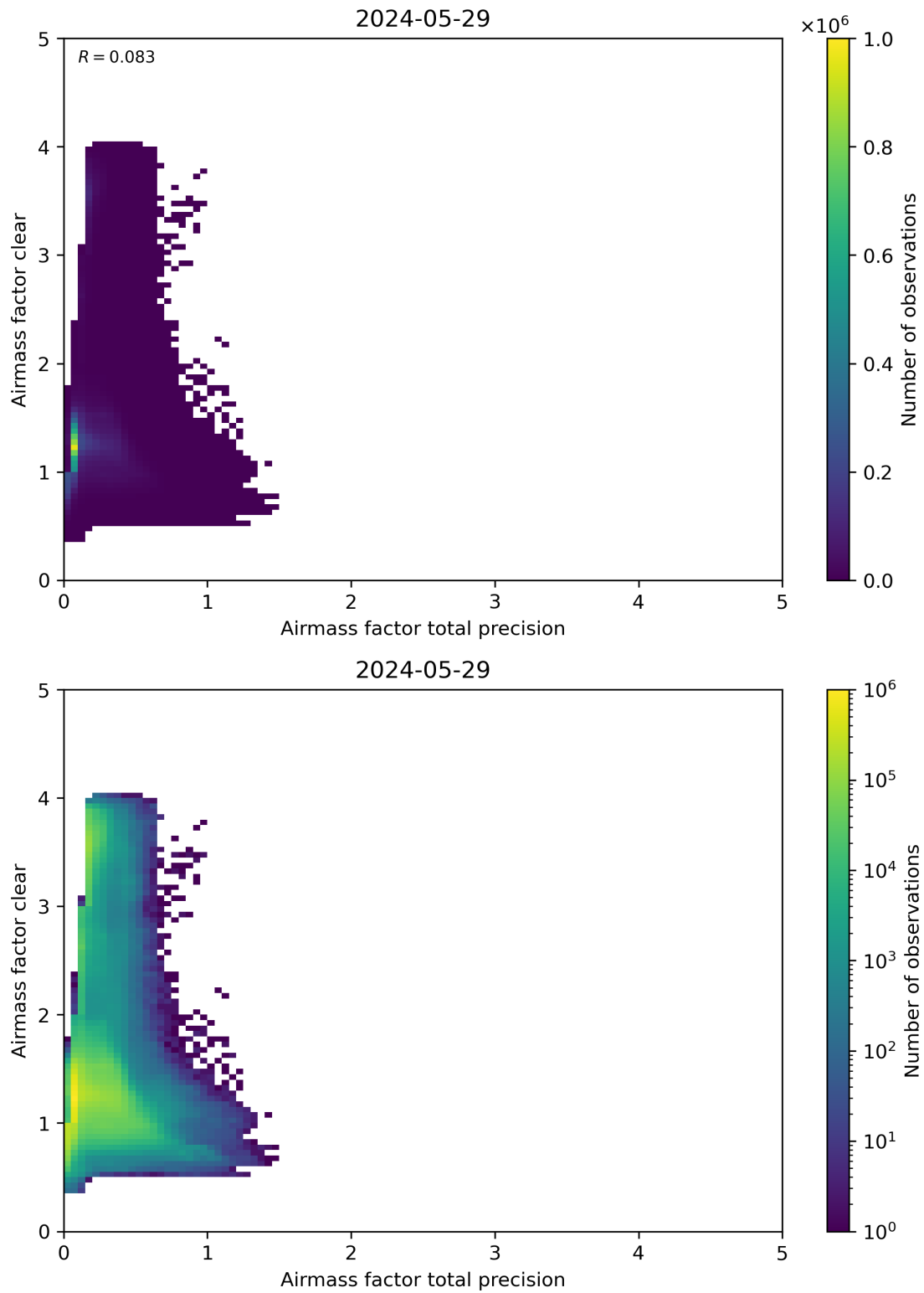
Figure 108: Scatter density plot of “Airmass factor total precision” against “Airmass factor clear” for 2024-05-28 to 2024-05-30.
