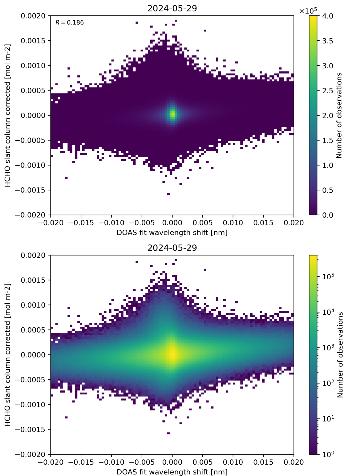
Figure 66: Scatter density plot of “DOAS fit wavelength shift” against “HCHO slant column corrected” for 2024-05-28 to 2024-05-30.
