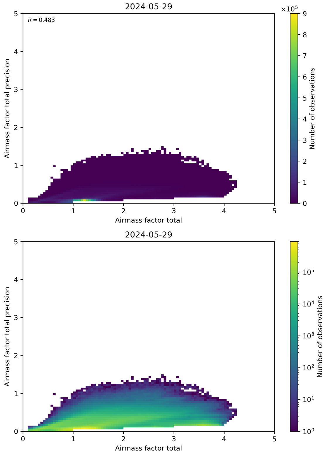
Figure 103: Scatter density plot of “Airmass factor total” against “Airmass factor total precision” for 2024-05-28 to 2024-05-30.
