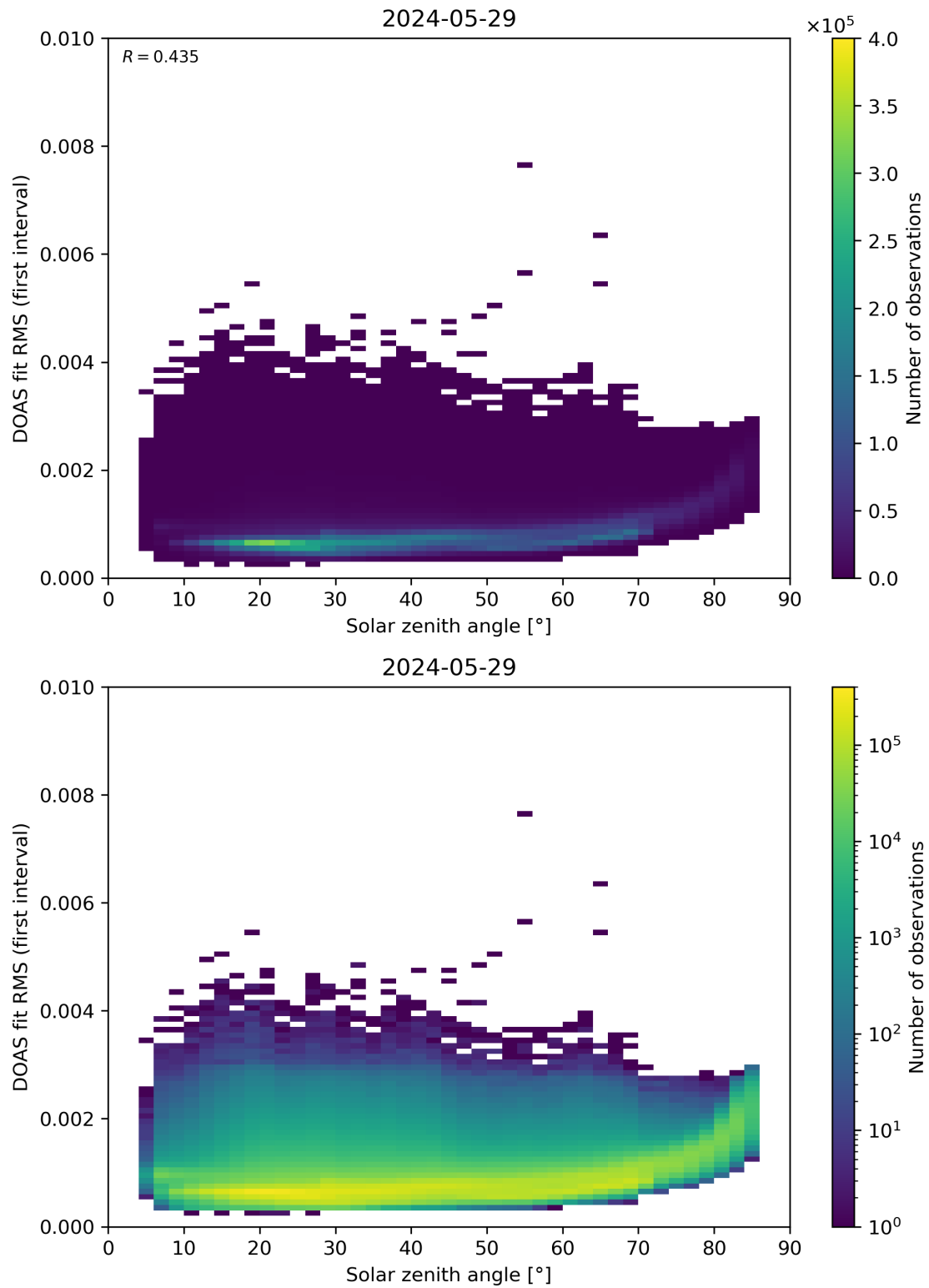
Figure 167: Scatter density plot of “Solar zenith angle” against “DOAS fit RMS (first interval)” for 2024-05-28 to 2024-05-30.
