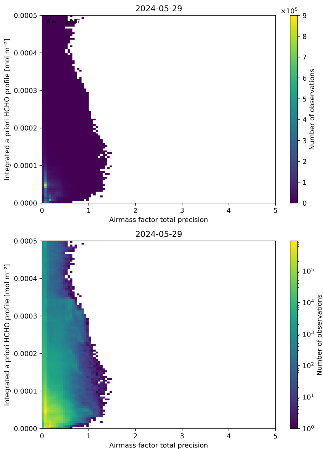
Figure 111: Scatter density plot of “Airmass factor total precision” against “Integrated a priori HCHO profile” for 2024-05-28 to 2024-05-30.
