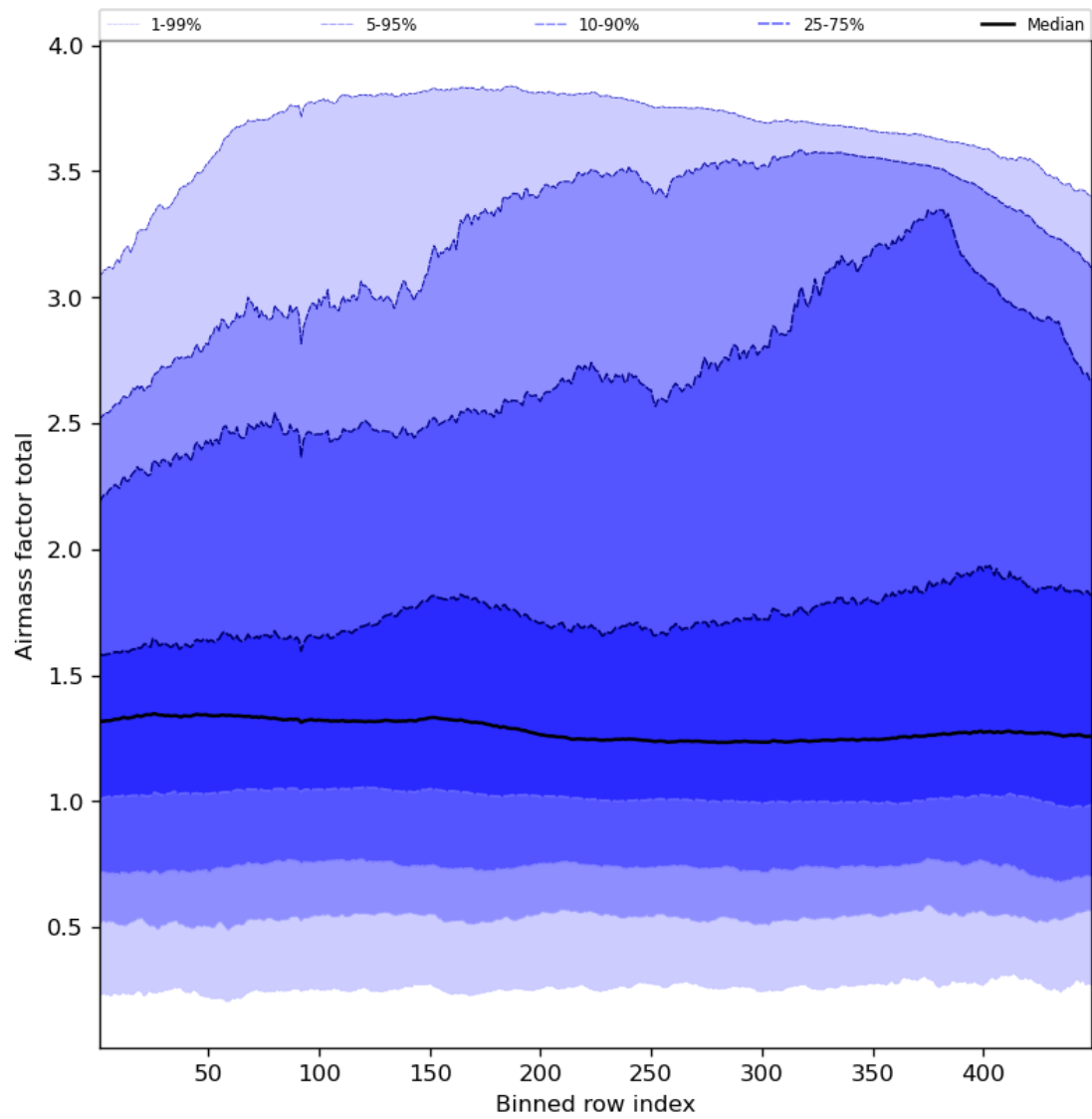
Figure 54: Along track statistics of “Airmass factor total” for 2024-05-28 to 2024-05-30
