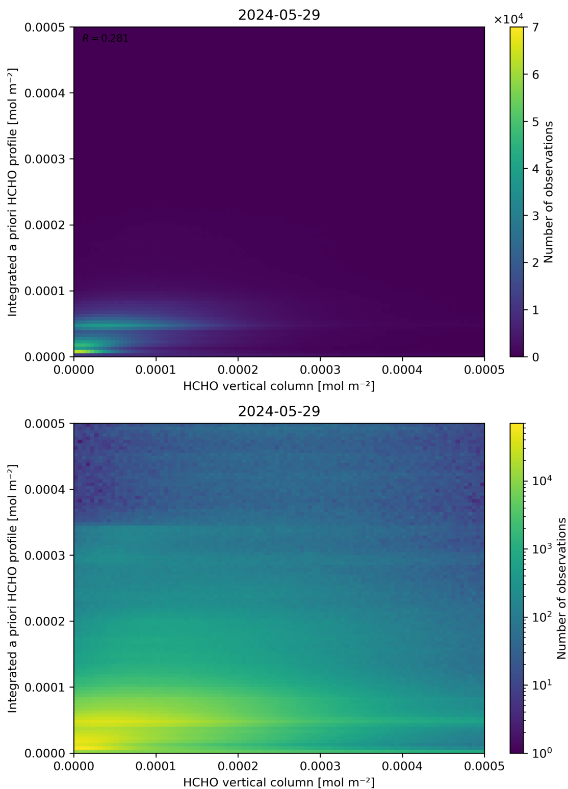
Figure 135: Scatter density plot of “HCHO vertical column” against “Integrated a priori HCHO profile” for 2024-05-28 to 2024-05-30.
