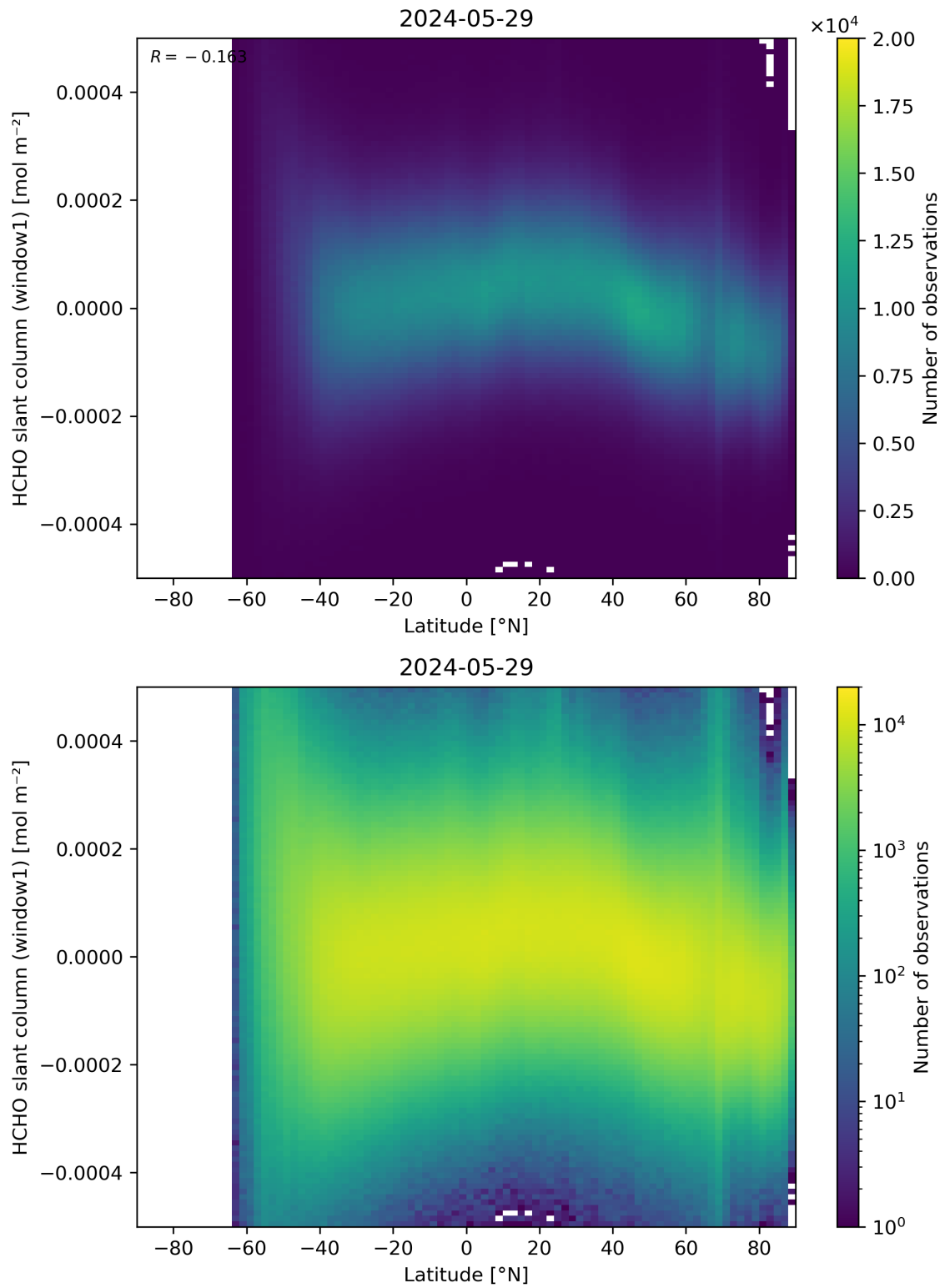
Figure 159: Scatter density plot of “Latitude” against “HCHO slant column (window1)” for 2024-05-28 to 2024-05-30.
