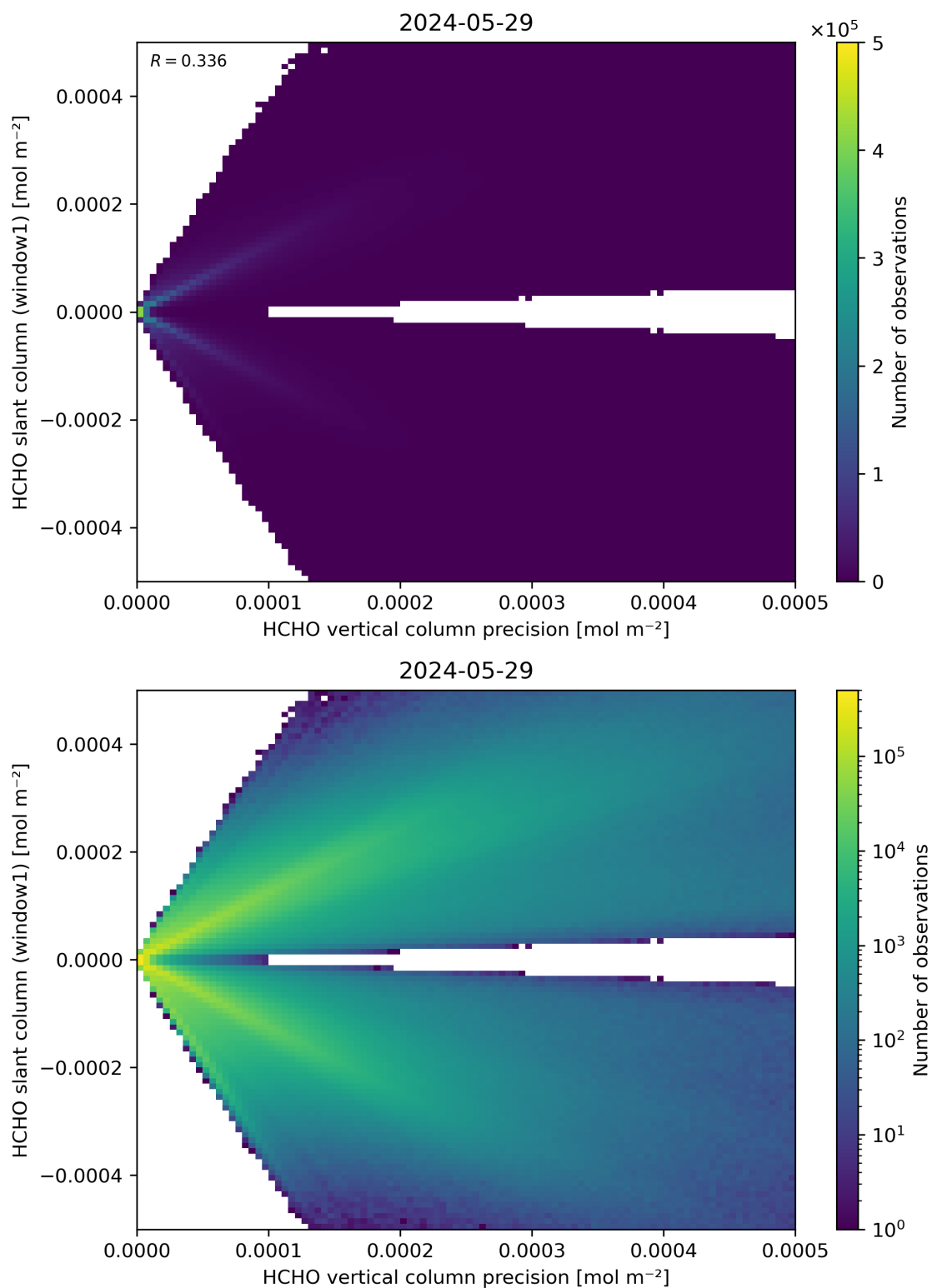
Figure 142: Scatter density plot of “HCHO vertical column precision” against “HCHO slant column (window1)” for 2024-05-28 to 2024-05-30.
