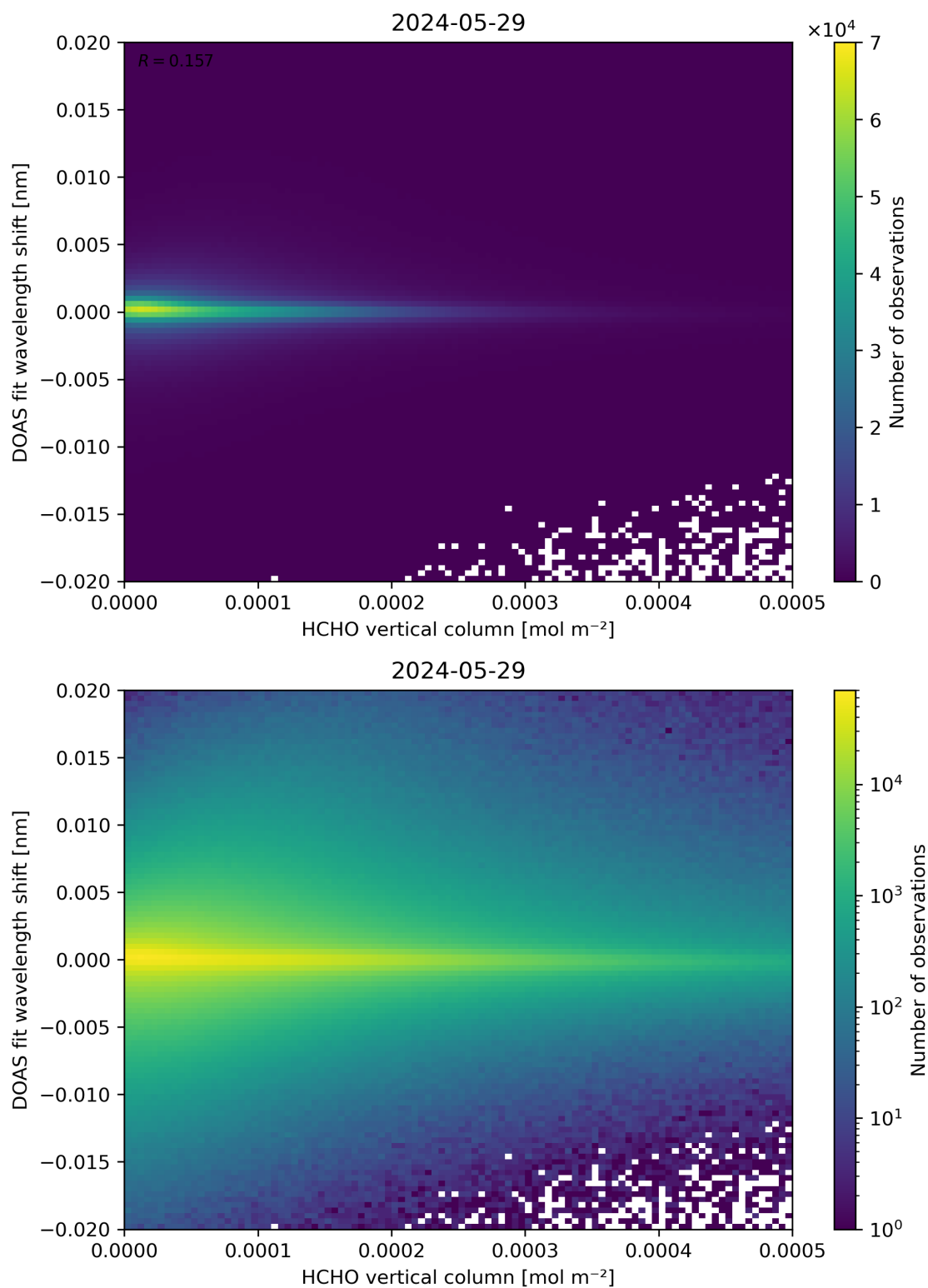
Figure 124: Scatter density plot of “HCHO vertical column” against “DOAS fit wavelength shift” for 2024-05-28 to 2024-05-30.
