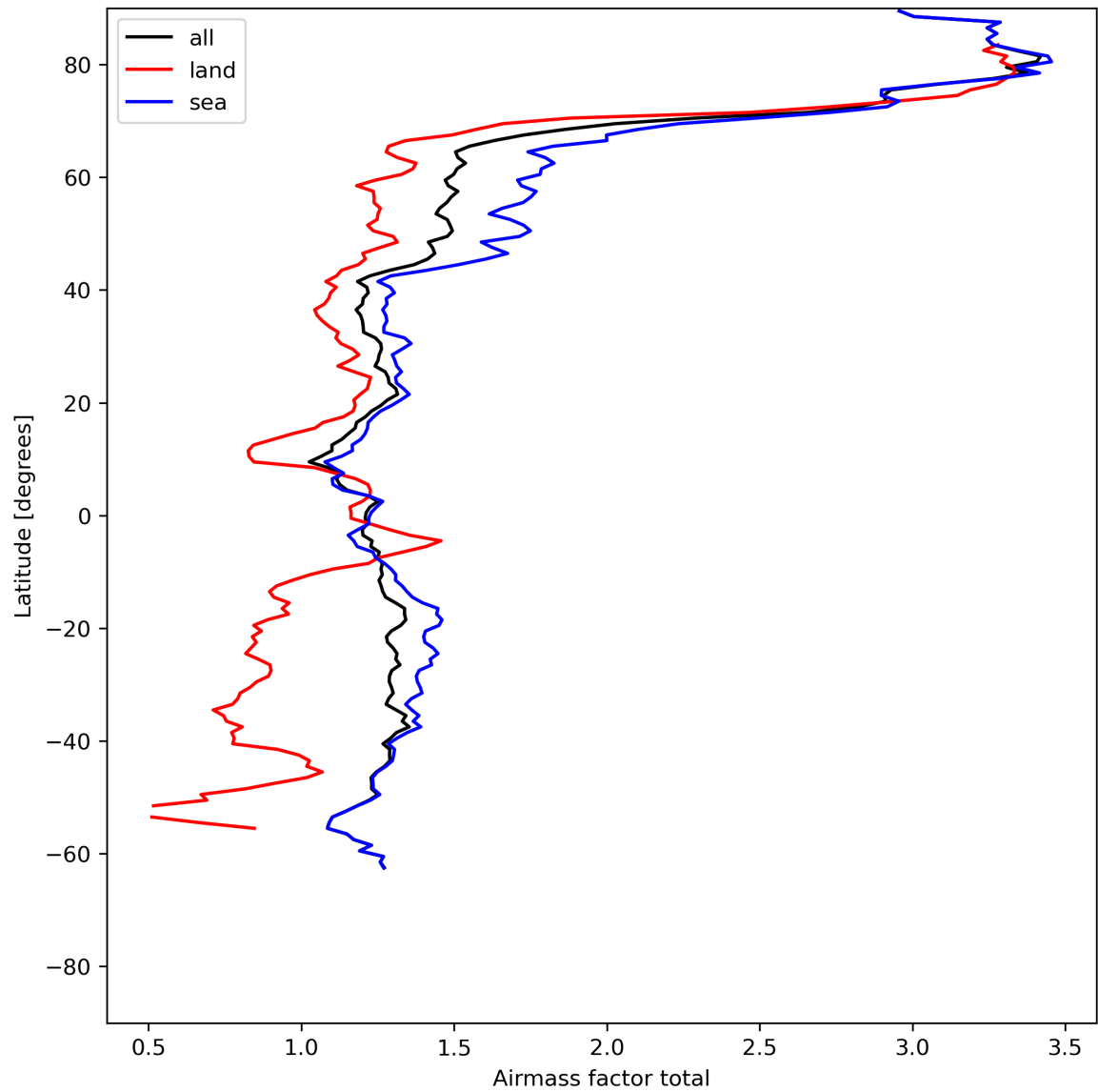
Figure 26: Zonal average of “Airmass factor total” for 2024-05-28 to 2024-05-30.
