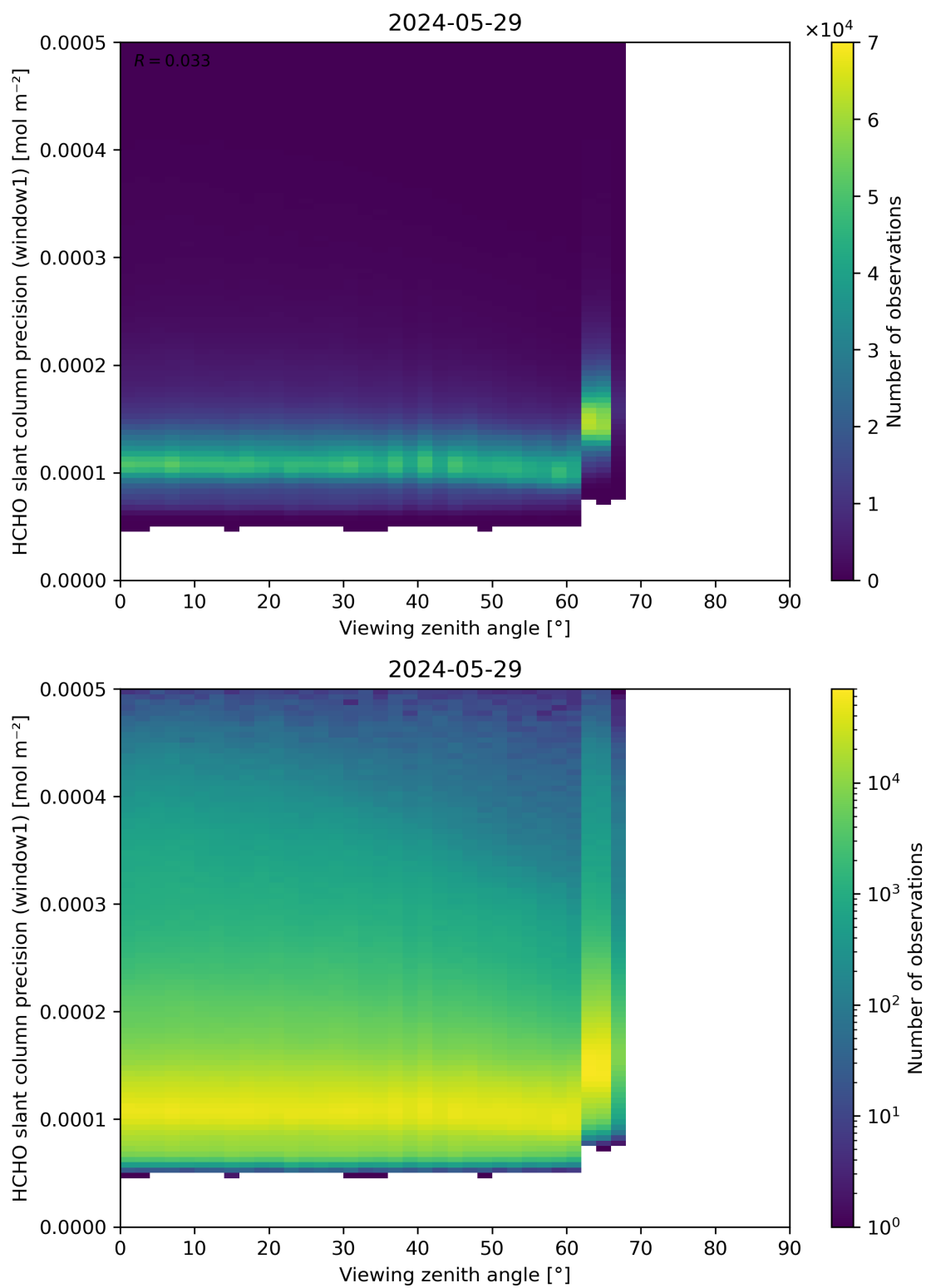
Figure 189: Scatter density plot of “Viewing zenith angle” against “HCHO slant column precision (window1)” for 2024-05-28 to 2024-05-30.
