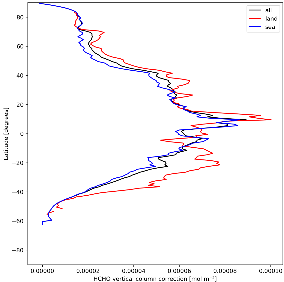
Figure 23: Zonal average of “HCHO vertical column correction” for 2024-05-28 to 2024-05-30.
