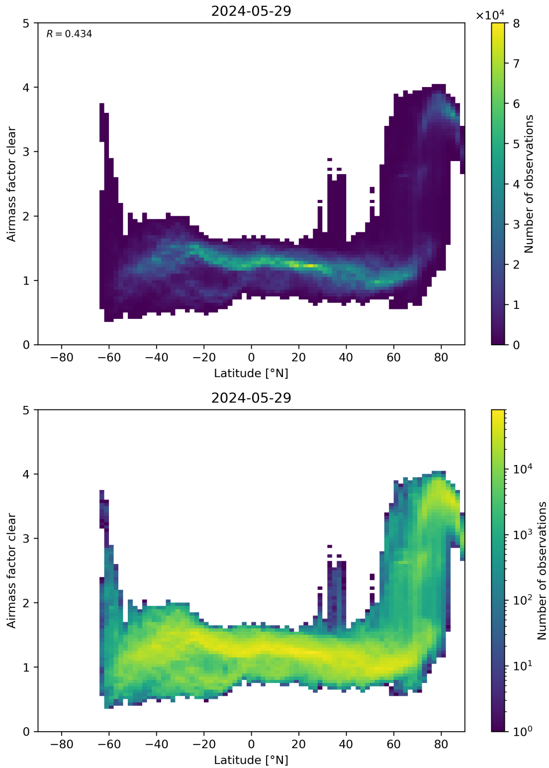
Figure 156: Scatter density plot of “Latitude” against “Airmass factor clear” for 2024-05-28 to 2024-05-30.
