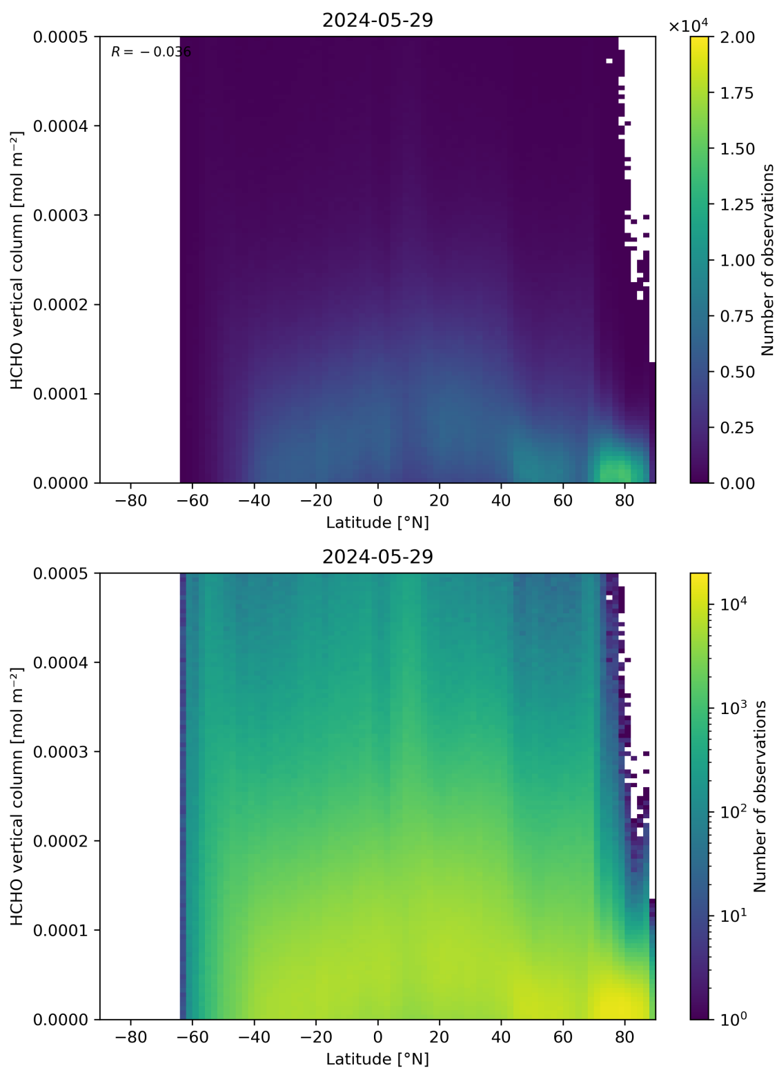
Figure 163: Scatter density plot of “Latitude” against “HCHO vertical column” for 2024-05-28 to 2024-05-30.
