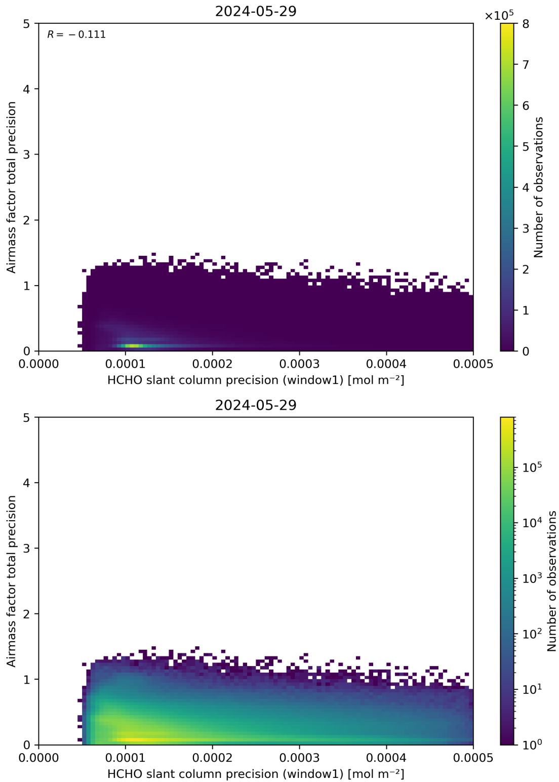
Figure 95: Scatter density plot of “HCHO slant column precision (window1)” against “Airmass factor total precision” for 2024-05-28 to 2024-05-30.
