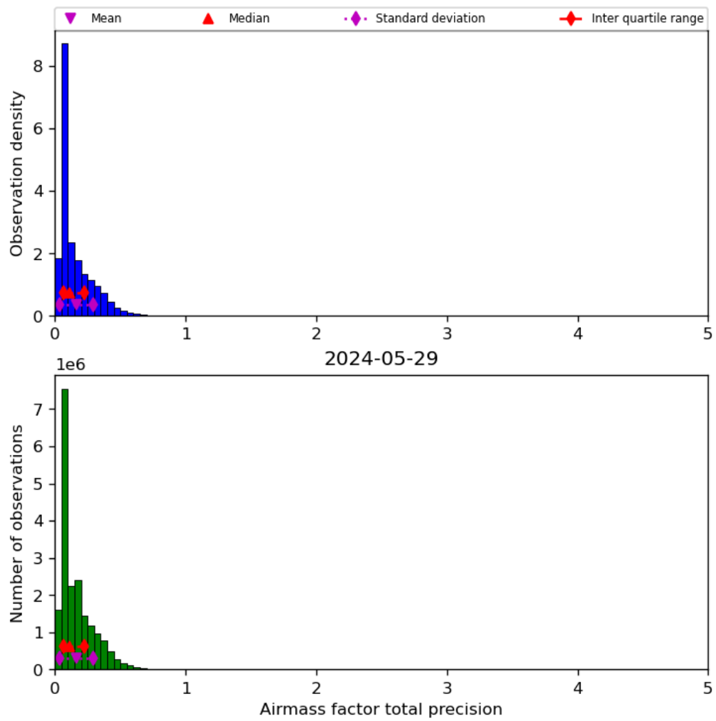
Figure 41: Histogram of “Airmass factor total precision” for 2024-05-28 to 2024-05-30
