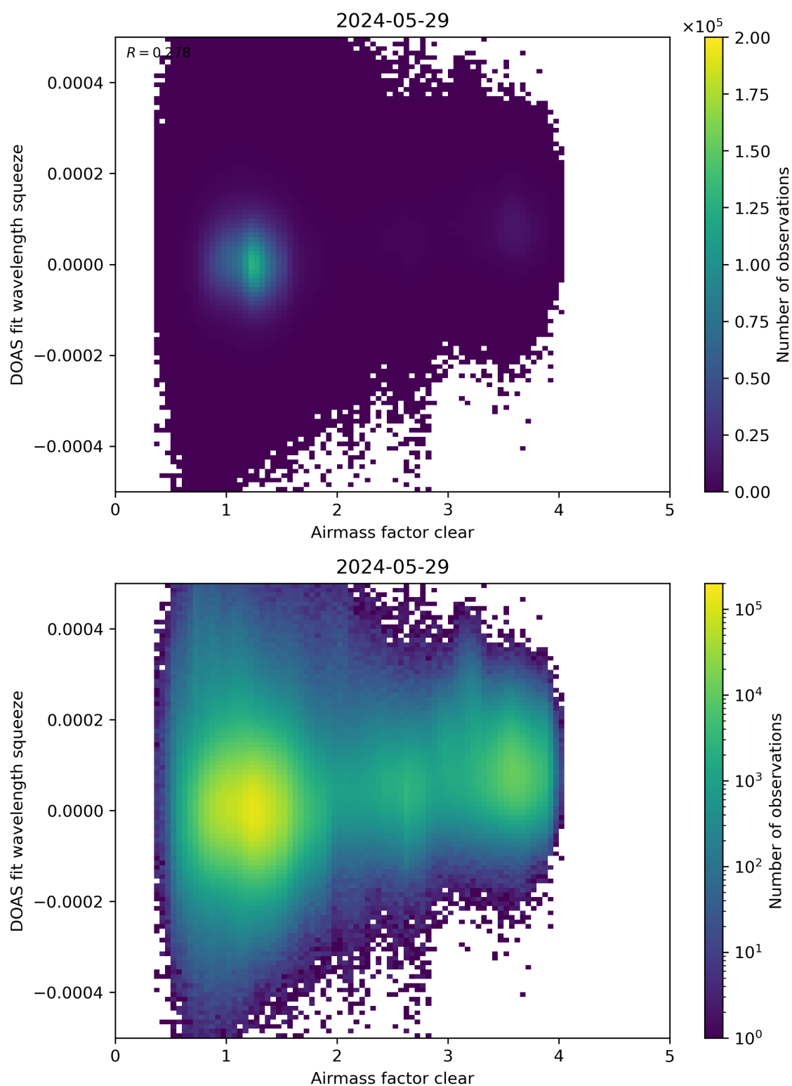
Figure 73: Scatter density plot of “Airmass factor clear” against “DOAS fit wavelength squeeze” for 2024-05-28 to 2024-05-30.
