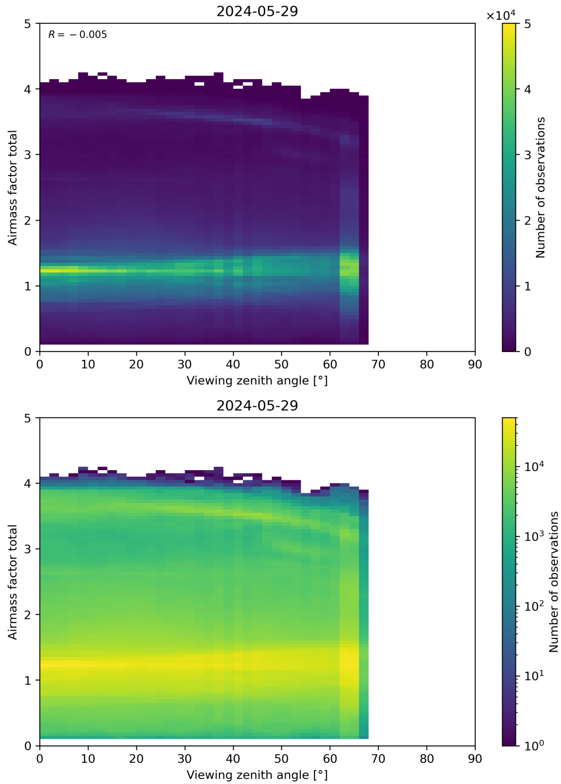
Figure 190: Scatter density plot of “Viewing zenith angle” against “Airmass factor total” for 2024-05-28 to 2024-05-30.
