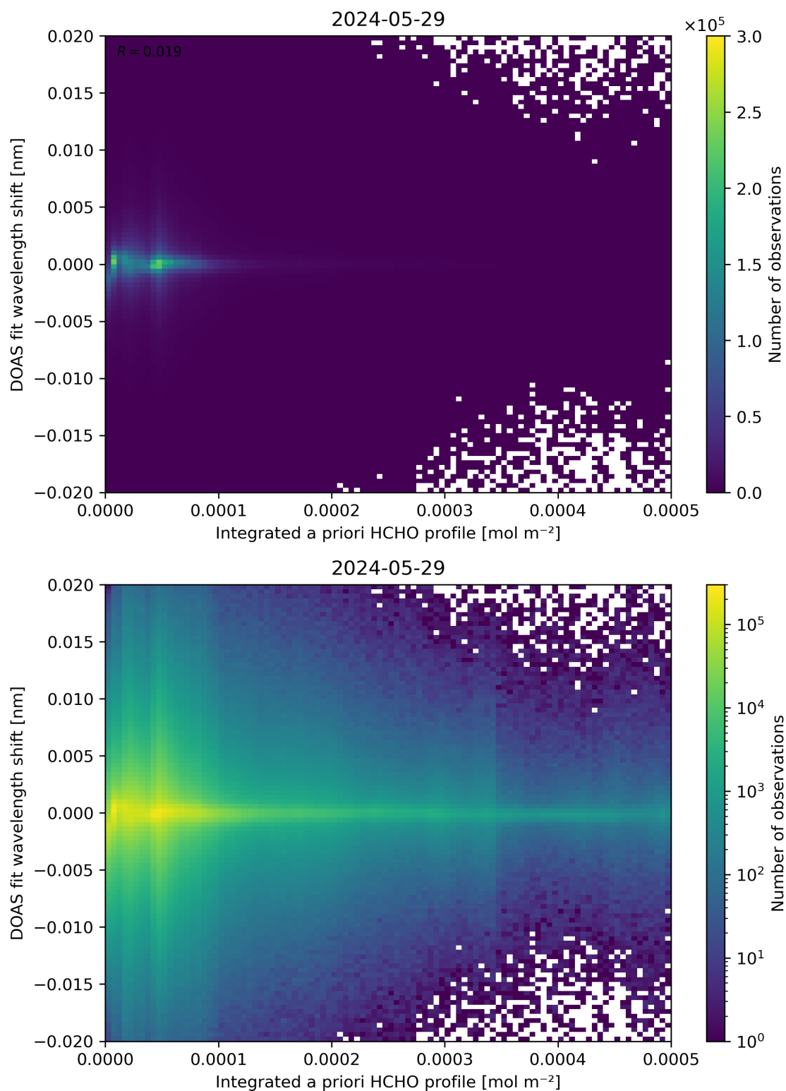
Figure 149: Scatter density plot of “Integrated a priori HCHO profile” against “DOAS fit wavelength shift” for 2024-05-28 to 2024-05-30.
