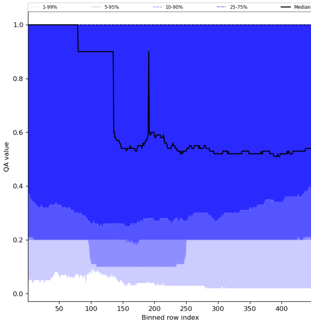
Figure 48: Along track statistics of “QA value” for 2024-05-28 to 2024-05-30
