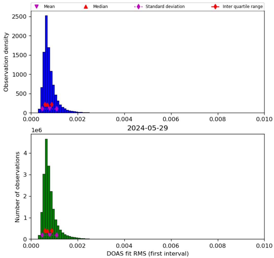
Figure 46: Histogram of “DOAS fit RMS (first interval)” for 2024-05-28 to 2024-05-30
