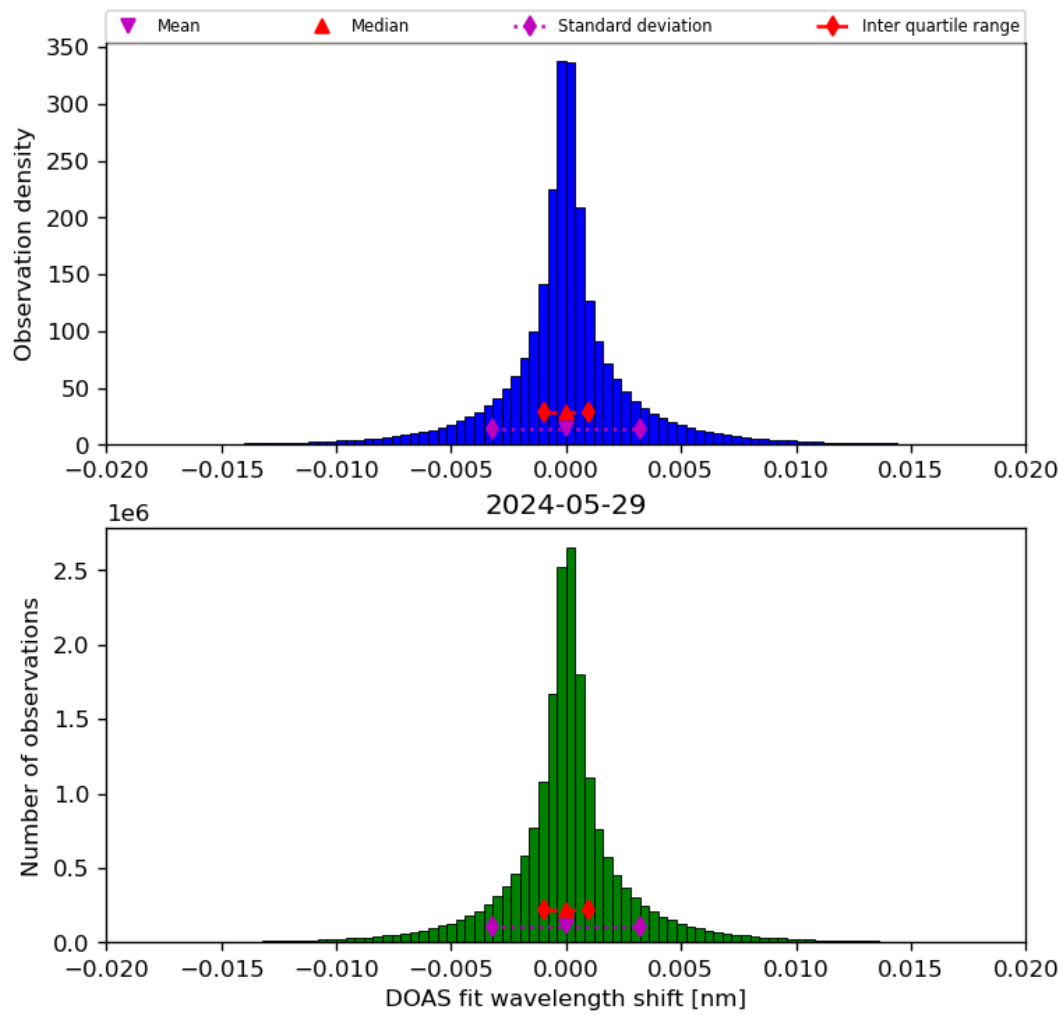
Figure 44: Histogram of “DOAS fit wavelength shift” for 2024-05-28 to 2024-05-30
