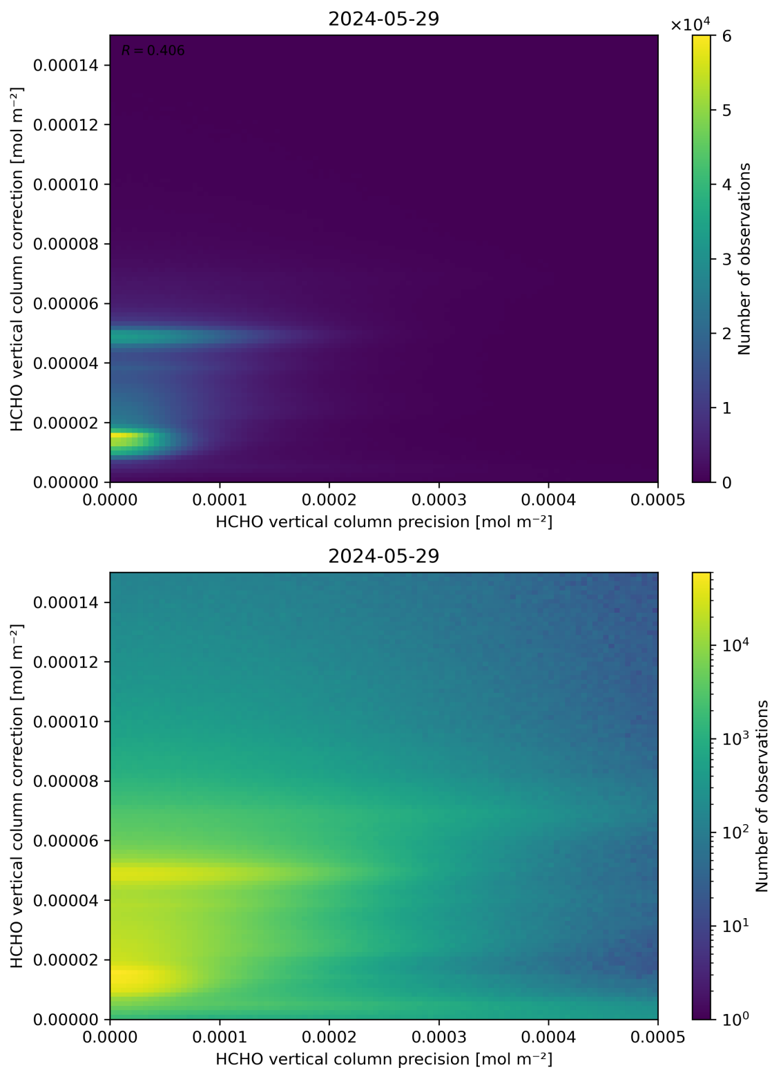
Figure 146: Scatter density plot of “HCHO vertical column precision” against “HCHO vertical column correction” for 2024-05-28 to 2024-05-30.
