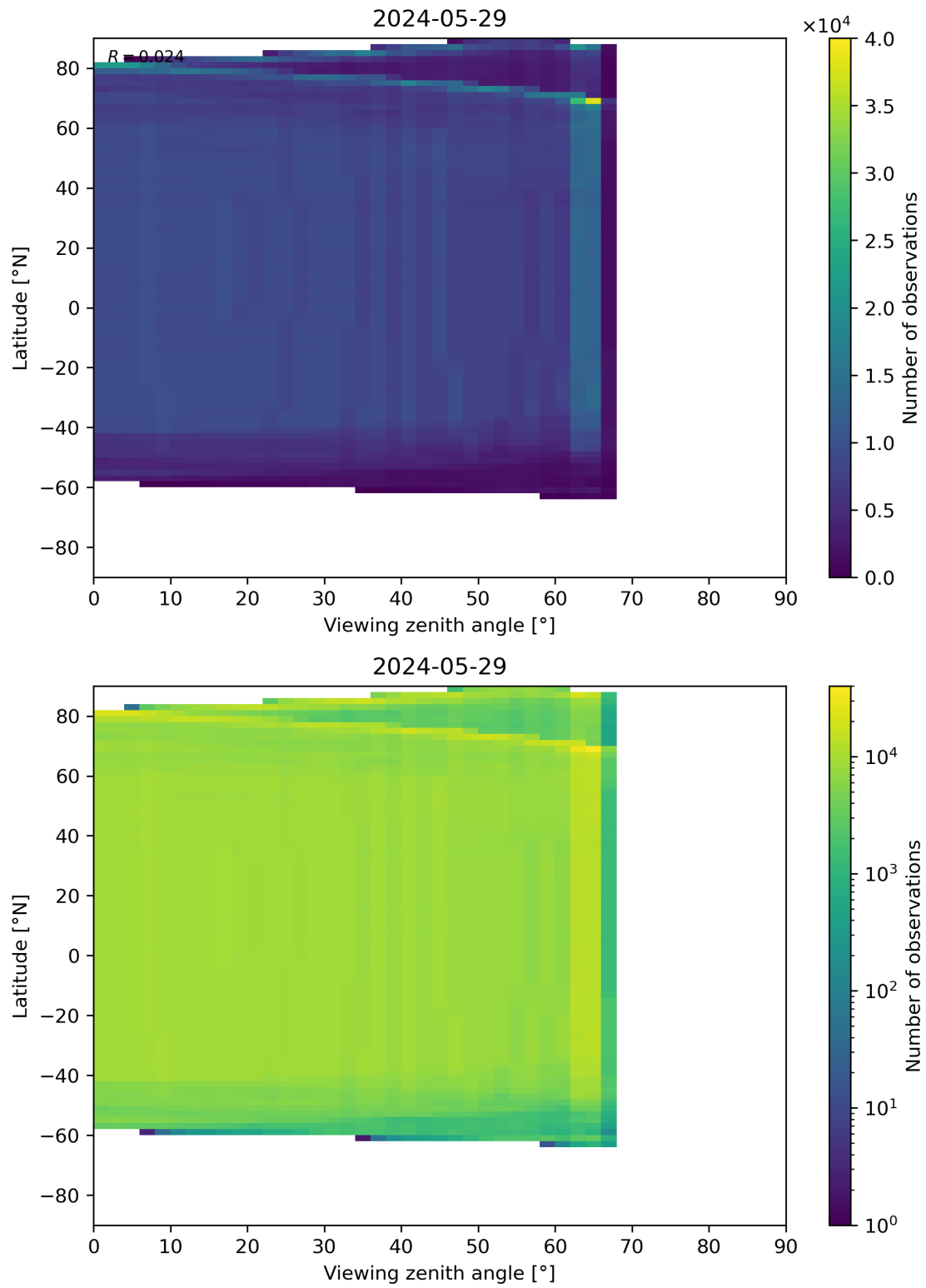
Figure 196: Scatter density plot of “Viewing zenith angle” against “Latitude” for 2024-05-28 to 2024-05-30.
