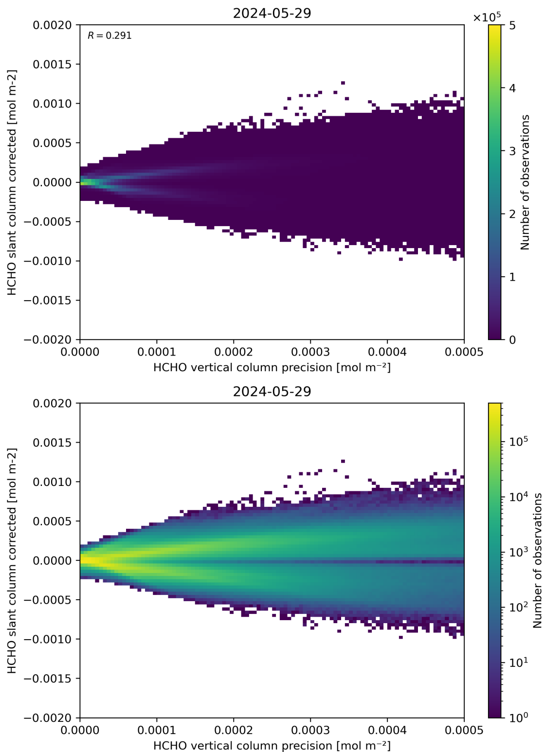
Figure 140: Scatter density plot of “HCHO vertical column precision” against “HCHO slant column corrected” for 2024-05-28 to 2024-05-30.
