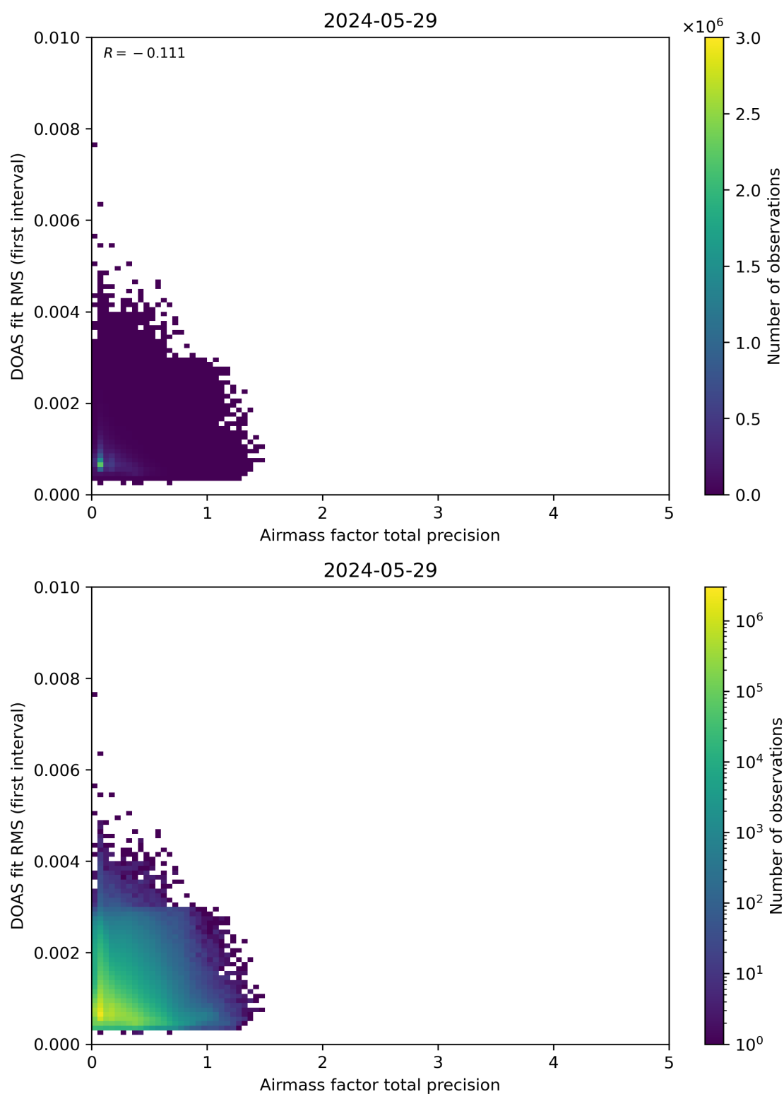
Figure 105: Scatter density plot of “Airmass factor total precision” against “DOAS fit RMS (first interval)” for 2024-05-28 to 2024-05-30.
