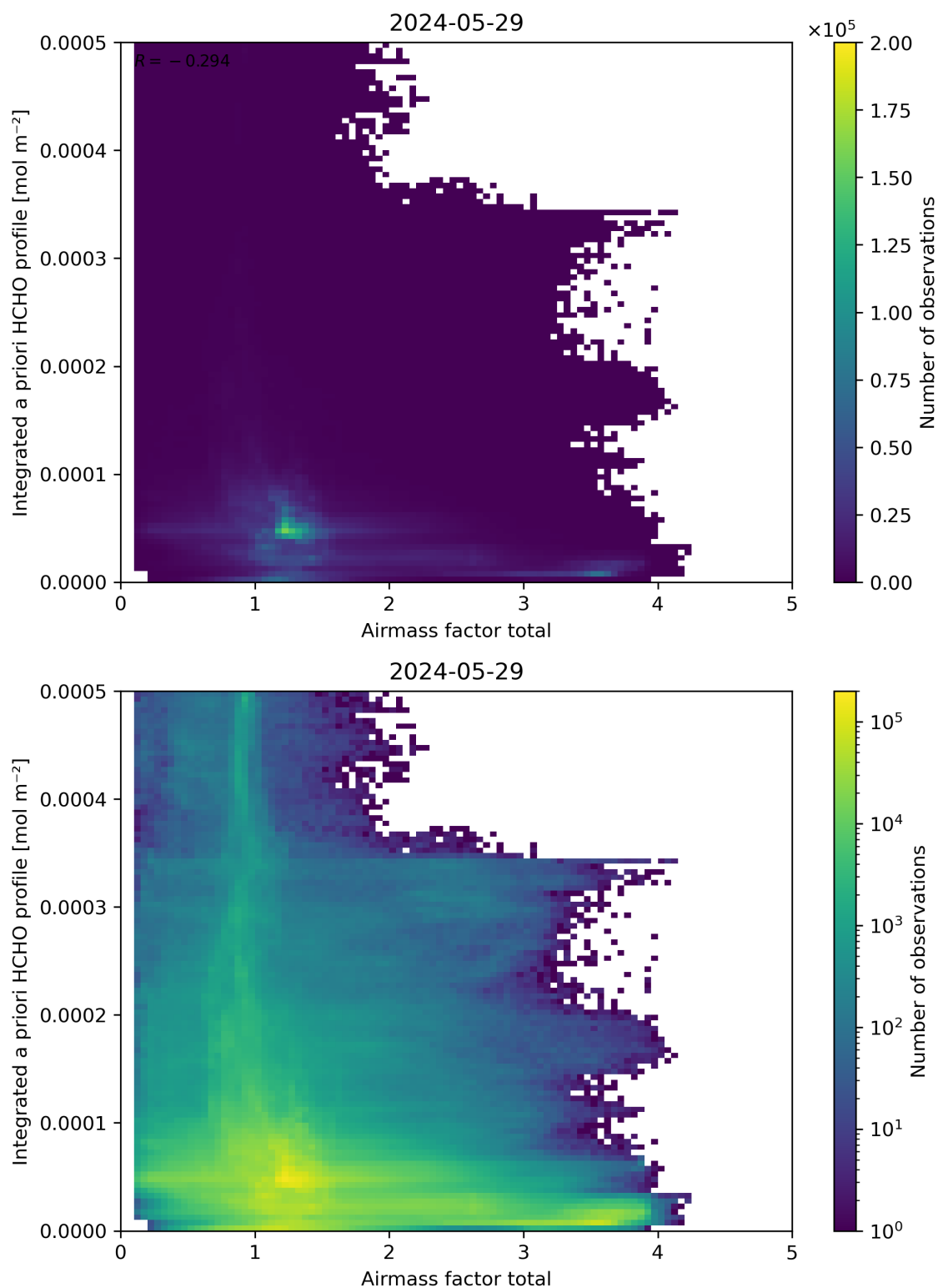
Figure 104: Scatter density plot of “Airmass factor total” against “Integrated a priori HCHO profile” for 2024-05-28 to 2024-05-30.
