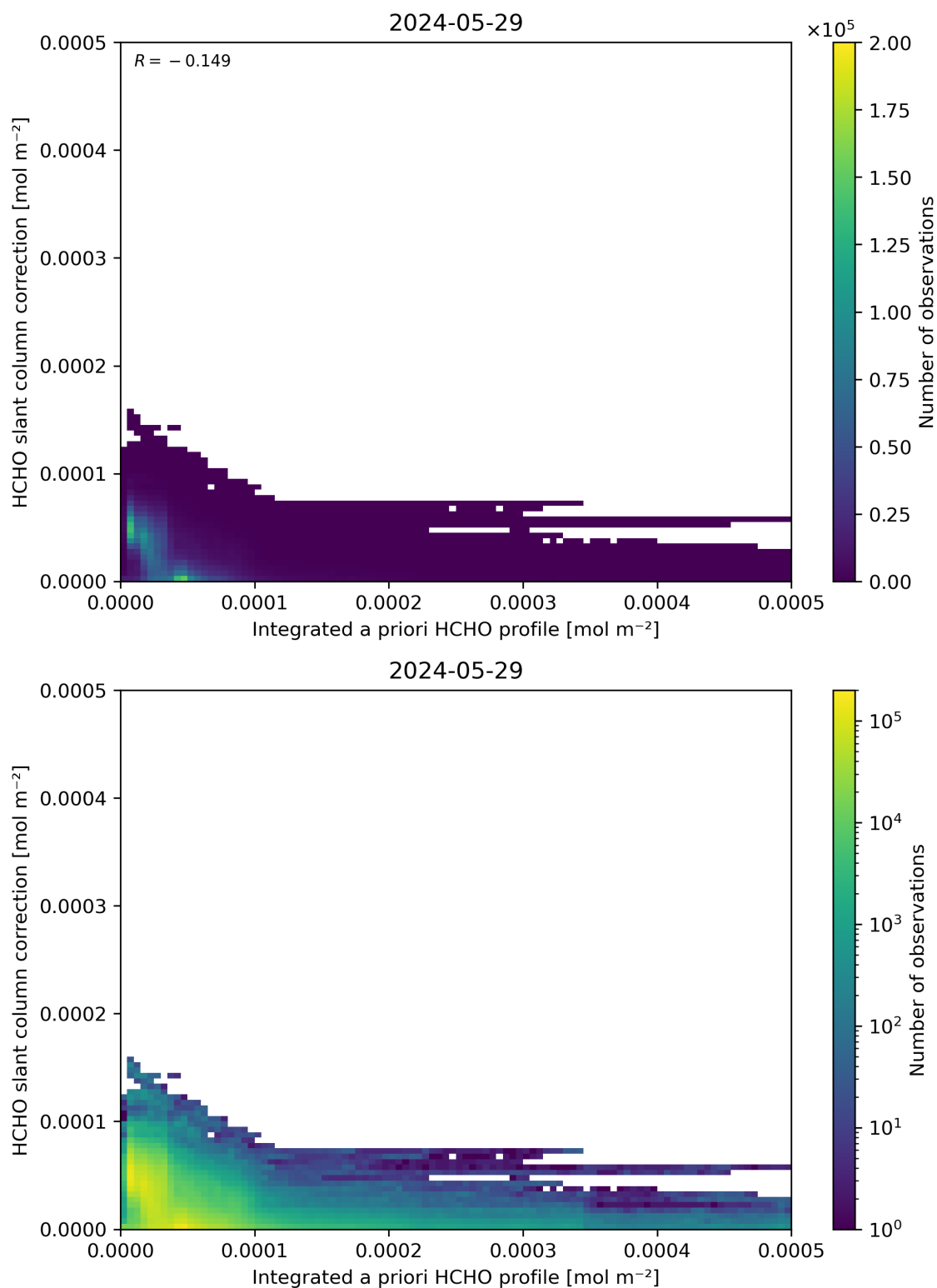
Figure 152: Scatter density plot of “Integrated a priori HCHO profile” against “HCHO slant column correction” for 2024-05-28 to 2024-05-30.
