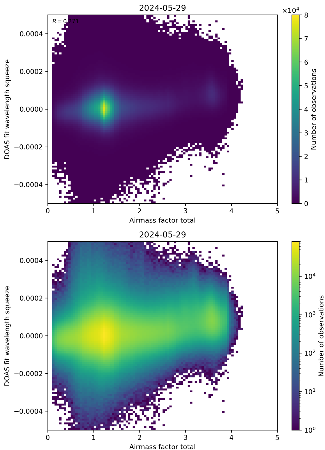
Figure 99: Scatter density plot of “Airmass factor total” against “DOAS fit wavelength squeeze” for 2024-05-28 to 2024-05-30.
