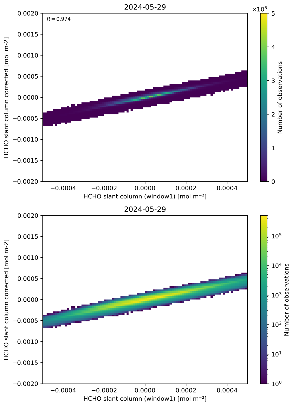
Figure 82: Scatter density plot of “HCHO slant column (window1)” against “HCHO slant column corrected” for 2024-05-28 to 2024-05-30.
