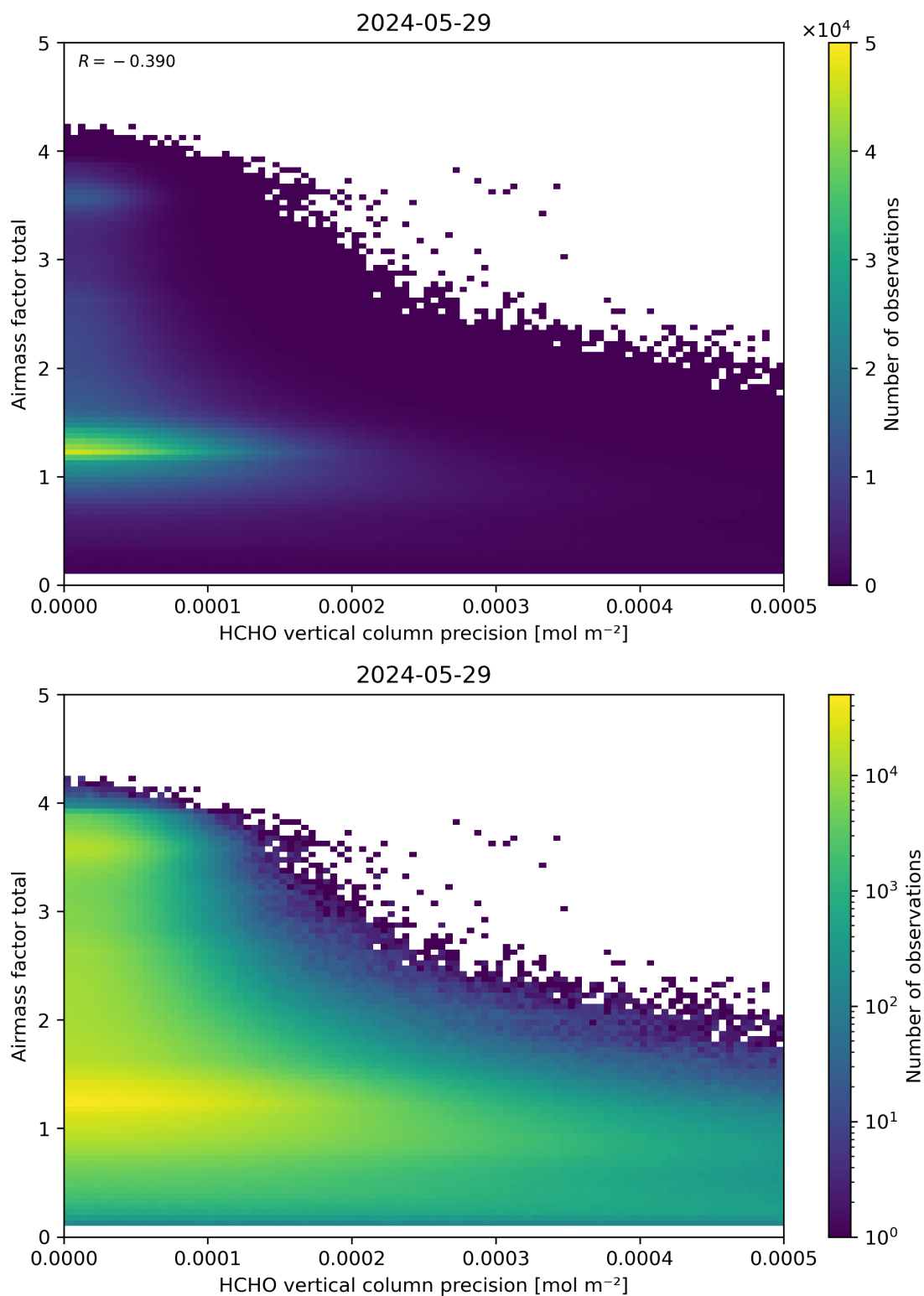
Figure 144: Scatter density plot of “HCHO vertical column precision” against “Airmass factor total” for 2024-05-28 to 2024-05-30.
