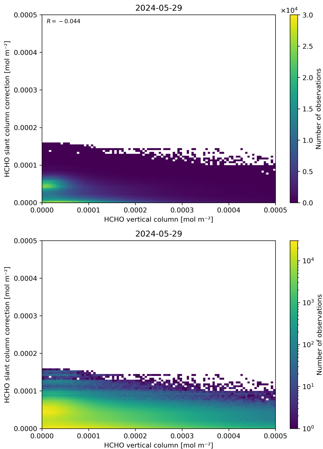
Figure 128: Scatter density plot of “HCHO vertical column” against “HCHO slant column correction” for 2024-05-28 to 2024-05-30.
