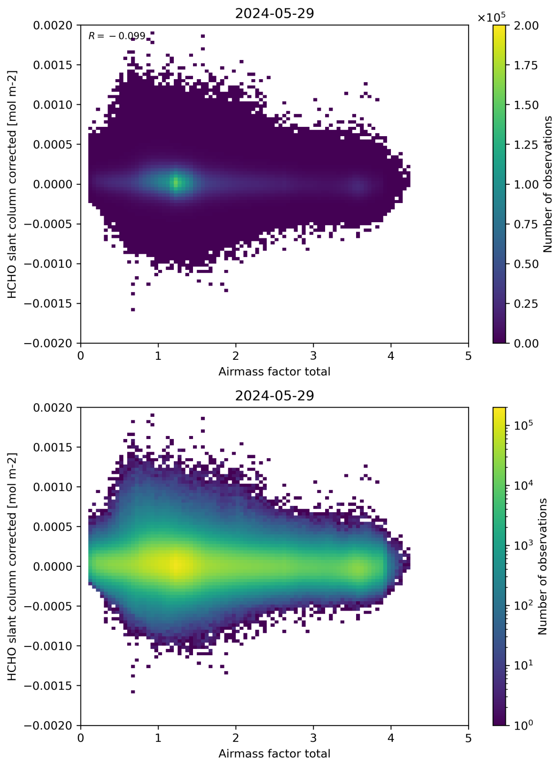
Figure 101: Scatter density plot of “Airmass factor total” against “HCHO slant column corrected” for 2024-05-28 to 2024-05-30.
