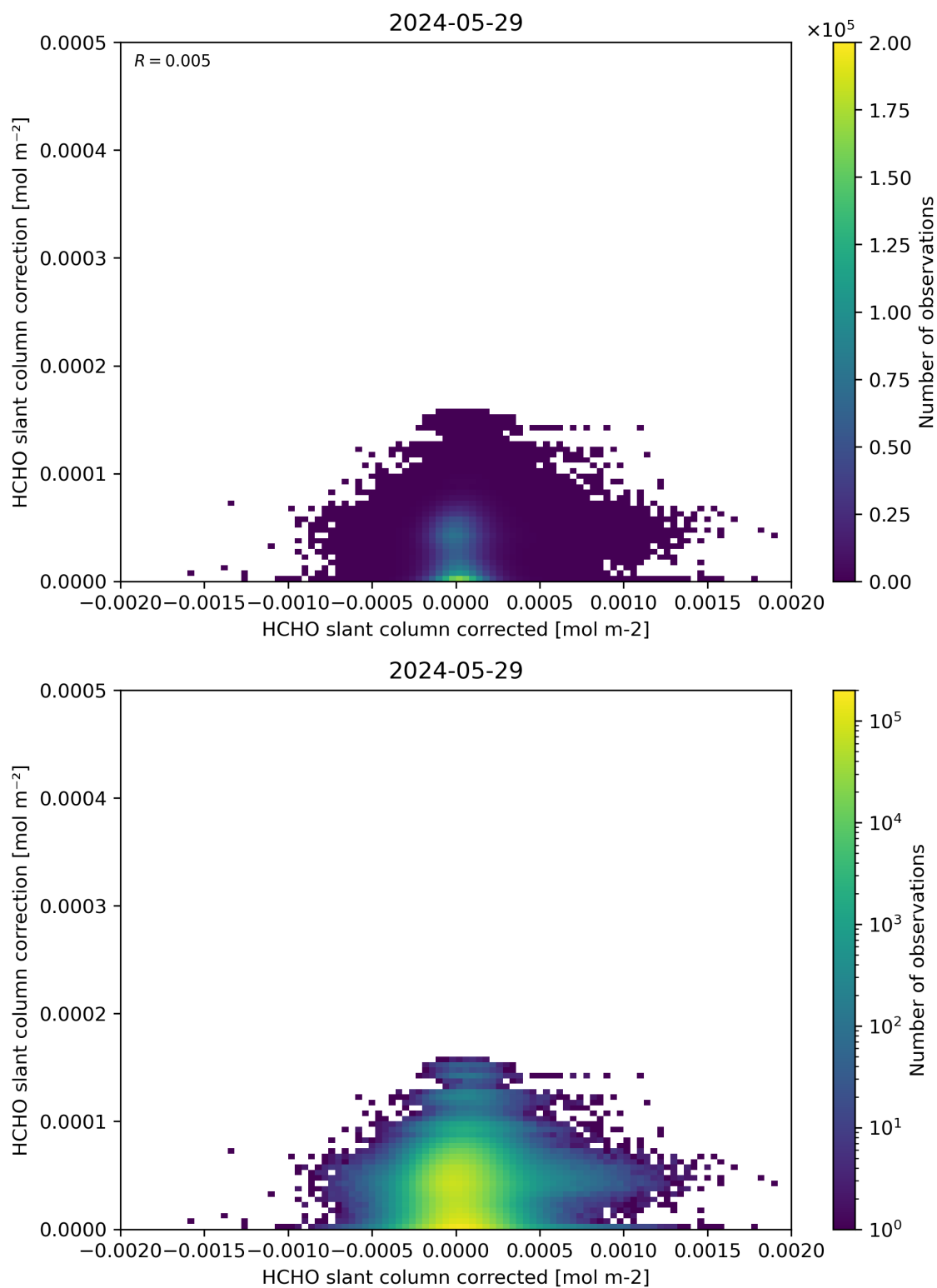
Figure 77: Scatter density plot of “HCHO slant column corrected” against “HCHO slant column correction” for 2024-05-28 to 2024-05-30.
