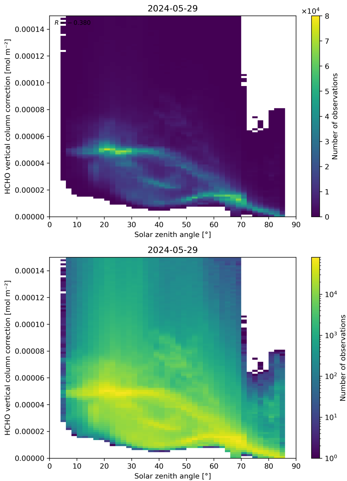
Figure 178: Scatter density plot of “Solar zenith angle” against “HCHO vertical column correction” for 2024-05-28 to 2024-05-30.
