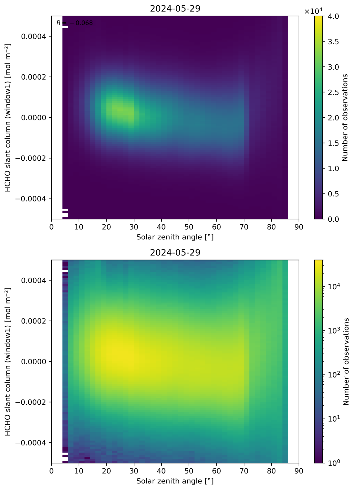
Figure 173: Scatter density plot of “Solar zenith angle” against “HCHO slant column (window1)” for 2024-05-28 to 2024-05-30.
