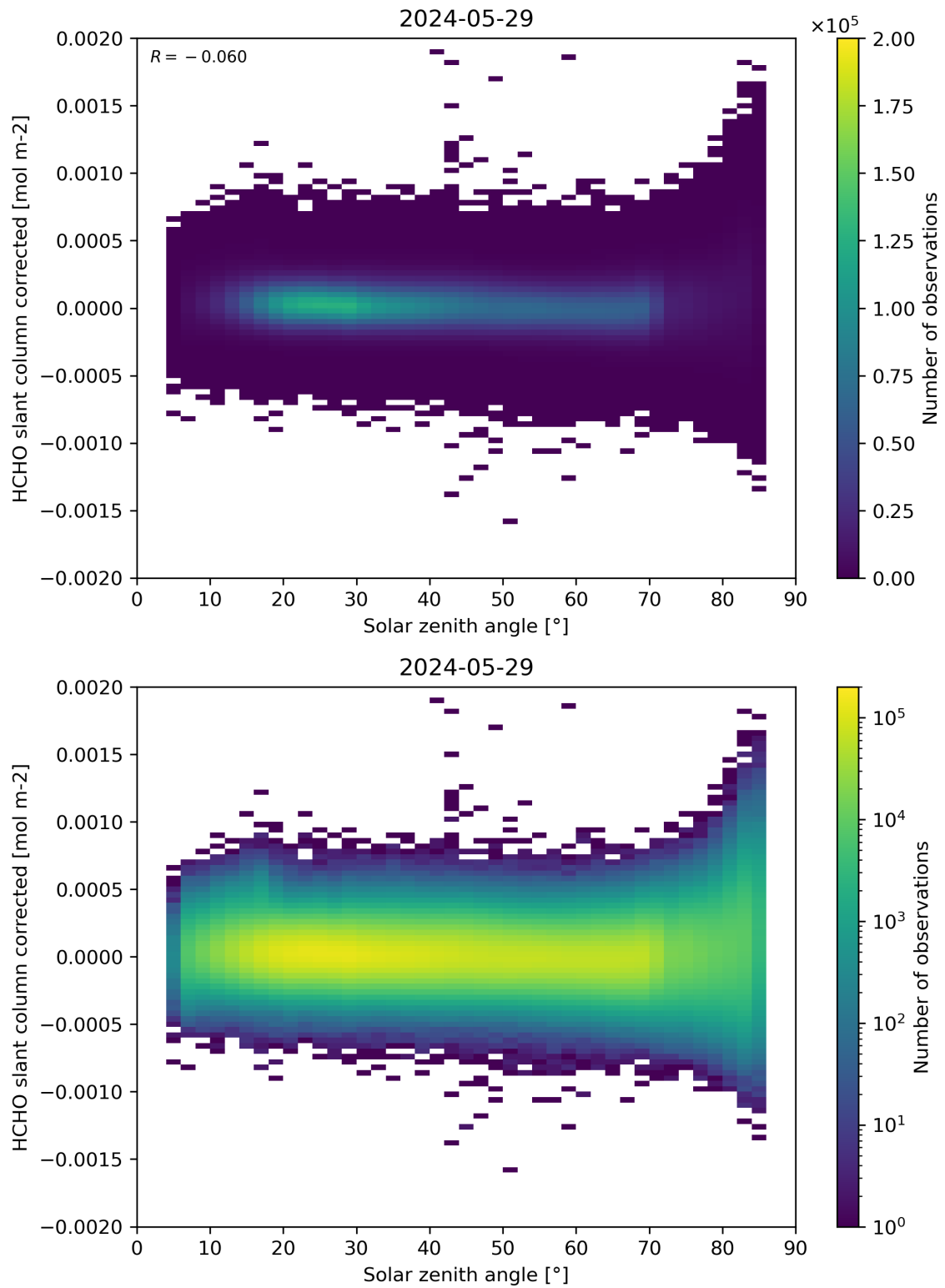
Figure 171: Scatter density plot of “Solar zenith angle” against “HCHO slant column corrected” for 2024-05-28 to 2024-05-30.
