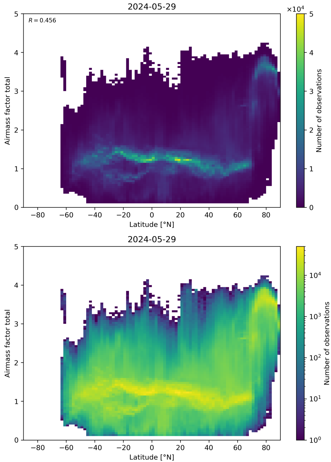
Figure 161: Scatter density plot of “Latitude” against “Airmass factor total” for 2024-05-28 to 2024-05-30.
