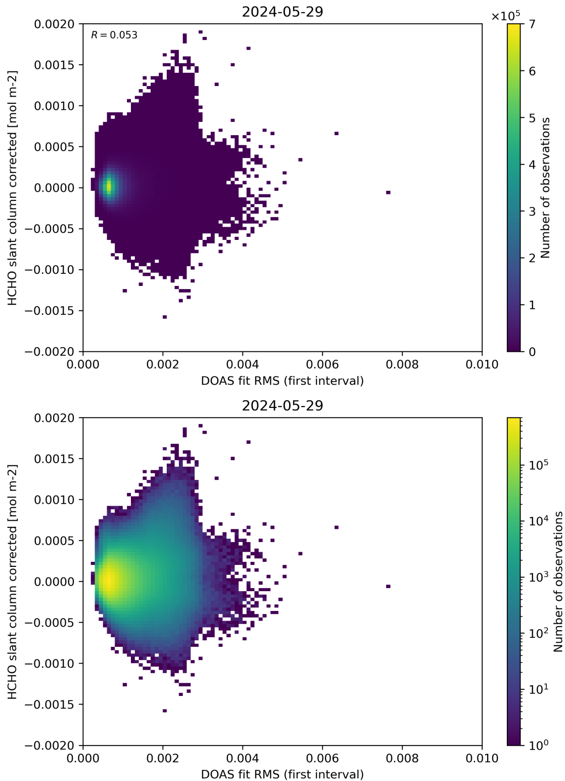
Figure 62: Scatter density plot of “DOAS fit RMS (first interval)” against “HCHO slant column corrected” for 2024-05-28 to 2024-05-30.
