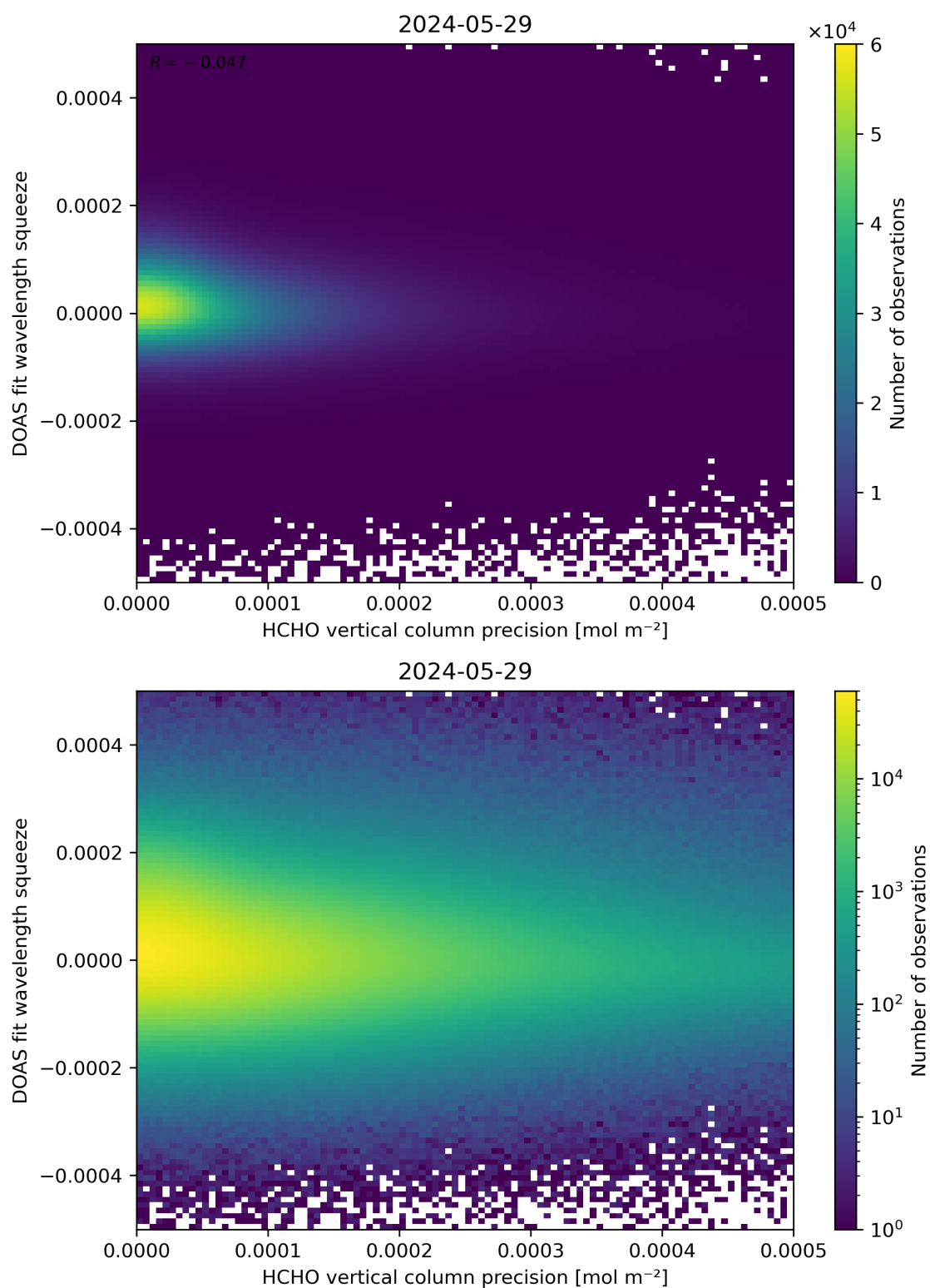
Figure 138: Scatter density plot of “HCHO vertical column precision” against “DOAS fit wavelength squeeze” for 2024-05-28 to 2024-05-30.
