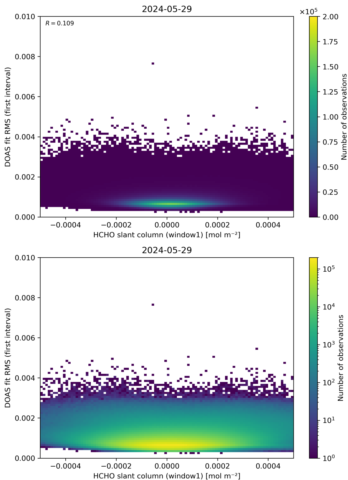
Figure 78: Scatter density plot of “HCHO slant column (window1)” against “DOAS fit RMS (first interval)” for 2024-05-28 to 2024-05-30.
