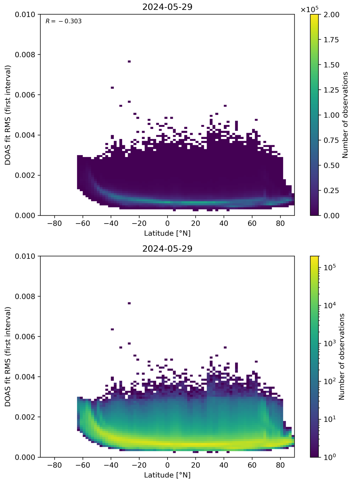
Figure 153: Scatter density plot of “Latitude” against “DOAS fit RMS (first interval)” for 2024-05-28 to 2024-05-30.
