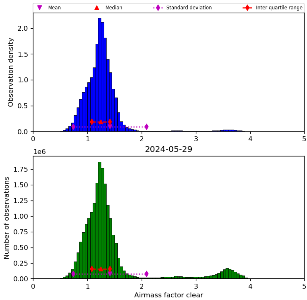
Figure 42: Histogram of “Airmass factor clear” for 2024-05-28 to 2024-05-30
