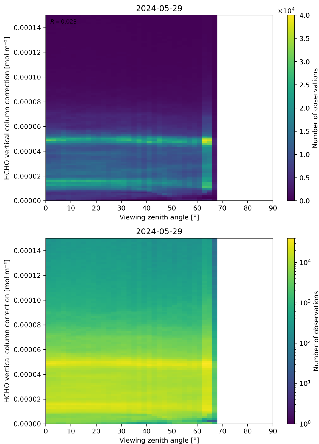
Figure 193: Scatter density plot of “Viewing zenith angle” against “HCHO vertical column correction” for 2024-05-28 to 2024-05-30.
