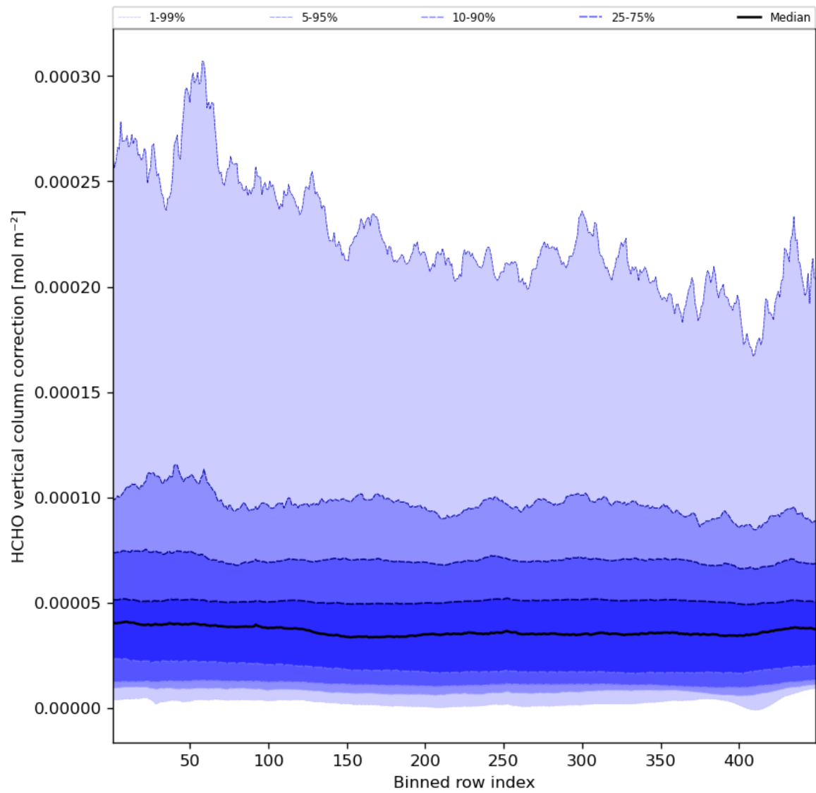
Figure 51: Along track statistics of “HCHO vertical column correction” for 2024-05-28 to 2024-05-30
