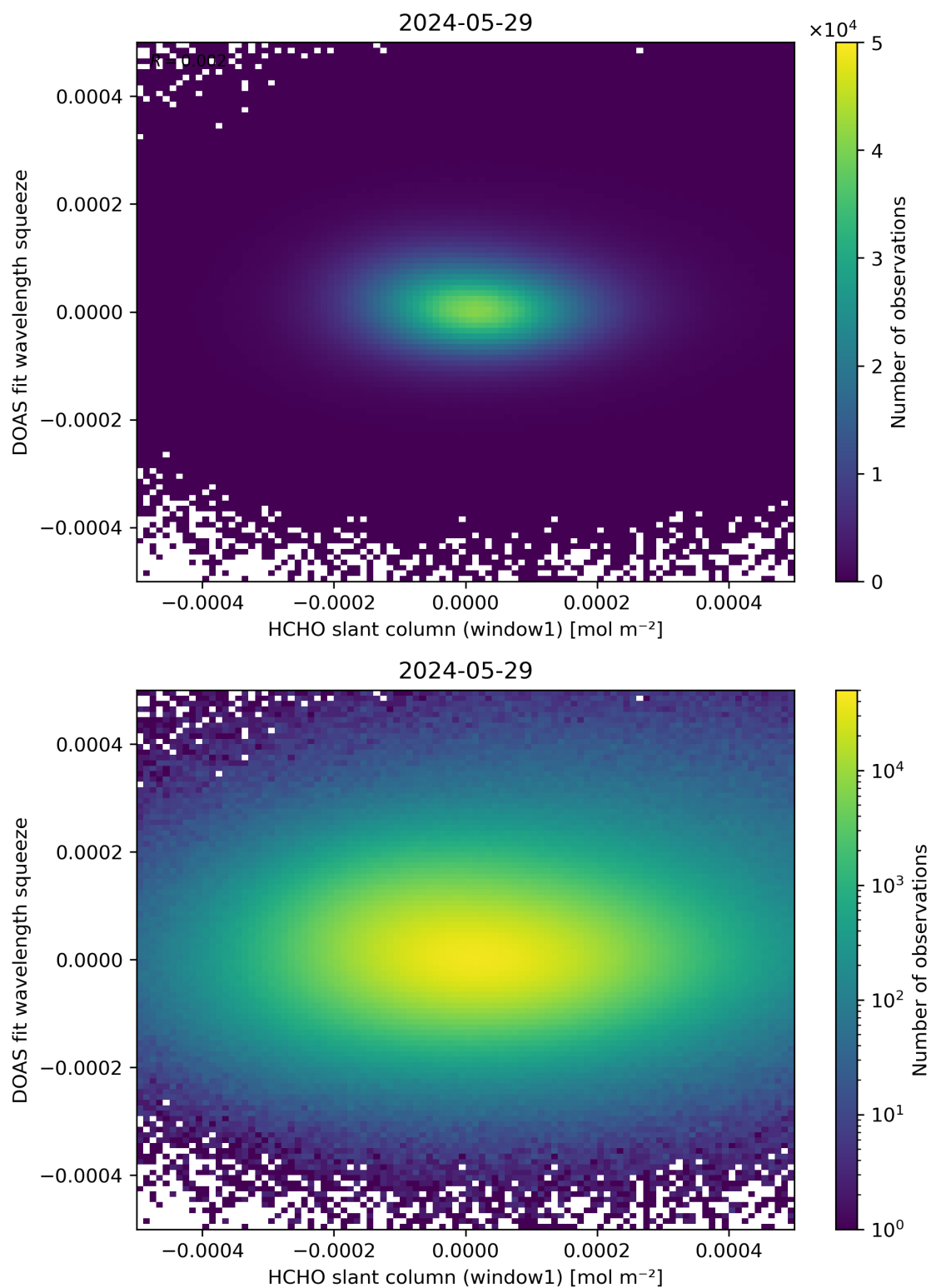
Figure 80: Scatter density plot of “HCHO slant column (window1)” against “DOAS fit wavelength squeeze” for 2024-05-28 to 2024-05-30.
