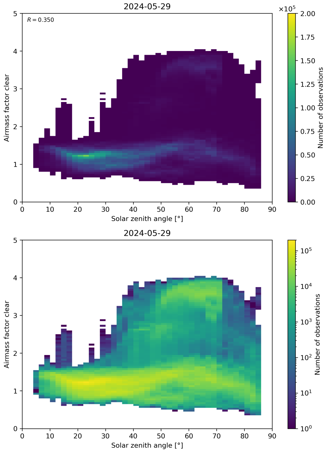
Figure 170: Scatter density plot of “Solar zenith angle” against “Airmass factor clear” for 2024-05-28 to 2024-05-30.
