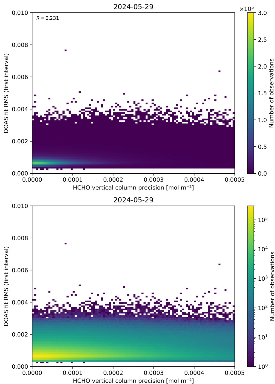
Figure 136: Scatter density plot of “HCHO vertical column precision” against “DOAS fit RMS (first interval)” for 2024-05-28 to 2024-05-30.
