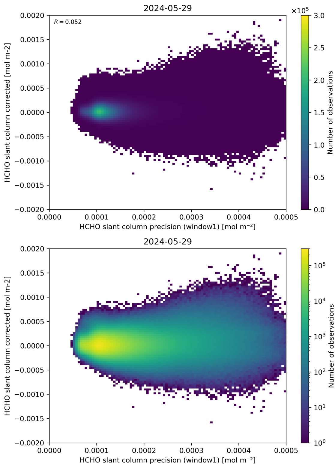
Figure 92: Scatter density plot of “HCHO slant column precision (window1)” against “HCHO slant column corrected” for 2024-05-28 to 2024-05-30.
