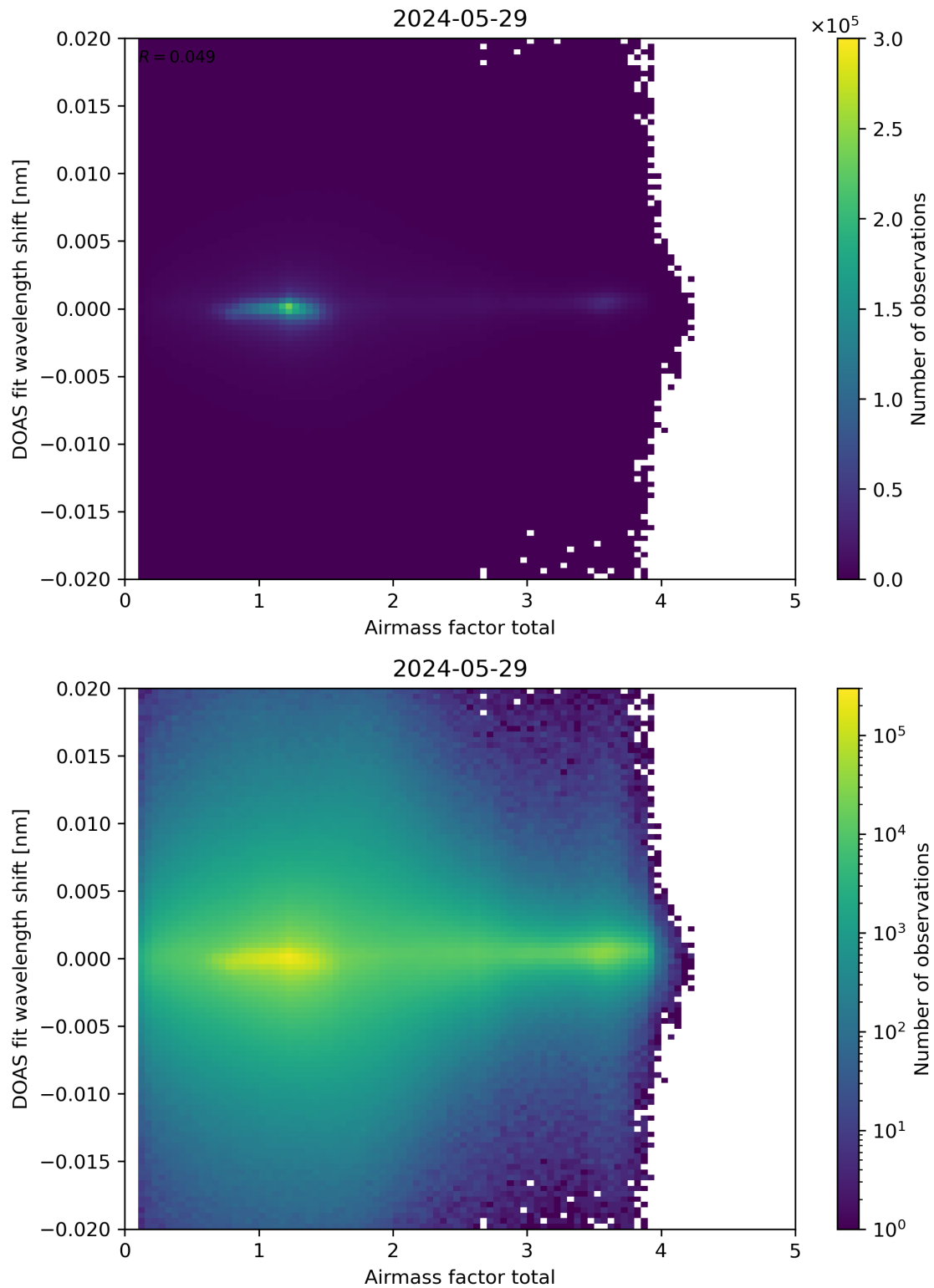
Figure 98: Scatter density plot of “Airmass factor total” against “DOAS fit wavelength shift” for 2024-05-28 to 2024-05-30.
