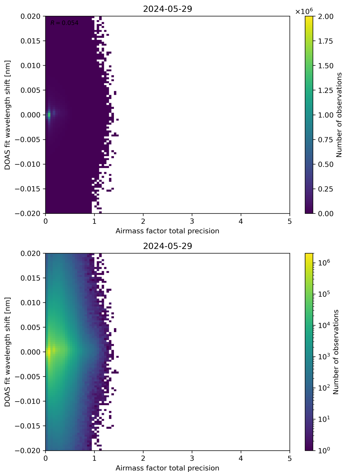
Figure 106: Scatter density plot of “Airmass factor total precision” against “DOAS fit wavelength shift” for 2024-05-28 to 2024-05-30.
