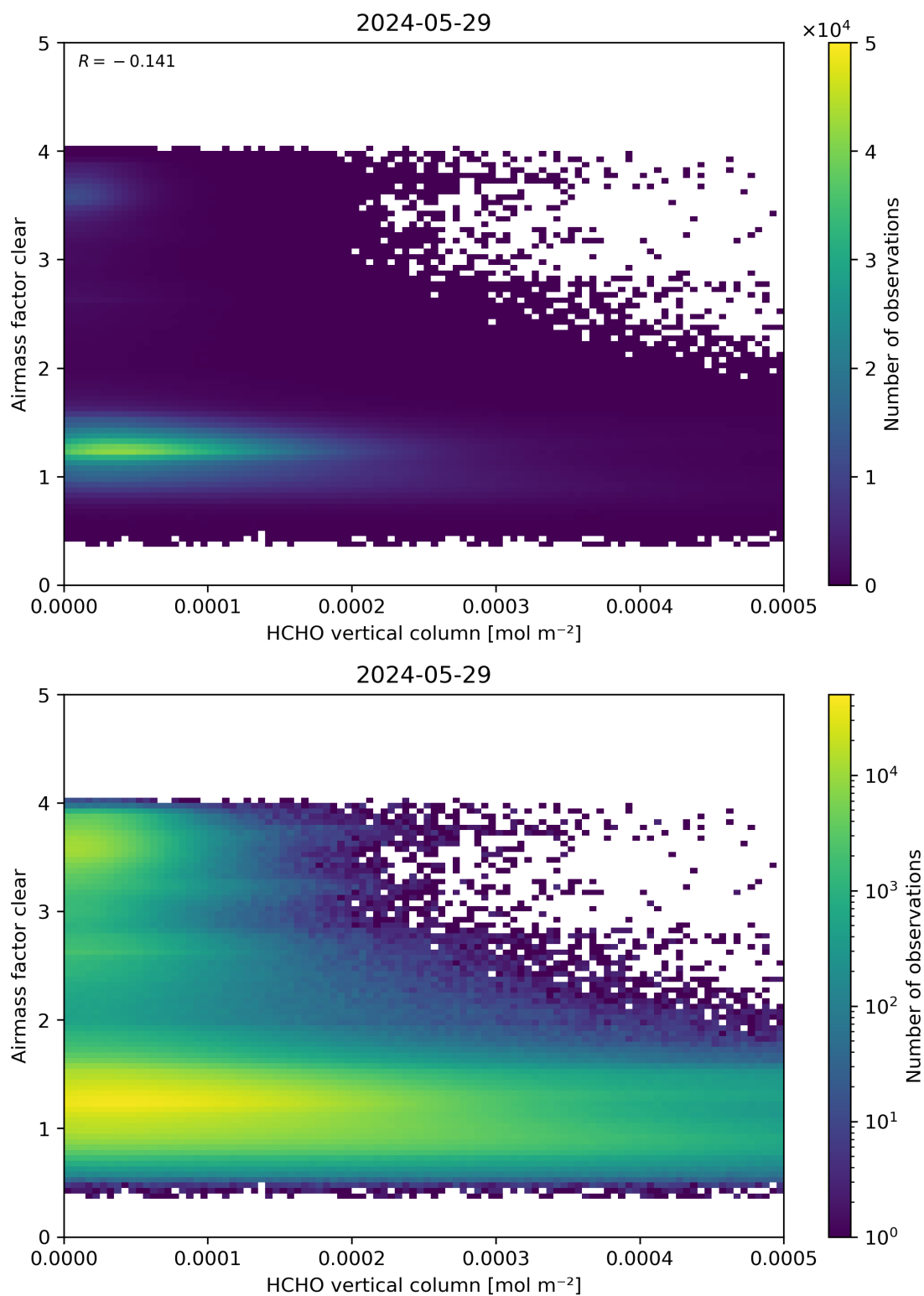
Figure 126: Scatter density plot of “HCHO vertical column” against “Airmass factor clear” for 2024-05-28 to 2024-05-30.
