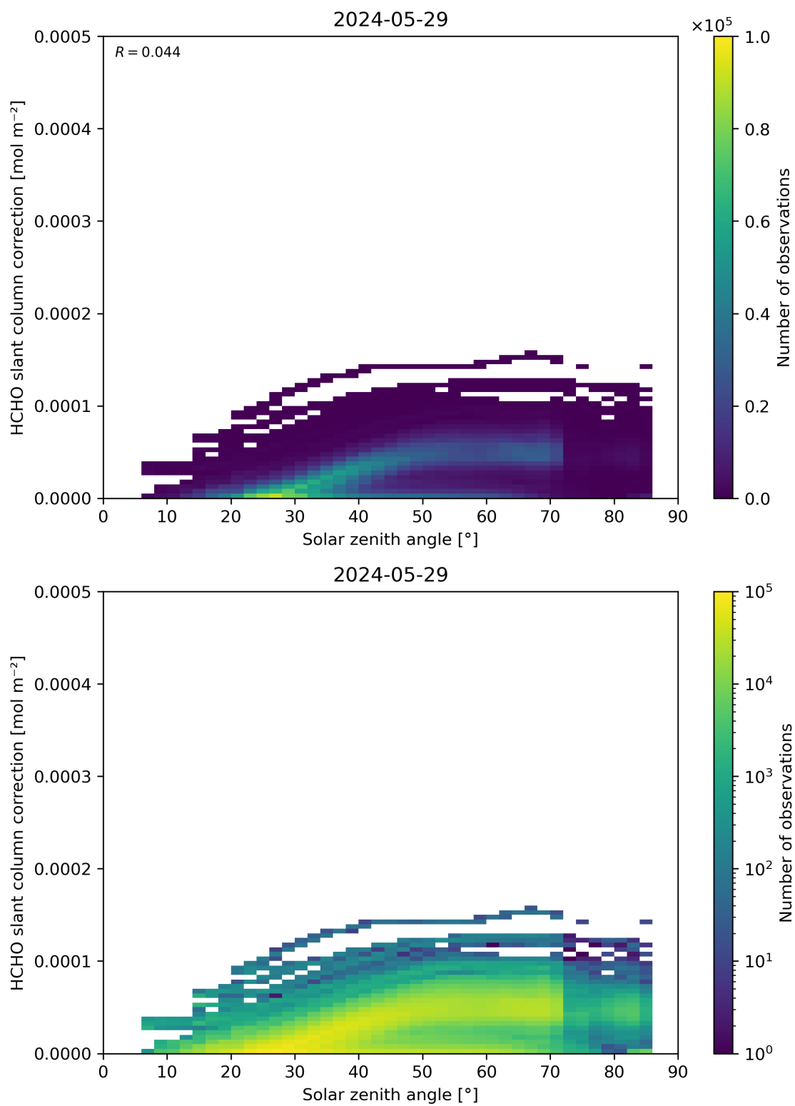
Figure 172: Scatter density plot of “Solar zenith angle” against “HCHO slant column correction” for 2024-05-28 to 2024-05-30.
