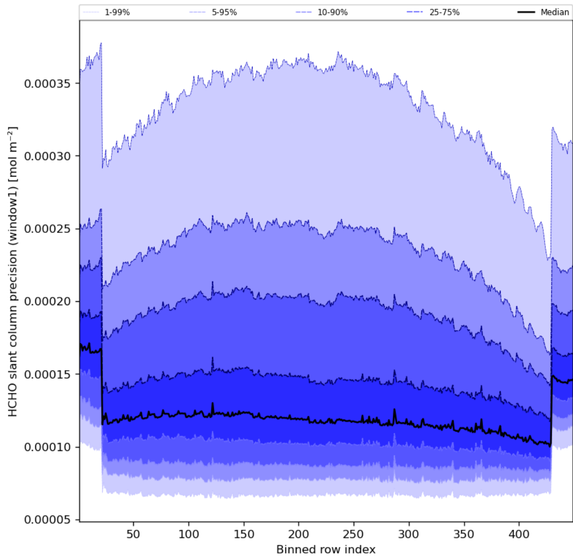
Figure 53: Along track statistics of “HCHO slant column precision (window1)” for 2024-05-28 to 2024-05-30
