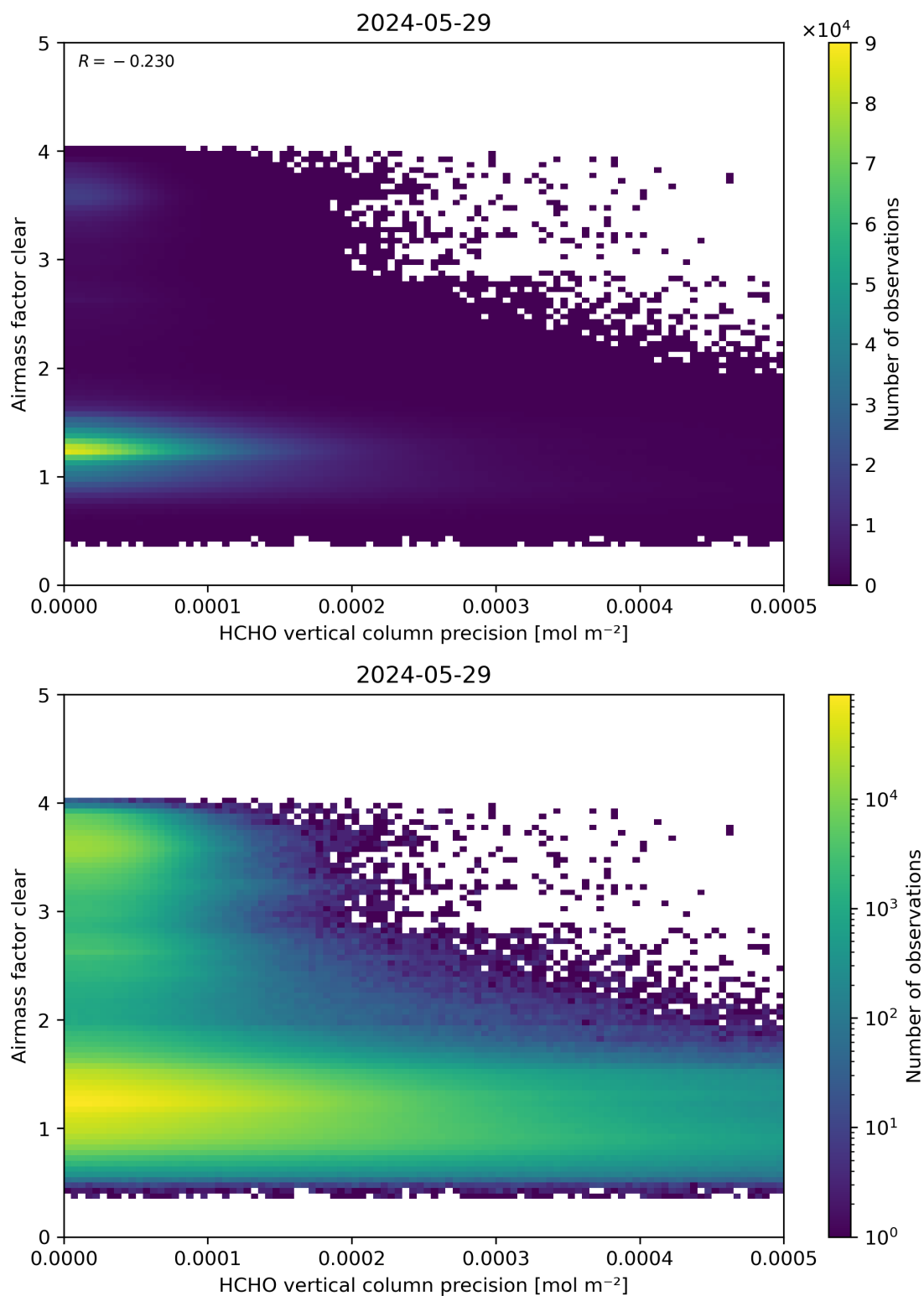
Figure 139: Scatter density plot of “HCHO vertical column precision” against “Airmass factor clear” for 2024-05-28 to 2024-05-30.
