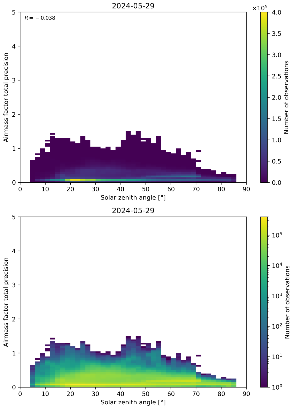
Figure 176: Scatter density plot of “Solar zenith angle” against “Airmass factor total precision” for 2024-05-28 to 2024-05-30.
