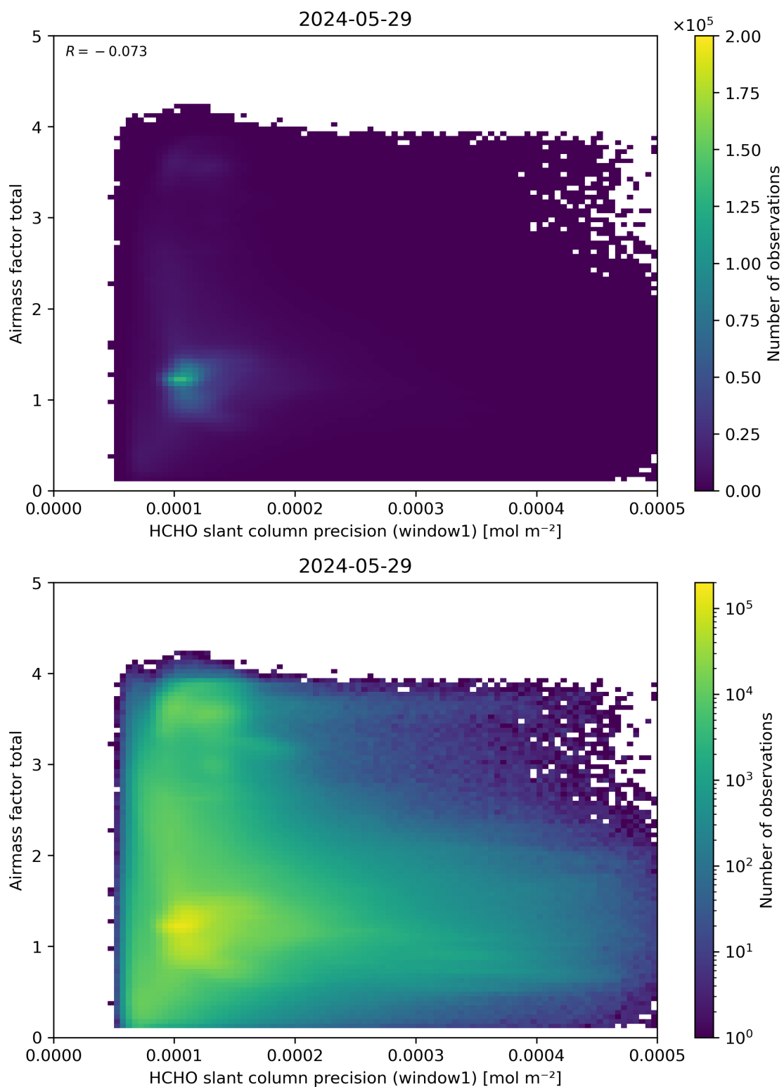
Figure 94: Scatter density plot of “HCHO slant column precision (window1)” against “Airmass factor total” for 2024-05-28 to 2024-05-30.
