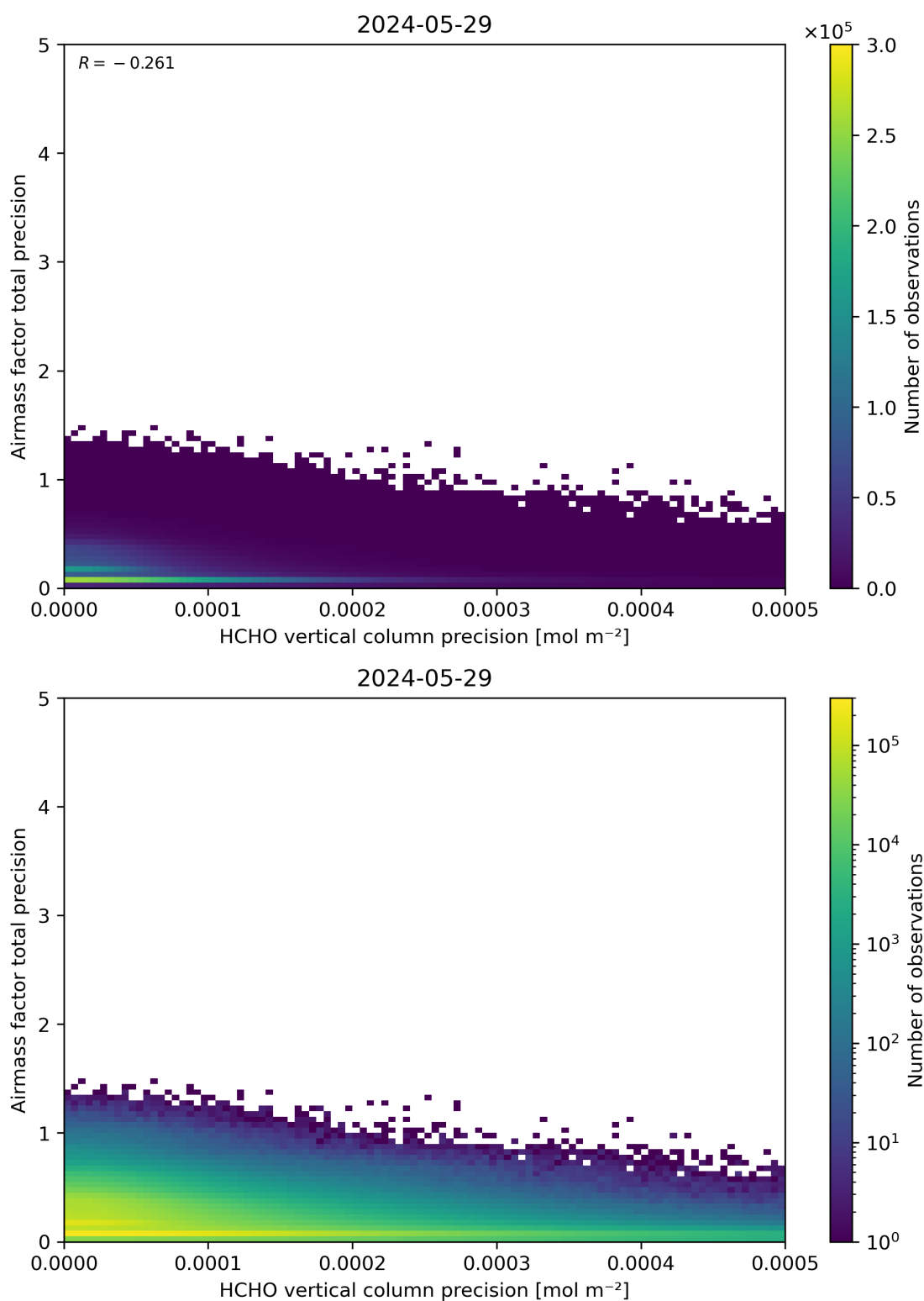
Figure 145: Scatter density plot of “HCHO vertical column precision” against “Airmass factor total precision” for 2024-05-28 to 2024-05-30.
