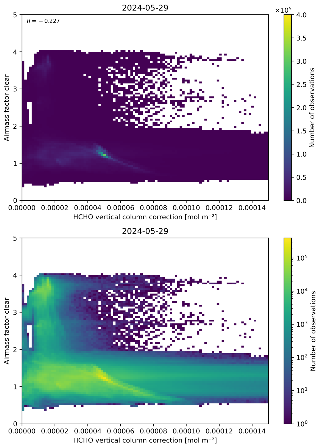
Figure 115: Scatter density plot of “HCHO vertical column correction” against “Airmass factor clear” for 2024-05-28 to 2024-05-30.
