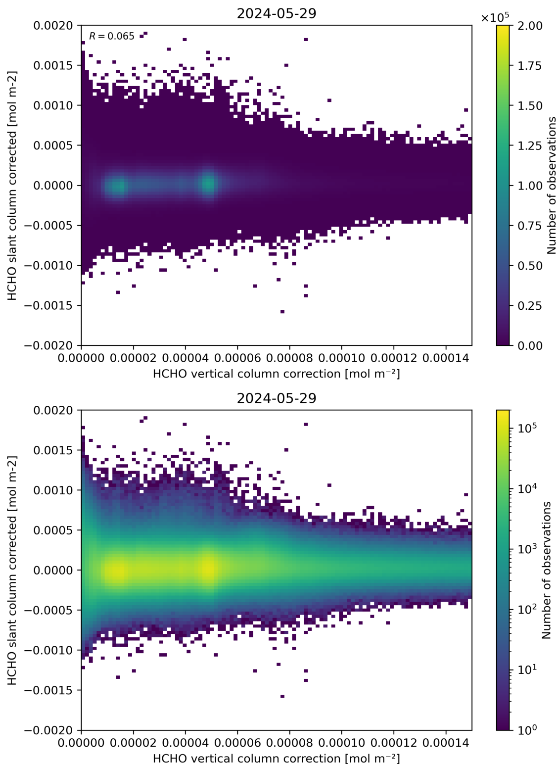
Figure 116: Scatter density plot of “HCHO vertical column correction” against “HCHO slant column corrected” for 2024-05-28 to 2024-05-30.
