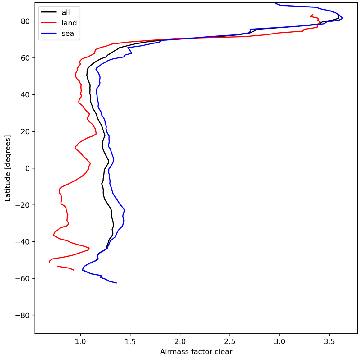
Figure 28: Zonal average of “Airmass factor clear” for 2024-05-28 to 2024-05-30.
