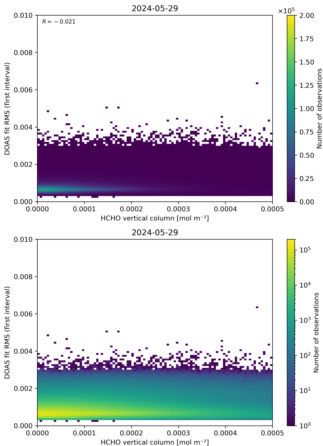
Figure 123: Scatter density plot of “HCHO vertical column” against “DOAS fit RMS (first interval)” for 2024-05-28 to 2024-05-30.
