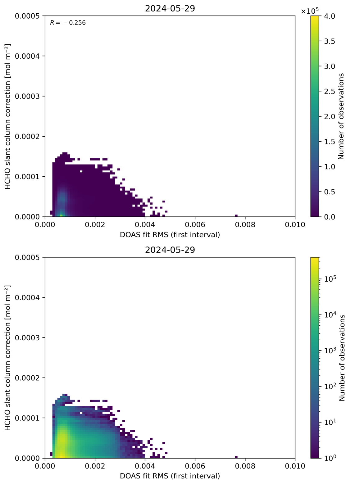
Figure 63: Scatter density plot of “DOAS fit RMS (first interval)” against “HCHO slant column correction” for 2024-05-28 to 2024-05-30.
