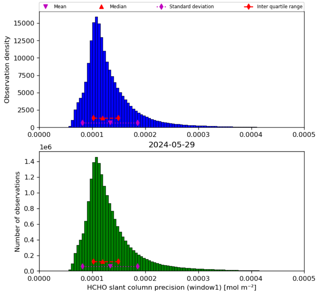
Figure 39: Histogram of “HCHO slant column precision (window1)” for 2024-05-28 to 2024-05-30
