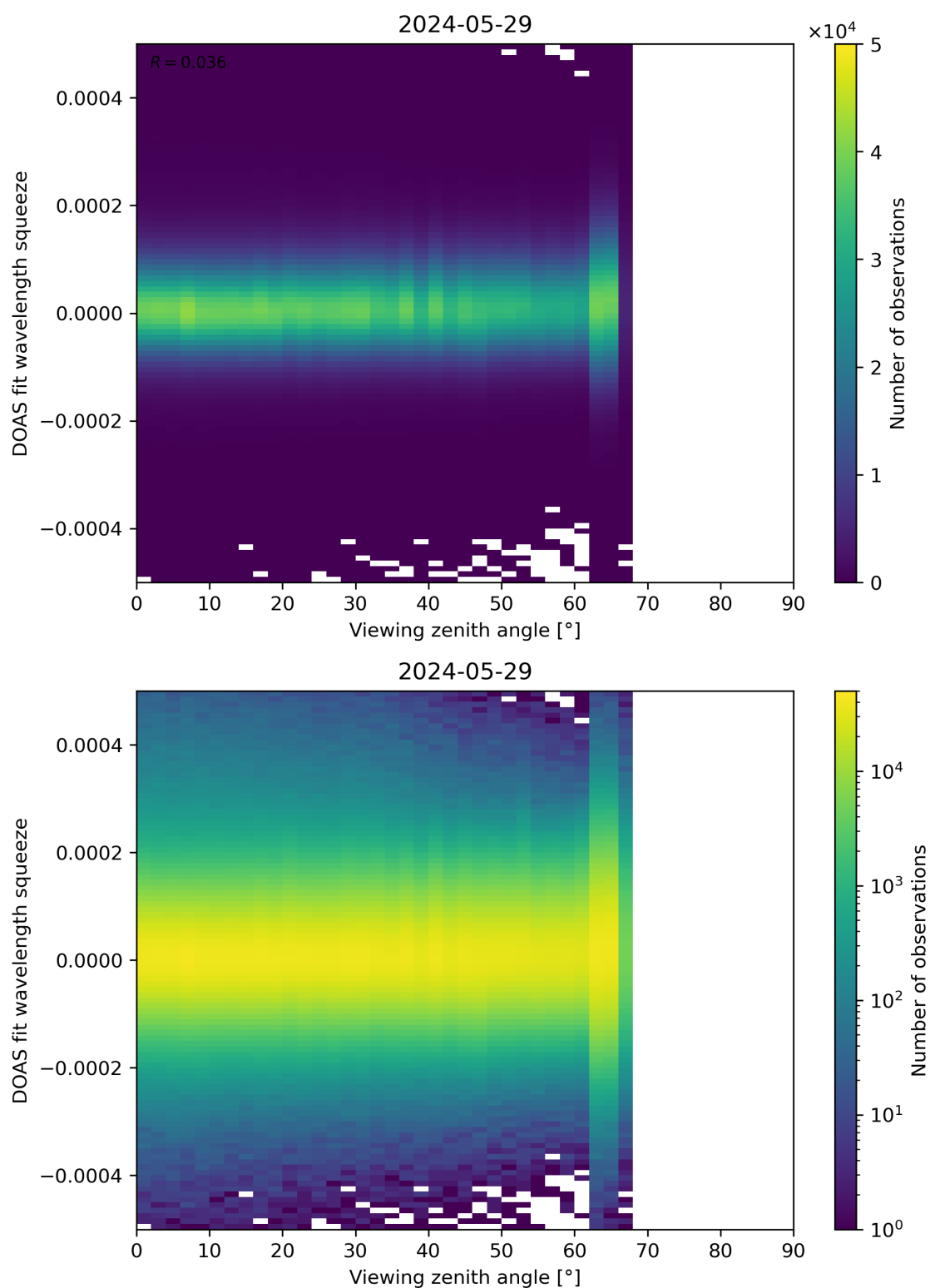
Figure 184: Scatter density plot of “Viewing zenith angle” against “DOAS fit wavelength squeeze” for 2024-05-28 to 2024-05-30.
