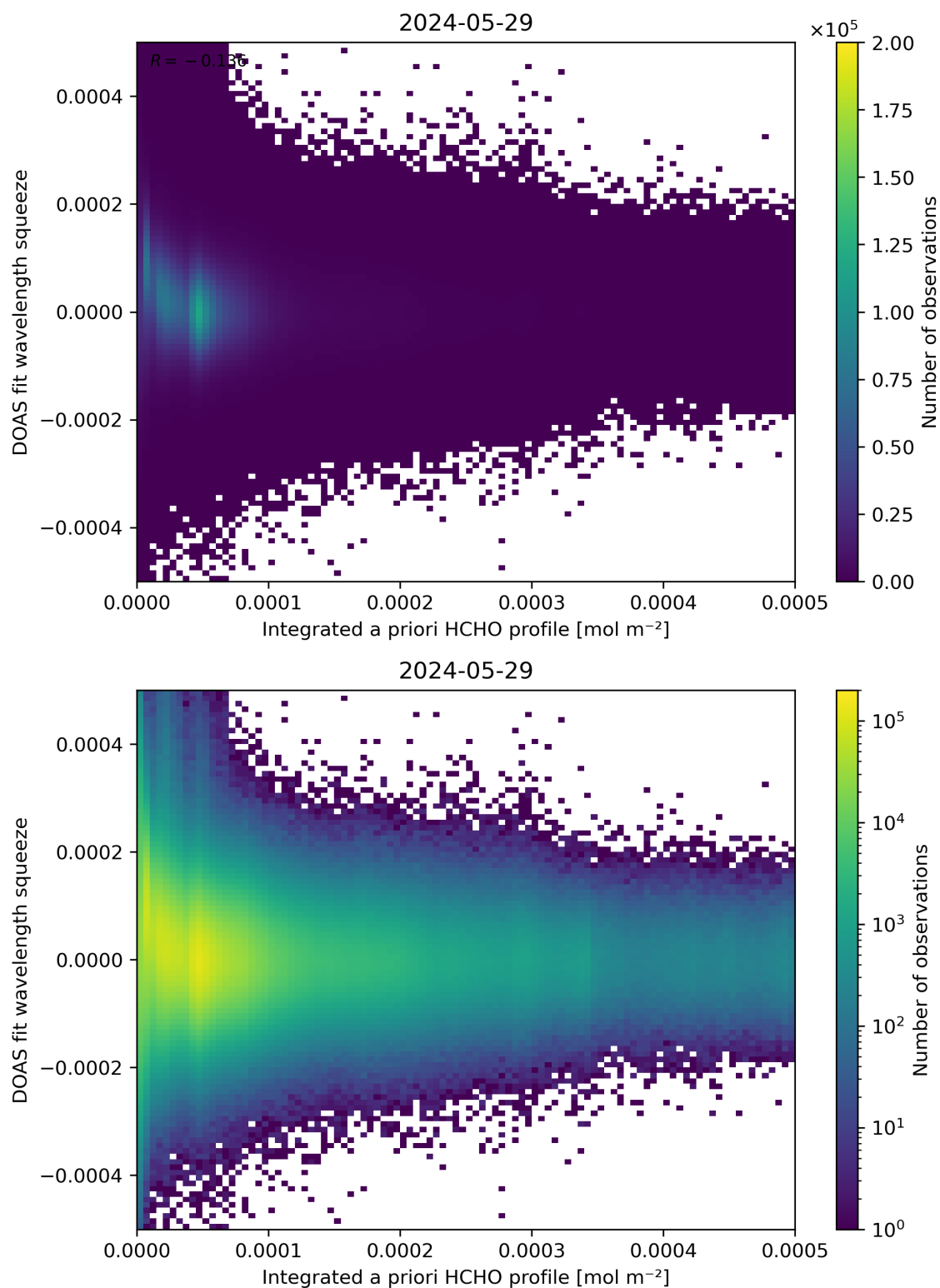
Figure 150: Scatter density plot of “Integrated a priori HCHO profile” against “DOAS fit wavelength squeeze” for 2024-05-28 to 2024-05-30.
