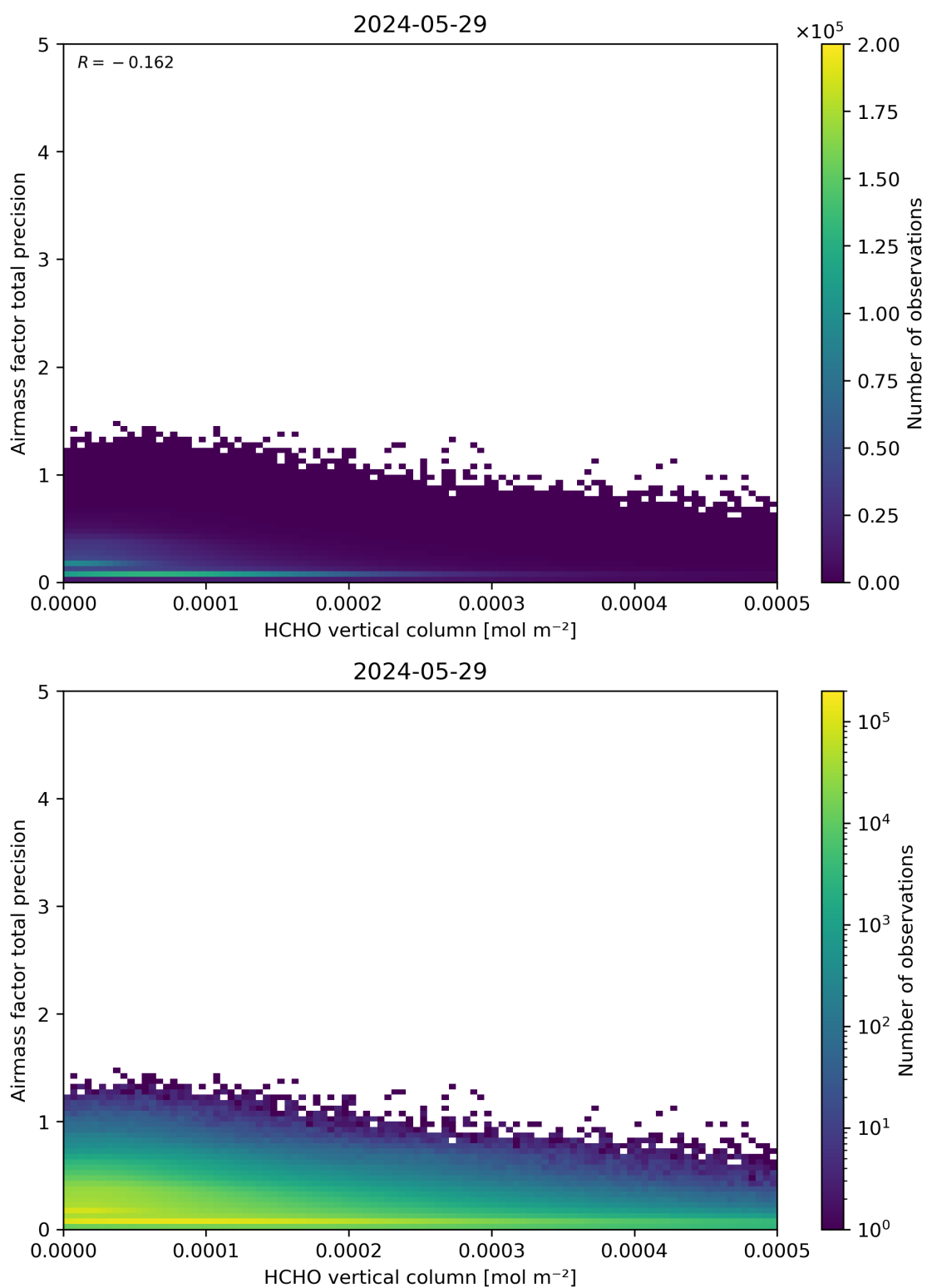
Figure 132: Scatter density plot of “HCHO vertical column” against “Airmass factor total precision” for 2024-05-28 to 2024-05-30.
