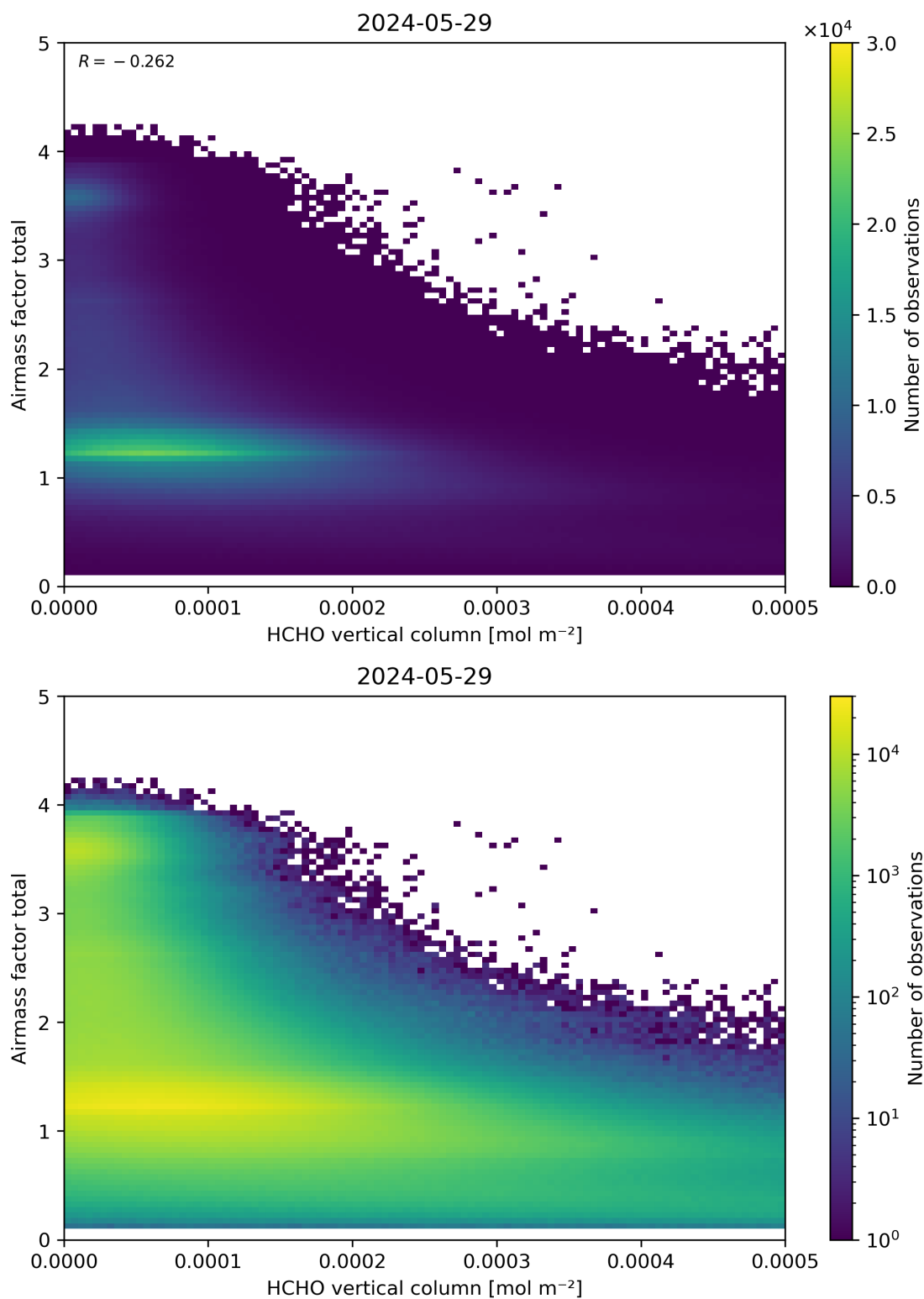
Figure 131: Scatter density plot of “HCHO vertical column” against “Airmass factor total” for 2024-05-28 to 2024-05-30.
