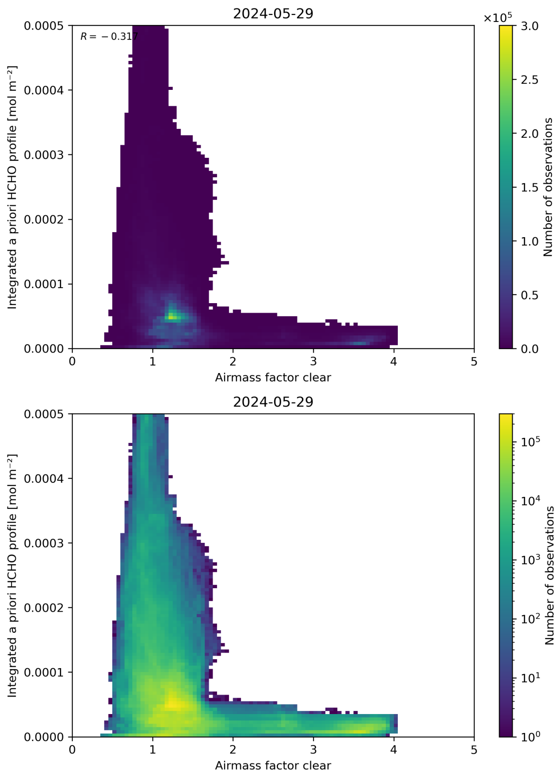
Figure 76: Scatter density plot of “Airmass factor clear” against “Integrated a priori HCHO profile” for 2024-05-28 to 2024-05-30.
