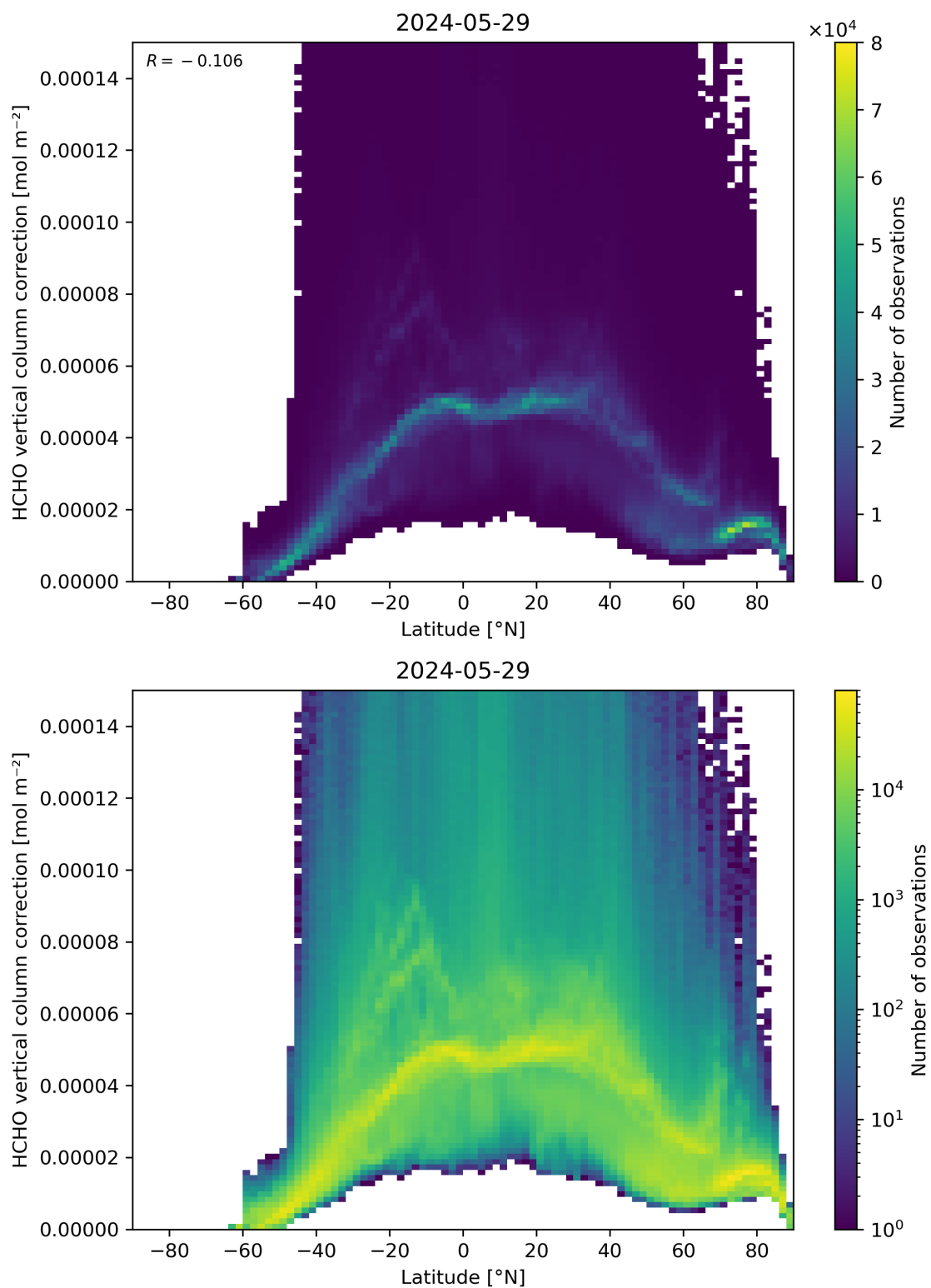
Figure 164: Scatter density plot of “Latitude” against “HCHO vertical column correction” for 2024-05-28 to 2024-05-30.
