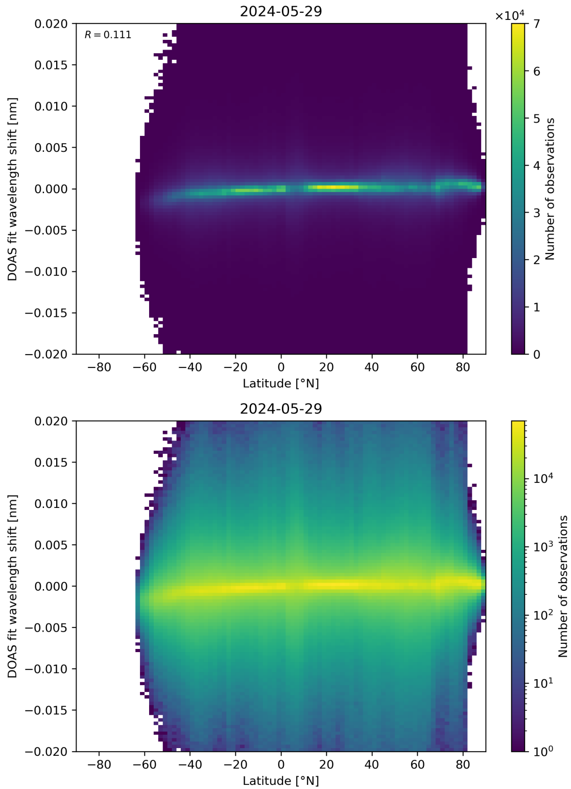
Figure 154: Scatter density plot of “Latitude” against “DOAS fit wavelength shift” for 2024-05-28 to 2024-05-30.
