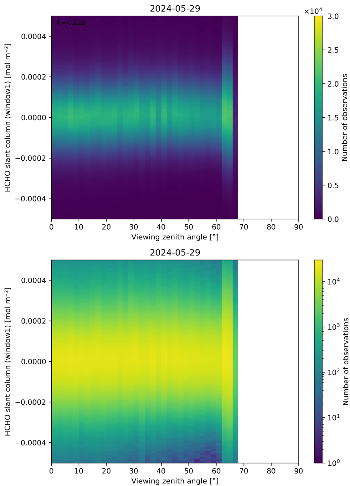
Figure 188: Scatter density plot of “Viewing zenith angle” against “HCHO slant column (window1)” for 2024-05-28 to 2024-05-30.
