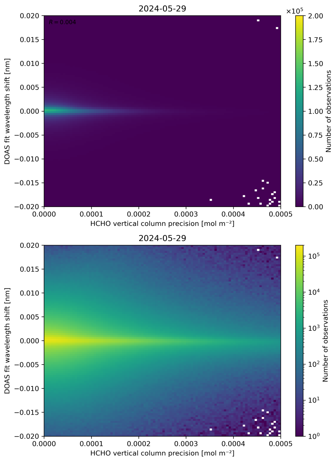
Figure 137: Scatter density plot of “HCHO vertical column precision” against “DOAS fit wavelength shift” for 2024-05-28 to 2024-05-30.
