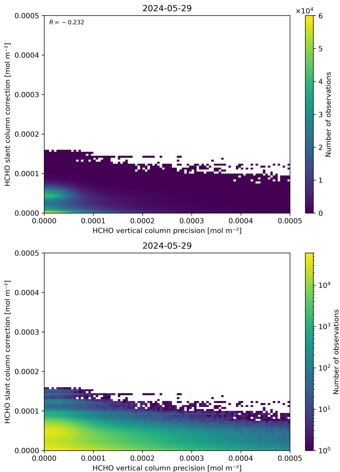
Figure 141: Scatter density plot of “HCHO vertical column precision” against “HCHO slant column correction” for 2024-05-28 to 2024-05-30.
