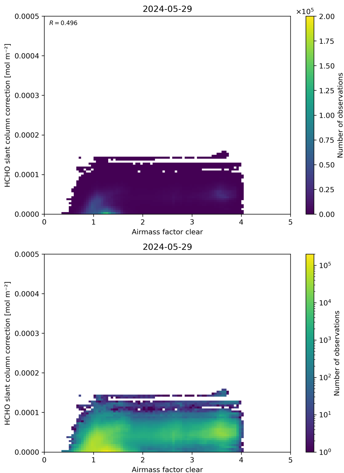
Figure 75: Scatter density plot of “Airmass factor clear” against “HCHO slant column correction” for 2024-05-28 to 2024-05-30.
