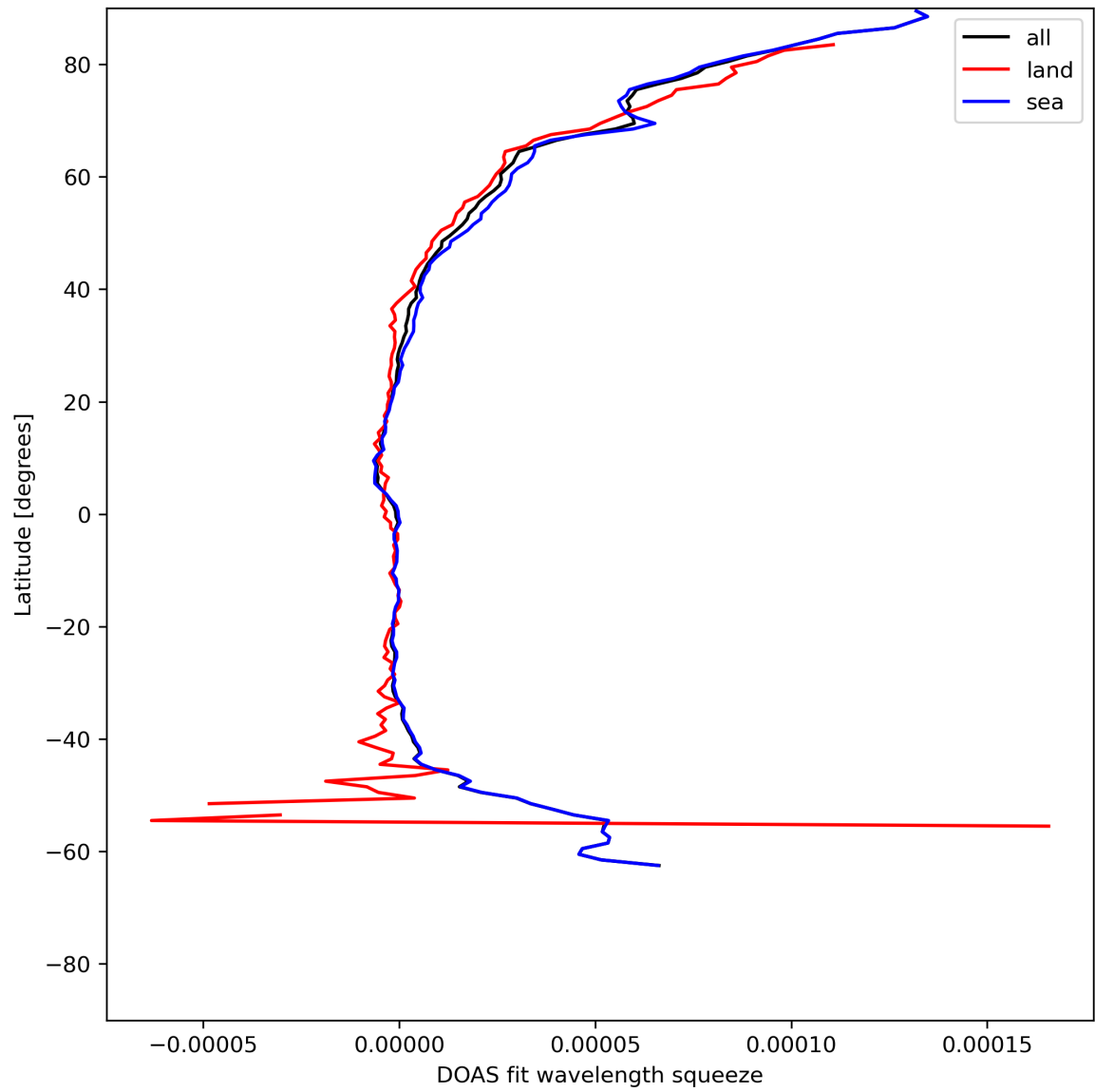
Figure 31: Zonal average of “DOAS fit wavelength squeeze” for 2024-05-28 to 2024-05-30.
