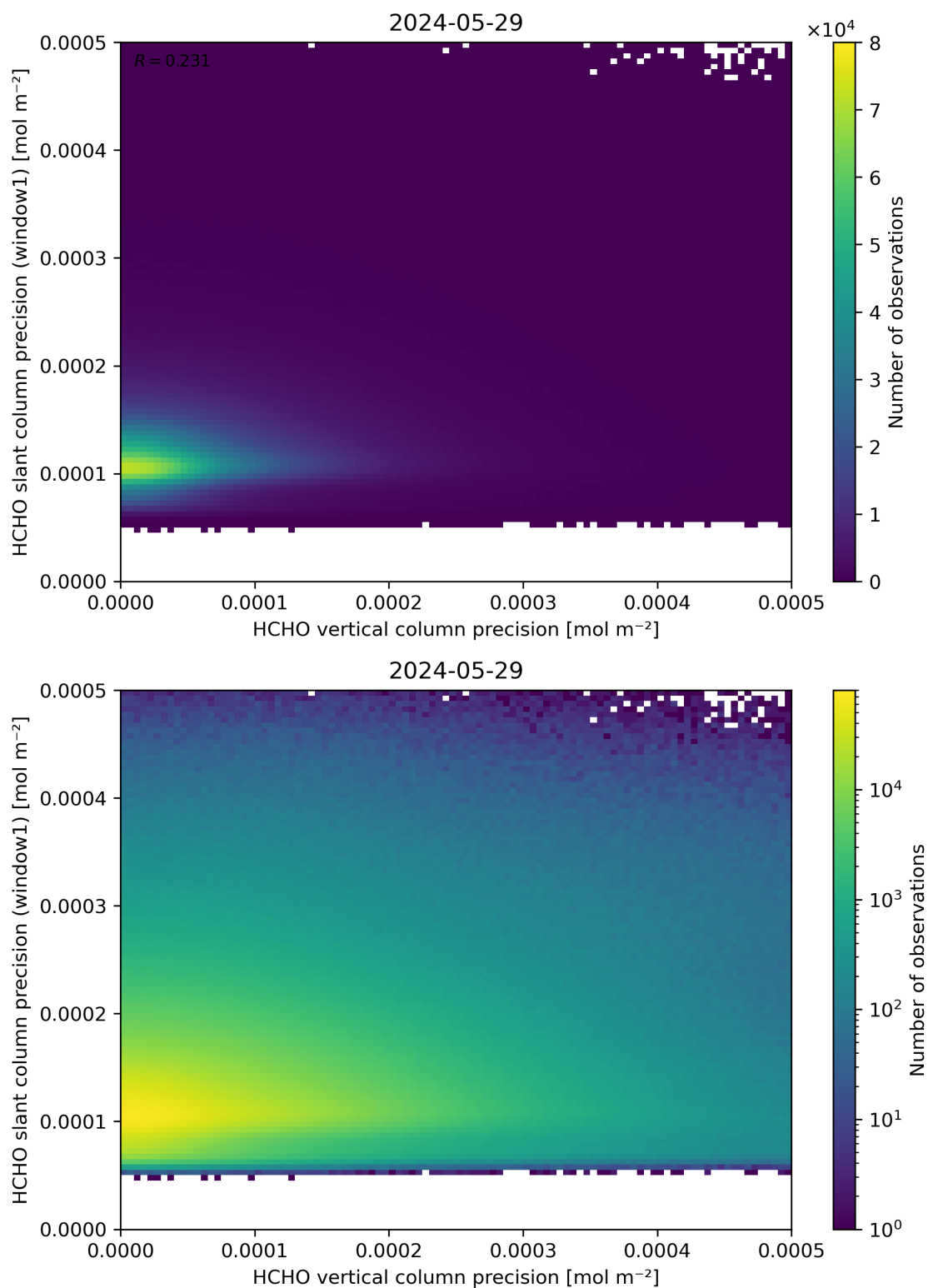
Figure 143: Scatter density plot of “HCHO vertical column precision” against “HCHO slant column precision (window1)” for 2024-05-28 to 2024-05-30.
