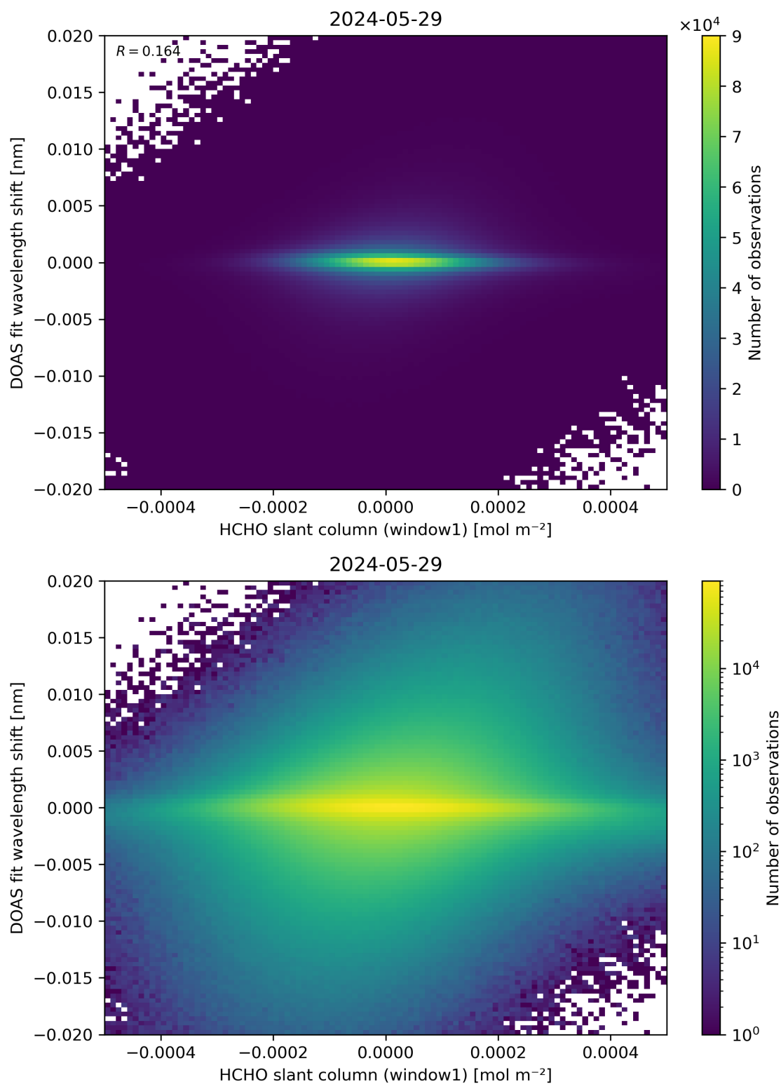
Figure 79: Scatter density plot of “HCHO slant column (window1)” against “DOAS fit wavelength shift” for 2024-05-28 to 2024-05-30.
