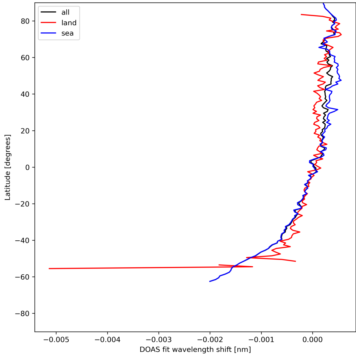
Figure 30: Zonal average of “DOAS fit wavelength shift” for 2024-05-28 to 2024-05-30.
