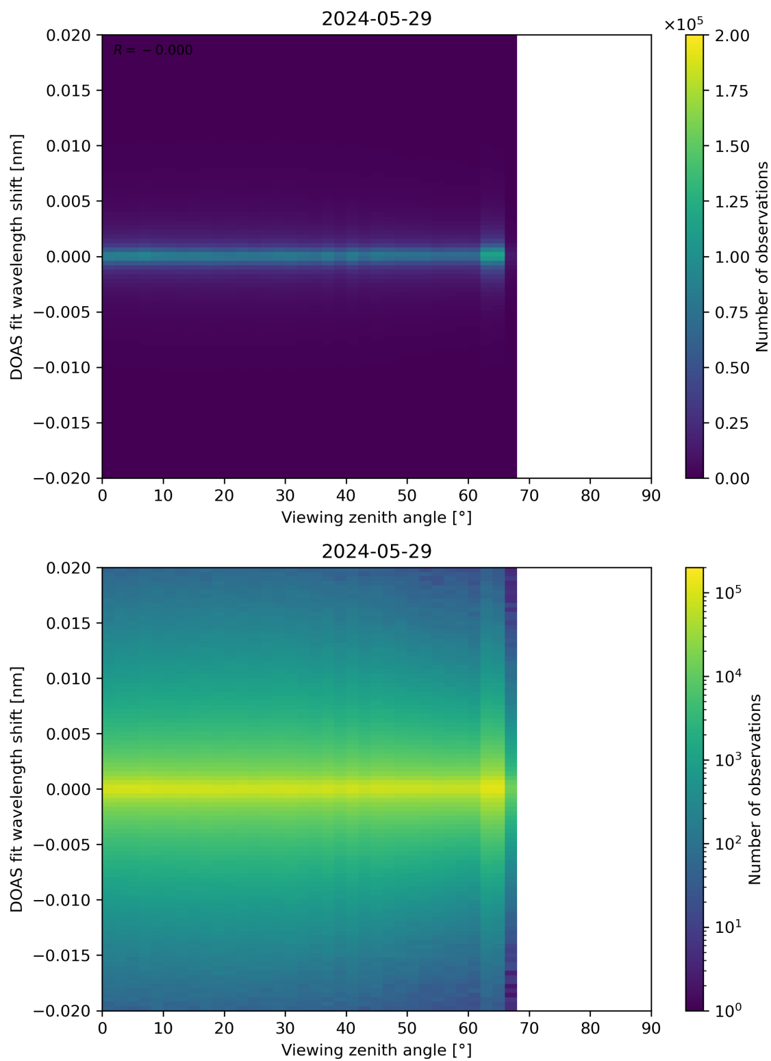
Figure 183: Scatter density plot of “Viewing zenith angle” against “DOAS fit wavelength shift” for 2024-05-28 to 2024-05-30.
