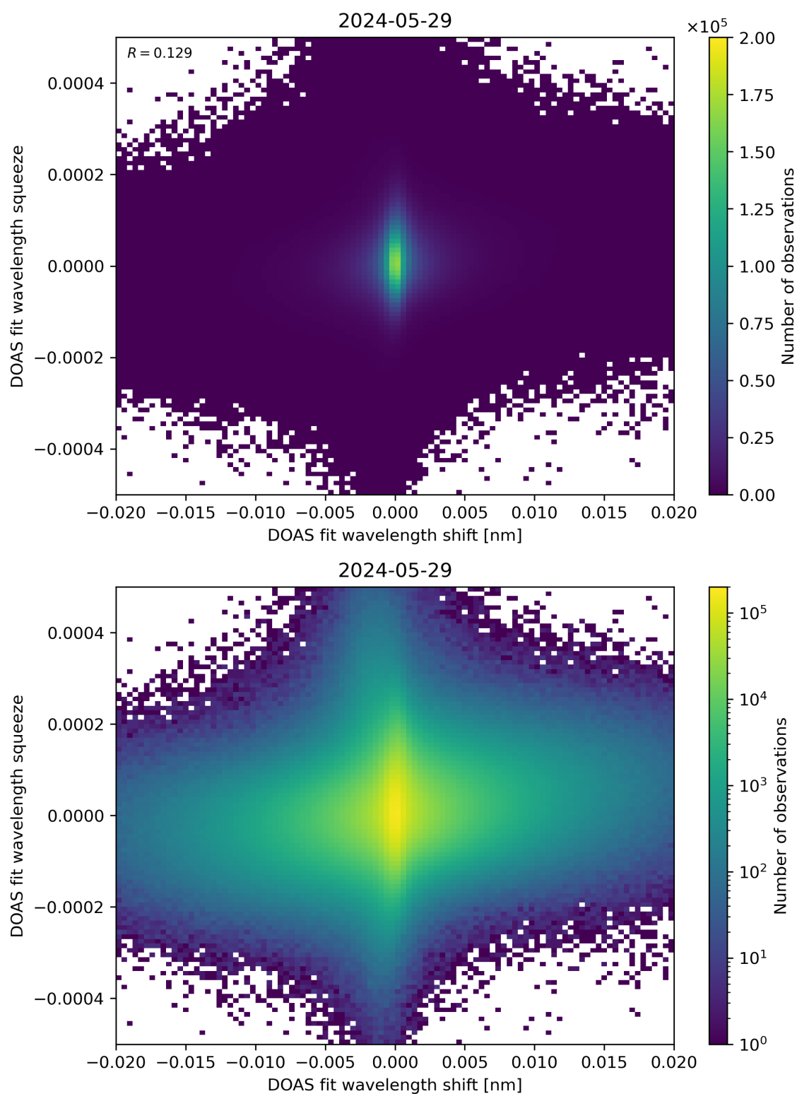
Figure 65: Scatter density plot of “DOAS fit wavelength shift” against “DOAS fit wavelength squeeze” for 2024-05-28 to 2024-05-30.
