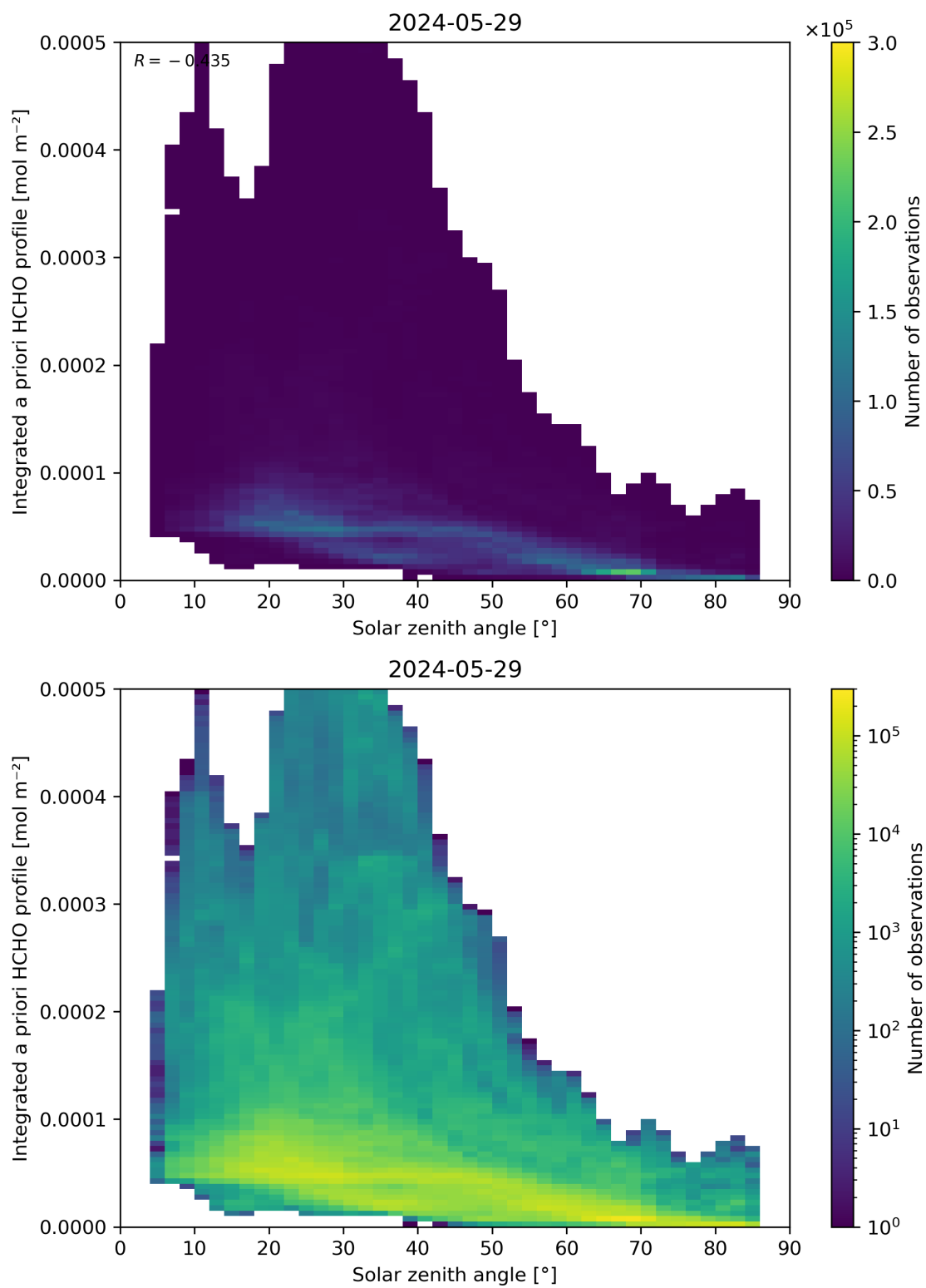
Figure 180: Scatter density plot of “Solar zenith angle” against “Integrated a priori HCHO profile” for 2024-05-28 to 2024-05-30.
