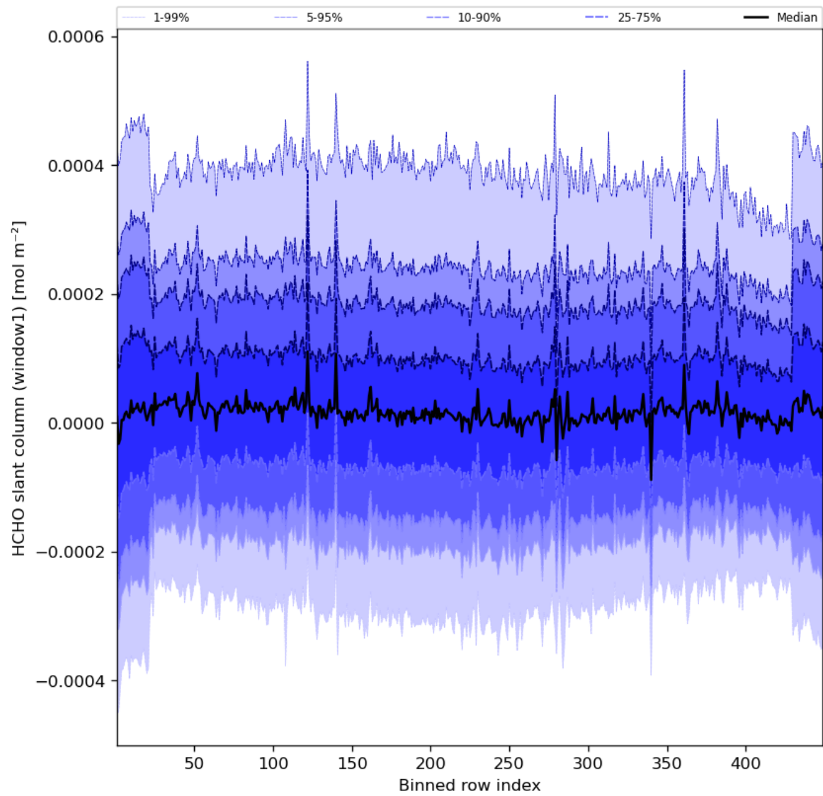
Figure 52: Along track statistics of “HCHO slant column (window1)” for 2024-05-28 to 2024-05-30
