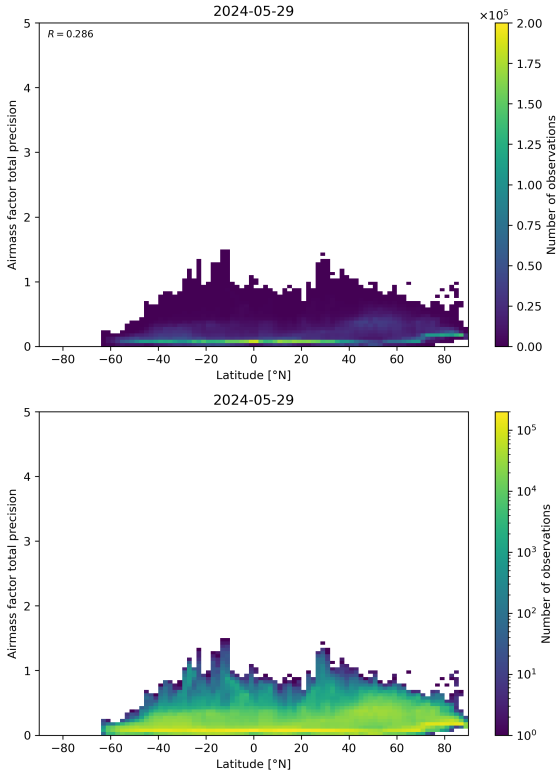
Figure 162: Scatter density plot of “Latitude” against “Airmass factor total precision” for 2024-05-28 to 2024-05-30.
