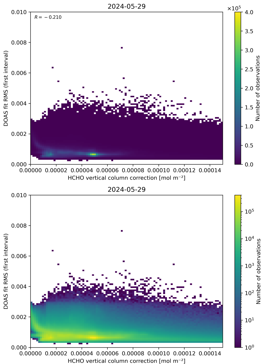
Figure 112: Scatter density plot of “HCHO vertical column correction” against “DOAS fit RMS (first interval)” for 2024-05-28 to 2024-05-30.
