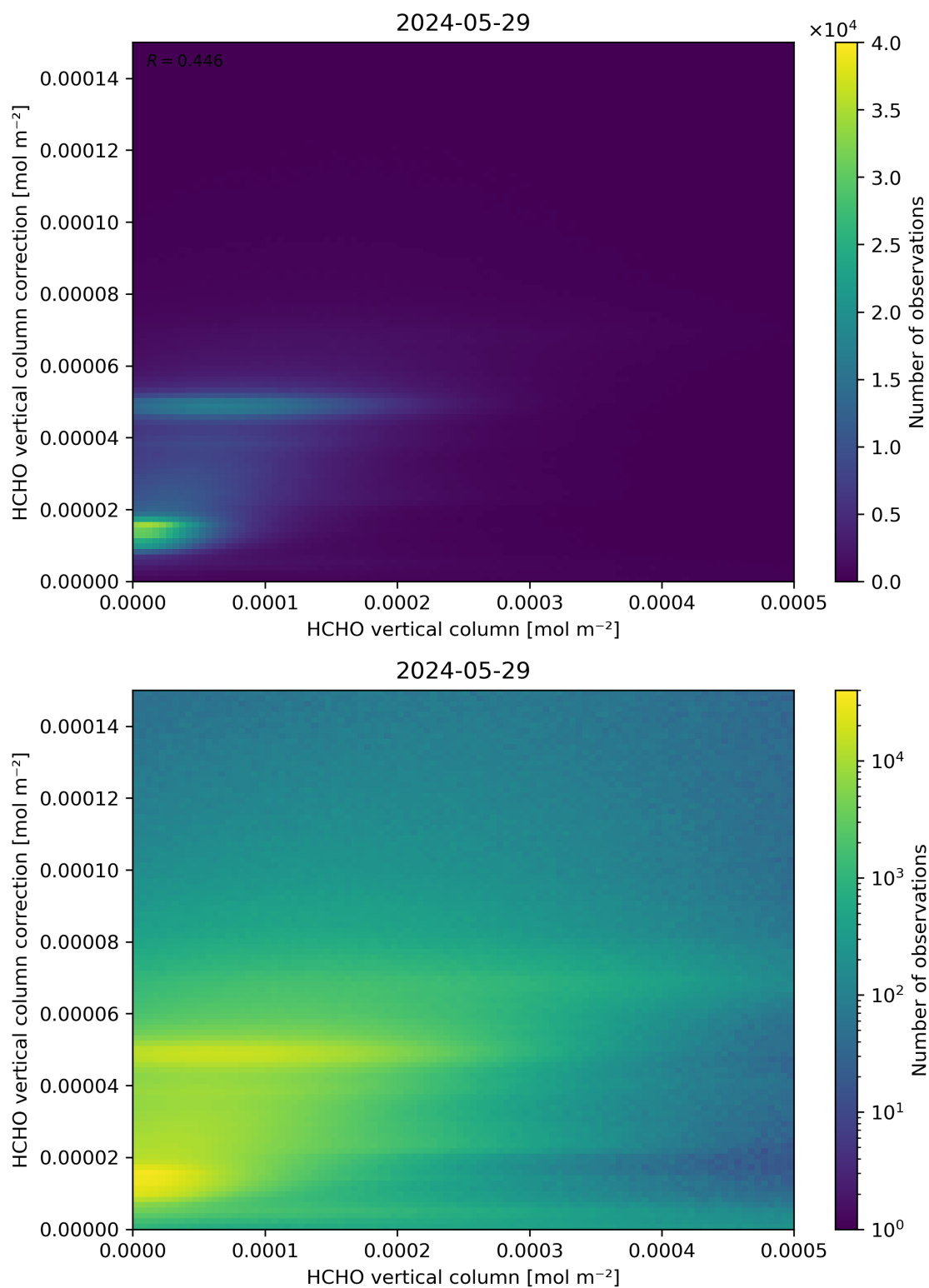
Figure 133: Scatter density plot of “HCHO vertical column” against “HCHO vertical column correction” for 2024-05-28 to 2024-05-30.
