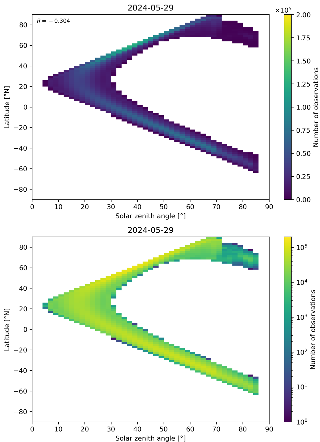
Figure 181: Scatter density plot of “Solar zenith angle” against “Latitude” for 2024-05-28 to 2024-05-30.
