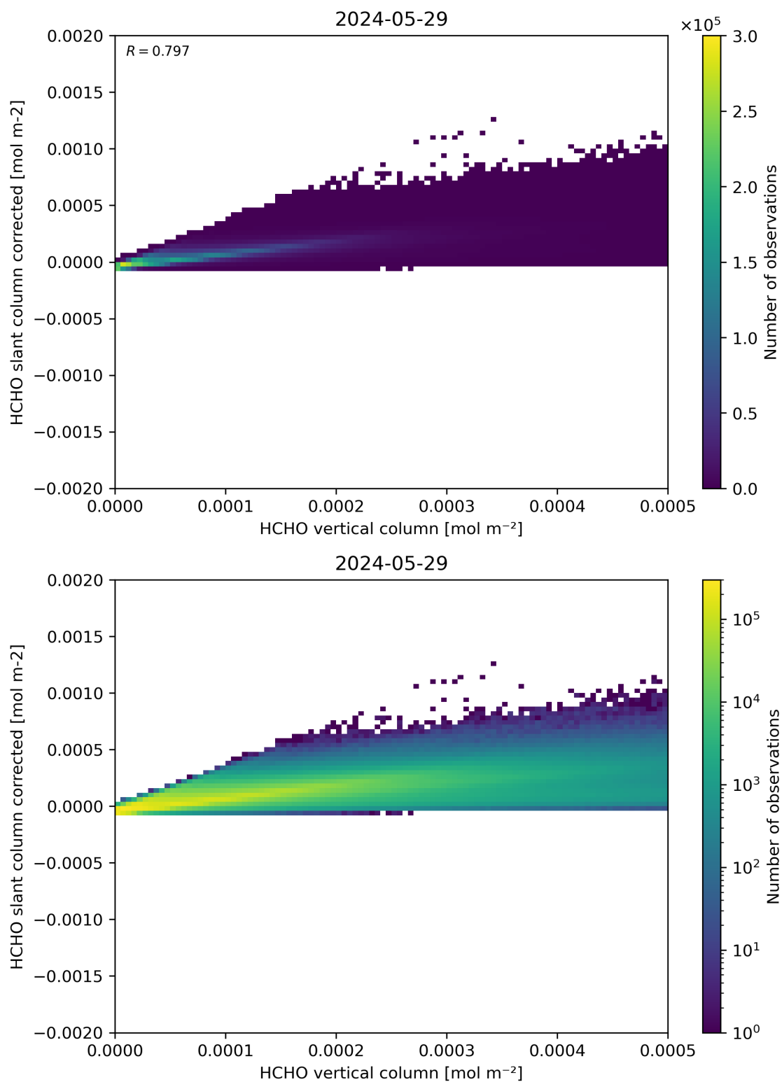
Figure 127: Scatter density plot of “HCHO vertical column” against “HCHO slant column corrected” for 2024-05-28 to 2024-05-30.
