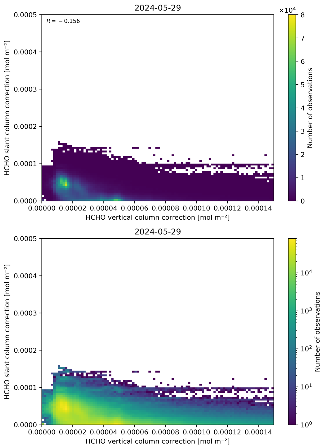
Figure 117: Scatter density plot of “HCHO vertical column correction” against “HCHO slant column correction” for 2024-05-28 to 2024-05-30.
