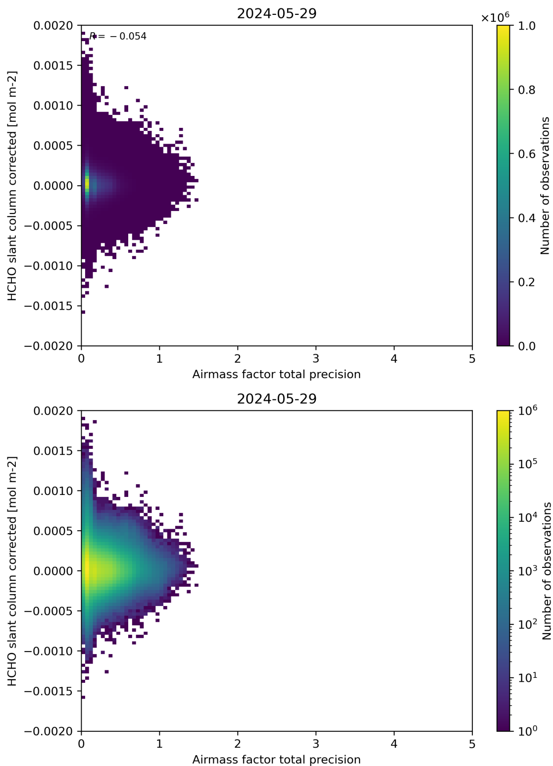
Figure 109: Scatter density plot of “Airmass factor total precision” against “HCHO slant column corrected” for 2024-05-28 to 2024-05-30.
