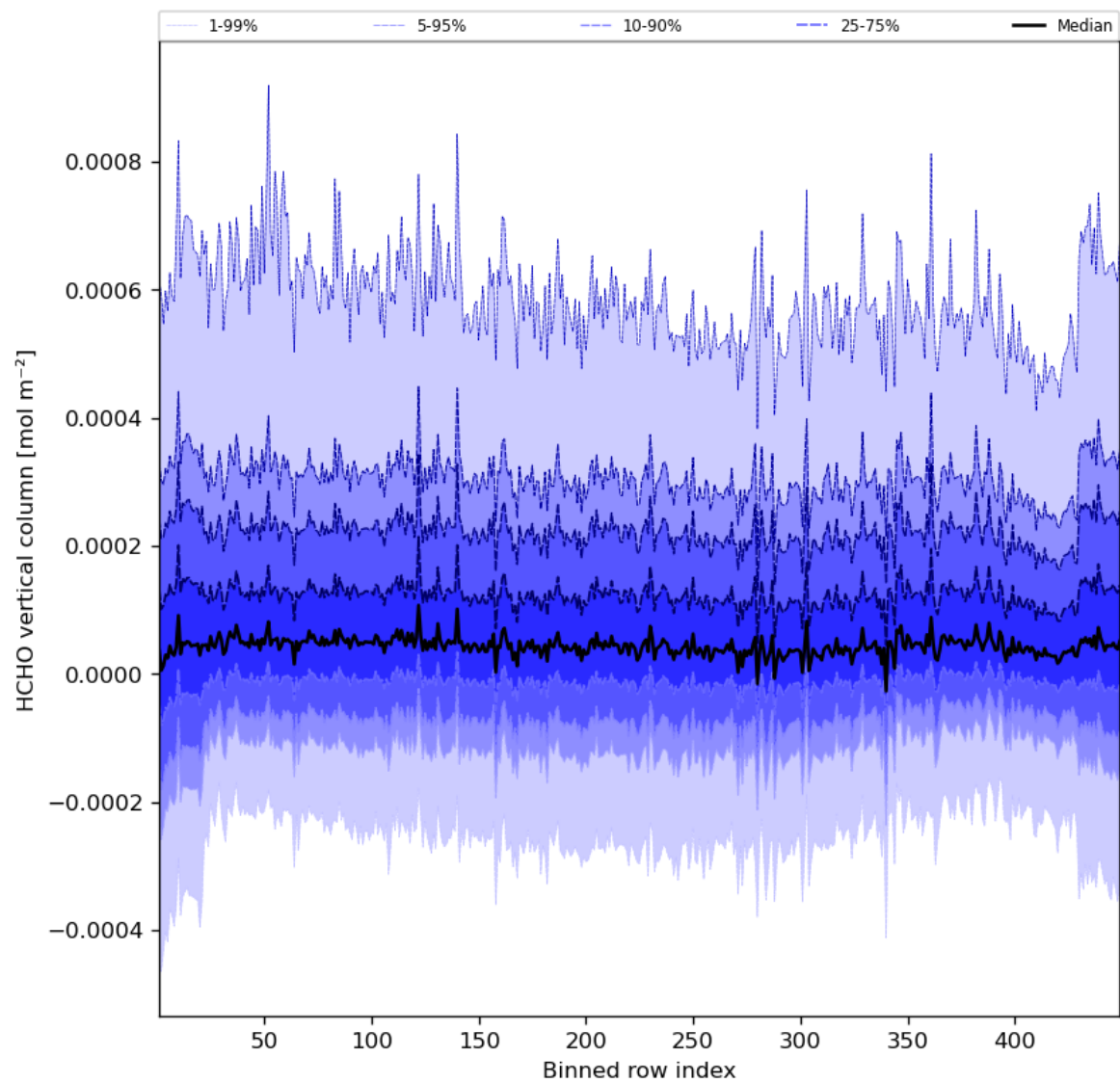
Figure 49: Along track statistics of “HCHO vertical column” for 2024-05-28 to 2024-05-30
