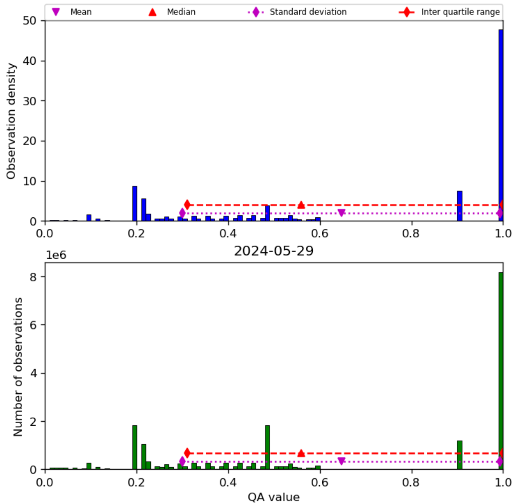
Figure 34: Histogram of “QA value” for 2024-05-28 to 2024-05-30
