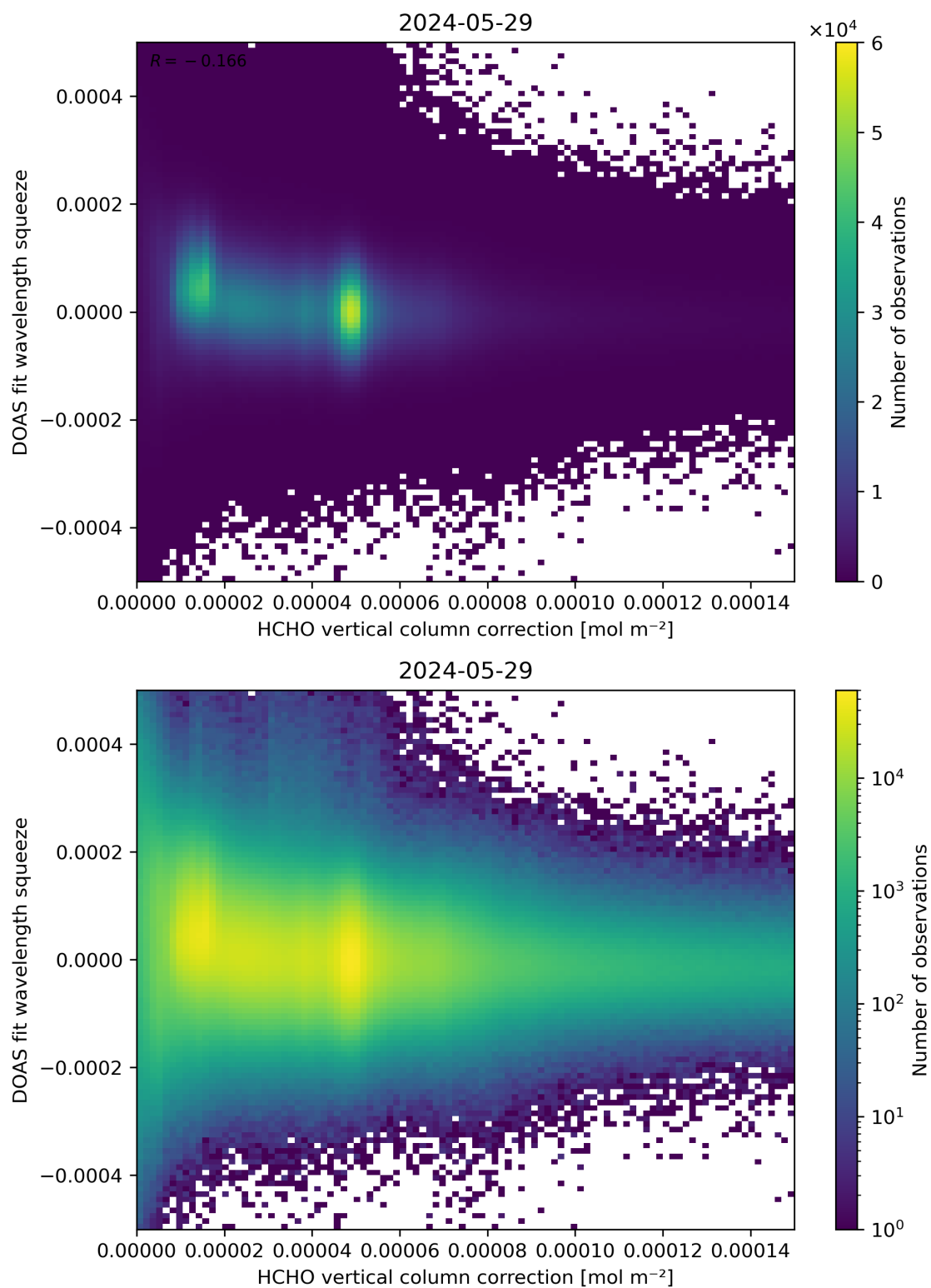
Figure 114: Scatter density plot of “HCHO vertical column correction” against “DOAS fit wavelength squeeze” for 2024-05-28 to 2024-05-30.
