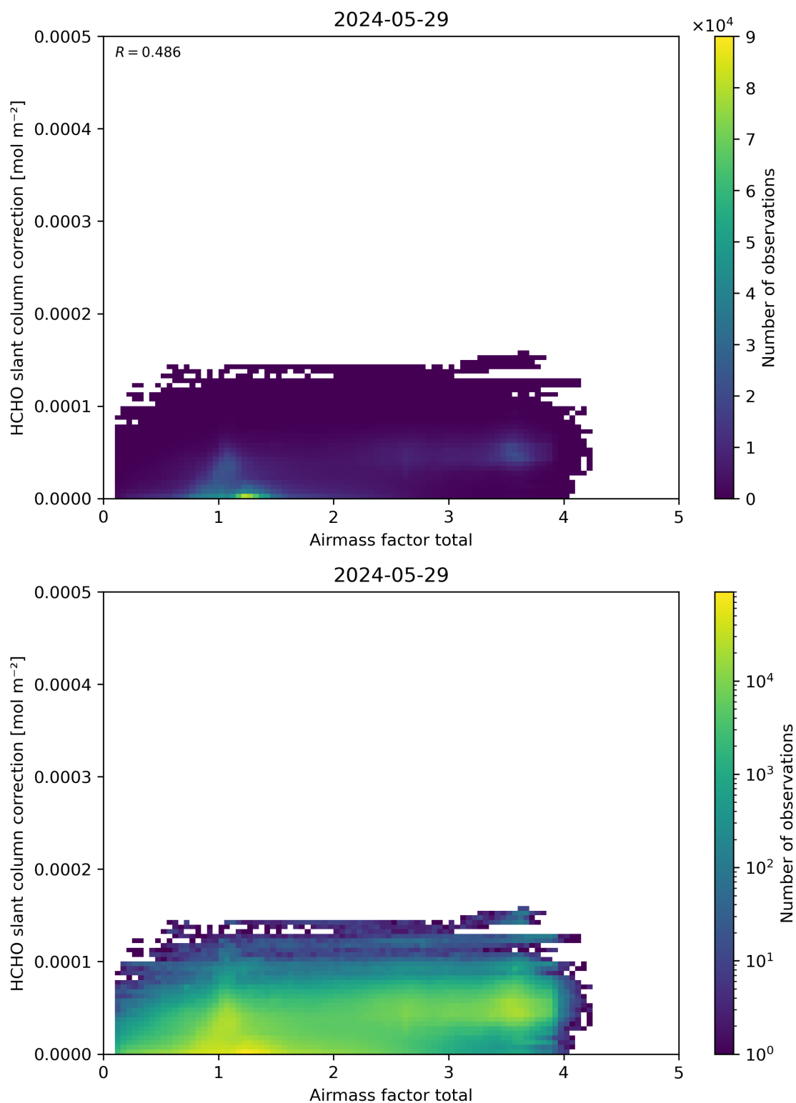
Figure 102: Scatter density plot of “Airmass factor total” against “HCHO slant column correction” for 2024-05-28 to 2024-05-30.
