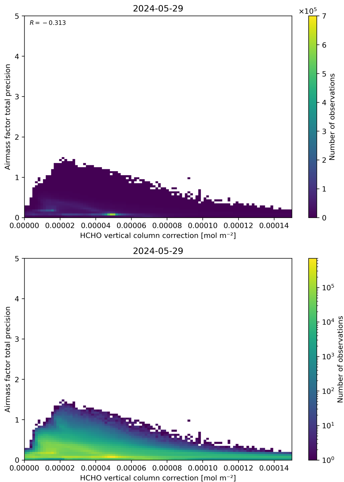
Figure 121: Scatter density plot of “HCHO vertical column correction” against “Airmass factor total precision” for 2024-05-28 to 2024-05-30.
