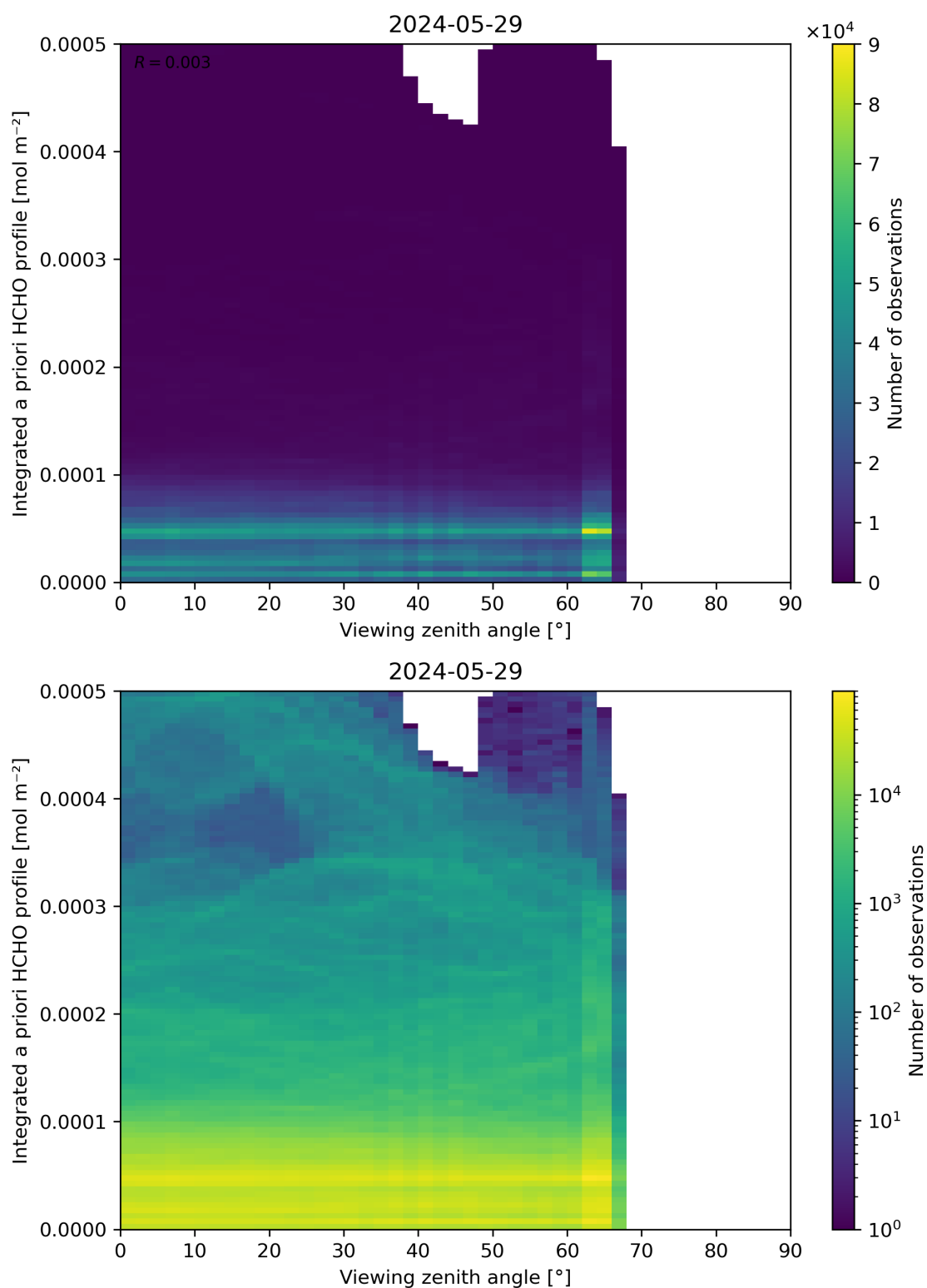
Figure 195: Scatter density plot of “Viewing zenith angle” against “Integrated a priori HCHO profile” for 2024-05-28 to 2024-05-30.
