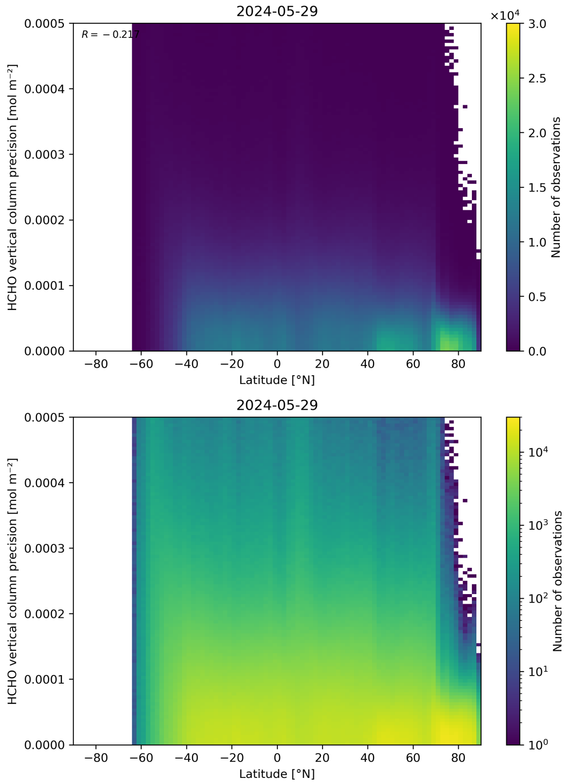
Figure 165: Scatter density plot of “Latitude” against “HCHO vertical column precision” for 2024-05-28 to 2024-05-30.
