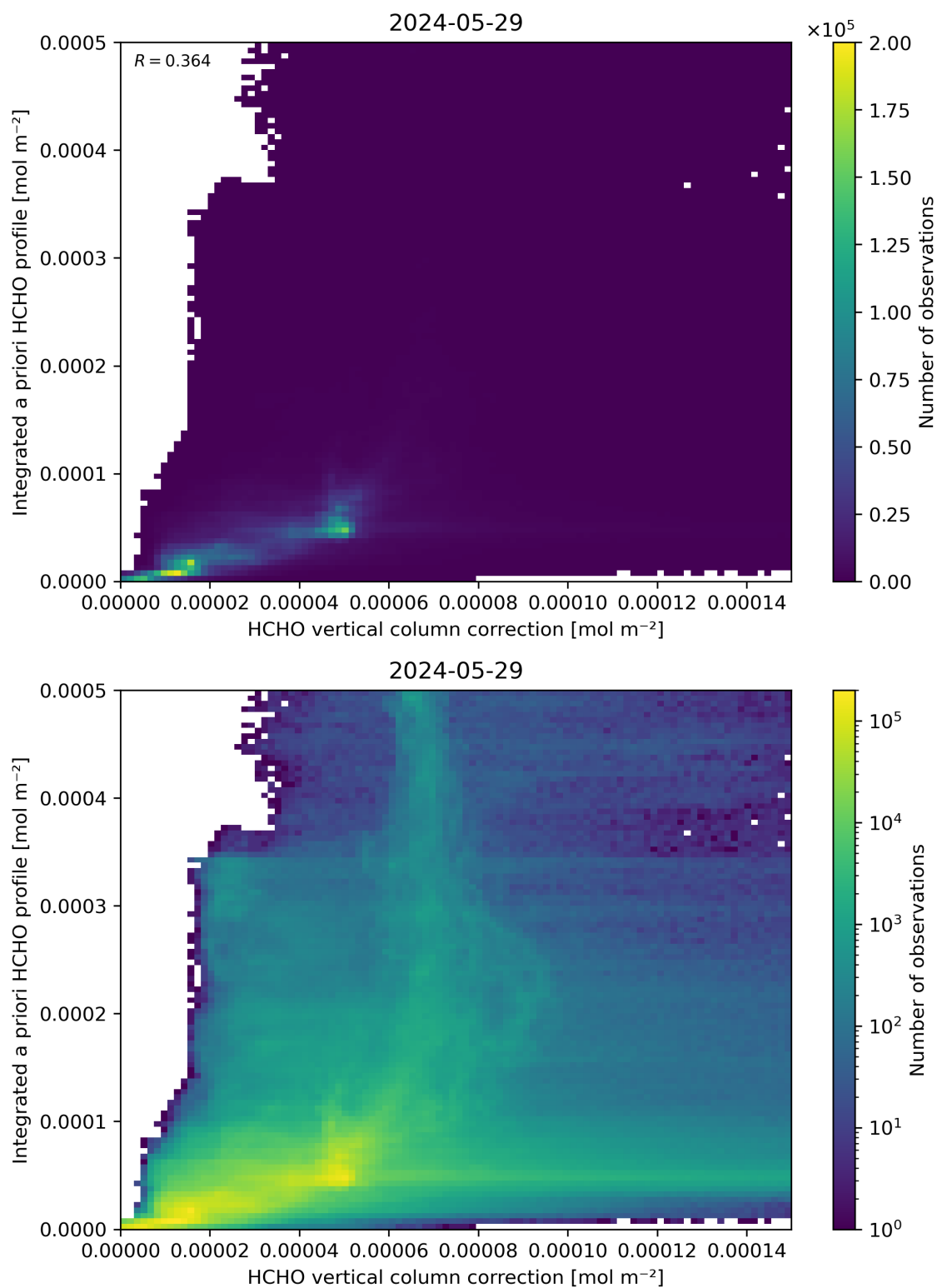
Figure 122: Scatter density plot of “HCHO vertical column correction” against “Integrated a priori HCHO profile” for 2024-05-28 to 2024-05-30.
