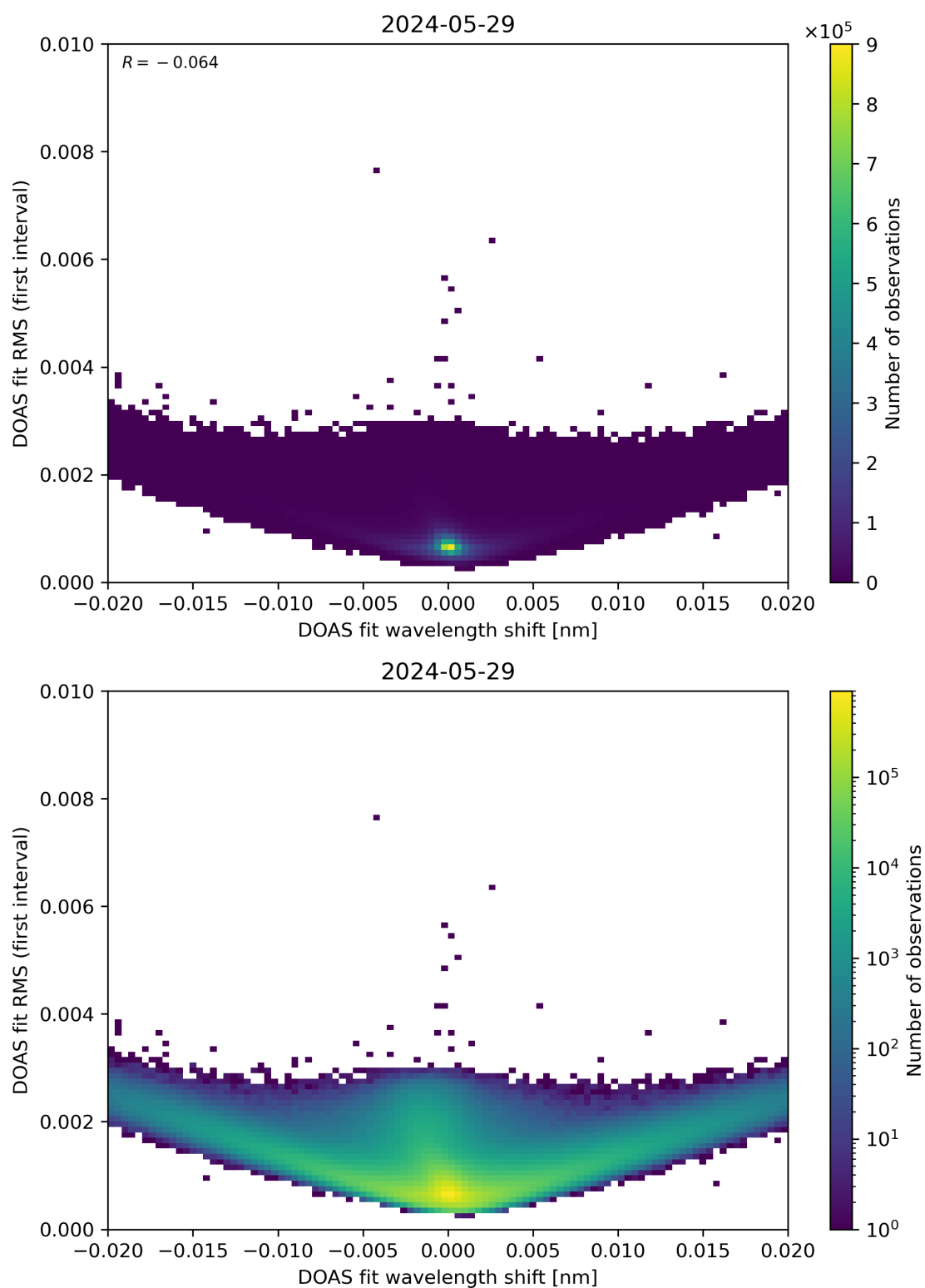
Figure 64: Scatter density plot of “DOAS fit wavelength shift” against “DOAS fit RMS (first interval)” for 2024-05-28 to 2024-05-30.
