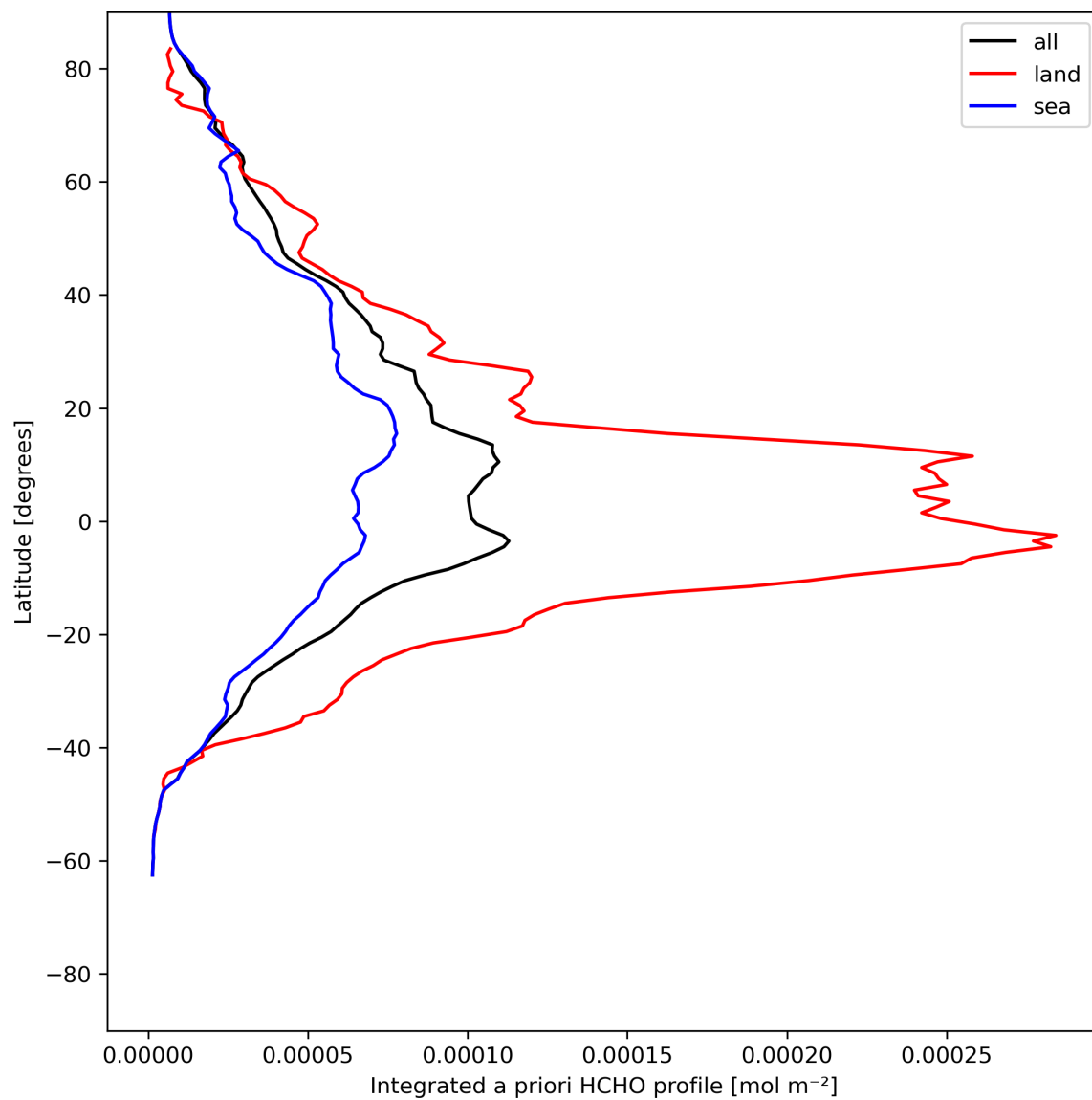
Figure 29: Zonal average of “Integrated a priori HCHO profile” for 2024-05-28 to 2024-05-30.
