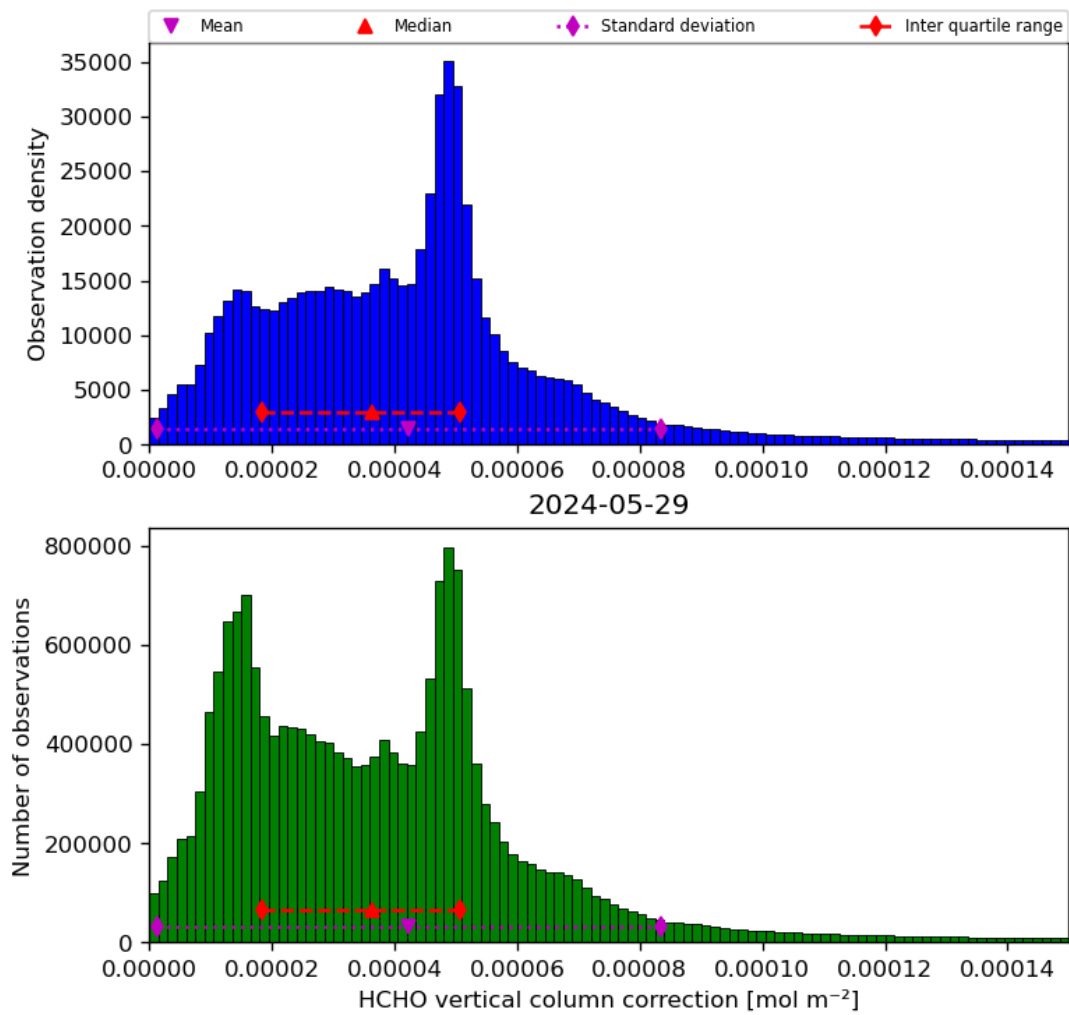
Figure 37: Histogram of “HCHO vertical column correction” for 2024-05-28 to 2024-05-30
