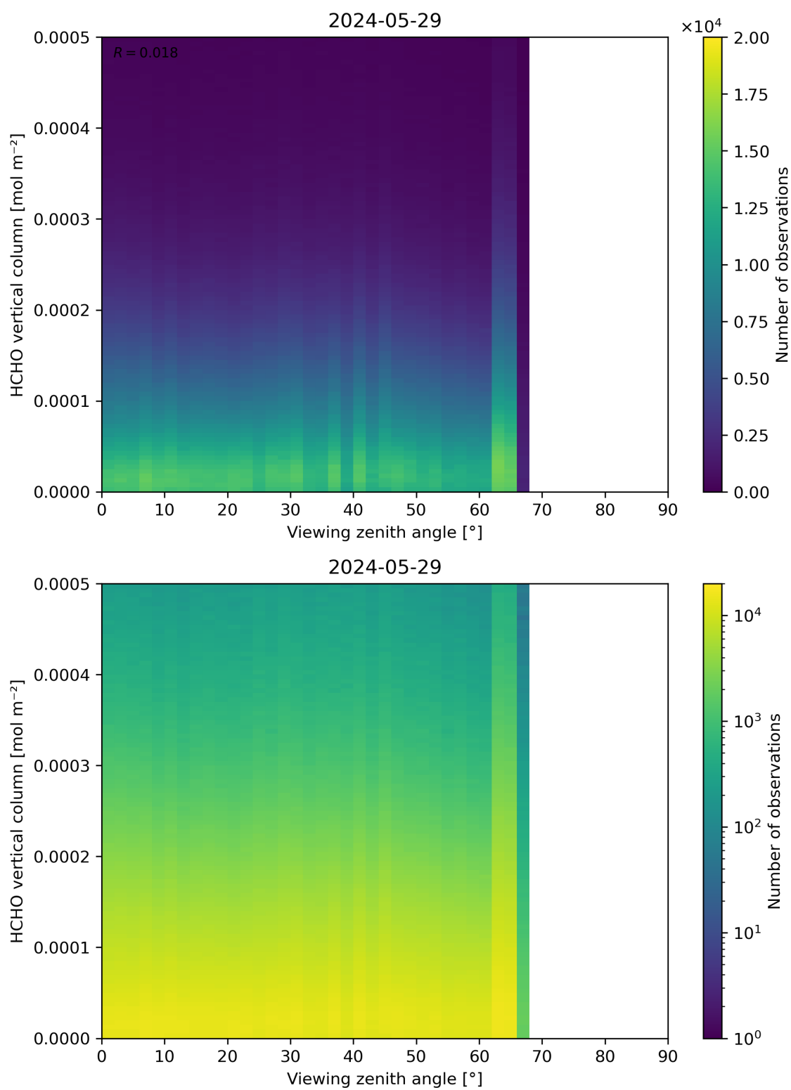
Figure 192: Scatter density plot of “Viewing zenith angle” against “HCHO vertical column” for 2024-05-28 to 2024-05-30.
