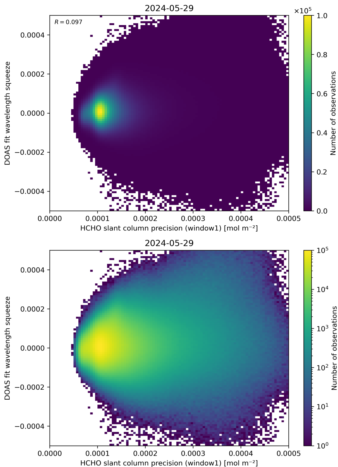
Figure 90: Scatter density plot of “HCHO slant column precision (window1)” against “DOAS fit wavelength squeeze” for 2024-05-28 to 2024-05-30.
