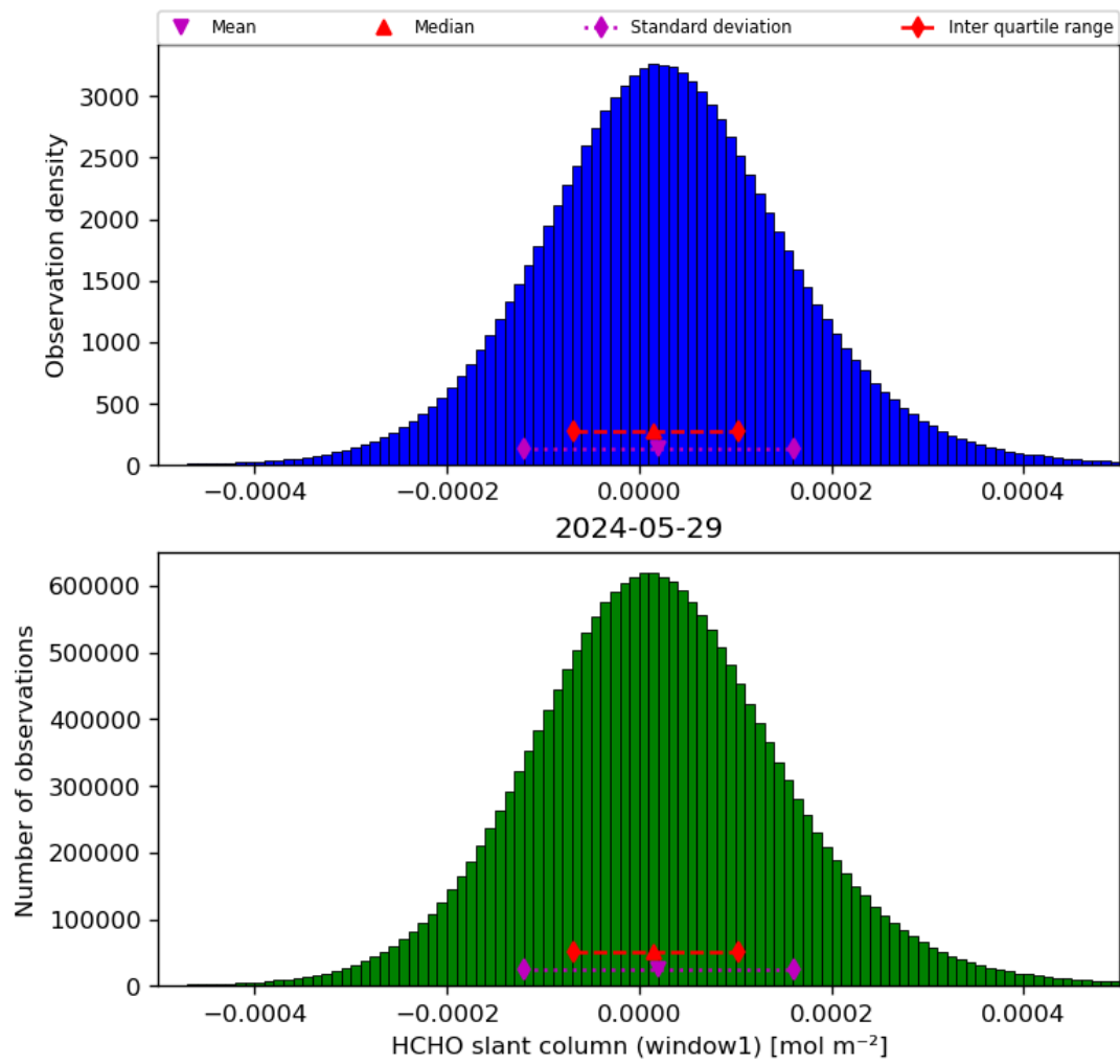
Figure 38: Histogram of “HCHO slant column (window1)” for 2024-05-28 to 2024-05-30
