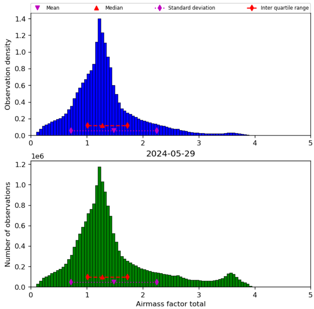
Figure 40: Histogram of “Airmass factor total” for 2024-05-28 to 2024-05-30
