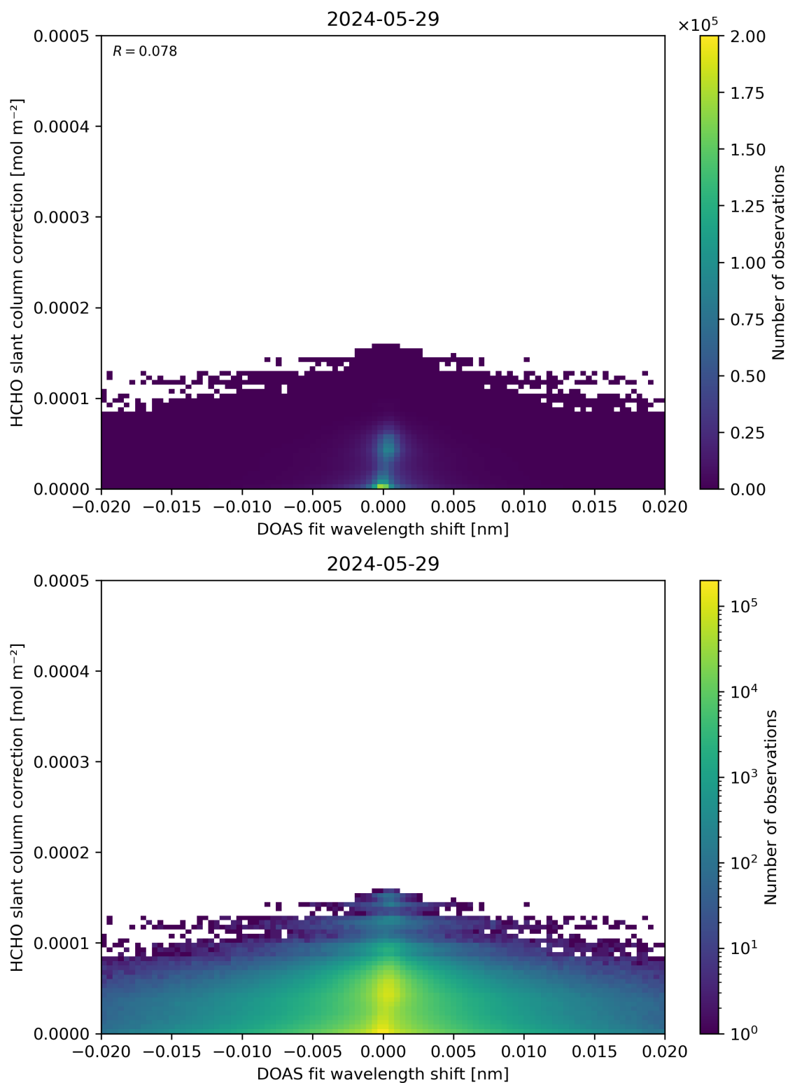
Figure 67: Scatter density plot of “DOAS fit wavelength shift” against “HCHO slant column correction” for 2024-05-28 to 2024-05-30.
