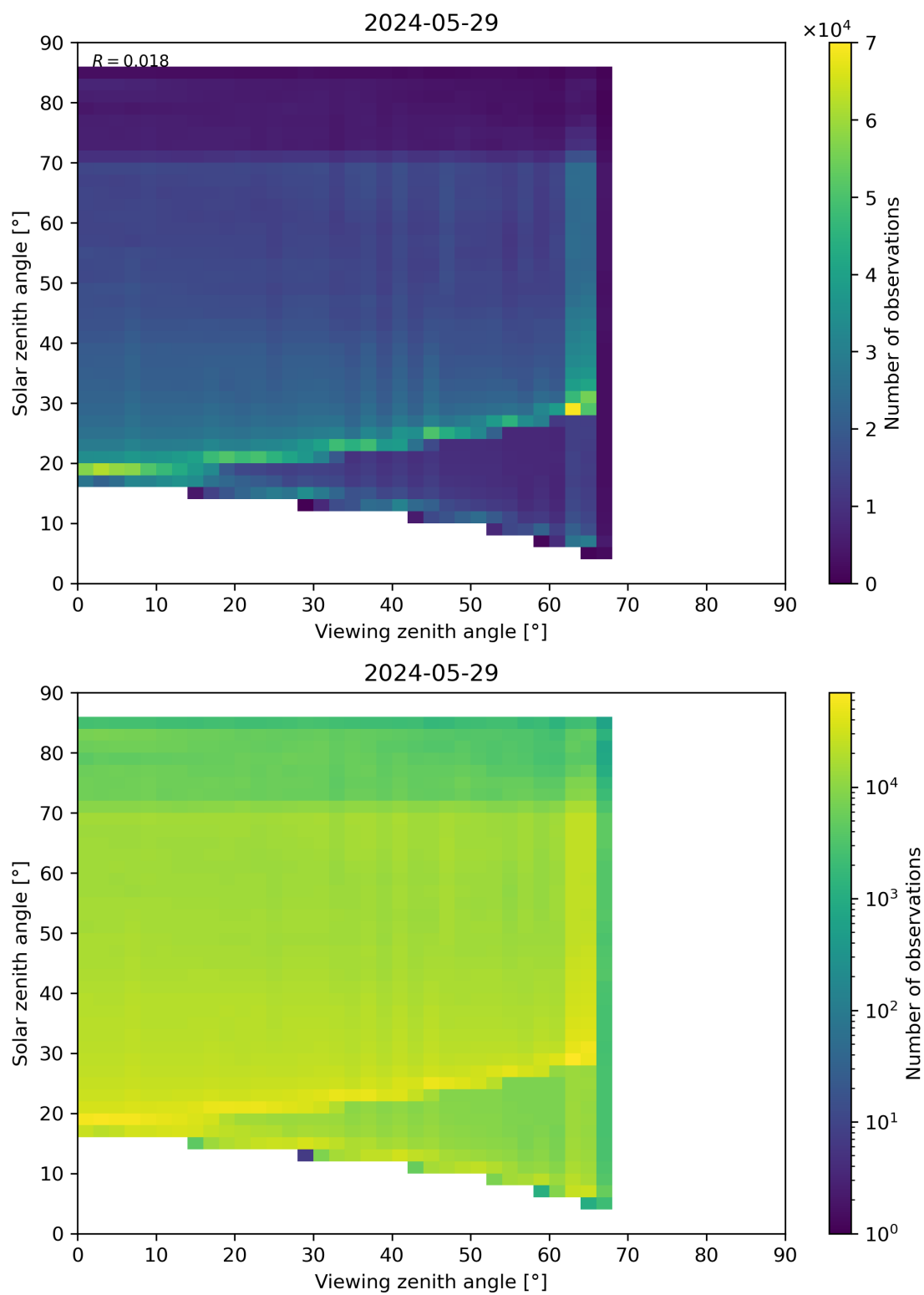
Figure 197: Scatter density plot of “Viewing zenith angle” against “Solar zenith angle” for 2024-05-28 to 2024-05-30.
