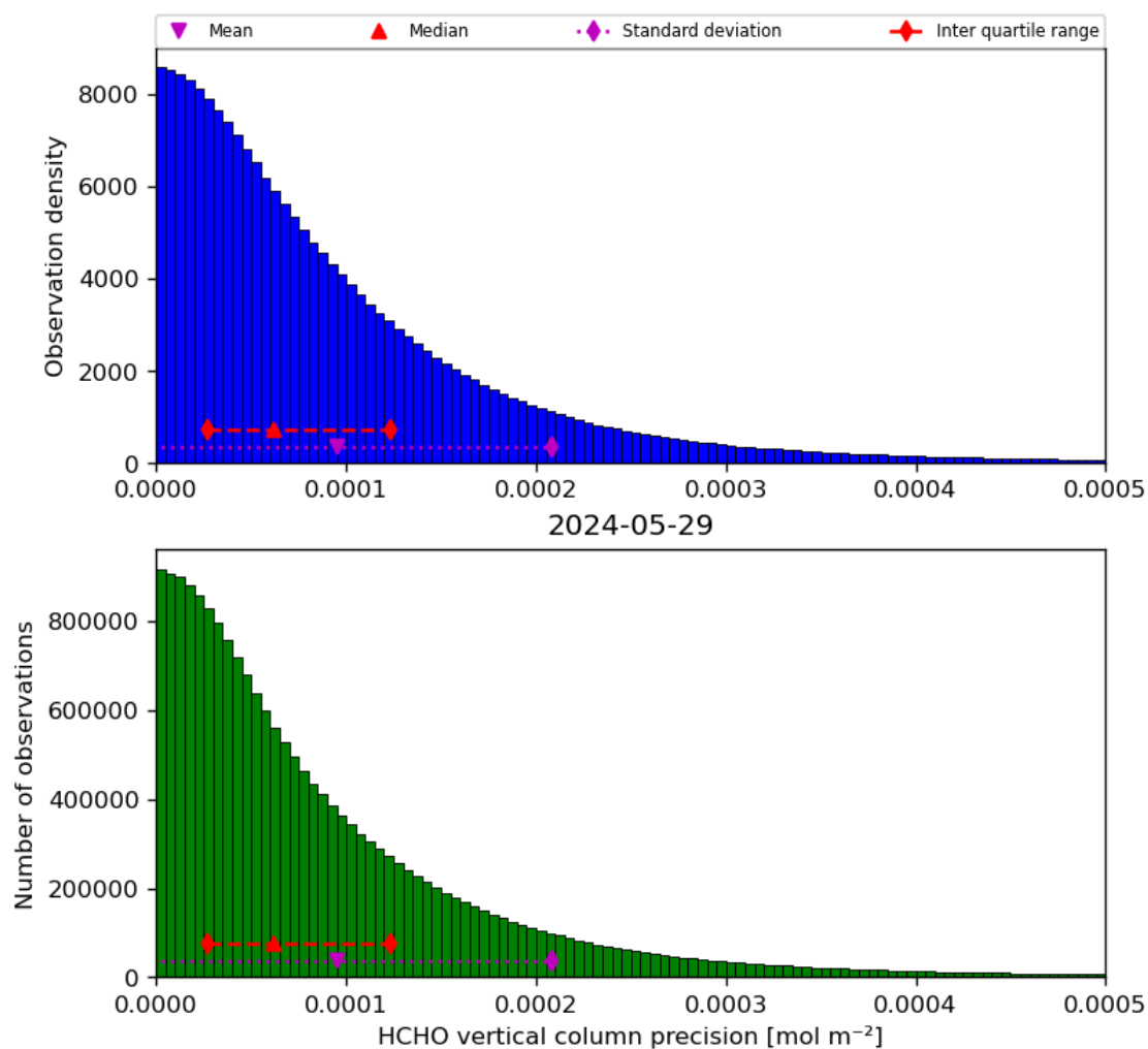
Figure 36: Histogram of “HCHO vertical column precision” for 2024-05-28 to 2024-05-30
