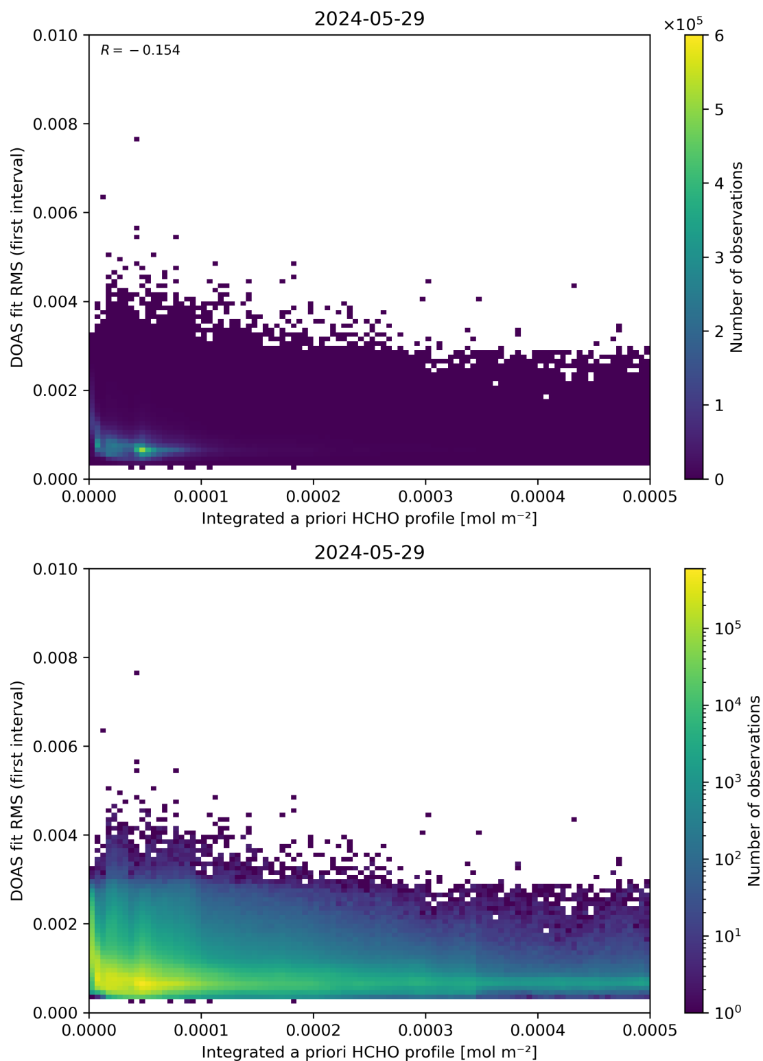
Figure 148: Scatter density plot of “Integrated a priori HCHO profile” against “DOAS fit RMS (first interval)” for 2024-05-28 to 2024-05-30.
