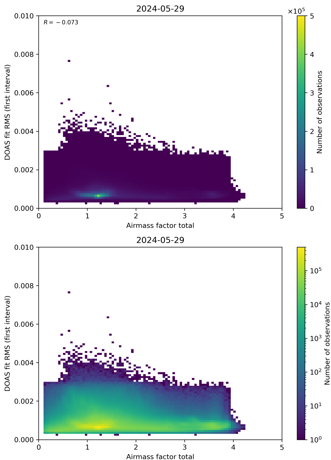
Figure 97: Scatter density plot of “Airmass factor total” against “DOAS fit RMS (first interval)” for 2024-05-28 to 2024-05-30.
