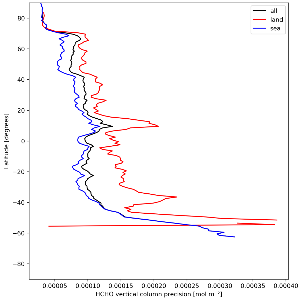
Figure 22: Zonal average of “HCHO vertical column precision” for 2024-05-28 to 2024-05-30.
