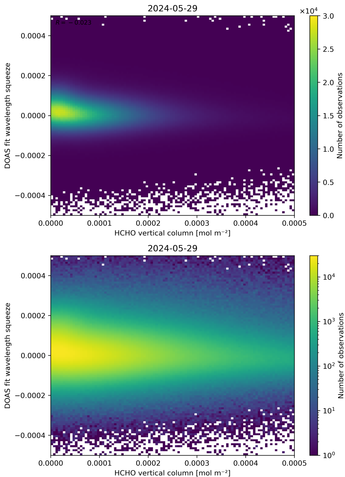
Figure 125: Scatter density plot of “HCHO vertical column” against “DOAS fit wavelength squeeze” for 2024-05-28 to 2024-05-30.
