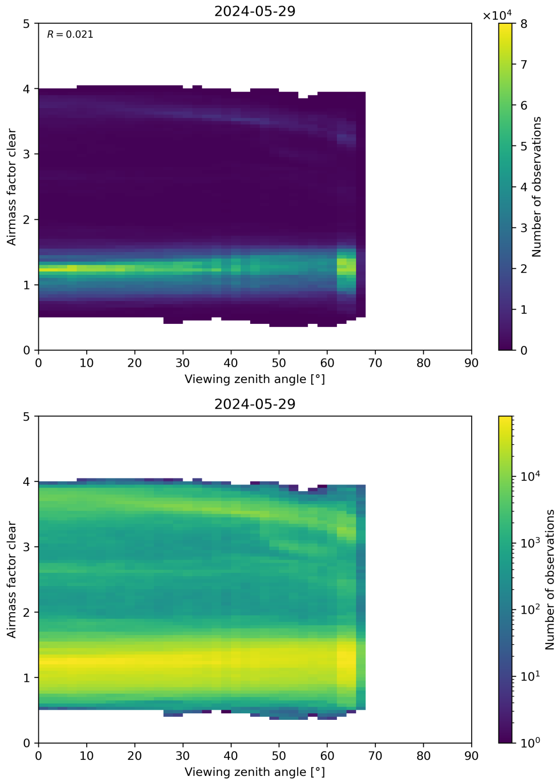
Figure 185: Scatter density plot of “Viewing zenith angle” against “Airmass factor clear” for 2024-05-28 to 2024-05-30.
