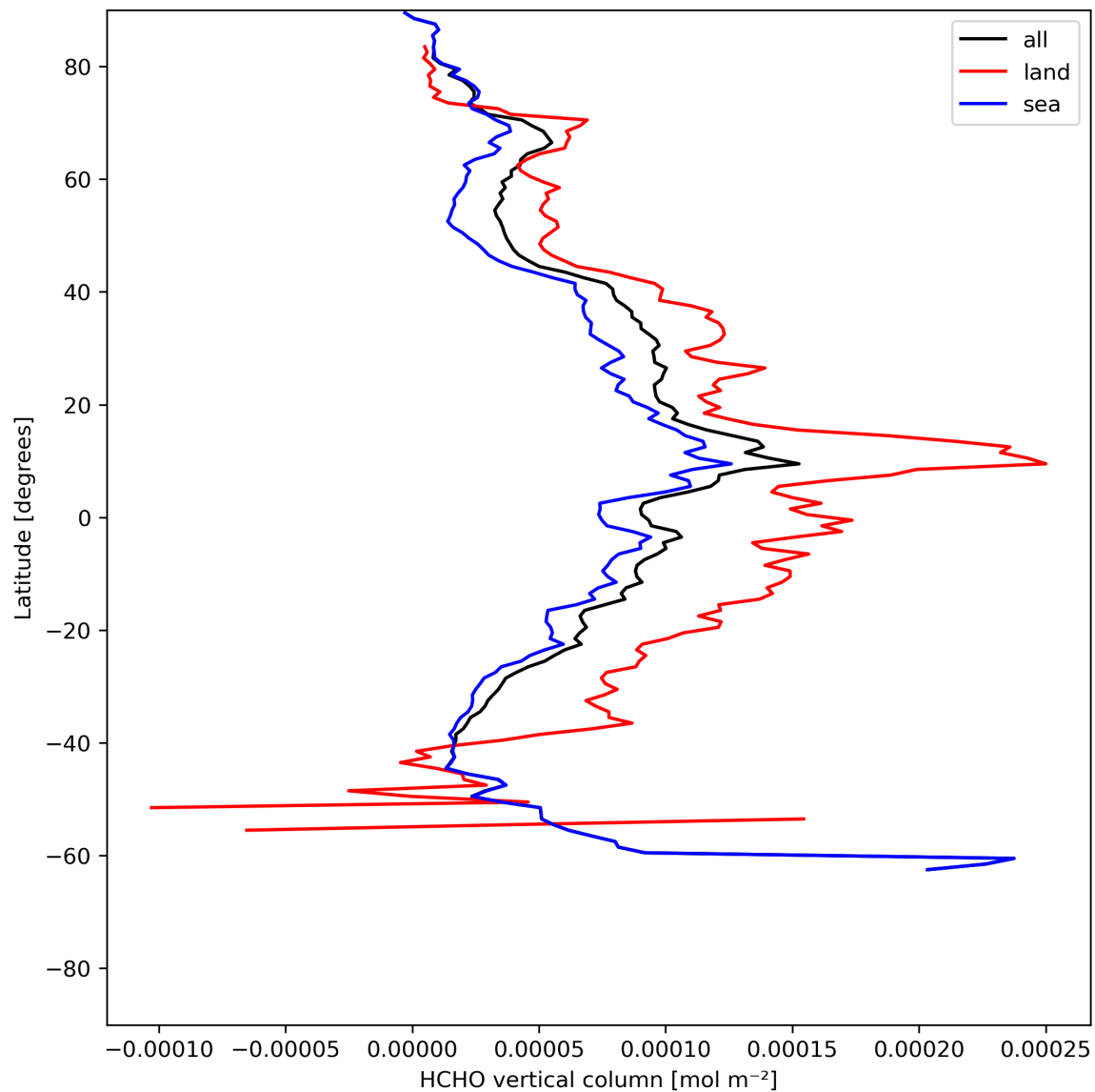
Figure 21: Zonal average of “HCHO vertical column” for 2024-05-28 to 2024-05-30.
