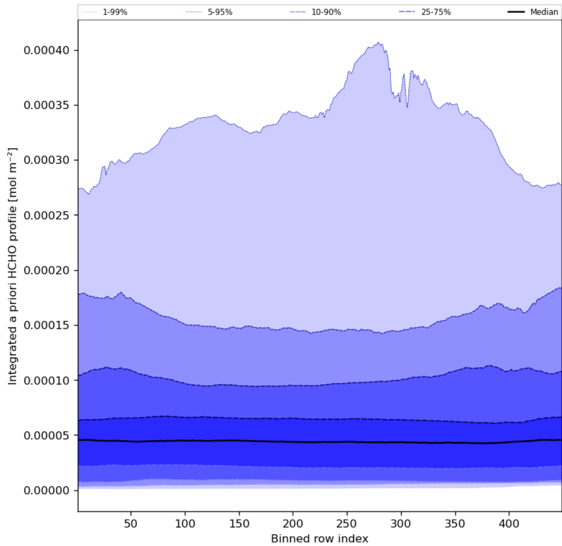
Figure 57: Along track statistics of “Integrated a priori HCHO profile” for 2024-05-28 to 2024-05-30
