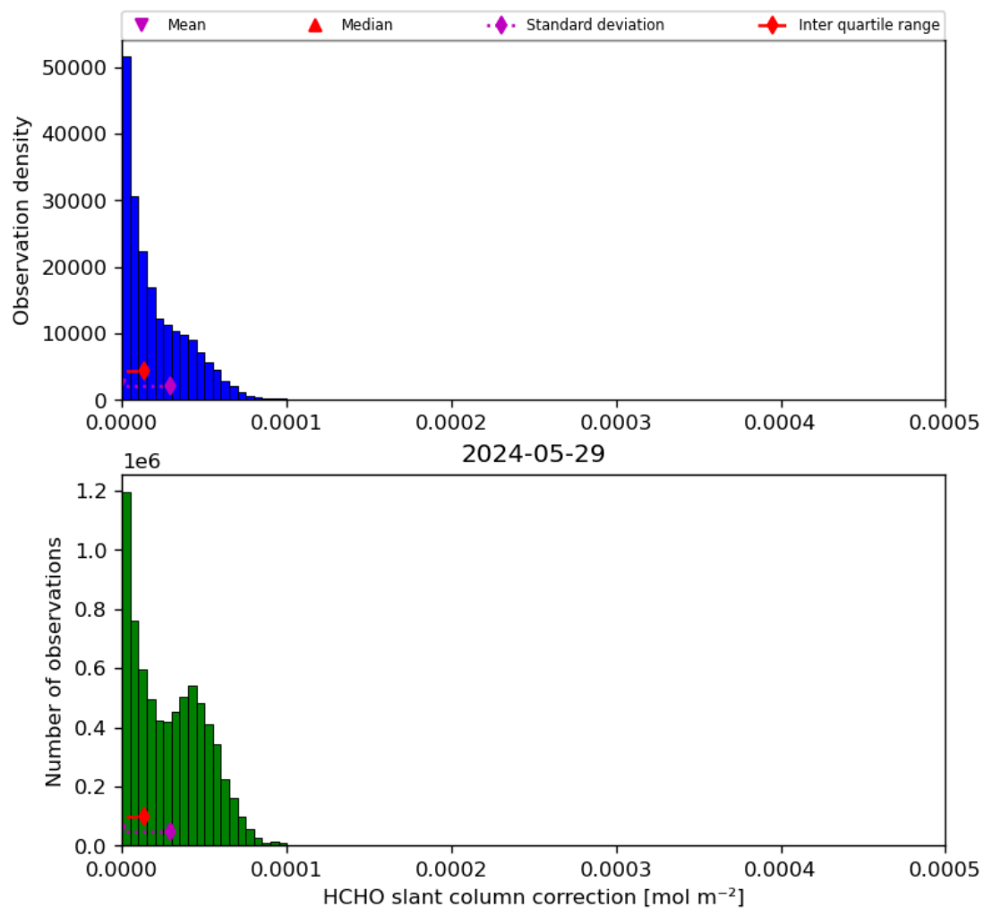
Figure 47: Histogram of “HCHO slant column correction” for 2024-05-28 to 2024-05-30
