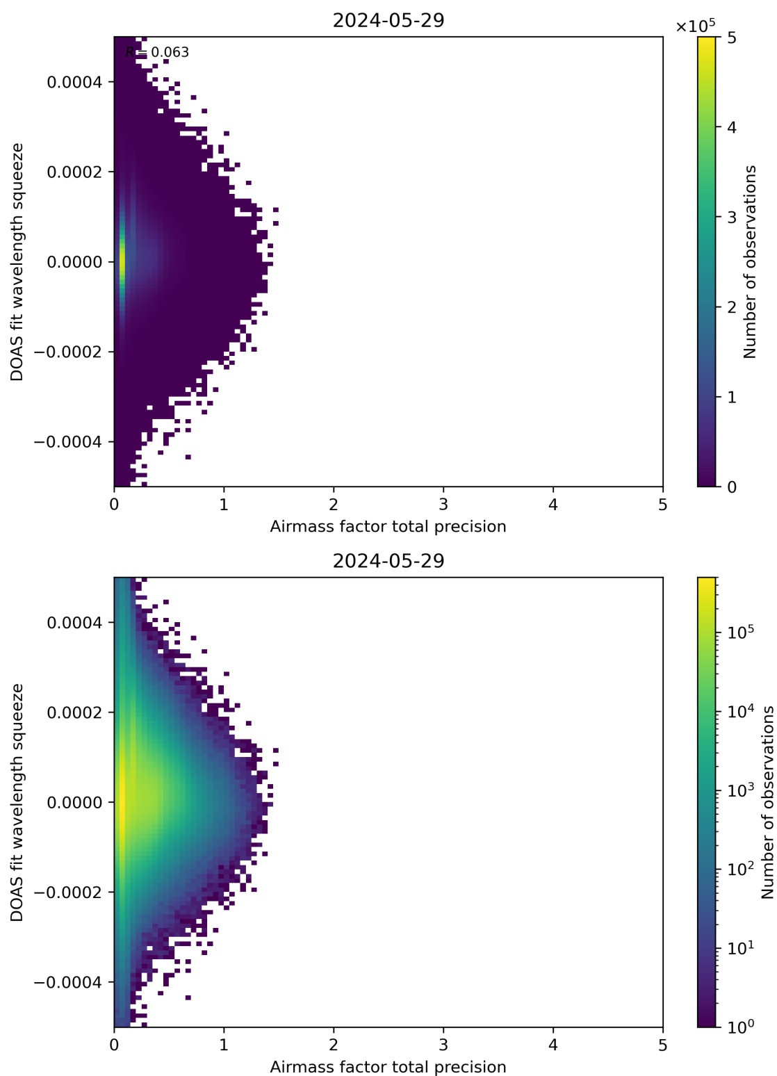
Figure 107: Scatter density plot of “Airmass factor total precision” against “DOAS fit wavelength squeeze” for 2024-05-28 to 2024-05-30.
