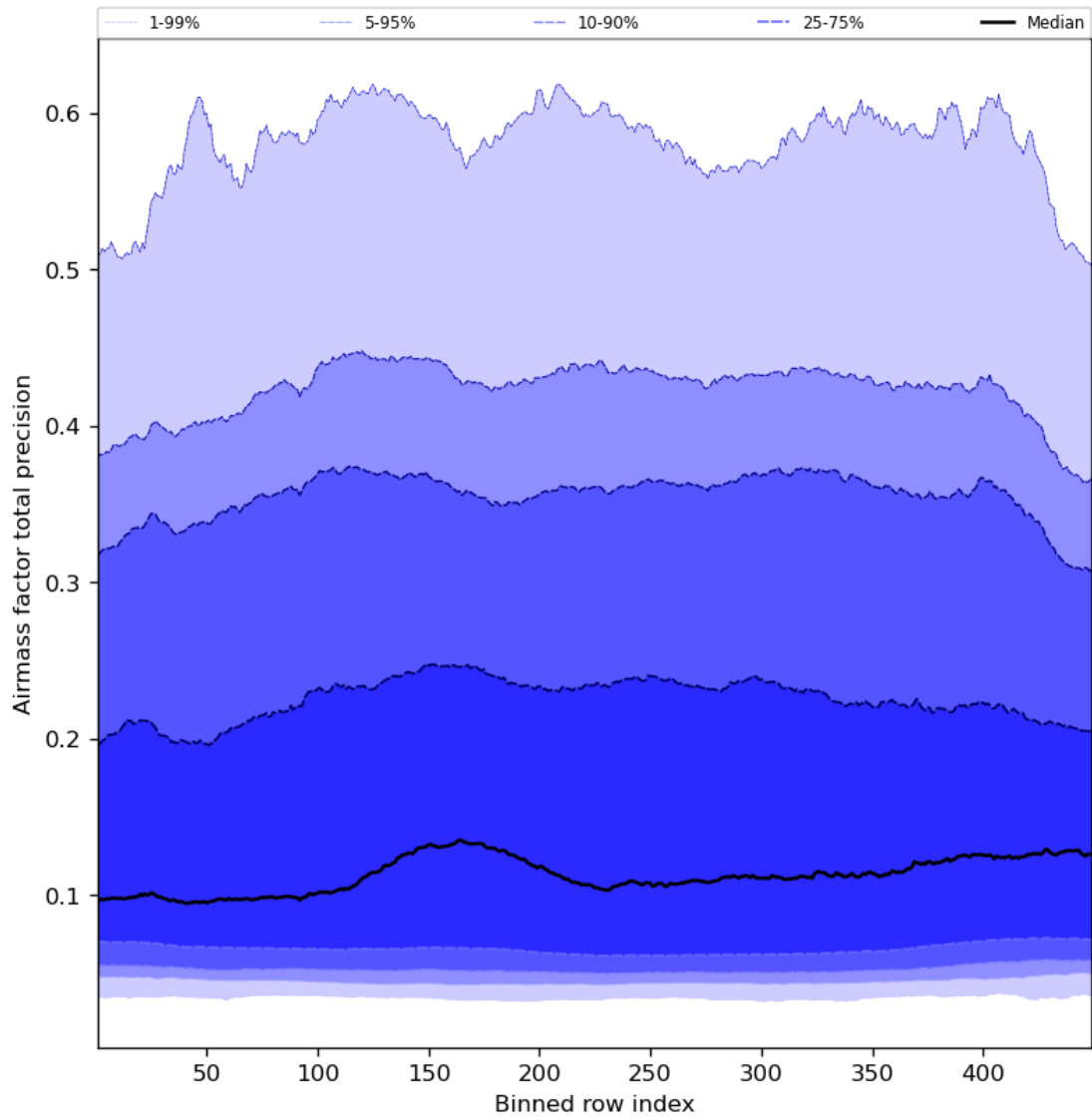
Figure 55: Along track statistics of “Airmass factor total precision” for 2024-05-28 to 2024-05-30
