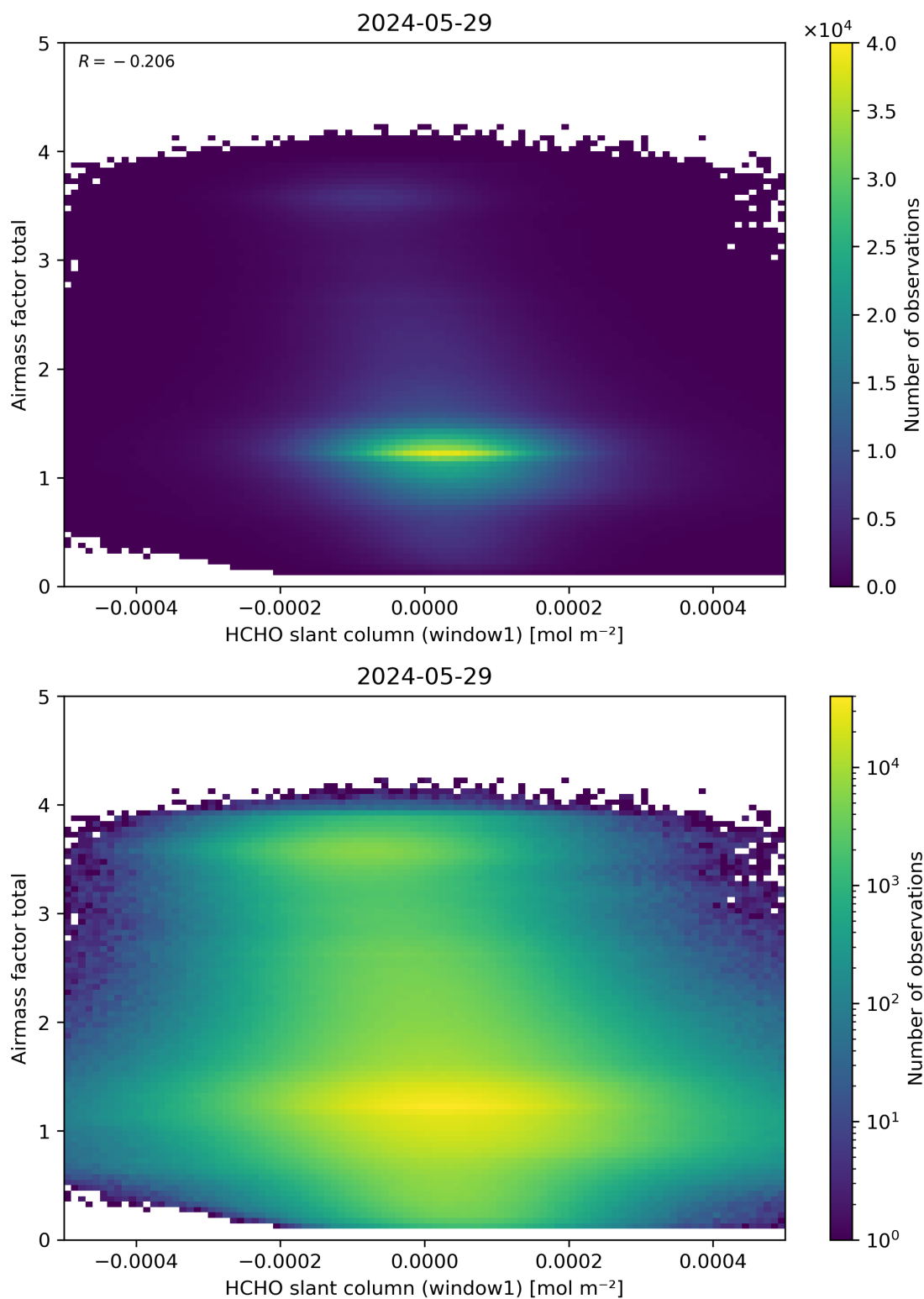
Figure 85: Scatter density plot of “HCHO slant column (window1)” against “Airmass factor total” for 2024-05-28 to 2024-05-30.
