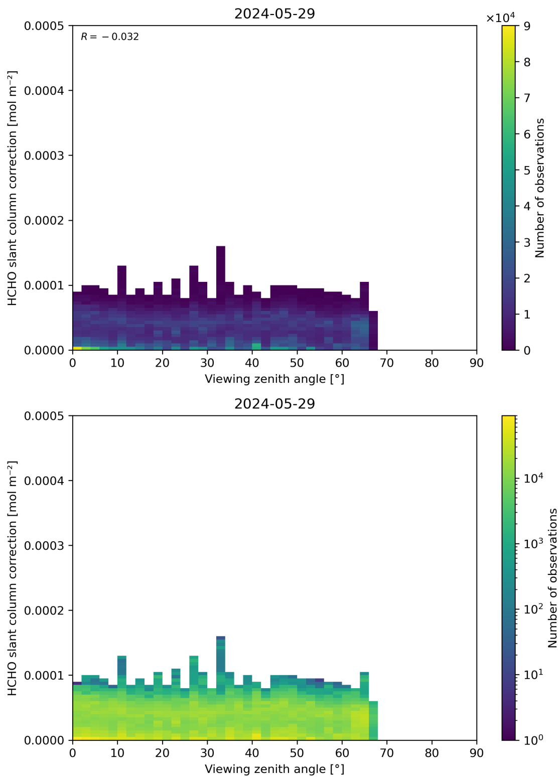
Figure 187: Scatter density plot of “Viewing zenith angle” against “HCHO slant column correction” for 2024-05-28 to 2024-05-30.
