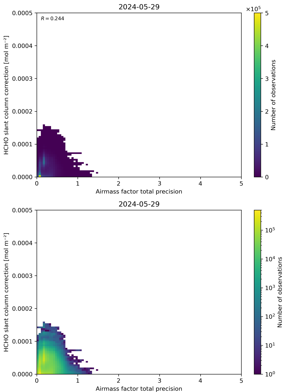
Figure 110: Scatter density plot of “Airmass factor total precision” against “HCHO slant column correction” for 2024-05-28 to 2024-05-30.
