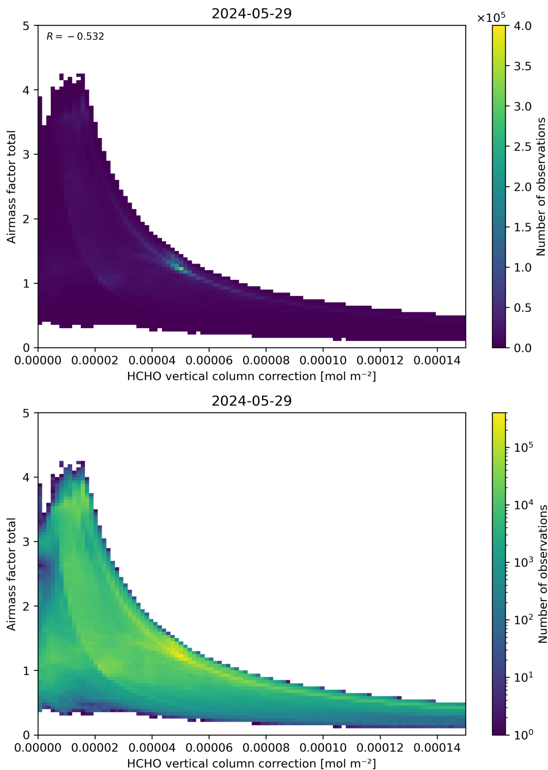
Figure 120: Scatter density plot of “HCHO vertical column correction” against “Airmass factor total” for 2024-05-28 to 2024-05-30.
