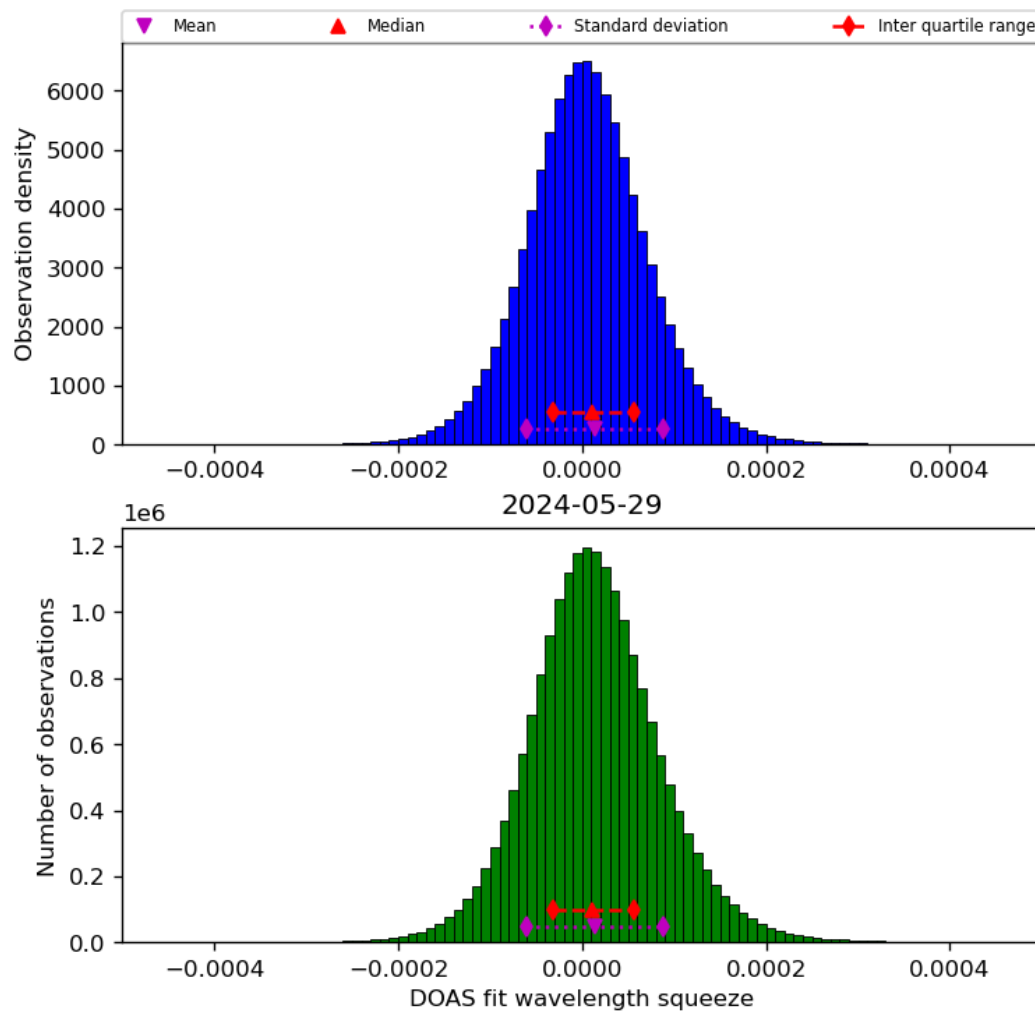
Figure 45: Histogram of “DOAS fit wavelength squeeze” for 2024-05-28 to 2024-05-30
