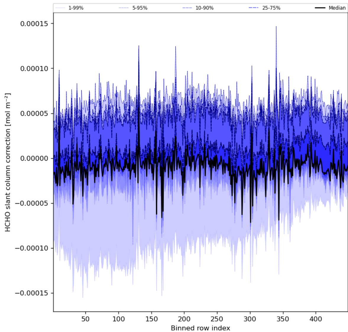
Figure 61: Along track statistics of “HCHO slant column correction” for 2024-05-28 to 2024-05-30
