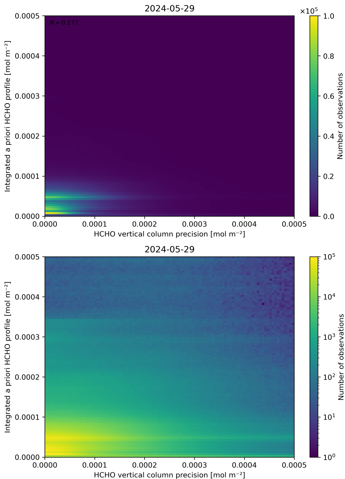
Figure 147: Scatter density plot of “HCHO vertical column precision” against “Integrated a priori HCHO profile” for 2024-05-28 to 2024-05-30.
