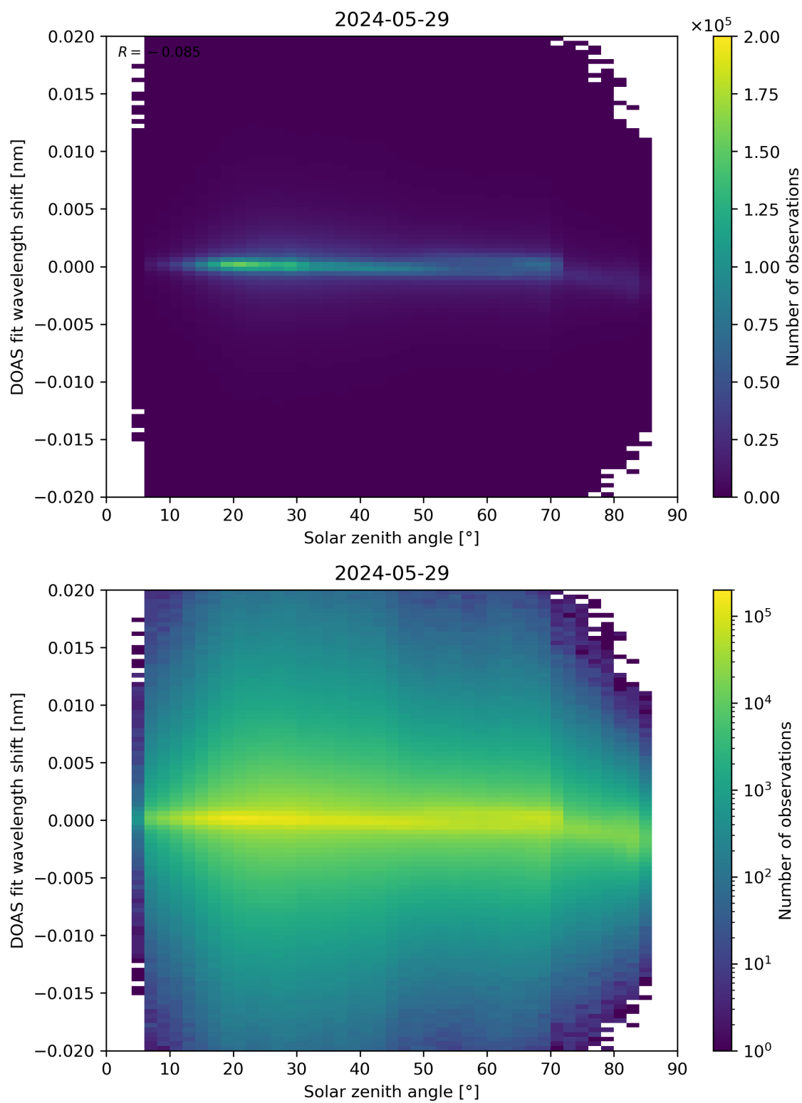
Figure 168: Scatter density plot of “Solar zenith angle” against “DOAS fit wavelength shift” for 2024-05-28 to 2024-05-30.
