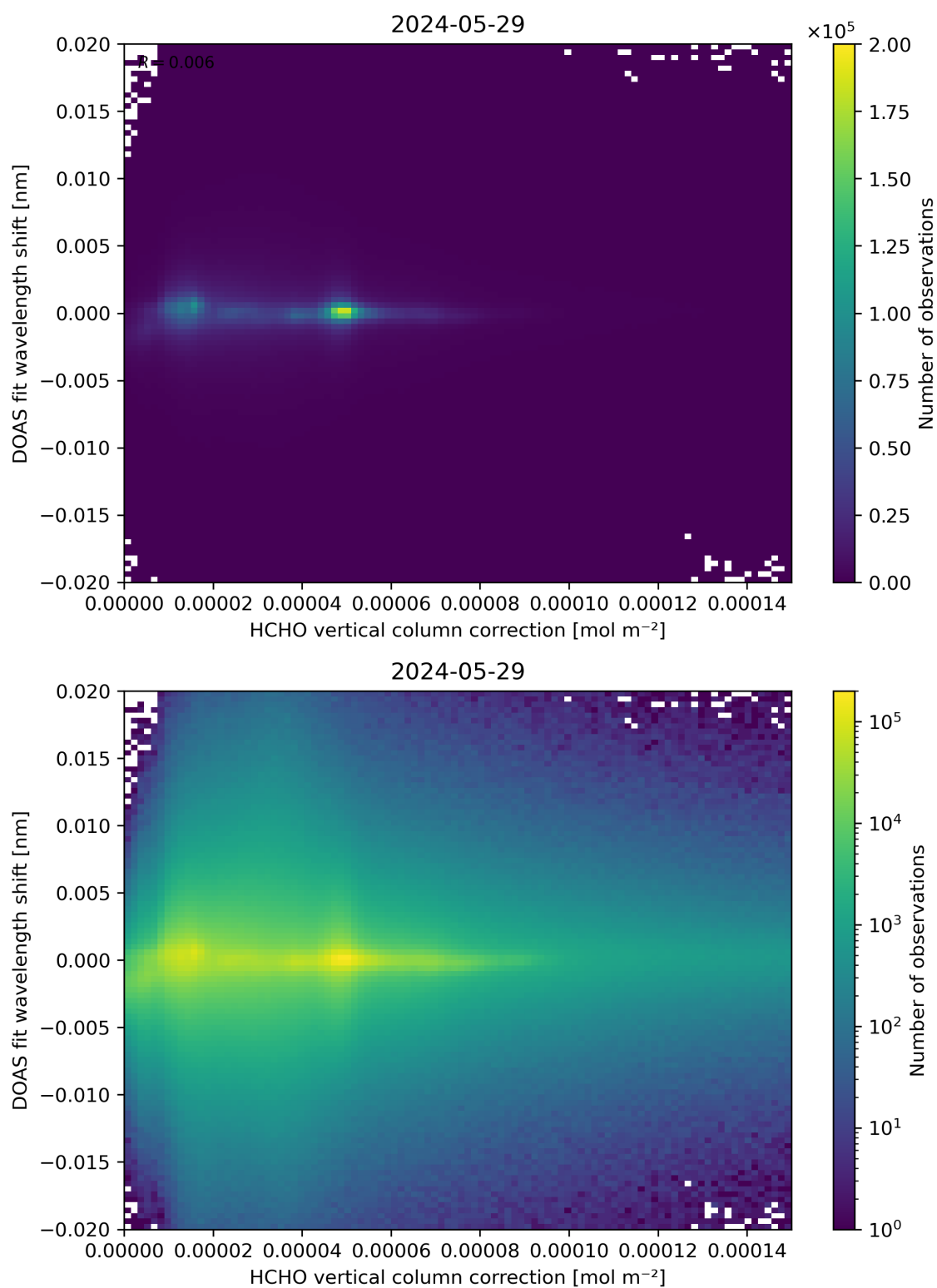
Figure 113: Scatter density plot of “HCHO vertical column correction” against “DOAS fit wavelength shift” for 2024-05-28 to 2024-05-30.
