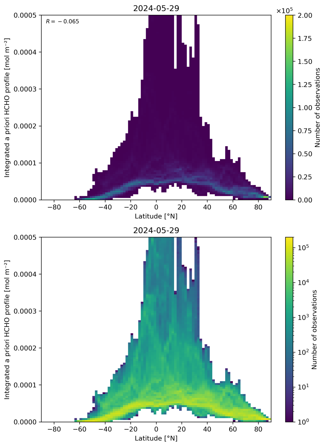
Figure 166: Scatter density plot of “Latitude” against “Integrated a priori HCHO profile” for 2024-05-28 to 2024-05-30.
