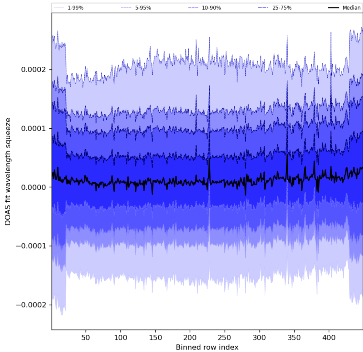
Figure 59: Along track statistics of “DOAS fit wavelength squeeze” for 2024-05-28 to 2024-05-30
