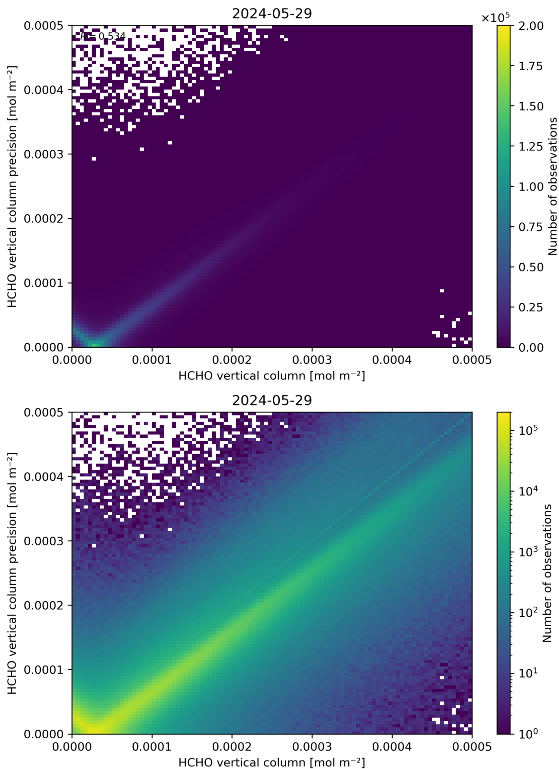
Figure 134: Scatter density plot of “HCHO vertical column” against “HCHO vertical column precision” for 2024-05-28 to 2024-05-30.
