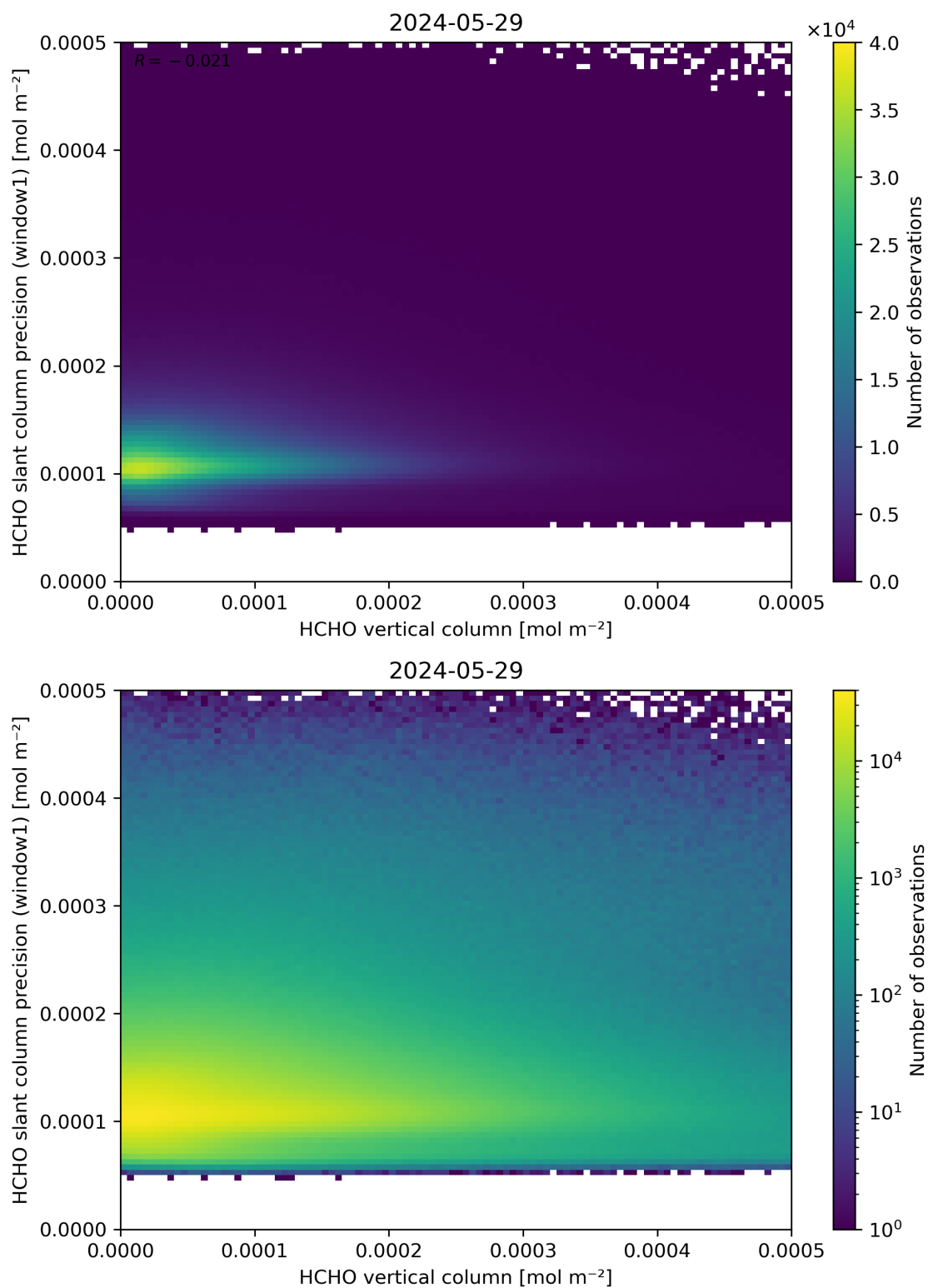
Figure 130: Scatter density plot of “HCHO vertical column” against “HCHO slant column precision (window1)” for 2024-05-28 to 2024-05-30.
