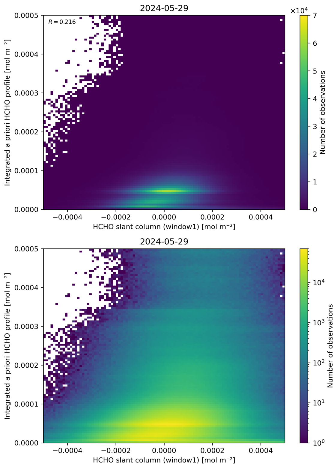
Figure 87: Scatter density plot of “HCHO slant column (window1)” against “Integrated a priori HCHO profile” for 2024-05-28 to 2024-05-30.
