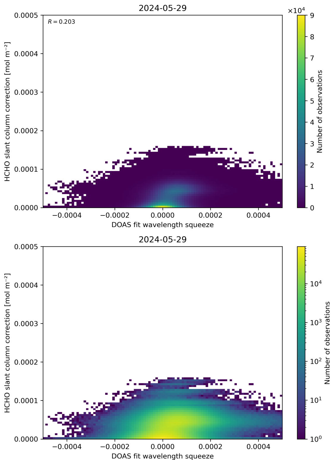
Figure 70: Scatter density plot of “DOAS fit wavelength squeeze” against “HCHO slant column correction” for 2024-05-28 to 2024-05-30.
