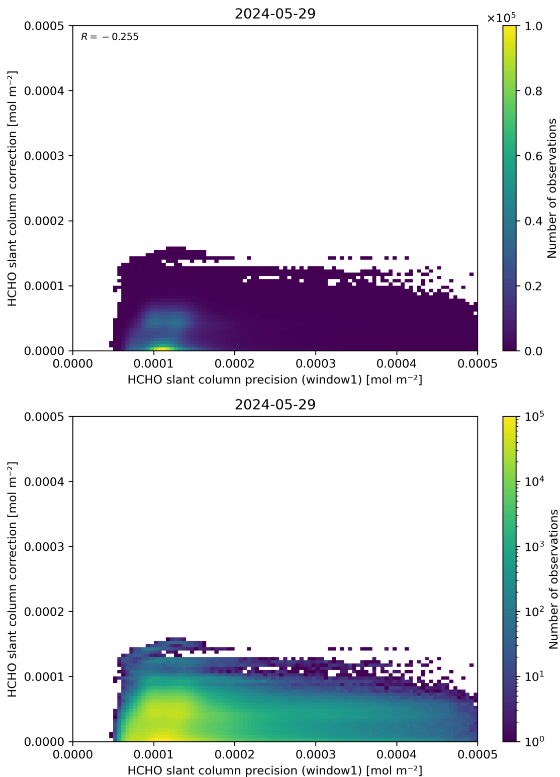
Figure 93: Scatter density plot of “HCHO slant column precision (window1)” against “HCHO slant column correction” for 2024-05-28 to 2024-05-30.
