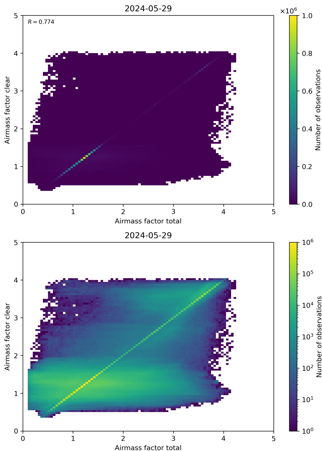
Figure 100: Scatter density plot of “Airmass factor total” against “Airmass factor clear” for 2024-05-28 to 2024-05-30.
