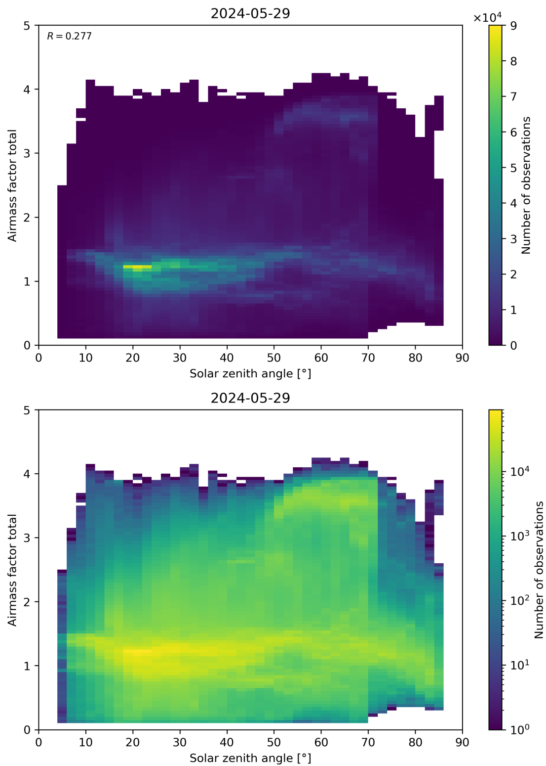
Figure 175: Scatter density plot of “Solar zenith angle” against “Airmass factor total” for 2024-05-28 to 2024-05-30.
