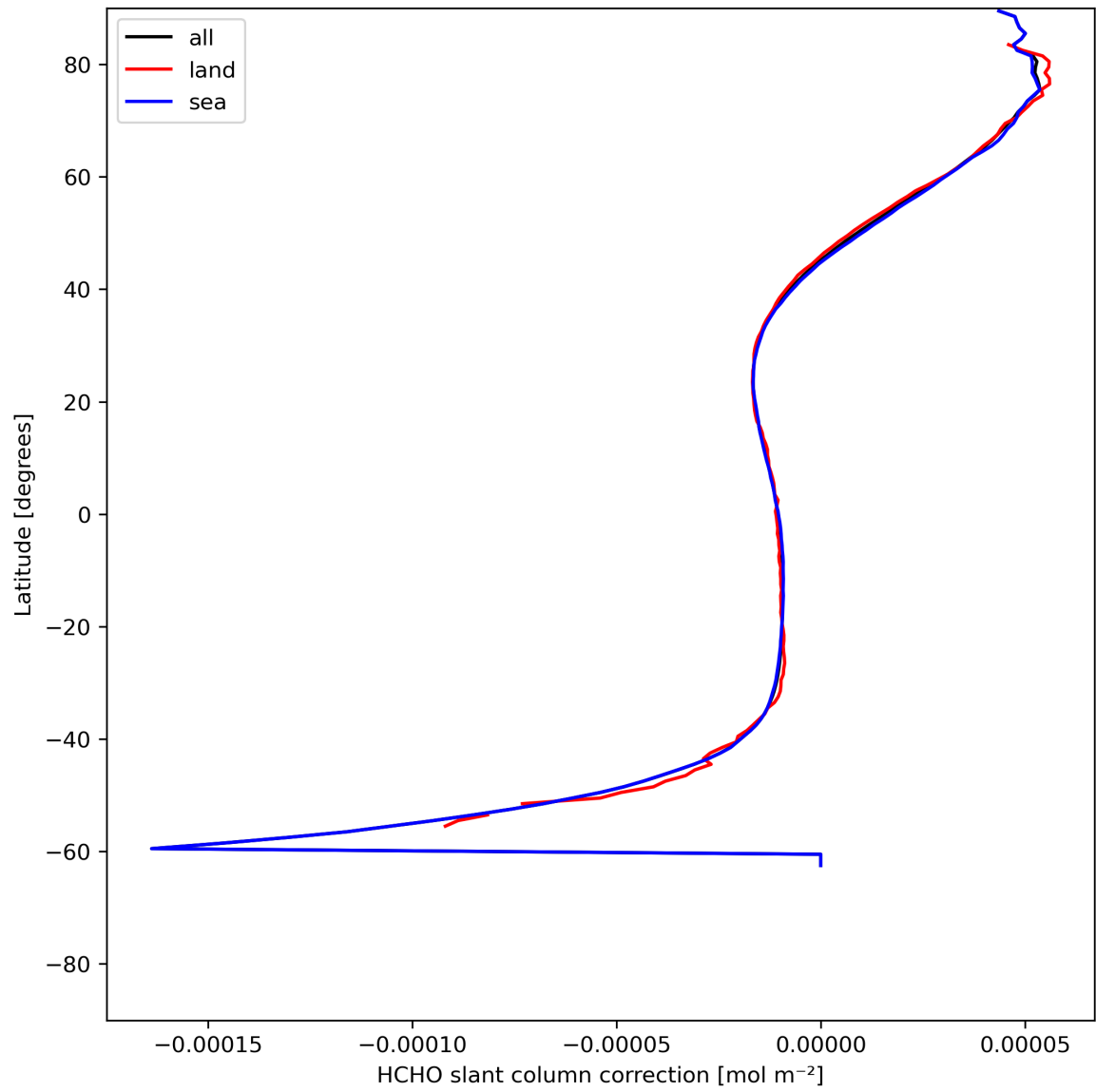
Figure 33: Zonal average of “HCHO slant column correction” for 2024-05-28 to 2024-05-30.
