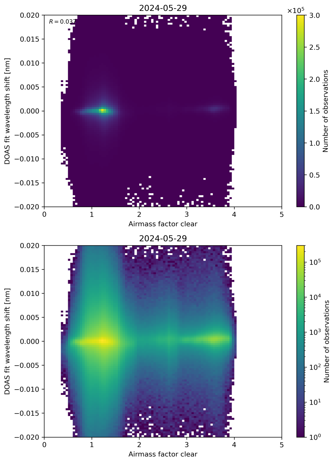
Figure 72: Scatter density plot of “Airmass factor clear” against “DOAS fit wavelength shift” for 2024-05-28 to 2024-05-30.
