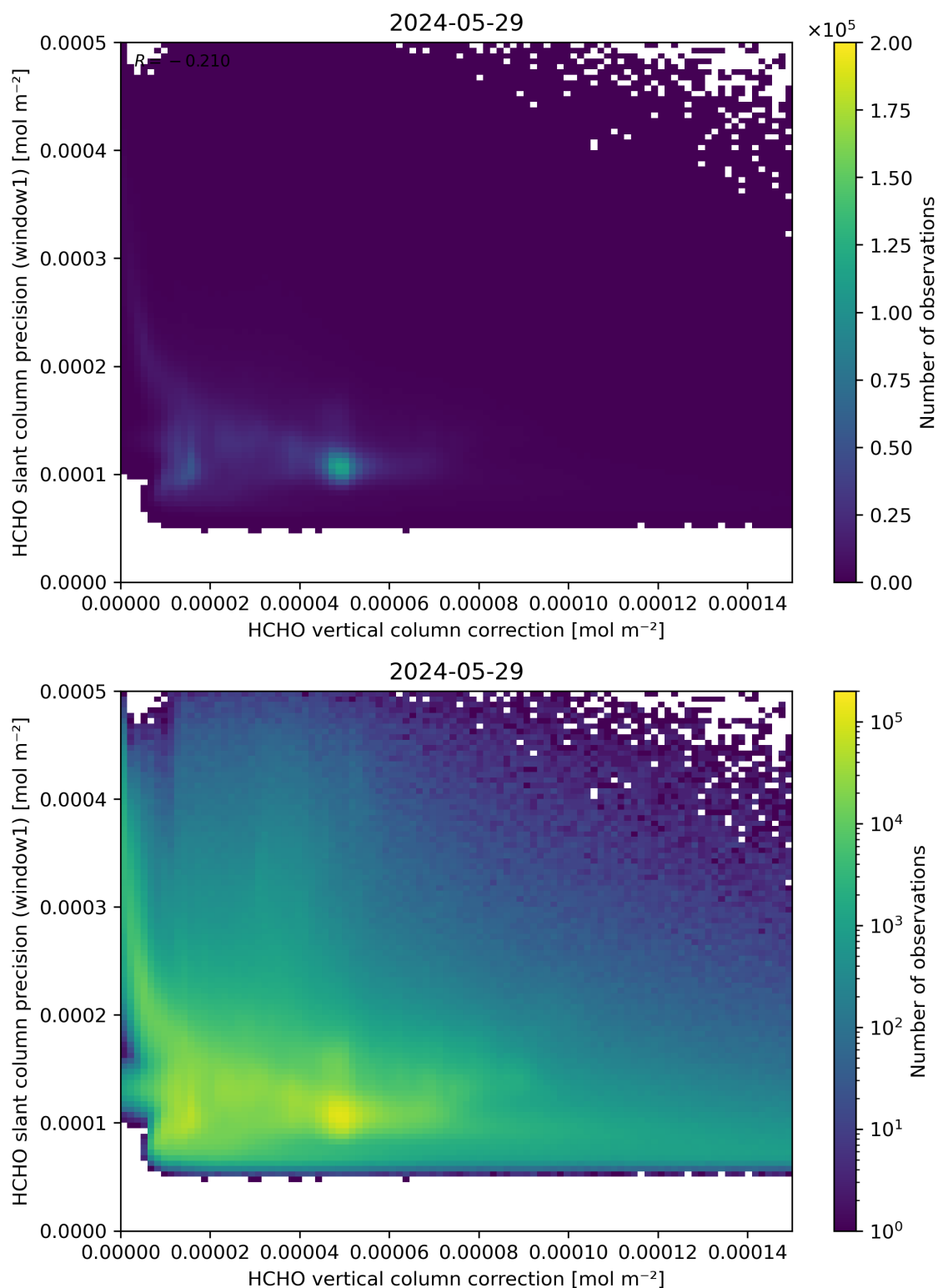
Figure 119: Scatter density plot of “HCHO vertical column correction” against “HCHO slant column precision (window1)” for 2024-05-28 to 2024-05-30.
