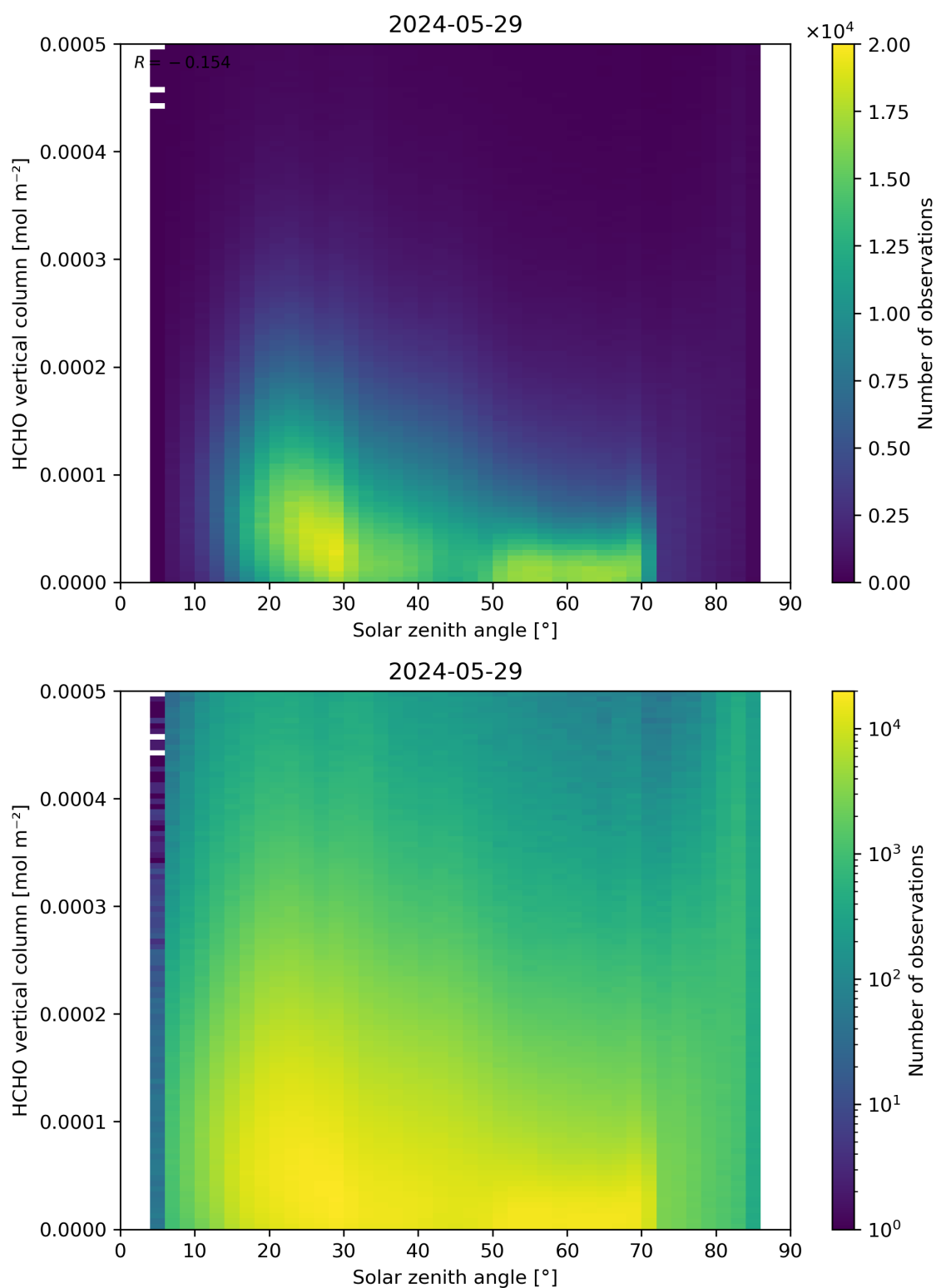
Figure 177: Scatter density plot of “Solar zenith angle” against “HCHO vertical column” for 2024-05-28 to 2024-05-30.
