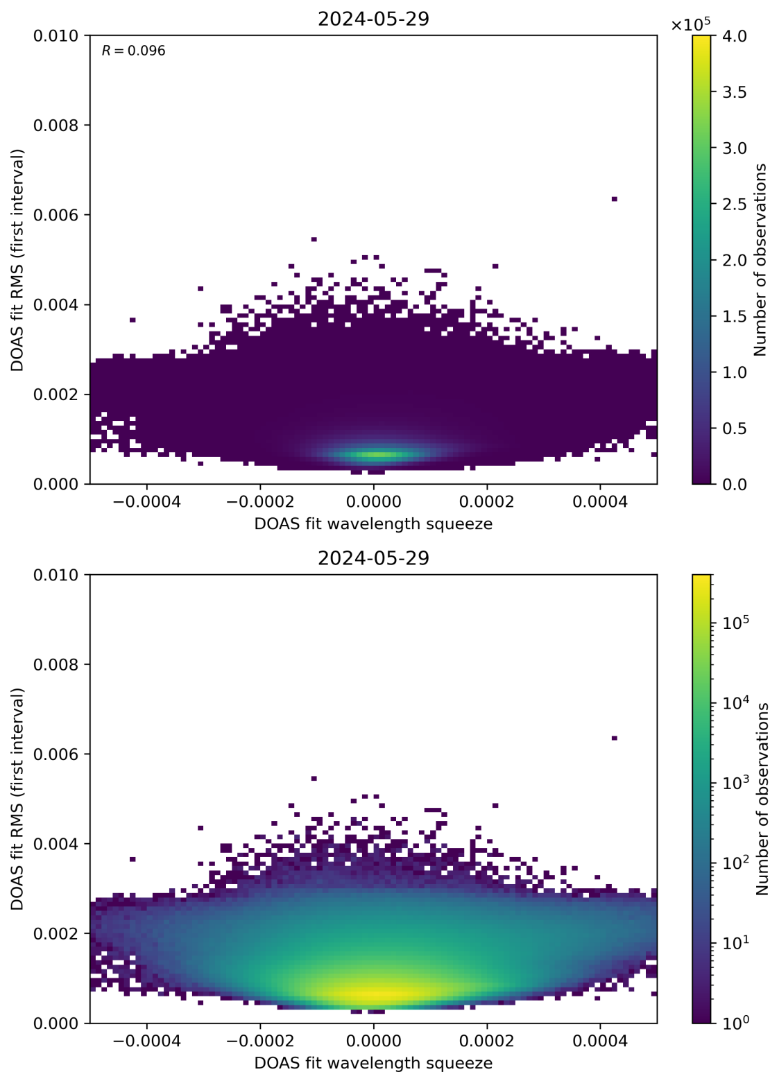
Figure 68: Scatter density plot of “DOAS fit wavelength squeeze” against “DOAS fit RMS (first interval)” for 2024-05-28 to 2024-05-30.
