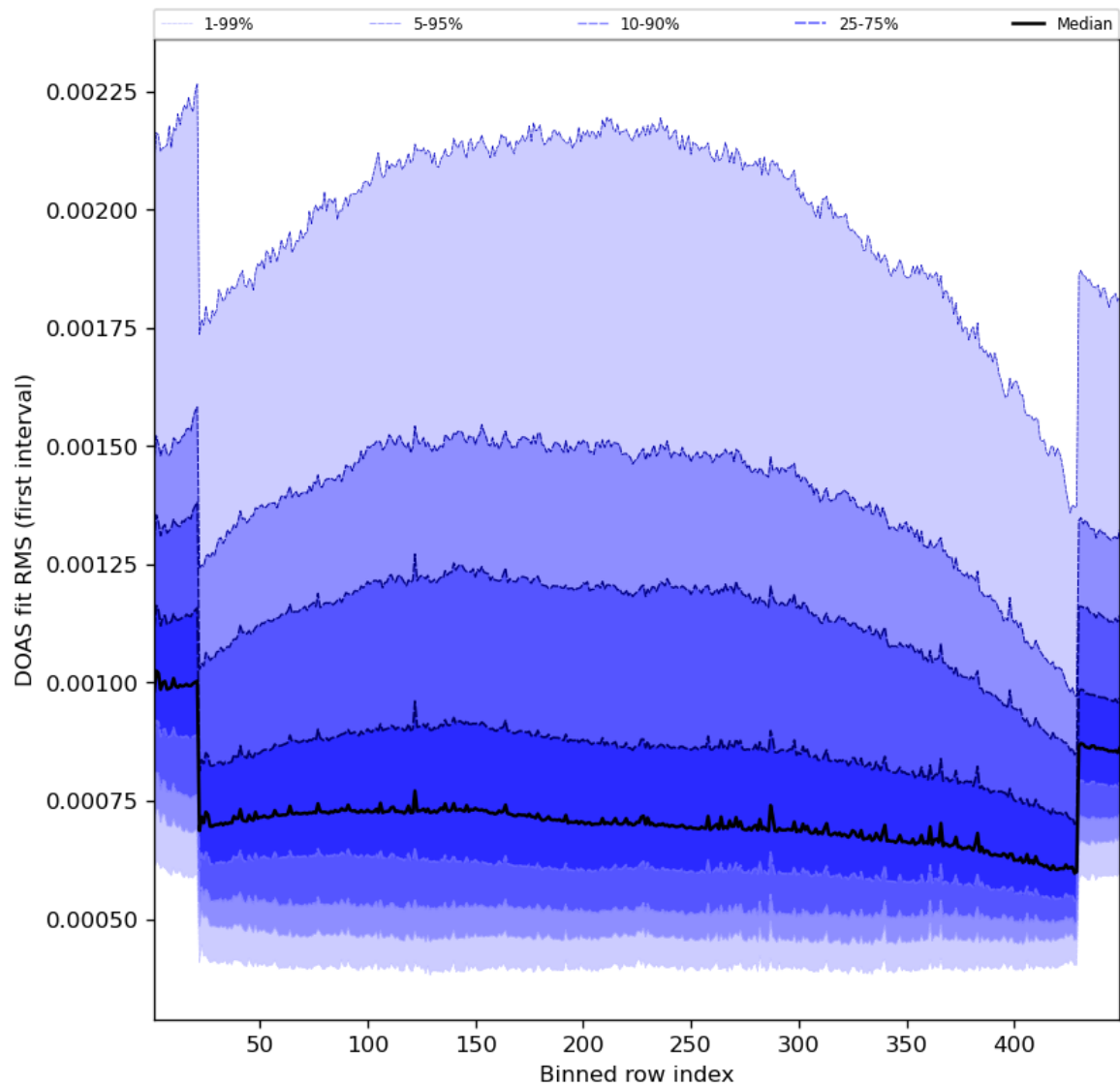
Figure 60: Along track statistics of “DOAS fit RMS (first interval)” for 2024-05-28 to 2024-05-30
