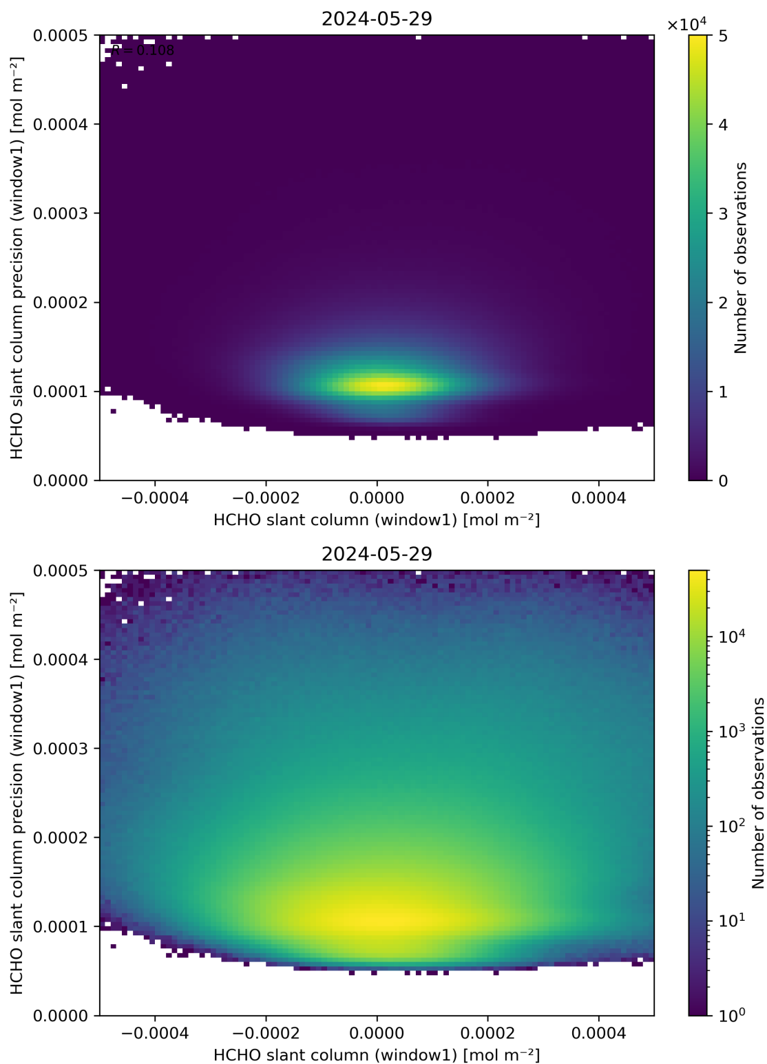
Figure 84: Scatter density plot of “HCHO slant column (window1)” against “HCHO slant column precision (window1)” for 2024-05-28 to 2024-05-30.
