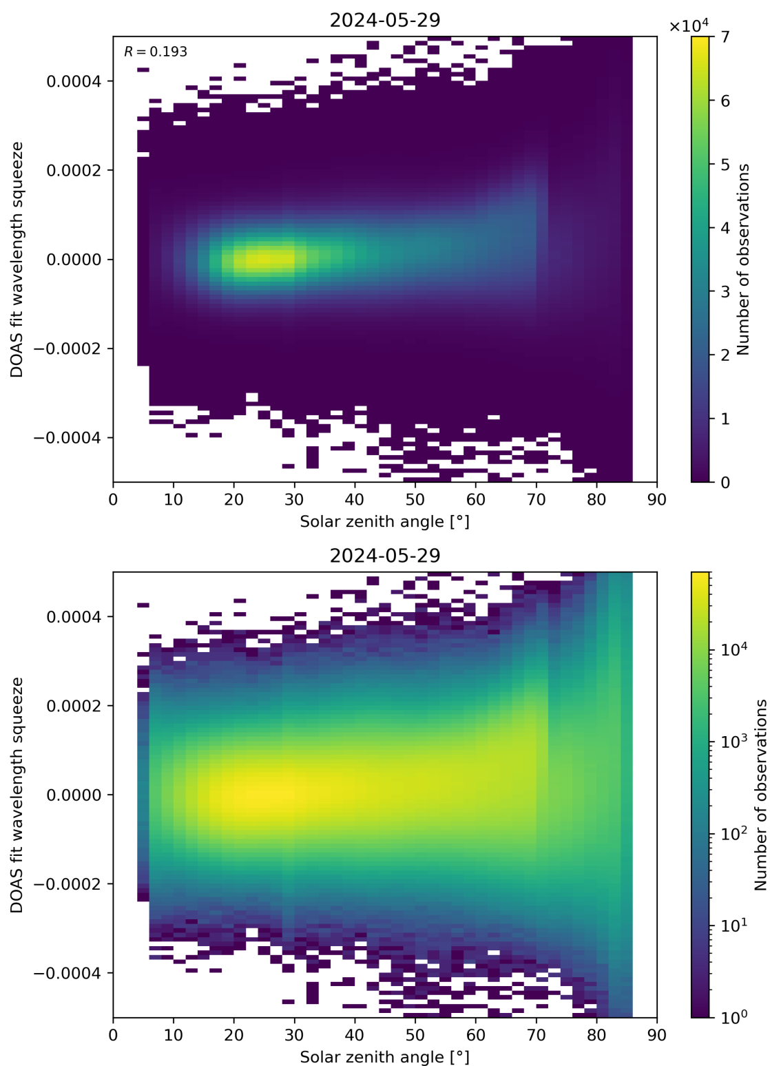
Figure 169: Scatter density plot of “Solar zenith angle” against “DOAS fit wavelength squeeze” for 2024-05-28 to 2024-05-30.
