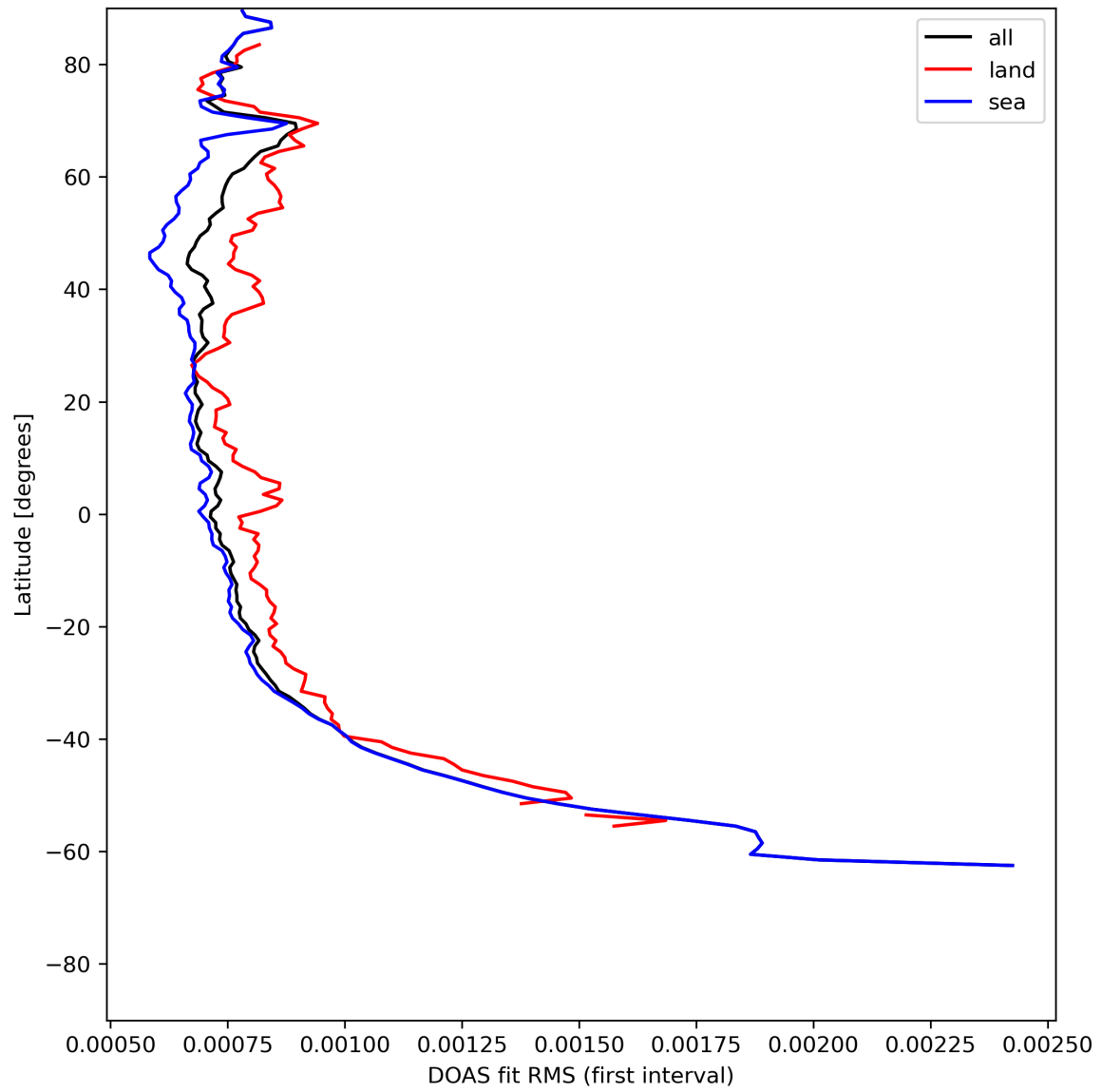
Figure 32: Zonal average of “DOAS fit RMS (first interval)” for 2024-05-28 to 2024-05-30.
