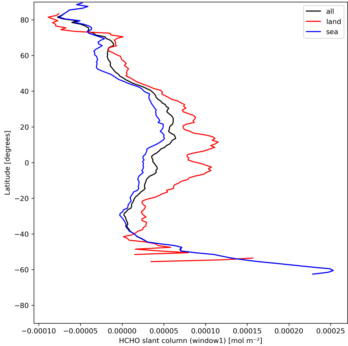
Figure 24: Zonal average of “HCHO slant column (window1)” for 2024-05-28 to 2024-05-30.
