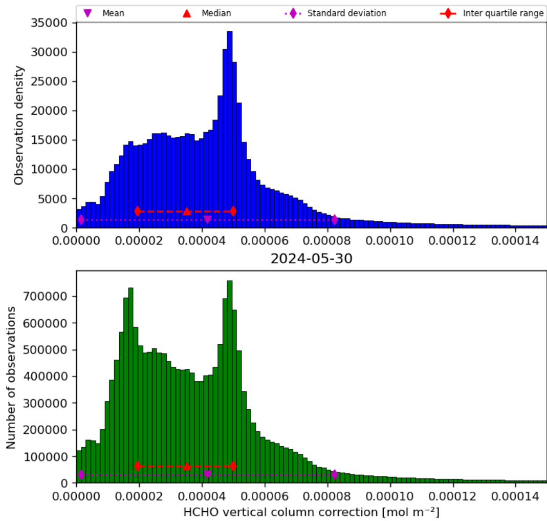
Figure 37: Histogram of “HCHO vertical column correction” for 2024-05-29 to 2024-05-31
