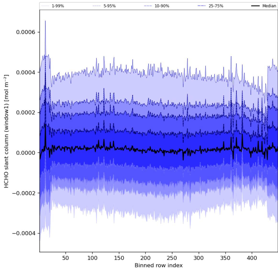
Figure 52: Along track statistics of “HCHO slant column (window1)” for 2024-05-29 to 2024-05-31
