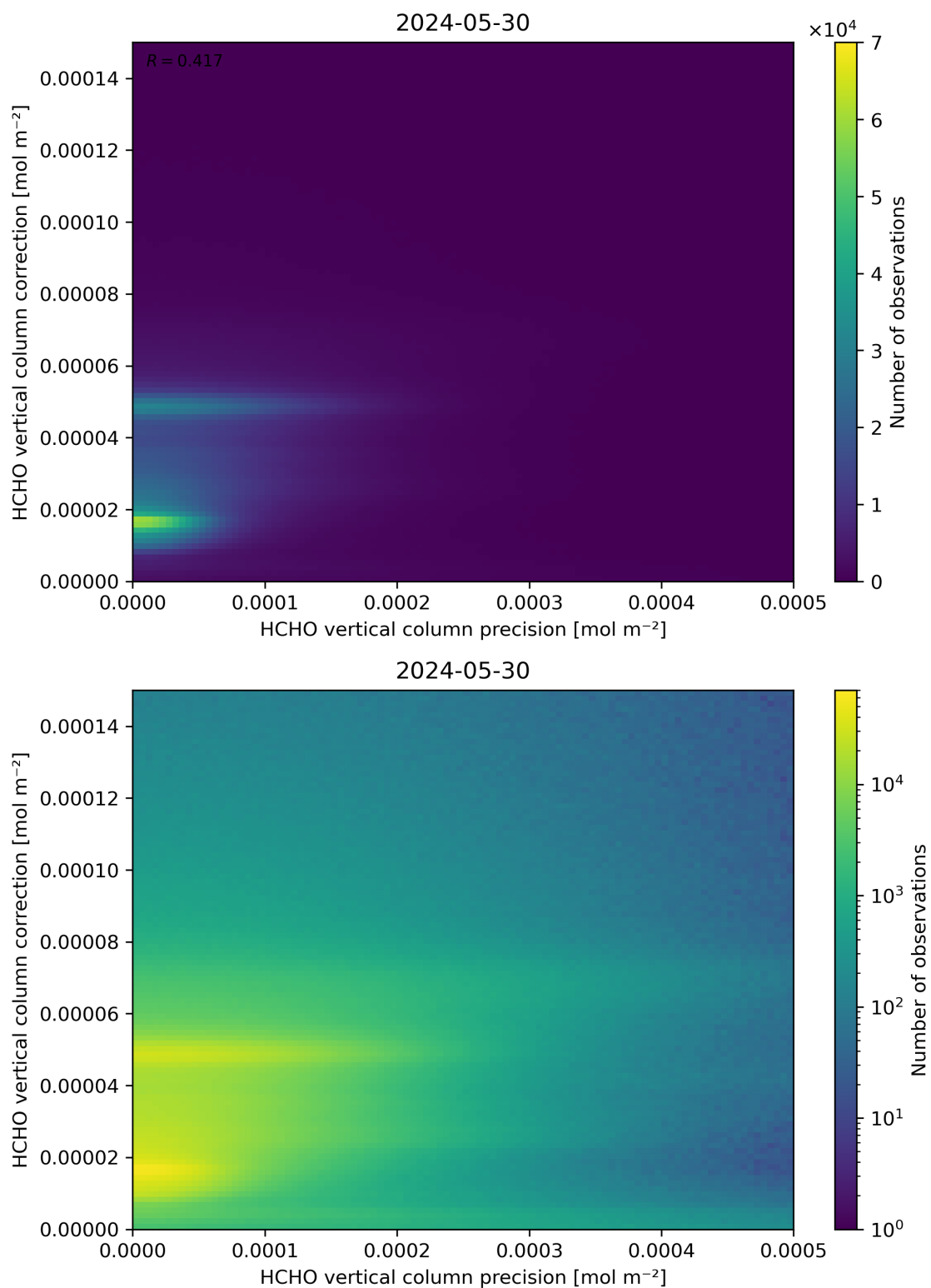
Figure 146: Scatter density plot of “HCHO vertical column precision” against “HCHO vertical column correction” for 2024-05-29 to 2024-05-31.
