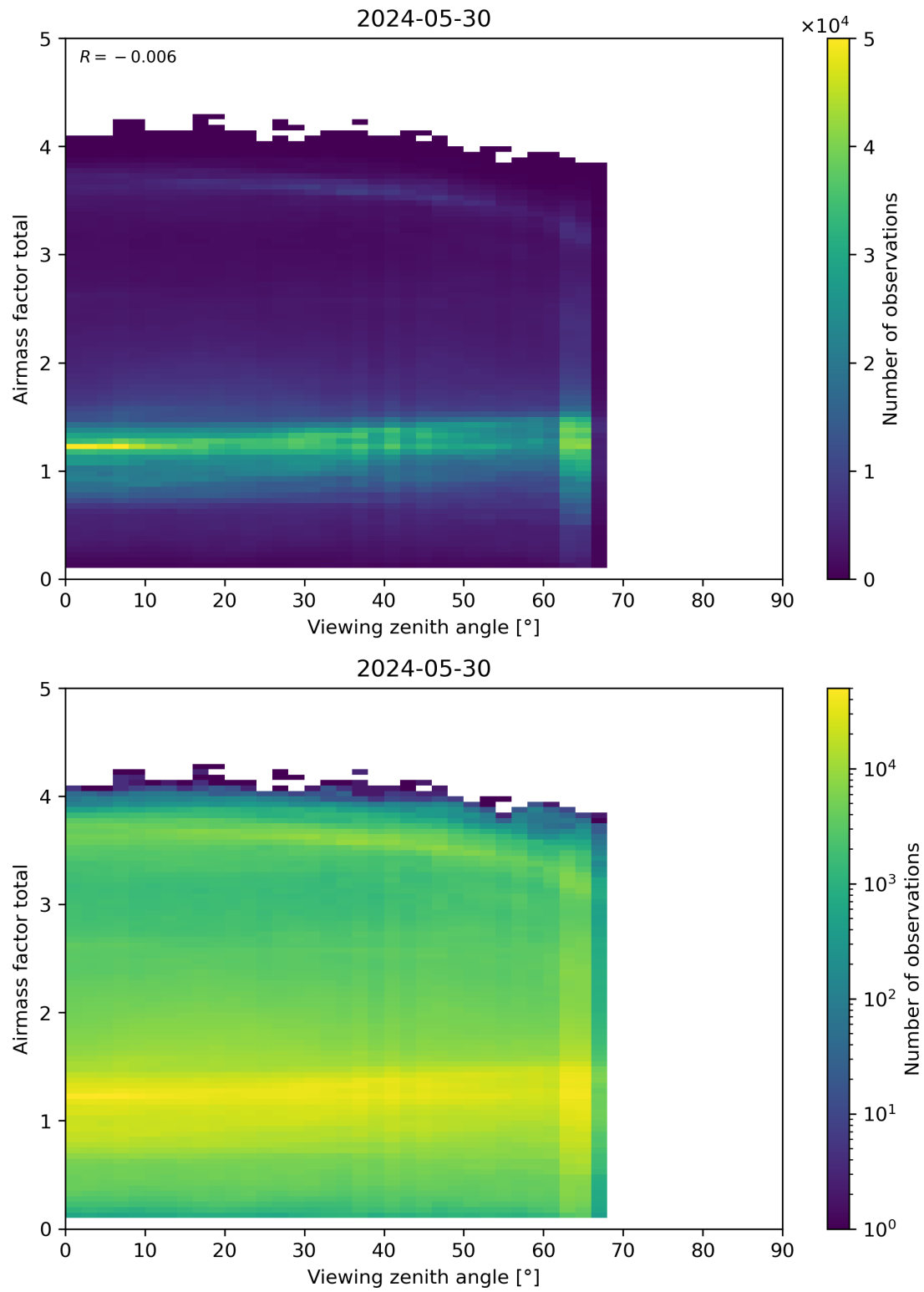
Figure 190: Scatter density plot of “Viewing zenith angle” against “Airmass factor total” for 2024-05-29 to 2024-05-31.
