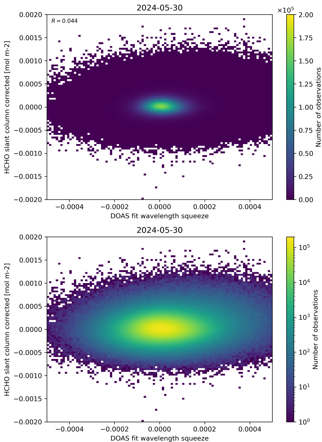
Figure 69: Scatter density plot of “DOAS fit wavelength squeeze” against “HCHO slant column corrected” for 2024-05-29 to 2024-05-31.
