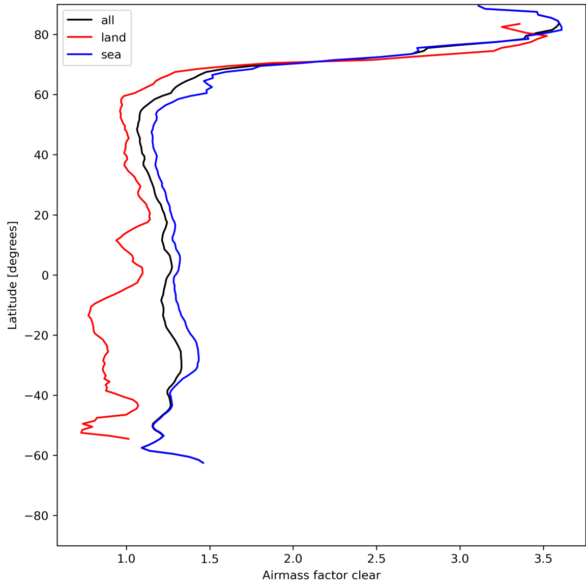
Figure 28: Zonal average of “Airmass factor clear” for 2024-05-29 to 2024-05-31.
