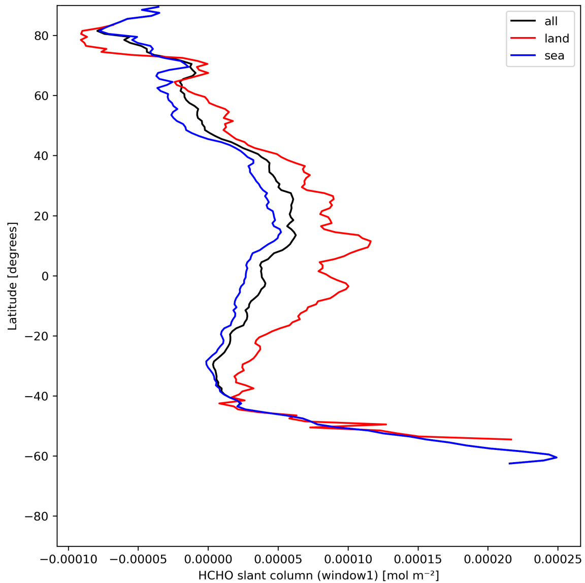
Figure 24: Zonal average of “HCHO slant column (window1)” for 2024-05-29 to 2024-05-31.
