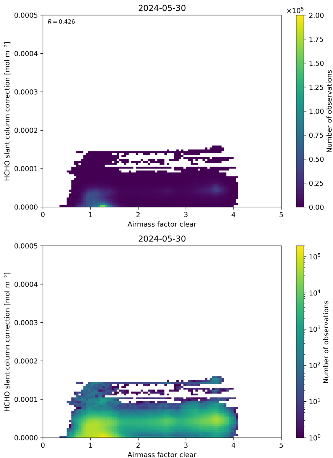
Figure 75: Scatter density plot of “Airmass factor clear” against “HCHO slant column correction” for 2024-05-29 to 2024-05-31.
