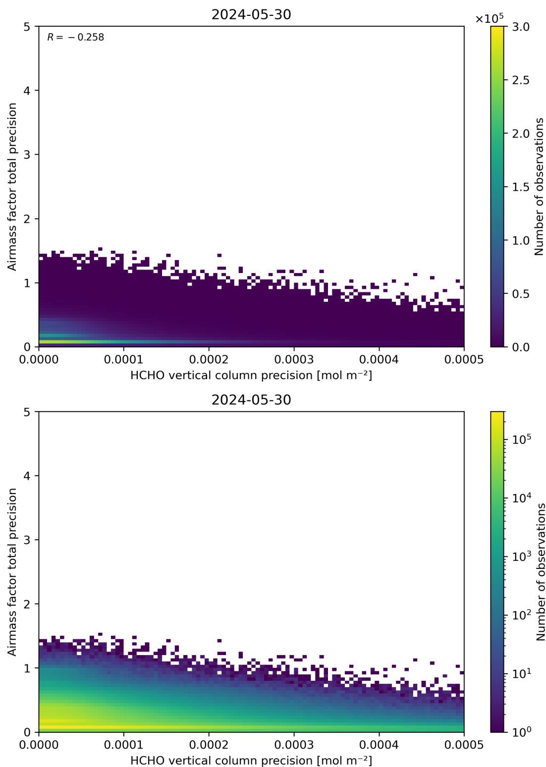
Figure 145: Scatter density plot of “HCHO vertical column precision” against “Airmass factor total precision” for 2024-05-29 to 2024-05-31.
