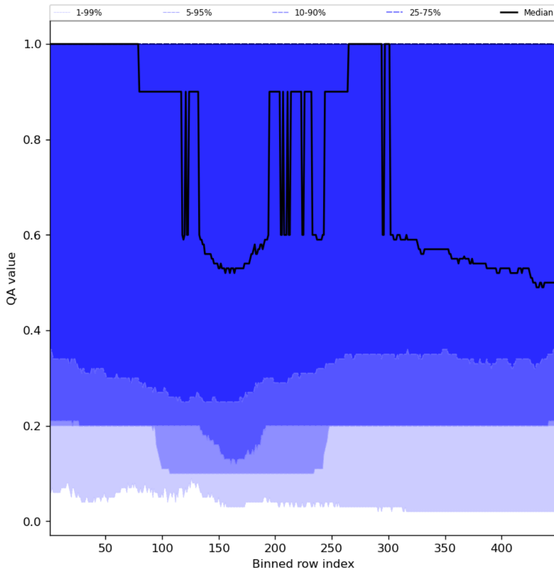
Figure 48: Along track statistics of “QA value” for 2024-05-29 to 2024-05-31
