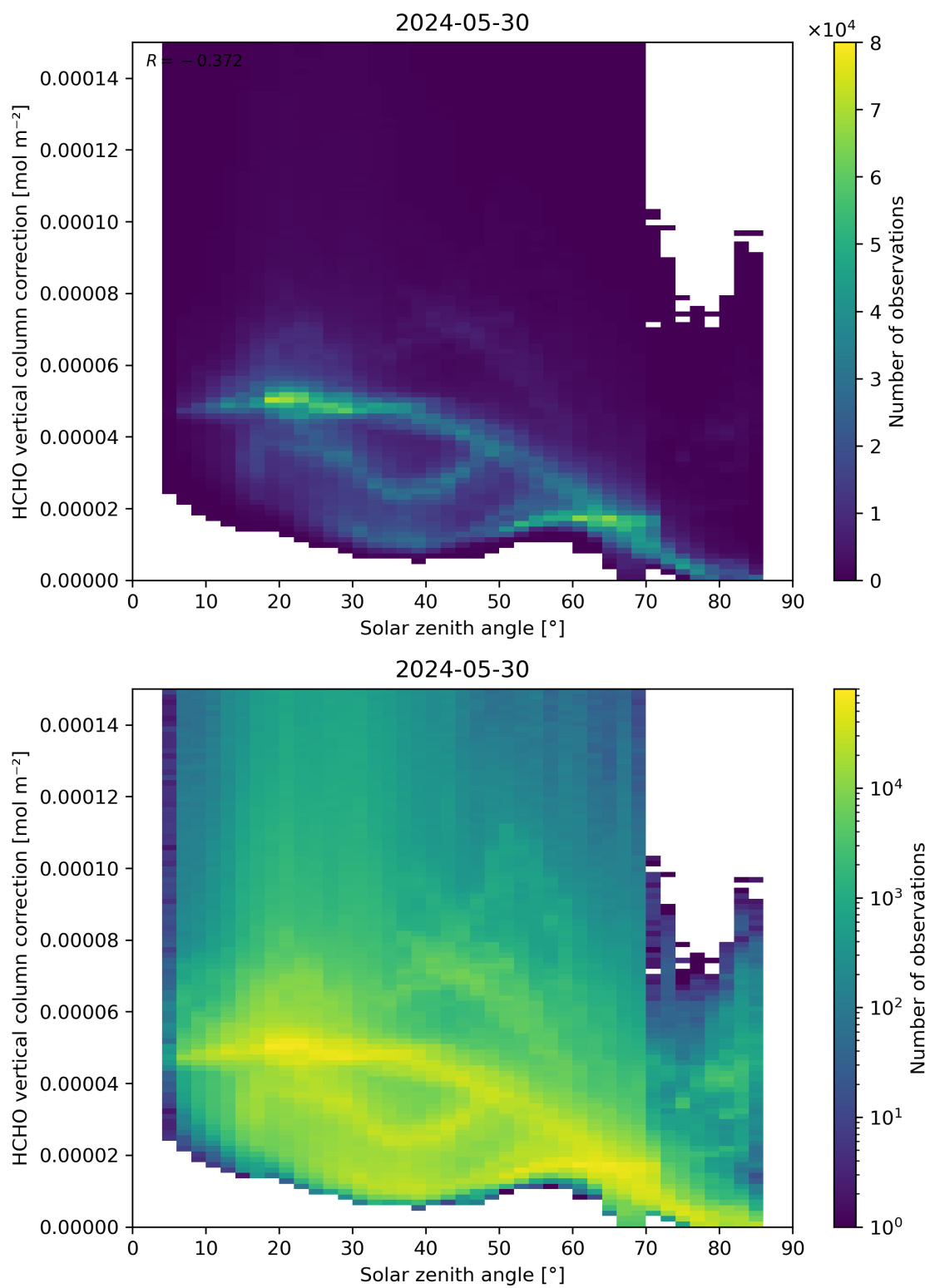
Figure 178: Scatter density plot of “Solar zenith angle” against “HCHO vertical column correction” for 2024-05-29 to 2024-05-31.
