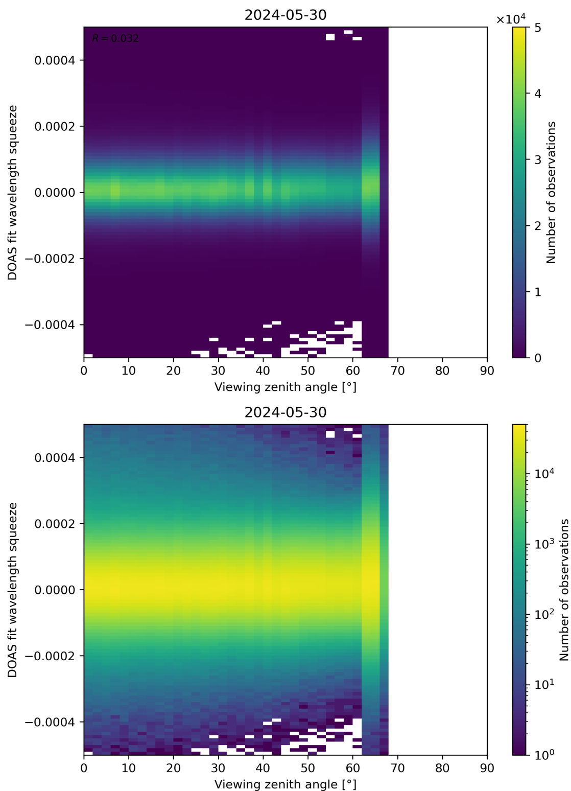
Figure 184: Scatter density plot of “Viewing zenith angle” against “DOAS fit wavelength squeeze” for 2024-05-29 to 2024-05-31.
