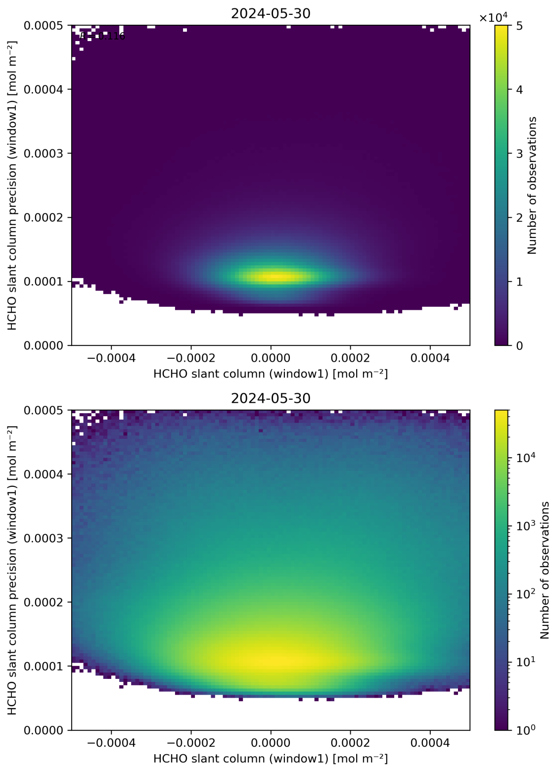
Figure 84: Scatter density plot of “HCHO slant column (window1)” against “HCHO slant column precision (window1)” for 2024-05-29 to 2024-05-31.
