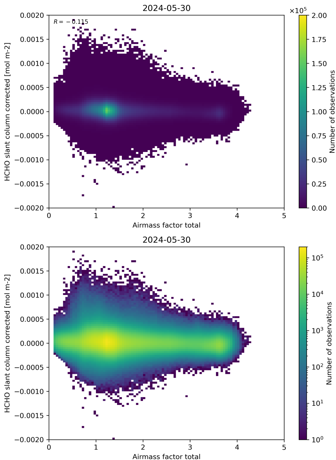
Figure 101: Scatter density plot of “Airmass factor total” against “HCHO slant column corrected” for 2024-05-29 to 2024-05-31.
