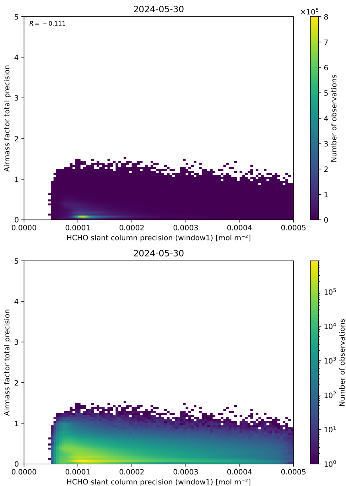
Figure 95: Scatter density plot of “HCHO slant column precision (window1)” against “Airmass factor total precision” for 2024-05-29 to 2024-05-31.
