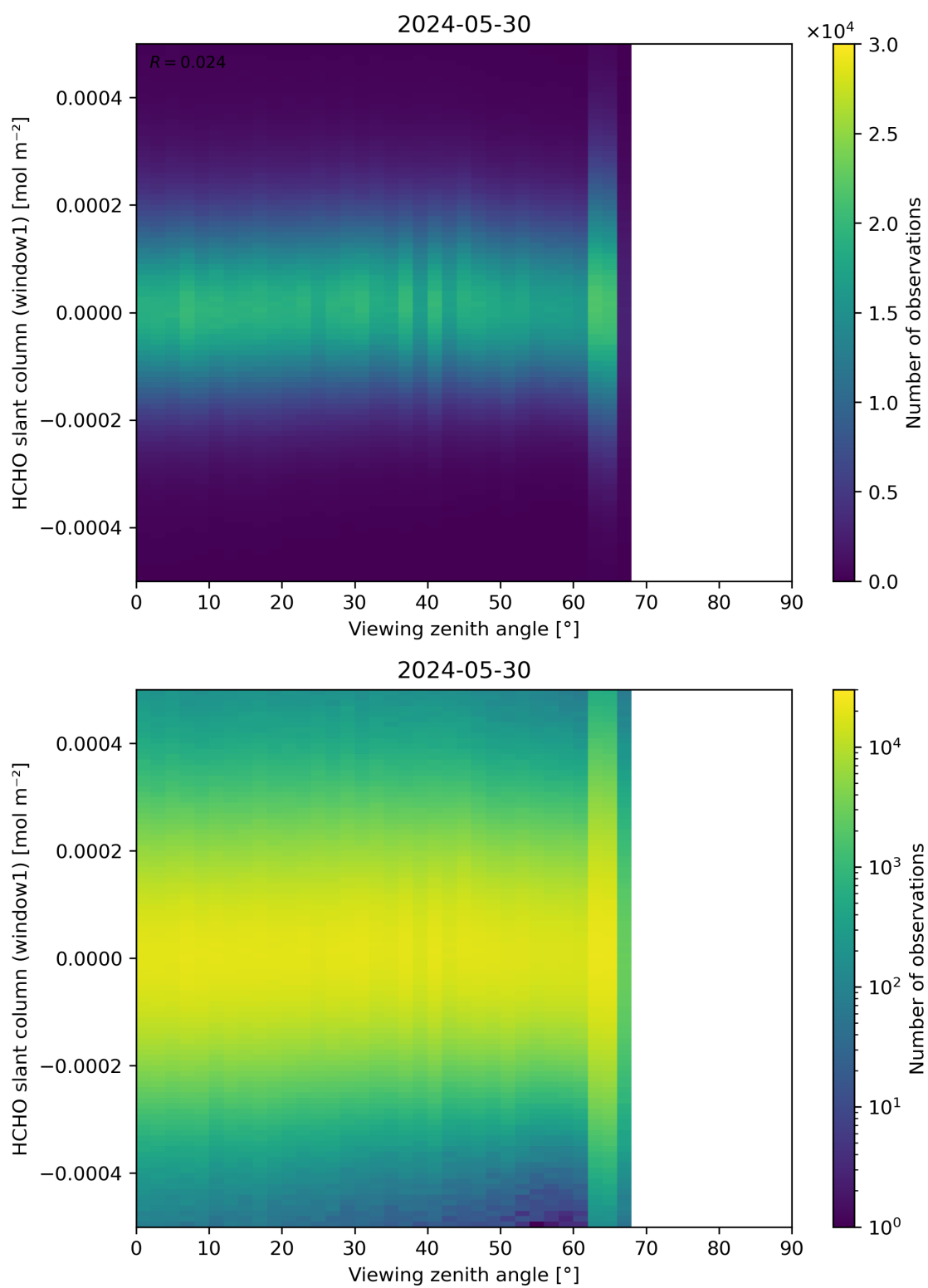
Figure 188: Scatter density plot of “Viewing zenith angle” against “HCHO slant column (window1)” for 2024-05-29 to 2024-05-31.
