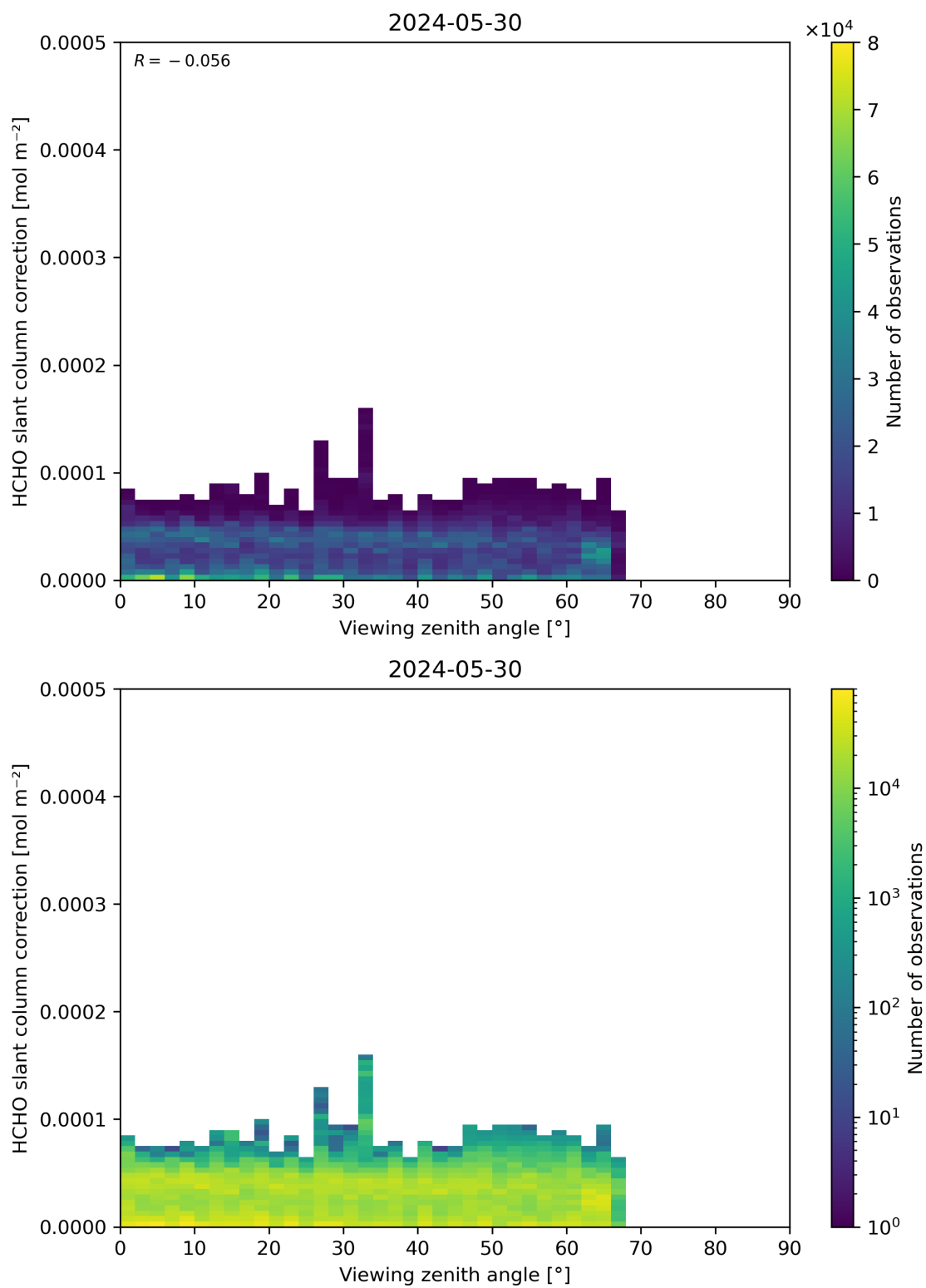
Figure 187: Scatter density plot of “Viewing zenith angle” against “HCHO slant column correction” for 2024-05-29 to 2024-05-31.
