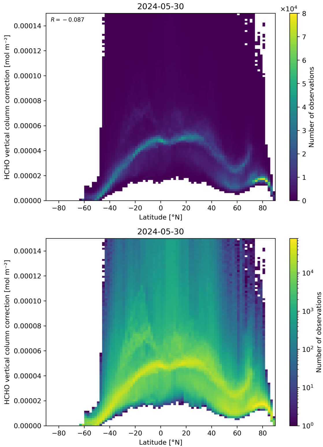
Figure 164: Scatter density plot of “Latitude” against “HCHO vertical column correction” for 2024-05-29 to 2024-05-31.
