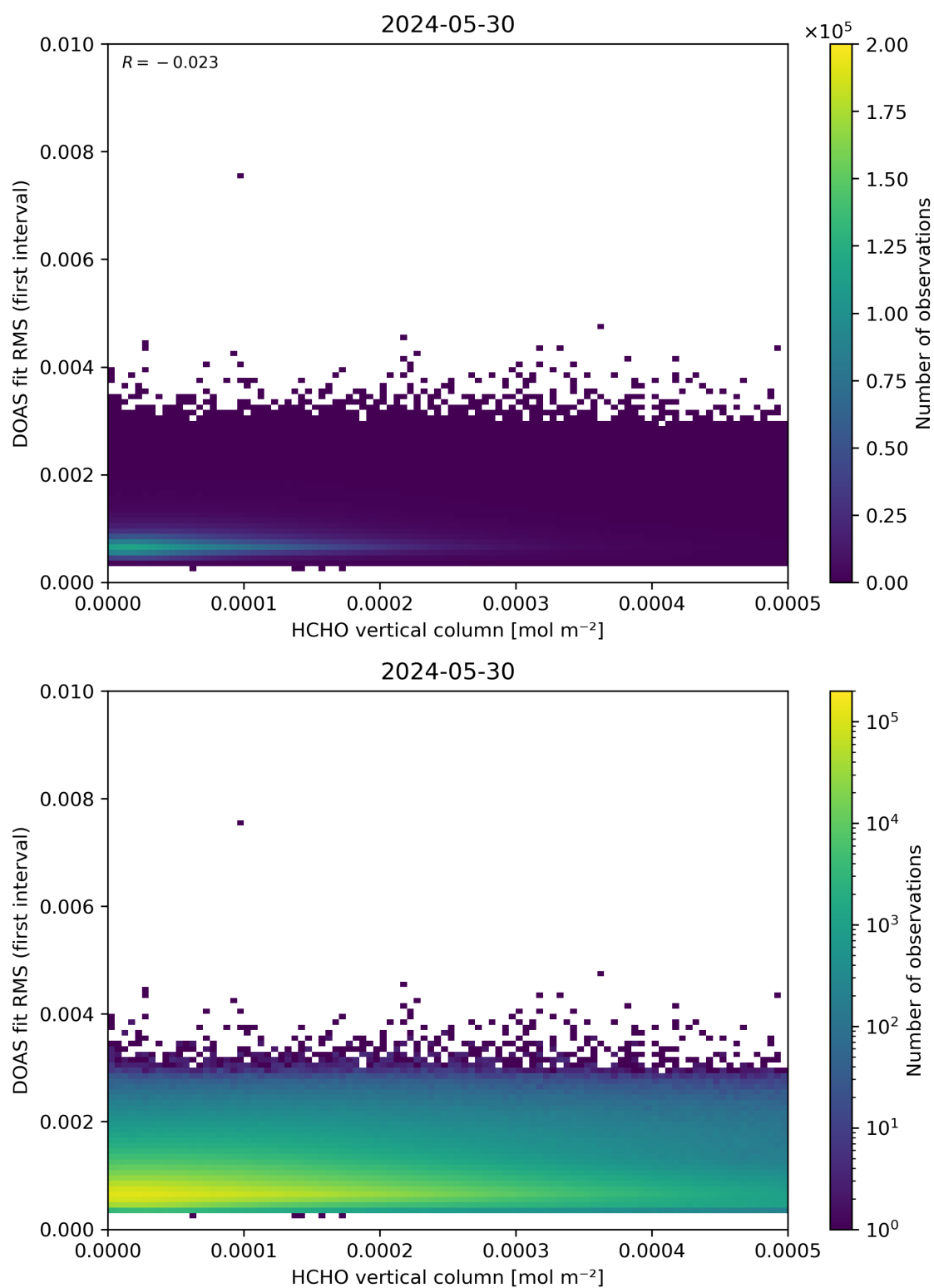
Figure 123: Scatter density plot of “HCHO vertical column” against “DOAS fit RMS (first interval)” for 2024-05-29 to 2024-05-31.
