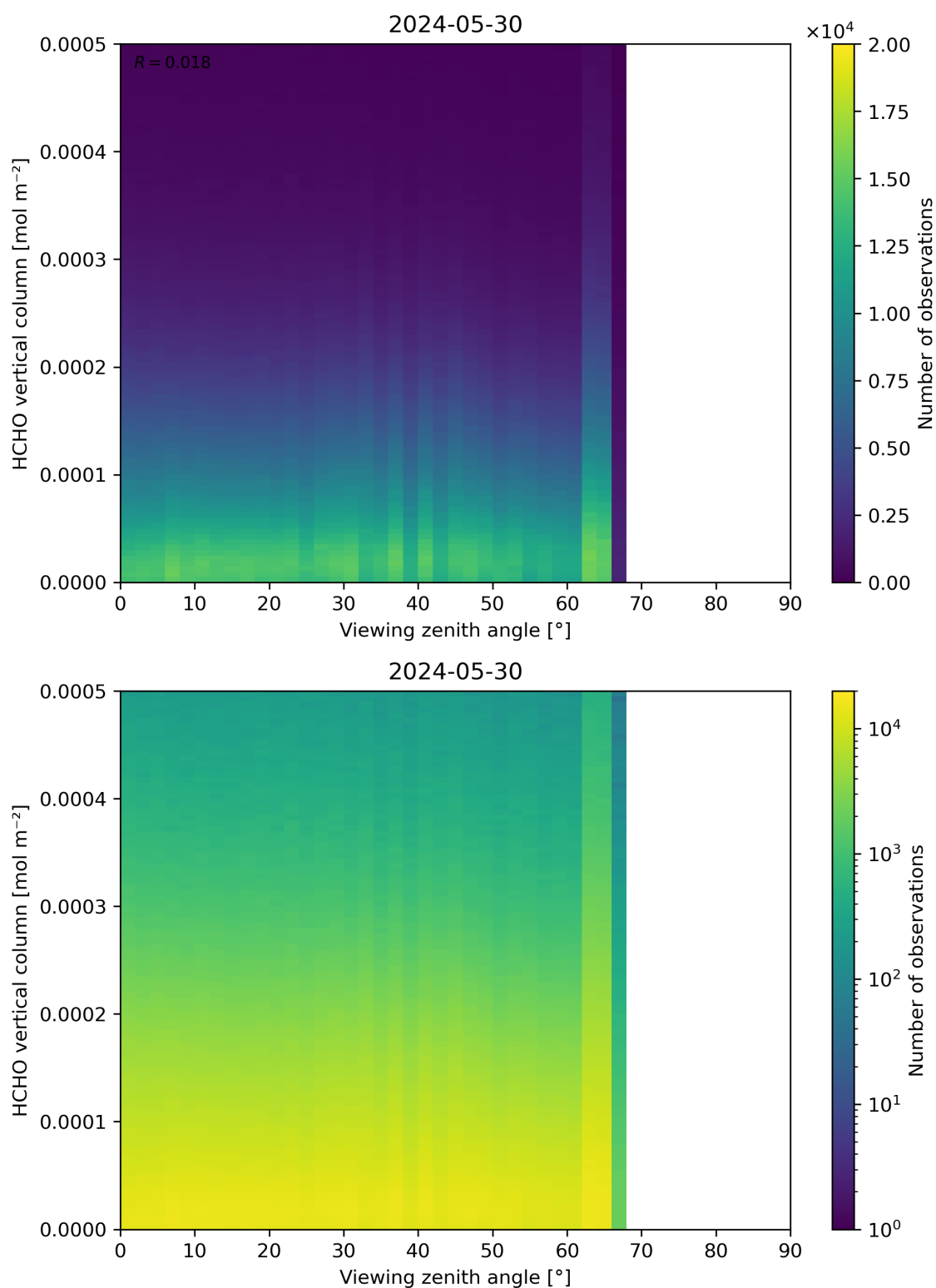
Figure 192: Scatter density plot of “Viewing zenith angle” against “HCHO vertical column” for 2024-05-29 to 2024-05-31.
