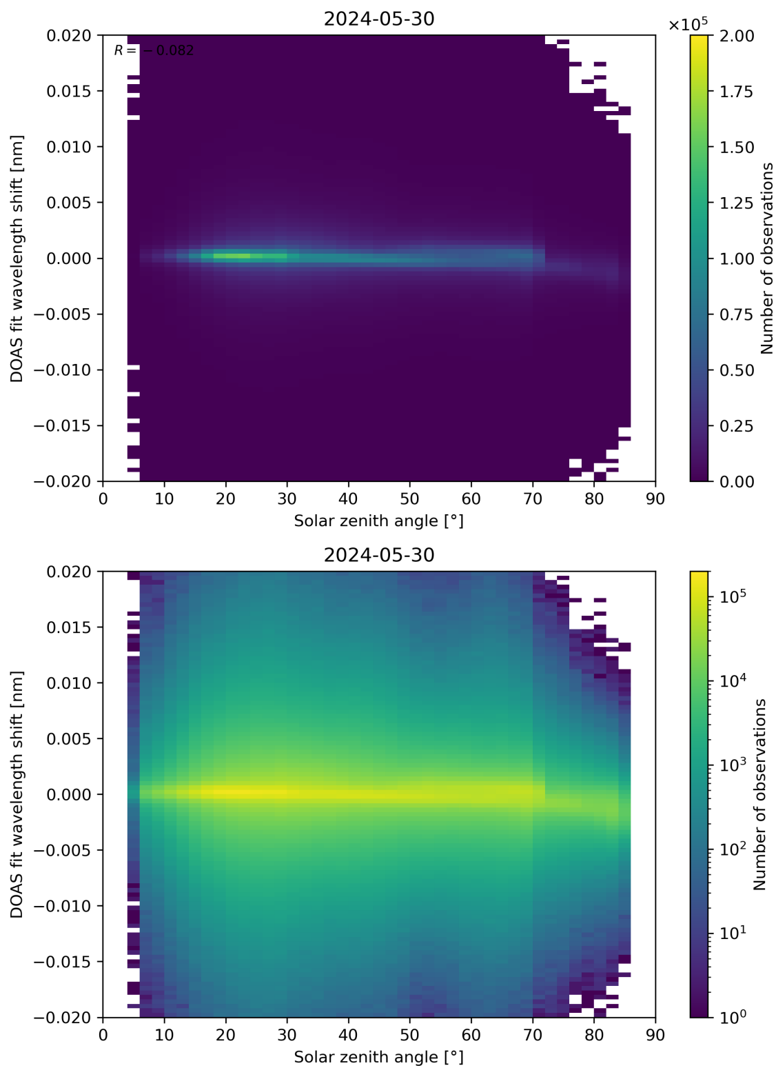
Figure 168: Scatter density plot of “Solar zenith angle” against “DOAS fit wavelength shift” for 2024-05-29 to 2024-05-31.
