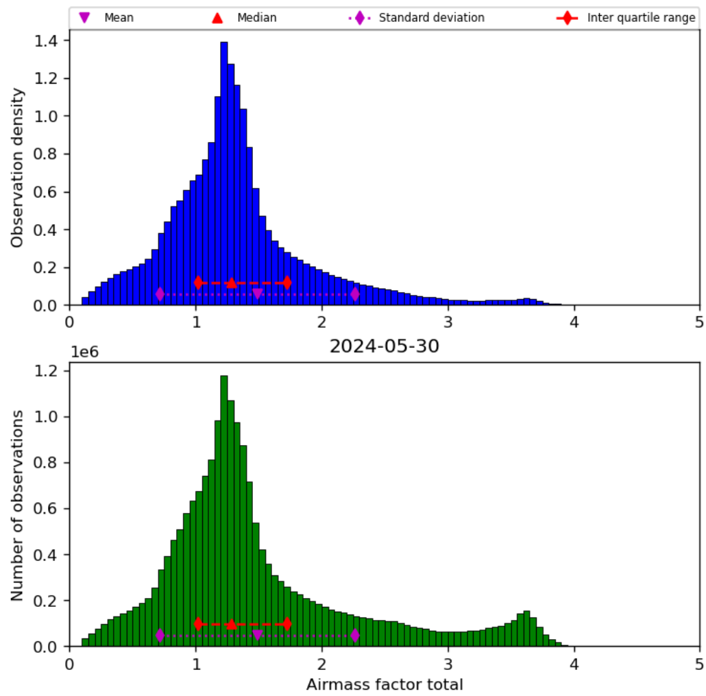
Figure 40: Histogram of “Airmass factor total” for 2024-05-29 to 2024-05-31
