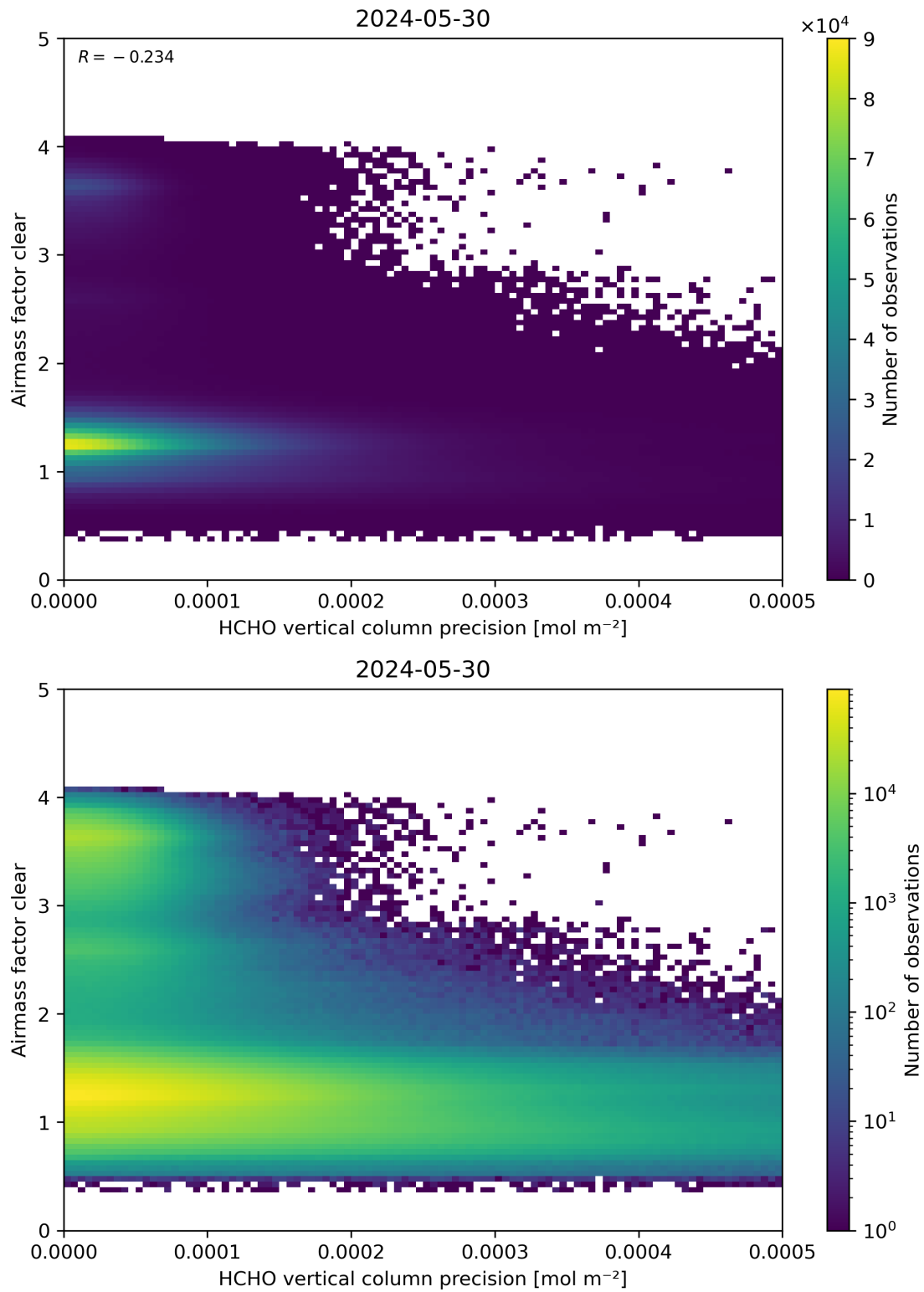
Figure 139: Scatter density plot of “HCHO vertical column precision” against “Airmass factor clear” for 2024-05-29 to 2024-05-31.
