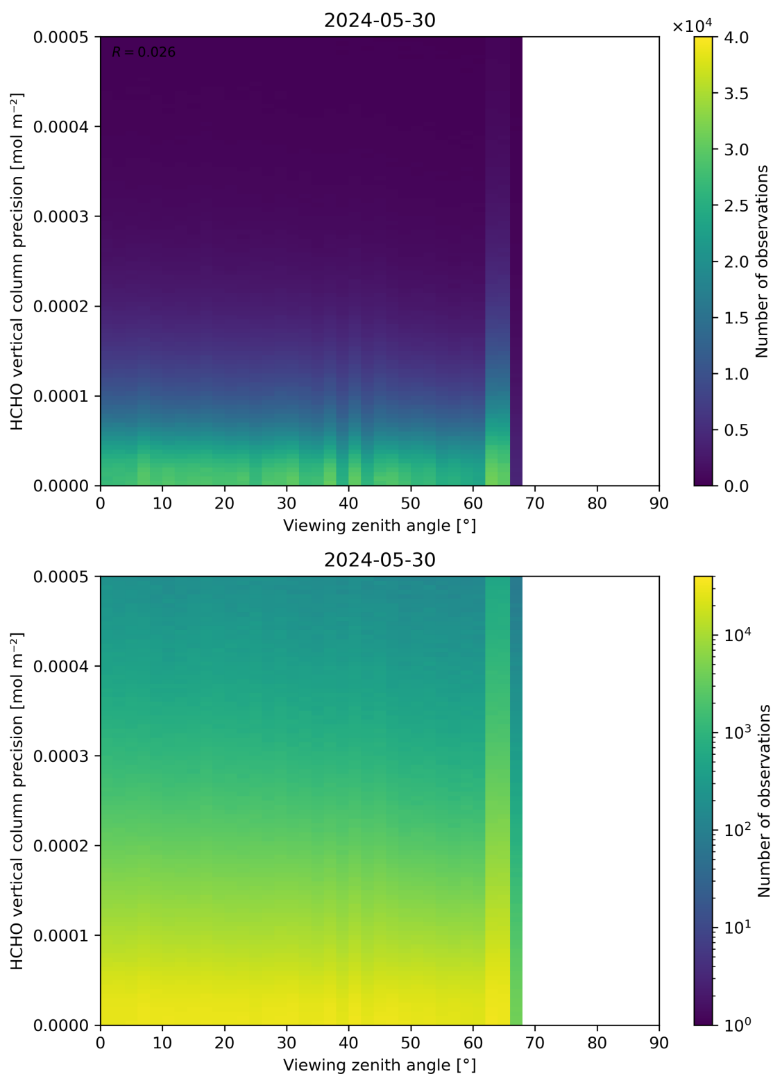
Figure 194: Scatter density plot of “Viewing zenith angle” against “HCHO vertical column precision” for 2024-05-29 to 2024-05-31.
