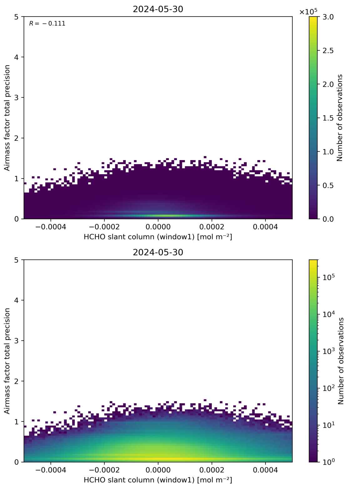
Figure 86: Scatter density plot of “HCHO slant column (window1)” against “Airmass factor total precision” for 2024-05-29 to 2024-05-31.
