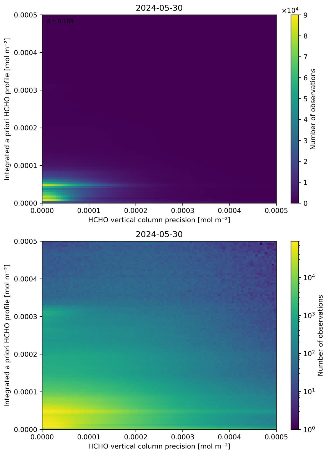
Figure 147: Scatter density plot of “HCHO vertical column precision” against “Integrated a priori HCHO profile” for 2024-05-29 to 2024-05-31.
