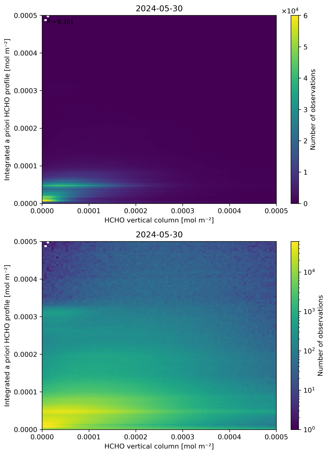
Figure 135: Scatter density plot of “HCHO vertical column” against “Integrated a priori HCHO profile” for 2024-05-29 to 2024-05-31.
