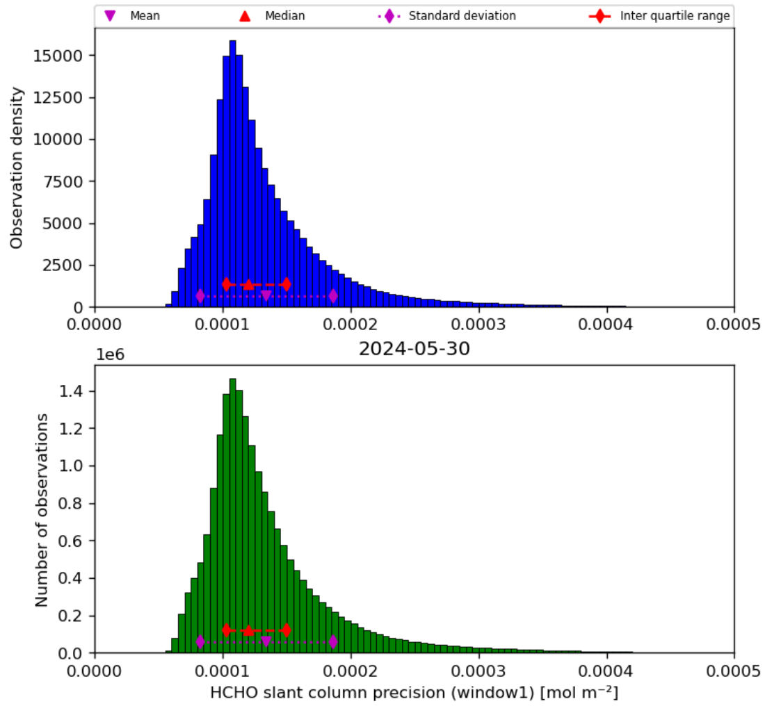
Figure 39: Histogram of “HCHO slant column precision (window1)” for 2024-05-29 to 2024-05-31
