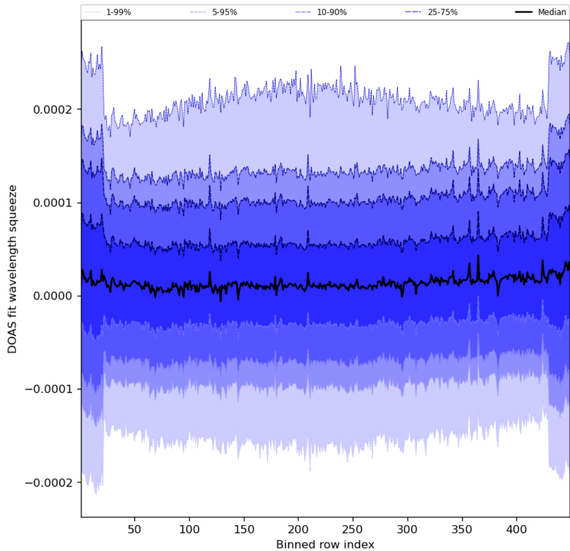
Figure 59: Along track statistics of “DOAS fit wavelength squeeze” for 2024-05-29 to 2024-05-31
