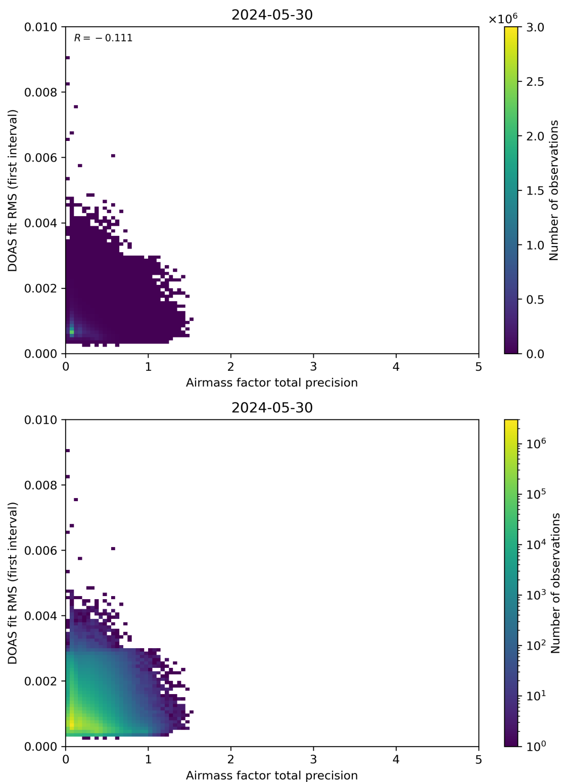
Figure 105: Scatter density plot of “Airmass factor total precision” against “DOAS fit RMS (first interval)” for 2024-05-29 to 2024-05-31.
