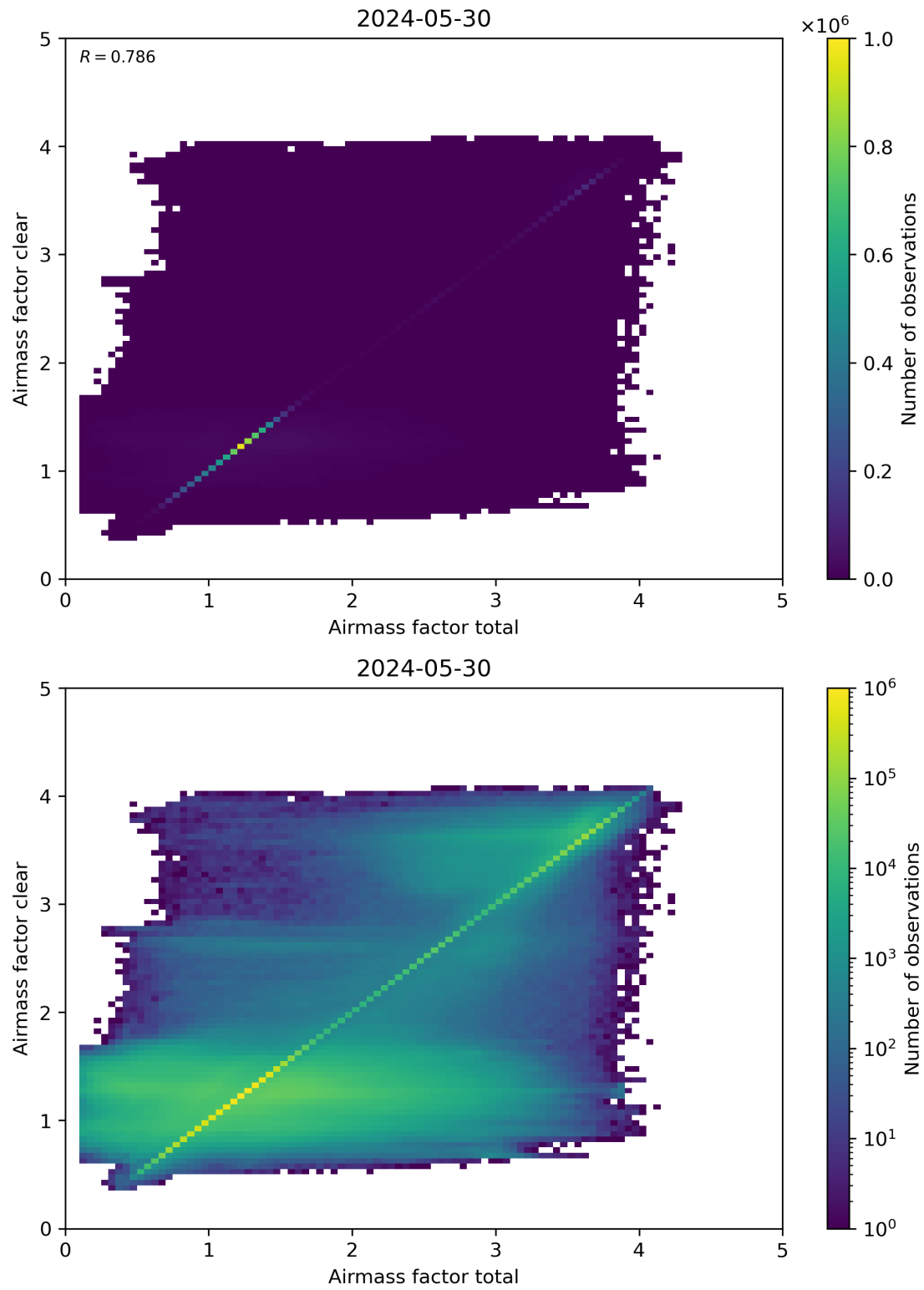
Figure 100: Scatter density plot of “Airmass factor total” against “Airmass factor clear” for 2024-05-29 to 2024-05-31.
