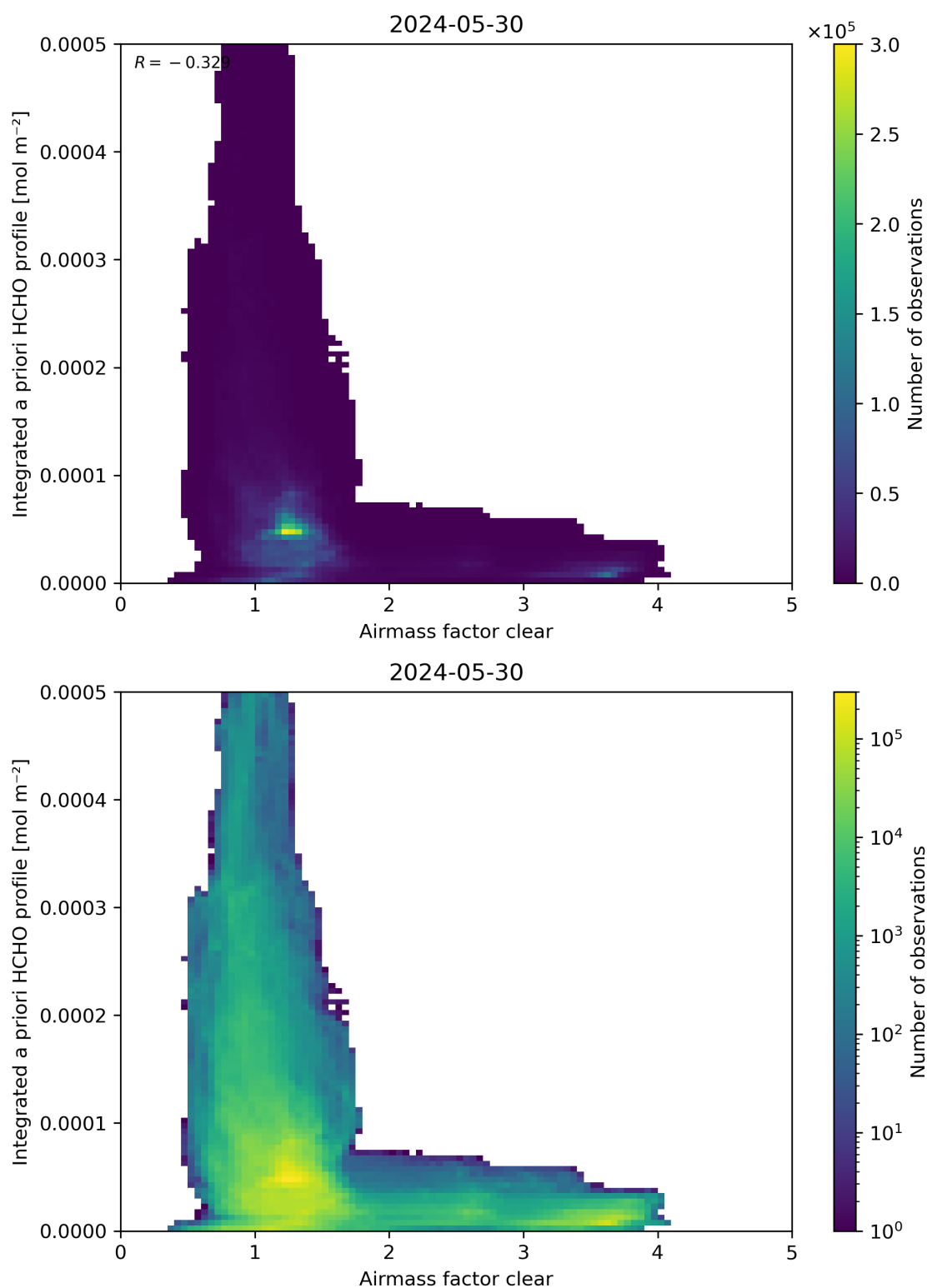
Figure 76: Scatter density plot of “Airmass factor clear” against “Integrated a priori HCHO profile” for 2024-05-29 to 2024-05-31.
