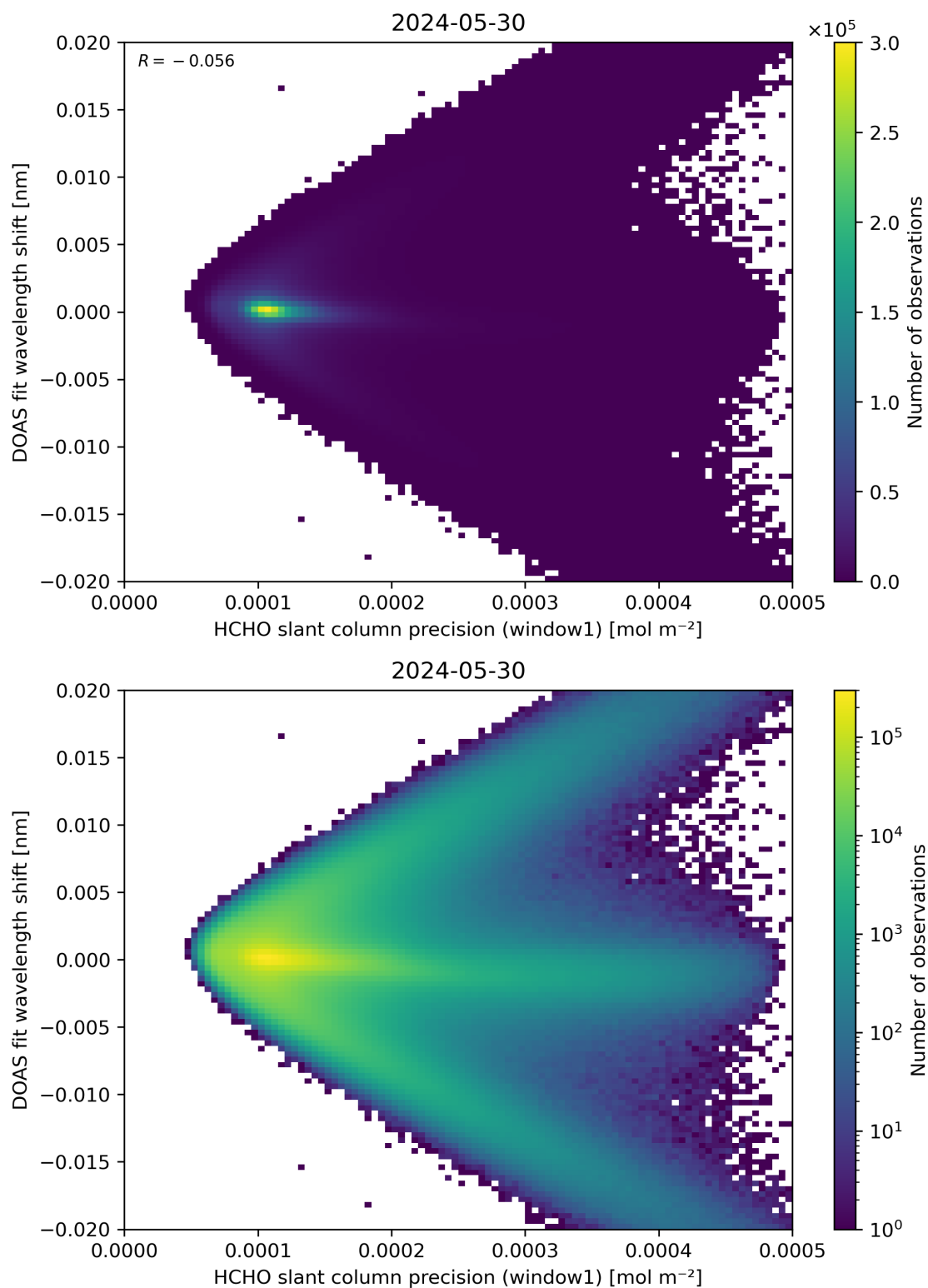
Figure 89: Scatter density plot of “HCHO slant column precision (window1)” against “DOAS fit wavelength shift” for 2024-05-29 to 2024-05-31.
