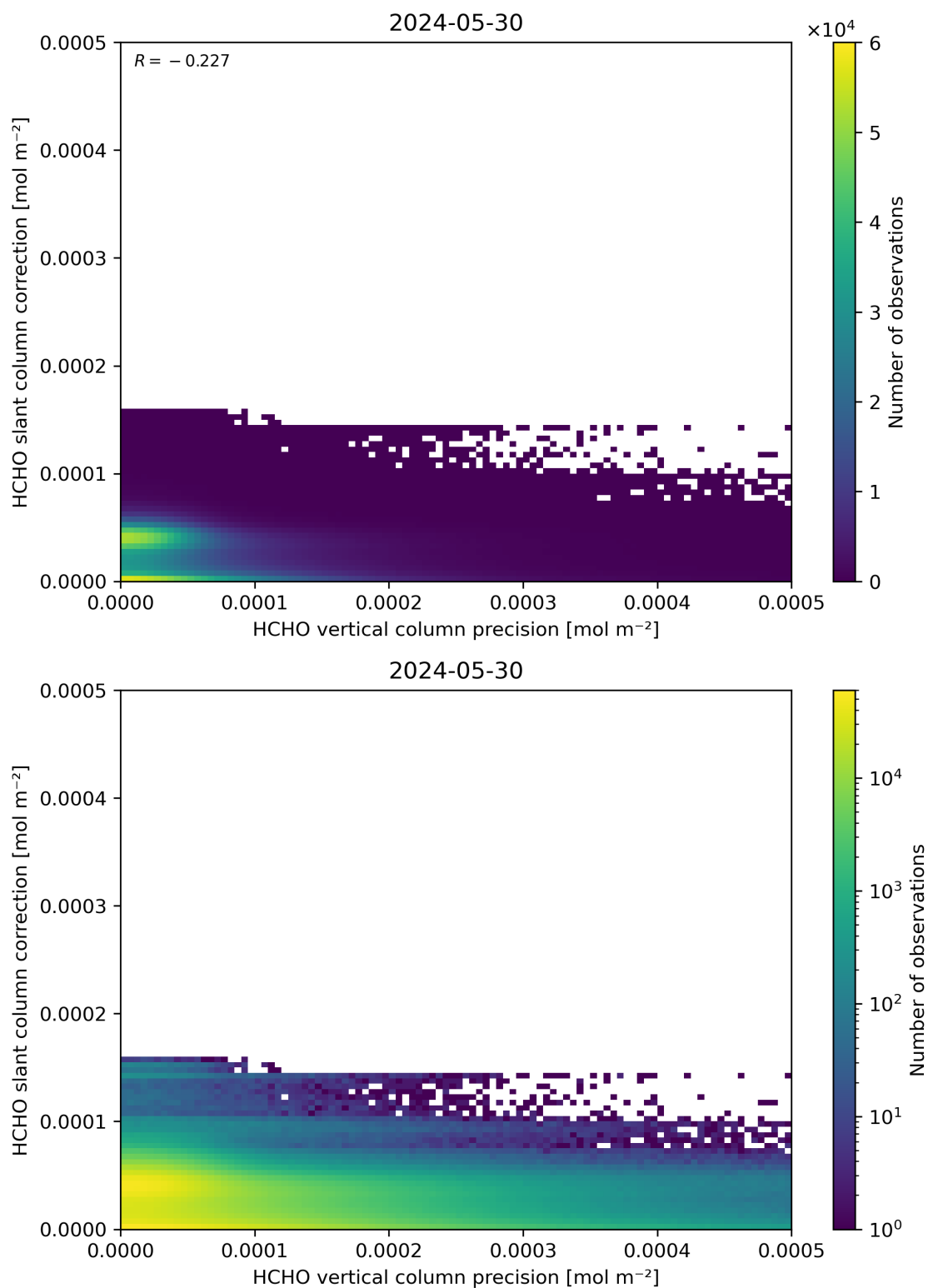
Figure 141: Scatter density plot of “HCHO vertical column precision” against “HCHO slant column correction” for 2024-05-29 to 2024-05-31.
