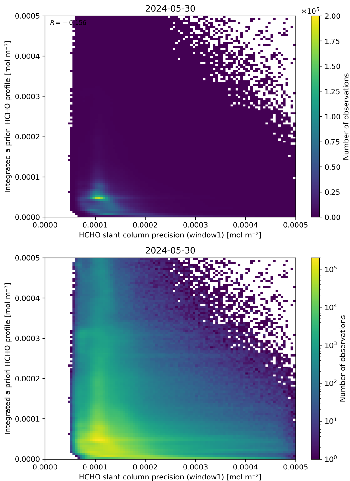
Figure 96: Scatter density plot of “HCHO slant column precision (window1)” against “Integrated a priori HCHO profile” for 2024-05-29 to 2024-05-31.
