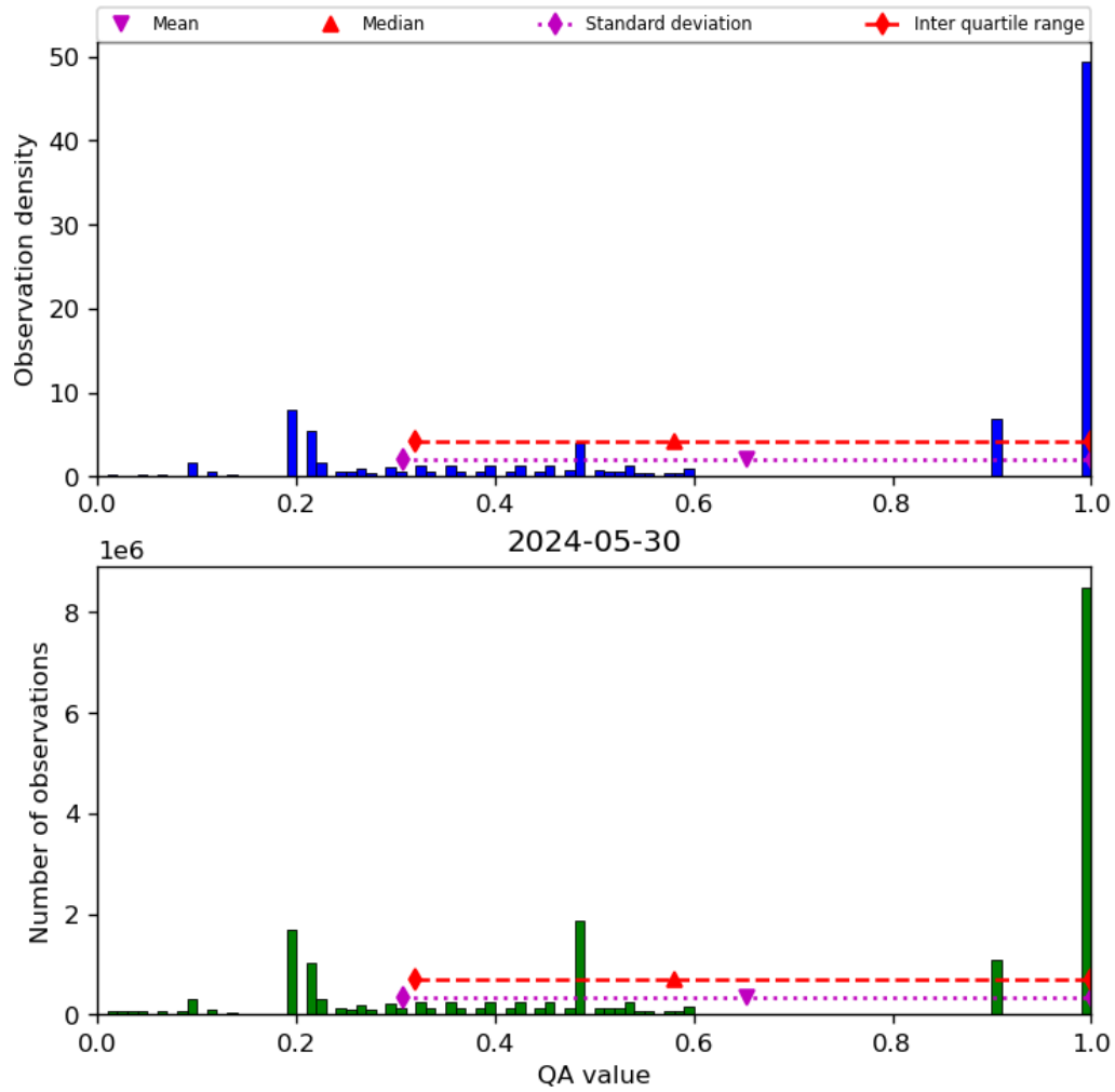
Figure 34: Histogram of “QA value” for 2024-05-29 to 2024-05-31
