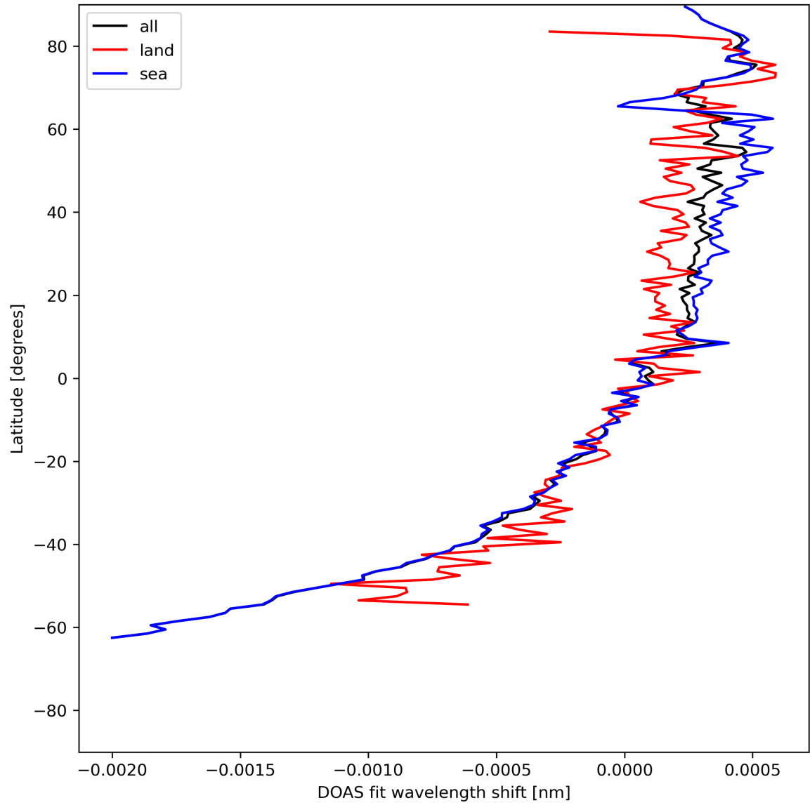
Figure 30: Zonal average of “DOAS fit wavelength shift” for 2024-05-29 to 2024-05-31.
