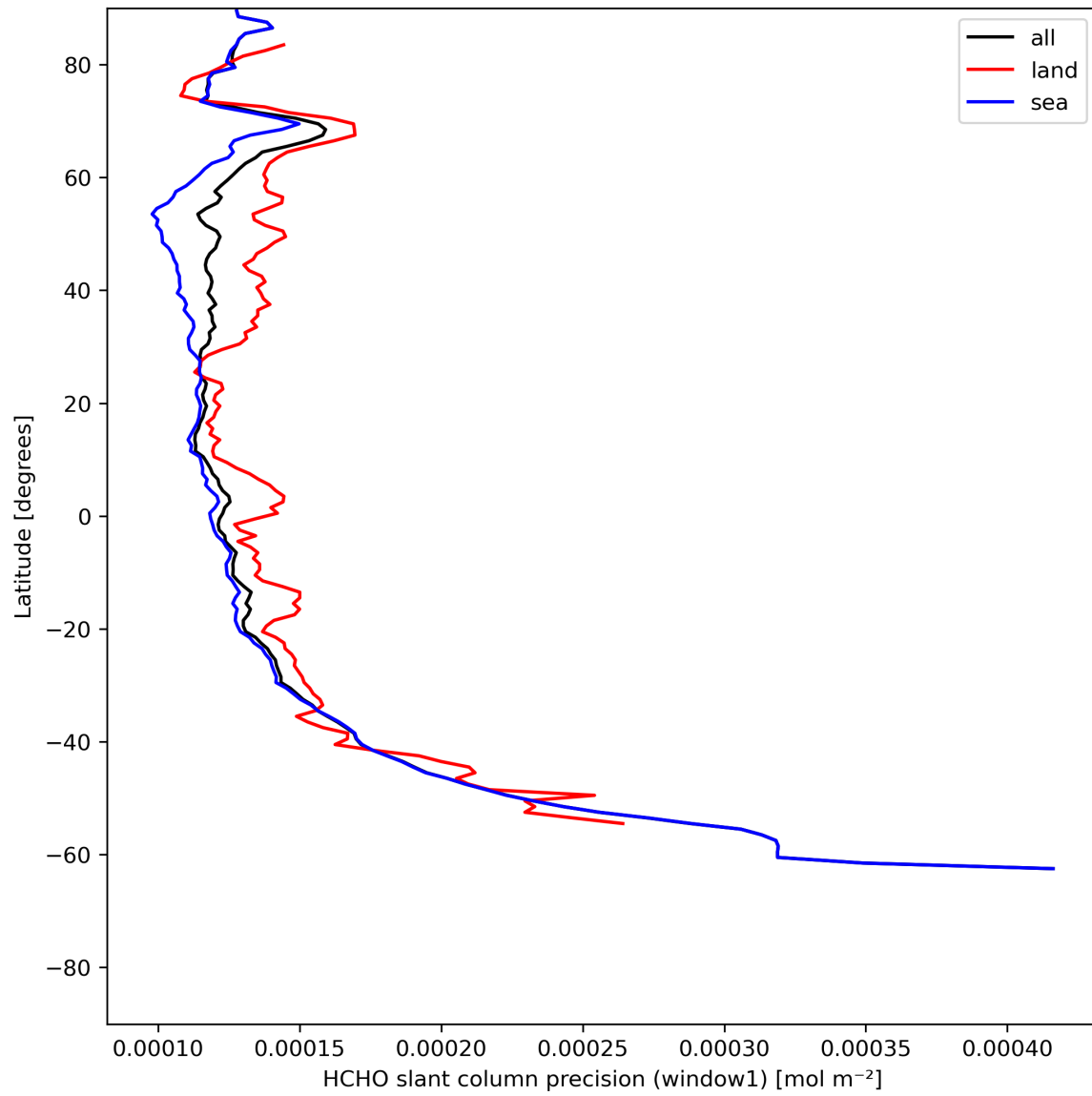
Figure 25: Zonal average of “HCHO slant column precision (window1)” for 2024-05-29 to 2024-05-31.
