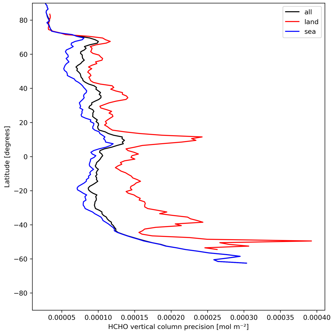
Figure 22: Zonal average of “HCHO vertical column precision” for 2024-05-29 to 2024-05-31.
