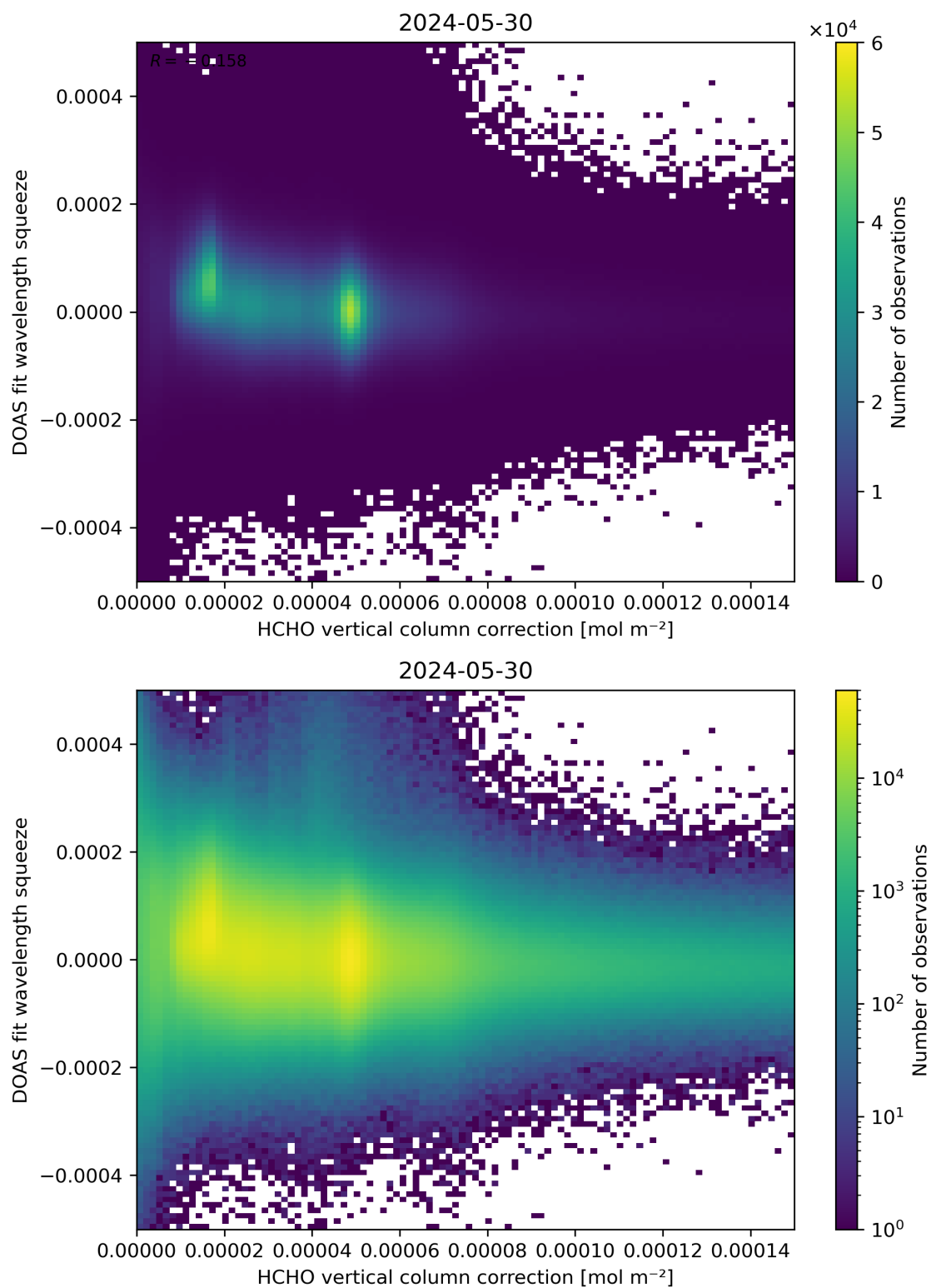
Figure 114: Scatter density plot of “HCHO vertical column correction” against “DOAS fit wavelength squeeze” for 2024-05-29 to 2024-05-31.
