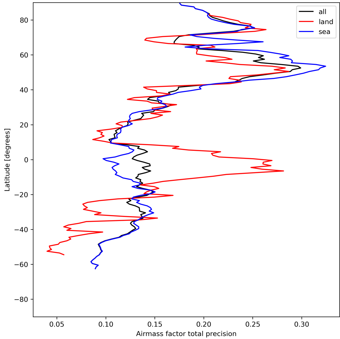
Figure 27: Zonal average of “Airmass factor total precision” for 2024-05-29 to 2024-05-31.
