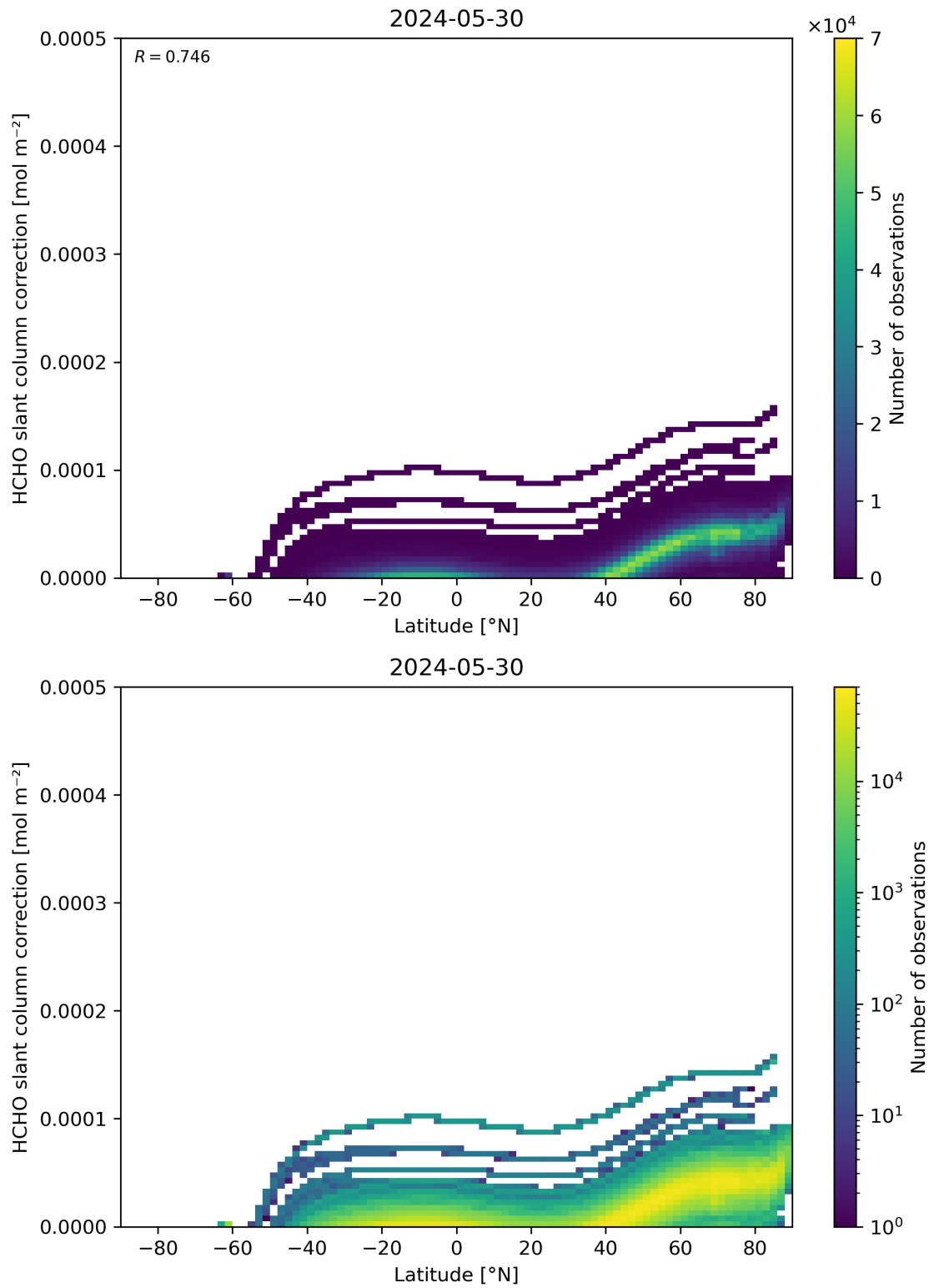
Figure 158: Scatter density plot of “Latitude” against “HCHO slant column correction” for 2024-05-29 to 2024-05-31.
