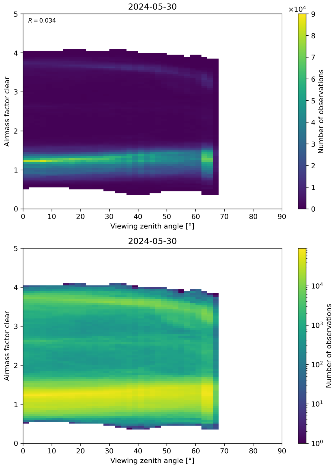
Figure 185: Scatter density plot of “Viewing zenith angle” against “Airmass factor clear” for 2024-05-29 to 2024-05-31.
