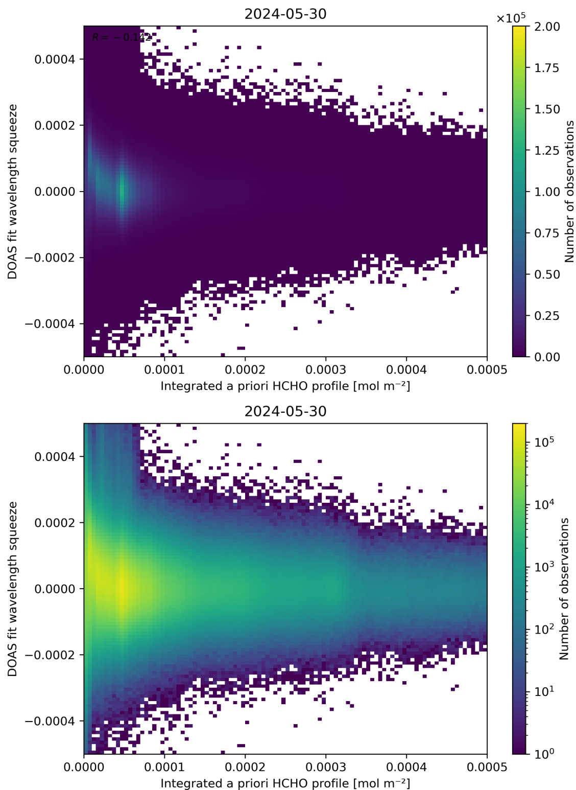
Figure 150: Scatter density plot of “Integrated a priori HCHO profile” against “DOAS fit wavelength squeeze” for 2024-05-29 to 2024-05-31.
