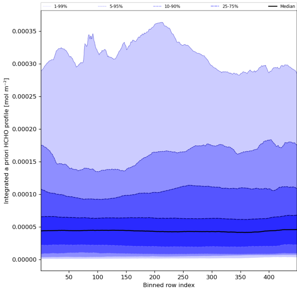
Figure 57: Along track statistics of “Integrated a priori HCHO profile” for 2024-05-29 to 2024-05-31
