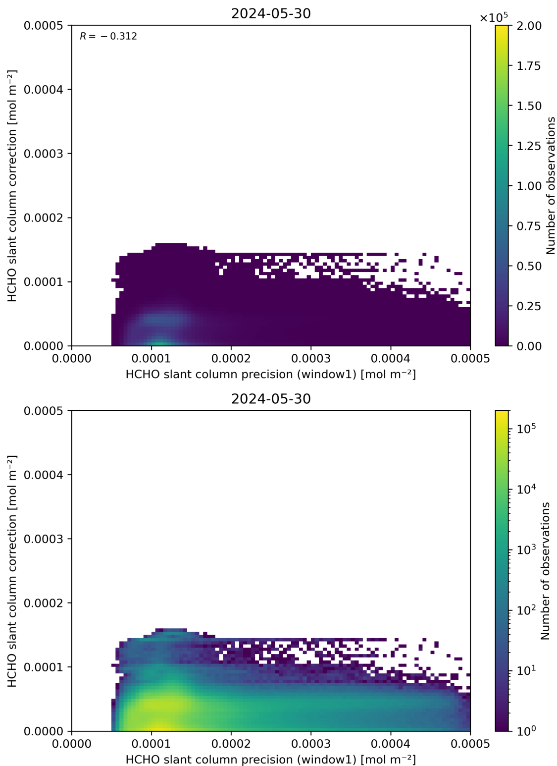
Figure 93: Scatter density plot of “HCHO slant column precision (window1)” against “HCHO slant column correction” for 2024-05-29 to 2024-05-31.
