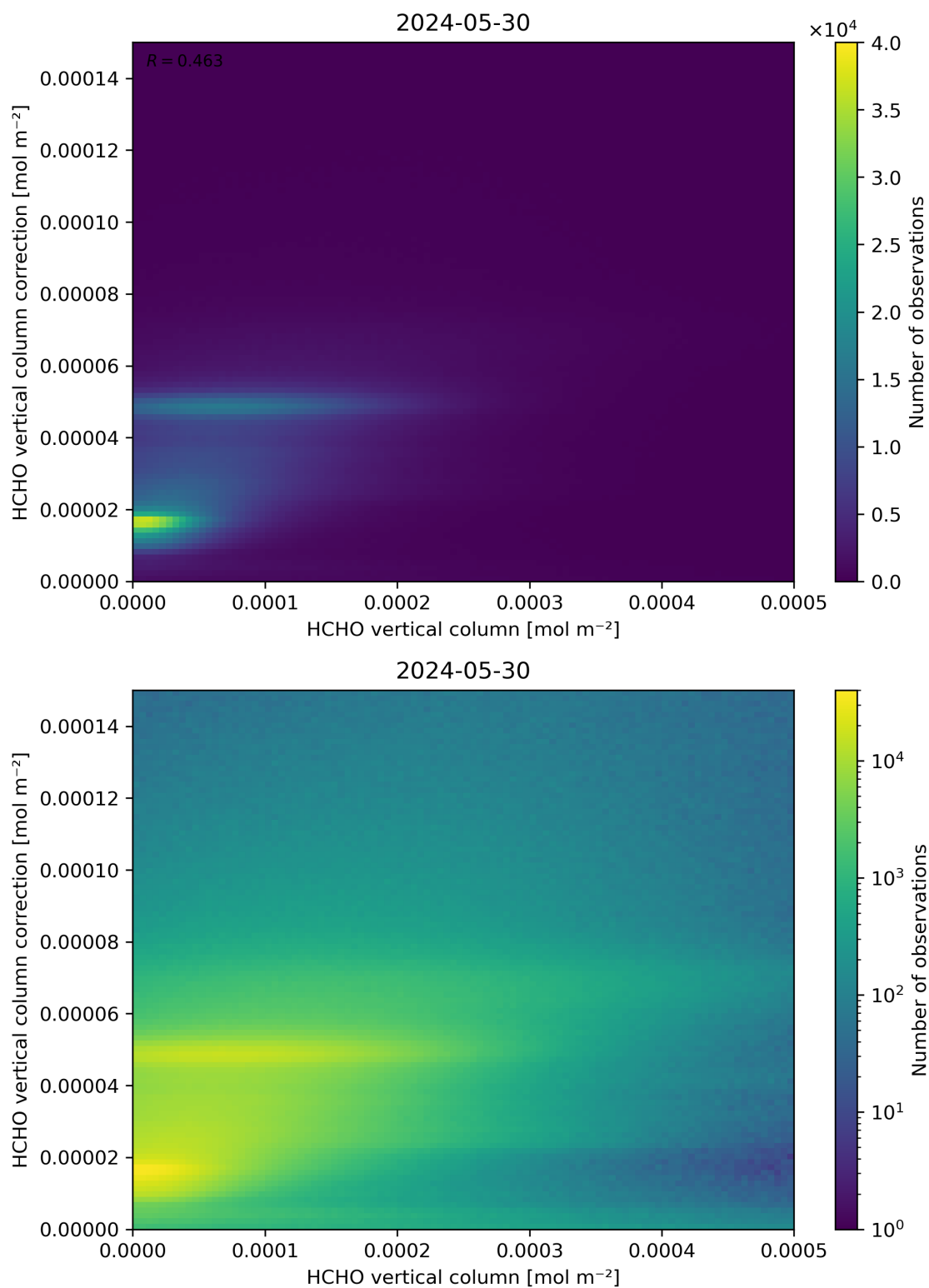
Figure 133: Scatter density plot of “HCHO vertical column” against “HCHO vertical column correction” for 2024-05-29 to 2024-05-31.
