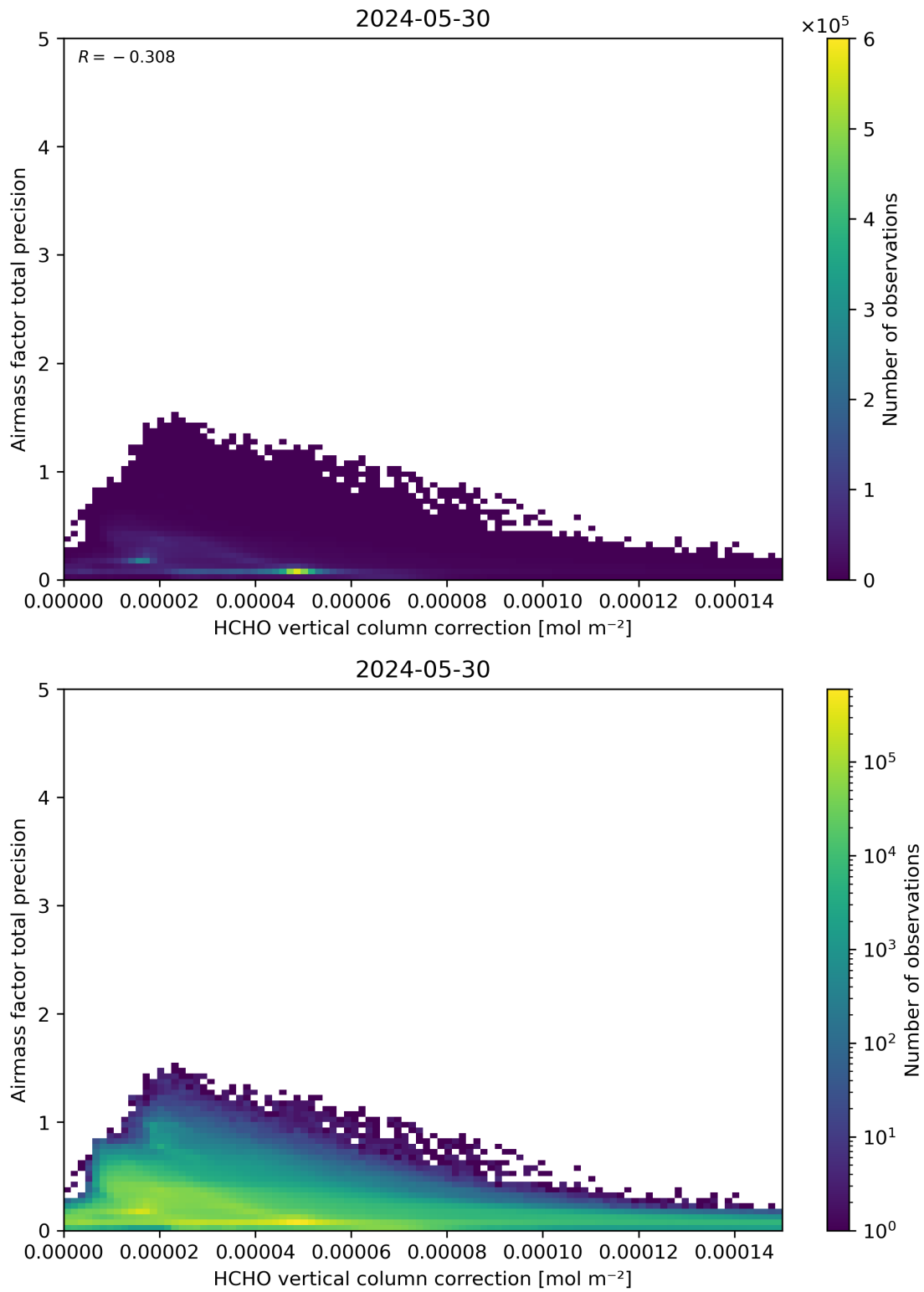
Figure 121: Scatter density plot of “HCHO vertical column correction” against “Airmass factor total precision” for 2024-05-29 to 2024-05-31.
