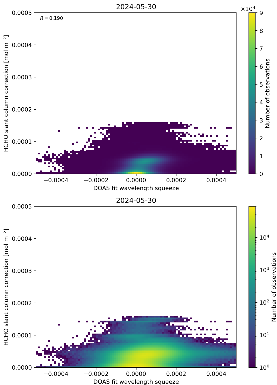
Figure 70: Scatter density plot of “DOAS fit wavelength squeeze” against “HCHO slant column correction” for 2024-05-29 to 2024-05-31.
