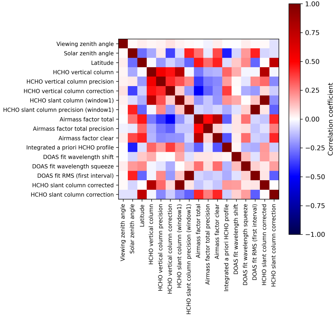
Figure 2: Map of correlation matrix for 2024-05-29 to 2024-05-31.
