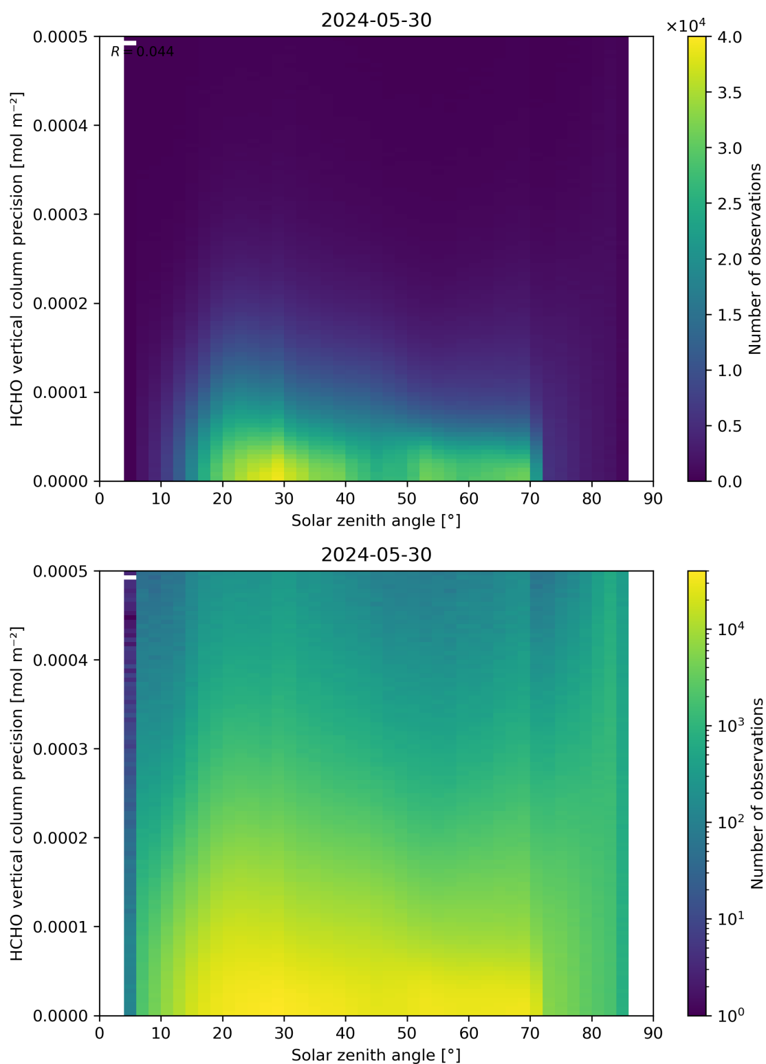
Figure 179: Scatter density plot of “Solar zenith angle” against “HCHO vertical column precision” for 2024-05-29 to 2024-05-31.
