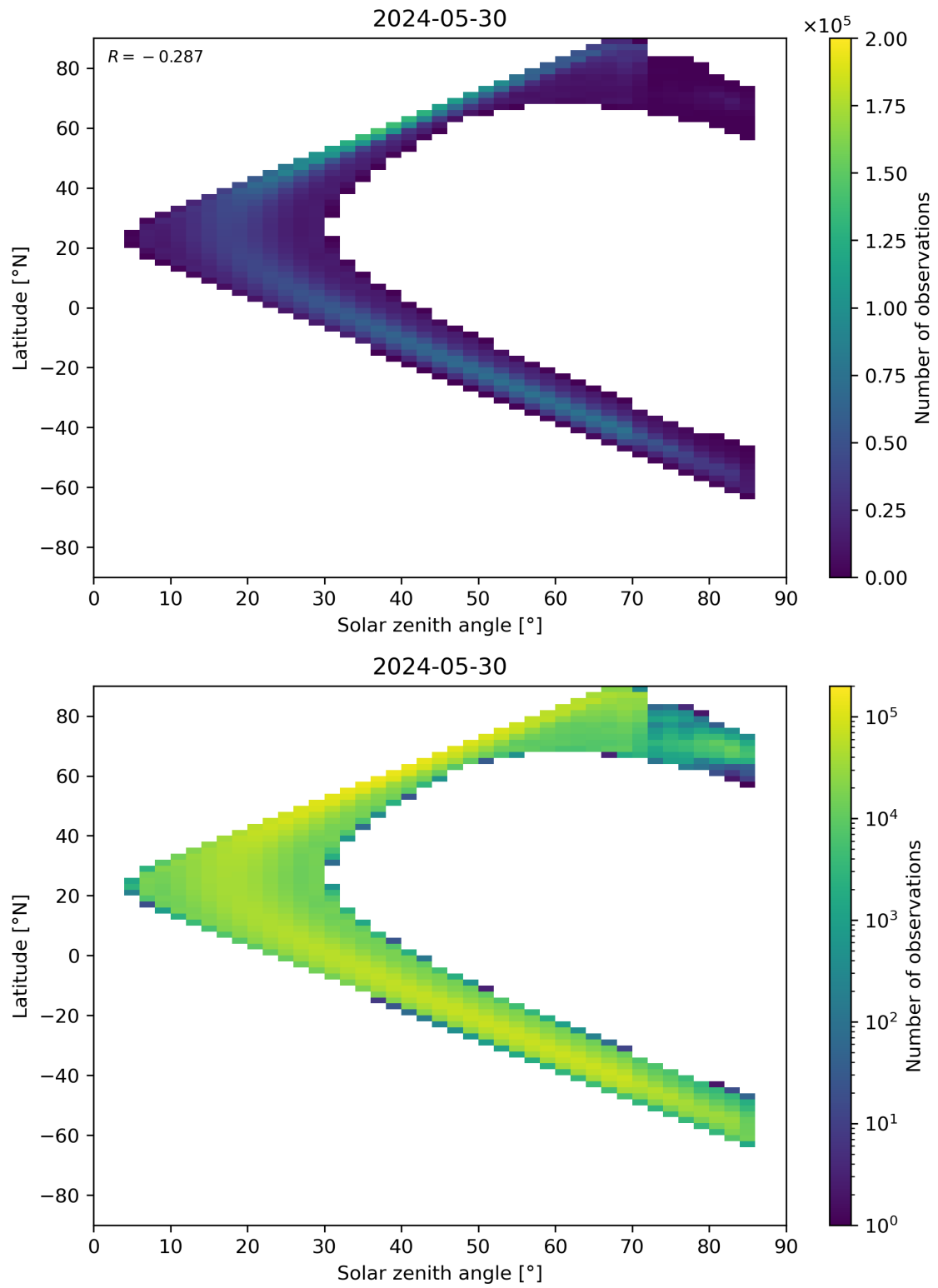
Figure 181: Scatter density plot of “Solar zenith angle” against “Latitude” for 2024-05-29 to 2024-05-31.
