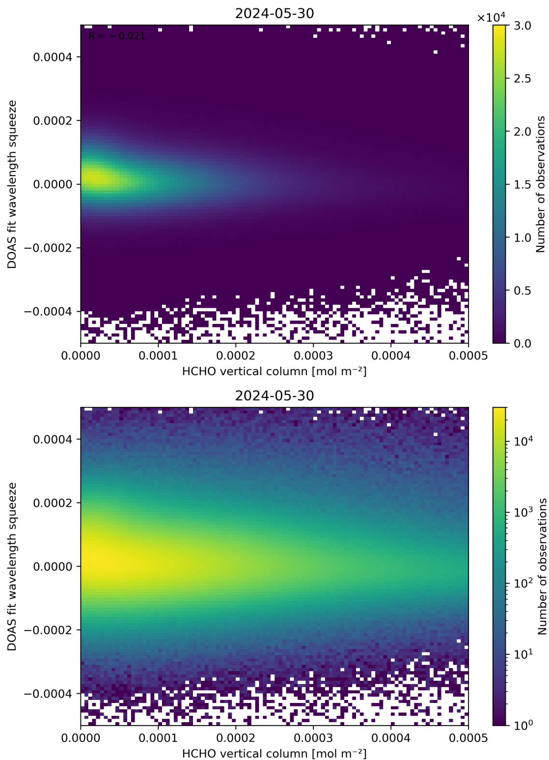
Figure 125: Scatter density plot of “HCHO vertical column” against “DOAS fit wavelength squeeze” for 2024-05-29 to 2024-05-31.
