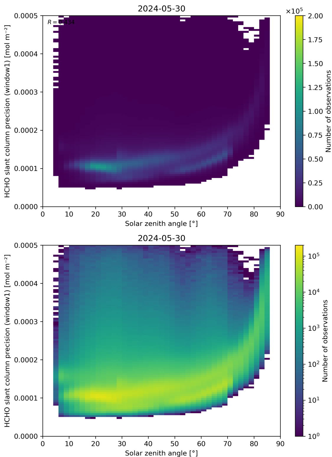
Figure 174: Scatter density plot of “Solar zenith angle” against “HCHO slant column precision (window1)” for 2024-05-29 to 2024-05-31.
