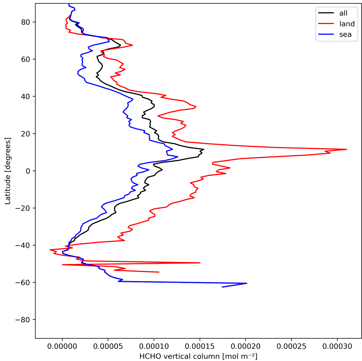
Figure 21: Zonal average of “HCHO vertical column” for 2024-05-29 to 2024-05-31.
