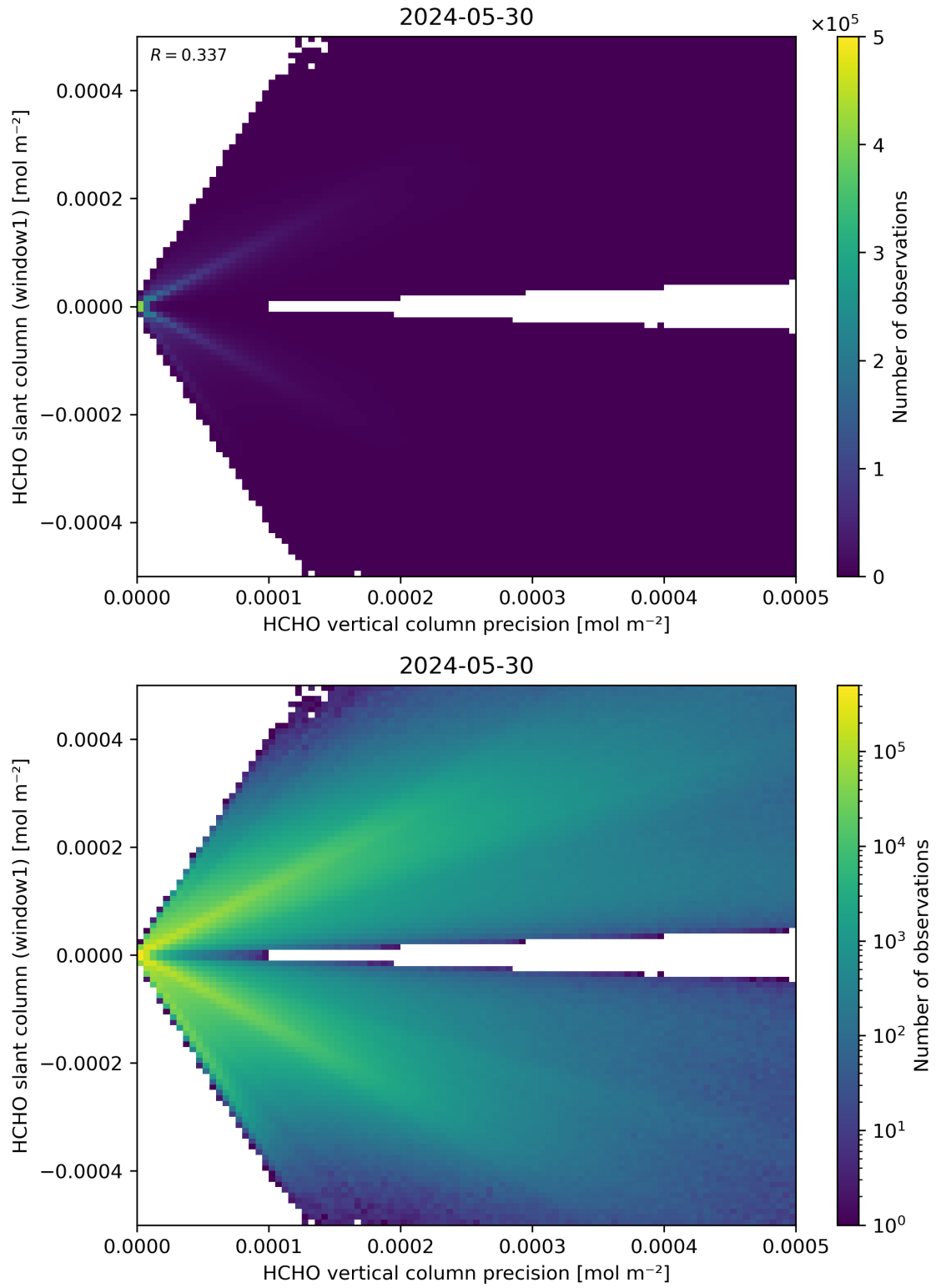
Figure 142: Scatter density plot of “HCHO vertical column precision” against “HCHO slant column (window1)” for 2024-05-29 to 2024-05-31.
