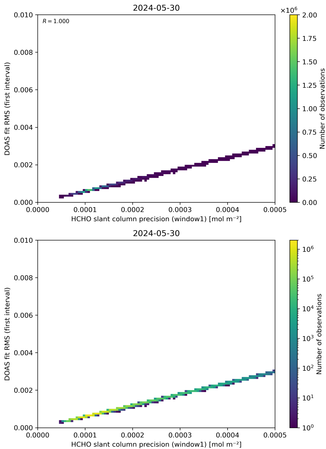
Figure 88: Scatter density plot of “HCHO slant column precision (window1)” against “DOAS fit RMS (first interval)” for 2024-05-29 to 2024-05-31.
