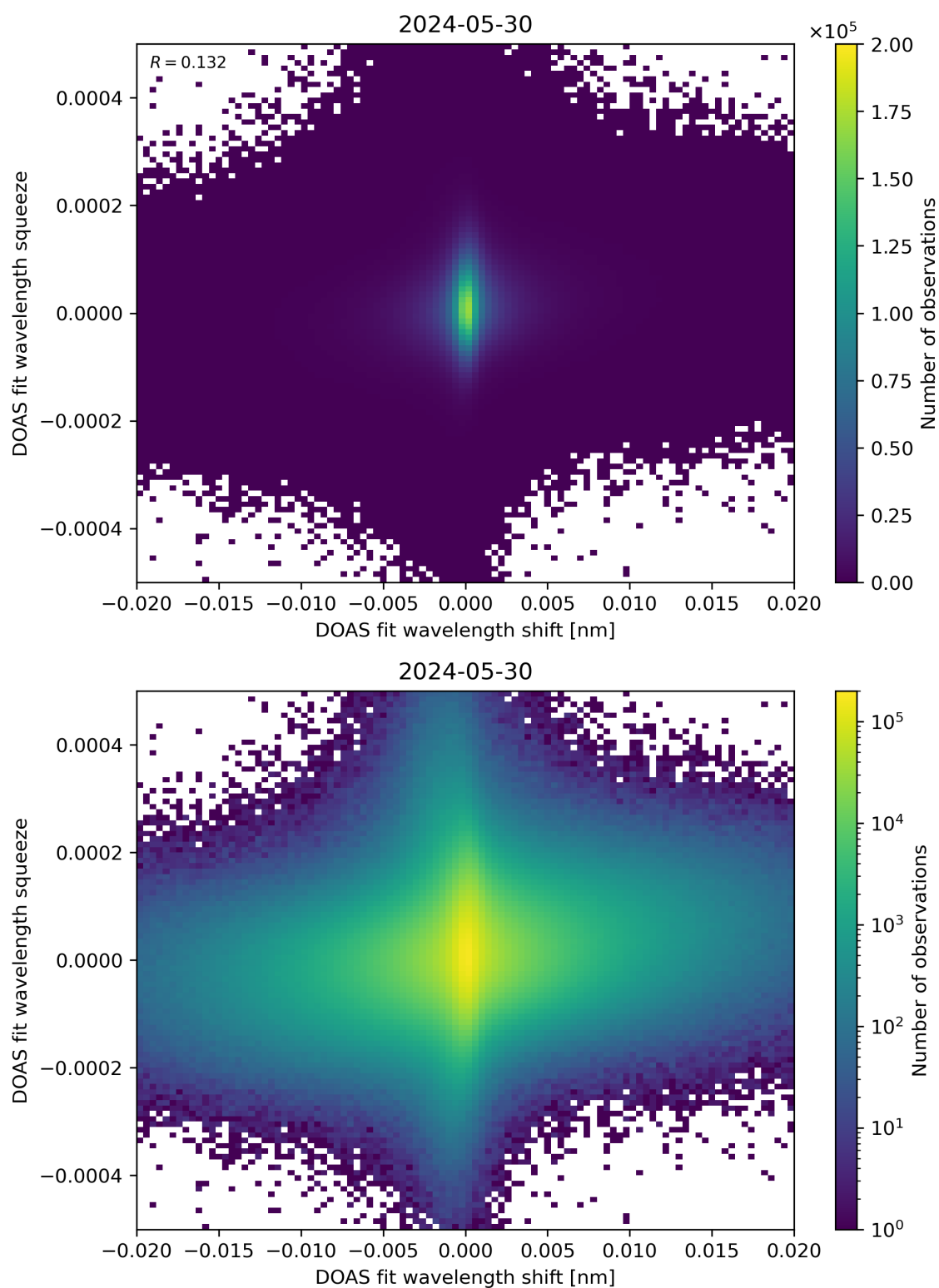
Figure 65: Scatter density plot of “DOAS fit wavelength shift” against “DOAS fit wavelength squeeze” for 2024-05-29 to 2024-05-31.
