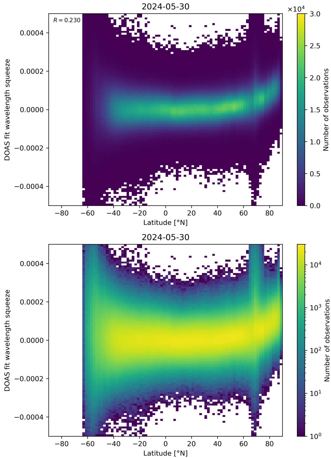
Figure 155: Scatter density plot of “Latitude” against “DOAS fit wavelength squeeze” for 2024-05-29 to 2024-05-31.
