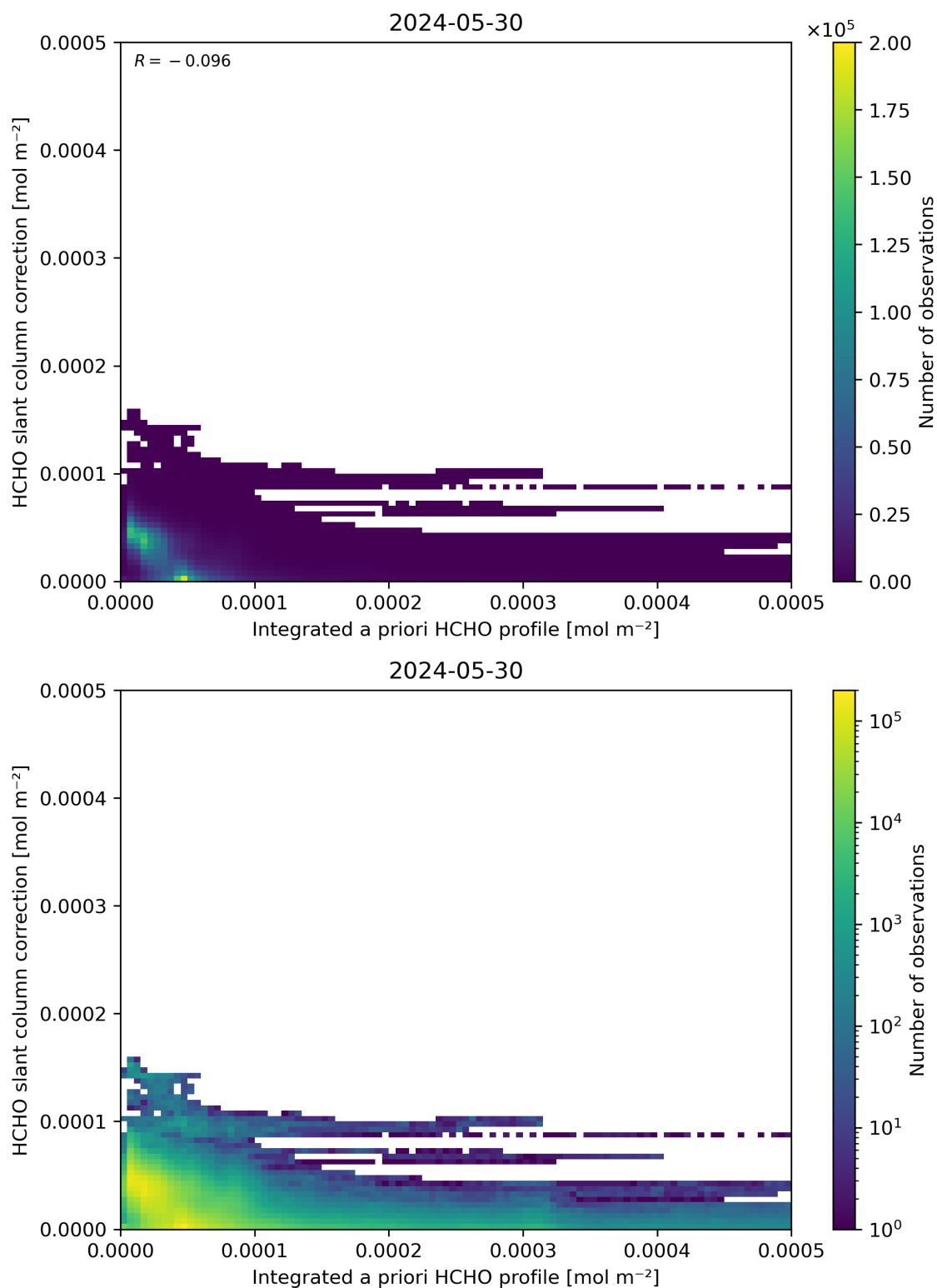
Figure 152: Scatter density plot of “Integrated a priori HCHO profile” against “HCHO slant column correction” for 2024-05-29 to 2024-05-31.
