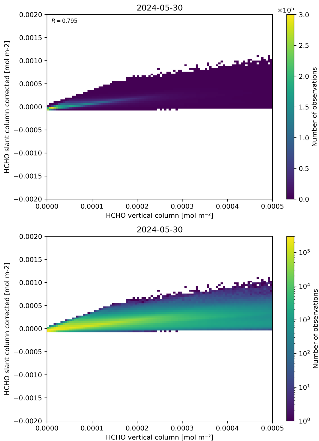
Figure 127: Scatter density plot of “HCHO vertical column” against “HCHO slant column corrected” for 2024-05-29 to 2024-05-31.
