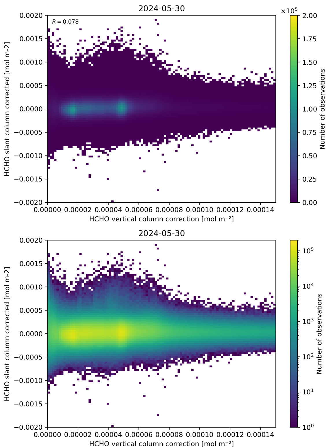
Figure 116: Scatter density plot of “HCHO vertical column correction” against “HCHO slant column corrected” for 2024-05-29 to 2024-05-31.
