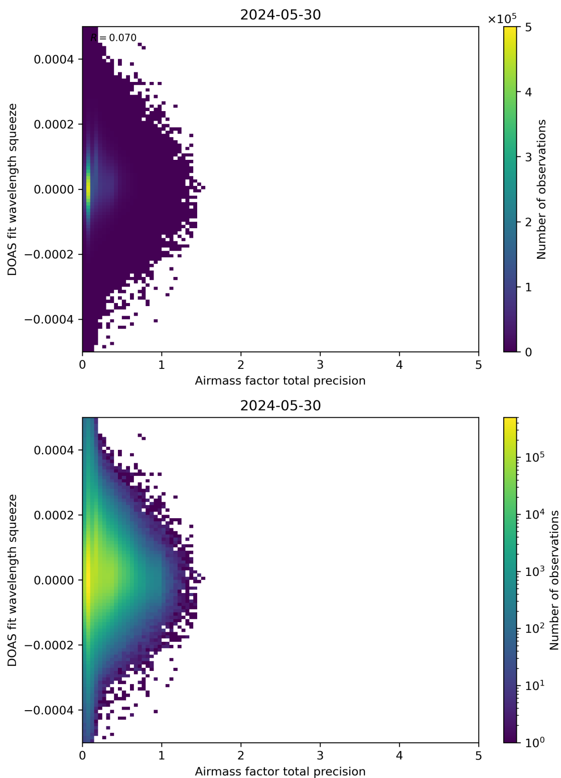
Figure 107: Scatter density plot of “Airmass factor total precision” against “DOAS fit wavelength squeeze” for 2024-05-29 to 2024-05-31.
