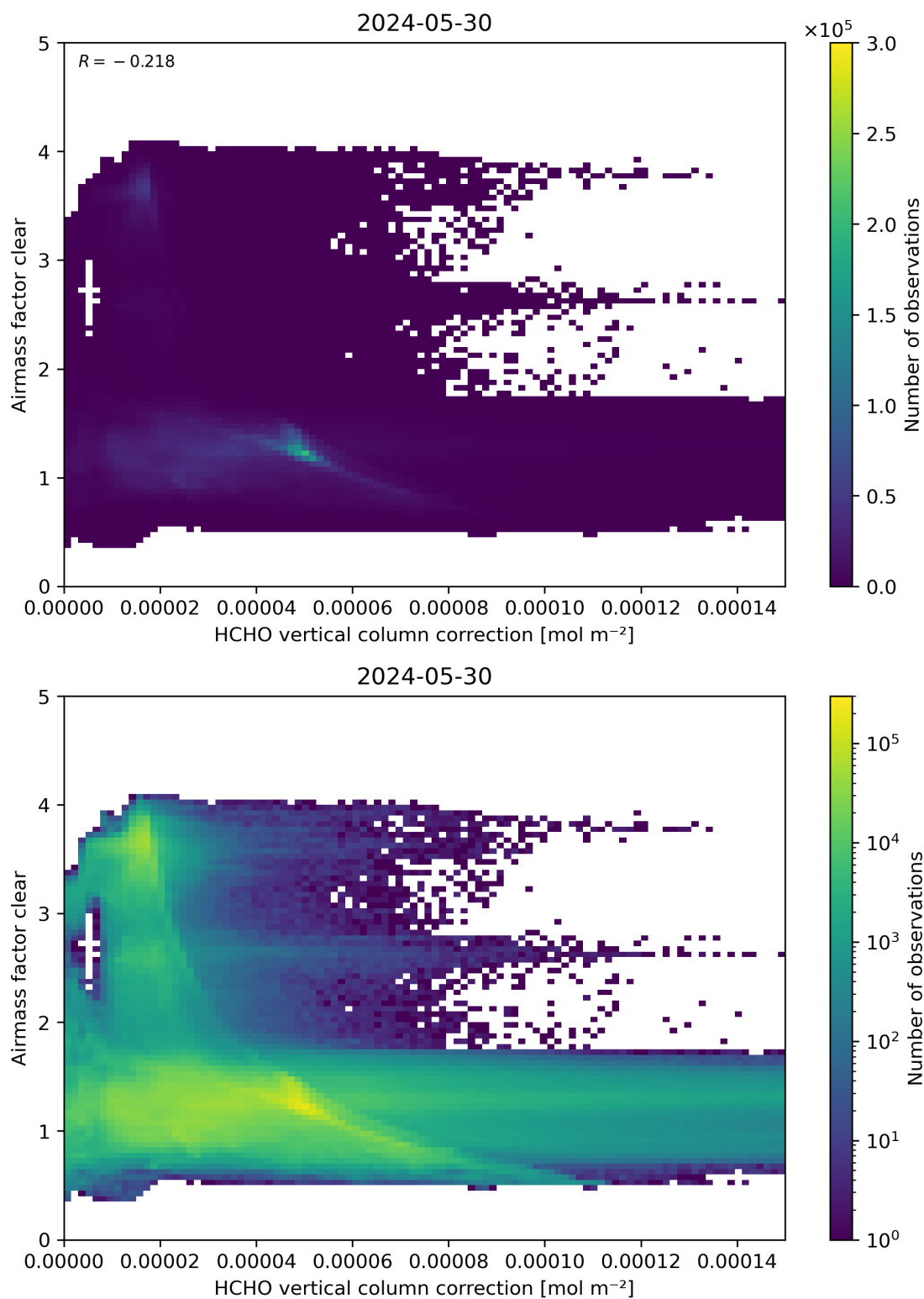
Figure 115: Scatter density plot of “HCHO vertical column correction” against “Airmass factor clear” for 2024-05-29 to 2024-05-31.
