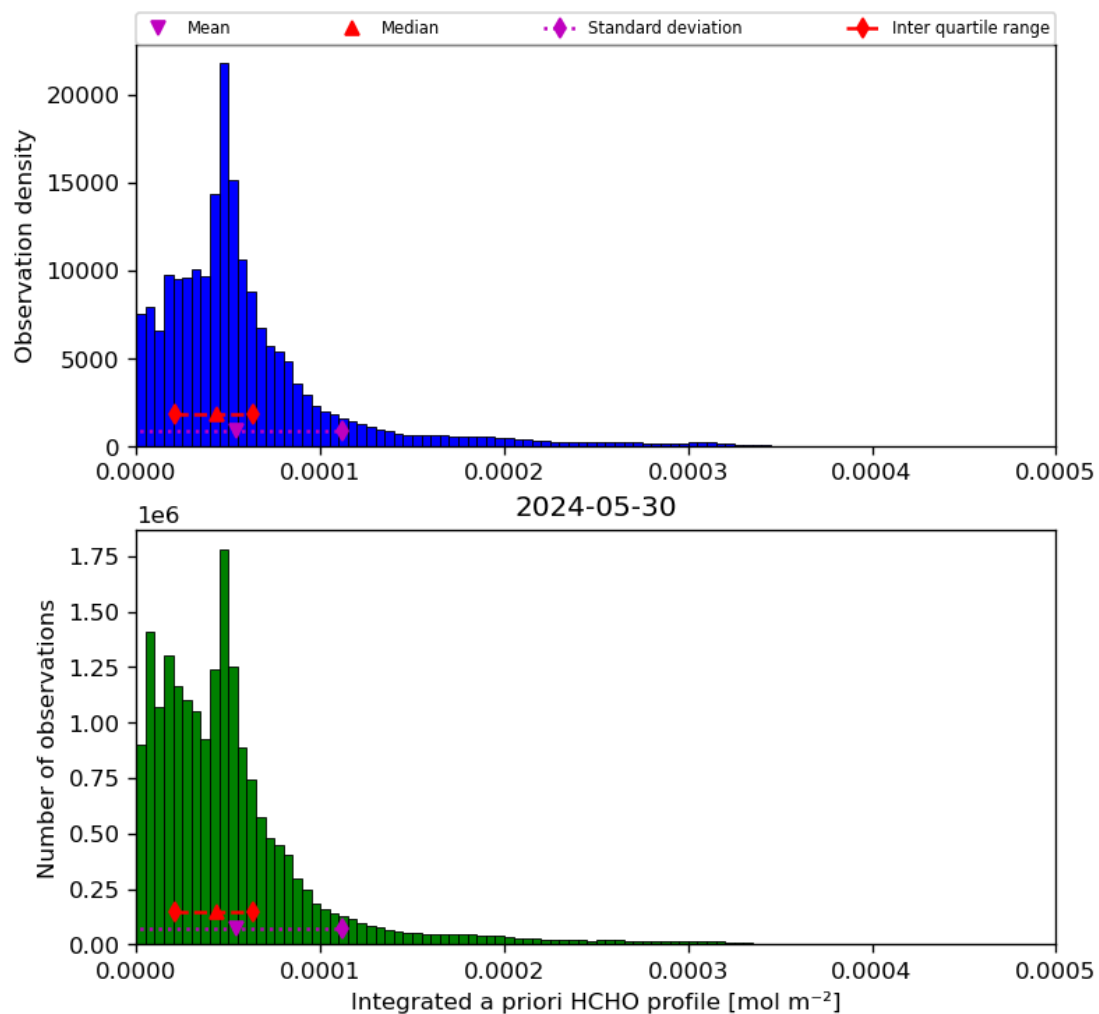
Figure 43: Histogram of “Integrated a priori HCHO profile” for 2024-05-29 to 2024-05-31
