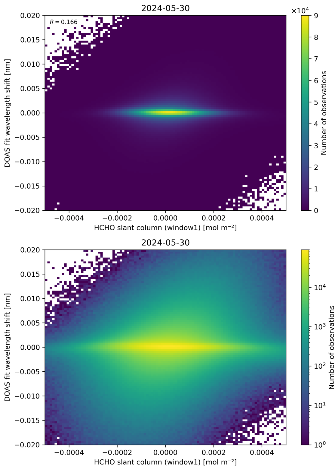
Figure 79: Scatter density plot of “HCHO slant column (window1)” against “DOAS fit wavelength shift” for 2024-05-29 to 2024-05-31.
