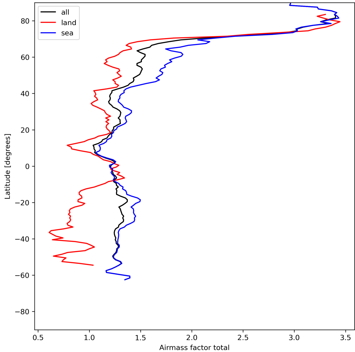
Figure 26: Zonal average of “Airmass factor total” for 2024-05-29 to 2024-05-31.
