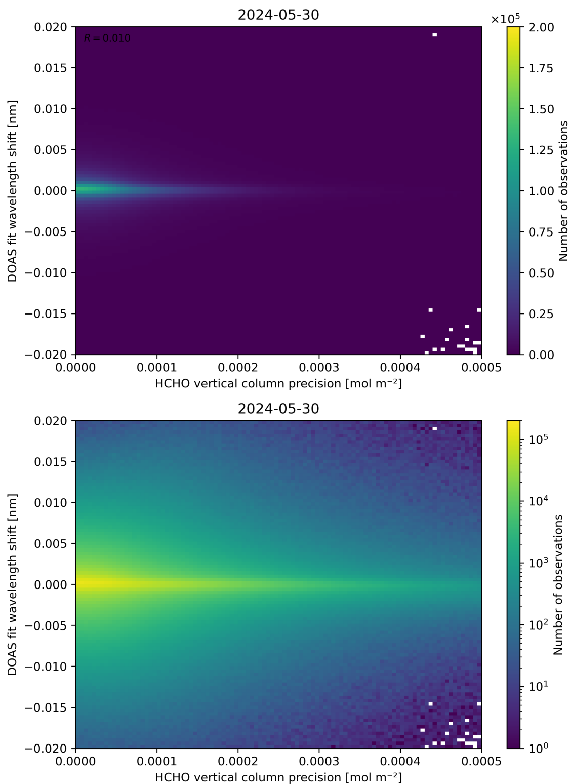
Figure 137: Scatter density plot of “HCHO vertical column precision” against “DOAS fit wavelength shift” for 2024-05-29 to 2024-05-31.
