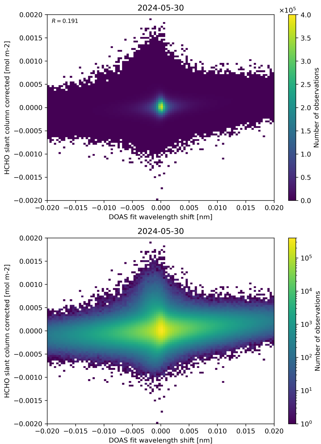
Figure 66: Scatter density plot of “DOAS fit wavelength shift” against “HCHO slant column corrected” for 2024-05-29 to 2024-05-31.
