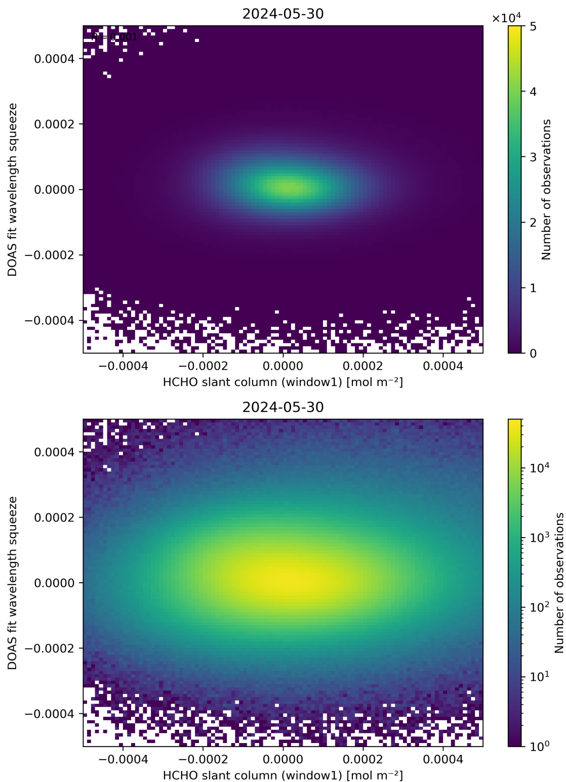
Figure 80: Scatter density plot of “HCHO slant column (window1)” against “DOAS fit wavelength squeeze” for 2024-05-29 to 2024-05-31.
