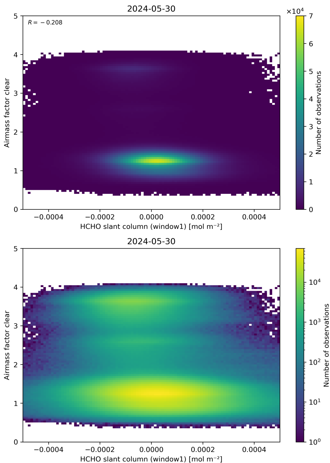
Figure 81: Scatter density plot of “HCHO slant column (window1)” against “Airmass factor clear” for 2024-05-29 to 2024-05-31.
