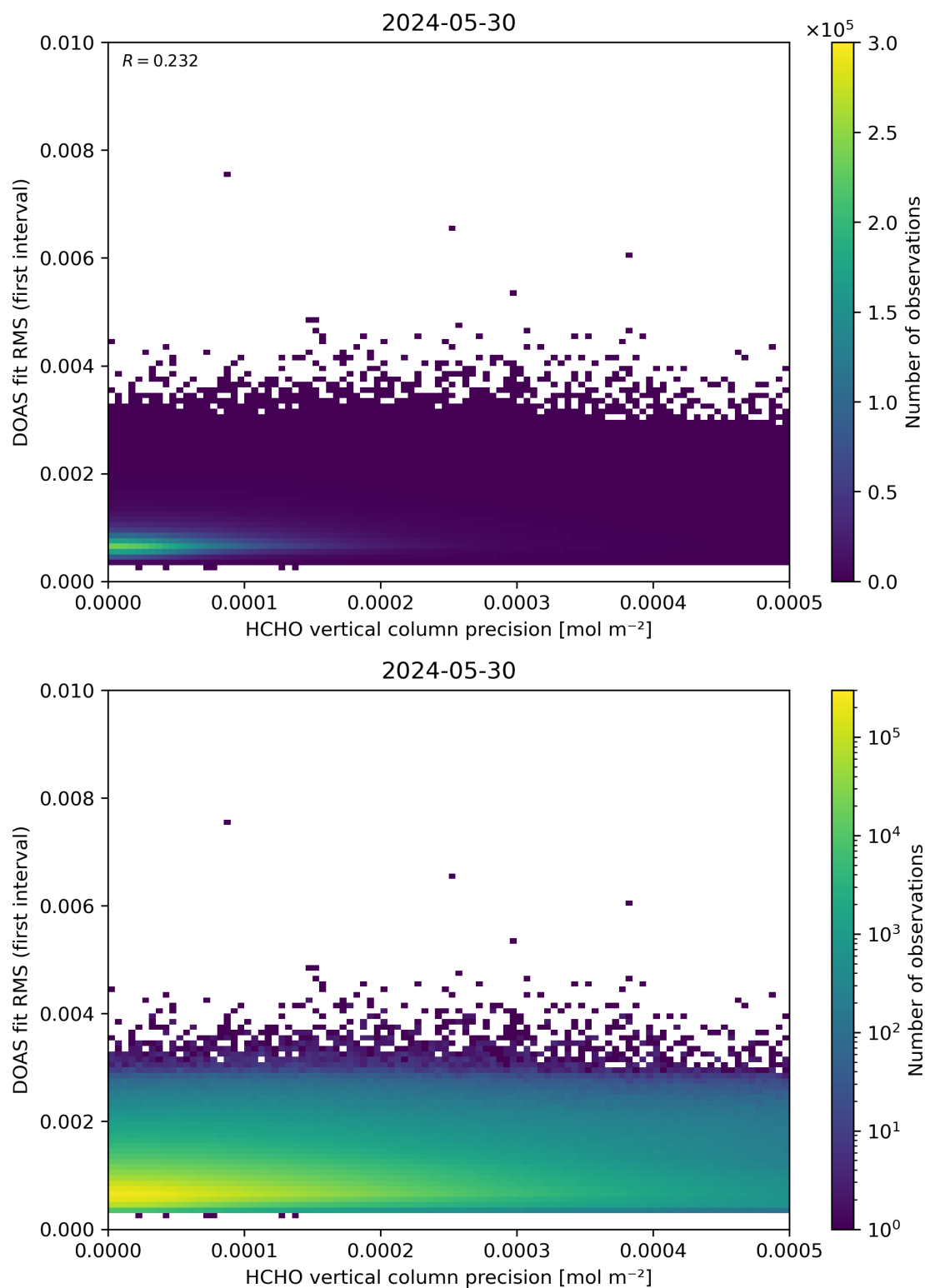
Figure 136: Scatter density plot of “HCHO vertical column precision” against “DOAS fit RMS (first interval)” for 2024-05-29 to 2024-05-31.
