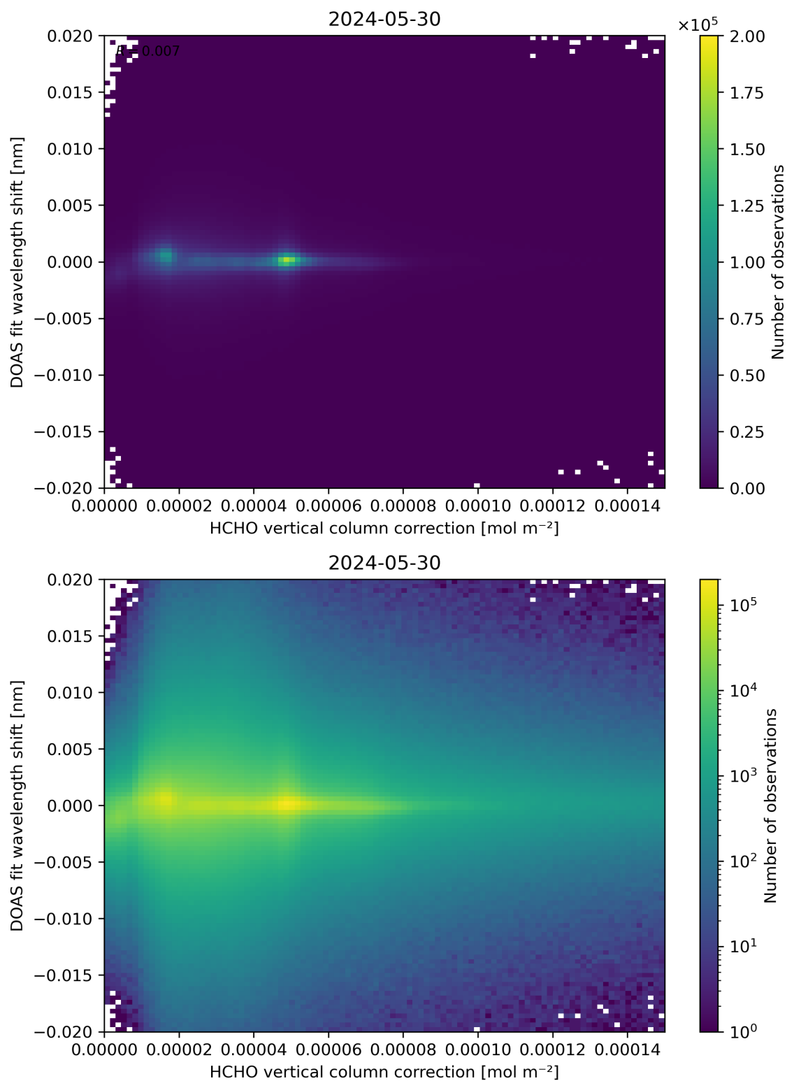
Figure 113: Scatter density plot of “HCHO vertical column correction” against “DOAS fit wavelength shift” for 2024-05-29 to 2024-05-31.
