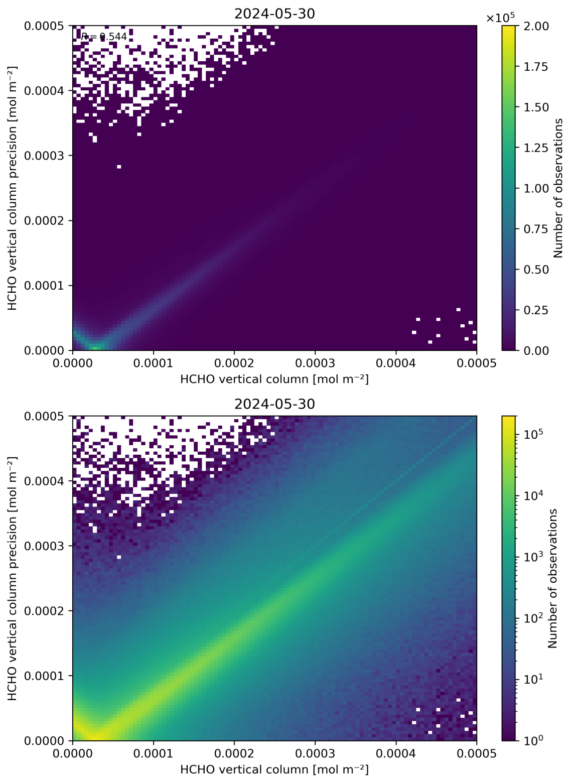
Figure 134: Scatter density plot of “HCHO vertical column” against “HCHO vertical column precision” for 2024-05-29 to 2024-05-31.
