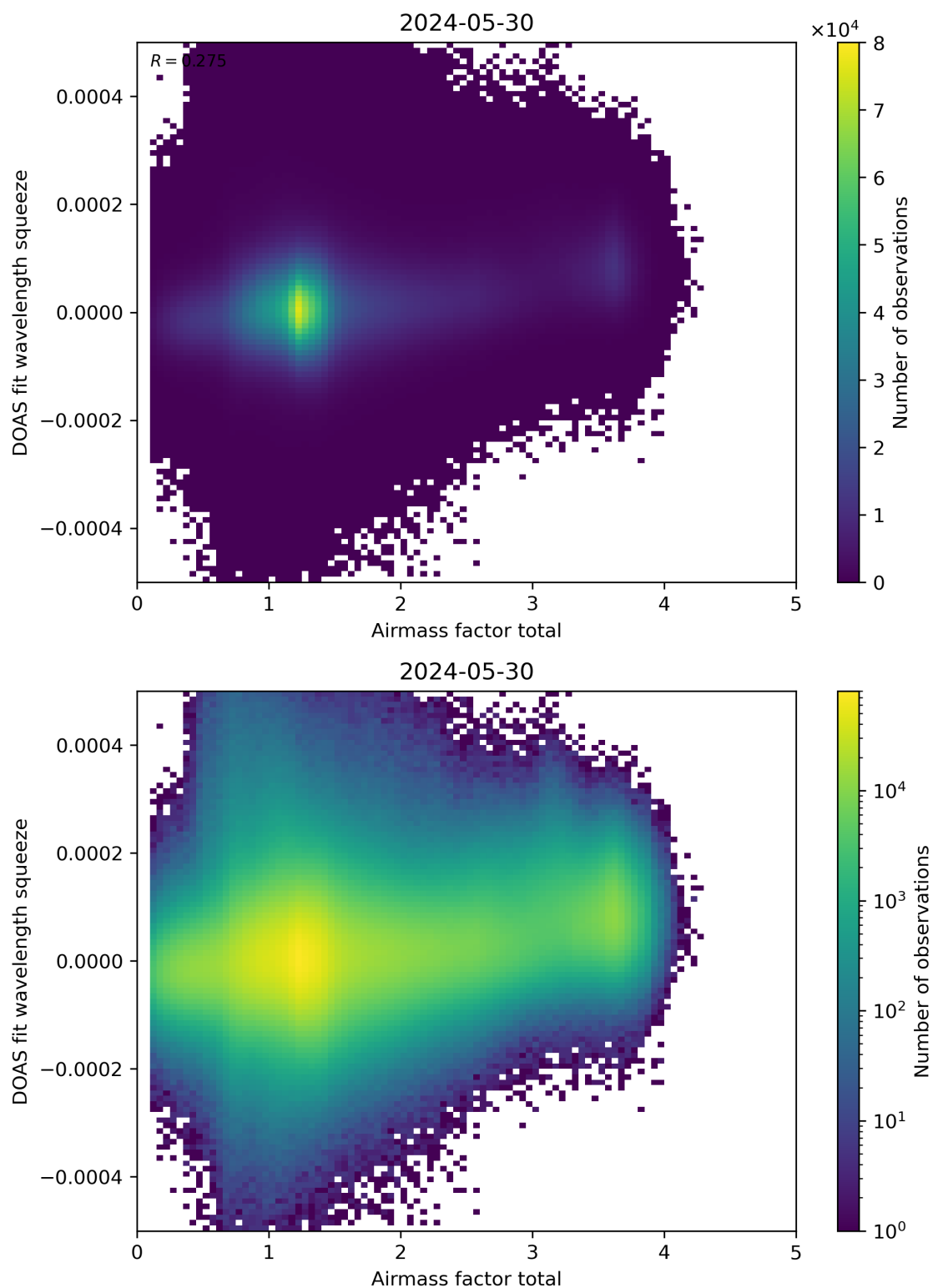
Figure 99: Scatter density plot of “Airmass factor total” against “DOAS fit wavelength squeeze” for 2024-05-29 to 2024-05-31.
