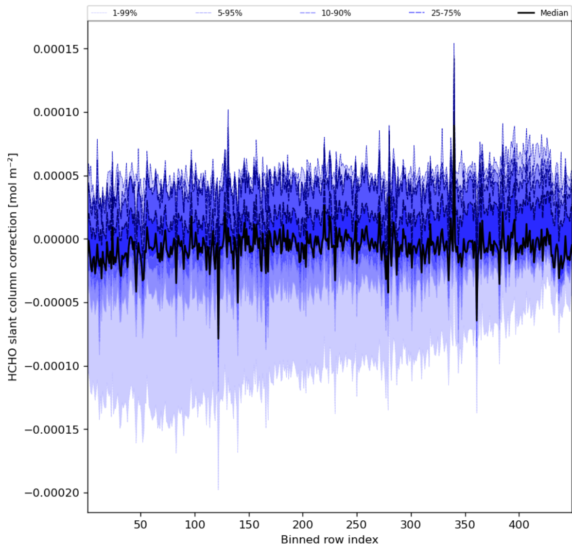
Figure 61: Along track statistics of “HCHO slant column correction” for 2024-05-29 to 2024-05-31
