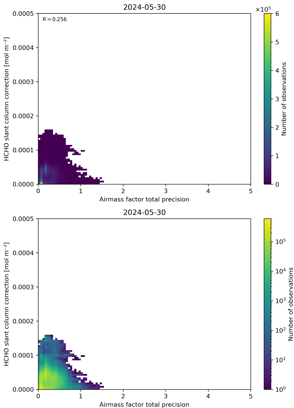
Figure 110: Scatter density plot of “Airmass factor total precision” against “HCHO slant column correction” for 2024-05-29 to 2024-05-31.
