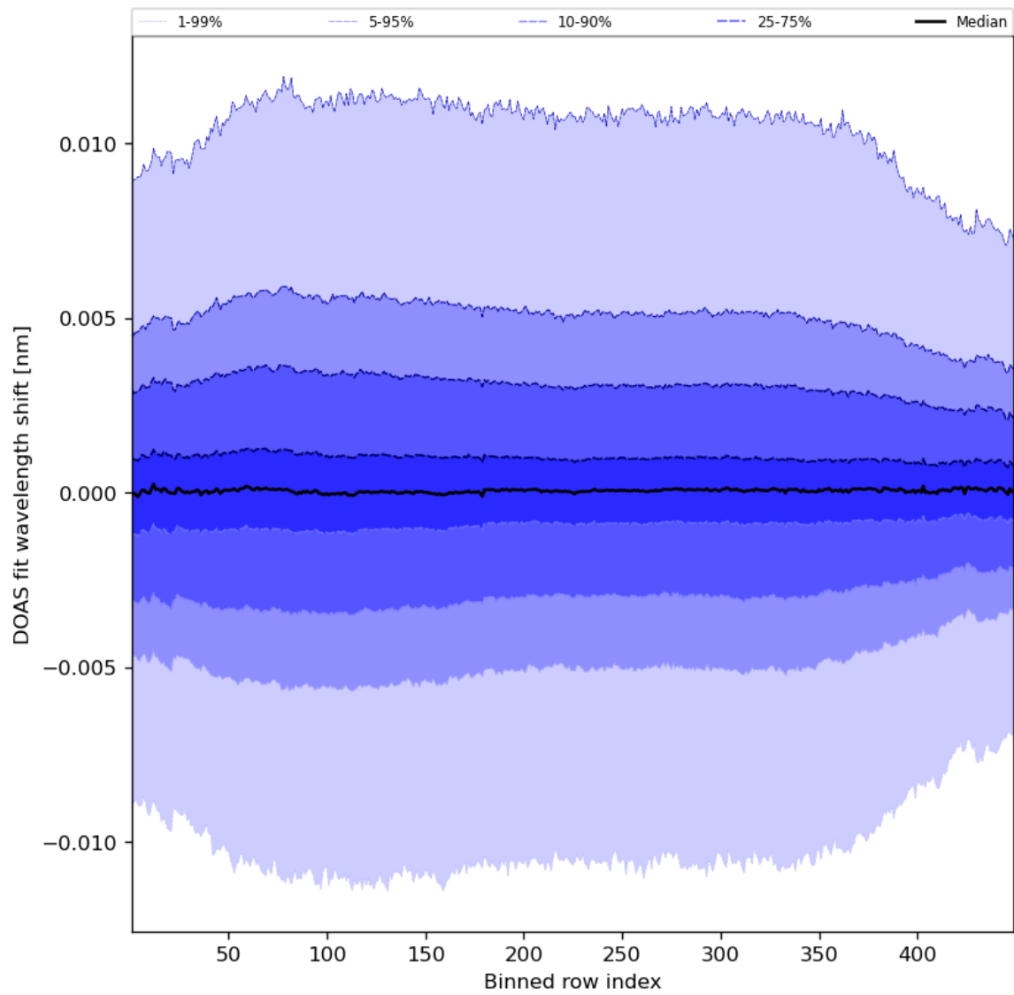
Figure 58: Along track statistics of “DOAS fit wavelength shift” for 2024-05-29 to 2024-05-31
