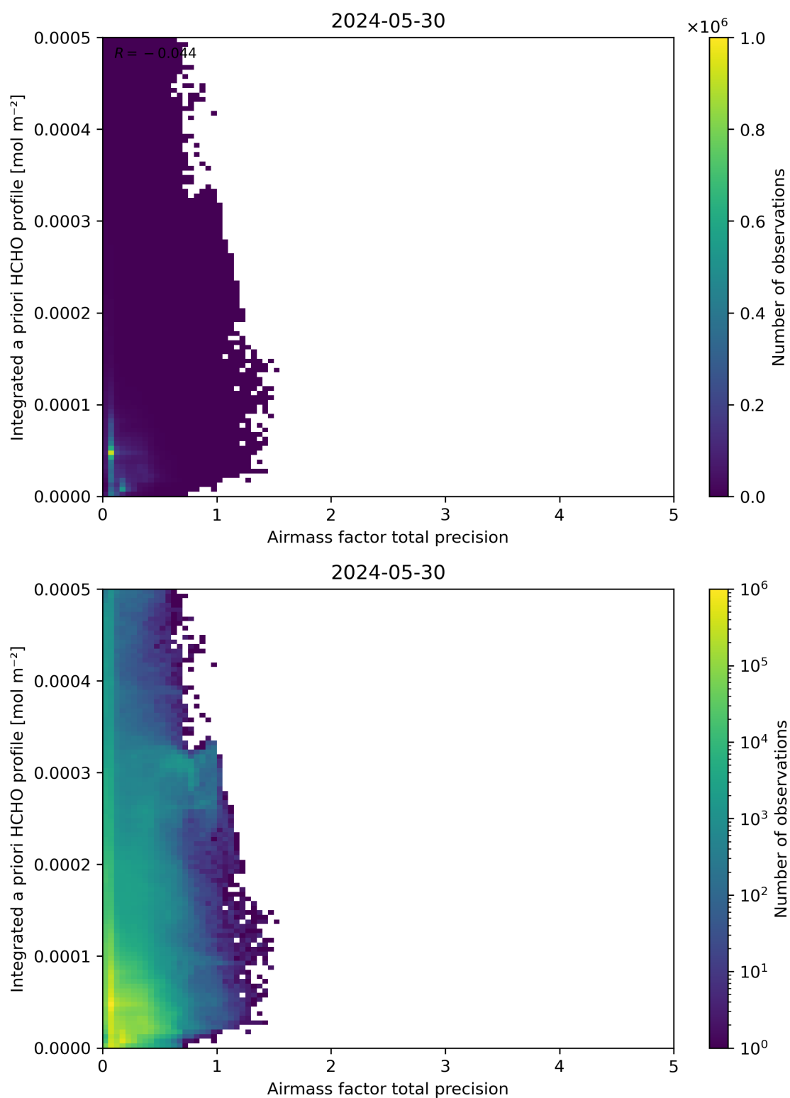
Figure 111: Scatter density plot of “Airmass factor total precision” against “Integrated a priori HCHO profile” for 2024-05-29 to 2024-05-31.
