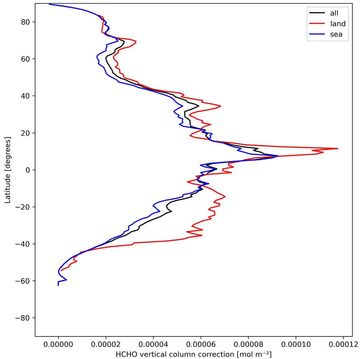
Figure 23: Zonal average of “HCHO vertical column correction” for 2024-05-29 to 2024-05-31.
