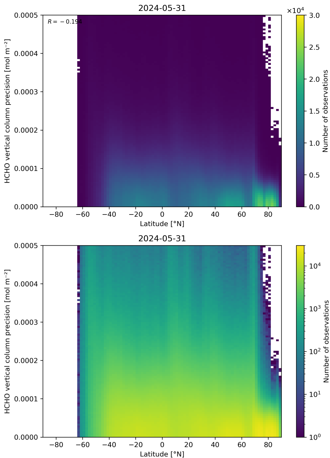
Figure 165: Scatter density plot of “Latitude” against “HCHO vertical column precision” for 2024-05-30 to 2024-06-01.
