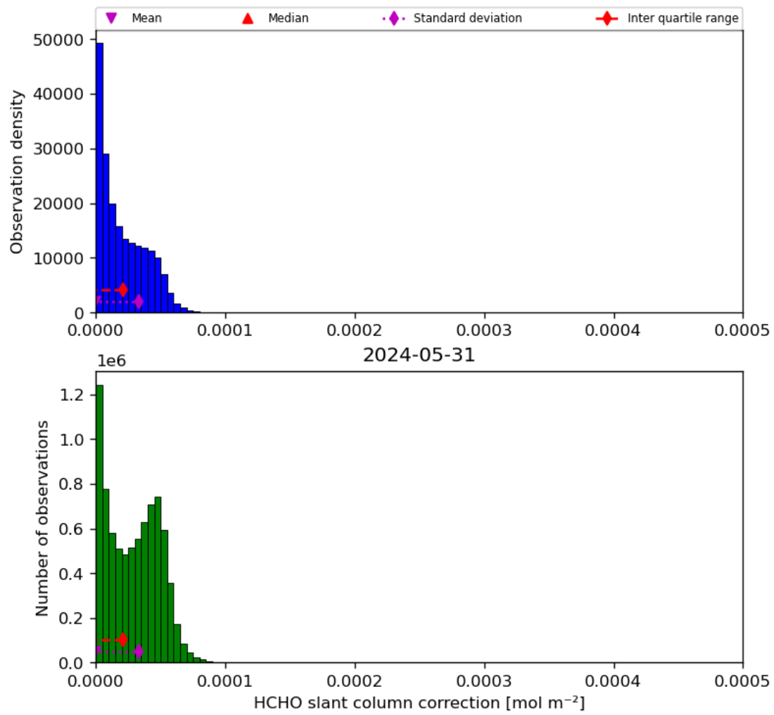
Figure 47: Histogram of “HCHO slant column correction” for 2024-05-30 to 2024-06-01
