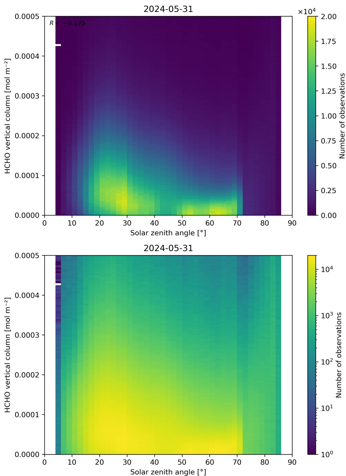
Figure 177: Scatter density plot of “Solar zenith angle” against “HCHO vertical column” for 2024-05-30 to 2024-06-01.
