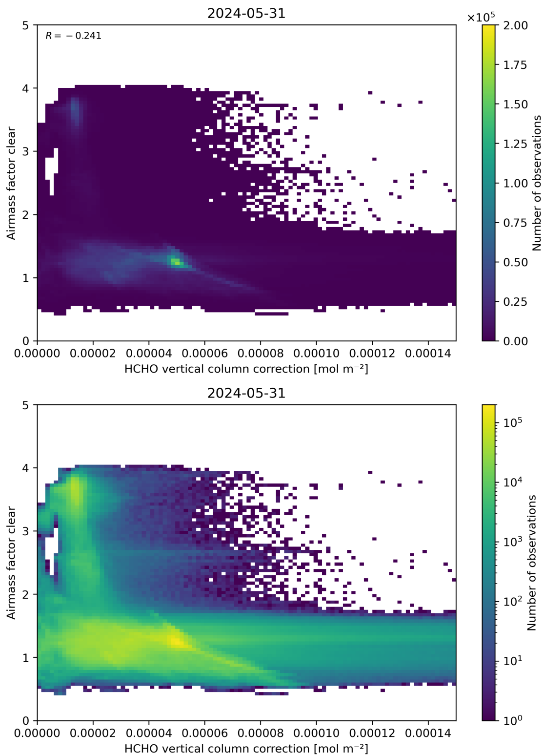
Figure 115: Scatter density plot of “HCHO vertical column correction” against “Airmass factor clear” for 2024-05-30 to 2024-06-01.
