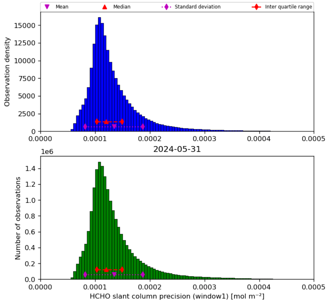
Figure 39: Histogram of “HCHO slant column precision (window1)” for 2024-05-30 to 2024-06-01
