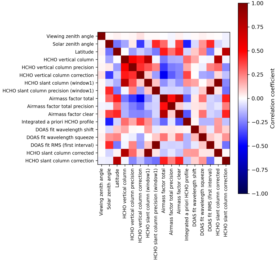
Figure 2: Map of correlation matrix for 2024-05-30 to 2024-06-01.
