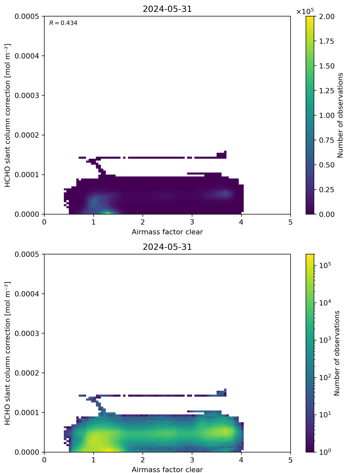
Figure 75: Scatter density plot of “Airmass factor clear” against “HCHO slant column correction” for 2024-05-30 to 2024-06-01.
