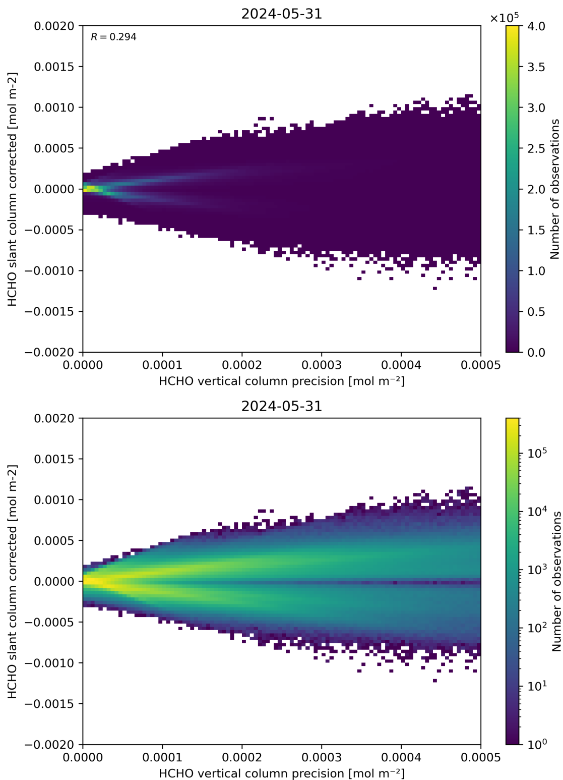
Figure 140: Scatter density plot of “HCHO vertical column precision” against “HCHO slant column corrected” for 2024-05-30 to 2024-06-01.
