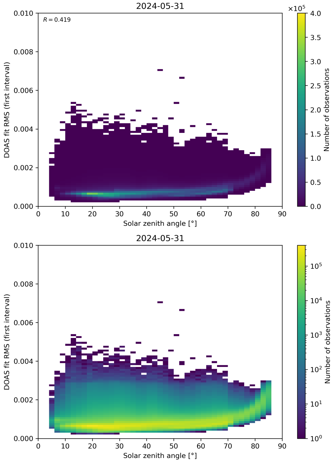
Figure 167: Scatter density plot of “Solar zenith angle” against “DOAS fit RMS (first interval)” for 2024-05-30 to 2024-06-01.
