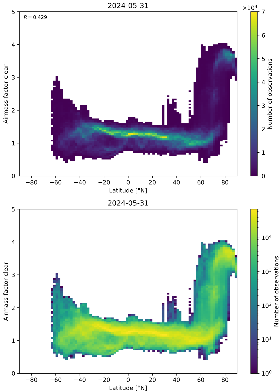
Figure 156: Scatter density plot of “Latitude” against “Airmass factor clear” for 2024-05-30 to 2024-06-01.
