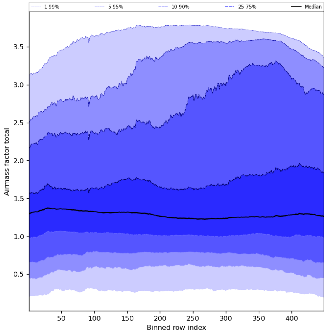
Figure 54: Along track statistics of “Airmass factor total” for 2024-05-30 to 2024-06-01
