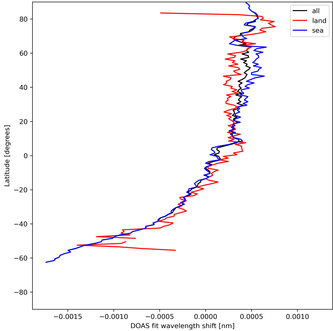
Figure 30: Zonal average of “DOAS fit wavelength shift” for 2024-05-30 to 2024-06-01.
