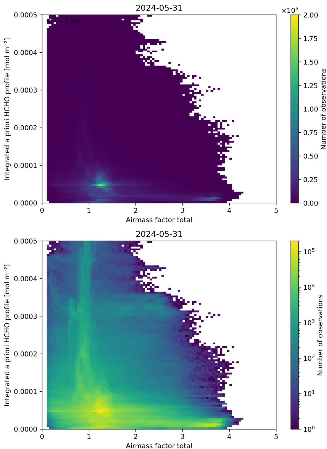
Figure 104: Scatter density plot of “Airmass factor total” against “Integrated a priori HCHO profile” for 2024-05-30 to 2024-06-01.
