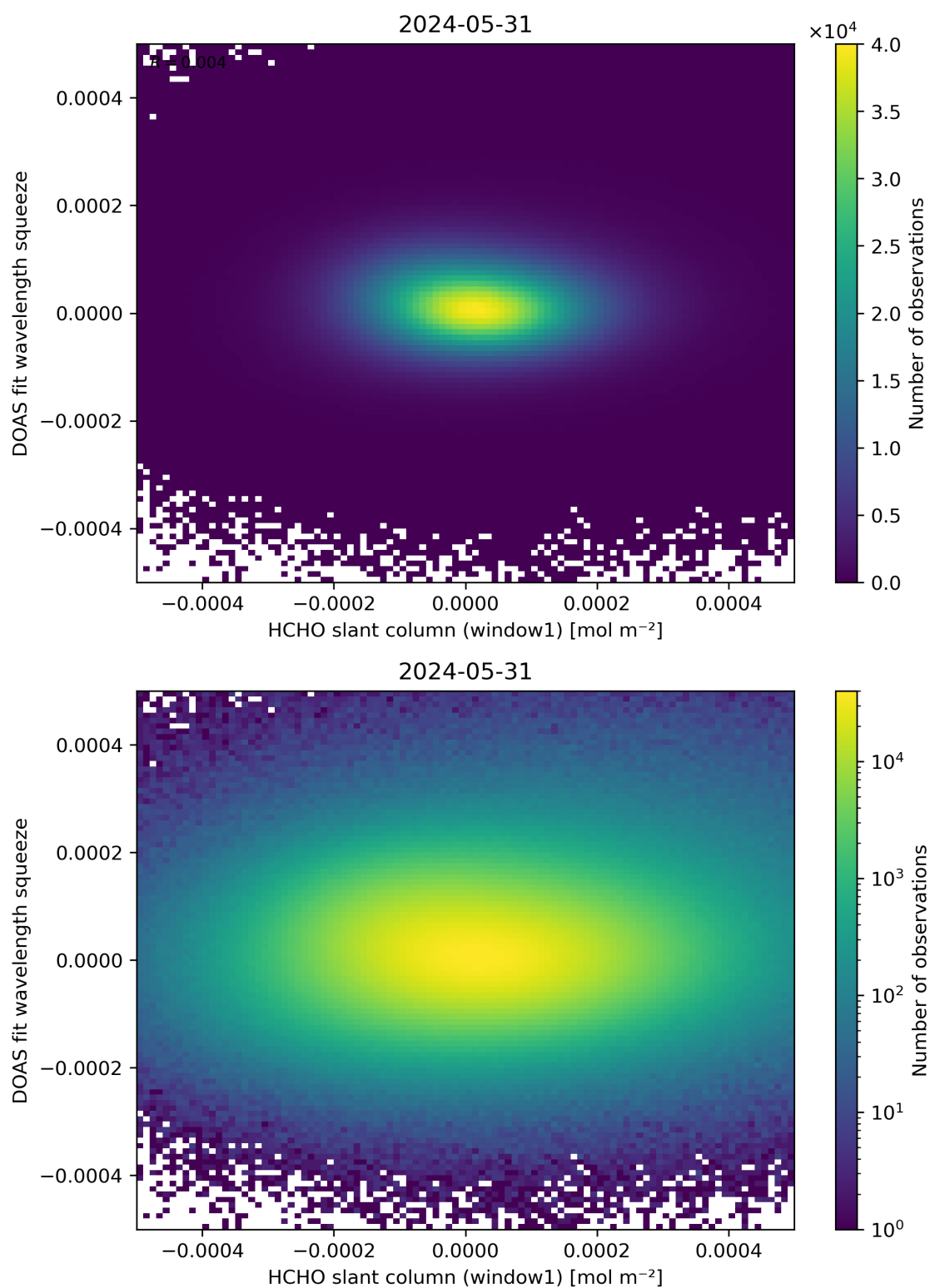
Figure 80: Scatter density plot of “HCHO slant column (window1)” against “DOAS fit wavelength squeeze” for 2024-05-30 to 2024-06-01.
