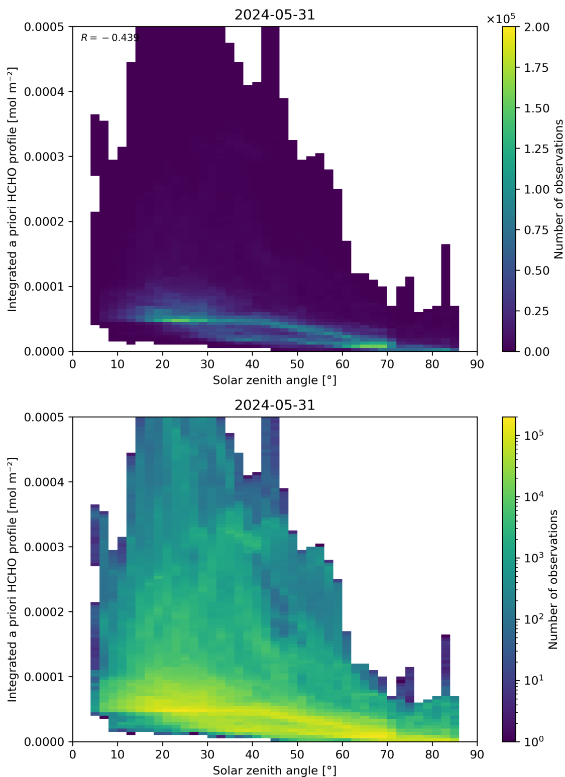
Figure 180: Scatter density plot of “Solar zenith angle” against “Integrated a priori HCHO profile” for 2024-05-30 to 2024-06-01.
