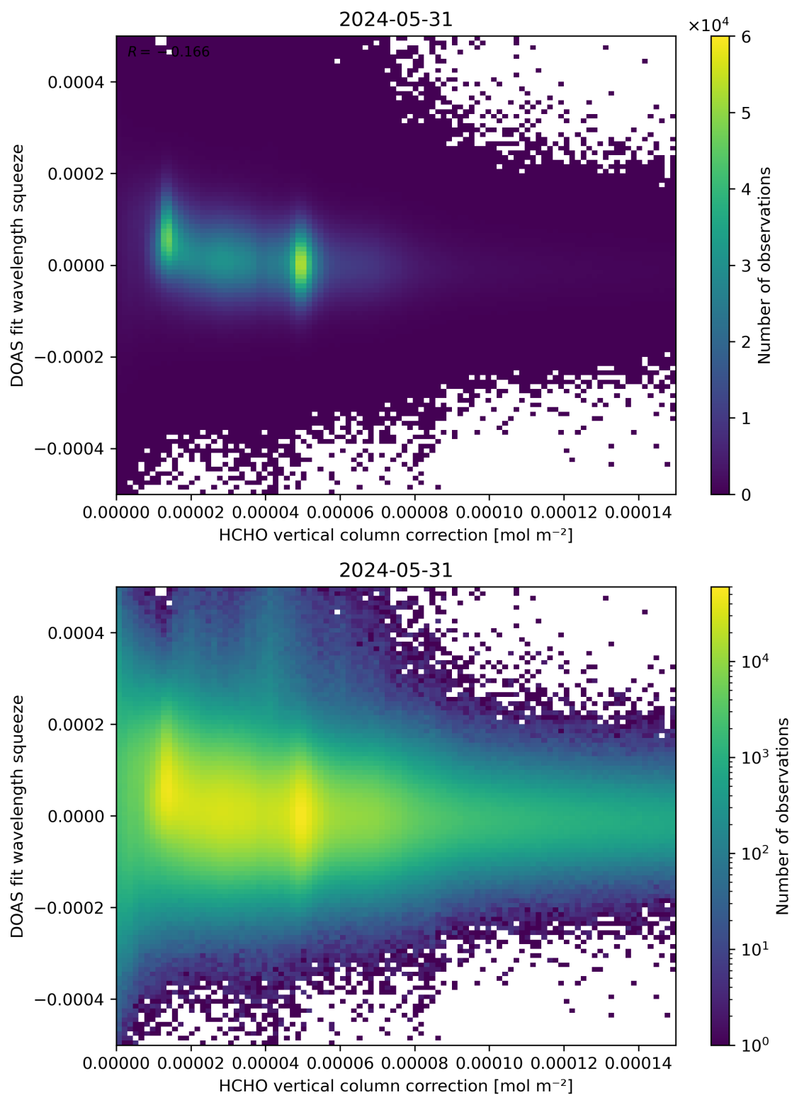
Figure 114: Scatter density plot of “HCHO vertical column correction” against “DOAS fit wavelength squeeze” for 2024-05-30 to 2024-06-01.
