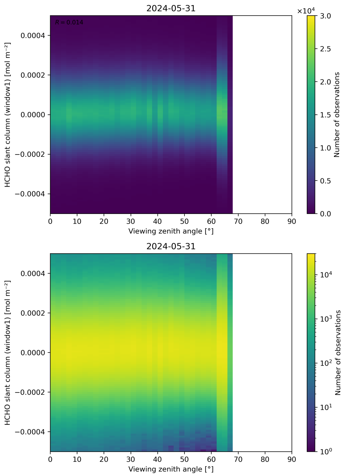
Figure 188: Scatter density plot of “Viewing zenith angle” against “HCHO slant column (window1)” for 2024-05-30 to 2024-06-01.
