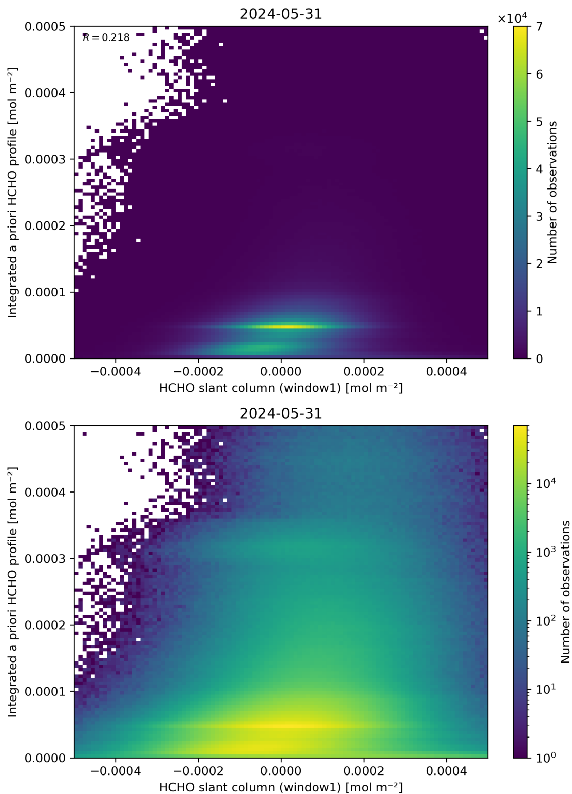
Figure 87: Scatter density plot of “HCHO slant column (window1)” against “Integrated a priori HCHO profile” for 2024-05-30 to 2024-06-01.
