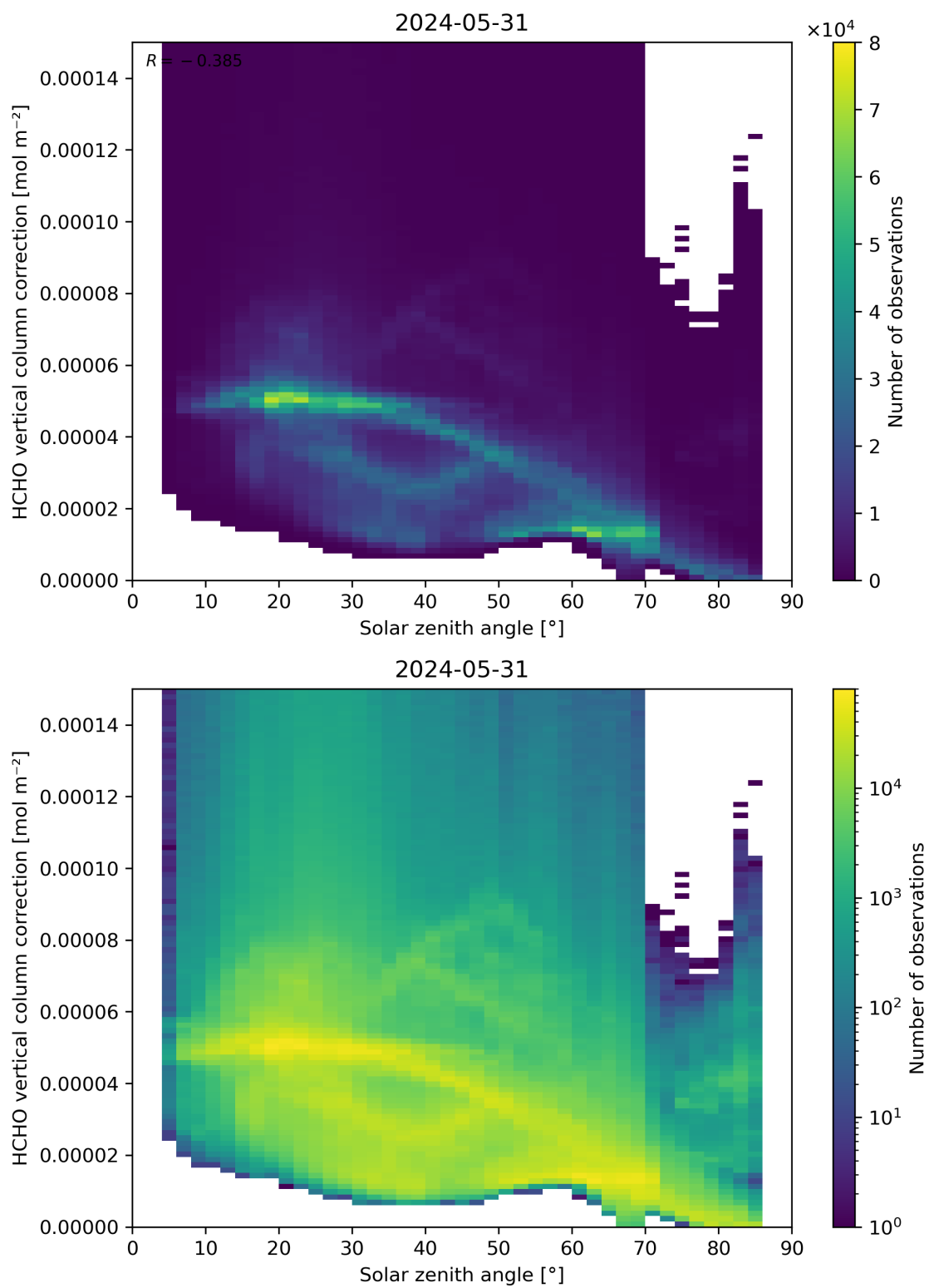
Figure 178: Scatter density plot of “Solar zenith angle” against “HCHO vertical column correction” for 2024-05-30 to 2024-06-01.
