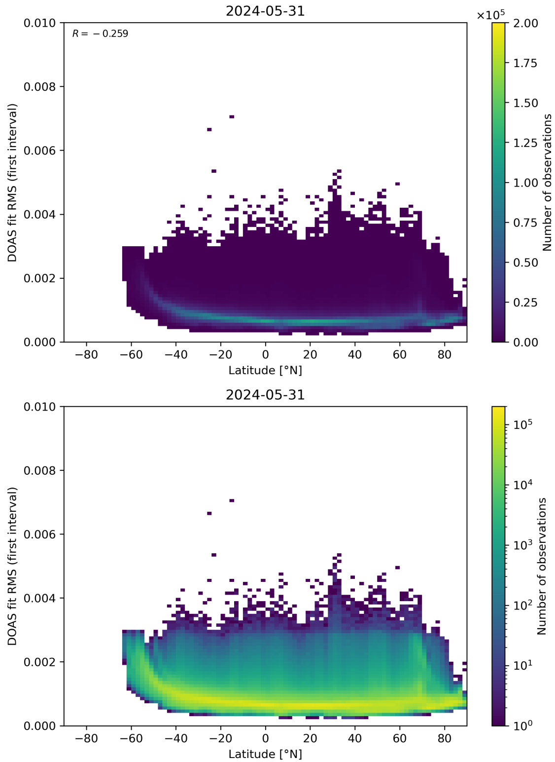
Figure 153: Scatter density plot of “Latitude” against “DOAS fit RMS (first interval)” for 2024-05-30 to 2024-06-01.
