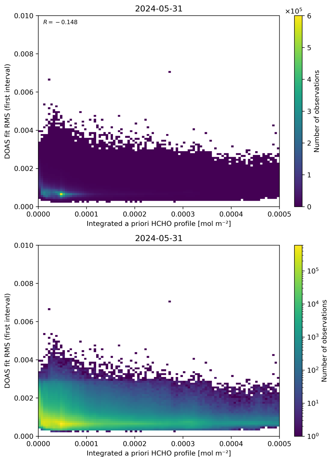
Figure 148: Scatter density plot of “Integrated a priori HCHO profile” against “DOAS fit RMS (first interval)” for 2024-05-30 to 2024-06-01.
