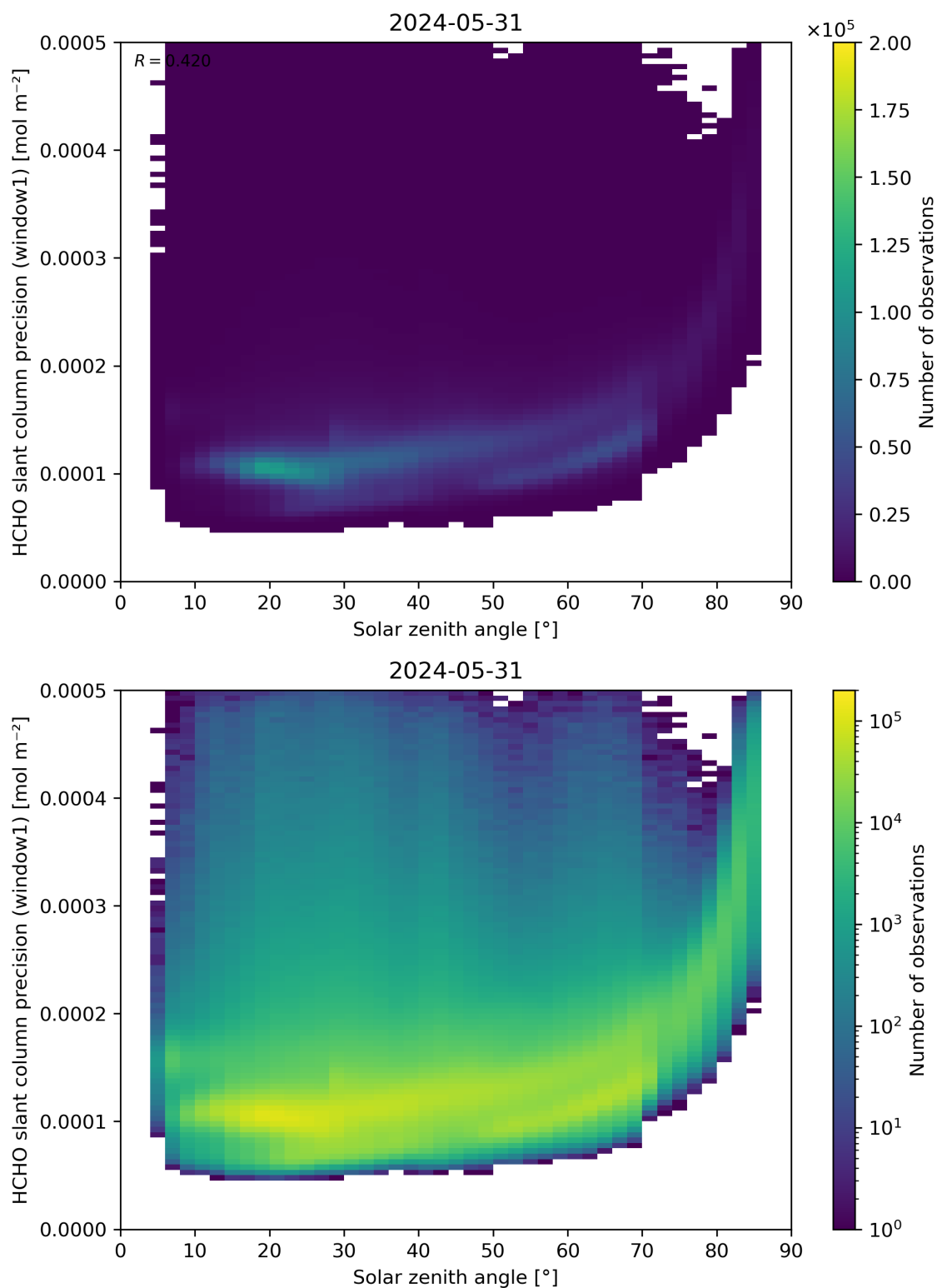
Figure 174: Scatter density plot of “Solar zenith angle” against “HCHO slant column precision (window1)” for 2024-05-30 to 2024-06-01.
