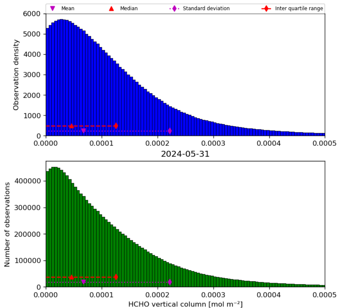
Figure 35: Histogram of “HCHO vertical column” for 2024-05-30 to 2024-06-01
