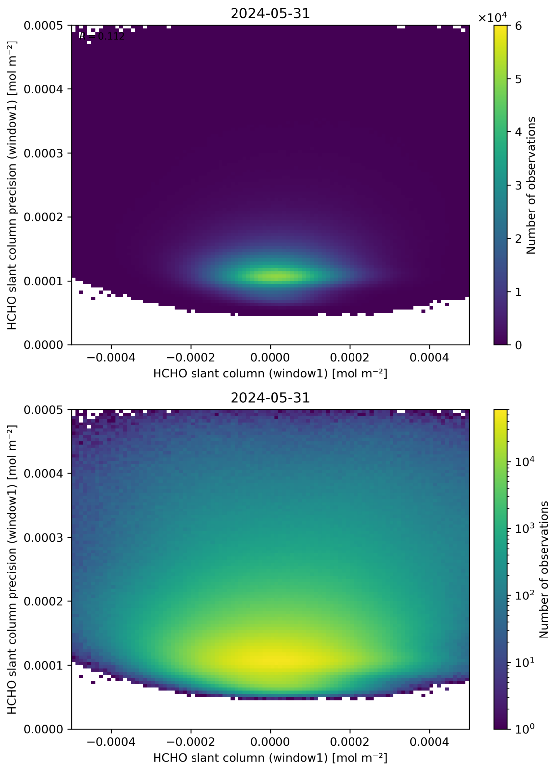
Figure 84: Scatter density plot of “HCHO slant column (window1)” against “HCHO slant column precision (window1)” for 2024-05-30 to 2024-06-01.
