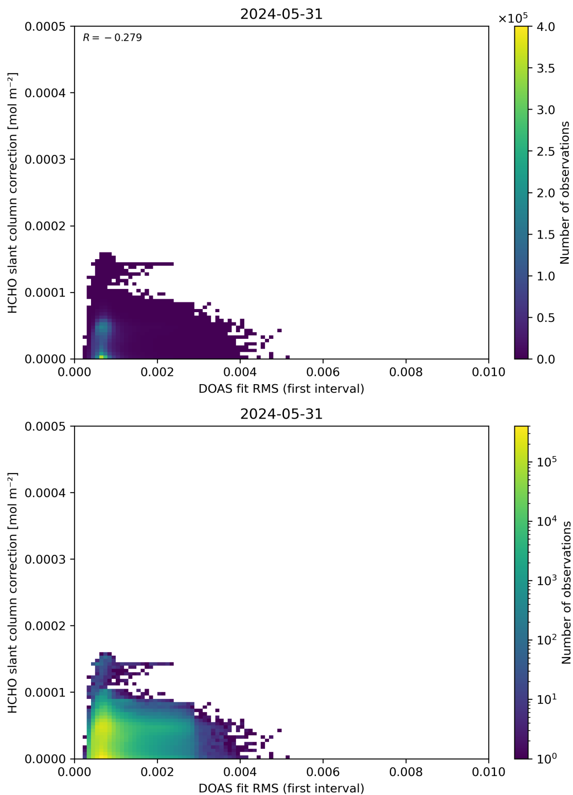
Figure 63: Scatter density plot of “DOAS fit RMS (first interval)” against “HCHO slant column correction” for 2024-05-30 to 2024-06-01.
