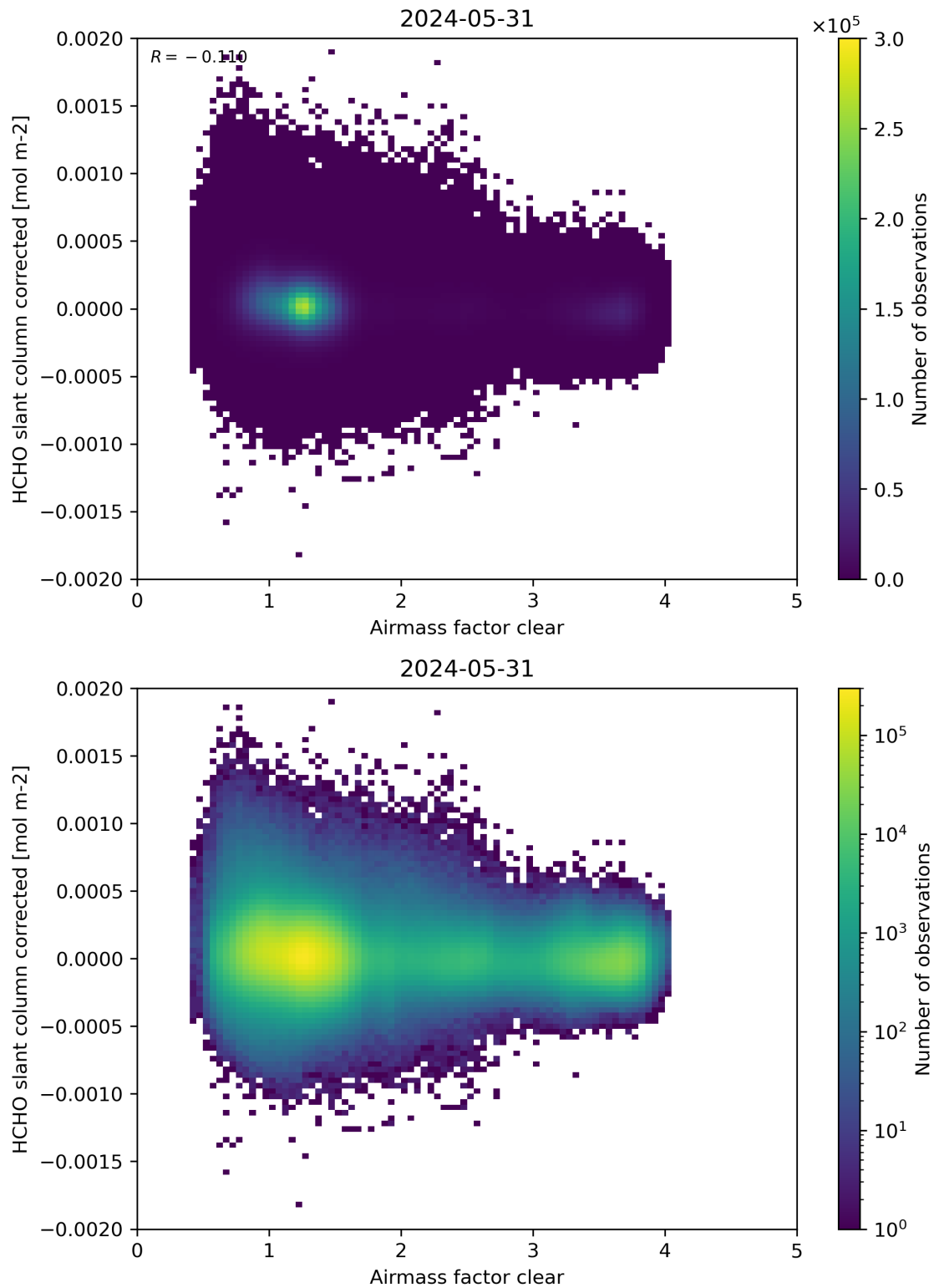
Figure 74: Scatter density plot of “Airmass factor clear” against “HCHO slant column corrected” for 2024-05-30 to 2024-06-01.
