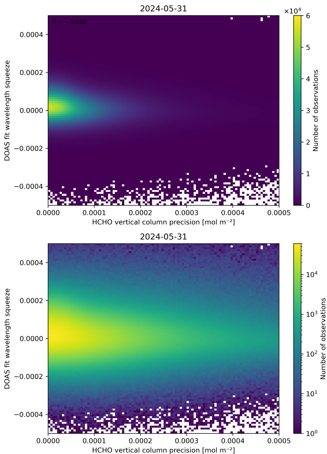
Figure 138: Scatter density plot of “HCHO vertical column precision” against “DOAS fit wavelength squeeze” for 2024-05-30 to 2024-06-01.
