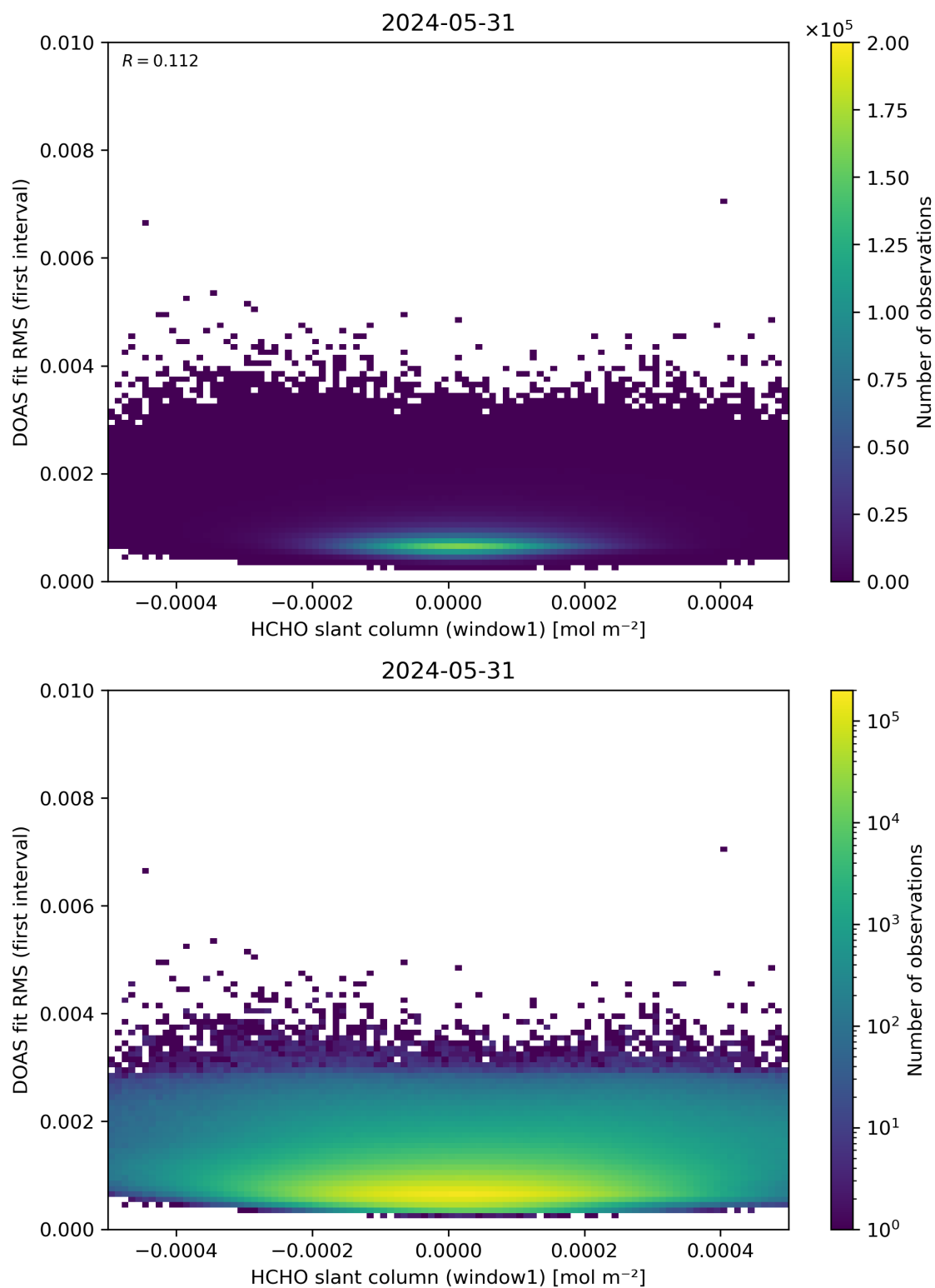
Figure 78: Scatter density plot of “HCHO slant column (window1)” against “DOAS fit RMS (first interval)” for 2024-05-30 to 2024-06-01.
