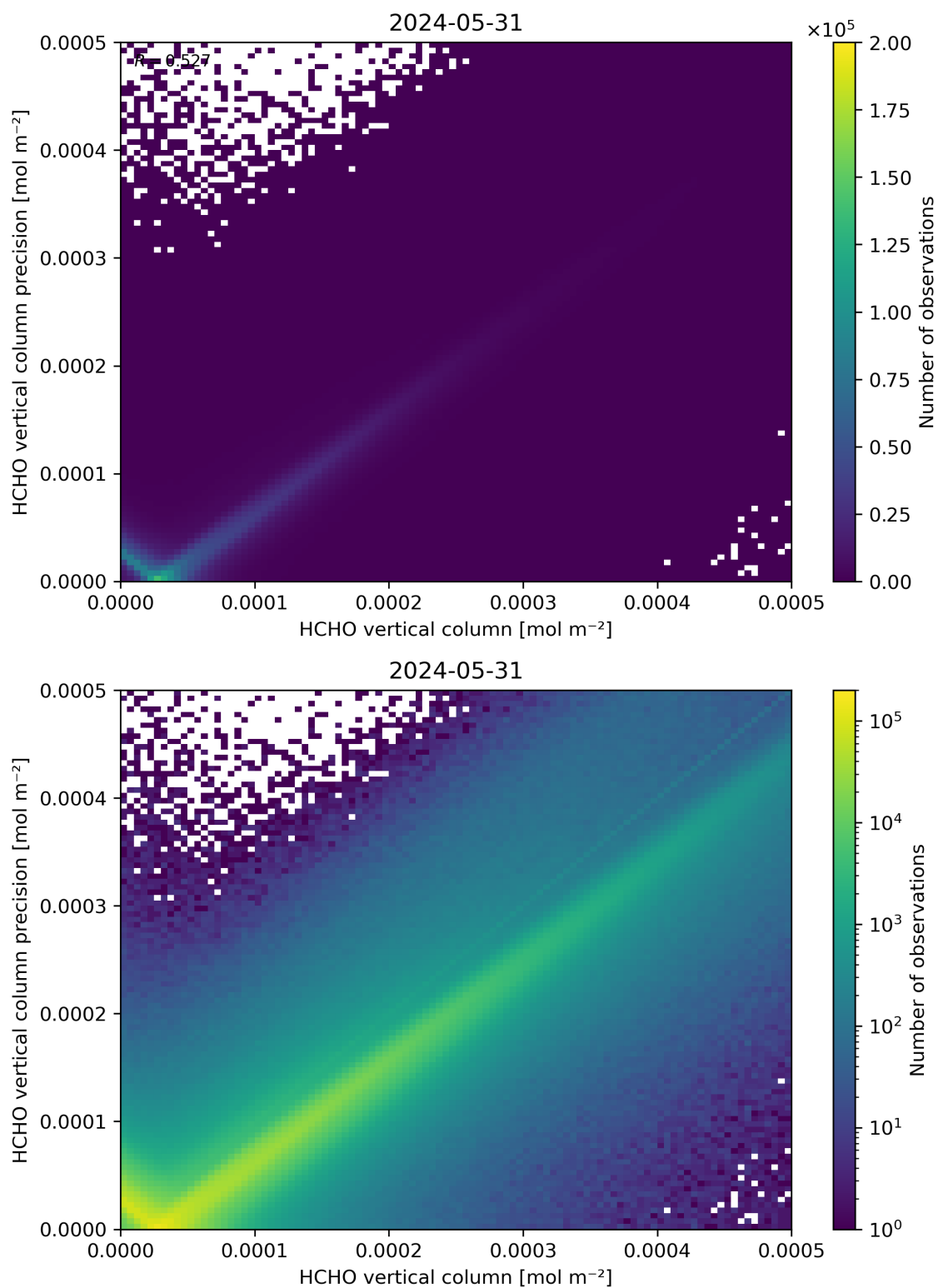
Figure 134: Scatter density plot of “HCHO vertical column” against “HCHO vertical column precision” for 2024-05-30 to 2024-06-01.
