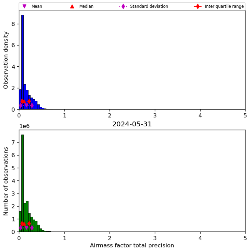
Figure 41: Histogram of “Airmass factor total precision” for 2024-05-30 to 2024-06-01
