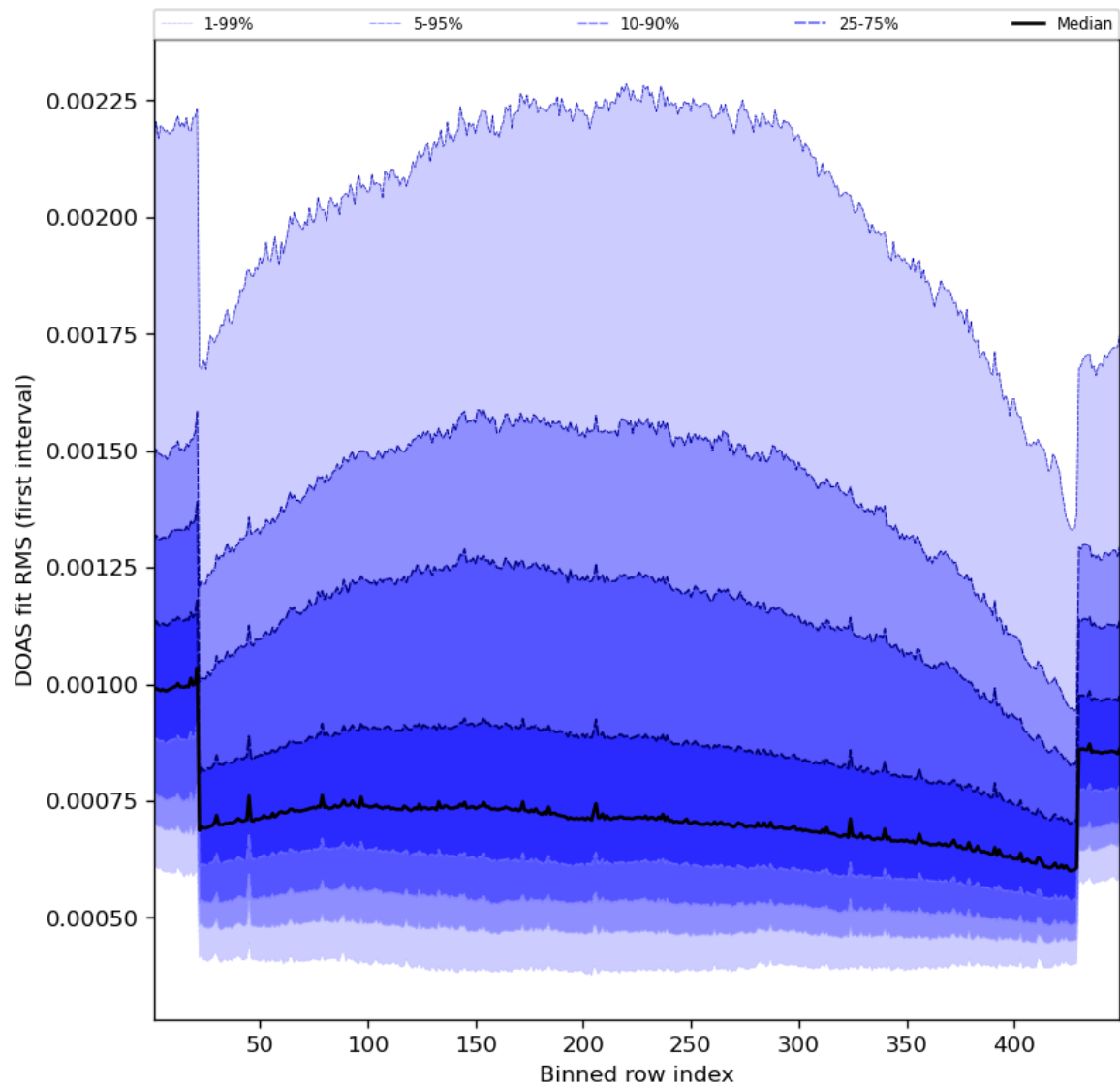
Figure 60: Along track statistics of “DOAS fit RMS (first interval)” for 2024-05-30 to 2024-06-01
