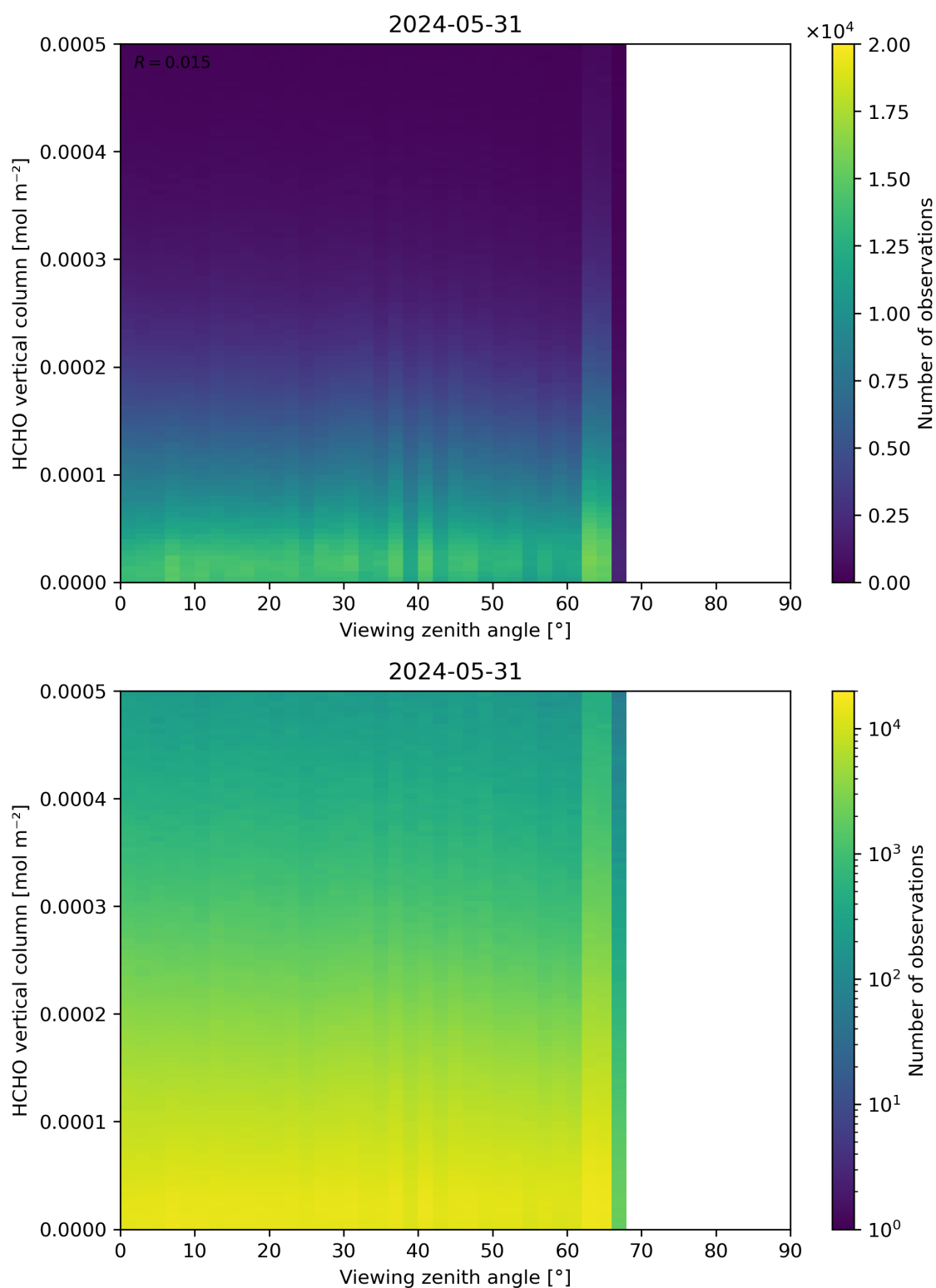
Figure 192: Scatter density plot of “Viewing zenith angle” against “HCHO vertical column” for 2024-05-30 to 2024-06-01.
