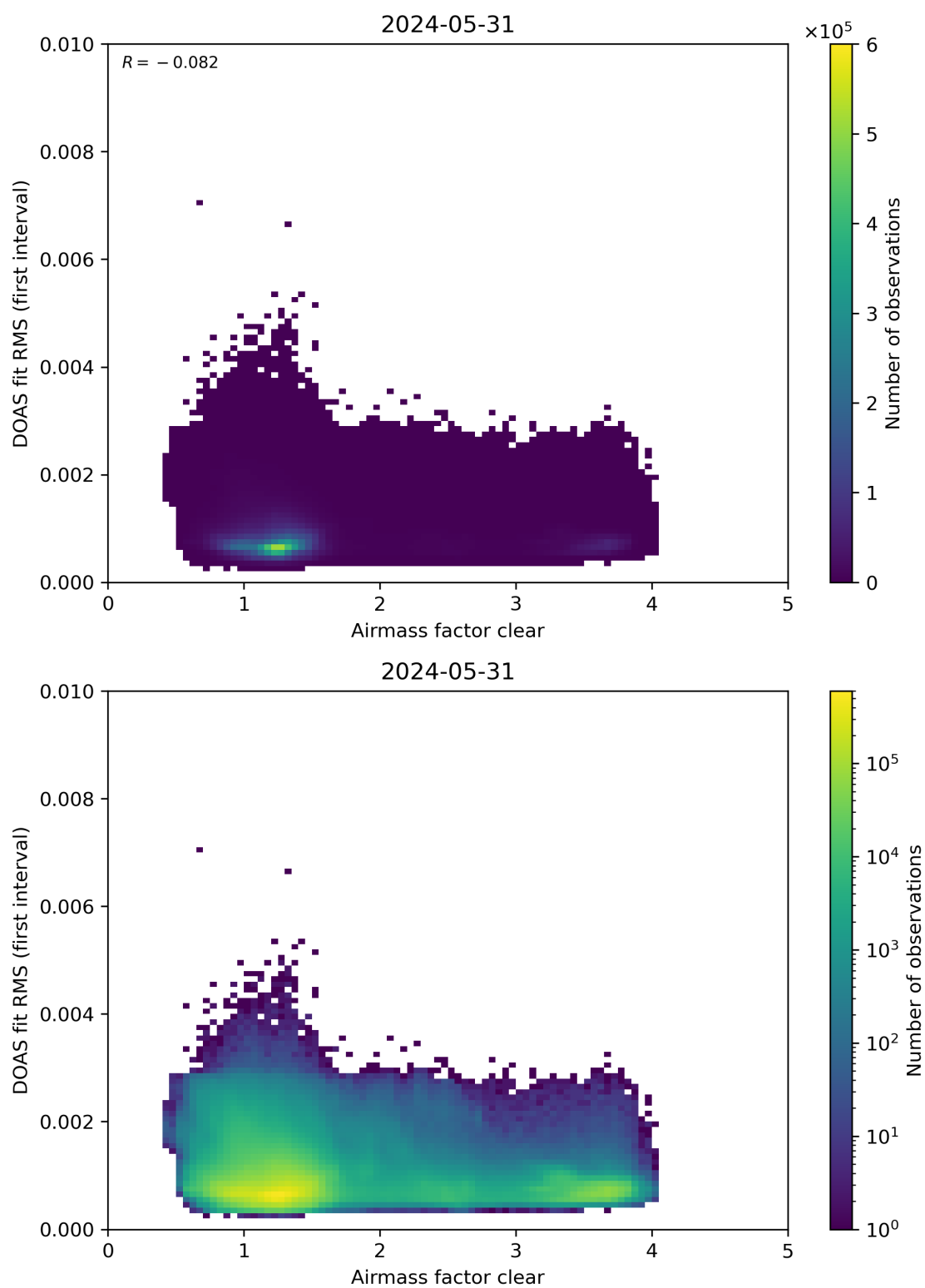
Figure 71: Scatter density plot of “Airmass factor clear” against “DOAS fit RMS (first interval)” for 2024-05-30 to 2024-06-01.
