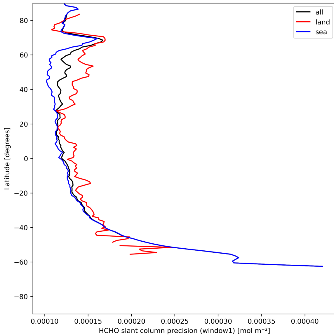
Figure 25: Zonal average of “HCHO slant column precision (window1)” for 2024-05-30 to 2024-06-01.
