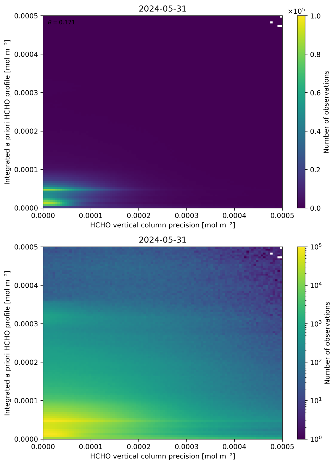
Figure 147: Scatter density plot of “HCHO vertical column precision” against “Integrated a priori HCHO profile” for 2024-05-30 to 2024-06-01.
