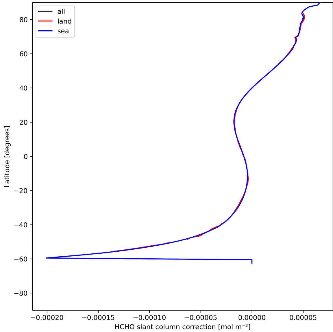
Figure 33: Zonal average of “HCHO slant column correction” for 2024-05-30 to 2024-06-01.
