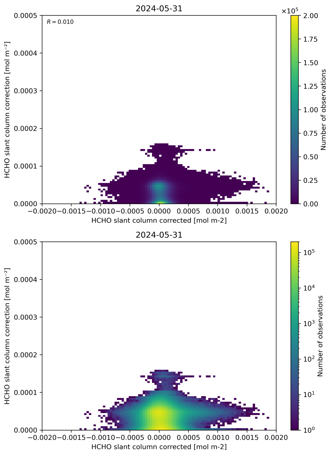
Figure 77: Scatter density plot of “HCHO slant column corrected” against “HCHO slant column correction” for 2024-05-30 to 2024-06-01.
