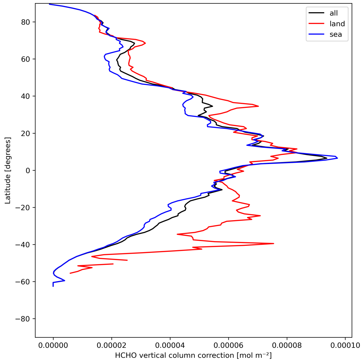
Figure 23: Zonal average of “HCHO vertical column correction” for 2024-05-30 to 2024-06-01.
