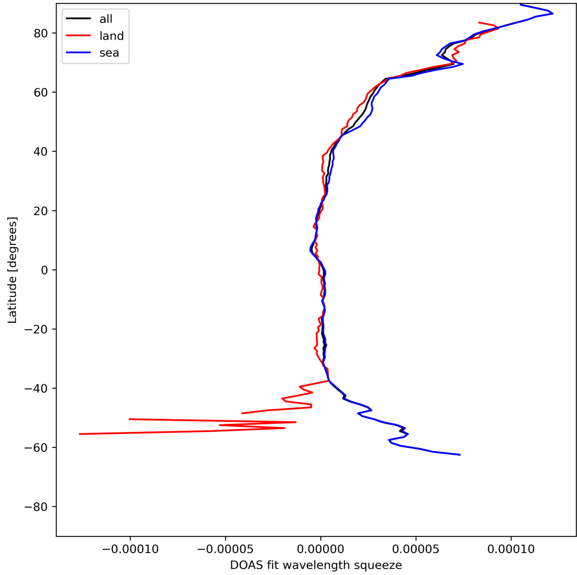
Figure 31: Zonal average of “DOAS fit wavelength squeeze” for 2024-05-30 to 2024-06-01.
