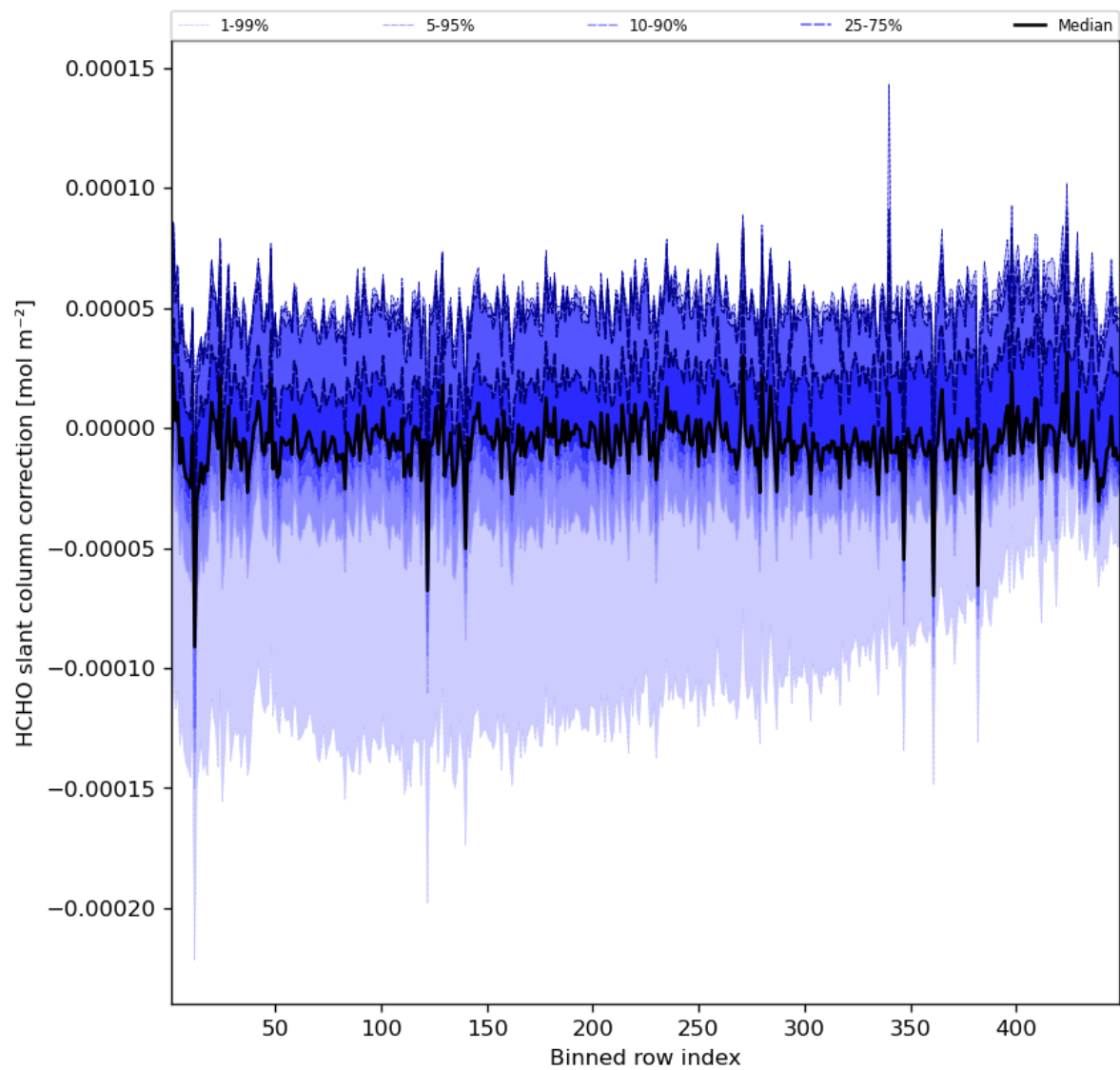
Figure 61: Along track statistics of “HCHO slant column correction” for 2024-05-30 to 2024-06-01
