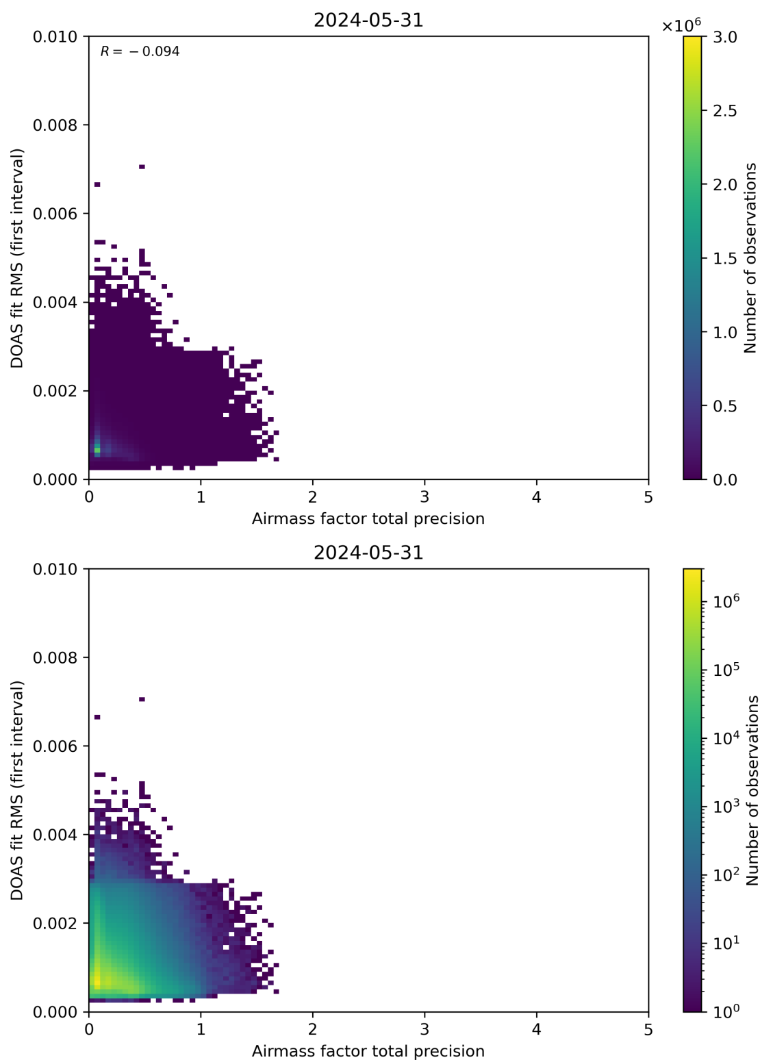
Figure 105: Scatter density plot of “Airmass factor total precision” against “DOAS fit RMS (first interval)” for 2024-05-30 to 2024-06-01.
