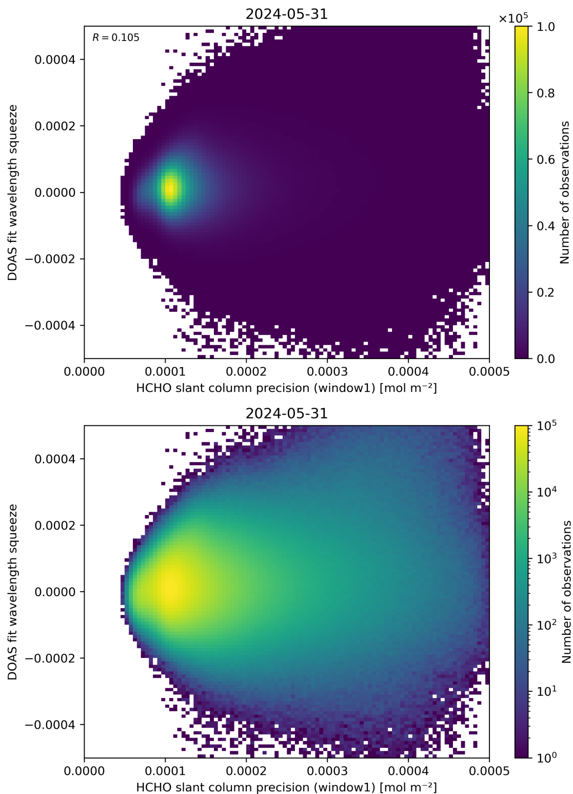
Figure 90: Scatter density plot of “HCHO slant column precision (window1)” against “DOAS fit wavelength squeeze” for 2024-05-30 to 2024-06-01.
