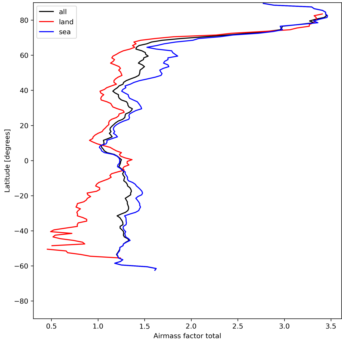
Figure 26: Zonal average of “Airmass factor total” for 2024-05-30 to 2024-06-01.
