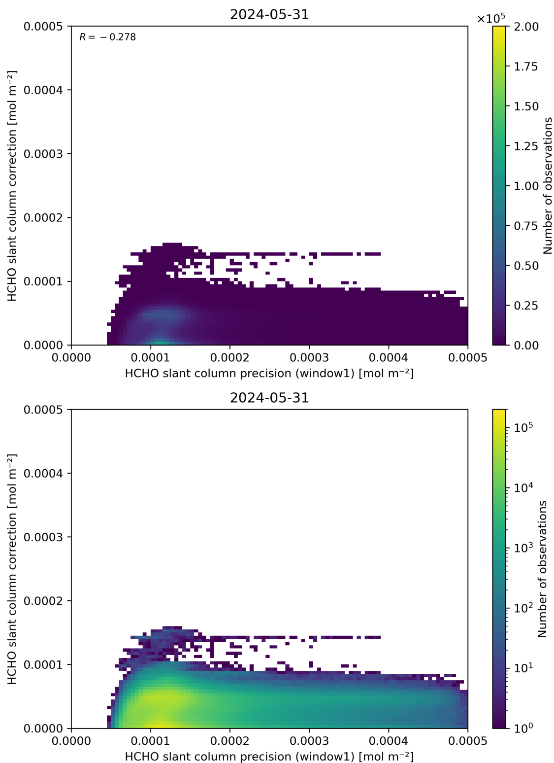
Figure 93: Scatter density plot of “HCHO slant column precision (window1)” against “HCHO slant column correction” for 2024-05-30 to 2024-06-01.
