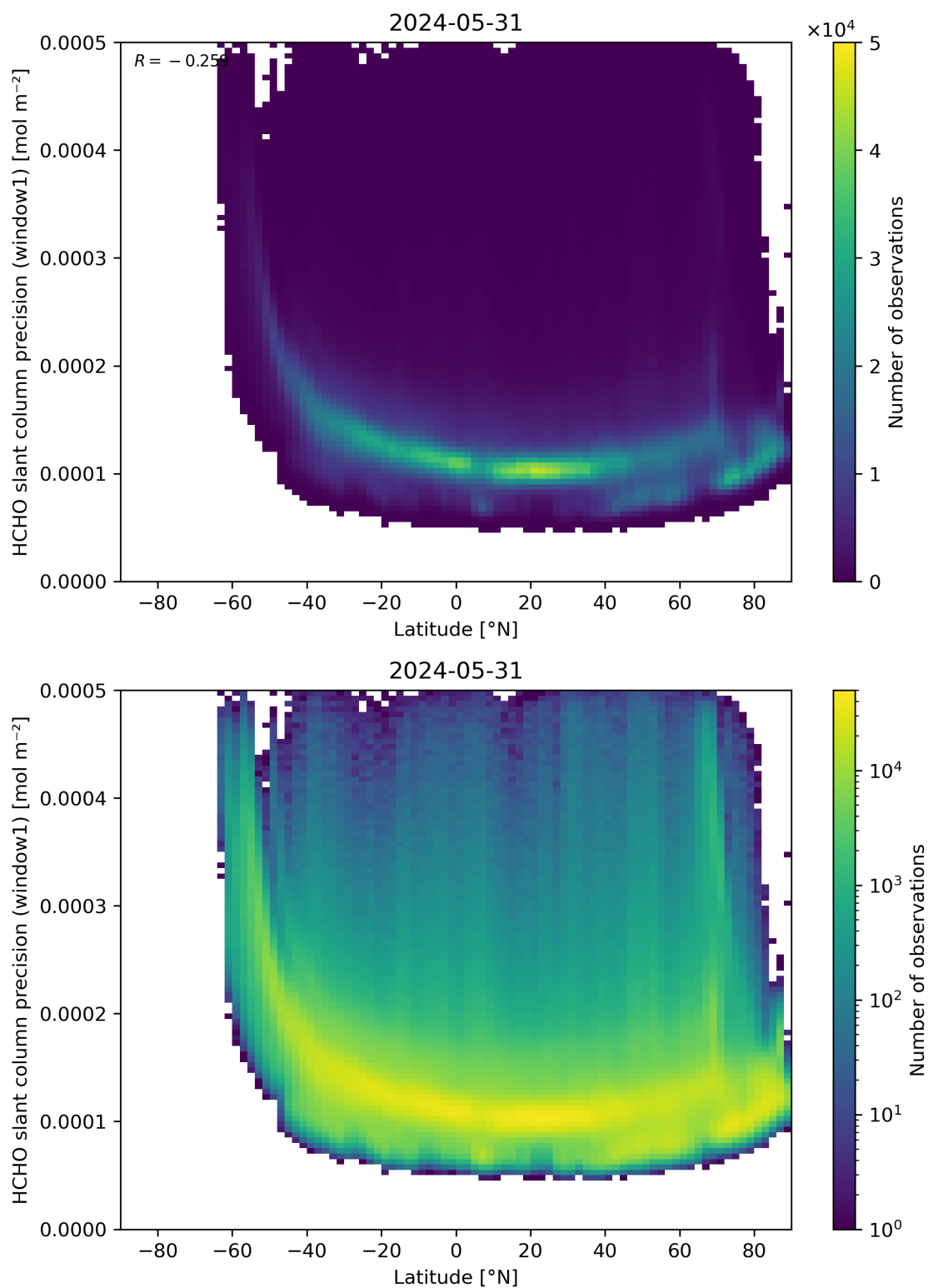
Figure 160: Scatter density plot of “Latitude” against “HCHO slant column precision (window1)” for 2024-05-30 to 2024-06-01.
