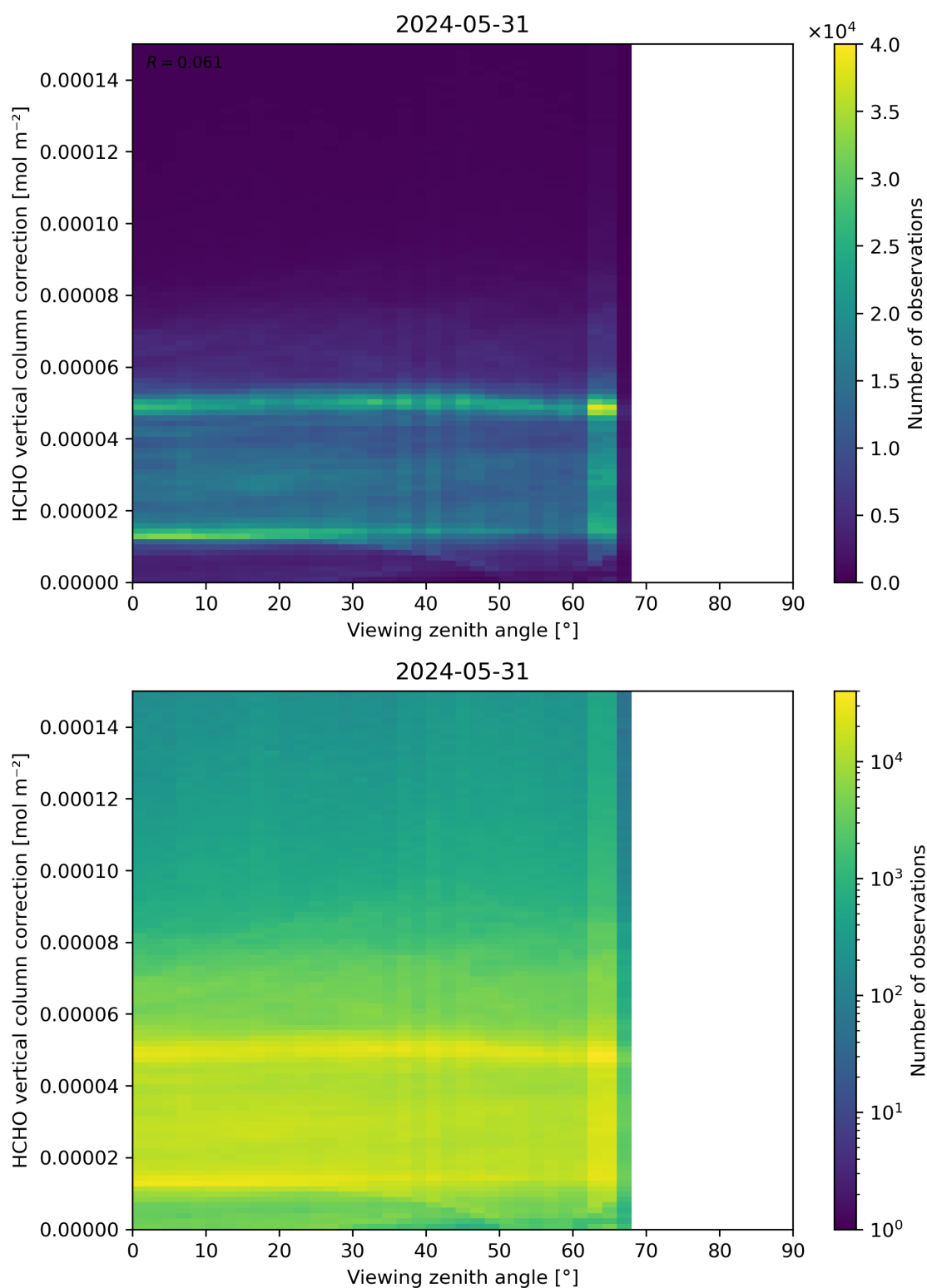
Figure 193: Scatter density plot of “Viewing zenith angle” against “HCHO vertical column correction” for 2024-05-30 to 2024-06-01.
