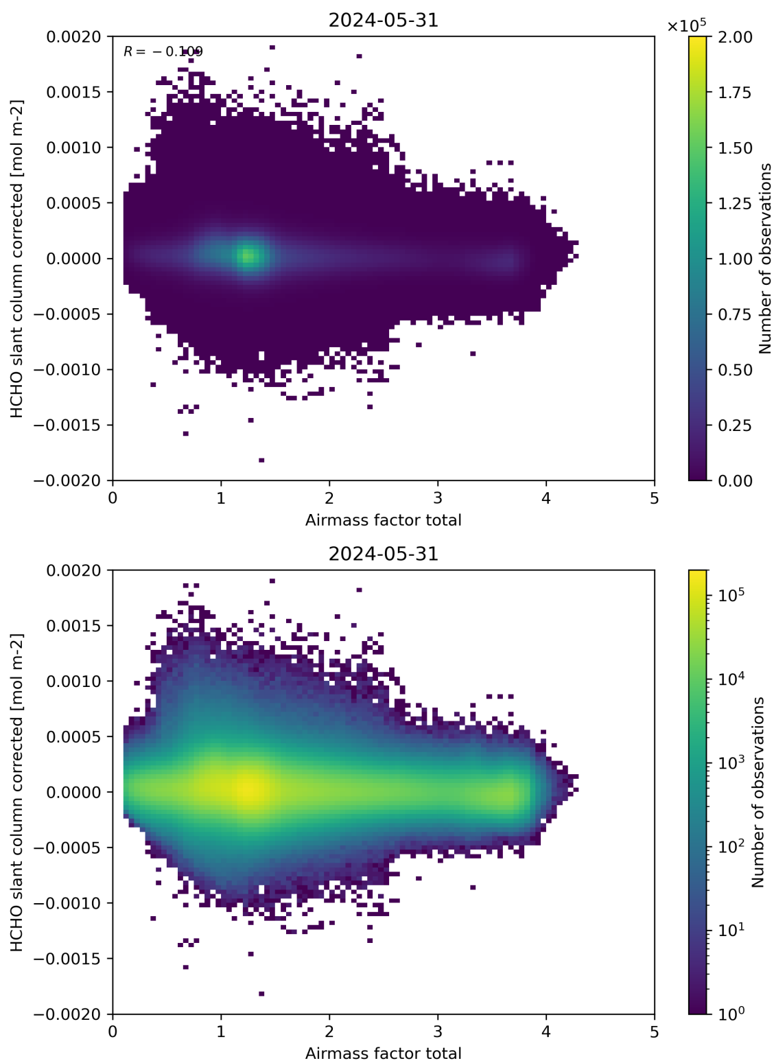
Figure 101: Scatter density plot of “Airmass factor total” against “HCHO slant column corrected” for 2024-05-30 to 2024-06-01.
