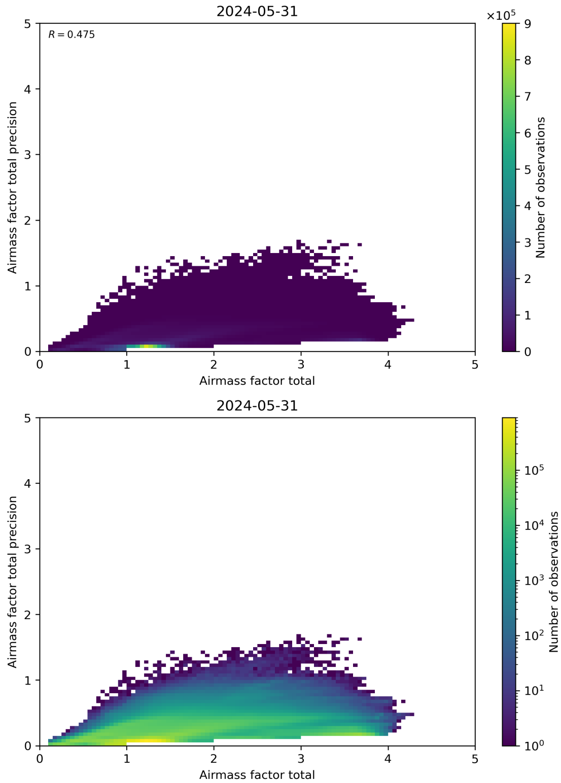
Figure 103: Scatter density plot of “Airmass factor total” against “Airmass factor total precision” for 2024-05-30 to 2024-06-01.
