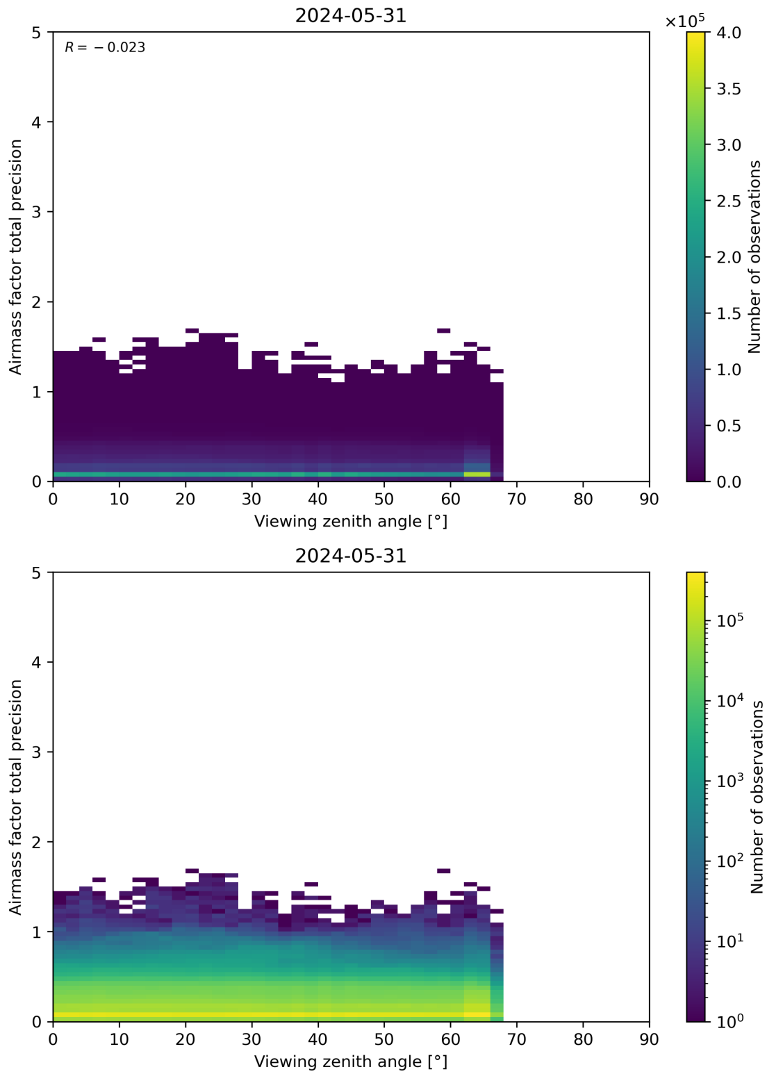
Figure 191: Scatter density plot of “Viewing zenith angle” against “Airmass factor total precision” for 2024-05-30 to 2024-06-01.
