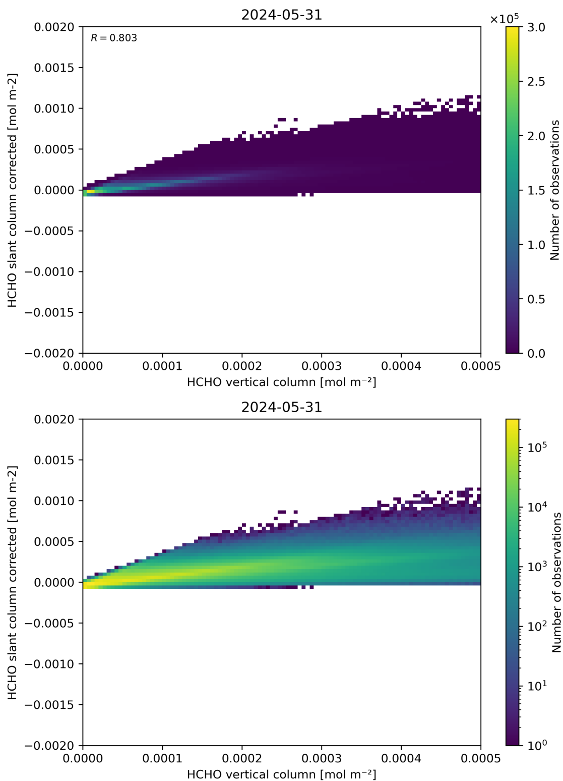
Figure 127: Scatter density plot of “HCHO vertical column” against “HCHO slant column corrected” for 2024-05-30 to 2024-06-01.
