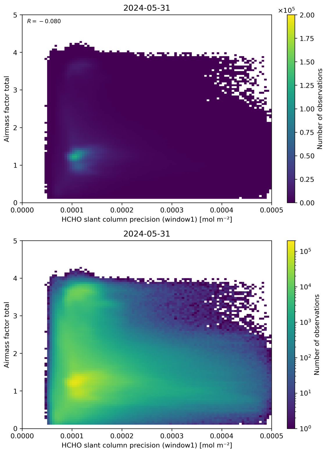
Figure 94: Scatter density plot of “HCHO slant column precision (window1)” against “Airmass factor total” for 2024-05-30 to 2024-06-01.
