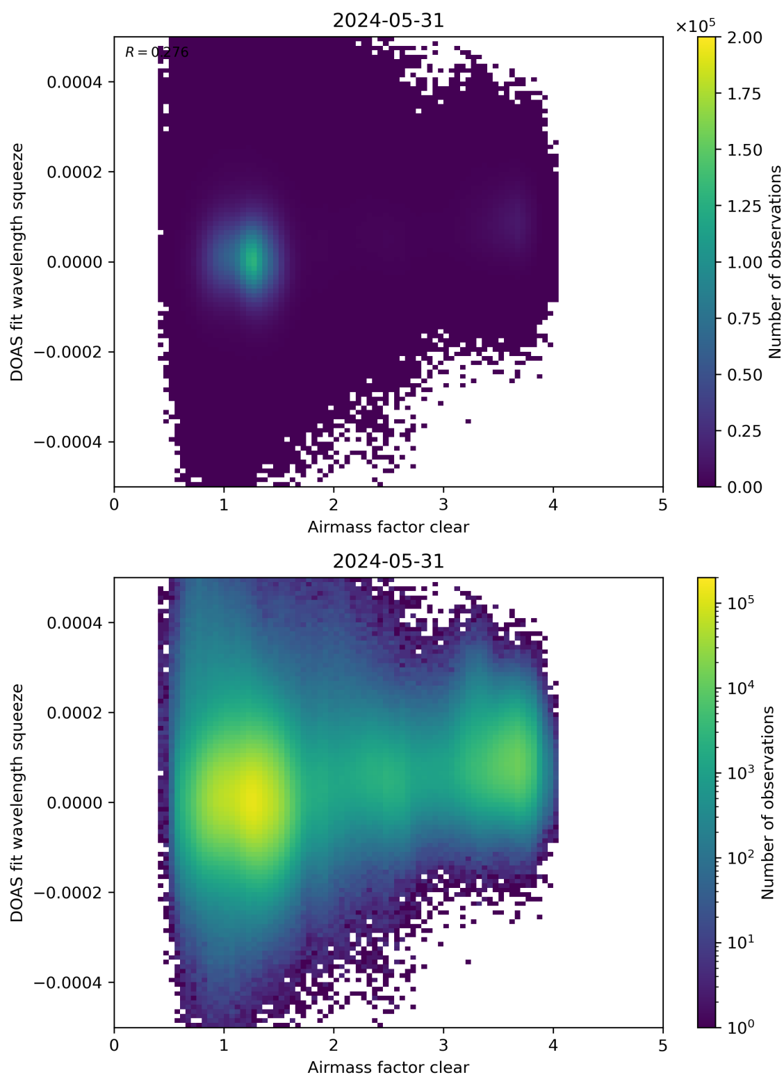
Figure 73: Scatter density plot of “Airmass factor clear” against “DOAS fit wavelength squeeze” for 2024-05-30 to 2024-06-01.
