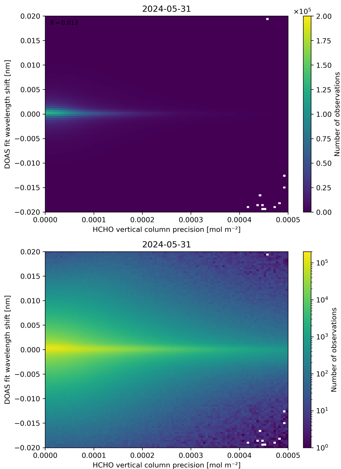
Figure 137: Scatter density plot of “HCHO vertical column precision” against “DOAS fit wavelength shift” for 2024-05-30 to 2024-06-01.
