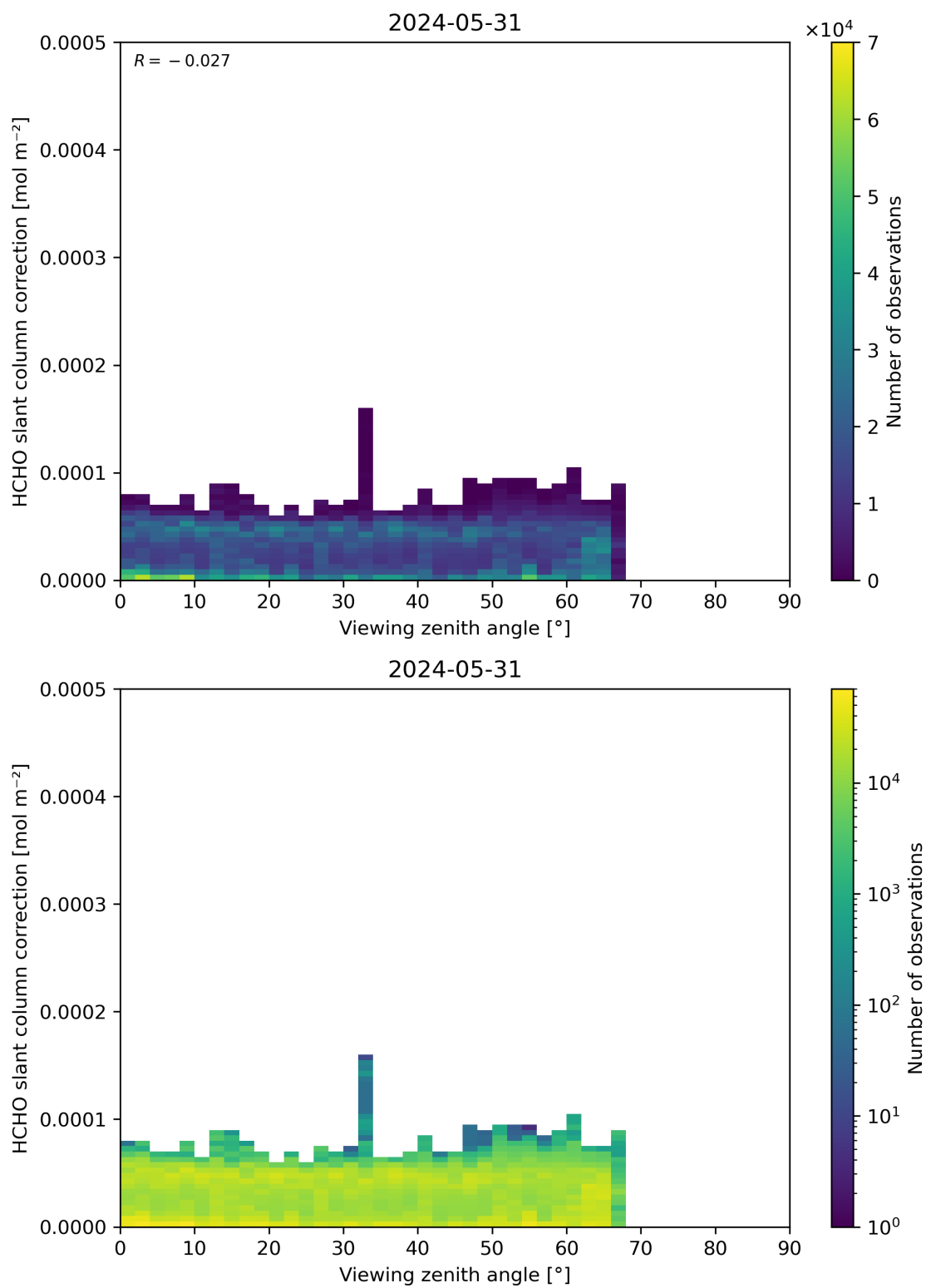
Figure 187: Scatter density plot of “Viewing zenith angle” against “HCHO slant column correction” for 2024-05-30 to 2024-06-01.
