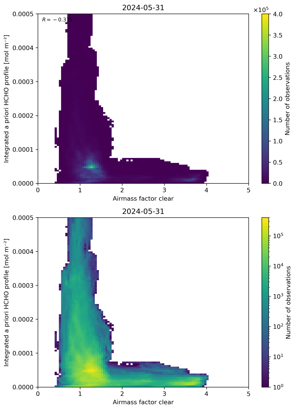
Figure 76: Scatter density plot of “Airmass factor clear” against “Integrated a priori HCHO profile” for 2024-05-30 to 2024-06-01.
