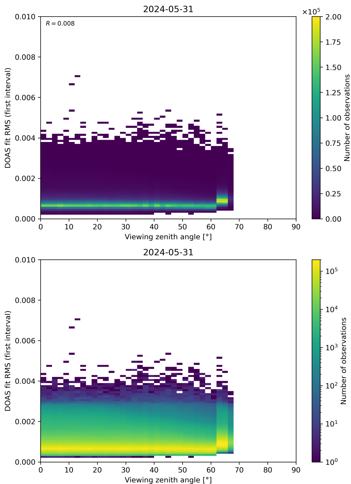
Figure 182: Scatter density plot of “Viewing zenith angle” against “DOAS fit RMS (first interval)” for 2024-05-30 to 2024-06-01.
