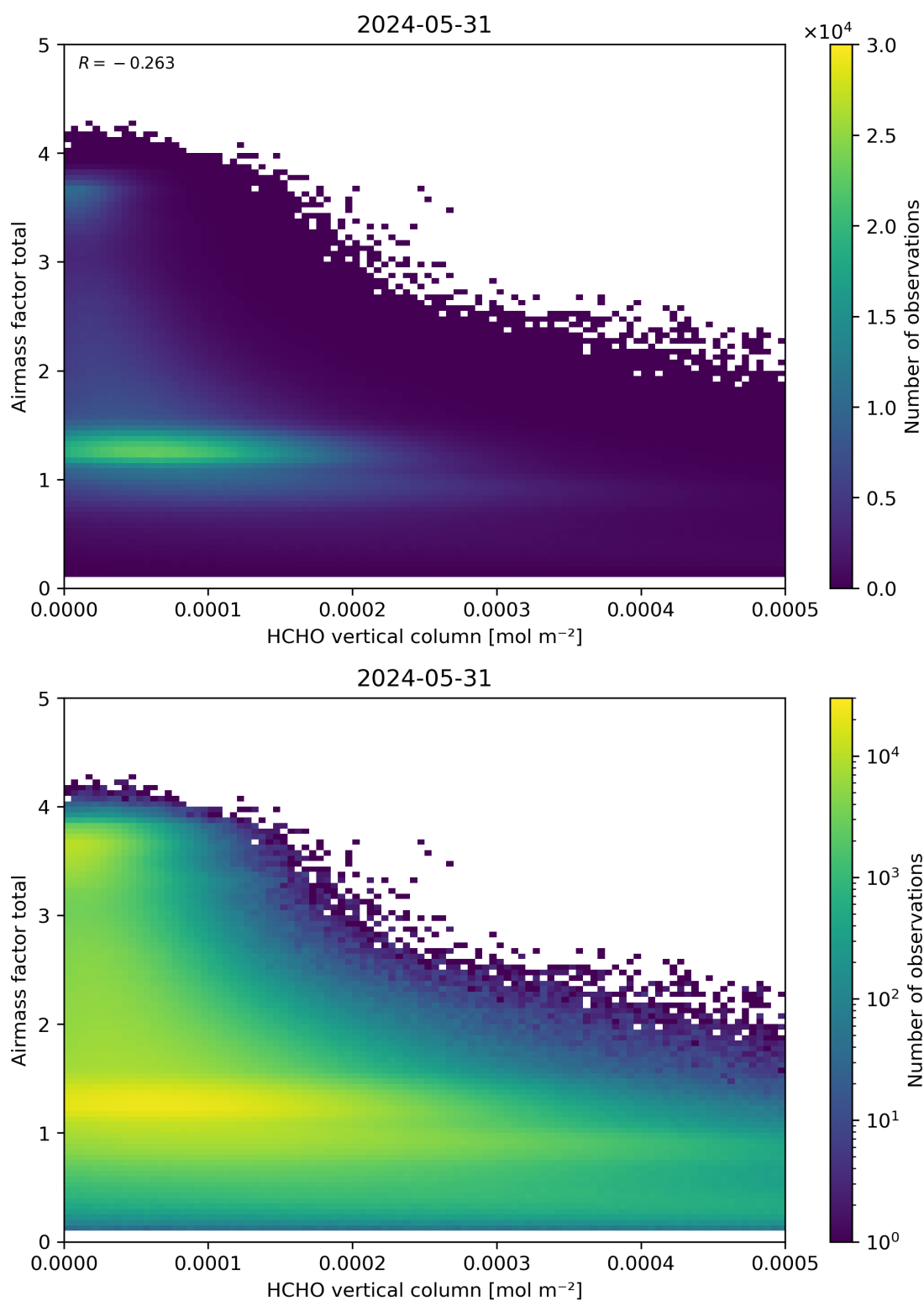
Figure 131: Scatter density plot of “HCHO vertical column” against “Airmass factor total” for 2024-05-30 to 2024-06-01.
