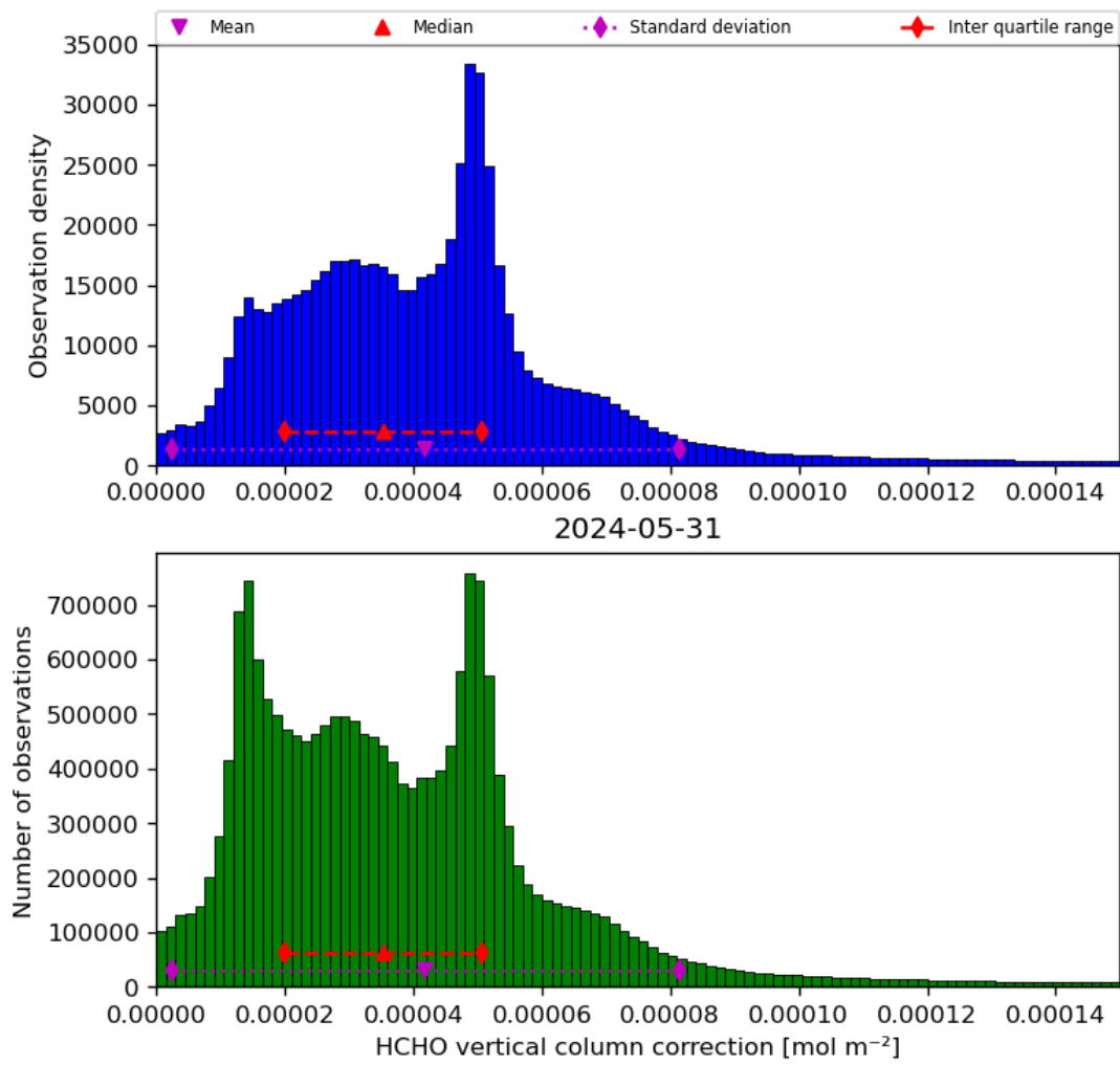
Figure 37: Histogram of “HCHO vertical column correction” for 2024-05-30 to 2024-06-01
