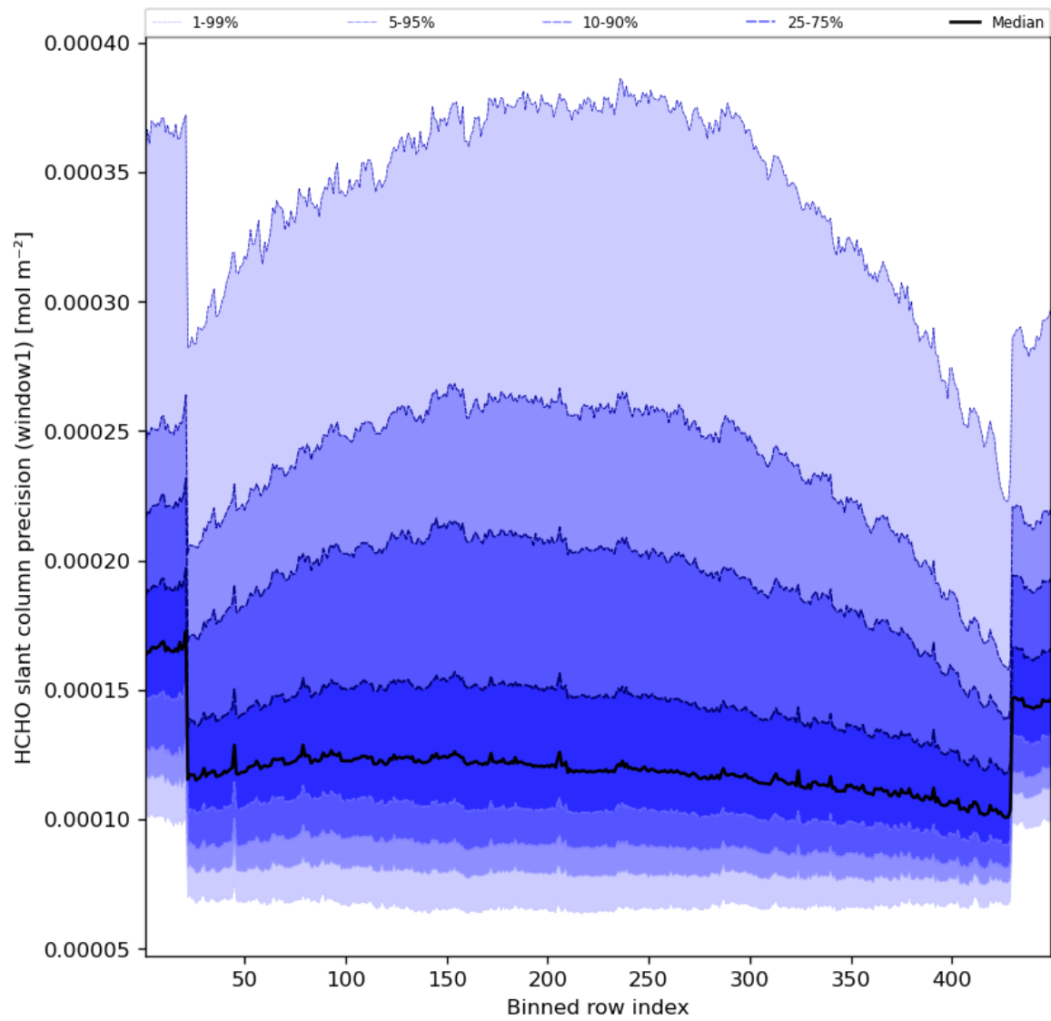
Figure 53: Along track statistics of “HCHO slant column precision (window1)” for 2024-05-30 to 2024-06-01
