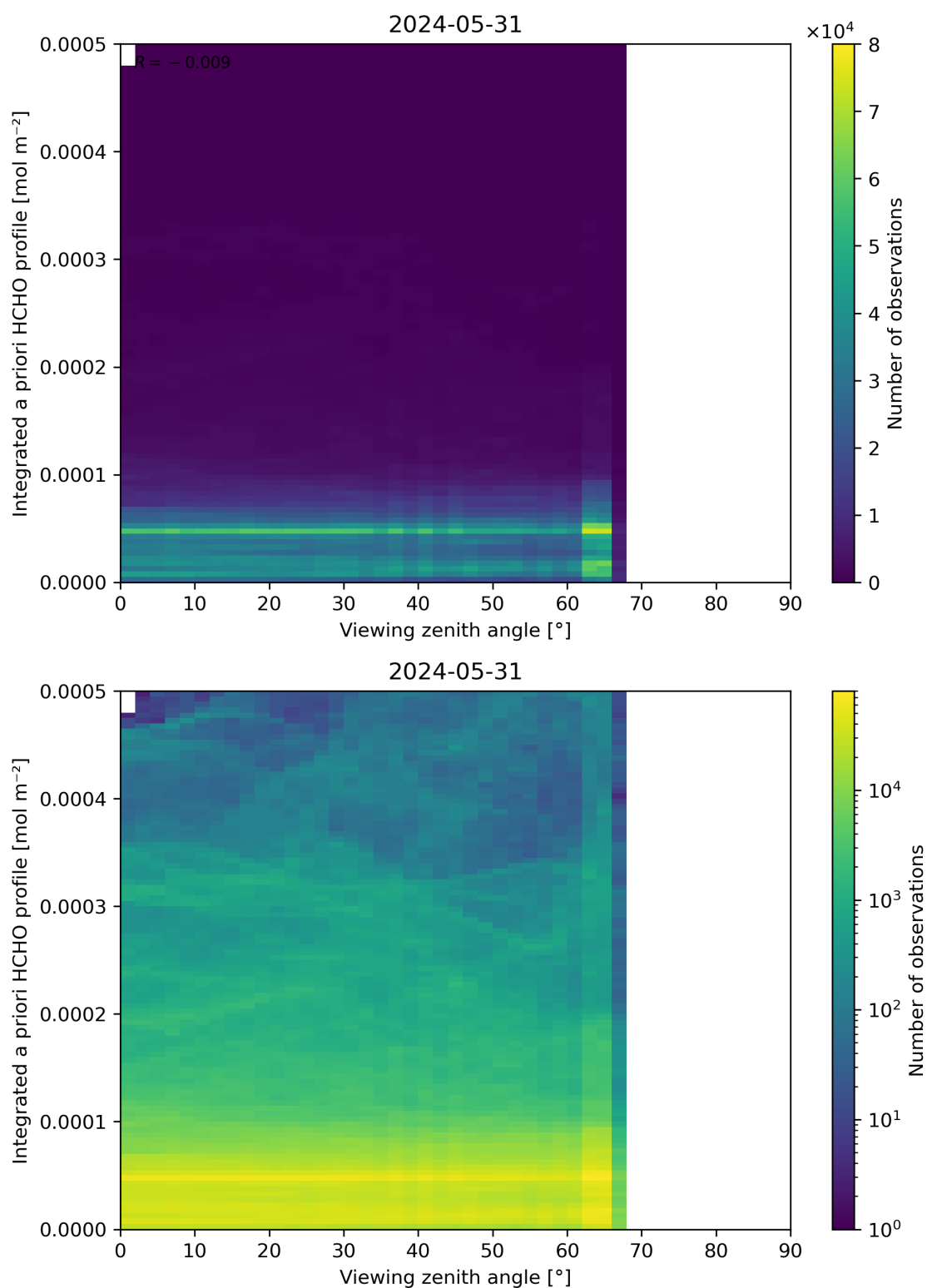
Figure 195: Scatter density plot of “Viewing zenith angle” against “Integrated a priori HCHO profile” for 2024-05-30 to 2024-06-01.
