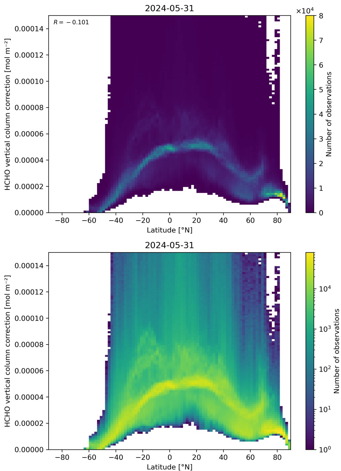
Figure 164: Scatter density plot of “Latitude” against “HCHO vertical column correction” for 2024-05-30 to 2024-06-01.
