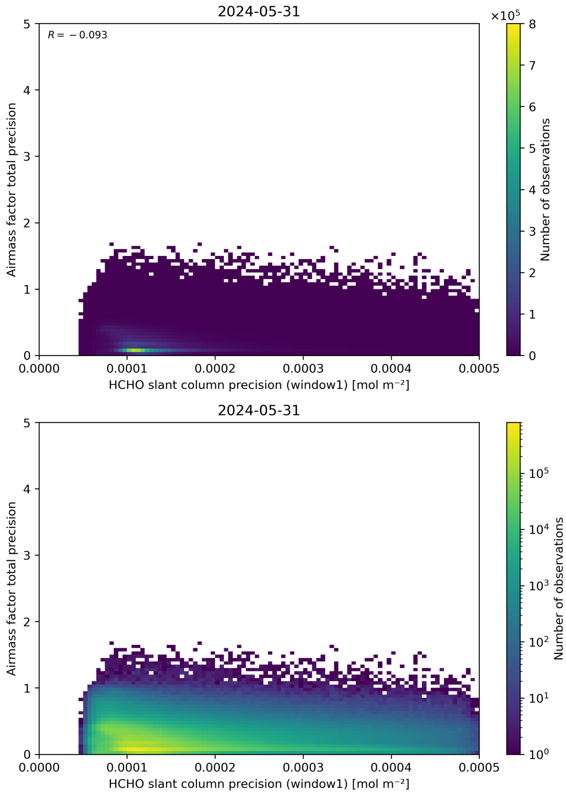
Figure 95: Scatter density plot of “HCHO slant column precision (window1)” against “Airmass factor total precision” for 2024-05-30 to 2024-06-01.
