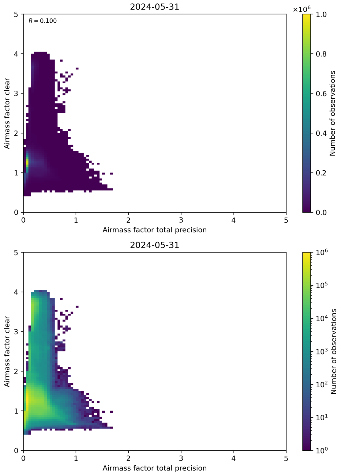
Figure 108: Scatter density plot of “Airmass factor total precision” against “Airmass factor clear” for 2024-05-30 to 2024-06-01.
