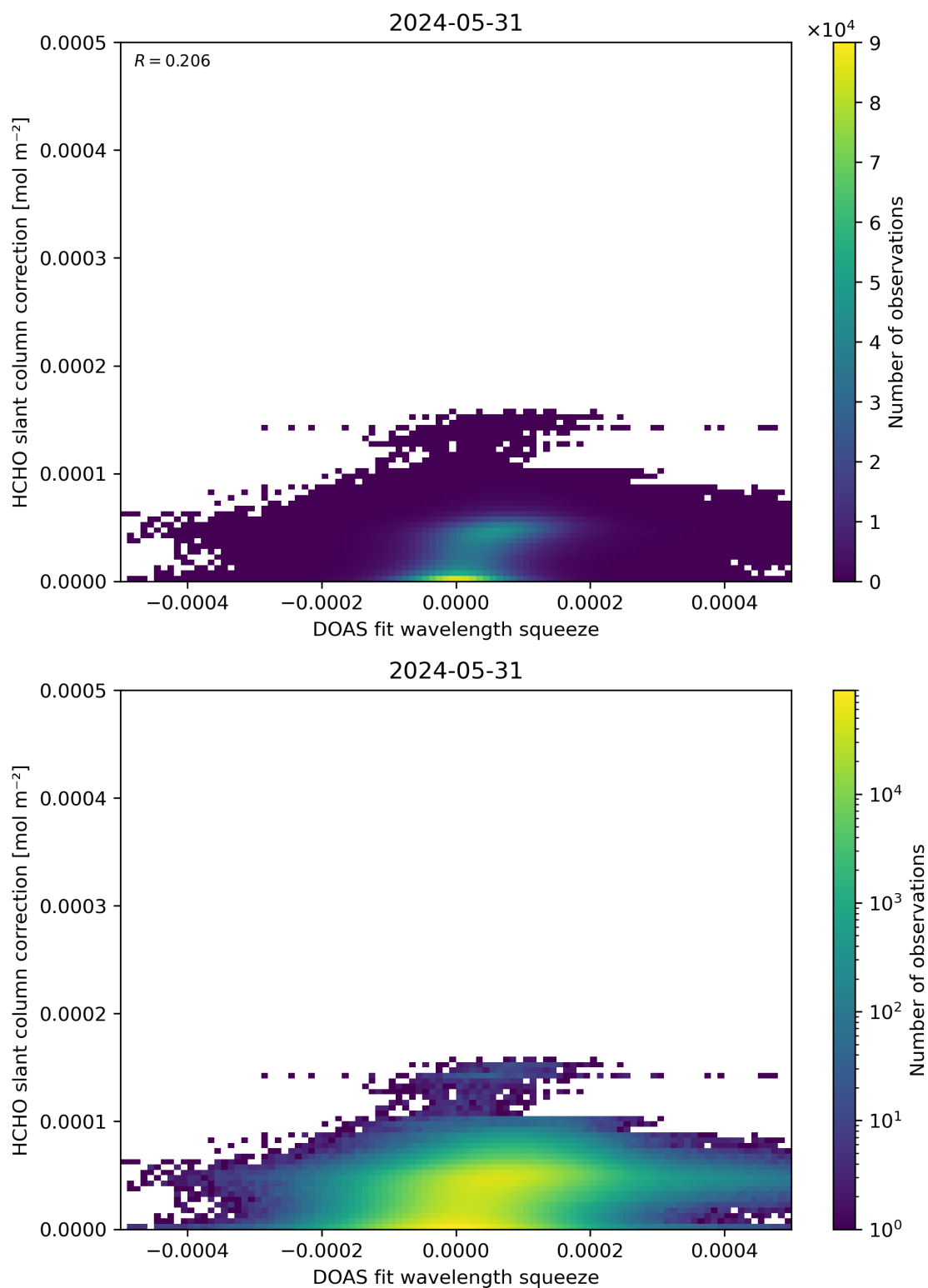
Figure 70: Scatter density plot of “DOAS fit wavelength squeeze” against “HCHO slant column correction” for 2024-05-30 to 2024-06-01.
