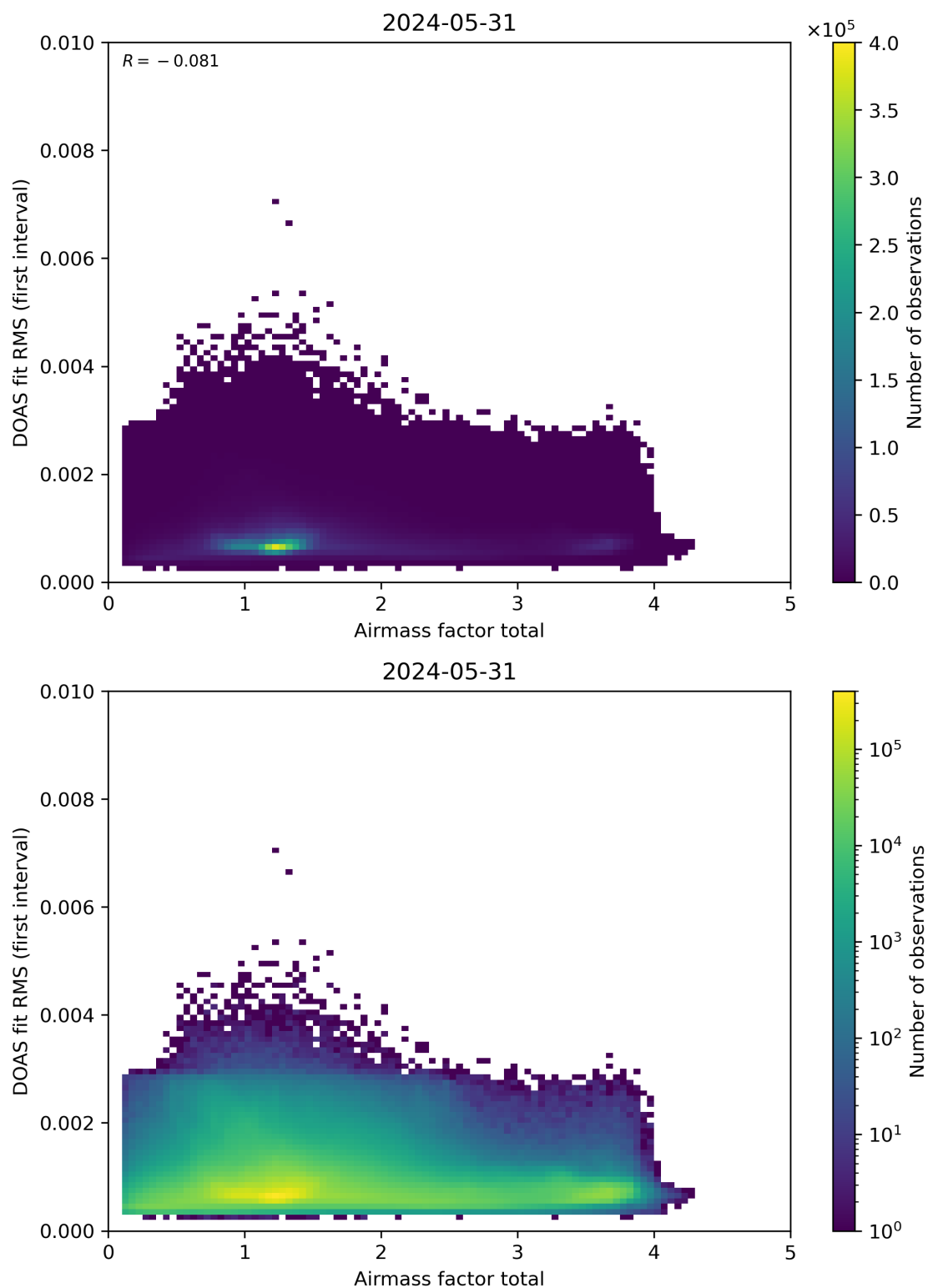
Figure 97: Scatter density plot of “Airmass factor total” against “DOAS fit RMS (first interval)” for 2024-05-30 to 2024-06-01.
