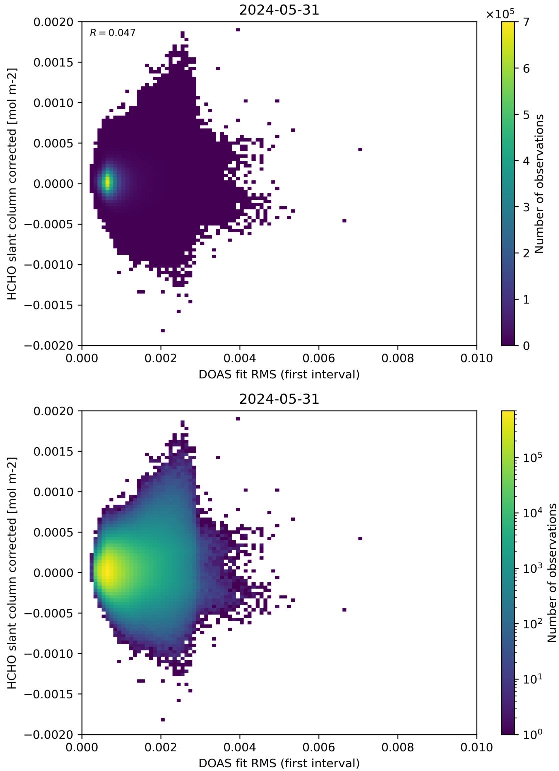
Figure 62: Scatter density plot of “DOAS fit RMS (first interval)” against “HCHO slant column corrected” for 2024-05-30 to 2024-06-01.
