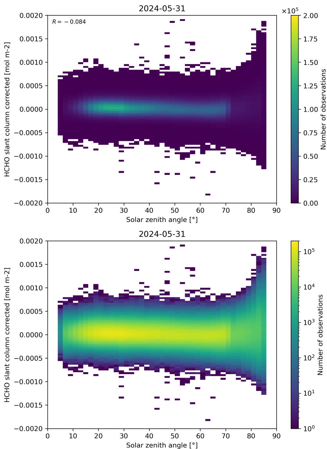
Figure 171: Scatter density plot of “Solar zenith angle” against “HCHO slant column corrected” for 2024-05-30 to 2024-06-01.
