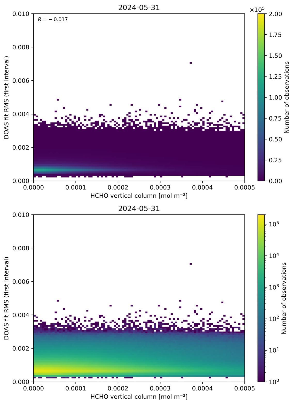
Figure 123: Scatter density plot of “HCHO vertical column” against “DOAS fit RMS (first interval)” for 2024-05-30 to 2024-06-01.
