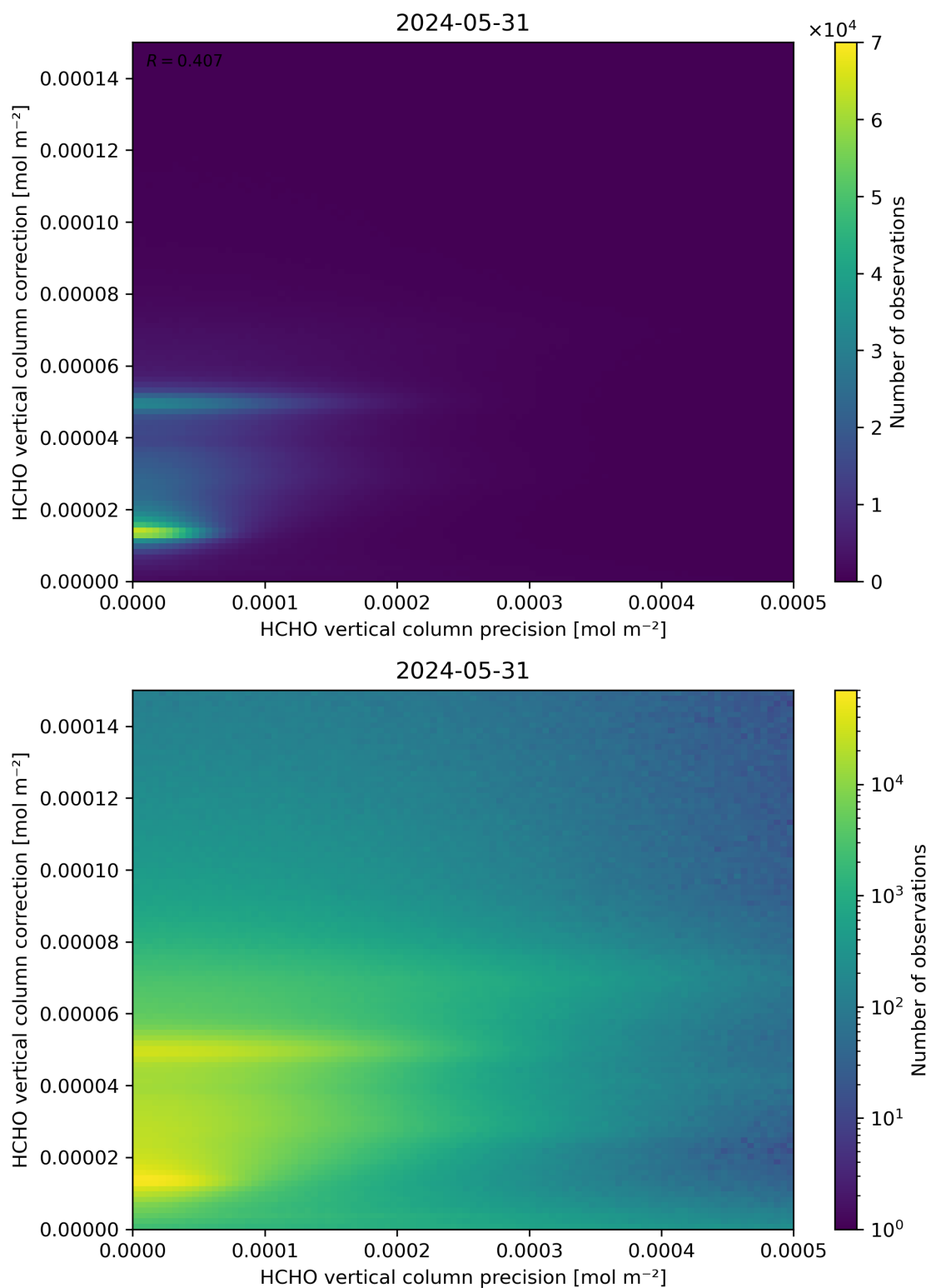
Figure 146: Scatter density plot of “HCHO vertical column precision” against “HCHO vertical column correction” for 2024-05-30 to 2024-06-01.
