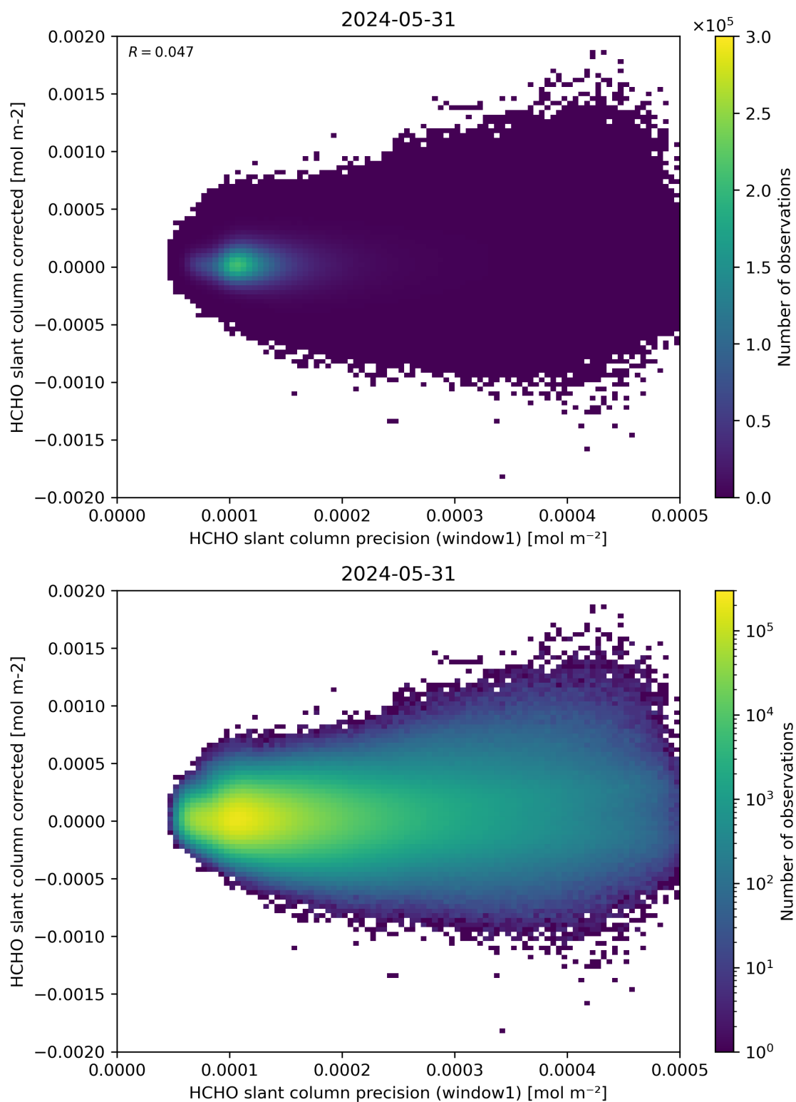
Figure 92: Scatter density plot of “HCHO slant column precision (window1)” against “HCHO slant column corrected” for 2024-05-30 to 2024-06-01.
