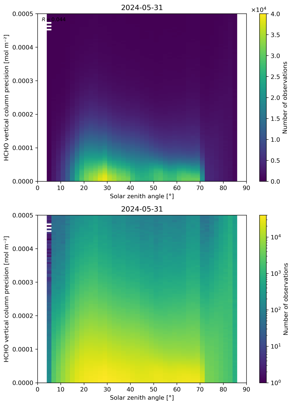
Figure 179: Scatter density plot of “Solar zenith angle” against “HCHO vertical column precision” for 2024-05-30 to 2024-06-01.
