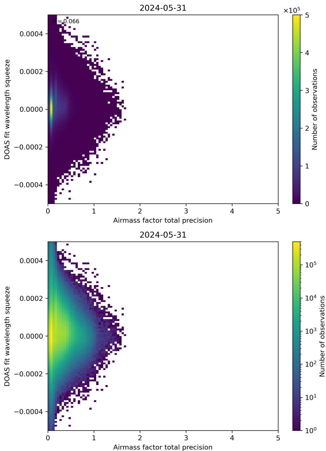
Figure 107: Scatter density plot of “Airmass factor total precision” against “DOAS fit wavelength squeeze” for 2024-05-30 to 2024-06-01.
