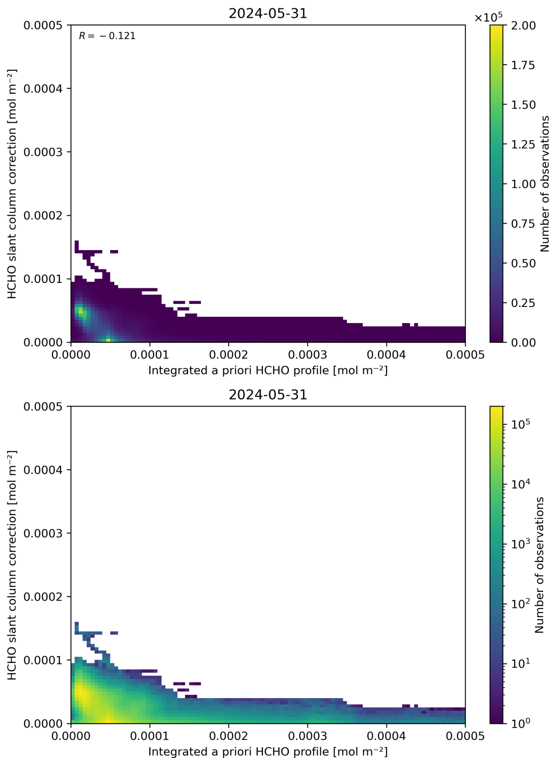
Figure 152: Scatter density plot of “Integrated a priori HCHO profile” against “HCHO slant column correction” for 2024-05-30 to 2024-06-01.
