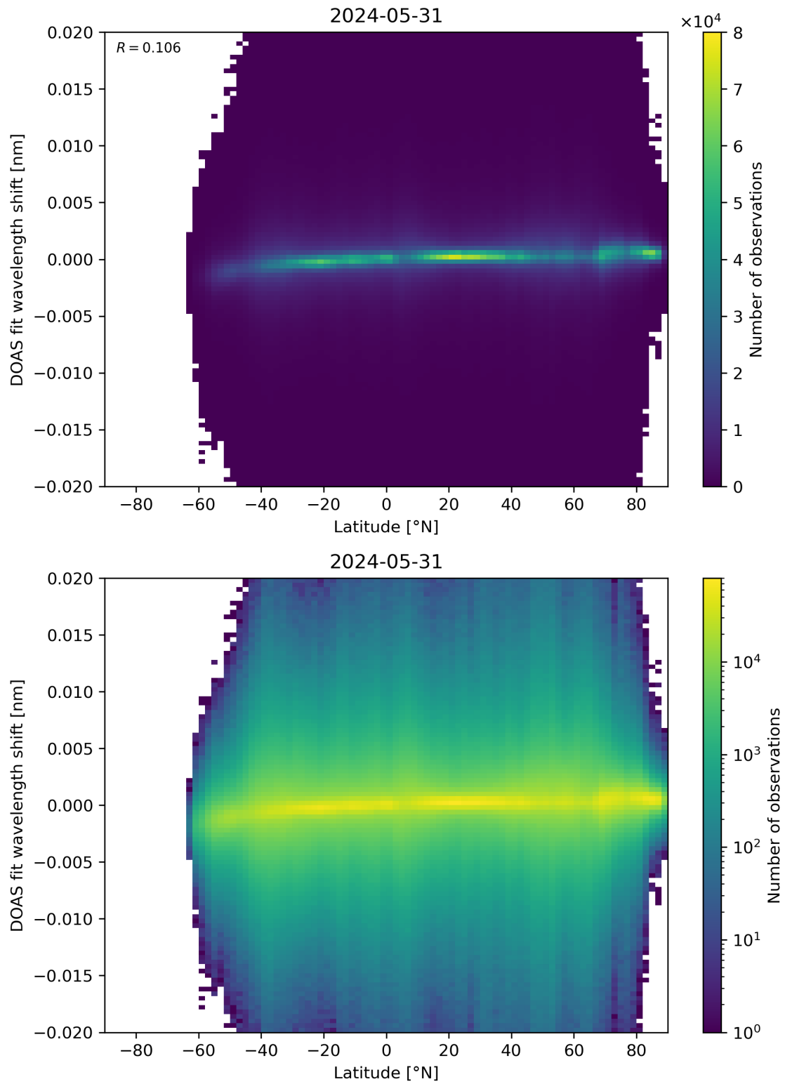
Figure 154: Scatter density plot of “Latitude” against “DOAS fit wavelength shift” for 2024-05-30 to 2024-06-01.
