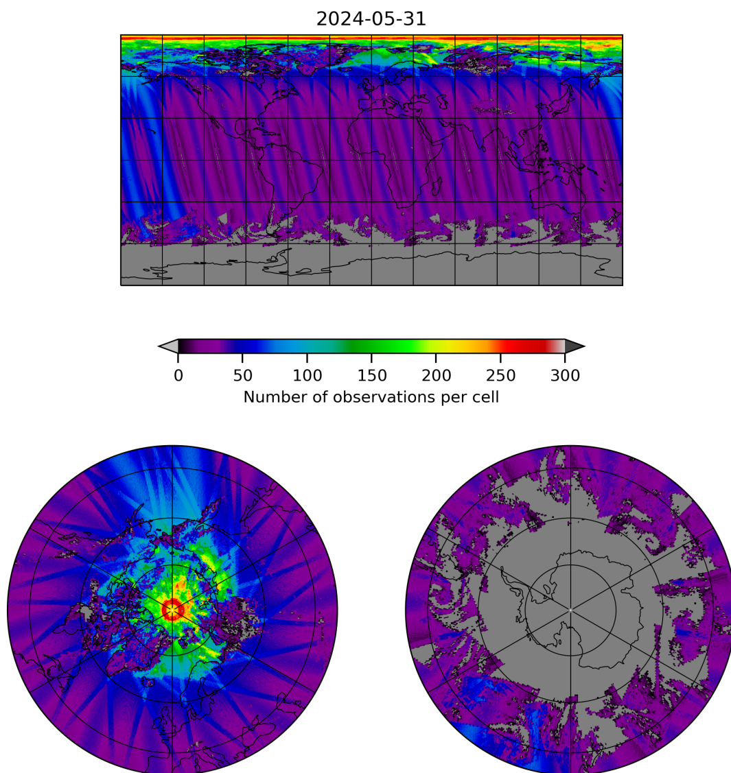
Figure 19: Map of the number of observations for 2024-05-30 to 2024-06-01
