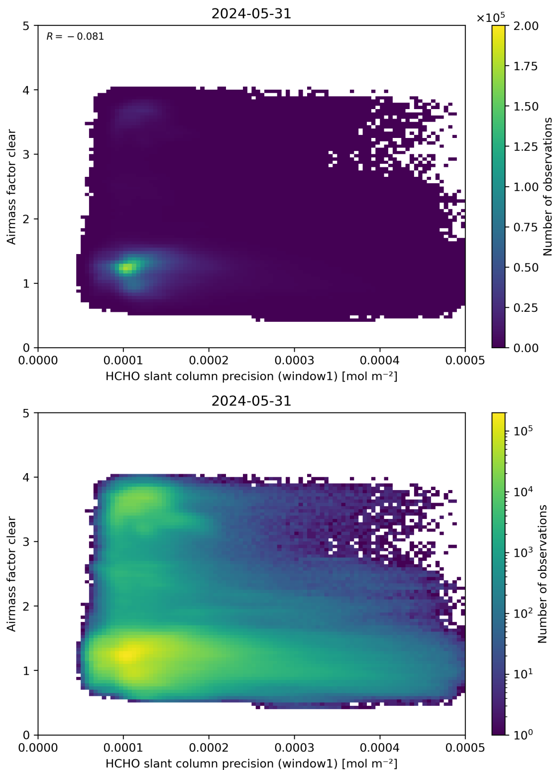
Figure 91: Scatter density plot of “HCHO slant column precision (window1)” against “Airmass factor clear” for 2024-05-30 to 2024-06-01.
