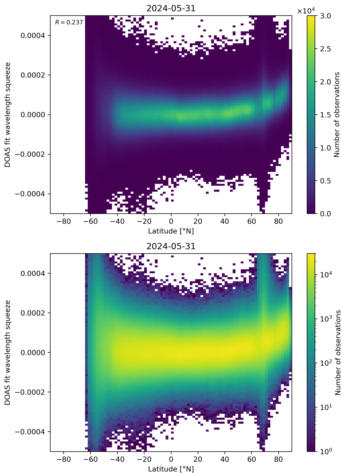
Figure 155: Scatter density plot of “Latitude” against “DOAS fit wavelength squeeze” for 2024-05-30 to 2024-06-01.
