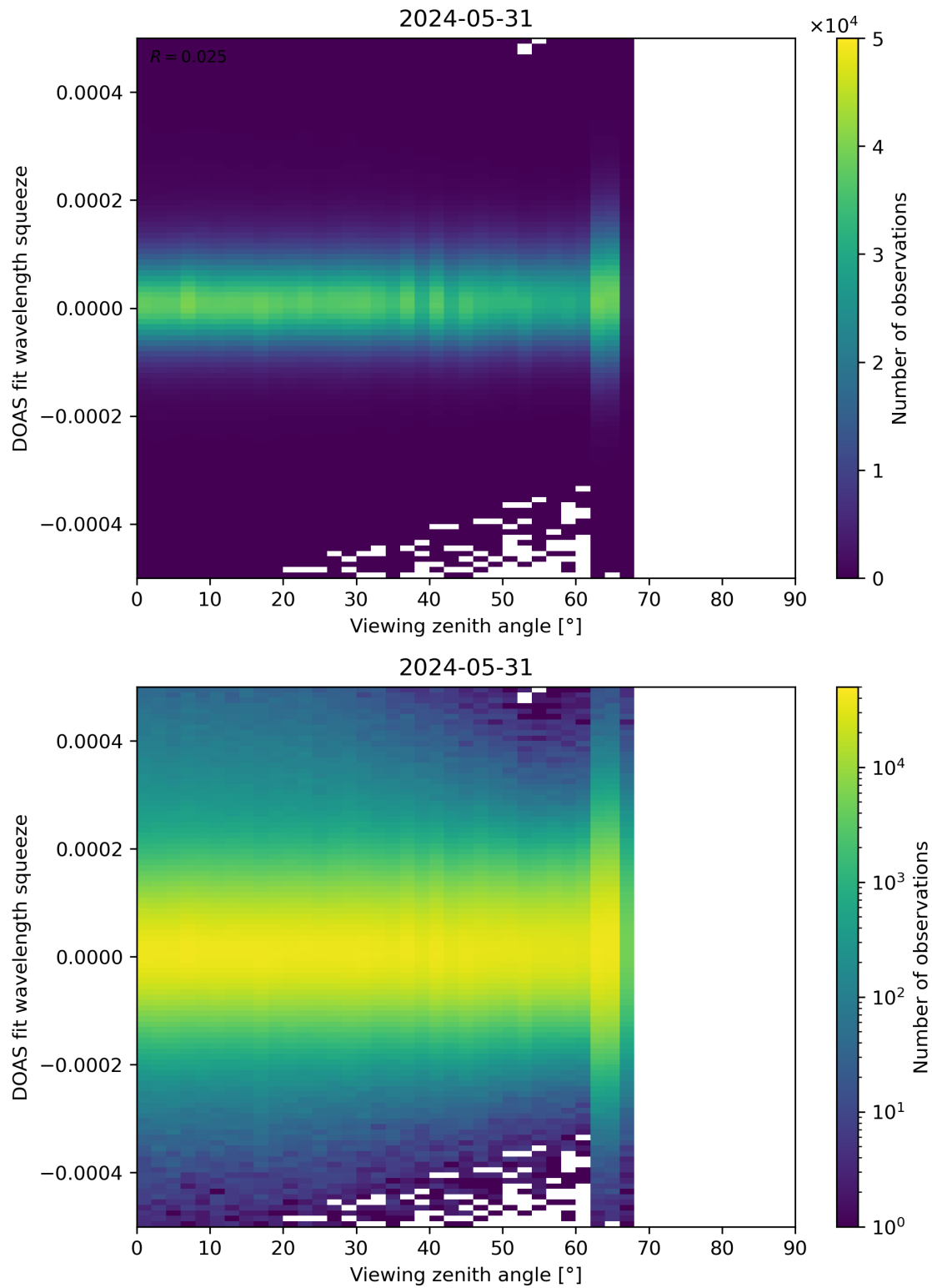
Figure 184: Scatter density plot of “Viewing zenith angle” against “DOAS fit wavelength squeeze” for 2024-05-30 to 2024-06-01.
