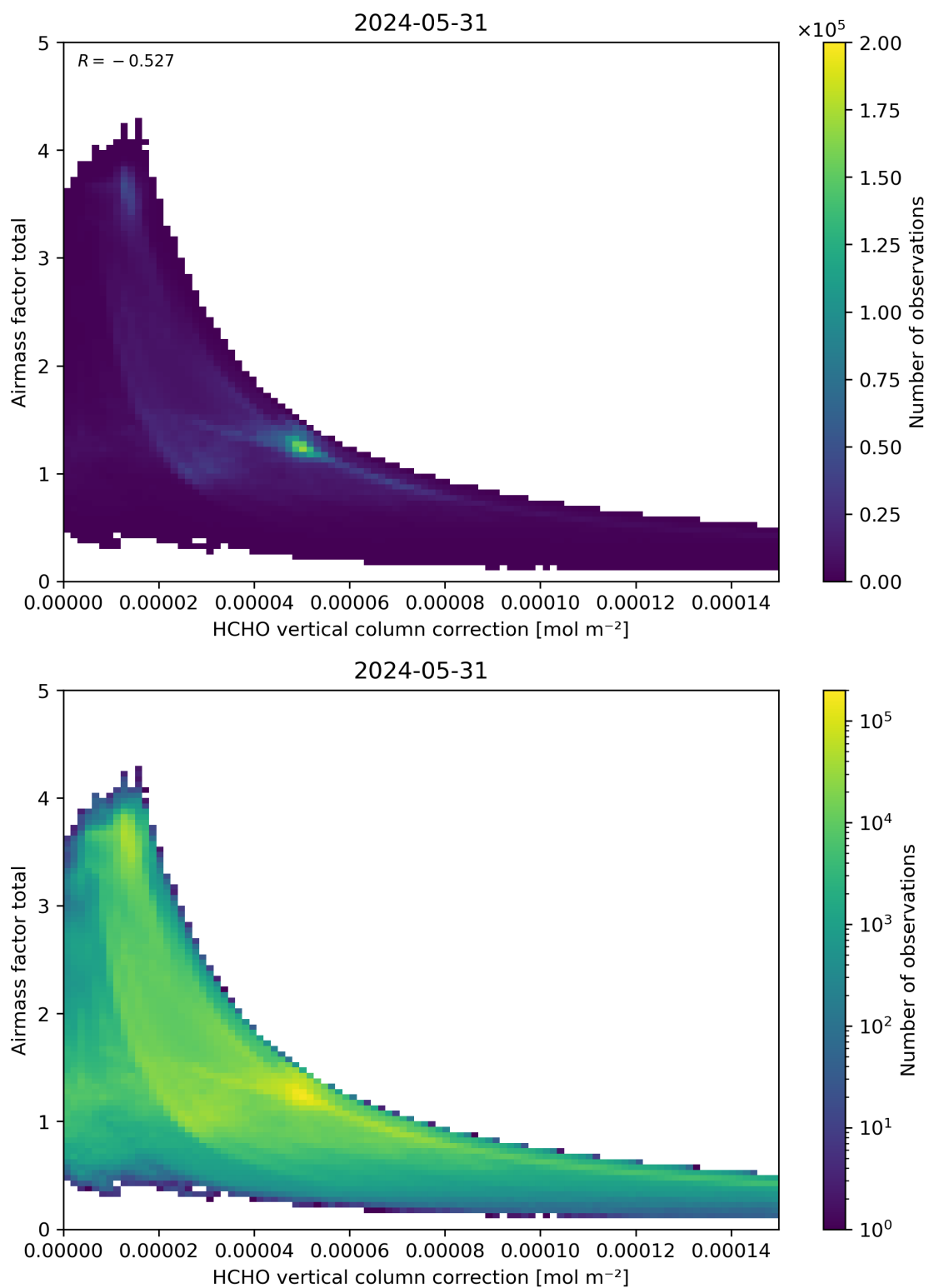
Figure 120: Scatter density plot of “HCHO vertical column correction” against “Airmass factor total” for 2024-05-30 to 2024-06-01.
