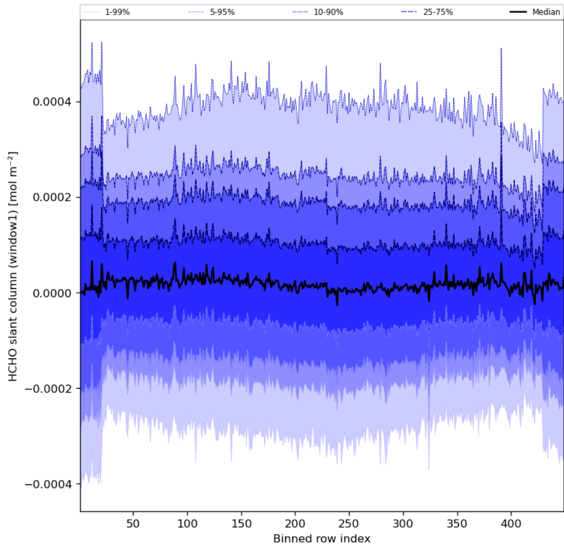
Figure 52: Along track statistics of “HCHO slant column (window1)” for 2024-05-30 to 2024-06-01
