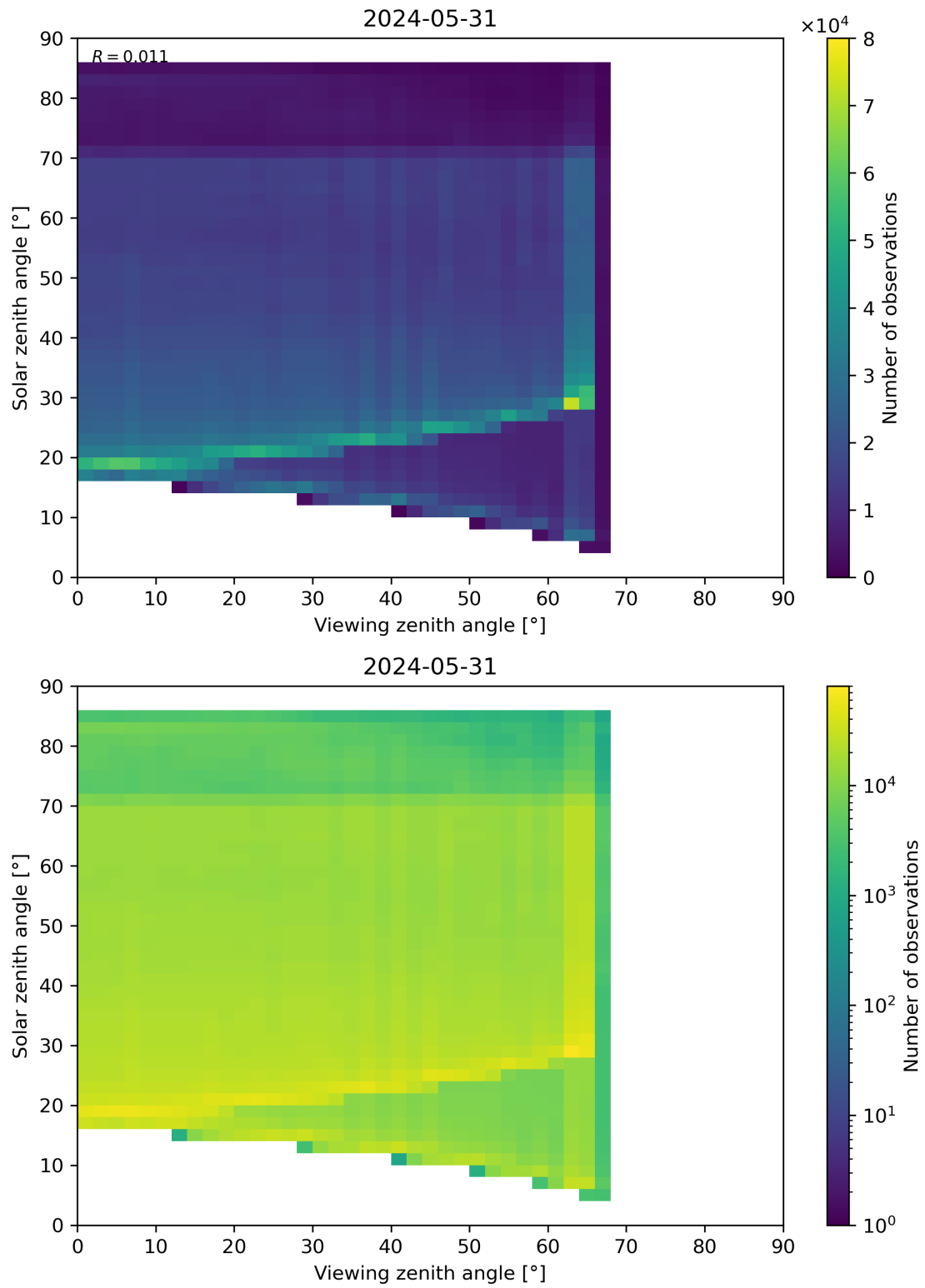
Figure 197: Scatter density plot of “Viewing zenith angle” against “Solar zenith angle” for 2024-05-30 to 2024-06-01.
