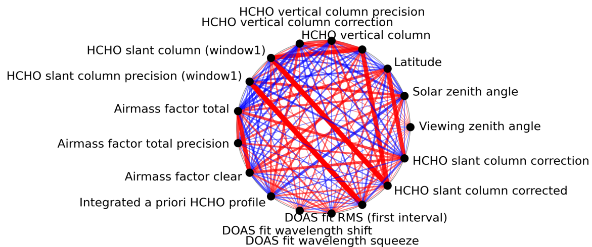
Figure 1: Map of correlation graph for 2024-05-30 to 2024-06-01.
