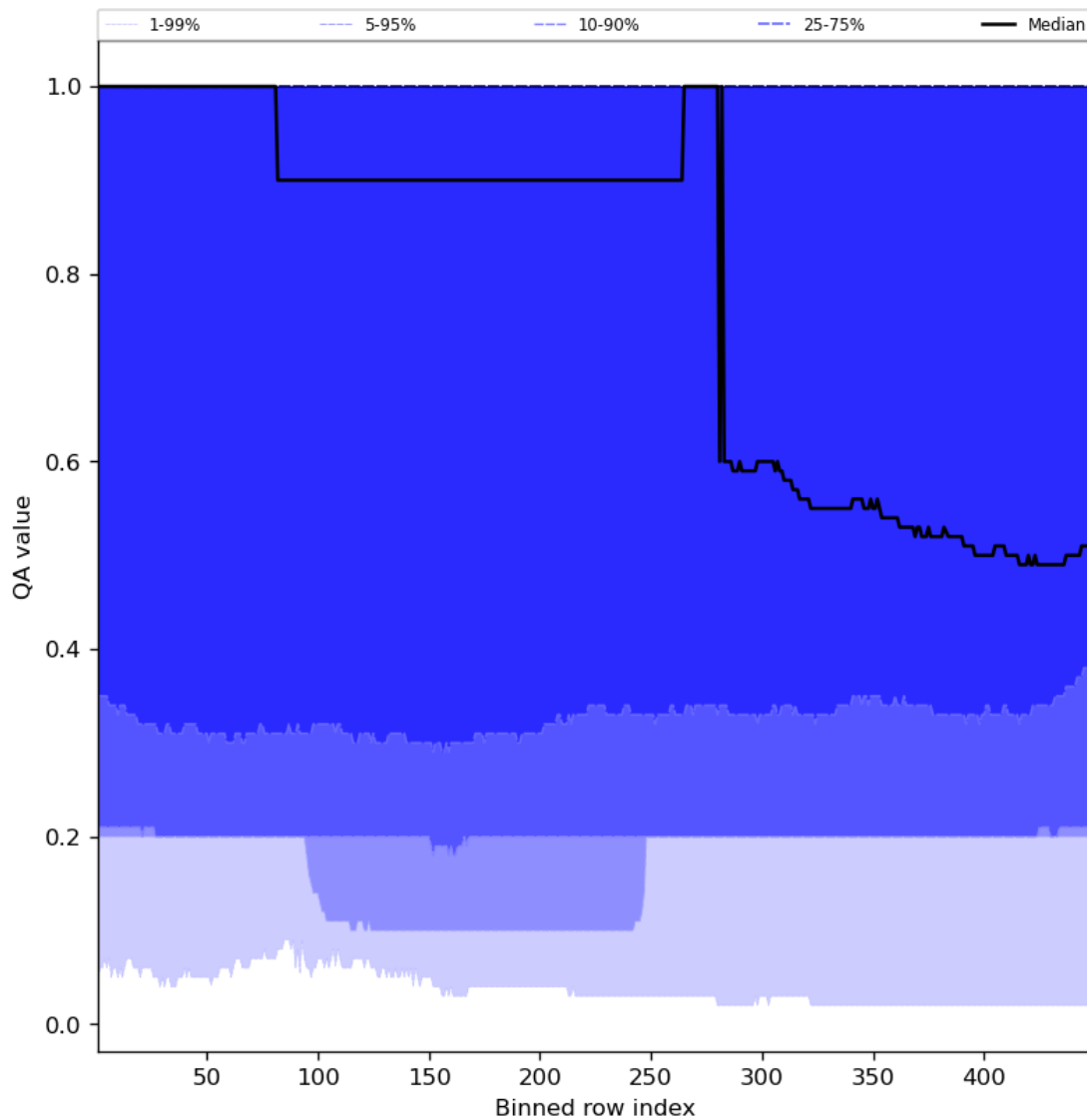
Figure 48: Along track statistics of “QA value” for 2024-05-30 to 2024-06-01
