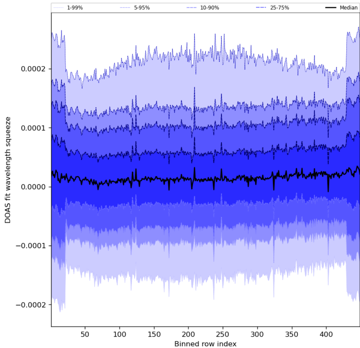
Figure 59: Along track statistics of “DOAS fit wavelength squeeze” for 2024-05-30 to 2024-06-01
