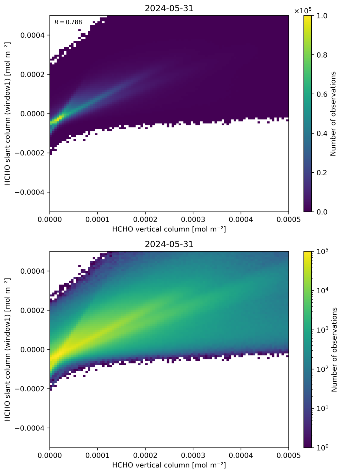
Figure 129: Scatter density plot of “HCHO vertical column” against “HCHO slant column (window1)” for 2024-05-30 to 2024-06-01.
