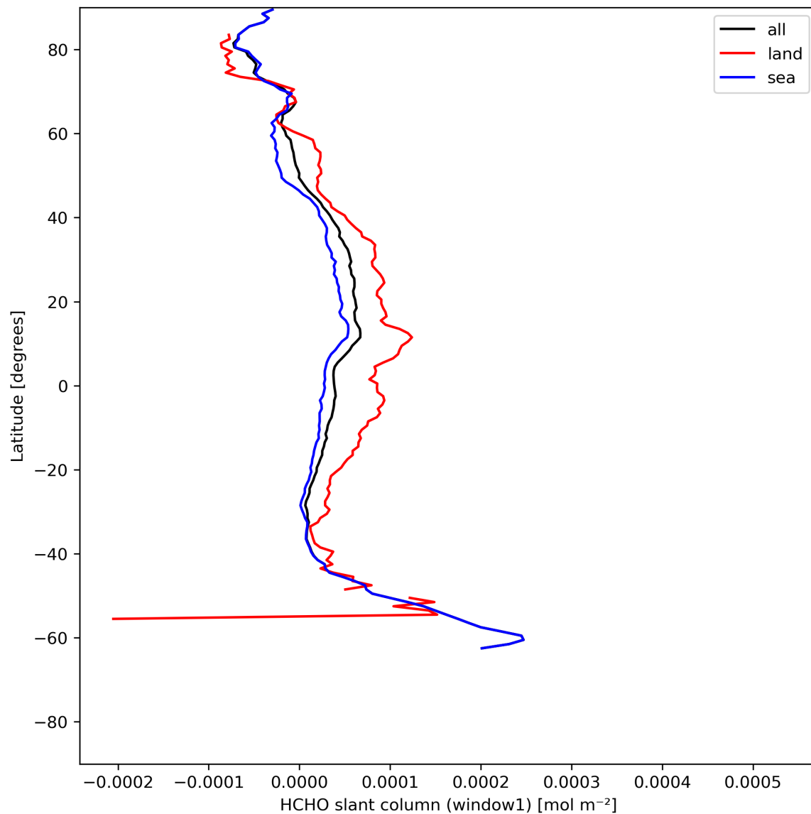
Figure 24: Zonal average of “HCHO slant column (window1)” for 2024-05-30 to 2024-06-01.
