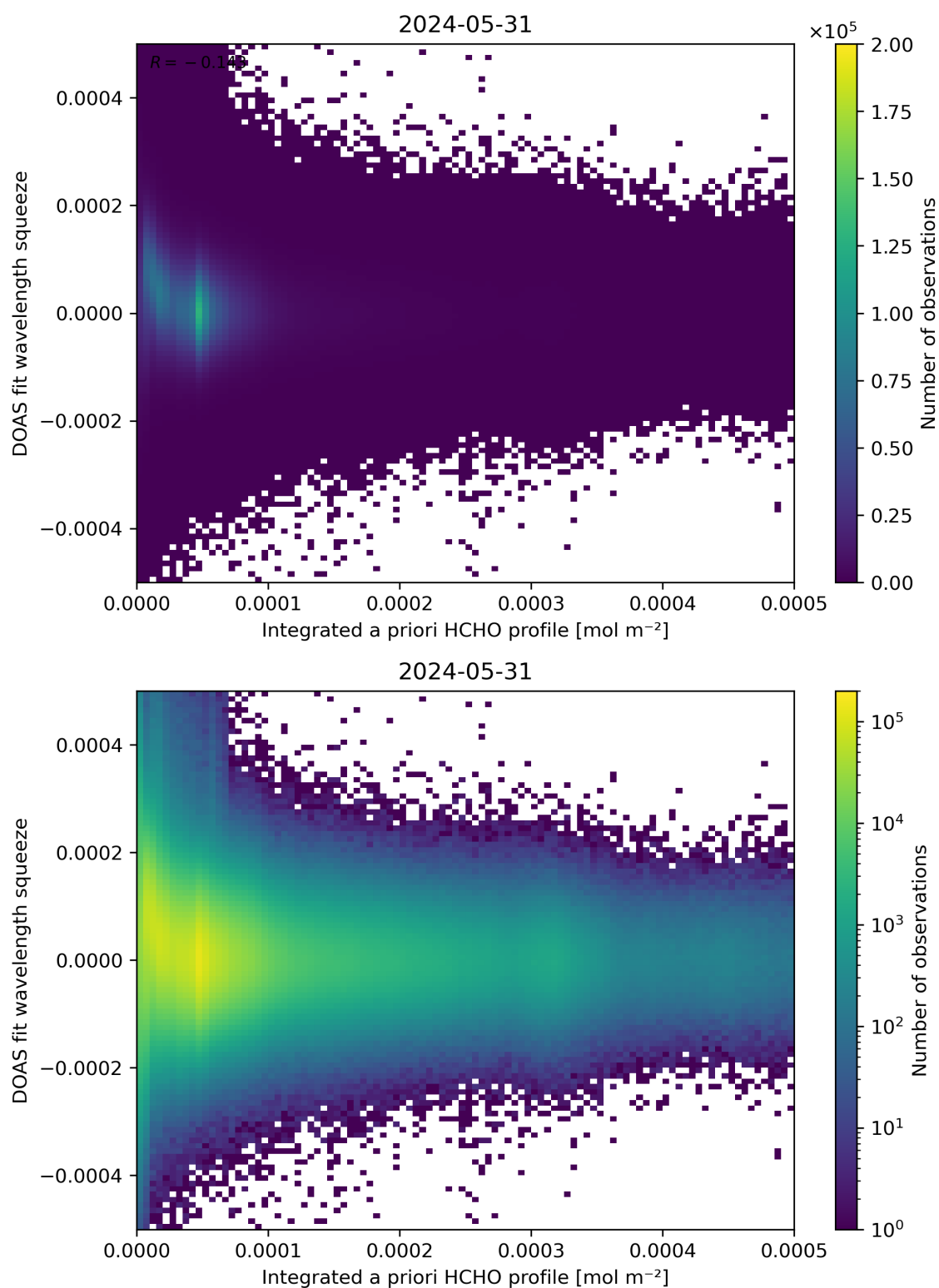
Figure 150: Scatter density plot of “Integrated a priori HCHO profile” against “DOAS fit wavelength squeeze” for 2024-05-30 to 2024-06-01.
