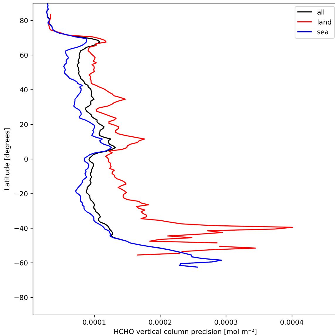
Figure 22: Zonal average of “HCHO vertical column precision” for 2024-05-30 to 2024-06-01.
