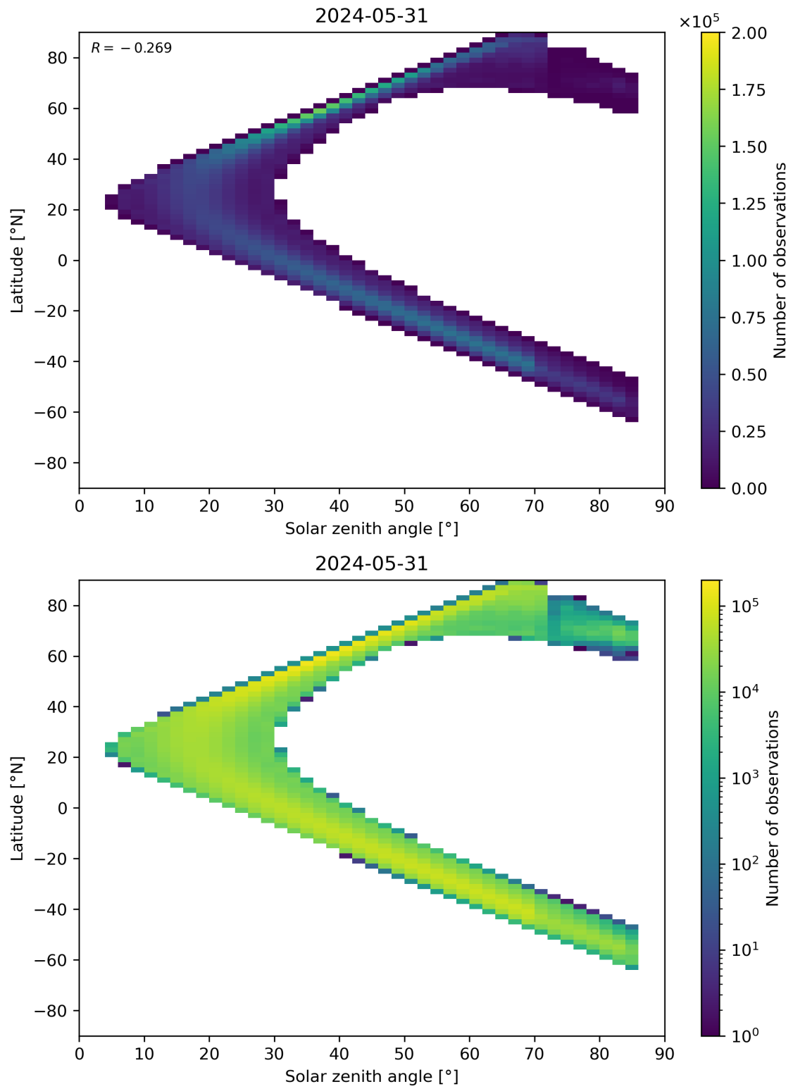
Figure 181: Scatter density plot of “Solar zenith angle” against “Latitude” for 2024-05-30 to 2024-06-01.
