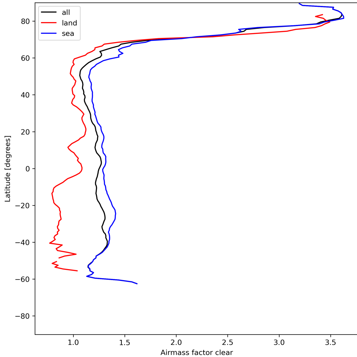
Figure 28: Zonal average of “Airmass factor clear” for 2024-05-30 to 2024-06-01.
