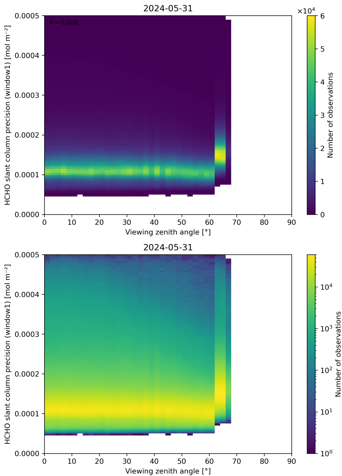
Figure 189: Scatter density plot of “Viewing zenith angle” against “HCHO slant column precision (window1)” for 2024-05-30 to 2024-06-01.
