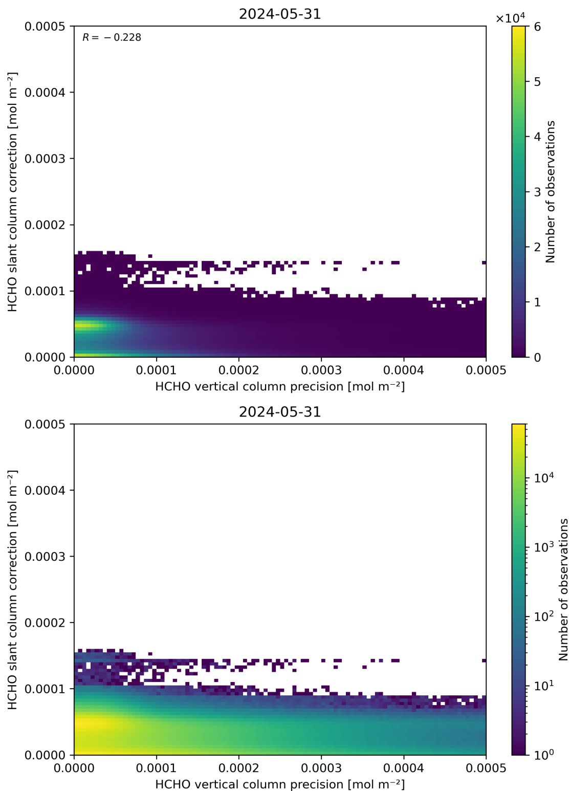
Figure 141: Scatter density plot of “HCHO vertical column precision” against “HCHO slant column correction” for 2024-05-30 to 2024-06-01.
