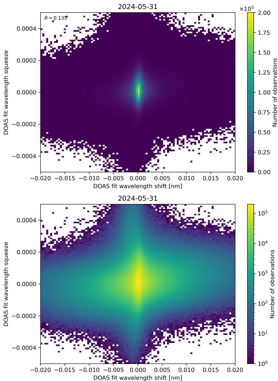
Figure 65: Scatter density plot of “DOAS fit wavelength shift” against “DOAS fit wavelength squeeze” for 2024-05-30 to 2024-06-01.
