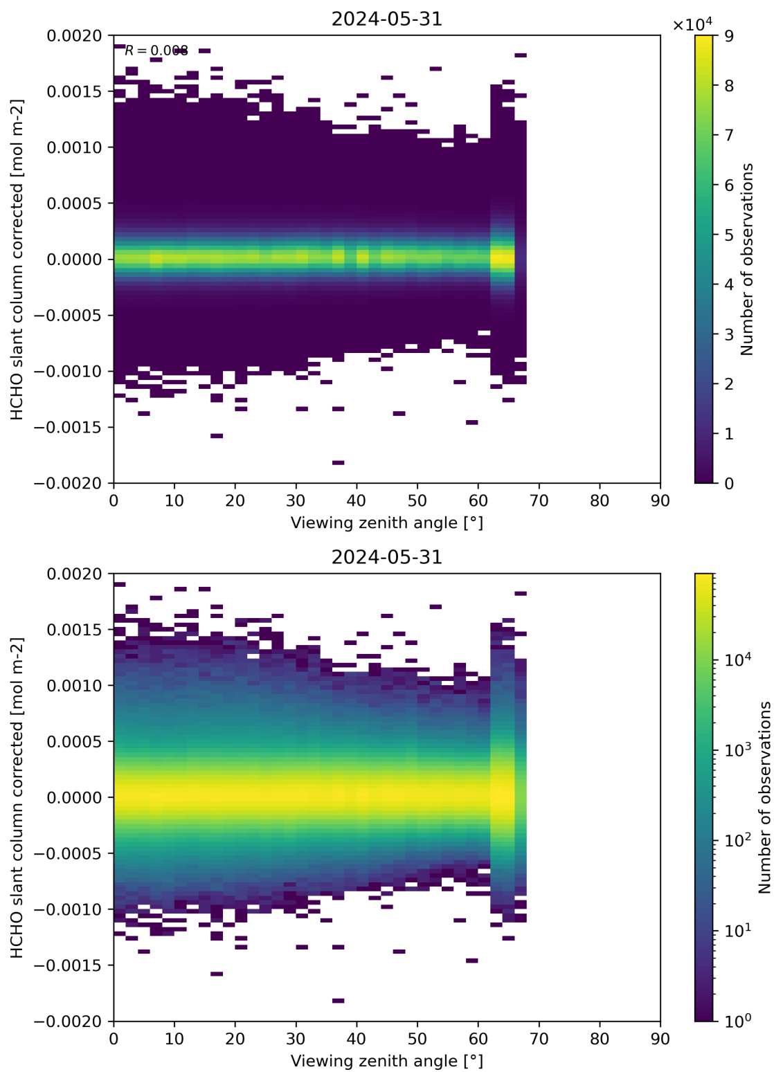
Figure 186: Scatter density plot of “Viewing zenith angle” against “HCHO slant column corrected” for 2024-05-30 to 2024-06-01.
