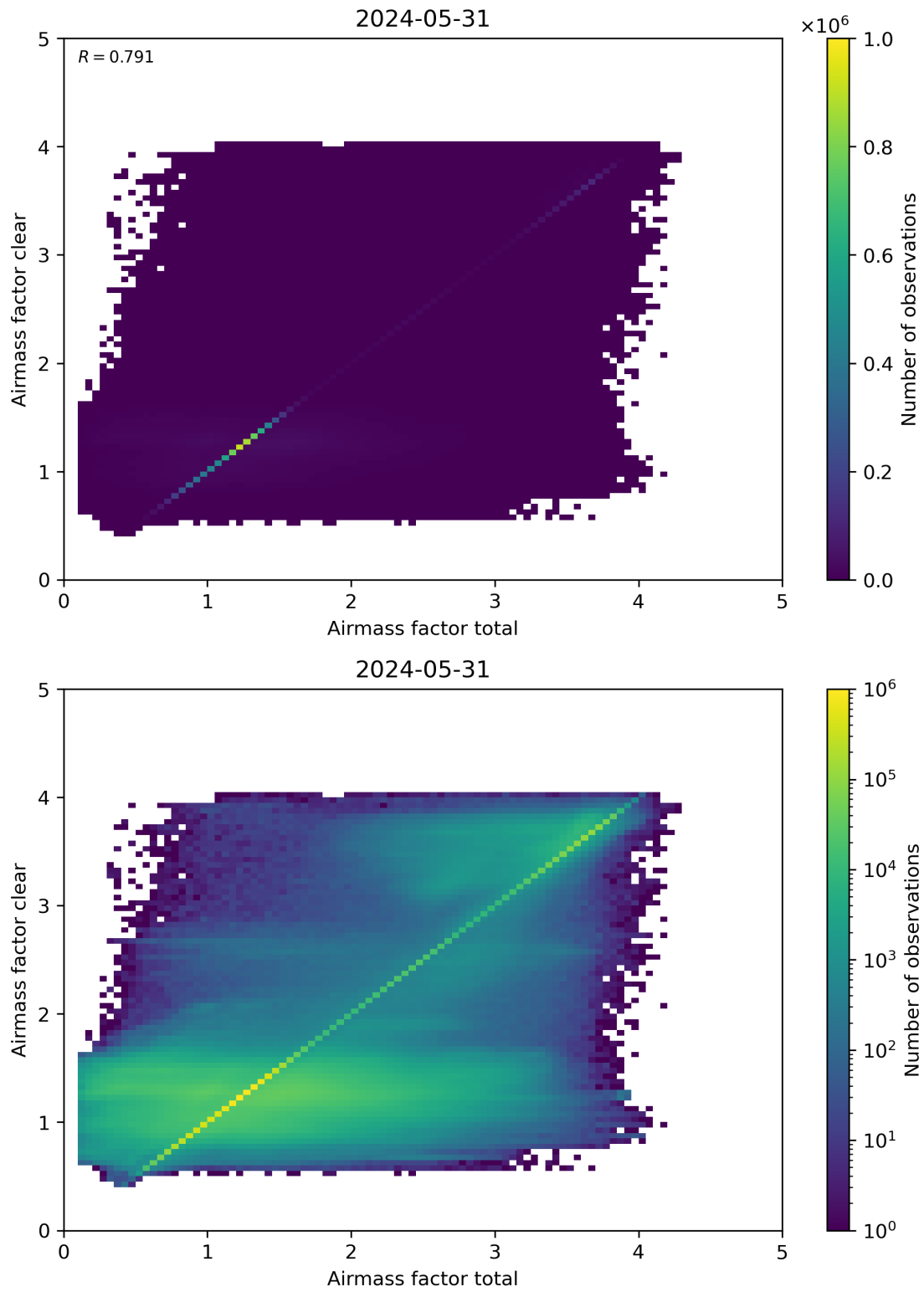
Figure 100: Scatter density plot of “Airmass factor total” against “Airmass factor clear” for 2024-05-30 to 2024-06-01.
