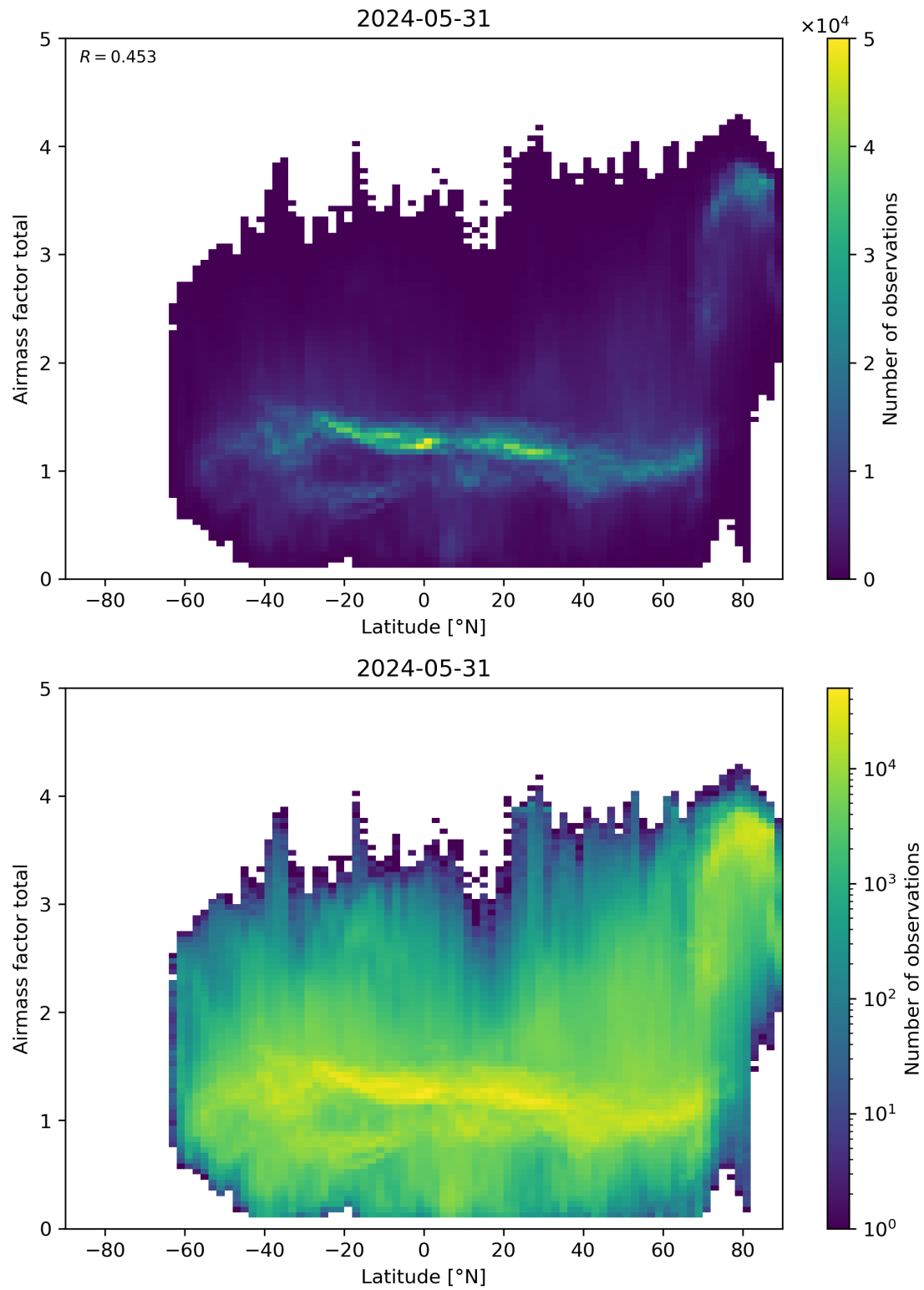
Figure 161: Scatter density plot of “Latitude” against “Airmass factor total” for 2024-05-30 to 2024-06-01.
