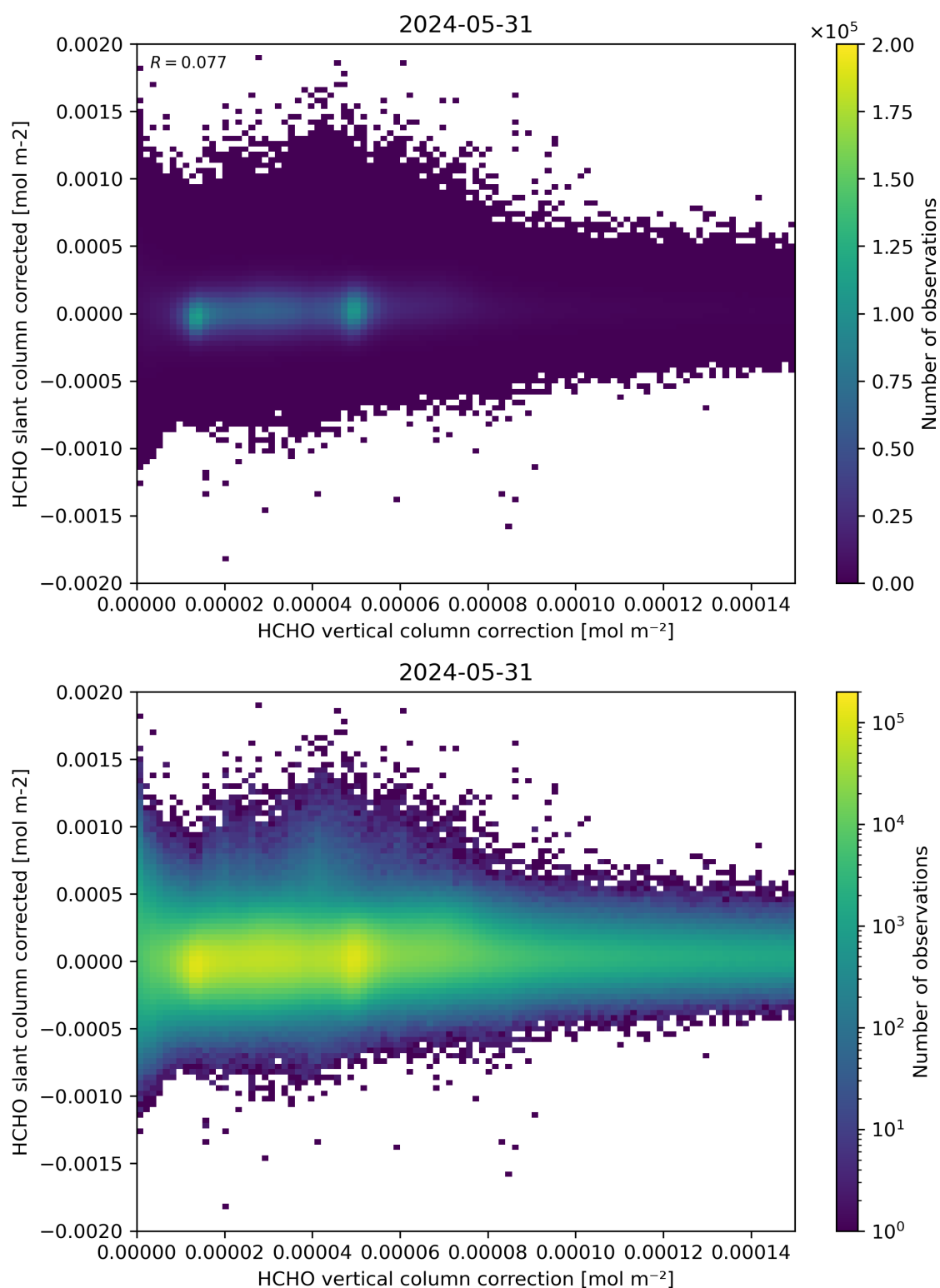
Figure 116: Scatter density plot of “HCHO vertical column correction” against “HCHO slant column corrected” for 2024-05-30 to 2024-06-01.
