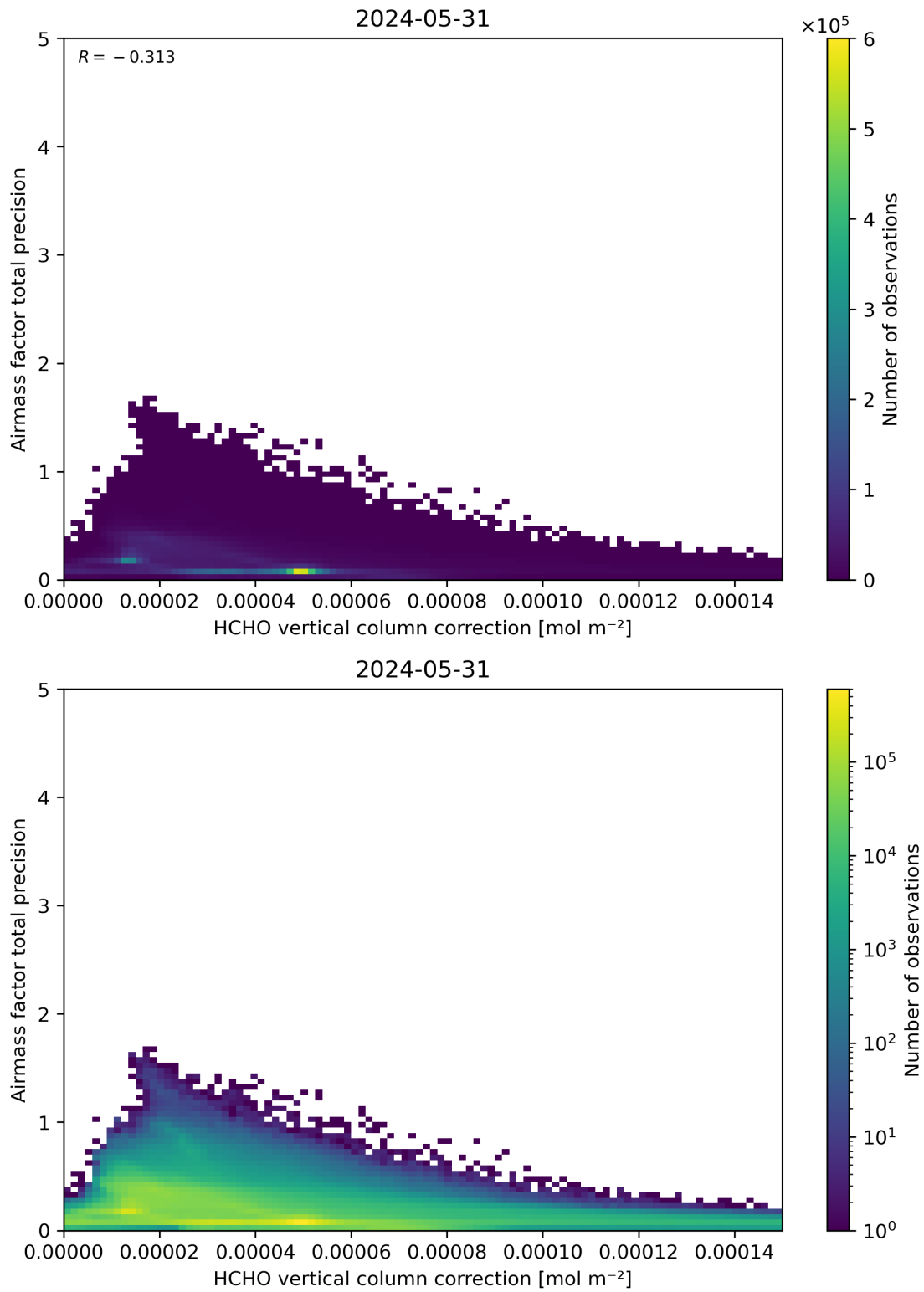
Figure 121: Scatter density plot of “HCHO vertical column correction” against “Airmass factor total precision” for 2024-05-30 to 2024-06-01.
