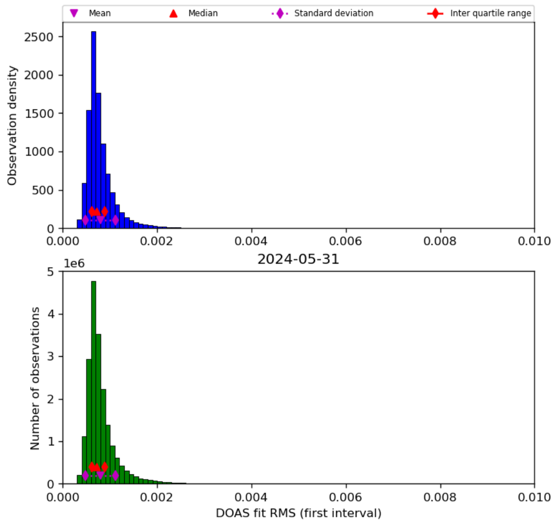
Figure 46: Histogram of “DOAS fit RMS (first interval)” for 2024-05-30 to 2024-06-01
