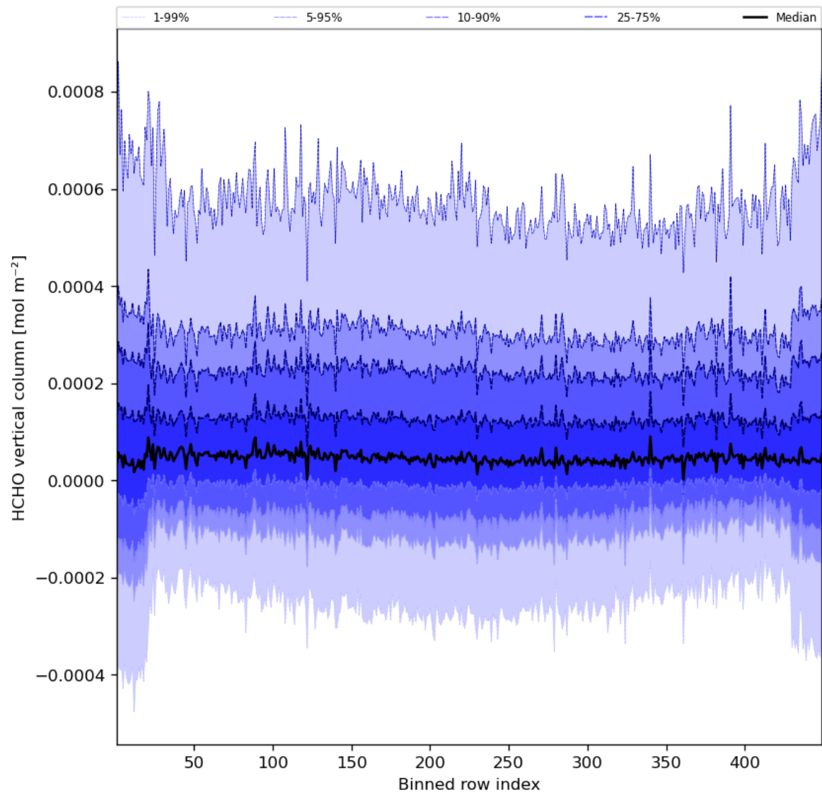
Figure 49: Along track statistics of “HCHO vertical column” for 2024-05-30 to 2024-06-01
