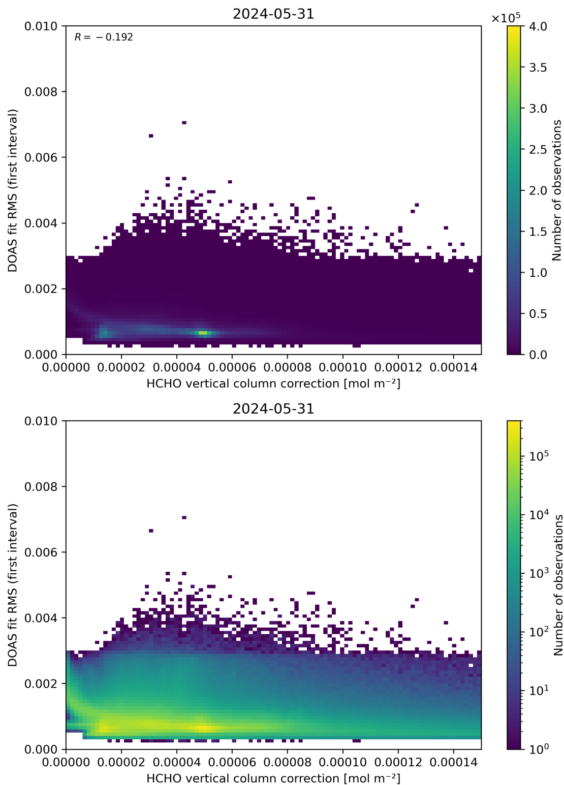
Figure 112: Scatter density plot of “HCHO vertical column correction” against “DOAS fit RMS (first interval)” for 2024-05-30 to 2024-06-01.
