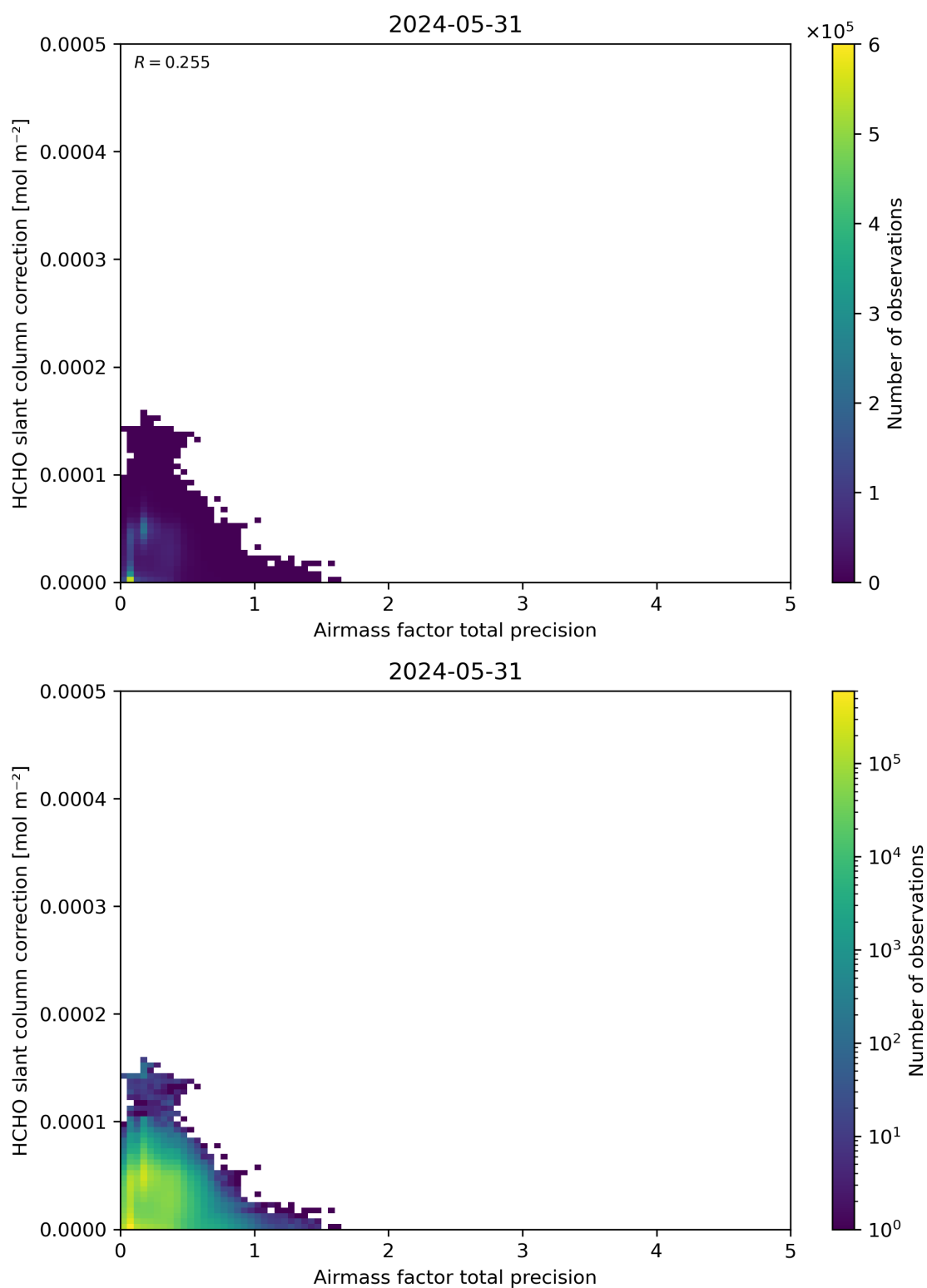
Figure 110: Scatter density plot of “Airmass factor total precision” against “HCHO slant column correction” for 2024-05-30 to 2024-06-01.
