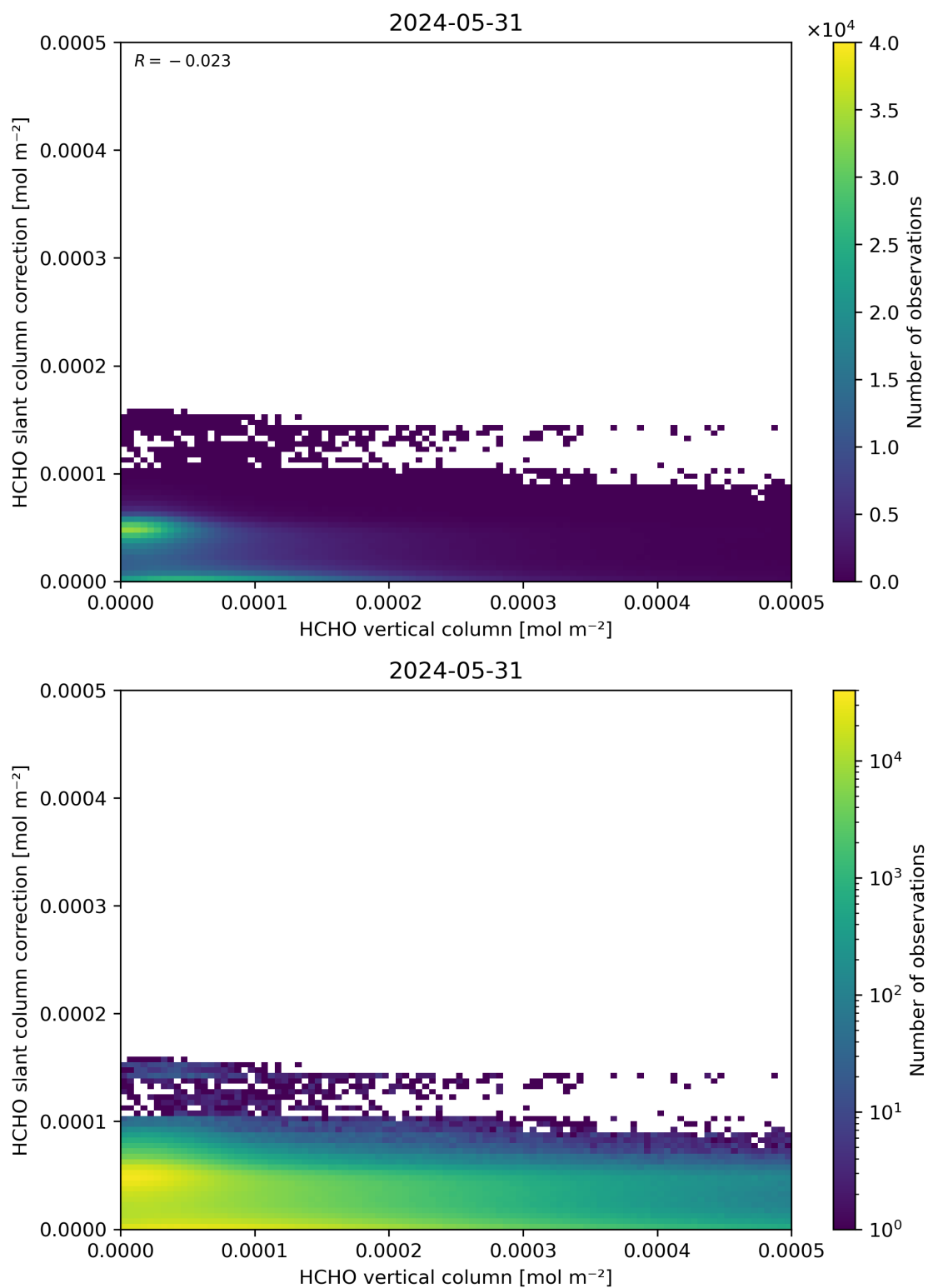
Figure 128: Scatter density plot of “HCHO vertical column” against “HCHO slant column correction” for 2024-05-30 to 2024-06-01.
