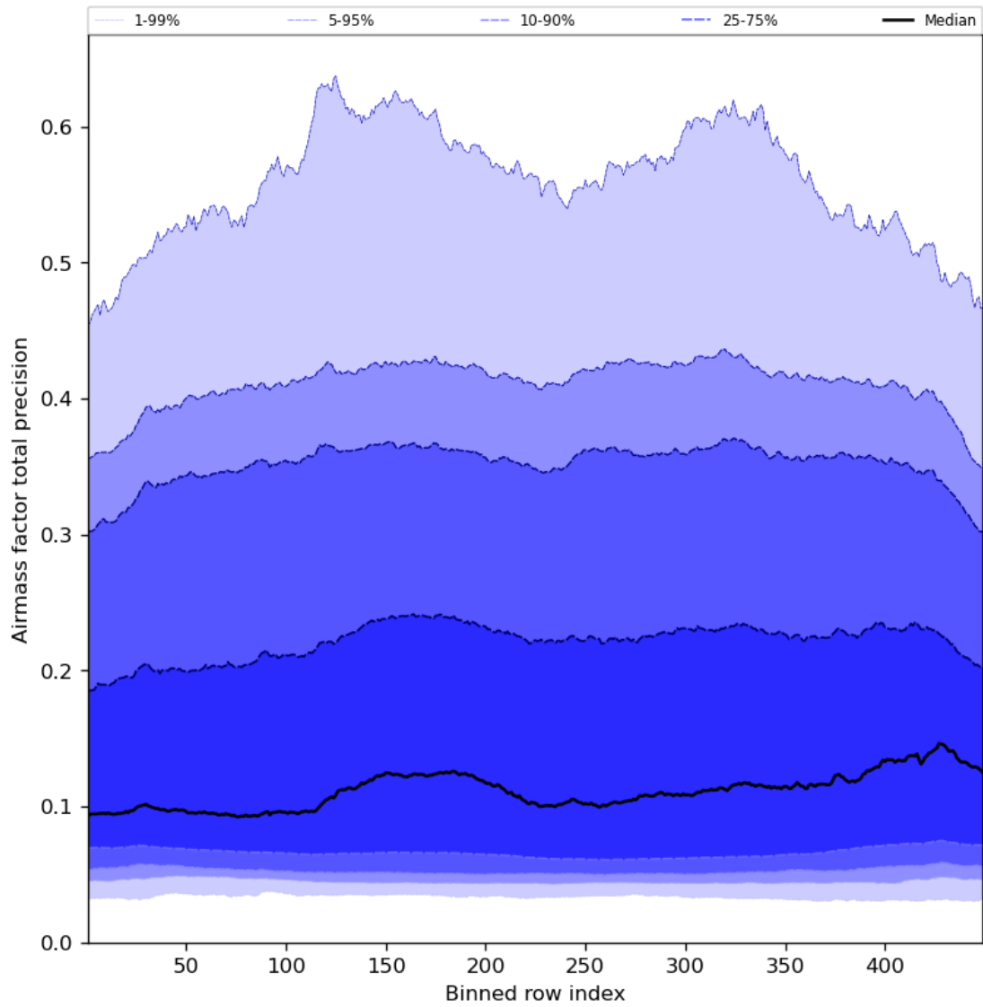
Figure 55: Along track statistics of “Airmass factor total precision” for 2024-05-30 to 2024-06-01
