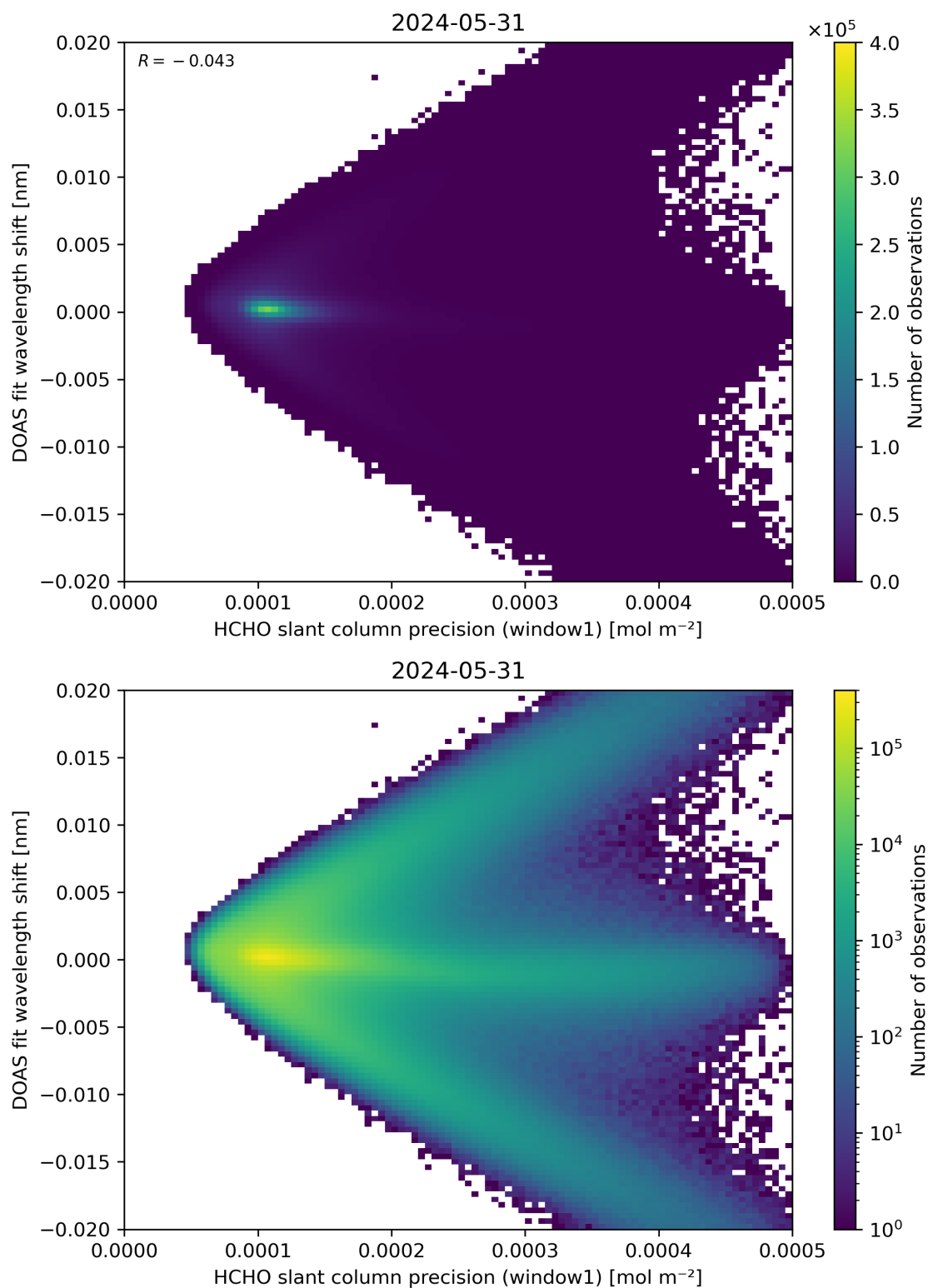
Figure 89: Scatter density plot of “HCHO slant column precision (window1)” against “DOAS fit wavelength shift” for 2024-05-30 to 2024-06-01.
