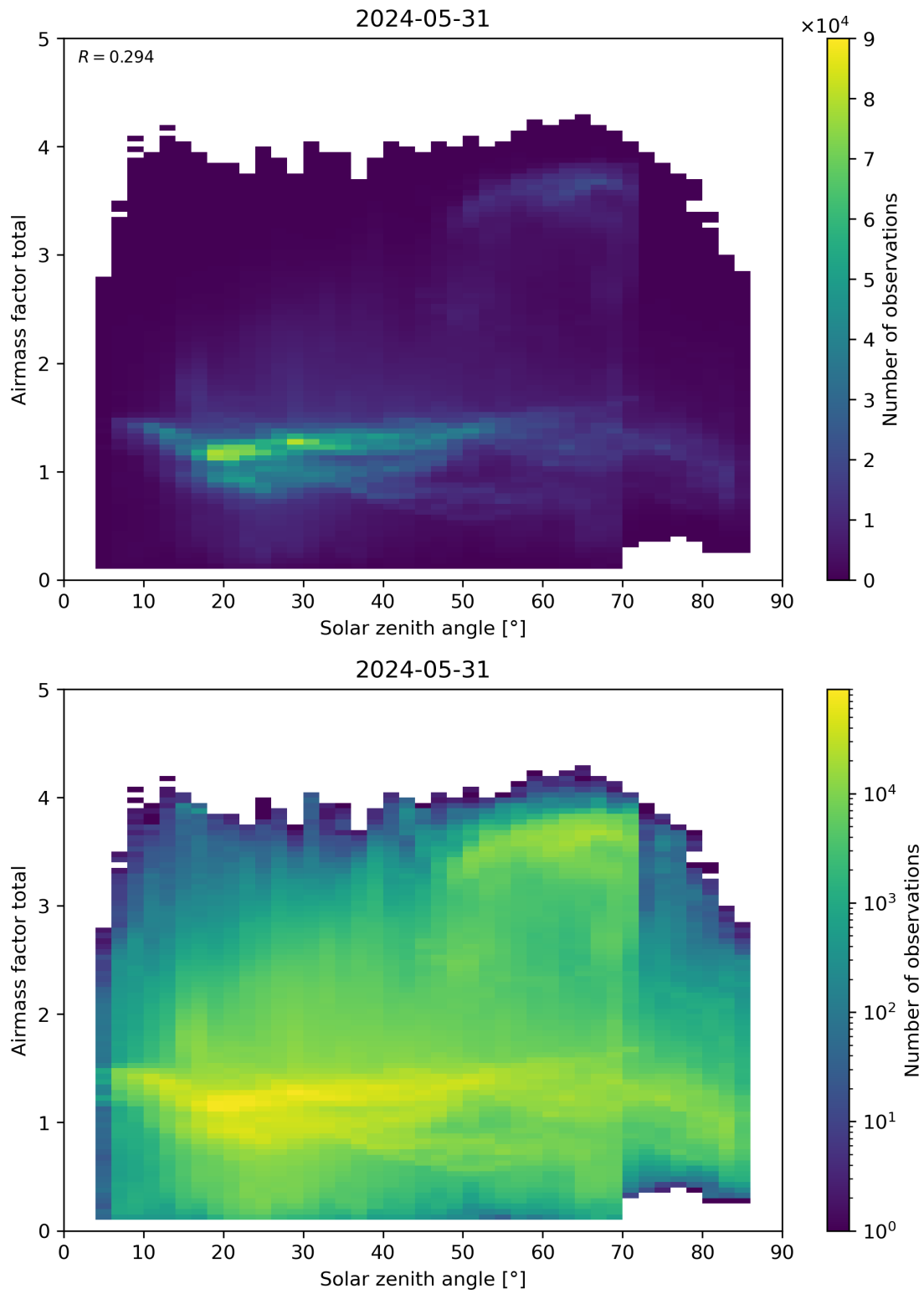
Figure 175: Scatter density plot of “Solar zenith angle” against “Airmass factor total” for 2024-05-30 to 2024-06-01.
