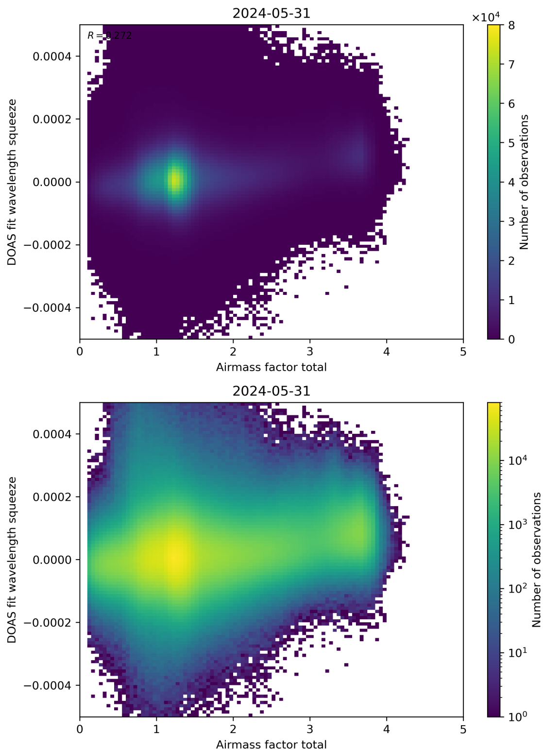
Figure 99: Scatter density plot of “Airmass factor total” against “DOAS fit wavelength squeeze” for 2024-05-30 to 2024-06-01.
