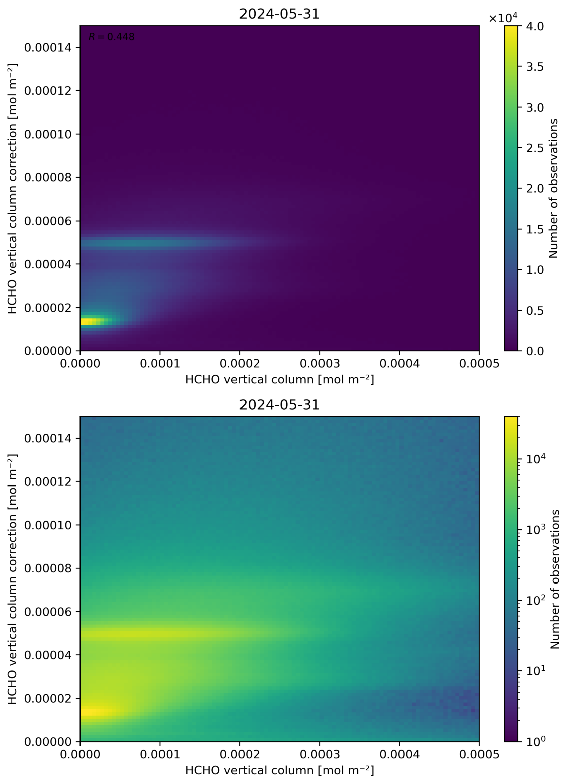
Figure 133: Scatter density plot of “HCHO vertical column” against “HCHO vertical column correction” for 2024-05-30 to 2024-06-01.
