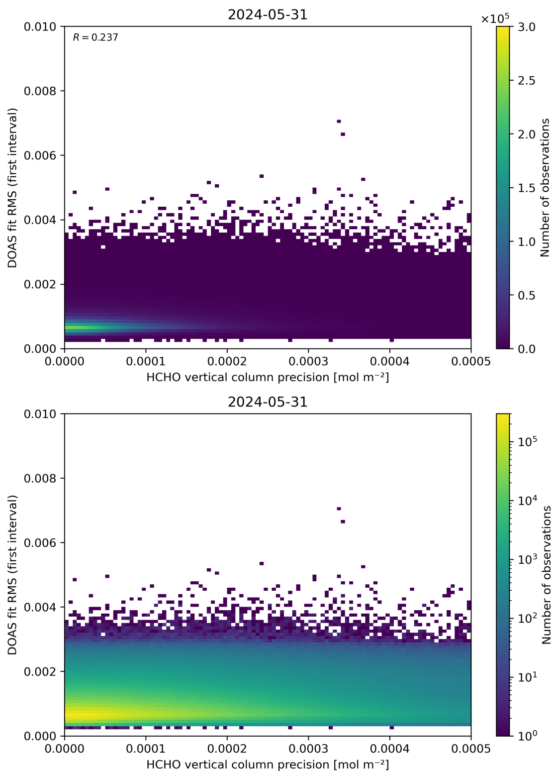
Figure 136: Scatter density plot of “HCHO vertical column precision” against “DOAS fit RMS (first interval)” for 2024-05-30 to 2024-06-01.
