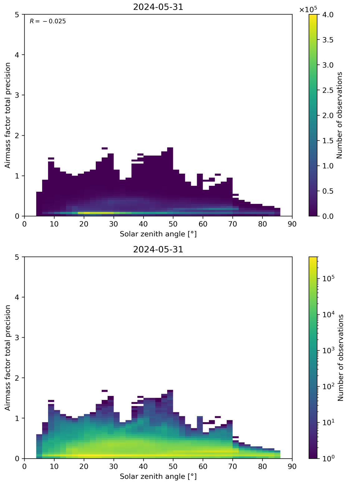
Figure 176: Scatter density plot of “Solar zenith angle” against “Airmass factor total precision” for 2024-05-30 to 2024-06-01.
