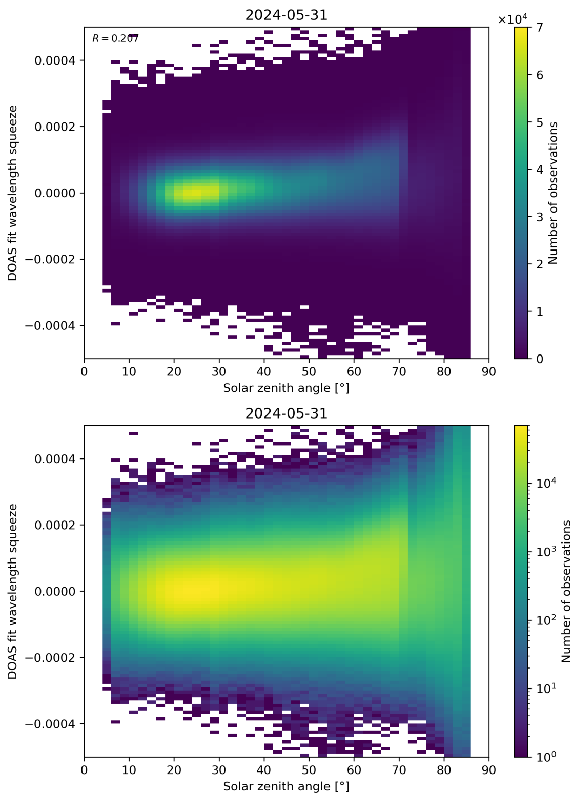
Figure 169: Scatter density plot of “Solar zenith angle” against “DOAS fit wavelength squeeze” for 2024-05-30 to 2024-06-01.
