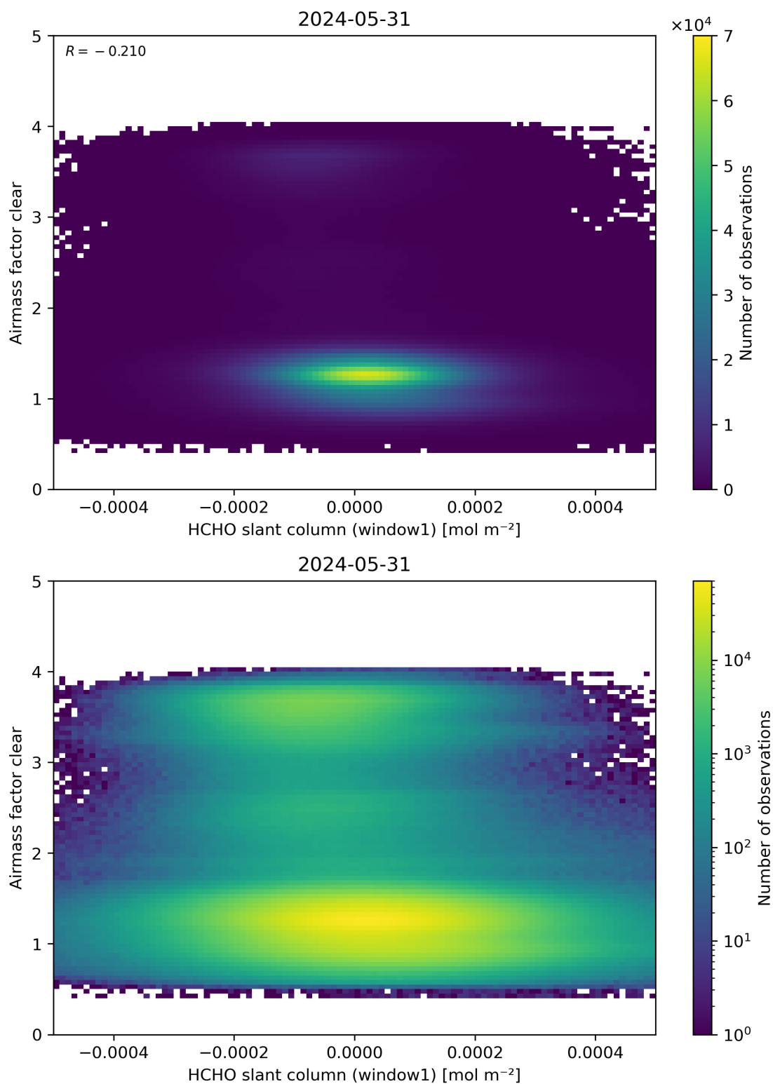
Figure 81: Scatter density plot of “HCHO slant column (window1)” against “Airmass factor clear” for 2024-05-30 to 2024-06-01.
