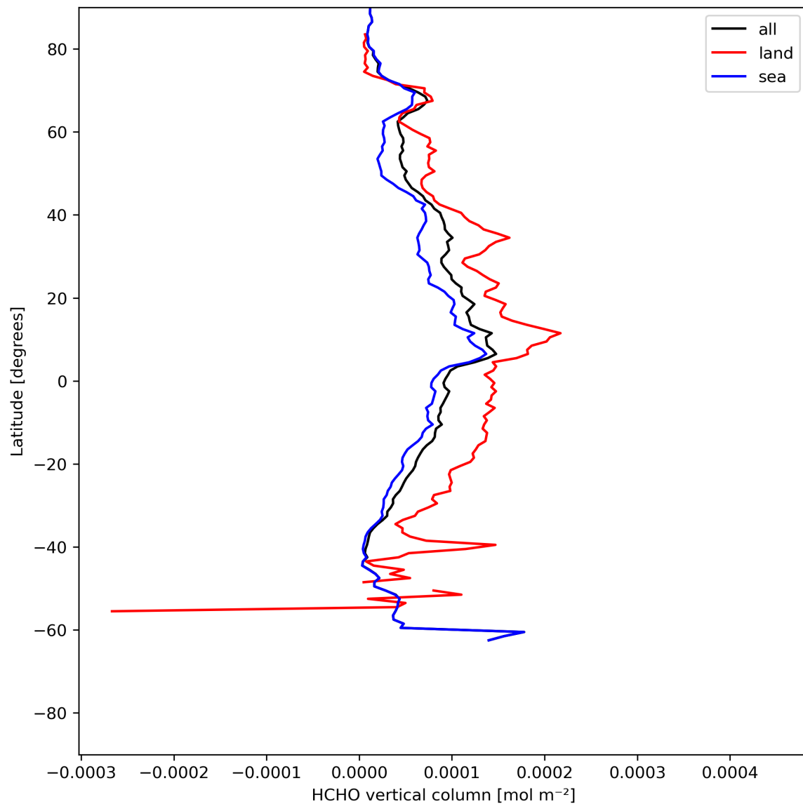
Figure 21: Zonal average of “HCHO vertical column” for 2024-05-30 to 2024-06-01.
