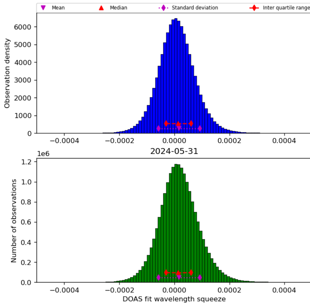
Figure 45: Histogram of “DOAS fit wavelength squeeze” for 2024-05-30 to 2024-06-01
