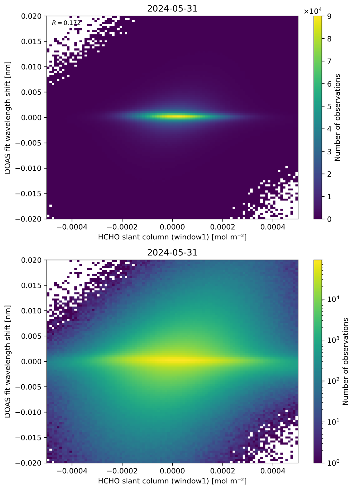
Figure 79: Scatter density plot of “HCHO slant column (window1)” against “DOAS fit wavelength shift” for 2024-05-30 to 2024-06-01.
