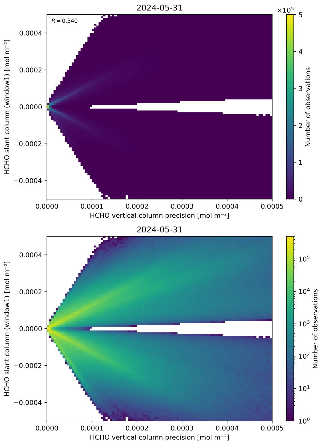
Figure 142: Scatter density plot of “HCHO vertical column precision” against “HCHO slant column (window1)” for 2024-05-30 to 2024-06-01.
