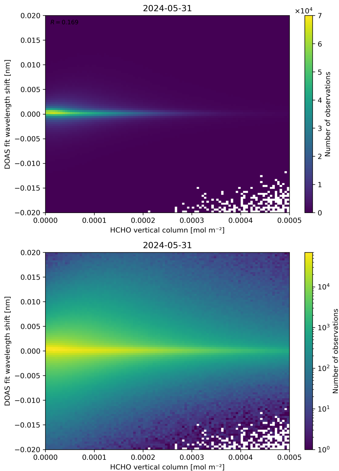
Figure 124: Scatter density plot of “HCHO vertical column” against “DOAS fit wavelength shift” for 2024-05-30 to 2024-06-01.
