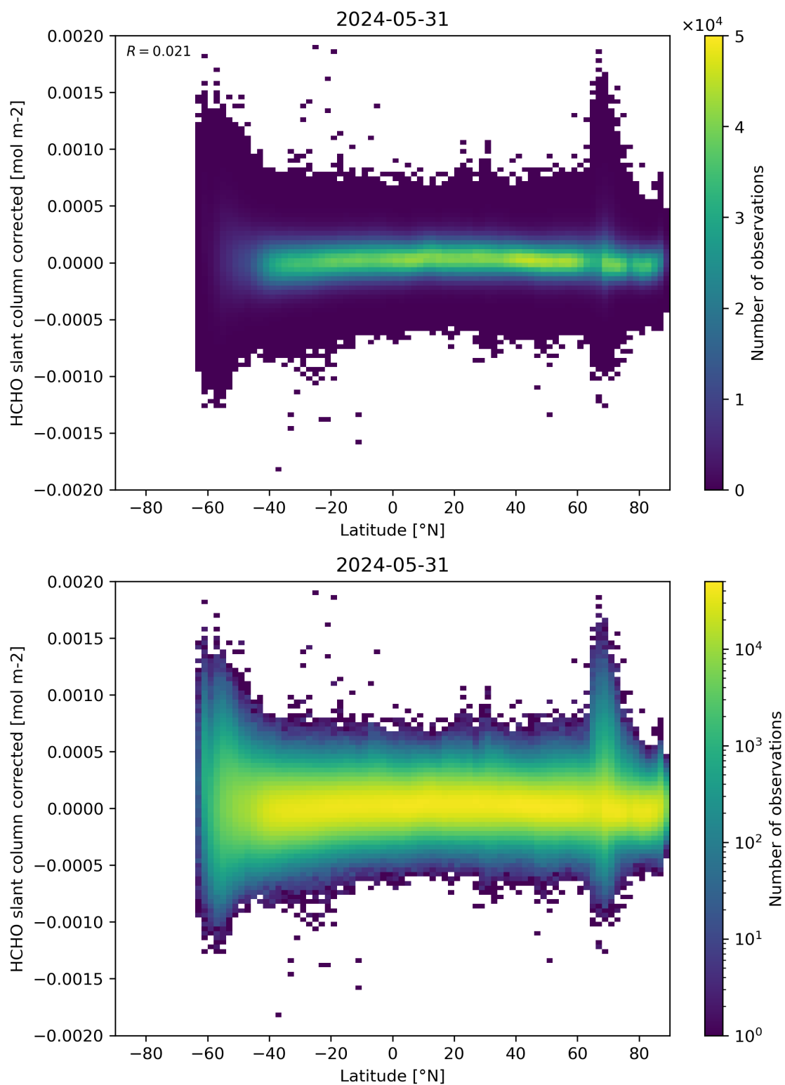
Figure 157: Scatter density plot of “Latitude” against “HCHO slant column corrected” for 2024-05-30 to 2024-06-01.
