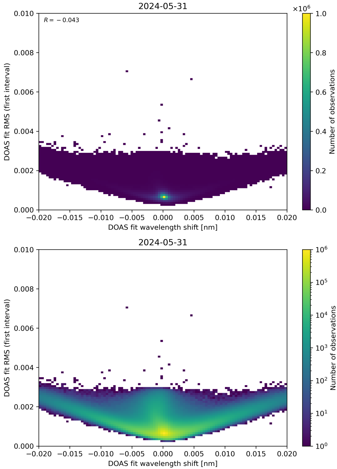
Figure 64: Scatter density plot of “DOAS fit wavelength shift” against “DOAS fit RMS (first interval)” for 2024-05-30 to 2024-06-01.
