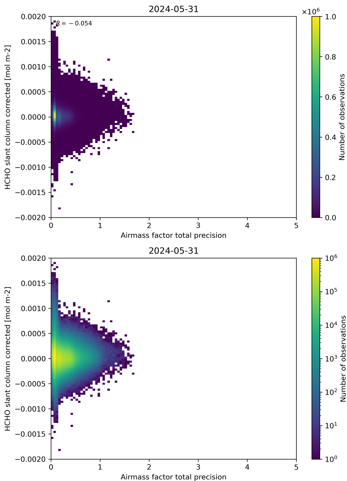
Figure 109: Scatter density plot of “Airmass factor total precision” against “HCHO slant column corrected” for 2024-05-30 to 2024-06-01.
