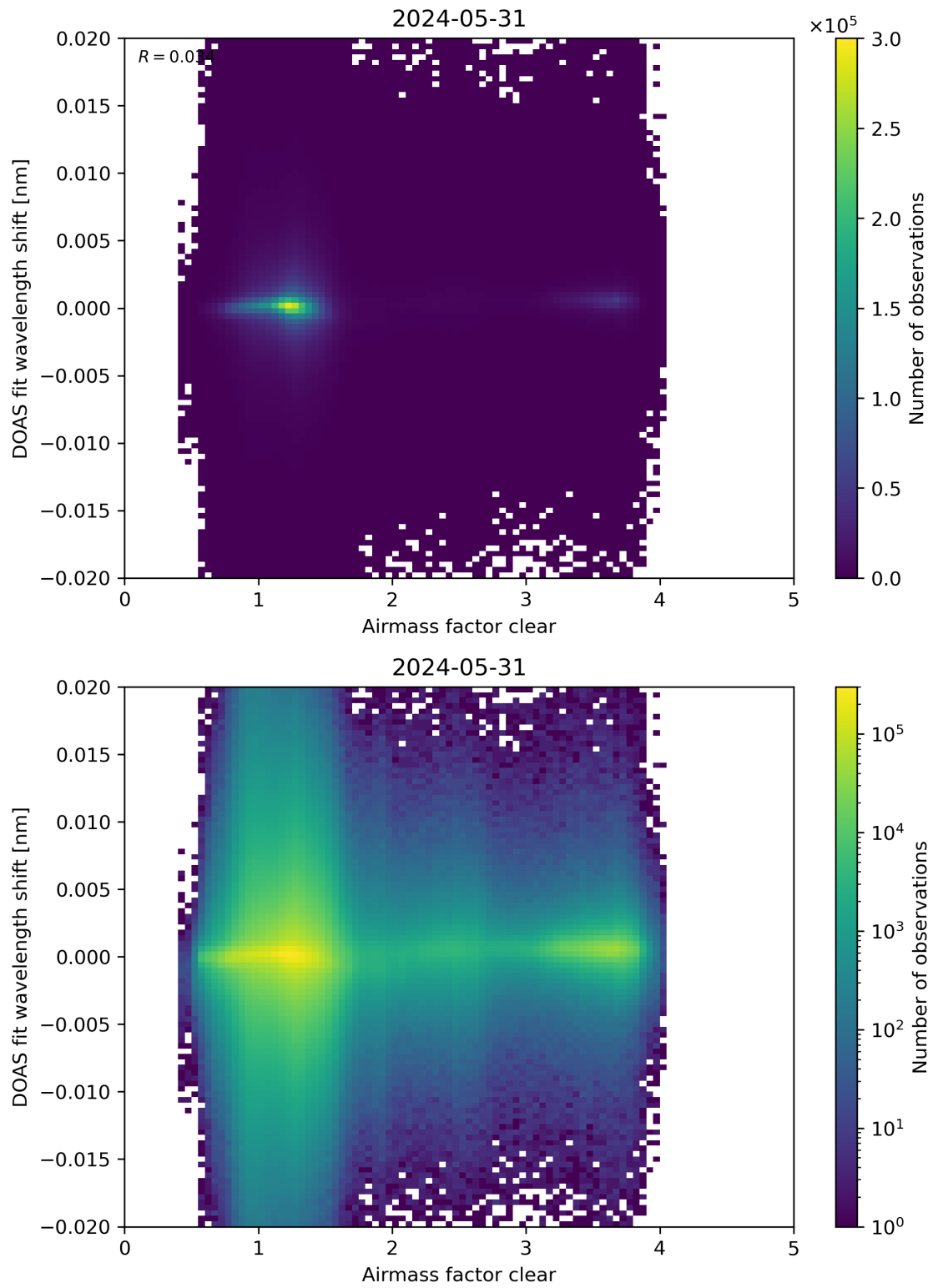
Figure 72: Scatter density plot of “Airmass factor clear” against “DOAS fit wavelength shift” for 2024-05-30 to 2024-06-01.
