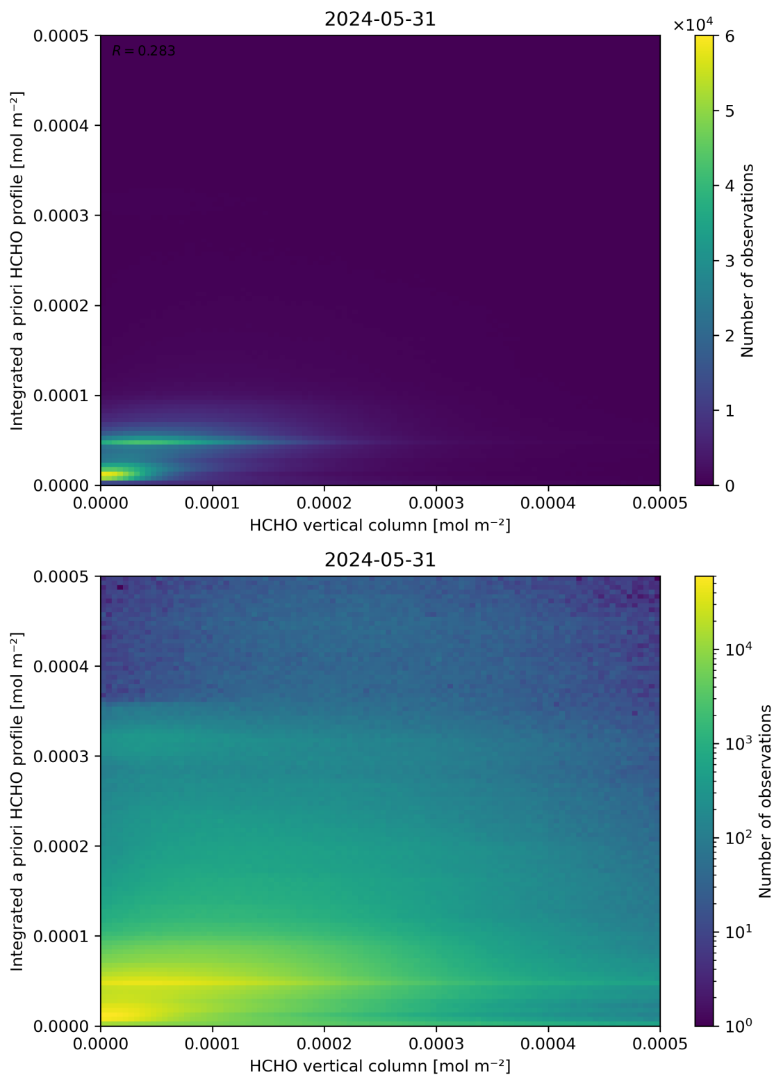
Figure 135: Scatter density plot of “HCHO vertical column” against “Integrated a priori HCHO profile” for 2024-05-30 to 2024-06-01.
