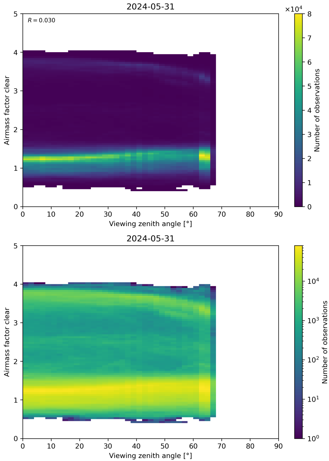
Figure 185: Scatter density plot of “Viewing zenith angle” against “Airmass factor clear” for 2024-05-30 to 2024-06-01.
