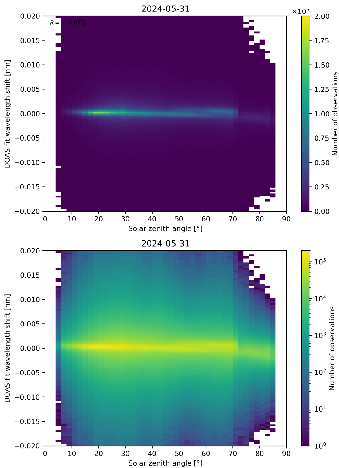
Figure 168: Scatter density plot of “Solar zenith angle” against “DOAS fit wavelength shift” for 2024-05-30 to 2024-06-01.
