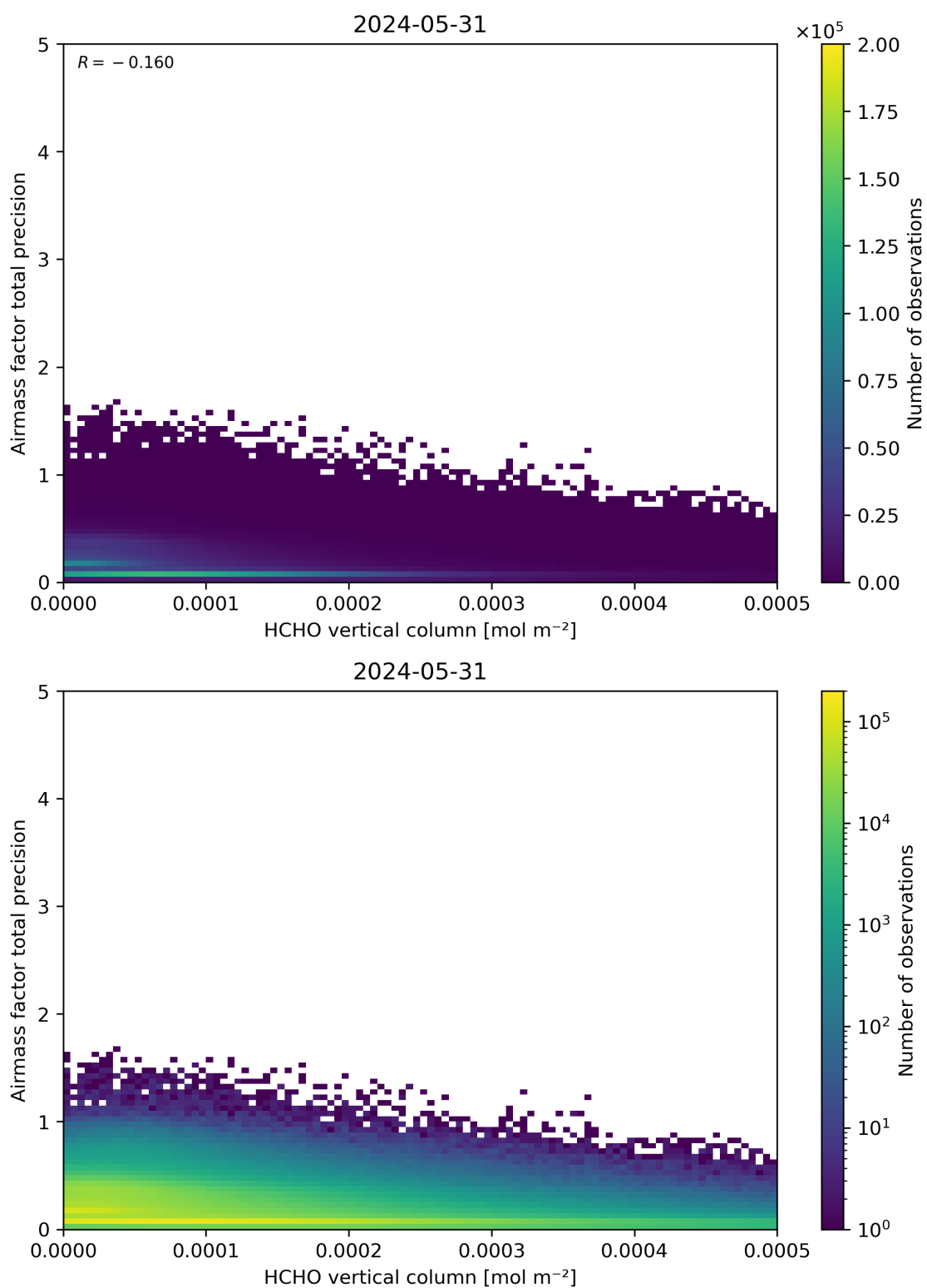
Figure 132: Scatter density plot of “HCHO vertical column” against “Airmass factor total precision” for 2024-05-30 to 2024-06-01.
