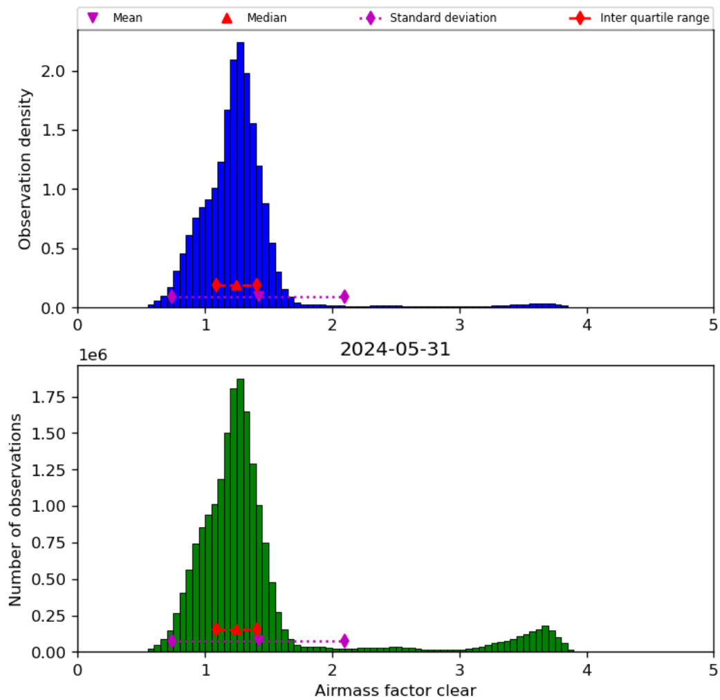
Figure 42: Histogram of “Airmass factor clear” for 2024-05-30 to 2024-06-01
