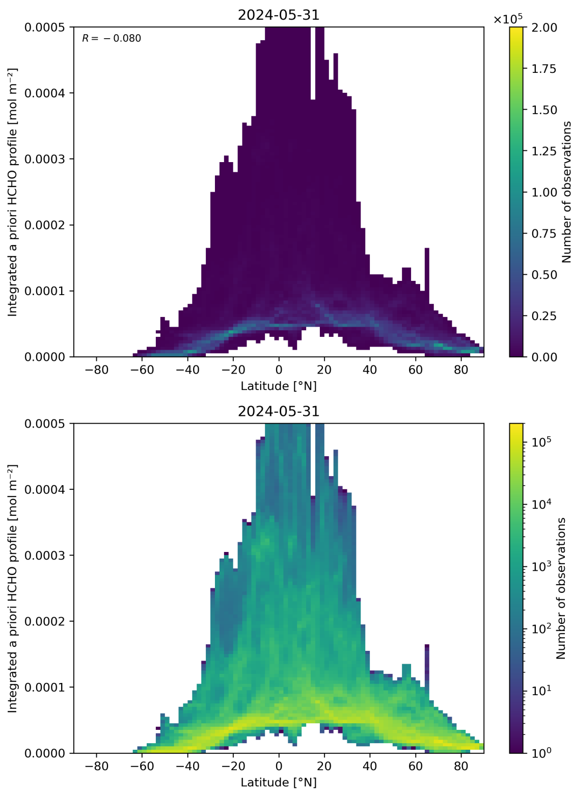
Figure 166: Scatter density plot of “Latitude” against “Integrated a priori HCHO profile” for 2024-05-30 to 2024-06-01.
