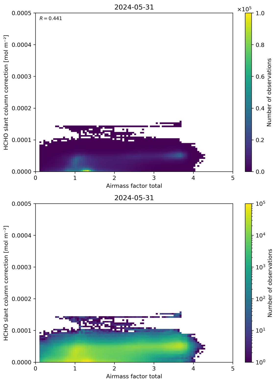
Figure 102: Scatter density plot of “Airmass factor total” against “HCHO slant column correction” for 2024-05-30 to 2024-06-01.
