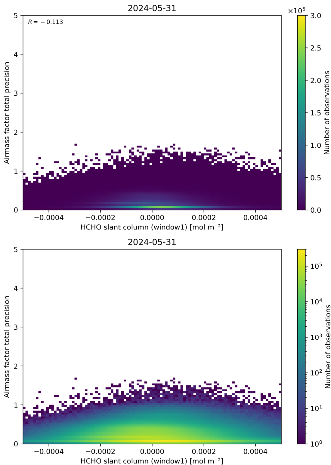
Figure 86: Scatter density plot of “HCHO slant column (window1)” against “Airmass factor total precision” for 2024-05-30 to 2024-06-01.
