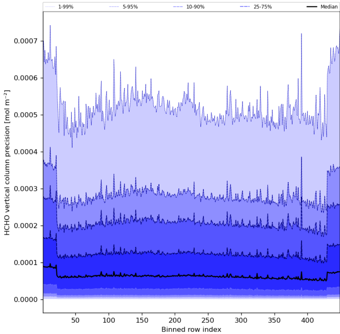
Figure 50: Along track statistics of “HCHO vertical column precision” for 2024-05-30 to 2024-06-01
