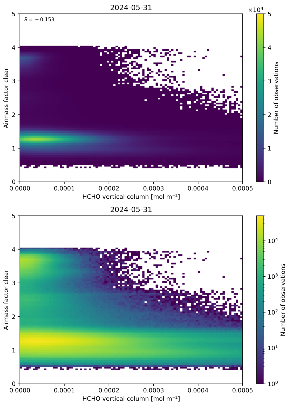
Figure 126: Scatter density plot of “HCHO vertical column” against “Airmass factor clear” for 2024-05-30 to 2024-06-01.
