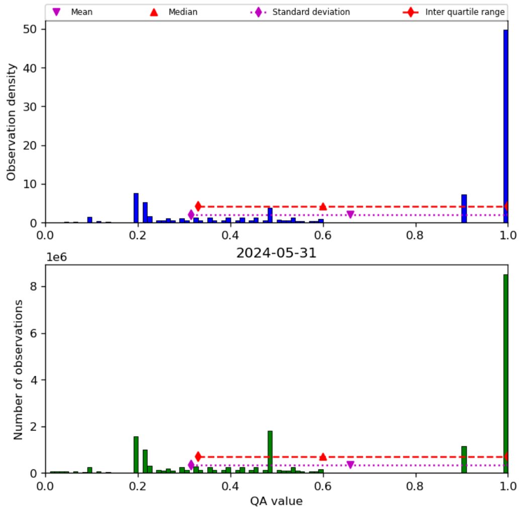
Figure 34: Histogram of “QA value” for 2024-05-30 to 2024-06-01
