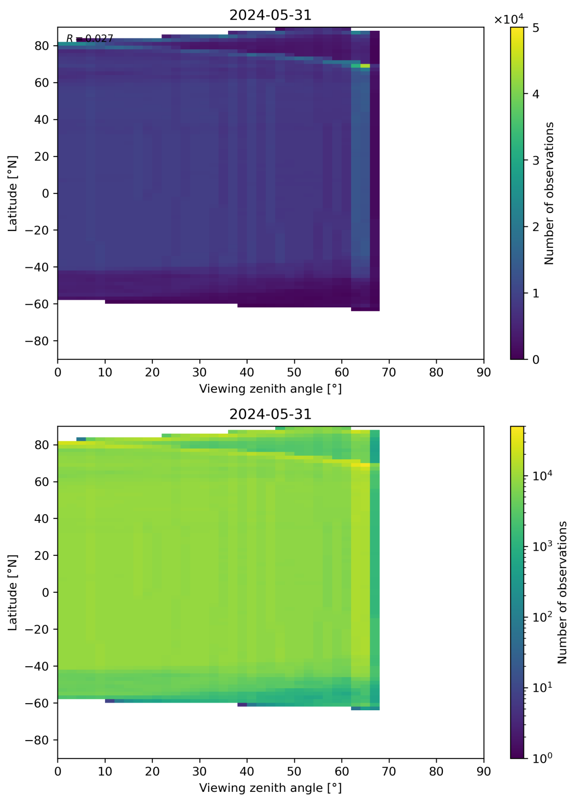
Figure 196: Scatter density plot of “Viewing zenith angle” against “Latitude” for 2024-05-30 to 2024-06-01.
