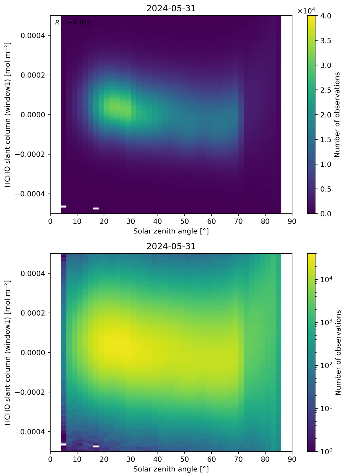
Figure 173: Scatter density plot of “Solar zenith angle” against “HCHO slant column (window1)” for 2024-05-30 to 2024-06-01.
