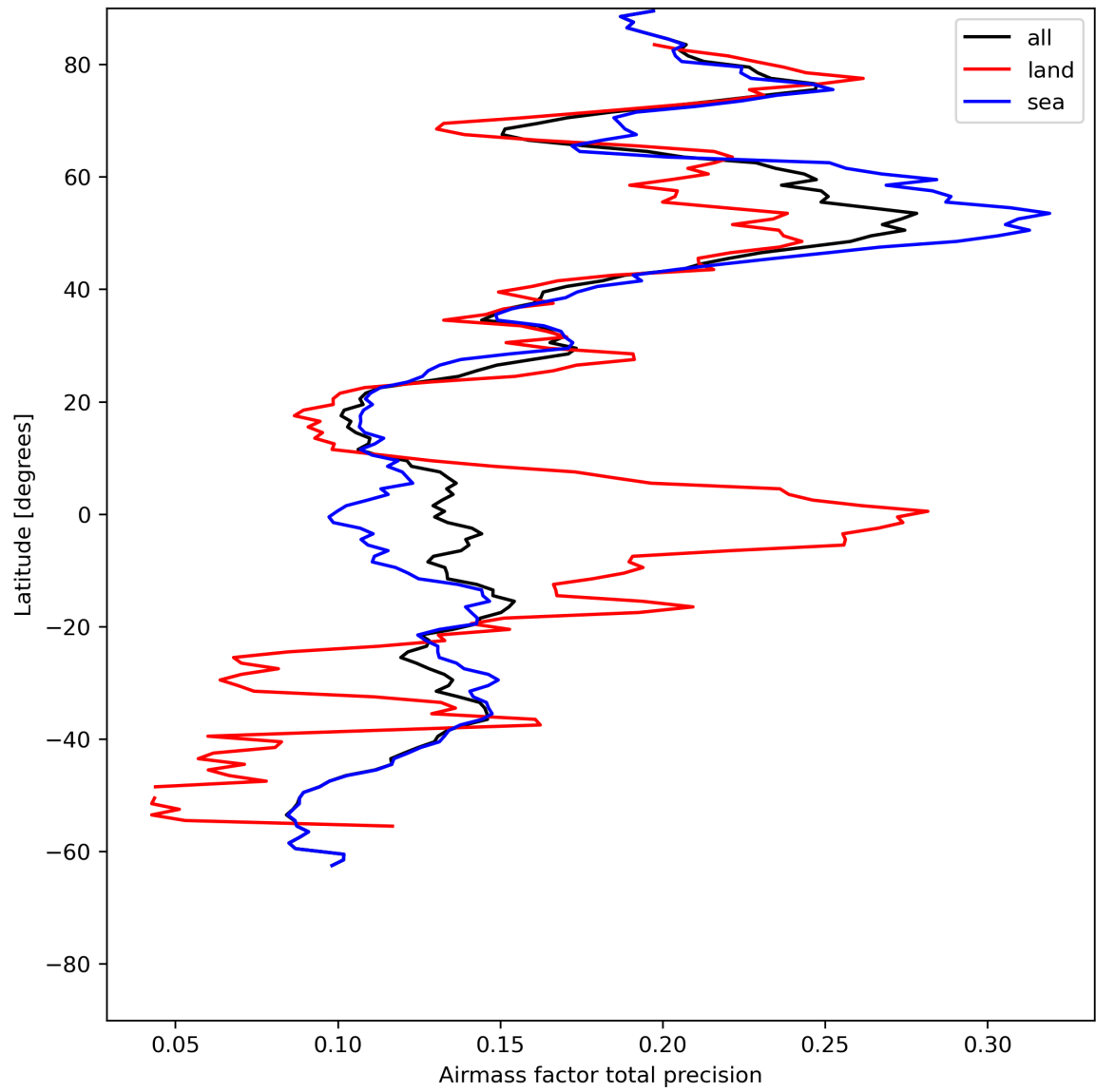
Figure 27: Zonal average of “Airmass factor total precision” for 2024-05-30 to 2024-06-01.
