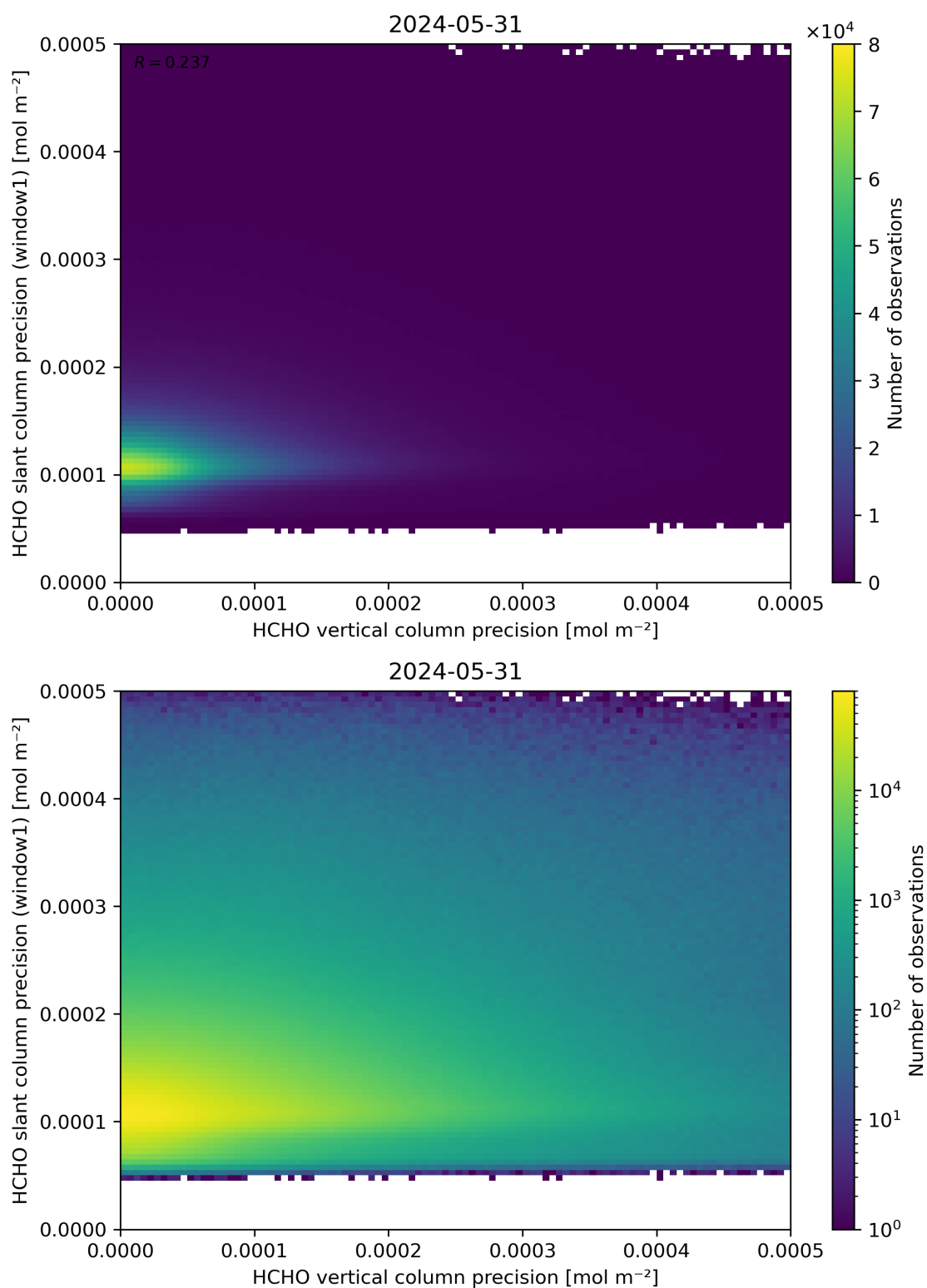
Figure 143: Scatter density plot of “HCHO vertical column precision” against “HCHO slant column precision (window1)” for 2024-05-30 to 2024-06-01.
