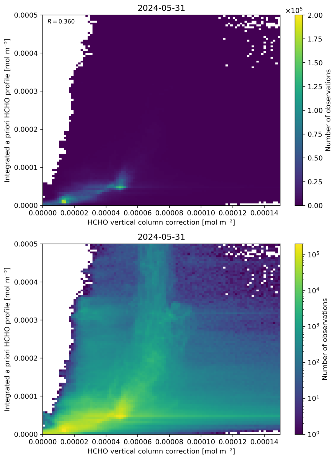
Figure 122: Scatter density plot of “HCHO vertical column correction” against “Integrated a priori HCHO profile” for 2024-05-30 to 2024-06-01.
