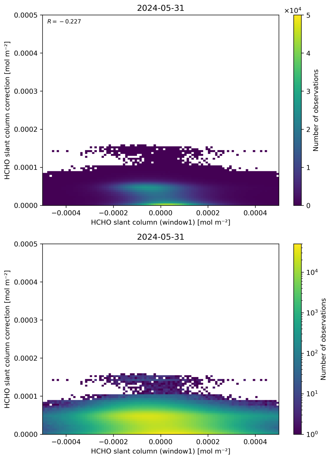
Figure 83: Scatter density plot of “HCHO slant column (window1)” against “HCHO slant column correction” for 2024-05-30 to 2024-06-01.
