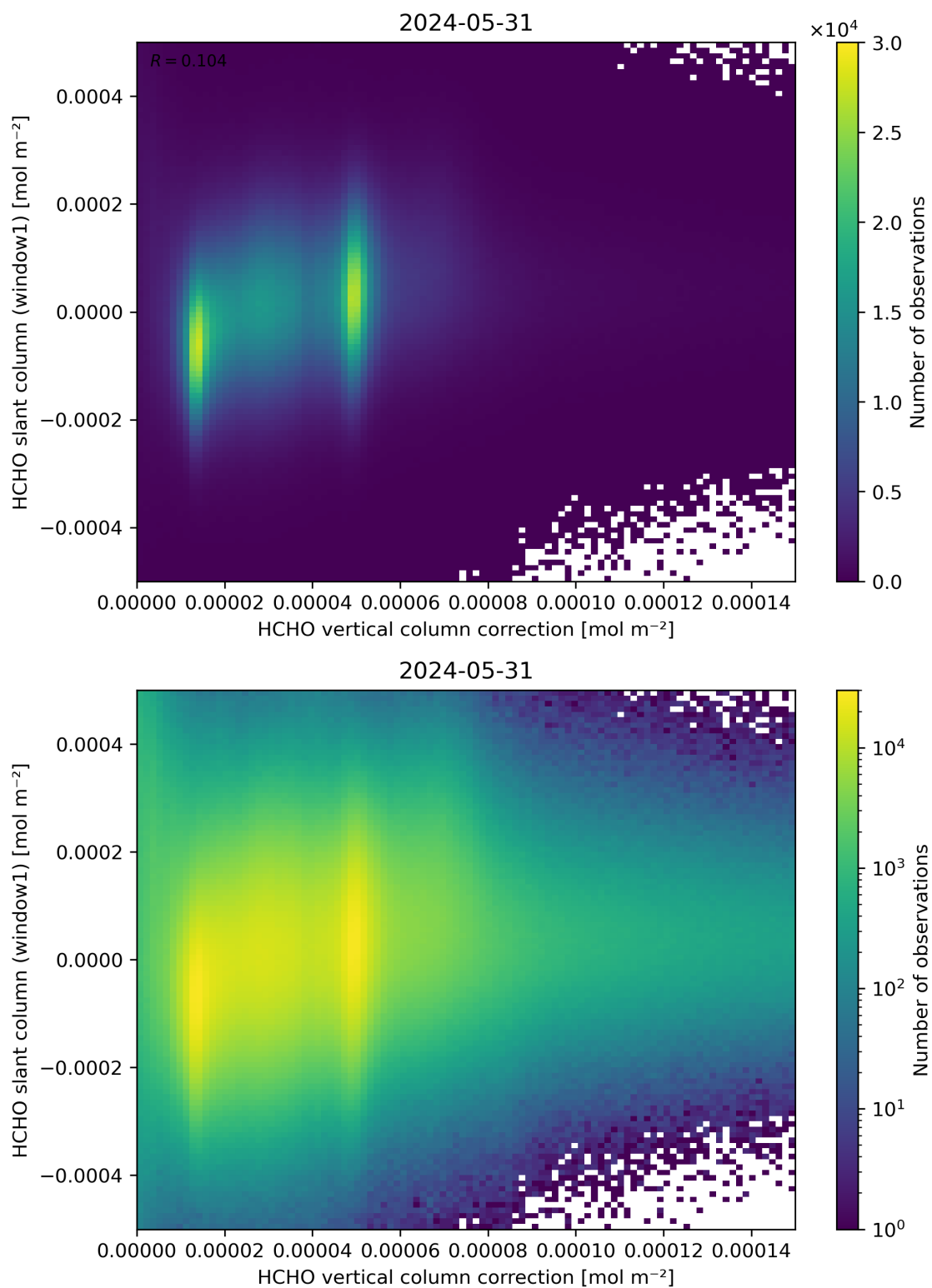
Figure 118: Scatter density plot of “HCHO vertical column correction” against “HCHO slant column (window1)” for 2024-05-30 to 2024-06-01.
