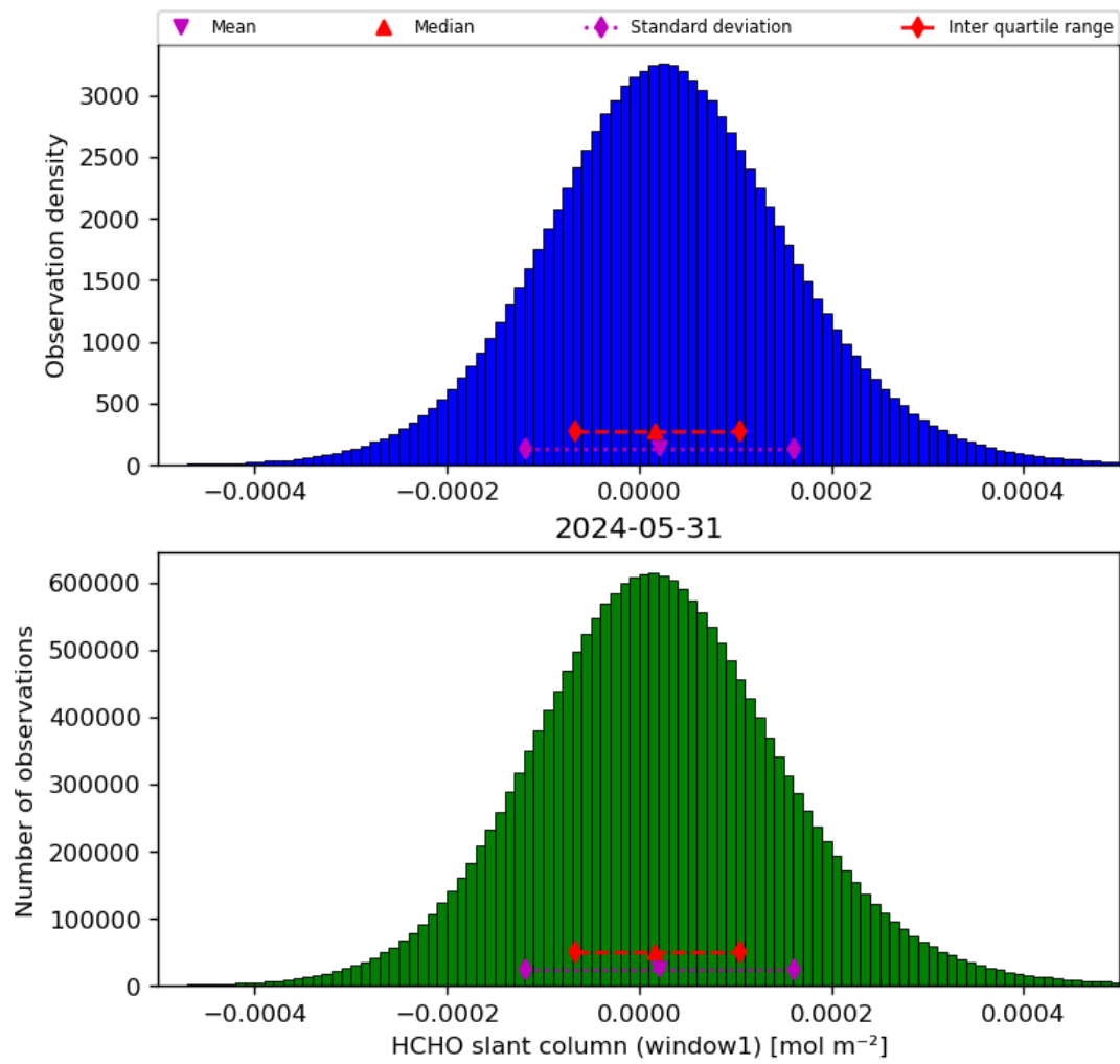
Figure 38: Histogram of “HCHO slant column (window1)” for 2024-05-30 to 2024-06-01
