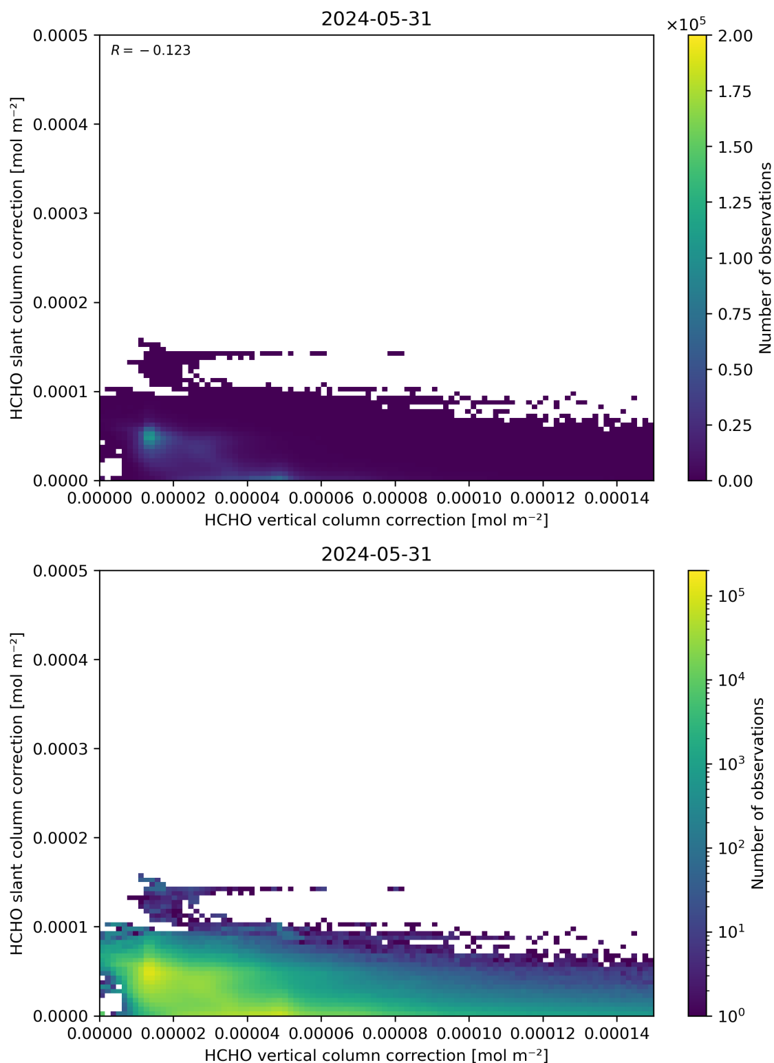
Figure 117: Scatter density plot of “HCHO vertical column correction” against “HCHO slant column correction” for 2024-05-30 to 2024-06-01.
