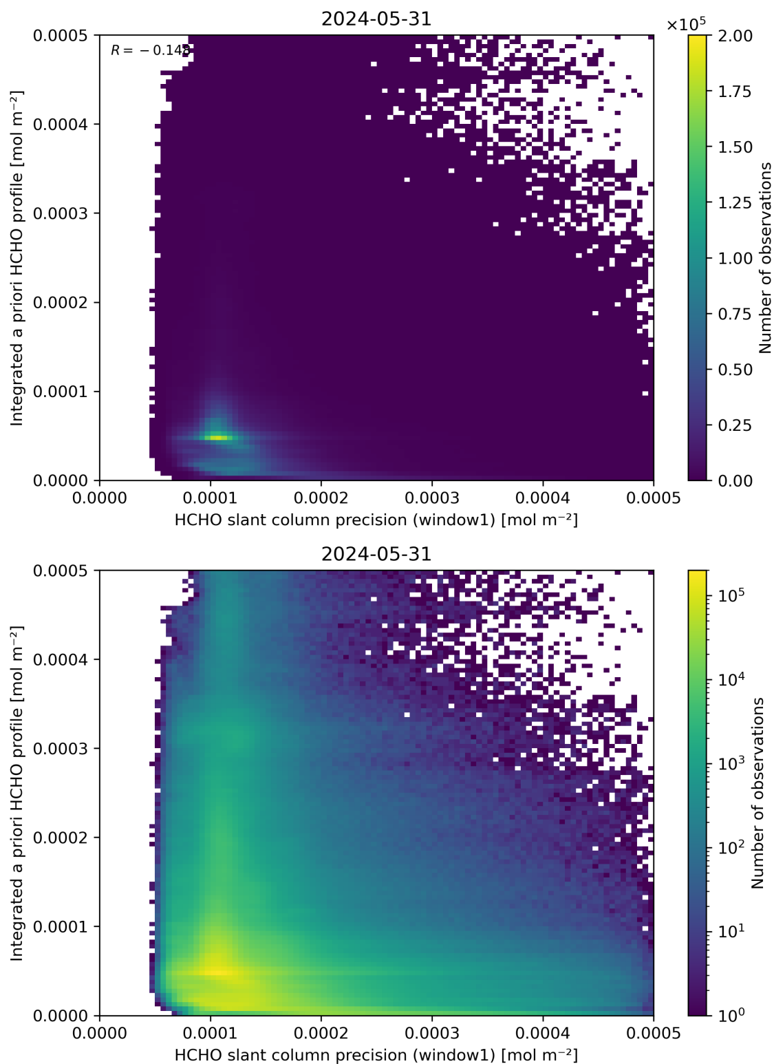
Figure 96: Scatter density plot of “HCHO slant column precision (window1)” against “Integrated a priori HCHO profile” for 2024-05-30 to 2024-06-01.
