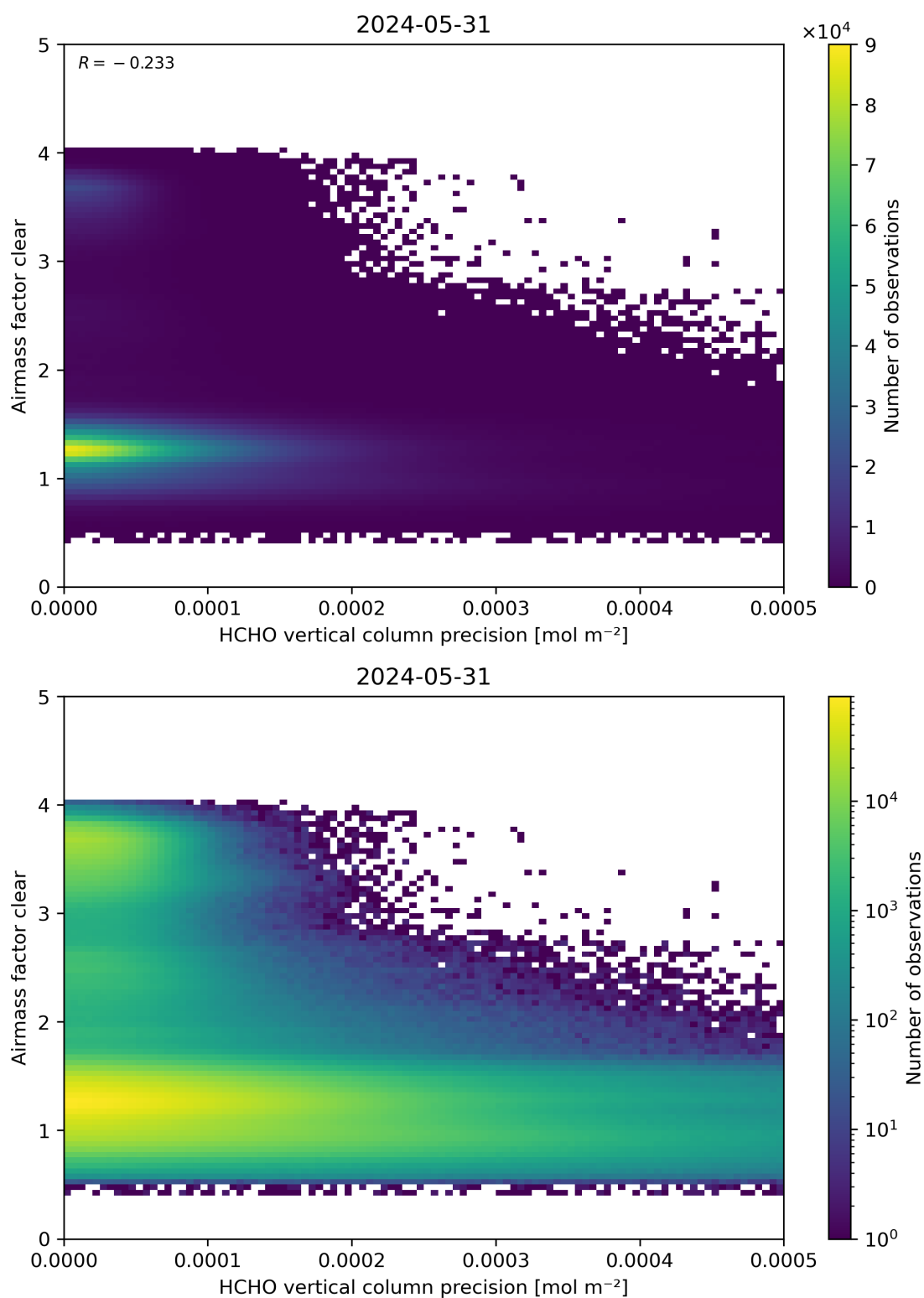
Figure 139: Scatter density plot of “HCHO vertical column precision” against “Airmass factor clear” for 2024-05-30 to 2024-06-01.
