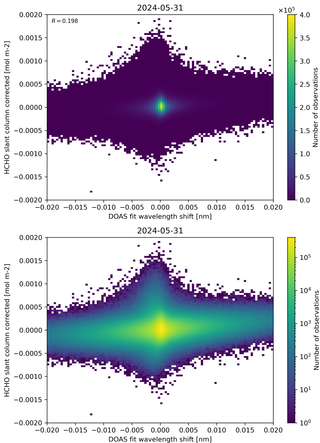
Figure 66: Scatter density plot of “DOAS fit wavelength shift” against “HCHO slant column corrected” for 2024-05-30 to 2024-06-01.
