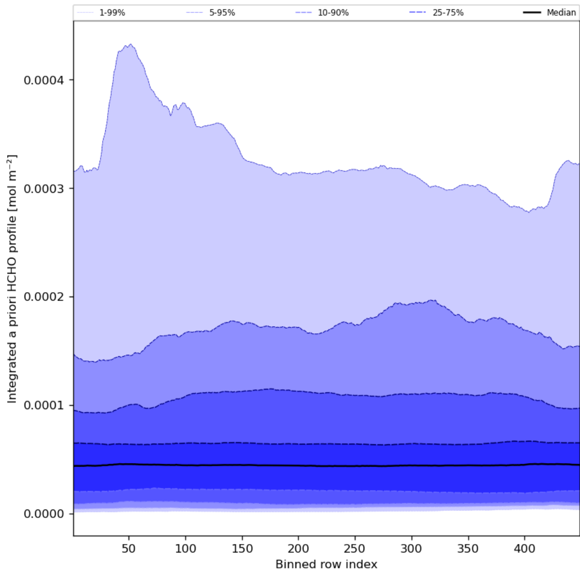
Figure 57: Along track statistics of “Integrated a priori HCHO profile” for 2024-05-30 to 2024-06-01
