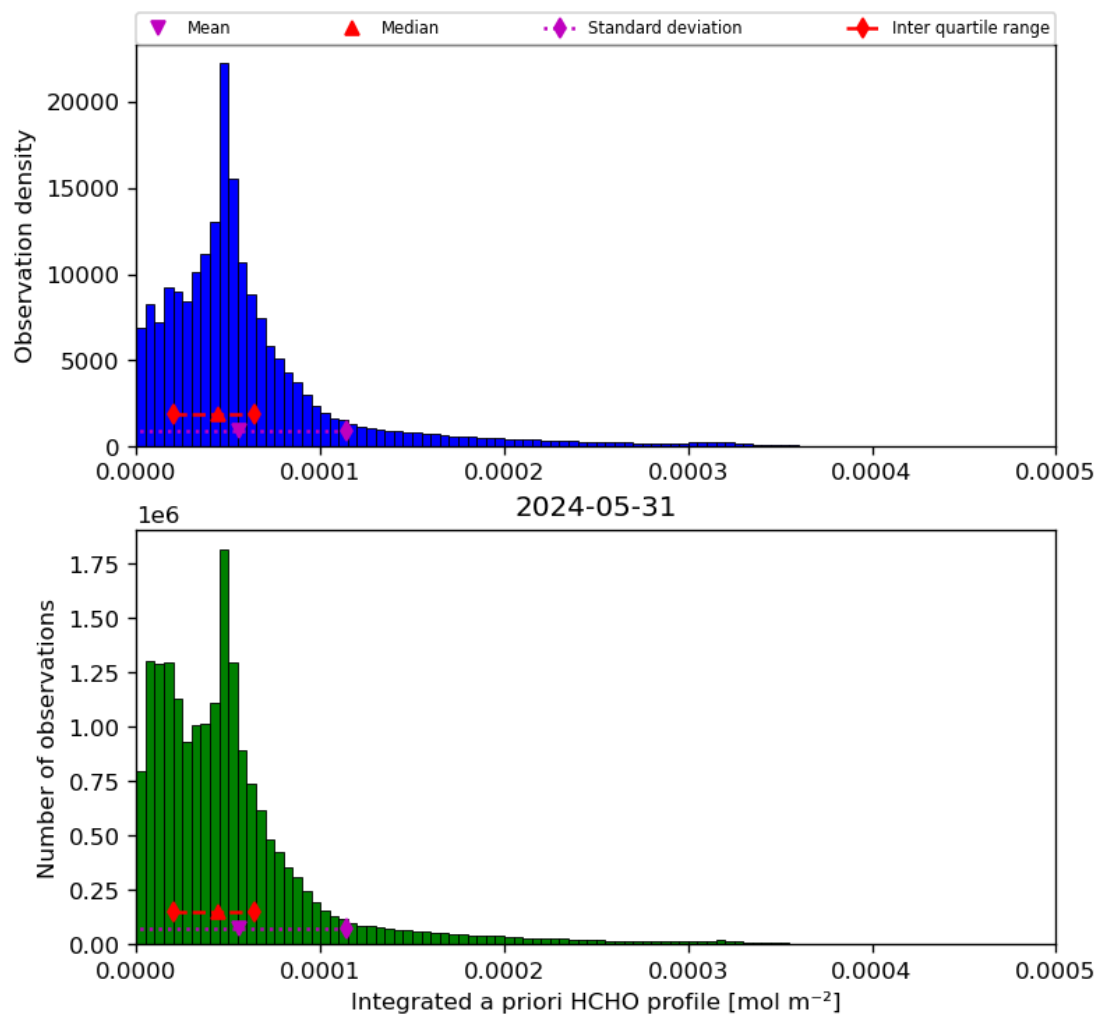
Figure 43: Histogram of “Integrated a priori HCHO profile” for 2024-05-30 to 2024-06-01
