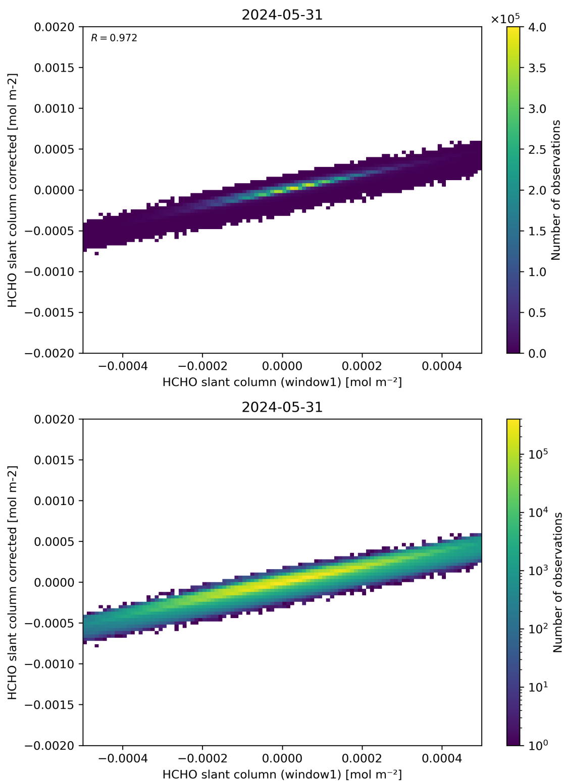
Figure 82: Scatter density plot of “HCHO slant column (window1)” against “HCHO slant column corrected” for 2024-05-30 to 2024-06-01.
