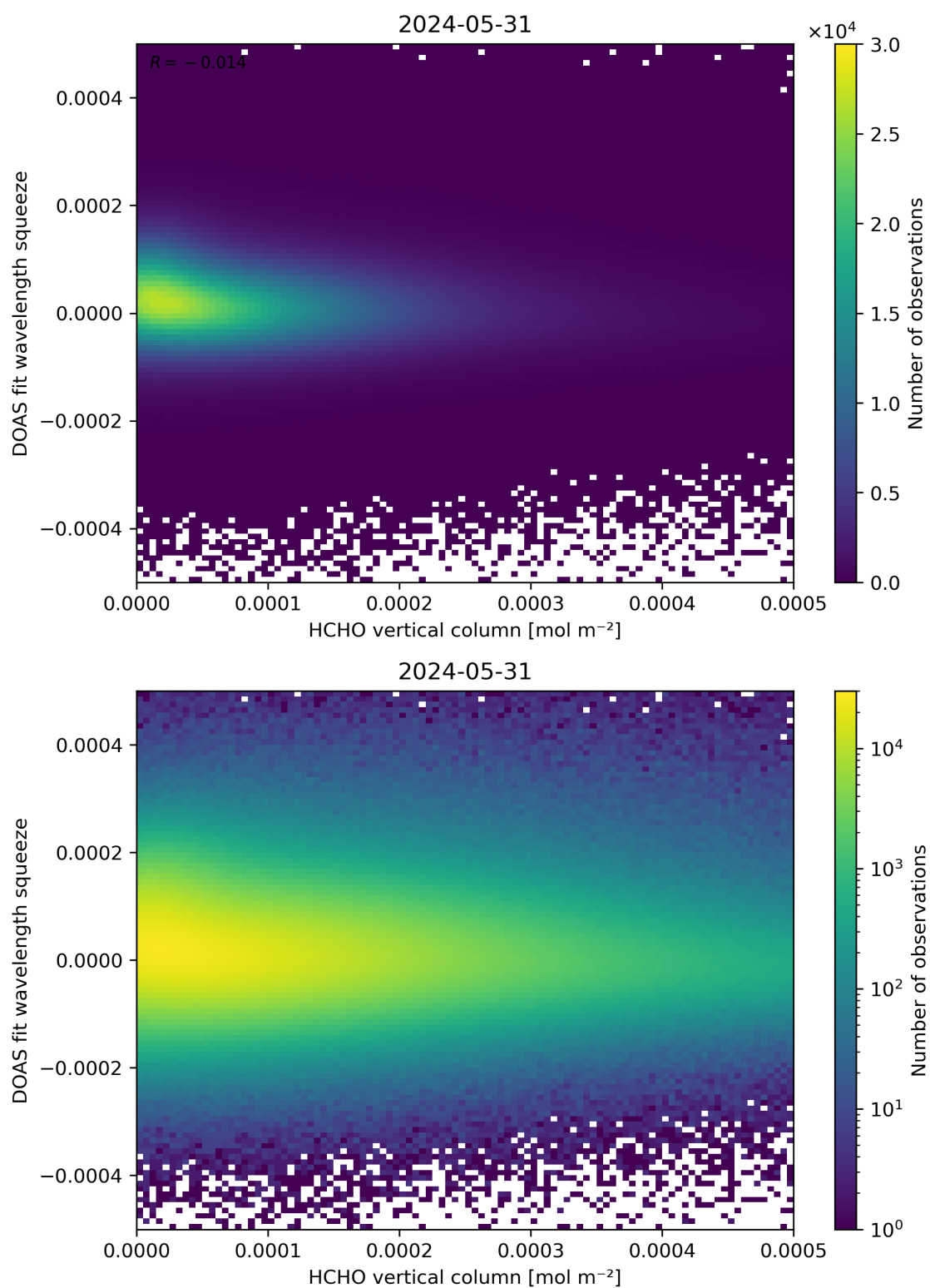
Figure 125: Scatter density plot of “HCHO vertical column” against “DOAS fit wavelength squeeze” for 2024-05-30 to 2024-06-01.
