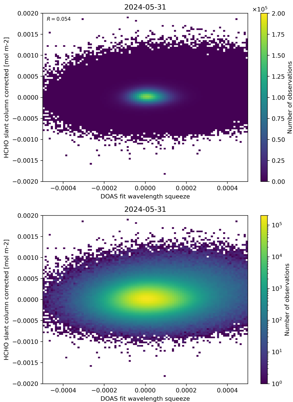
Figure 69: Scatter density plot of “DOAS fit wavelength squeeze” against “HCHO slant column corrected” for 2024-05-30 to 2024-06-01.
