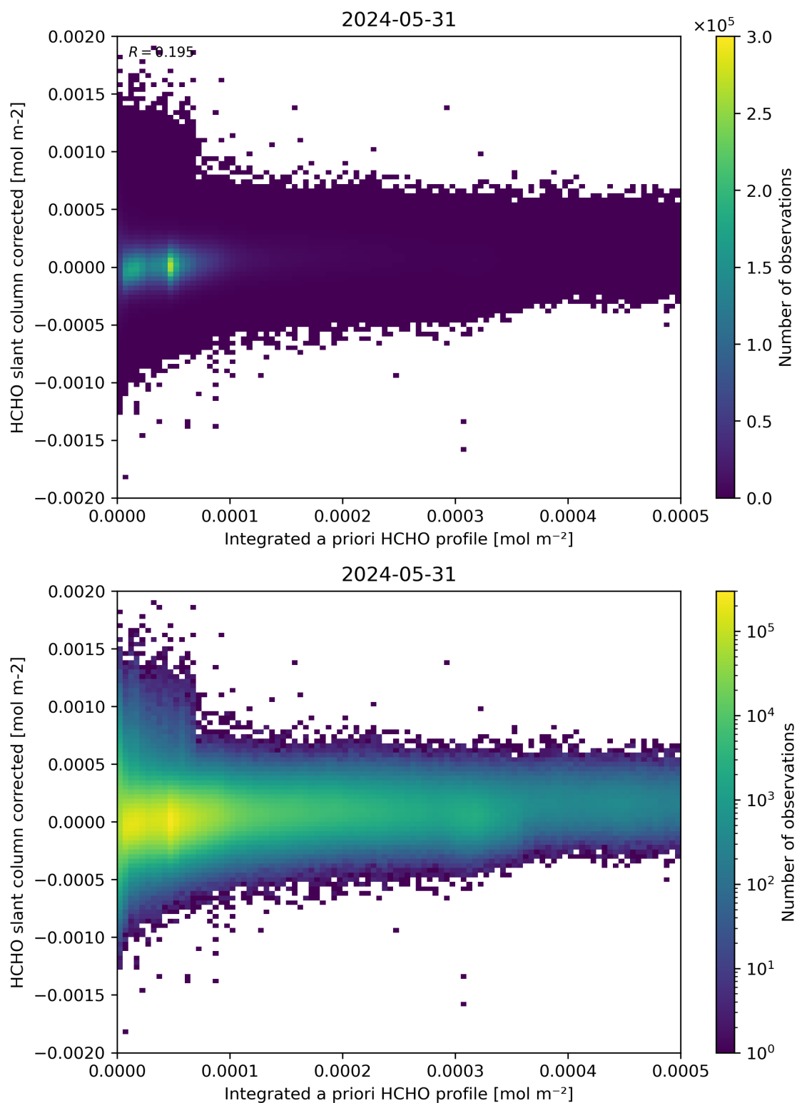
Figure 151: Scatter density plot of “Integrated a priori HCHO profile” against “HCHO slant column corrected” for 2024-05-30 to 2024-06-01.
