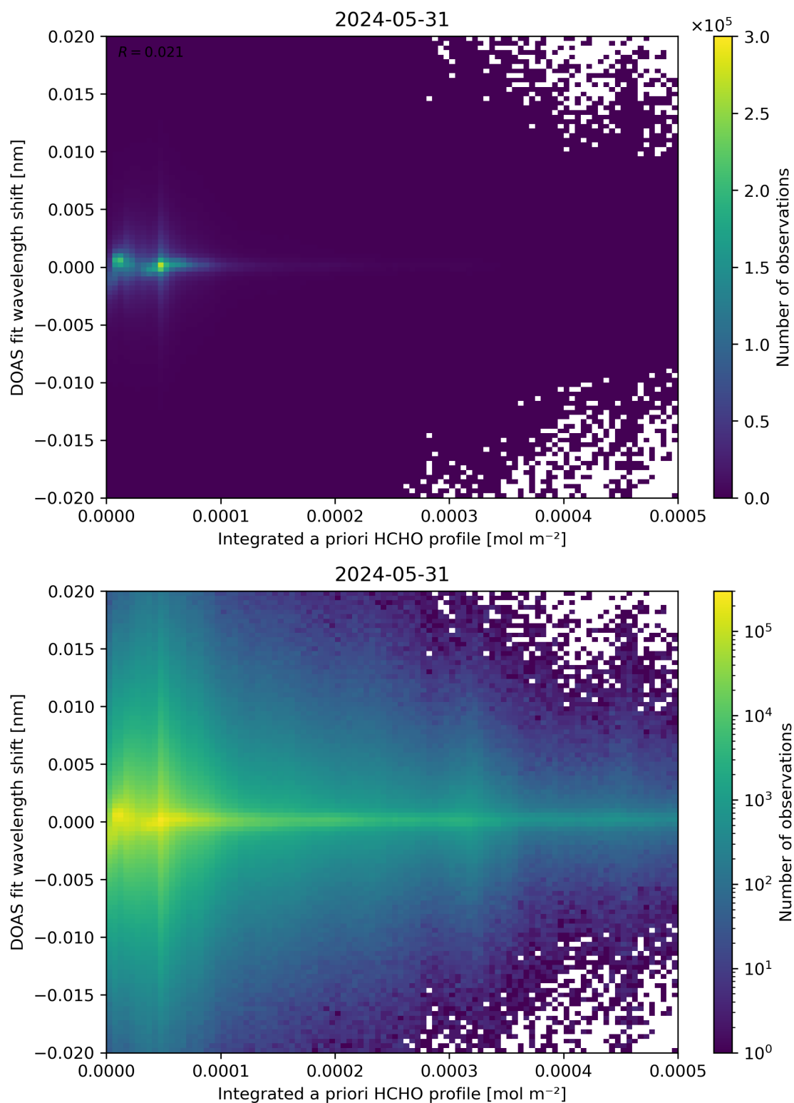
Figure 149: Scatter density plot of “Integrated a priori HCHO profile” against “DOAS fit wavelength shift” for 2024-05-30 to 2024-06-01.
