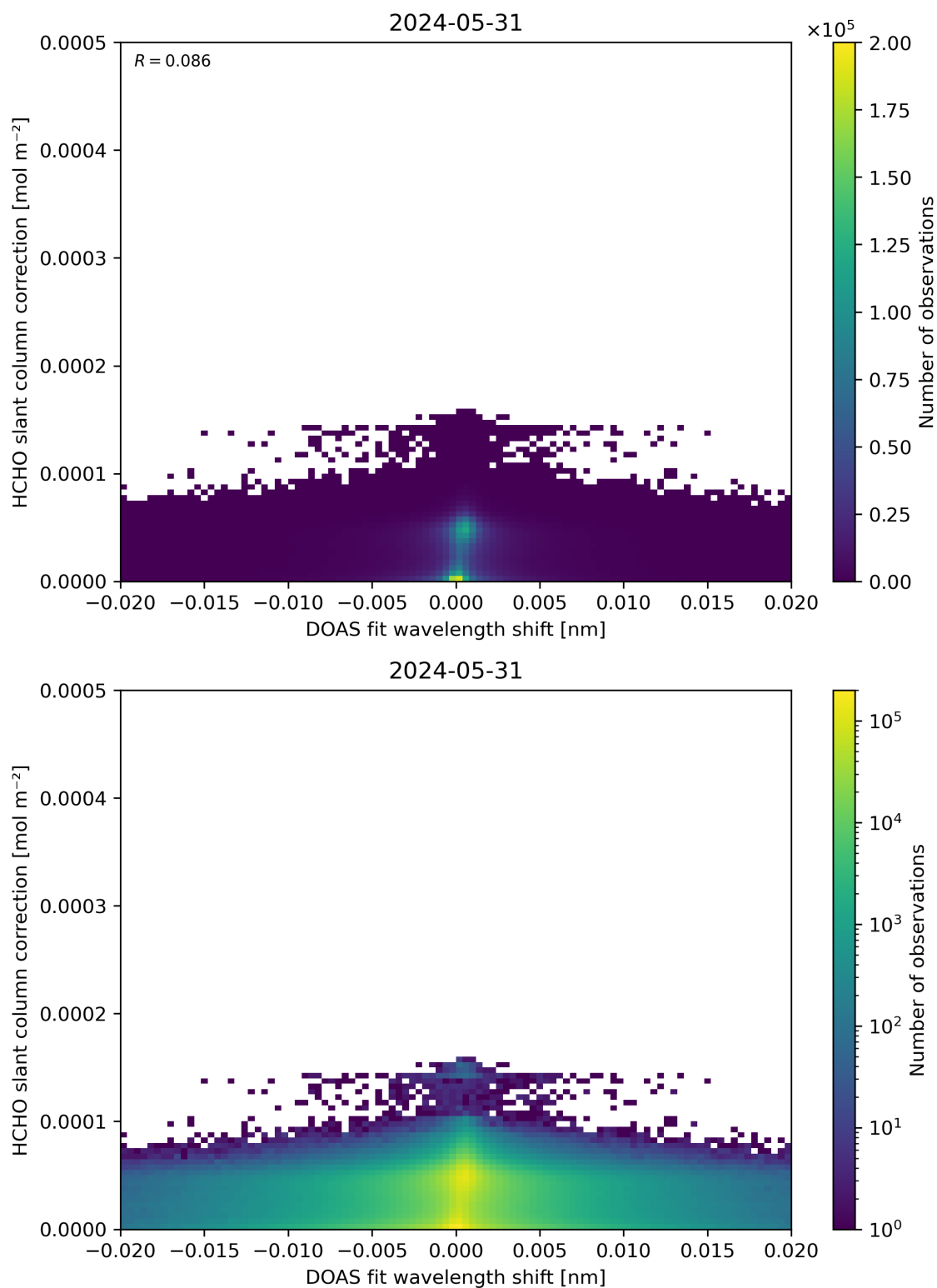
Figure 67: Scatter density plot of “DOAS fit wavelength shift” against “HCHO slant column correction” for 2024-05-30 to 2024-06-01.
