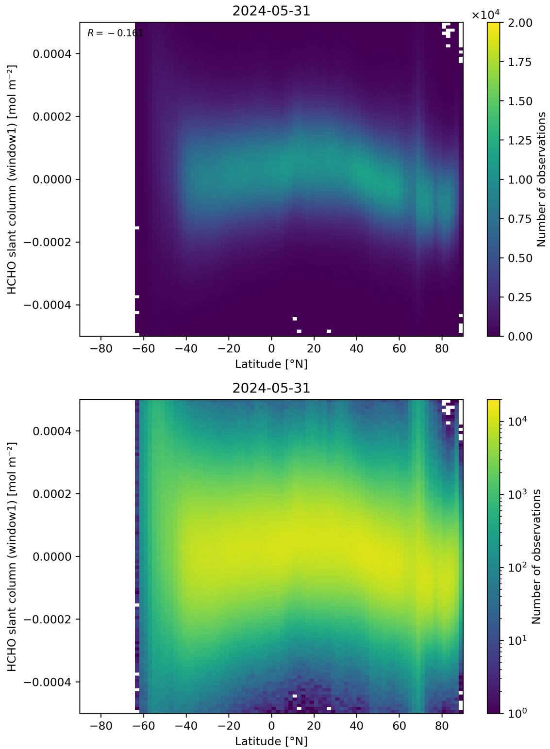
Figure 159: Scatter density plot of “Latitude” against “HCHO slant column (window1)” for 2024-05-30 to 2024-06-01.
