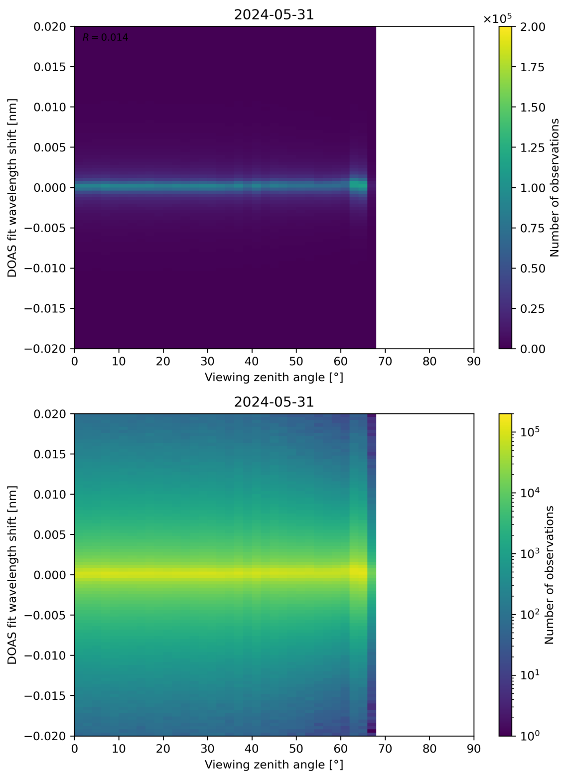
Figure 183: Scatter density plot of “Viewing zenith angle” against “DOAS fit wavelength shift” for 2024-05-30 to 2024-06-01.
