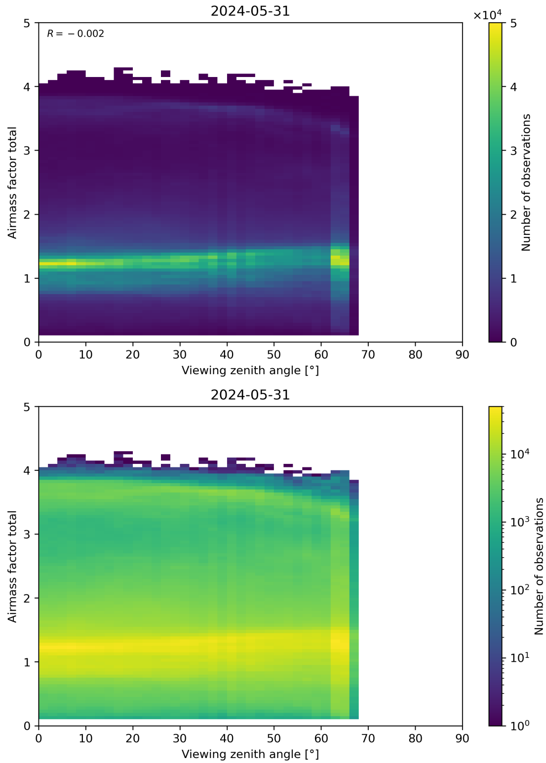
Figure 190: Scatter density plot of “Viewing zenith angle” against “Airmass factor total” for 2024-05-30 to 2024-06-01.
