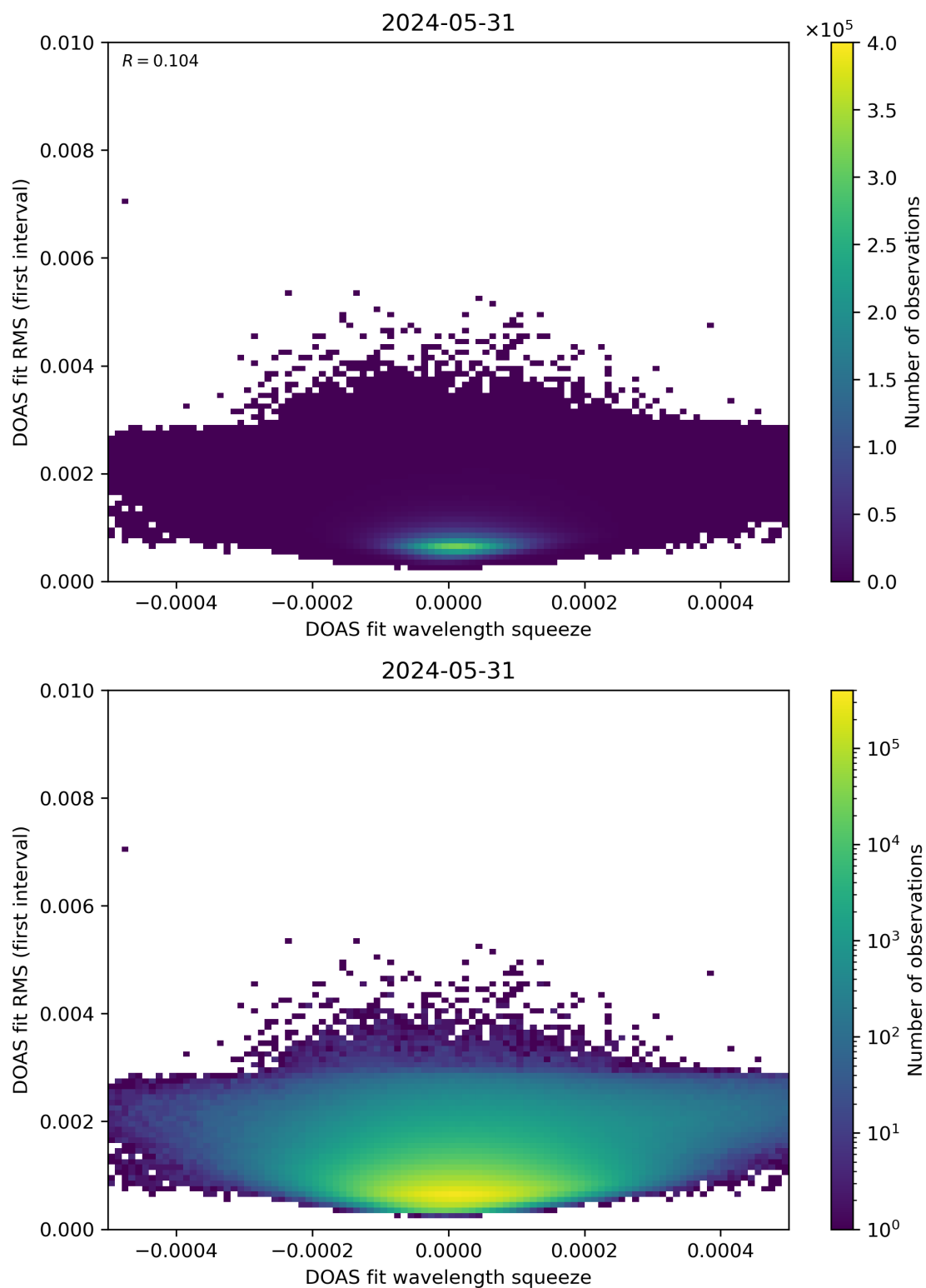
Figure 68: Scatter density plot of “DOAS fit wavelength squeeze” against “DOAS fit RMS (first interval)” for 2024-05-30 to 2024-06-01.
