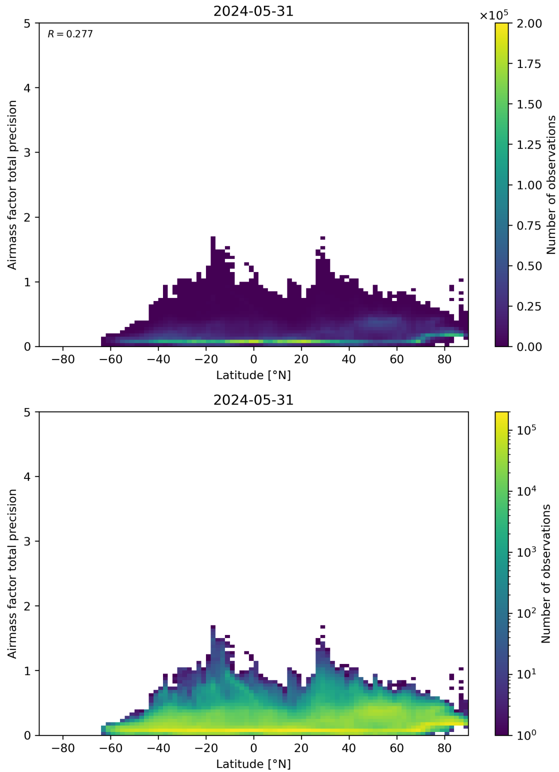
Figure 162: Scatter density plot of “Latitude” against “Airmass factor total precision” for 2024-05-30 to 2024-06-01.
