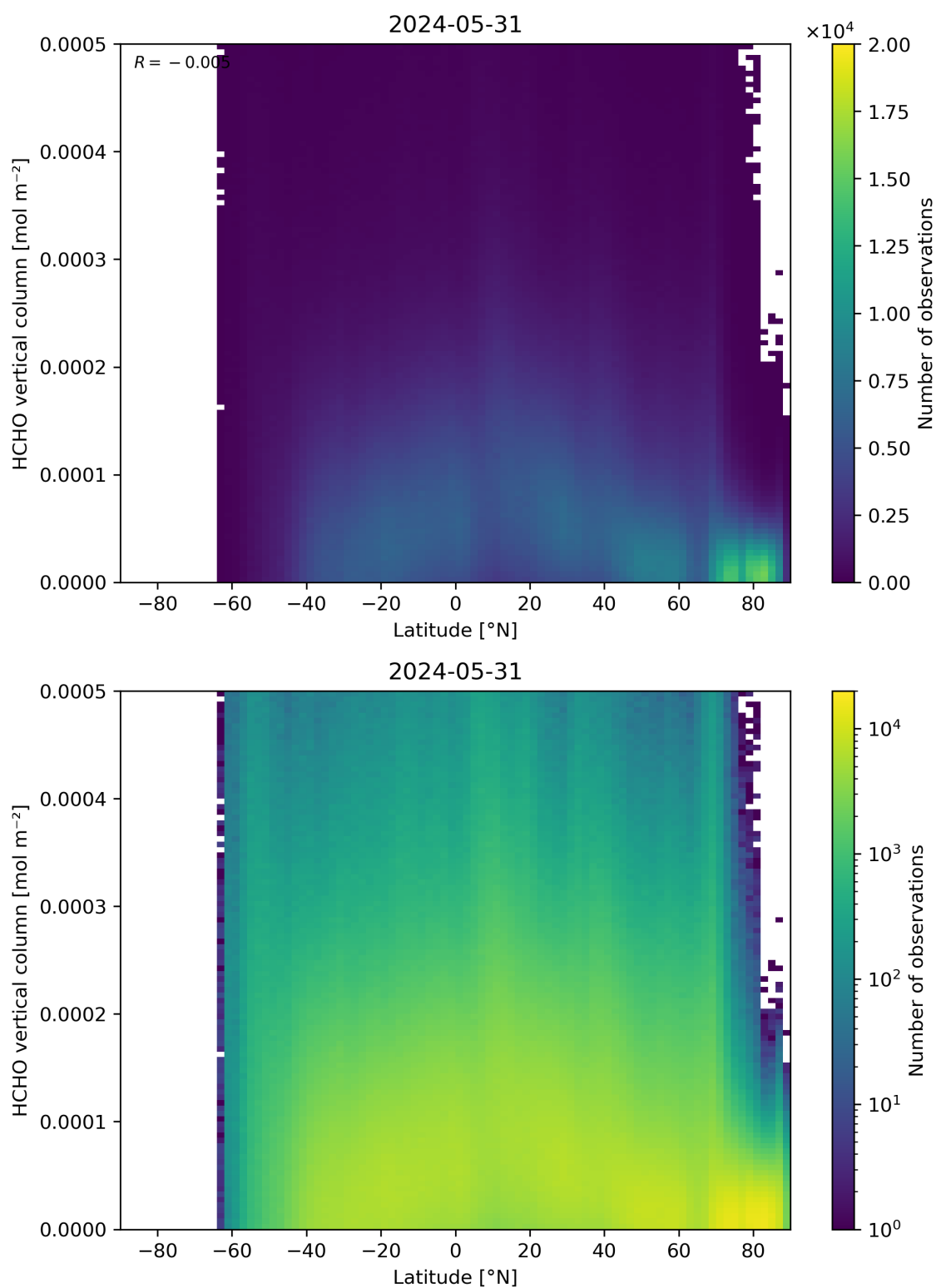
Figure 163: Scatter density plot of “Latitude” against “HCHO vertical column” for 2024-05-30 to 2024-06-01.
