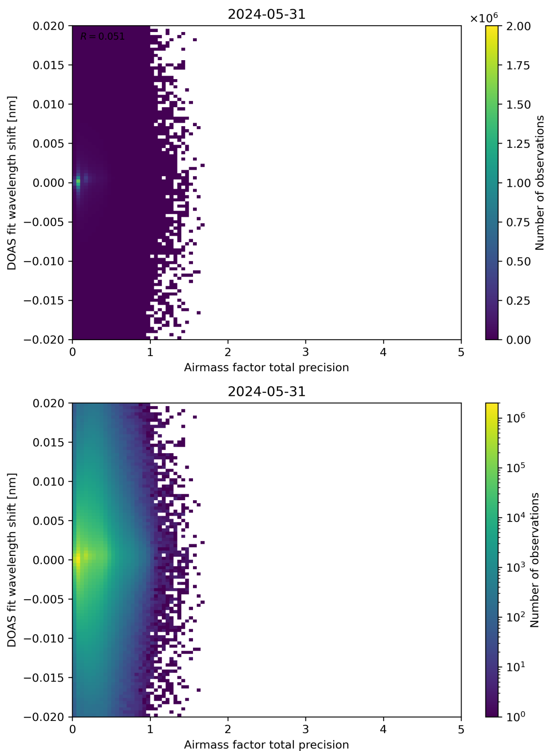
Figure 106: Scatter density plot of “Airmass factor total precision” against “DOAS fit wavelength shift” for 2024-05-30 to 2024-06-01.
