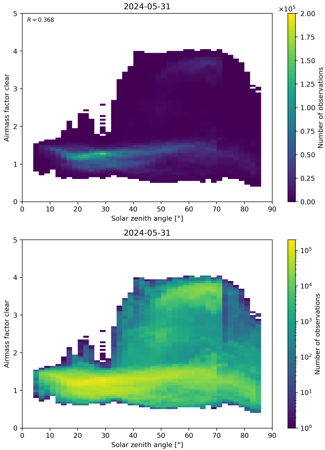
Figure 170: Scatter density plot of “Solar zenith angle” against “Airmass factor clear” for 2024-05-30 to 2024-06-01.
