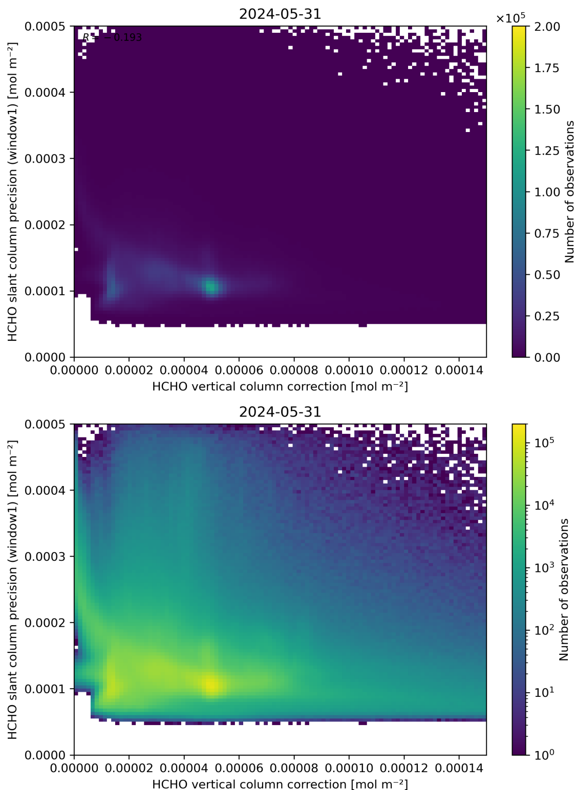
Figure 119: Scatter density plot of “HCHO vertical column correction” against “HCHO slant column precision (window1)” for 2024-05-30 to 2024-06-01.
