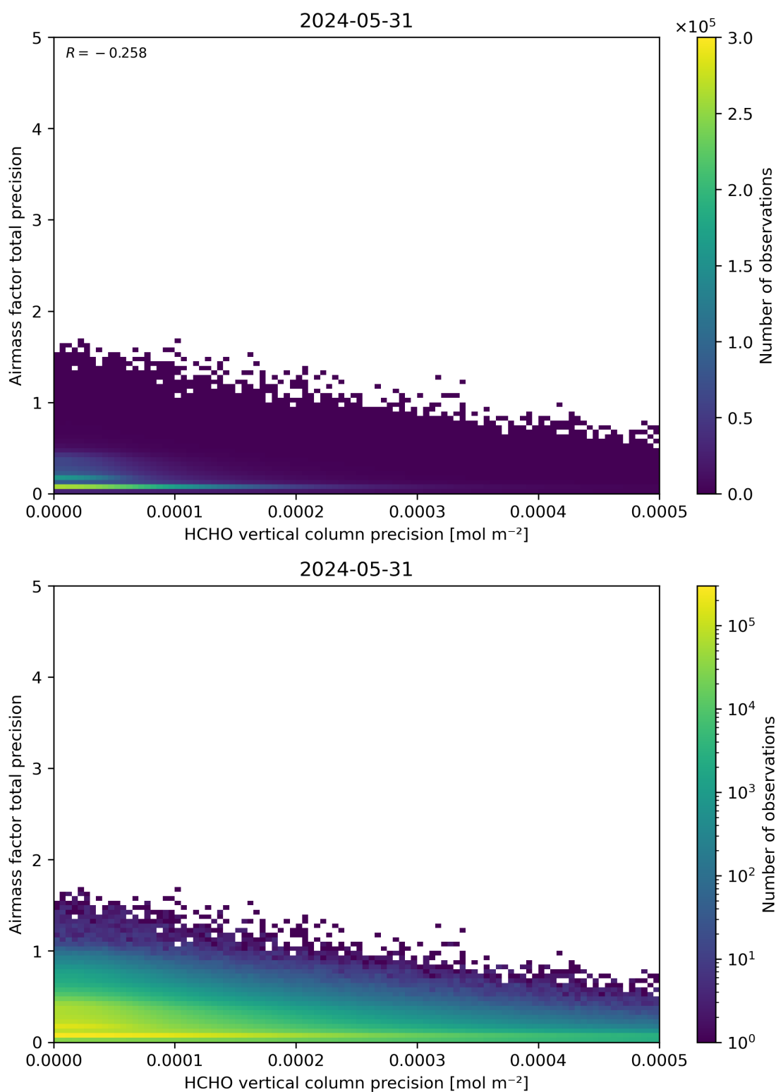
Figure 145: Scatter density plot of “HCHO vertical column precision” against “Airmass factor total precision” for 2024-05-30 to 2024-06-01.
