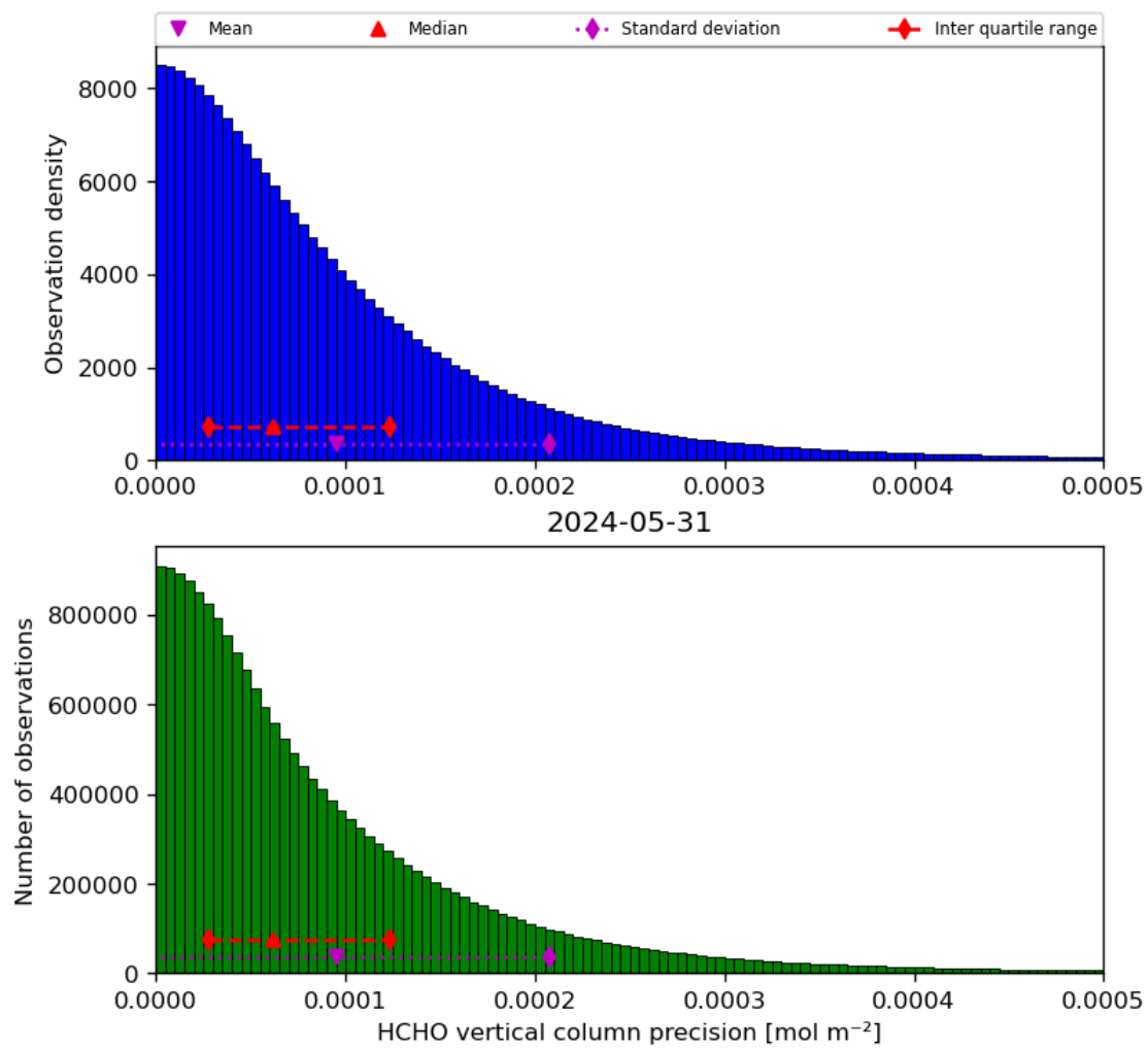
Figure 36: Histogram of “HCHO vertical column precision” for 2024-05-30 to 2024-06-01
