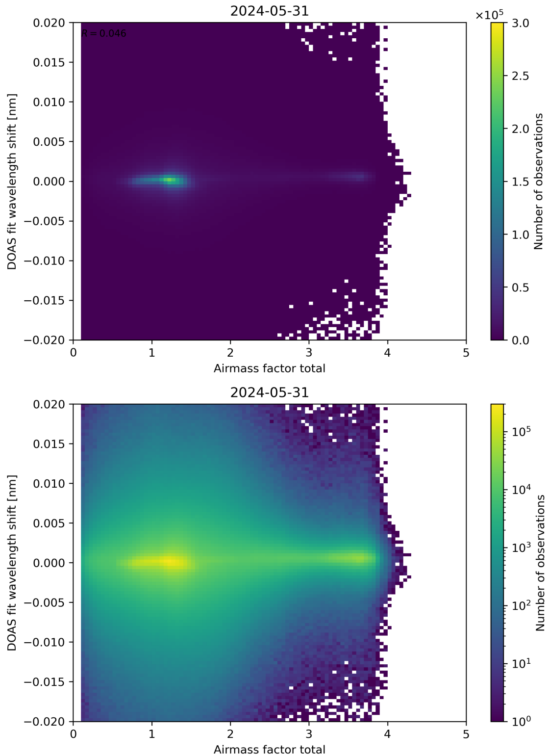
Figure 98: Scatter density plot of “Airmass factor total” against “DOAS fit wavelength shift” for 2024-05-30 to 2024-06-01.
