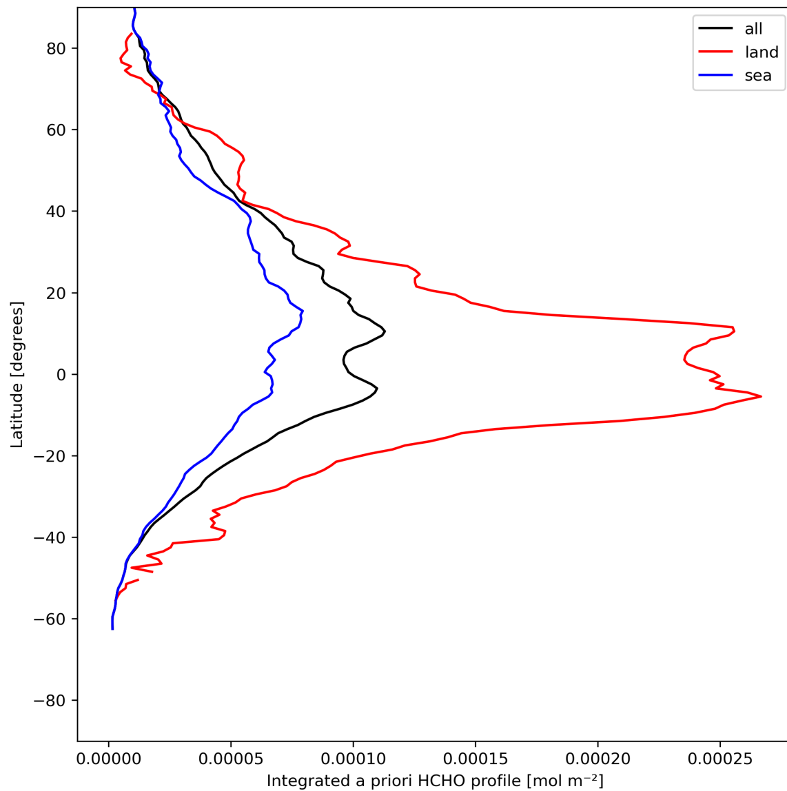
Figure 29: Zonal average of “Integrated a priori HCHO profile” for 2024-05-30 to 2024-06-01.
