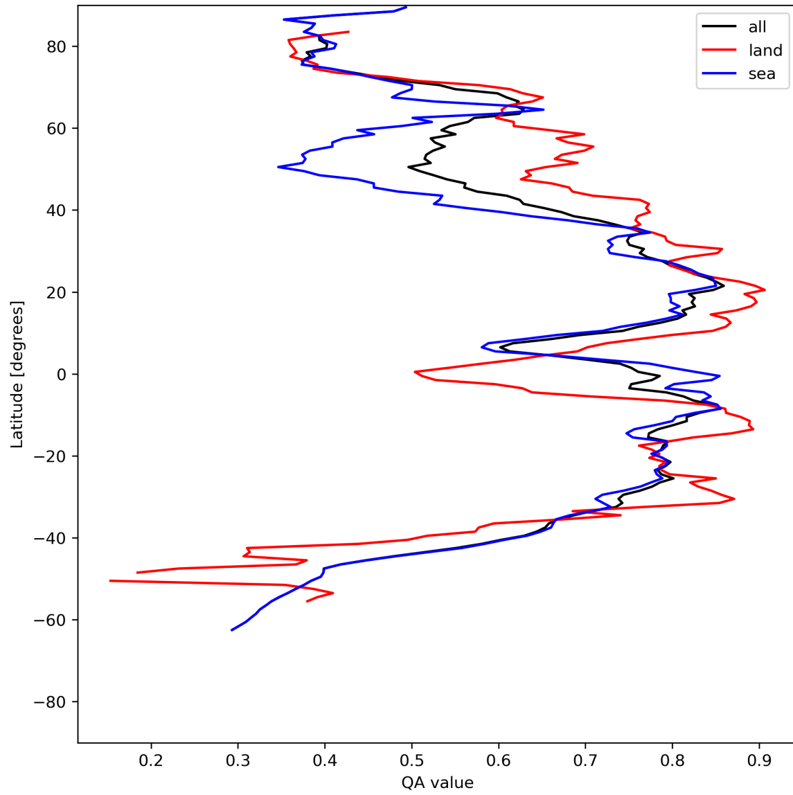
Figure 20: Zonal average of “QA value” for 2024-05-30 to 2024-06-01.
