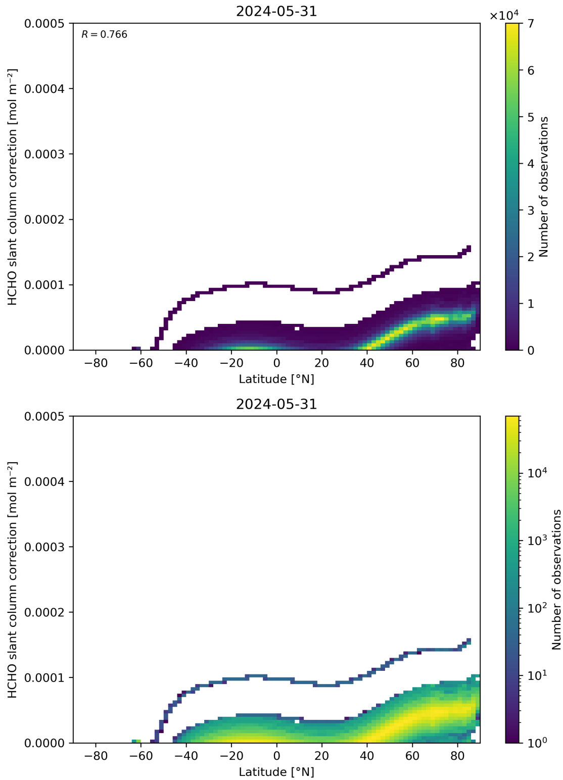
Figure 158: Scatter density plot of “Latitude” against “HCHO slant column correction” for 2024-05-30 to 2024-06-01.
