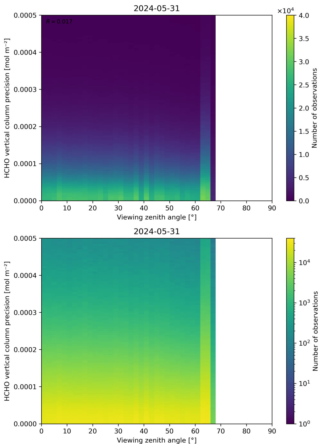
Figure 194: Scatter density plot of “Viewing zenith angle” against “HCHO vertical column precision” for 2024-05-30 to 2024-06-01.
