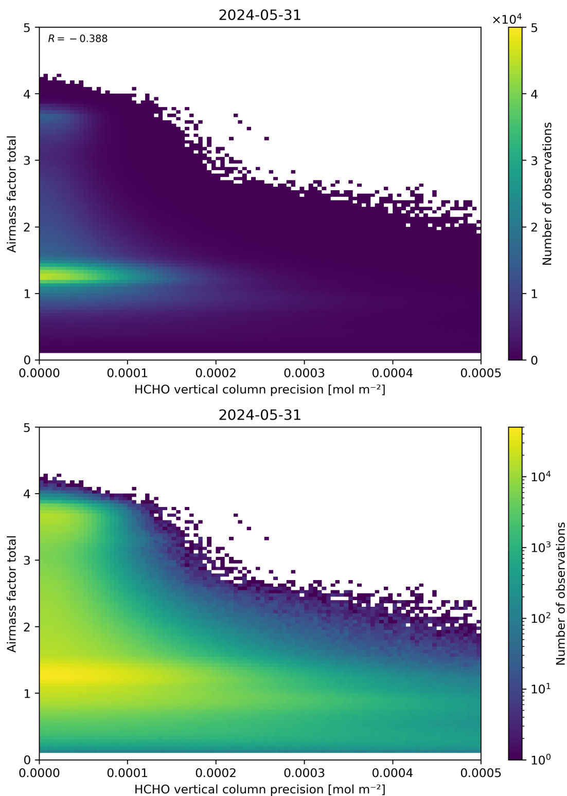
Figure 144: Scatter density plot of “HCHO vertical column precision” against “Airmass factor total” for 2024-05-30 to 2024-06-01.
