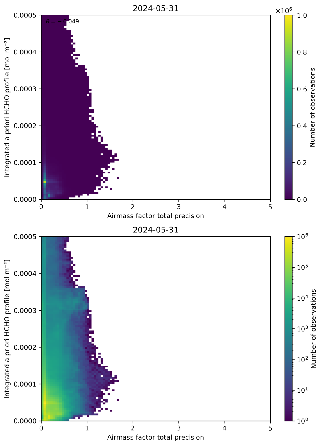
Figure 111: Scatter density plot of “Airmass factor total precision” against “Integrated a priori HCHO profile” for 2024-05-30 to 2024-06-01.
