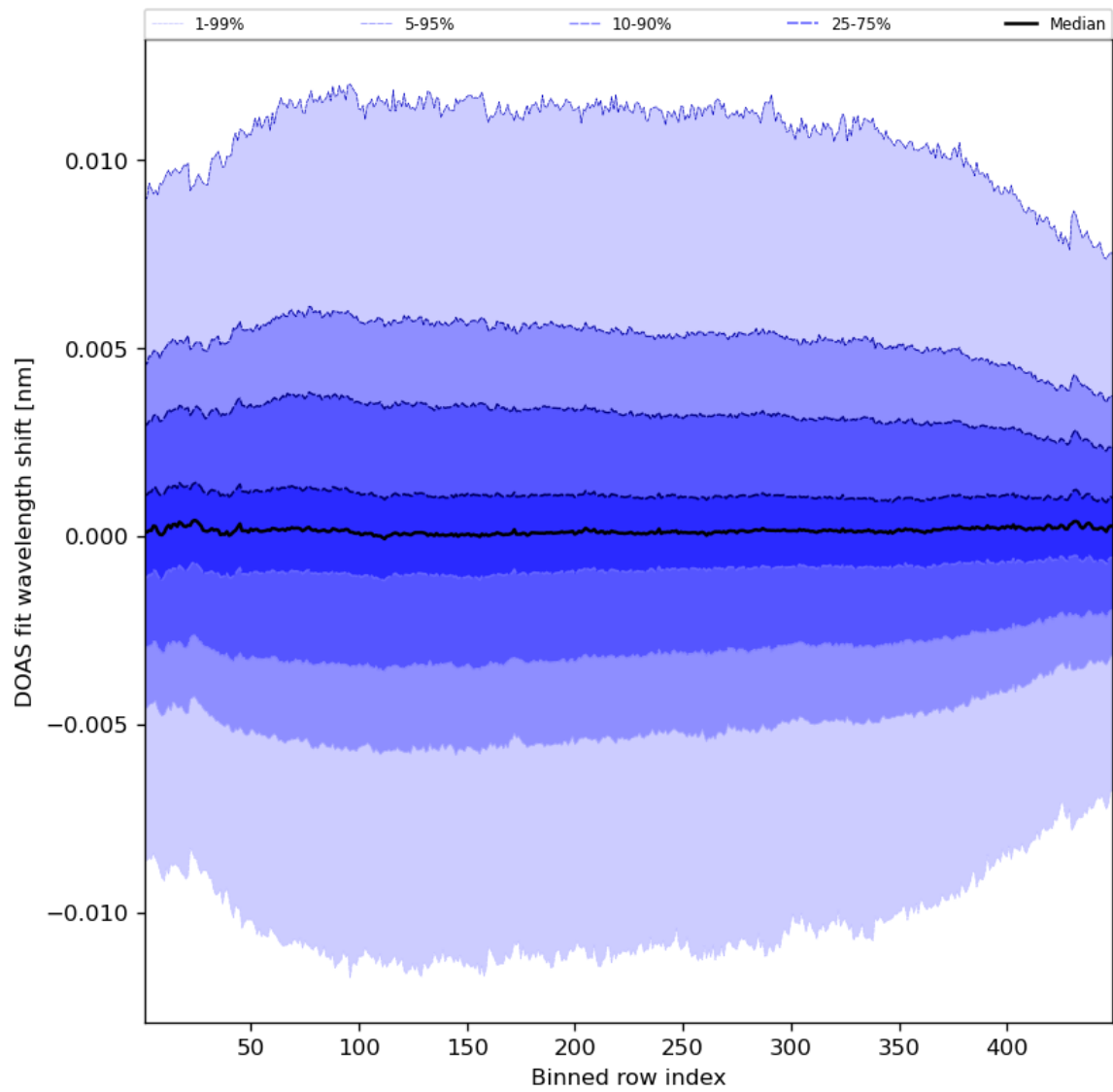
Figure 58: Along track statistics of “DOAS fit wavelength shift” for 2024-05-30 to 2024-06-01
