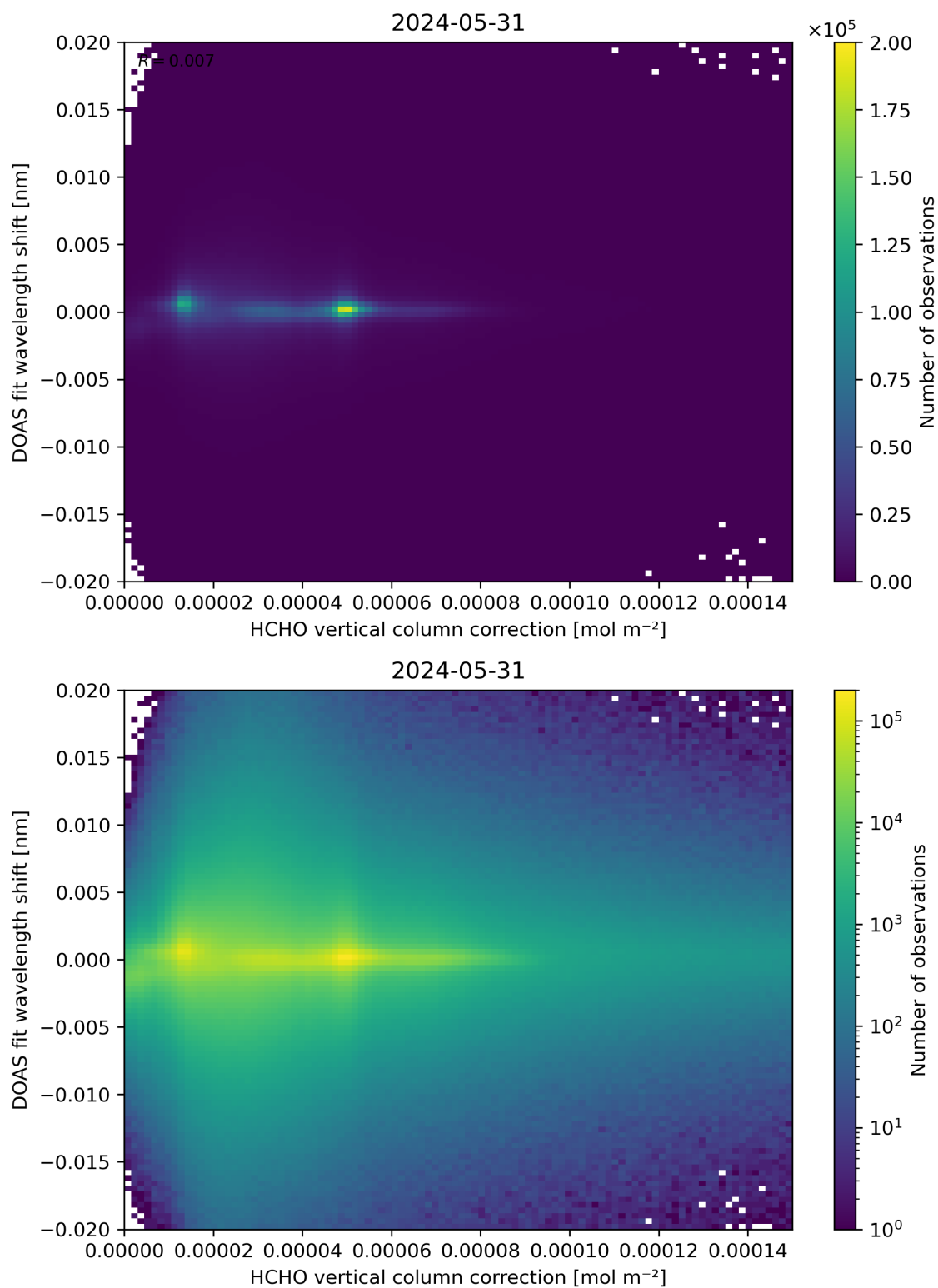
Figure 113: Scatter density plot of “HCHO vertical column correction” against “DOAS fit wavelength shift” for 2024-05-30 to 2024-06-01.
