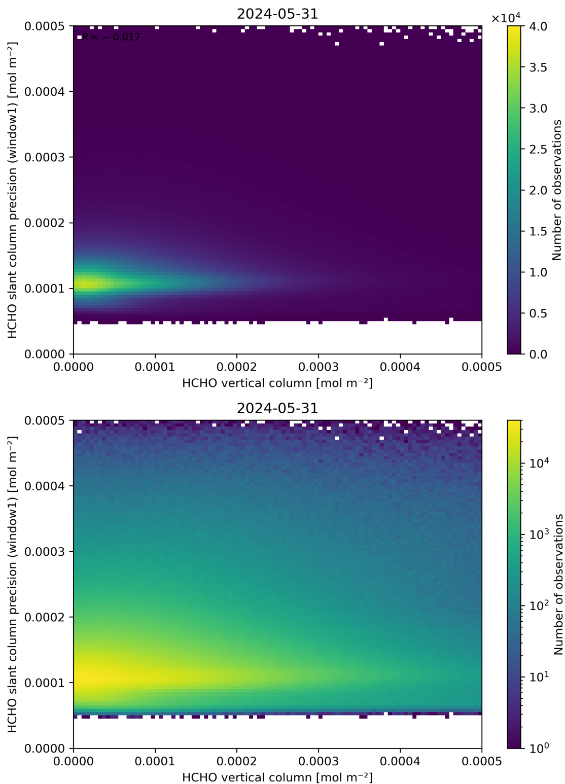
Figure 130: Scatter density plot of “HCHO vertical column” against “HCHO slant column precision (window1)” for 2024-05-30 to 2024-06-01.
