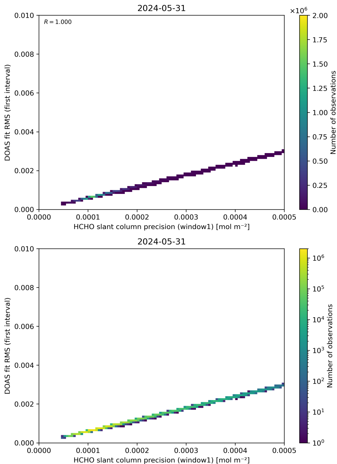
Figure 88: Scatter density plot of “HCHO slant column precision (window1)” against “DOAS fit RMS (first interval)” for 2024-05-30 to 2024-06-01.
