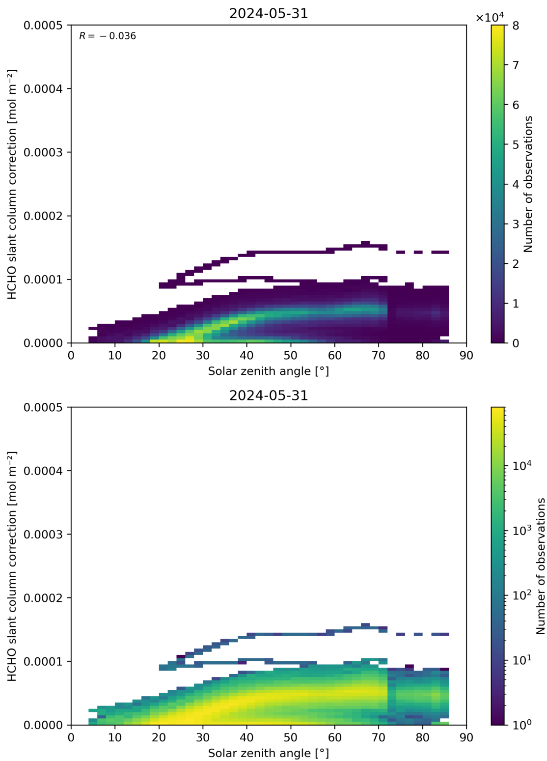
Figure 172: Scatter density plot of “Solar zenith angle” against “HCHO slant column correction” for 2024-05-30 to 2024-06-01.
