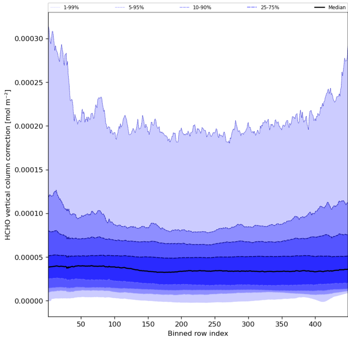
Figure 51: Along track statistics of “HCHO vertical column correction” for 2024-05-30 to 2024-06-01
