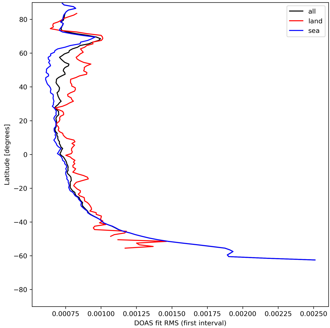
Figure 32: Zonal average of "DOAS fit RMS (first interval)" for 2024-05-30 to 2024-06-01.
