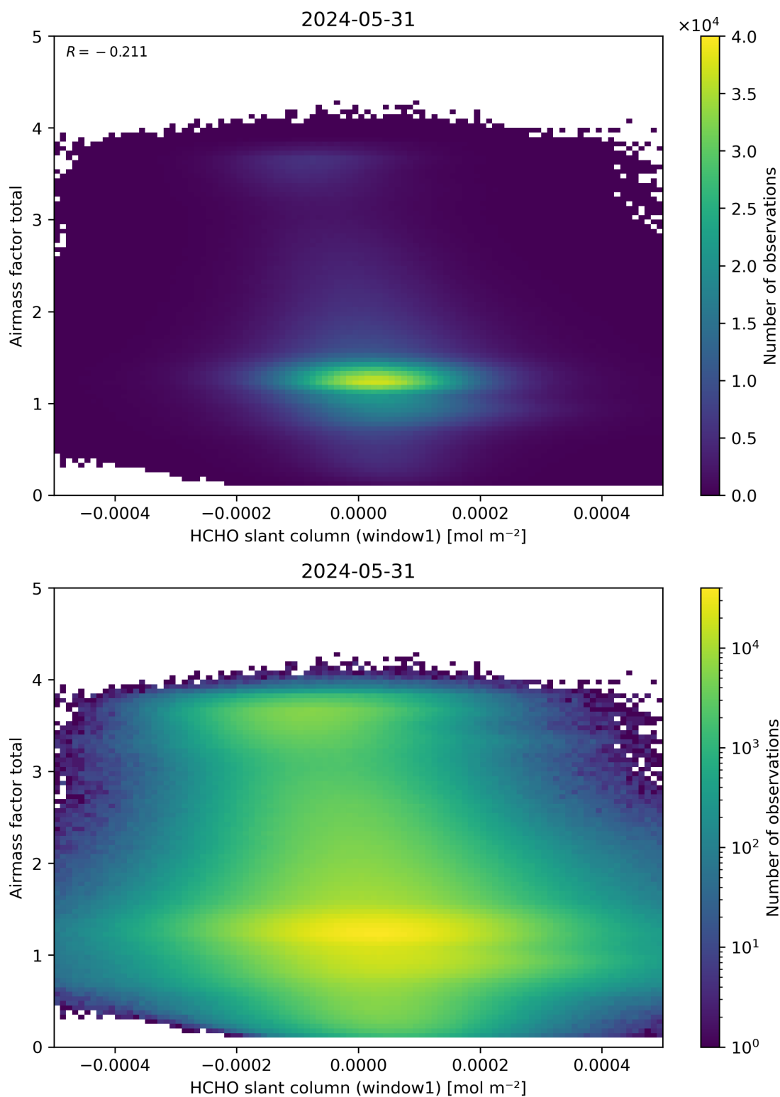
Figure 85: Scatter density plot of “HCHO slant column (window1)” against “Airmass factor total” for 2024-05-30 to 2024-06-01.
