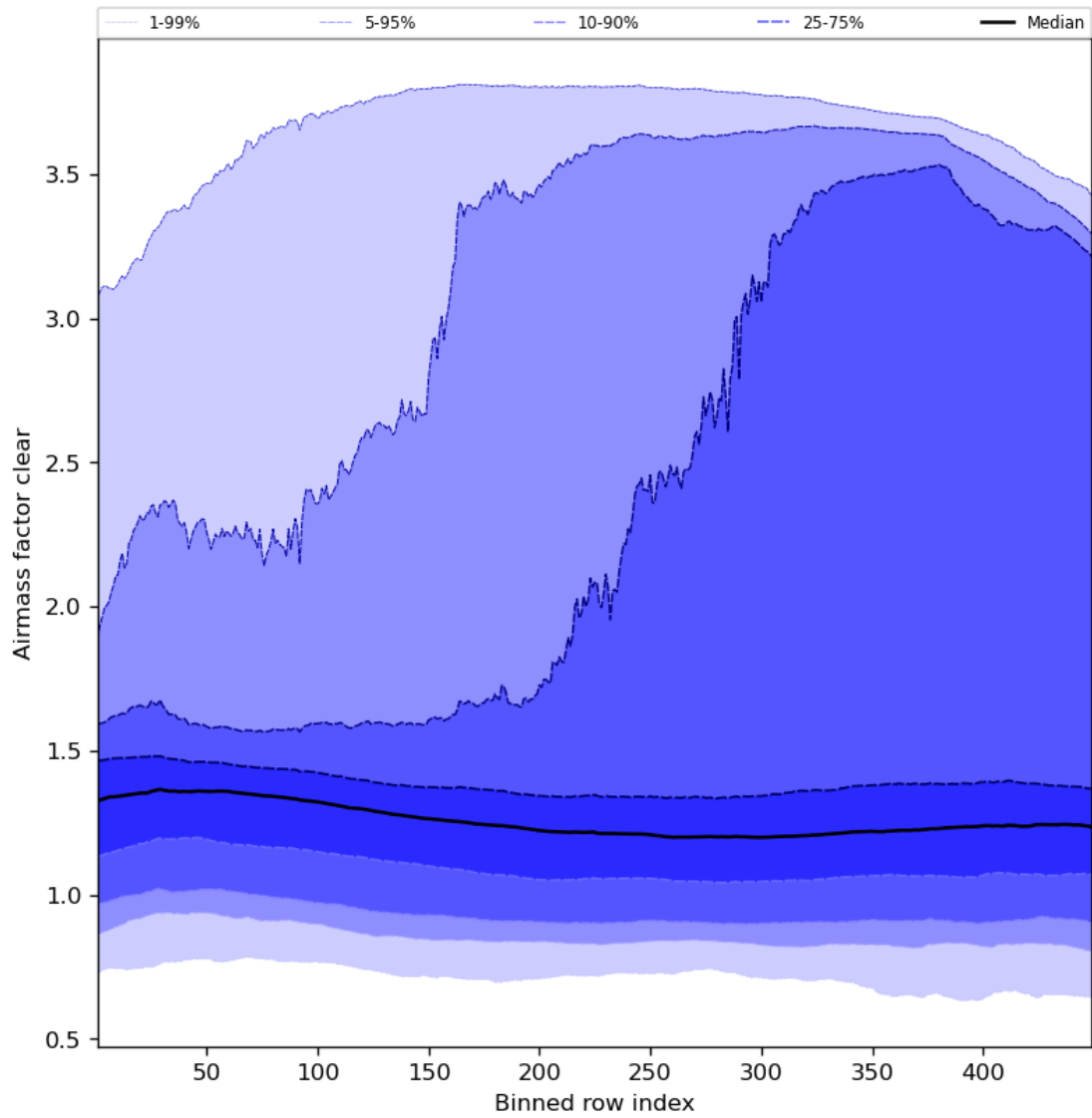
Figure 56: Along track statistics of “Airmass factor clear” for 2024-05-30 to 2024-06-01
