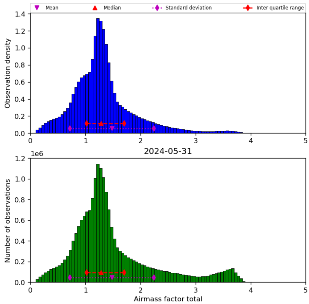
Figure 40: Histogram of “Airmass factor total” for 2024-05-30 to 2024-06-01
