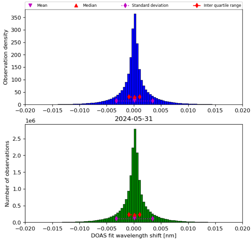
Figure 44: Histogram of “DOAS fit wavelength shift” for 2024-05-30 to 2024-06-01
