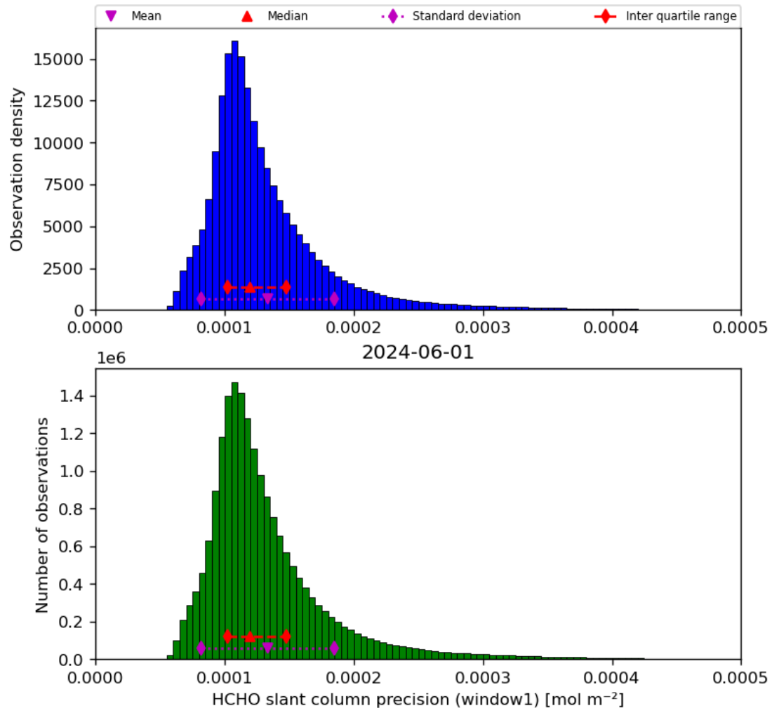
Figure 39: Histogram of “HCHO slant column precision (window1)” for 2024-05-31 to 2024-06-02
