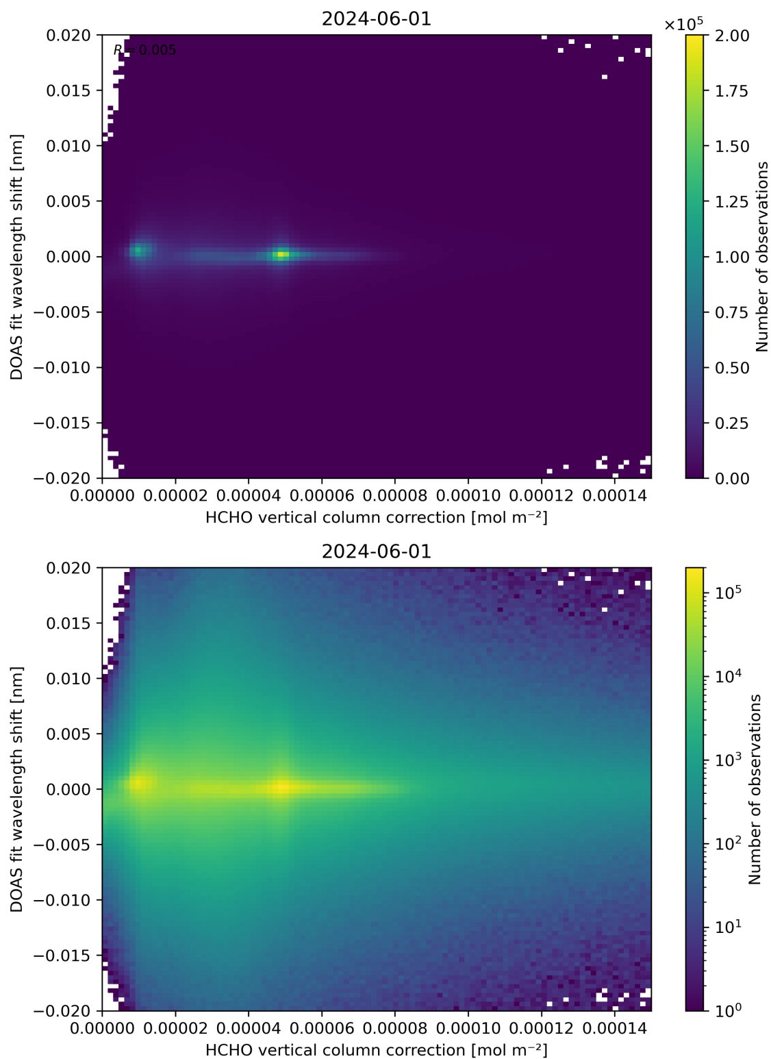
Figure 113: Scatter density plot of “HCHO vertical column correction” against “DOAS fit wavelength shift” for 2024-05-31 to 2024-06-02.
