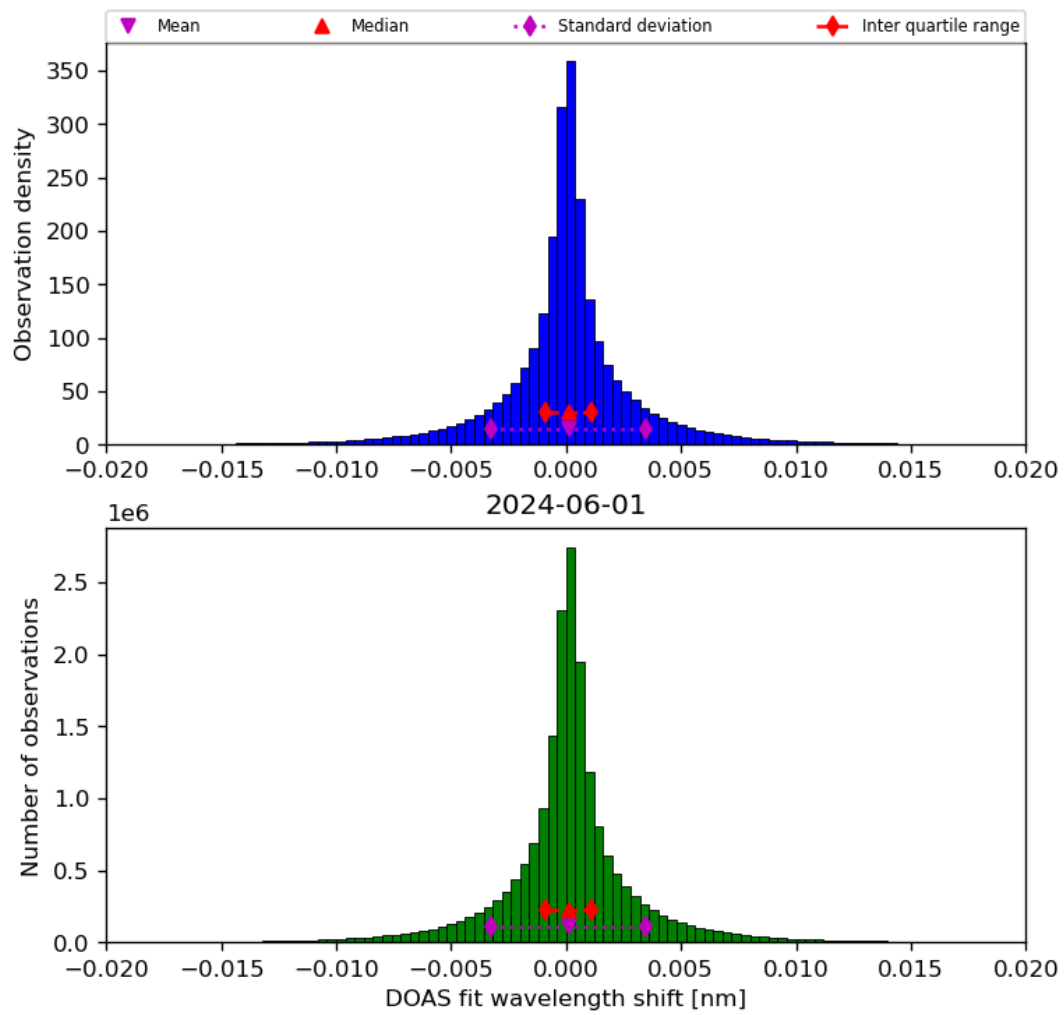
Figure 44: Histogram of “DOAS fit wavelength shift” for 2024-05-31 to 2024-06-02
