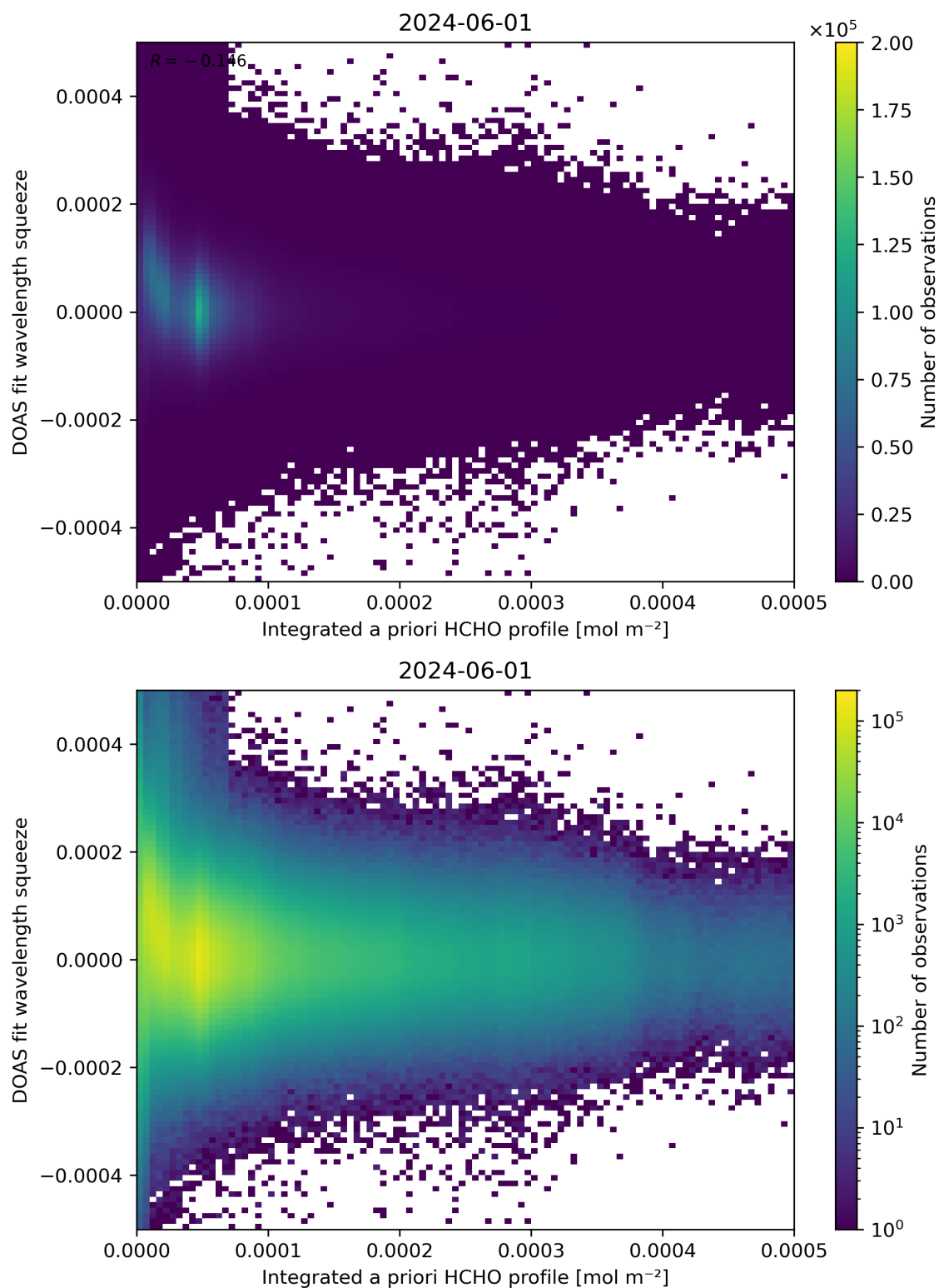
Figure 150: Scatter density plot of “Integrated a priori HCHO profile” against “DOAS fit wavelength squeeze” for 2024-05-31 to 2024-06-02.
