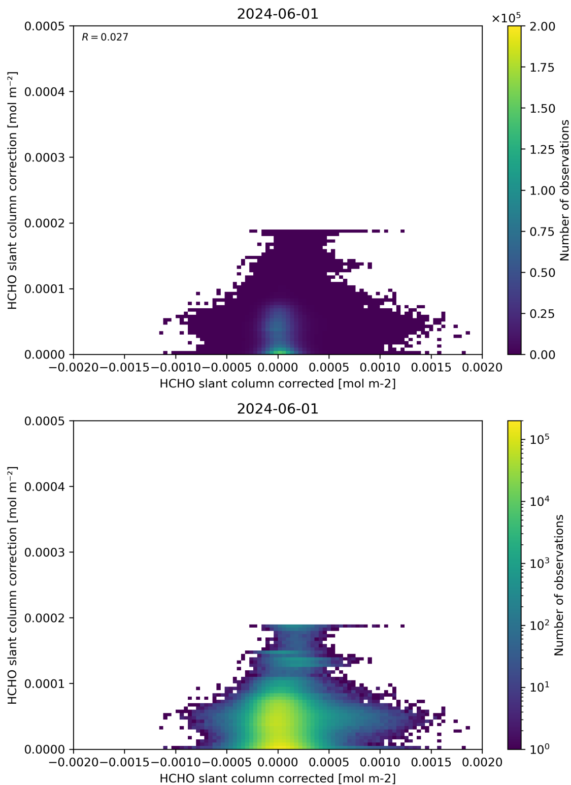
Figure 77: Scatter density plot of “HCHO slant column corrected” against “HCHO slant column correction” for 2024-05-31 to 2024-06-02.
