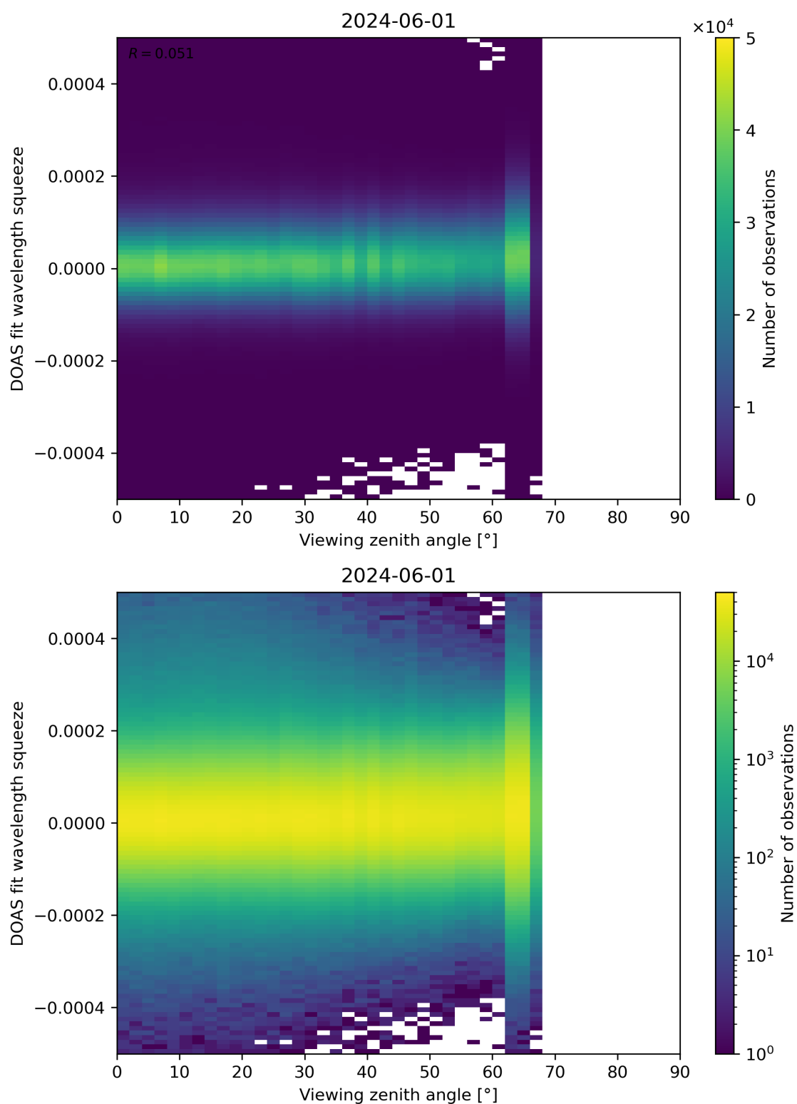
Figure 184: Scatter density plot of “Viewing zenith angle” against “DOAS fit wavelength squeeze” for 2024-05-31 to 2024-06-02.
