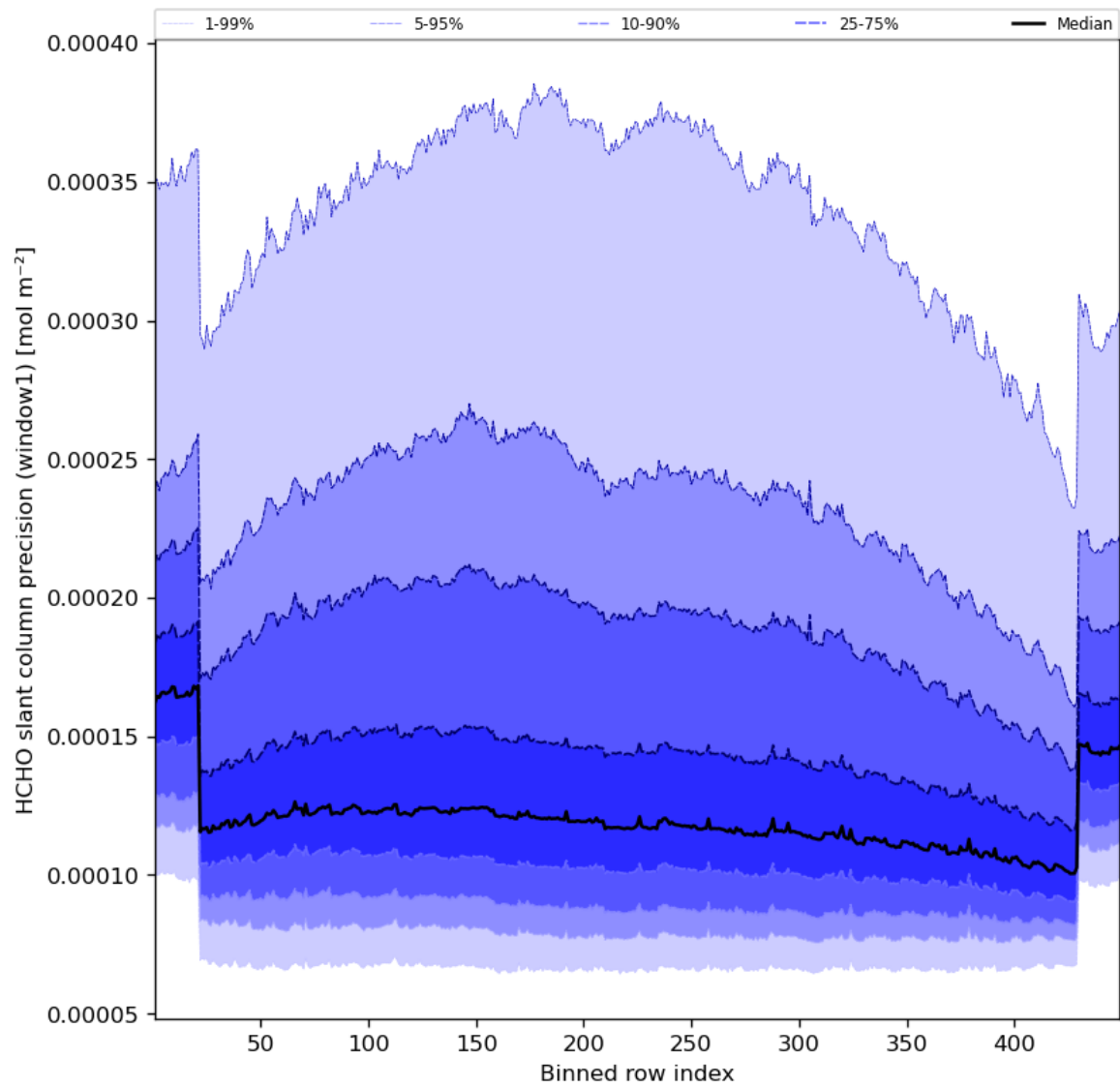
Figure 53: Along track statistics of “HCHO slant column precision (window1)” for 2024-05-31 to 2024-06-02
