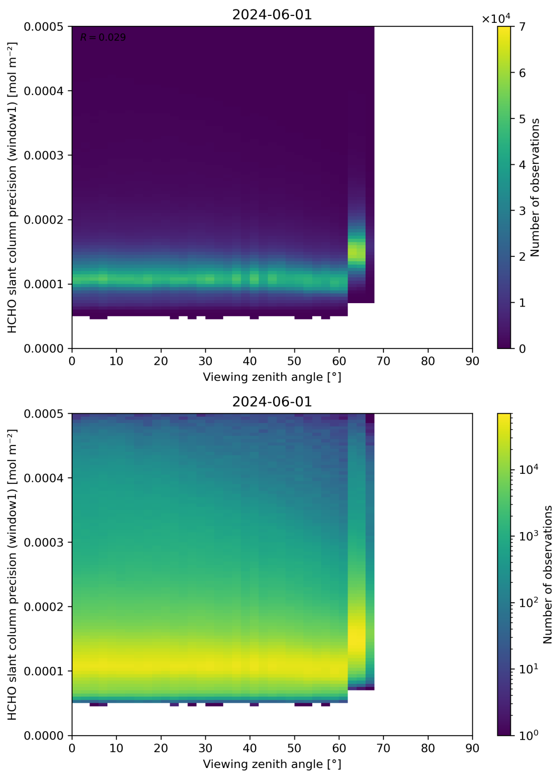
Figure 189: Scatter density plot of “Viewing zenith angle” against “HCHO slant column precision (window1)” for 2024-05-31 to 2024-06-02.
