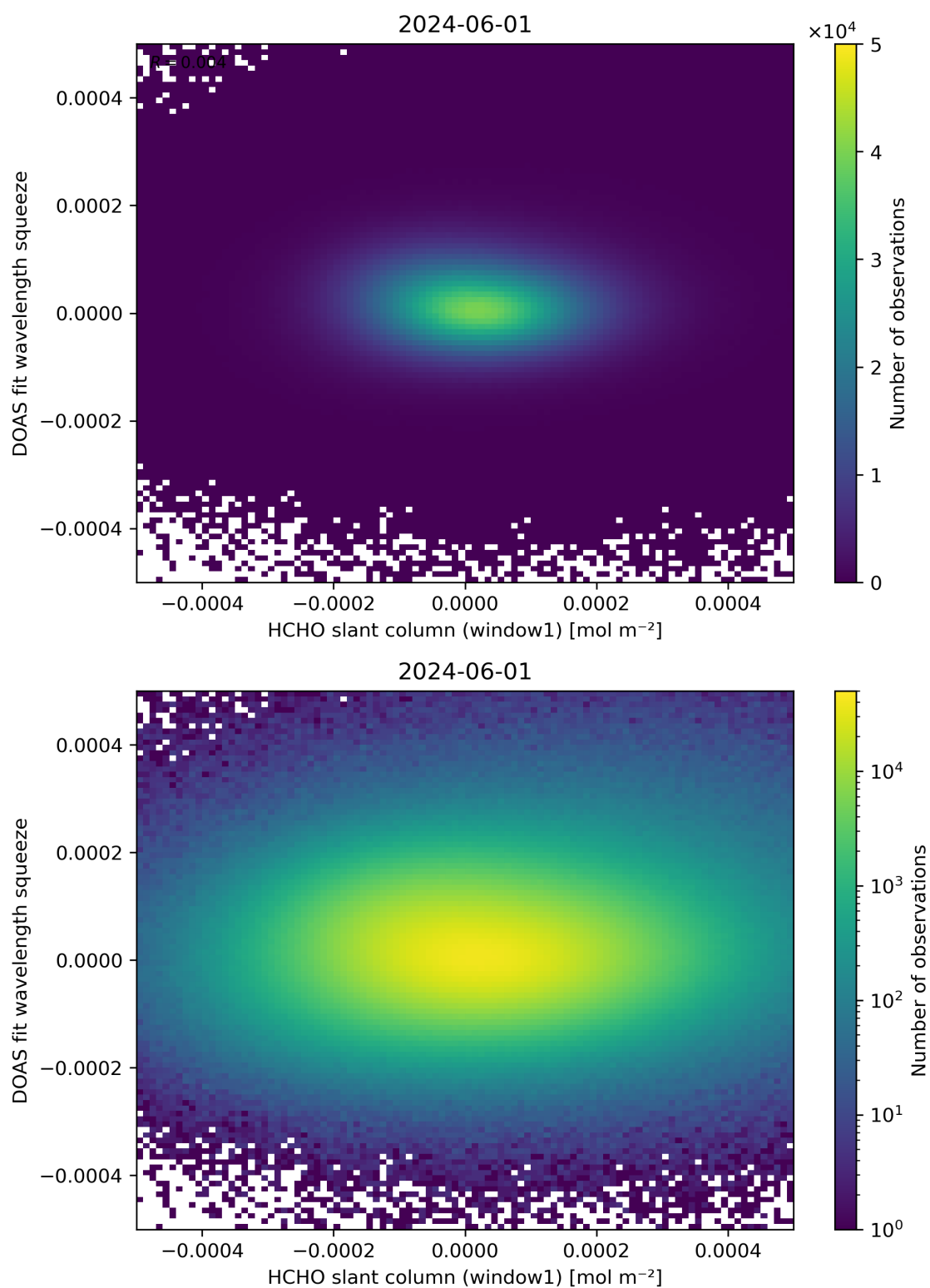
Figure 80: Scatter density plot of “HCHO slant column (window1)” against “DOAS fit wavelength squeeze” for 2024-05-31 to 2024-06-02.
