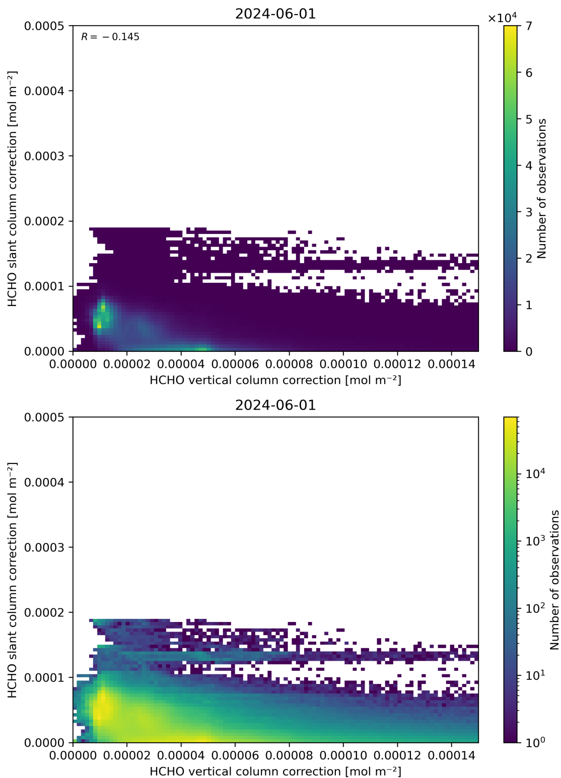
Figure 117: Scatter density plot of “HCHO vertical column correction” against “HCHO slant column correction” for 2024-05-31 to 2024-06-02.
