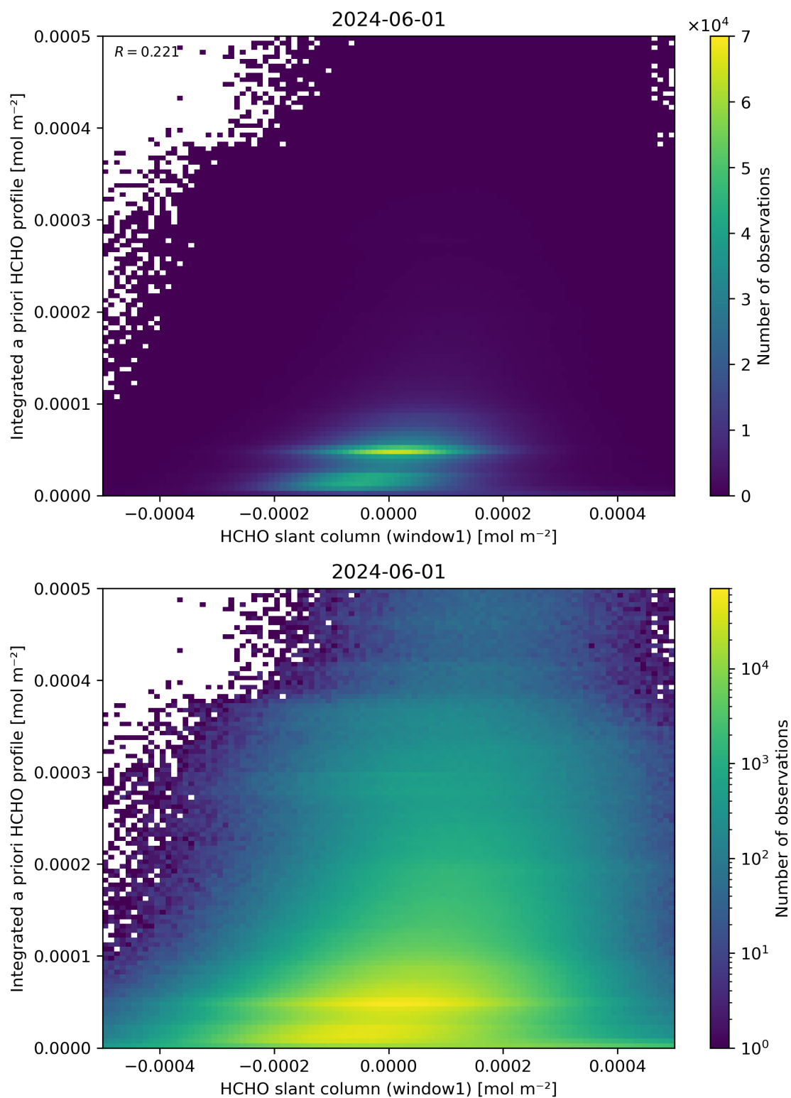
Figure 87: Scatter density plot of “HCHO slant column (window1)” against “Integrated a priori HCHO profile” for 2024-05-31 to 2024-06-02.
