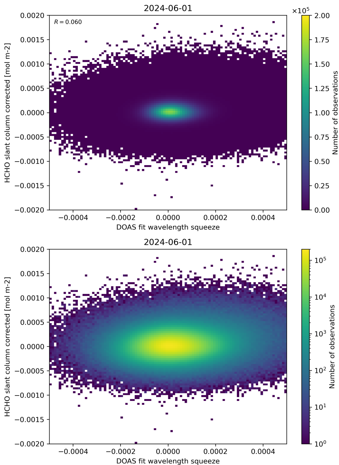
Figure 69: Scatter density plot of “DOAS fit wavelength squeeze” against “HCHO slant column corrected” for 2024-05-31 to 2024-06-02.
