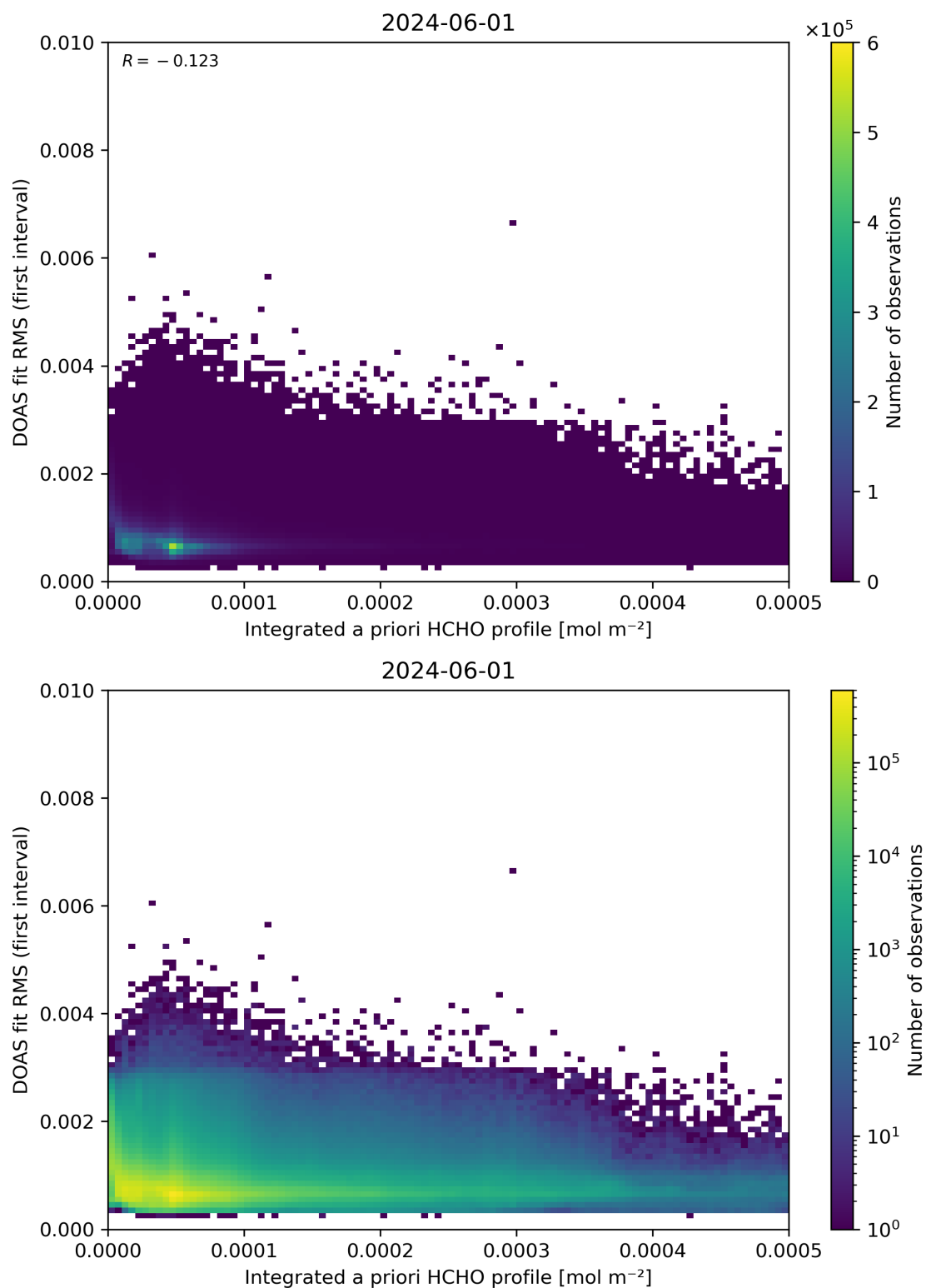
Figure 148: Scatter density plot of “Integrated a priori HCHO profile” against “DOAS fit RMS (first interval)” for 2024-05-31 to 2024-06-02.
