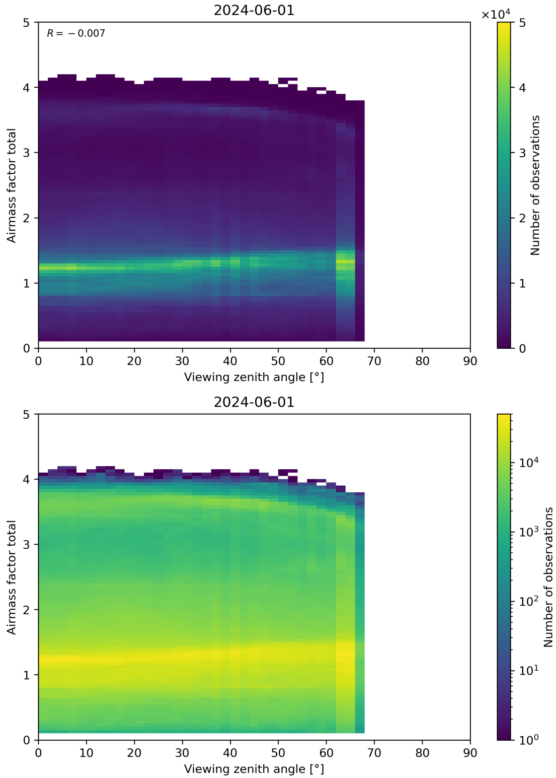
Figure 190: Scatter density plot of “Viewing zenith angle” against “Airmass factor total” for 2024-05-31 to 2024-06-02.
