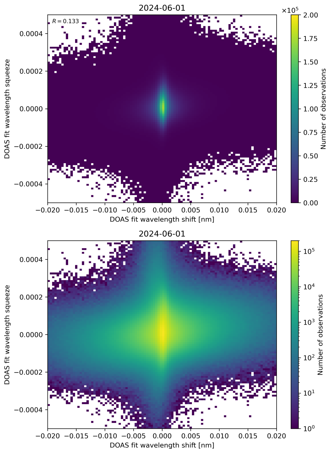
Figure 65: Scatter density plot of “DOAS fit wavelength shift” against “DOAS fit wavelength squeeze” for 2024-05-31 to 2024-06-02.
