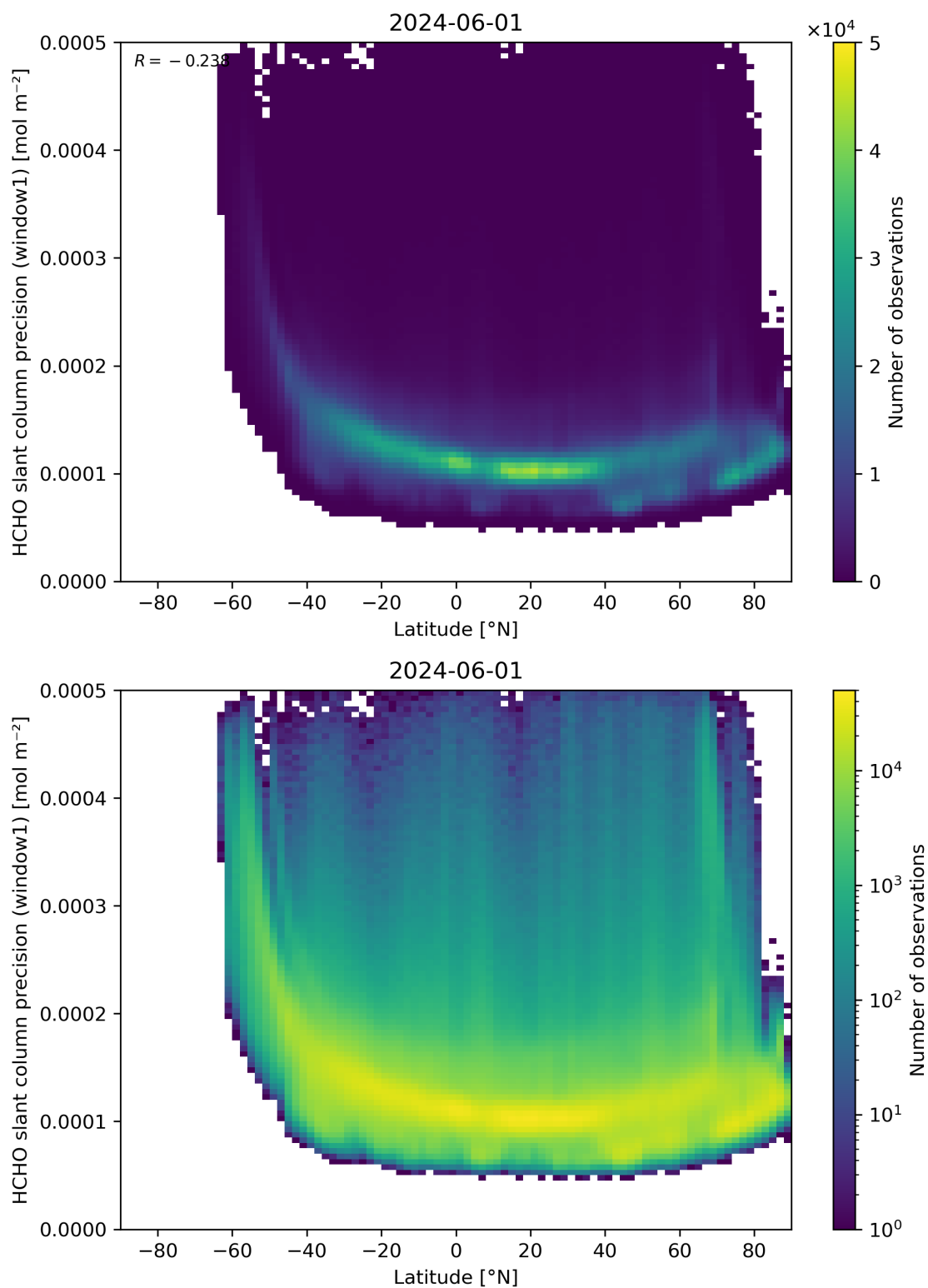
Figure 160: Scatter density plot of “Latitude” against “HCHO slant column precision (window1)” for 2024-05-31 to 2024-06-02.
