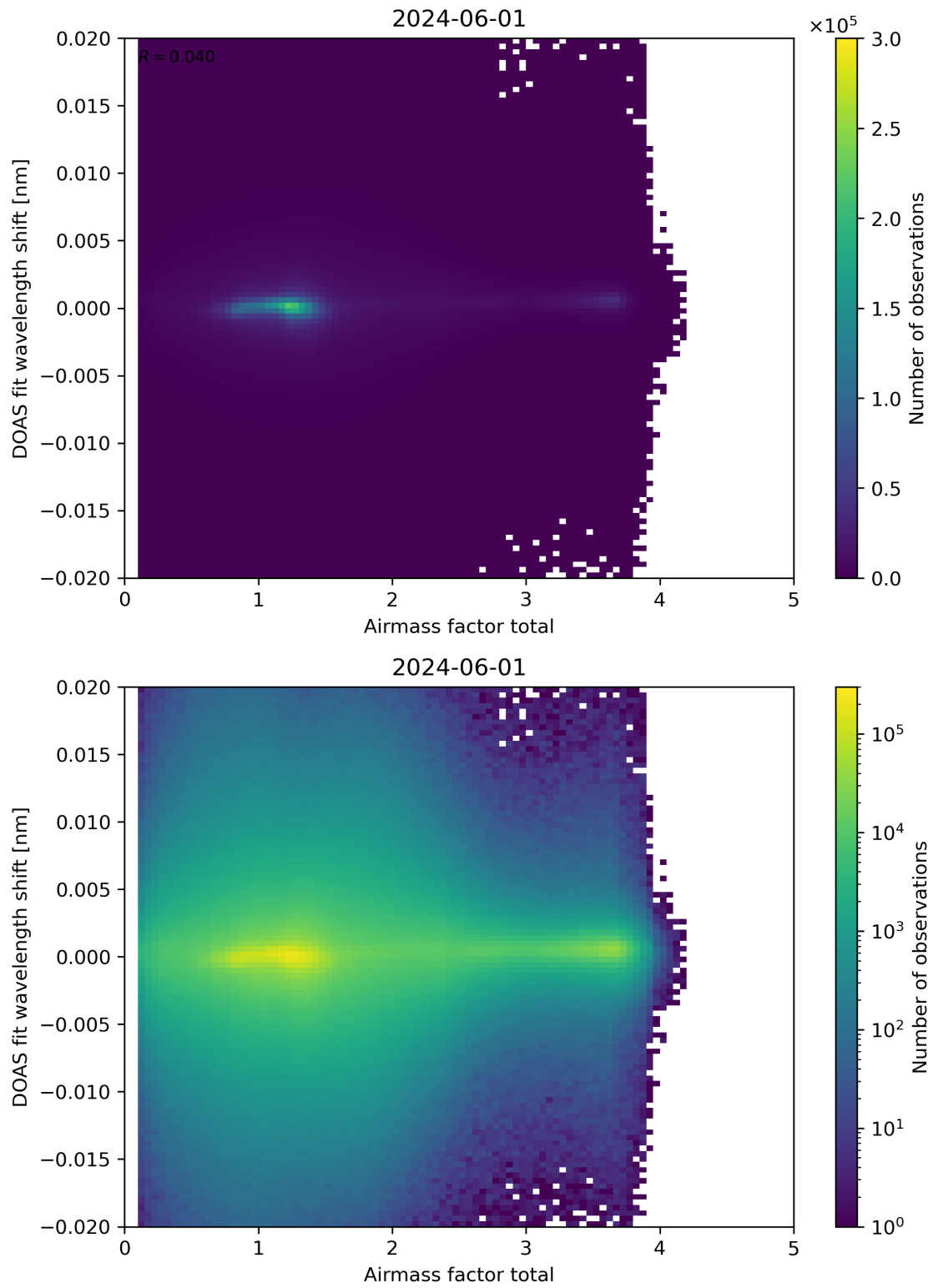
Figure 98: Scatter density plot of “Airmass factor total” against “DOAS fit wavelength shift” for 2024-05-31 to 2024-06-02.
