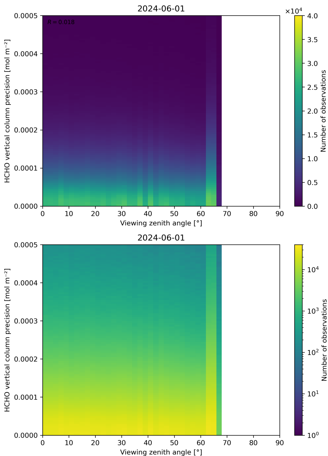
Figure 194: Scatter density plot of “Viewing zenith angle” against “HCHO vertical column precision” for 2024-05-31 to 2024-06-02.
