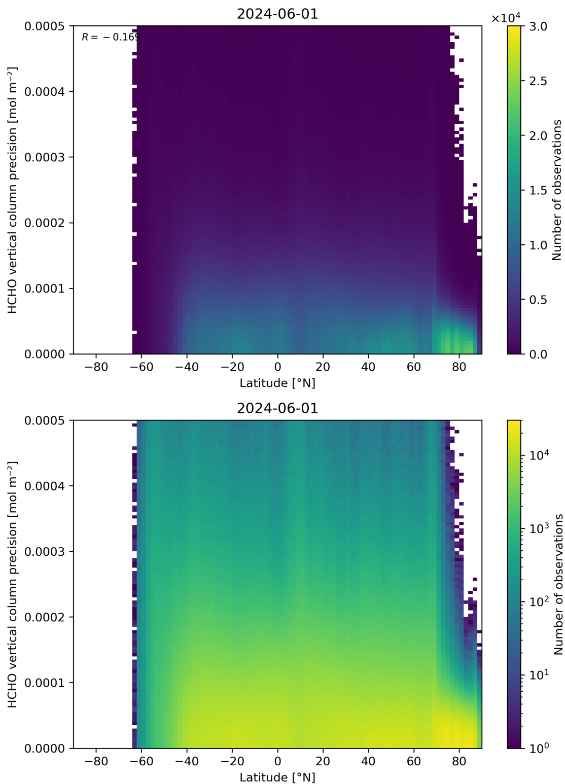
Figure 165: Scatter density plot of “Latitude” against “HCHO vertical column precision” for 2024-05-31 to 2024-06-02.
