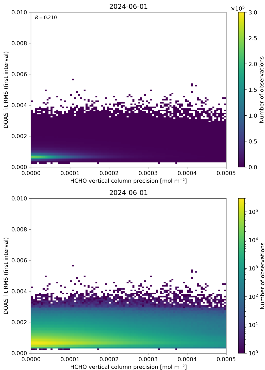
Figure 136: Scatter density plot of “HCHO vertical column precision” against “DOAS fit RMS (first interval)” for 2024-05-31 to 2024-06-02.
