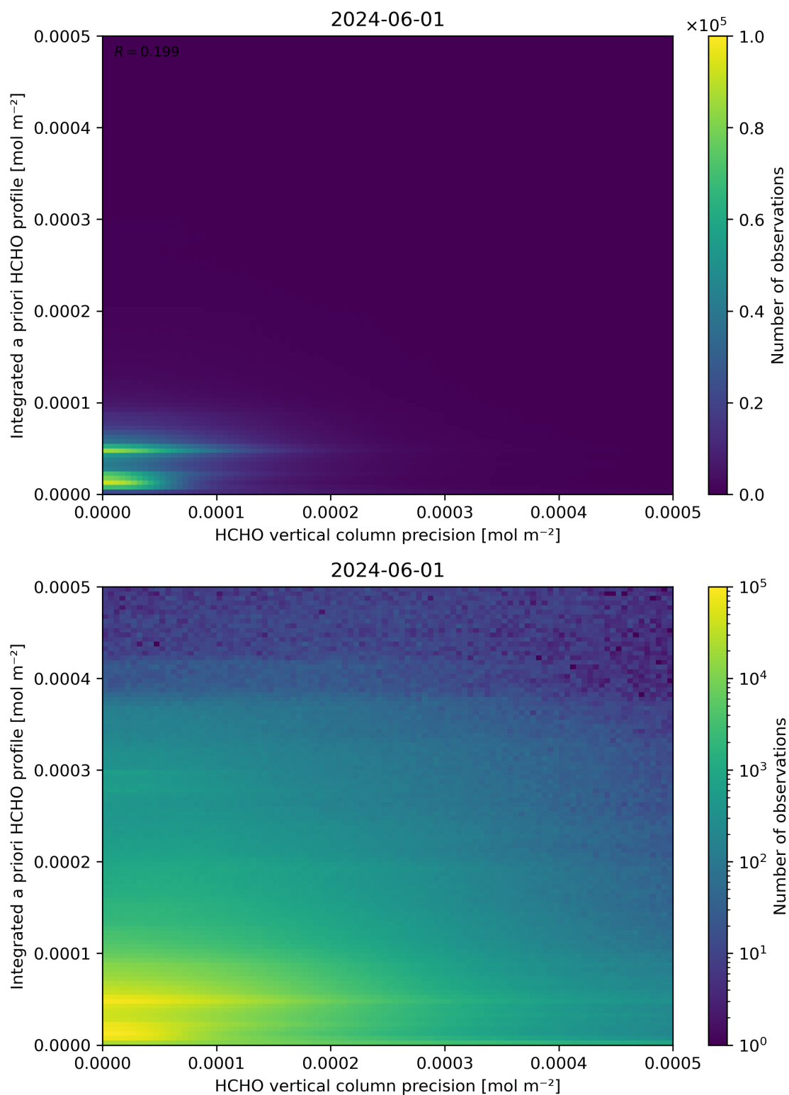
Figure 147: Scatter density plot of “HCHO vertical column precision” against “Integrated a priori HCHO profile” for 2024-05-31 to 2024-06-02.
