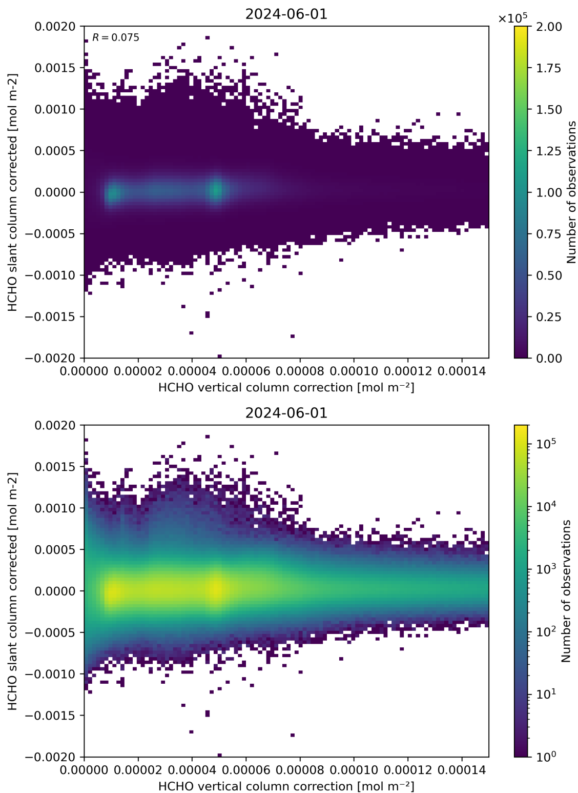
Figure 116: Scatter density plot of “HCHO vertical column correction” against “HCHO slant column corrected” for 2024-05-31 to 2024-06-02.
