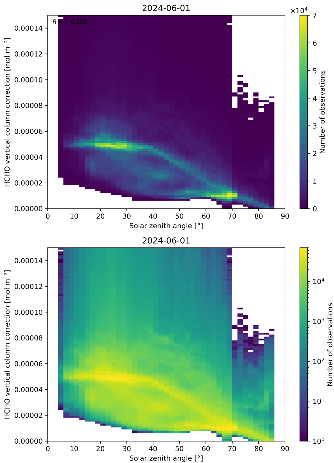
Figure 178: Scatter density plot of “Solar zenith angle” against “HCHO vertical column correction” for 2024-05-31 to 2024-06-02.
