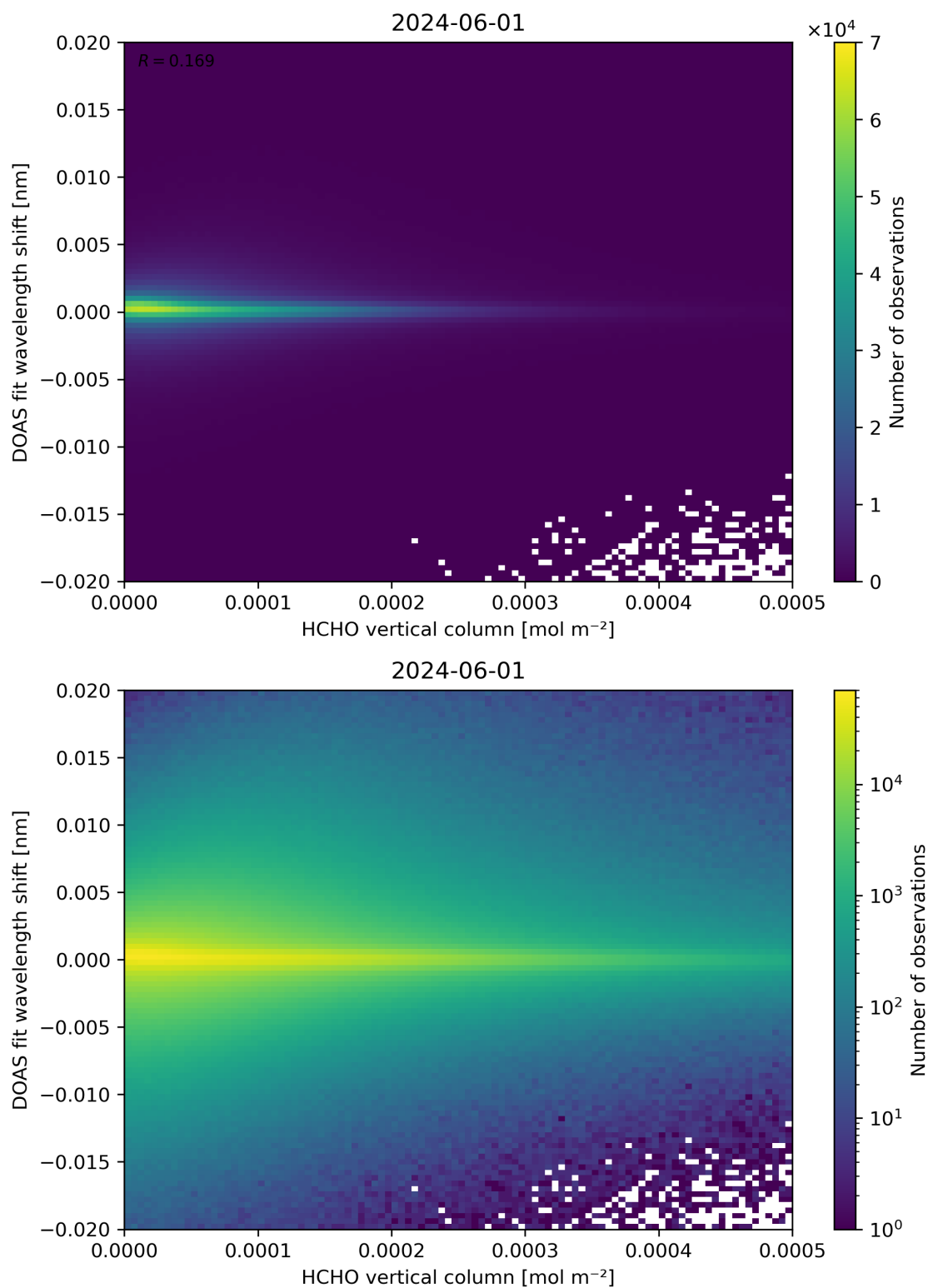
Figure 124: Scatter density plot of “HCHO vertical column” against “DOAS fit wavelength shift” for 2024-05-31 to 2024-06-02.
