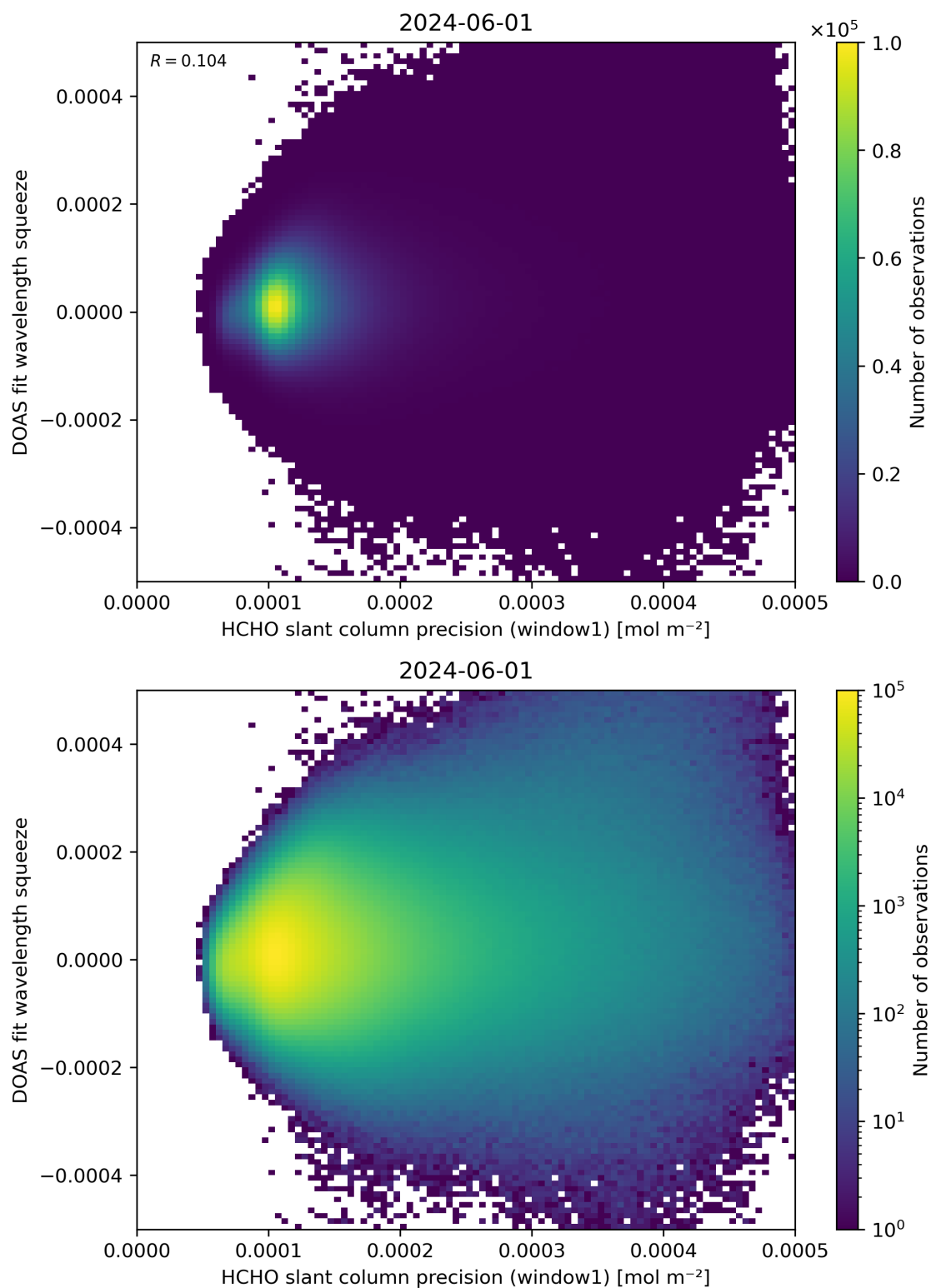
Figure 90: Scatter density plot of “HCHO slant column precision (window1)” against “DOAS fit wavelength squeeze” for 2024-05-31 to 2024-06-02.
