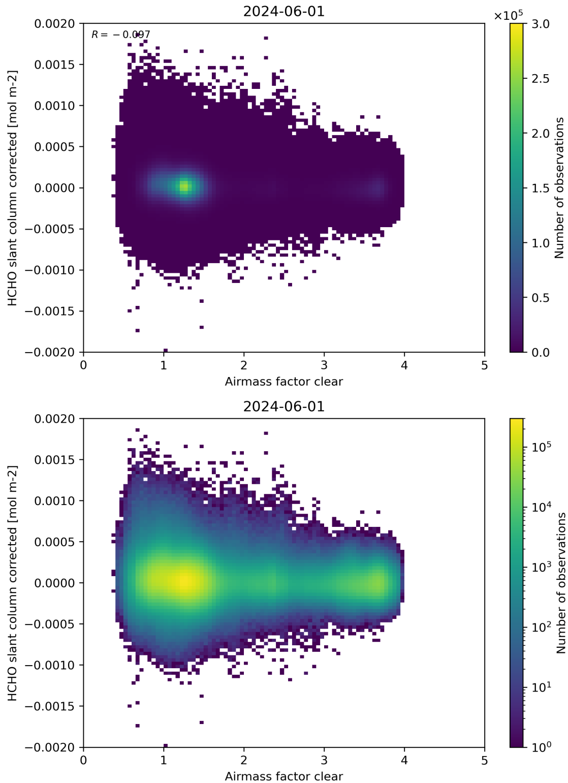
Figure 74: Scatter density plot of “Airmass factor clear” against “HCHO slant column corrected” for 2024-05-31 to 2024-06-02.
