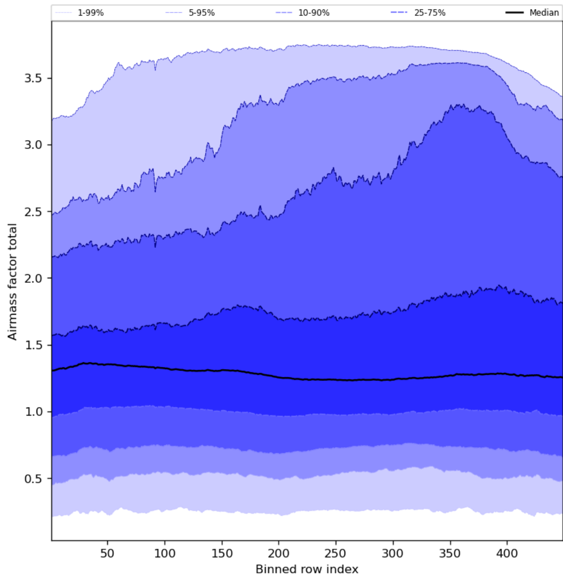
Figure 54: Along track statistics of “Airmass factor total” for 2024-05-31 to 2024-06-02
