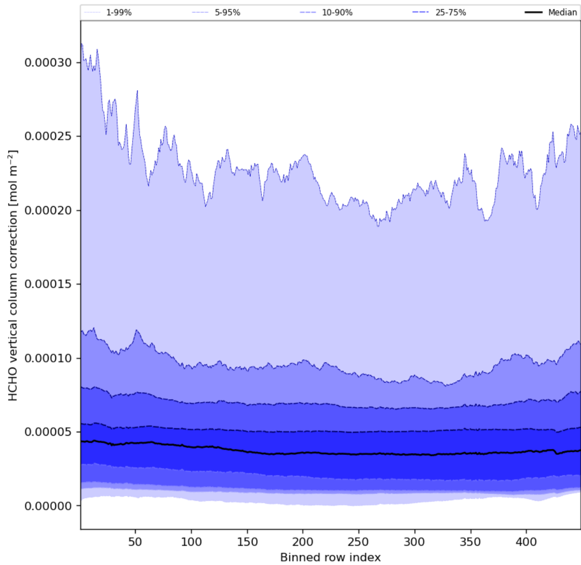
Figure 51: Along track statistics of “HCHO vertical column correction” for 2024-05-31 to 2024-06-02
