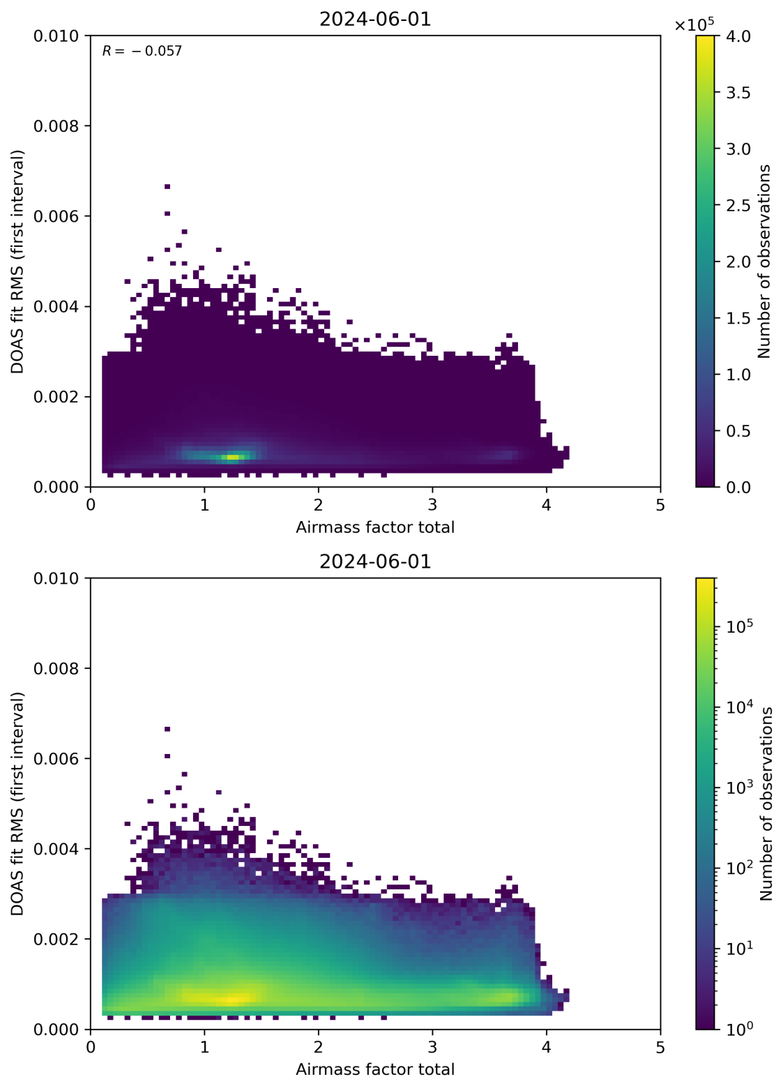
Figure 97: Scatter density plot of “Airmass factor total” against “DOAS fit RMS (first interval)” for 2024-05-31 to 2024-06-02.
