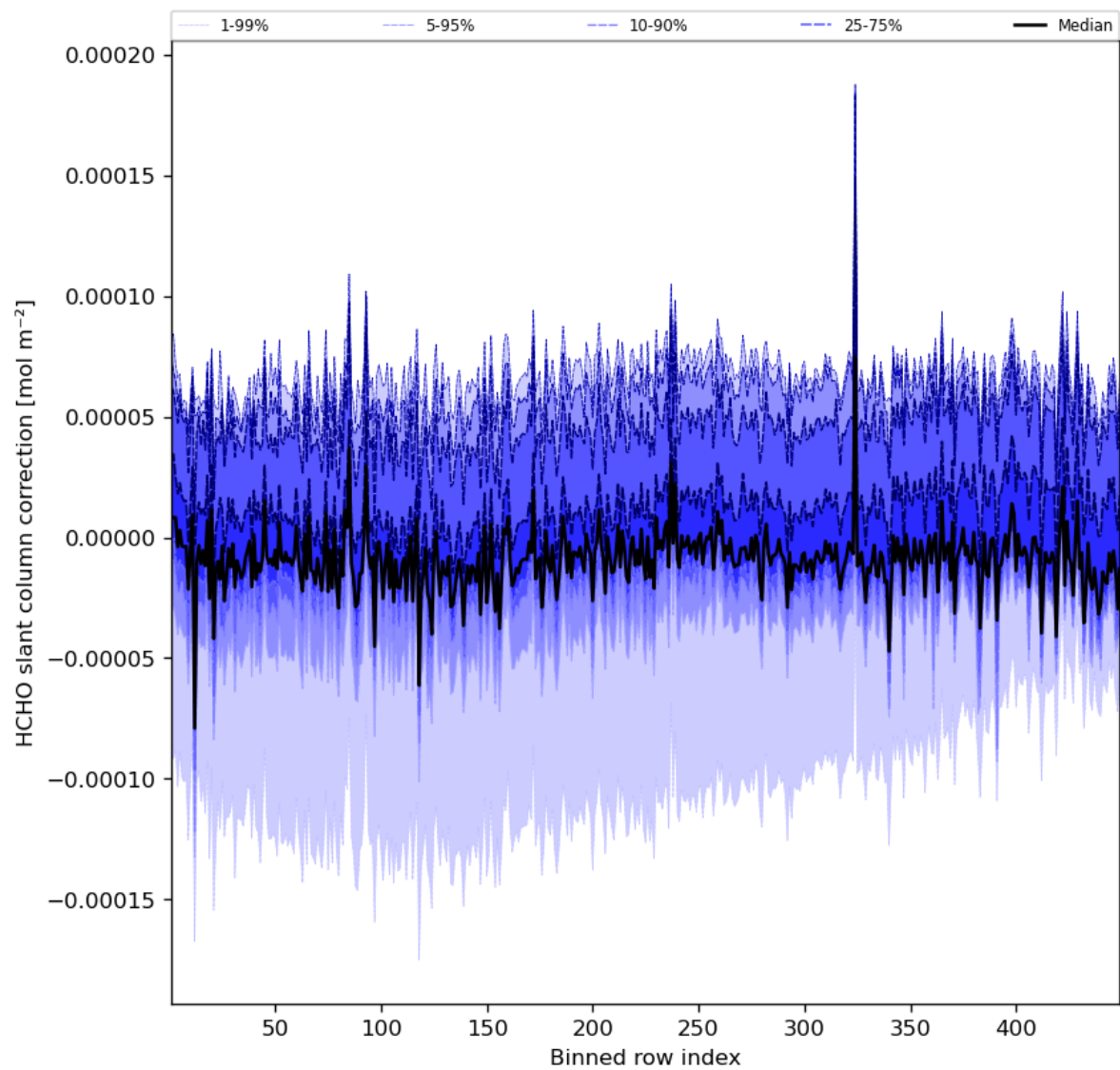
Figure 61: Along track statistics of “HCHO slant column correction” for 2024-05-31 to 2024-06-02
