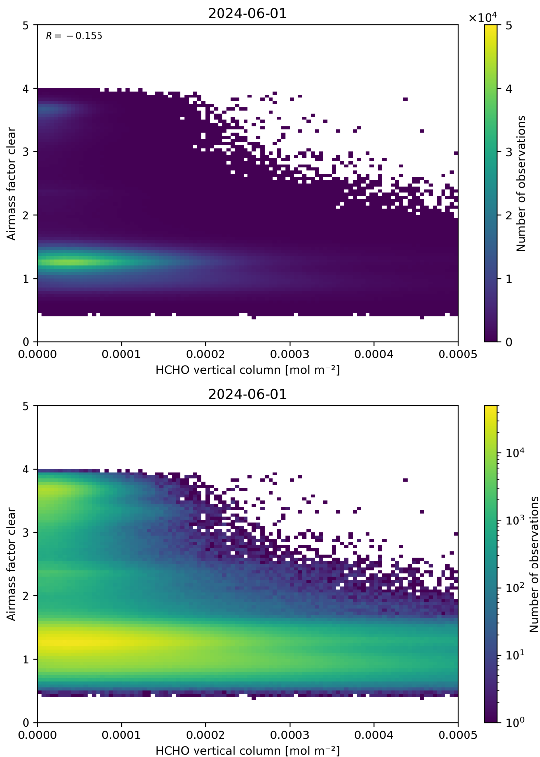
Figure 126: Scatter density plot of “HCHO vertical column” against “Airmass factor clear” for 2024-05-31 to 2024-06-02.
