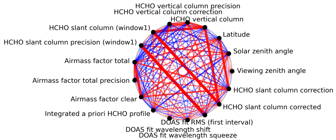
Figure 1: Map of correlation graph for 2024-05-31 to 2024-06-02.
