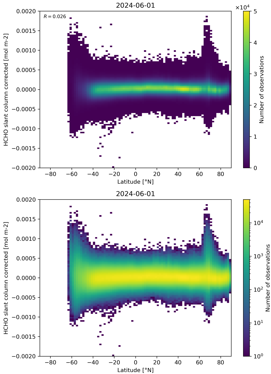
Figure 157: Scatter density plot of “Latitude” against “HCHO slant column corrected” for 2024-05-31 to 2024-06-02.
