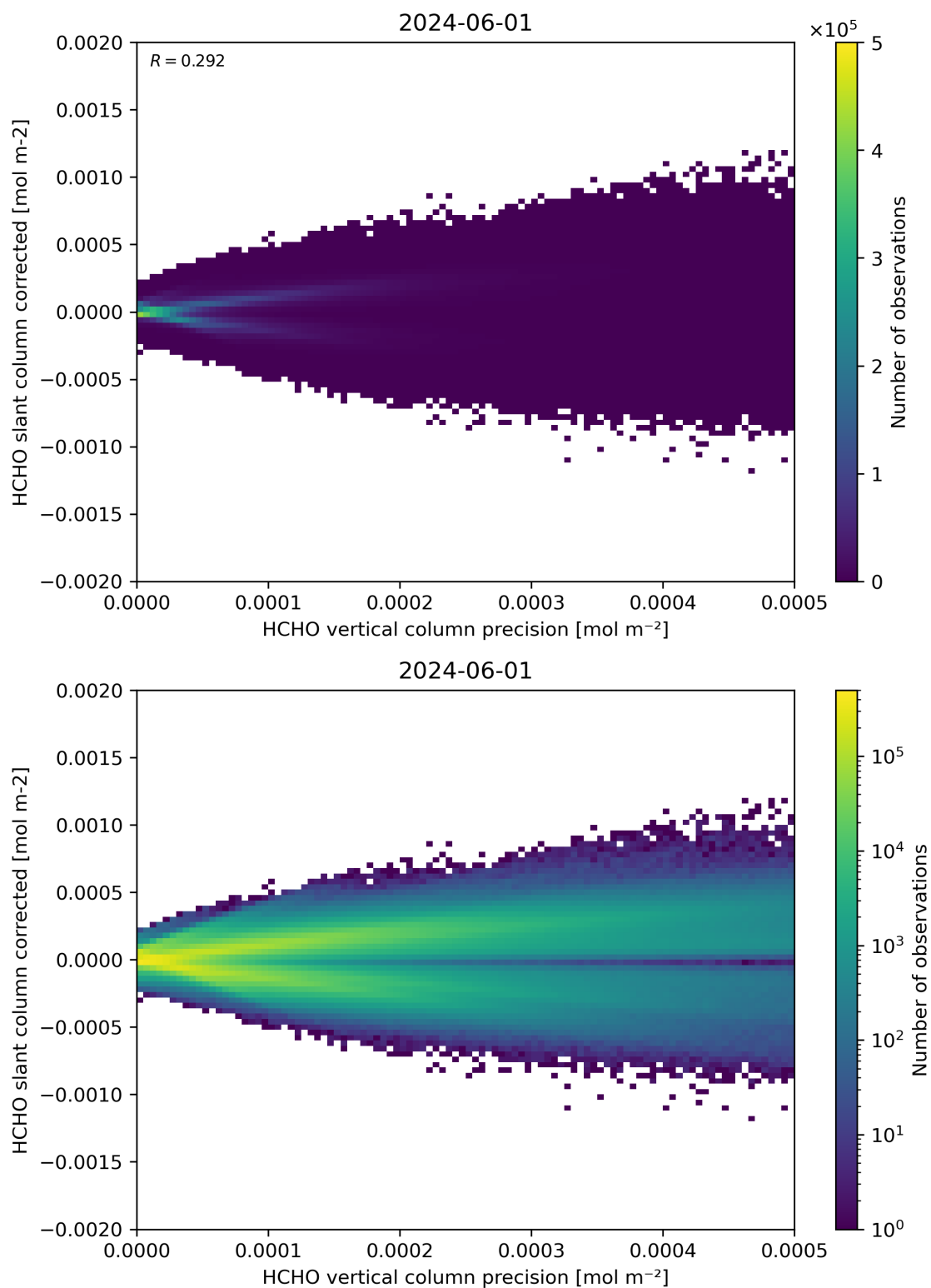
Figure 140: Scatter density plot of “HCHO vertical column precision” against “HCHO slant column corrected” for 2024-05-31 to 2024-06-02.
