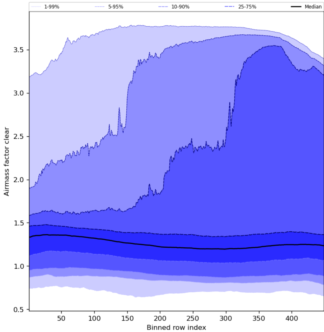
Figure 56: Along track statistics of “Airmass factor clear” for 2024-05-31 to 2024-06-02
