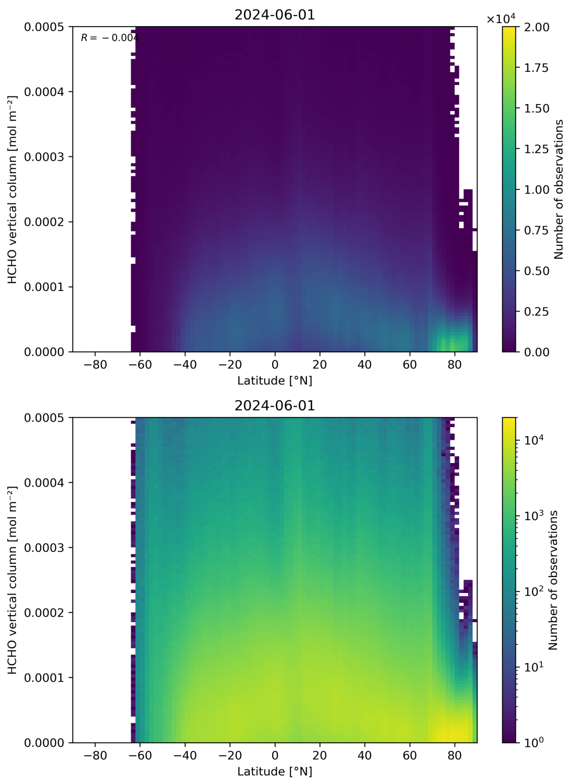
Figure 163: Scatter density plot of “Latitude” against “HCHO vertical column” for 2024-05-31 to 2024-06-02.
