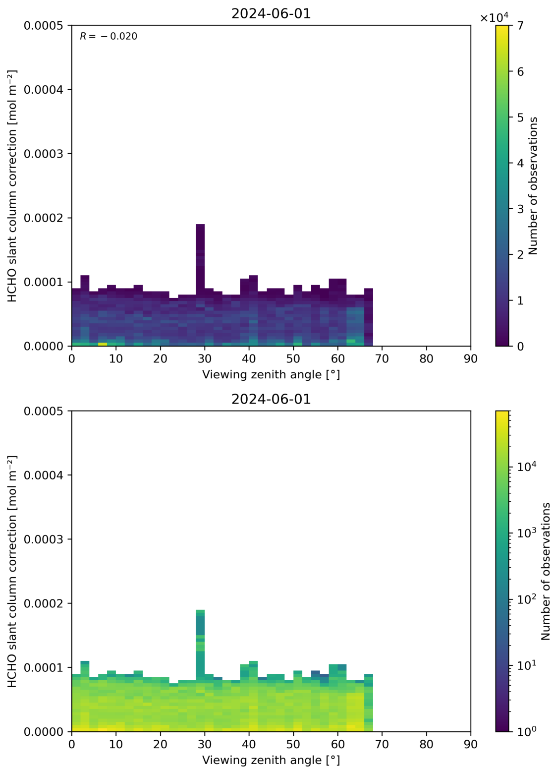
Figure 187: Scatter density plot of “Viewing zenith angle” against “HCHO slant column correction” for 2024-05-31 to 2024-06-02.
