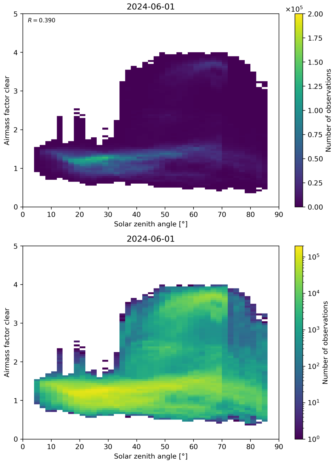
Figure 170: Scatter density plot of “Solar zenith angle” against “Airmass factor clear” for 2024-05-31 to 2024-06-02.
