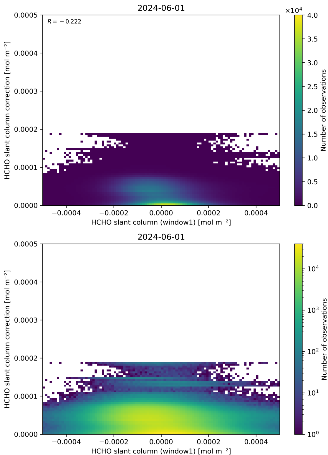
Figure 83: Scatter density plot of “HCHO slant column (window1)” against “HCHO slant column correction” for 2024-05-31 to 2024-06-02.
