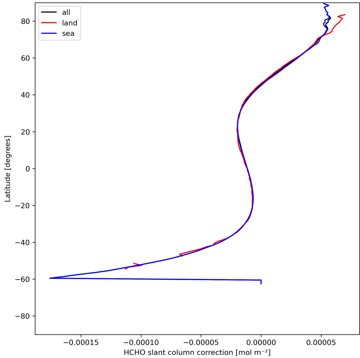
Figure 33: Zonal average of “HCHO slant column correction” for 2024-05-31 to 2024-06-02.
