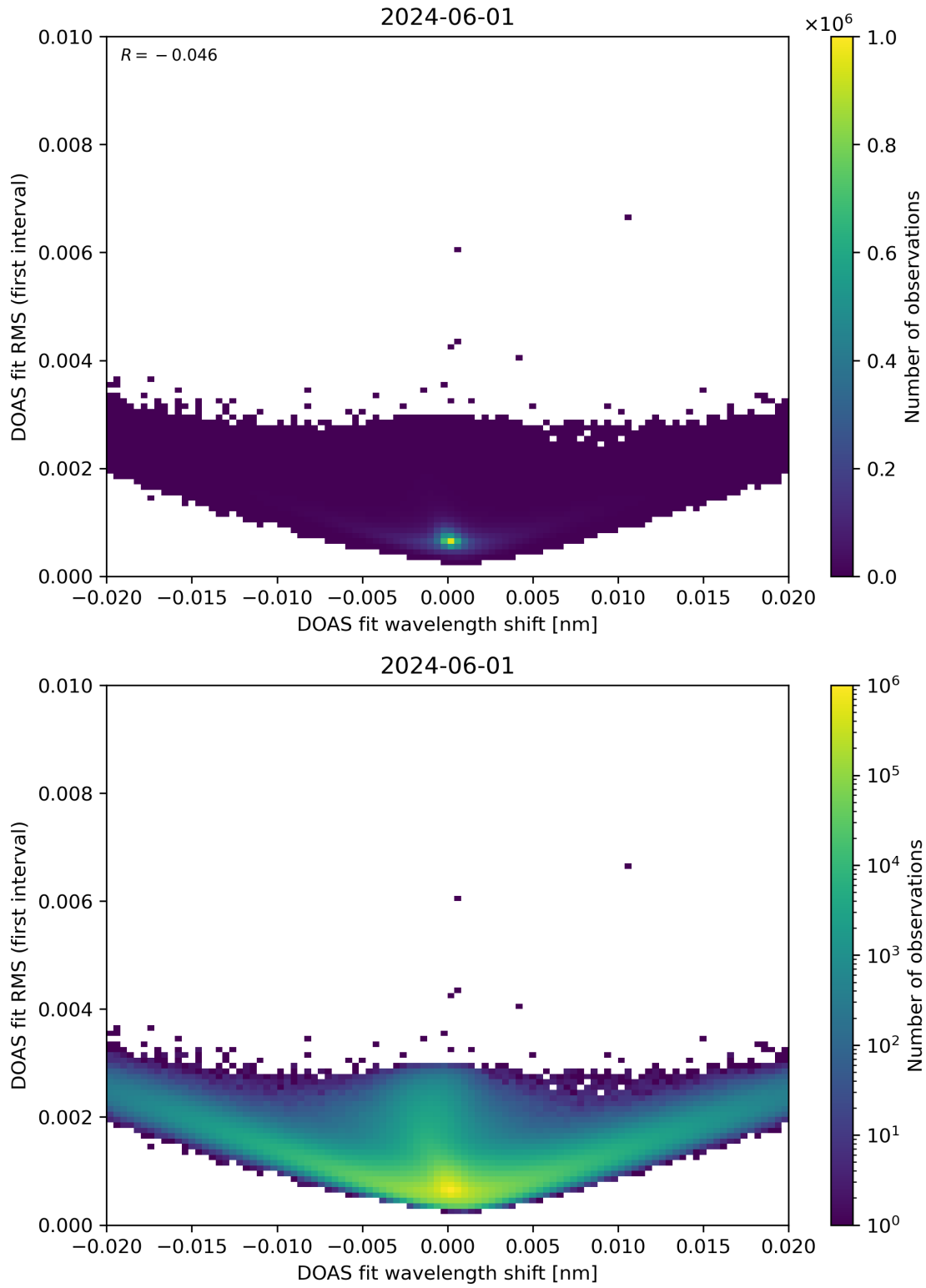
Figure 64: Scatter density plot of “DOAS fit wavelength shift” against “DOAS fit RMS (first interval)” for 2024-05-31 to 2024-06-02.
