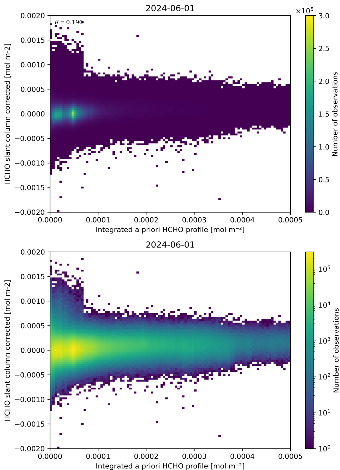
Figure 151: Scatter density plot of “Integrated a priori HCHO profile” against “HCHO slant column corrected” for 2024-05-31 to 2024-06-02.
