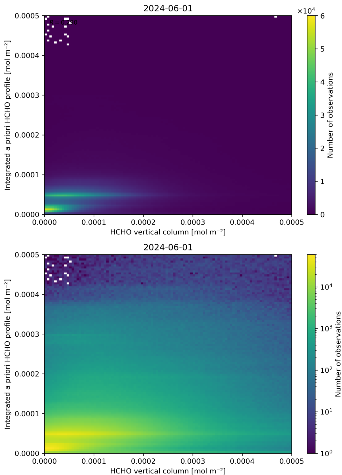
Figure 135: Scatter density plot of “HCHO vertical column” against “Integrated a priori HCHO profile” for 2024-05-31 to 2024-06-02.
