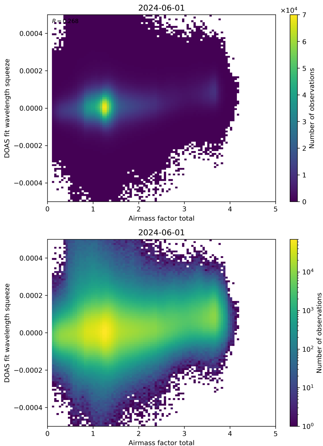
Figure 99: Scatter density plot of “Airmass factor total” against “DOAS fit wavelength squeeze” for 2024-05-31 to 2024-06-02.
