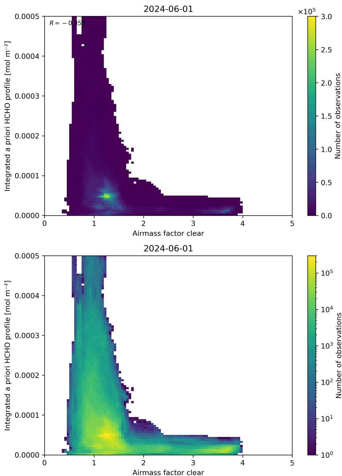
Figure 76: Scatter density plot of “Airmass factor clear” against “Integrated a priori HCHO profile” for 2024-05-31 to 2024-06-02.
