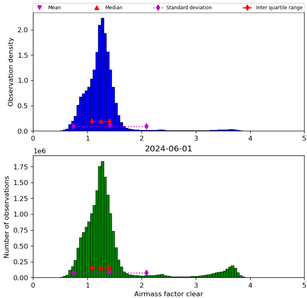
Figure 42: Histogram of “Airmass factor clear” for 2024-05-31 to 2024-06-02
