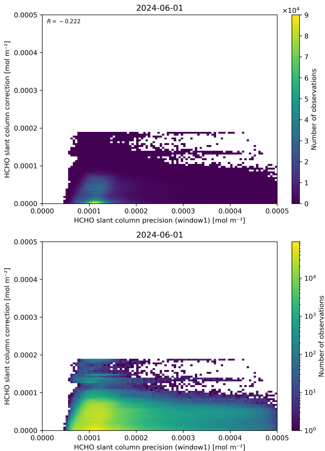
Figure 93: Scatter density plot of “HCHO slant column precision (window1)” against “HCHO slant column correction” for 2024-05-31 to 2024-06-02.
