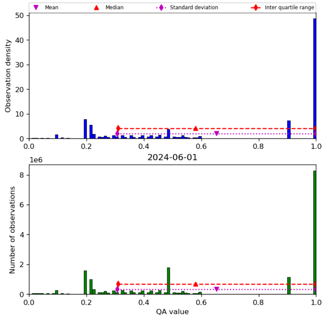
Figure 34: Histogram of “QA value” for 2024-05-31 to 2024-06-02
