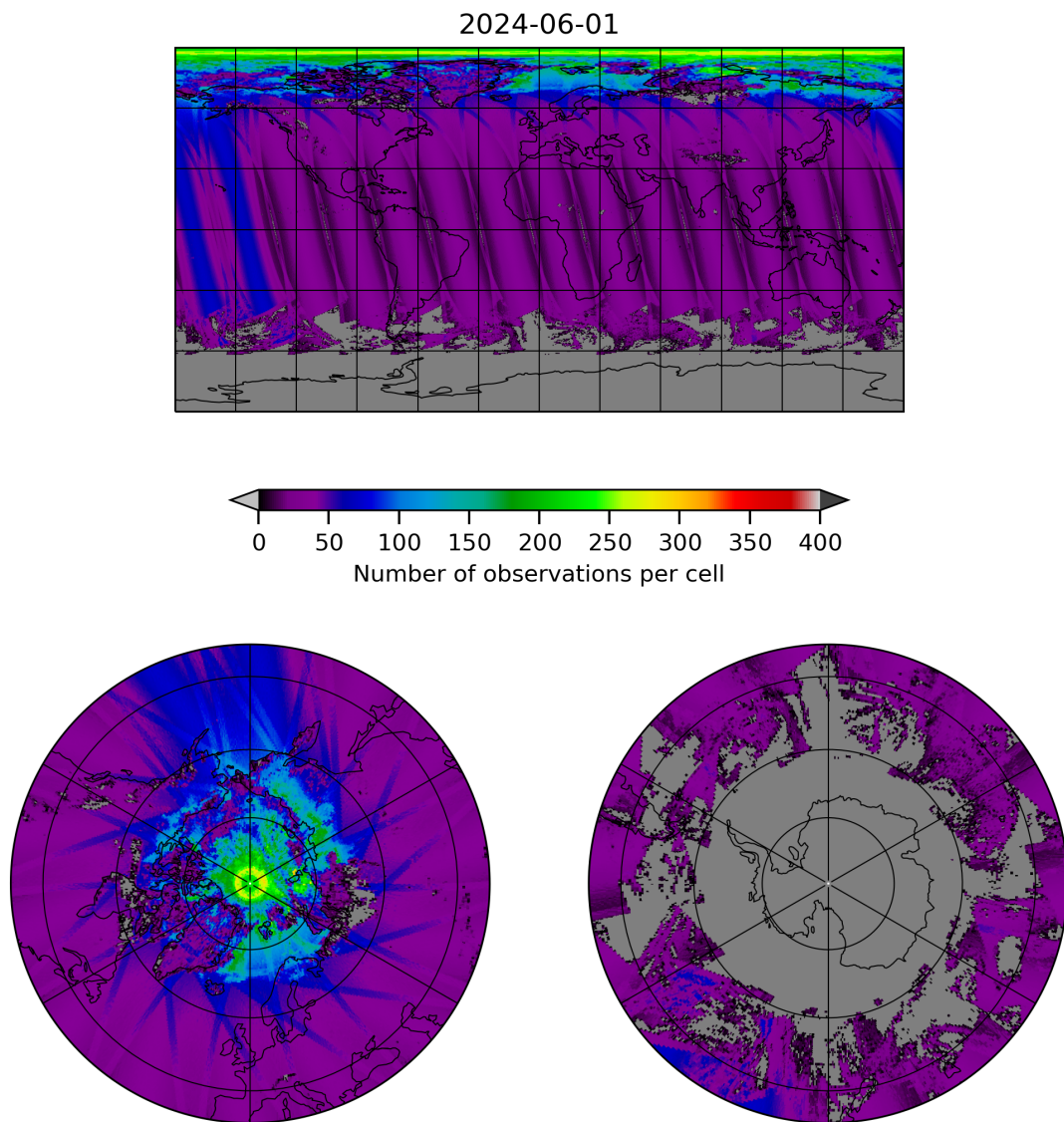
Figure 19: Map of the number of observations for 2024-05-31 to 2024-06-02
