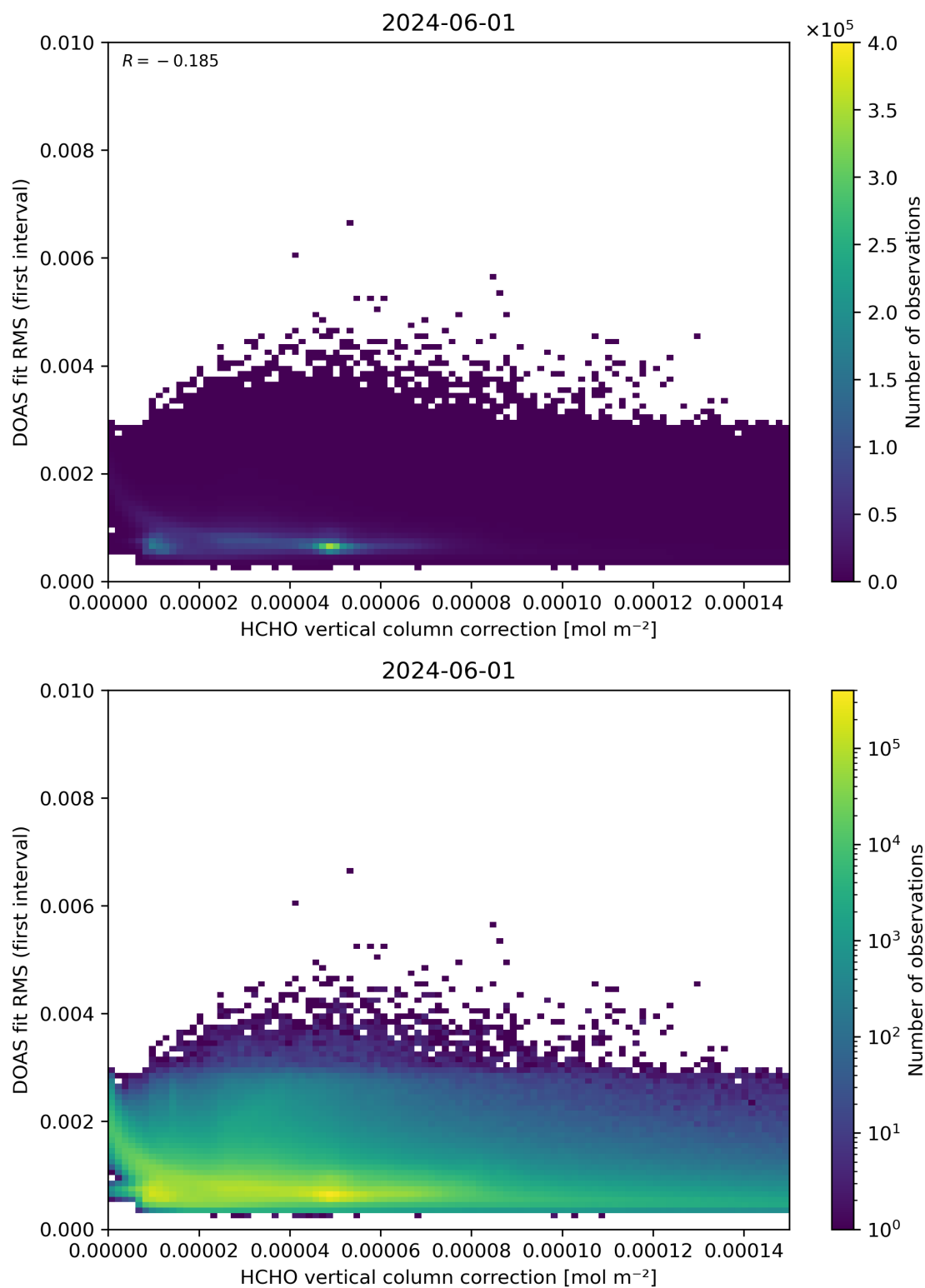
Figure 112: Scatter density plot of “HCHO vertical column correction” against “DOAS fit RMS (first interval)” for 2024-05-31 to 2024-06-02.
