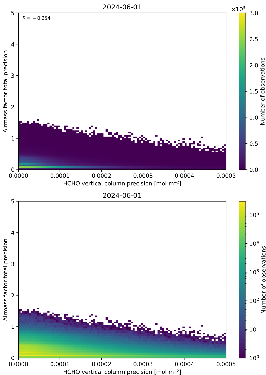
Figure 145: Scatter density plot of “HCHO vertical column precision” against “Airmass factor total precision” for 2024-05-31 to 2024-06-02.
