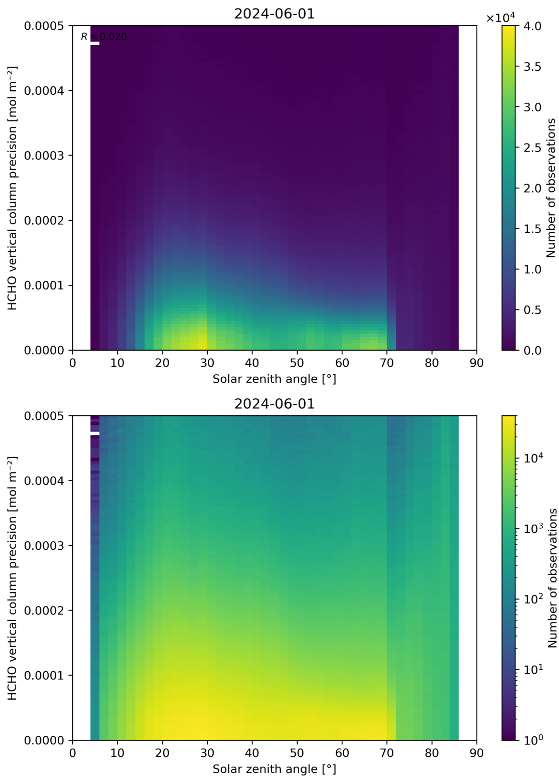
Figure 179: Scatter density plot of “Solar zenith angle” against “HCHO vertical column precision” for 2024-05-31 to 2024-06-02.
