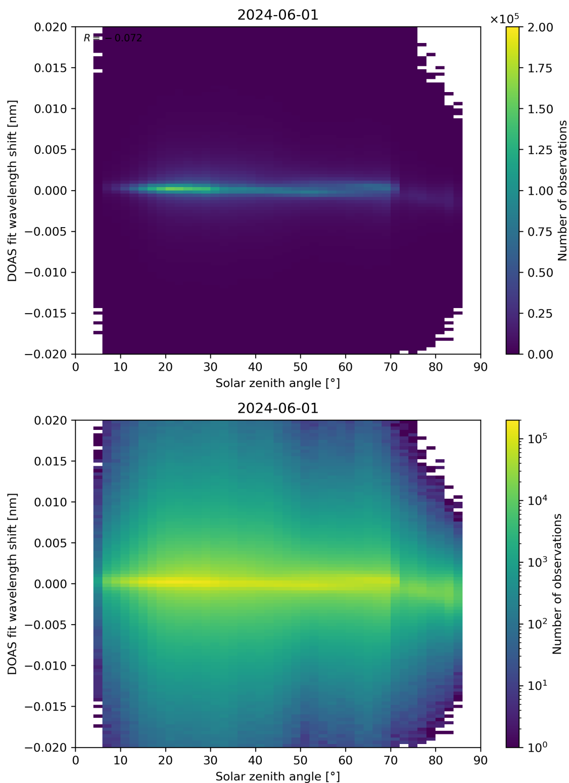
Figure 168: Scatter density plot of “Solar zenith angle” against “DOAS fit wavelength shift” for 2024-05-31 to 2024-06-02.
