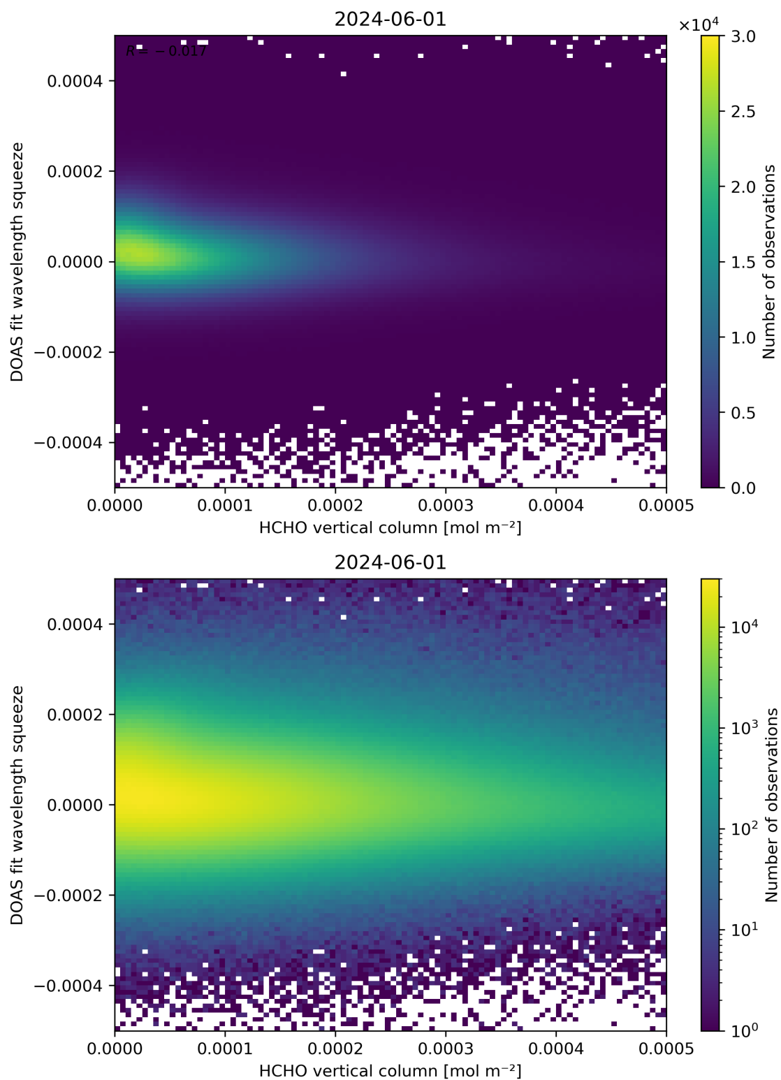
Figure 125: Scatter density plot of “HCHO vertical column” against “DOAS fit wavelength squeeze” for 2024-05-31 to 2024-06-02.
