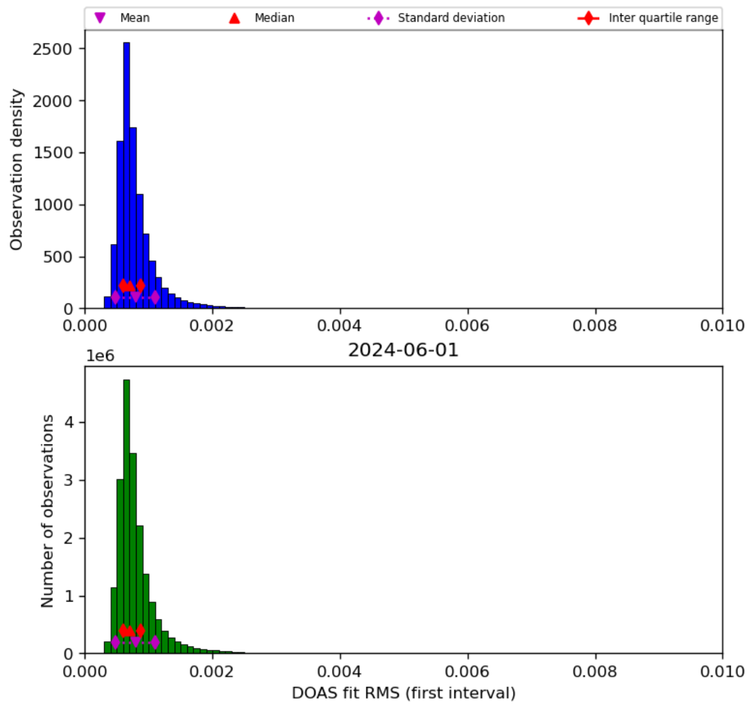
Figure 46: Histogram of “DOAS fit RMS (first interval)” for 2024-05-31 to 2024-06-02
