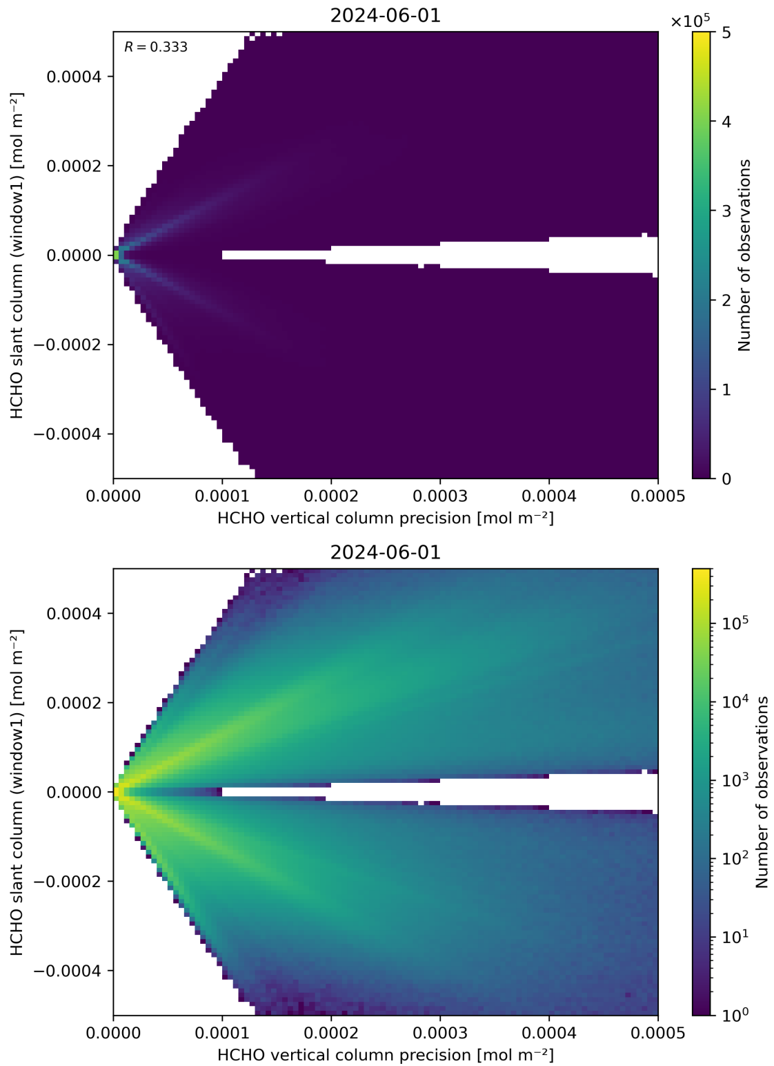
Figure 142: Scatter density plot of “HCHO vertical column precision” against “HCHO slant column (window1)” for 2024-05-31 to 2024-06-02.
