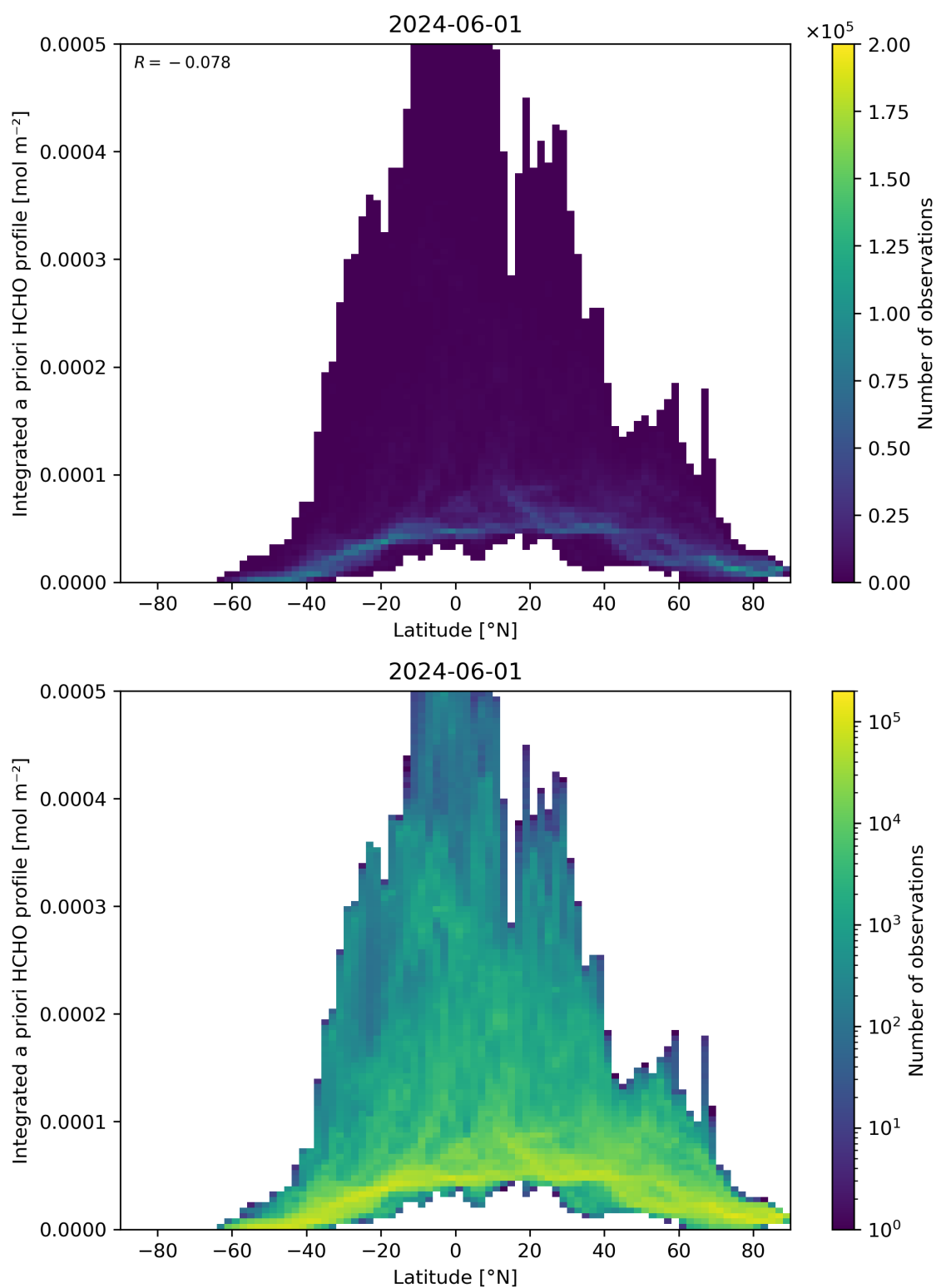
Figure 166: Scatter density plot of “Latitude” against “Integrated a priori HCHO profile” for 2024-05-31 to 2024-06-02.
