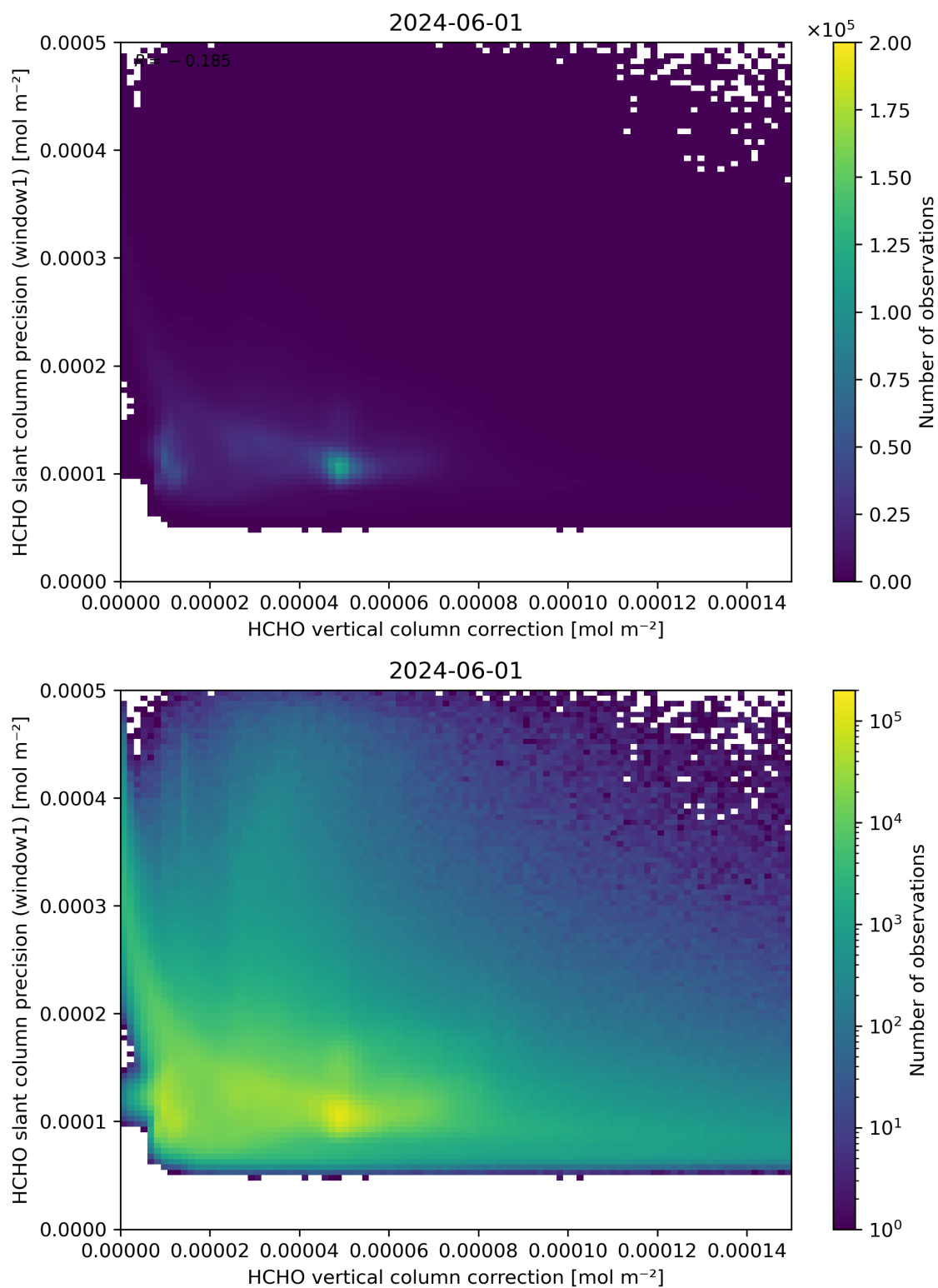
Figure 119: Scatter density plot of “HCHO vertical column correction” against “HCHO slant column precision (window1)” for 2024-05-31 to 2024-06-02.
