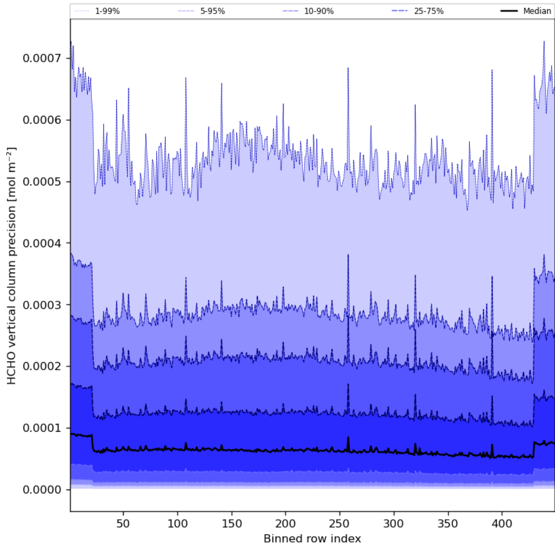
Figure 50: Along track statistics of “HCHO vertical column precision” for 2024-05-31 to 2024-06-02
