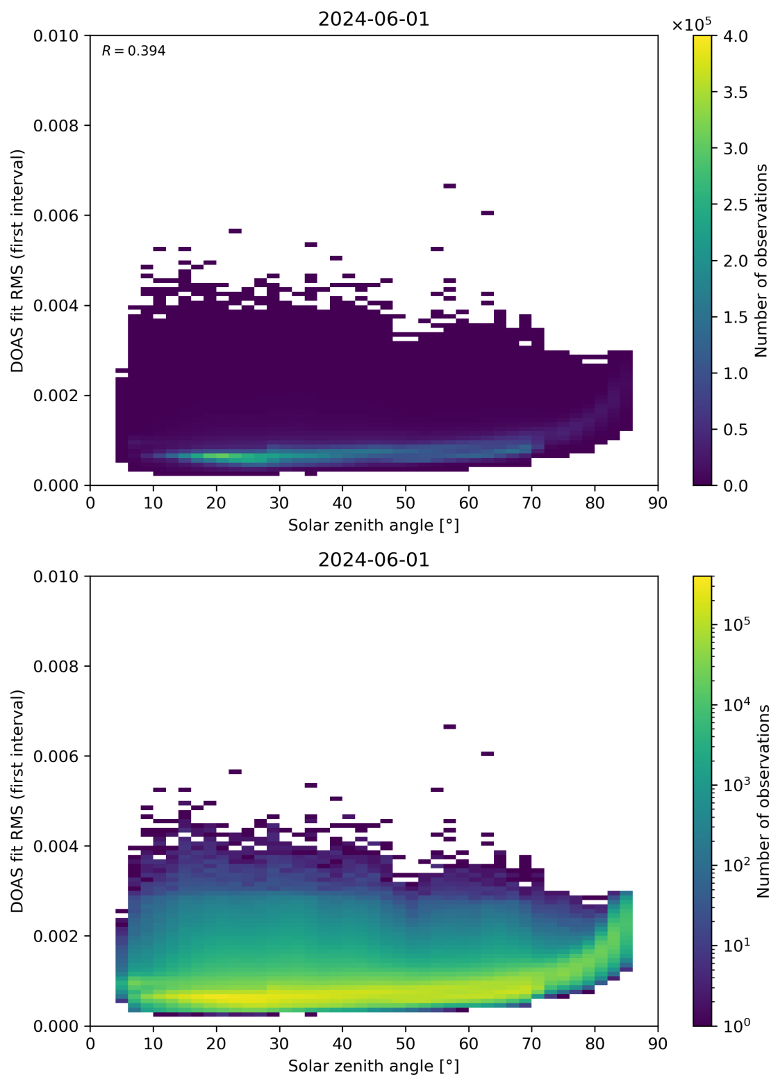
Figure 167: Scatter density plot of “Solar zenith angle” against “DOAS fit RMS (first interval)” for 2024-05-31 to 2024-06-02.
