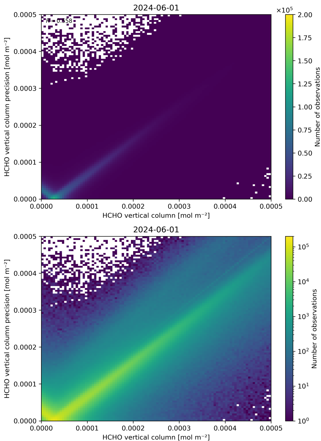
Figure 134: Scatter density plot of “HCHO vertical column” against “HCHO vertical column precision” for 2024-05-31 to 2024-06-02.
