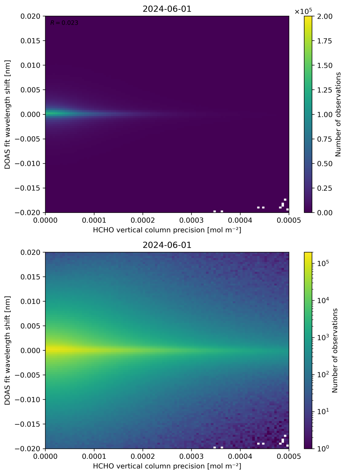
Figure 137: Scatter density plot of “HCHO vertical column precision” against “DOAS fit wavelength shift” for 2024-05-31 to 2024-06-02.
