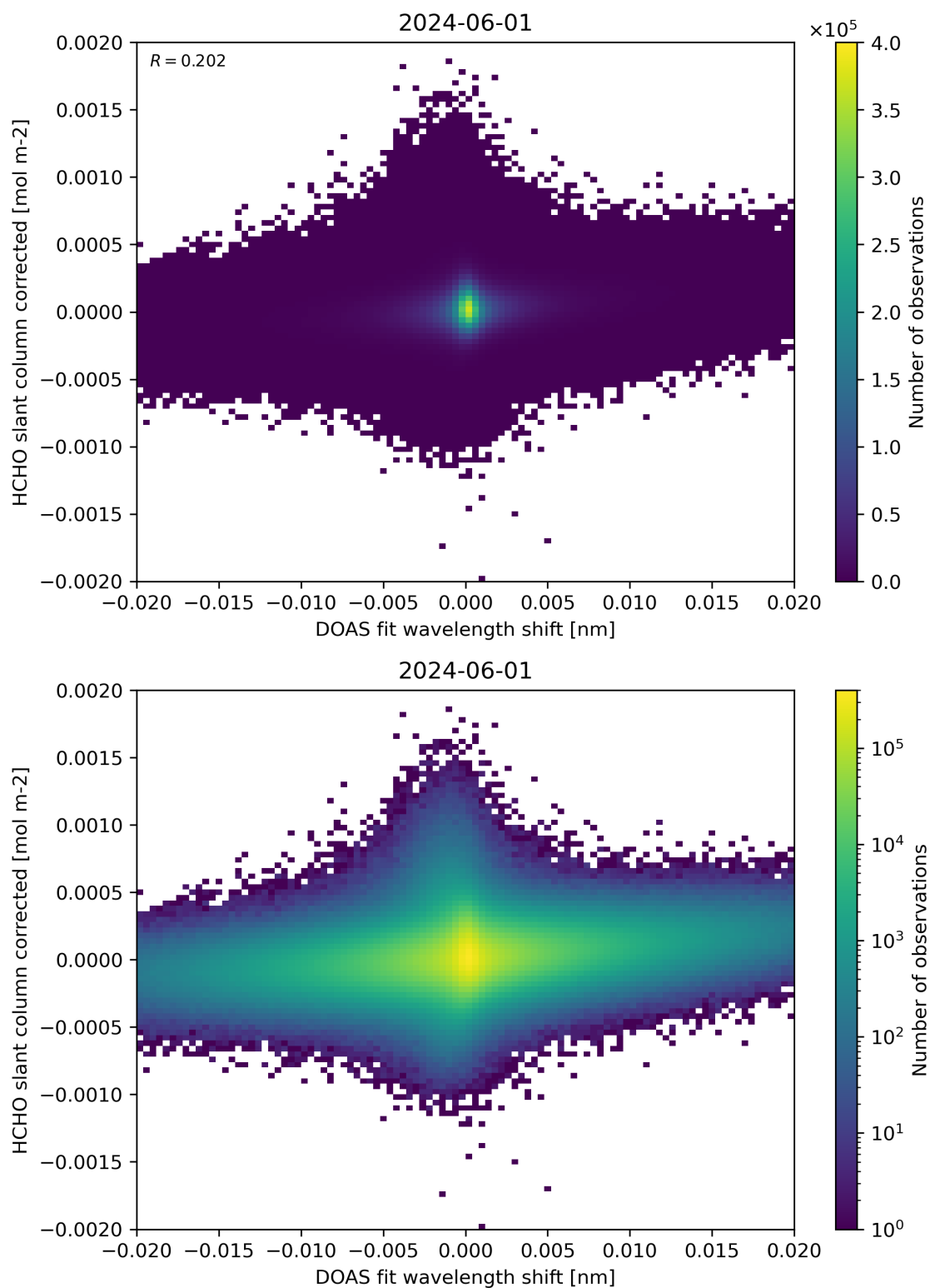
Figure 66: Scatter density plot of “DOAS fit wavelength shift” against “HCHO slant column corrected” for 2024-05-31 to 2024-06-02.
