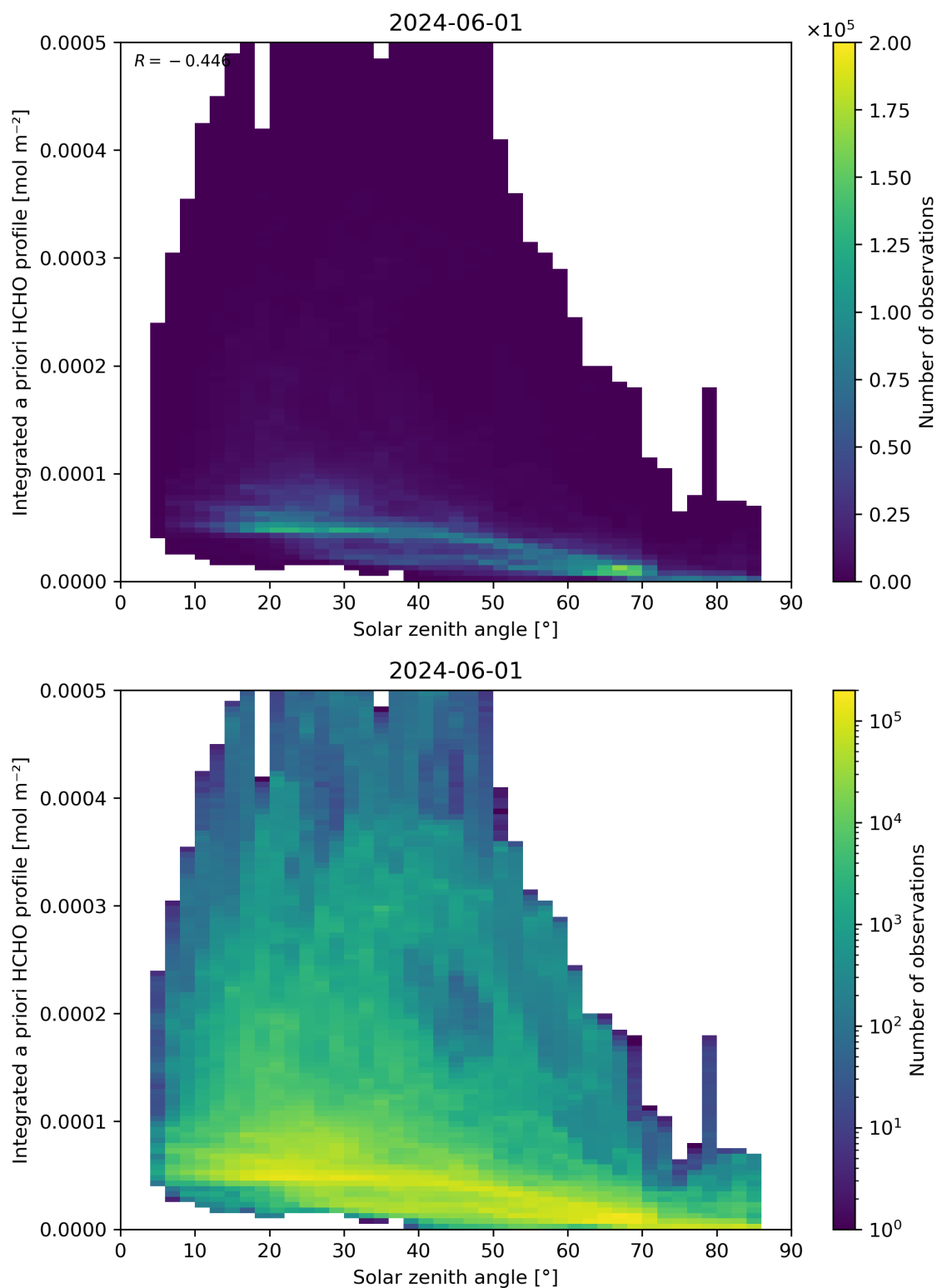
Figure 180: Scatter density plot of “Solar zenith angle” against “Integrated a priori HCHO profile” for 2024-05-31 to 2024-06-02.
