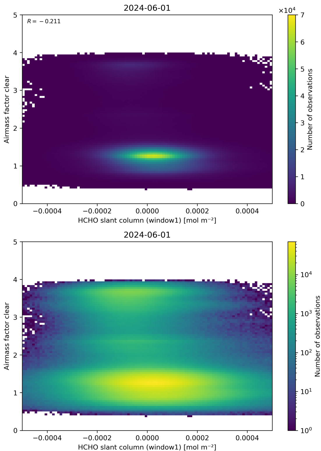
Figure 81: Scatter density plot of “HCHO slant column (window1)” against “Airmass factor clear” for 2024-05-31 to 2024-06-02.
