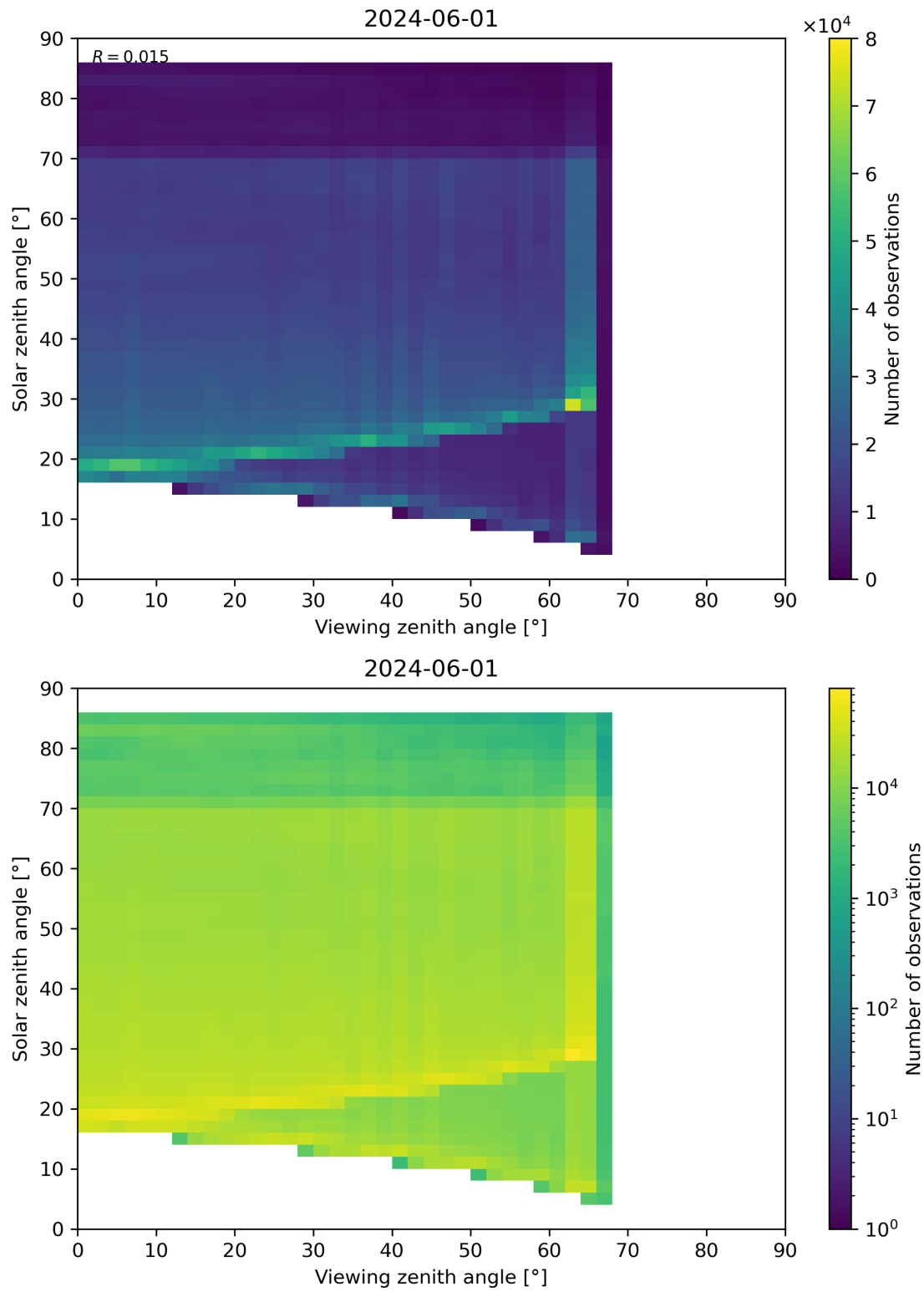
Figure 197: Scatter density plot of “Viewing zenith angle” against “Solar zenith angle” for 2024-05-31 to 2024-06-02.
