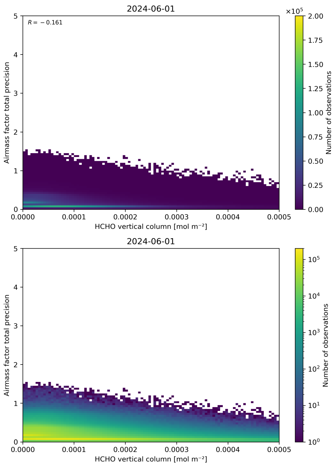
Figure 132: Scatter density plot of “HCHO vertical column” against “Airmass factor total precision” for 2024-05-31 to 2024-06-02.
