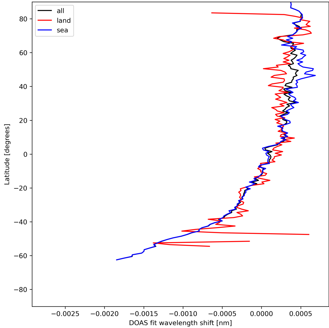
Figure 30: Zonal average of “DOAS fit wavelength shift” for 2024-05-31 to 2024-06-02.
