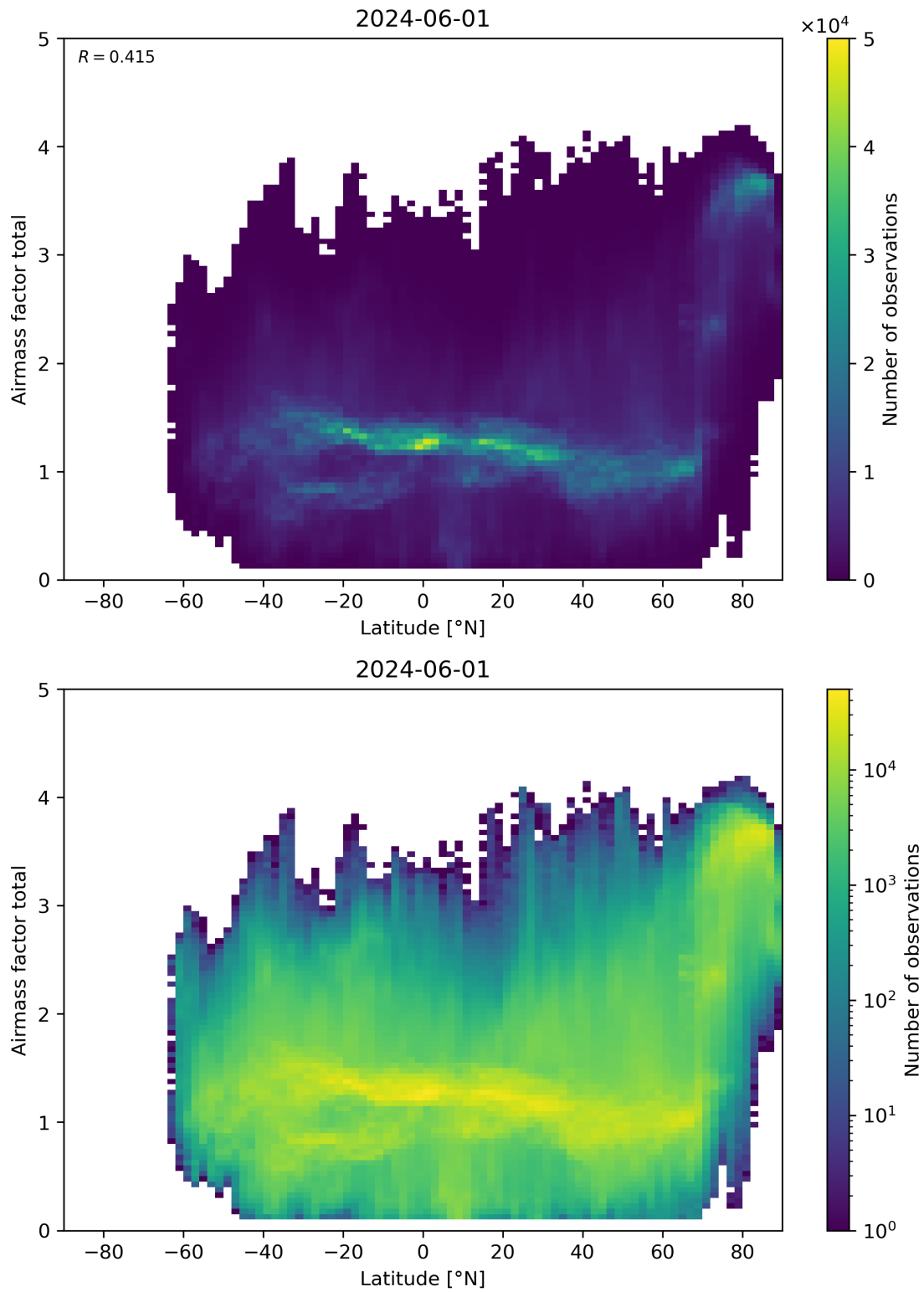
Figure 161: Scatter density plot of “Latitude” against “Airmass factor total” for 2024-05-31 to 2024-06-02.
