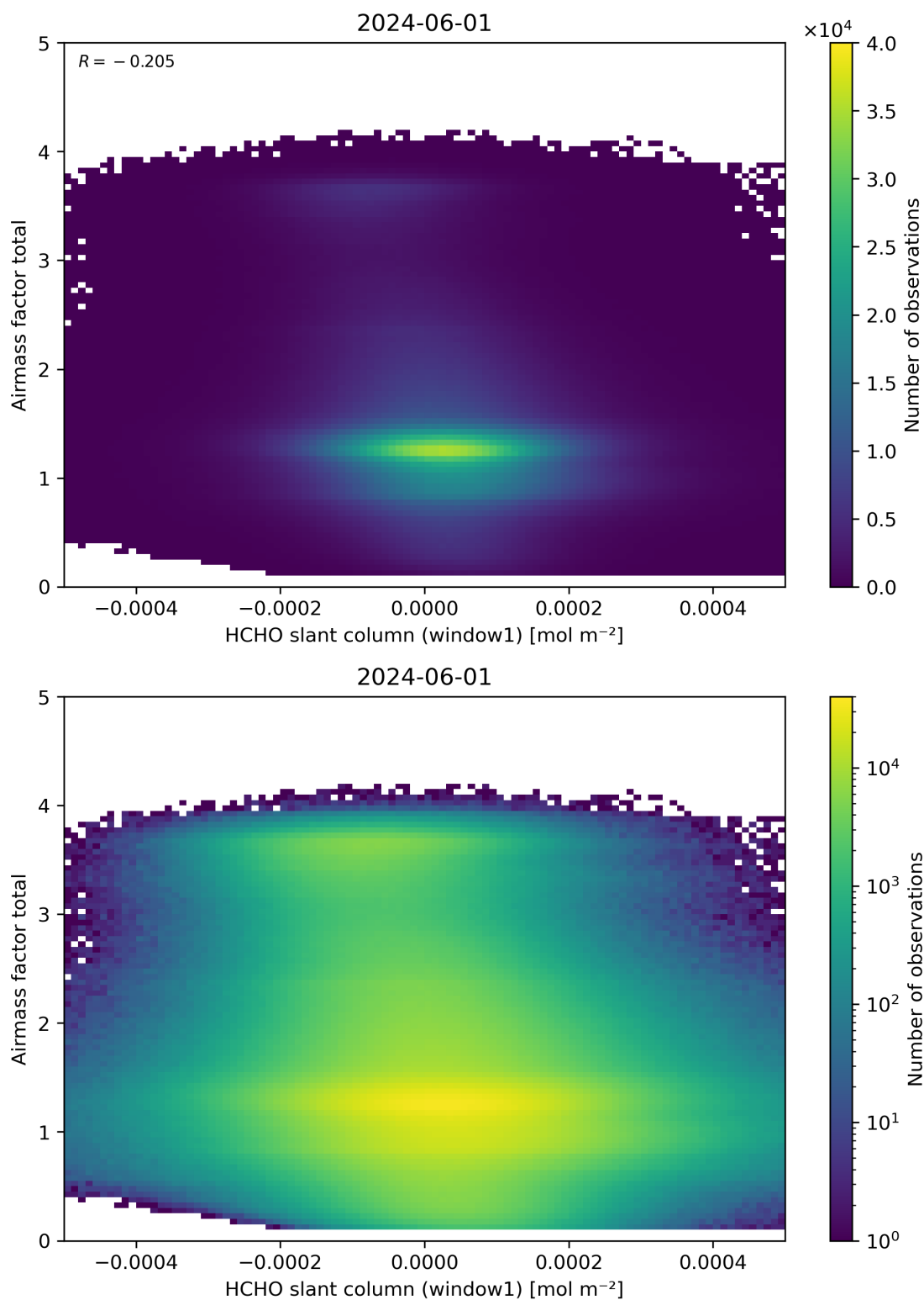
Figure 85: Scatter density plot of “HCHO slant column (window1)” against “Airmass factor total” for 2024-05-31 to 2024-06-02.
