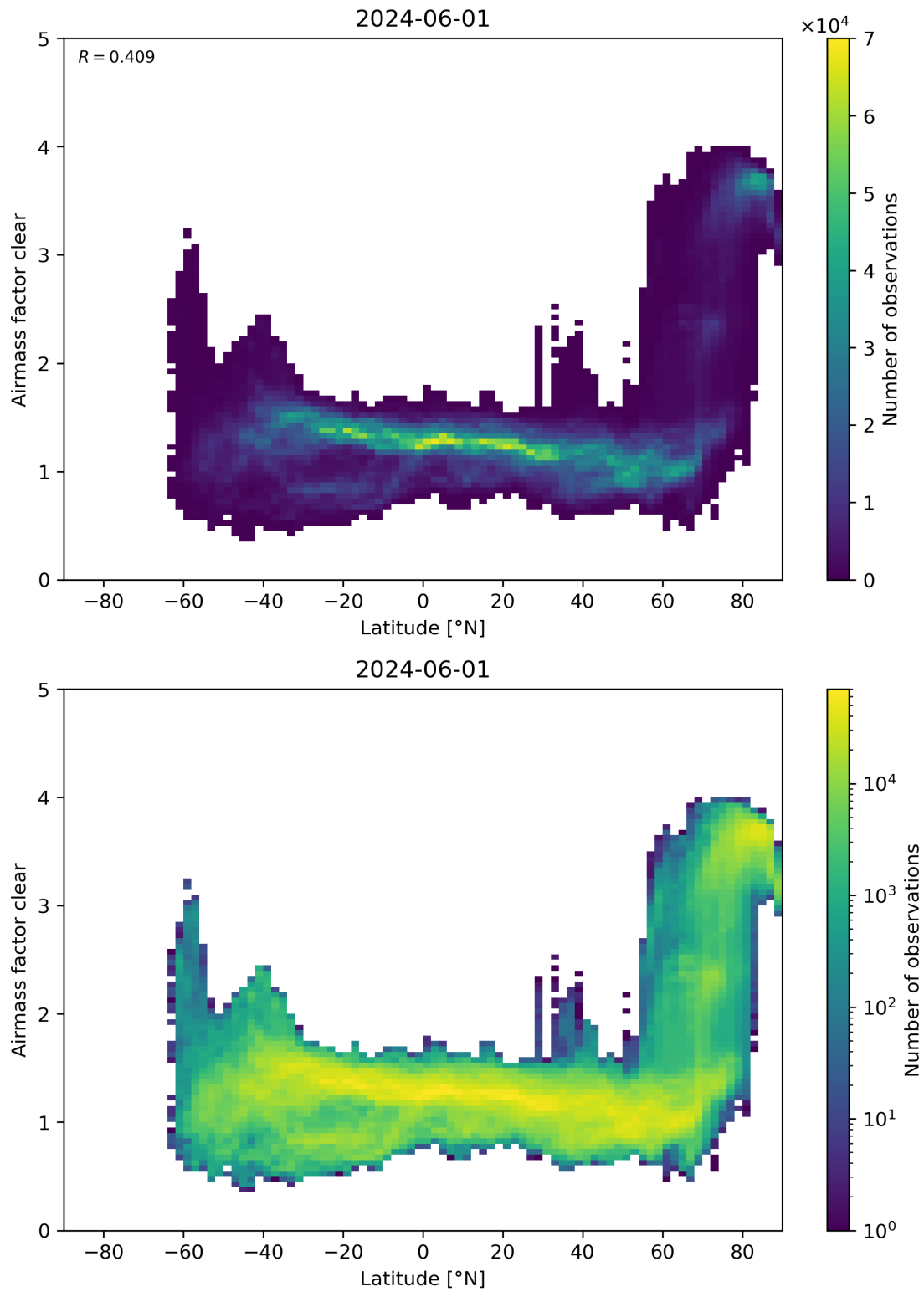
Figure 156: Scatter density plot of “Latitude” against “Airmass factor clear” for 2024-05-31 to 2024-06-02.
