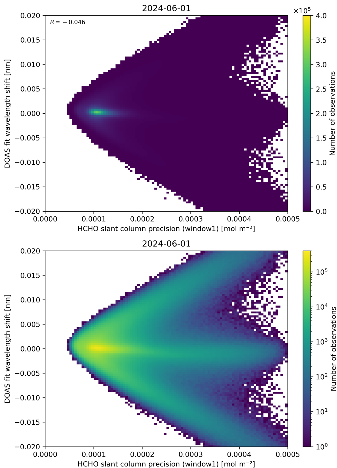
Figure 89: Scatter density plot of “HCHO slant column precision (window1)” against “DOAS fit wavelength shift” for 2024-05-31 to 2024-06-02.
