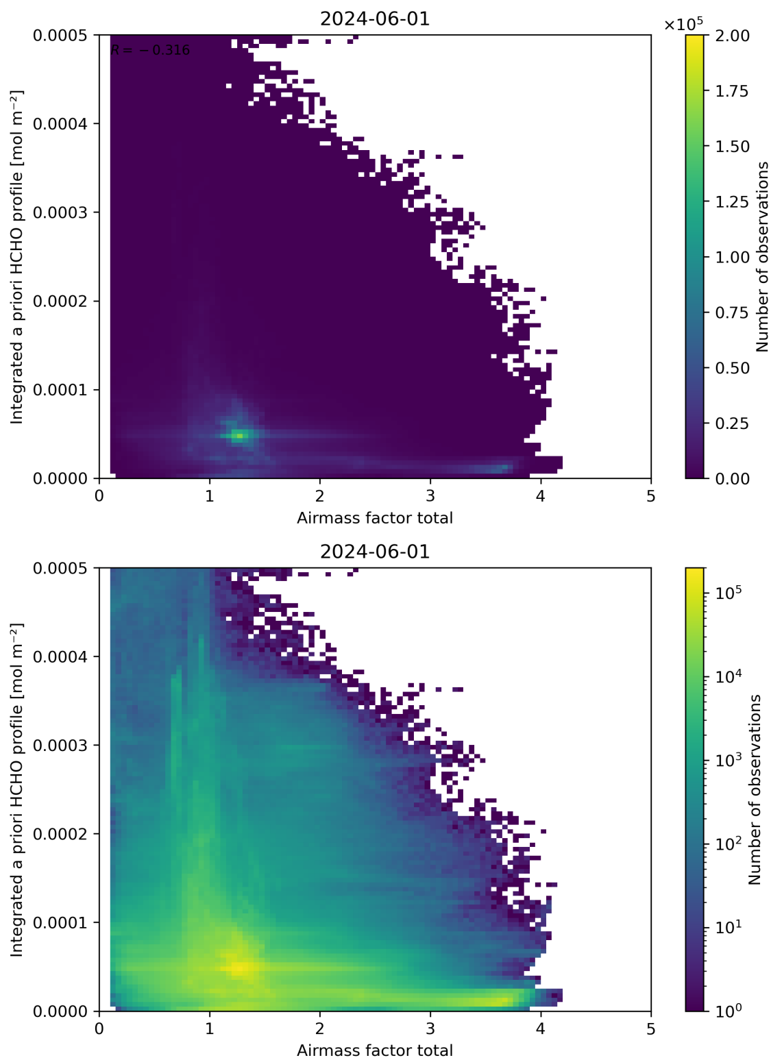
Figure 104: Scatter density plot of “Airmass factor total” against “Integrated a priori HCHO profile” for 2024-05-31 to 2024-06-02.
