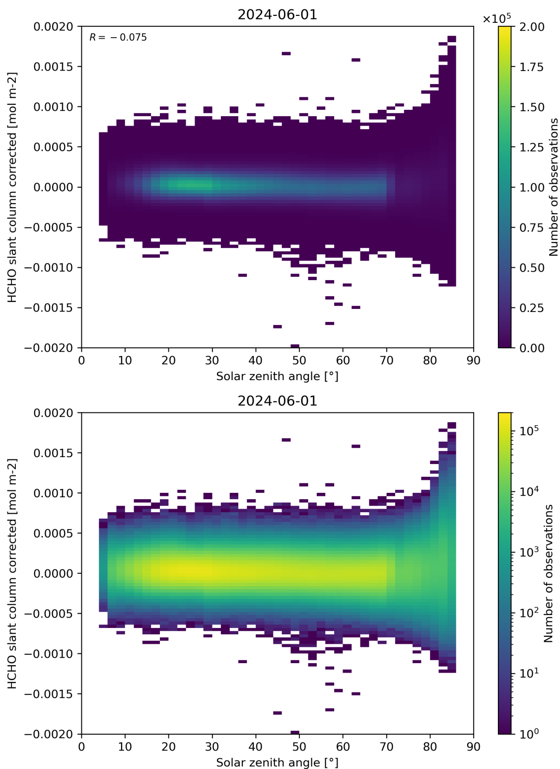
Figure 171: Scatter density plot of “Solar zenith angle” against “HCHO slant column corrected” for 2024-05-31 to 2024-06-02.
