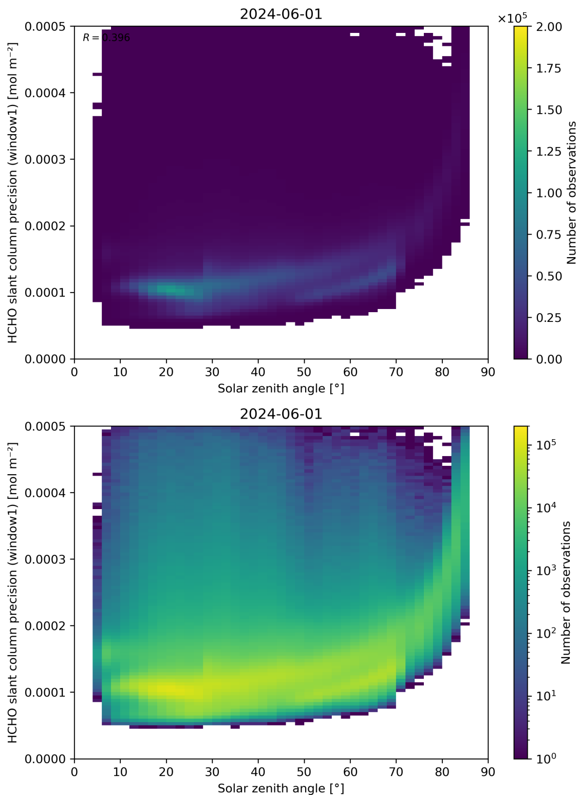
Figure 174: Scatter density plot of “Solar zenith angle” against “HCHO slant column precision (window1)” for 2024-05-31 to 2024-06-02.
