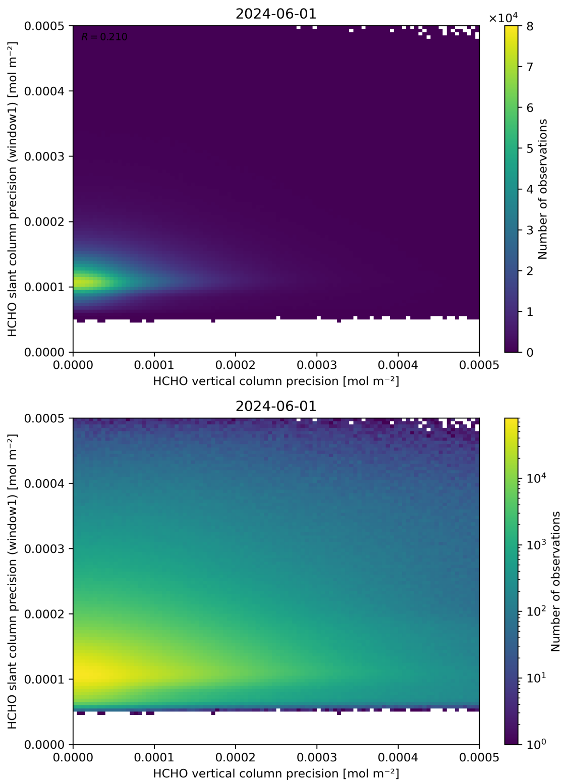
Figure 143: Scatter density plot of “HCHO vertical column precision” against “HCHO slant column precision (window1)” for 2024-05-31 to 2024-06-02.
