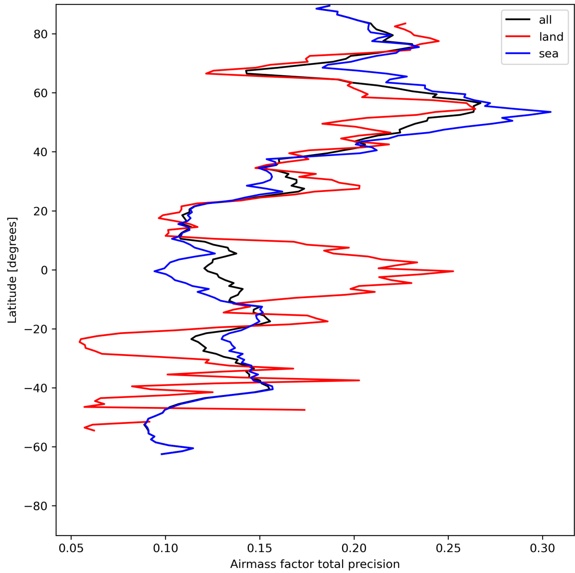
Figure 27: Zonal average of “Airmass factor total precision” for 2024-05-31 to 2024-06-02.
