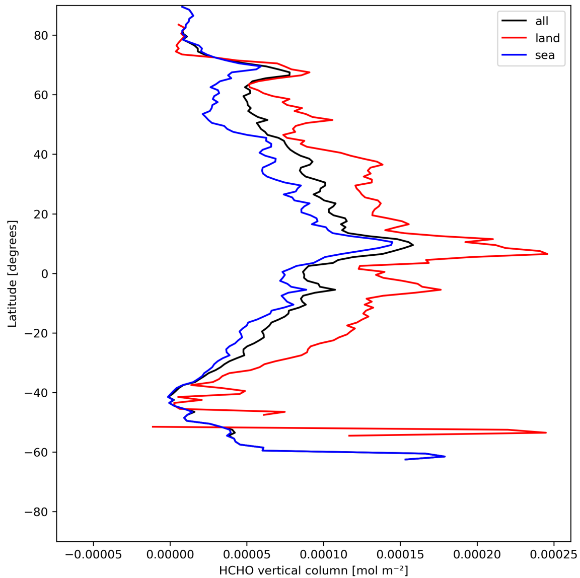
Figure 21: Zonal average of “HCHO vertical column” for 2024-05-31 to 2024-06-02.
