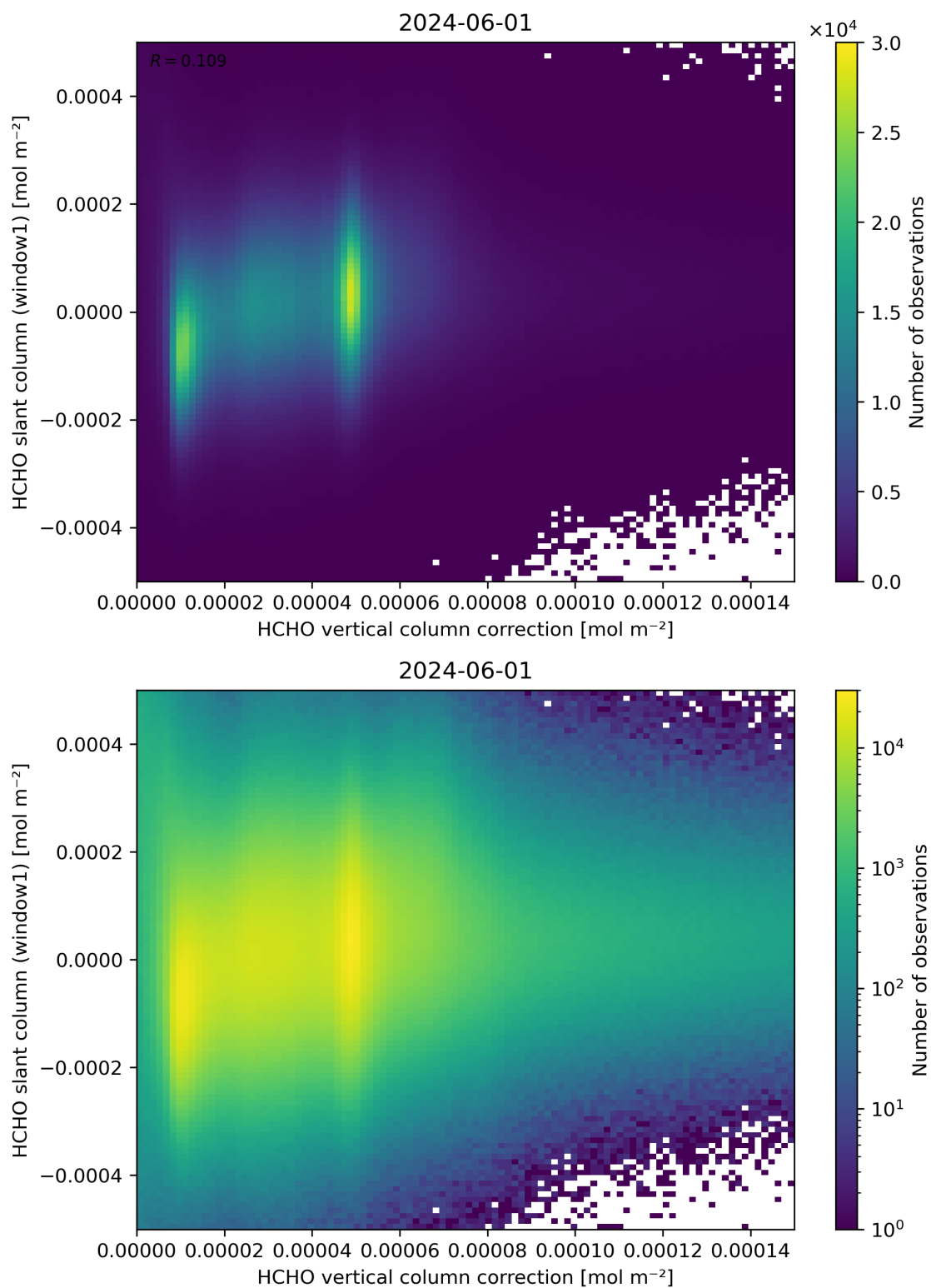
Figure 118: Scatter density plot of “HCHO vertical column correction” against “HCHO slant column (window1)” for 2024-05-31 to 2024-06-02.
