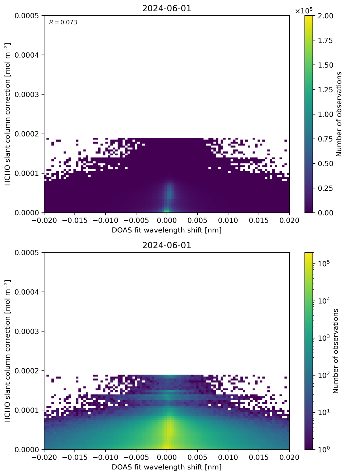
Figure 67: Scatter density plot of “DOAS fit wavelength shift” against “HCHO slant column correction” for 2024-05-31 to 2024-06-02.
