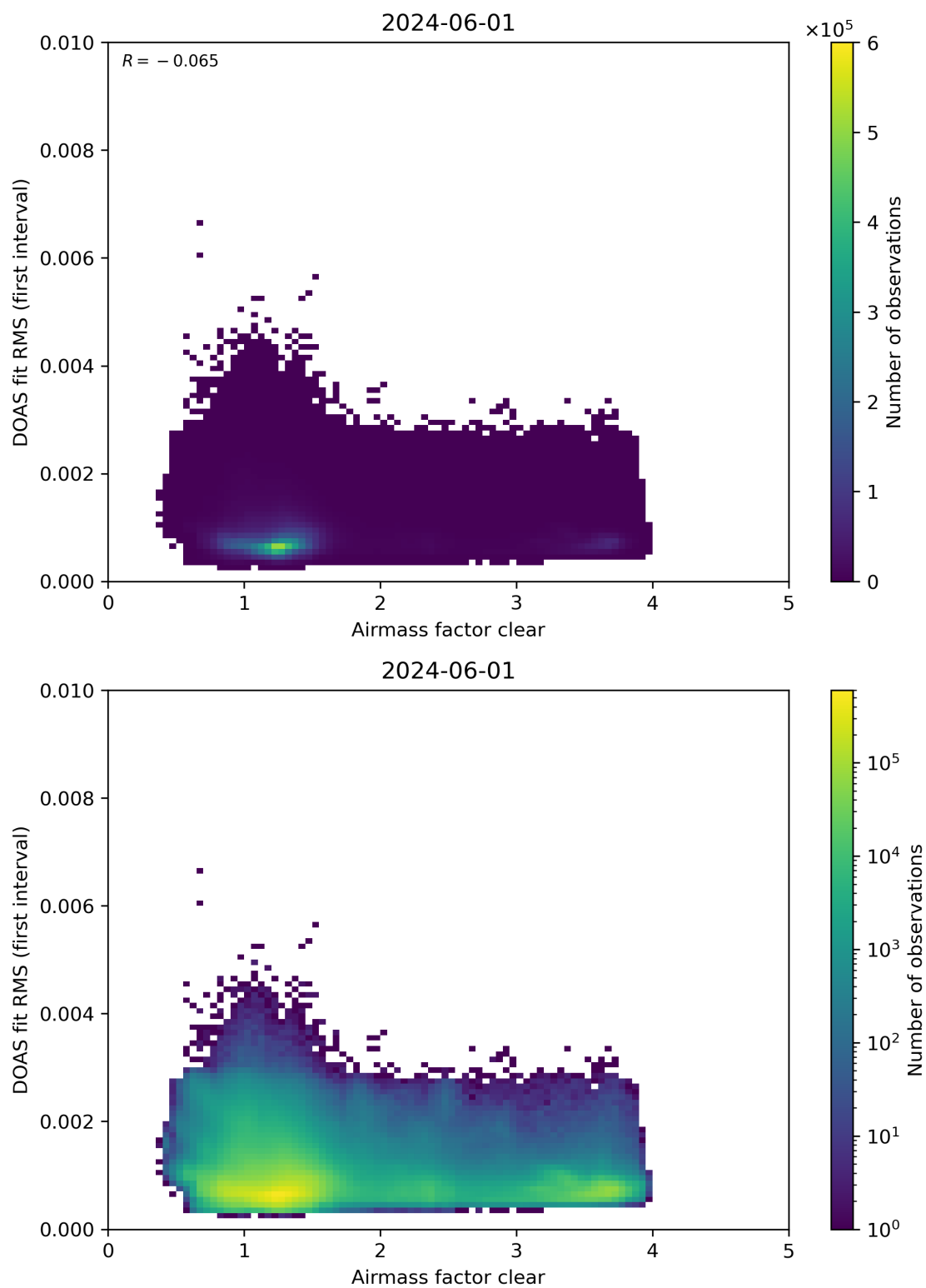
Figure 71: Scatter density plot of “Airmass factor clear” against “DOAS fit RMS (first interval)” for 2024-05-31 to 2024-06-02.
