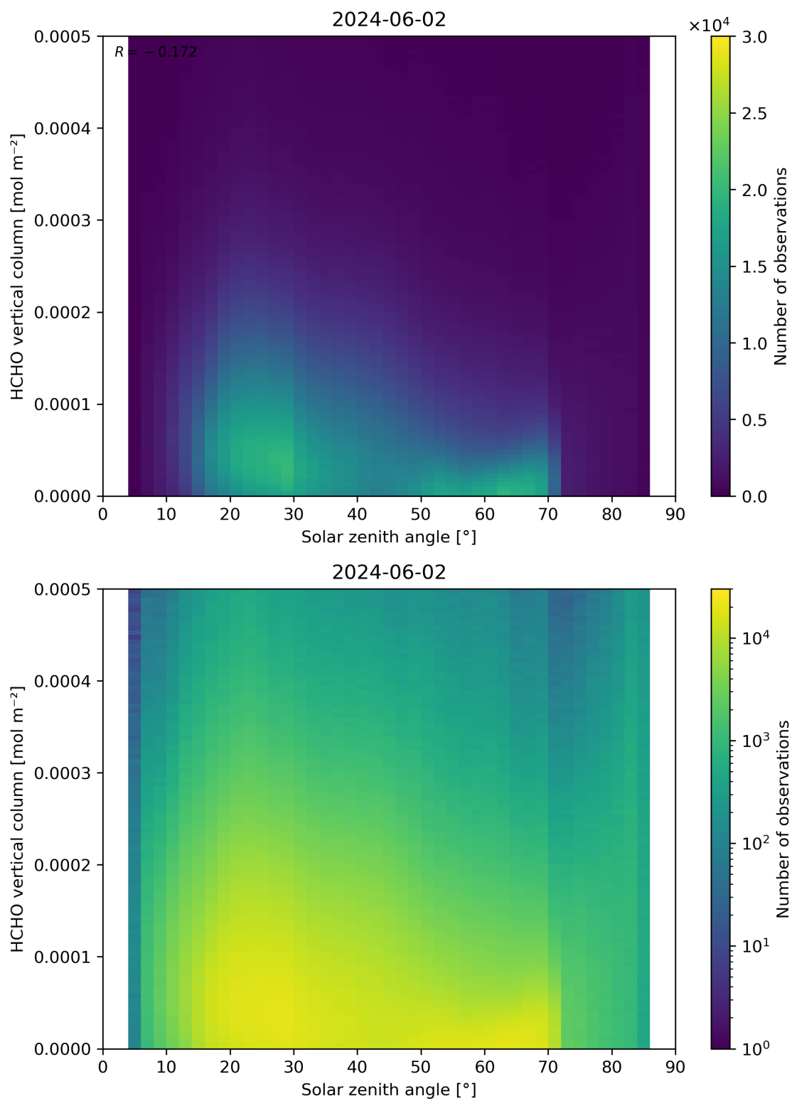
Figure 177: Scatter density plot of “Solar zenith angle” against “HCHO vertical column” for 2024-06-01 to 2024-06-03.
