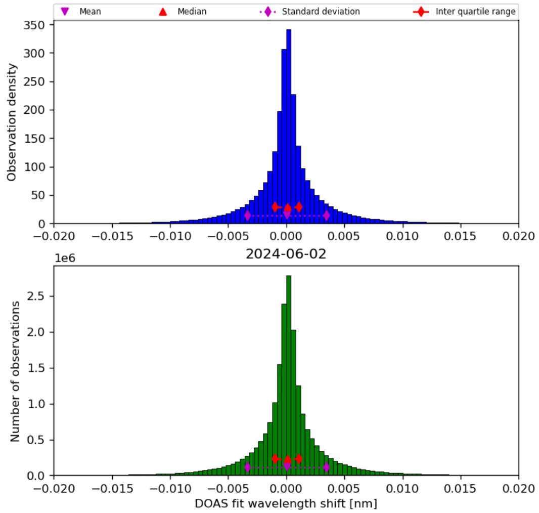
Figure 44: Histogram of “DOAS fit wavelength shift” for 2024-06-01 to 2024-06-03
