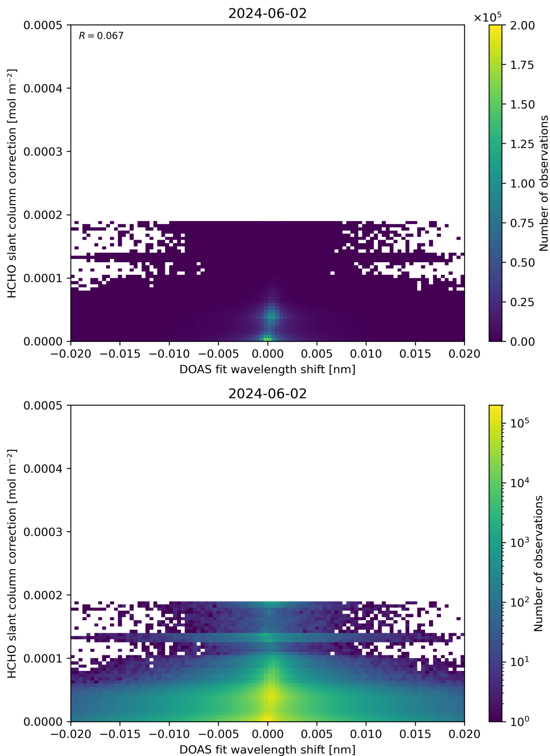
Figure 67: Scatter density plot of “DOAS fit wavelength shift” against “HCHO slant column correction” for 2024-06-01 to 2024-06-03.
