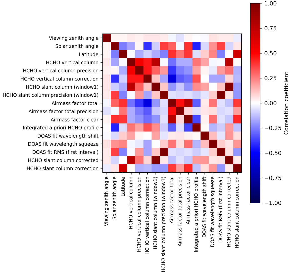
Figure 2: Map of correlation matrix for 2024-06-01 to 2024-06-03.
