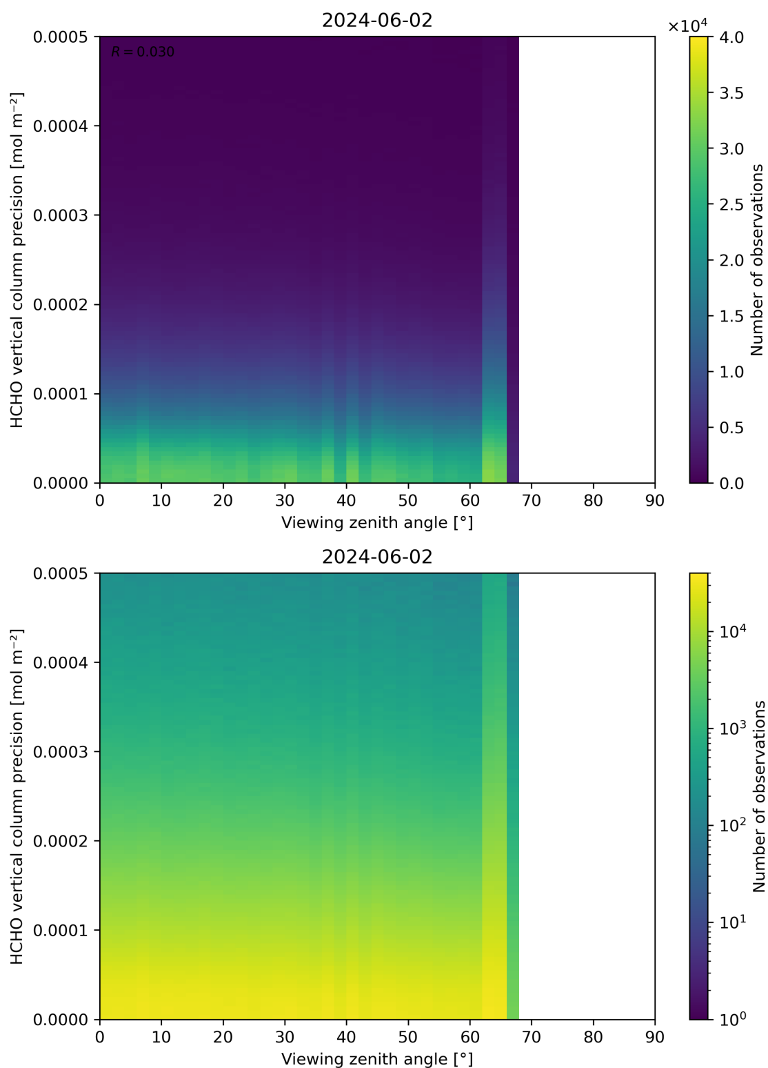
Figure 194: Scatter density plot of “Viewing zenith angle” against “HCHO vertical column precision” for 2024-06-01 to 2024-06-03.
