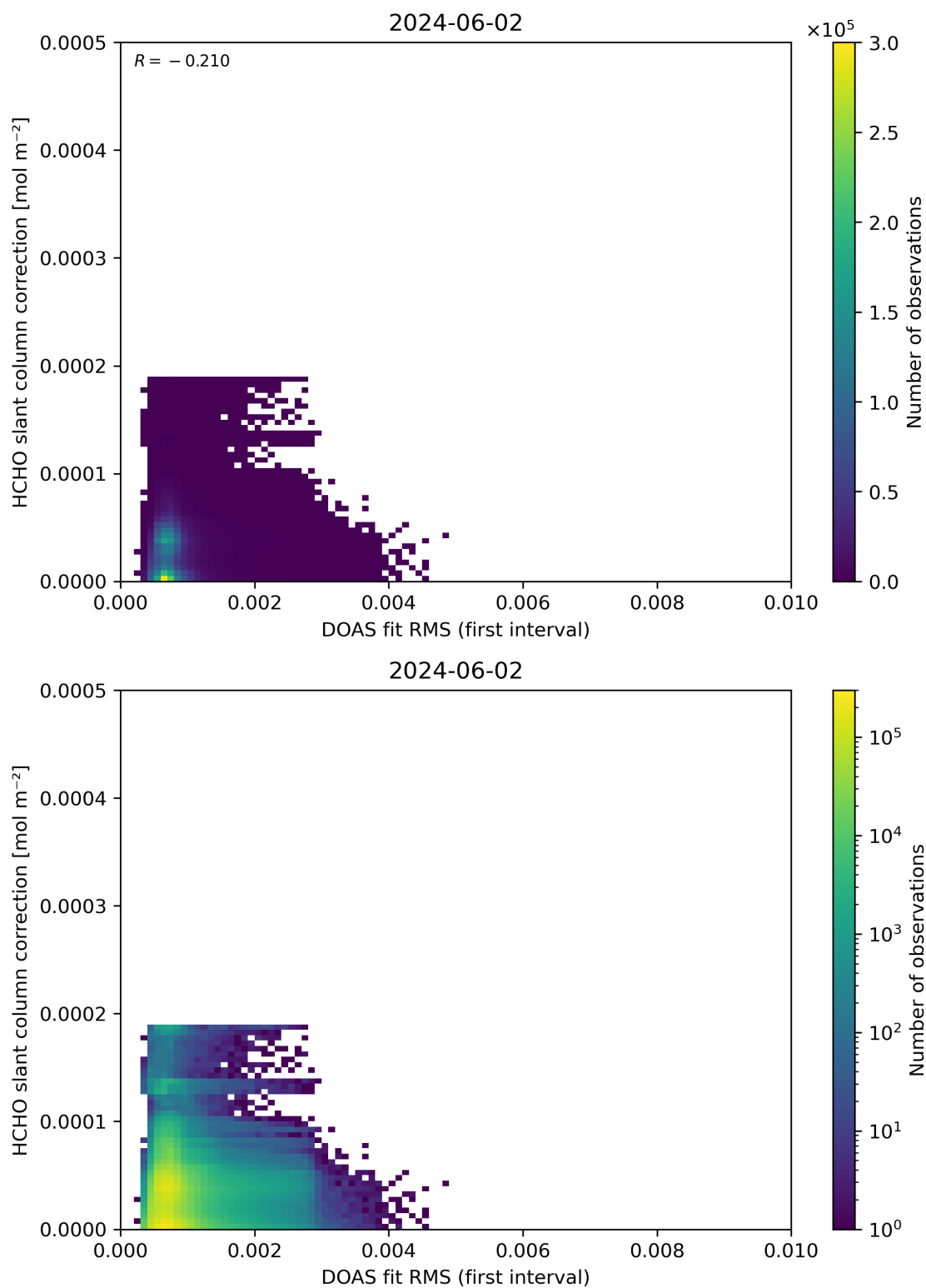
Figure 63: Scatter density plot of “DOAS fit RMS (first interval)” against “HCHO slant column correction” for 2024-06-01 to 2024-06-03.
