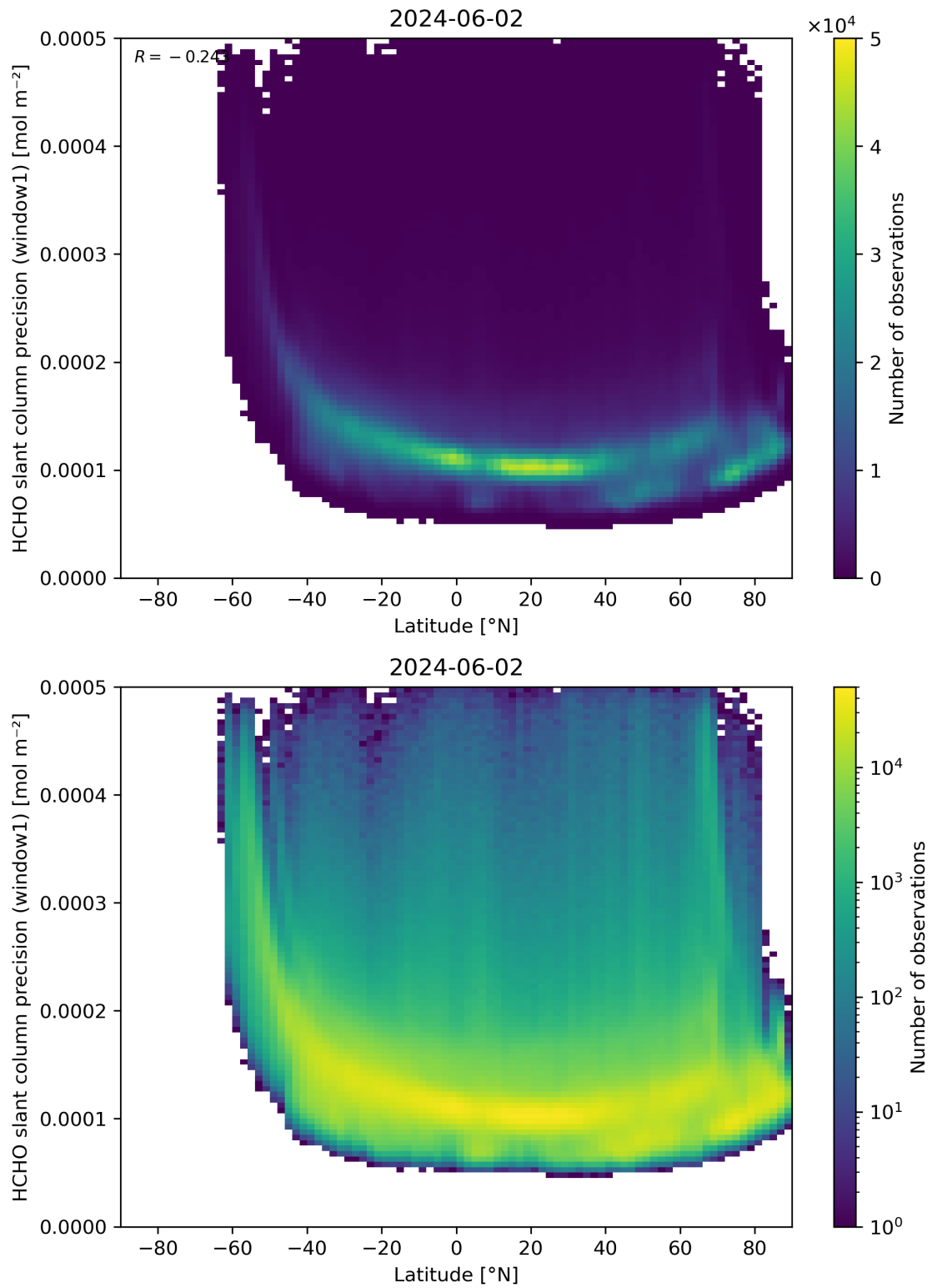
Figure 160: Scatter density plot of “Latitude” against “HCHO slant column precision (window1)” for 2024-06-01 to 2024-06-03.
