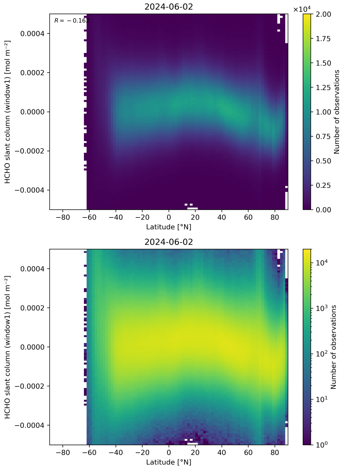
Figure 159: Scatter density plot of “Latitude” against “HCHO slant column (window1)” for 2024-06-01 to 2024-06-03.
