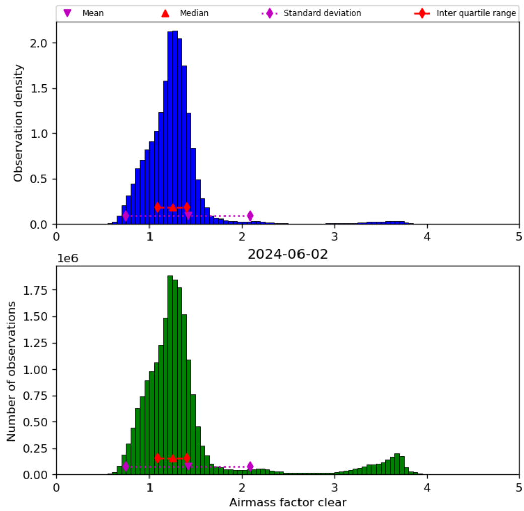
Figure 42: Histogram of “Airmass factor clear” for 2024-06-01 to 2024-06-03
