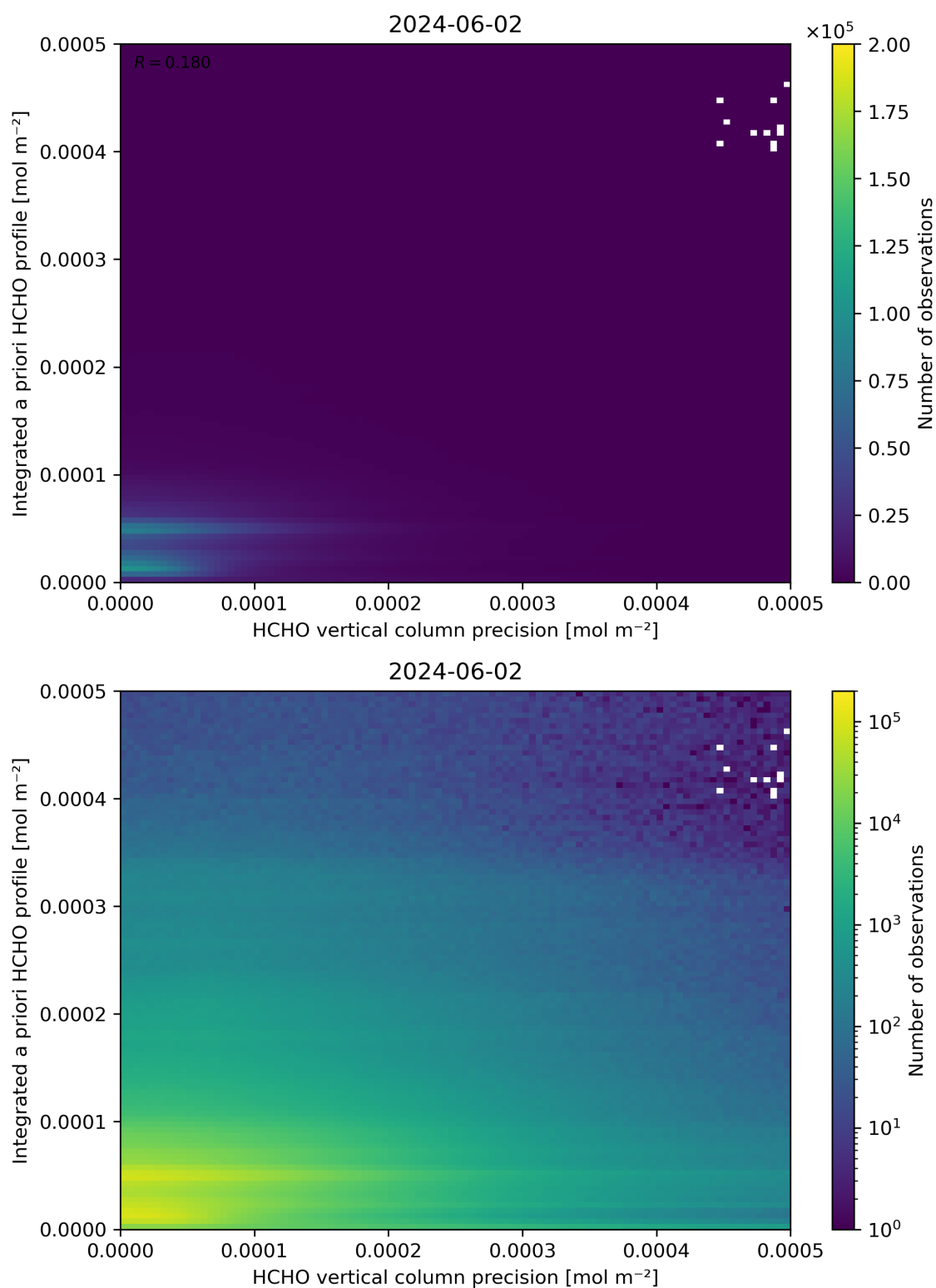
Figure 147: Scatter density plot of “HCHO vertical column precision” against “Integrated a priori HCHO profile” for 2024-06-01 to 2024-06-03.
