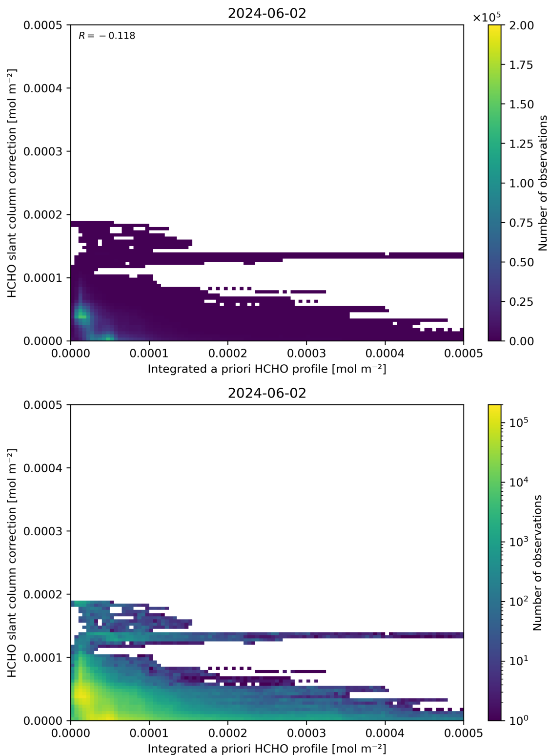
Figure 152: Scatter density plot of “Integrated a priori HCHO profile” against “HCHO slant column correction” for 2024-06-01 to 2024-06-03.
