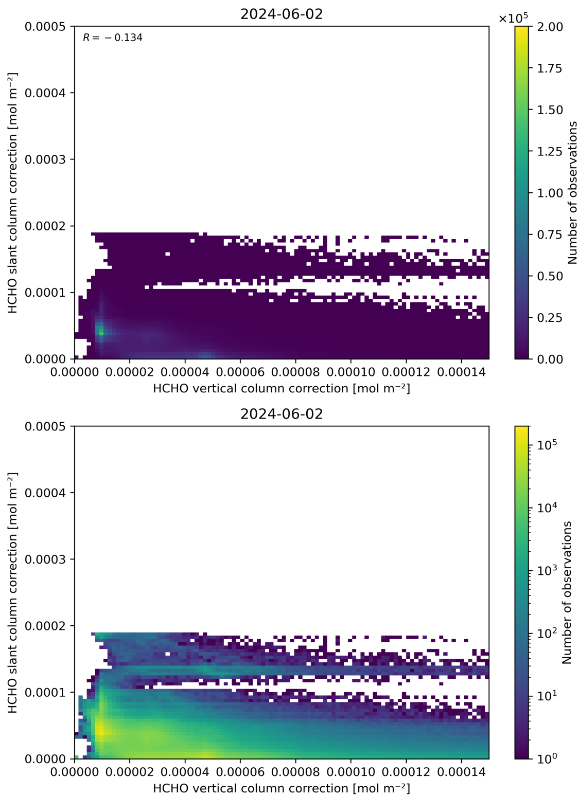
Figure 117: Scatter density plot of “HCHO vertical column correction” against “HCHO slant column correction” for 2024-06-01 to 2024-06-03.
