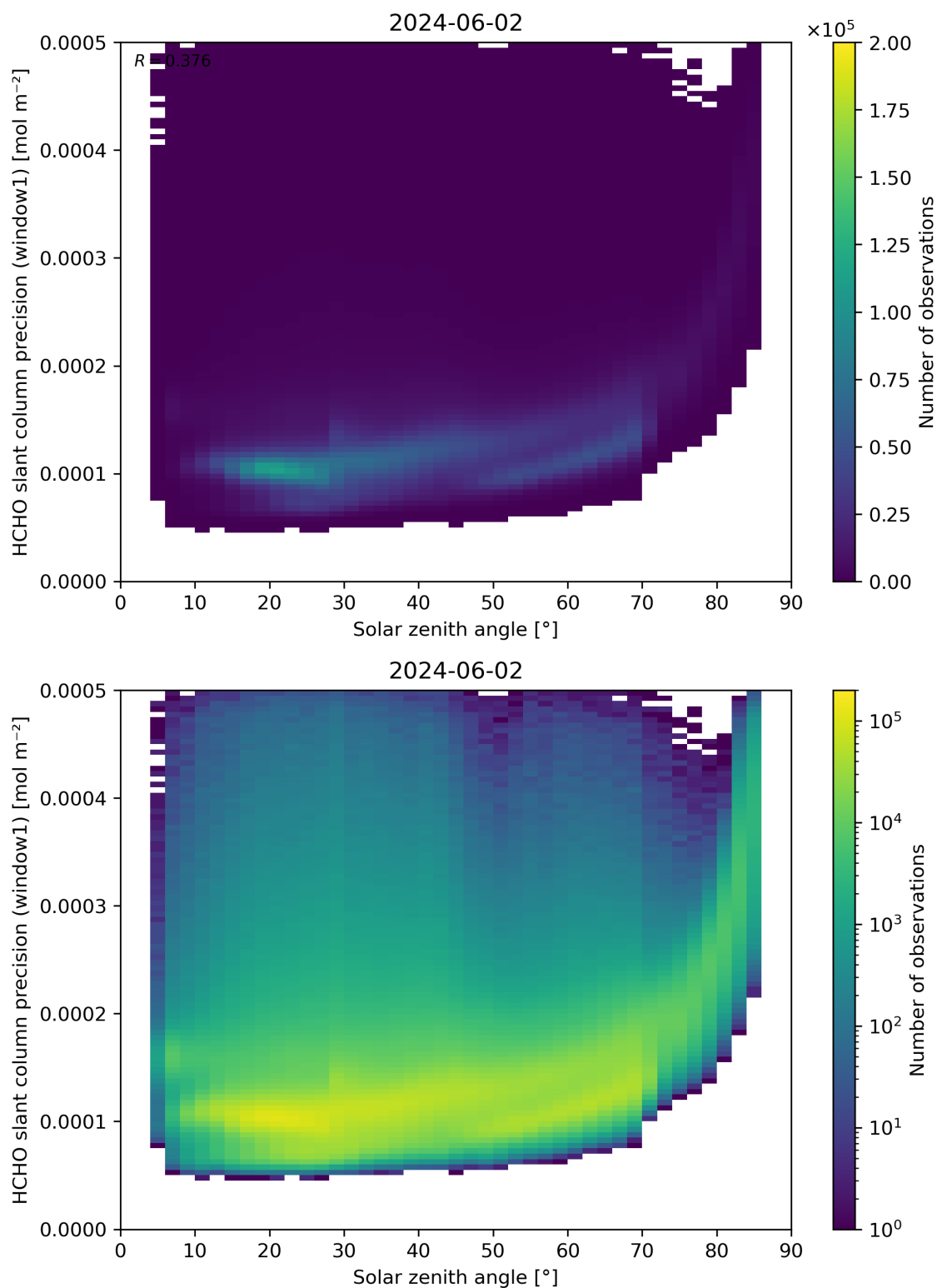
Figure 174: Scatter density plot of “Solar zenith angle” against “HCHO slant column precision (window1)” for 2024-06-01 to 2024-06-03.
