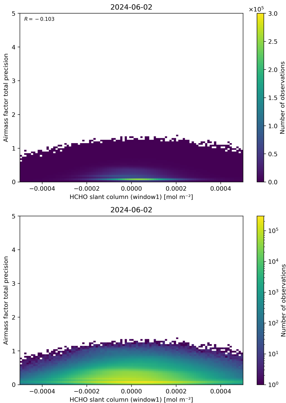
Figure 86: Scatter density plot of “HCHO slant column (window1)” against “Airmass factor total precision” for 2024-06-01 to 2024-06-03.
