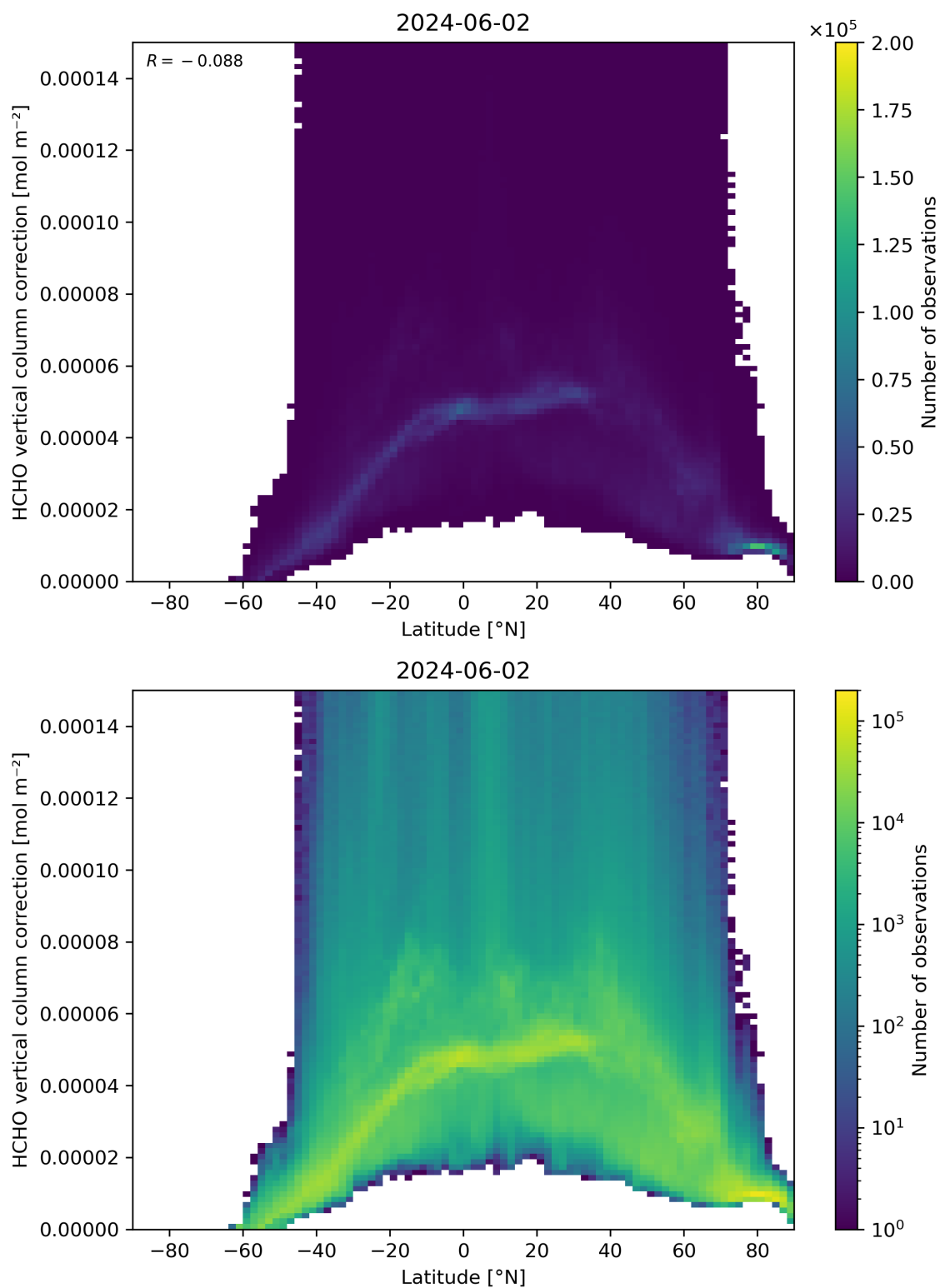
Figure 164: Scatter density plot of “Latitude” against “HCHO vertical column correction” for 2024-06-01 to 2024-06-03.
