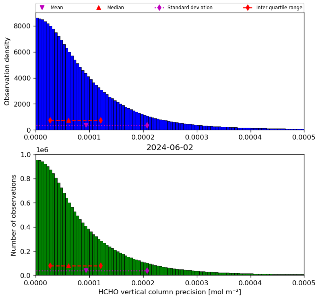
Figure 36: Histogram of “HCHO vertical column precision” for 2024-06-01 to 2024-06-03
