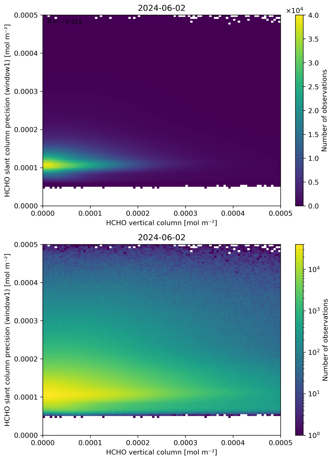
Figure 130: Scatter density plot of “HCHO vertical column” against “HCHO slant column precision (window1)” for 2024-06-01 to 2024-06-03.
