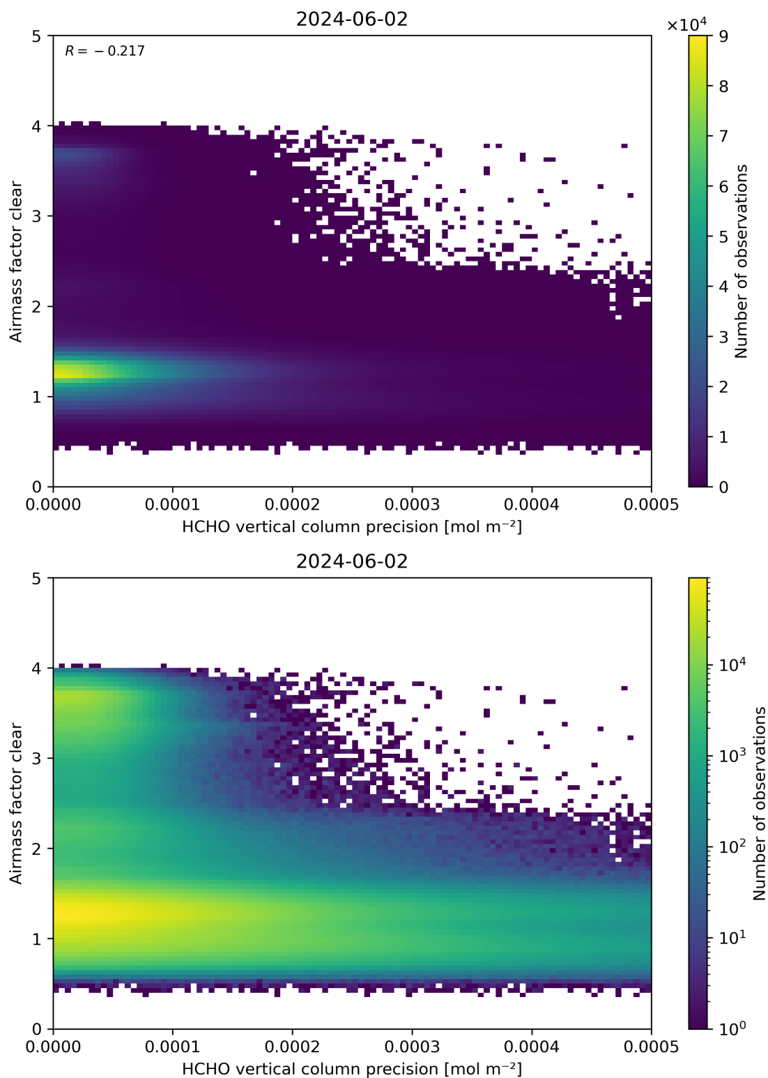
Figure 139: Scatter density plot of “HCHO vertical column precision” against “Airmass factor clear” for 2024-06-01 to 2024-06-03.
