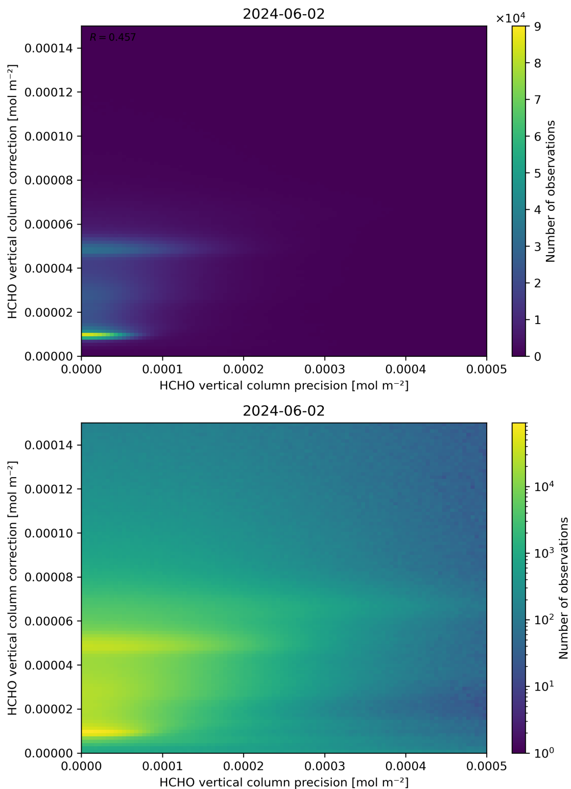
Figure 146: Scatter density plot of “HCHO vertical column precision” against “HCHO vertical column correction” for 2024-06-01 to 2024-06-03.
