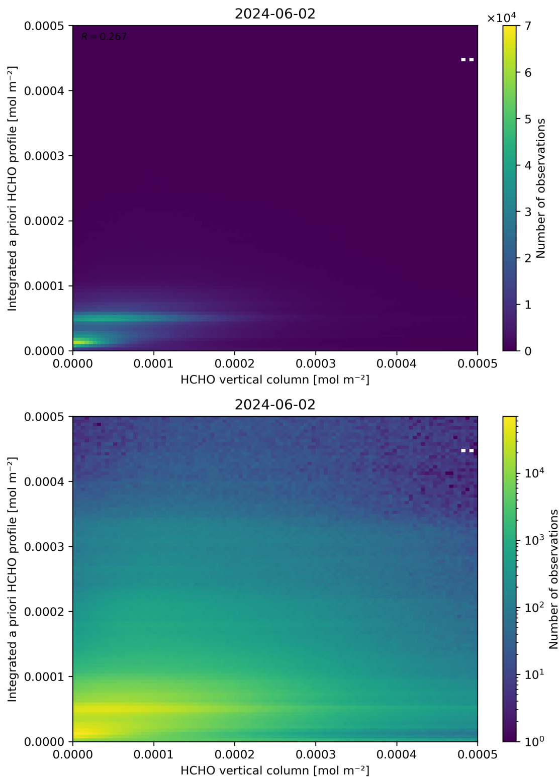
Figure 135: Scatter density plot of “HCHO vertical column” against “Integrated a priori HCHO profile” for 2024-06-01 to 2024-06-03.
