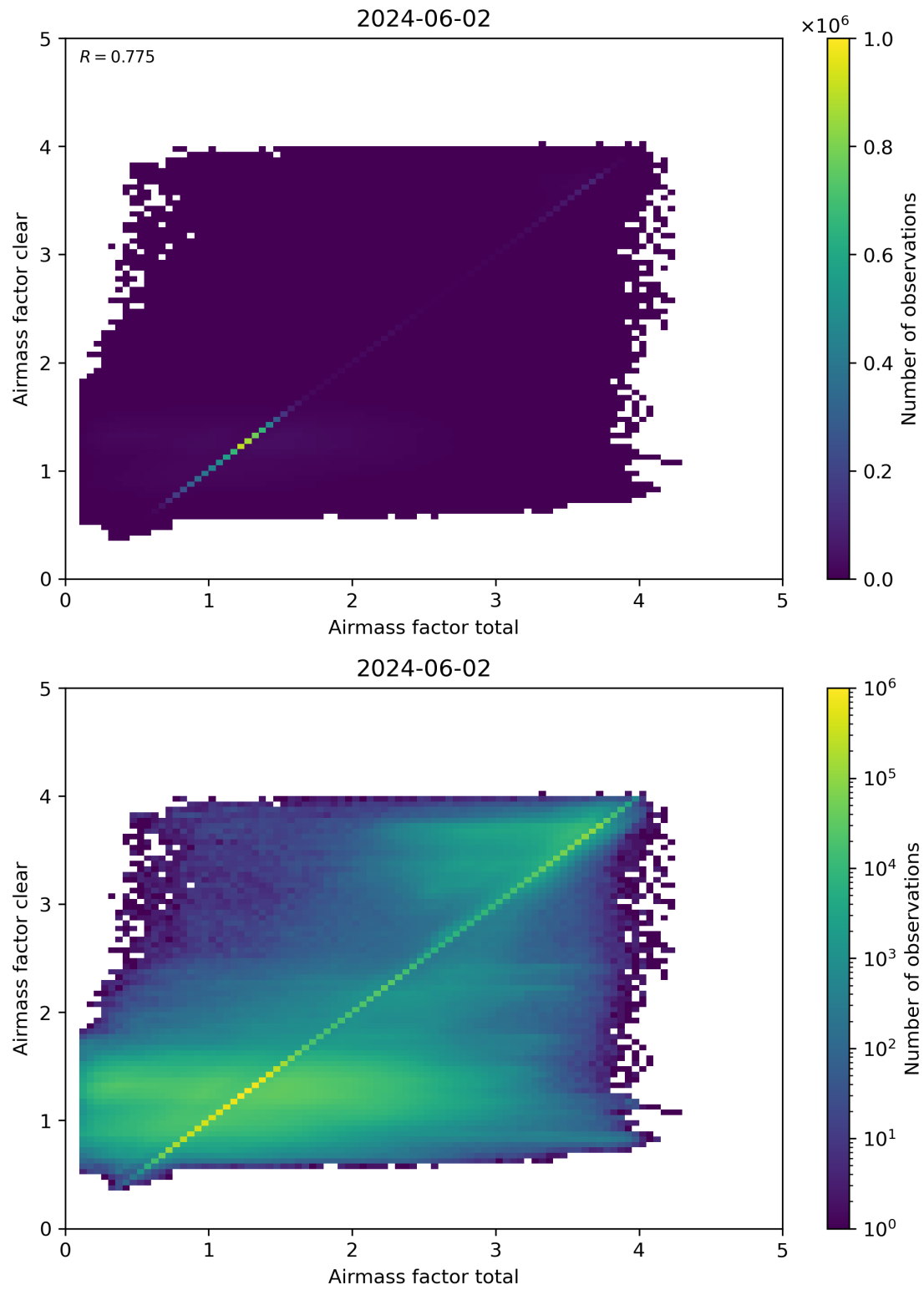
Figure 100: Scatter density plot of “Airmass factor total” against “Airmass factor clear” for 2024-06-01 to 2024-06-03.
