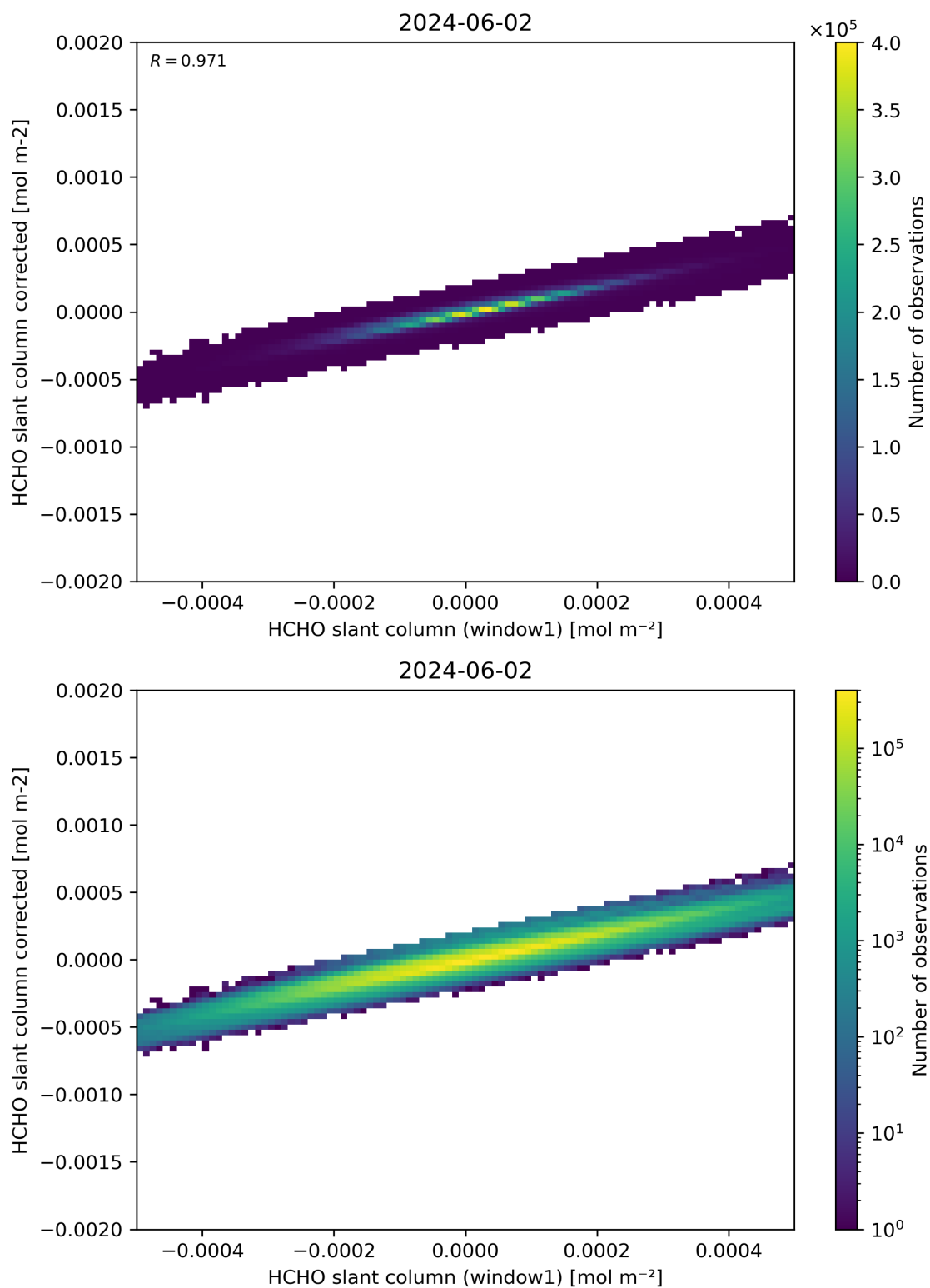
Figure 82: Scatter density plot of “HCHO slant column (window1)” against “HCHO slant column corrected” for 2024-06-01 to 2024-06-03.
