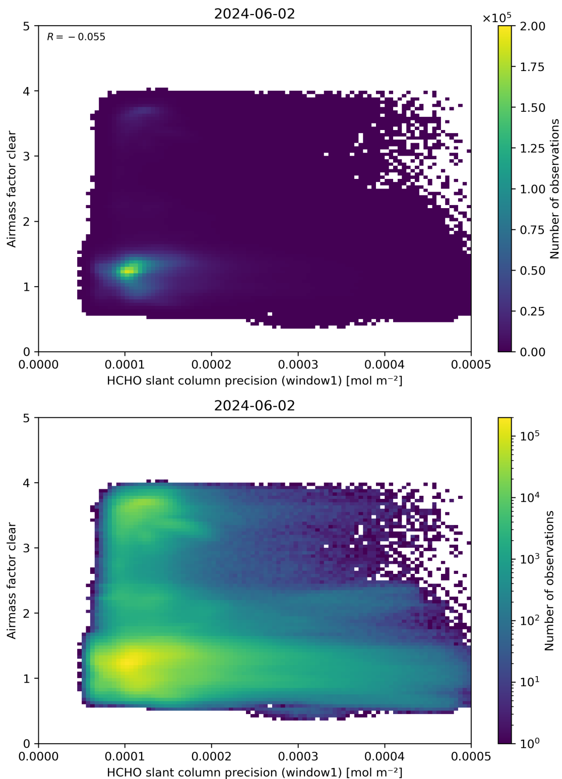
Figure 91: Scatter density plot of “HCHO slant column precision (window1)” against “Airmass factor clear” for 2024-06-01 to 2024-06-03.
