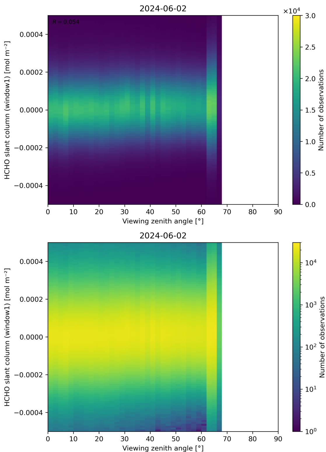
Figure 188: Scatter density plot of “Viewing zenith angle” against “HCHO slant column (window1)” for 2024-06-01 to 2024-06-03.
