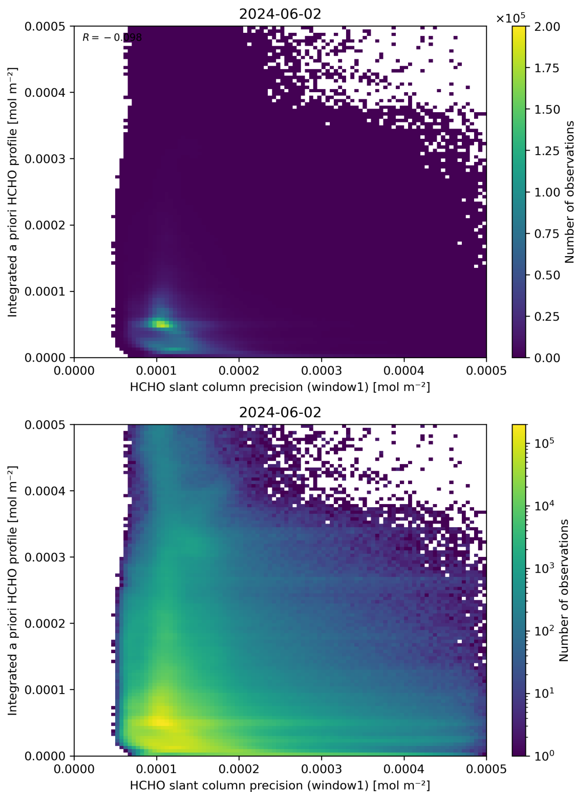
Figure 96: Scatter density plot of “HCHO slant column precision (window1)” against “Integrated a priori HCHO profile” for 2024-06-01 to 2024-06-03.
