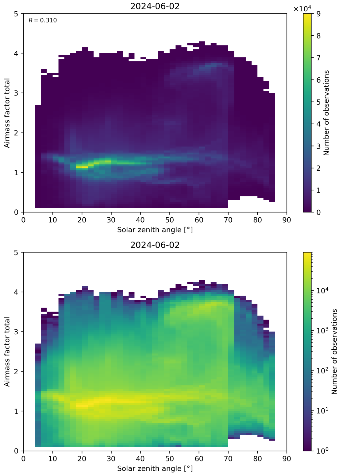
Figure 175: Scatter density plot of “Solar zenith angle” against “Airmass factor total” for 2024-06-01 to 2024-06-03.
