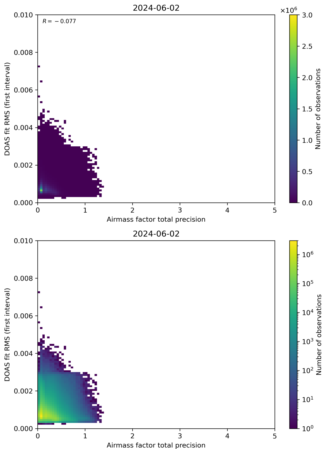
Figure 105: Scatter density plot of “Airmass factor total precision” against “DOAS fit RMS (first interval)” for 2024-06-01 to 2024-06-03.
