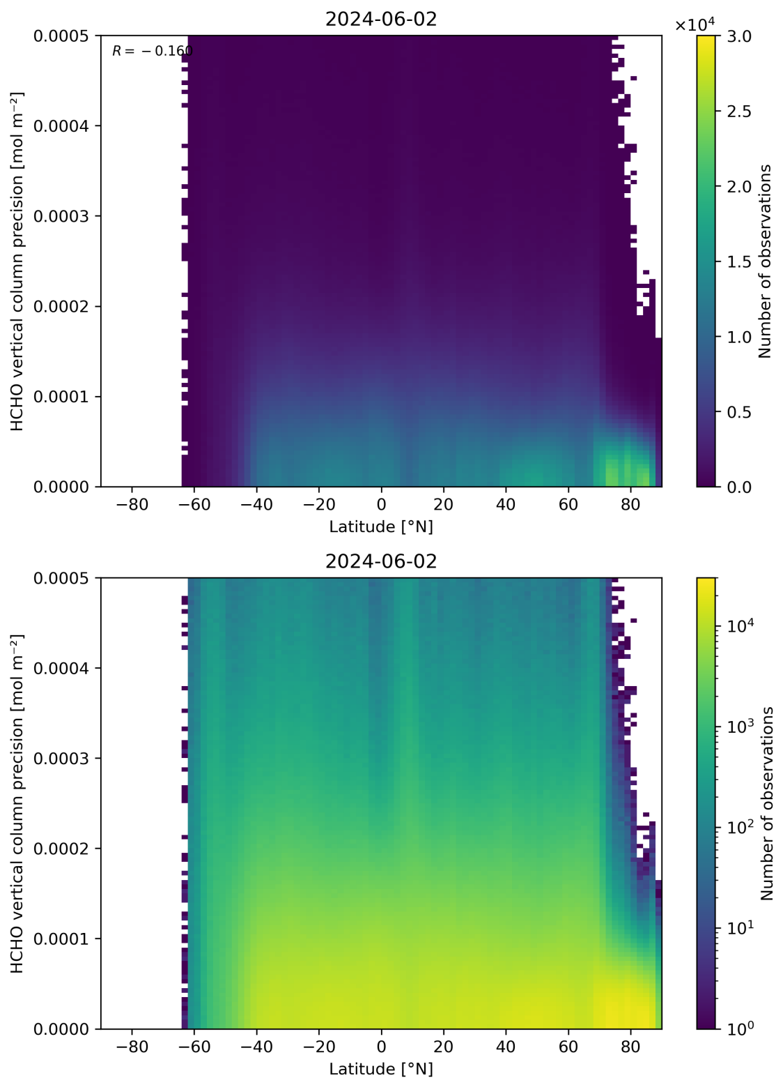
Figure 165: Scatter density plot of “Latitude” against “HCHO vertical column precision” for 2024-06-01 to 2024-06-03.
