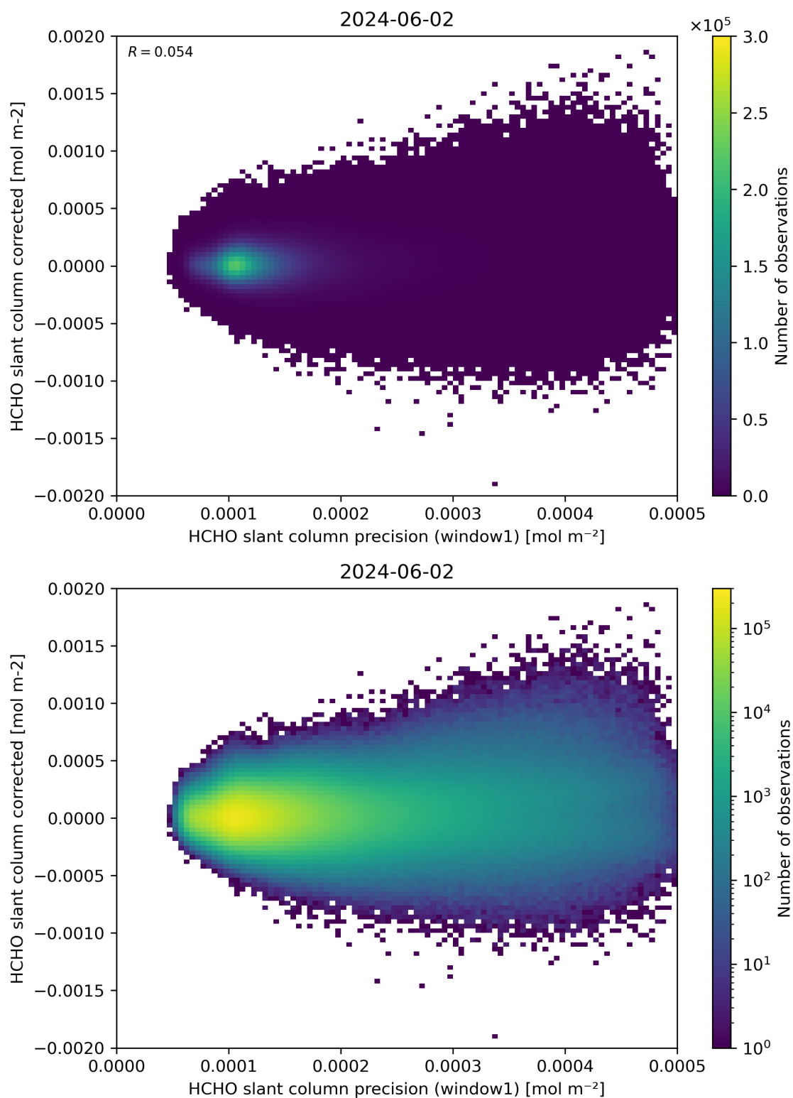
Figure 92: Scatter density plot of “HCHO slant column precision (window1)” against “HCHO slant column corrected” for 2024-06-01 to 2024-06-03.
