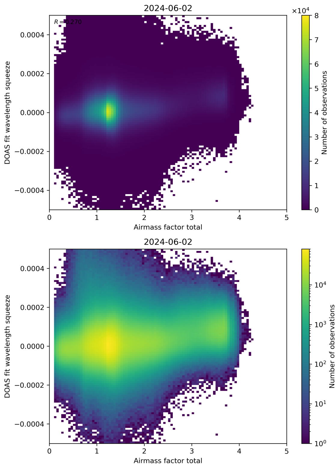
Figure 99: Scatter density plot of “Airmass factor total” against “DOAS fit wavelength squeeze” for 2024-06-01 to 2024-06-03.
