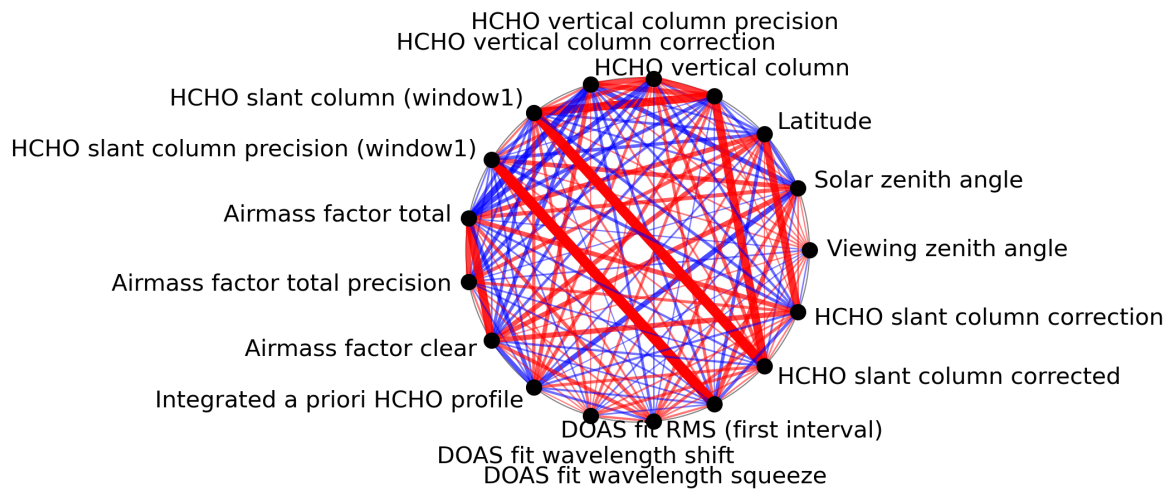
Figure 1: Map of correlation graph for 2024-06-01 to 2024-06-03.
