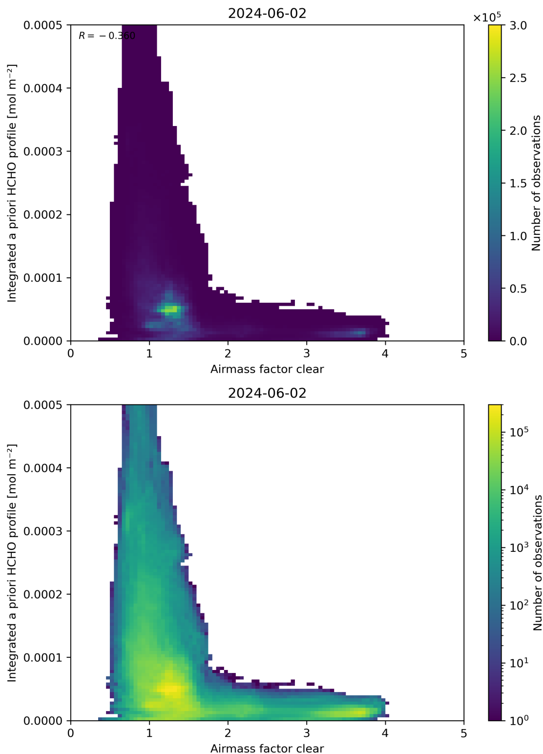
Figure 76: Scatter density plot of “Airmass factor clear” against “Integrated a priori HCHO profile” for 2024-06-01 to 2024-06-03.
