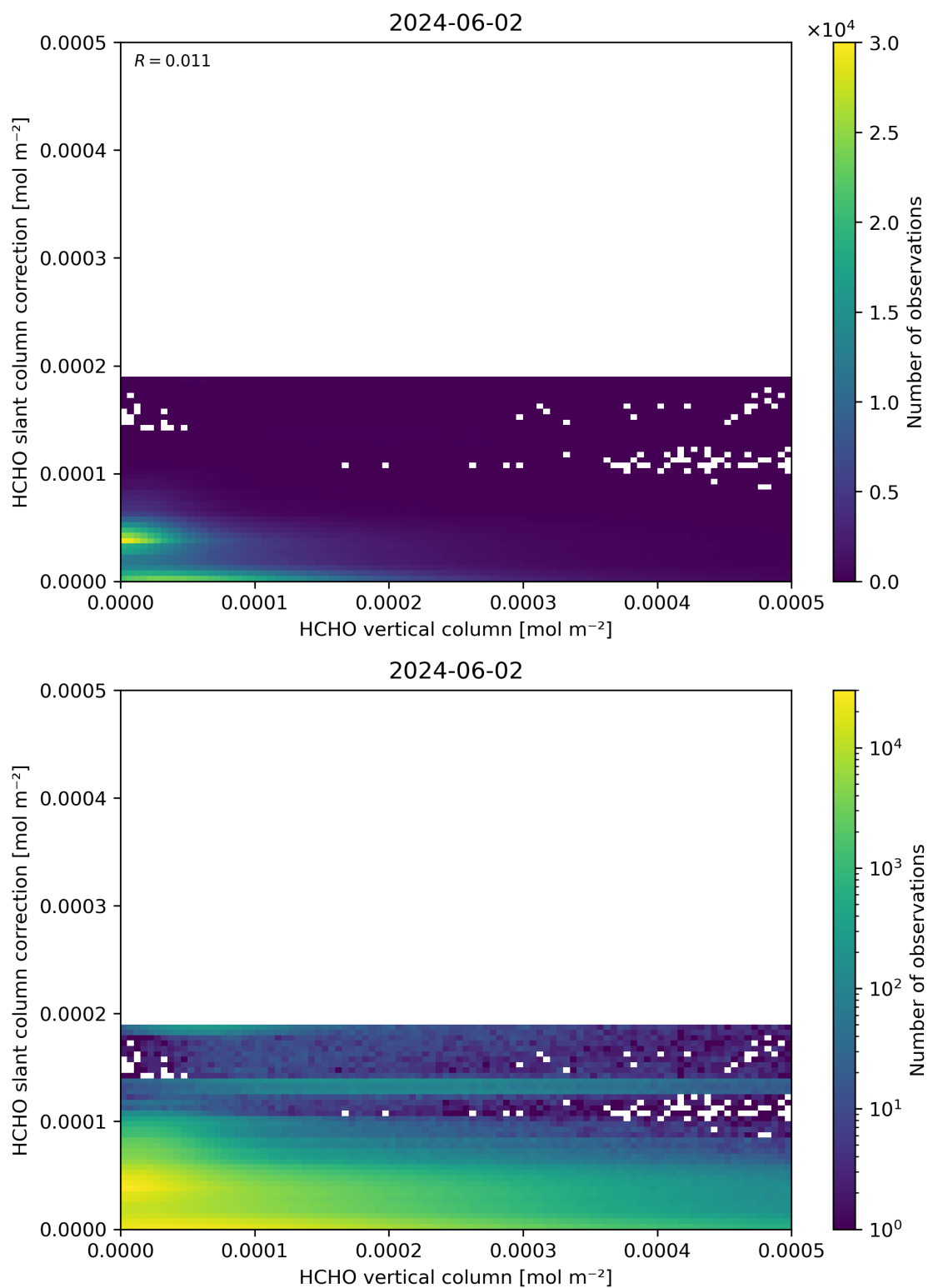
Figure 128: Scatter density plot of “HCHO vertical column” against “HCHO slant column correction” for 2024-06-01 to 2024-06-03.
