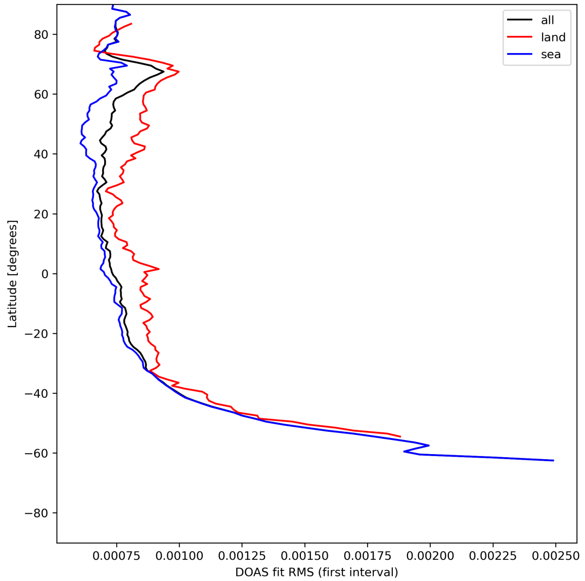
Figure 32: Zonal average of "DOAS fit RMS (first interval)" for 2024-06-01 to 2024-06-03.
