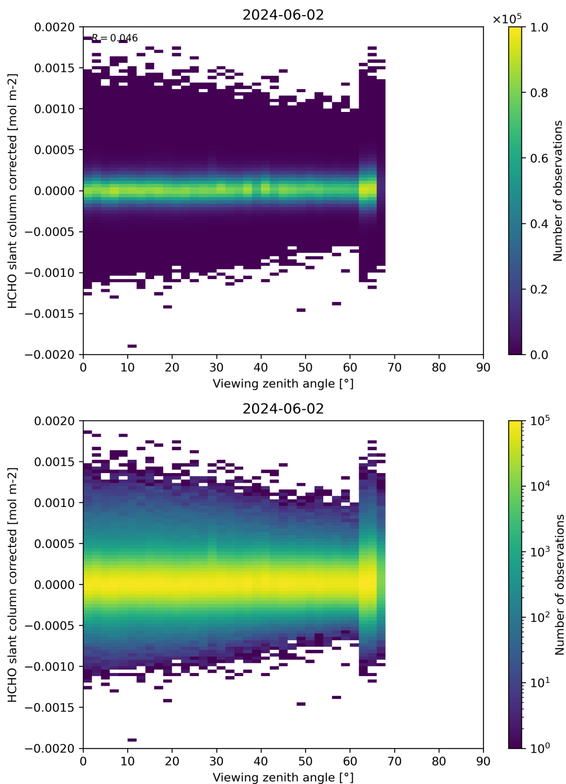
Figure 186: Scatter density plot of “Viewing zenith angle” against “HCHO slant column corrected” for 2024-06-01 to 2024-06-03.
