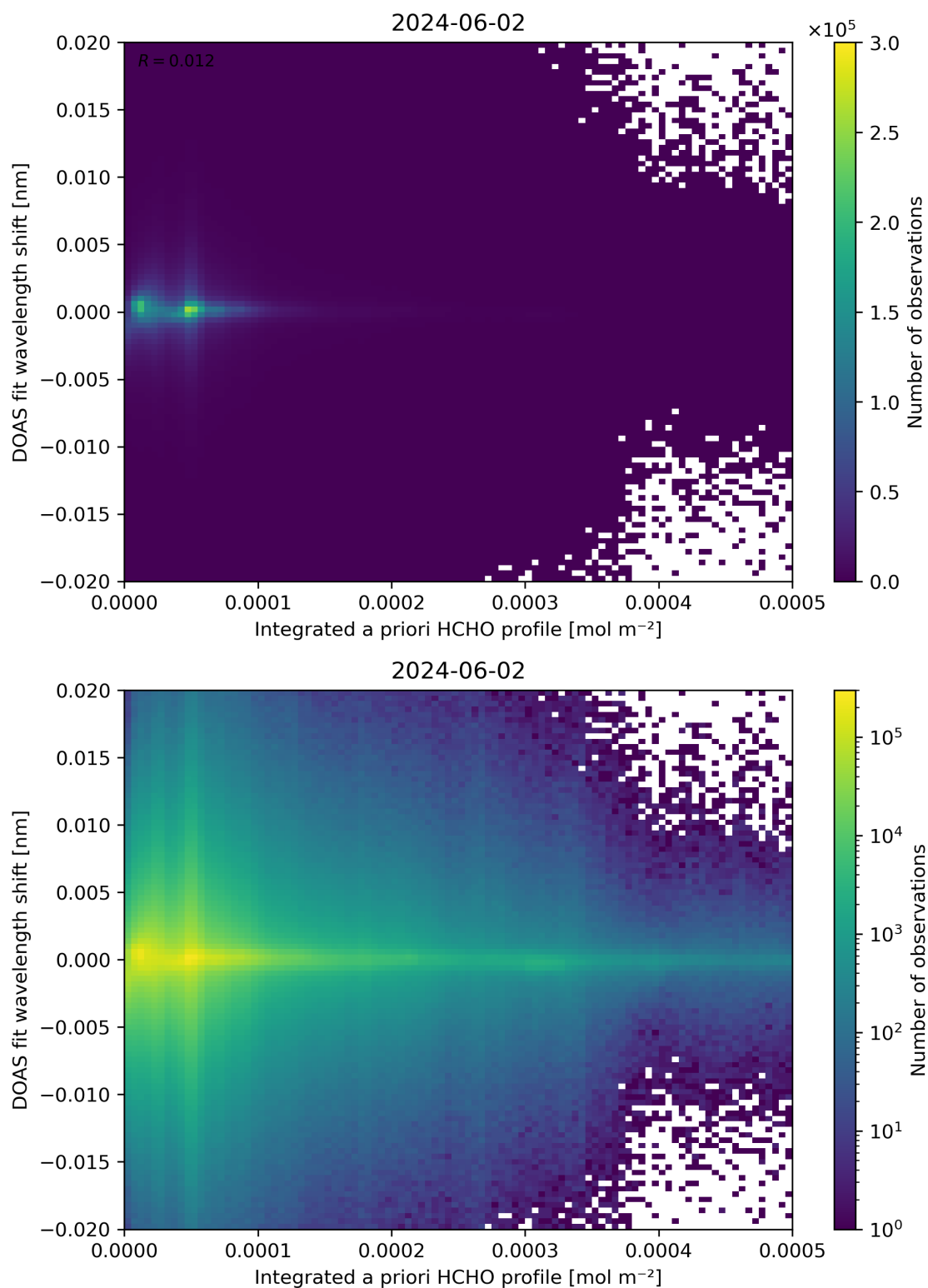
Figure 149: Scatter density plot of “Integrated a priori HCHO profile” against “DOAS fit wavelength shift” for 2024-06-01 to 2024-06-03.
