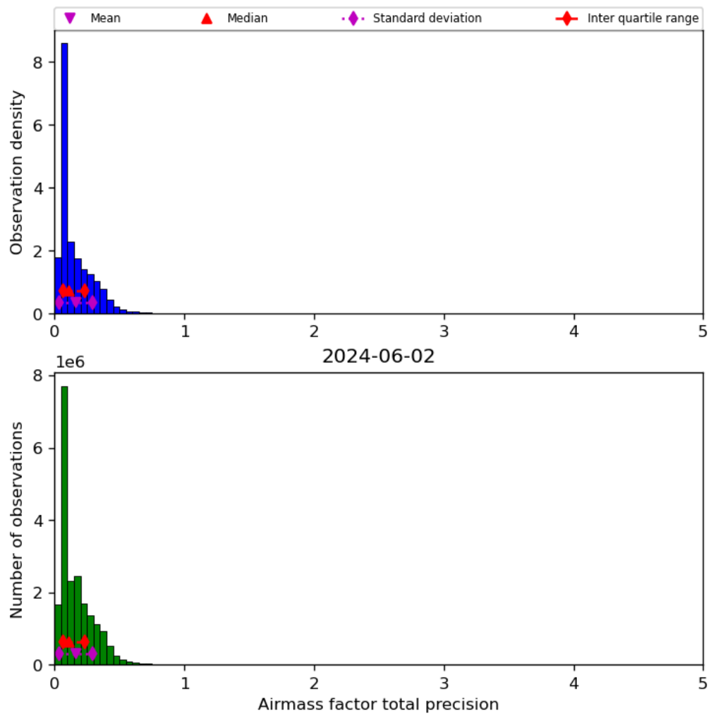
Figure 41: Histogram of “Airmass factor total precision” for 2024-06-01 to 2024-06-03
