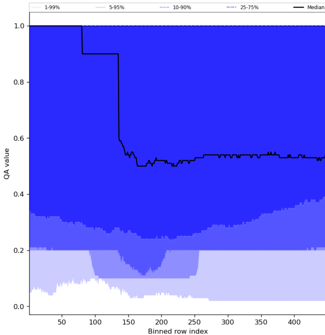
Figure 48: Along track statistics of “QA value” for 2024-06-01 to 2024-06-03
