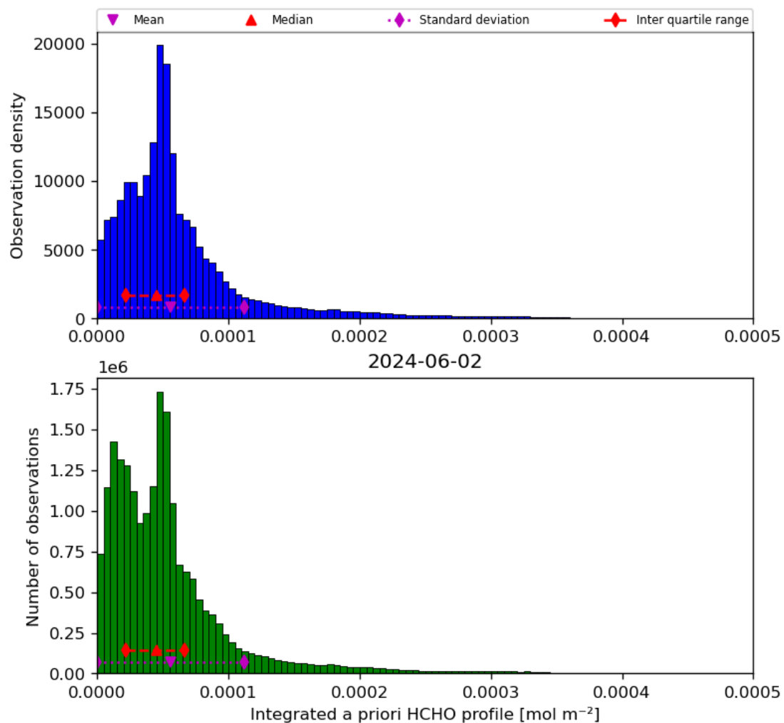
Figure 43: Histogram of “Integrated a priori HCHO profile” for 2024-06-01 to 2024-06-03
