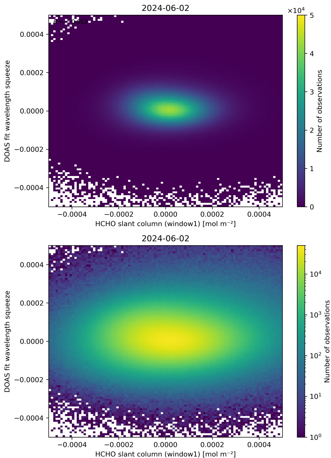
Figure 80: Scatter density plot of “HCHO slant column (window1)” against “DOAS fit wavelength squeeze” for 2024-06-01 to 2024-06-03.
