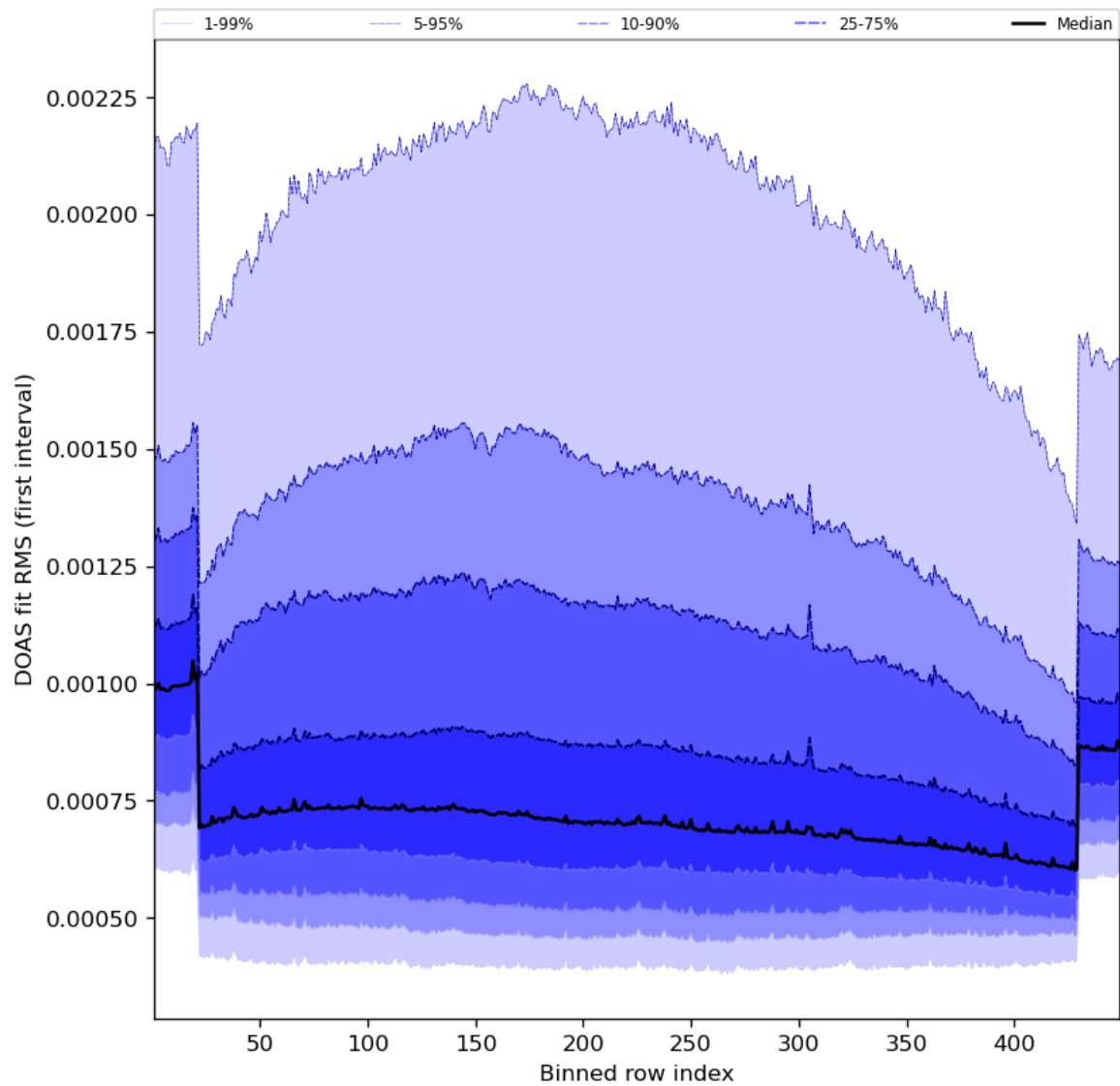
Figure 60: Along track statistics of “DOAS fit RMS (first interval)” for 2024-06-01 to 2024-06-03
