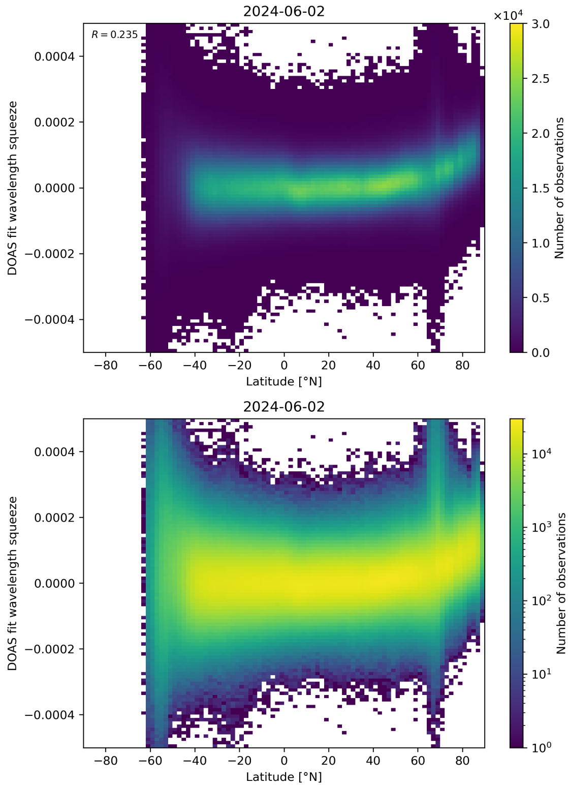
Figure 155: Scatter density plot of “Latitude” against “DOAS fit wavelength squeeze” for 2024-06-01 to 2024-06-03.
