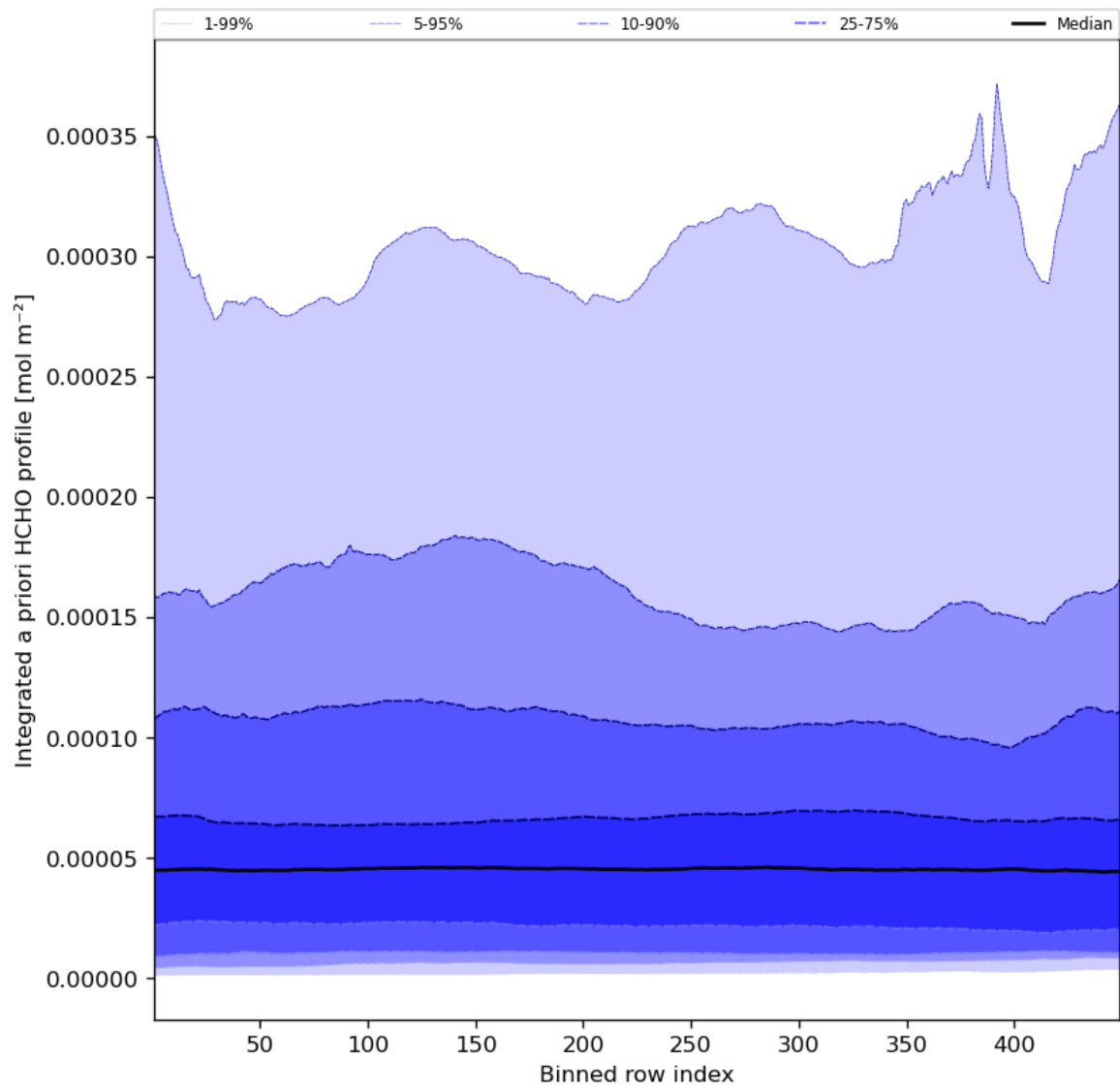
Figure 57: Along track statistics of “Integrated a priori HCHO profile” for 2024-06-01 to 2024-06-03
