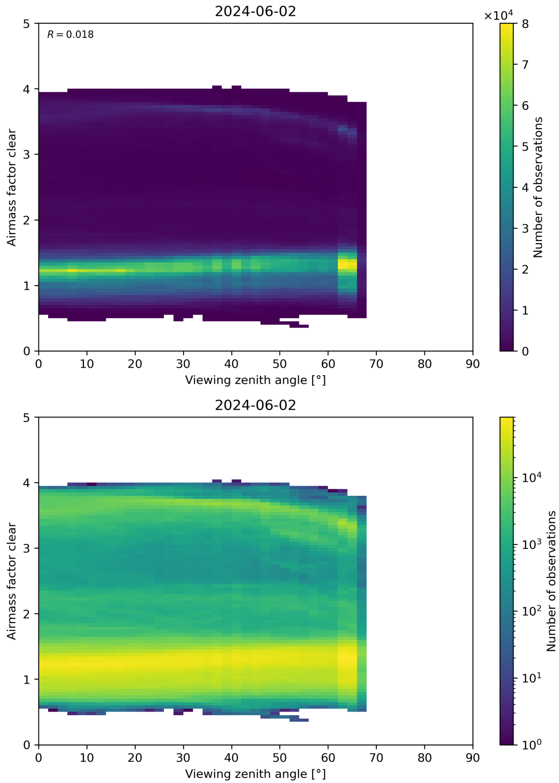
Figure 185: Scatter density plot of “Viewing zenith angle” against “Airmass factor clear” for 2024-06-01 to 2024-06-03.
