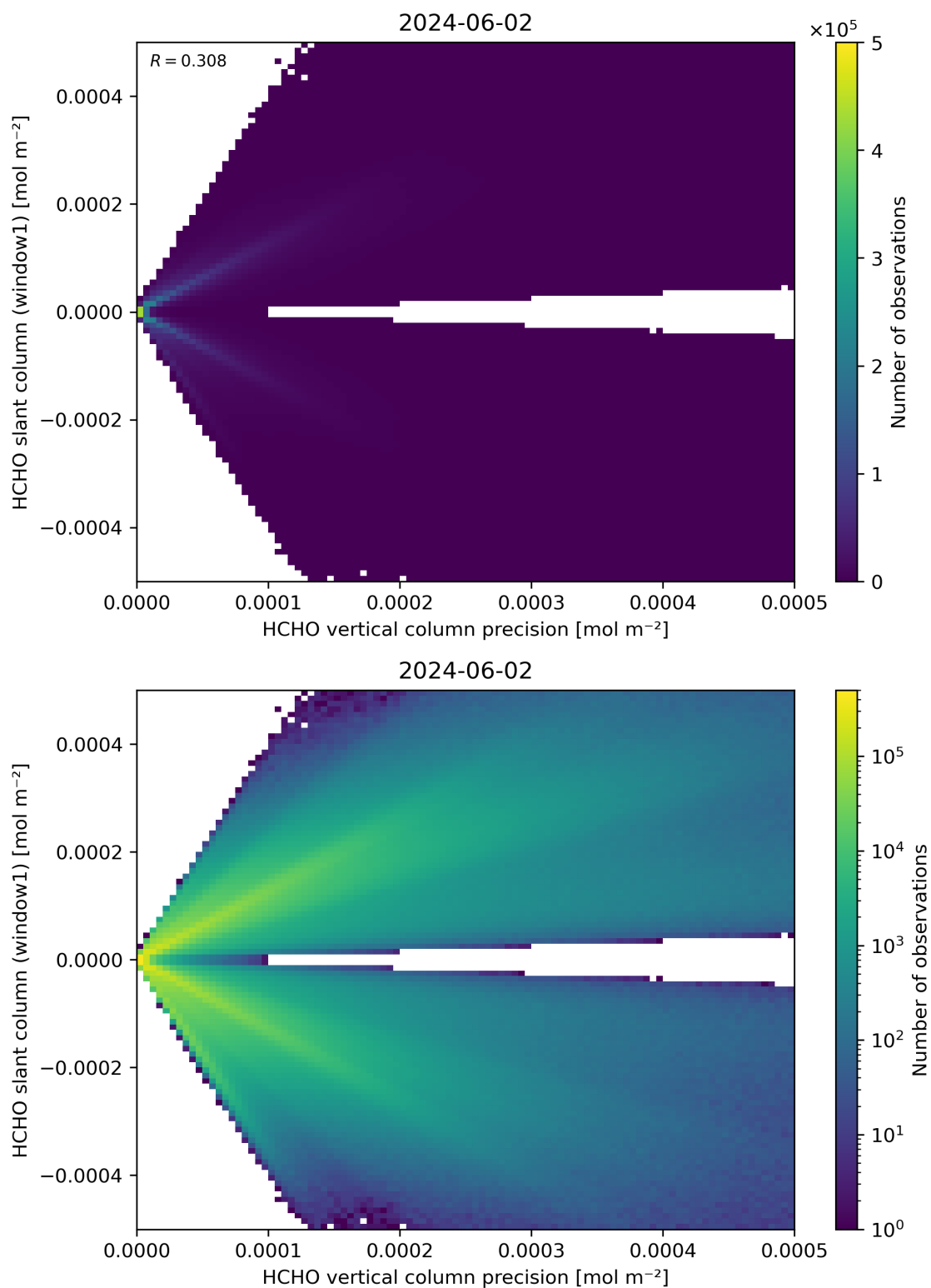
Figure 142: Scatter density plot of “HCHO vertical column precision” against “HCHO slant column (window1)” for 2024-06-01 to 2024-06-03.
