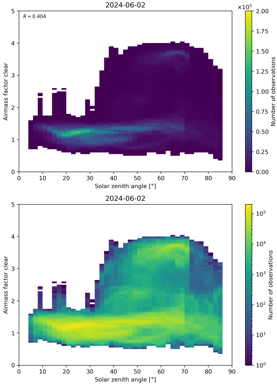
Figure 170: Scatter density plot of “Solar zenith angle” against “Airmass factor clear” for 2024-06-01 to 2024-06-03.
