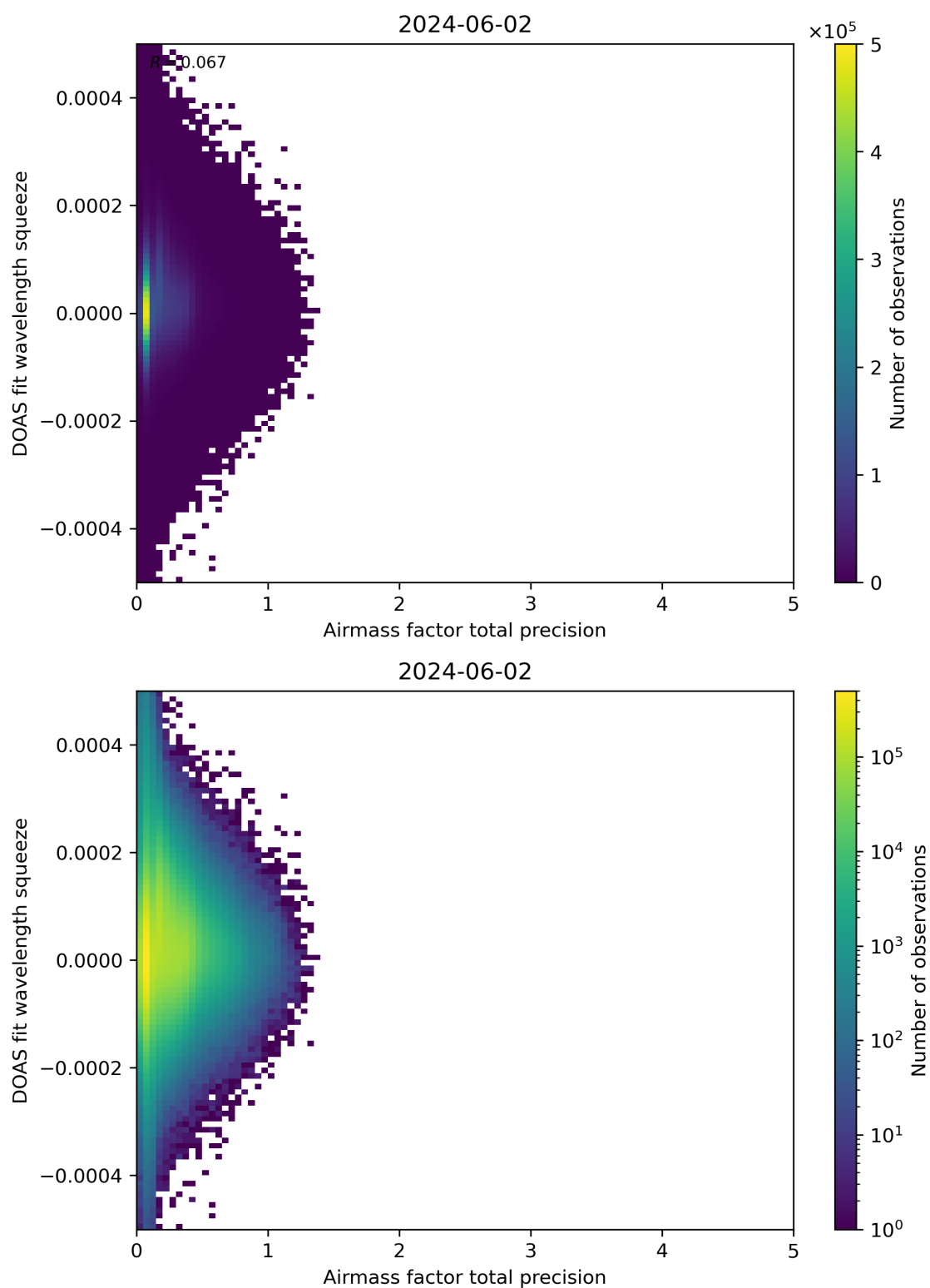
Figure 107: Scatter density plot of “Airmass factor total precision” against “DOAS fit wavelength squeeze” for 2024-06-01 to 2024-06-03.
