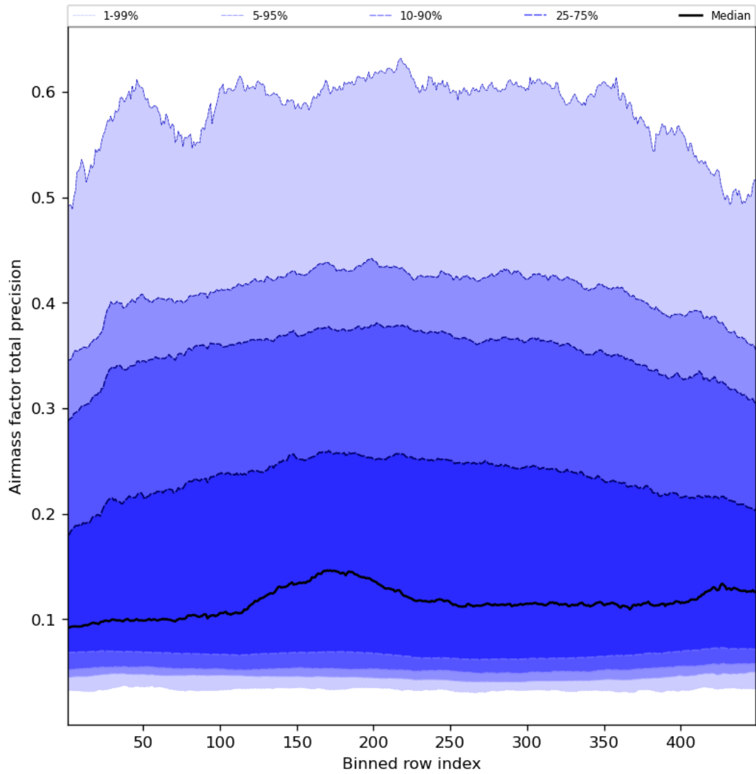
Figure 55: Along track statistics of “Airmass factor total precision” for 2024-06-01 to 2024-06-03
