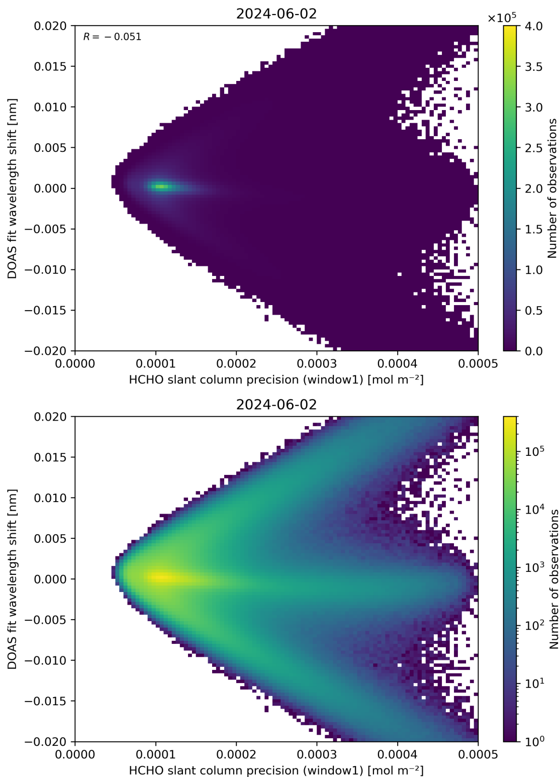
Figure 89: Scatter density plot of “HCHO slant column precision (window1)” against “DOAS fit wavelength shift” for 2024-06-01 to 2024-06-03.
