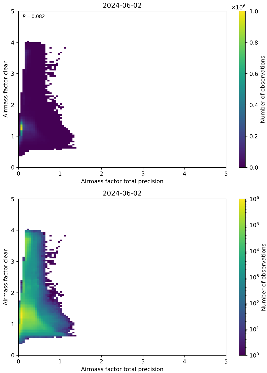
Figure 108: Scatter density plot of “Airmass factor total precision” against “Airmass factor clear” for 2024-06-01 to 2024-06-03.
