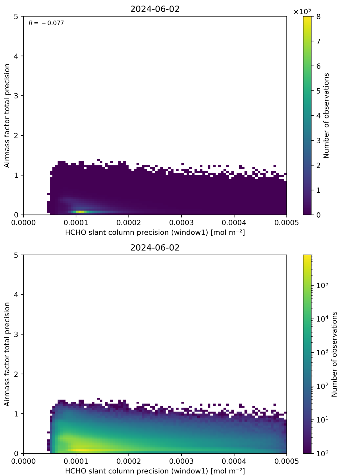
Figure 95: Scatter density plot of “HCHO slant column precision (window1)” against “Airmass factor total precision” for 2024-06-01 to 2024-06-03.
