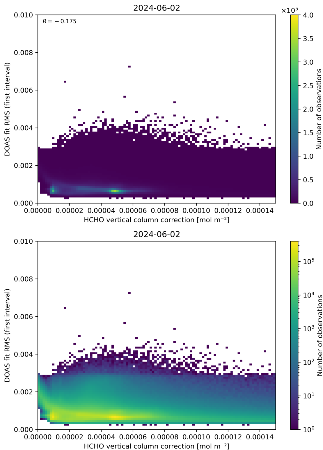
Figure 112: Scatter density plot of “HCHO vertical column correction” against “DOAS fit RMS (first interval)” for 2024-06-01 to 2024-06-03.
