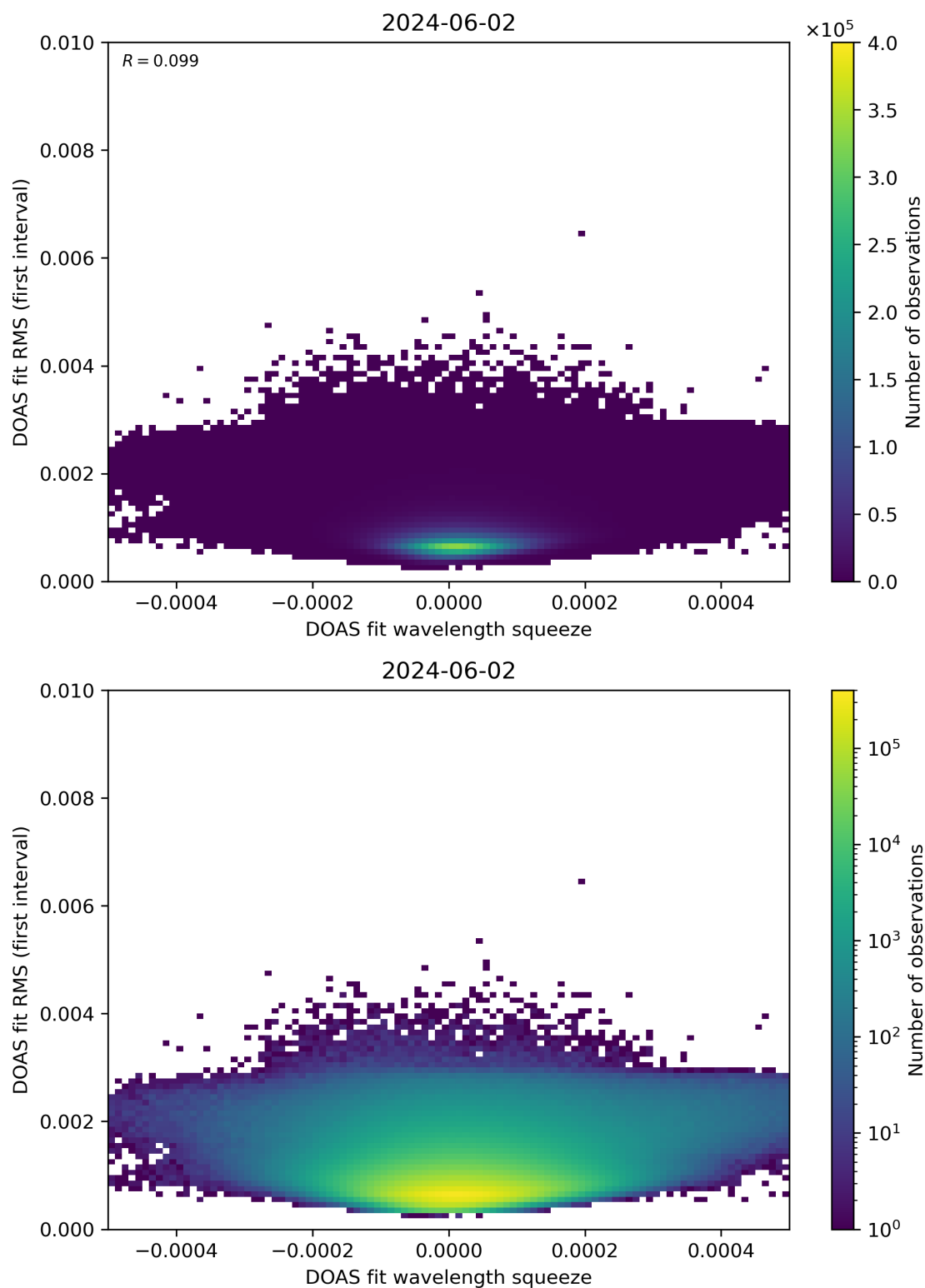
Figure 68: Scatter density plot of “DOAS fit wavelength squeeze” against “DOAS fit RMS (first interval)” for 2024-06-01 to 2024-06-03.
