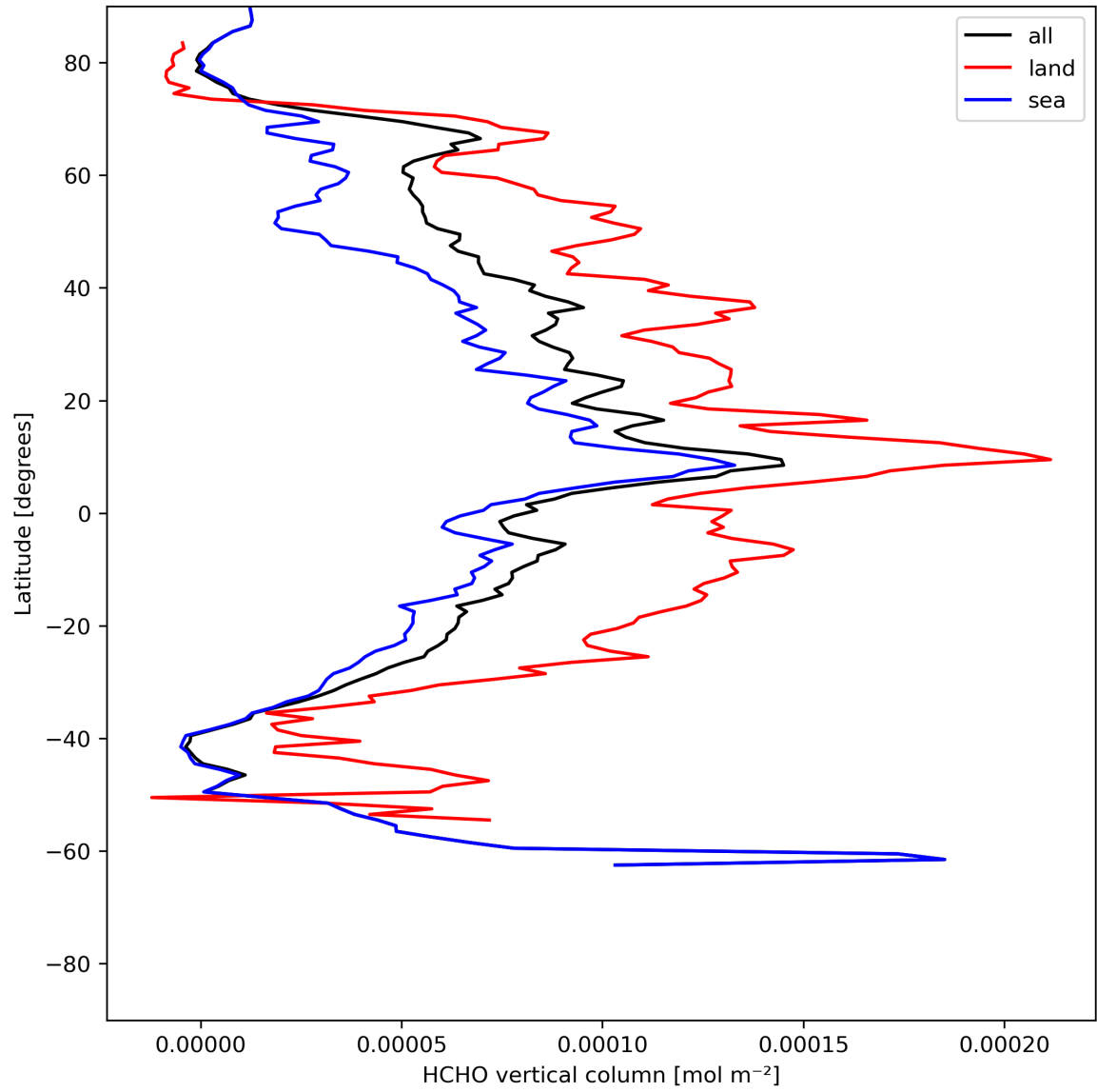
Figure 21: Zonal average of “HCHO vertical column” for 2024-06-01 to 2024-06-03.
