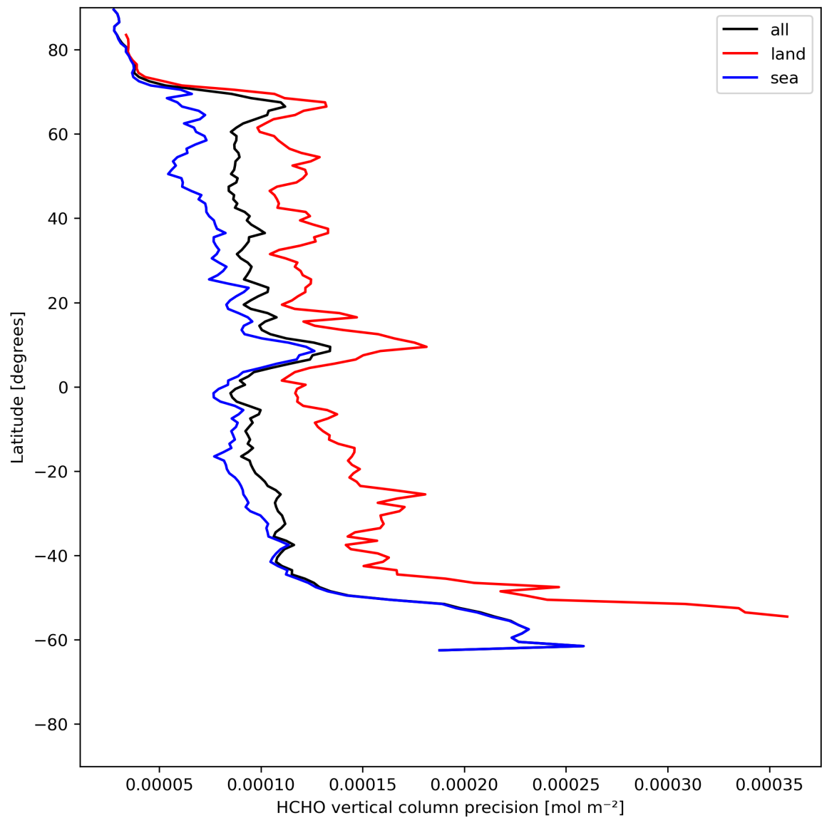
Figure 22: Zonal average of “HCHO vertical column precision” for 2024-06-01 to 2024-06-03.
