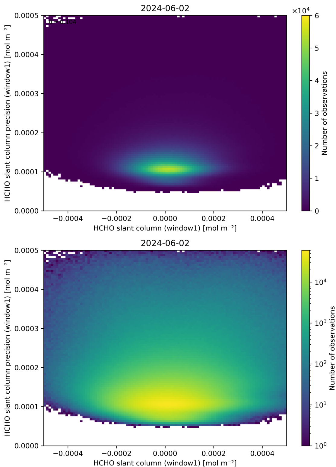
Figure 84: Scatter density plot of “HCHO slant column (window1)” against “HCHO slant column precision (window1)” for 2024-06-01 to 2024-06-03.
