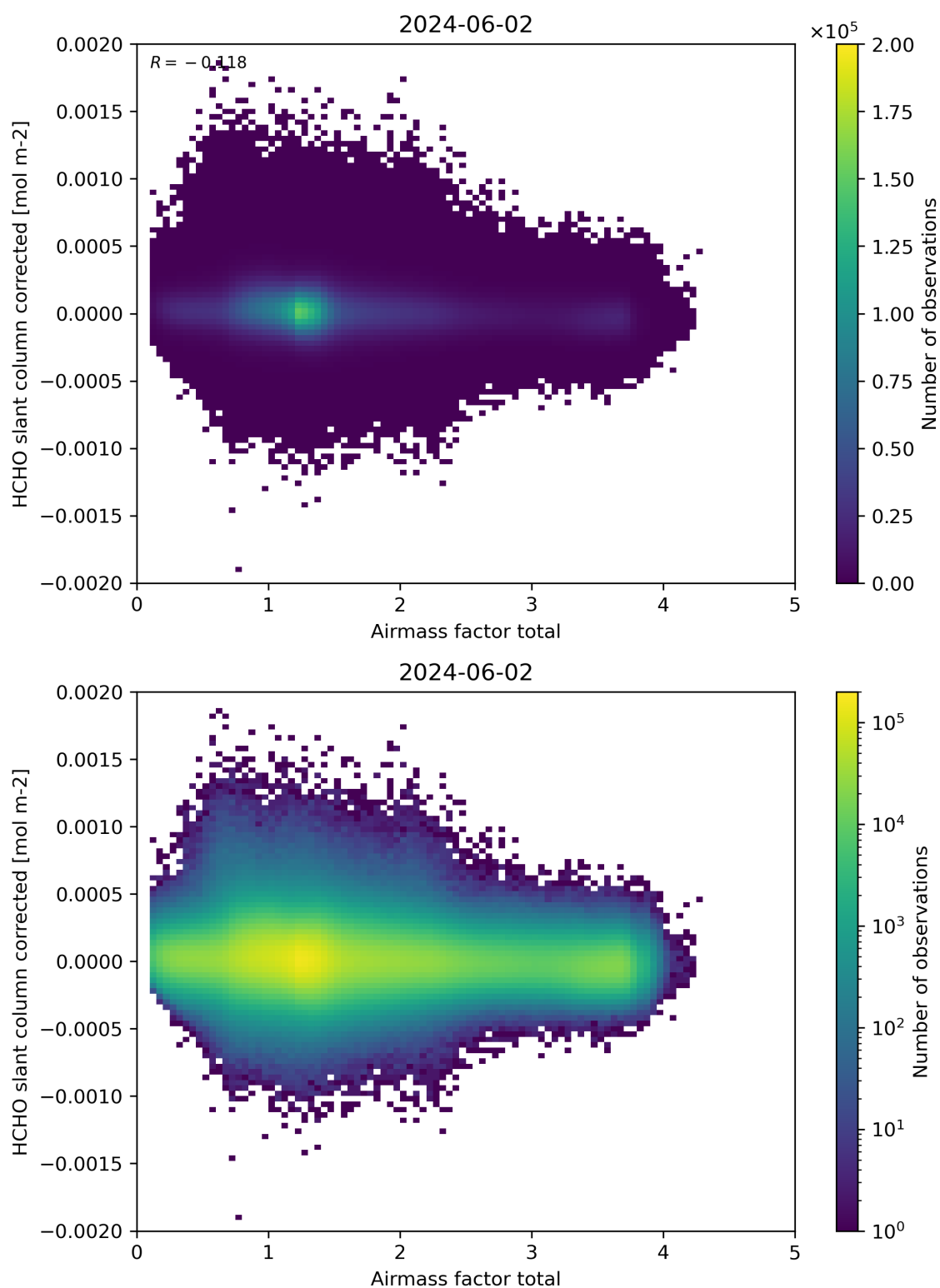
Figure 101: Scatter density plot of “Airmass factor total” against “HCHO slant column corrected” for 2024-06-01 to 2024-06-03.
