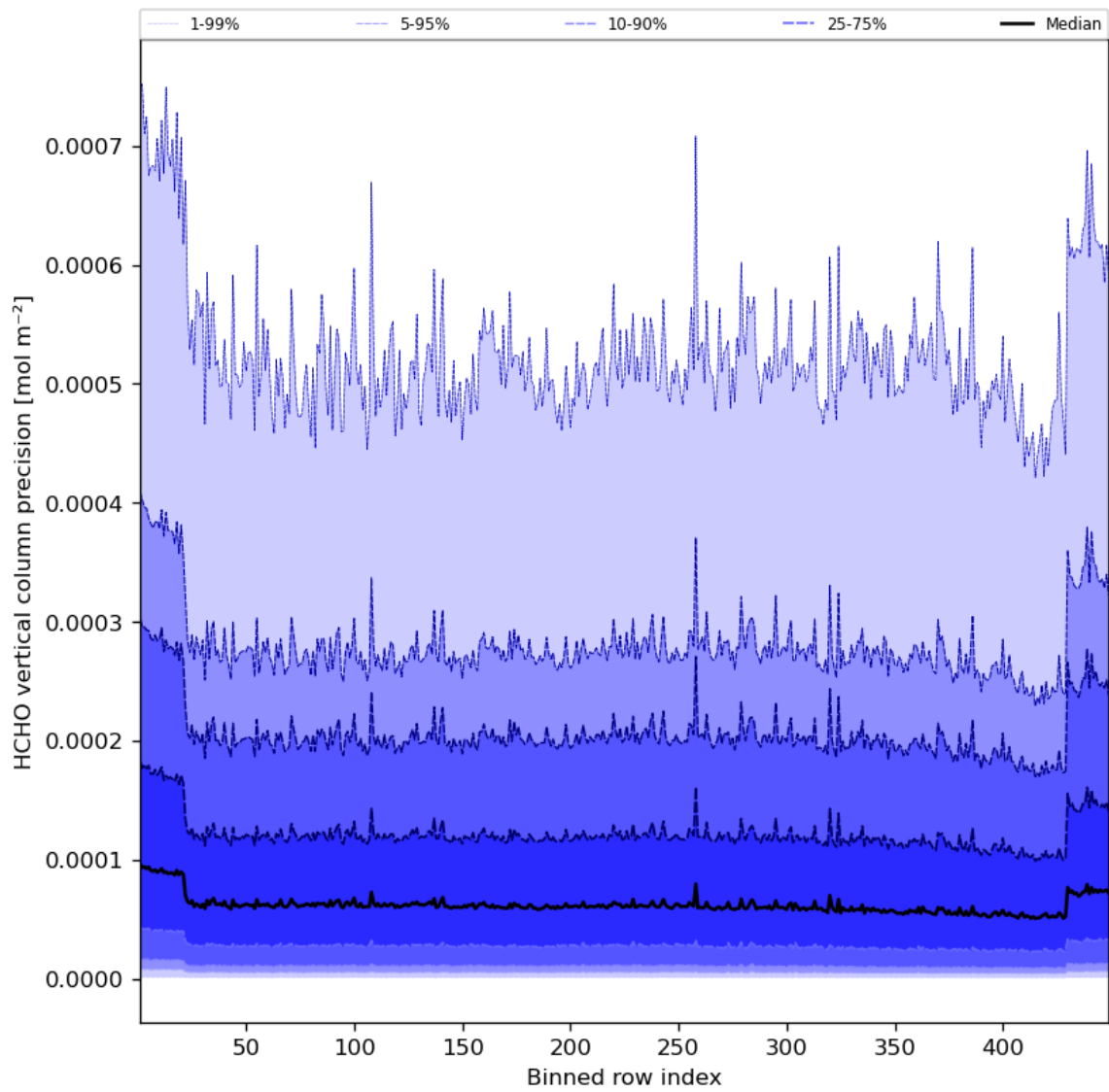
Figure 50: Along track statistics of “HCHO vertical column precision” for 2024-06-01 to 2024-06-03
