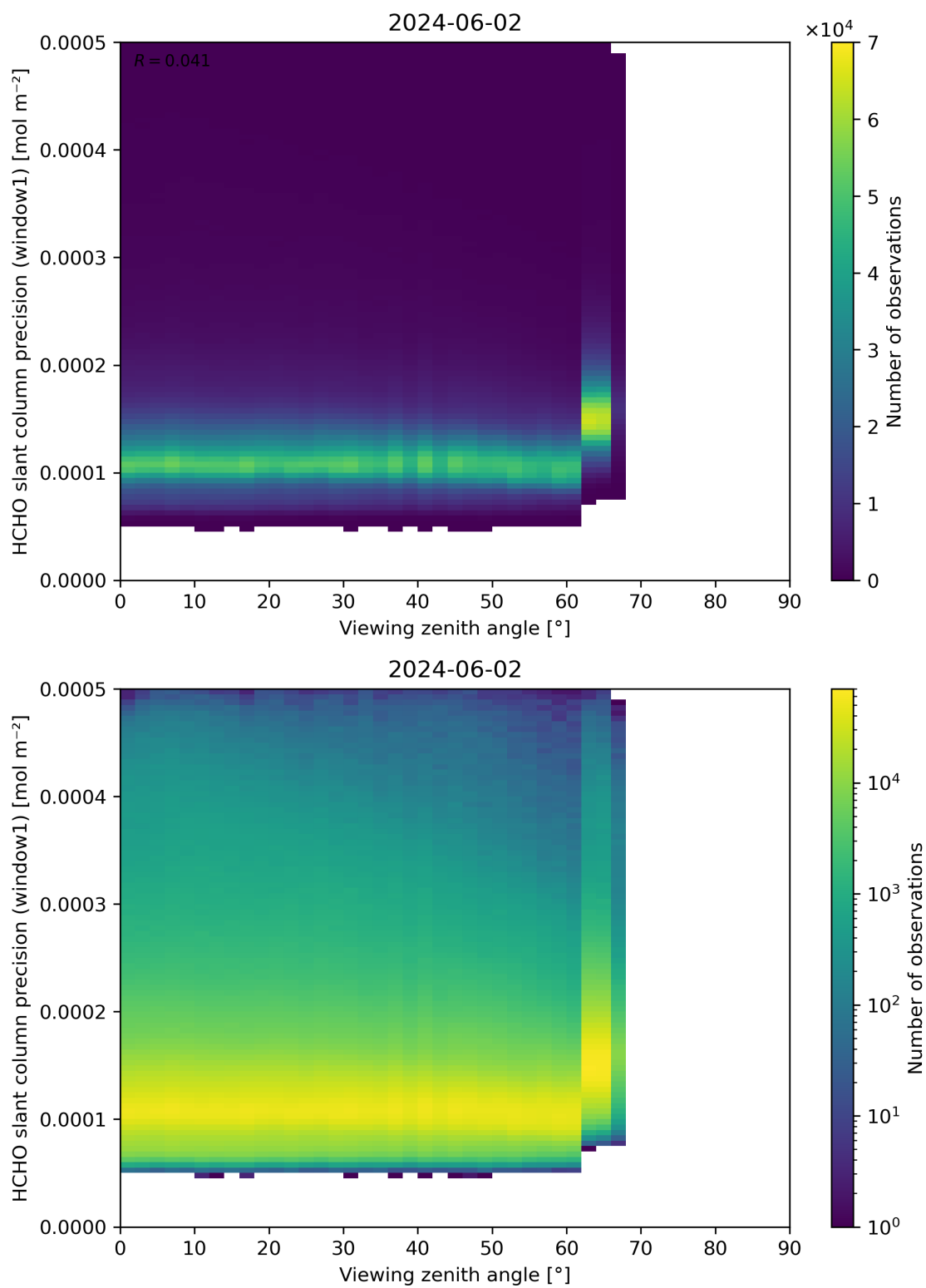
Figure 189: Scatter density plot of “Viewing zenith angle” against “HCHO slant column precision (window1)” for 2024-06-01 to 2024-06-03.
