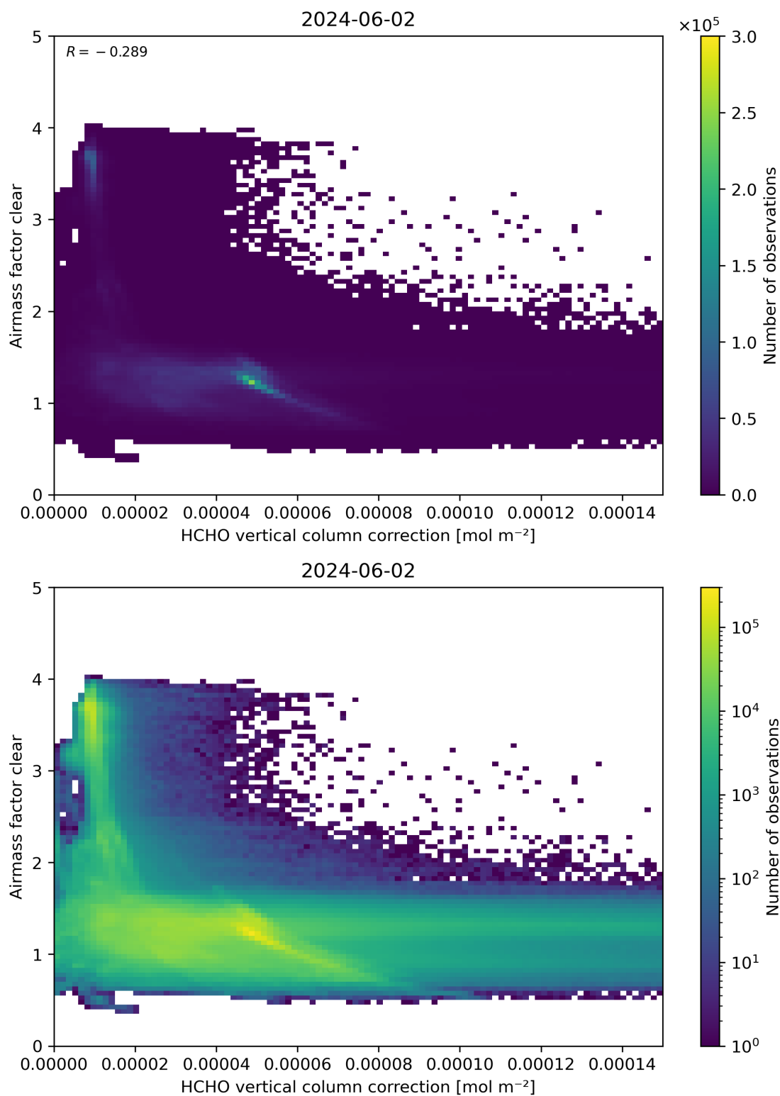
Figure 115: Scatter density plot of “HCHO vertical column correction” against “Airmass factor clear” for 2024-06-01 to 2024-06-03.
