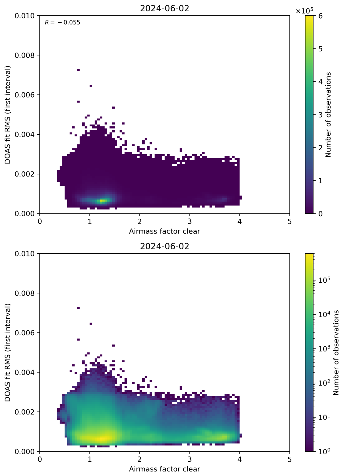
Figure 71: Scatter density plot of “Airmass factor clear” against “DOAS fit RMS (first interval)” for 2024-06-01 to 2024-06-03.
