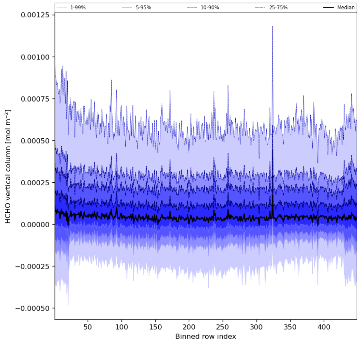
Figure 49: Along track statistics of “HCHO vertical column” for 2024-06-01 to 2024-06-03
