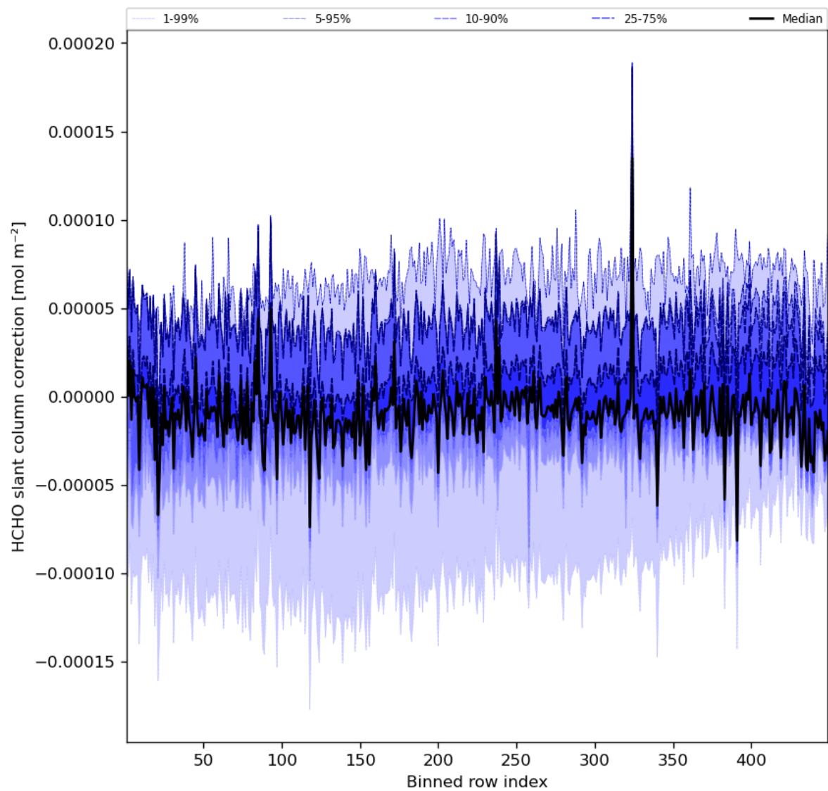
Figure 61: Along track statistics of “HCHO slant column correction” for 2024-06-01 to 2024-06-03
