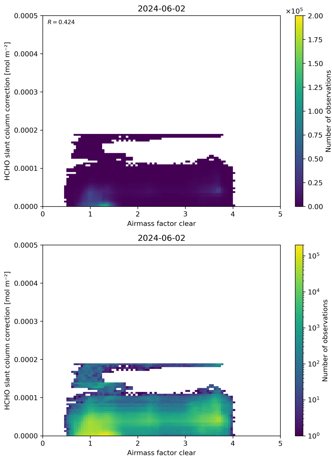
Figure 75: Scatter density plot of “Airmass factor clear” against “HCHO slant column correction” for 2024-06-01 to 2024-06-03.
