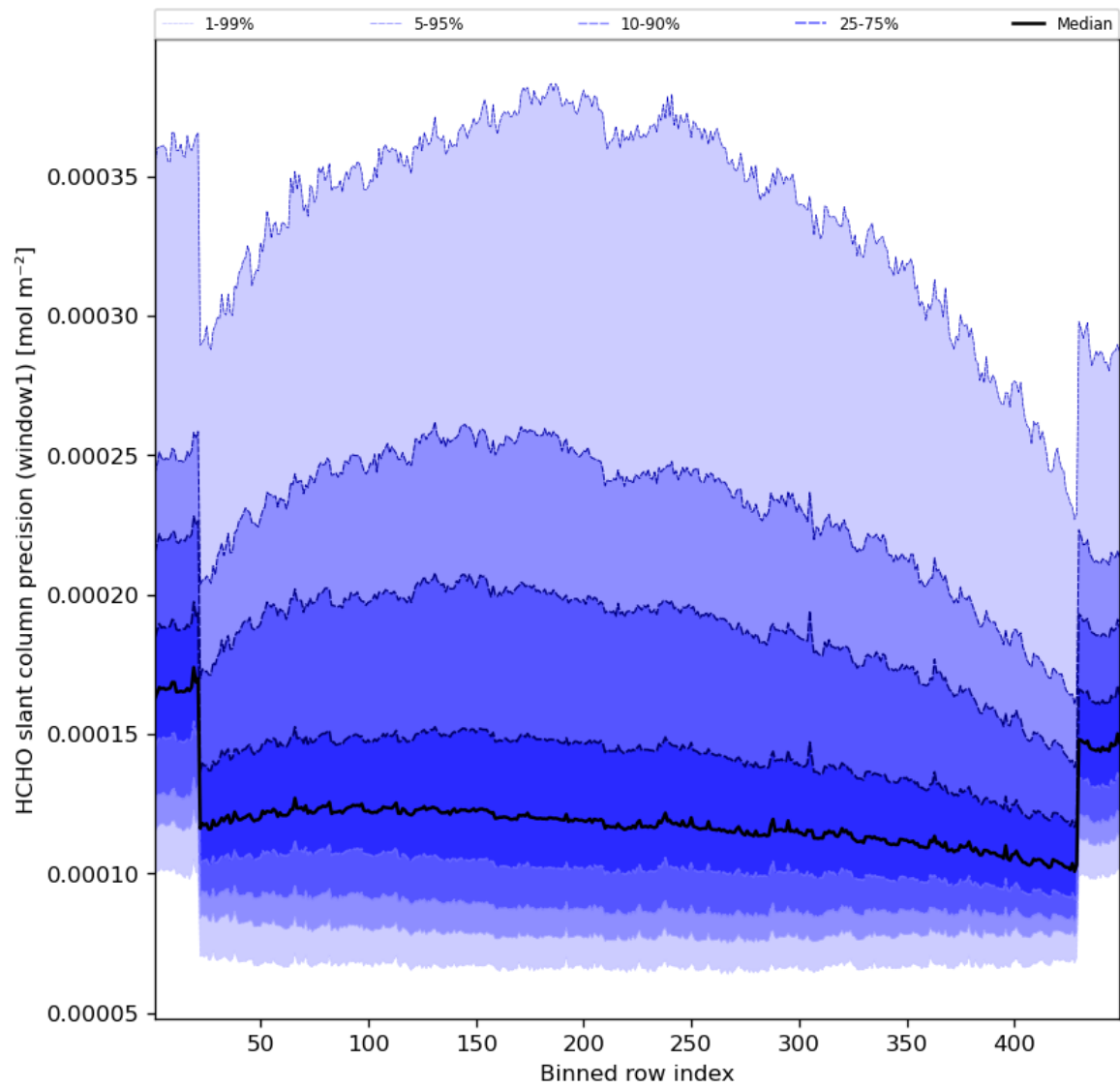
Figure 53: Along track statistics of “HCHO slant column precision (window1)” for 2024-06-01 to 2024-06-03
