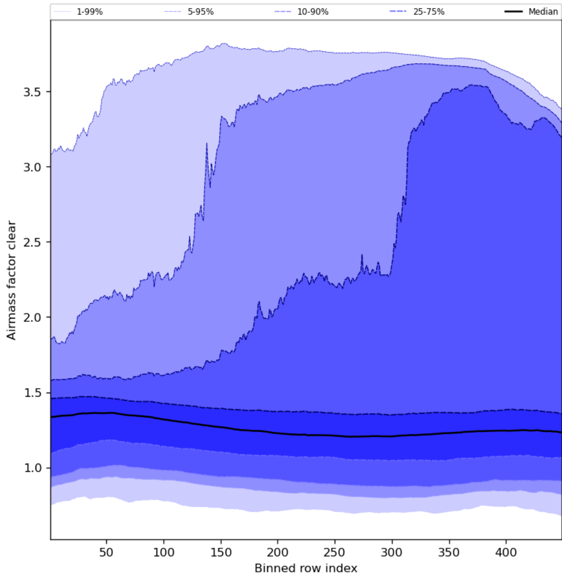
Figure 56: Along track statistics of “Airmass factor clear” for 2024-06-01 to 2024-06-03
