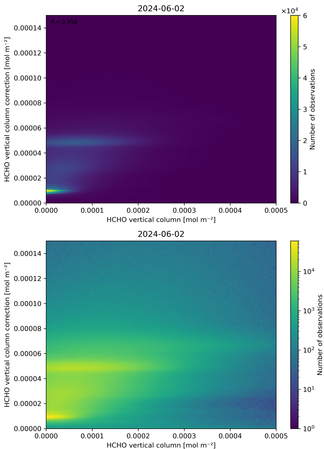
Figure 133: Scatter density plot of “HCHO vertical column” against “HCHO vertical column correction” for 2024-06-01 to 2024-06-03.
