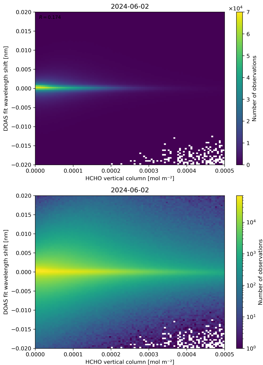
Figure 124: Scatter density plot of “HCHO vertical column” against “DOAS fit wavelength shift” for 2024-06-01 to 2024-06-03.
