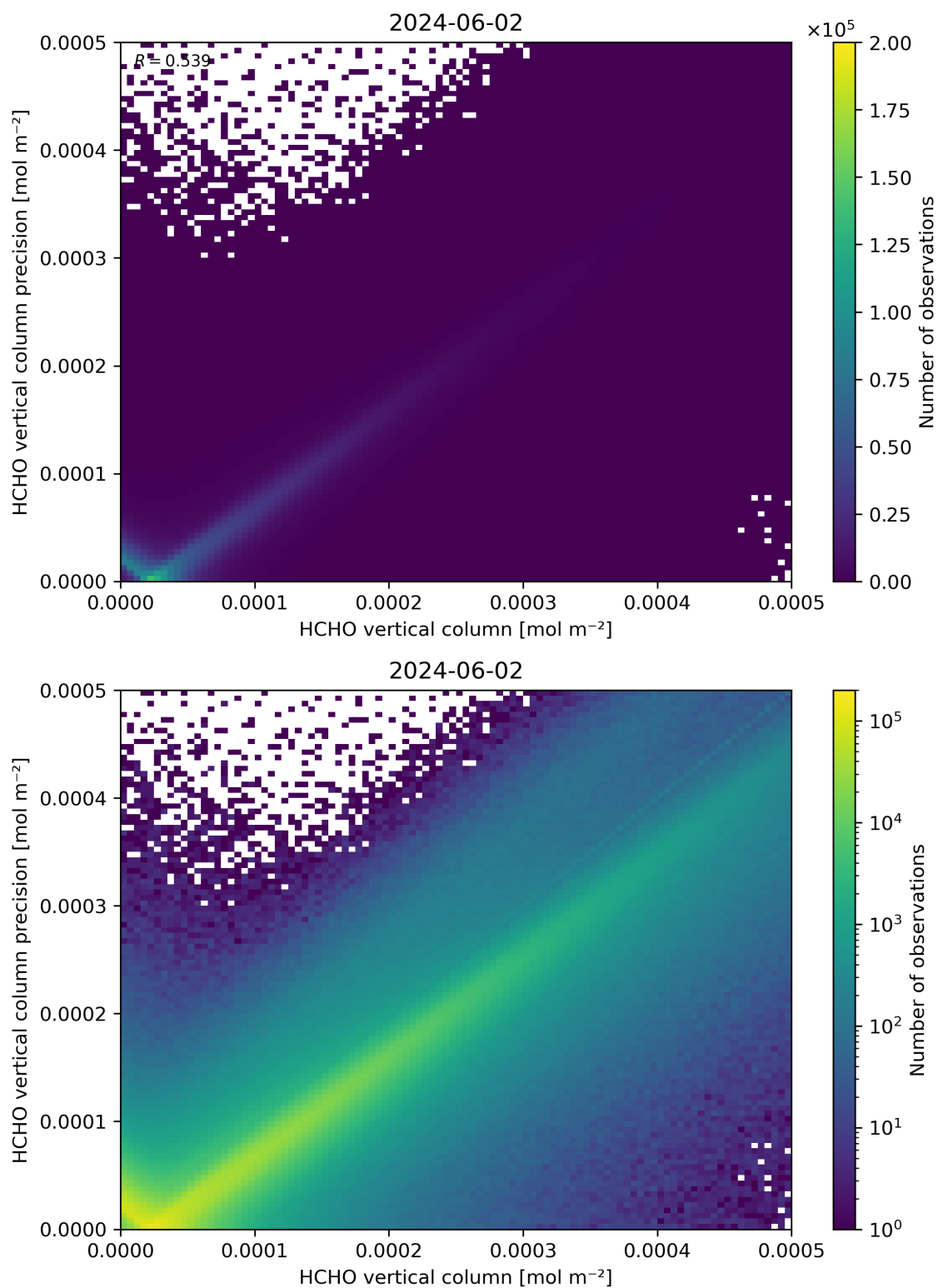
Figure 134: Scatter density plot of “HCHO vertical column” against “HCHO vertical column precision” for 2024-06-01 to 2024-06-03.
