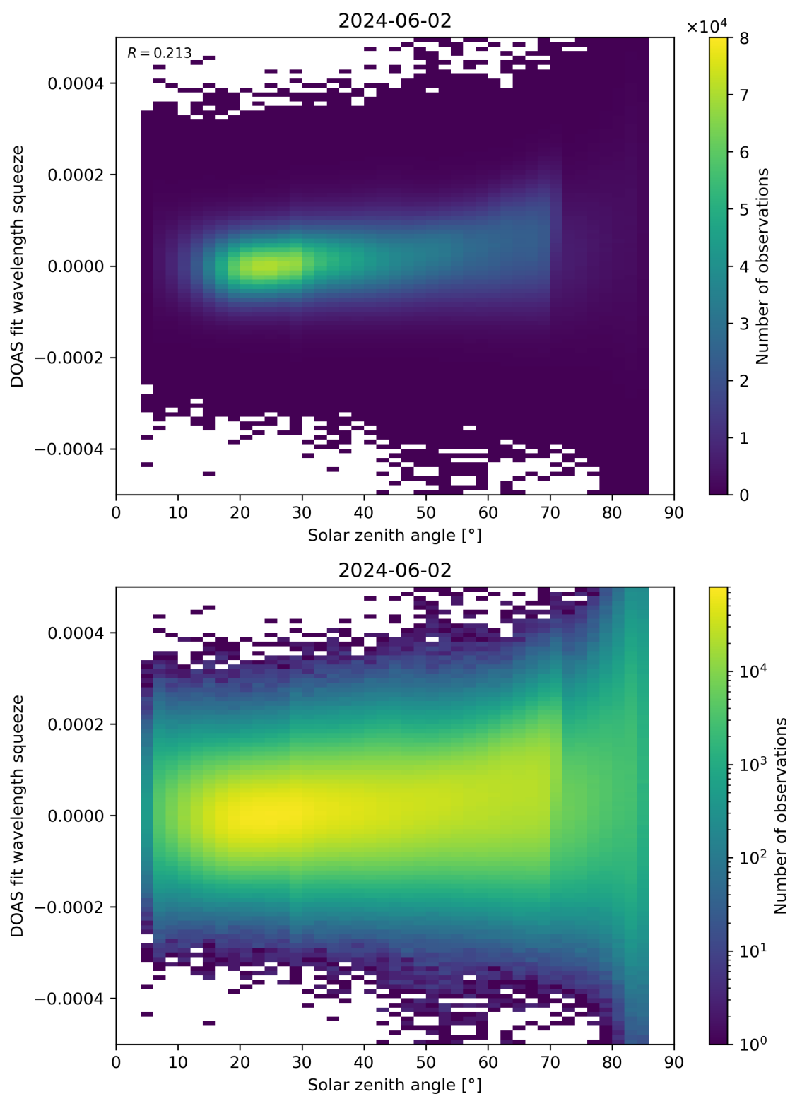
Figure 169: Scatter density plot of “Solar zenith angle” against “DOAS fit wavelength squeeze” for 2024-06-01 to 2024-06-03.
