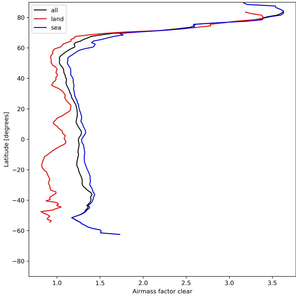
Figure 28: Zonal average of “Airmass factor clear” for 2024-06-01 to 2024-06-03.
