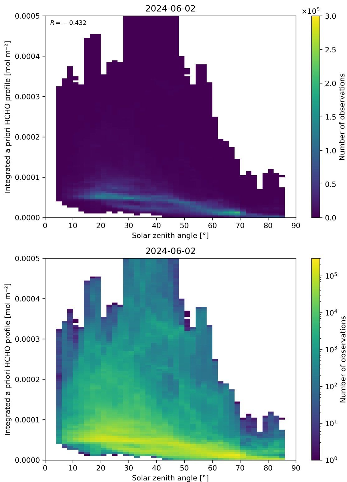
Figure 180: Scatter density plot of “Solar zenith angle” against “Integrated a priori HCHO profile” for 2024-06-01 to 2024-06-03.
