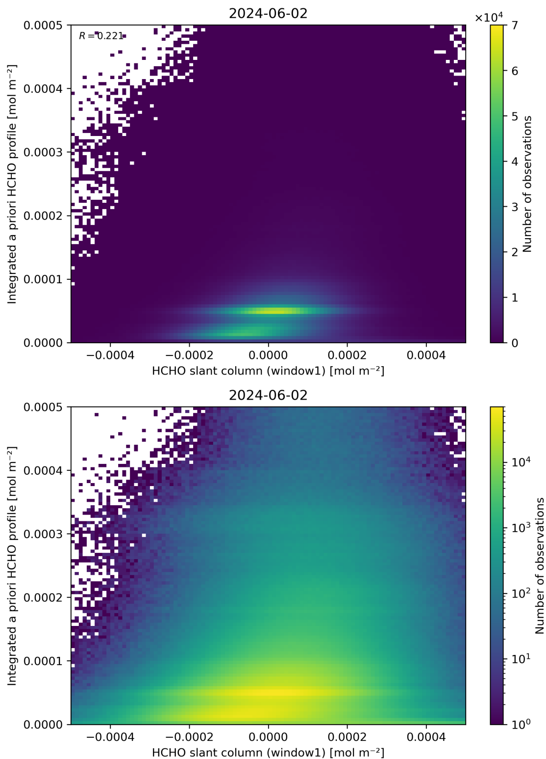
Figure 87: Scatter density plot of “HCHO slant column (window1)” against “Integrated a priori HCHO profile” for 2024-06-01 to 2024-06-03.
