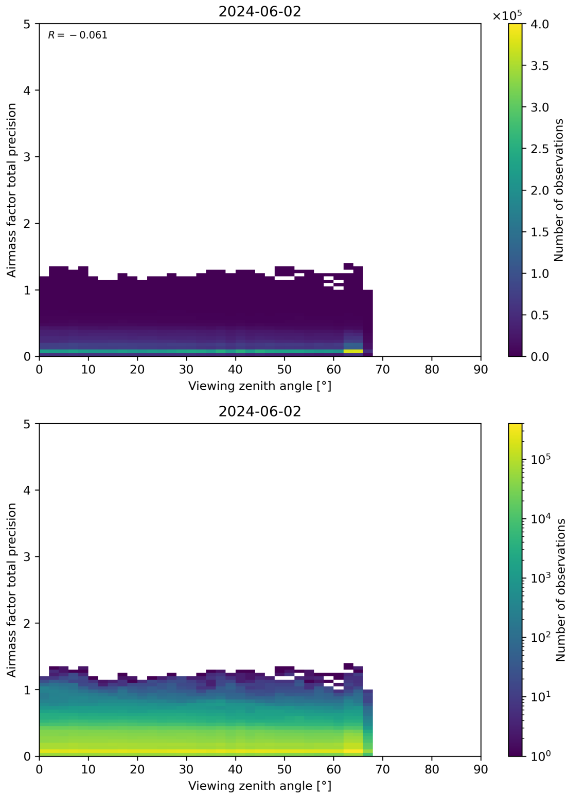
Figure 191: Scatter density plot of “Viewing zenith angle” against “Airmass factor total precision” for 2024-06-01 to 2024-06-03.
