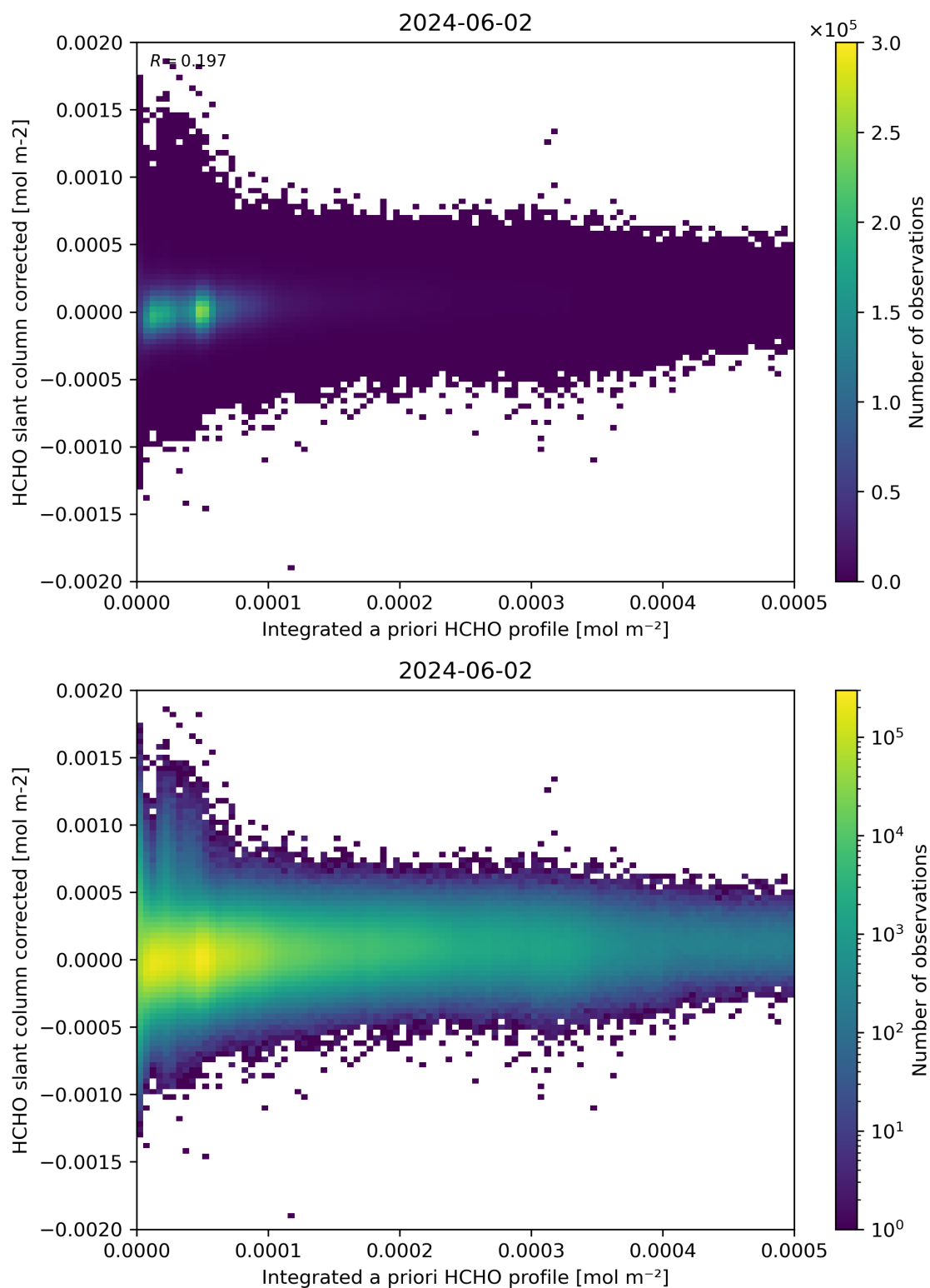
Figure 151: Scatter density plot of “Integrated a priori HCHO profile” against “HCHO slant column corrected” for 2024-06-01 to 2024-06-03.
