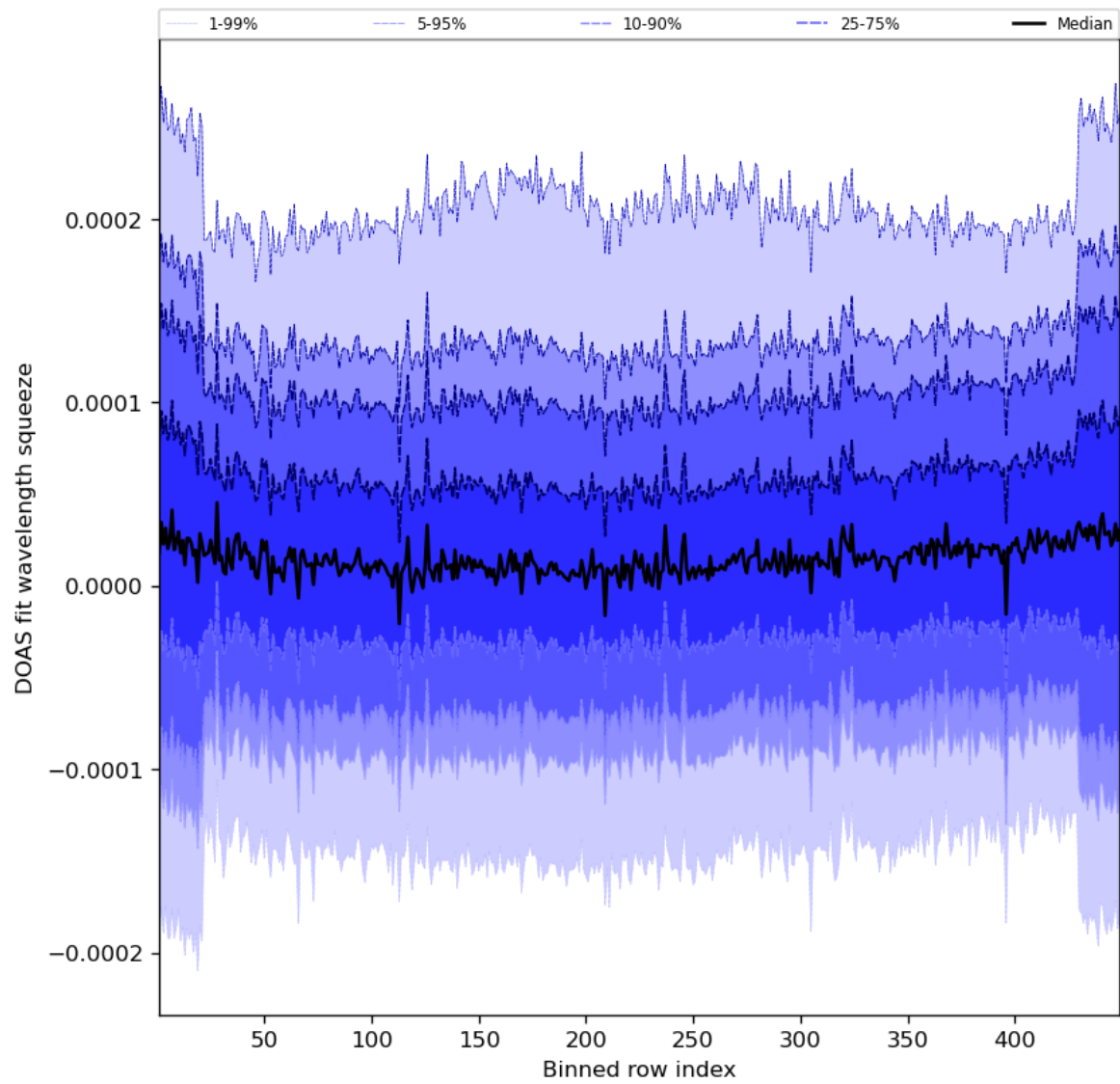
Figure 59: Along track statistics of “DOAS fit wavelength squeeze” for 2024-06-01 to 2024-06-03
