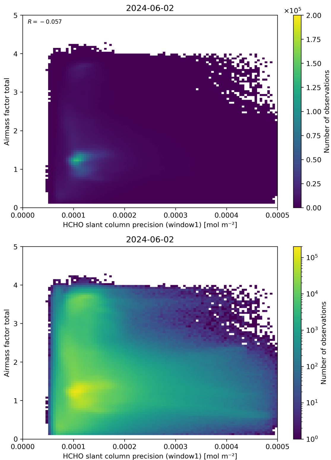
Figure 94: Scatter density plot of “HCHO slant column precision (window1)” against “Airmass factor total” for 2024-06-01 to 2024-06-03.
