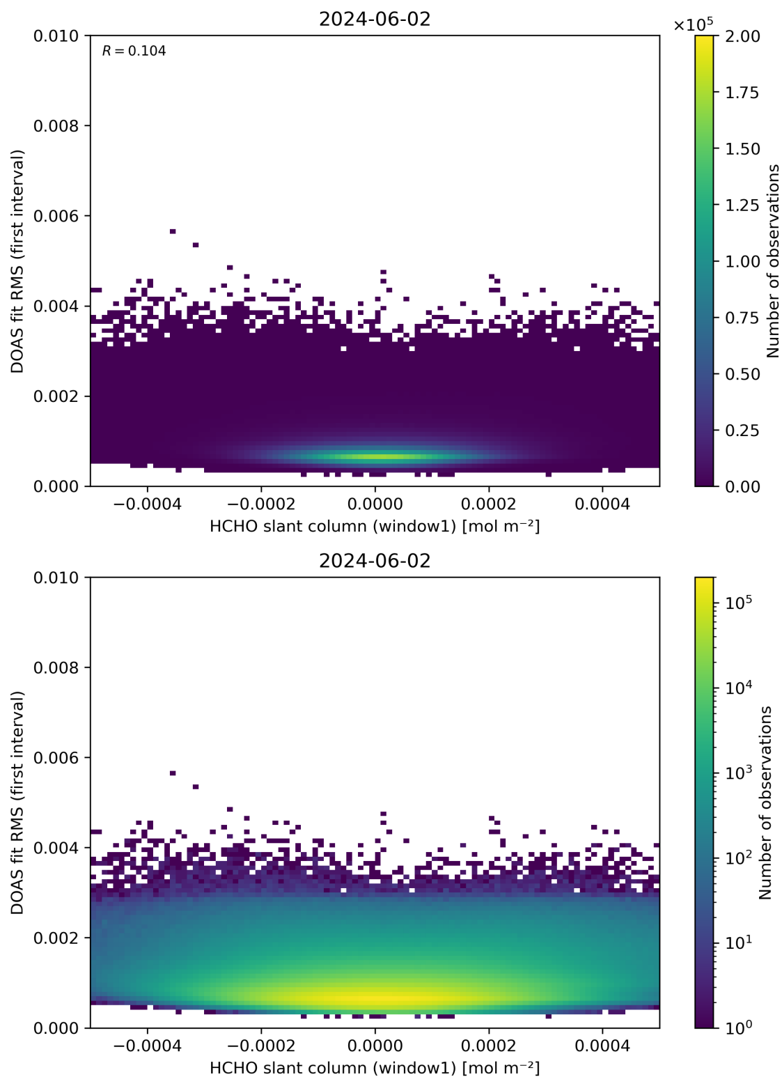
Figure 78: Scatter density plot of “HCHO slant column (window1)” against “DOAS fit RMS (first interval)” for 2024-06-01 to 2024-06-03.
