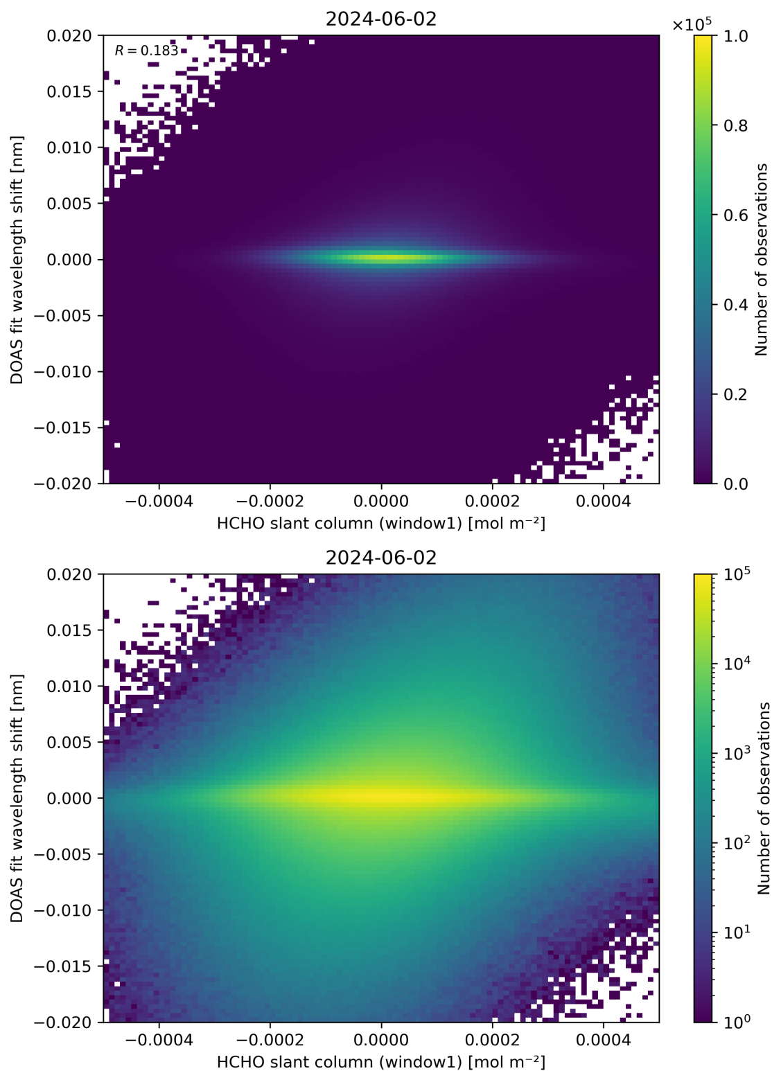
Figure 79: Scatter density plot of “HCHO slant column (window1)” against “DOAS fit wavelength shift” for 2024-06-01 to 2024-06-03.
