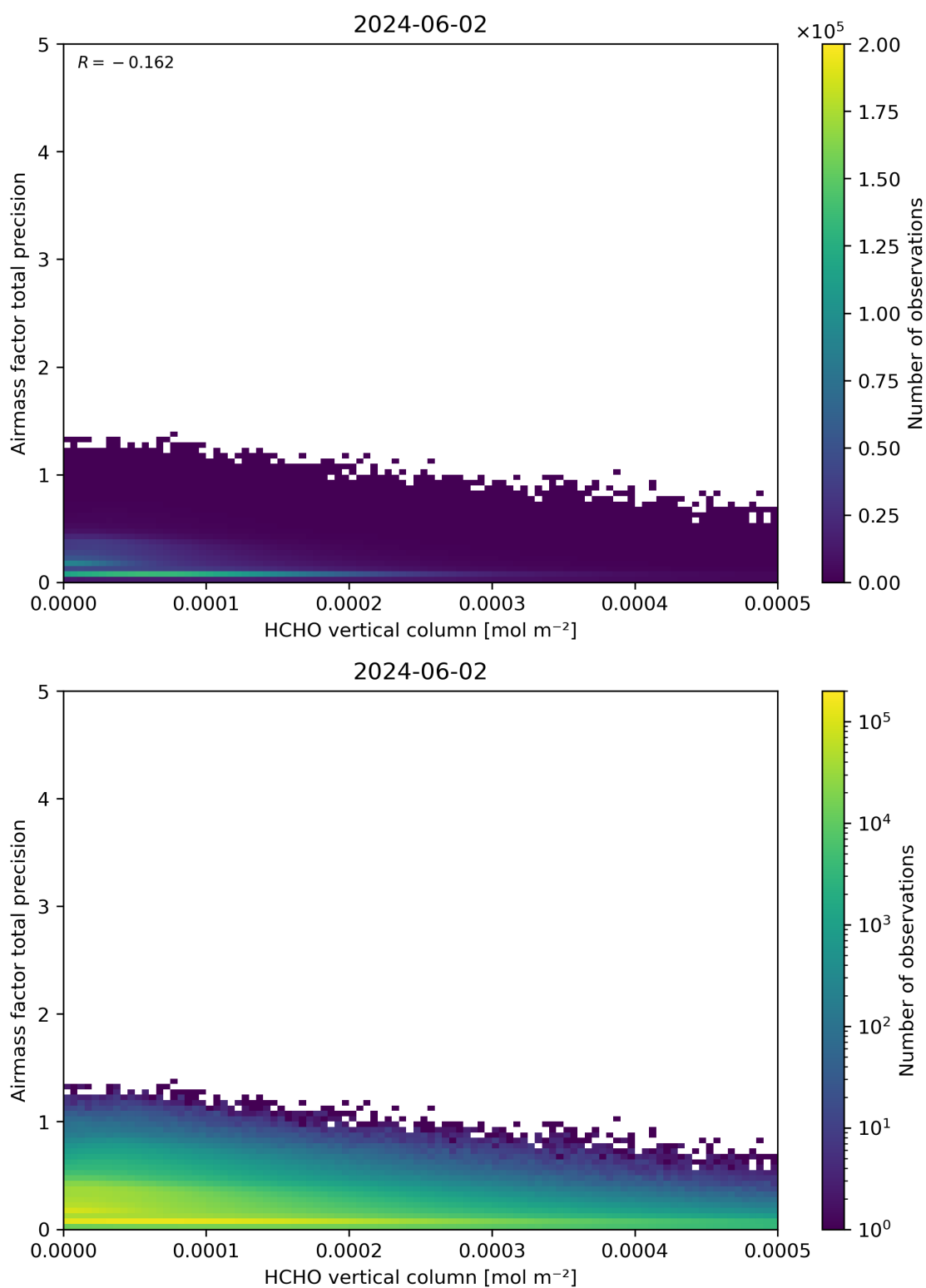
Figure 132: Scatter density plot of “HCHO vertical column” against “Airmass factor total precision” for 2024-06-01 to 2024-06-03.
