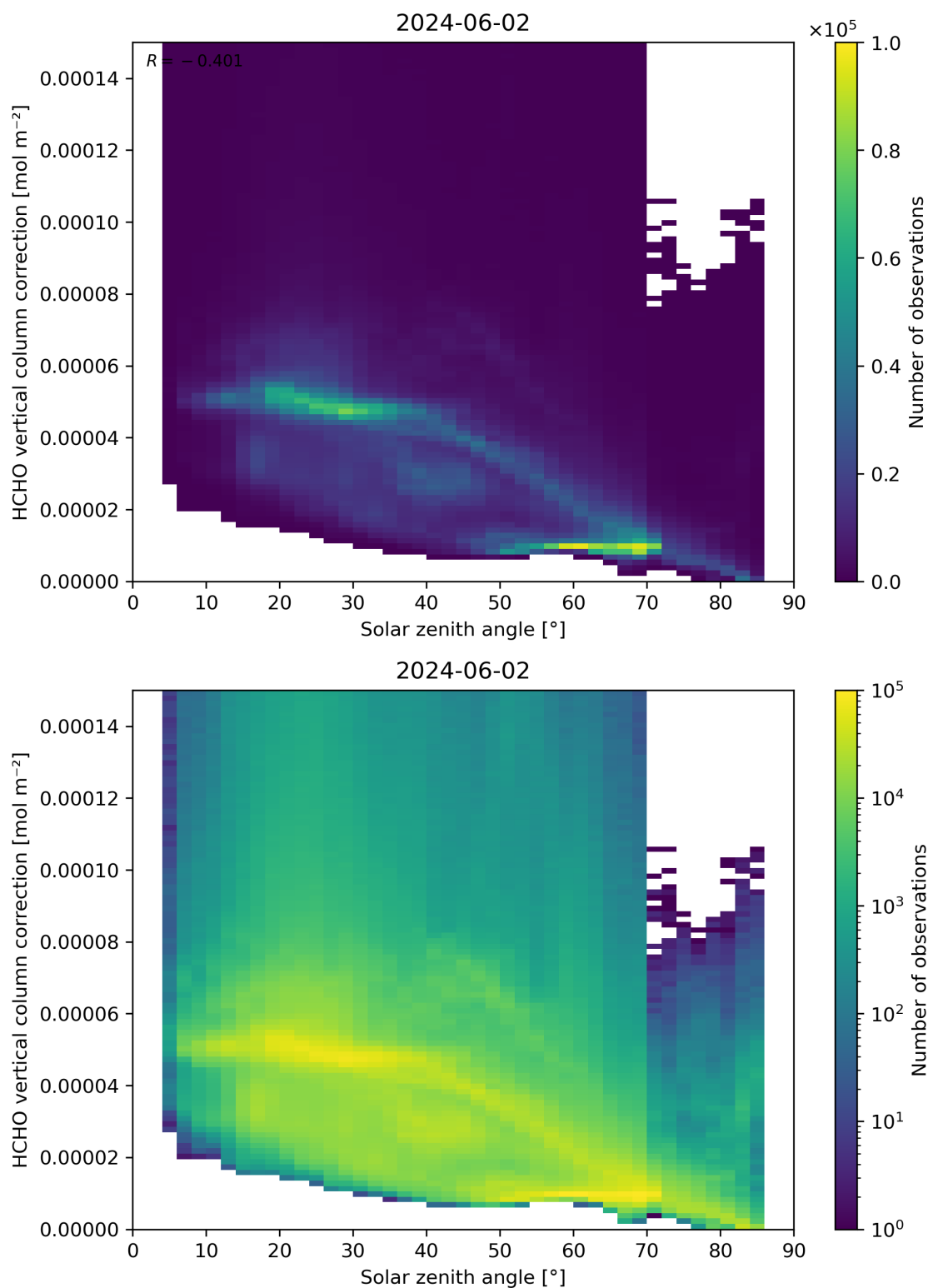
Figure 178: Scatter density plot of “Solar zenith angle” against “HCHO vertical column correction” for 2024-06-01 to 2024-06-03.
