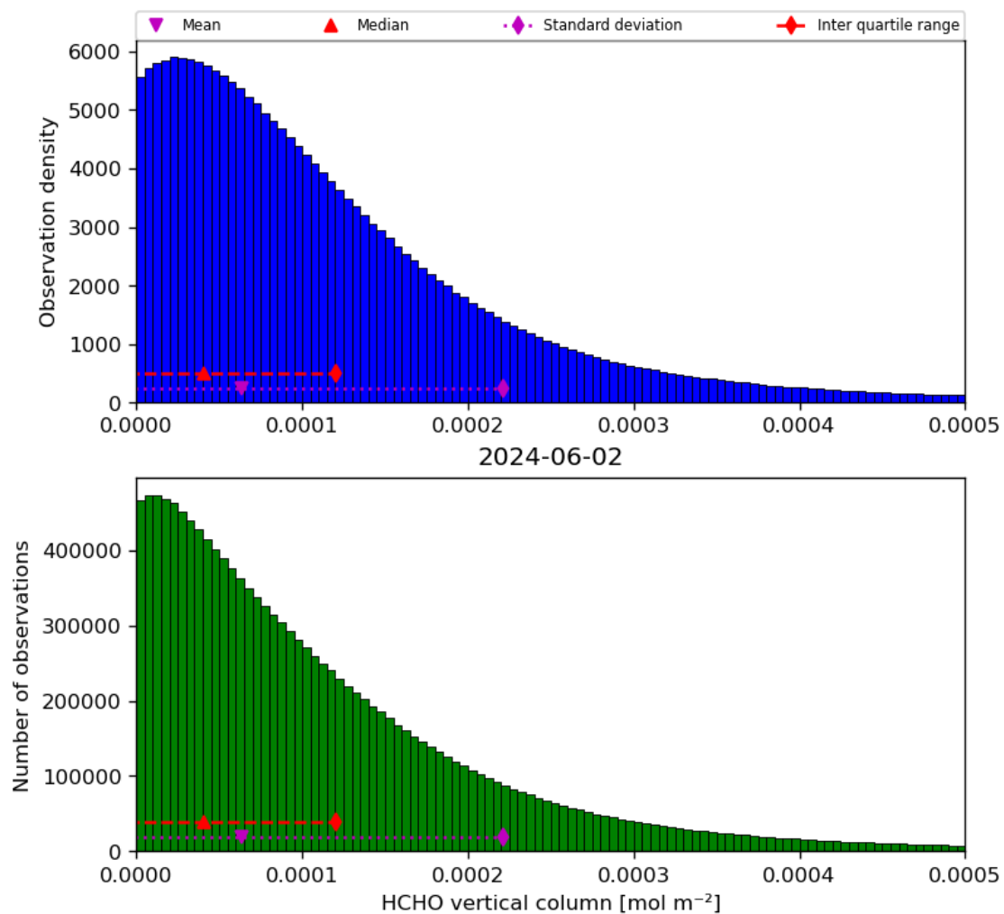
Figure 35: Histogram of “HCHO vertical column” for 2024-06-01 to 2024-06-03
