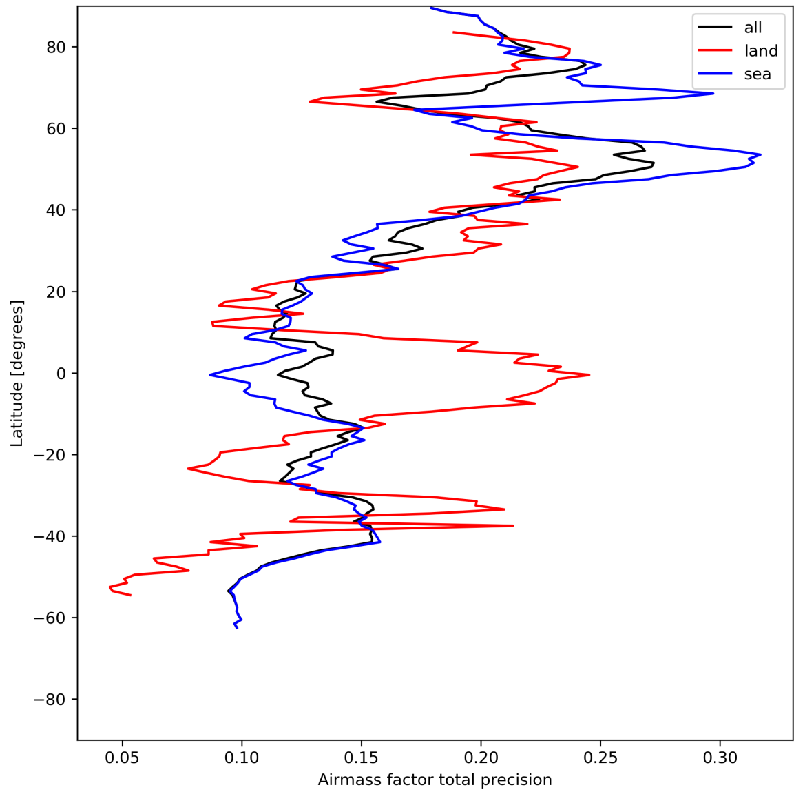
Figure 27: Zonal average of “Airmass factor total precision” for 2024-06-01 to 2024-06-03.
