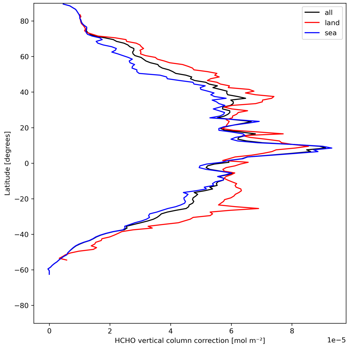
Figure 23: Zonal average of “HCHO vertical column correction” for 2024-06-01 to 2024-06-03.
