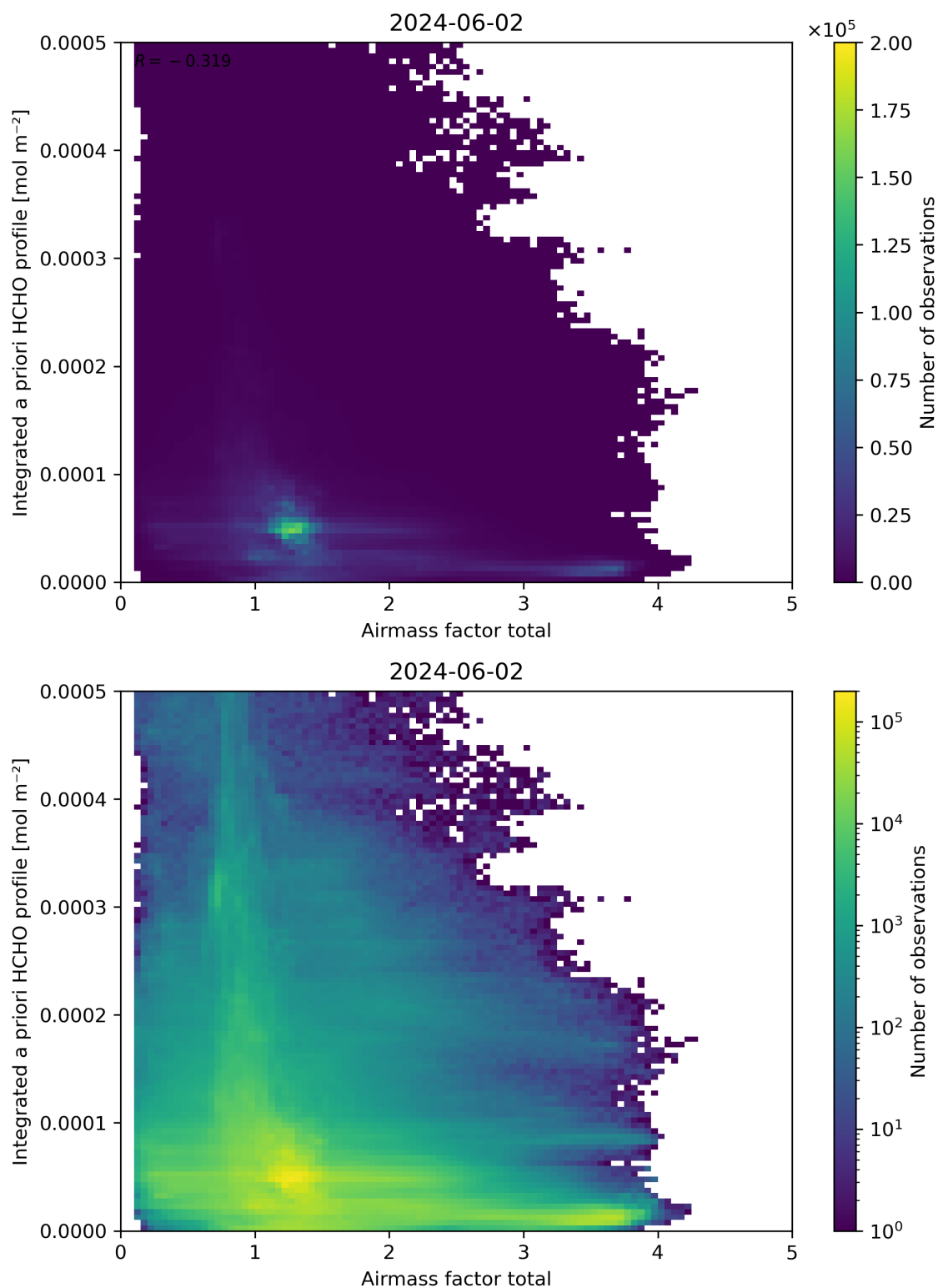
Figure 104: Scatter density plot of “Airmass factor total” against “Integrated a priori HCHO profile” for 2024-06-01 to 2024-06-03.
