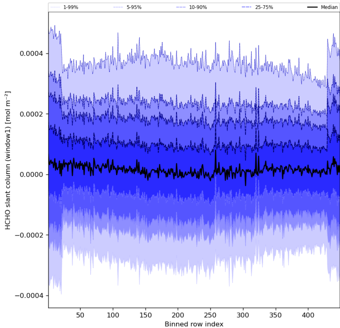
Figure 52: Along track statistics of “HCHO slant column (window1)” for 2024-06-01 to 2024-06-03
