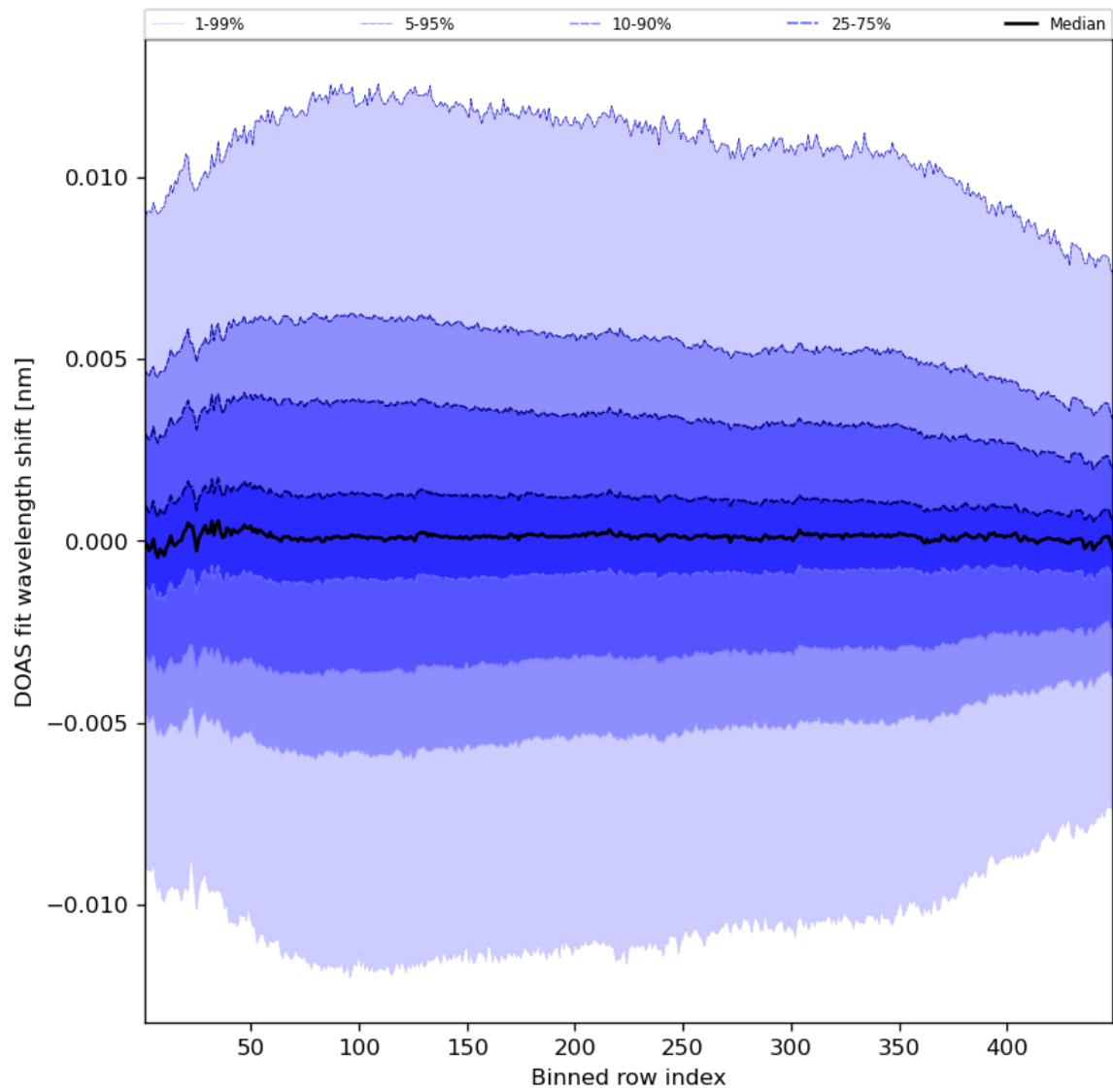
Figure 58: Along track statistics of “DOAS fit wavelength shift” for 2024-06-01 to 2024-06-03
