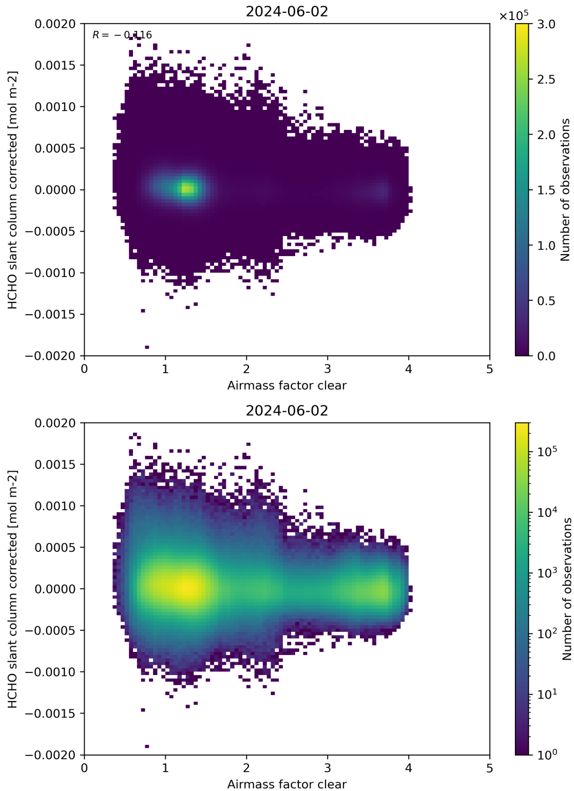
Figure 74: Scatter density plot of “Airmass factor clear” against “HCHO slant column corrected” for 2024-06-01 to 2024-06-03.
