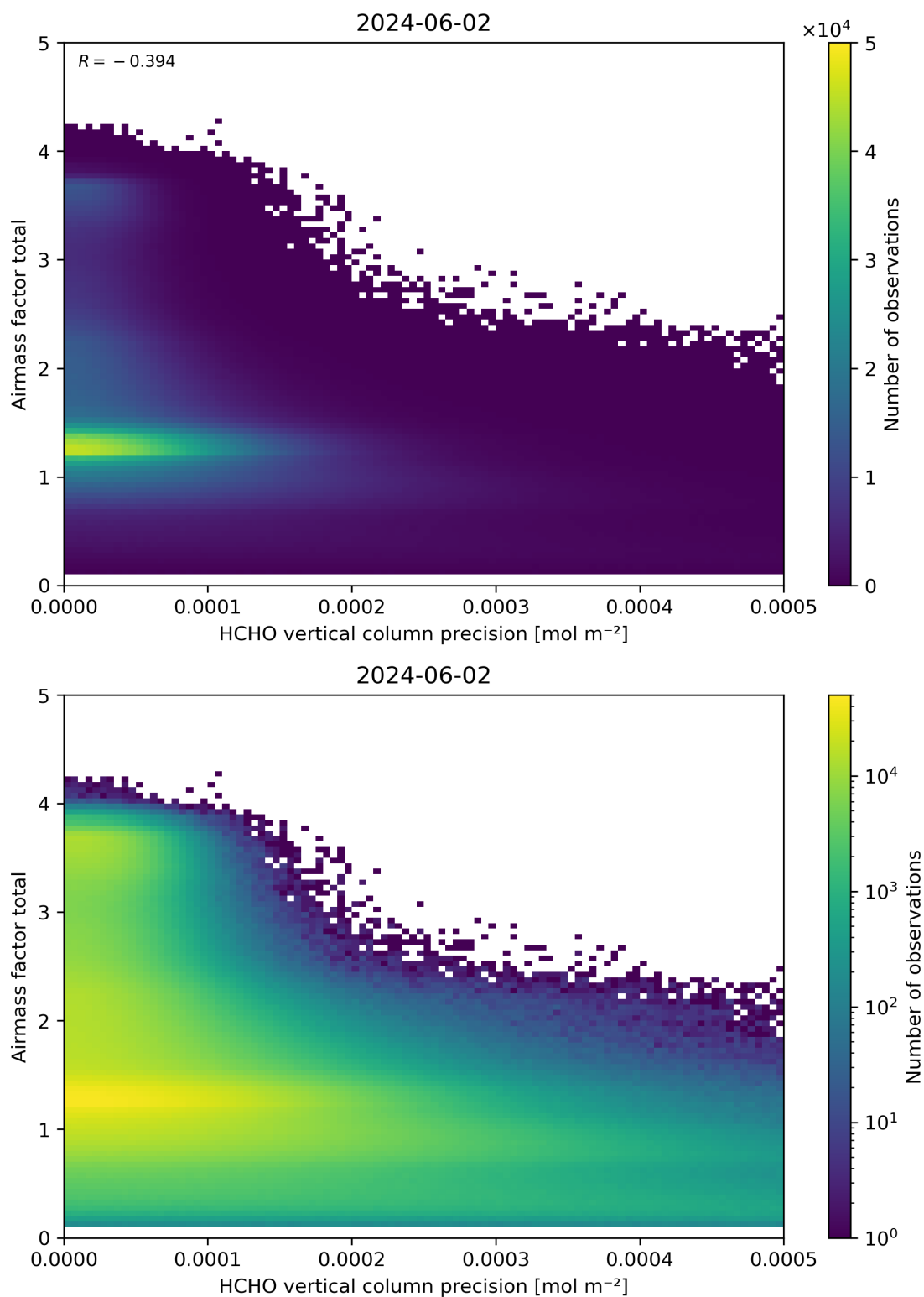
Figure 144: Scatter density plot of “HCHO vertical column precision” against “Airmass factor total” for 2024-06-01 to 2024-06-03.
