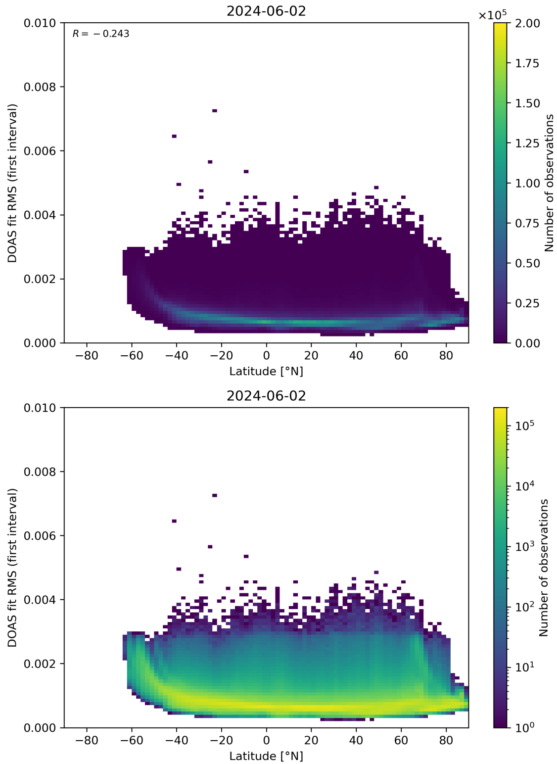
Figure 153: Scatter density plot of “Latitude” against “DOAS fit RMS (first interval)” for 2024-06-01 to 2024-06-03.
