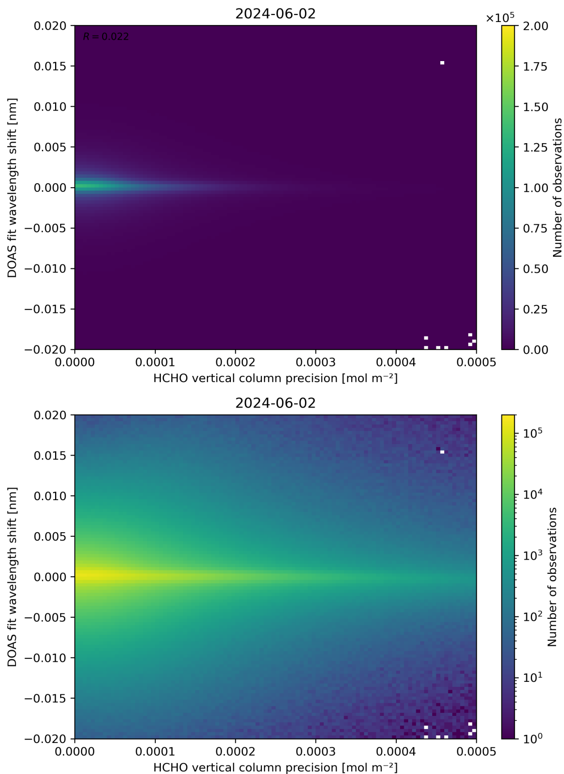
Figure 137: Scatter density plot of “HCHO vertical column precision” against “DOAS fit wavelength shift” for 2024-06-01 to 2024-06-03.
