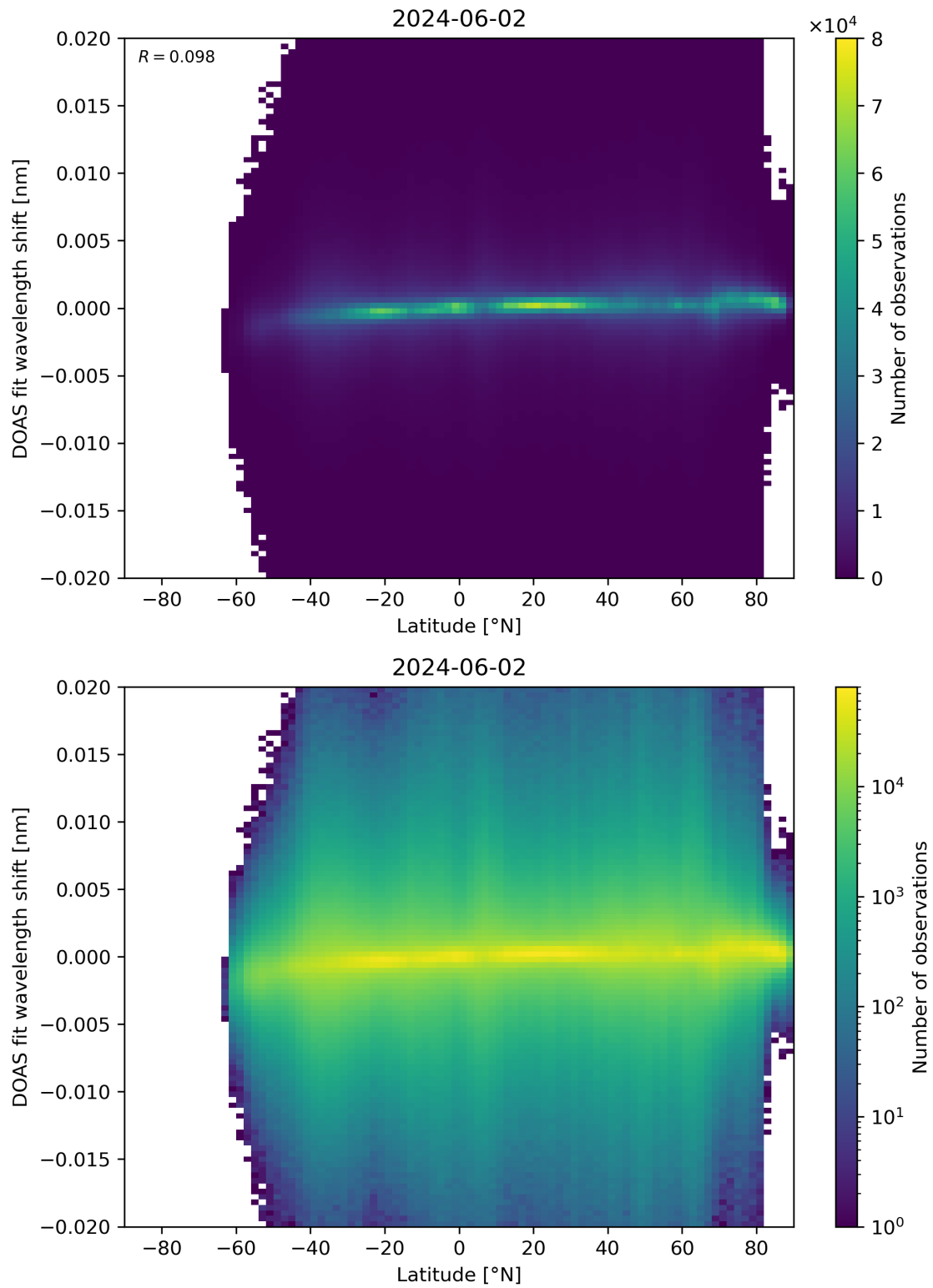
Figure 154: Scatter density plot of “Latitude” against “DOAS fit wavelength shift” for 2024-06-01 to 2024-06-03.
