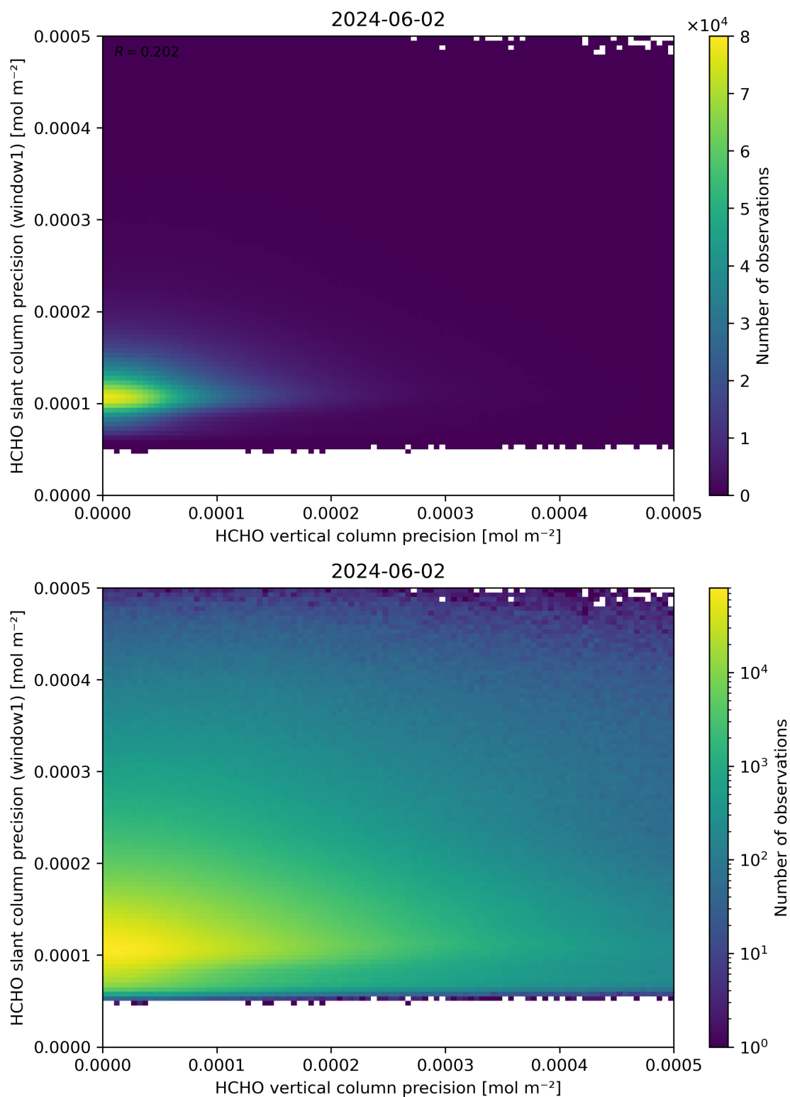
Figure 143: Scatter density plot of “HCHO vertical column precision” against “HCHO slant column precision (window1)” for 2024-06-01 to 2024-06-03.
