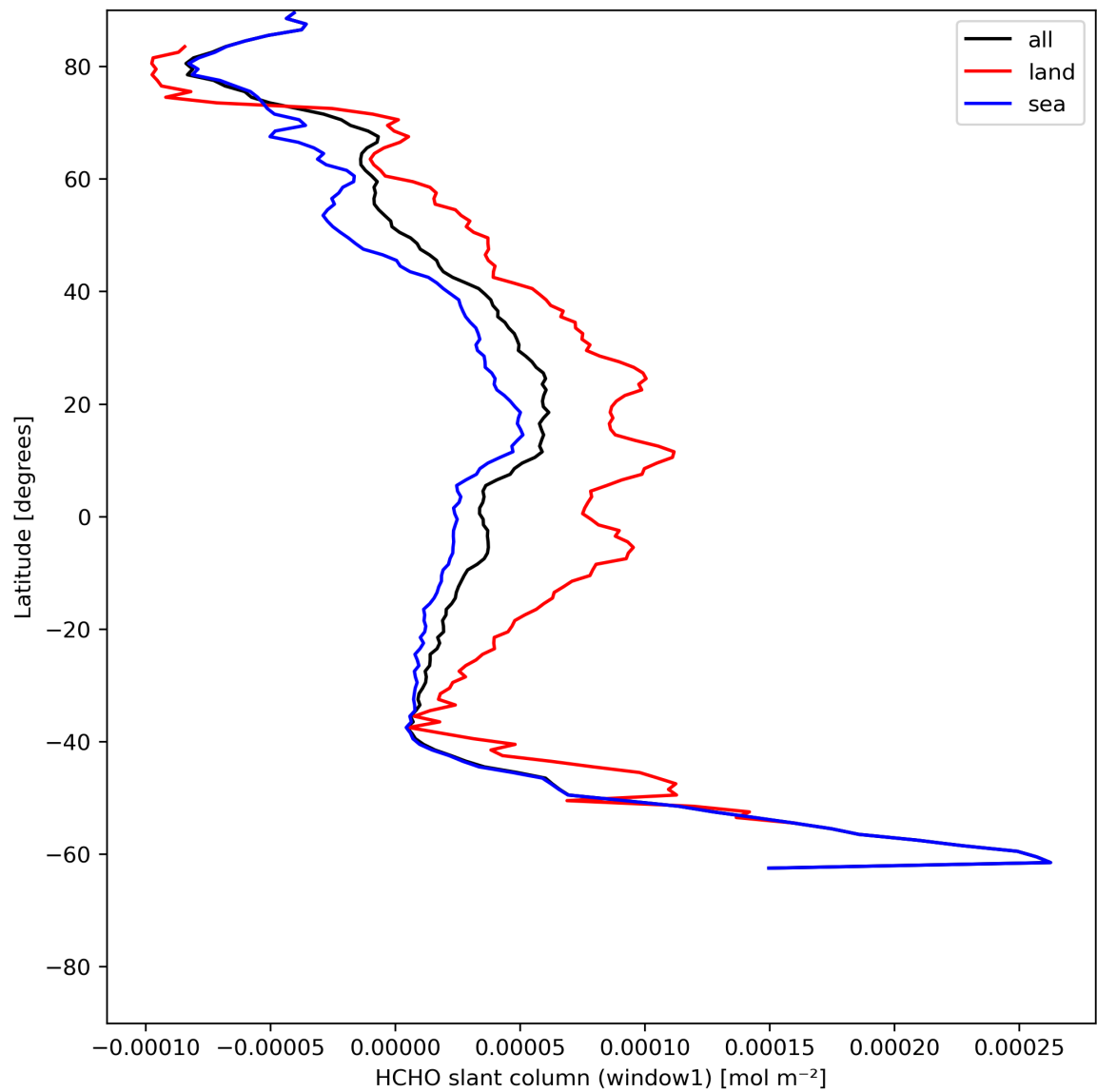
Figure 24: Zonal average of “HCHO slant column (window1)” for 2024-06-01 to 2024-06-03.
