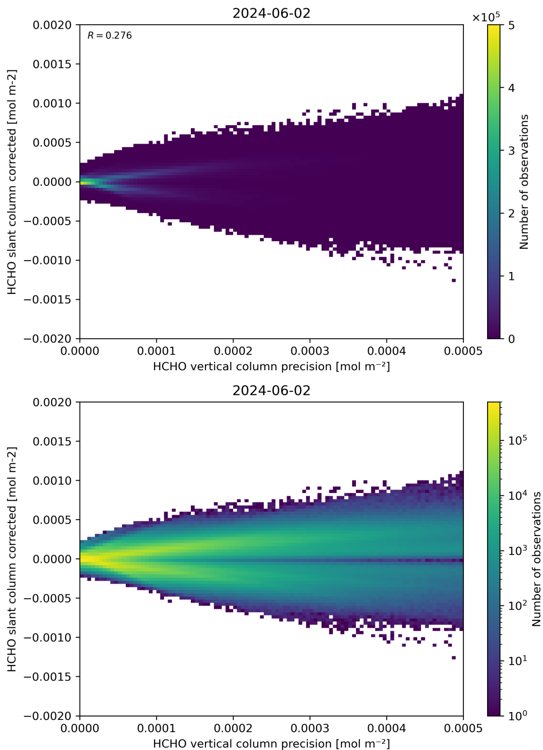
Figure 140: Scatter density plot of “HCHO vertical column precision” against “HCHO slant column corrected” for 2024-06-01 to 2024-06-03.
