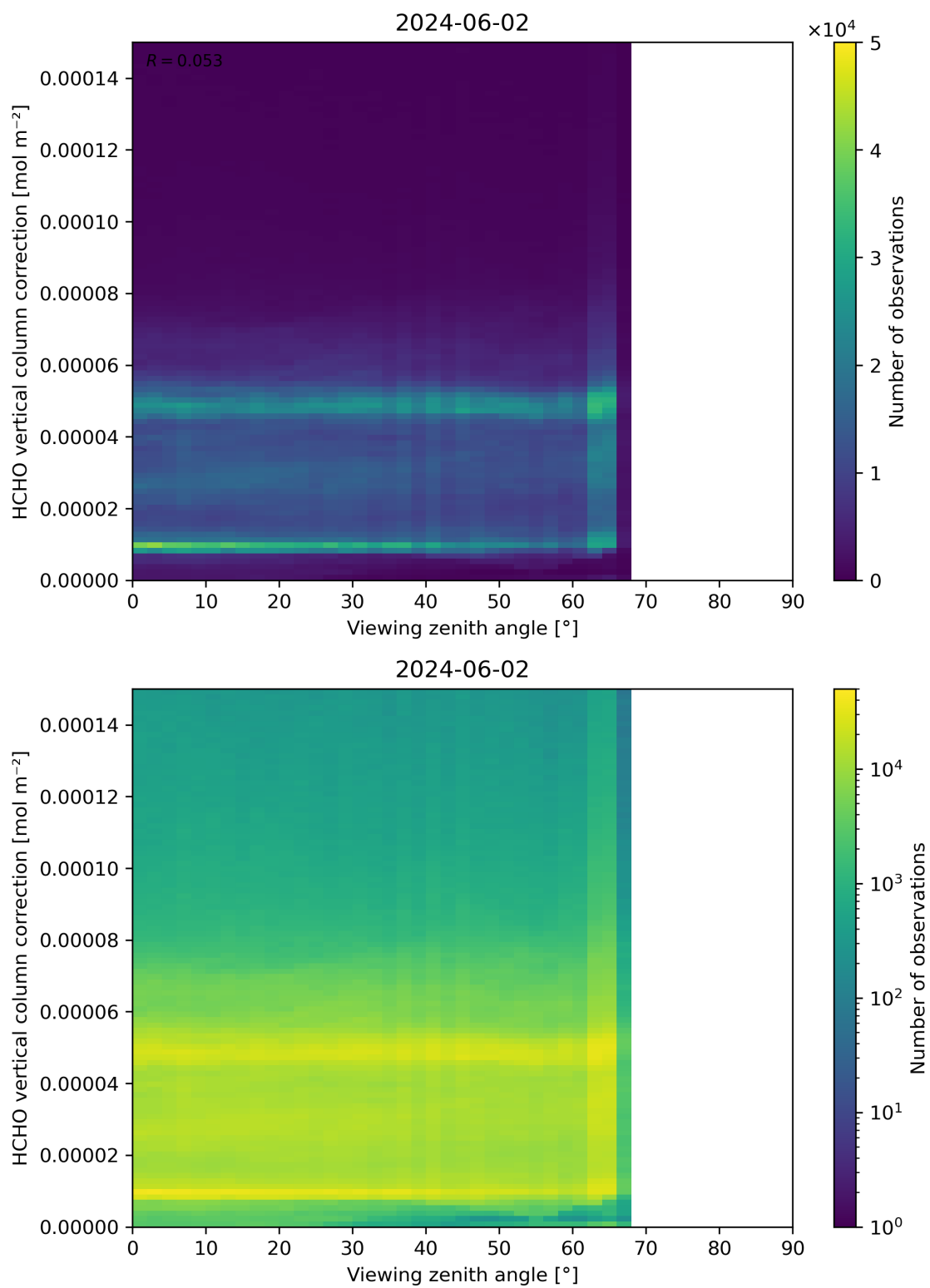
Figure 193: Scatter density plot of “Viewing zenith angle” against “HCHO vertical column correction” for 2024-06-01 to 2024-06-03.
