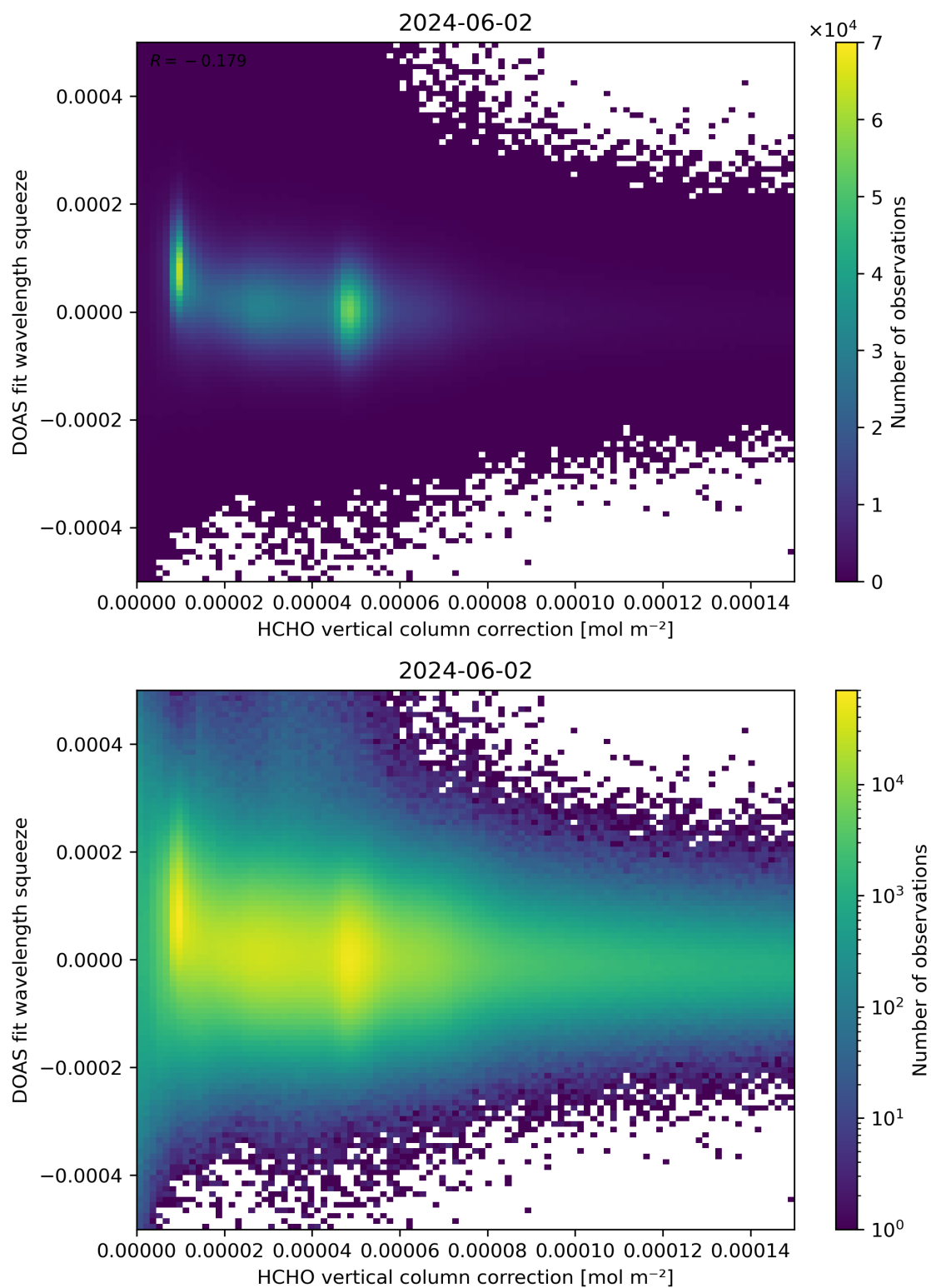
Figure 114: Scatter density plot of “HCHO vertical column correction” against “DOAS fit wavelength squeeze” for 2024-06-01 to 2024-06-03.
