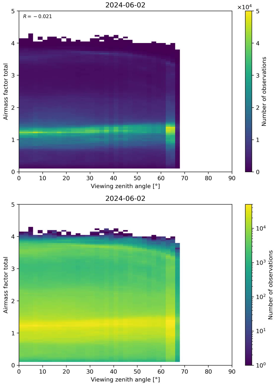
Figure 190: Scatter density plot of “Viewing zenith angle” against “Airmass factor total” for 2024-06-01 to 2024-06-03.
