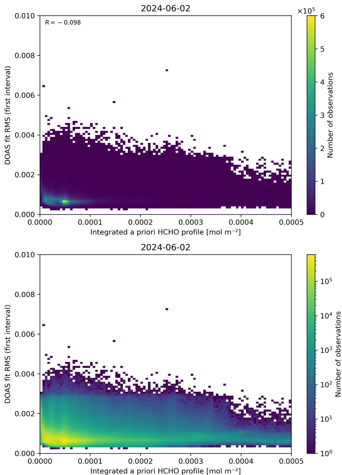
Figure 148: Scatter density plot of “Integrated a priori HCHO profile” against “DOAS fit RMS (first interval)” for 2024-06-01 to 2024-06-03.
