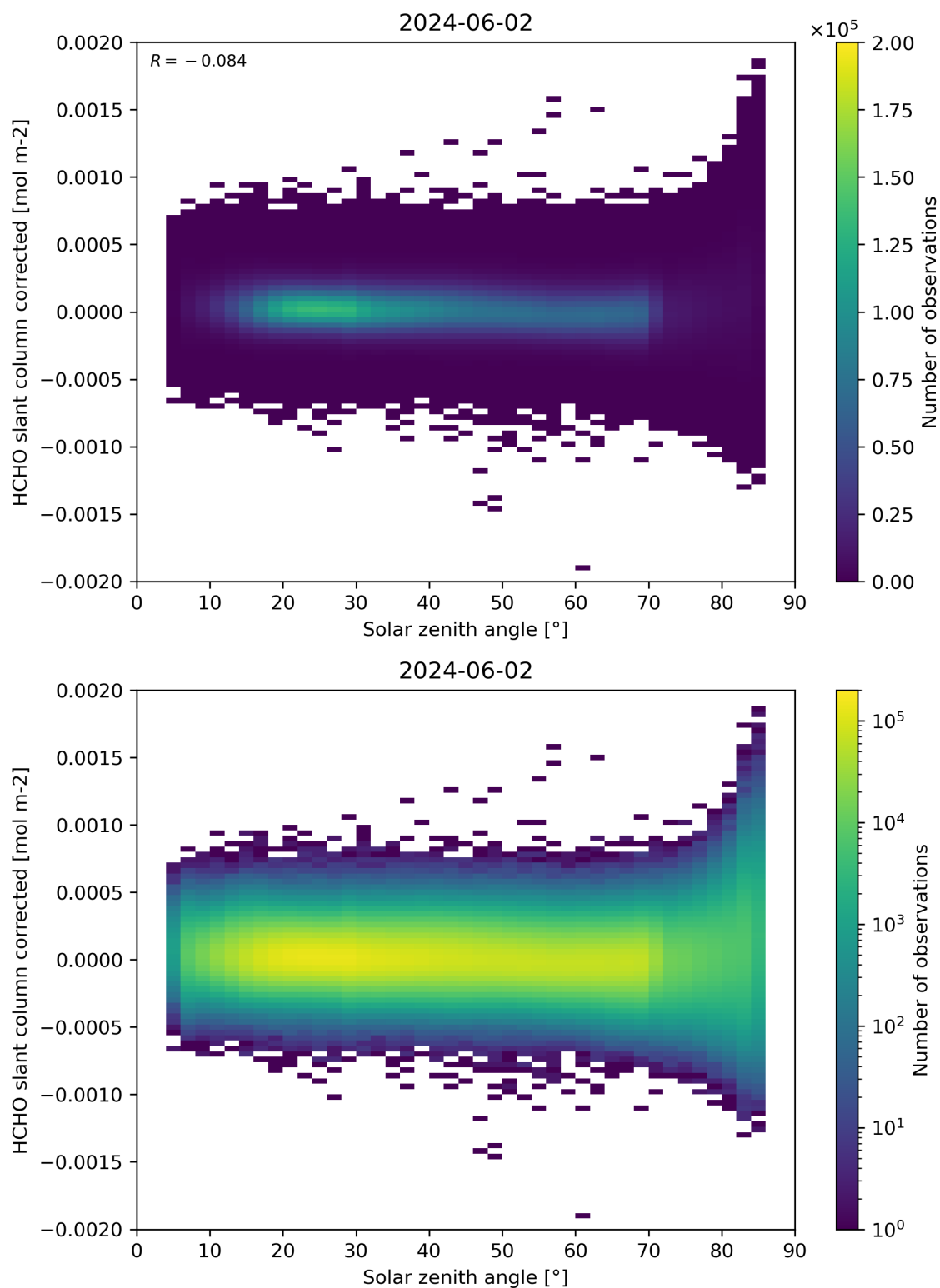
Figure 171: Scatter density plot of “Solar zenith angle” against “HCHO slant column corrected” for 2024-06-01 to 2024-06-03.
