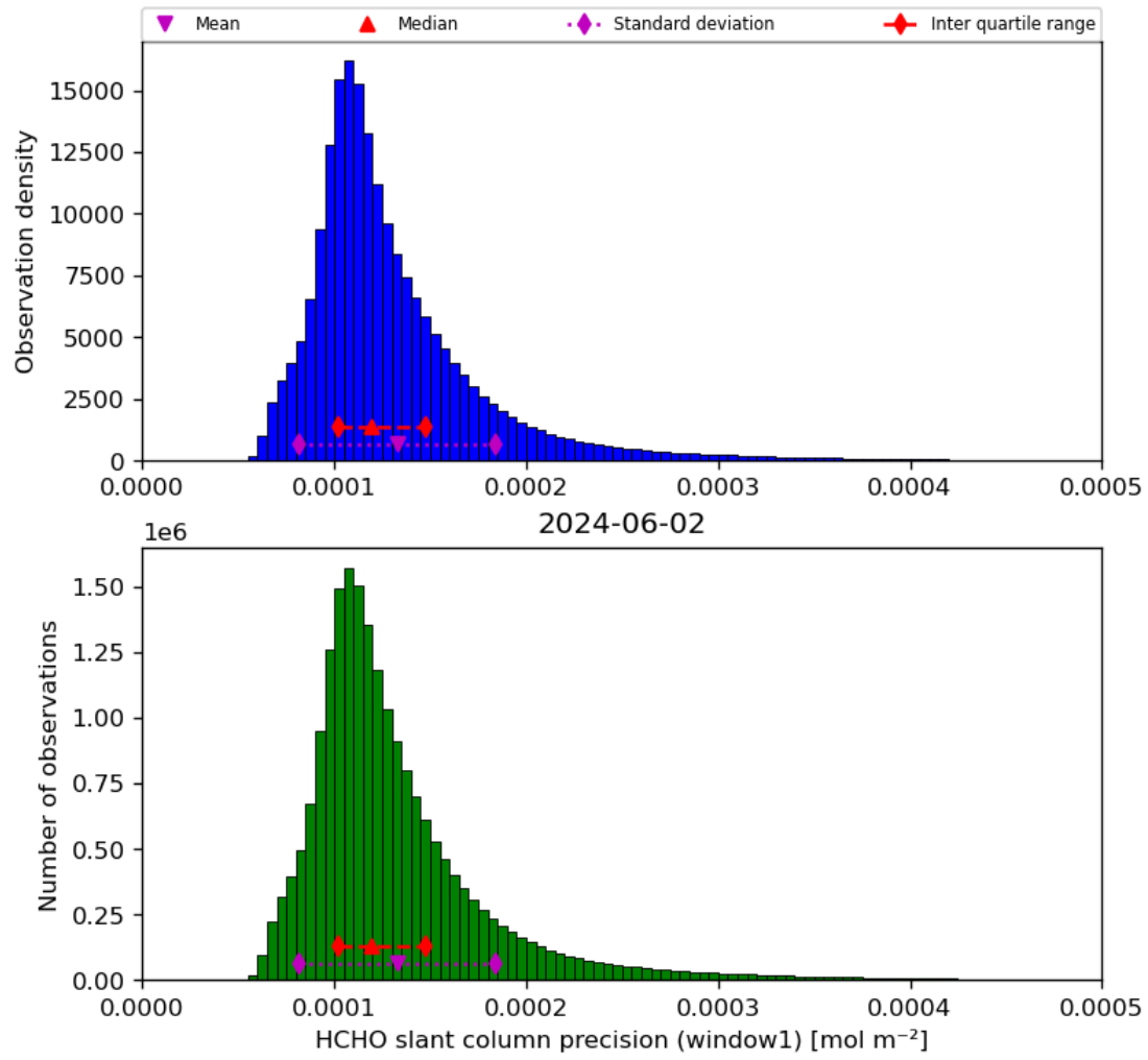
Figure 39: Histogram of “HCHO slant column precision (window1)” for 2024-06-01 to 2024-06-03
