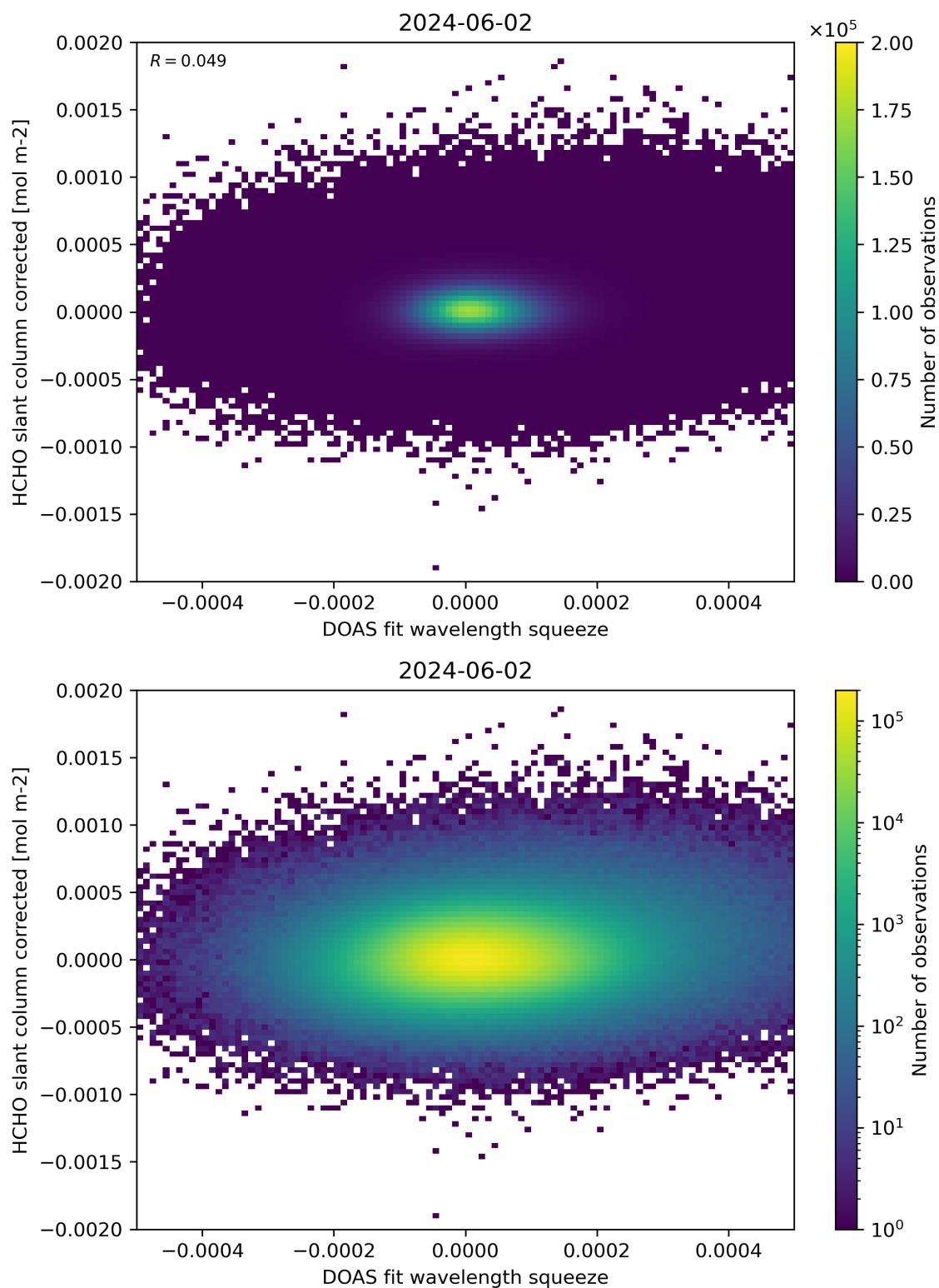
Figure 69: Scatter density plot of “DOAS fit wavelength squeeze” against “HCHO slant column corrected” for 2024-06-01 to 2024-06-03.
