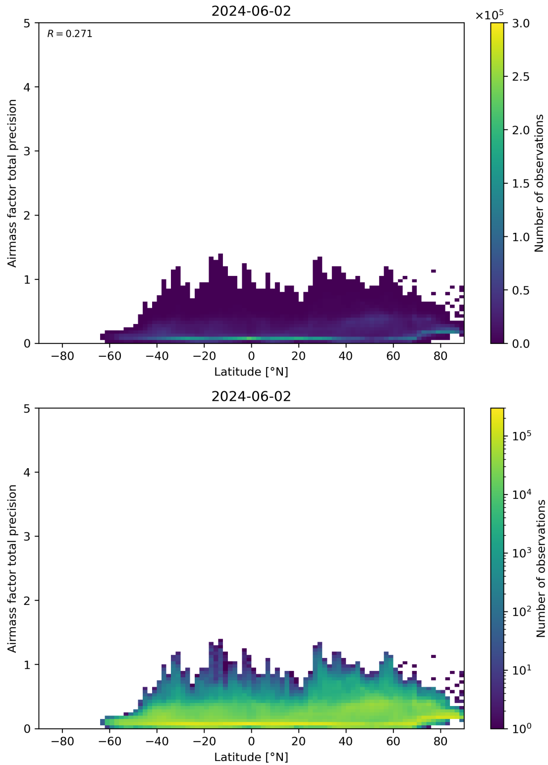
Figure 162: Scatter density plot of “Latitude” against “Airmass factor total precision” for 2024-06-01 to 2024-06-03.
