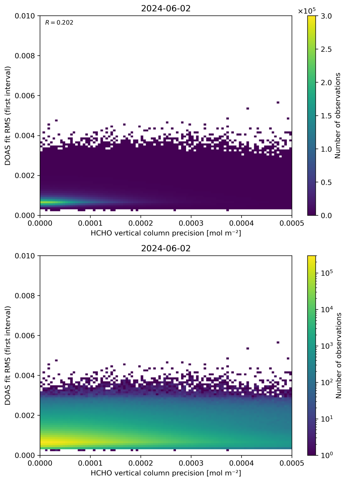
Figure 136: Scatter density plot of “HCHO vertical column precision” against “DOAS fit RMS (first interval)” for 2024-06-01 to 2024-06-03.
