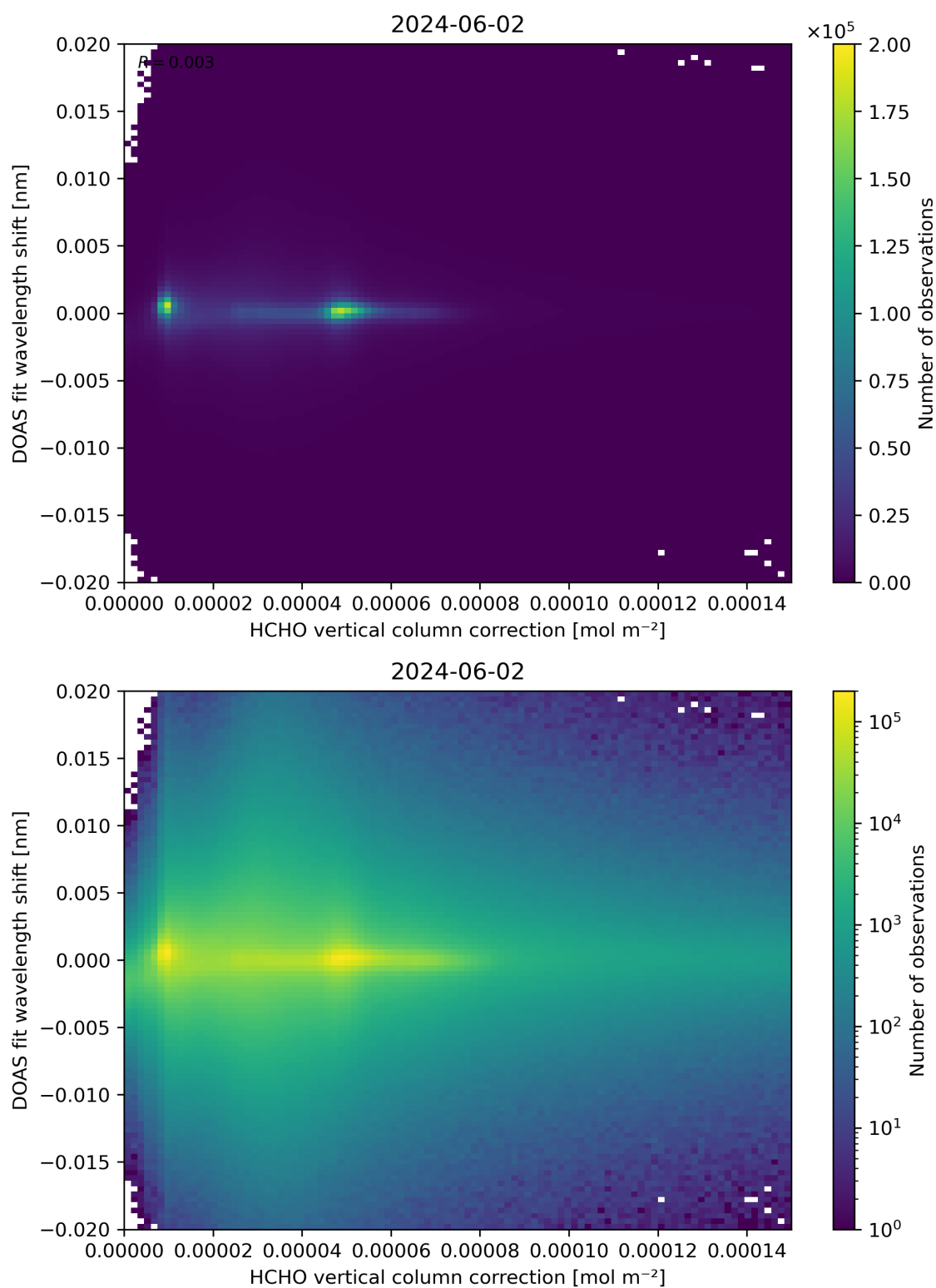
Figure 113: Scatter density plot of “HCHO vertical column correction” against “DOAS fit wavelength shift” for 2024-06-01 to 2024-06-03.
