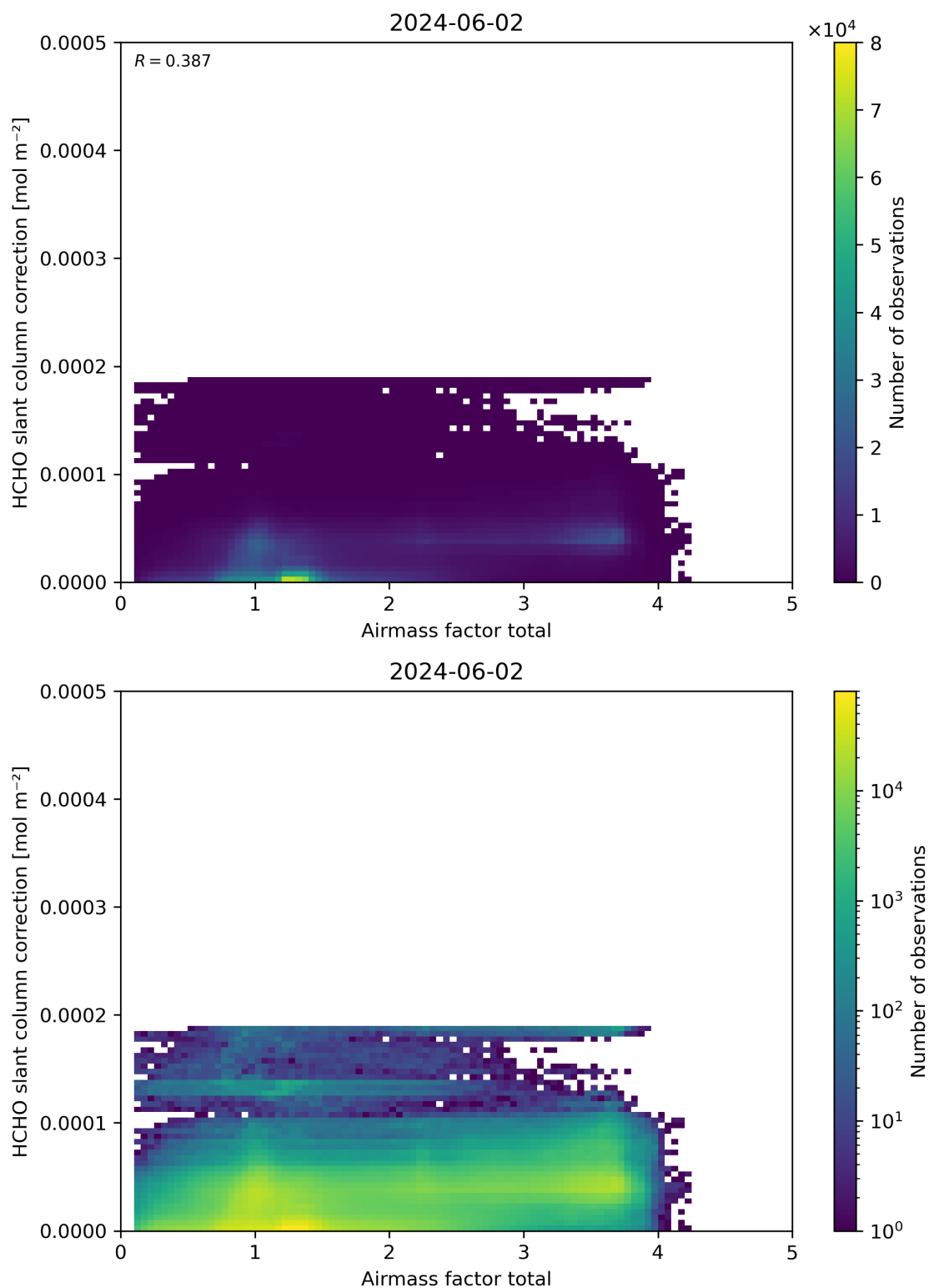
Figure 102: Scatter density plot of “Airmass factor total” against “HCHO slant column correction” for 2024-06-01 to 2024-06-03.
