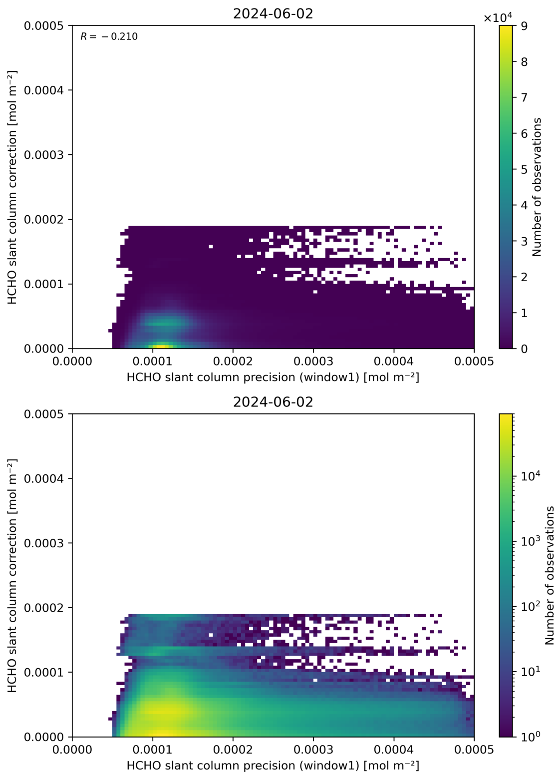
Figure 93: Scatter density plot of “HCHO slant column precision (window1)” against “HCHO slant column correction” for 2024-06-01 to 2024-06-03.
