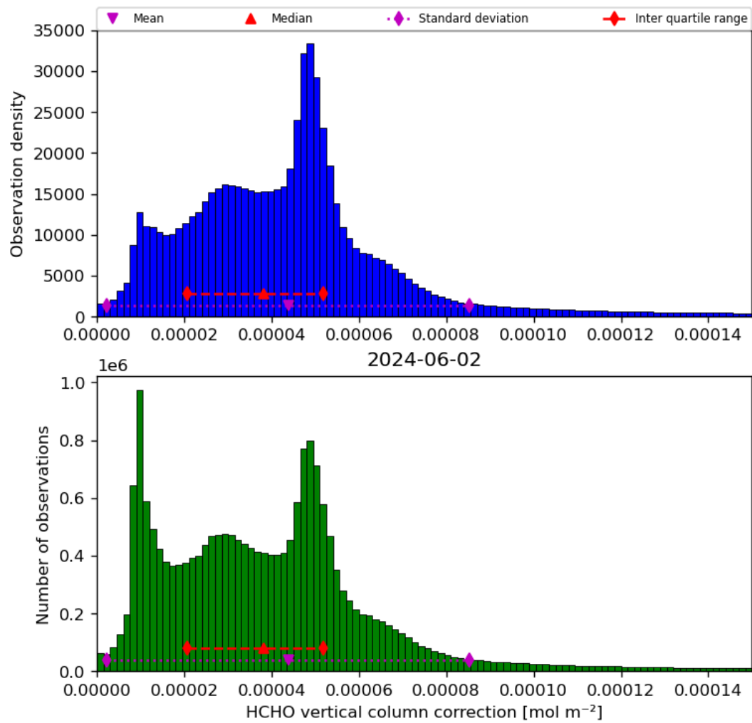
Figure 37: Histogram of “HCHO vertical column correction” for 2024-06-01 to 2024-06-03
