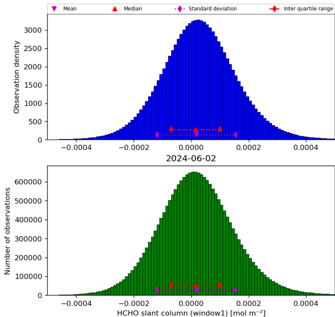
Figure 38: Histogram of “HCHO slant column (window1)” for 2024-06-01 to 2024-06-03
