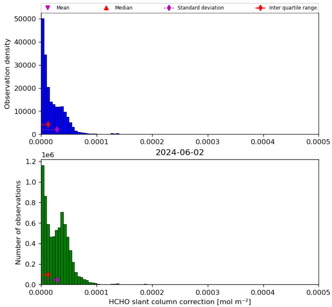
Figure 47: Histogram of “HCHO slant column correction” for 2024-06-01 to 2024-06-03
