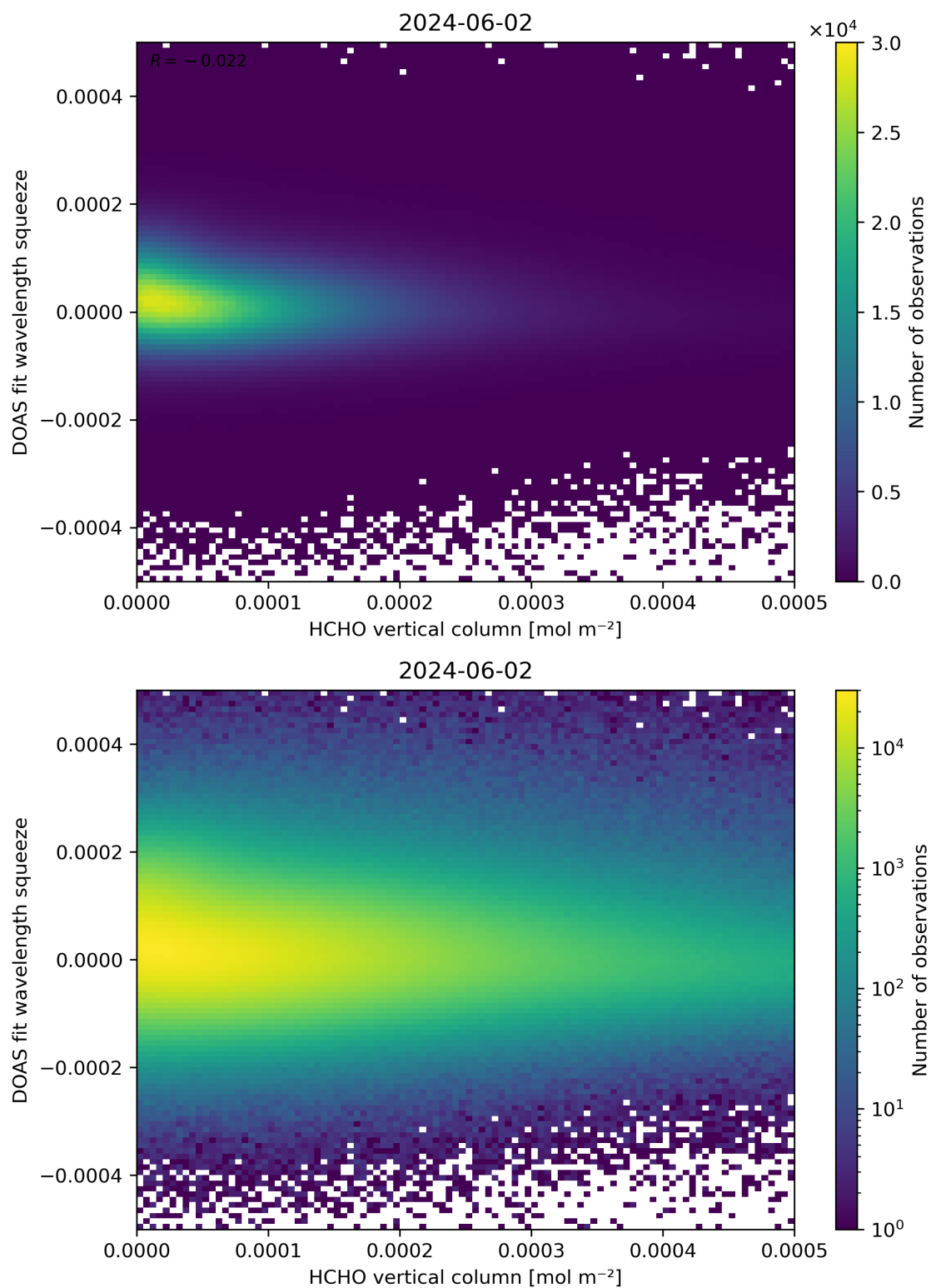
Figure 125: Scatter density plot of “HCHO vertical column” against “DOAS fit wavelength squeeze” for 2024-06-01 to 2024-06-03.
