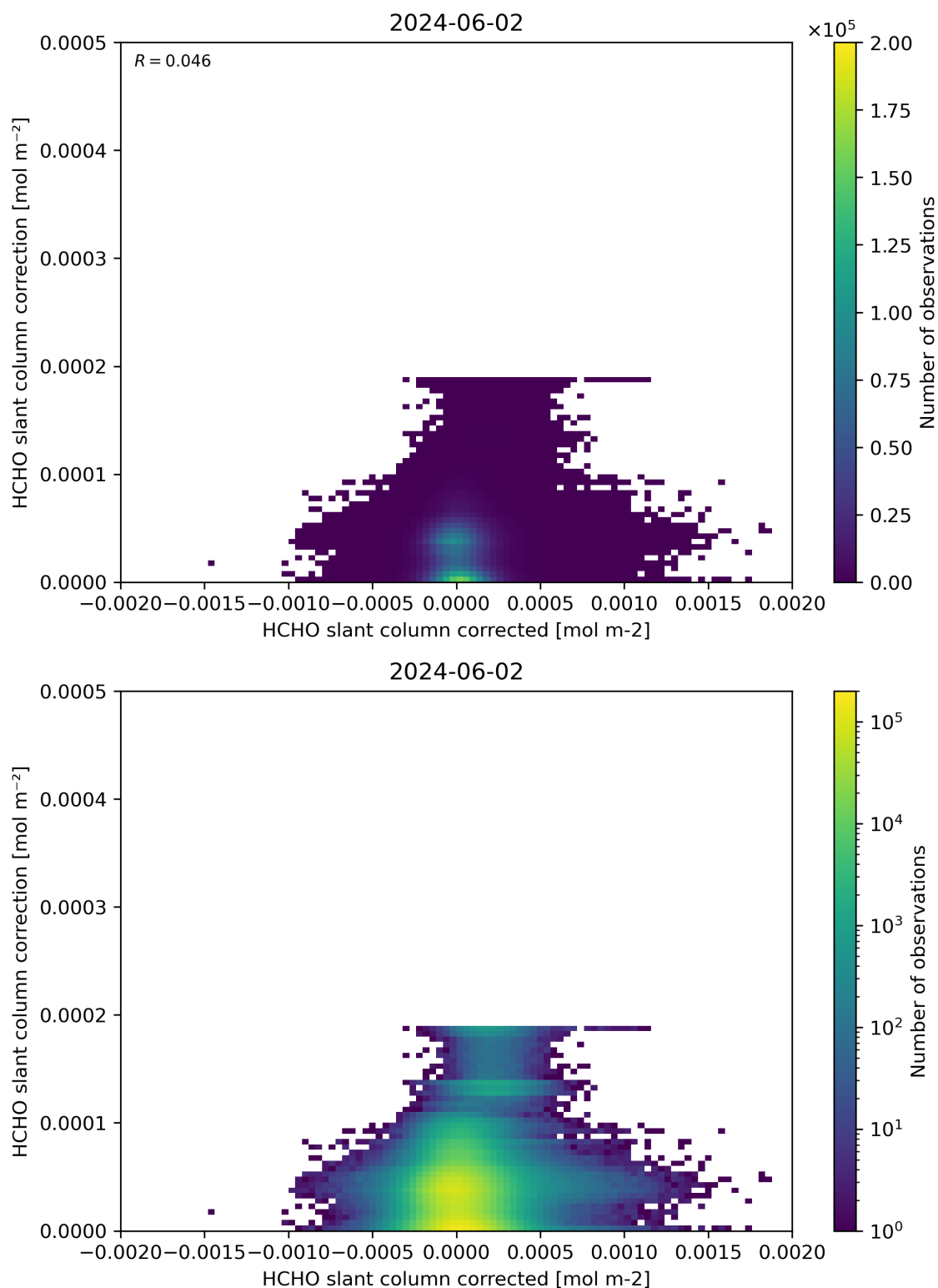
Figure 77: Scatter density plot of “HCHO slant column corrected” against “HCHO slant column correction” for 2024-06-01 to 2024-06-03.
