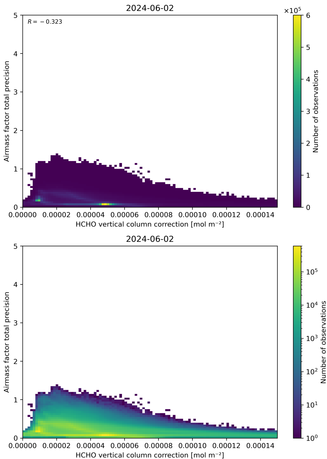
Figure 121: Scatter density plot of “HCHO vertical column correction” against “Airmass factor total precision” for 2024-06-01 to 2024-06-03.
