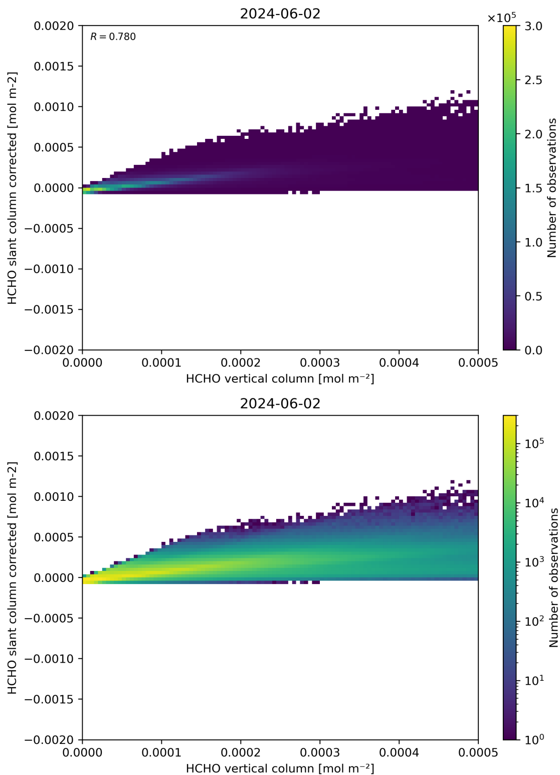
Figure 127: Scatter density plot of “HCHO vertical column” against “HCHO slant column corrected” for 2024-06-01 to 2024-06-03.
