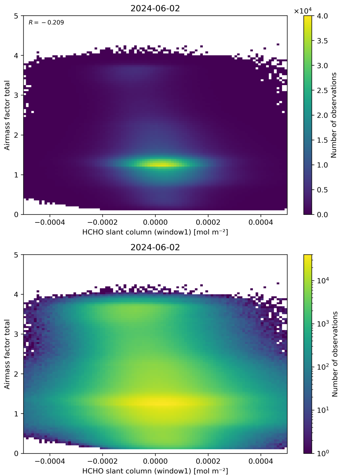
Figure 85: Scatter density plot of “HCHO slant column (window1)” against “Airmass factor total” for 2024-06-01 to 2024-06-03.
