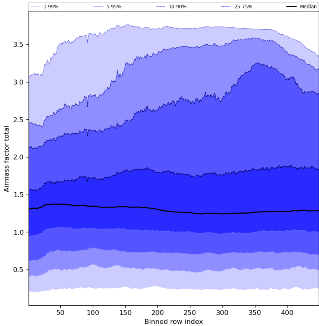
Figure 54: Along track statistics of “Airmass factor total” for 2024-06-01 to 2024-06-03
