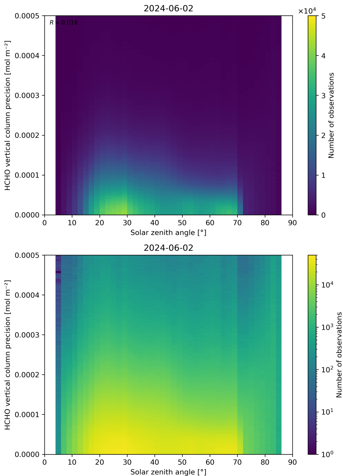
Figure 179: Scatter density plot of “Solar zenith angle” against “HCHO vertical column precision” for 2024-06-01 to 2024-06-03.
