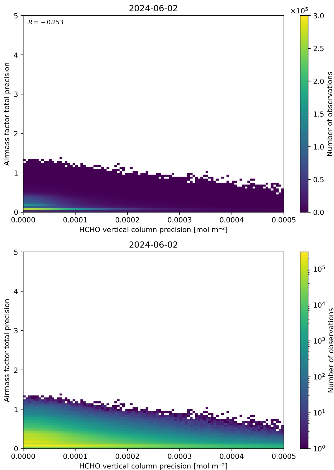
Figure 145: Scatter density plot of “HCHO vertical column precision” against “Airmass factor total precision” for 2024-06-01 to 2024-06-03.
