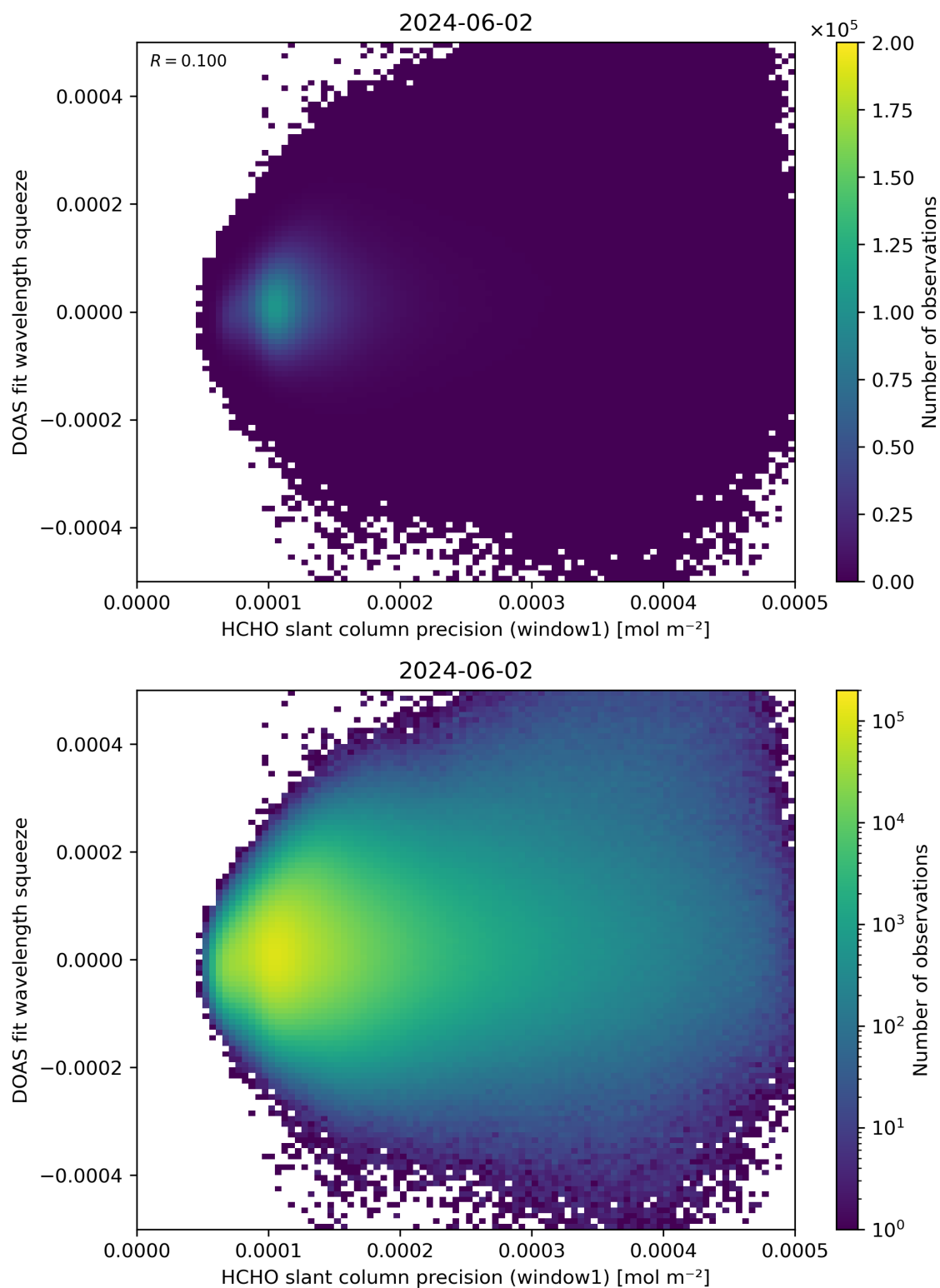
Figure 90: Scatter density plot of “HCHO slant column precision (window1)” against “DOAS fit wavelength squeeze” for 2024-06-01 to 2024-06-03.
