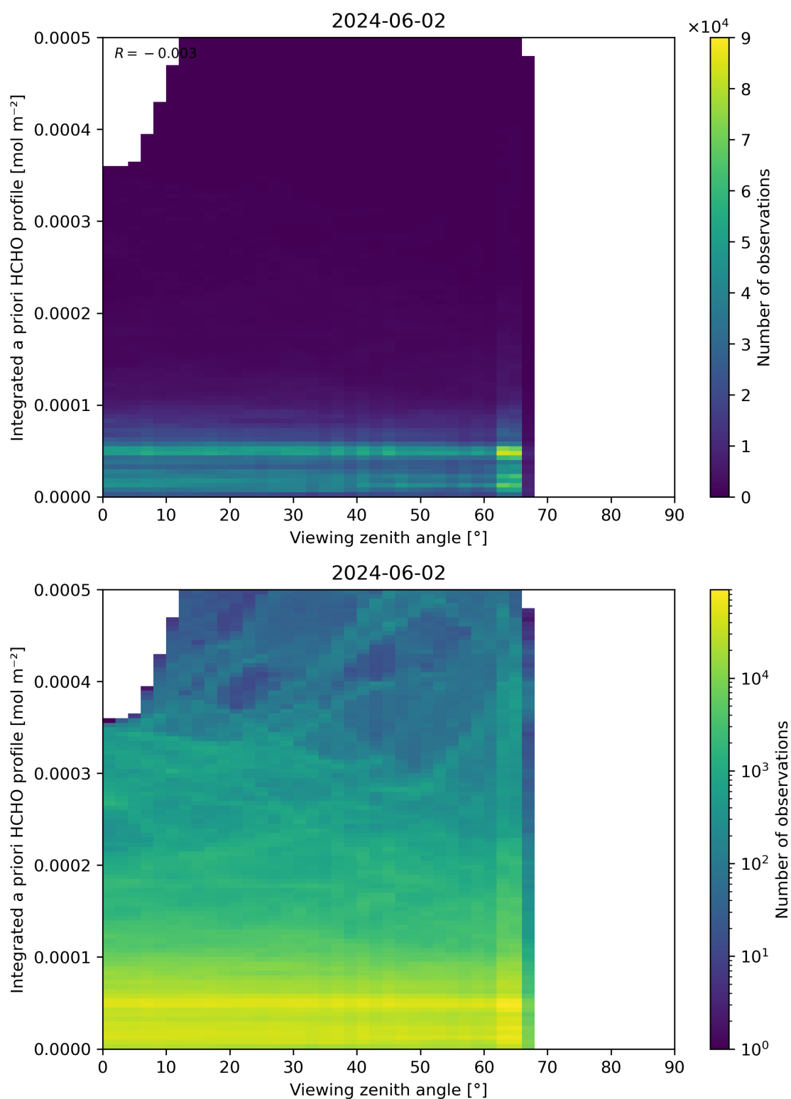
Figure 195: Scatter density plot of “Viewing zenith angle” against “Integrated a priori HCHO profile” for 2024-06-01 to 2024-06-03.
