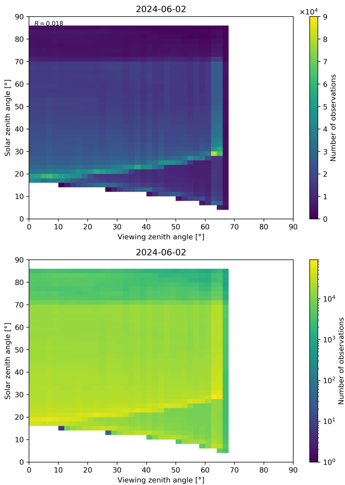
Figure 197: Scatter density plot of “Viewing zenith angle” against “Solar zenith angle” for 2024-06-01 to 2024-06-03.
