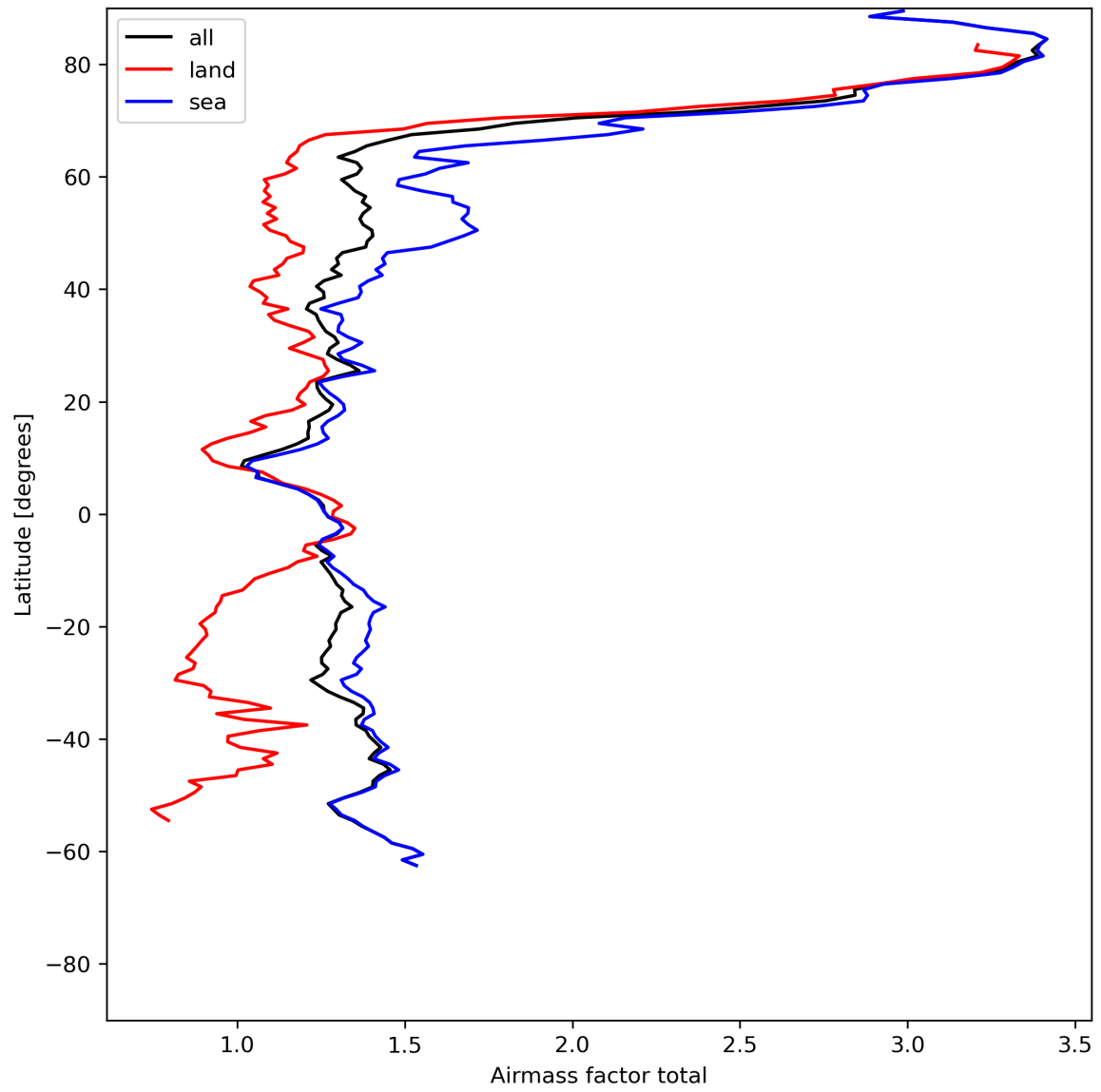
Figure 26: Zonal average of “Airmass factor total” for 2024-06-01 to 2024-06-03.
