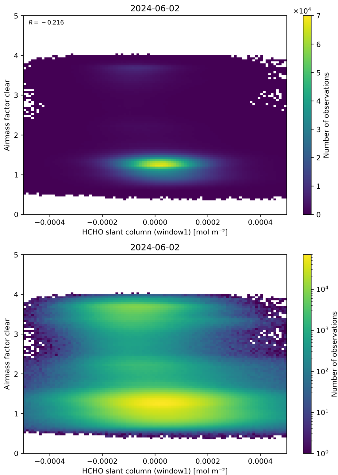
Figure 81: Scatter density plot of “HCHO slant column (window1)” against “Airmass factor clear” for 2024-06-01 to 2024-06-03.
