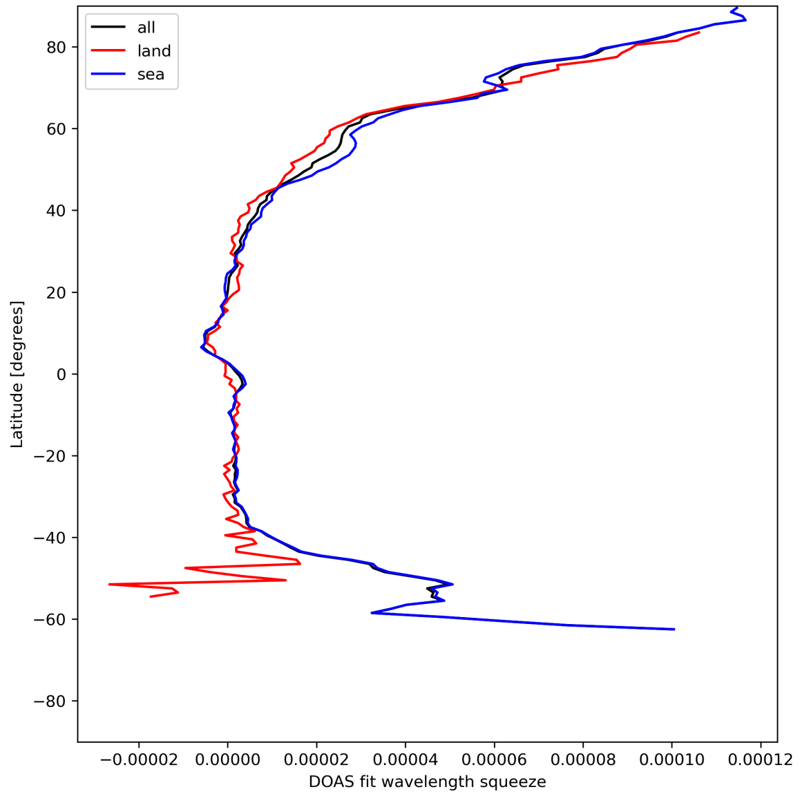
Figure 31: Zonal average of “DOAS fit wavelength squeeze” for 2024-06-01 to 2024-06-03.
