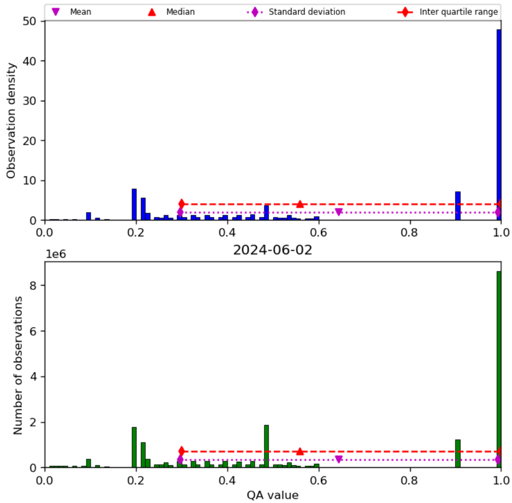
Figure 34: Histogram of “QA value” for 2024-06-01 to 2024-06-03
