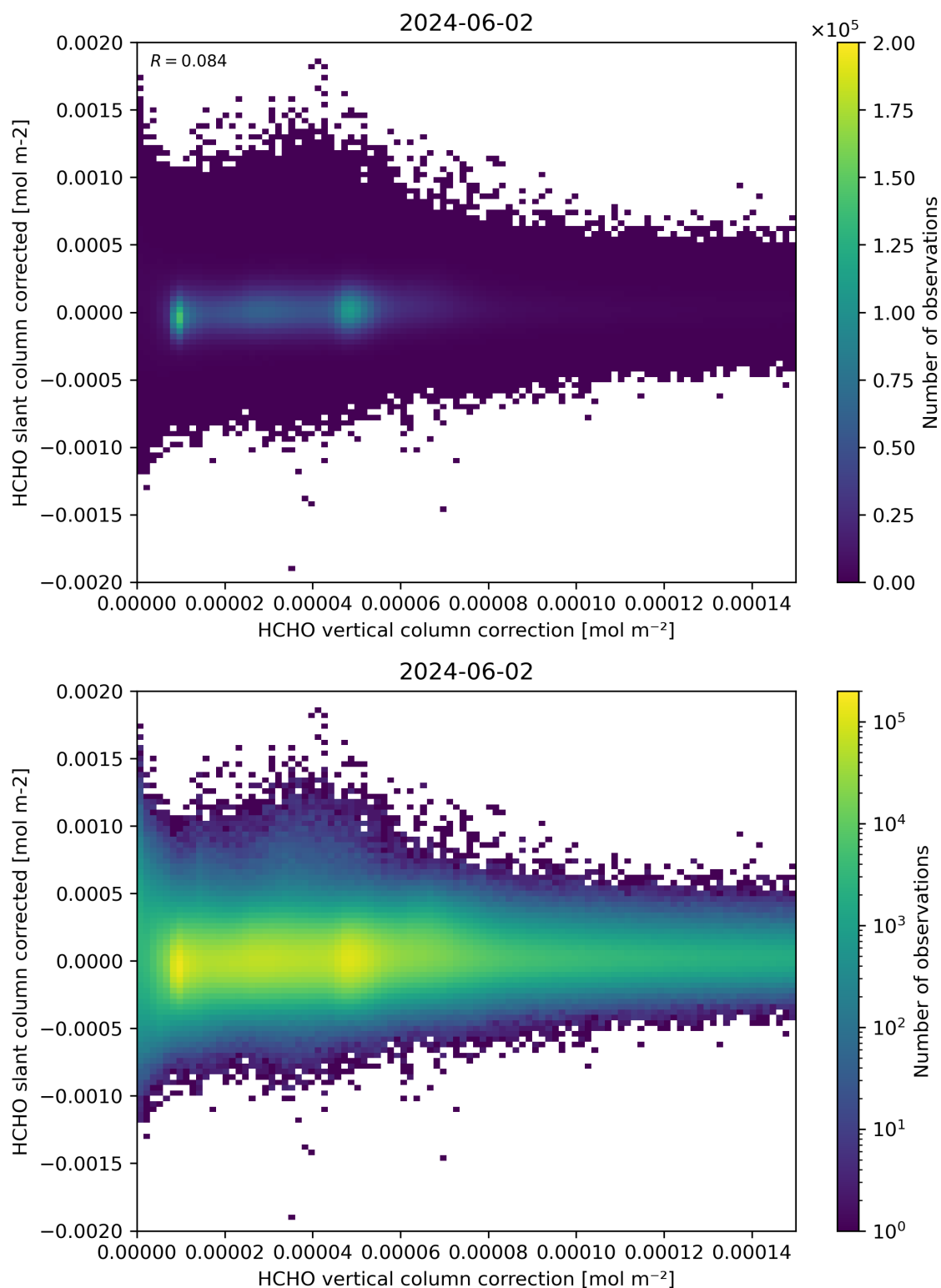
Figure 116: Scatter density plot of “HCHO vertical column correction” against “HCHO slant column corrected” for 2024-06-01 to 2024-06-03.
