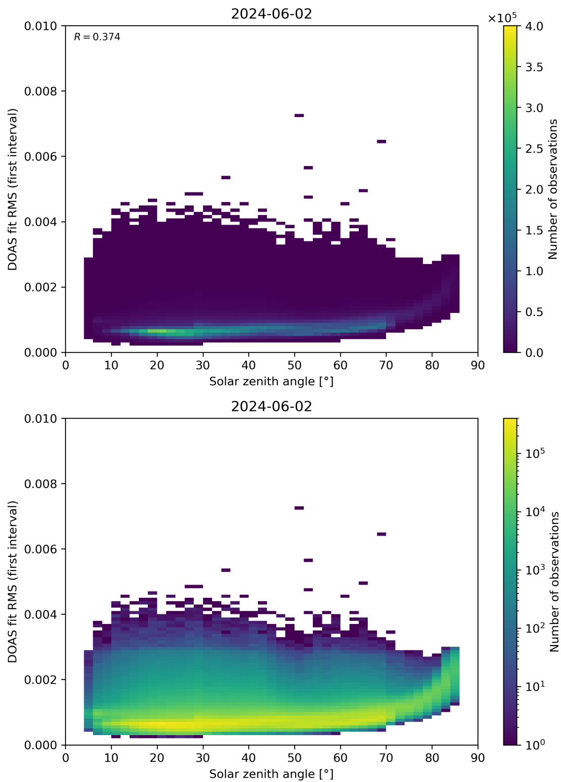
Figure 167: Scatter density plot of “Solar zenith angle” against “DOAS fit RMS (first interval)” for 2024-06-01 to 2024-06-03.
