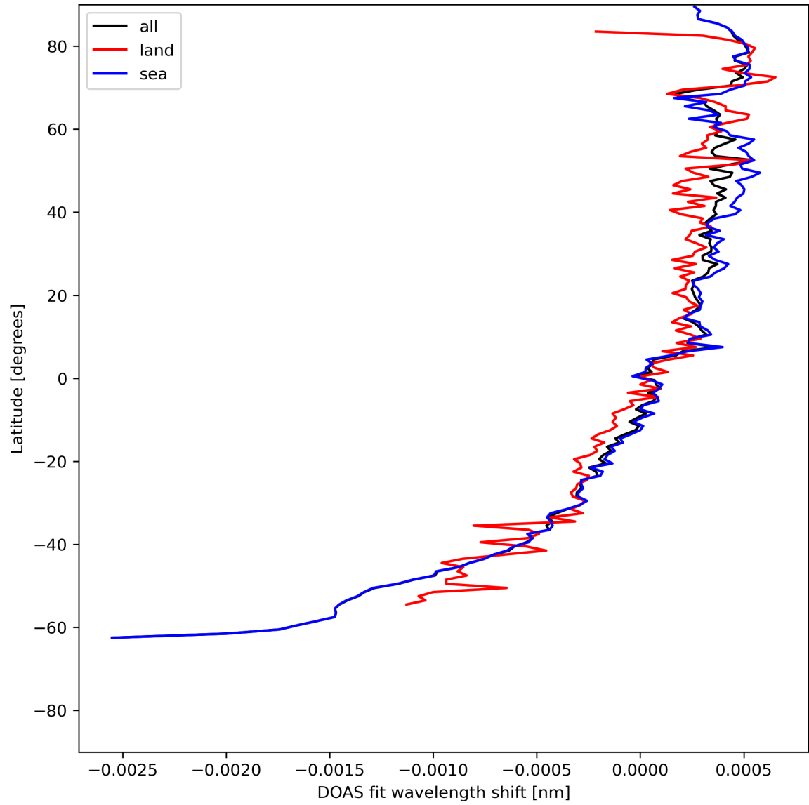
Figure 30: Zonal average of “DOAS fit wavelength shift” for 2024-06-01 to 2024-06-03.
