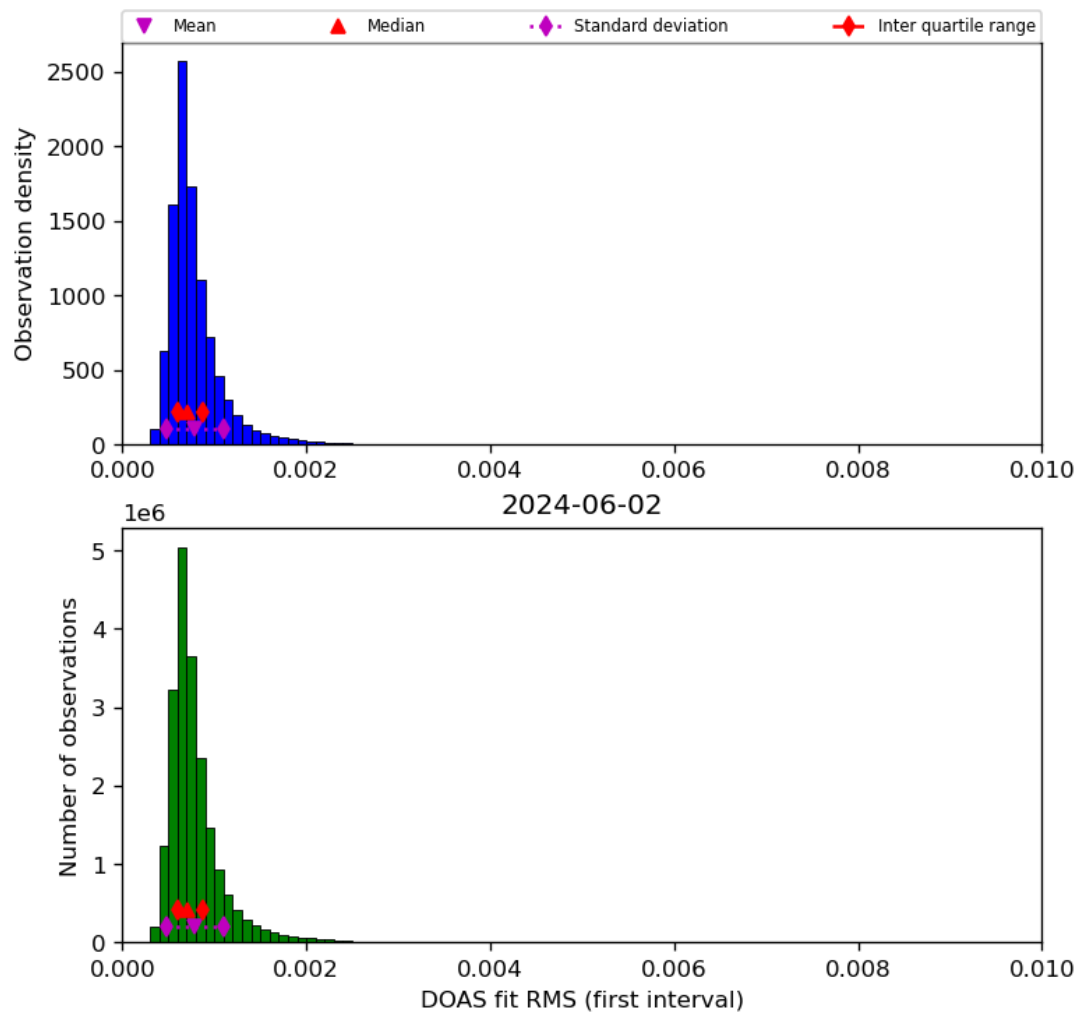
Figure 46: Histogram of “DOAS fit RMS (first interval)” for 2024-06-01 to 2024-06-03
