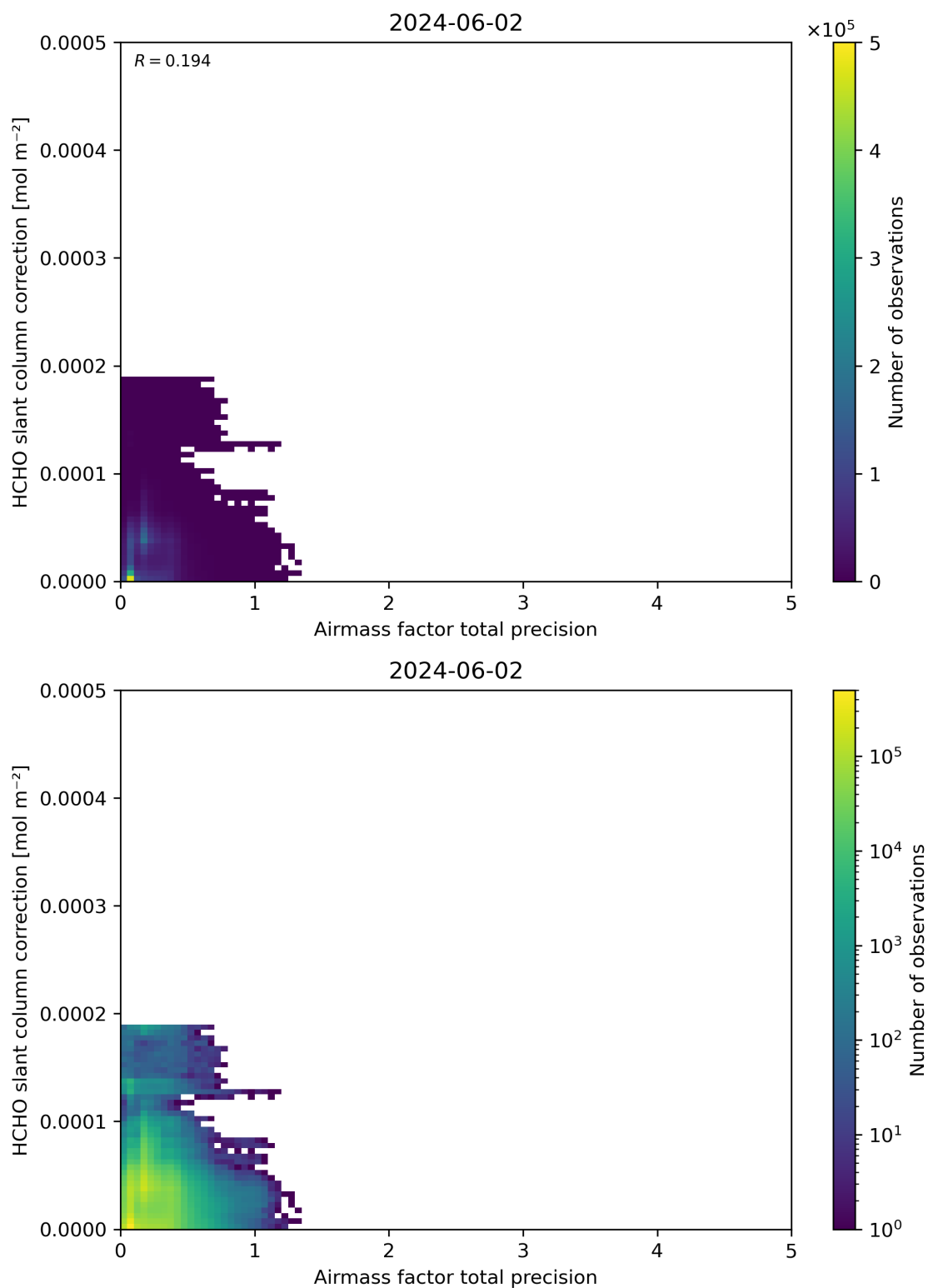
Figure 110: Scatter density plot of “Airmass factor total precision” against “HCHO slant column correction” for 2024-06-01 to 2024-06-03.
