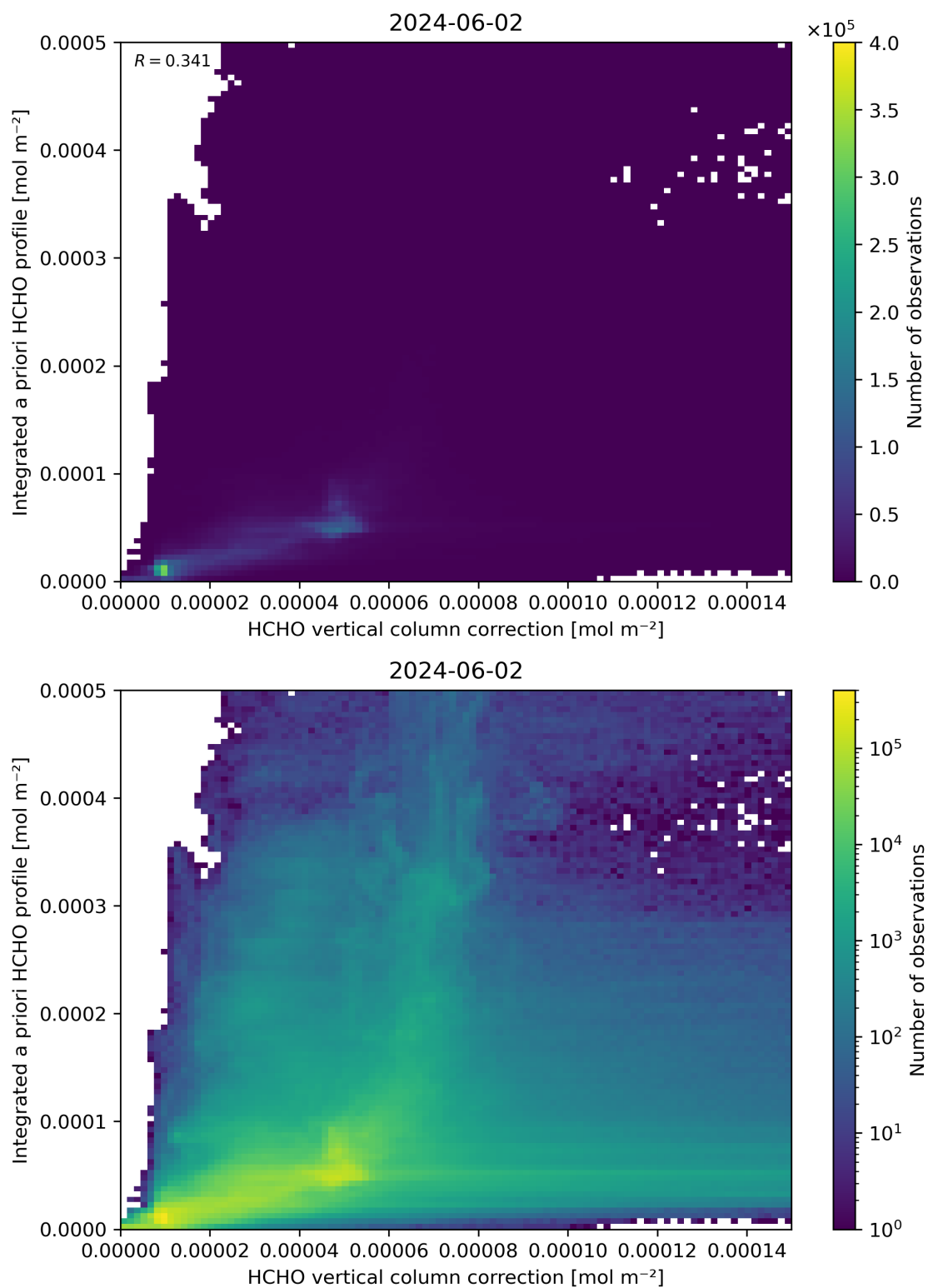
Figure 122: Scatter density plot of “HCHO vertical column correction” against “Integrated a priori HCHO profile” for 2024-06-01 to 2024-06-03.
