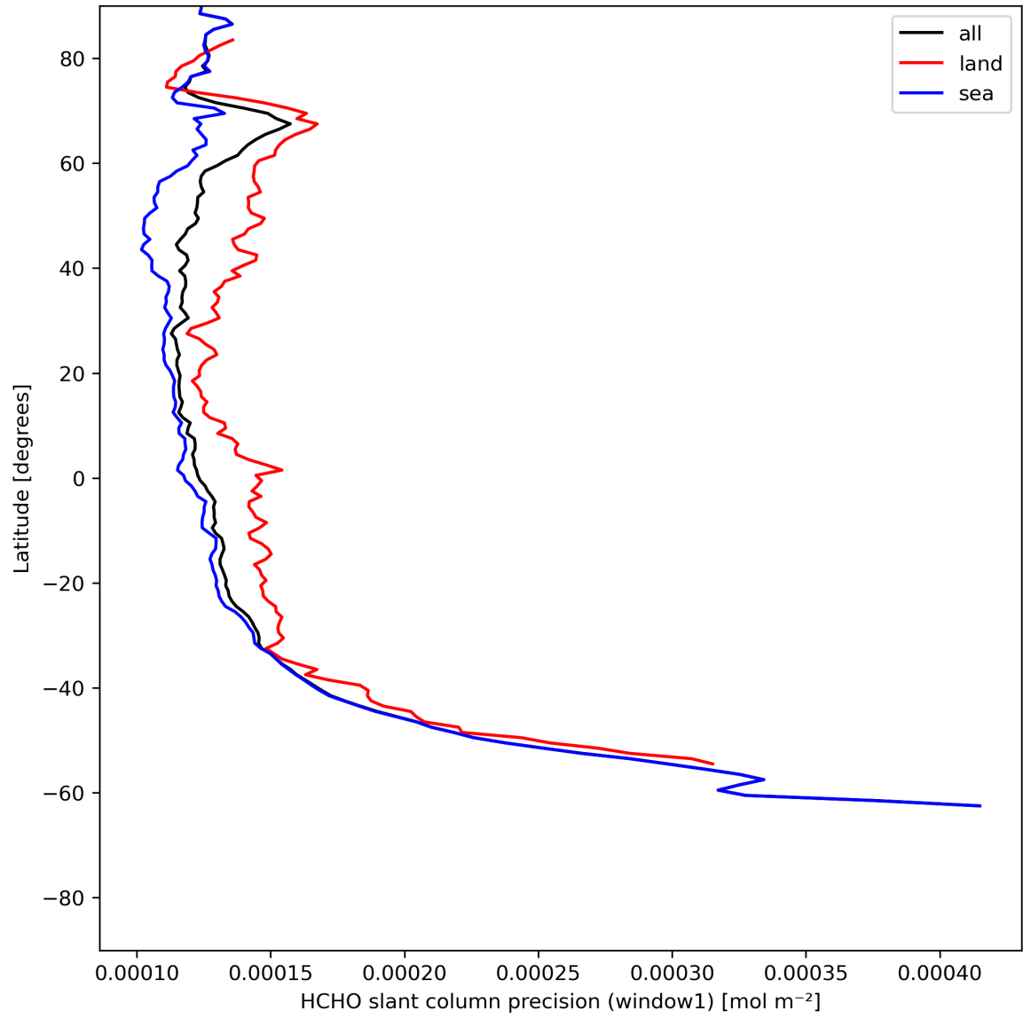
Figure 25: Zonal average of “HCHO slant column precision (window1)” for 2024-06-01 to 2024-06-03.
