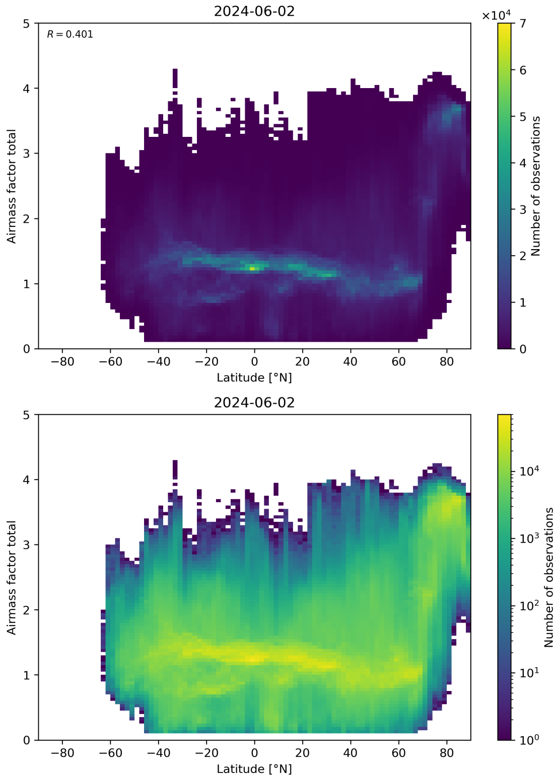
Figure 161: Scatter density plot of “Latitude” against “Airmass factor total” for 2024-06-01 to 2024-06-03.
