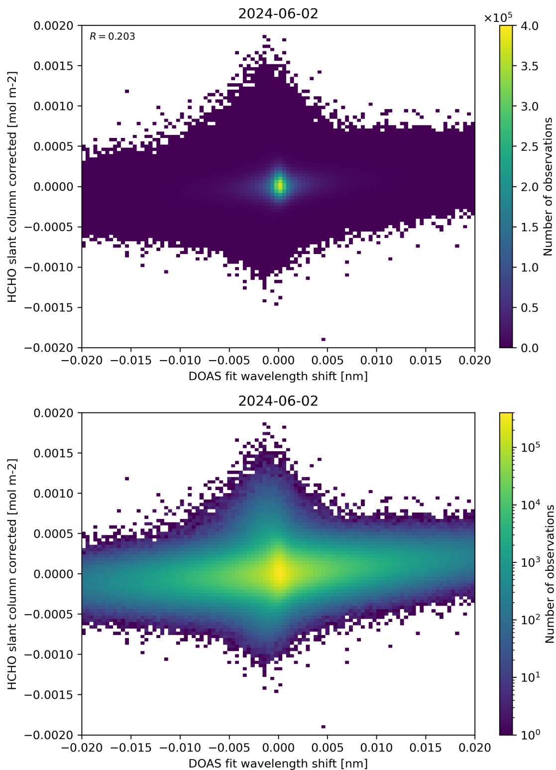
Figure 66: Scatter density plot of “DOAS fit wavelength shift” against “HCHO slant column corrected” for 2024-06-01 to 2024-06-03.
