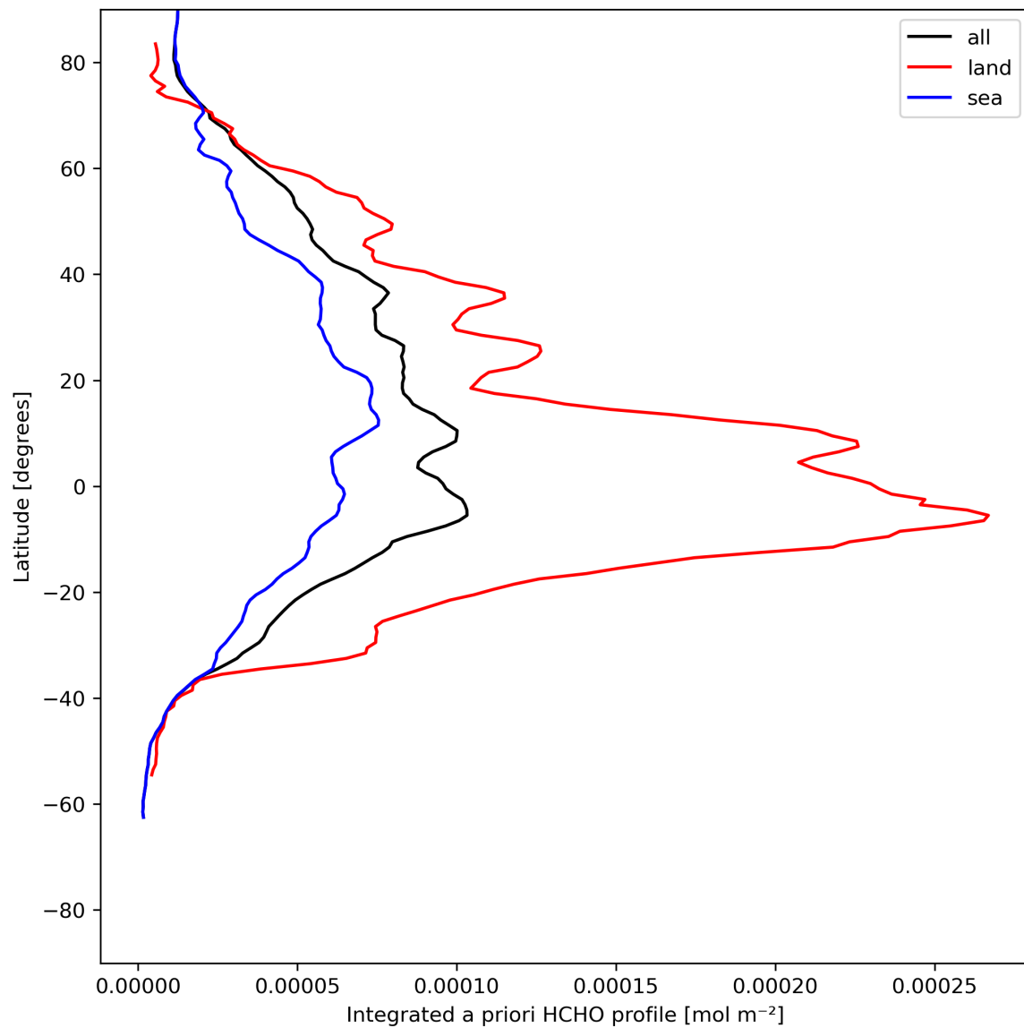
Figure 29: Zonal average of “Integrated a priori HCHO profile” for 2024-06-01 to 2024-06-03.
