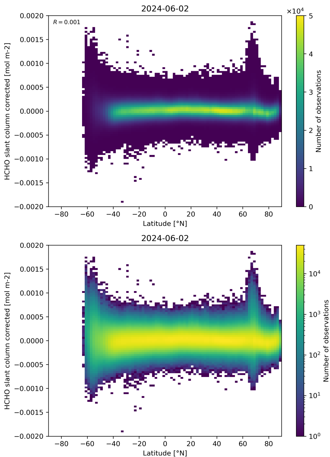
Figure 157: Scatter density plot of “Latitude” against “HCHO slant column corrected” for 2024-06-01 to 2024-06-03.
