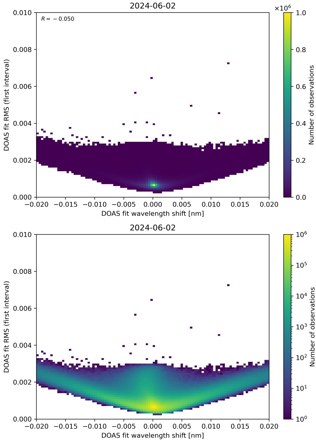
Figure 64: Scatter density plot of “DOAS fit wavelength shift” against “DOAS fit RMS (first interval)” for 2024-06-01 to 2024-06-03.
