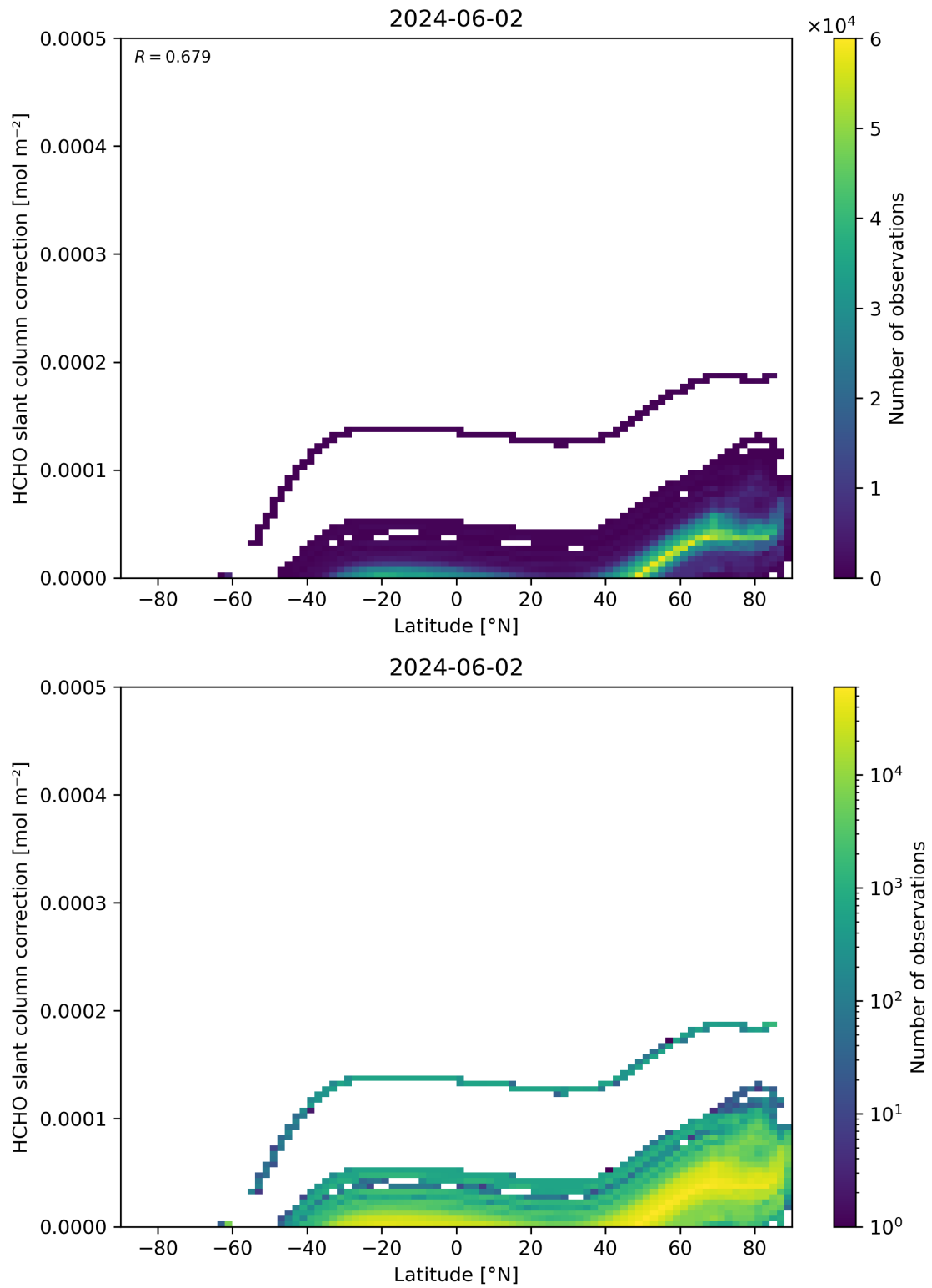
Figure 158: Scatter density plot of “Latitude” against “HCHO slant column correction” for 2024-06-01 to 2024-06-03.
