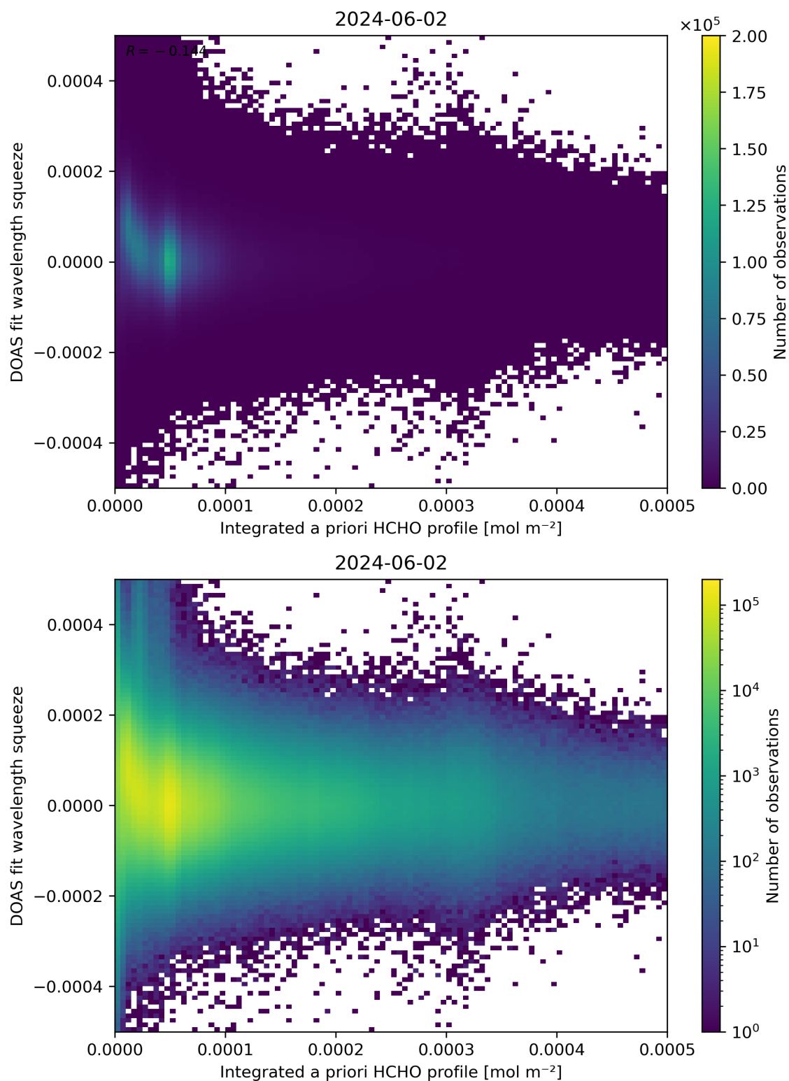
Figure 150: Scatter density plot of “Integrated a priori HCHO profile” against “DOAS fit wavelength squeeze” for 2024-06-01 to 2024-06-03.
