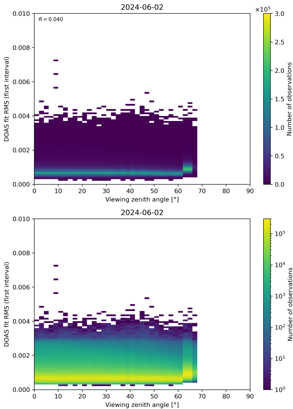
Figure 182: Scatter density plot of “Viewing zenith angle” against “DOAS fit RMS (first interval)” for 2024-06-01 to 2024-06-03.
