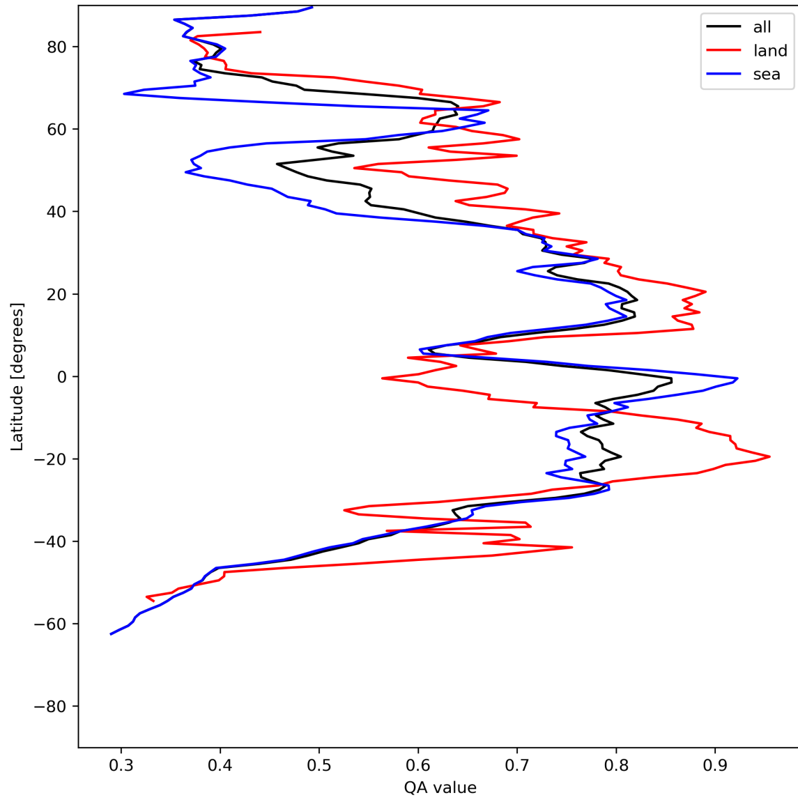
Figure 20: Zonal average of “QA value” for 2024-06-01 to 2024-06-03.
