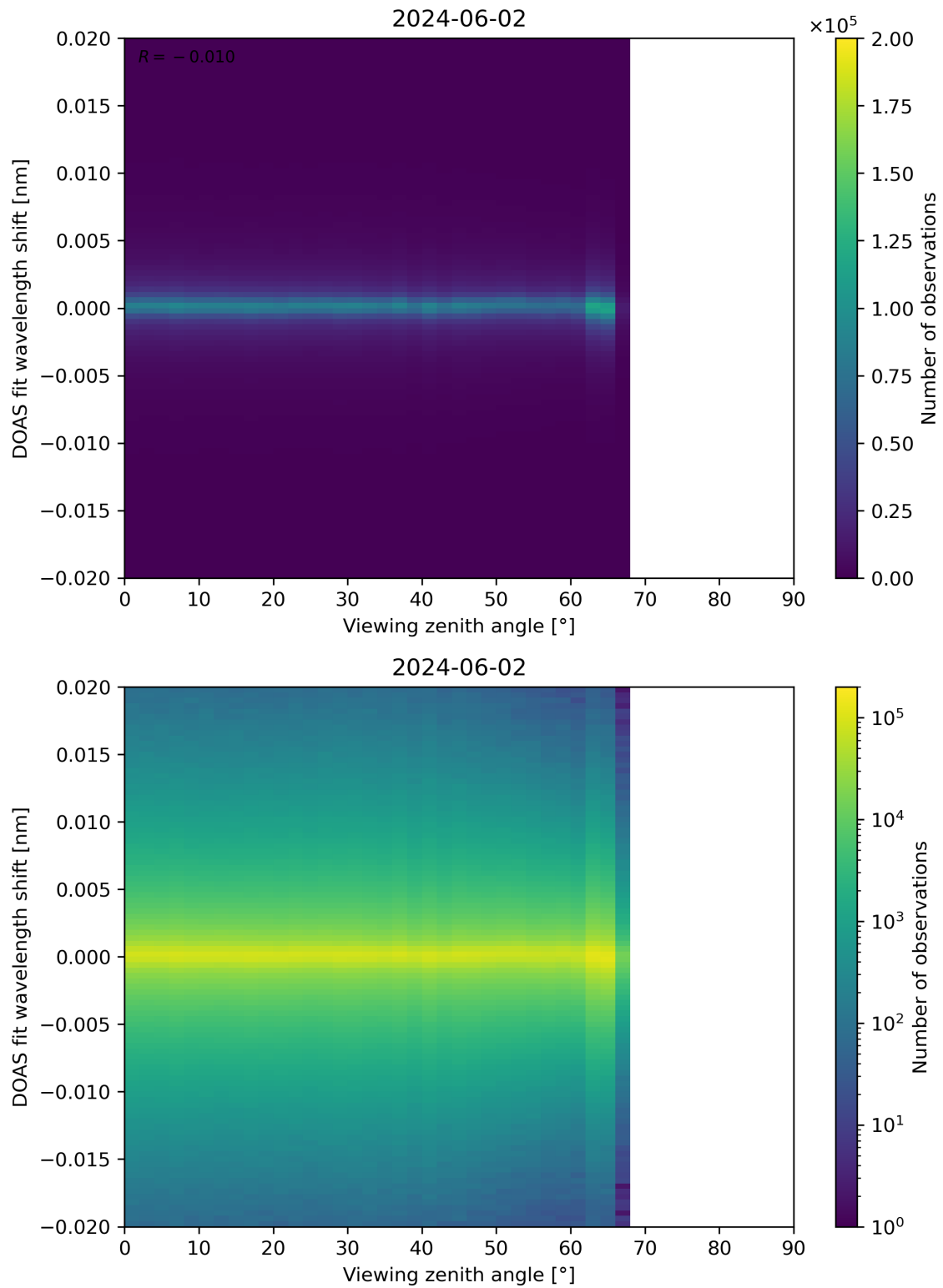
Figure 183: Scatter density plot of “Viewing zenith angle” against “DOAS fit wavelength shift” for 2024-06-01 to 2024-06-03.
