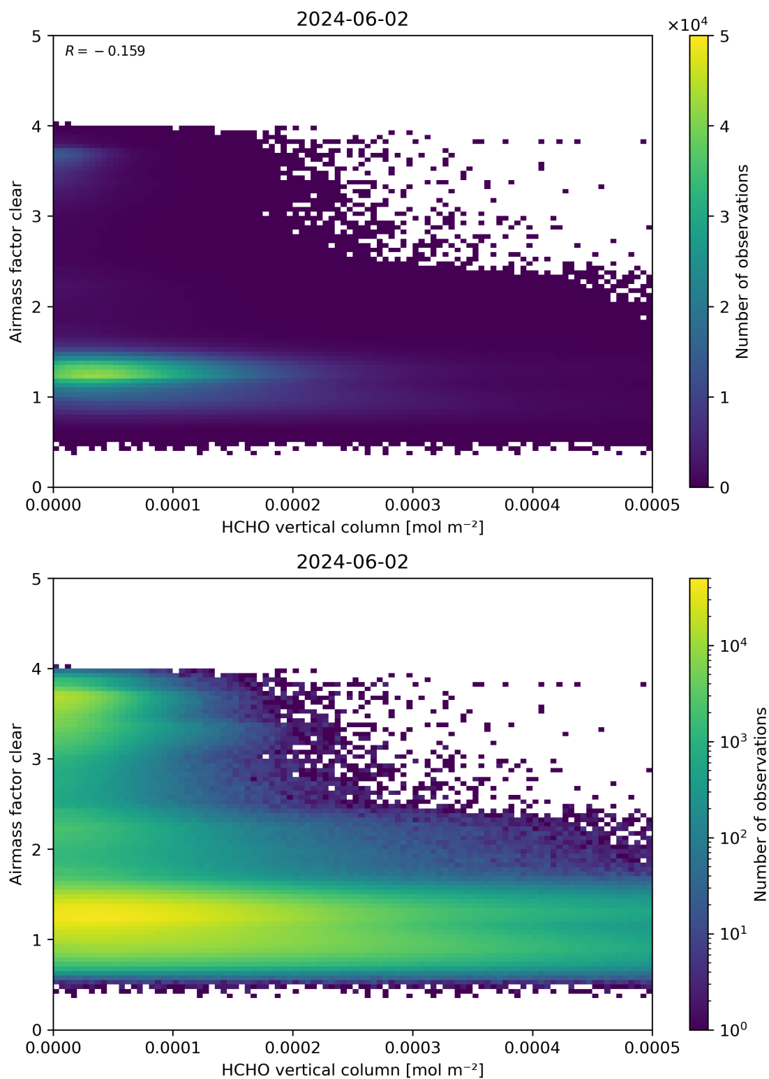
Figure 126: Scatter density plot of “HCHO vertical column” against “Airmass factor clear” for 2024-06-01 to 2024-06-03.
