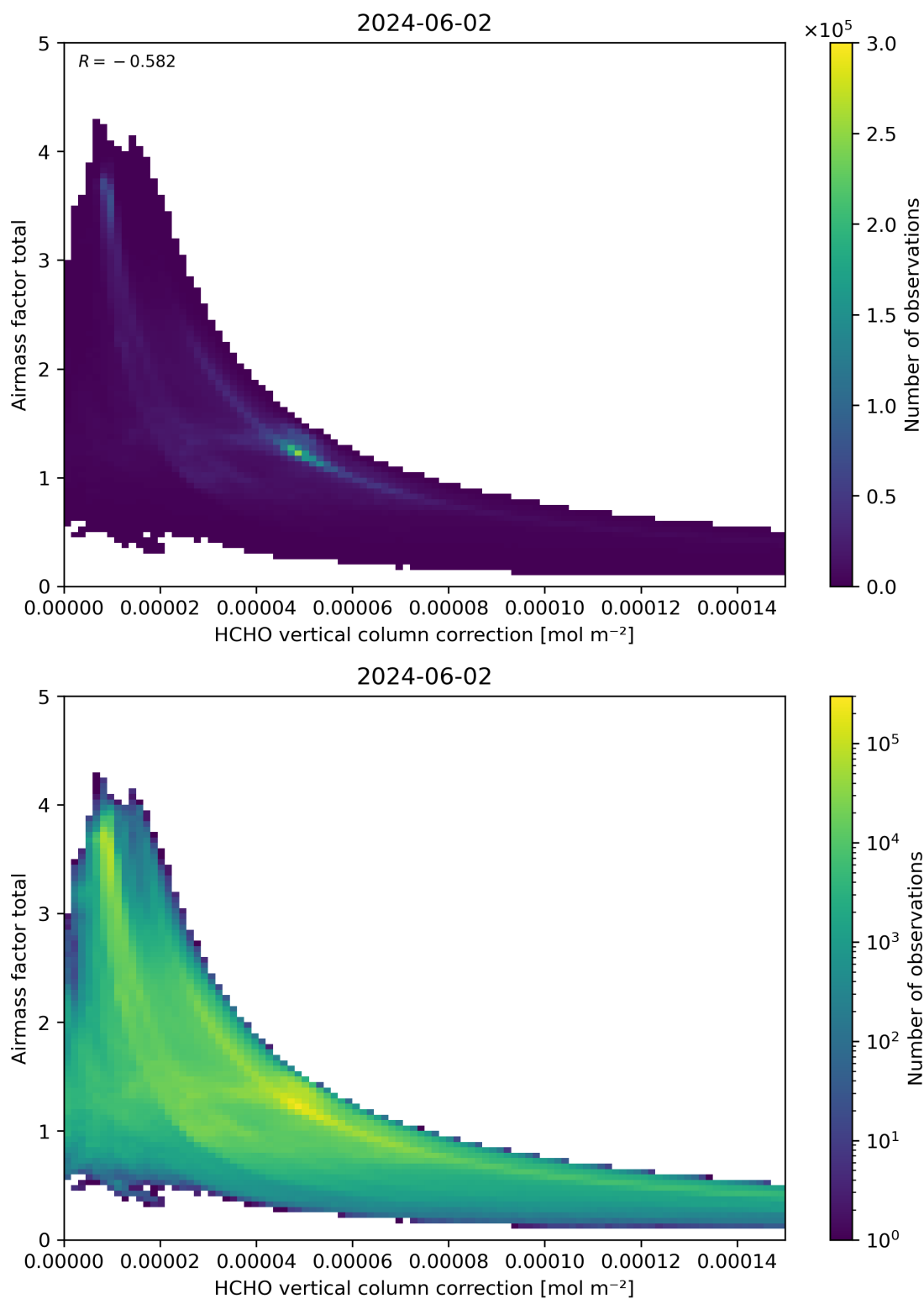
Figure 120: Scatter density plot of “HCHO vertical column correction” against “Airmass factor total” for 2024-06-01 to 2024-06-03.
