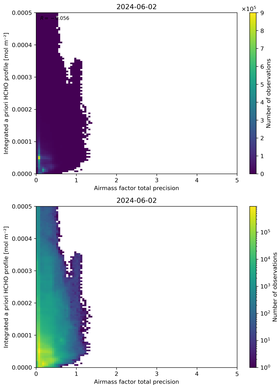
Figure 111: Scatter density plot of “Airmass factor total precision” against “Integrated a priori HCHO profile” for 2024-06-01 to 2024-06-03.
