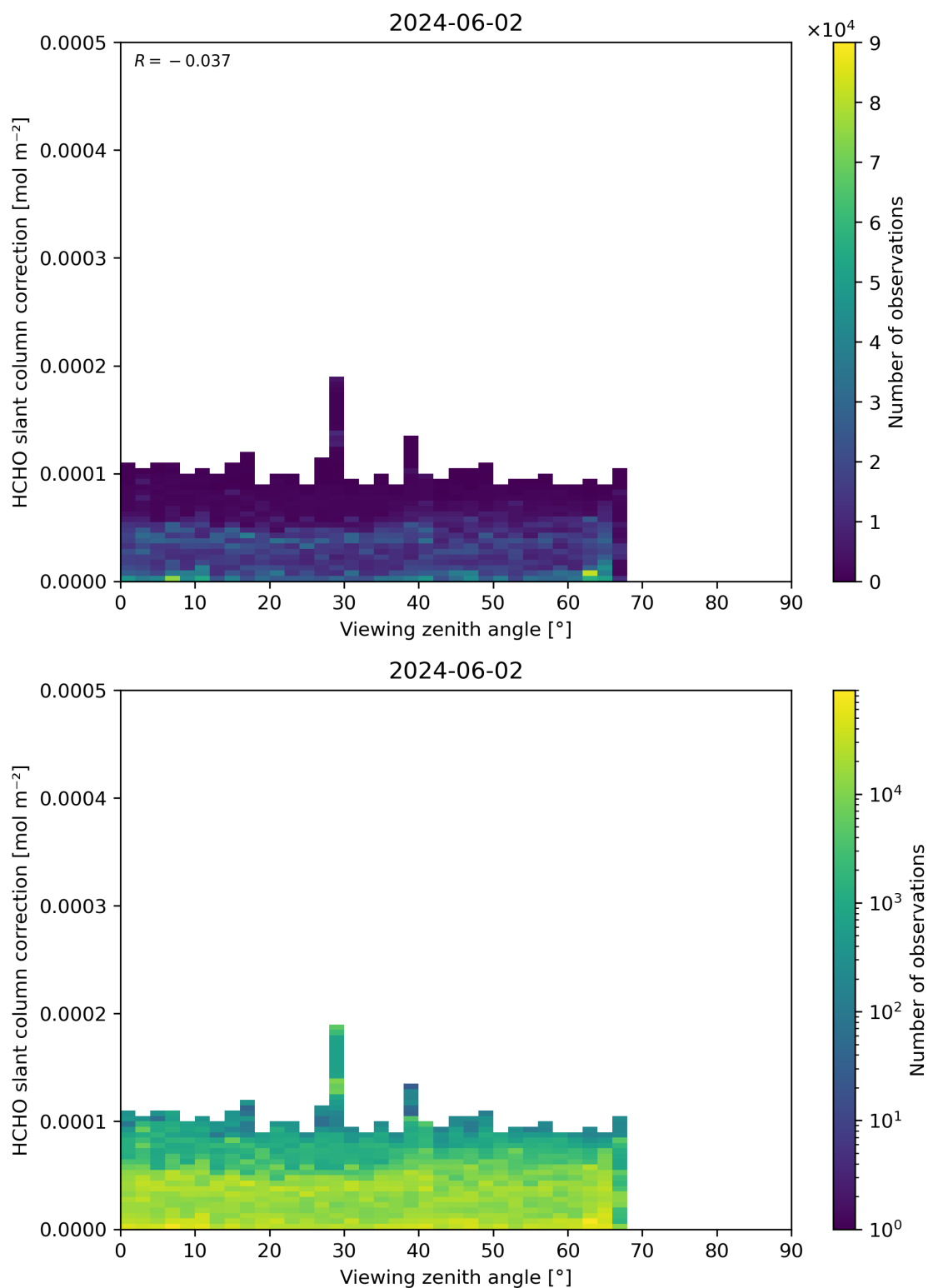
Figure 187: Scatter density plot of “Viewing zenith angle” against “HCHO slant column correction” for 2024-06-01 to 2024-06-03.
