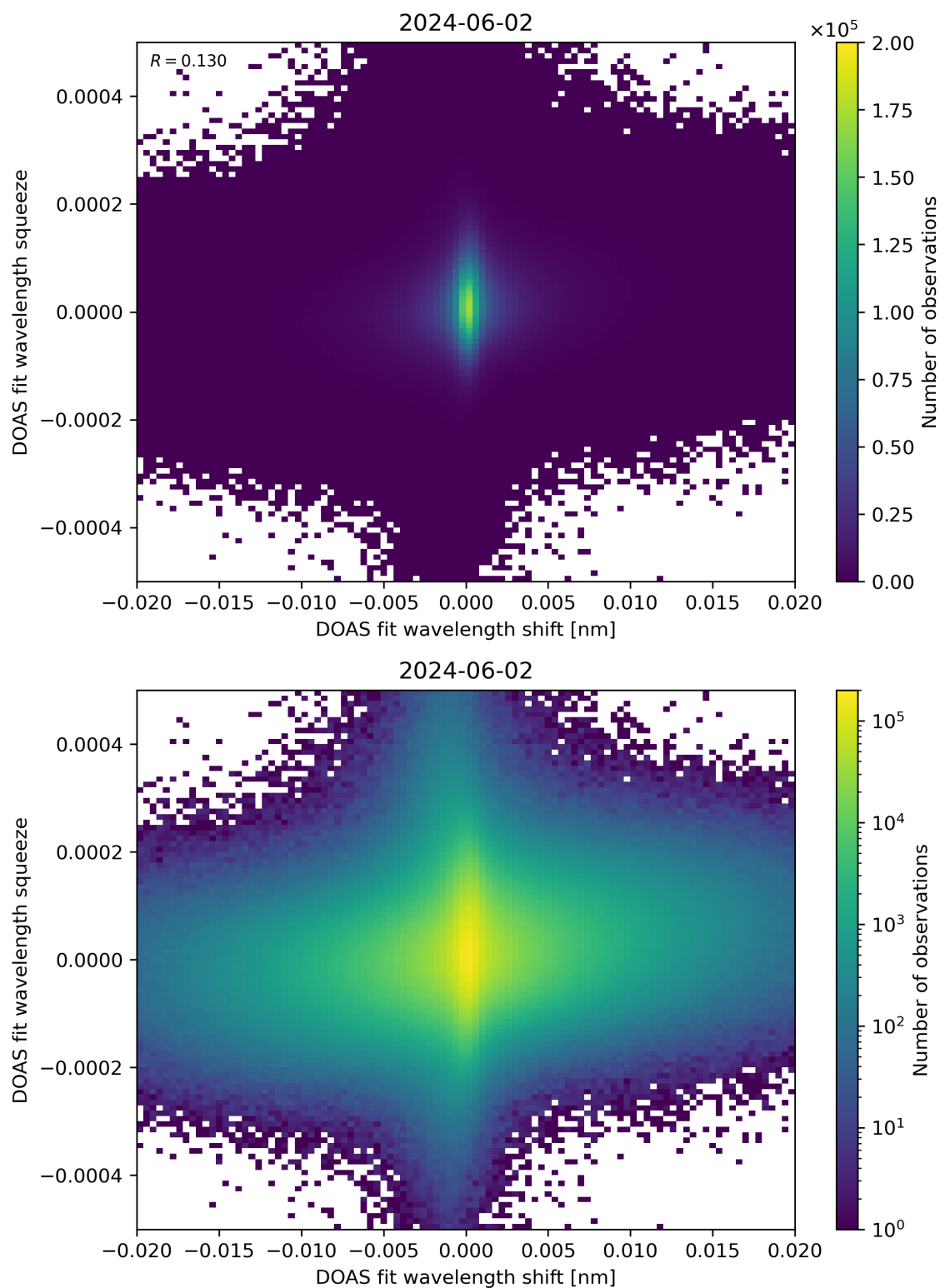
Figure 65: Scatter density plot of “DOAS fit wavelength shift” against “DOAS fit wavelength squeeze” for 2024-06-01 to 2024-06-03.
