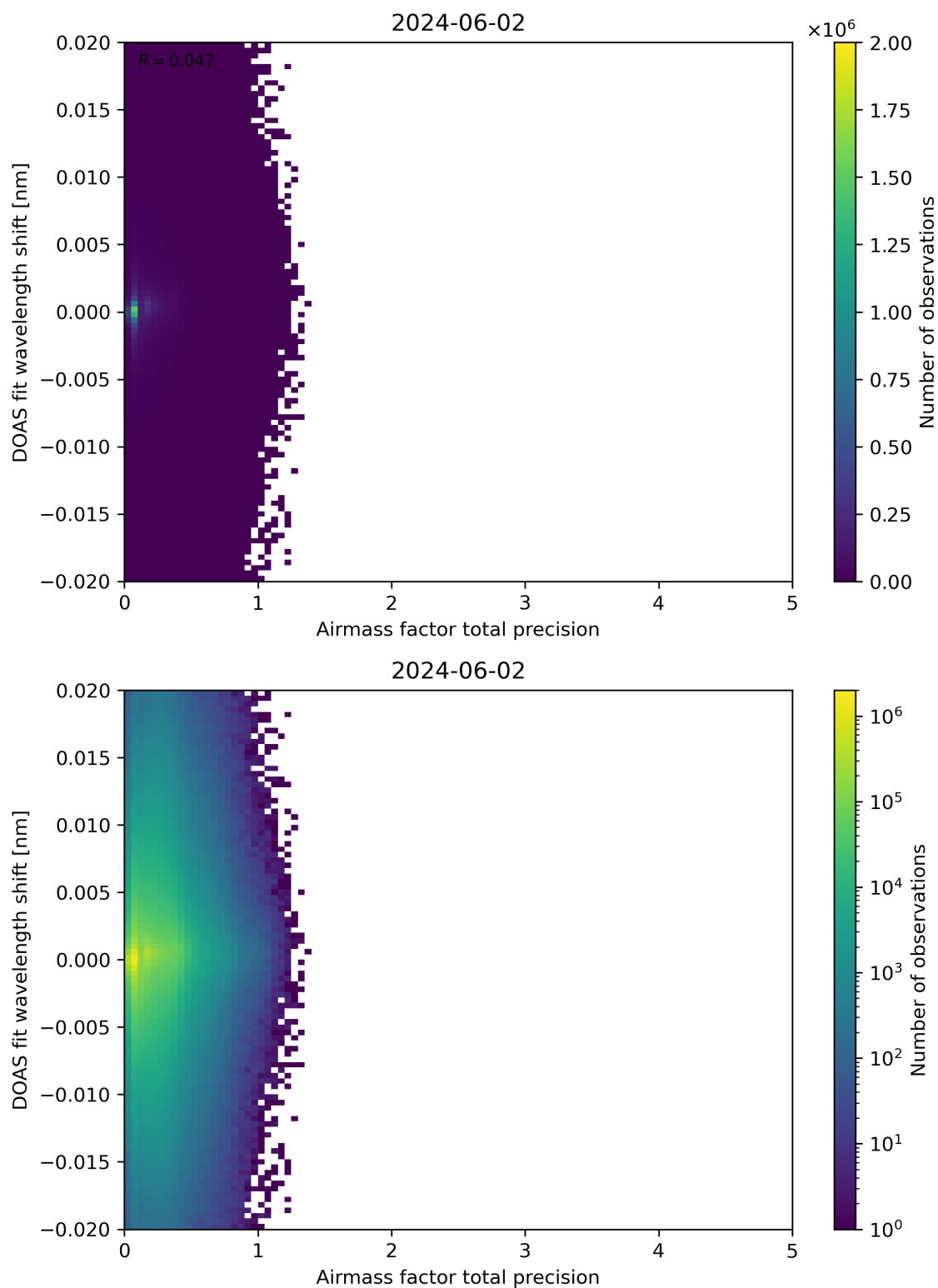
Figure 106: Scatter density plot of “Airmass factor total precision” against “DOAS fit wavelength shift” for 2024-06-01 to 2024-06-03.
