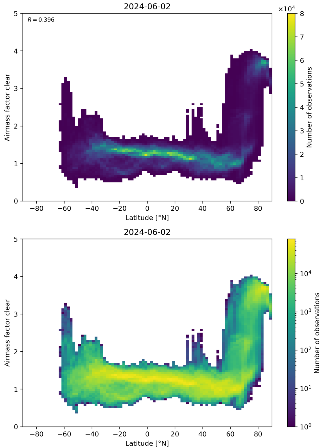
Figure 156: Scatter density plot of “Latitude” against “Airmass factor clear” for 2024-06-01 to 2024-06-03.
