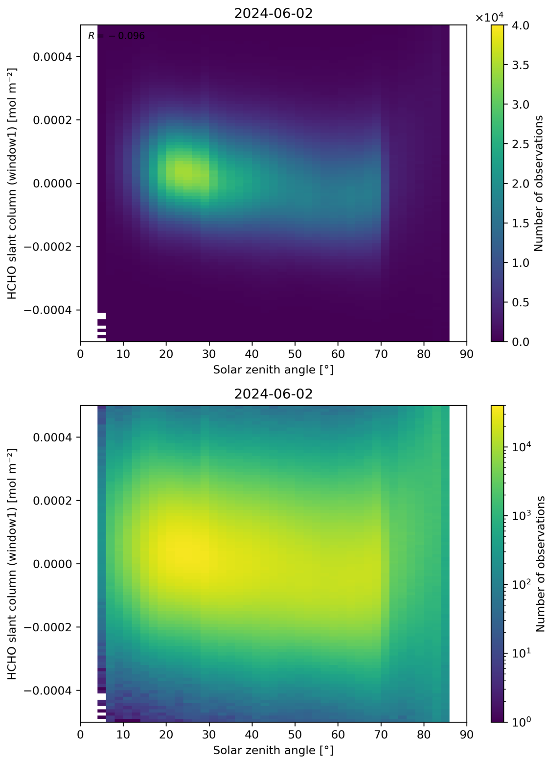
Figure 173: Scatter density plot of “Solar zenith angle” against “HCHO slant column (window1)” for 2024-06-01 to 2024-06-03.
