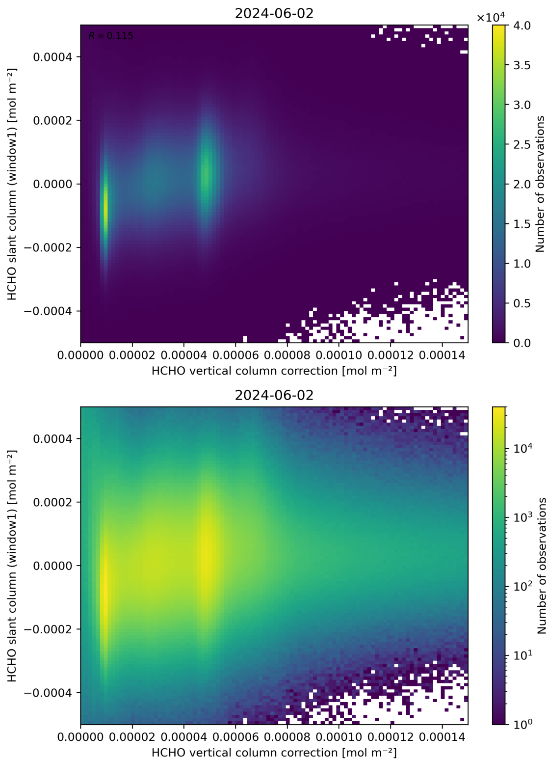
Figure 118: Scatter density plot of “HCHO vertical column correction” against “HCHO slant column (window1)” for 2024-06-01 to 2024-06-03.
