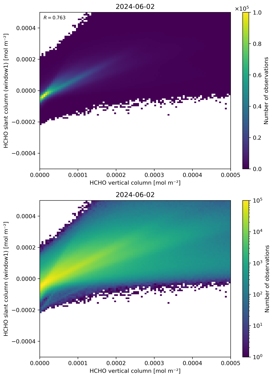
Figure 129: Scatter density plot of “HCHO vertical column” against “HCHO slant column (window1)” for 2024-06-01 to 2024-06-03.
