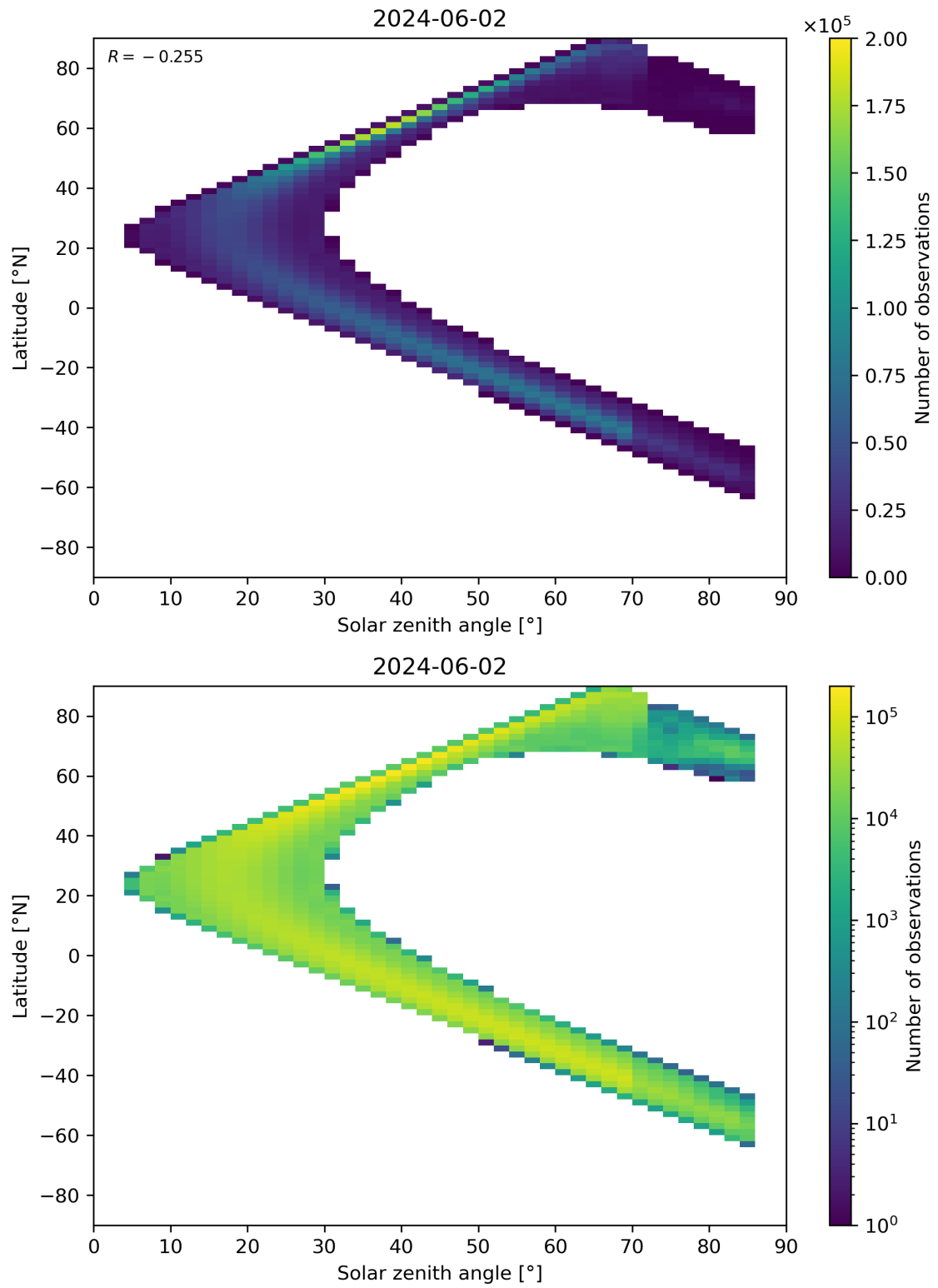
Figure 181: Scatter density plot of “Solar zenith angle” against “Latitude” for 2024-06-01 to 2024-06-03.
