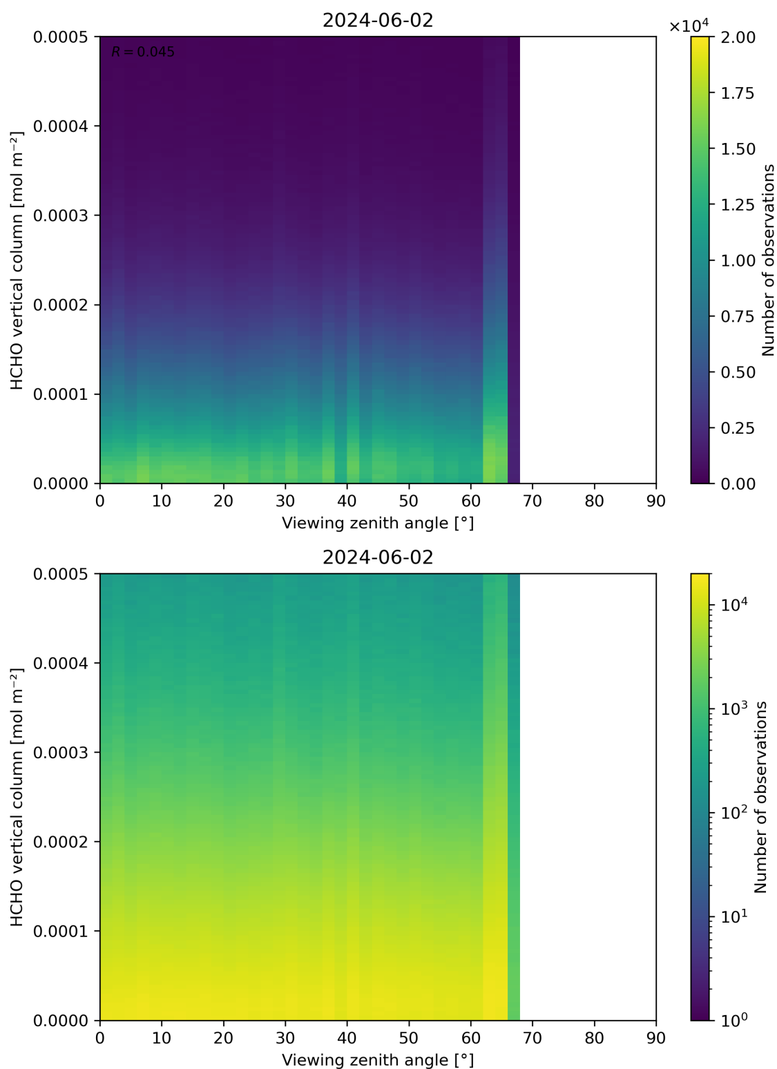
Figure 192: Scatter density plot of “Viewing zenith angle” against “HCHO vertical column” for 2024-06-01 to 2024-06-03.
