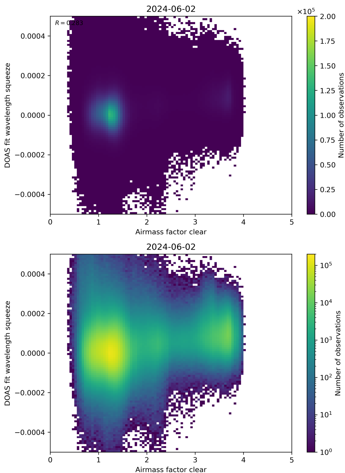
Figure 73: Scatter density plot of “Airmass factor clear” against “DOAS fit wavelength squeeze” for 2024-06-01 to 2024-06-03.
