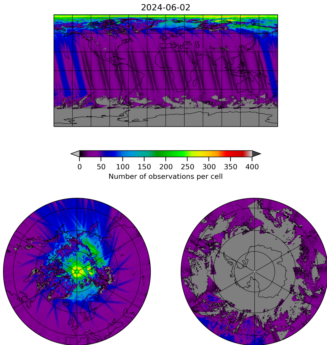
Figure 19: Map of the number of observations for 2024-06-01 to 2024-06-03
