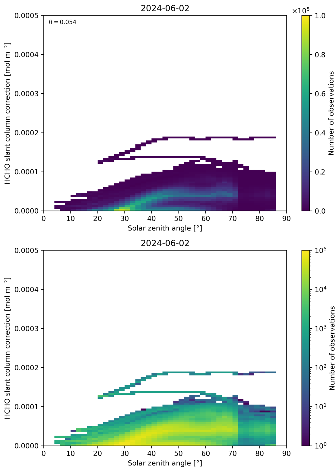
Figure 172: Scatter density plot of “Solar zenith angle” against “HCHO slant column correction” for 2024-06-01 to 2024-06-03.
