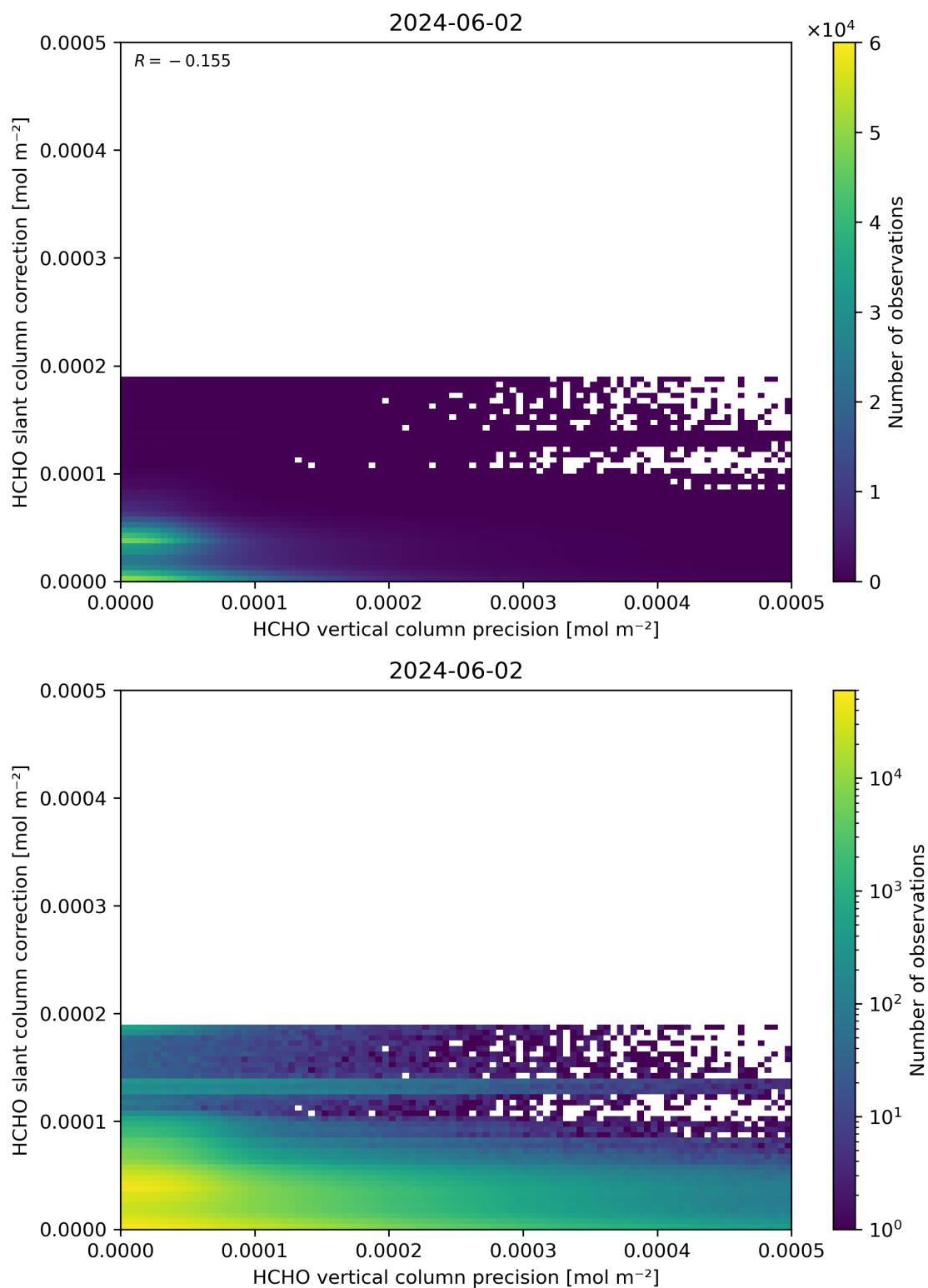
Figure 141: Scatter density plot of “HCHO vertical column precision” against “HCHO slant column correction” for 2024-06-01 to 2024-06-03.
