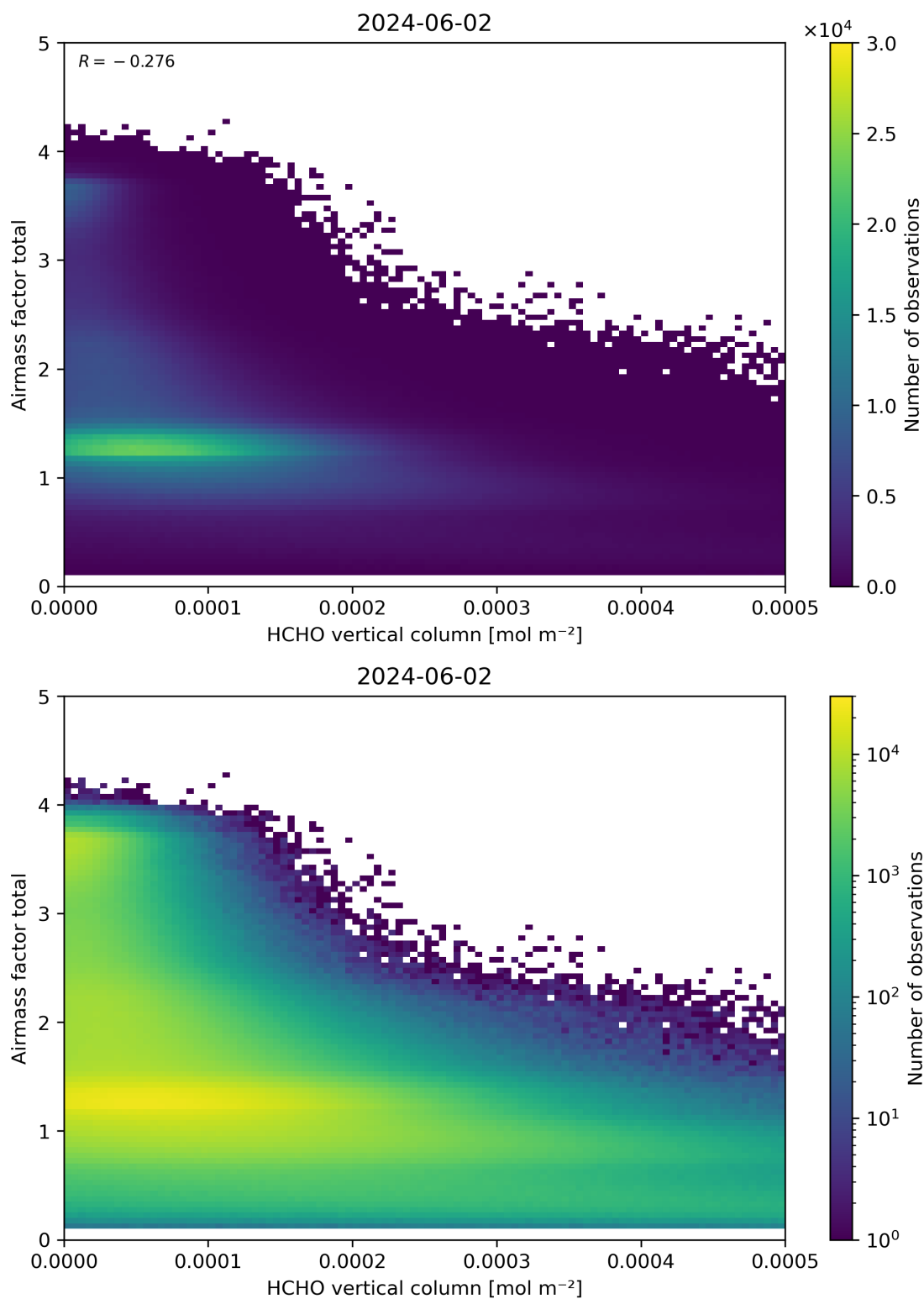
Figure 131: Scatter density plot of “HCHO vertical column” against “Airmass factor total” for 2024-06-01 to 2024-06-03.
