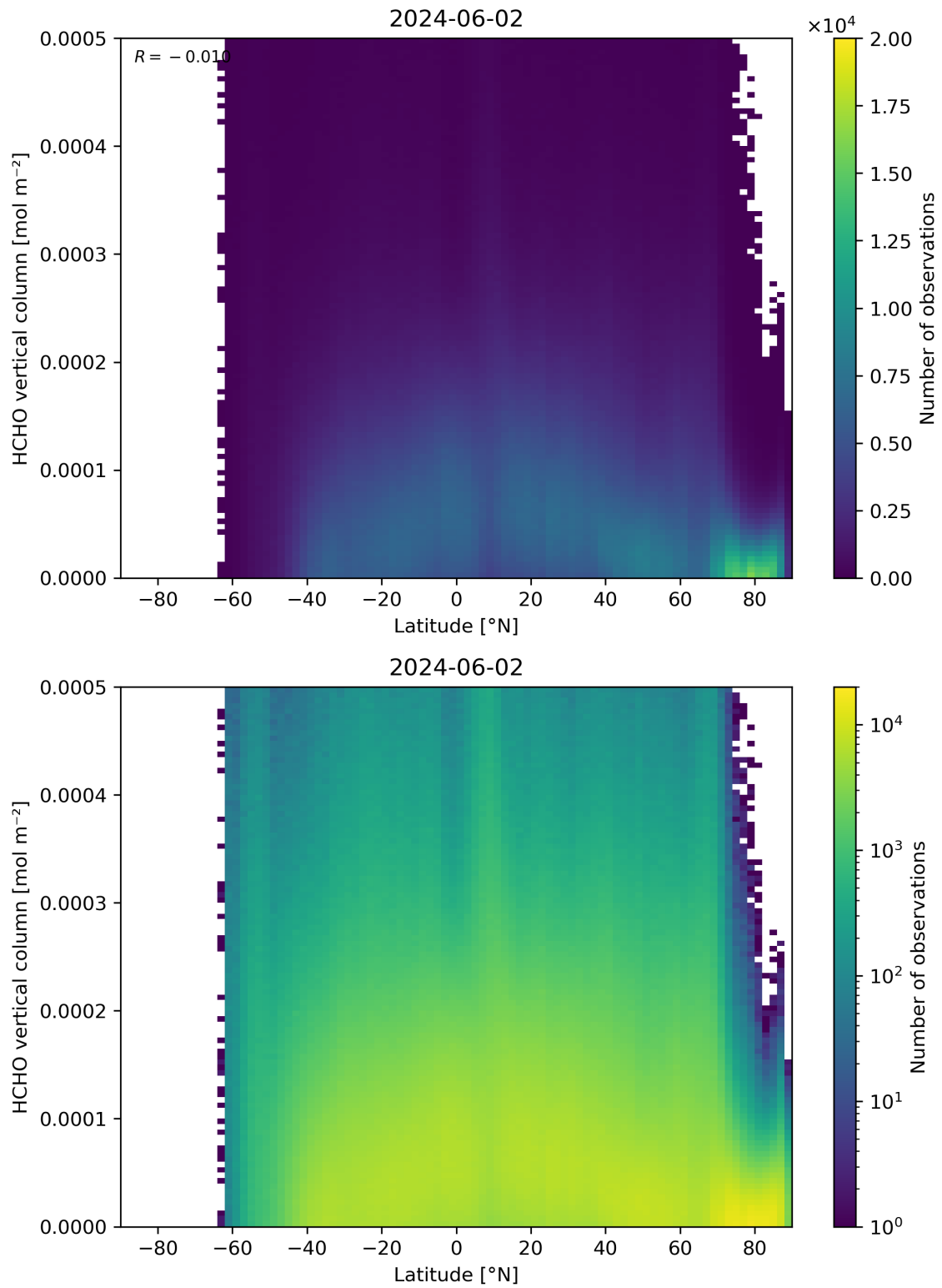
Figure 163: Scatter density plot of “Latitude” against “HCHO vertical column” for 2024-06-01 to 2024-06-03.
