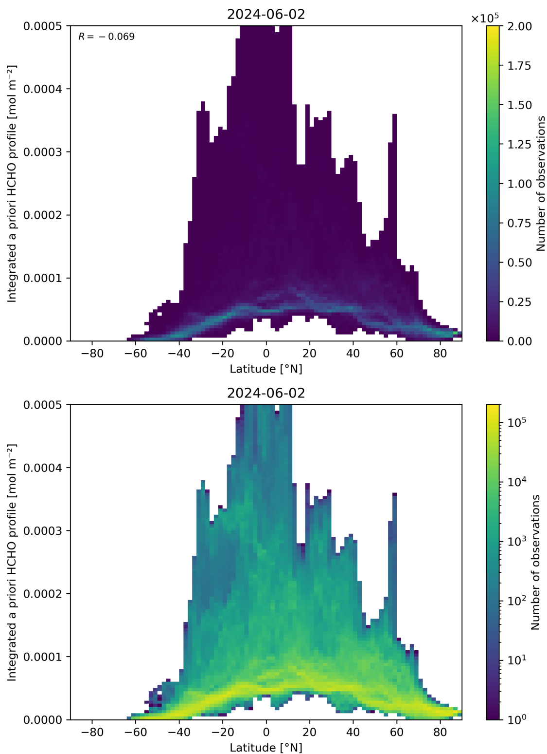
Figure 166: Scatter density plot of “Latitude” against “Integrated a priori HCHO profile” for 2024-06-01 to 2024-06-03.
