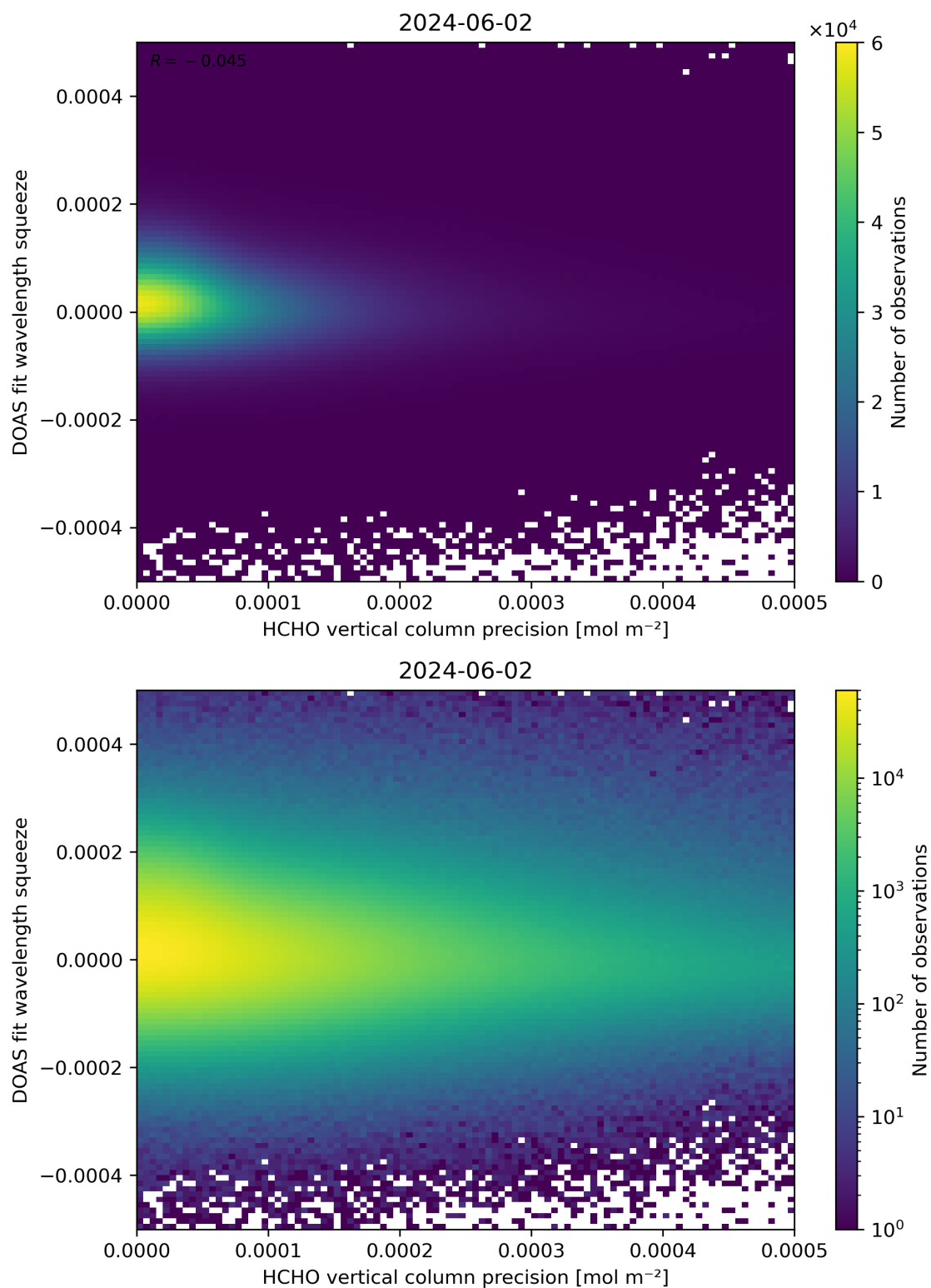
Figure 138: Scatter density plot of “HCHO vertical column precision” against “DOAS fit wavelength squeeze” for 2024-06-01 to 2024-06-03.
