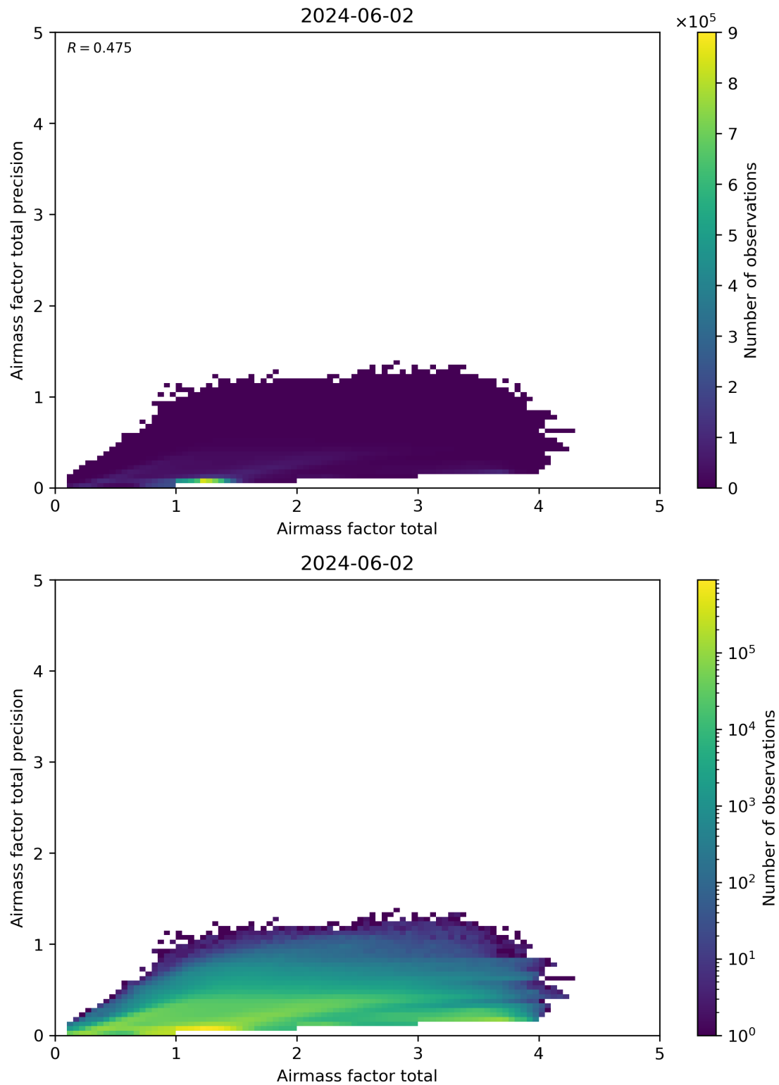
Figure 103: Scatter density plot of “Airmass factor total” against “Airmass factor total precision” for 2024-06-01 to 2024-06-03.
