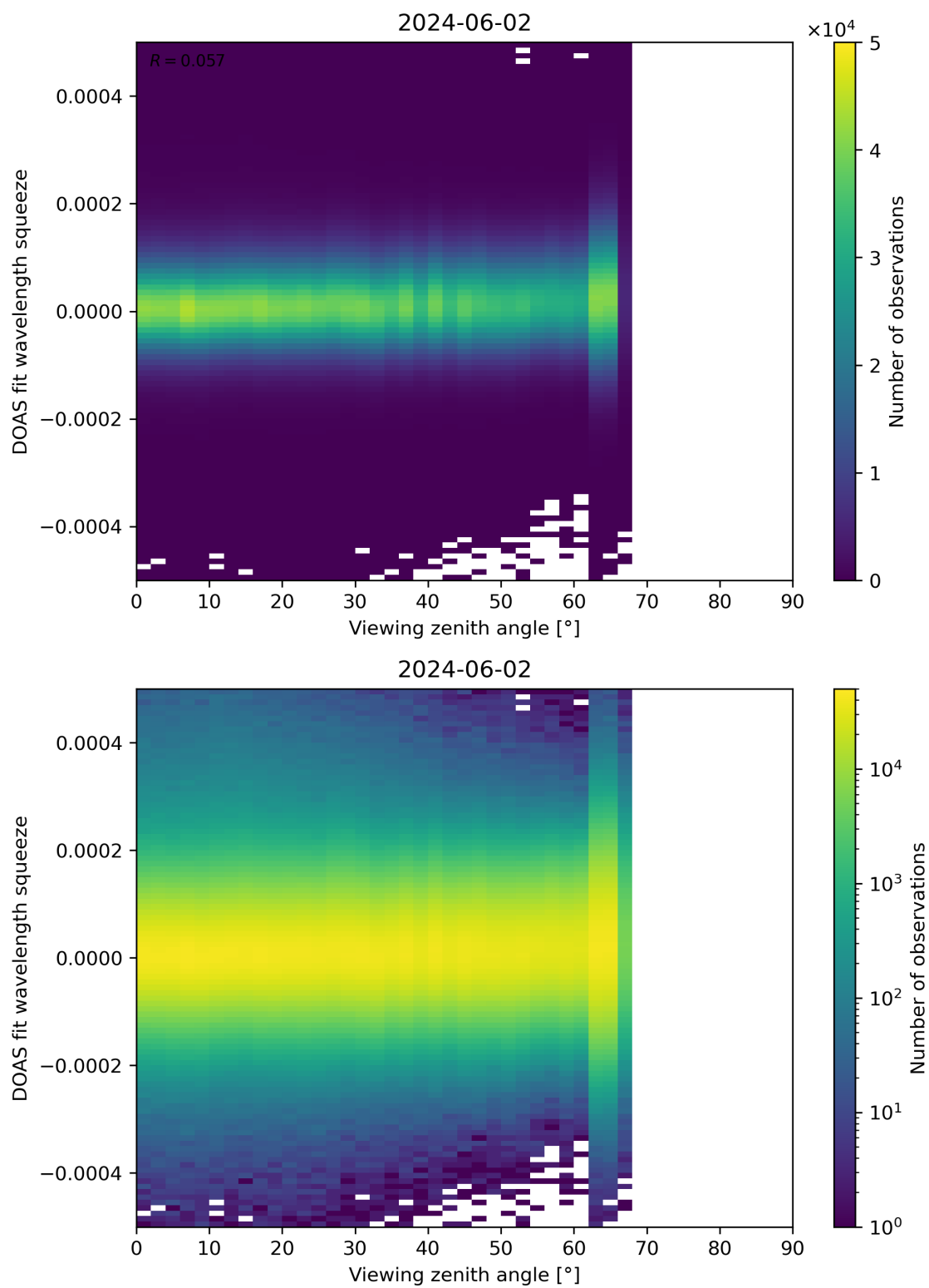
Figure 184: Scatter density plot of “Viewing zenith angle” against “DOAS fit wavelength squeeze” for 2024-06-01 to 2024-06-03.
