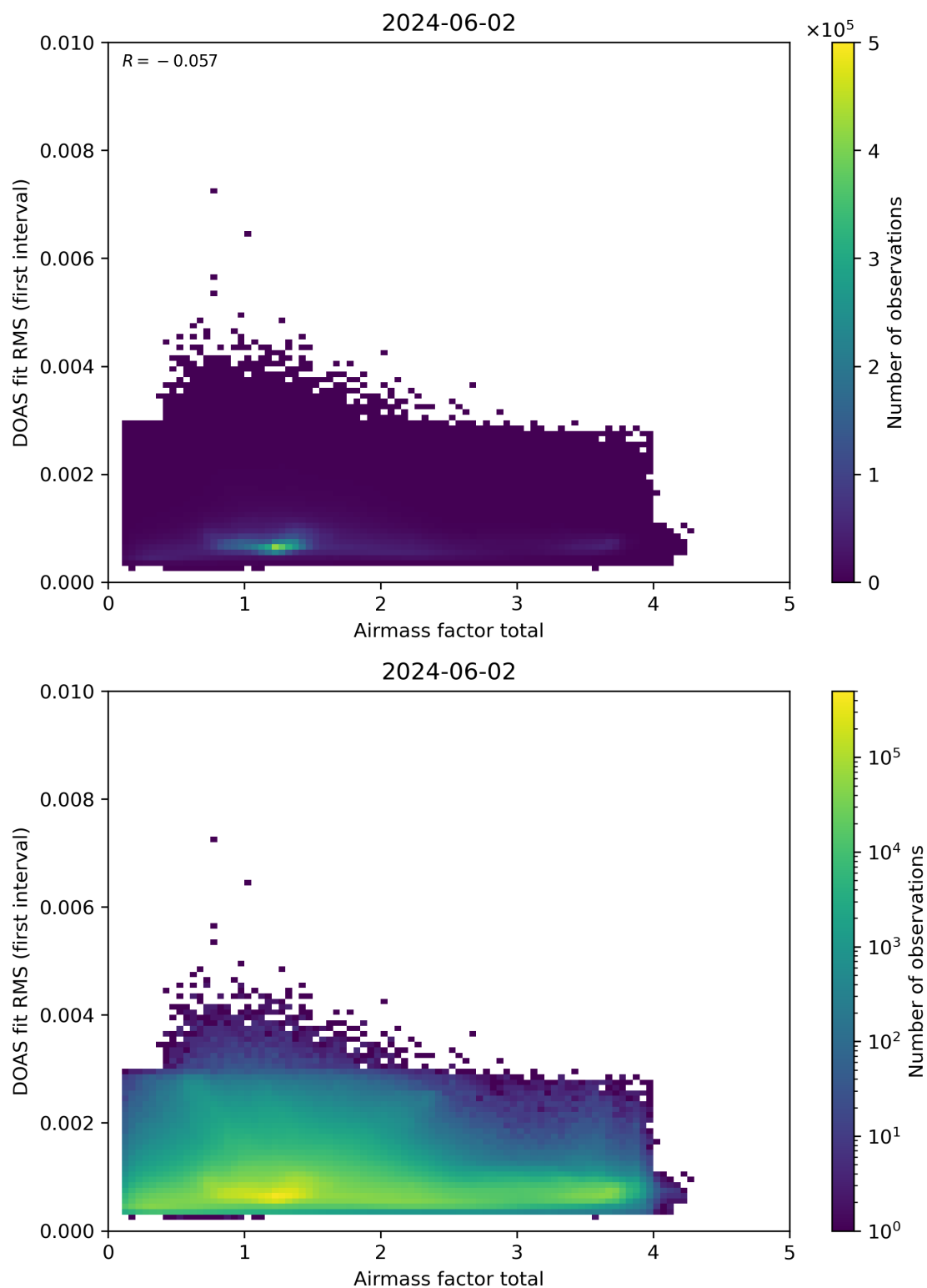
Figure 97: Scatter density plot of “Airmass factor total” against “DOAS fit RMS (first interval)” for 2024-06-01 to 2024-06-03.
