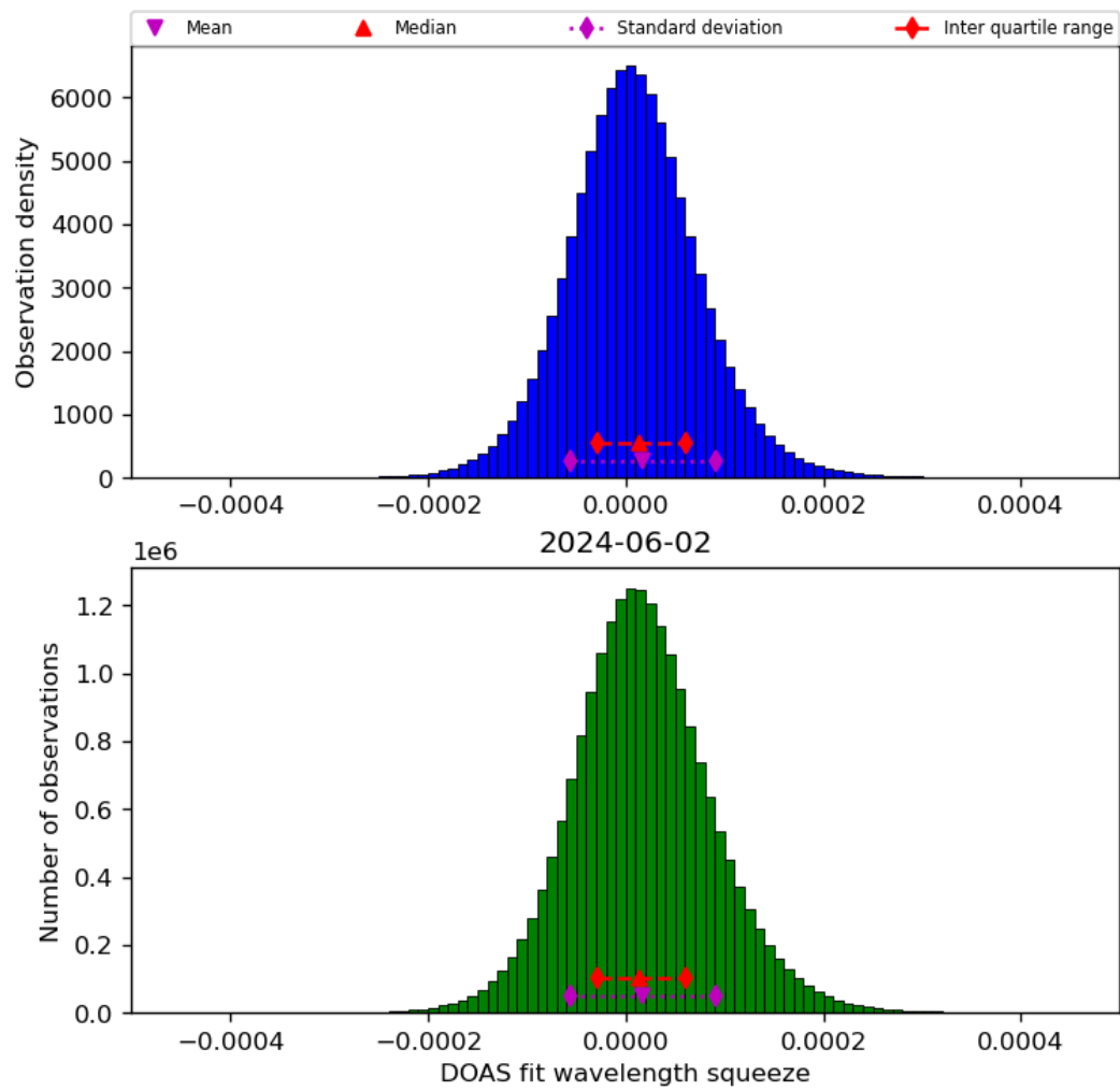
Figure 45: Histogram of “DOAS fit wavelength squeeze” for 2024-06-01 to 2024-06-03
