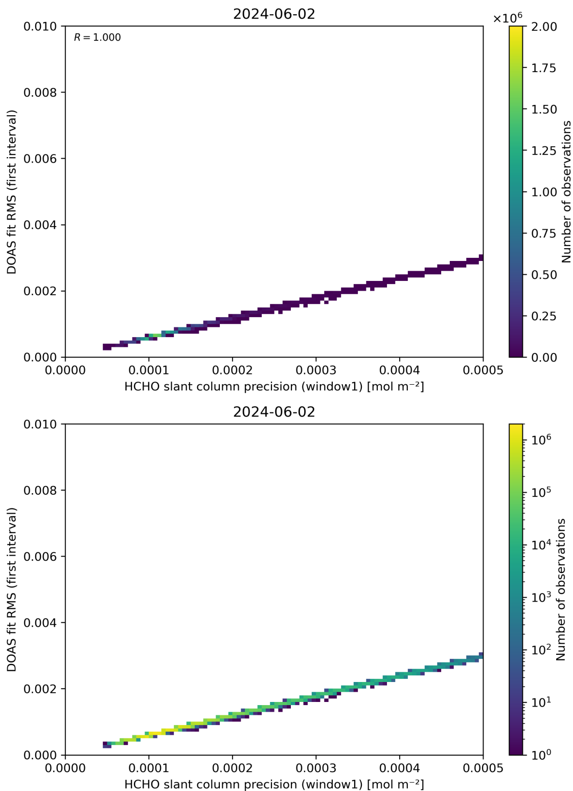
Figure 88: Scatter density plot of “HCHO slant column precision (window1)” against “DOAS fit RMS (first interval)” for 2024-06-01 to 2024-06-03.
