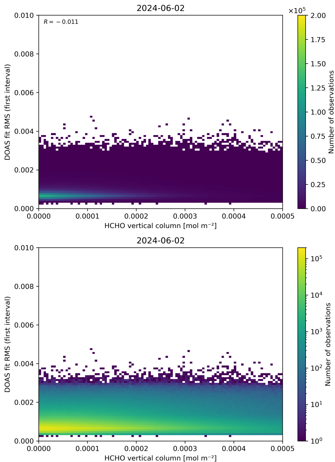
Figure 123: Scatter density plot of “HCHO vertical column” against “DOAS fit RMS (first interval)” for 2024-06-01 to 2024-06-03.
