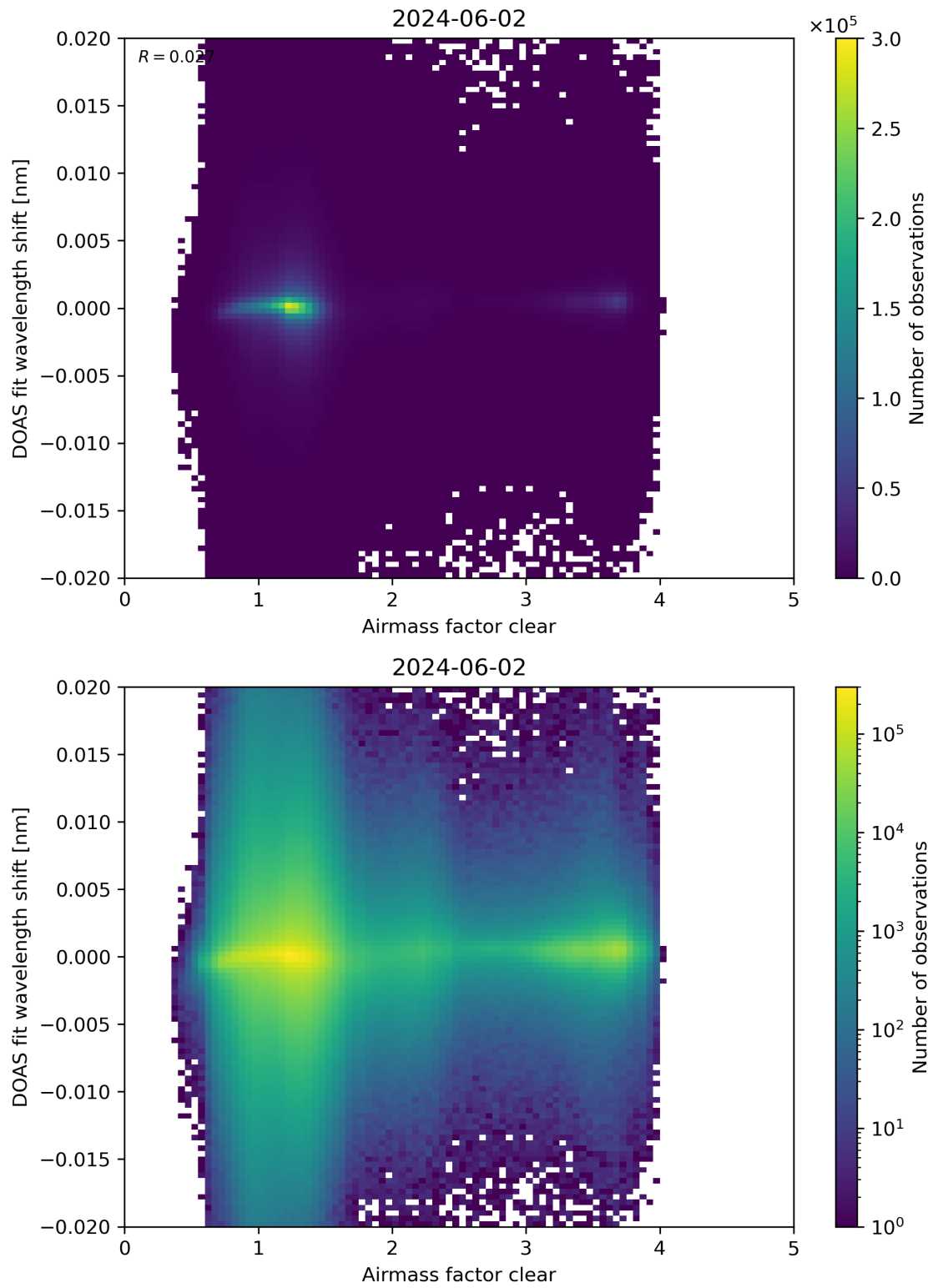
Figure 72: Scatter density plot of “Airmass factor clear” against “DOAS fit wavelength shift” for 2024-06-01 to 2024-06-03.
