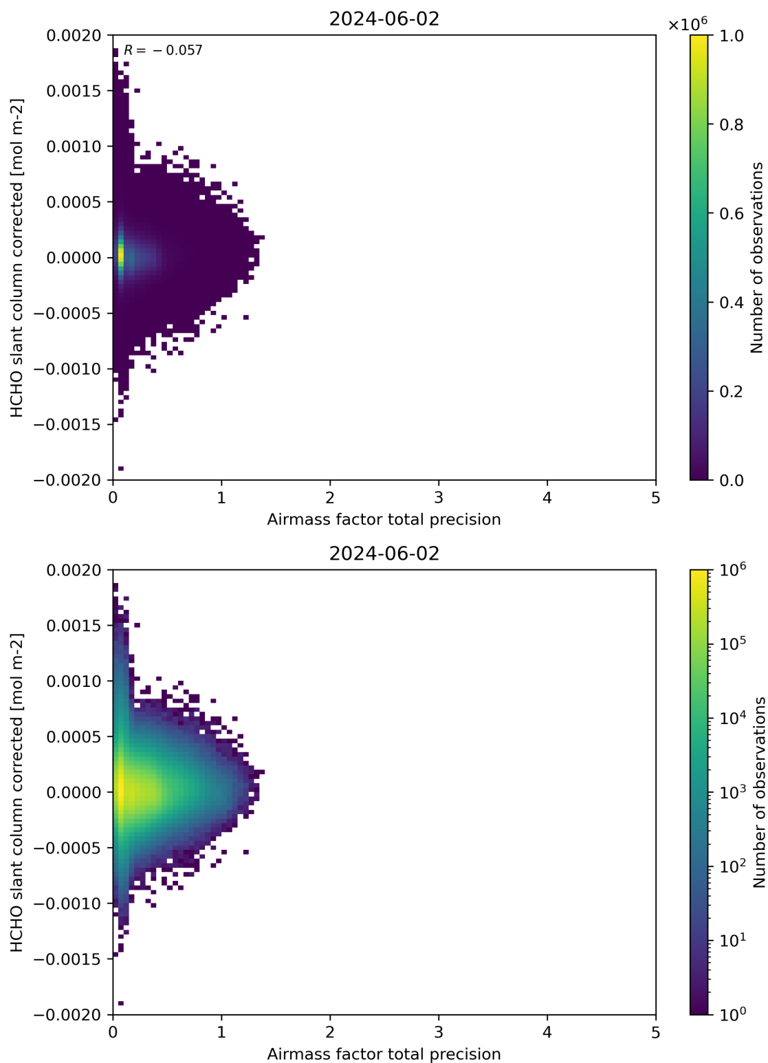
Figure 109: Scatter density plot of “Airmass factor total precision” against “HCHO slant column corrected” for 2024-06-01 to 2024-06-03.
