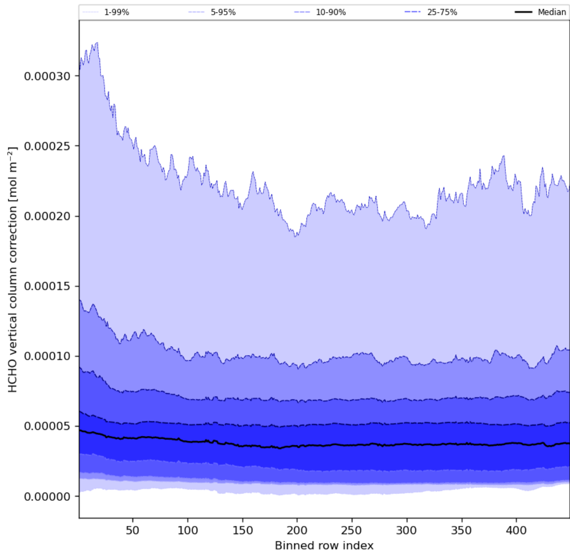
Figure 51: Along track statistics of “HCHO vertical column correction” for 2024-06-01 to 2024-06-03
