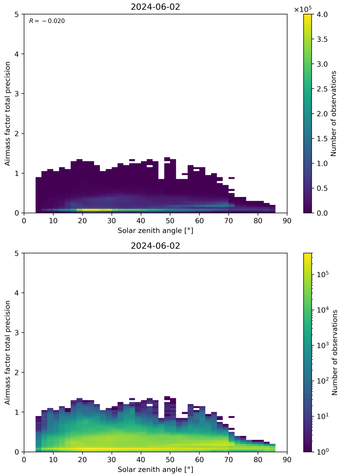
Figure 176: Scatter density plot of “Solar zenith angle” against “Airmass factor total precision” for 2024-06-01 to 2024-06-03.
