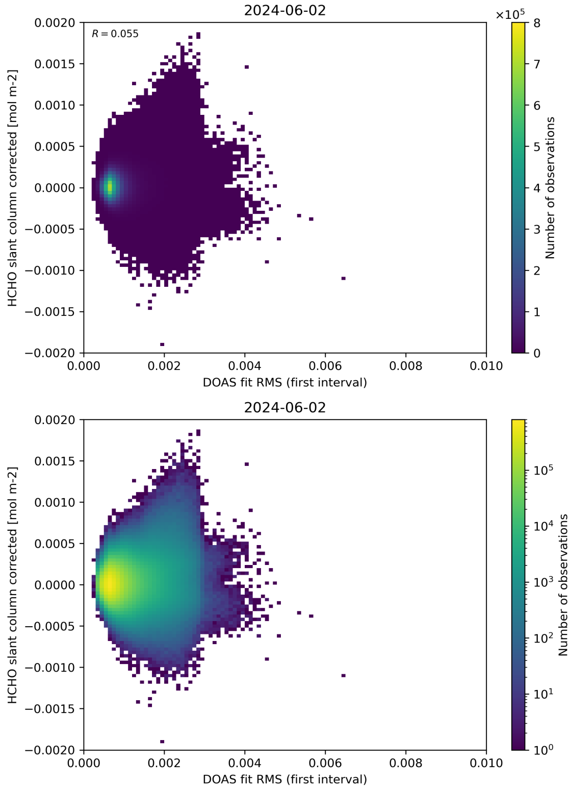
Figure 62: Scatter density plot of “DOAS fit RMS (first interval)” against “HCHO slant column corrected” for 2024-06-01 to 2024-06-03.
