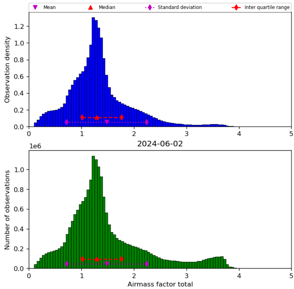
Figure 40: Histogram of “Airmass factor total” for 2024-06-01 to 2024-06-03
