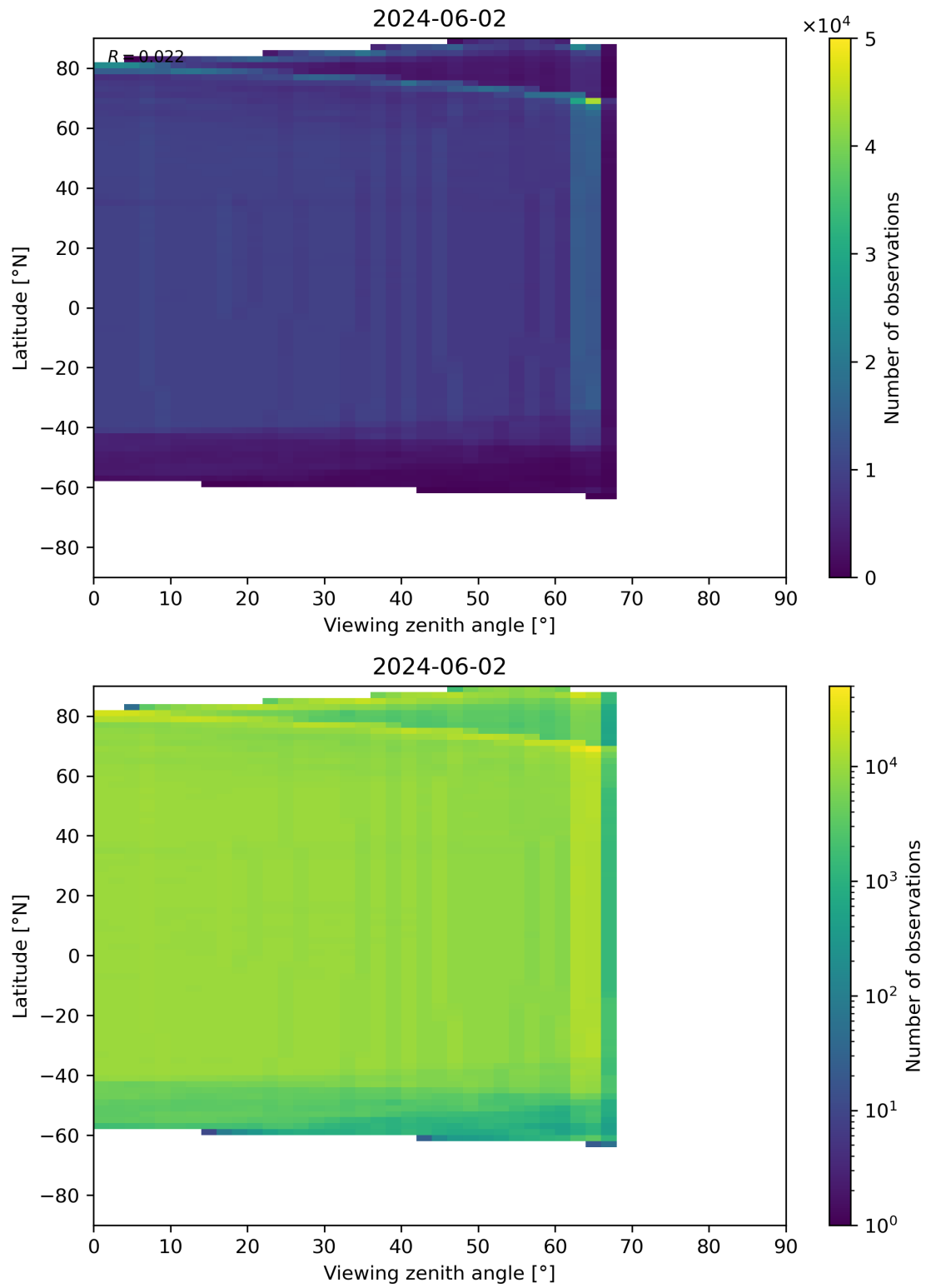
Figure 196: Scatter density plot of “Viewing zenith angle” against “Latitude” for 2024-06-01 to 2024-06-03.
