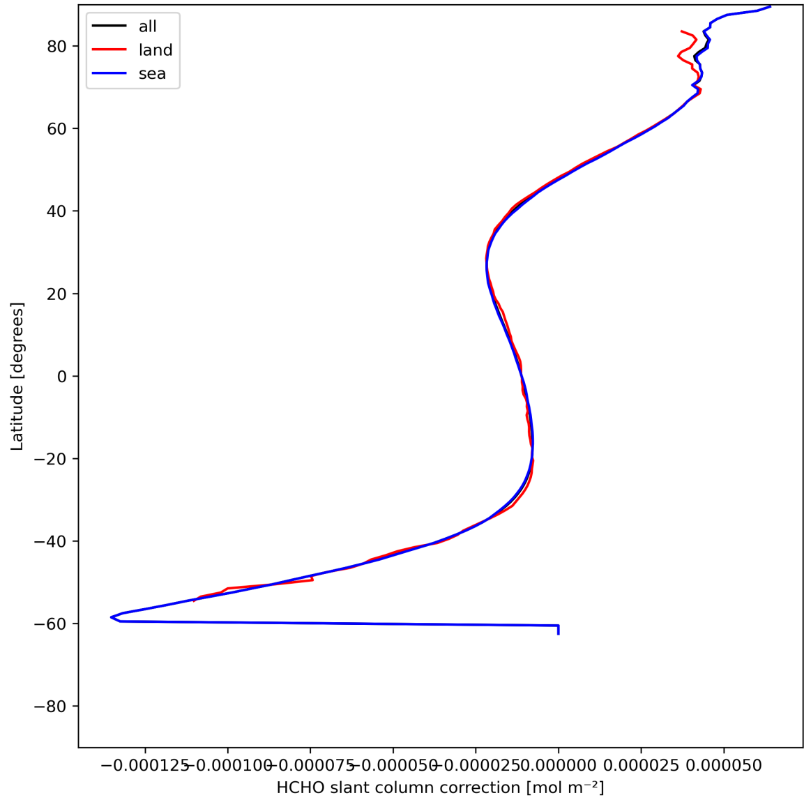
Figure 33: Zonal average of “HCHO slant column correction” for 2024-06-01 to 2024-06-03.
