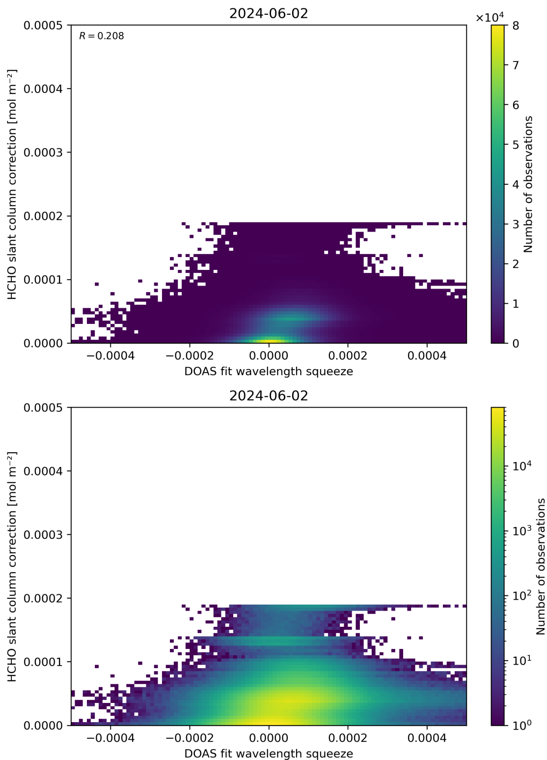
Figure 70: Scatter density plot of “DOAS fit wavelength squeeze” against “HCHO slant column correction” for 2024-06-01 to 2024-06-03.
