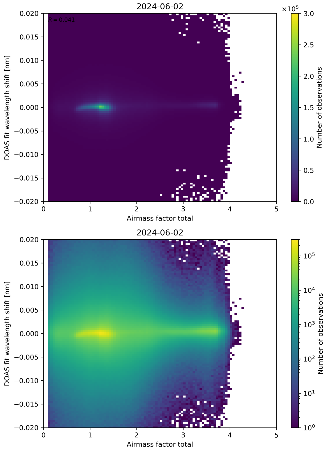
Figure 98: Scatter density plot of “Airmass factor total” against “DOAS fit wavelength shift” for 2024-06-01 to 2024-06-03.
