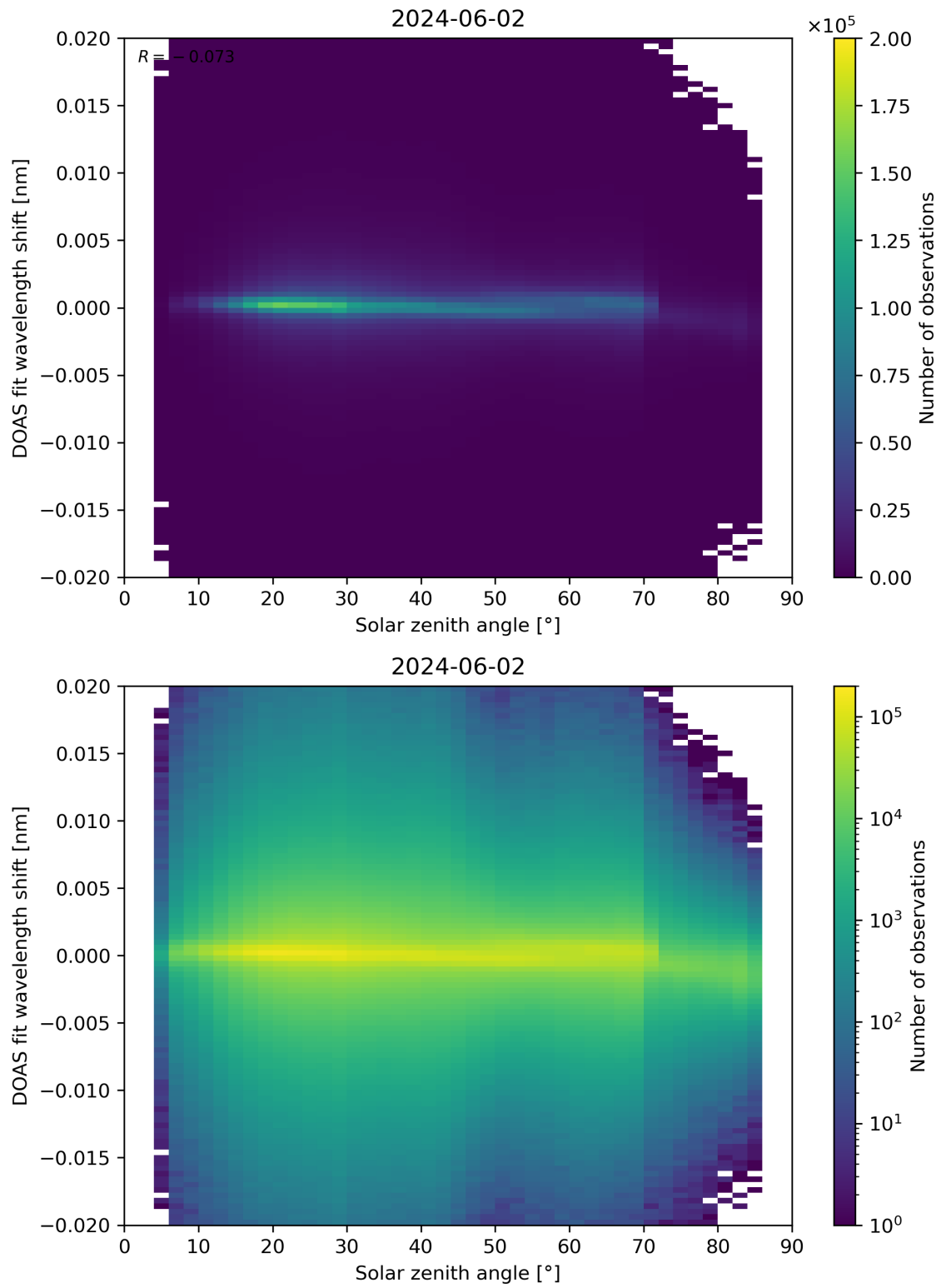
Figure 168: Scatter density plot of “Solar zenith angle” against “DOAS fit wavelength shift” for 2024-06-01 to 2024-06-03.
