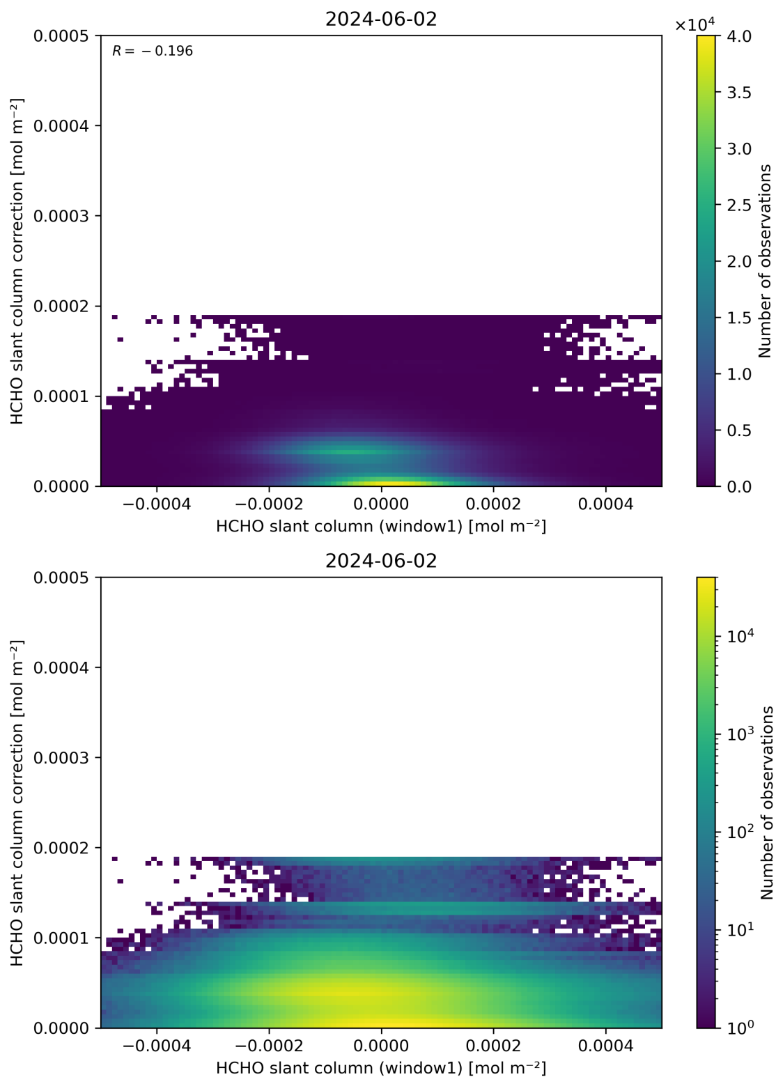
Figure 83: Scatter density plot of “HCHO slant column (window1)” against “HCHO slant column correction” for 2024-06-01 to 2024-06-03.
