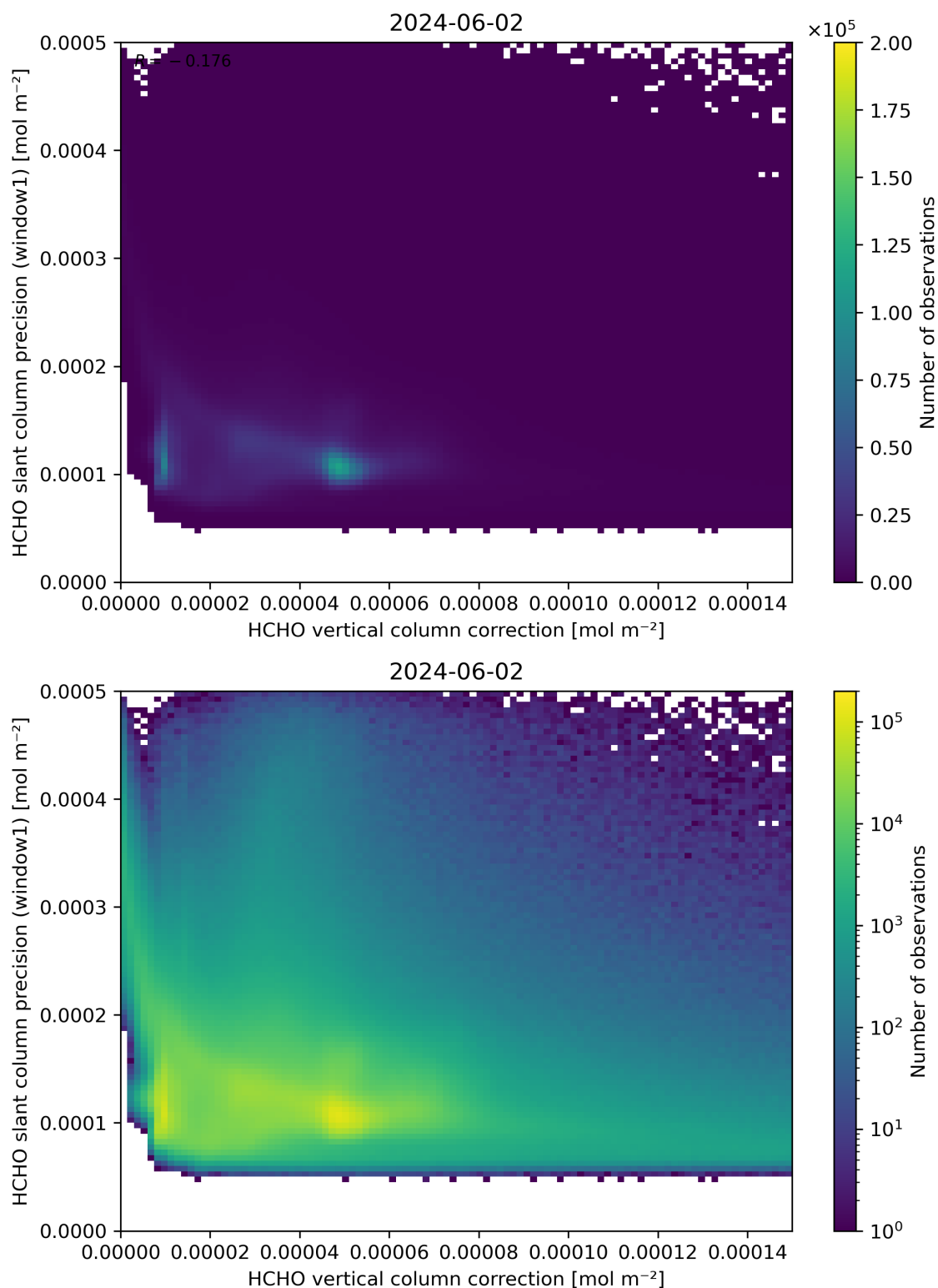
Figure 119: Scatter density plot of “HCHO vertical column correction” against “HCHO slant column precision (window1)” for 2024-06-01 to 2024-06-03.
