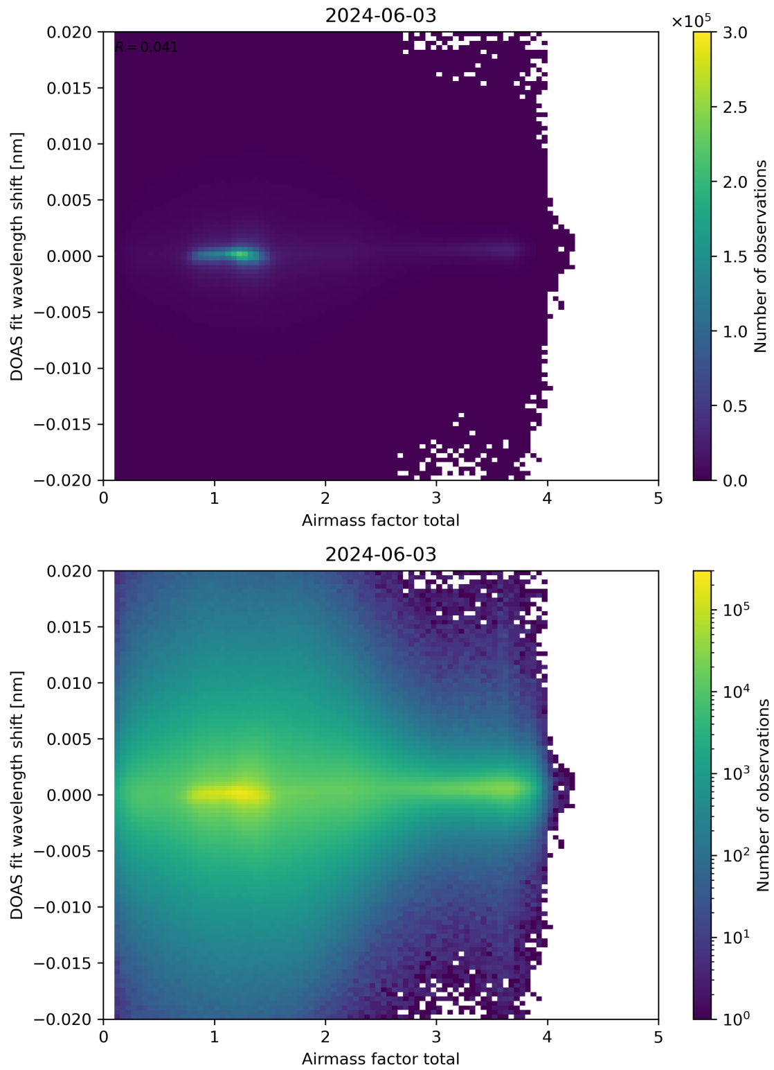
Figure 98: Scatter density plot of “Airmass factor total” against “DOAS fit wavelength shift” for 2024-06-03 to 2024-06-04.
