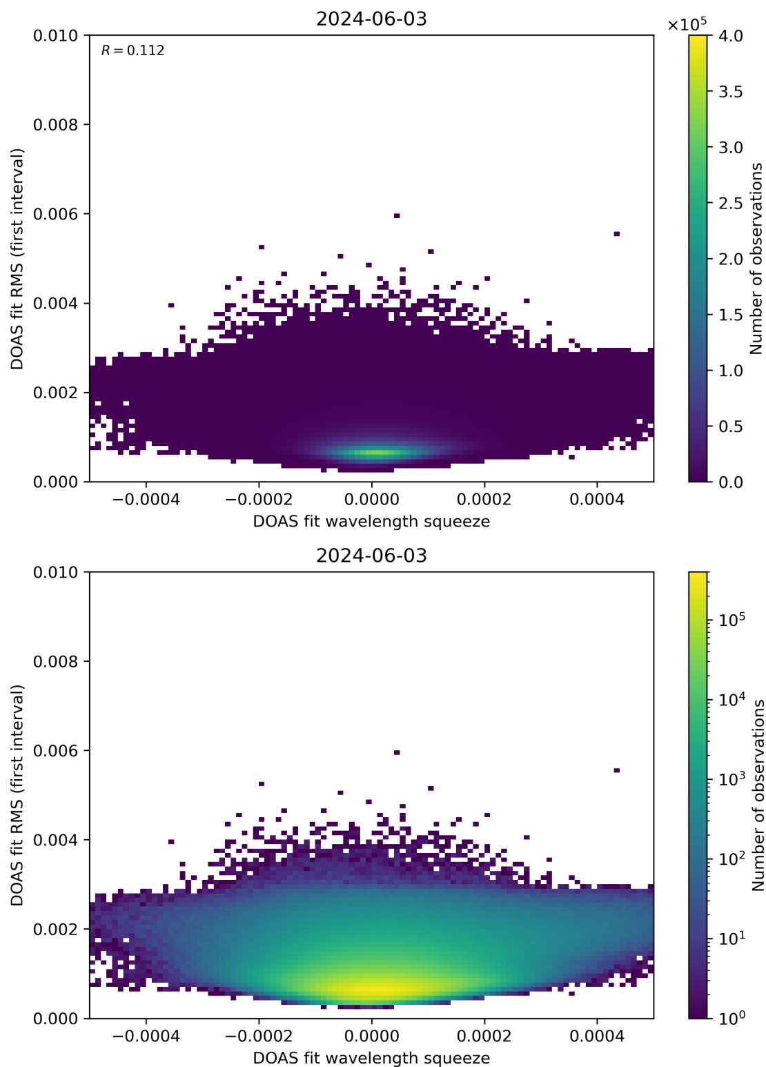
Figure 68: Scatter density plot of “DOAS fit wavelength squeeze” against “DOAS fit RMS (first interval)” for 2024-06-03 to 2024-06-04.
