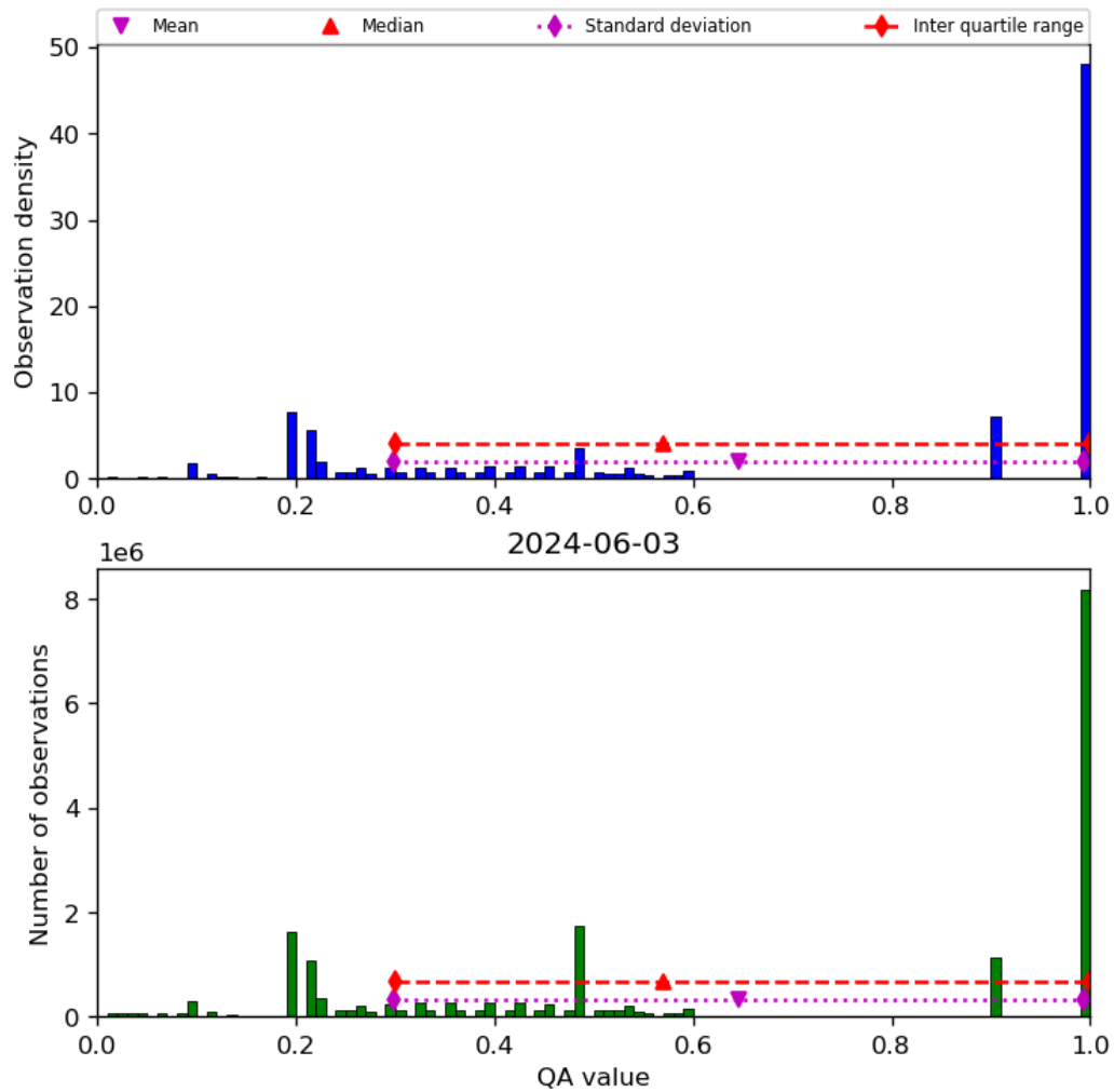
Figure 34: Histogram of “QA value” for 2024-06-03 to 2024-06-04
