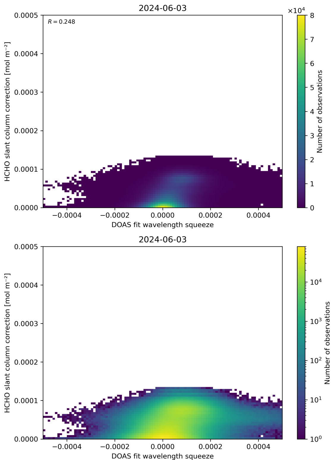
Figure 70: Scatter density plot of “DOAS fit wavelength squeeze” against “HCHO slant column correction” for 2024-06-03 to 2024-06-04.
