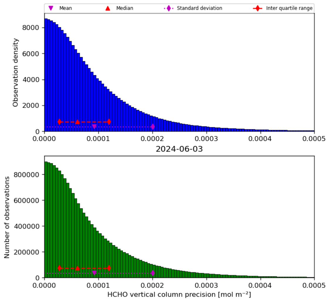
Figure 36: Histogram of “HCHO vertical column precision” for 2024-06-03 to 2024-06-04
