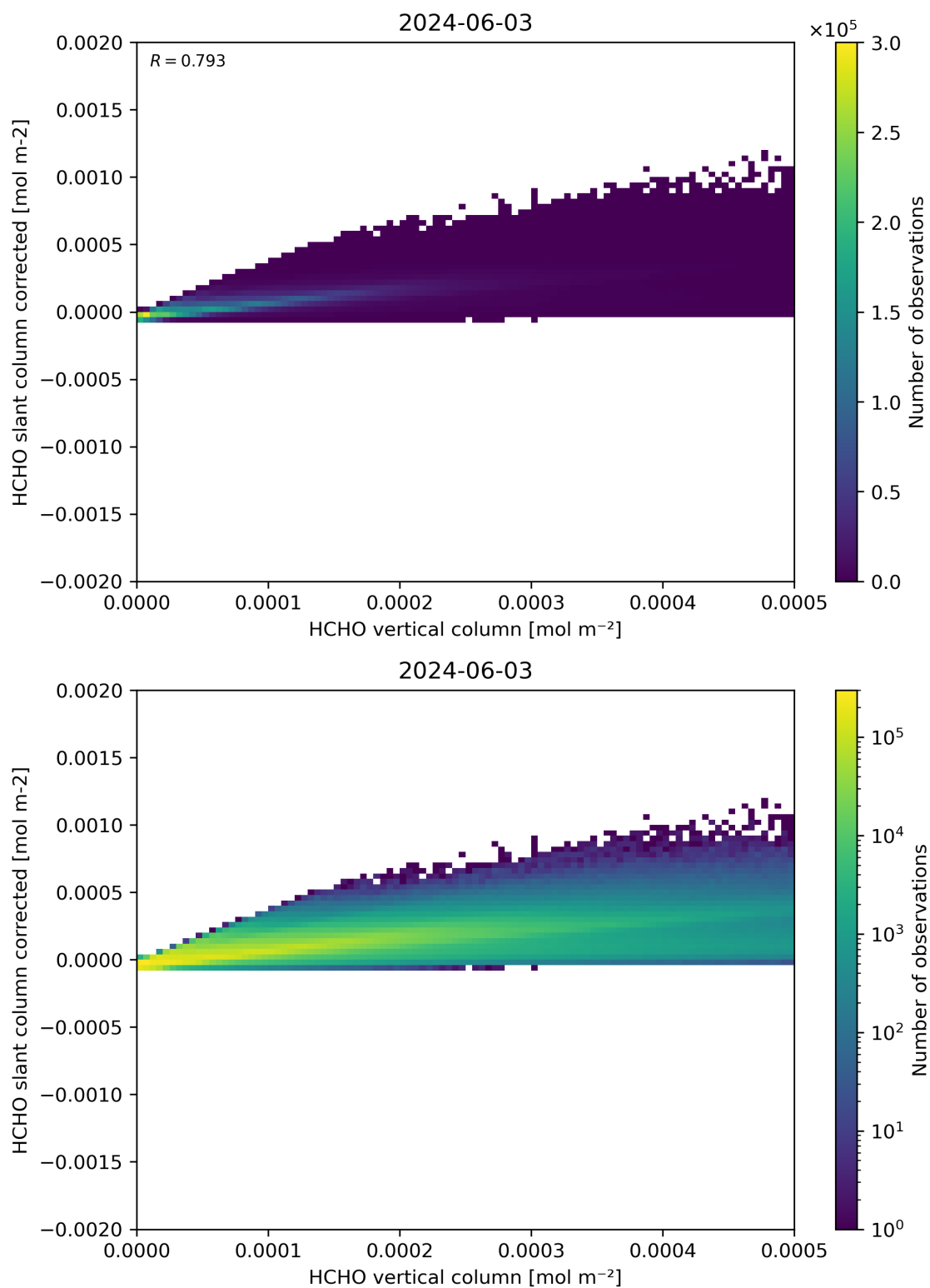
Figure 127: Scatter density plot of “HCHO vertical column” against “HCHO slant column corrected” for 2024-06-03 to 2024-06-04.
