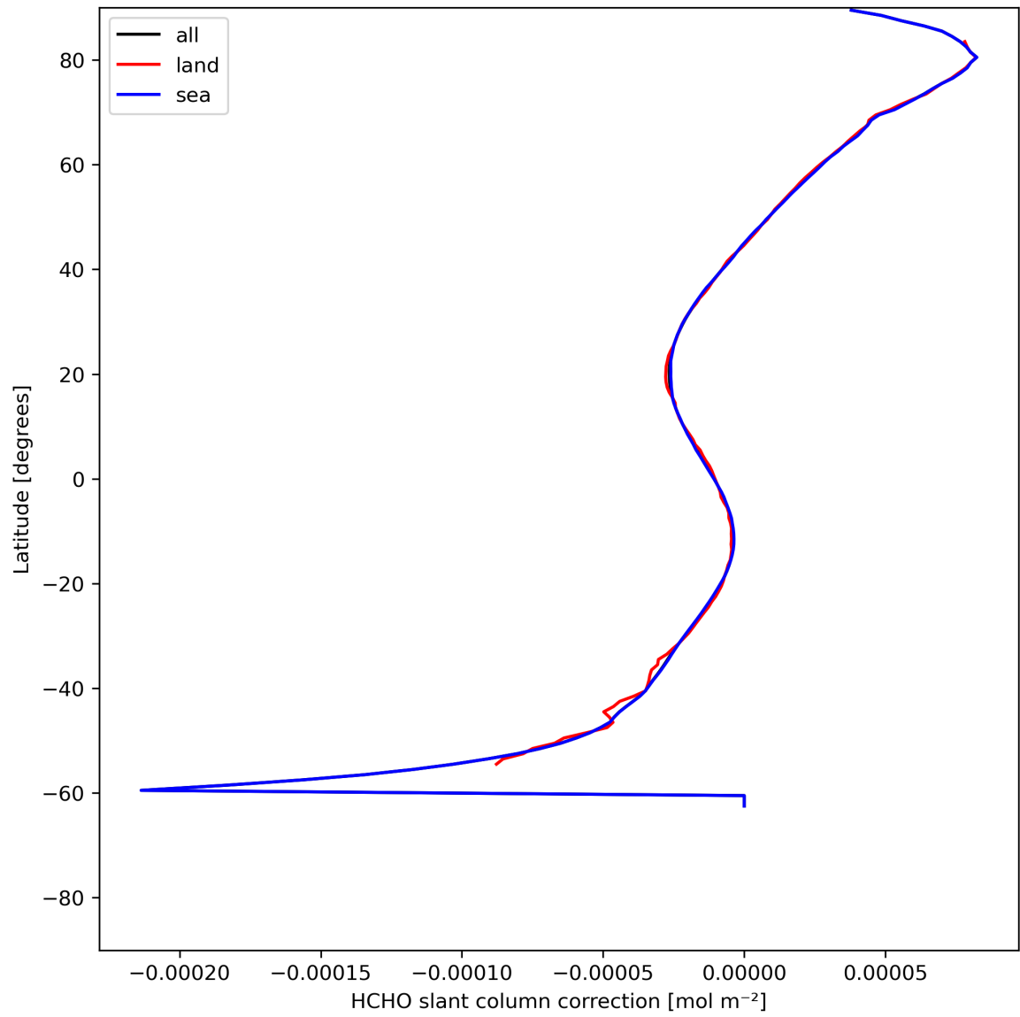
Figure 33: Zonal average of “HCHO slant column correction” for 2024-06-03 to 2024-06-04.
