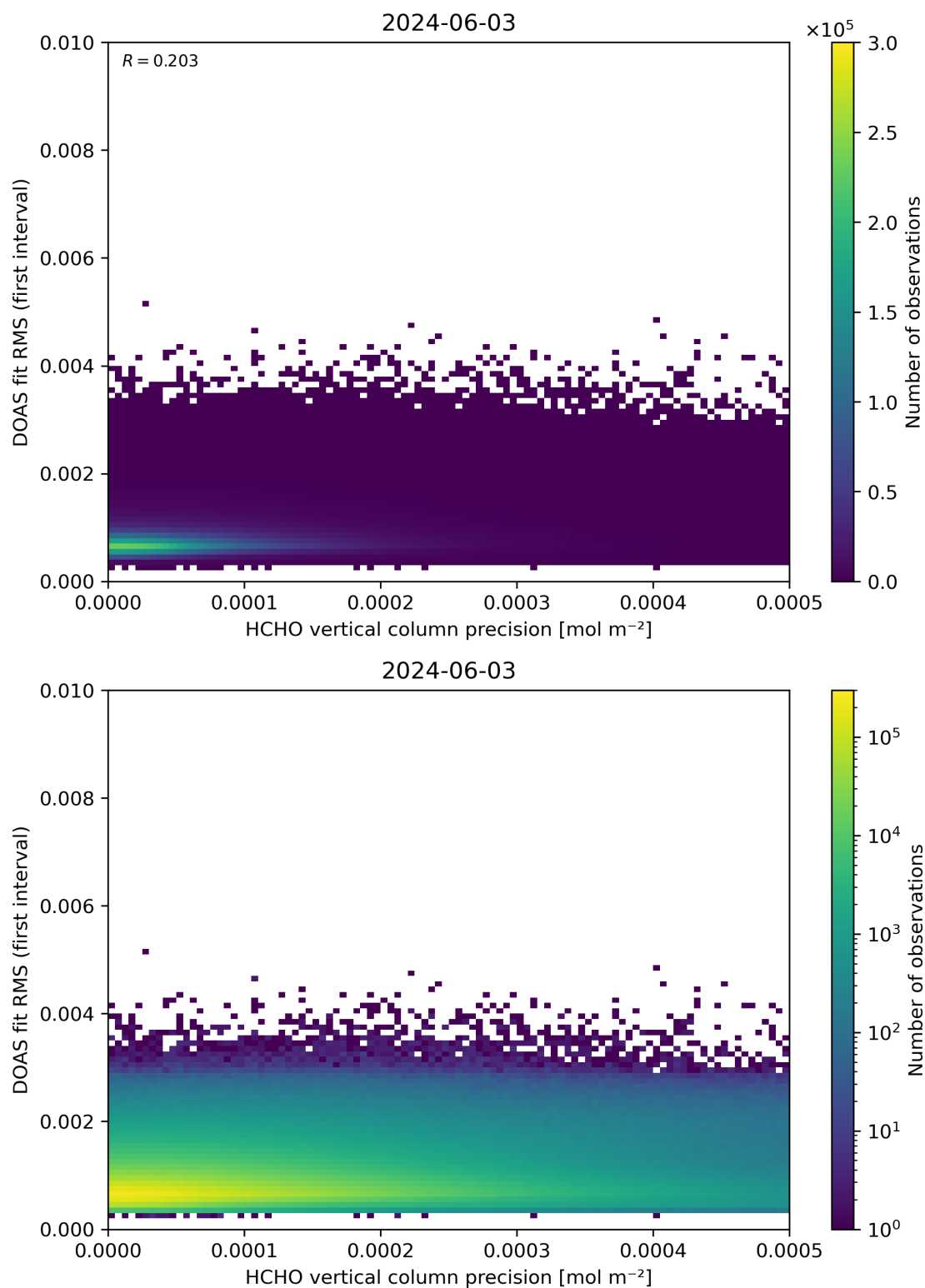
Figure 136: Scatter density plot of “HCHO vertical column precision” against “DOAS fit RMS (first interval)” for 2024-06-03 to 2024-06-04.
