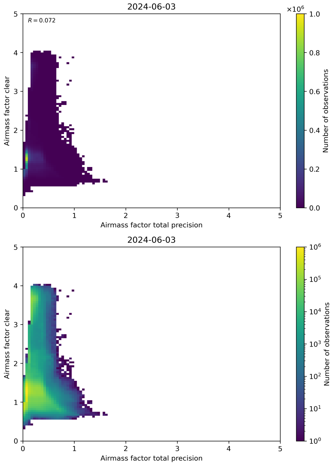
Figure 108: Scatter density plot of “Airmass factor total precision” against “Airmass factor clear” for 2024-06-03 to 2024-06-04.
