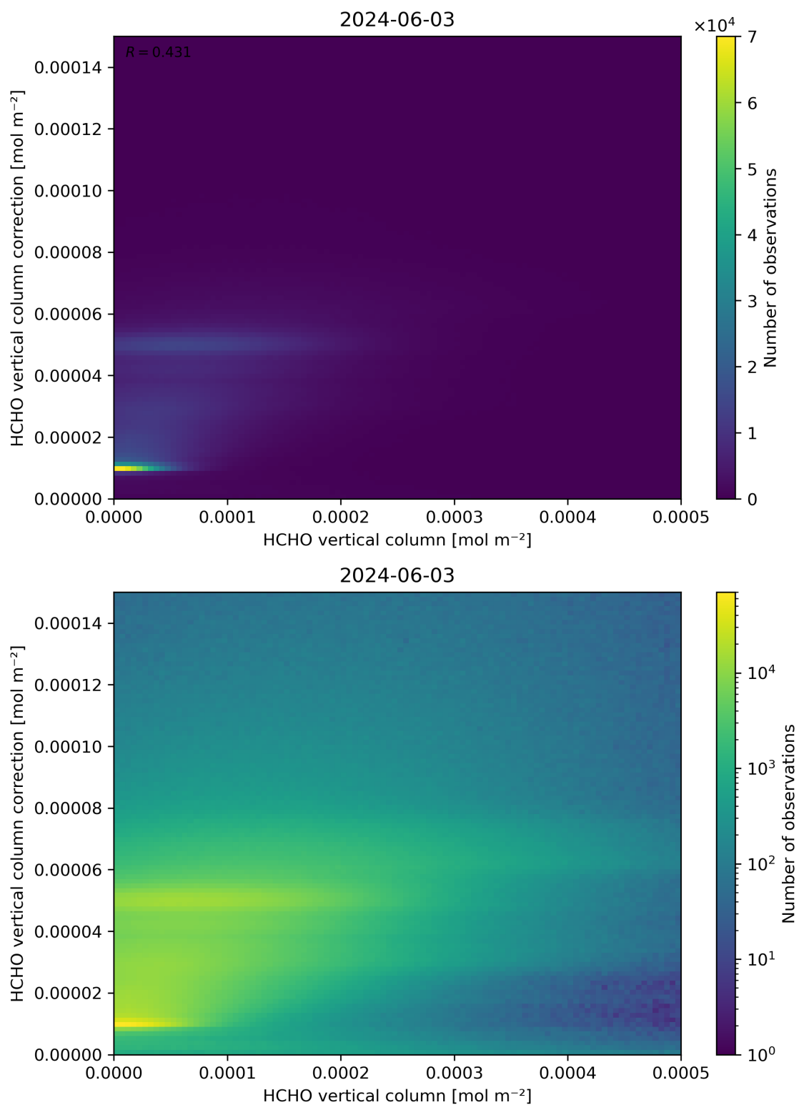
Figure 133: Scatter density plot of “HCHO vertical column” against “HCHO vertical column correction” for 2024-06-03 to 2024-06-04.
