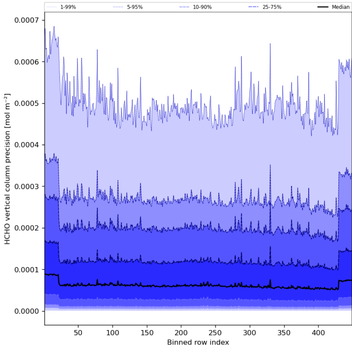
Figure 50: Along track statistics of “HCHO vertical column precision” for 2024-06-03 to 2024-06-04
