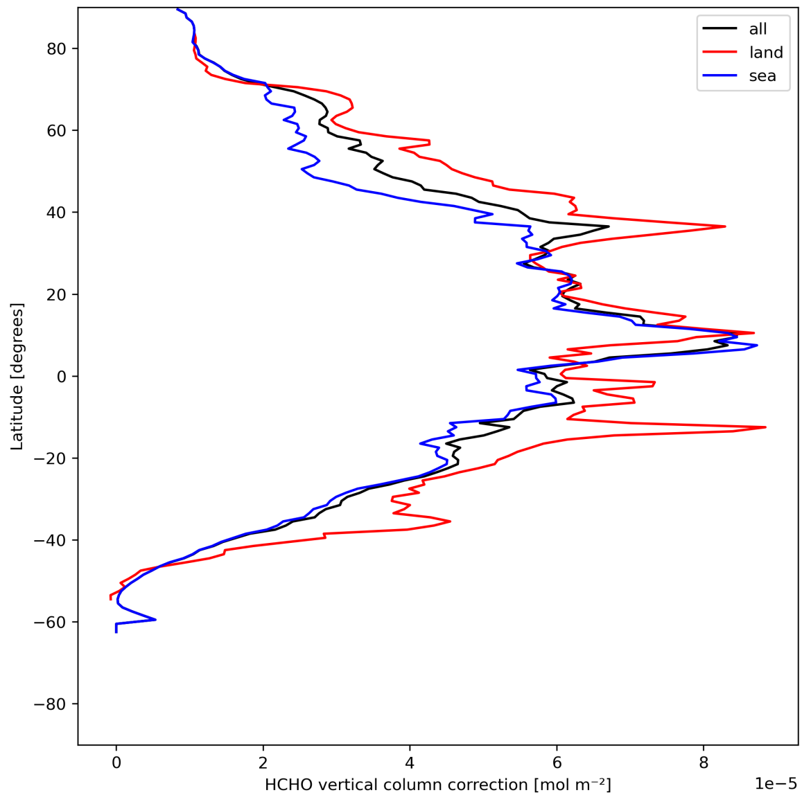
Figure 23: Zonal average of “HCHO vertical column correction” for 2024-06-03 to 2024-06-04.
