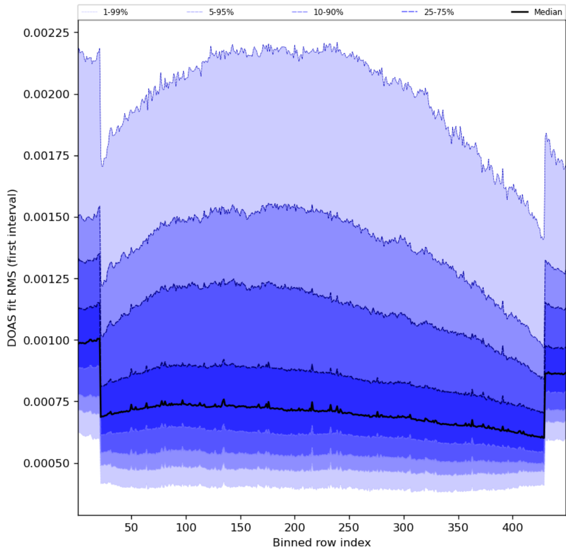
Figure 60: Along track statistics of “DOAS fit RMS (first interval)” for 2024-06-03 to 2024-06-04
