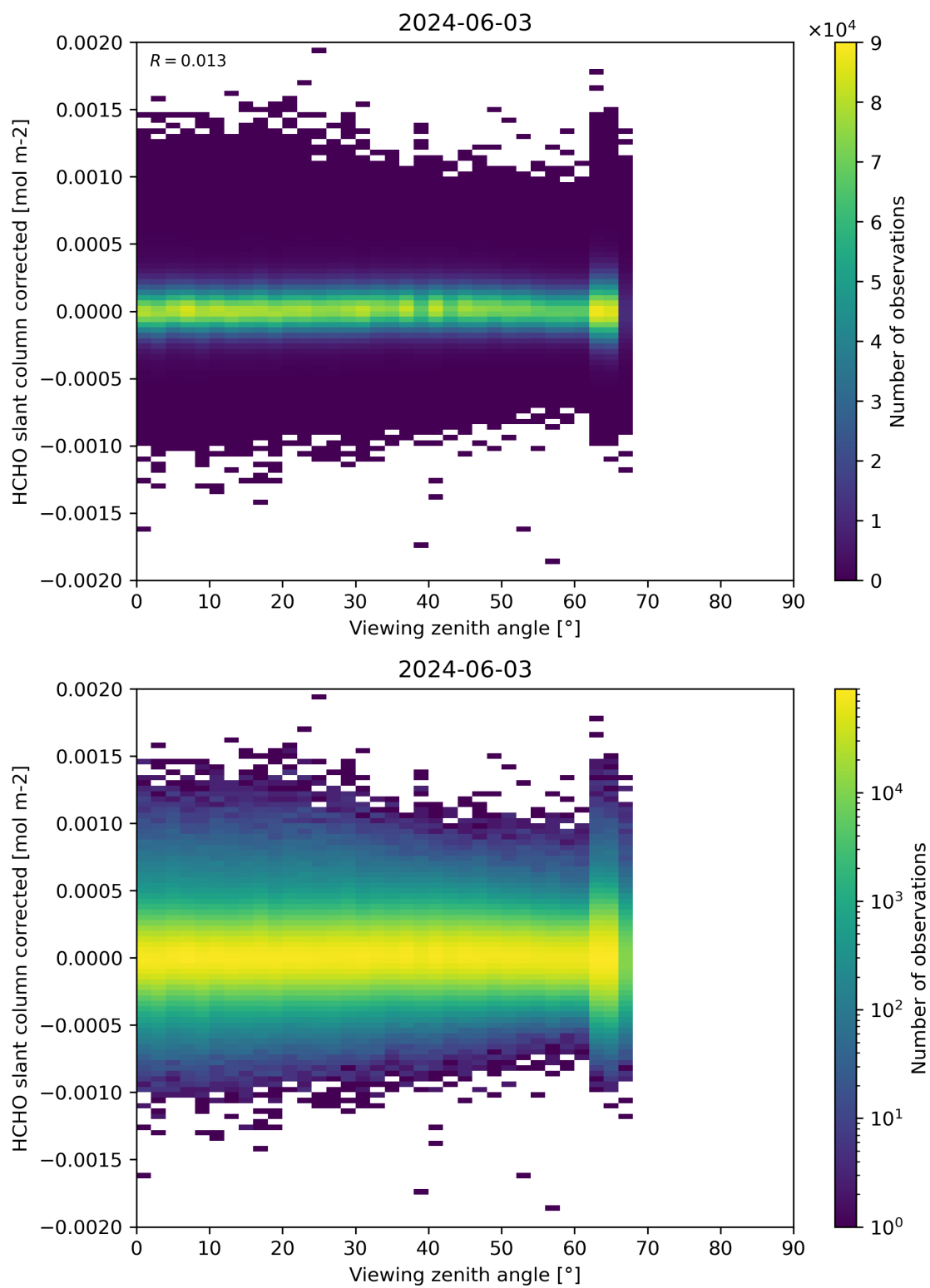
Figure 186: Scatter density plot of “Viewing zenith angle” against “HCHO slant column corrected” for 2024-06-03 to 2024-06-04.
