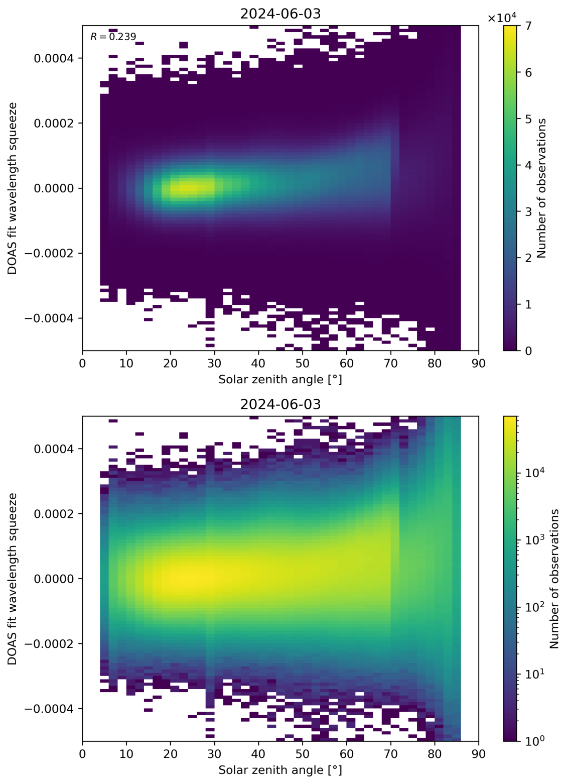
Figure 169: Scatter density plot of “Solar zenith angle” against “DOAS fit wavelength squeeze” for 2024-06-03 to 2024-06-04.
