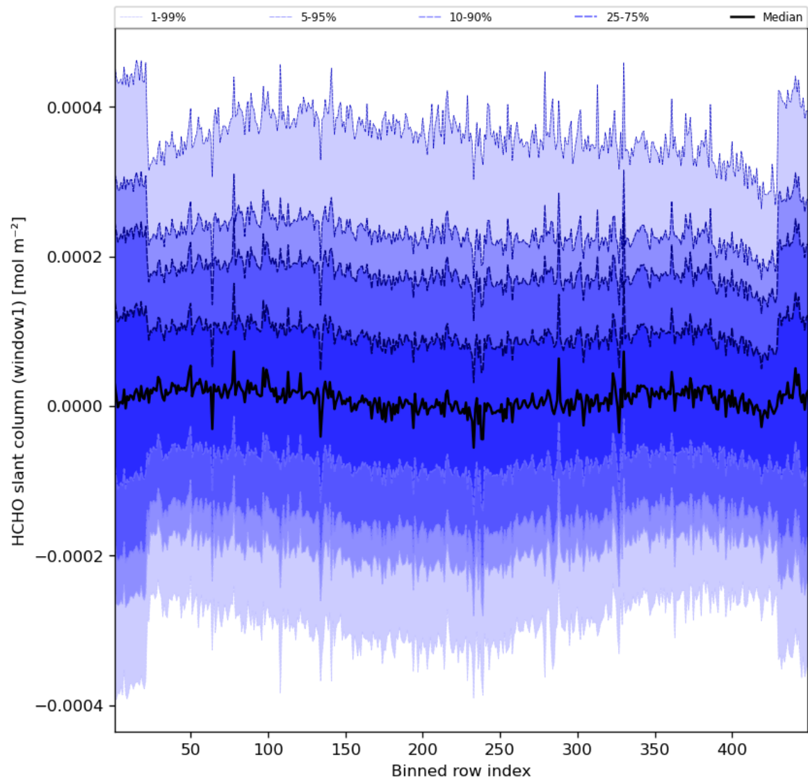
Figure 52: Along track statistics of “HCHO slant column (window1)” for 2024-06-03 to 2024-06-04
