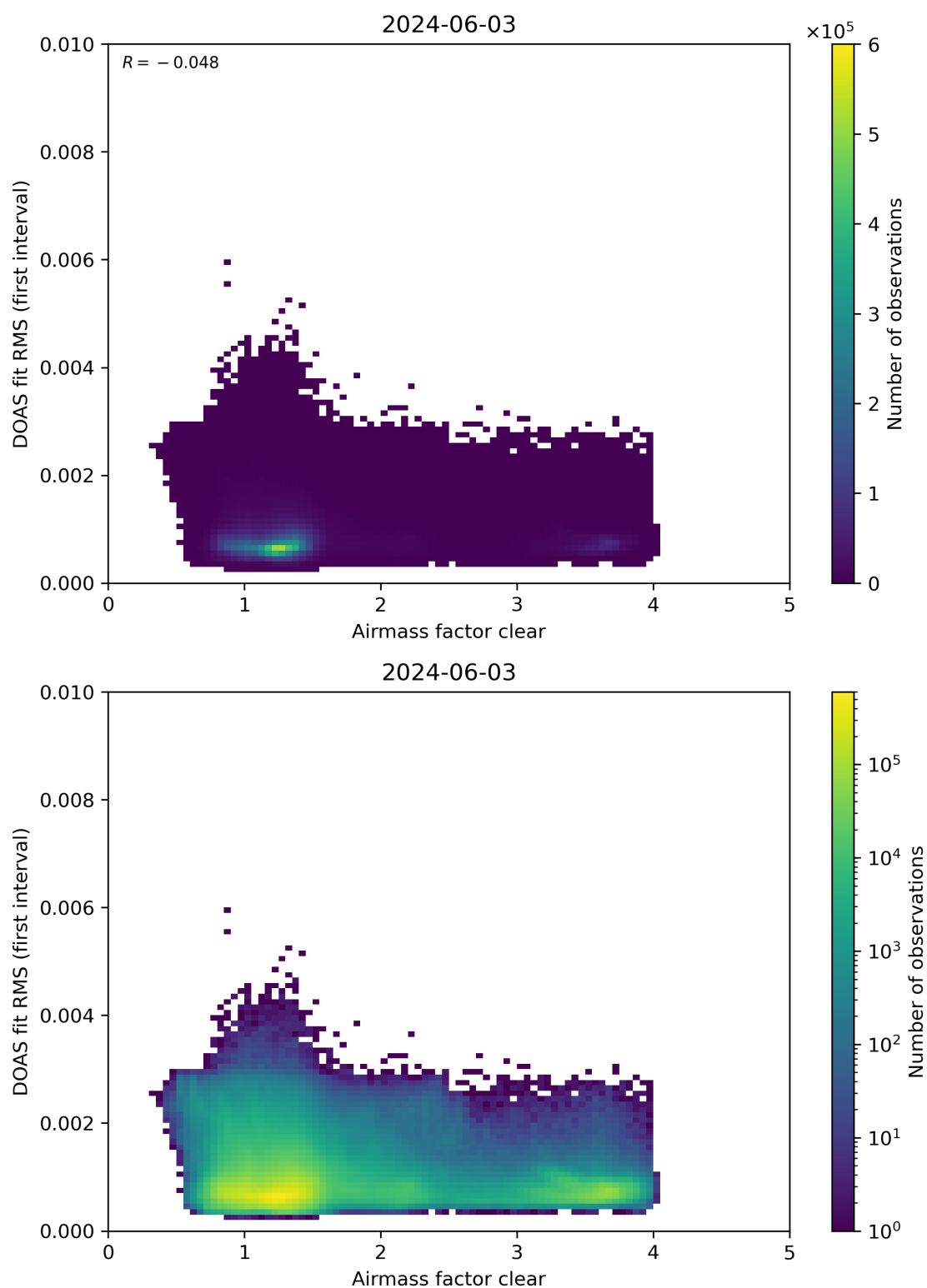
Figure 71: Scatter density plot of “Airmass factor clear” against “DOAS fit RMS (first interval)” for 2024-06-03 to 2024-06-04.
