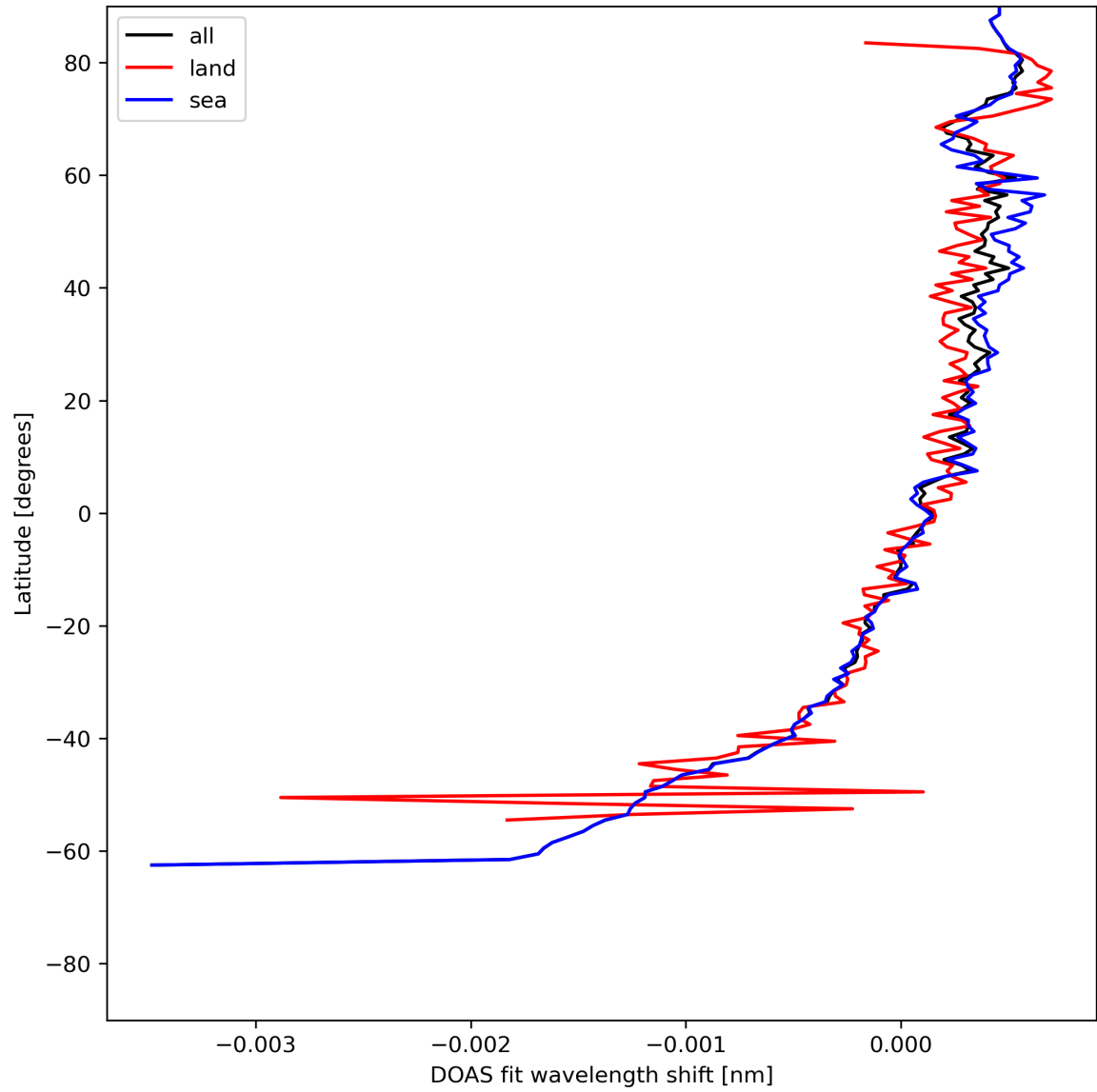
Figure 30: Zonal average of “DOAS fit wavelength shift” for 2024-06-03 to 2024-06-04.
