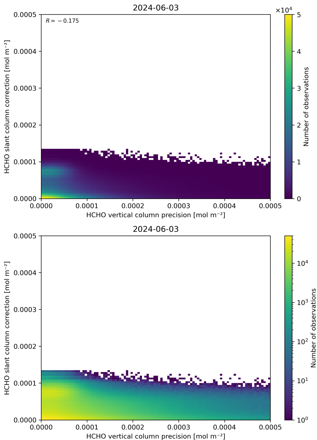
Figure 141: Scatter density plot of “HCHO vertical column precision” against “HCHO slant column correction” for 2024-06-03 to 2024-06-04.
