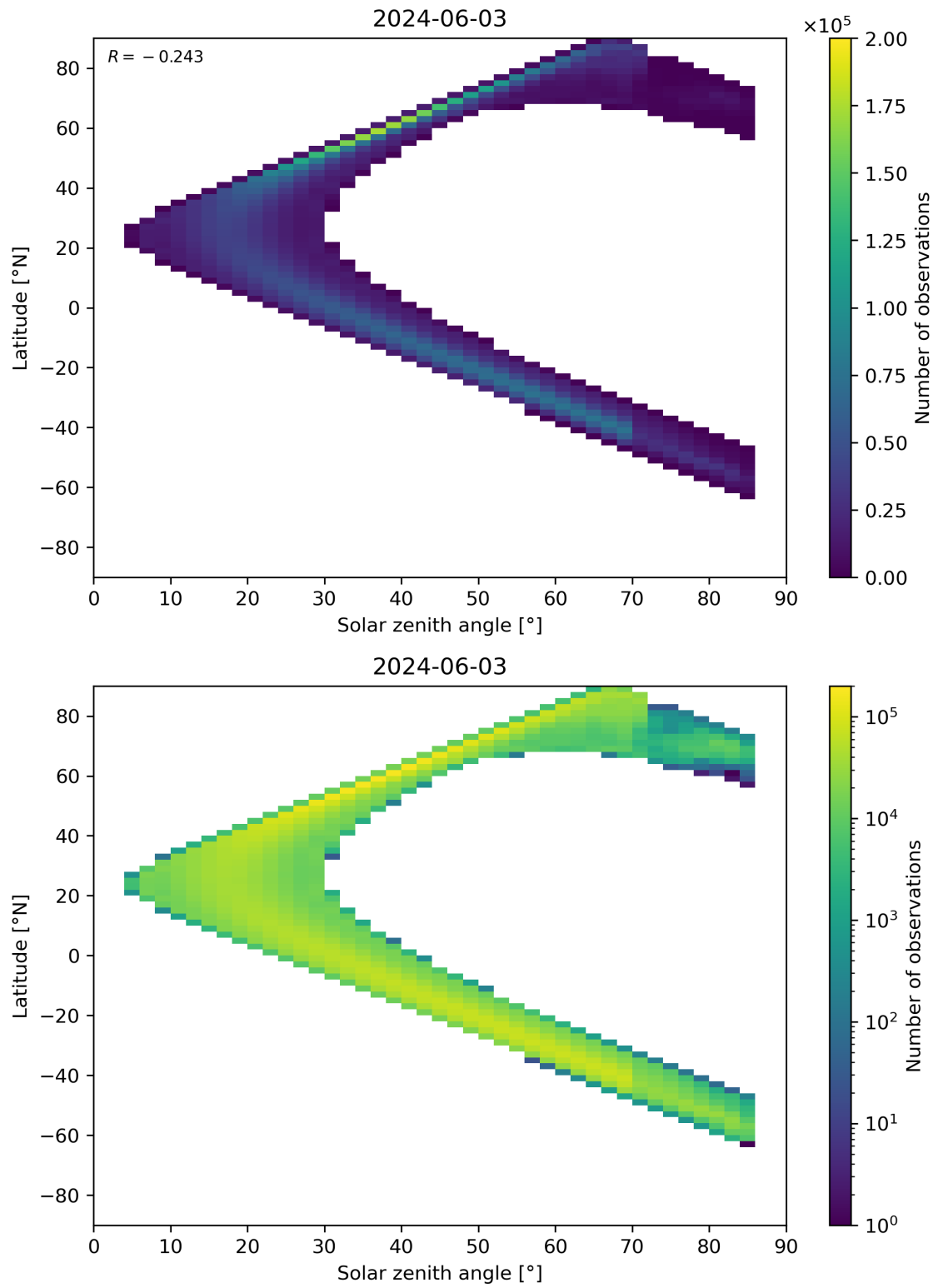
Figure 181: Scatter density plot of “Solar zenith angle” against “Latitude” for 2024-06-03 to 2024-06-04.
