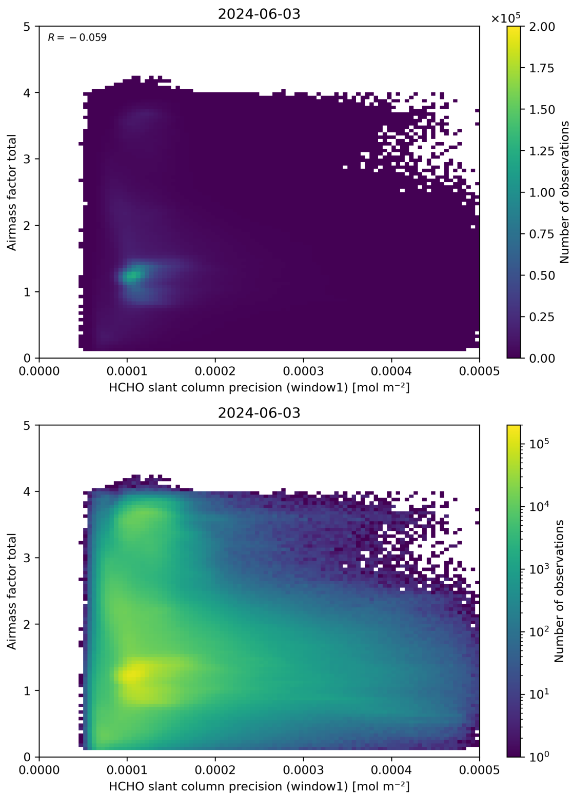
Figure 94: Scatter density plot of “HCHO slant column precision (window1)” against “Airmass factor total” for 2024-06-03 to 2024-06-04.
