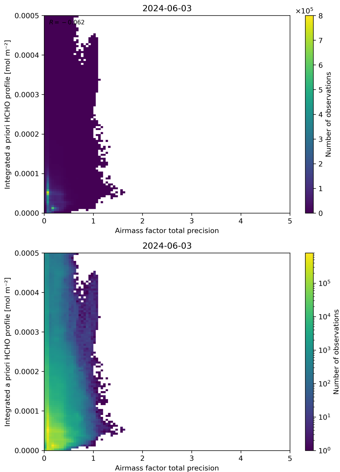
Figure 111: Scatter density plot of “Airmass factor total precision” against “Integrated a priori HCHO profile” for 2024-06-03 to 2024-06-04.
