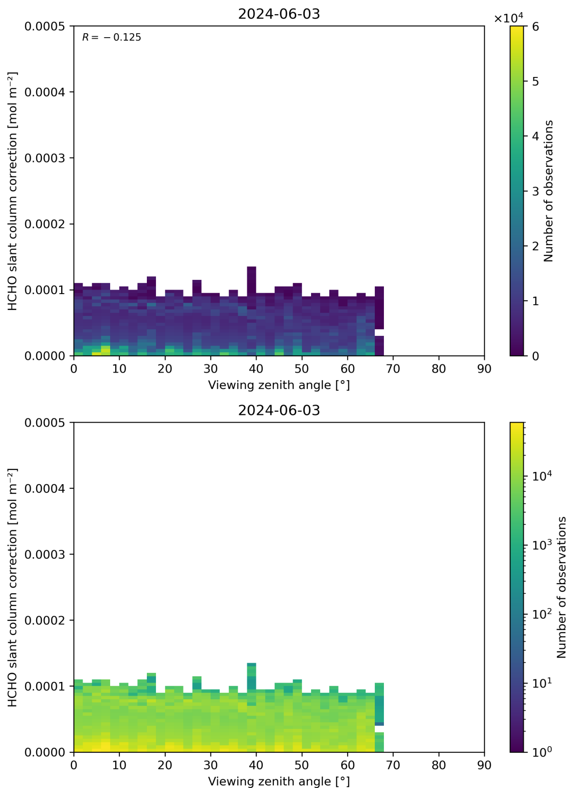
Figure 187: Scatter density plot of “Viewing zenith angle” against “HCHO slant column correction” for 2024-06-03 to 2024-06-04.
