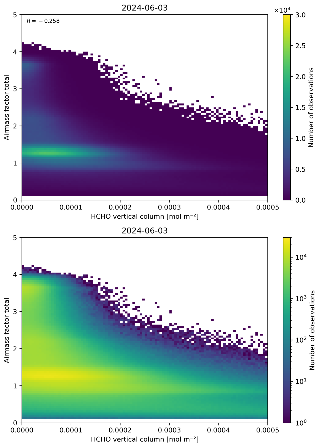
Figure 131: Scatter density plot of “HCHO vertical column” against “Airmass factor total” for 2024-06-03 to 2024-06-04.
