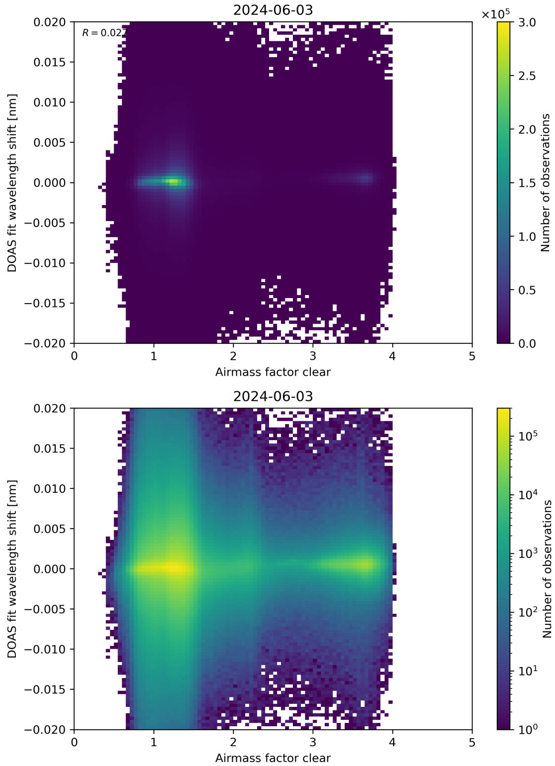
Figure 72: Scatter density plot of “Airmass factor clear” against “DOAS fit wavelength shift” for 2024-06-03 to 2024-06-04.
