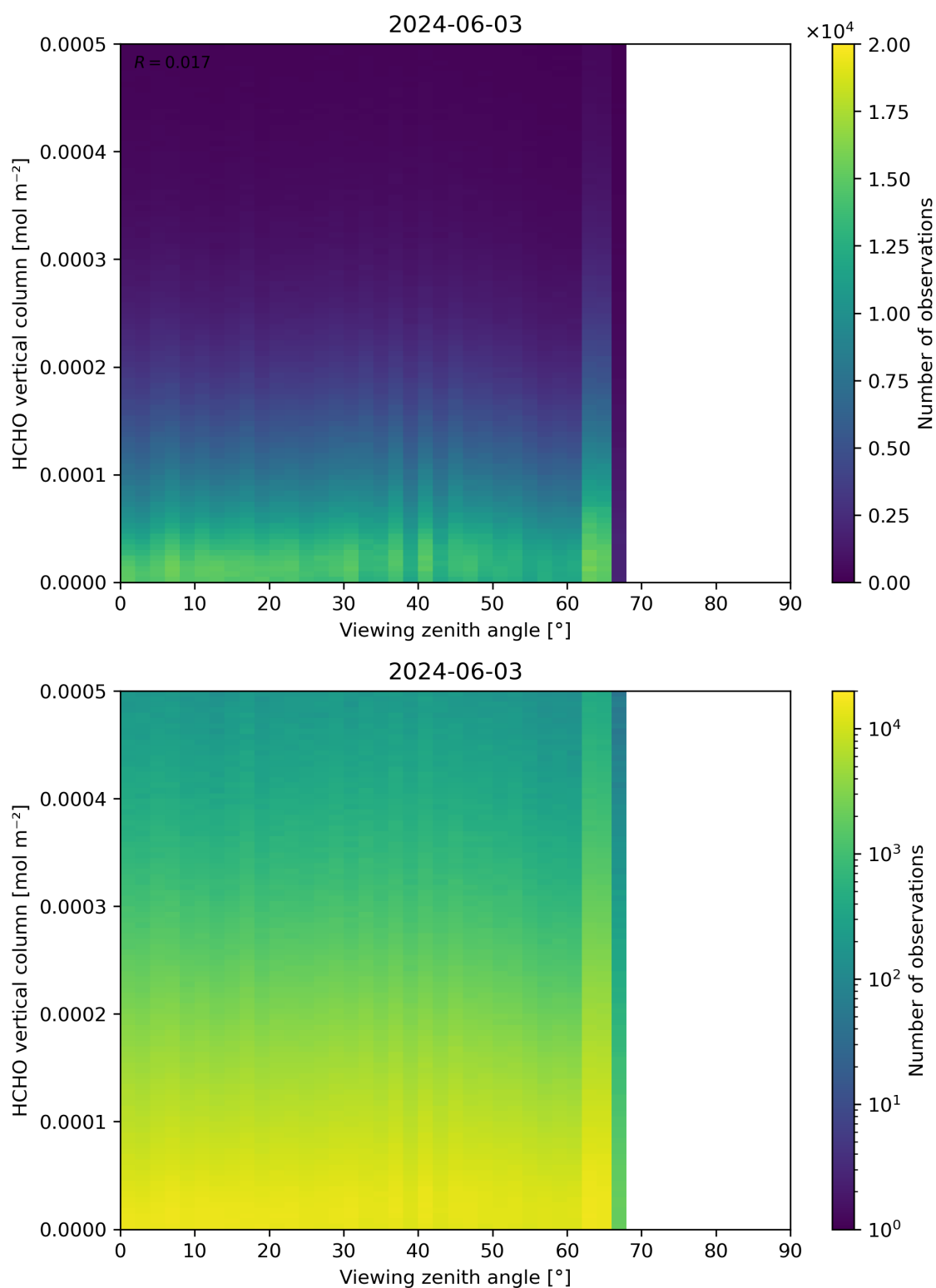
Figure 192: Scatter density plot of “Viewing zenith angle” against “HCHO vertical column” for 2024-06-03 to 2024-06-04.
