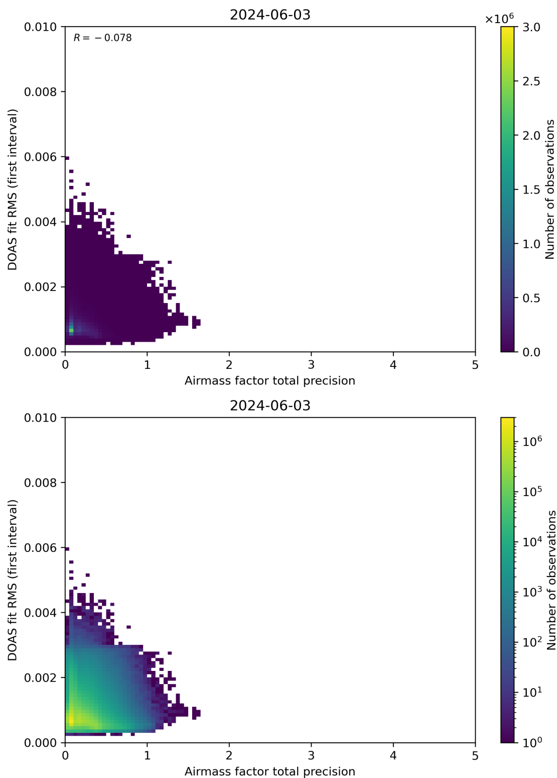
Figure 105: Scatter density plot of “Airmass factor total precision” against “DOAS fit RMS (first interval)” for 2024-06-03 to 2024-06-04.
