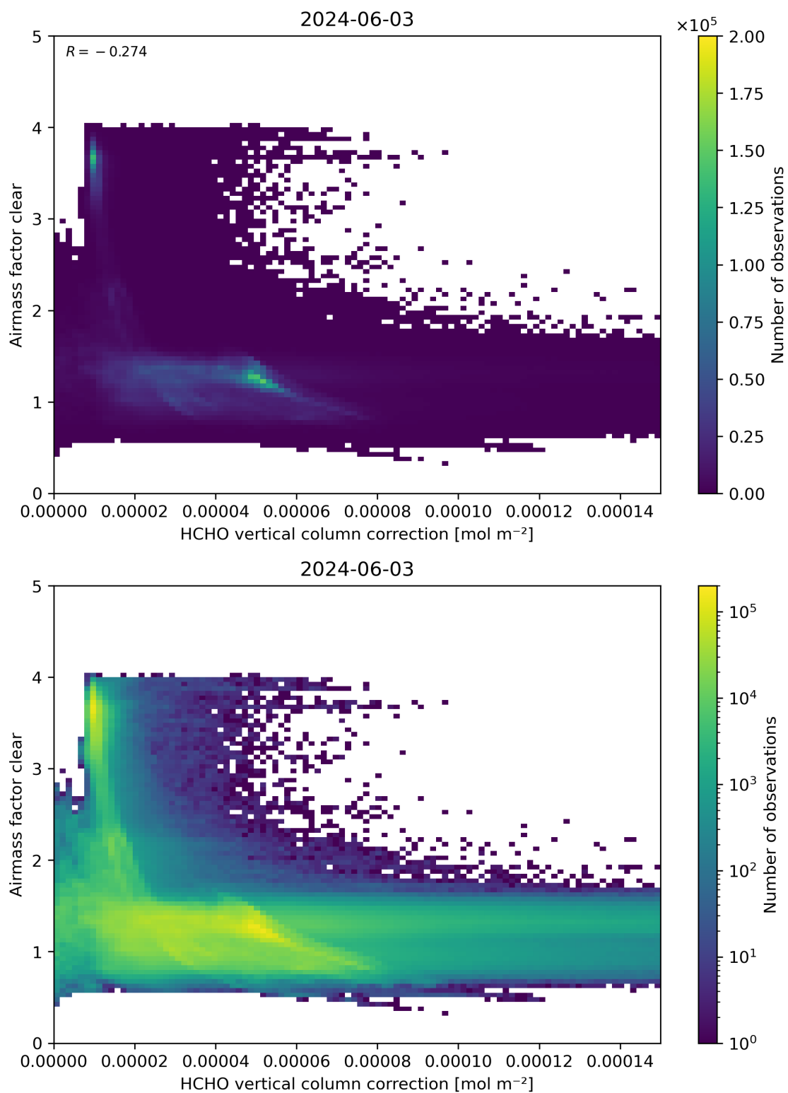
Figure 115: Scatter density plot of “HCHO vertical column correction” against “Airmass factor clear” for 2024-06-03 to 2024-06-04.
