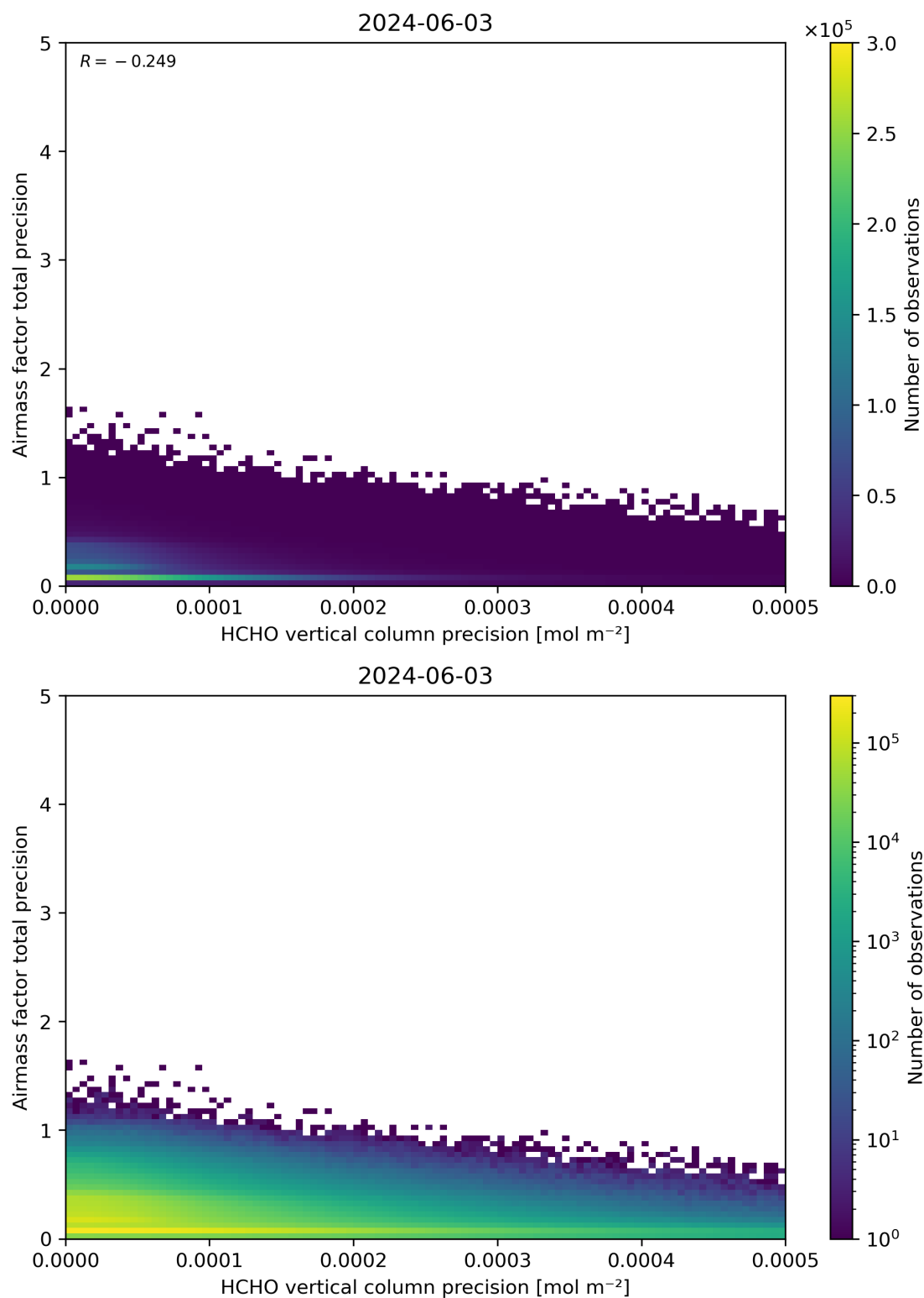
Figure 145: Scatter density plot of “HCHO vertical column precision” against “Airmass factor total precision” for 2024-06-03 to 2024-06-04.
