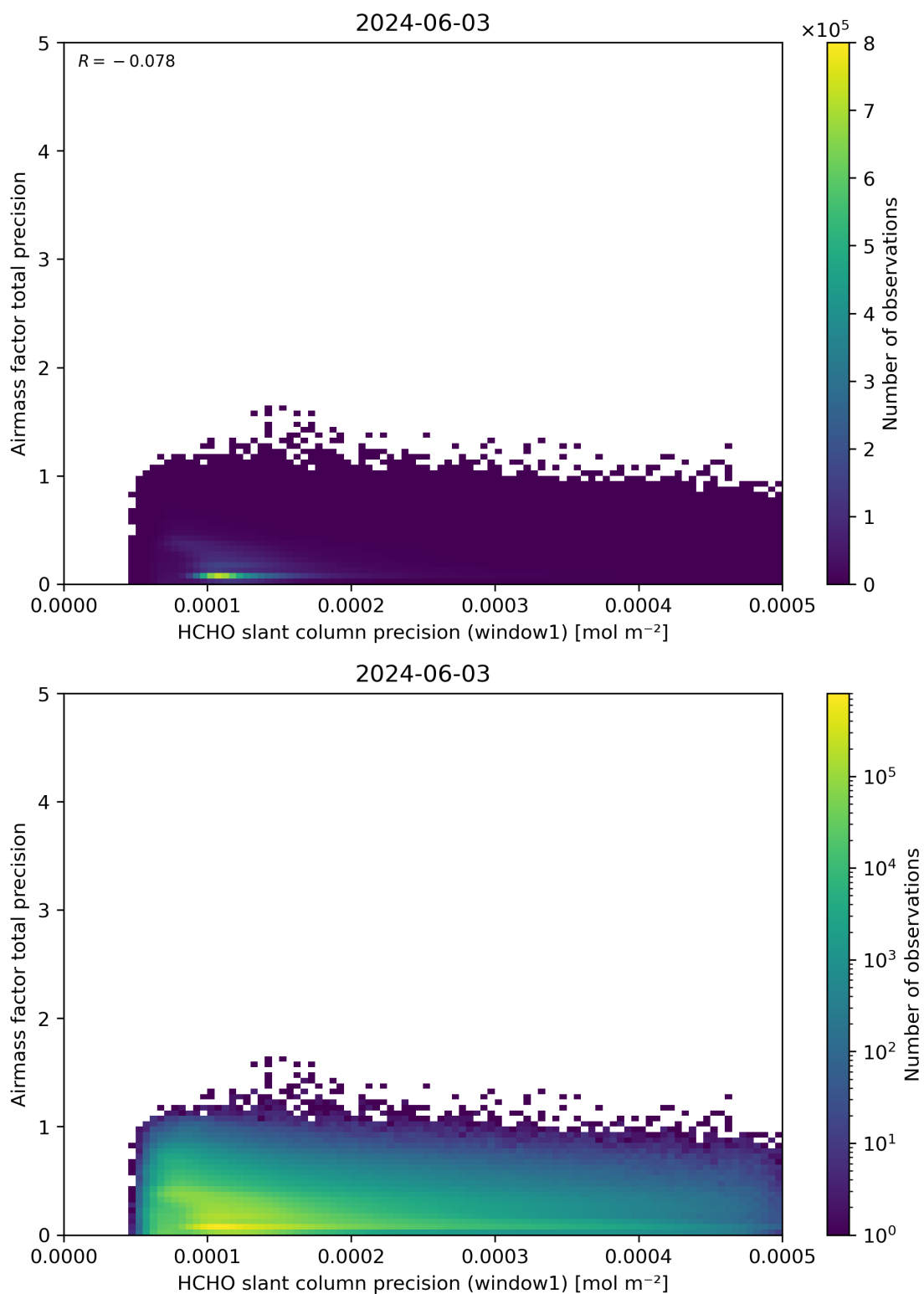
Figure 95: Scatter density plot of “HCHO slant column precision (window1)” against “Airmass factor total precision” for 2024-06-03 to 2024-06-04.
