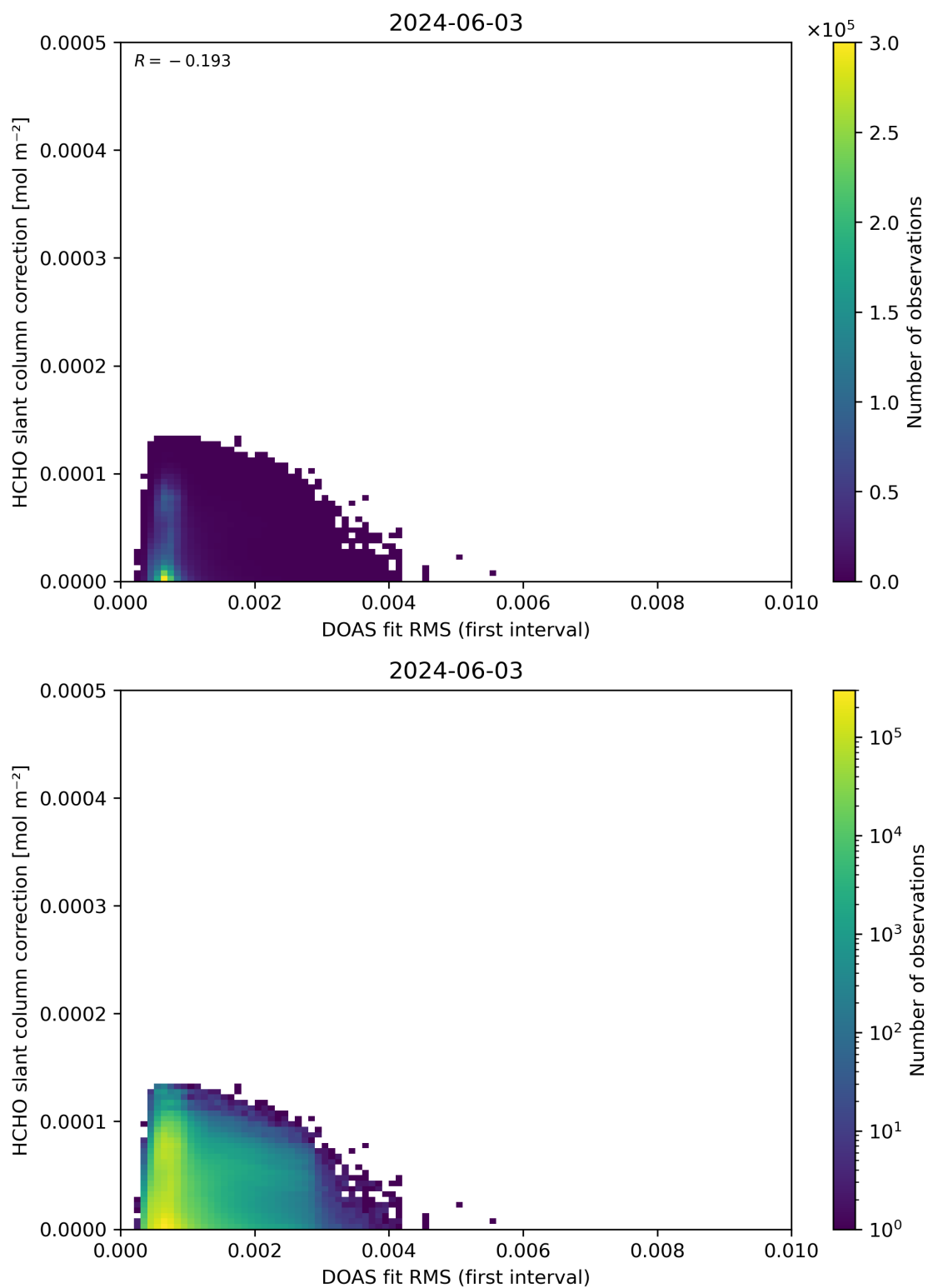
Figure 63: Scatter density plot of “DOAS fit RMS (first interval)” against “HCHO slant column correction” for 2024-06-03 to 2024-06-04.
