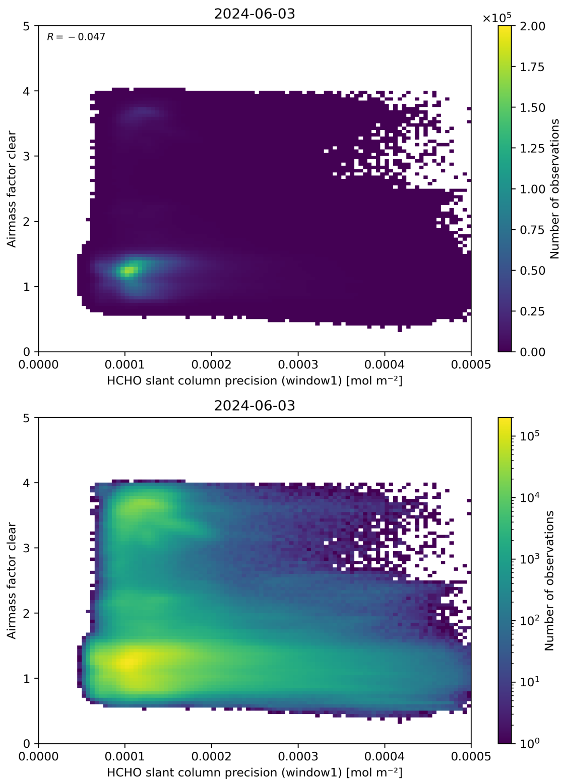
Figure 91: Scatter density plot of “HCHO slant column precision (window1)” against “Airmass factor clear” for 2024-06-03 to 2024-06-04.
