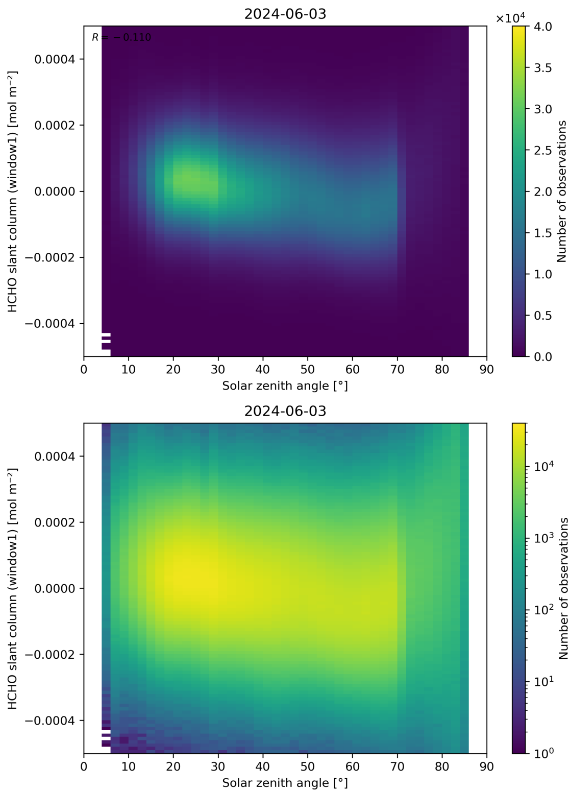
Figure 173: Scatter density plot of “Solar zenith angle” against “HCHO slant column (window1)” for 2024-06-03 to 2024-06-04.
