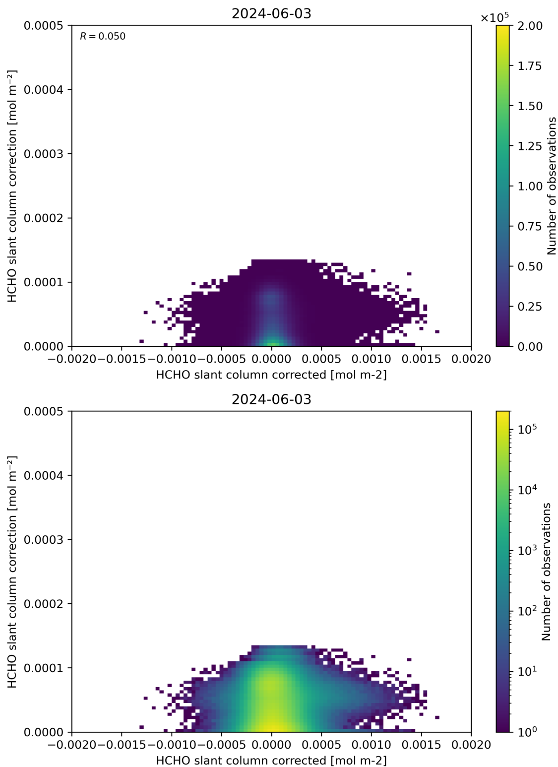
Figure 77: Scatter density plot of “HCHO slant column corrected” against “HCHO slant column correction” for 2024-06-03 to 2024-06-04.
