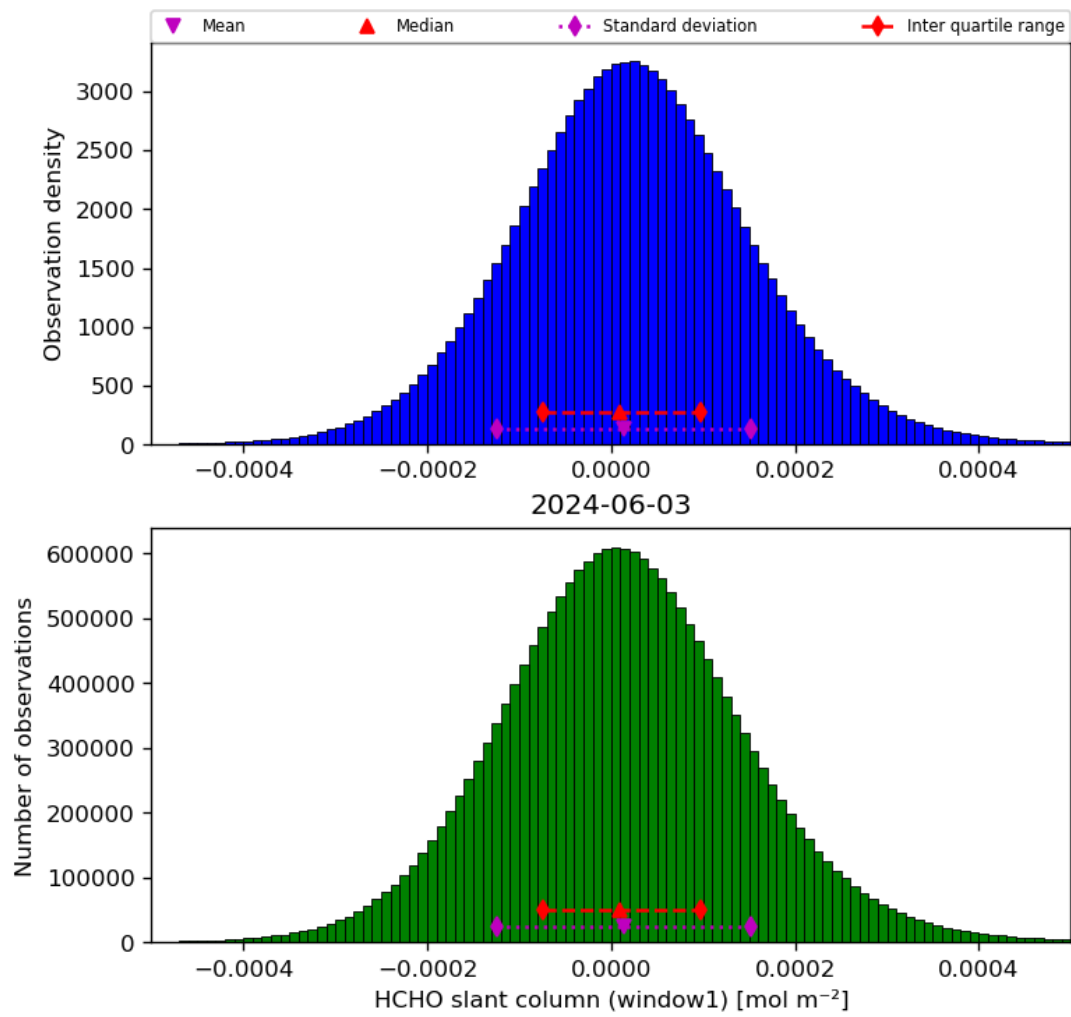
Figure 38: Histogram of “HCHO slant column (window1)” for 2024-06-03 to 2024-06-04
