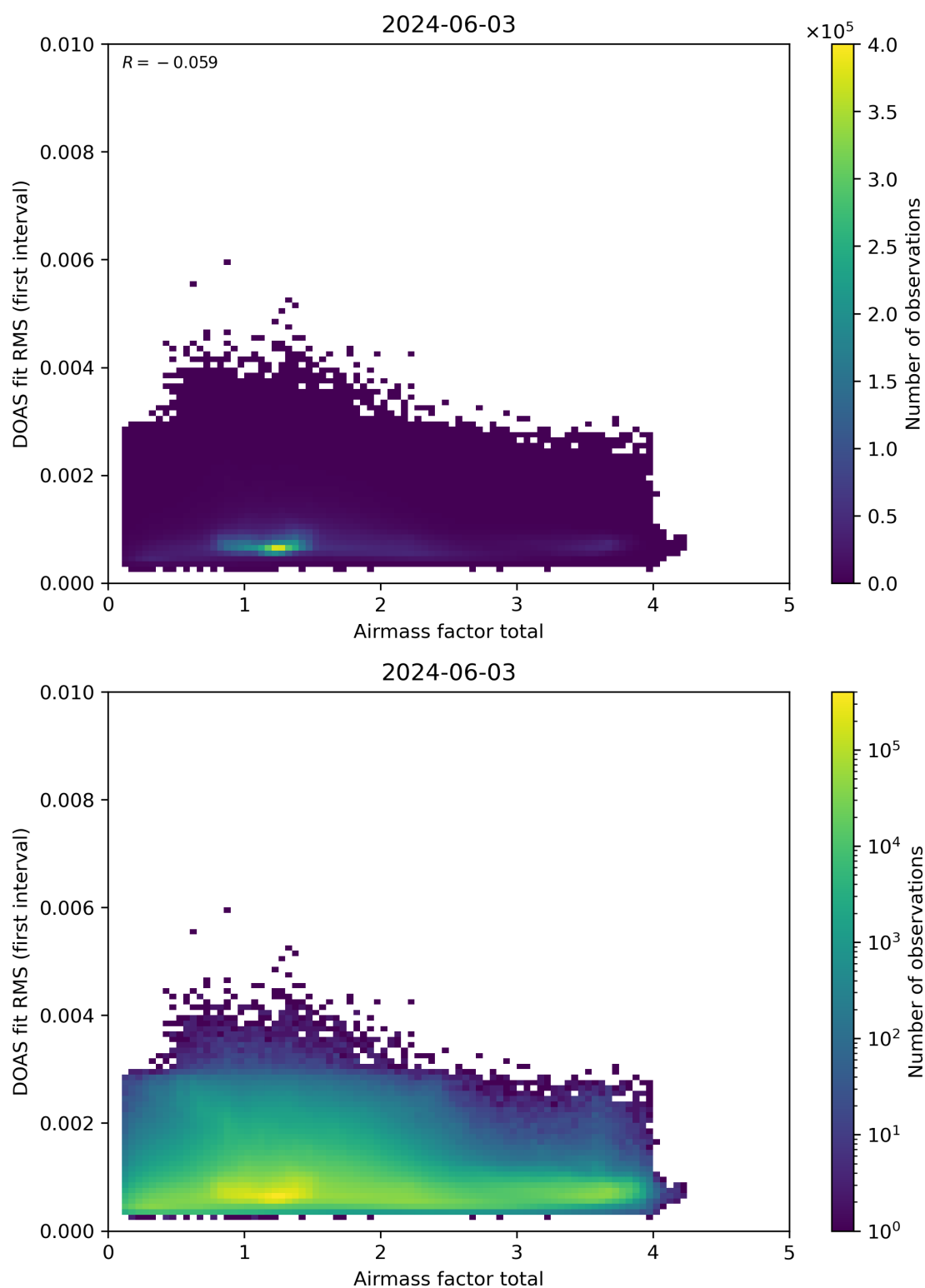
Figure 97: Scatter density plot of “Airmass factor total” against “DOAS fit RMS (first interval)” for 2024-06-03 to 2024-06-04.
