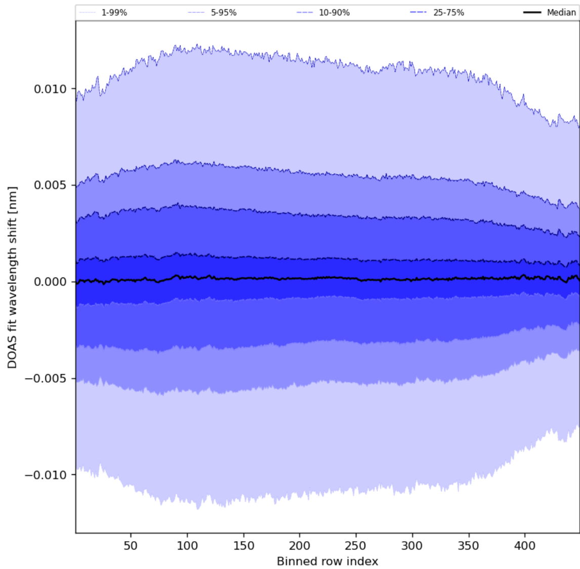
Figure 58: Along track statistics of “DOAS fit wavelength shift” for 2024-06-03 to 2024-06-04
