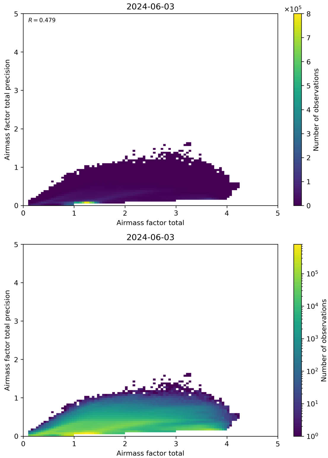
Figure 103: Scatter density plot of “Airmass factor total” against “Airmass factor total precision” for 2024-06-03 to 2024-06-04.
