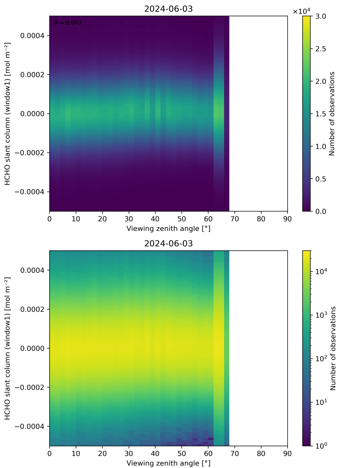
Figure 188: Scatter density plot of “Viewing zenith angle” against “HCHO slant column (window1)” for 2024-06-03 to 2024-06-04.
