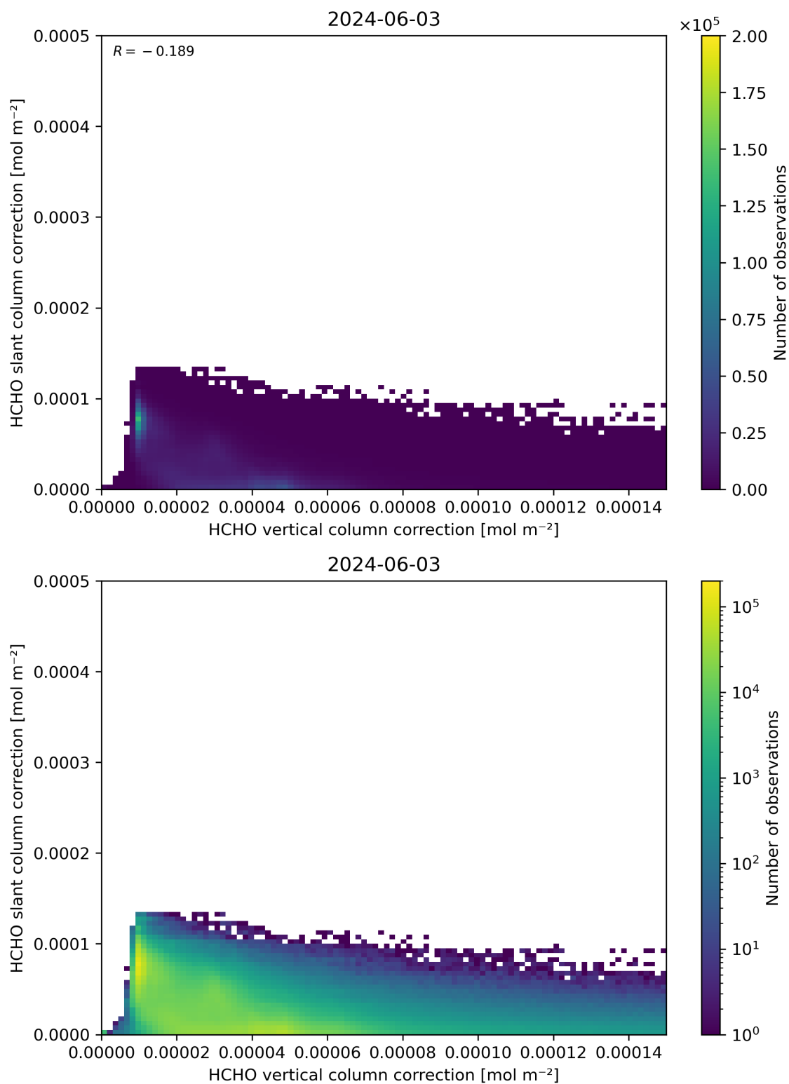
Figure 117: Scatter density plot of “HCHO vertical column correction” against “HCHO slant column correction” for 2024-06-03 to 2024-06-04.
