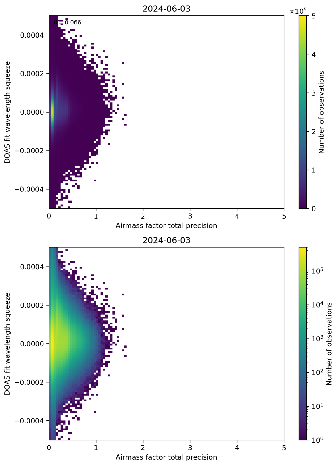
Figure 107: Scatter density plot of “Airmass factor total precision” against “DOAS fit wavelength squeeze” for 2024-06-03 to 2024-06-04.
