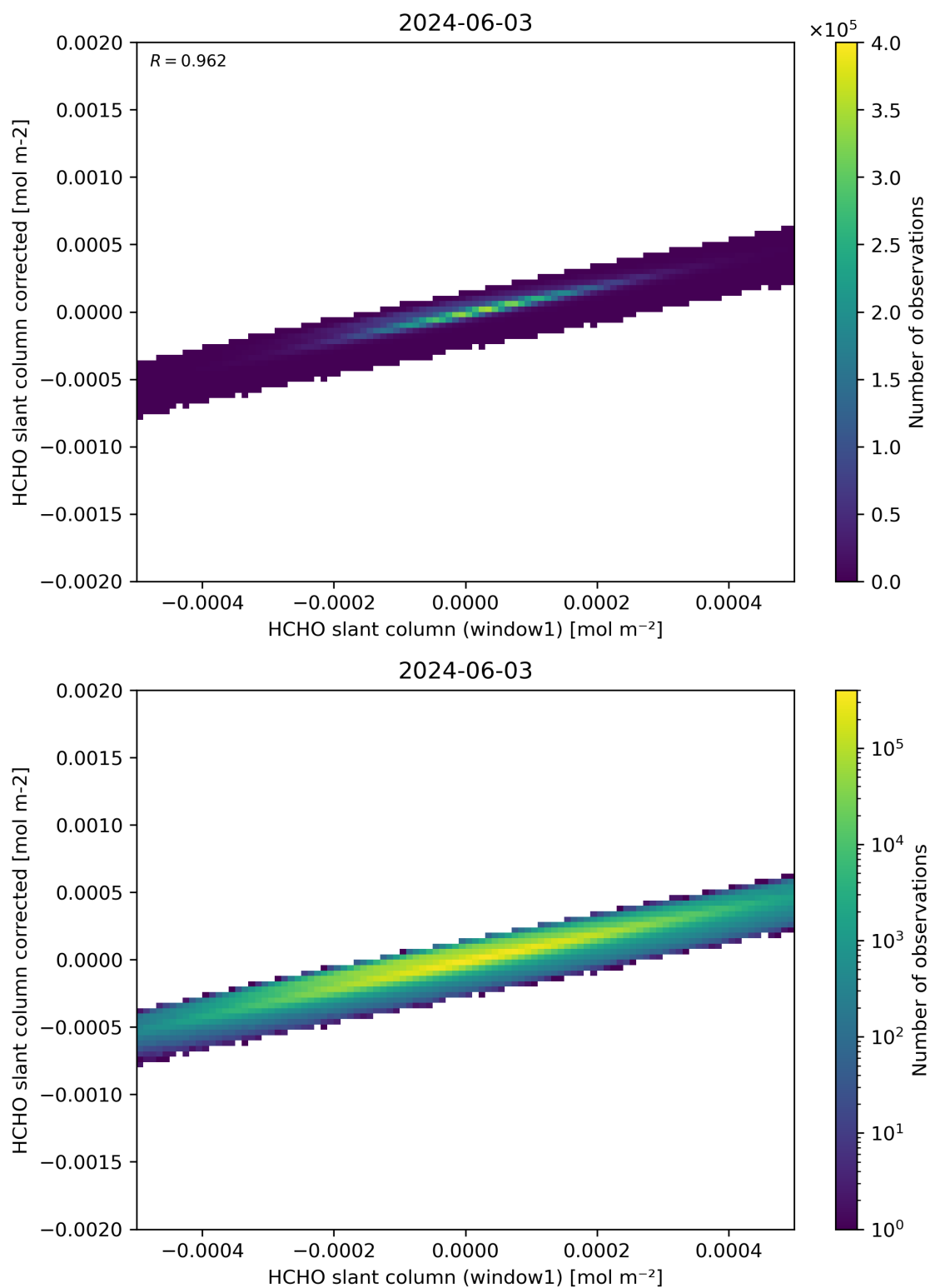
Figure 82: Scatter density plot of “HCHO slant column (window1)” against “HCHO slant column corrected” for 2024-06-03 to 2024-06-04.
