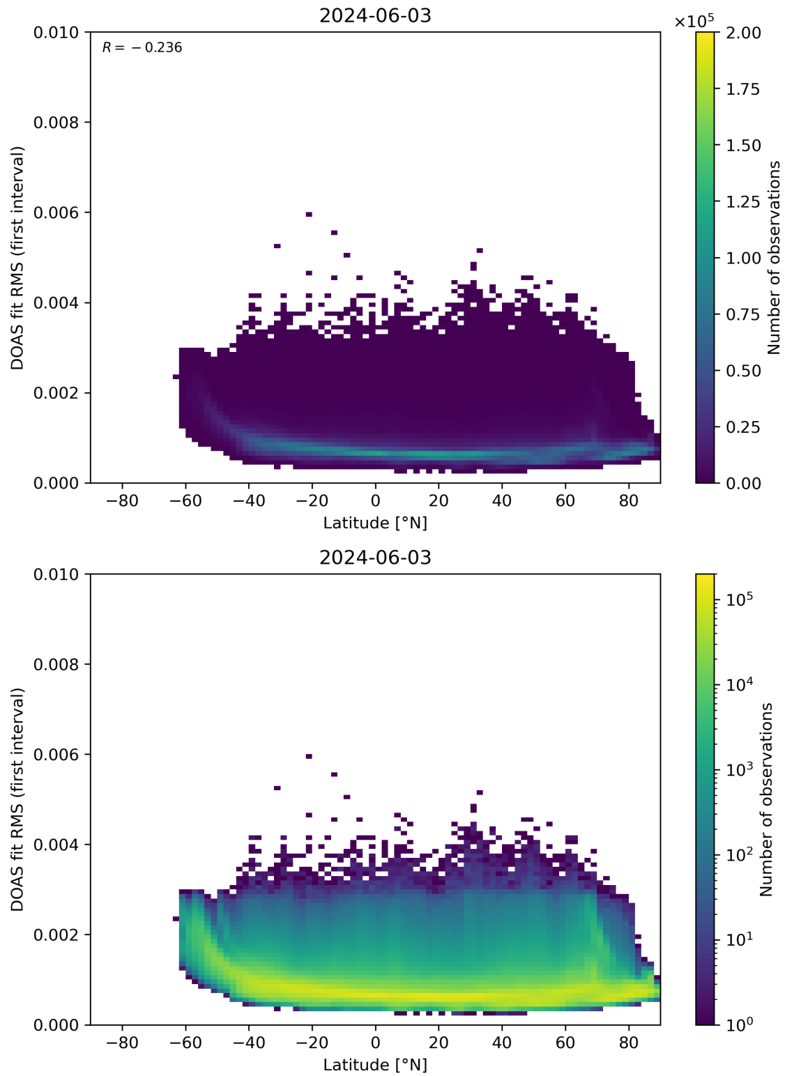
Figure 153: Scatter density plot of “Latitude” against “DOAS fit RMS (first interval)” for 2024-06-03 to 2024-06-04.
