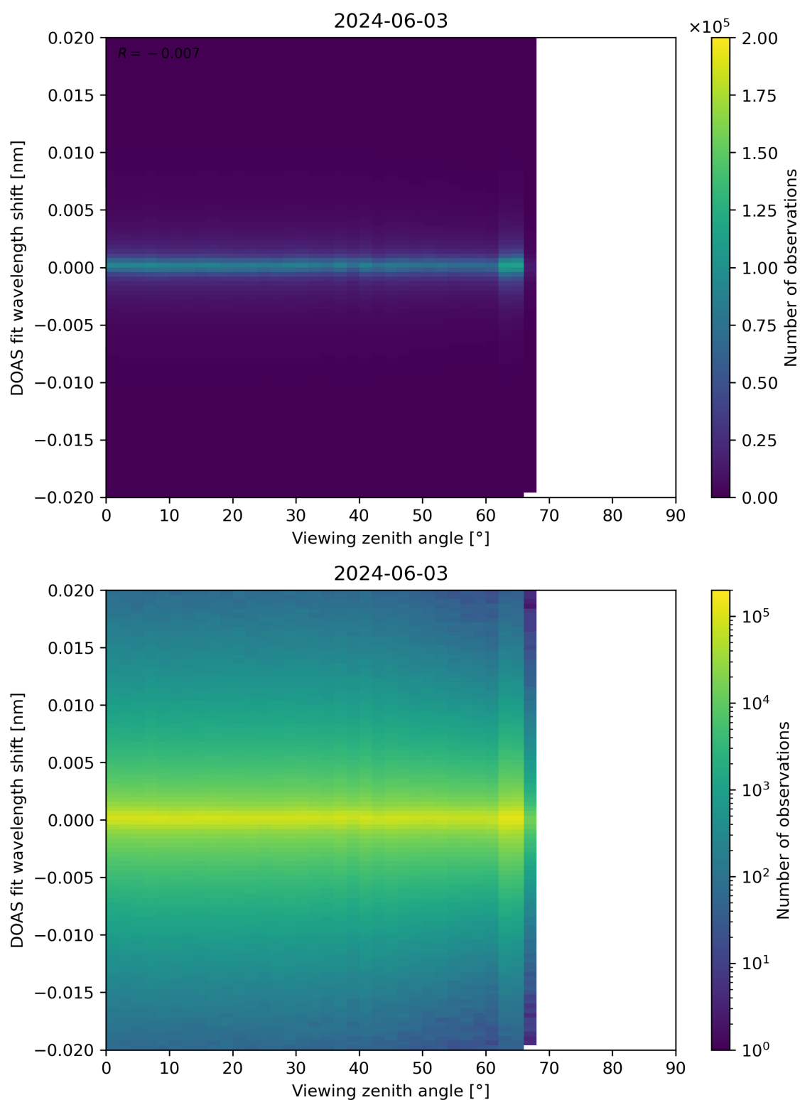
Figure 183: Scatter density plot of “Viewing zenith angle” against “DOAS fit wavelength shift” for 2024-06-03 to 2024-06-04.
