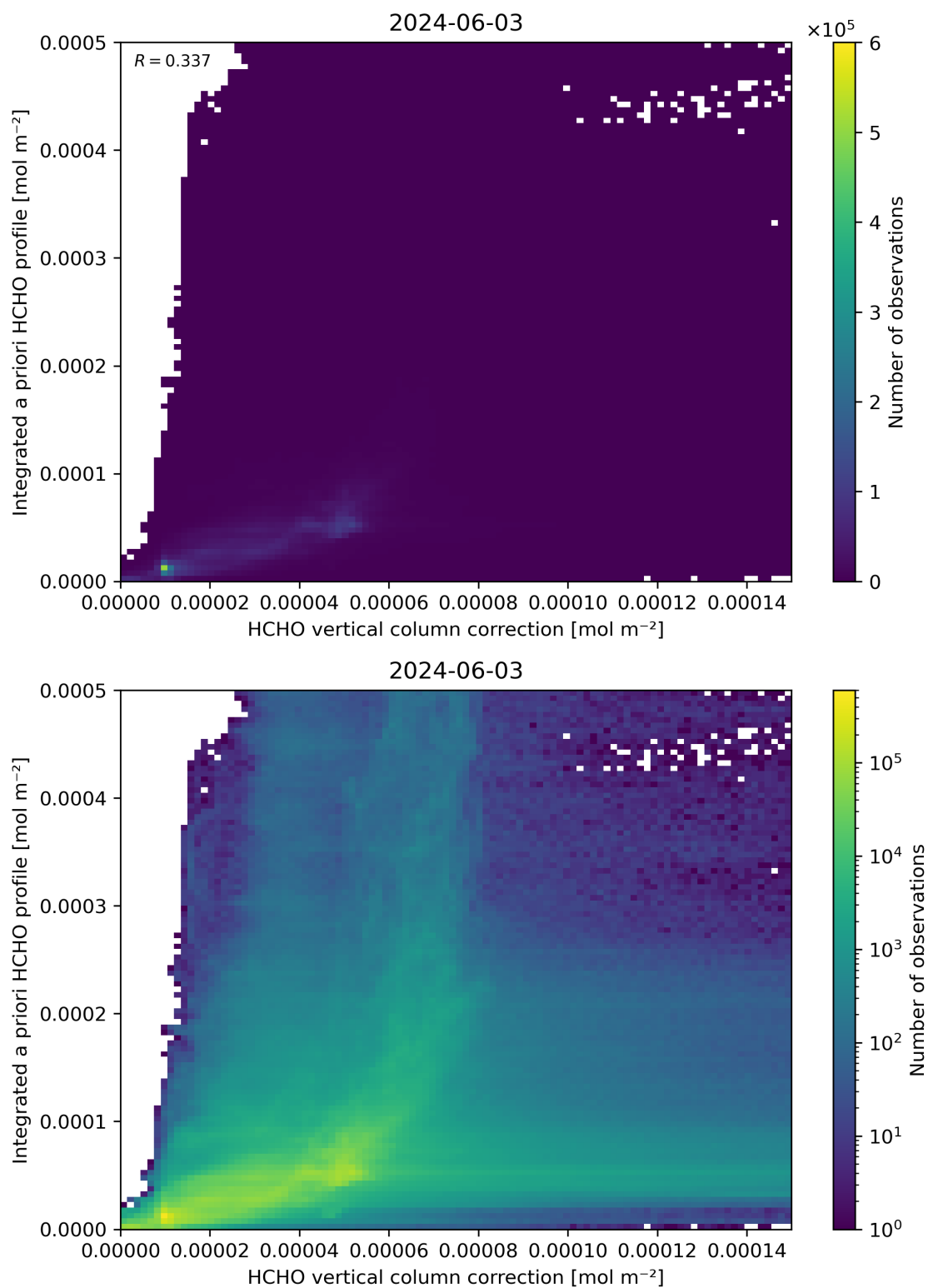
Figure 122: Scatter density plot of “HCHO vertical column correction” against “Integrated a priori HCHO profile” for 2024-06-03 to 2024-06-04.
