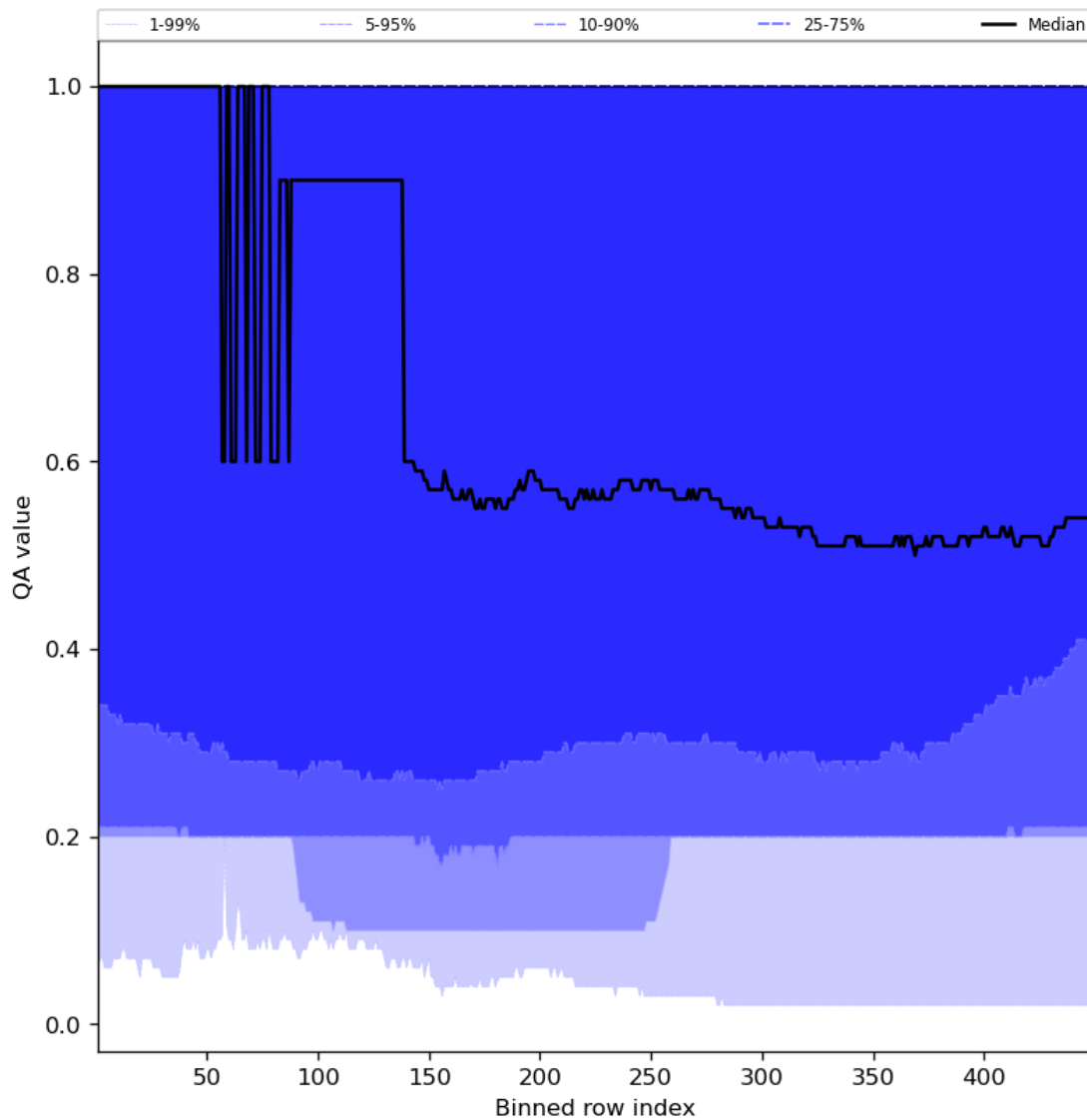
Figure 48: Along track statistics of “QA value” for 2024-06-03 to 2024-06-04
