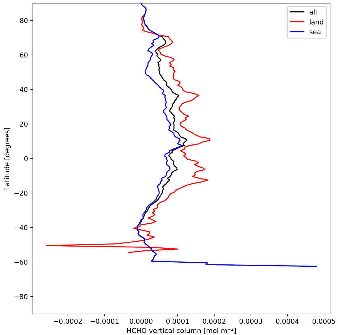
Figure 21: Zonal average of “HCHO vertical column” for 2024-06-03 to 2024-06-04.
