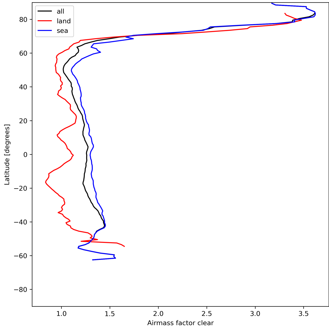
Figure 28: Zonal average of “Airmass factor clear” for 2024-06-03 to 2024-06-04.
