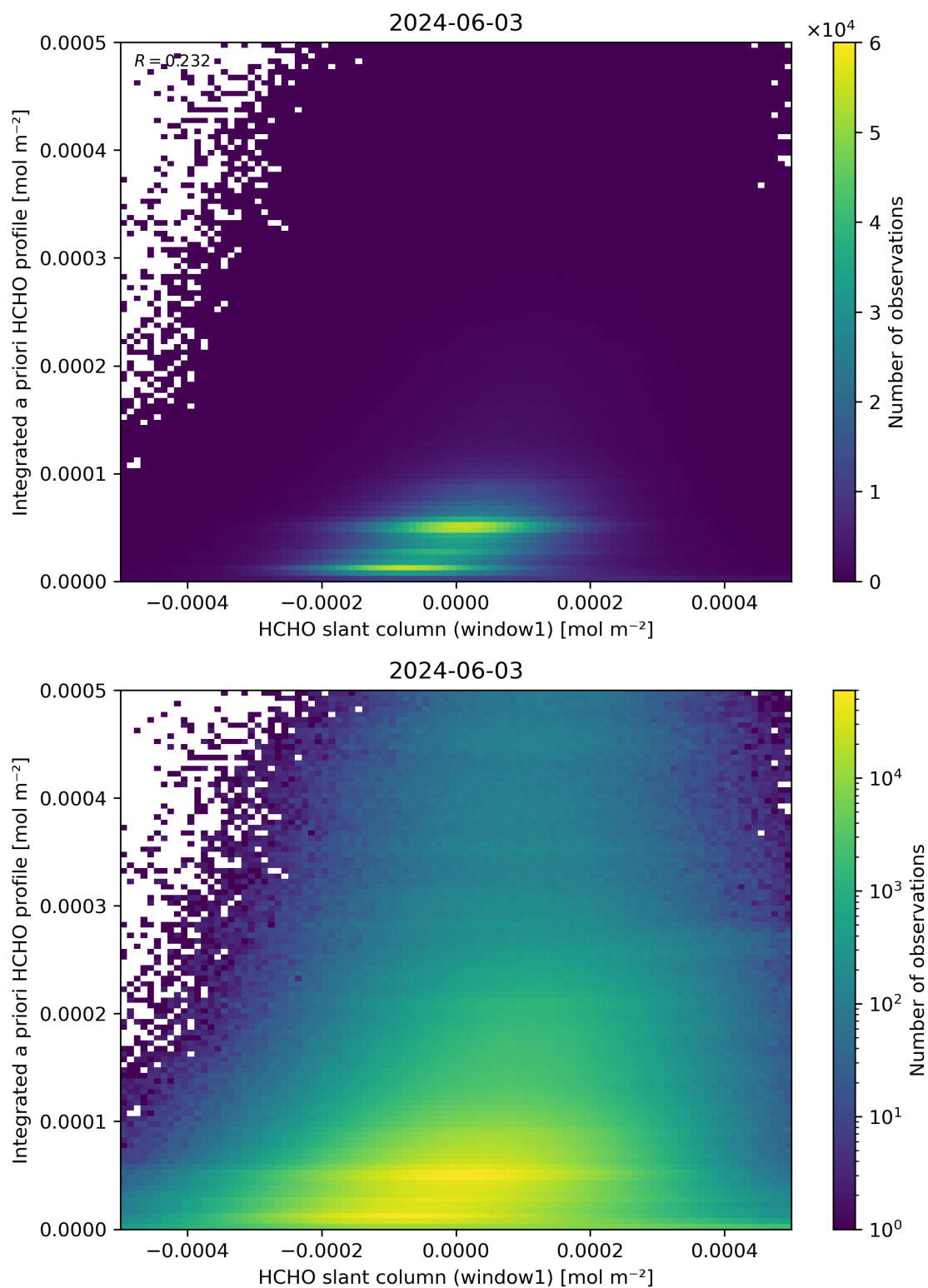
Figure 87: Scatter density plot of “HCHO slant column (window1)” against “Integrated a priori HCHO profile” for 2024-06-03 to 2024-06-04.
