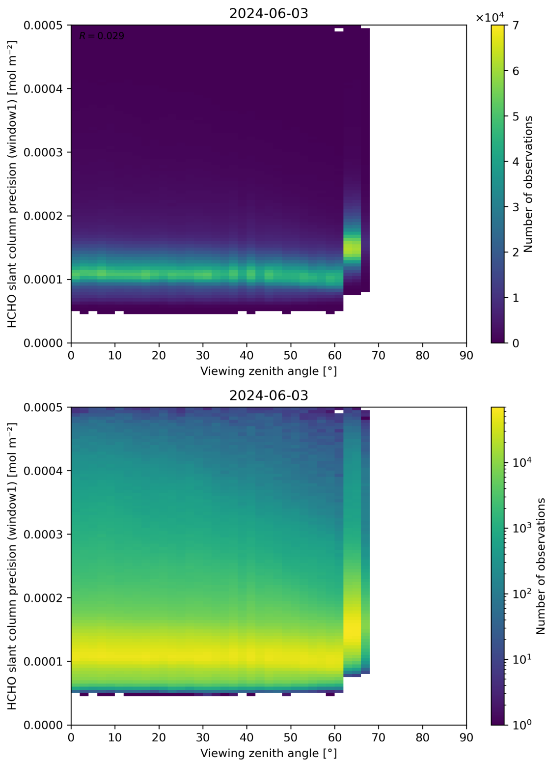
Figure 189: Scatter density plot of “Viewing zenith angle” against “HCHO slant column precision (window1)” for 2024-06-03 to 2024-06-04.
