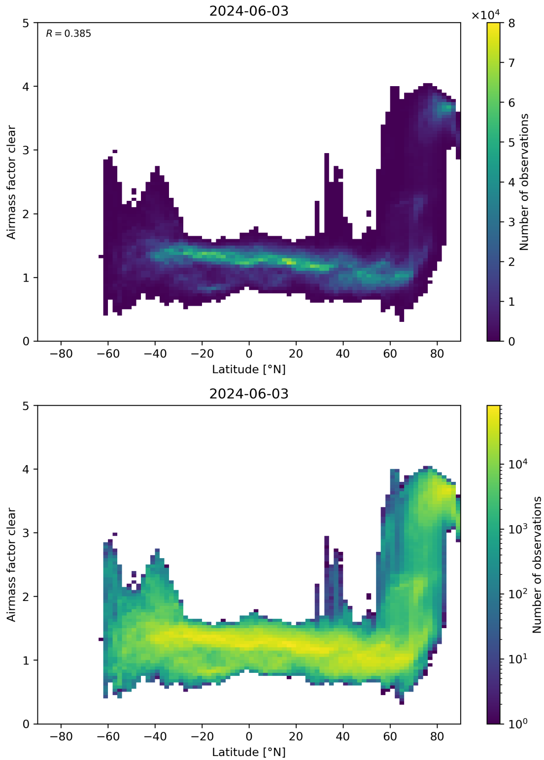
Figure 156: Scatter density plot of “Latitude” against “Airmass factor clear” for 2024-06-03 to 2024-06-04.
