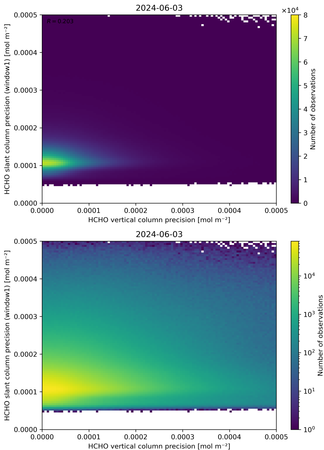
Figure 143: Scatter density plot of “HCHO vertical column precision” against “HCHO slant column precision (window1)” for 2024-06-03 to 2024-06-04.
