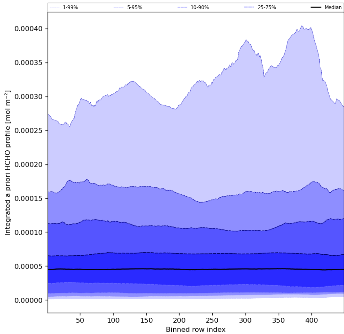
Figure 57: Along track statistics of “Integrated a priori HCHO profile” for 2024-06-03 to 2024-06-04
