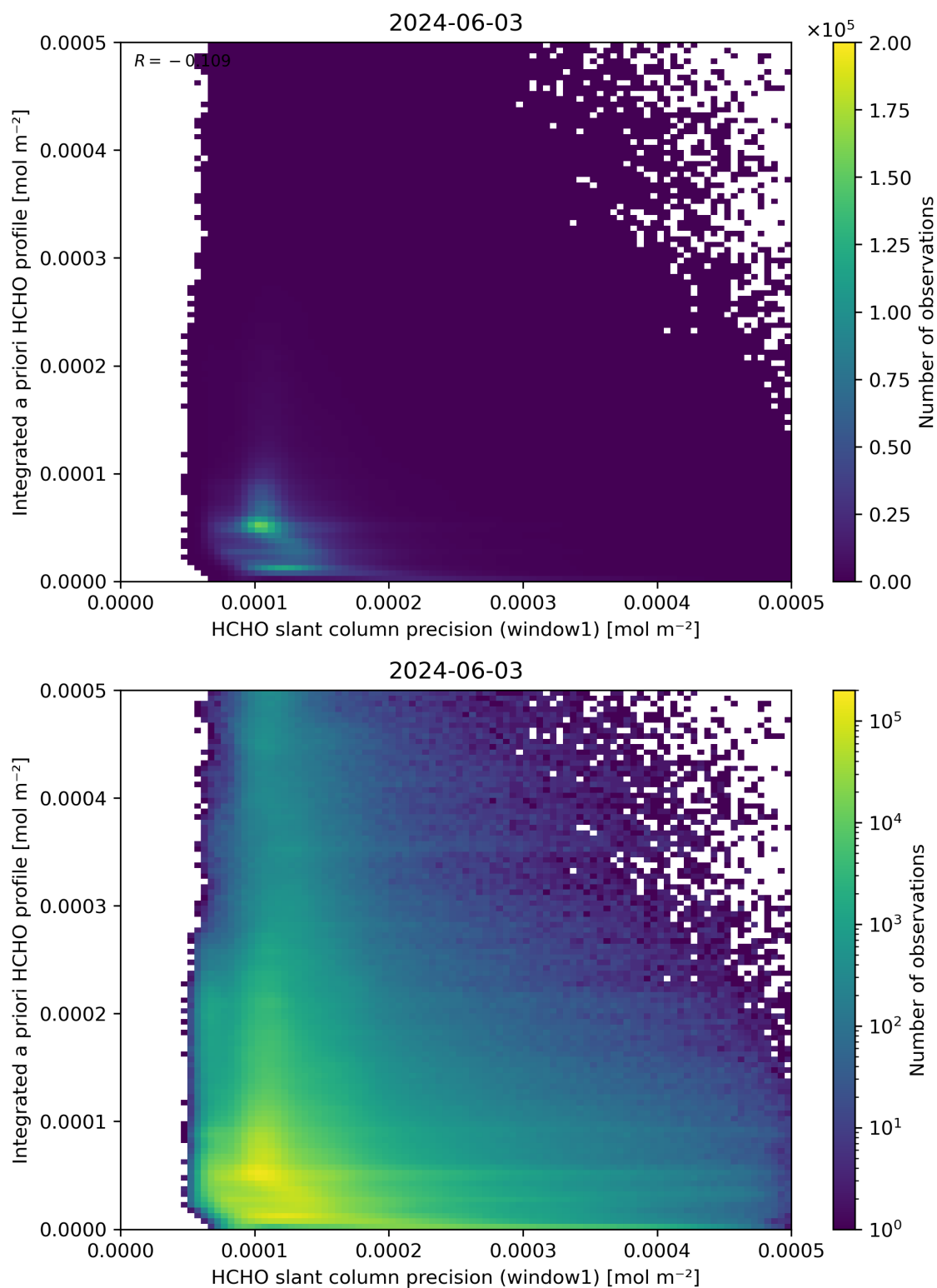
Figure 96: Scatter density plot of “HCHO slant column precision (window1)” against “Integrated a priori HCHO profile” for 2024-06-03 to 2024-06-04.
