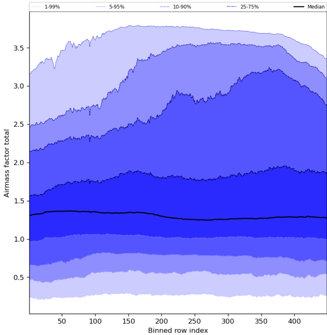
Figure 54: Along track statistics of “Airmass factor total” for 2024-06-03 to 2024-06-04
