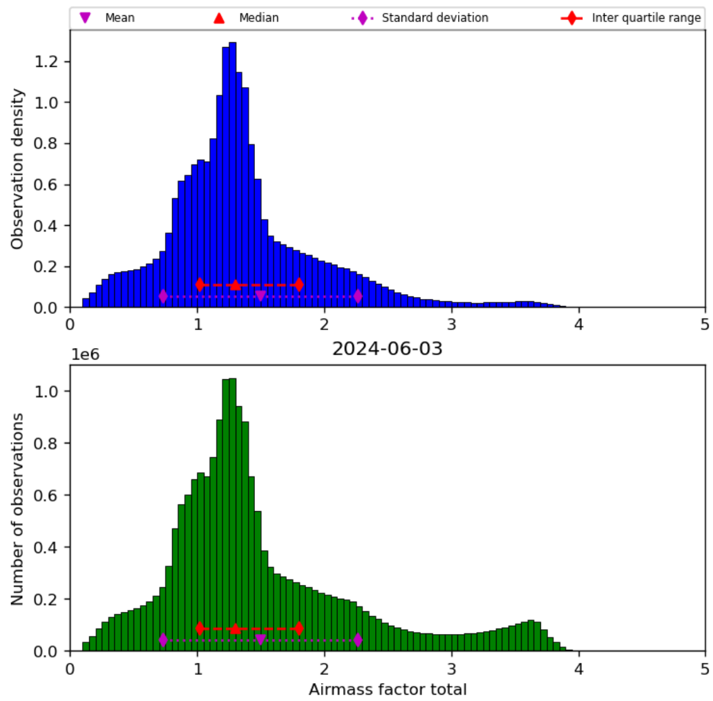
Figure 40: Histogram of “Airmass factor total” for 2024-06-03 to 2024-06-04
