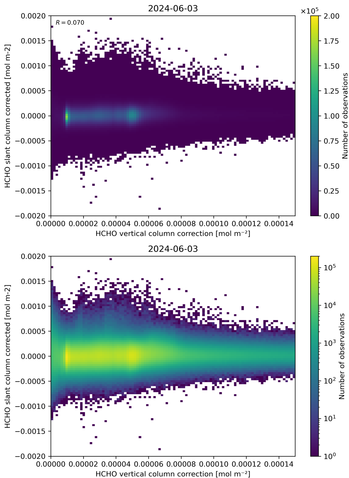
Figure 116: Scatter density plot of “HCHO vertical column correction” against “HCHO slant column corrected” for 2024-06-03 to 2024-06-04.
