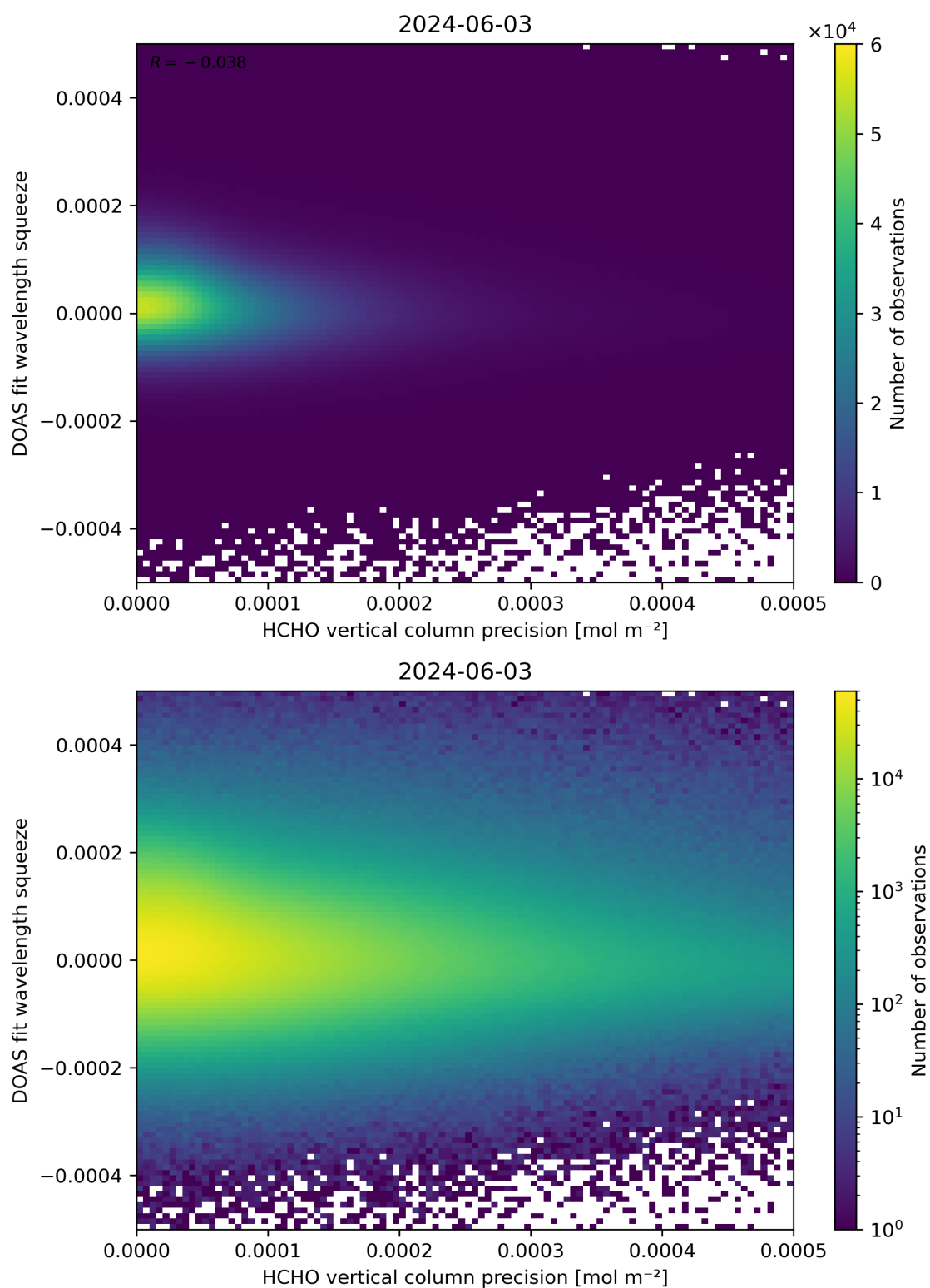
Figure 138: Scatter density plot of “HCHO vertical column precision” against “DOAS fit wavelength squeeze” for 2024-06-03 to 2024-06-04.
