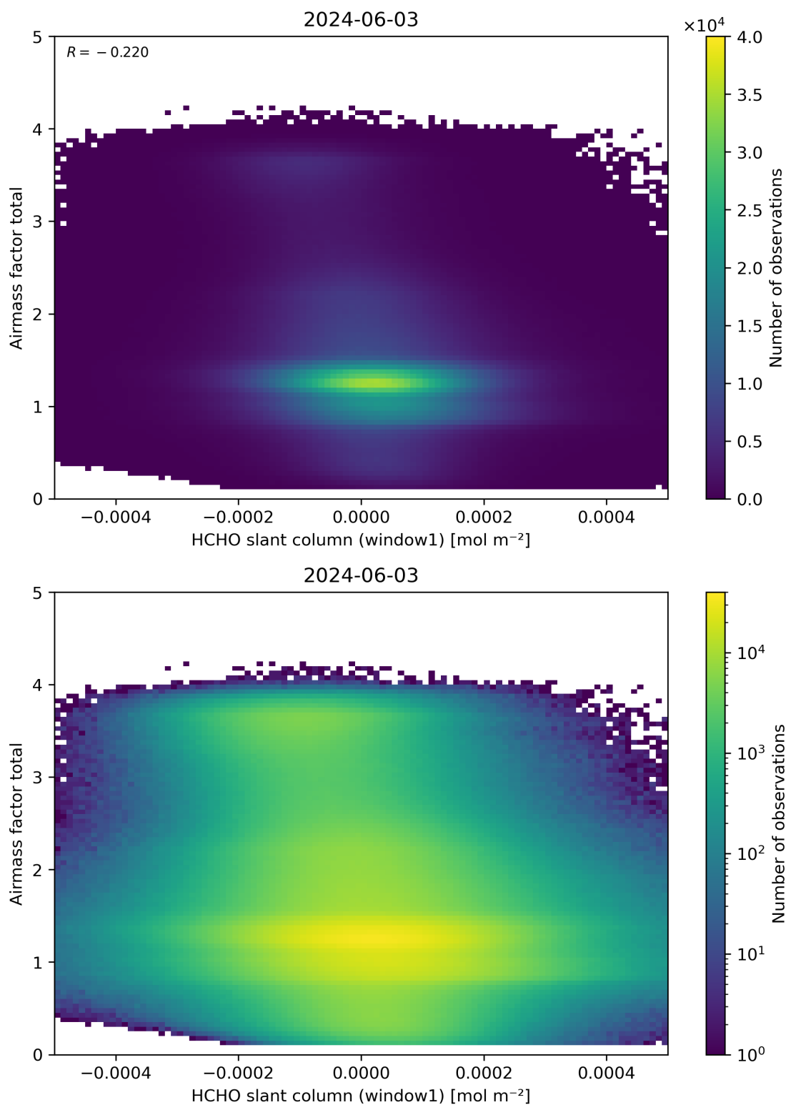
Figure 85: Scatter density plot of “HCHO slant column (window1)” against “Airmass factor total” for 2024-06-03 to 2024-06-04.
