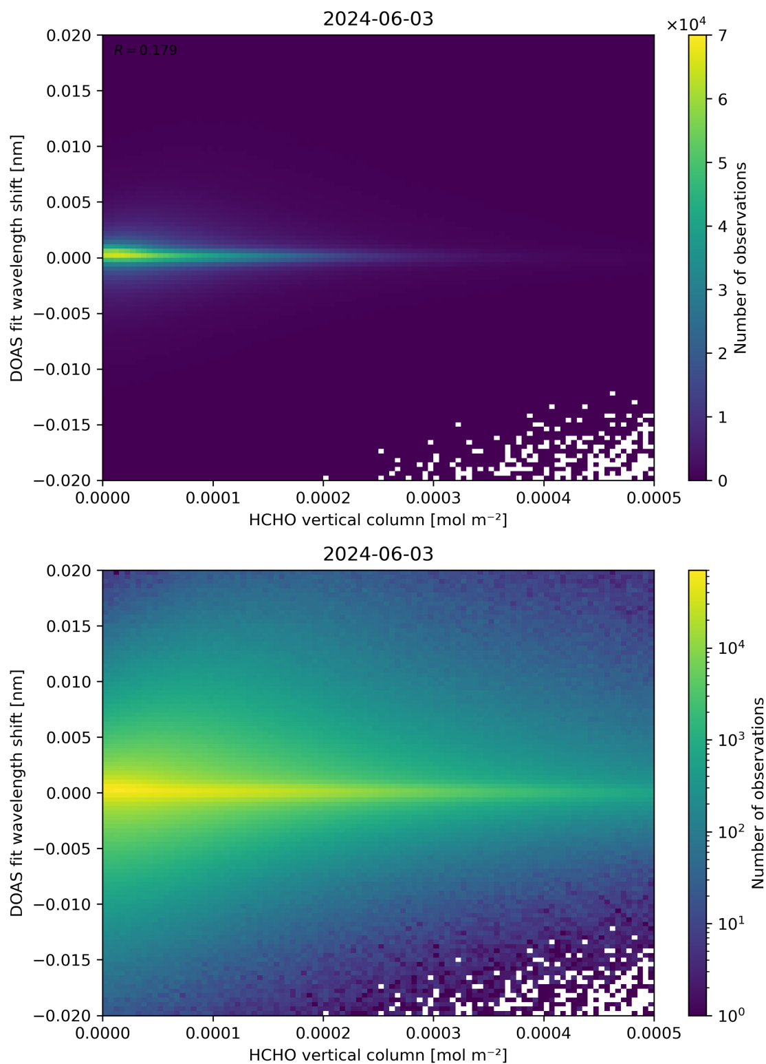
Figure 124: Scatter density plot of “HCHO vertical column” against “DOAS fit wavelength shift” for 2024-06-03 to 2024-06-04.
