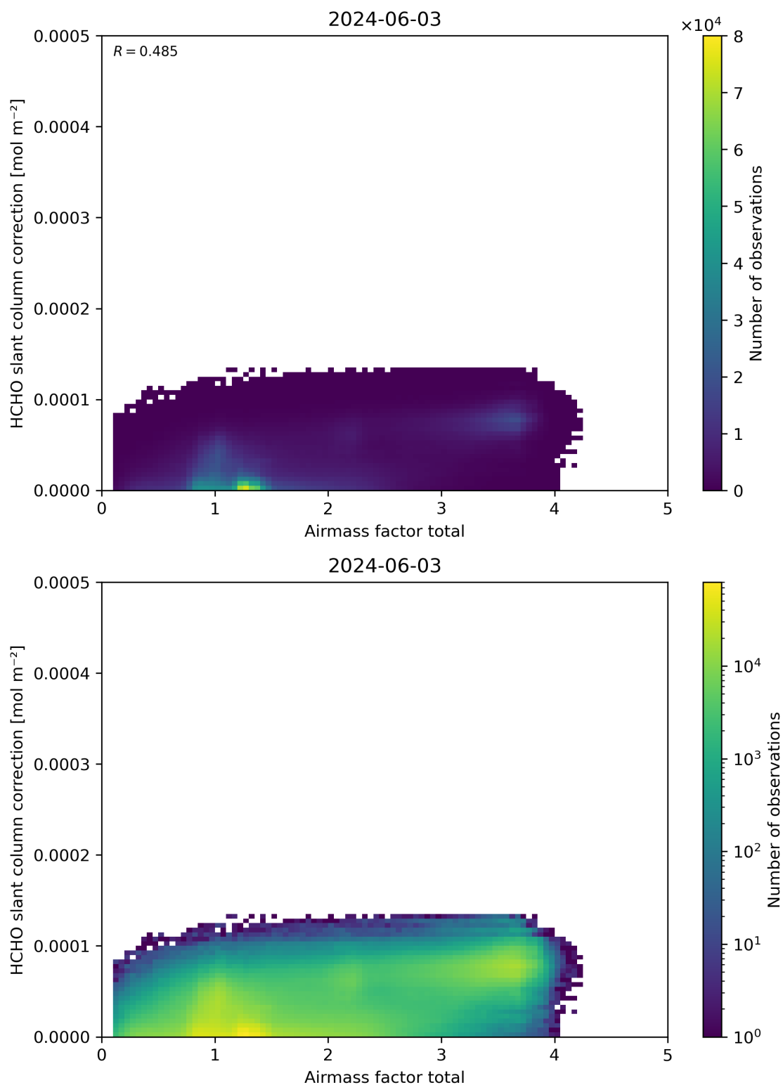
Figure 102: Scatter density plot of “Airmass factor total” against “HCHO slant column correction” for 2024-06-03 to 2024-06-04.
