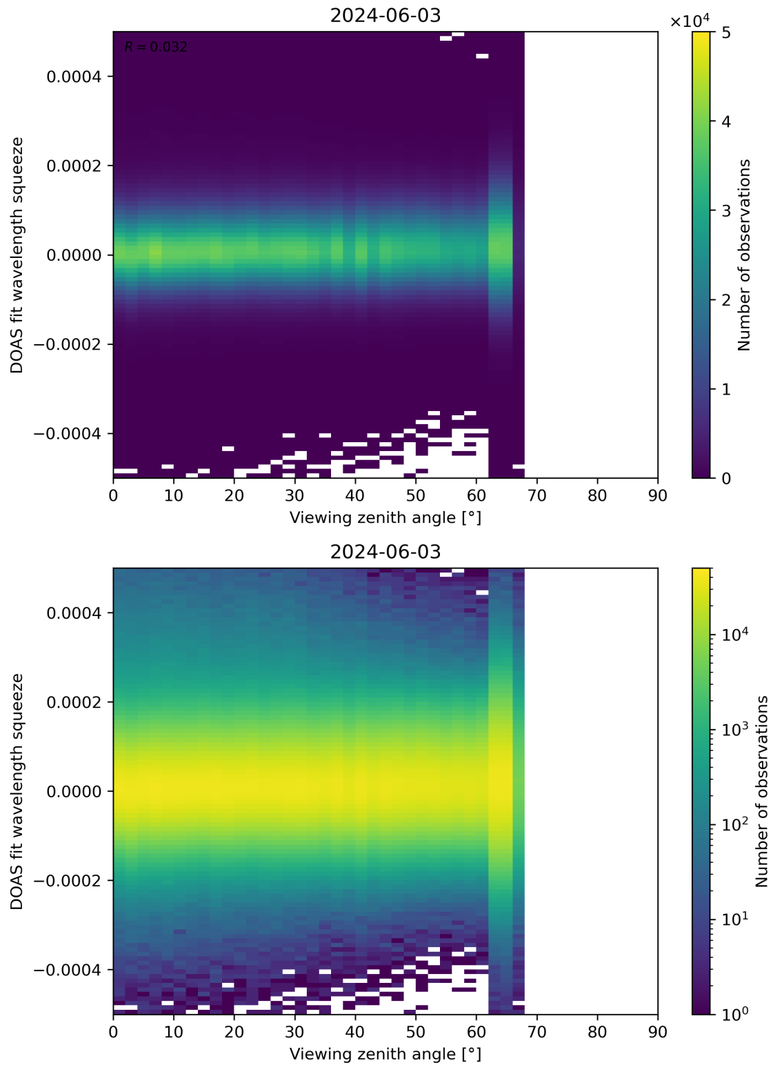
Figure 184: Scatter density plot of “Viewing zenith angle” against “DOAS fit wavelength squeeze” for 2024-06-03 to 2024-06-04.
