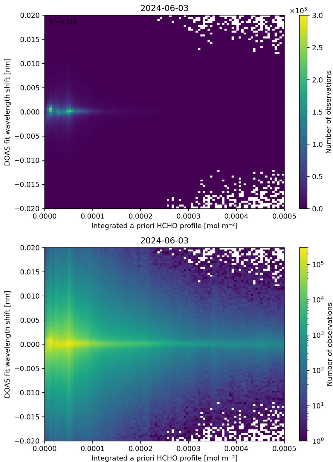
Figure 149: Scatter density plot of “Integrated a priori HCHO profile” against “DOAS fit wavelength shift” for 2024-06-03 to 2024-06-04.
