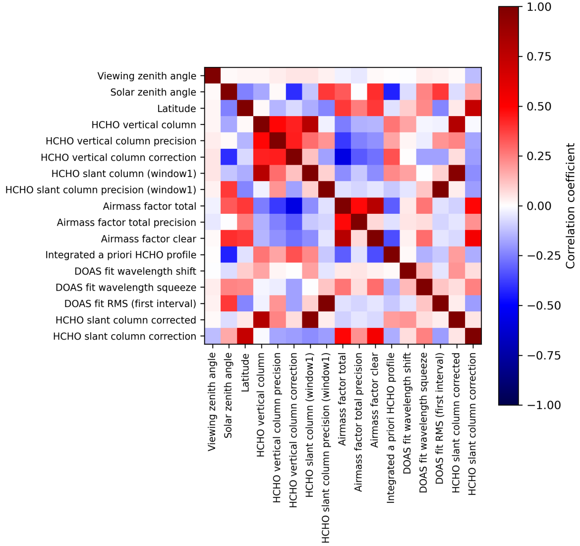
Figure 2: Map of correlation matrix for 2024-06-03 to 2024-06-04.
