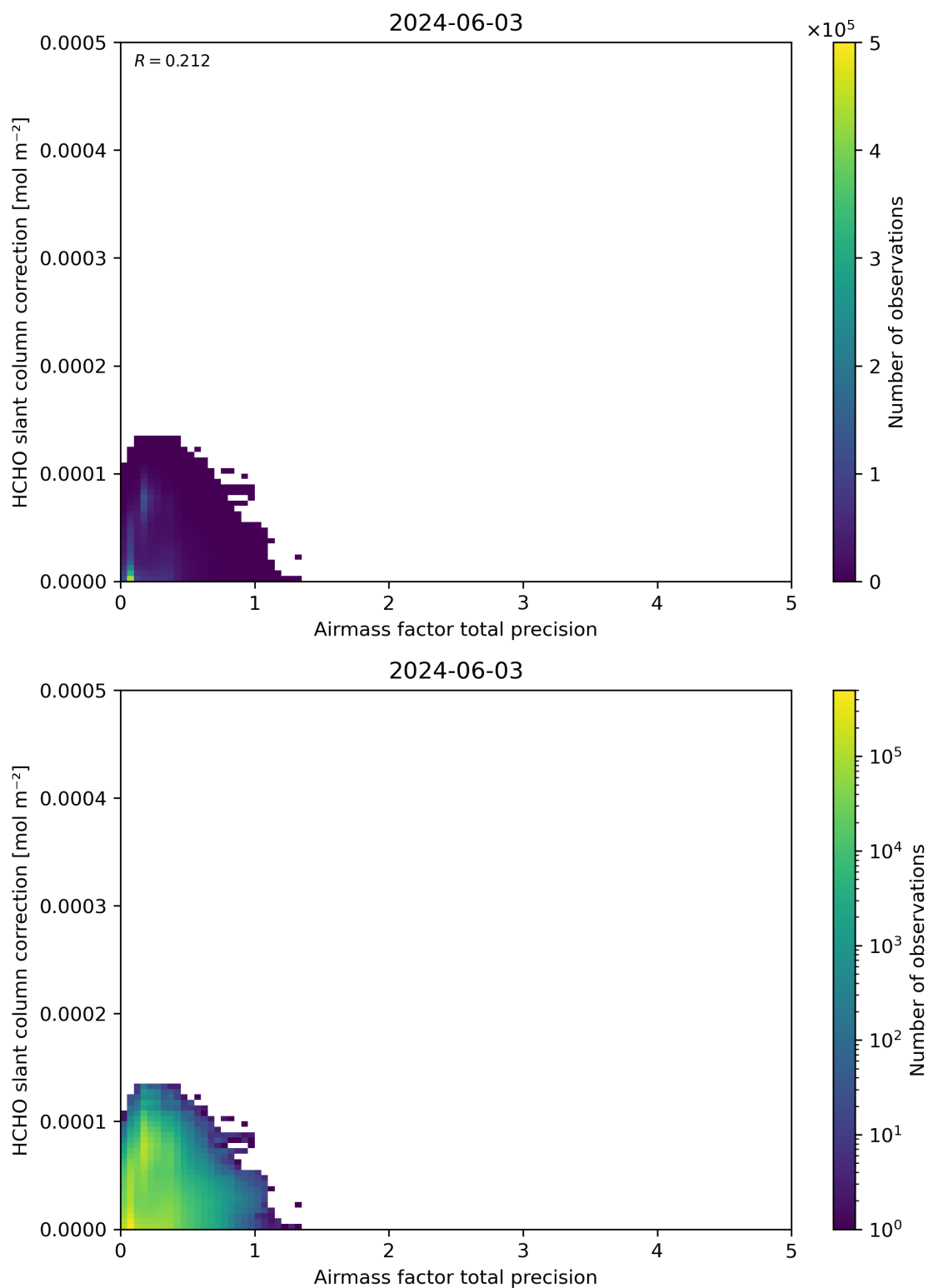
Figure 110: Scatter density plot of “Airmass factor total precision” against “HCHO slant column correction” for 2024-06-03 to 2024-06-04.
