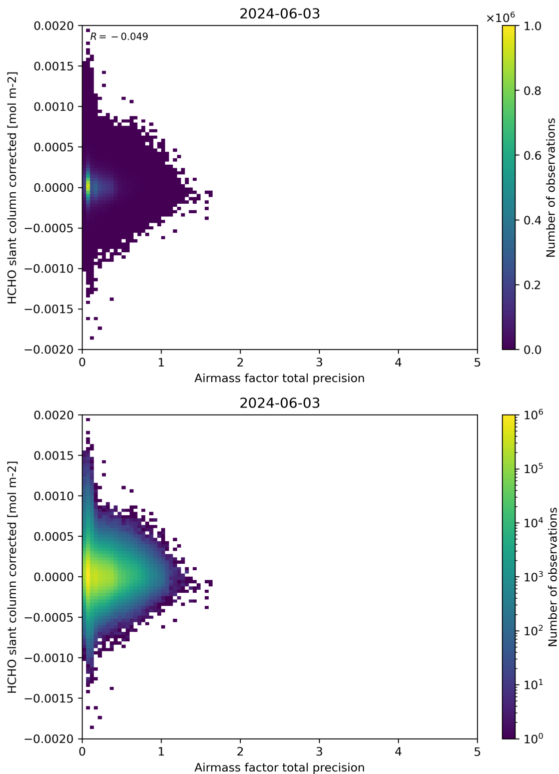
Figure 109: Scatter density plot of “Airmass factor total precision” against “HCHO slant column corrected” for 2024-06-03 to 2024-06-04.
