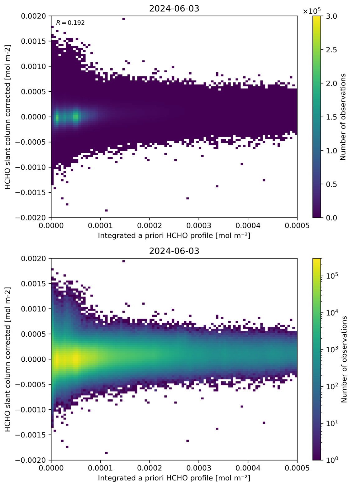
Figure 151: Scatter density plot of “Integrated a priori HCHO profile” against “HCHO slant column corrected” for 2024-06-03 to 2024-06-04.
