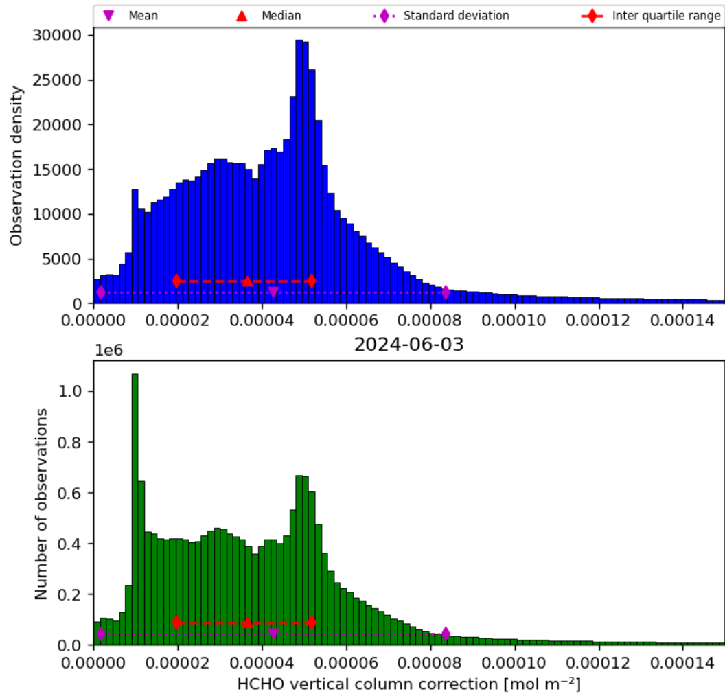
Figure 37: Histogram of “HCHO vertical column correction” for 2024-06-03 to 2024-06-04
