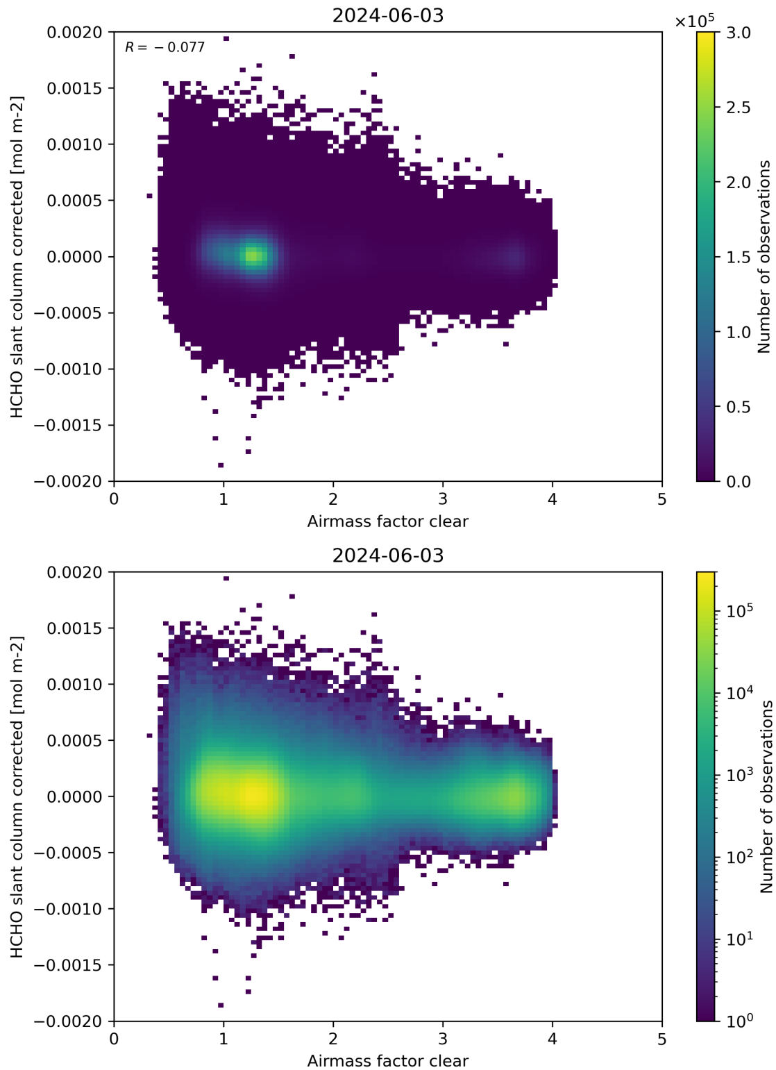
Figure 74: Scatter density plot of “Airmass factor clear” against “HCHO slant column corrected” for 2024-06-03 to 2024-06-04.
