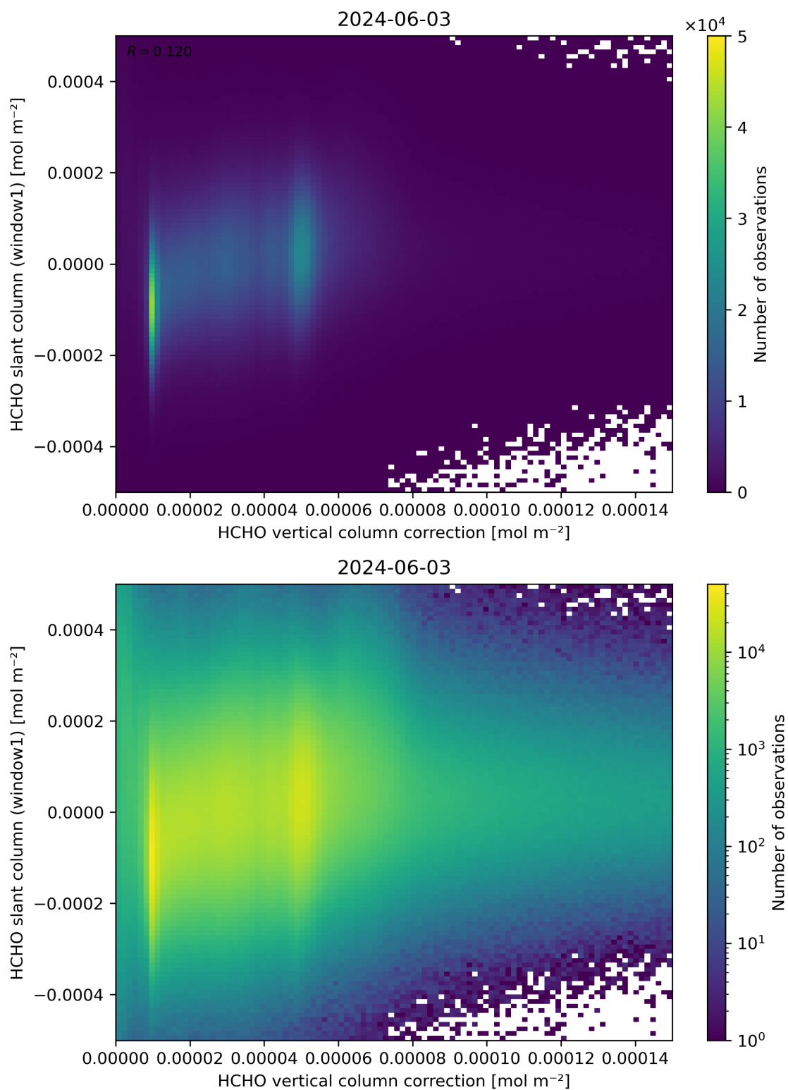
Figure 118: Scatter density plot of “HCHO vertical column correction” against “HCHO slant column (window1)” for 2024-06-03 to 2024-06-04.
