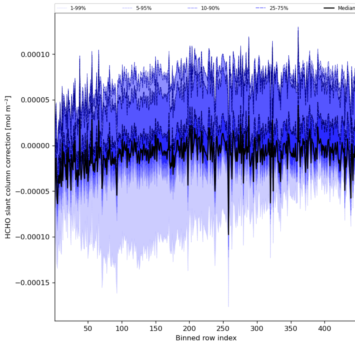
Figure 61: Along track statistics of “HCHO slant column correction” for 2024-06-03 to 2024-06-04
