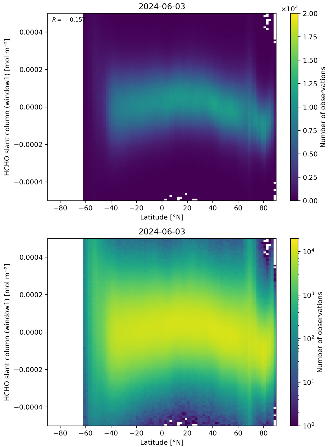
Figure 159: Scatter density plot of “Latitude” against “HCHO slant column (window1)” for 2024-06-03 to 2024-06-04.
