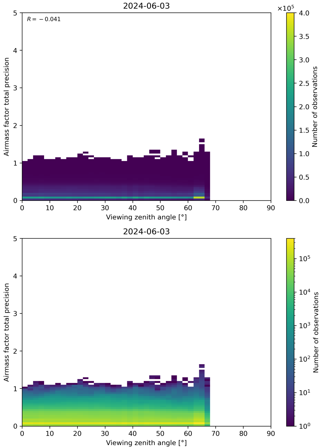
Figure 191: Scatter density plot of “Viewing zenith angle” against “Airmass factor total precision” for 2024-06-03 to 2024-06-04.
