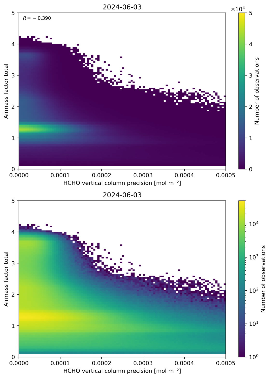
Figure 144: Scatter density plot of “HCHO vertical column precision” against “Airmass factor total” for 2024-06-03 to 2024-06-04.
