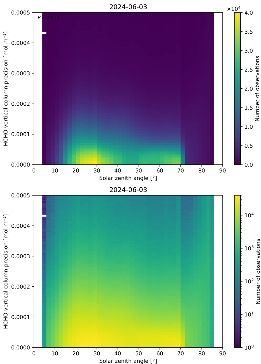
Figure 179: Scatter density plot of “Solar zenith angle” against “HCHO vertical column precision” for 2024-06-03 to 2024-06-04.
