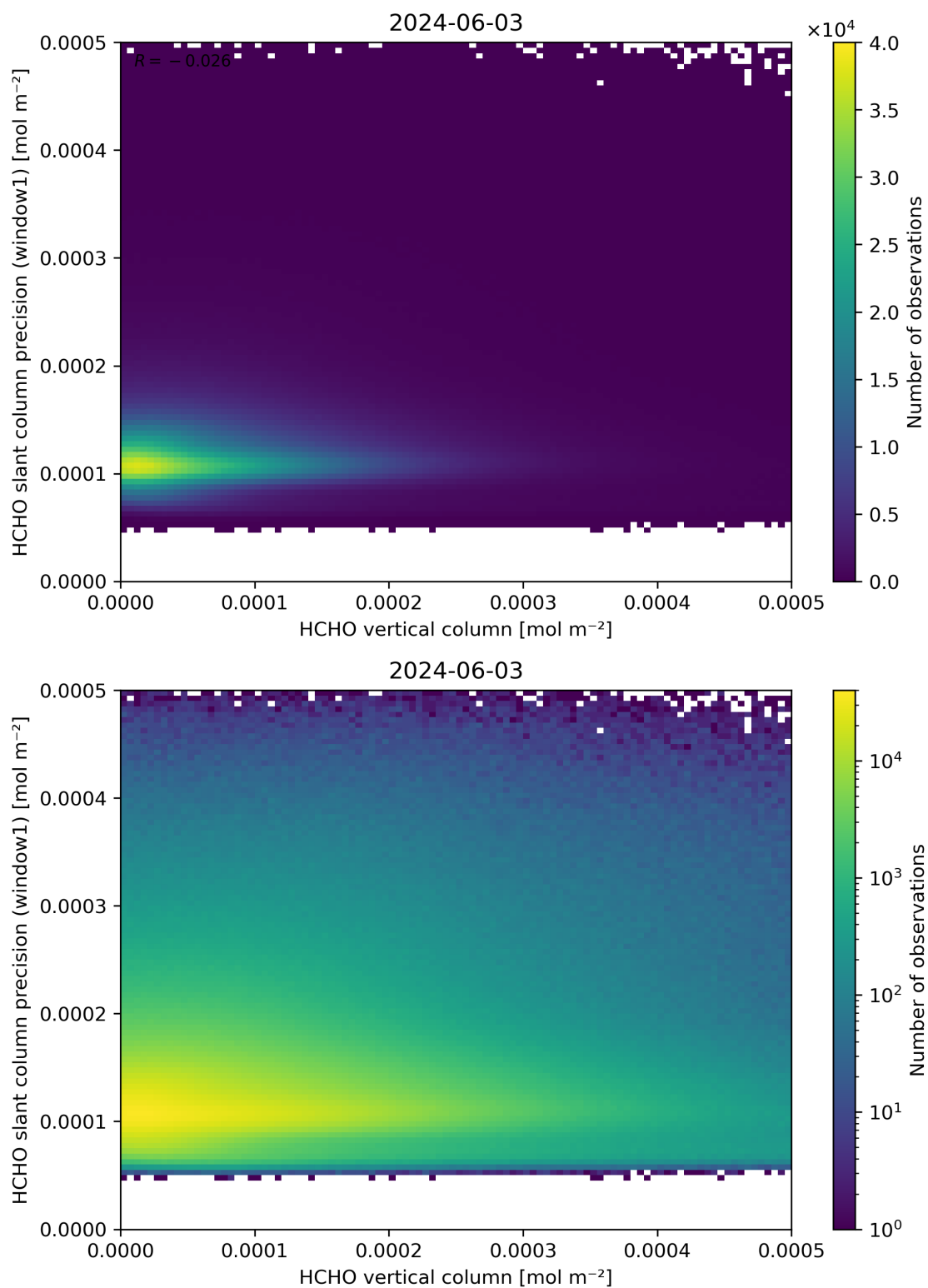
Figure 130: Scatter density plot of “HCHO vertical column” against “HCHO slant column precision (window1)” for 2024-06-03 to 2024-06-04.
