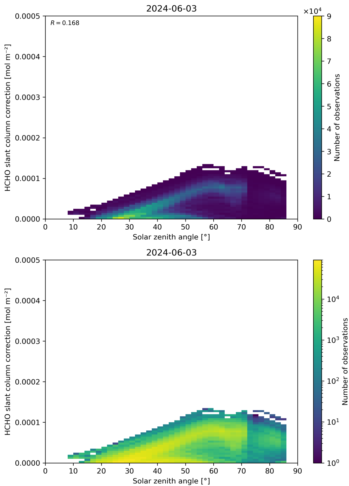
Figure 172: Scatter density plot of “Solar zenith angle” against “HCHO slant column correction” for 2024-06-03 to 2024-06-04.
