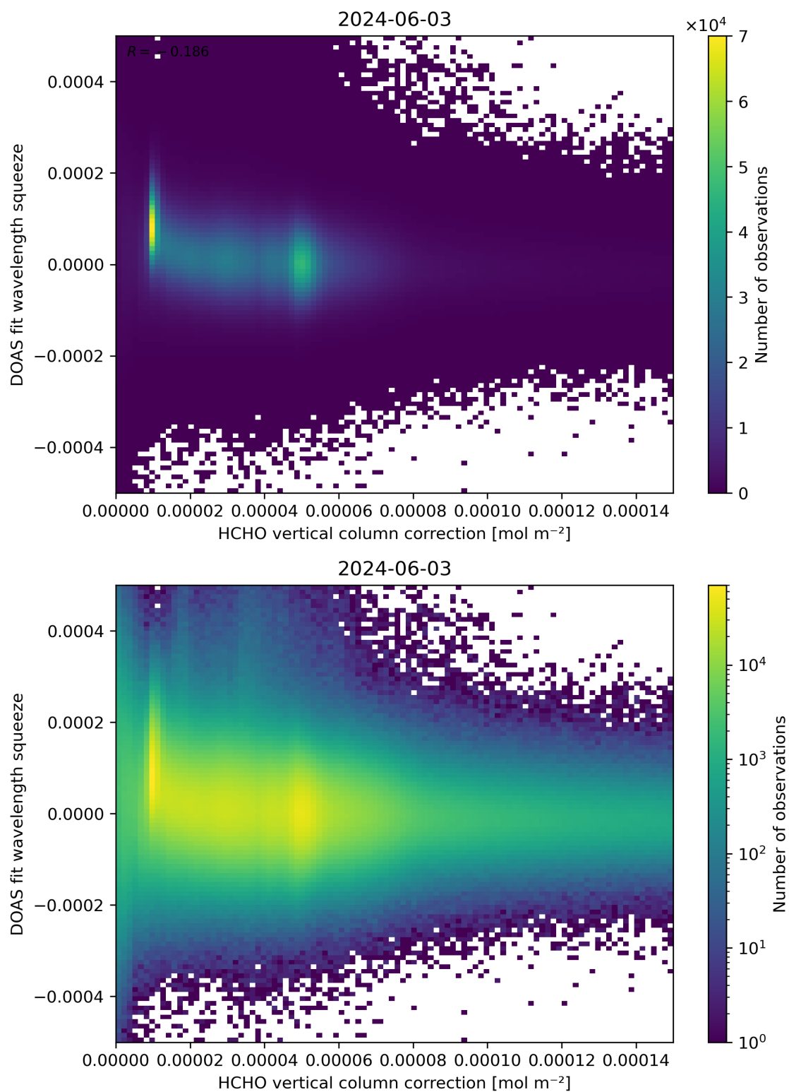
Figure 114: Scatter density plot of “HCHO vertical column correction” against “DOAS fit wavelength squeeze” for 2024-06-03 to 2024-06-04.
