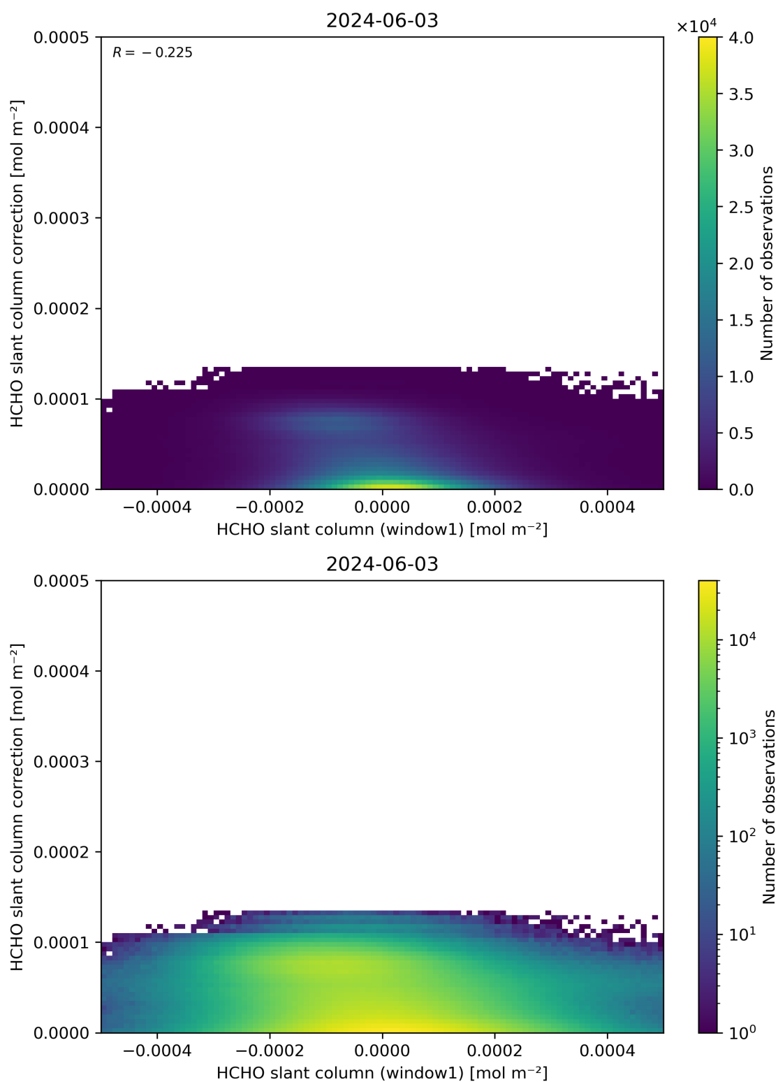
Figure 83: Scatter density plot of “HCHO slant column (window1)” against “HCHO slant column correction” for 2024-06-03 to 2024-06-04.
