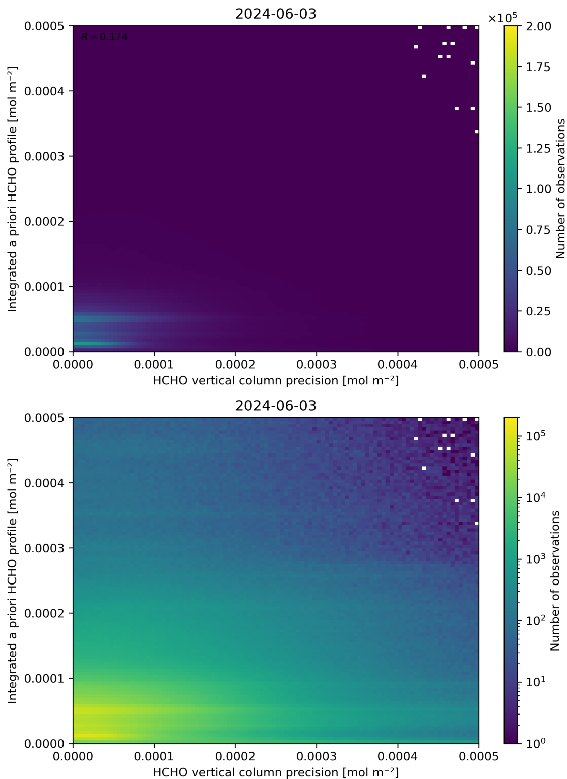
Figure 147: Scatter density plot of “HCHO vertical column precision” against “Integrated a priori HCHO profile” for 2024-06-03 to 2024-06-04.
