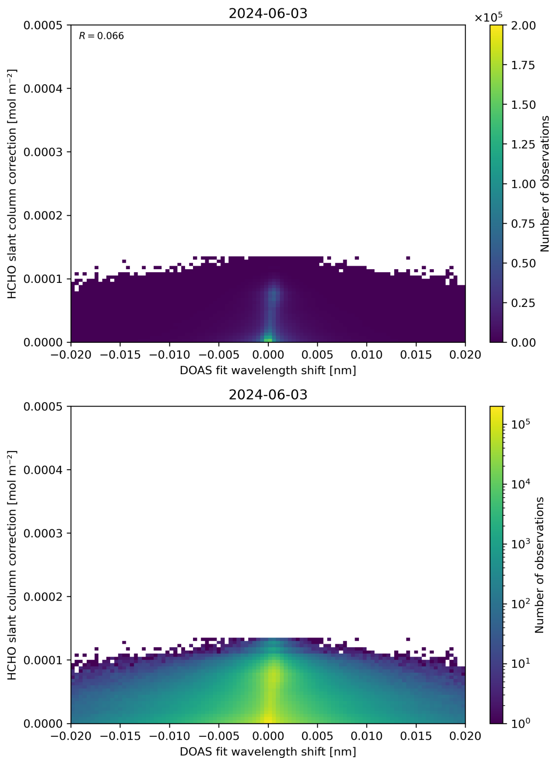
Figure 67: Scatter density plot of “DOAS fit wavelength shift” against “HCHO slant column correction” for 2024-06-03 to 2024-06-04.
