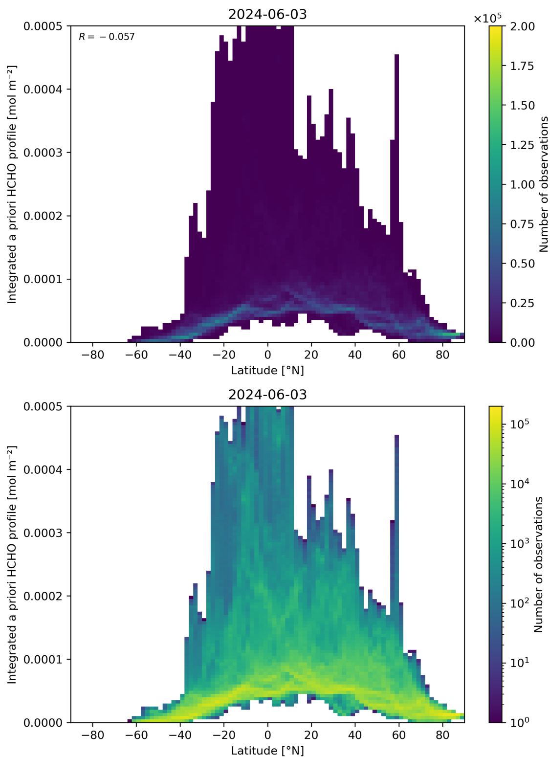
Figure 166: Scatter density plot of “Latitude” against “Integrated a priori HCHO profile” for 2024-06-03 to 2024-06-04.
