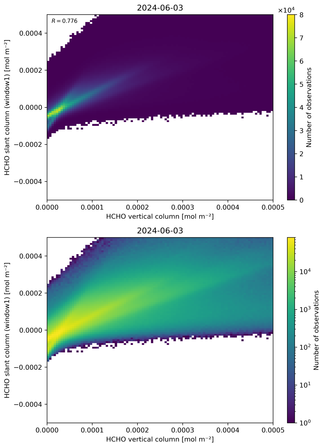
Figure 129: Scatter density plot of “HCHO vertical column” against “HCHO slant column (window1)” for 2024-06-03 to 2024-06-04.
