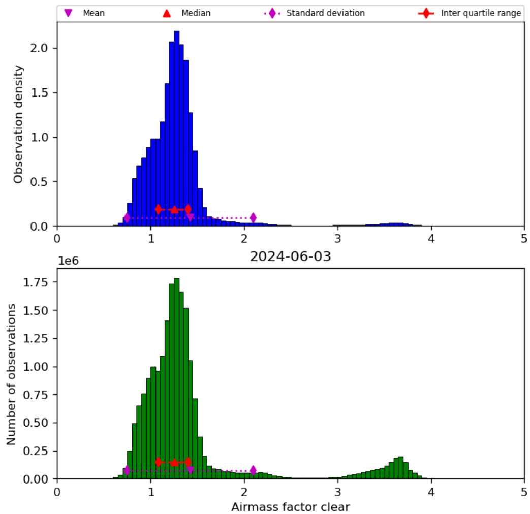
Figure 42: Histogram of “Airmass factor clear” for 2024-06-03 to 2024-06-04
