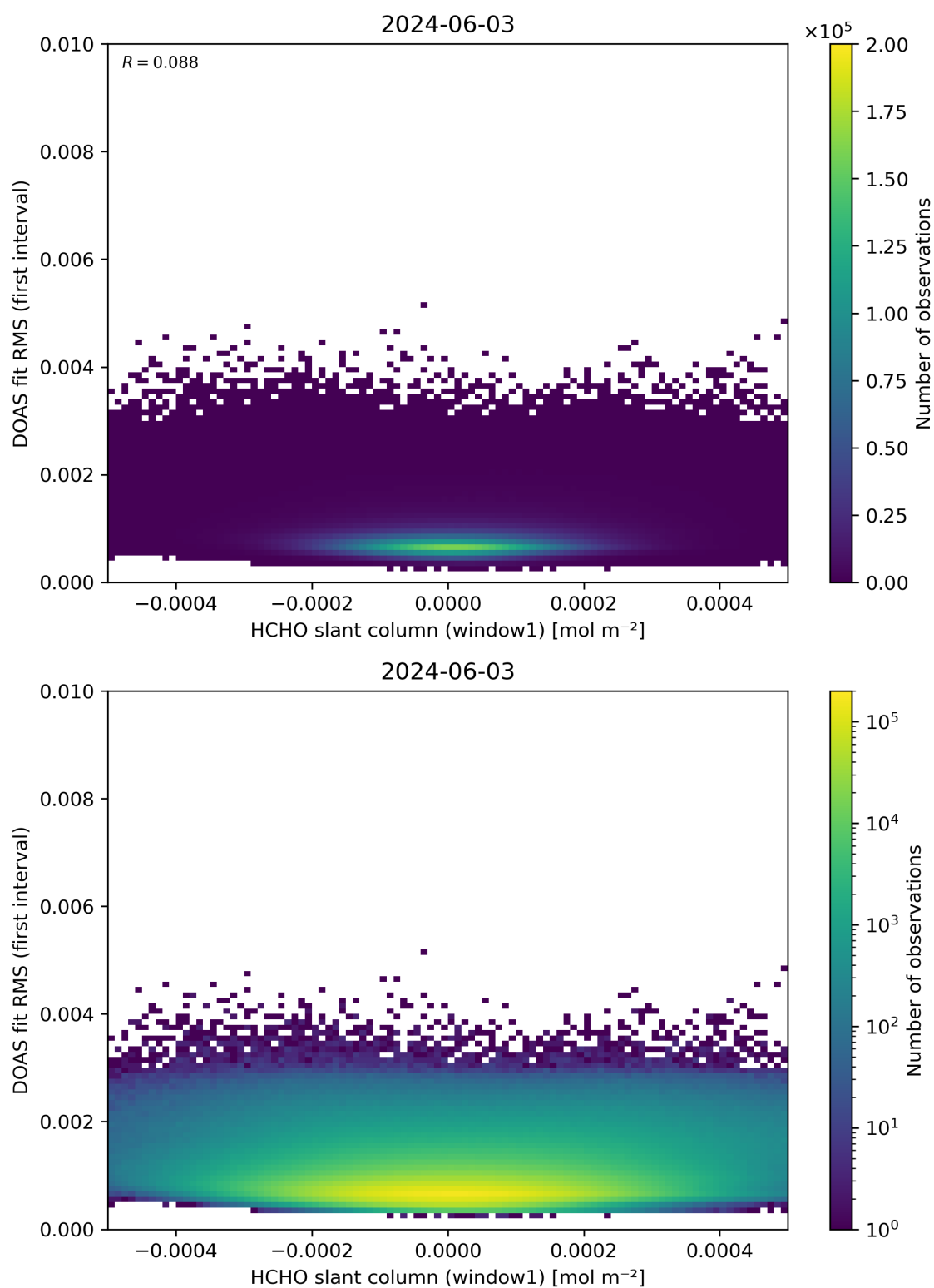
Figure 78: Scatter density plot of “HCHO slant column (window1)” against “DOAS fit RMS (first interval)” for 2024-06-03 to 2024-06-04.
