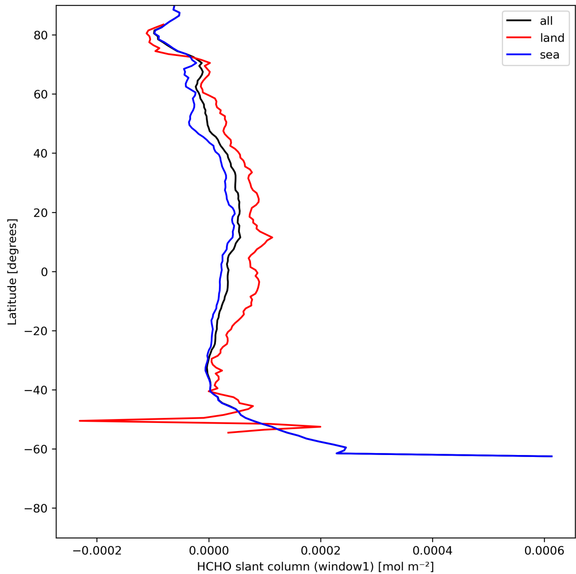
Figure 24: Zonal average of “HCHO slant column (window1)” for 2024-06-03 to 2024-06-04.
