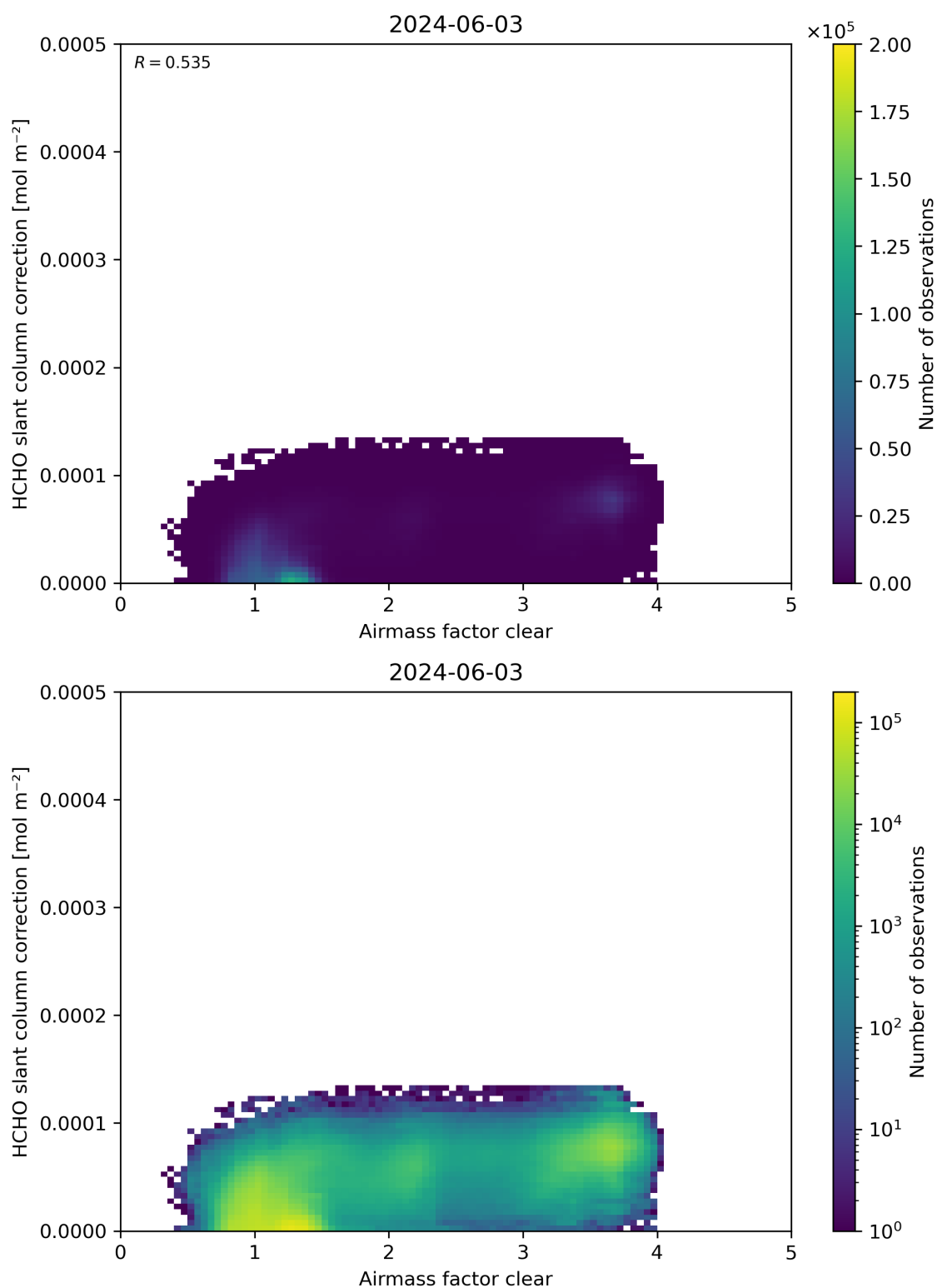
Figure 75: Scatter density plot of “Airmass factor clear” against “HCHO slant column correction” for 2024-06-03 to 2024-06-04.
