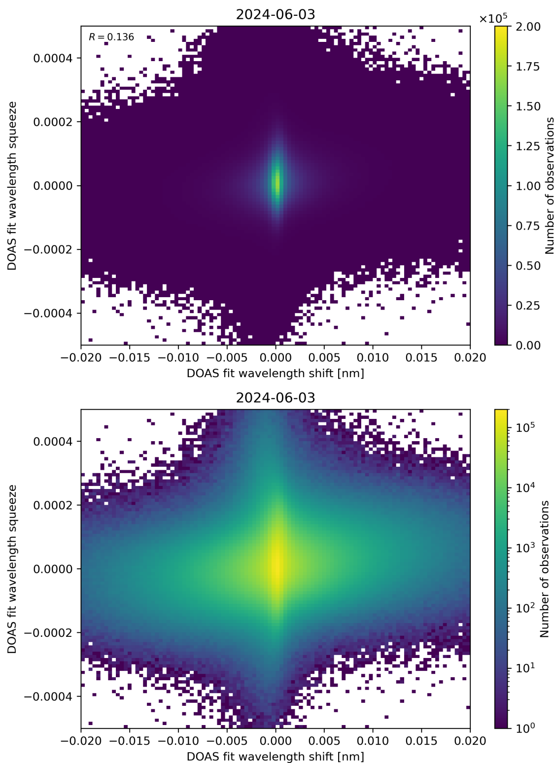
Figure 65: Scatter density plot of “DOAS fit wavelength shift” against “DOAS fit wavelength squeeze” for 2024-06-03 to 2024-06-04.
