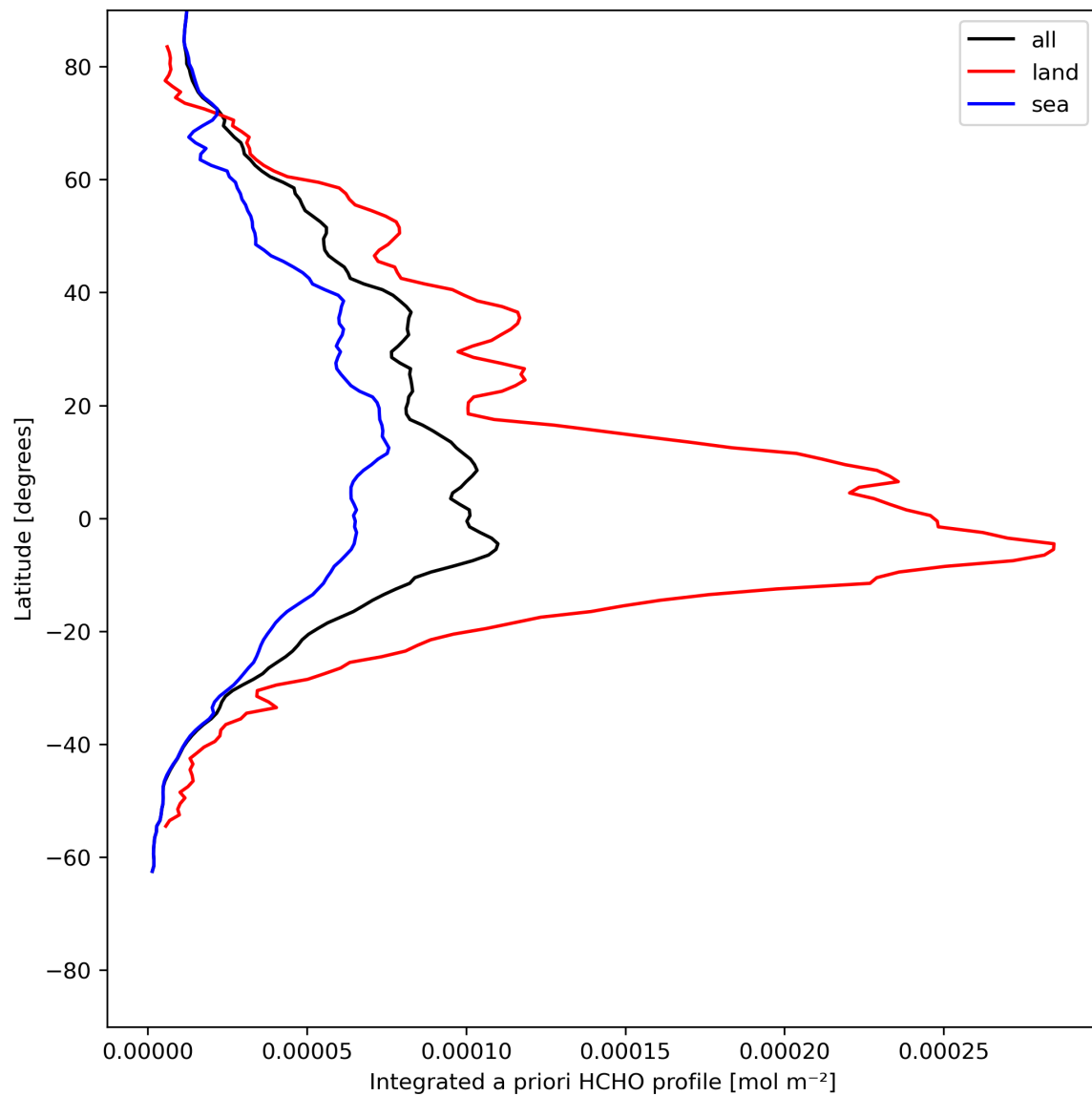
Figure 29: Zonal average of “Integrated a priori HCHO profile” for 2024-06-03 to 2024-06-04.
