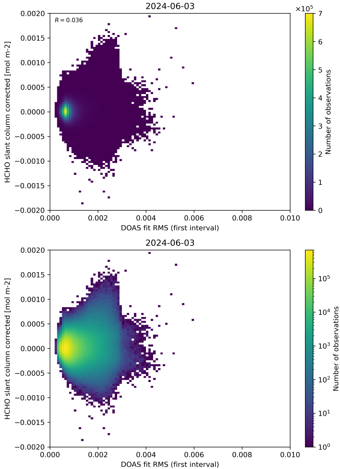
Figure 62: Scatter density plot of “DOAS fit RMS (first interval)” against “HCHO slant column corrected” for 2024-06-03 to 2024-06-04.
