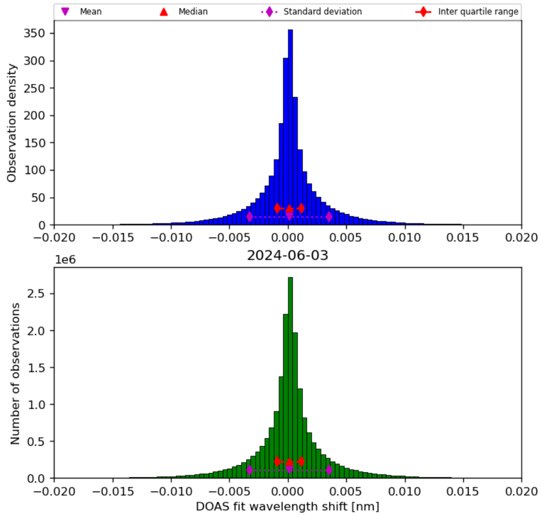
Figure 44: Histogram of “DOAS fit wavelength shift” for 2024-06-03 to 2024-06-04
