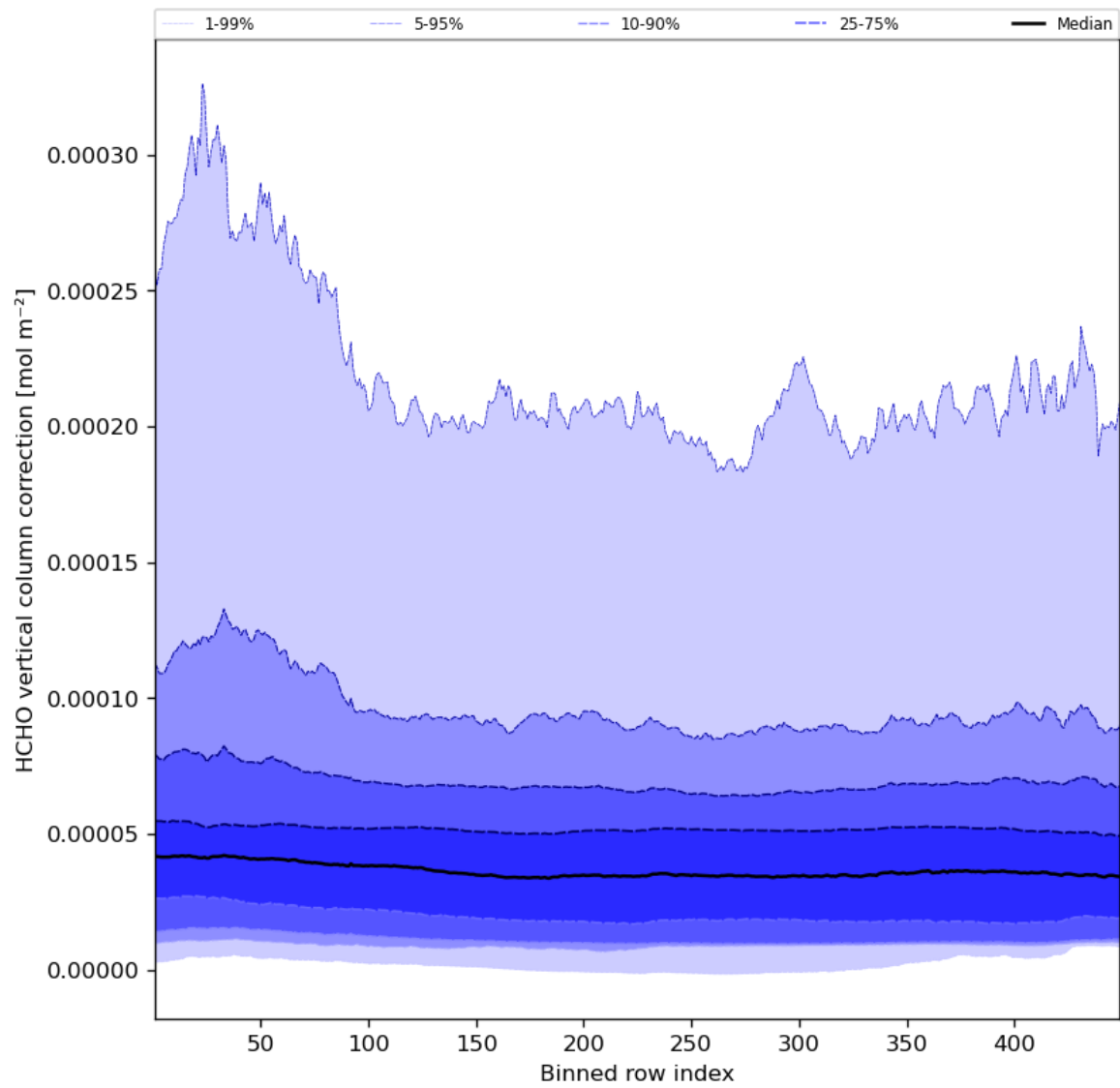
Figure 51: Along track statistics of “HCHO vertical column correction” for 2024-06-03 to 2024-06-04
