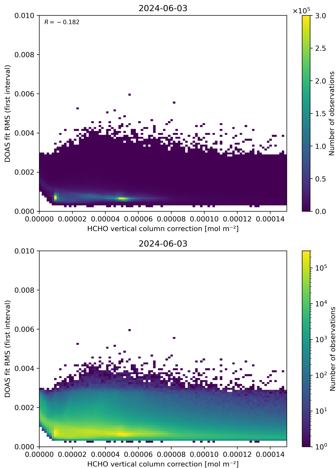
Figure 112: Scatter density plot of “HCHO vertical column correction” against “DOAS fit RMS (first interval)” for 2024-06-03 to 2024-06-04.
