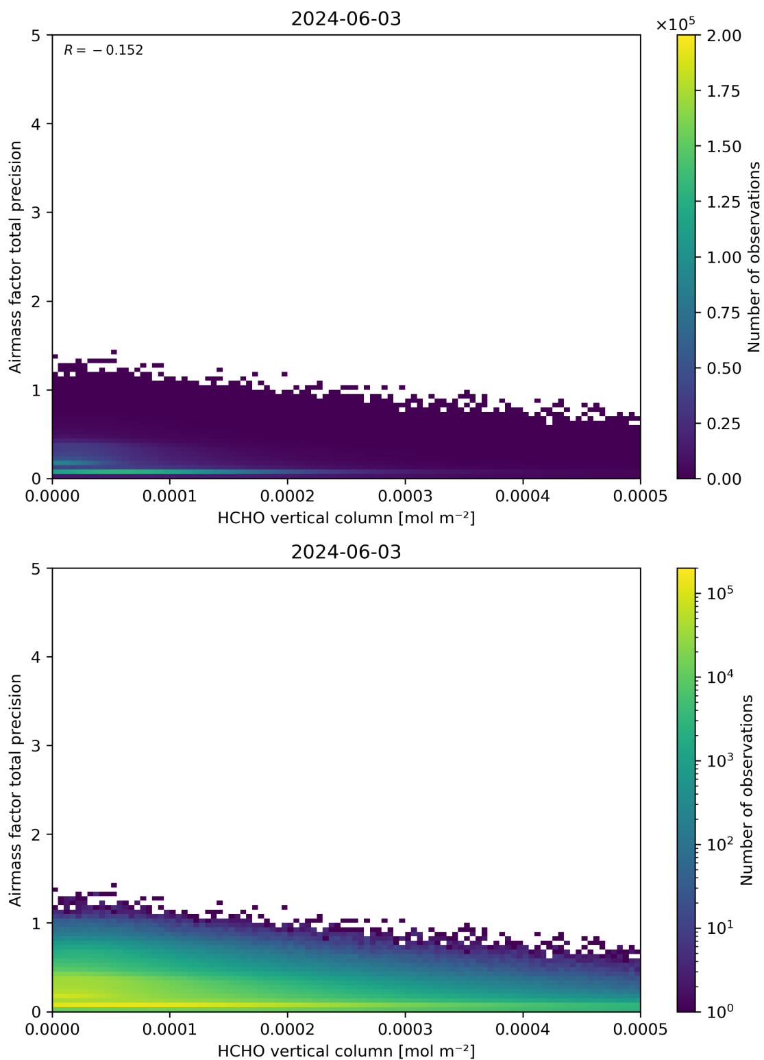
Figure 132: Scatter density plot of “HCHO vertical column” against “Airmass factor total precision” for 2024-06-03 to 2024-06-04.
