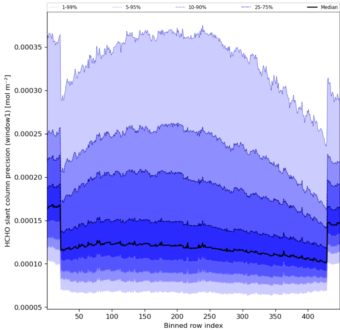
Figure 53: Along track statistics of “HCHO slant column precision (window1)” for 2024-06-03 to 2024-06-04
