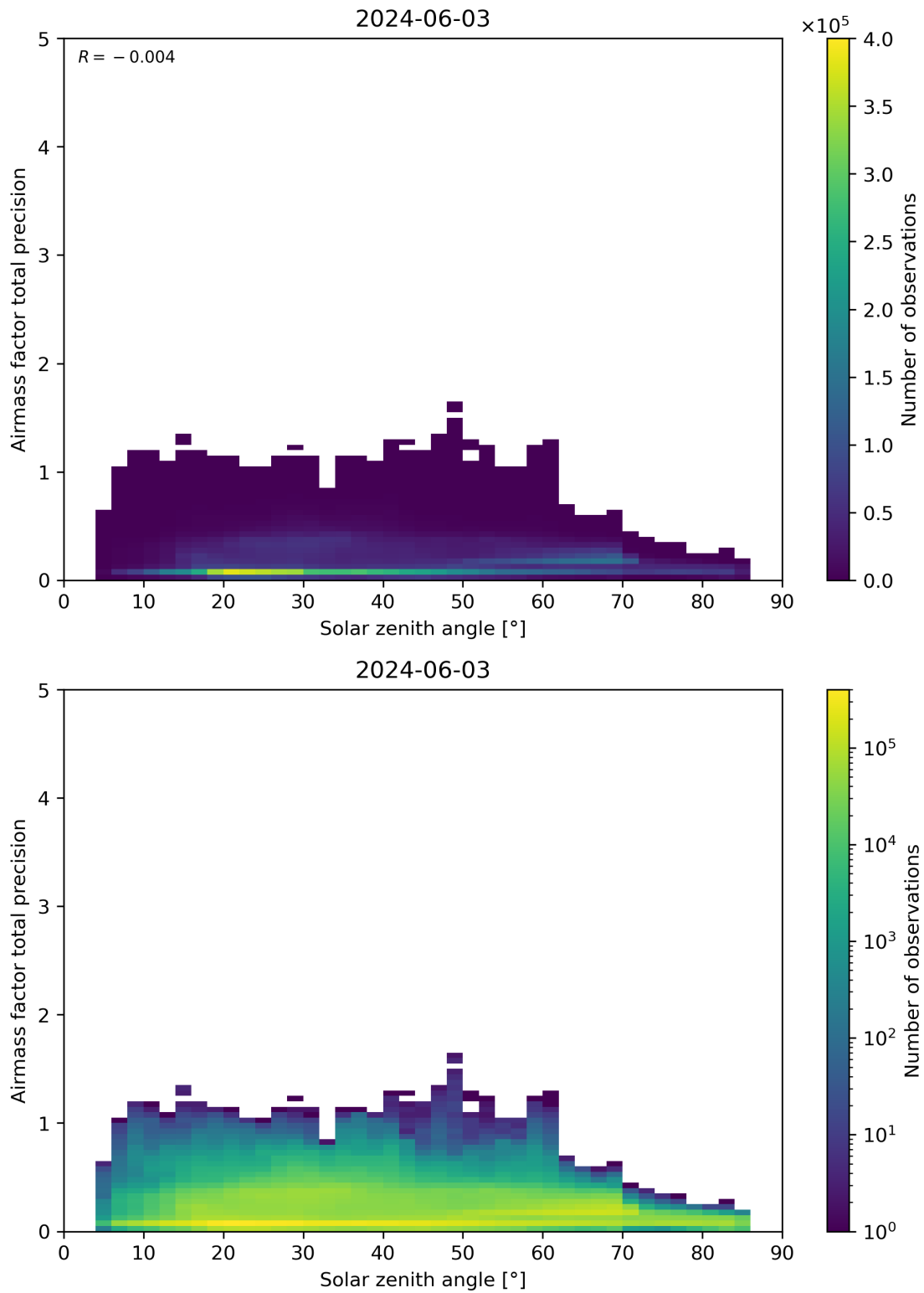
Figure 176: Scatter density plot of “Solar zenith angle” against “Airmass factor total precision” for 2024-06-03 to 2024-06-04.
