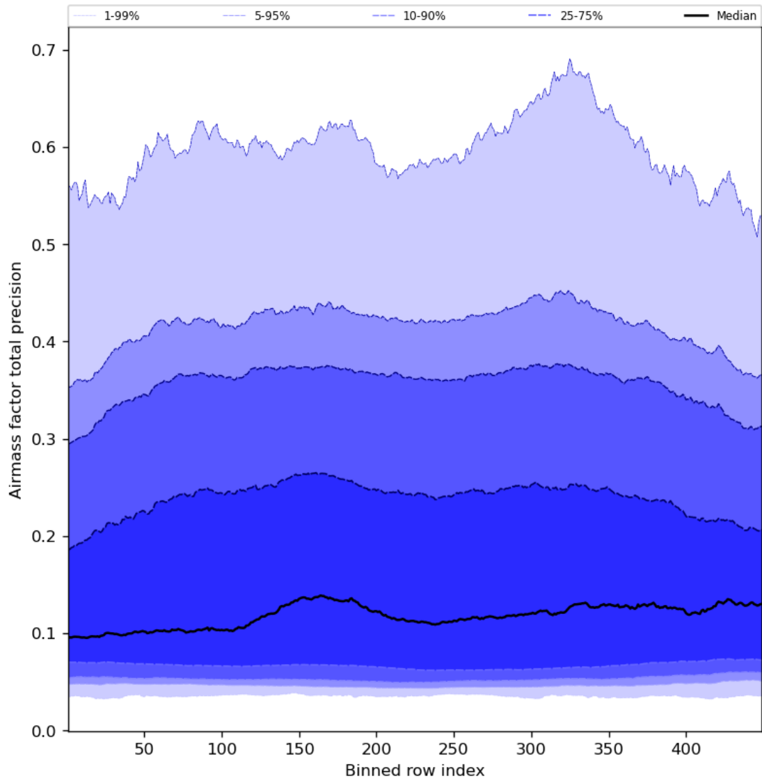
Figure 55: Along track statistics of “Airmass factor total precision” for 2024-06-03 to 2024-06-04
