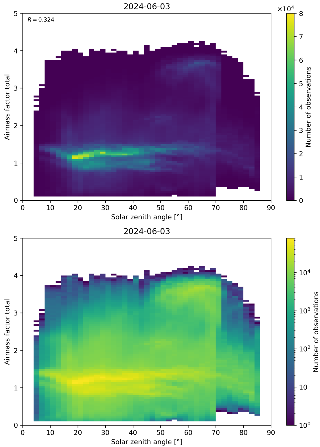
Figure 175: Scatter density plot of “Solar zenith angle” against “Airmass factor total” for 2024-06-03 to 2024-06-04.
