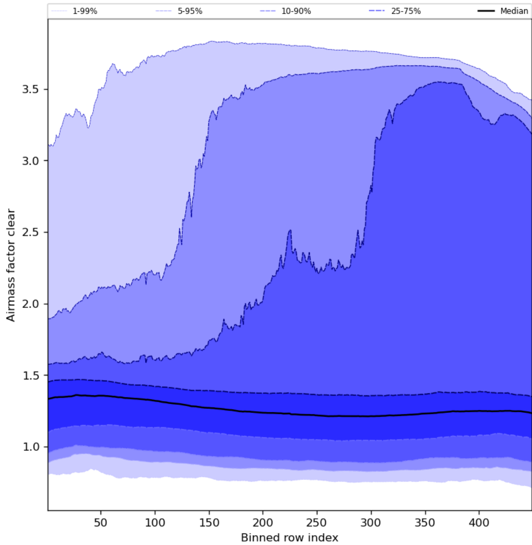
Figure 56: Along track statistics of “Airmass factor clear” for 2024-06-03 to 2024-06-04
