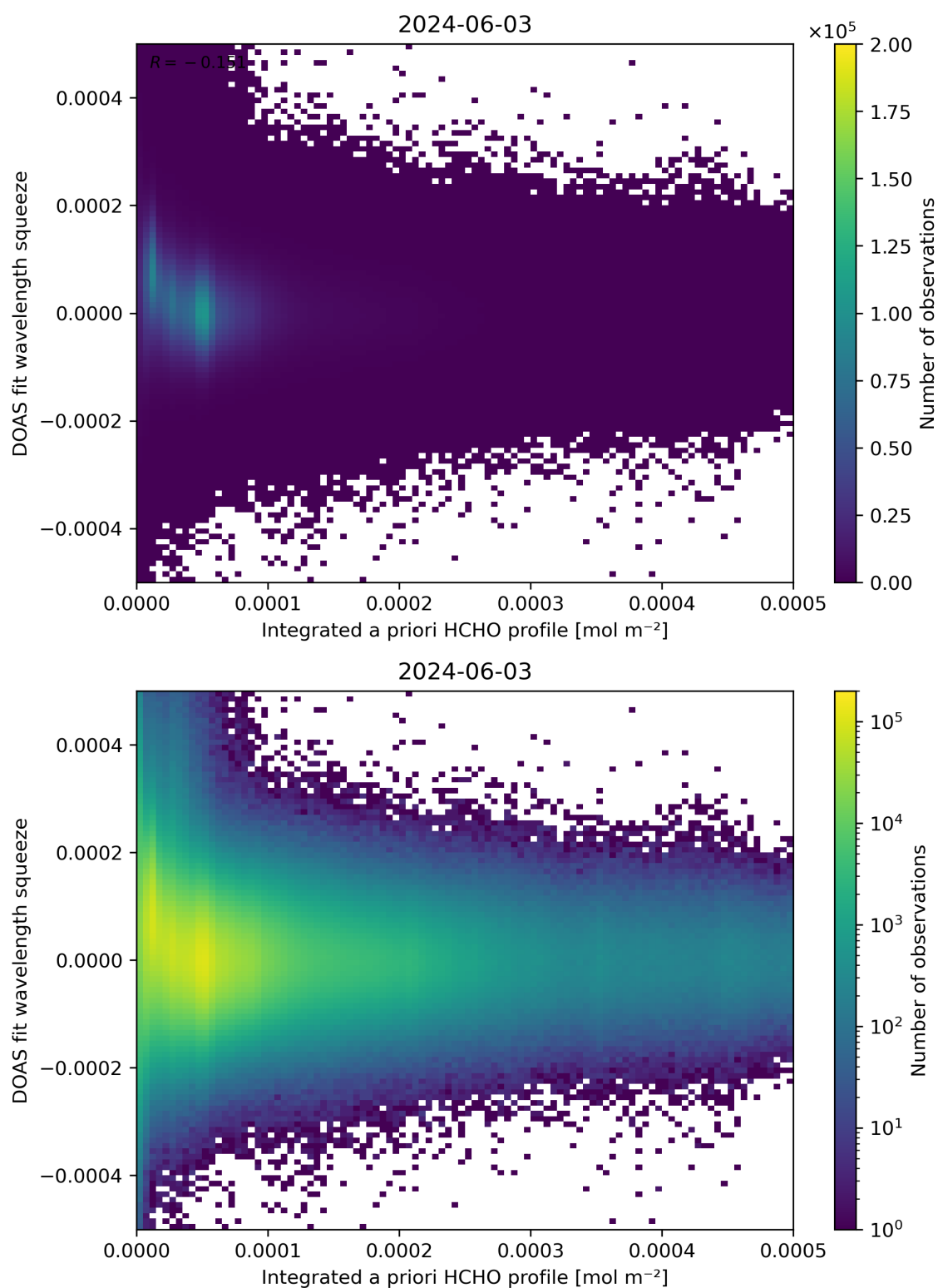
Figure 150: Scatter density plot of “Integrated a priori HCHO profile” against “DOAS fit wavelength squeeze” for 2024-06-03 to 2024-06-04.
