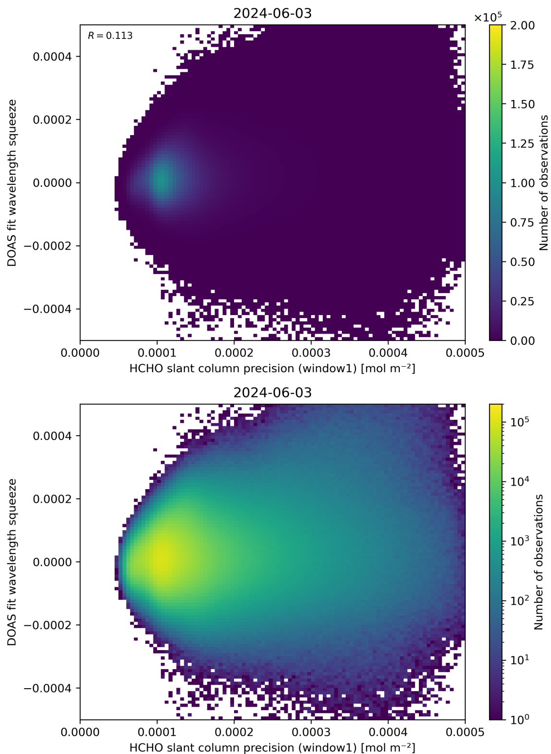
Figure 90: Scatter density plot of “HCHO slant column precision (window1)” against “DOAS fit wavelength squeeze” for 2024-06-03 to 2024-06-04.
