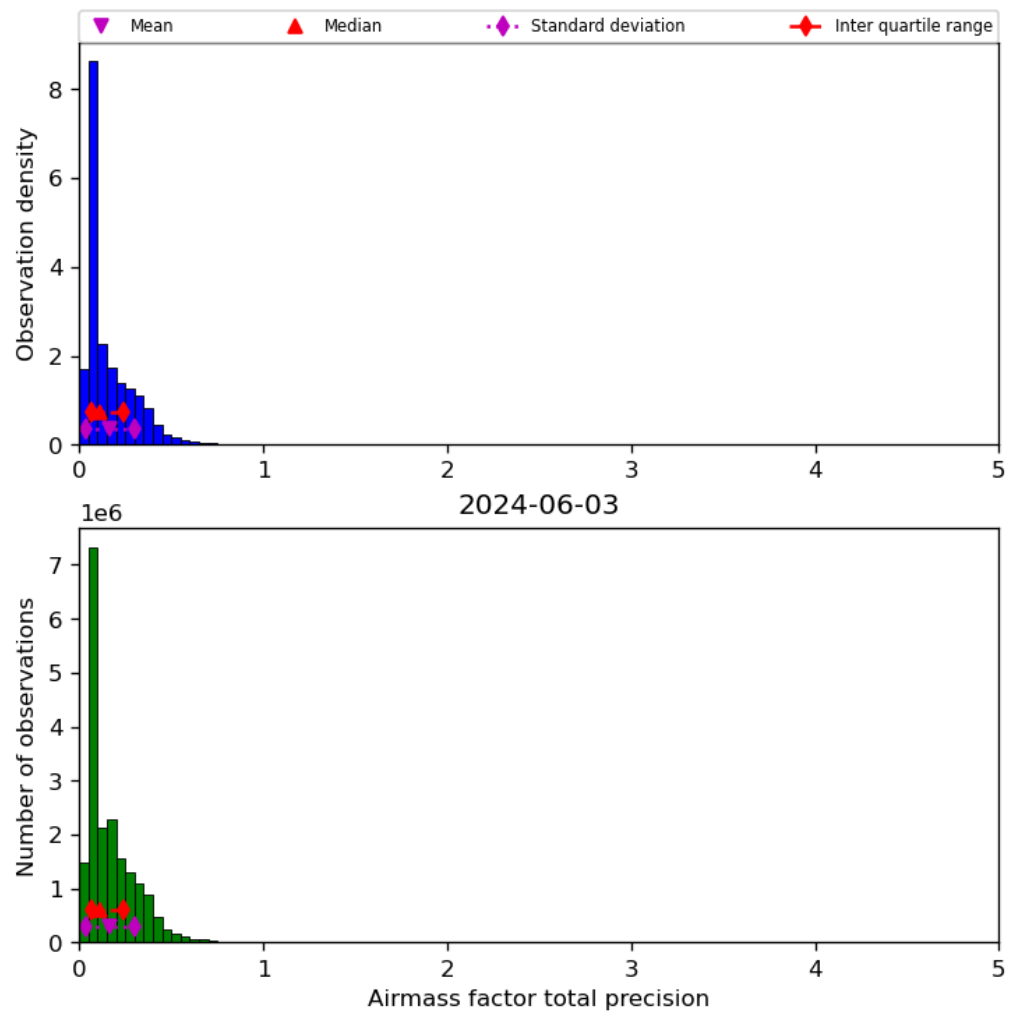
Figure 41: Histogram of “Airmass factor total precision” for 2024-06-03 to 2024-06-04
