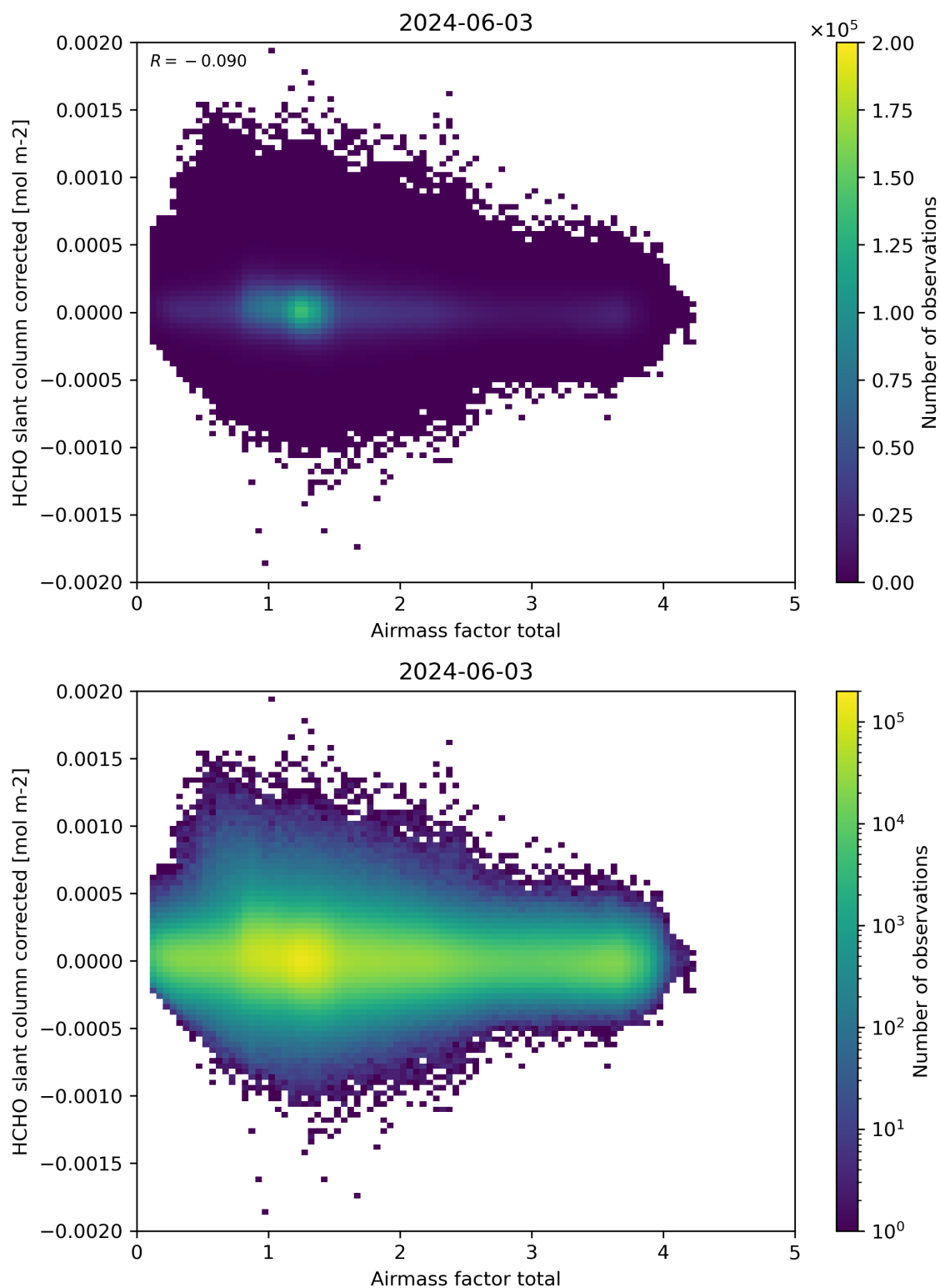
Figure 101: Scatter density plot of “Airmass factor total” against “HCHO slant column corrected” for 2024-06-03 to 2024-06-04.
