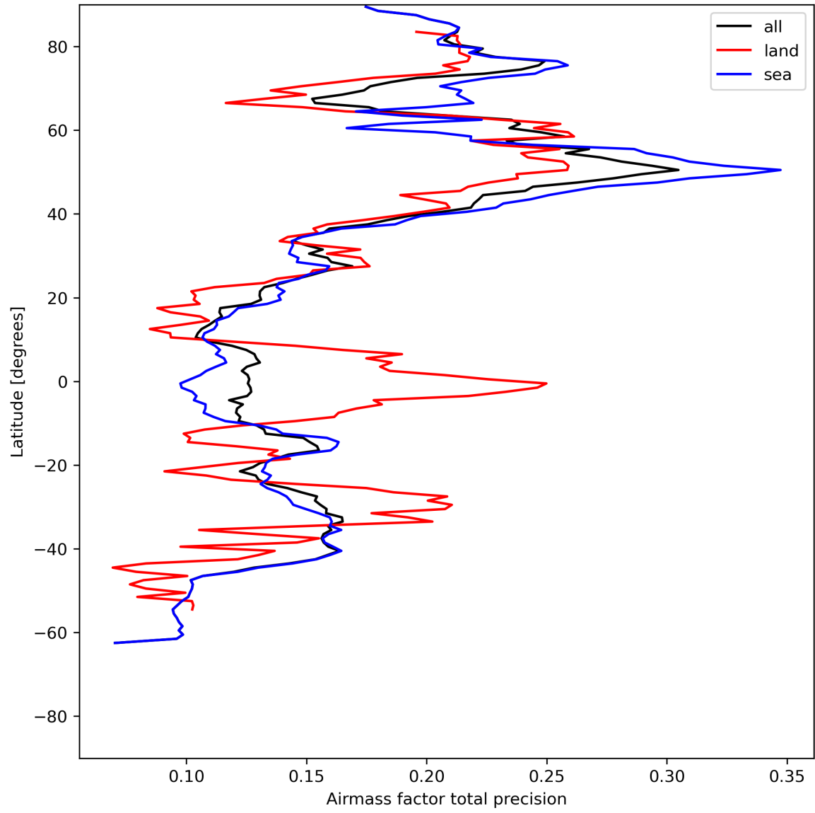
Figure 27: Zonal average of “Airmass factor total precision” for 2024-06-03 to 2024-06-04.
