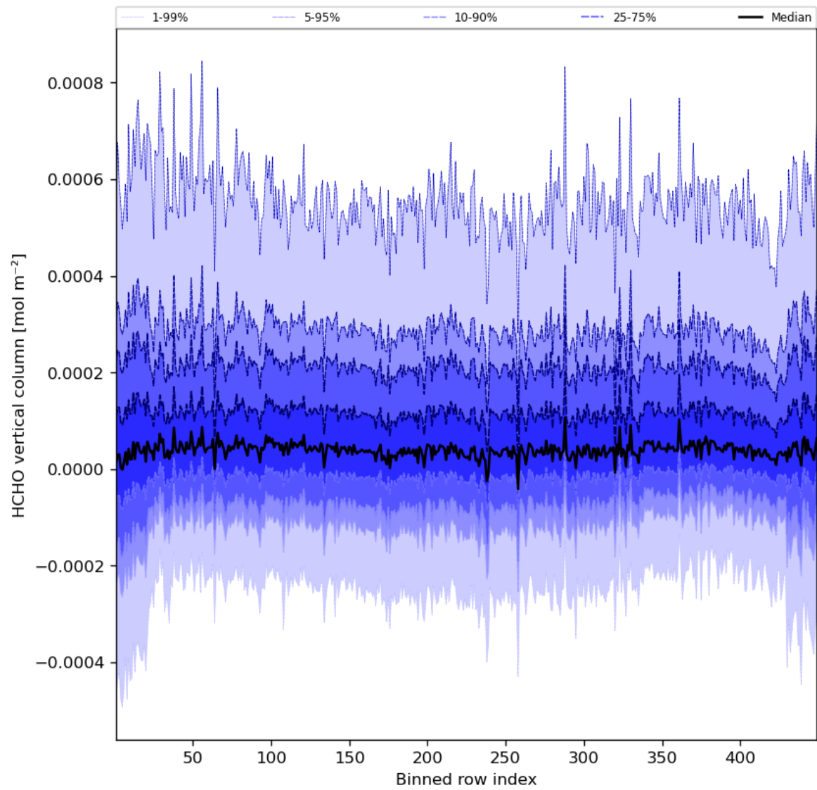
Figure 49: Along track statistics of “HCHO vertical column” for 2024-06-03 to 2024-06-04
