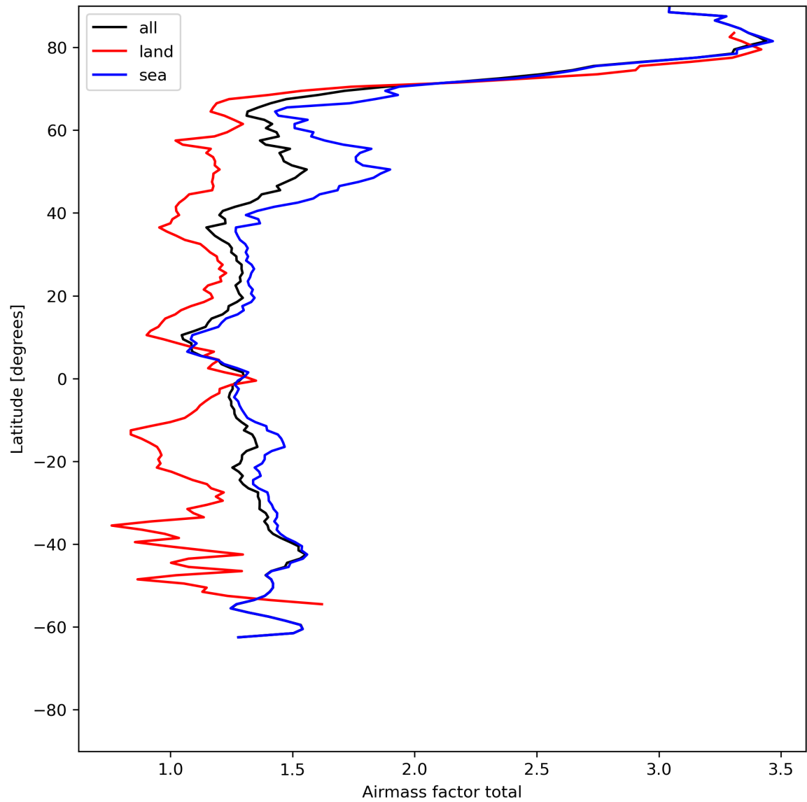
Figure 26: Zonal average of “Airmass factor total” for 2024-06-03 to 2024-06-04.
