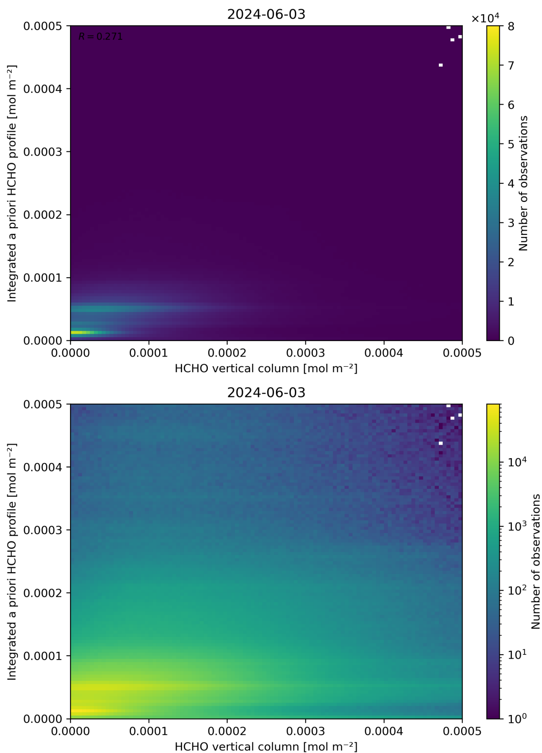
Figure 135: Scatter density plot of “HCHO vertical column” against “Integrated a priori HCHO profile” for 2024-06-03 to 2024-06-04.
