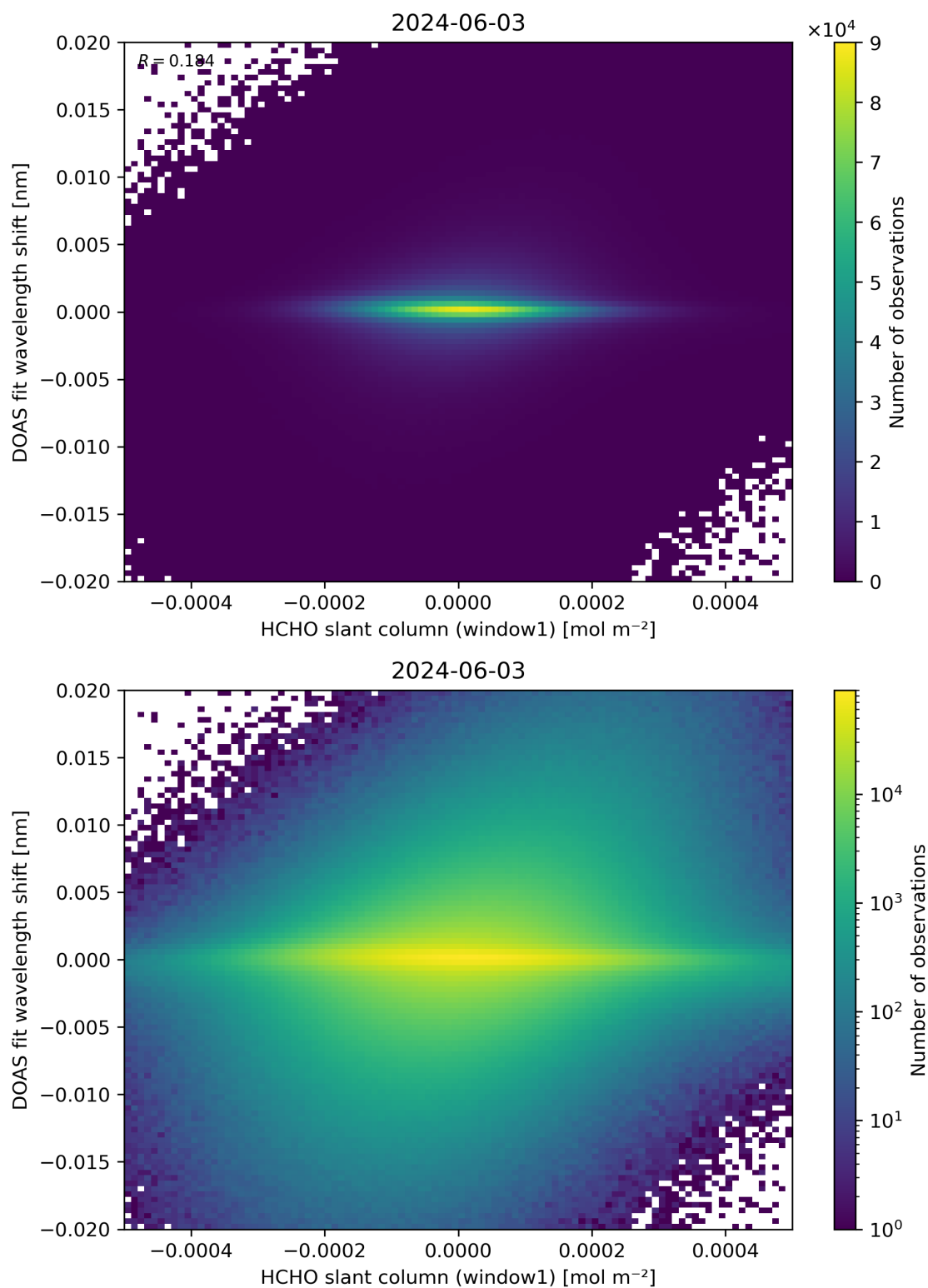
Figure 79: Scatter density plot of “HCHO slant column (window1)” against “DOAS fit wavelength shift” for 2024-06-03 to 2024-06-04.
