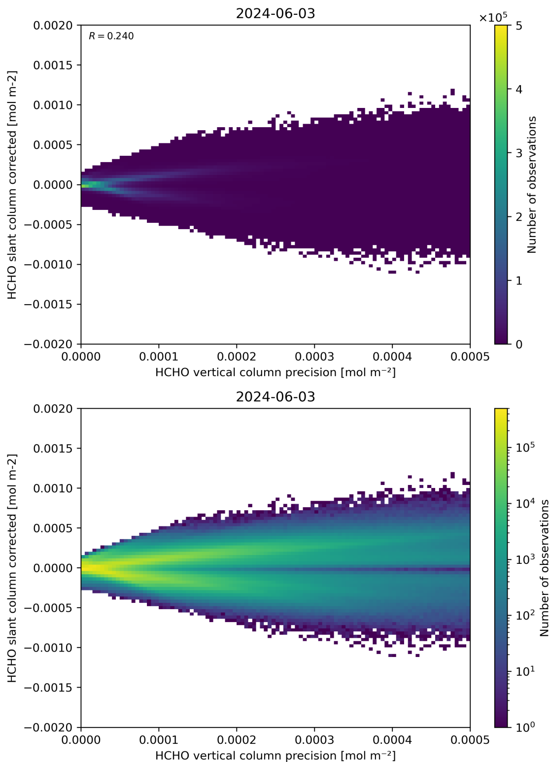
Figure 140: Scatter density plot of “HCHO vertical column precision” against “HCHO slant column corrected” for 2024-06-03 to 2024-06-04.
