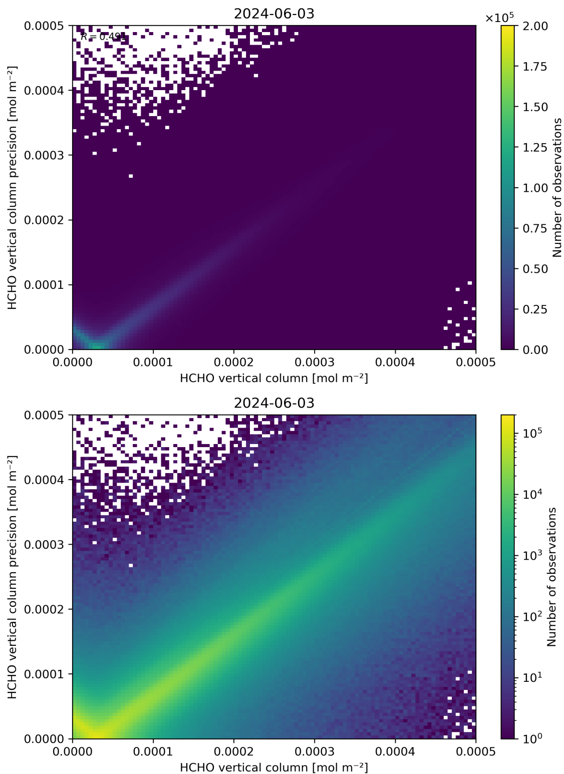
Figure 134: Scatter density plot of “HCHO vertical column” against “HCHO vertical column precision” for 2024-06-03 to 2024-06-04.
