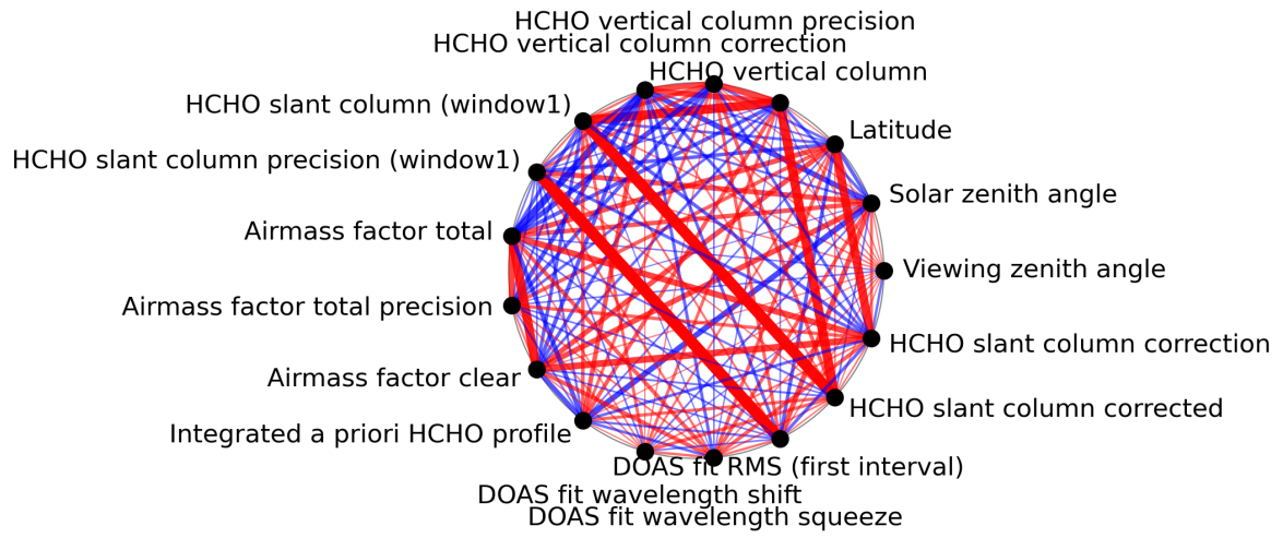
Figure 1: Map of correlation graph for 2024-06-03 to 2024-06-04.
