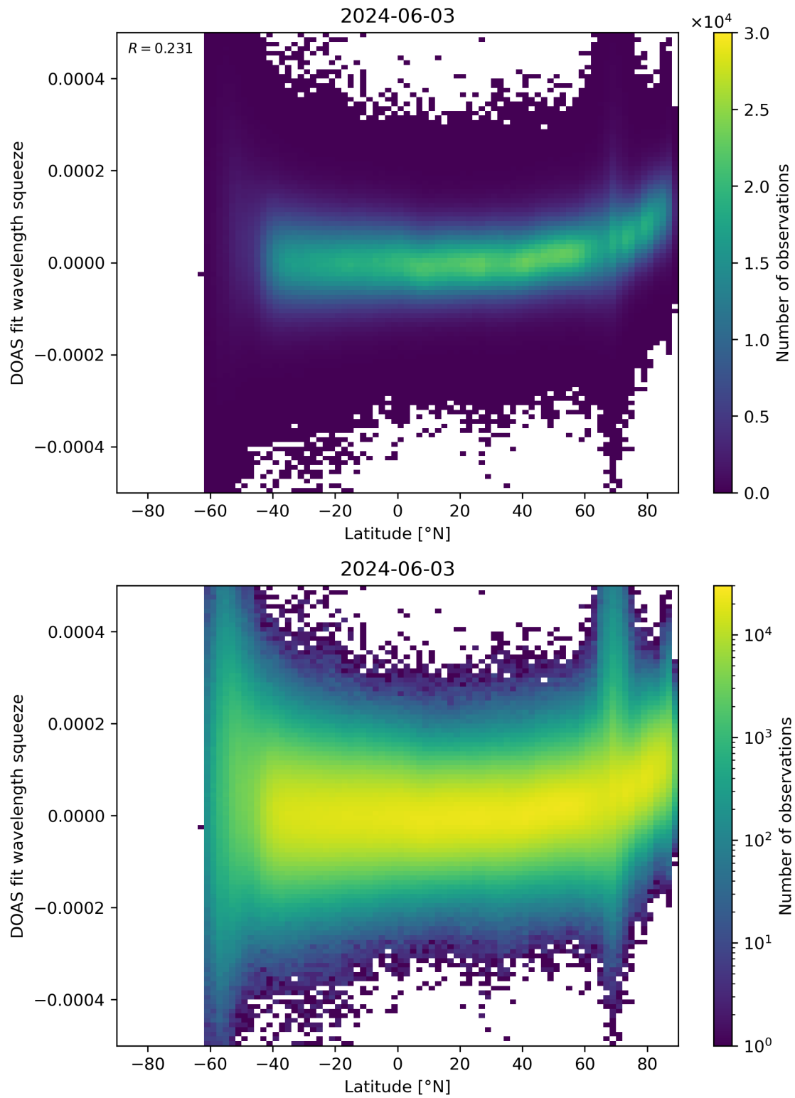
Figure 155: Scatter density plot of “Latitude” against “DOAS fit wavelength squeeze” for 2024-06-03 to 2024-06-04.
