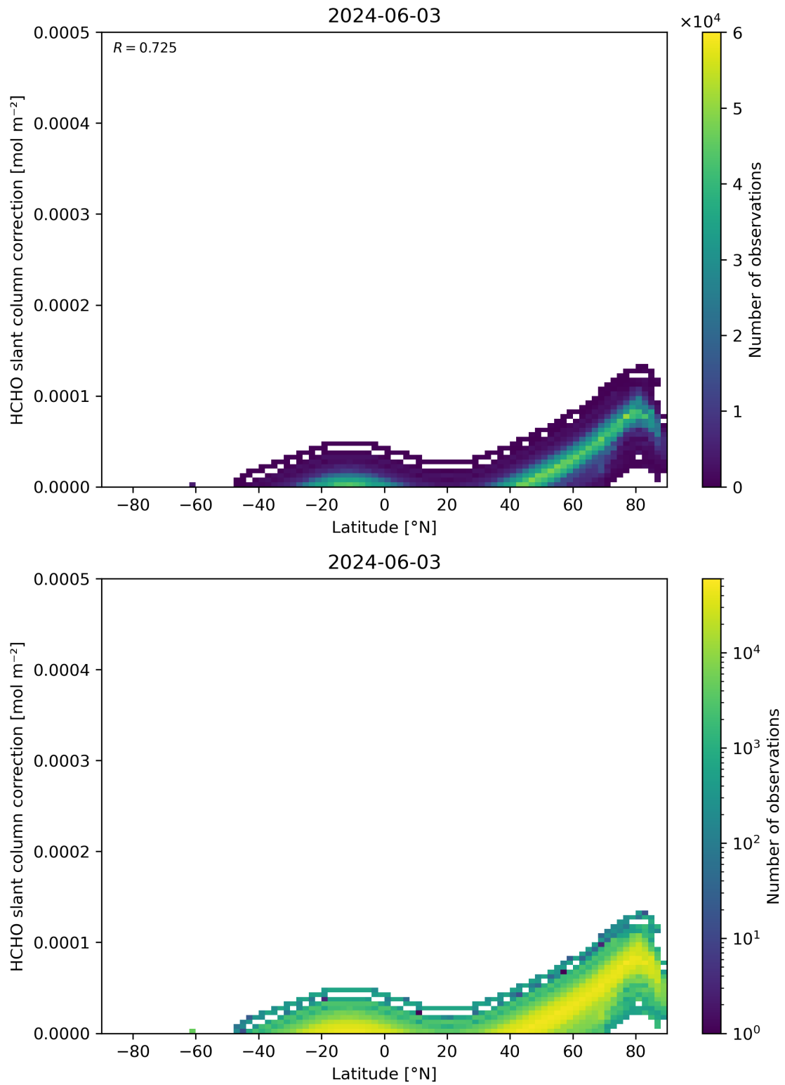
Figure 158: Scatter density plot of “Latitude” against “HCHO slant column correction” for 2024-06-03 to 2024-06-04.
