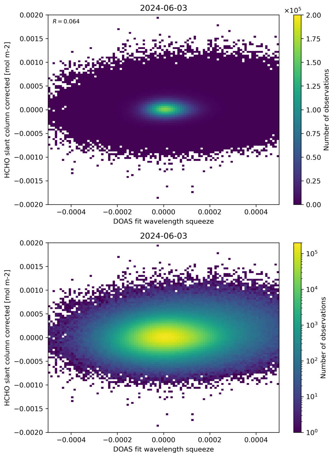
Figure 69: Scatter density plot of “DOAS fit wavelength squeeze” against “HCHO slant column corrected” for 2024-06-03 to 2024-06-04.
