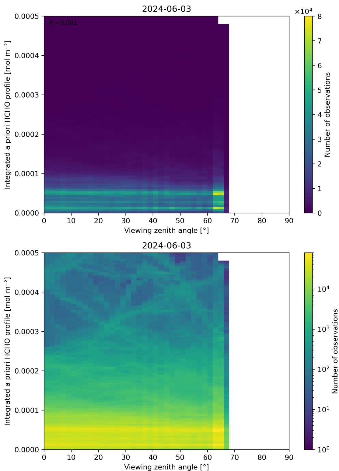
Figure 195: Scatter density plot of “Viewing zenith angle” against “Integrated a priori HCHO profile” for 2024-06-03 to 2024-06-04.
