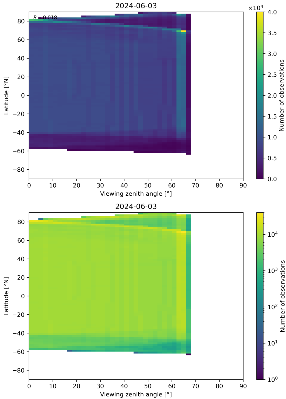
Figure 196: Scatter density plot of “Viewing zenith angle” against “Latitude” for 2024-06-03 to 2024-06-04.
