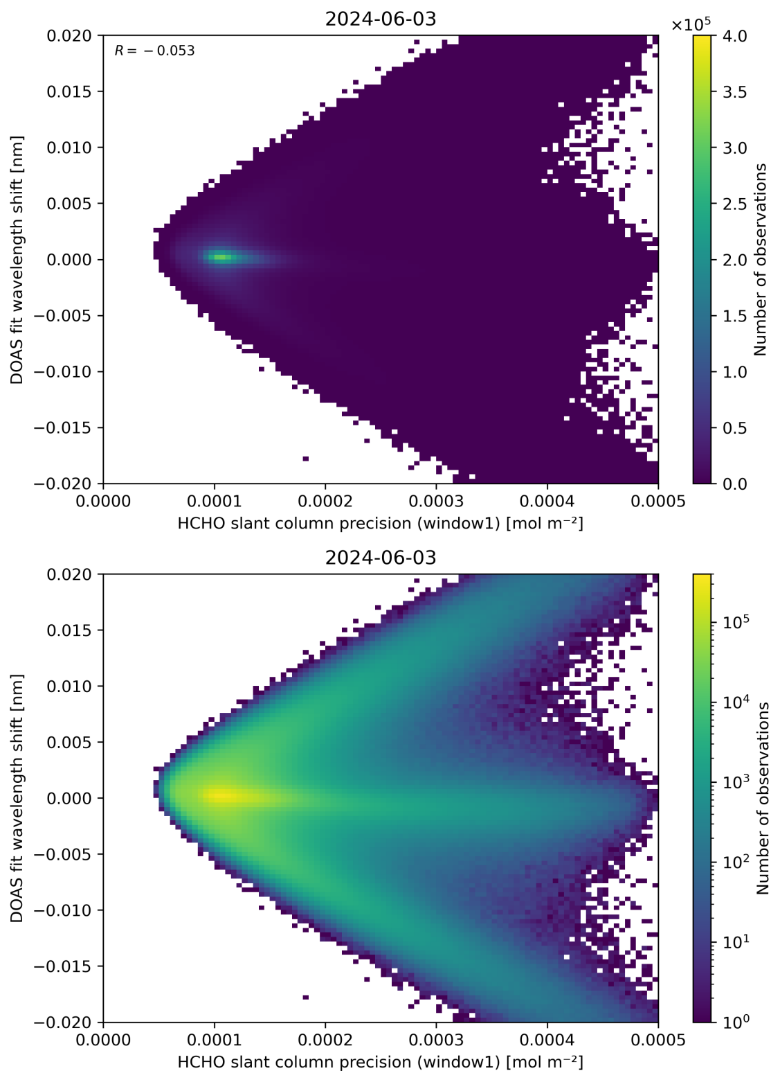
Figure 89: Scatter density plot of “HCHO slant column precision (window1)” against “DOAS fit wavelength shift” for 2024-06-03 to 2024-06-04.
