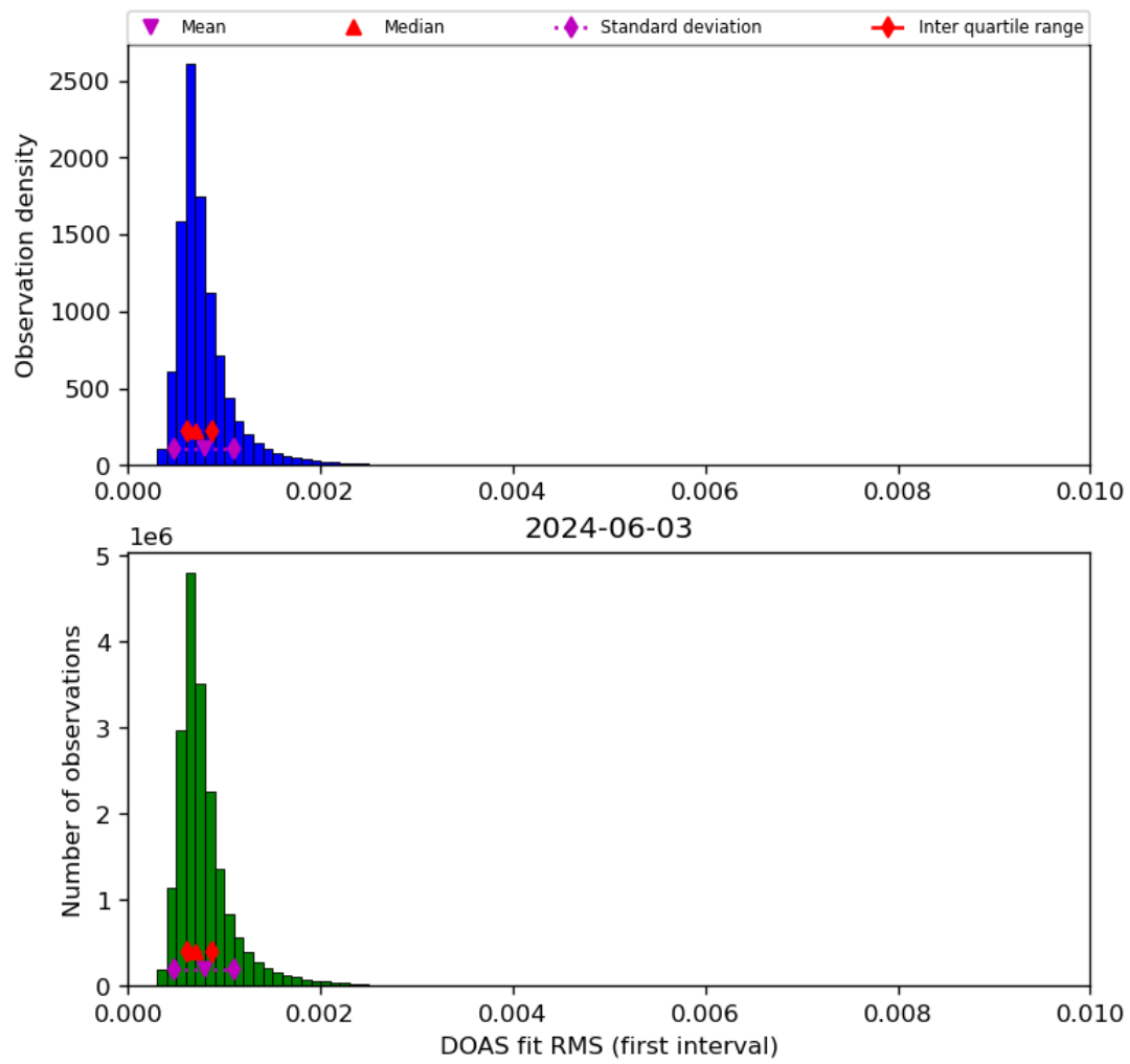
Figure 46: Histogram of “DOAS fit RMS (first interval)” for 2024-06-03 to 2024-06-04
