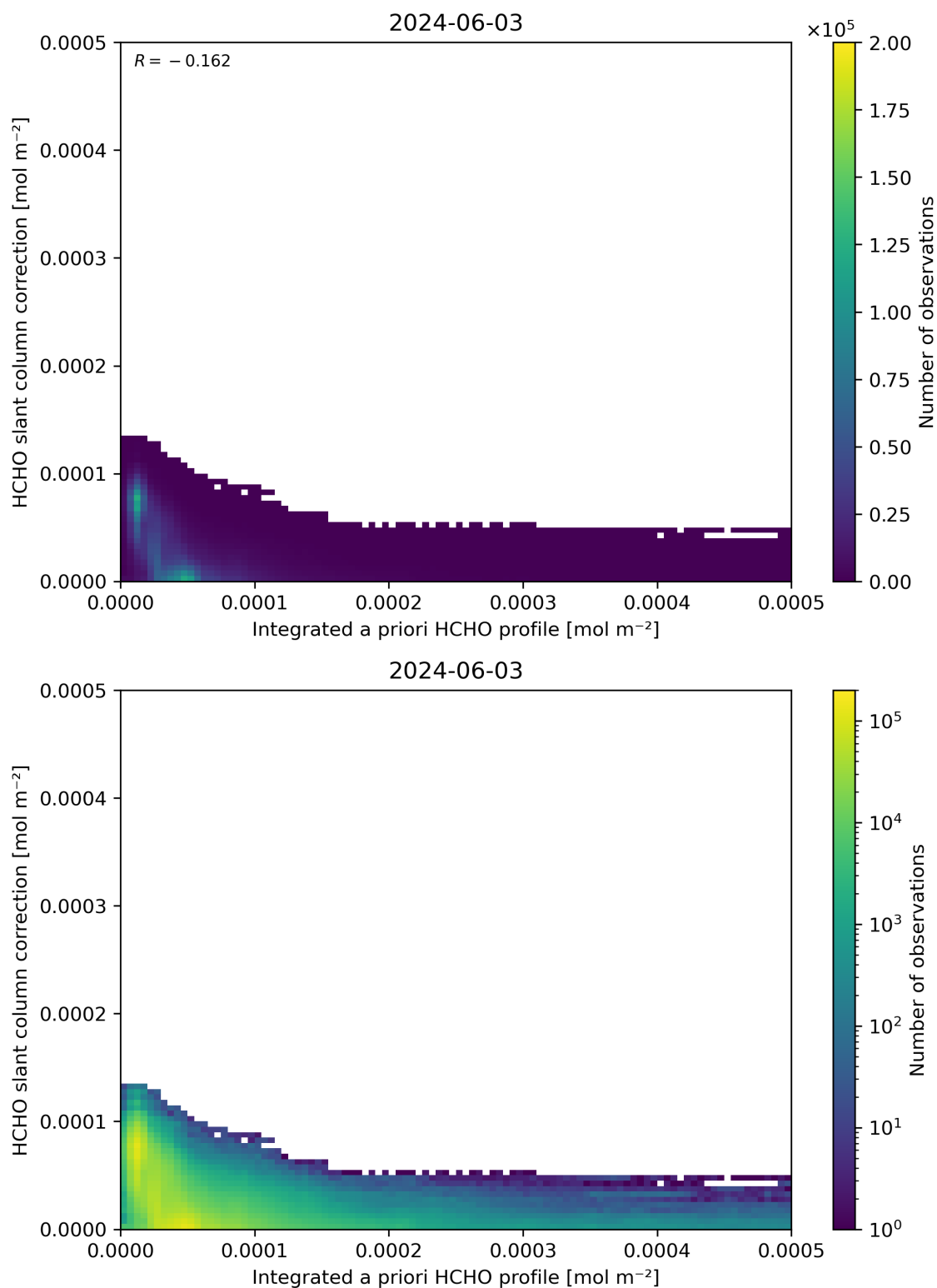
Figure 152: Scatter density plot of “Integrated a priori HCHO profile” against “HCHO slant column correction” for 2024-06-03 to 2024-06-04.
