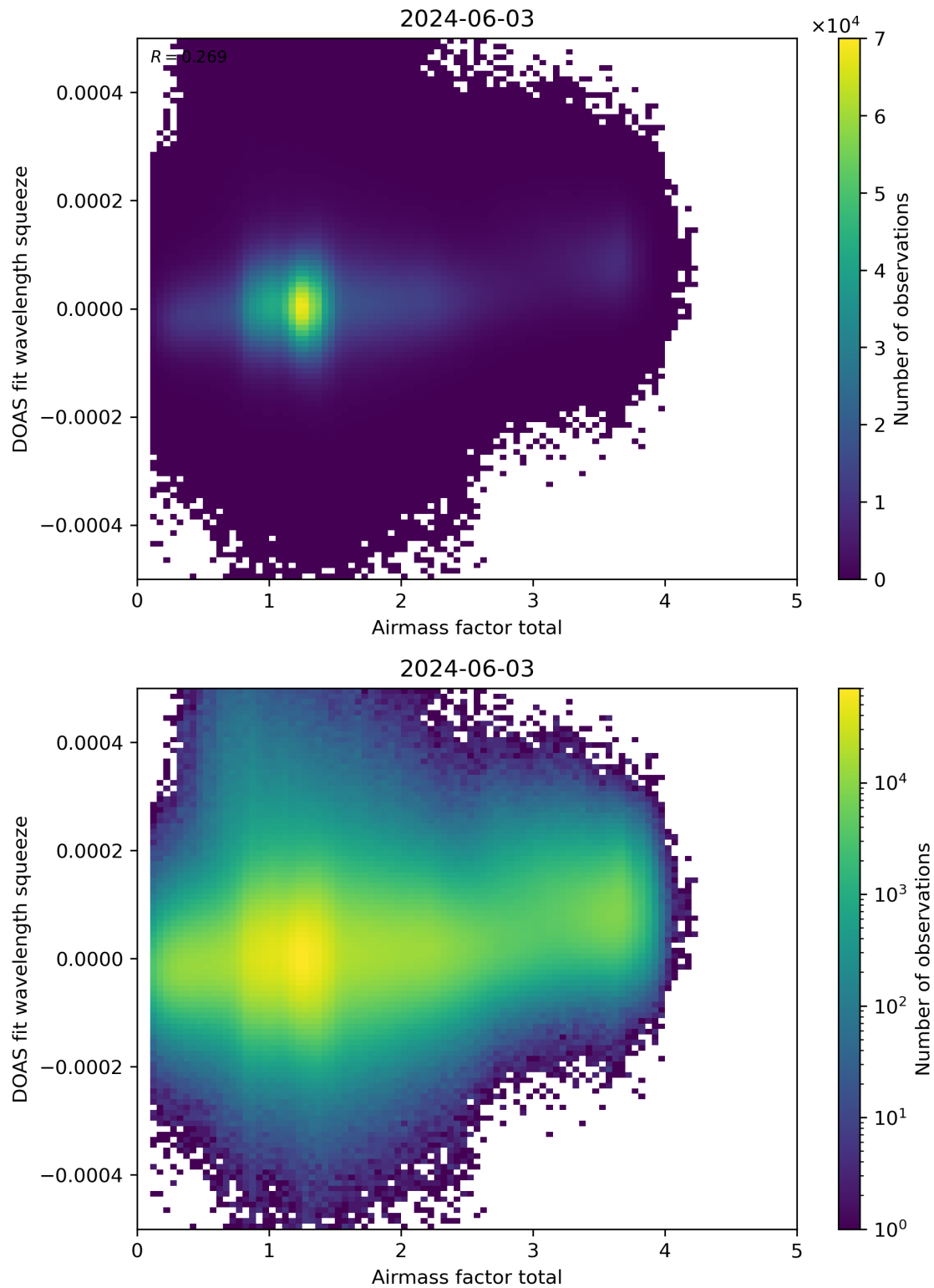
Figure 99: Scatter density plot of “Airmass factor total” against “DOAS fit wavelength squeeze” for 2024-06-03 to 2024-06-04.
