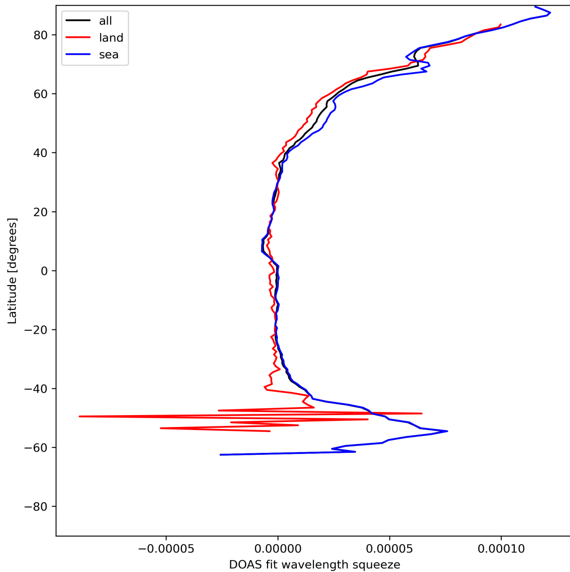
Figure 31: Zonal average of "DOAS fit wavelength squeeze" for 2024-06-03 to 2024-06-04.
