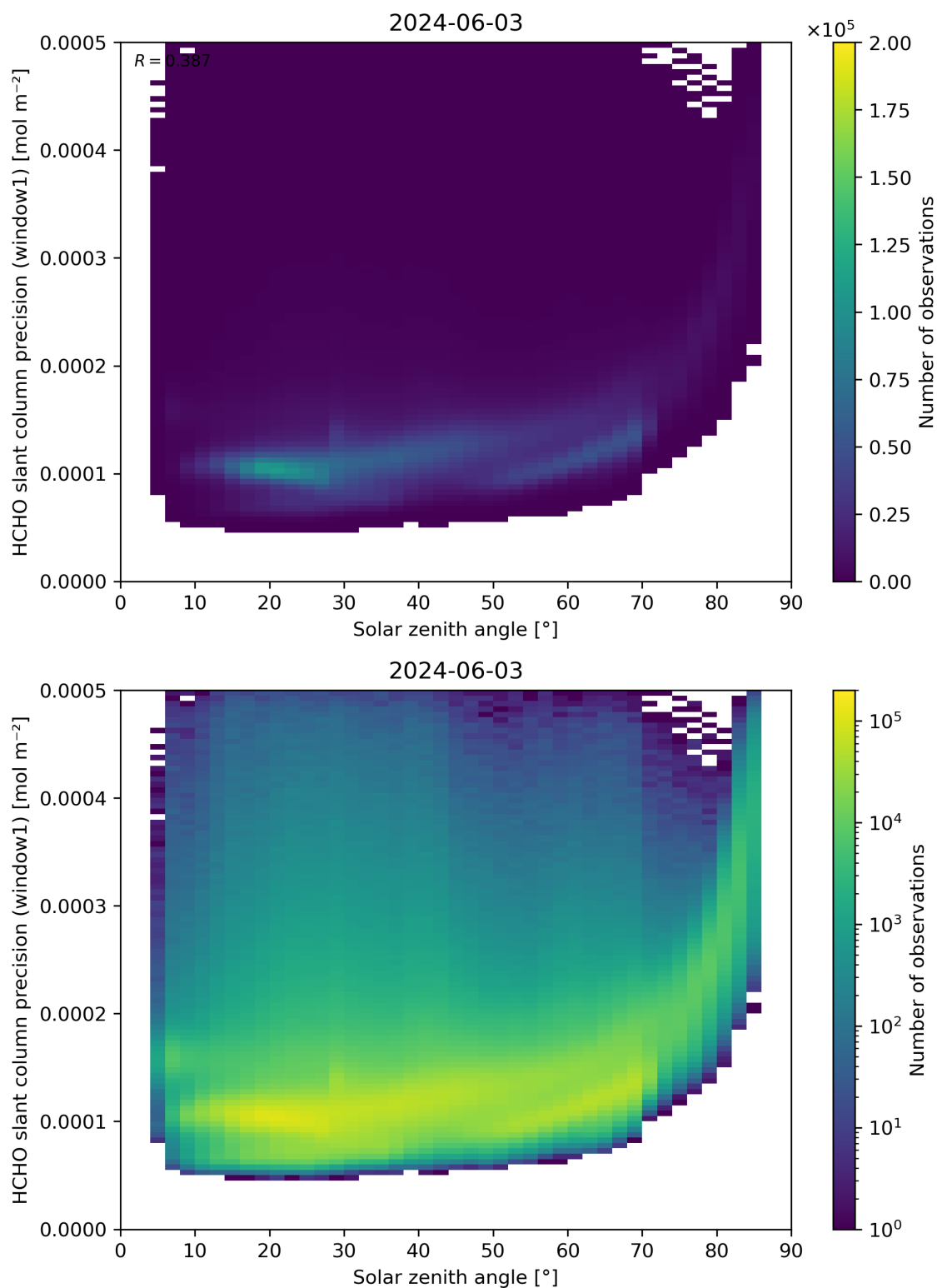
Figure 174: Scatter density plot of “Solar zenith angle” against “HCHO slant column precision (window1)” for 2024-06-03 to 2024-06-04.
