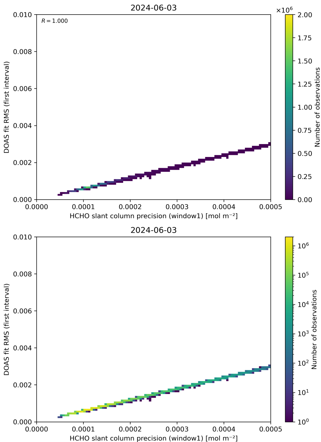
Figure 88: Scatter density plot of “HCHO slant column precision (window1)” against “DOAS fit RMS (first interval)” for 2024-06-03 to 2024-06-04.
