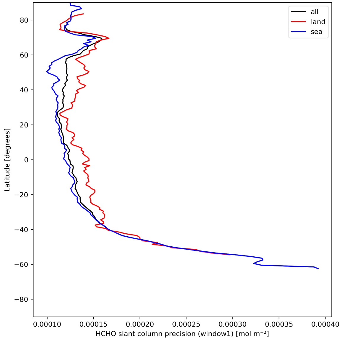
Figure 25: Zonal average of “HCHO slant column precision (window1)” for 2024-06-03 to 2024-06-04.
