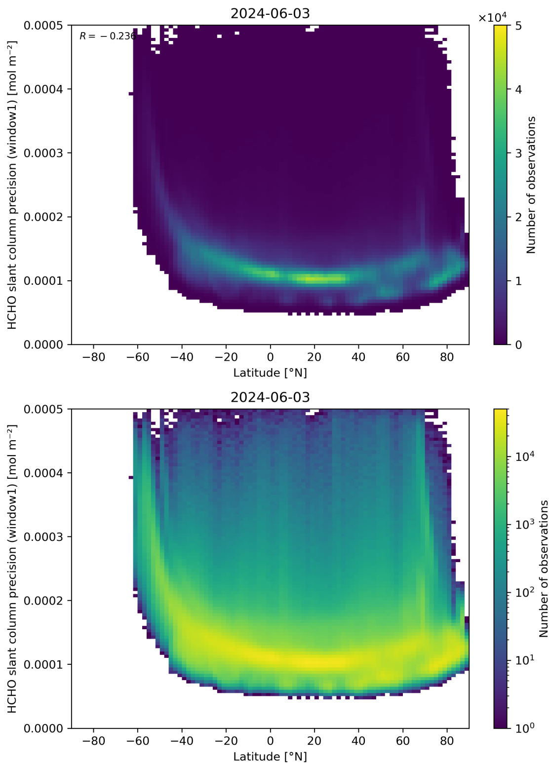
Figure 160: Scatter density plot of “Latitude” against “HCHO slant column precision (window1)” for 2024-06-03 to 2024-06-04.
