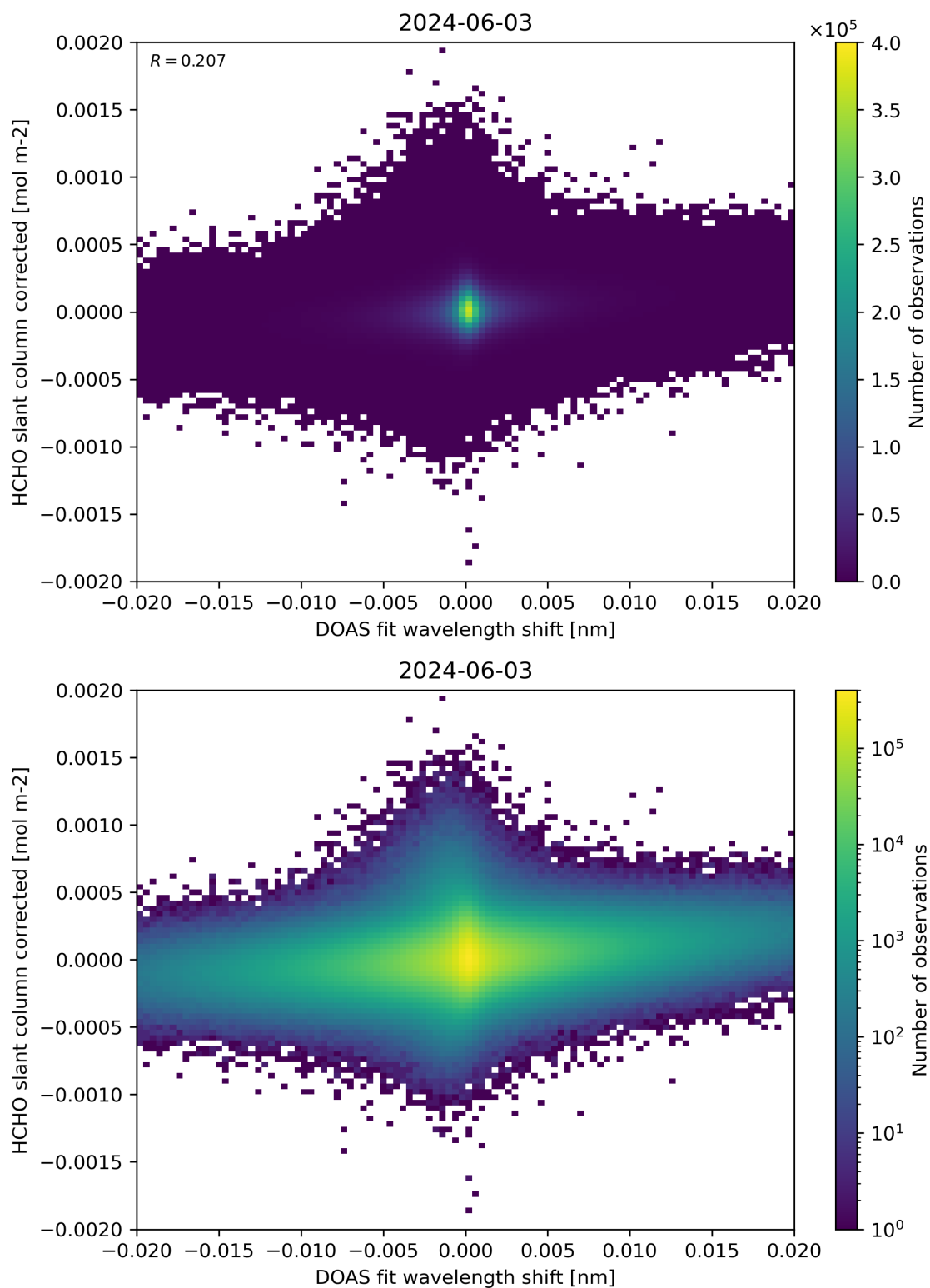
Figure 66: Scatter density plot of “DOAS fit wavelength shift” against “HCHO slant column corrected” for 2024-06-03 to 2024-06-04.
