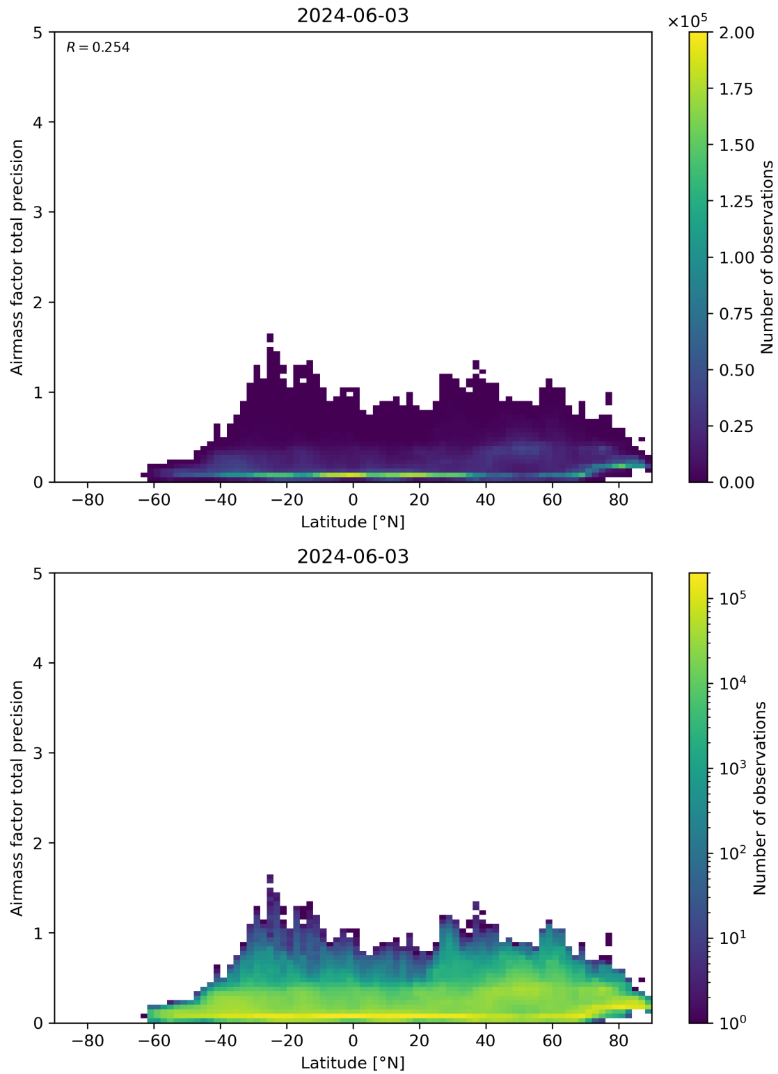
Figure 162: Scatter density plot of “Latitude” against “Airmass factor total precision” for 2024-06-03 to 2024-06-04.
