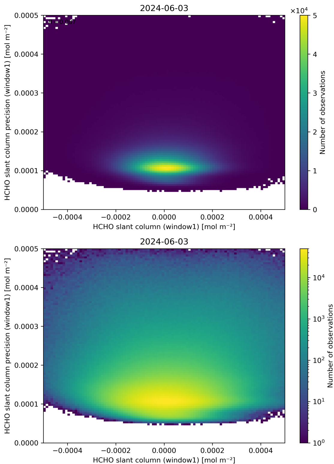
Figure 84: Scatter density plot of “HCHO slant column (window1)” against “HCHO slant column precision (window1)” for 2024-06-03 to 2024-06-04.
