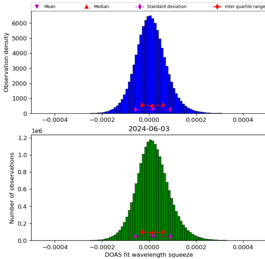
Figure 45: Histogram of “DOAS fit wavelength squeeze” for 2024-06-03 to 2024-06-04
