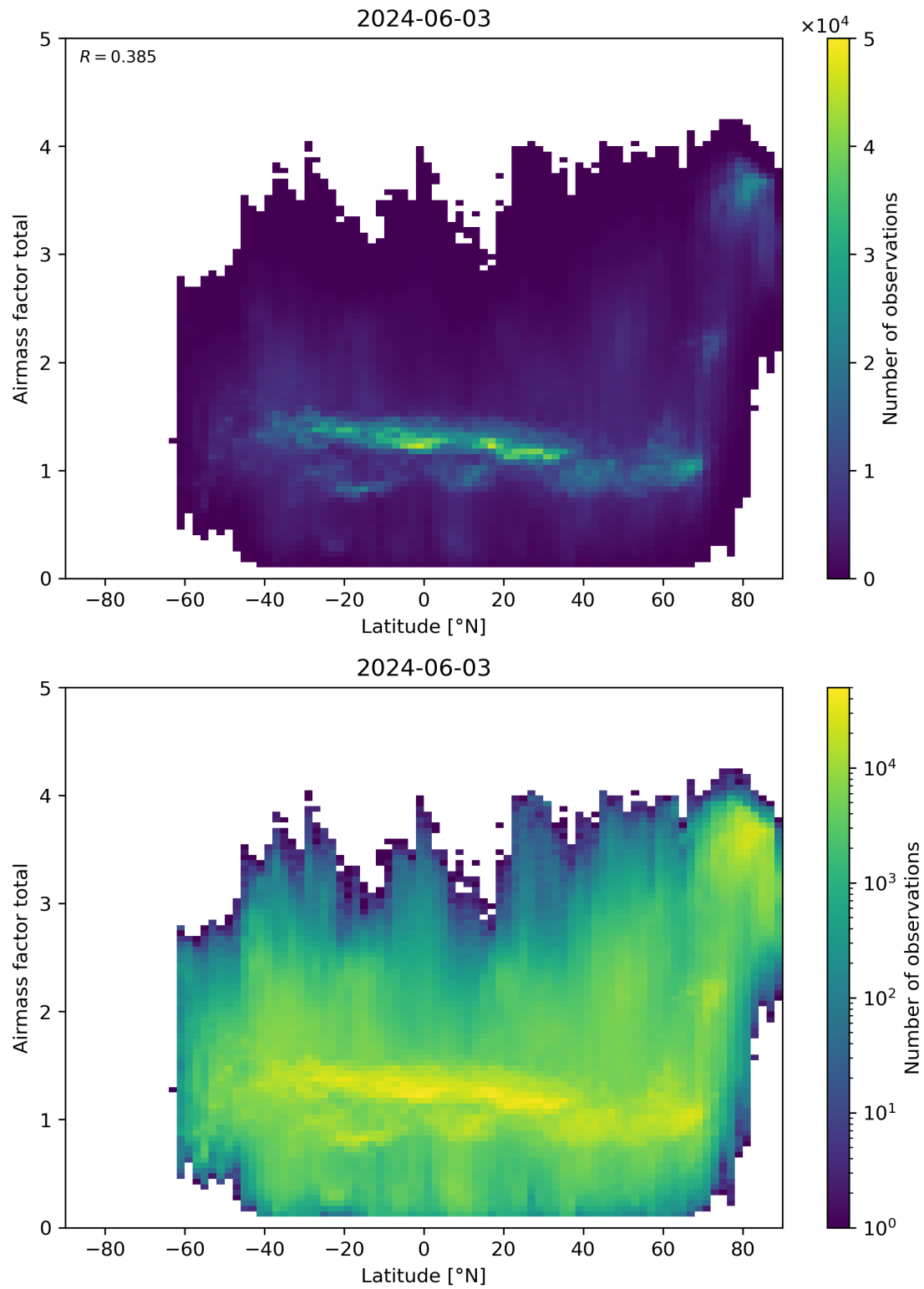
Figure 161: Scatter density plot of “Latitude” against “Airmass factor total” for 2024-06-03 to 2024-06-04.
