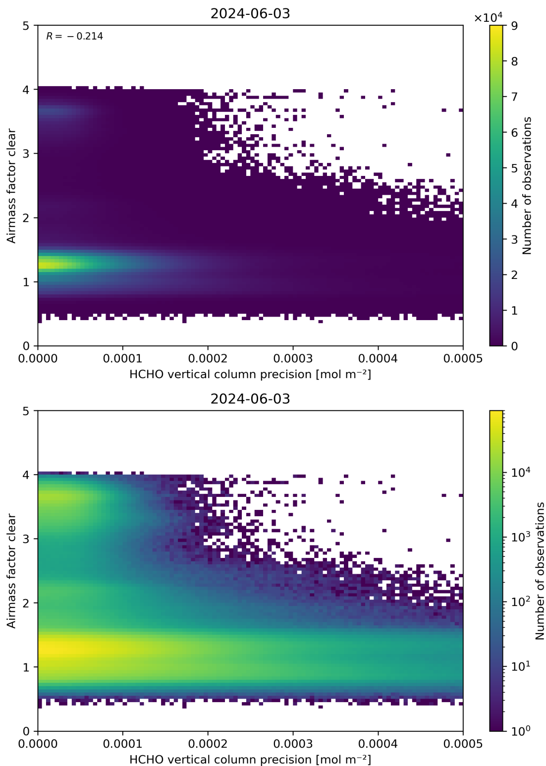
Figure 139: Scatter density plot of “HCHO vertical column precision” against “Airmass factor clear” for 2024-06-03 to 2024-06-04.
