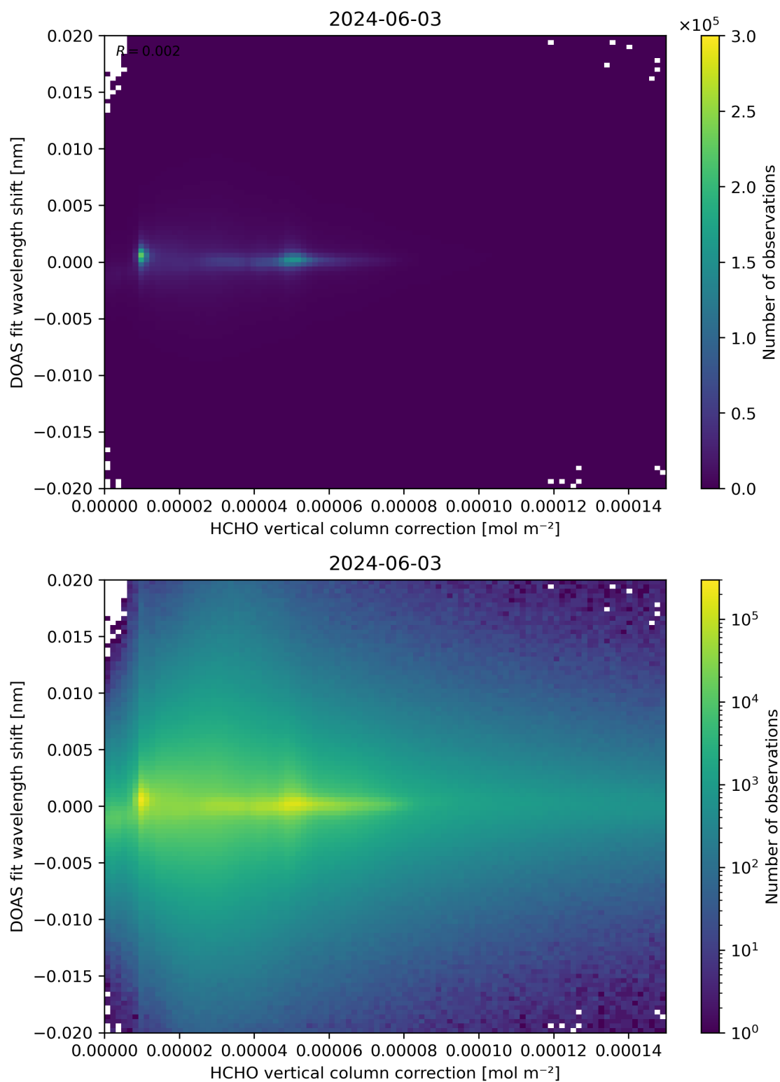
Figure 113: Scatter density plot of “HCHO vertical column correction” against “DOAS fit wavelength shift” for 2024-06-03 to 2024-06-04.
