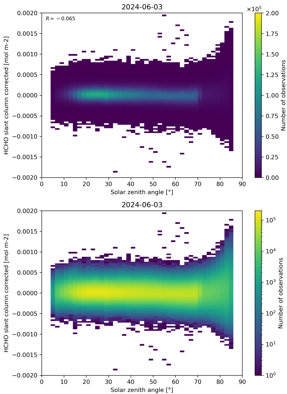
Figure 171: Scatter density plot of “Solar zenith angle” against “HCHO slant column corrected” for 2024-06-03 to 2024-06-04.
