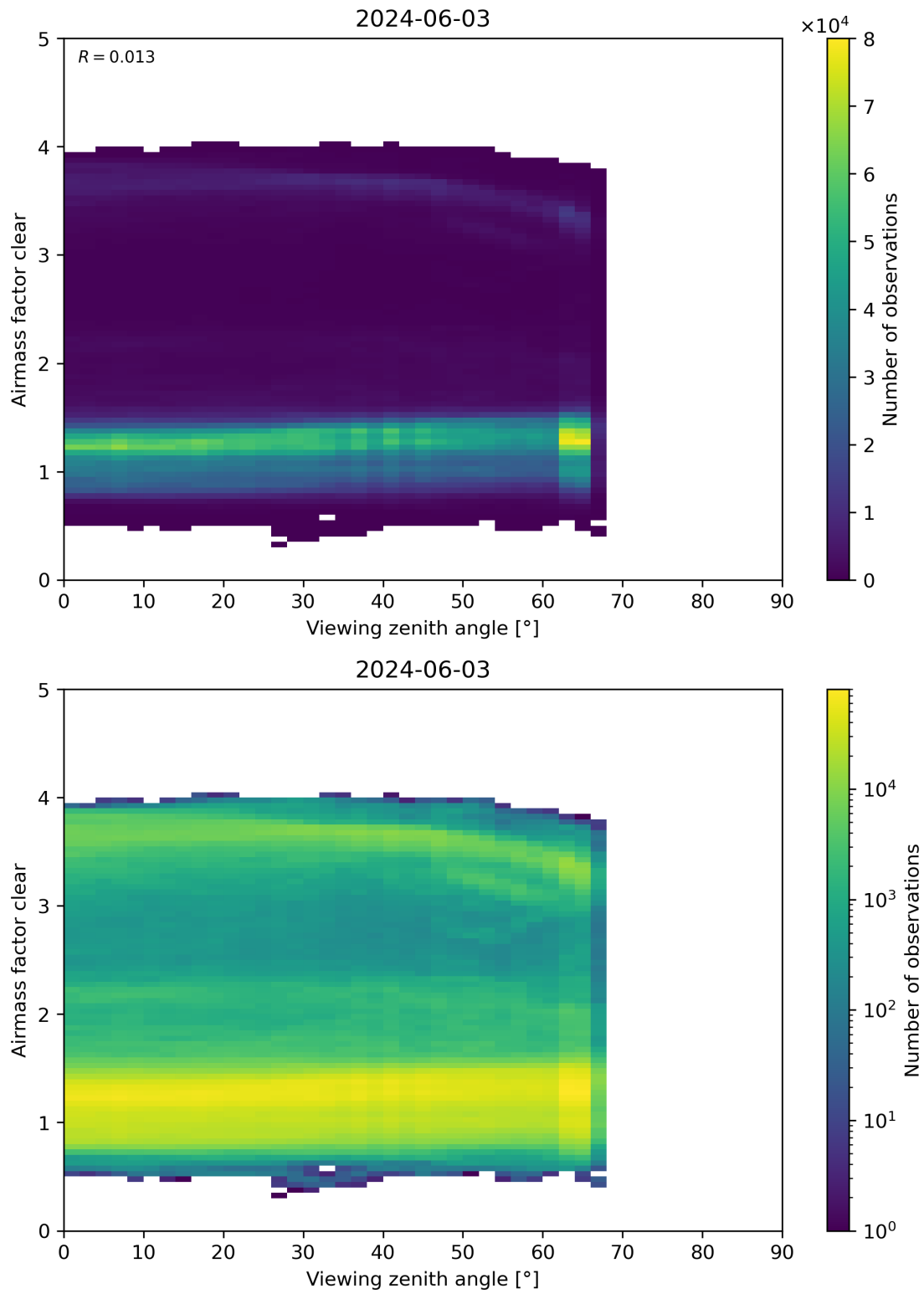
Figure 185: Scatter density plot of “Viewing zenith angle” against “Airmass factor clear” for 2024-06-03 to 2024-06-04.
