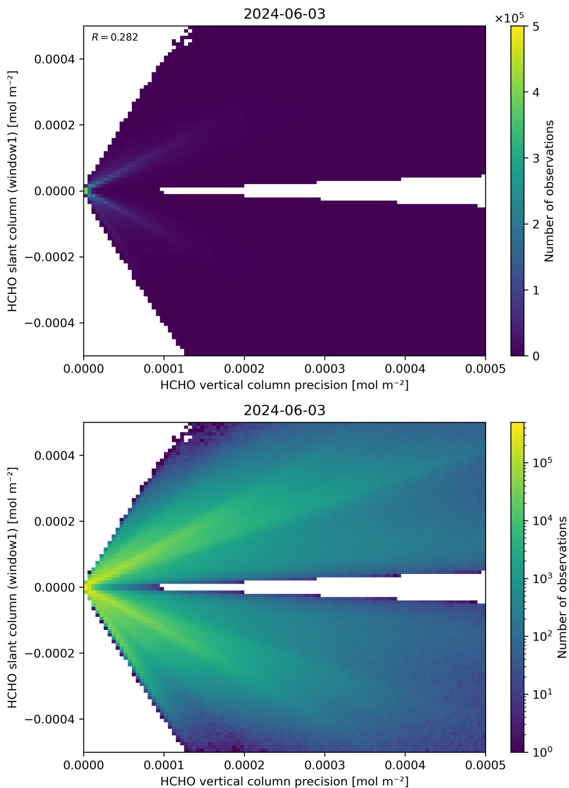
Figure 142: Scatter density plot of “HCHO vertical column precision” against “HCHO slant column (window1)” for 2024-06-03 to 2024-06-04.
