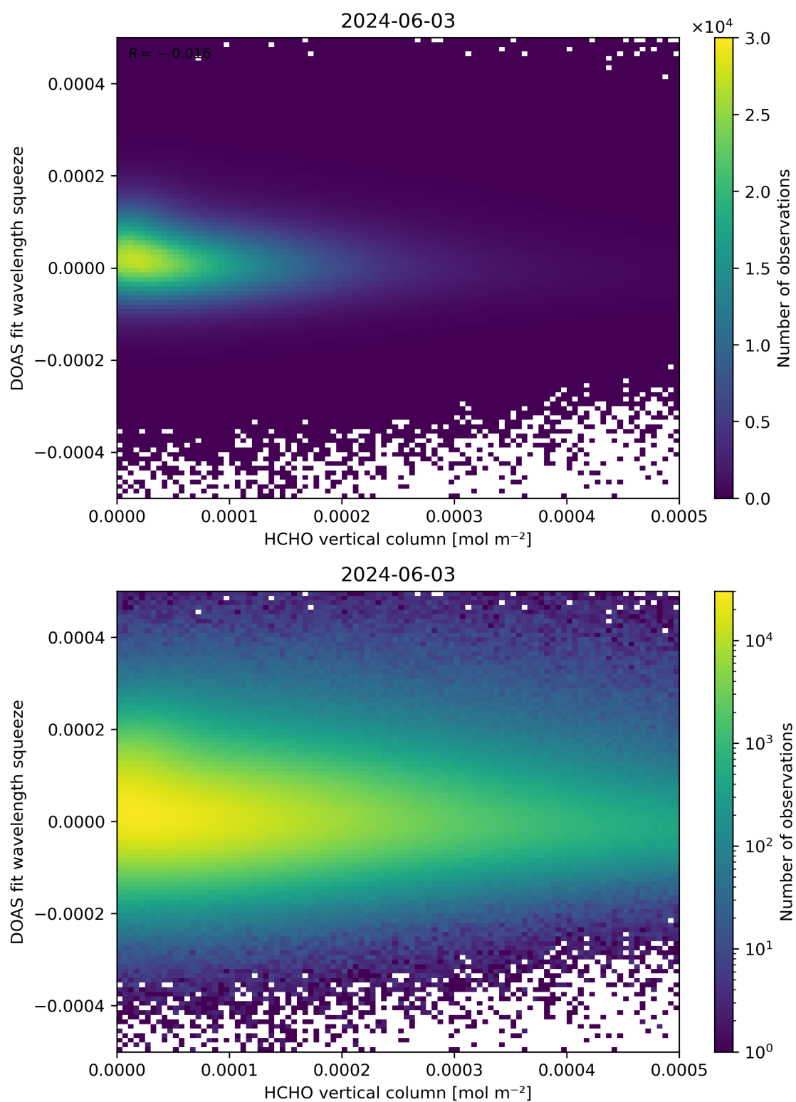
Figure 125: Scatter density plot of “HCHO vertical column” against “DOAS fit wavelength squeeze” for 2024-06-03 to 2024-06-04.
