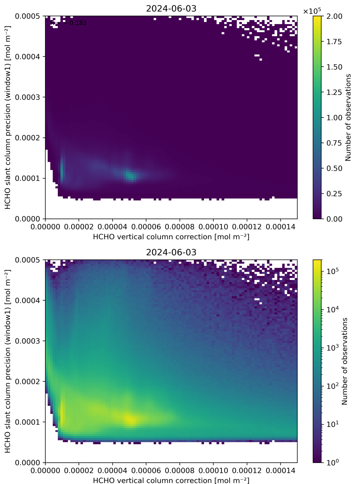
Figure 119: Scatter density plot of “HCHO vertical column correction” against “HCHO slant column precision (window1)” for 2024-06-03 to 2024-06-04.
