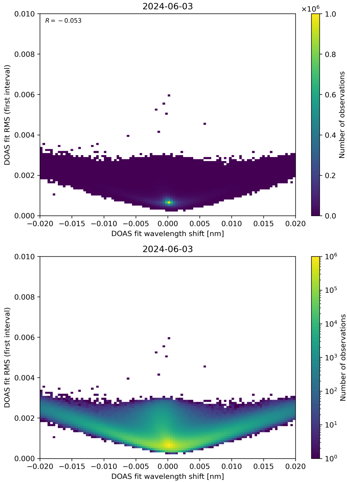
Figure 64: Scatter density plot of “DOAS fit wavelength shift” against “DOAS fit RMS (first interval)” for 2024-06-03 to 2024-06-04.
