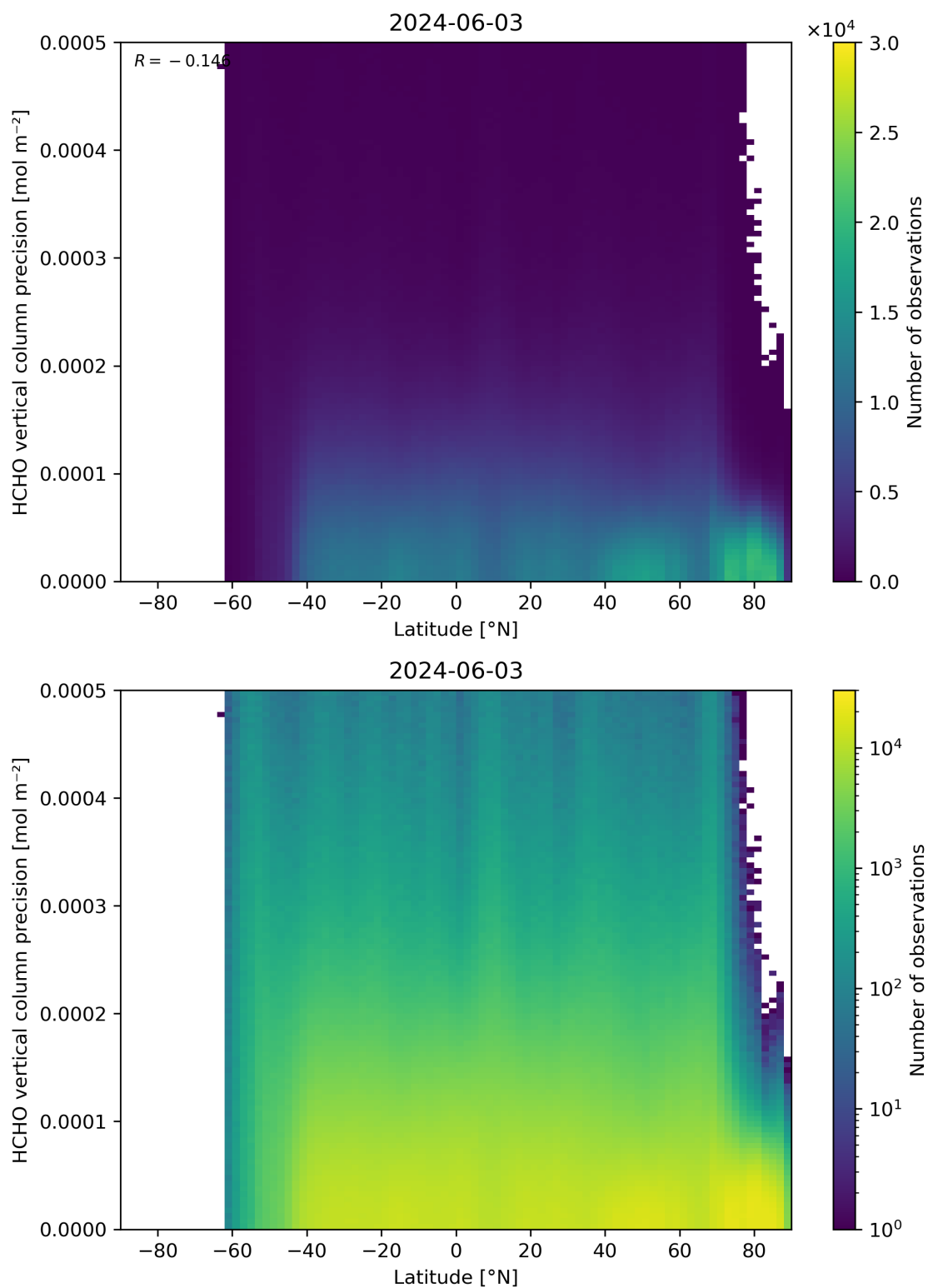
Figure 165: Scatter density plot of “Latitude” against “HCHO vertical column precision” for 2024-06-03 to 2024-06-04.
