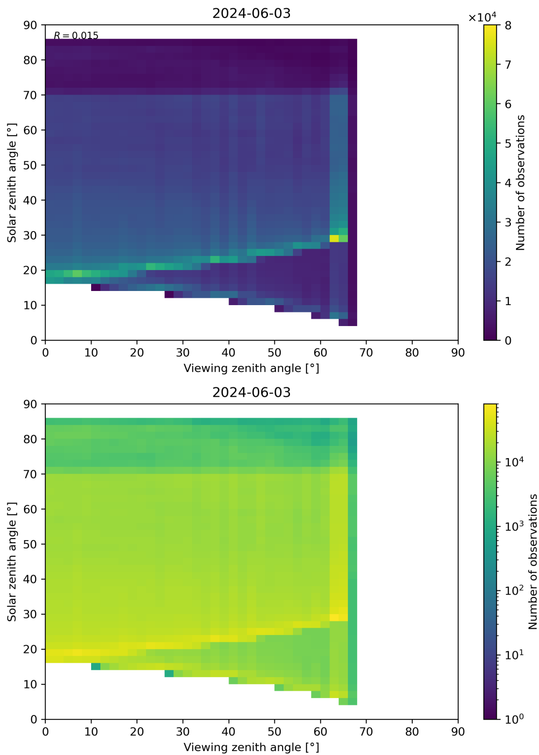
Figure 197: Scatter density plot of “Viewing zenith angle” against “Solar zenith angle” for 2024-06-03 to 2024-06-04.
