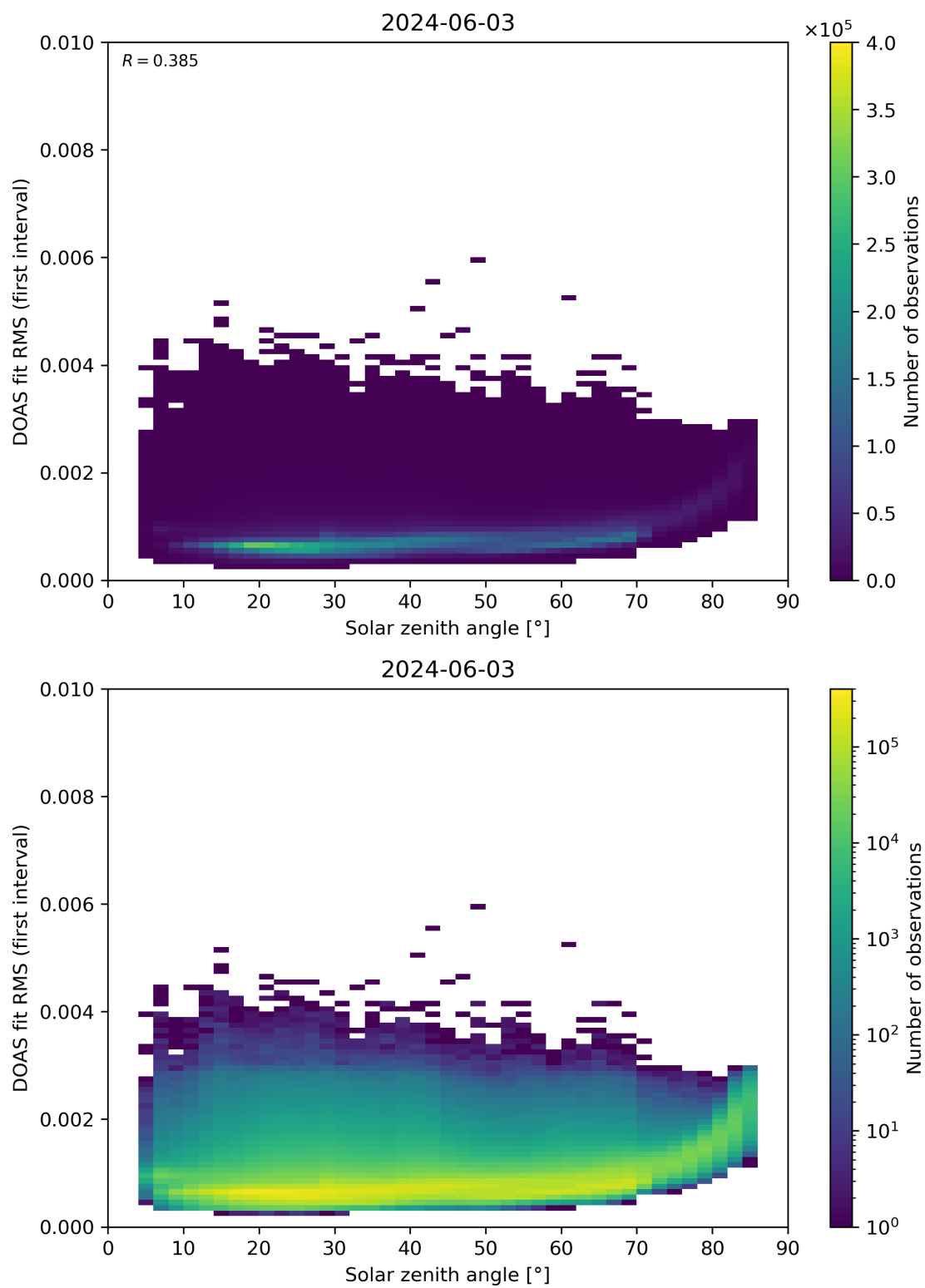
Figure 167: Scatter density plot of “Solar zenith angle” against “DOAS fit RMS (first interval)” for 2024-06-03 to 2024-06-04.
