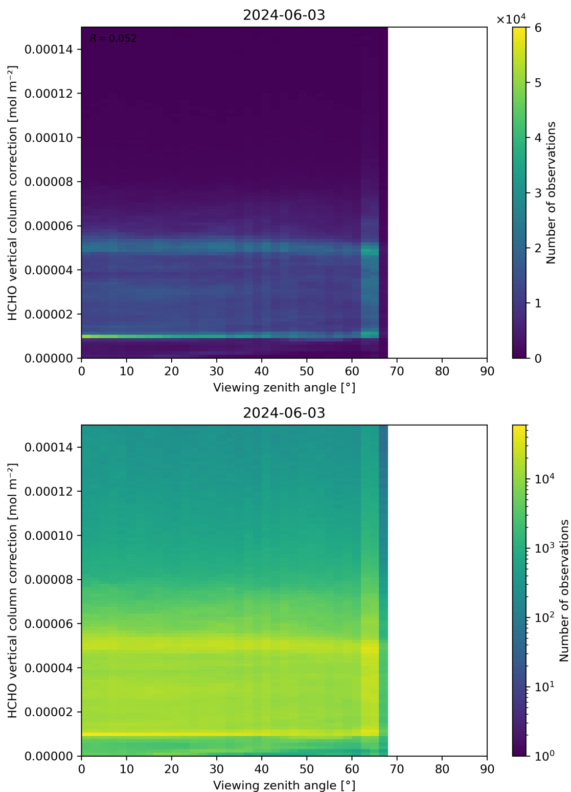
Figure 193: Scatter density plot of “Viewing zenith angle” against “HCHO vertical column correction” for 2024-06-03 to 2024-06-04.
