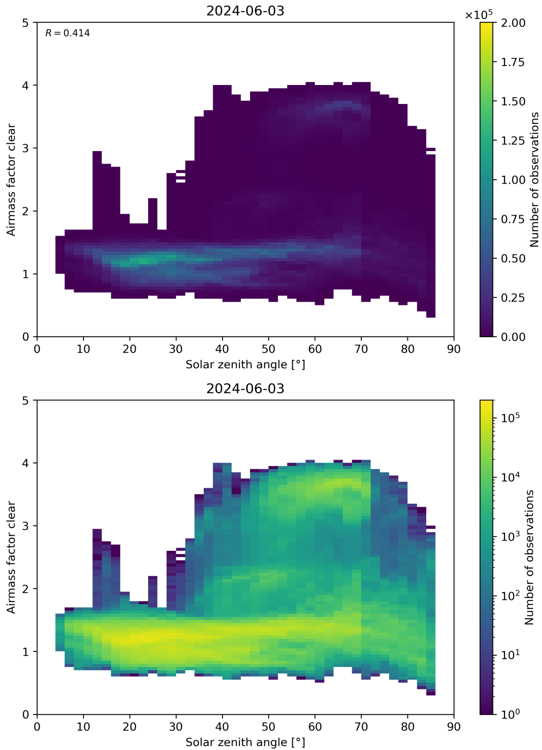
Figure 170: Scatter density plot of “Solar zenith angle” against “Airmass factor clear” for 2024-06-03 to 2024-06-04.
