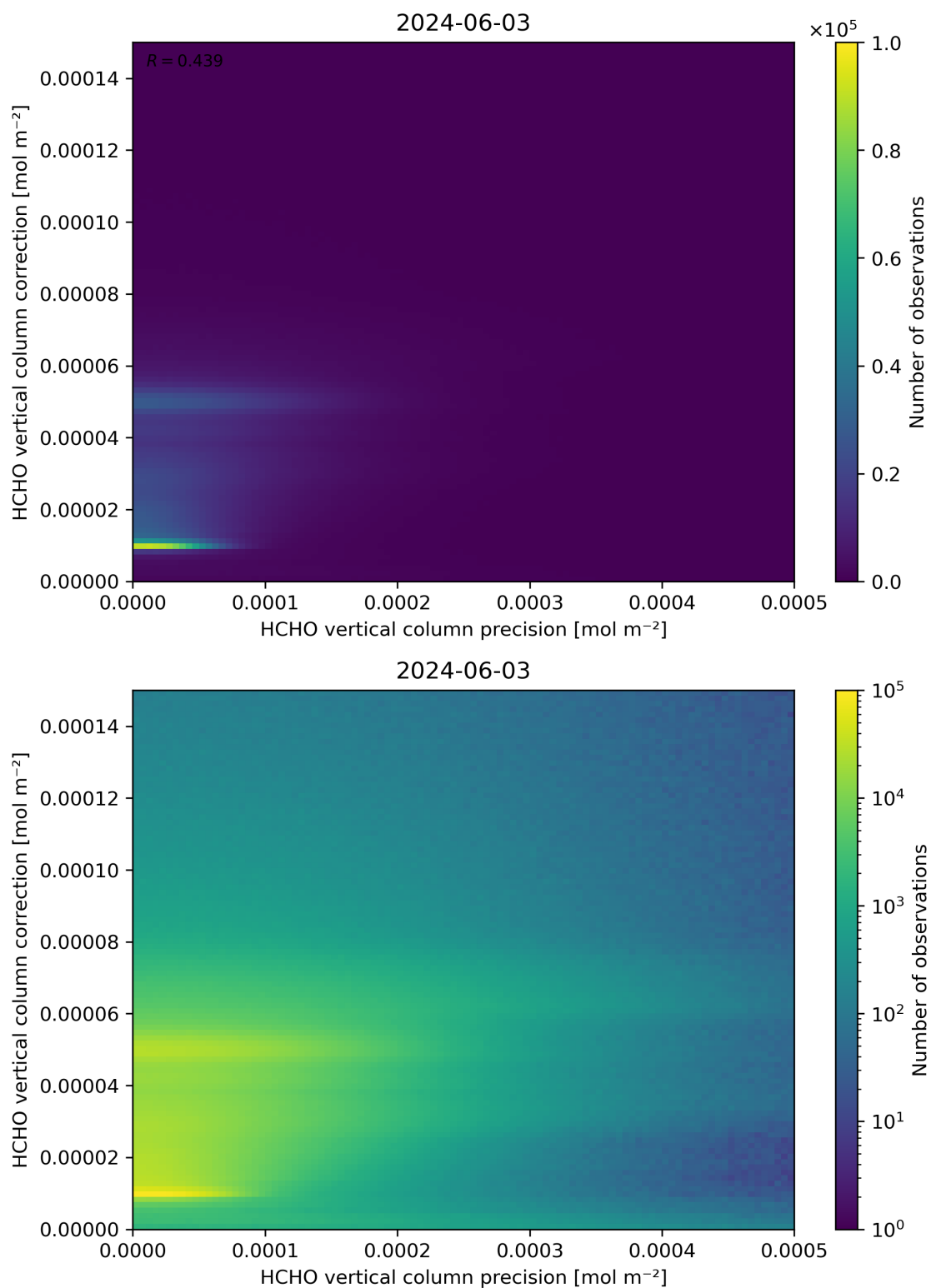
Figure 146: Scatter density plot of “HCHO vertical column precision” against “HCHO vertical column correction” for 2024-06-03 to 2024-06-04.
