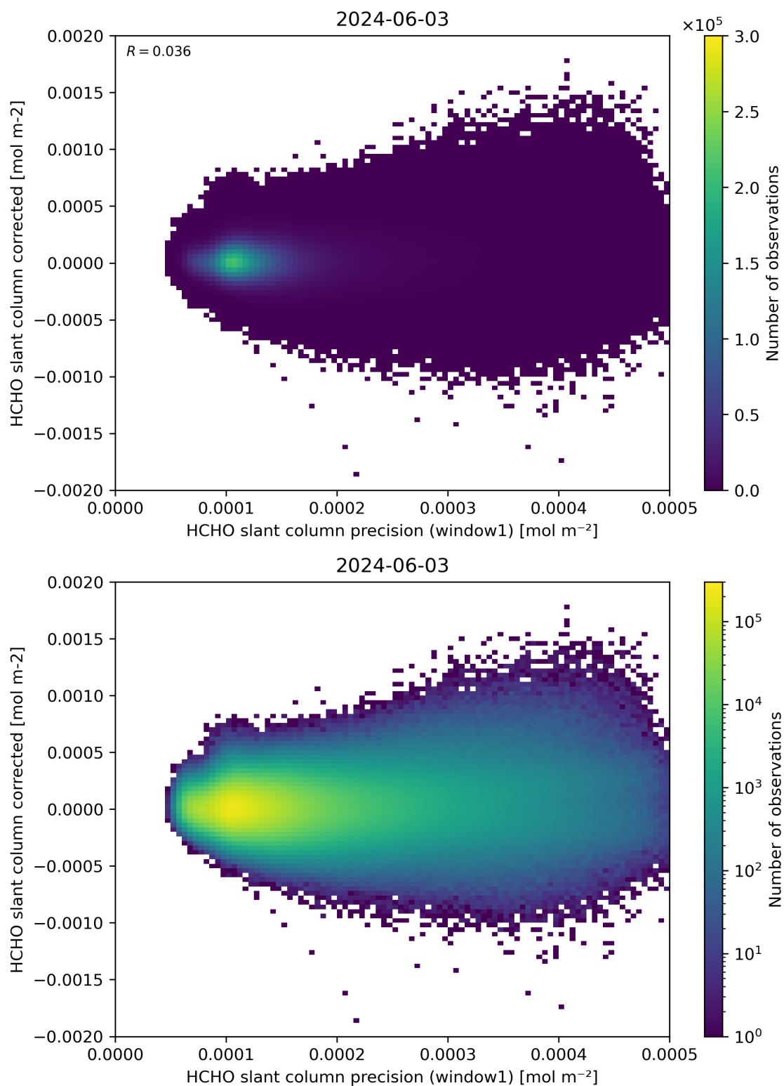
Figure 92: Scatter density plot of “HCHO slant column precision (window1)” against “HCHO slant column corrected” for 2024-06-03 to 2024-06-04.
