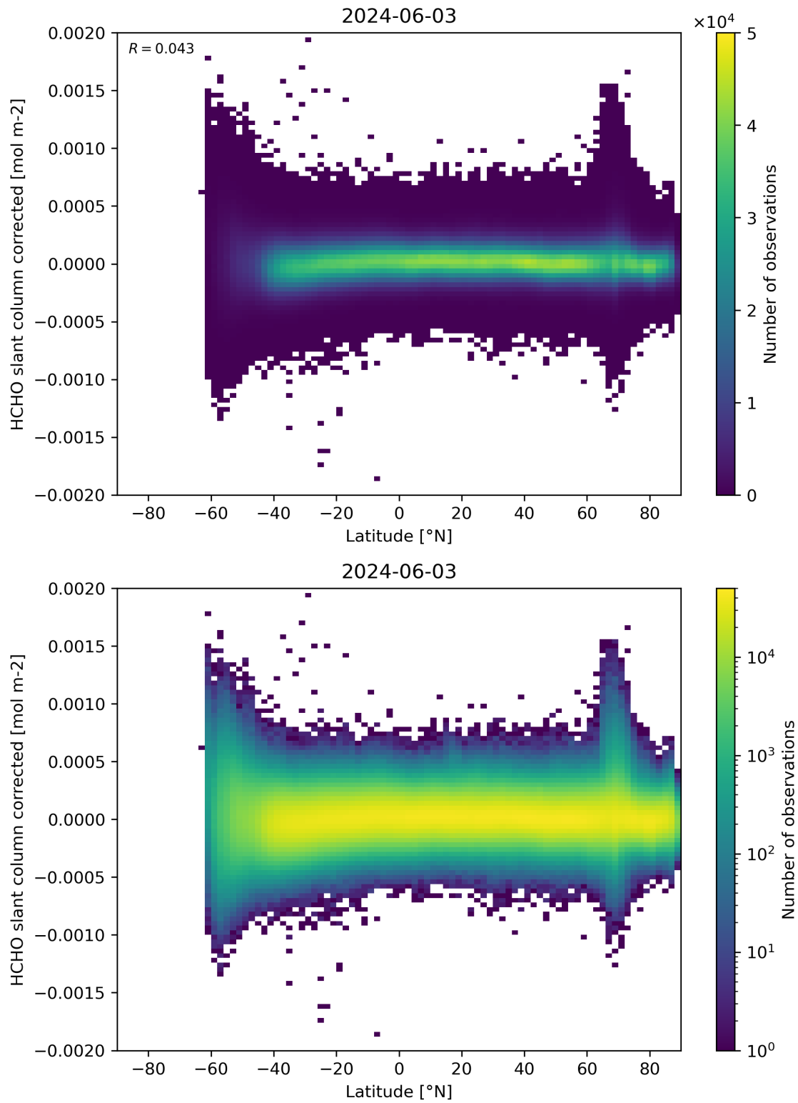
Figure 157: Scatter density plot of “Latitude” against “HCHO slant column corrected” for 2024-06-03 to 2024-06-04.
