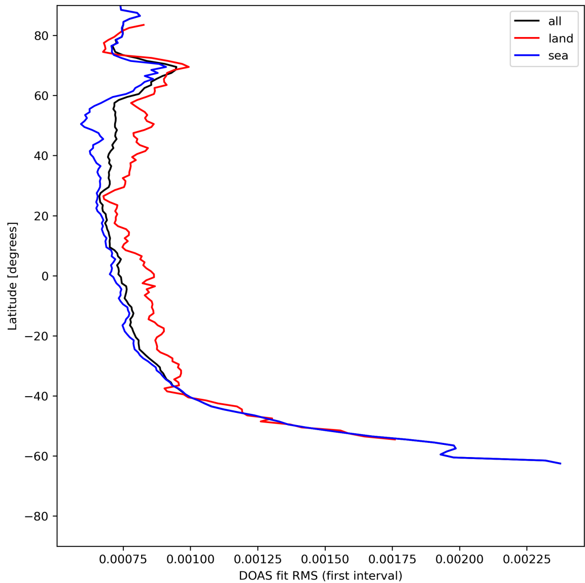
Figure 32: Zonal average of “DOAS fit RMS (first interval)” for 2024-06-03 to 2024-06-04.
