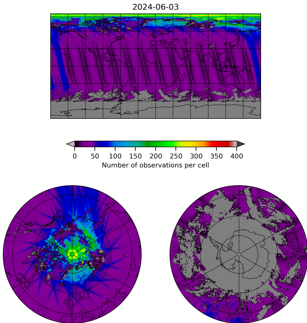
Figure 19: Map of the number of observations for 2024-06-03 to 2024-06-04
