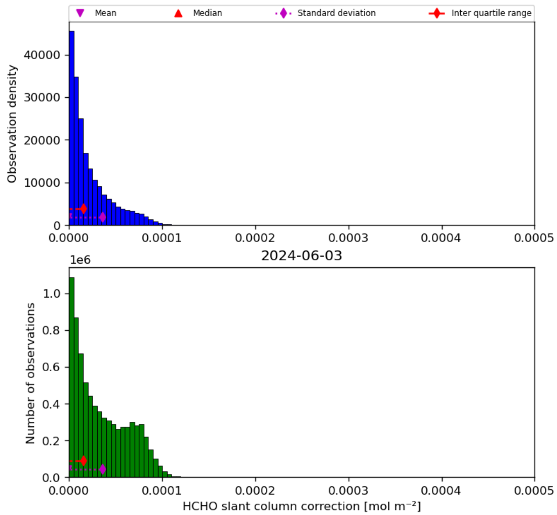
Figure 47: Histogram of “HCHO slant column correction” for 2024-06-03 to 2024-06-04
