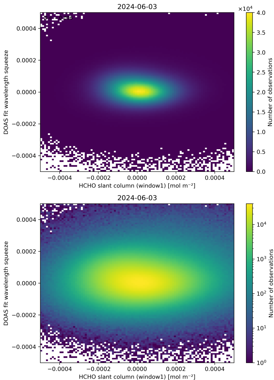
Figure 80: Scatter density plot of “HCHO slant column (window1)” against “DOAS fit wavelength squeeze” for 2024-06-03 to 2024-06-04.
