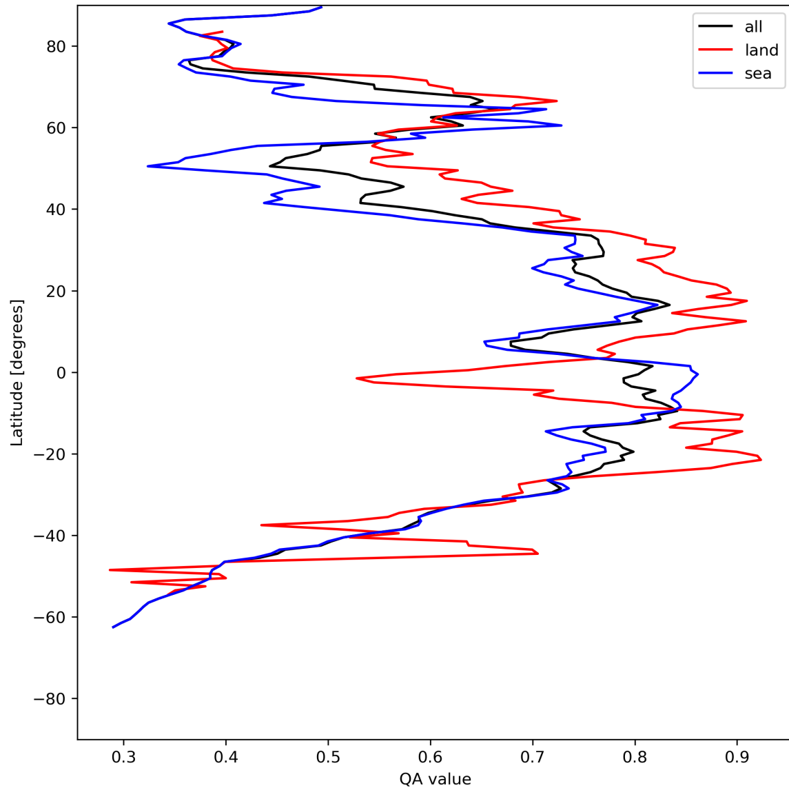
Figure 20: Zonal average of “QA value” for 2024-06-03 to 2024-06-04.
