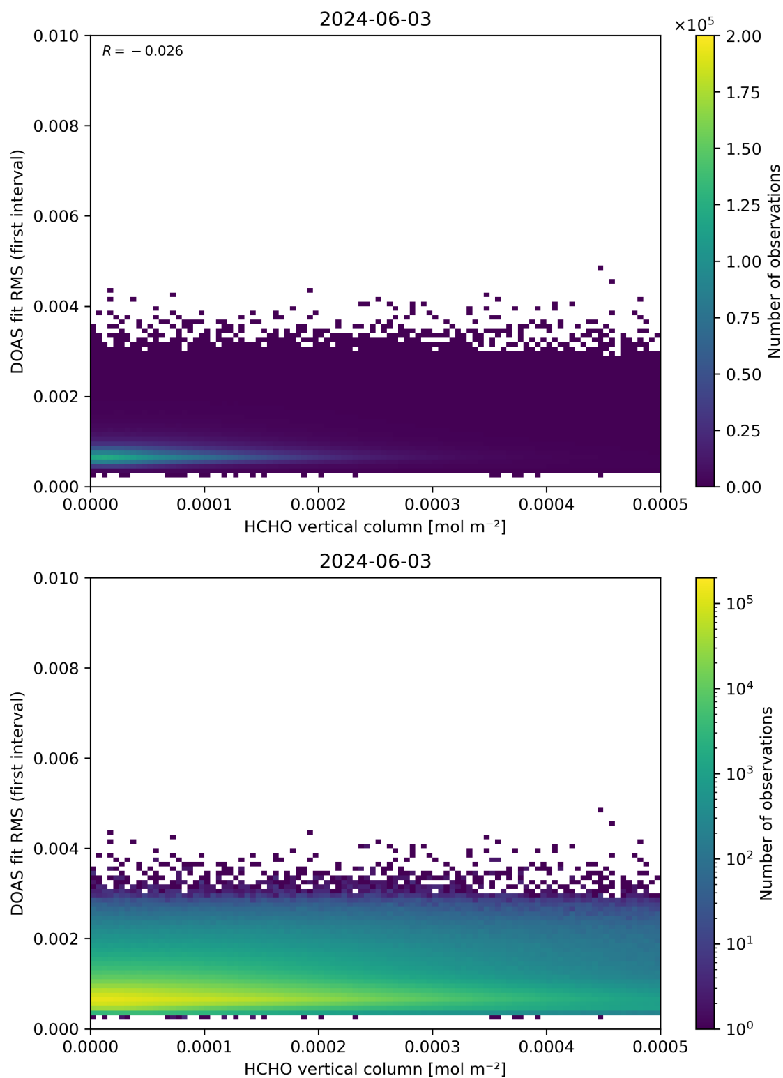
Figure 123: Scatter density plot of “HCHO vertical column” against “DOAS fit RMS (first interval)” for 2024-06-03 to 2024-06-04.
