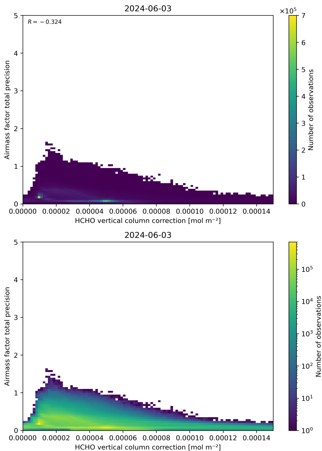
Figure 121: Scatter density plot of “HCHO vertical column correction” against “Airmass factor total precision” for 2024-06-03 to 2024-06-04.
