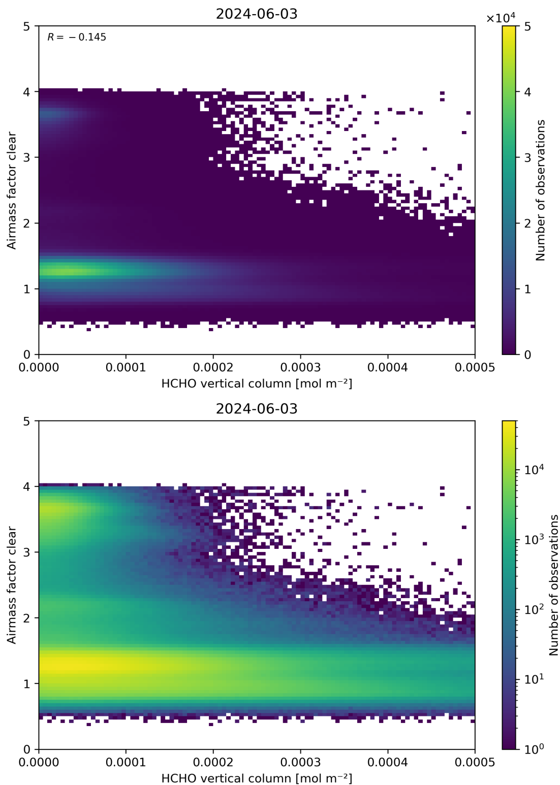
Figure 126: Scatter density plot of “HCHO vertical column” against “Airmass factor clear” for 2024-06-03 to 2024-06-04.
