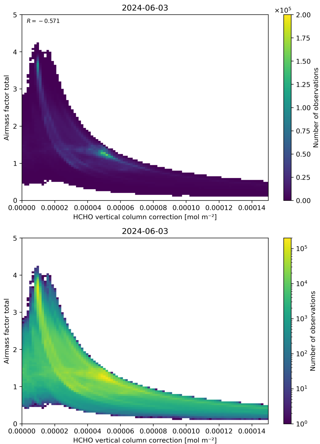
Figure 120: Scatter density plot of “HCHO vertical column correction” against “Airmass factor total” for 2024-06-03 to 2024-06-04.
