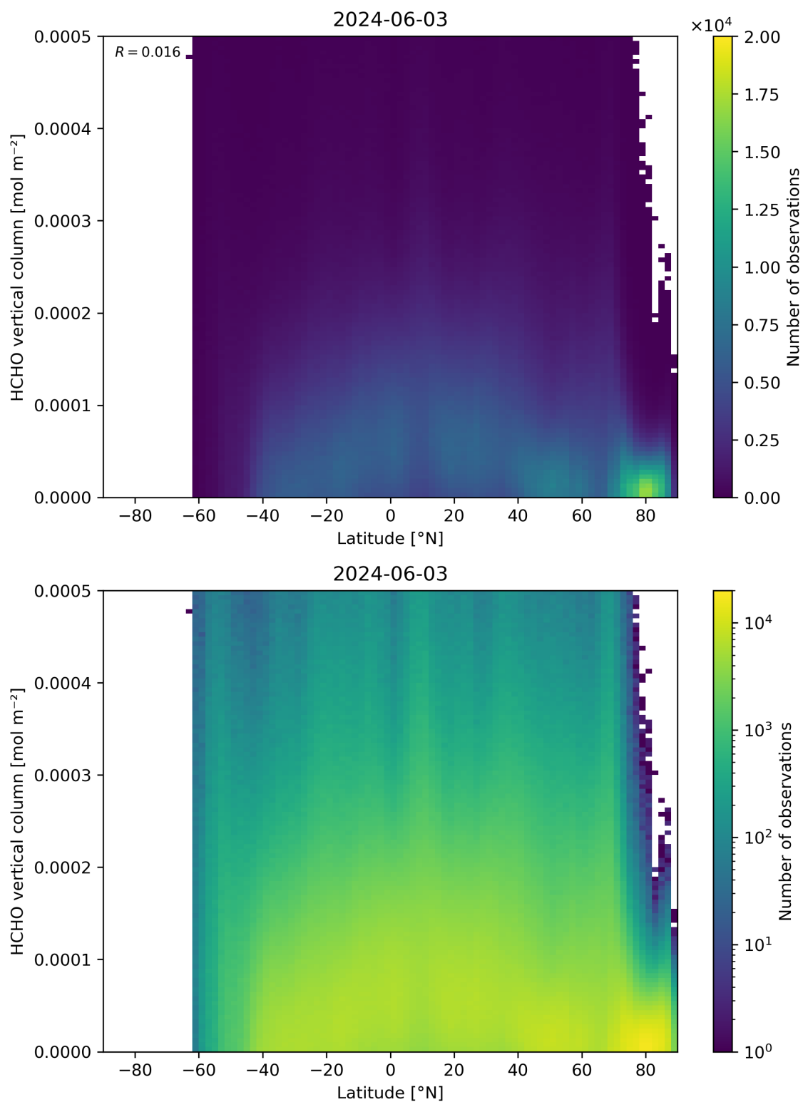
Figure 163: Scatter density plot of “Latitude” against “HCHO vertical column” for 2024-06-03 to 2024-06-04.
