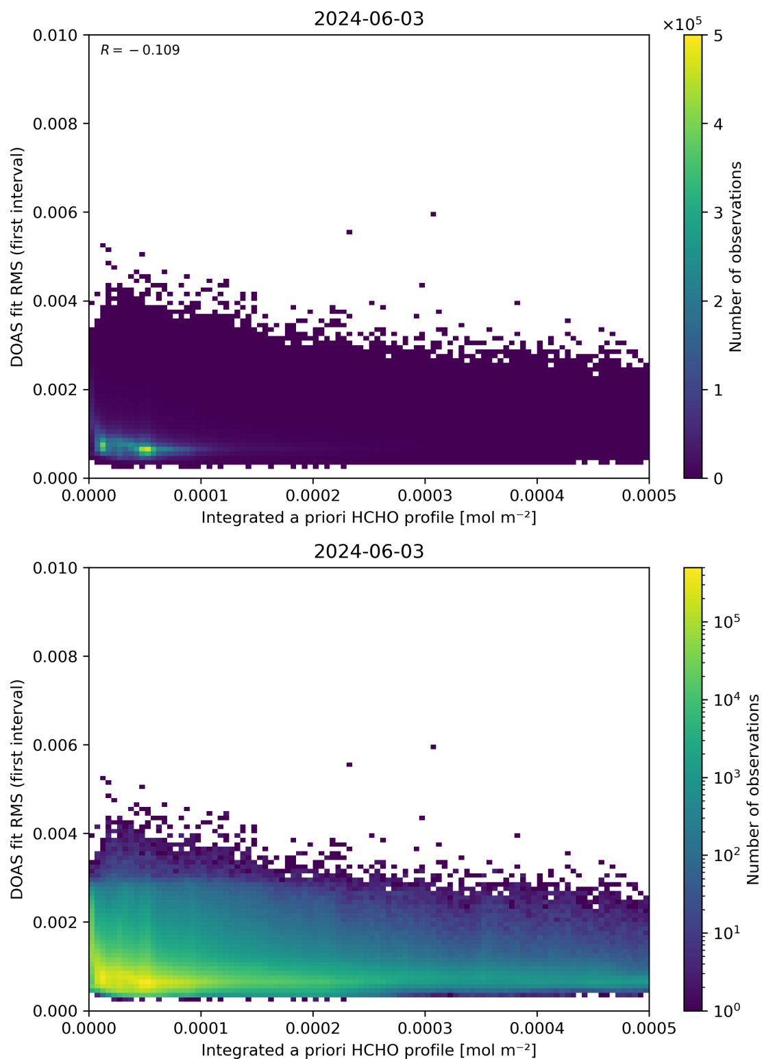
Figure 148: Scatter density plot of “Integrated a priori HCHO profile” against “DOAS fit RMS (first interval)” for 2024-06-03 to 2024-06-04.
