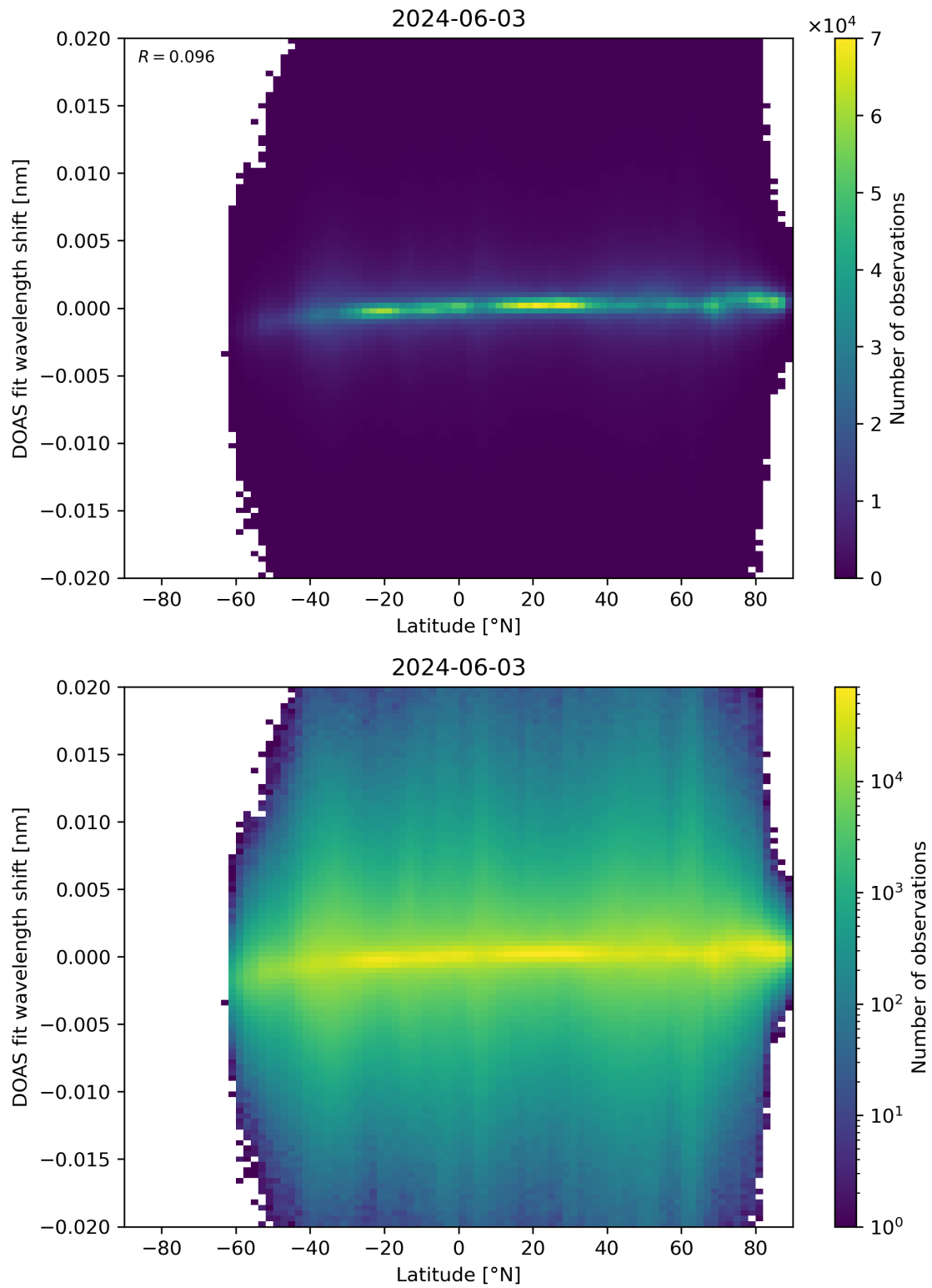
Figure 154: Scatter density plot of “Latitude” against “DOAS fit wavelength shift” for 2024-06-03 to 2024-06-04.
