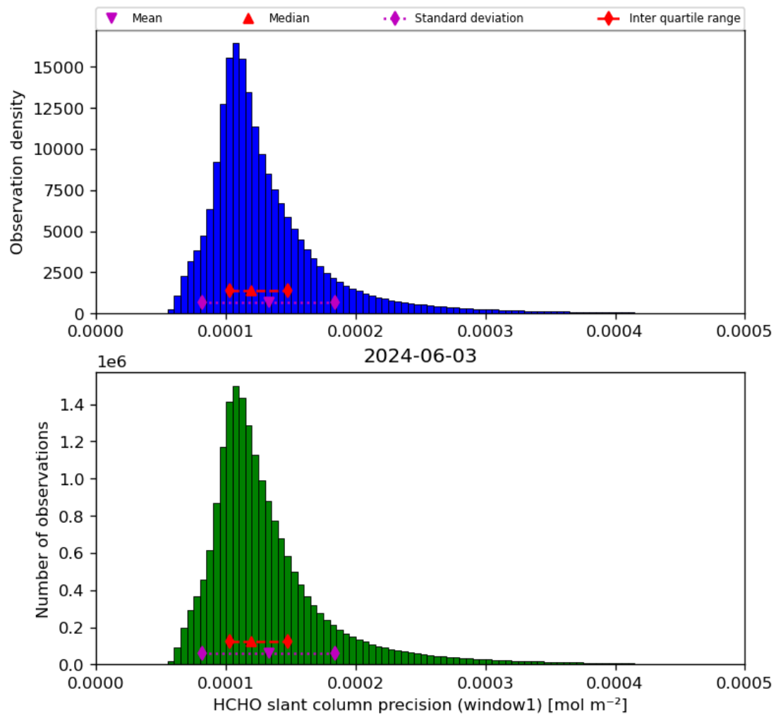
Figure 39: Histogram of “HCHO slant column precision (window1)” for 2024-06-03 to 2024-06-04
