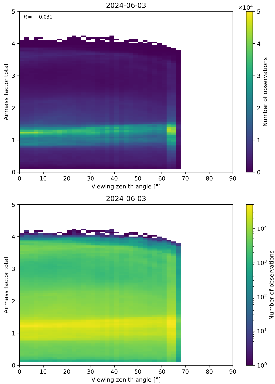
Figure 190: Scatter density plot of “Viewing zenith angle” against “Airmass factor total” for 2024-06-03 to 2024-06-04.
