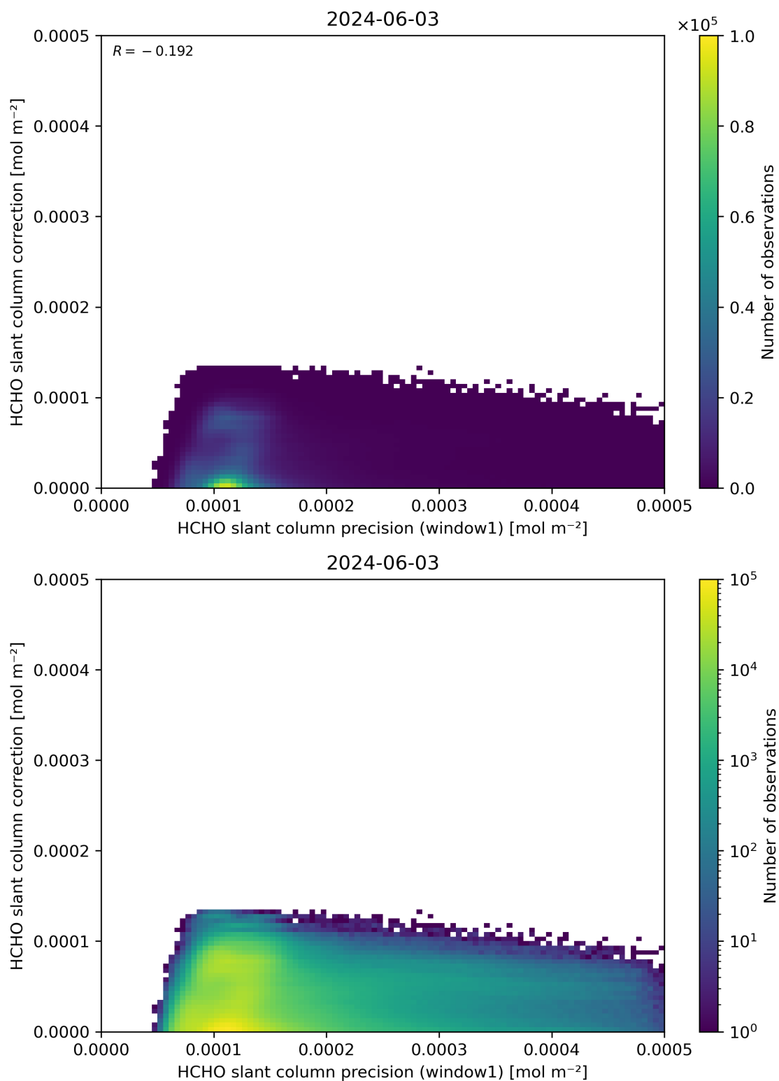
Figure 93: Scatter density plot of “HCHO slant column precision (window1)” against “HCHO slant column correction” for 2024-06-03 to 2024-06-04.
