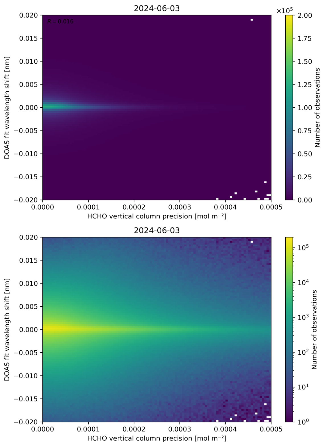
Figure 137: Scatter density plot of “HCHO vertical column precision” against “DOAS fit wavelength shift” for 2024-06-03 to 2024-06-04.
