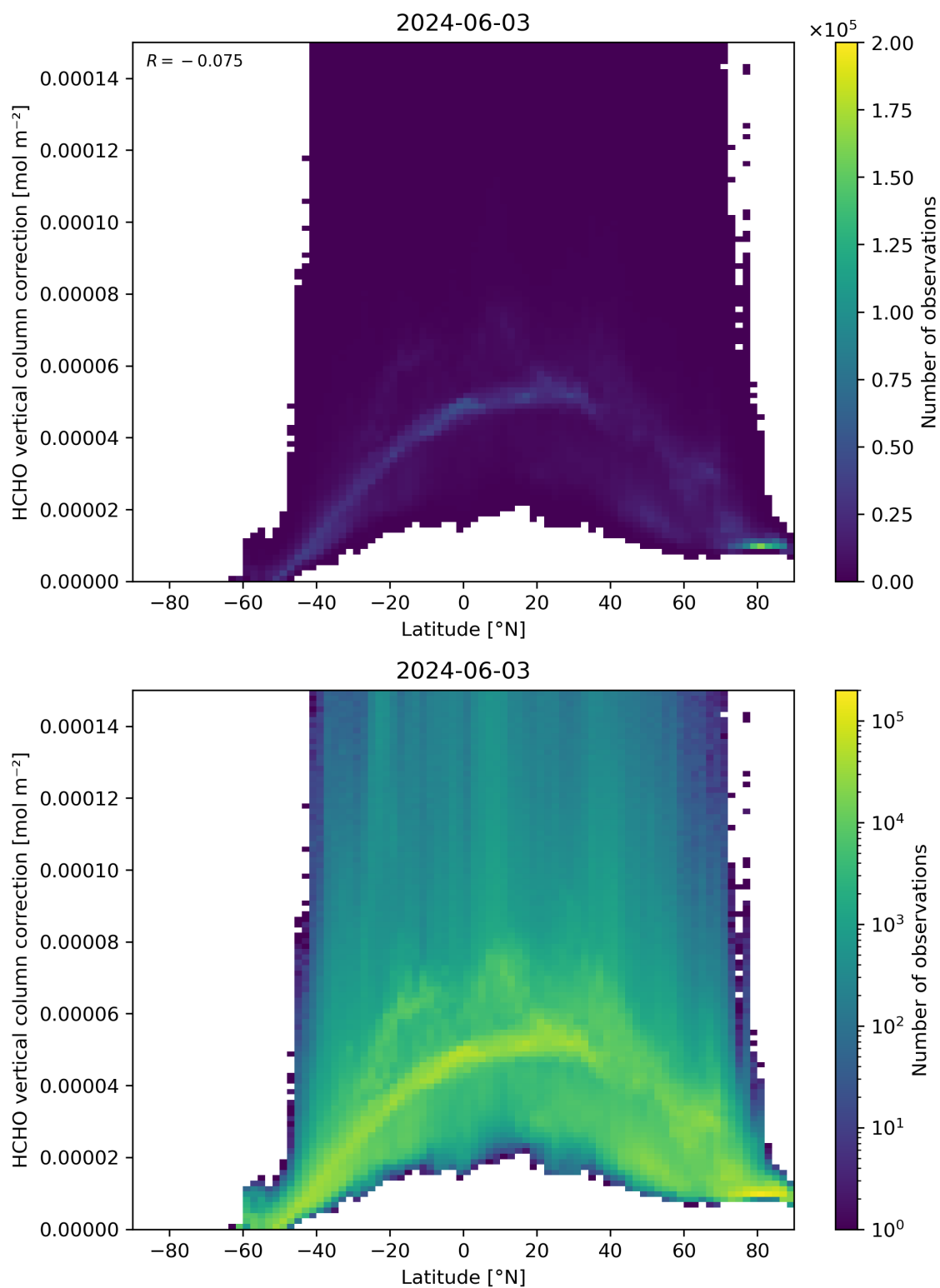
Figure 164: Scatter density plot of “Latitude” against “HCHO vertical column correction” for 2024-06-03 to 2024-06-04.
