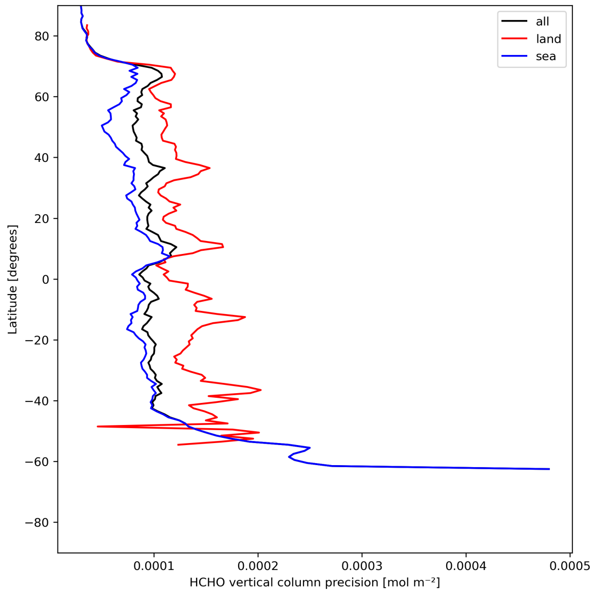
Figure 22: Zonal average of “HCHO vertical column precision” for 2024-06-03 to 2024-06-04.
