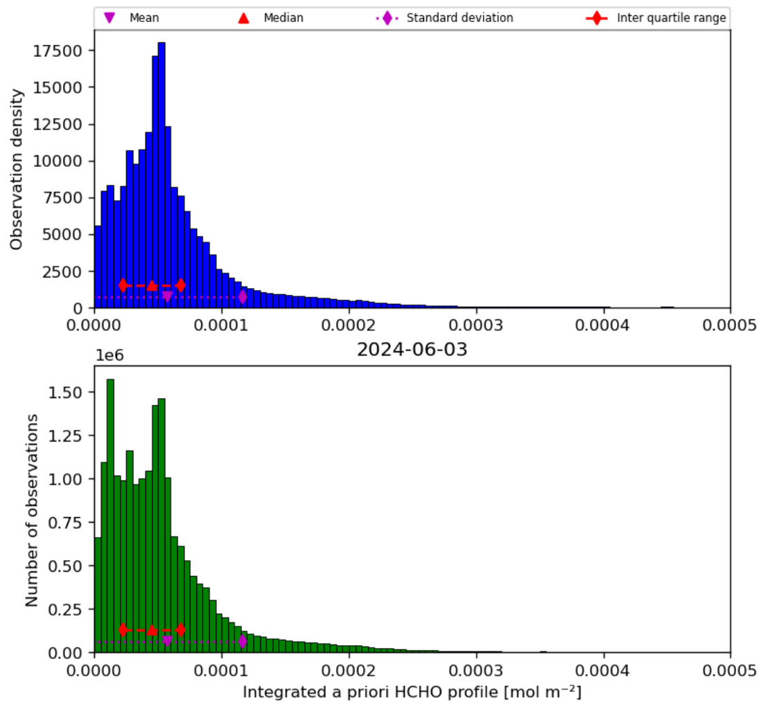
Figure 43: Histogram of “Integrated a priori HCHO profile” for 2024-06-03 to 2024-06-04
