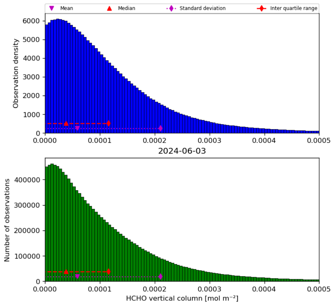
Figure 35: Histogram of “HCHO vertical column” for 2024-06-03 to 2024-06-04
