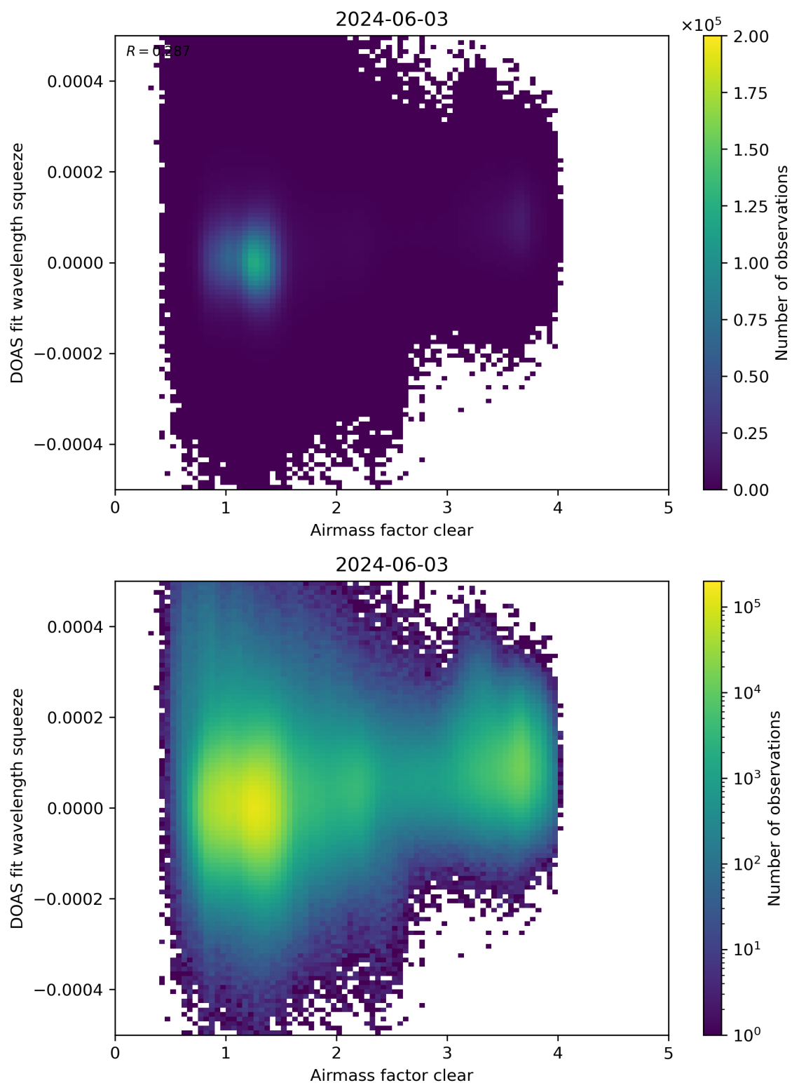
Figure 73: Scatter density plot of “Airmass factor clear” against “DOAS fit wavelength squeeze” for 2024-06-03 to 2024-06-04.
