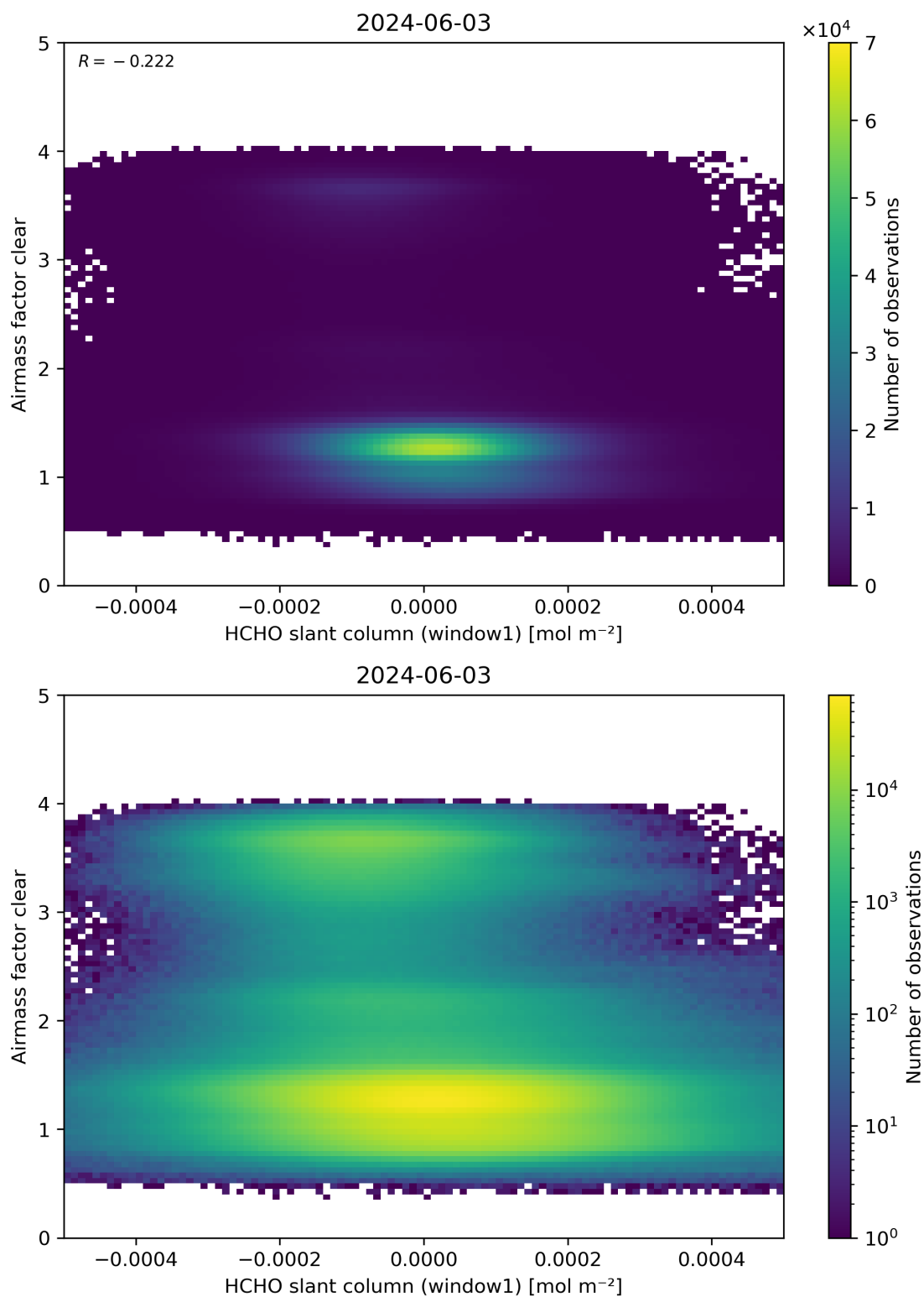
Figure 81: Scatter density plot of “HCHO slant column (window1)” against “Airmass factor clear” for 2024-06-03 to 2024-06-04.
