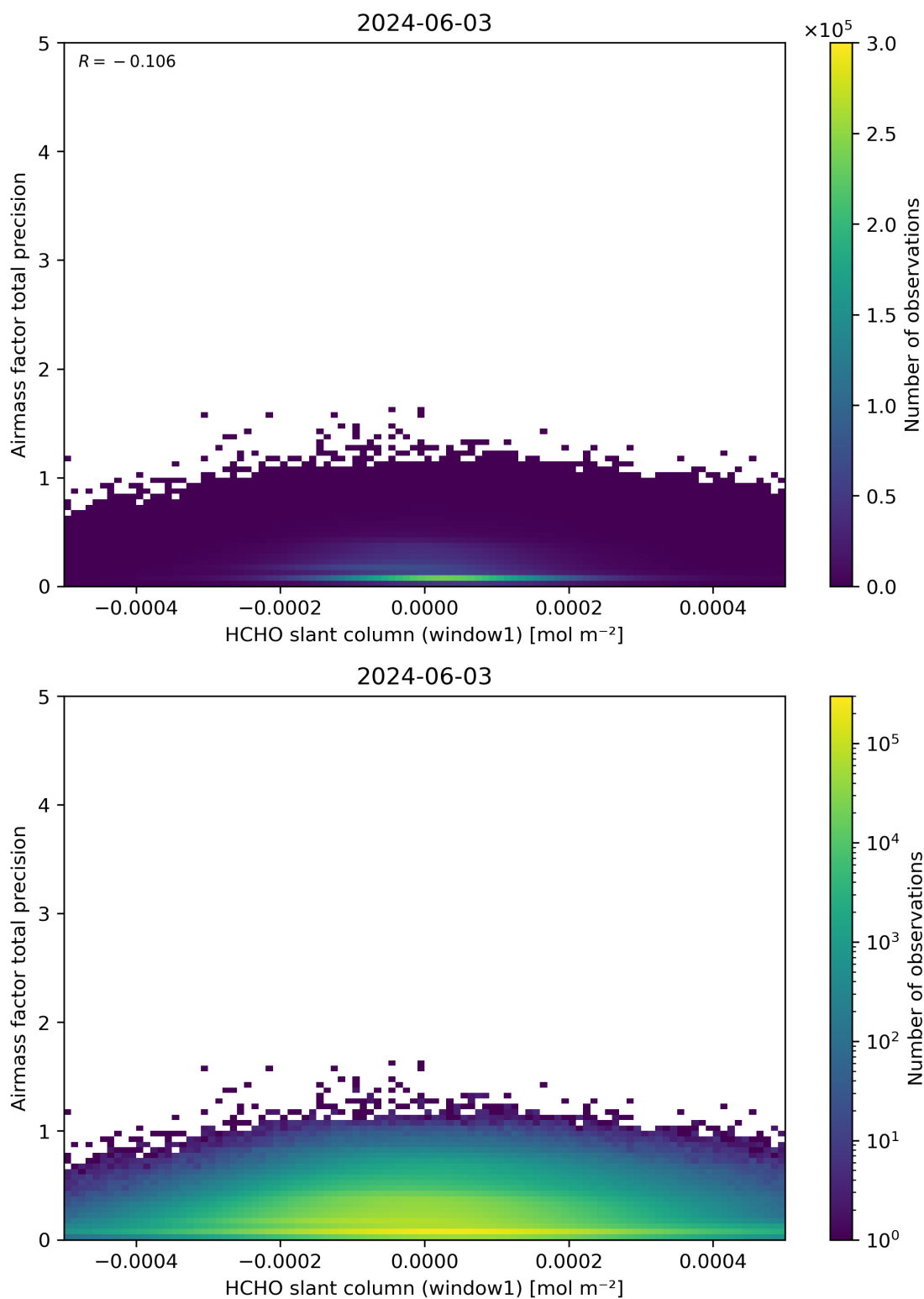
Figure 86: Scatter density plot of “HCHO slant column (window1)” against “Airmass factor total precision” for 2024-06-03 to 2024-06-04.
