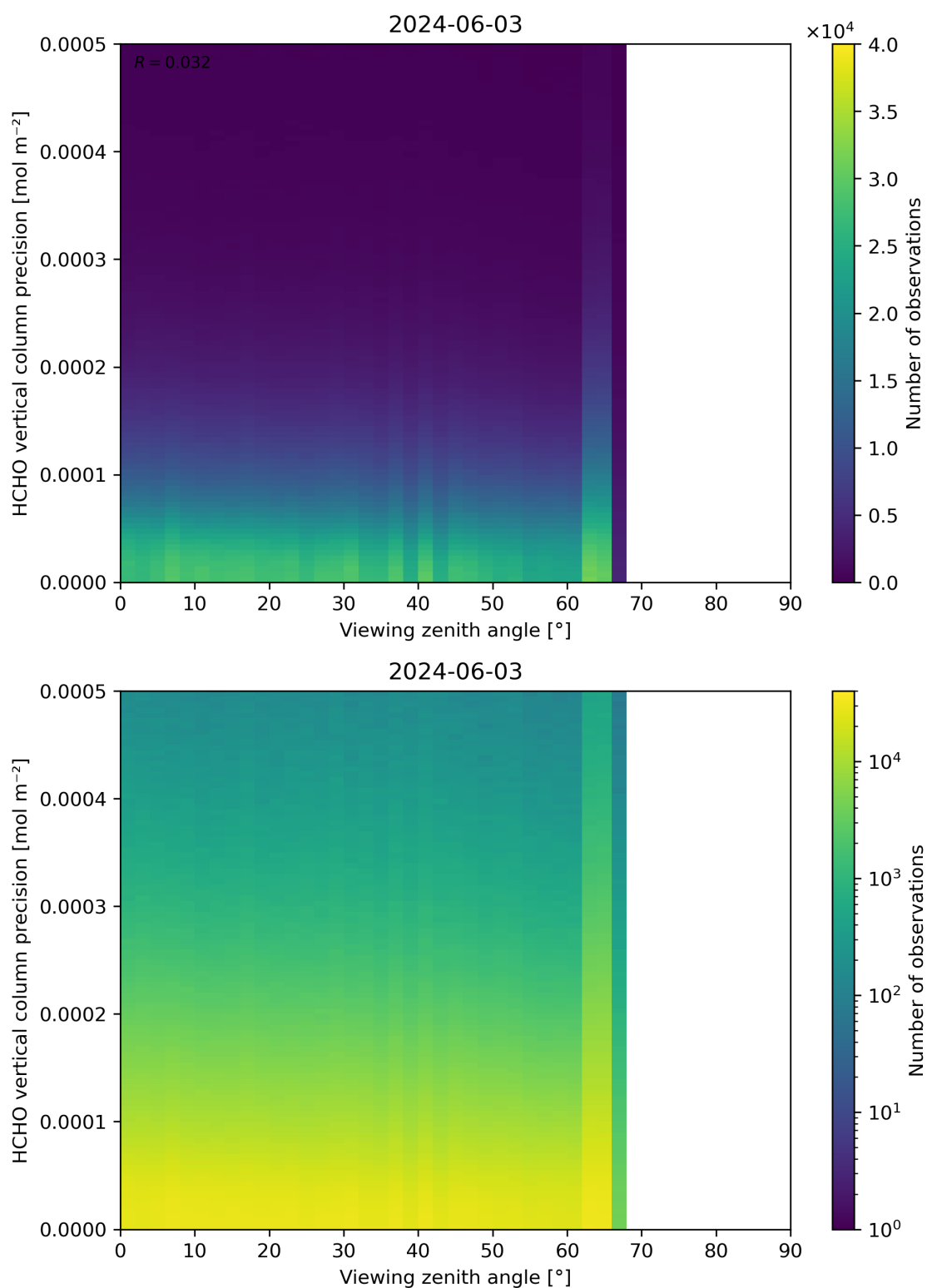
Figure 194: Scatter density plot of “Viewing zenith angle” against “HCHO vertical column precision” for 2024-06-03 to 2024-06-04.
