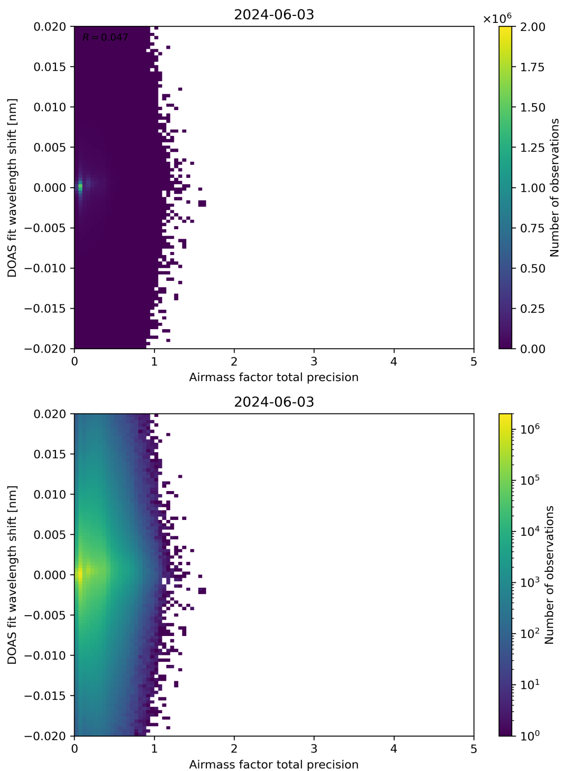
Figure 106: Scatter density plot of “Airmass factor total precision” against “DOAS fit wavelength shift” for 2024-06-03 to 2024-06-04.
