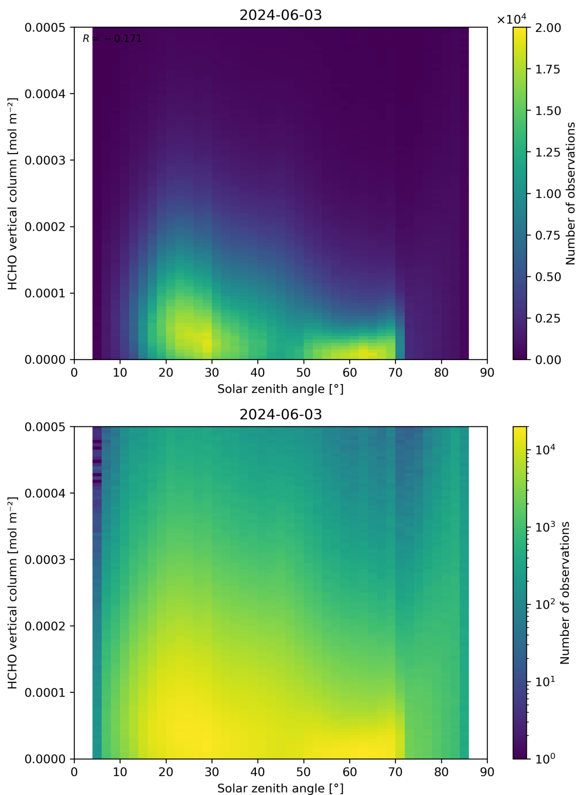
Figure 177: Scatter density plot of “Solar zenith angle” against “HCHO vertical column” for 2024-06-03 to 2024-06-04.
