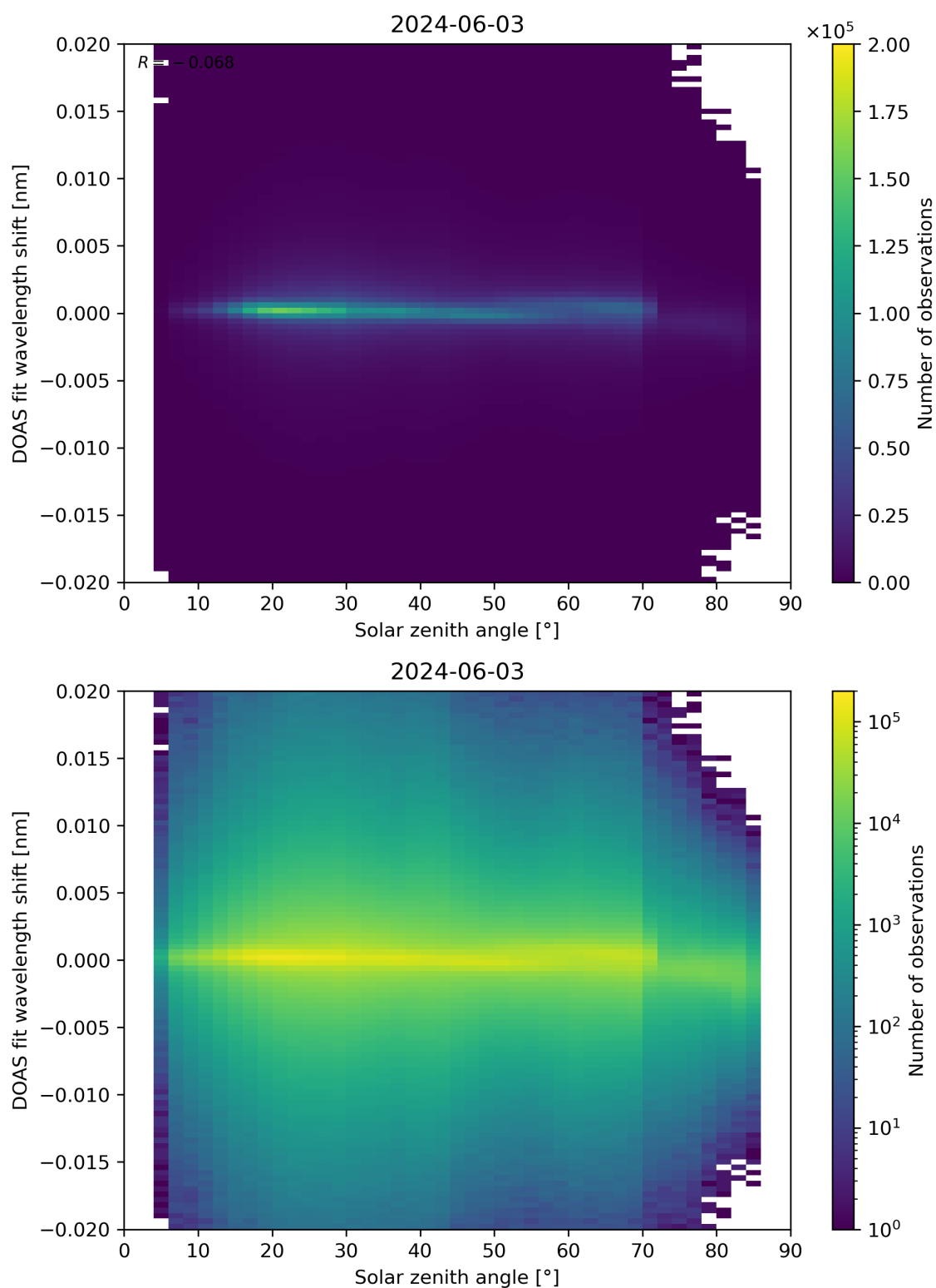
Figure 168: Scatter density plot of “Solar zenith angle” against “DOAS fit wavelength shift” for 2024-06-03 to 2024-06-04.
