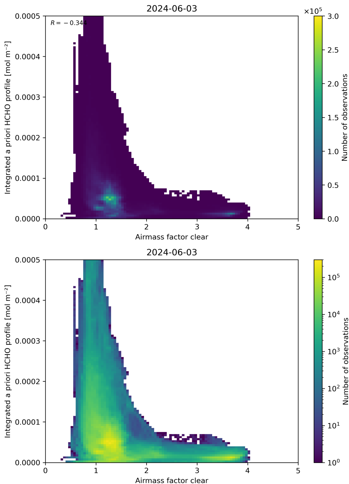
Figure 76: Scatter density plot of “Airmass factor clear” against “Integrated a priori HCHO profile” for 2024-06-03 to 2024-06-04.
