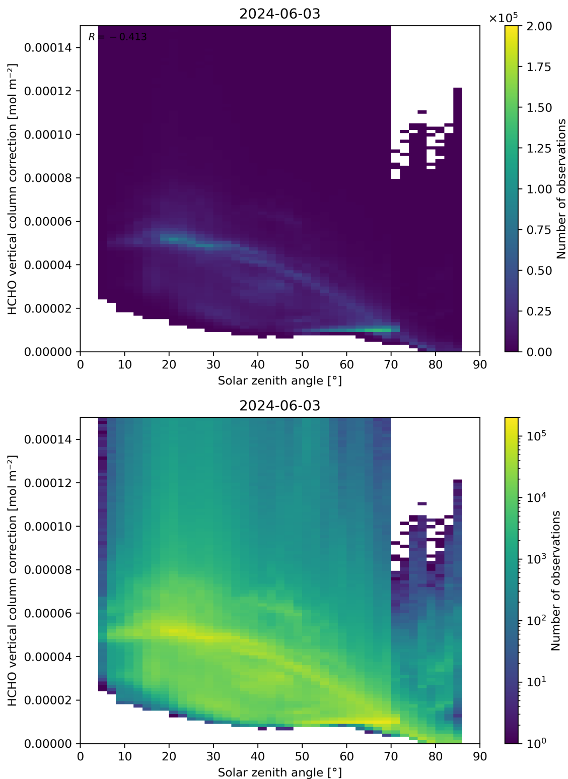
Figure 178: Scatter density plot of “Solar zenith angle” against “HCHO vertical column correction” for 2024-06-03 to 2024-06-04.
