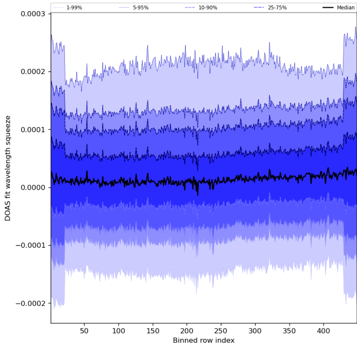
Figure 59: Along track statistics of “DOAS fit wavelength squeeze” for 2024-06-03 to 2024-06-04
