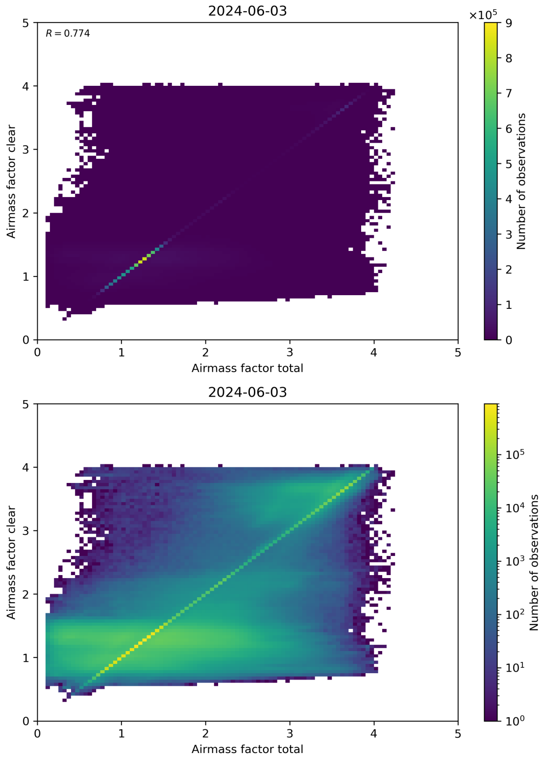
Figure 100: Scatter density plot of “Airmass factor total” against “Airmass factor clear” for 2024-06-03 to 2024-06-04.
