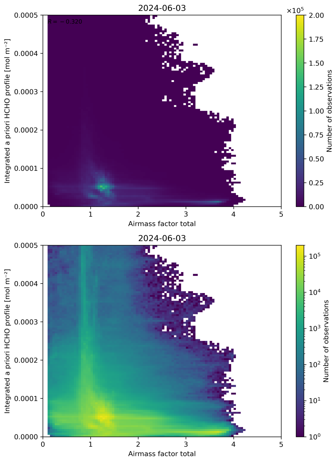
Figure 104: Scatter density plot of “Airmass factor total” against “Integrated a priori HCHO profile” for 2024-06-03 to 2024-06-04.
