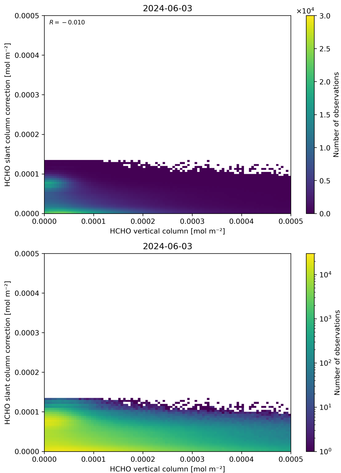
Figure 128: Scatter density plot of “HCHO vertical column” against “HCHO slant column correction” for 2024-06-03 to 2024-06-04.
