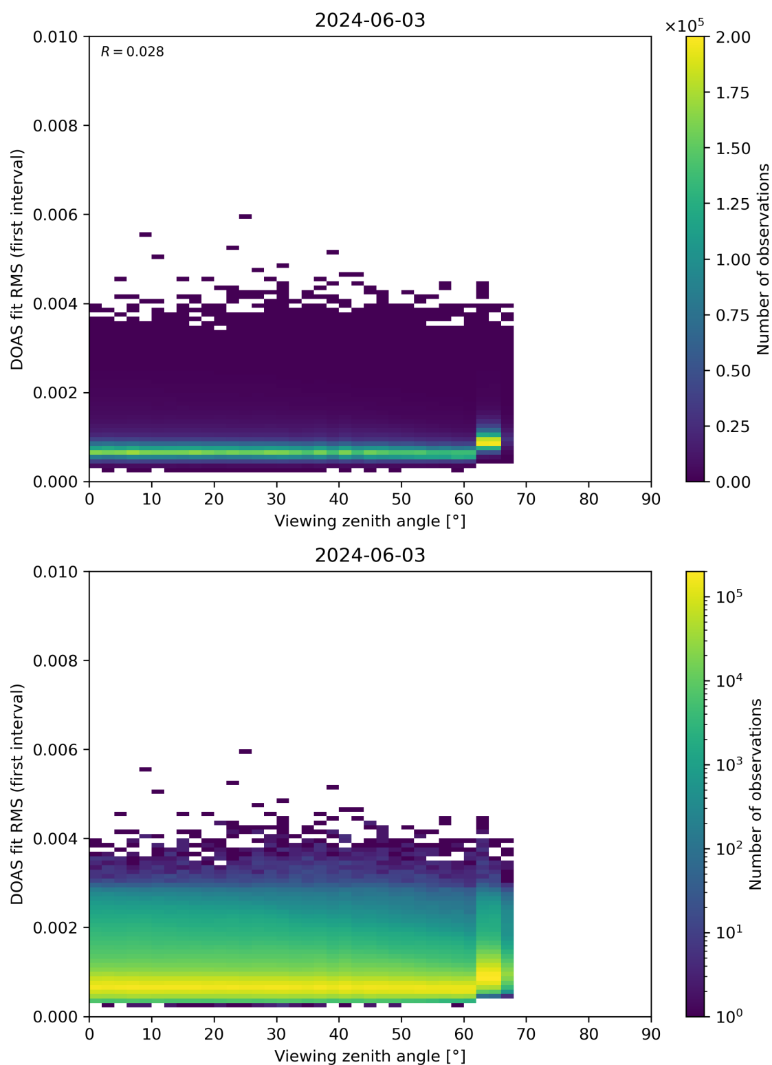
Figure 182: Scatter density plot of “Viewing zenith angle” against “DOAS fit RMS (first interval)” for 2024-06-03 to 2024-06-04.
