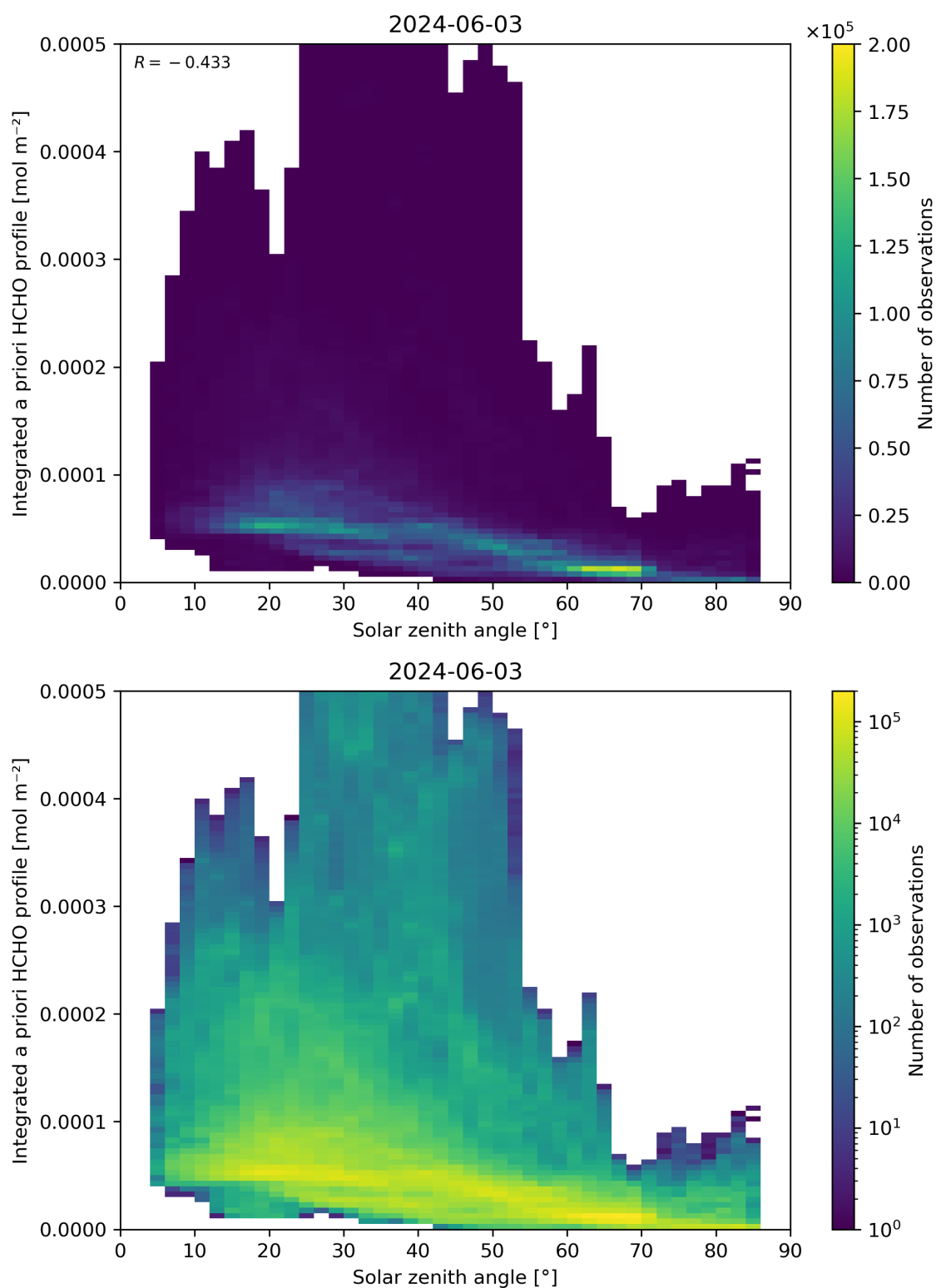
Figure 180: Scatter density plot of “Solar zenith angle” against “Integrated a priori HCHO profile” for 2024-06-03 to 2024-06-04.
