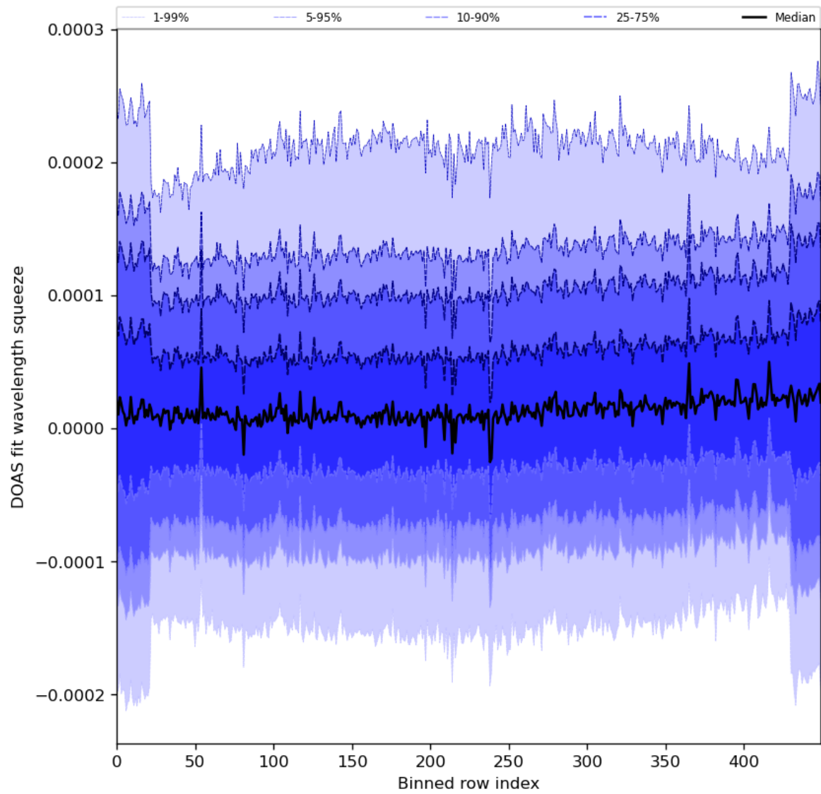
Figure 59: Along track statistics of “DOAS fit wavelength squeeze” for 2024-06-03 to 2024-06-05
