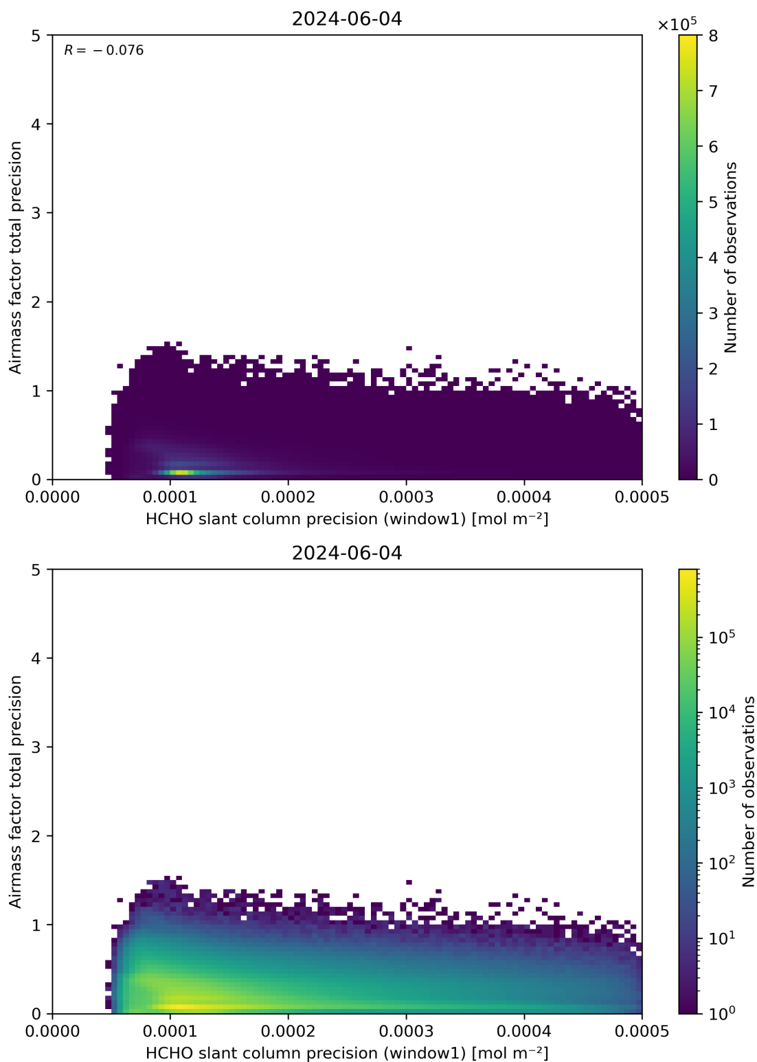
Figure 95: Scatter density plot of “HCHO slant column precision (window1)” against “Airmass factor total precision” for 2024-06-03 to 2024-06-05.
