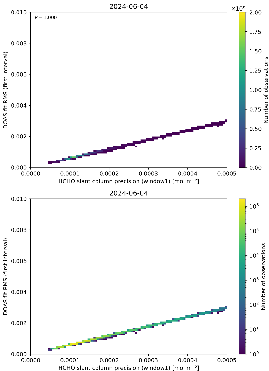
Figure 88: Scatter density plot of “HCHO slant column precision (window1)” against “DOAS fit RMS (first interval)” for 2024-06-03 to 2024-06-05.
