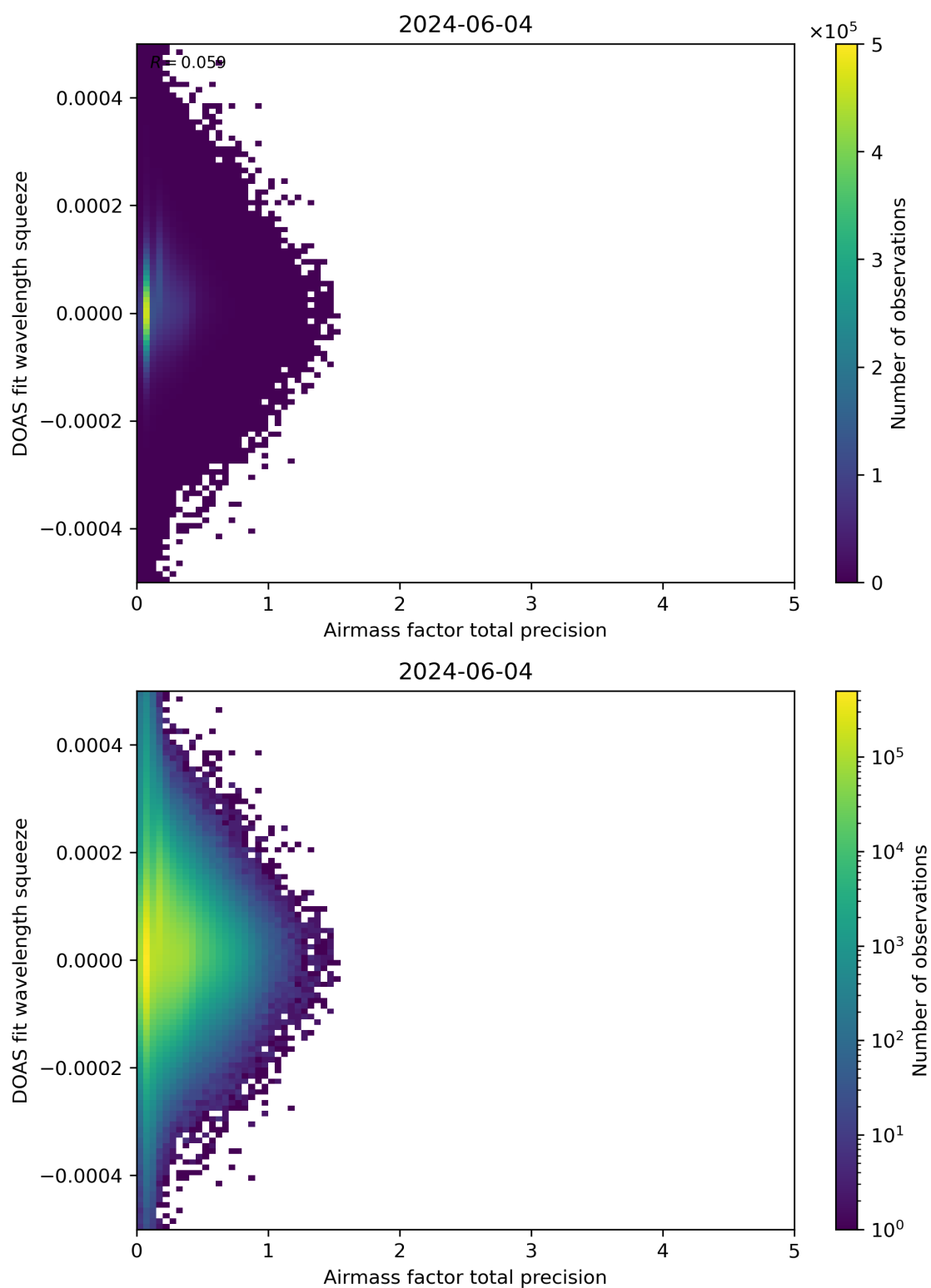
Figure 107: Scatter density plot of “Airmass factor total precision” against “DOAS fit wavelength squeeze” for 2024-06-03 to 2024-06-05.
