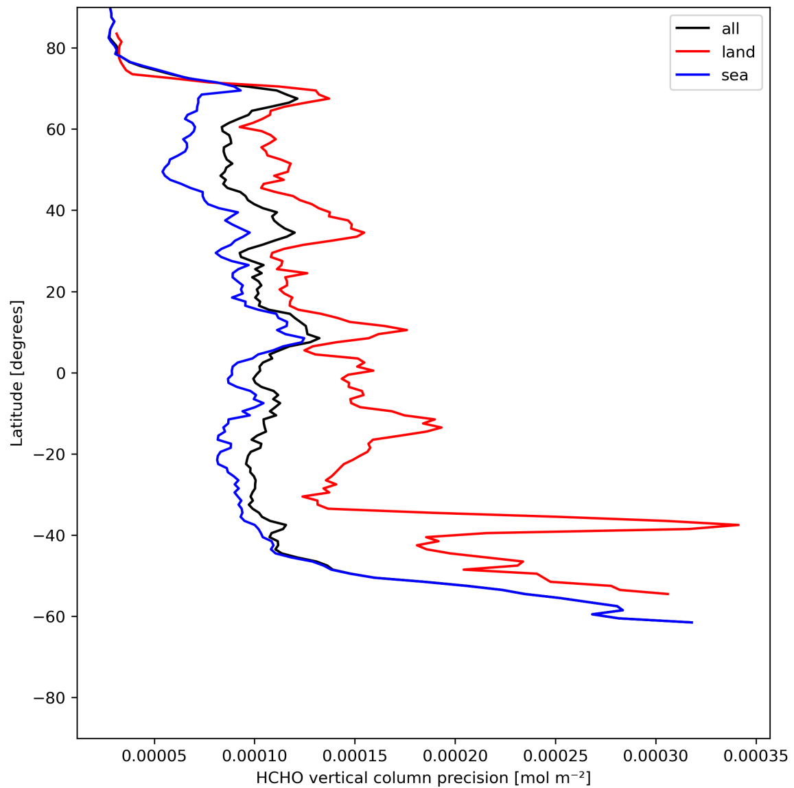
Figure 22: Zonal average of “HCHO vertical column precision” for 2024-06-03 to 2024-06-05.
