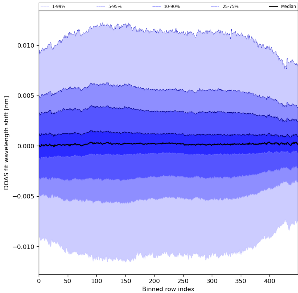
Figure 58: Along track statistics of “DOAS fit wavelength shift” for 2024-06-03 to 2024-06-05
