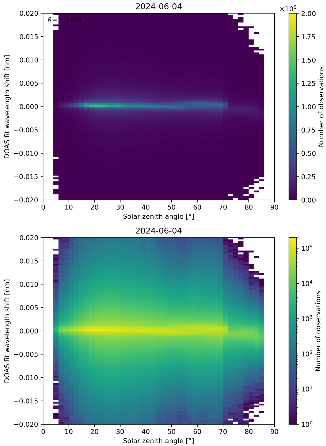
Figure 168: Scatter density plot of “Solar zenith angle” against “DOAS fit wavelength shift” for 2024-06-03 to 2024-06-05.
