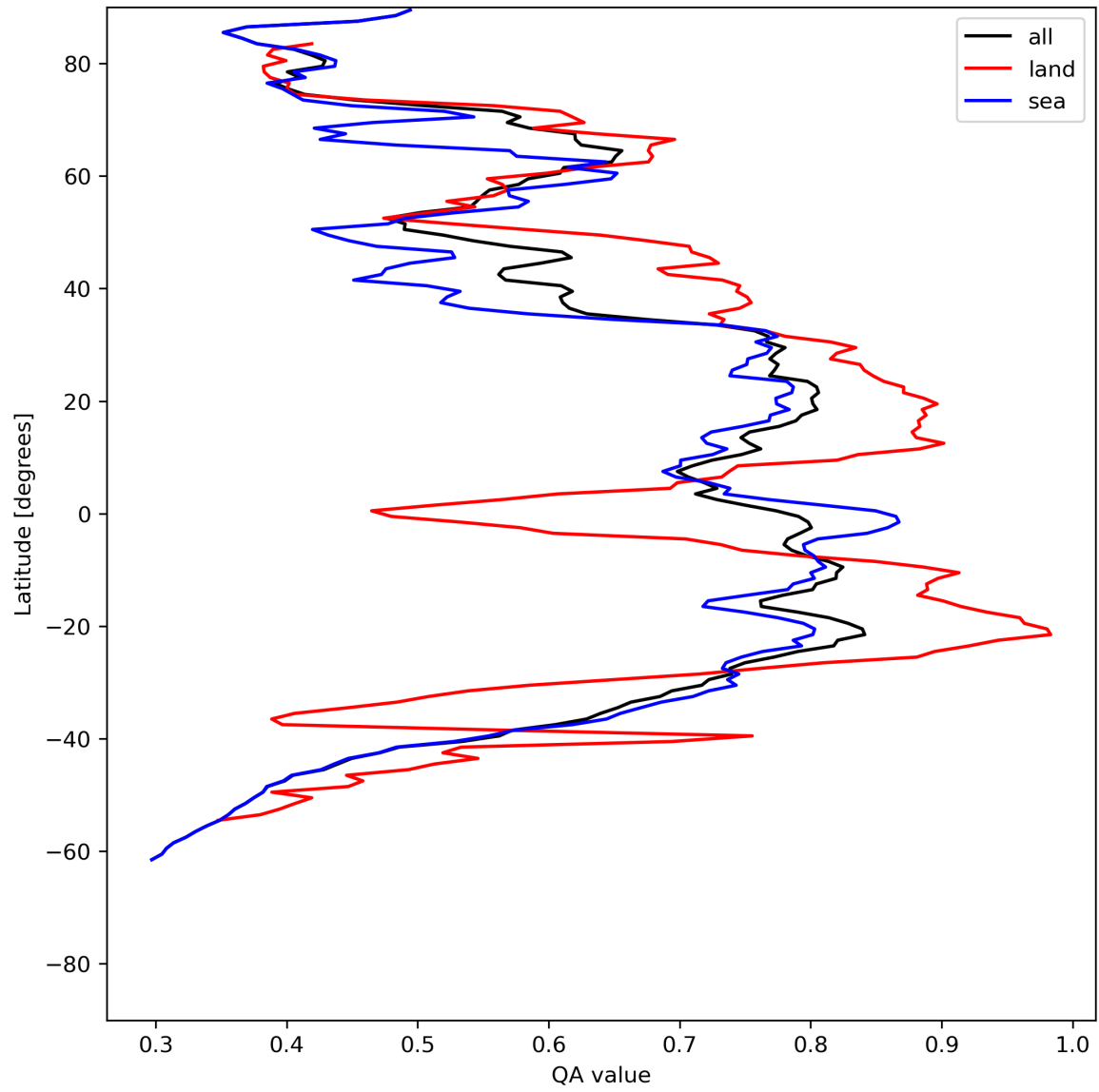
Figure 20: Zonal average of “QA value” for 2024-06-03 to 2024-06-05.
