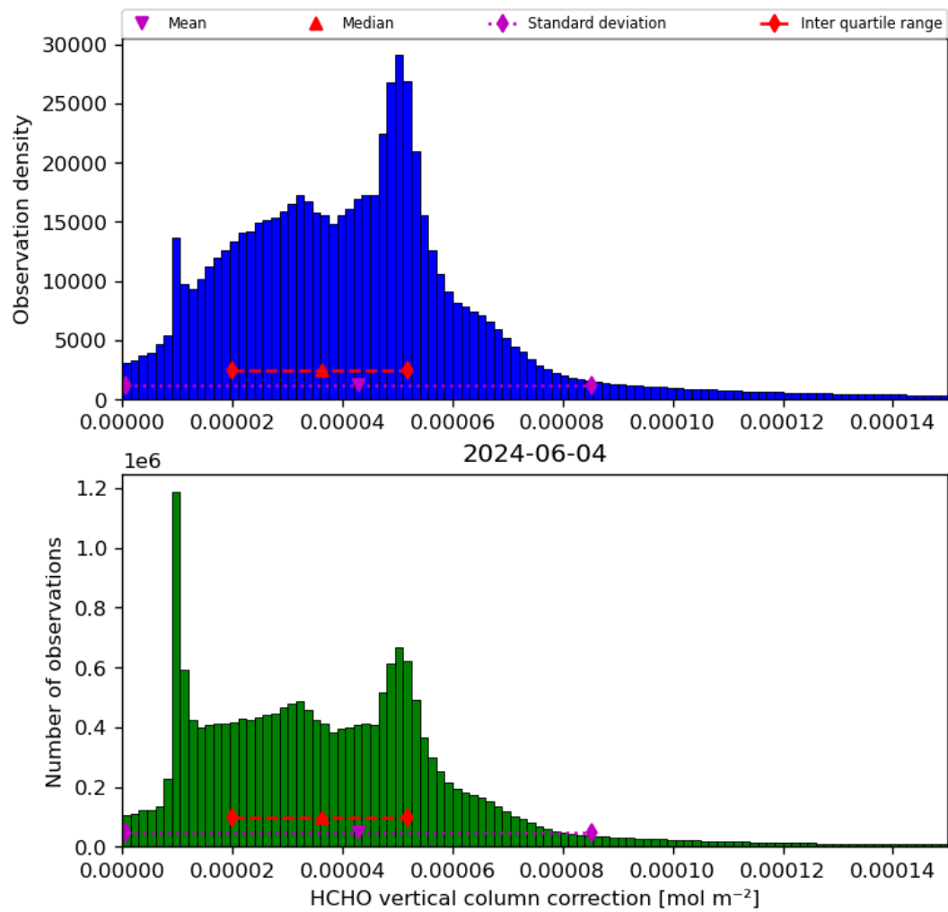
Figure 37: Histogram of “HCHO vertical column correction” for 2024-06-03 to 2024-06-05
