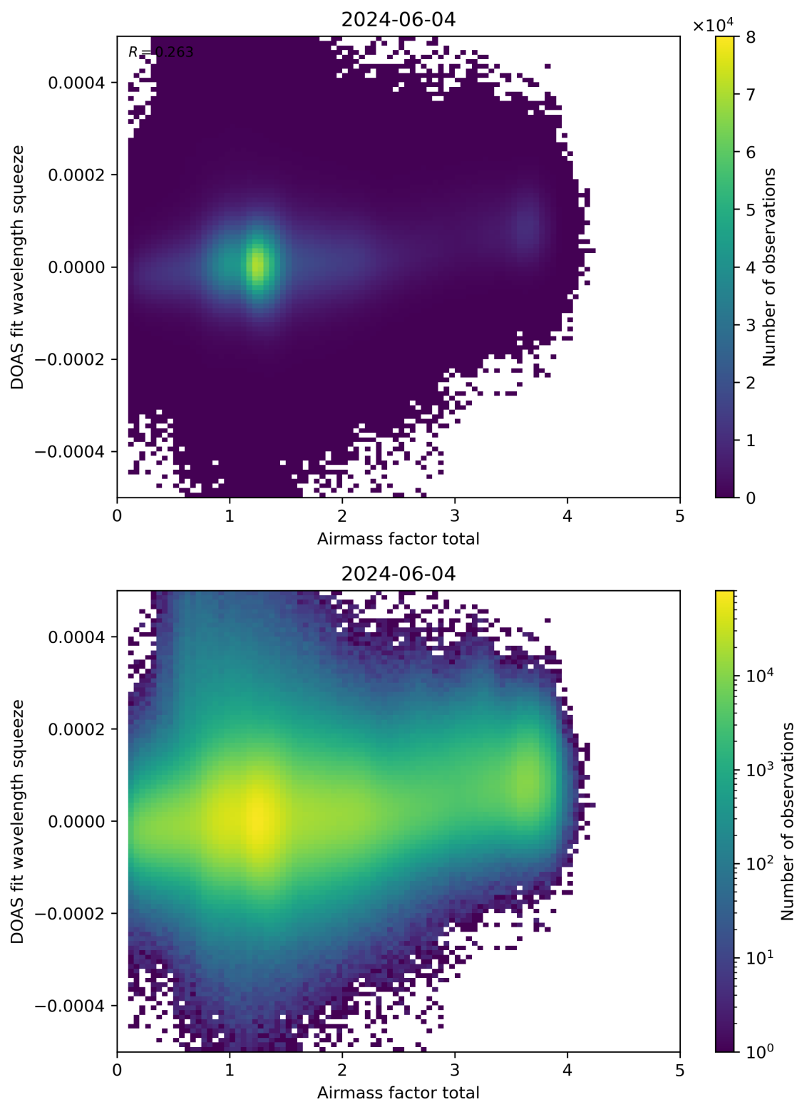
Figure 99: Scatter density plot of “Airmass factor total” against “DOAS fit wavelength squeeze” for 2024-06-03 to 2024-06-05.
