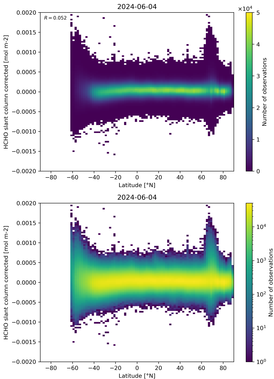
Figure 157: Scatter density plot of “Latitude” against “HCHO slant column corrected” for 2024-06-03 to 2024-06-05.
