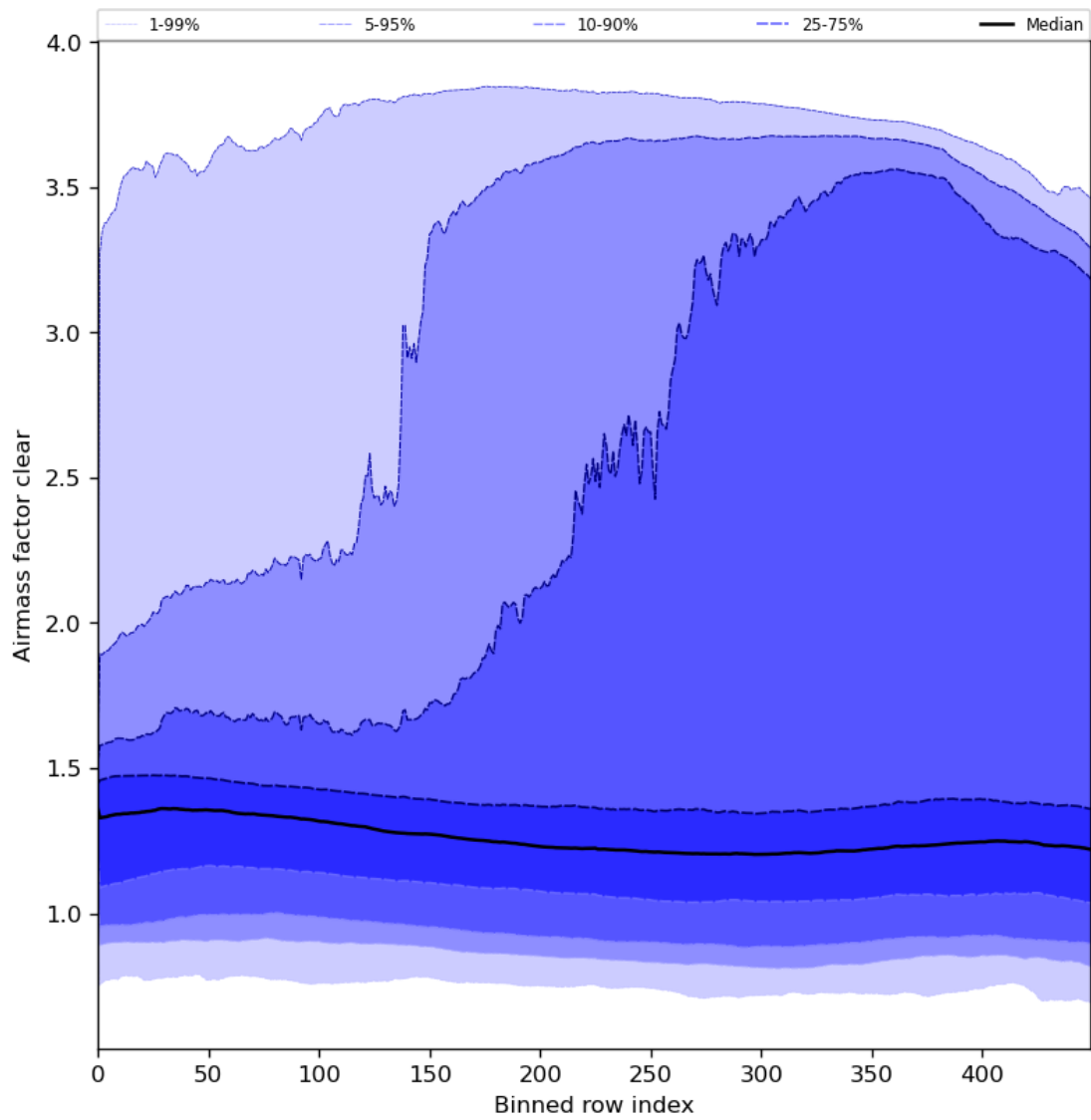
Figure 56: Along track statistics of “Airmass factor clear” for 2024-06-03 to 2024-06-05
