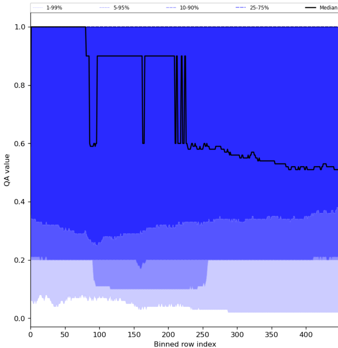
Figure 48: Along track statistics of “QA value” for 2024-06-03 to 2024-06-05
