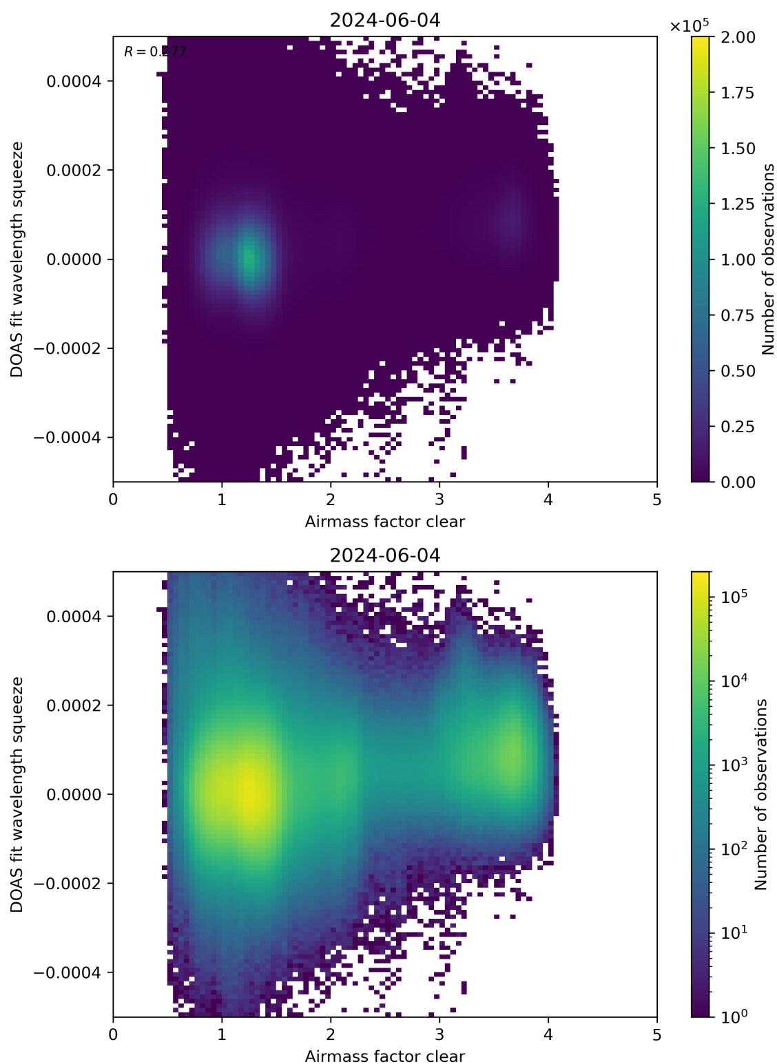
Figure 73: Scatter density plot of “Airmass factor clear” against “DOAS fit wavelength squeeze” for 2024-06-03 to 2024-06-05.
