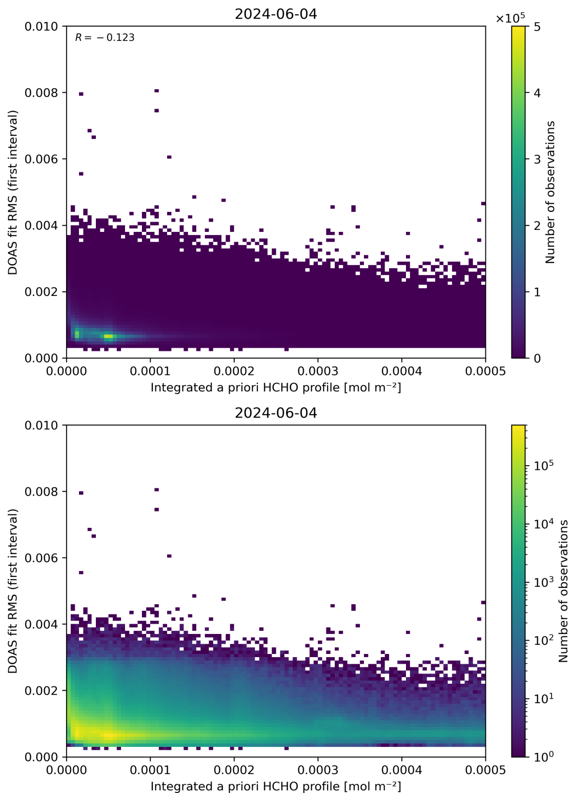
Figure 148: Scatter density plot of “Integrated a priori HCHO profile” against “DOAS fit RMS (first interval)” for 2024-06-03 to 2024-06-05.
