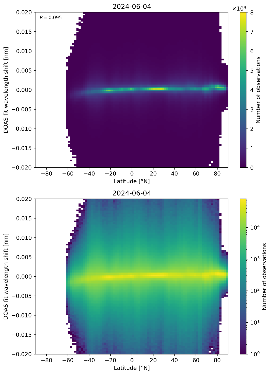
Figure 154: Scatter density plot of “Latitude” against “DOAS fit wavelength shift” for 2024-06-03 to 2024-06-05.
