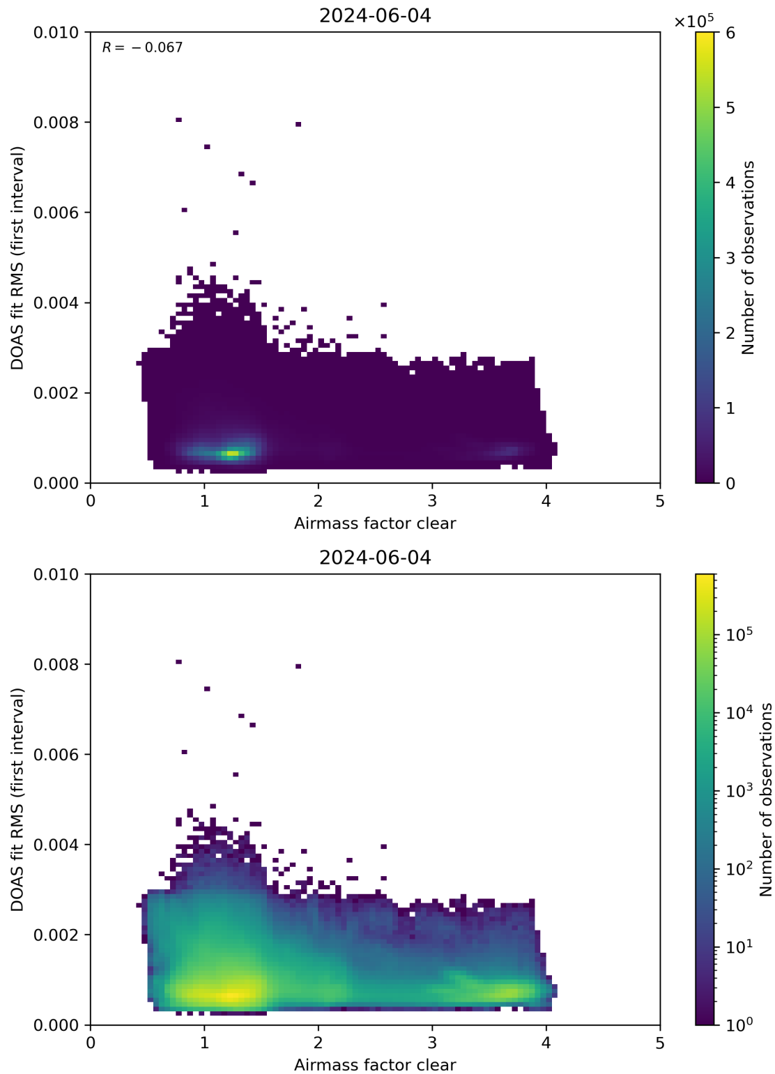
Figure 71: Scatter density plot of “Airmass factor clear” against “DOAS fit RMS (first interval)” for 2024-06-03 to 2024-06-05.
