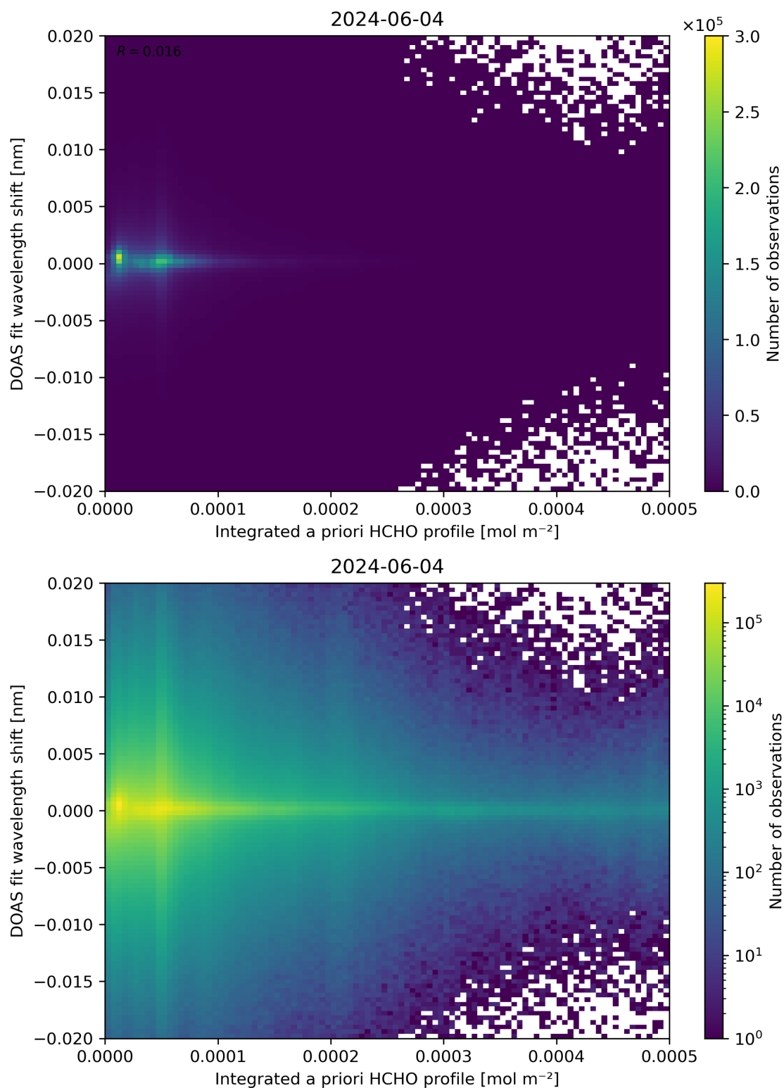
Figure 149: Scatter density plot of “Integrated a priori HCHO profile” against “DOAS fit wavelength shift” for 2024-06-03 to 2024-06-05.
