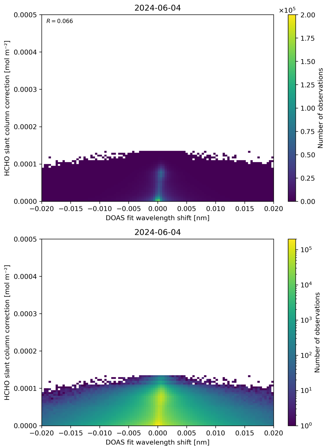
Figure 67: Scatter density plot of “DOAS fit wavelength shift” against “HCHO slant column correction” for 2024-06-03 to 2024-06-05.
