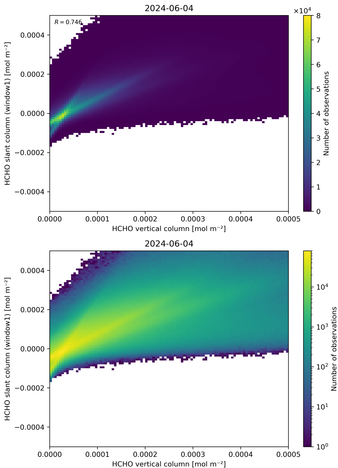
Figure 129: Scatter density plot of “HCHO vertical column” against “HCHO slant column (window1)” for 2024-06-03 to 2024-06-05.
