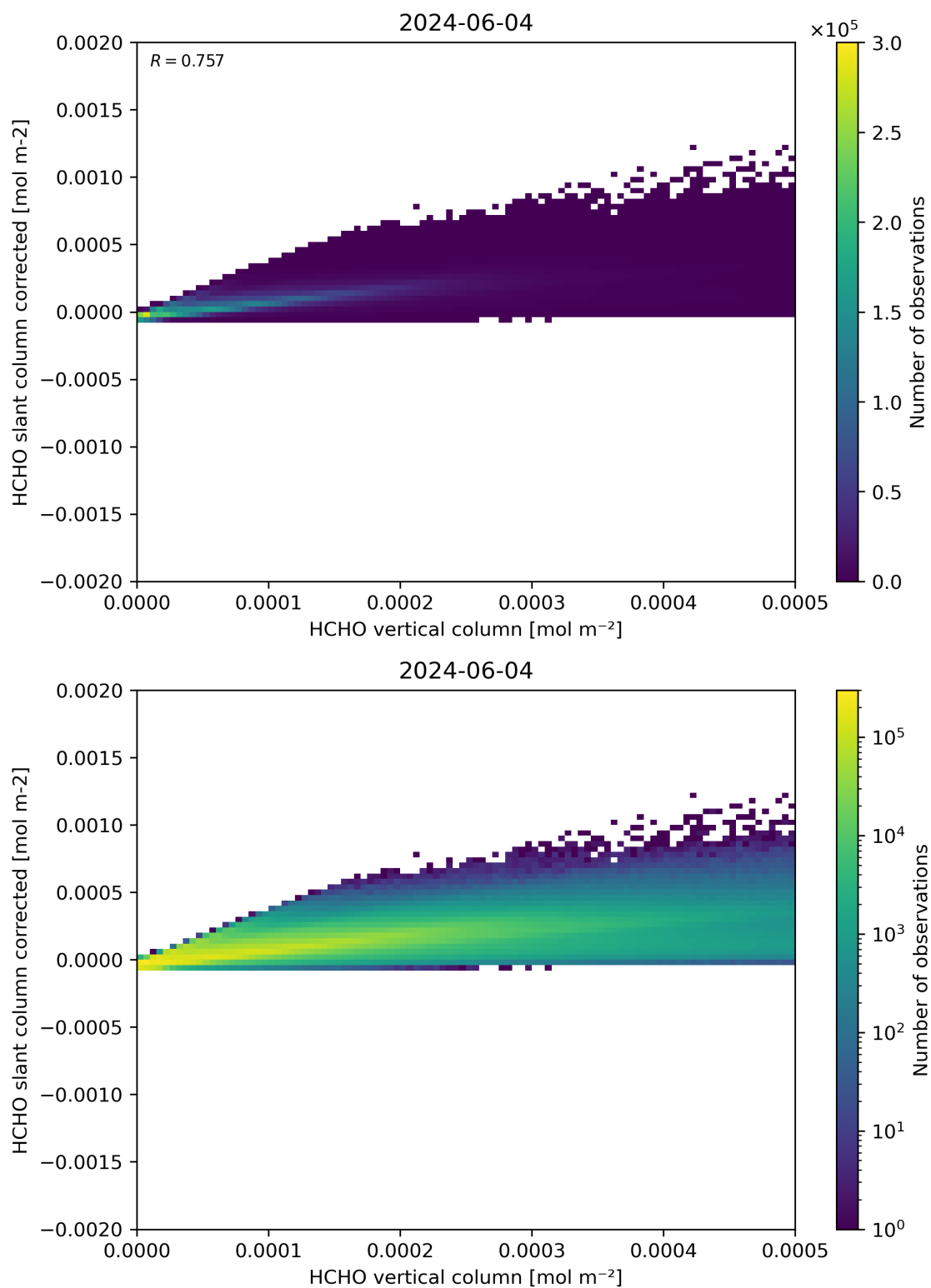
Figure 127: Scatter density plot of “HCHO vertical column” against “HCHO slant column corrected” for 2024-06-03 to 2024-06-05.
