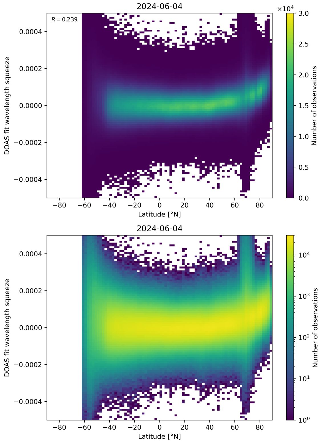
Figure 155: Scatter density plot of “Latitude” against “DOAS fit wavelength squeeze” for 2024-06-03 to 2024-06-05.
