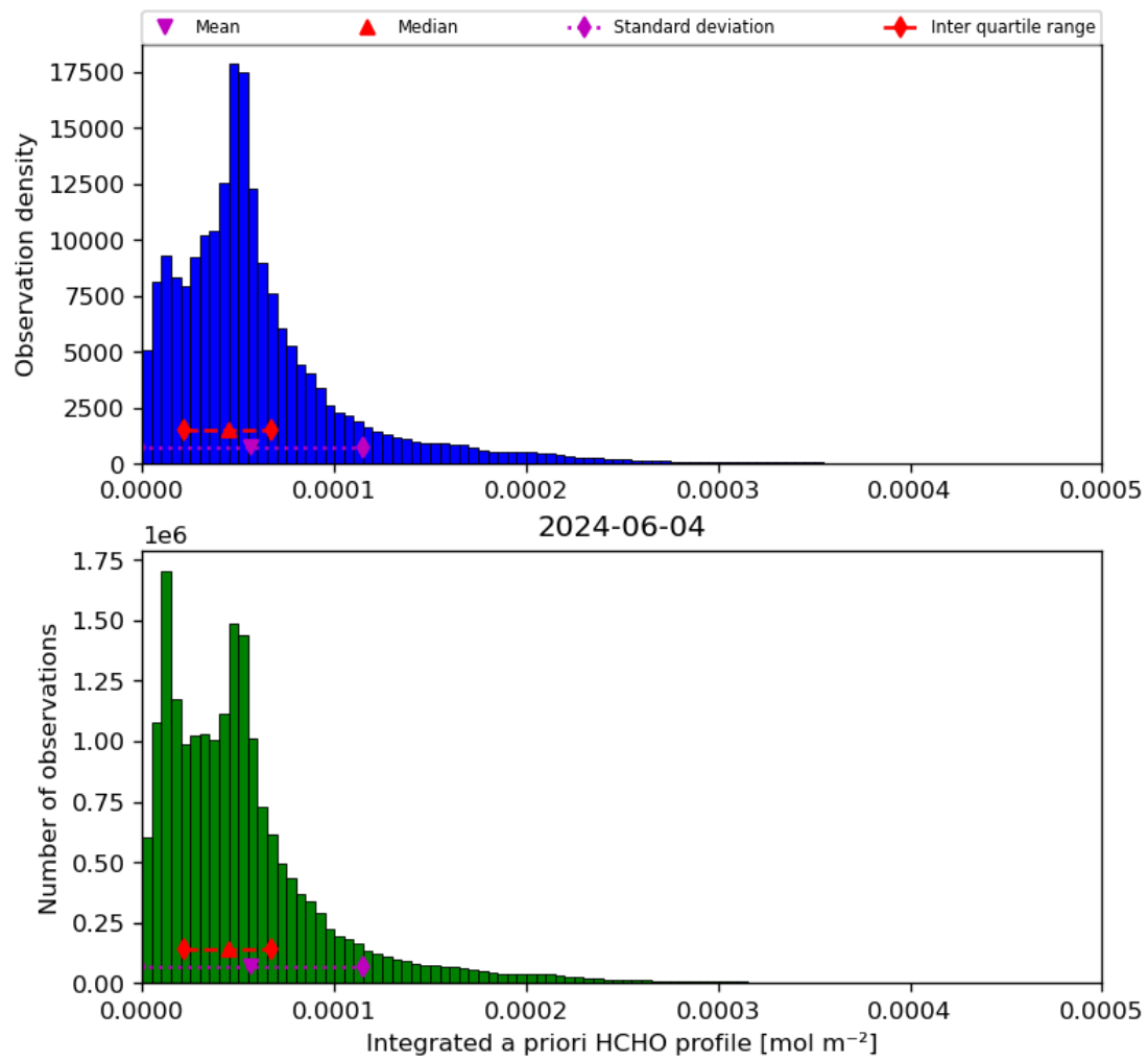
Figure 43: Histogram of “Integrated a priori HCHO profile” for 2024-06-03 to 2024-06-05
