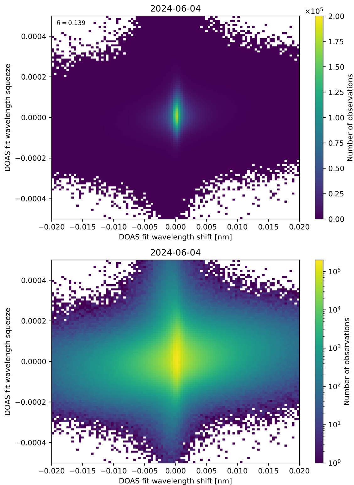
Figure 65: Scatter density plot of “DOAS fit wavelength shift” against “DOAS fit wavelength squeeze” for 2024-06-03 to 2024-06-05.
