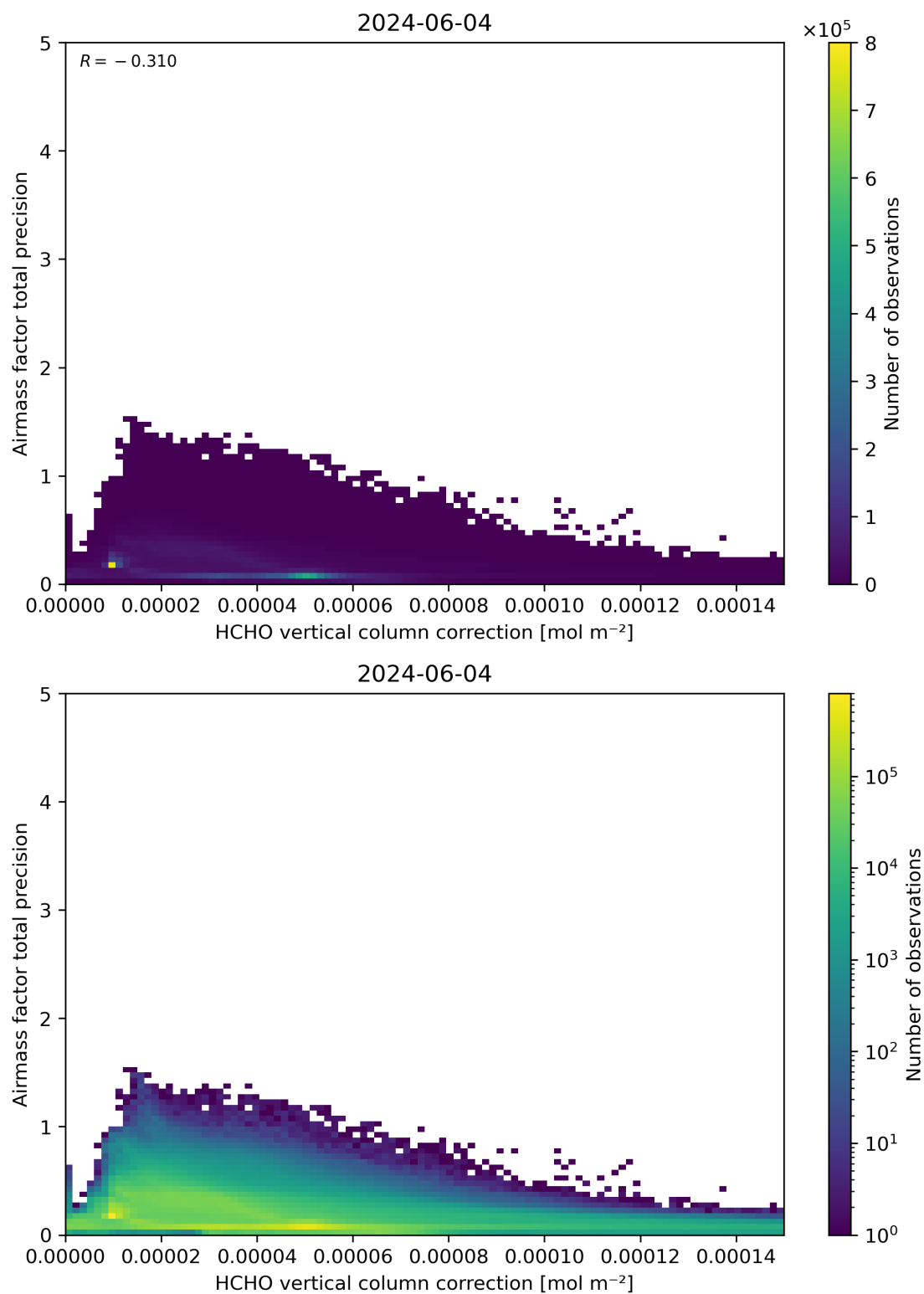
Figure 121: Scatter density plot of “HCHO vertical column correction” against “Airmass factor total precision” for 2024-06-03 to 2024-06-05.
