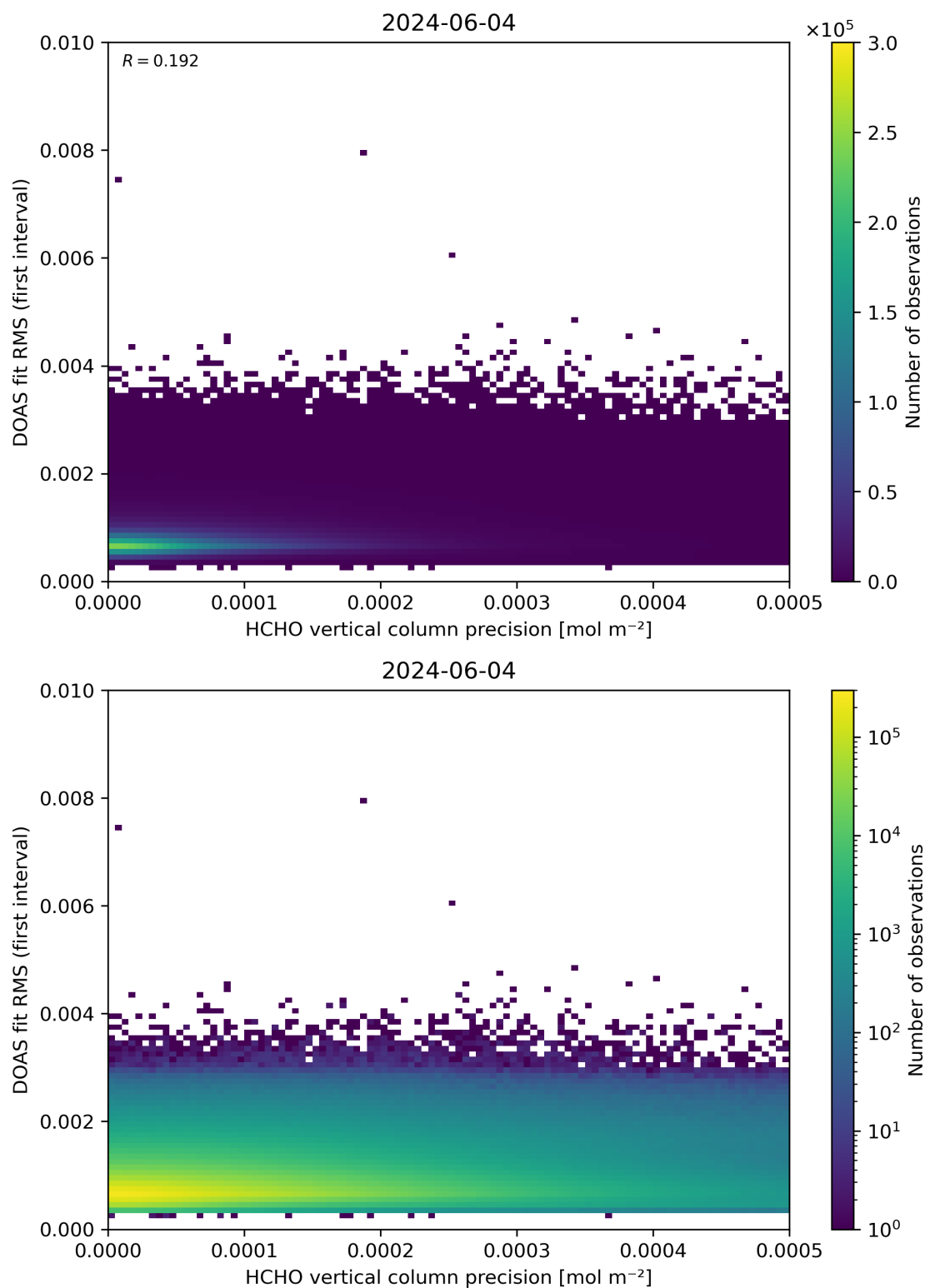
Figure 136: Scatter density plot of “HCHO vertical column precision” against “DOAS fit RMS (first interval)” for 2024-06-03 to 2024-06-05.
