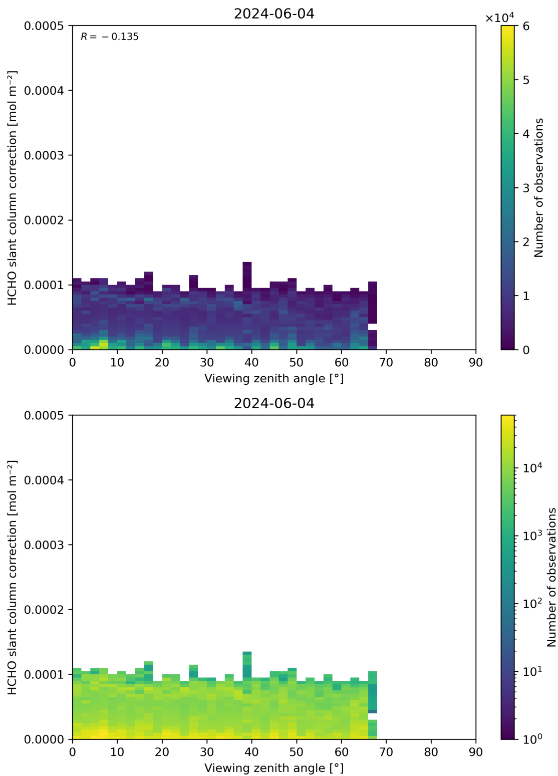
Figure 187: Scatter density plot of “Viewing zenith angle” against “HCHO slant column correction” for 2024-06-03 to 2024-06-05.
