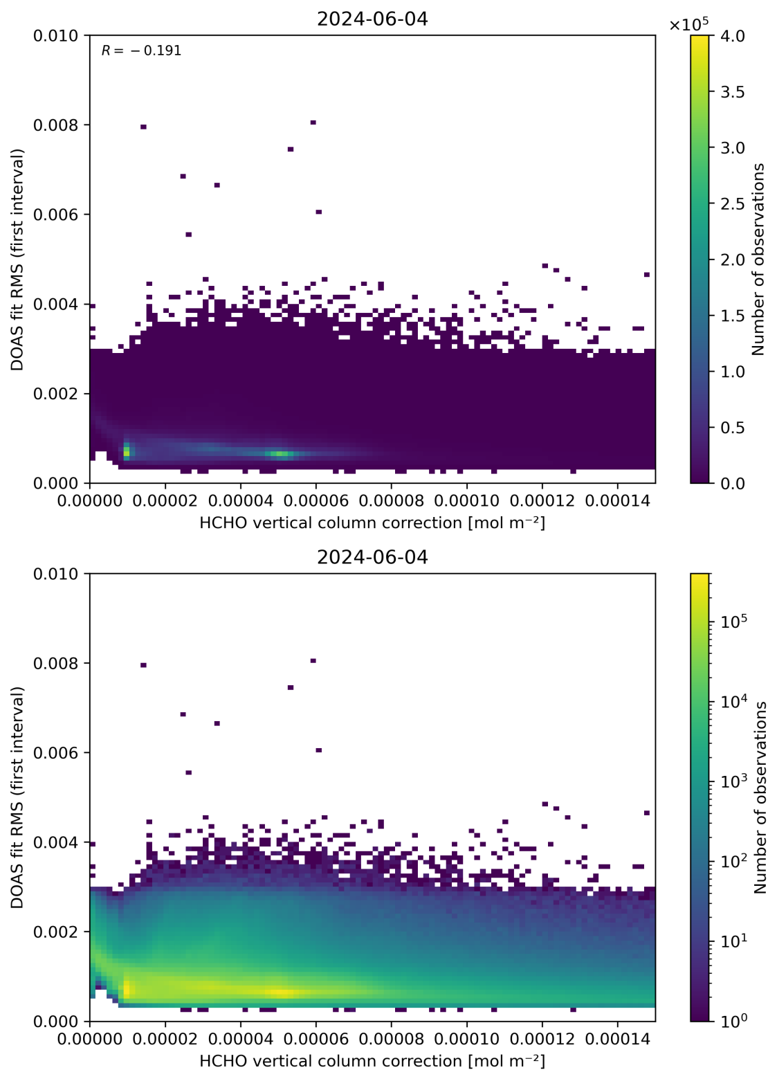
Figure 112: Scatter density plot of “HCHO vertical column correction” against “DOAS fit RMS (first interval)” for 2024-06-03 to 2024-06-05.
