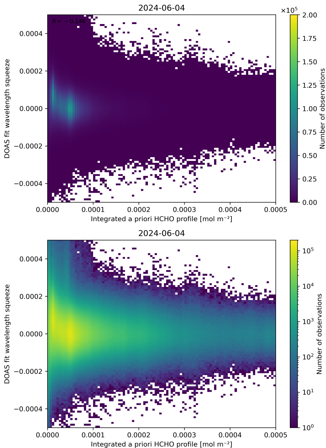
Figure 150: Scatter density plot of “Integrated a priori HCHO profile” against “DOAS fit wavelength squeeze” for 2024-06-03 to 2024-06-05.
