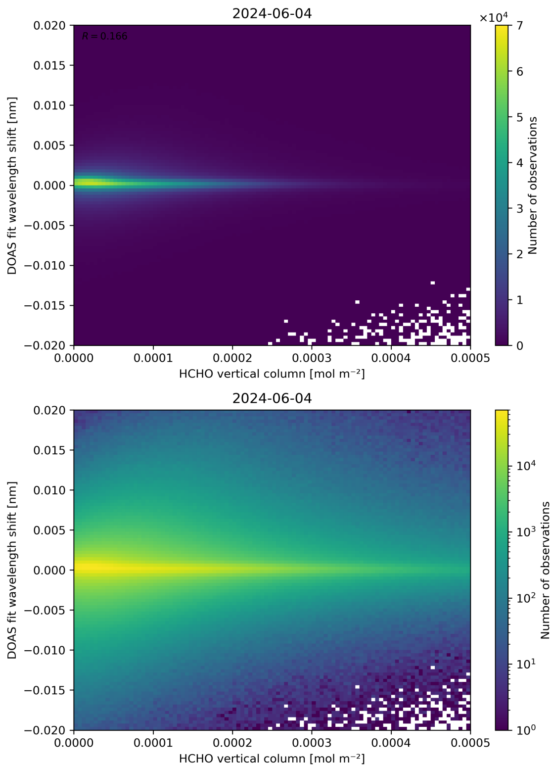
Figure 124: Scatter density plot of “HCHO vertical column” against “DOAS fit wavelength shift” for 2024-06-03 to 2024-06-05.
