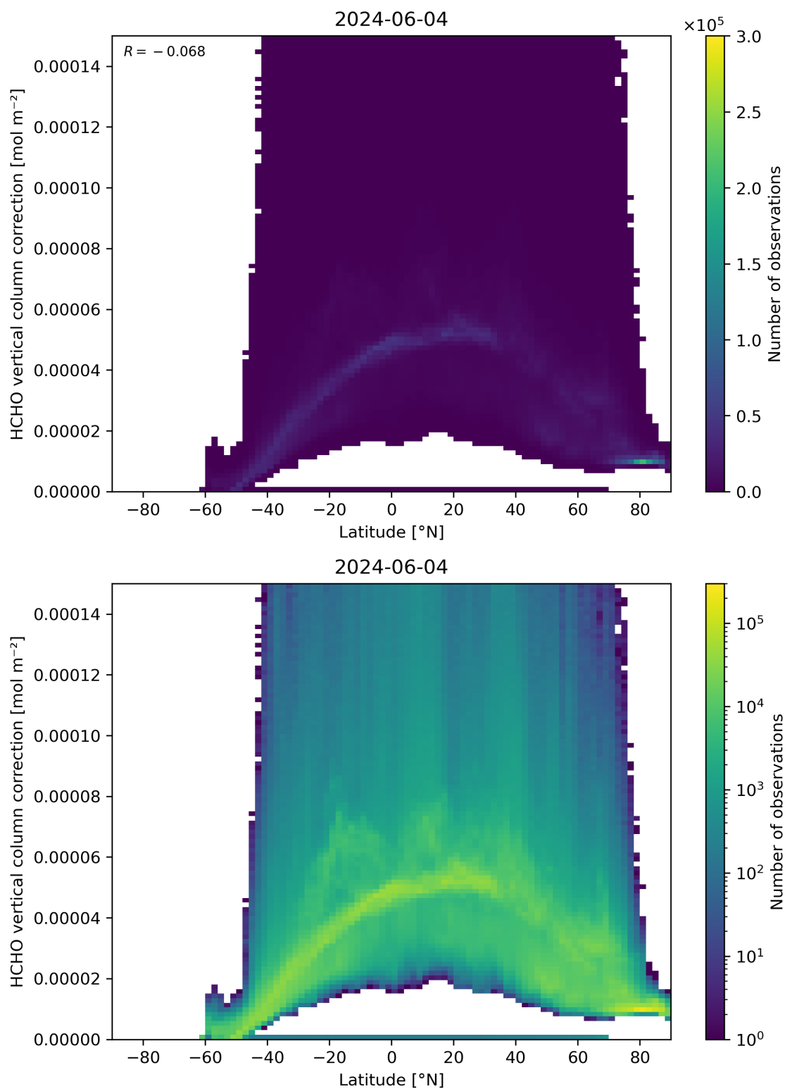
Figure 164: Scatter density plot of “Latitude” against “HCHO vertical column correction” for 2024-06-03 to 2024-06-05.
