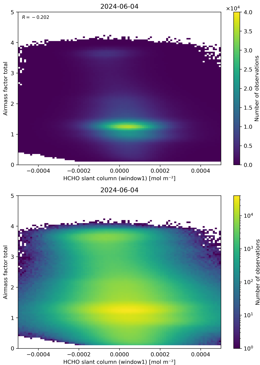
Figure 85: Scatter density plot of “HCHO slant column (window1)” against “Airmass factor total” for 2024-06-03 to 2024-06-05.
