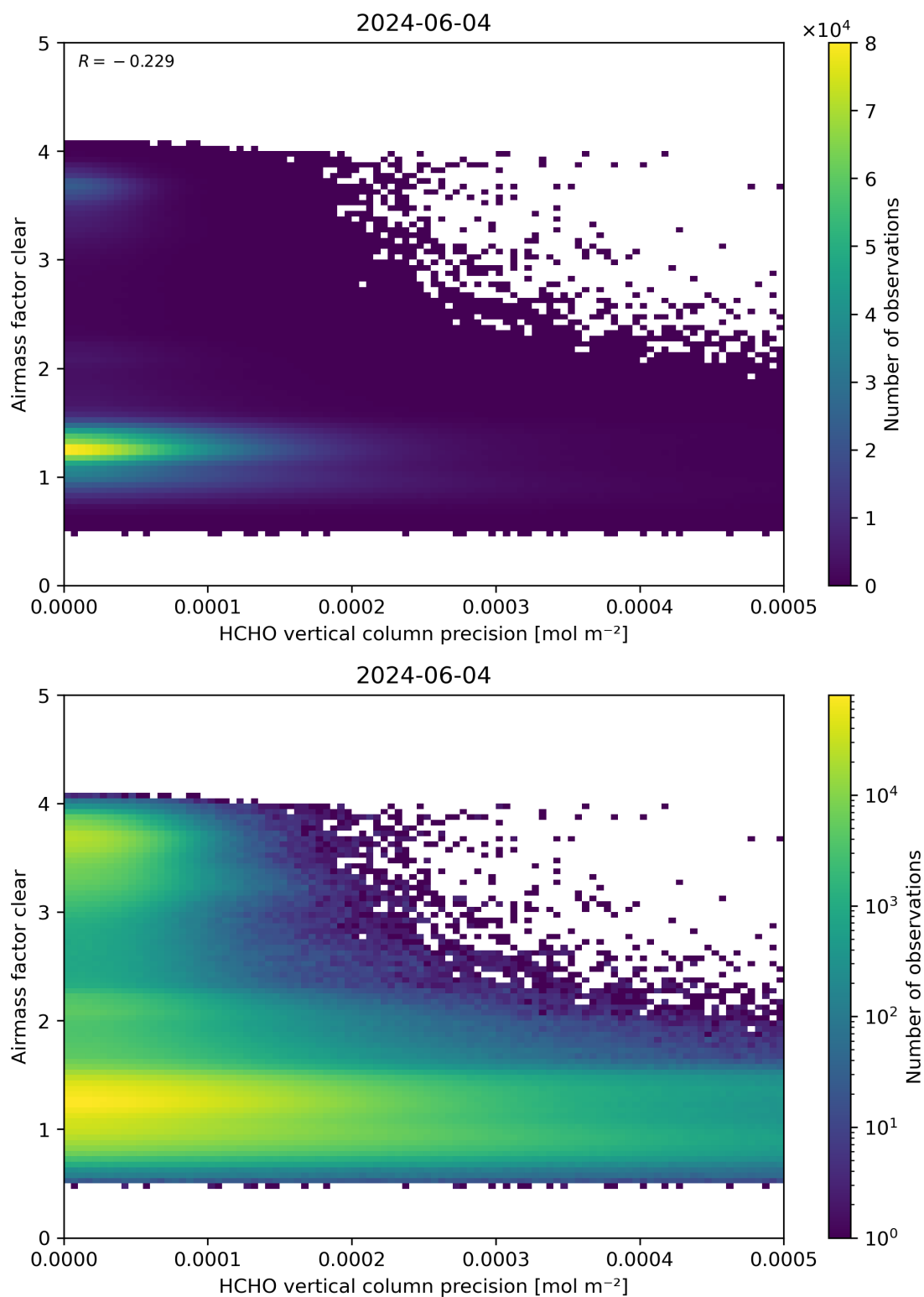
Figure 139: Scatter density plot of “HCHO vertical column precision” against “Airmass factor clear” for 2024-06-03 to 2024-06-05.
