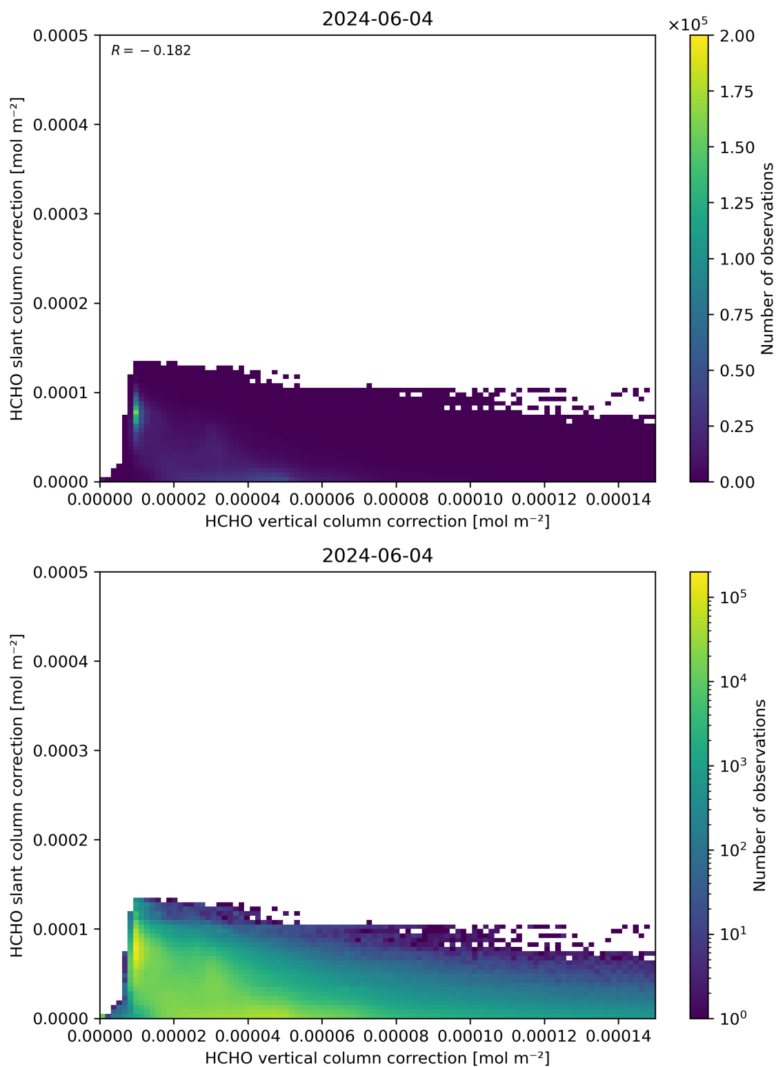
Figure 117: Scatter density plot of “HCHO vertical column correction” against “HCHO slant column correction” for 2024-06-03 to 2024-06-05.
