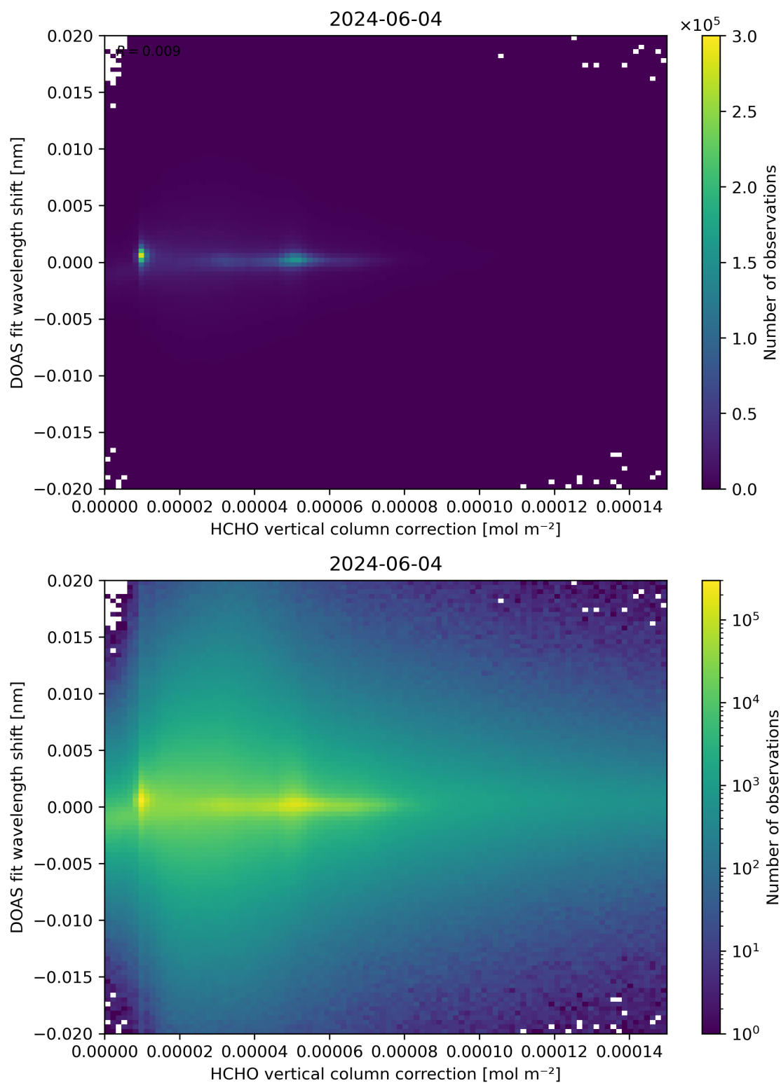
Figure 113: Scatter density plot of “HCHO vertical column correction” against “DOAS fit wavelength shift” for 2024-06-03 to 2024-06-05.
