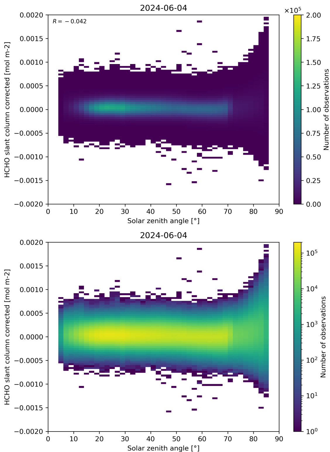
Figure 171: Scatter density plot of “Solar zenith angle” against “HCHO slant column corrected” for 2024-06-03 to 2024-06-05.
