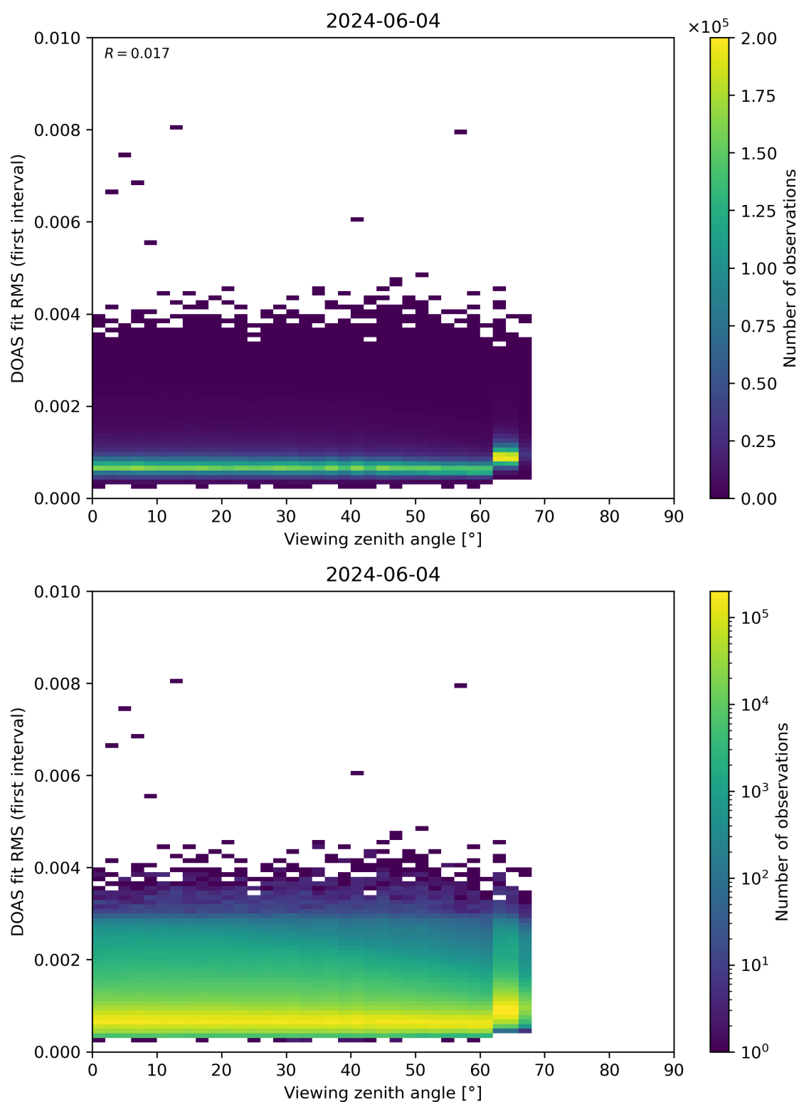
Figure 182: Scatter density plot of “Viewing zenith angle” against “DOAS fit RMS (first interval)” for 2024-06-03 to 2024-06-05.
