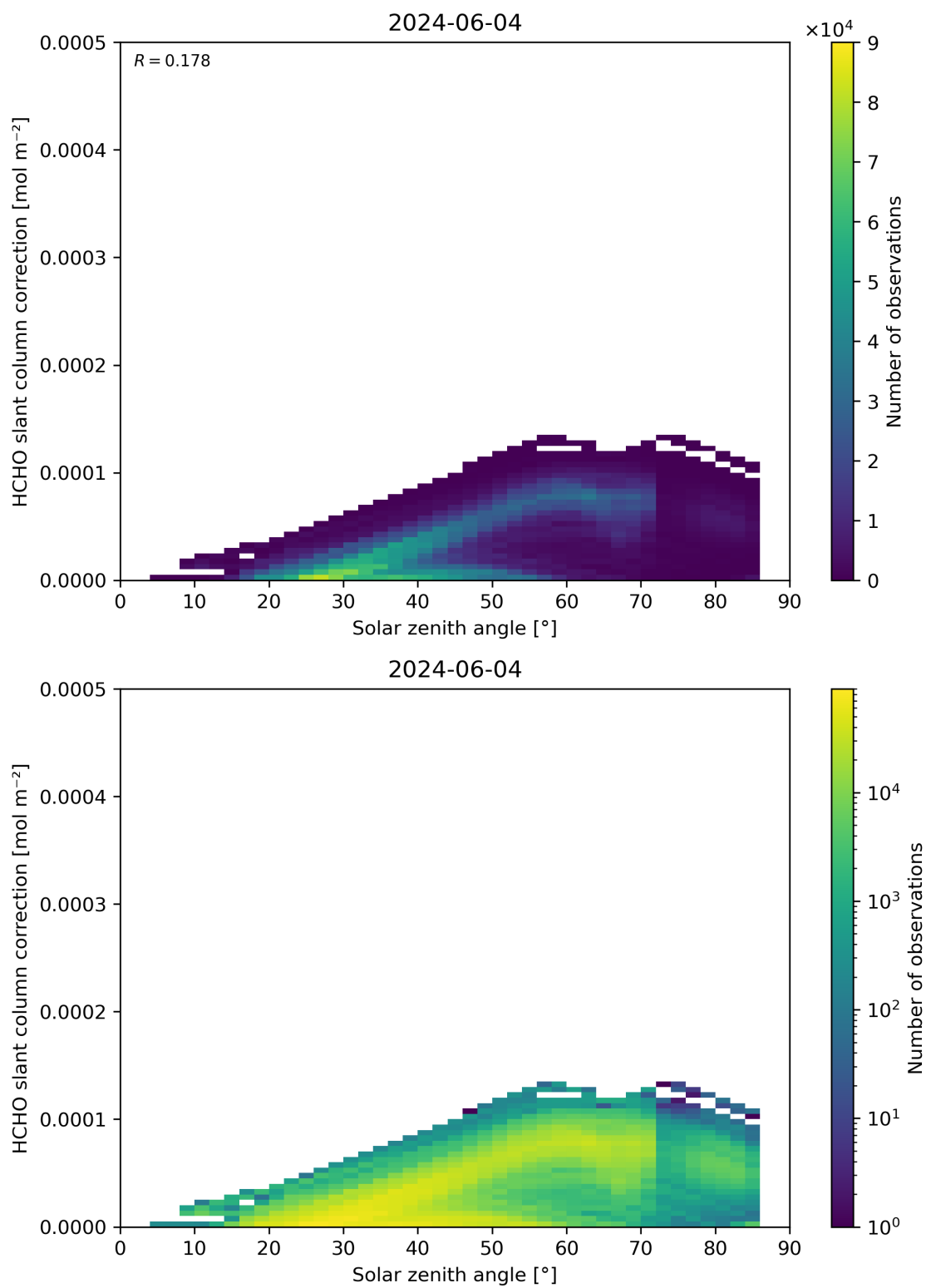
Figure 172: Scatter density plot of “Solar zenith angle” against “HCHO slant column correction” for 2024-06-03 to 2024-06-05.
