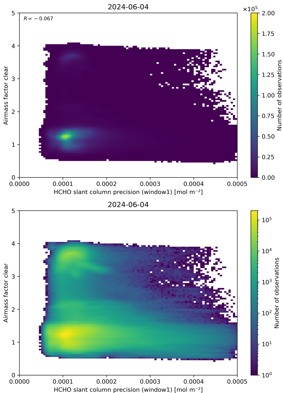
Figure 91: Scatter density plot of “HCHO slant column precision (window1)” against “Airmass factor clear” for 2024-06-03 to 2024-06-05.
