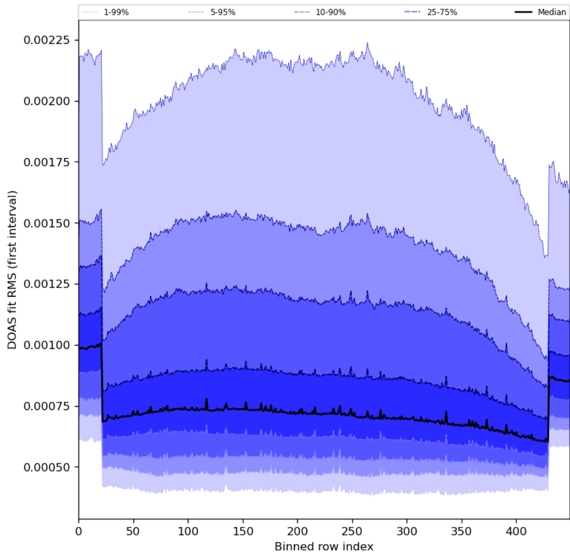
Figure 60: Along track statistics of “DOAS fit RMS (first interval)” for 2024-06-03 to 2024-06-05
