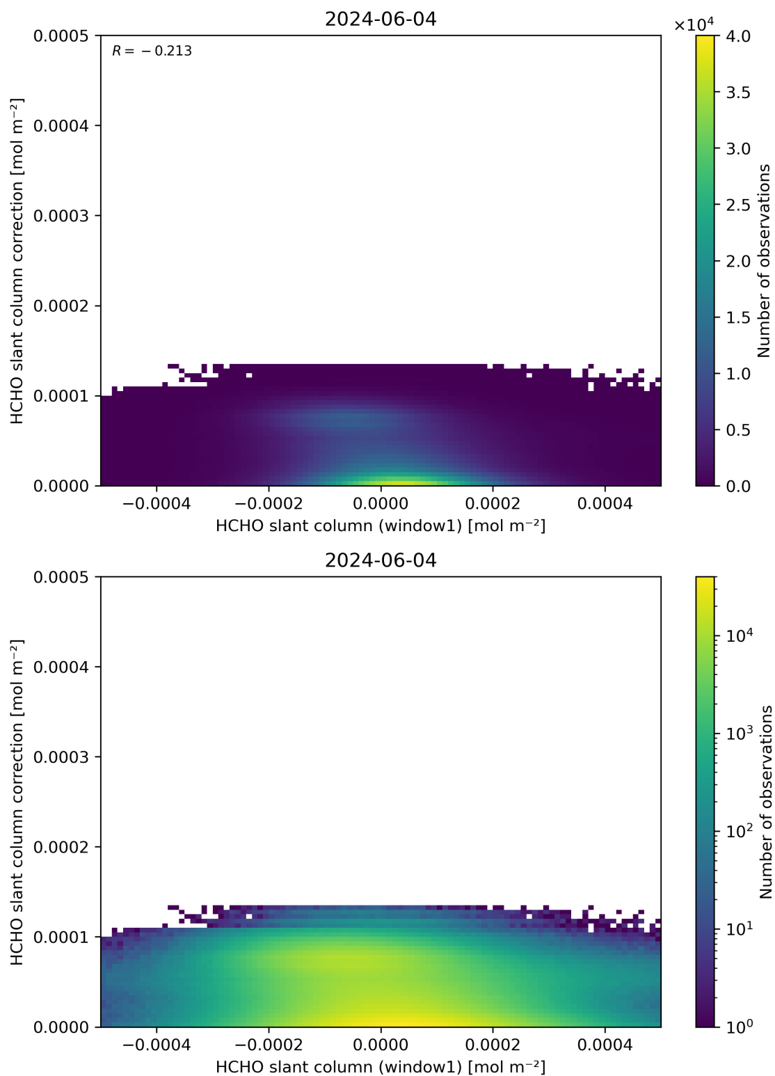
Figure 83: Scatter density plot of “HCHO slant column (window1)” against “HCHO slant column correction” for 2024-06-03 to 2024-06-05.
