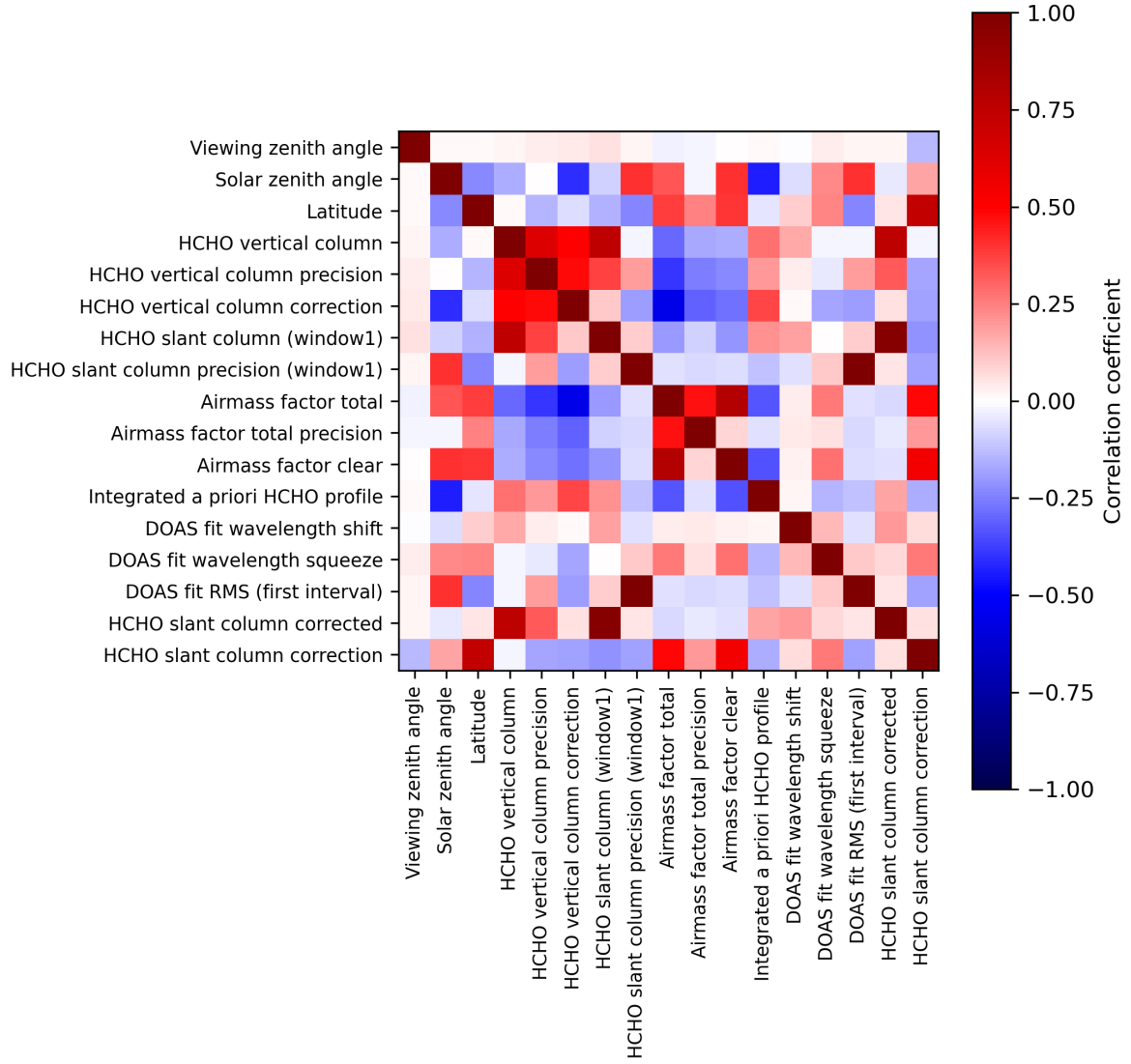
Figure 2: Map of correlation matrix for 2024-06-03 to 2024-06-05.
