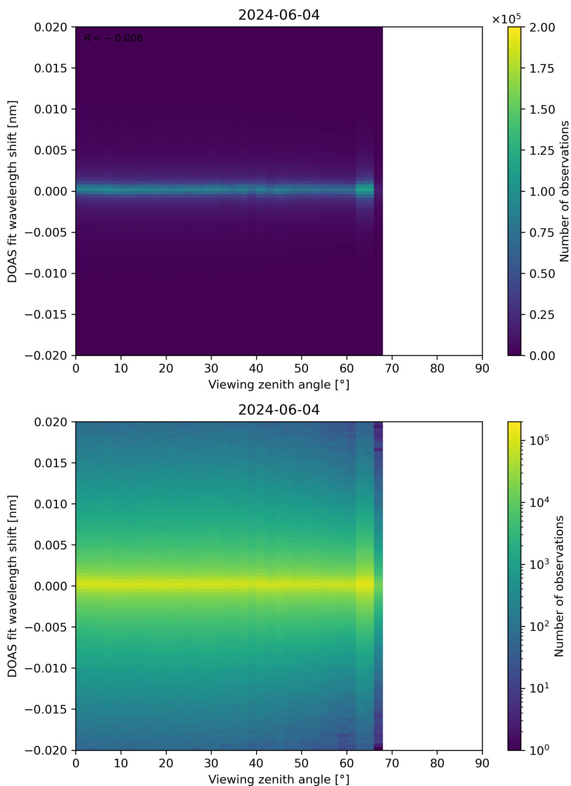
Figure 183: Scatter density plot of “Viewing zenith angle” against “DOAS fit wavelength shift” for 2024-06-03 to 2024-06-05.
