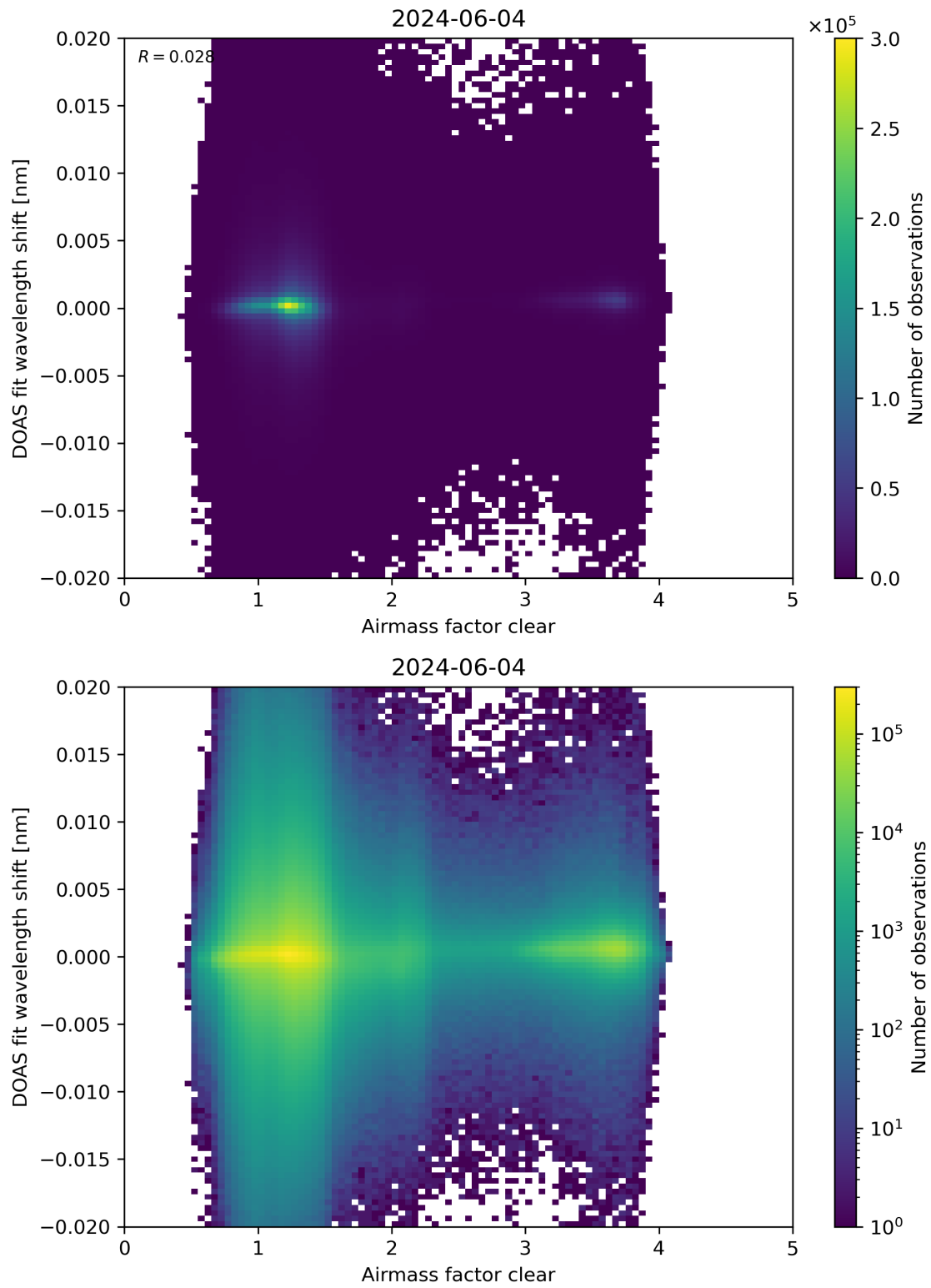
Figure 72: Scatter density plot of “Airmass factor clear” against “DOAS fit wavelength shift” for 2024-06-03 to 2024-06-05.
