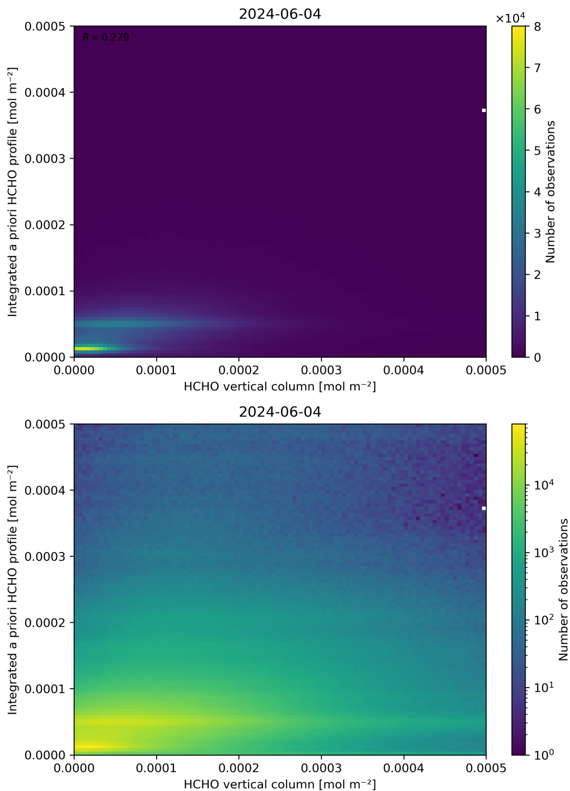
Figure 135: Scatter density plot of “HCHO vertical column” against “Integrated a priori HCHO profile” for 2024-06-03 to 2024-06-05.
