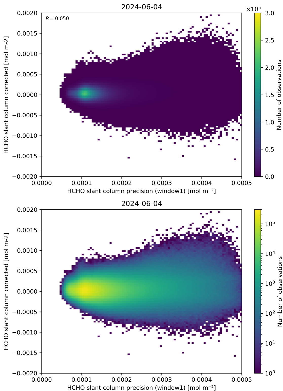
Figure 92: Scatter density plot of “HCHO slant column precision (window1)” against “HCHO slant column corrected” for 2024-06-03 to 2024-06-05.
