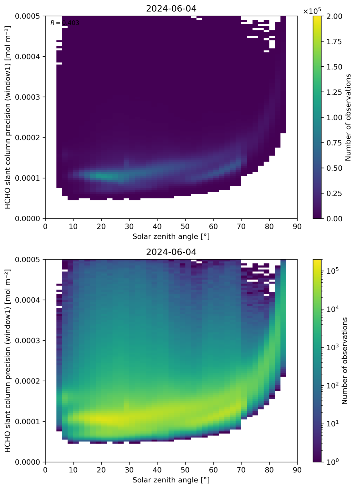
Figure 174: Scatter density plot of “Solar zenith angle” against “HCHO slant column precision (window1)” for 2024-06-03 to 2024-06-05.
