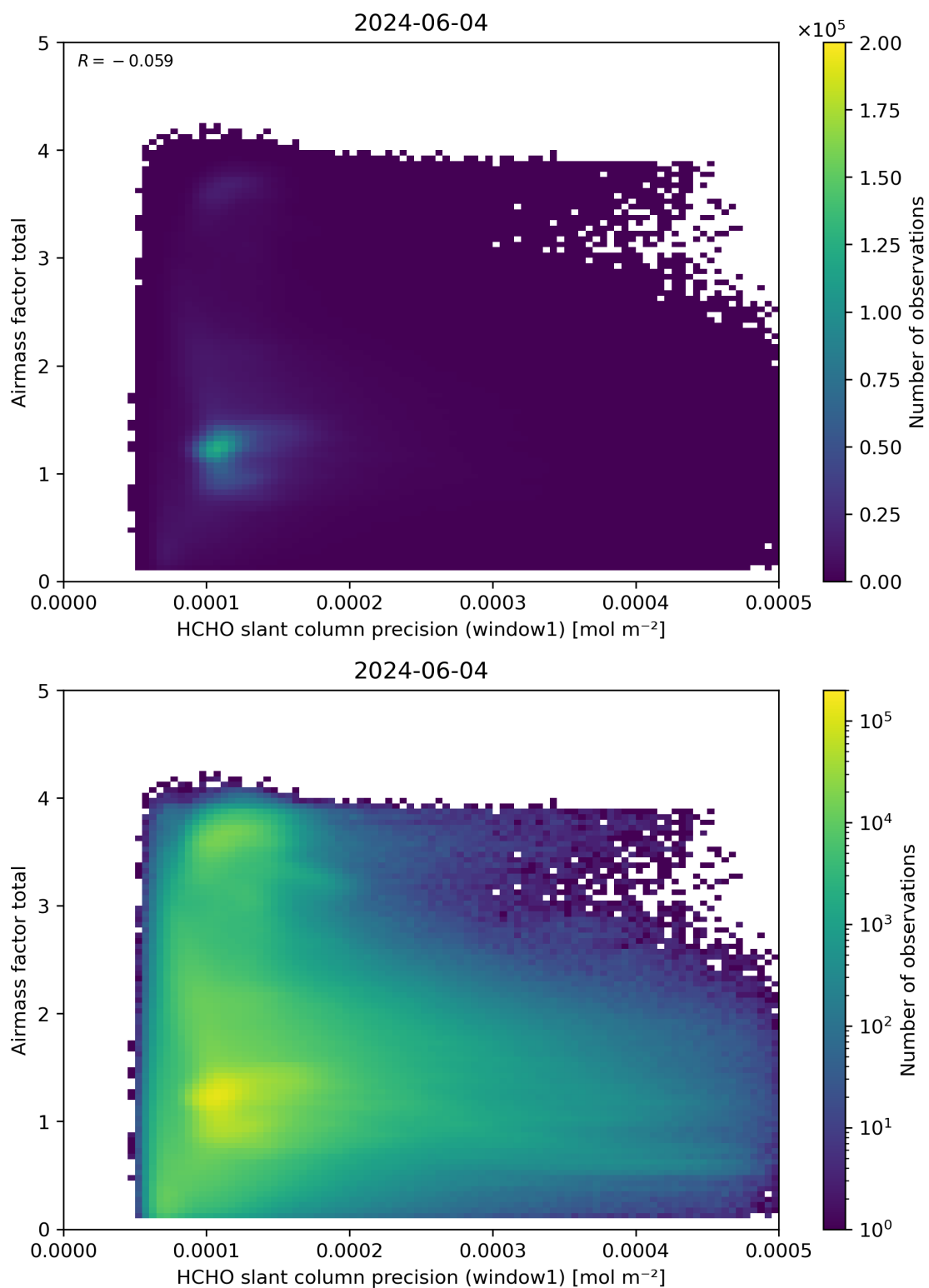
Figure 94: Scatter density plot of “HCHO slant column precision (window1)” against “Airmass factor total” for 2024-06-03 to 2024-06-05.
