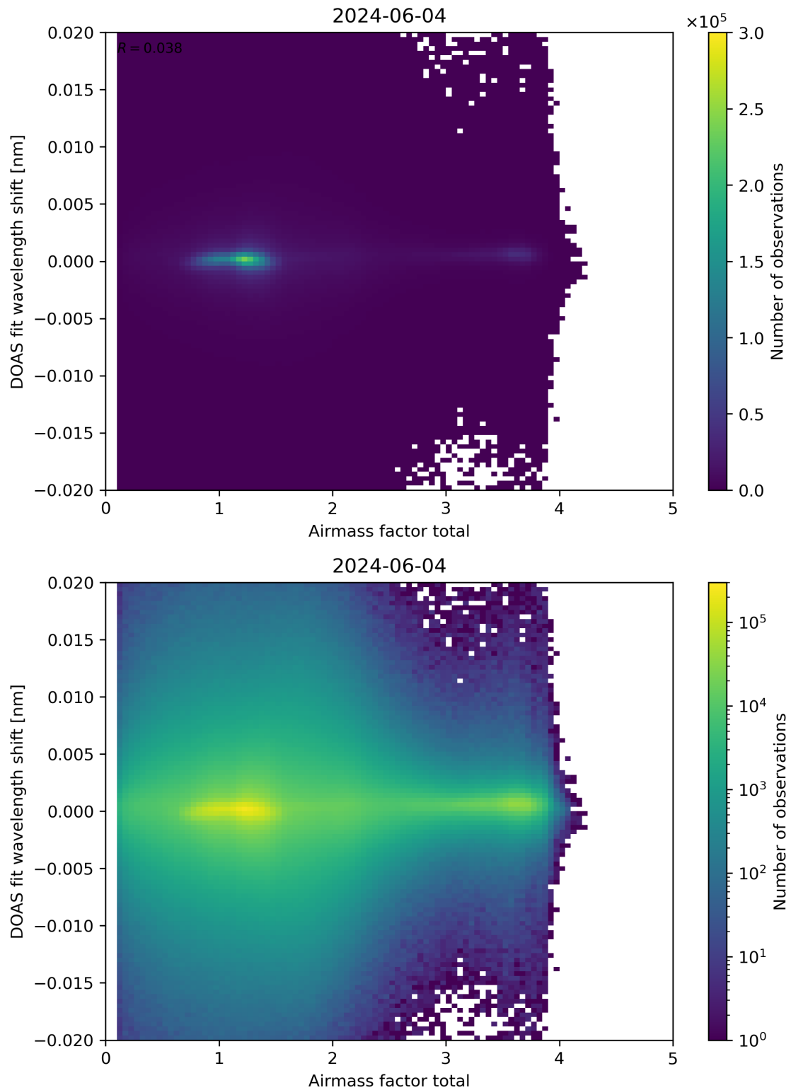
Figure 98: Scatter density plot of “Airmass factor total” against “DOAS fit wavelength shift” for 2024-06-03 to 2024-06-05.
