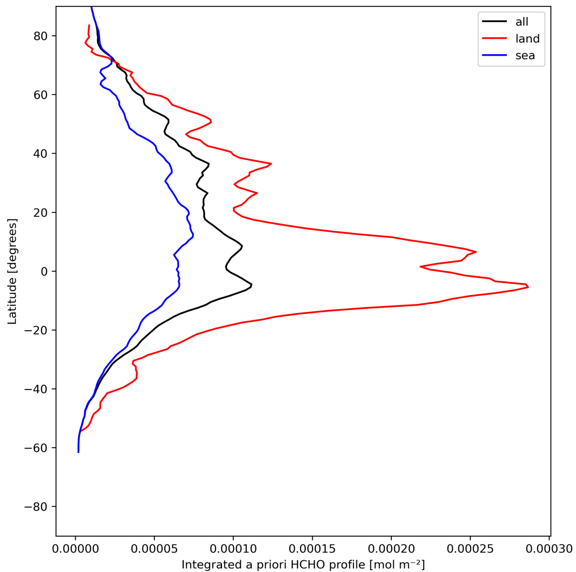
Figure 29: Zonal average of “Integrated a priori HCHO profile” for 2024-06-03 to 2024-06-05.
