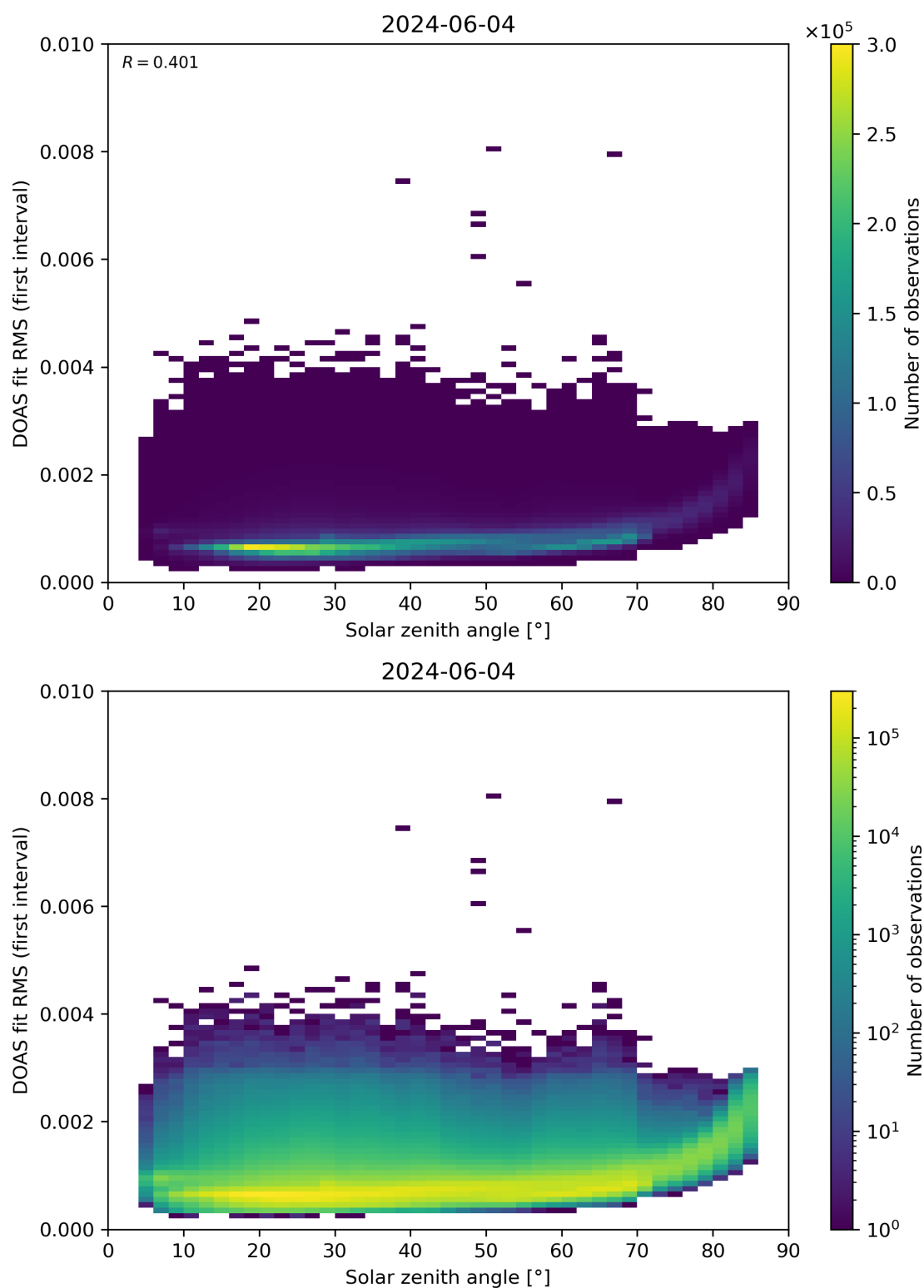
Figure 167: Scatter density plot of “Solar zenith angle” against “DOAS fit RMS (first interval)” for 2024-06-03 to 2024-06-05.
