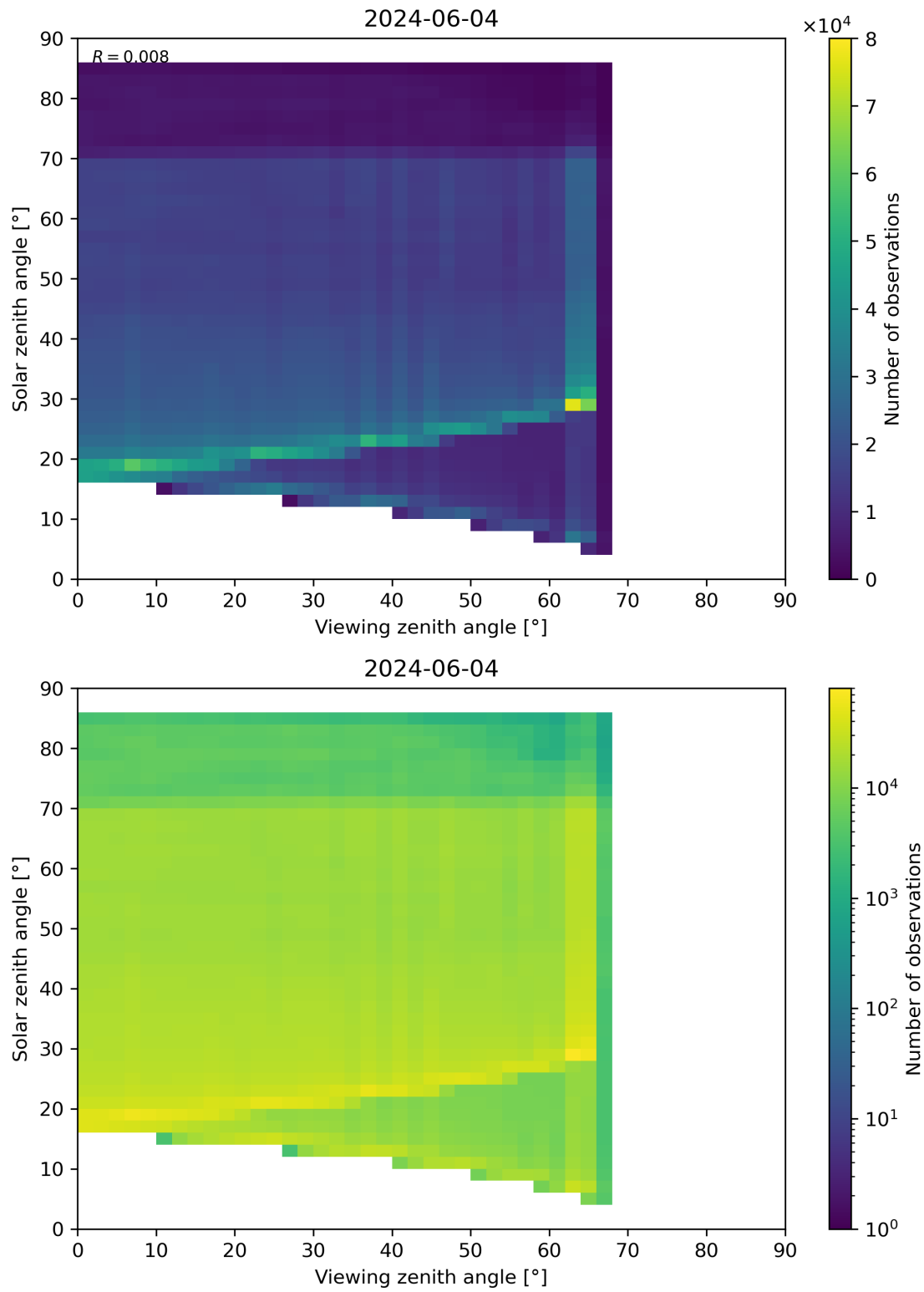
Figure 197: Scatter density plot of “Viewing zenith angle” against “Solar zenith angle” for 2024-06-03 to 2024-06-05.
