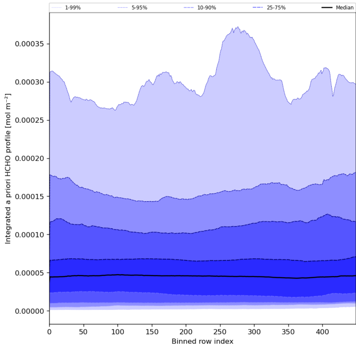
Figure 57: Along track statistics of “Integrated a priori HCHO profile” for 2024-06-03 to 2024-06-05
