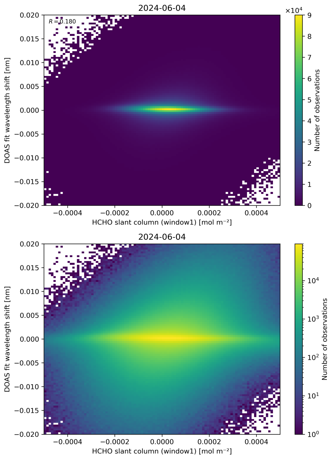
Figure 79: Scatter density plot of “HCHO slant column (window1)” against “DOAS fit wavelength shift” for 2024-06-03 to 2024-06-05.
