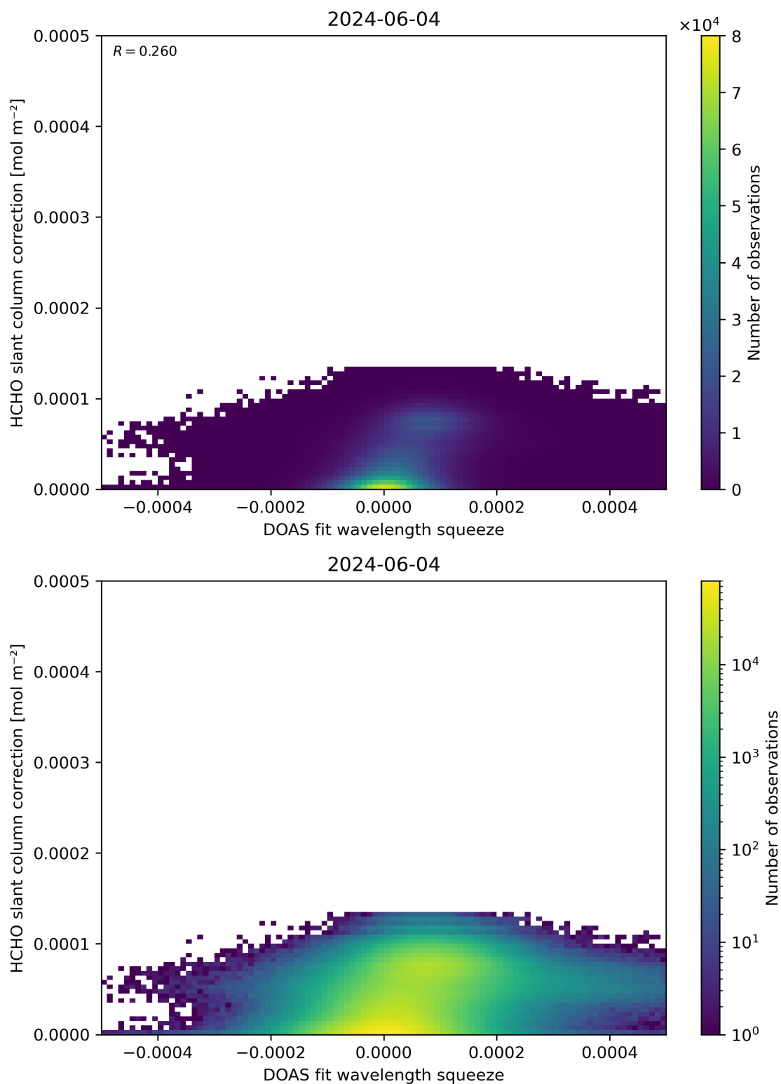
Figure 70: Scatter density plot of “DOAS fit wavelength squeeze” against “HCHO slant column correction” for 2024-06-03 to 2024-06-05.
