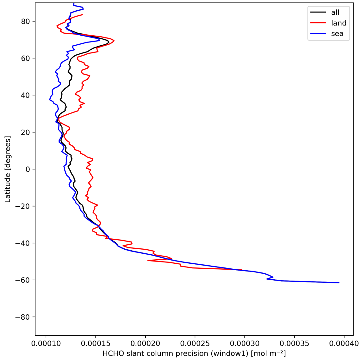
Figure 25: Zonal average of "HCHO slant column precision (window1)" for 2024-06-03 to 2024-06-05.
