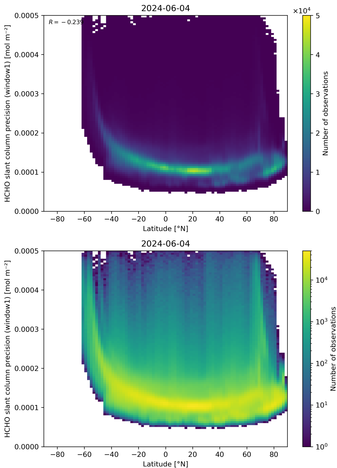
Figure 160: Scatter density plot of “Latitude” against “HCHO slant column precision (window1)” for 2024-06-03 to 2024-06-05.
