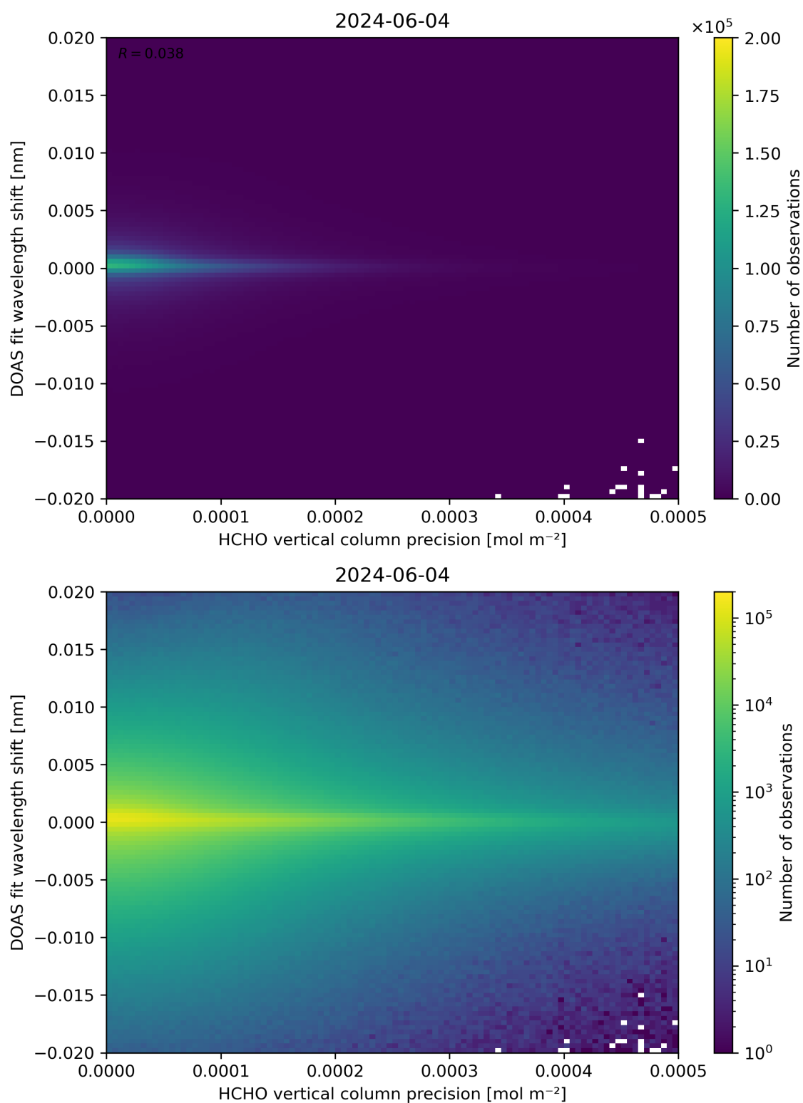
Figure 137: Scatter density plot of “HCHO vertical column precision” against “DOAS fit wavelength shift” for 2024-06-03 to 2024-06-05.
