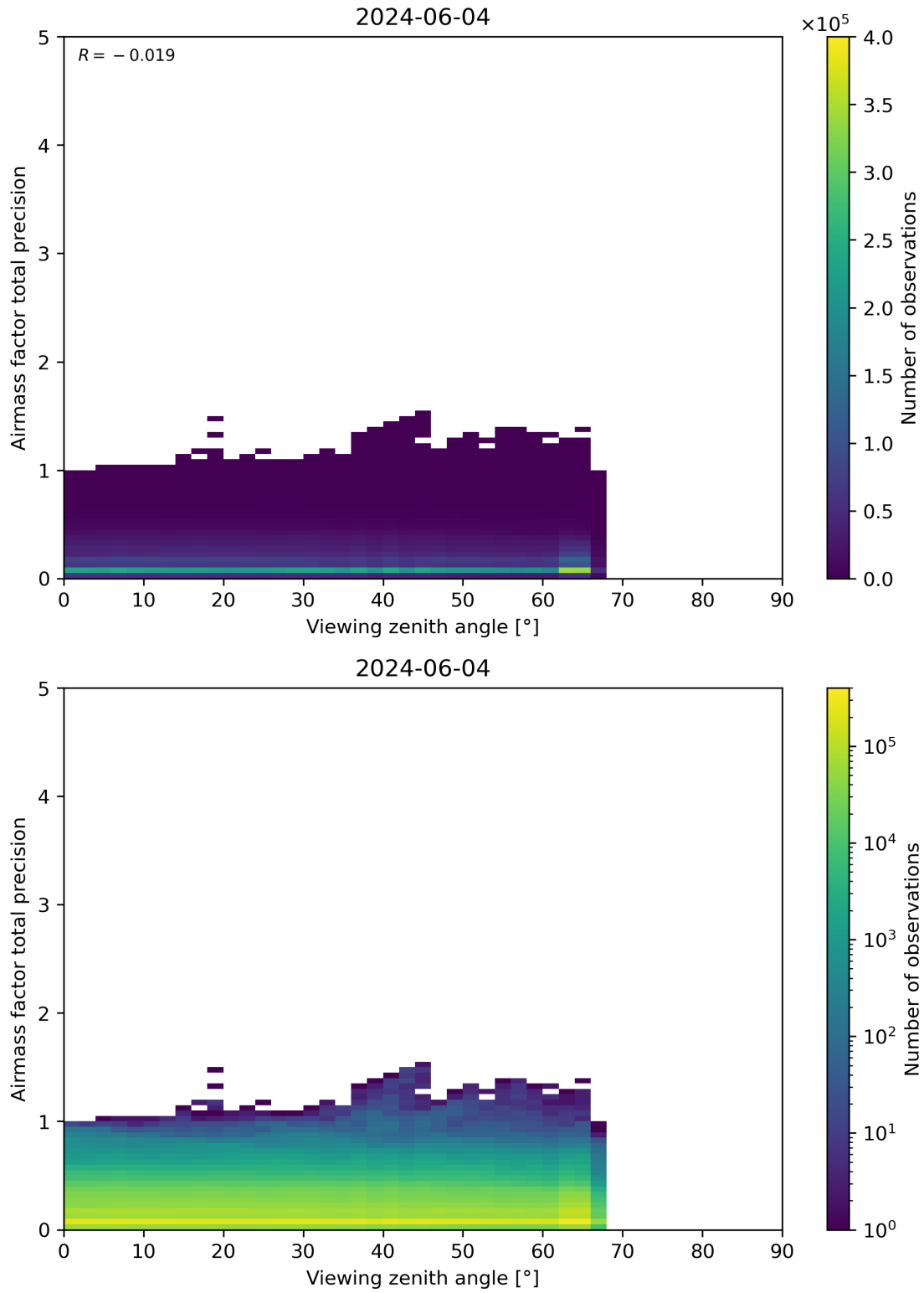
Figure 191: Scatter density plot of “Viewing zenith angle” against “Airmass factor total precision” for 2024-06-03 to 2024-06-05.
