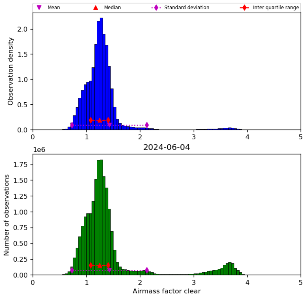
Figure 42: Histogram of “Airmass factor clear” for 2024-06-03 to 2024-06-05
