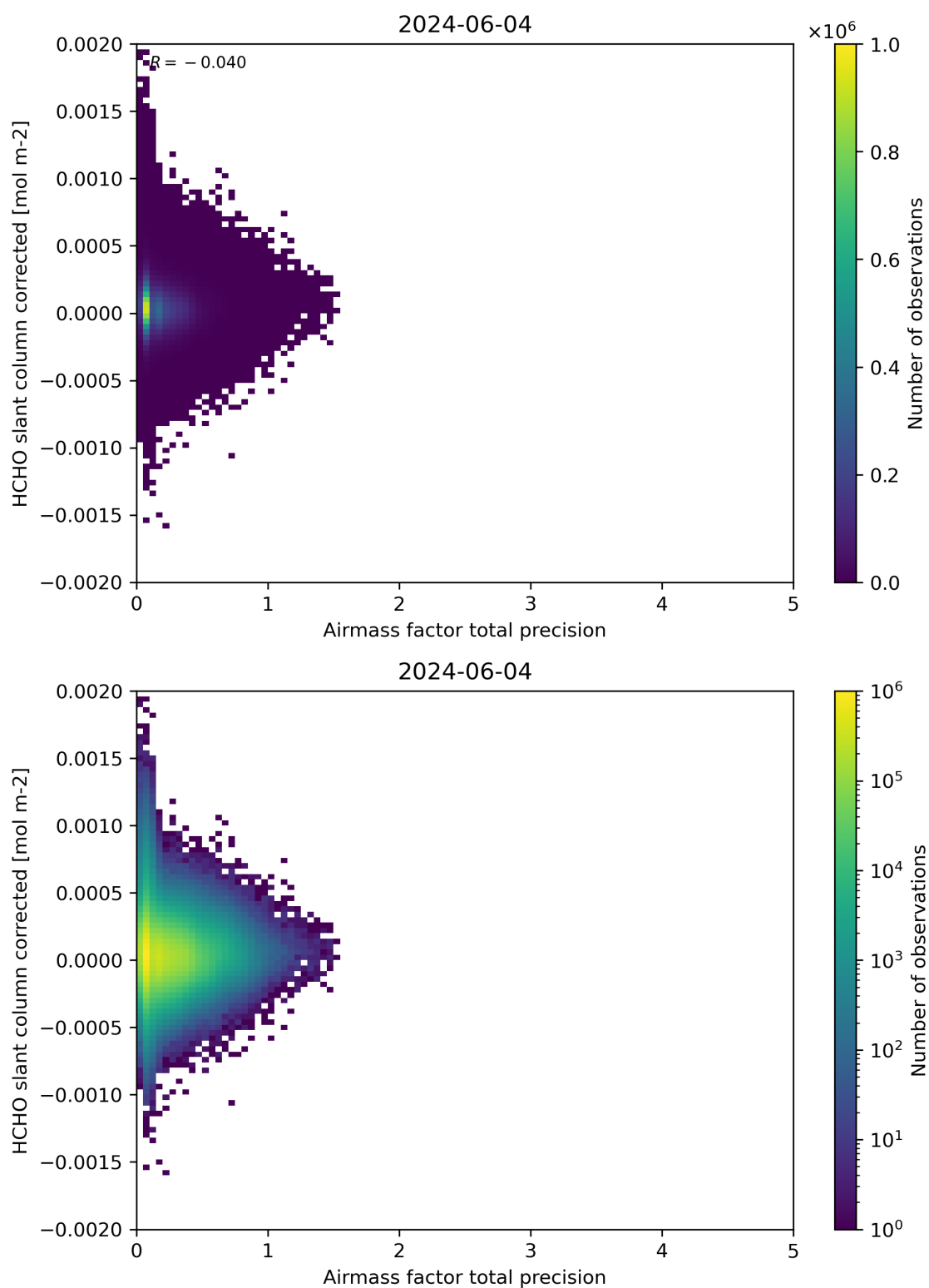
Figure 109: Scatter density plot of “Airmass factor total precision” against “HCHO slant column corrected” for 2024-06-03 to 2024-06-05.
