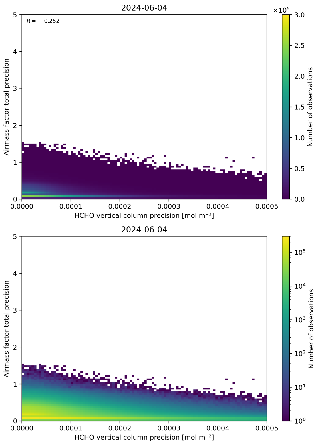
Figure 145: Scatter density plot of “HCHO vertical column precision” against “Airmass factor total precision” for 2024-06-03 to 2024-06-05.
