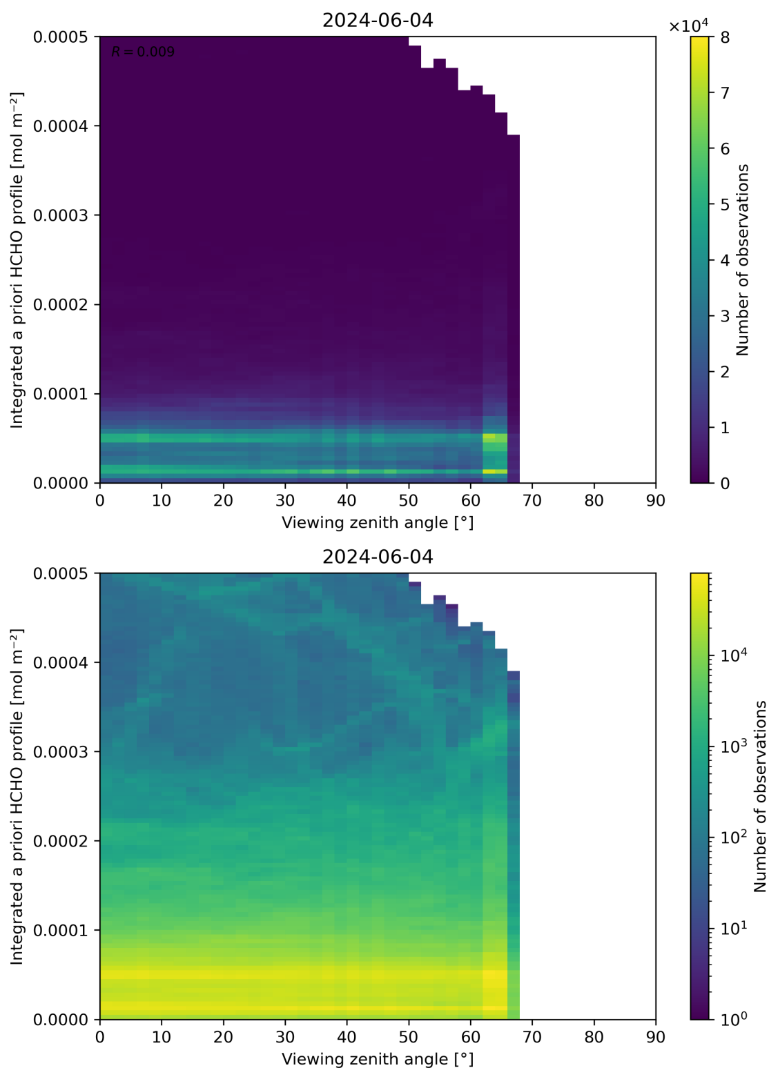
Figure 195: Scatter density plot of “Viewing zenith angle” against “Integrated a priori HCHO profile” for 2024-06-03 to 2024-06-05.
