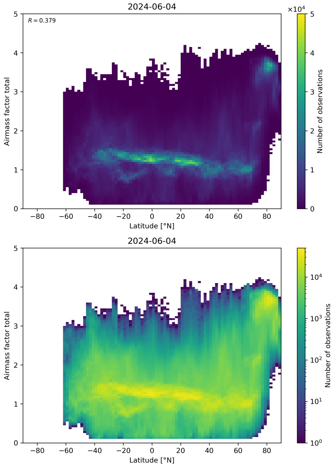
Figure 161: Scatter density plot of “Latitude” against “Airmass factor total” for 2024-06-03 to 2024-06-05.
