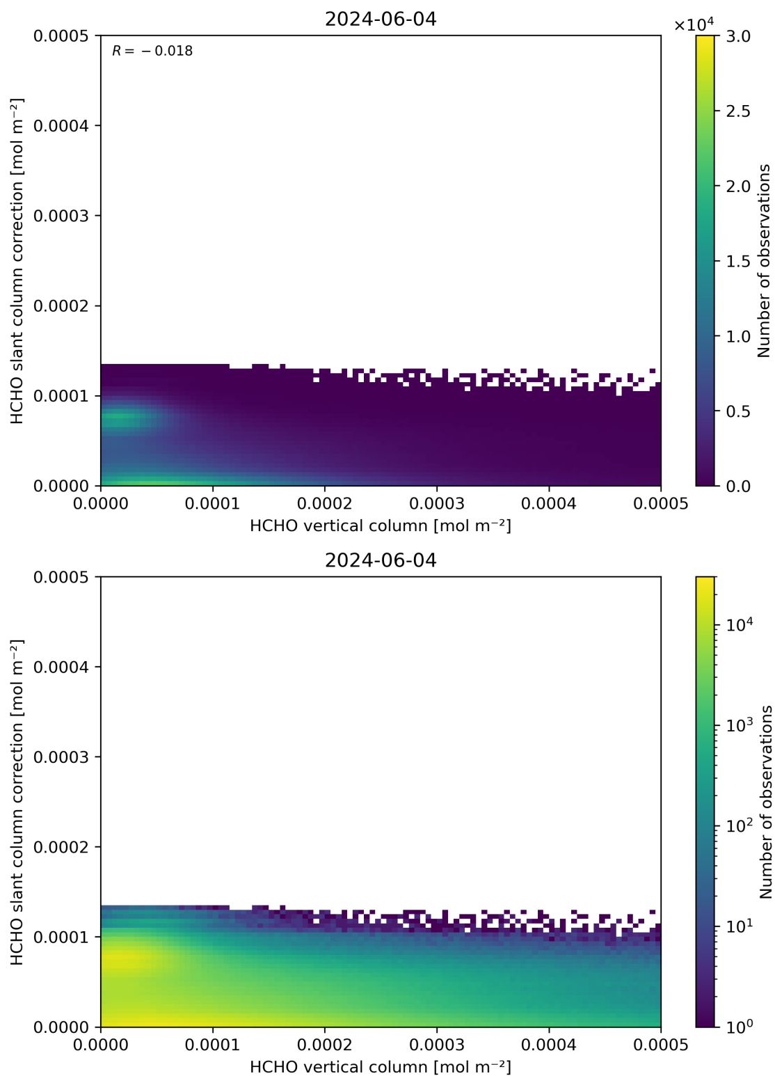
Figure 128: Scatter density plot of “HCHO vertical column” against “HCHO slant column correction” for 2024-06-03 to 2024-06-05.
