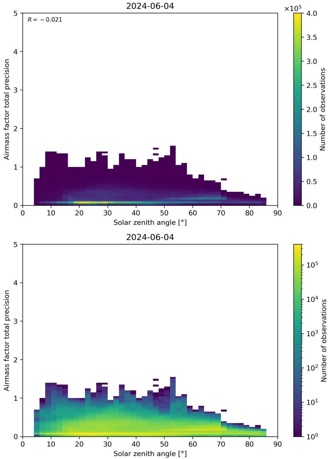
Figure 176: Scatter density plot of “Solar zenith angle” against “Airmass factor total precision” for 2024-06-03 to 2024-06-05.
