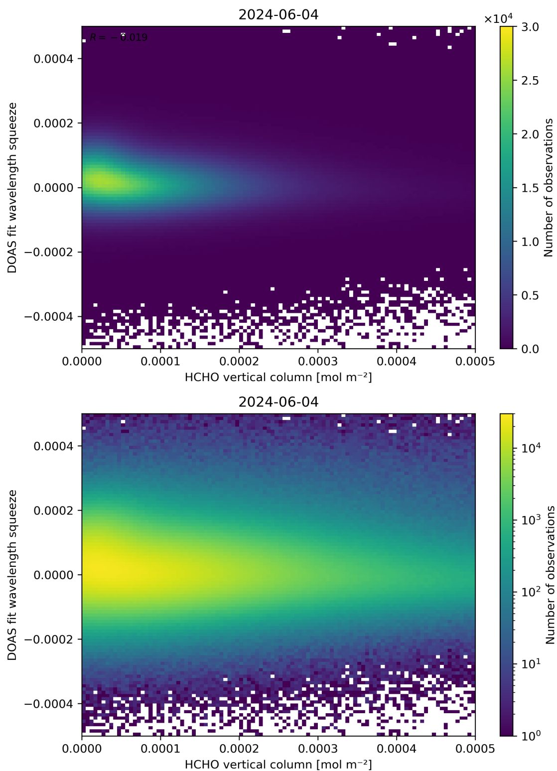
Figure 125: Scatter density plot of “HCHO vertical column” against “DOAS fit wavelength squeeze” for 2024-06-03 to 2024-06-05.
