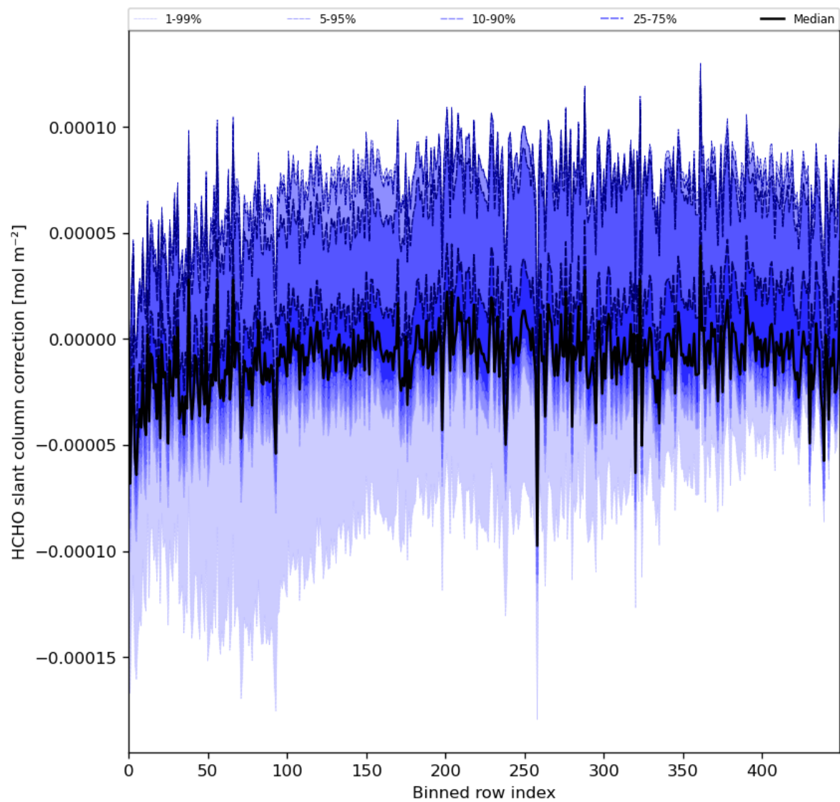
Figure 61: Along track statistics of “HCHO slant column correction” for 2024-06-03 to 2024-06-05
