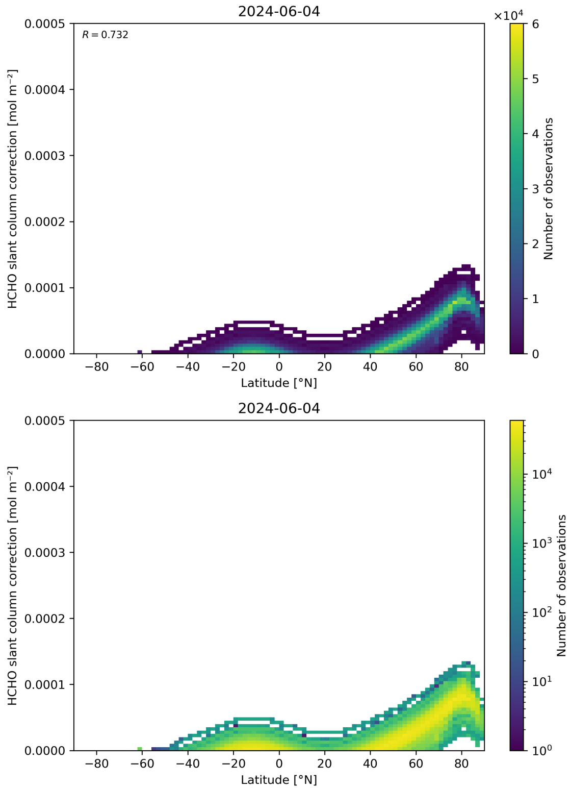
Figure 158: Scatter density plot of “Latitude” against “HCHO slant column correction” for 2024-06-03 to 2024-06-05.
