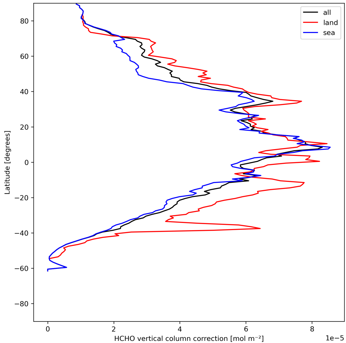
Figure 23: Zonal average of “HCHO vertical column correction” for 2024-06-03 to 2024-06-05.
