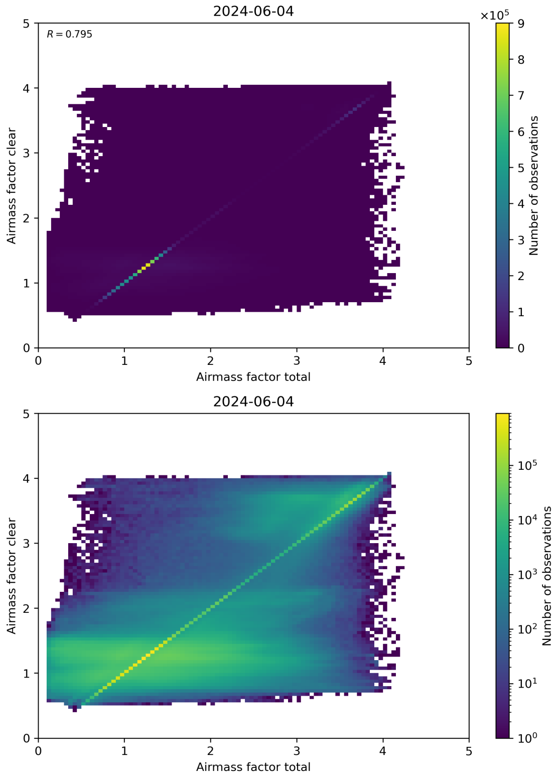
Figure 100: Scatter density plot of “Airmass factor total” against “Airmass factor clear” for 2024-06-03 to 2024-06-05.
