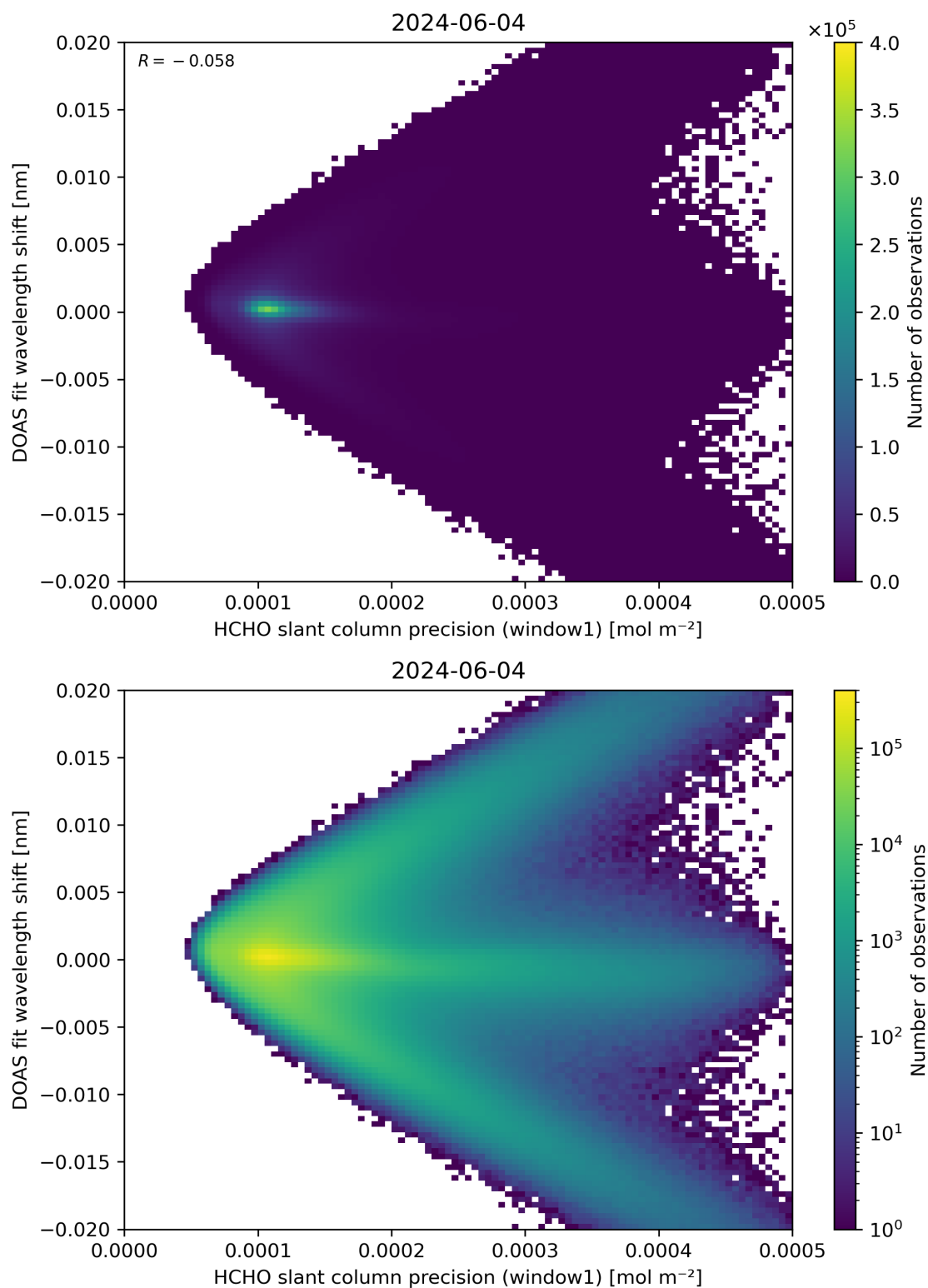
Figure 89: Scatter density plot of “HCHO slant column precision (window1)” against “DOAS fit wavelength shift” for 2024-06-03 to 2024-06-05.
