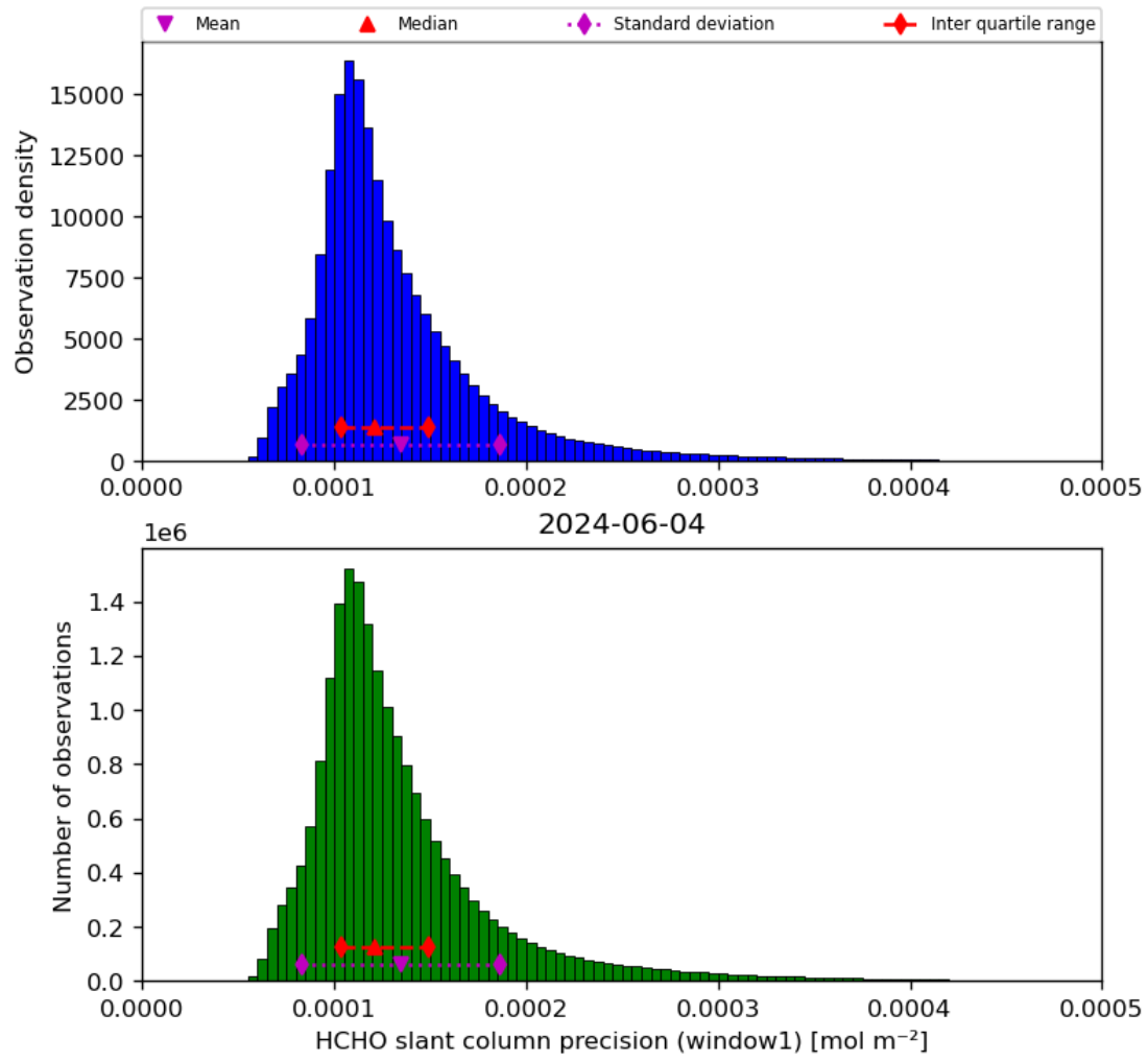
Figure 39: Histogram of “HCHO slant column precision (window1)” for 2024-06-03 to 2024-06-05
