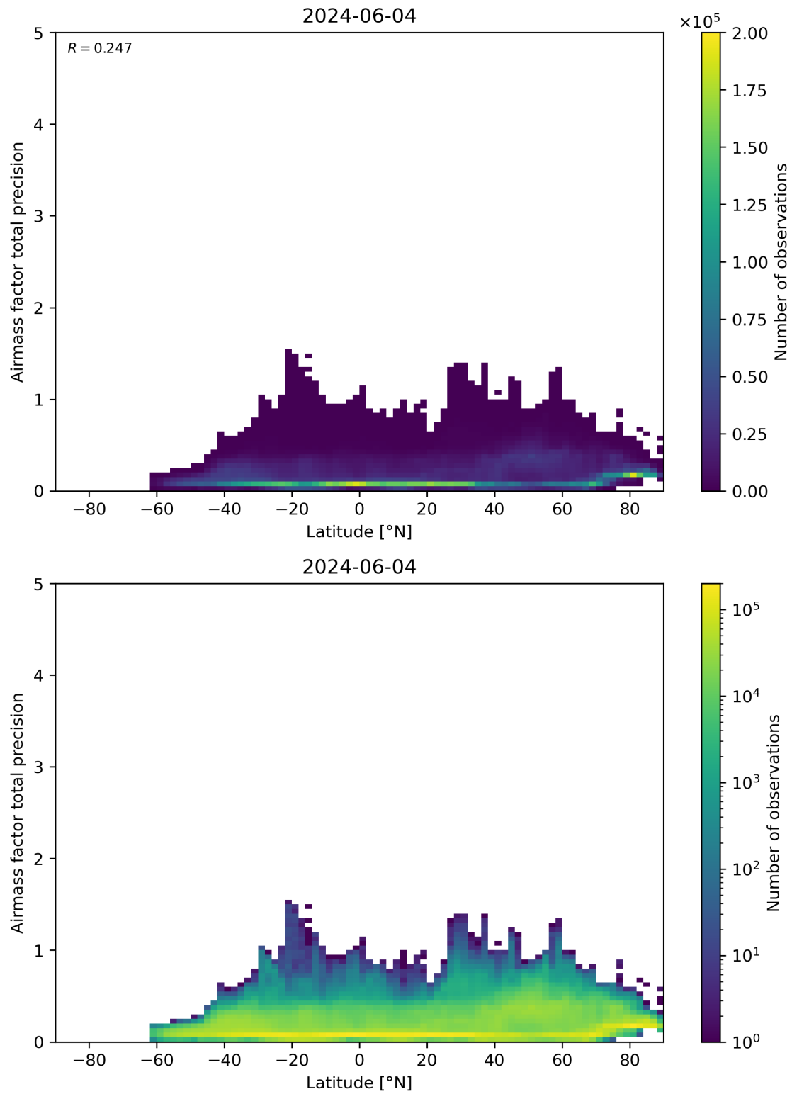
Figure 162: Scatter density plot of “Latitude” against “Airmass factor total precision” for 2024-06-03 to 2024-06-05.
