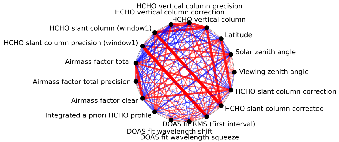
Figure 1: Map of correlation graph for 2024-06-03 to 2024-06-05.
