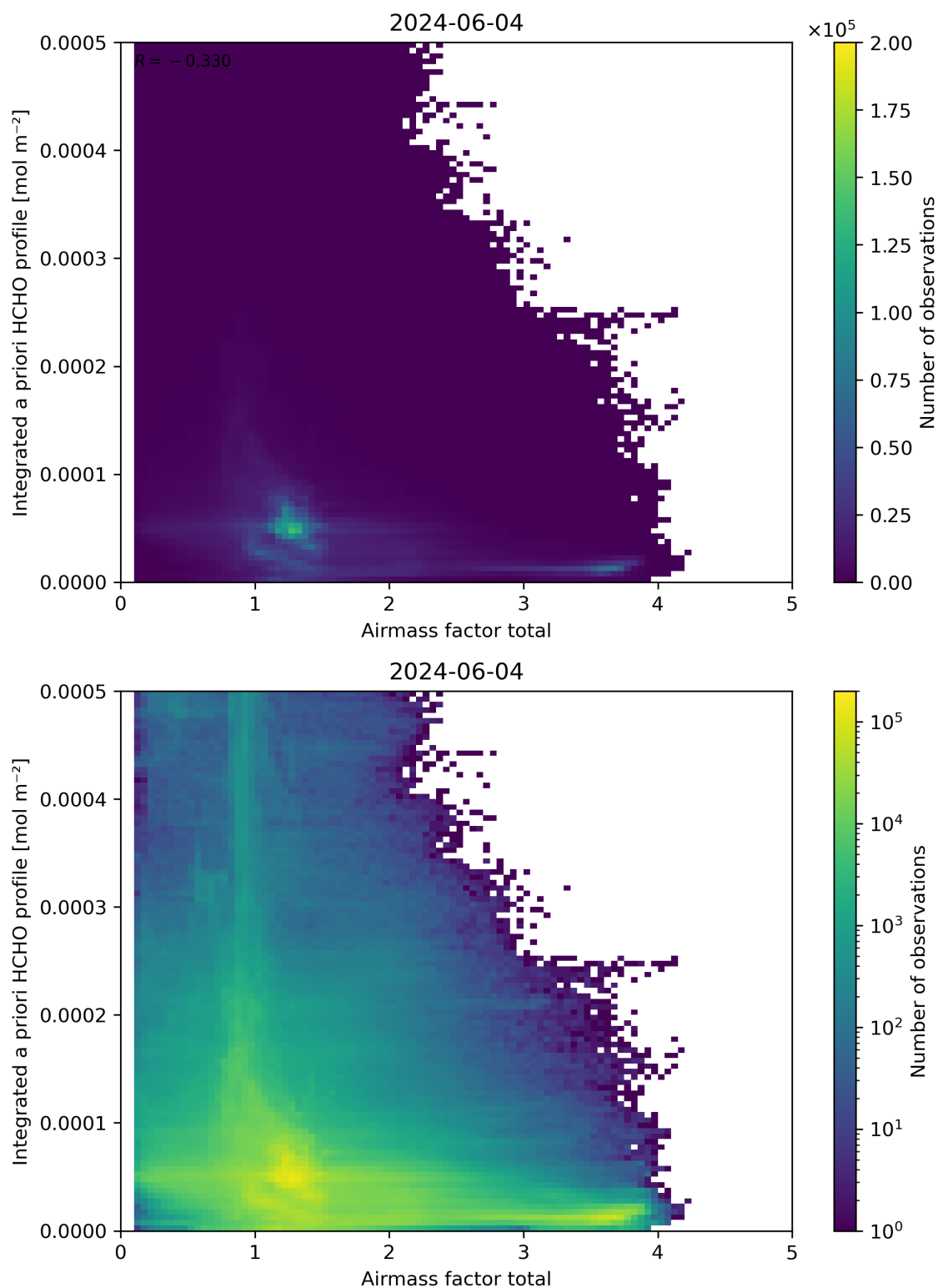
Figure 104: Scatter density plot of “Airmass factor total” against “Integrated a priori HCHO profile” for 2024-06-03 to 2024-06-05.
