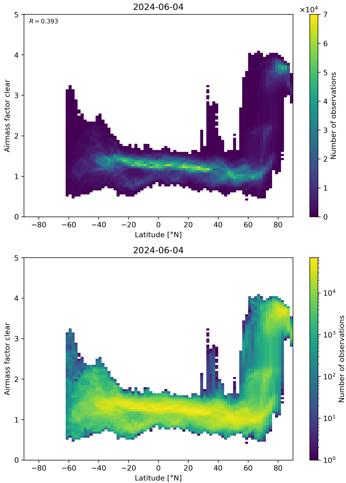
Figure 156: Scatter density plot of “Latitude” against “Airmass factor clear” for 2024-06-03 to 2024-06-05.
