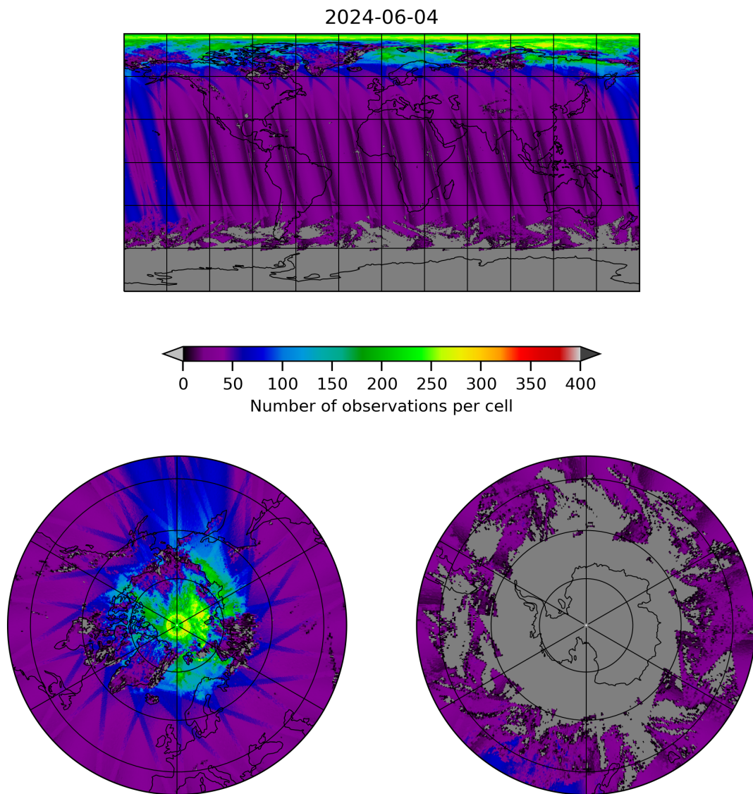
Figure 19: Map of the number of observations for 2024-06-03 to 2024-06-05
