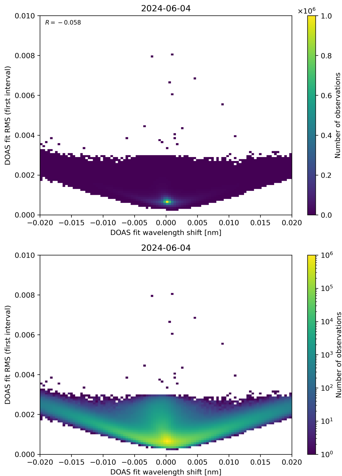
Figure 64: Scatter density plot of “DOAS fit wavelength shift” against “DOAS fit RMS (first interval)” for 2024-06-03 to 2024-06-05.
