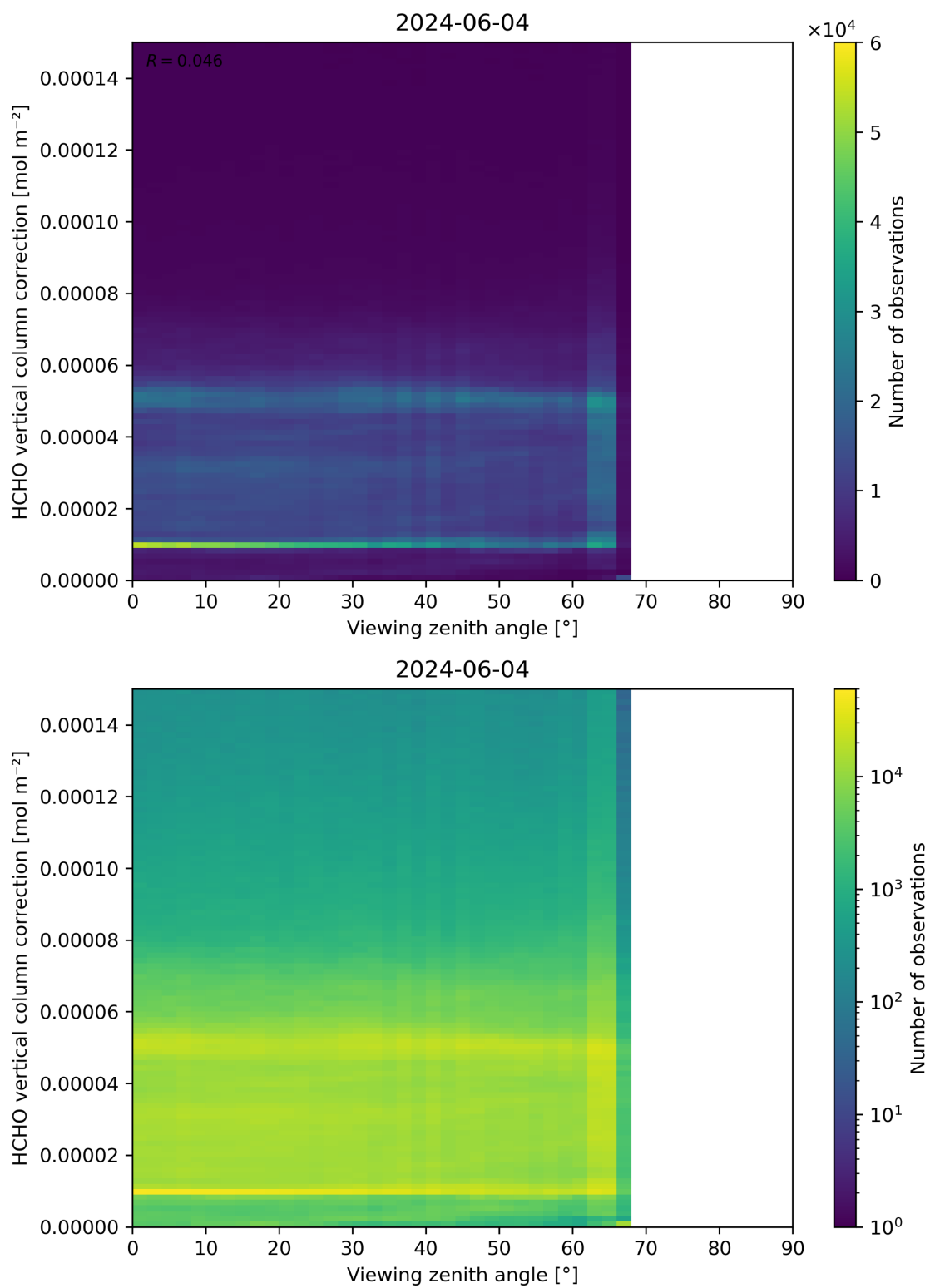
Figure 193: Scatter density plot of “Viewing zenith angle” against “HCHO vertical column correction” for 2024-06-03 to 2024-06-05.
