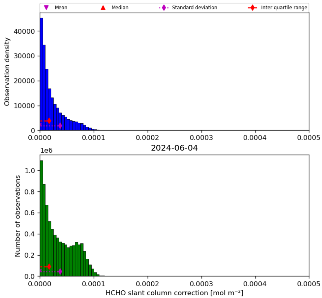
Figure 47: Histogram of "HCHO slant column correction" for 2024-06-03 to 2024-06-05
