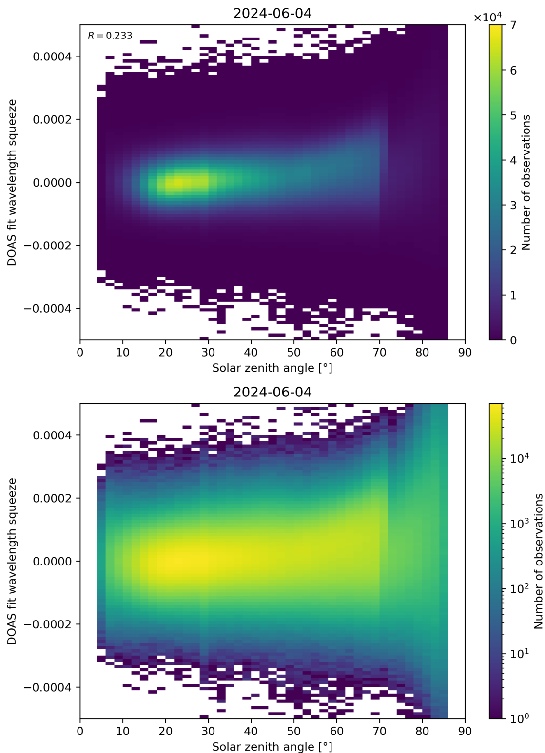
Figure 169: Scatter density plot of “Solar zenith angle” against “DOAS fit wavelength squeeze” for 2024-06-03 to 2024-06-05.
