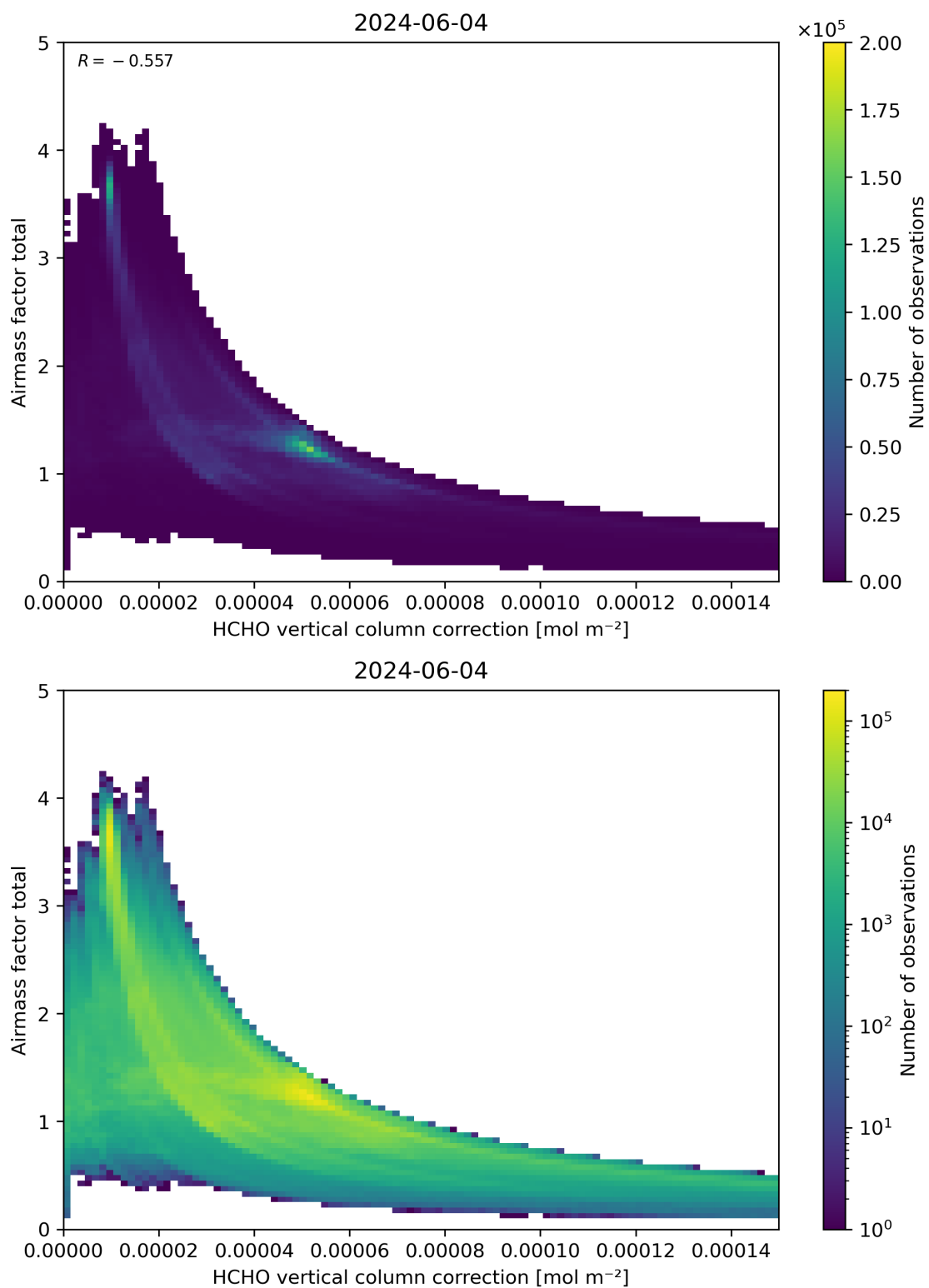
Figure 120: Scatter density plot of “HCHO vertical column correction” against “Airmass factor total” for 2024-06-03 to 2024-06-05.
