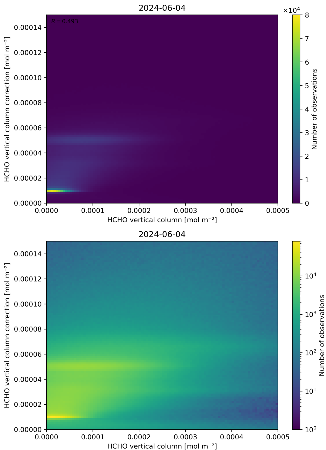
Figure 133: Scatter density plot of “HCHO vertical column” against “HCHO vertical column correction” for 2024-06-03 to 2024-06-05.
