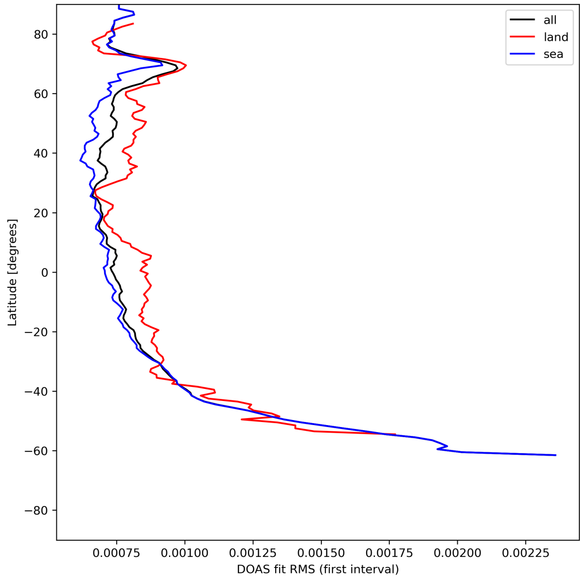
Figure 32: Zonal average of “DOAS fit RMS (first interval)” for 2024-06-03 to 2024-06-05.
