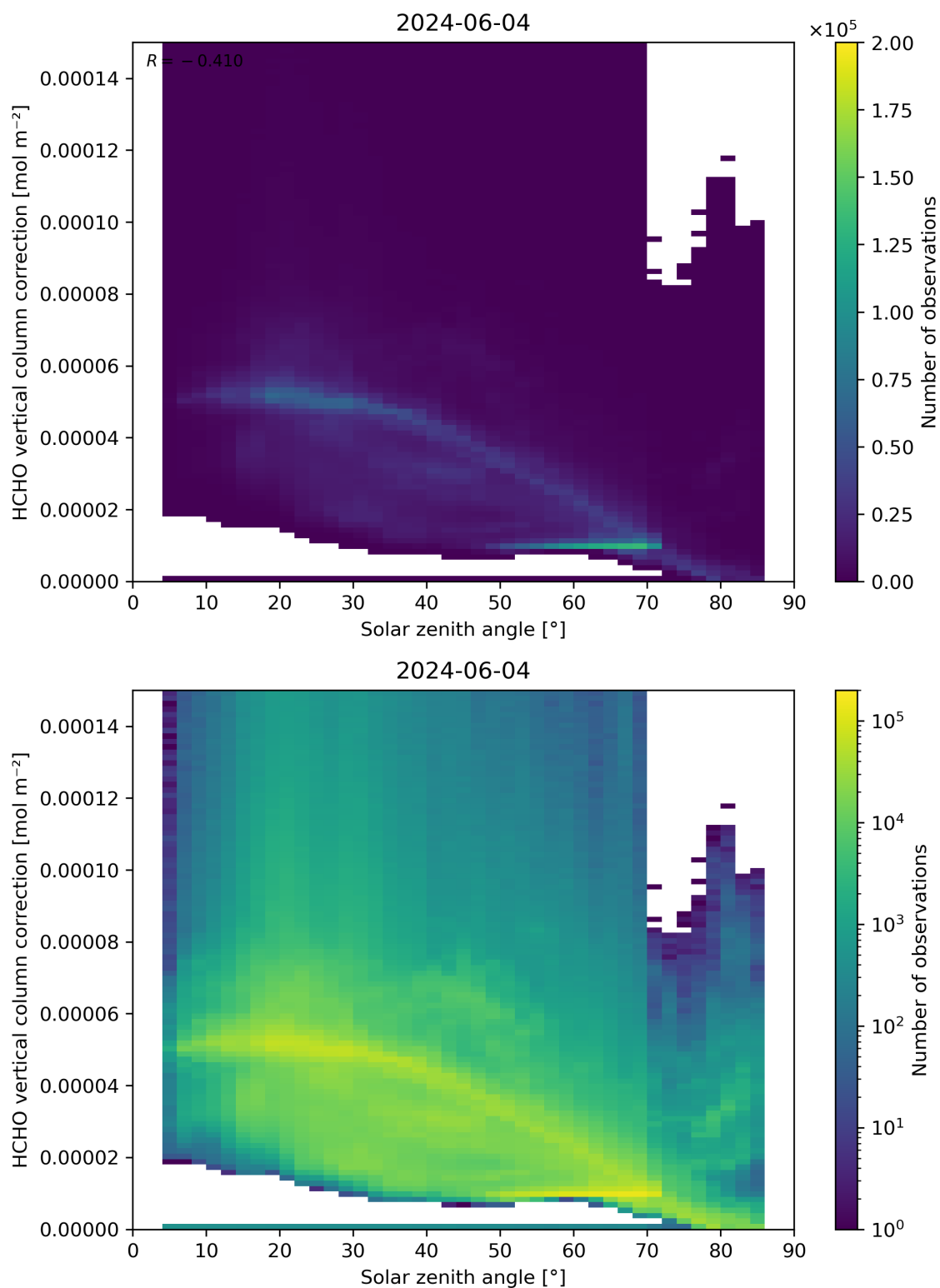
Figure 178: Scatter density plot of “Solar zenith angle” against “HCHO vertical column correction” for 2024-06-03 to 2024-06-05.
