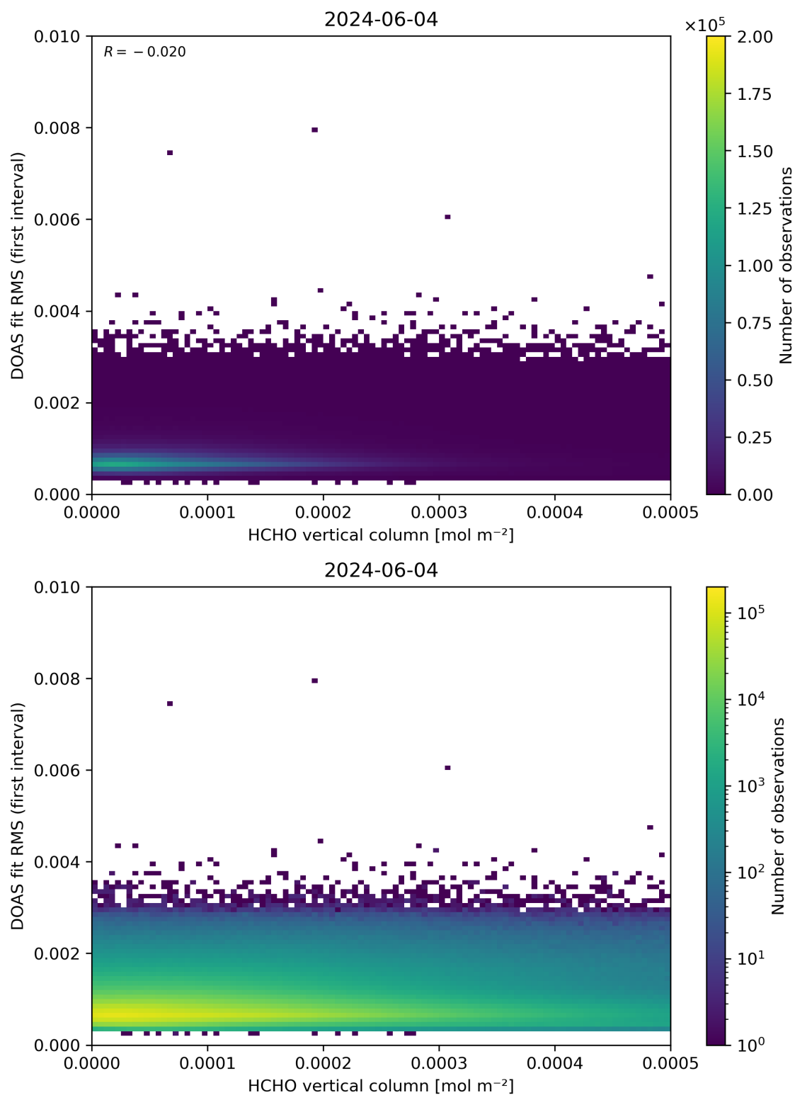
Figure 123: Scatter density plot of “HCHO vertical column” against “DOAS fit RMS (first interval)” for 2024-06-03 to 2024-06-05.
