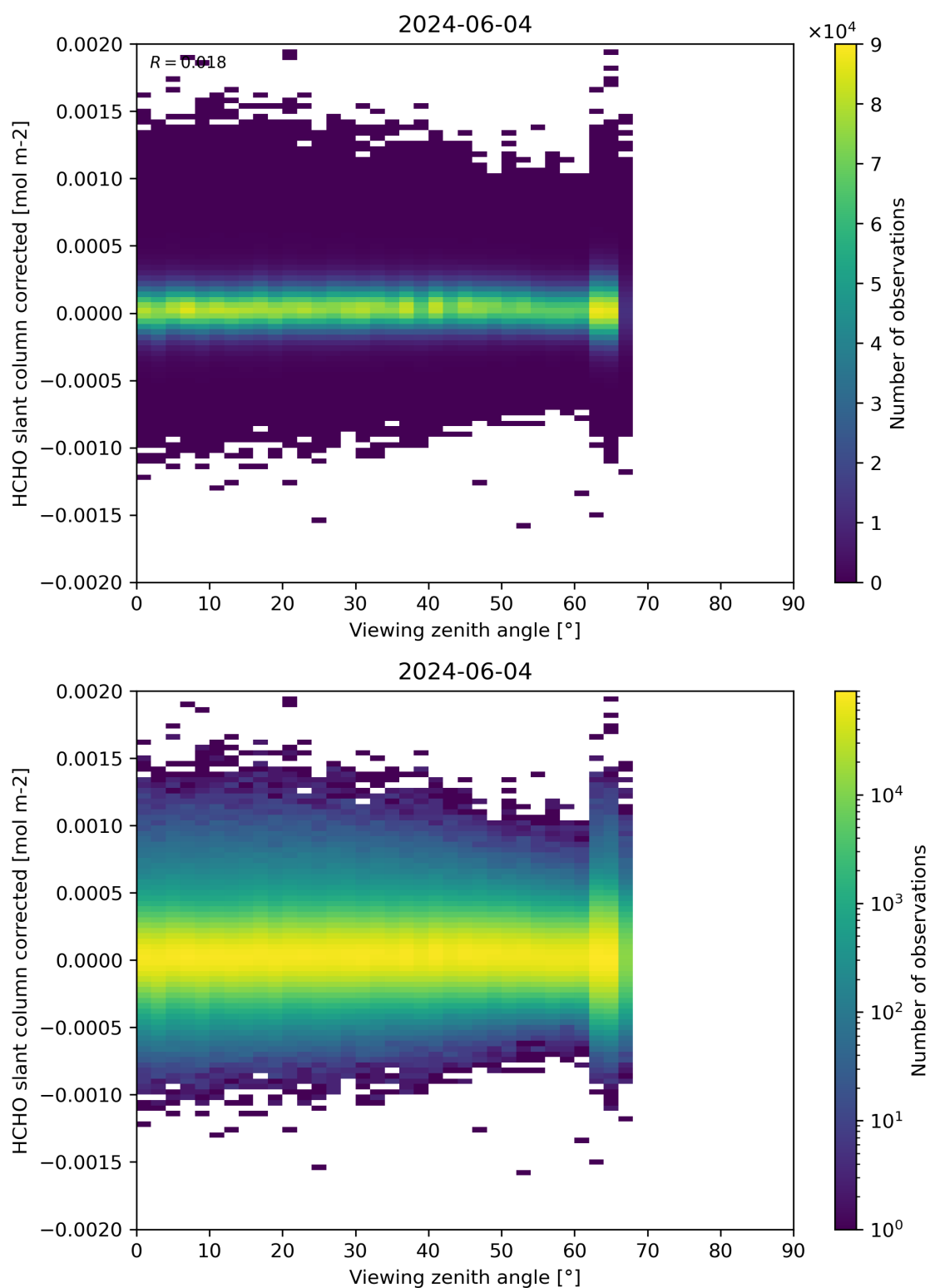
Figure 186: Scatter density plot of “Viewing zenith angle” against “HCHO slant column corrected” for 2024-06-03 to 2024-06-05.
