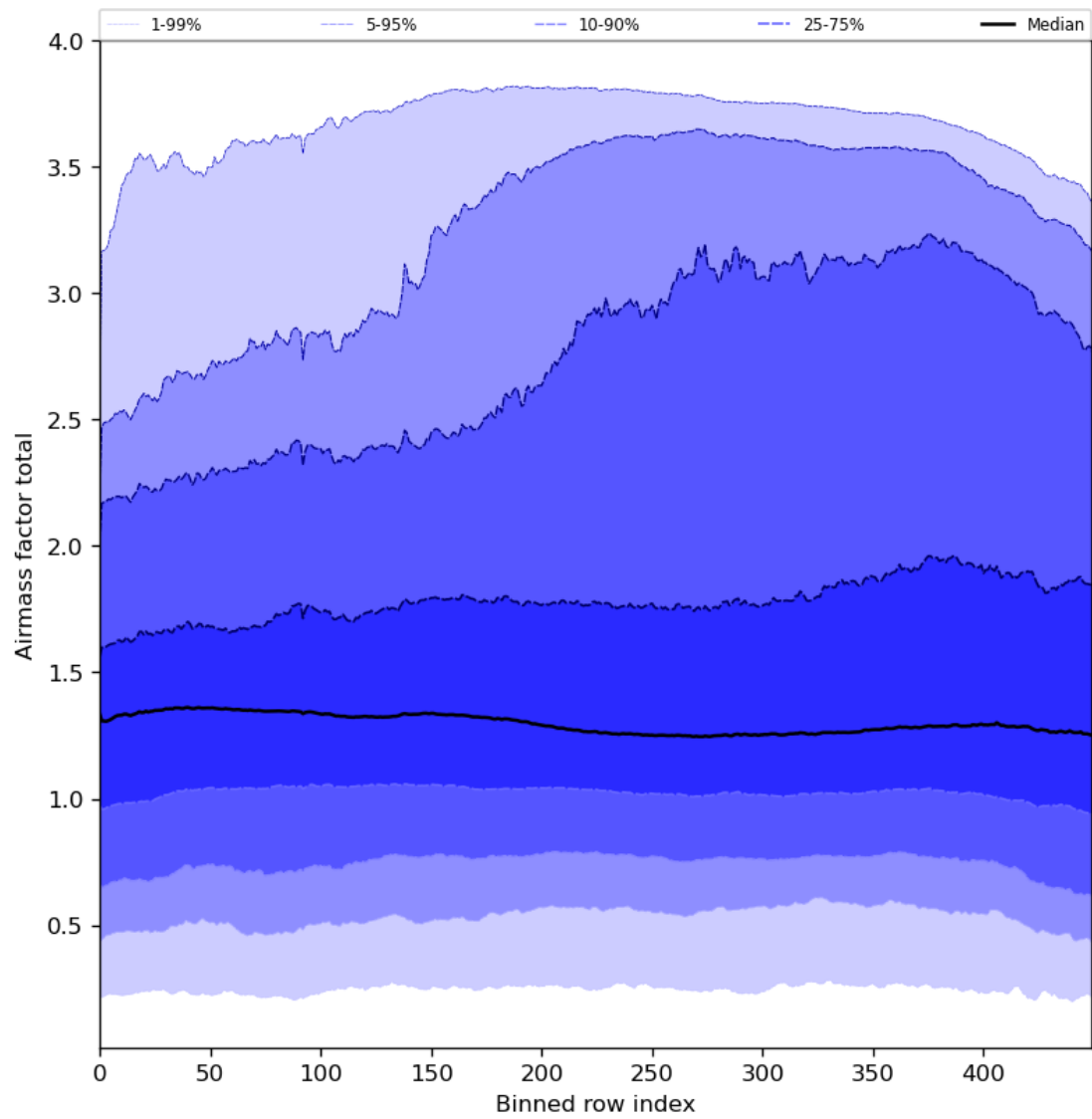
Figure 54: Along track statistics of “Airmass factor total” for 2024-06-03 to 2024-06-05
