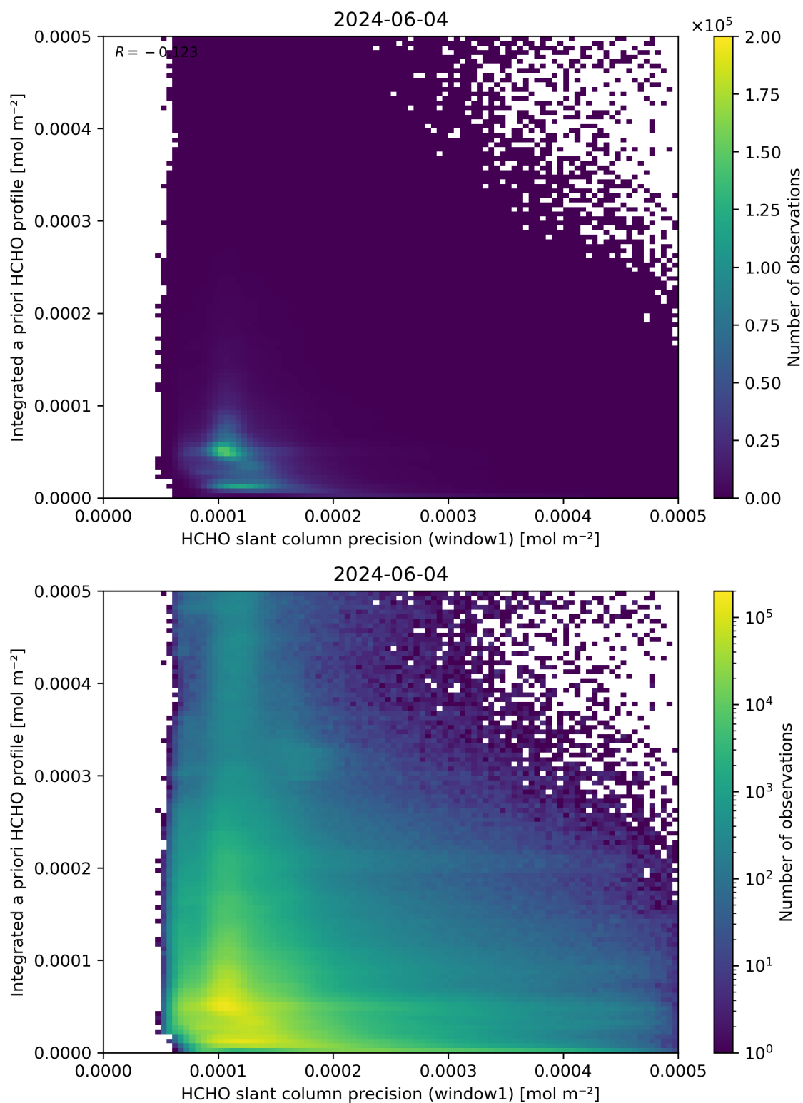
Figure 96: Scatter density plot of “HCHO slant column precision (window1)” against “Integrated a priori HCHO profile” for 2024-06-03 to 2024-06-05.
