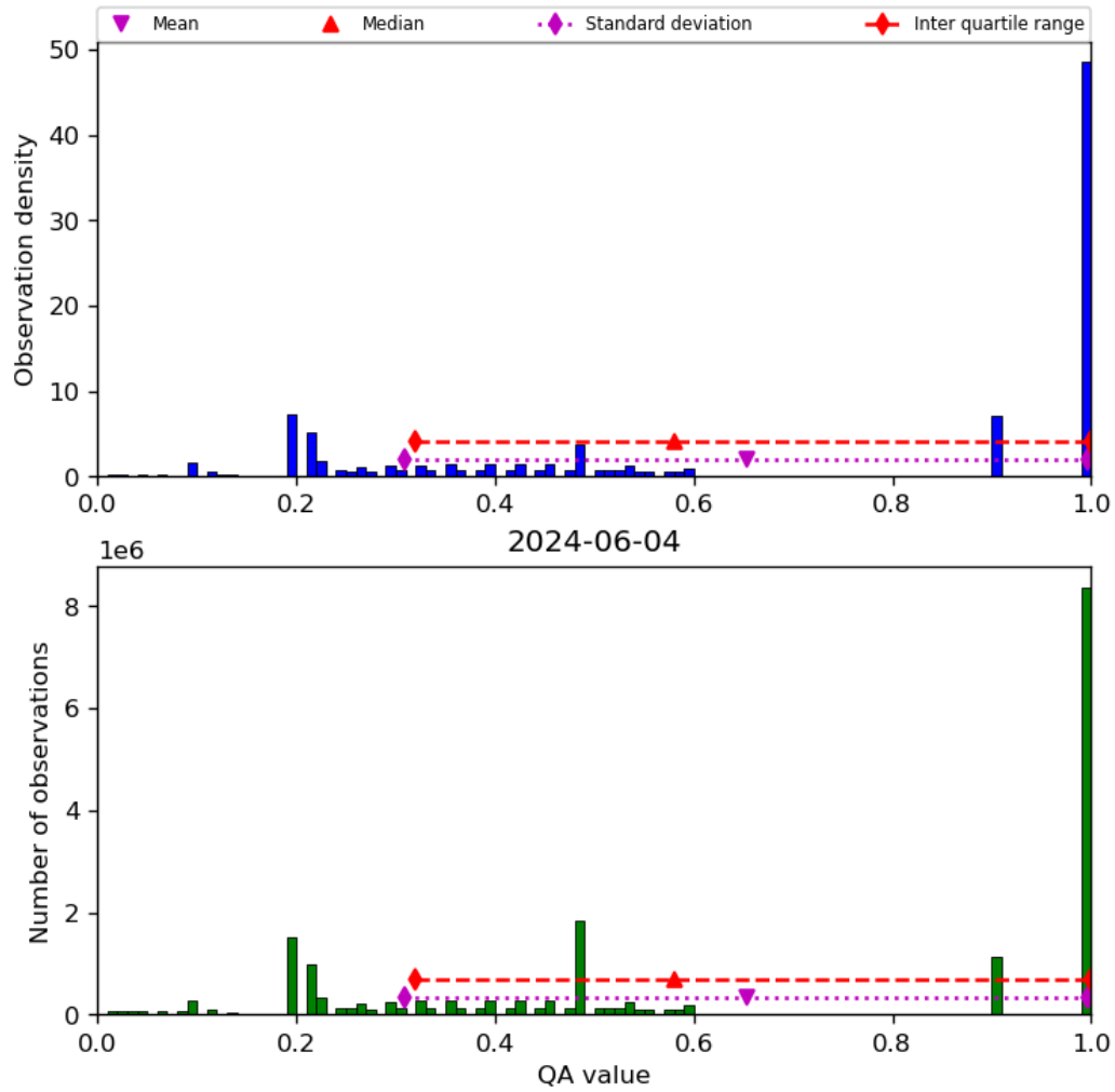
Figure 34: Histogram of “QA value” for 2024-06-03 to 2024-06-05
