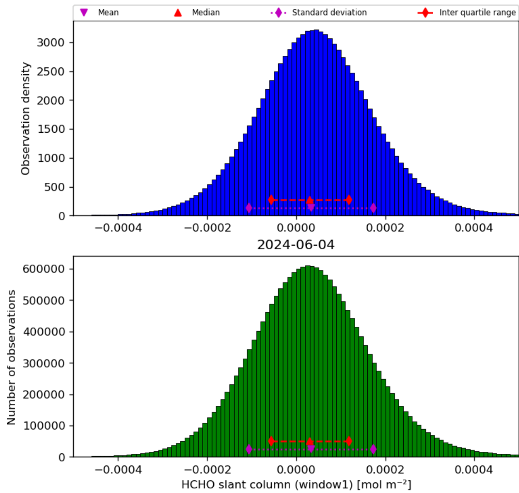
Figure 38: Histogram of “HCHO slant column (window1)” for 2024-06-03 to 2024-06-05
