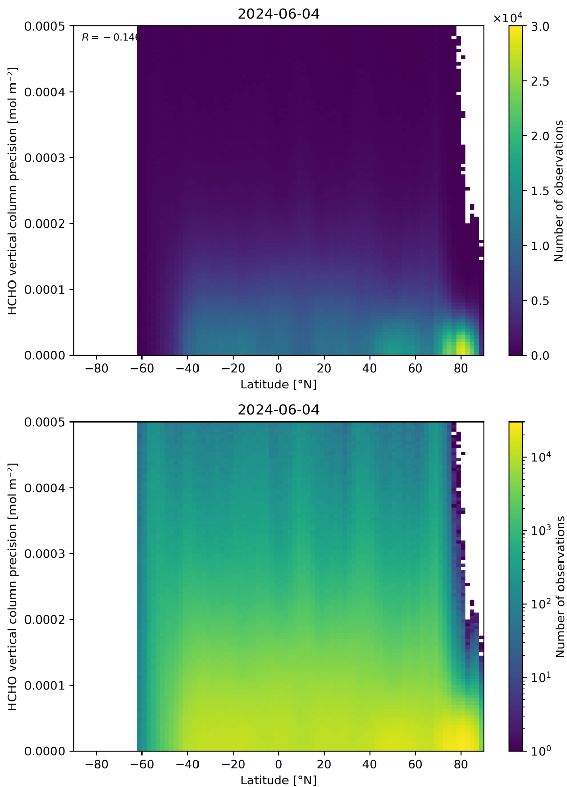
Figure 165: Scatter density plot of “Latitude” against “HCHO vertical column precision” for 2024-06-03 to 2024-06-05.
