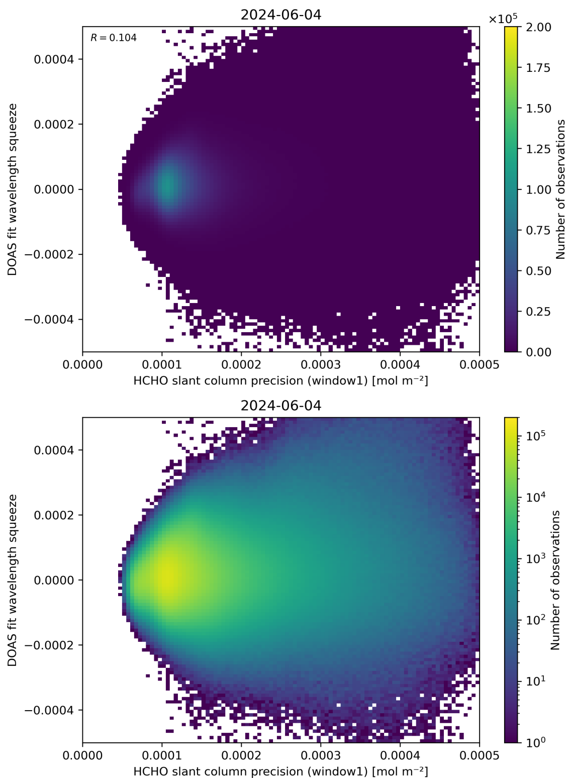
Figure 90: Scatter density plot of “HCHO slant column precision (window1)” against “DOAS fit wavelength squeeze” for 2024-06-03 to 2024-06-05.
