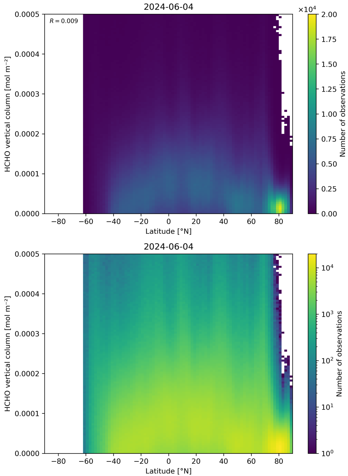
Figure 163: Scatter density plot of “Latitude” against “HCHO vertical column” for 2024-06-03 to 2024-06-05.
