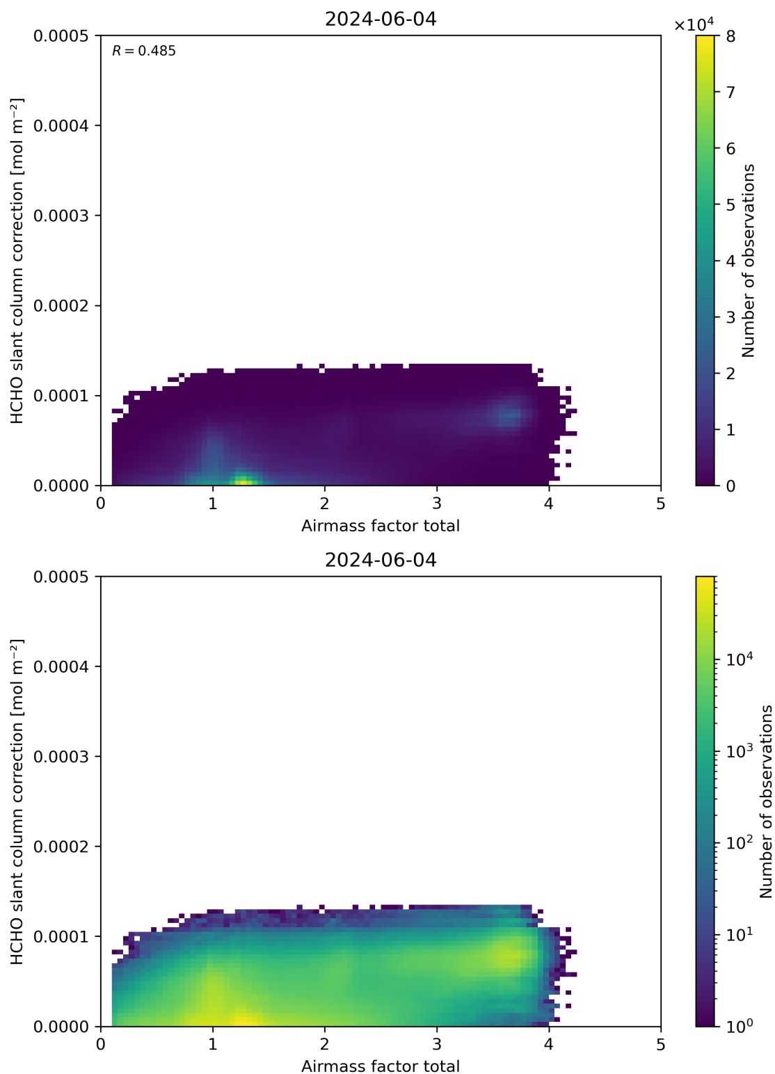
Figure 102: Scatter density plot of “Airmass factor total” against “HCHO slant column correction” for 2024-06-03 to 2024-06-05.
