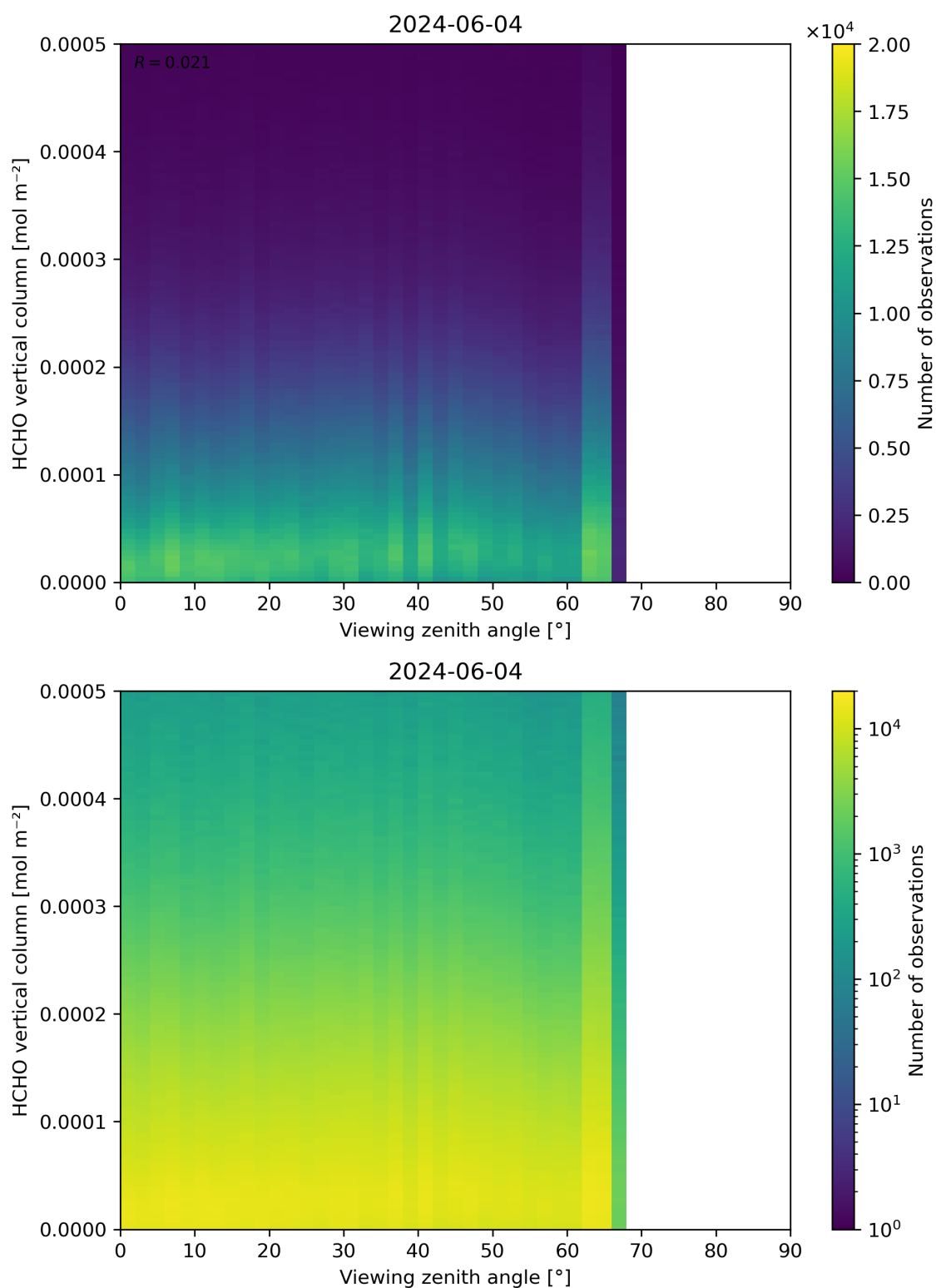
Figure 192: Scatter density plot of “Viewing zenith angle” against “HCHO vertical column” for 2024-06-03 to 2024-06-05.
