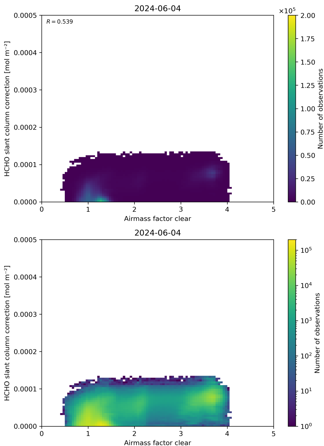
Figure 75: Scatter density plot of “Airmass factor clear” against “HCHO slant column correction” for 2024-06-03 to 2024-06-05.
