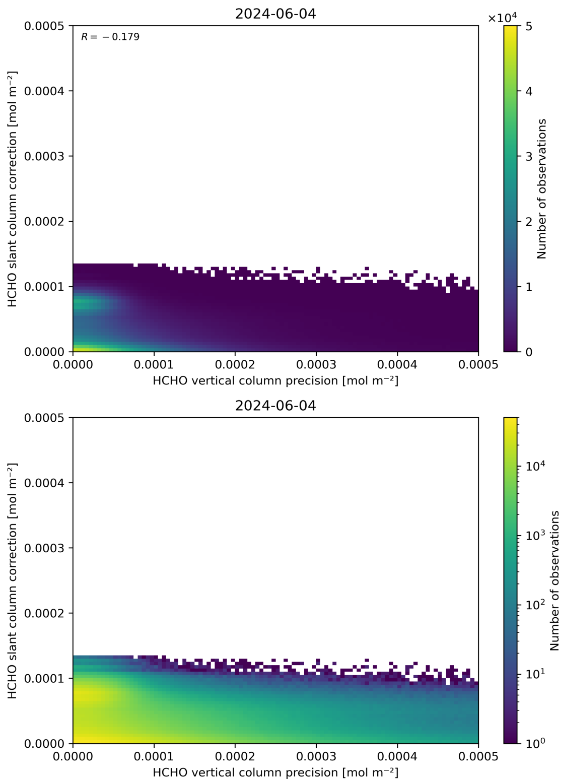
Figure 141: Scatter density plot of “HCHO vertical column precision” against “HCHO slant column correction” for 2024-06-03 to 2024-06-05.
