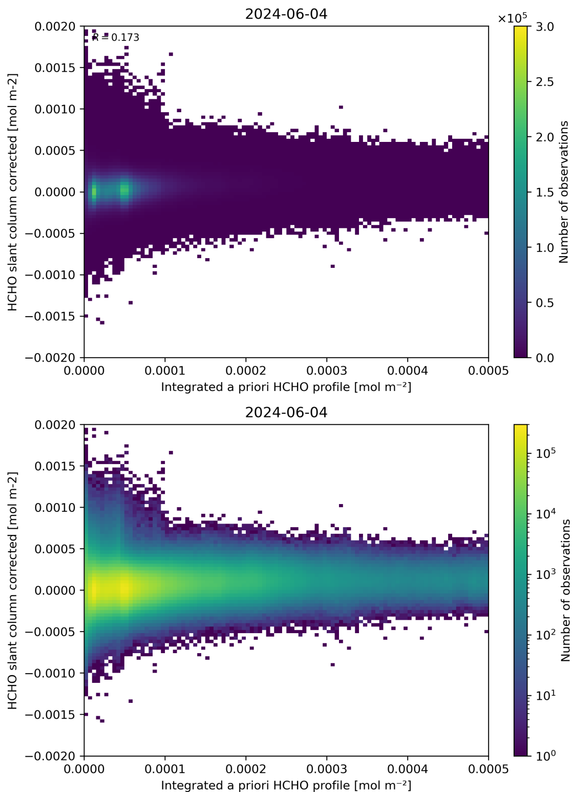
Figure 151: Scatter density plot of “Integrated a priori HCHO profile” against “HCHO slant column corrected” for 2024-06-03 to 2024-06-05.
