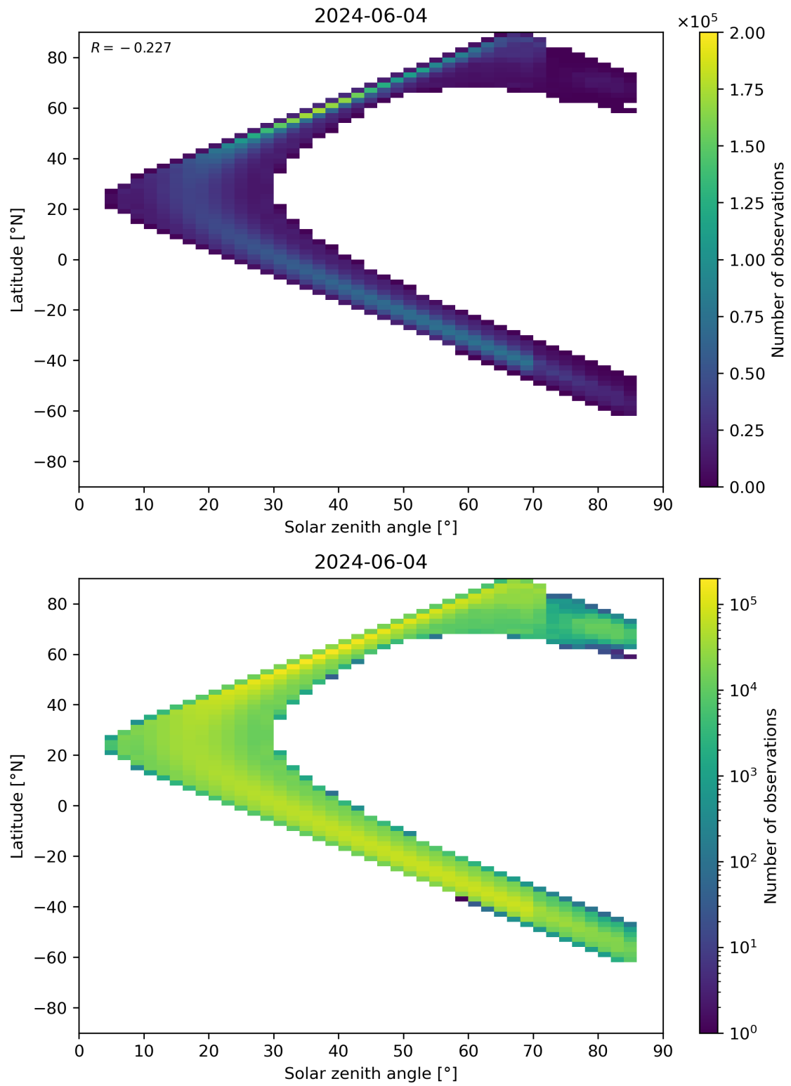
Figure 181: Scatter density plot of “Solar zenith angle” against “Latitude” for 2024-06-03 to 2024-06-05.
