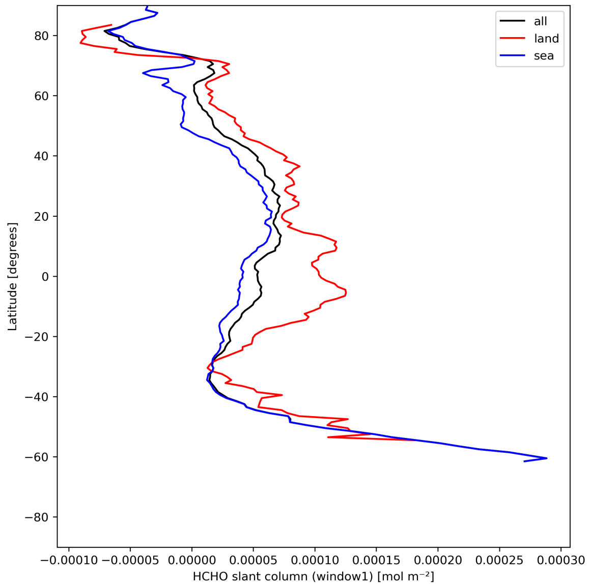
Figure 24: Zonal average of “HCHO slant column (window1)” for 2024-06-03 to 2024-06-05.
