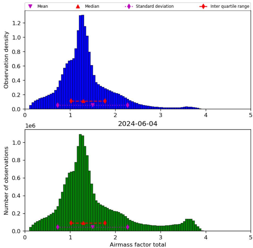
Figure 40: Histogram of “Airmass factor total” for 2024-06-03 to 2024-06-05
