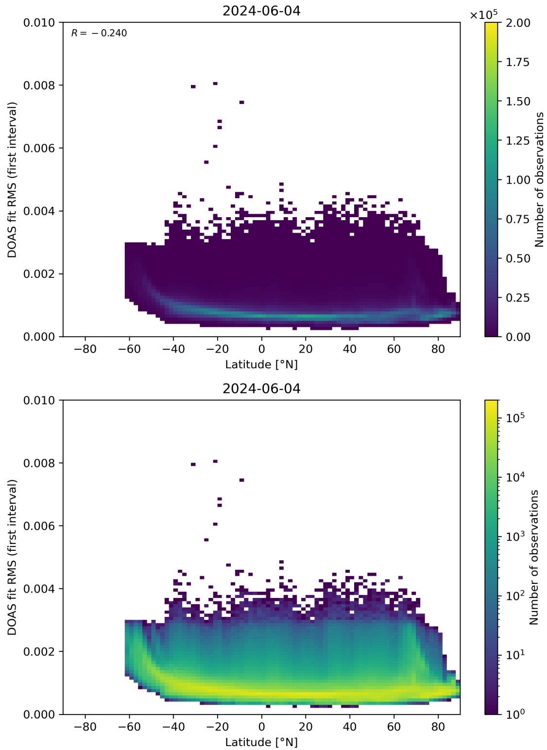
Figure 153: Scatter density plot of “Latitude” against “DOAS fit RMS (first interval)” for 2024-06-03 to 2024-06-05.
