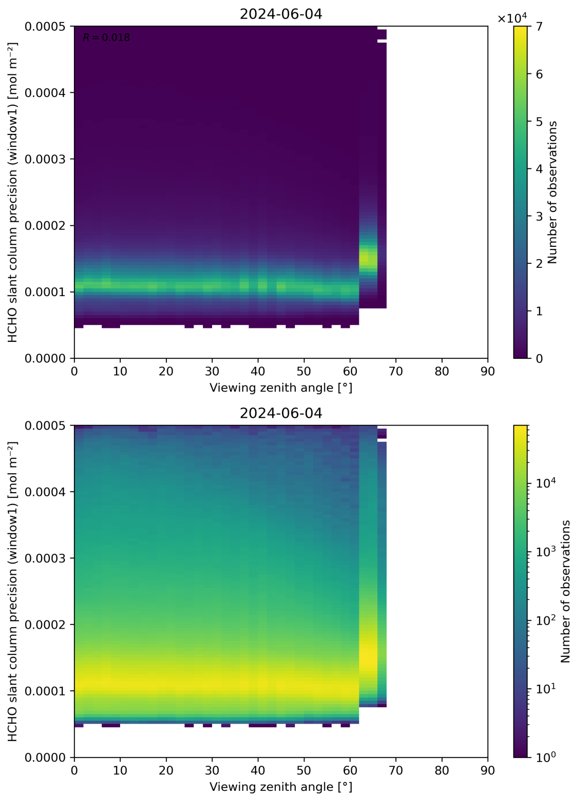
Figure 189: Scatter density plot of “Viewing zenith angle” against “HCHO slant column precision (window1)” for 2024-06-03 to 2024-06-05.
