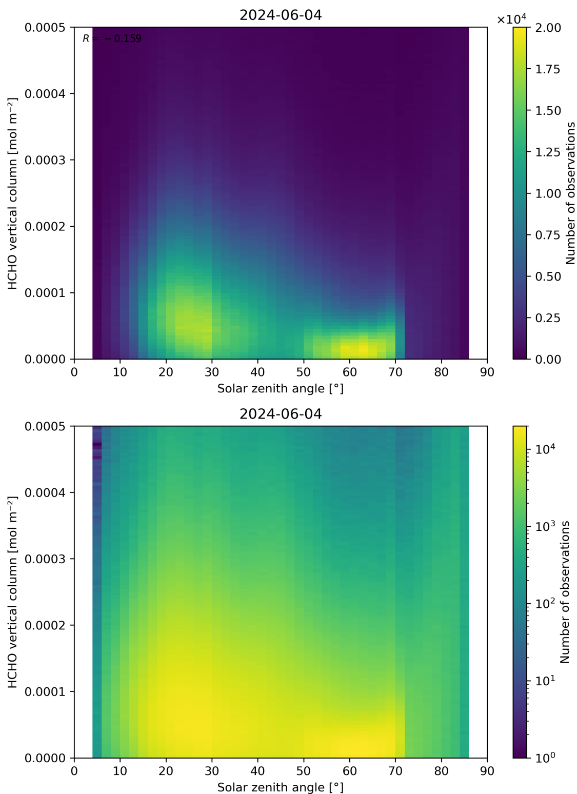
Figure 177: Scatter density plot of “Solar zenith angle” against “HCHO vertical column” for 2024-06-03 to 2024-06-05.
