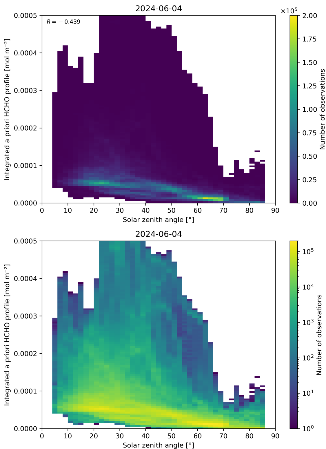
Figure 180: Scatter density plot of “Solar zenith angle” against “Integrated a priori HCHO profile” for 2024-06-03 to 2024-06-05.
