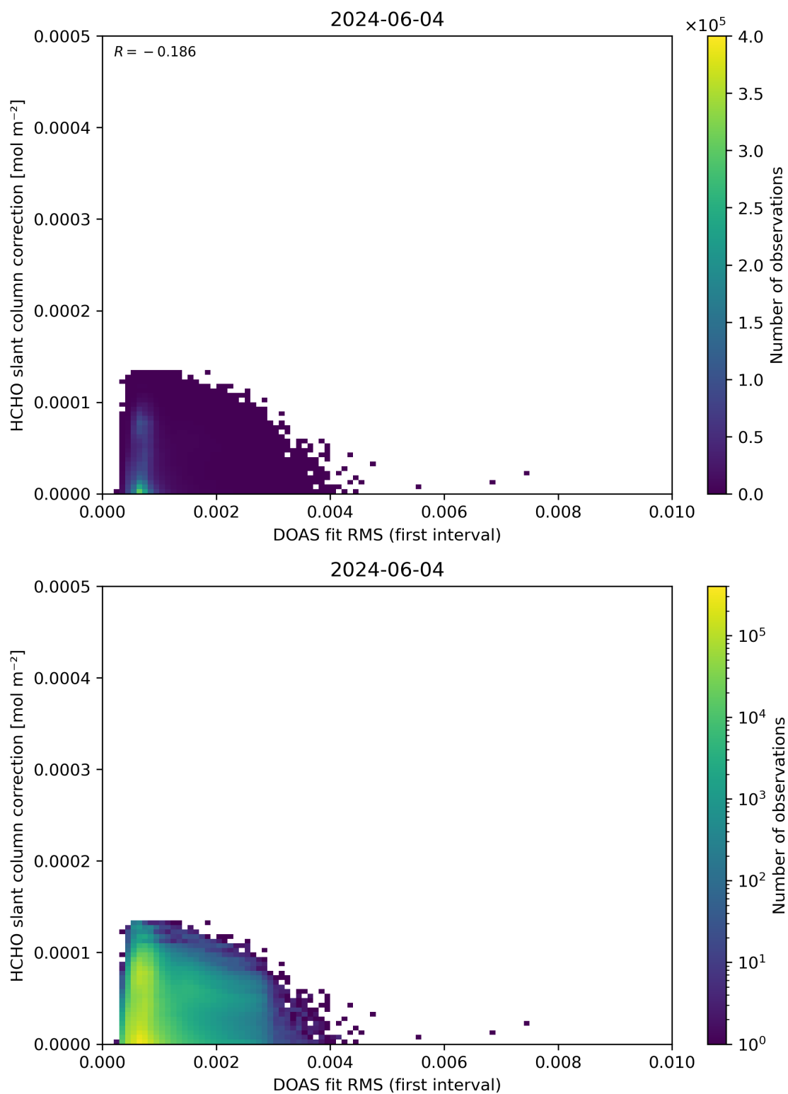
Figure 63: Scatter density plot of “DOAS fit RMS (first interval)” against “HCHO slant column correction” for 2024-06-03 to 2024-06-05.
