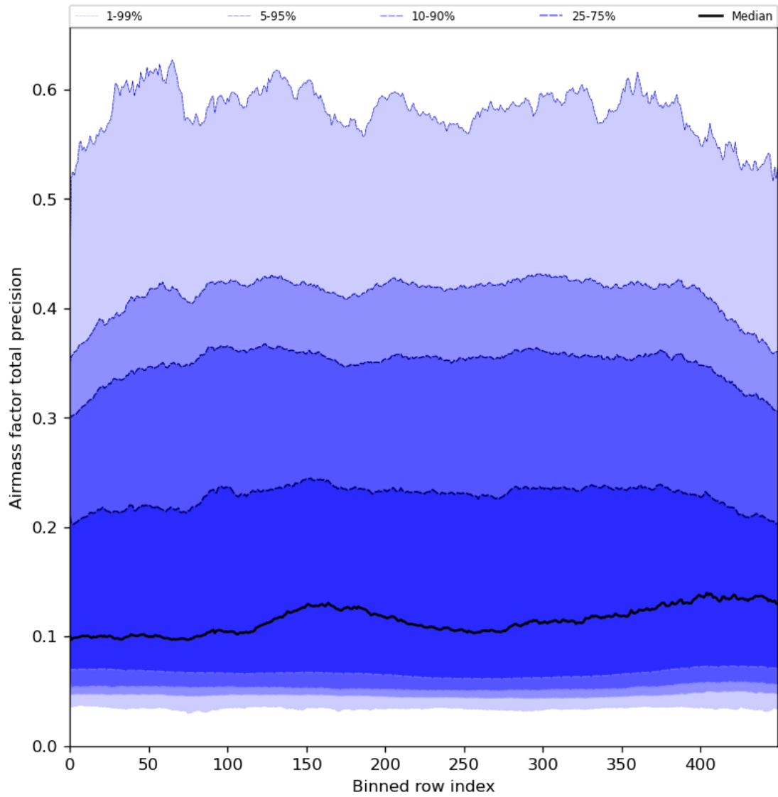
Figure 55: Along track statistics of “Airmass factor total precision” for 2024-06-03 to 2024-06-05
