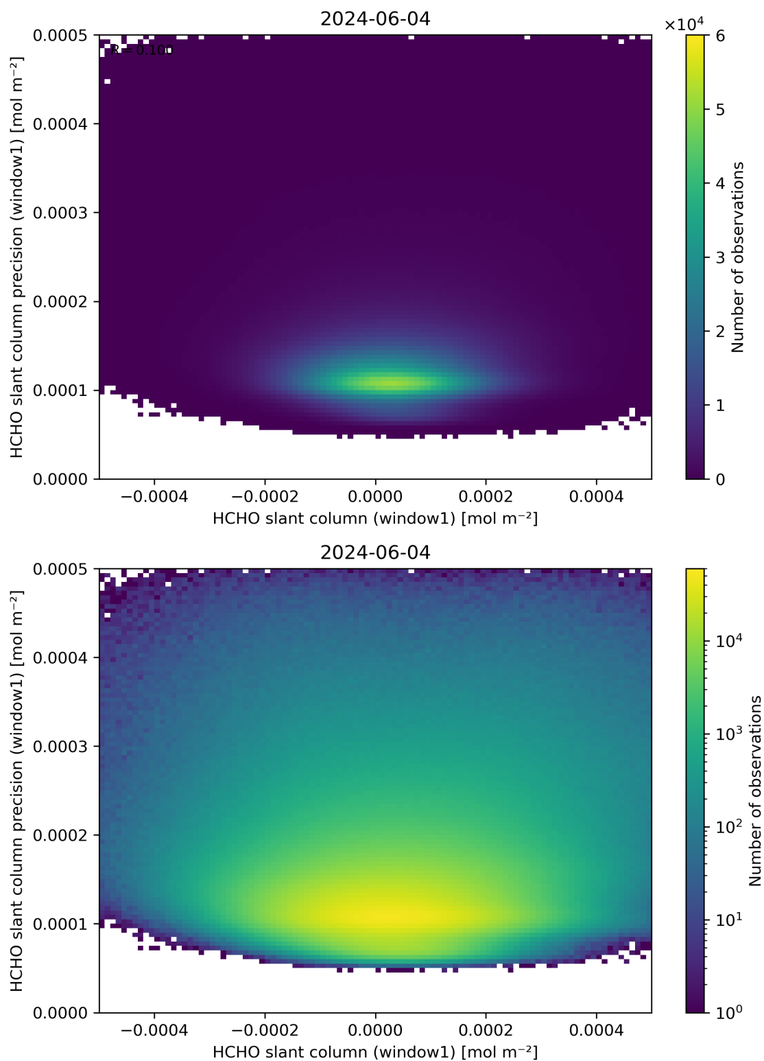
Figure 84: Scatter density plot of “HCHO slant column (window1)” against “HCHO slant column precision (window1)” for 2024-06-03 to 2024-06-05.
