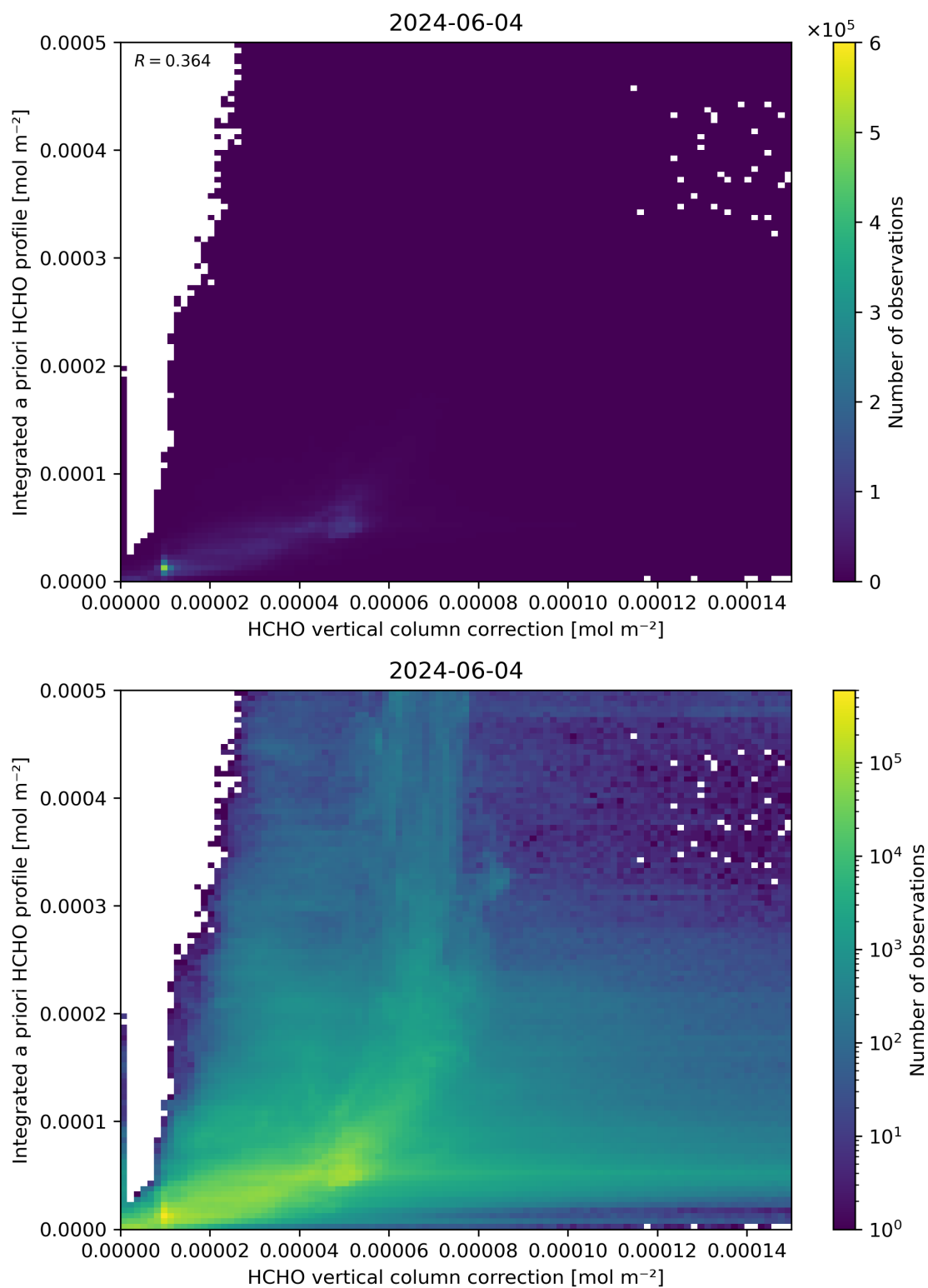
Figure 122: Scatter density plot of “HCHO vertical column correction” against “Integrated a priori HCHO profile” for 2024-06-03 to 2024-06-05.
