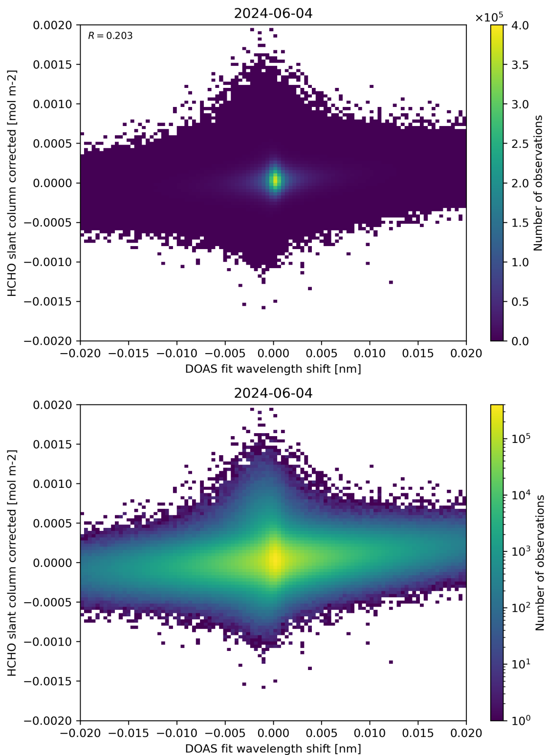
Figure 66: Scatter density plot of “DOAS fit wavelength shift” against “HCHO slant column corrected” for 2024-06-03 to 2024-06-05.
