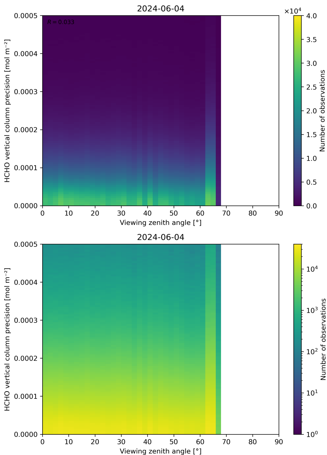
Figure 194: Scatter density plot of “Viewing zenith angle” against “HCHO vertical column precision” for 2024-06-03 to 2024-06-05.
