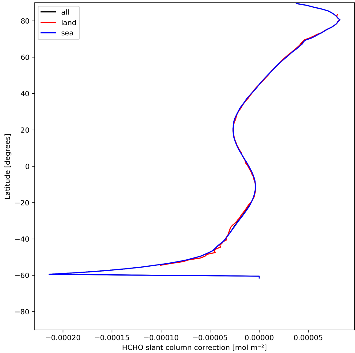
Figure 33: Zonal average of “HCHO slant column correction” for 2024-06-03 to 2024-06-05.
