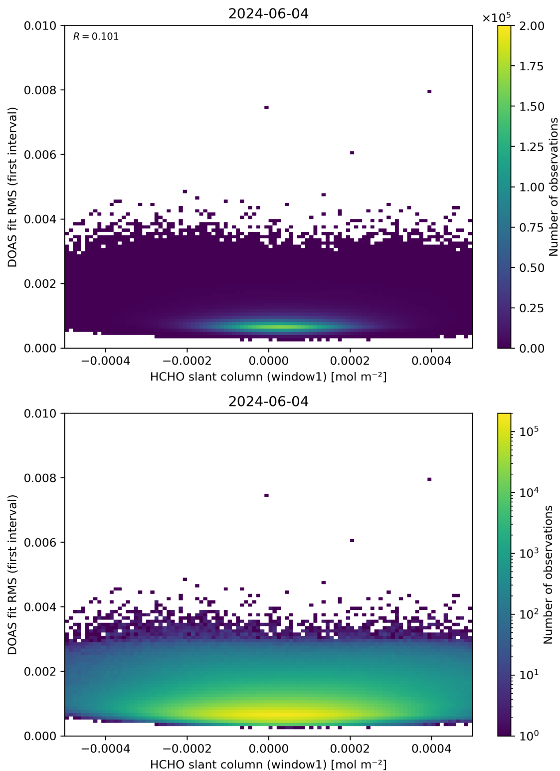
Figure 78: Scatter density plot of “HCHO slant column (window1)” against “DOAS fit RMS (first interval)” for 2024-06-03 to 2024-06-05.
