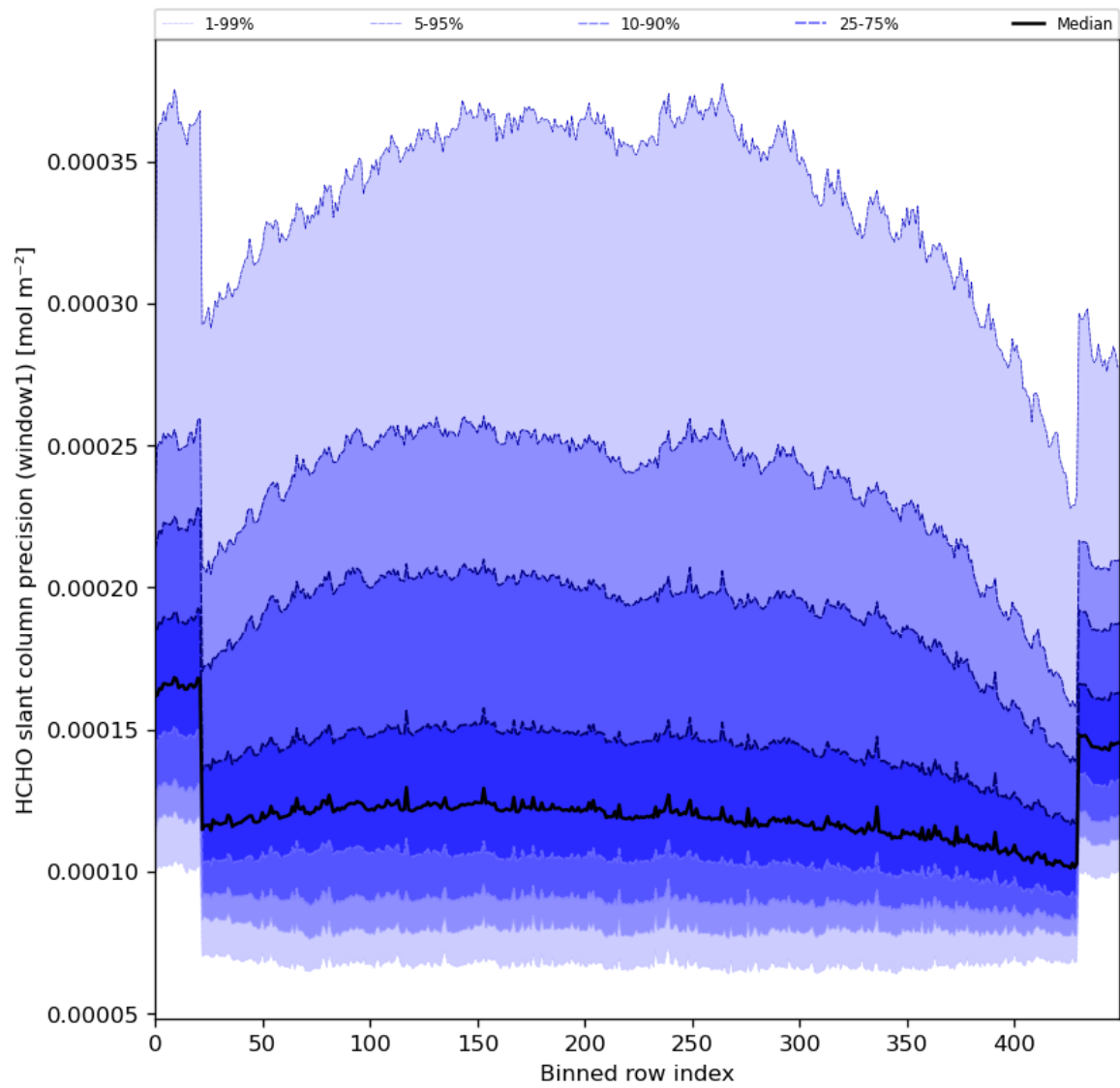
Figure 53: Along track statistics of “HCHO slant column precision (window1)” for 2024-06-03 to 2024-06-05
