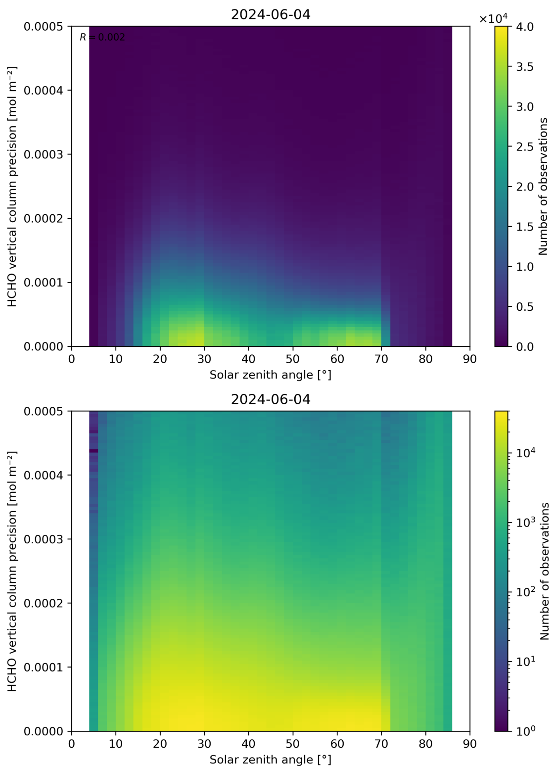
Figure 179: Scatter density plot of “Solar zenith angle” against “HCHO vertical column precision” for 2024-06-03 to 2024-06-05.
