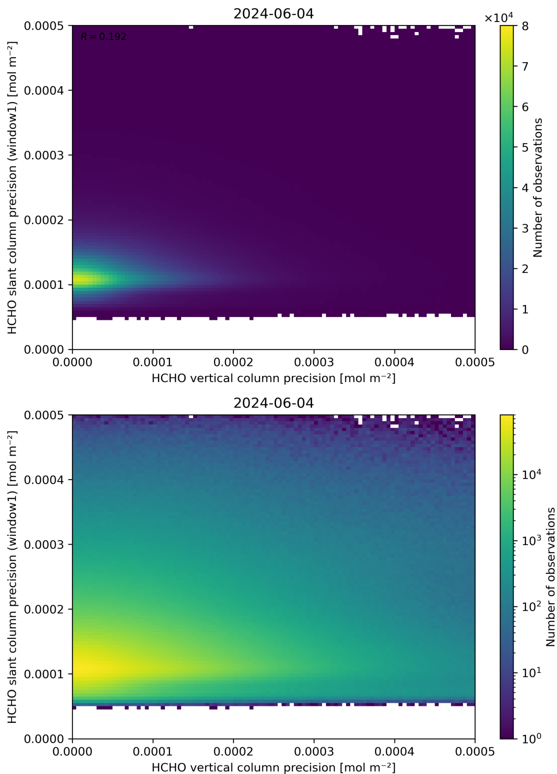
Figure 143: Scatter density plot of “HCHO vertical column precision” against “HCHO slant column precision (window1)” for 2024-06-03 to 2024-06-05.
