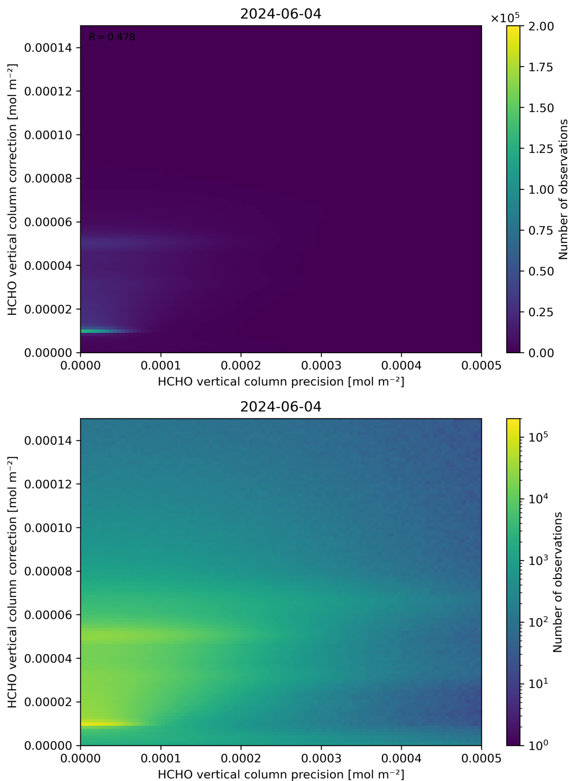
Figure 146: Scatter density plot of “HCHO vertical column precision” against “HCHO vertical column correction” for 2024-06-03 to 2024-06-05.
