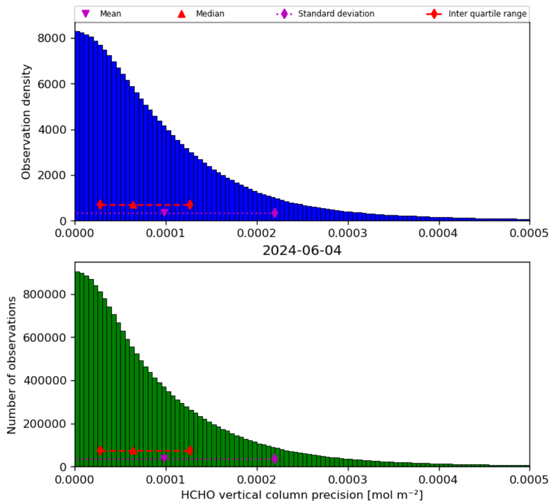
Figure 36: Histogram of “HCHO vertical column precision” for 2024-06-03 to 2024-06-05
