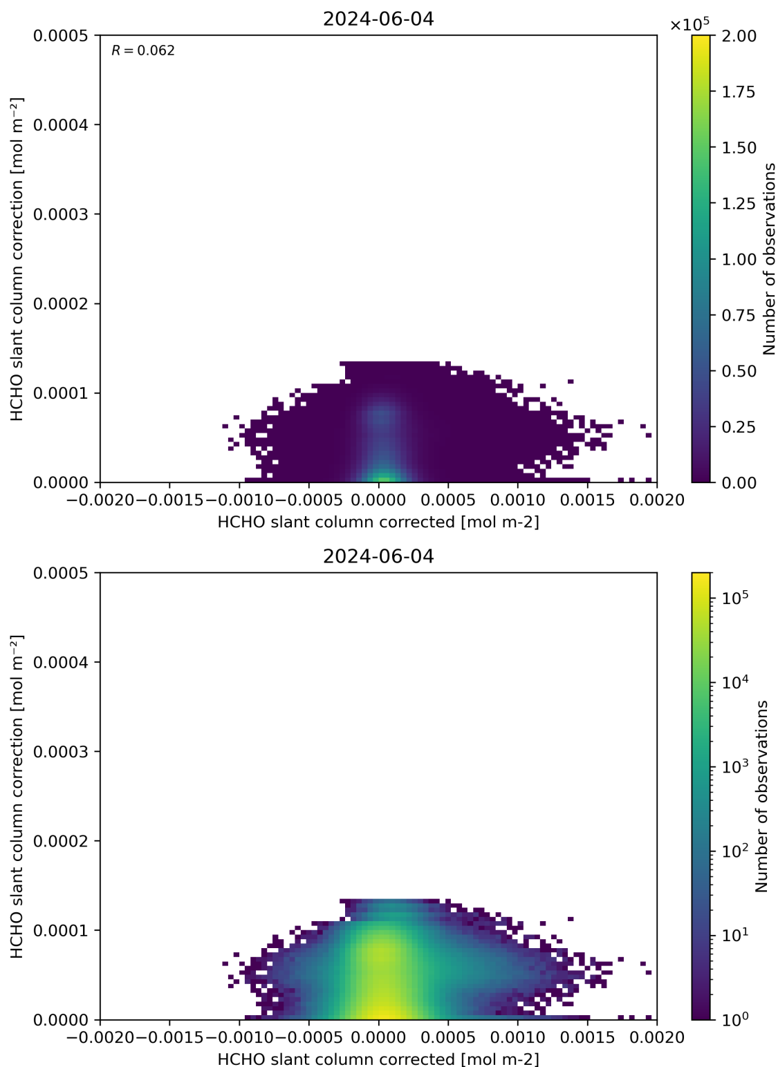
Figure 77: Scatter density plot of “HCHO slant column corrected” against “HCHO slant column correction” for 2024-06-03 to 2024-06-05.
