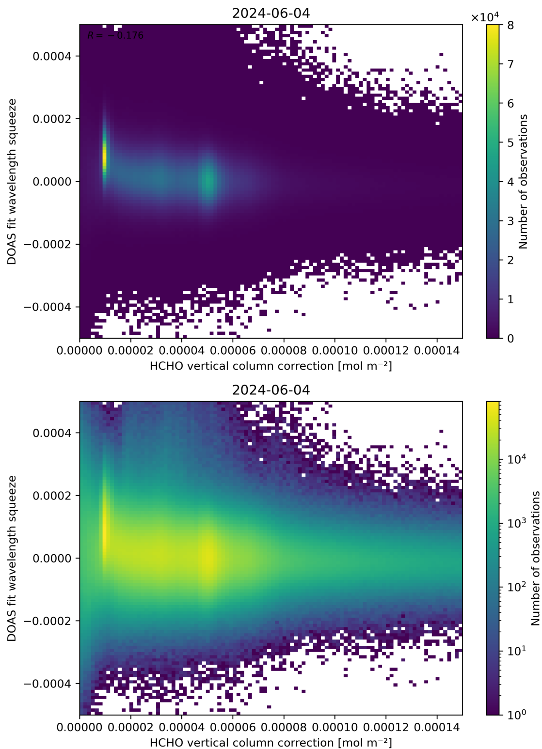
Figure 114: Scatter density plot of “HCHO vertical column correction” against “DOAS fit wavelength squeeze” for 2024-06-03 to 2024-06-05.
