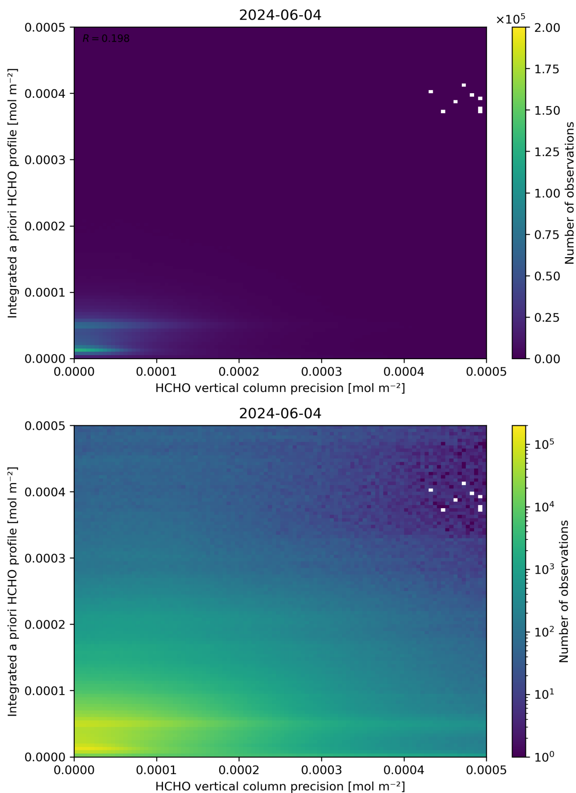
Figure 147: Scatter density plot of “HCHO vertical column precision” against “Integrated a priori HCHO profile” for 2024-06-03 to 2024-06-05.
