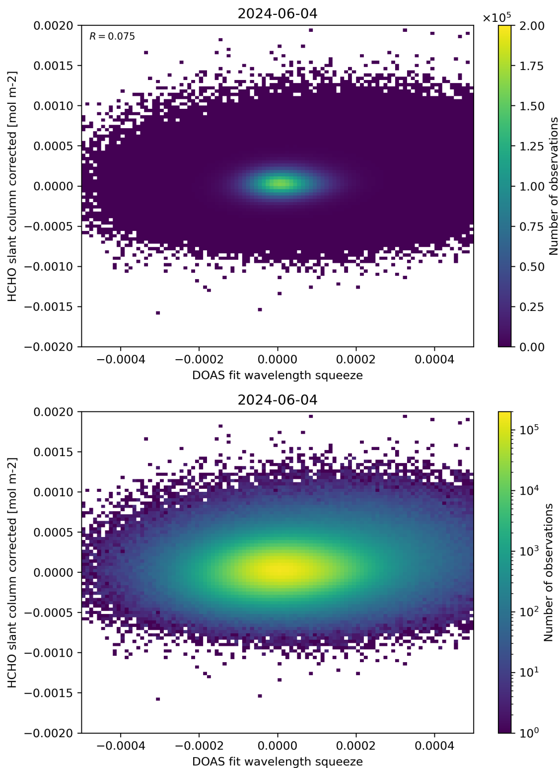
Figure 69: Scatter density plot of “DOAS fit wavelength squeeze” against “HCHO slant column corrected” for 2024-06-03 to 2024-06-05.
