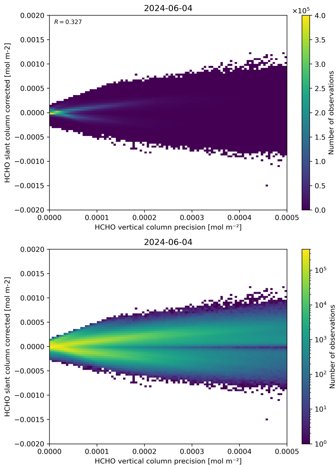
Figure 140: Scatter density plot of “HCHO vertical column precision” against “HCHO slant column corrected” for 2024-06-03 to 2024-06-05.
