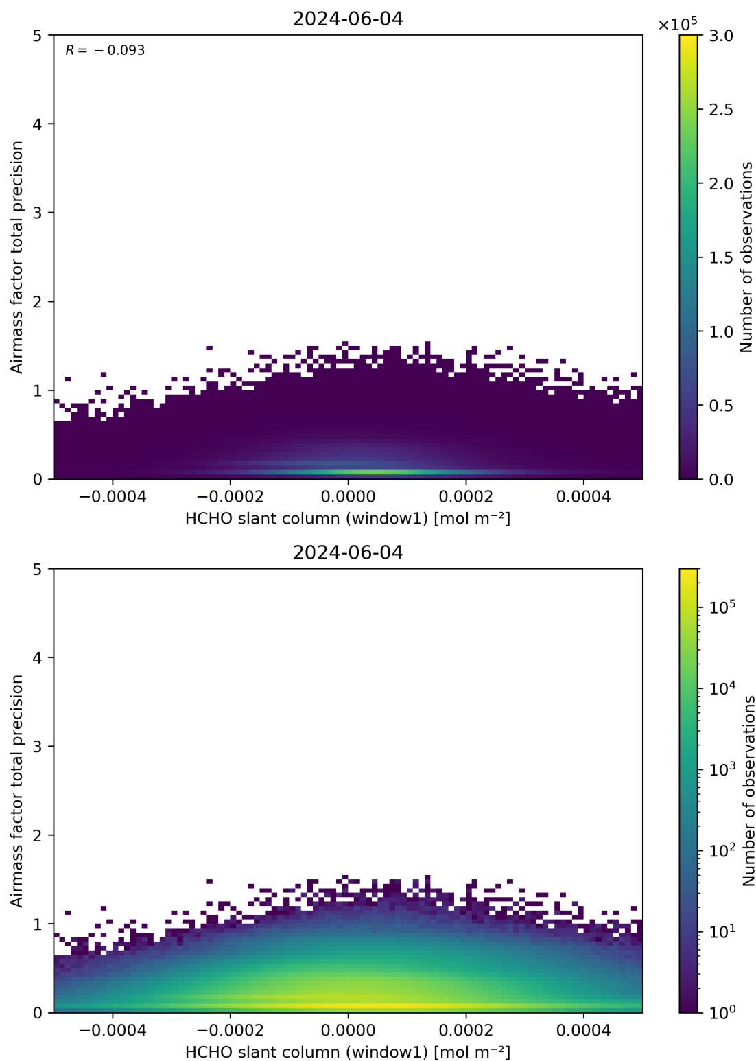
Figure 86: Scatter density plot of “HCHO slant column (window1)” against “Airmass factor total precision” for 2024-06-03 to 2024-06-05.
