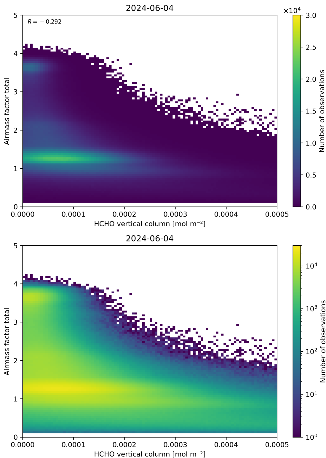
Figure 131: Scatter density plot of “HCHO vertical column” against “Airmass factor total” for 2024-06-03 to 2024-06-05.
