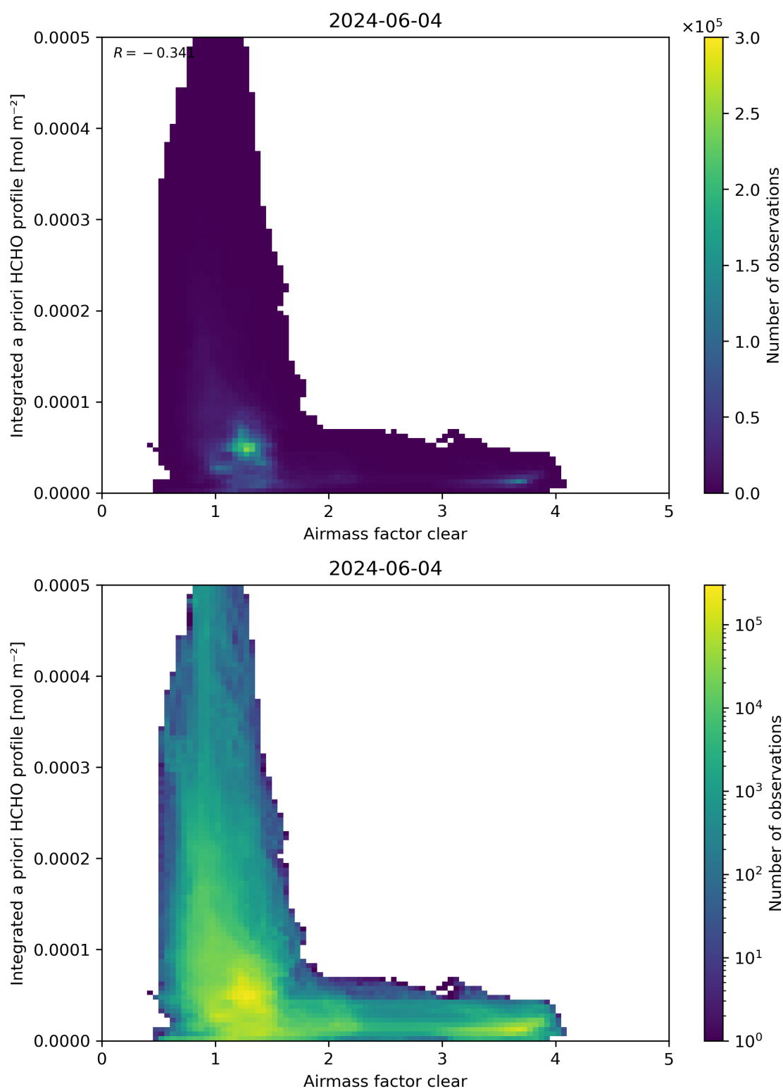
Figure 76: Scatter density plot of “Airmass factor clear” against “Integrated a priori HCHO profile” for 2024-06-03 to 2024-06-05.
