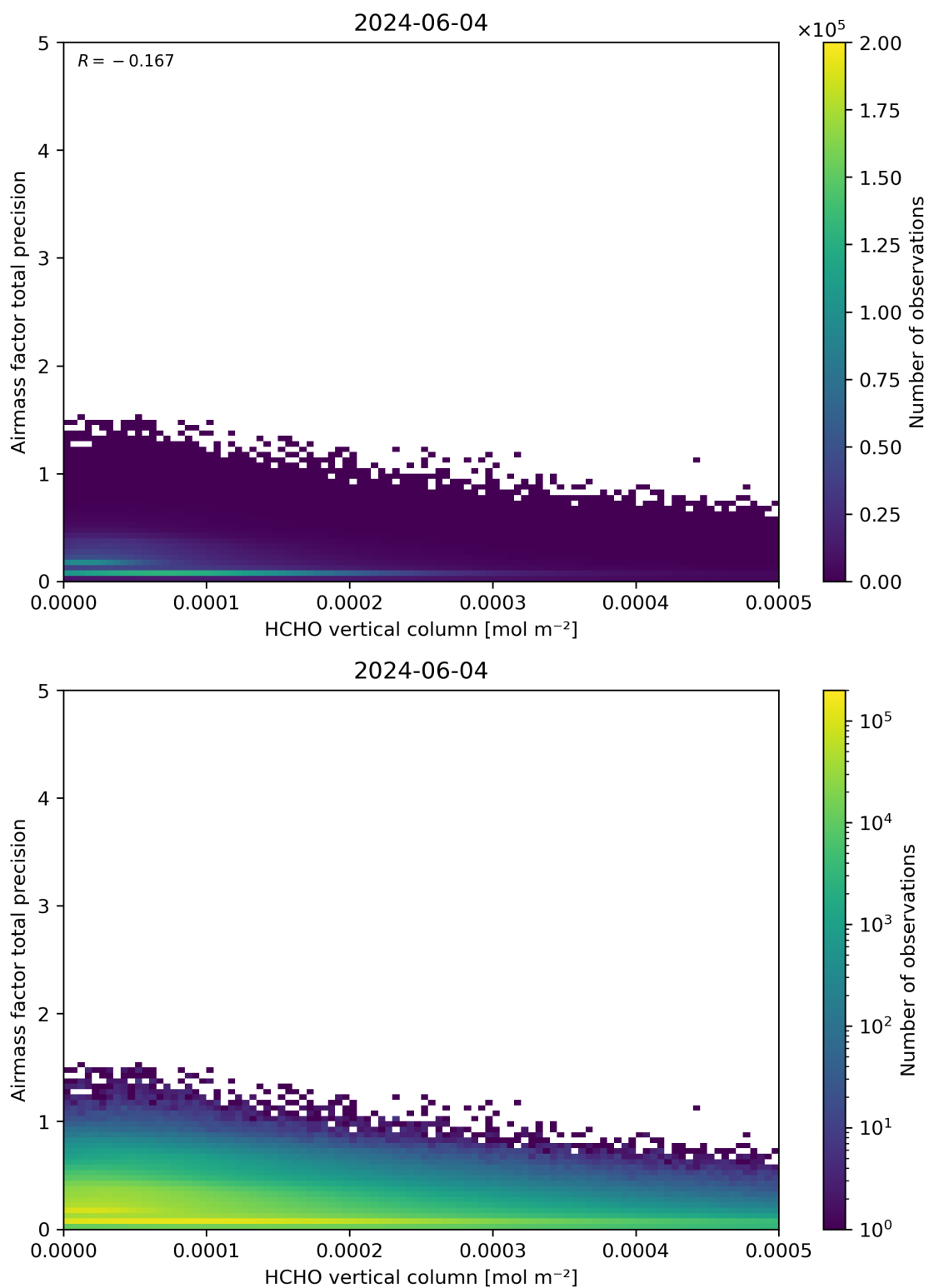
Figure 132: Scatter density plot of “HCHO vertical column” against “Airmass factor total precision” for 2024-06-03 to 2024-06-05.
