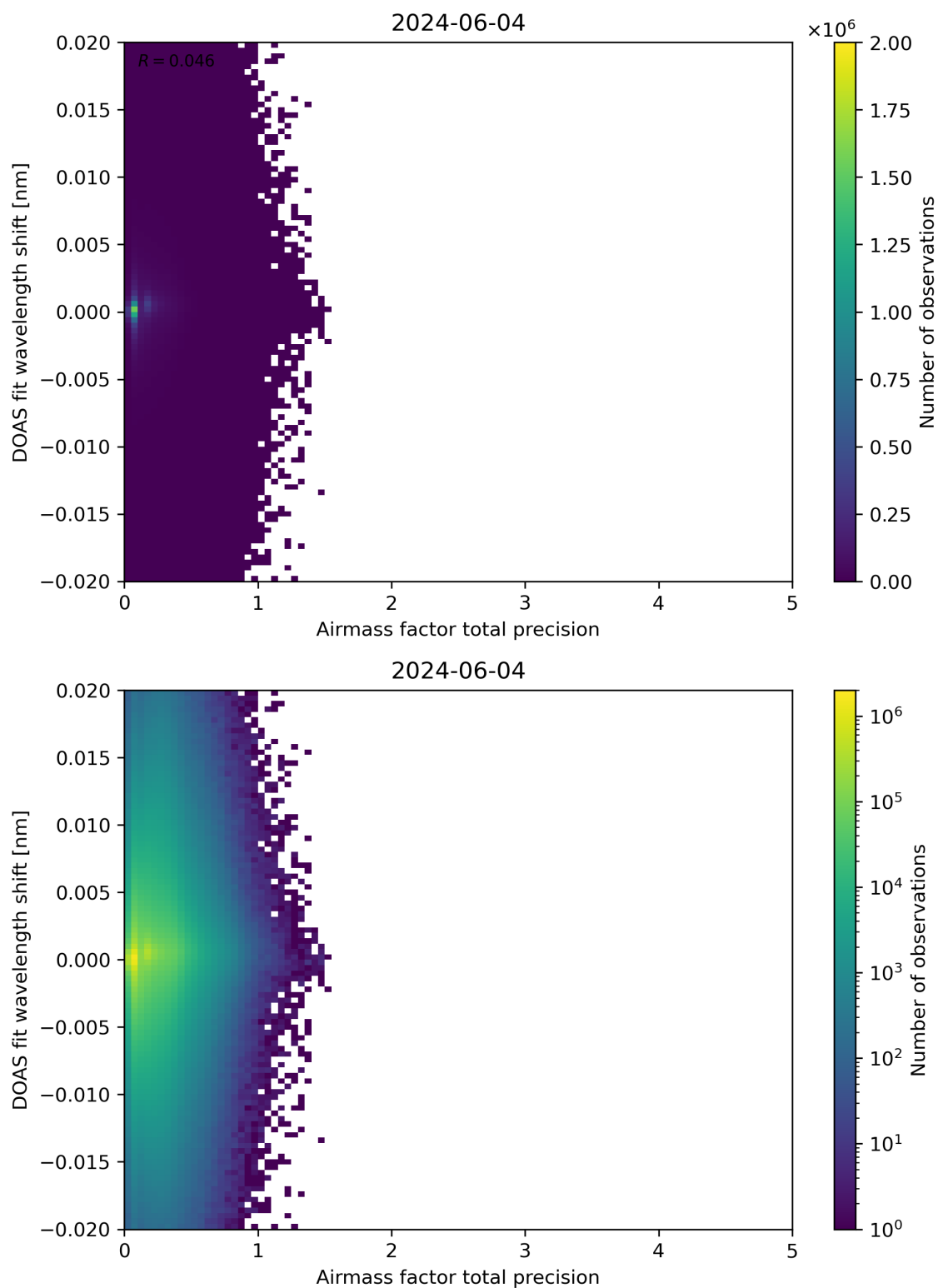
Figure 106: Scatter density plot of “Airmass factor total precision” against “DOAS fit wavelength shift” for 2024-06-03 to 2024-06-05.
