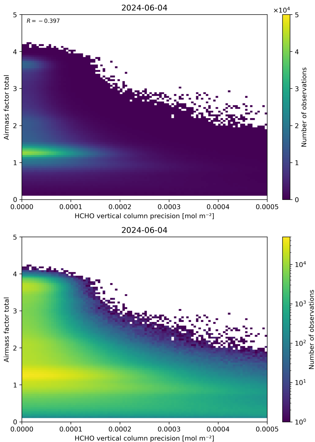
Figure 144: Scatter density plot of “HCHO vertical column precision” against “Airmass factor total” for 2024-06-03 to 2024-06-05.
