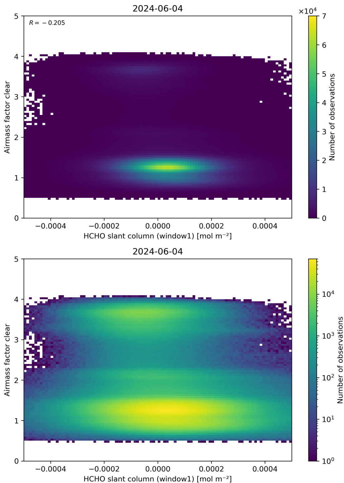
Figure 81: Scatter density plot of “HCHO slant column (window1)” against “Airmass factor clear” for 2024-06-03 to 2024-06-05.
