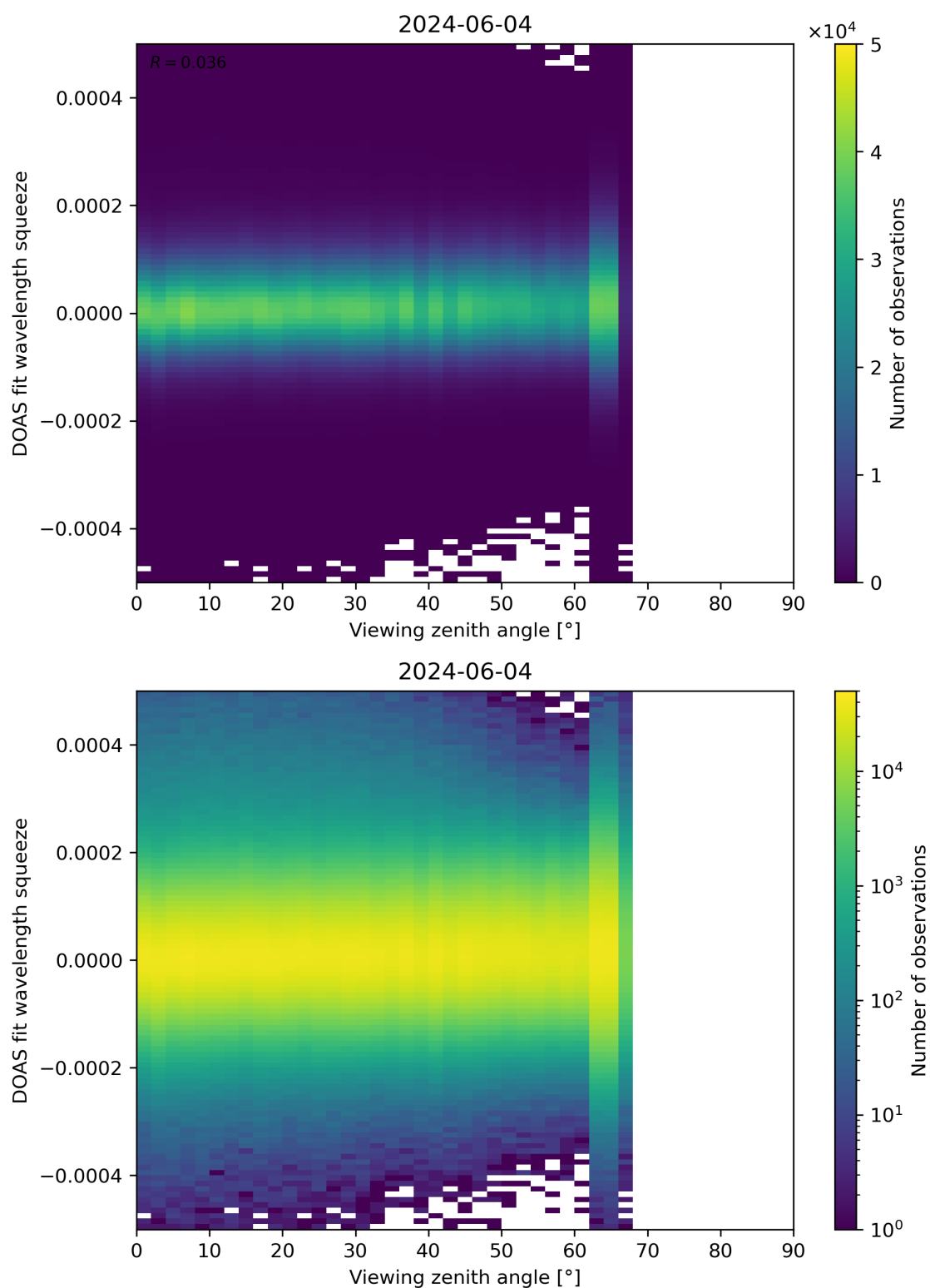
Figure 184: Scatter density plot of “Viewing zenith angle” against “DOAS fit wavelength squeeze” for 2024-06-03 to 2024-06-05.
