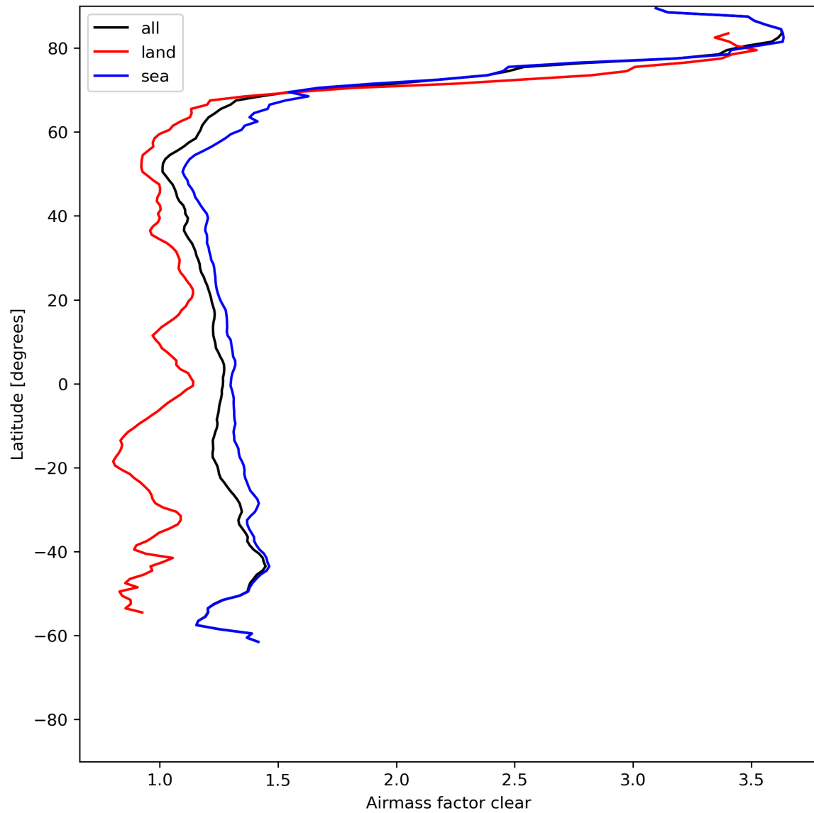
Figure 28: Zonal average of “Airmass factor clear” for 2024-06-03 to 2024-06-05.
