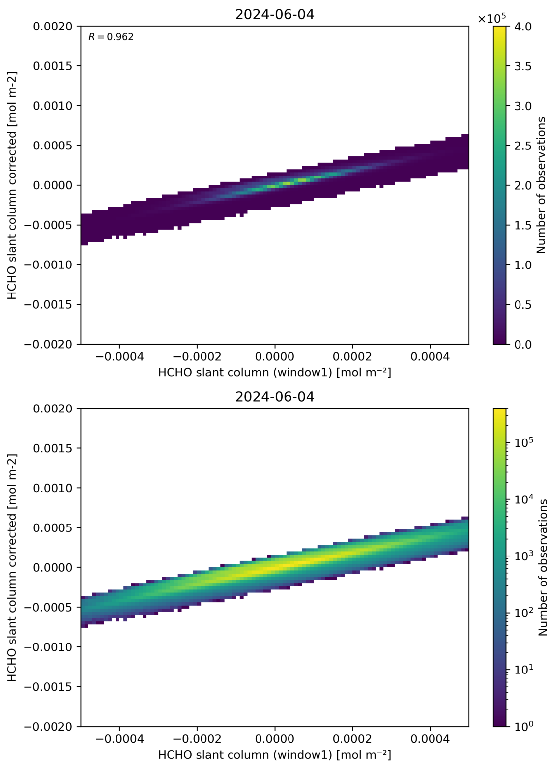
Figure 82: Scatter density plot of “HCHO slant column (window1)” against “HCHO slant column corrected” for 2024-06-03 to 2024-06-05.
