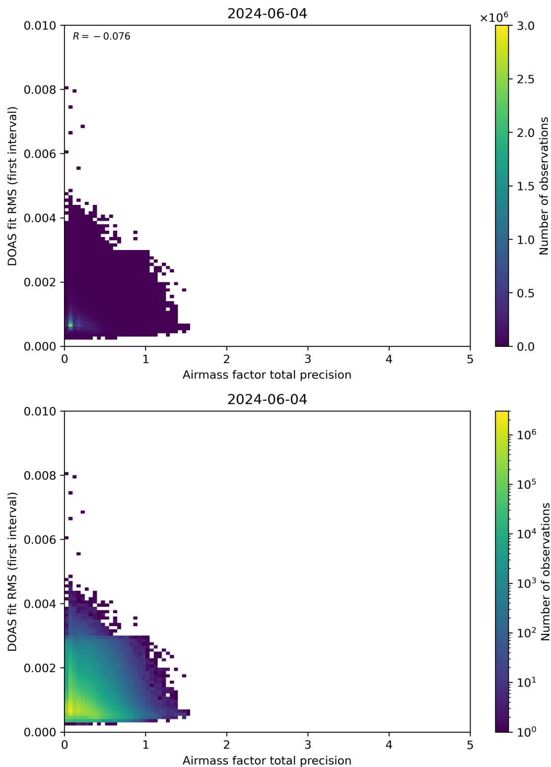
Figure 105: Scatter density plot of “Airmass factor total precision” against “DOAS fit RMS (first interval)” for 2024-06-03 to 2024-06-05.
