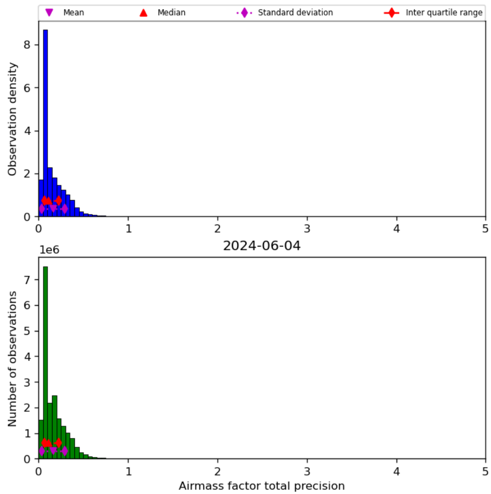
Figure 41: Histogram of “Airmass factor total precision” for 2024-06-03 to 2024-06-05
