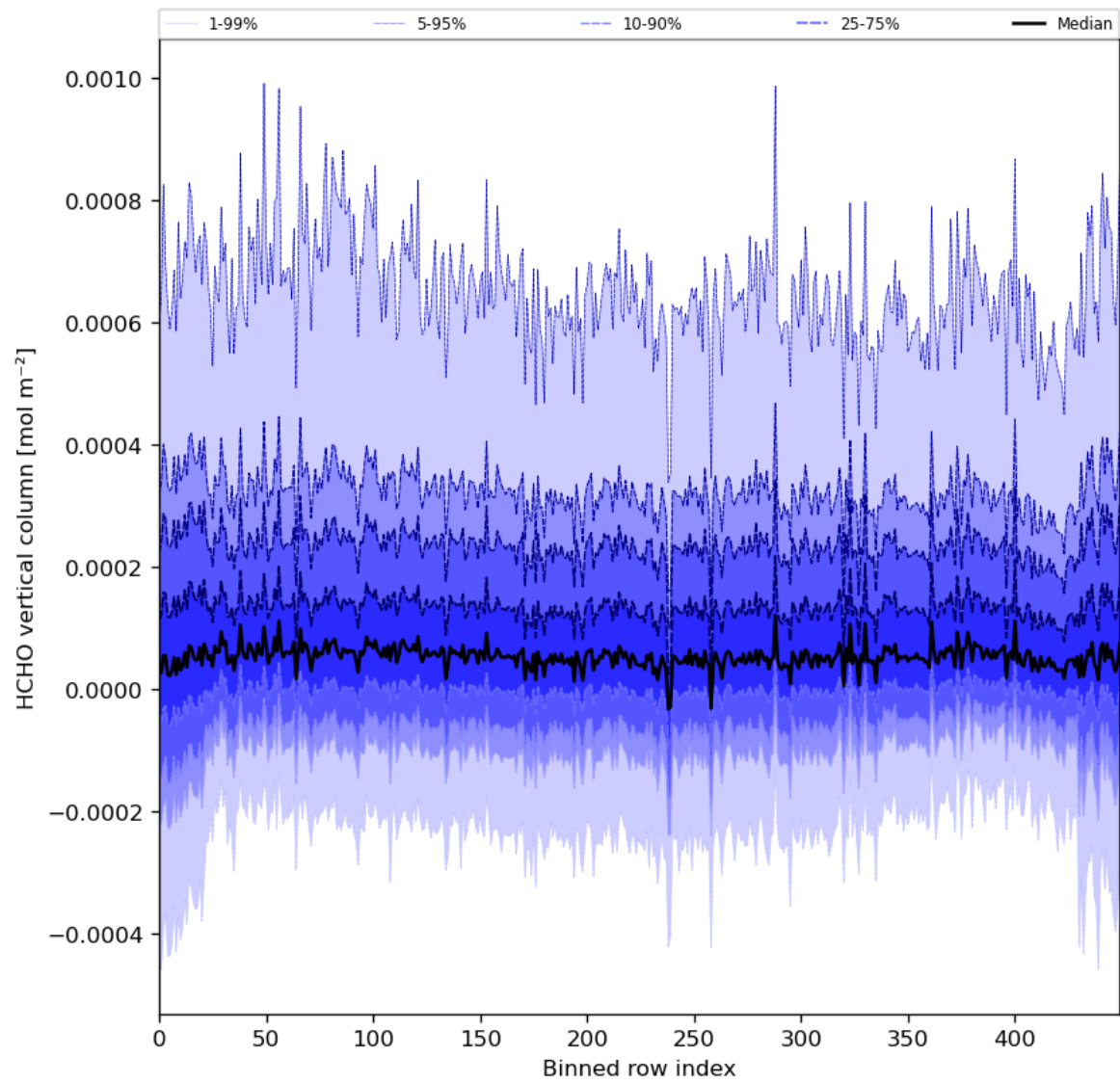
Figure 49: Along track statistics of “HCHO vertical column” for 2024-06-03 to 2024-06-05
