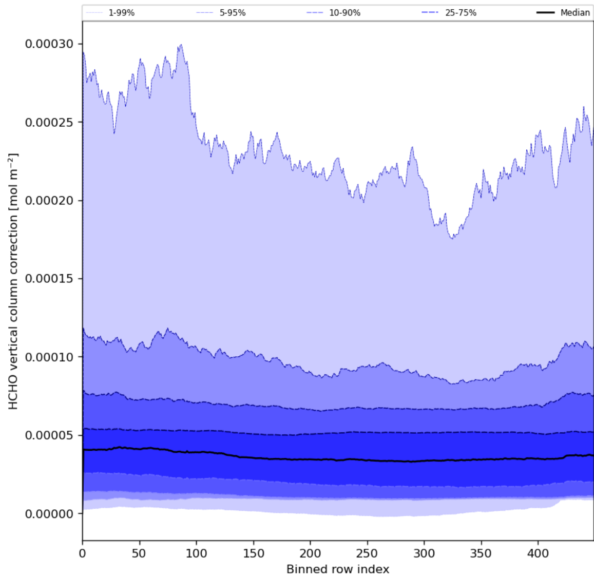
Figure 51: Along track statistics of “HCHO vertical column correction” for 2024-06-03 to 2024-06-05
