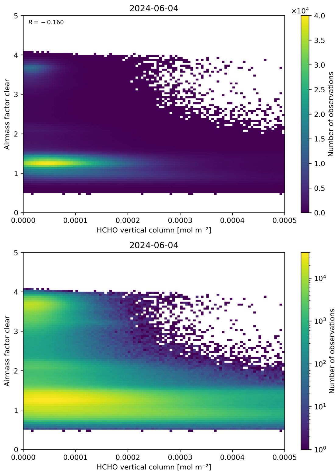
Figure 126: Scatter density plot of “HCHO vertical column” against “Airmass factor clear” for 2024-06-03 to 2024-06-05.
