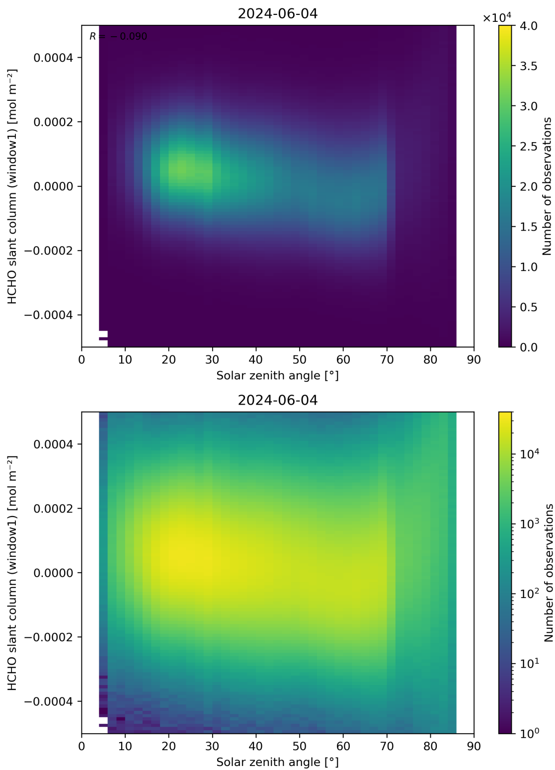
Figure 173: Scatter density plot of “Solar zenith angle” against “HCHO slant column (window1)” for 2024-06-03 to 2024-06-05.
