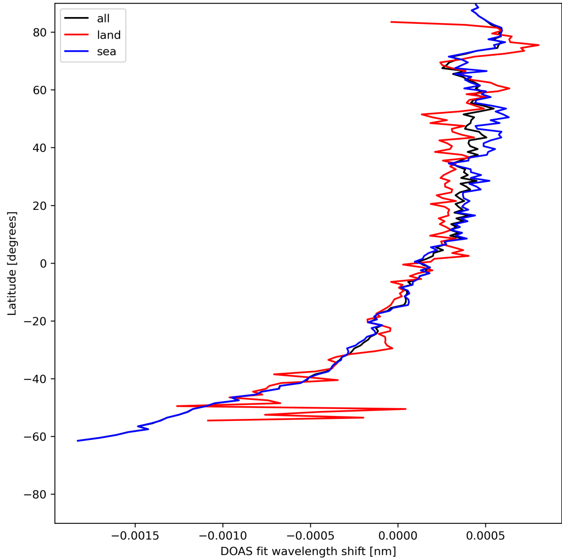
Figure 30: Zonal average of “DOAS fit wavelength shift” for 2024-06-03 to 2024-06-05.
