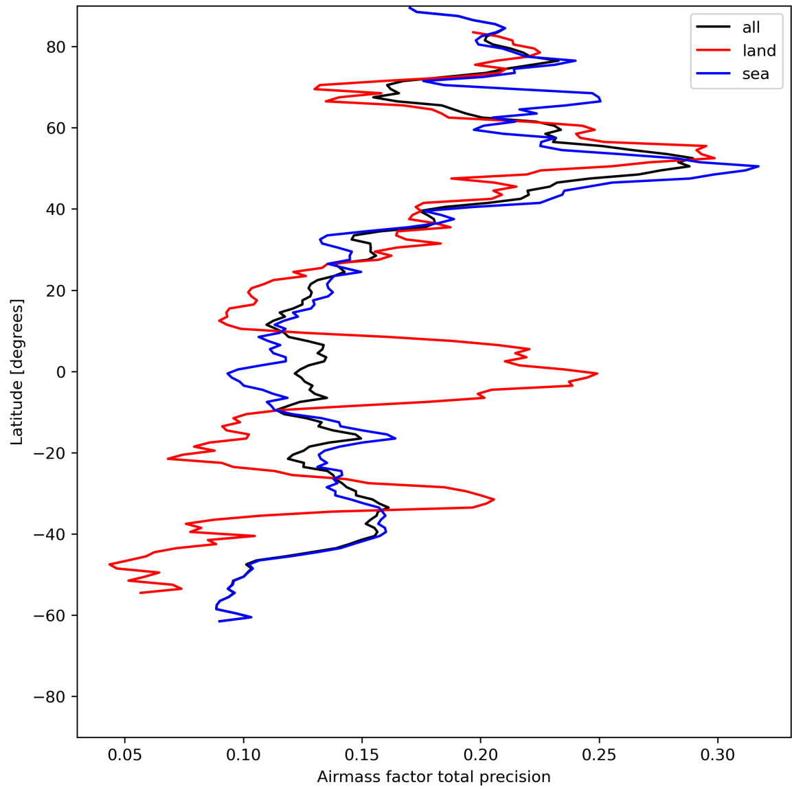
Figure 27: Zonal average of “Airmass factor total precision” for 2024-06-03 to 2024-06-05.
