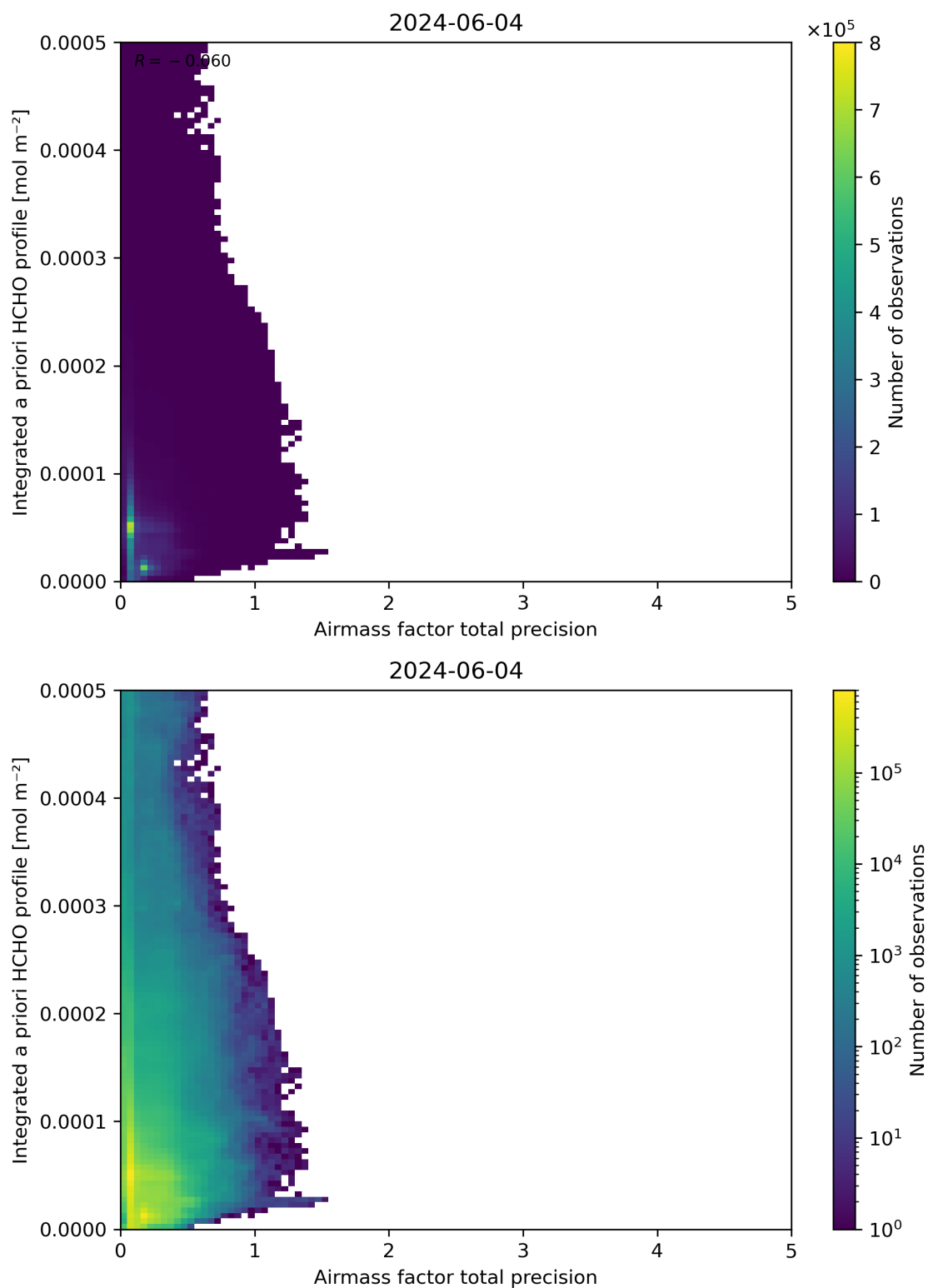
Figure 111: Scatter density plot of “Airmass factor total precision” against “Integrated a priori HCHO profile” for 2024-06-03 to 2024-06-05.
