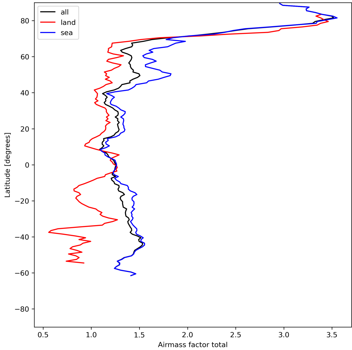
Figure 26: Zonal average of “Airmass factor total” for 2024-06-03 to 2024-06-05.
