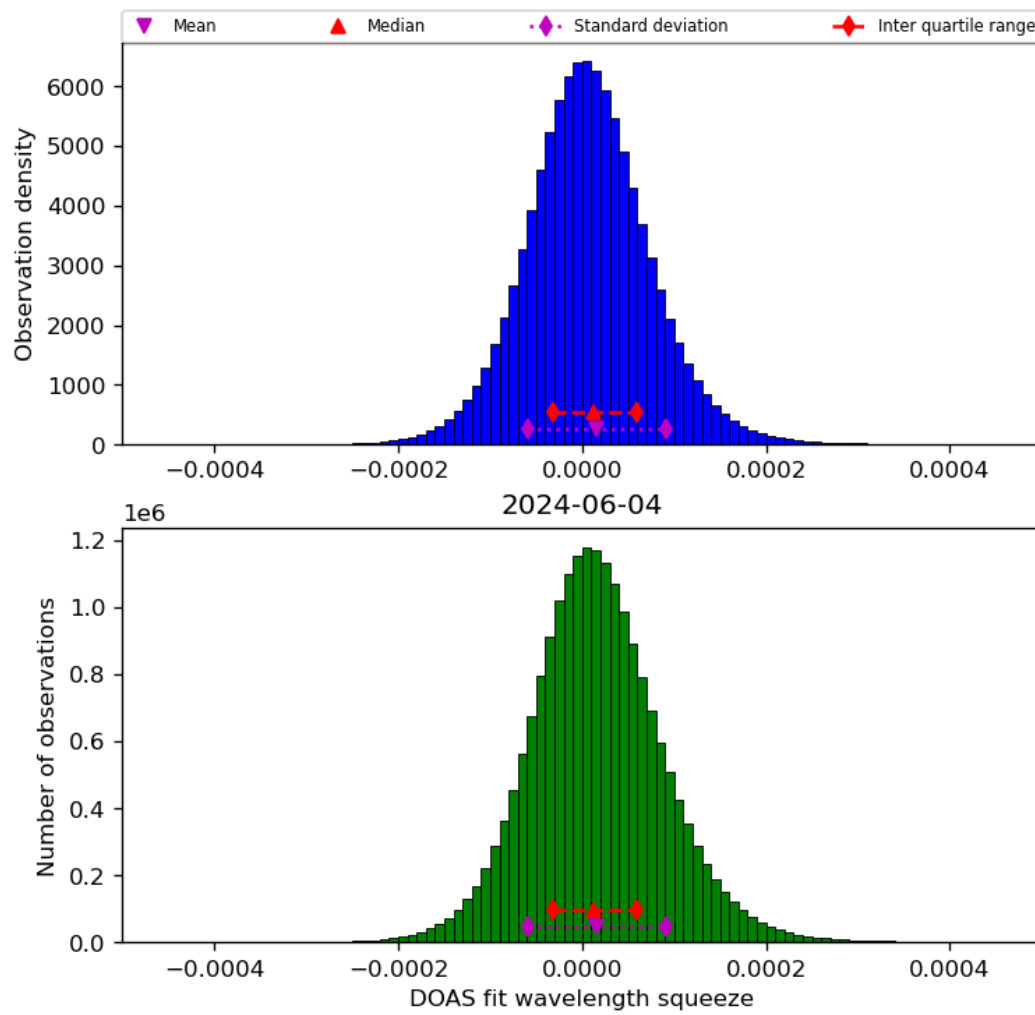
Figure 45: Histogram of “DOAS fit wavelength squeeze” for 2024-06-03 to 2024-06-05
