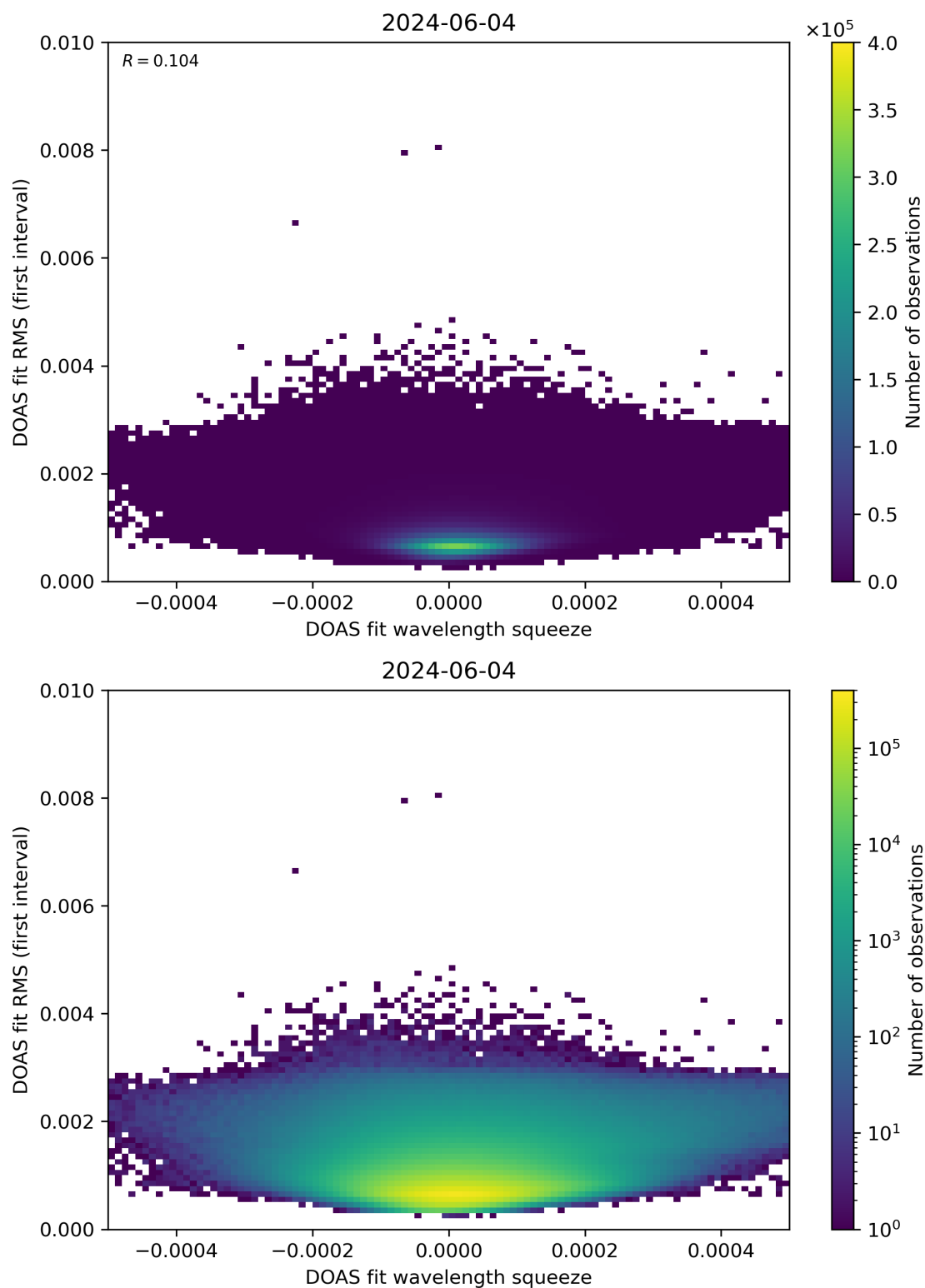
Figure 68: Scatter density plot of “DOAS fit wavelength squeeze” against “DOAS fit RMS (first interval)” for 2024-06-03 to 2024-06-05.
