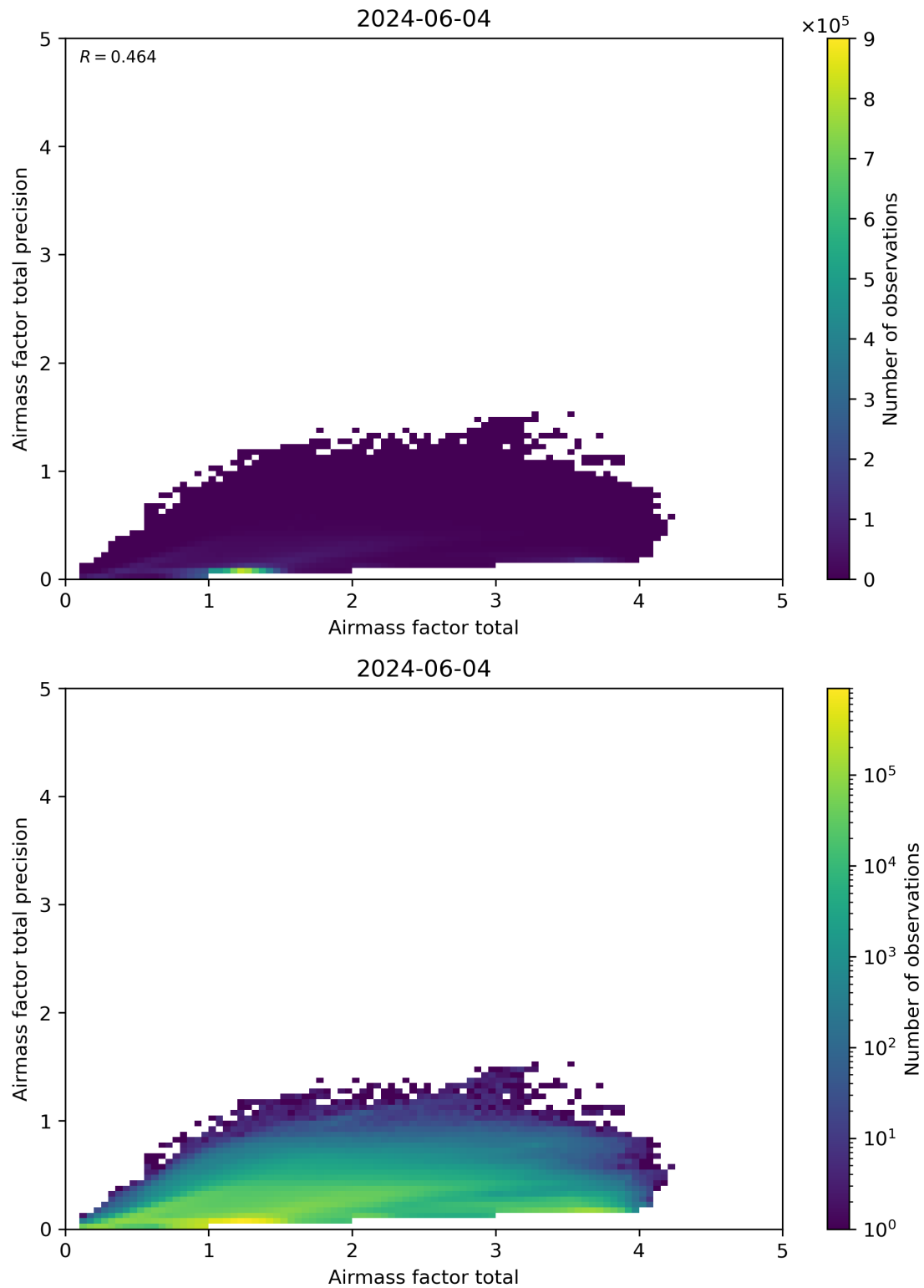
Figure 103: Scatter density plot of “Airmass factor total” against “Airmass factor total precision” for 2024-06-03 to 2024-06-05.
