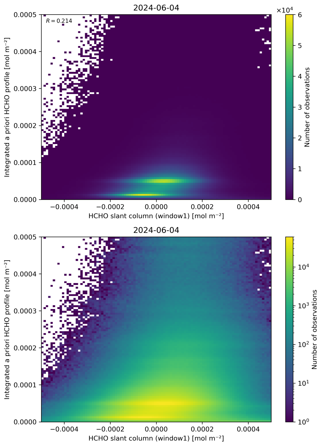
Figure 87: Scatter density plot of “HCHO slant column (window1)” against “Integrated a priori HCHO profile” for 2024-06-03 to 2024-06-05.
