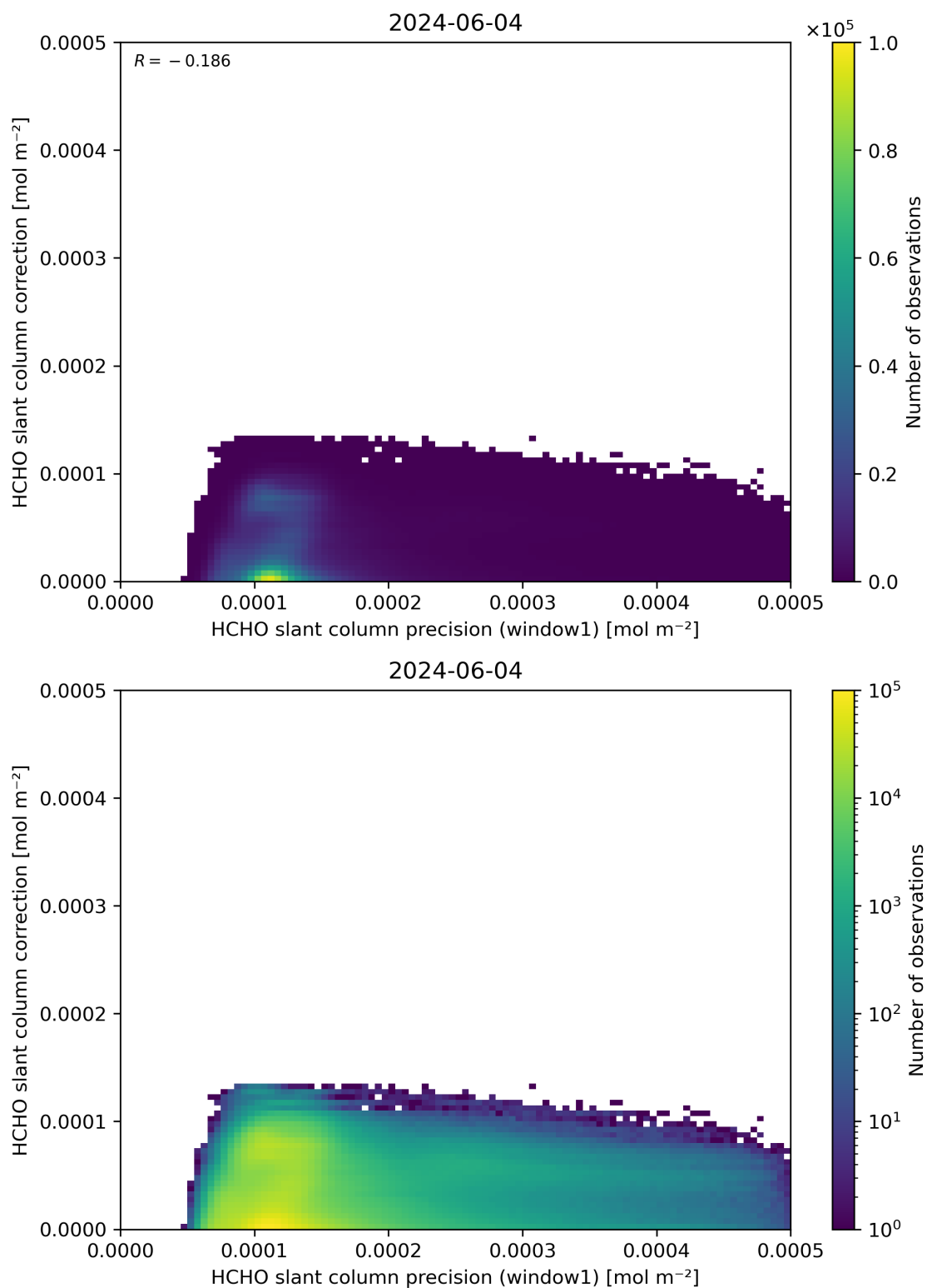
Figure 93: Scatter density plot of “HCHO slant column precision (window1)” against “HCHO slant column correction” for 2024-06-03 to 2024-06-05.
