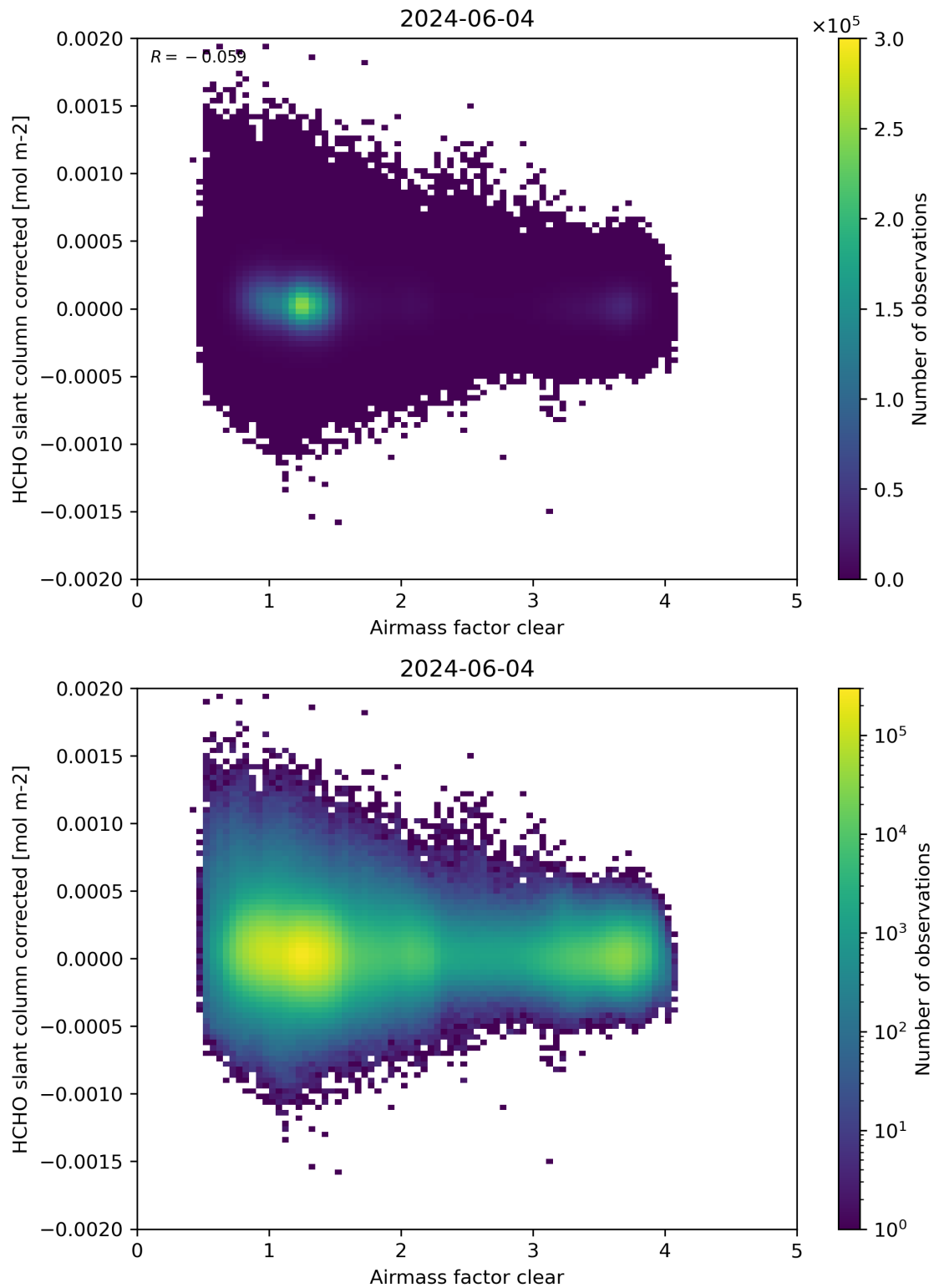
Figure 74: Scatter density plot of “Airmass factor clear” against “HCHO slant column corrected” for 2024-06-03 to 2024-06-05.
