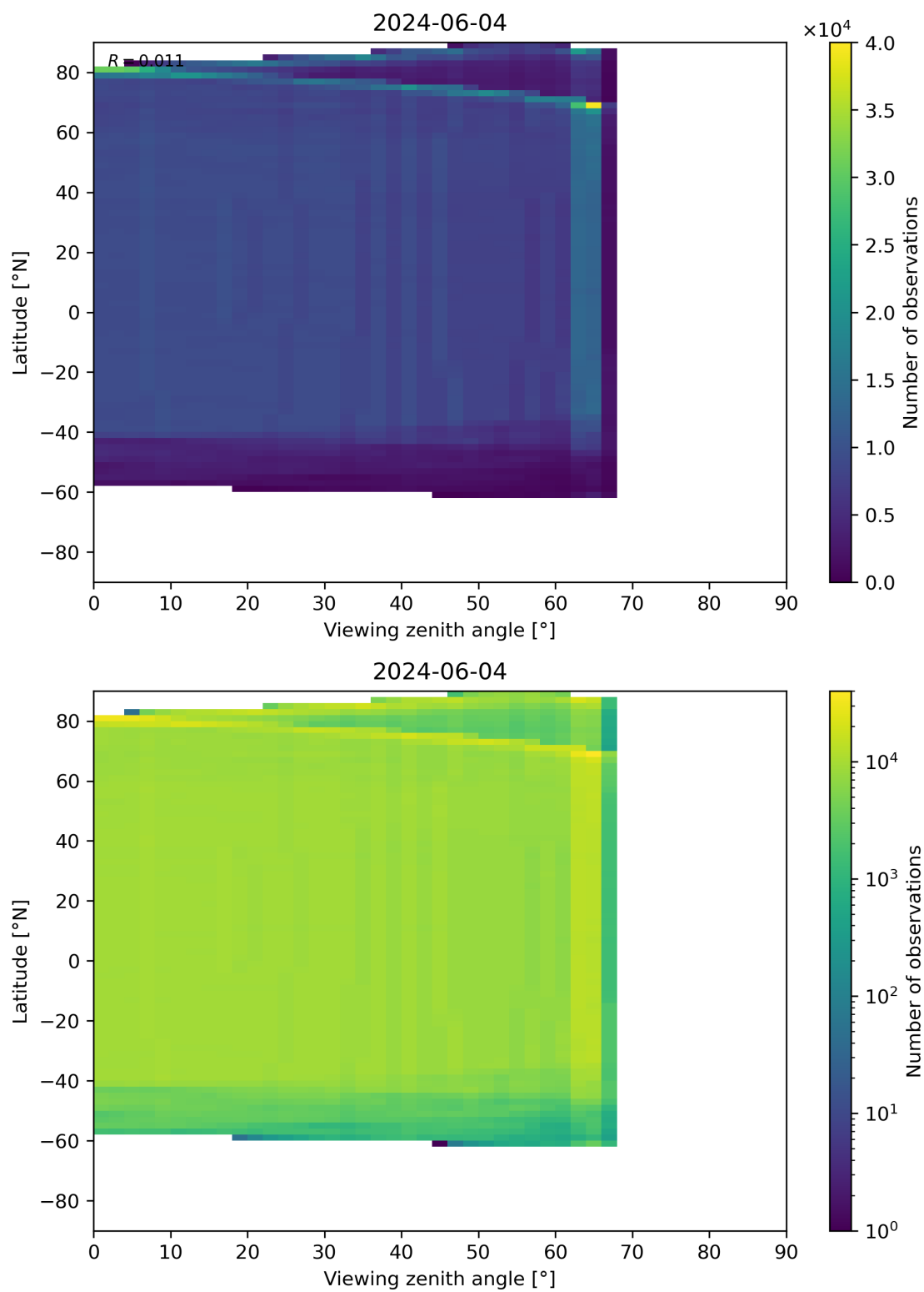
Figure 196: Scatter density plot of “Viewing zenith angle” against “Latitude” for 2024-06-03 to 2024-06-05.
