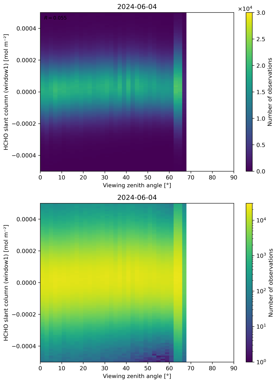
Figure 188: Scatter density plot of “Viewing zenith angle” against “HCHO slant column (window1)” for 2024-06-03 to 2024-06-05.
