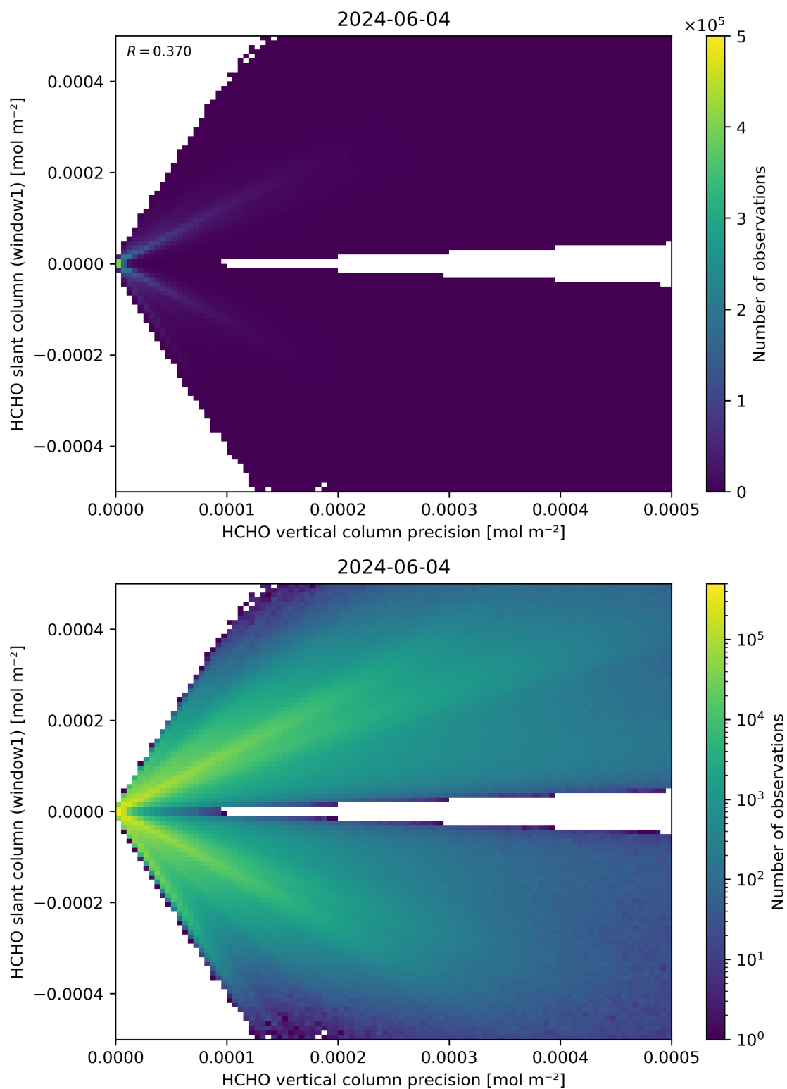
Figure 142: Scatter density plot of “HCHO vertical column precision” against “HCHO slant column (window1)” for 2024-06-03 to 2024-06-05.
