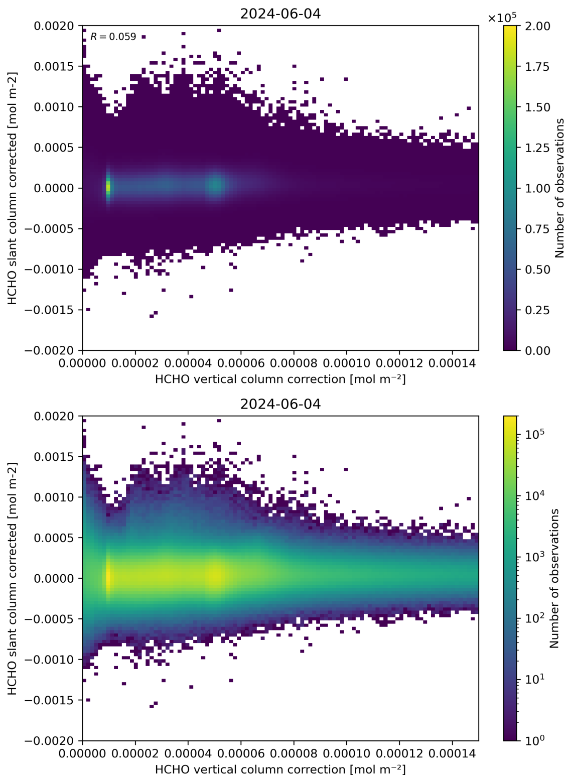
Figure 116: Scatter density plot of “HCHO vertical column correction” against “HCHO slant column corrected” for 2024-06-03 to 2024-06-05.
