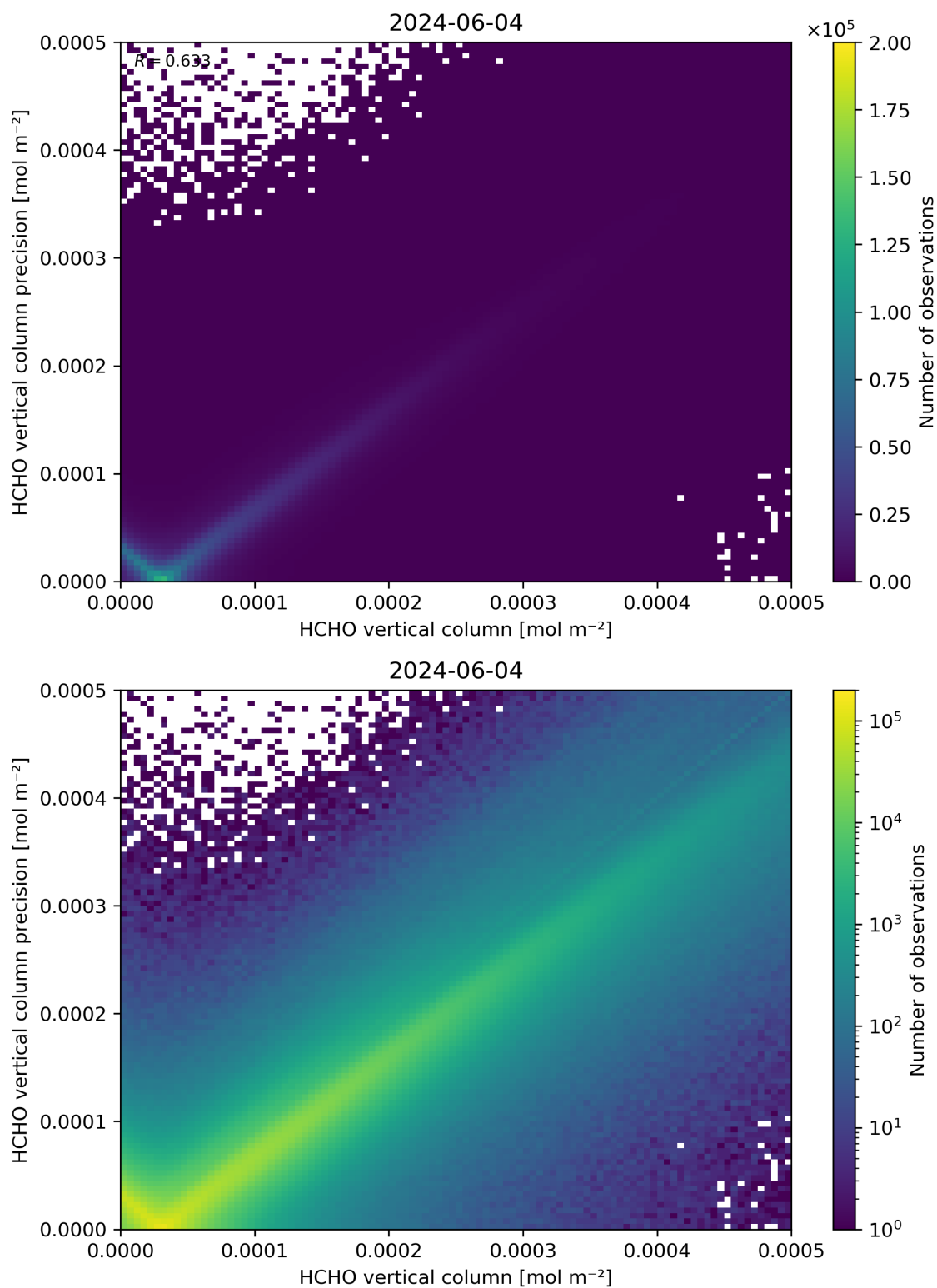
Figure 134: Scatter density plot of “HCHO vertical column” against “HCHO vertical column precision” for 2024-06-03 to 2024-06-05.
