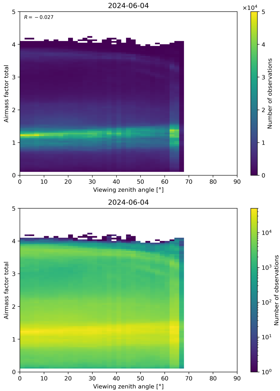
Figure 190: Scatter density plot of “Viewing zenith angle” against “Airmass factor total” for 2024-06-03 to 2024-06-05.
