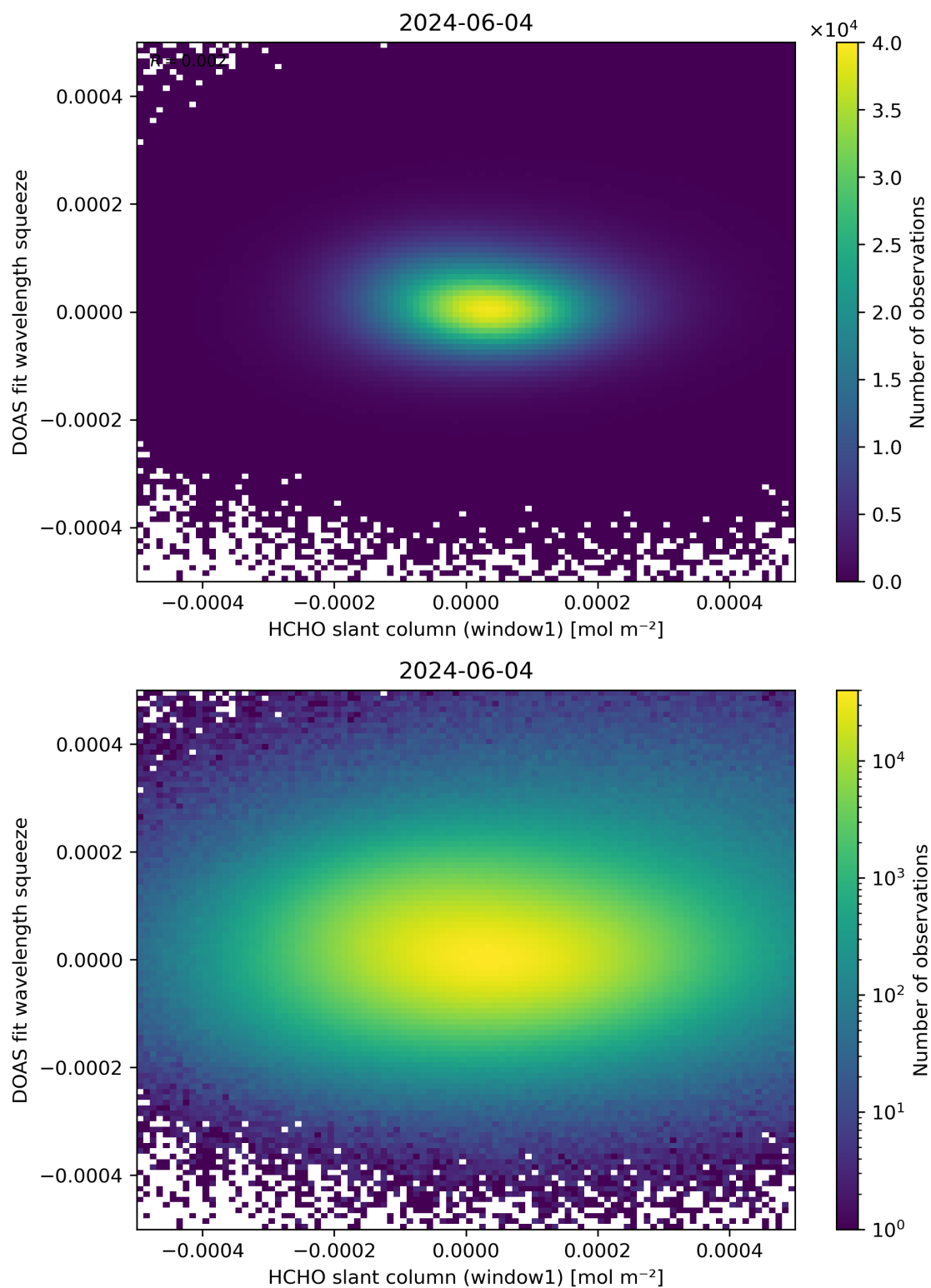
Figure 80: Scatter density plot of “HCHO slant column (window1)” against “DOAS fit wavelength squeeze” for 2024-06-03 to 2024-06-05.
