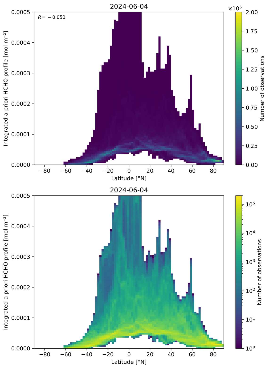
Figure 166: Scatter density plot of “Latitude” against “Integrated a priori HCHO profile” for 2024-06-03 to 2024-06-05.
