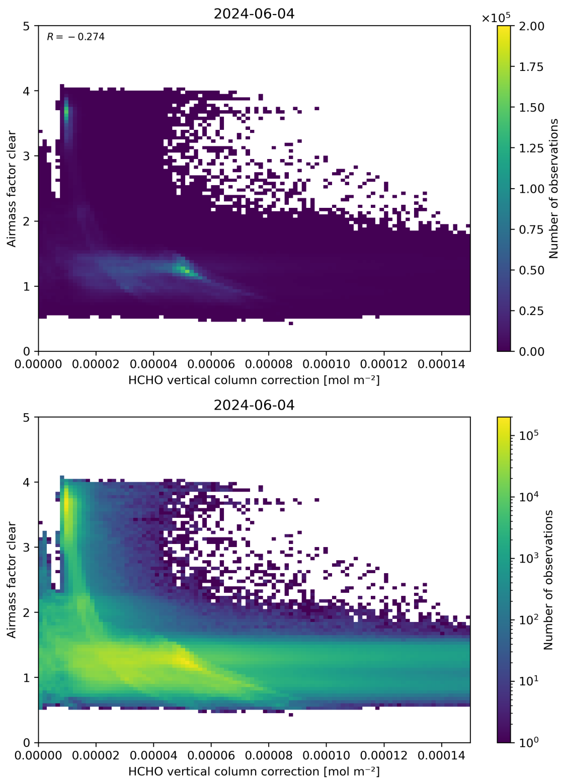
Figure 115: Scatter density plot of “HCHO vertical column correction” against “Airmass factor clear” for 2024-06-03 to 2024-06-05.
