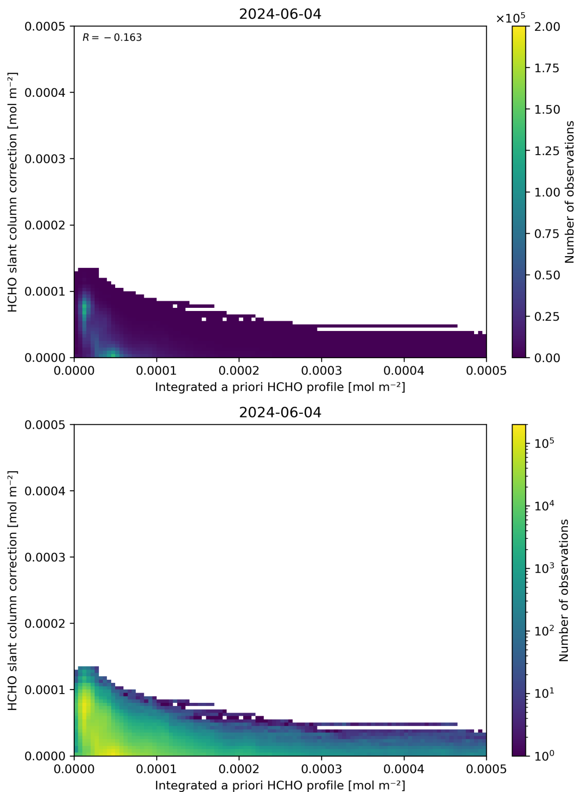
Figure 152: Scatter density plot of “Integrated a priori HCHO profile” against “HCHO slant column correction” for 2024-06-03 to 2024-06-05.
