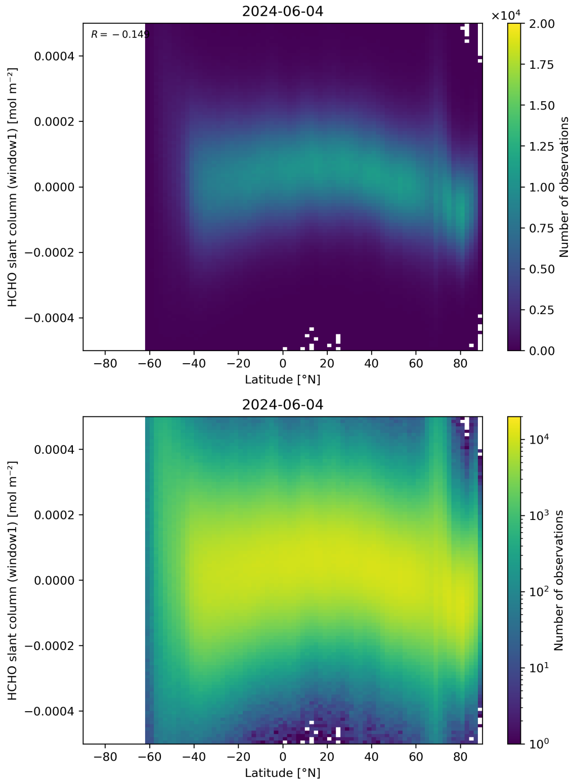
Figure 159: Scatter density plot of “Latitude” against “HCHO slant column (window1)” for 2024-06-03 to 2024-06-05.
