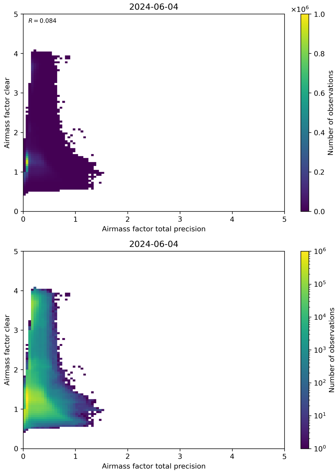
Figure 108: Scatter density plot of “Airmass factor total precision” against “Airmass factor clear” for 2024-06-03 to 2024-06-05.
