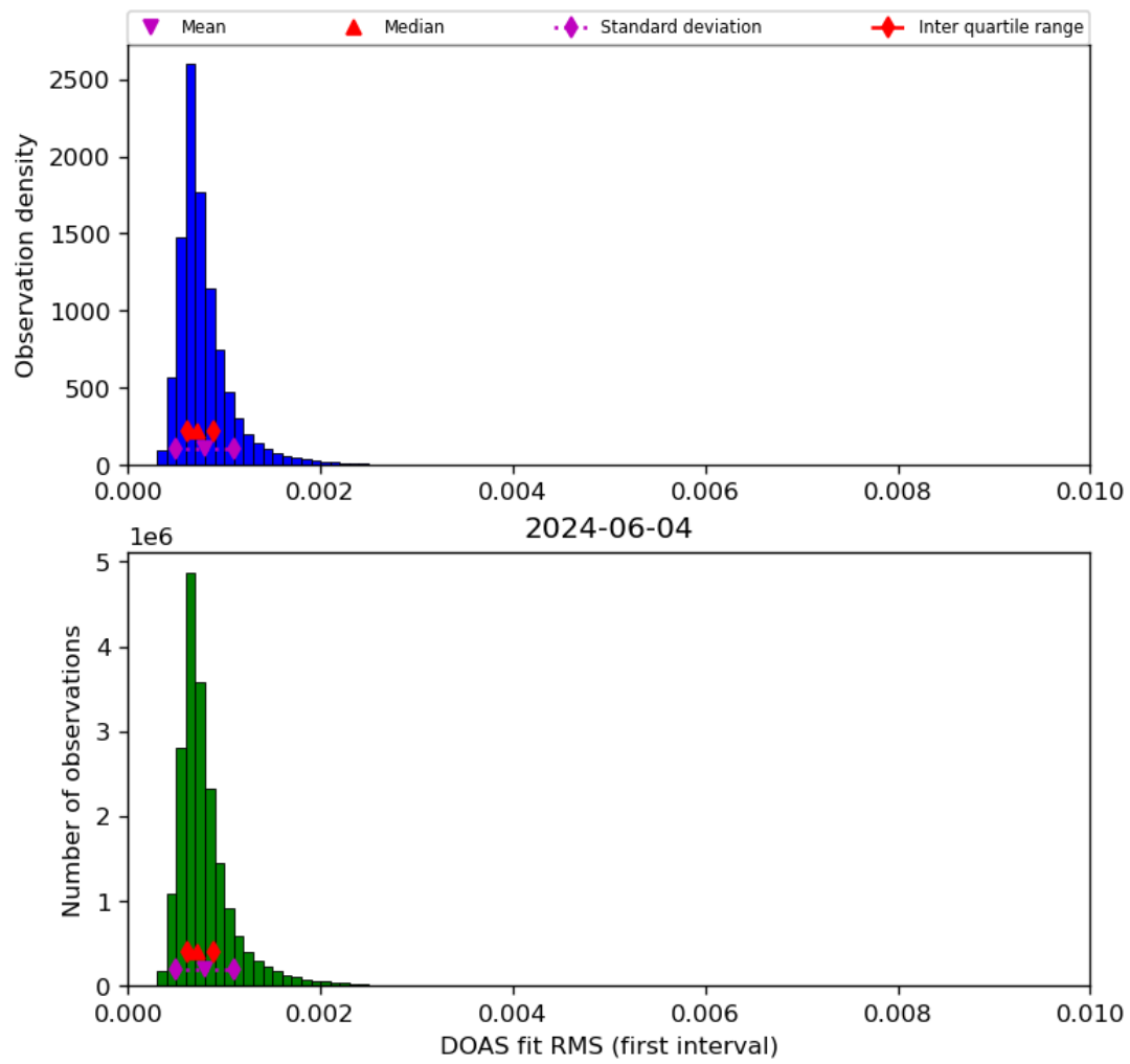
Figure 46: Histogram of “DOAS fit RMS (first interval)” for 2024-06-03 to 2024-06-05
