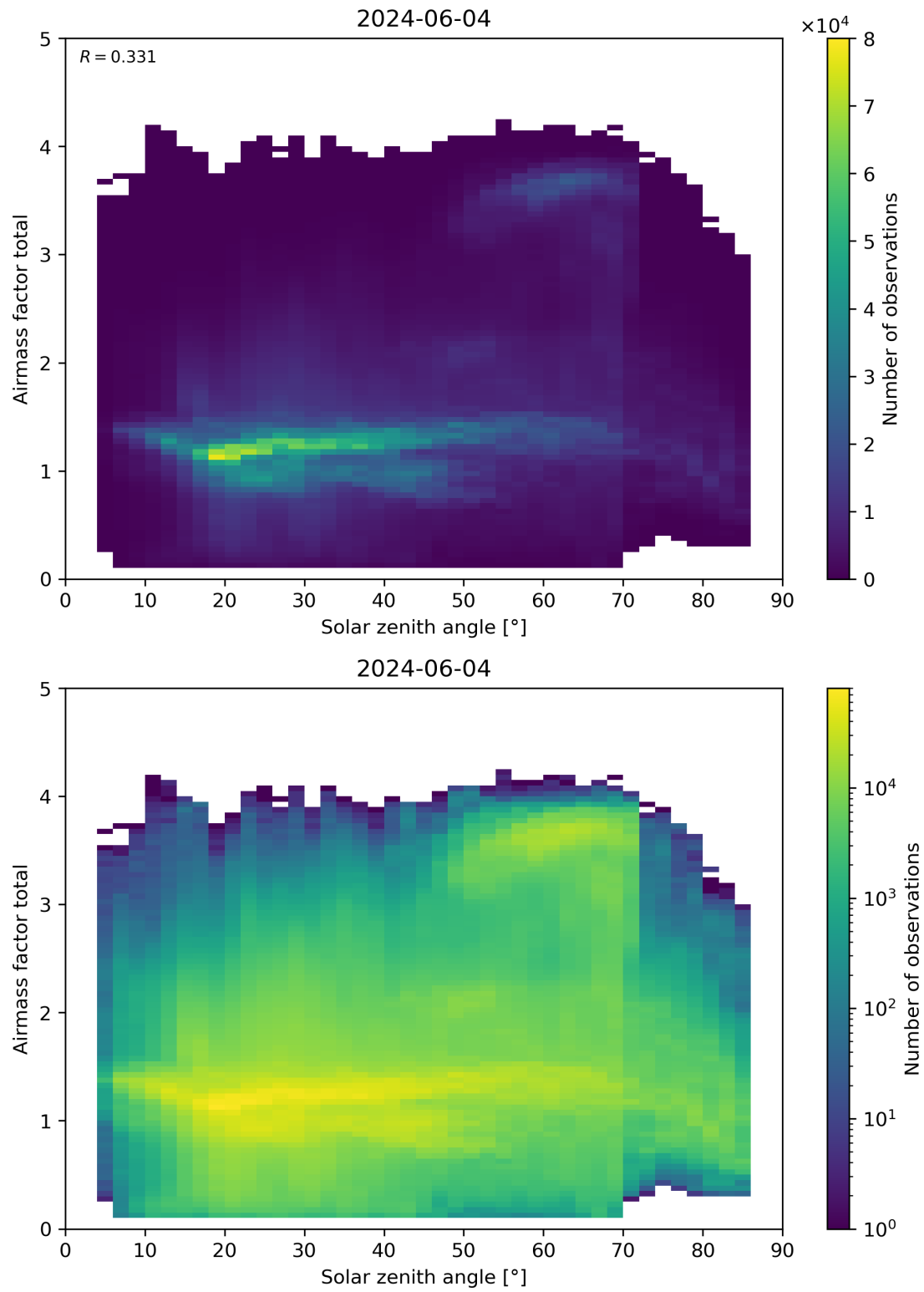
Figure 175: Scatter density plot of “Solar zenith angle” against “Airmass factor total” for 2024-06-03 to 2024-06-05.
