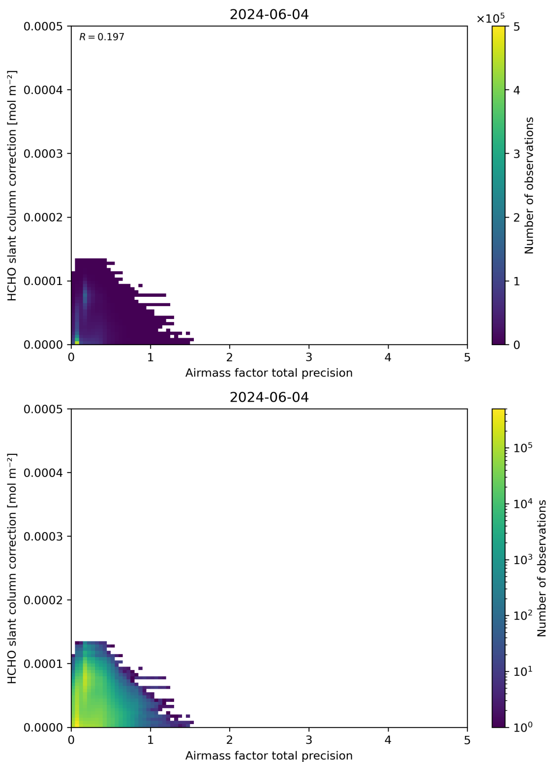
Figure 110: Scatter density plot of “Airmass factor total precision” against “HCHO slant column correction” for 2024-06-03 to 2024-06-05.
