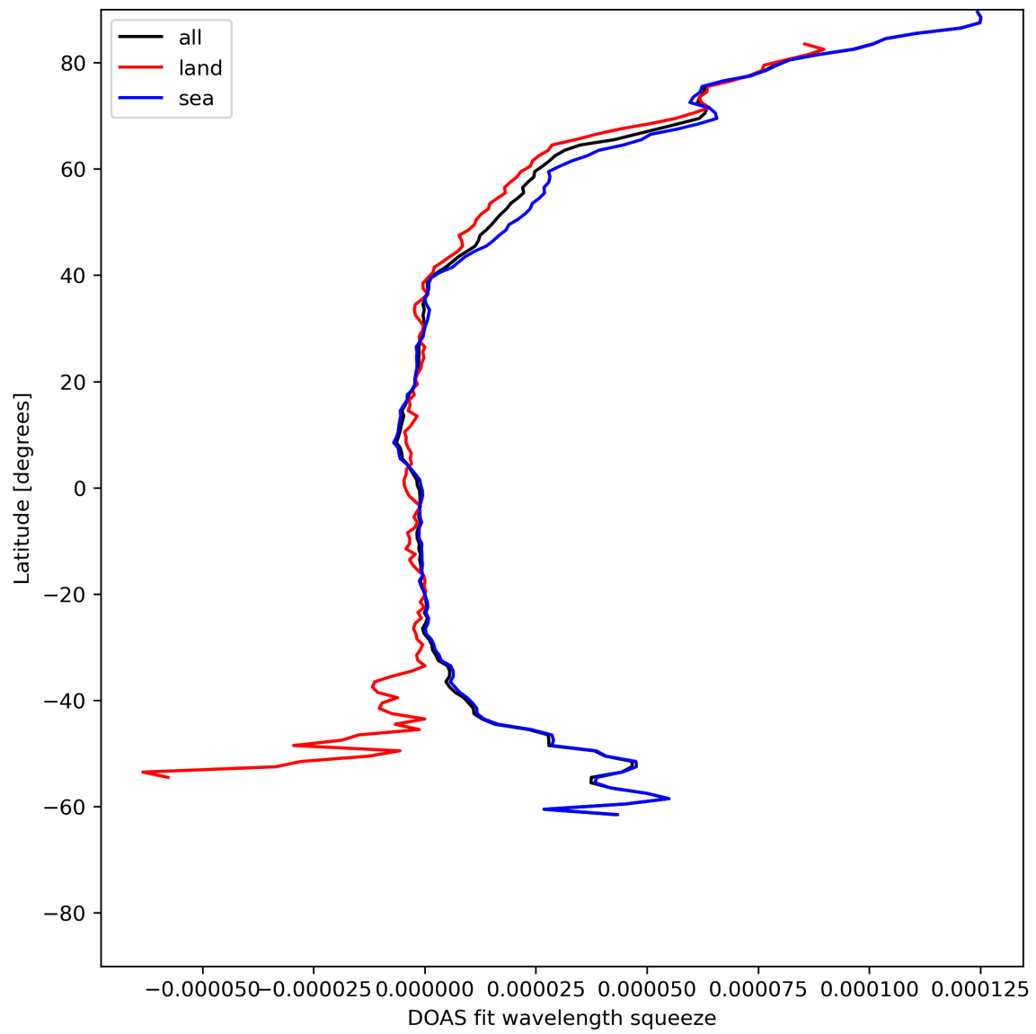
Figure 31: Zonal average of “DOAS fit wavelength squeeze” for 2024-06-03 to 2024-06-05.
