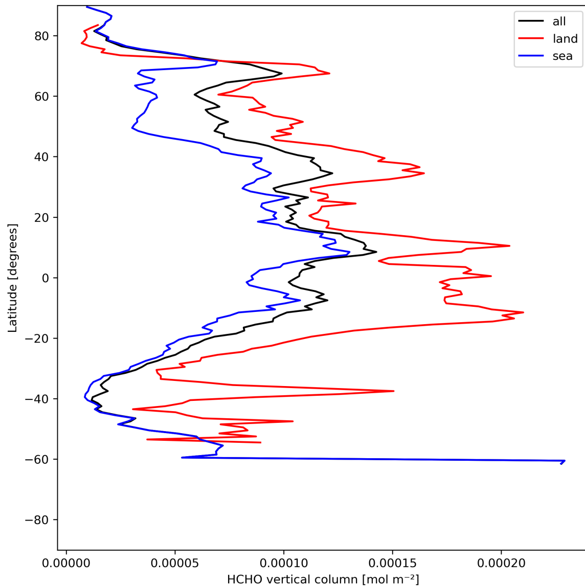
Figure 21: Zonal average of “HCHO vertical column” for 2024-06-03 to 2024-06-05.
