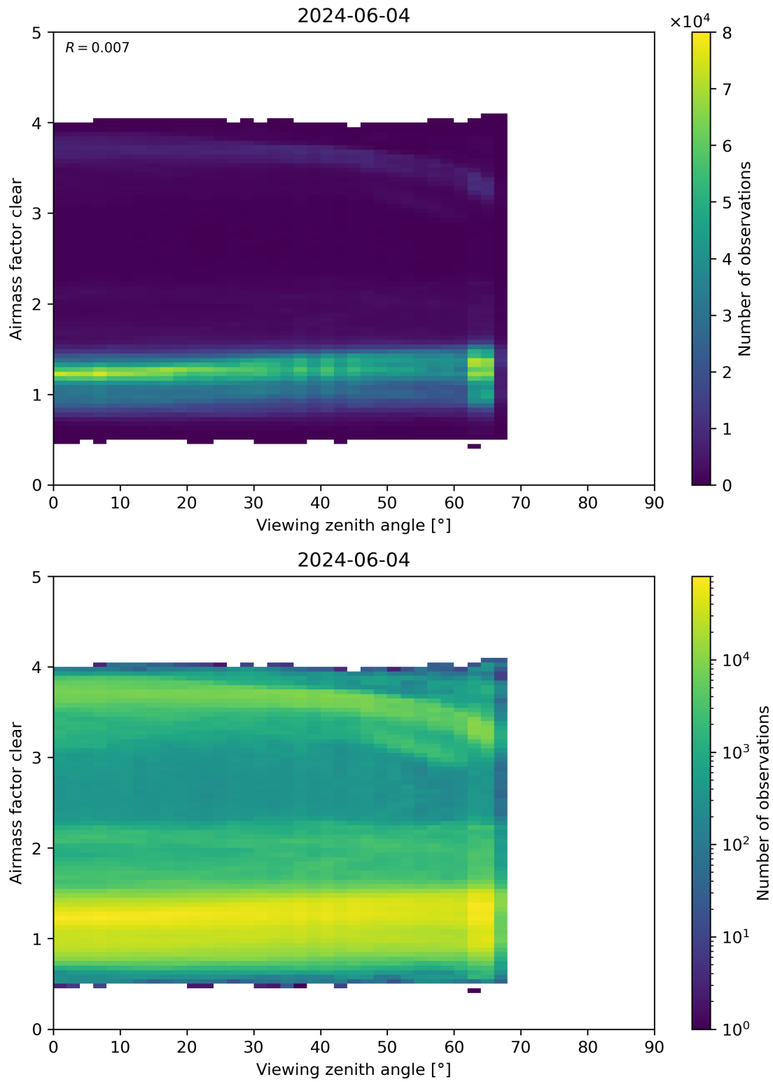
Figure 185: Scatter density plot of “Viewing zenith angle” against “Airmass factor clear” for 2024-06-03 to 2024-06-05.
