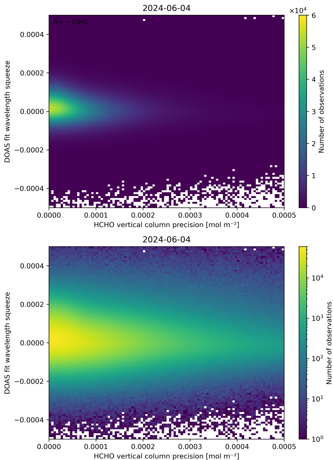
Figure 138: Scatter density plot of “HCHO vertical column precision” against “DOAS fit wavelength squeeze” for 2024-06-03 to 2024-06-05.
