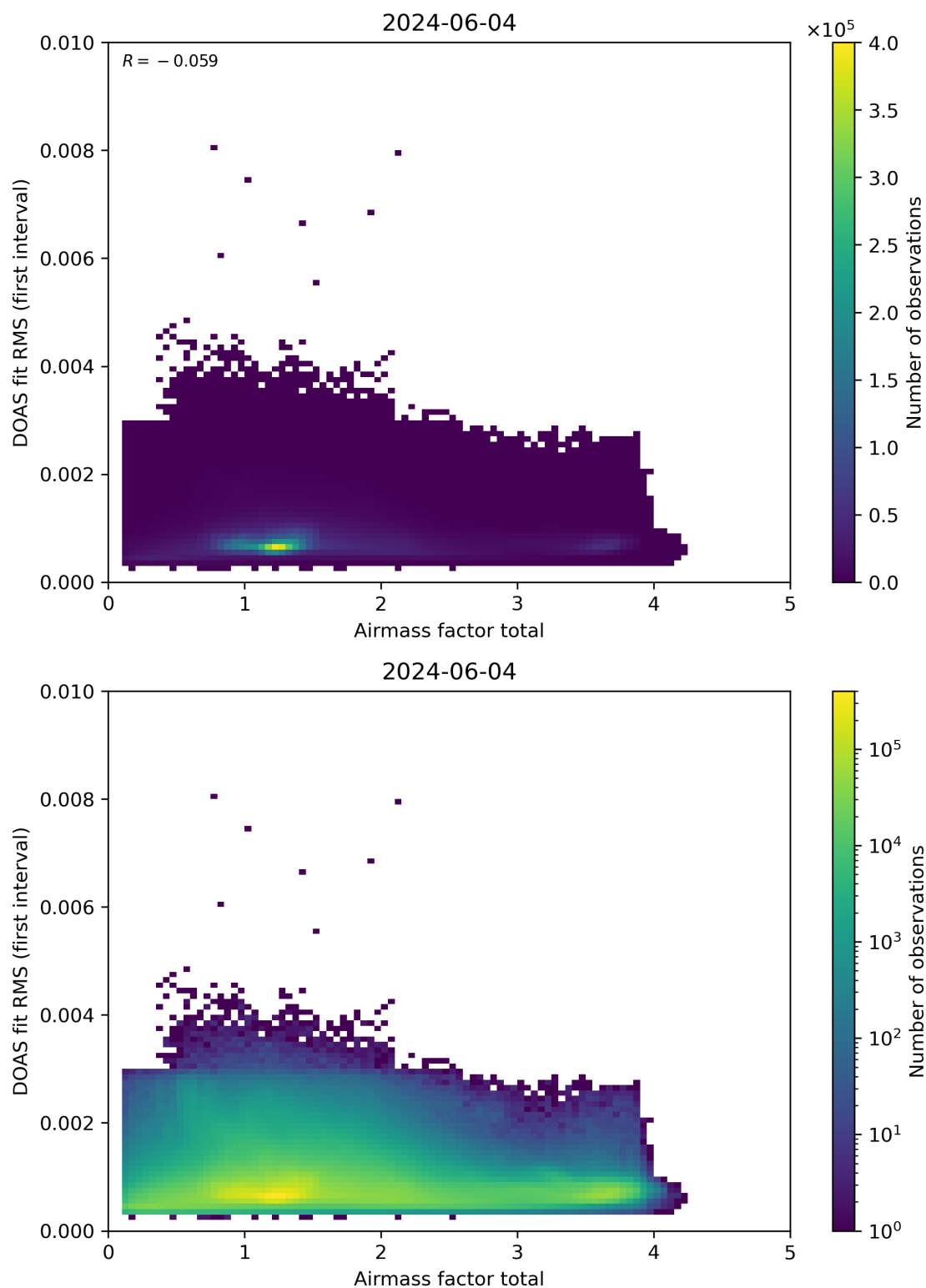
Figure 97: Scatter density plot of “Airmass factor total” against “DOAS fit RMS (first interval)” for 2024-06-03 to 2024-06-05.
