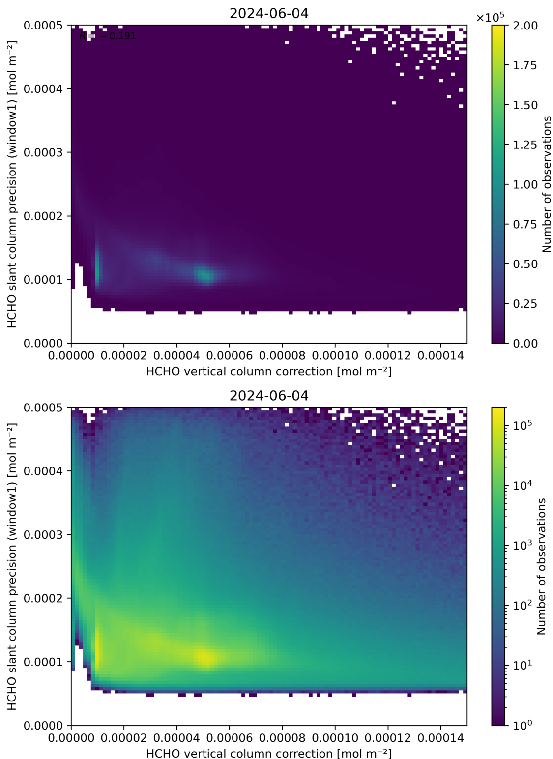
Figure 119: Scatter density plot of “HCHO vertical column correction” against “HCHO slant column precision (window1)” for 2024-06-03 to 2024-06-05.
