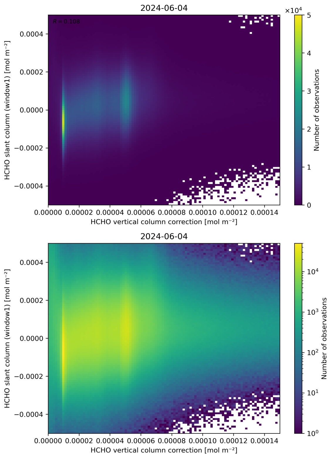
Figure 118: Scatter density plot of “HCHO vertical column correction” against “HCHO slant column (window1)” for 2024-06-03 to 2024-06-05.
