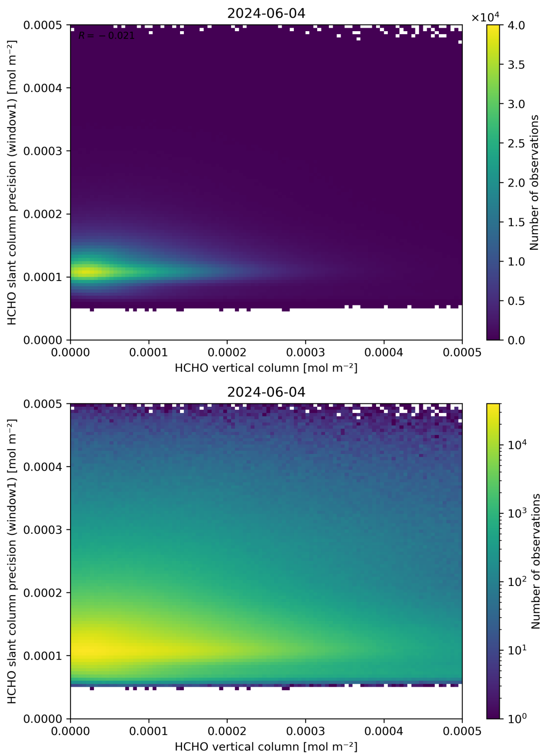
Figure 130: Scatter density plot of “HCHO vertical column” against “HCHO slant column precision (window1)” for 2024-06-03 to 2024-06-05.
