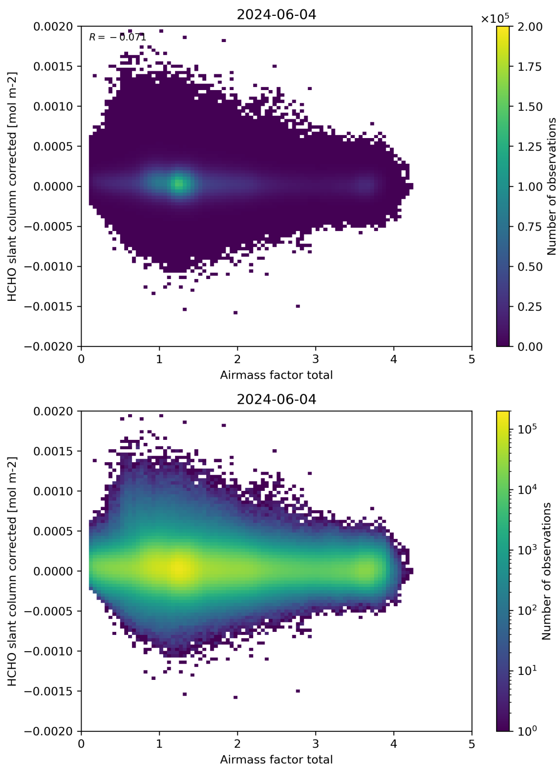
Figure 101: Scatter density plot of “Airmass factor total” against “HCHO slant column corrected” for 2024-06-03 to 2024-06-05.
