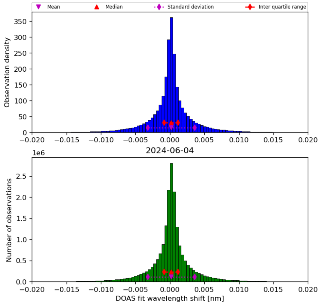
Figure 44: Histogram of “DOAS fit wavelength shift” for 2024-06-03 to 2024-06-05
