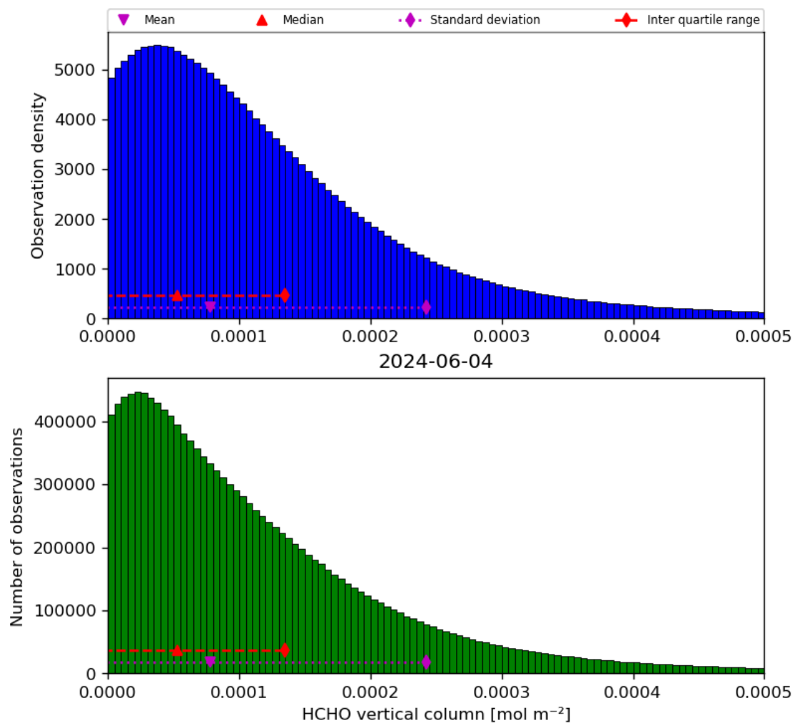
Figure 35: Histogram of “HCHO vertical column” for 2024-06-03 to 2024-06-05
