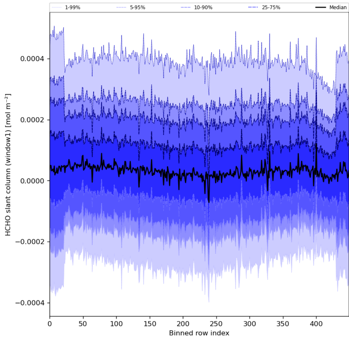
Figure 52: Along track statistics of “HCHO slant column (window1)” for 2024-06-03 to 2024-06-05
