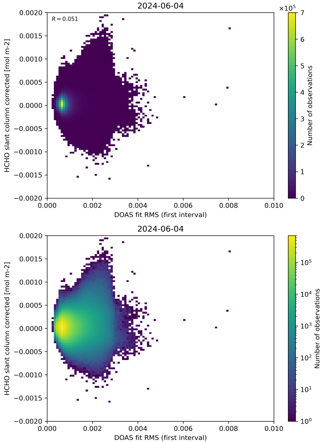
Figure 62: Scatter density plot of “DOAS fit RMS (first interval)” against “HCHO slant column corrected” for 2024-06-03 to 2024-06-05.
