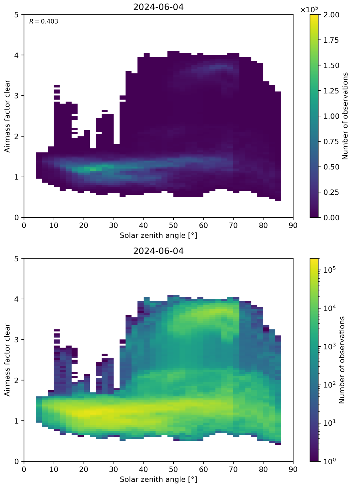
Figure 170: Scatter density plot of “Solar zenith angle” against “Airmass factor clear” for 2024-06-03 to 2024-06-05.
