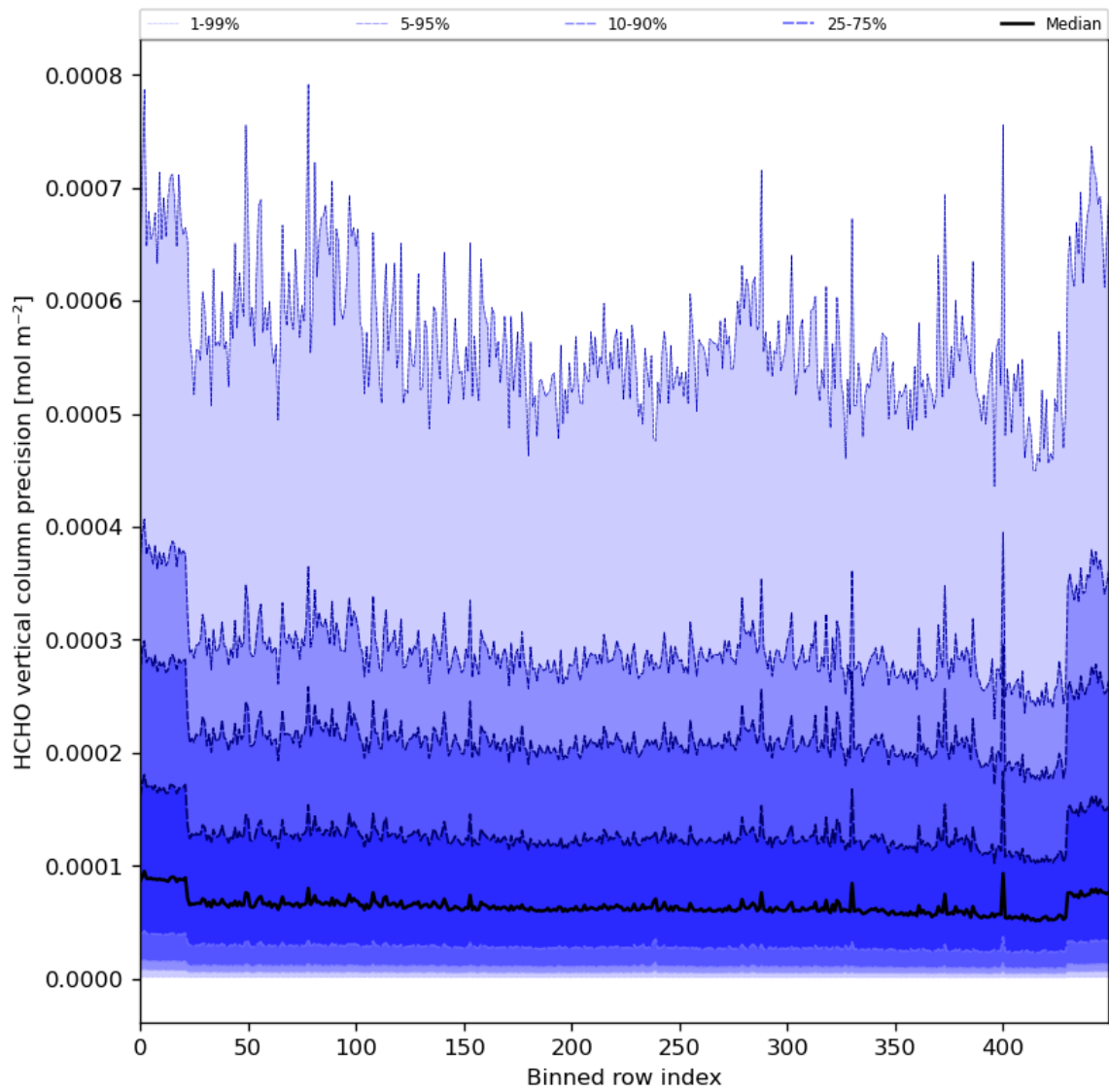
Figure 50: Along track statistics of “HCHO vertical column precision” for 2024-06-03 to 2024-06-05
