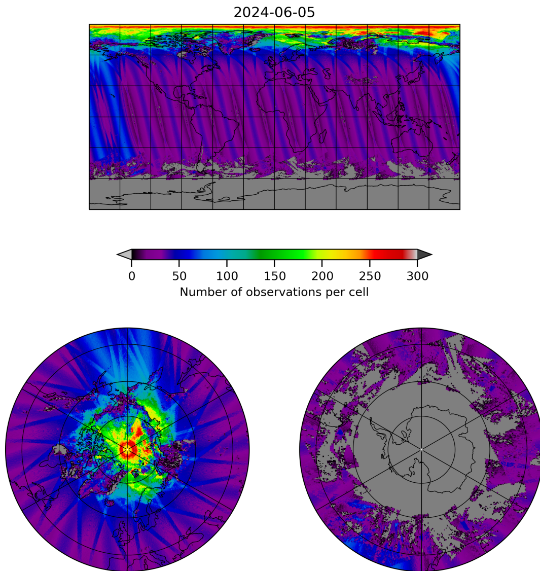
Figure 19: Map of the number of observations for 2024-06-04 to 2024-06-06
