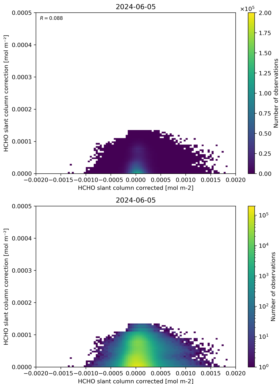
Figure 77: Scatter density plot of “HCHO slant column corrected” against “HCHO slant column correction” for 2024-06-04 to 2024-06-06.
