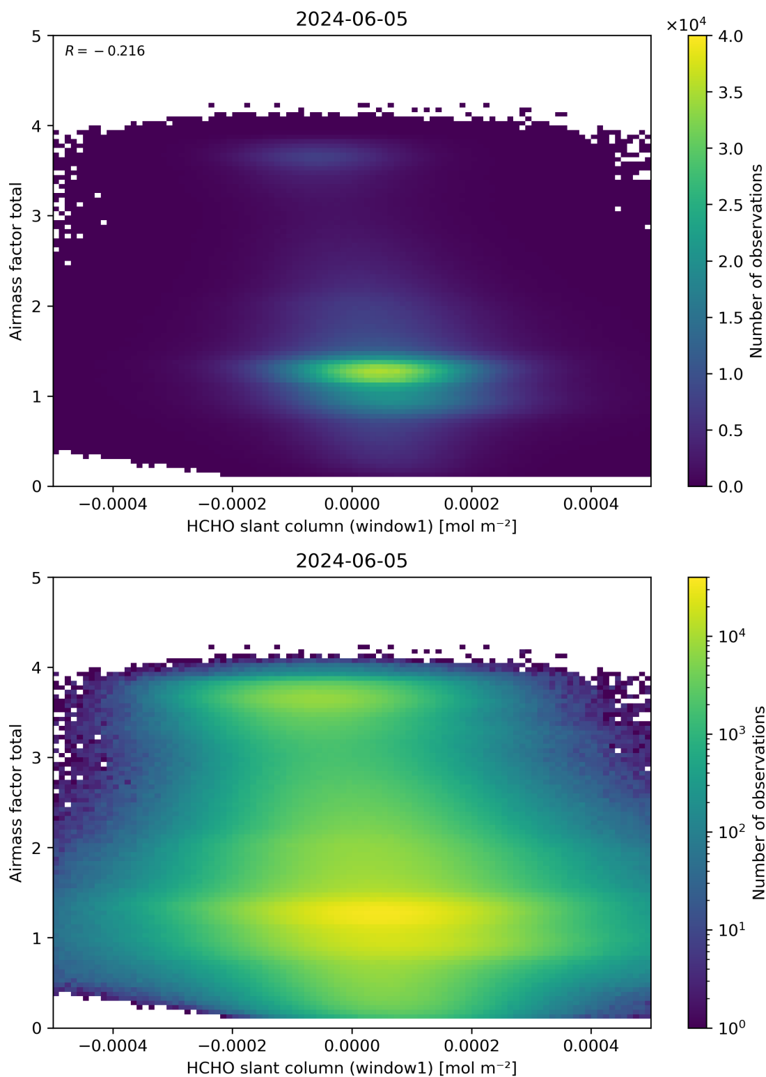
Figure 85: Scatter density plot of “HCHO slant column (window1)” against “Airmass factor total” for 2024-06-04 to 2024-06-06.
