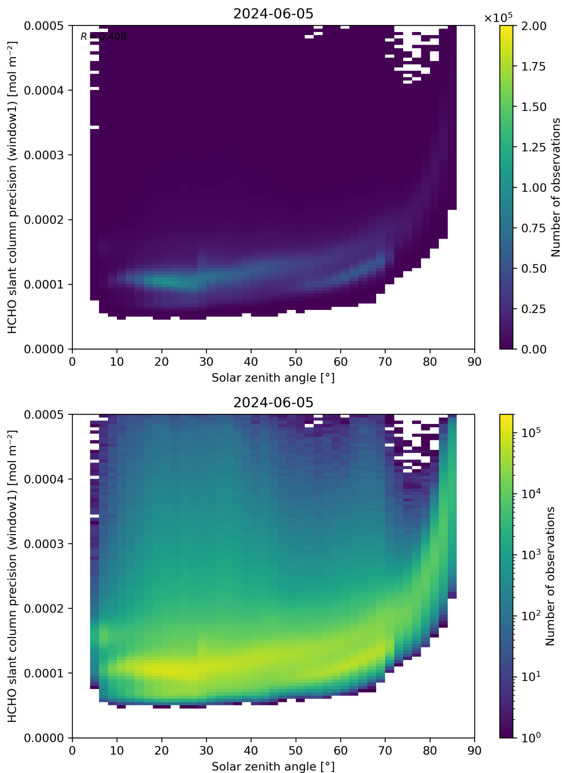
Figure 174: Scatter density plot of “Solar zenith angle” against “HCHO slant column precision (window1)” for 2024-06-04 to 2024-06-06.
