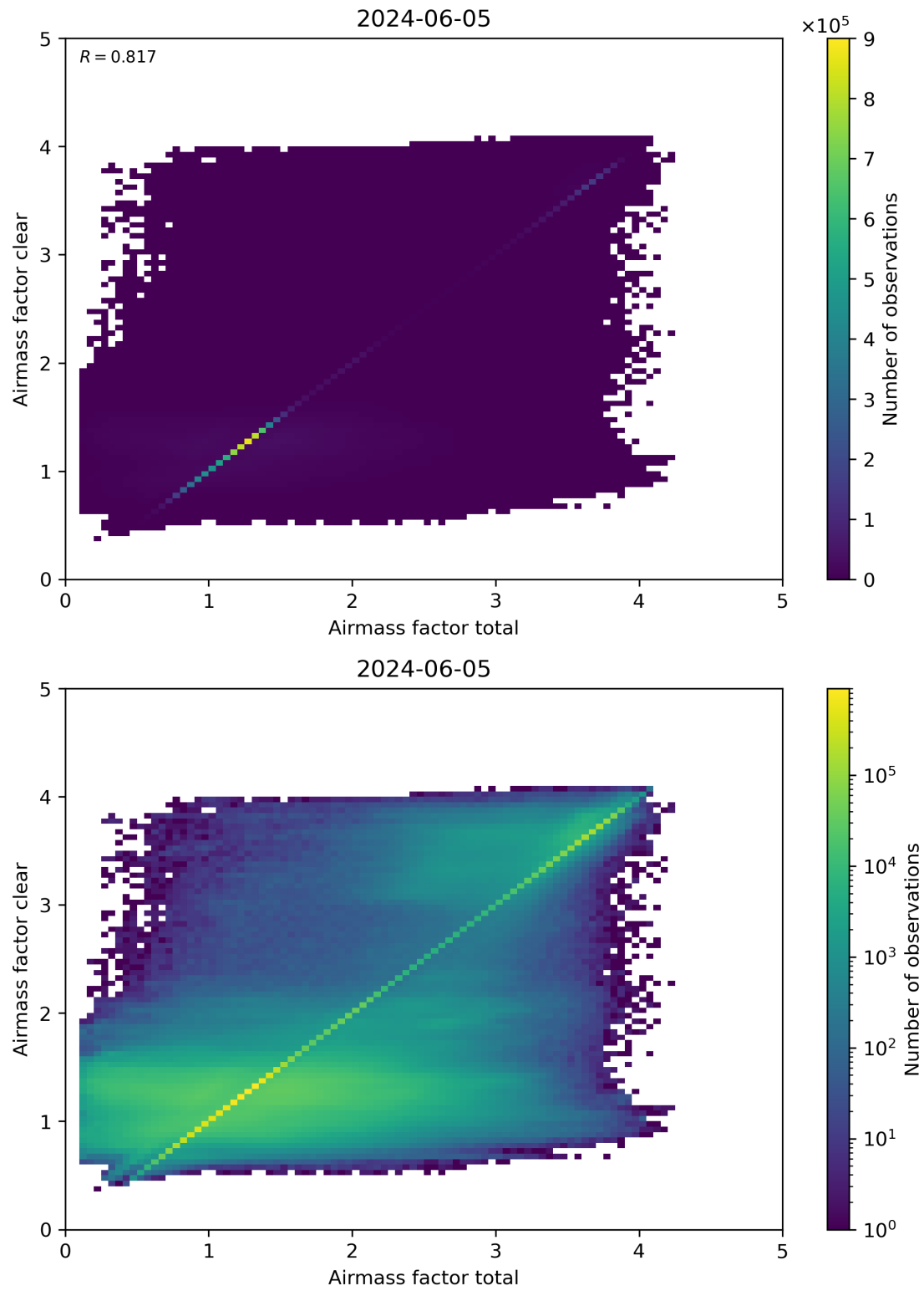
Figure 100: Scatter density plot of “Airmass factor total” against “Airmass factor clear” for 2024-06-04 to 2024-06-06.
