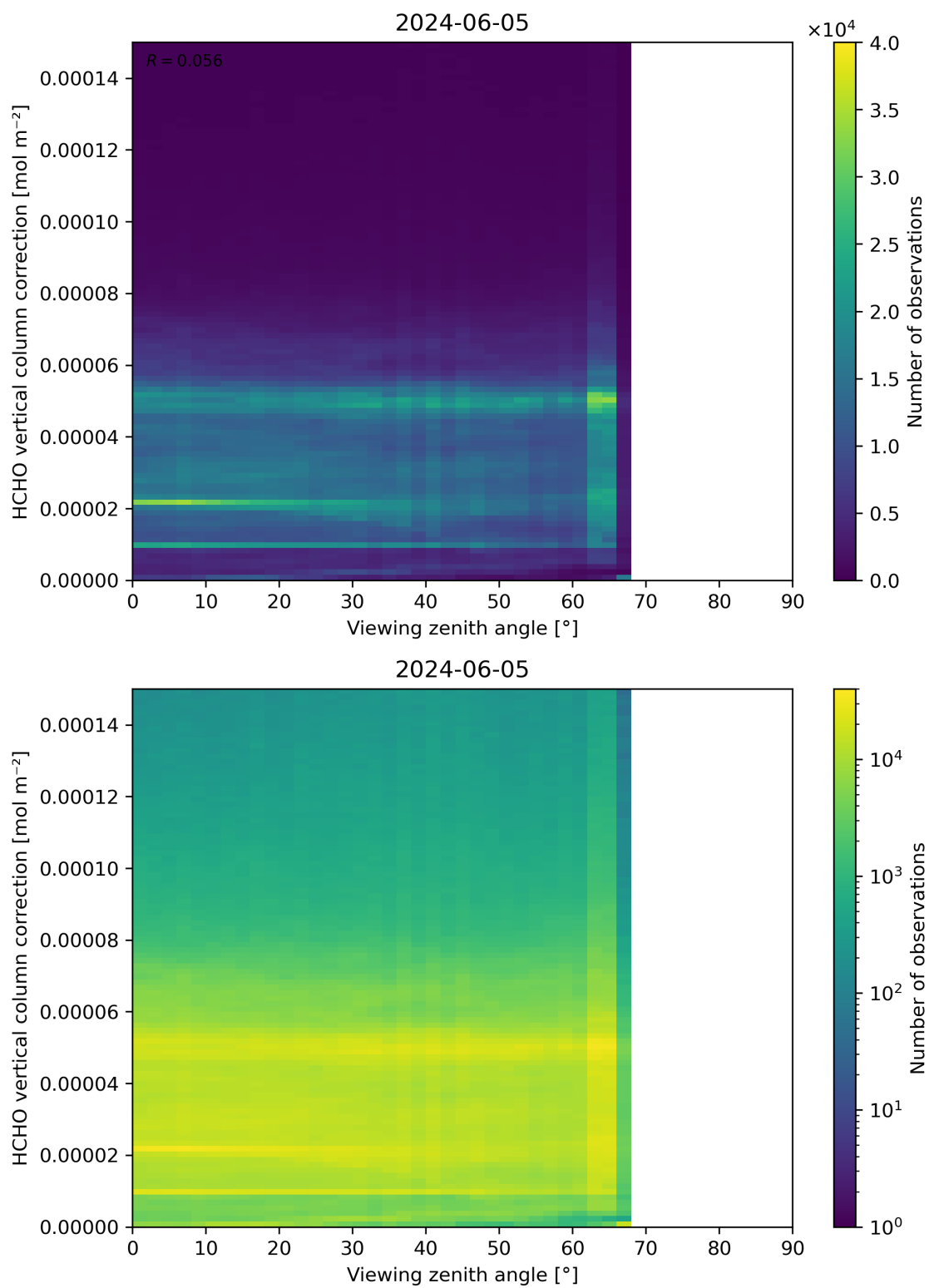
Figure 193: Scatter density plot of “Viewing zenith angle” against “HCHO vertical column correction” for 2024-06-04 to 2024-06-06.
