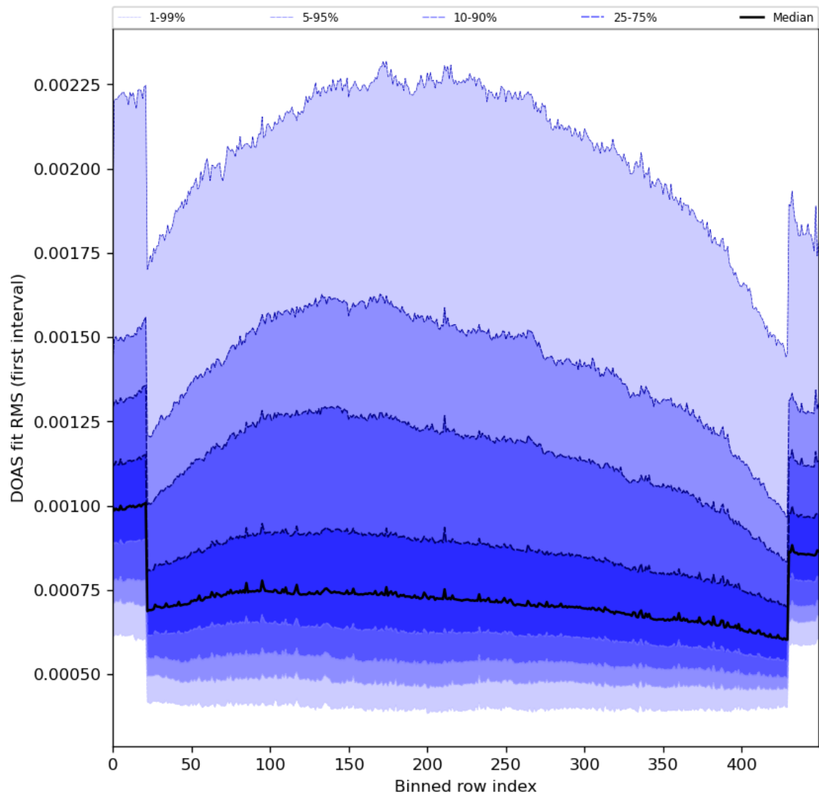
Figure 60: Along track statistics of “DOAS fit RMS (first interval)” for 2024-06-04 to 2024-06-06
