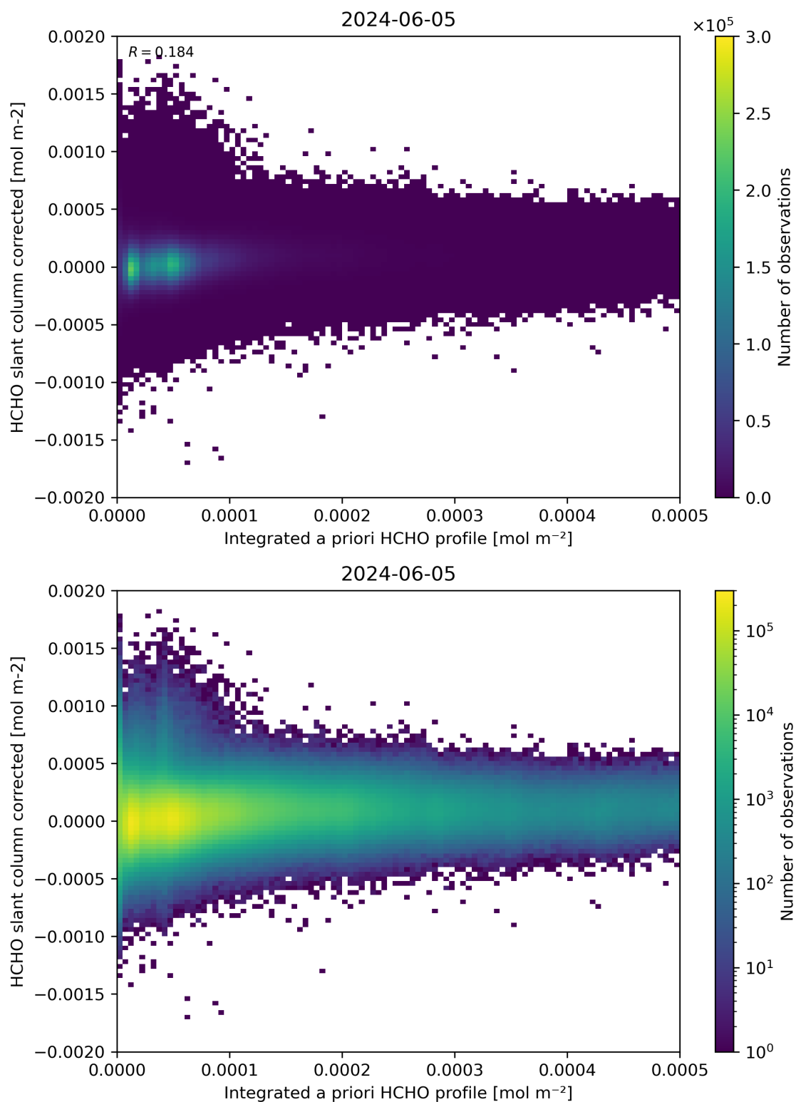
Figure 151: Scatter density plot of “Integrated a priori HCHO profile” against “HCHO slant column corrected” for 2024-06-04 to 2024-06-06.
