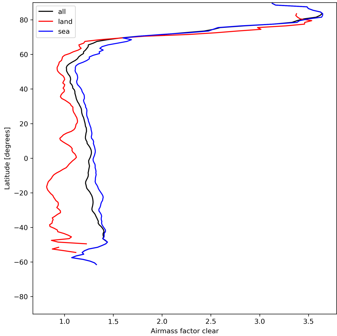
Figure 28: Zonal average of “Airmass factor clear” for 2024-06-04 to 2024-06-06.
