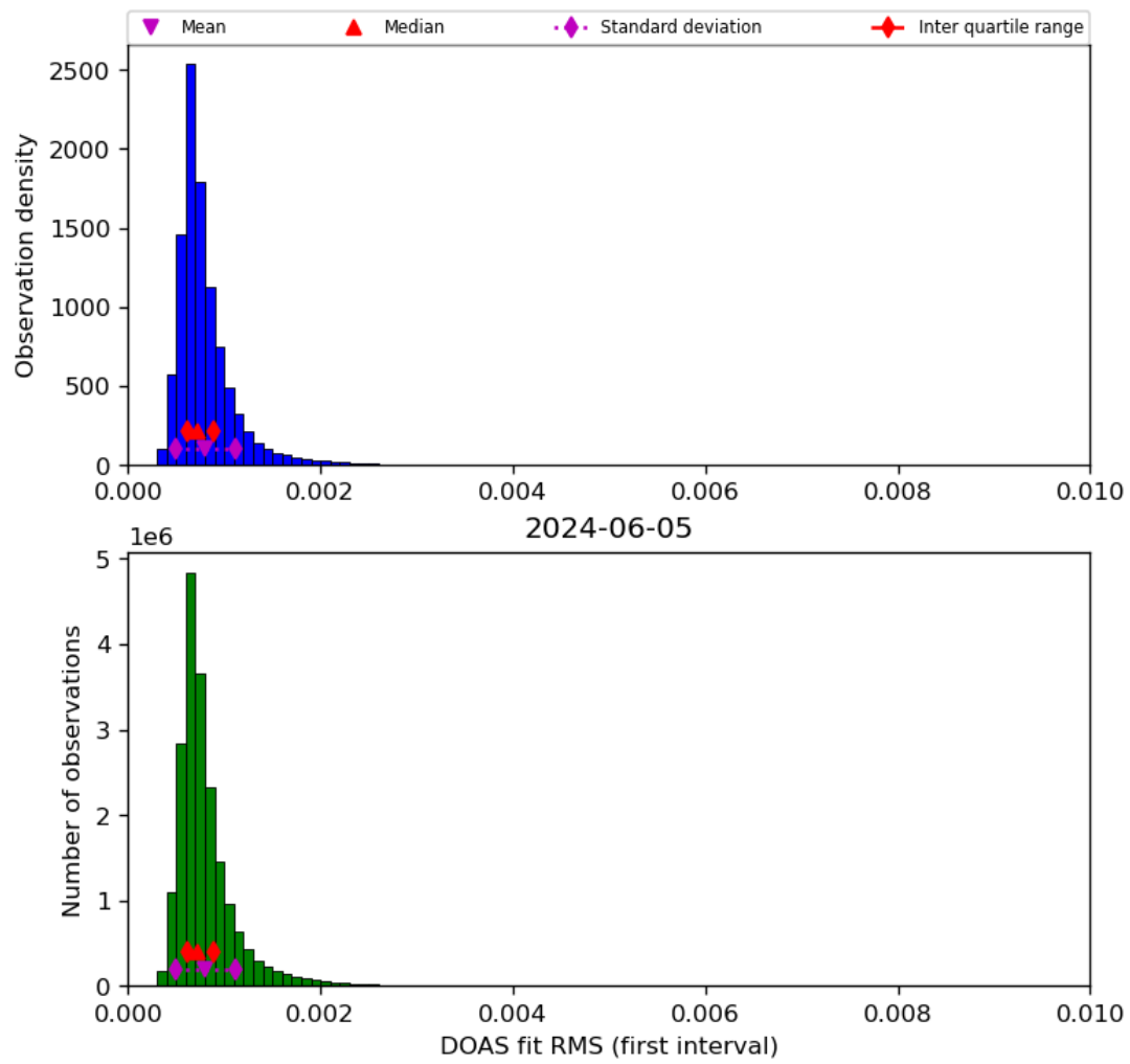
Figure 46: Histogram of “DOAS fit RMS (first interval)” for 2024-06-04 to 2024-06-06
