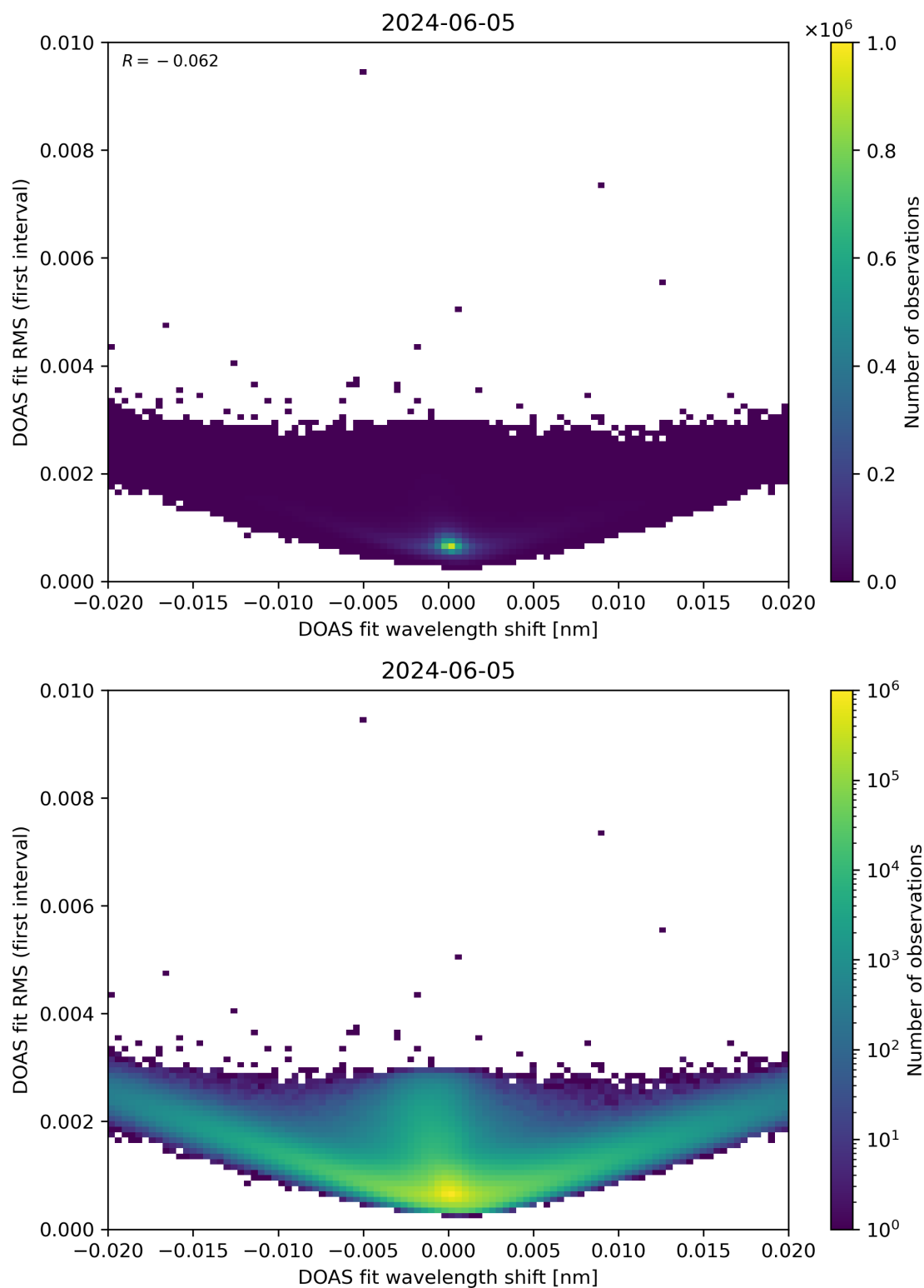
Figure 64: Scatter density plot of “DOAS fit wavelength shift” against “DOAS fit RMS (first interval)” for 2024-06-04 to 2024-06-06.
