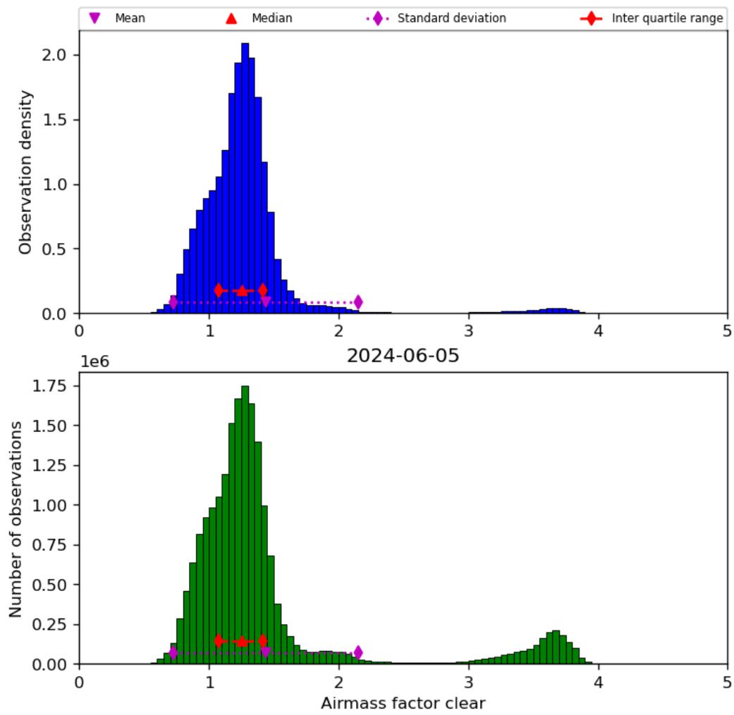
Figure 42: Histogram of “Airmass factor clear” for 2024-06-04 to 2024-06-06
