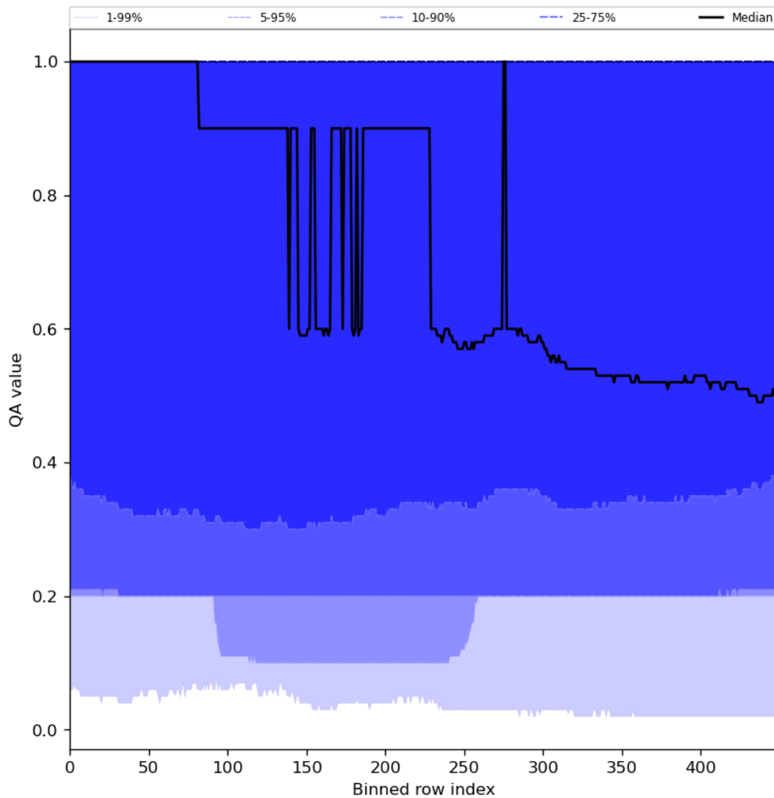
Figure 48: Along track statistics of “QA value” for 2024-06-04 to 2024-06-06
