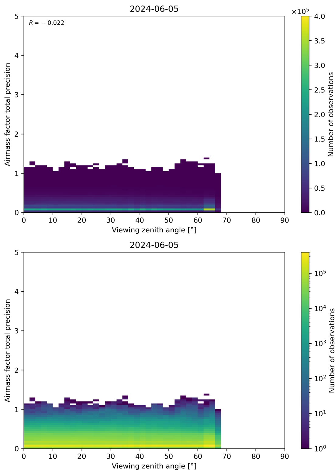
Figure 191: Scatter density plot of “Viewing zenith angle” against “Airmass factor total precision” for 2024-06-04 to 2024-06-06.
