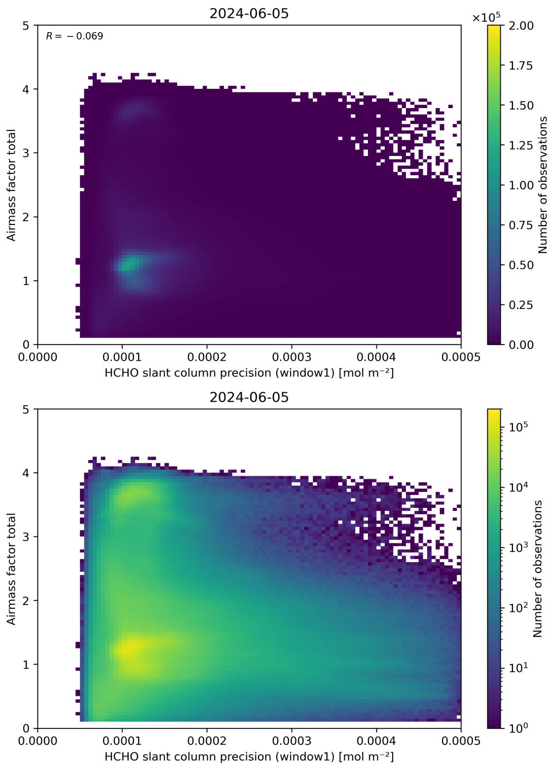
Figure 94: Scatter density plot of “HCHO slant column precision (window1)” against “Airmass factor total” for 2024-06-04 to 2024-06-06.
