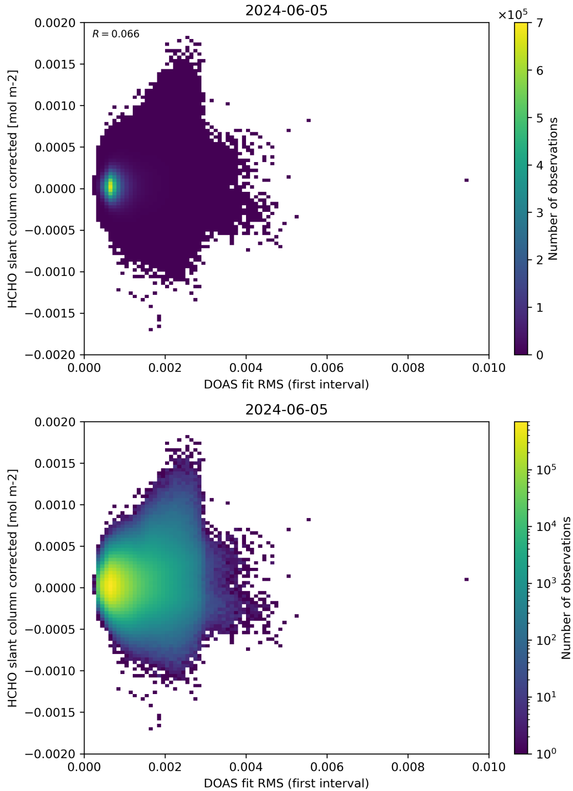
Figure 62: Scatter density plot of “DOAS fit RMS (first interval)” against “HCHO slant column corrected” for 2024-06-04 to 2024-06-06.
