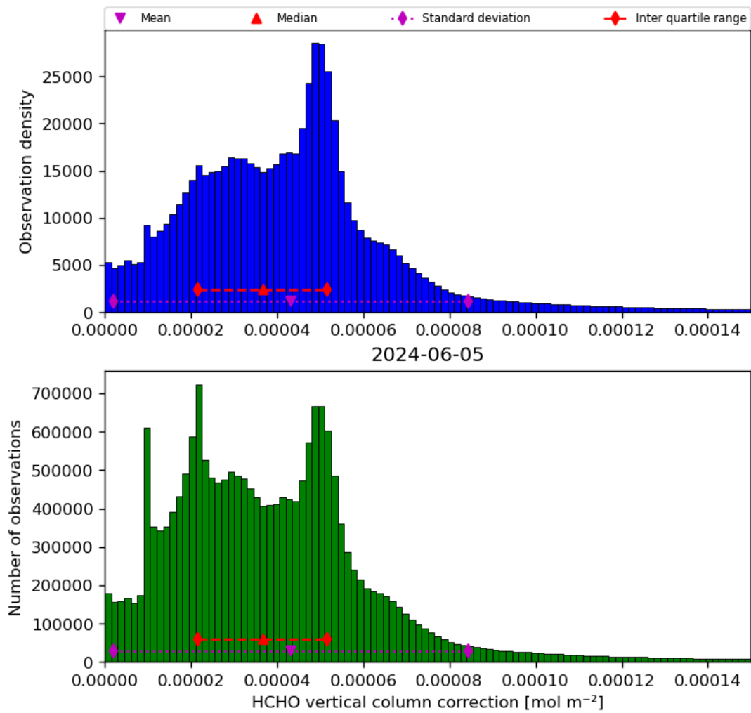
Figure 37: Histogram of “HCHO vertical column correction” for 2024-06-04 to 2024-06-06
