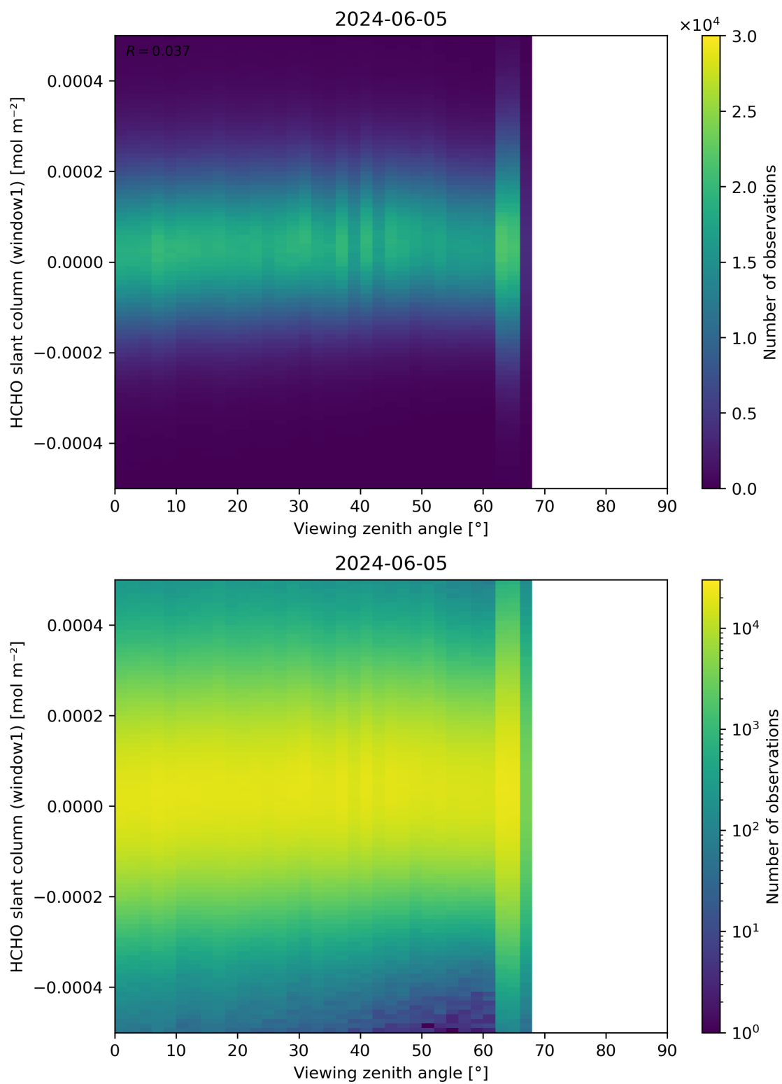
Figure 188: Scatter density plot of “Viewing zenith angle” against “HCHO slant column (window1)” for 2024-06-04 to 2024-06-06.
