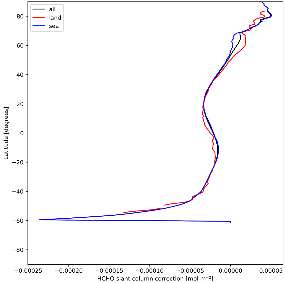
Figure 33: Zonal average of “HCHO slant column correction” for 2024-06-04 to 2024-06-06.
