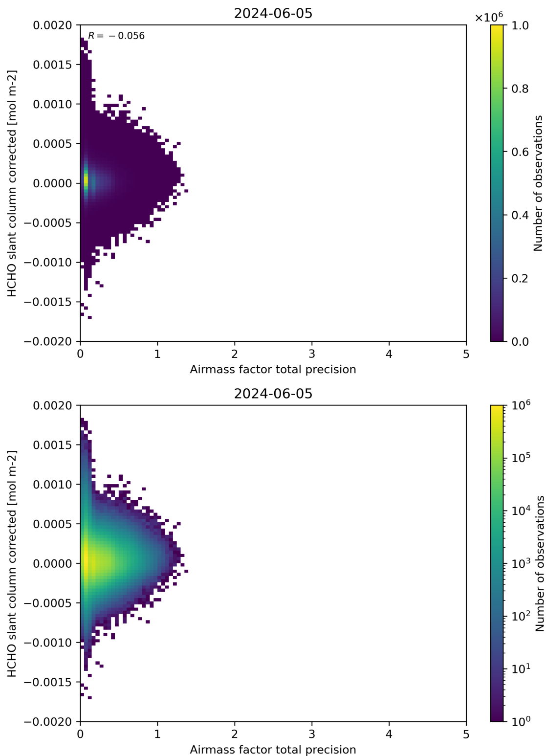
Figure 109: Scatter density plot of “Airmass factor total precision” against “HCHO slant column corrected” for 2024-06-04 to 2024-06-06.
