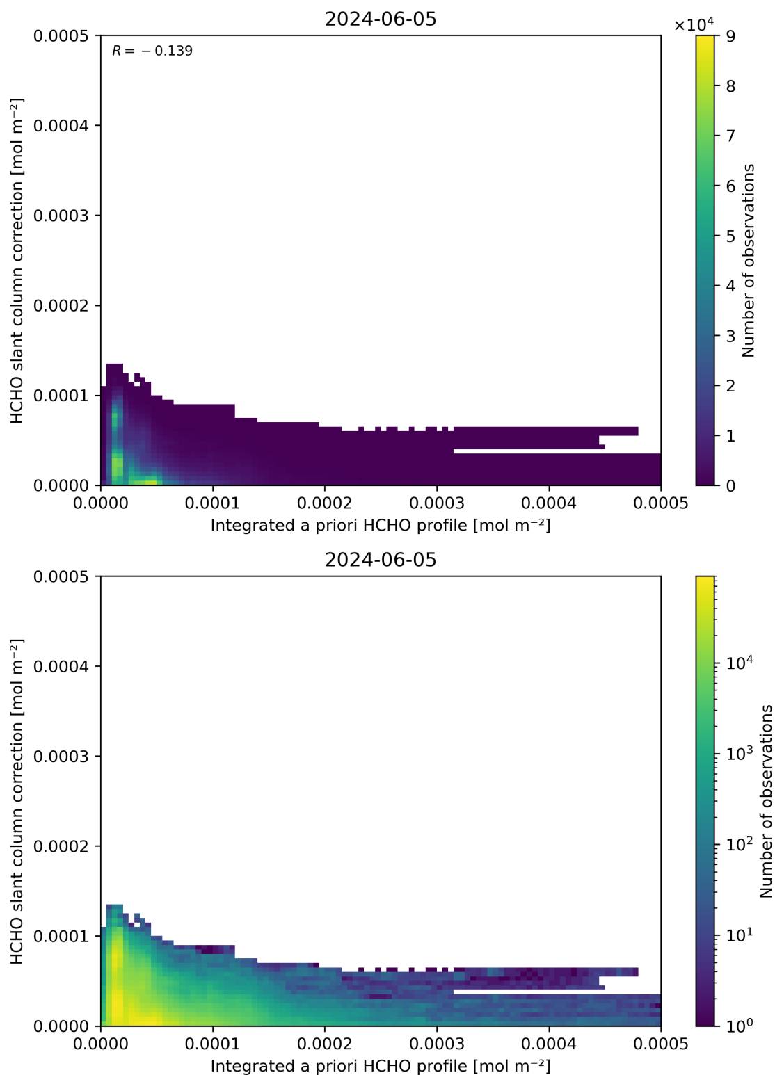
Figure 152: Scatter density plot of “Integrated a priori HCHO profile” against “HCHO slant column correction” for 2024-06-04 to 2024-06-06.
