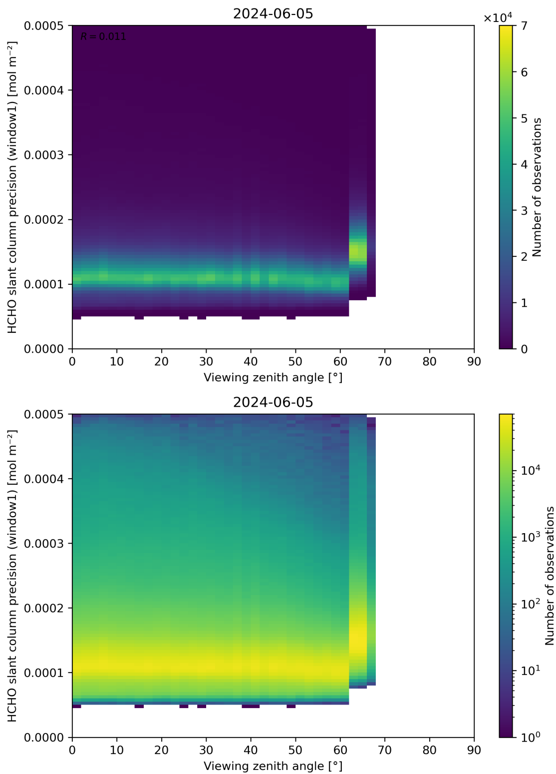
Figure 189: Scatter density plot of “Viewing zenith angle” against “HCHO slant column precision (window1)” for 2024-06-04 to 2024-06-06.
