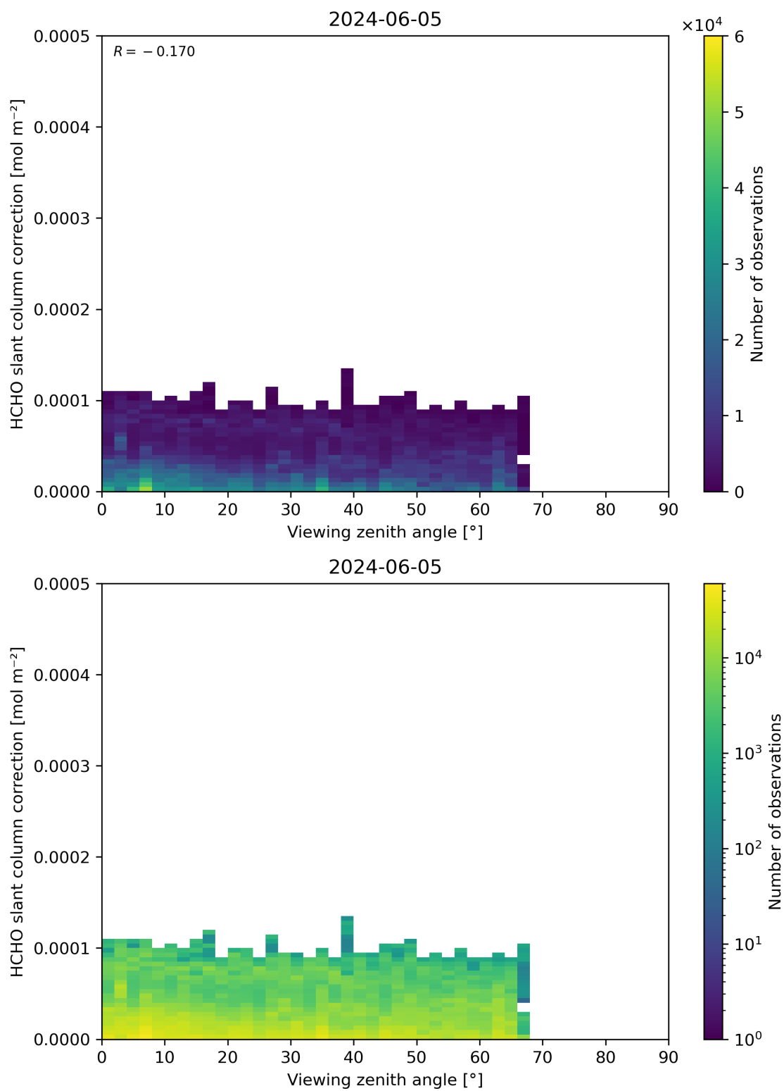
Figure 187: Scatter density plot of “Viewing zenith angle” against “HCHO slant column correction” for 2024-06-04 to 2024-06-06.
