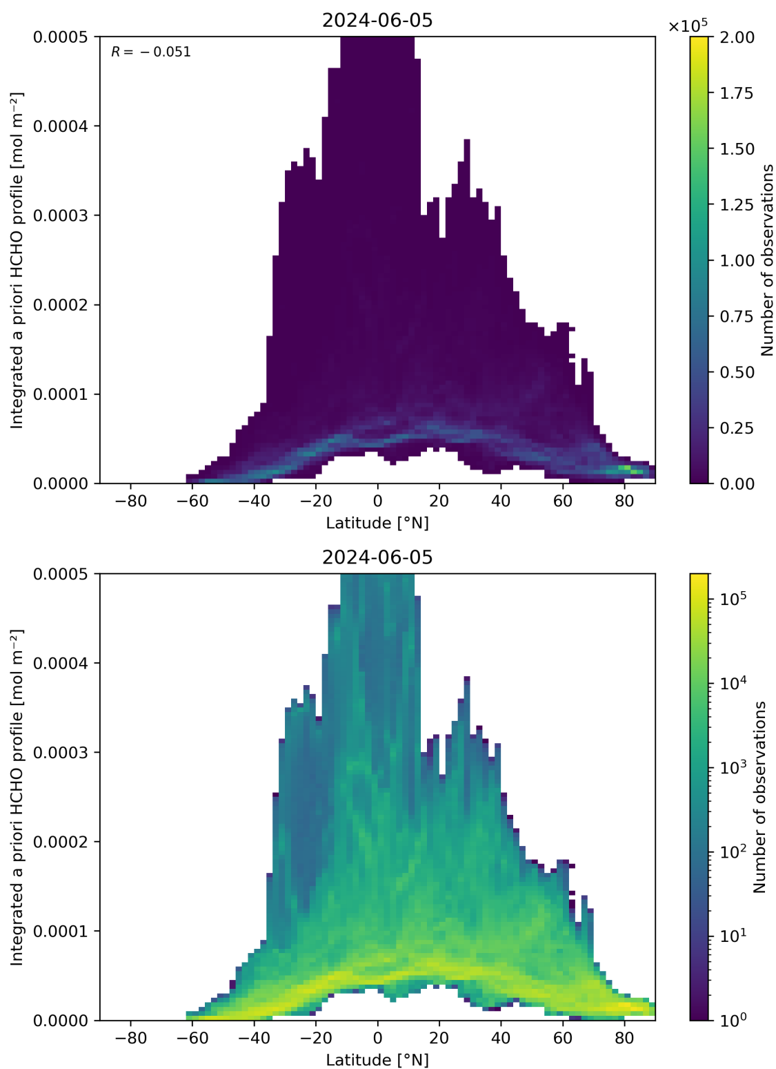
Figure 166: Scatter density plot of “Latitude” against “Integrated a priori HCHO profile” for 2024-06-04 to 2024-06-06.
