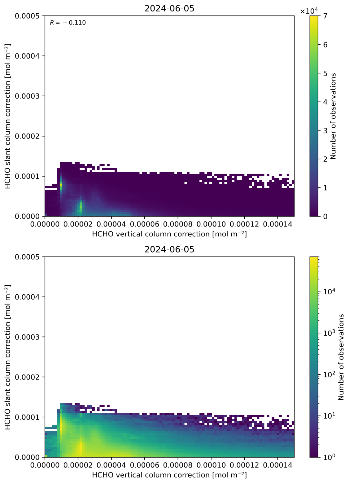
Figure 117: Scatter density plot of “HCHO vertical column correction” against “HCHO slant column correction” for 2024-06-04 to 2024-06-06.
