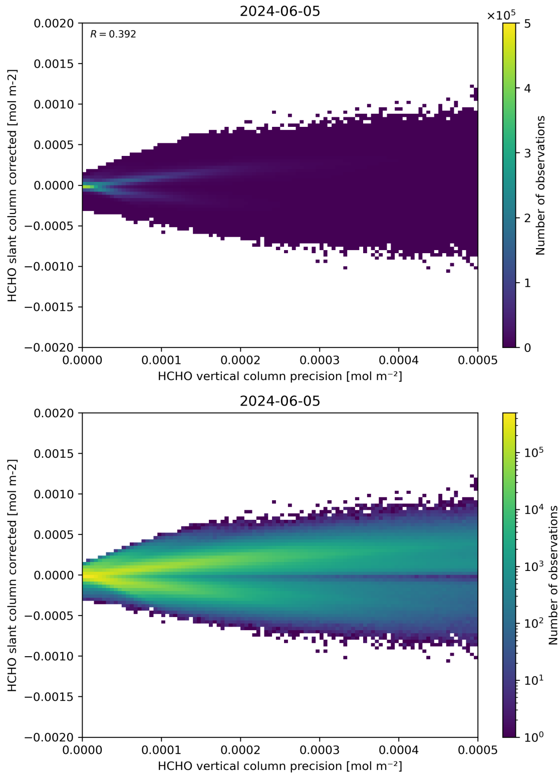
Figure 140: Scatter density plot of “HCHO vertical column precision” against “HCHO slant column corrected” for 2024-06-04 to 2024-06-06.
