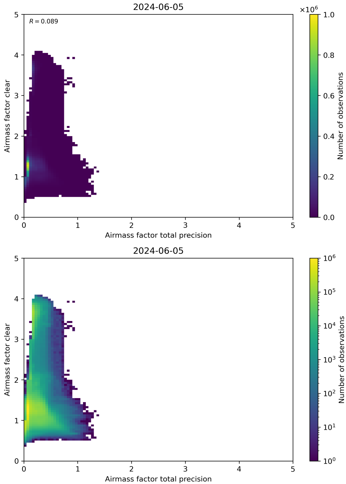
Figure 108: Scatter density plot of “Airmass factor total precision” against “Airmass factor clear” for 2024-06-04 to 2024-06-06.
