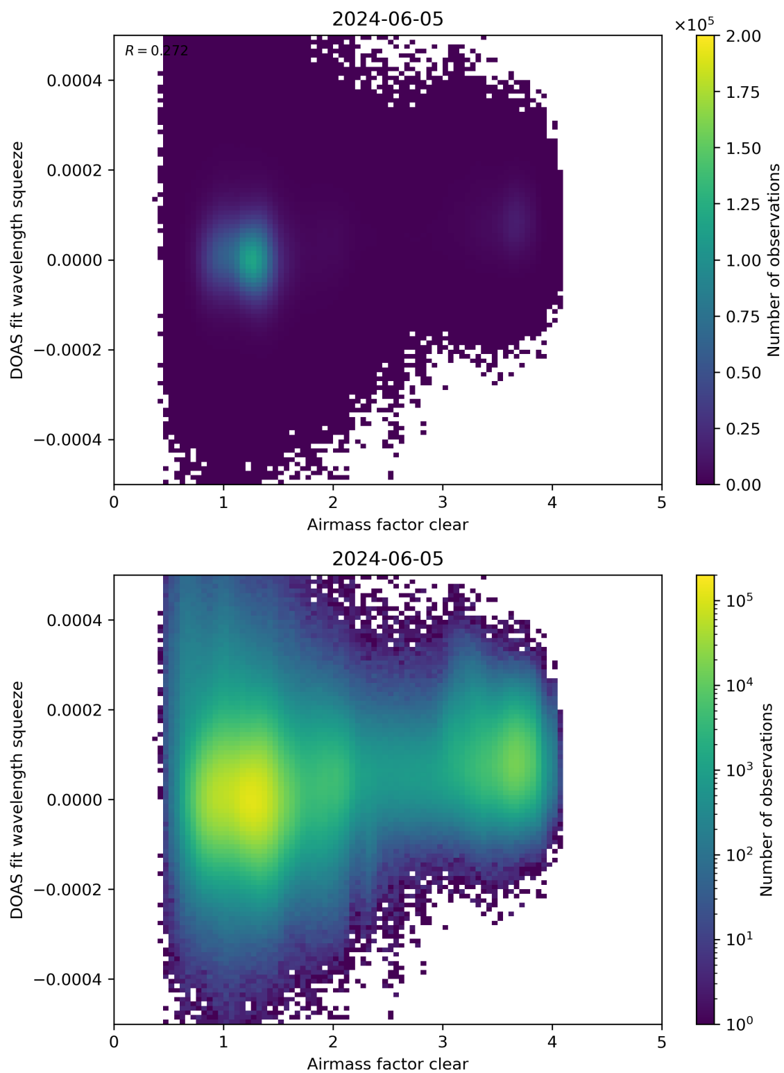
Figure 73: Scatter density plot of “Airmass factor clear” against “DOAS fit wavelength squeeze” for 2024-06-04 to 2024-06-06.
