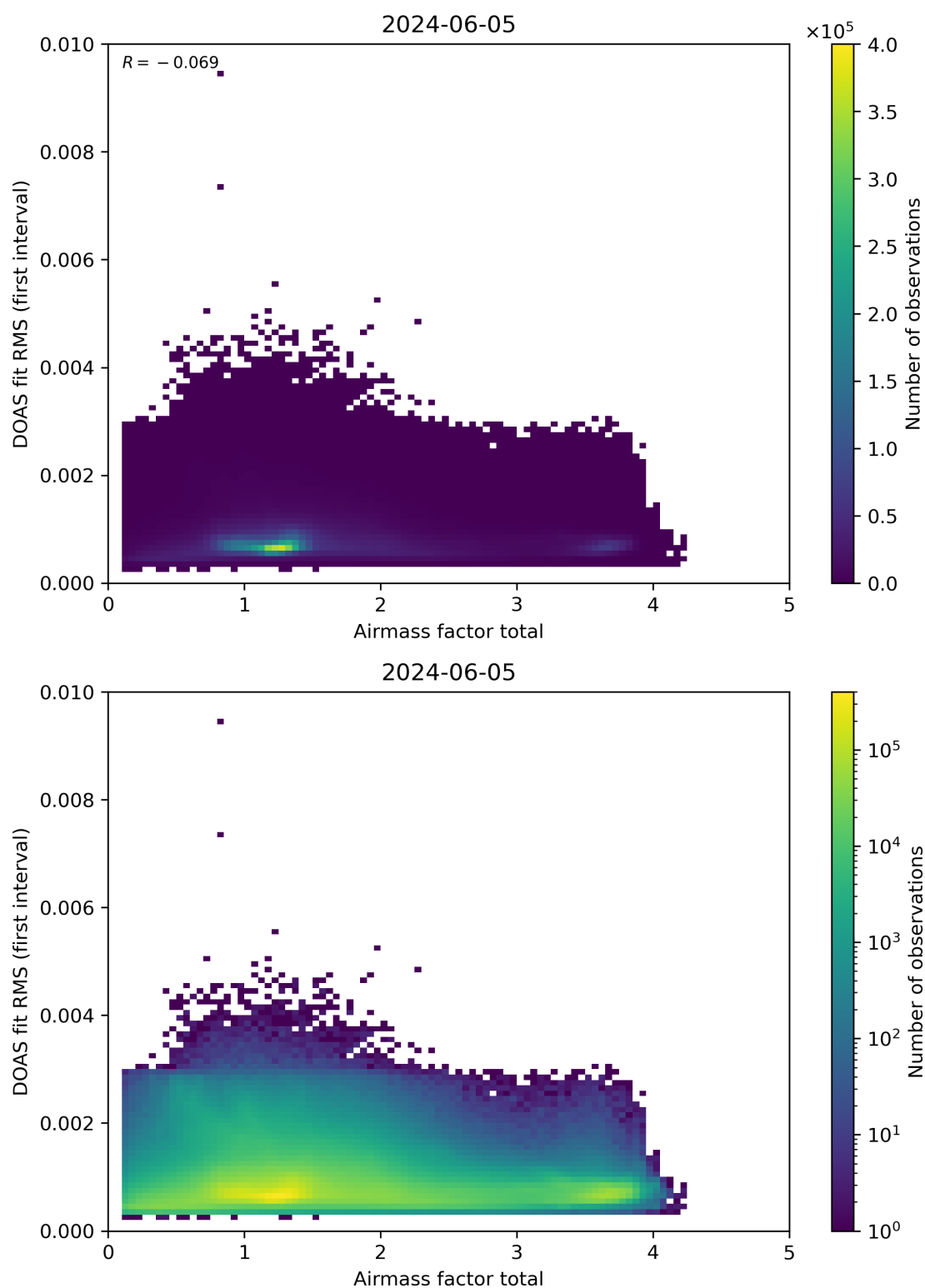
Figure 97: Scatter density plot of “Airmass factor total” against “DOAS fit RMS (first interval)” for 2024-06-04 to 2024-06-06.
