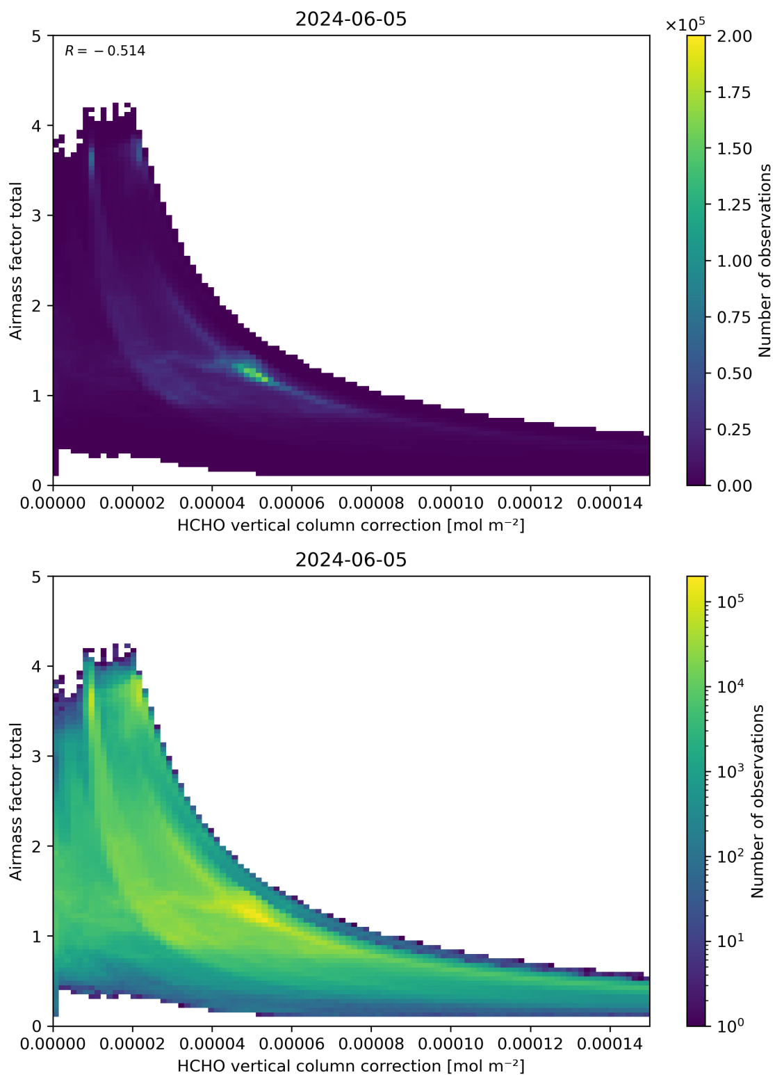
Figure 120: Scatter density plot of “HCHO vertical column correction” against “Airmass factor total” for 2024-06-04 to 2024-06-06.
