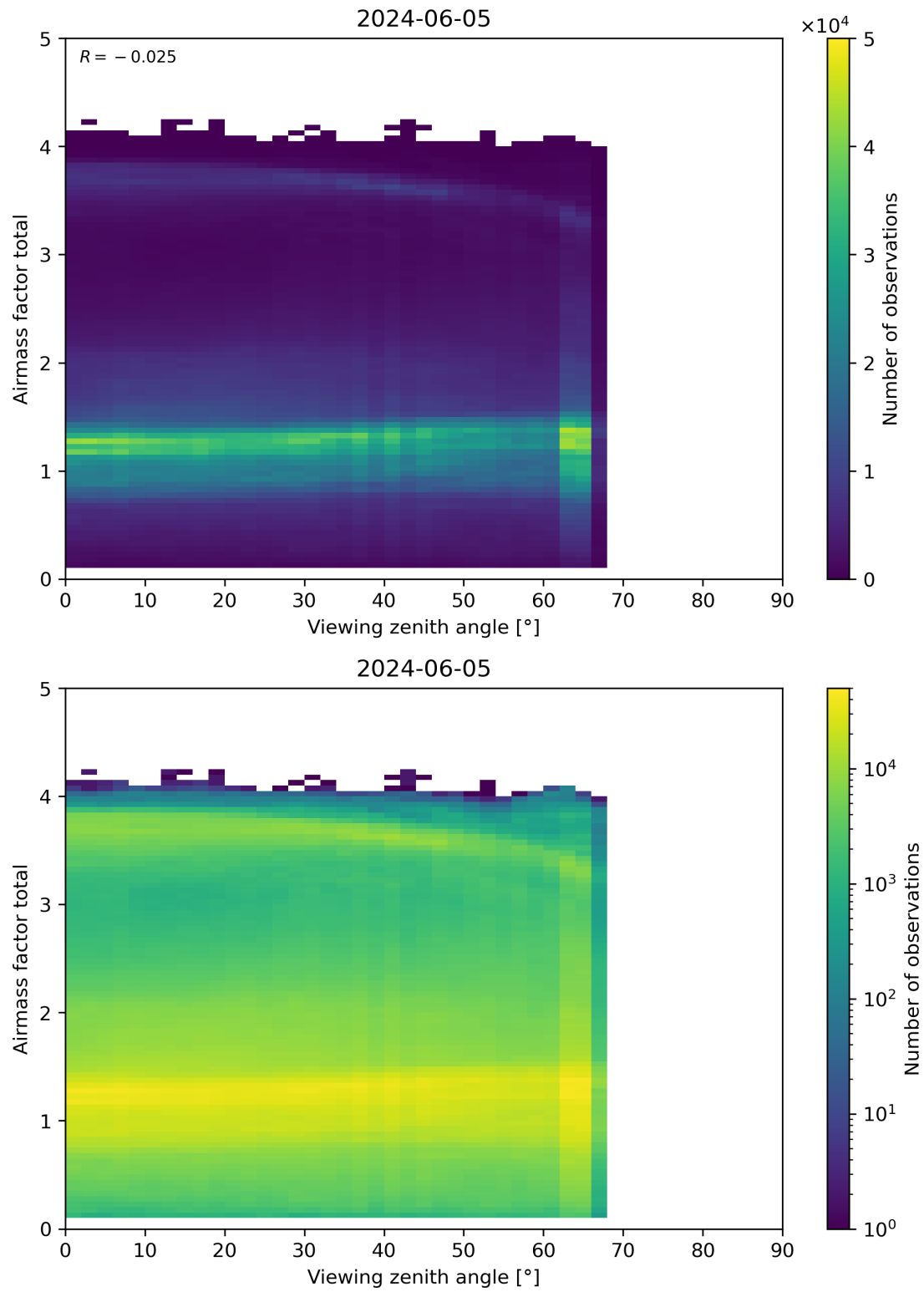
Figure 190: Scatter density plot of “Viewing zenith angle” against “Airmass factor total” for 2024-06-04 to 2024-06-06.
