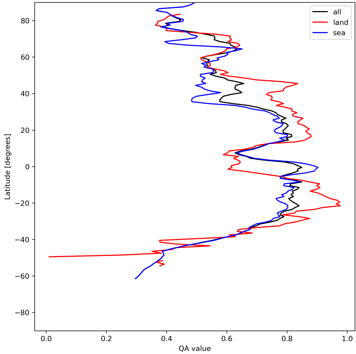
Figure 20: Zonal average of “QA value” for 2024-06-04 to 2024-06-06.
