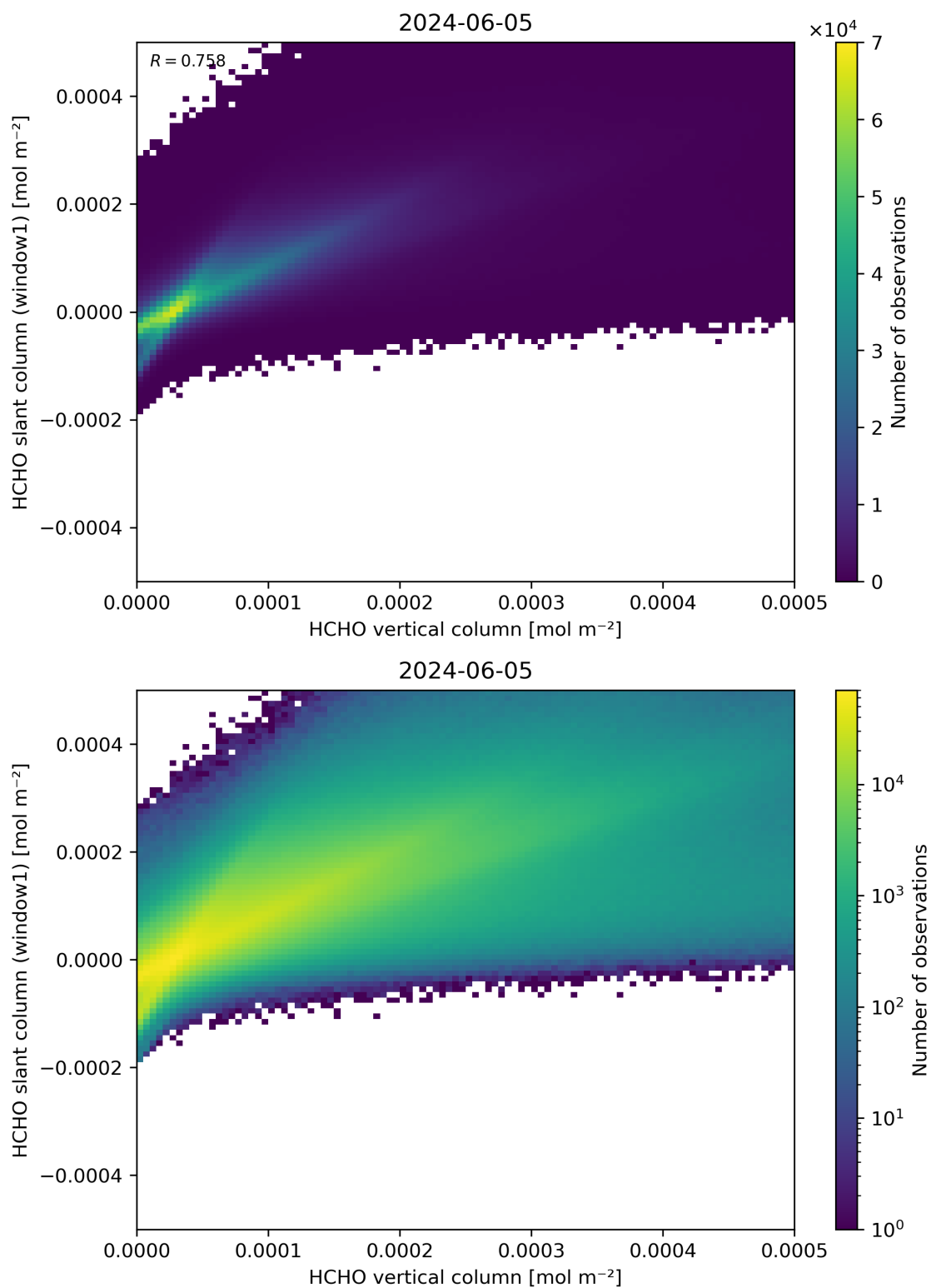
Figure 129: Scatter density plot of “HCHO vertical column” against “HCHO slant column (window1)” for 2024-06-04 to 2024-06-06.
