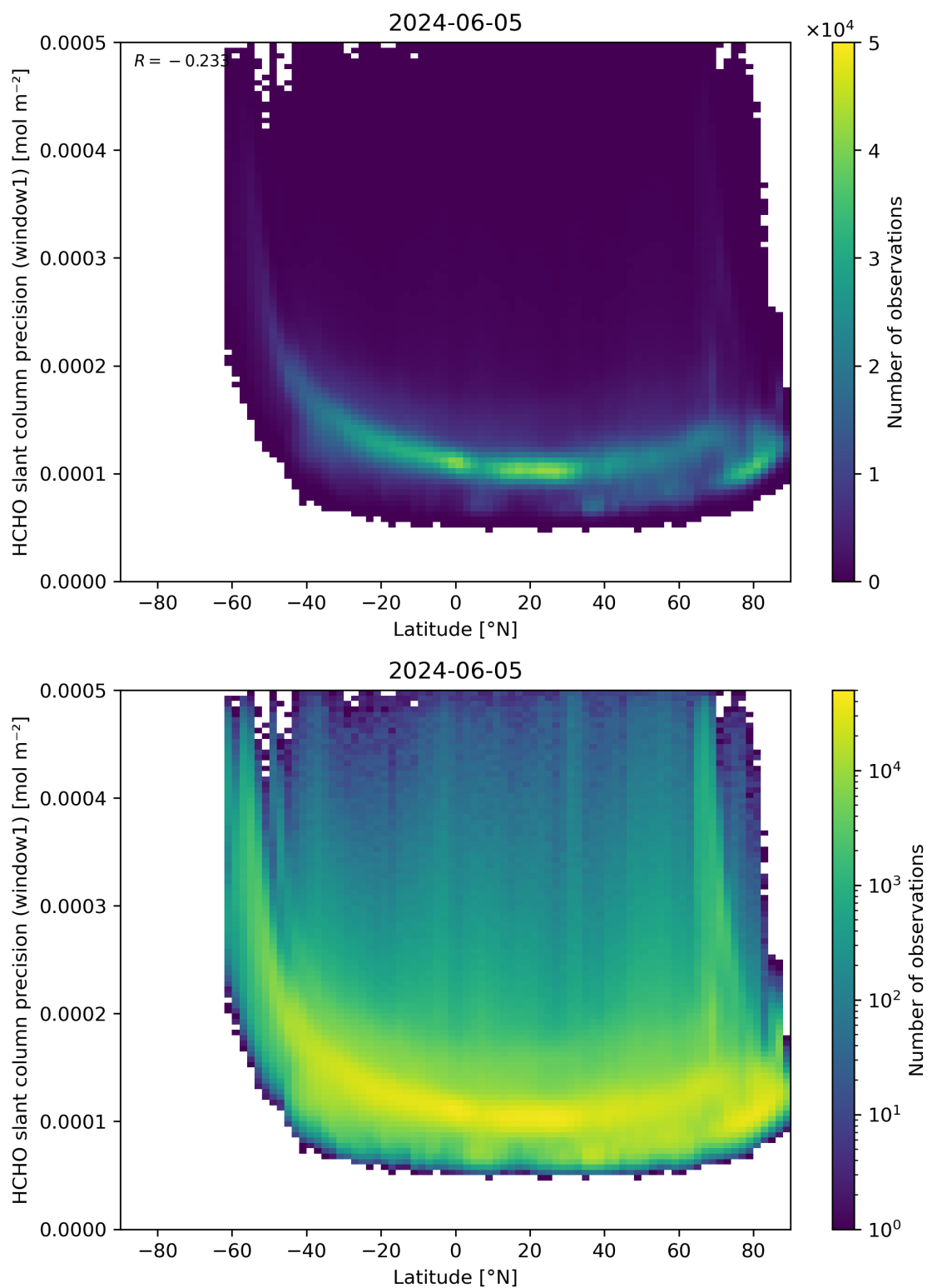
Figure 160: Scatter density plot of “Latitude” against “HCHO slant column precision (window1)” for 2024-06-04 to 2024-06-06.
