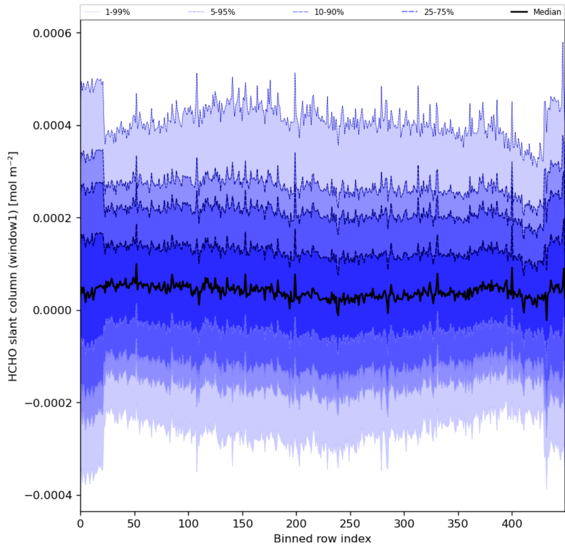
Figure 52: Along track statistics of “HCHO slant column (window1)” for 2024-06-04 to 2024-06-06
