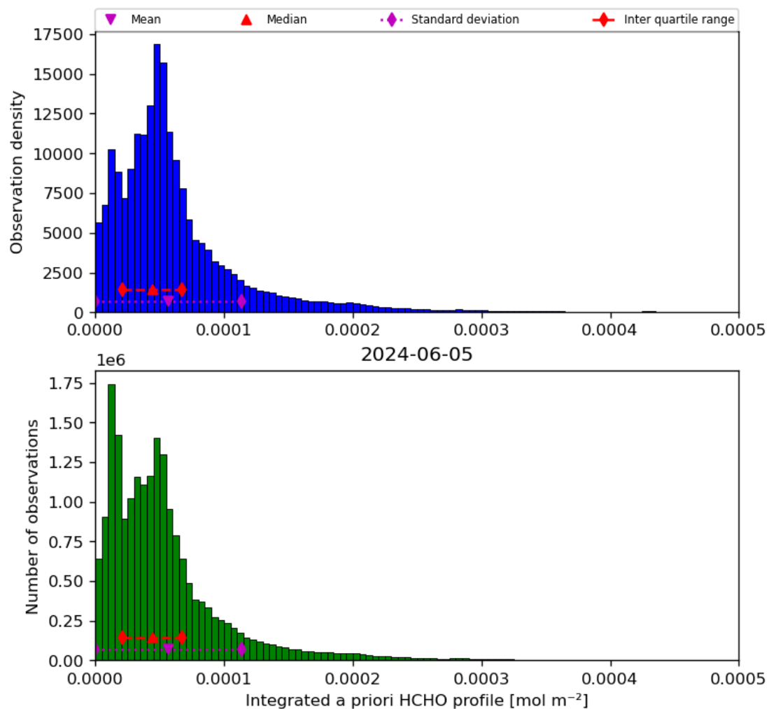
Figure 43: Histogram of “Integrated a priori HCHO profile” for 2024-06-04 to 2024-06-06
