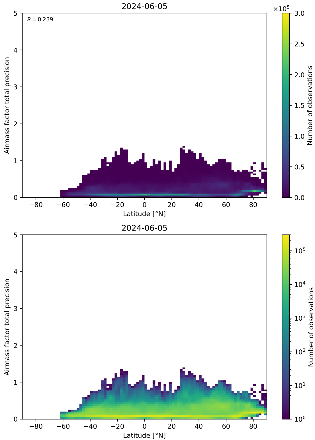
Figure 162: Scatter density plot of “Latitude” against “Airmass factor total precision” for 2024-06-04 to 2024-06-06.
