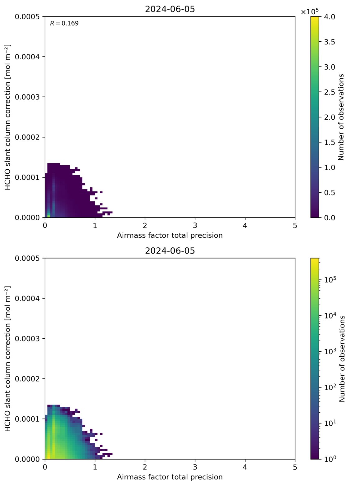
Figure 110: Scatter density plot of “Airmass factor total precision” against “HCHO slant column correction” for 2024-06-04 to 2024-06-06.
