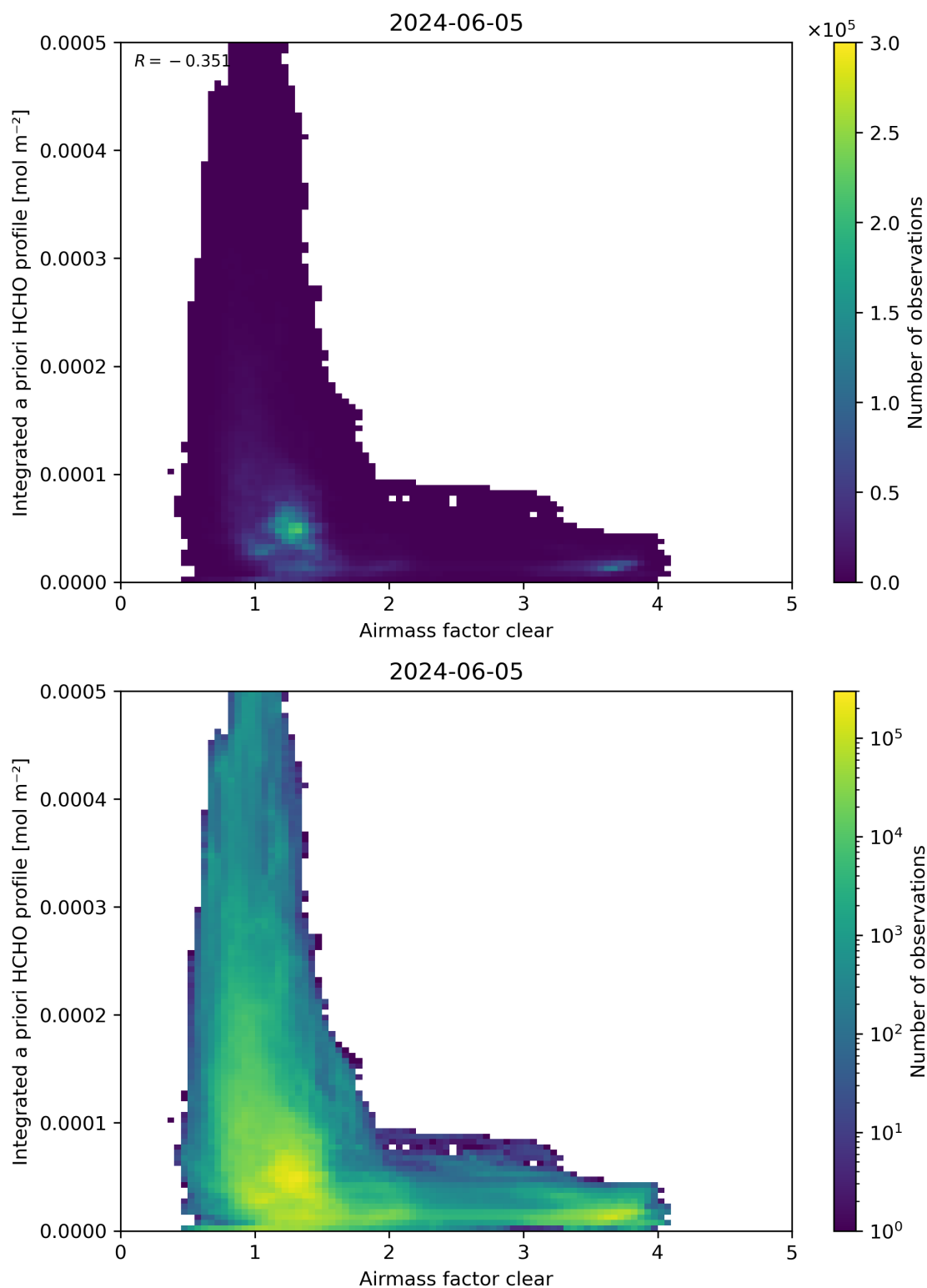
Figure 76: Scatter density plot of “Airmass factor clear” against “Integrated a priori HCHO profile” for 2024-06-04 to 2024-06-06.
