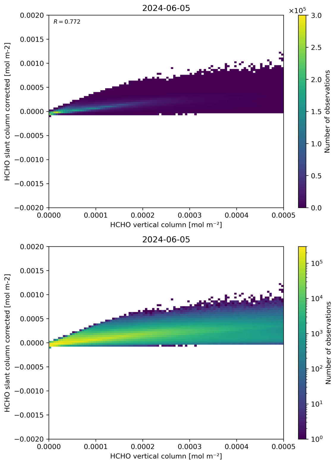
Figure 127: Scatter density plot of “HCHO vertical column” against “HCHO slant column corrected” for 2024-06-04 to 2024-06-06.
