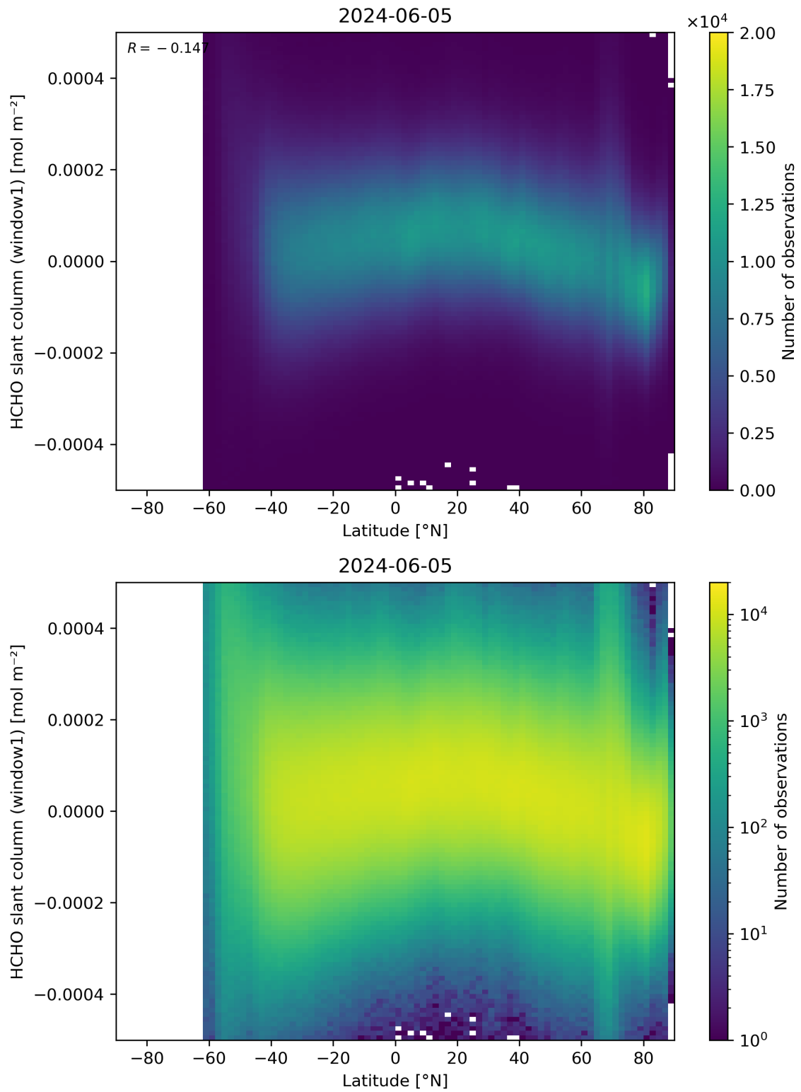
Figure 159: Scatter density plot of “Latitude” against “HCHO slant column (window1)” for 2024-06-04 to 2024-06-06.
