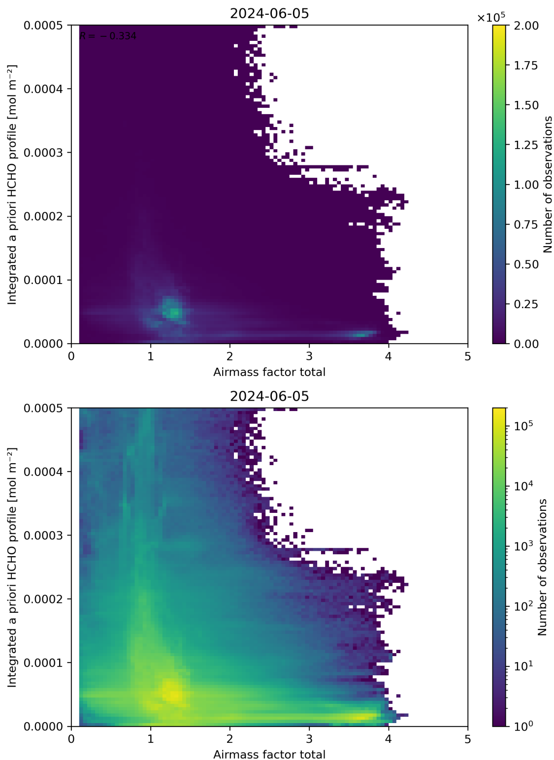
Figure 104: Scatter density plot of “Airmass factor total” against “Integrated a priori HCHO profile” for 2024-06-04 to 2024-06-06.
