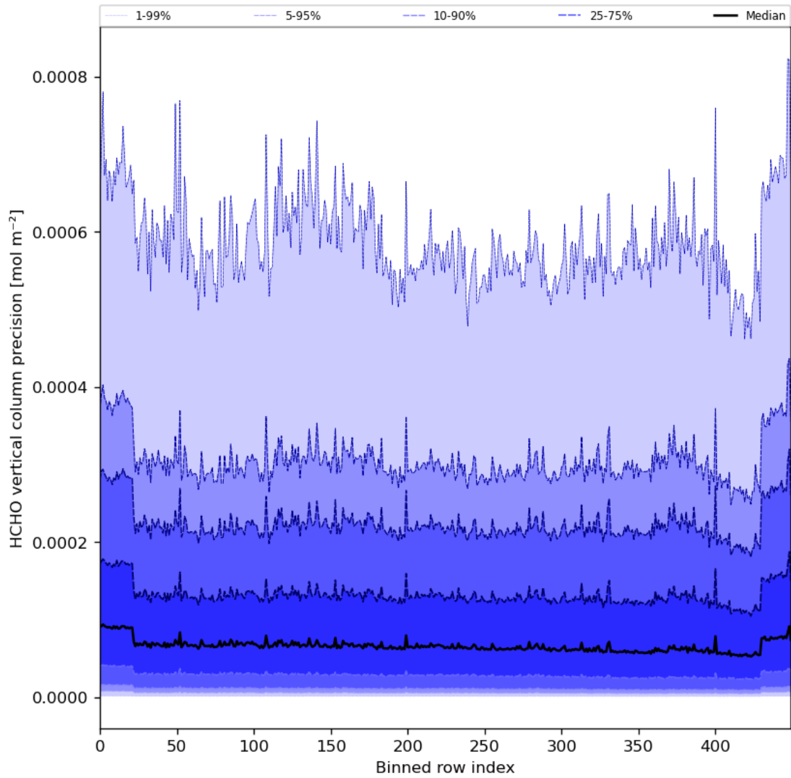
Figure 50: Along track statistics of “HCHO vertical column precision” for 2024-06-04 to 2024-06-06
