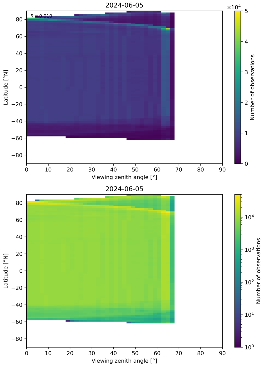
Figure 196: Scatter density plot of “Viewing zenith angle” against “Latitude” for 2024-06-04 to 2024-06-06.
