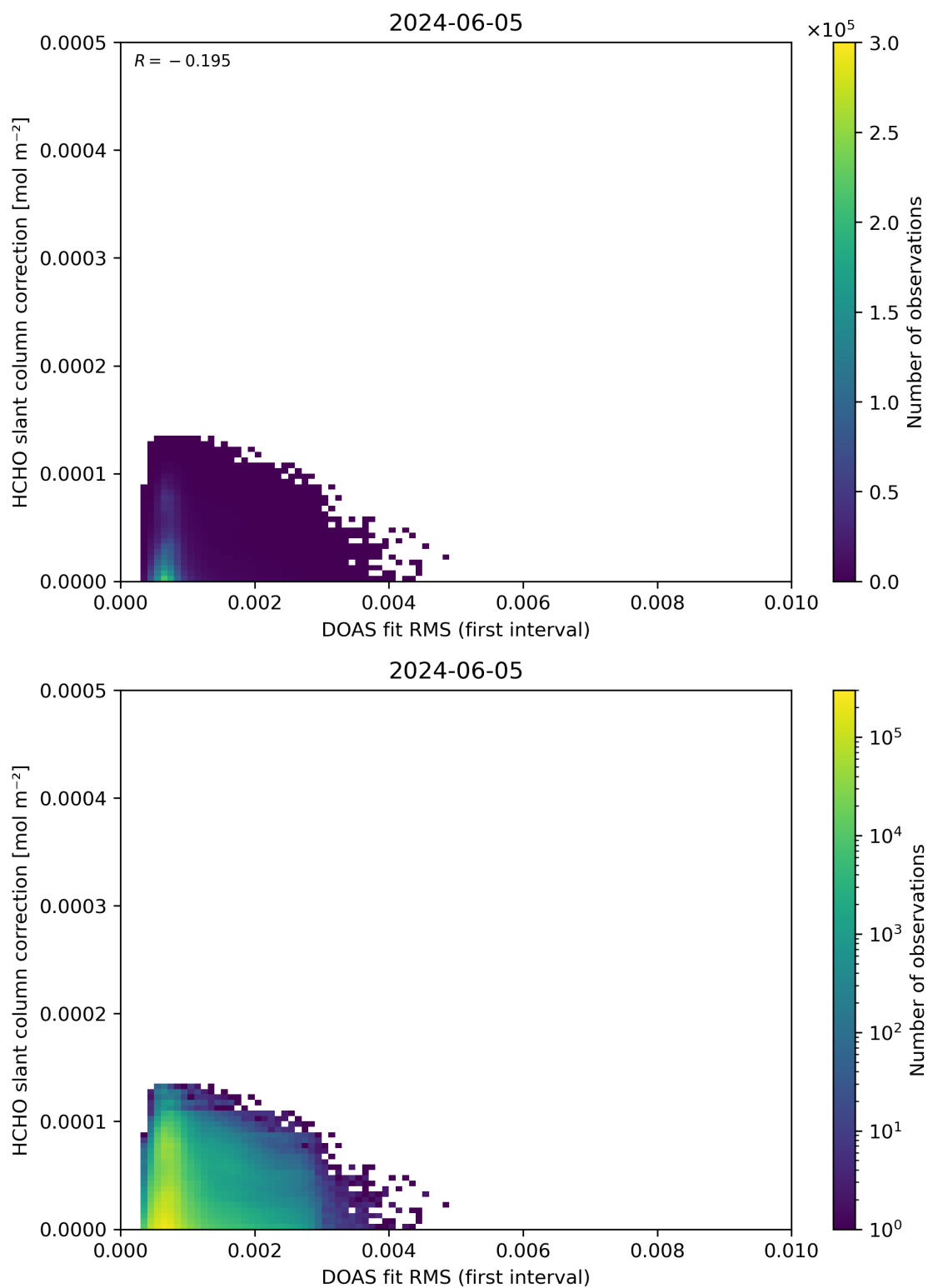
Figure 63: Scatter density plot of “DOAS fit RMS (first interval)” against “HCHO slant column correction” for 2024-06-04 to 2024-06-06.
