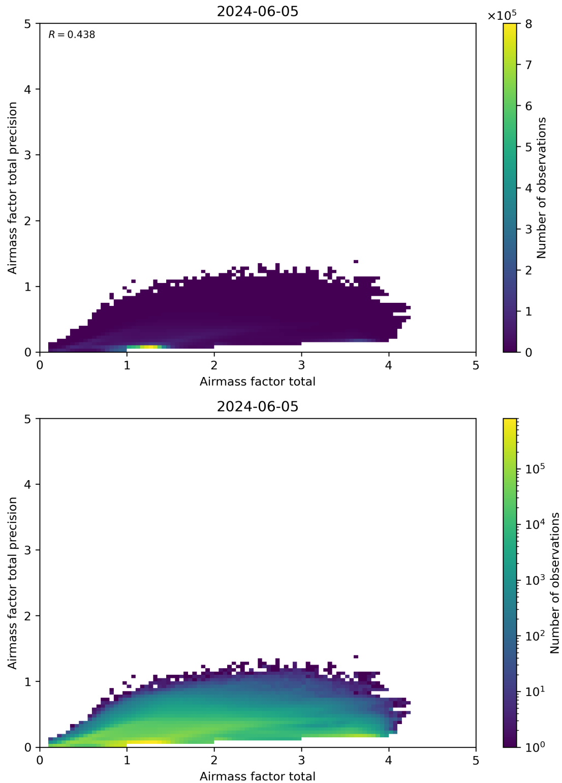
Figure 103: Scatter density plot of “Airmass factor total” against “Airmass factor total precision” for 2024-06-04 to 2024-06-06.
