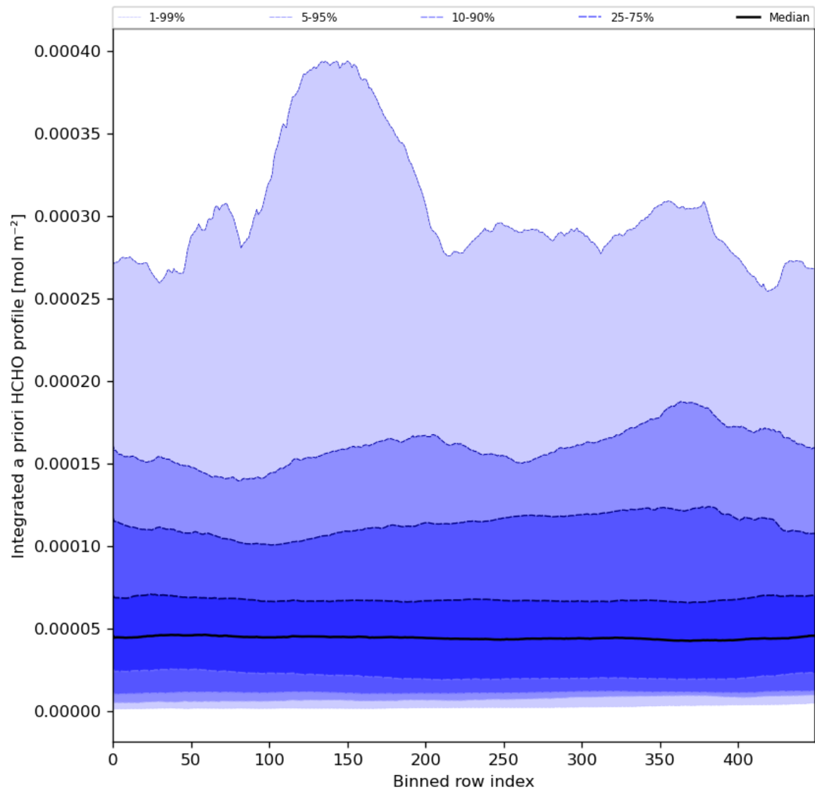
Figure 57: Along track statistics of “Integrated a priori HCHO profile” for 2024-06-04 to 2024-06-06
