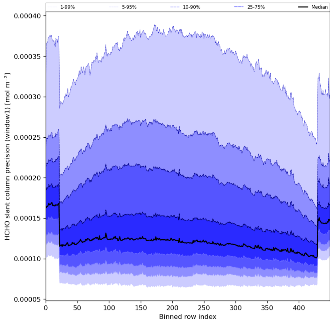
Figure 53: Along track statistics of “HCHO slant column precision (window1)” for 2024-06-04 to 2024-06-06
