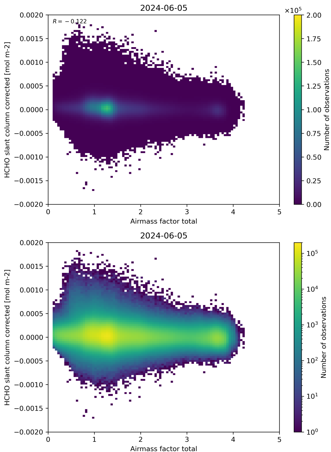
Figure 101: Scatter density plot of “Airmass factor total” against “HCHO slant column corrected” for 2024-06-04 to 2024-06-06.
