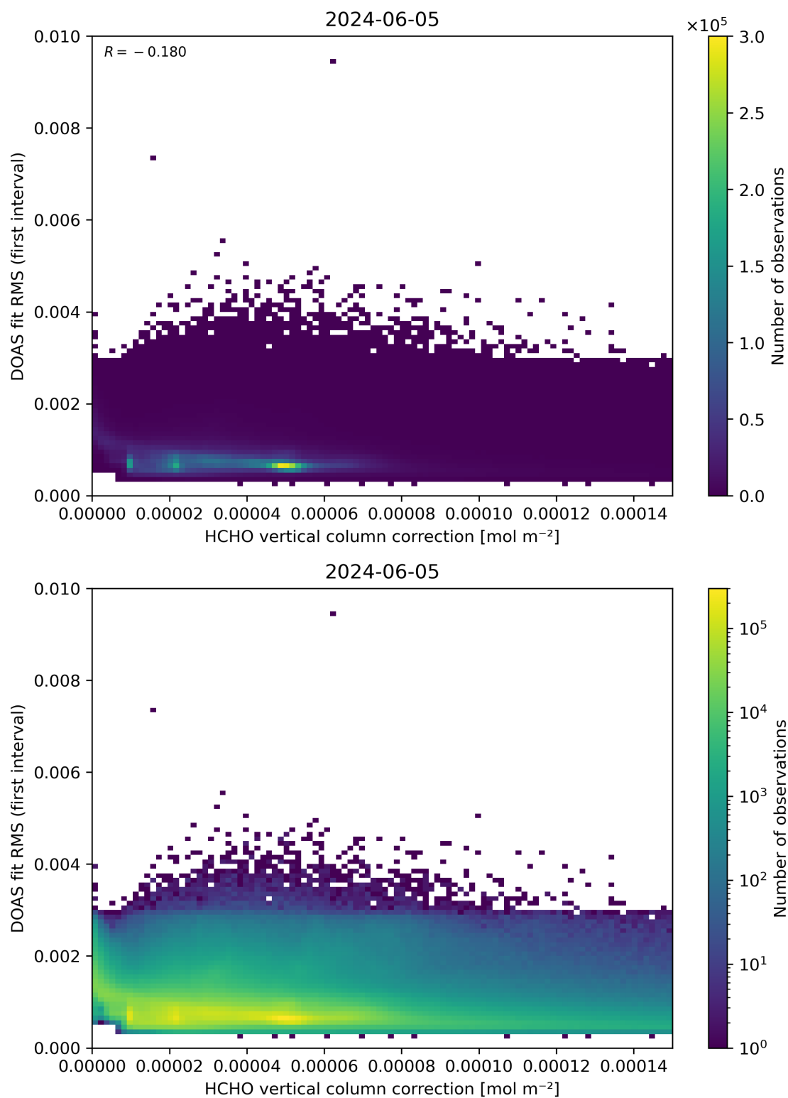
Figure 112: Scatter density plot of “HCHO vertical column correction” against “DOAS fit RMS (first interval)” for 2024-06-04 to 2024-06-06.
