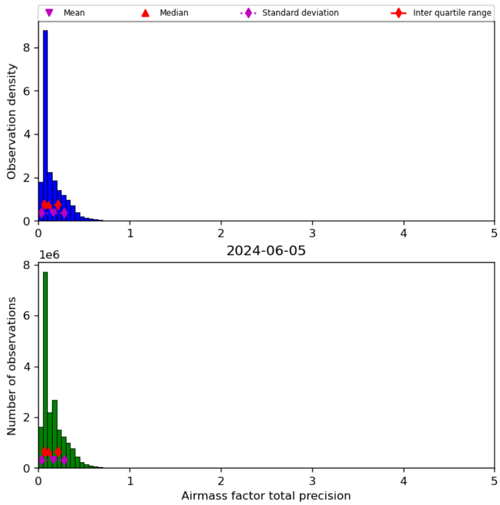
Figure 41: Histogram of “Airmass factor total precision” for 2024-06-04 to 2024-06-06
