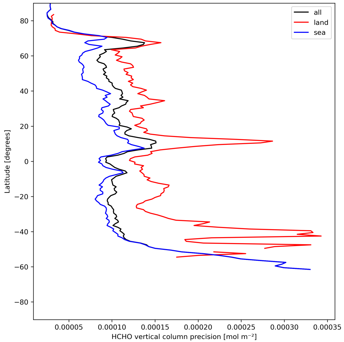
Figure 22: Zonal average of “HCHO vertical column precision” for 2024-06-04 to 2024-06-06.
