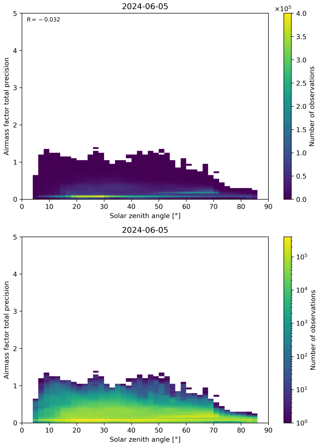
Figure 176: Scatter density plot of “Solar zenith angle” against “Airmass factor total precision” for 2024-06-04 to 2024-06-06.
