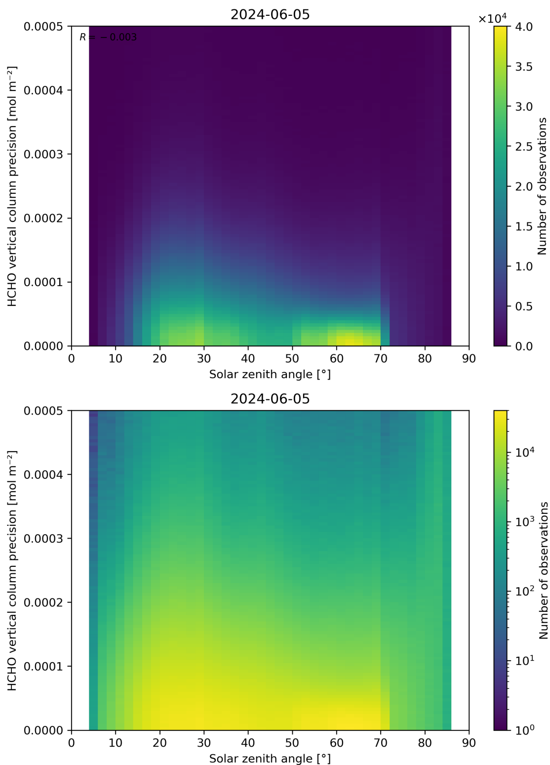
Figure 179: Scatter density plot of “Solar zenith angle” against “HCHO vertical column precision” for 2024-06-04 to 2024-06-06.
