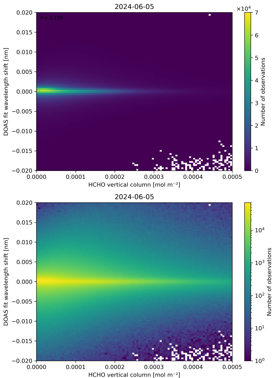
Figure 124: Scatter density plot of “HCHO vertical column” against “DOAS fit wavelength shift” for 2024-06-04 to 2024-06-06.
