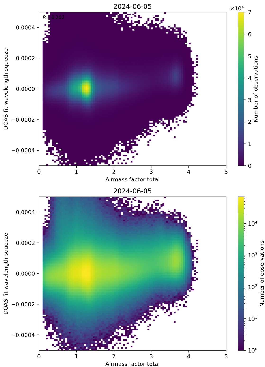
Figure 99: Scatter density plot of “Airmass factor total” against “DOAS fit wavelength squeeze” for 2024-06-04 to 2024-06-06.
