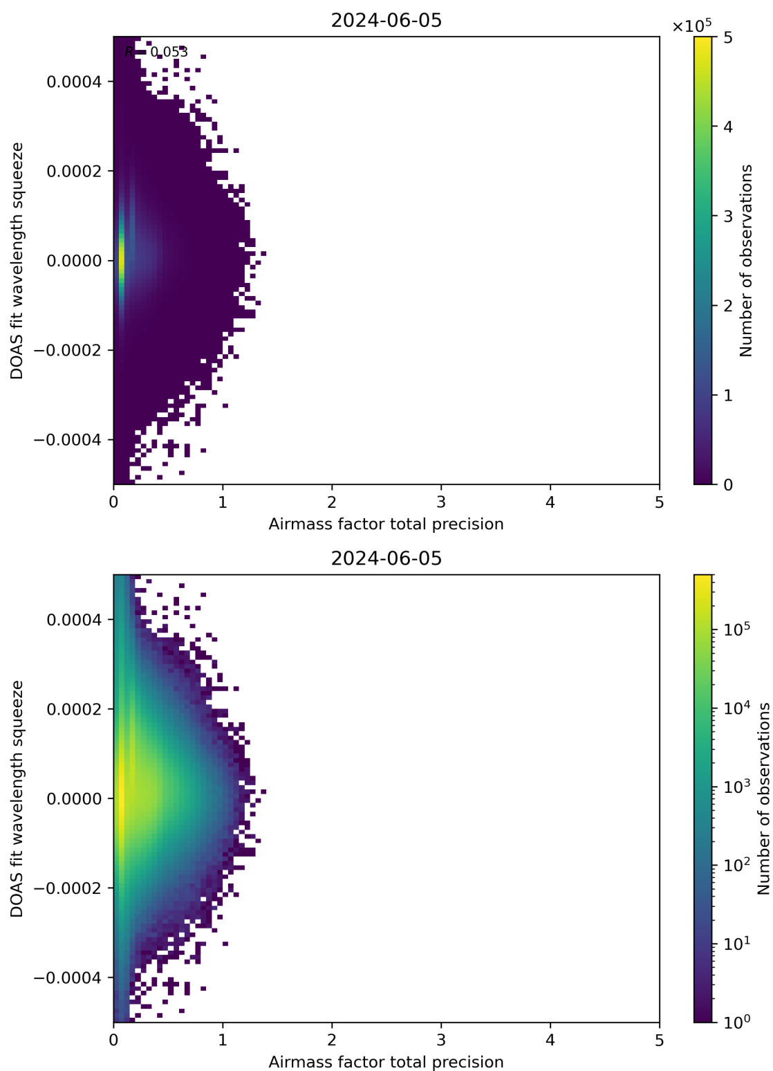
Figure 107: Scatter density plot of “Airmass factor total precision” against “DOAS fit wavelength squeeze” for 2024-06-04 to 2024-06-06.
