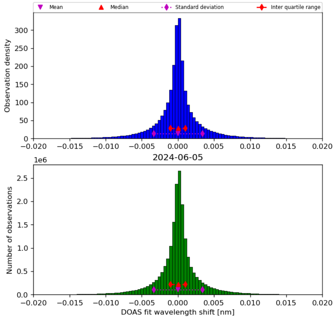
Figure 44: Histogram of “DOAS fit wavelength shift” for 2024-06-04 to 2024-06-06
