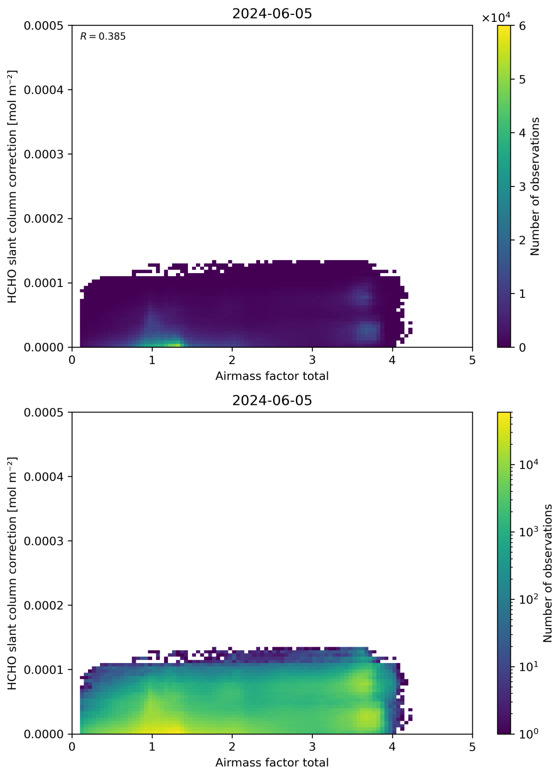
Figure 102: Scatter density plot of “Airmass factor total” against “HCHO slant column correction” for 2024-06-04 to 2024-06-06.
