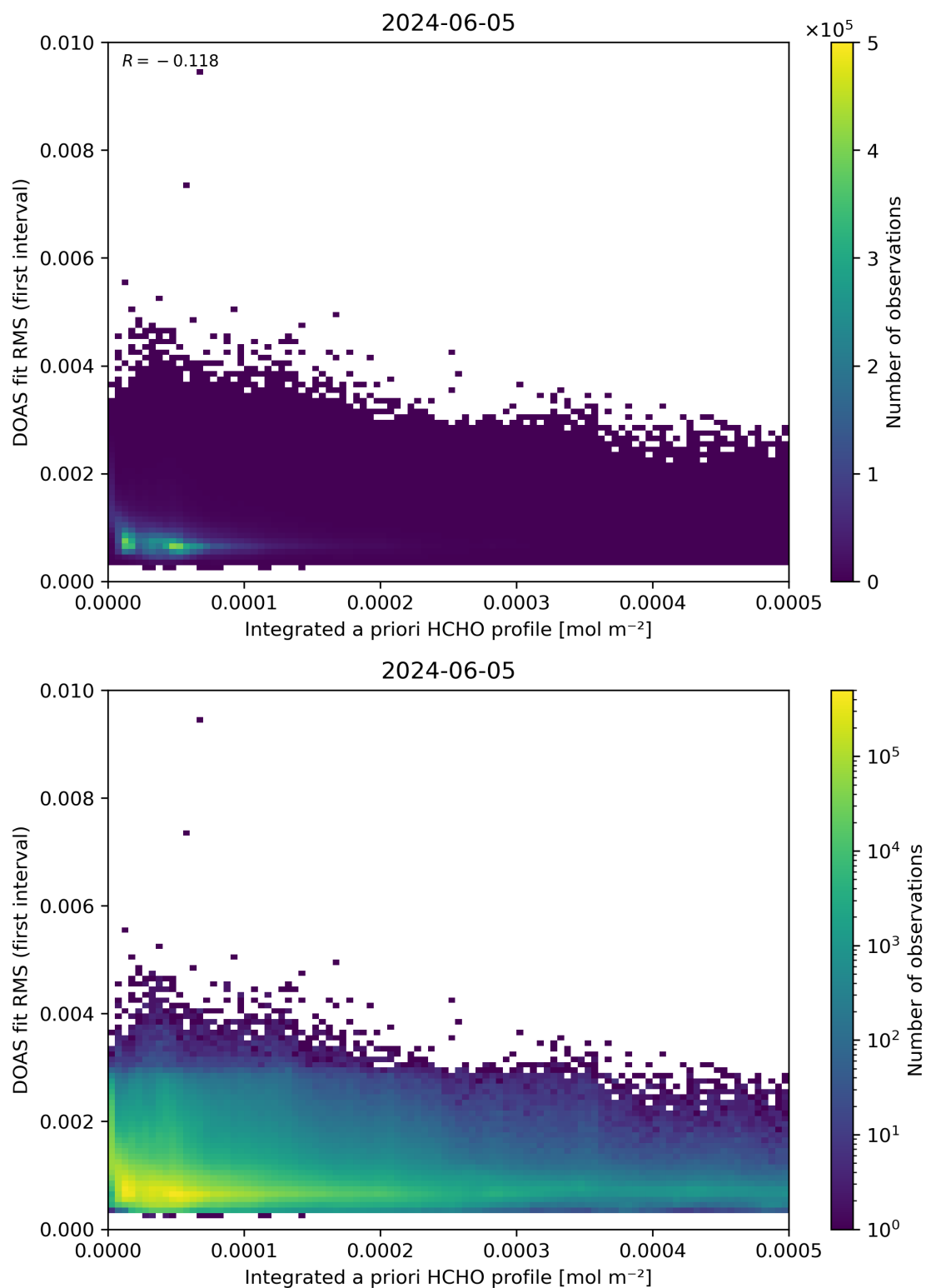
Figure 148: Scatter density plot of “Integrated a priori HCHO profile” against “DOAS fit RMS (first interval)” for 2024-06-04 to 2024-06-06.
