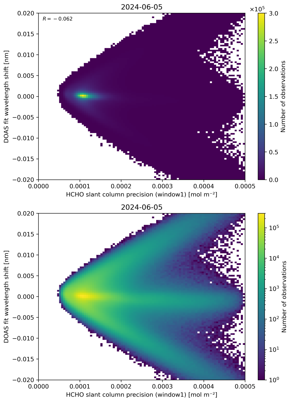
Figure 89: Scatter density plot of “HCHO slant column precision (window1)” against “DOAS fit wavelength shift” for 2024-06-04 to 2024-06-06.
