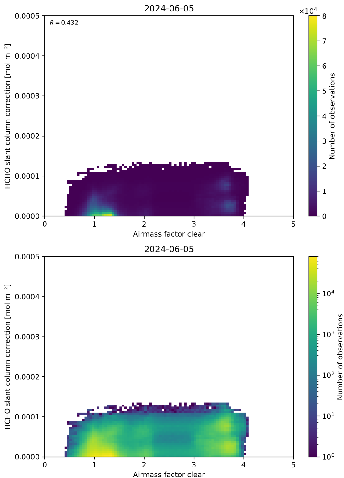
Figure 75: Scatter density plot of “Airmass factor clear” against “HCHO slant column correction” for 2024-06-04 to 2024-06-06.
