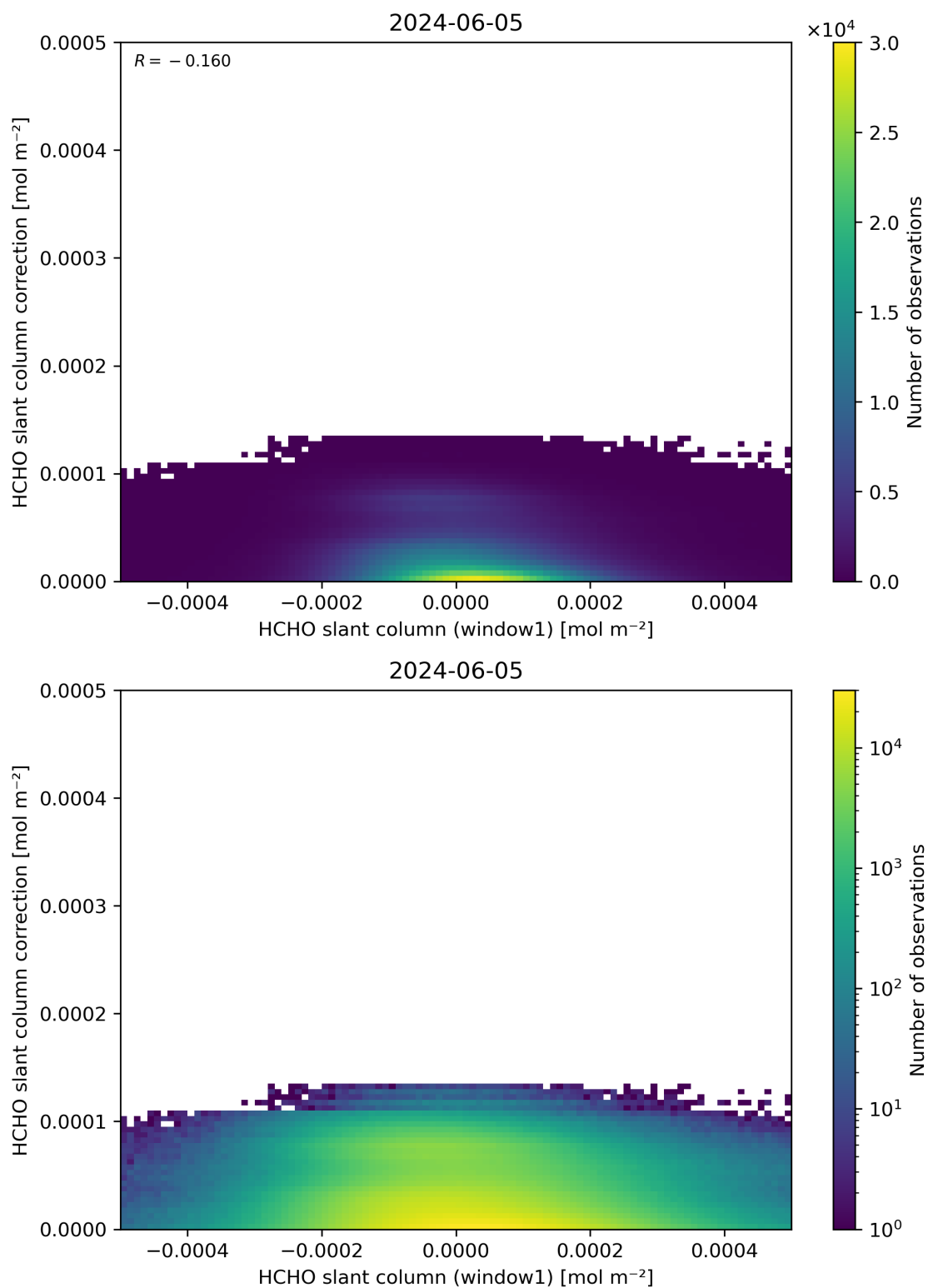
Figure 83: Scatter density plot of “HCHO slant column (window1)” against “HCHO slant column correction” for 2024-06-04 to 2024-06-06.
