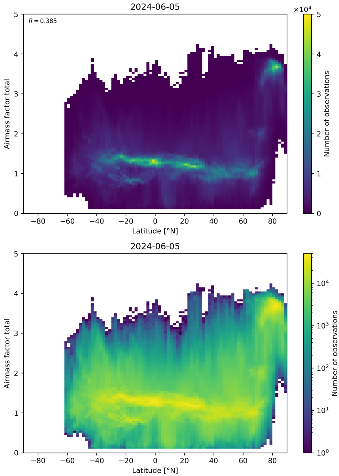
Figure 161: Scatter density plot of “Latitude” against “Airmass factor total” for 2024-06-04 to 2024-06-06.
