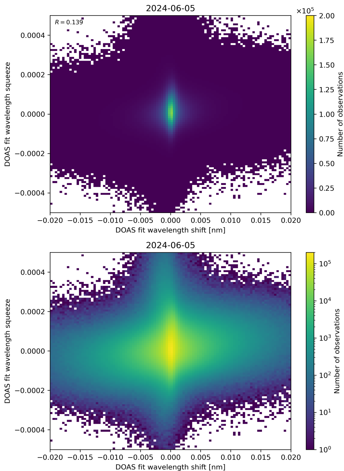
Figure 65: Scatter density plot of “DOAS fit wavelength shift” against “DOAS fit wavelength squeeze” for 2024-06-04 to 2024-06-06.
