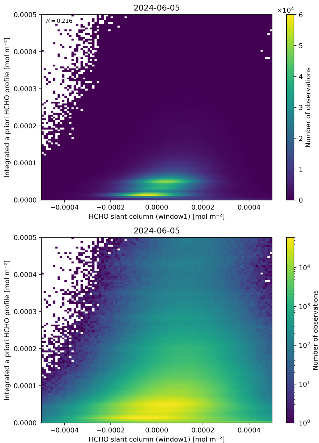
Figure 87: Scatter density plot of “HCHO slant column (window1)” against “Integrated a priori HCHO profile” for 2024-06-04 to 2024-06-06.
