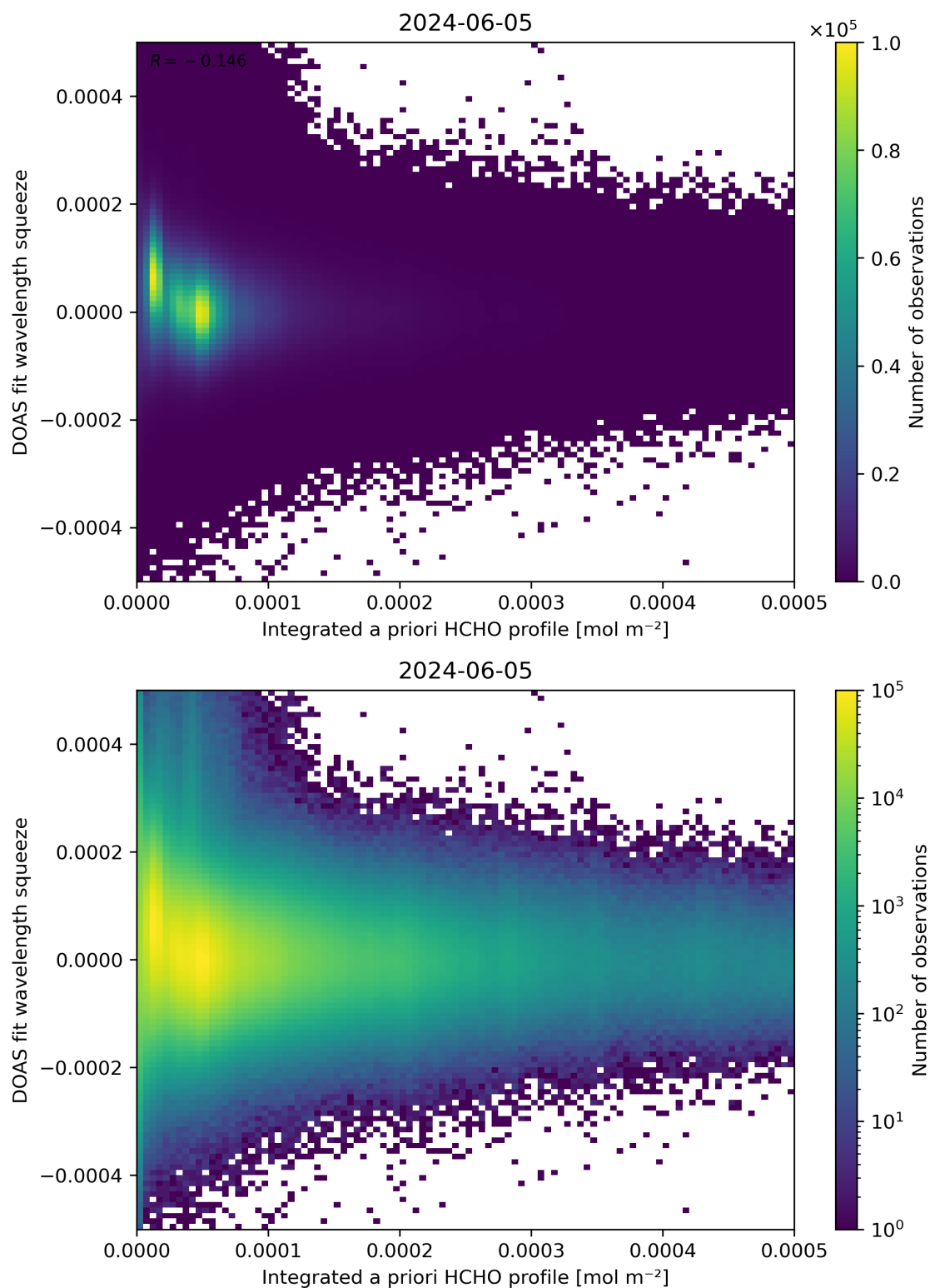
Figure 150: Scatter density plot of “Integrated a priori HCHO profile” against “DOAS fit wavelength squeeze” for 2024-06-04 to 2024-06-06.
