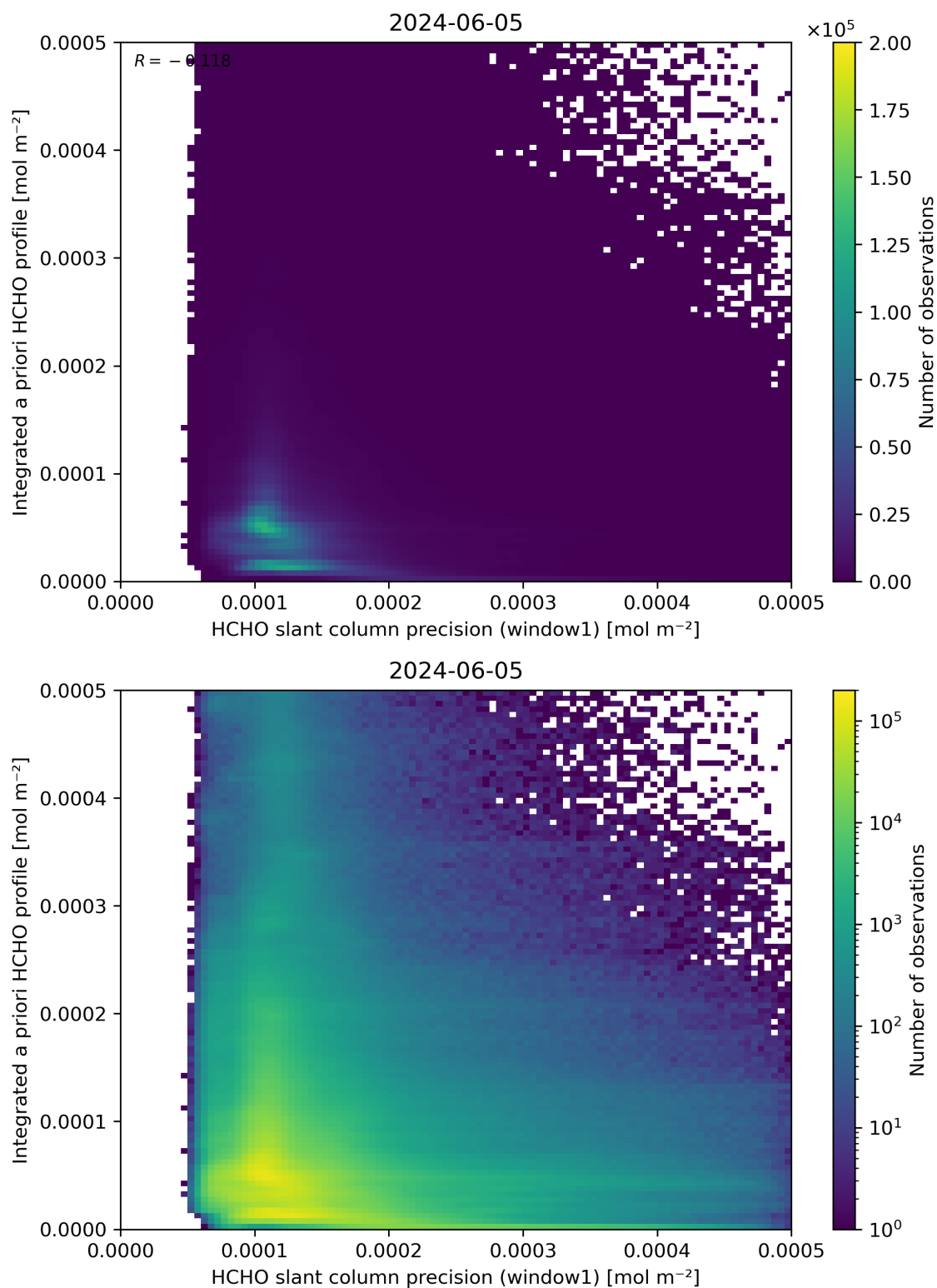
Figure 96: Scatter density plot of “HCHO slant column precision (window1)” against “Integrated a priori HCHO profile” for 2024-06-04 to 2024-06-06.
