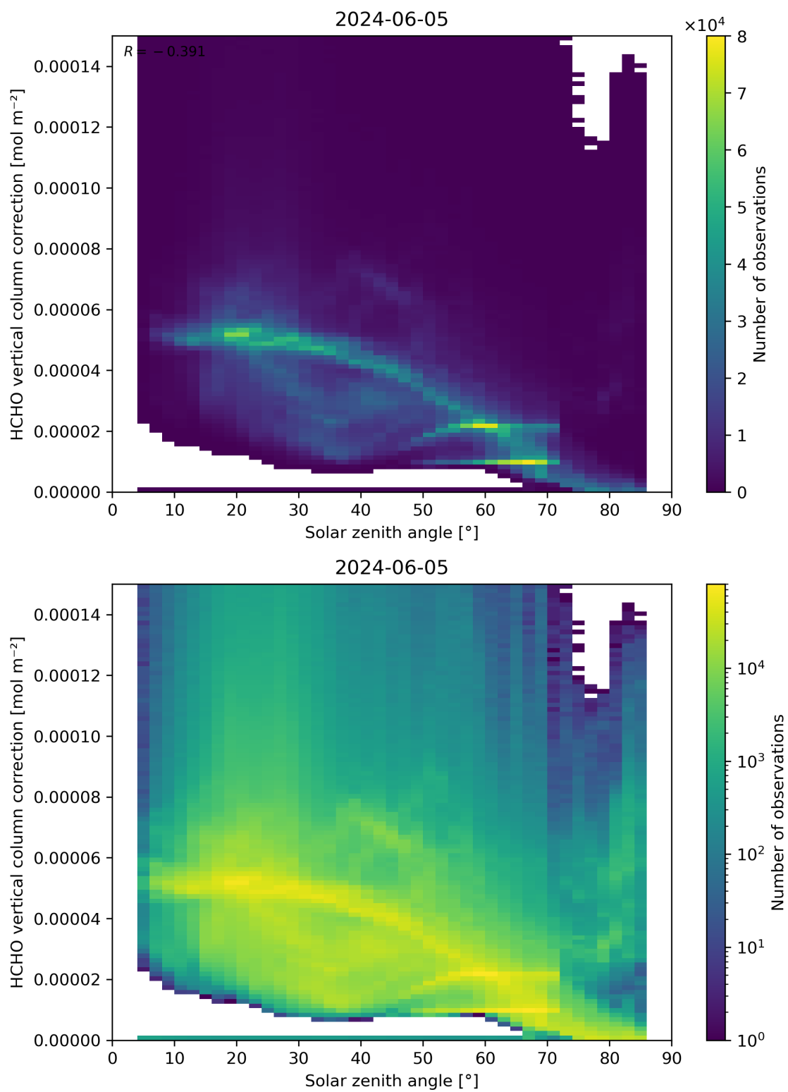
Figure 178: Scatter density plot of “Solar zenith angle” against “HCHO vertical column correction” for 2024-06-04 to 2024-06-06.
