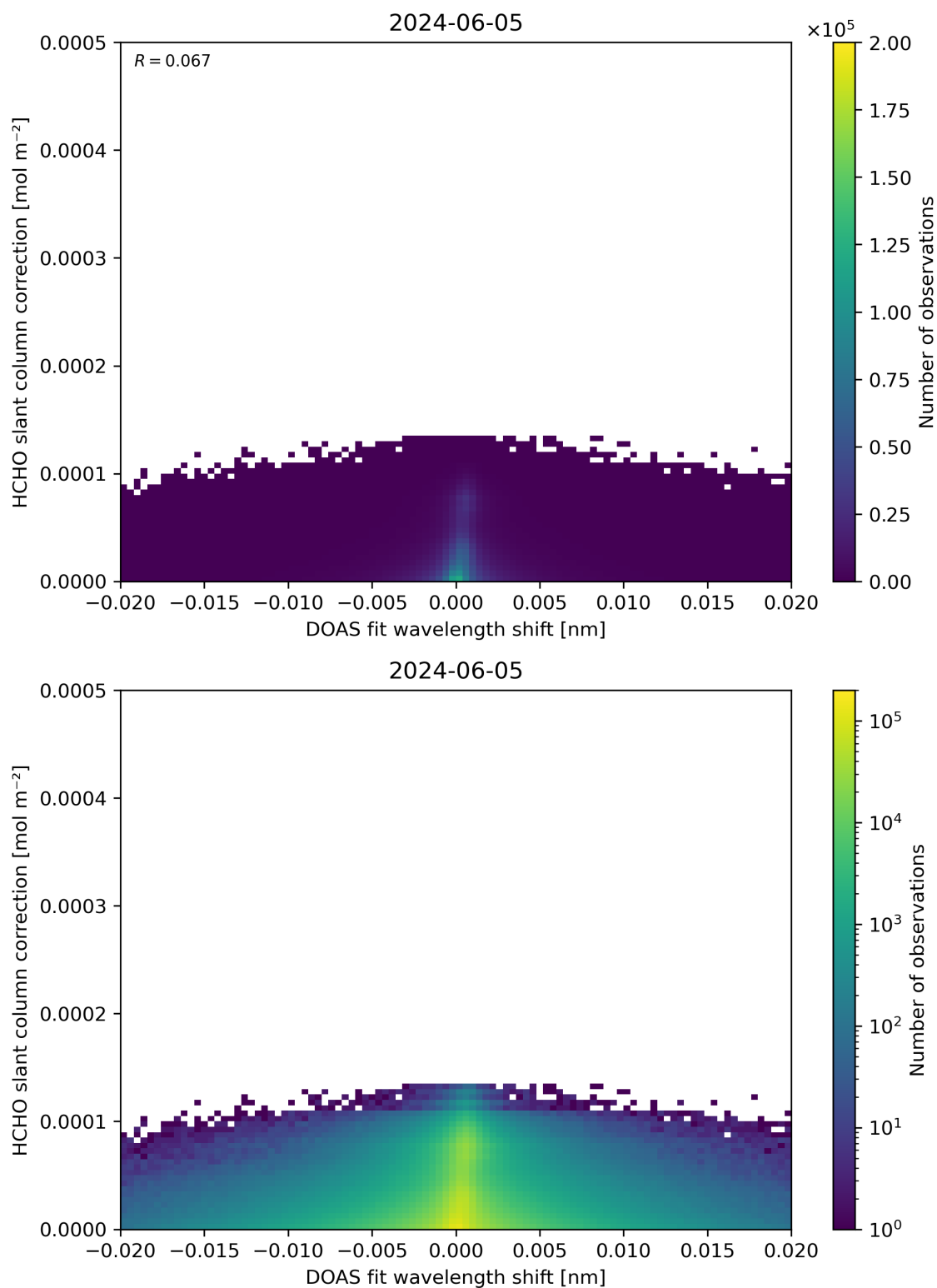
Figure 67: Scatter density plot of “DOAS fit wavelength shift” against “HCHO slant column correction” for 2024-06-04 to 2024-06-06.
