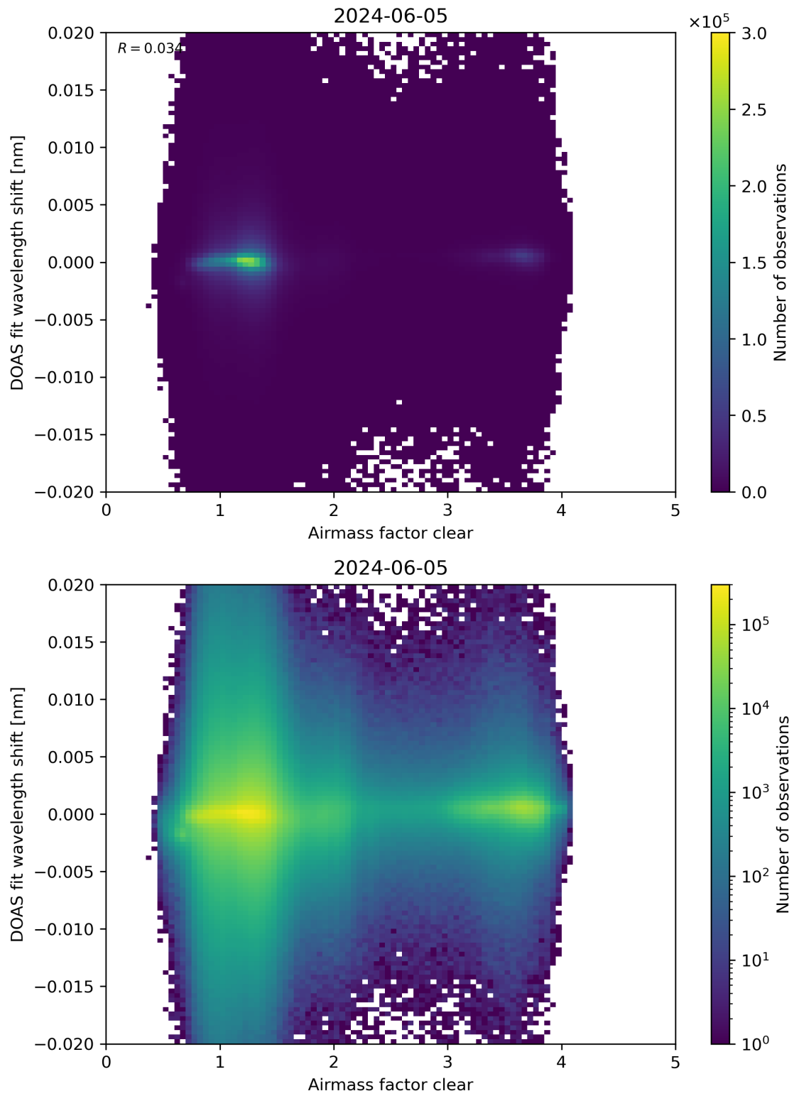
Figure 72: Scatter density plot of “Airmass factor clear” against “DOAS fit wavelength shift” for 2024-06-04 to 2024-06-06.
