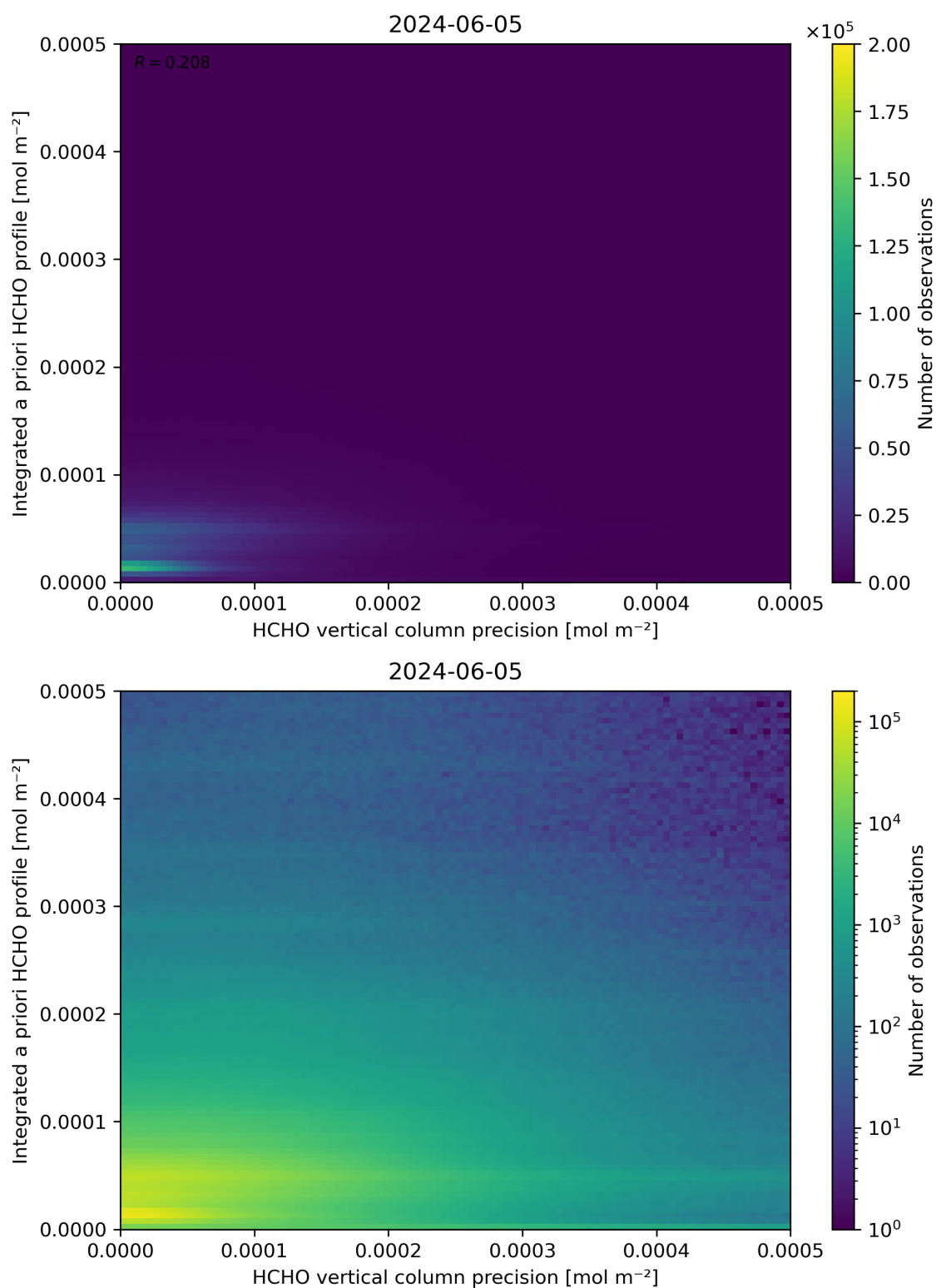
Figure 147: Scatter density plot of “HCHO vertical column precision” against “Integrated a priori HCHO profile” for 2024-06-04 to 2024-06-06.
