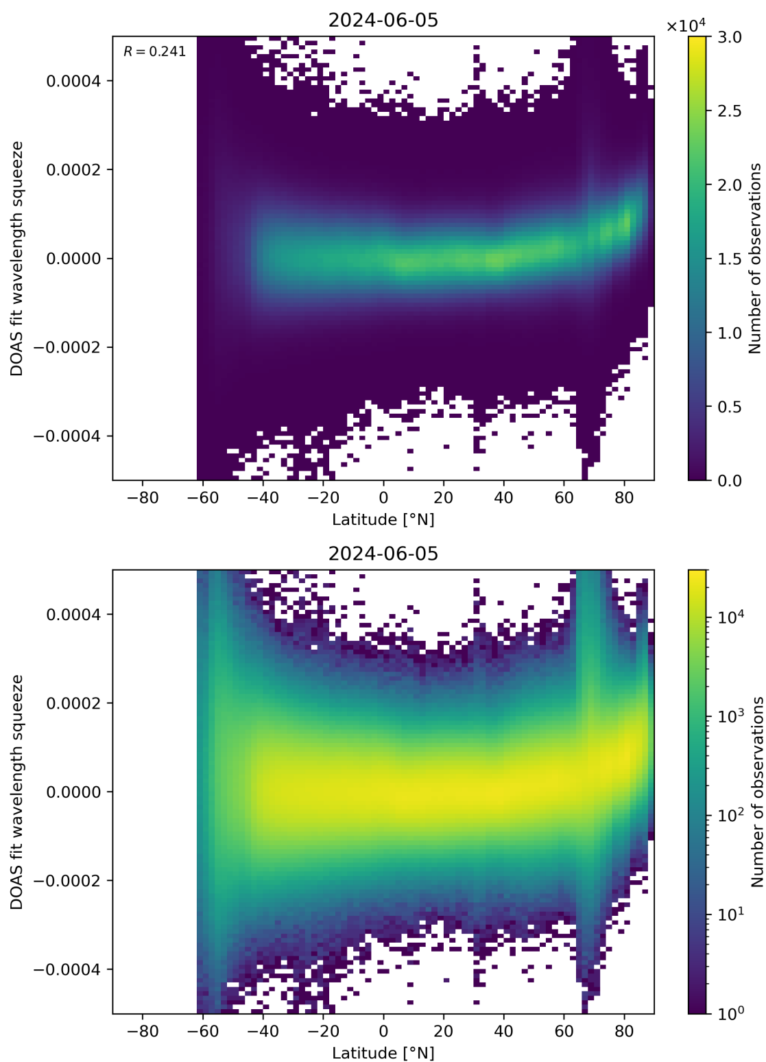
Figure 155: Scatter density plot of “Latitude” against “DOAS fit wavelength squeeze” for 2024-06-04 to 2024-06-06.
