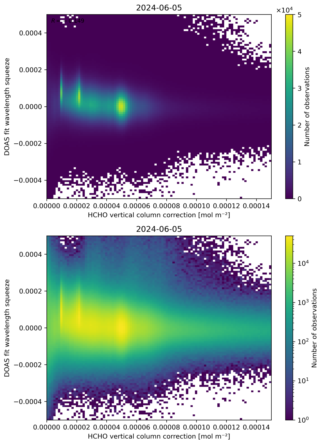
Figure 114: Scatter density plot of “HCHO vertical column correction” against “DOAS fit wavelength squeeze” for 2024-06-04 to 2024-06-06.
