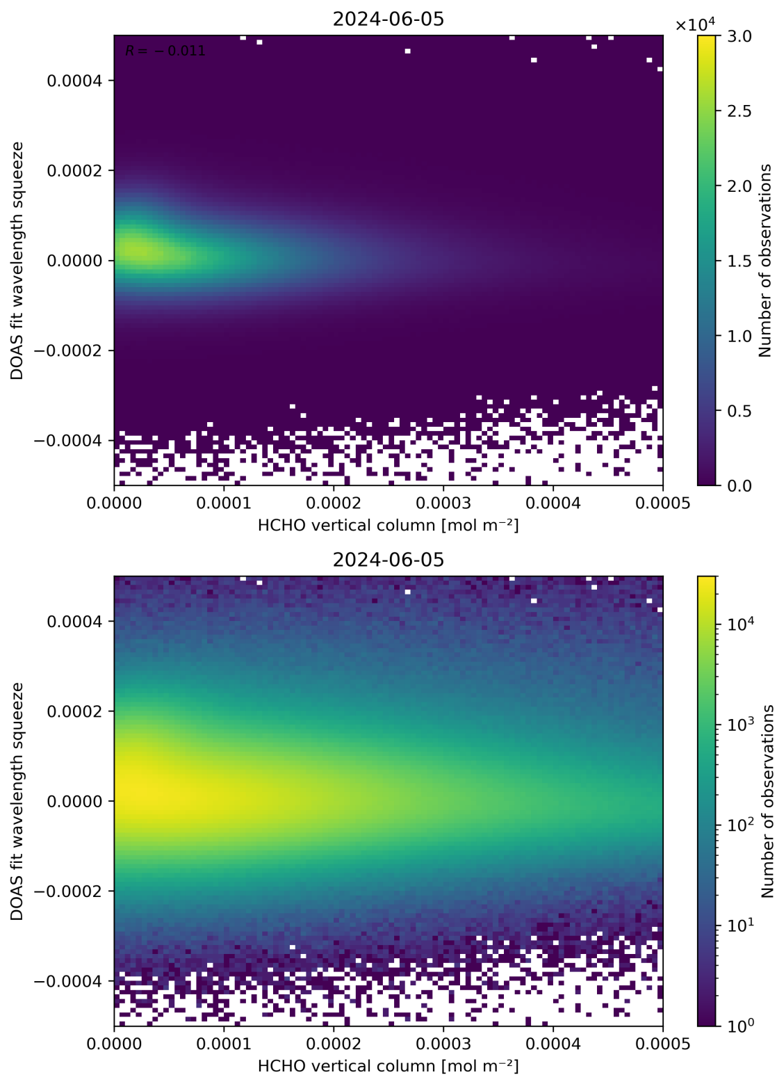
Figure 125: Scatter density plot of “HCHO vertical column” against “DOAS fit wavelength squeeze” for 2024-06-04 to 2024-06-06.
