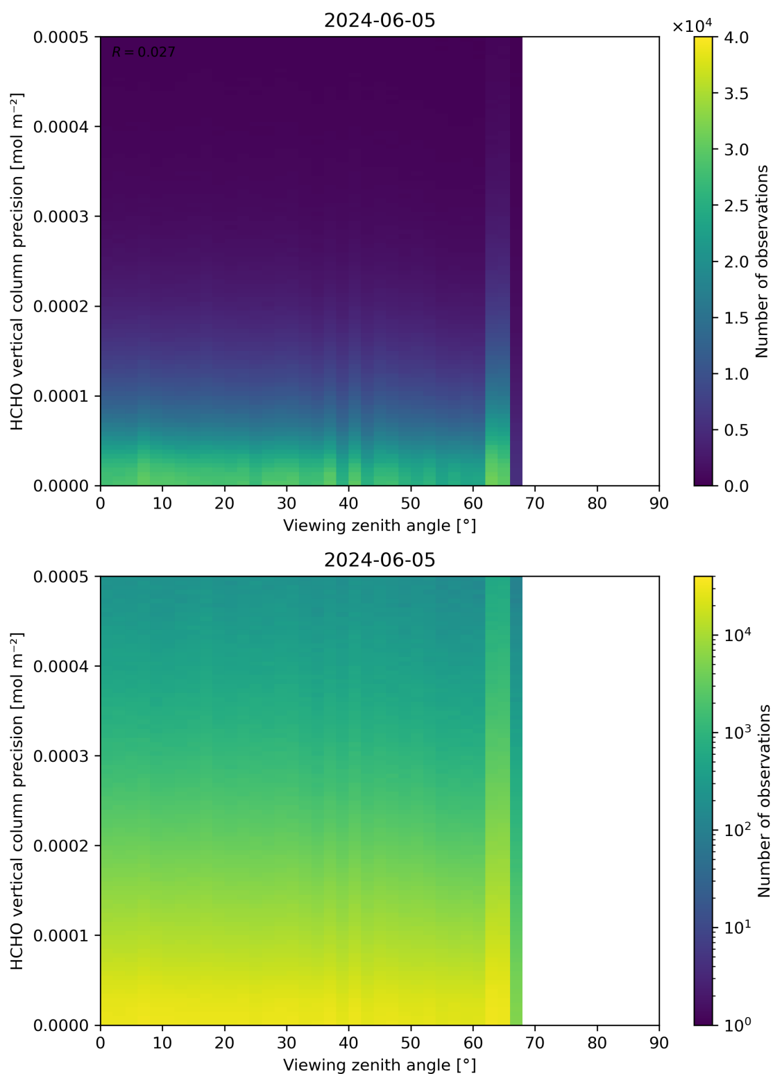
Figure 194: Scatter density plot of “Viewing zenith angle” against “HCHO vertical column precision” for 2024-06-04 to 2024-06-06.
