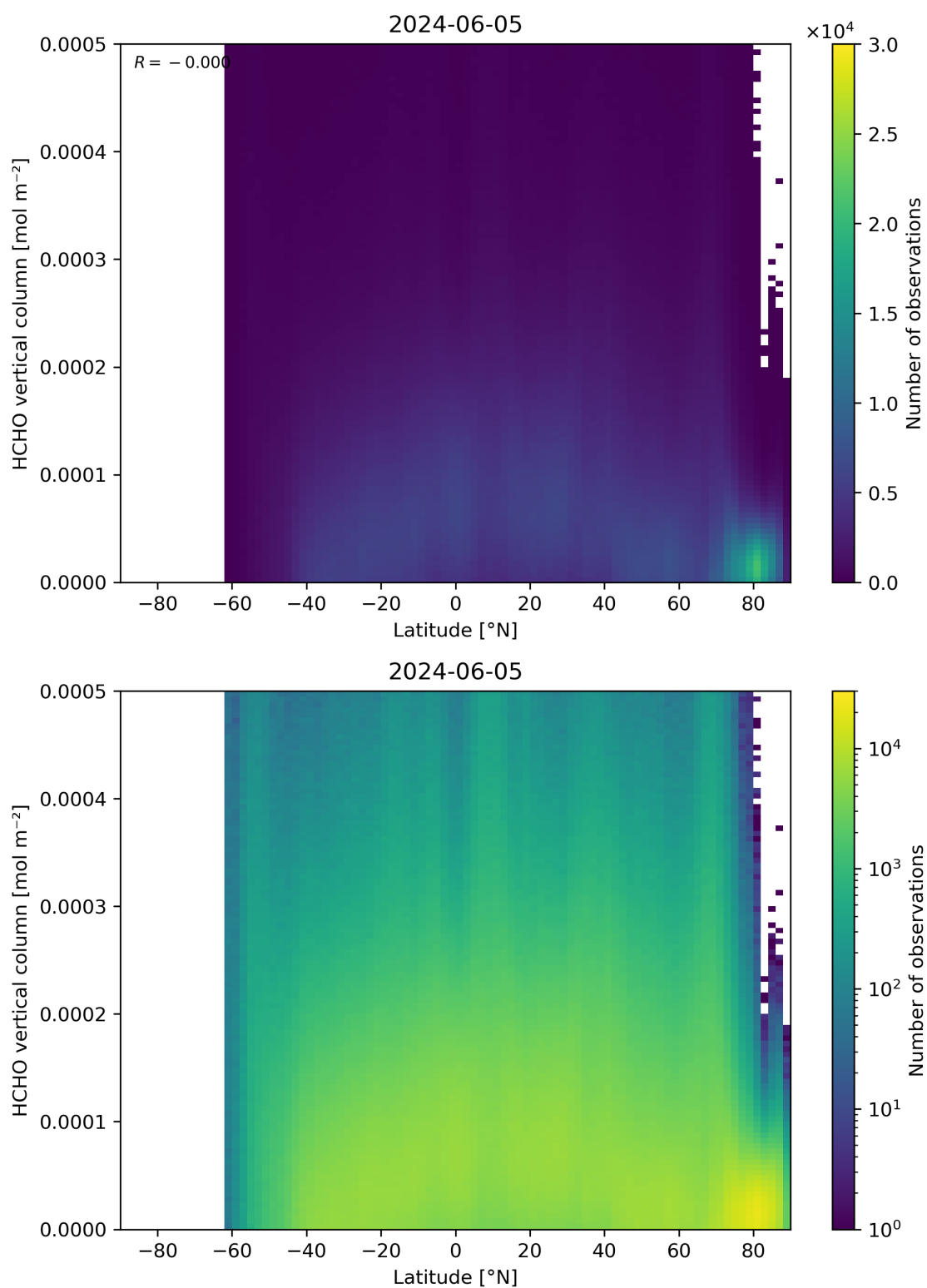
Figure 163: Scatter density plot of “Latitude” against “HCHO vertical column” for 2024-06-04 to 2024-06-06.
