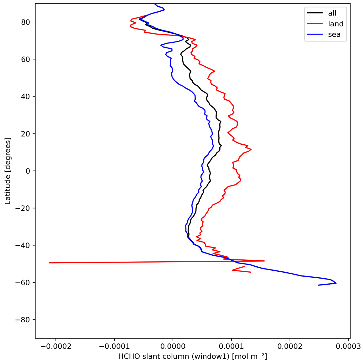
Figure 24: Zonal average of “HCHO slant column (window1)” for 2024-06-04 to 2024-06-06.
