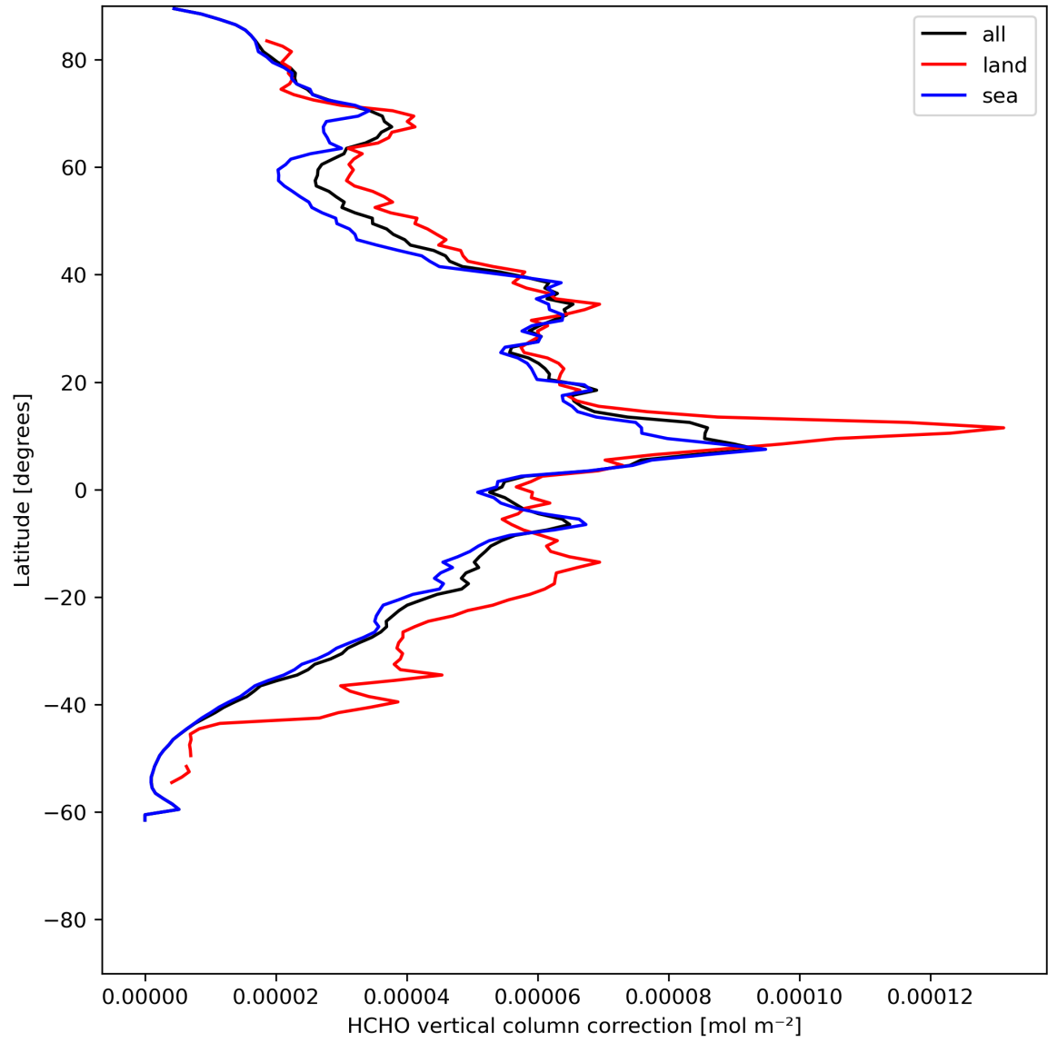
Figure 23: Zonal average of “HCHO vertical column correction” for 2024-06-04 to 2024-06-06.
