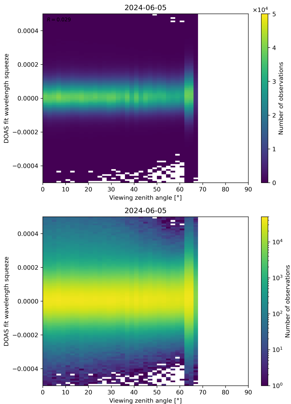
Figure 184: Scatter density plot of “Viewing zenith angle” against “DOAS fit wavelength squeeze” for 2024-06-04 to 2024-06-06.
