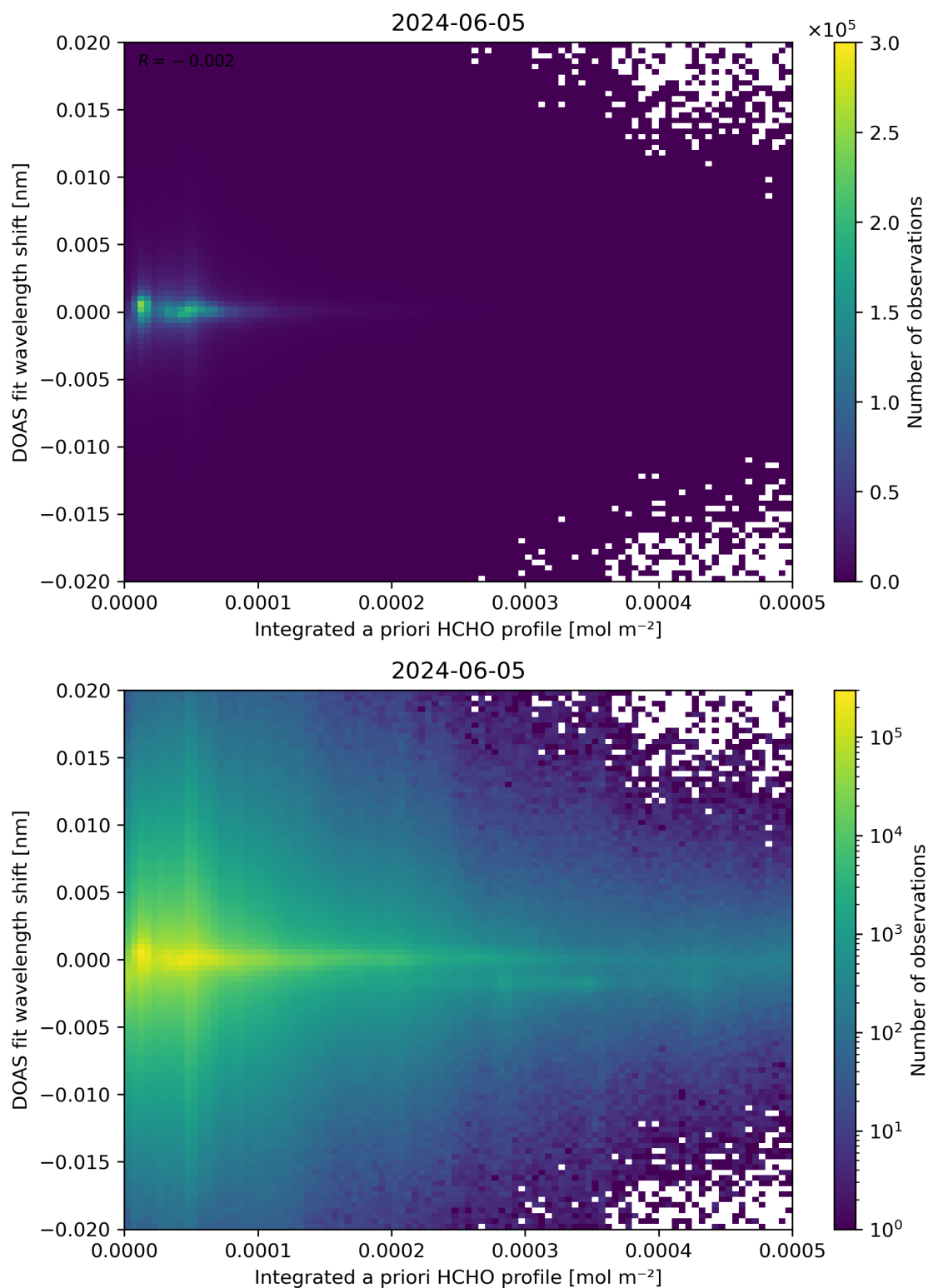
Figure 149: Scatter density plot of “Integrated a priori HCHO profile” against “DOAS fit wavelength shift” for 2024-06-04 to 2024-06-06.
