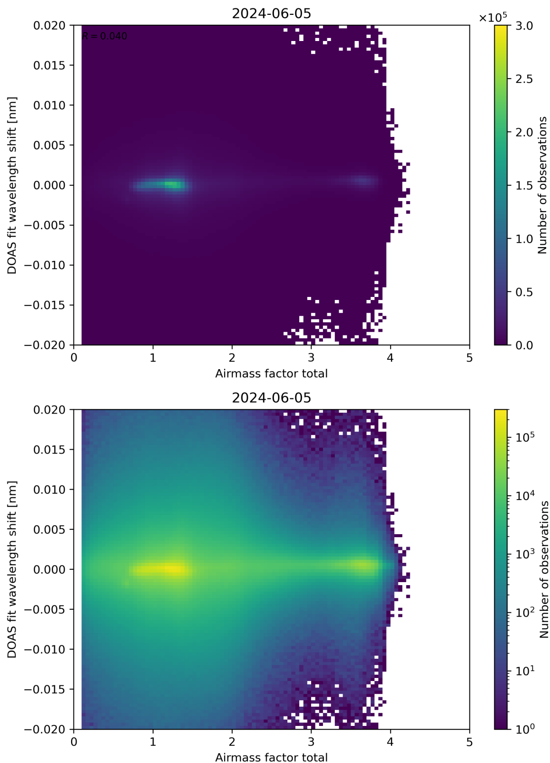
Figure 98: Scatter density plot of “Airmass factor total” against “DOAS fit wavelength shift” for 2024-06-04 to 2024-06-06.
