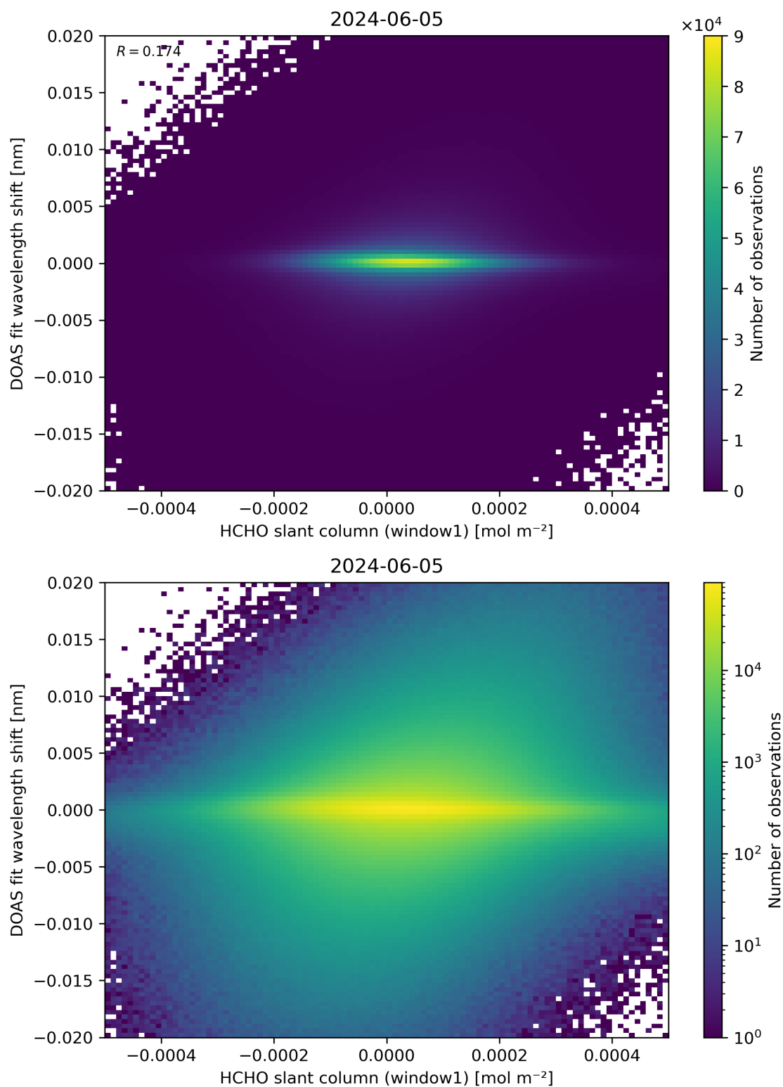
Figure 79: Scatter density plot of “HCHO slant column (window1)” against “DOAS fit wavelength shift” for 2024-06-04 to 2024-06-06.
