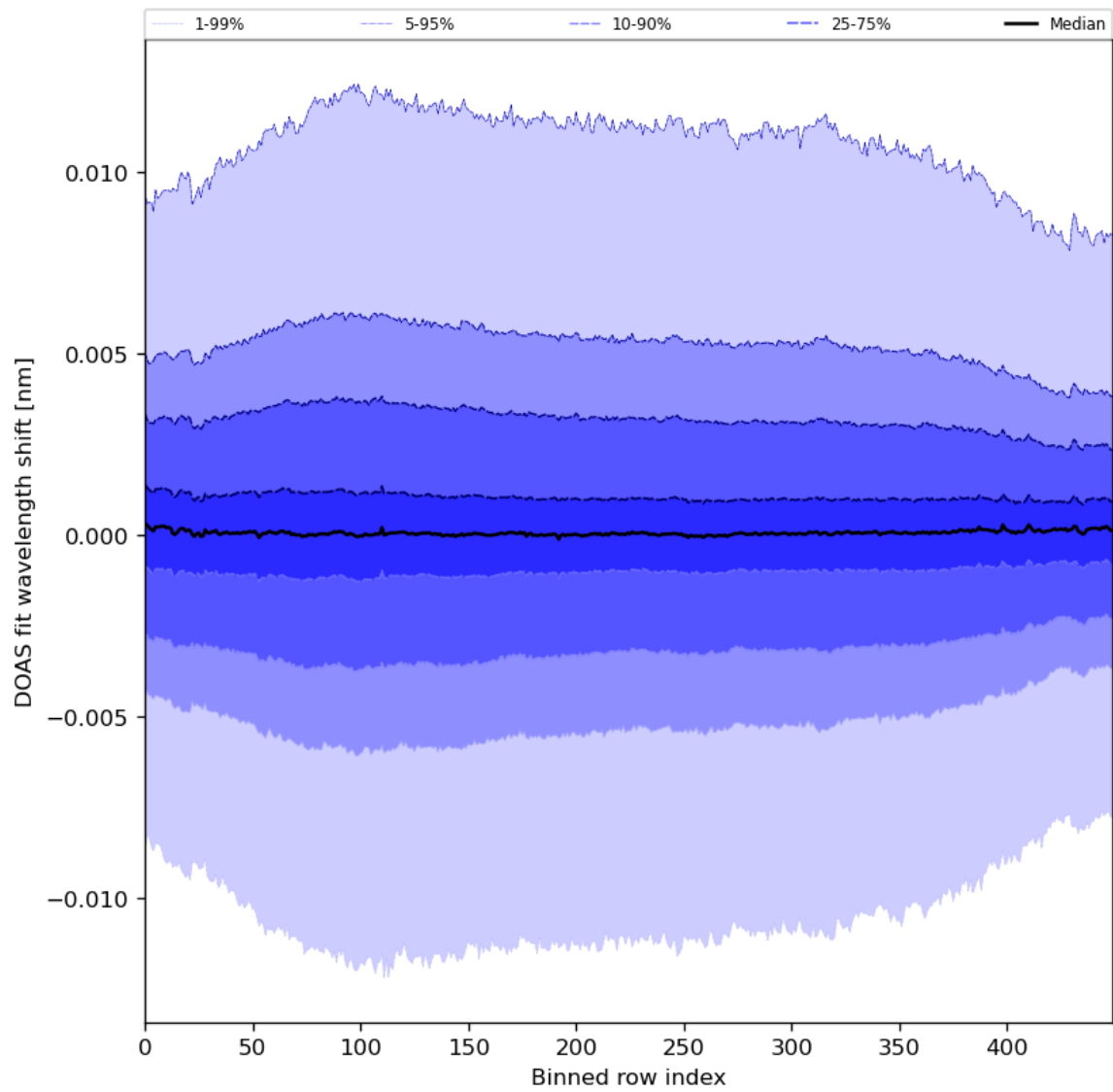
Figure 58: Along track statistics of “DOAS fit wavelength shift” for 2024-06-04 to 2024-06-06
