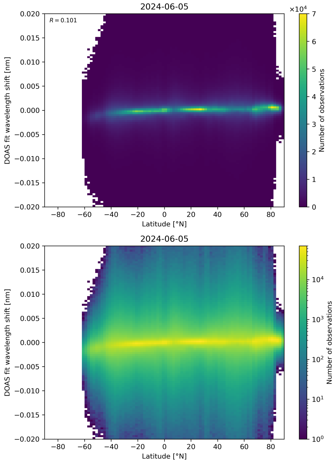
Figure 154: Scatter density plot of “Latitude” against “DOAS fit wavelength shift” for 2024-06-04 to 2024-06-06.
