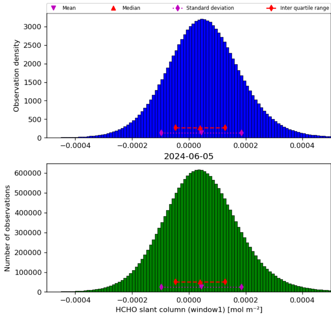
Figure 38: Histogram of “HCHO slant column (window1)” for 2024-06-04 to 2024-06-06
