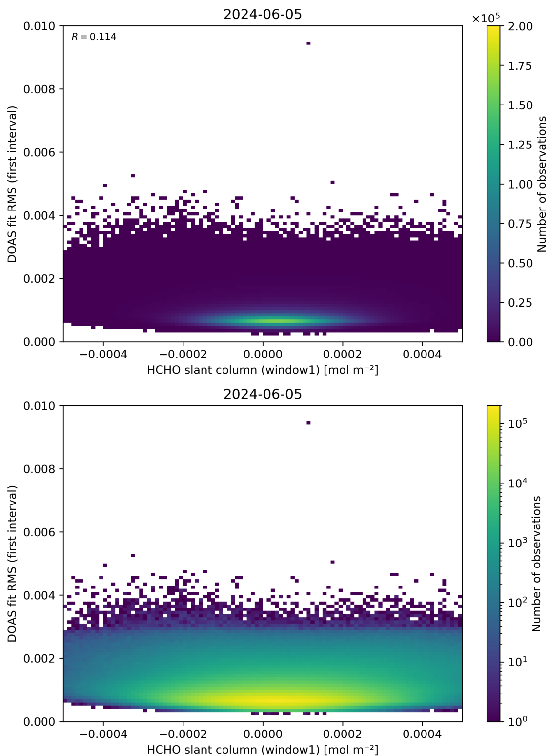
Figure 78: Scatter density plot of “HCHO slant column (window1)” against “DOAS fit RMS (first interval)” for 2024-06-04 to 2024-06-06.
