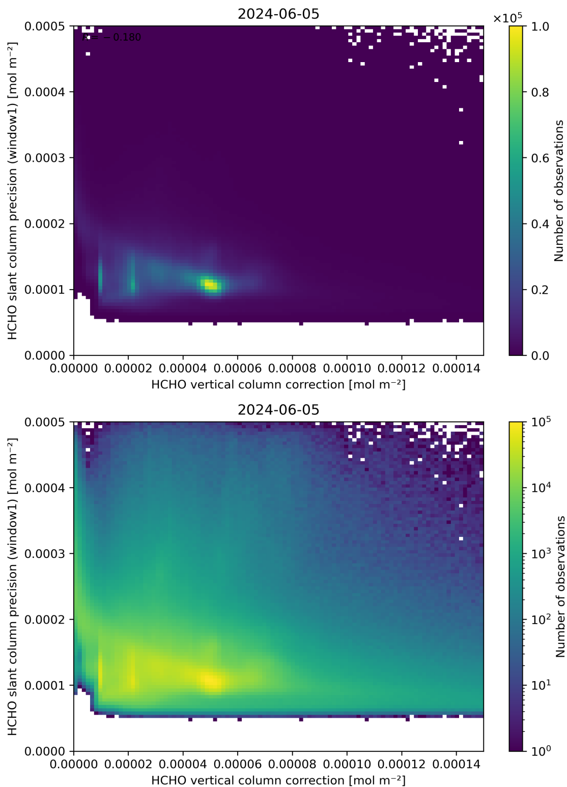
Figure 119: Scatter density plot of “HCHO vertical column correction” against “HCHO slant column precision (window1)” for 2024-06-04 to 2024-06-06.
