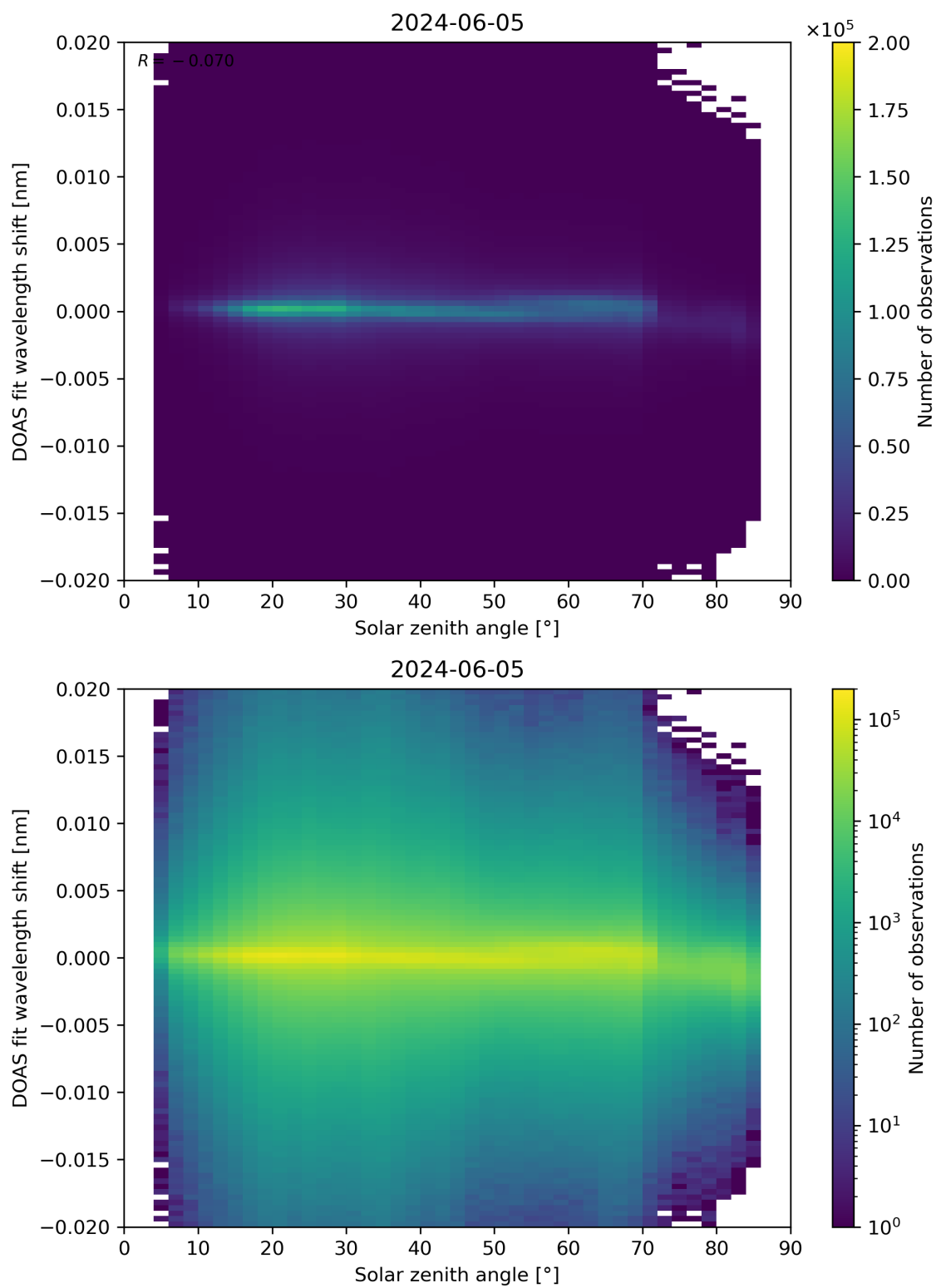
Figure 168: Scatter density plot of “Solar zenith angle” against “DOAS fit wavelength shift” for 2024-06-04 to 2024-06-06.
