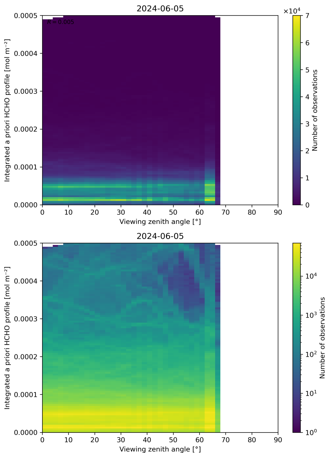
Figure 195: Scatter density plot of “Viewing zenith angle” against “Integrated a priori HCHO profile” for 2024-06-04 to 2024-06-06.
