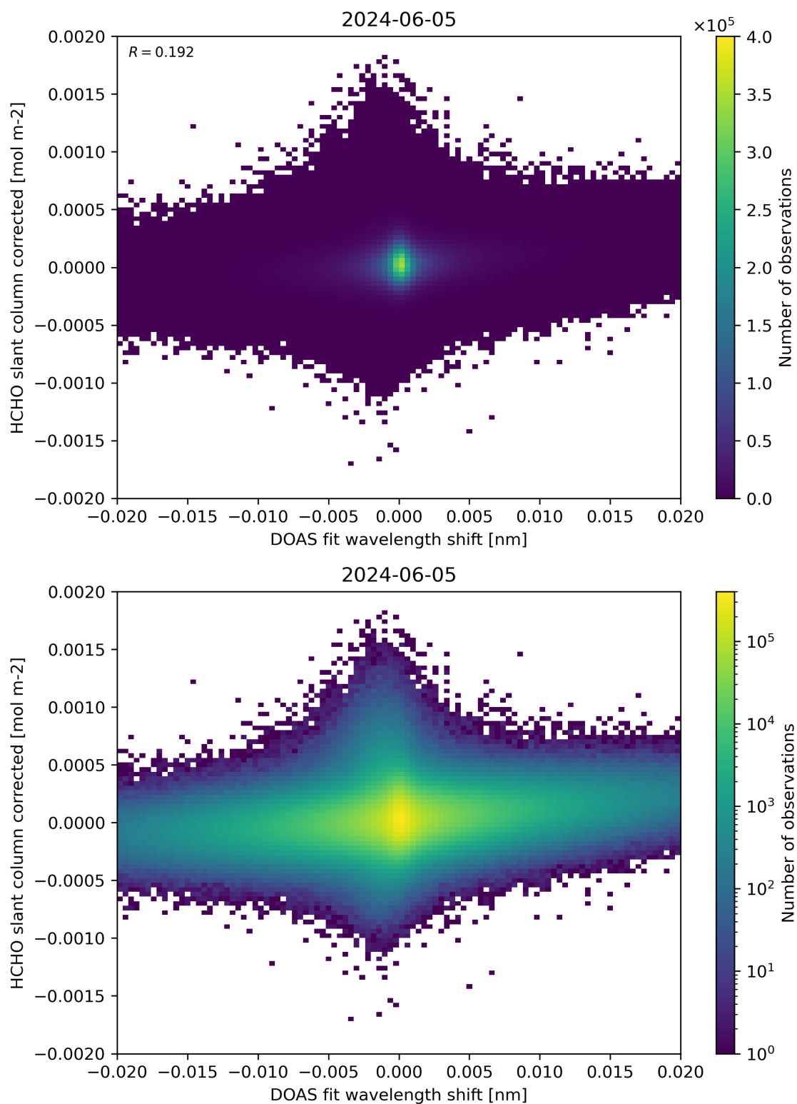
Figure 66: Scatter density plot of “DOAS fit wavelength shift” against “HCHO slant column corrected” for 2024-06-04 to 2024-06-06.
