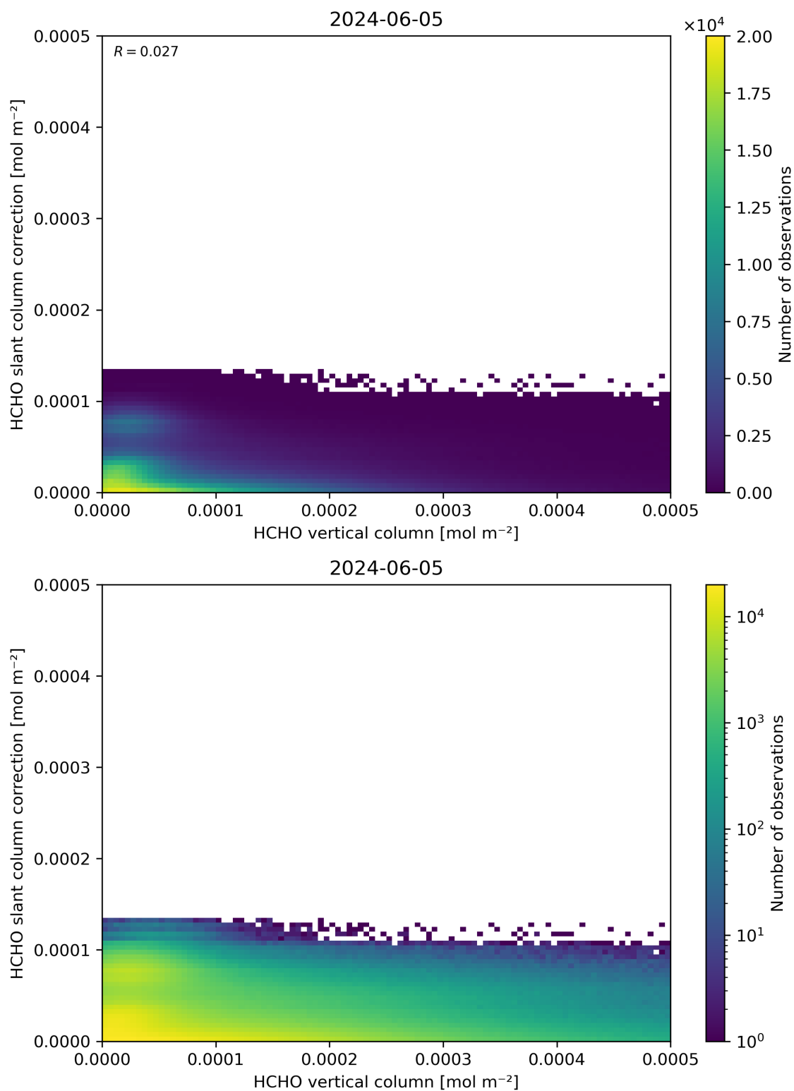
Figure 128: Scatter density plot of “HCHO vertical column” against “HCHO slant column correction” for 2024-06-04 to 2024-06-06.
