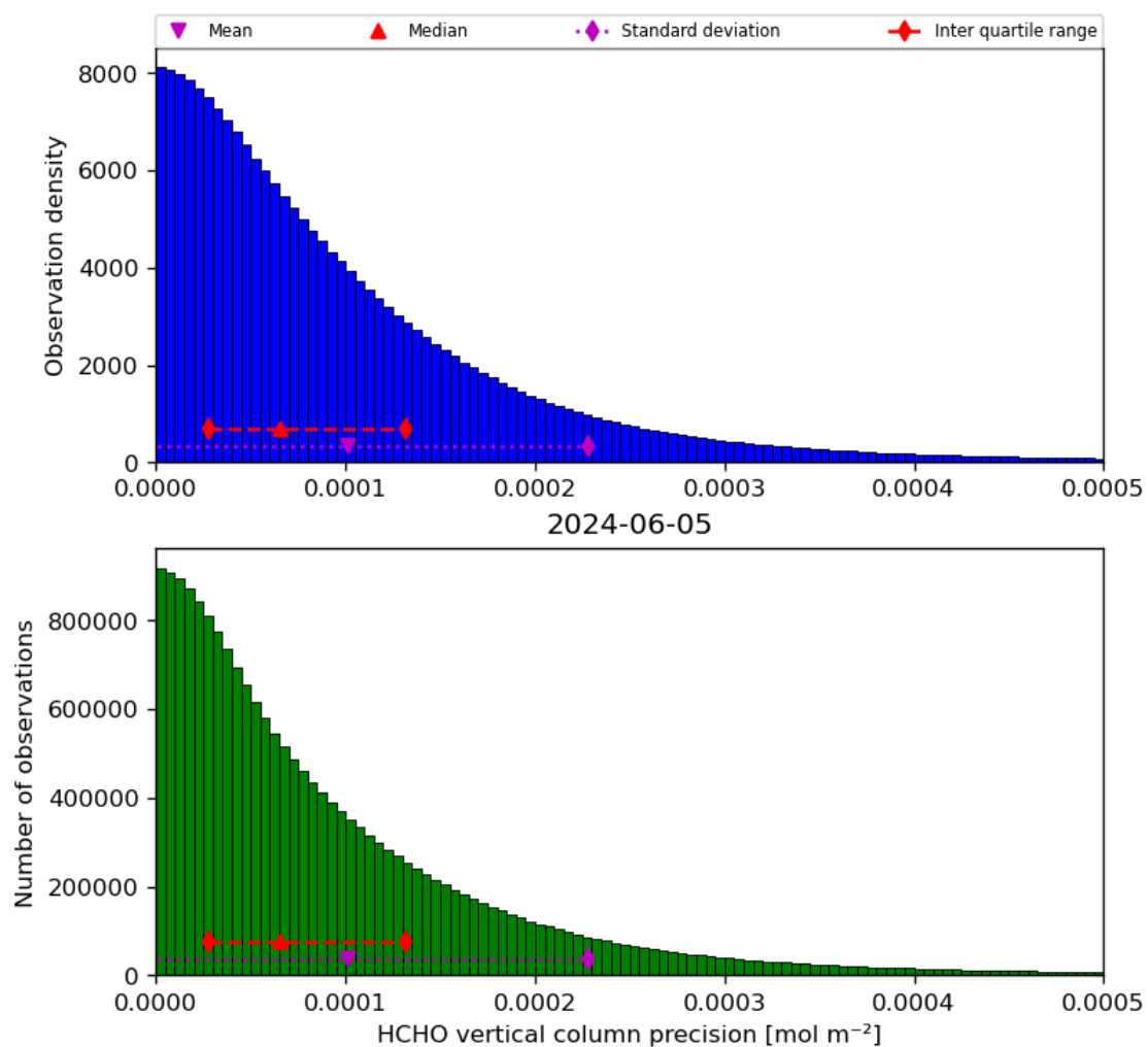
Figure 36: Histogram of “HCHO vertical column precision” for 2024-06-04 to 2024-06-06
