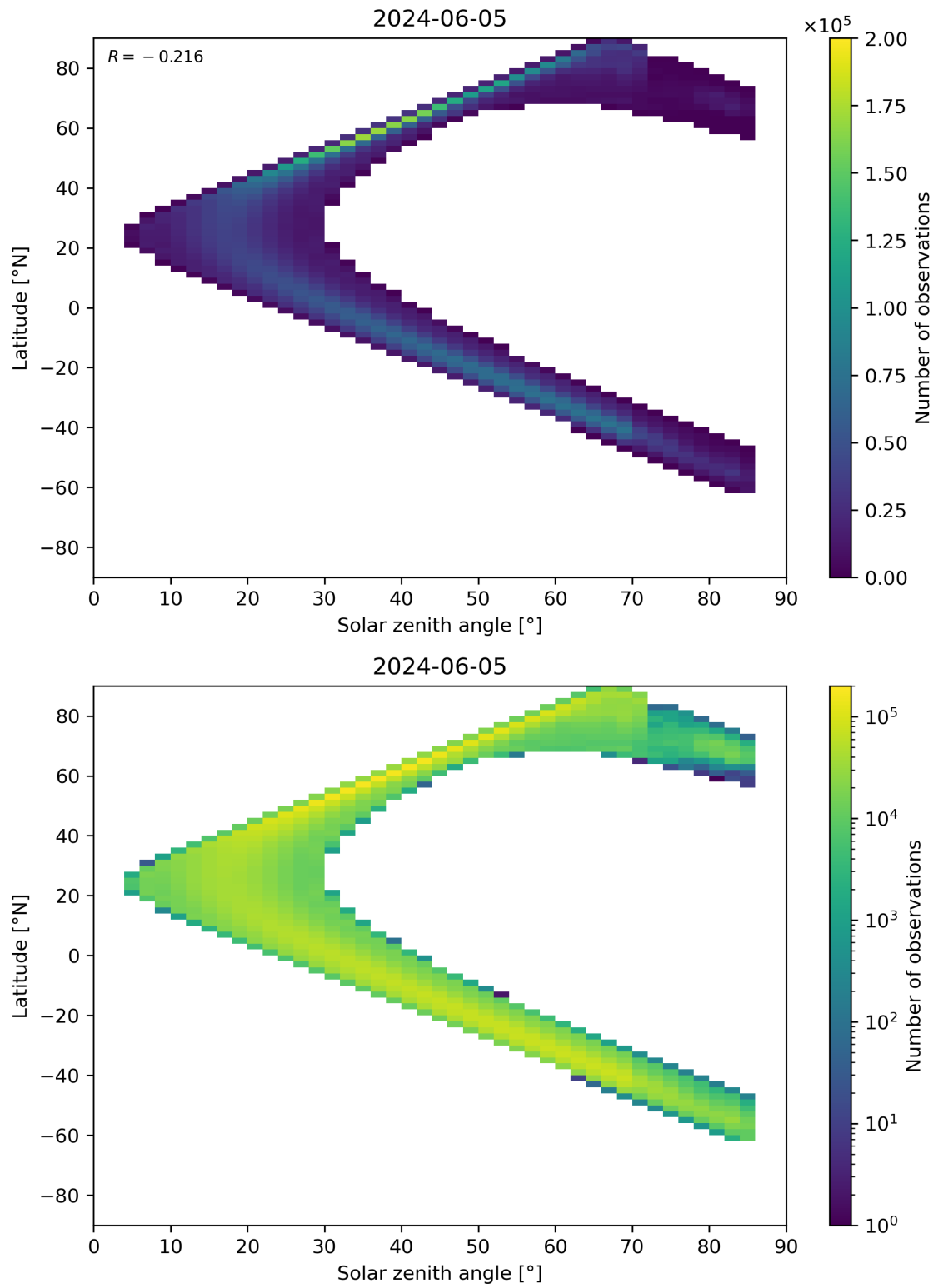
Figure 181: Scatter density plot of “Solar zenith angle” against “Latitude” for 2024-06-04 to 2024-06-06.
