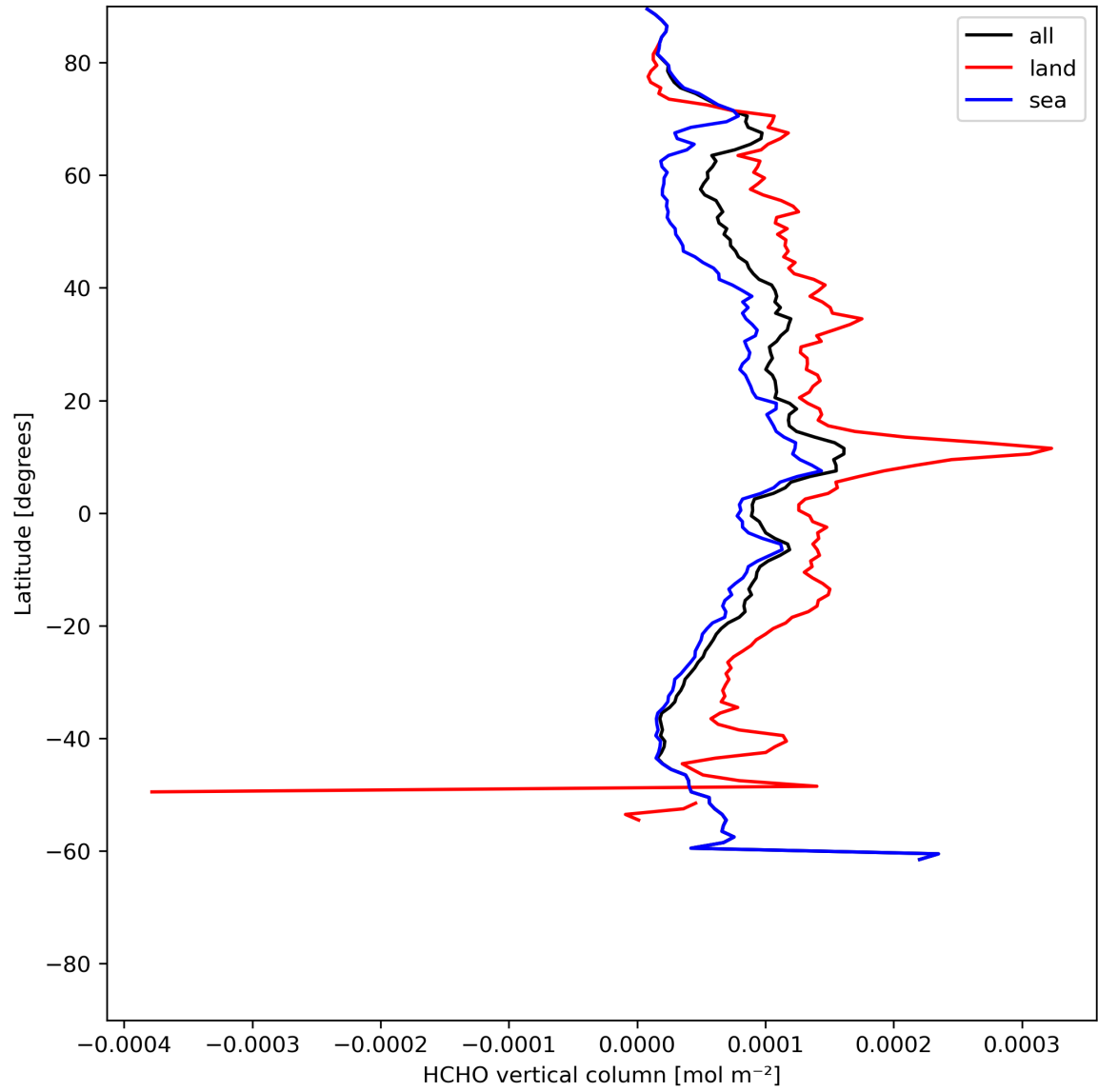
Figure 21: Zonal average of “HCHO vertical column” for 2024-06-04 to 2024-06-06.
