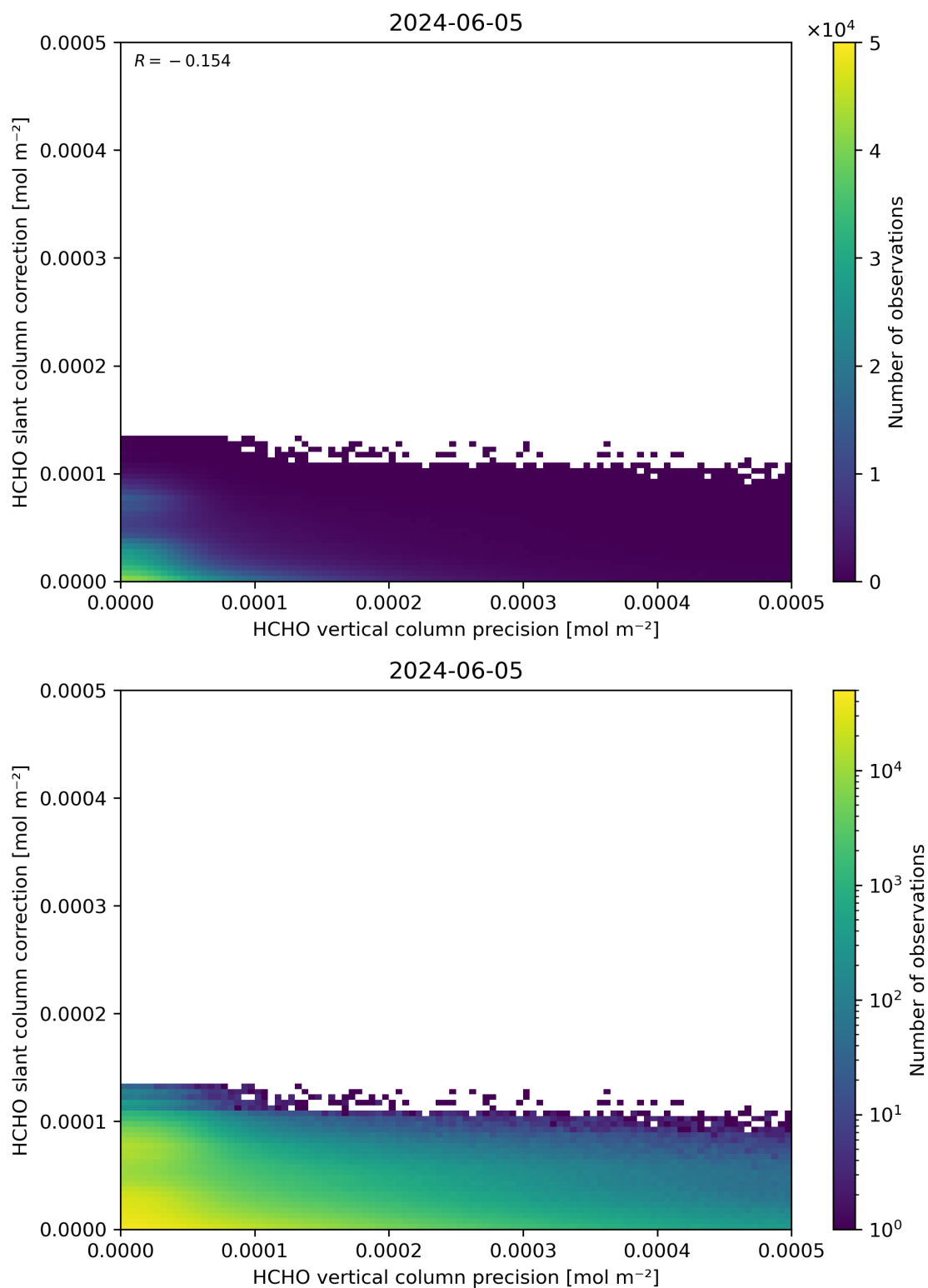
Figure 141: Scatter density plot of “HCHO vertical column precision” against “HCHO slant column correction” for 2024-06-04 to 2024-06-06.
