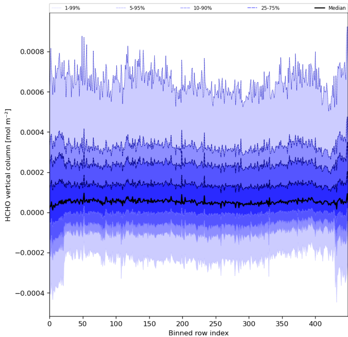
Figure 49: Along track statistics of “HCHO vertical column” for 2024-06-04 to 2024-06-06
