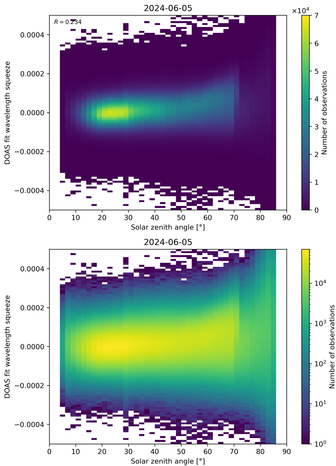
Figure 169: Scatter density plot of “Solar zenith angle” against “DOAS fit wavelength squeeze” for 2024-06-04 to 2024-06-06.
