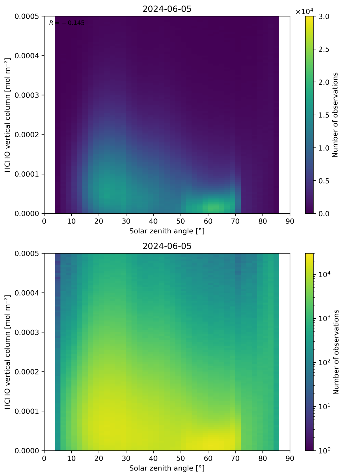
Figure 177: Scatter density plot of “Solar zenith angle” against “HCHO vertical column” for 2024-06-04 to 2024-06-06.
