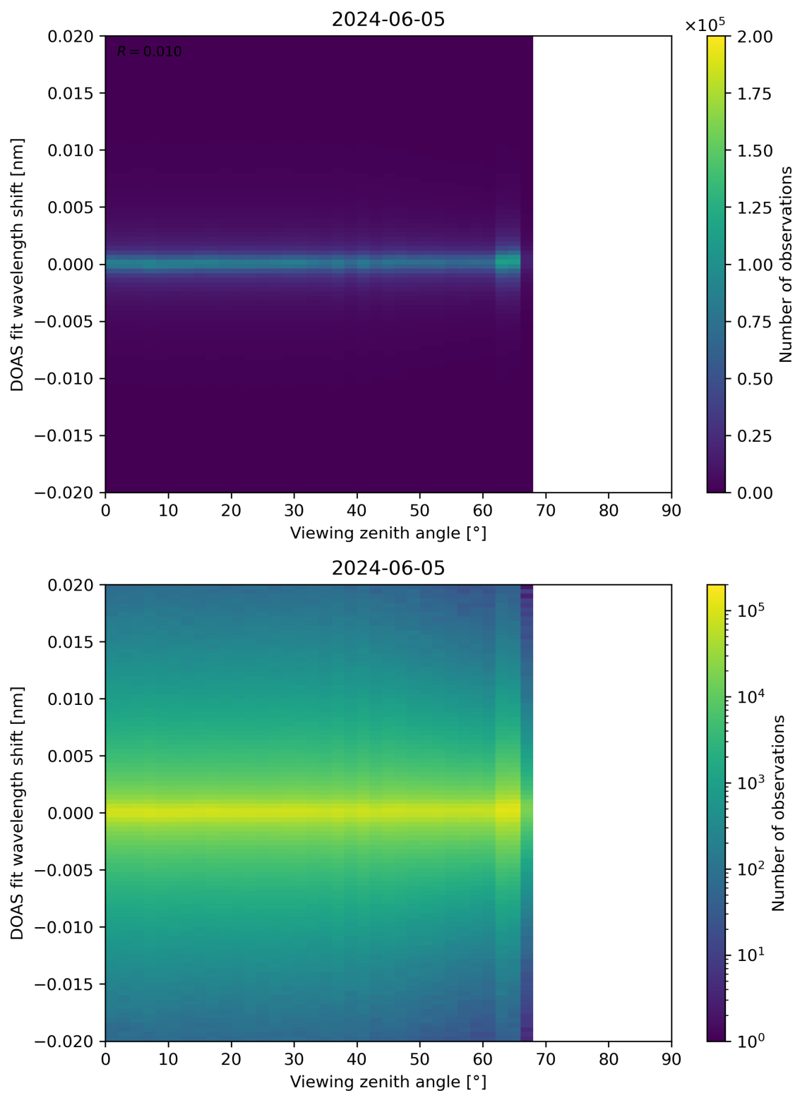
Figure 183: Scatter density plot of “Viewing zenith angle” against “DOAS fit wavelength shift” for 2024-06-04 to 2024-06-06.
