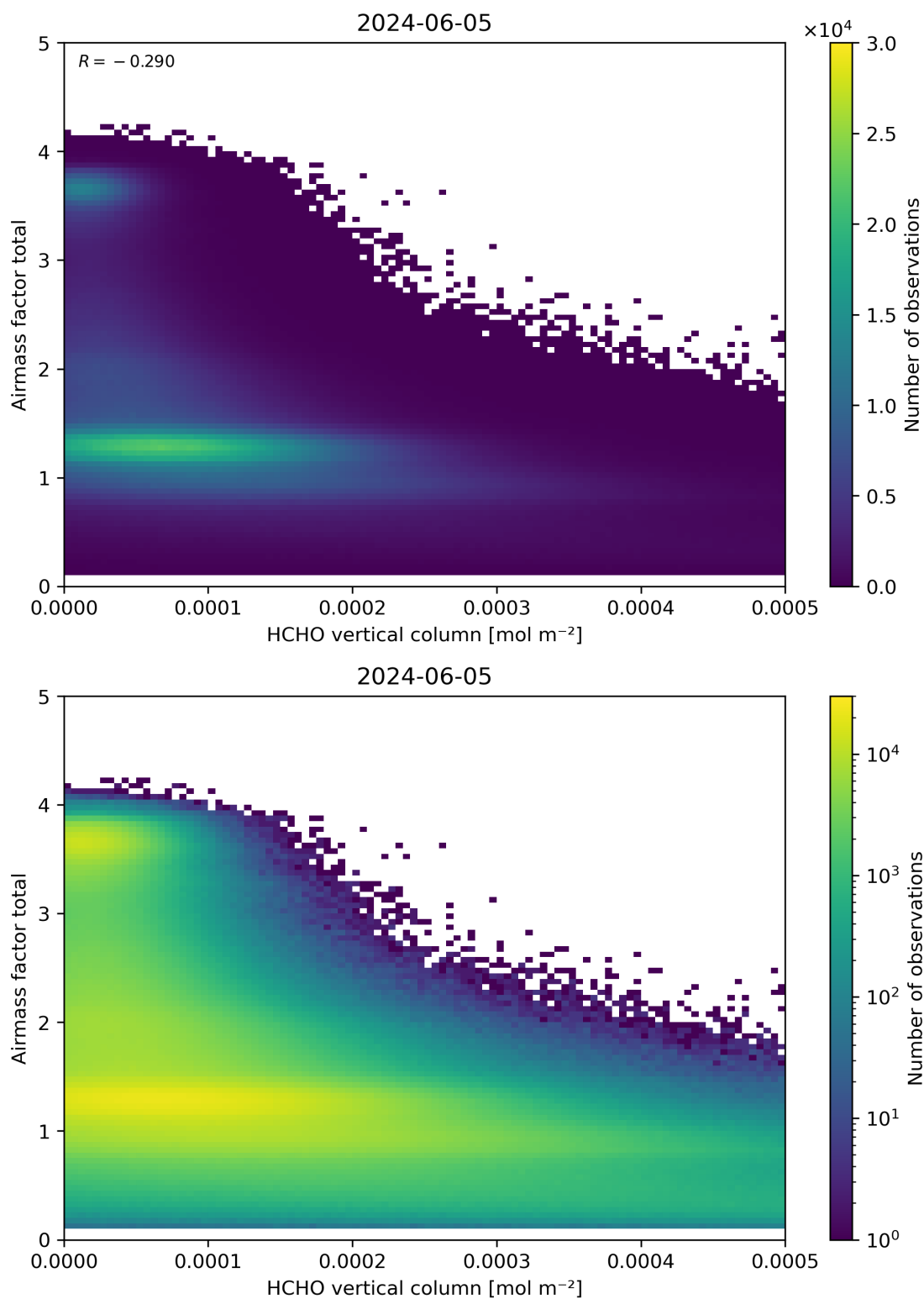
Figure 131: Scatter density plot of “HCHO vertical column” against “Airmass factor total” for 2024-06-04 to 2024-06-06.
