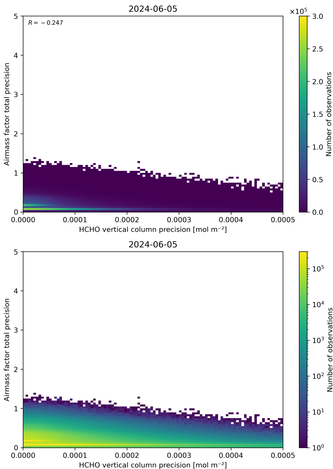
Figure 145: Scatter density plot of “HCHO vertical column precision” against “Airmass factor total precision” for 2024-06-04 to 2024-06-06.
