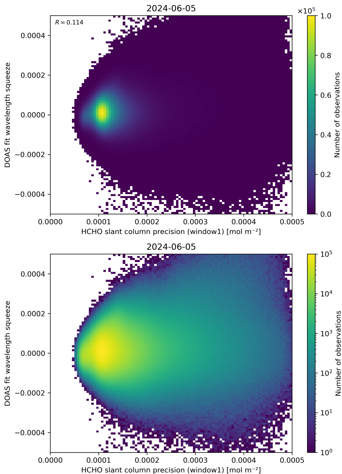
Figure 90: Scatter density plot of “HCHO slant column precision (window1)” against “DOAS fit wavelength squeeze” for 2024-06-04 to 2024-06-06.
