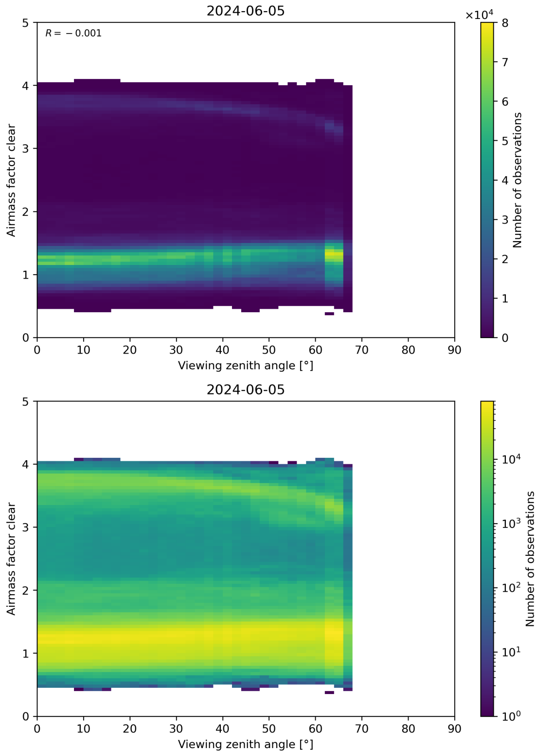
Figure 185: Scatter density plot of “Viewing zenith angle” against “Airmass factor clear” for 2024-06-04 to 2024-06-06.
