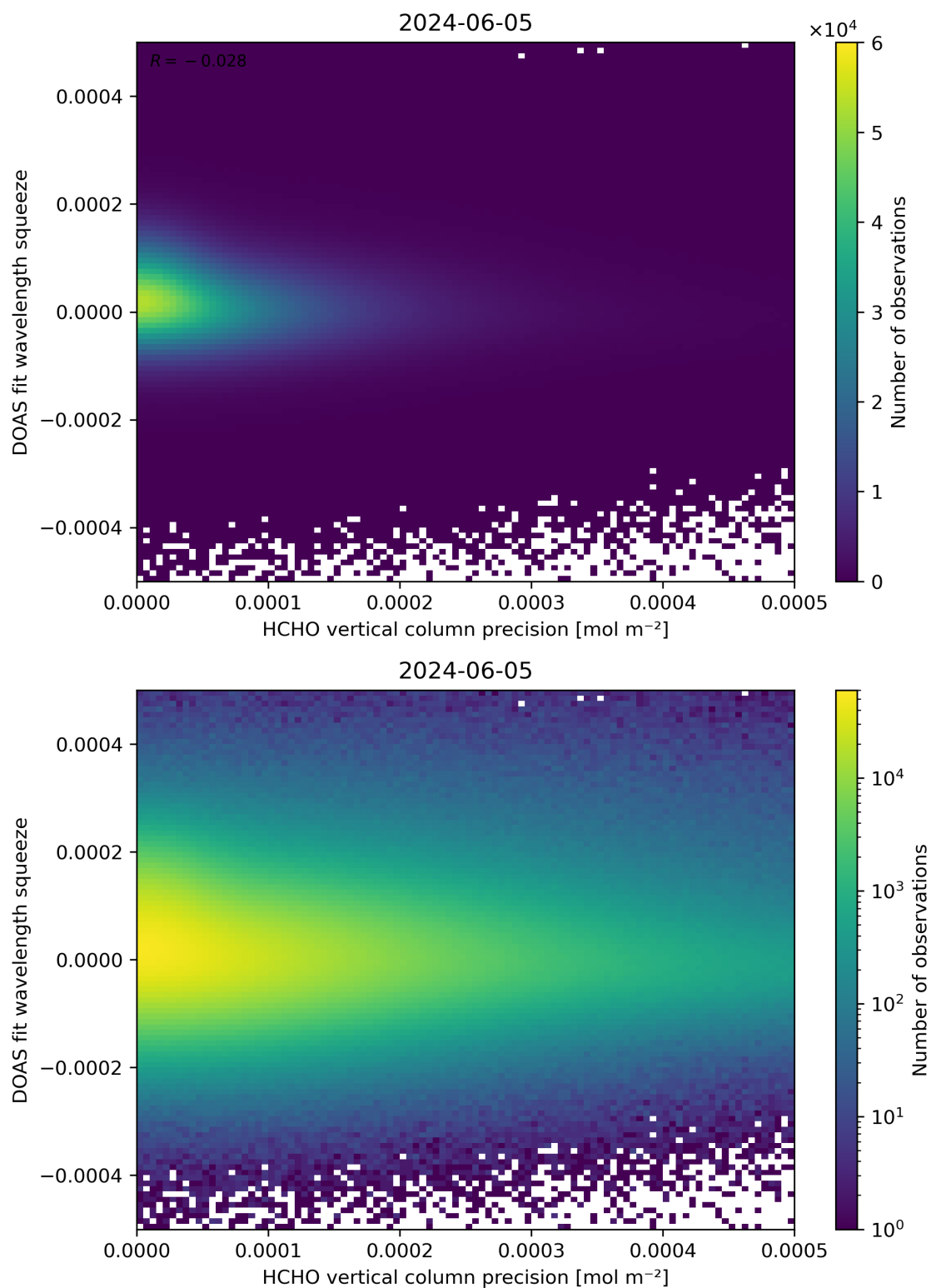
Figure 138: Scatter density plot of “HCHO vertical column precision” against “DOAS fit wavelength squeeze” for 2024-06-04 to 2024-06-06.
