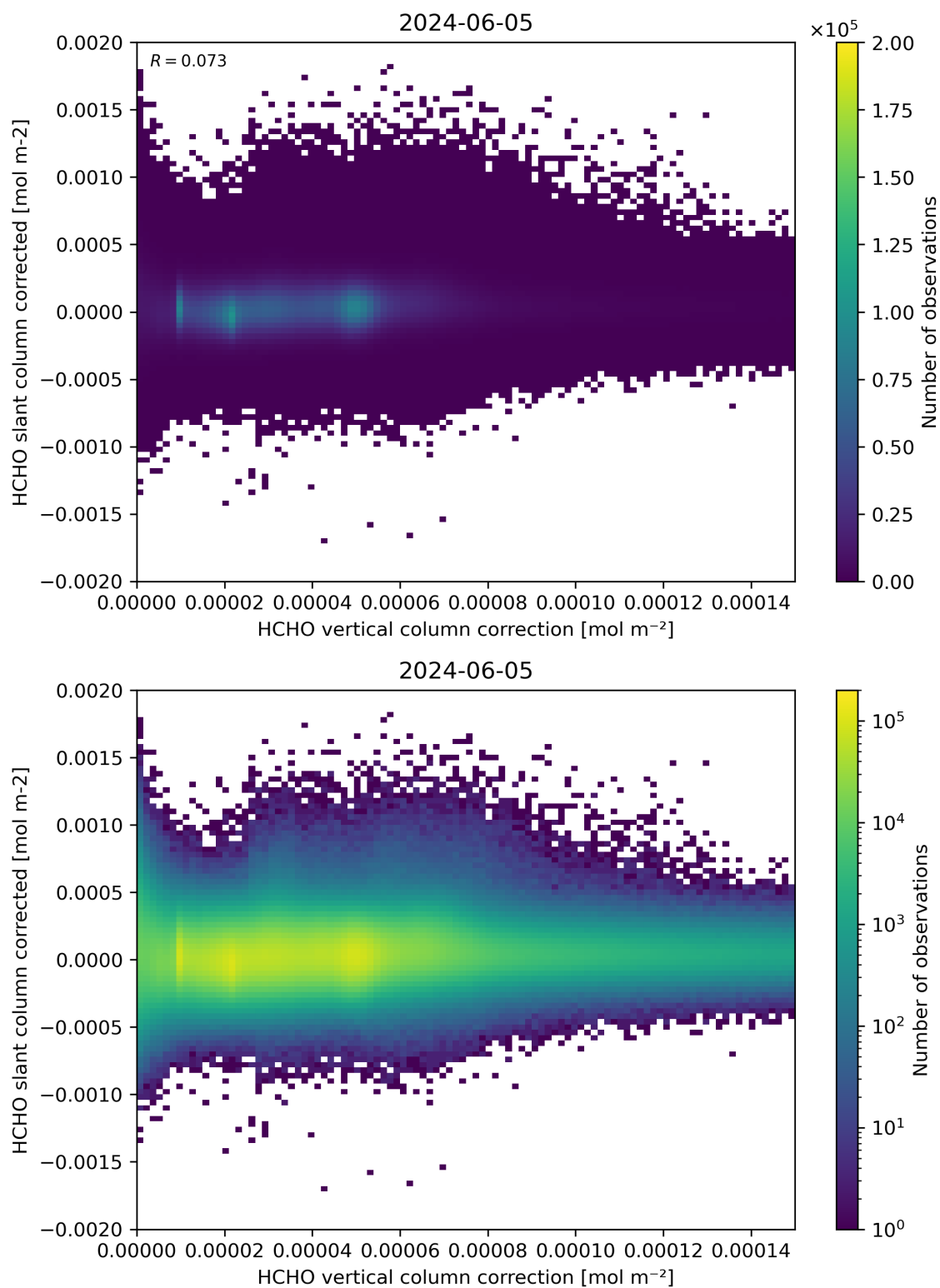
Figure 116: Scatter density plot of “HCHO vertical column correction” against “HCHO slant column corrected” for 2024-06-04 to 2024-06-06.
