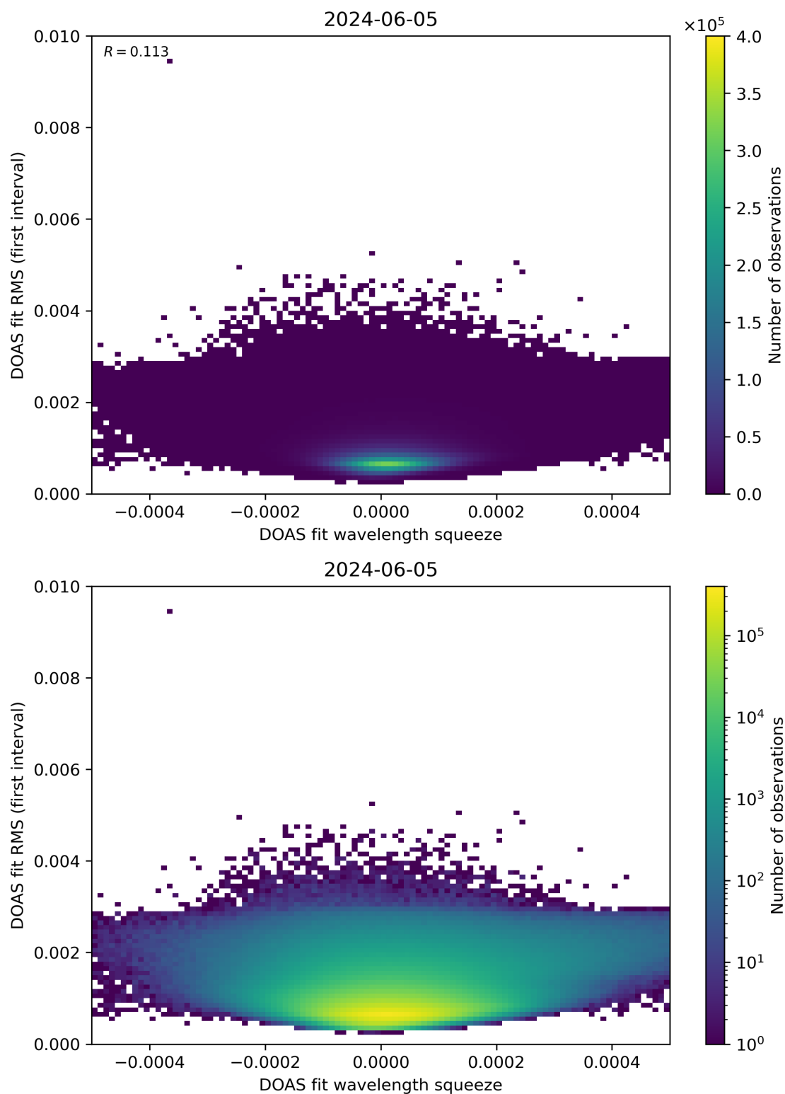
Figure 68: Scatter density plot of “DOAS fit wavelength squeeze” against “DOAS fit RMS (first interval)” for 2024-06-04 to 2024-06-06.
