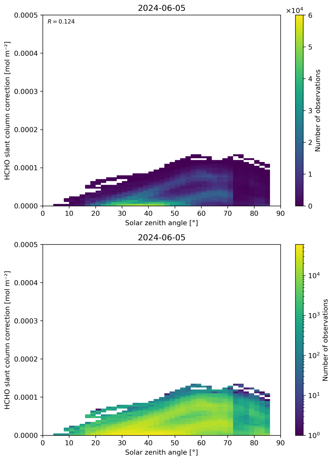
Figure 172: Scatter density plot of “Solar zenith angle” against “HCHO slant column correction” for 2024-06-04 to 2024-06-06.
