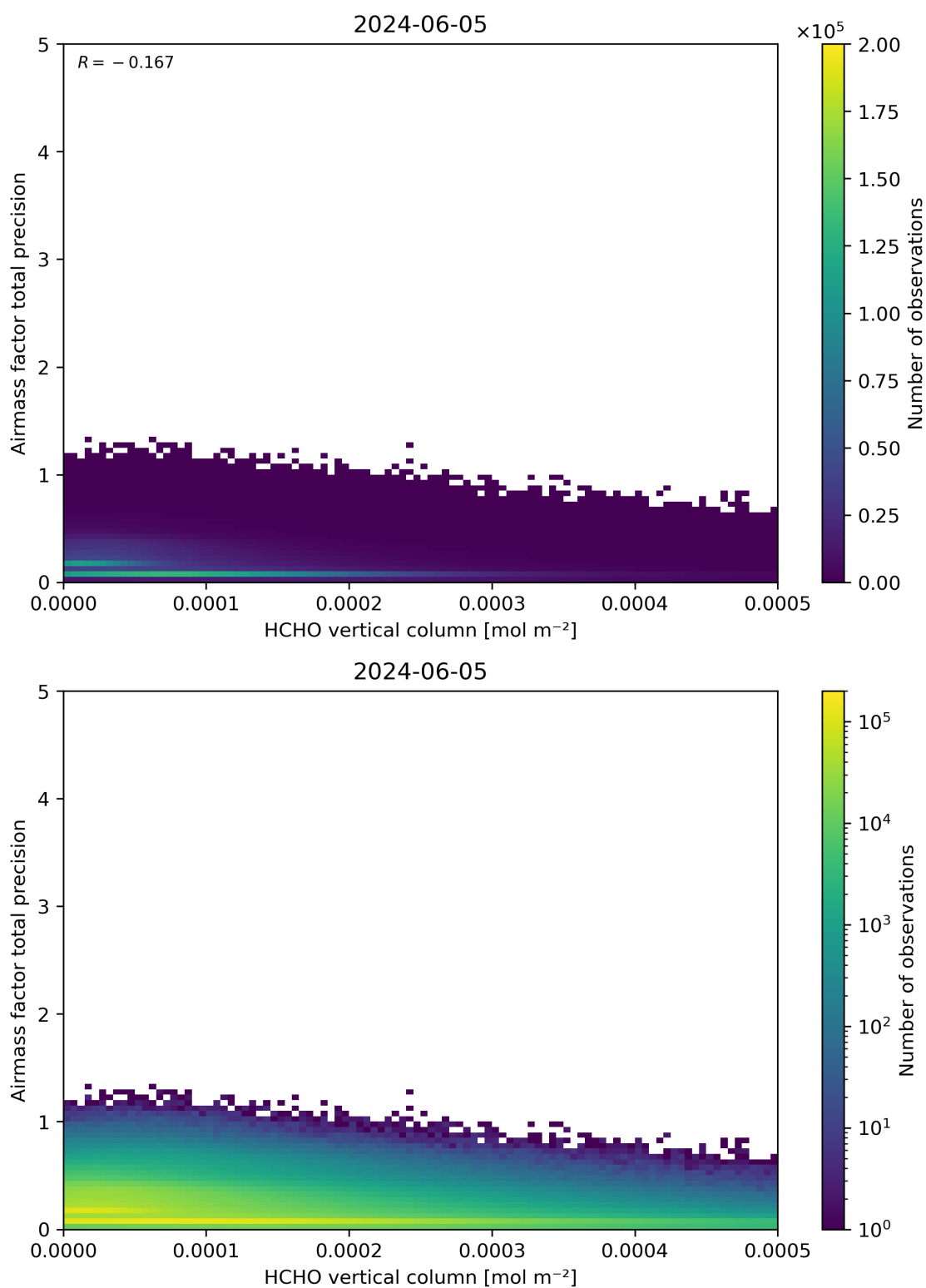
Figure 132: Scatter density plot of “HCHO vertical column” against “Airmass factor total precision” for 2024-06-04 to 2024-06-06.
