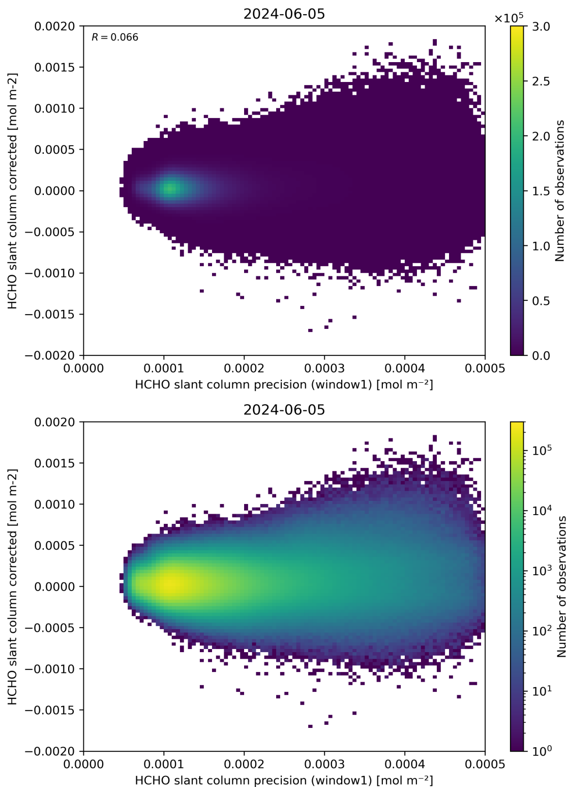
Figure 92: Scatter density plot of “HCHO slant column precision (window1)” against “HCHO slant column corrected” for 2024-06-04 to 2024-06-06.
