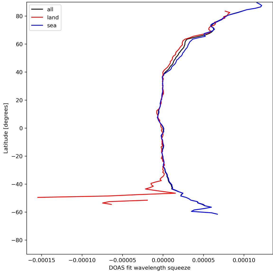
Figure 31: Zonal average of “DOAS fit wavelength squeeze” for 2024-06-04 to 2024-06-06.
