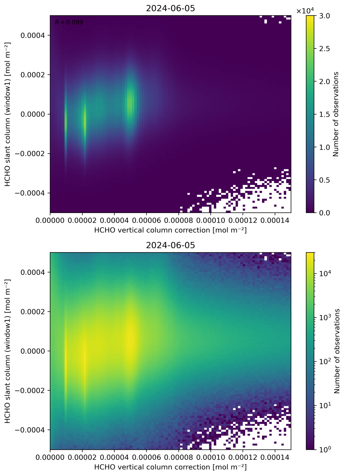
Figure 118: Scatter density plot of “HCHO vertical column correction” against “HCHO slant column (window1)” for 2024-06-04 to 2024-06-06.
