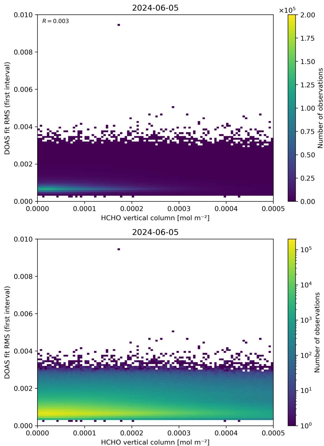
Figure 123: Scatter density plot of “HCHO vertical column” against “DOAS fit RMS (first interval)” for 2024-06-04 to 2024-06-06.
