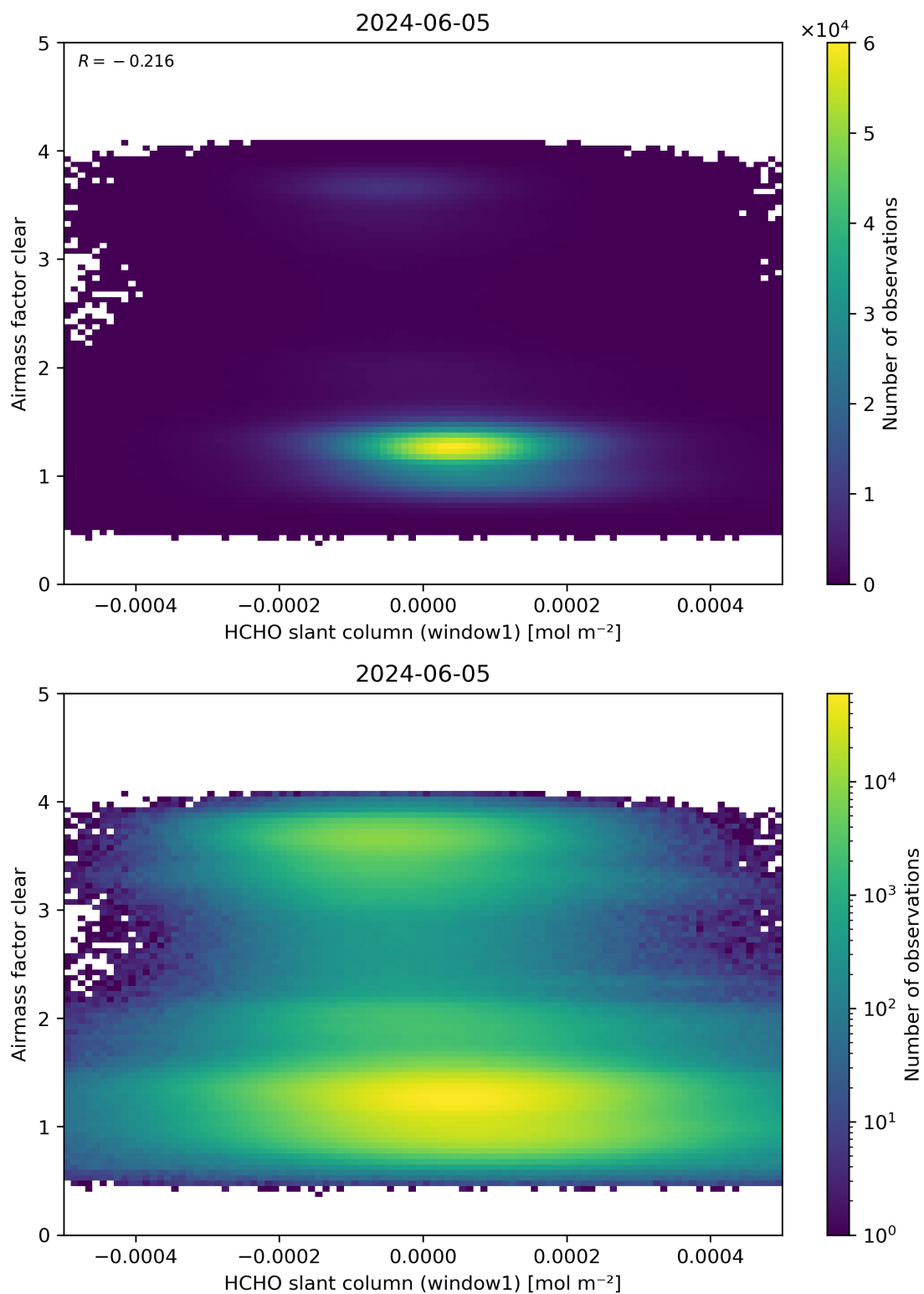
Figure 81: Scatter density plot of “HCHO slant column (window1)” against “Airmass factor clear” for 2024-06-04 to 2024-06-06.
