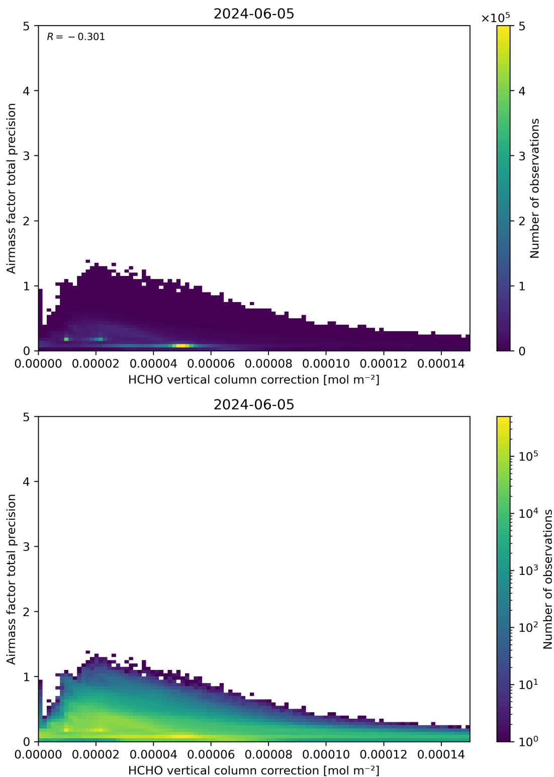
Figure 121: Scatter density plot of “HCHO vertical column correction” against “Airmass factor total precision” for 2024-06-04 to 2024-06-06.
