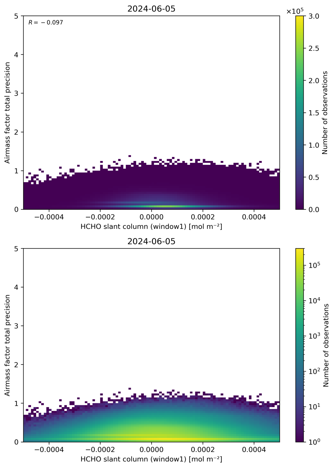
Figure 86: Scatter density plot of “HCHO slant column (window1)” against “Airmass factor total precision” for 2024-06-04 to 2024-06-06.
