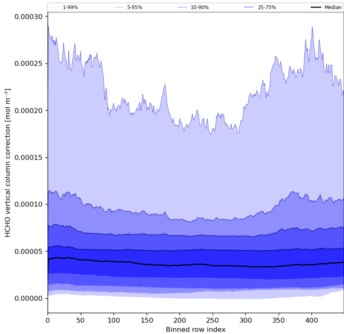
Figure 51: Along track statistics of “HCHO vertical column correction” for 2024-06-04 to 2024-06-06
