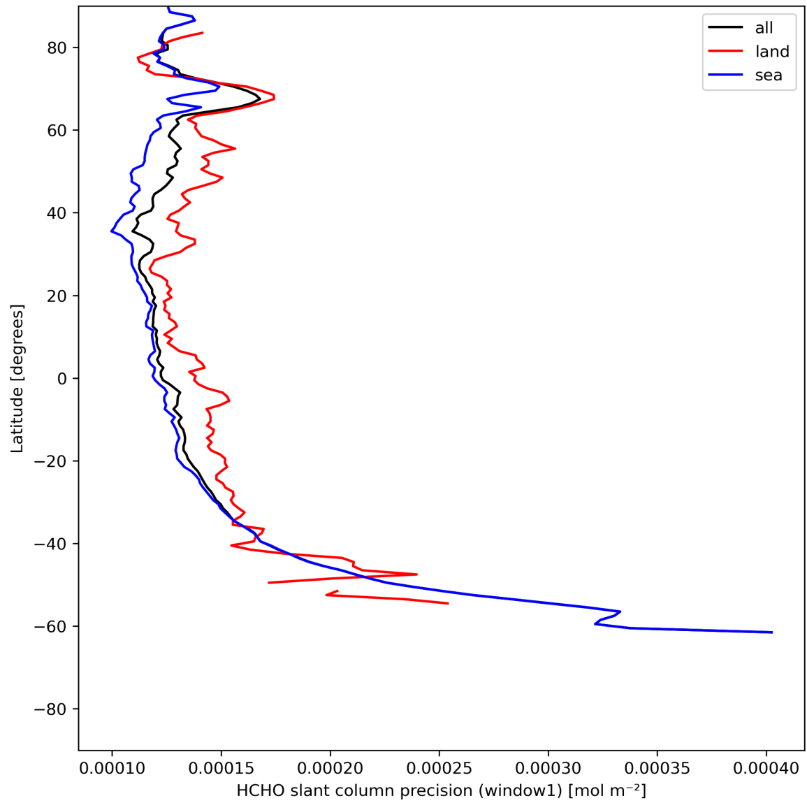
Figure 25: Zonal average of “HCHO slant column precision (window1)” for 2024-06-04 to 2024-06-06.
