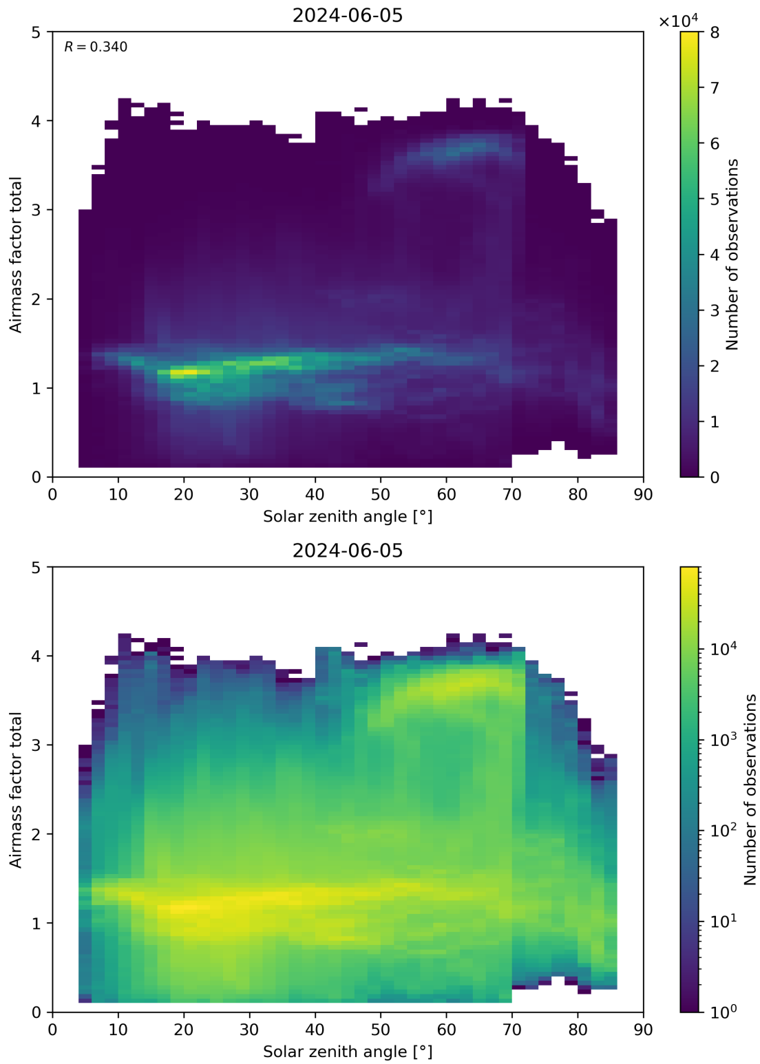
Figure 175: Scatter density plot of “Solar zenith angle” against “Airmass factor total” for 2024-06-04 to 2024-06-06.
