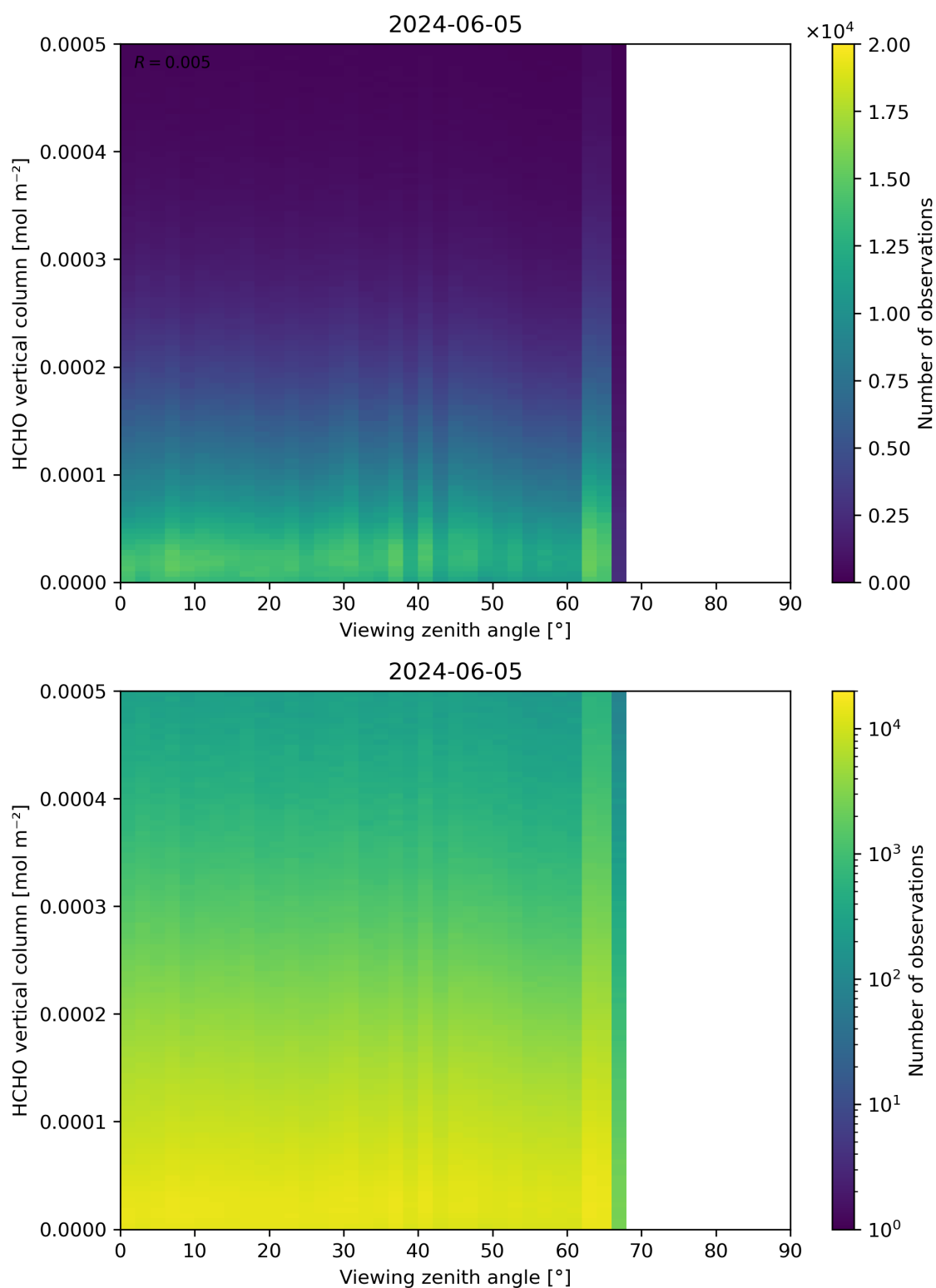
Figure 192: Scatter density plot of “Viewing zenith angle” against “HCHO vertical column” for 2024-06-04 to 2024-06-06.
