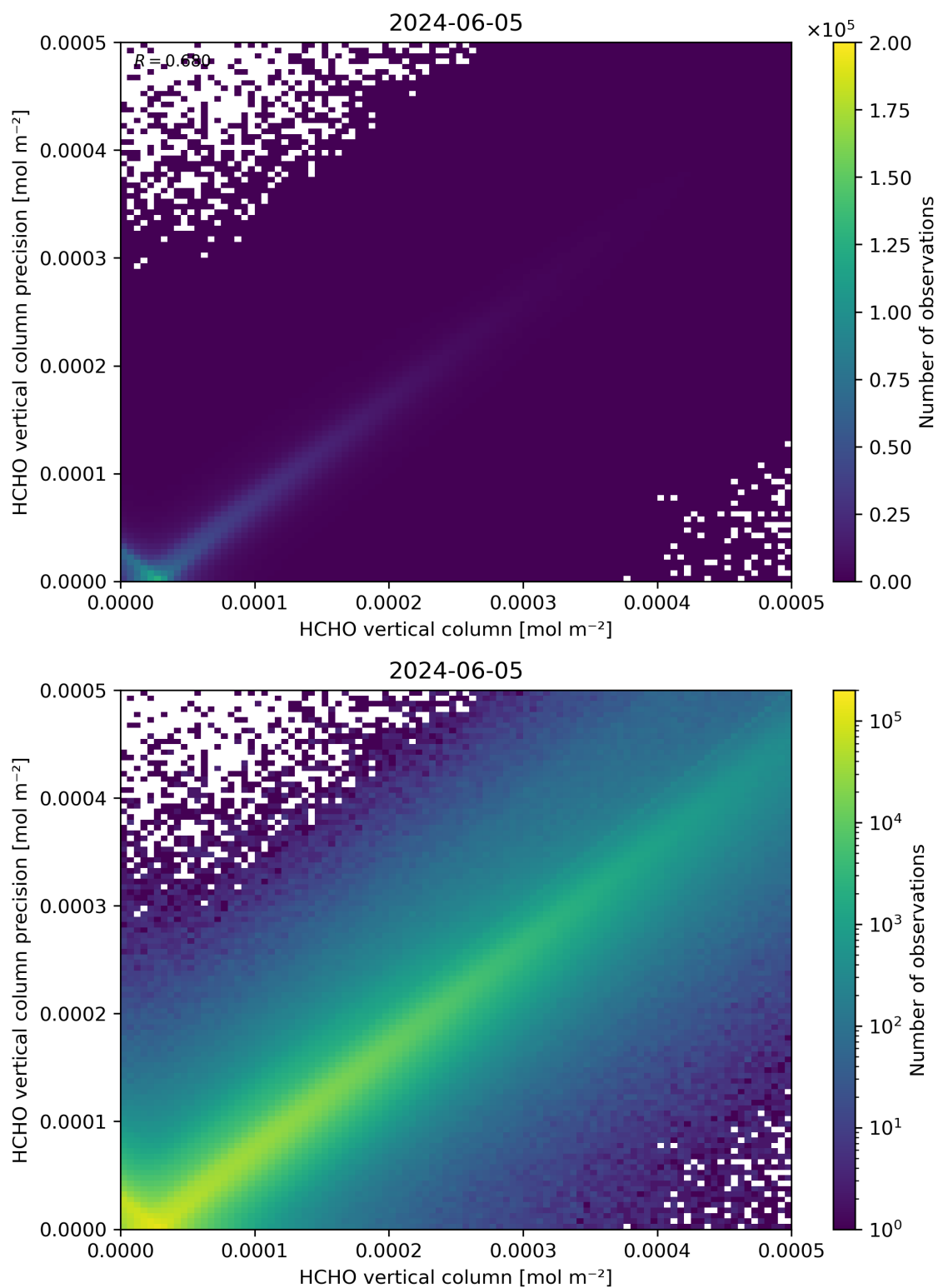
Figure 134: Scatter density plot of “HCHO vertical column” against “HCHO vertical column precision” for 2024-06-04 to 2024-06-06.
