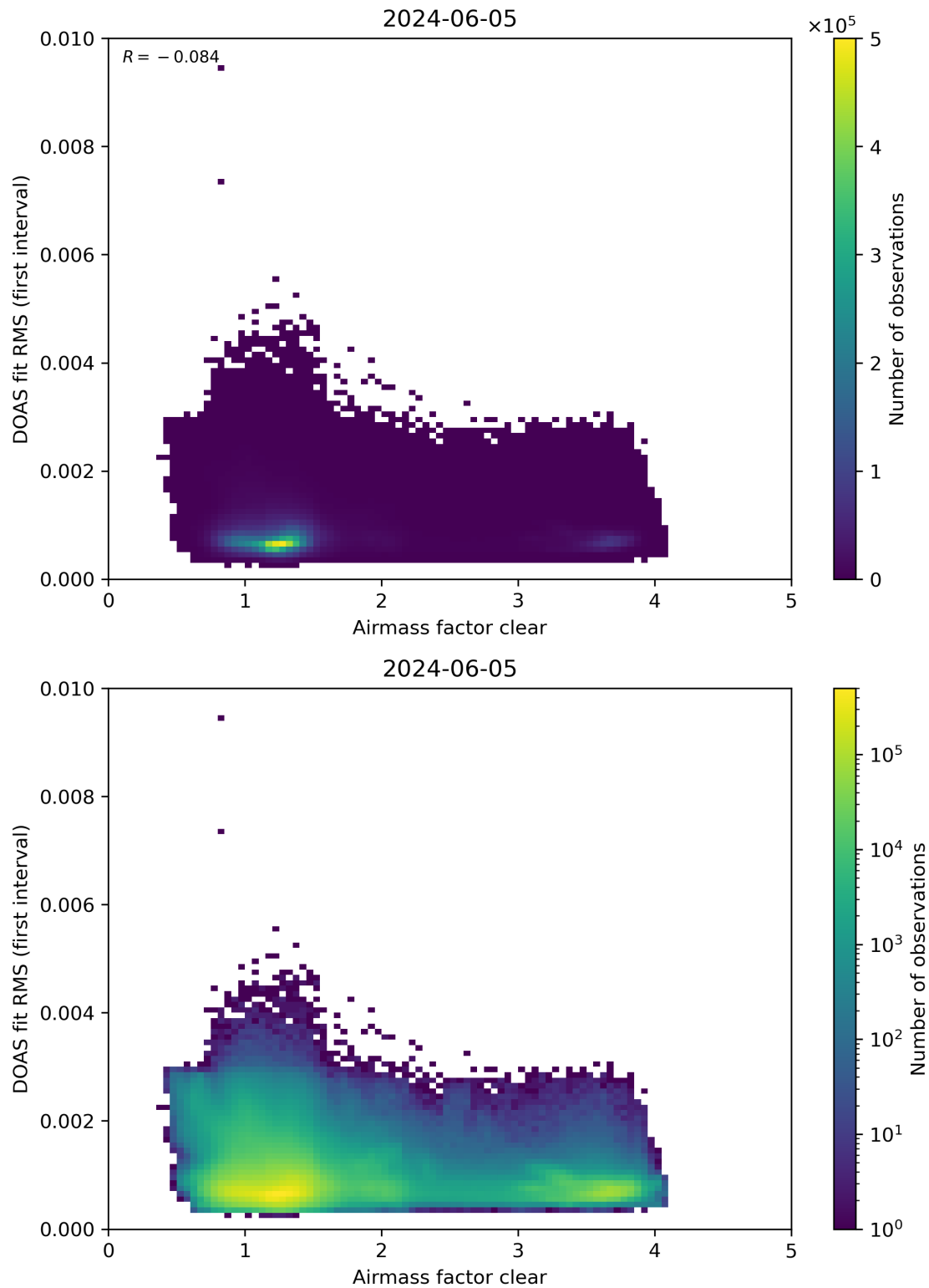
Figure 71: Scatter density plot of “Airmass factor clear” against “DOAS fit RMS (first interval)” for 2024-06-04 to 2024-06-06.
