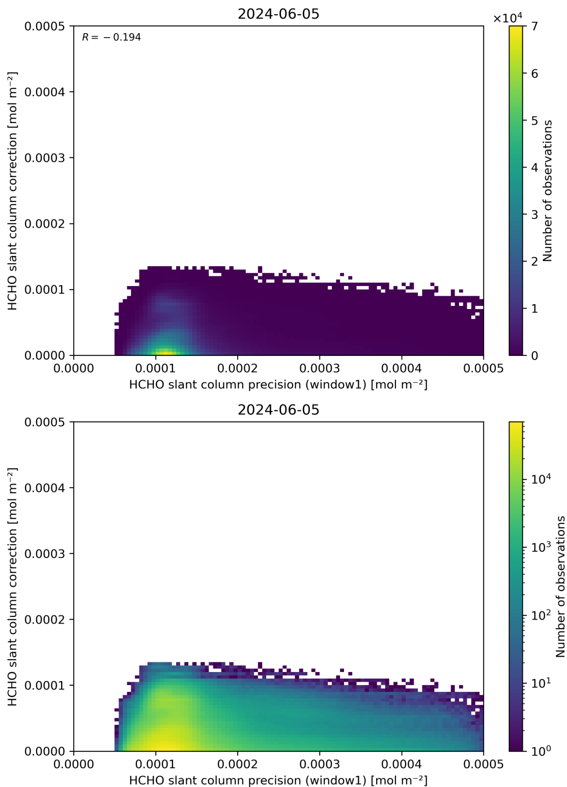
Figure 93: Scatter density plot of “HCHO slant column precision (window1)” against “HCHO slant column correction” for 2024-06-04 to 2024-06-06.
