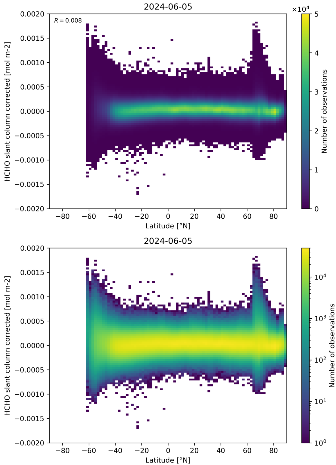
Figure 157: Scatter density plot of “Latitude” against “HCHO slant column corrected” for 2024-06-04 to 2024-06-06.
