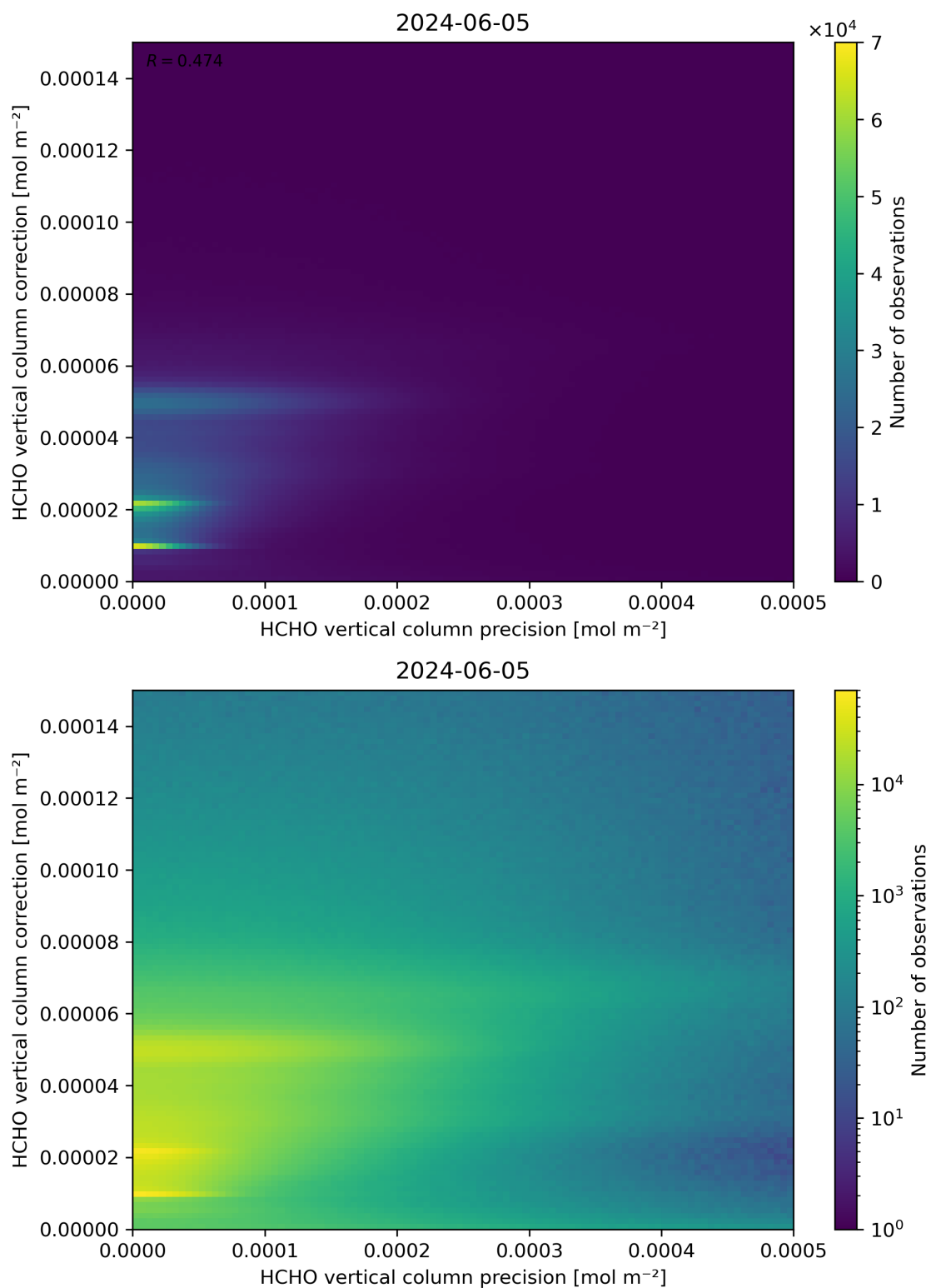
Figure 146: Scatter density plot of “HCHO vertical column precision” against “HCHO vertical column correction” for 2024-06-04 to 2024-06-06.
