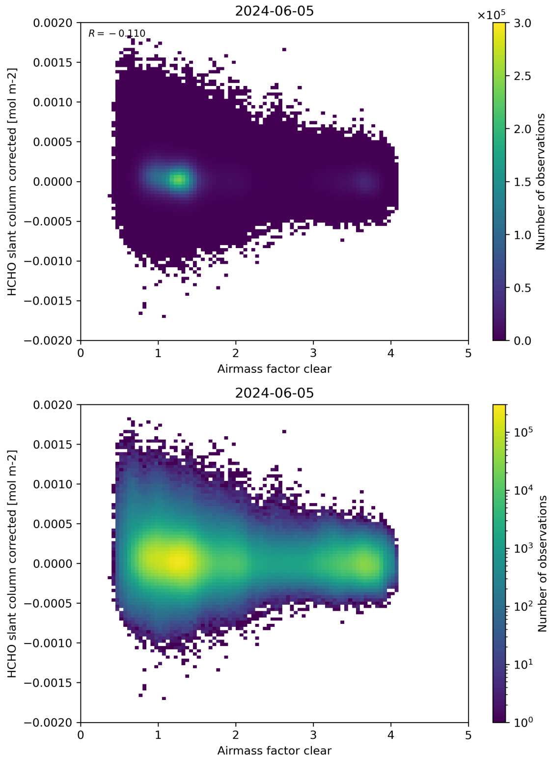
Figure 74: Scatter density plot of “Airmass factor clear” against “HCHO slant column corrected” for 2024-06-04 to 2024-06-06.
