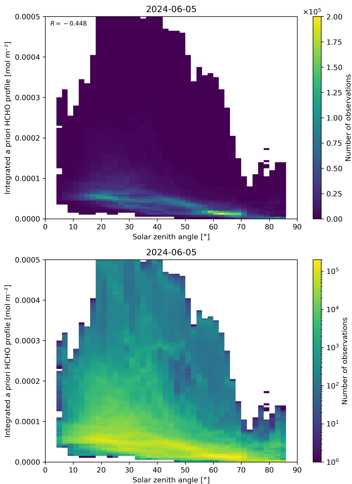
Figure 180: Scatter density plot of “Solar zenith angle” against “Integrated a priori HCHO profile” for 2024-06-04 to 2024-06-06.
