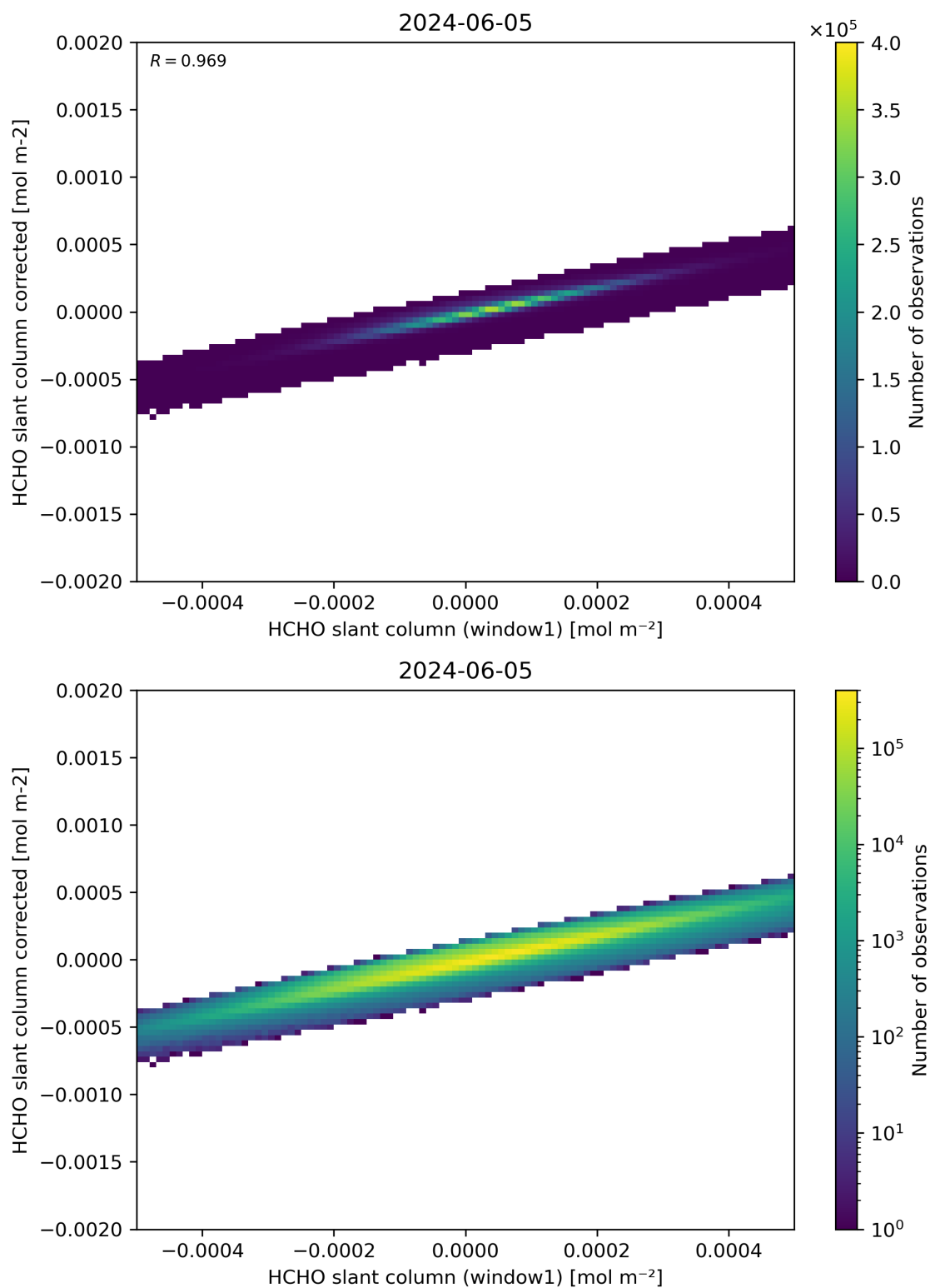
Figure 82: Scatter density plot of “HCHO slant column (window1)” against “HCHO slant column corrected” for 2024-06-04 to 2024-06-06.
