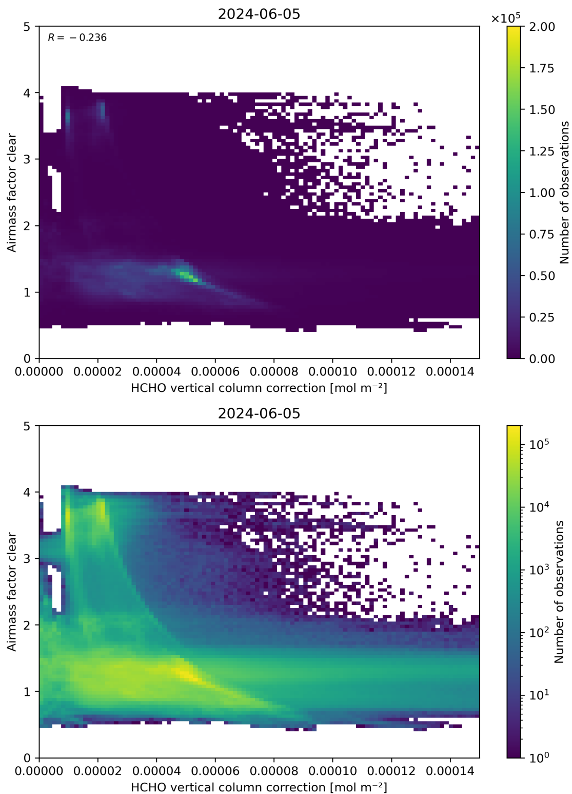
Figure 115: Scatter density plot of “HCHO vertical column correction” against “Airmass factor clear” for 2024-06-04 to 2024-06-06.
