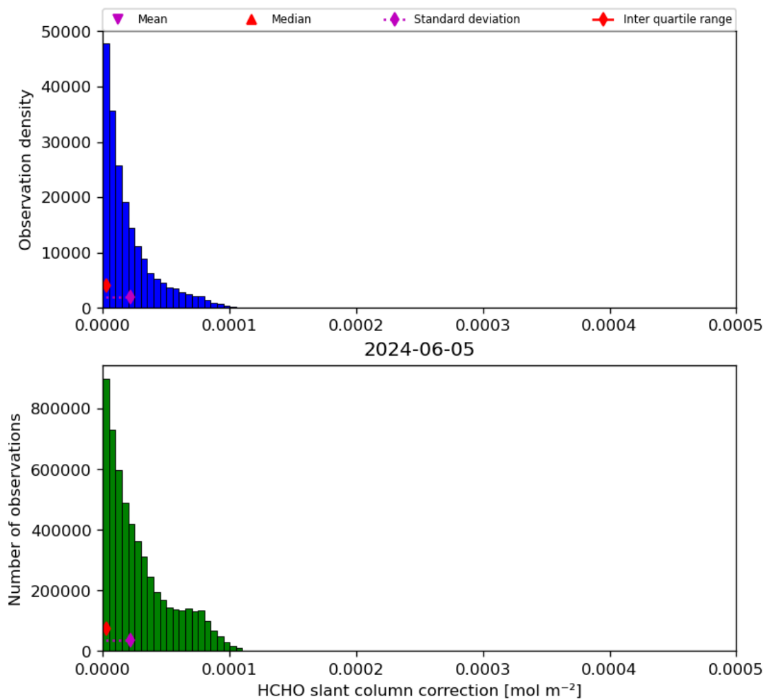
Figure 47: Histogram of “HCHO slant column correction” for 2024-06-04 to 2024-06-06
