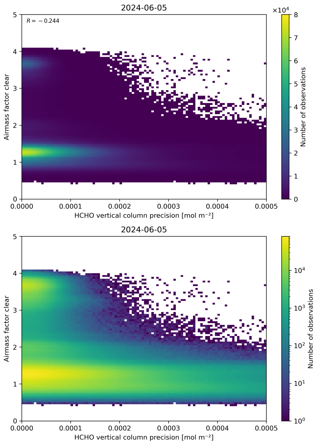
Figure 139: Scatter density plot of “HCHO vertical column precision” against “Airmass factor clear” for 2024-06-04 to 2024-06-06.
