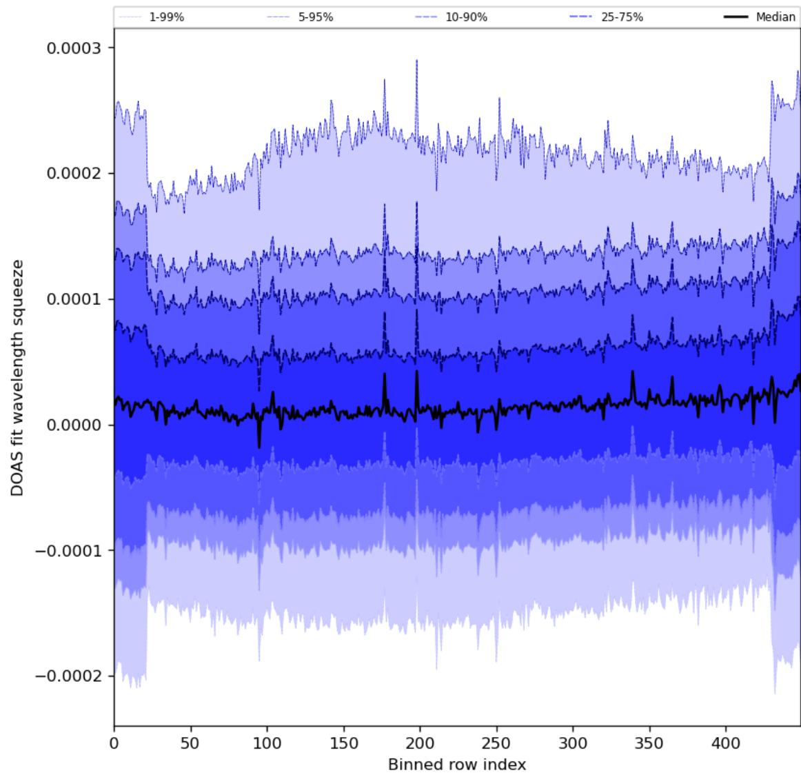
Figure 59: Along track statistics of “DOAS fit wavelength squeeze” for 2024-06-04 to 2024-06-06
