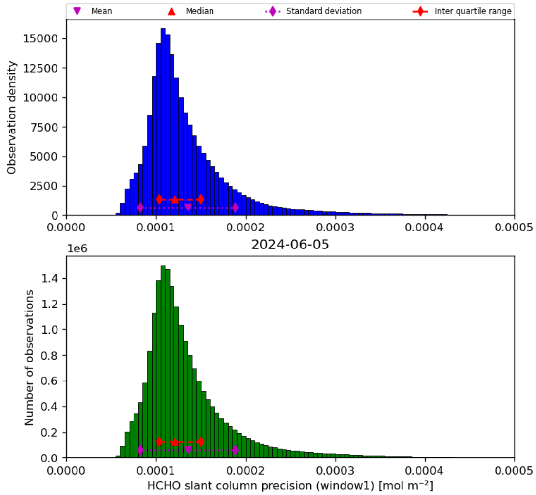
Figure 39: Histogram of “HCHO slant column precision (window1)” for 2024-06-04 to 2024-06-06
