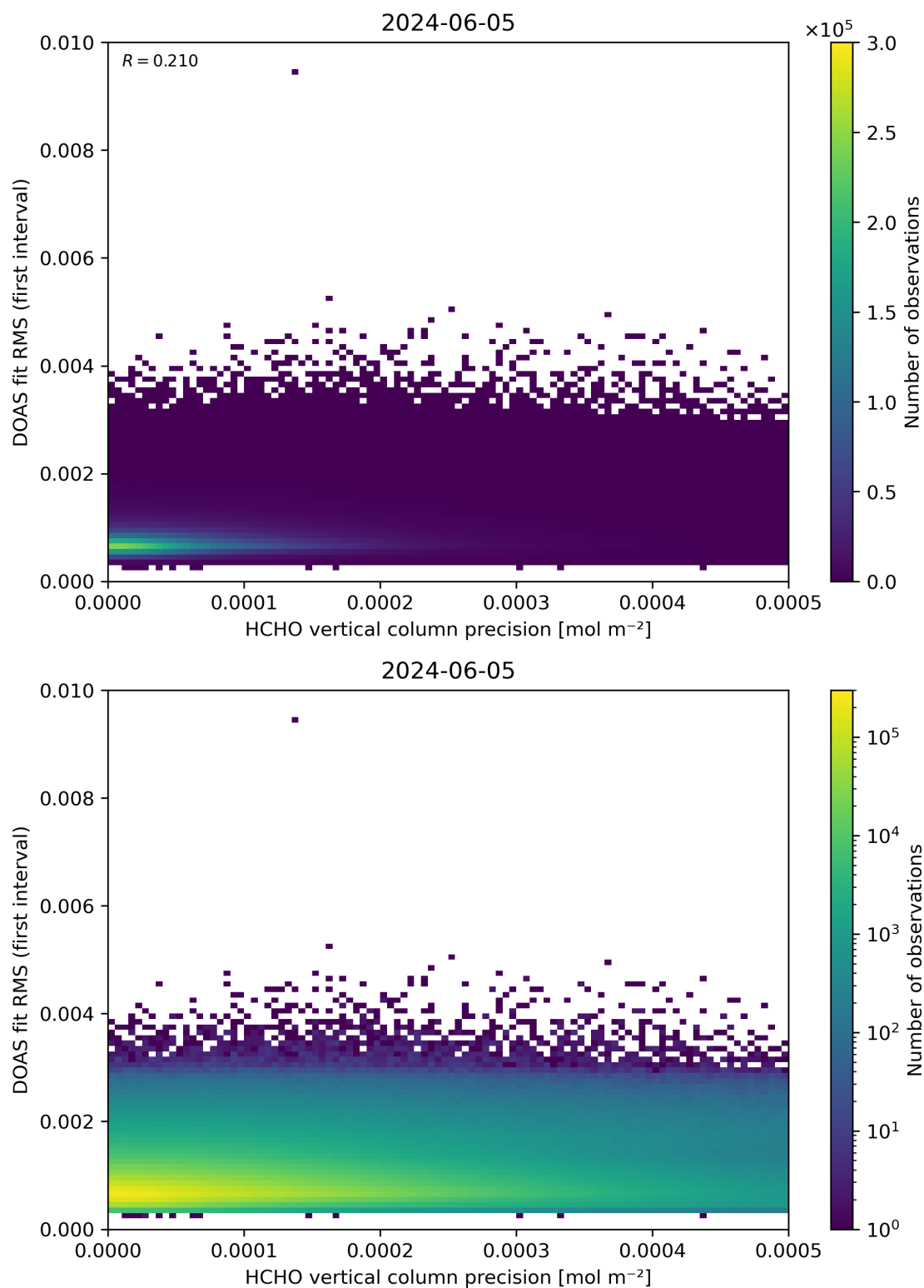
Figure 136: Scatter density plot of “HCHO vertical column precision” against “DOAS fit RMS (first interval)” for 2024-06-04 to 2024-06-06.
