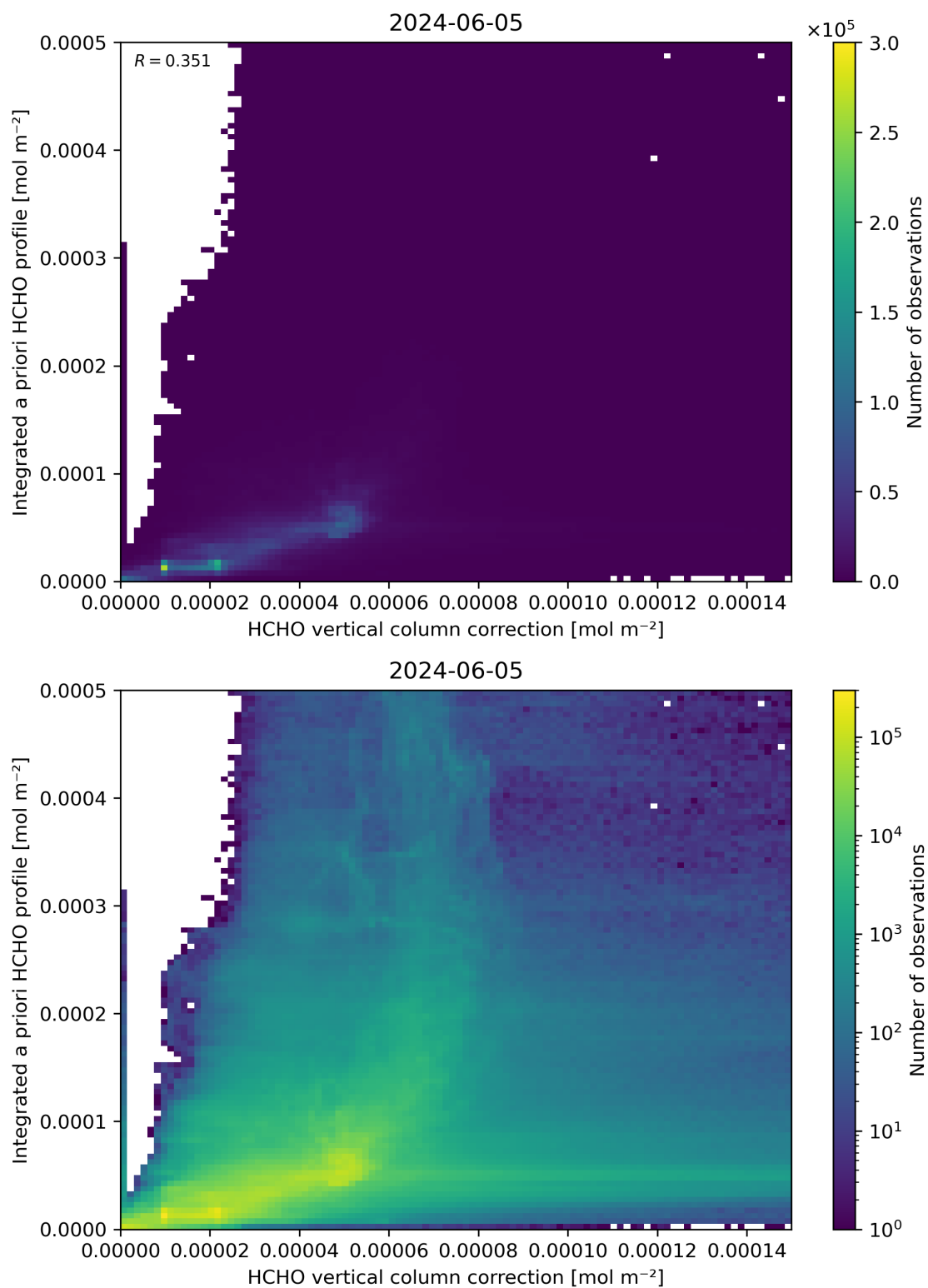
Figure 122: Scatter density plot of “HCHO vertical column correction” against “Integrated a priori HCHO profile” for 2024-06-04 to 2024-06-06.
