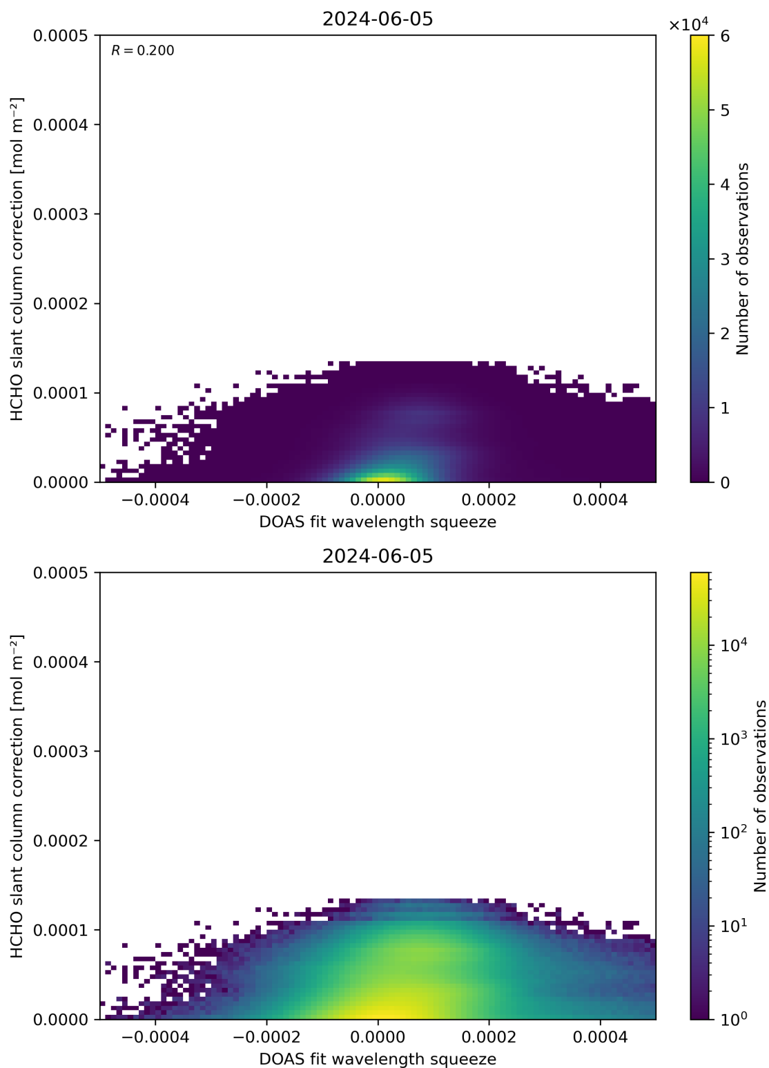
Figure 70: Scatter density plot of “DOAS fit wavelength squeeze” against “HCHO slant column correction” for 2024-06-04 to 2024-06-06.
