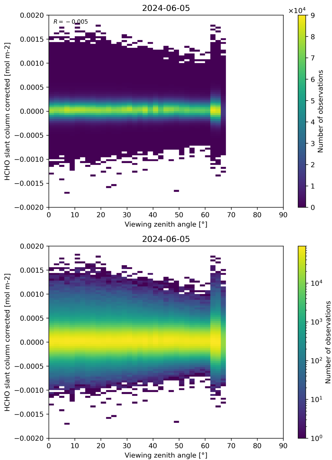
Figure 186: Scatter density plot of “Viewing zenith angle” against “HCHO slant column corrected” for 2024-06-04 to 2024-06-06.
