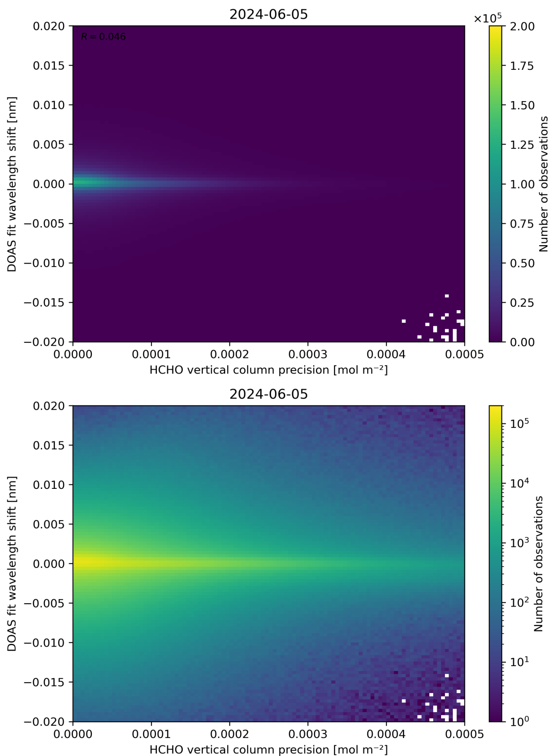
Figure 137: Scatter density plot of “HCHO vertical column precision” against “DOAS fit wavelength shift” for 2024-06-04 to 2024-06-06.
