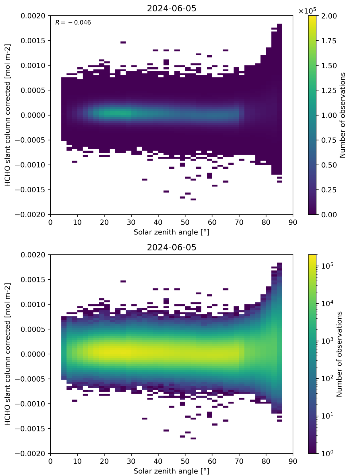
Figure 171: Scatter density plot of “Solar zenith angle” against “HCHO slant column corrected” for 2024-06-04 to 2024-06-06.
