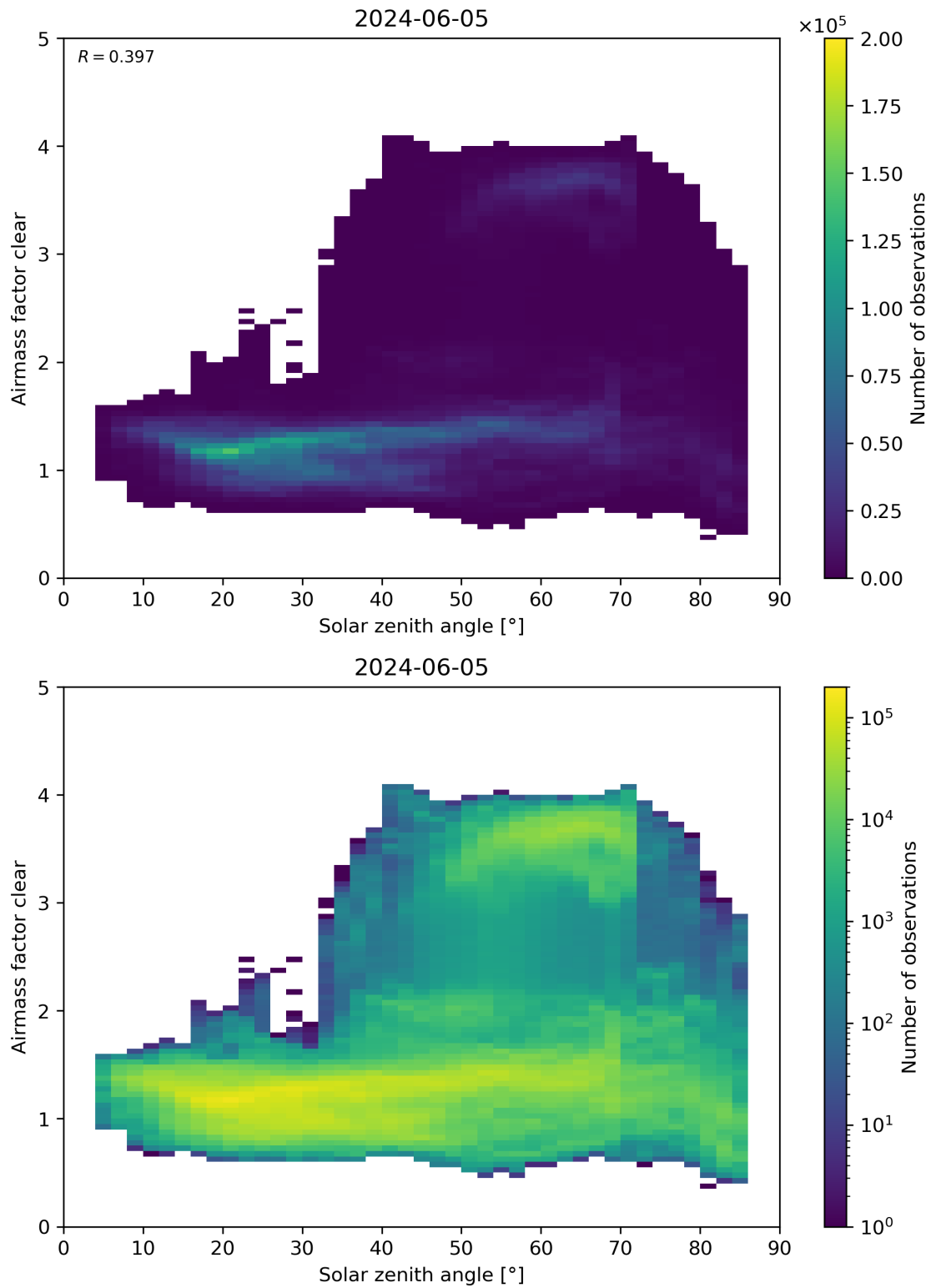
Figure 170: Scatter density plot of “Solar zenith angle” against “Airmass factor clear” for 2024-06-04 to 2024-06-06.
