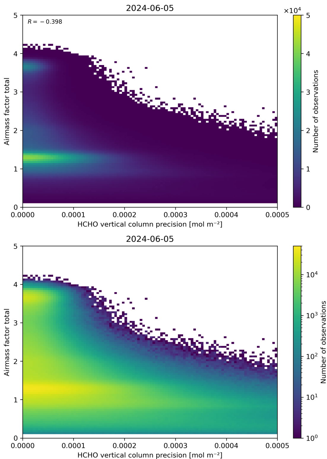
Figure 144: Scatter density plot of “HCHO vertical column precision” against “Airmass factor total” for 2024-06-04 to 2024-06-06.
