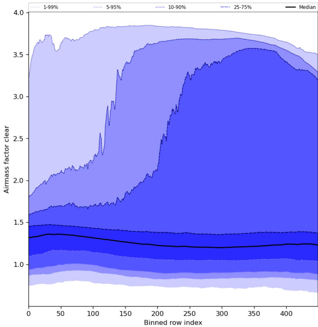
Figure 56: Along track statistics of “Airmass factor clear” for 2024-06-04 to 2024-06-06
