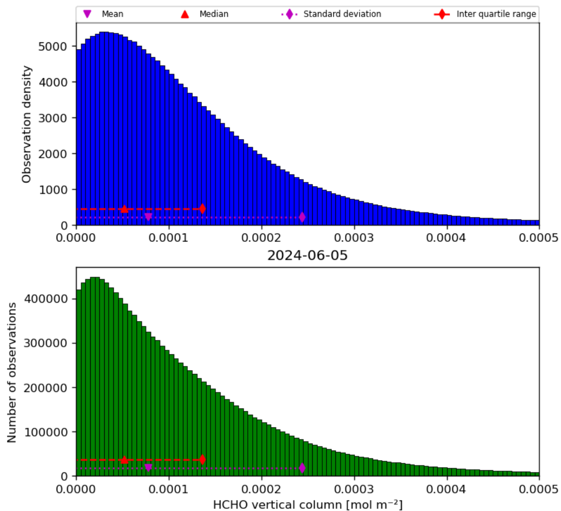
Figure 35: Histogram of “HCHO vertical column” for 2024-06-04 to 2024-06-06
