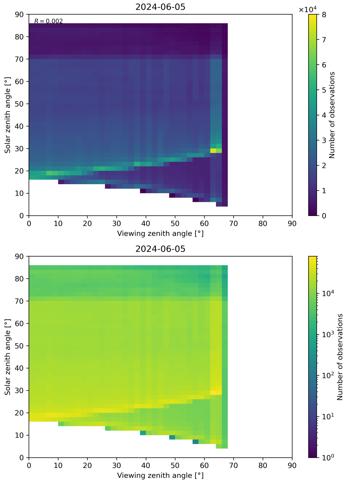
Figure 197: Scatter density plot of “Viewing zenith angle” against “Solar zenith angle” for 2024-06-04 to 2024-06-06.
