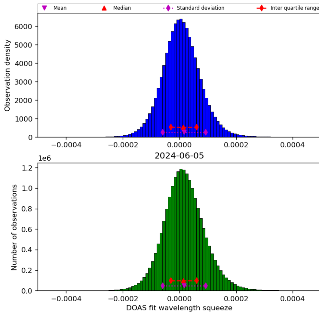
Figure 45: Histogram of “DOAS fit wavelength squeeze” for 2024-06-04 to 2024-06-06
