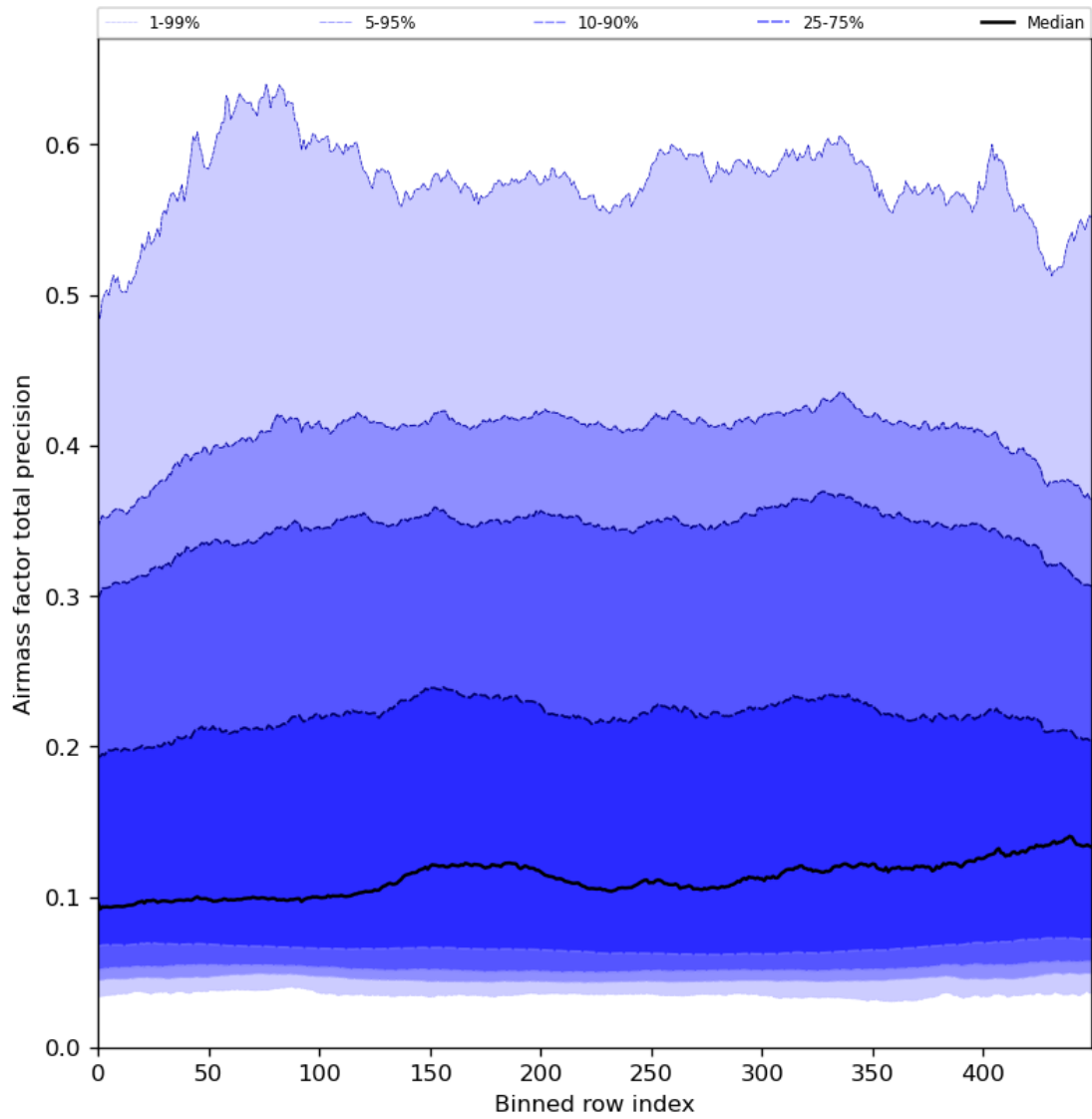
Figure 55: Along track statistics of “Airmass factor total precision” for 2024-06-04 to 2024-06-06
