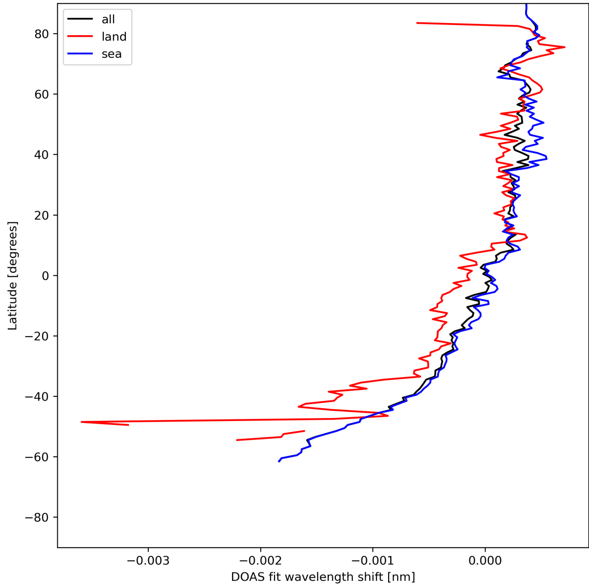
Figure 30: Zonal average of “DOAS fit wavelength shift” for 2024-06-04 to 2024-06-06.
