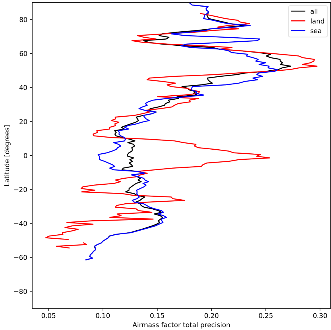
Figure 27: Zonal average of “Airmass factor total precision” for 2024-06-04 to 2024-06-06.
