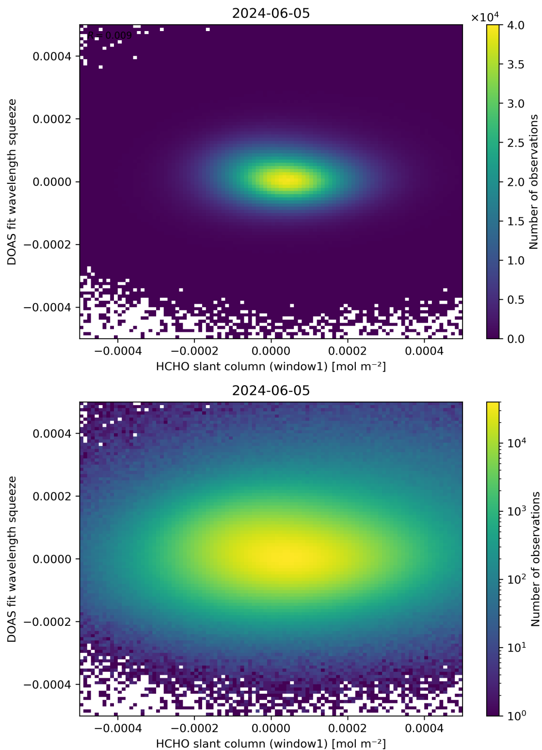
Figure 80: Scatter density plot of “HCHO slant column (window1)” against “DOAS fit wavelength squeeze” for 2024-06-04 to 2024-06-06.
