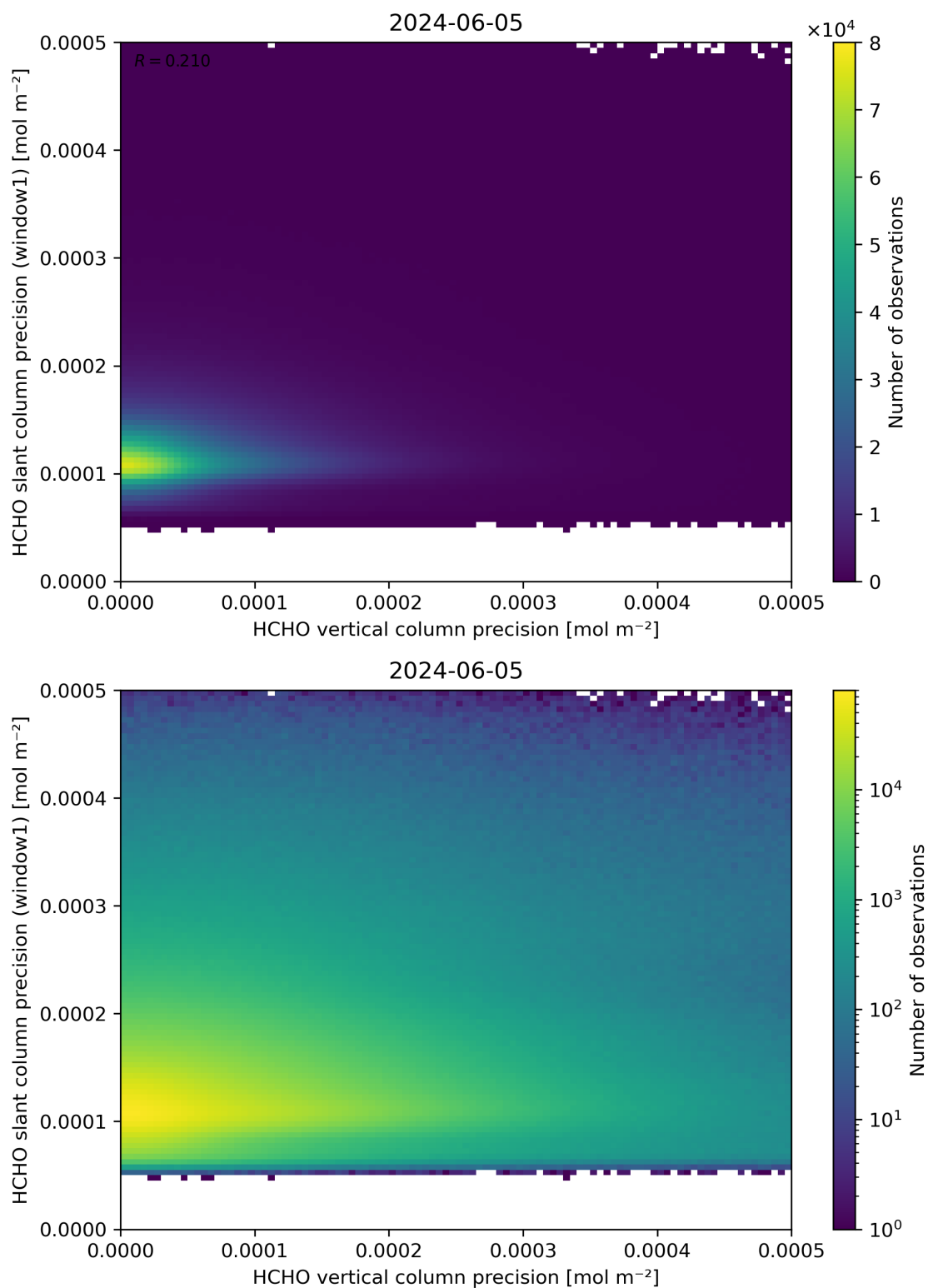
Figure 143: Scatter density plot of “HCHO vertical column precision” against “HCHO slant column precision (window1)” for 2024-06-04 to 2024-06-06.
