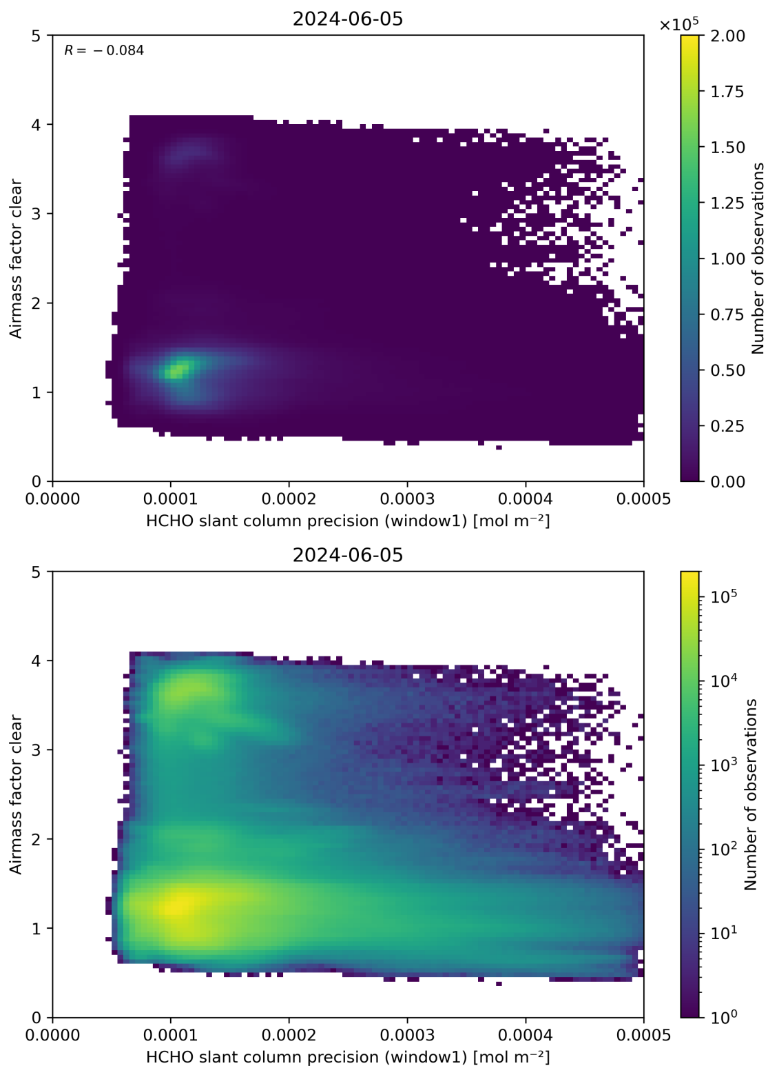
Figure 91: Scatter density plot of “HCHO slant column precision (window1)” against “Airmass factor clear” for 2024-06-04 to 2024-06-06.
