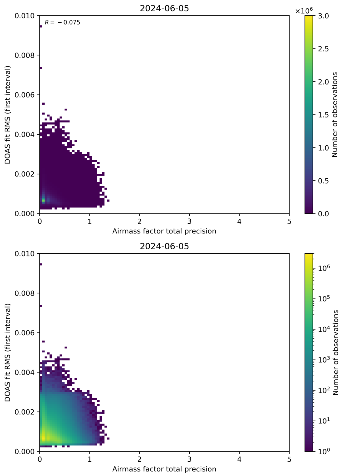
Figure 105: Scatter density plot of “Airmass factor total precision” against “DOAS fit RMS (first interval)” for 2024-06-04 to 2024-06-06.
