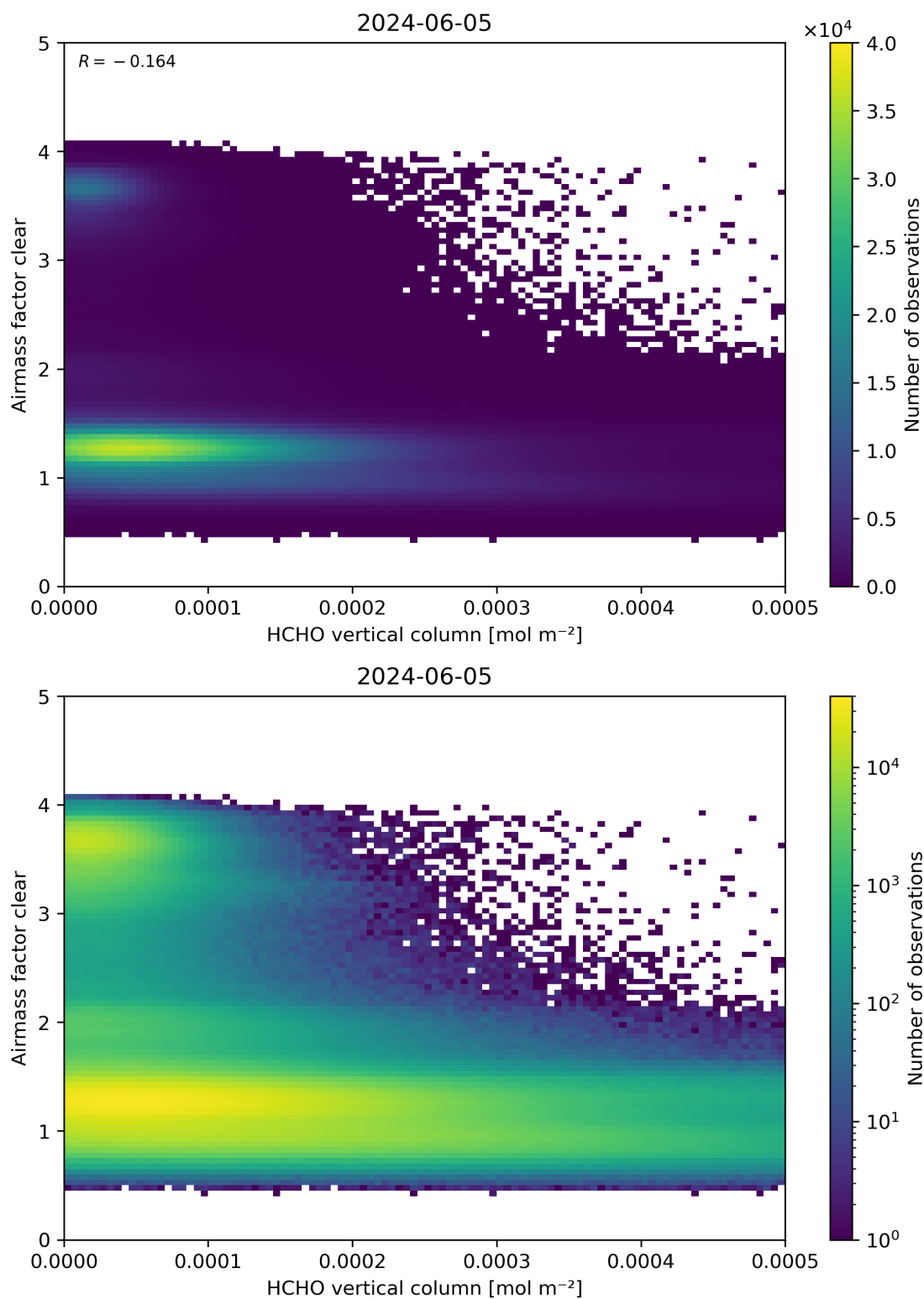
Figure 126: Scatter density plot of “HCHO vertical column” against “Airmass factor clear” for 2024-06-04 to 2024-06-06.
