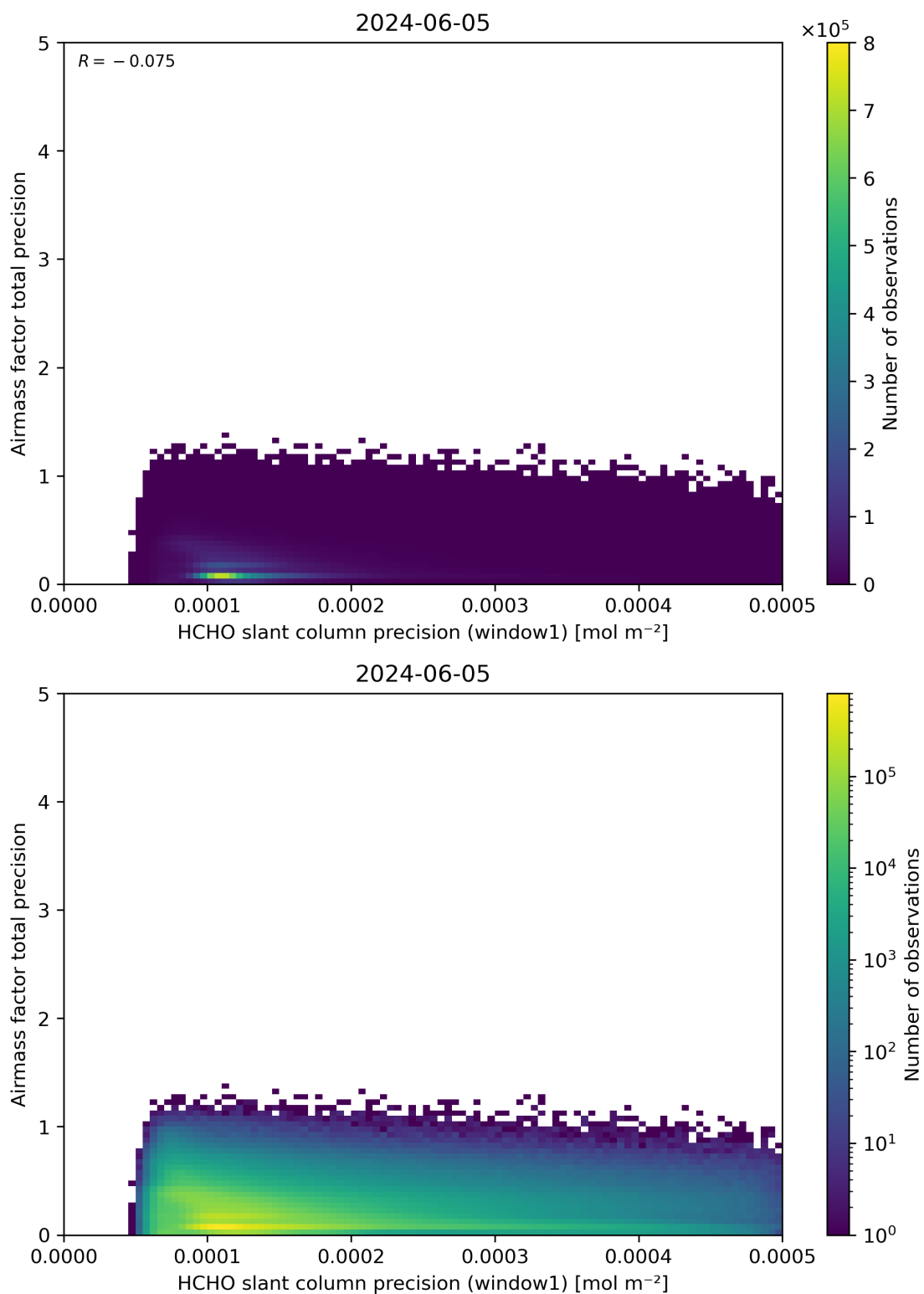
Figure 95: Scatter density plot of “HCHO slant column precision (window1)” against “Airmass factor total precision” for 2024-06-04 to 2024-06-06.
