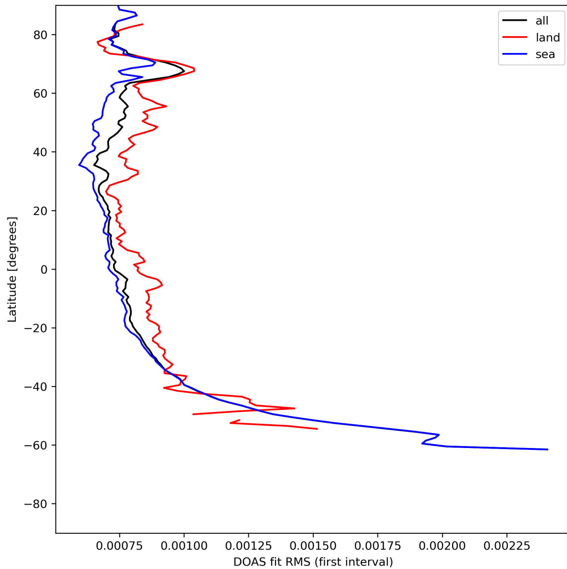
Figure 32: Zonal average of “DOAS fit RMS (first interval)” for 2024-06-04 to 2024-06-06.
