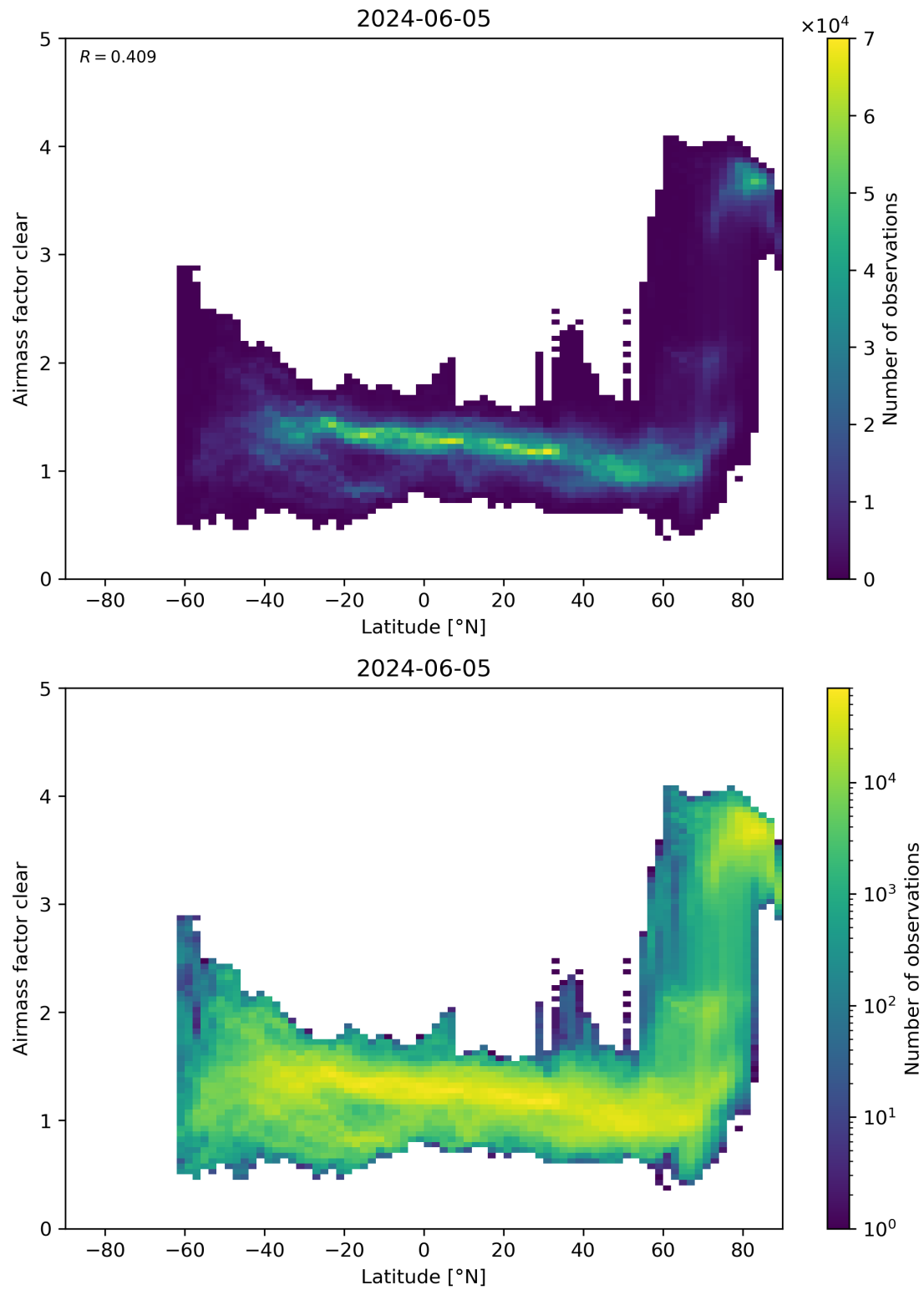
Figure 156: Scatter density plot of “Latitude” against “Airmass factor clear” for 2024-06-04 to 2024-06-06.
