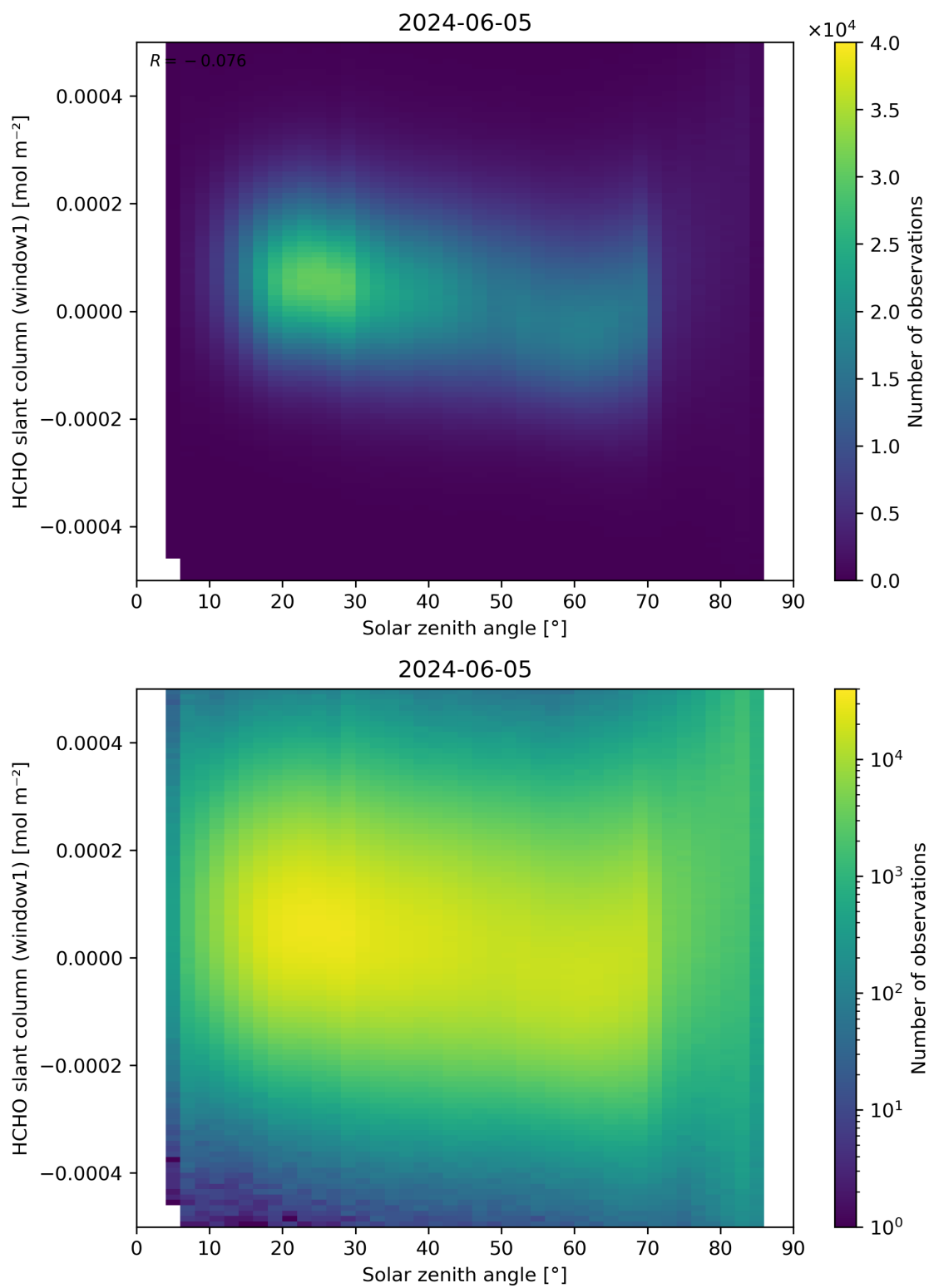
Figure 173: Scatter density plot of “Solar zenith angle” against “HCHO slant column (window1)” for 2024-06-04 to 2024-06-06.
