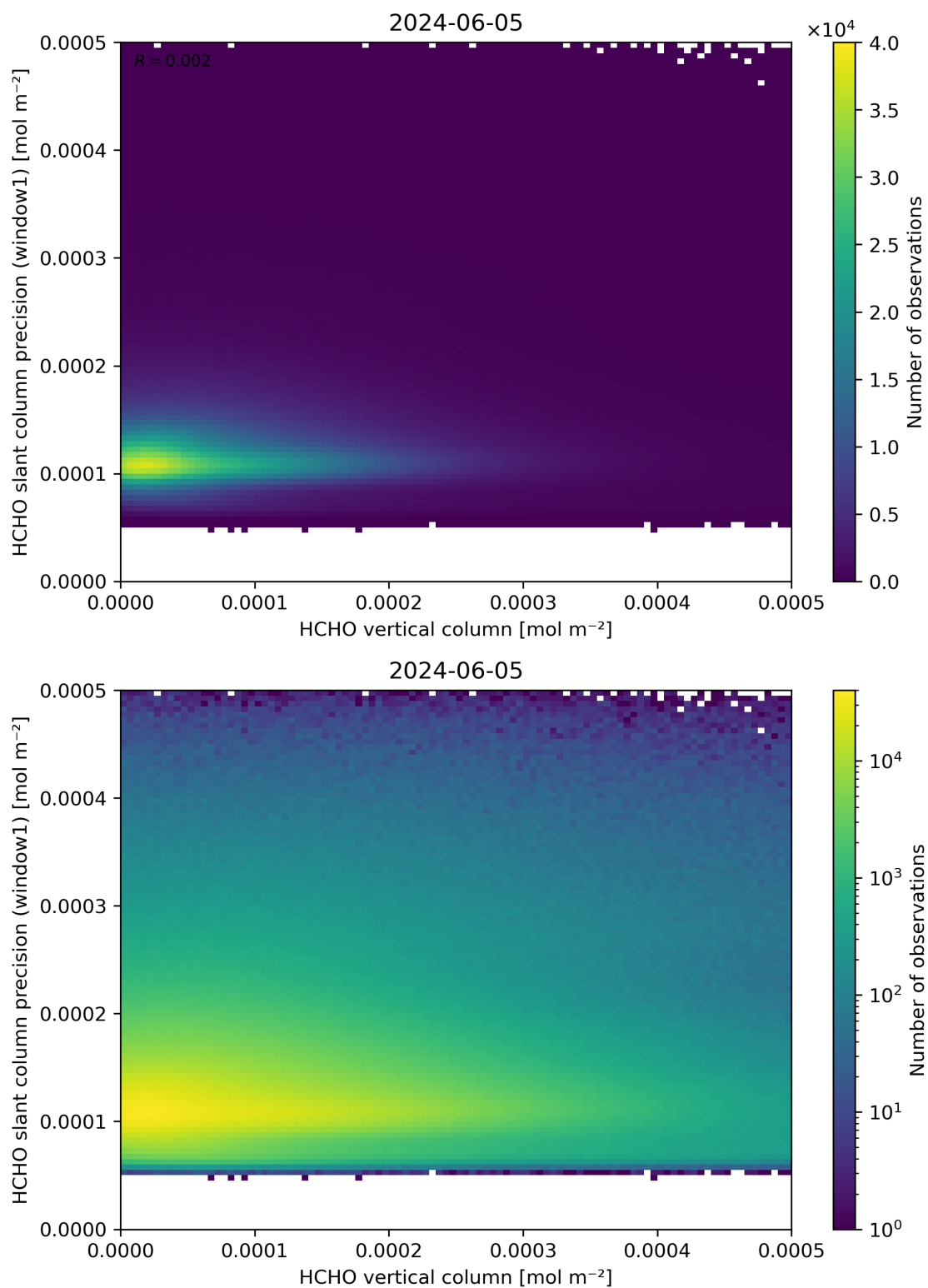
Figure 130: Scatter density plot of “HCHO vertical column” against “HCHO slant column precision (window1)” for 2024-06-04 to 2024-06-06.
