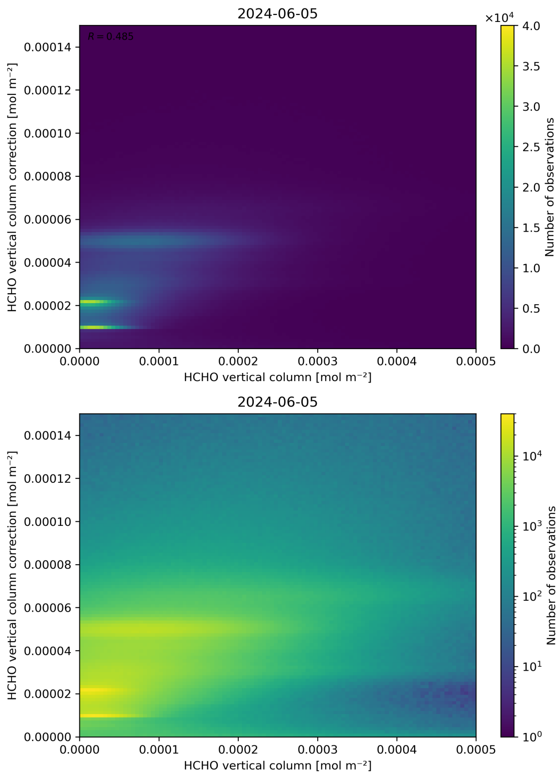
Figure 133: Scatter density plot of “HCHO vertical column” against “HCHO vertical column correction” for 2024-06-04 to 2024-06-06.
