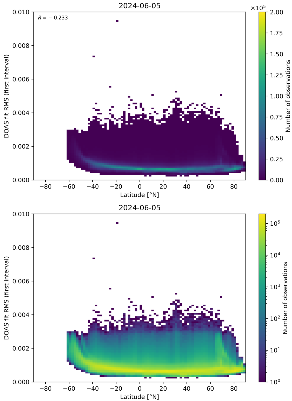
Figure 153: Scatter density plot of “Latitude” against “DOAS fit RMS (first interval)” for 2024-06-04 to 2024-06-06.
