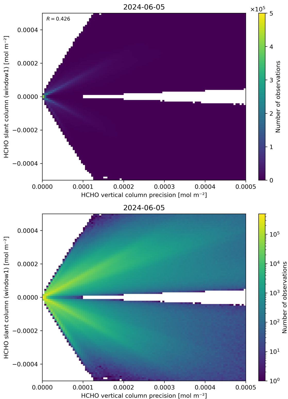
Figure 142: Scatter density plot of “HCHO vertical column precision” against “HCHO slant column (window1)” for 2024-06-04 to 2024-06-06.
