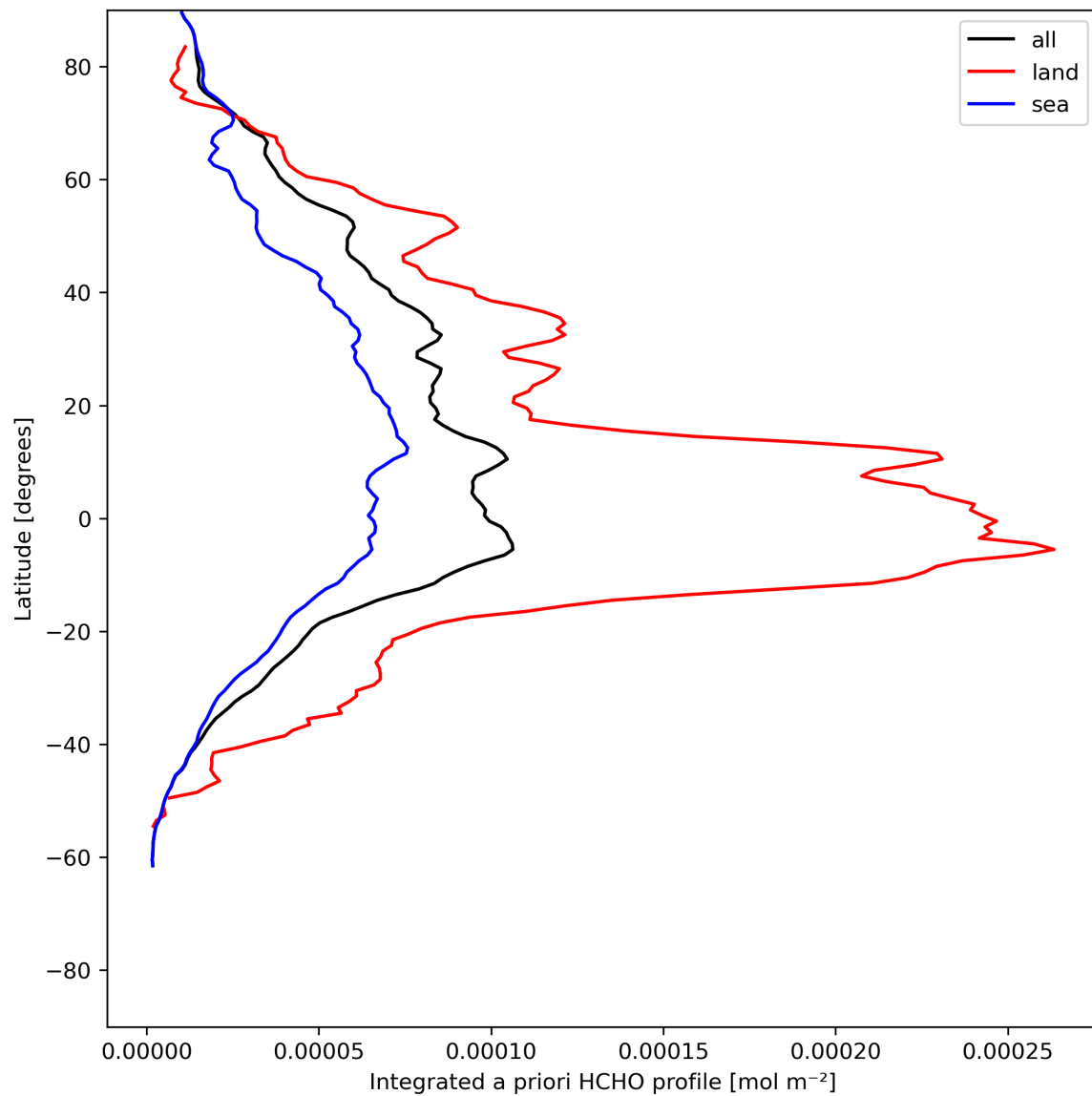
Figure 29: Zonal average of “Integrated a priori HCHO profile” for 2024-06-04 to 2024-06-06.
