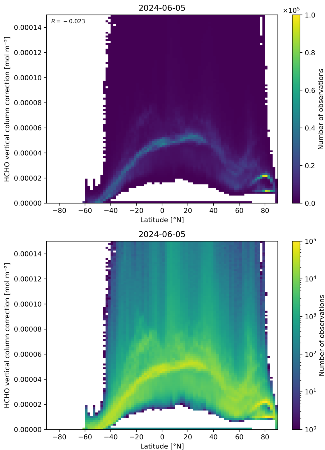
Figure 164: Scatter density plot of “Latitude” against “HCHO vertical column correction” for 2024-06-04 to 2024-06-06.
