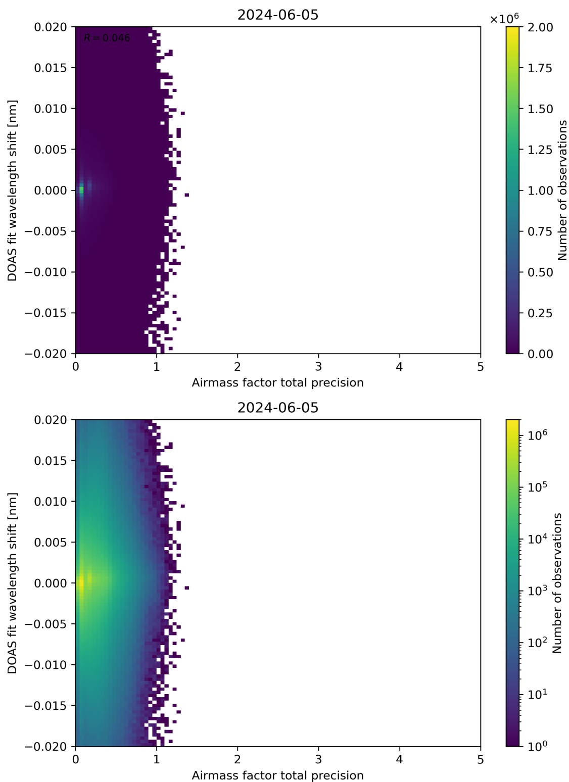
Figure 106: Scatter density plot of “Airmass factor total precision” against “DOAS fit wavelength shift” for 2024-06-04 to 2024-06-06.
