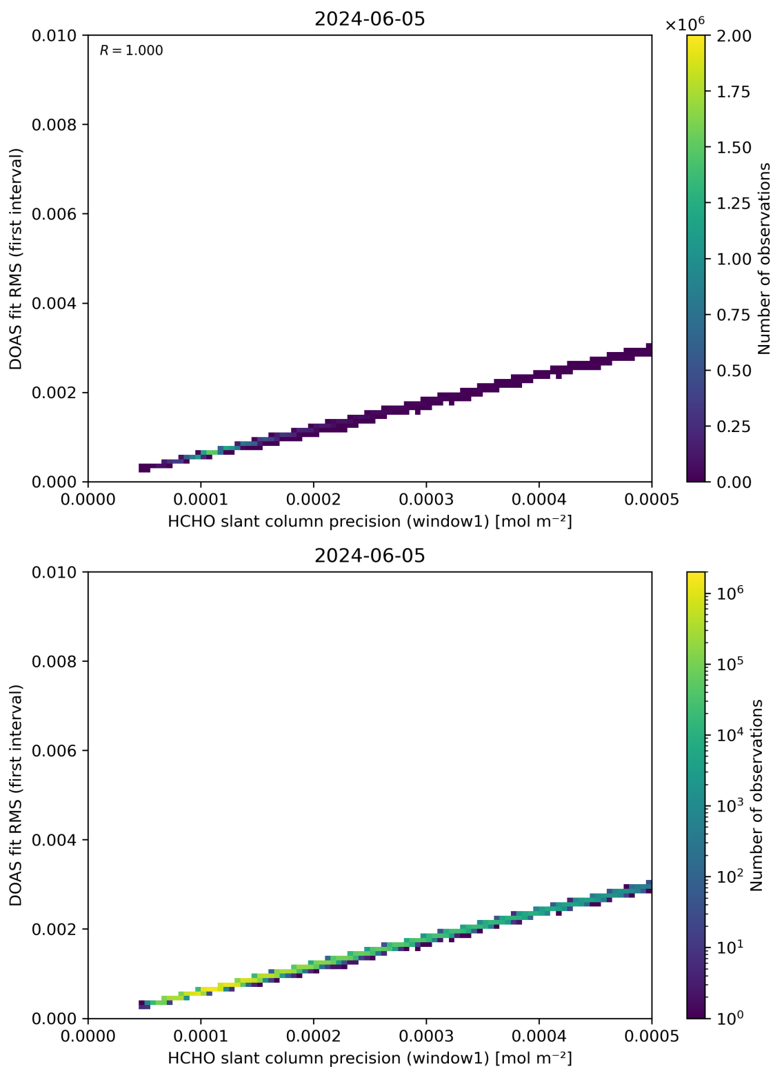
Figure 88: Scatter density plot of “HCHO slant column precision (window1)” against “DOAS fit RMS (first interval)” for 2024-06-04 to 2024-06-06.
