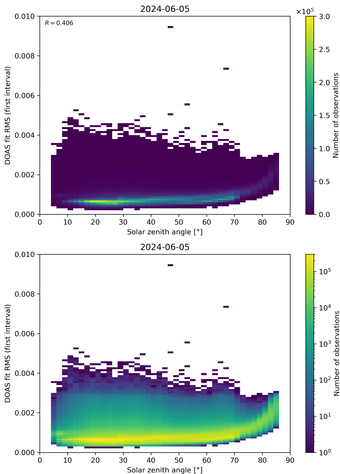
Figure 167: Scatter density plot of “Solar zenith angle” against “DOAS fit RMS (first interval)” for 2024-06-04 to 2024-06-06.
