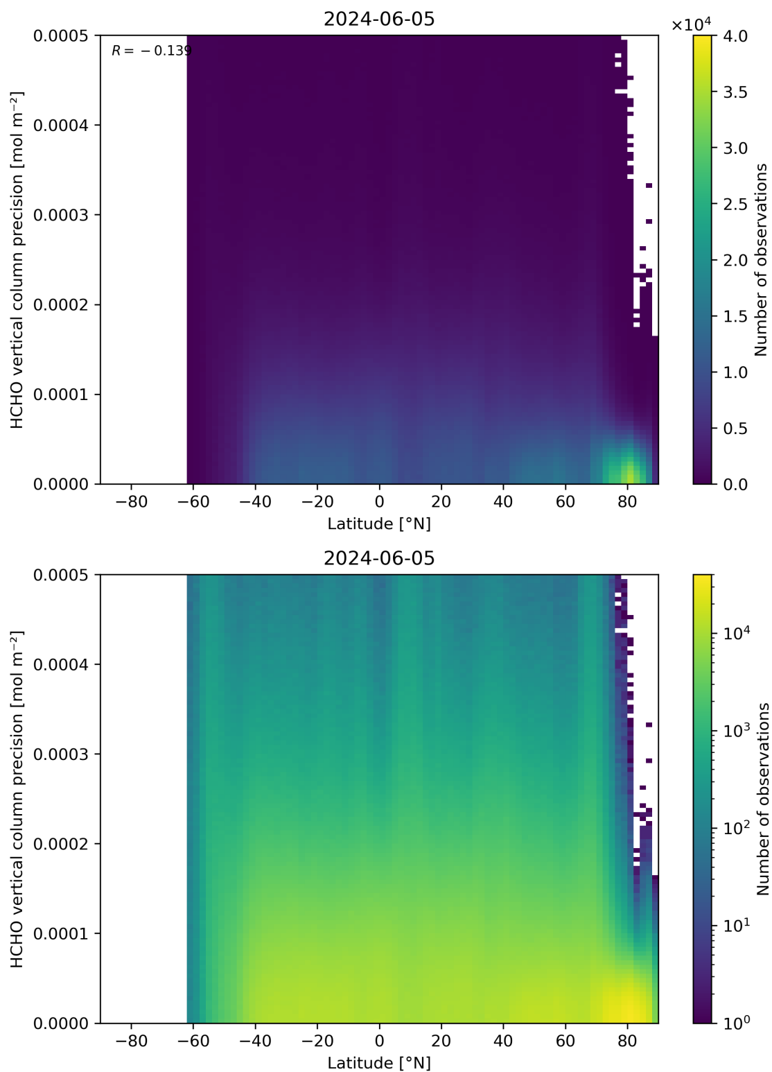
Figure 165: Scatter density plot of “Latitude” against “HCHO vertical column precision” for 2024-06-04 to 2024-06-06.
