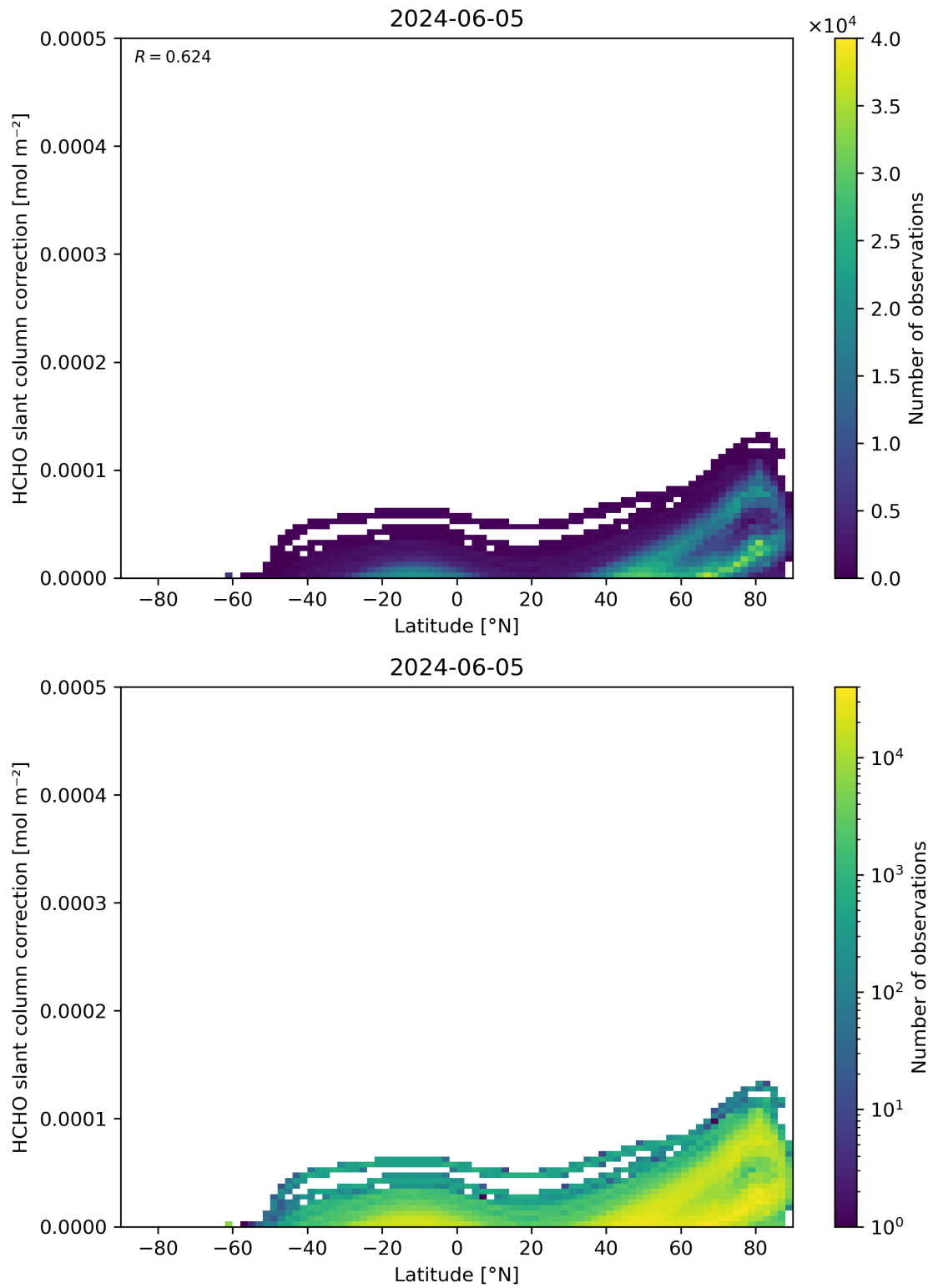
Figure 158: Scatter density plot of “Latitude” against “HCHO slant column correction” for 2024-06-04 to 2024-06-06.
