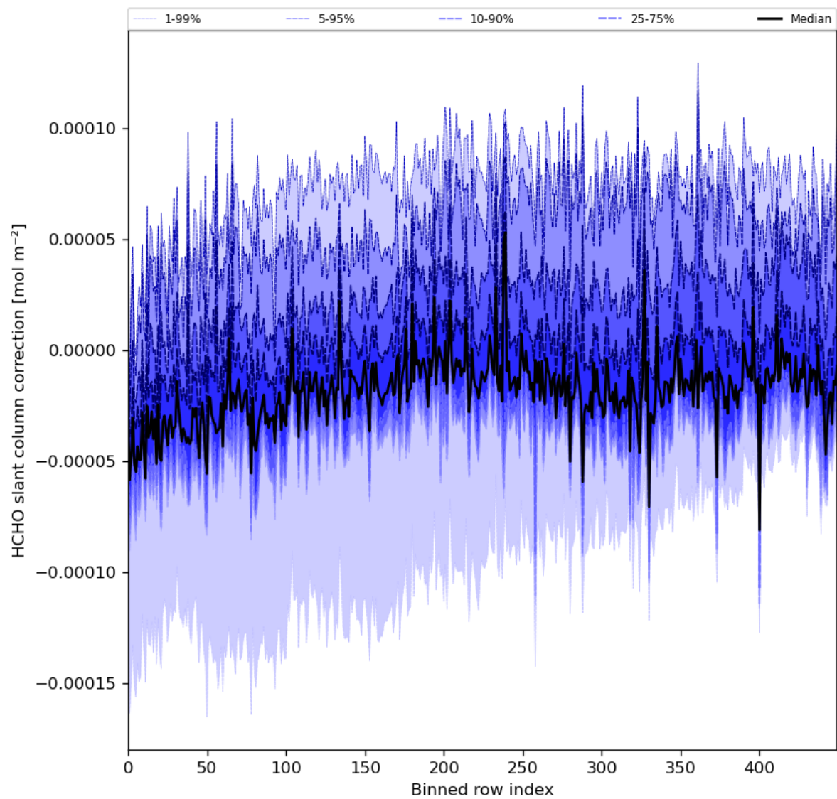
Figure 61: Along track statistics of “HCHO slant column correction” for 2024-06-04 to 2024-06-06
