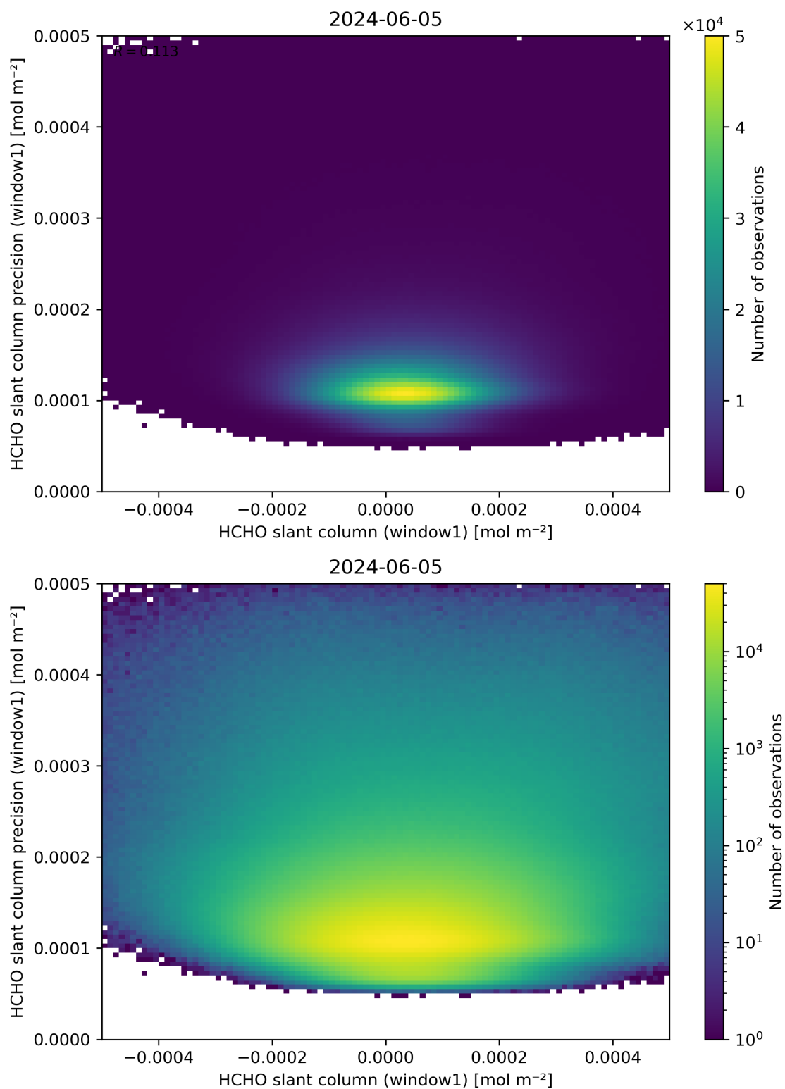
Figure 84: Scatter density plot of “HCHO slant column (window1)” against “HCHO slant column precision (window1)” for 2024-06-04 to 2024-06-06.
