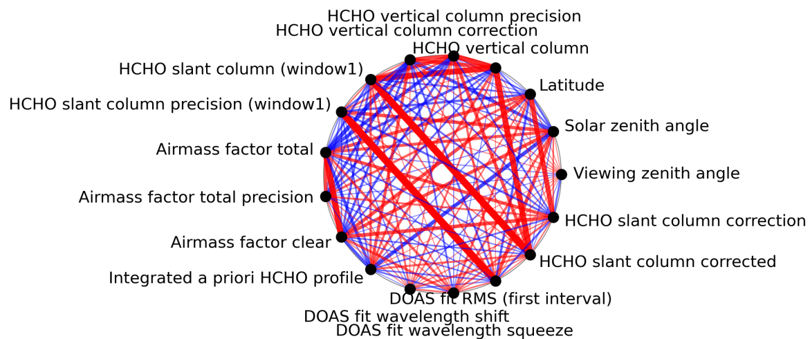
Figure 1: Map of correlation graph for 2024-06-04 to 2024-06-06.
