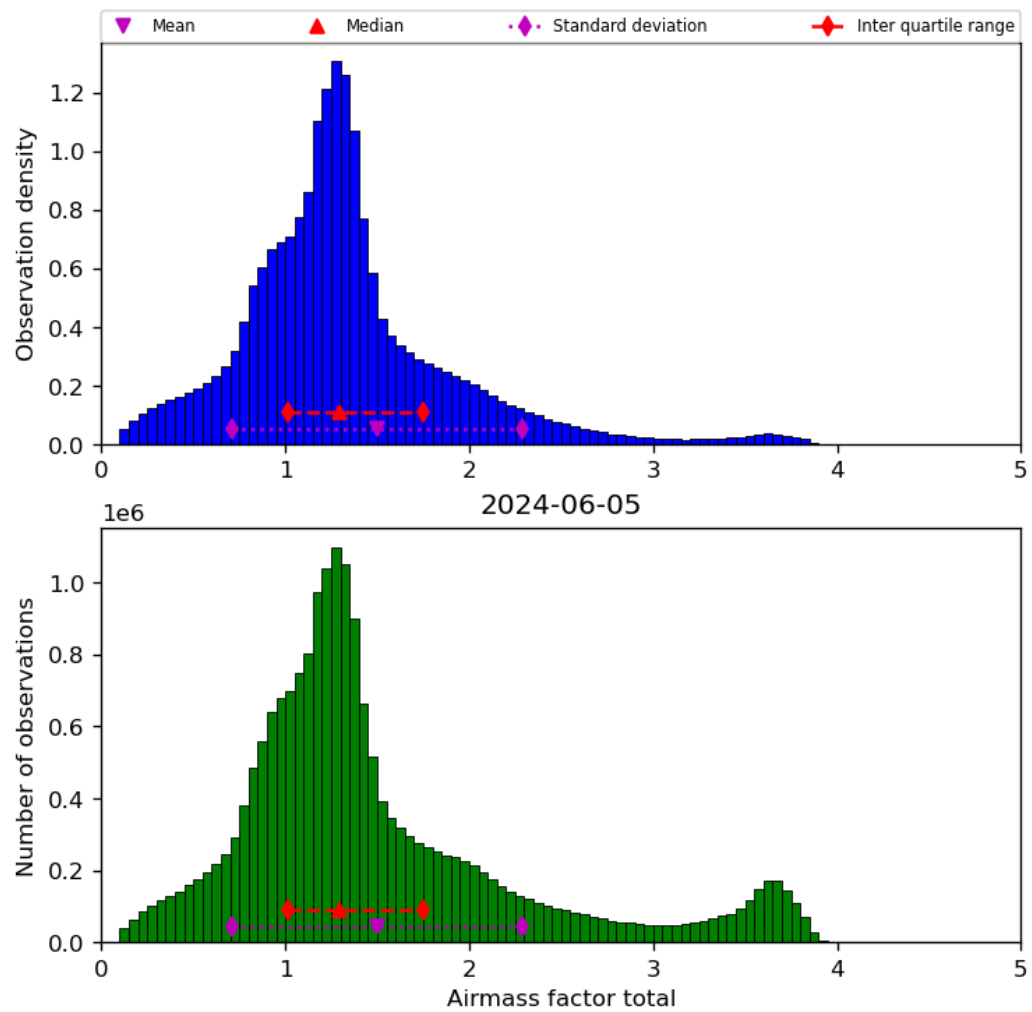
Figure 40: Histogram of “Airmass factor total” for 2024-06-04 to 2024-06-06
