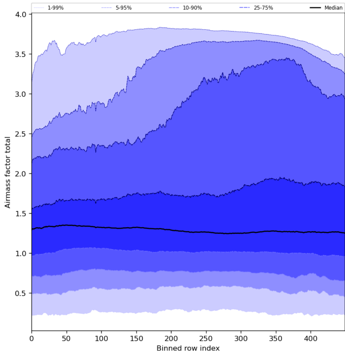
Figure 54: Along track statistics of “Airmass factor total” for 2024-06-04 to 2024-06-06
