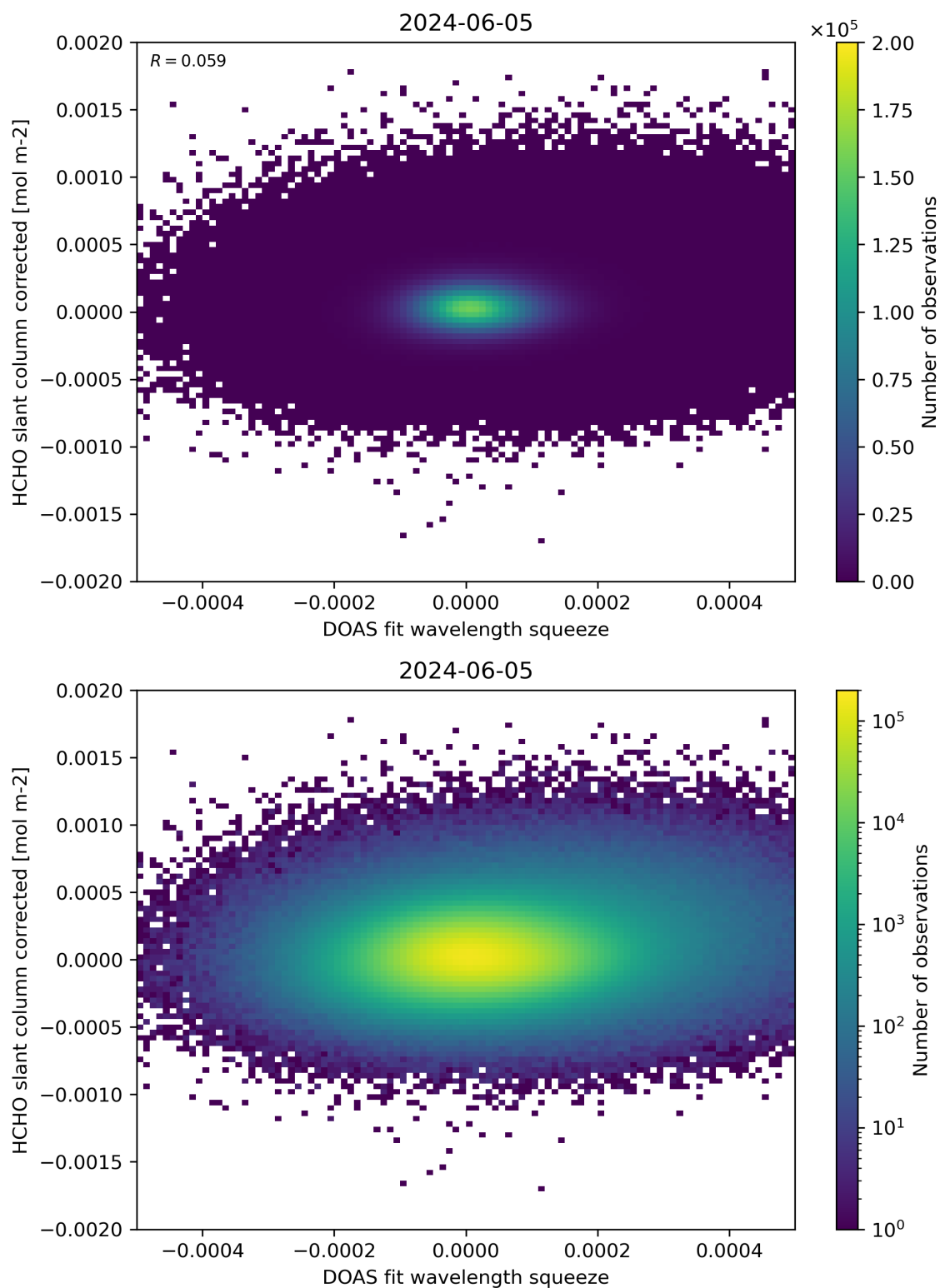
Figure 69: Scatter density plot of “DOAS fit wavelength squeeze” against “HCHO slant column corrected” for 2024-06-04 to 2024-06-06.
