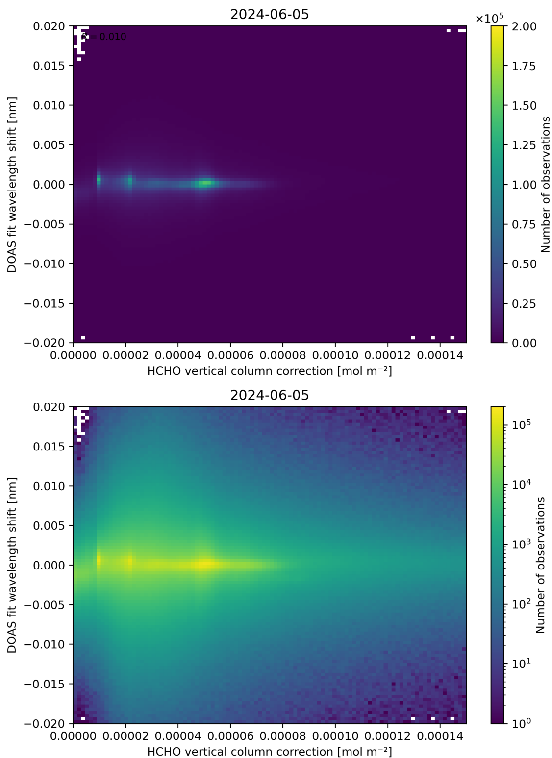
Figure 113: Scatter density plot of “HCHO vertical column correction” against “DOAS fit wavelength shift” for 2024-06-04 to 2024-06-06.
