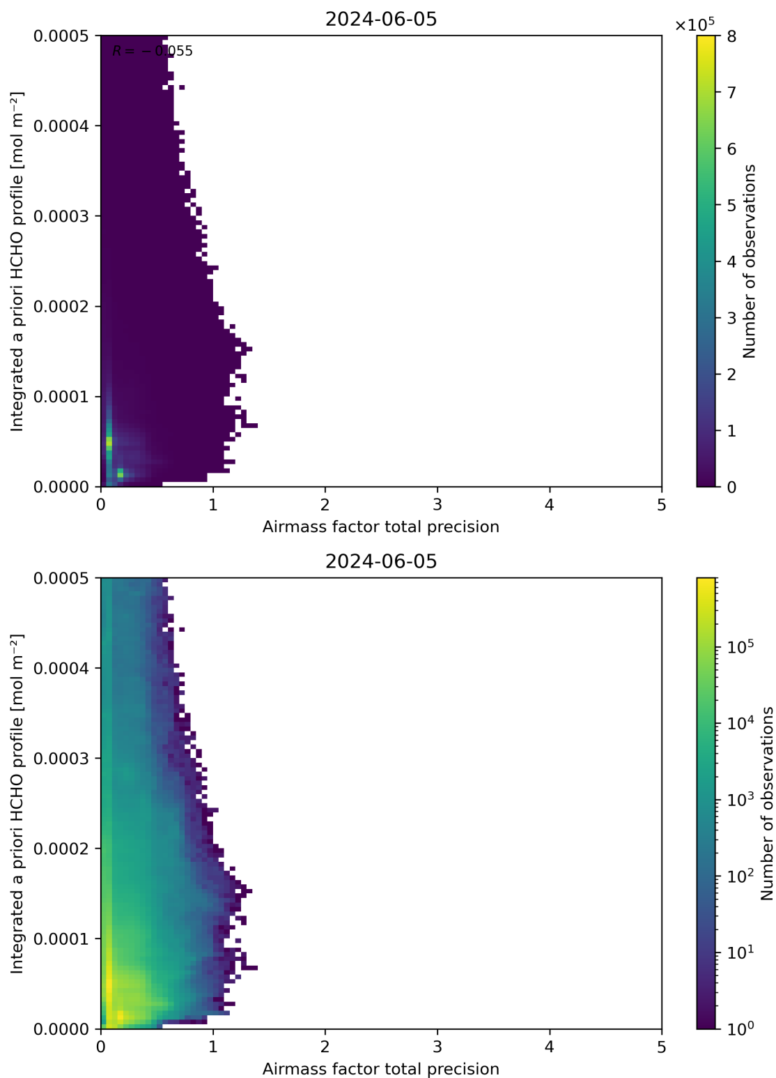
Figure 111: Scatter density plot of “Airmass factor total precision” against “Integrated a priori HCHO profile” for 2024-06-04 to 2024-06-06.
