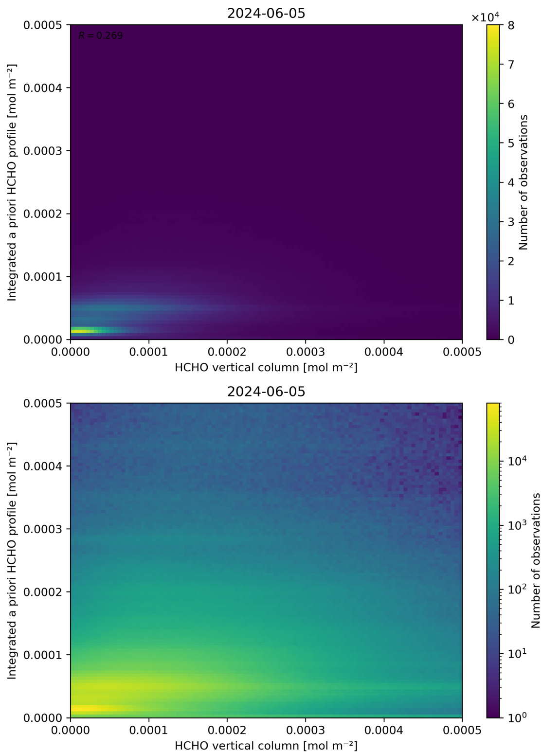
Figure 135: Scatter density plot of “HCHO vertical column” against “Integrated a priori HCHO profile” for 2024-06-04 to 2024-06-06.
