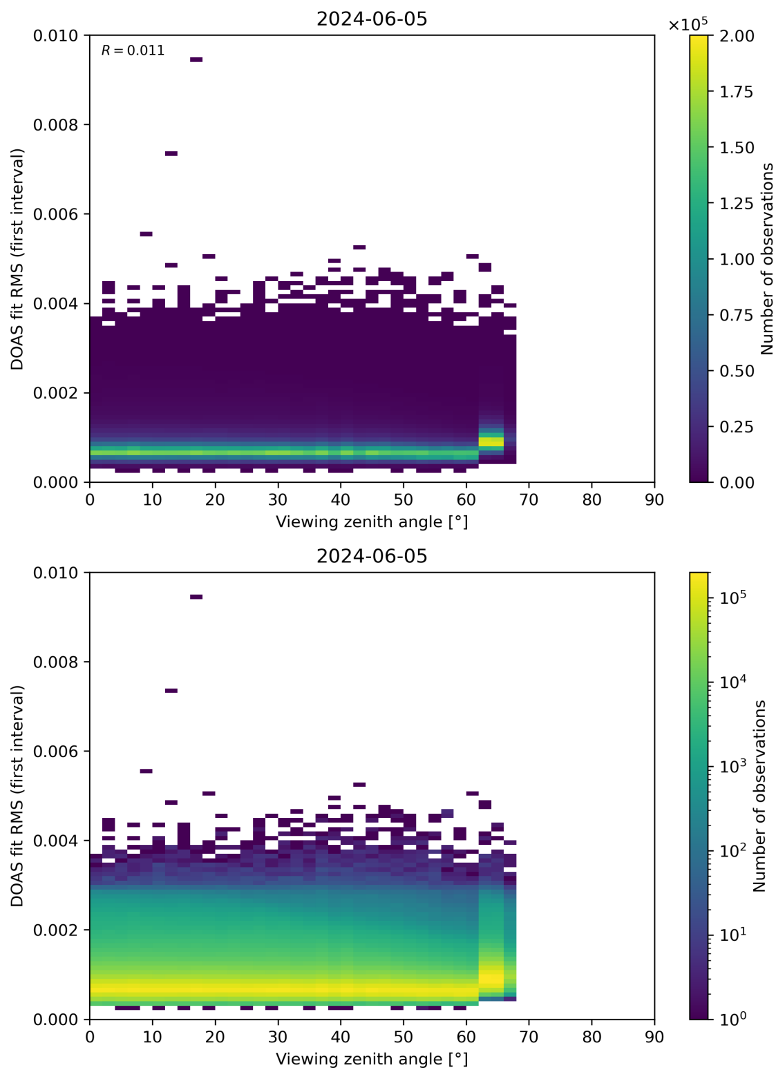
Figure 182: Scatter density plot of “Viewing zenith angle” against “DOAS fit RMS (first interval)” for 2024-06-04 to 2024-06-06.
