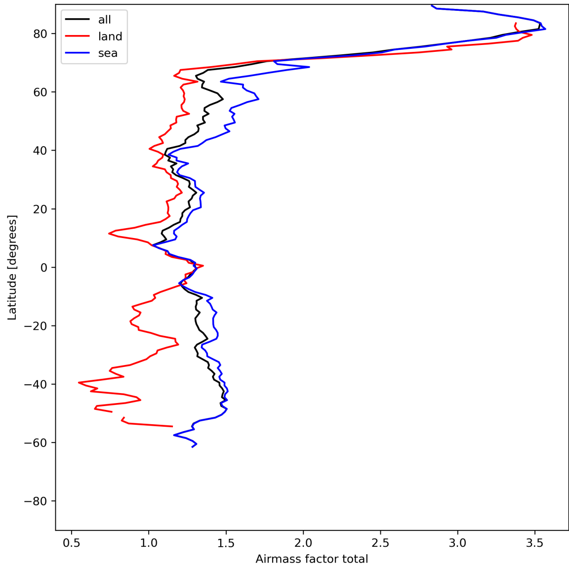
Figure 26: Zonal average of “Airmass factor total” for 2024-06-04 to 2024-06-06.
