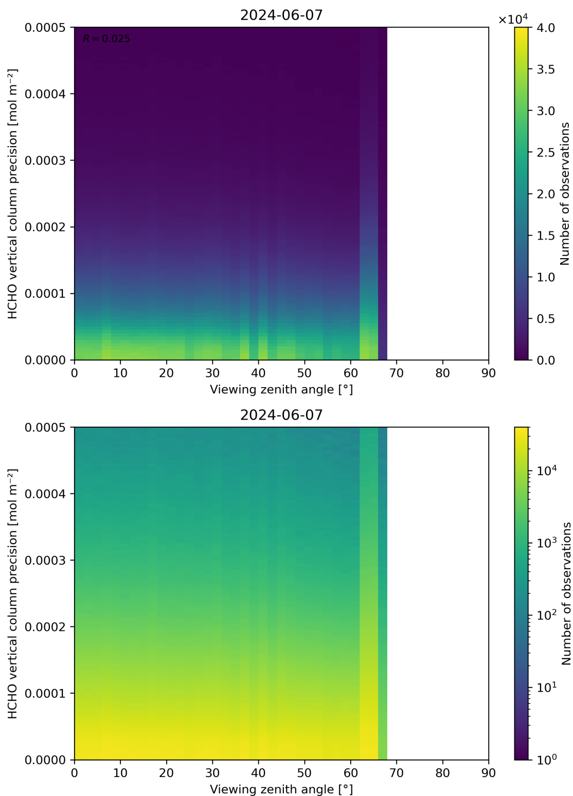
Figure 194: Scatter density plot of “Viewing zenith angle” against “HCHO vertical column precision” for 2024-06-06 to 2024-06-08.
