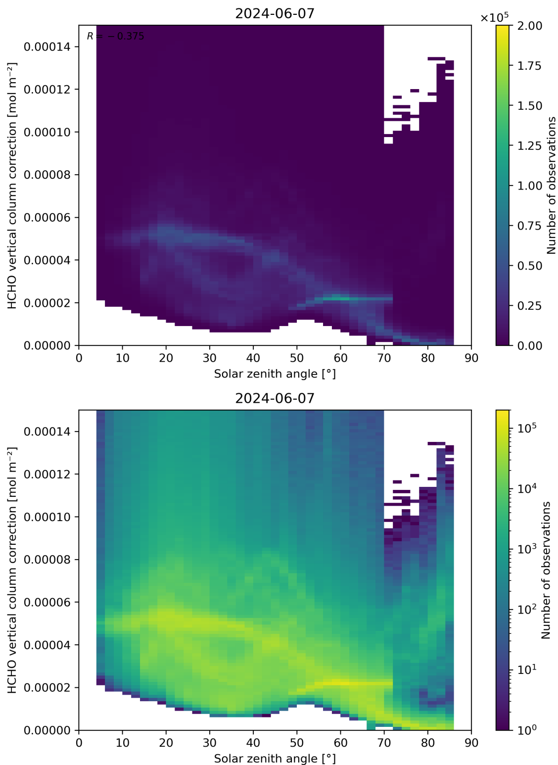
Figure 178: Scatter density plot of “Solar zenith angle” against “HCHO vertical column correction” for 2024-06-06 to 2024-06-08.
