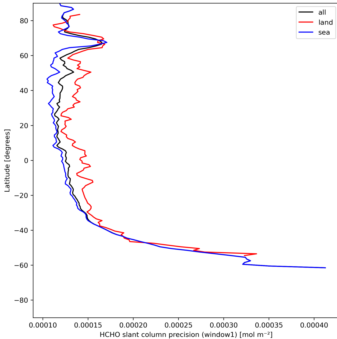
Figure 25: Zonal average of “HCHO slant column precision (window1)” for 2024-06-06 to 2024-06-08.
