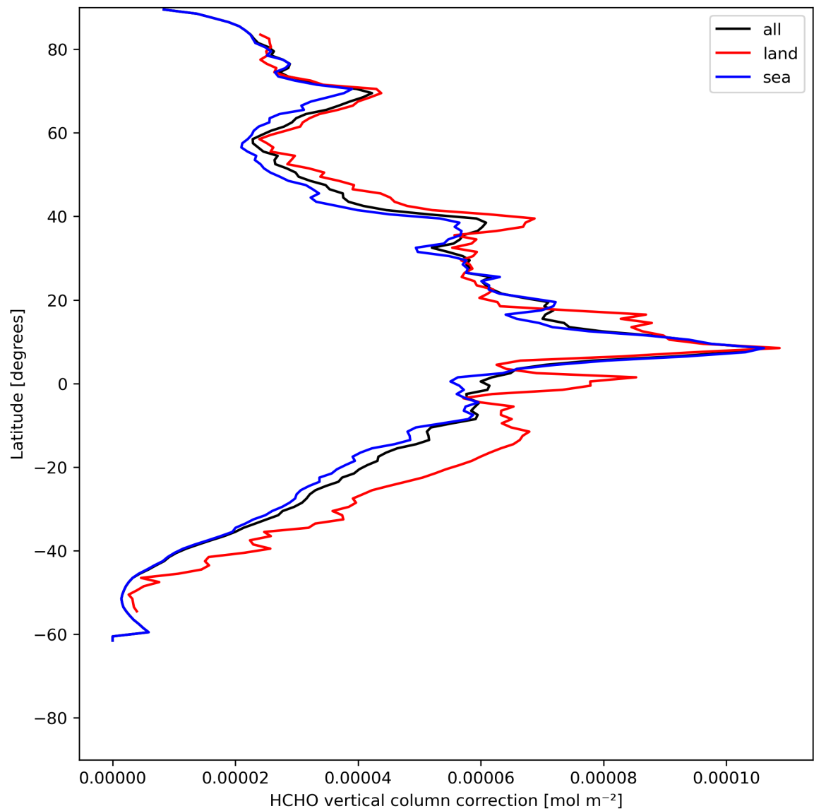
Figure 23: Zonal average of “HCHO vertical column correction” for 2024-06-06 to 2024-06-08.
