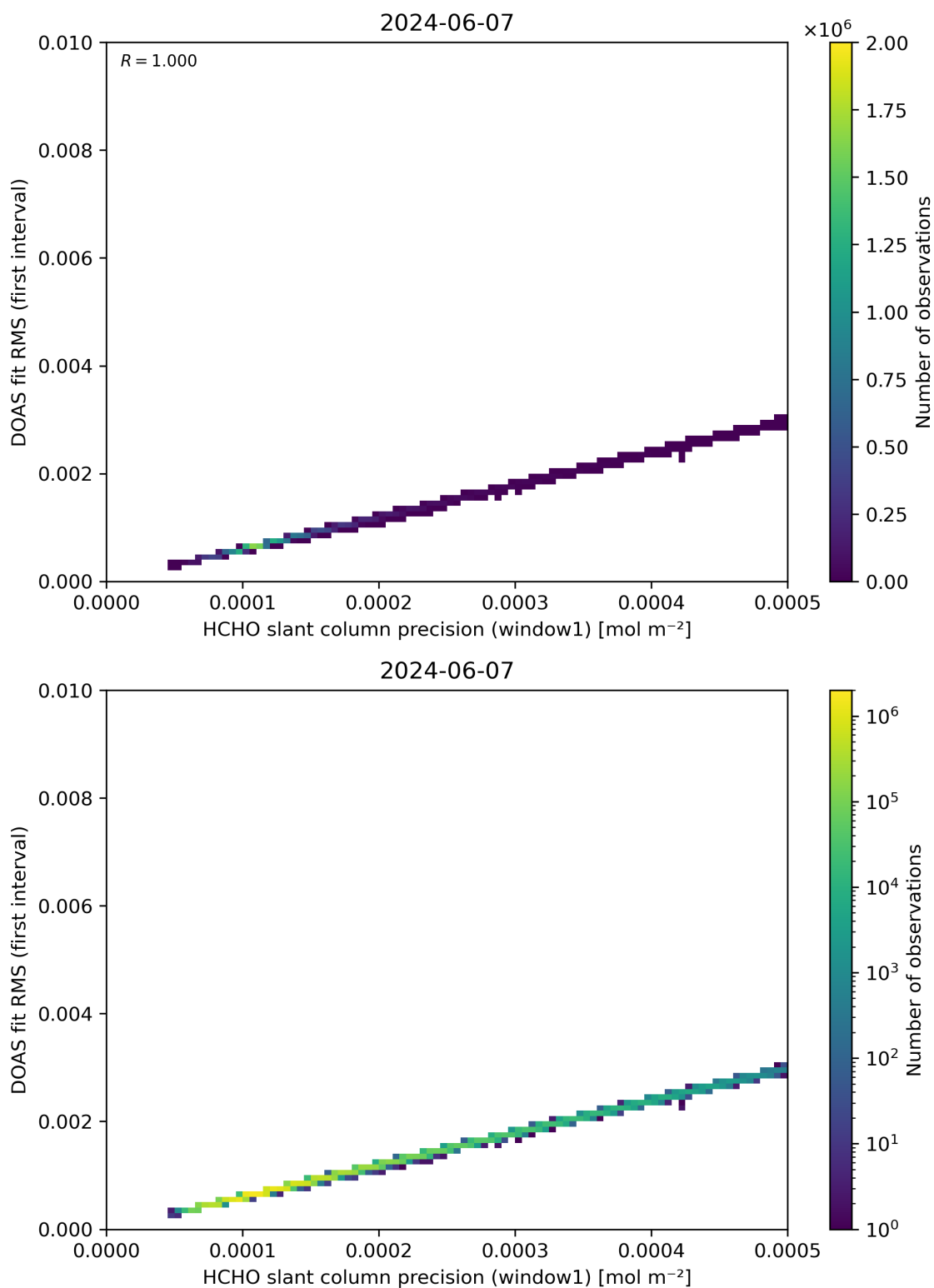
Figure 88: Scatter density plot of “HCHO slant column precision (window1)” against “DOAS fit RMS (first interval)” for 2024-06-06 to 2024-06-08.
