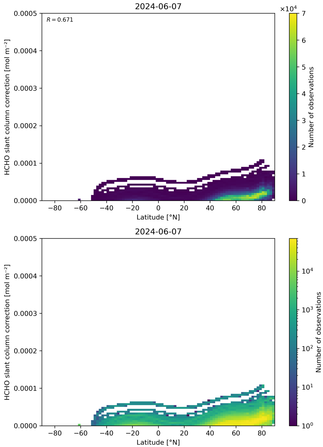
Figure 158: Scatter density plot of “Latitude” against “HCHO slant column correction” for 2024-06-06 to 2024-06-08.
