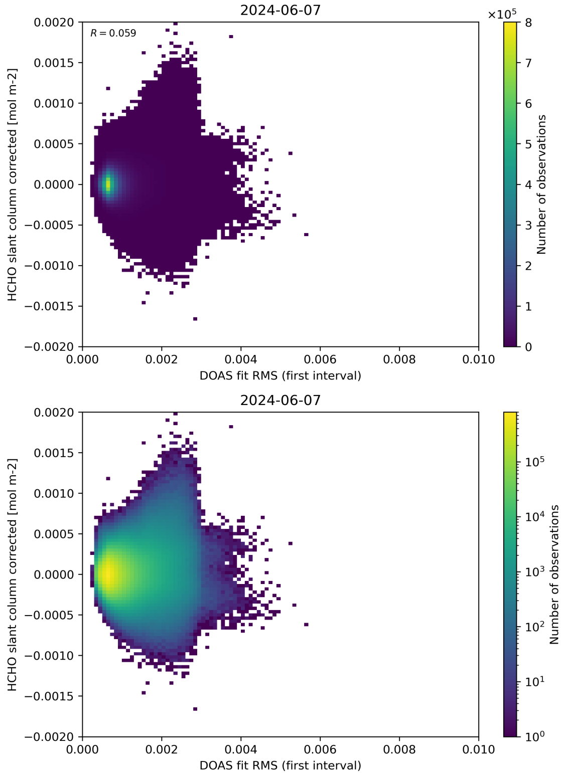
Figure 62: Scatter density plot of “DOAS fit RMS (first interval)” against “HCHO slant column corrected” for 2024-06-06 to 2024-06-08.
