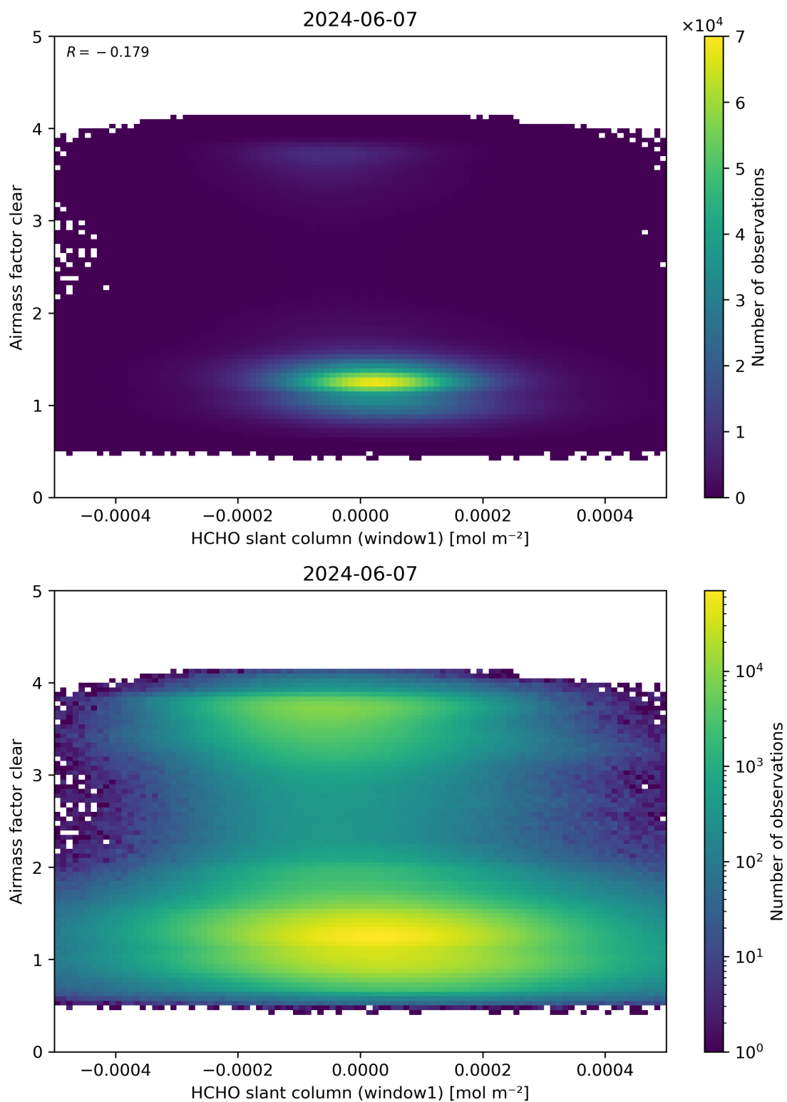
Figure 81: Scatter density plot of “HCHO slant column (window1)” against “Airmass factor clear” for 2024-06-06 to 2024-06-08.
