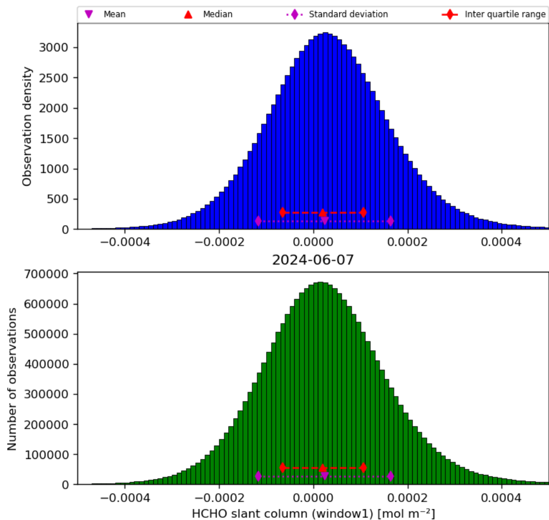
Figure 38: Histogram of “HCHO slant column (window1)” for 2024-06-06 to 2024-06-08
