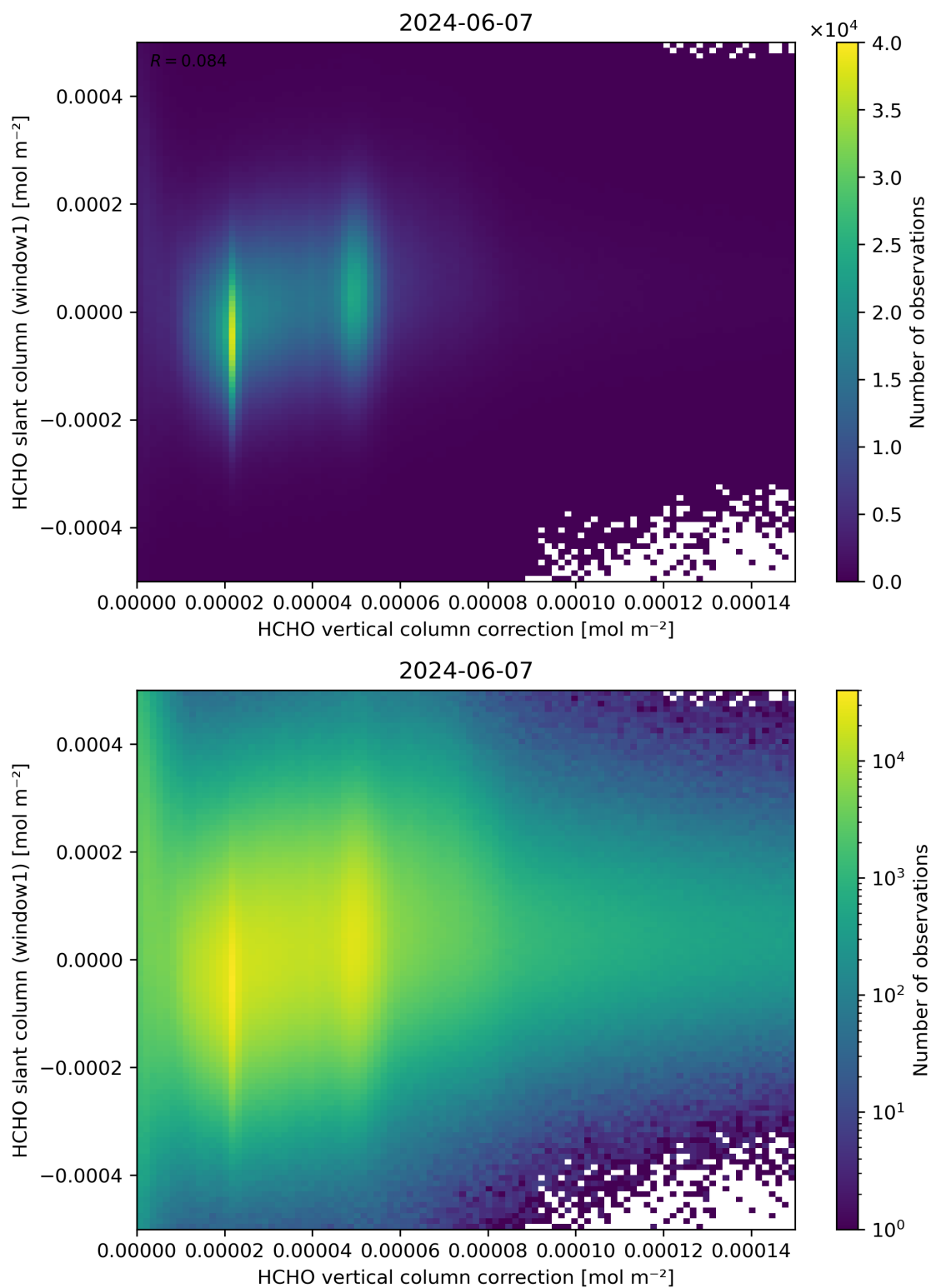
Figure 118: Scatter density plot of “HCHO vertical column correction” against “HCHO slant column (window1)” for 2024-06-06 to 2024-06-08.
