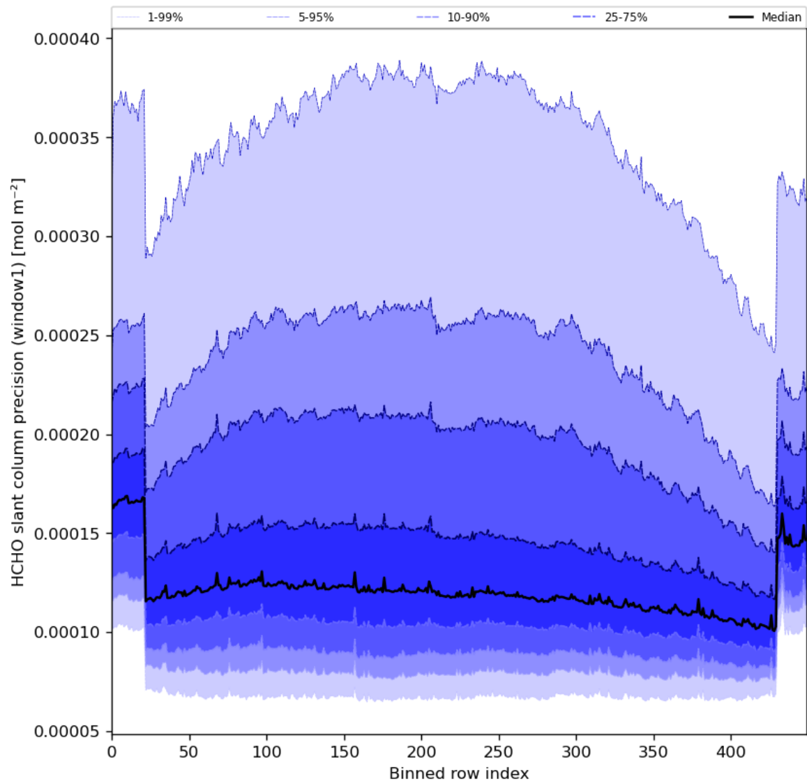
Figure 53: Along track statistics of “HCHO slant column precision (window1)” for 2024-06-06 to 2024-06-08
