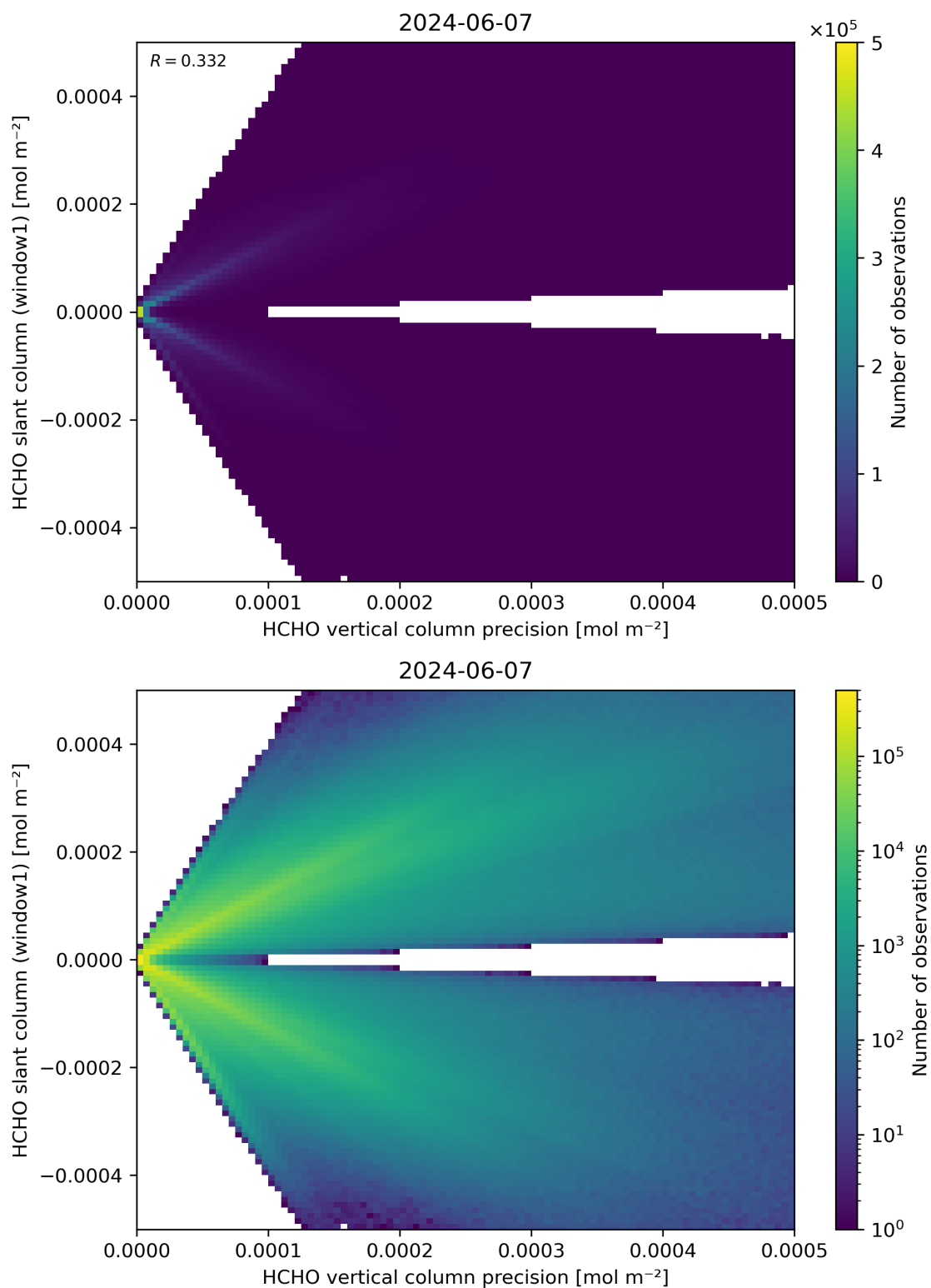
Figure 142: Scatter density plot of “HCHO vertical column precision” against “HCHO slant column (window1)” for 2024-06-06 to 2024-06-08.
