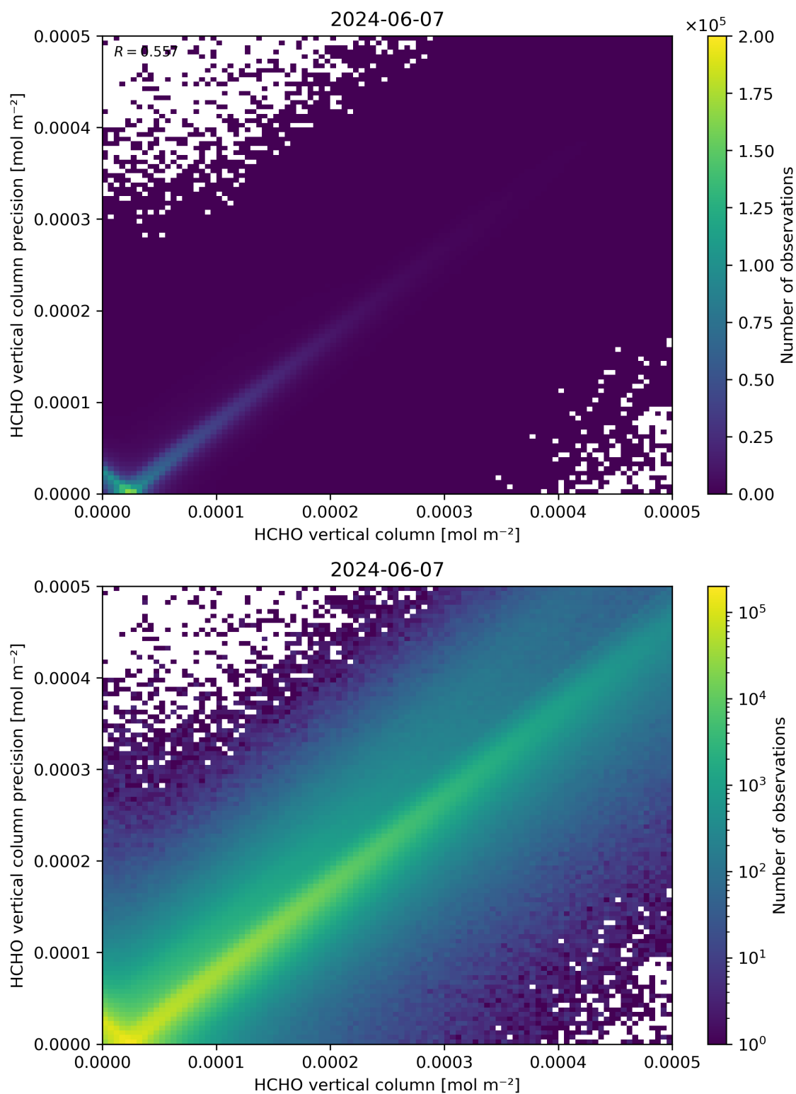
Figure 134: Scatter density plot of “HCHO vertical column” against “HCHO vertical column precision” for 2024-06-06 to 2024-06-08.
