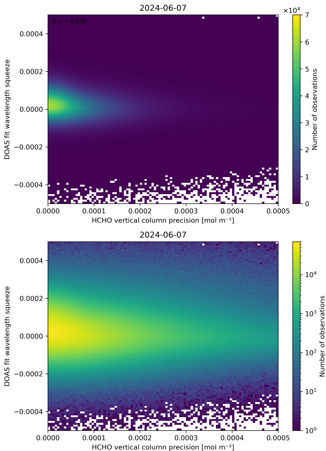
Figure 138: Scatter density plot of “HCHO vertical column precision” against “DOAS fit wavelength squeeze” for 2024-06-06 to 2024-06-08.
