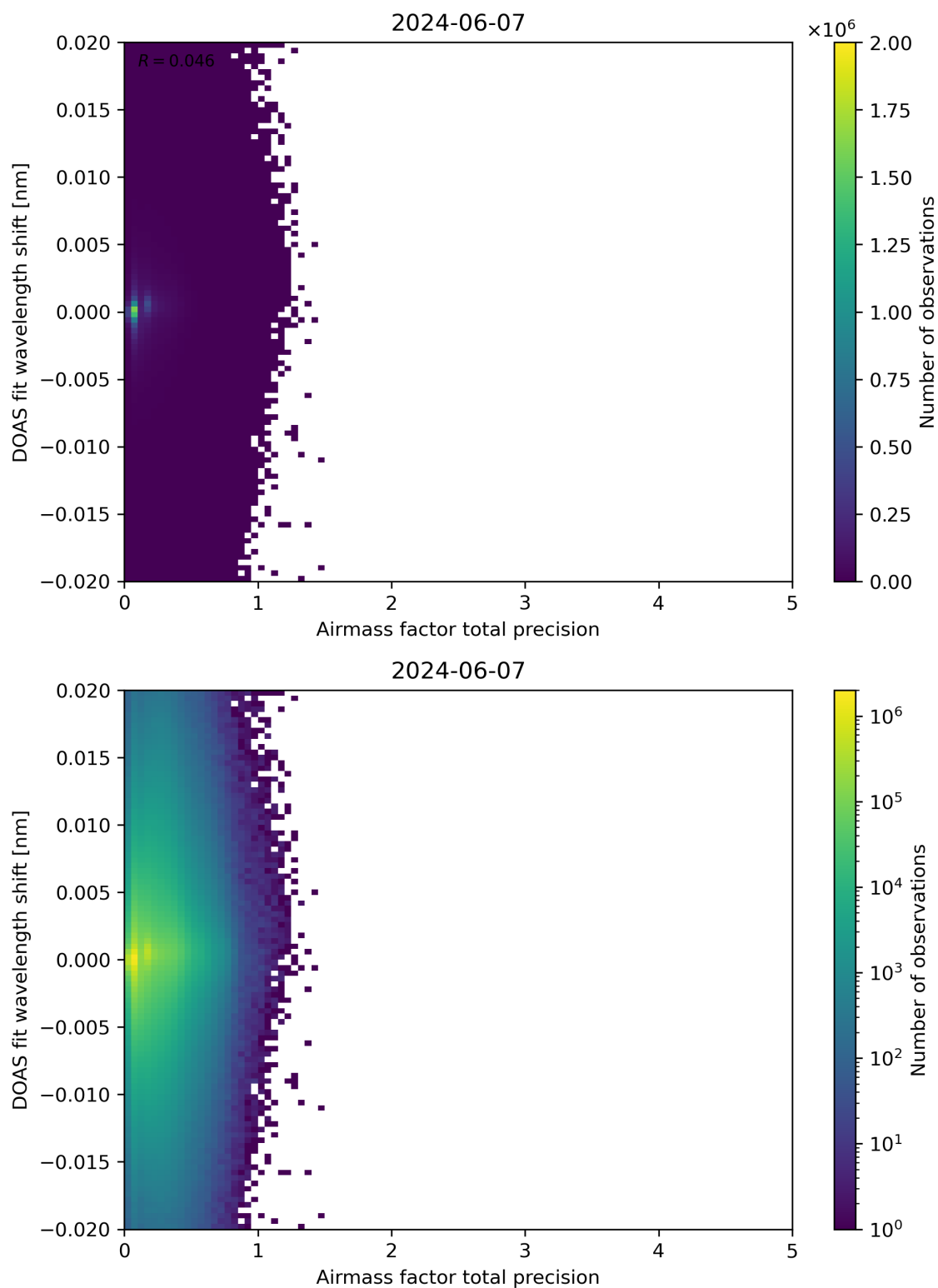
Figure 106: Scatter density plot of “Airmass factor total precision” against “DOAS fit wavelength shift” for 2024-06-06 to 2024-06-08.
