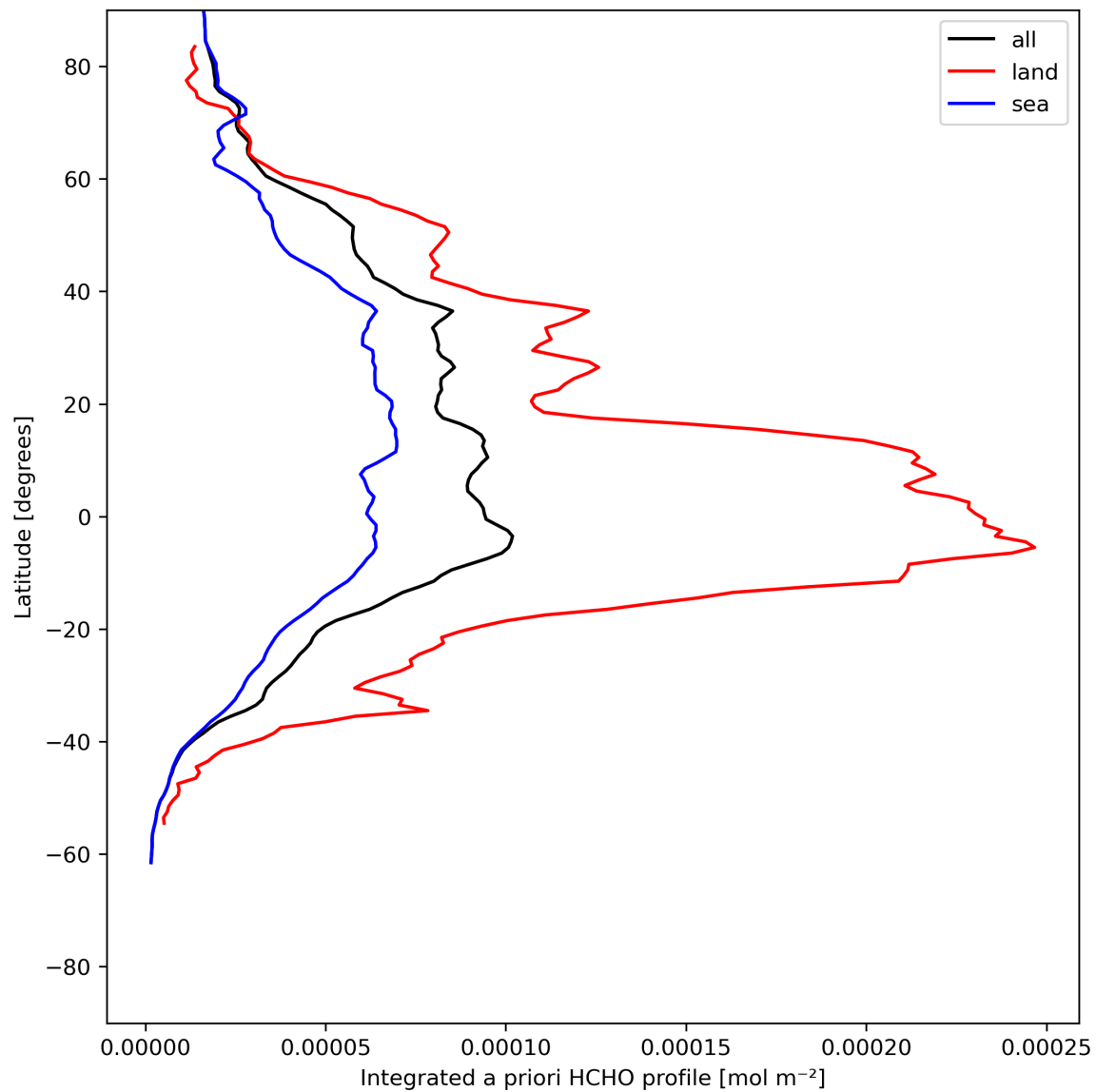
Figure 29: Zonal average of “Integrated a priori HCHO profile” for 2024-06-06 to 2024-06-08.
