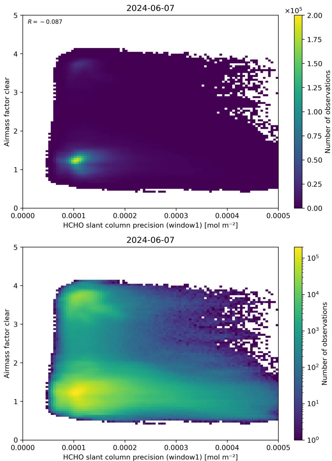
Figure 91: Scatter density plot of “HCHO slant column precision (window1)” against “Airmass factor clear” for 2024-06-06 to 2024-06-08.
