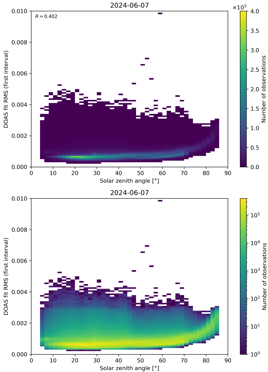
Figure 167: Scatter density plot of “Solar zenith angle” against “DOAS fit RMS (first interval)” for 2024-06-06 to 2024-06-08.
