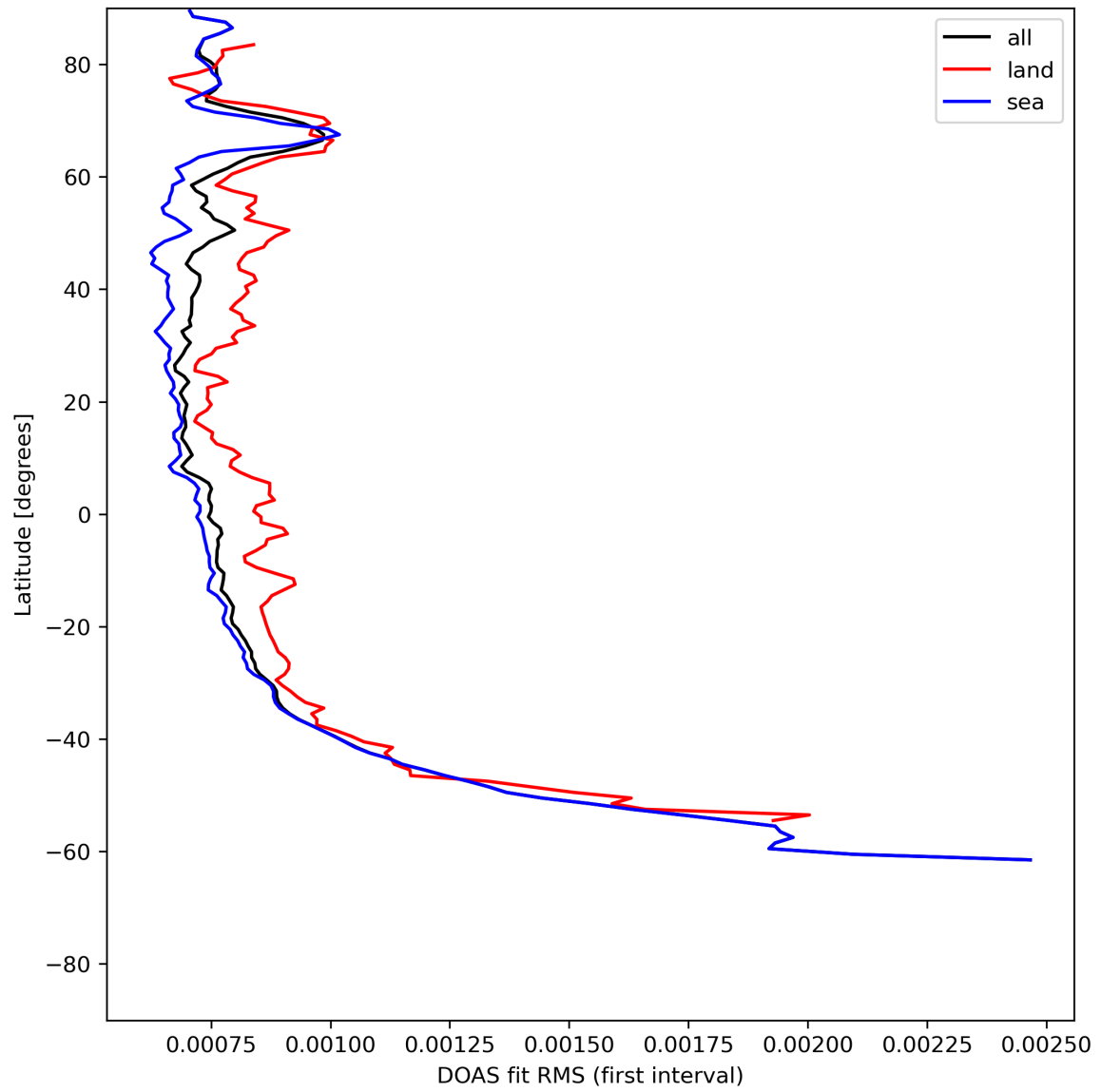
Figure 32: Zonal average of "DOAS fit RMS (first interval)" for 2024-06-06 to 2024-06-08.
