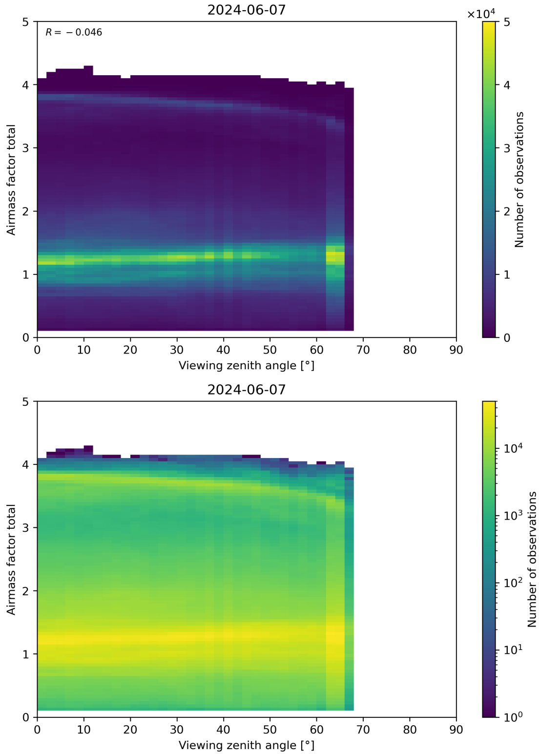
Figure 190: Scatter density plot of “Viewing zenith angle” against “Airmass factor total” for 2024-06-06 to 2024-06-08.
