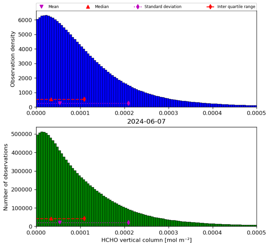
Figure 35: Histogram of “HCHO vertical column” for 2024-06-06 to 2024-06-08
