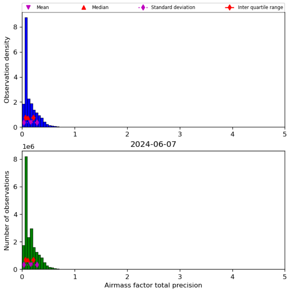
Figure 41: Histogram of “Airmass factor total precision” for 2024-06-06 to 2024-06-08
