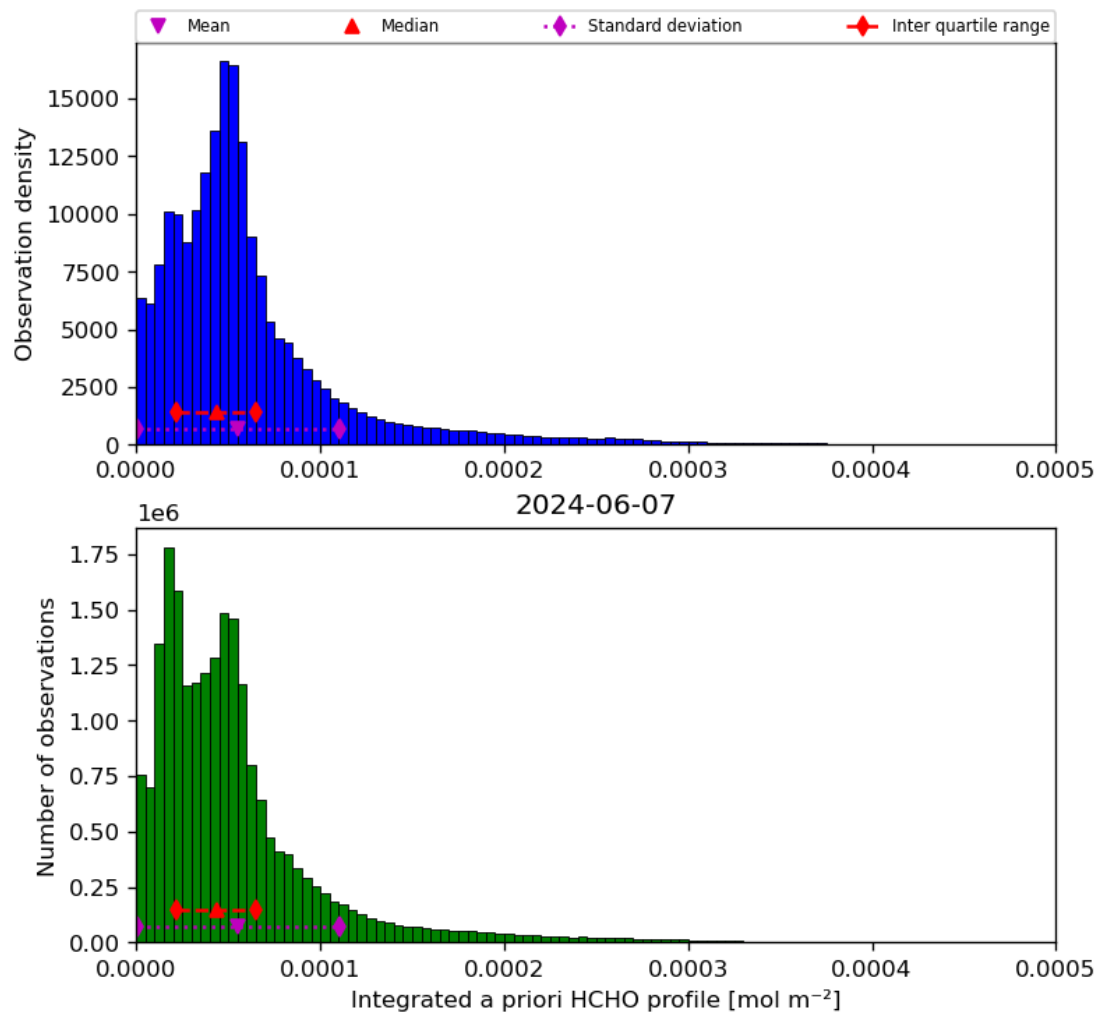
Figure 43: Histogram of “Integrated a priori HCHO profile” for 2024-06-06 to 2024-06-08
