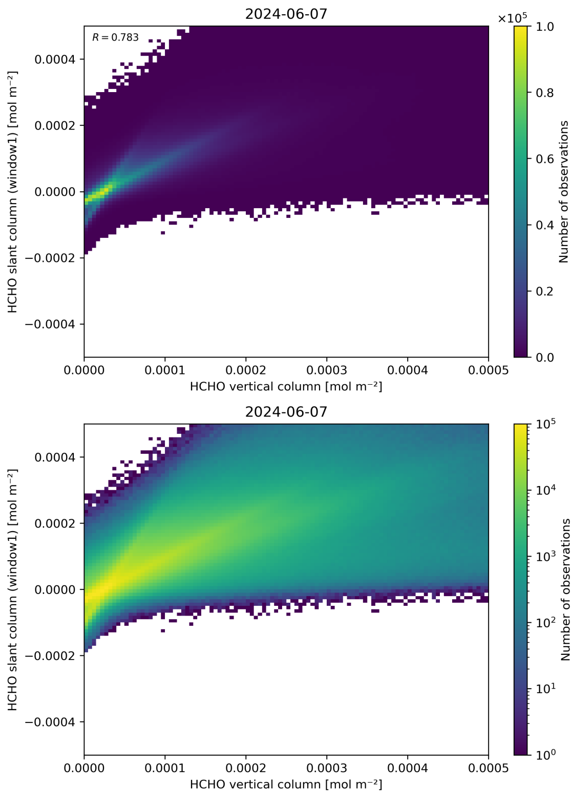
Figure 129: Scatter density plot of “HCHO vertical column” against “HCHO slant column (window1)” for 2024-06-06 to 2024-06-08.
