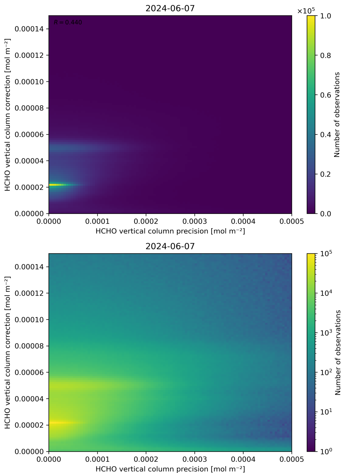
Figure 146: Scatter density plot of “HCHO vertical column precision” against “HCHO vertical column correction” for 2024-06-06 to 2024-06-08.
