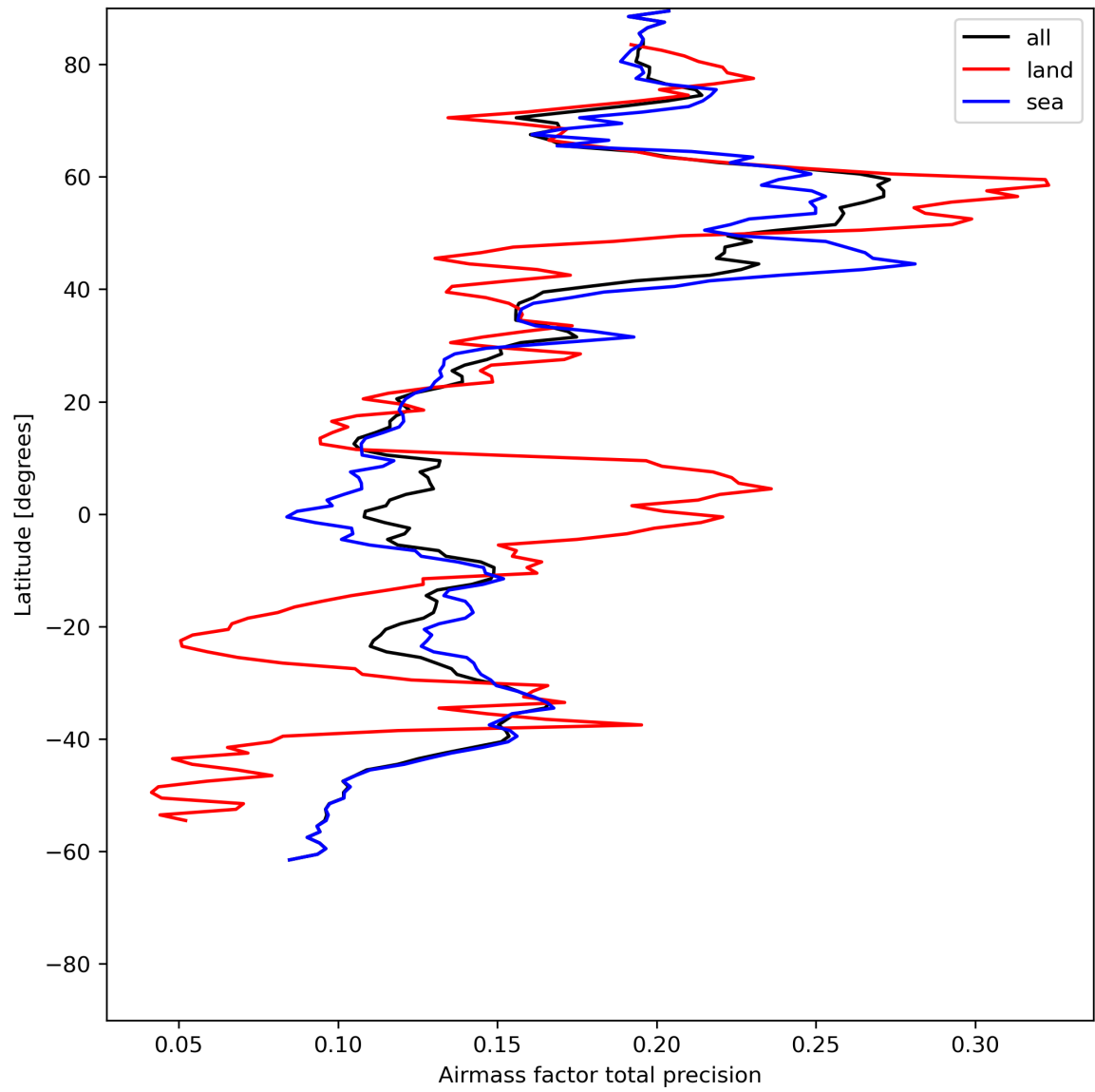
Figure 27: Zonal average of “Airmass factor total precision” for 2024-06-06 to 2024-06-08.
