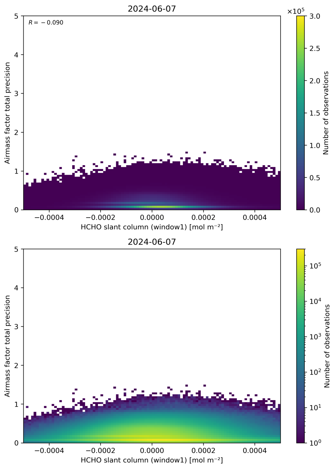
Figure 86: Scatter density plot of “HCHO slant column (window1)” against “Airmass factor total precision” for 2024-06-06 to 2024-06-08.
