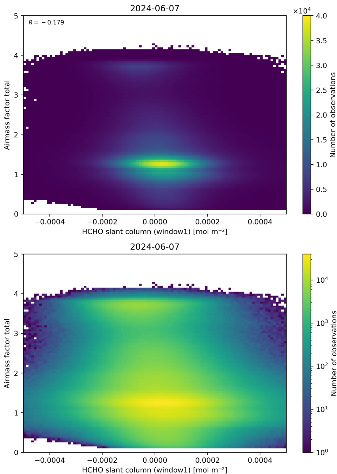
Figure 85: Scatter density plot of “HCHO slant column (window1)” against “Airmass factor total” for 2024-06-06 to 2024-06-08.
