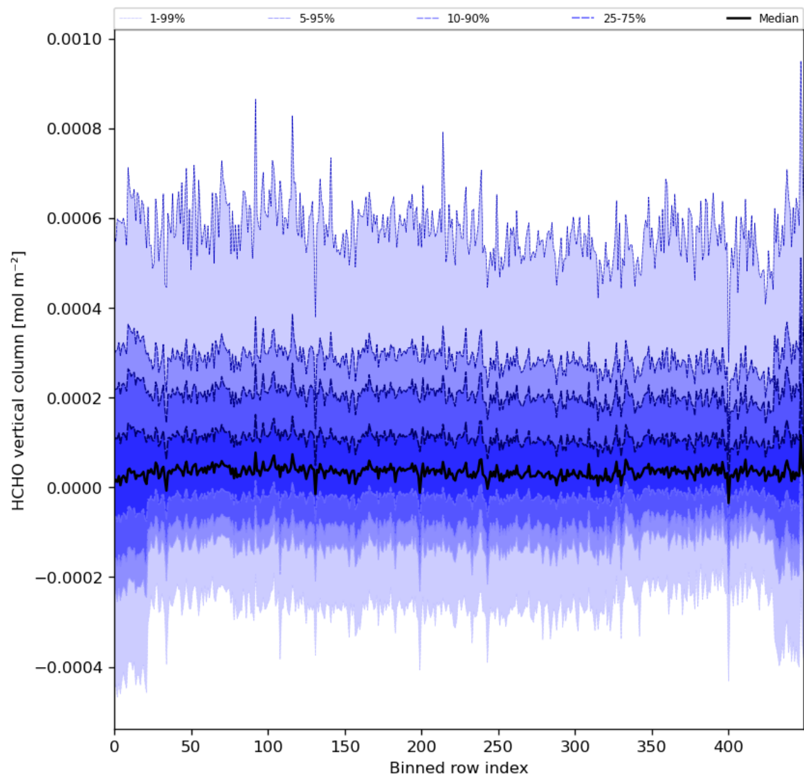
Figure 49: Along track statistics of “HCHO vertical column” for 2024-06-06 to 2024-06-08
