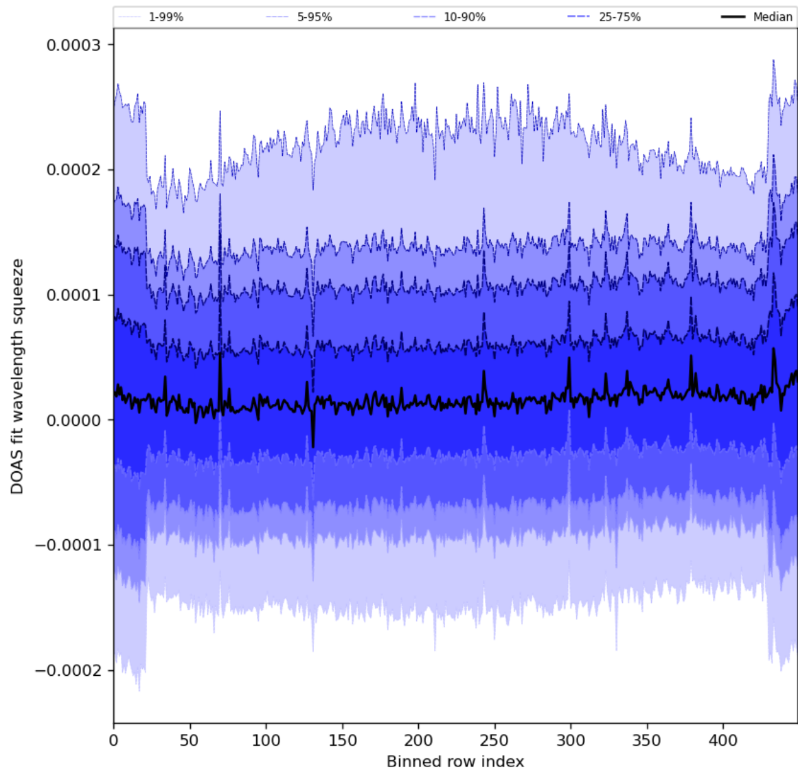
Figure 59: Along track statistics of “DOAS fit wavelength squeeze” for 2024-06-06 to 2024-06-08
