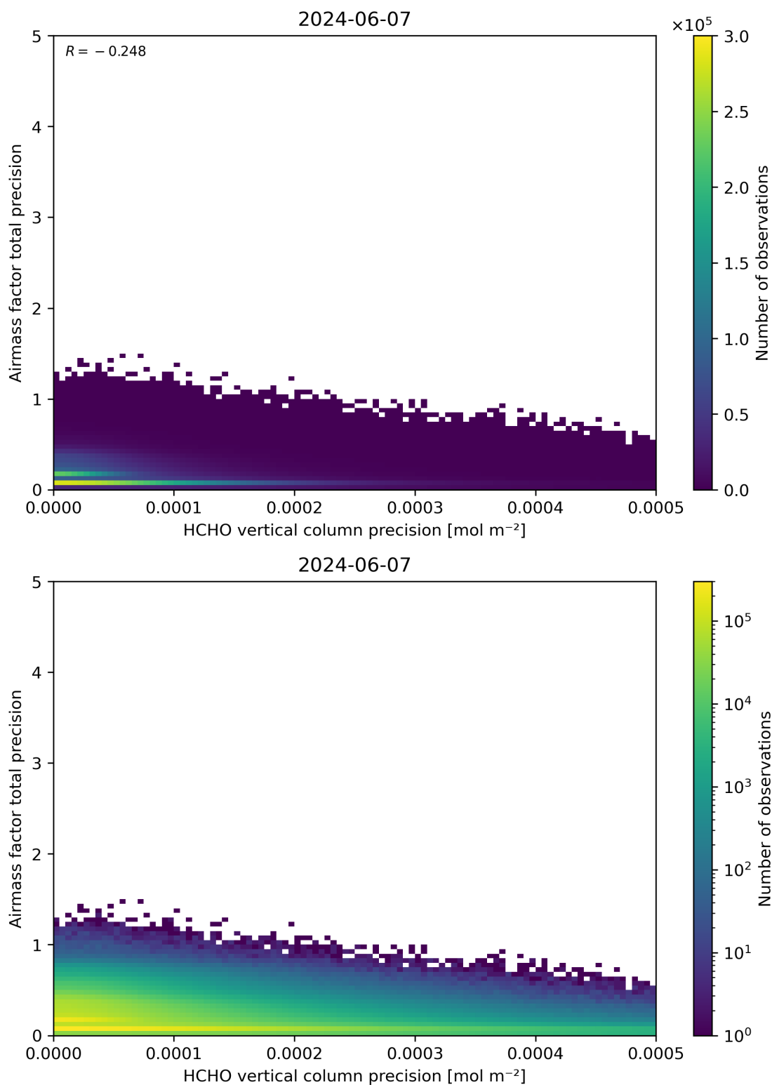
Figure 145: Scatter density plot of “HCHO vertical column precision” against “Airmass factor total precision” for 2024-06-06 to 2024-06-08.
