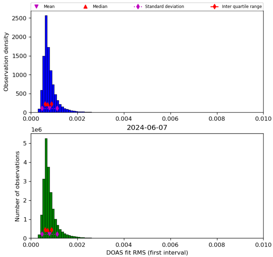
Figure 46: Histogram of “DOAS fit RMS (first interval)” for 2024-06-06 to 2024-06-08
