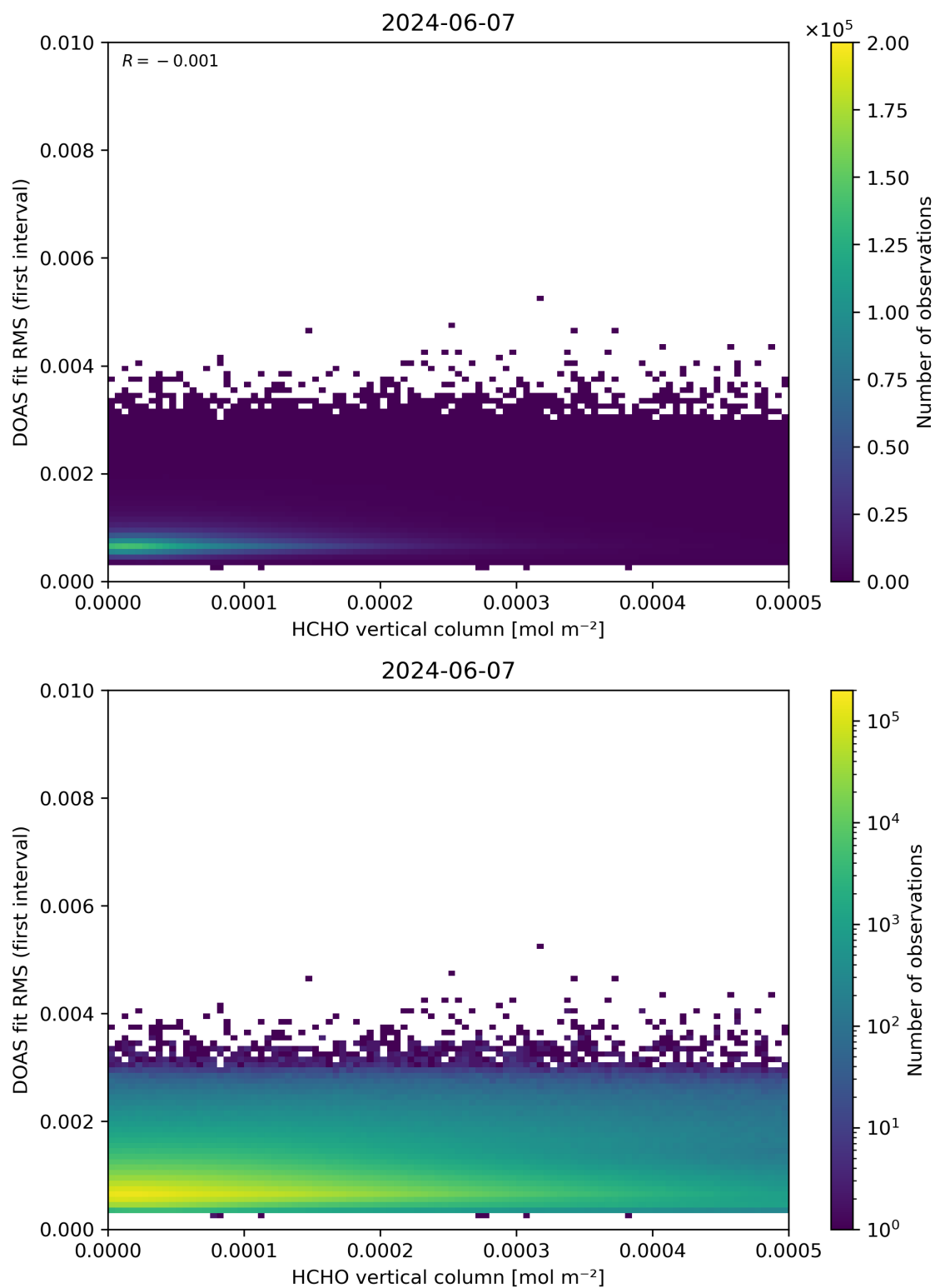
Figure 123: Scatter density plot of “HCHO vertical column” against “DOAS fit RMS (first interval)” for 2024-06-06 to 2024-06-08.
