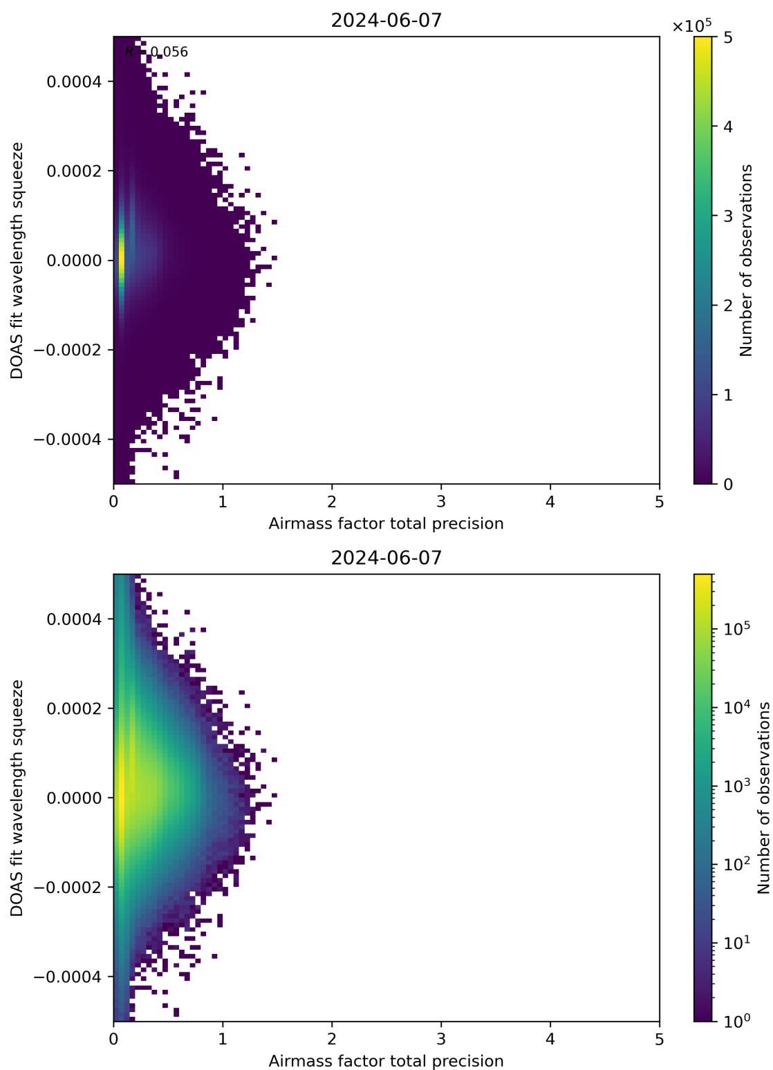
Figure 107: Scatter density plot of “Airmass factor total precision” against “DOAS fit wavelength squeeze” for 2024-06-06 to 2024-06-08.
