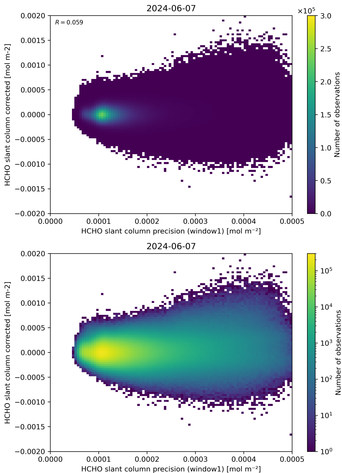
Figure 92: Scatter density plot of “HCHO slant column precision (window1)” against “HCHO slant column corrected” for 2024-06-06 to 2024-06-08.
