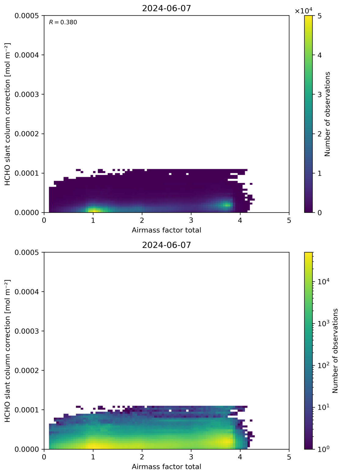
Figure 102: Scatter density plot of “Airmass factor total” against “HCHO slant column correction” for 2024-06-06 to 2024-06-08.
