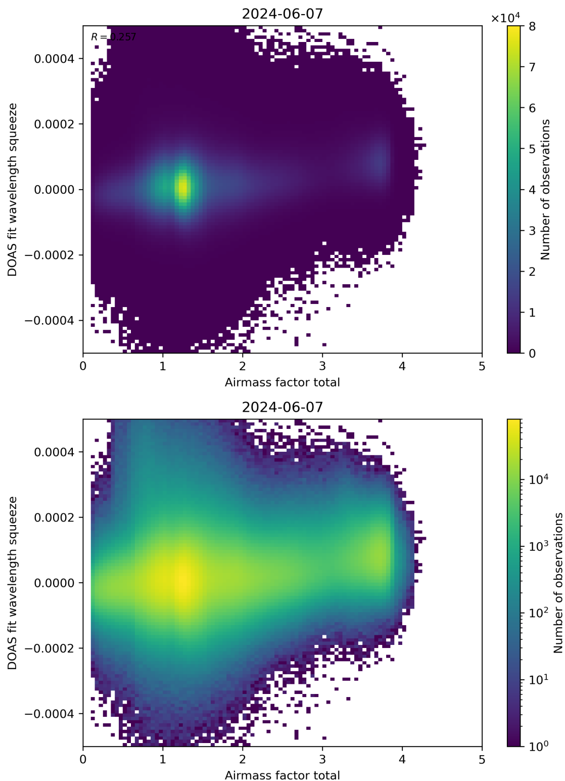
Figure 99: Scatter density plot of “Airmass factor total” against “DOAS fit wavelength squeeze” for 2024-06-06 to 2024-06-08.
