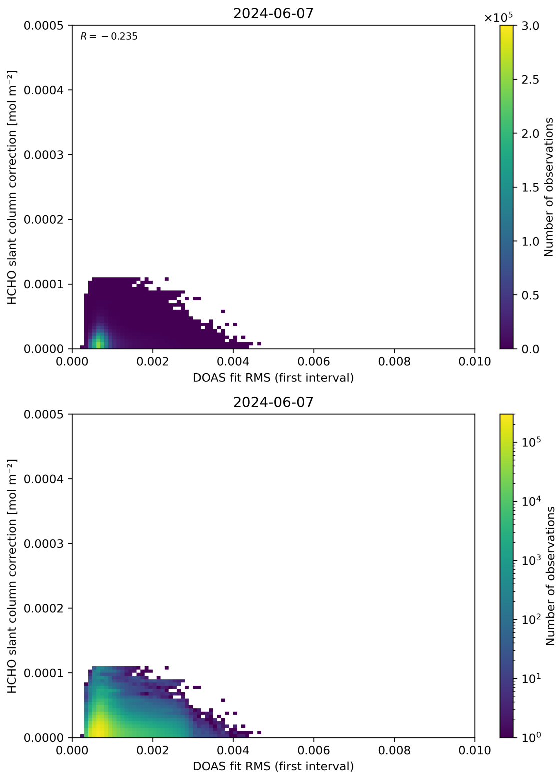
Figure 63: Scatter density plot of “DOAS fit RMS (first interval)” against “HCHO slant column correction” for 2024-06-06 to 2024-06-08.
