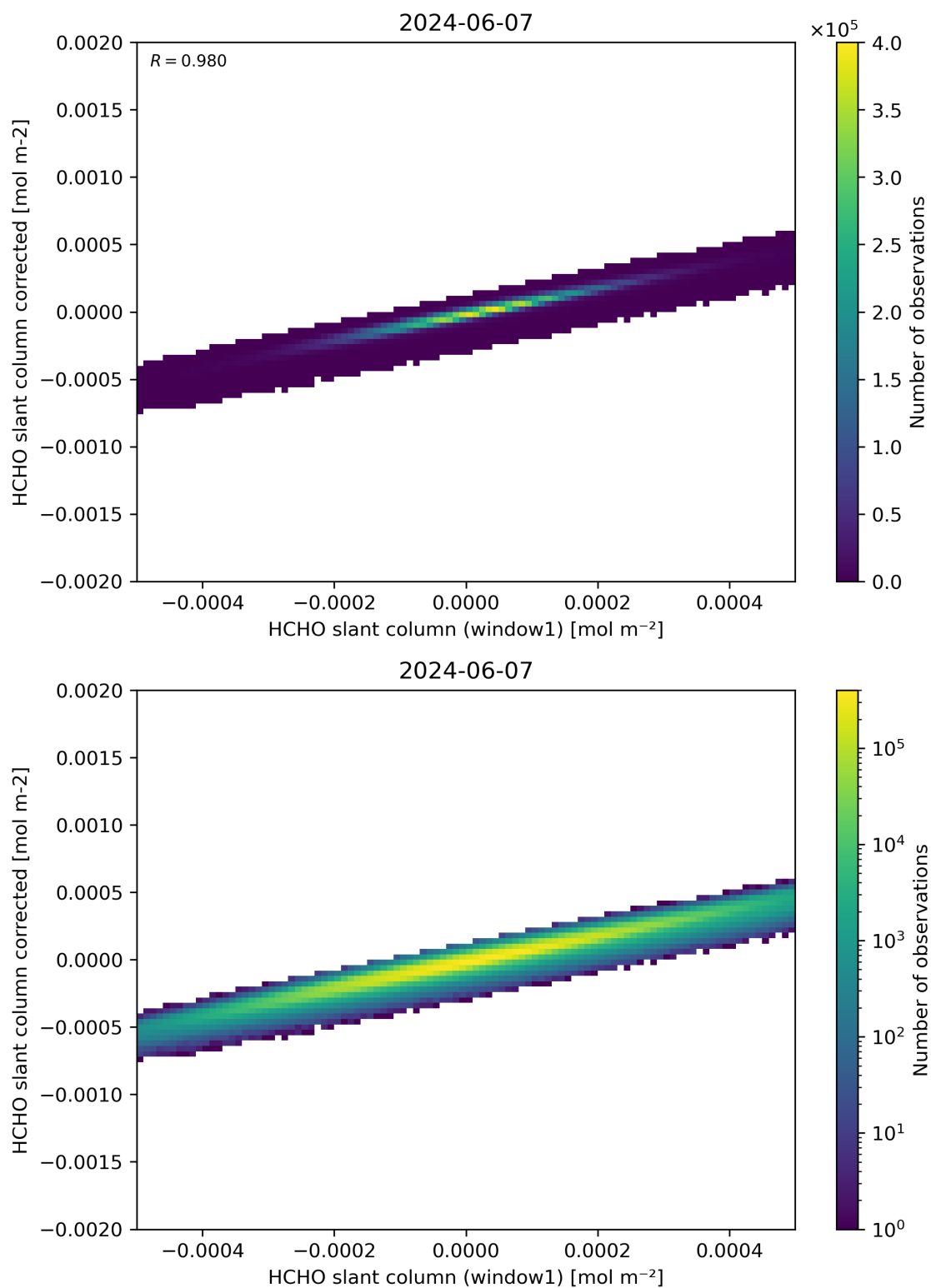
Figure 82: Scatter density plot of “HCHO slant column (window1)” against “HCHO slant column corrected” for 2024-06-06 to 2024-06-08.
