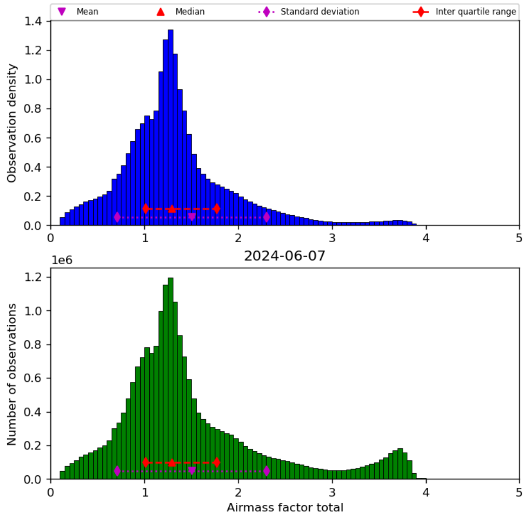
Figure 40: Histogram of “Airmass factor total” for 2024-06-06 to 2024-06-08
