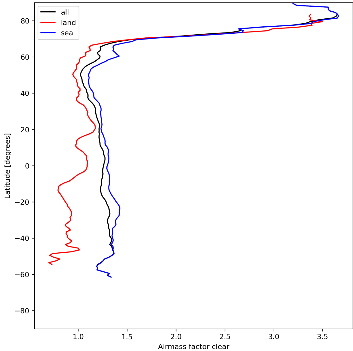
Figure 28: Zonal average of “Airmass factor clear” for 2024-06-06 to 2024-06-08.
