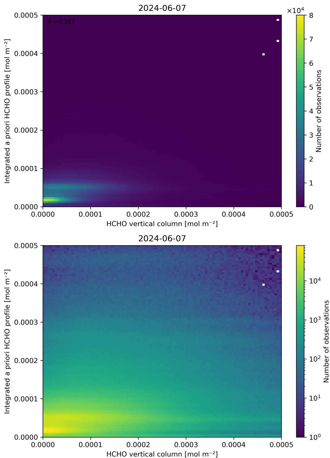
Figure 135: Scatter density plot of “HCHO vertical column” against “Integrated a priori HCHO profile” for 2024-06-06 to 2024-06-08.
