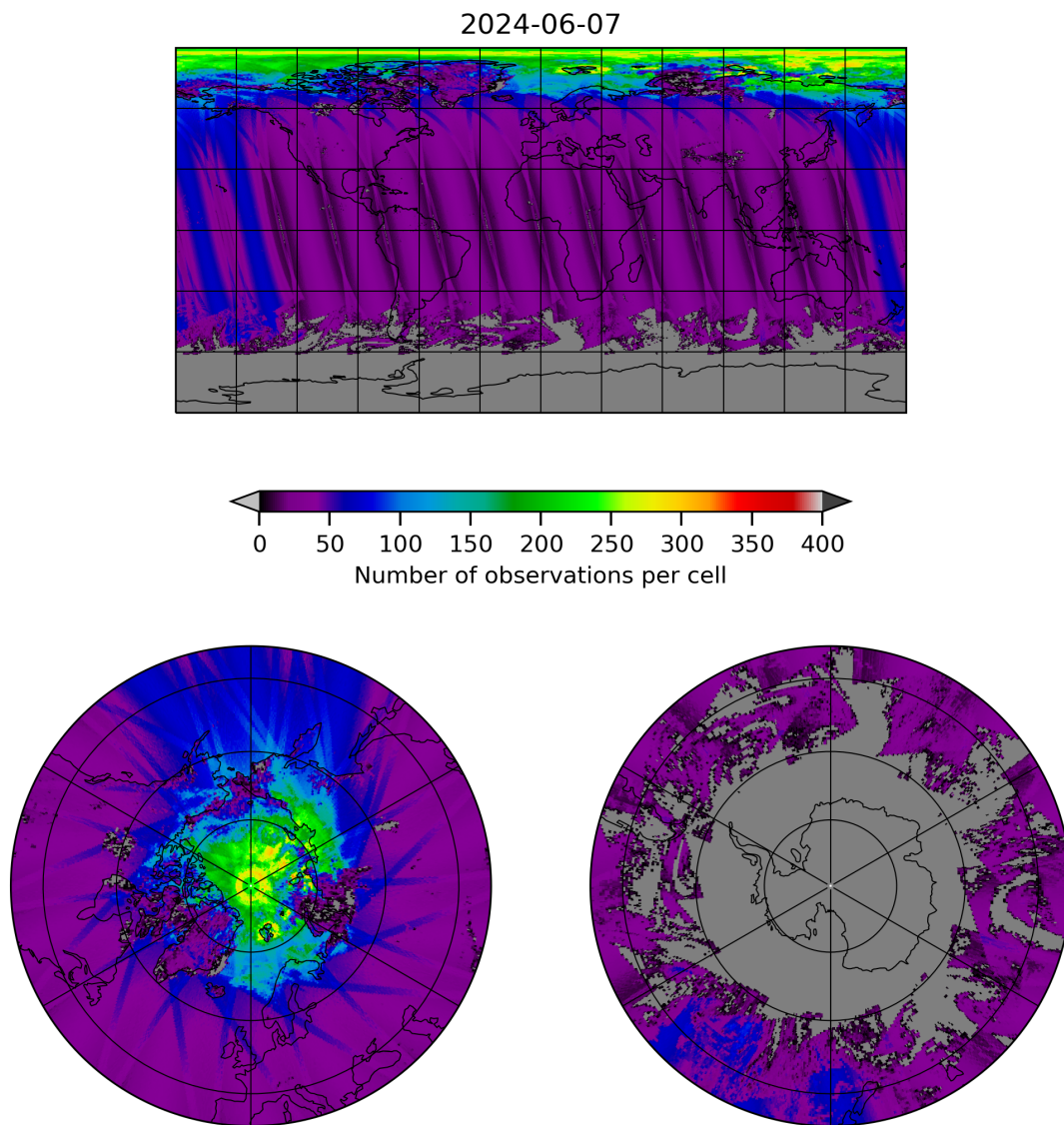
Figure 19: Map of the number of observations for 2024-06-06 to 2024-06-08
