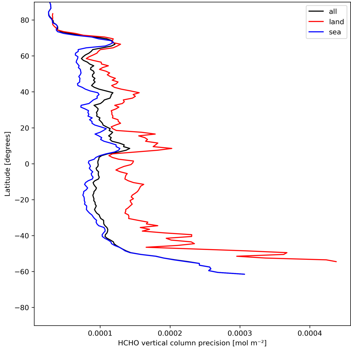
Figure 22: Zonal average of “HCHO vertical column precision” for 2024-06-06 to 2024-06-08.
