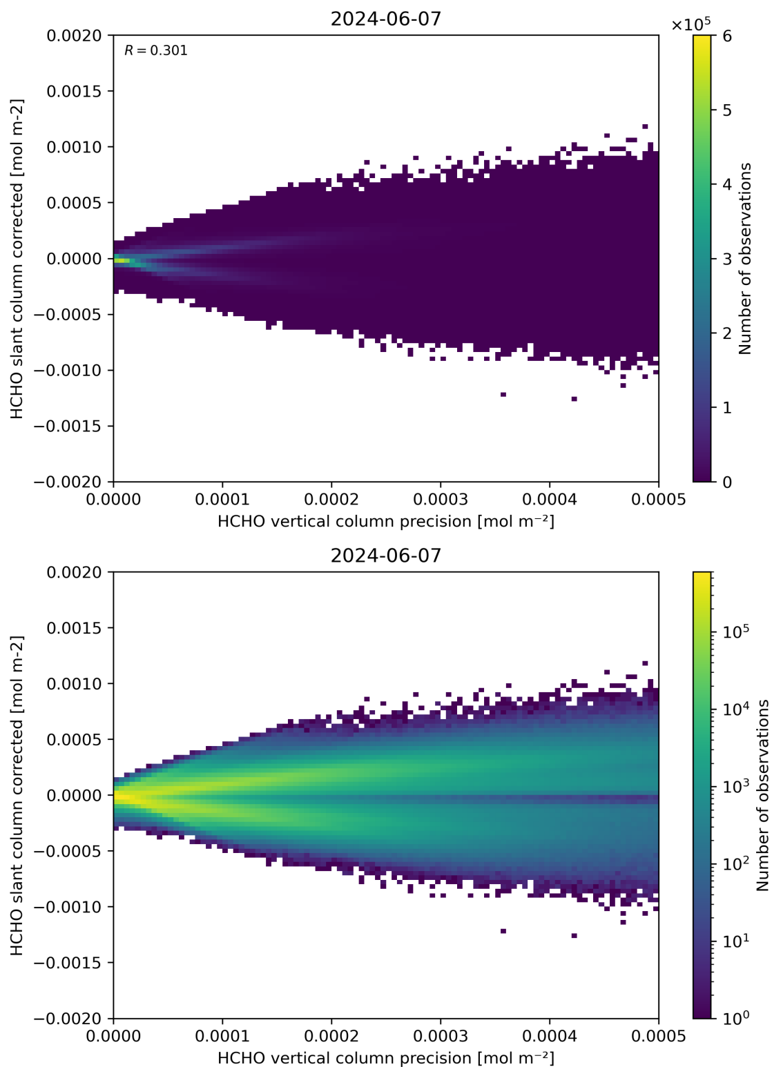
Figure 140: Scatter density plot of “HCHO vertical column precision” against “HCHO slant column corrected” for 2024-06-06 to 2024-06-08.
