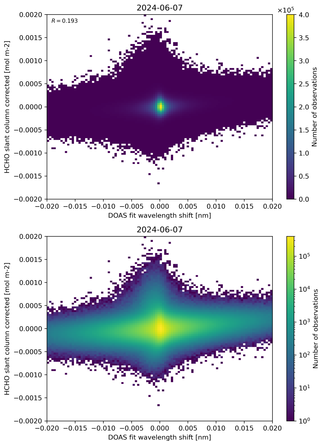
Figure 66: Scatter density plot of “DOAS fit wavelength shift” against “HCHO slant column corrected” for 2024-06-06 to 2024-06-08.
