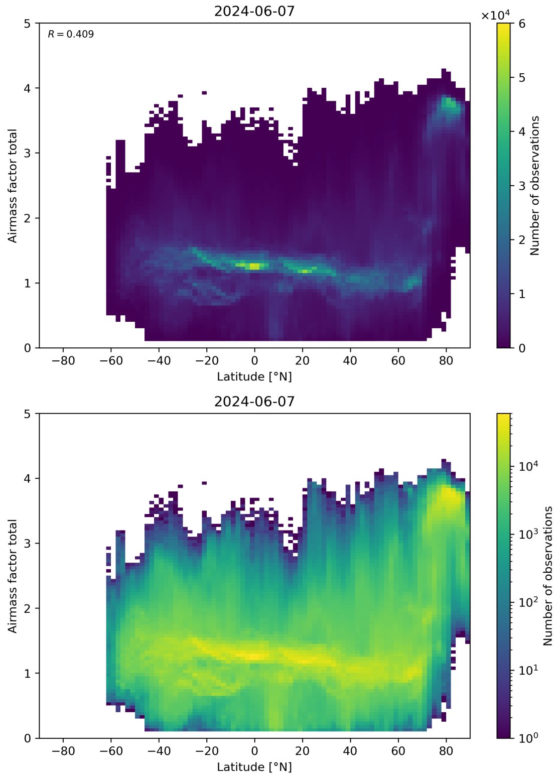
Figure 161: Scatter density plot of “Latitude” against “Airmass factor total” for 2024-06-06 to 2024-06-08.
