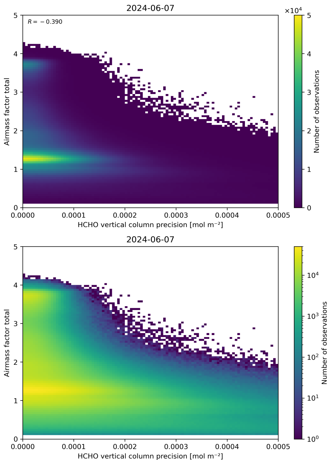
Figure 144: Scatter density plot of “HCHO vertical column precision” against “Airmass factor total” for 2024-06-06 to 2024-06-08.
