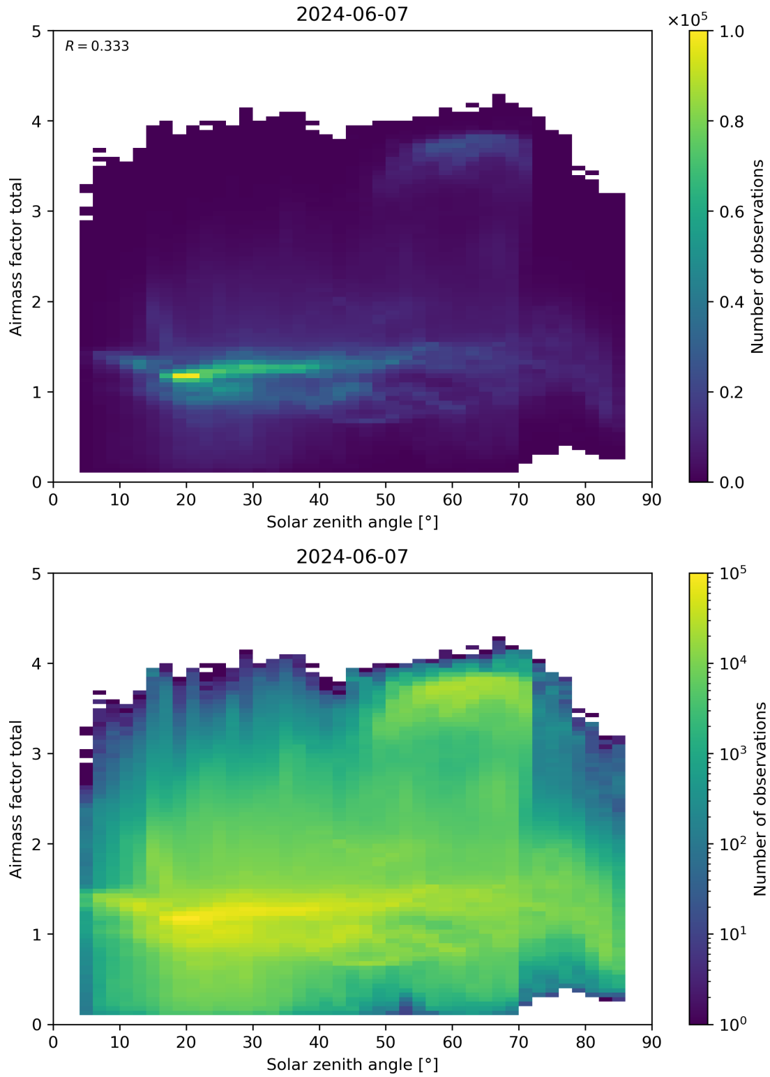
Figure 175: Scatter density plot of “Solar zenith angle” against “Airmass factor total” for 2024-06-06 to 2024-06-08.
