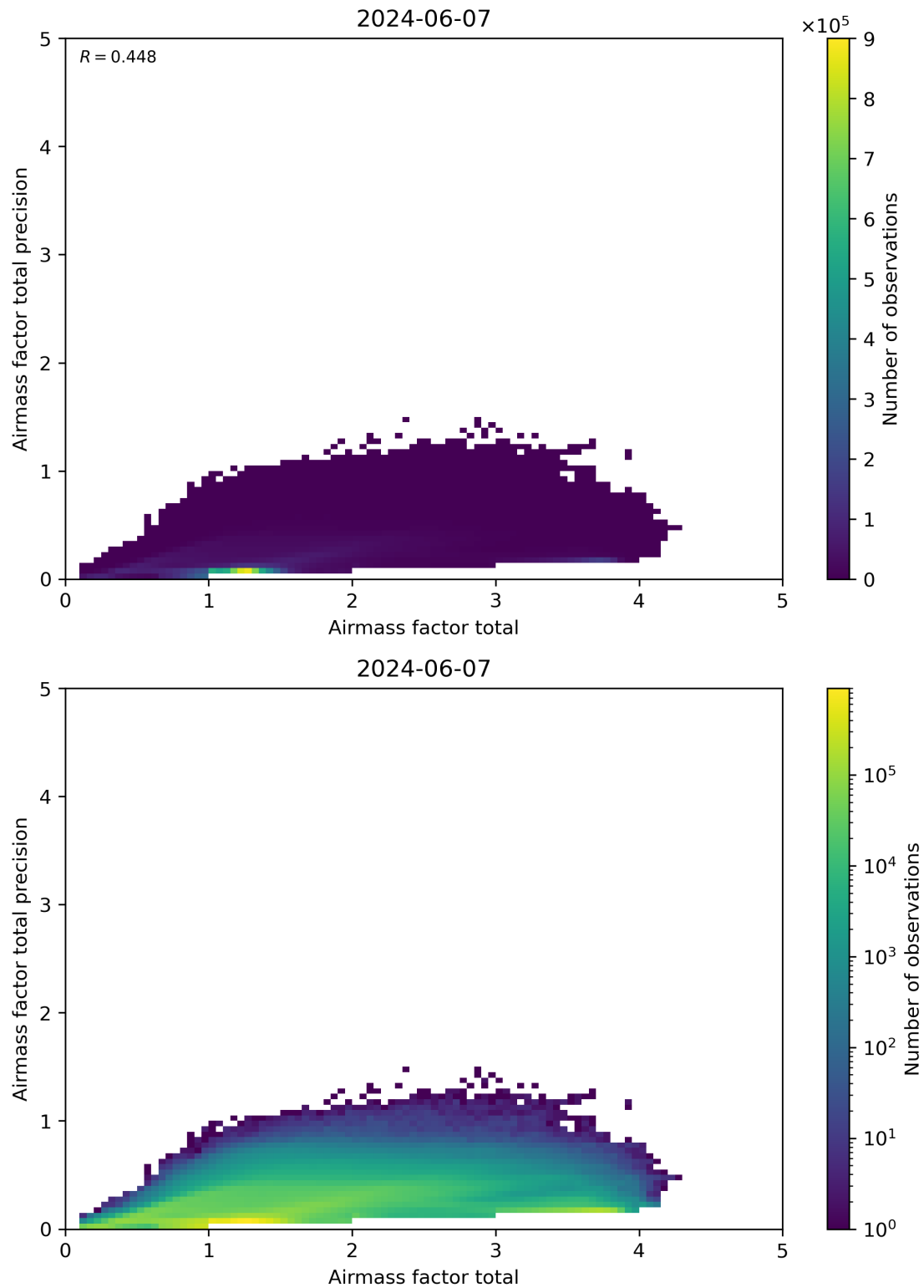
Figure 103: Scatter density plot of “Airmass factor total” against “Airmass factor total precision” for 2024-06-06 to 2024-06-08.
