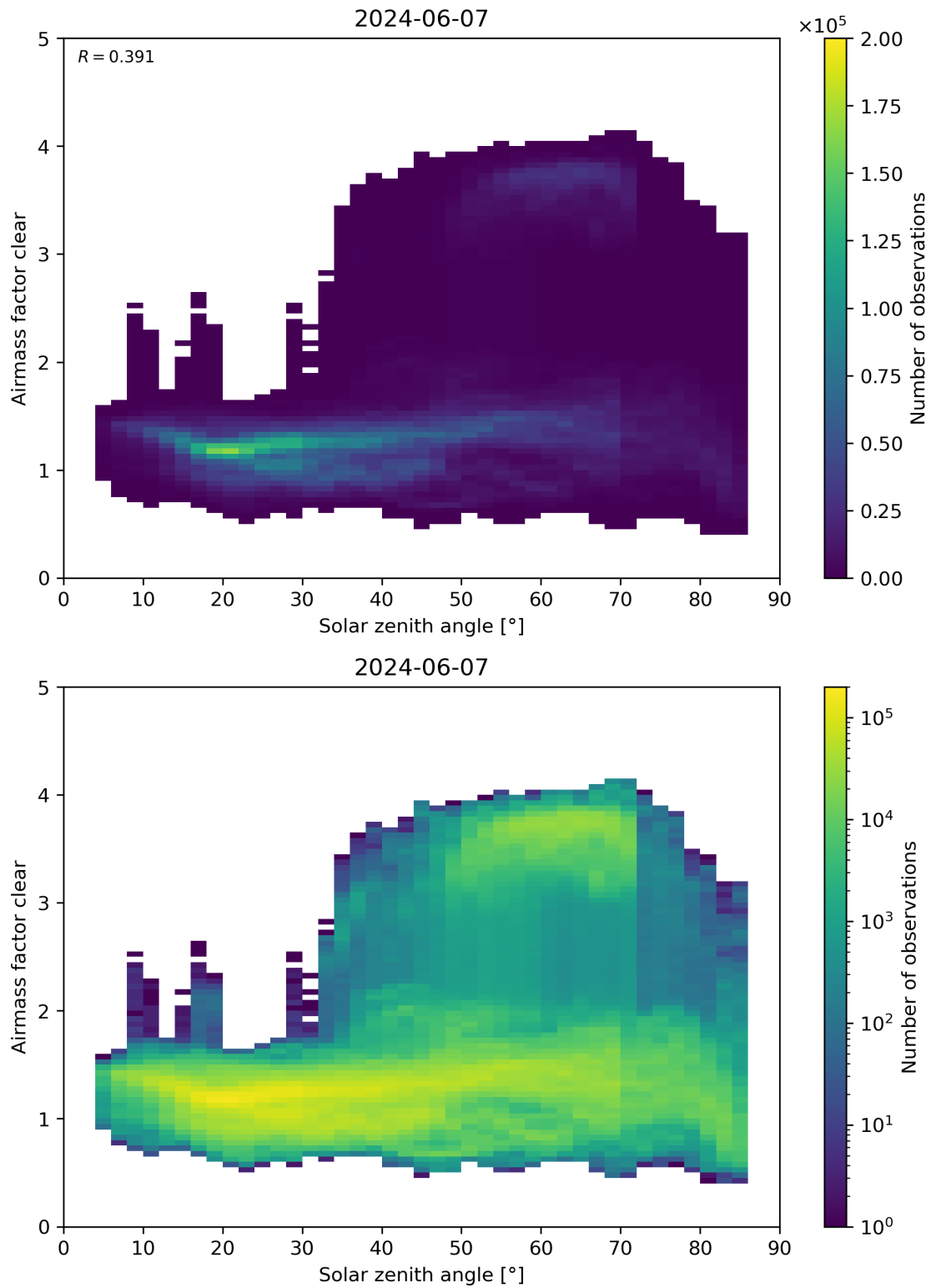
Figure 170: Scatter density plot of “Solar zenith angle” against “Airmass factor clear” for 2024-06-06 to 2024-06-08.
