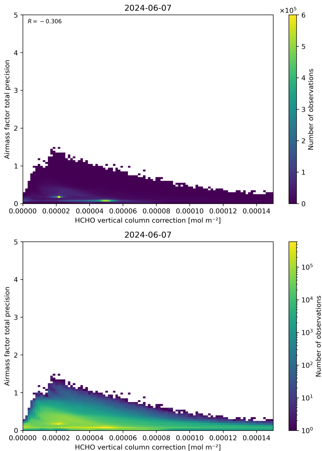
Figure 121: Scatter density plot of “HCHO vertical column correction” against “Airmass factor total precision” for 2024-06-06 to 2024-06-08.
