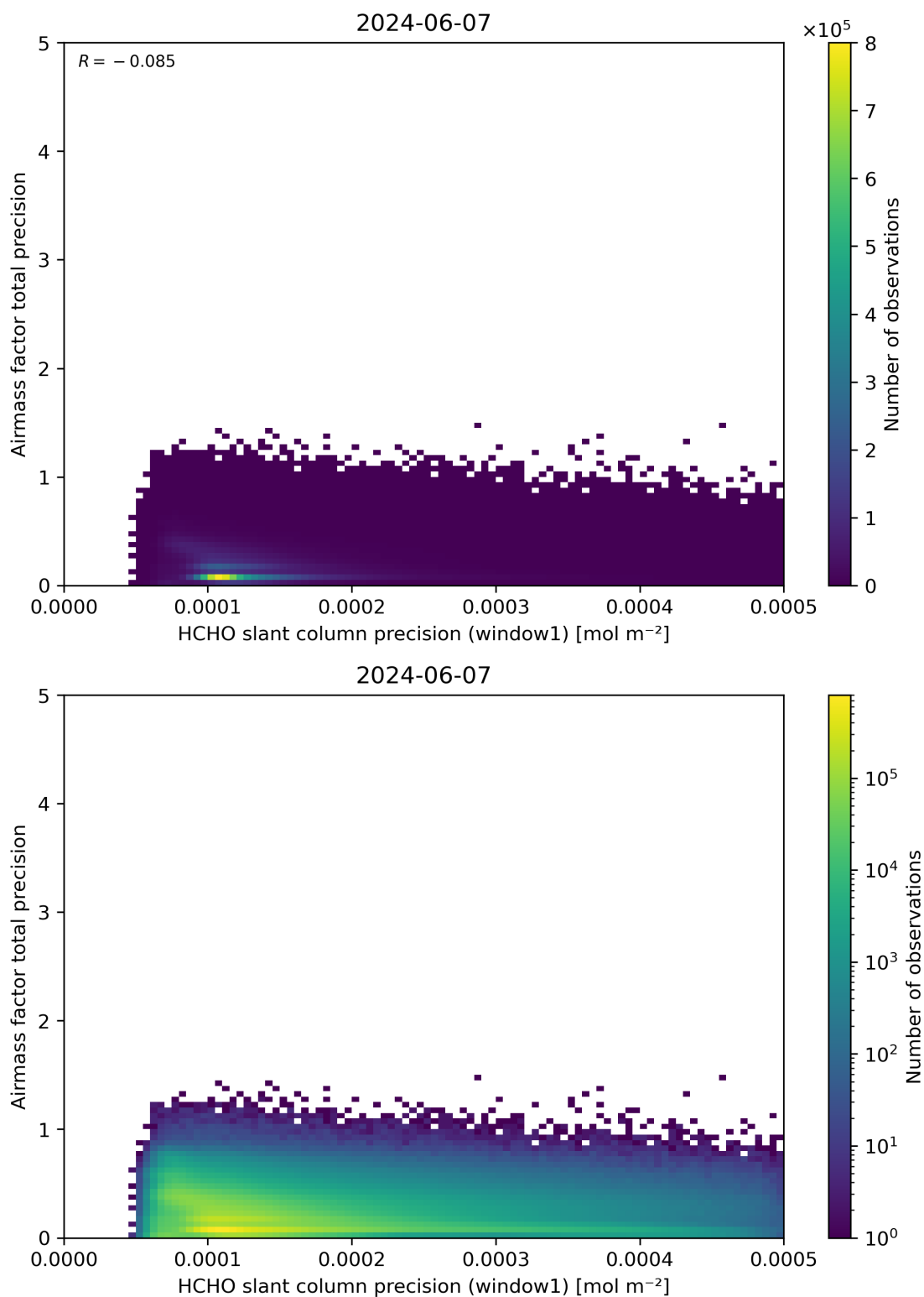
Figure 95: Scatter density plot of “HCHO slant column precision (window1)” against “Airmass factor total precision” for 2024-06-06 to 2024-06-08.
