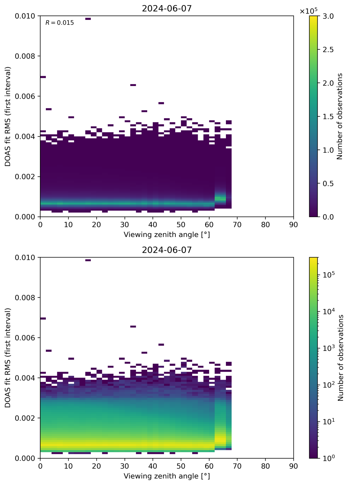
Figure 182: Scatter density plot of “Viewing zenith angle” against “DOAS fit RMS (first interval)” for 2024-06-06 to 2024-06-08.
