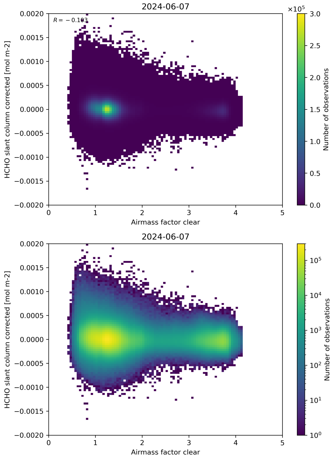
Figure 74: Scatter density plot of “Airmass factor clear” against “HCHO slant column corrected” for 2024-06-06 to 2024-06-08.
