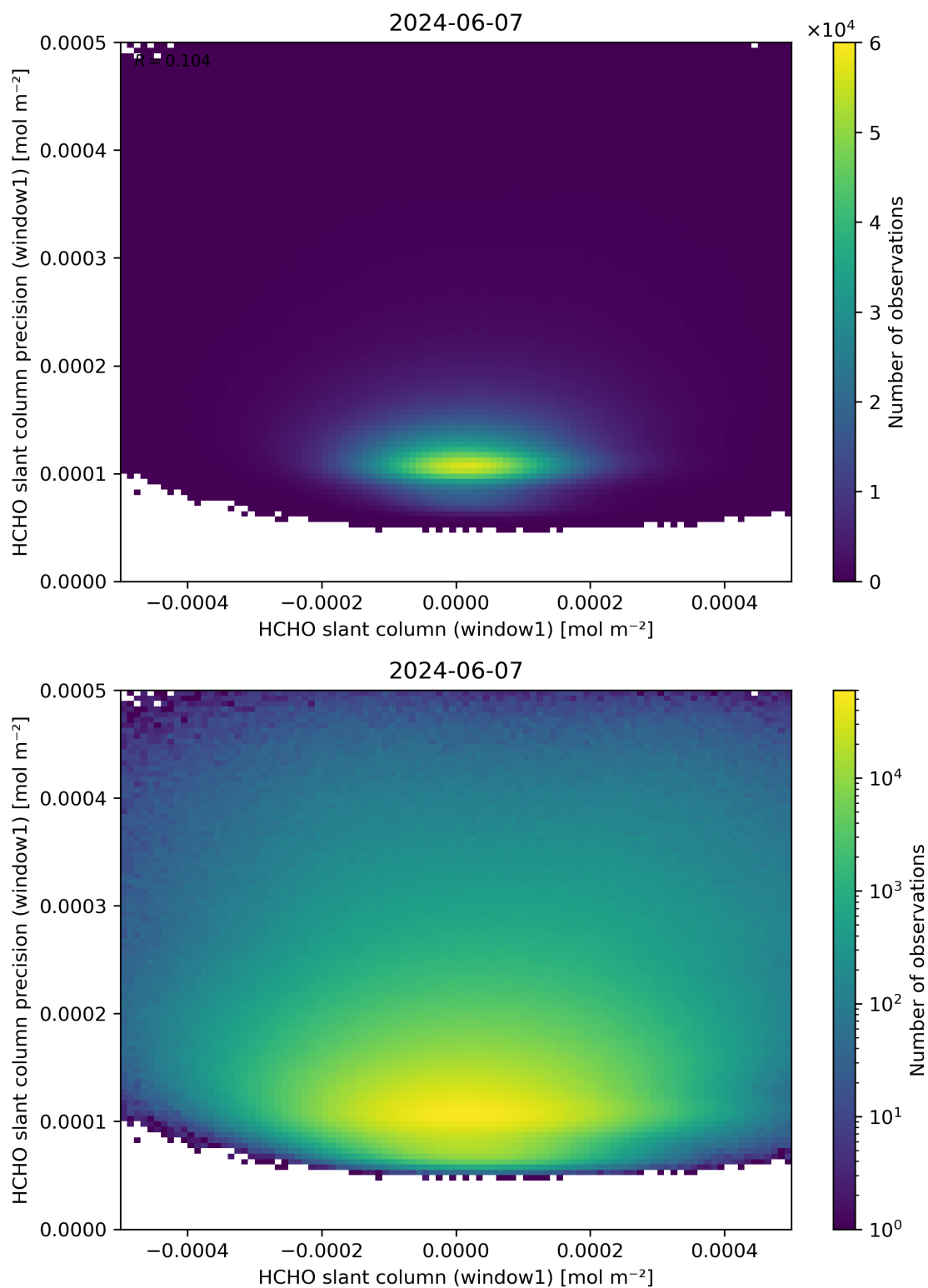
Figure 84: Scatter density plot of “HCHO slant column (window1)” against “HCHO slant column precision (window1)” for 2024-06-06 to 2024-06-08.
