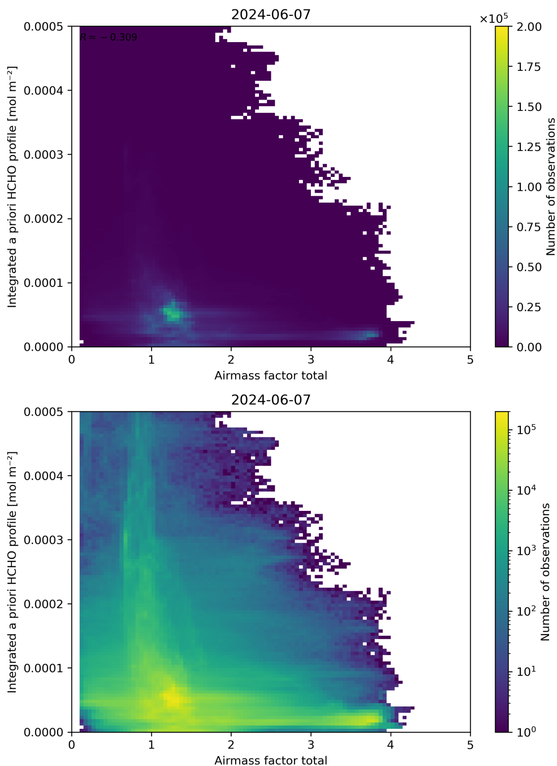
Figure 104: Scatter density plot of “Airmass factor total” against “Integrated a priori HCHO profile” for 2024-06-06 to 2024-06-08.
