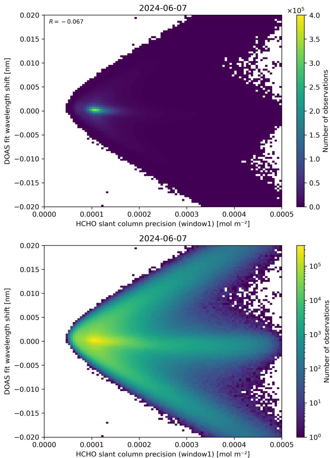
Figure 89: Scatter density plot of “HCHO slant column precision (window1)” against “DOAS fit wavelength shift” for 2024-06-06 to 2024-06-08.
