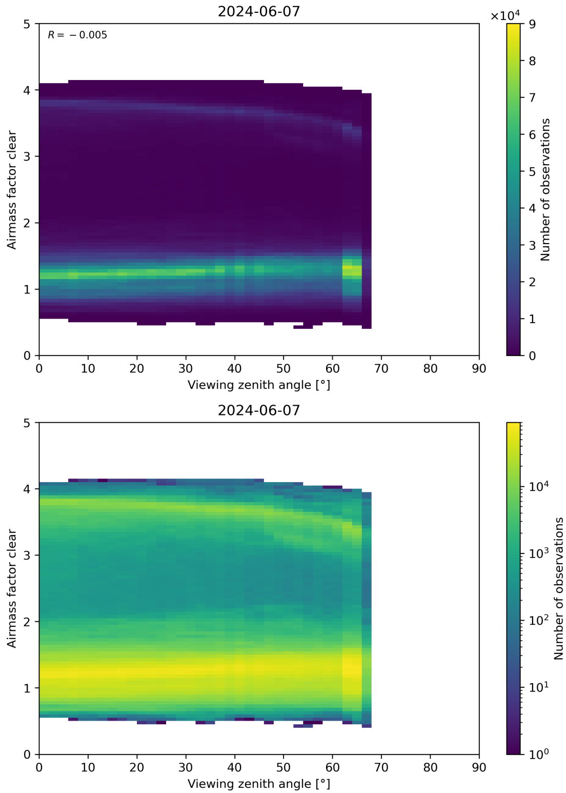
Figure 185: Scatter density plot of “Viewing zenith angle” against “Airmass factor clear” for 2024-06-06 to 2024-06-08.
