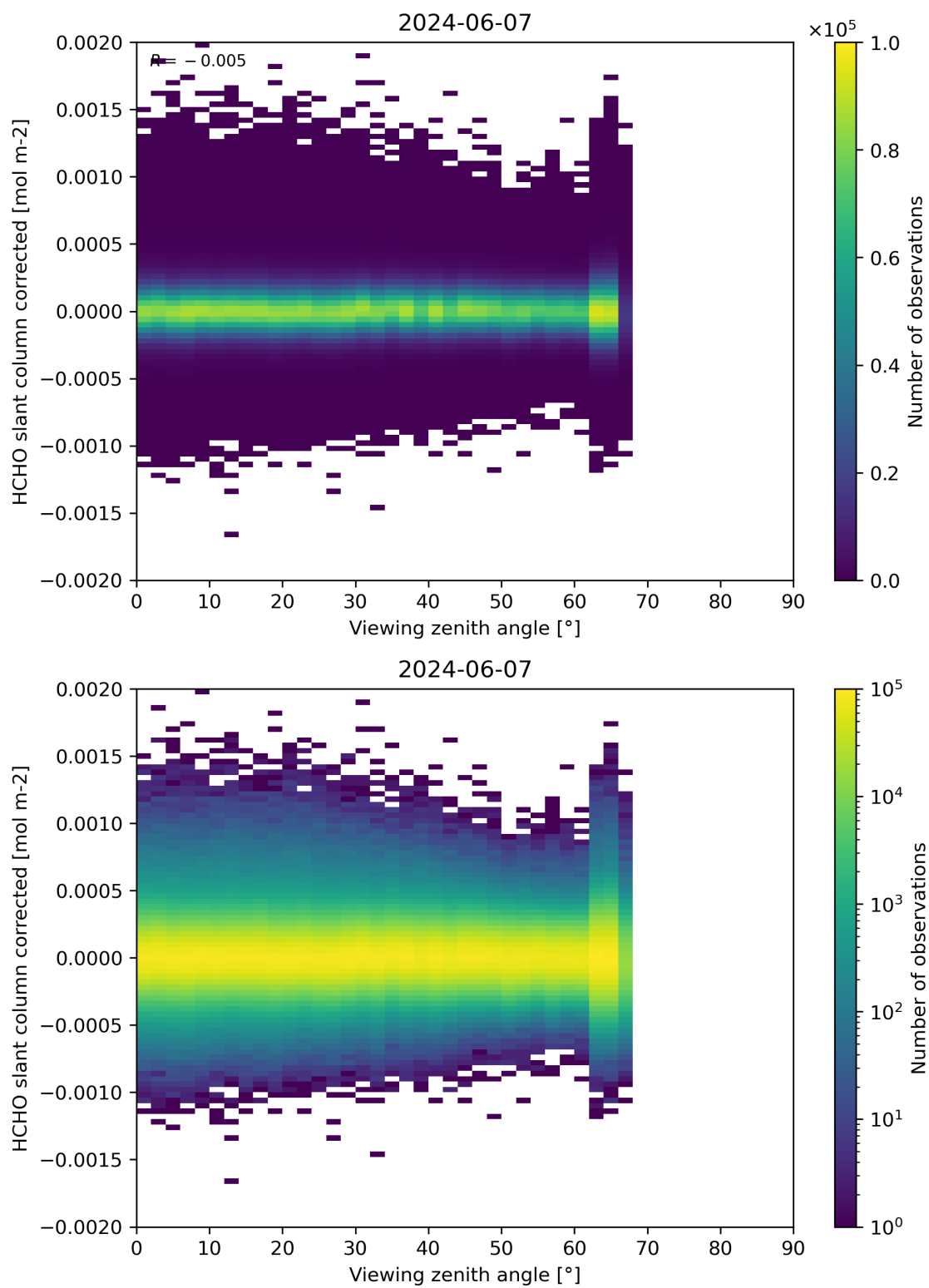
Figure 186: Scatter density plot of “Viewing zenith angle” against “HCHO slant column corrected” for 2024-06-06 to 2024-06-08.
