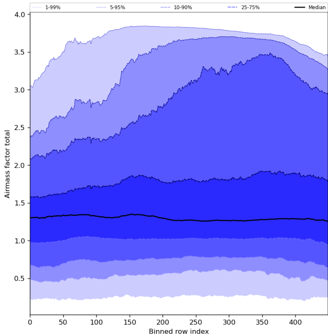
Figure 54: Along track statistics of “Airmass factor total” for 2024-06-06 to 2024-06-08
