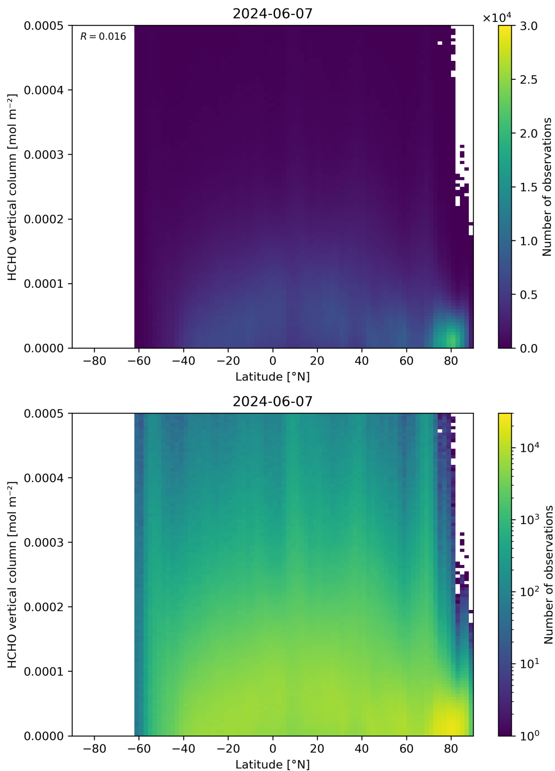
Figure 163: Scatter density plot of “Latitude” against “HCHO vertical column” for 2024-06-06 to 2024-06-08.
