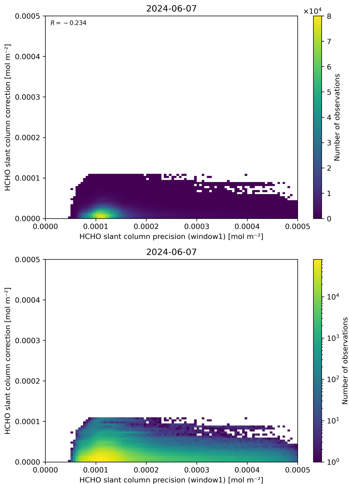
Figure 93: Scatter density plot of “HCHO slant column precision (window1)” against “HCHO slant column correction” for 2024-06-06 to 2024-06-08.
