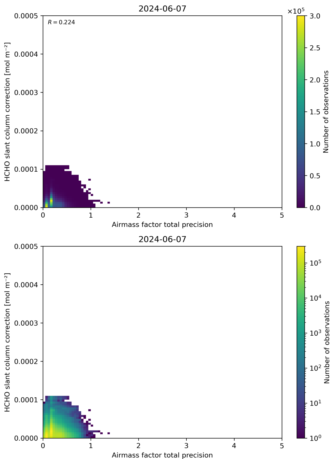
Figure 110: Scatter density plot of “Airmass factor total precision” against “HCHO slant column correction” for 2024-06-06 to 2024-06-08.
