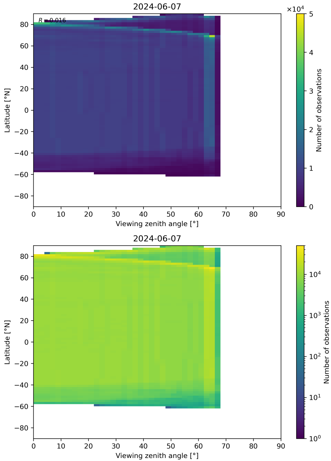
Figure 196: Scatter density plot of “Viewing zenith angle” against “Latitude” for 2024-06-06 to 2024-06-08.
