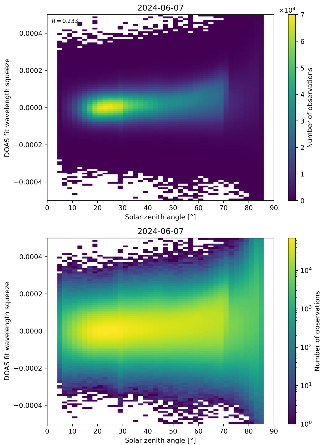
Figure 169: Scatter density plot of “Solar zenith angle” against “DOAS fit wavelength squeeze” for 2024-06-06 to 2024-06-08.
