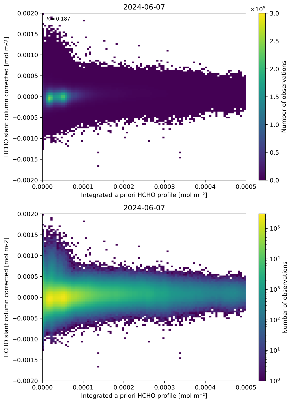
Figure 151: Scatter density plot of “Integrated a priori HCHO profile” against “HCHO slant column corrected” for 2024-06-06 to 2024-06-08.
