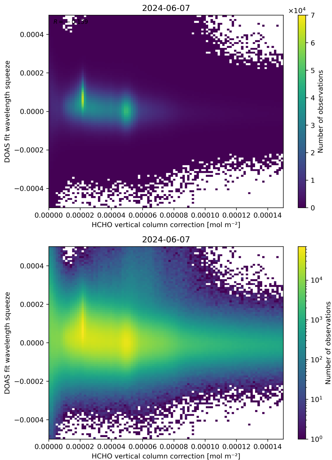
Figure 114: Scatter density plot of “HCHO vertical column correction” against “DOAS fit wavelength squeeze” for 2024-06-06 to 2024-06-08.
