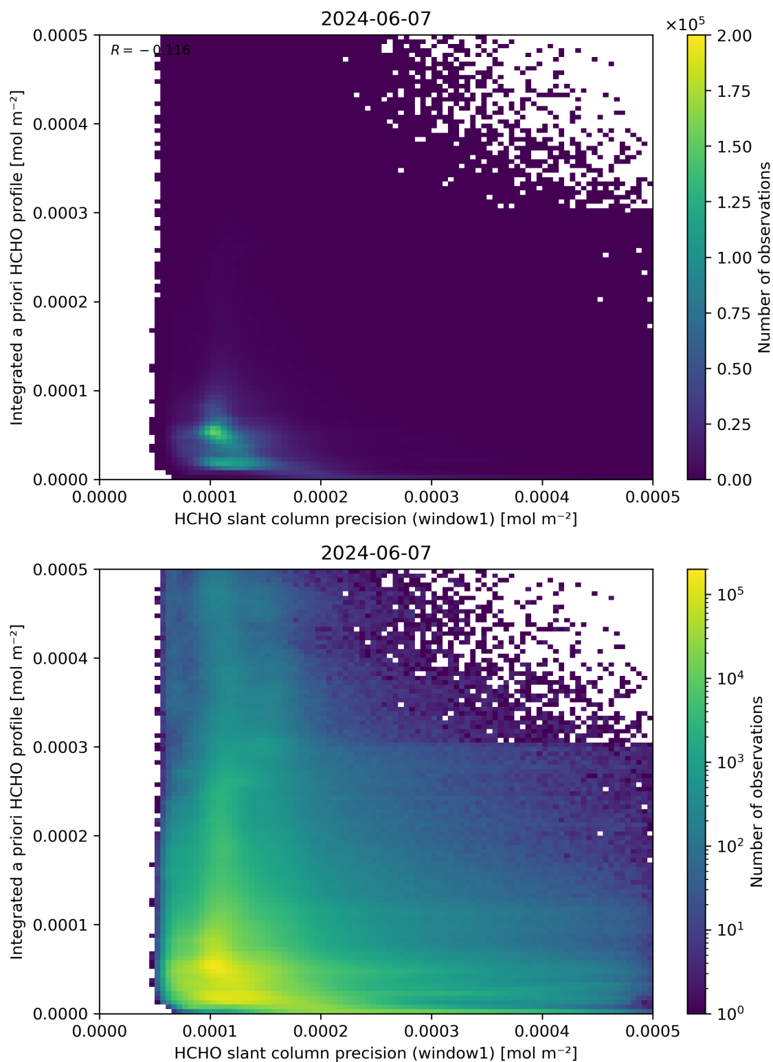
Figure 96: Scatter density plot of “HCHO slant column precision (window1)” against “Integrated a priori HCHO profile” for 2024-06-06 to 2024-06-08.
