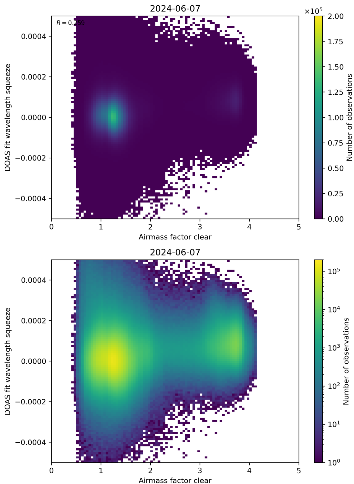
Figure 73: Scatter density plot of “Airmass factor clear” against “DOAS fit wavelength squeeze” for 2024-06-06 to 2024-06-08.
