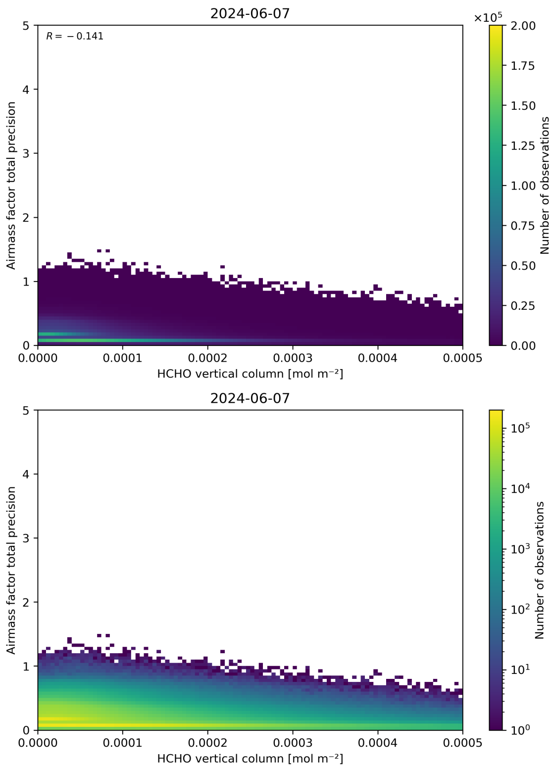
Figure 132: Scatter density plot of “HCHO vertical column” against “Airmass factor total precision” for 2024-06-06 to 2024-06-08.
