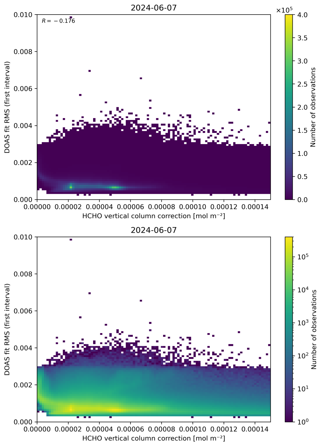
Figure 112: Scatter density plot of “HCHO vertical column correction” against “DOAS fit RMS (first interval)” for 2024-06-06 to 2024-06-08.
