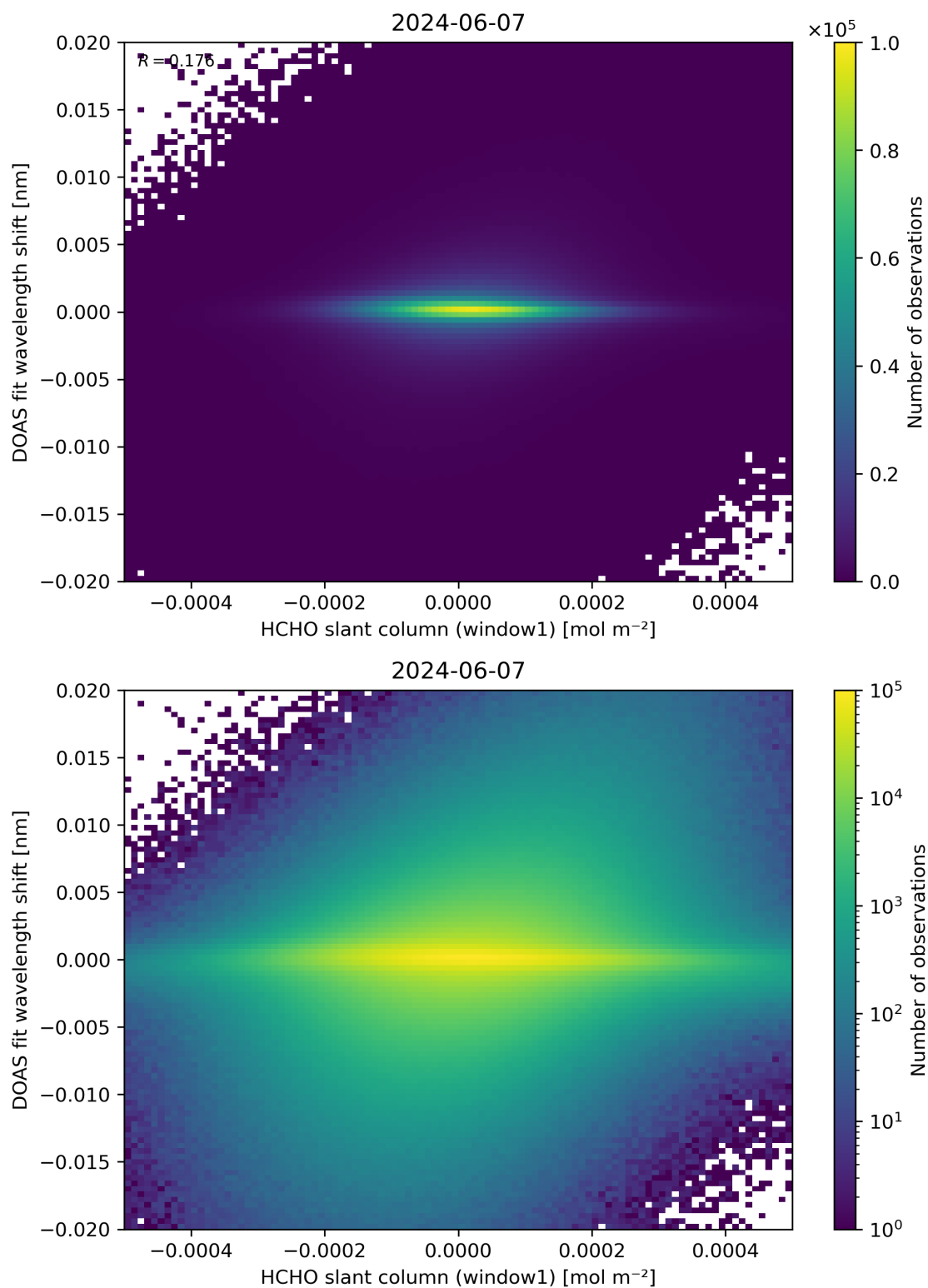
Figure 79: Scatter density plot of “HCHO slant column (window1)” against “DOAS fit wavelength shift” for 2024-06-06 to 2024-06-08.
