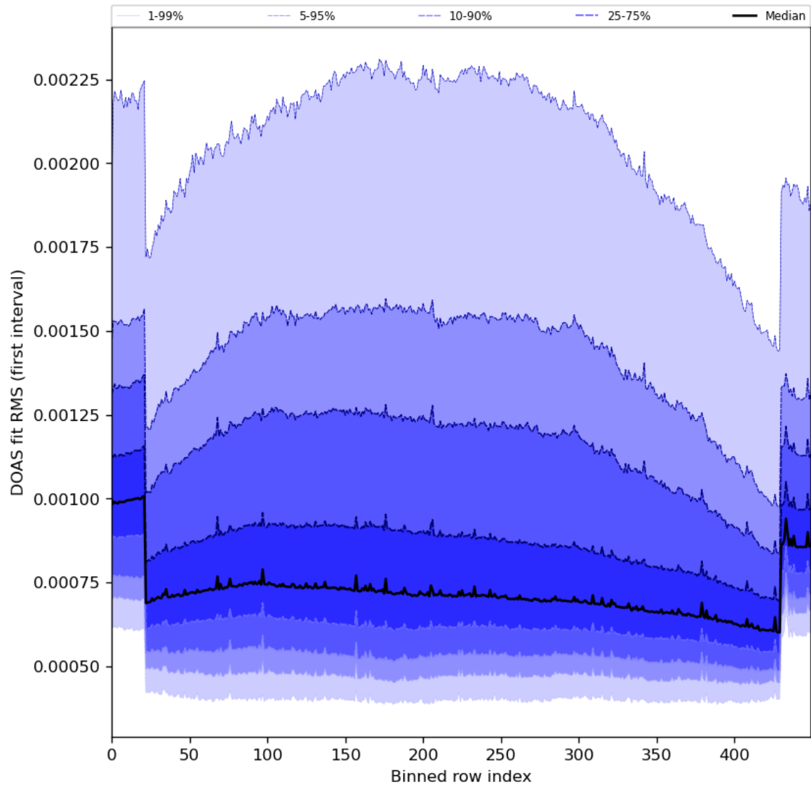
Figure 60: Along track statistics of “DOAS fit RMS (first interval)” for 2024-06-06 to 2024-06-08
