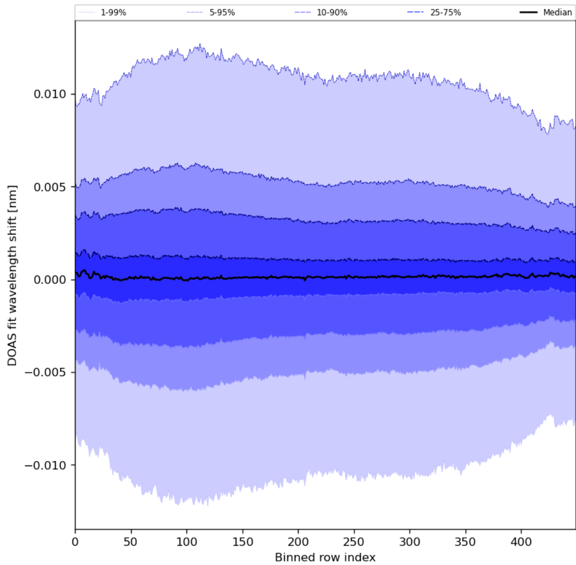
Figure 58: Along track statistics of “DOAS fit wavelength shift” for 2024-06-06 to 2024-06-08
