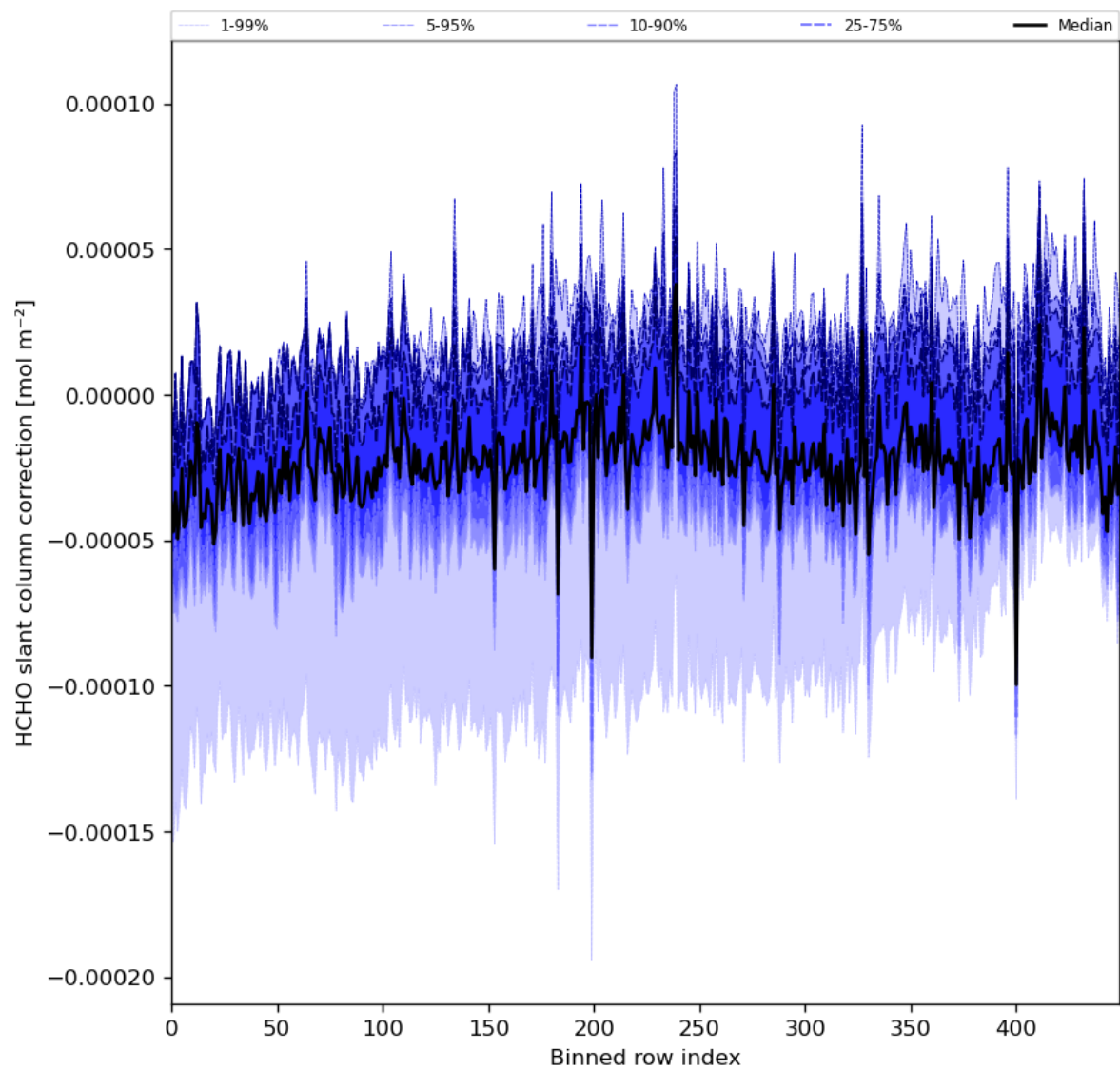
Figure 61: Along track statistics of “HCHO slant column correction” for 2024-06-06 to 2024-06-08
