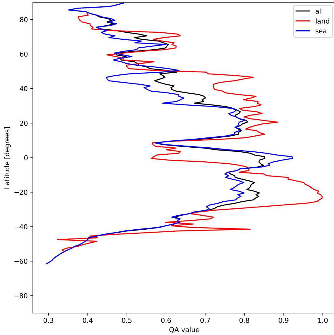
Figure 20: Zonal average of “QA value” for 2024-06-06 to 2024-06-08.
