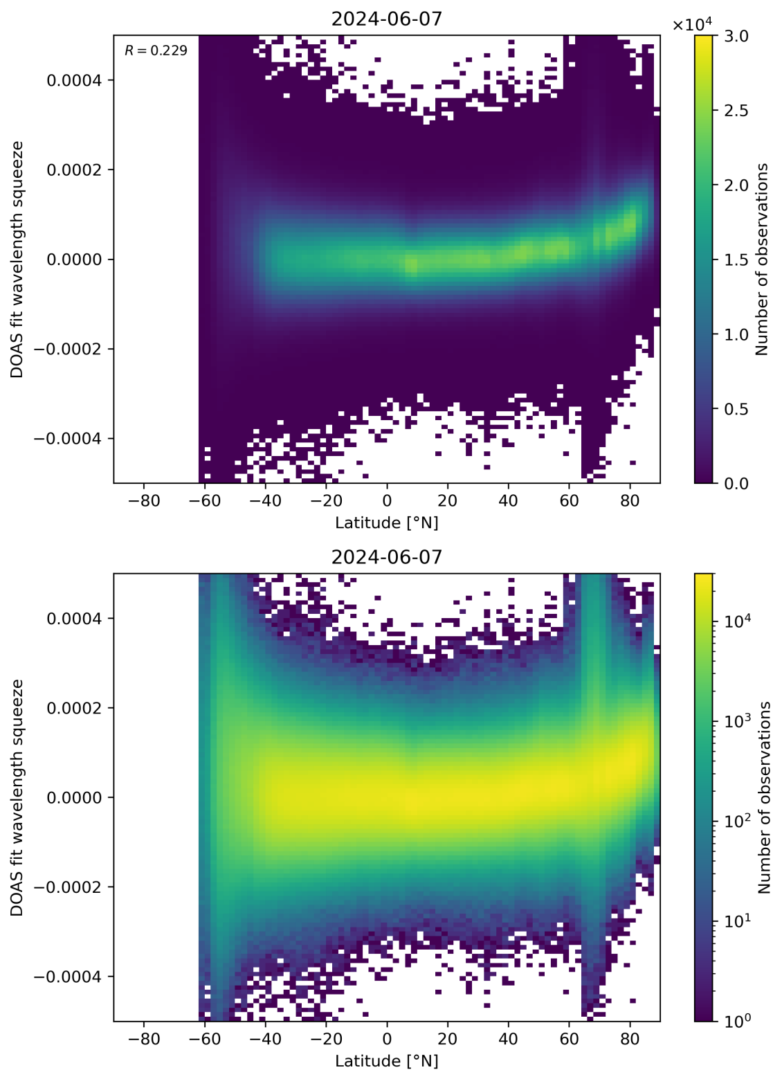
Figure 155: Scatter density plot of “Latitude” against “DOAS fit wavelength squeeze” for 2024-06-06 to 2024-06-08.
