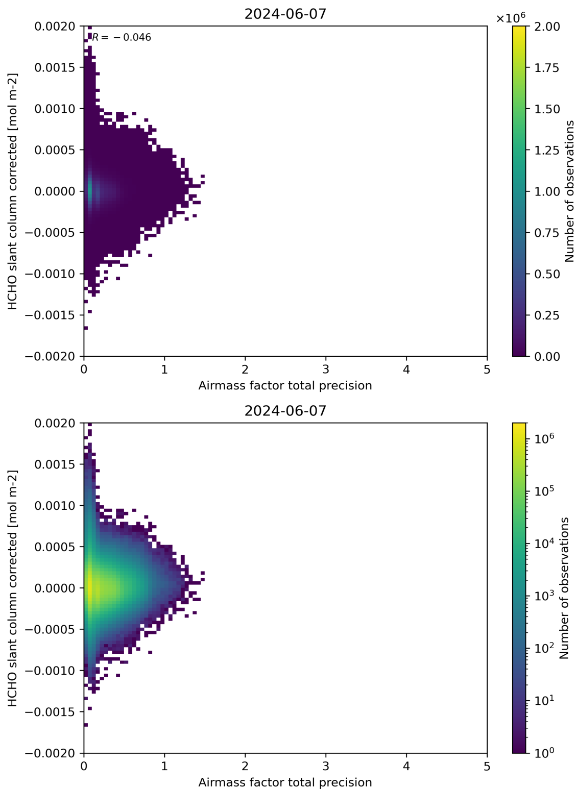
Figure 109: Scatter density plot of “Airmass factor total precision” against “HCHO slant column corrected” for 2024-06-06 to 2024-06-08.
