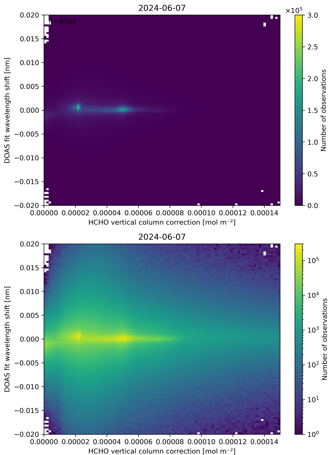
Figure 113: Scatter density plot of “HCHO vertical column correction” against “DOAS fit wavelength shift” for 2024-06-06 to 2024-06-08.
