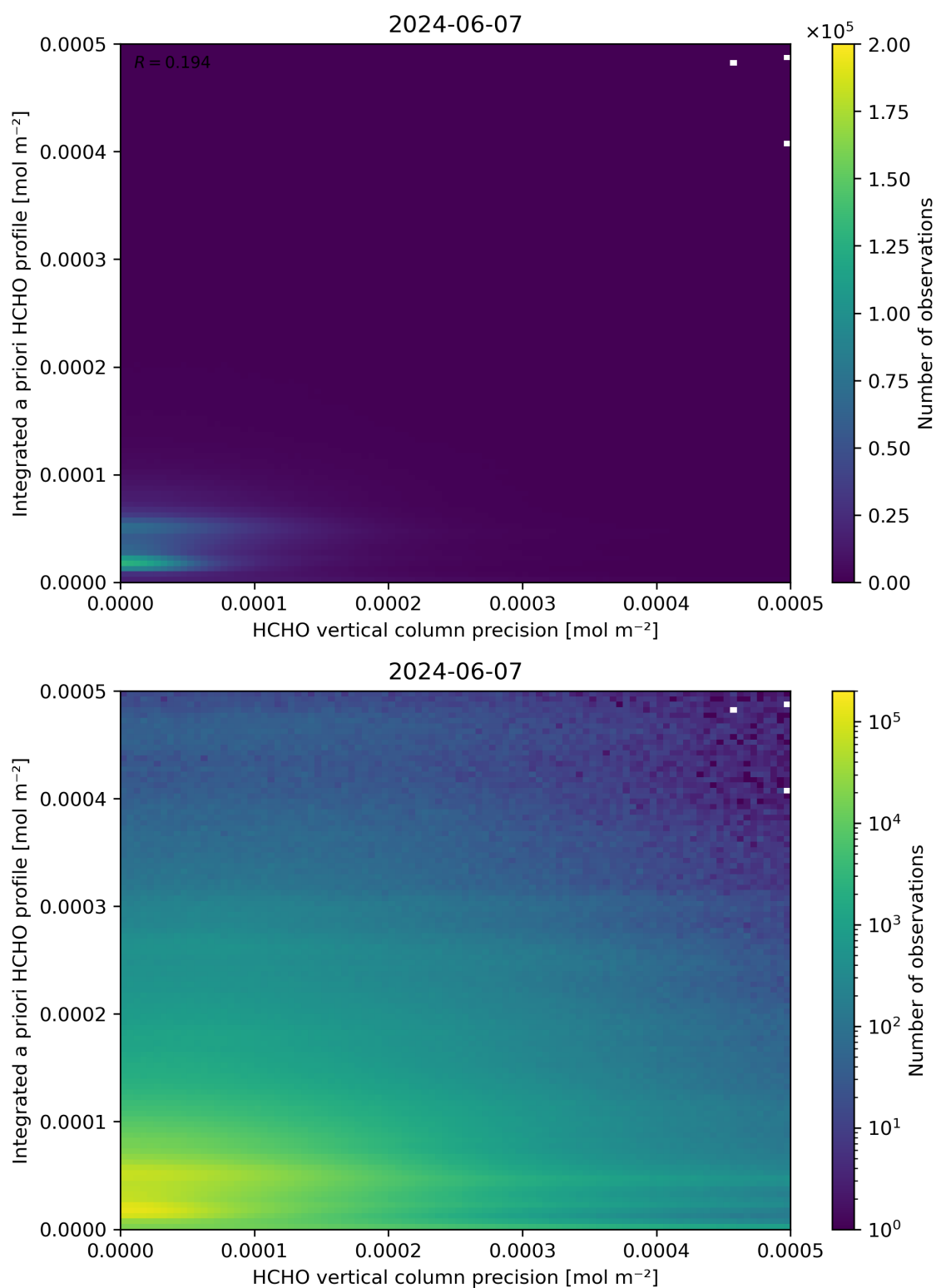
Figure 147: Scatter density plot of “HCHO vertical column precision” against “Integrated a priori HCHO profile” for 2024-06-06 to 2024-06-08.
