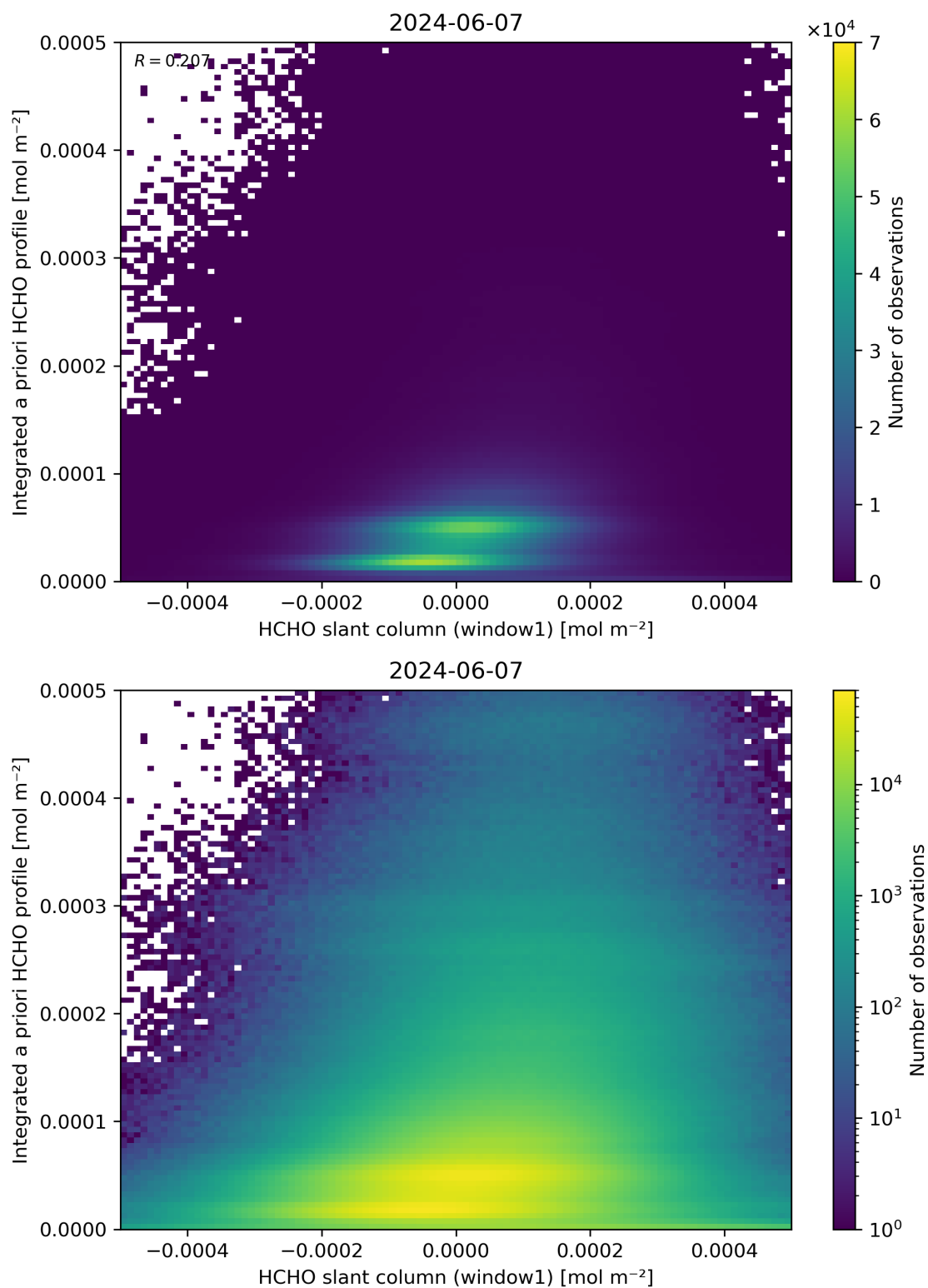
Figure 87: Scatter density plot of “HCHO slant column (window1)” against “Integrated a priori HCHO profile” for 2024-06-06 to 2024-06-08.
