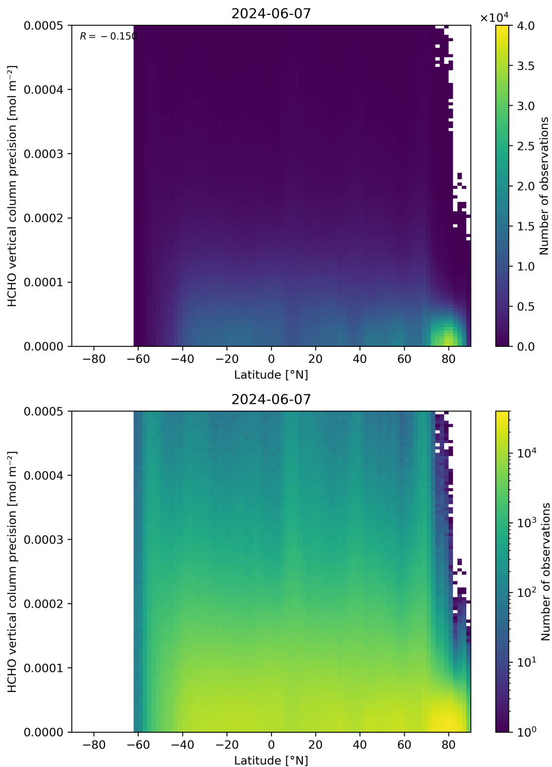
Figure 165: Scatter density plot of “Latitude” against “HCHO vertical column precision” for 2024-06-06 to 2024-06-08.
