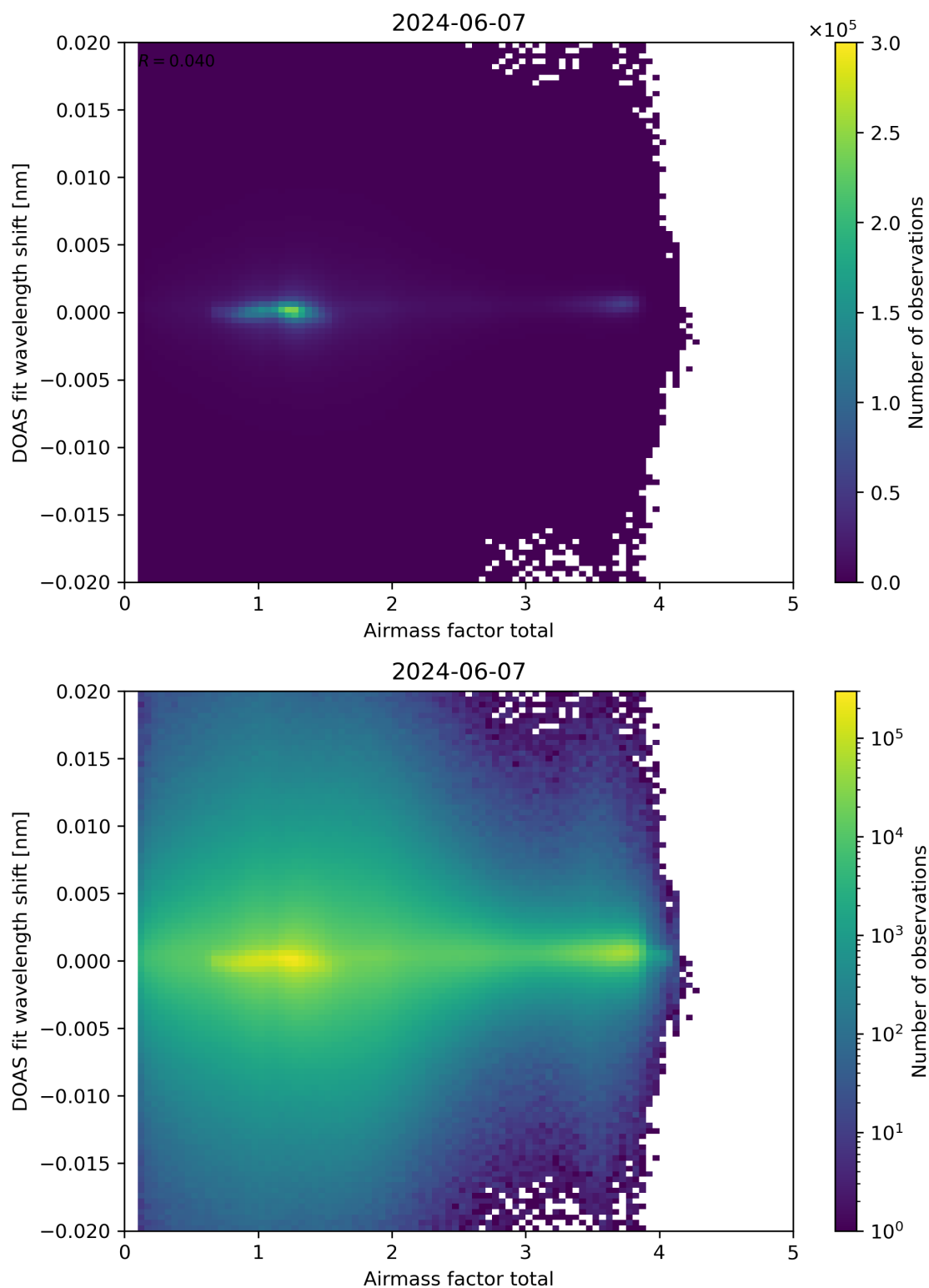
Figure 98: Scatter density plot of “Airmass factor total” against “DOAS fit wavelength shift” for 2024-06-06 to 2024-06-08.
