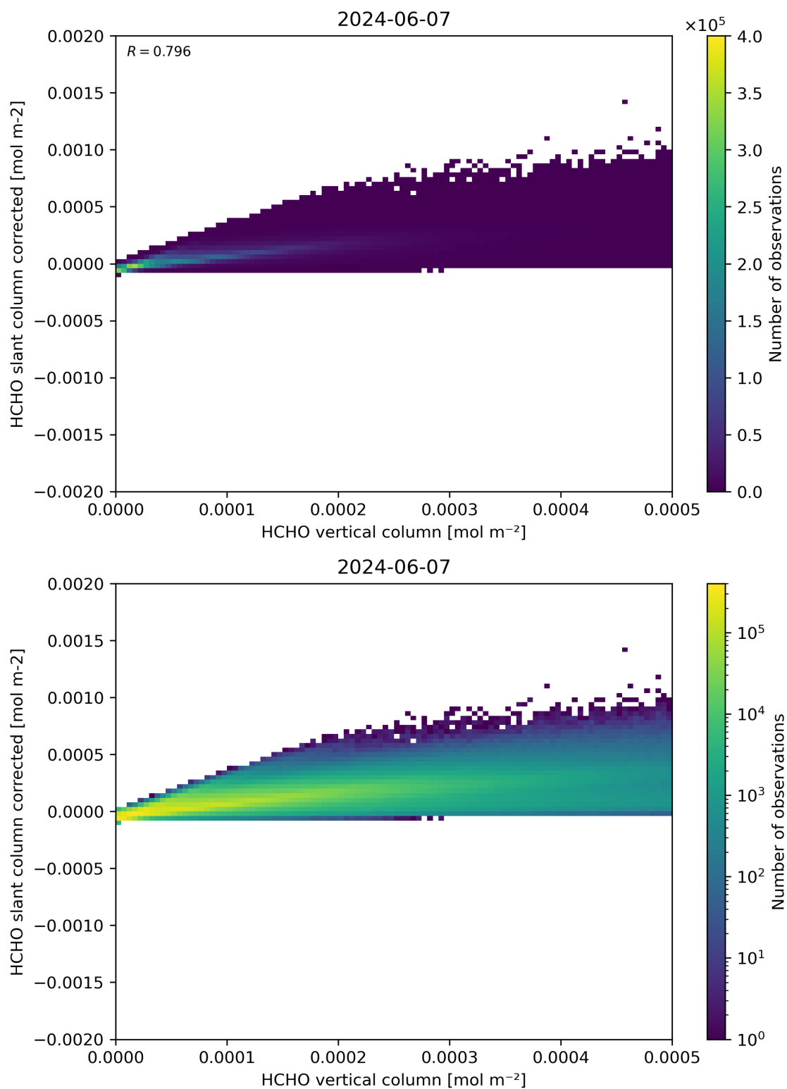
Figure 127: Scatter density plot of “HCHO vertical column” against “HCHO slant column corrected” for 2024-06-06 to 2024-06-08.
