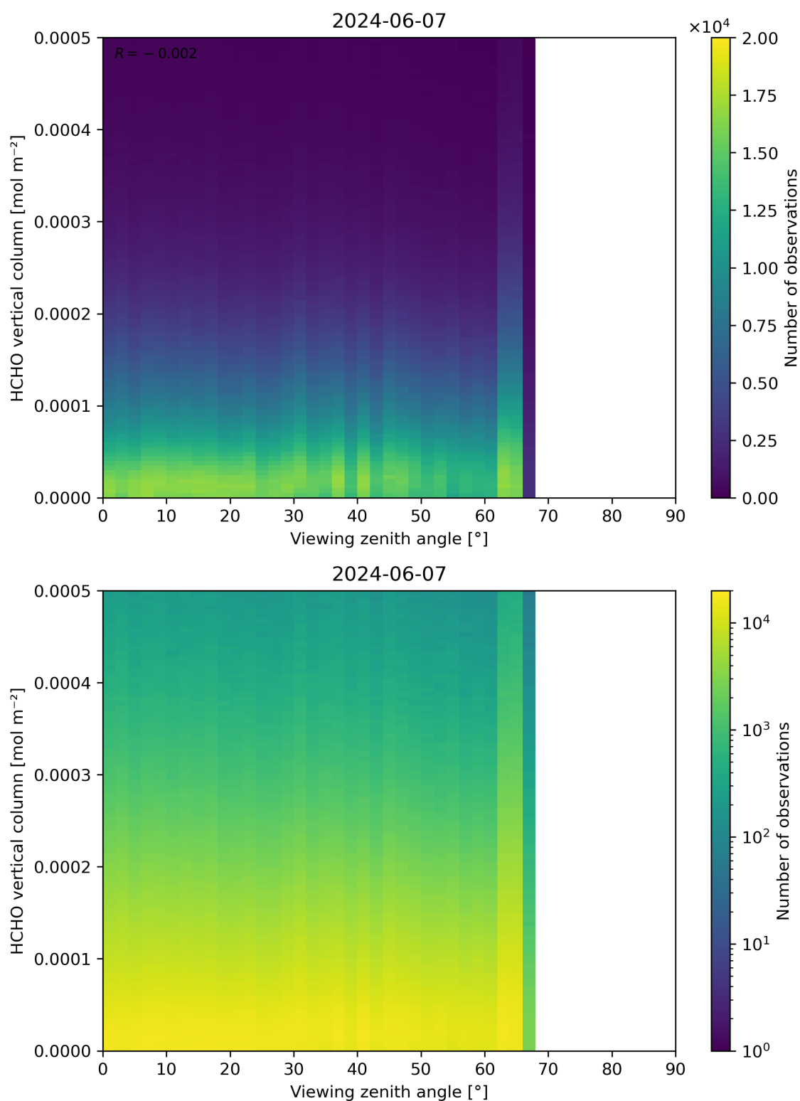
Figure 192: Scatter density plot of “Viewing zenith angle” against “HCHO vertical column” for 2024-06-06 to 2024-06-08.
