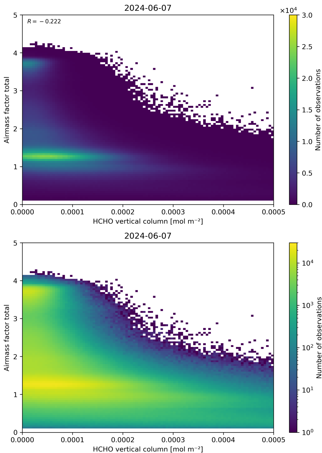
Figure 131: Scatter density plot of “HCHO vertical column” against “Airmass factor total” for 2024-06-06 to 2024-06-08.
