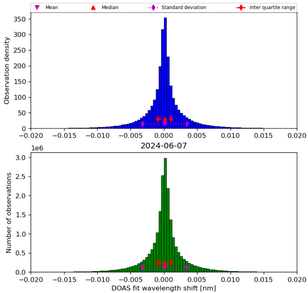
Figure 44: Histogram of “DOAS fit wavelength shift” for 2024-06-06 to 2024-06-08
