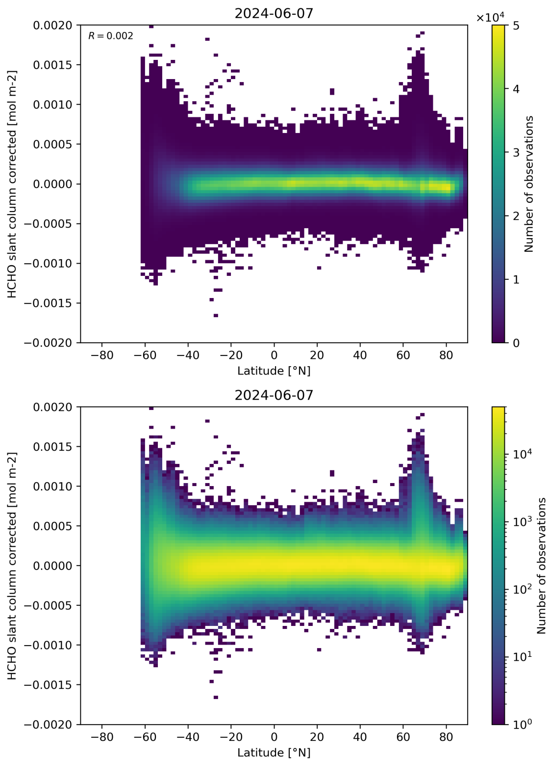
Figure 157: Scatter density plot of “Latitude” against “HCHO slant column corrected” for 2024-06-06 to 2024-06-08.
