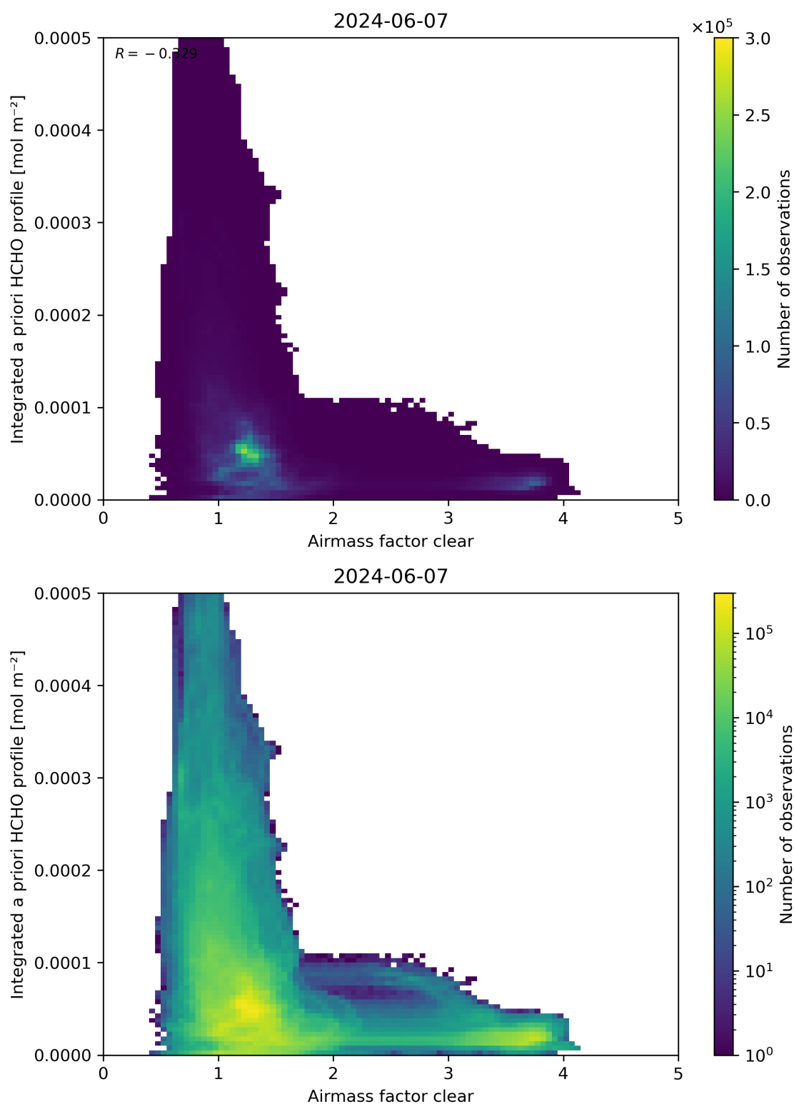
Figure 76: Scatter density plot of “Airmass factor clear” against “Integrated a priori HCHO profile” for 2024-06-06 to 2024-06-08.
