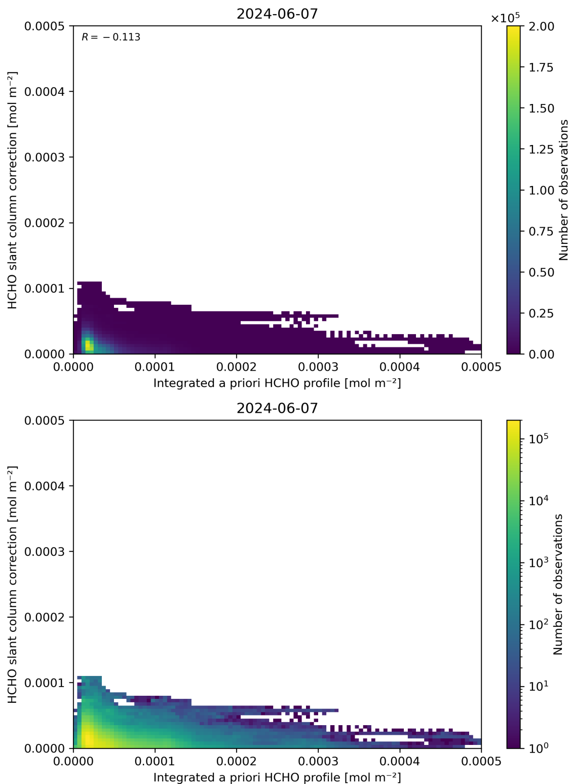
Figure 152: Scatter density plot of “Integrated a priori HCHO profile” against “HCHO slant column correction” for 2024-06-06 to 2024-06-08.
