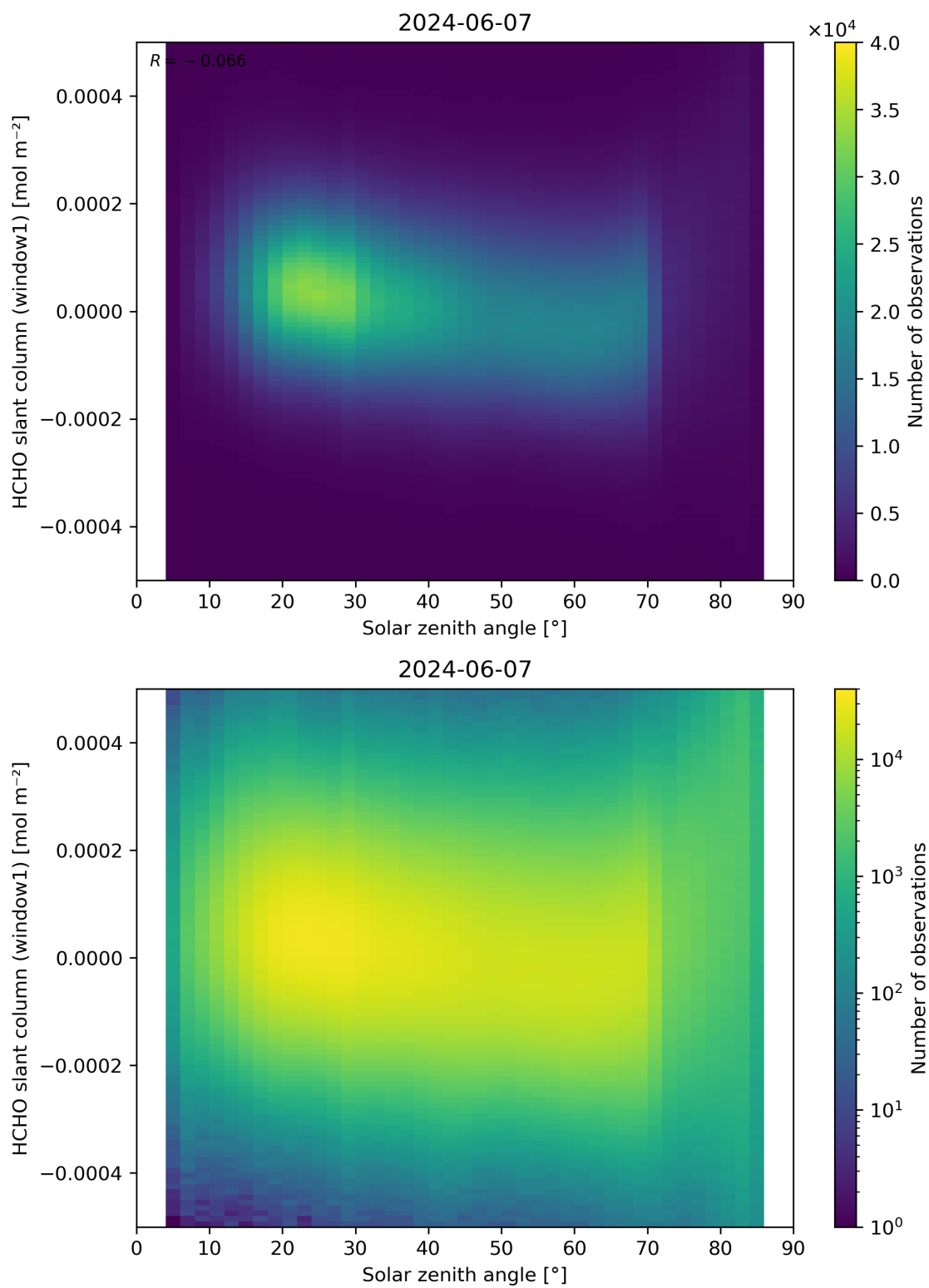
Figure 173: Scatter density plot of “Solar zenith angle” against “HCHO slant column (window1)” for 2024-06-06 to 2024-06-08.
