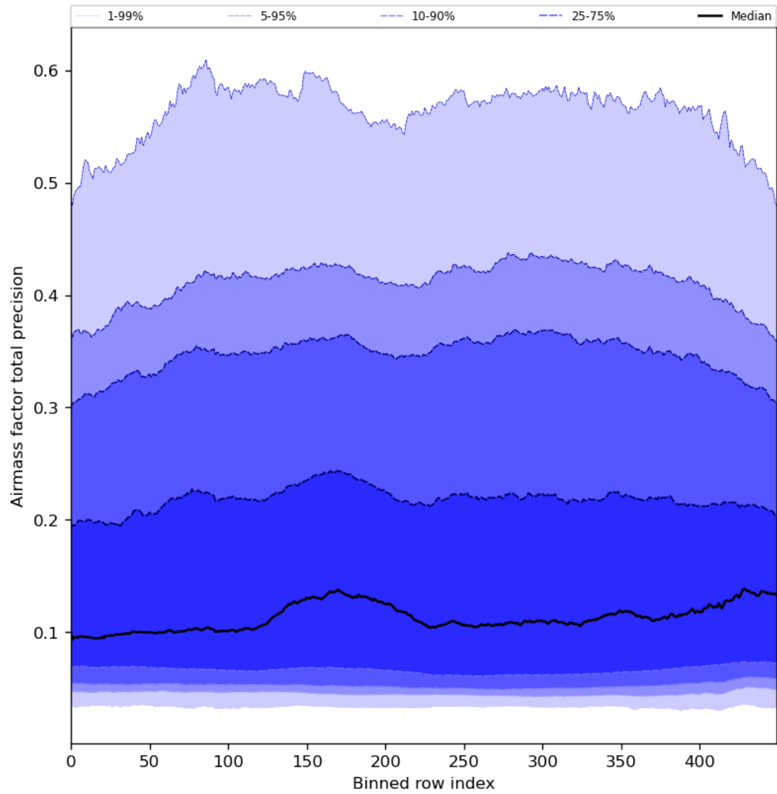
Figure 55: Along track statistics of “Airmass factor total precision” for 2024-06-06 to 2024-06-08
