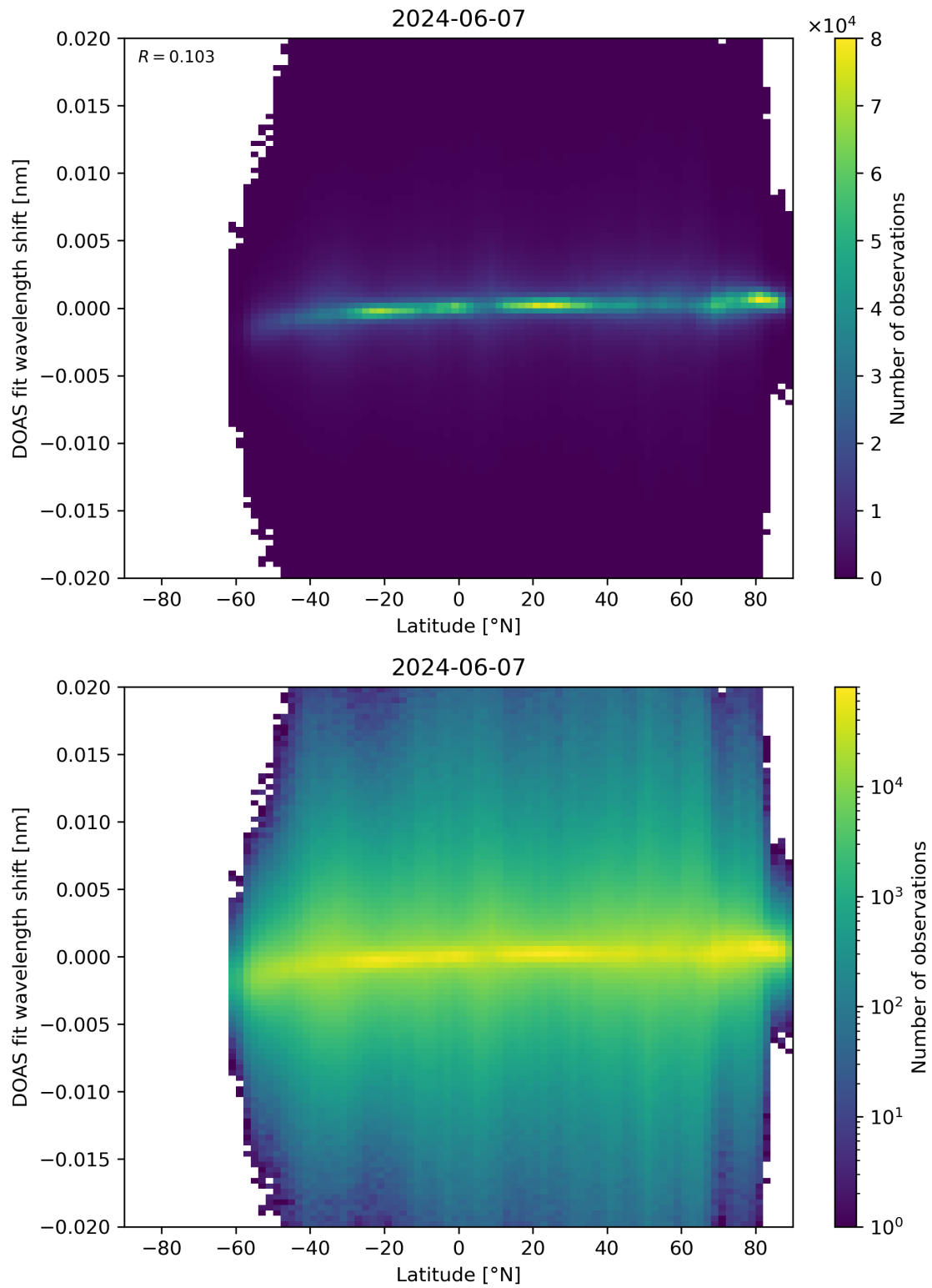
Figure 154: Scatter density plot of “Latitude” against “DOAS fit wavelength shift” for 2024-06-06 to 2024-06-08.
