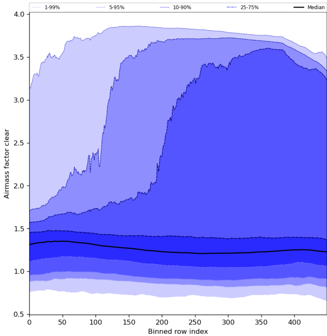
Figure 56: Along track statistics of “Airmass factor clear” for 2024-06-06 to 2024-06-08
