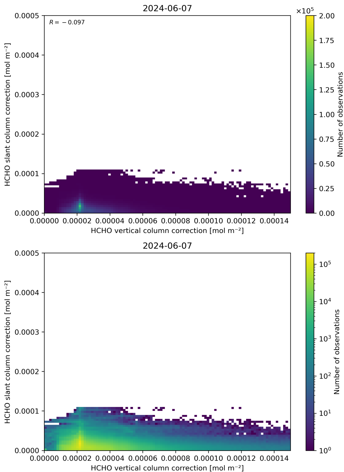
Figure 117: Scatter density plot of “HCHO vertical column correction” against “HCHO slant column correction” for 2024-06-06 to 2024-06-08.
