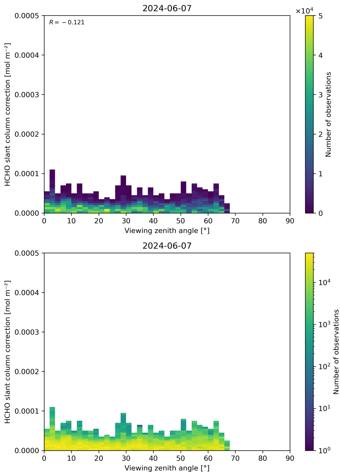
Figure 187: Scatter density plot of “Viewing zenith angle” against “HCHO slant column correction” for 2024-06-06 to 2024-06-08.
