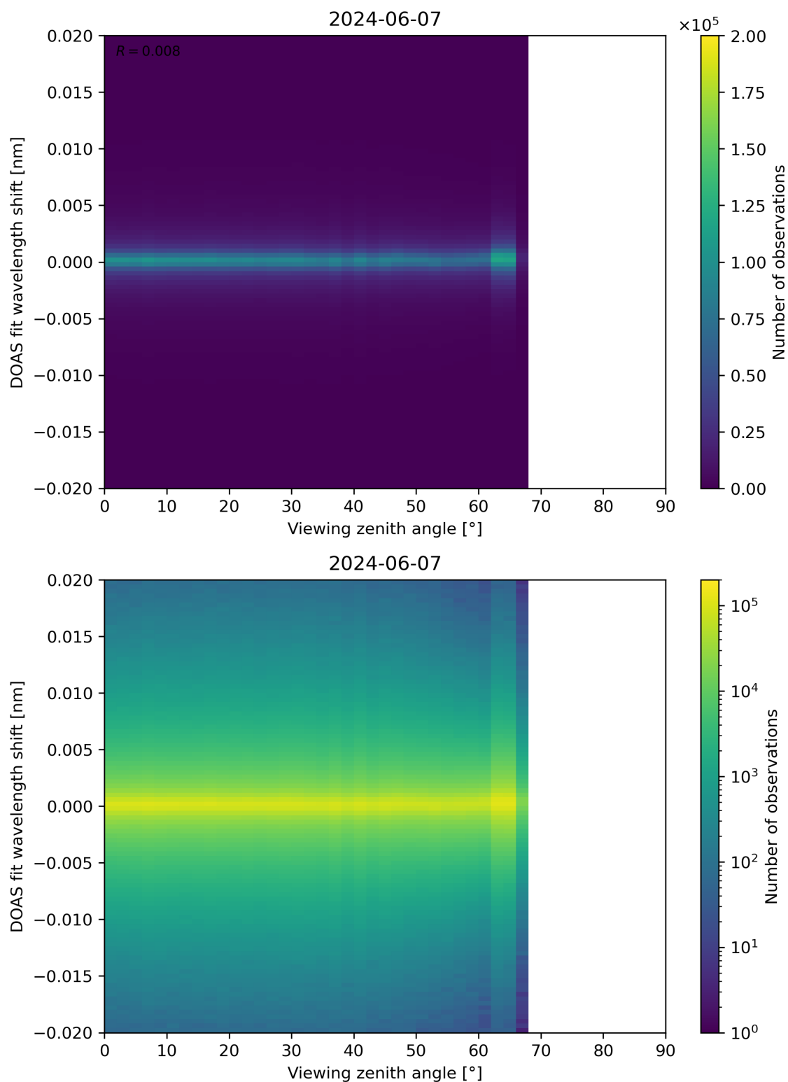
Figure 183: Scatter density plot of “Viewing zenith angle” against “DOAS fit wavelength shift” for 2024-06-06 to 2024-06-08.
