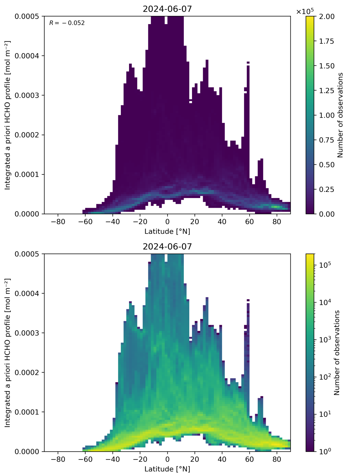
Figure 166: Scatter density plot of “Latitude” against “Integrated a priori HCHO profile” for 2024-06-06 to 2024-06-08.
