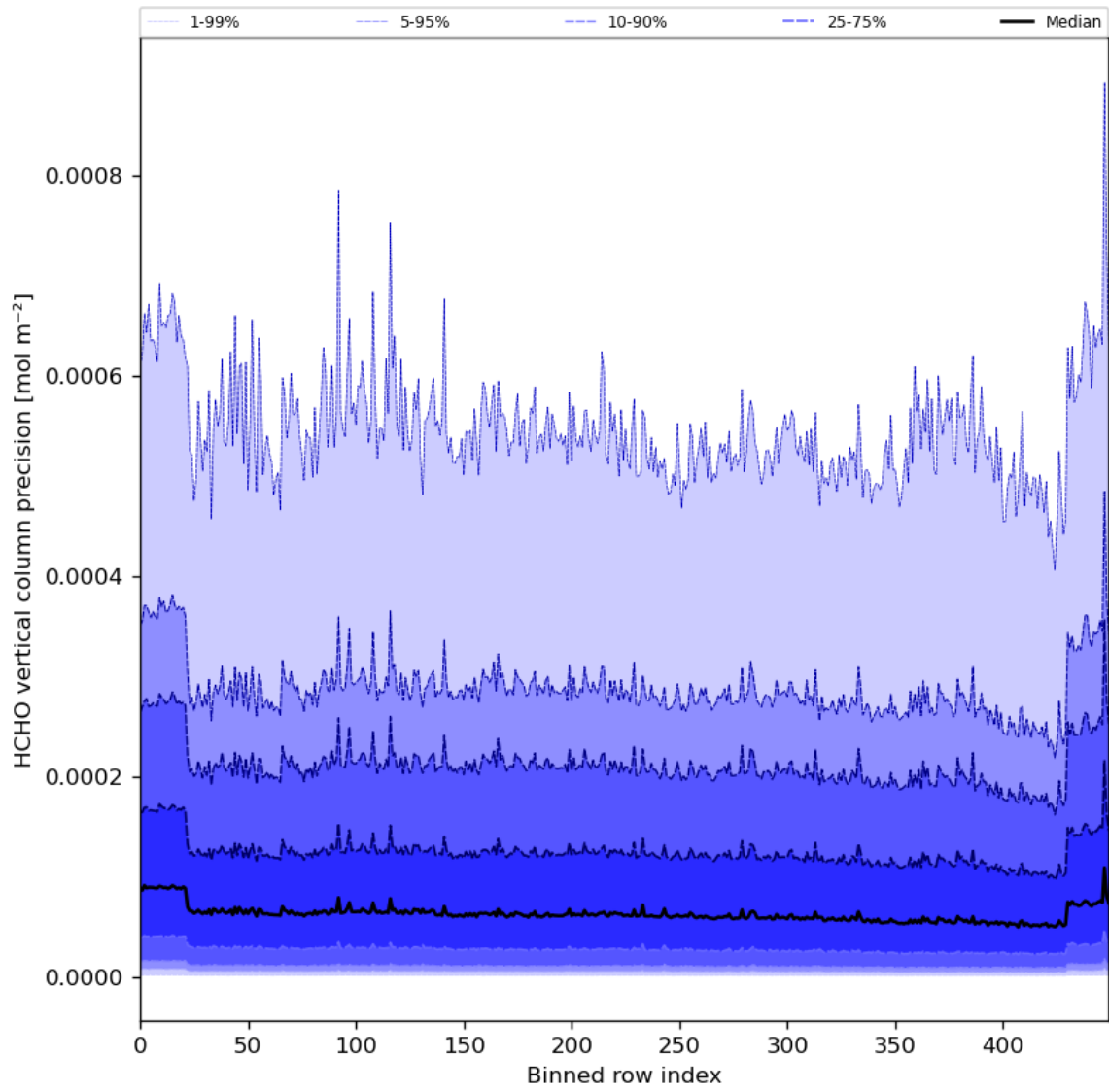
Figure 50: Along track statistics of “HCHO vertical column precision” for 2024-06-06 to 2024-06-08
