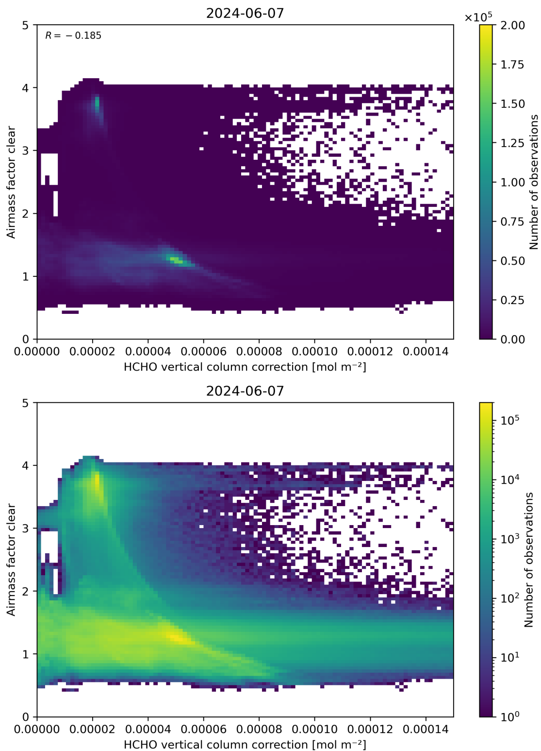
Figure 115: Scatter density plot of “HCHO vertical column correction” against “Airmass factor clear” for 2024-06-06 to 2024-06-08.
