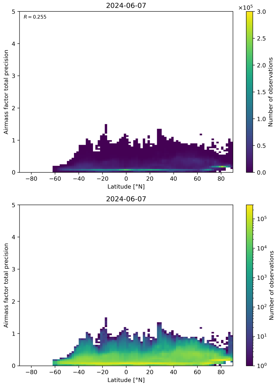
Figure 162: Scatter density plot of “Latitude” against “Airmass factor total precision” for 2024-06-06 to 2024-06-08.
