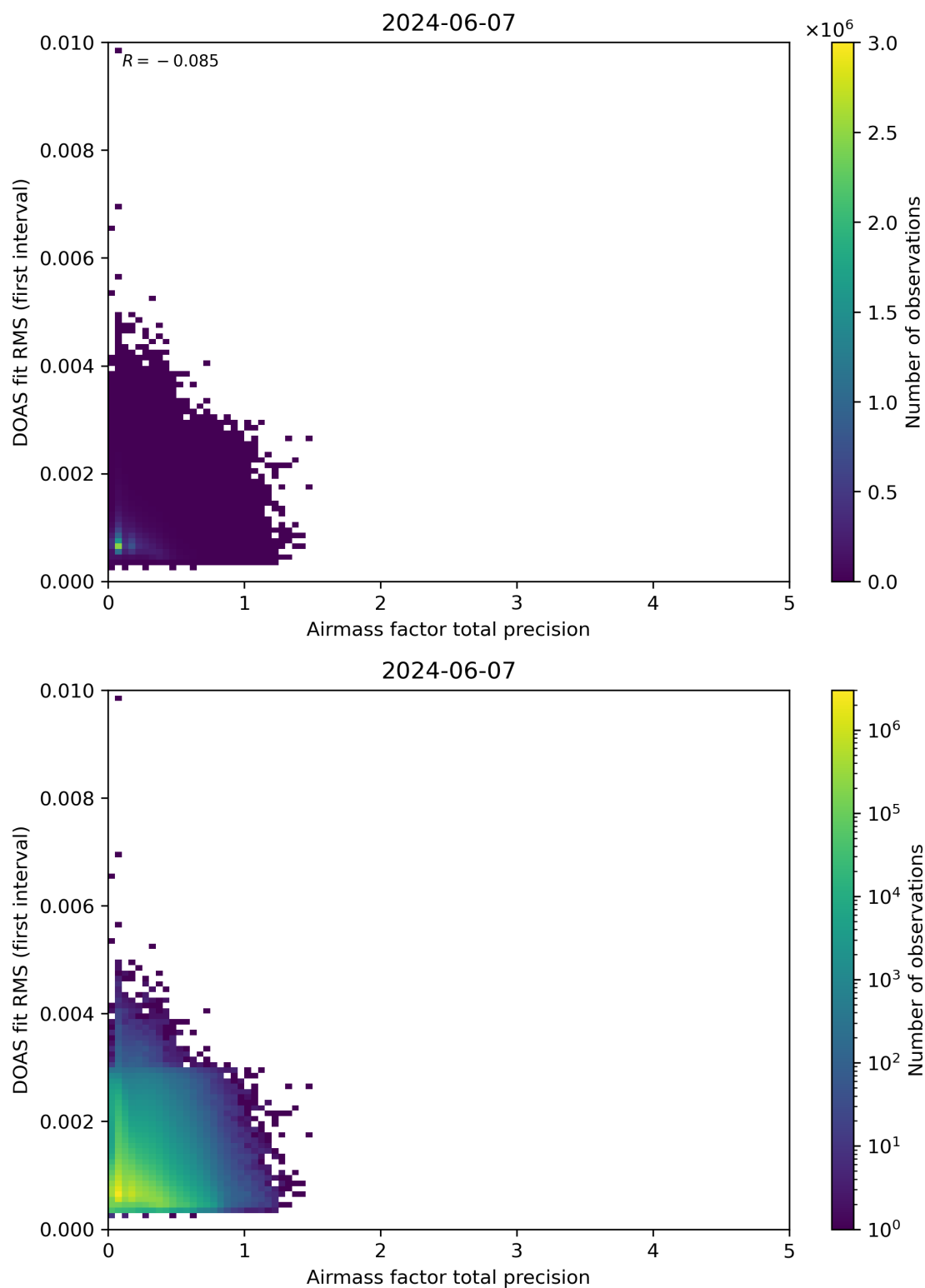
Figure 105: Scatter density plot of “Airmass factor total precision” against “DOAS fit RMS (first interval)” for 2024-06-06 to 2024-06-08.
