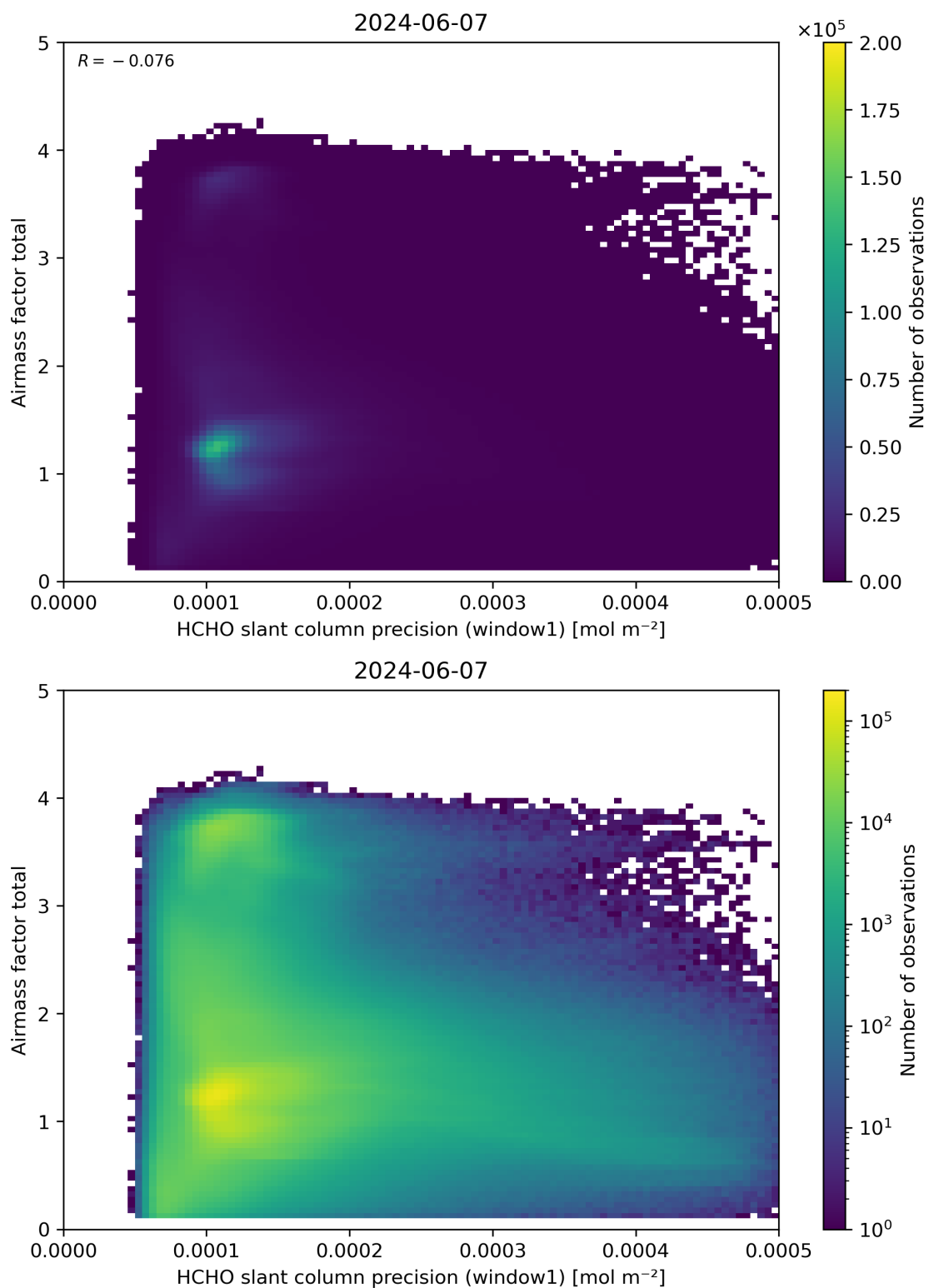
Figure 94: Scatter density plot of “HCHO slant column precision (window1)” against “Airmass factor total” for 2024-06-06 to 2024-06-08.
