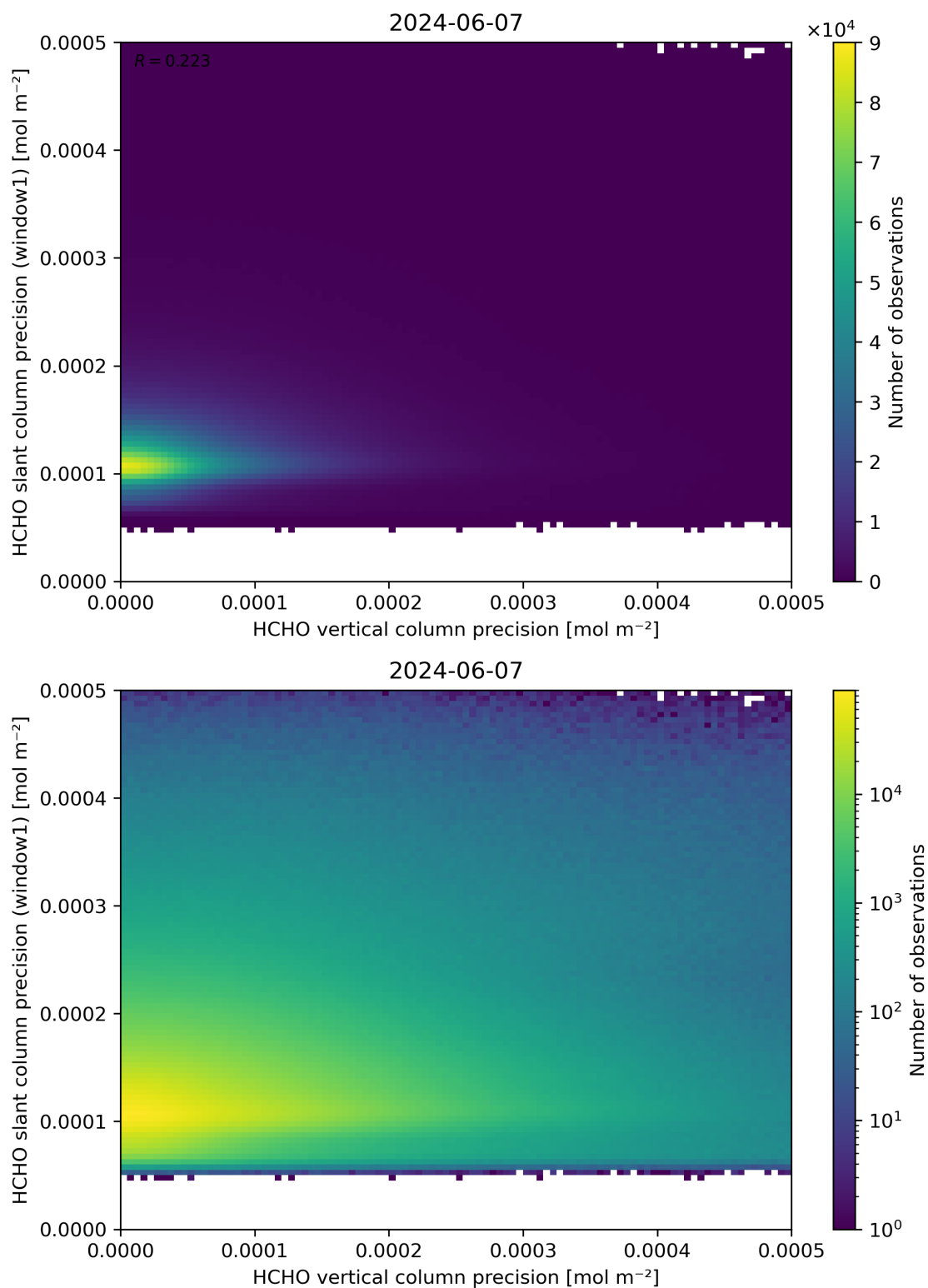
Figure 143: Scatter density plot of “HCHO vertical column precision” against “HCHO slant column precision (window1)” for 2024-06-06 to 2024-06-08.
