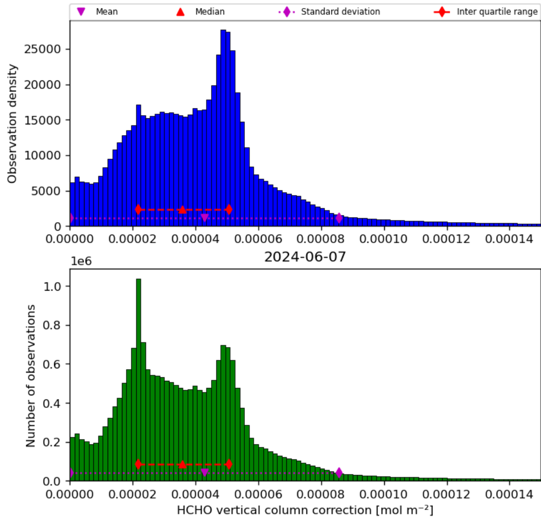
Figure 37: Histogram of “HCHO vertical column correction” for 2024-06-06 to 2024-06-08
