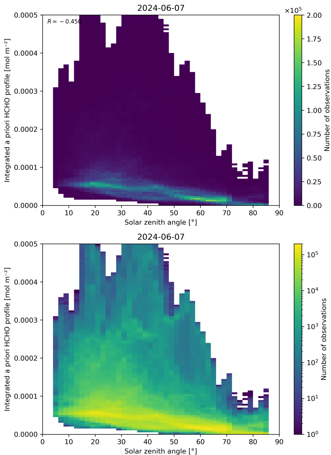
Figure 180: Scatter density plot of “Solar zenith angle” against “Integrated a priori HCHO profile” for 2024-06-06 to 2024-06-08.
