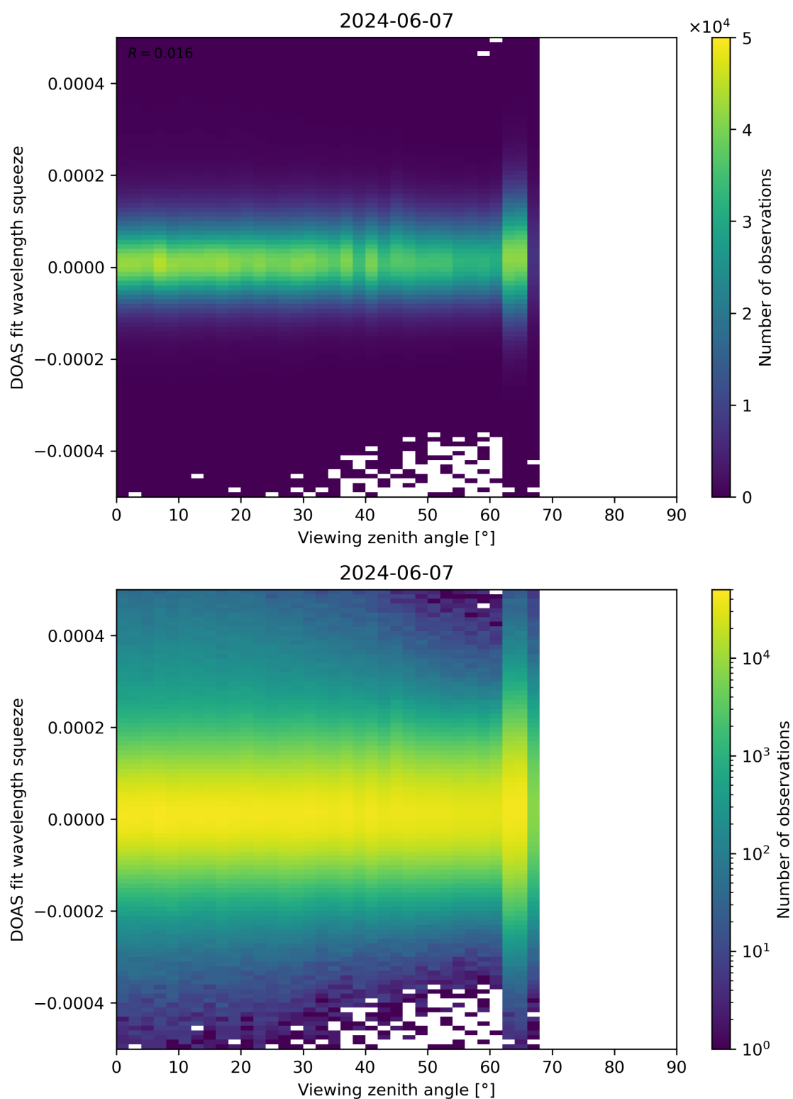
Figure 184: Scatter density plot of “Viewing zenith angle” against “DOAS fit wavelength squeeze” for 2024-06-06 to 2024-06-08.
