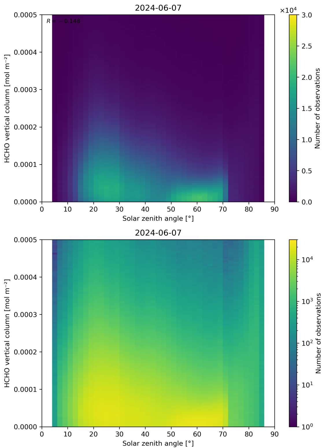
Figure 177: Scatter density plot of “Solar zenith angle” against “HCHO vertical column” for 2024-06-06 to 2024-06-08.
