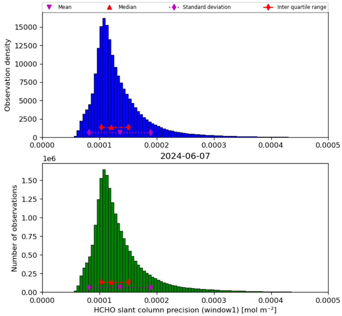
Figure 39: Histogram of “HCHO slant column precision (window1)” for 2024-06-06 to 2024-06-08
