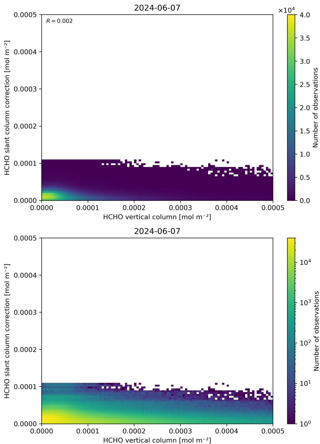
Figure 128: Scatter density plot of “HCHO vertical column” against “HCHO slant column correction” for 2024-06-06 to 2024-06-08.
