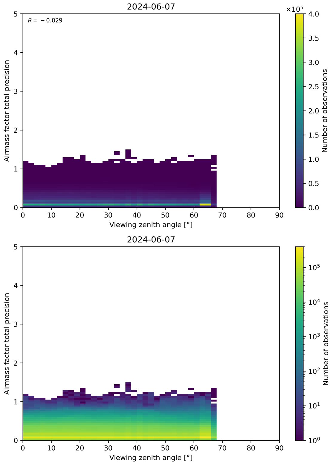
Figure 191: Scatter density plot of “Viewing zenith angle” against “Airmass factor total precision” for 2024-06-06 to 2024-06-08.
