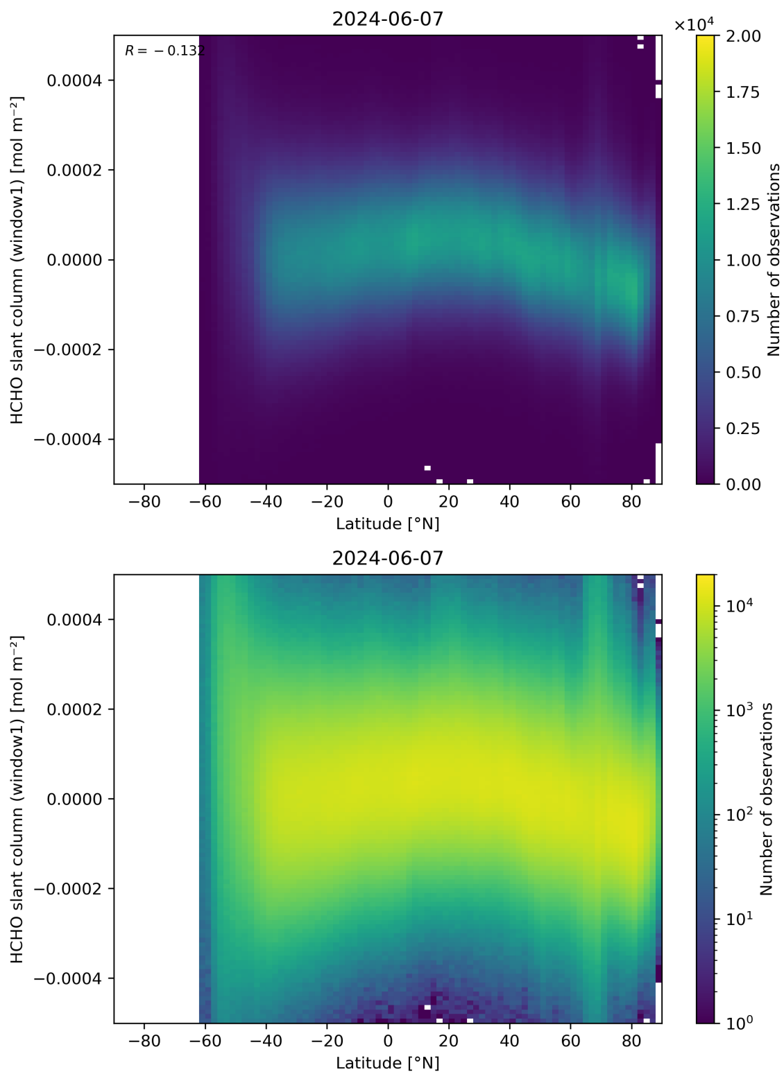
Figure 159: Scatter density plot of “Latitude” against “HCHO slant column (window1)” for 2024-06-06 to 2024-06-08.
