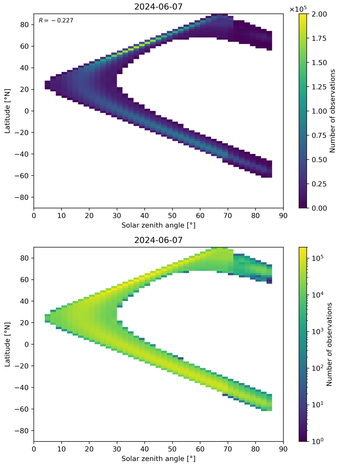
Figure 181: Scatter density plot of “Solar zenith angle” against “Latitude” for 2024-06-06 to 2024-06-08.
