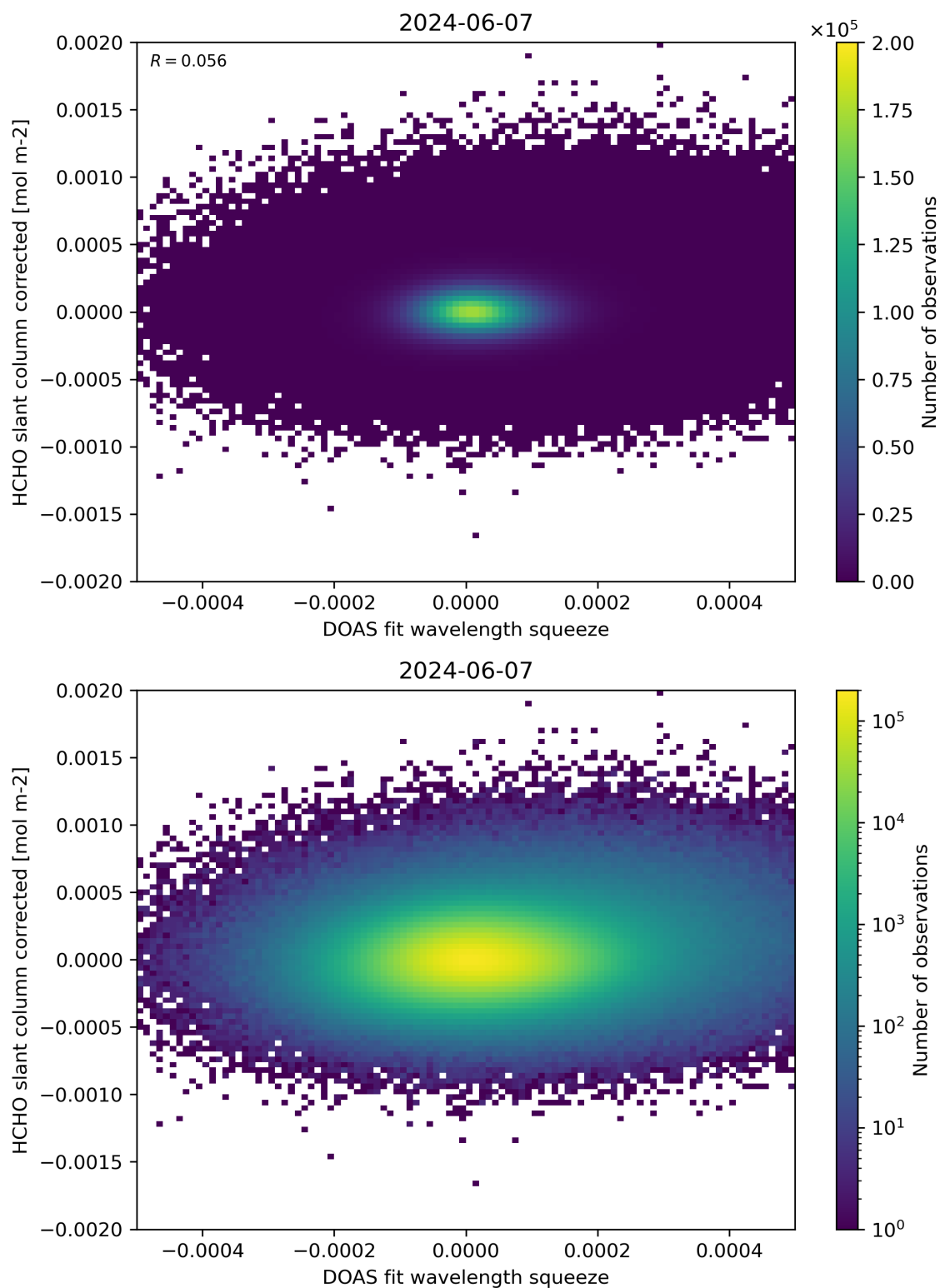
Figure 69: Scatter density plot of “DOAS fit wavelength squeeze” against “HCHO slant column corrected” for 2024-06-06 to 2024-06-08.
