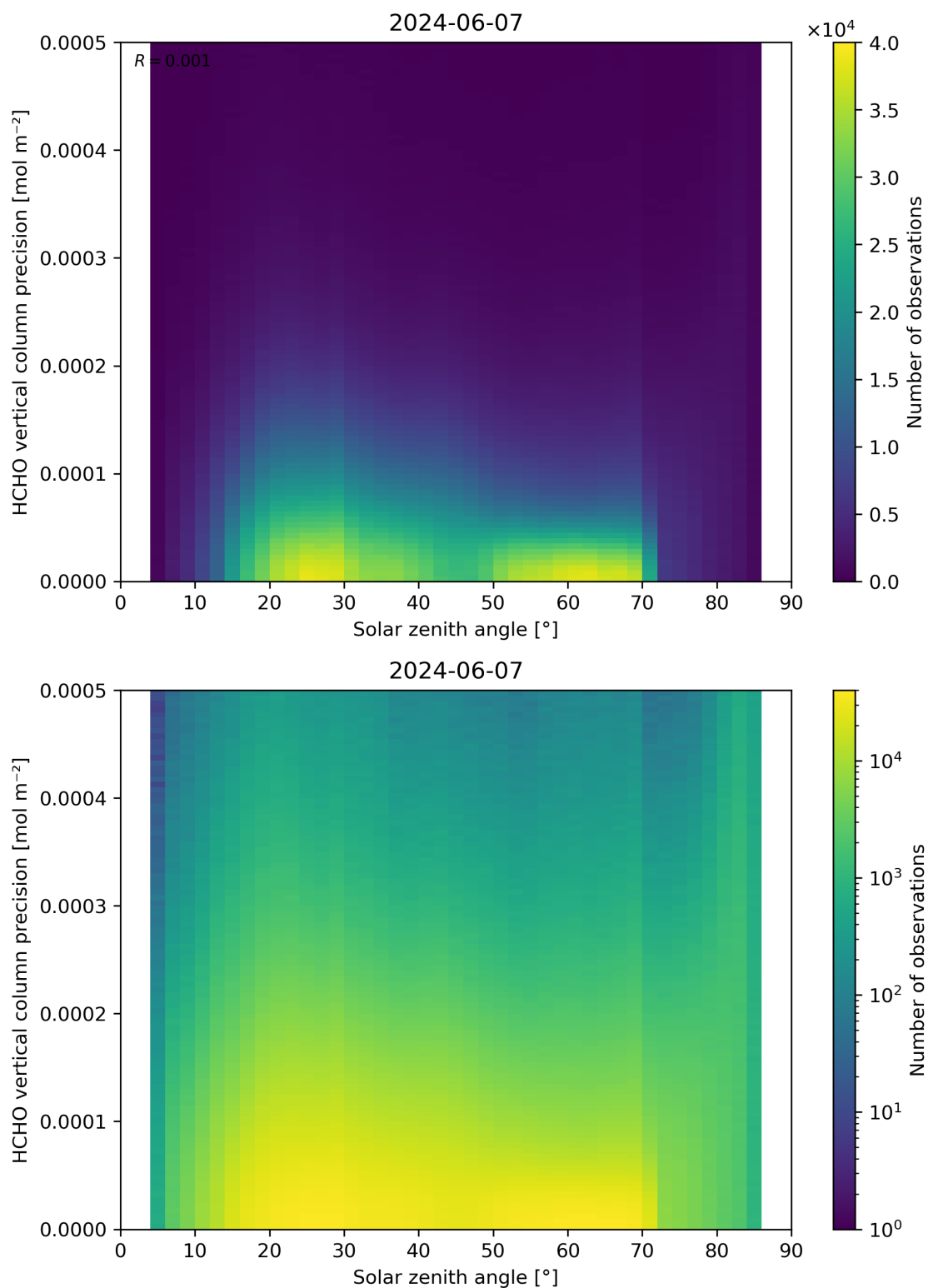
Figure 179: Scatter density plot of “Solar zenith angle” against “HCHO vertical column precision” for 2024-06-06 to 2024-06-08.
