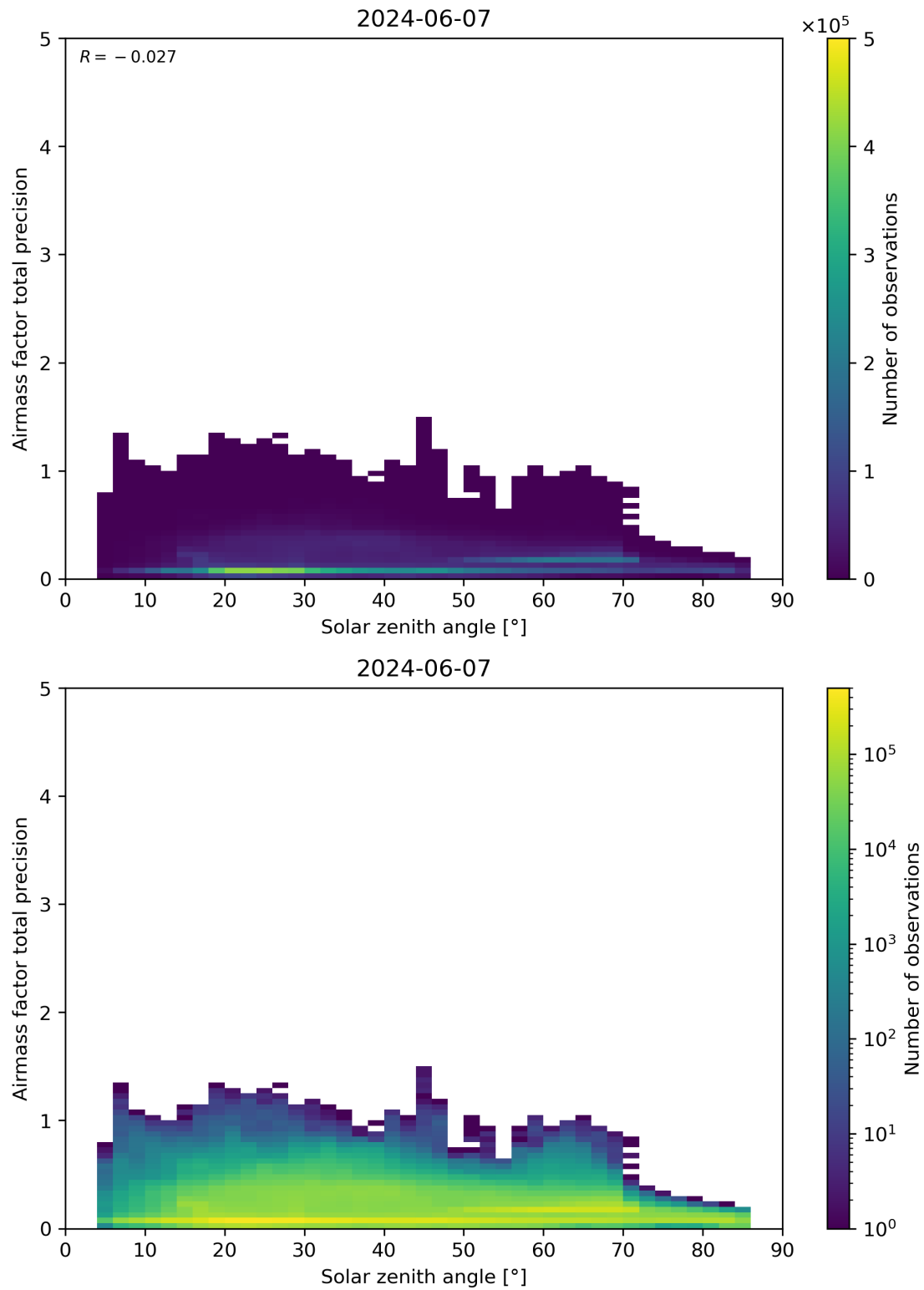
Figure 176: Scatter density plot of “Solar zenith angle” against “Airmass factor total precision” for 2024-06-06 to 2024-06-08.
