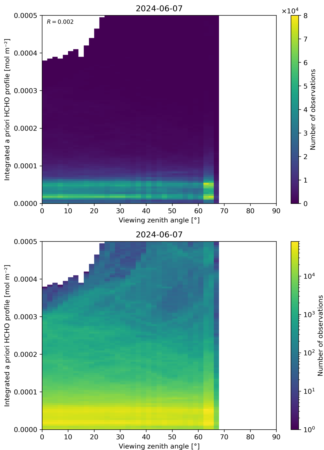
Figure 195: Scatter density plot of “Viewing zenith angle” against “Integrated a priori HCHO profile” for 2024-06-06 to 2024-06-08.
