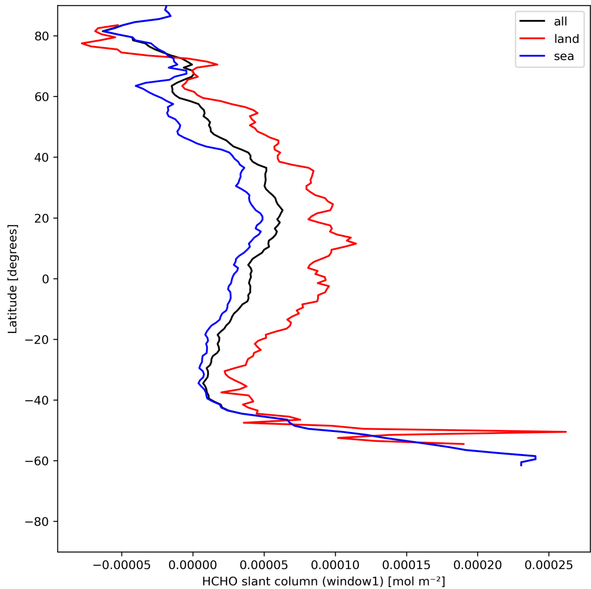
Figure 24: Zonal average of “HCHO slant column (window1)” for 2024-06-06 to 2024-06-08.
