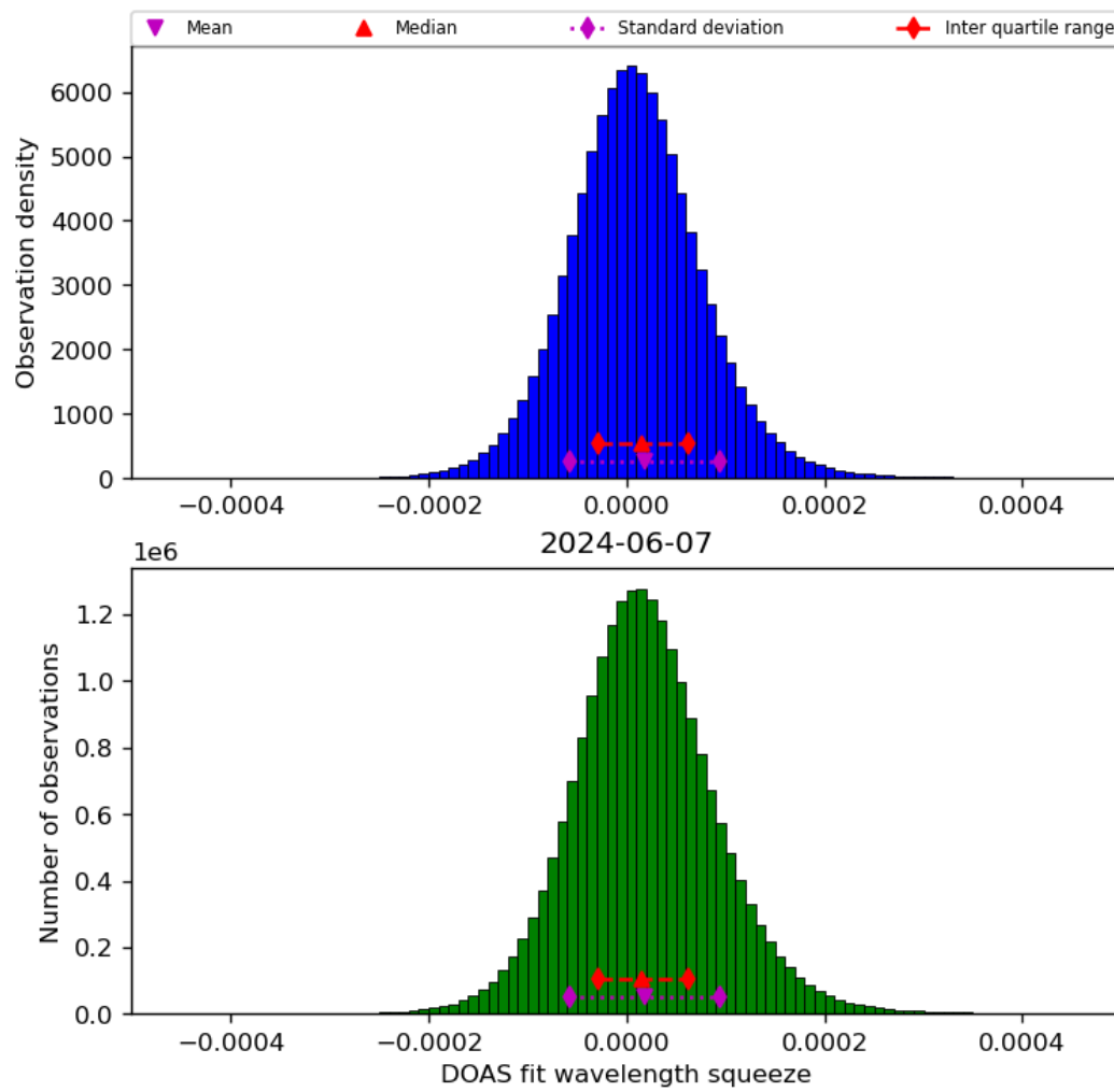
Figure 45: Histogram of “DOAS fit wavelength squeeze” for 2024-06-06 to 2024-06-08
