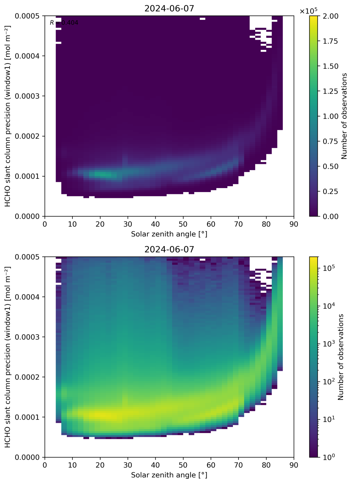
Figure 174: Scatter density plot of “Solar zenith angle” against “HCHO slant column precision (window1)” for 2024-06-06 to 2024-06-08.
