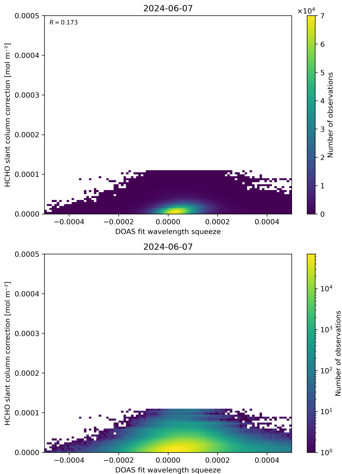
Figure 70: Scatter density plot of “DOAS fit wavelength squeeze” against “HCHO slant column correction” for 2024-06-06 to 2024-06-08.
