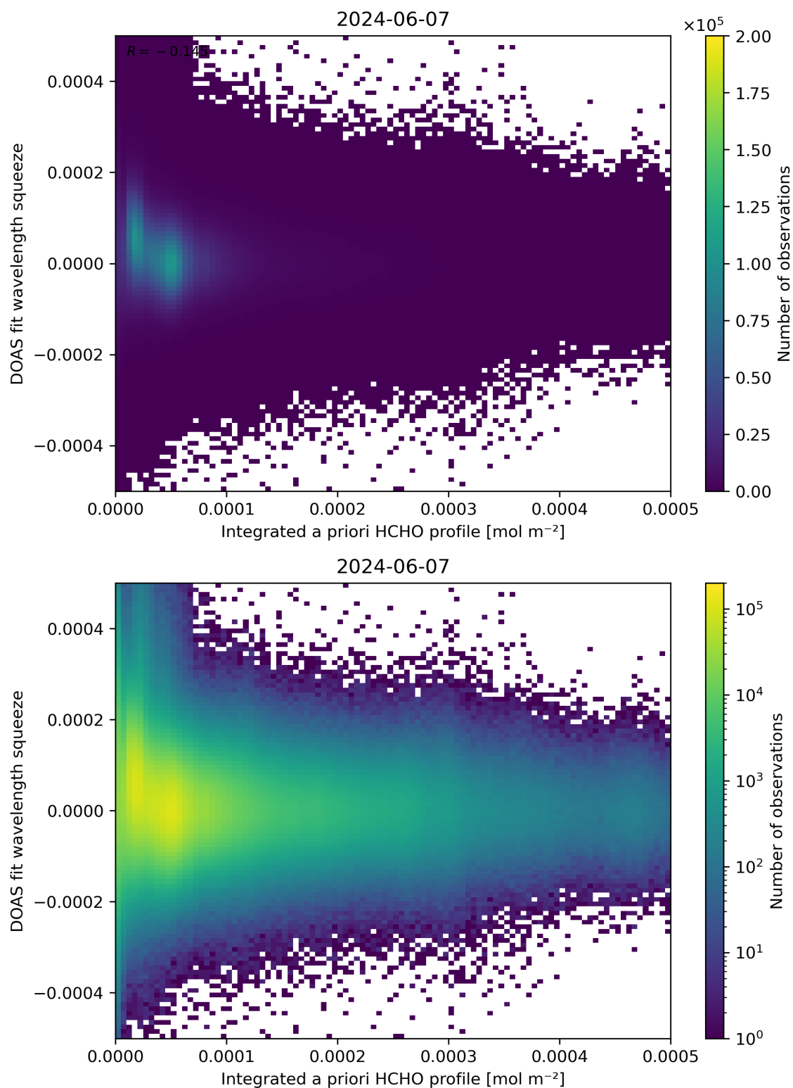
Figure 150: Scatter density plot of “Integrated a priori HCHO profile” against “DOAS fit wavelength squeeze” for 2024-06-06 to 2024-06-08.
