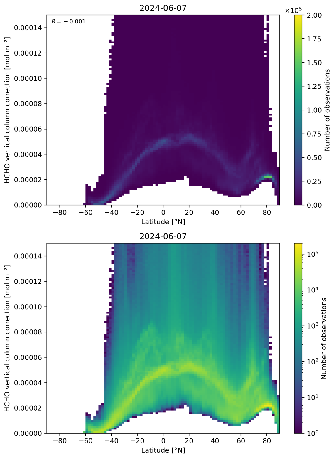
Figure 164: Scatter density plot of “Latitude” against “HCHO vertical column correction” for 2024-06-06 to 2024-06-08.
