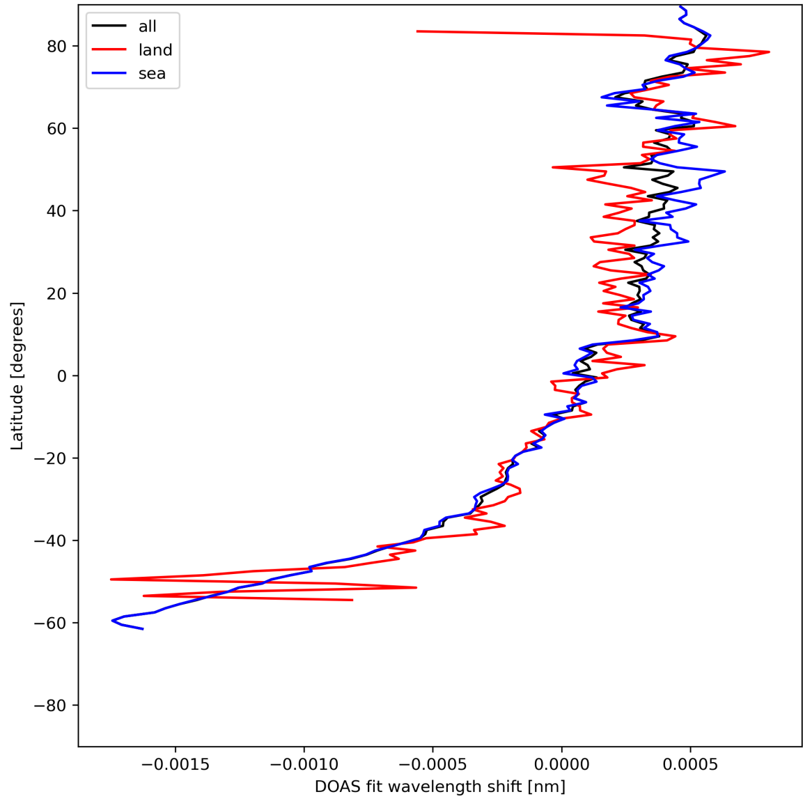
Figure 30: Zonal average of “DOAS fit wavelength shift” for 2024-06-06 to 2024-06-08.
