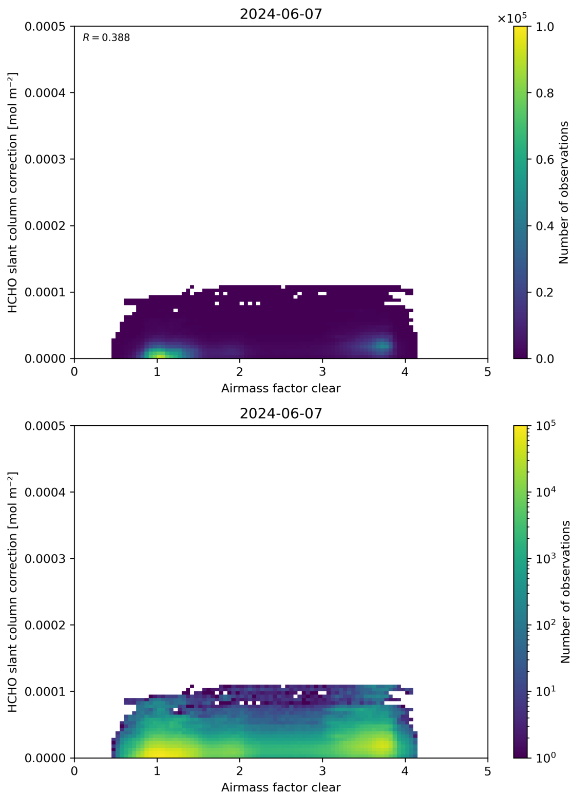
Figure 75: Scatter density plot of “Airmass factor clear” against “HCHO slant column correction” for 2024-06-06 to 2024-06-08.
