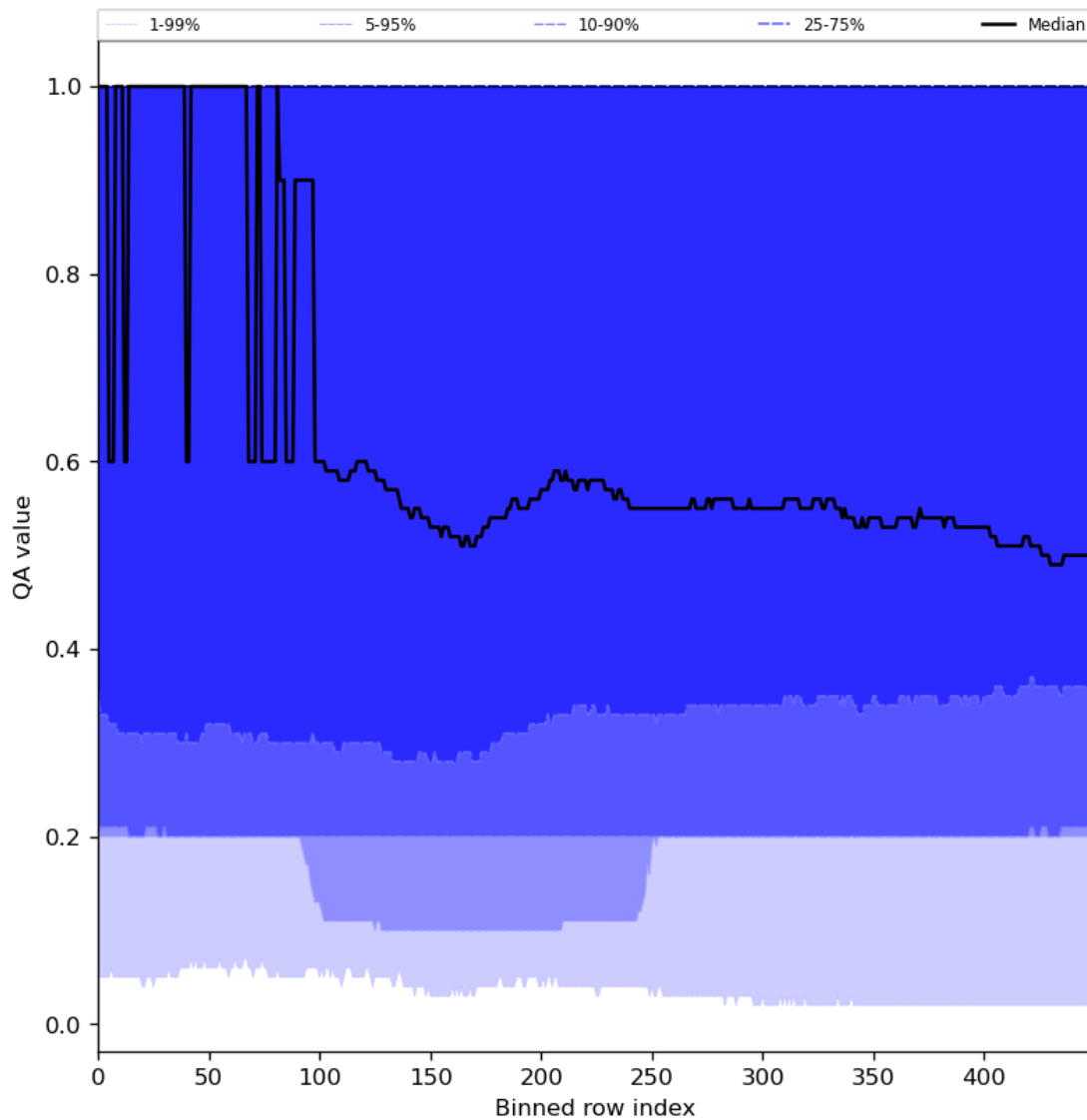
Figure 48: Along track statistics of “QA value” for 2024-06-06 to 2024-06-08
