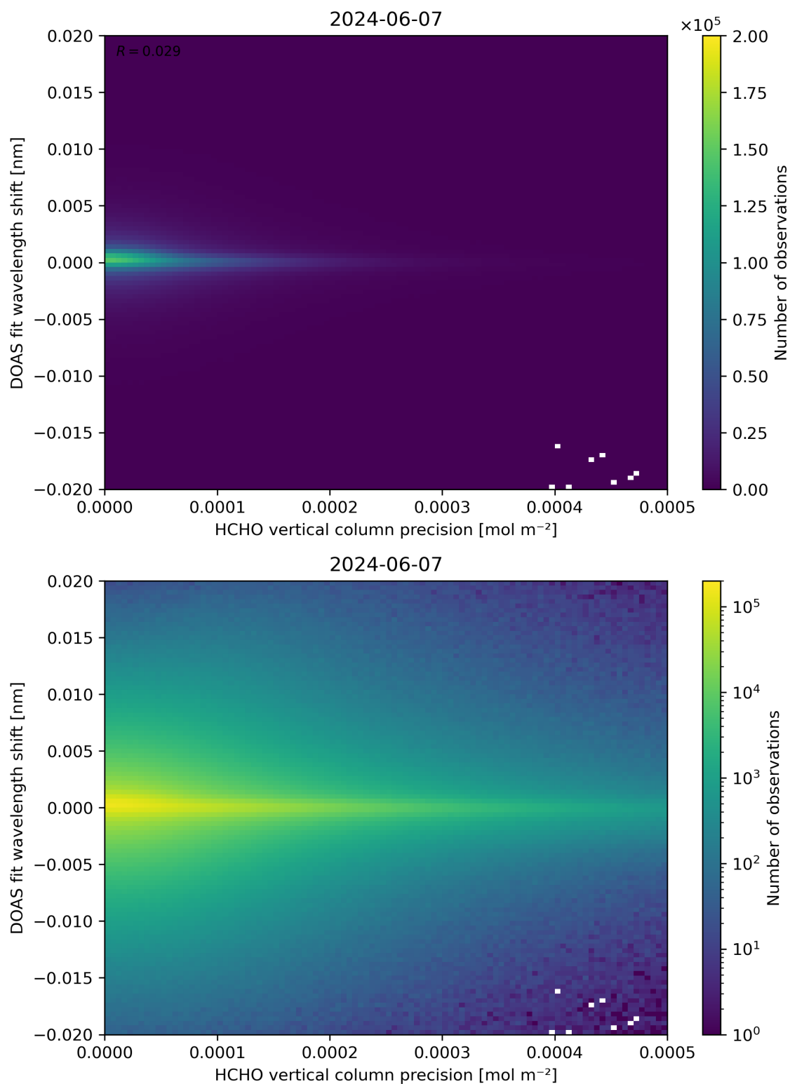
Figure 137: Scatter density plot of “HCHO vertical column precision” against “DOAS fit wavelength shift” for 2024-06-06 to 2024-06-08.
