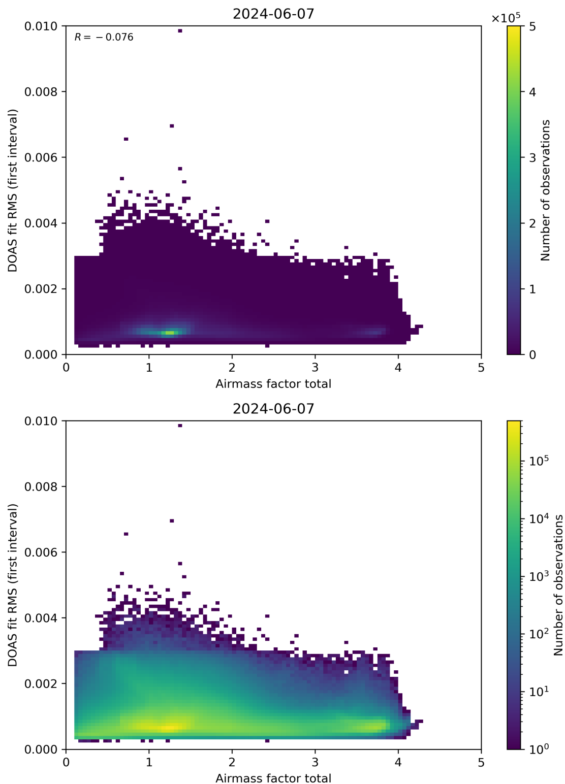
Figure 97: Scatter density plot of “Airmass factor total” against “DOAS fit RMS (first interval)” for 2024-06-06 to 2024-06-08.
