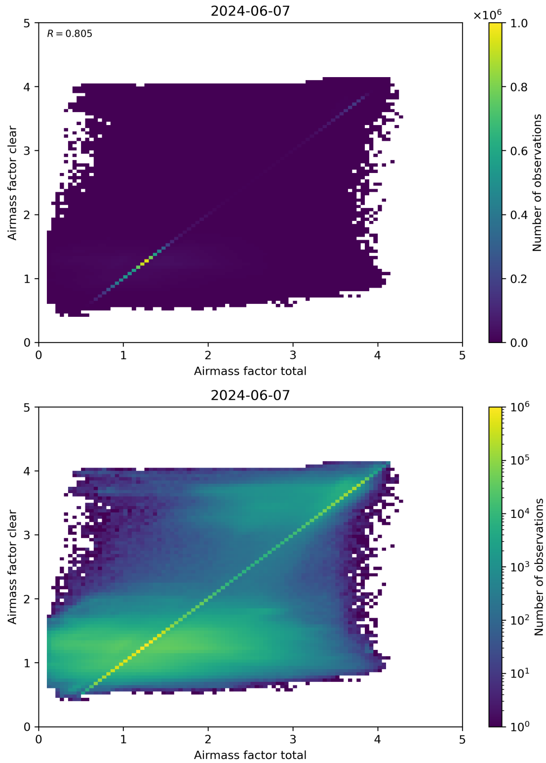
Figure 100: Scatter density plot of “Airmass factor total” against “Airmass factor clear” for 2024-06-06 to 2024-06-08.
