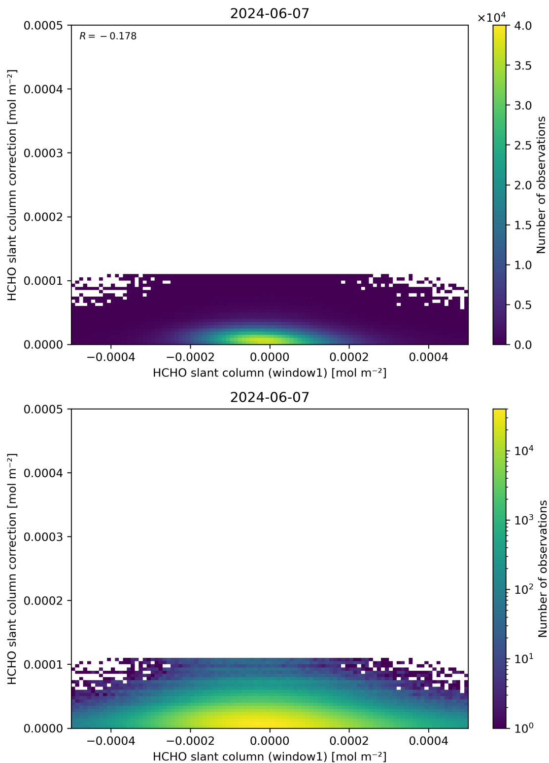
Figure 83: Scatter density plot of “HCHO slant column (window1)” against “HCHO slant column correction” for 2024-06-06 to 2024-06-08.
