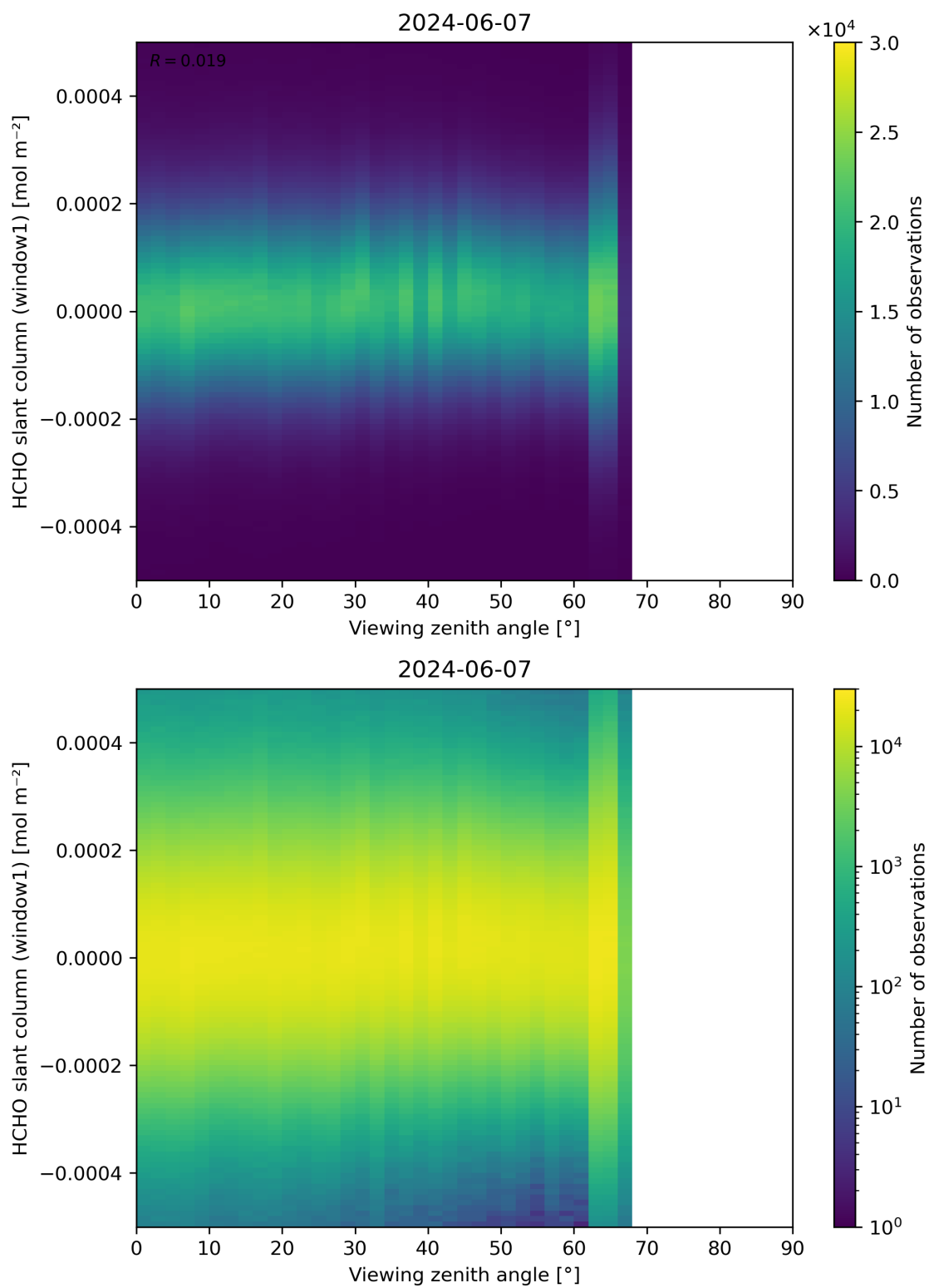
Figure 188: Scatter density plot of “Viewing zenith angle” against “HCHO slant column (window1)” for 2024-06-06 to 2024-06-08.
