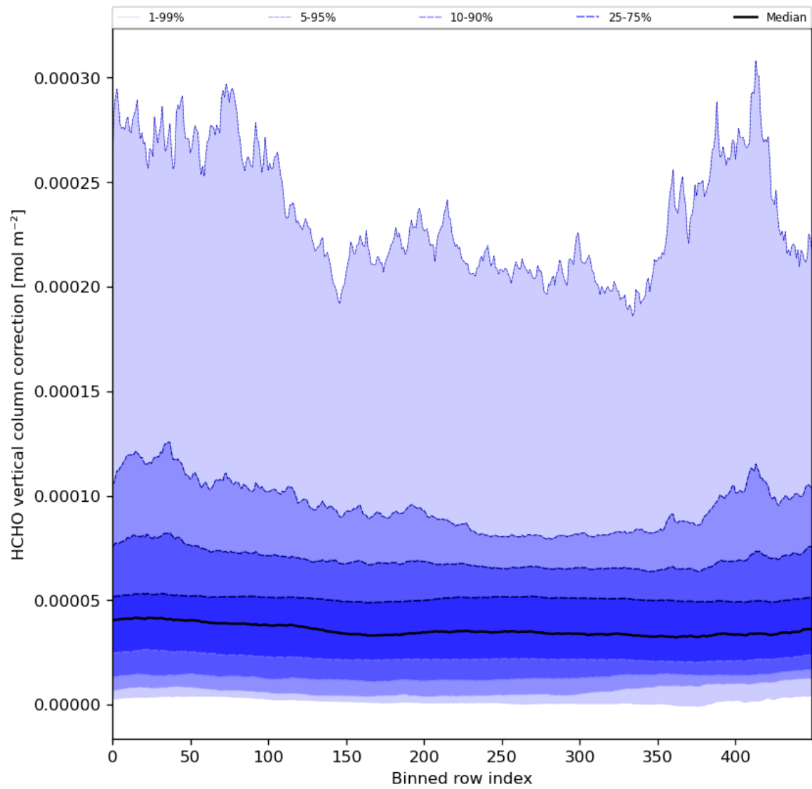
Figure 51: Along track statistics of “HCHO vertical column correction” for 2024-06-06 to 2024-06-08
