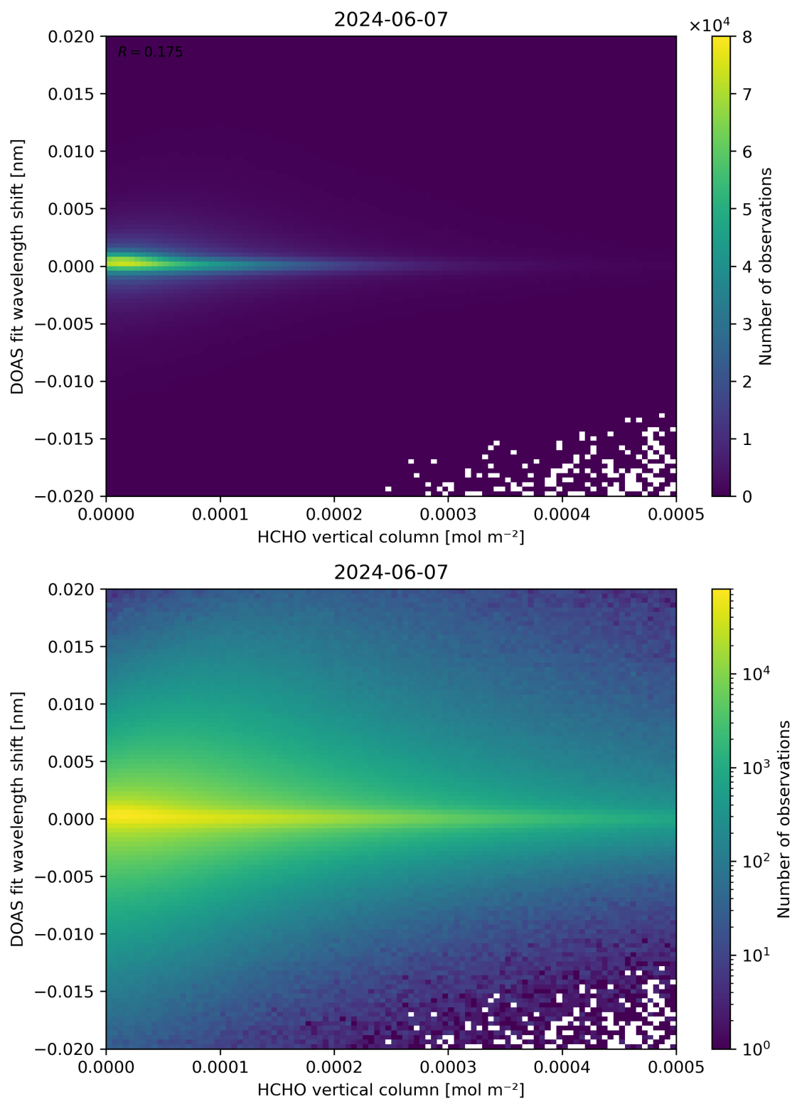
Figure 124: Scatter density plot of “HCHO vertical column” against “DOAS fit wavelength shift” for 2024-06-06 to 2024-06-08.
