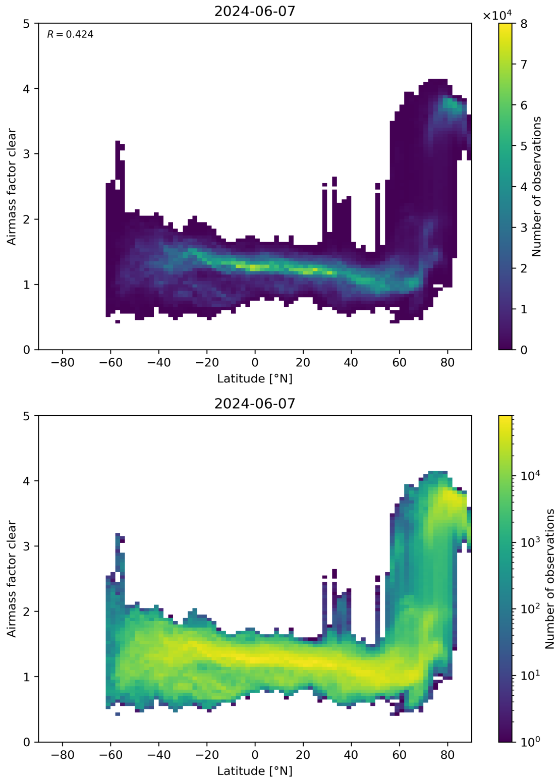
Figure 156: Scatter density plot of “Latitude” against “Airmass factor clear” for 2024-06-06 to 2024-06-08.
