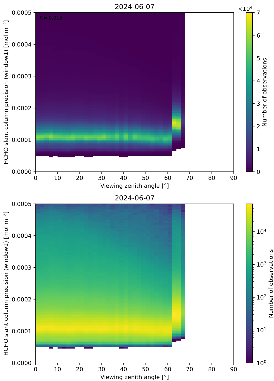
Figure 189: Scatter density plot of “Viewing zenith angle” against “HCHO slant column precision (window1)” for 2024-06-06 to 2024-06-08.
