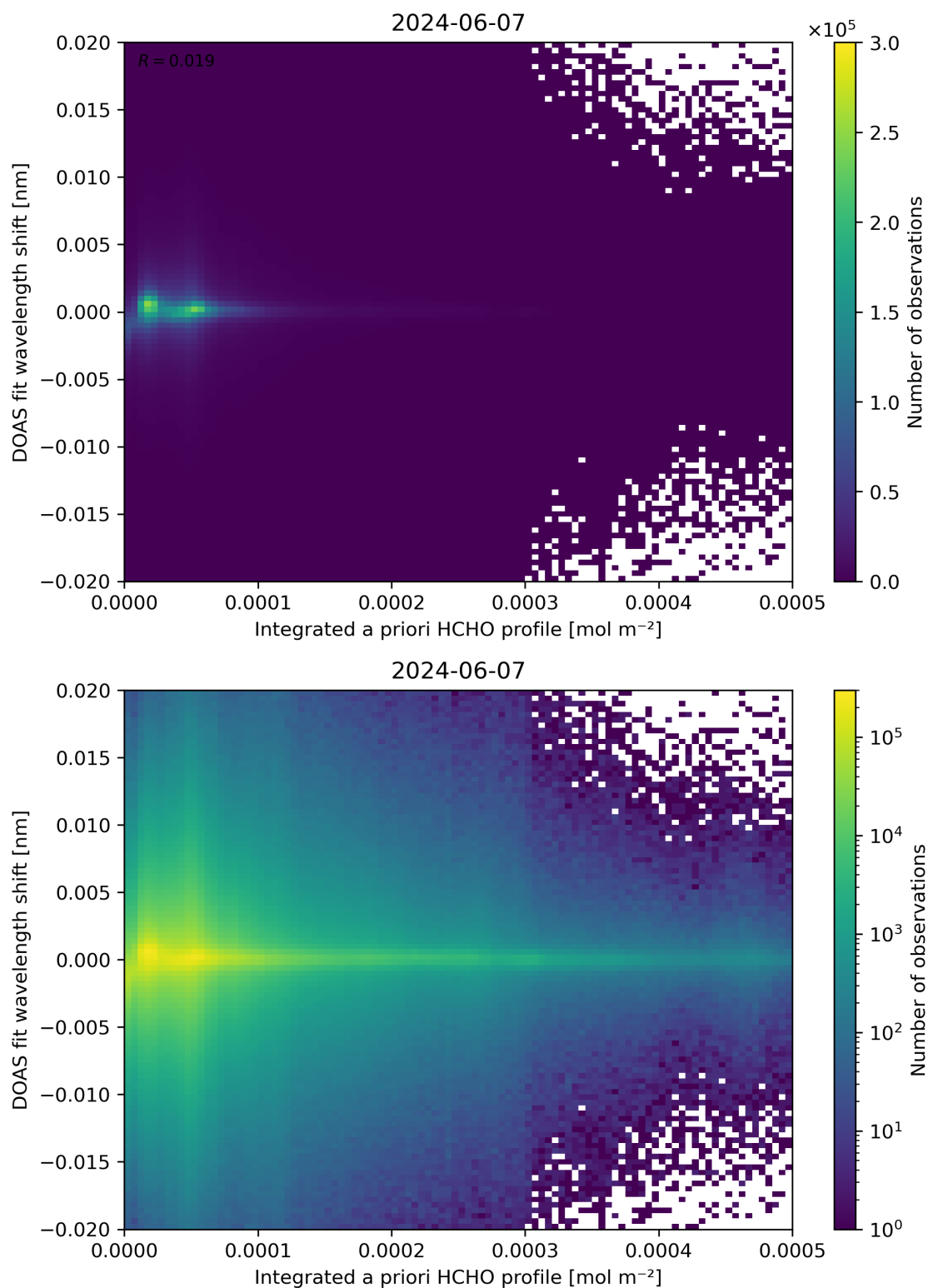
Figure 149: Scatter density plot of “Integrated a priori HCHO profile” against “DOAS fit wavelength shift” for 2024-06-06 to 2024-06-08.
