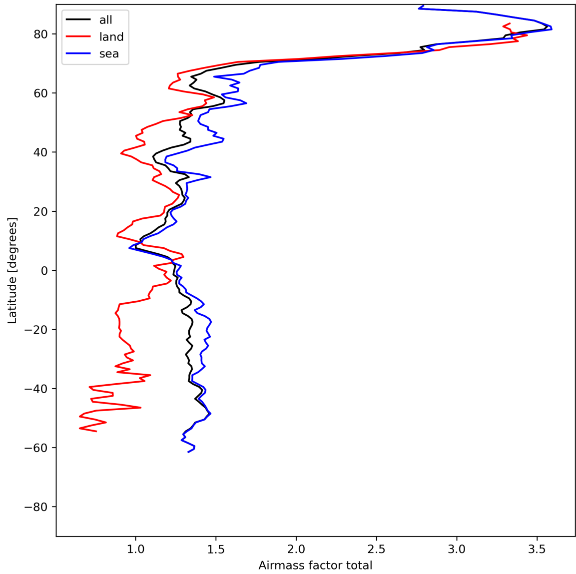
Figure 26: Zonal average of “Airmass factor total” for 2024-06-06 to 2024-06-08.
