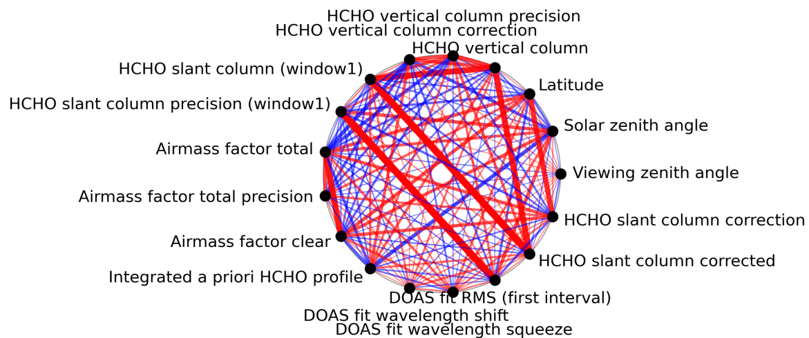
Figure 1: Map of correlation graph for 2024-06-06 to 2024-06-08.
