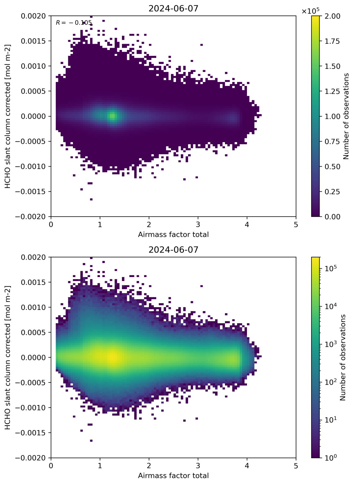
Figure 101: Scatter density plot of “Airmass factor total” against “HCHO slant column corrected” for 2024-06-06 to 2024-06-08.
