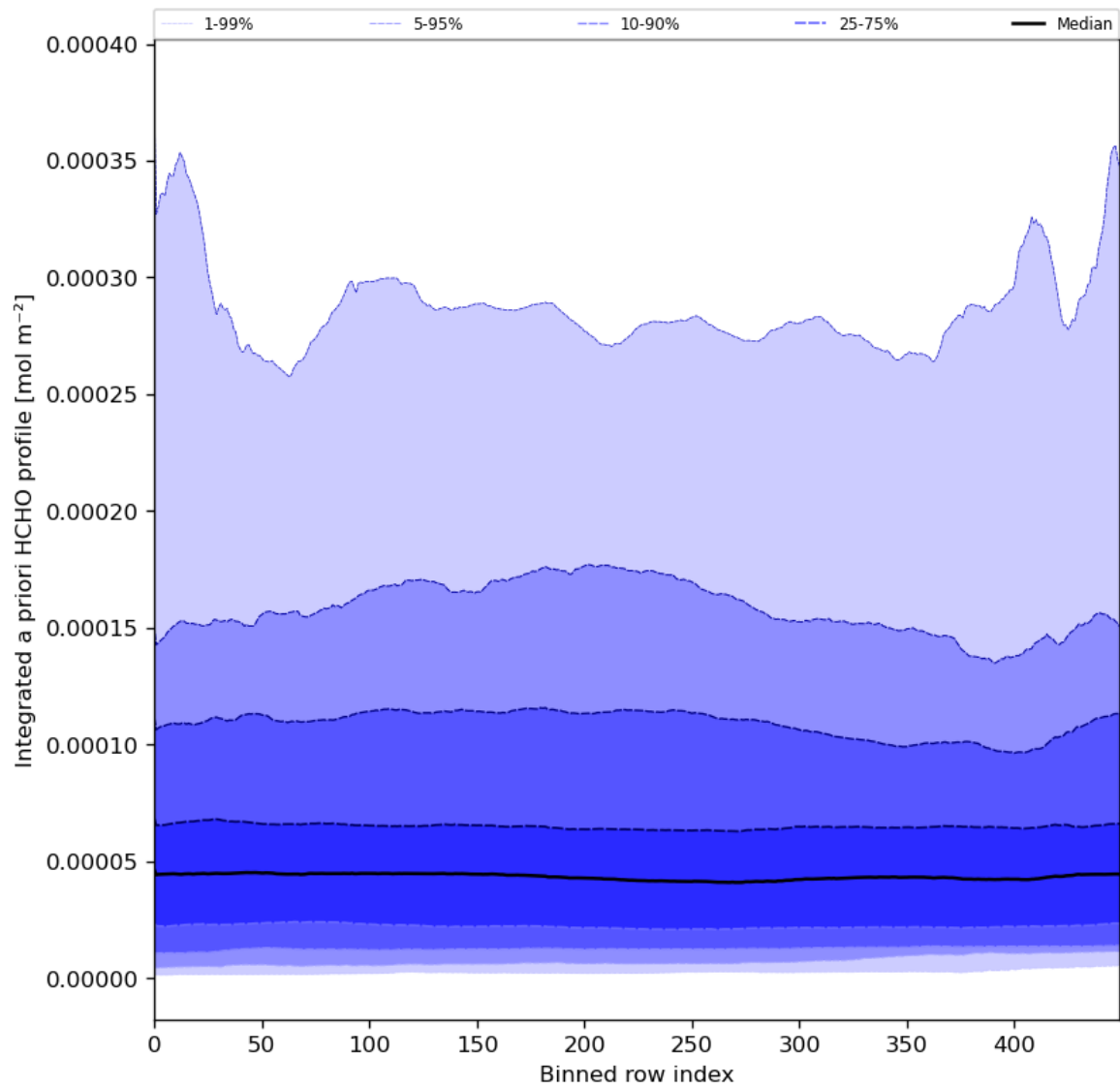
Figure 57: Along track statistics of “Integrated a priori HCHO profile” for 2024-06-06 to 2024-06-08
