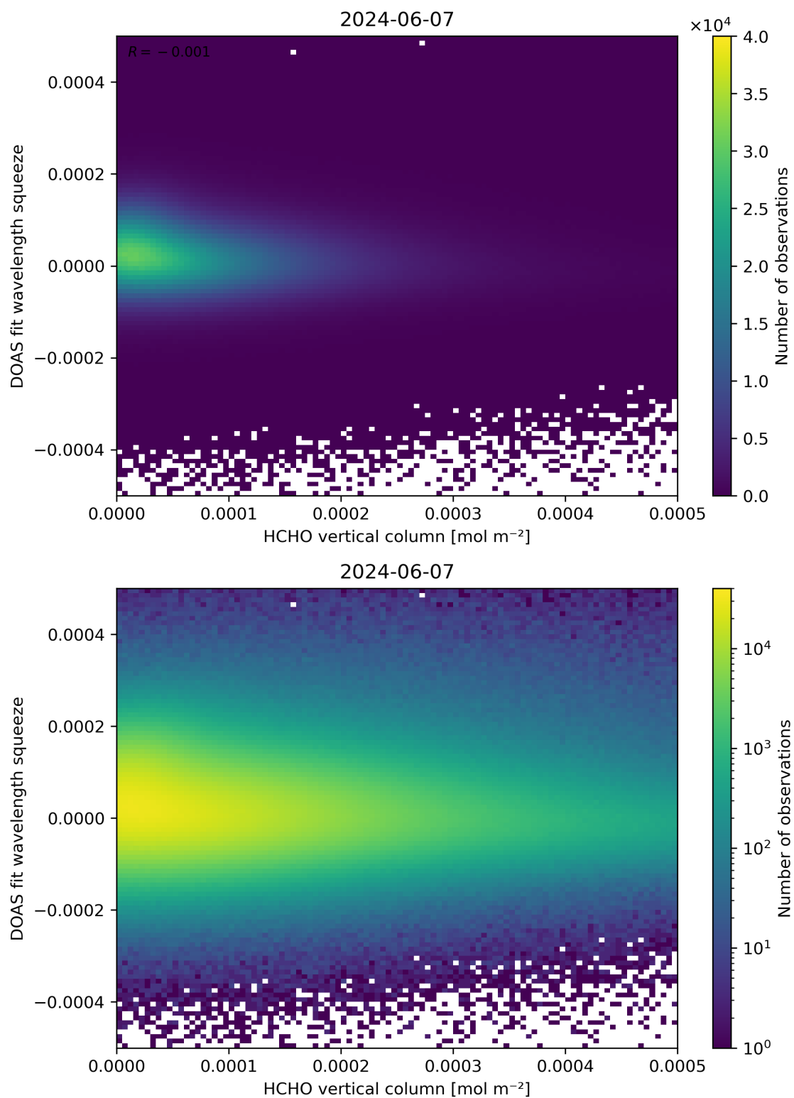
Figure 125: Scatter density plot of “HCHO vertical column” against “DOAS fit wavelength squeeze” for 2024-06-06 to 2024-06-08.
