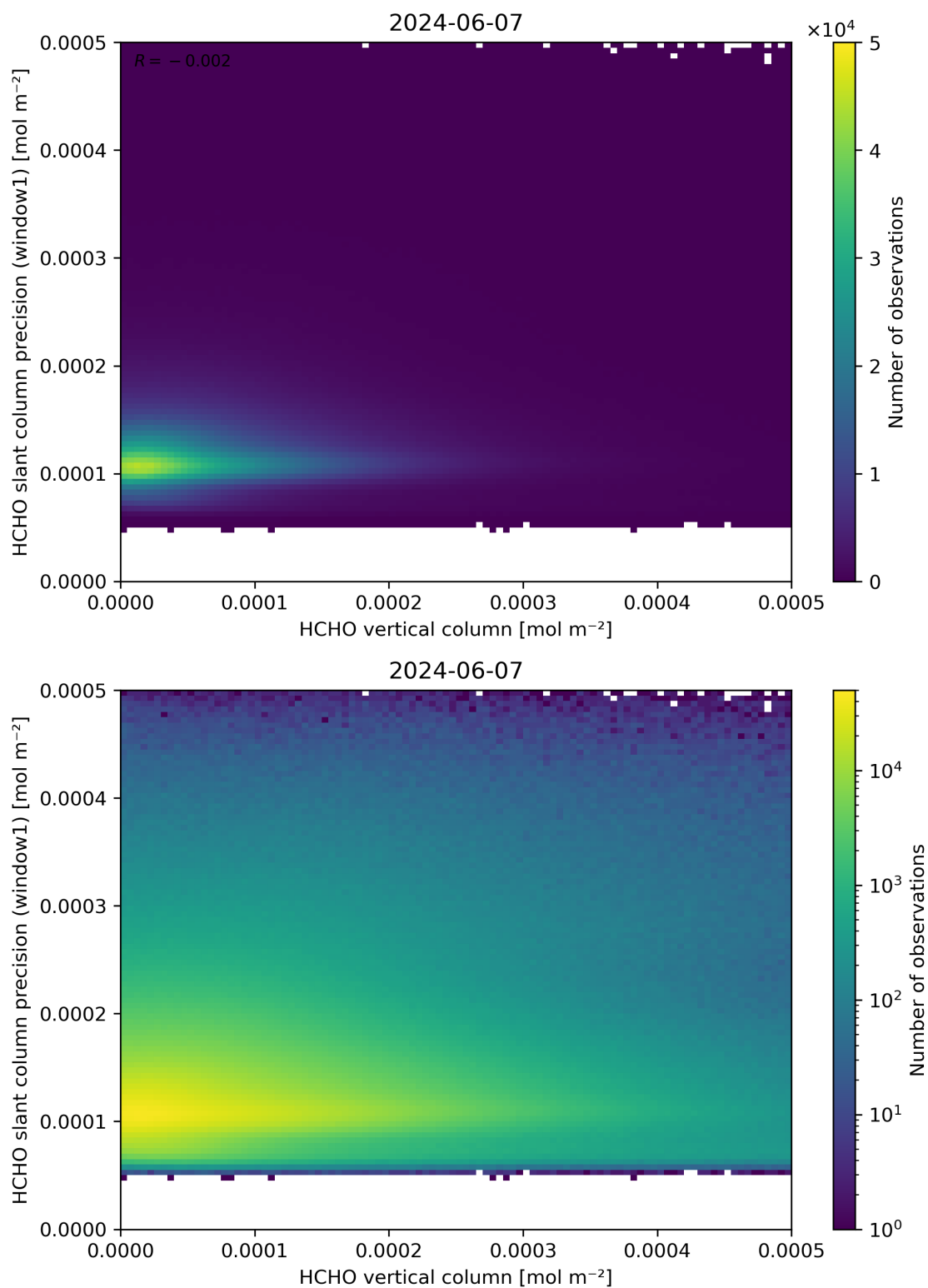
Figure 130: Scatter density plot of “HCHO vertical column” against “HCHO slant column precision (window1)” for 2024-06-06 to 2024-06-08.
