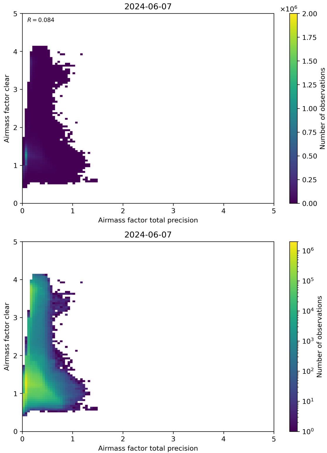
Figure 108: Scatter density plot of “Airmass factor total precision” against “Airmass factor clear” for 2024-06-06 to 2024-06-08.
