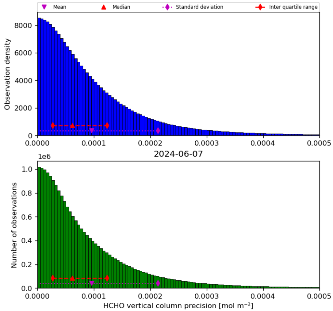
Figure 36: Histogram of “HCHO vertical column precision” for 2024-06-06 to 2024-06-08
