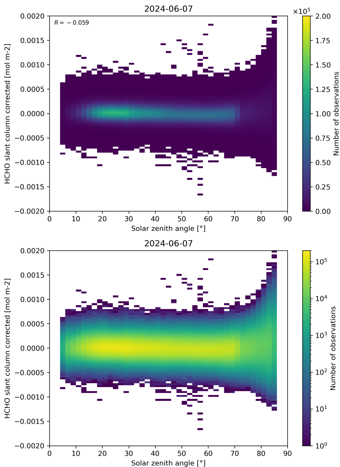
Figure 171: Scatter density plot of “Solar zenith angle” against “HCHO slant column corrected” for 2024-06-06 to 2024-06-08.
