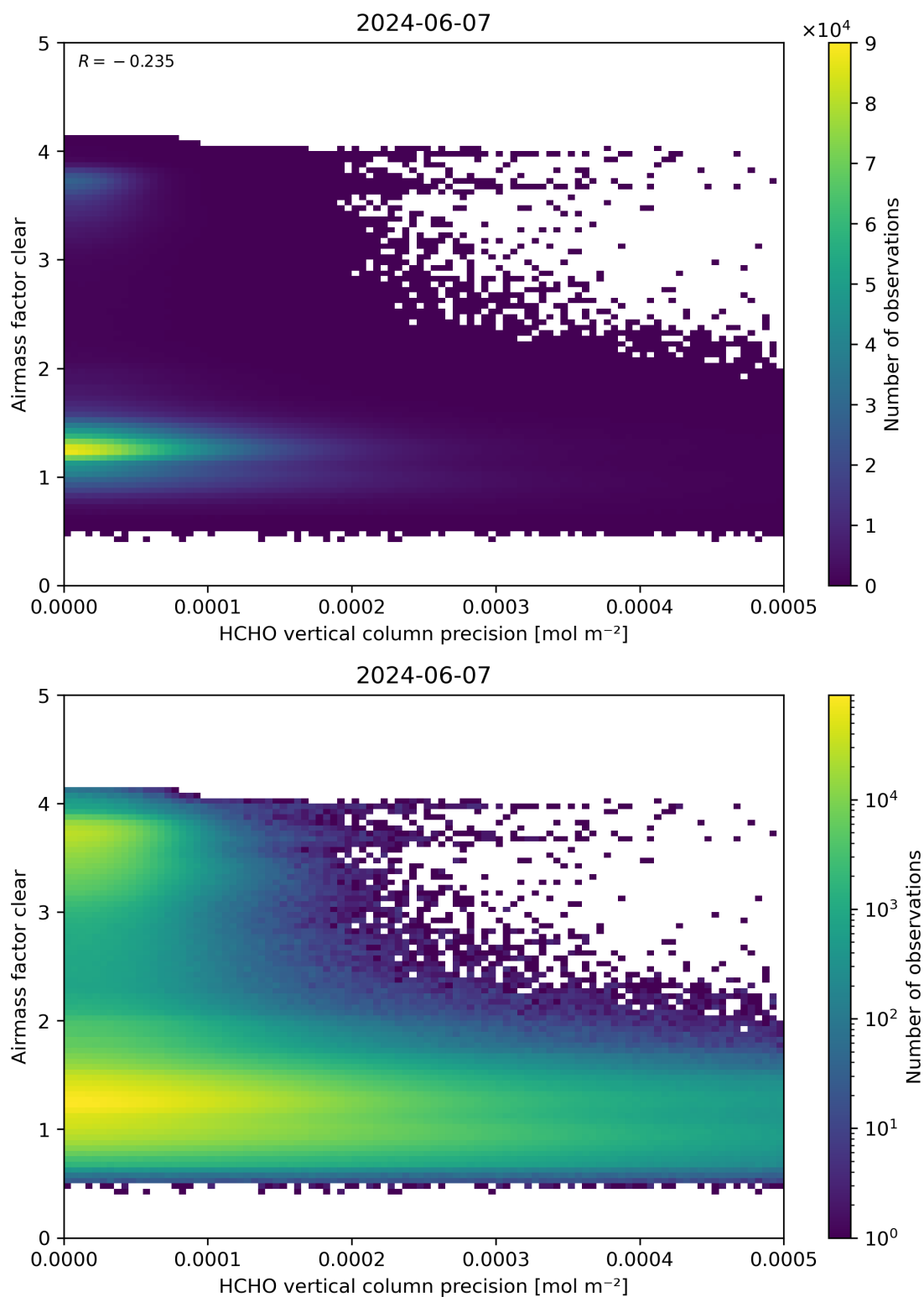
Figure 139: Scatter density plot of “HCHO vertical column precision” against “Airmass factor clear” for 2024-06-06 to 2024-06-08.
