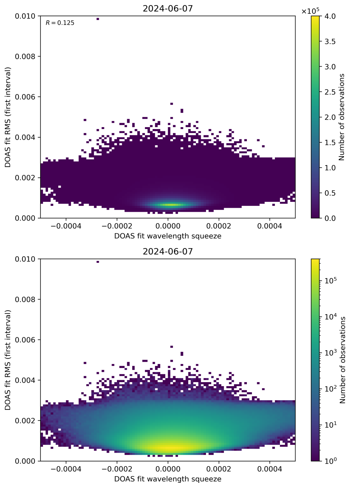
Figure 68: Scatter density plot of “DOAS fit wavelength squeeze” against “DOAS fit RMS (first interval)” for 2024-06-06 to 2024-06-08.
