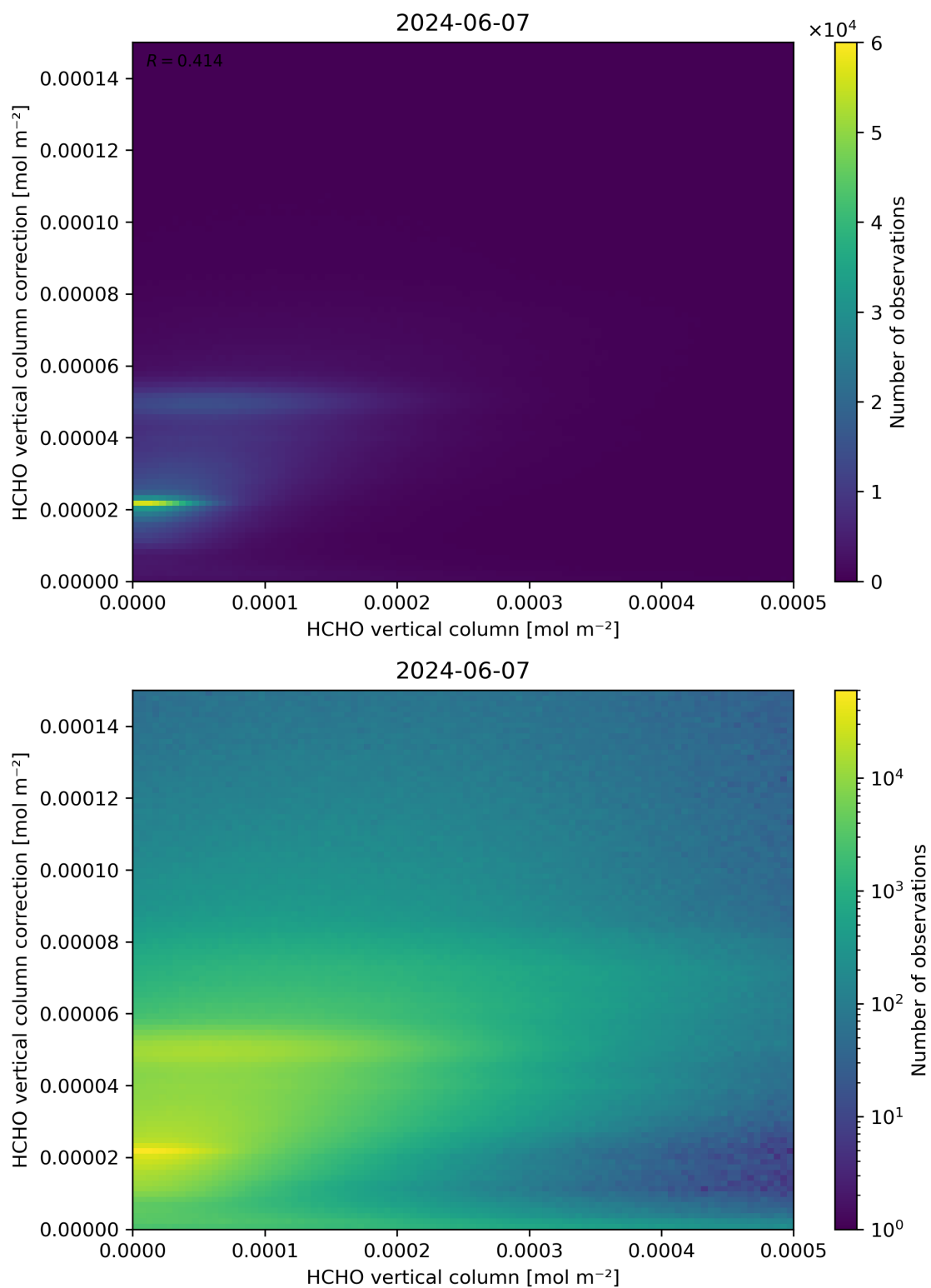
Figure 133: Scatter density plot of “HCHO vertical column” against “HCHO vertical column correction” for 2024-06-06 to 2024-06-08.
