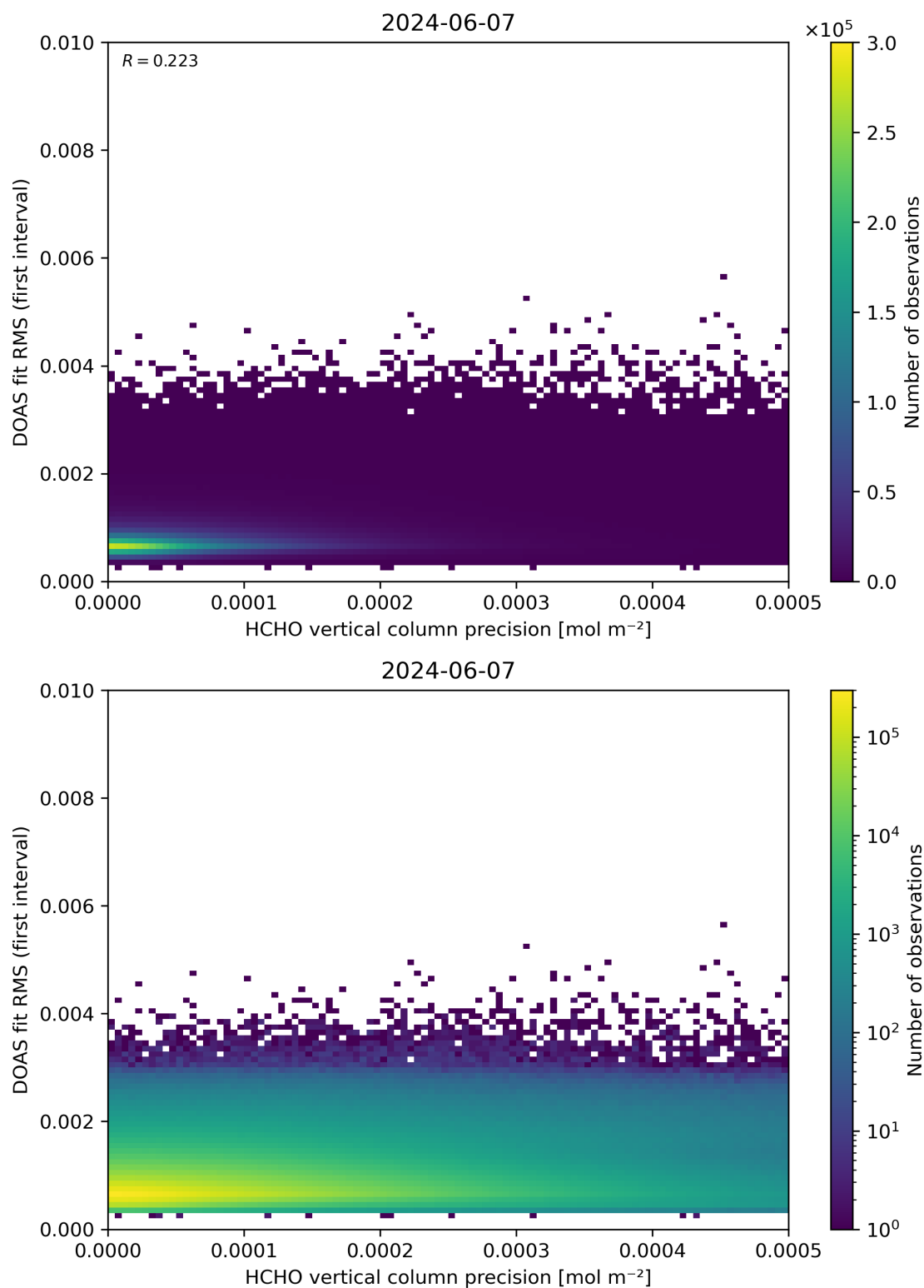
Figure 136: Scatter density plot of “HCHO vertical column precision” against “DOAS fit RMS (first interval)” for 2024-06-06 to 2024-06-08.
