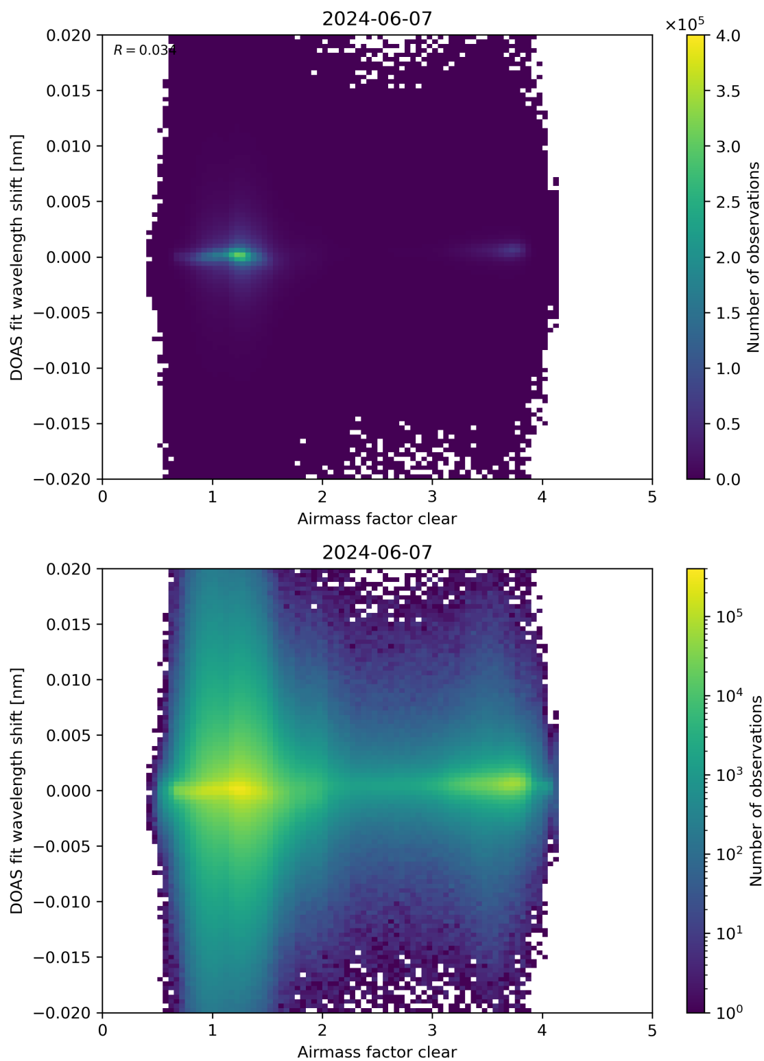
Figure 72: Scatter density plot of “Airmass factor clear” against “DOAS fit wavelength shift” for 2024-06-06 to 2024-06-08.
