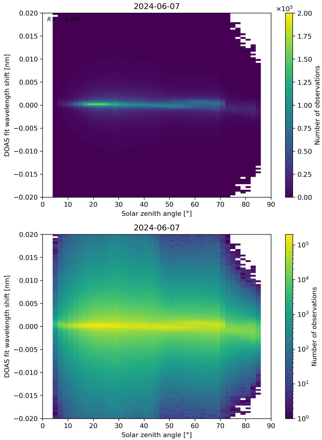
Figure 168: Scatter density plot of “Solar zenith angle” against “DOAS fit wavelength shift” for 2024-06-06 to 2024-06-08.
