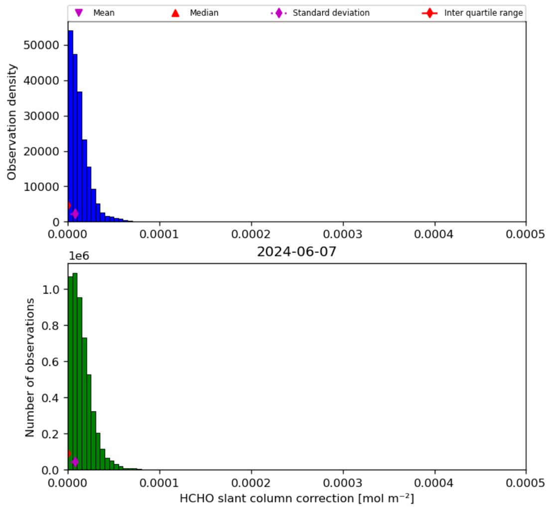
Figure 47: Histogram of “HCHO slant column correction” for 2024-06-06 to 2024-06-08
