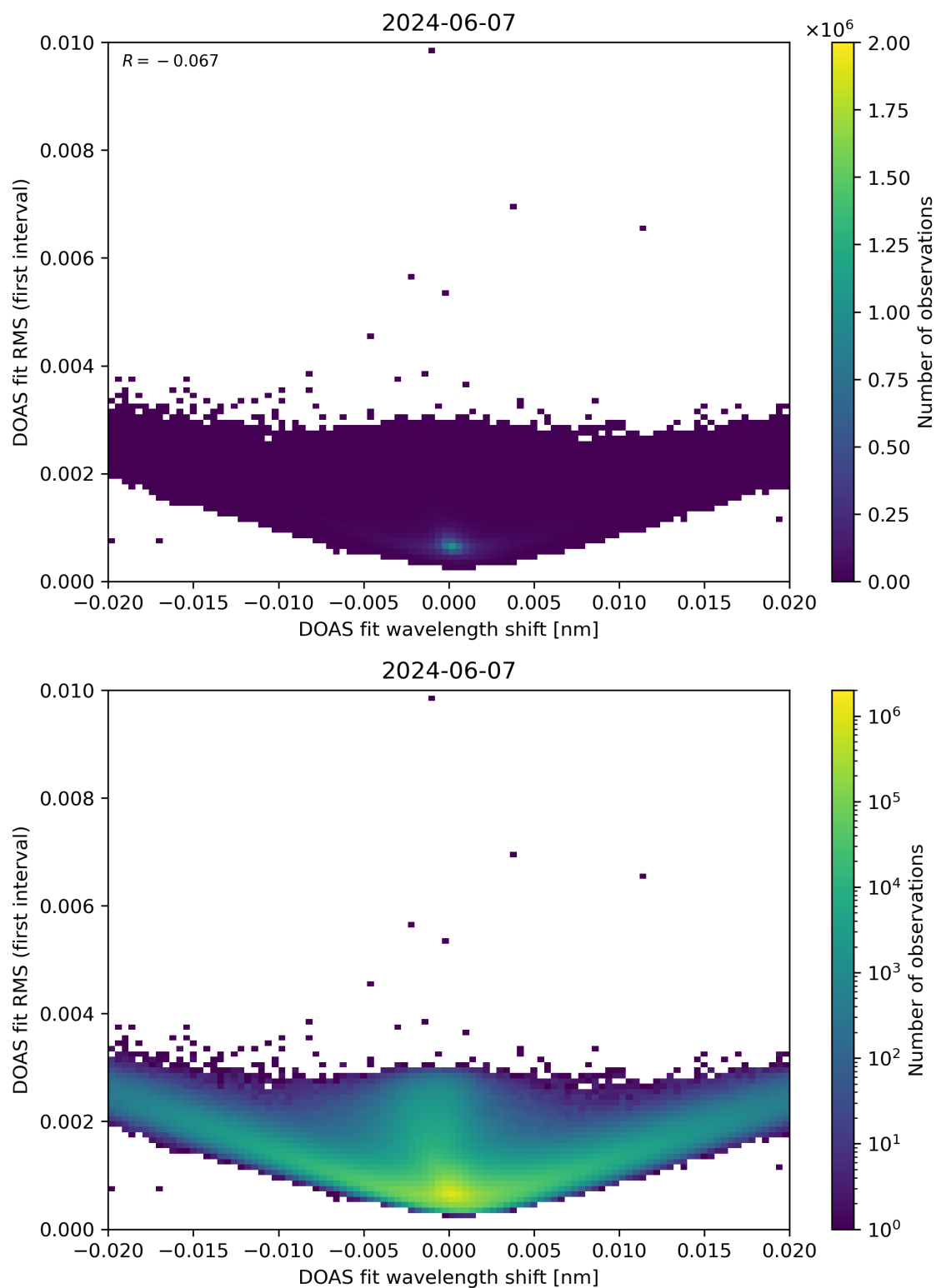
Figure 64: Scatter density plot of “DOAS fit wavelength shift” against “DOAS fit RMS (first interval)” for 2024-06-06 to 2024-06-08.
