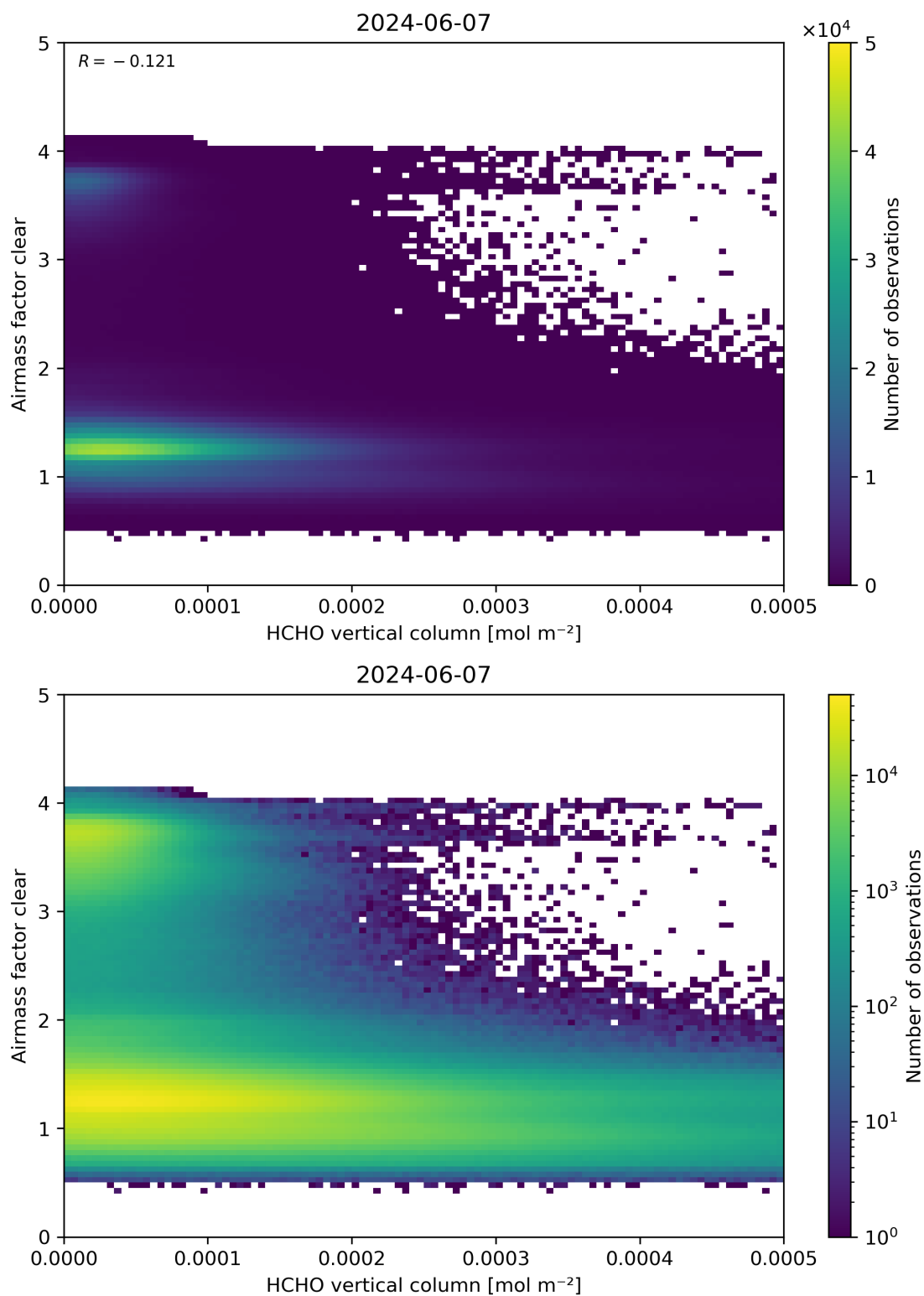
Figure 126: Scatter density plot of “HCHO vertical column” against “Airmass factor clear” for 2024-06-06 to 2024-06-08.
