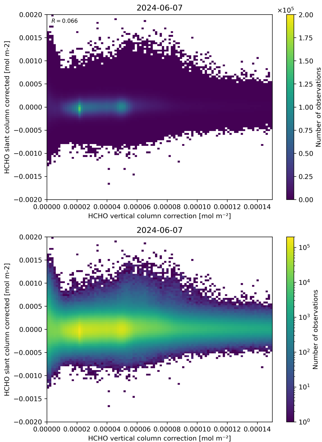
Figure 116: Scatter density plot of “HCHO vertical column correction” against “HCHO slant column corrected” for 2024-06-06 to 2024-06-08.
