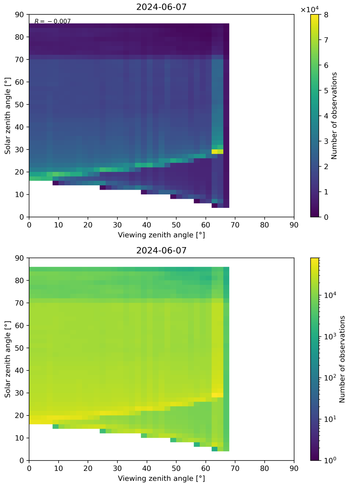
Figure 197: Scatter density plot of “Viewing zenith angle” against “Solar zenith angle” for 2024-06-06 to 2024-06-08.
