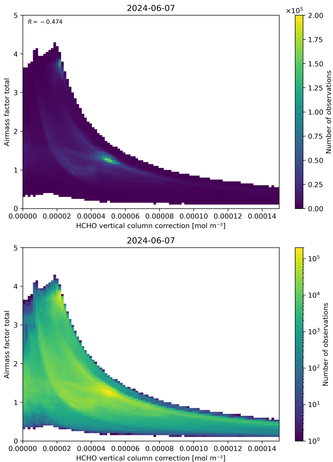
Figure 120: Scatter density plot of “HCHO vertical column correction” against “Airmass factor total” for 2024-06-06 to 2024-06-08.
