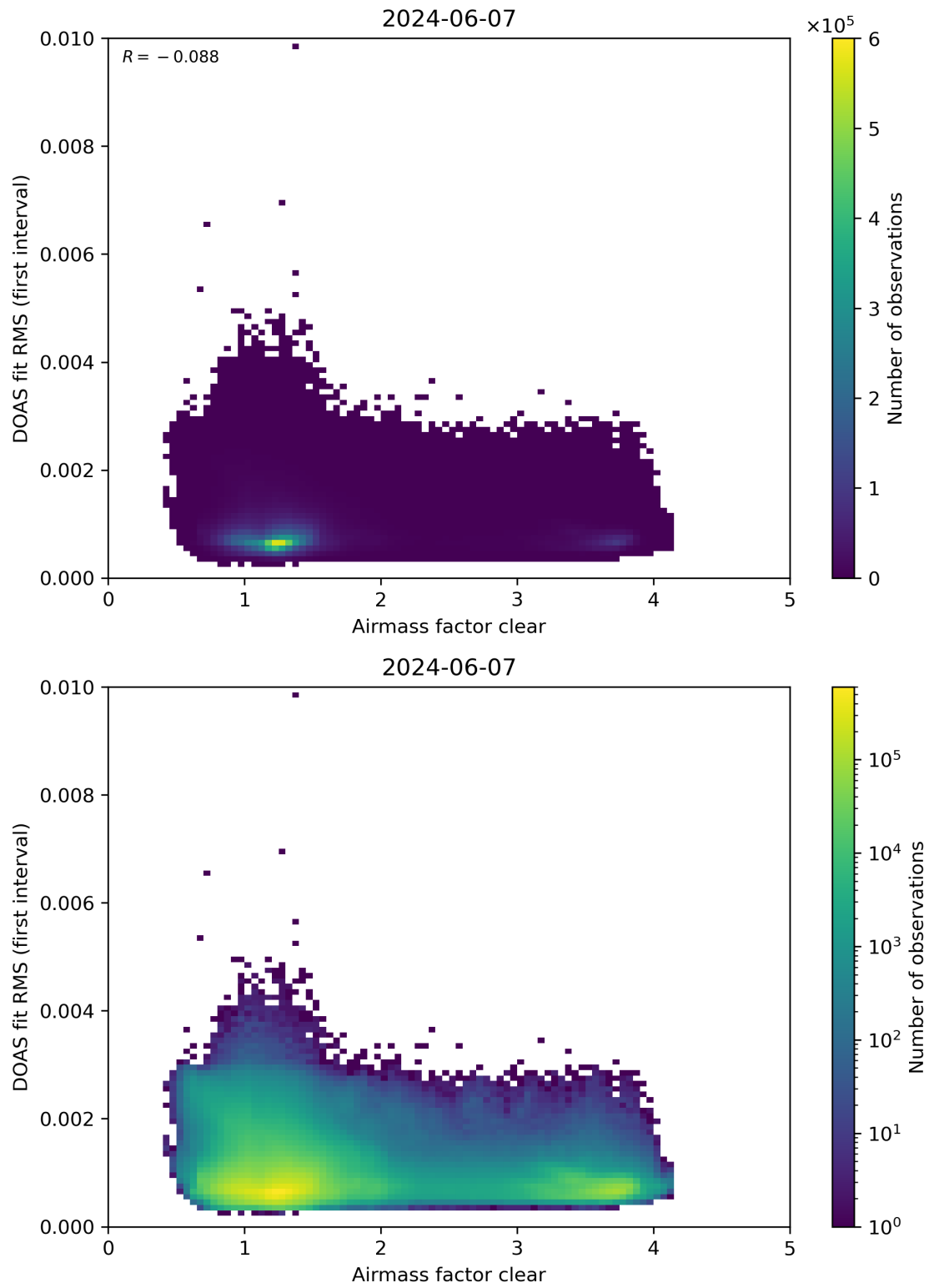
Figure 71: Scatter density plot of “Airmass factor clear” against “DOAS fit RMS (first interval)” for 2024-06-06 to 2024-06-08.
