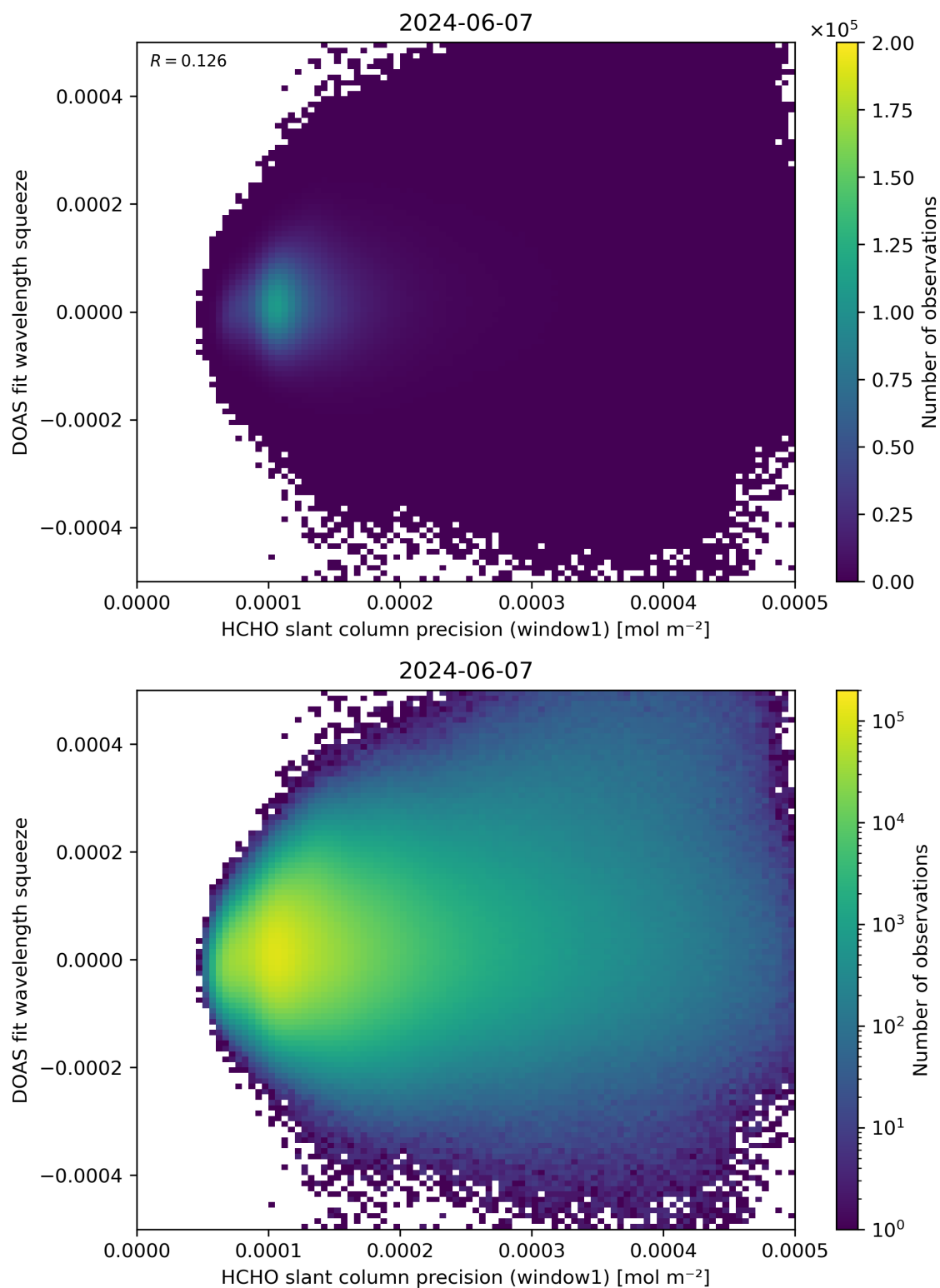
Figure 90: Scatter density plot of “HCHO slant column precision (window1)” against “DOAS fit wavelength squeeze” for 2024-06-06 to 2024-06-08.
