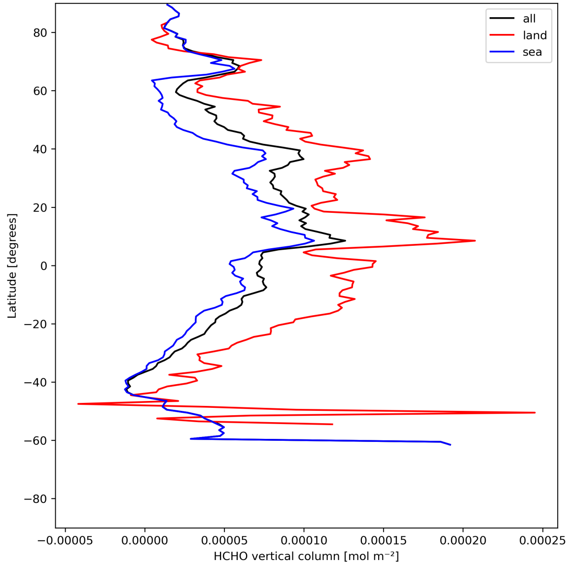
Figure 21: Zonal average of “HCHO vertical column” for 2024-06-06 to 2024-06-08.
