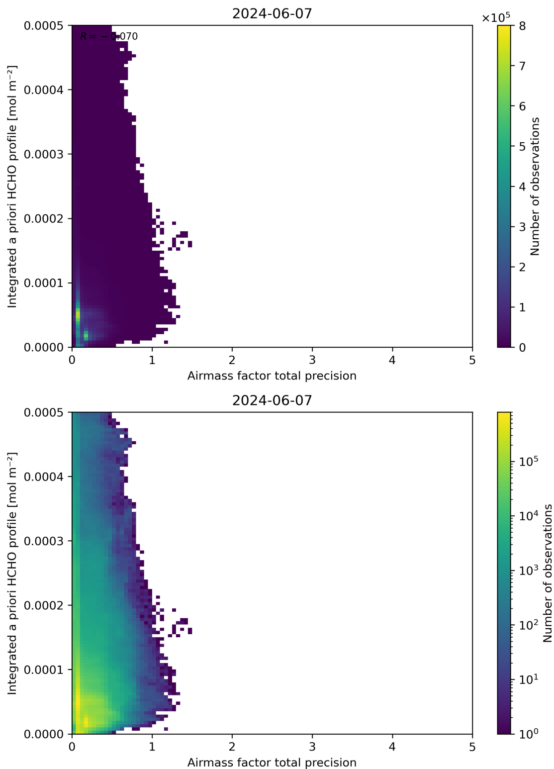
Figure 111: Scatter density plot of “Airmass factor total precision” against “Integrated a priori HCHO profile” for 2024-06-06 to 2024-06-08.
