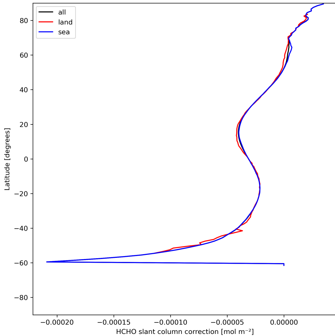
Figure 33: Zonal average of “HCHO slant column correction” for 2024-06-06 to 2024-06-08.
