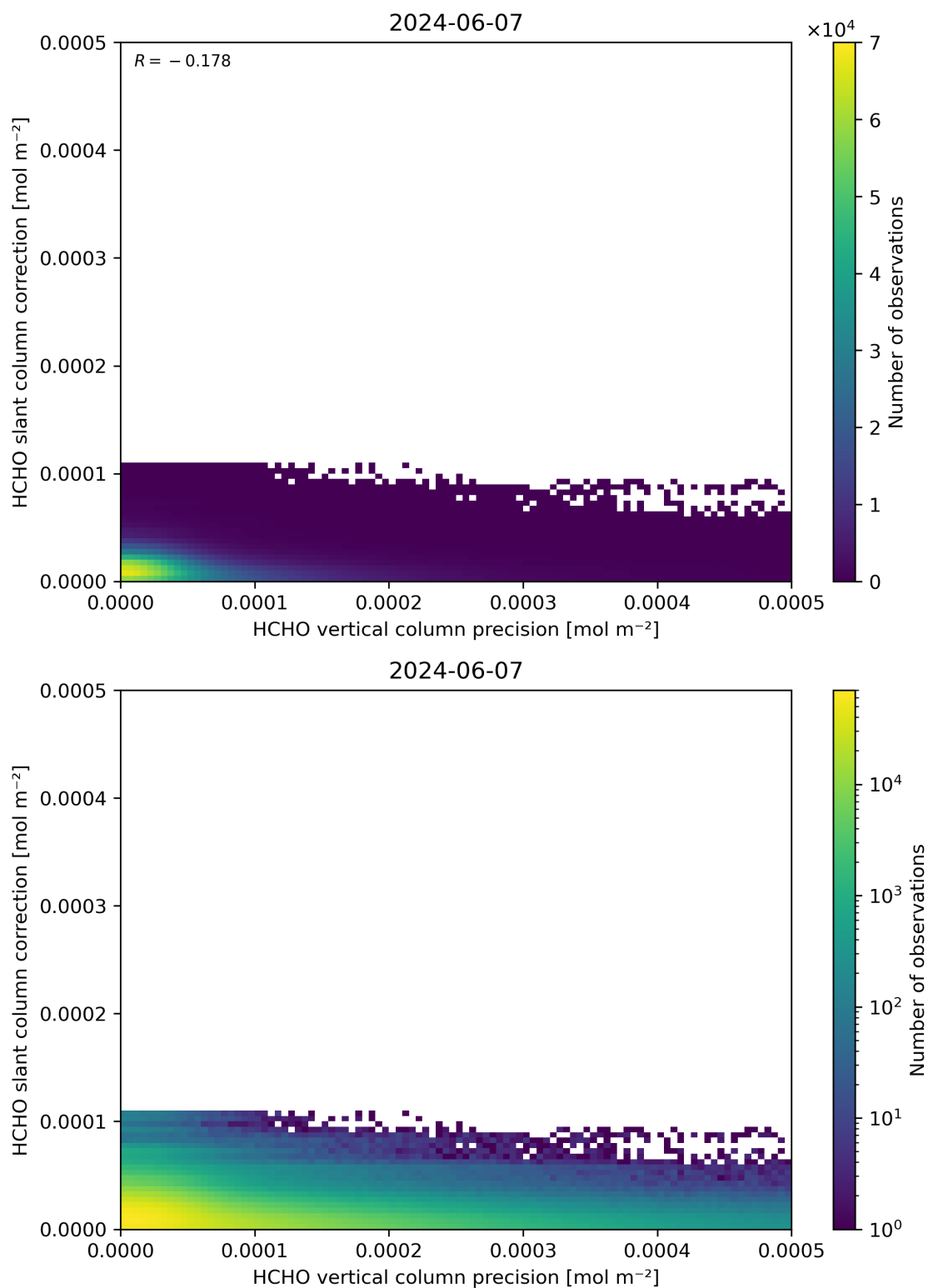
Figure 141: Scatter density plot of “HCHO vertical column precision” against “HCHO slant column correction” for 2024-06-06 to 2024-06-08.
