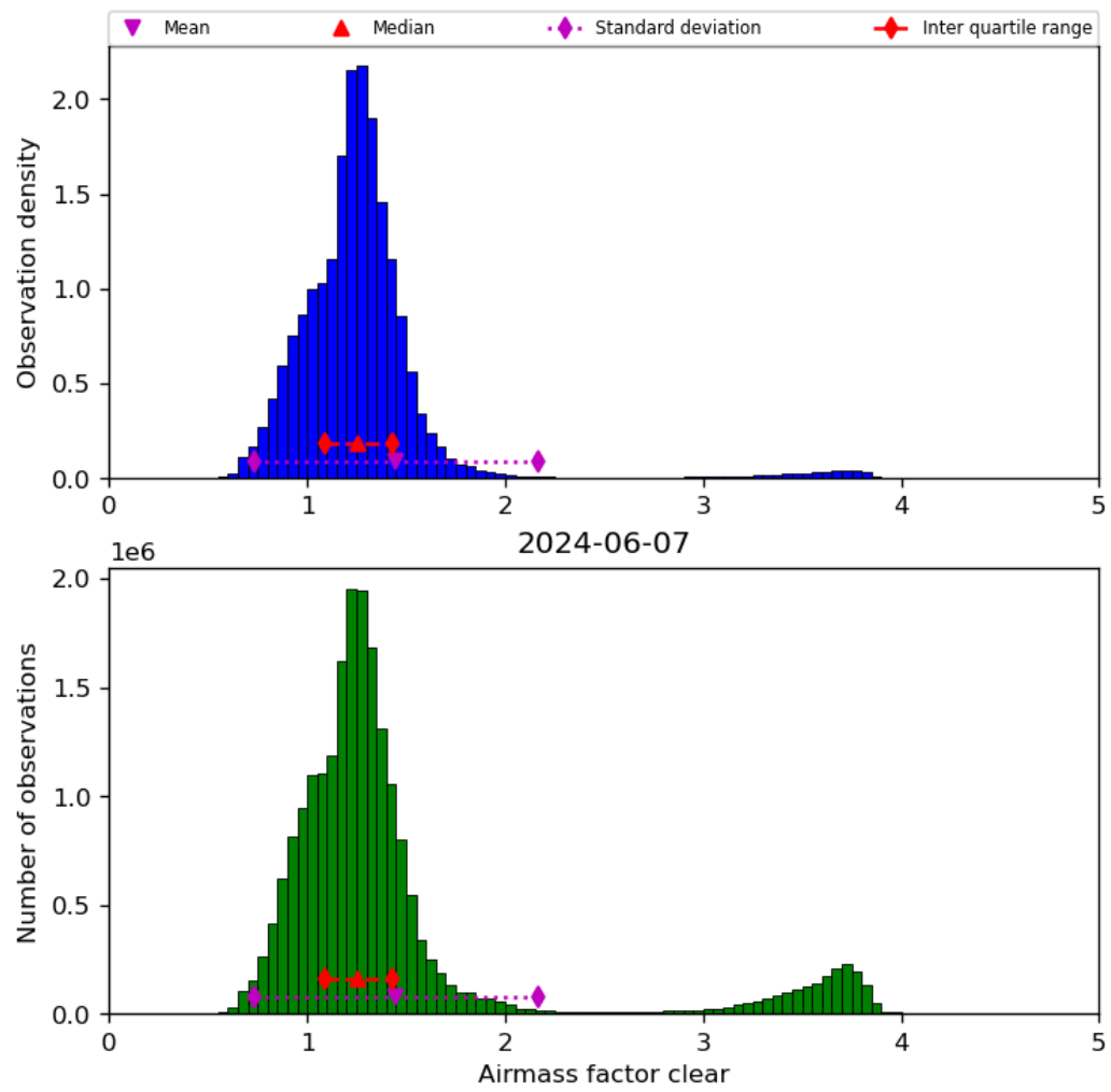
Figure 42: Histogram of “Airmass factor clear” for 2024-06-06 to 2024-06-08
