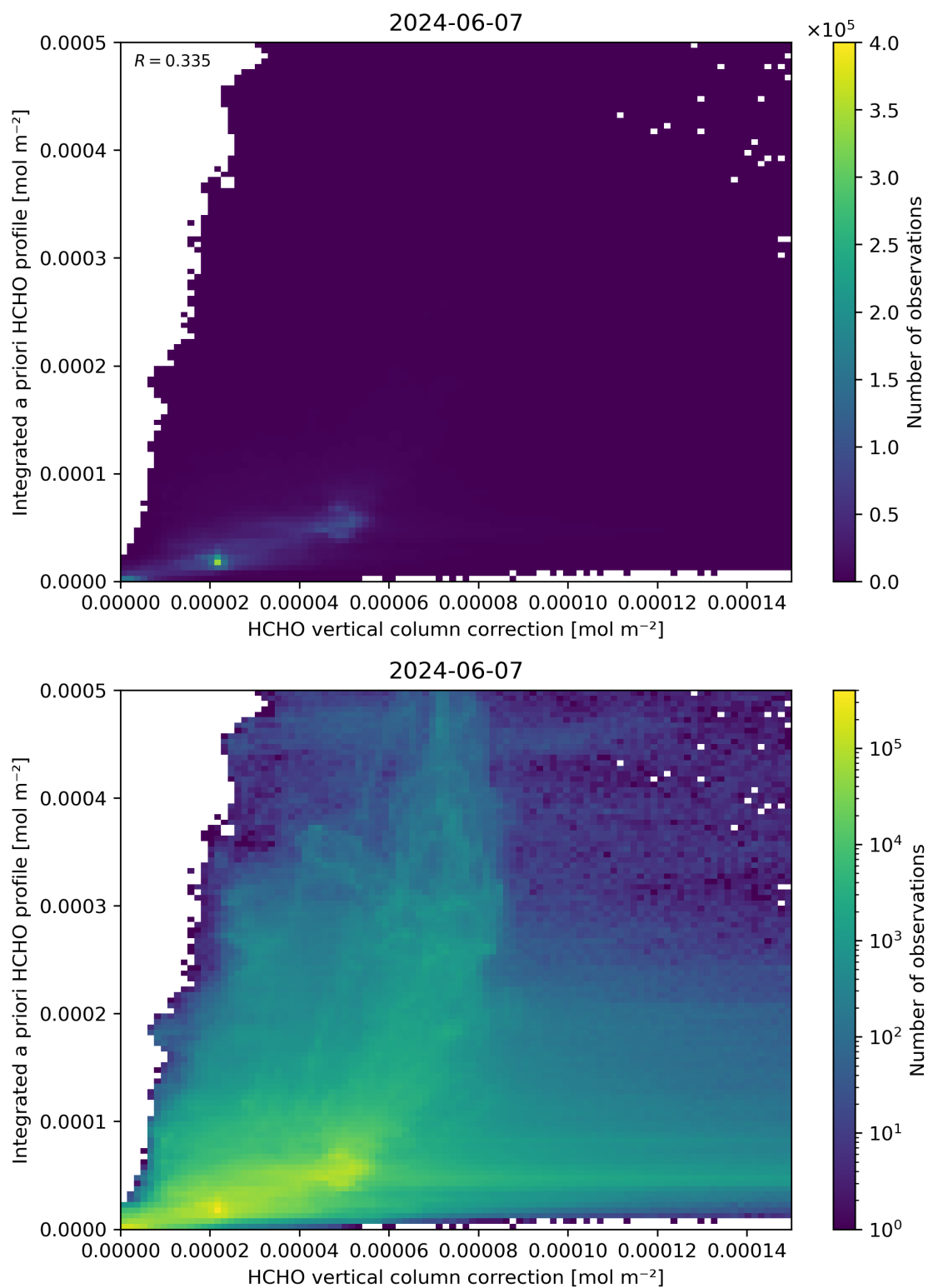
Figure 122: Scatter density plot of “HCHO vertical column correction” against “Integrated a priori HCHO profile” for 2024-06-06 to 2024-06-08.
