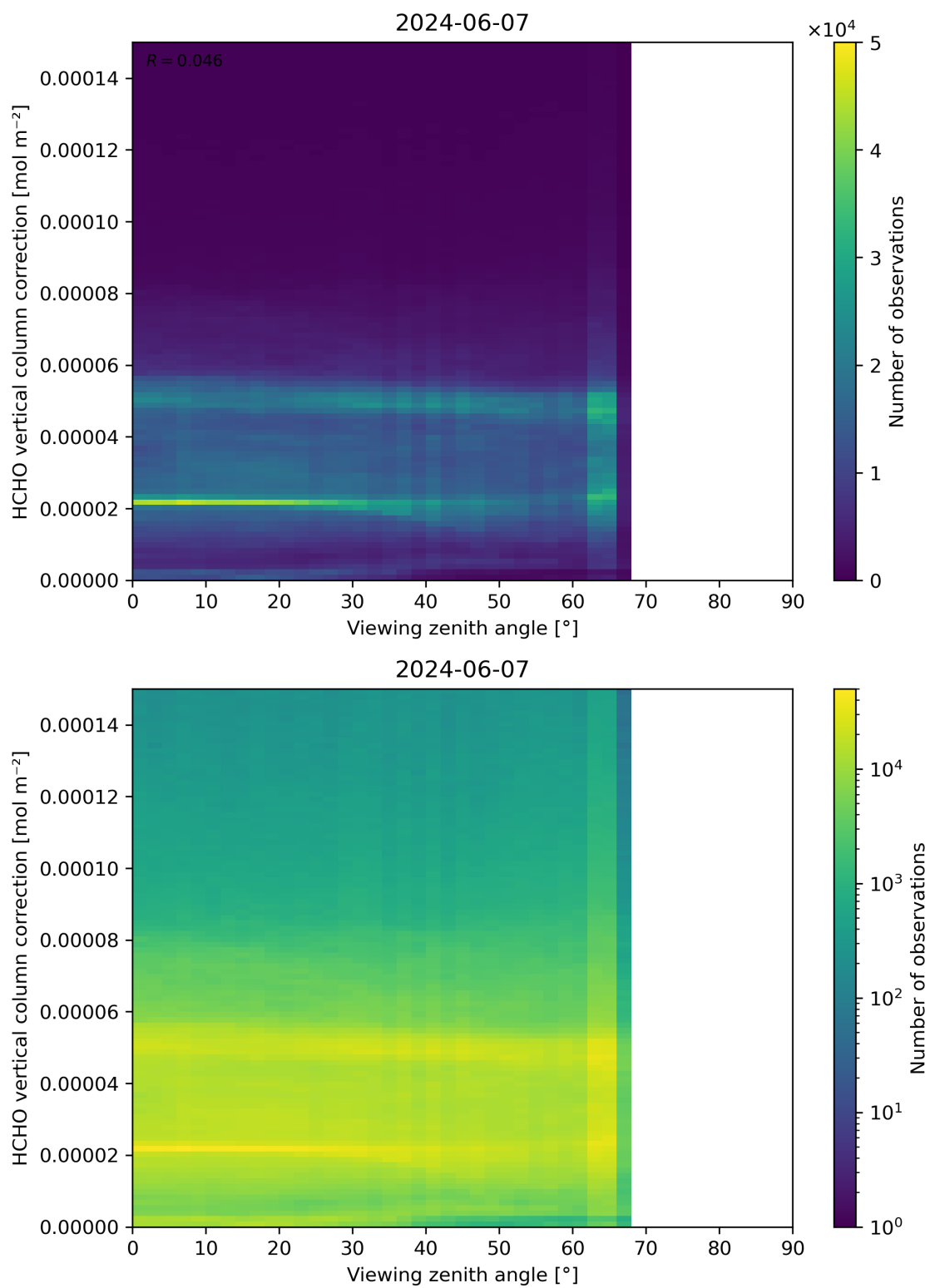
Figure 193: Scatter density plot of “Viewing zenith angle” against “HCHO vertical column correction” for 2024-06-06 to 2024-06-08.
