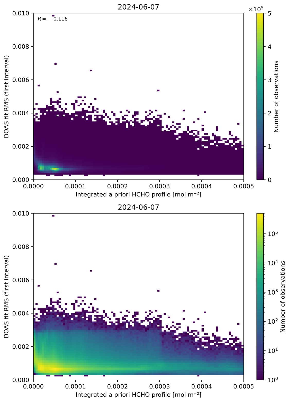
Figure 148: Scatter density plot of “Integrated a priori HCHO profile” against “DOAS fit RMS (first interval)” for 2024-06-06 to 2024-06-08.
