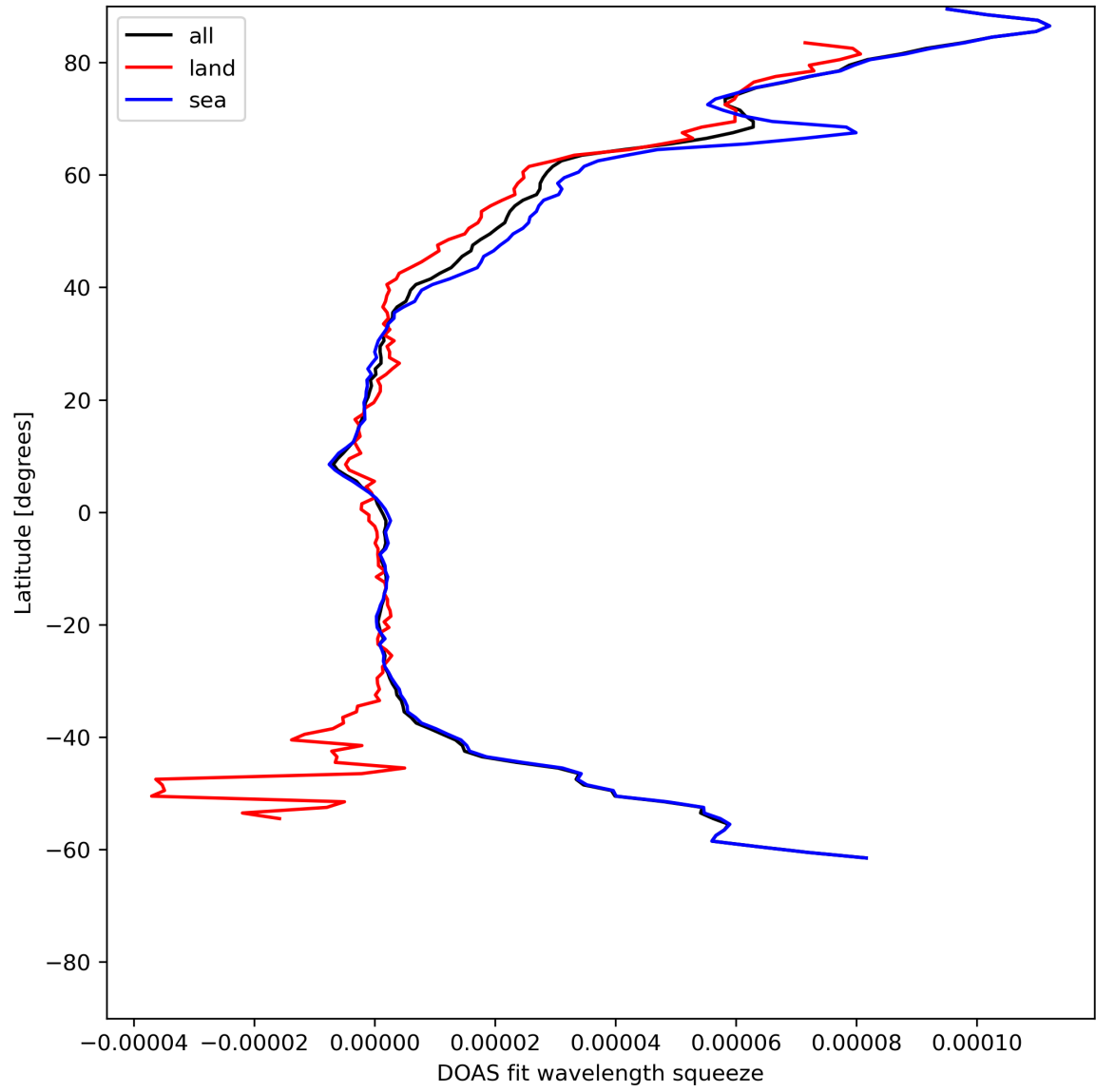
Figure 31: Zonal average of “DOAS fit wavelength squeeze” for 2024-06-06 to 2024-06-08.
