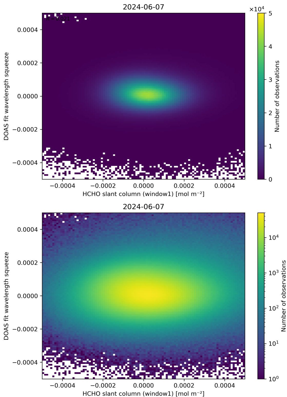
Figure 80: Scatter density plot of “HCHO slant column (window1)” against “DOAS fit wavelength squeeze” for 2024-06-06 to 2024-06-08.
