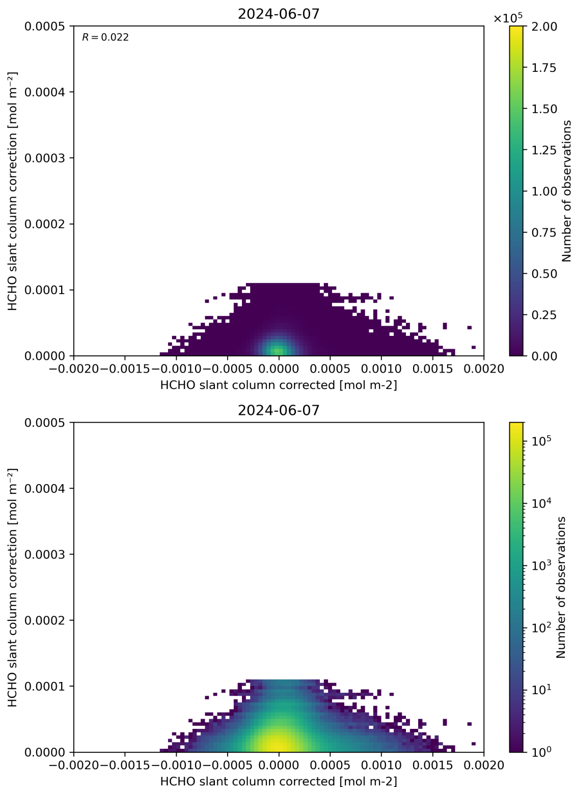
Figure 77: Scatter density plot of “HCHO slant column corrected” against “HCHO slant column correction” for 2024-06-06 to 2024-06-08.
