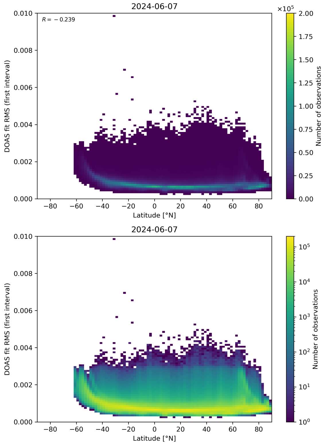
Figure 153: Scatter density plot of “Latitude” against “DOAS fit RMS (first interval)” for 2024-06-06 to 2024-06-08.
