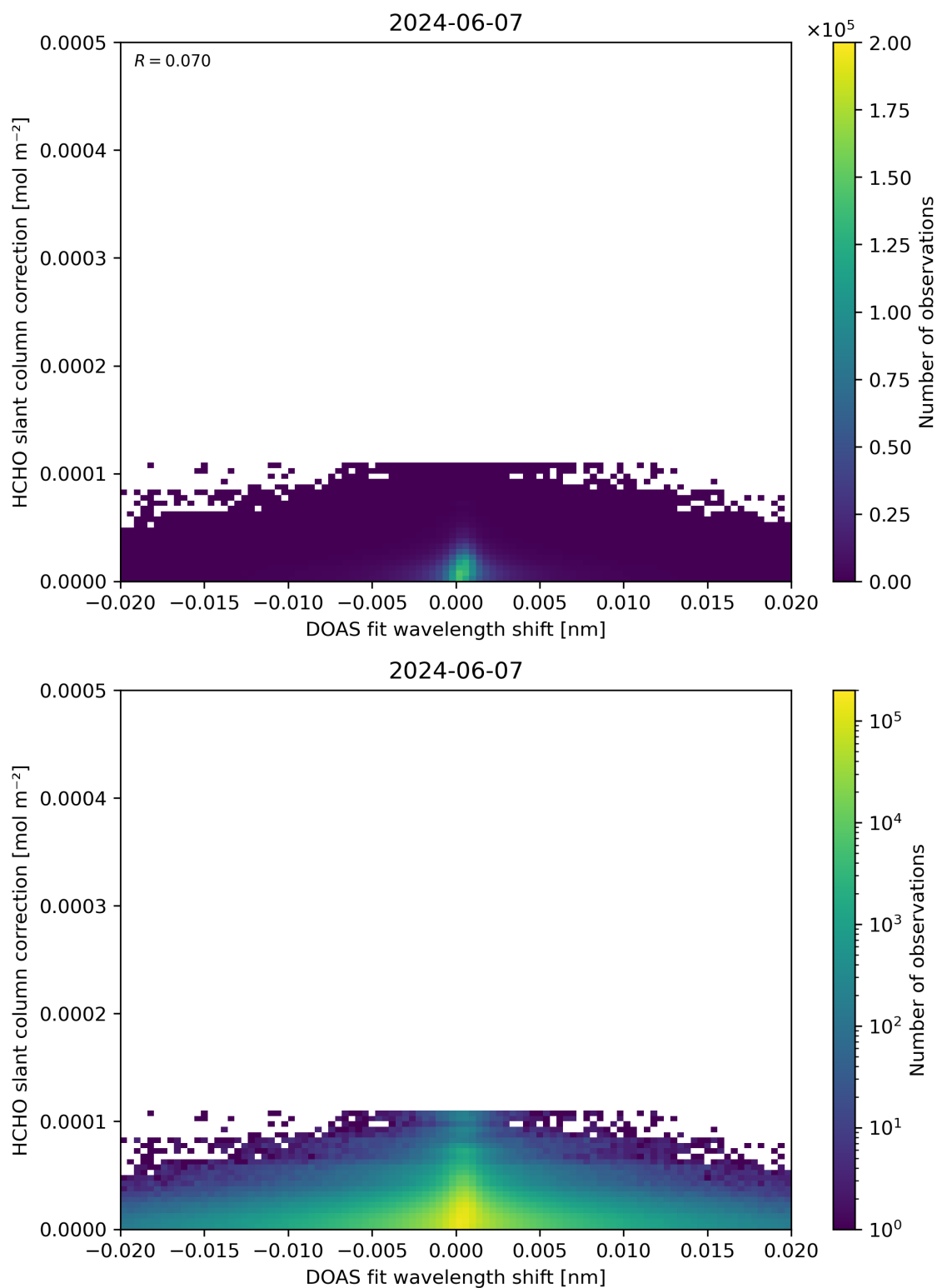
Figure 67: Scatter density plot of “DOAS fit wavelength shift” against “HCHO slant column correction” for 2024-06-06 to 2024-06-08.
