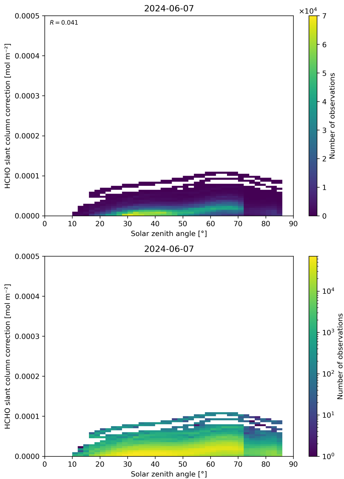
Figure 172: Scatter density plot of “Solar zenith angle” against “HCHO slant column correction” for 2024-06-06 to 2024-06-08.
