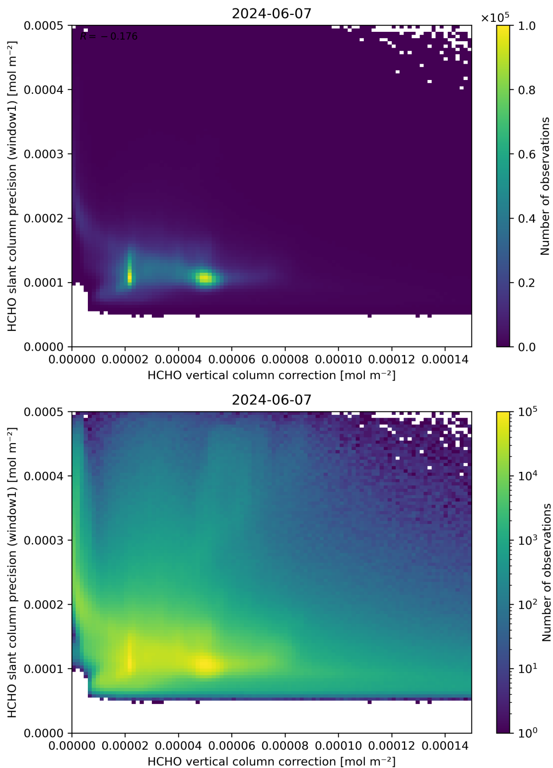
Figure 119: Scatter density plot of “HCHO vertical column correction” against “HCHO slant column precision (window1)” for 2024-06-06 to 2024-06-08.
