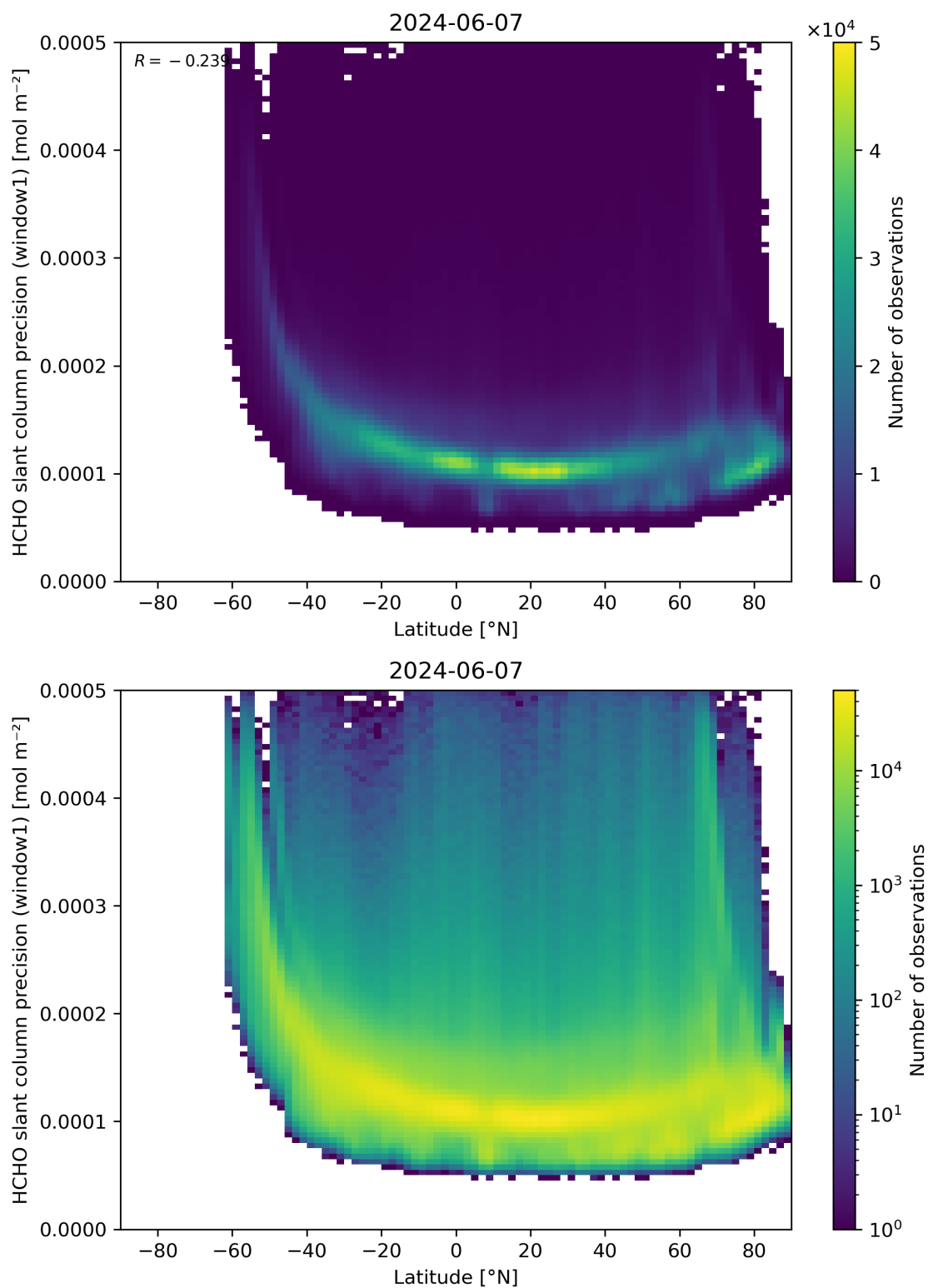
Figure 160: Scatter density plot of “Latitude” against “HCHO slant column precision (window1)” for 2024-06-06 to 2024-06-08.
