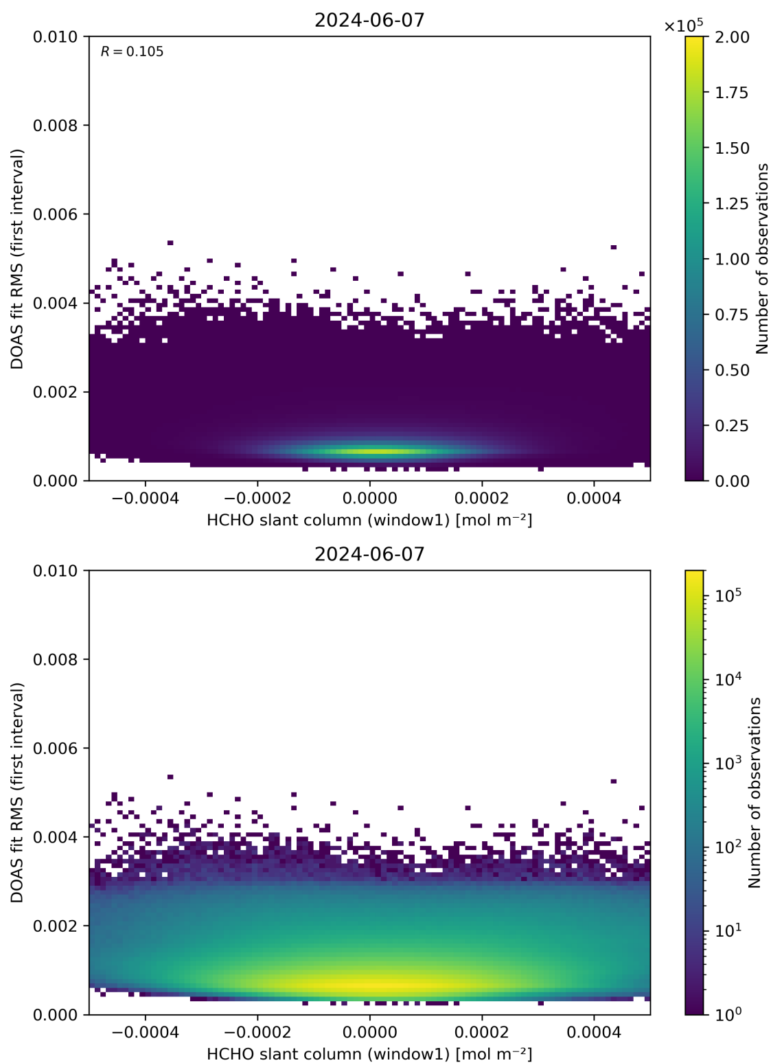
Figure 78: Scatter density plot of “HCHO slant column (window1)” against “DOAS fit RMS (first interval)” for 2024-06-06 to 2024-06-08.
