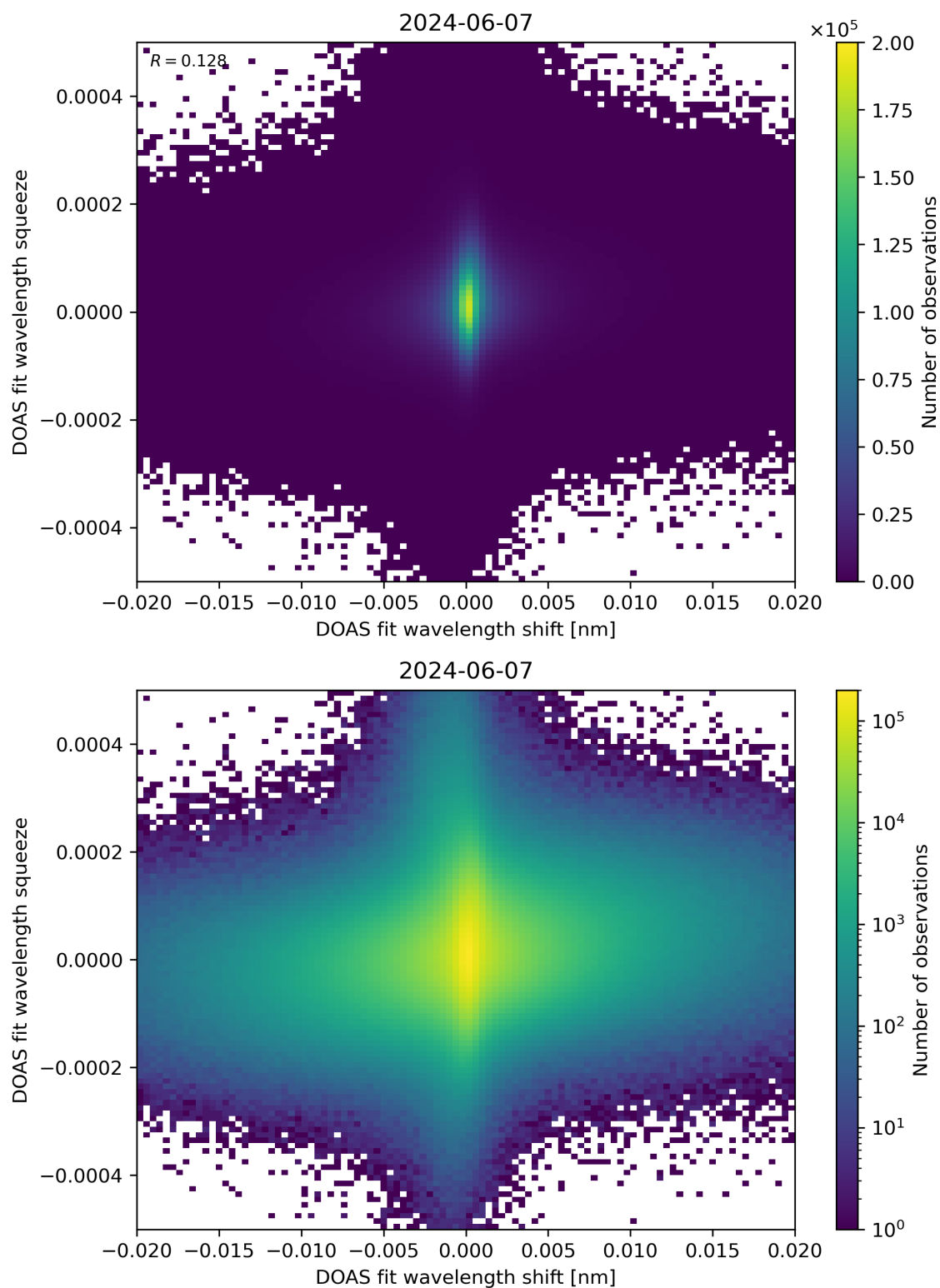
Figure 65: Scatter density plot of “DOAS fit wavelength shift” against “DOAS fit wavelength squeeze” for 2024-06-06 to 2024-06-08.
