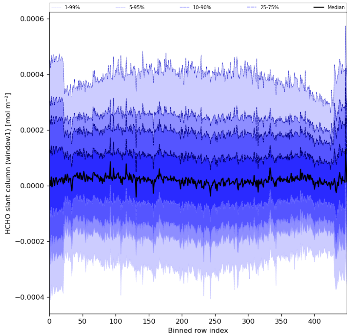
Figure 52: Along track statistics of “HCHO slant column (window1)” for 2024-06-06 to 2024-06-08
