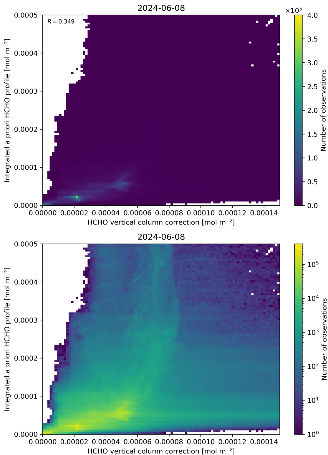
Figure 122: Scatter density plot of “HCHO vertical column correction” against “Integrated a priori HCHO profile” for 2024-06-08 to 2024-06-09.
