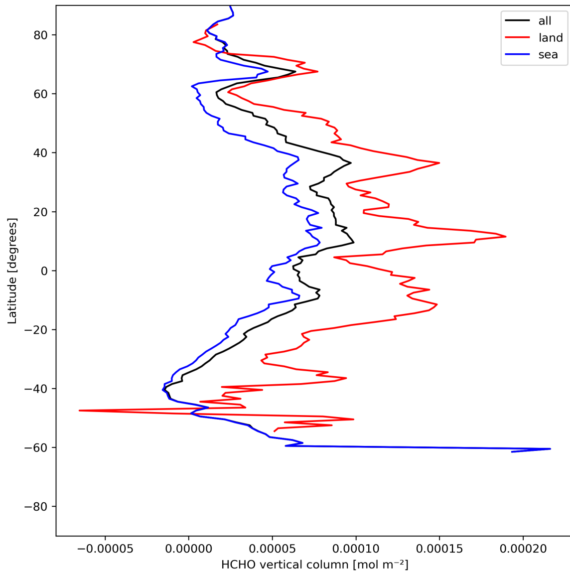
Figure 21: Zonal average of “HCHO vertical column” for 2024-06-08 to 2024-06-09.
