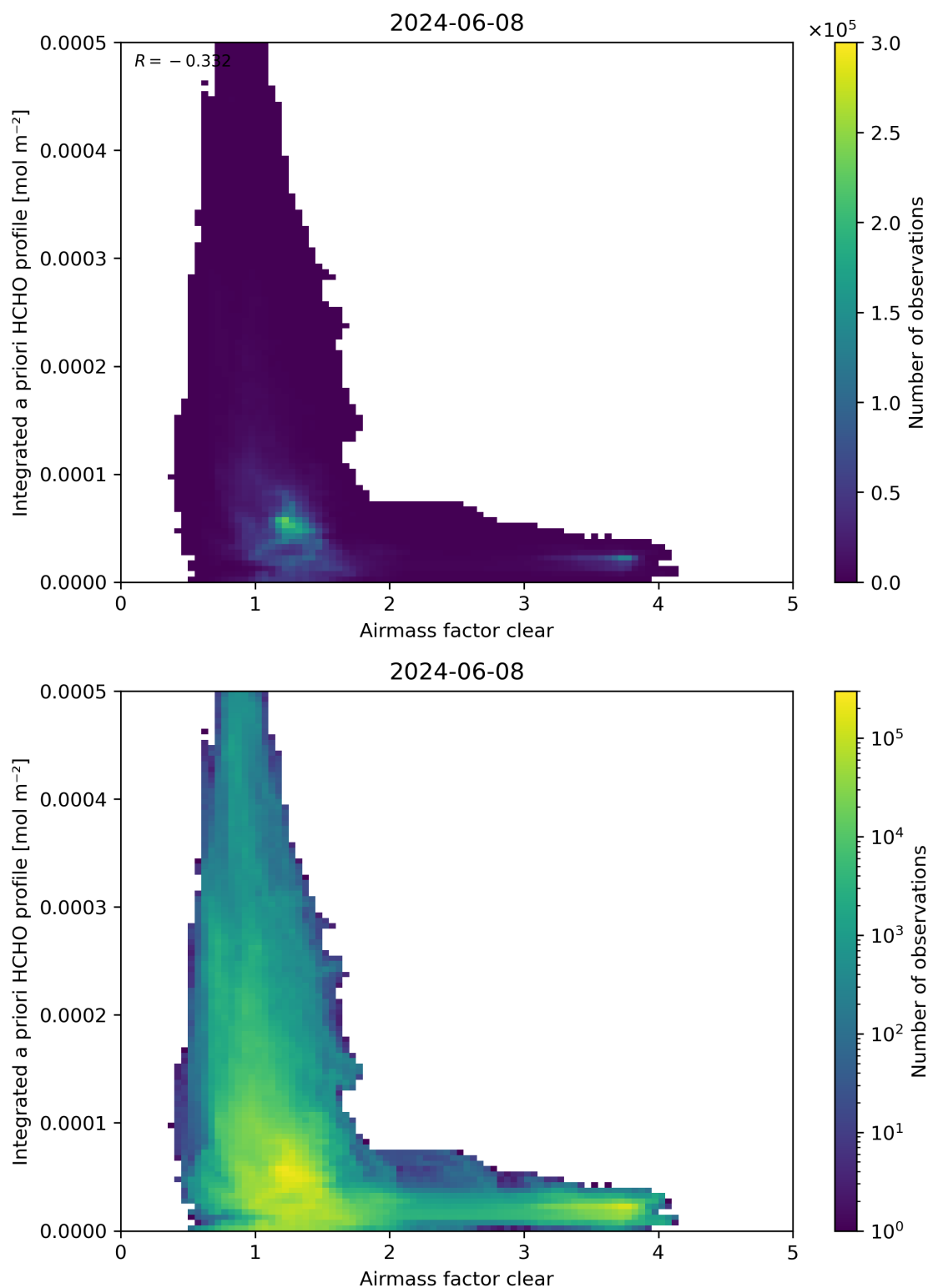
Figure 76: Scatter density plot of “Airmass factor clear” against “Integrated a priori HCHO profile” for 2024-06-08 to 2024-06-09.
