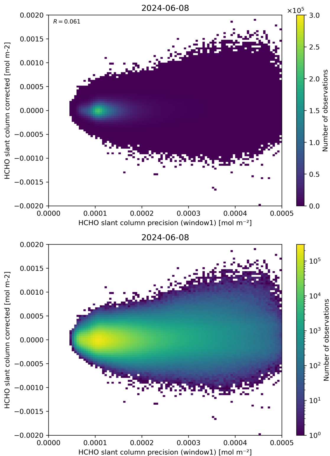
Figure 92: Scatter density plot of “HCHO slant column precision (window1)” against “HCHO slant column corrected” for 2024-06-08 to 2024-06-09.
