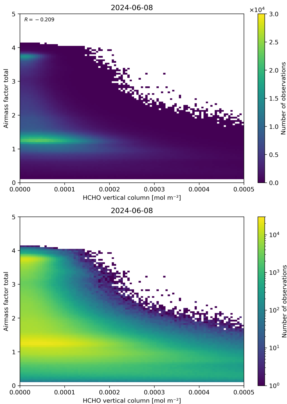
Figure 131: Scatter density plot of “HCHO vertical column” against “Airmass factor total” for 2024-06-08 to 2024-06-09.
