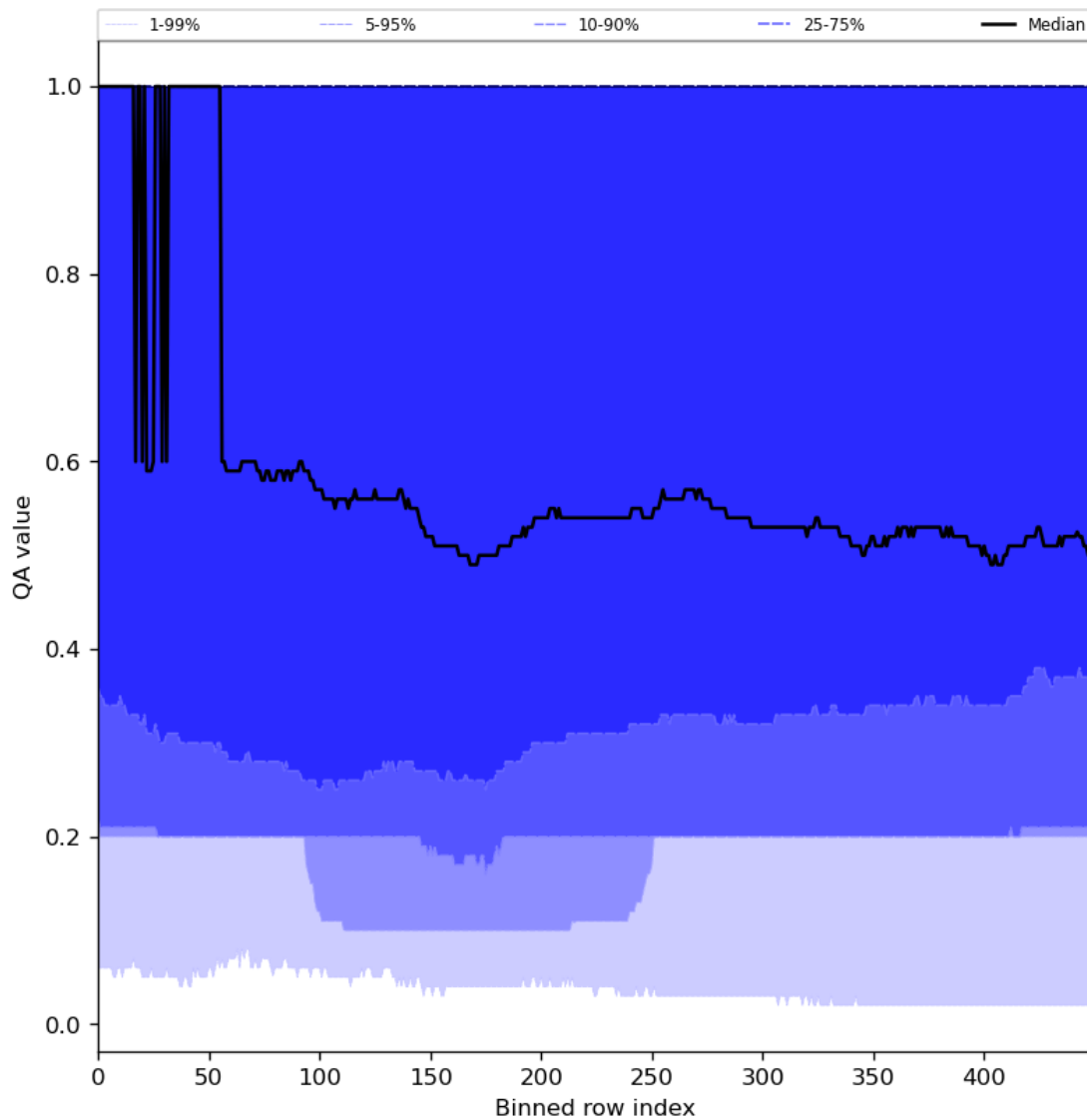
Figure 48: Along track statistics of “QA value” for 2024-06-08 to 2024-06-09
