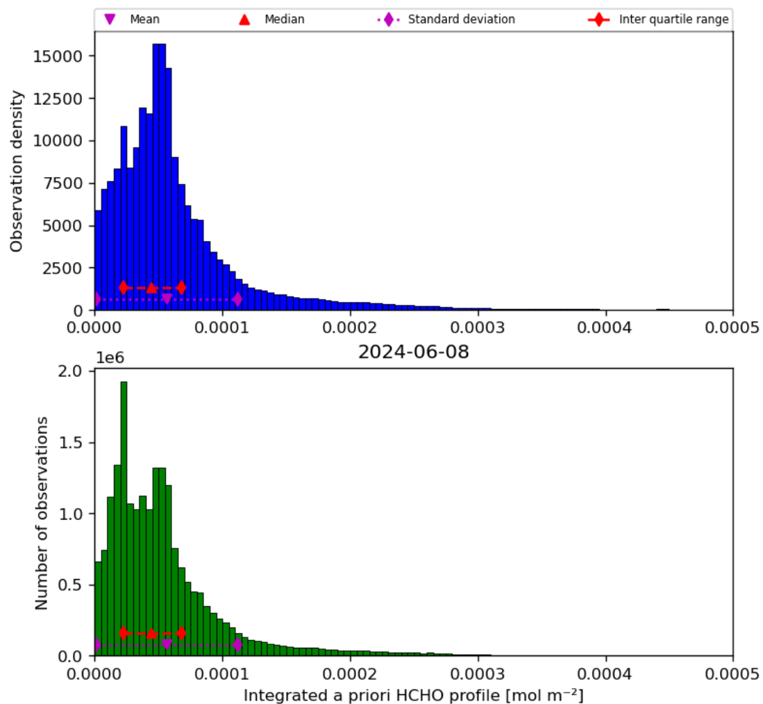
Figure 43: Histogram of “Integrated a priori HCHO profile” for 2024-06-08 to 2024-06-09
