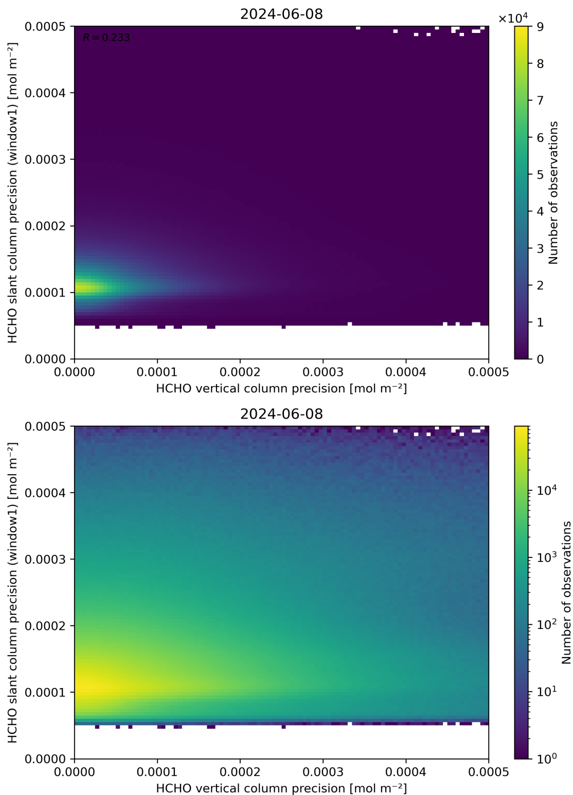
Figure 143: Scatter density plot of “HCHO vertical column precision” against “HCHO slant column precision (window1)” for 2024-06-08 to 2024-06-09.
