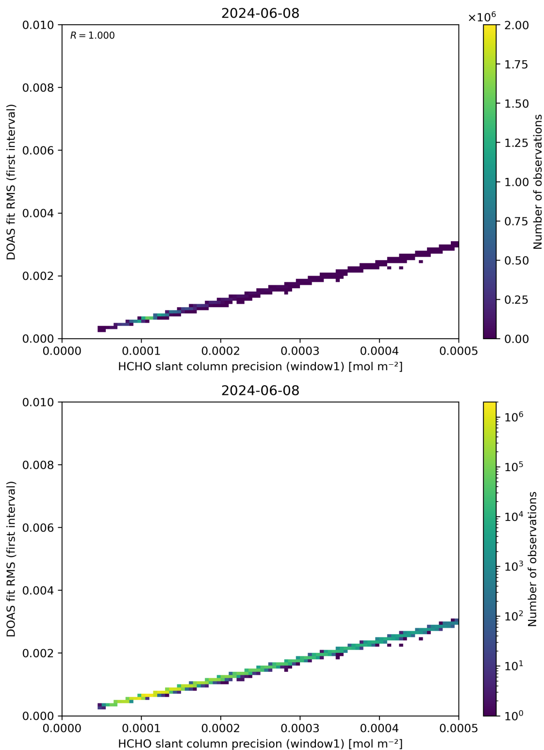
Figure 88: Scatter density plot of “HCHO slant column precision (window1)” against “DOAS fit RMS (first interval)” for 2024-06-08 to 2024-06-09.
