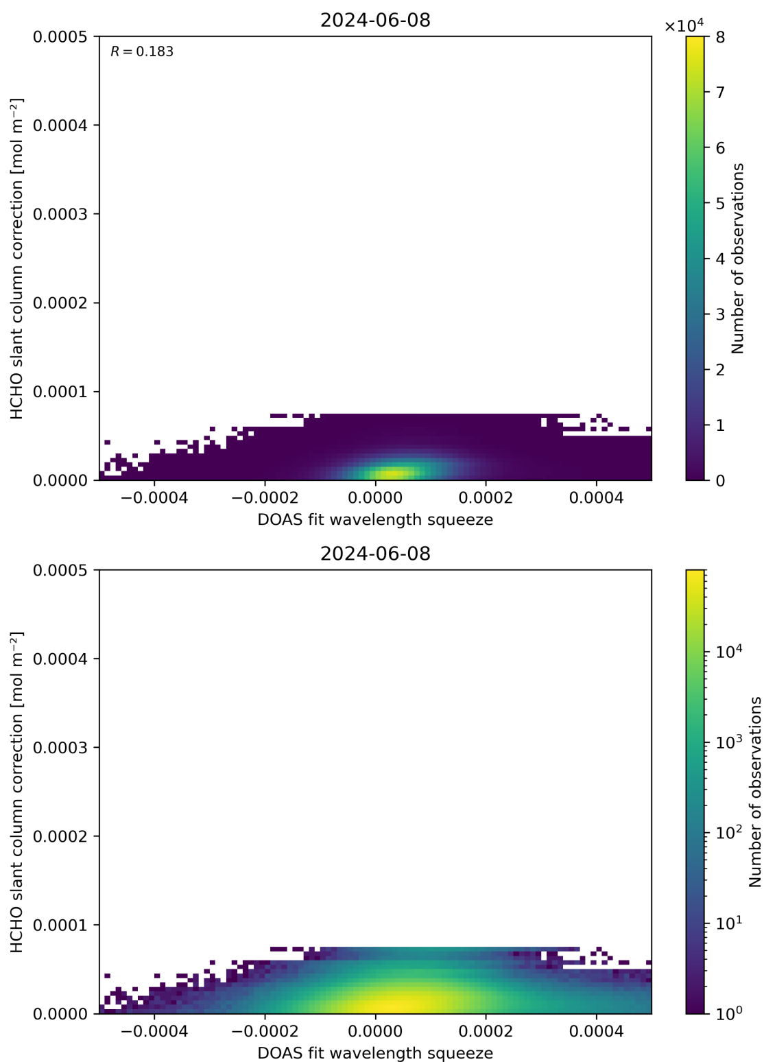
Figure 70: Scatter density plot of “DOAS fit wavelength squeeze” against “HCHO slant column correction” for 2024-06-08 to 2024-06-09.
