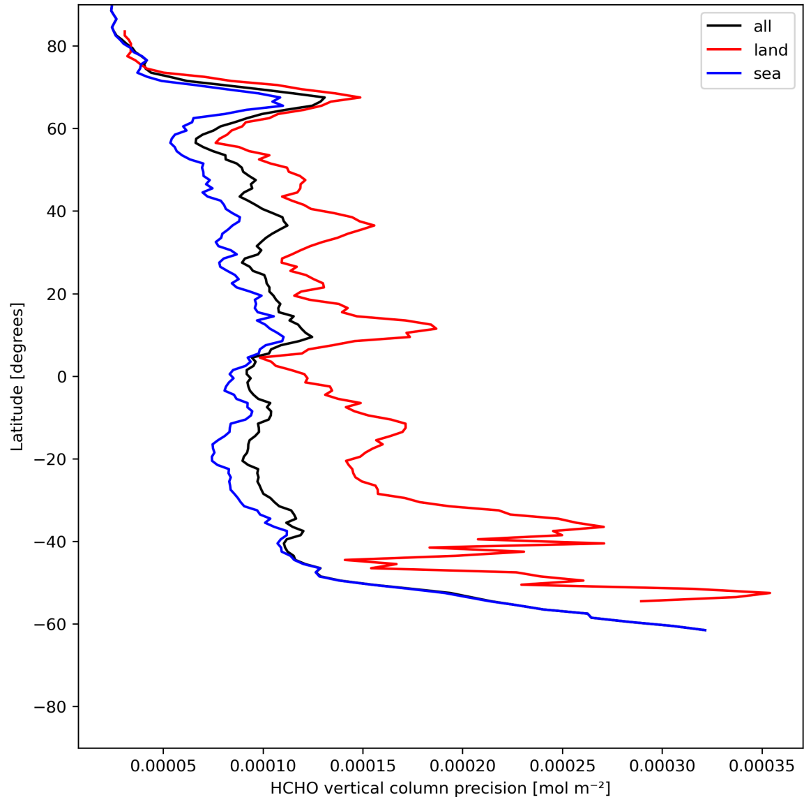
Figure 22: Zonal average of “HCHO vertical column precision” for 2024-06-08 to 2024-06-09.
