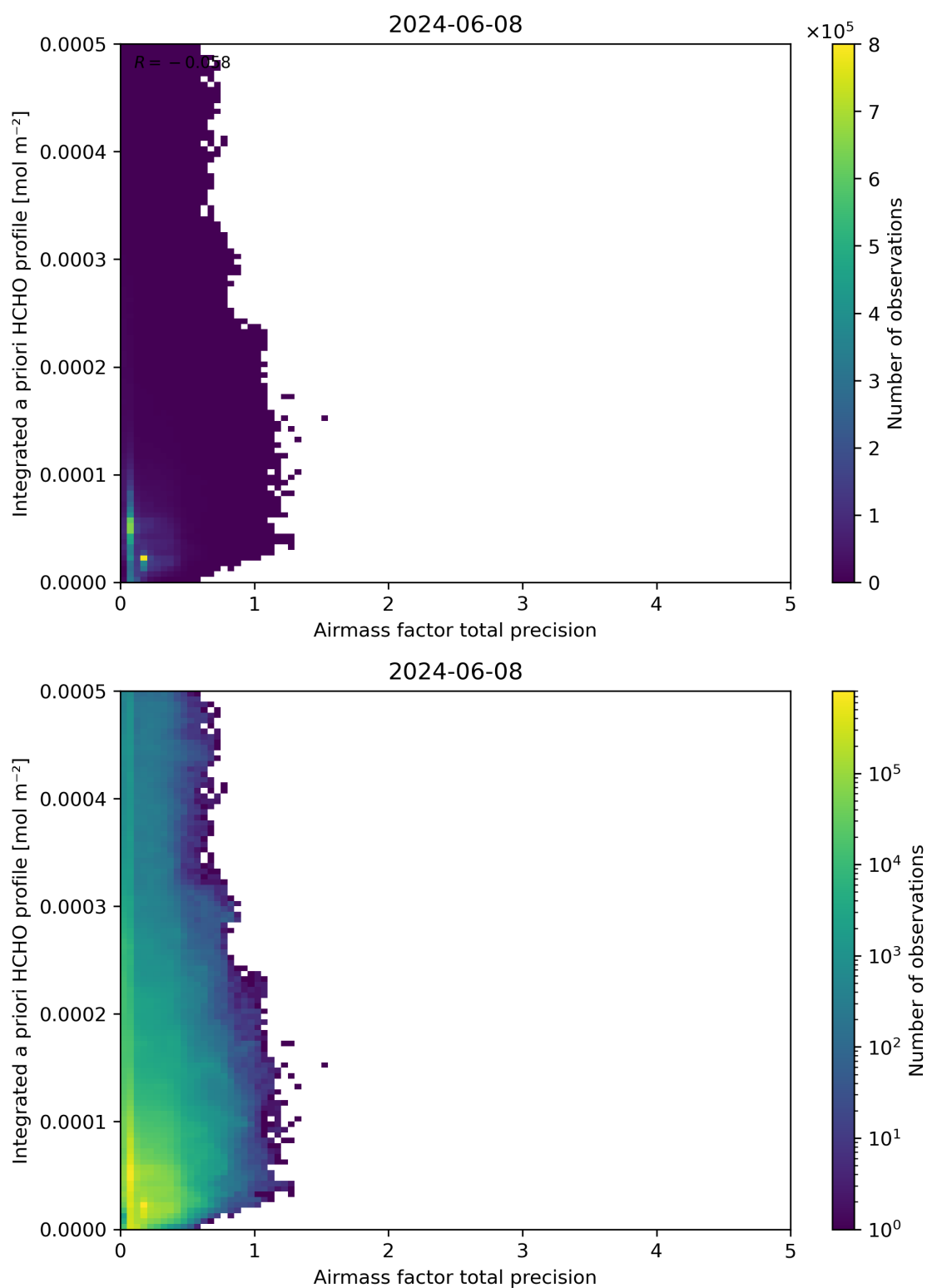
Figure 111: Scatter density plot of “Airmass factor total precision” against “Integrated a priori HCHO profile” for 2024-06-08 to 2024-06-09.
