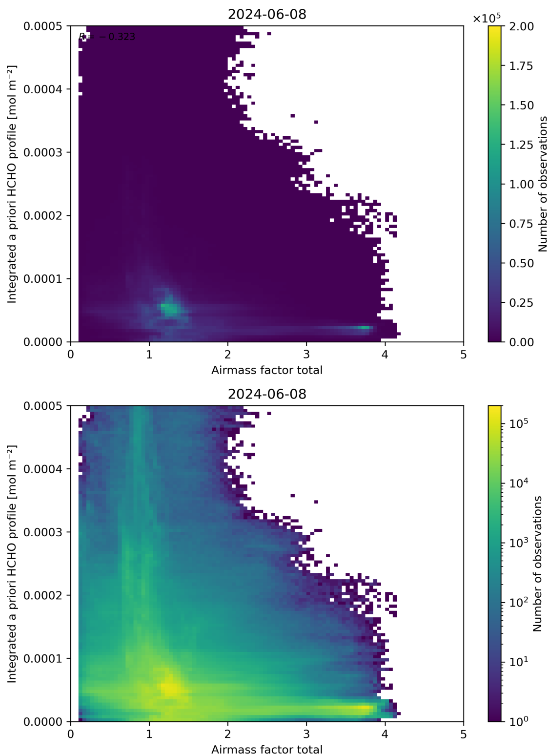
Figure 104: Scatter density plot of “Airmass factor total” against “Integrated a priori HCHO profile” for 2024-06-08 to 2024-06-09.
