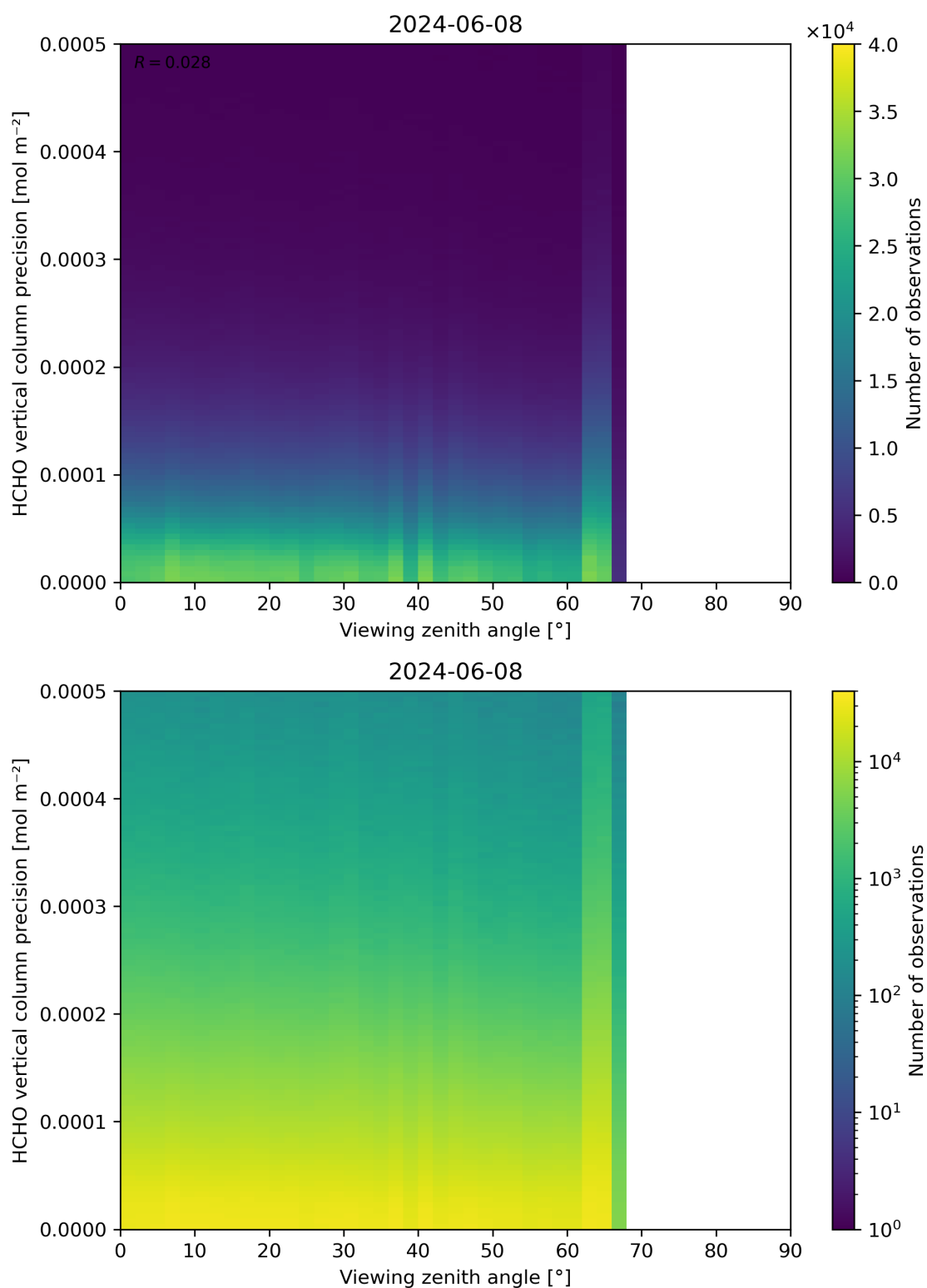
Figure 194: Scatter density plot of “Viewing zenith angle” against “HCHO vertical column precision” for 2024-06-08 to 2024-06-09.
