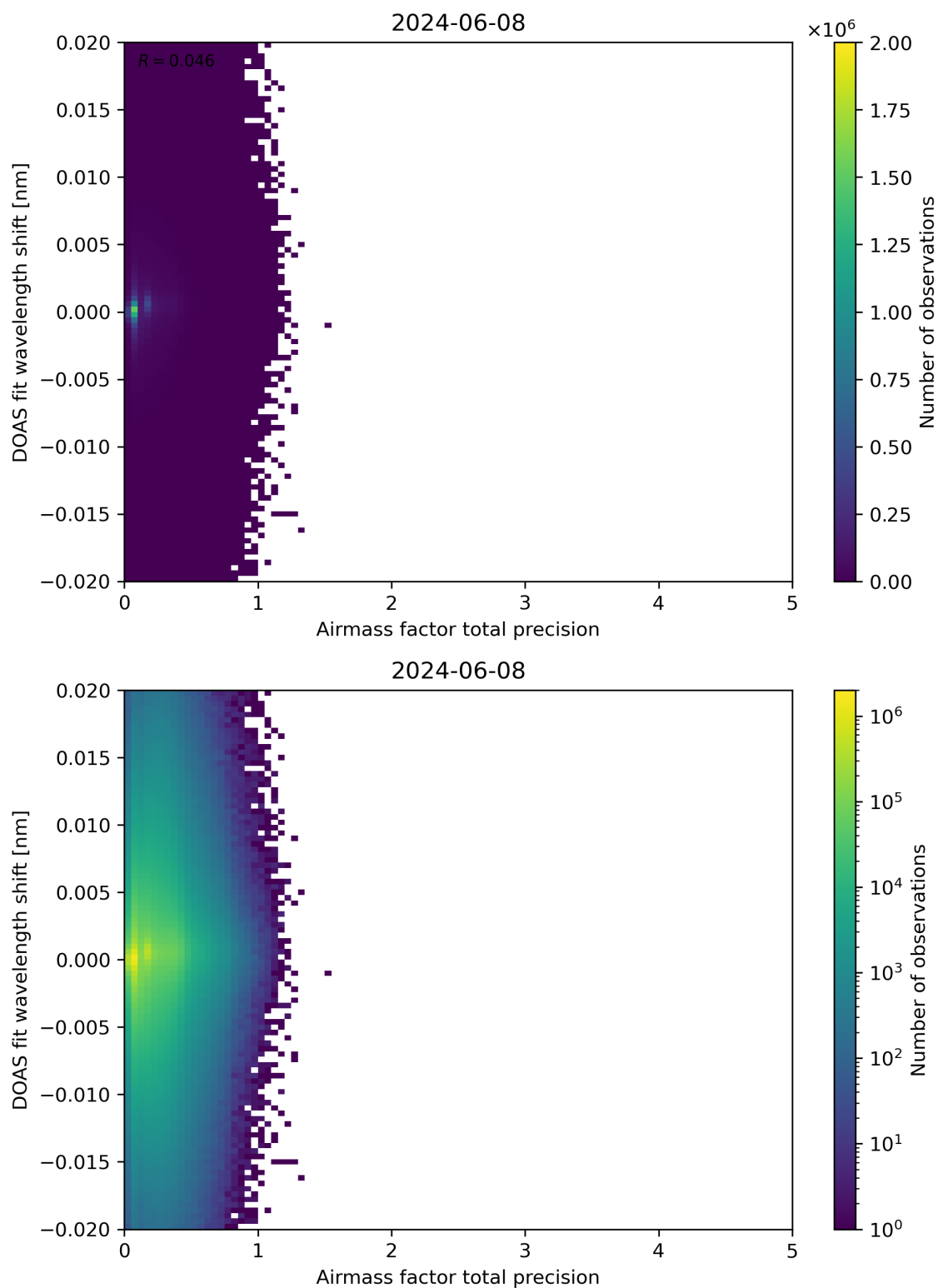
Figure 106: Scatter density plot of “Airmass factor total precision” against “DOAS fit wavelength shift” for 2024-06-08 to 2024-06-09.
