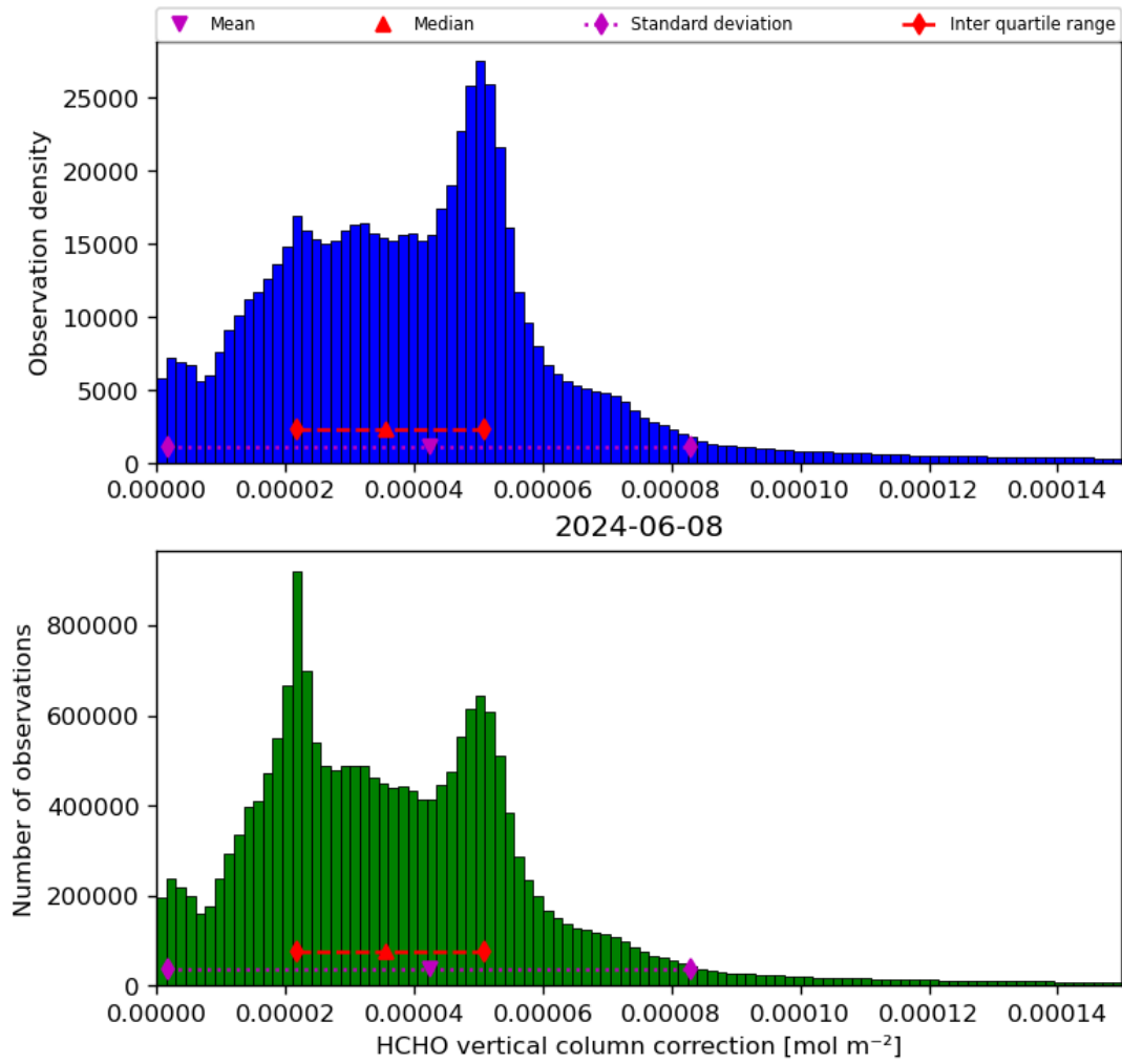
Figure 37: Histogram of “HCHO vertical column correction” for 2024-06-08 to 2024-06-09
