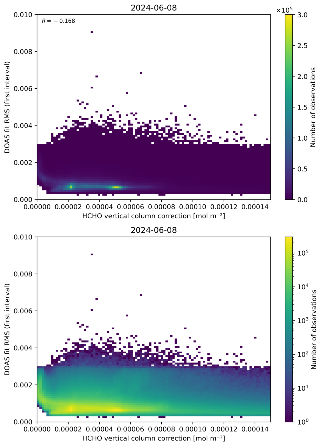
Figure 112: Scatter density plot of “HCHO vertical column correction” against “DOAS fit RMS (first interval)” for 2024-06-08 to 2024-06-09.
