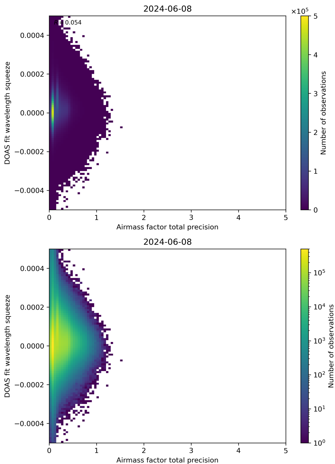
Figure 107: Scatter density plot of “Airmass factor total precision” against “DOAS fit wavelength squeeze” for 2024-06-08 to 2024-06-09.
