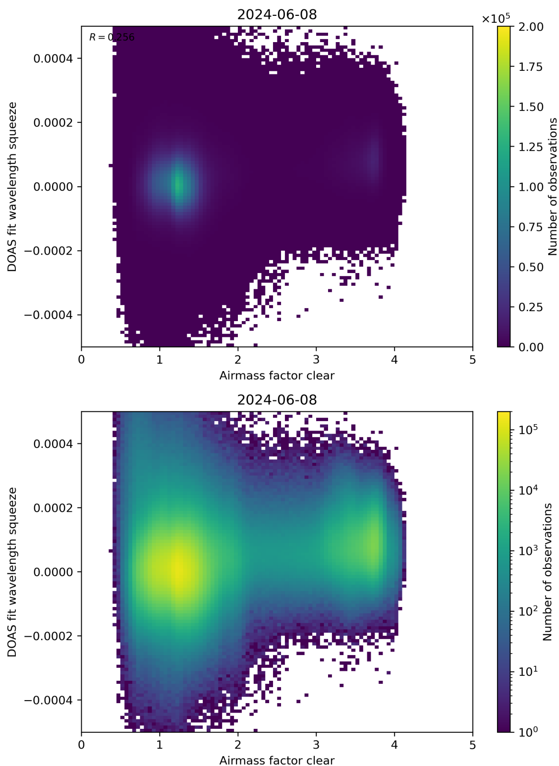
Figure 73: Scatter density plot of “Airmass factor clear” against “DOAS fit wavelength squeeze” for 2024-06-08 to 2024-06-09.
