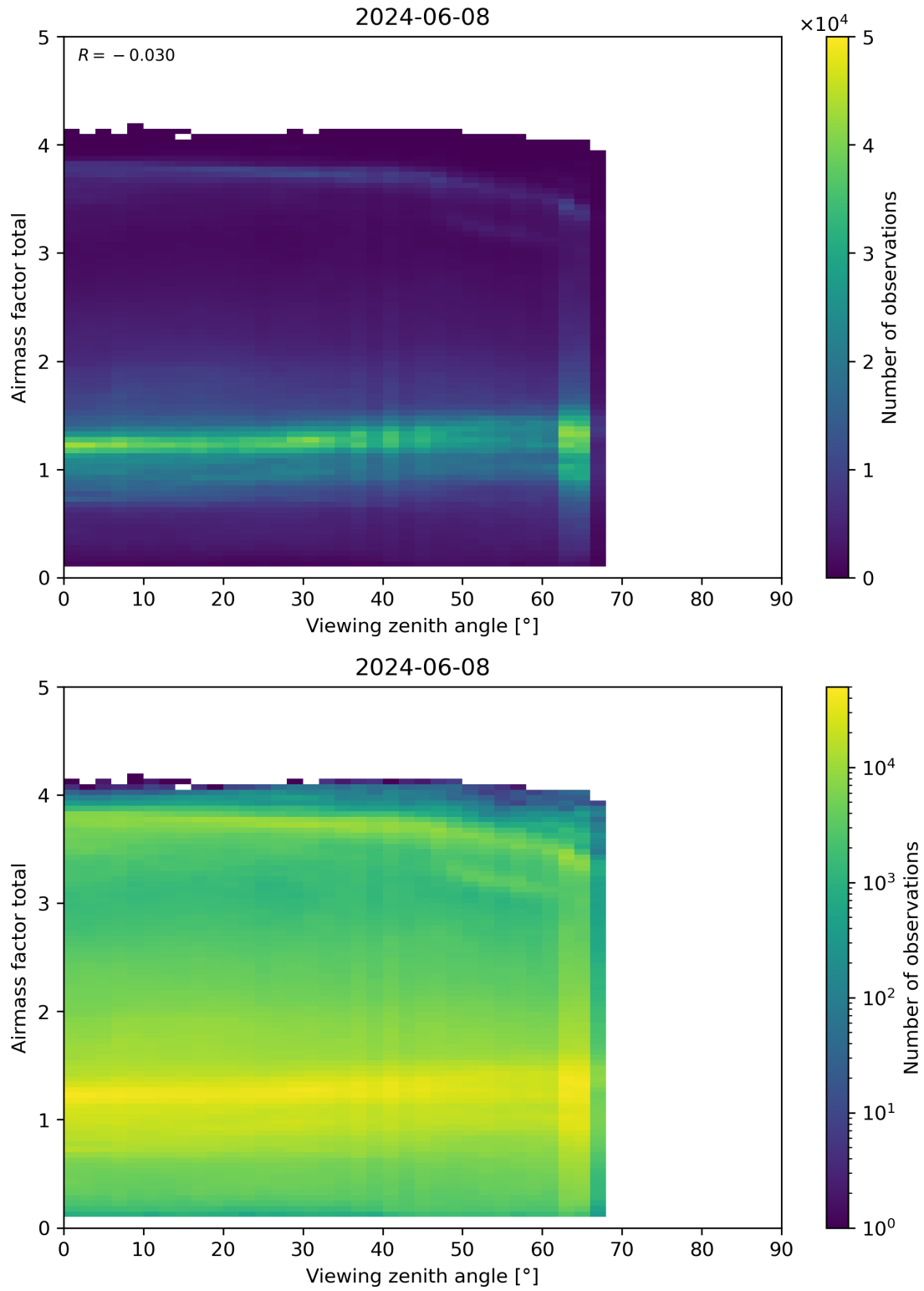
Figure 190: Scatter density plot of “Viewing zenith angle” against “Airmass factor total” for 2024-06-08 to 2024-06-09.
