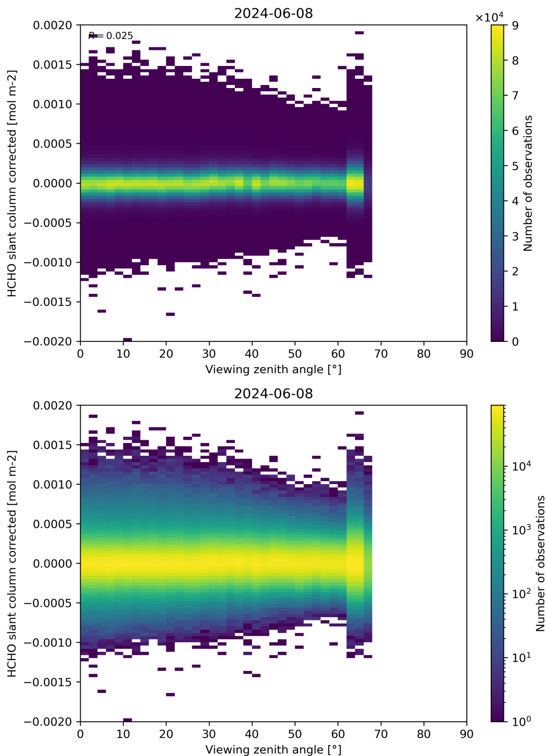
Figure 186: Scatter density plot of “Viewing zenith angle” against “HCHO slant column corrected” for 2024-06-08 to 2024-06-09.
