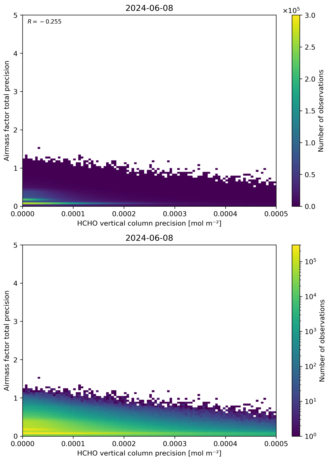
Figure 145: Scatter density plot of “HCHO vertical column precision” against “Airmass factor total precision” for 2024-06-08 to 2024-06-09.
