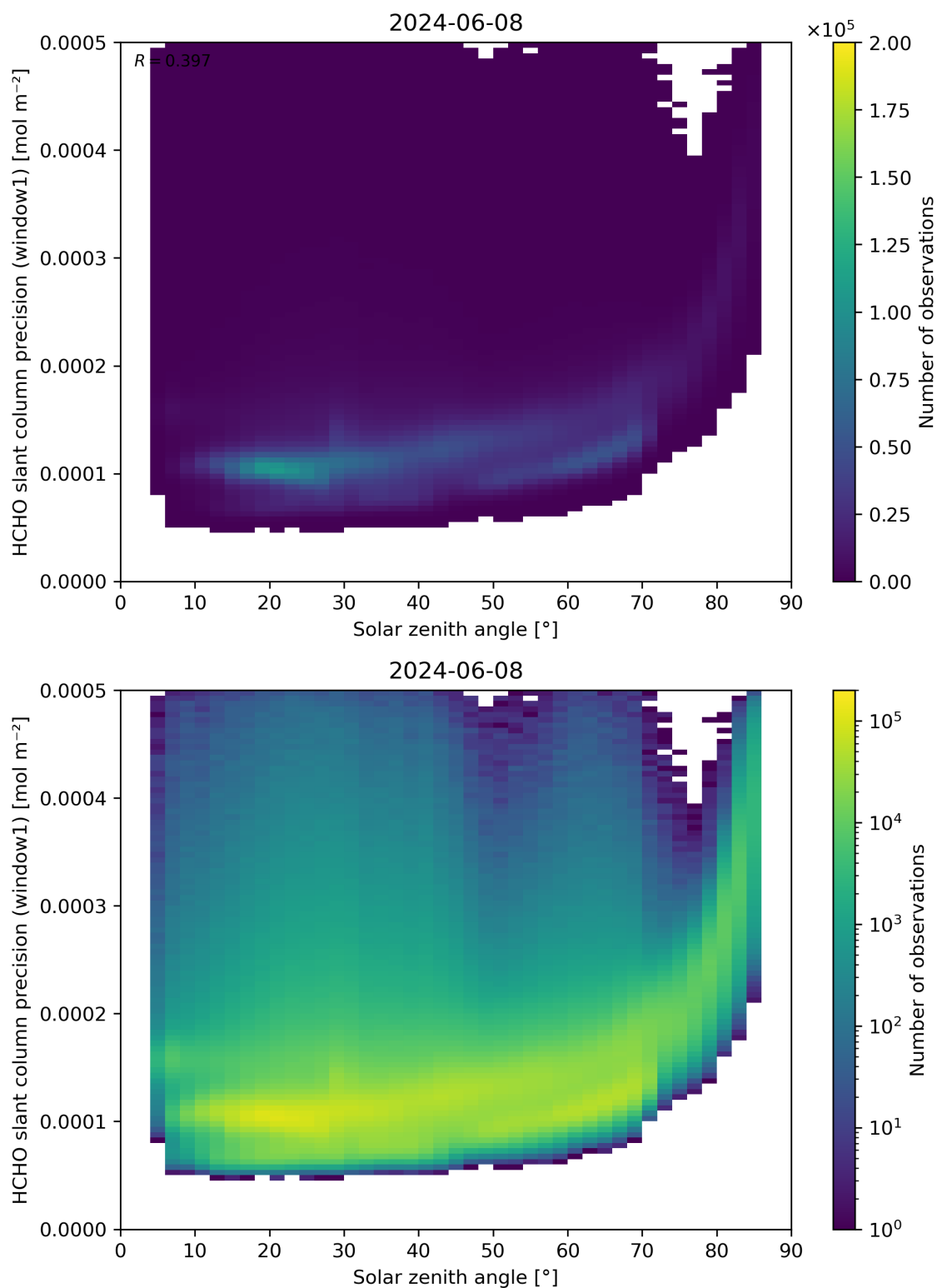
Figure 174: Scatter density plot of “Solar zenith angle” against “HCHO slant column precision (window1)” for 2024-06-08 to 2024-06-09.
