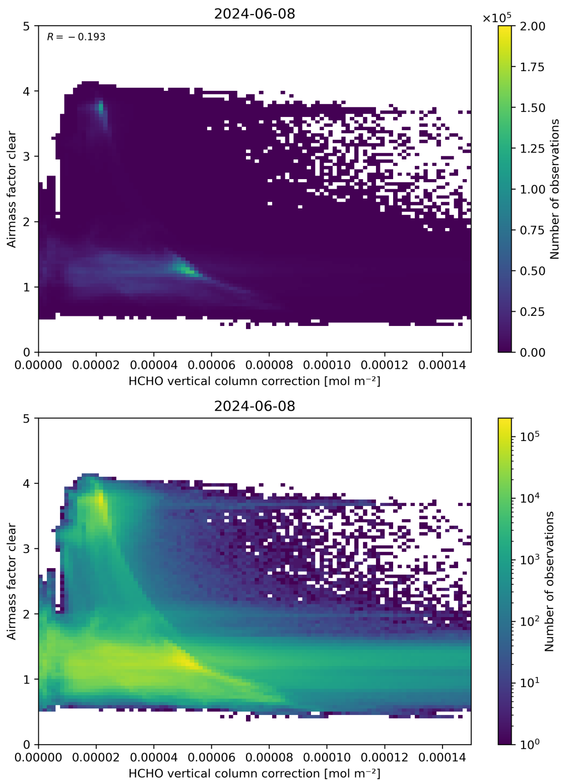
Figure 115: Scatter density plot of “HCHO vertical column correction” against “Airmass factor clear” for 2024-06-08 to 2024-06-09.
