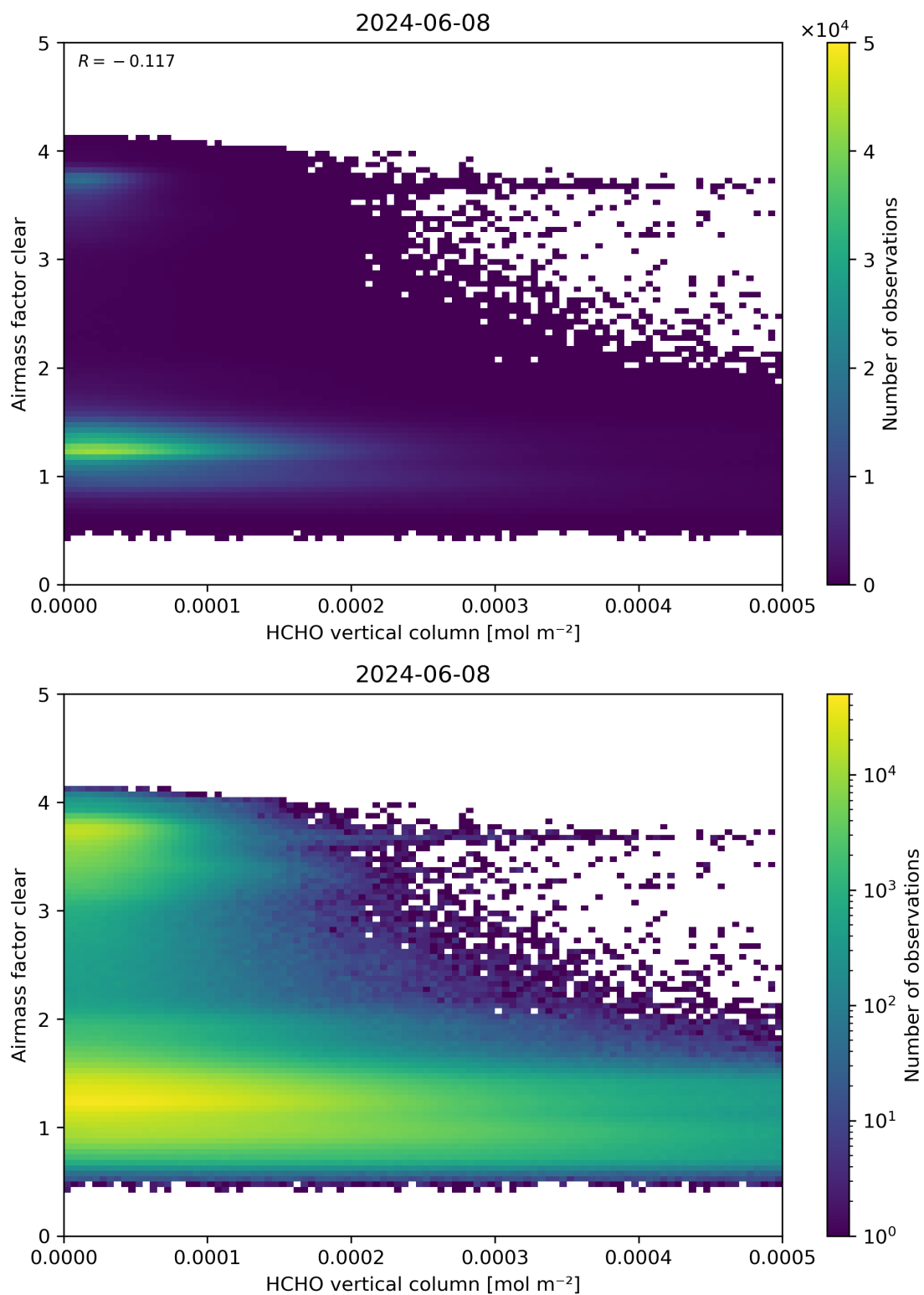
Figure 126: Scatter density plot of “HCHO vertical column” against “Airmass factor clear” for 2024-06-08 to 2024-06-09.
