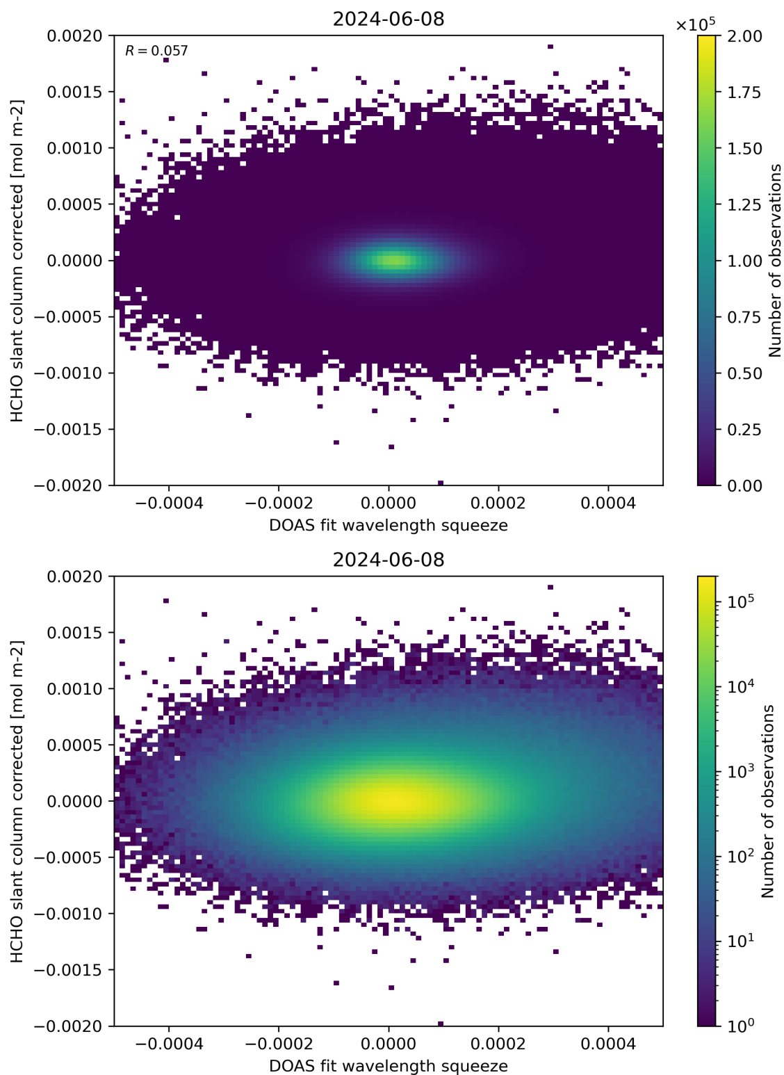
Figure 69: Scatter density plot of “DOAS fit wavelength squeeze” against “HCHO slant column corrected” for 2024-06-08 to 2024-06-09.
