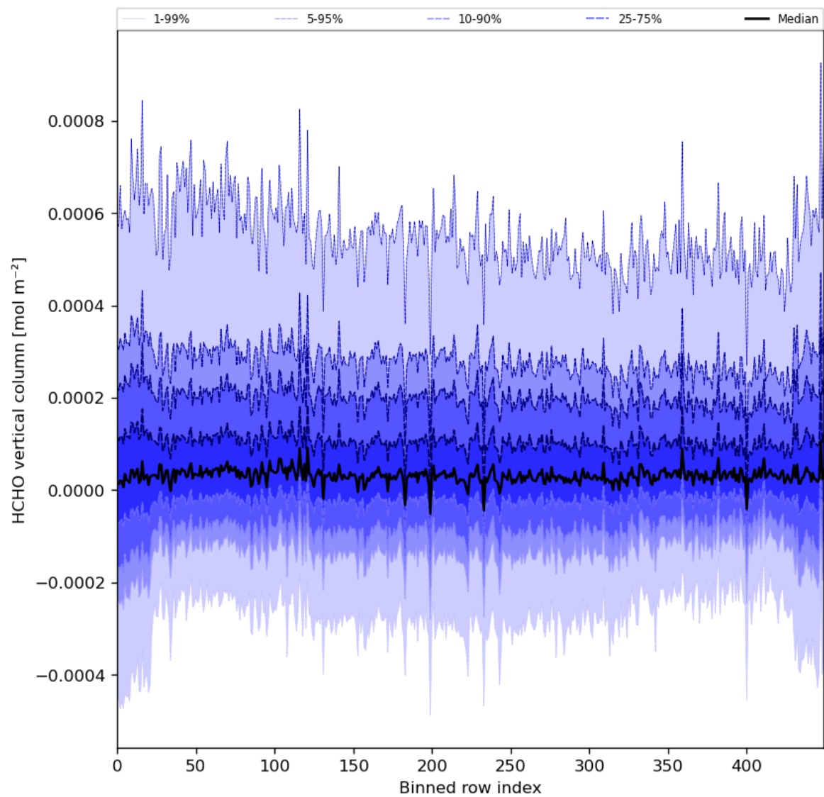
Figure 49: Along track statistics of “HCHO vertical column” for 2024-06-08 to 2024-06-09
