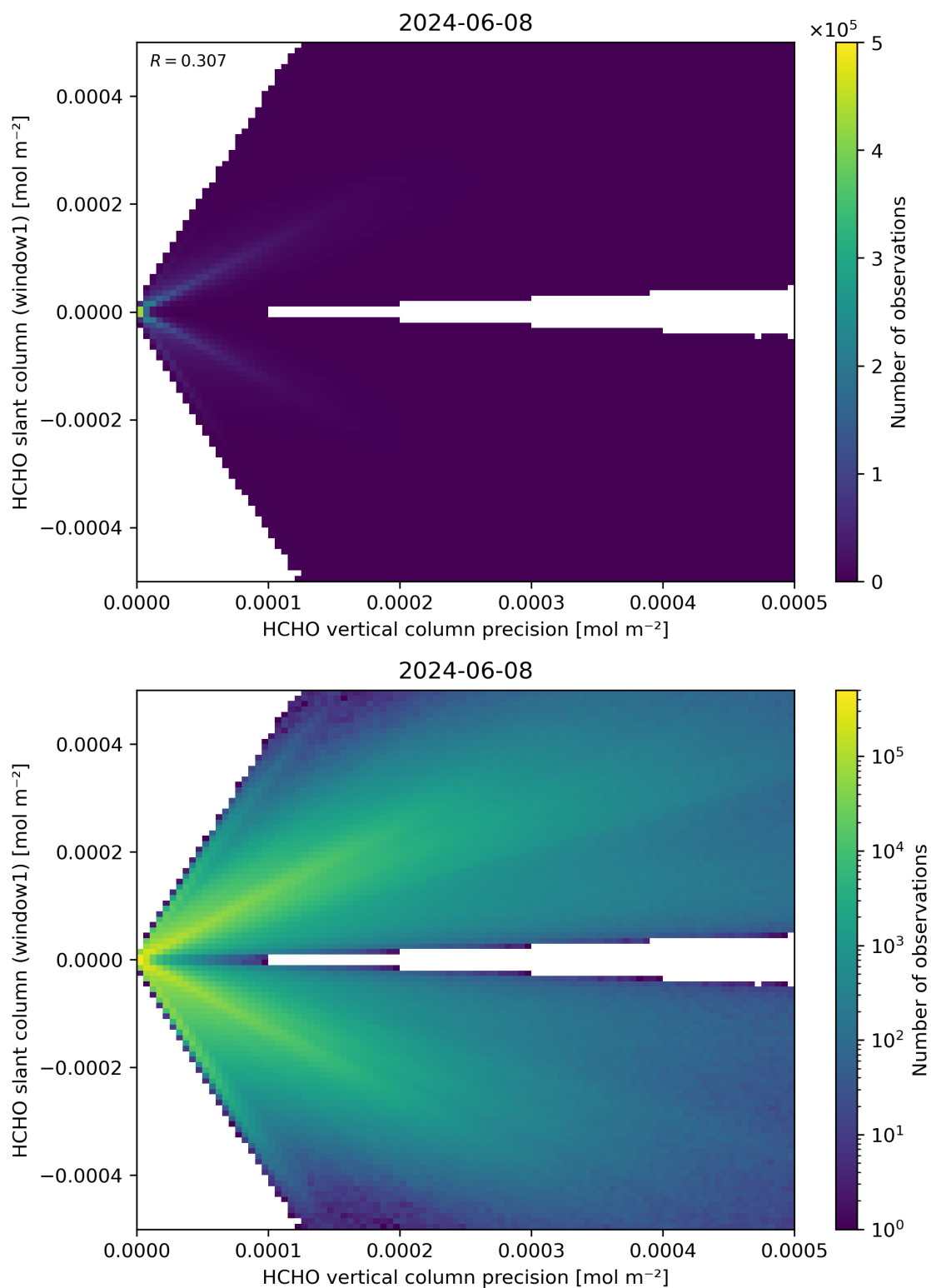
Figure 142: Scatter density plot of “HCHO vertical column precision” against “HCHO slant column (window1)” for 2024-06-08 to 2024-06-09.
