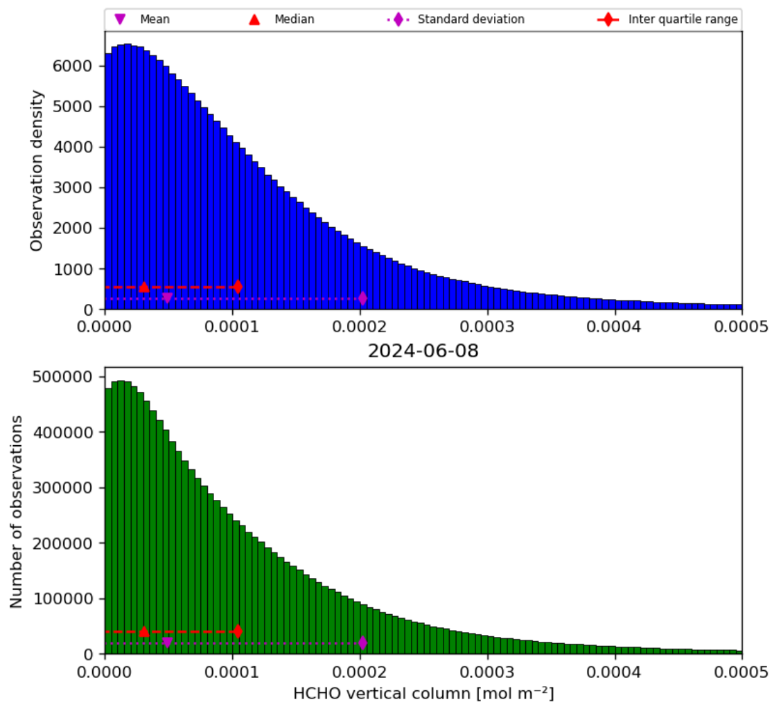
Figure 35: Histogram of “HCHO vertical column” for 2024-06-08 to 2024-06-09
