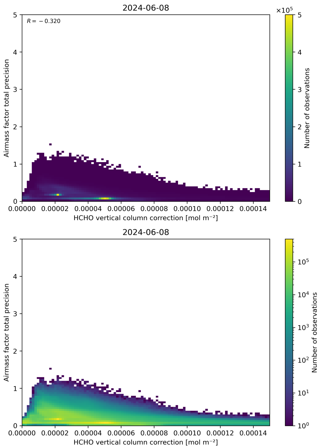
Figure 121: Scatter density plot of “HCHO vertical column correction” against “Airmass factor total precision” for 2024-06-08 to 2024-06-09.
