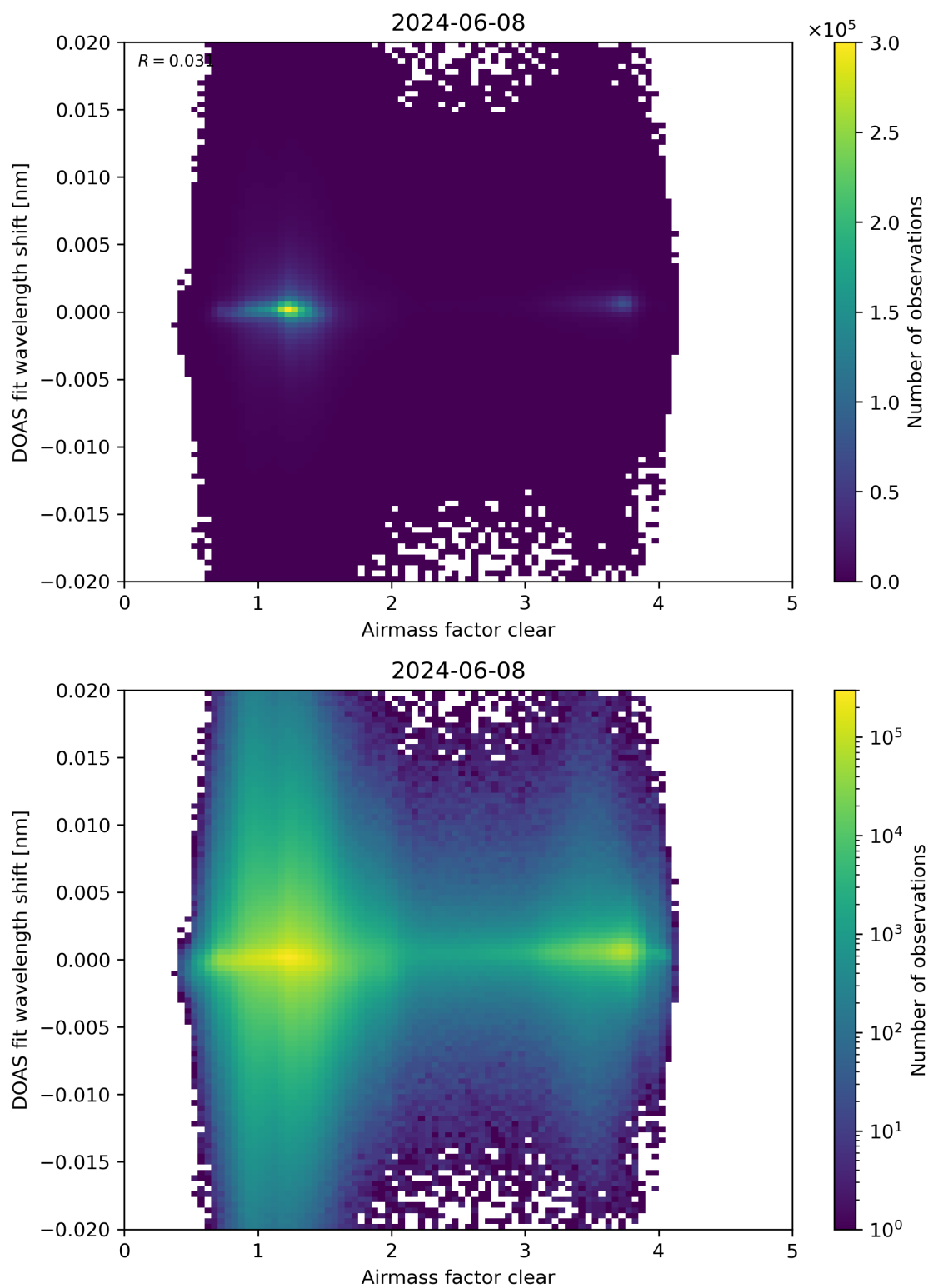
Figure 72: Scatter density plot of “Airmass factor clear” against “DOAS fit wavelength shift” for 2024-06-08 to 2024-06-09.
