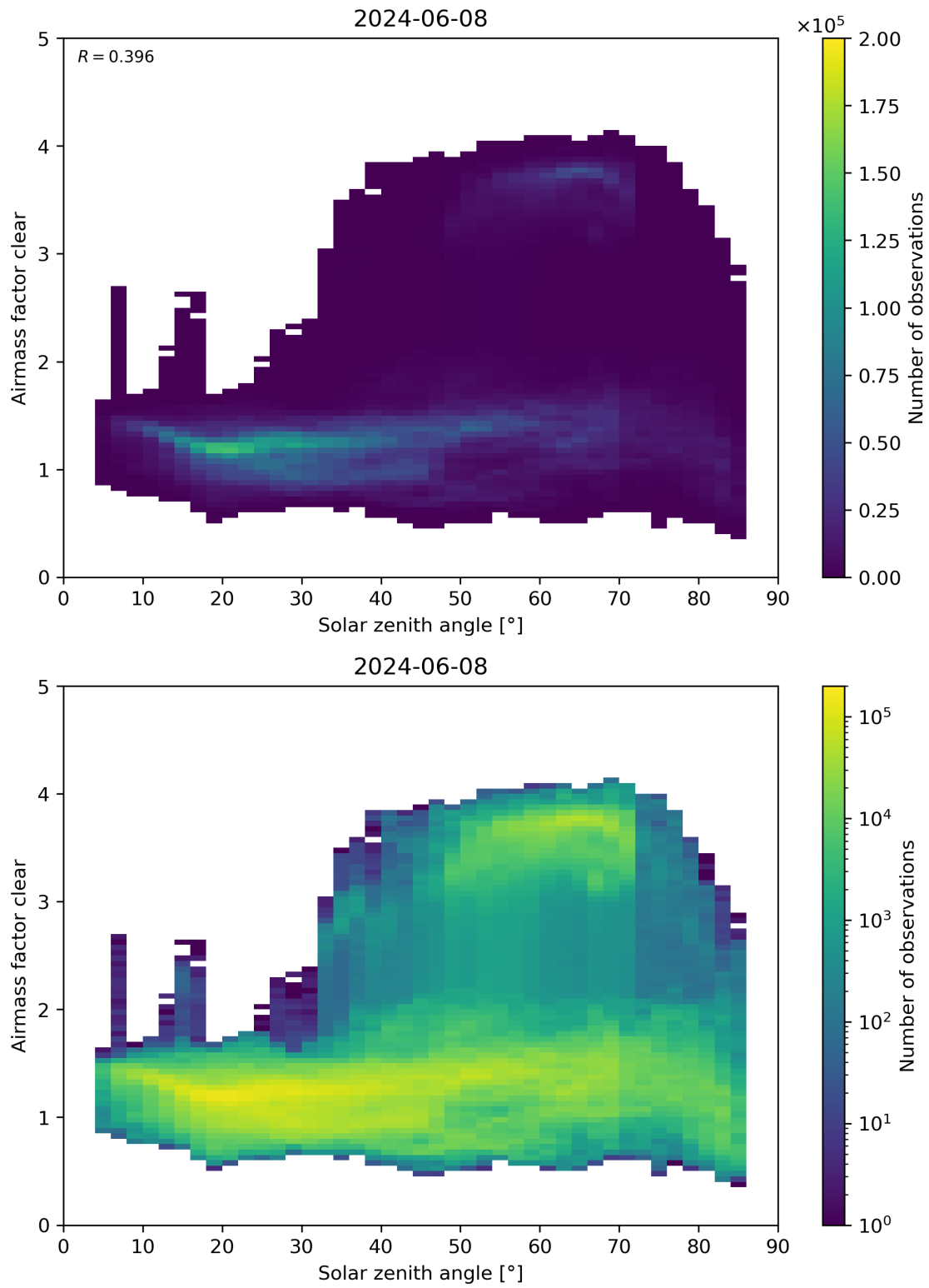
Figure 170: Scatter density plot of “Solar zenith angle” against “Airmass factor clear” for 2024-06-08 to 2024-06-09.
