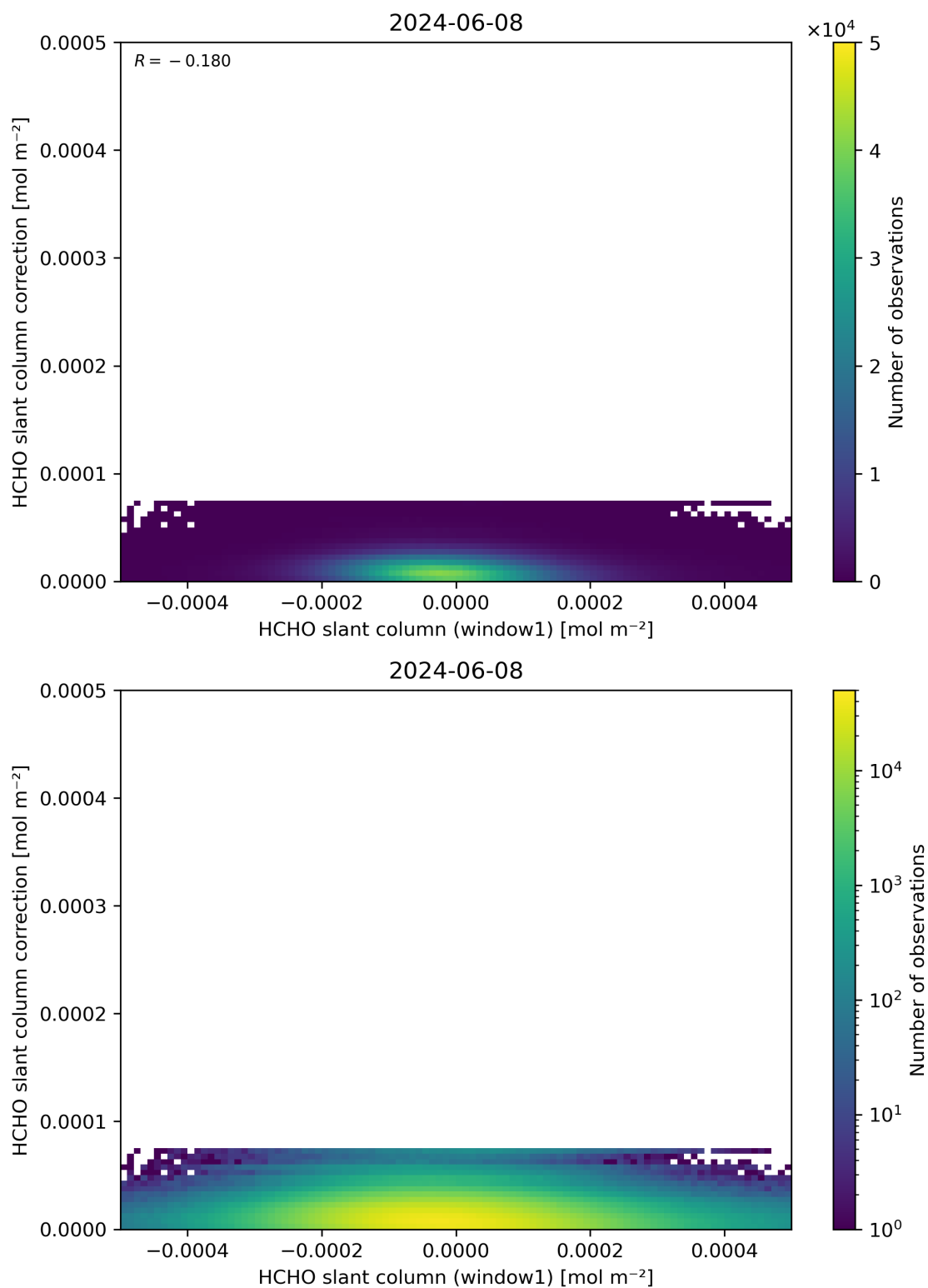
Figure 83: Scatter density plot of “HCHO slant column (window1)” against “HCHO slant column correction” for 2024-06-08 to 2024-06-09.
