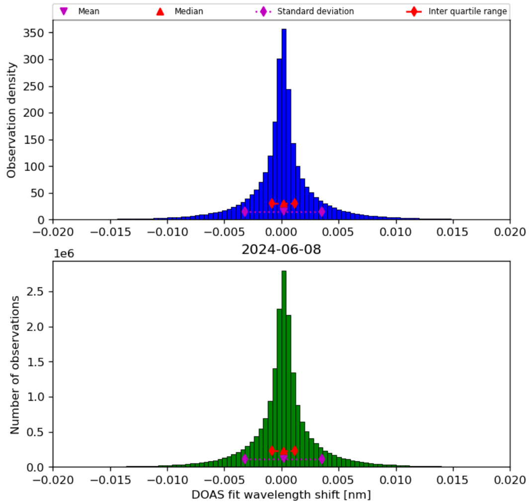
Figure 44: Histogram of “DOAS fit wavelength shift” for 2024-06-08 to 2024-06-09
