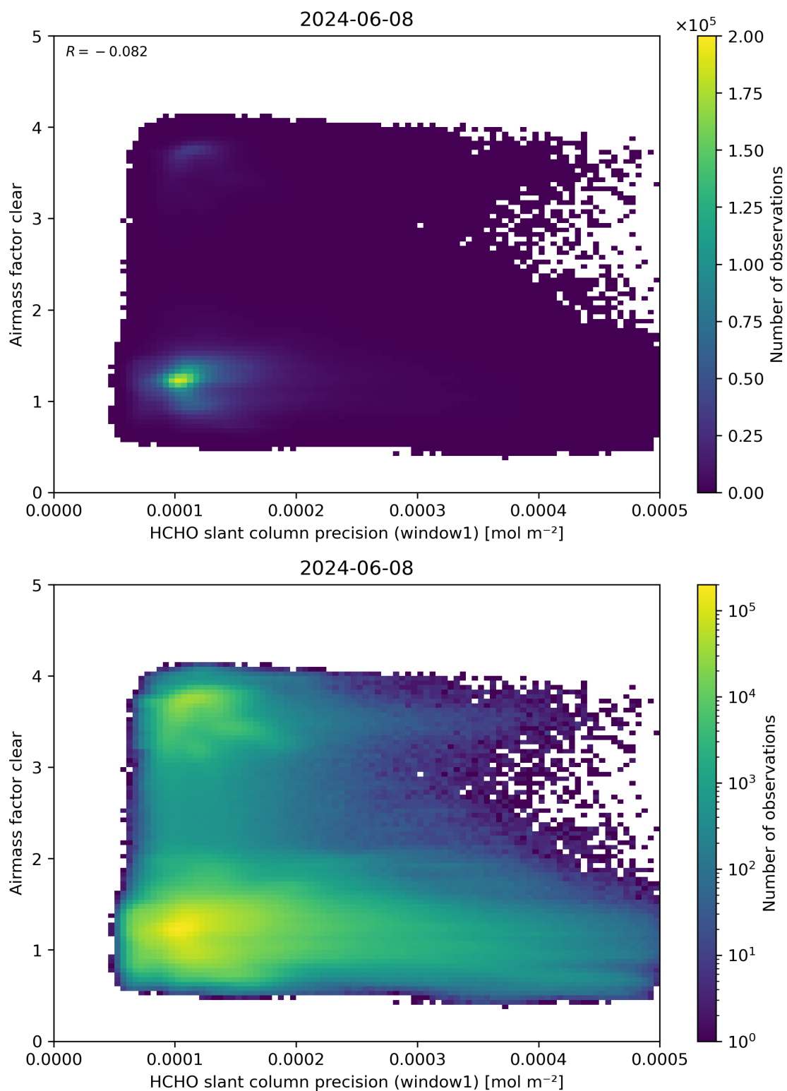
Figure 91: Scatter density plot of “HCHO slant column precision (window1)” against “Airmass factor clear” for 2024-06-08 to 2024-06-09.
