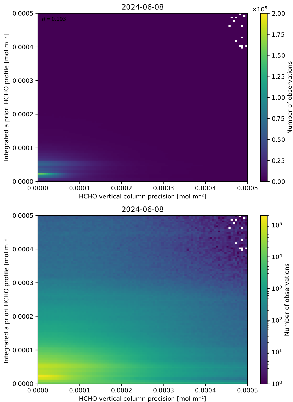
Figure 147: Scatter density plot of “HCHO vertical column precision” against “Integrated a priori HCHO profile” for 2024-06-08 to 2024-06-09.
