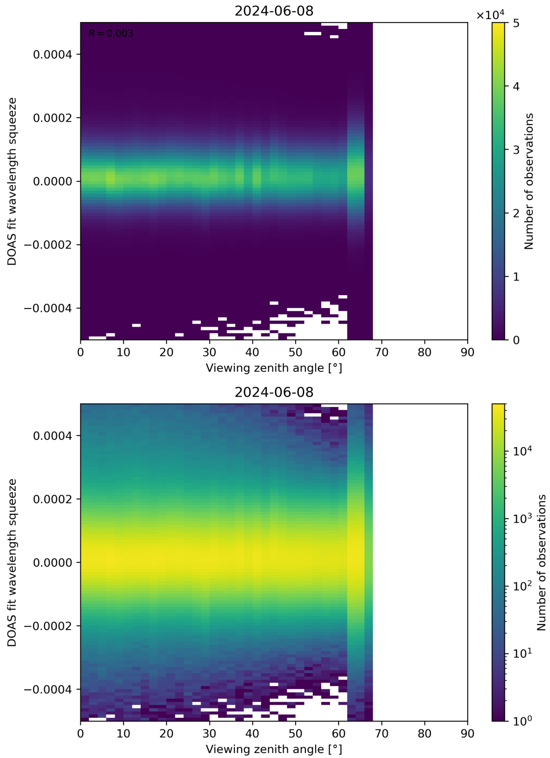
Figure 184: Scatter density plot of “Viewing zenith angle” against “DOAS fit wavelength squeeze” for 2024-06-08 to 2024-06-09.
