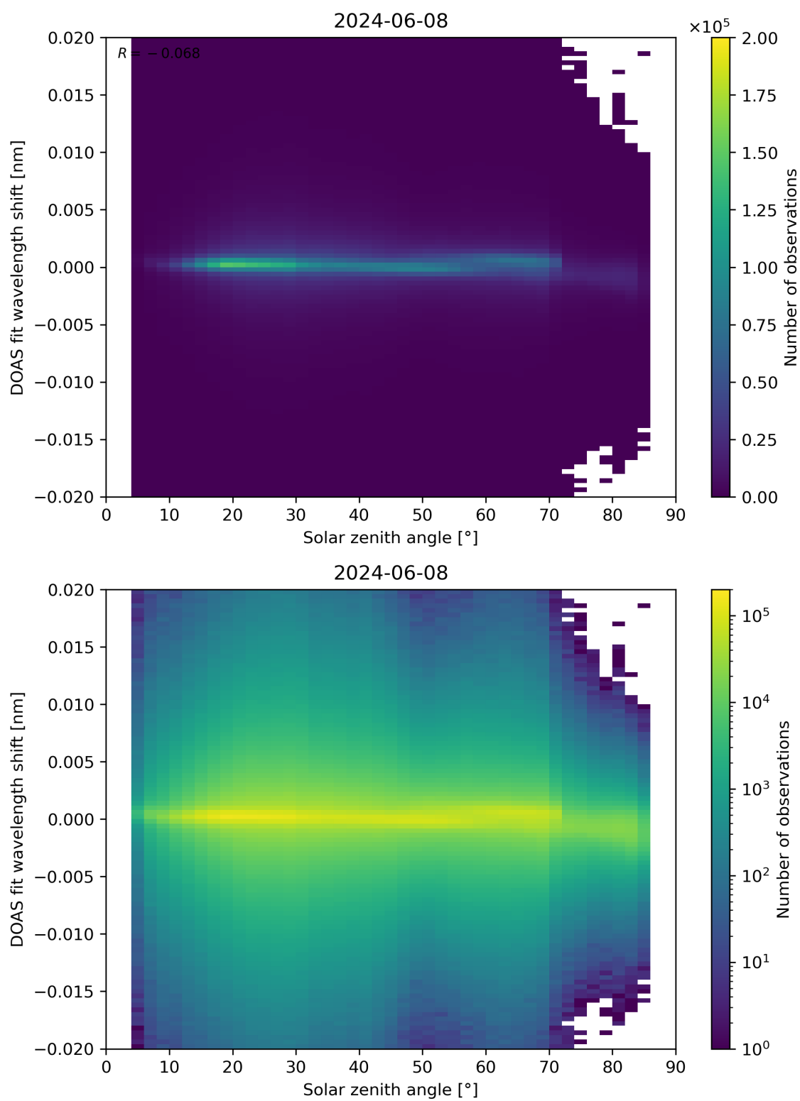
Figure 168: Scatter density plot of “Solar zenith angle” against “DOAS fit wavelength shift” for 2024-06-08 to 2024-06-09.
