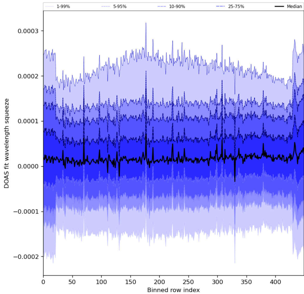
Figure 59: Along track statistics of “DOAS fit wavelength squeeze” for 2024-06-08 to 2024-06-09
