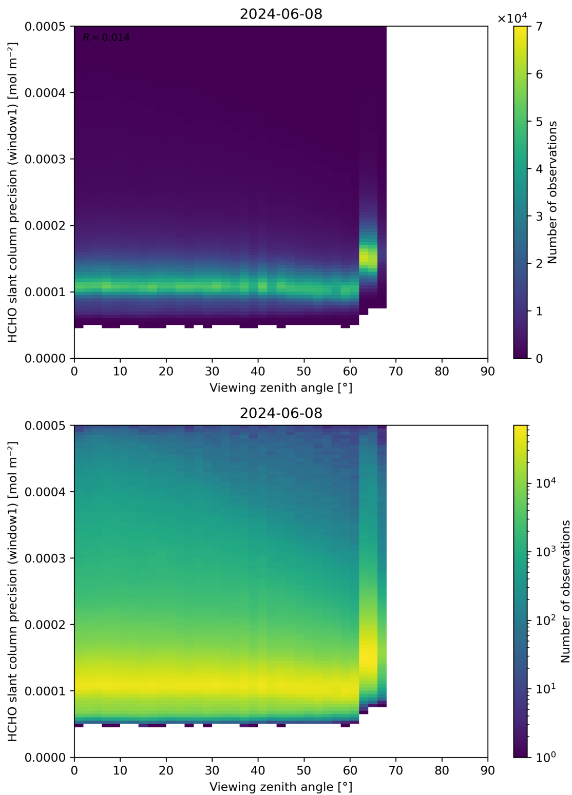
Figure 189: Scatter density plot of “Viewing zenith angle” against “HCHO slant column precision (window1)” for 2024-06-08 to 2024-06-09.
