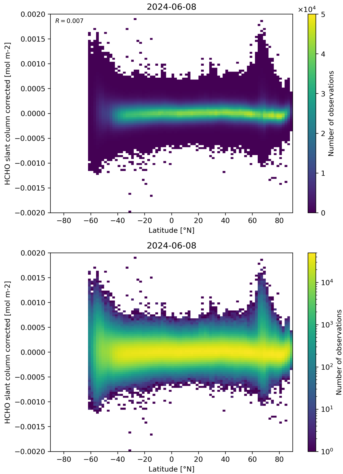
Figure 157: Scatter density plot of “Latitude” against “HCHO slant column corrected” for 2024-06-08 to 2024-06-09.
