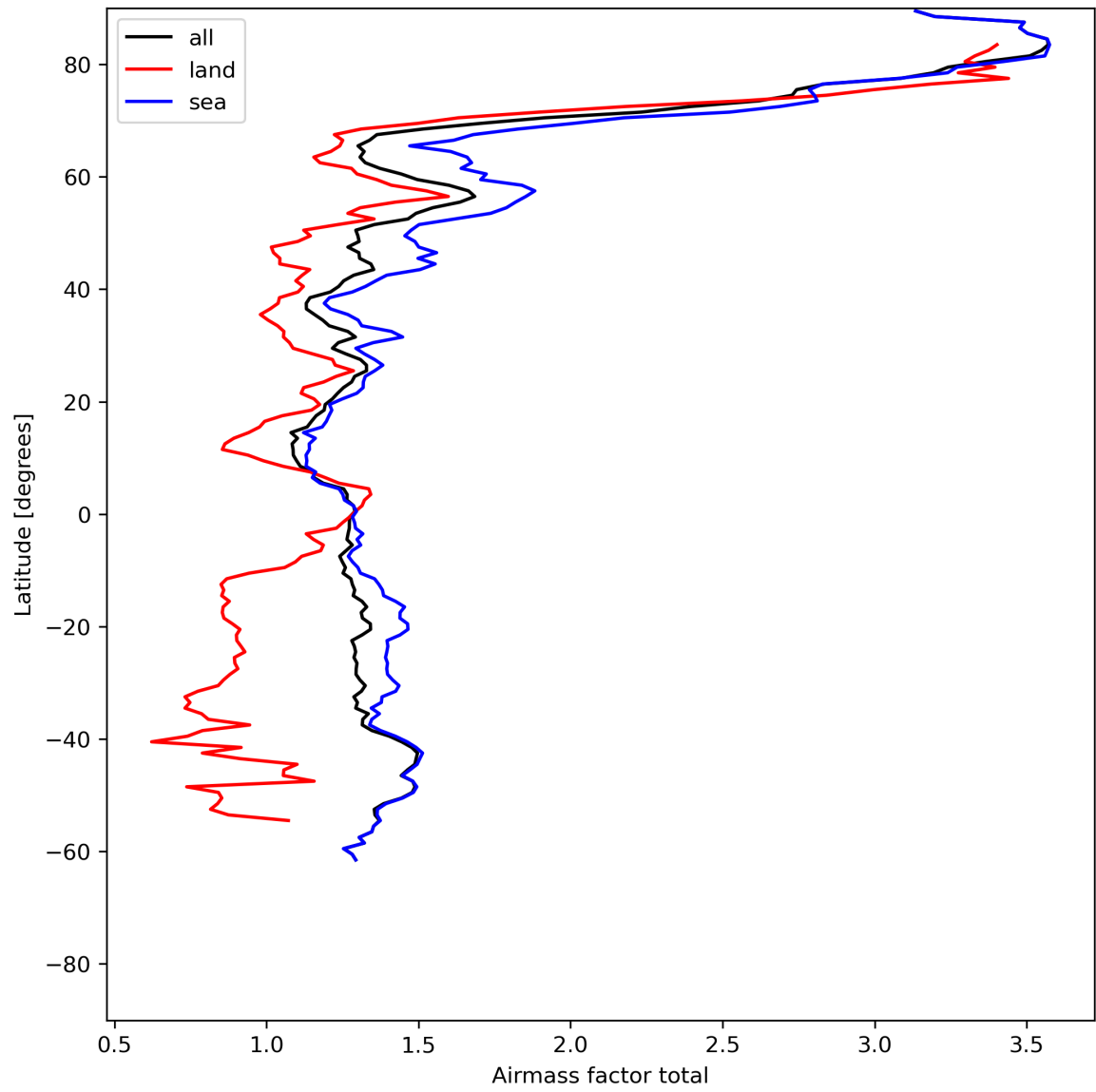
Figure 26: Zonal average of “Airmass factor total” for 2024-06-08 to 2024-06-09.
