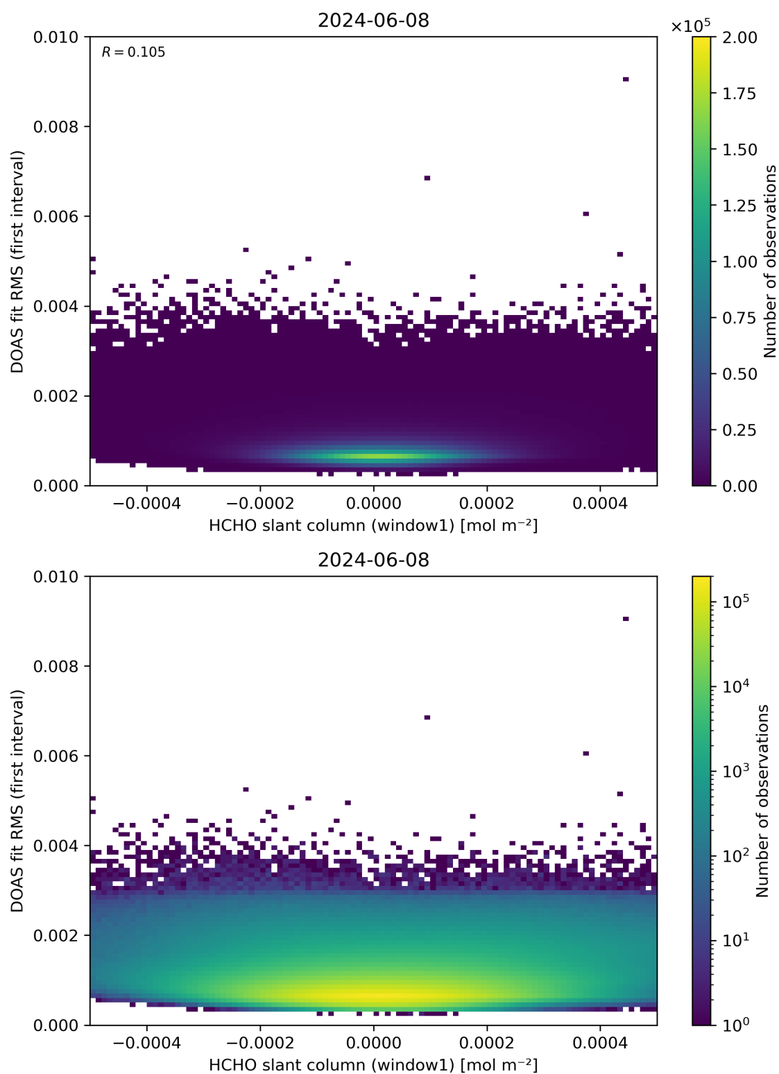
Figure 78: Scatter density plot of “HCHO slant column (window1)” against “DOAS fit RMS (first interval)” for 2024-06-08 to 2024-06-09.
