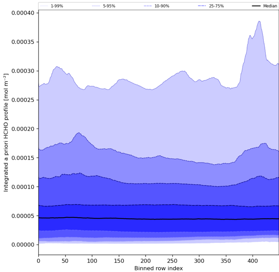
Figure 57: Along track statistics of “Integrated a priori HCHO profile” for 2024-06-08 to 2024-06-09
