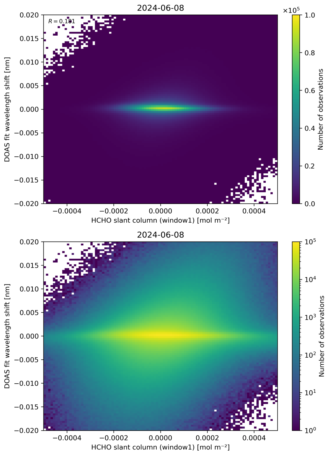
Figure 79: Scatter density plot of “HCHO slant column (window1)” against “DOAS fit wavelength shift” for 2024-06-08 to 2024-06-09.
