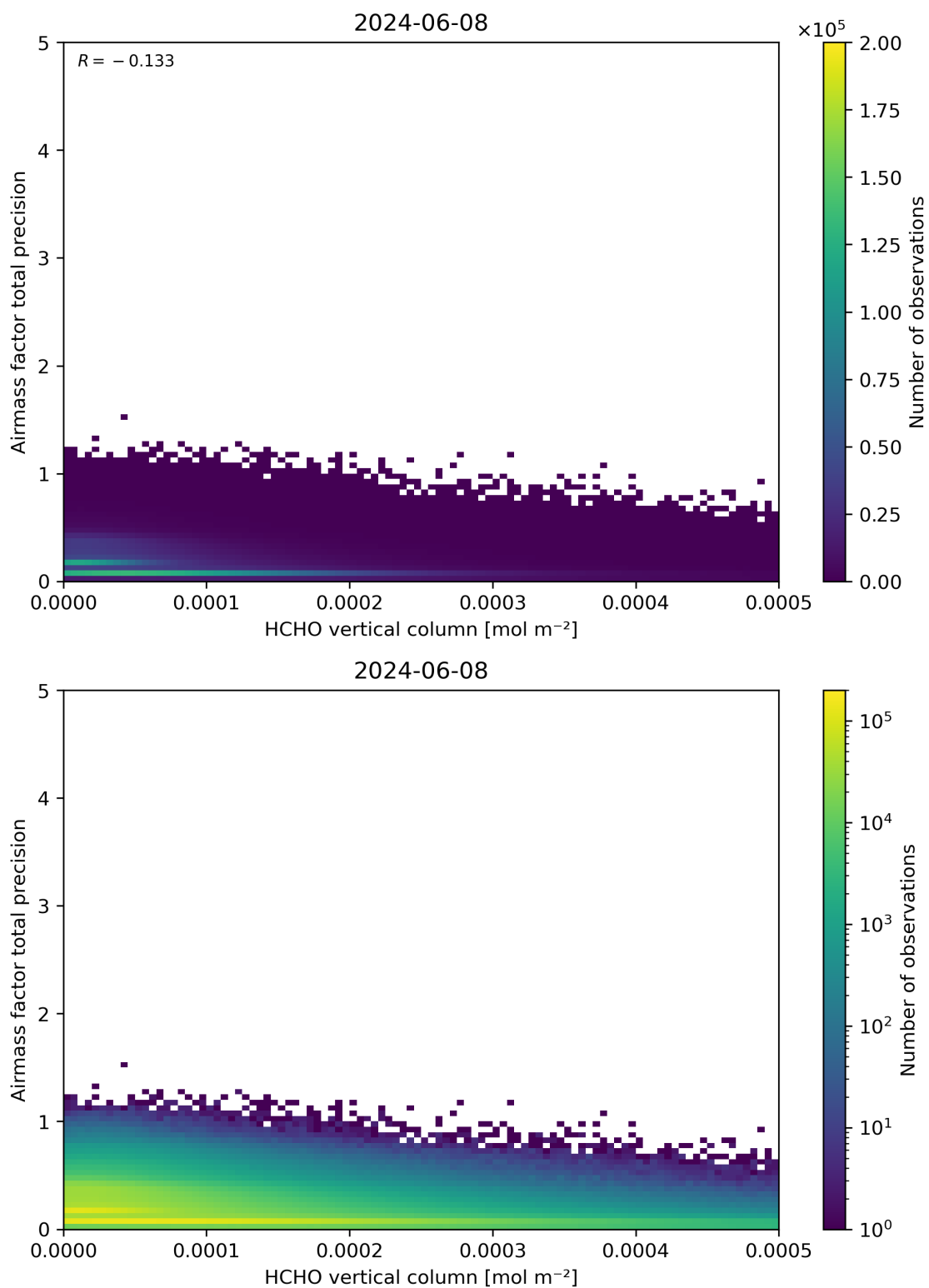
Figure 132: Scatter density plot of “HCHO vertical column” against “Airmass factor total precision” for 2024-06-08 to 2024-06-09.
