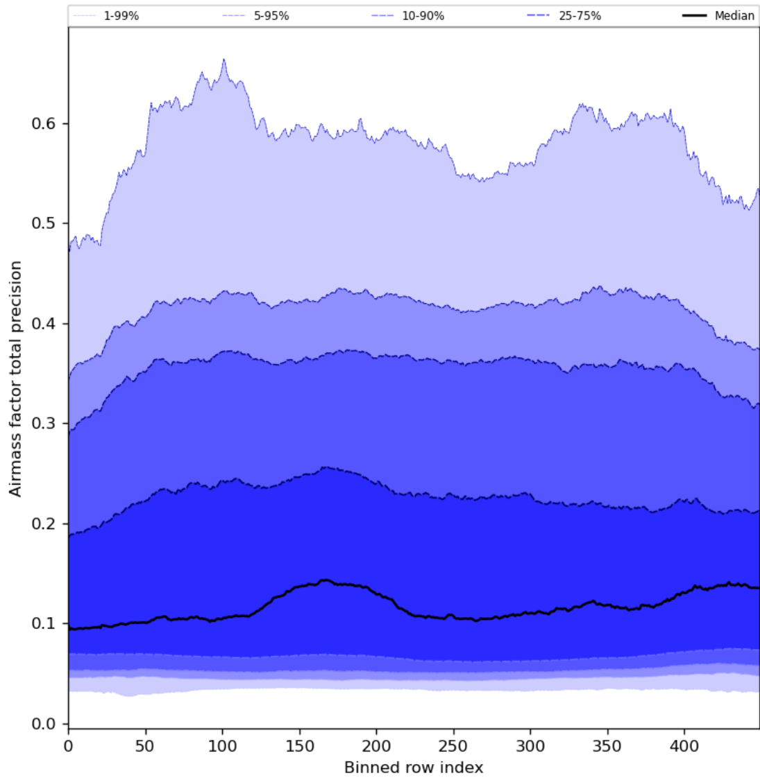
Figure 55: Along track statistics of “Airmass factor total precision” for 2024-06-08 to 2024-06-09
