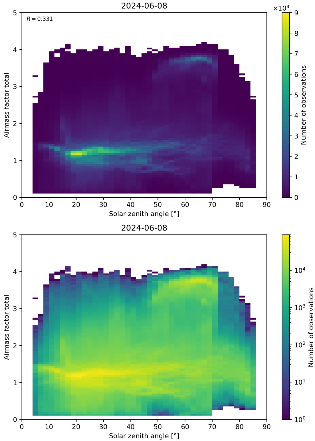
Figure 175: Scatter density plot of “Solar zenith angle” against “Airmass factor total” for 2024-06-08 to 2024-06-09.
