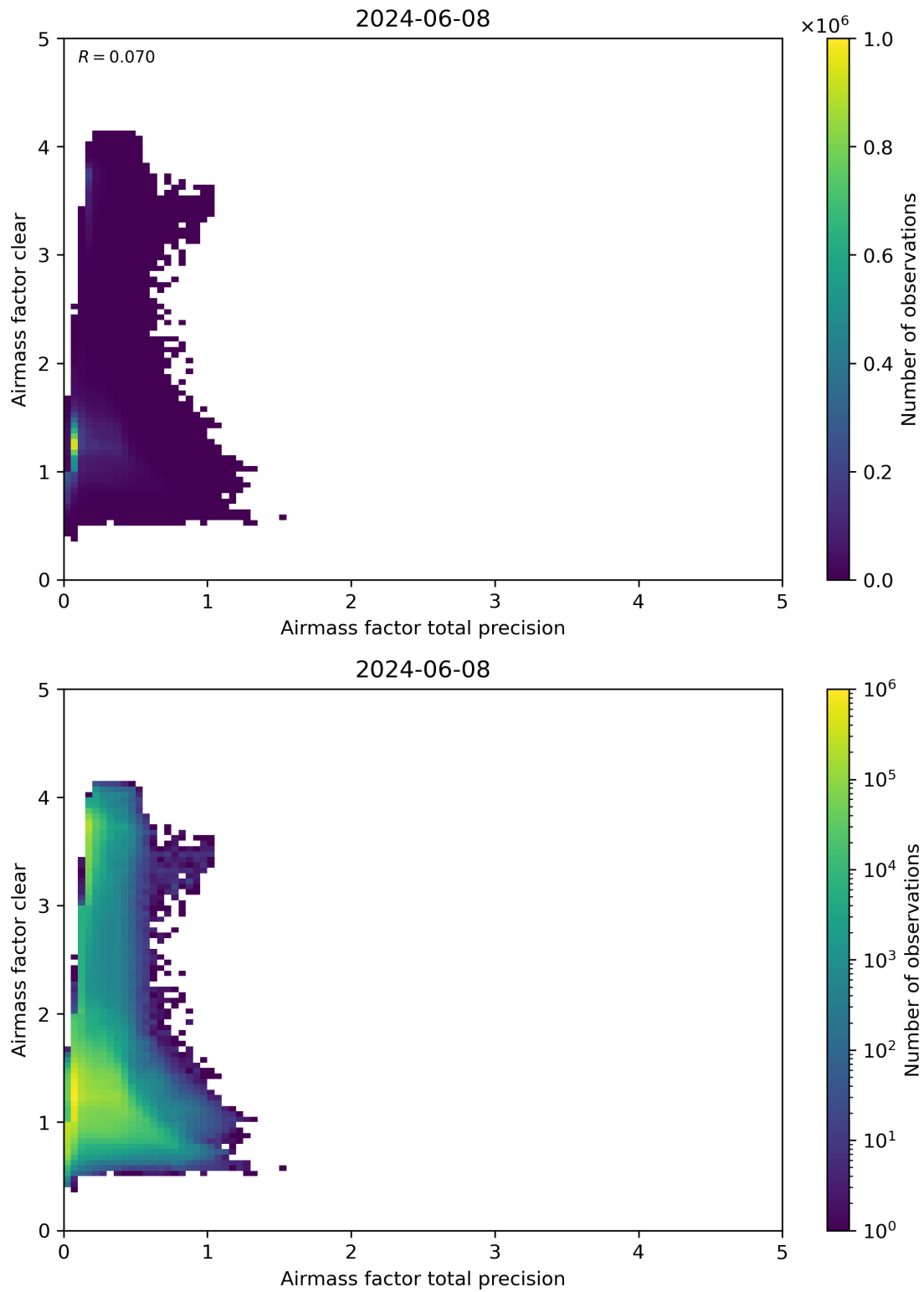
Figure 108: Scatter density plot of “Airmass factor total precision” against “Airmass factor clear” for 2024-06-08 to 2024-06-09.
