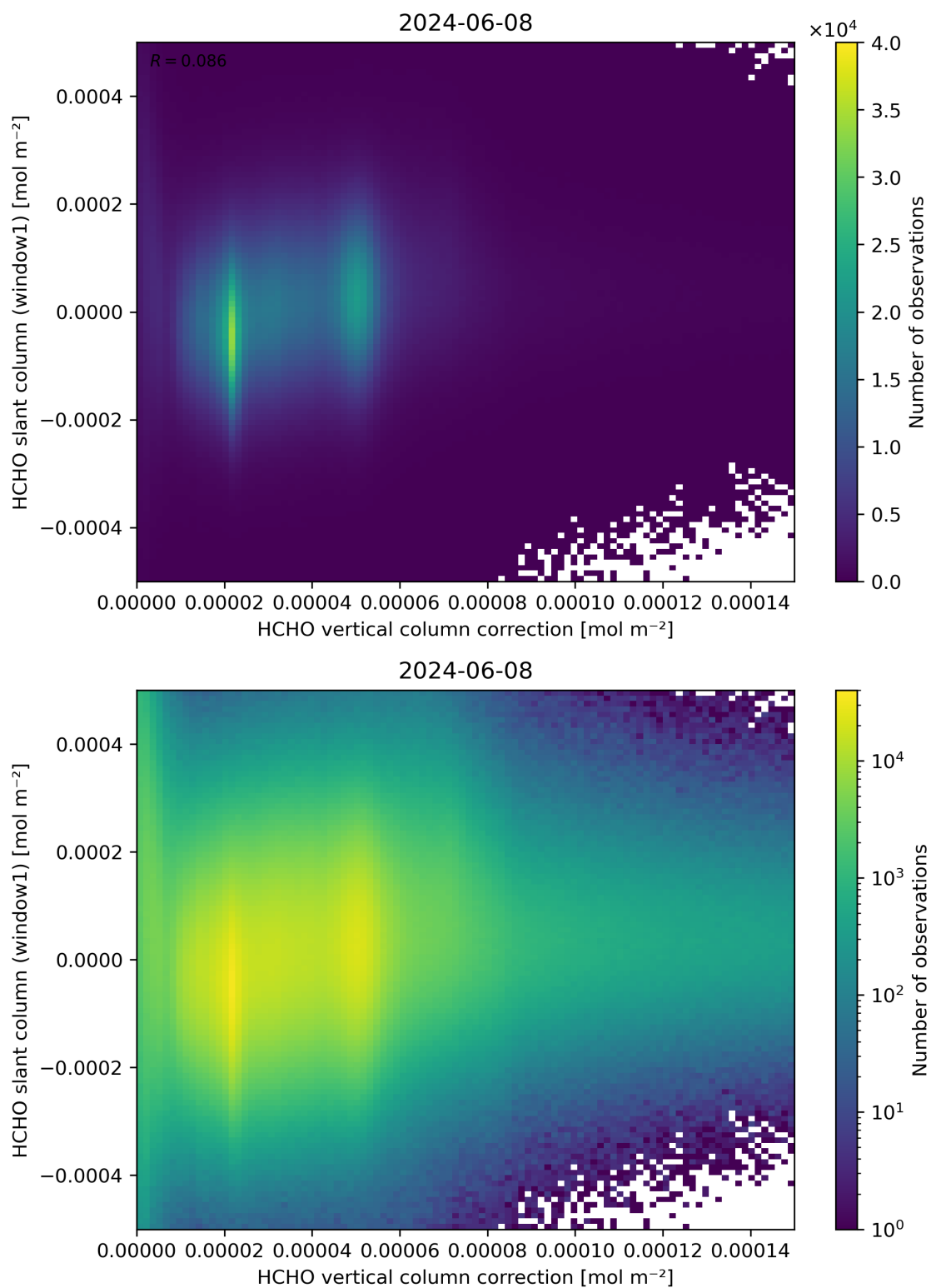
Figure 118: Scatter density plot of “HCHO vertical column correction” against “HCHO slant column (window1)” for 2024-06-08 to 2024-06-09.
