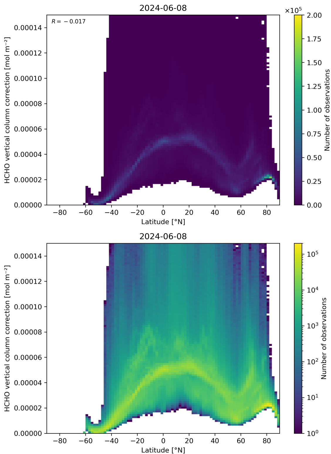
Figure 164: Scatter density plot of “Latitude” against “HCHO vertical column correction” for 2024-06-08 to 2024-06-09.
