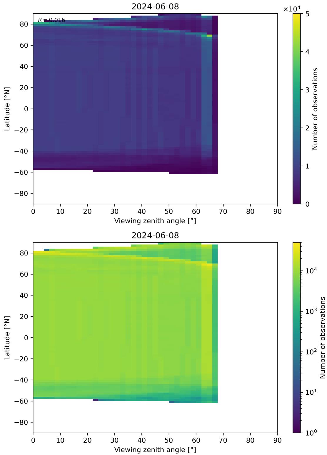
Figure 196: Scatter density plot of “Viewing zenith angle” against “Latitude” for 2024-06-08 to 2024-06-09.
