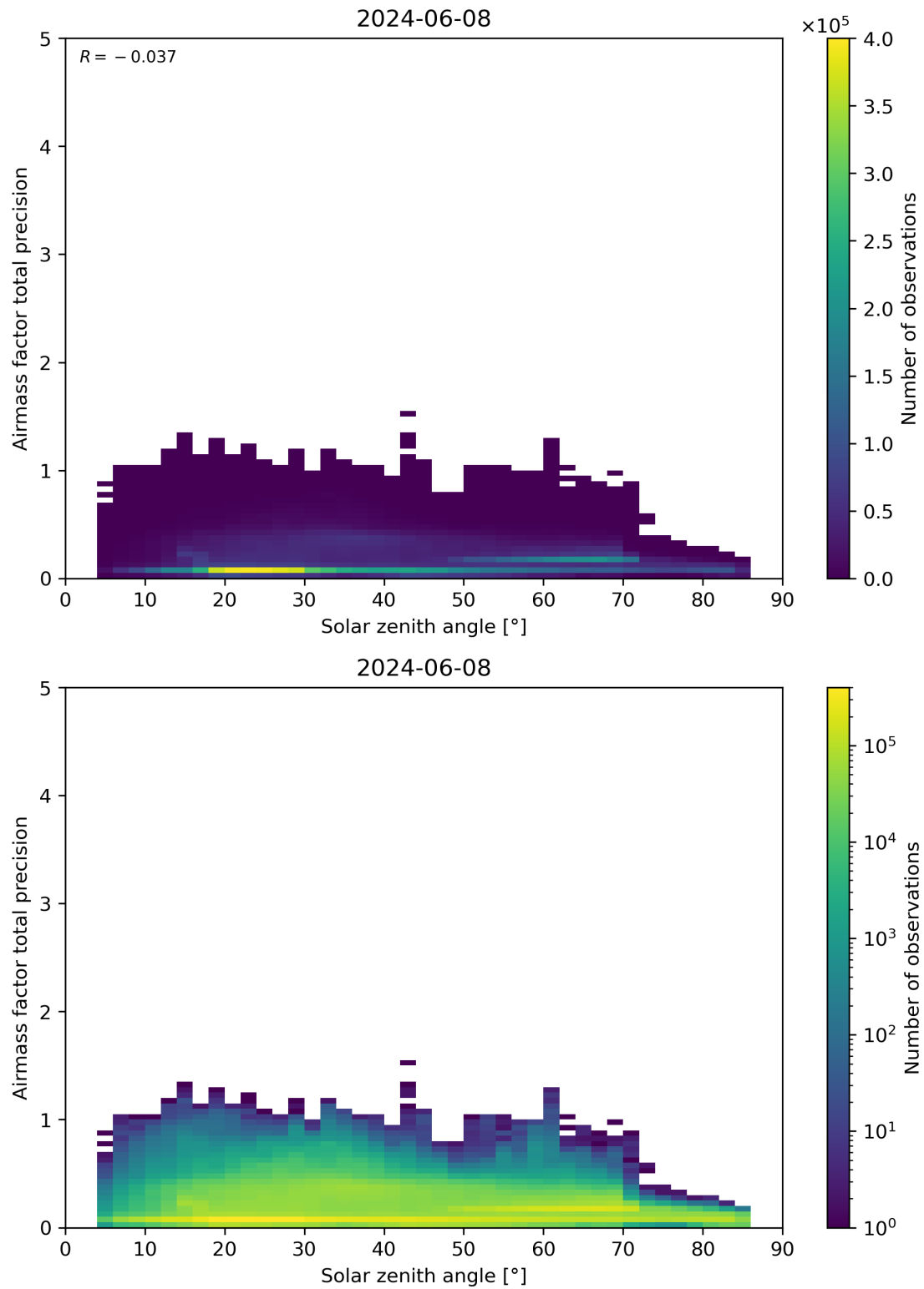
Figure 176: Scatter density plot of “Solar zenith angle” against “Airmass factor total precision” for 2024-06-08 to 2024-06-09.
