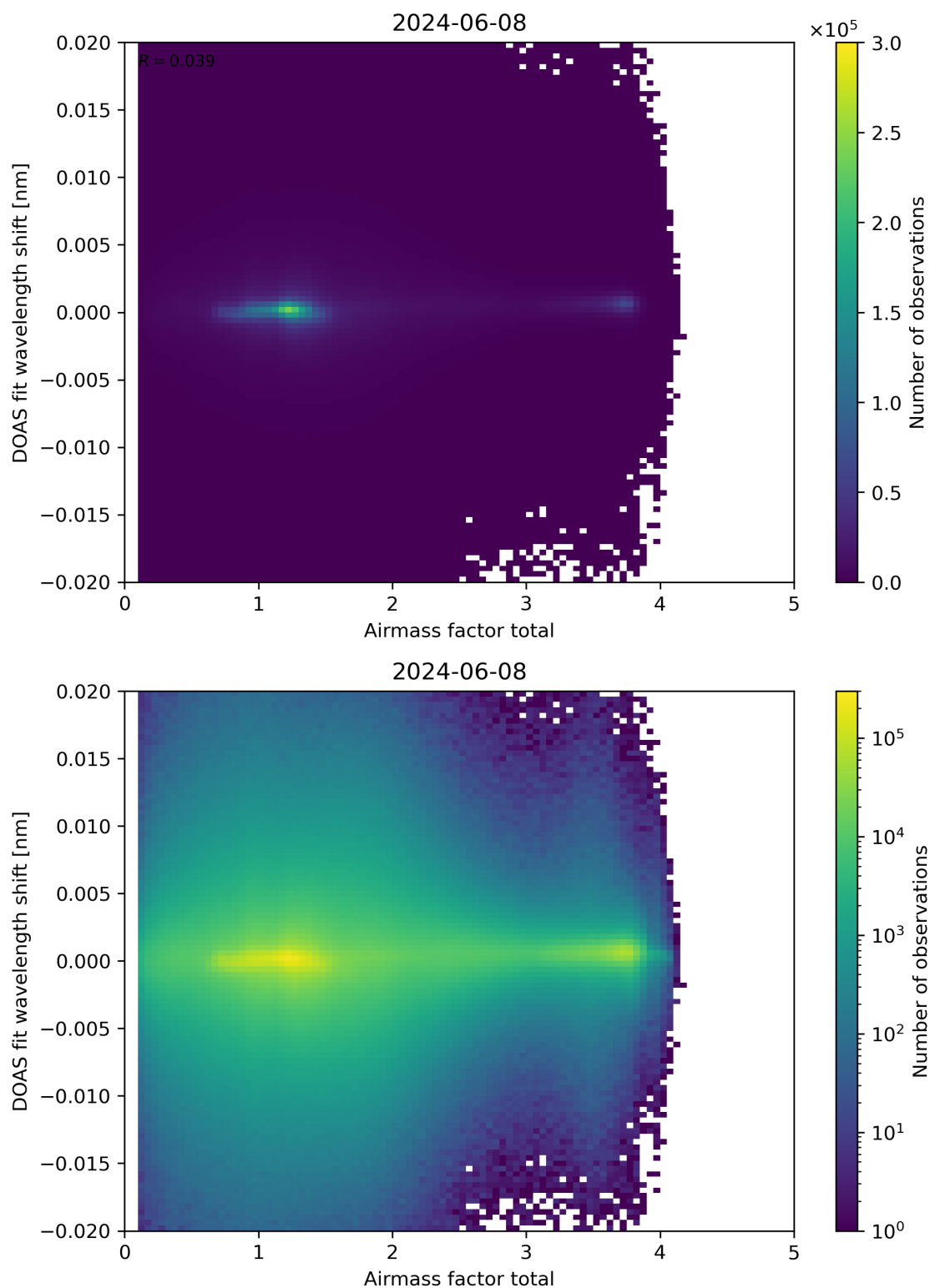
Figure 98: Scatter density plot of “Airmass factor total” against “DOAS fit wavelength shift” for 2024-06-08 to 2024-06-09.
