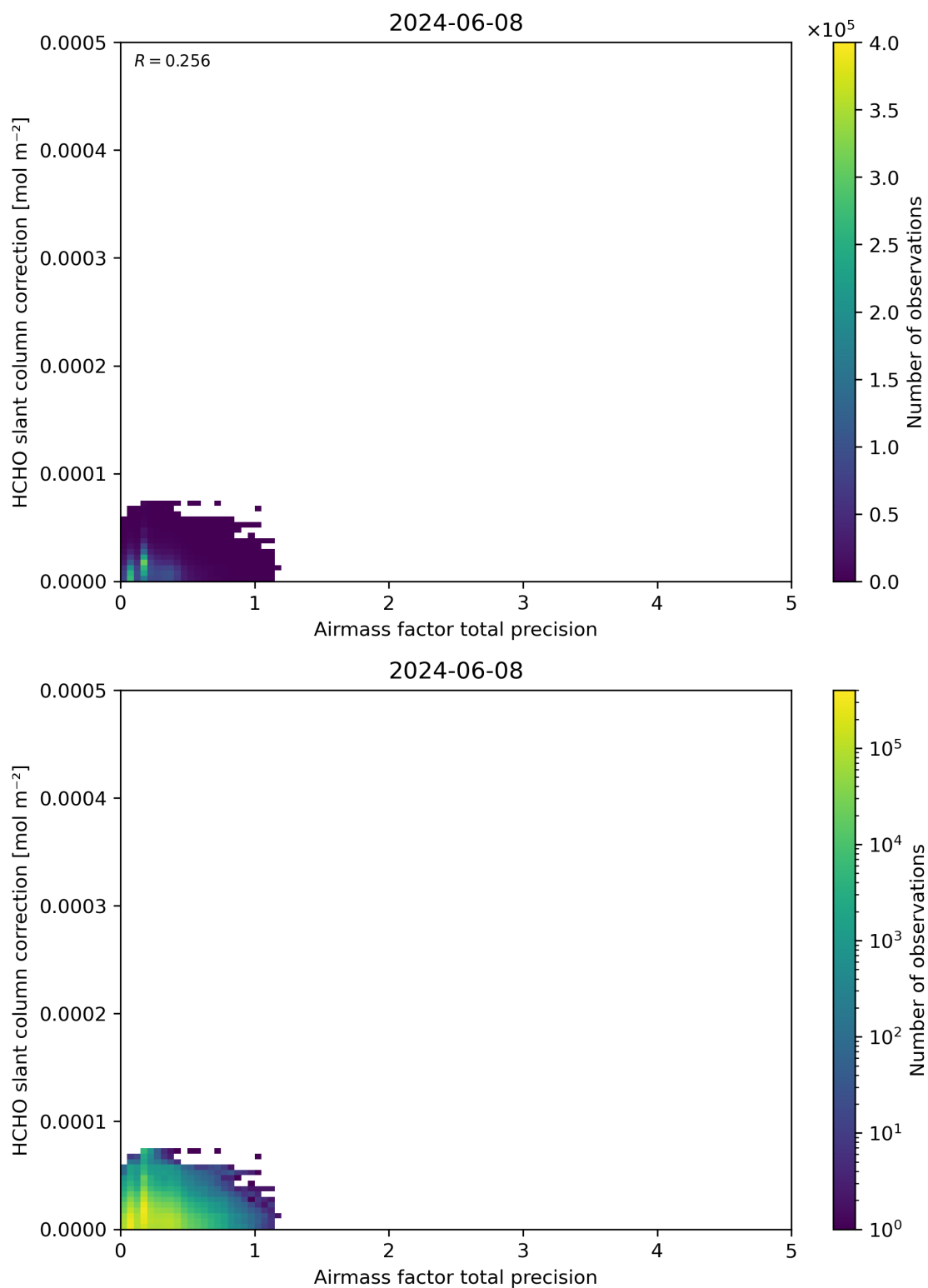
Figure 110: Scatter density plot of “Airmass factor total precision” against “HCHO slant column correction” for 2024-06-08 to 2024-06-09.
