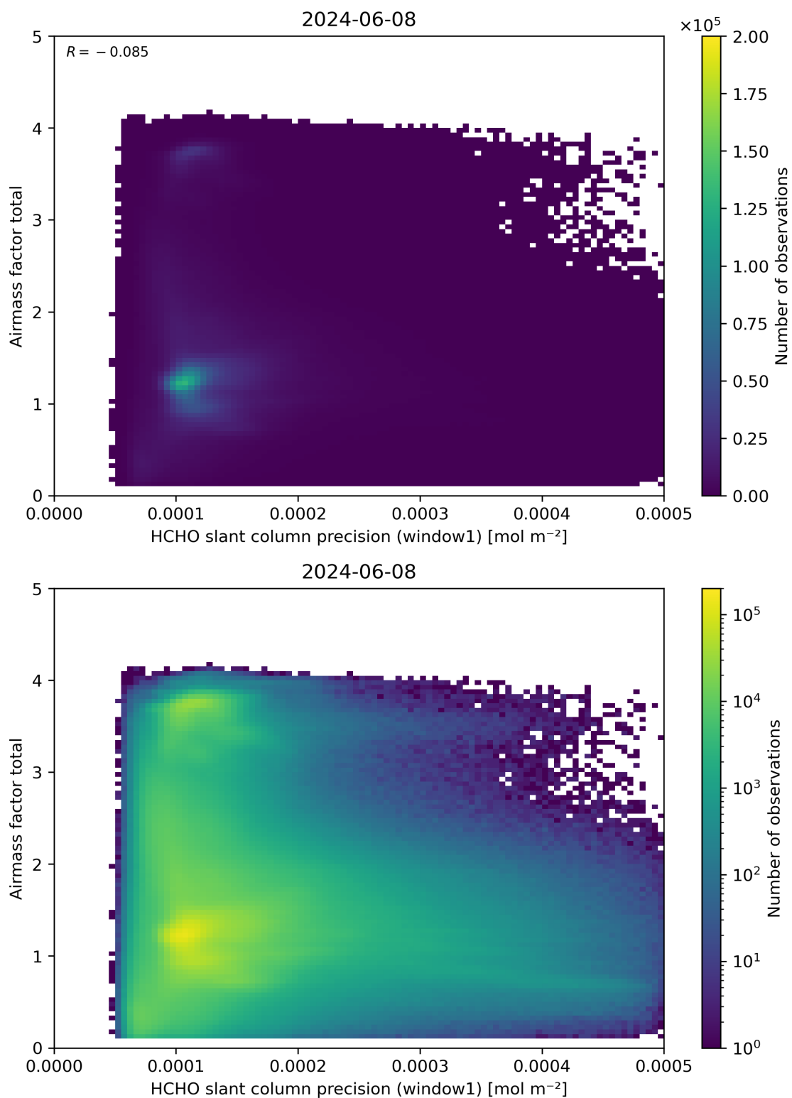
Figure 94: Scatter density plot of “HCHO slant column precision (window1)” against “Airmass factor total” for 2024-06-08 to 2024-06-09.
