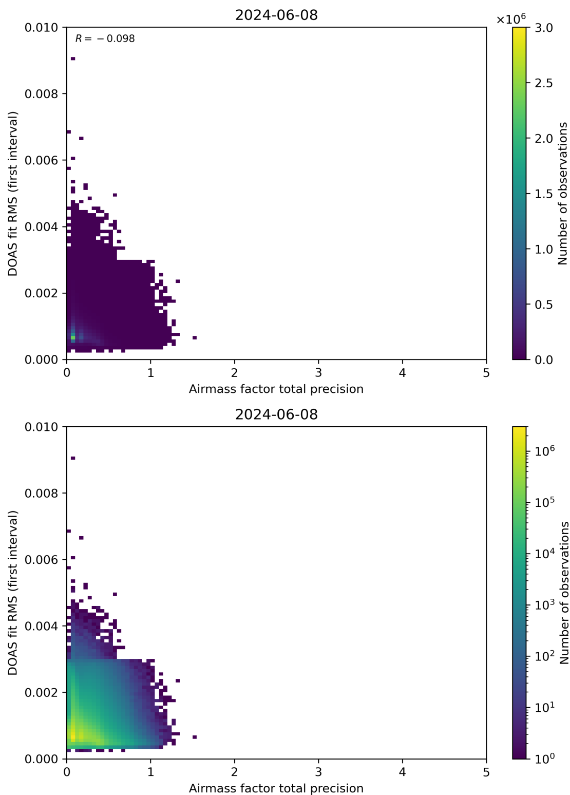
Figure 105: Scatter density plot of “Airmass factor total precision” against “DOAS fit RMS (first interval)” for 2024-06-08 to 2024-06-09.
