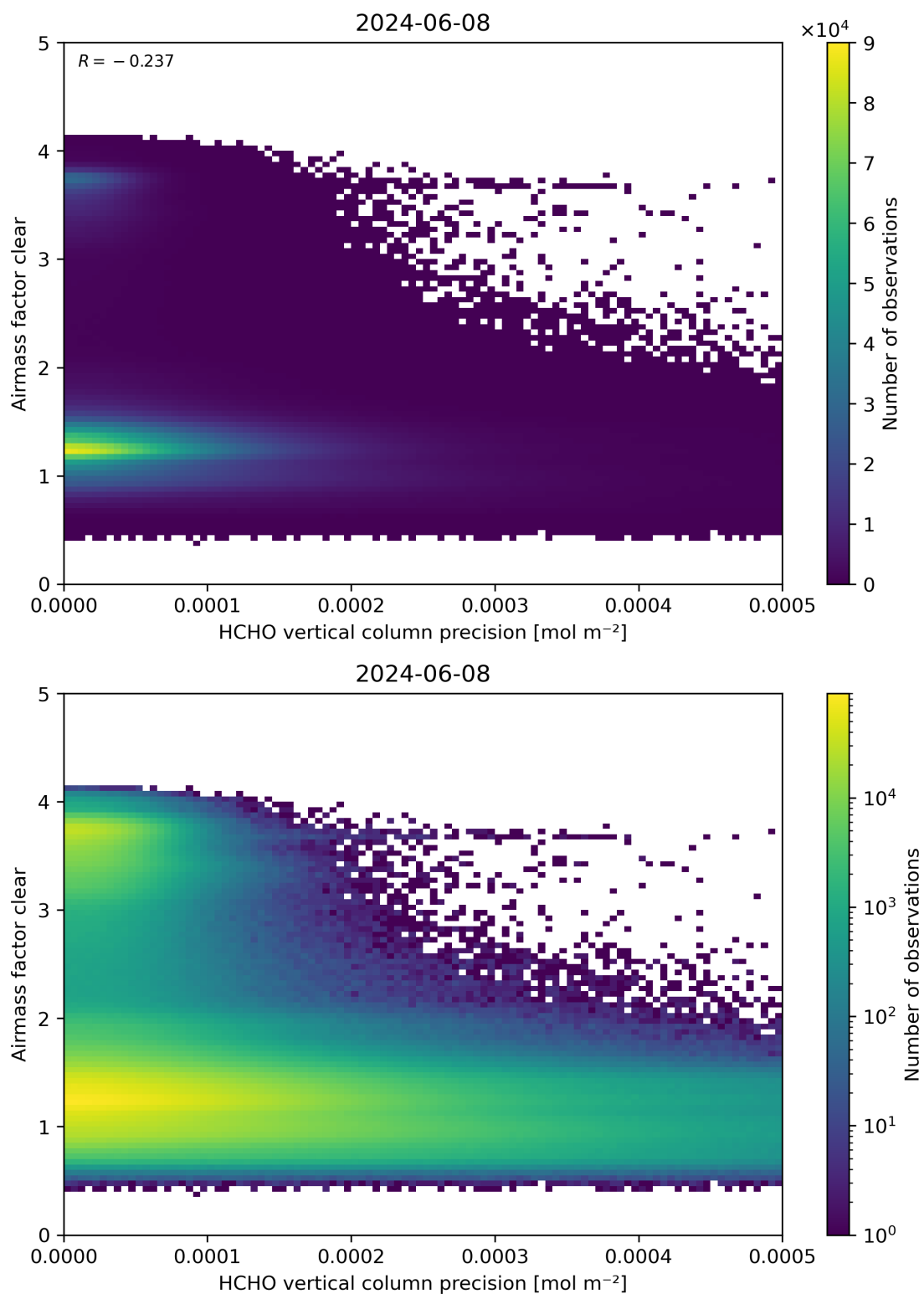
Figure 139: Scatter density plot of “HCHO vertical column precision” against “Airmass factor clear” for 2024-06-08 to 2024-06-09.
