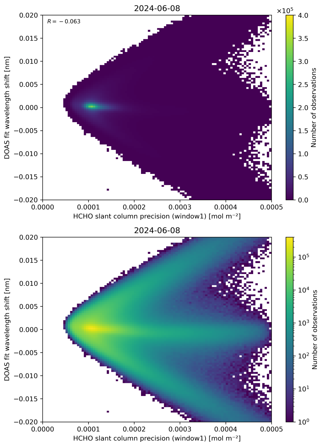
Figure 89: Scatter density plot of “HCHO slant column precision (window1)” against “DOAS fit wavelength shift” for 2024-06-08 to 2024-06-09.
