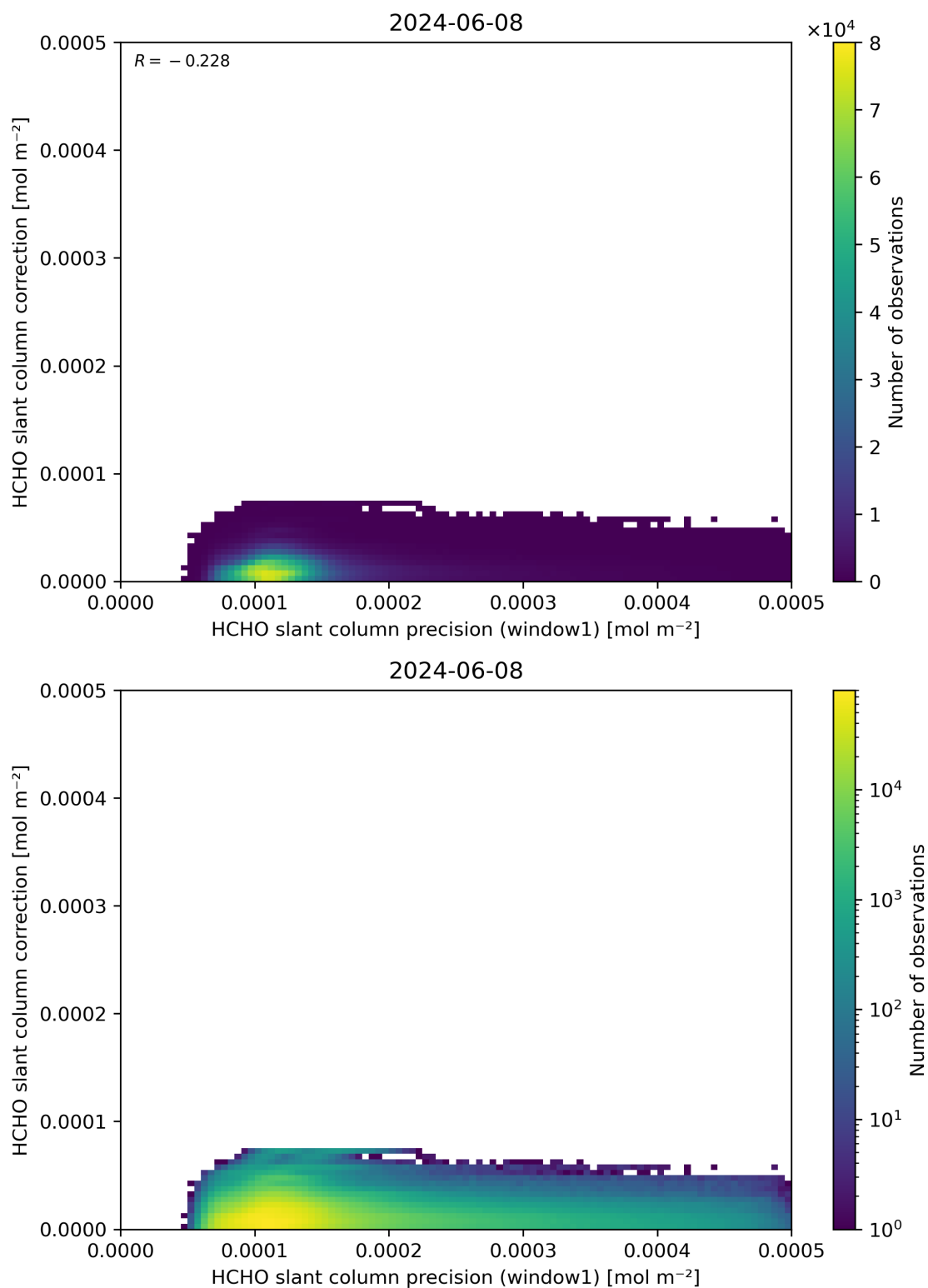
Figure 93: Scatter density plot of “HCHO slant column precision (window1)” against “HCHO slant column correction” for 2024-06-08 to 2024-06-09.
