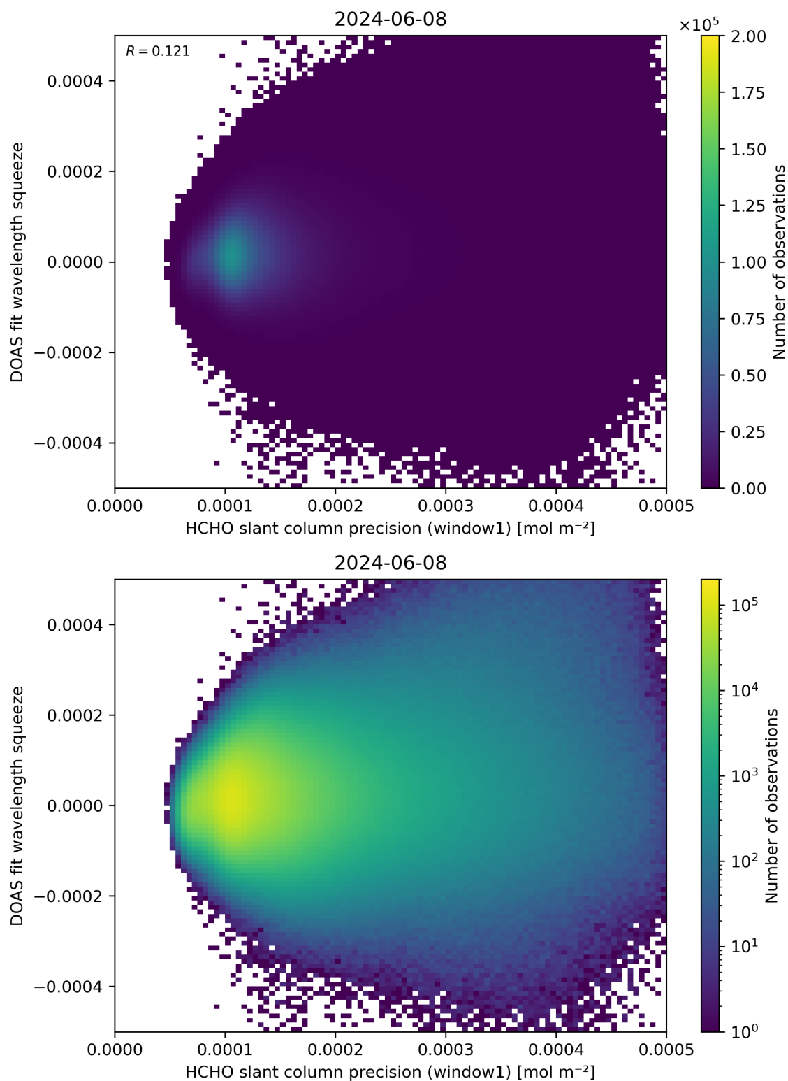
Figure 90: Scatter density plot of “HCHO slant column precision (window1)” against “DOAS fit wavelength squeeze” for 2024-06-08 to 2024-06-09.
