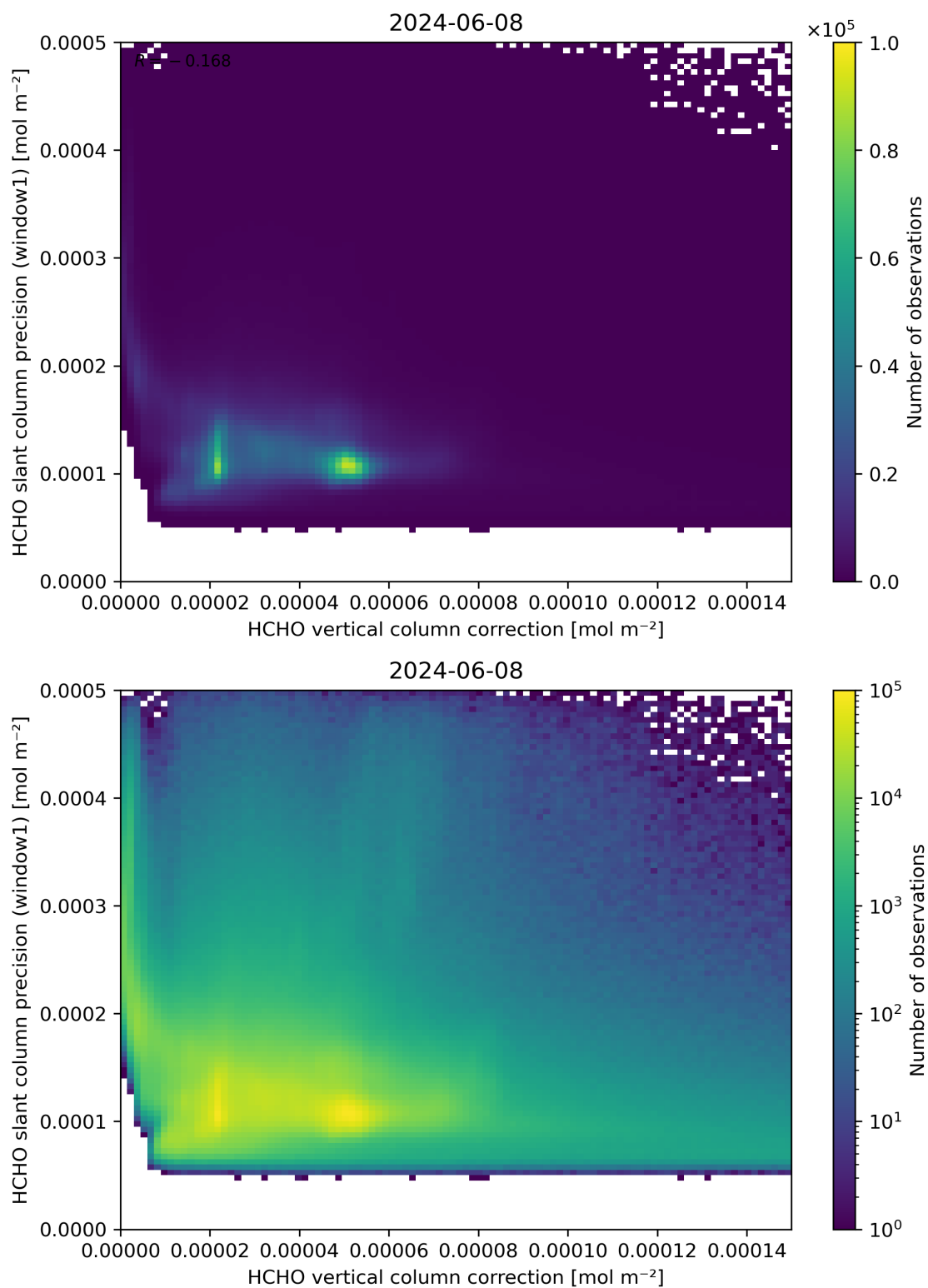
Figure 119: Scatter density plot of “HCHO vertical column correction” against “HCHO slant column precision (window1)” for 2024-06-08 to 2024-06-09.
