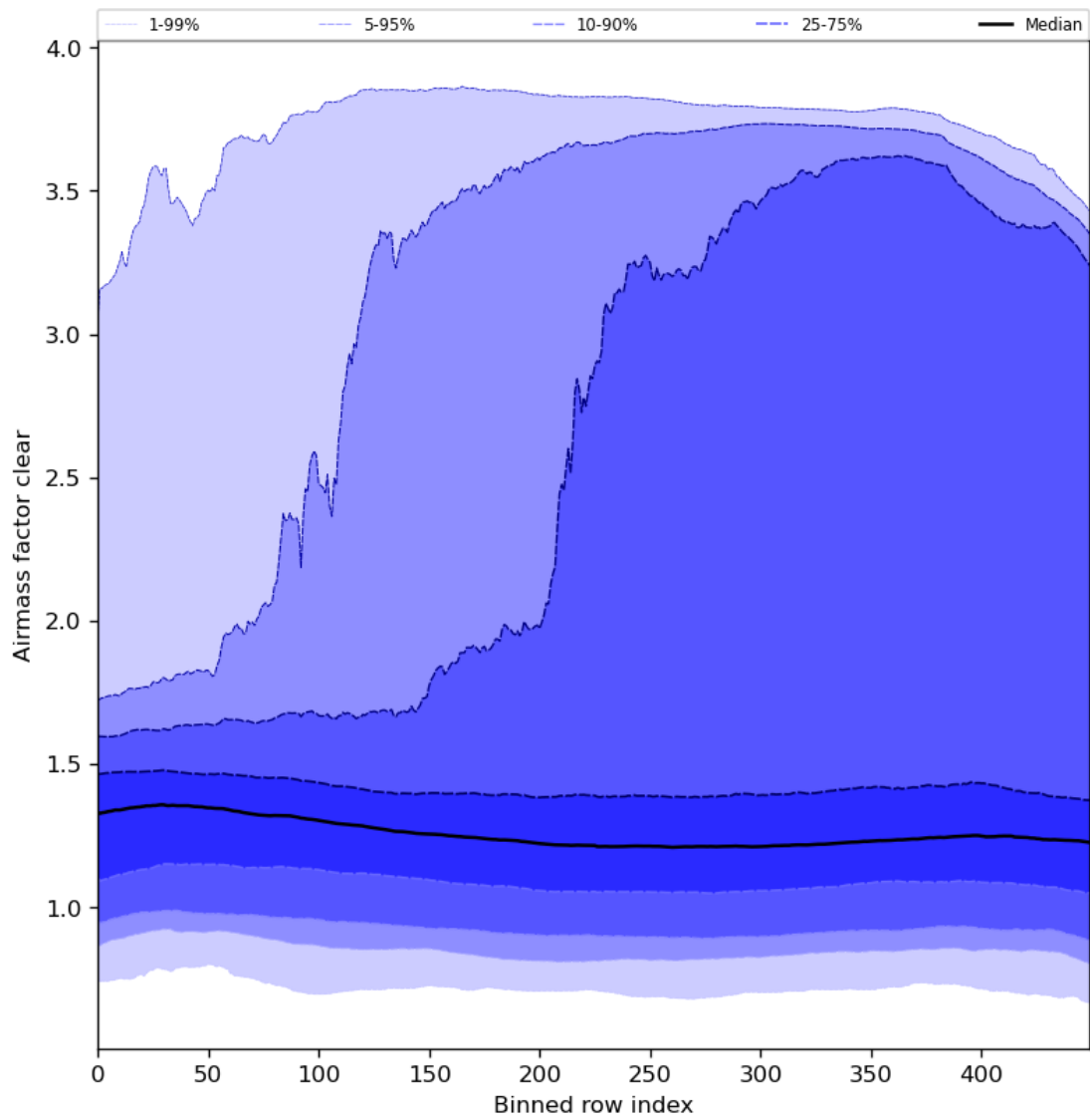
Figure 56: Along track statistics of “Airmass factor clear” for 2024-06-08 to 2024-06-09
