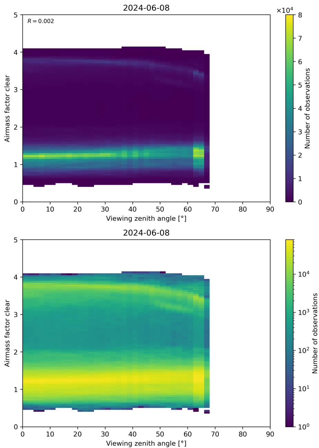
Figure 185: Scatter density plot of “Viewing zenith angle” against “Airmass factor clear” for 2024-06-08 to 2024-06-09.
