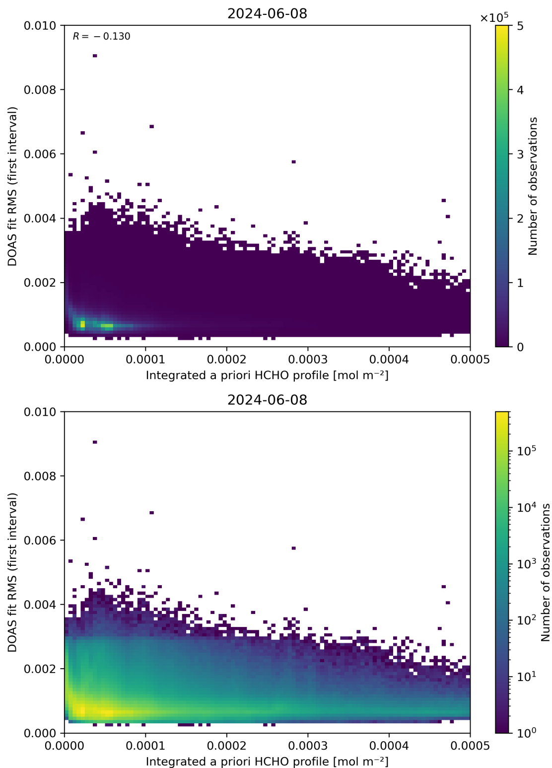
Figure 148: Scatter density plot of “Integrated a priori HCHO profile” against “DOAS fit RMS (first interval)” for 2024-06-08 to 2024-06-09.
