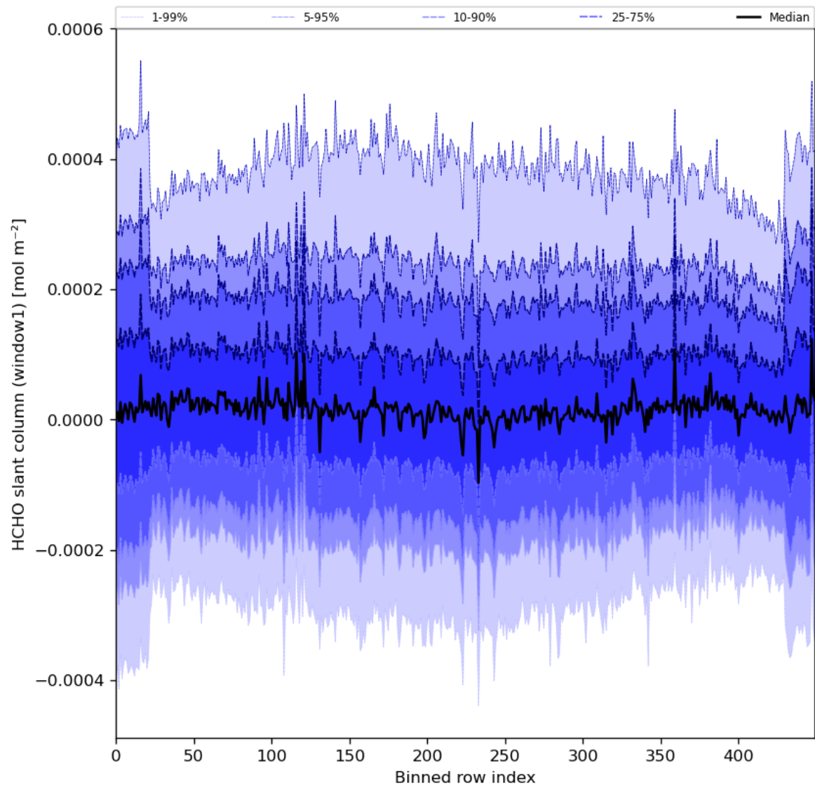
Figure 52: Along track statistics of “HCHO slant column (window1)” for 2024-06-08 to 2024-06-09
