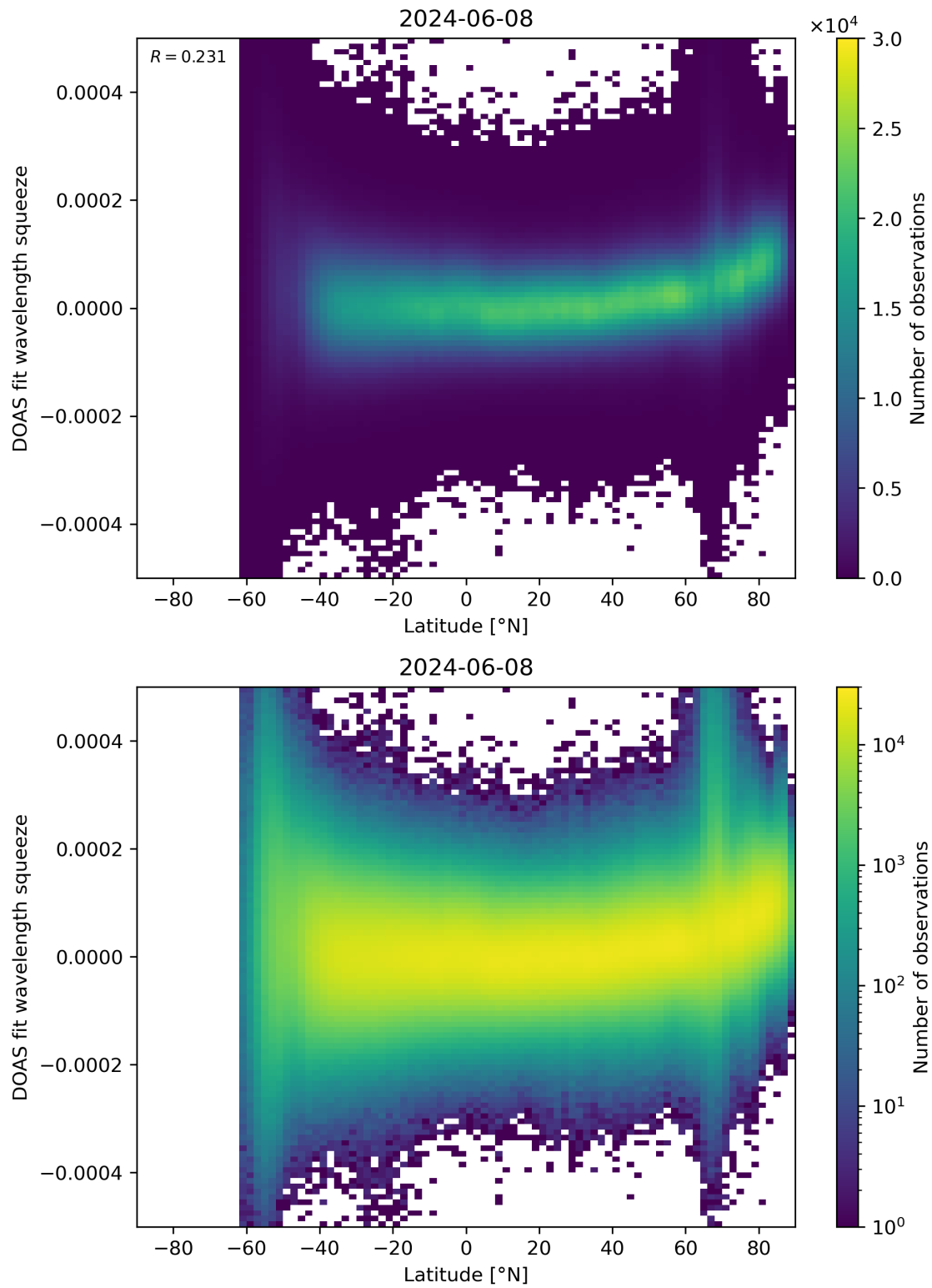
Figure 155: Scatter density plot of “Latitude” against “DOAS fit wavelength squeeze” for 2024-06-08 to 2024-06-09.
