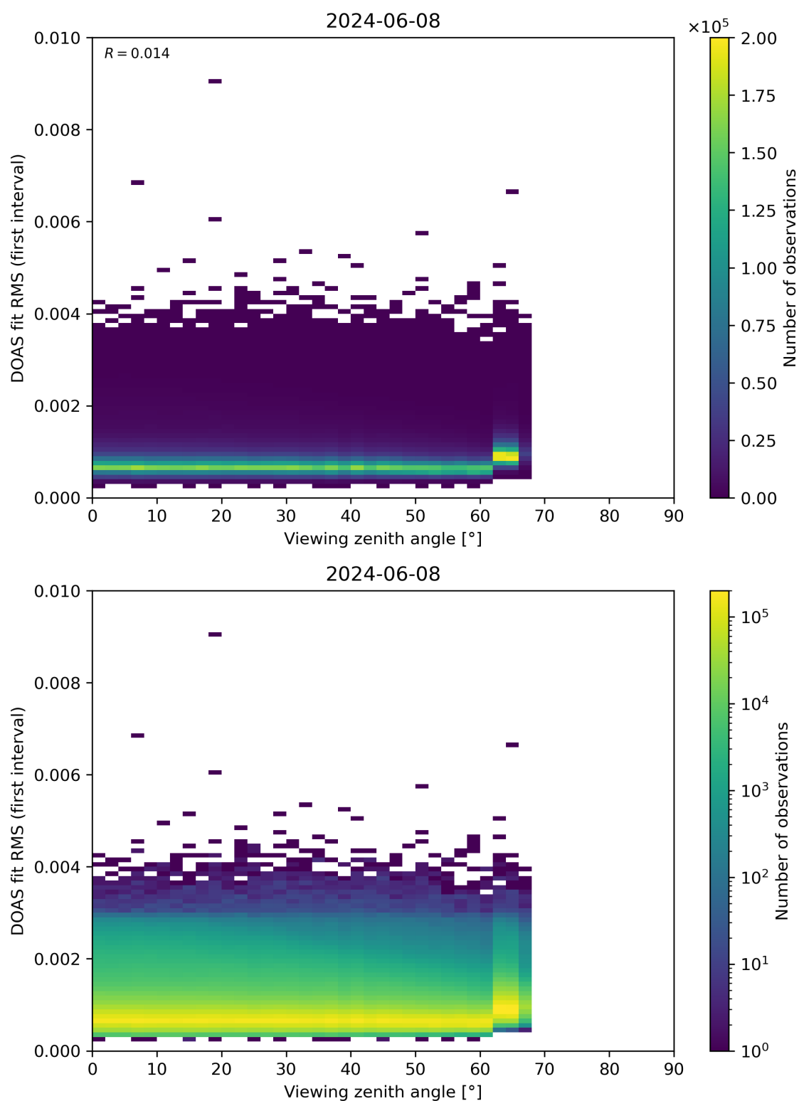
Figure 182: Scatter density plot of “Viewing zenith angle” against “DOAS fit RMS (first interval)” for 2024-06-08 to 2024-06-09.
