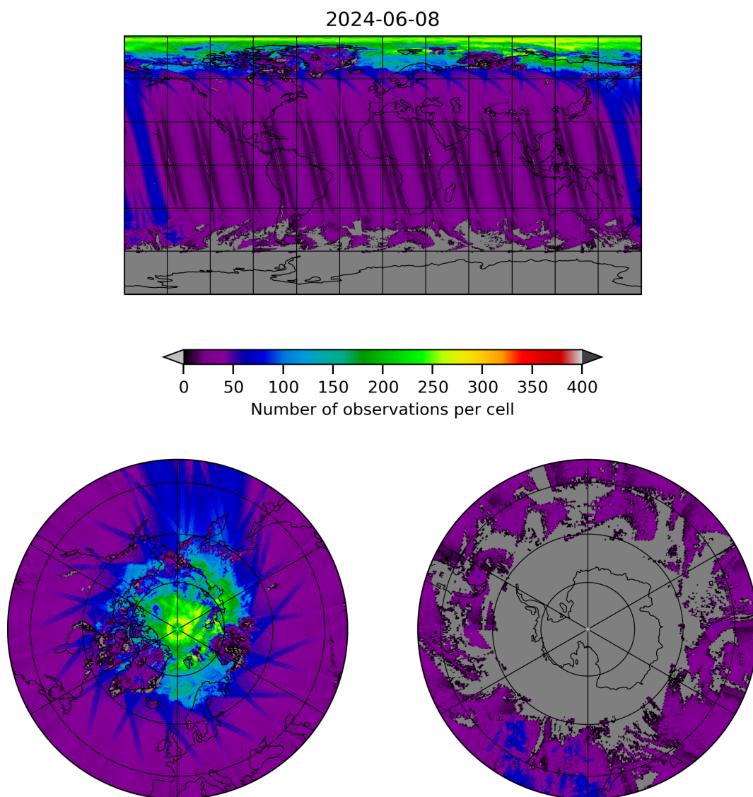
Figure 19: Map of the number of observations for 2024-06-08 to 2024-06-09
