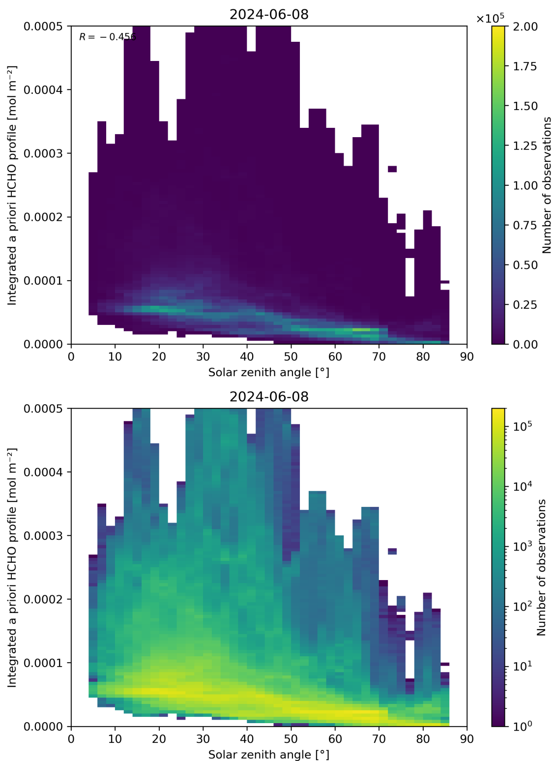
Figure 180: Scatter density plot of “Solar zenith angle” against “Integrated a priori HCHO profile” for 2024-06-08 to 2024-06-09.
