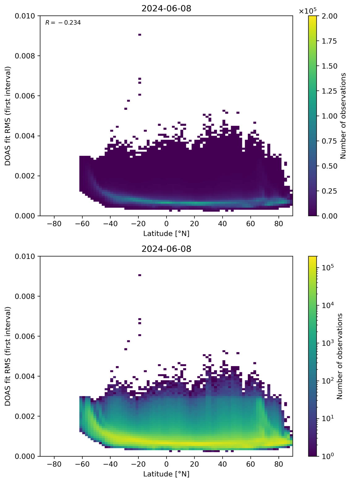
Figure 153: Scatter density plot of “Latitude” against “DOAS fit RMS (first interval)” for 2024-06-08 to 2024-06-09.
