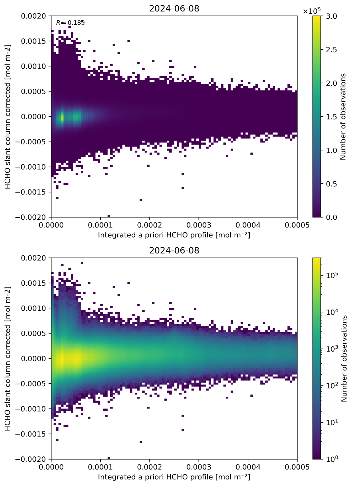
Figure 151: Scatter density plot of “Integrated a priori HCHO profile” against “HCHO slant column corrected” for 2024-06-08 to 2024-06-09.
