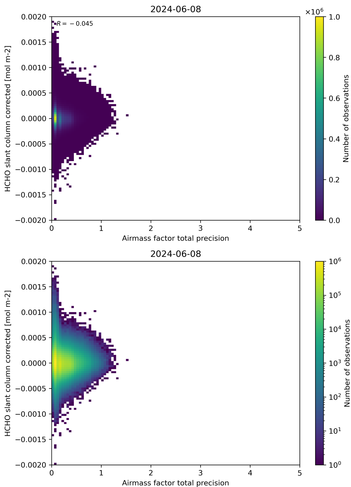
Figure 109: Scatter density plot of “Airmass factor total precision” against “HCHO slant column corrected” for 2024-06-08 to 2024-06-09.
