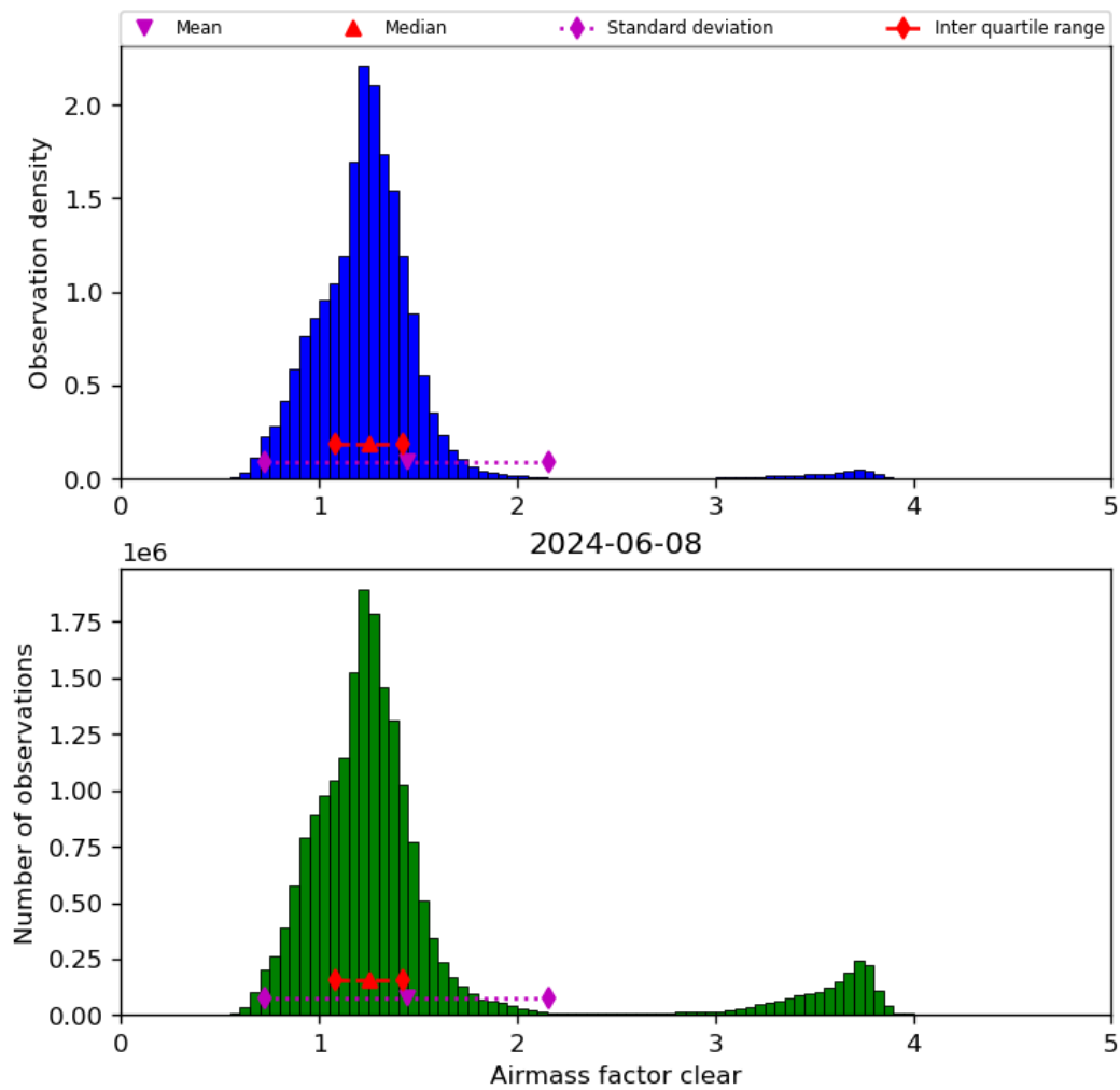
Figure 42: Histogram of “Airmass factor clear” for 2024-06-08 to 2024-06-09
