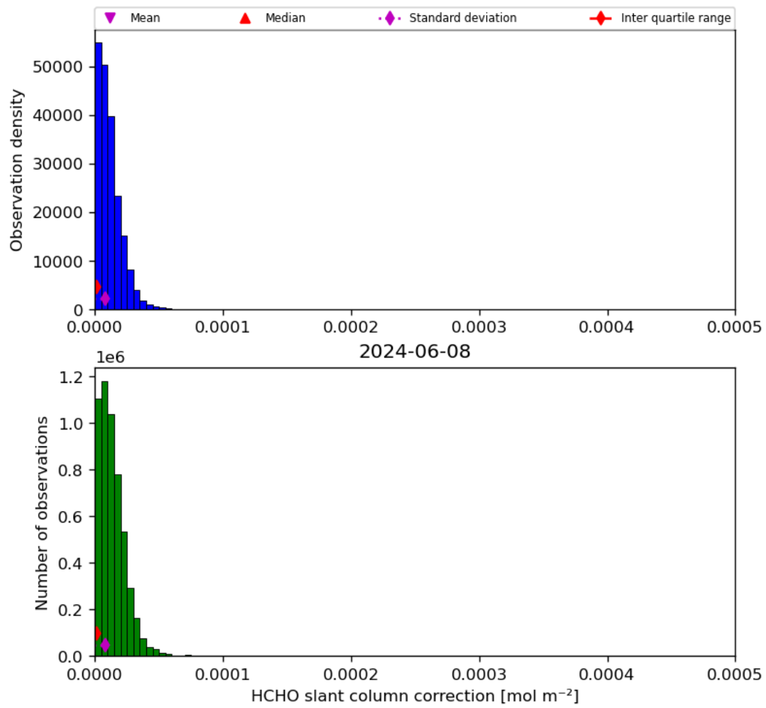
Figure 47: Histogram of “HCHO slant column correction” for 2024-06-08 to 2024-06-09
