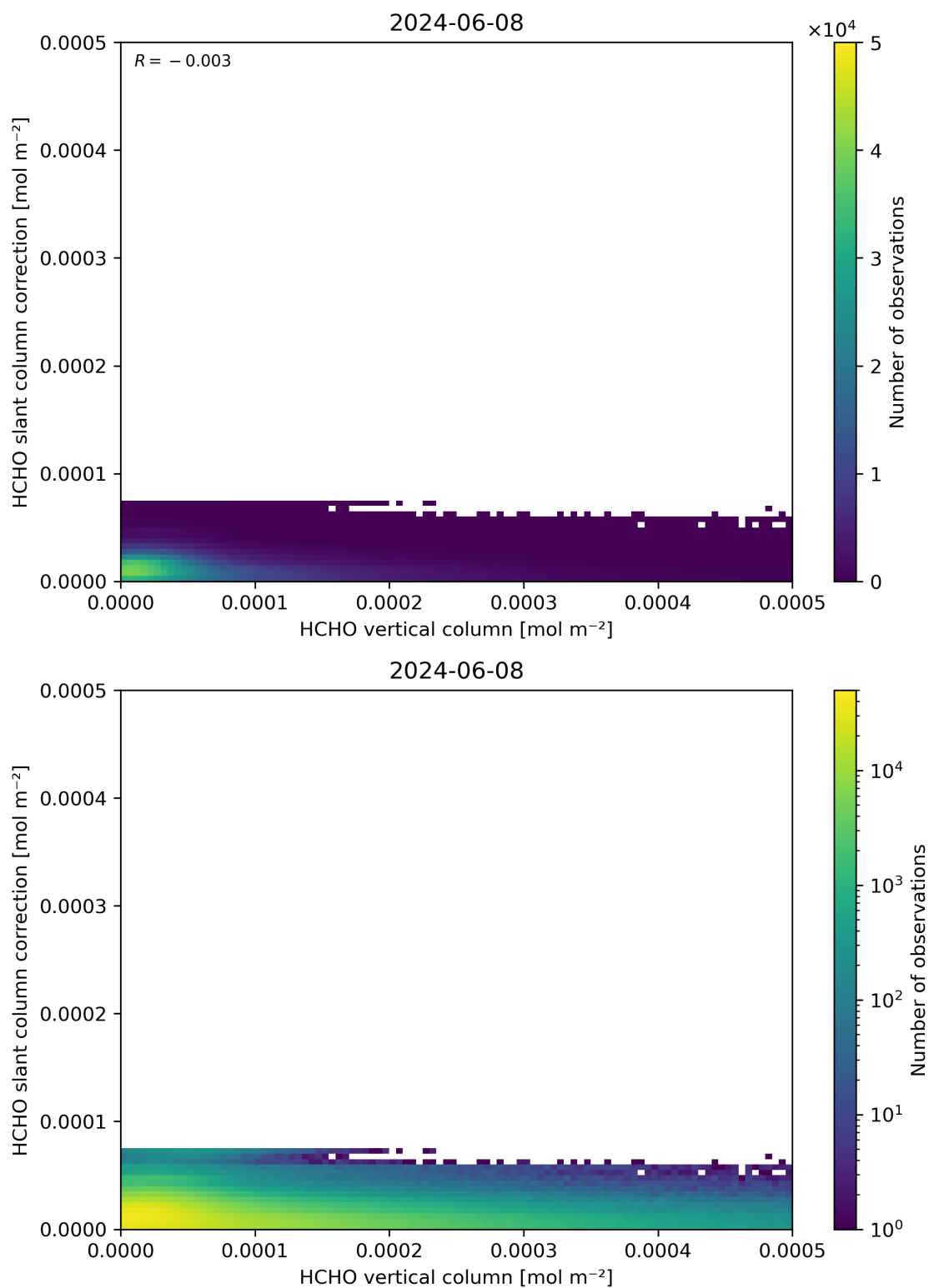
Figure 128: Scatter density plot of “HCHO vertical column” against “HCHO slant column correction” for 2024-06-08 to 2024-06-09.
