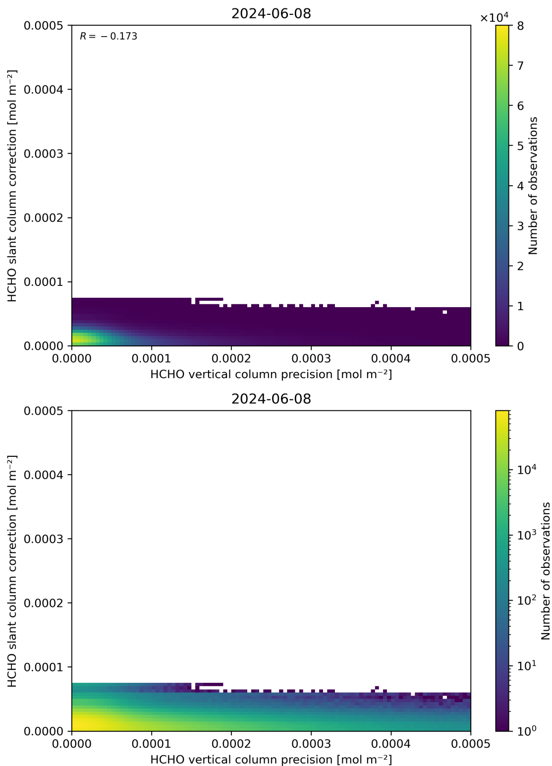
Figure 141: Scatter density plot of “HCHO vertical column precision” against “HCHO slant column correction” for 2024-06-08 to 2024-06-09.
