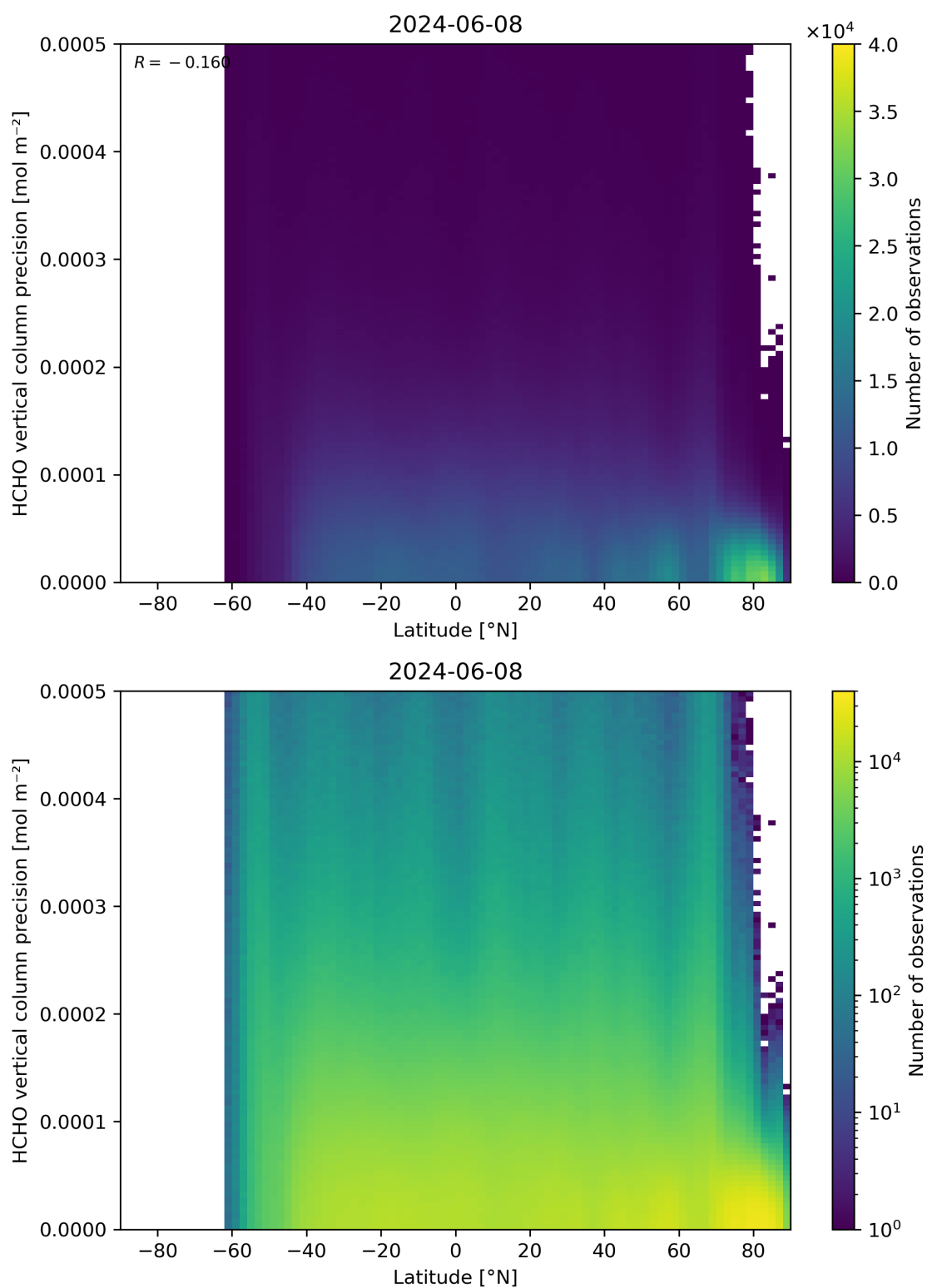
Figure 165: Scatter density plot of “Latitude” against “HCHO vertical column precision” for 2024-06-08 to 2024-06-09.
