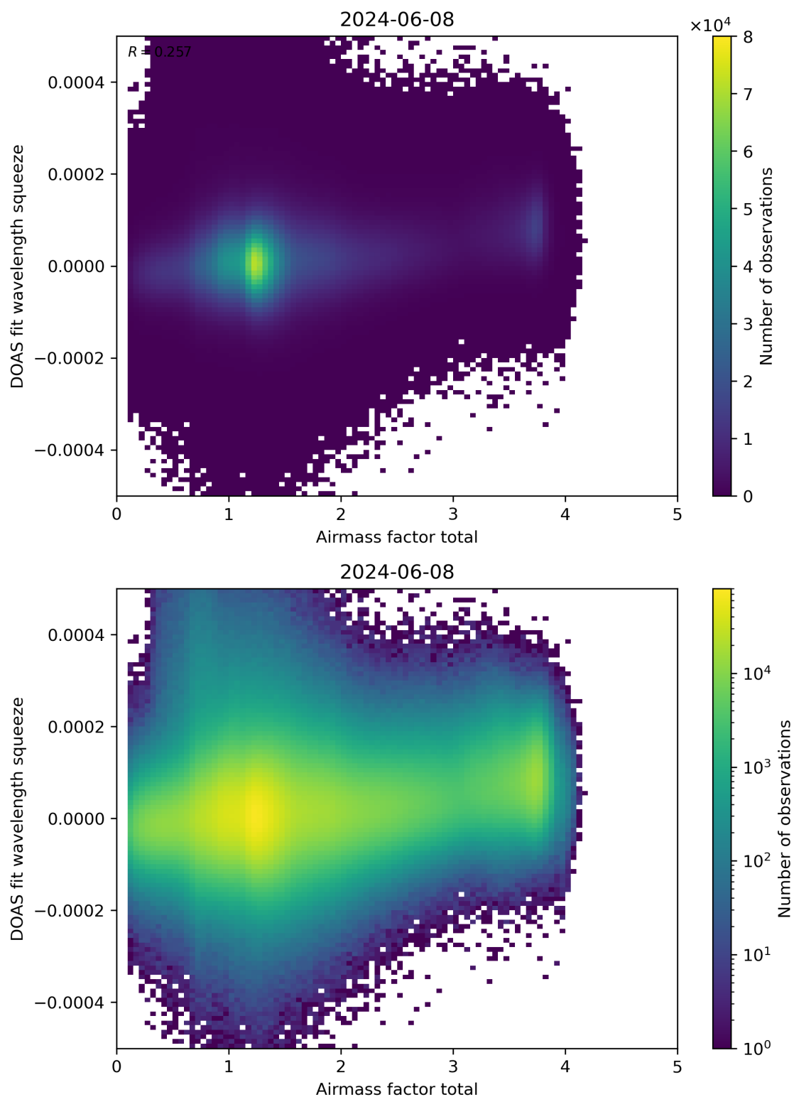
Figure 99: Scatter density plot of “Airmass factor total” against “DOAS fit wavelength squeeze” for 2024-06-08 to 2024-06-09.
