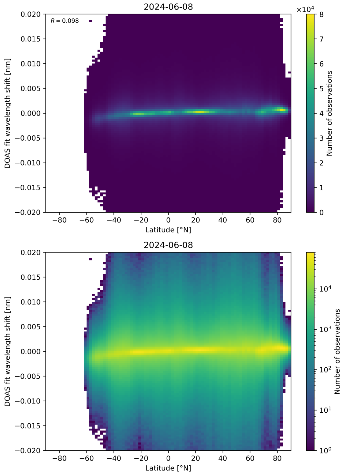
Figure 154: Scatter density plot of “Latitude” against “DOAS fit wavelength shift” for 2024-06-08 to 2024-06-09.
