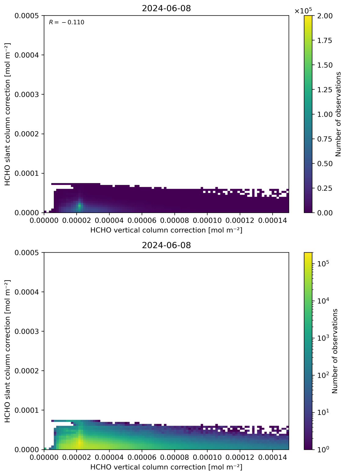
Figure 117: Scatter density plot of “HCHO vertical column correction” against “HCHO slant column correction” for 2024-06-08 to 2024-06-09.
