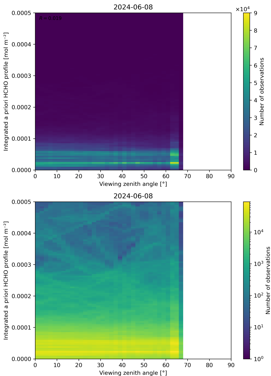
Figure 195: Scatter density plot of “Viewing zenith angle” against “Integrated a priori HCHO profile” for 2024-06-08 to 2024-06-09.
