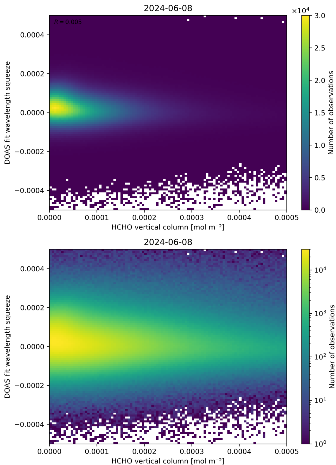
Figure 125: Scatter density plot of “HCHO vertical column” against “DOAS fit wavelength squeeze” for 2024-06-08 to 2024-06-09.
