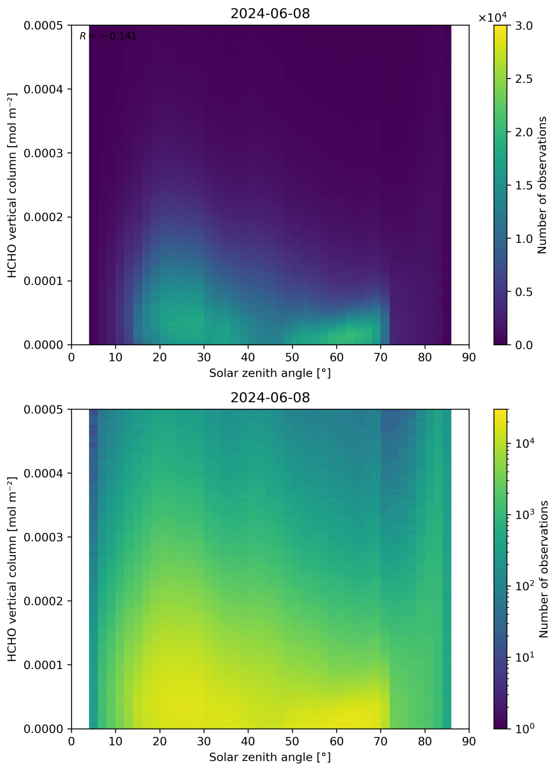
Figure 177: Scatter density plot of “Solar zenith angle” against “HCHO vertical column” for 2024-06-08 to 2024-06-09.
