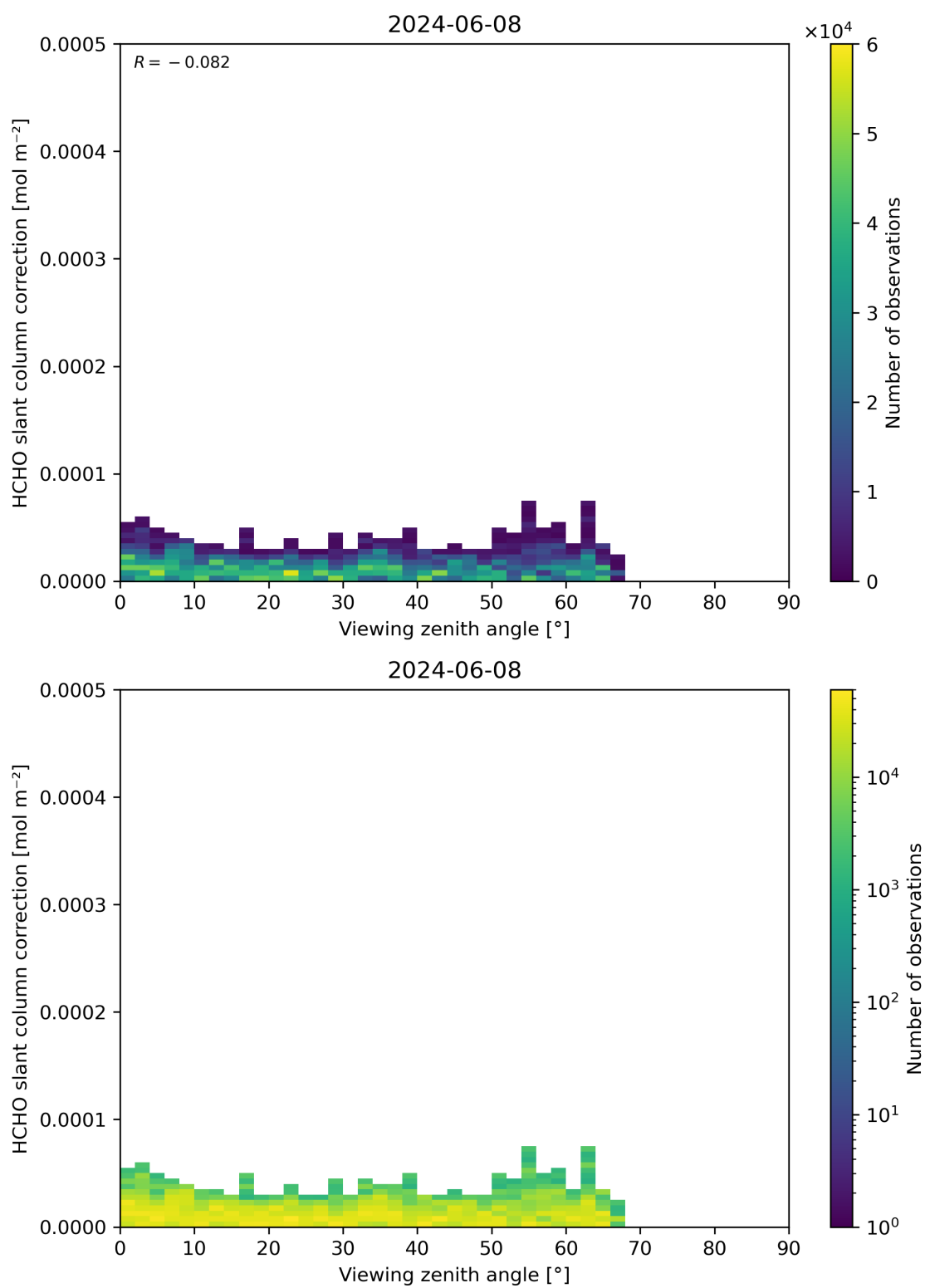
Figure 187: Scatter density plot of “Viewing zenith angle” against “HCHO slant column correction” for 2024-06-08 to 2024-06-09.
