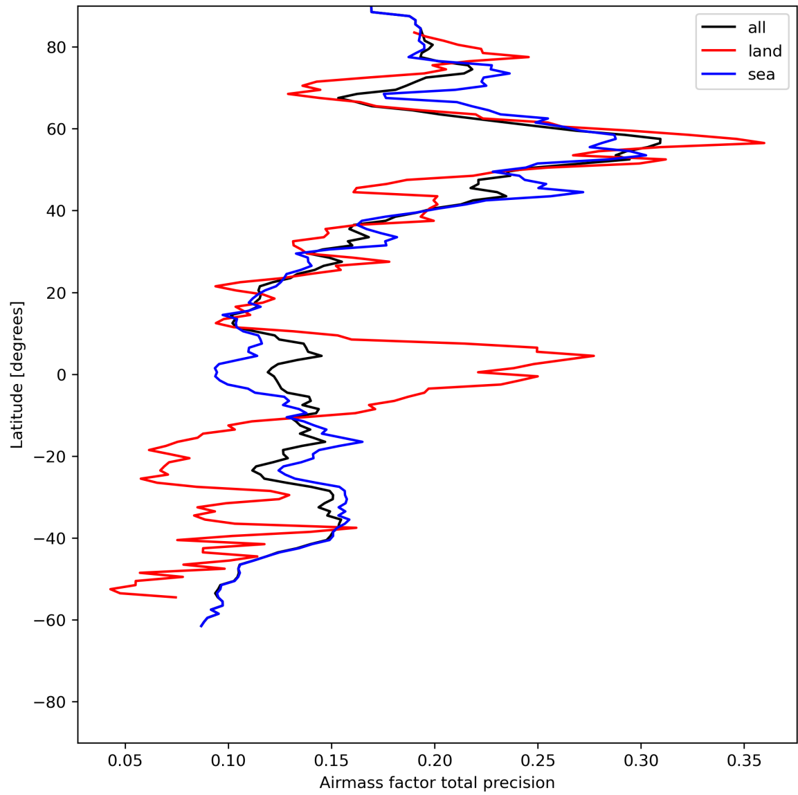
Figure 27: Zonal average of “Airmass factor total precision” for 2024-06-08 to 2024-06-09.
