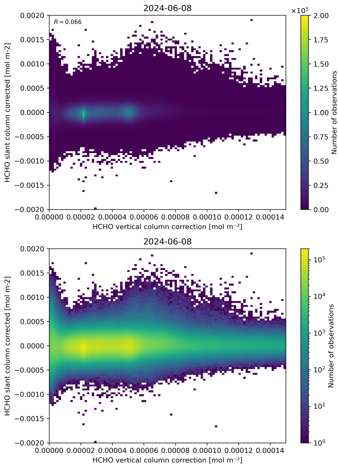
Figure 116: Scatter density plot of “HCHO vertical column correction” against “HCHO slant column corrected” for 2024-06-08 to 2024-06-09.
