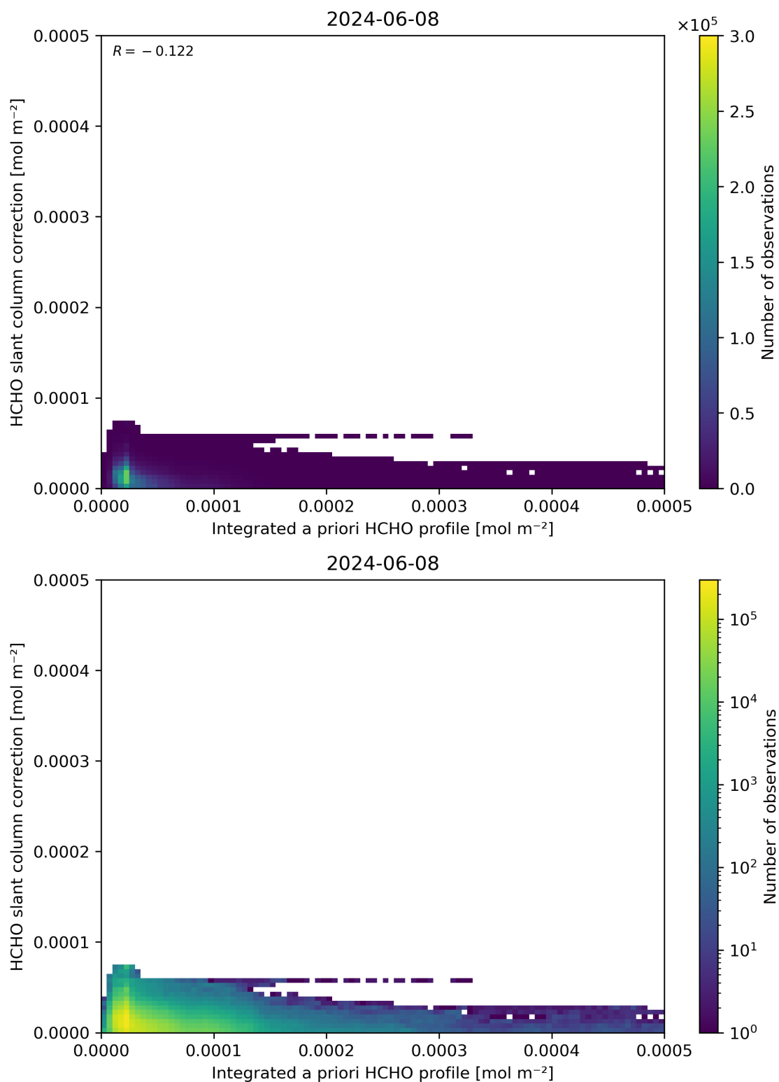
Figure 152: Scatter density plot of “Integrated a priori HCHO profile” against “HCHO slant column correction” for 2024-06-08 to 2024-06-09.
