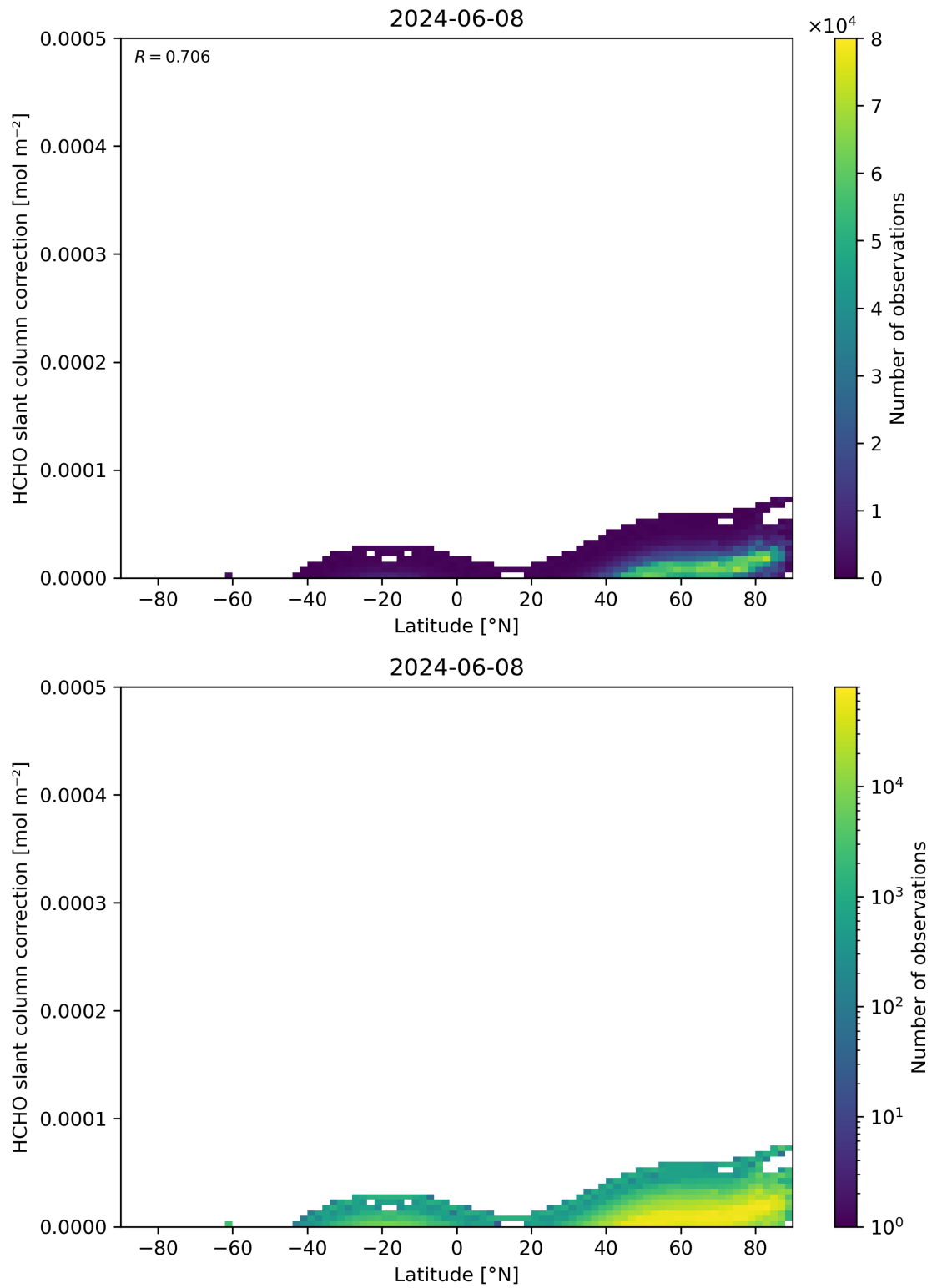
Figure 158: Scatter density plot of “Latitude” against “HCHO slant column correction” for 2024-06-08 to 2024-06-09.
