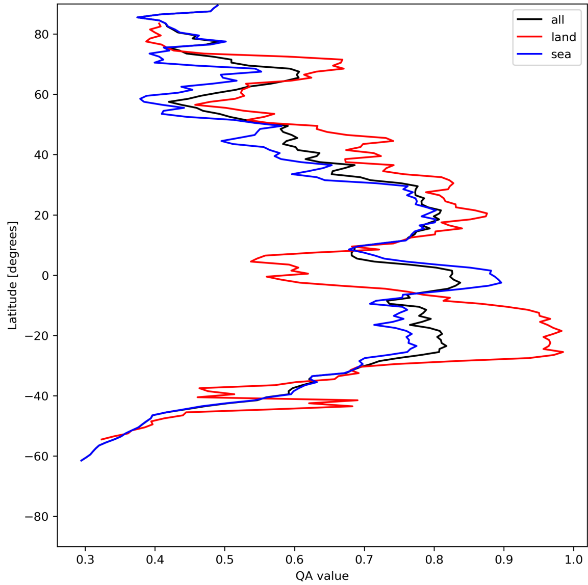
Figure 20: Zonal average of “QA value” for 2024-06-08 to 2024-06-09.
