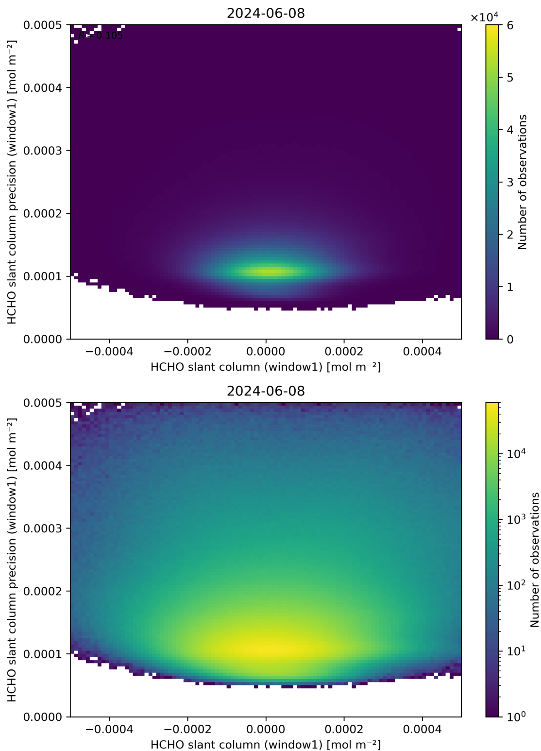
Figure 84: Scatter density plot of “HCHO slant column (window1)” against “HCHO slant column precision (window1)” for 2024-06-08 to 2024-06-09.
