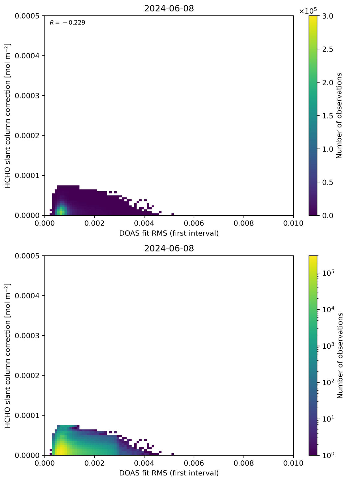
Figure 63: Scatter density plot of “DOAS fit RMS (first interval)” against “HCHO slant column correction” for 2024-06-08 to 2024-06-09.
