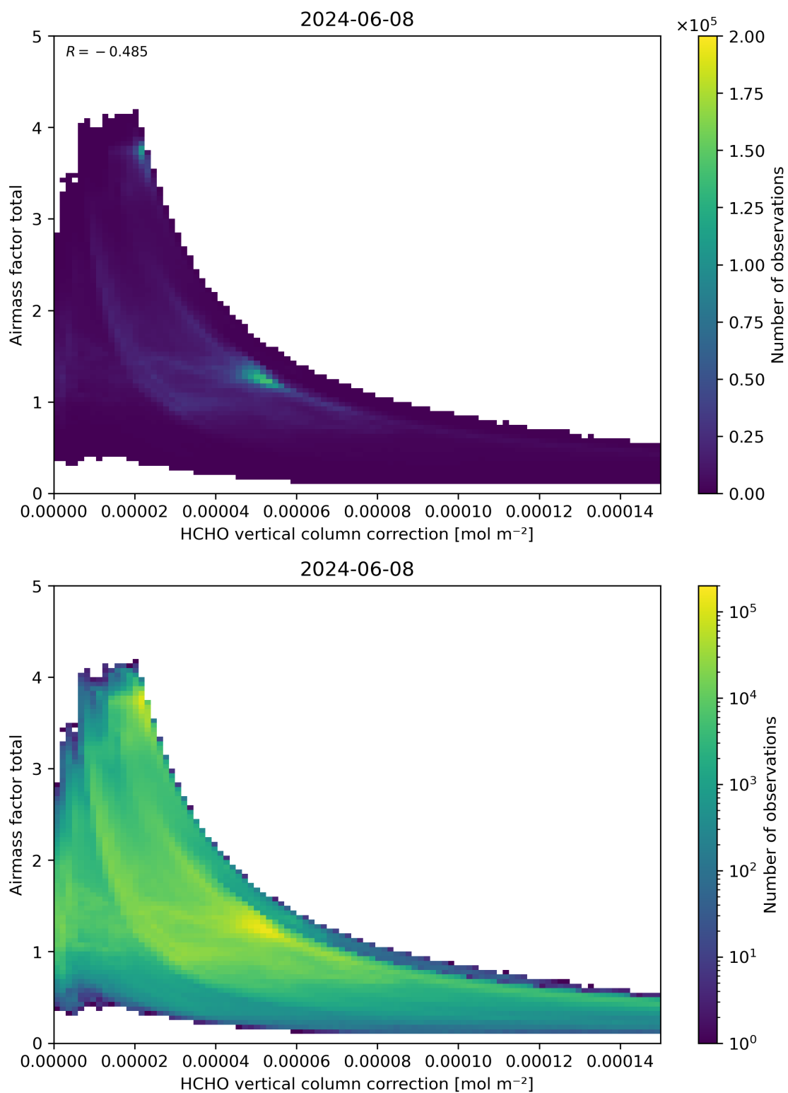
Figure 120: Scatter density plot of “HCHO vertical column correction” against “Airmass factor total” for 2024-06-08 to 2024-06-09.
