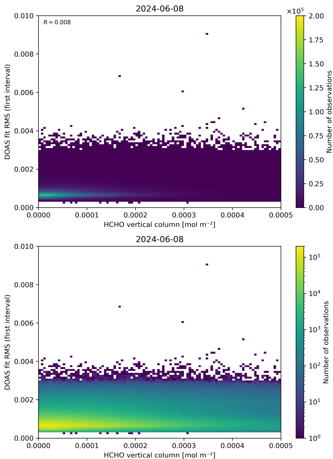
Figure 123: Scatter density plot of “HCHO vertical column” against “DOAS fit RMS (first interval)” for 2024-06-08 to 2024-06-09.
