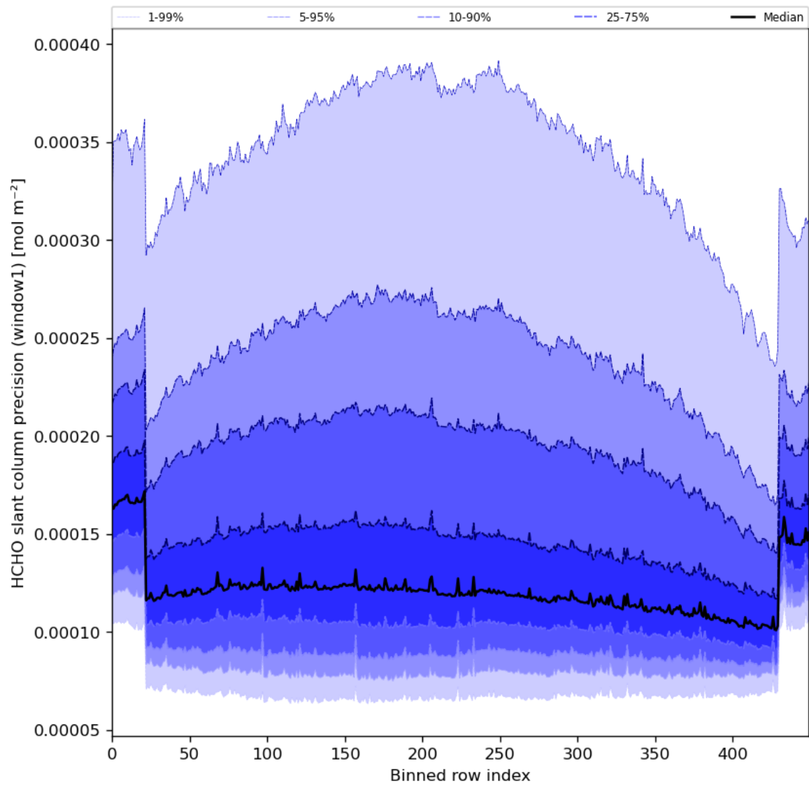
Figure 53: Along track statistics of “HCHO slant column precision (window1)” for 2024-06-08 to 2024-06-09
