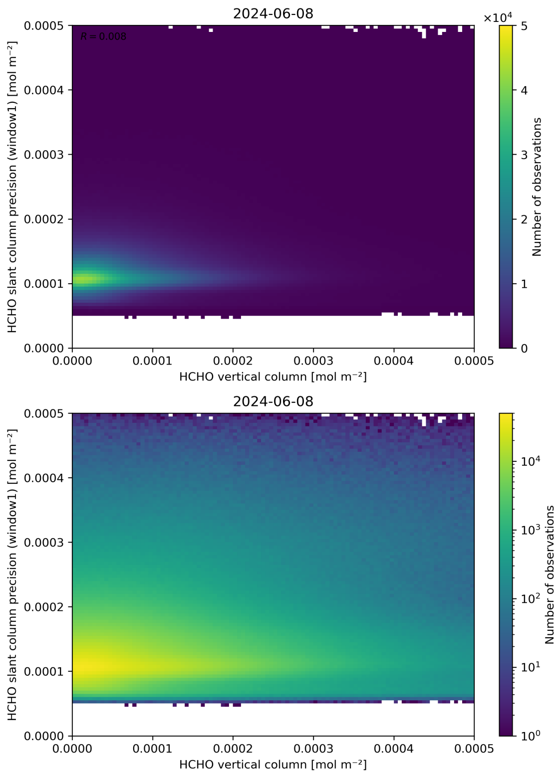
Figure 130: Scatter density plot of “HCHO vertical column” against “HCHO slant column precision (window1)” for 2024-06-08 to 2024-06-09.
