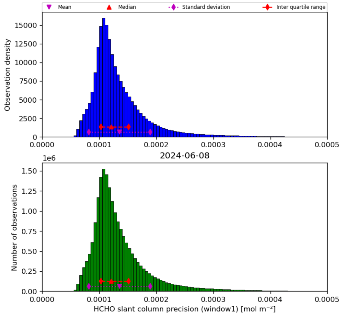
Figure 39: Histogram of “HCHO slant column precision (window1)” for 2024-06-08 to 2024-06-09
