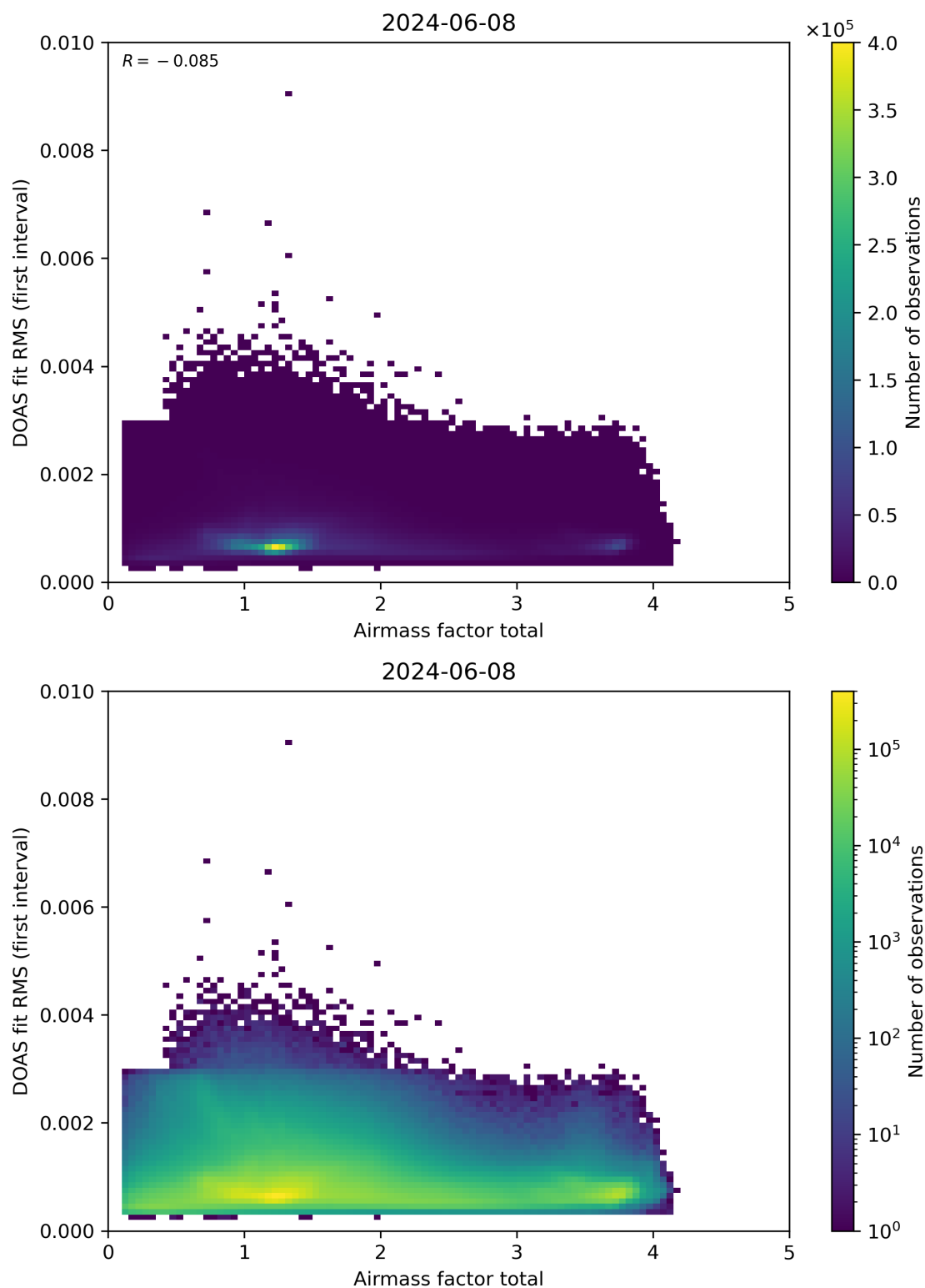
Figure 97: Scatter density plot of “Airmass factor total” against “DOAS fit RMS (first interval)” for 2024-06-08 to 2024-06-09.
