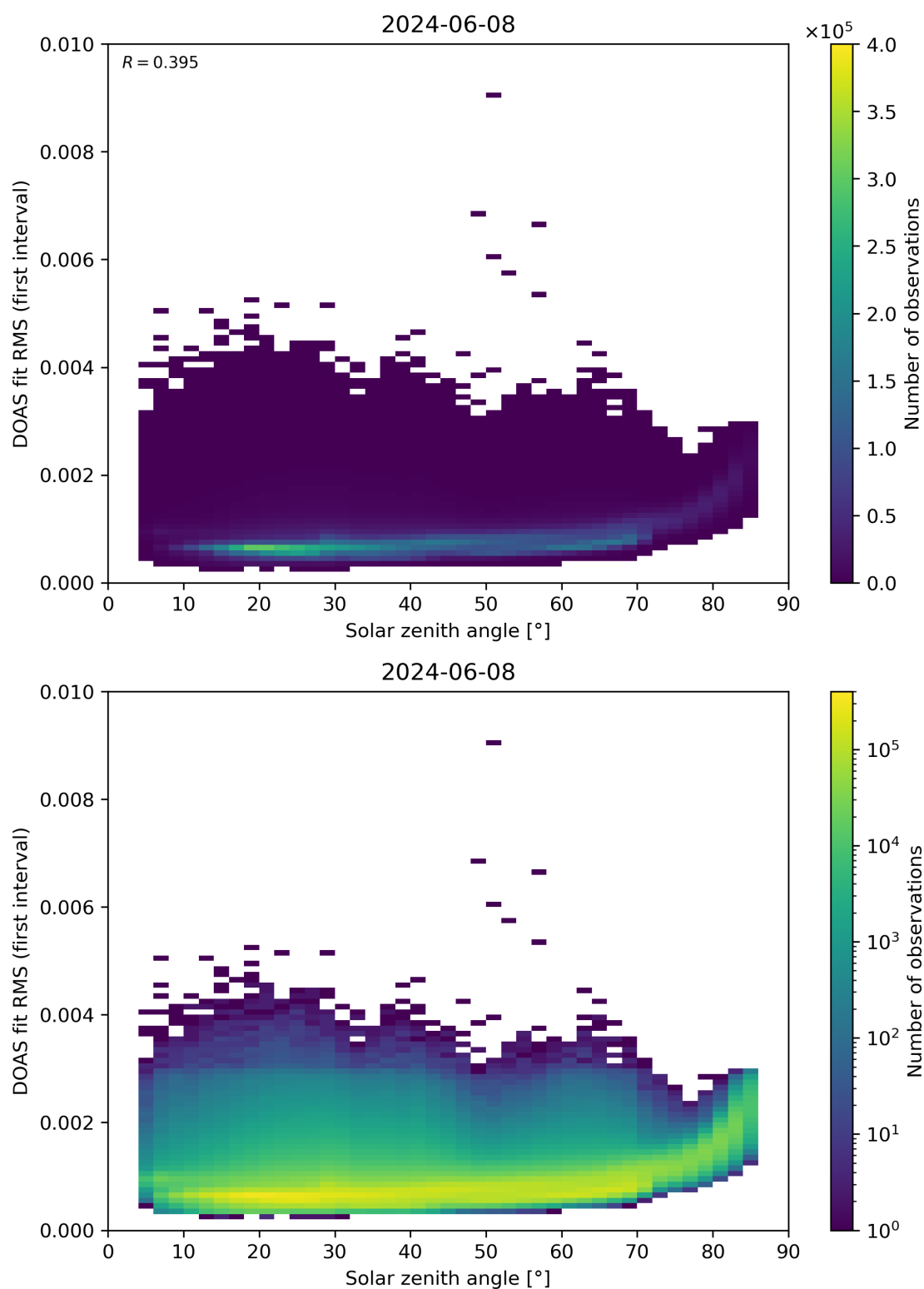
Figure 167: Scatter density plot of “Solar zenith angle” against “DOAS fit RMS (first interval)” for 2024-06-08 to 2024-06-09.
