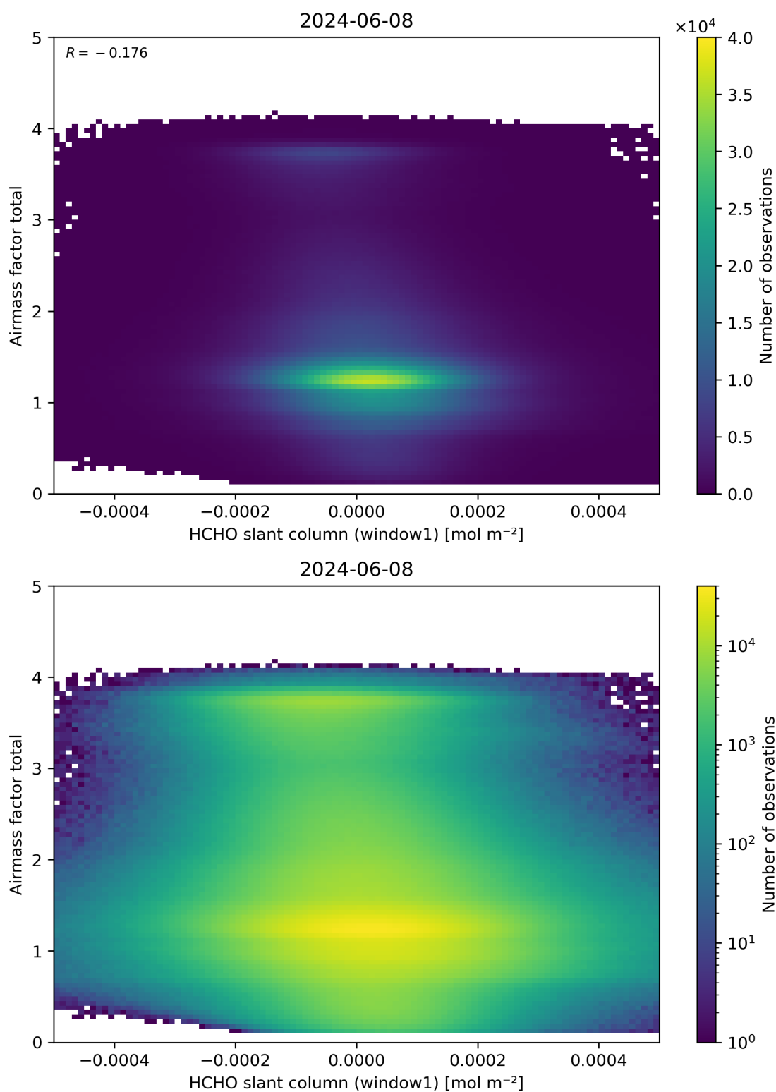
Figure 85: Scatter density plot of “HCHO slant column (window1)” against “Airmass factor total” for 2024-06-08 to 2024-06-09.
