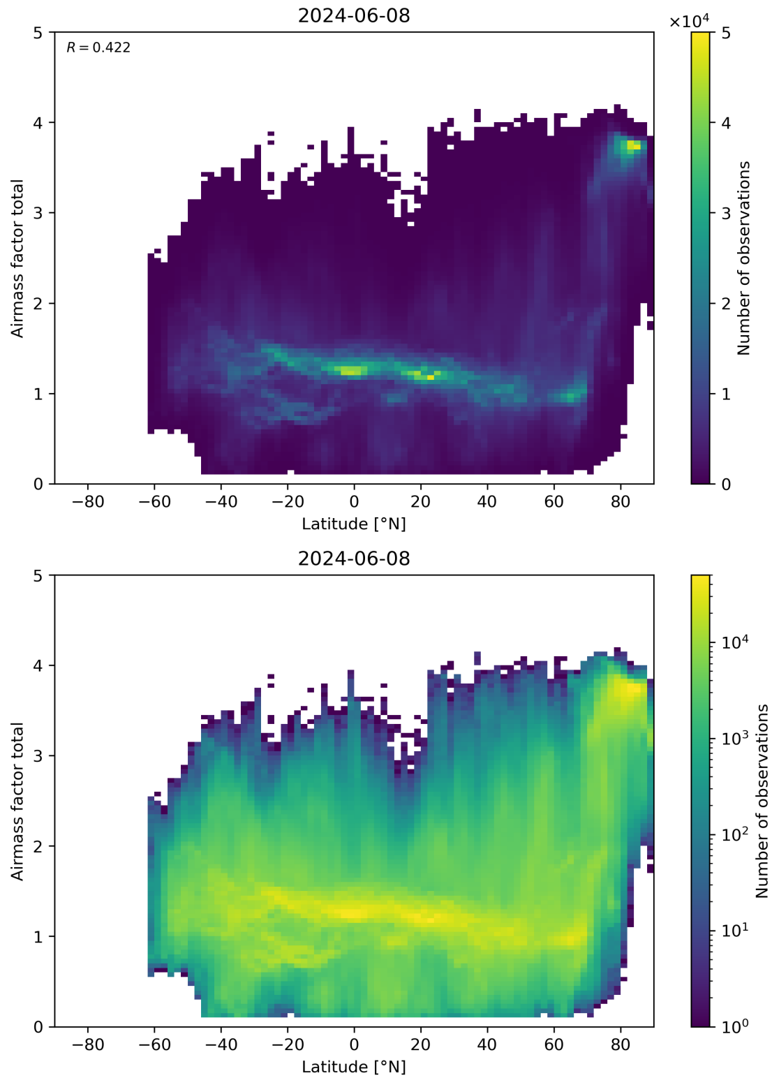
Figure 161: Scatter density plot of “Latitude” against “Airmass factor total” for 2024-06-08 to 2024-06-09.
