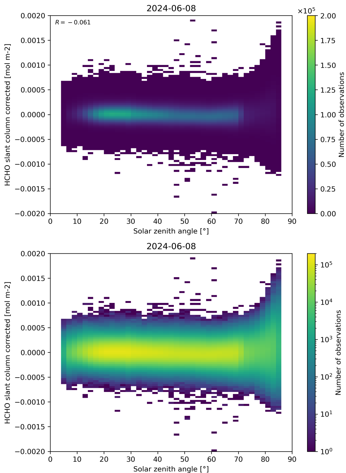
Figure 171: Scatter density plot of “Solar zenith angle” against “HCHO slant column corrected” for 2024-06-08 to 2024-06-09.
