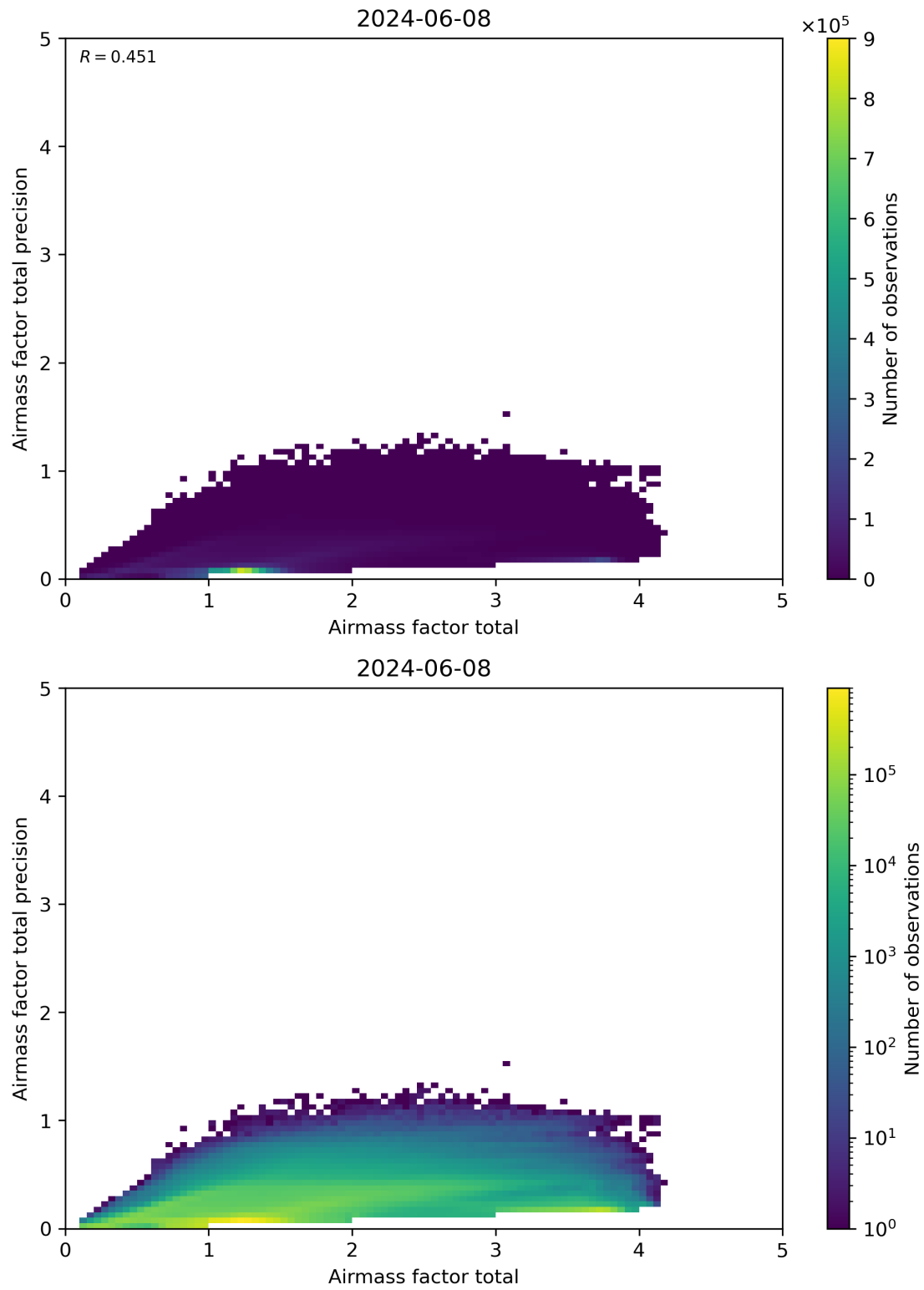
Figure 103: Scatter density plot of “Airmass factor total” against “Airmass factor total precision” for 2024-06-08 to 2024-06-09.
