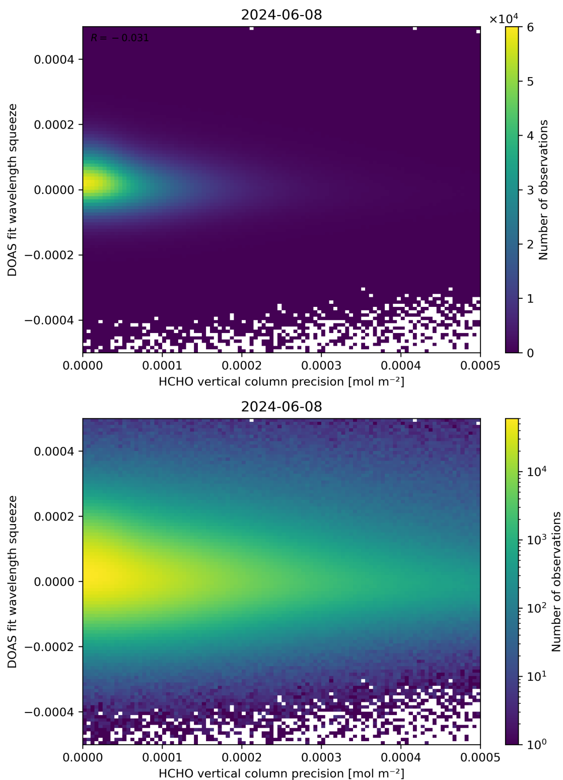
Figure 138: Scatter density plot of “HCHO vertical column precision” against “DOAS fit wavelength squeeze” for 2024-06-08 to 2024-06-09.
