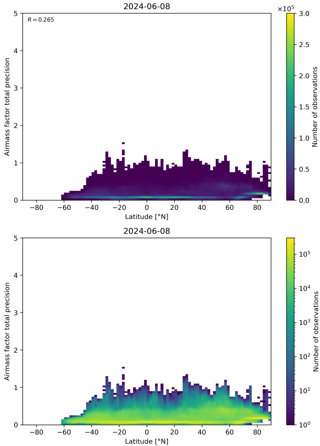
Figure 162: Scatter density plot of “Latitude” against “Airmass factor total precision” for 2024-06-08 to 2024-06-09.
