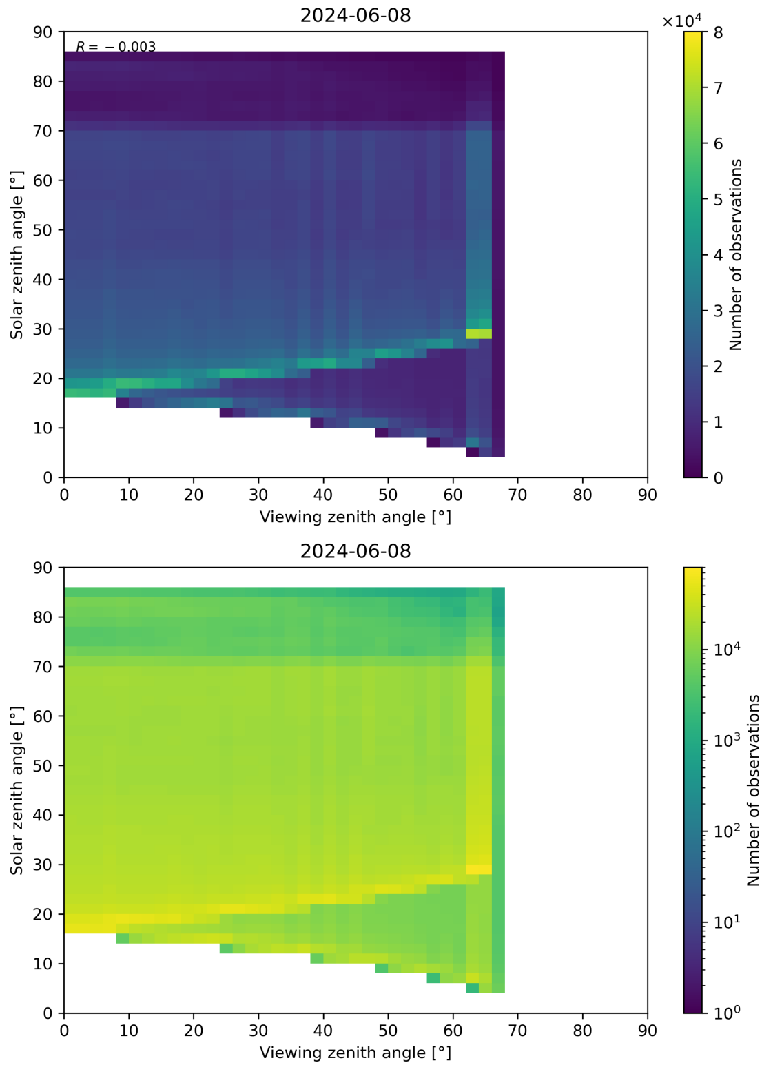
Figure 197: Scatter density plot of “Viewing zenith angle” against “Solar zenith angle” for 2024-06-08 to 2024-06-09.
