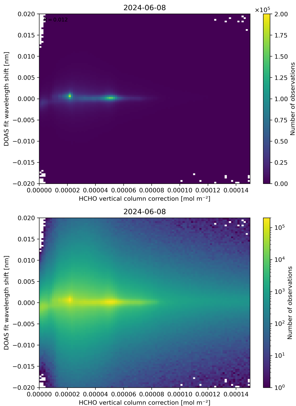
Figure 113: Scatter density plot of “HCHO vertical column correction” against “DOAS fit wavelength shift” for 2024-06-08 to 2024-06-09.
