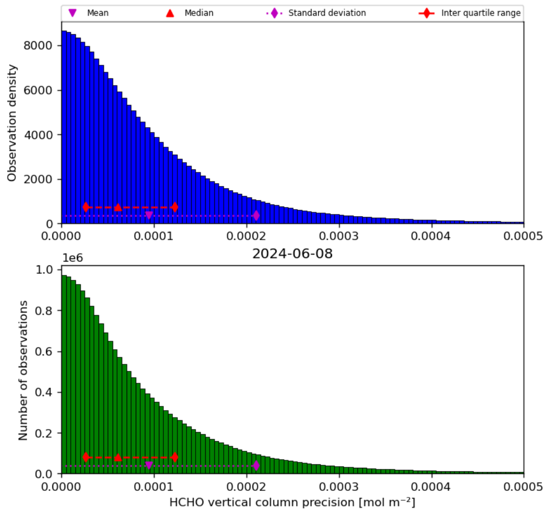
Figure 36: Histogram of “HCHO vertical column precision” for 2024-06-08 to 2024-06-09
