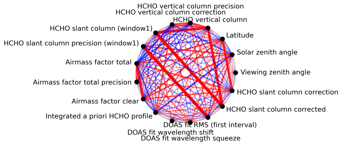
Figure 1: Map of correlation graph for 2024-06-08 to 2024-06-09.
