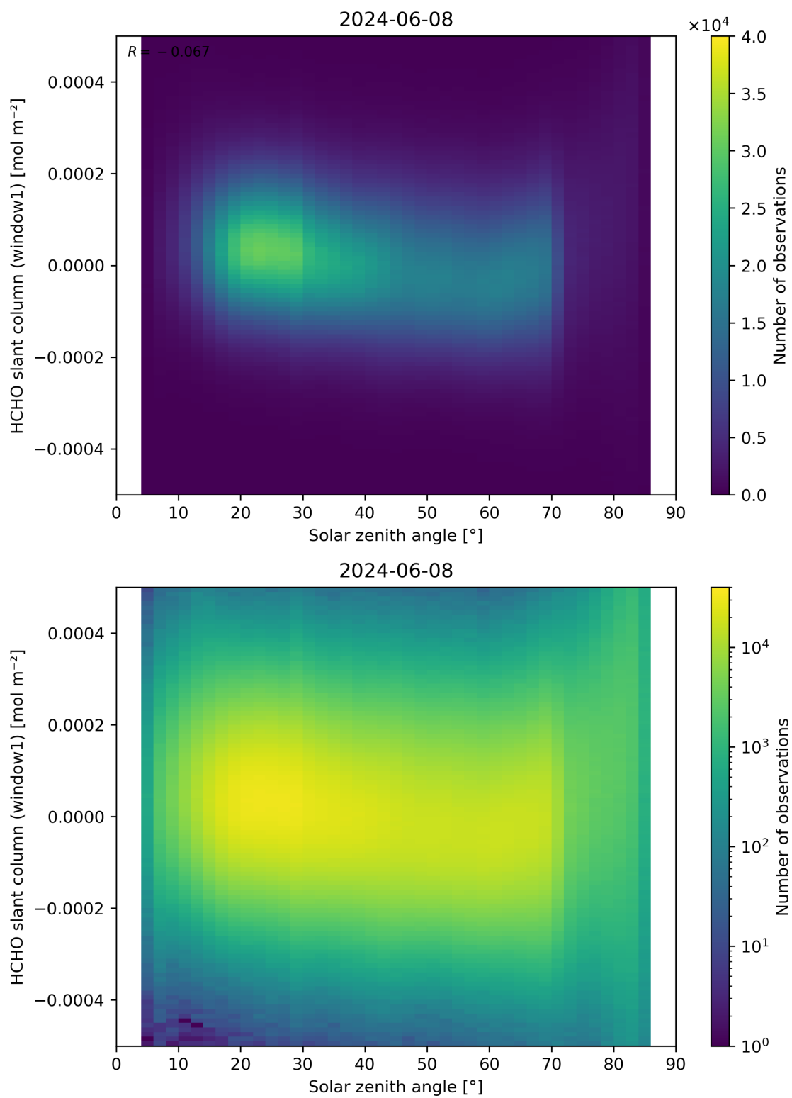
Figure 173: Scatter density plot of “Solar zenith angle” against “HCHO slant column (window1)” for 2024-06-08 to 2024-06-09.
