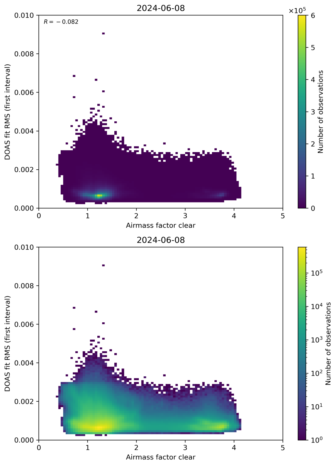
Figure 71: Scatter density plot of “Airmass factor clear” against “DOAS fit RMS (first interval)” for 2024-06-08 to 2024-06-09.
