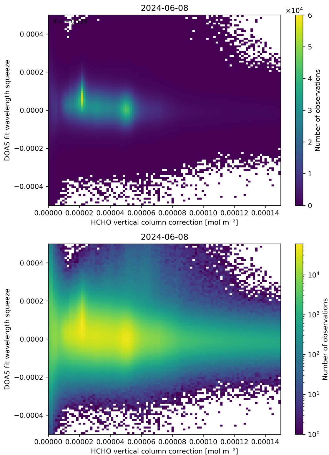
Figure 114: Scatter density plot of “HCHO vertical column correction” against “DOAS fit wavelength squeeze” for 2024-06-08 to 2024-06-09.
