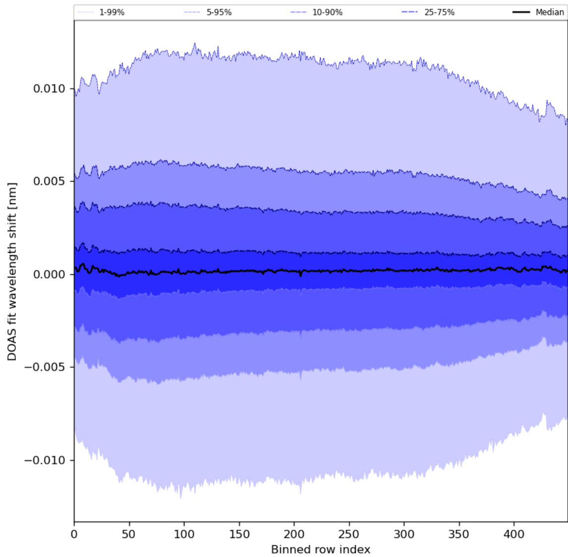
Figure 58: Along track statistics of “DOAS fit wavelength shift” for 2024-06-08 to 2024-06-09
