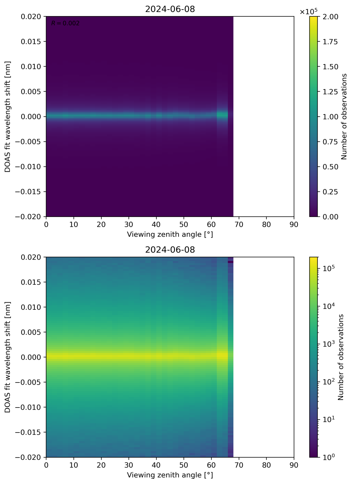
Figure 183: Scatter density plot of “Viewing zenith angle” against “DOAS fit wavelength shift” for 2024-06-08 to 2024-06-09.
