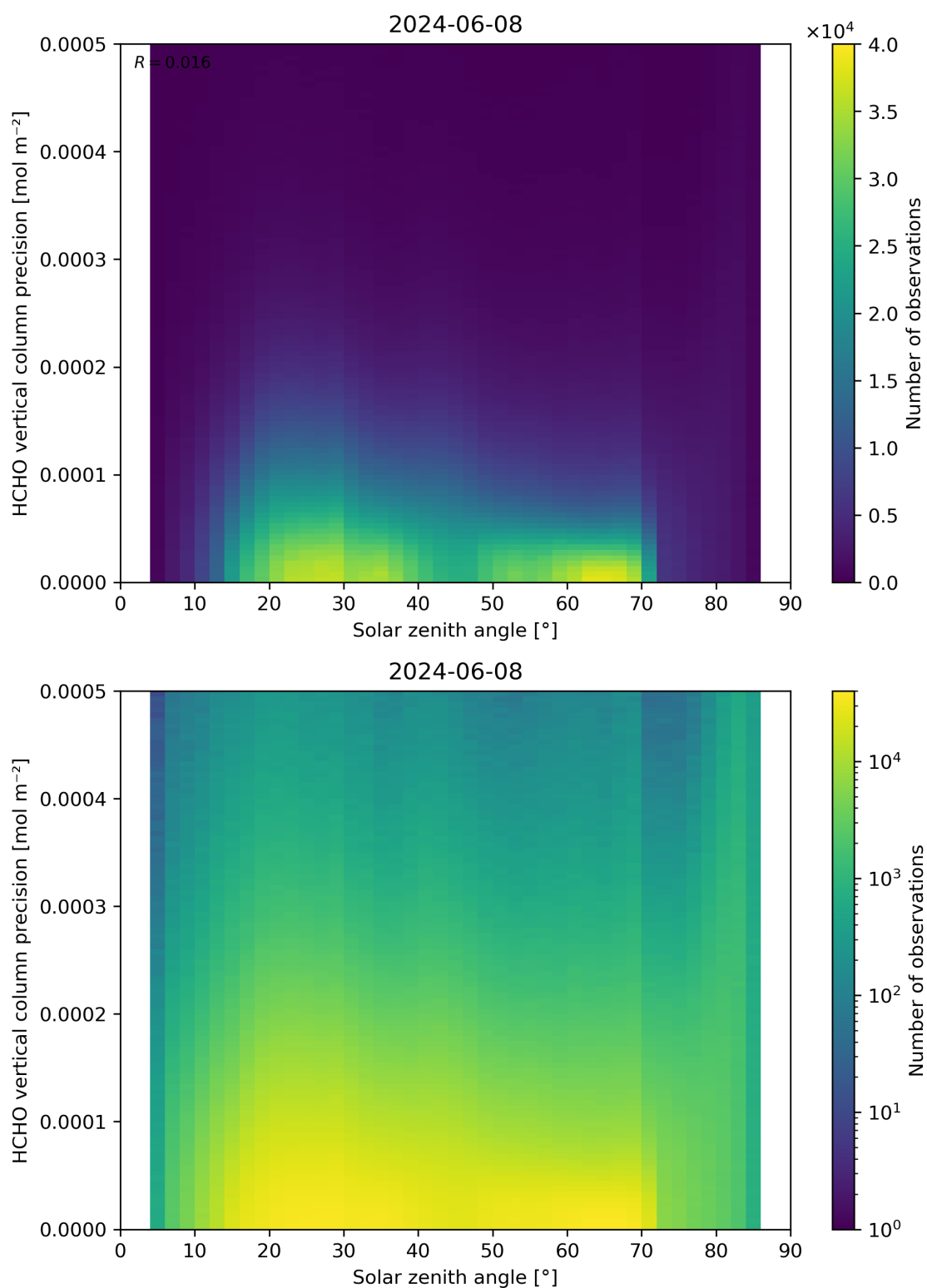
Figure 179: Scatter density plot of “Solar zenith angle” against “HCHO vertical column precision” for 2024-06-08 to 2024-06-09.
