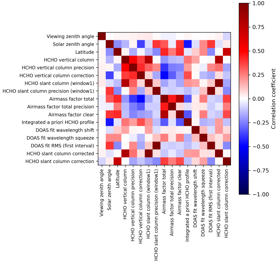
Figure 2: Map of correlation matrix for 2024-06-08 to 2024-06-09.
