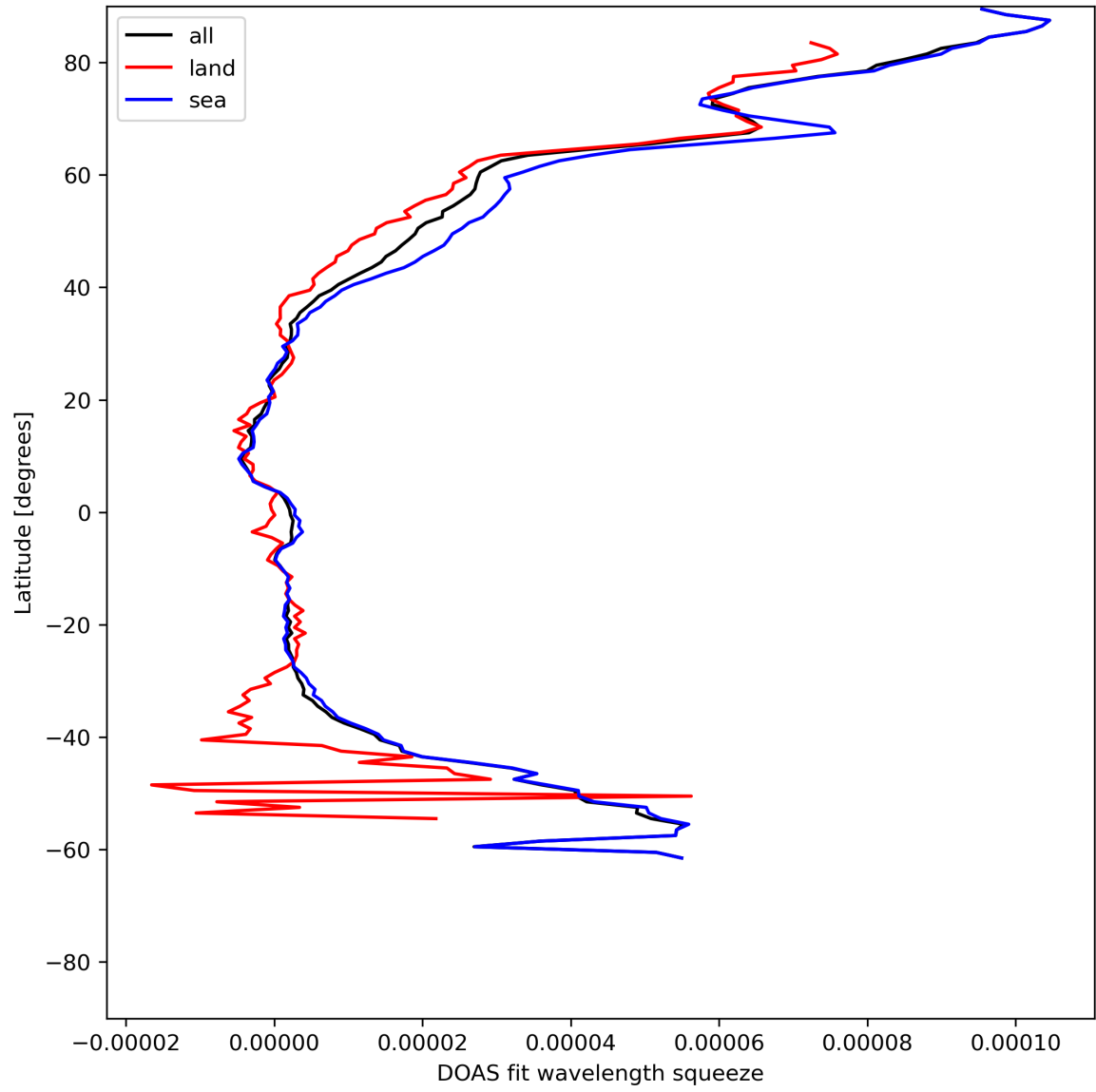
Figure 31: Zonal average of “DOAS fit wavelength squeeze” for 2024-06-08 to 2024-06-09.
