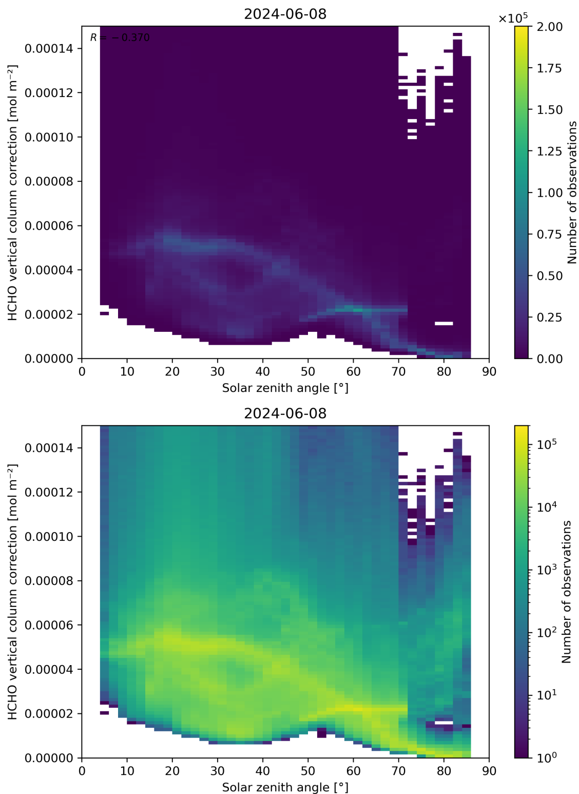
Figure 178: Scatter density plot of “Solar zenith angle” against “HCHO vertical column correction” for 2024-06-08 to 2024-06-09.
