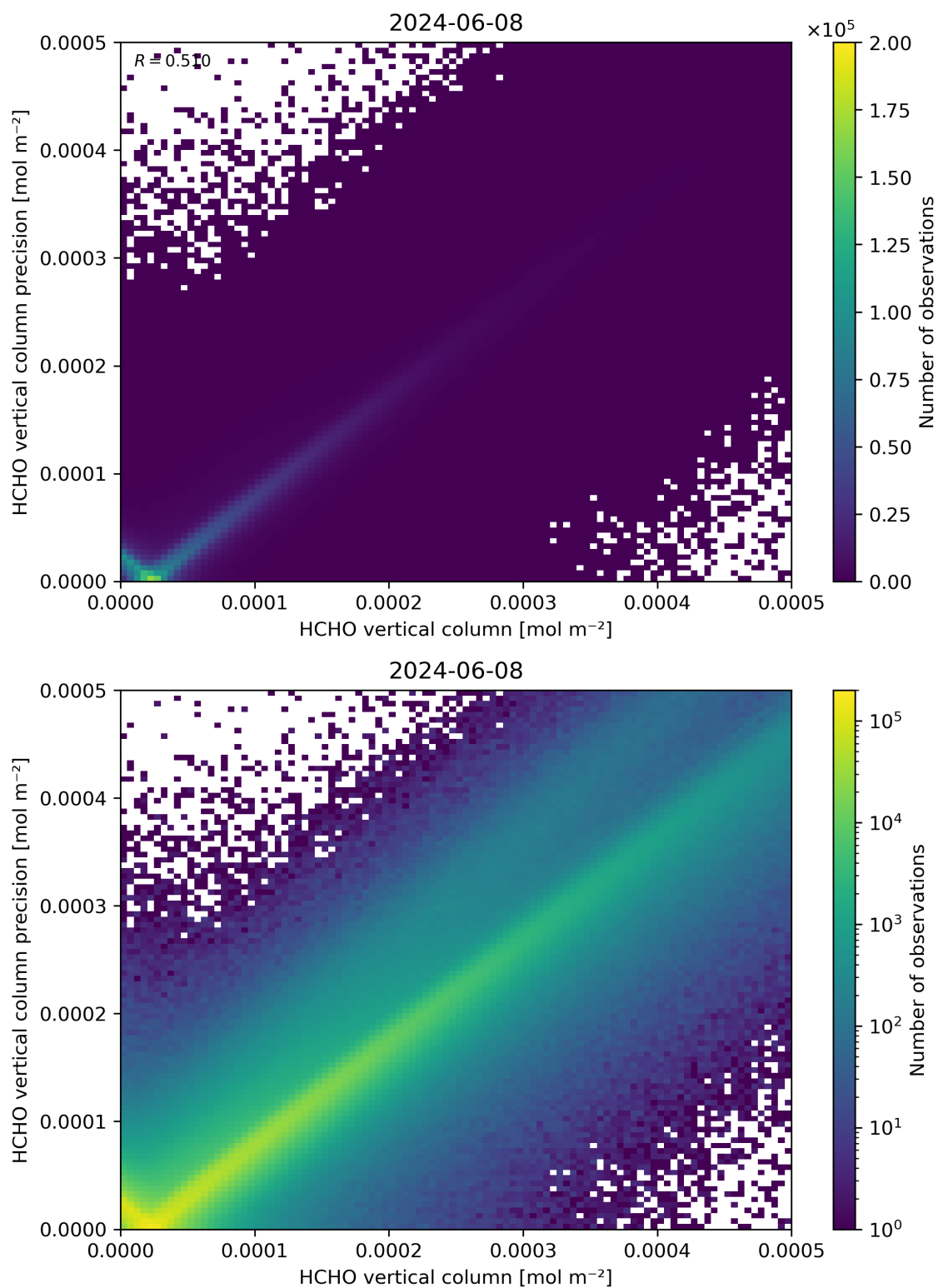
Figure 134: Scatter density plot of “HCHO vertical column” against “HCHO vertical column precision” for 2024-06-08 to 2024-06-09.
