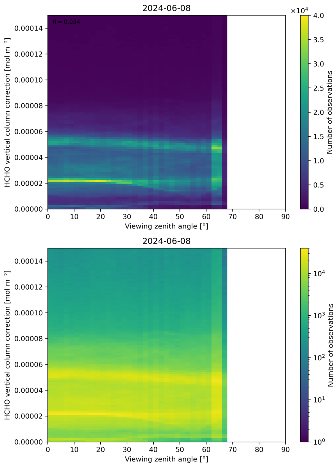
Figure 193: Scatter density plot of “Viewing zenith angle” against “HCHO vertical column correction” for 2024-06-08 to 2024-06-09.
