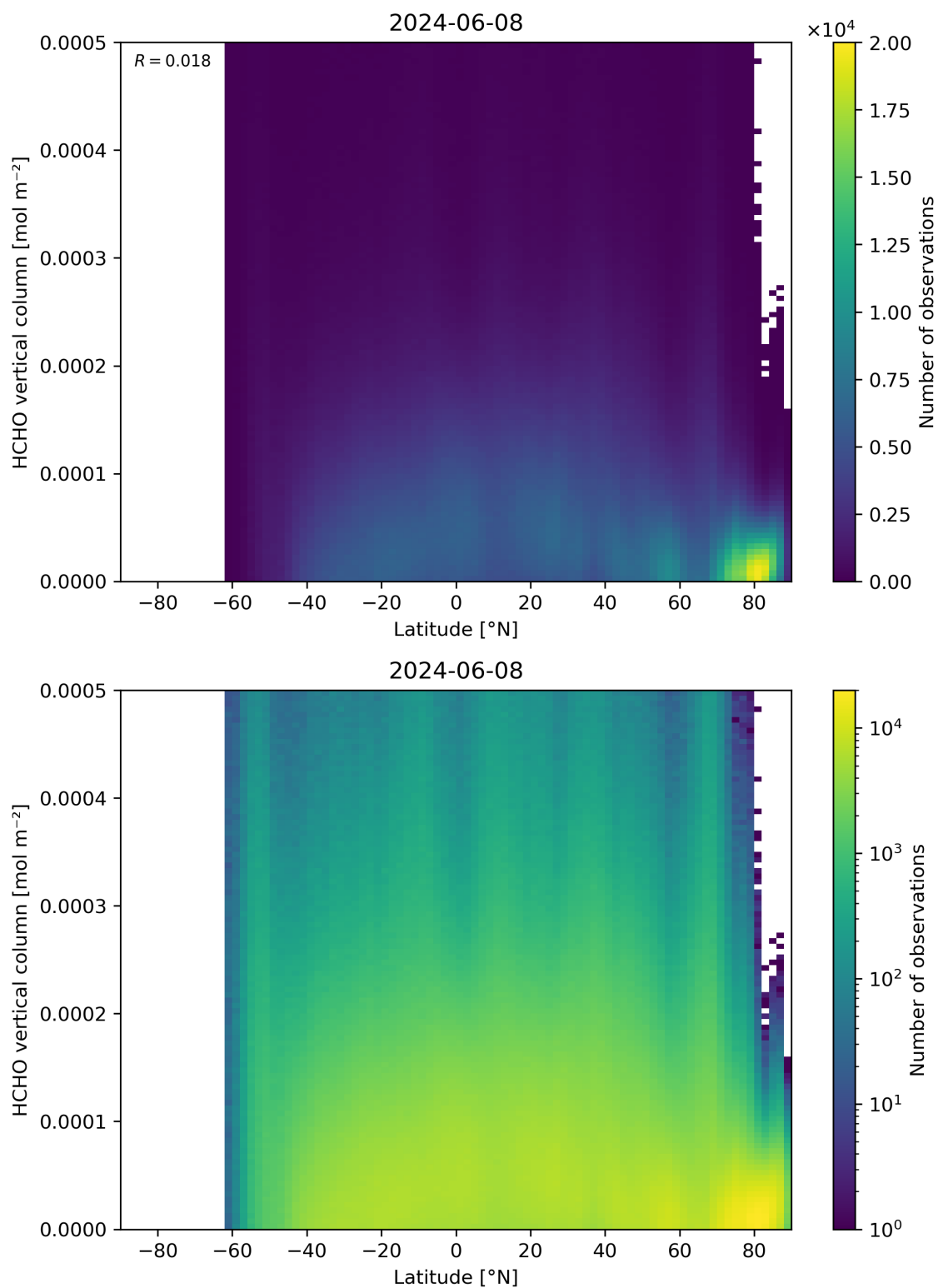
Figure 163: Scatter density plot of “Latitude” against “HCHO vertical column” for 2024-06-08 to 2024-06-09.
