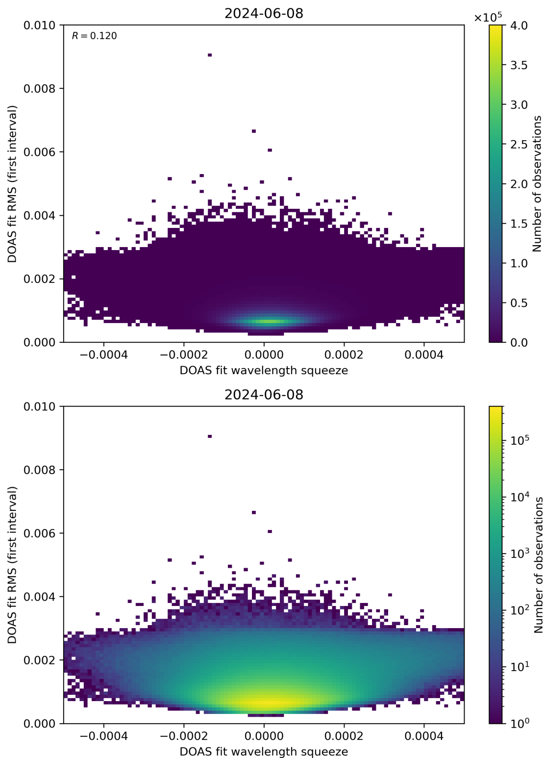
Figure 68: Scatter density plot of “DOAS fit wavelength squeeze” against “DOAS fit RMS (first interval)” for 2024-06-08 to 2024-06-09.
