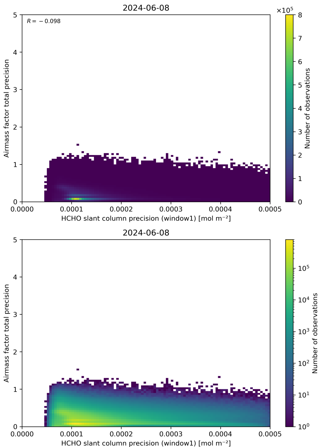
Figure 95: Scatter density plot of “HCHO slant column precision (window1)” against “Airmass factor total precision” for 2024-06-08 to 2024-06-09.
