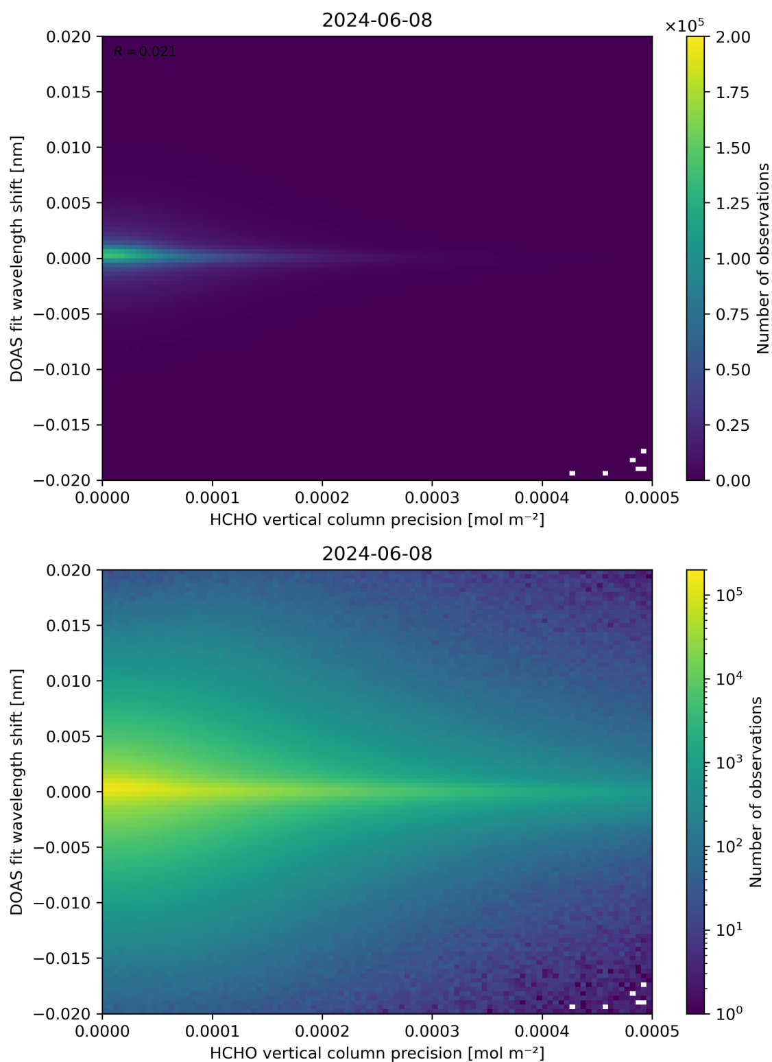
Figure 137: Scatter density plot of “HCHO vertical column precision” against “DOAS fit wavelength shift” for 2024-06-08 to 2024-06-09.
