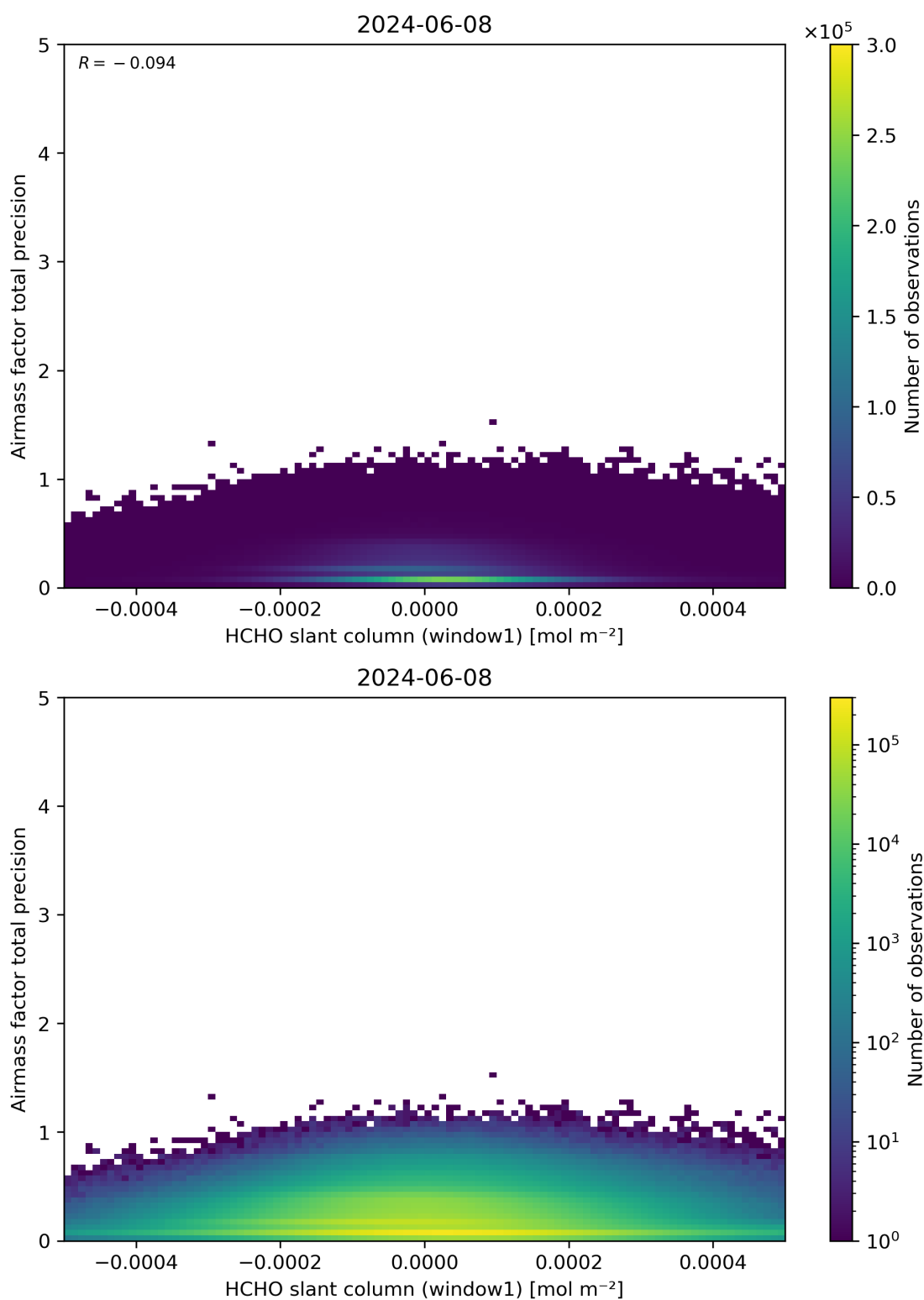
Figure 86: Scatter density plot of “HCHO slant column (window1)” against “Airmass factor total precision” for 2024-06-08 to 2024-06-09.
