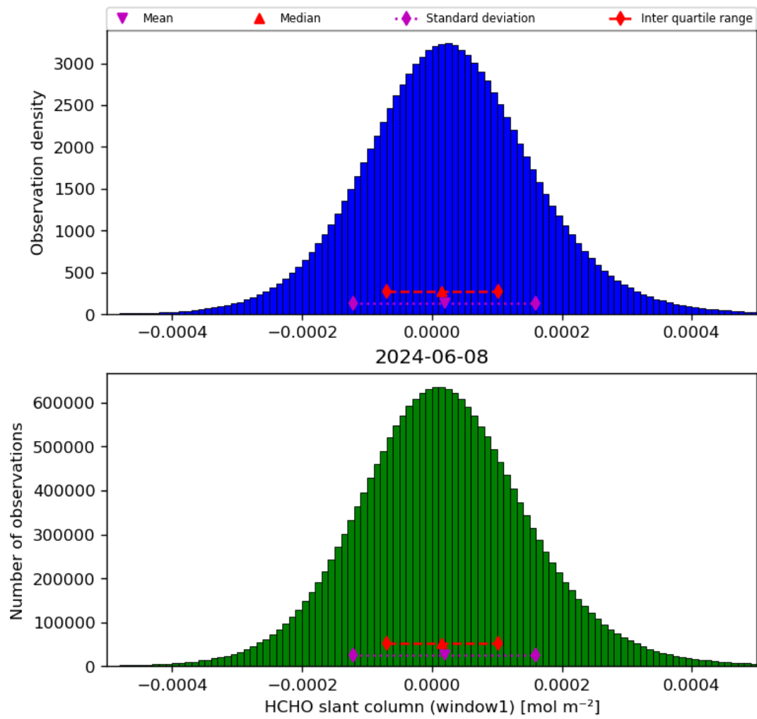
Figure 38: Histogram of “HCHO slant column (window1)” for 2024-06-08 to 2024-06-09
