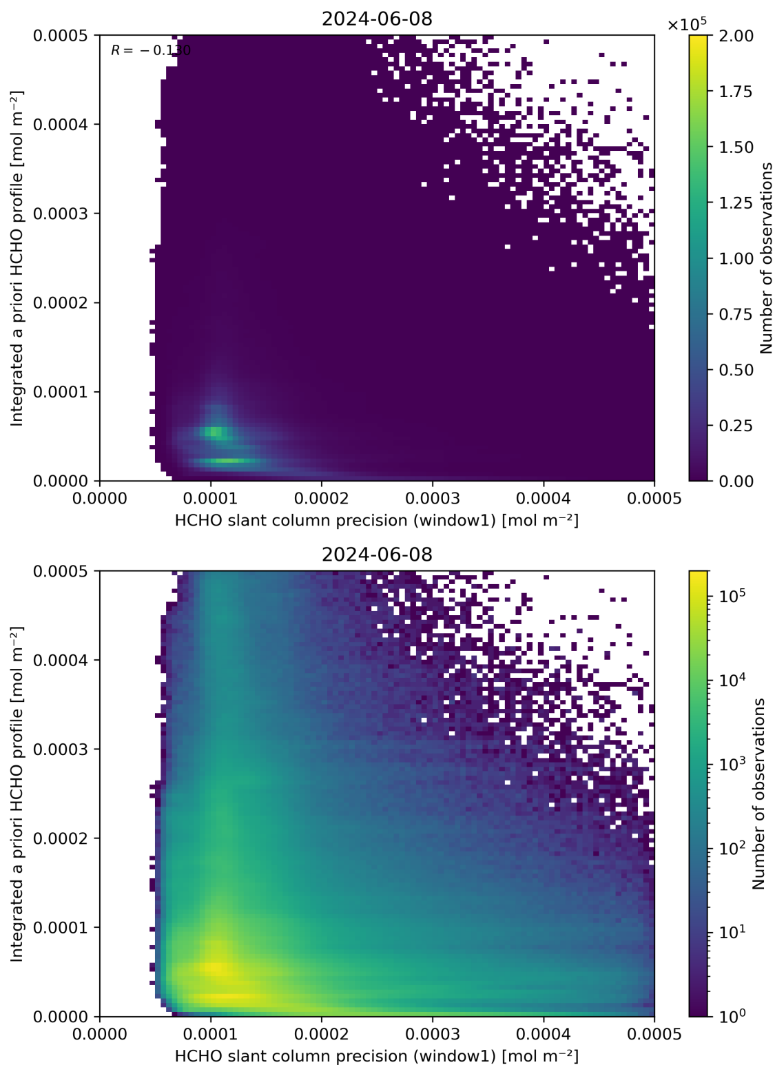
Figure 96: Scatter density plot of “HCHO slant column precision (window1)” against “Integrated a priori HCHO profile” for 2024-06-08 to 2024-06-09.
