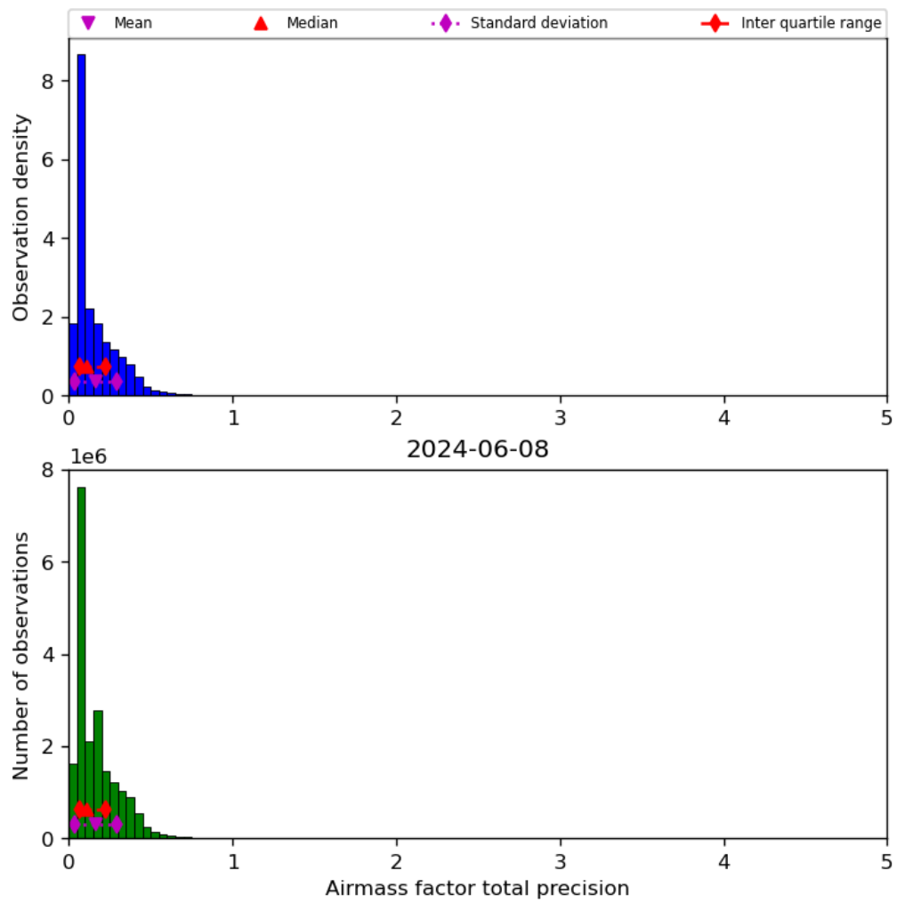
Figure 41: Histogram of “Airmass factor total precision” for 2024-06-08 to 2024-06-09
