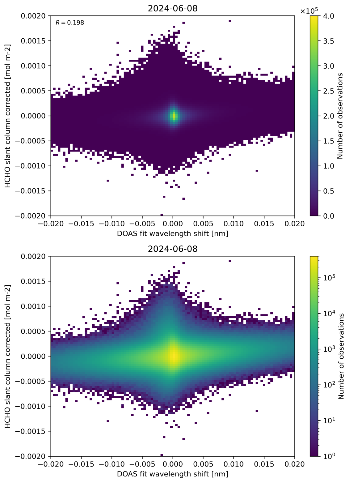
Figure 66: Scatter density plot of “DOAS fit wavelength shift” against “HCHO slant column corrected” for 2024-06-08 to 2024-06-09.
