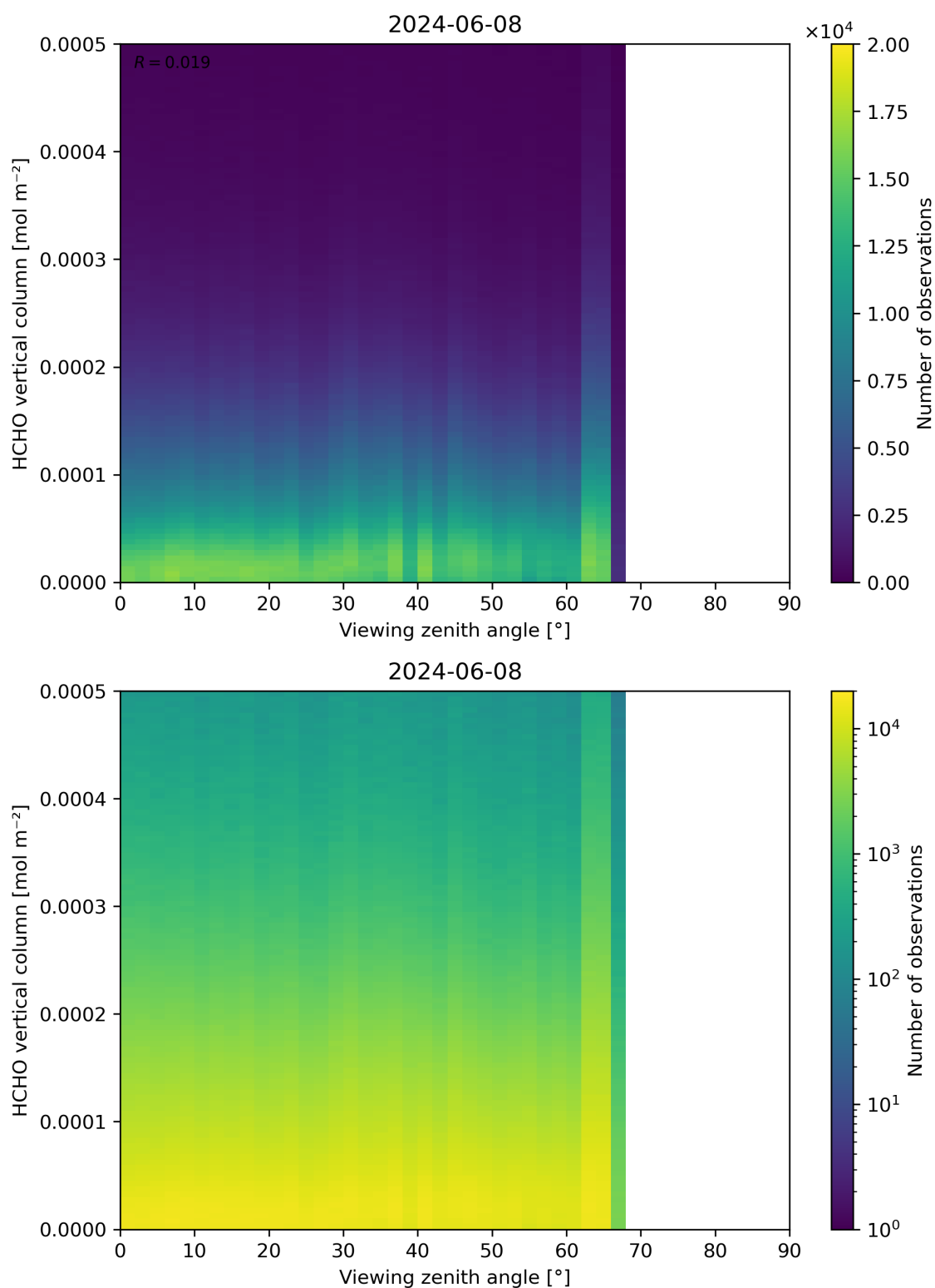
Figure 192: Scatter density plot of “Viewing zenith angle” against “HCHO vertical column” for 2024-06-08 to 2024-06-09.
