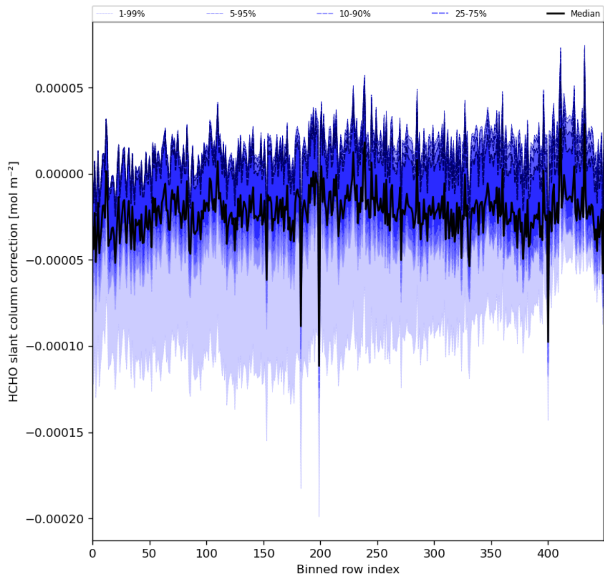
Figure 61: Along track statistics of “HCHO slant column correction” for 2024-06-08 to 2024-06-09
