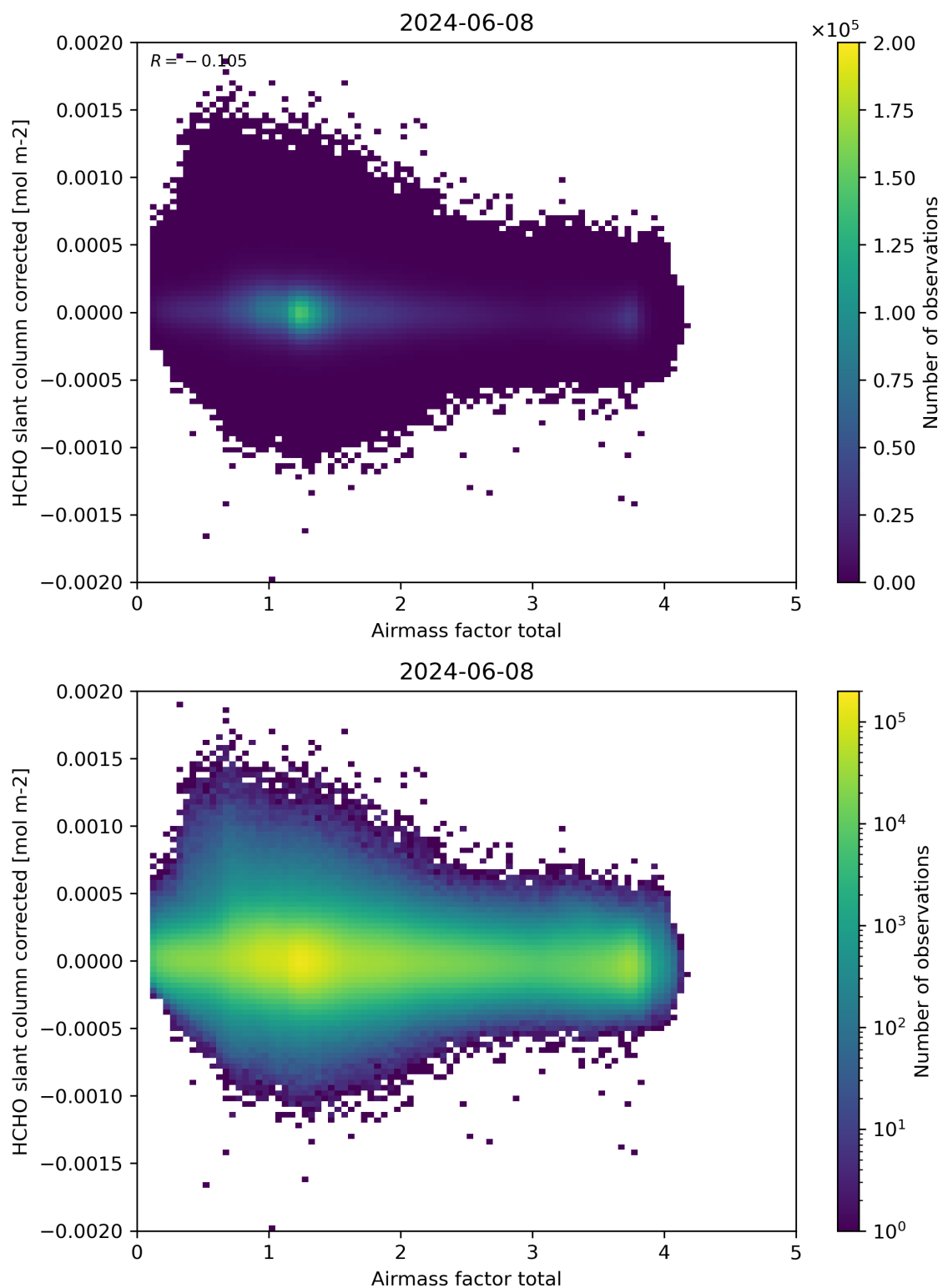
Figure 101: Scatter density plot of “Airmass factor total” against “HCHO slant column corrected” for 2024-06-08 to 2024-06-09.
