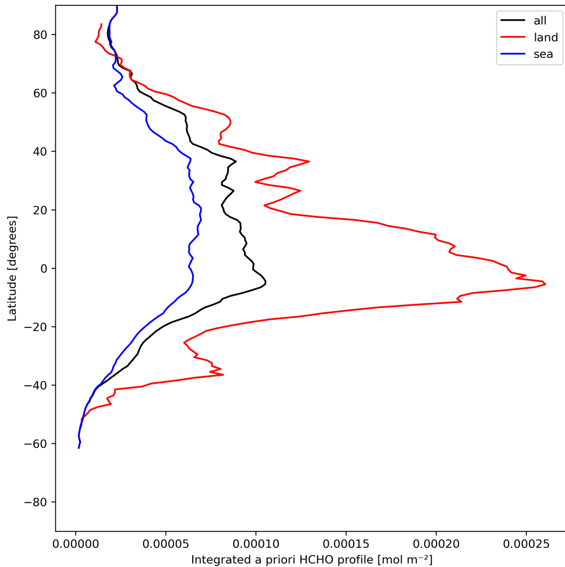
Figure 29: Zonal average of “Integrated a priori HCHO profile” for 2024-06-08 to 2024-06-09.
