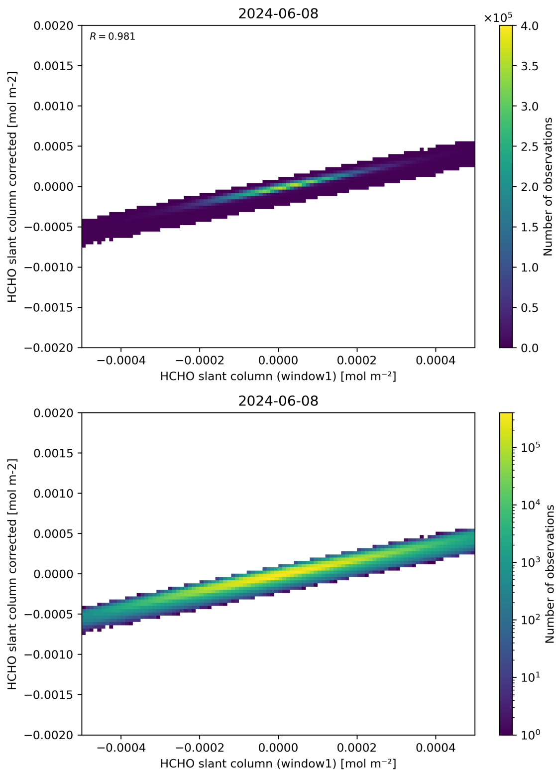
Figure 82: Scatter density plot of “HCHO slant column (window1)” against “HCHO slant column corrected” for 2024-06-08 to 2024-06-09.
