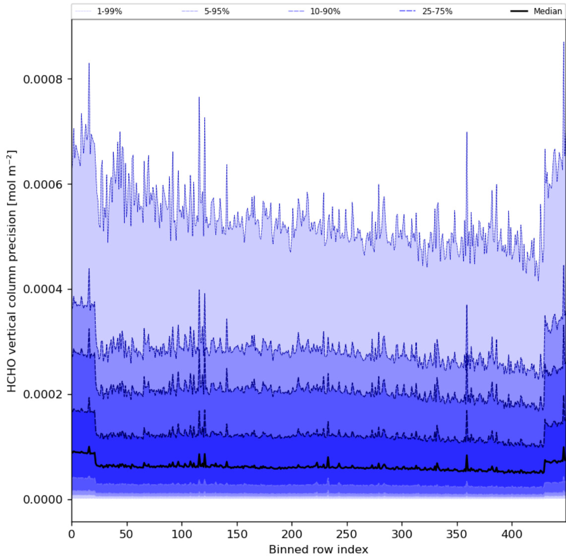
Figure 50: Along track statistics of “HCHO vertical column precision” for 2024-06-08 to 2024-06-09
