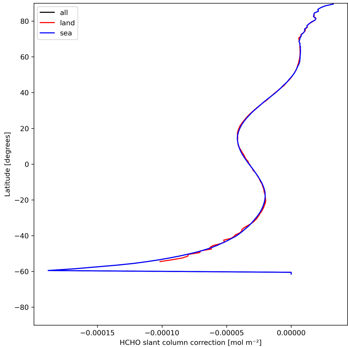
Figure 33: Zonal average of “HCHO slant column correction” for 2024-06-08 to 2024-06-09.
