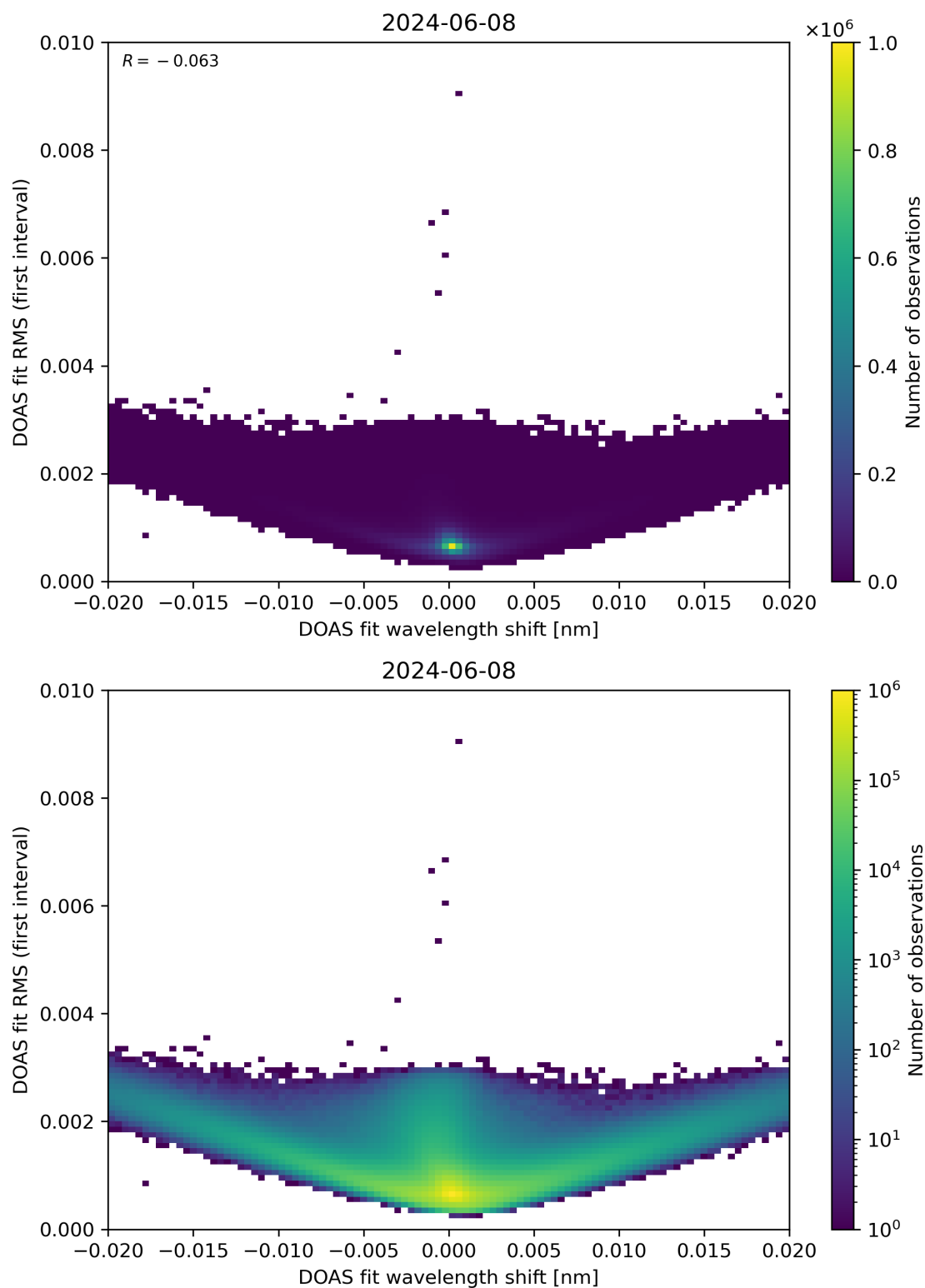
Figure 64: Scatter density plot of “DOAS fit wavelength shift” against “DOAS fit RMS (first interval)” for 2024-06-08 to 2024-06-09.
