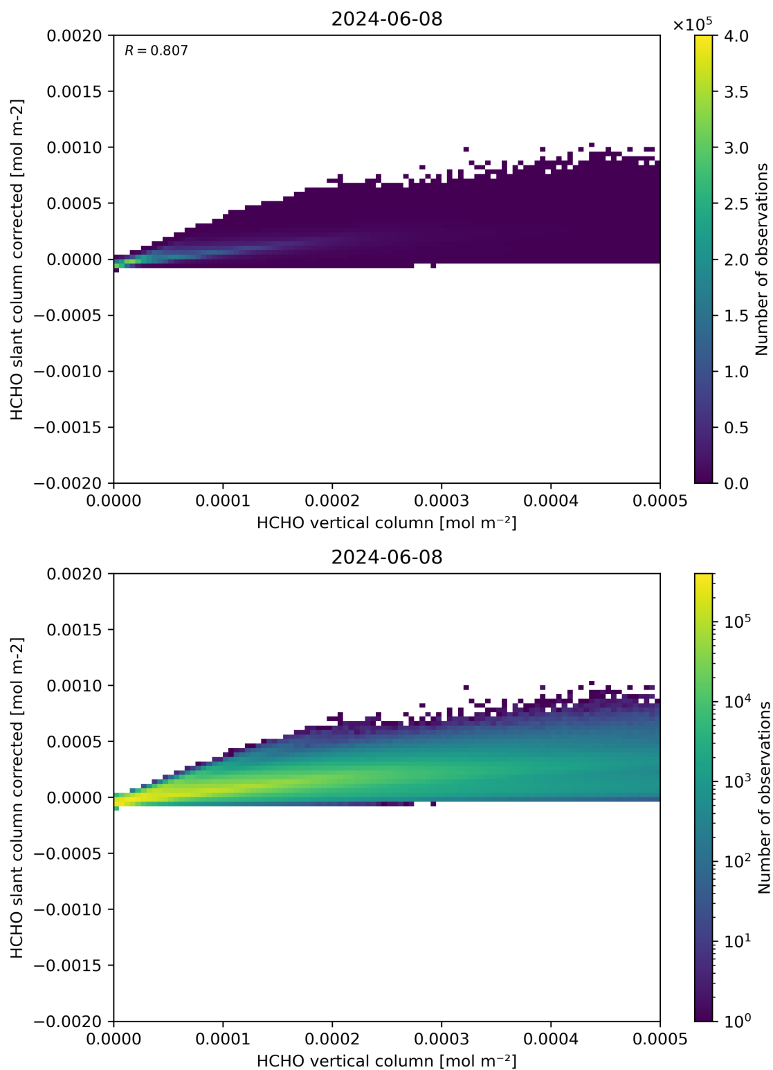
Figure 127: Scatter density plot of “HCHO vertical column” against “HCHO slant column corrected” for 2024-06-08 to 2024-06-09.
