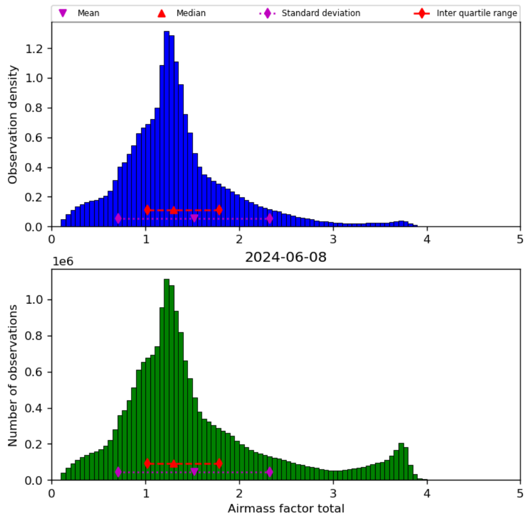
Figure 40: Histogram of “Airmass factor total” for 2024-06-08 to 2024-06-09
