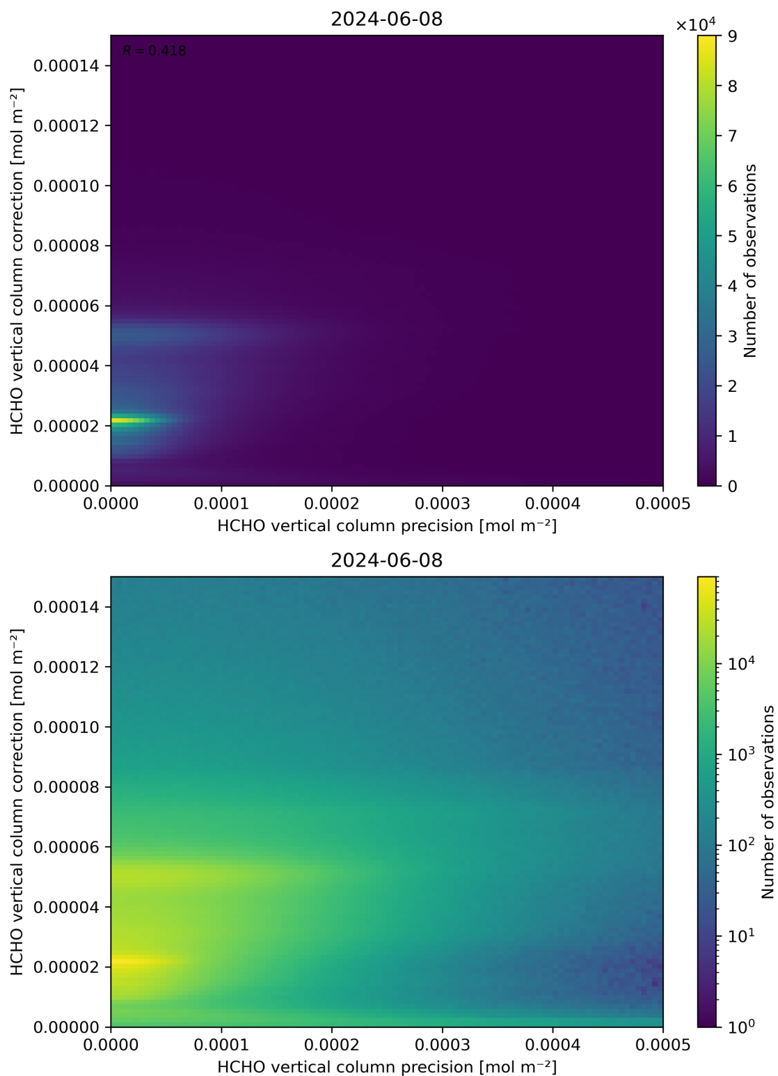
Figure 146: Scatter density plot of “HCHO vertical column precision” against “HCHO vertical column correction” for 2024-06-08 to 2024-06-09.
