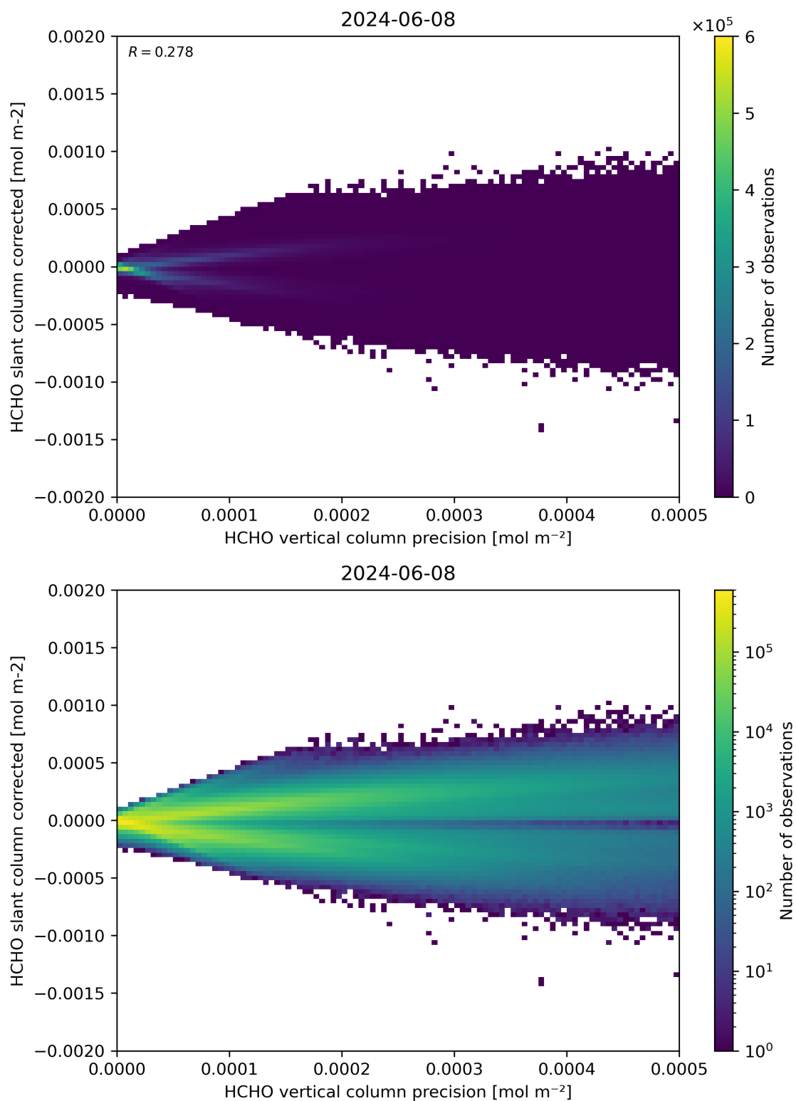
Figure 140: Scatter density plot of “HCHO vertical column precision” against “HCHO slant column corrected” for 2024-06-08 to 2024-06-09.
