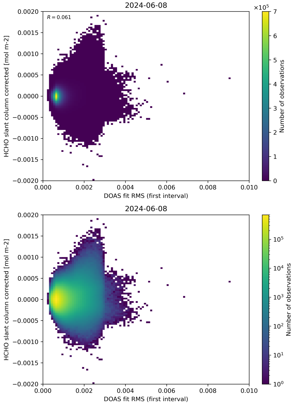
Figure 62: Scatter density plot of “DOAS fit RMS (first interval)” against “HCHO slant column corrected” for 2024-06-08 to 2024-06-09.
