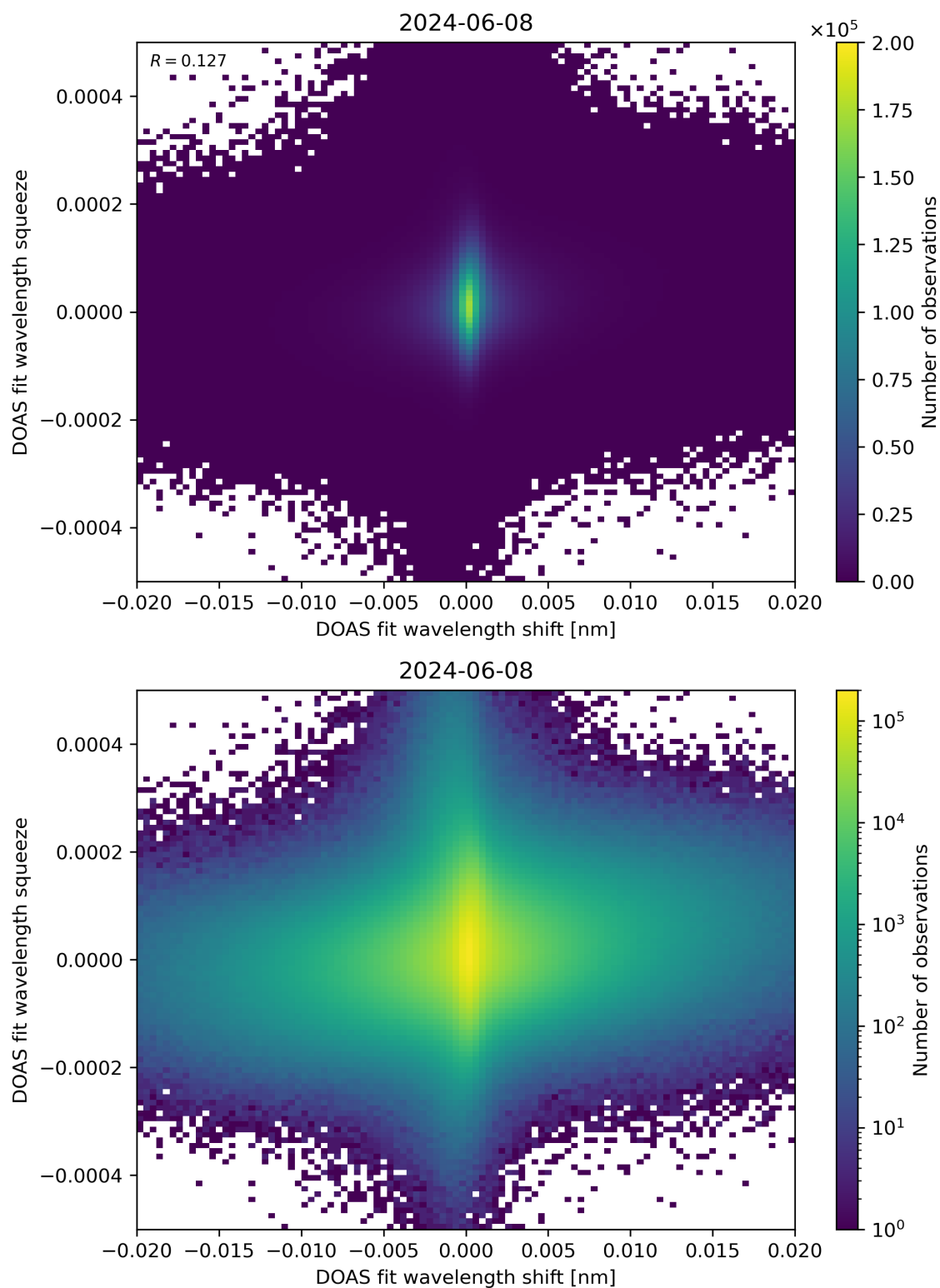
Figure 65: Scatter density plot of “DOAS fit wavelength shift” against “DOAS fit wavelength squeeze” for 2024-06-08 to 2024-06-09.
