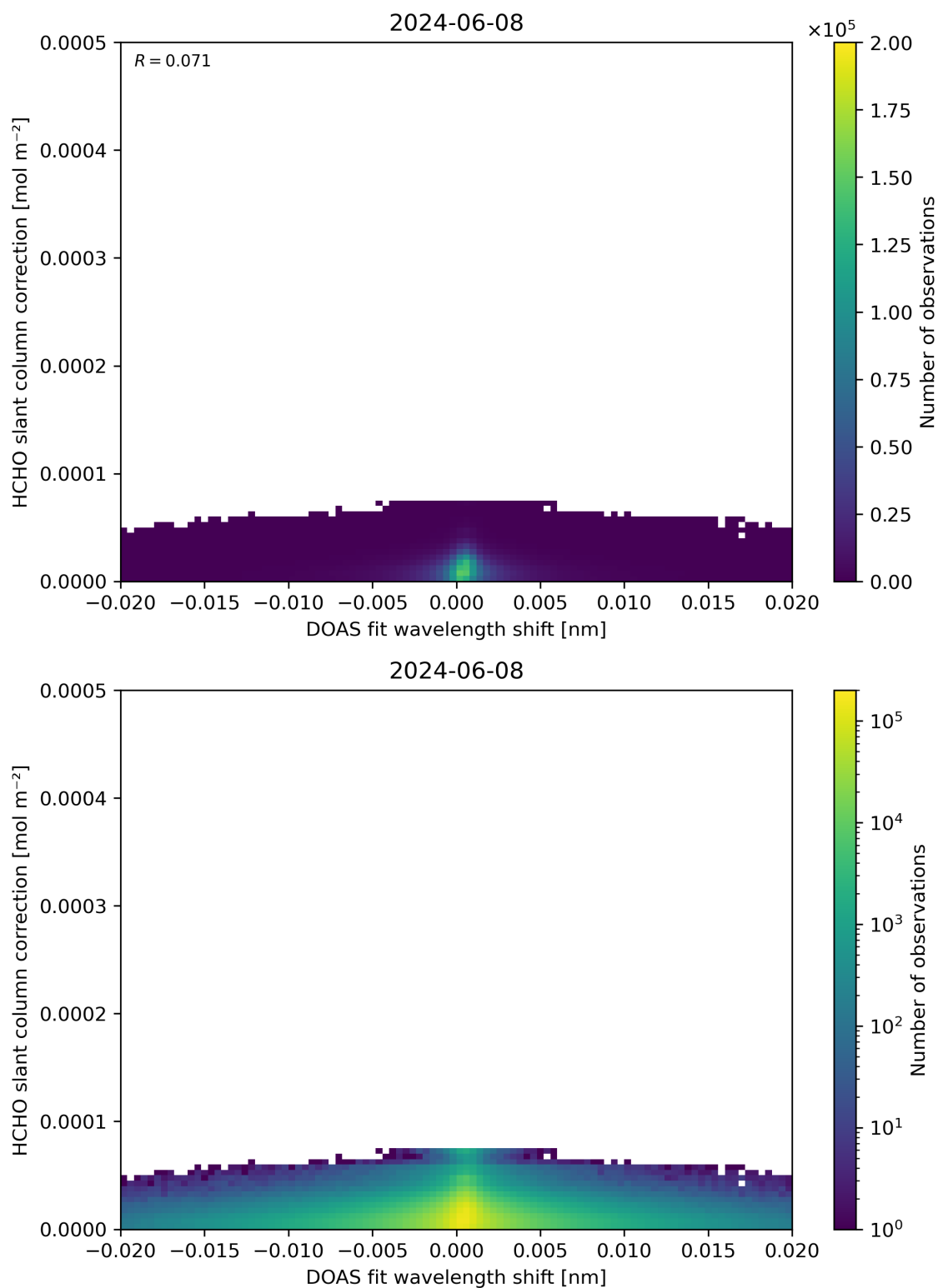
Figure 67: Scatter density plot of “DOAS fit wavelength shift” against “HCHO slant column correction” for 2024-06-08 to 2024-06-09.
