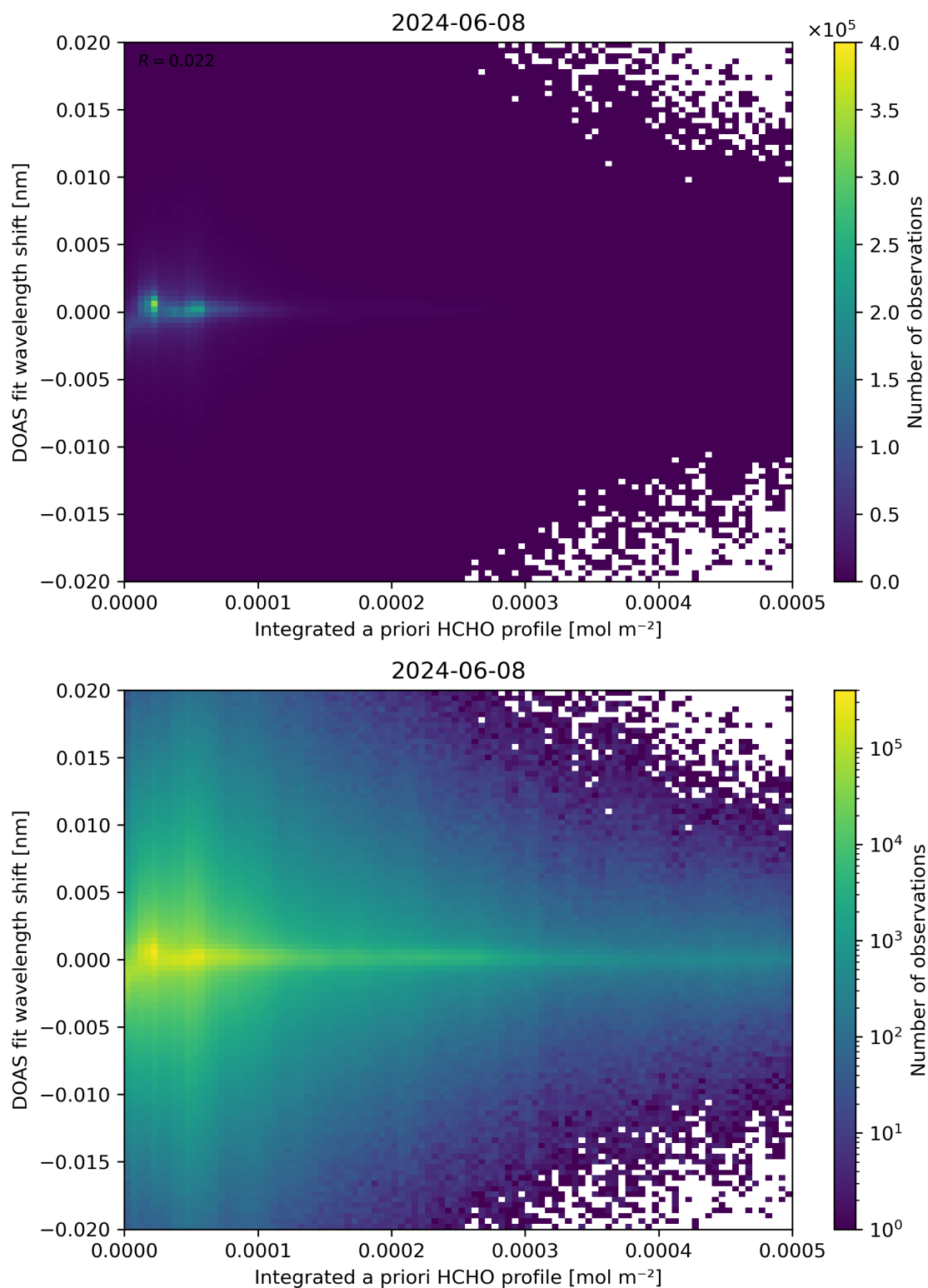
Figure 149: Scatter density plot of “Integrated a priori HCHO profile” against “DOAS fit wavelength shift” for 2024-06-08 to 2024-06-09.
