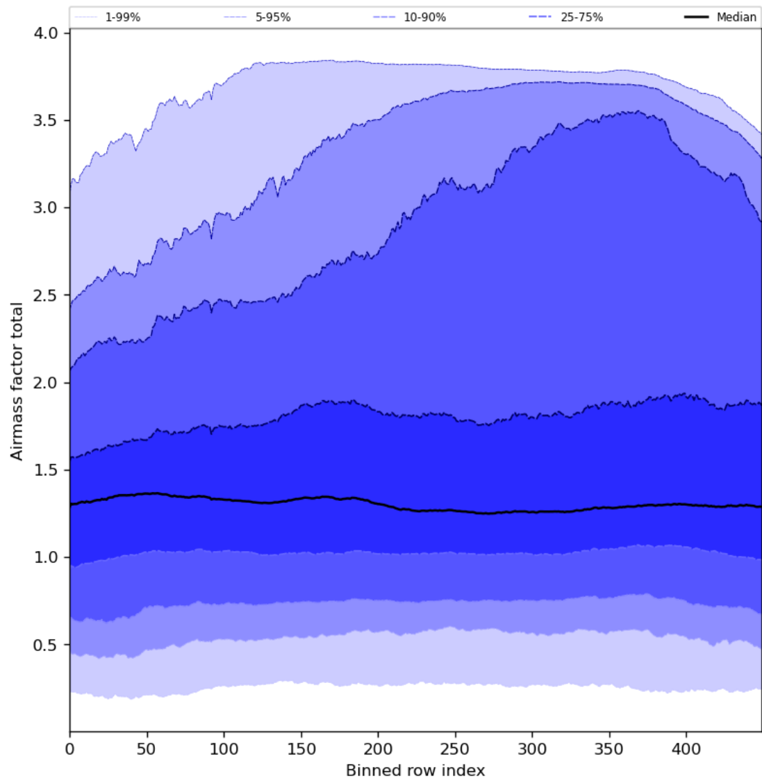
Figure 54: Along track statistics of “Airmass factor total” for 2024-06-08 to 2024-06-09
