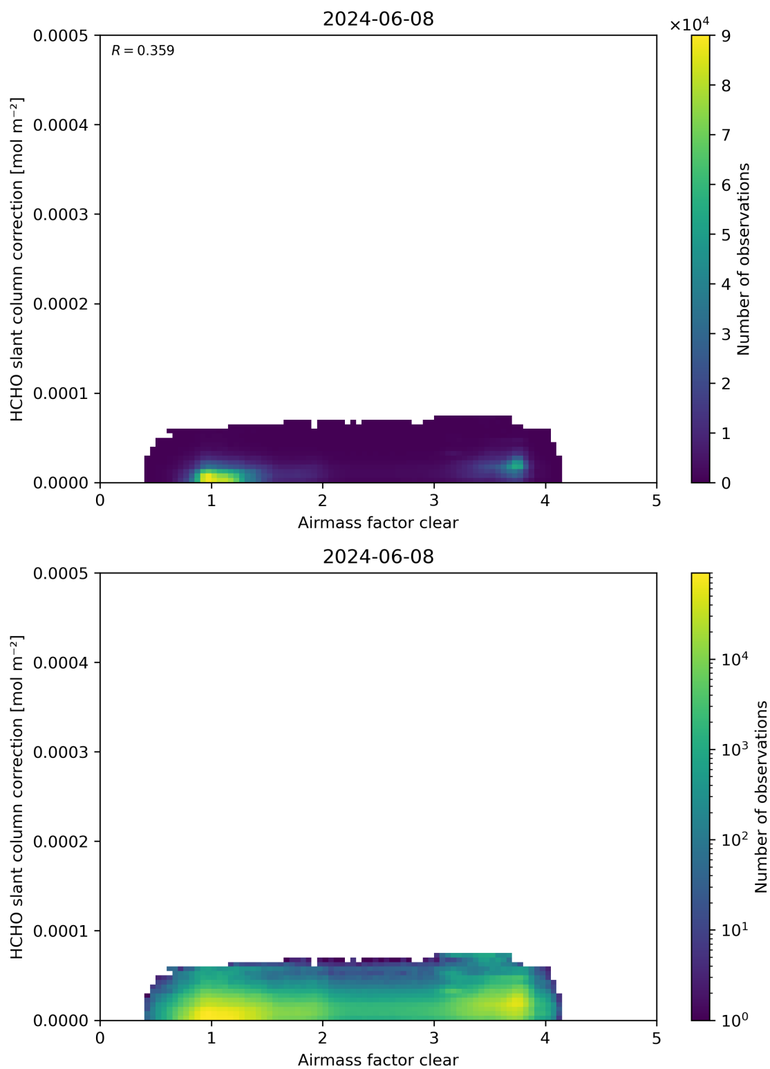
Figure 75: Scatter density plot of “Airmass factor clear” against “HCHO slant column correction” for 2024-06-08 to 2024-06-09.
