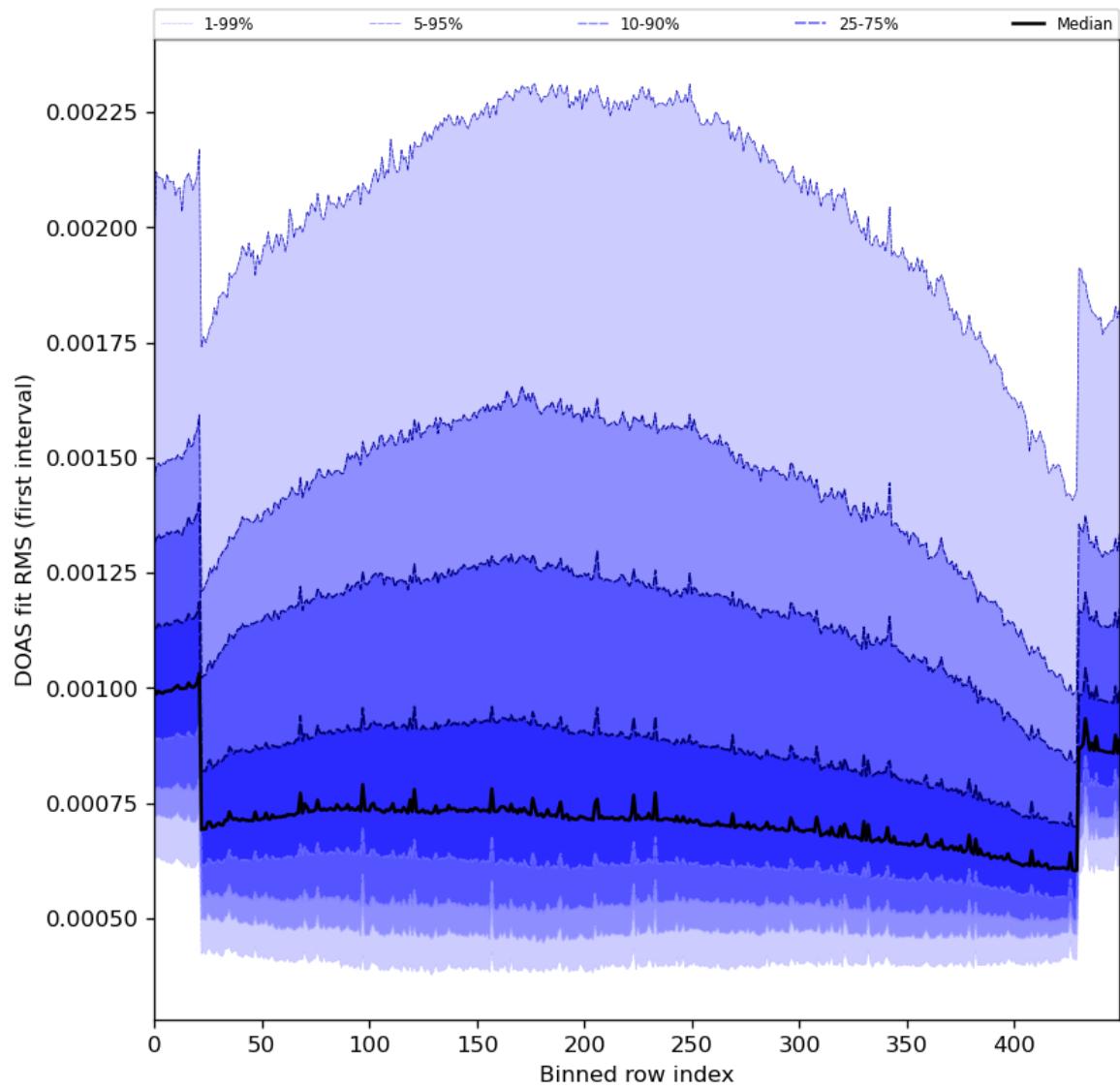
Figure 60: Along track statistics of “DOAS fit RMS (first interval)” for 2024-06-08 to 2024-06-09
