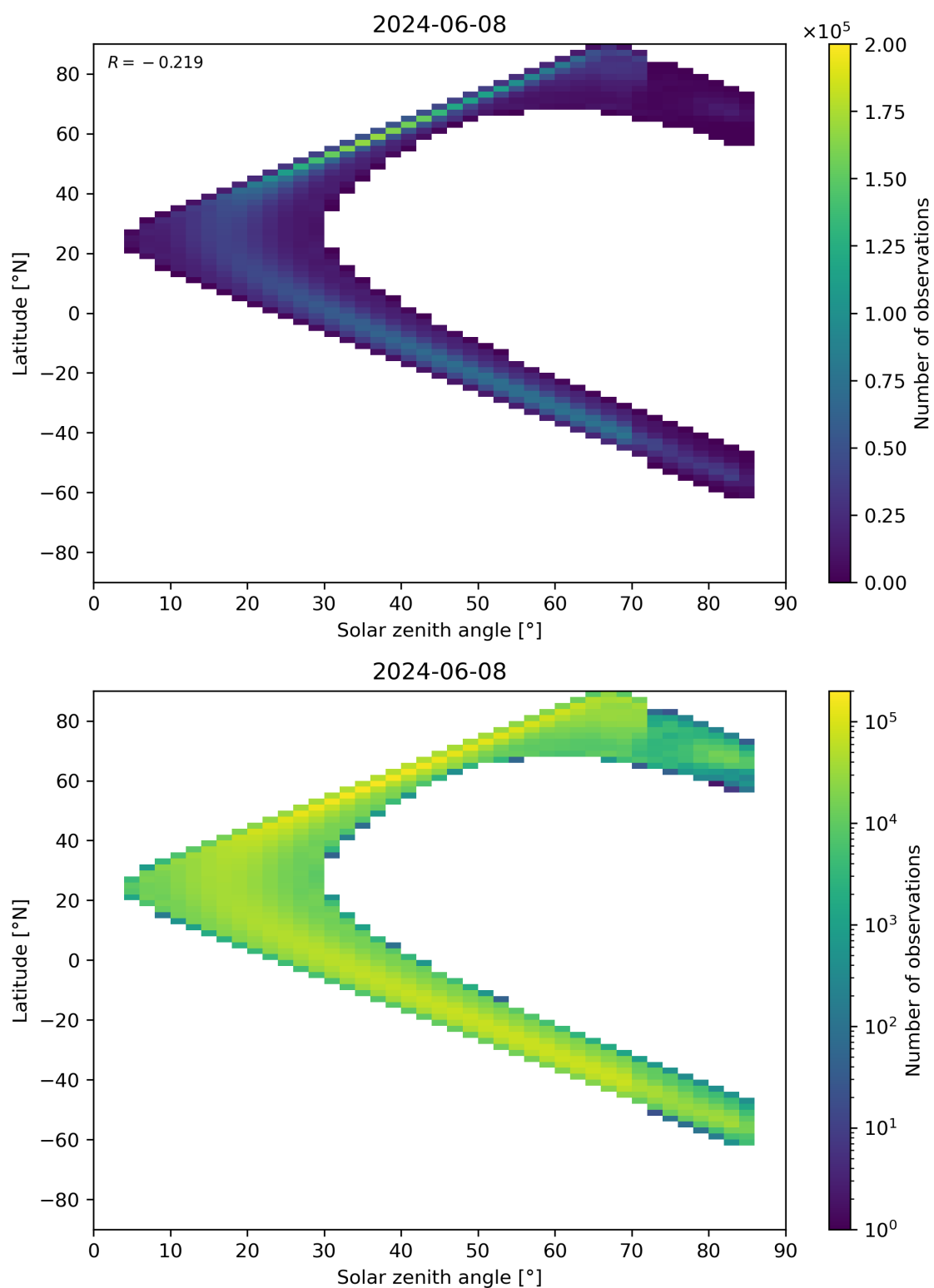
Figure 181: Scatter density plot of “Solar zenith angle” against “Latitude” for 2024-06-08 to 2024-06-09.
