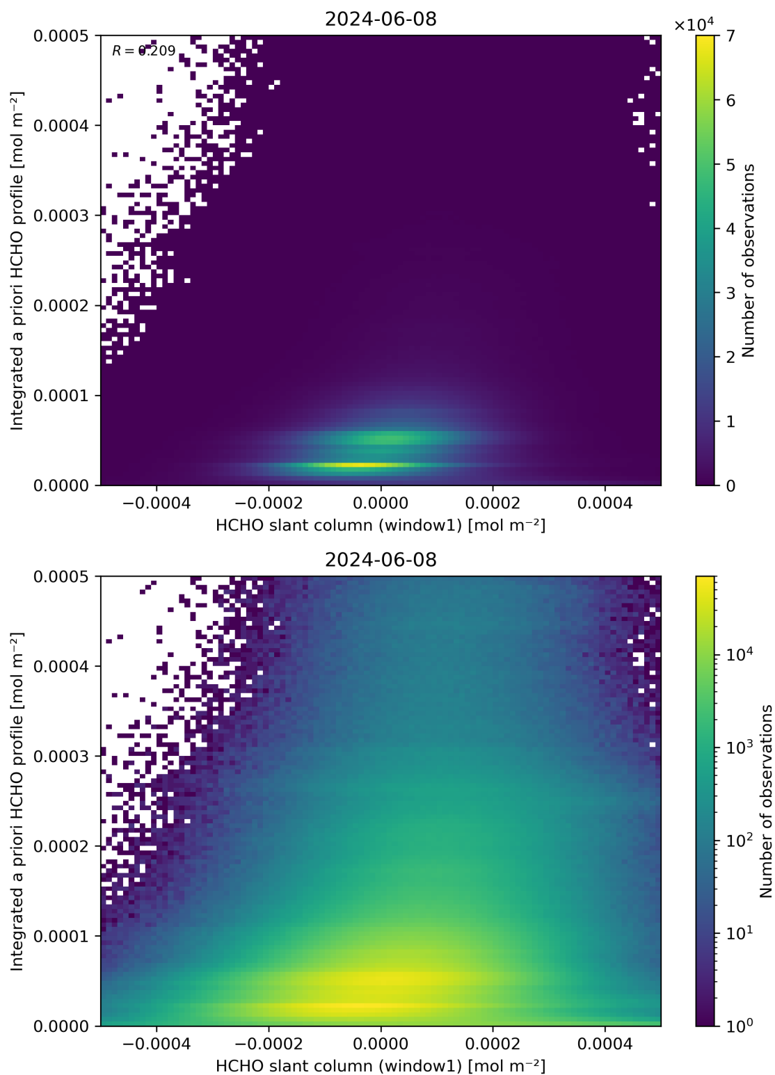
Figure 87: Scatter density plot of “HCHO slant column (window1)” against “Integrated a priori HCHO profile” for 2024-06-08 to 2024-06-09.
