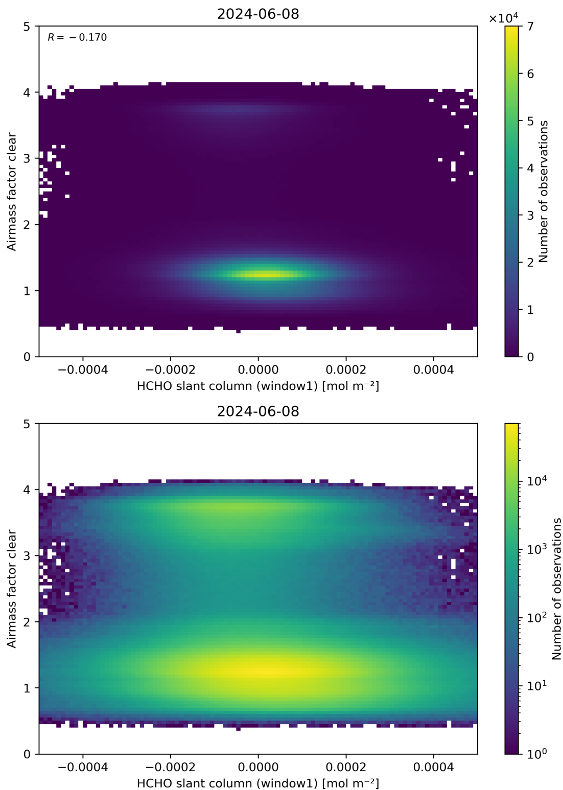
Figure 81: Scatter density plot of “HCHO slant column (window1)” against “Airmass factor clear” for 2024-06-08 to 2024-06-09.
