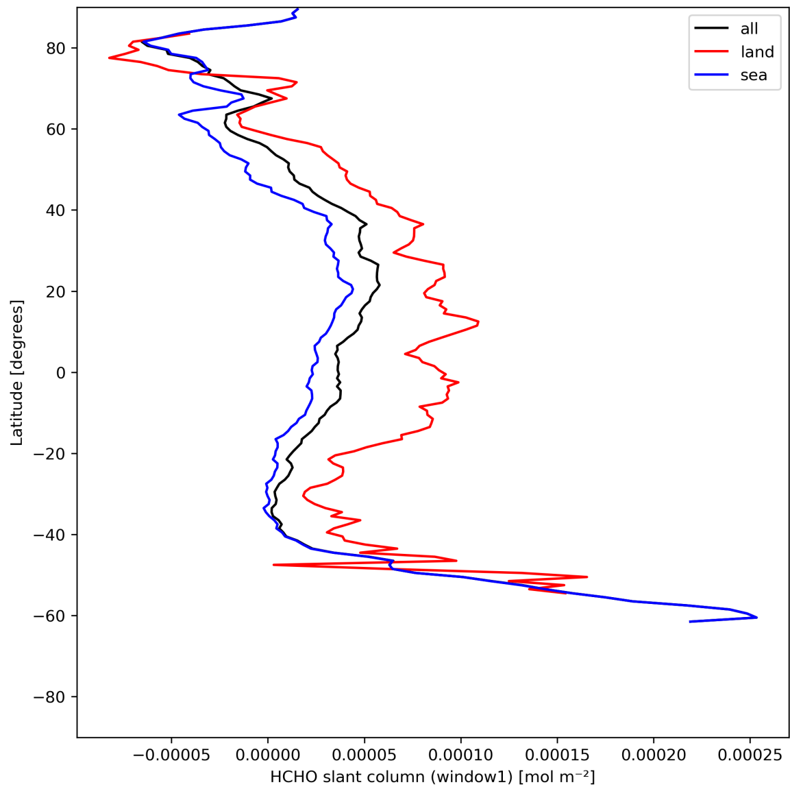
Figure 24: Zonal average of “HCHO slant column (window1)” for 2024-06-08 to 2024-06-09.
