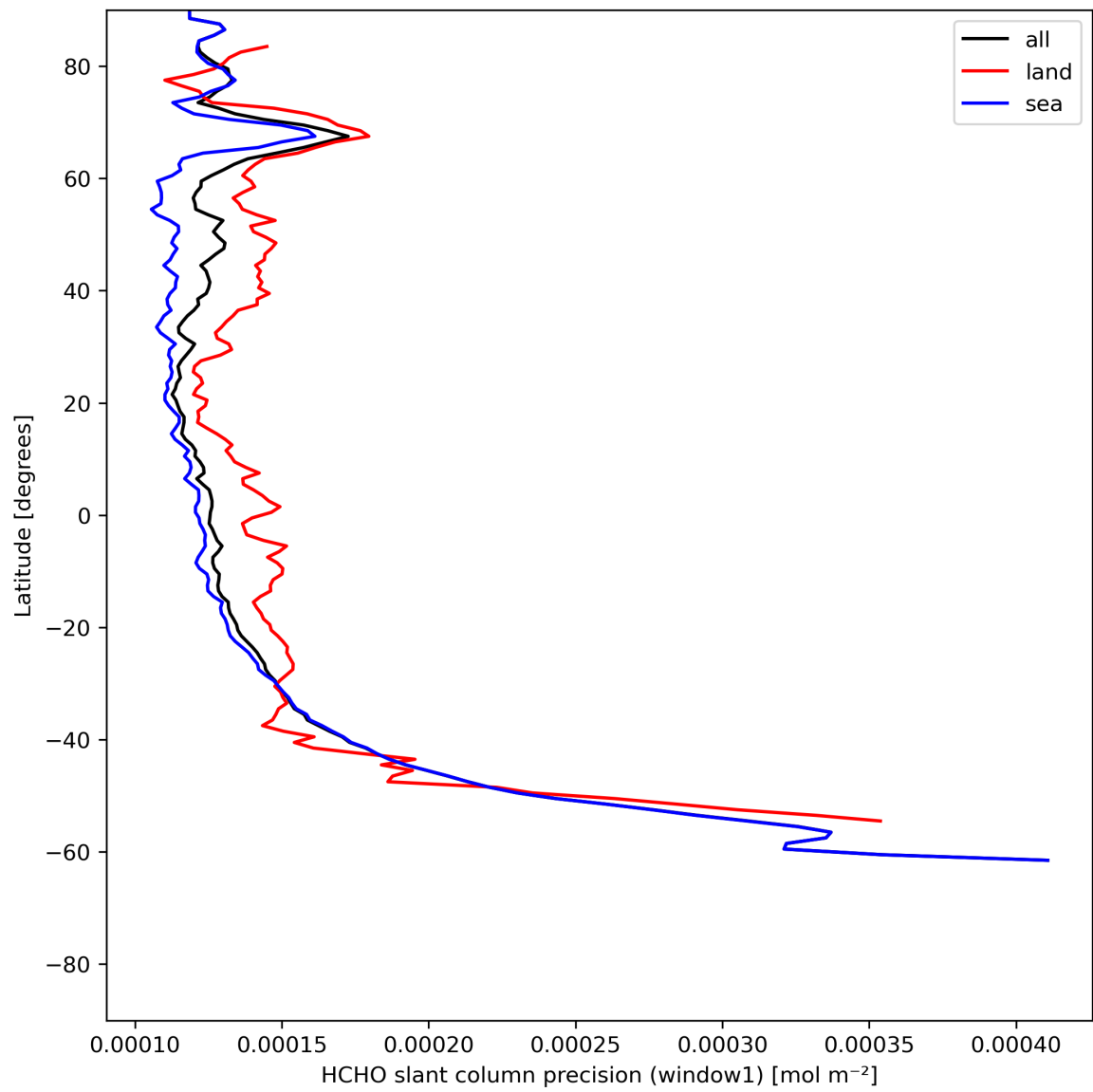
Figure 25: Zonal average of “HCHO slant column precision (window1)” for 2024-06-08 to 2024-06-09.
