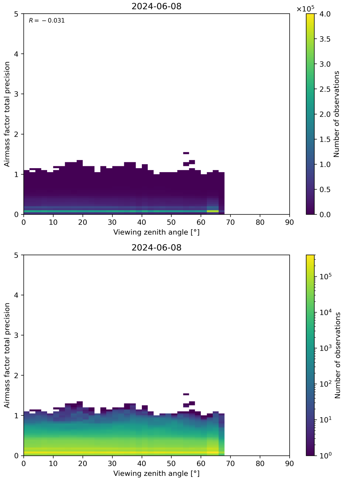
Figure 191: Scatter density plot of “Viewing zenith angle” against “Airmass factor total precision” for 2024-06-08 to 2024-06-09.
