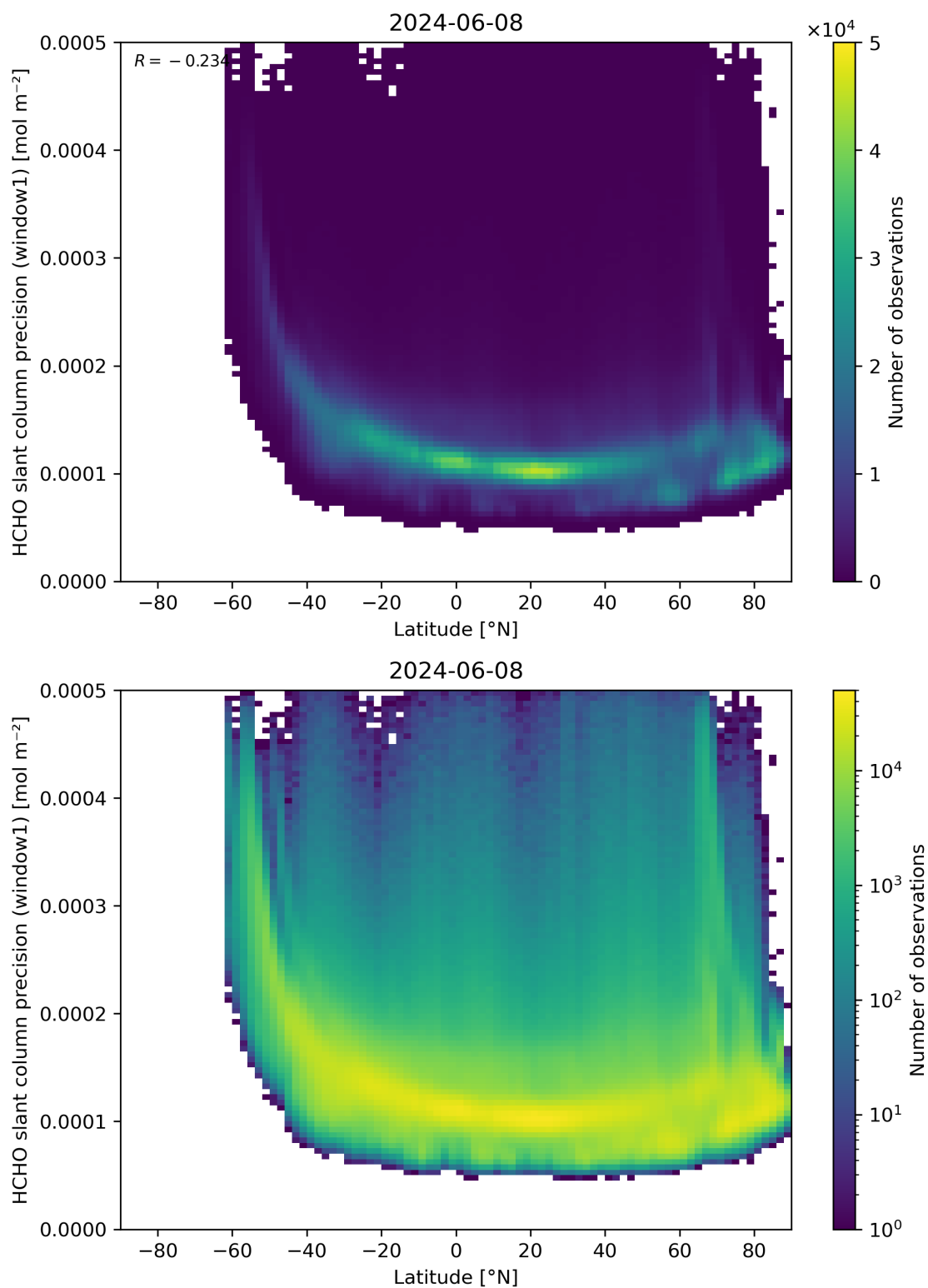
Figure 160: Scatter density plot of “Latitude” against “HCHO slant column precision (window1)” for 2024-06-08 to 2024-06-09.
