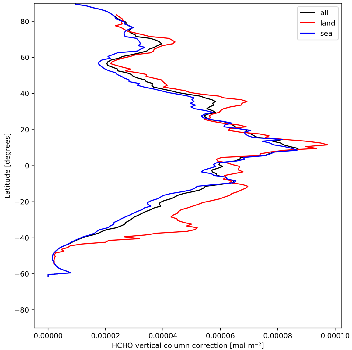
Figure 23: Zonal average of "HCHO vertical column correction" for 2024-06-08 to 2024-06-09.
