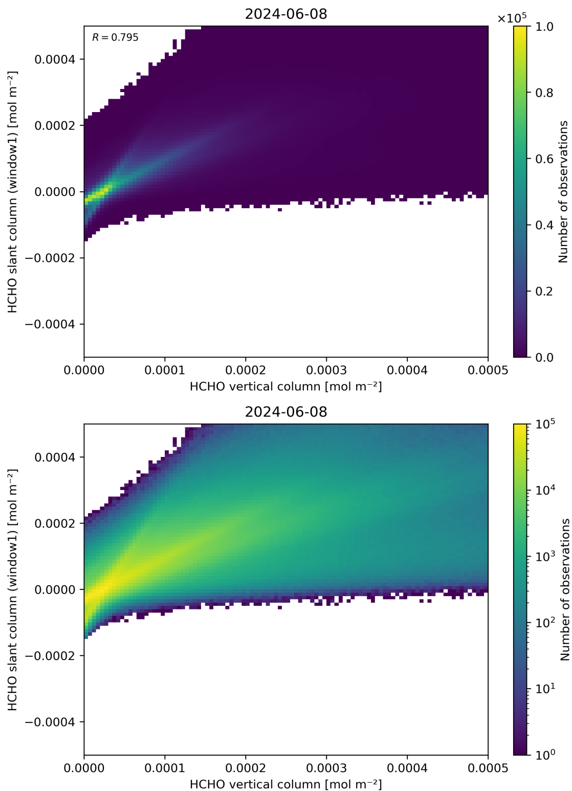
Figure 129: Scatter density plot of “HCHO vertical column” against “HCHO slant column (window1)” for 2024-06-08 to 2024-06-09.
