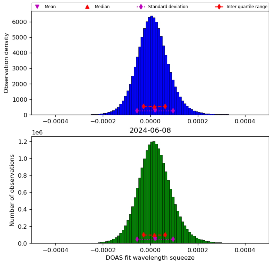
Figure 45: Histogram of “DOAS fit wavelength squeeze” for 2024-06-08 to 2024-06-09
