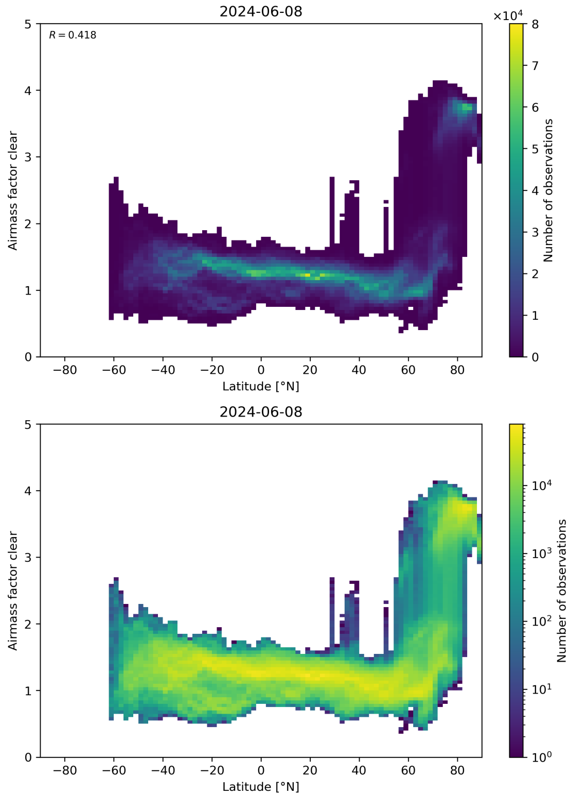
Figure 156: Scatter density plot of “Latitude” against “Airmass factor clear” for 2024-06-08 to 2024-06-09.
