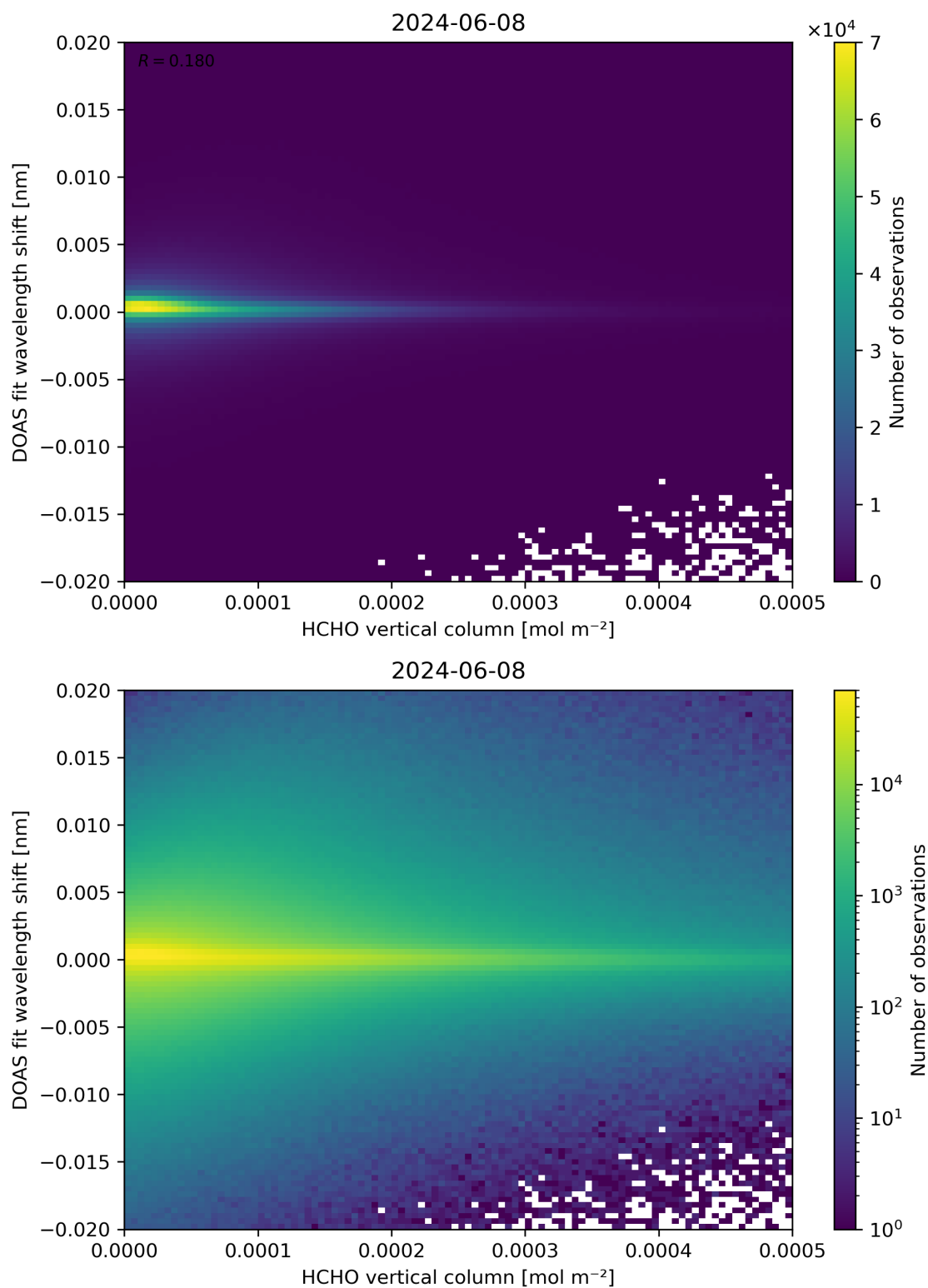
Figure 124: Scatter density plot of “HCHO vertical column” against “DOAS fit wavelength shift” for 2024-06-08 to 2024-06-09.
