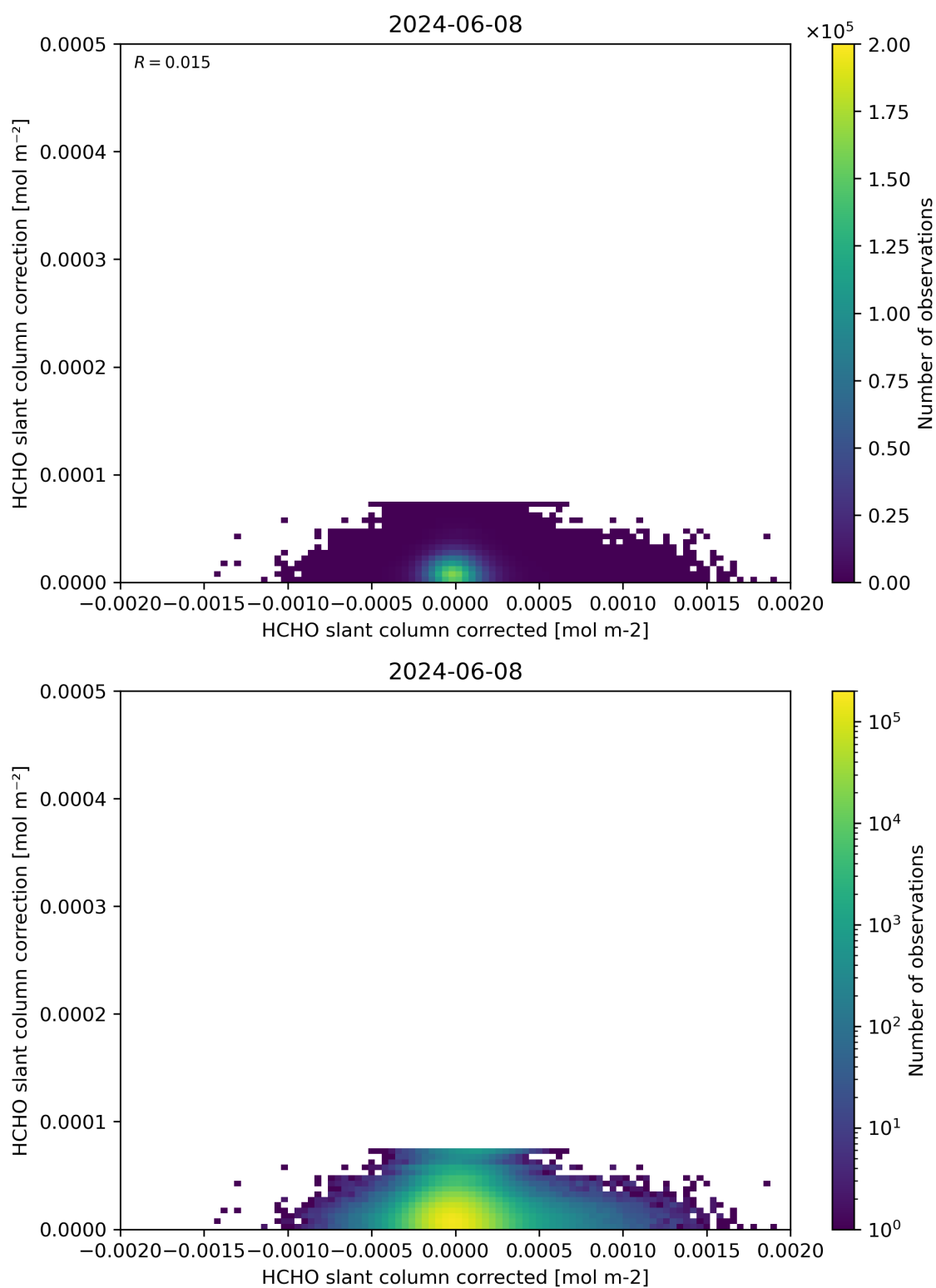
Figure 77: Scatter density plot of “HCHO slant column corrected” against “HCHO slant column correction” for 2024-06-08 to 2024-06-09.
