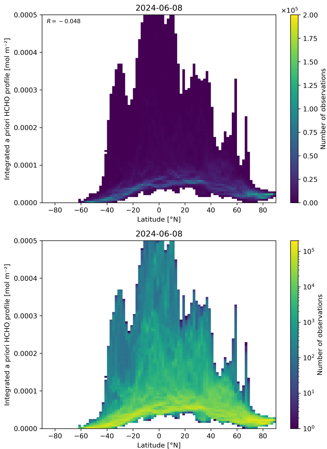
Figure 166: Scatter density plot of “Latitude” against “Integrated a priori HCHO profile” for 2024-06-08 to 2024-06-09.
