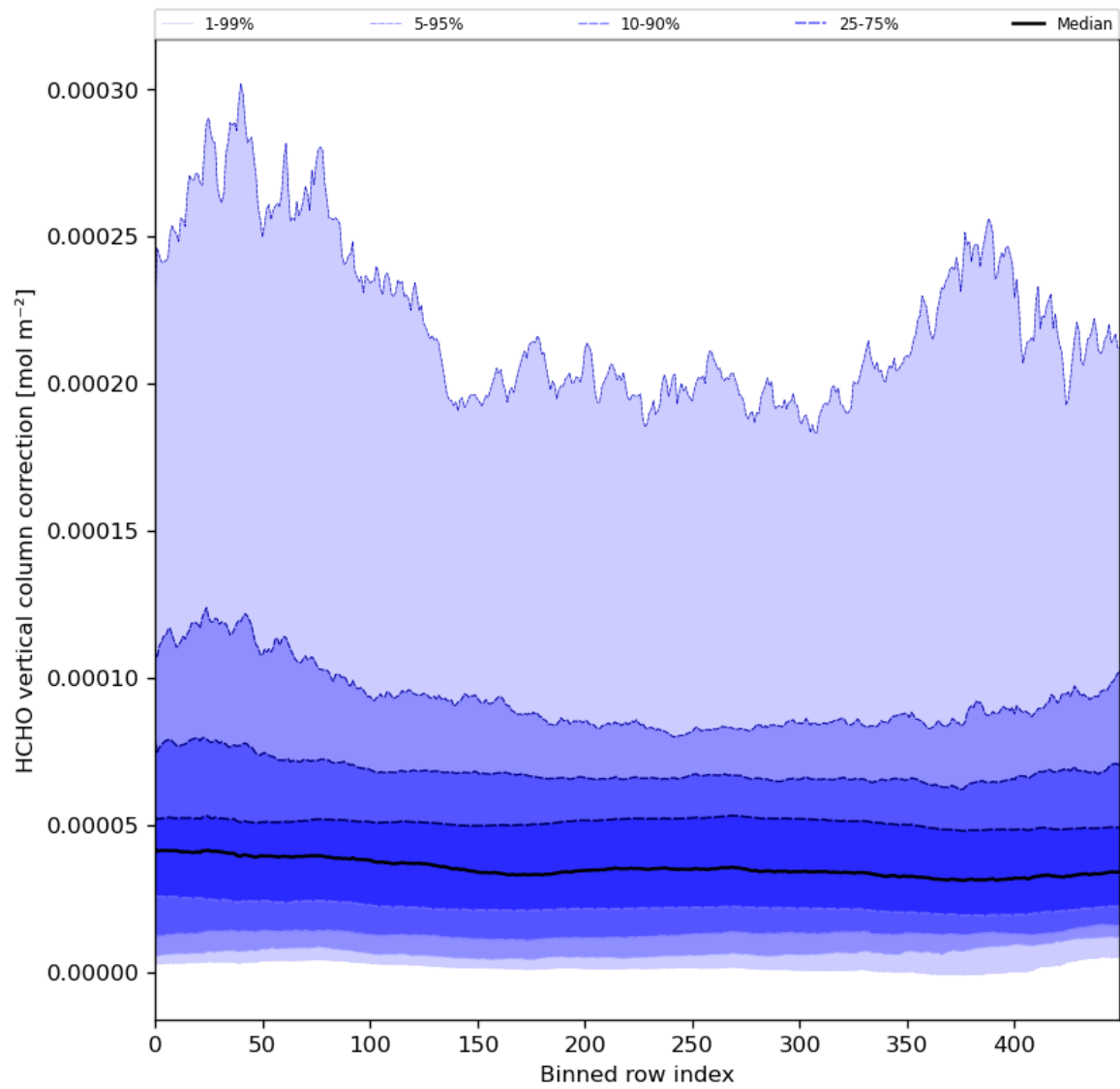
Figure 51: Along track statistics of “HCHO vertical column correction” for 2024-06-08 to 2024-06-09
