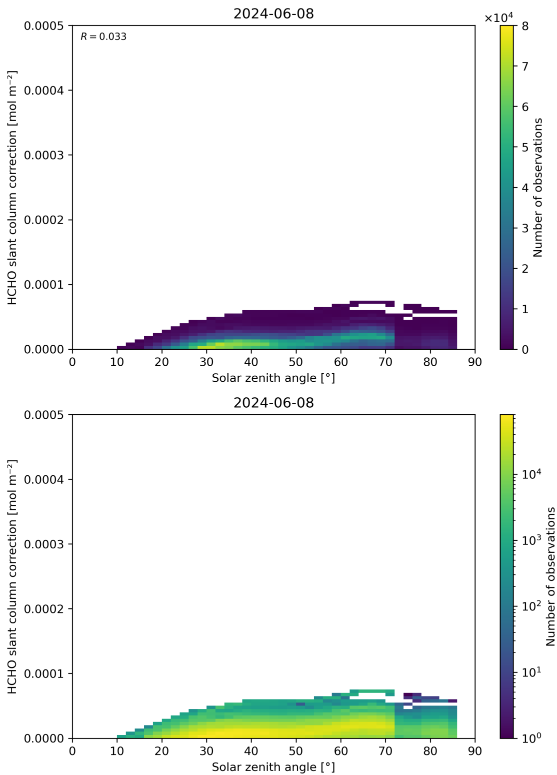
Figure 172: Scatter density plot of “Solar zenith angle” against “HCHO slant column correction” for 2024-06-08 to 2024-06-09.
