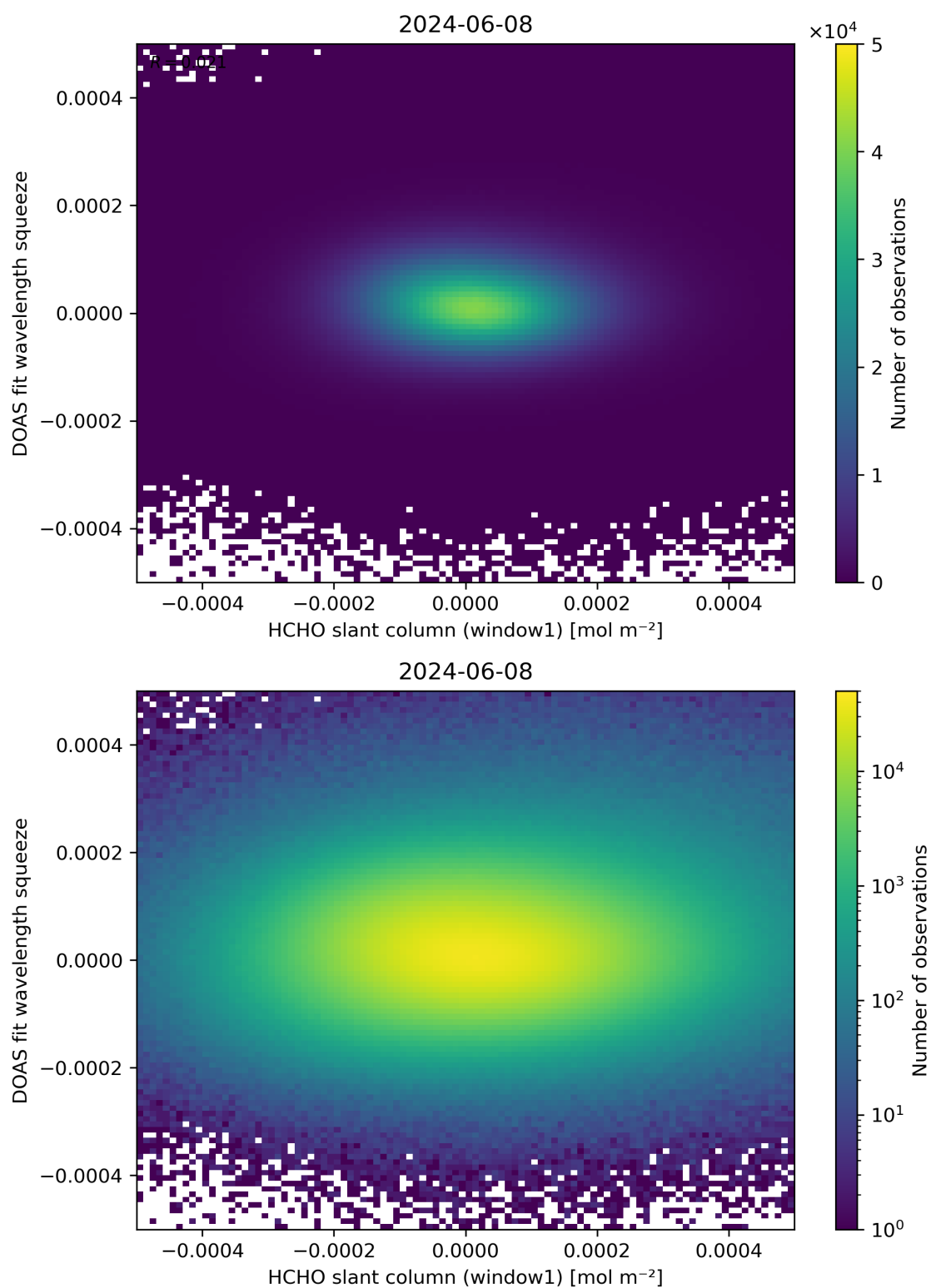
Figure 80: Scatter density plot of “HCHO slant column (window1)” against “DOAS fit wavelength squeeze” for 2024-06-08 to 2024-06-09.
