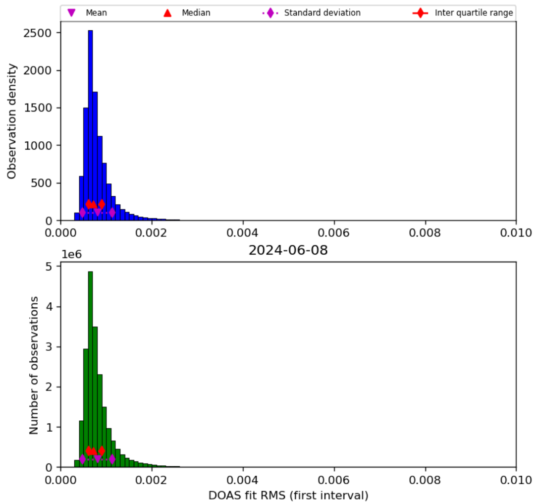
Figure 46: Histogram of “DOAS fit RMS (first interval)” for 2024-06-08 to 2024-06-09
