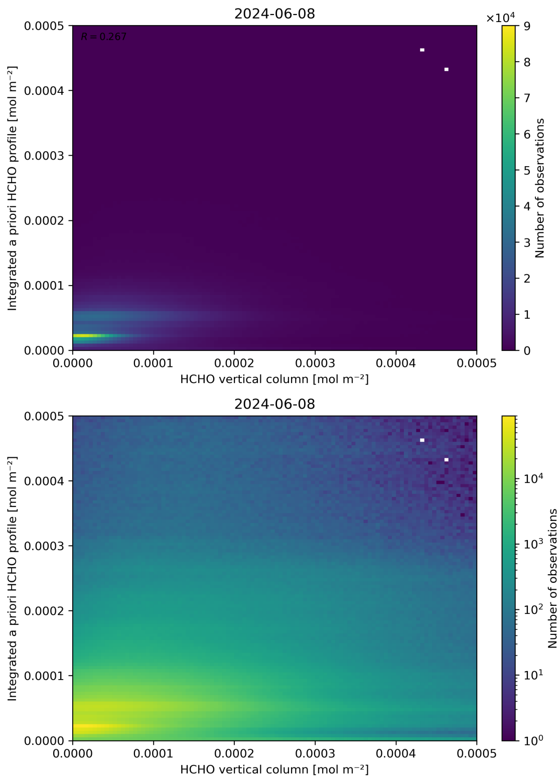
Figure 135: Scatter density plot of “HCHO vertical column” against “Integrated a priori HCHO profile” for 2024-06-08 to 2024-06-09.
