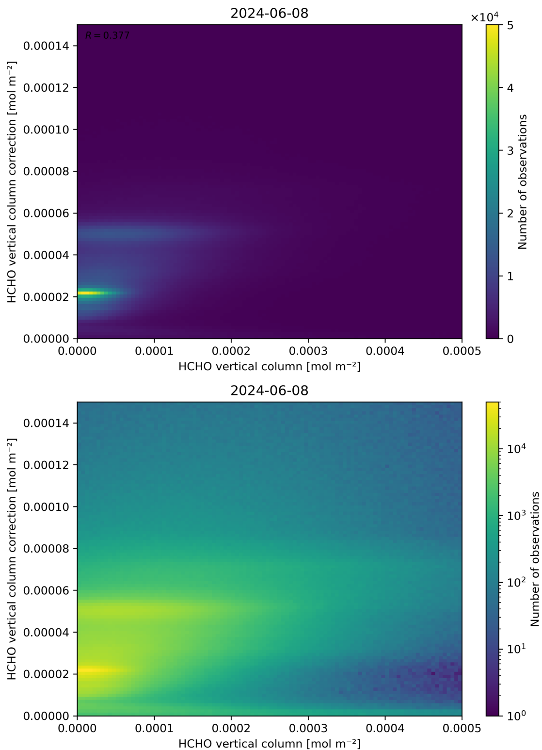
Figure 133: Scatter density plot of “HCHO vertical column” against “HCHO vertical column correction” for 2024-06-08 to 2024-06-09.
