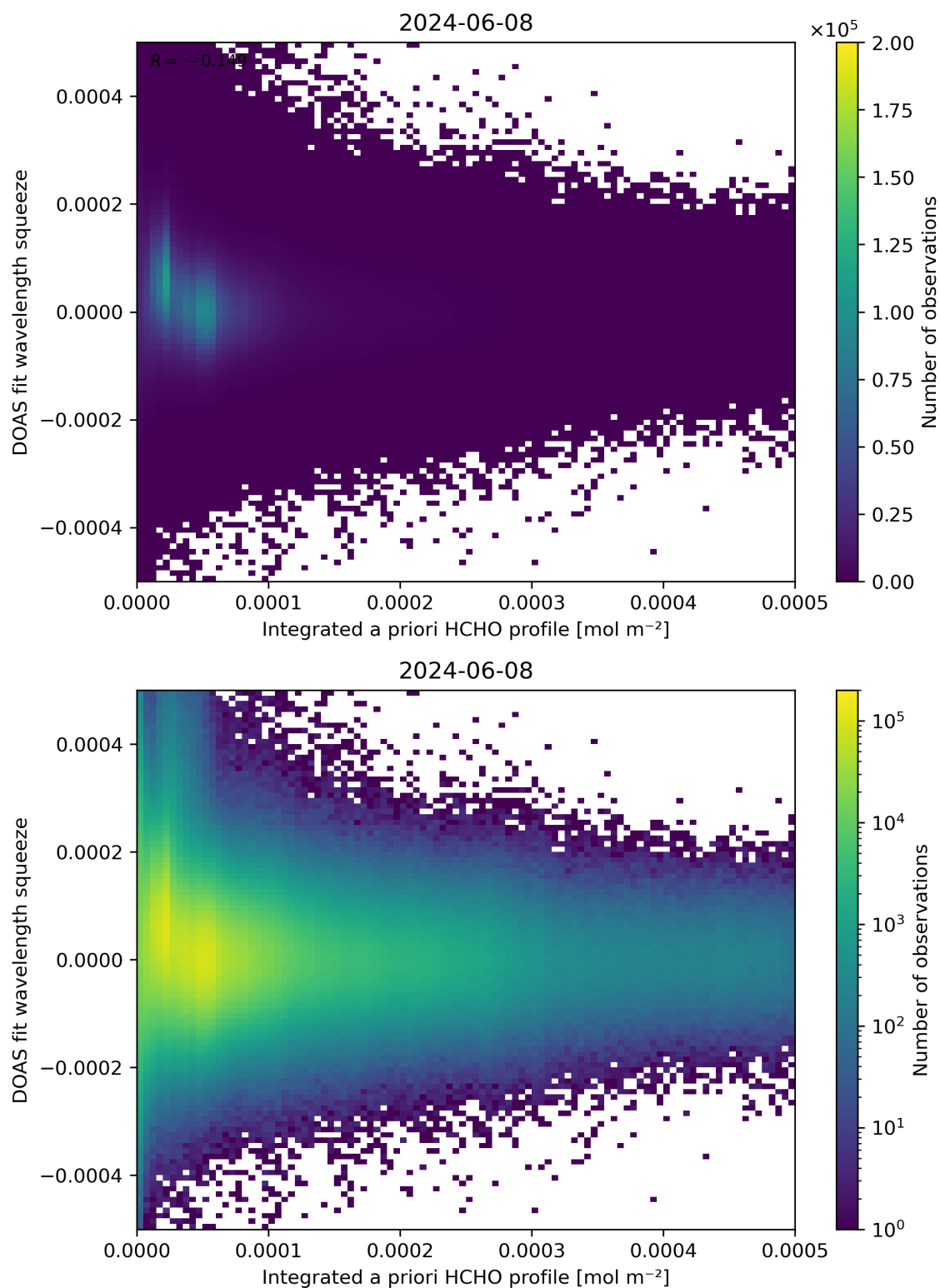
Figure 150: Scatter density plot of “Integrated a priori HCHO profile” against “DOAS fit wavelength squeeze” for 2024-06-08 to 2024-06-09.
