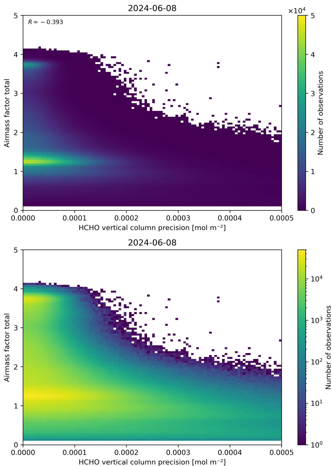
Figure 144: Scatter density plot of “HCHO vertical column precision” against “Airmass factor total” for 2024-06-08 to 2024-06-09.
