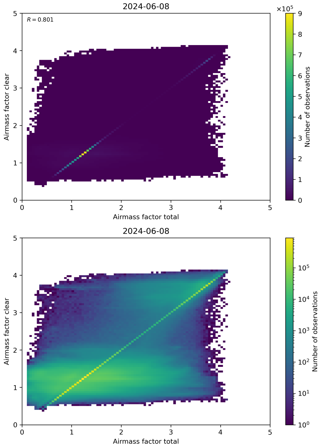
Figure 100: Scatter density plot of “Airmass factor total” against “Airmass factor clear” for 2024-06-08 to 2024-06-09.
