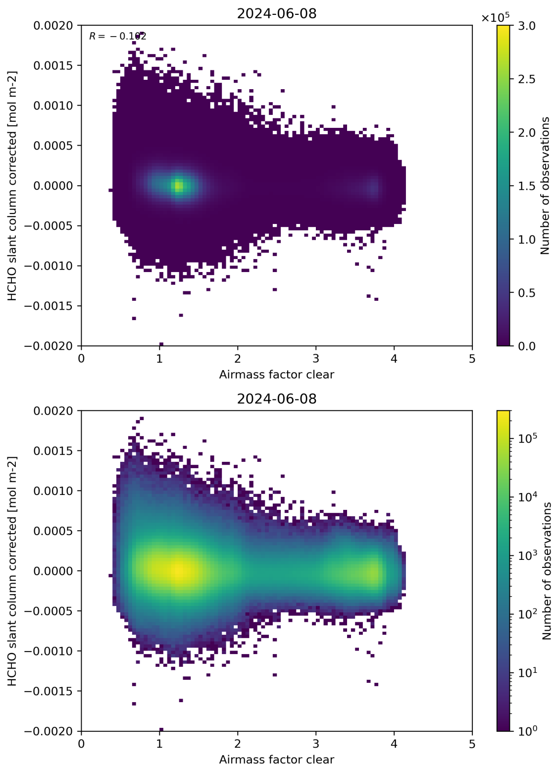
Figure 74: Scatter density plot of “Airmass factor clear” against “HCHO slant column corrected” for 2024-06-08 to 2024-06-09.
