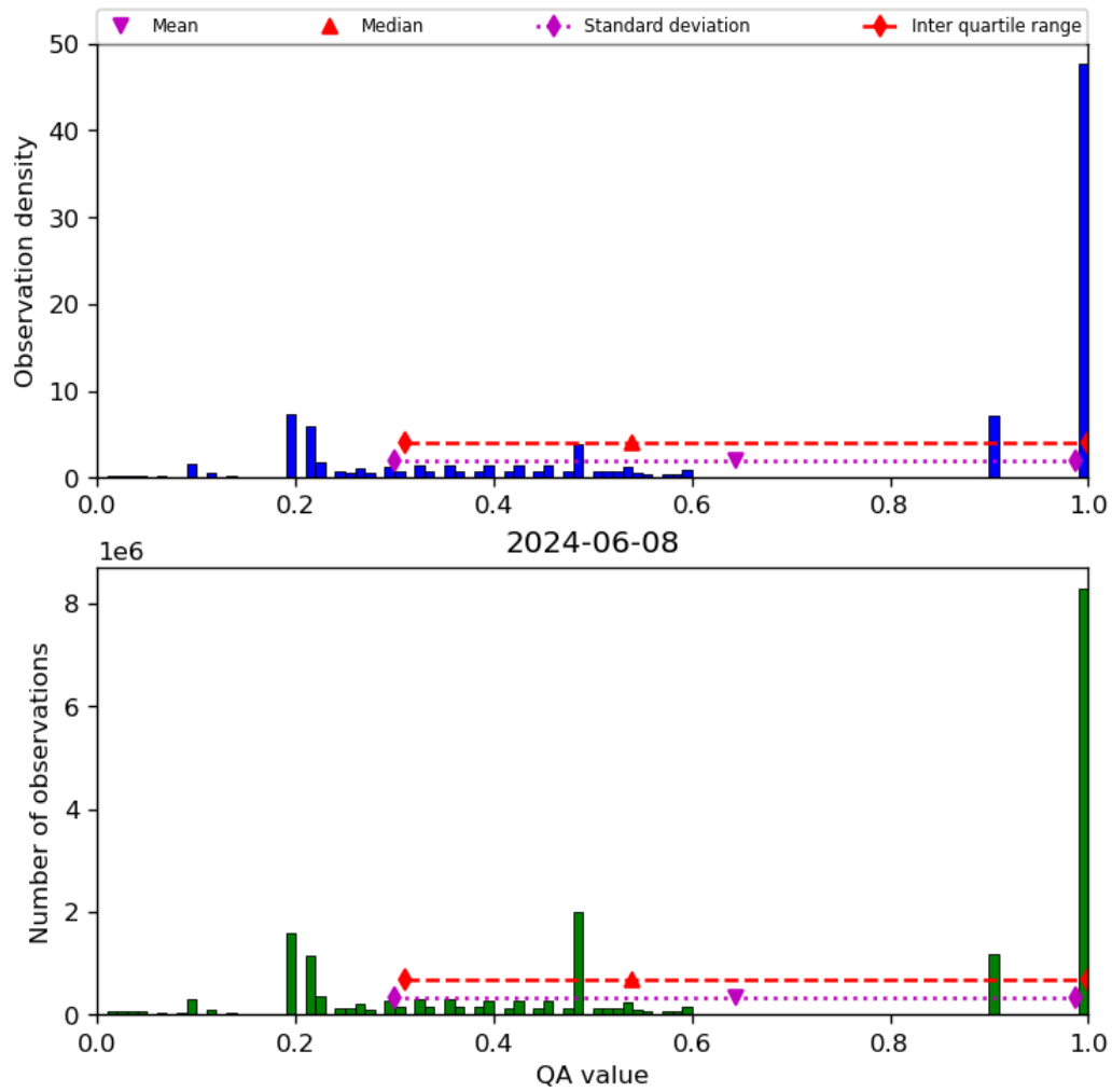
Figure 34: Histogram of “QA value” for 2024-06-08 to 2024-06-09
