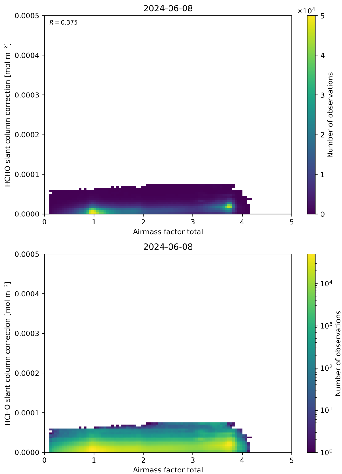
Figure 102: Scatter density plot of “Air mass factor total” against “HCHO slant column correction” for 2024-06-08 to 2024-06-09.
