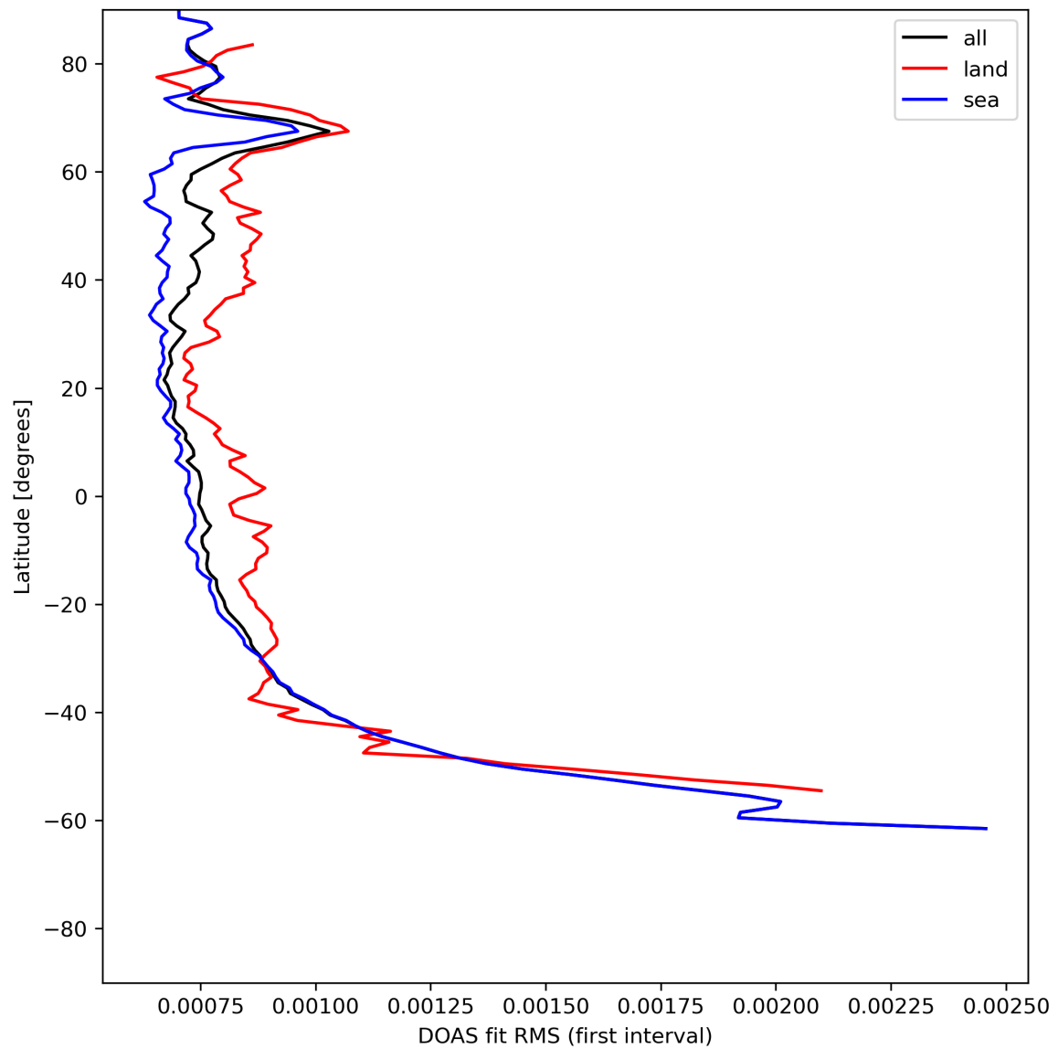
Figure 32: Zonal average of “DOAS fit RMS (first interval)” for 2024-06-08 to 2024-06-09.
