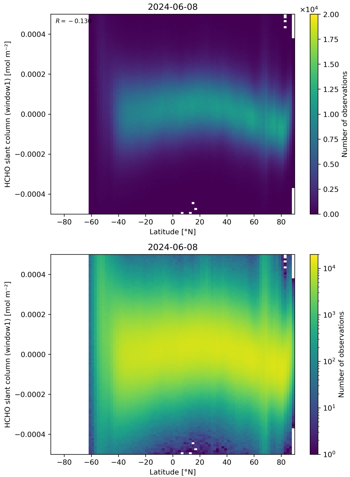
Figure 159: Scatter density plot of “Latitude” against “HCHO slant column (window1)” for 2024-06-08 to 2024-06-09.
