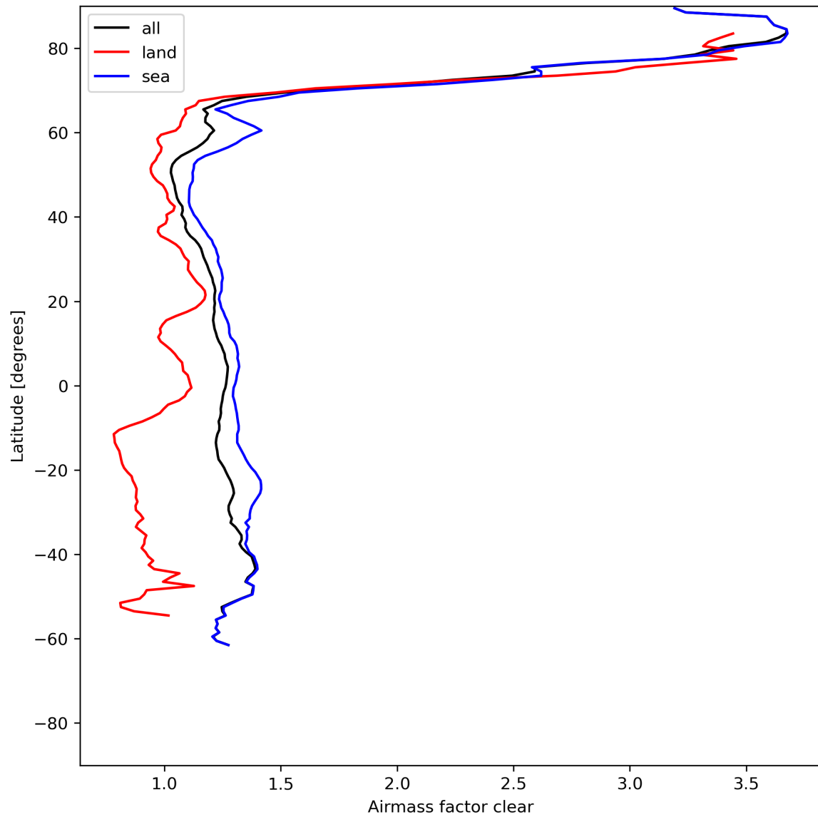
Figure 28: Zonal average of “Airmass factor clear” for 2024-06-08 to 2024-06-09.
