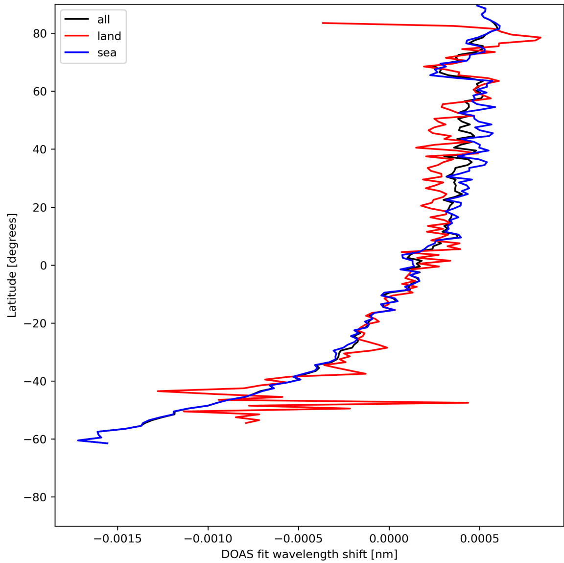
Figure 30: Zonal average of “DOAS fit wavelength shift” for 2024-06-08 to 2024-06-09.
