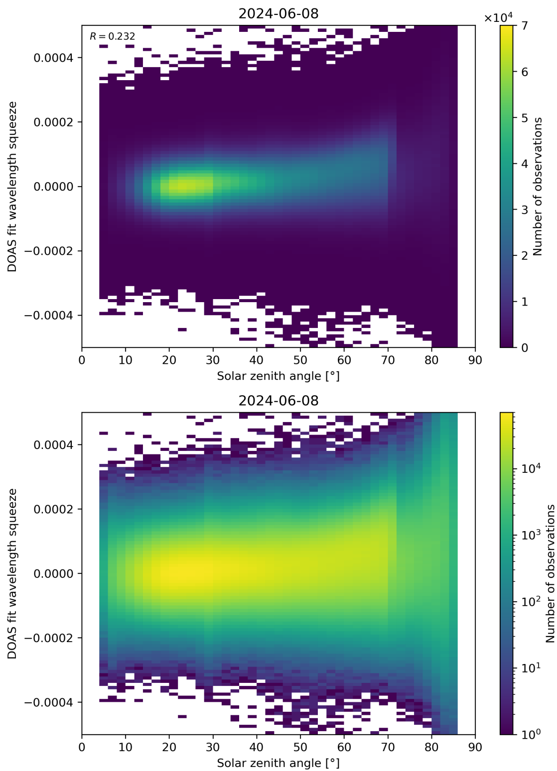
Figure 169: Scatter density plot of “Solar zenith angle” against “DOAS fit wavelength squeeze” for 2024-06-08 to 2024-06-09.
