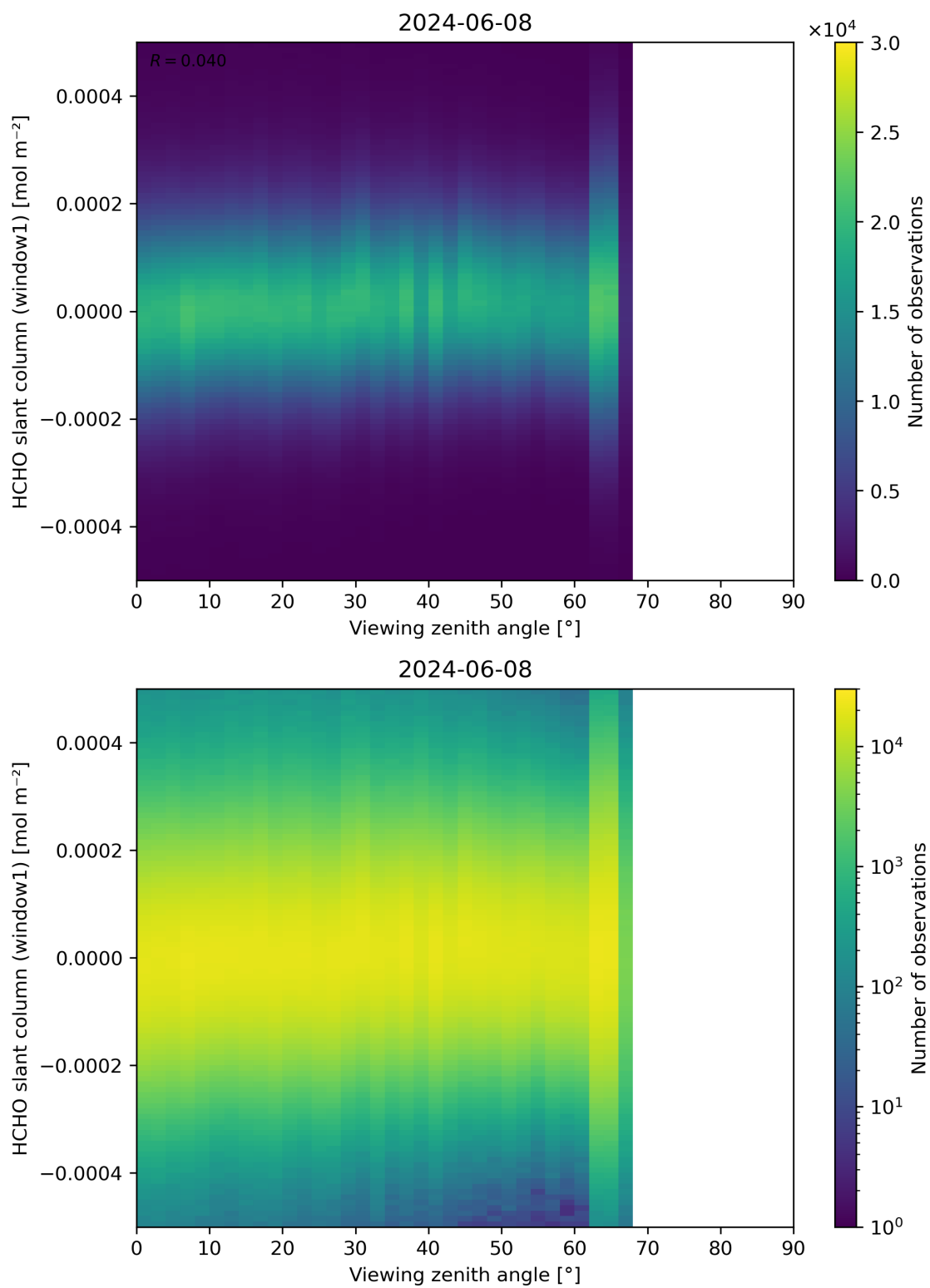
Figure 188: Scatter density plot of “Viewing zenith angle” against “HCHO slant column (window1)” for 2024-06-08 to 2024-06-09.
