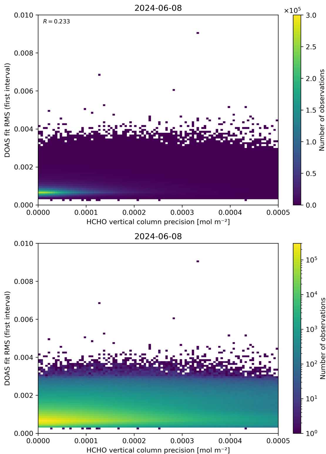
Figure 136: Scatter density plot of “HCHO vertical column precision” against “DOAS fit RMS (first interval)” for 2024-06-08 to 2024-06-09.
