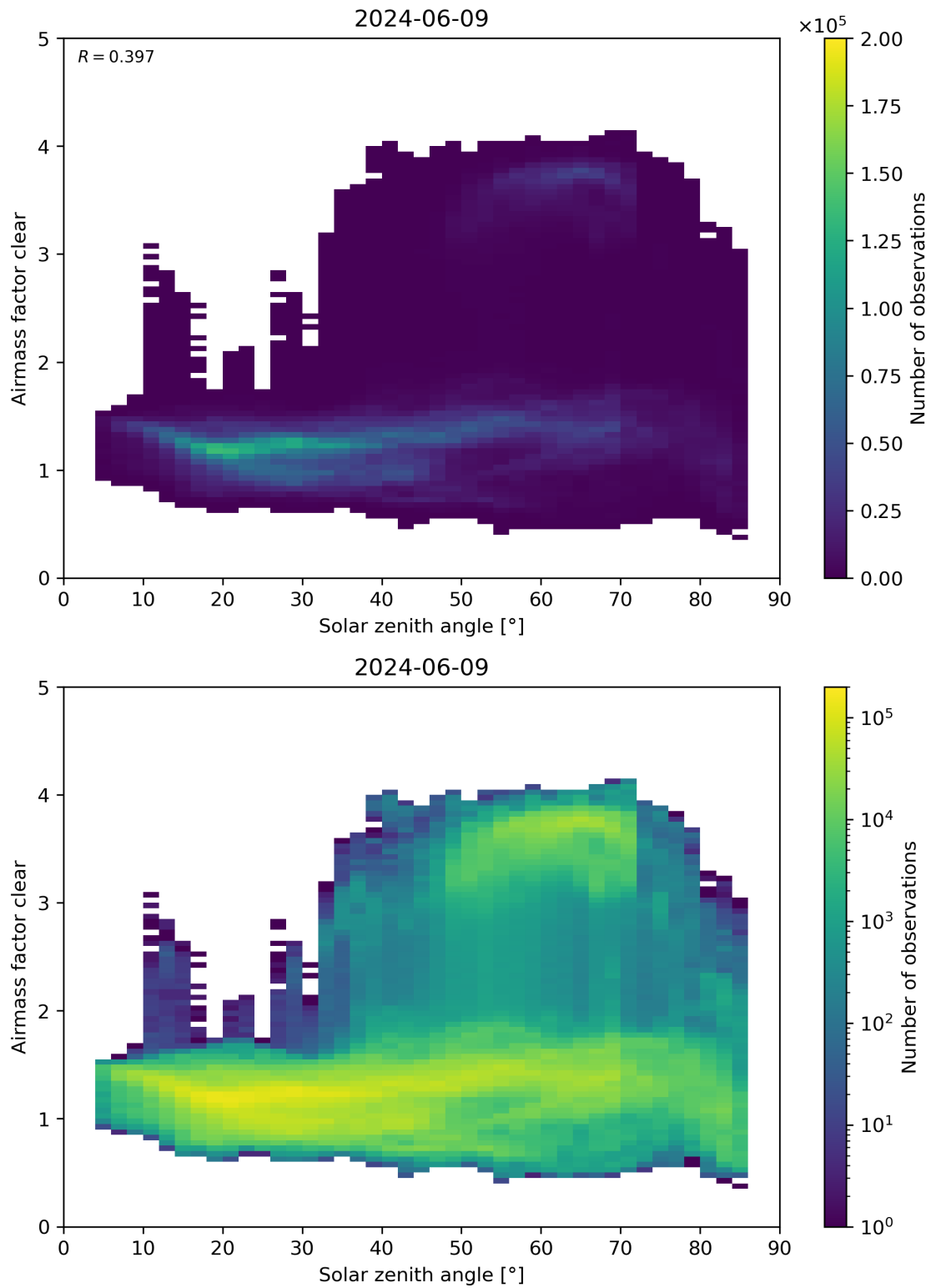
Figure 170: Scatter density plot of “Solar zenith angle” against “Airmass factor clear” for 2024-06-08 to 2024-06-10.
