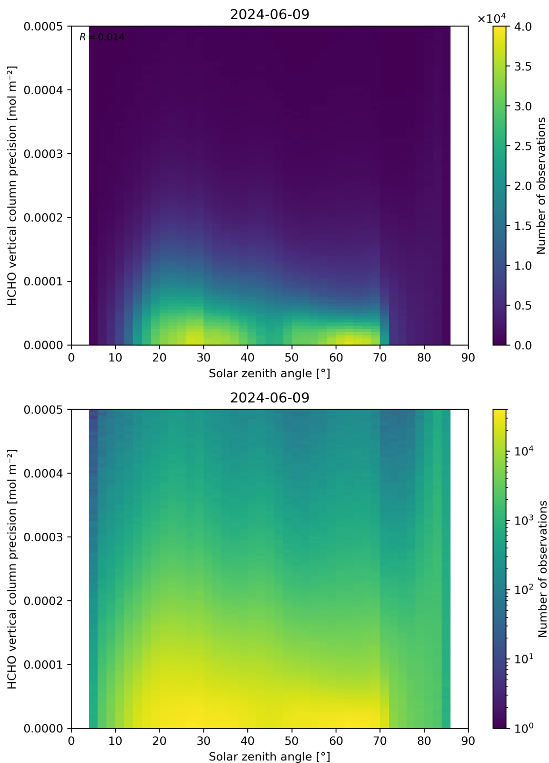
Figure 179: Scatter density plot of “Solar zenith angle” against “HCHO vertical column precision” for 2024-06-08 to 2024-06-10.
