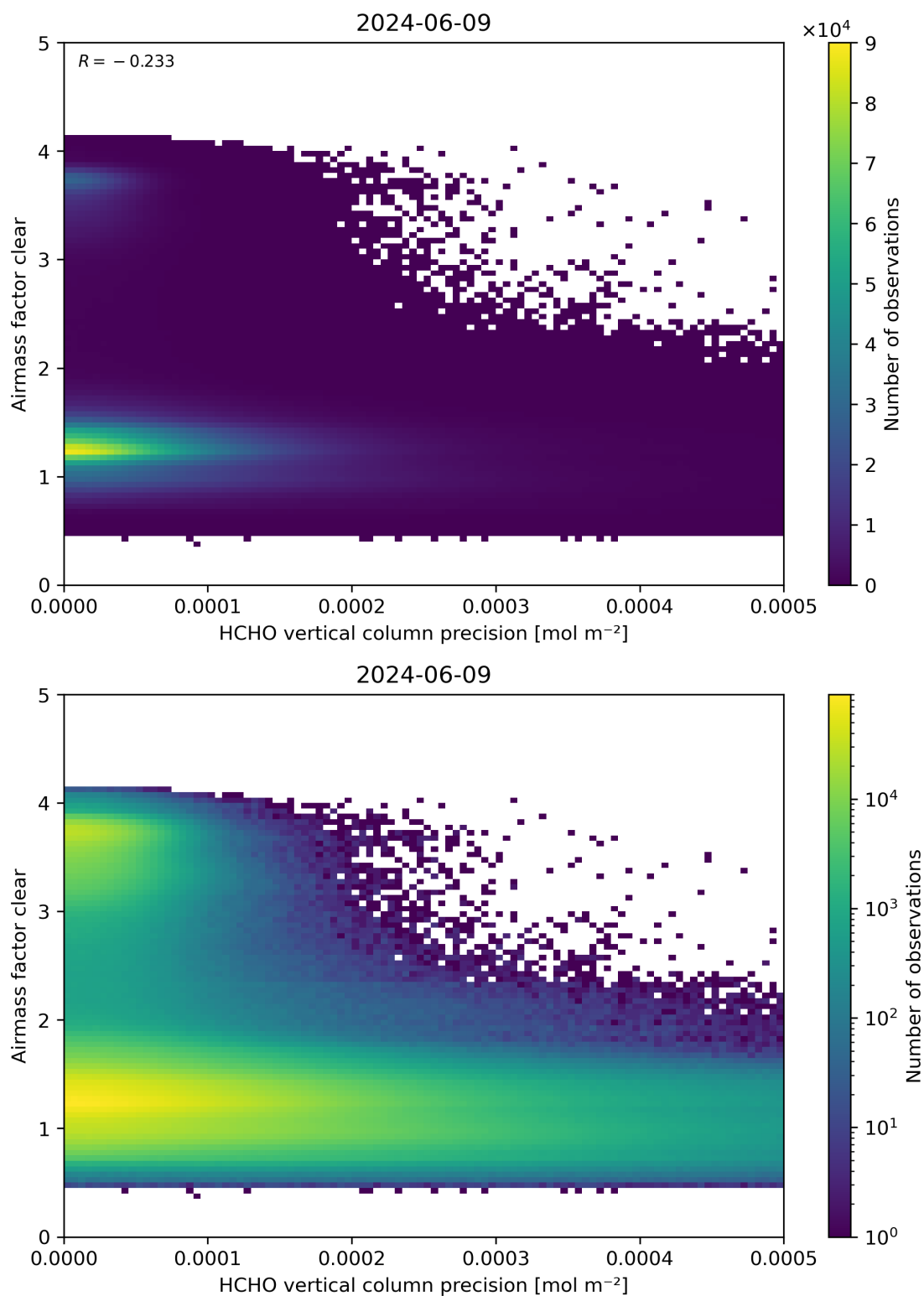
Figure 139: Scatter density plot of “HCHO vertical column precision” against “Airmass factor clear” for 2024-06-08 to 2024-06-10.
