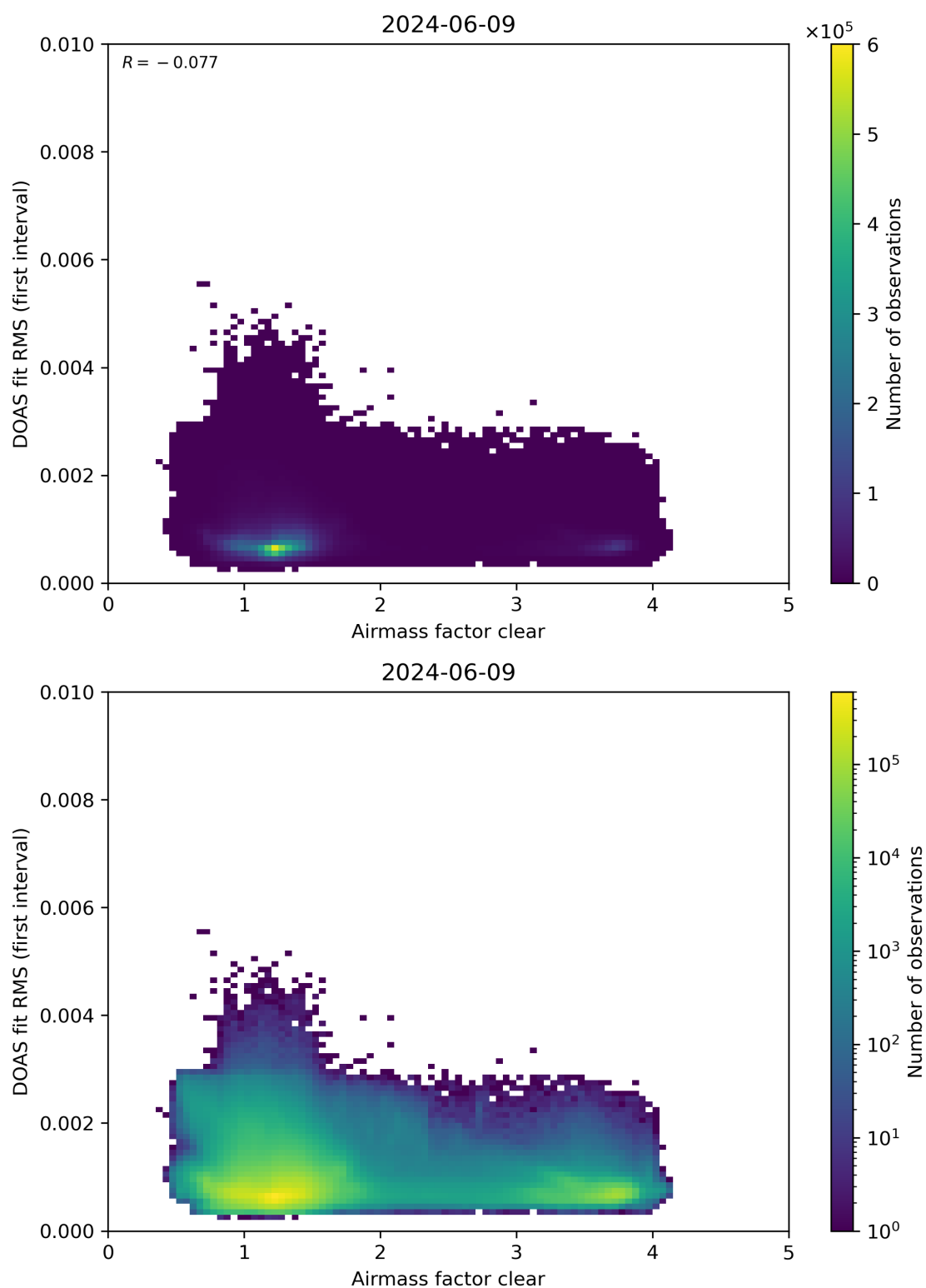
Figure 71: Scatter density plot of “Airmass factor clear” against “DOAS fit RMS (first interval)” for 2024-06-08 to 2024-06-10.
