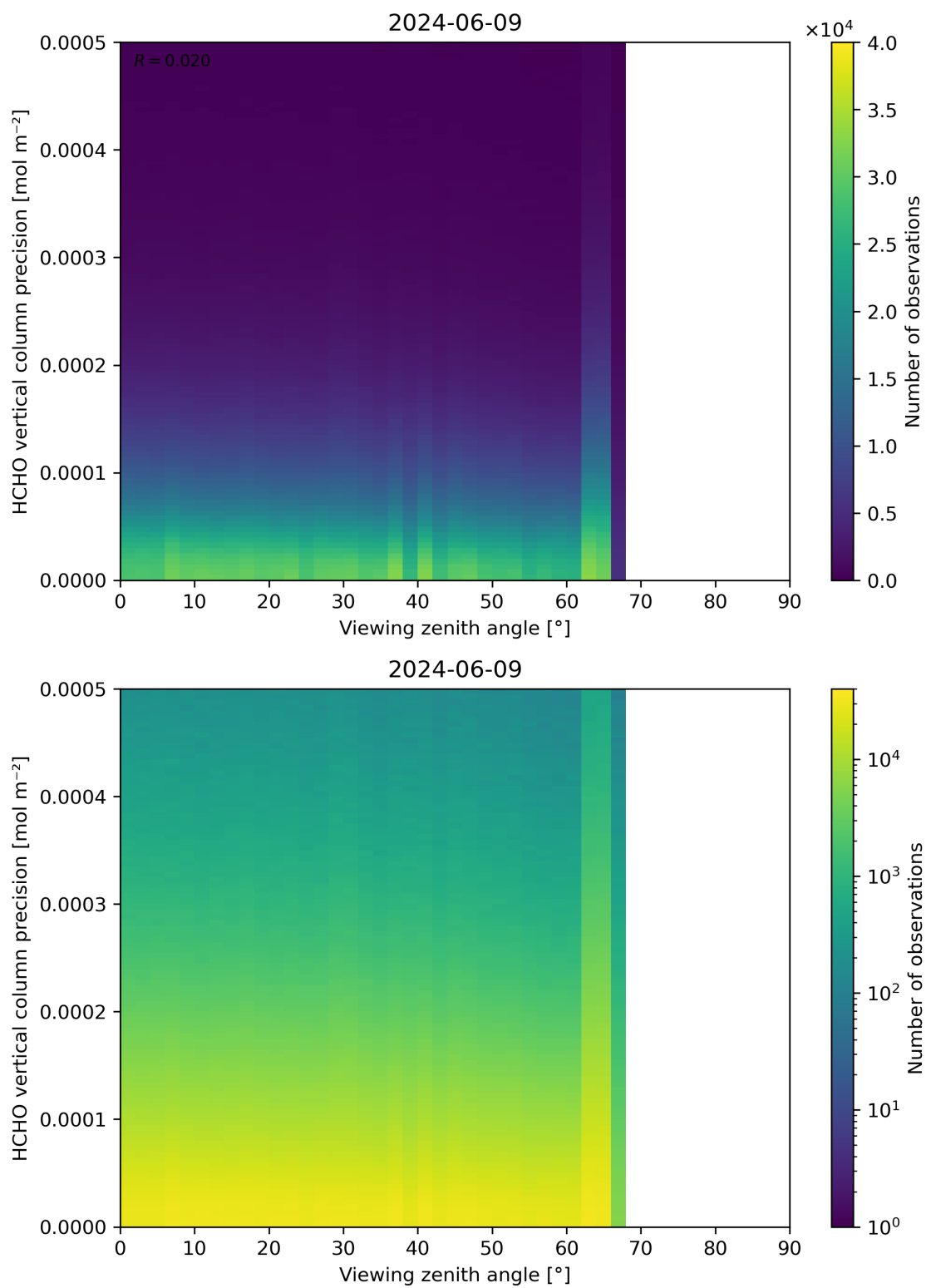
Figure 194: Scatter density plot of “Viewing zenith angle” against “HCHO vertical column precision” for 2024-06-08 to 2024-06-10.
