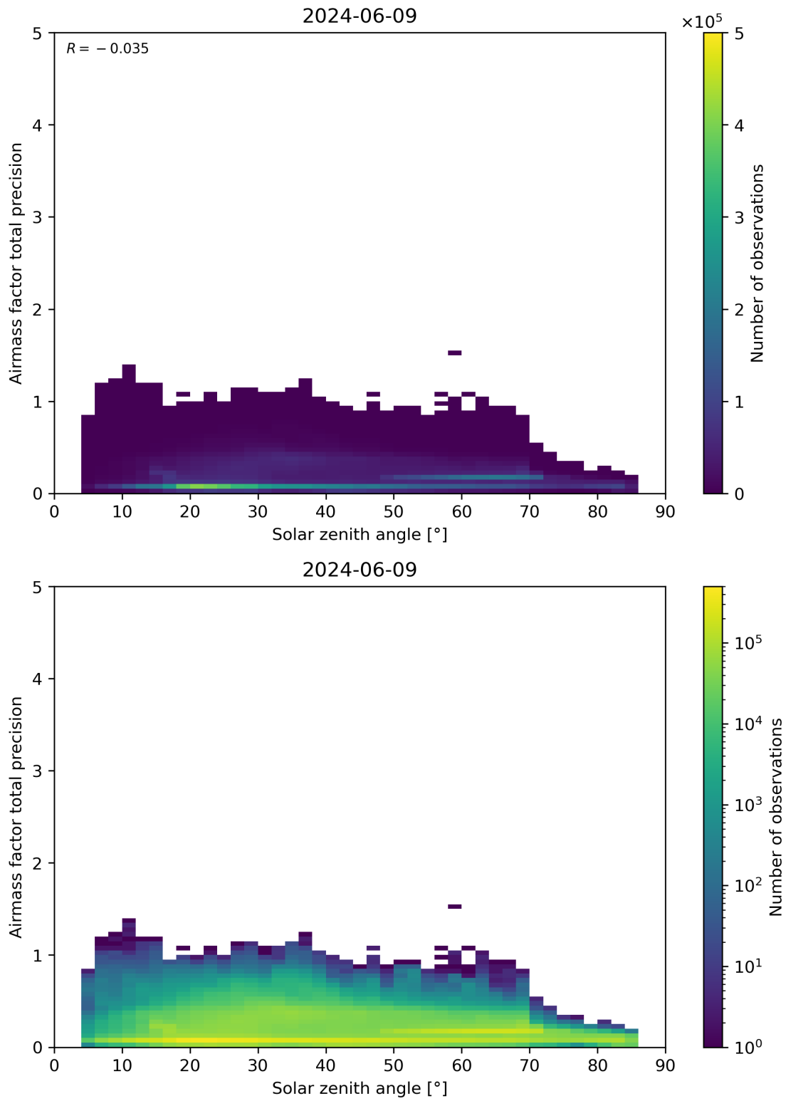
Figure 176: Scatter density plot of “Solar zenith angle” against “Airmass factor total precision” for 2024-06-08 to 2024-06-10.
