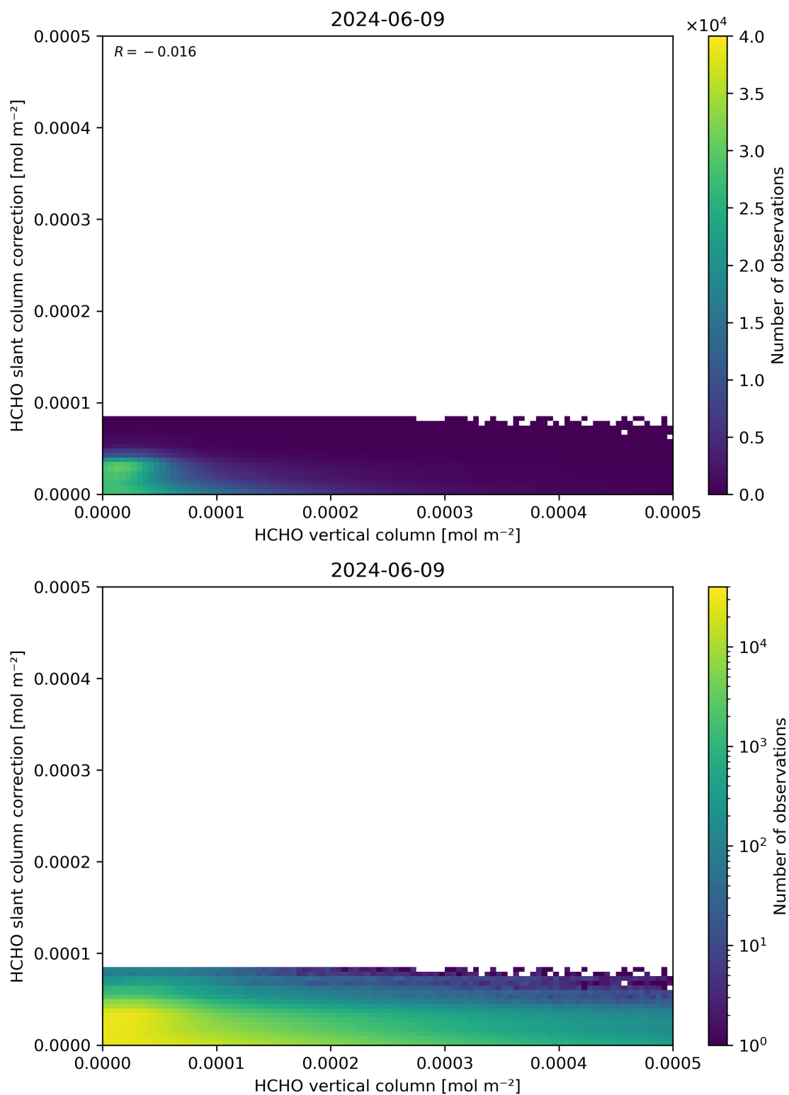
Figure 128: Scatter density plot of “HCHO vertical column” against “HCHO slant column correction” for 2024-06-08 to 2024-06-10.
