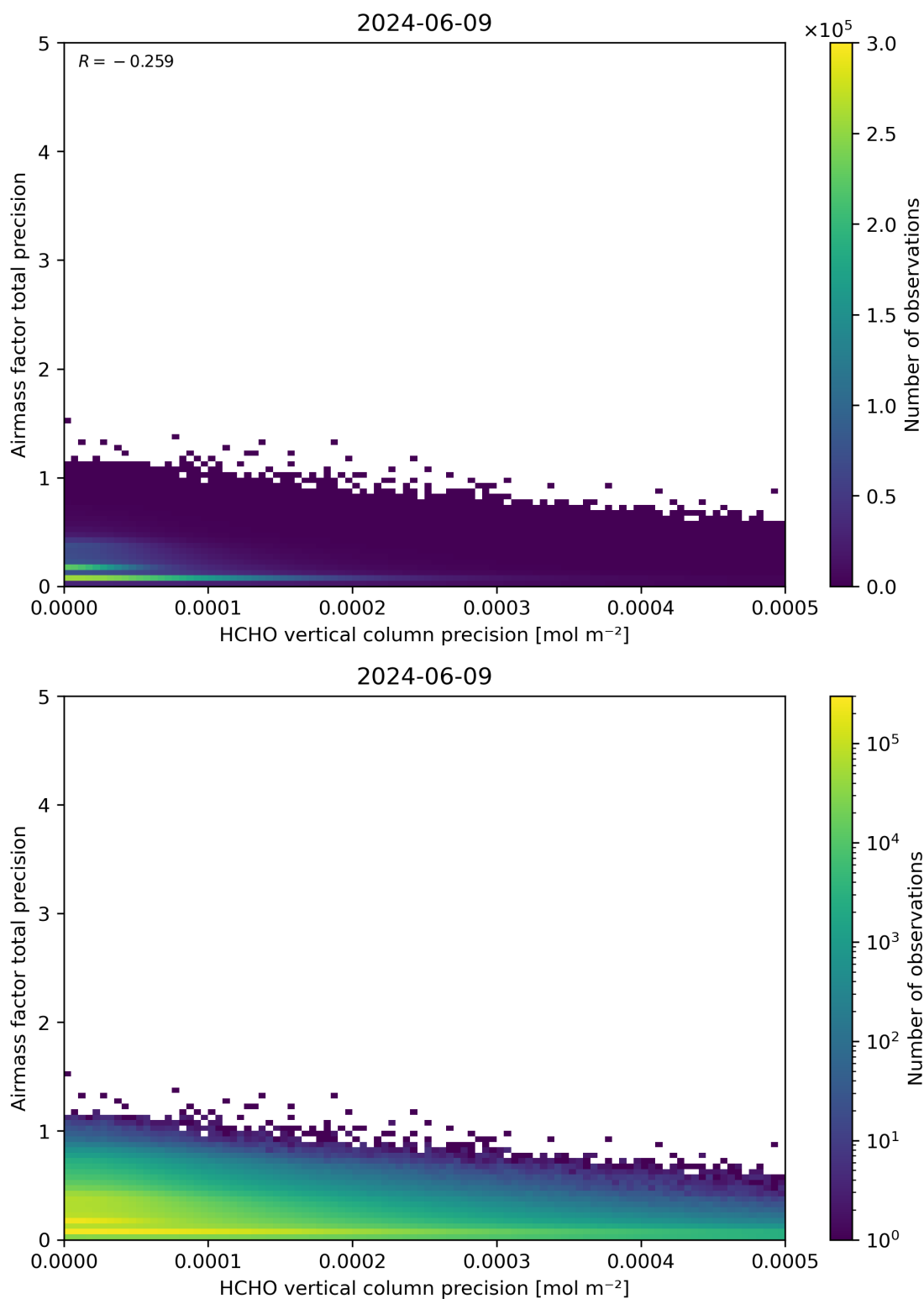
Figure 145: Scatter density plot of “HCHO vertical column precision” against “Airmass factor total precision” for 2024-06-08 to 2024-06-10.
