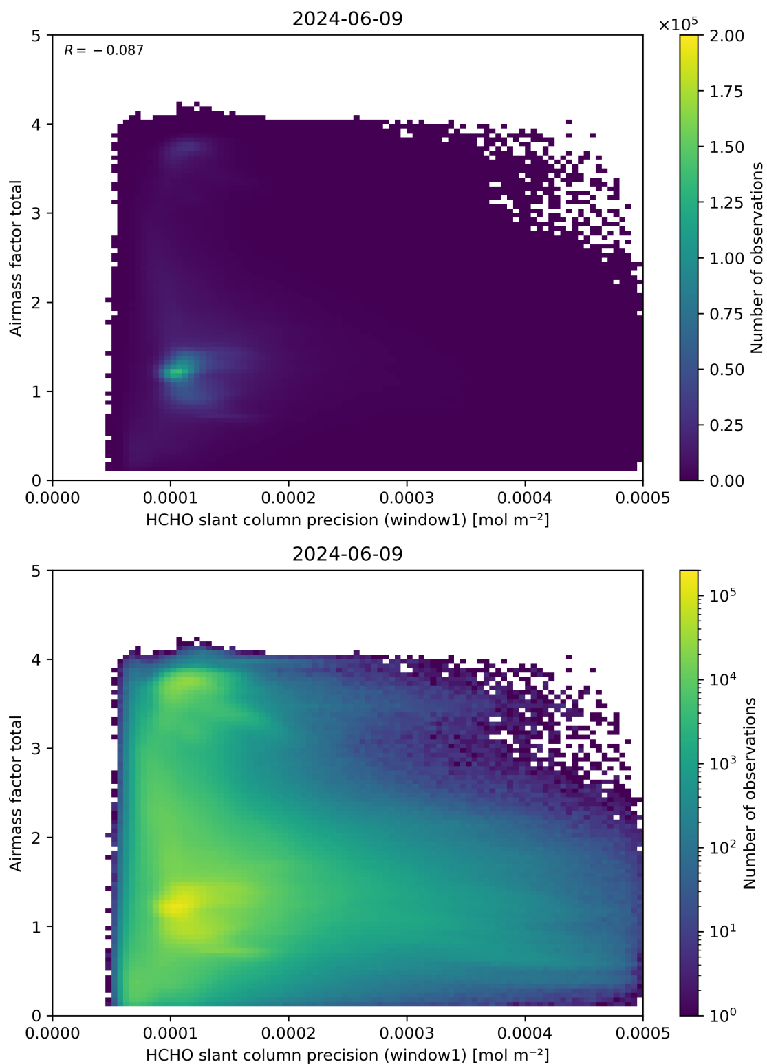
Figure 94: Scatter density plot of “HCHO slant column precision (window1)” against “Airmass factor total” for 2024-06-08 to 2024-06-10.
