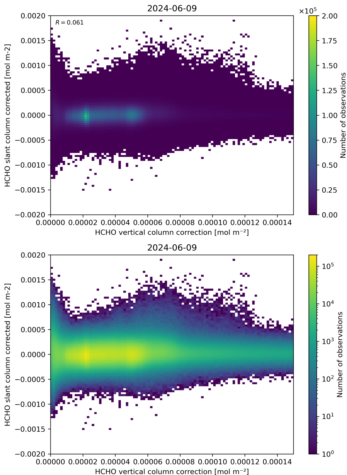
Figure 116: Scatter density plot of “HCHO vertical column correction” against “HCHO slant column corrected” for 2024-06-08 to 2024-06-10.
