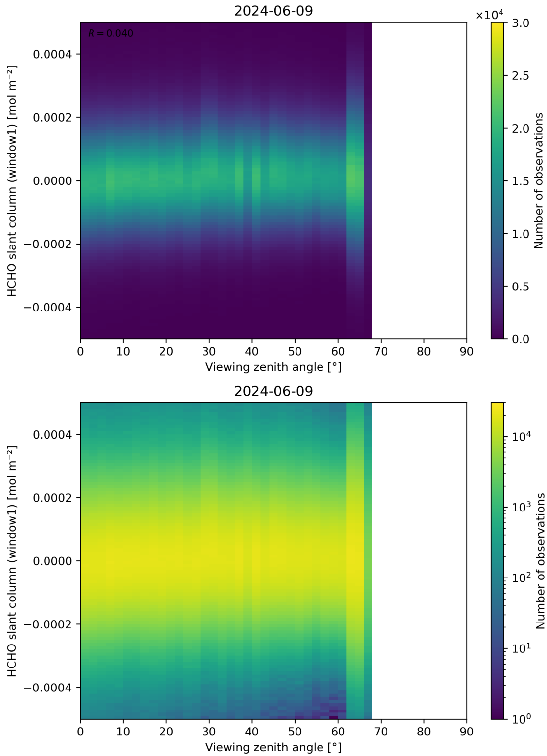
Figure 188: Scatter density plot of “Viewing zenith angle” against “HCHO slant column (window1)” for 2024-06-08 to 2024-06-10.
