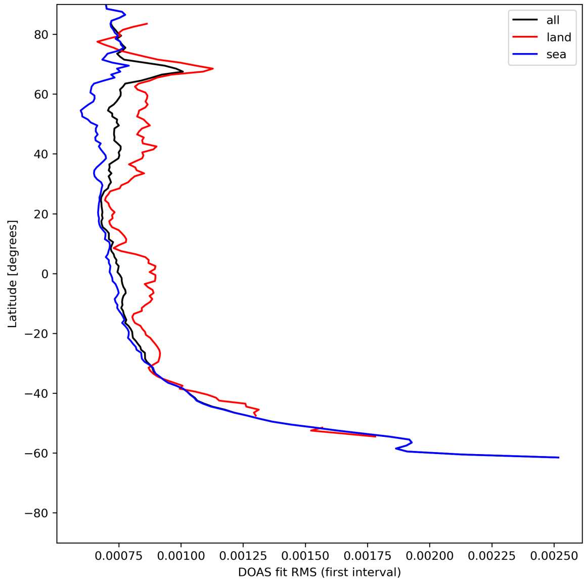
Figure 32: Zonal average of "DOAS fit RMS (first interval)" for 2024-06-08 to 2024-06-10.
