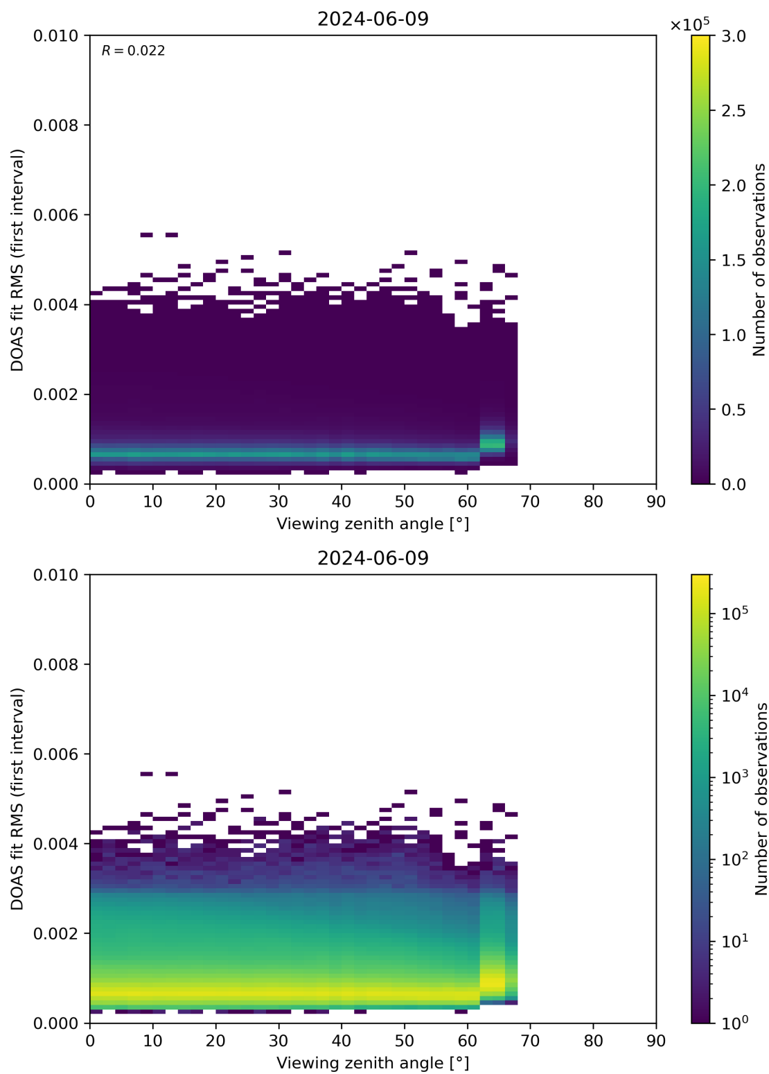
Figure 182: Scatter density plot of “Viewing zenith angle” against “DOAS fit RMS (first interval)” for 2024-06-08 to 2024-06-10.
