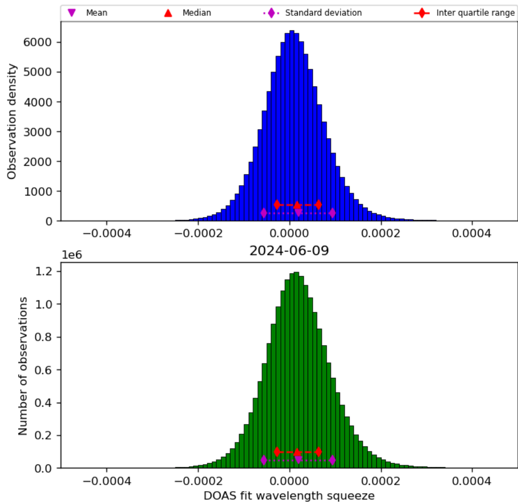
Figure 45: Histogram of “DOAS fit wavelength squeeze” for 2024-06-08 to 2024-06-10
