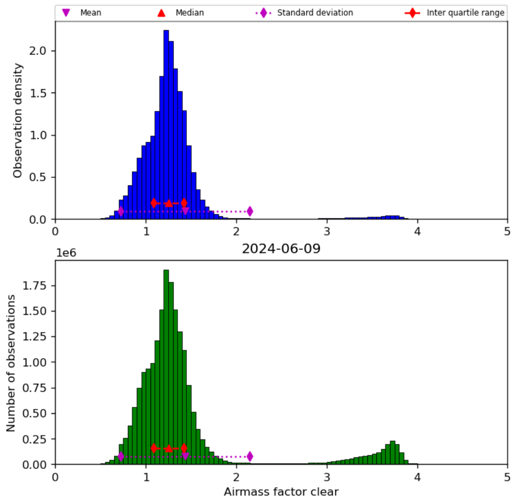
Figure 42: Histogram of “Airmass factor clear” for 2024-06-08 to 2024-06-10
