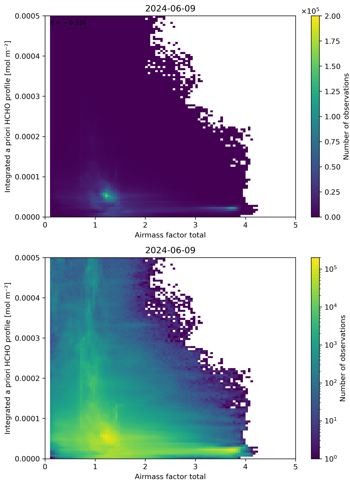
Figure 104: Scatter density plot of “Air mass factor total” against “Integrated a priori HCHO profile” for 2024-06-08 to 2024-06-10.
