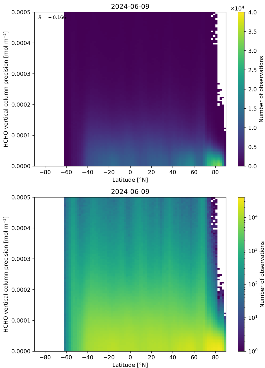
Figure 165: Scatter density plot of “Latitude” against “HCHO vertical column precision” for 2024-06-08 to 2024-06-10.
