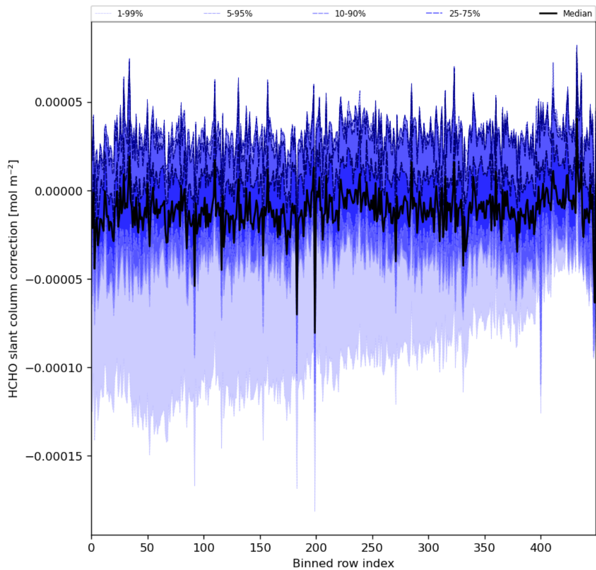
Figure 61: Along track statistics of “HCHO slant column correction” for 2024-06-08 to 2024-06-10
