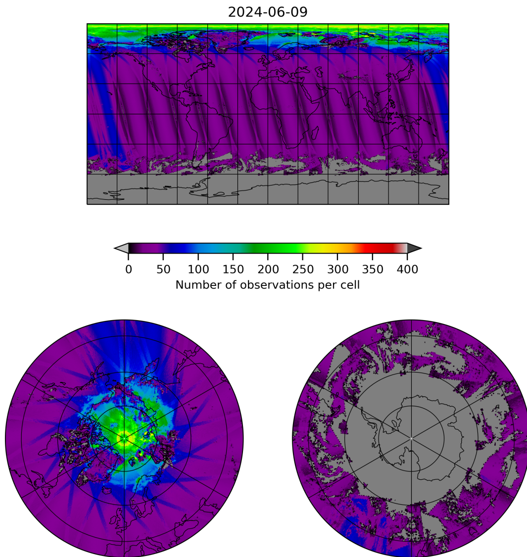
Figure 19: Map of the number of observations for 2024-06-08 to 2024-06-10
