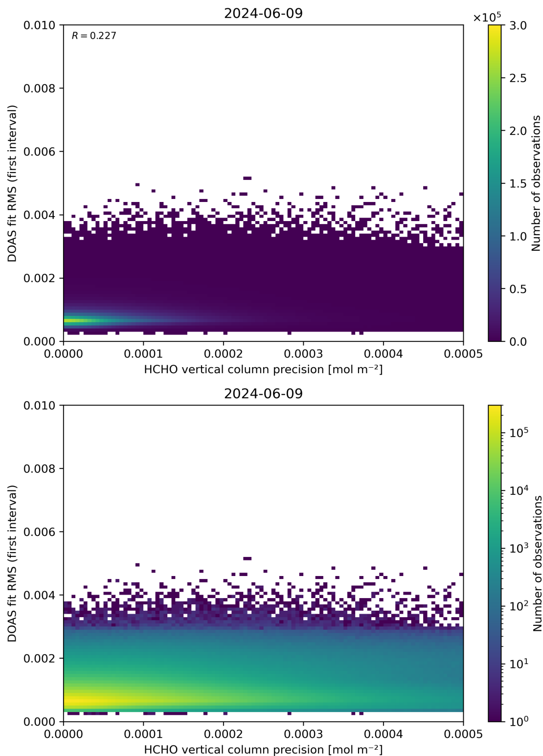
Figure 136: Scatter density plot of “HCHO vertical column precision” against “DOAS fit RMS (first interval)” for 2024-06-08 to 2024-06-10.
