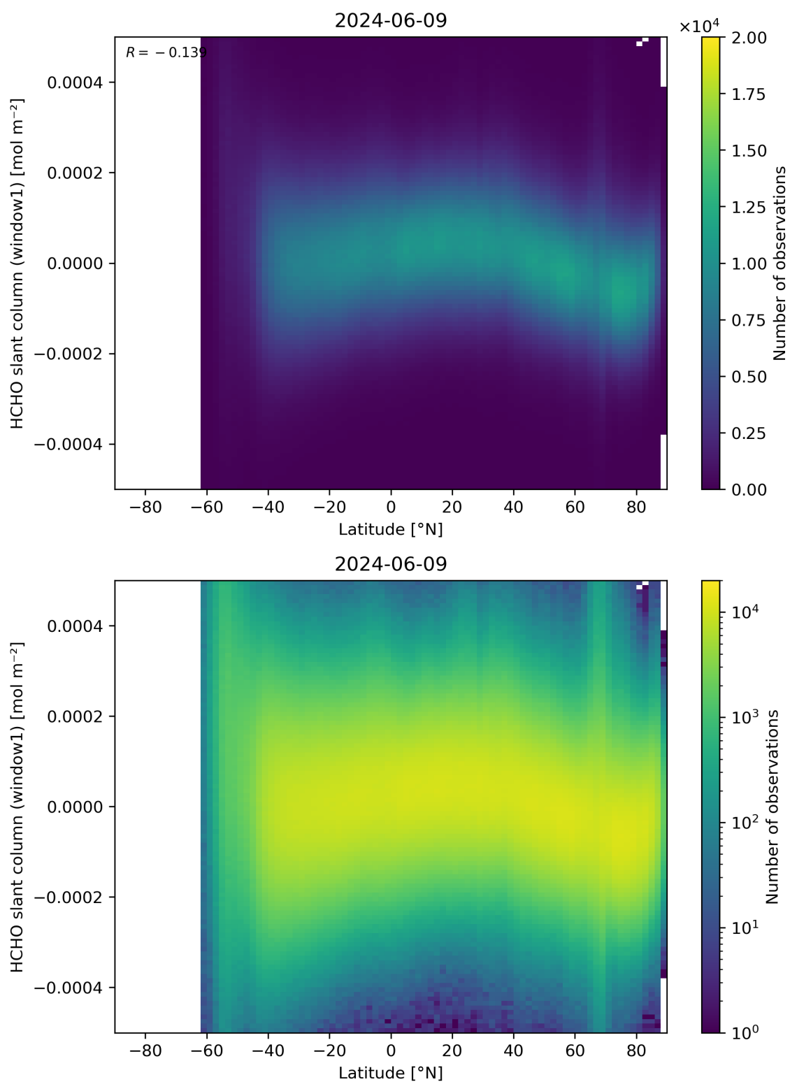
Figure 159: Scatter density plot of “Latitude” against “HCHO slant column (window1)” for 2024-06-08 to 2024-06-10.
