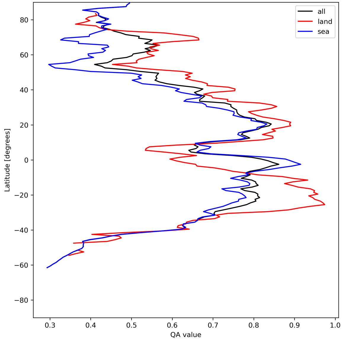
Figure 20: Zonal average of “QA value” for 2024-06-08 to 2024-06-10.
