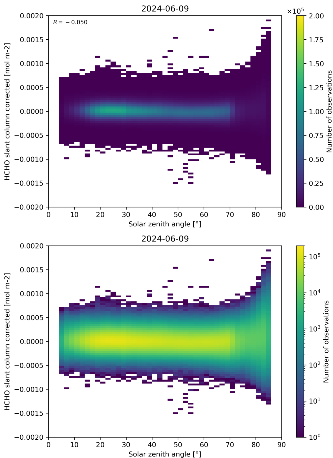
Figure 171: Scatter density plot of “Solar zenith angle” against “HCHO slant column corrected” for 2024-06-08 to 2024-06-10.
