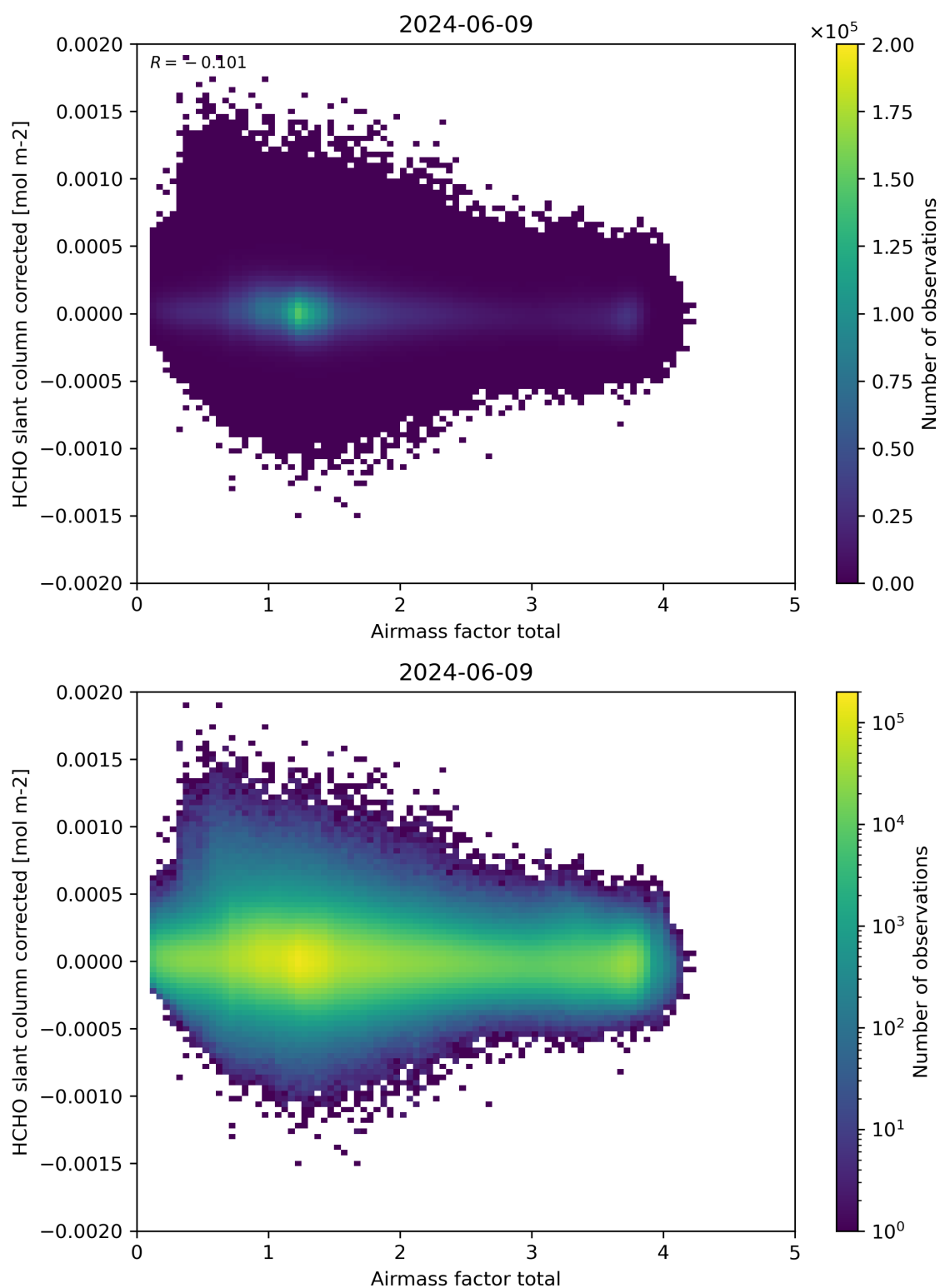
Figure 101: Scatter density plot of “Airmass factor total” against “HCHO slant column corrected” for 2024-06-08 to 2024-06-10.
