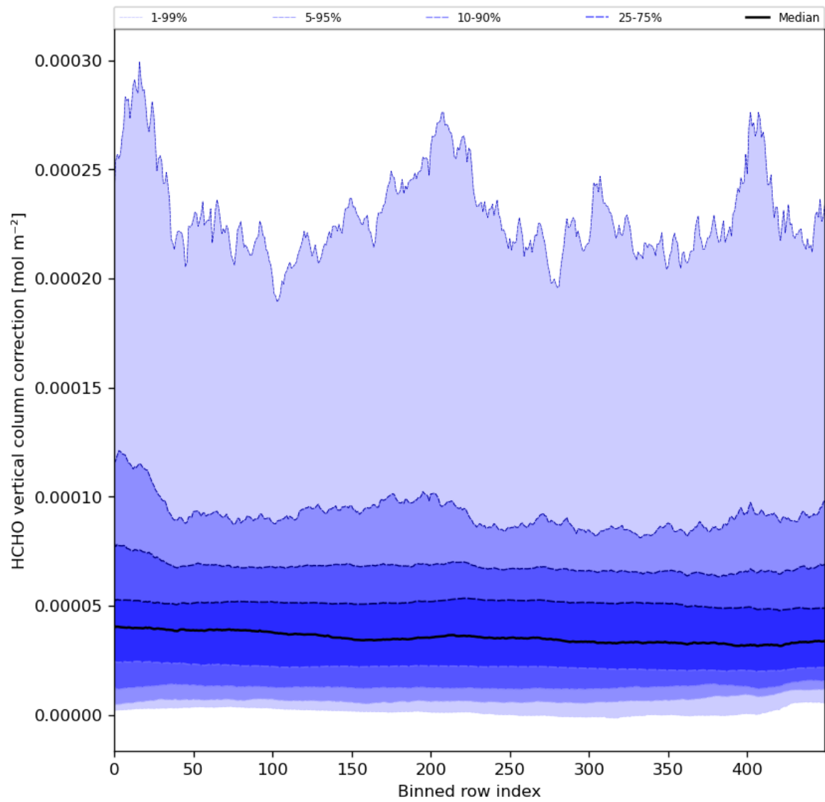
Figure 51: Along track statistics of "HCHO vertical column correction" for 2024-06-08 to 2024-06-10
