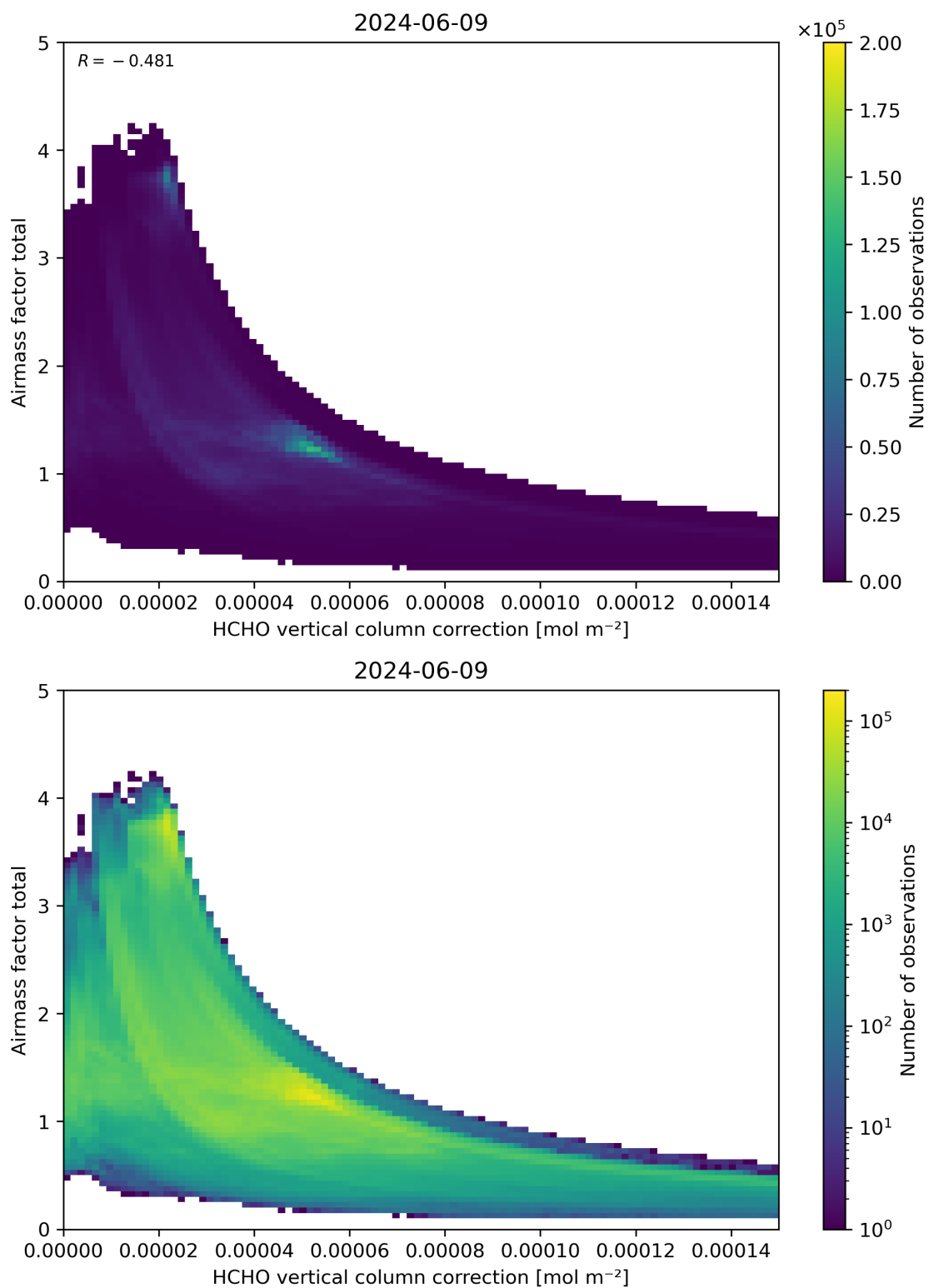
Figure 120: Scatter density plot of “HCHO vertical column correction” against “Airmass factor total” for 2024-06-08 to 2024-06-10.
