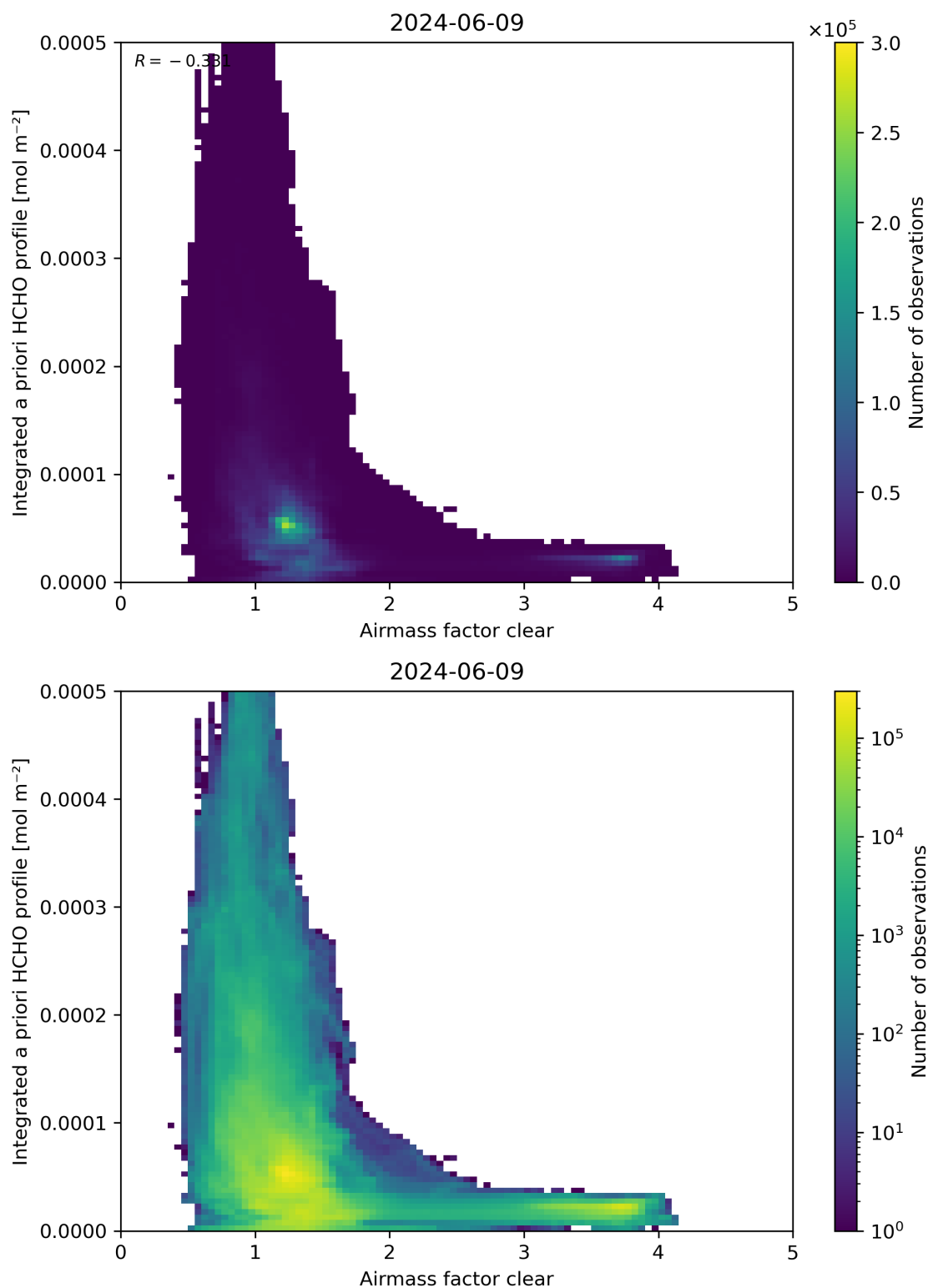
Figure 76: Scatter density plot of “Airmass factor clear” against “Integrated a priori HCHO profile” for 2024-06-08 to 2024-06-10.
