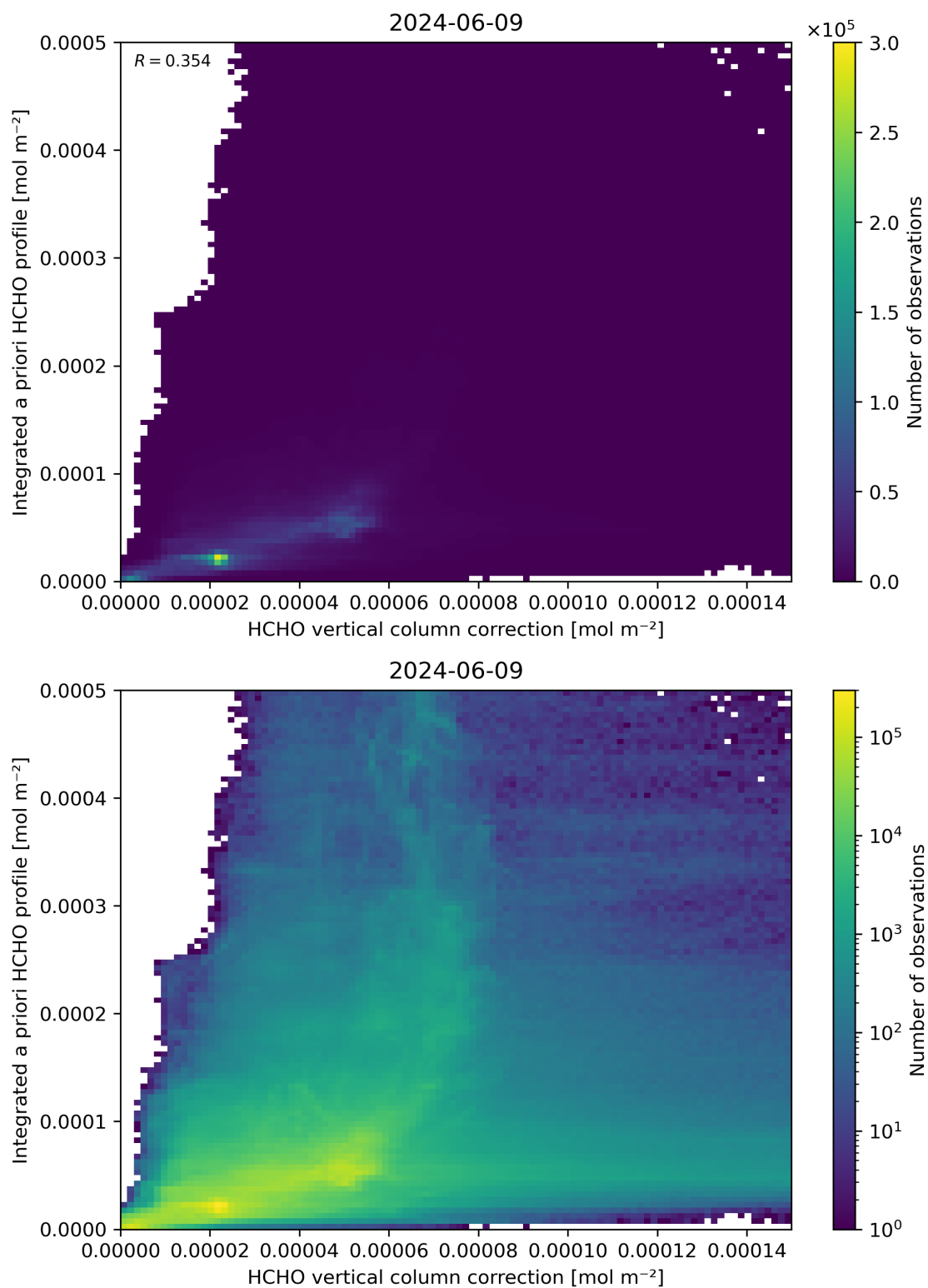
Figure 122: Scatter density plot of “HCHO vertical column correction” against “Integrated a priori HCHO profile” for 2024-06-08 to 2024-06-10.
