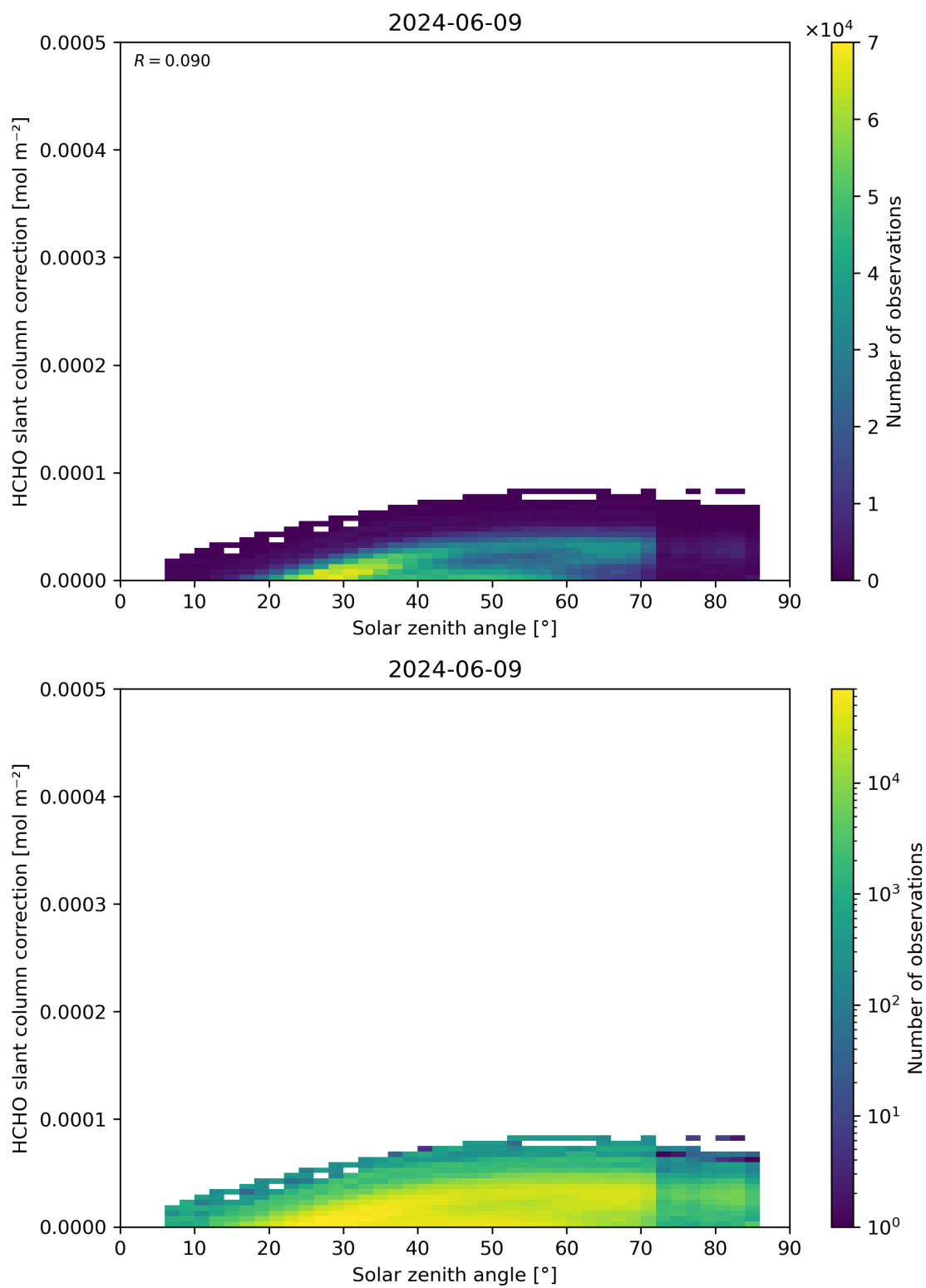
Figure 172: Scatter density plot of “Solar zenith angle” against “HCHO slant column correction” for 2024-06-08 to 2024-06-10.
