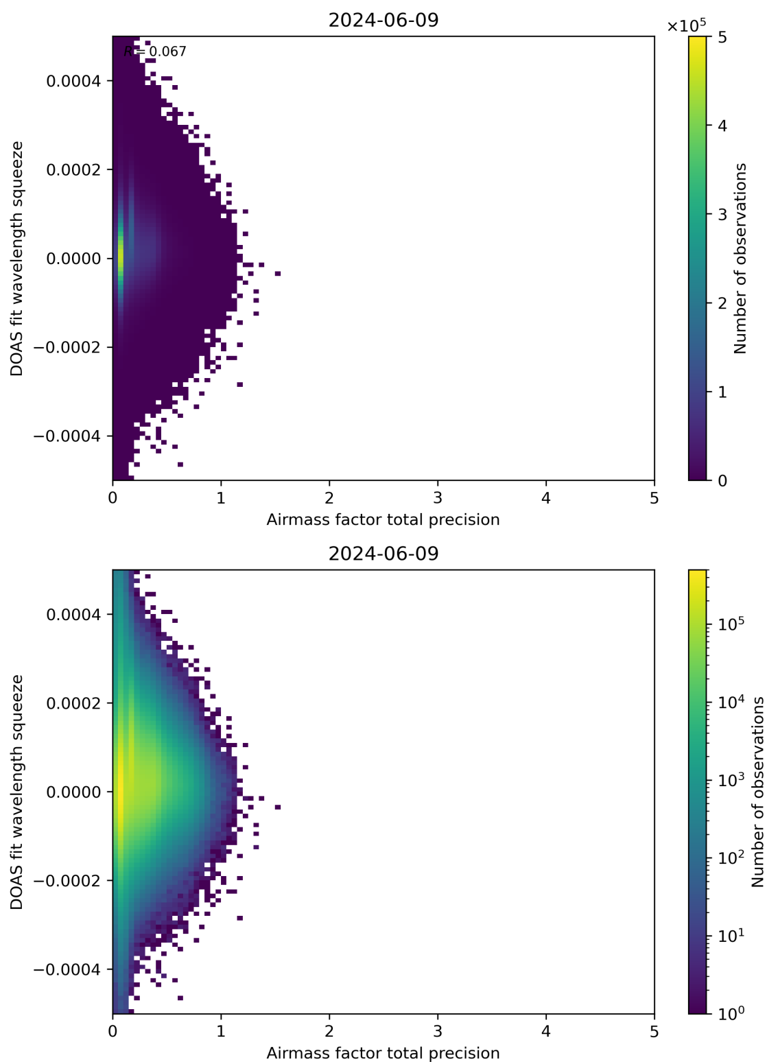
Figure 107: Scatter density plot of “Airmass factor total precision” against “DOAS fit wavelength squeeze” for 2024-06-08 to 2024-06-10.
