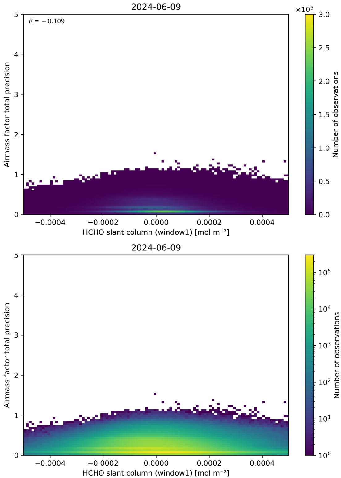
Figure 86: Scatter density plot of “HCHO slant column (window1)” against “Airmass factor total precision” for 2024-06-08 to 2024-06-10.
