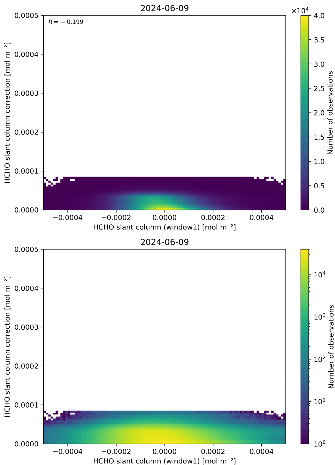
Figure 83: Scatter density plot of “HCHO slant column (window1)” against “HCHO slant column correction” for 2024-06-08 to 2024-06-10.
