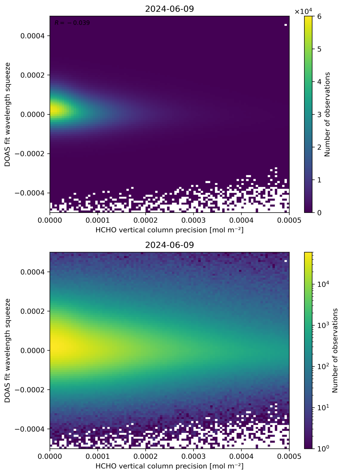
Figure 138: Scatter density plot of “HCHO vertical column precision” against “DOAS fit wavelength squeeze” for 2024-06-08 to 2024-06-10.
