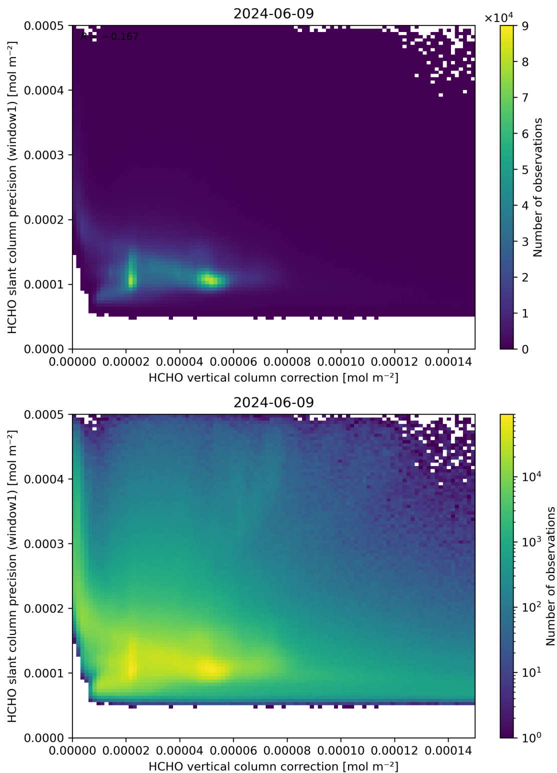
Figure 119: Scatter density plot of “HCHO vertical column correction” against “HCHO slant column precision (window1)” for 2024-06-08 to 2024-06-10.
