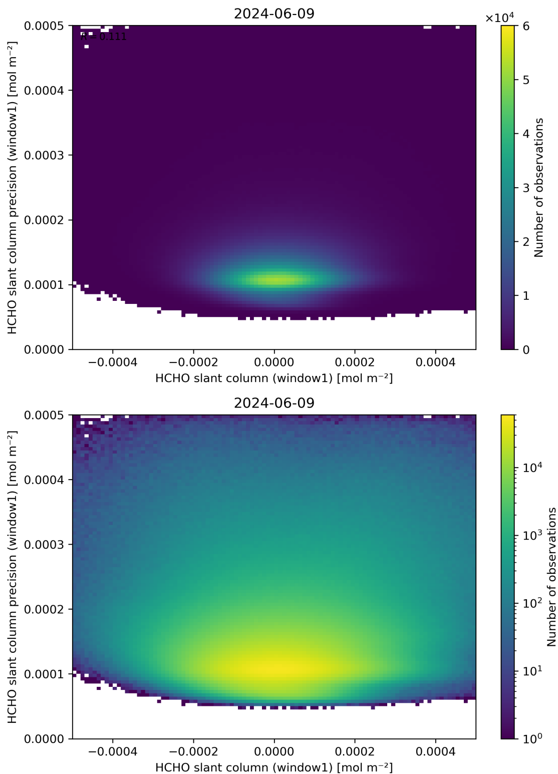
Figure 84: Scatter density plot of “HCHO slant column (window1)” against “HCHO slant column precision (window1)” for 2024-06-08 to 2024-06-10.
