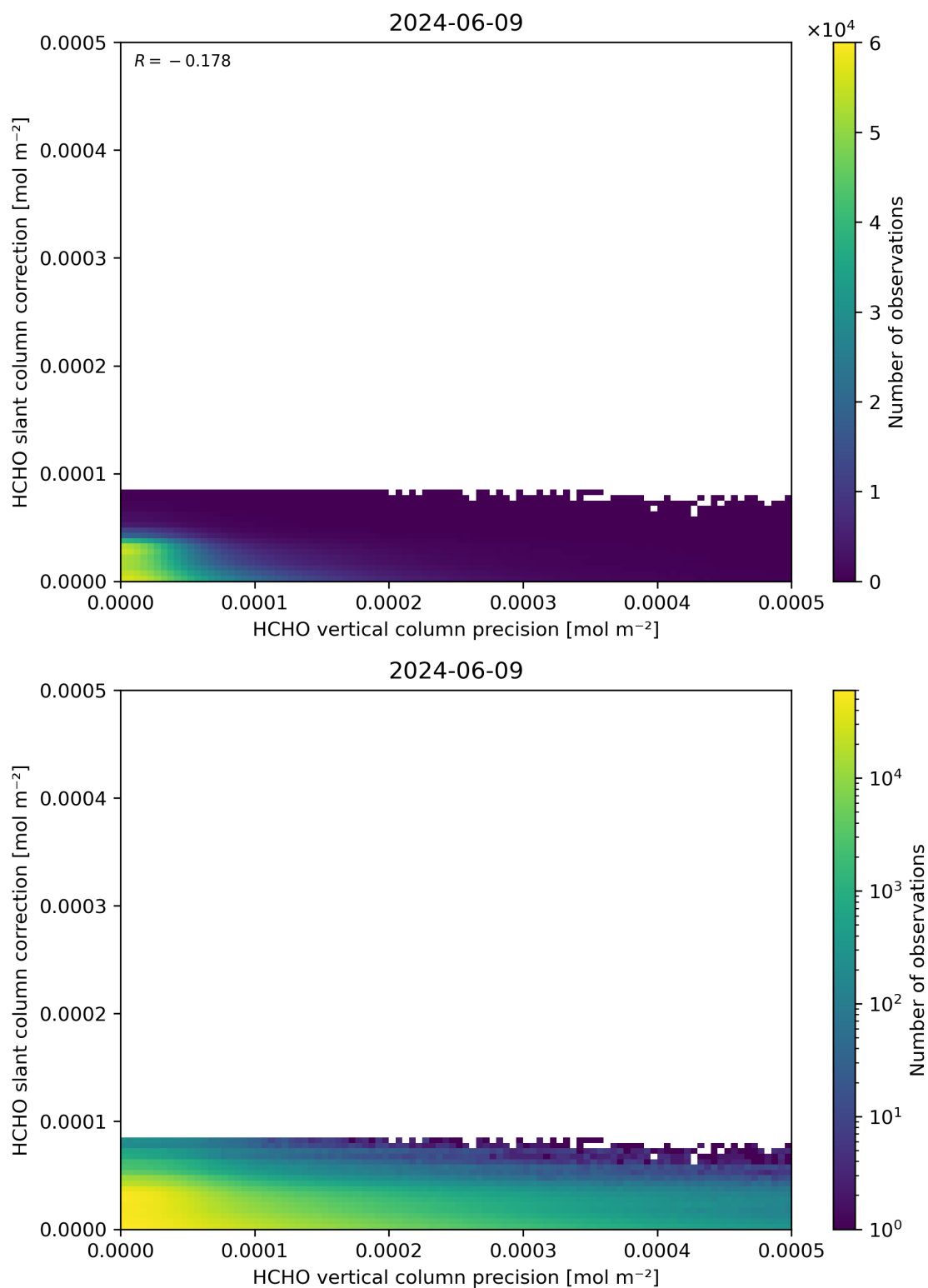
Figure 141: Scatter density plot of “HCHO vertical column precision” against “HCHO slant column correction” for 2024-06-08 to 2024-06-10.
