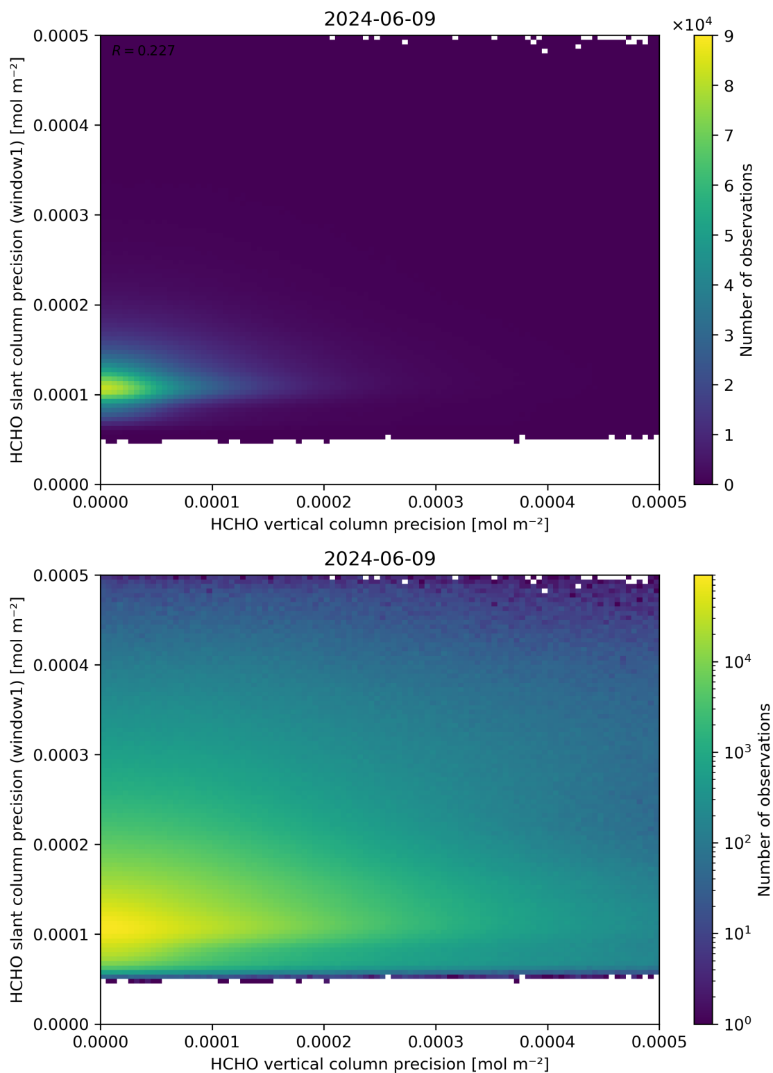
Figure 143: Scatter density plot of “HCHO vertical column precision” against “HCHO slant column precision (window1)” for 2024-06-08 to 2024-06-10.
