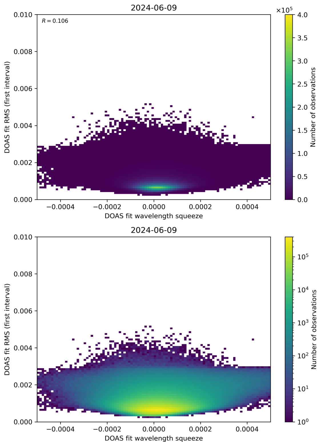
Figure 68: Scatter density plot of “DOAS fit wavelength squeeze” against “DOAS fit RMS (first interval)” for 2024-06-08 to 2024-06-10.
