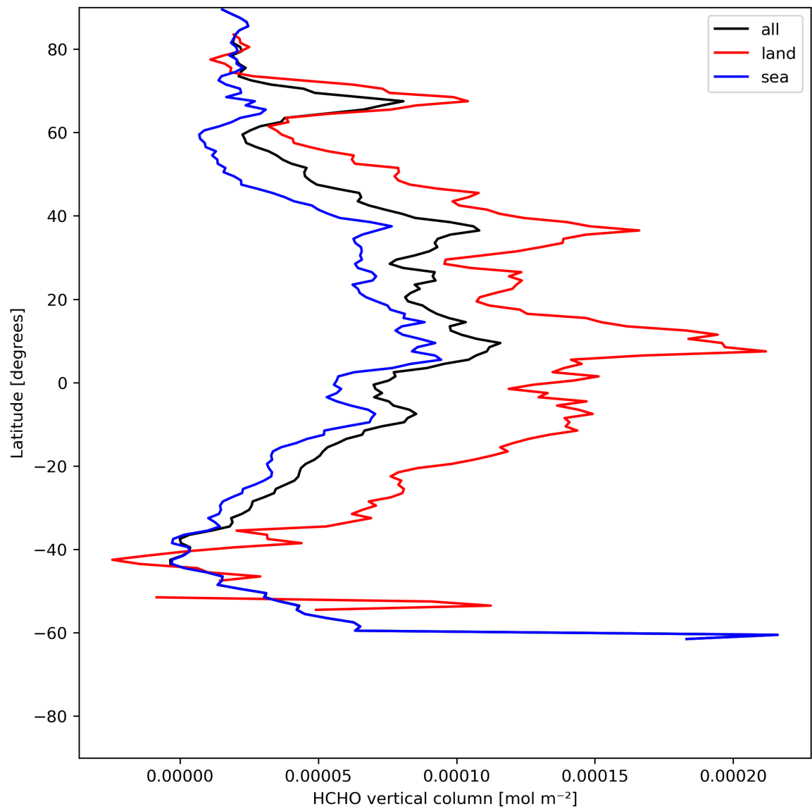
Figure 21: Zonal average of “HCHO vertical column” for 2024-06-08 to 2024-06-10.
