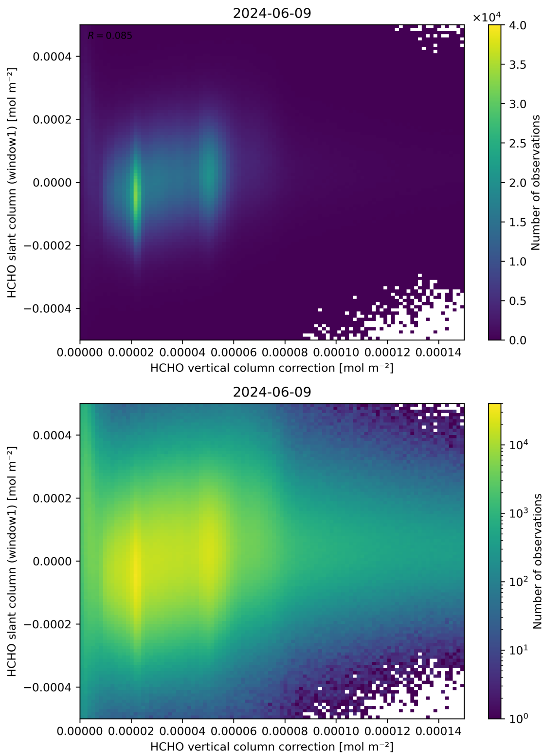
Figure 118: Scatter density plot of “HCHO vertical column correction” against “HCHO slant column (window1)” for 2024-06-08 to 2024-06-10.
