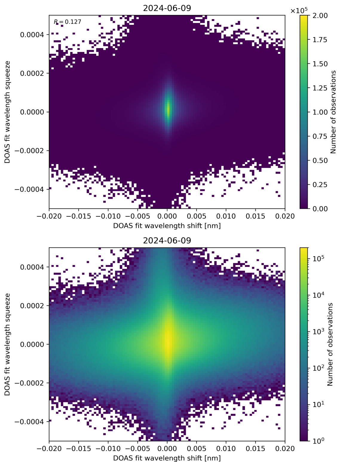
Figure 65: Scatter density plot of “DOAS fit wavelength shift” against “DOAS fit wavelength squeeze” for 2024-06-08 to 2024-06-10.
