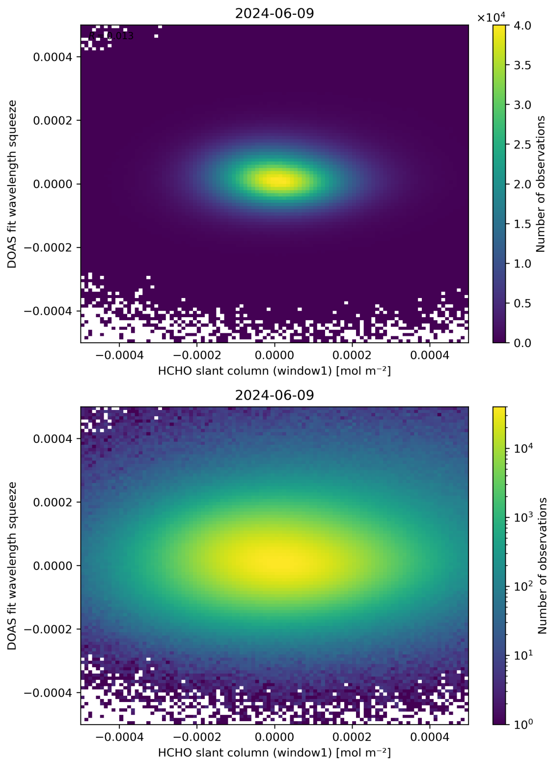
Figure 80: Scatter density plot of “HCHO slant column (window1)” against “DOAS fit wavelength squeeze” for 2024-06-08 to 2024-06-10.
