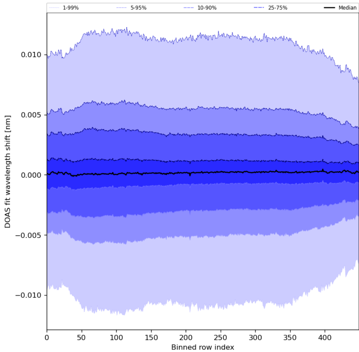
Figure 58: Along track statistics of “DOAS fit wavelength shift” for 2024-06-08 to 2024-06-10
