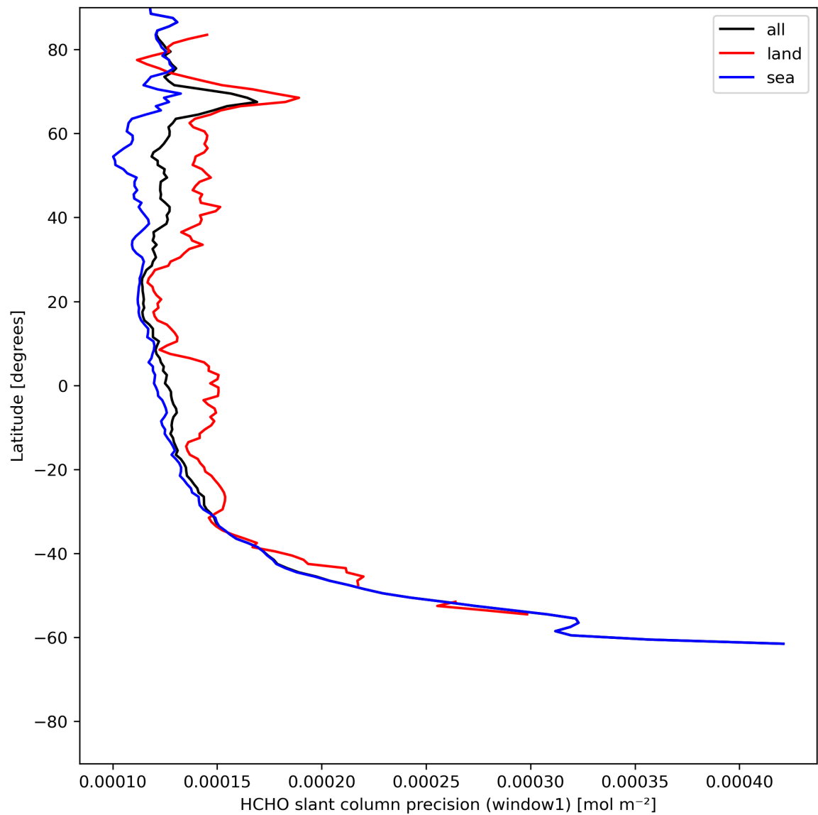
Figure 25: Zonal average of “HCHO slant column precision (window1)” for 2024-06-08 to 2024-06-10.
