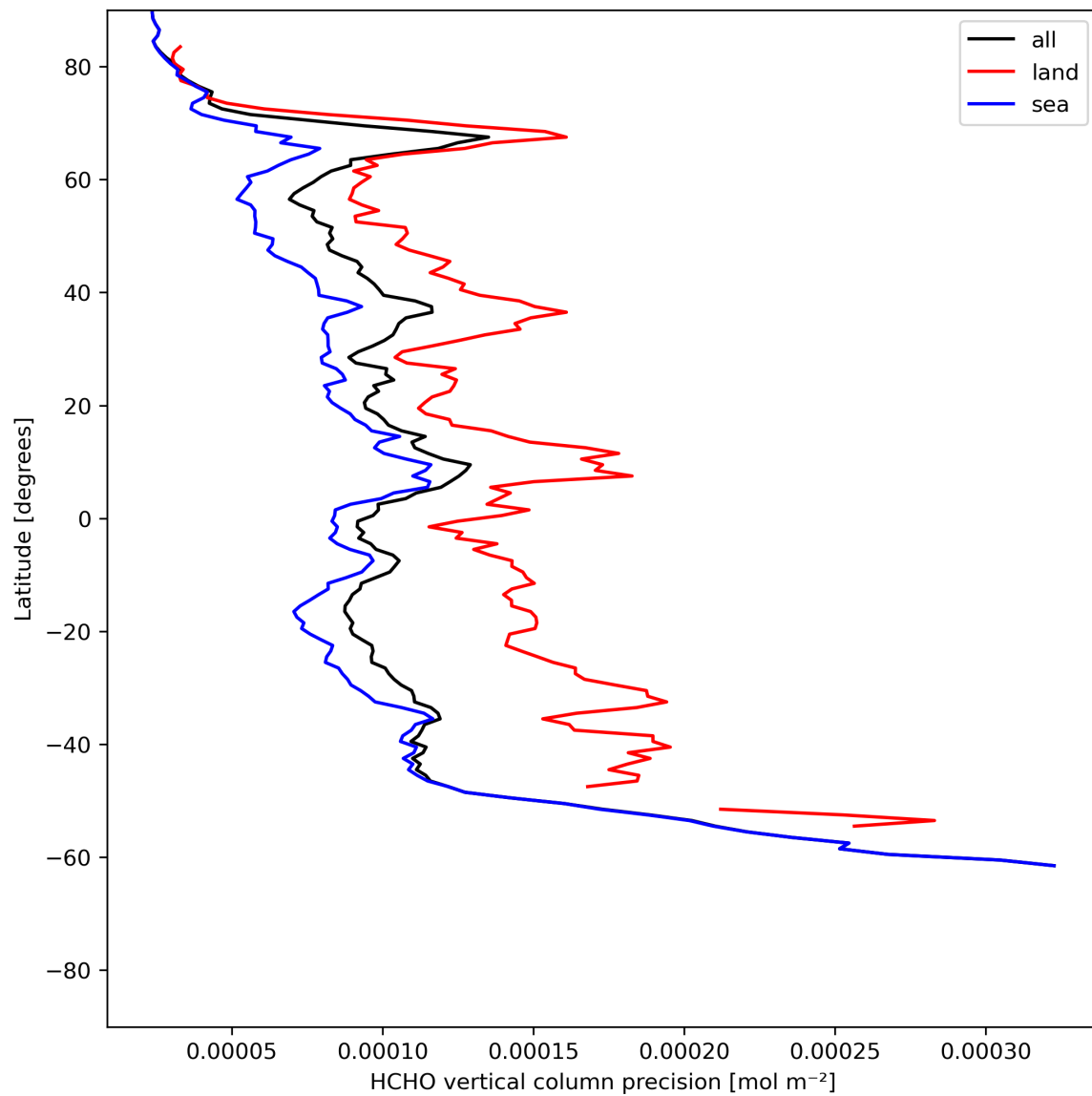
Figure 22: Zonal average of “HCHO vertical column precision” for 2024-06-08 to 2024-06-10.
