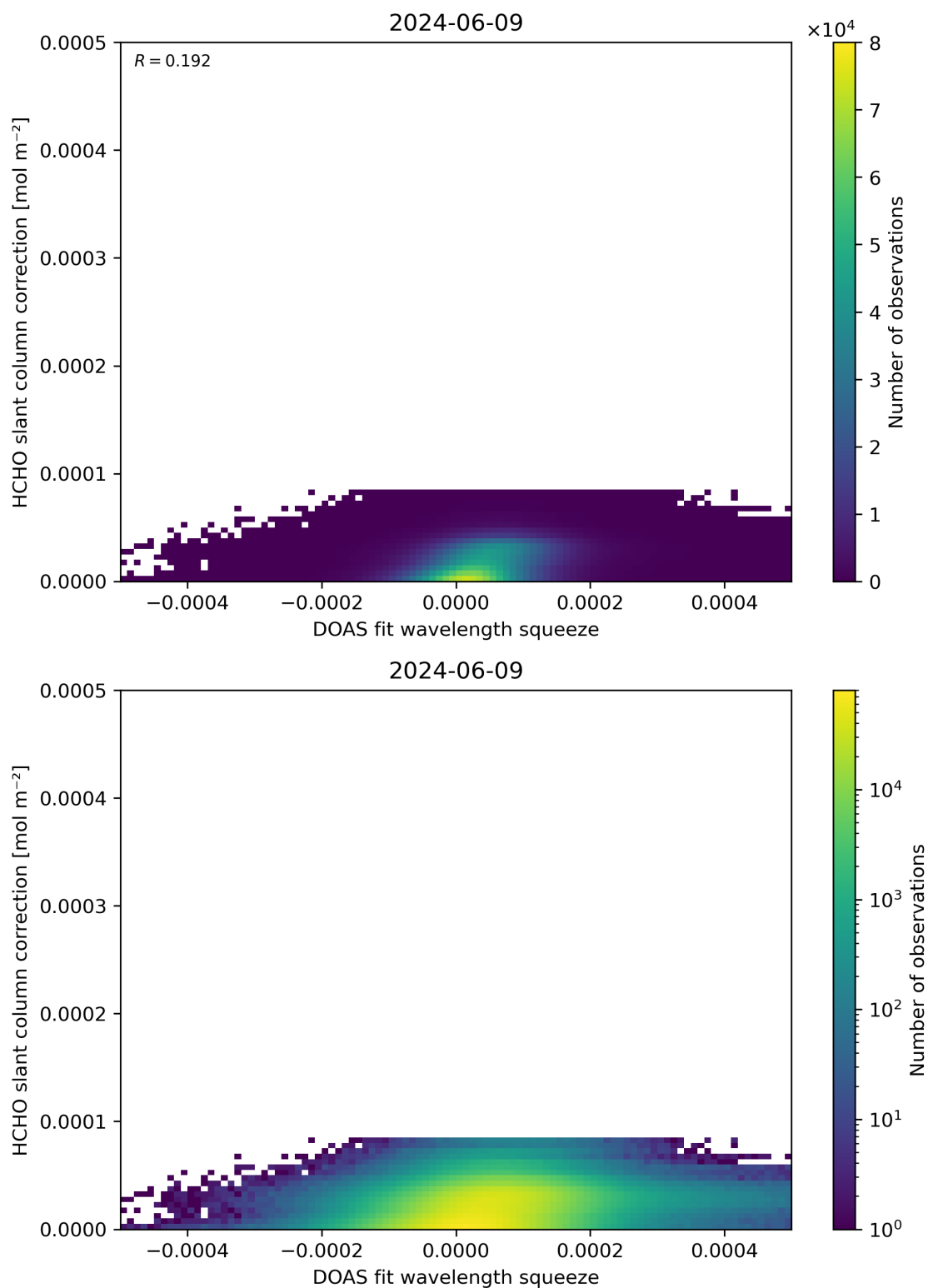
Figure 70: Scatter density plot of “DOAS fit wavelength squeeze” against “HCHO slant column correction” for 2024-06-08 to 2024-06-10.
