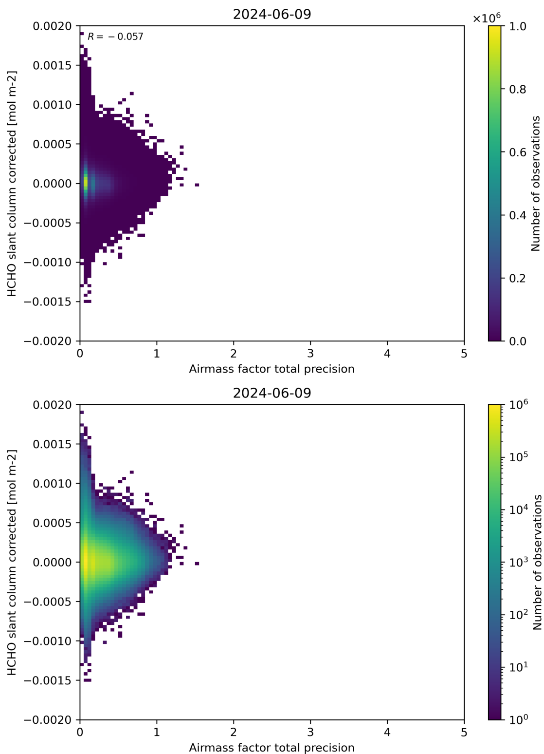
Figure 109: Scatter density plot of “Airmass factor total precision” against “HCHO slant column corrected” for 2024-06-08 to 2024-06-10.
