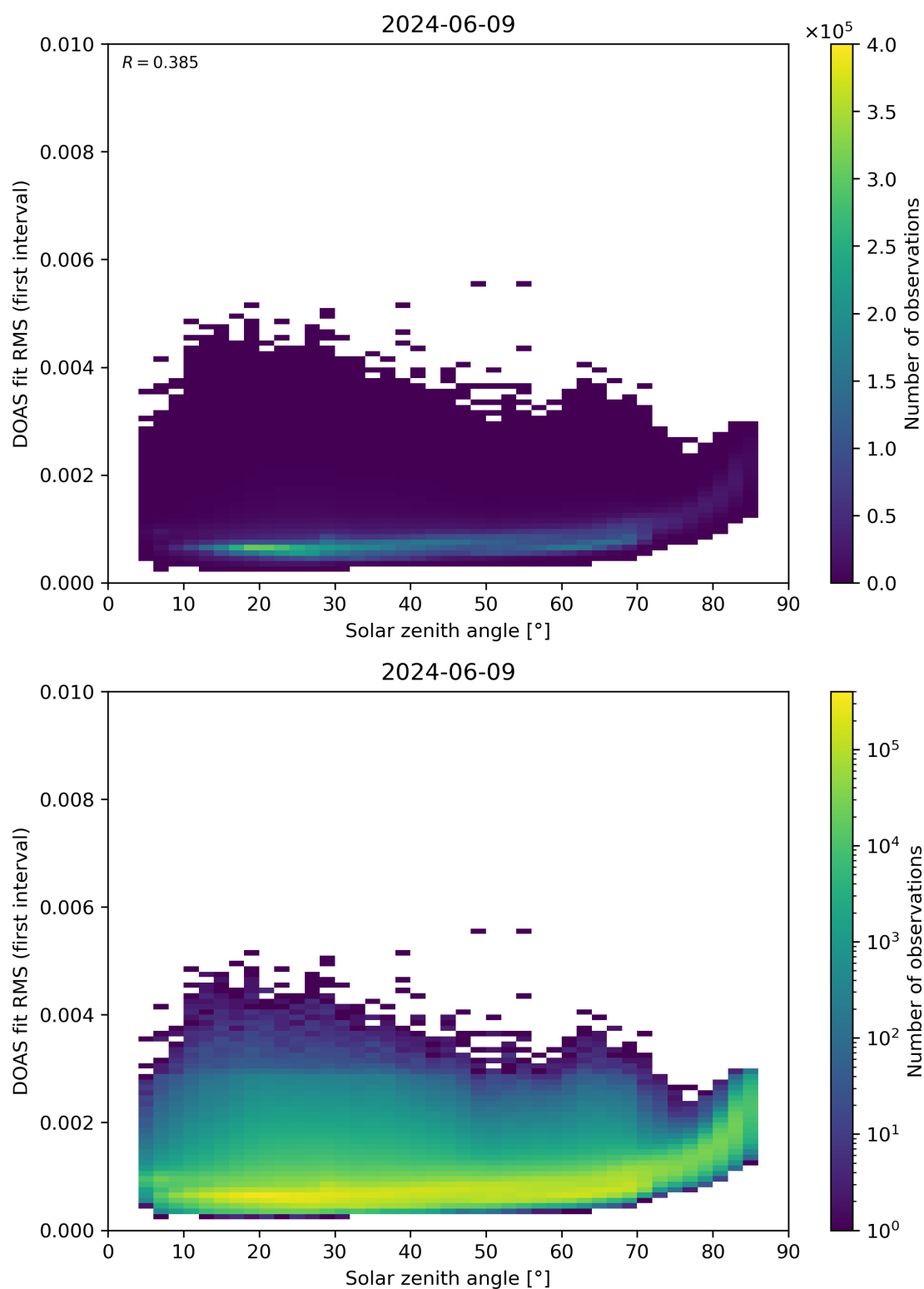
Figure 167: Scatter density plot of “Solar zenith angle” against “DOAS fit RMS (first interval)” for 2024-06-08 to 2024-06-10.
