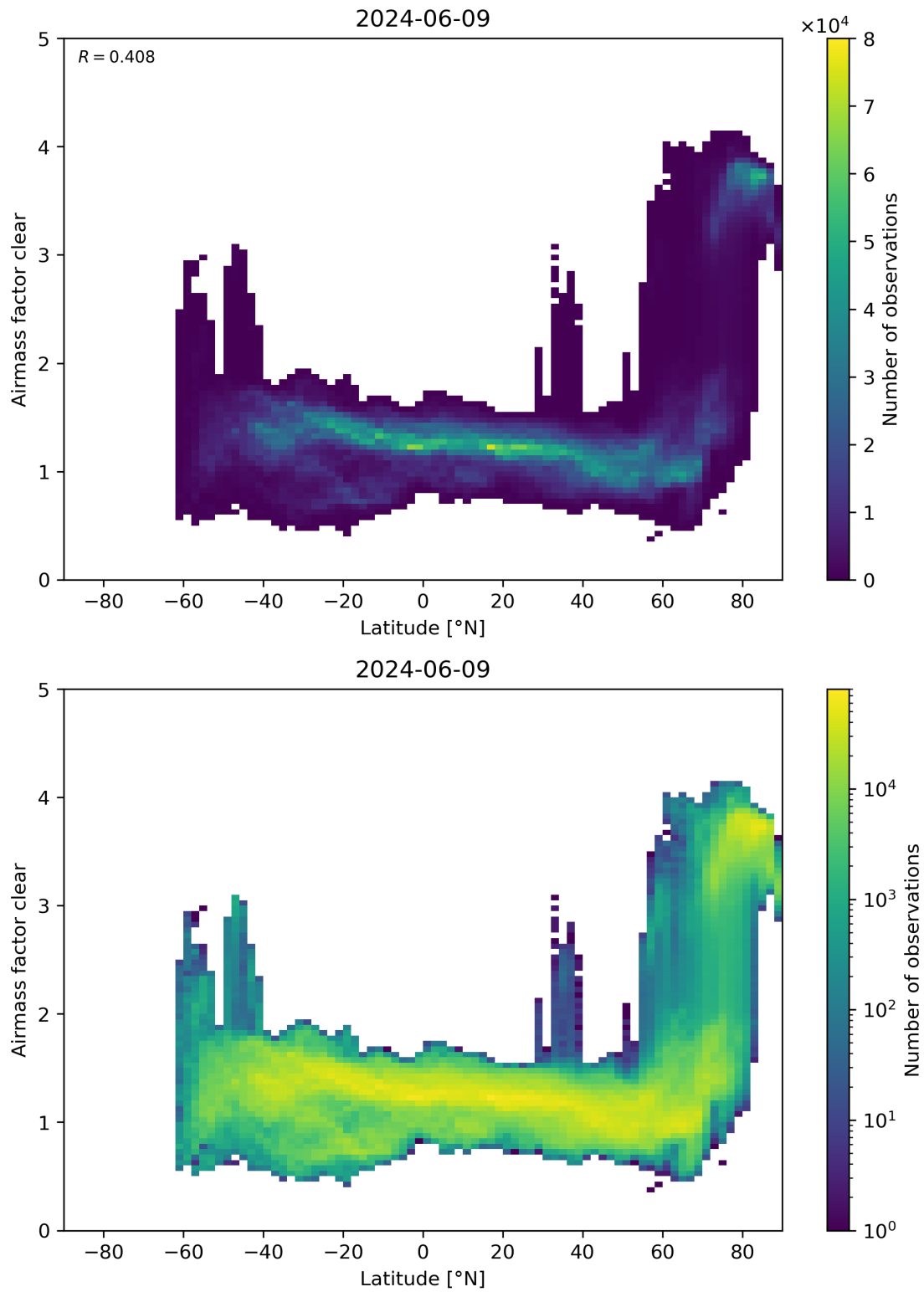
Figure 156: Scatter density plot of “Latitude” against “Airmass factor clear” for 2024-06-08 to 2024-06-10.
