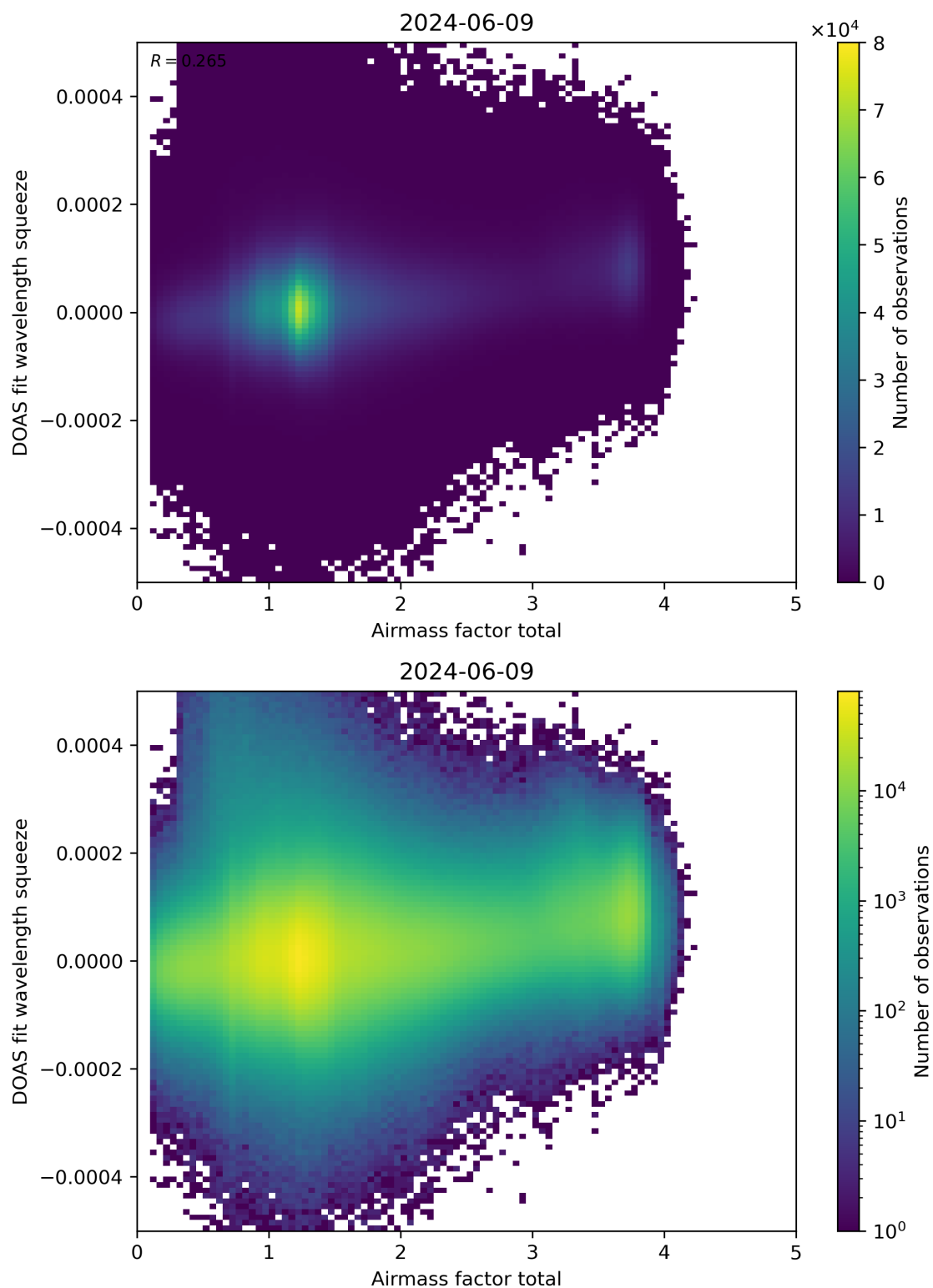
Figure 99: Scatter density plot of “Airmass factor total” against “DOAS fit wavelength squeeze” for 2024-06-08 to 2024-06-10.
