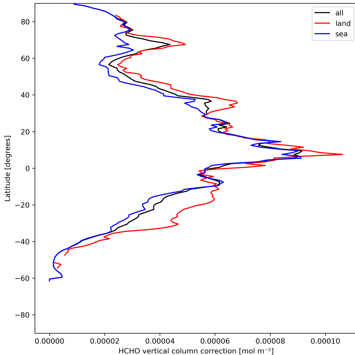
Figure 23: Zonal average of “HCHO vertical column correction” for 2024-06-08 to 2024-06-10.
