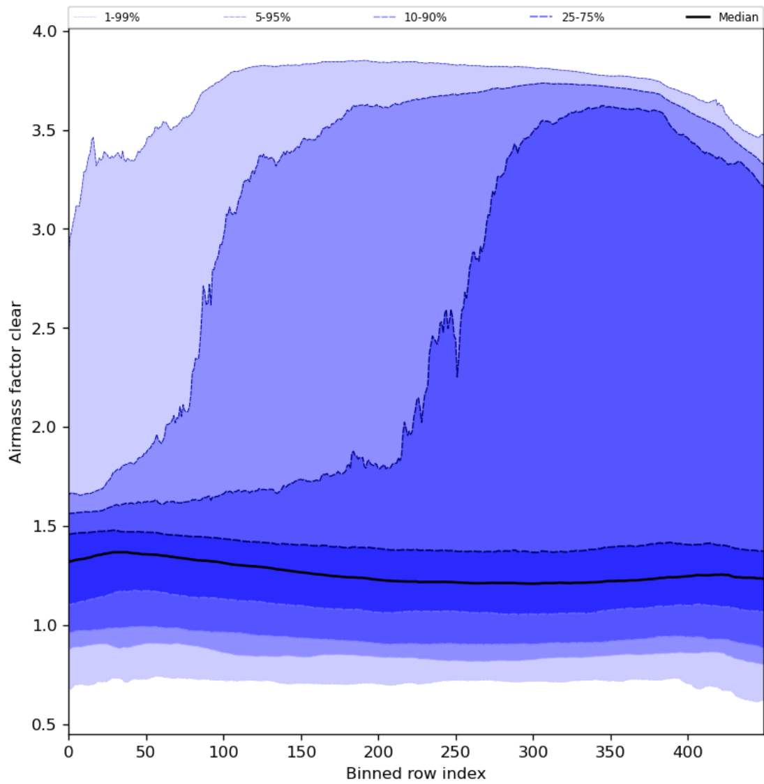
Figure 56: Along track statistics of “Airmass factor clear” for 2024-06-08 to 2024-06-10
