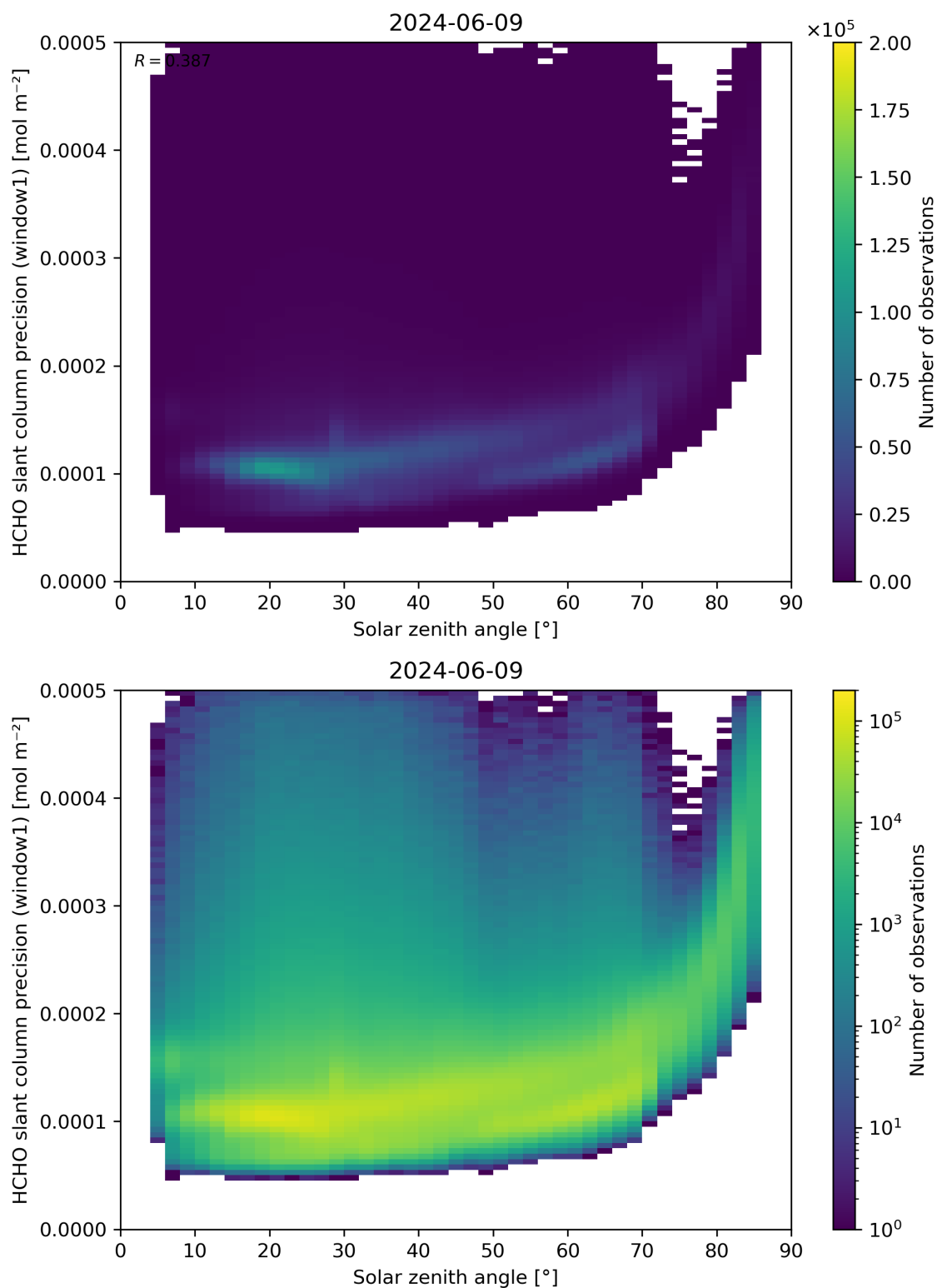
Figure 174: Scatter density plot of “Solar zenith angle” against “HCHO slant column precision (window1)” for 2024-06-08 to 2024-06-10.
