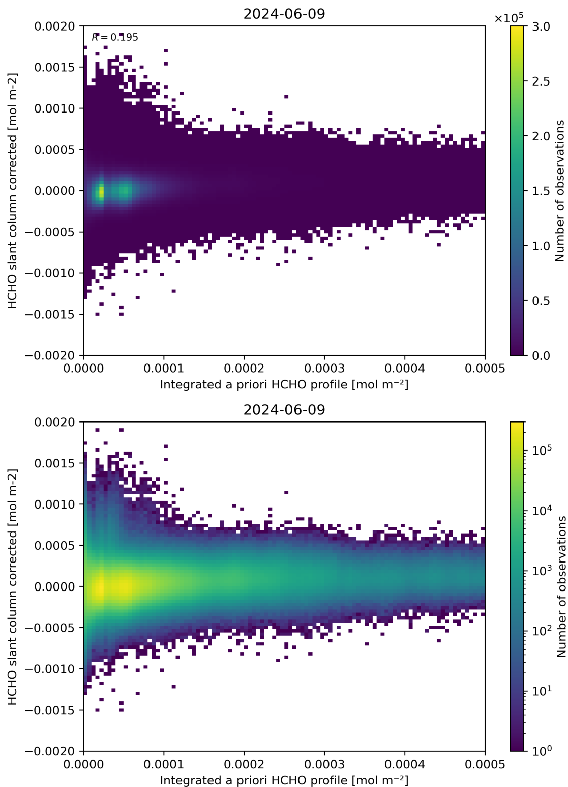
Figure 151: Scatter density plot of “Integrated a priori HCHO profile” against “HCHO slant column corrected” for 2024-06-08 to 2024-06-10.
