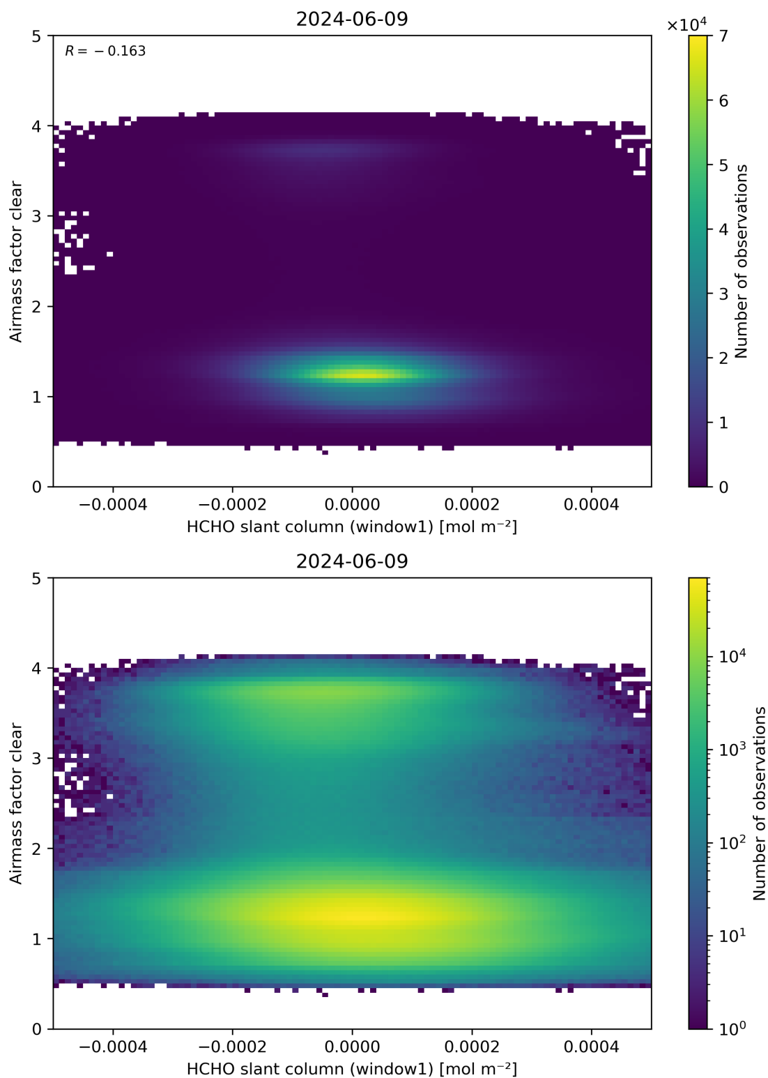
Figure 81: Scatter density plot of “HCHO slant column (window1)” against “Airmass factor clear” for 2024-06-08 to 2024-06-10.
