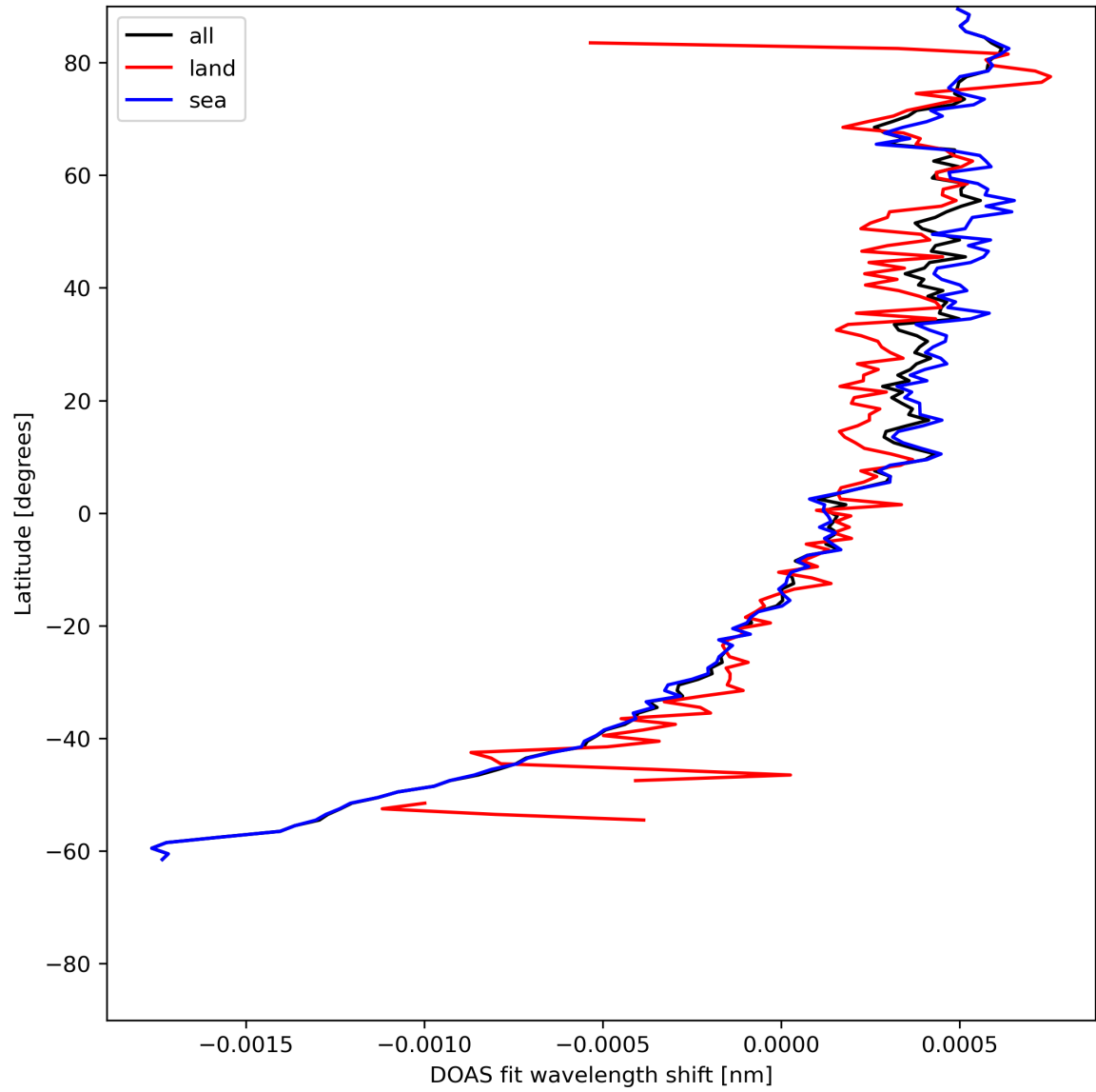
Figure 30: Zonal average of “DOAS fit wavelength shift” for 2024-06-08 to 2024-06-10.
