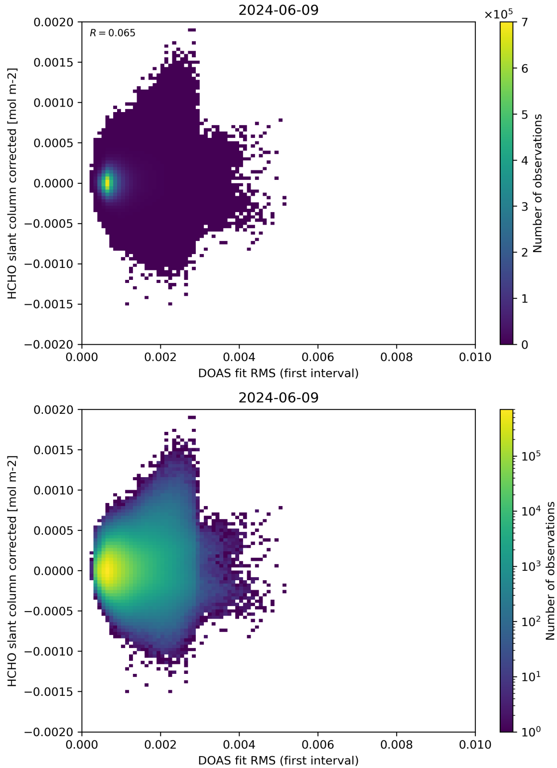
Figure 62: Scatter density plot of “DOAS fit RMS (first interval)” against “HCHO slant column corrected” for 2024-06-08 to 2024-06-10.
