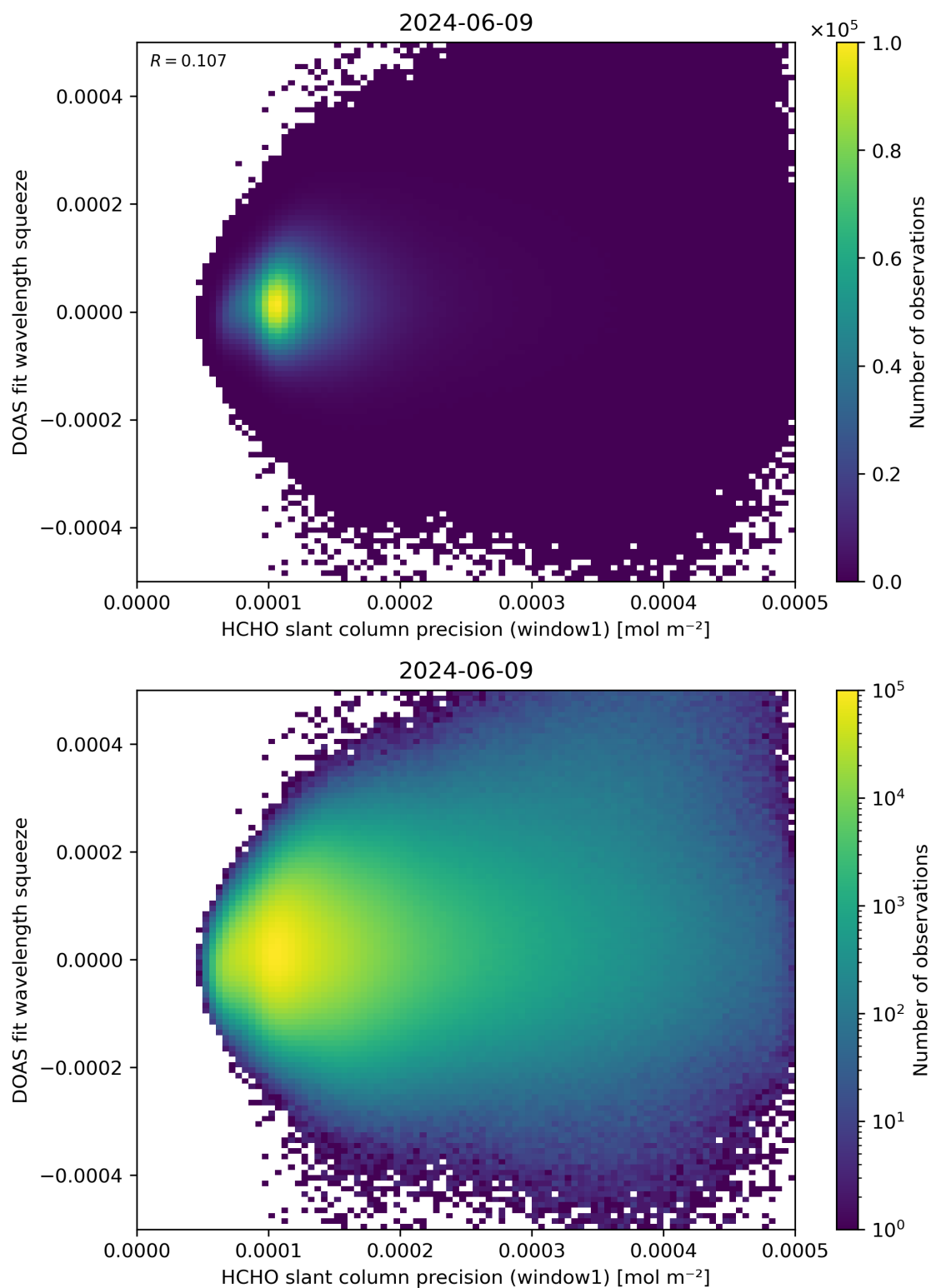
Figure 90: Scatter density plot of “HCHO slant column precision (window1)” against “DOAS fit wavelength squeeze” for 2024-06-08 to 2024-06-10.
