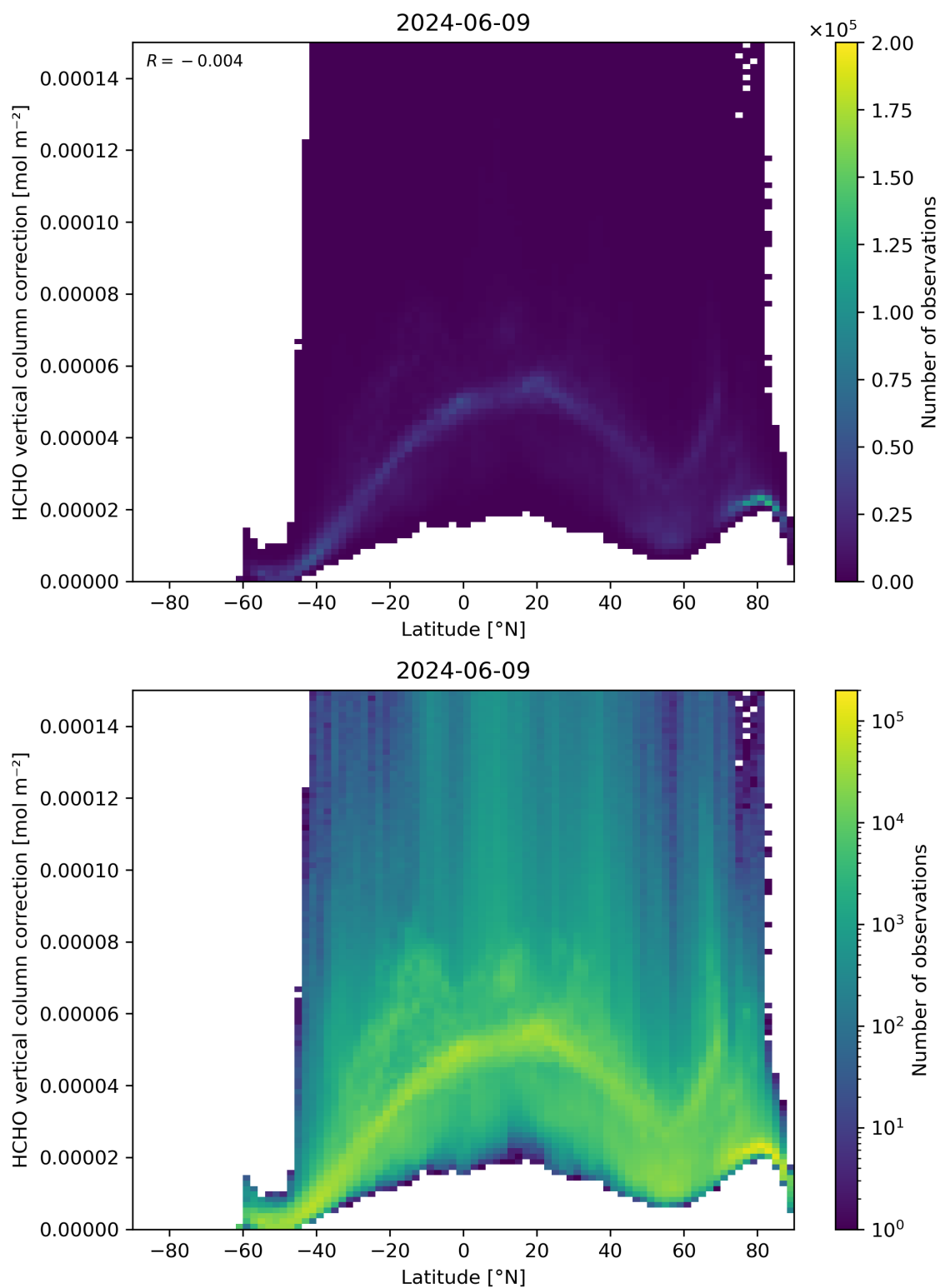
Figure 164: Scatter density plot of “Latitude” against “HCHO vertical column correction” for 2024-06-08 to 2024-06-10.
