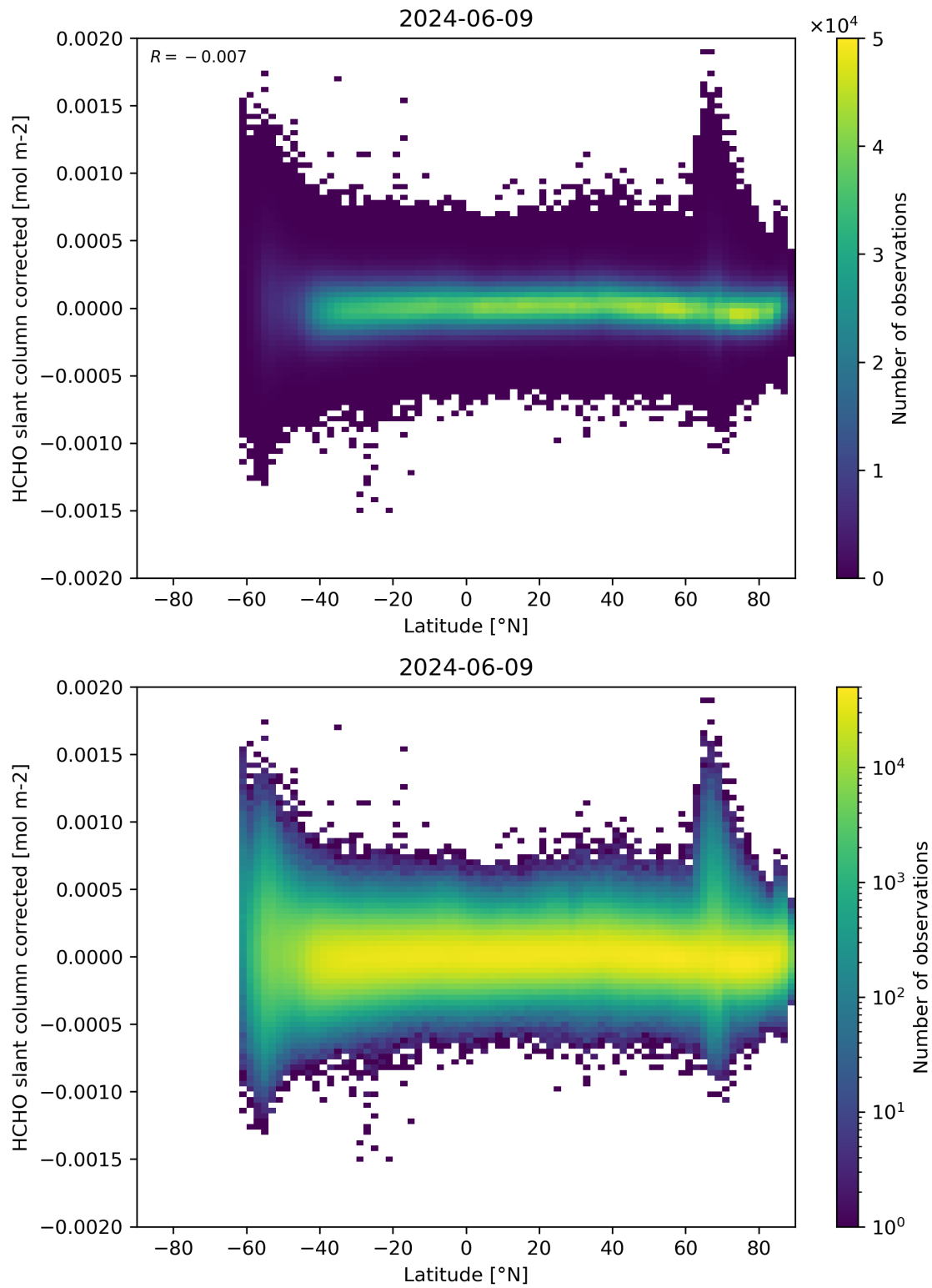
Figure 157: Scatter density plot of “Latitude” against “HCHO slant column corrected” for 2024-06-08 to 2024-06-10.
