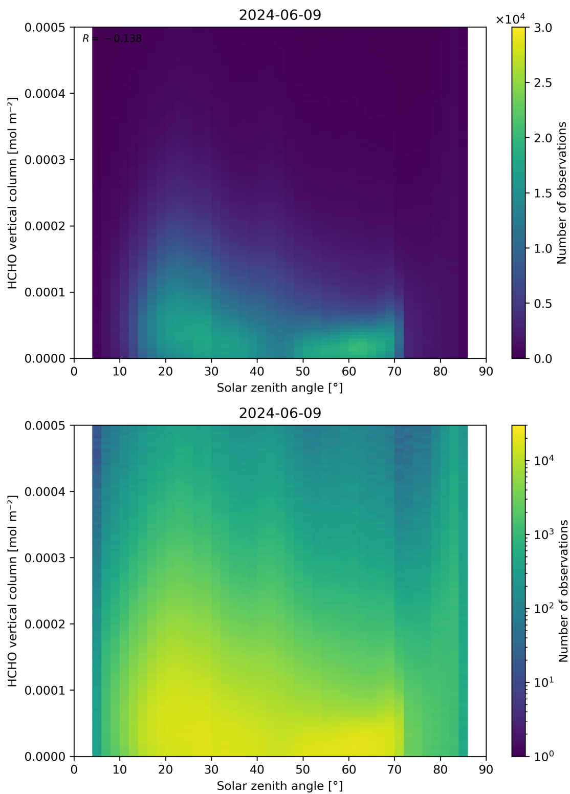
Figure 177: Scatter density plot of “Solar zenith angle” against “HCHO vertical column” for 2024-06-08 to 2024-06-10.
