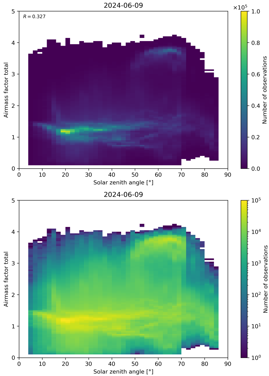
Figure 175: Scatter density plot of “Solar zenith angle” against “Airmass factor total” for 2024-06-08 to 2024-06-10.
