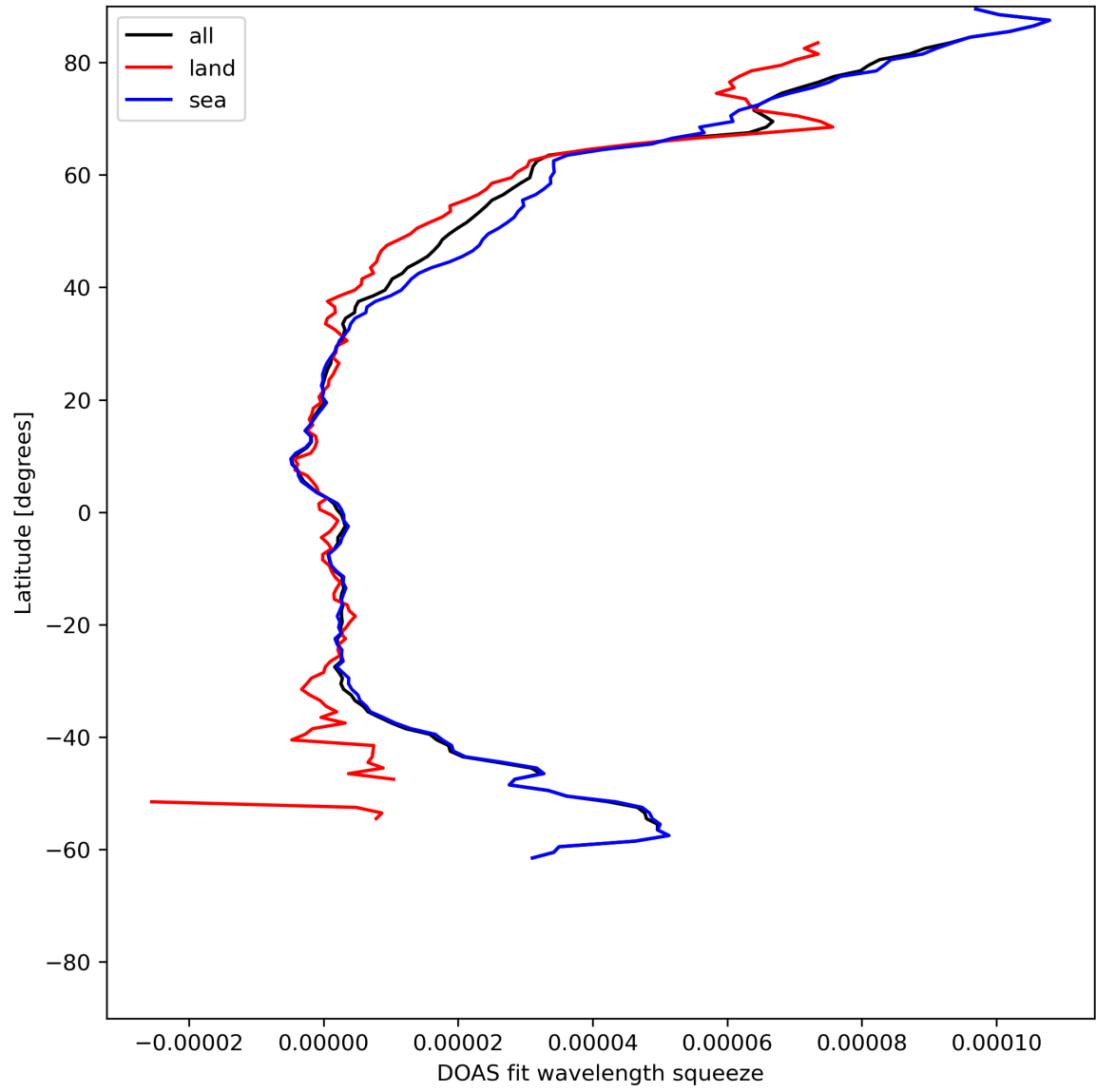
Figure 31: Zonal average of “DOAS fit wavelength squeeze” for 2024-06-08 to 2024-06-10.
