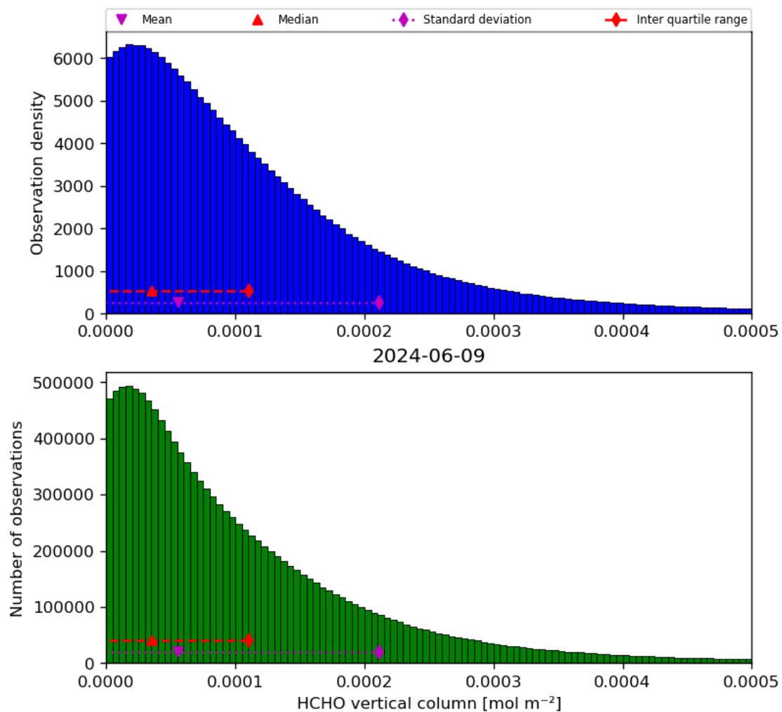
Figure 35: Histogram of “HCHO vertical column” for 2024-06-08 to 2024-06-10
