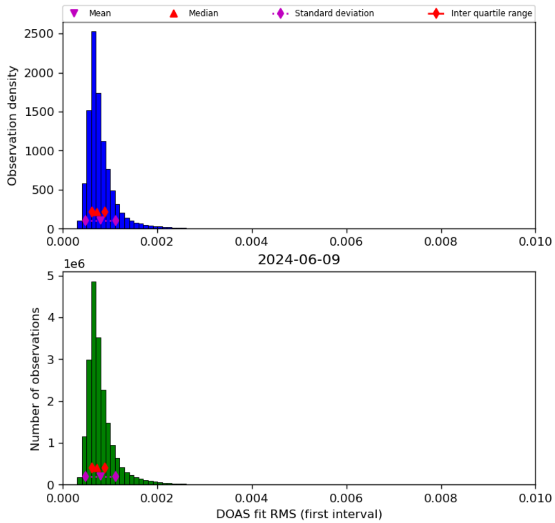
Figure 46: Histogram of “DOAS fit RMS (first interval)” for 2024-06-08 to 2024-06-10
