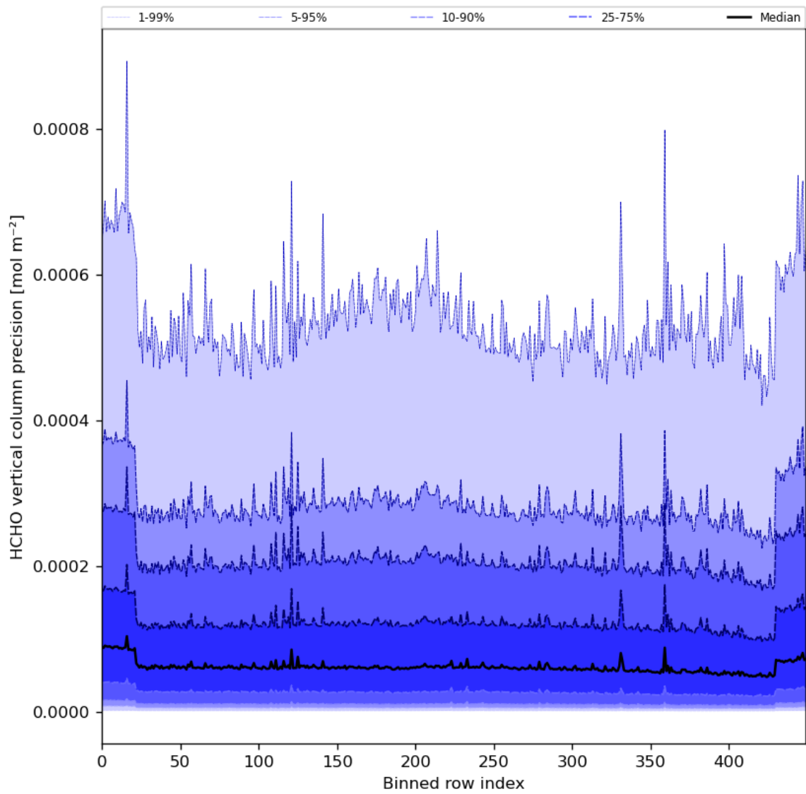
Figure 50: Along track statistics of “HCHO vertical column precision” for 2024-06-08 to 2024-06-10
