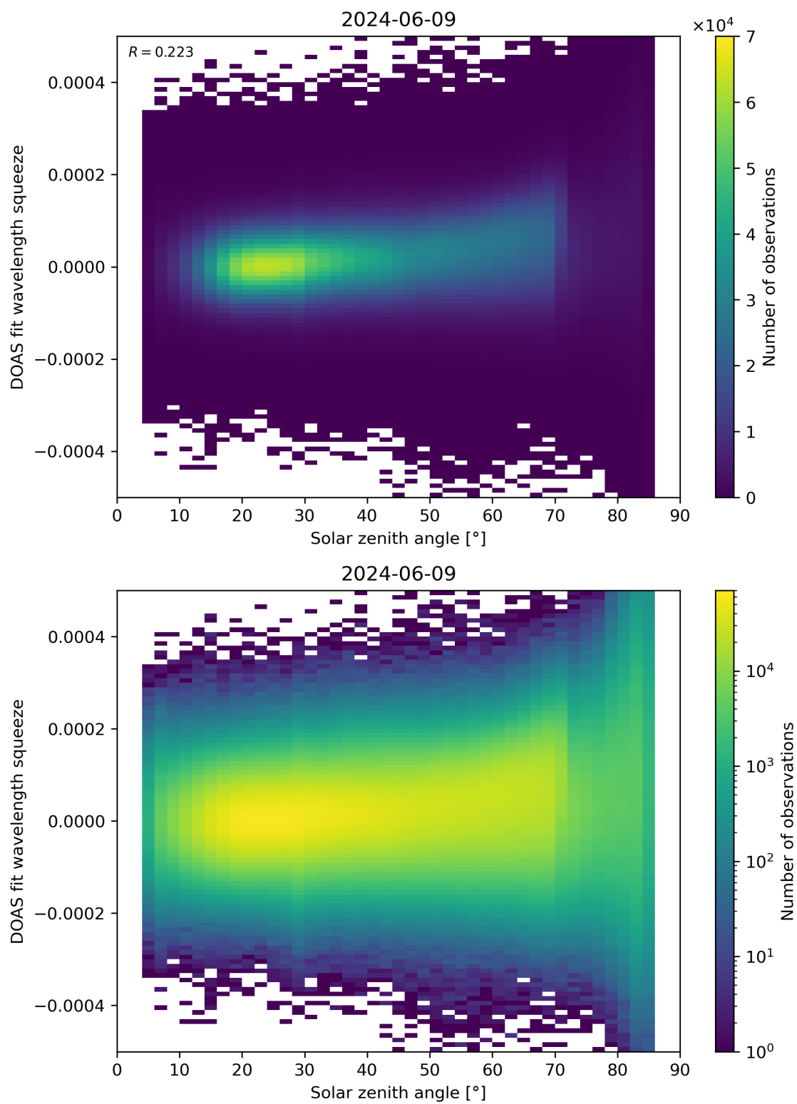
Figure 169: Scatter density plot of “Solar zenith angle” against “DOAS fit wavelength squeeze” for 2024-06-08 to 2024-06-10.
