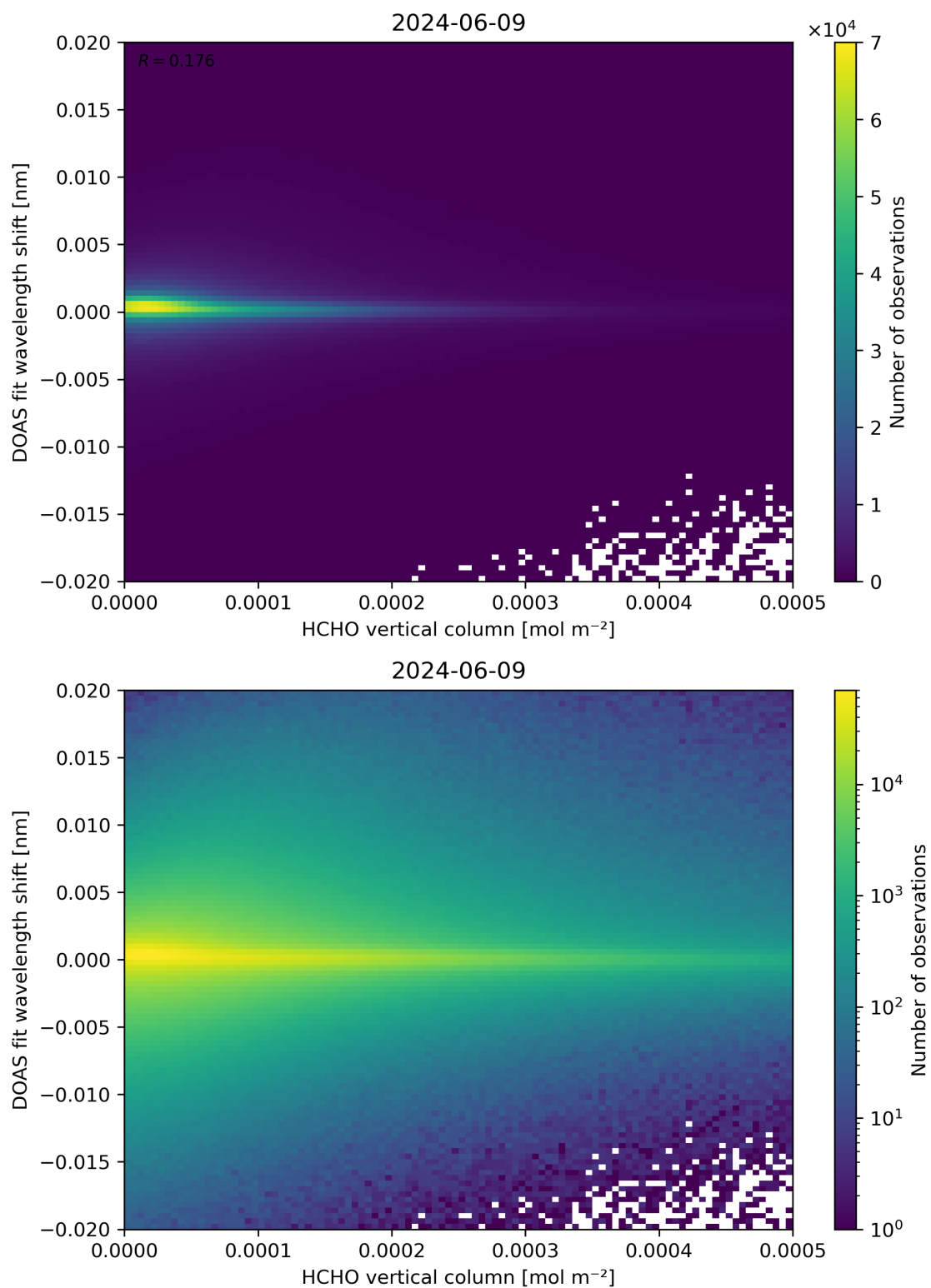
Figure 124: Scatter density plot of “HCHO vertical column” against “DOAS fit wavelength shift” for 2024-06-08 to 2024-06-10.
