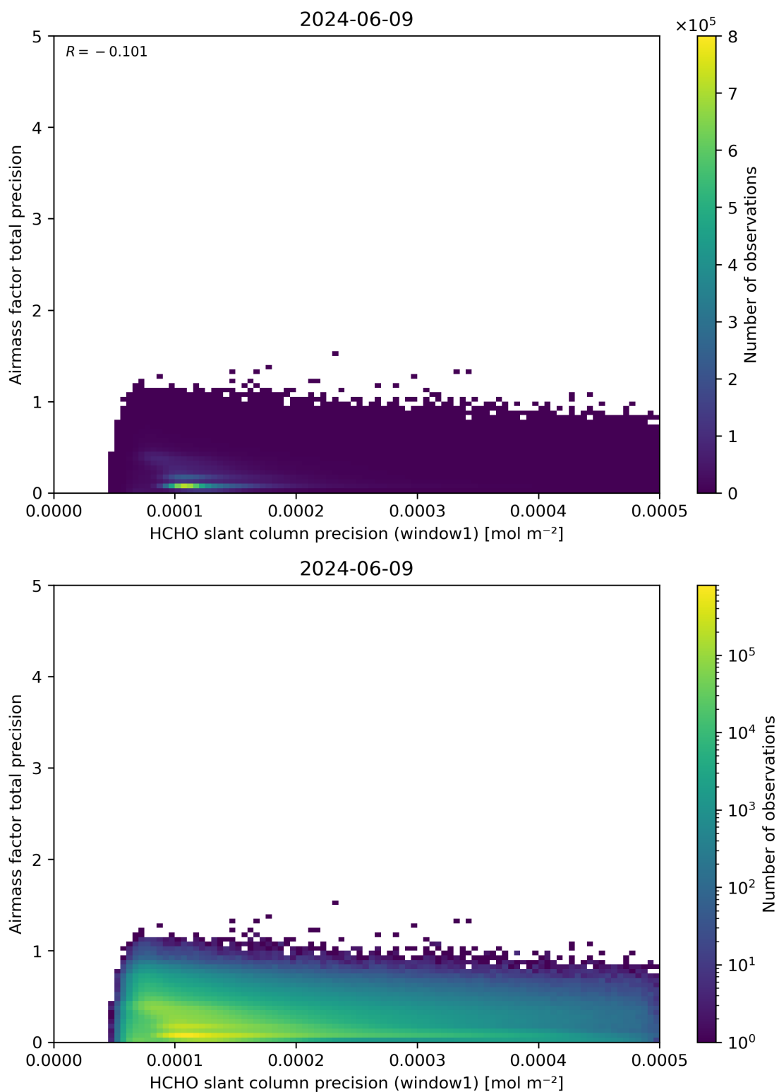
Figure 95: Scatter density plot of “HCHO slant column precision (window1)” against “Airmass factor total precision” for 2024-06-08 to 2024-06-10.
