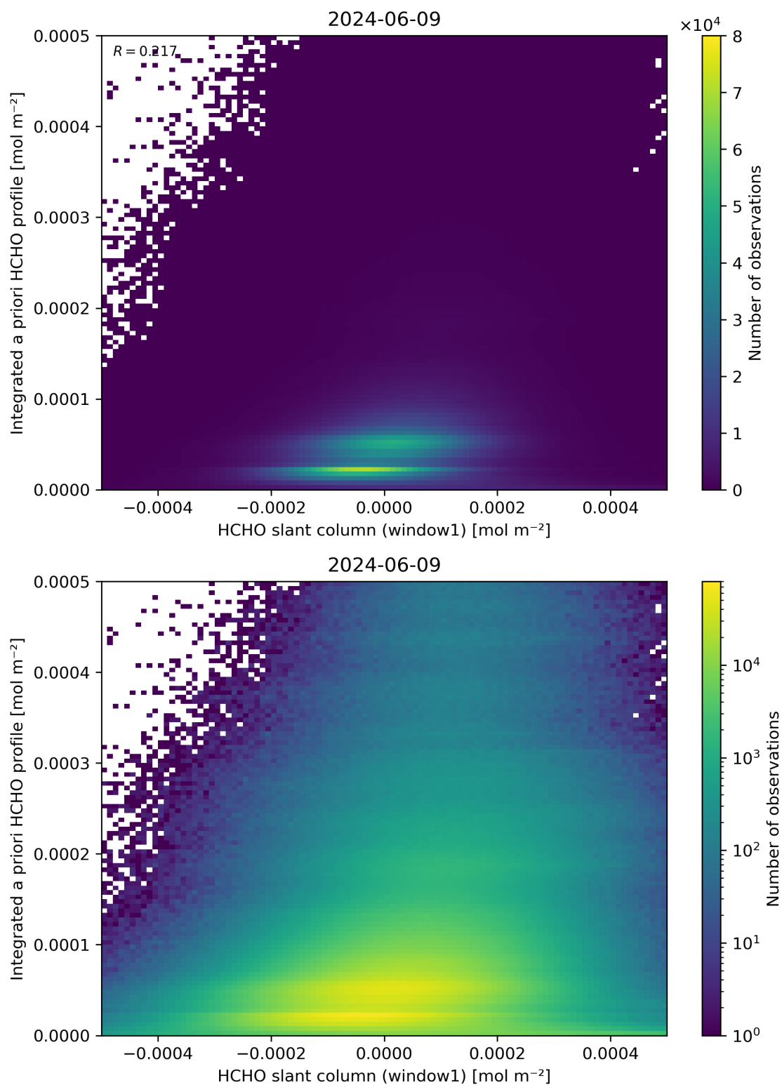
Figure 87: Scatter density plot of “HCHO slant column (window1)” against “Integrated a priori HCHO profile” for 2024-06-08 to 2024-06-10.
