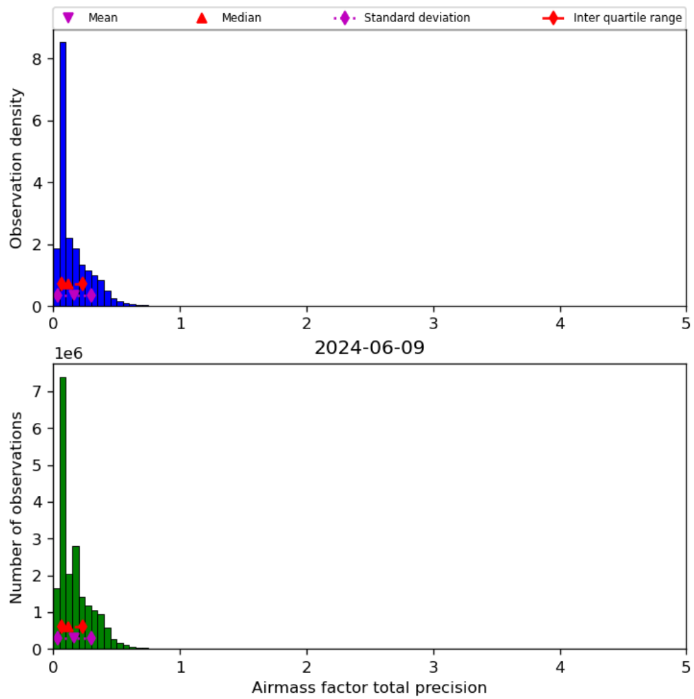
Figure 41: Histogram of “Airmass factor total precision” for 2024-06-08 to 2024-06-10
