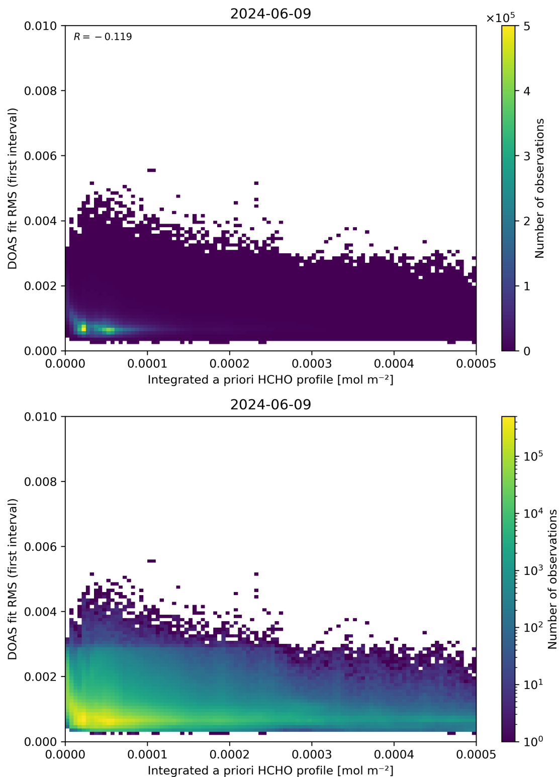
Figure 148: Scatter density plot of “Integrated a priori HCHO profile” against “DOAS fit RMS (first interval)” for 2024-06-08 to 2024-06-10.
