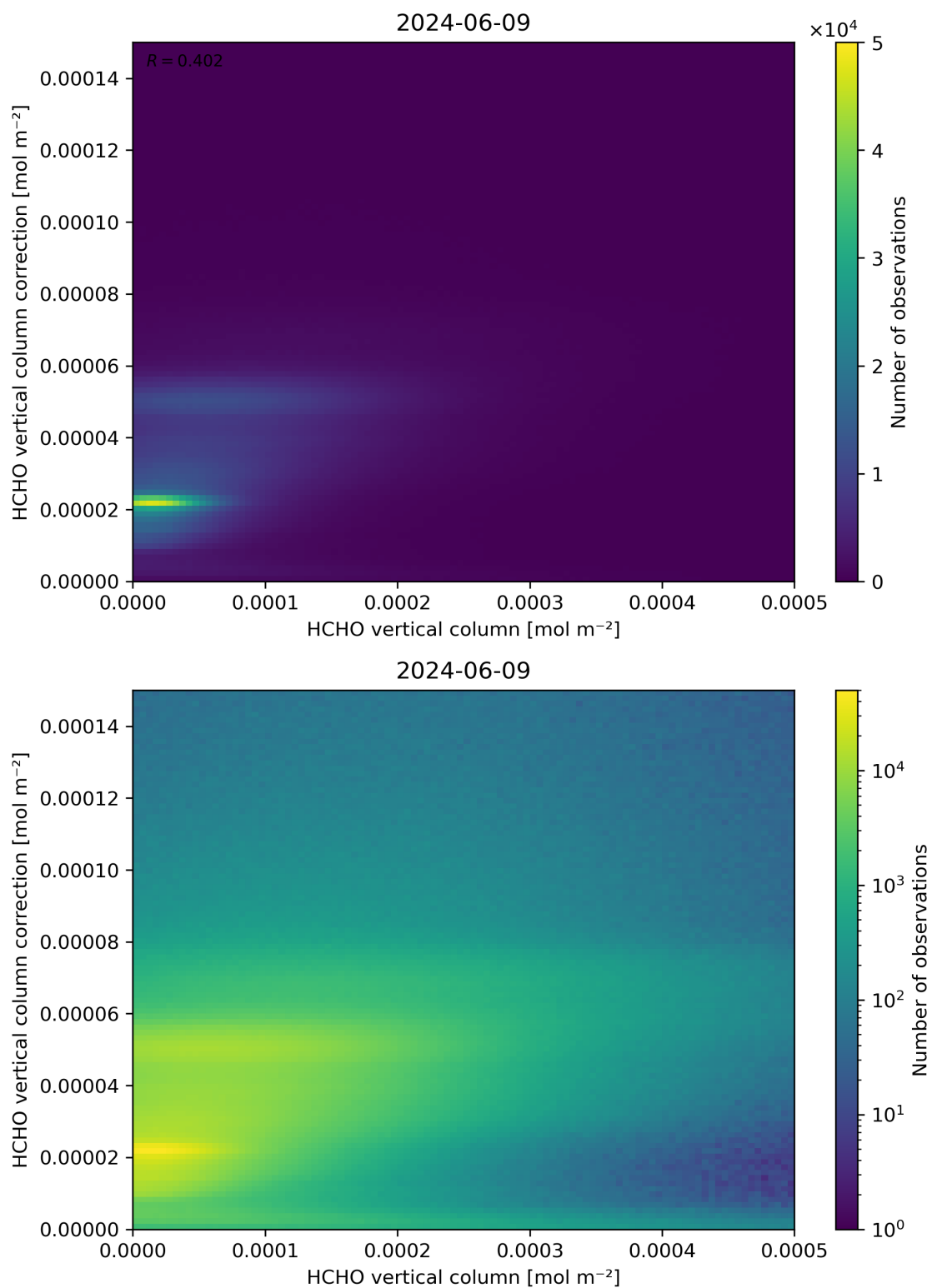
Figure 133: Scatter density plot of “HCHO vertical column” against “HCHO vertical column correction” for 2024-06-08 to 2024-06-10.
