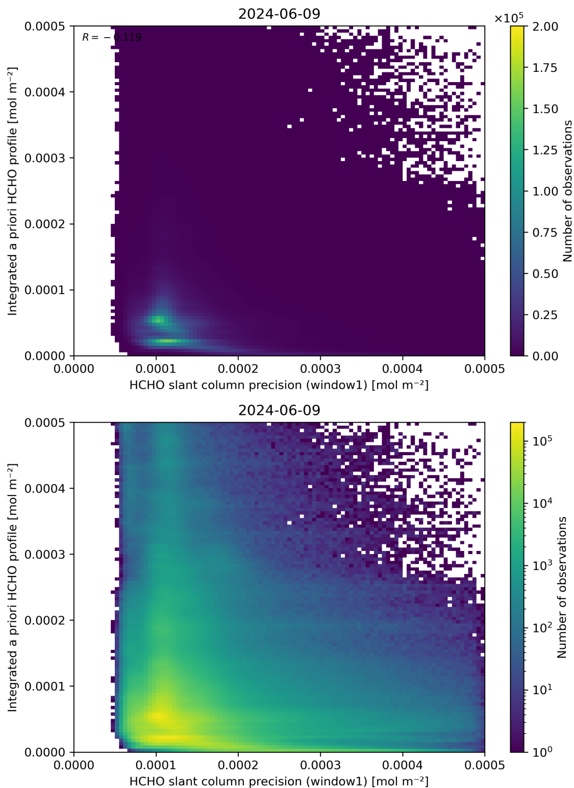
Figure 96: Scatter density plot of “HCHO slant column precision (window1)” against “Integrated a priori HCHO profile” for 2024-06-08 to 2024-06-10.
