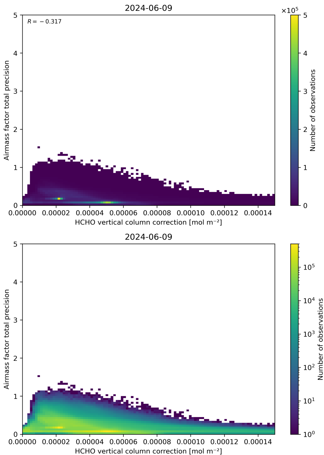
Figure 121: Scatter density plot of “HCHO vertical column correction” against “Airmass factor total precision” for 2024-06-08 to 2024-06-10.
