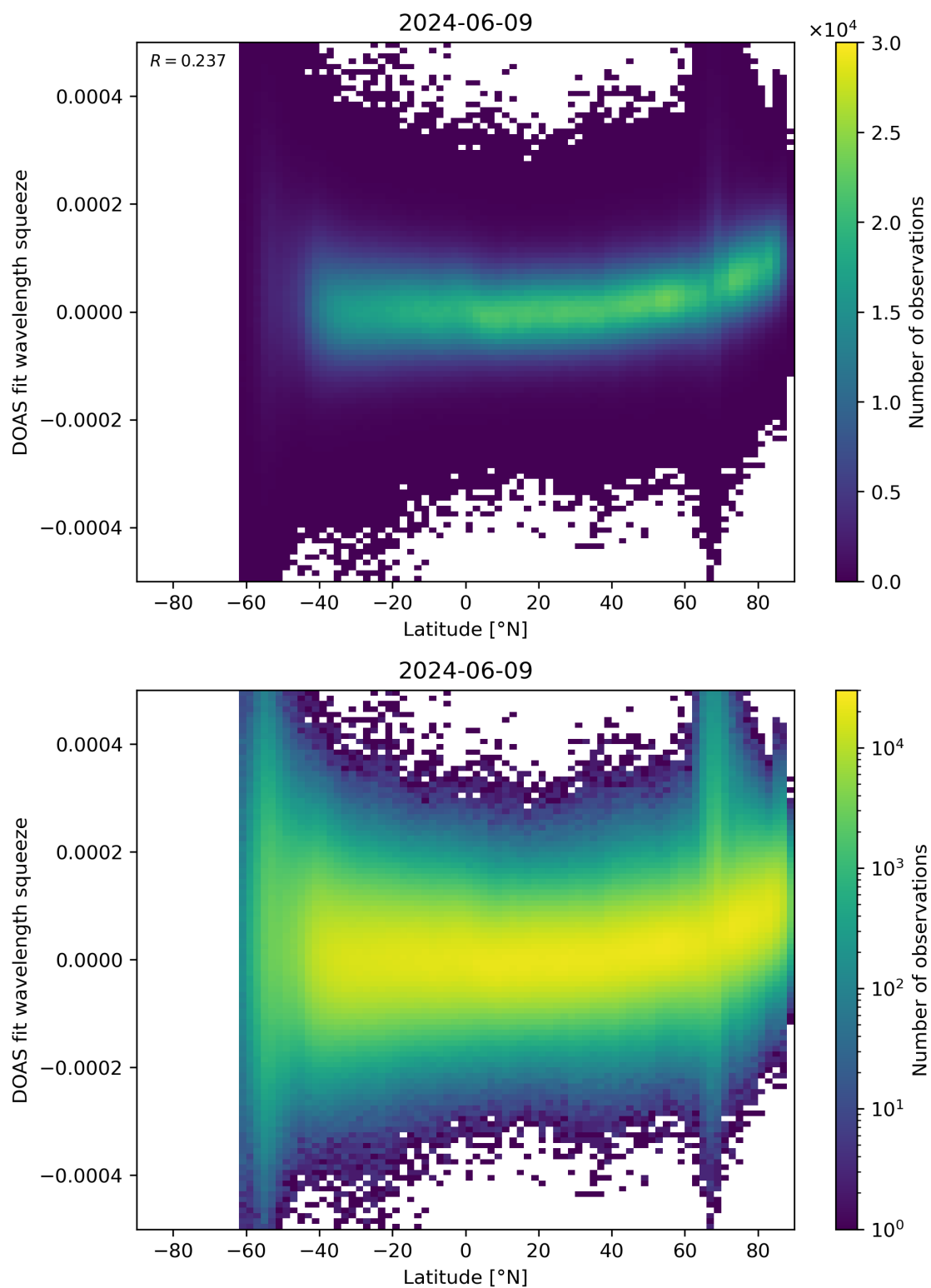
Figure 155: Scatter density plot of “Latitude” against “DOAS fit wavelength squeeze” for 2024-06-08 to 2024-06-10.
