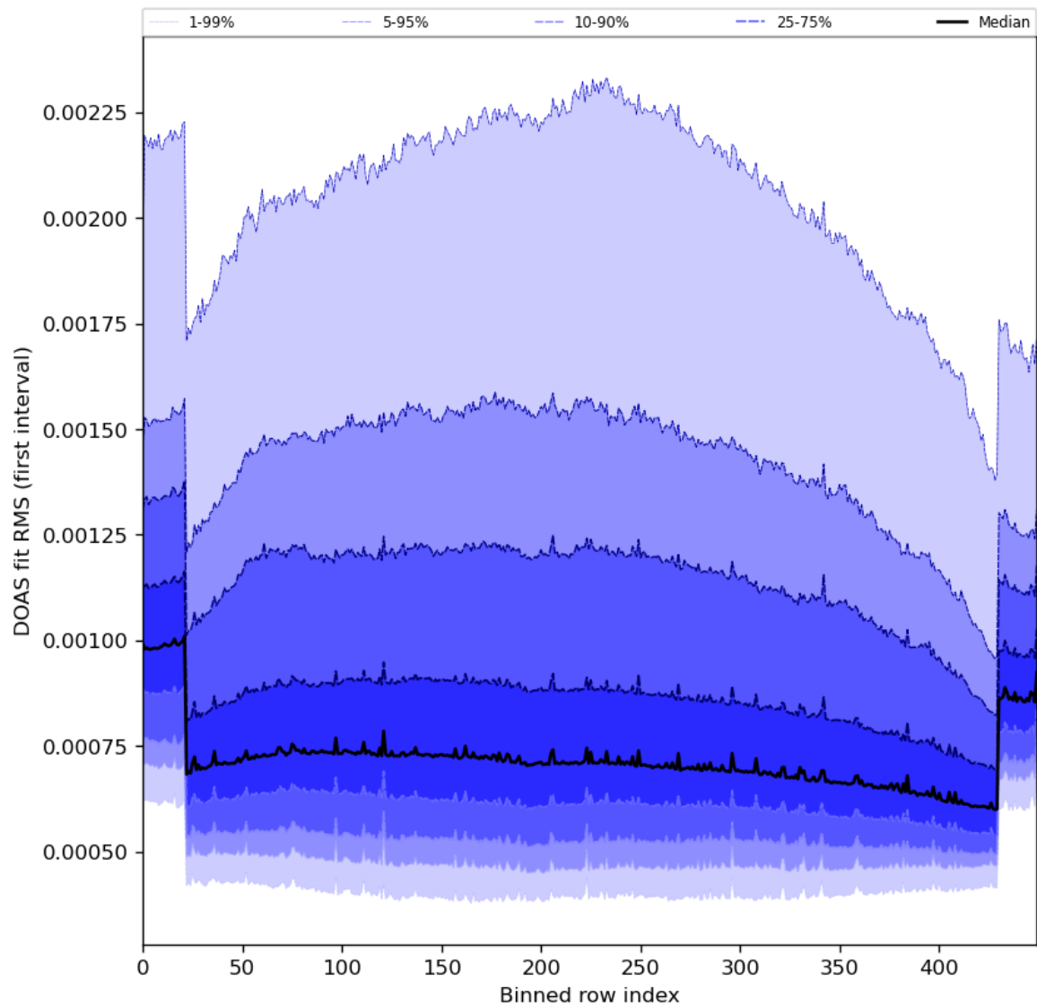
Figure 60: Along track statistics of “DOAS fit RMS (first interval)” for 2024-06-08 to 2024-06-10
