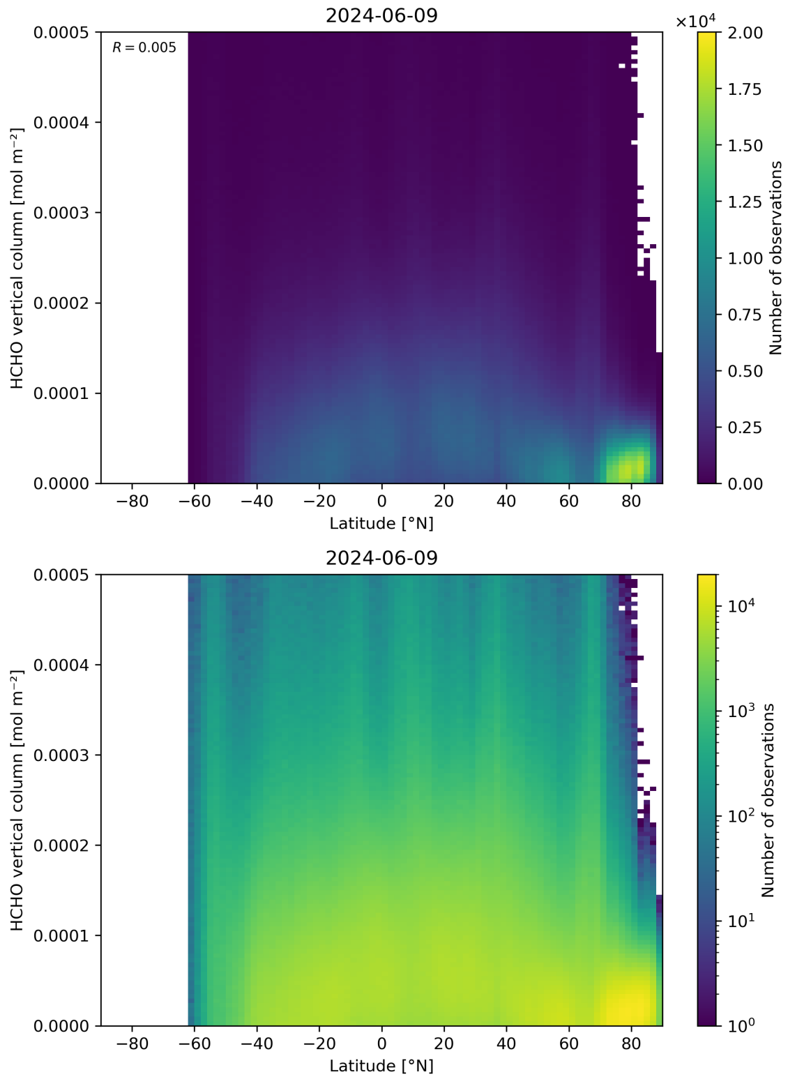
Figure 163: Scatter density plot of “Latitude” against “HCHO vertical column” for 2024-06-08 to 2024-06-10.
