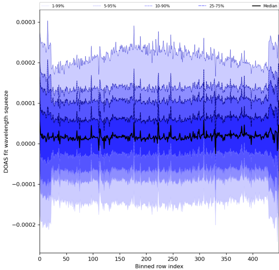
Figure 59: Along track statistics of “DOAS fit wavelength squeeze” for 2024-06-08 to 2024-06-10
