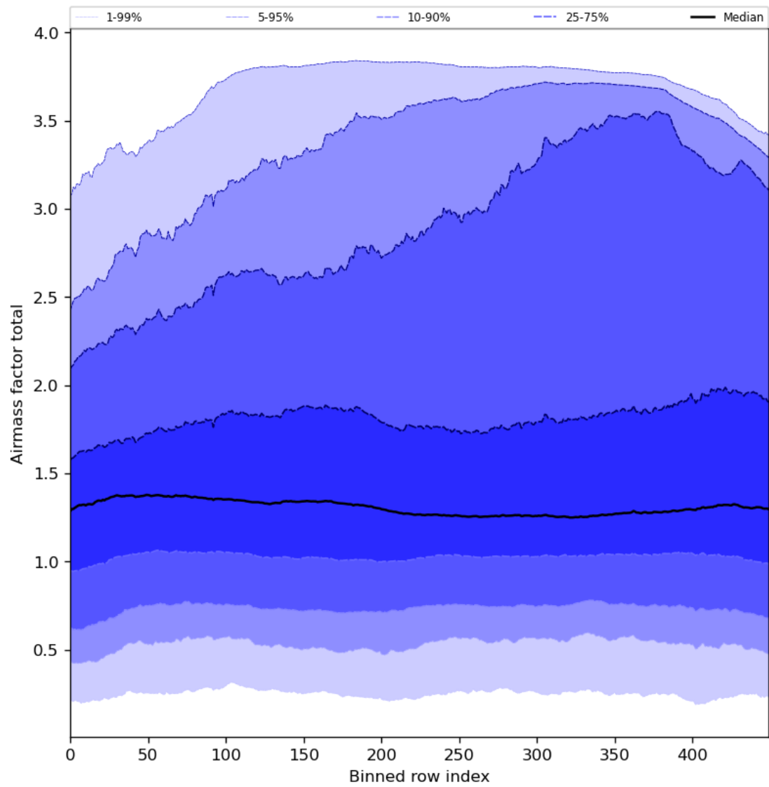
Figure 54: Along track statistics of “Airmass factor total” for 2024-06-08 to 2024-06-10
