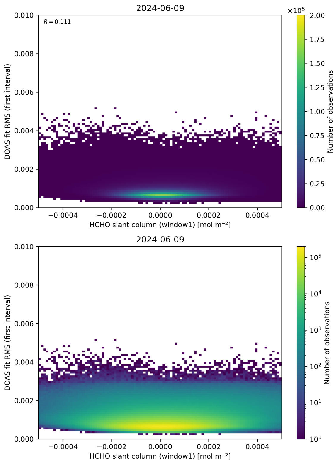
Figure 78: Scatter density plot of “HCHO slant column (window1)” against “DOAS fit RMS (first interval)” for 2024-06-08 to 2024-06-10.
