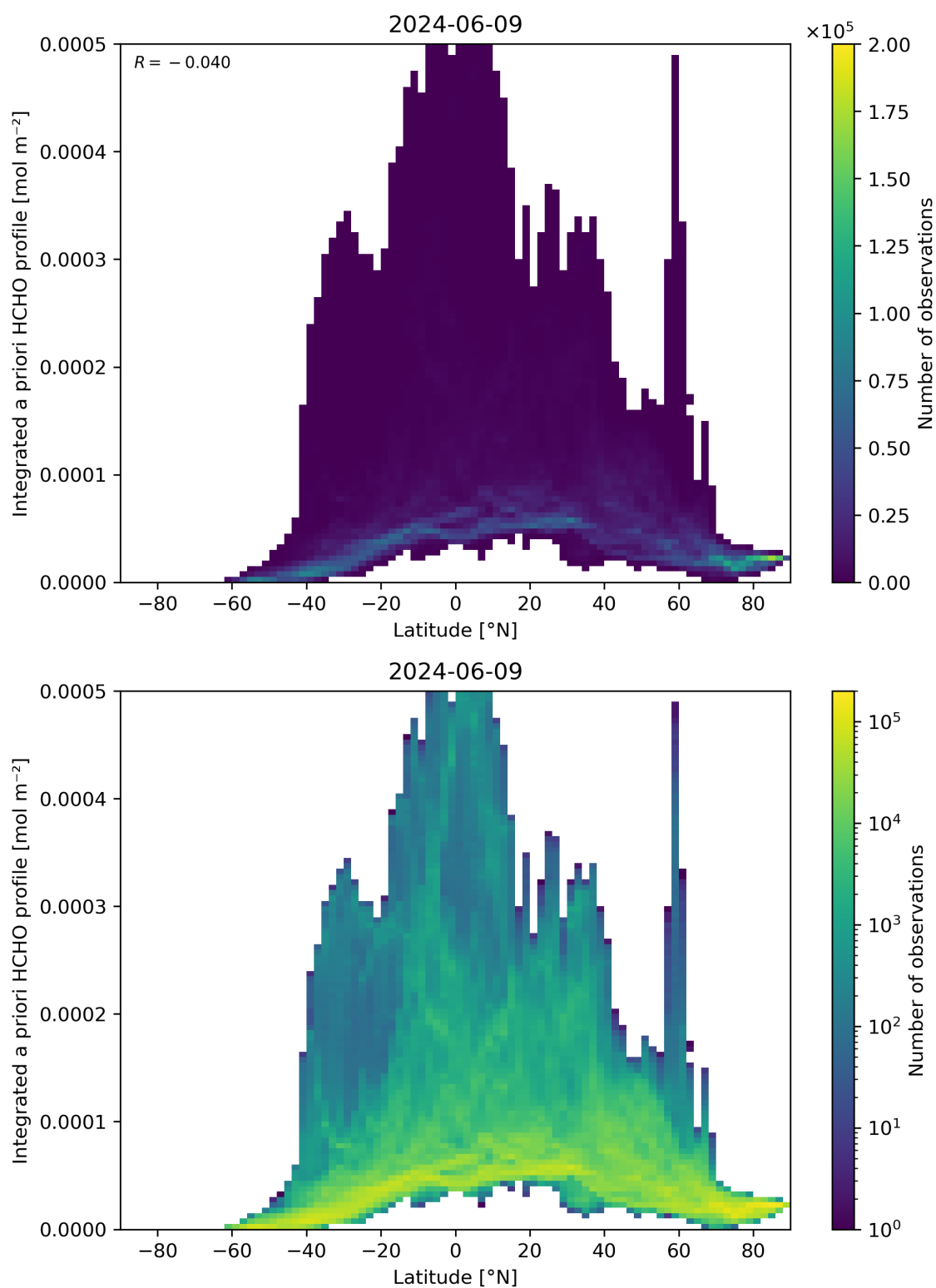
Figure 166: Scatter density plot of “Latitude” against “Integrated a priori HCHO profile” for 2024-06-08 to 2024-06-10.
