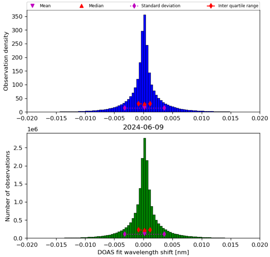
Figure 44: Histogram of “DOAS fit wavelength shift” for 2024-06-08 to 2024-06-10
