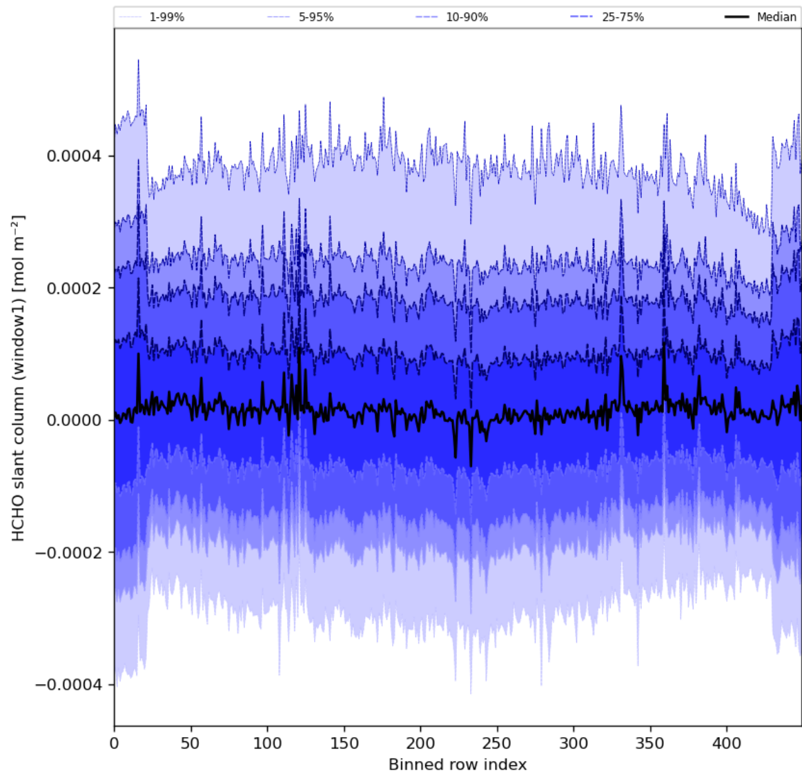
Figure 52: Along track statistics of “HCHO slant column (window1)” for 2024-06-08 to 2024-06-10
