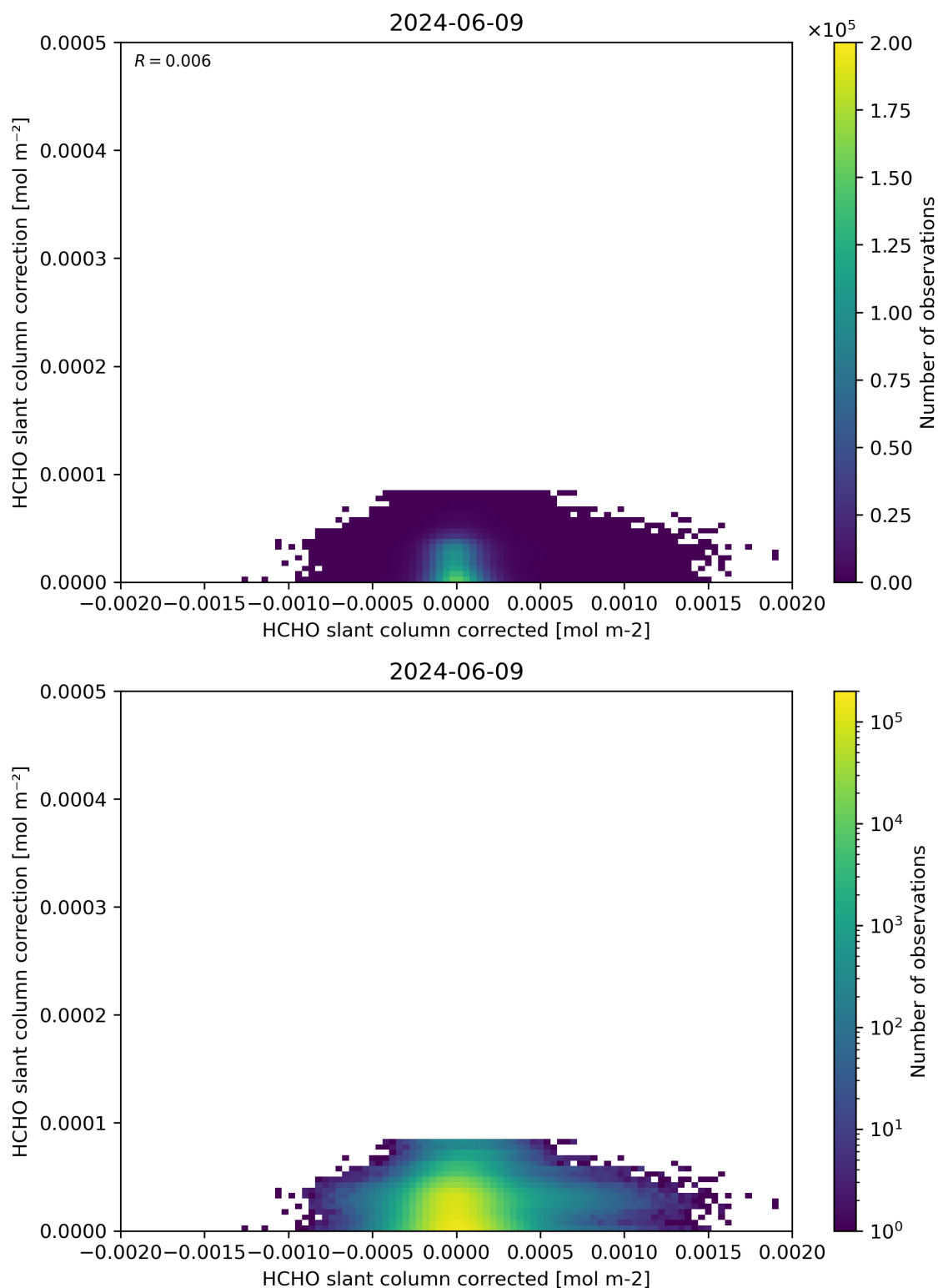
Figure 77: Scatter density plot of “HCHO slant column corrected” against “HCHO slant column correction” for 2024-06-08 to 2024-06-10.
