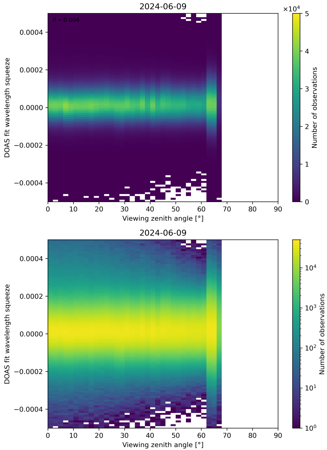
Figure 184: Scatter density plot of “Viewing zenith angle” against “DOAS fit wavelength squeeze” for 2024-06-08 to 2024-06-10.
