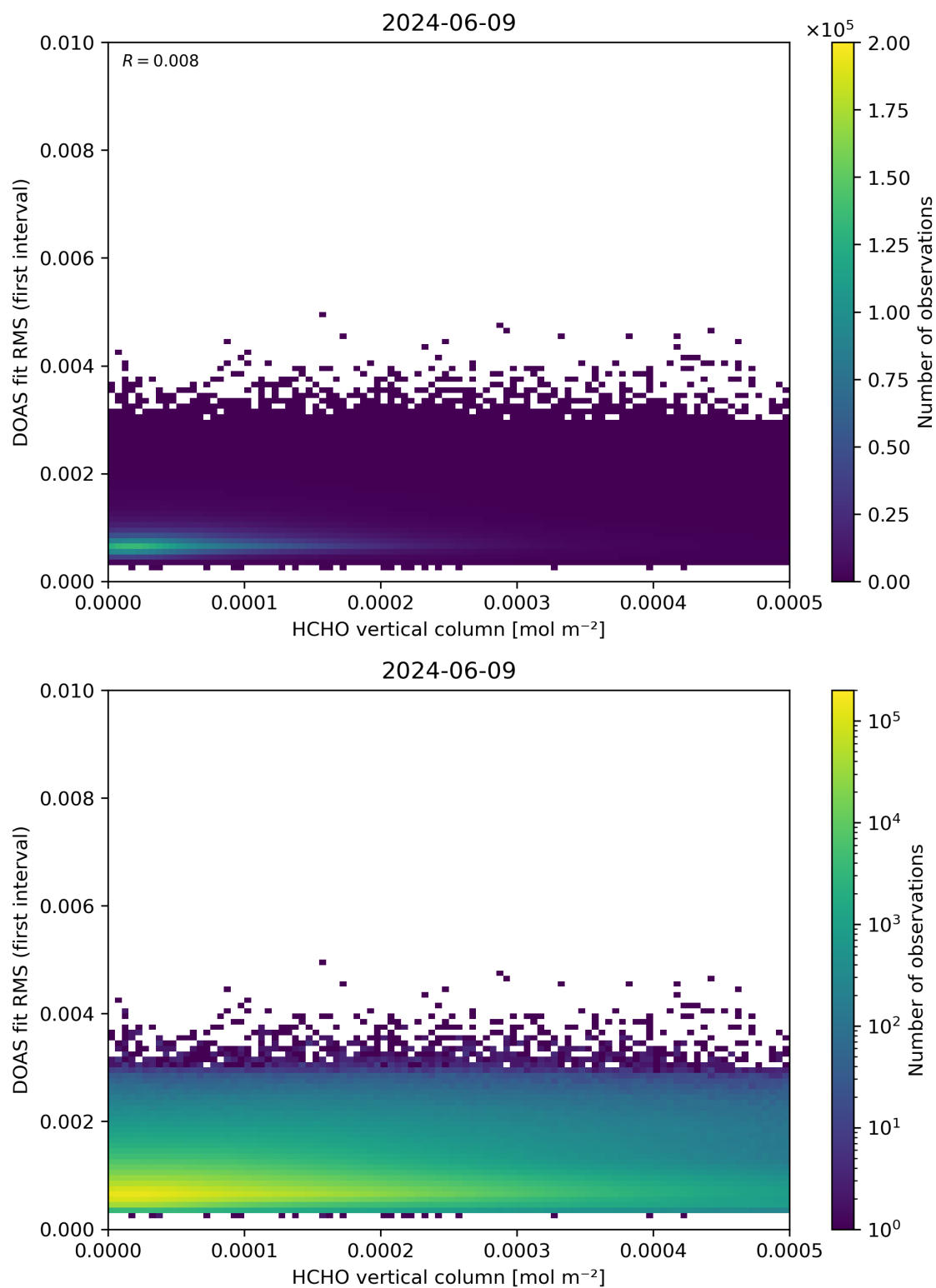
Figure 123: Scatter density plot of “HCHO vertical column” against “DOAS fit RMS (first interval)” for 2024-06-08 to 2024-06-10.
