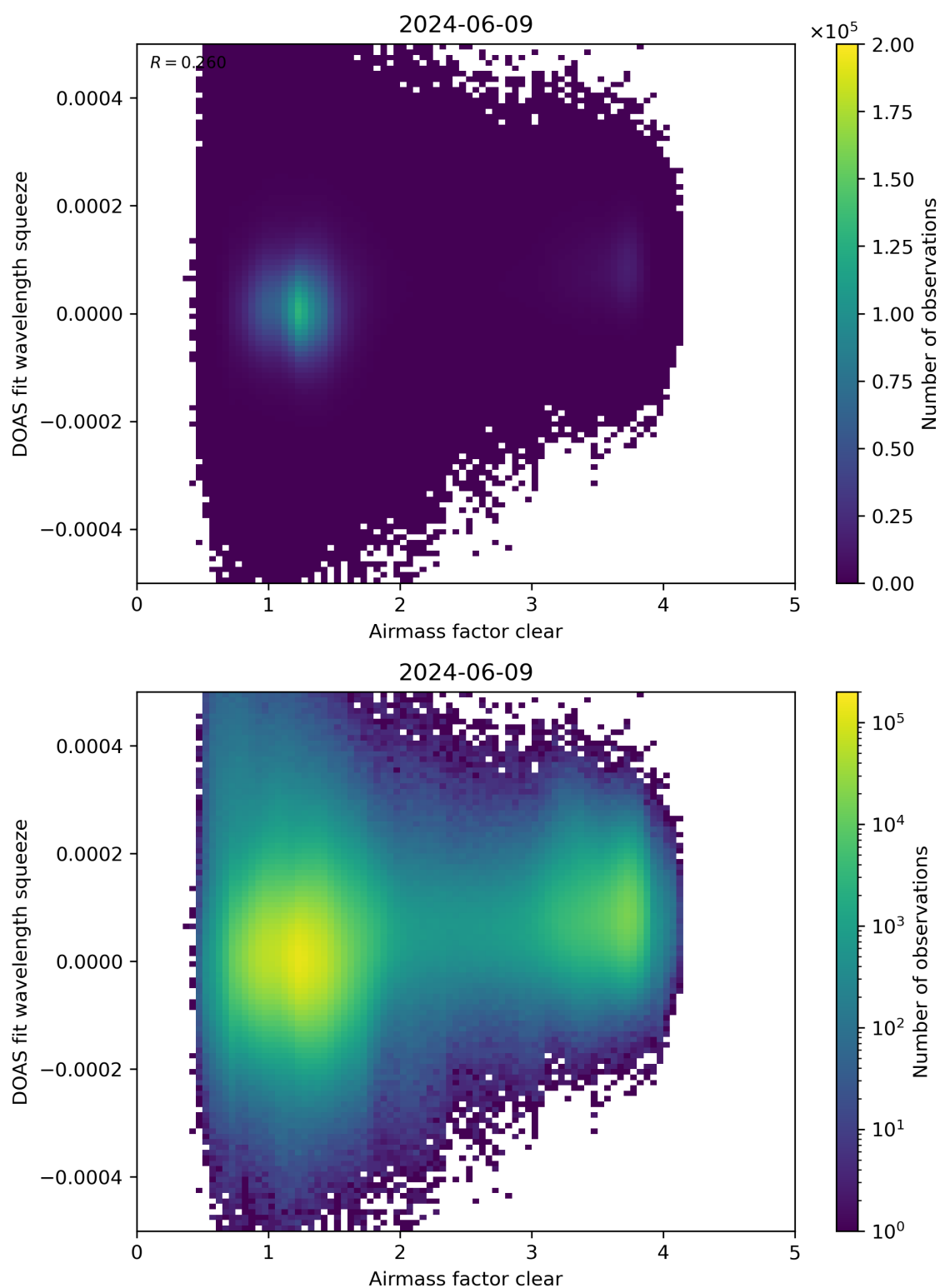
Figure 73: Scatter density plot of “Airmass factor clear” against “DOAS fit wavelength squeeze” for 2024-06-08 to 2024-06-10.
