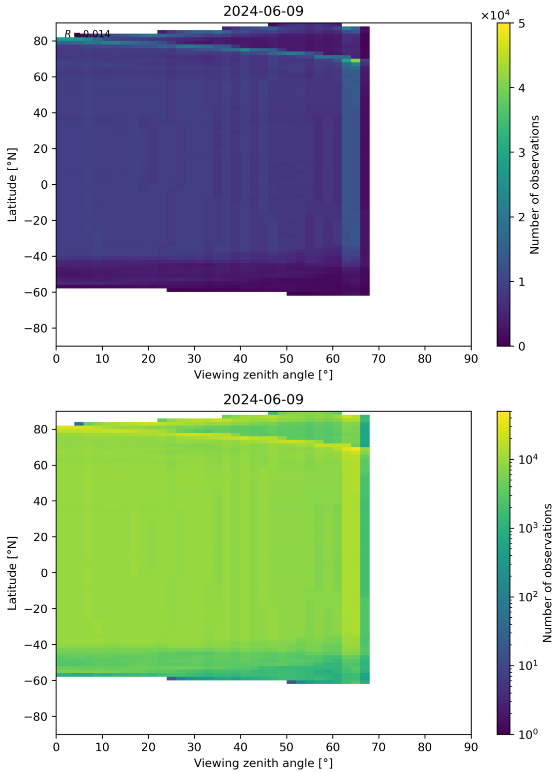
Figure 196: Scatter density plot of “Viewing zenith angle” against “Latitude” for 2024-06-08 to 2024-06-10.
