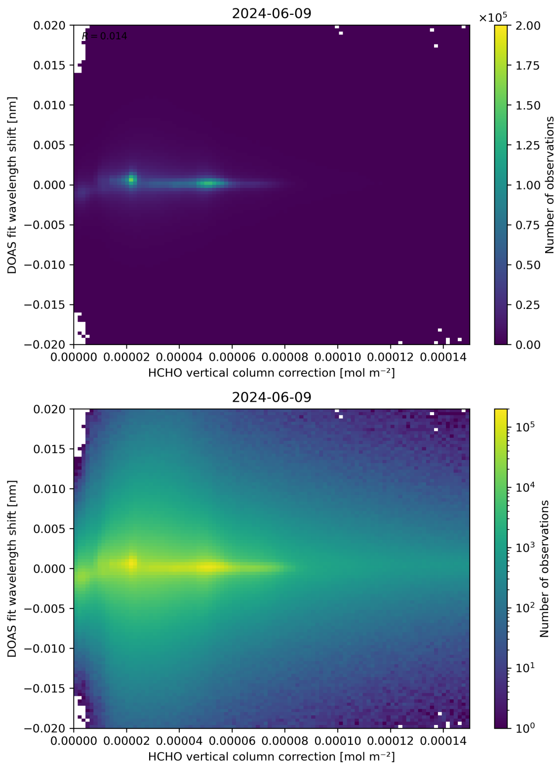
Figure 113: Scatter density plot of “HCHO vertical column correction” against “DOAS fit wavelength shift” for 2024-06-08 to 2024-06-10.
