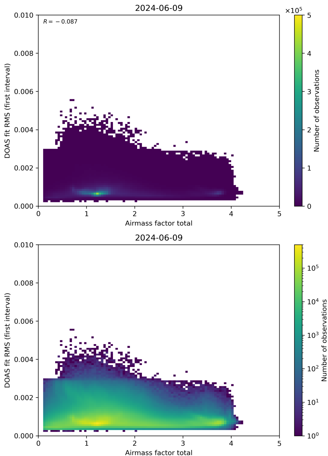
Figure 97: Scatter density plot of “Airmass factor total” against “DOAS fit RMS (first interval)” for 2024-06-08 to 2024-06-10.
