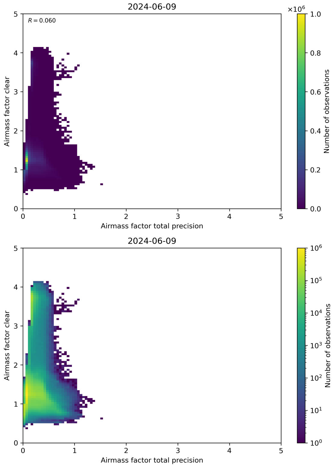
Figure 108: Scatter density plot of “Airmass factor total precision” against “Airmass factor clear” for 2024-06-08 to 2024-06-10.
