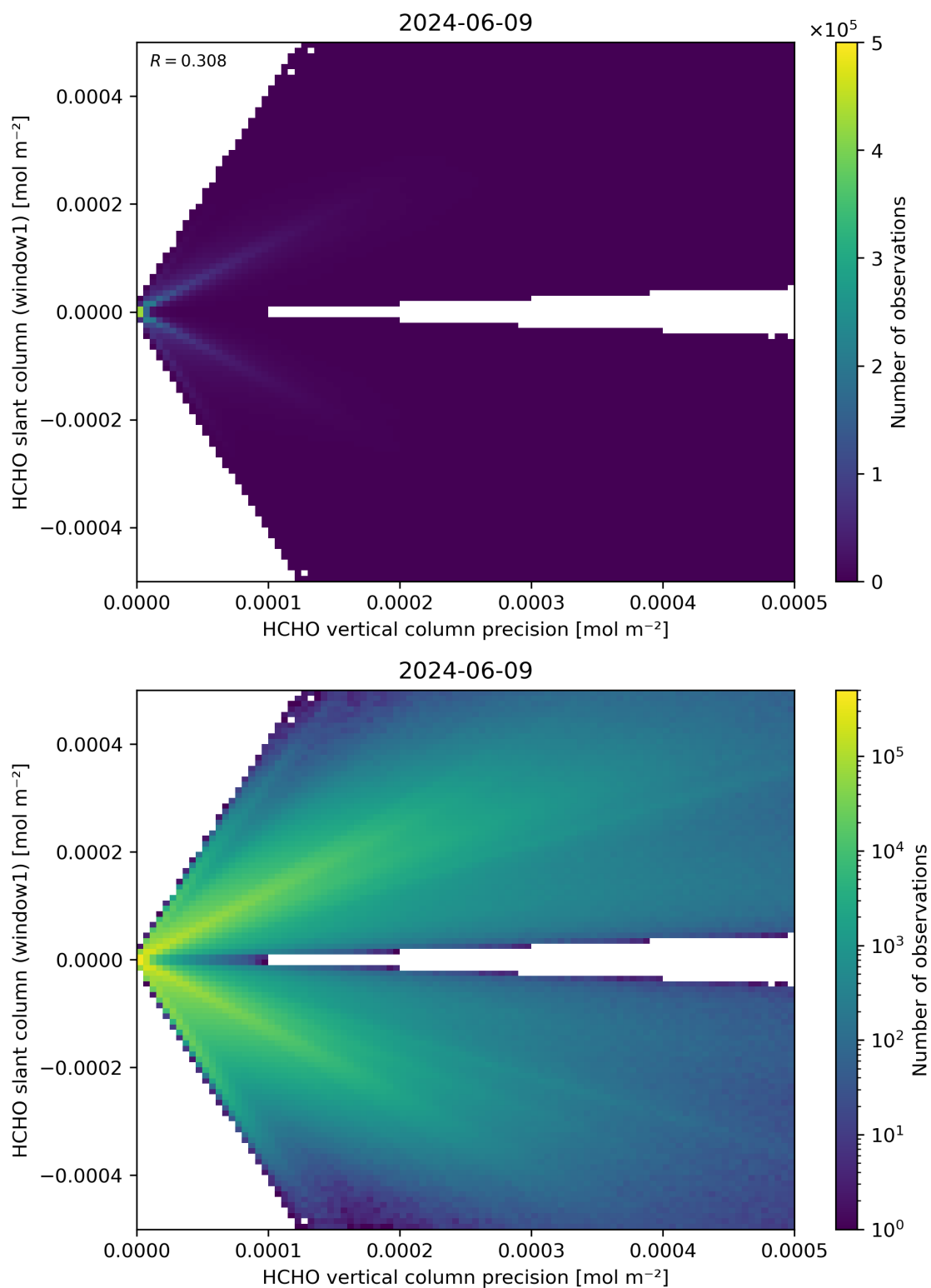
Figure 142: Scatter density plot of “HCHO vertical column precision” against “HCHO slant column (window1)” for 2024-06-08 to 2024-06-10.
