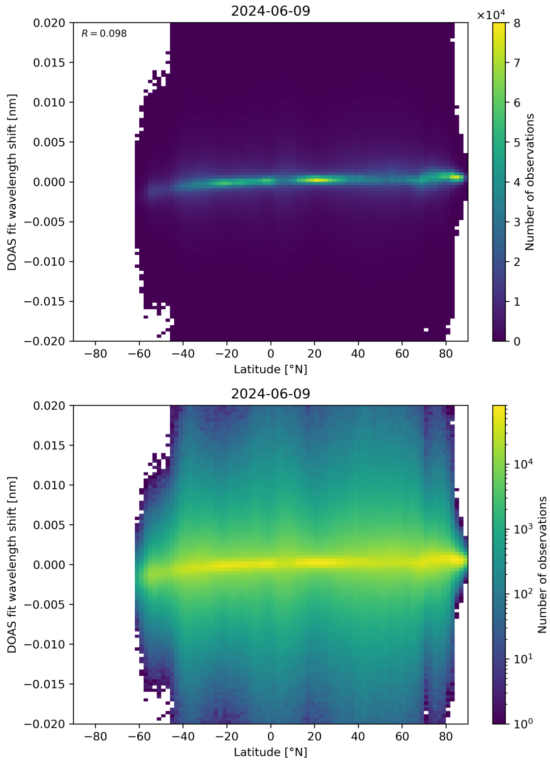
Figure 154: Scatter density plot of “Latitude” against “DOAS fit wavelength shift” for 2024-06-08 to 2024-06-10.
