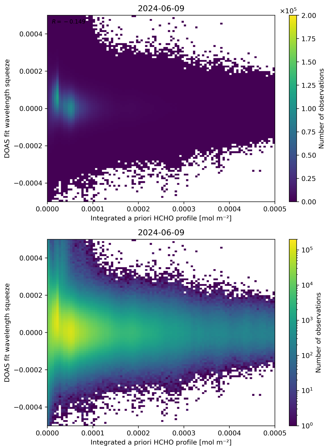
Figure 150: Scatter density plot of “Integrated a priori HCHO profile” against “DOAS fit wavelength squeeze” for 2024-06-08 to 2024-06-10.
