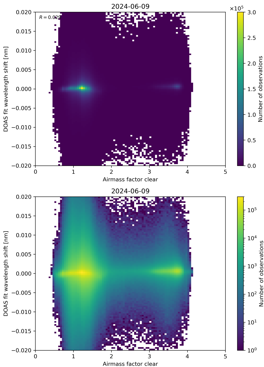
Figure 72: Scatter density plot of “Airmass factor clear” against “DOAS fit wavelength shift” for 2024-06-08 to 2024-06-10.
