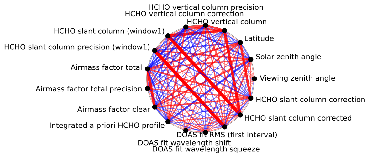
Figure 1: Map of correlation graph for 2024-06-08 to 2024-06-10.
