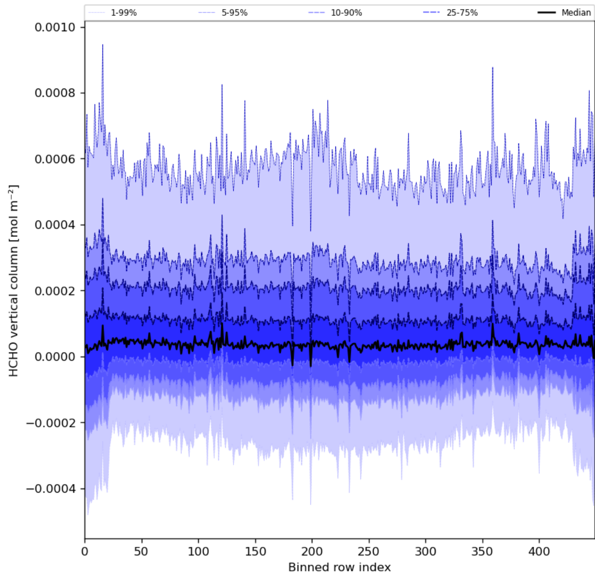
Figure 49: Along track statistics of “HCHO vertical column” for 2024-06-08 to 2024-06-10
