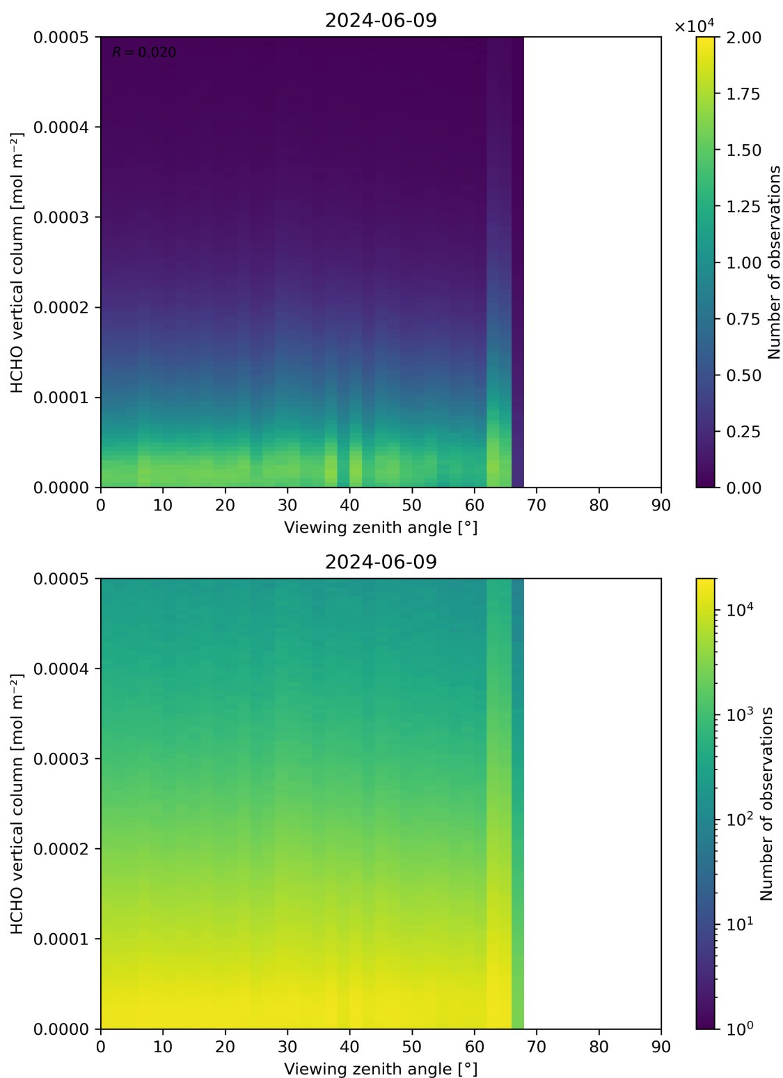
Figure 192: Scatter density plot of “Viewing zenith angle” against “HCHO vertical column” for 2024-06-08 to 2024-06-10.
