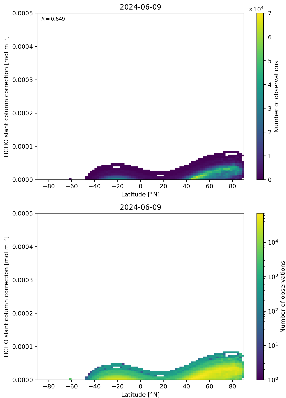
Figure 158: Scatter density plot of “Latitude” against “HCHO slant column correction” for 2024-06-08 to 2024-06-10.
