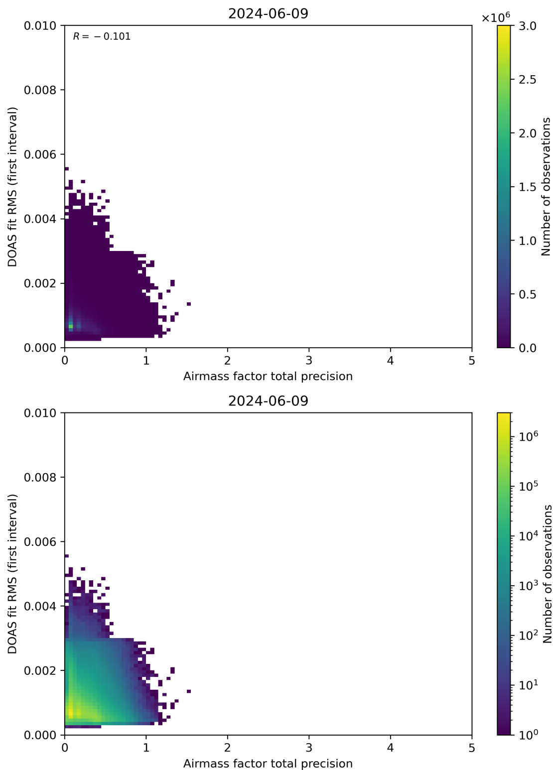
Figure 105: Scatter density plot of “Airmass factor total precision” against “DOAS fit RMS (first interval)” for 2024-06-08 to 2024-06-10.
