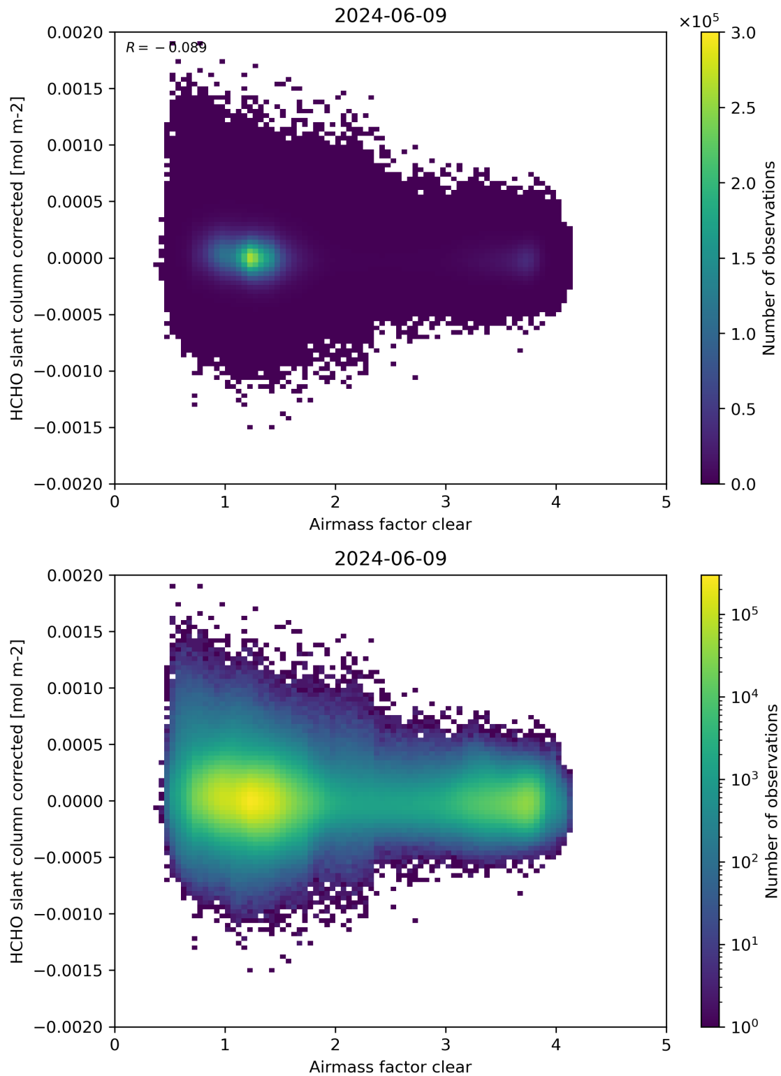
Figure 74: Scatter density plot of “Airmass factor clear” against “HCHO slant column corrected” for 2024-06-08 to 2024-06-10.
