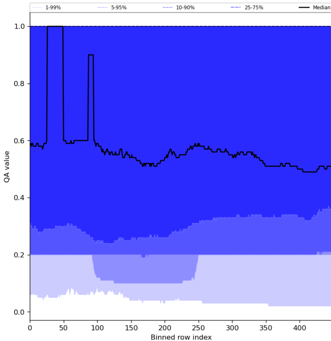
Figure 48: Along track statistics of “QA value” for 2024-06-08 to 2024-06-10
