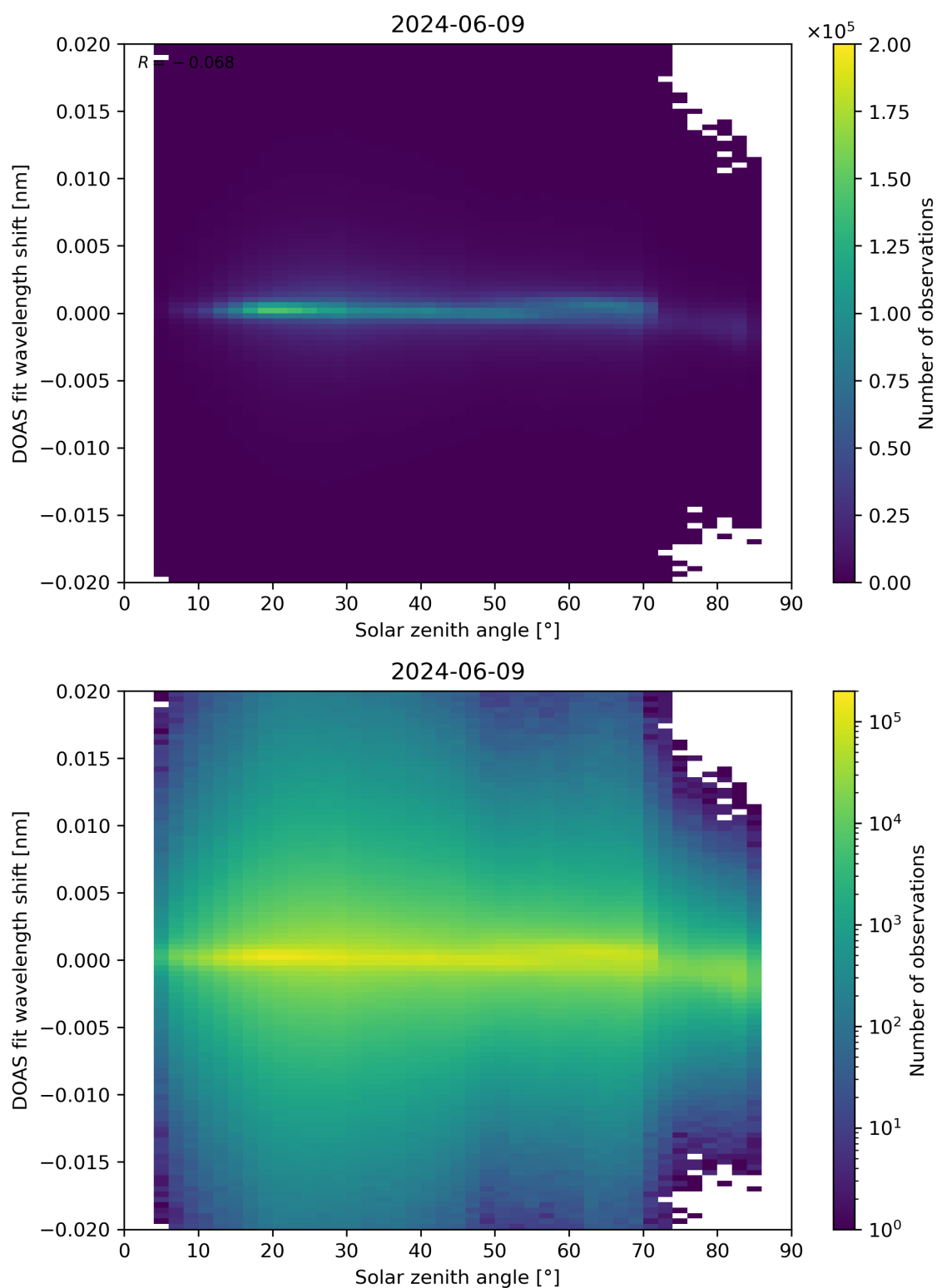
Figure 168: Scatter density plot of “Solar zenith angle” against “DOAS fit wavelength shift” for 2024-06-08 to 2024-06-10.
