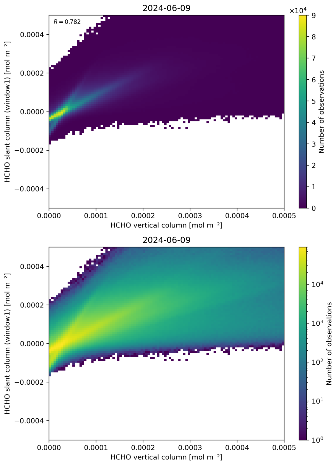
Figure 129: Scatter density plot of “HCHO vertical column” against “HCHO slant column (window1)” for 2024-06-08 to 2024-06-10.
