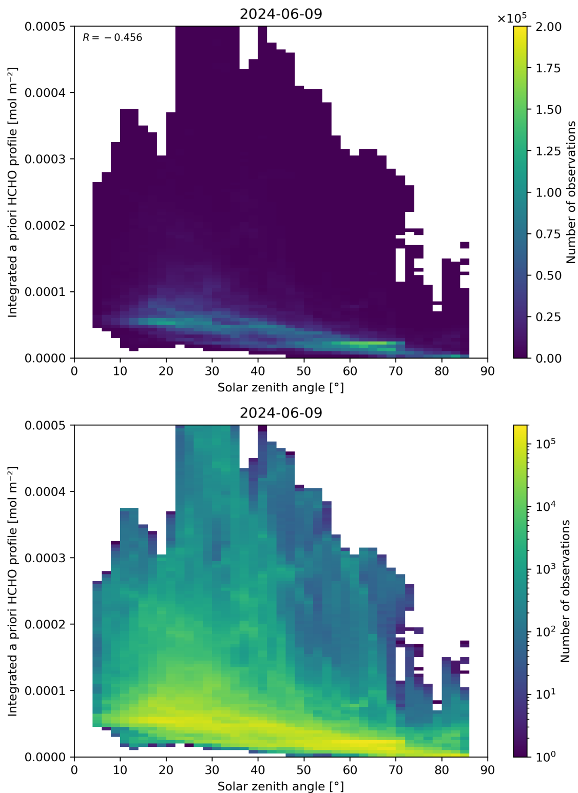
Figure 180: Scatter density plot of “Solar zenith angle” against “Integrated a priori HCHO profile” for 2024-06-08 to 2024-06-10.
