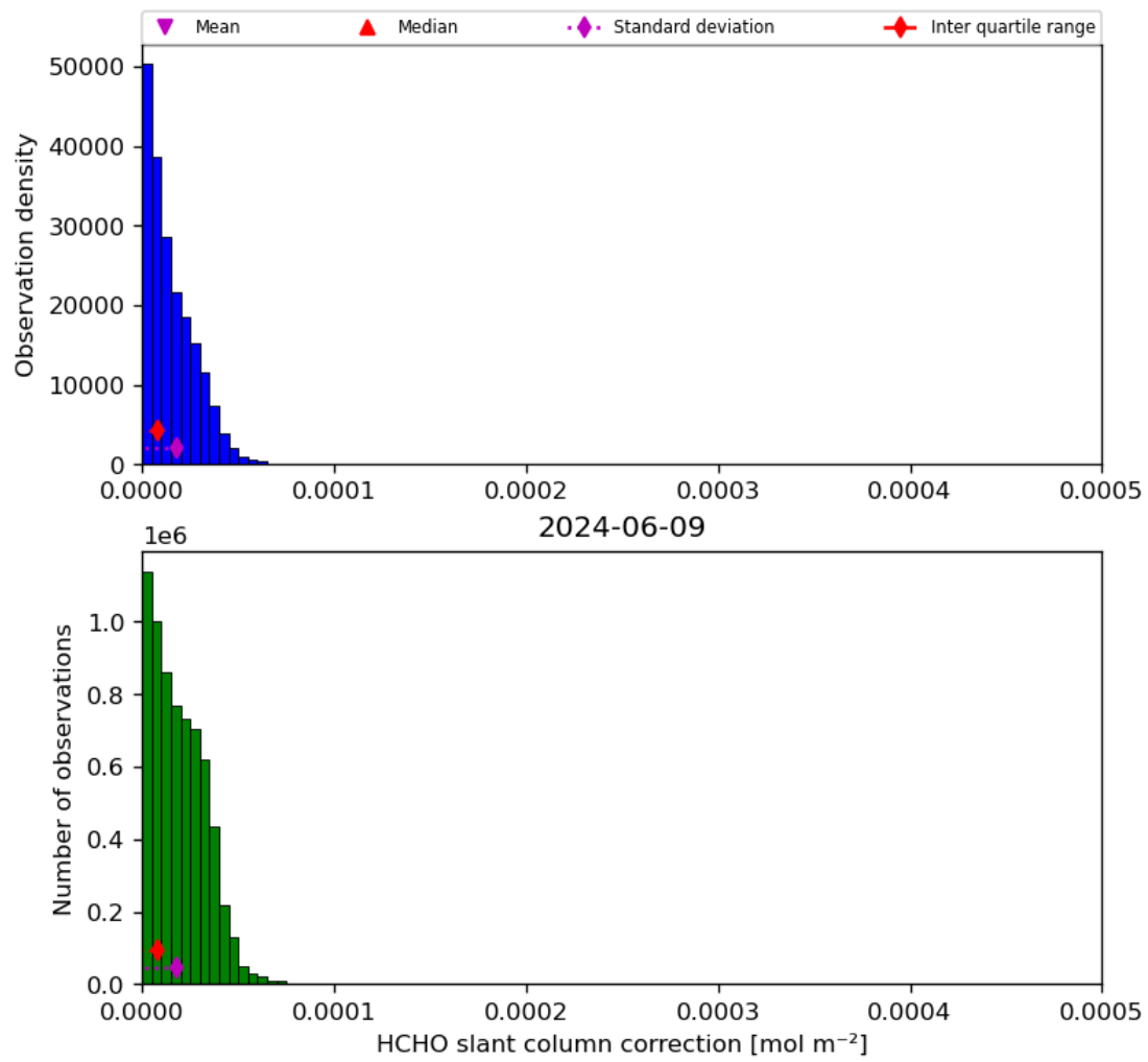
Figure 47: Histogram of “HCHO slant column correction” for 2024-06-08 to 2024-06-10
