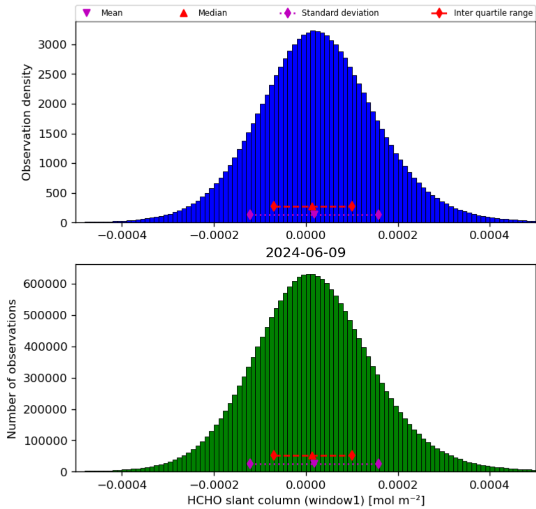
Figure 38: Histogram of “HCHO slant column (window1)” for 2024-06-08 to 2024-06-10
