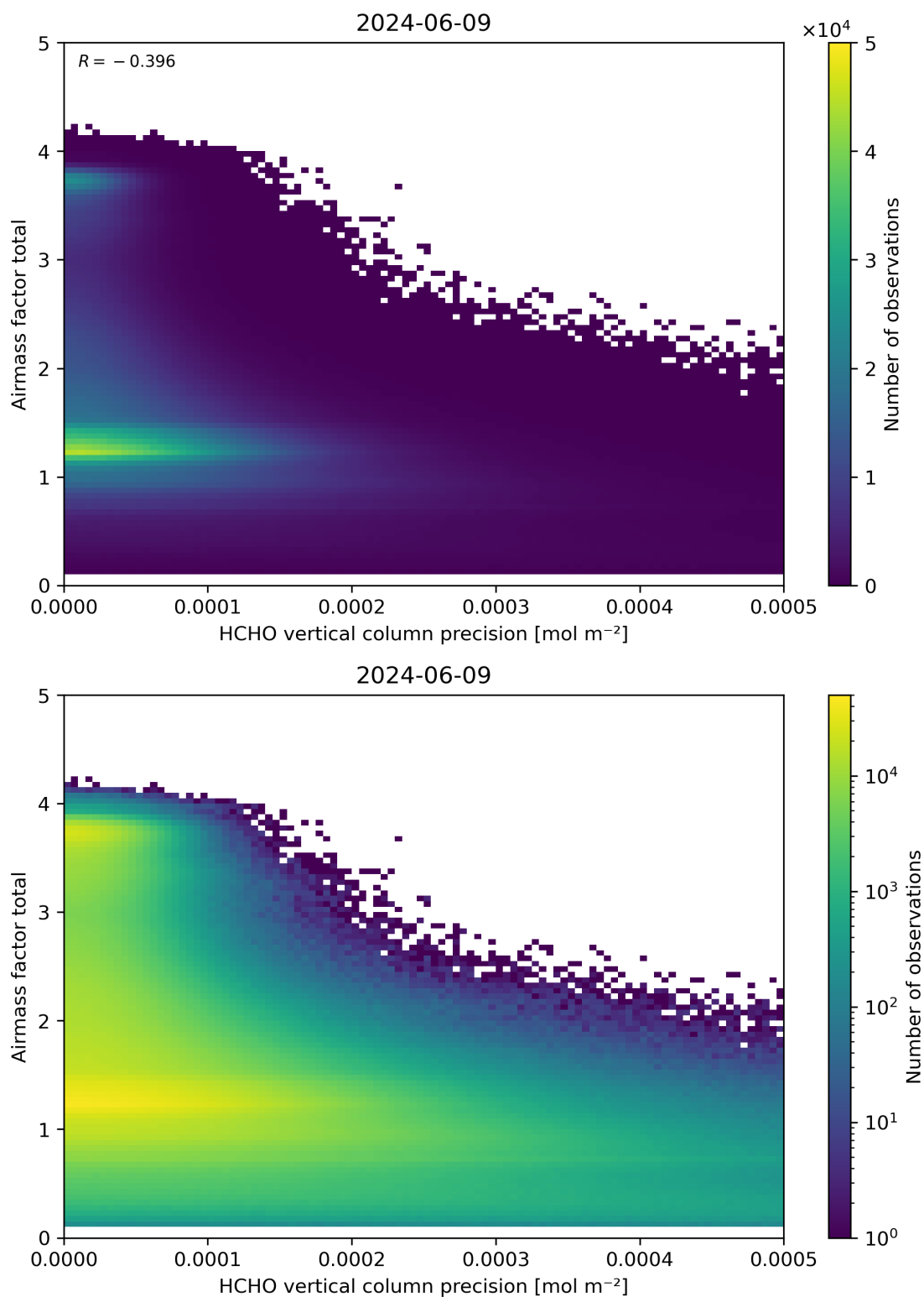
Figure 144: Scatter density plot of “HCHO vertical column precision” against “Airmass factor total” for 2024-06-08 to 2024-06-10.
