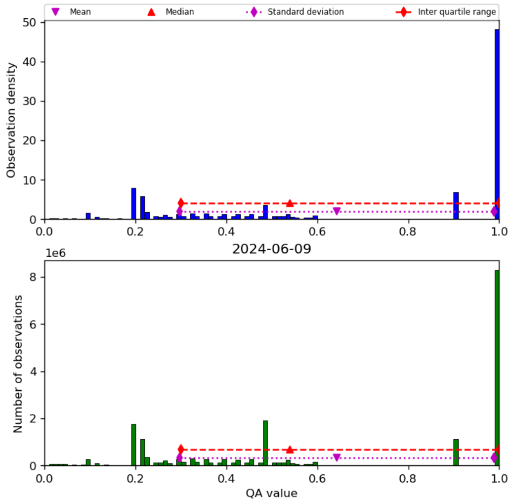
Figure 34: Histogram of “QA value” for 2024-06-08 to 2024-06-10
