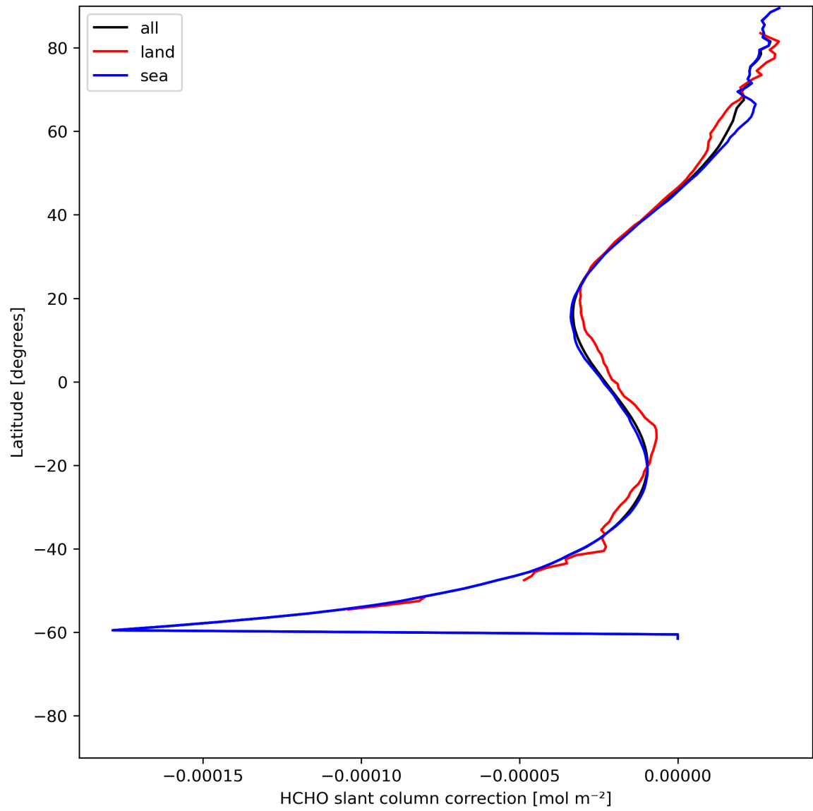
Figure 33: Zonal average of “HCHO slant column correction” for 2024-06-08 to 2024-06-10.
