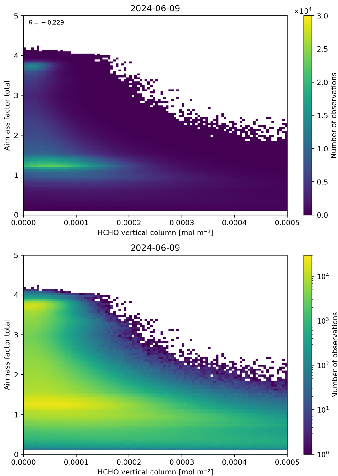
Figure 131: Scatter density plot of “HCHO vertical column” against “Airmass factor total” for 2024-06-08 to 2024-06-10.
