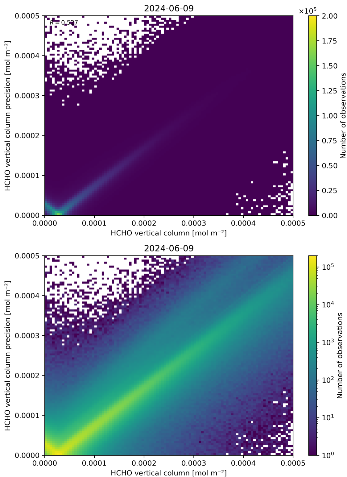
Figure 134: Scatter density plot of “HCHO vertical column” against “HCHO vertical column precision” for 2024-06-08 to 2024-06-10.
