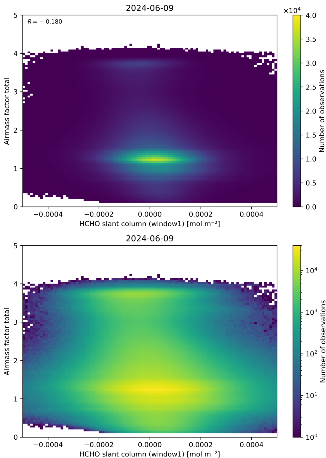
Figure 85: Scatter density plot of “HCHO slant column (window1)” against “Airmass factor total” for 2024-06-08 to 2024-06-10.
