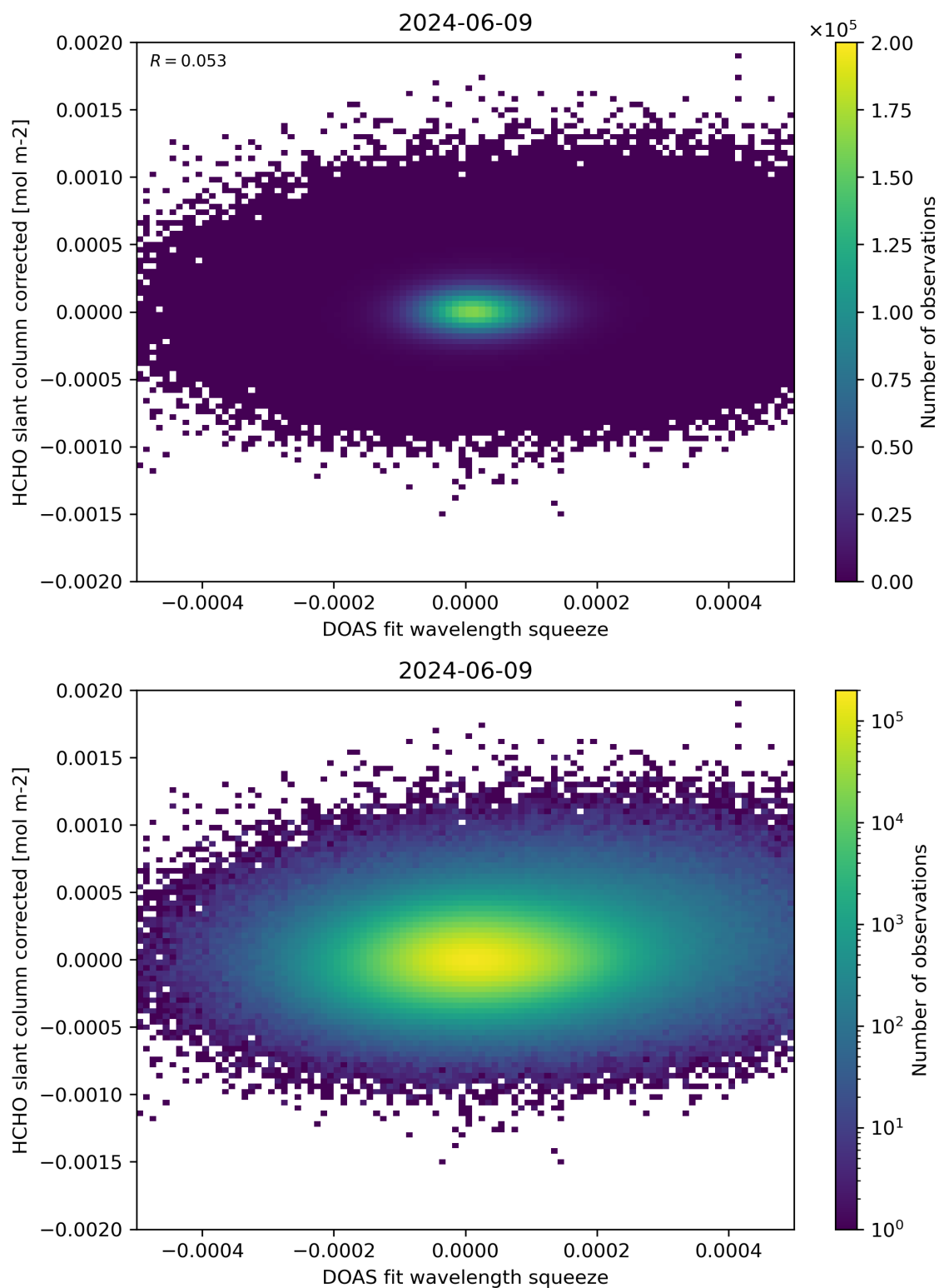
Figure 69: Scatter density plot of “DOAS fit wavelength squeeze” against “HCHO slant column corrected” for 2024-06-08 to 2024-06-10.
