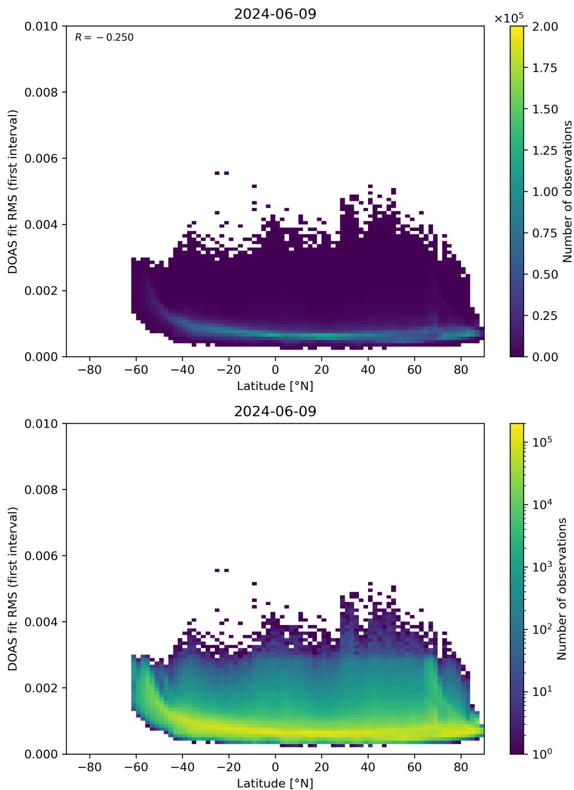
Figure 153: Scatter density plot of “Latitude” against “DOAS fit RMS (first interval)” for 2024-06-08 to 2024-06-10.
