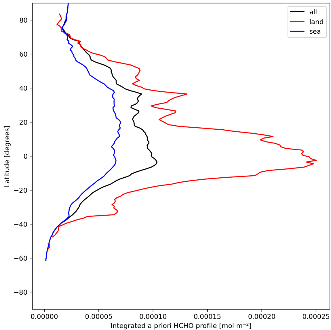
Figure 29: Zonal average of “Integrated a priori HCHO profile” for 2024-06-08 to 2024-06-10.
