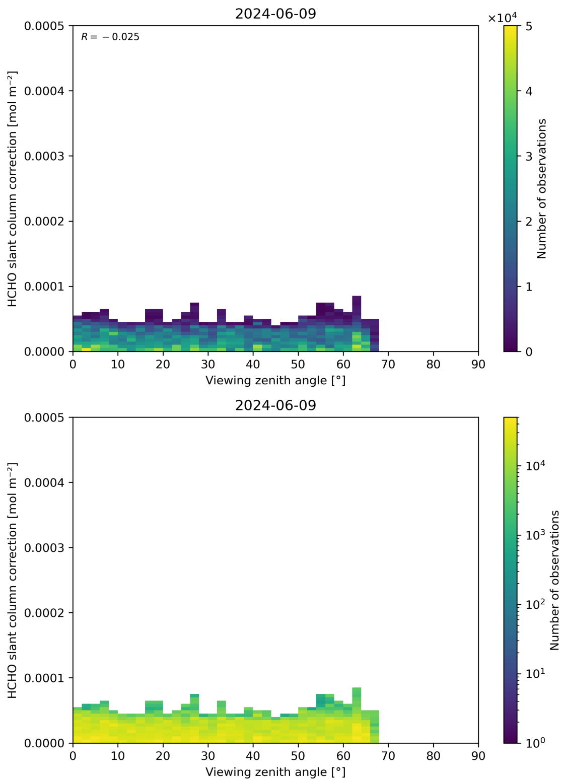
Figure 187: Scatter density plot of “Viewing zenith angle” against “HCHO slant column correction” for 2024-06-08 to 2024-06-10.
