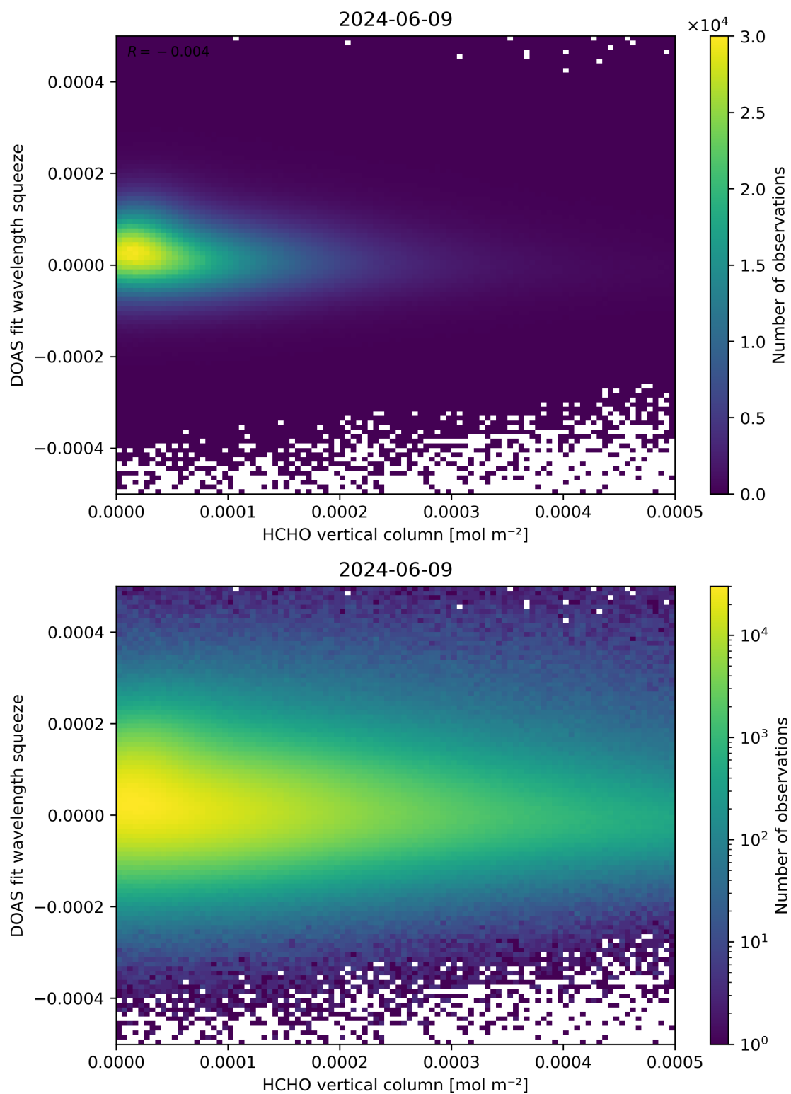
Figure 125: Scatter density plot of “HCHO vertical column” against “DOAS fit wavelength squeeze” for 2024-06-08 to 2024-06-10.
