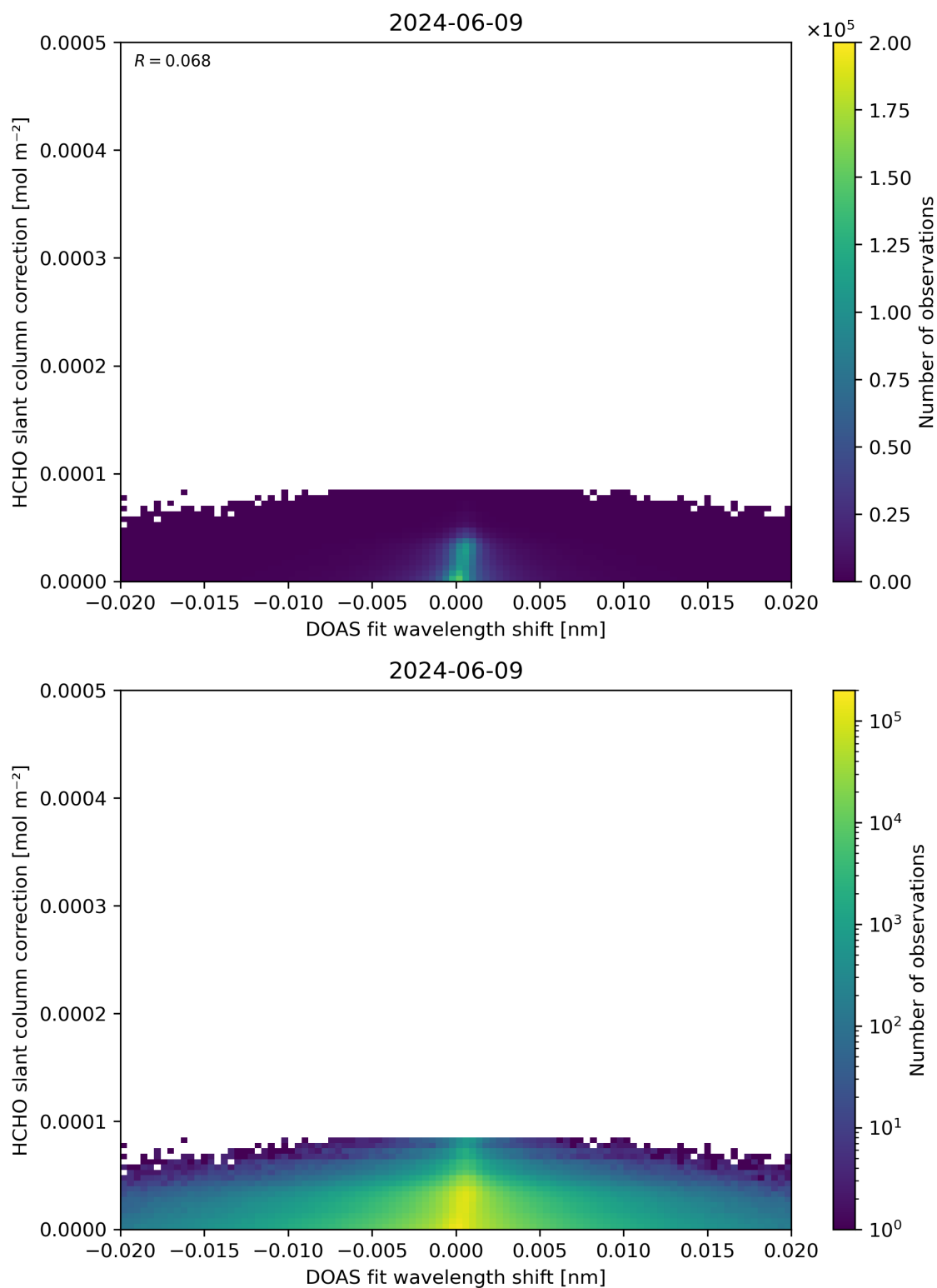
Figure 67: Scatter density plot of “DOAS fit wavelength shift” against “HCHO slant column correction” for 2024-06-08 to 2024-06-10.
