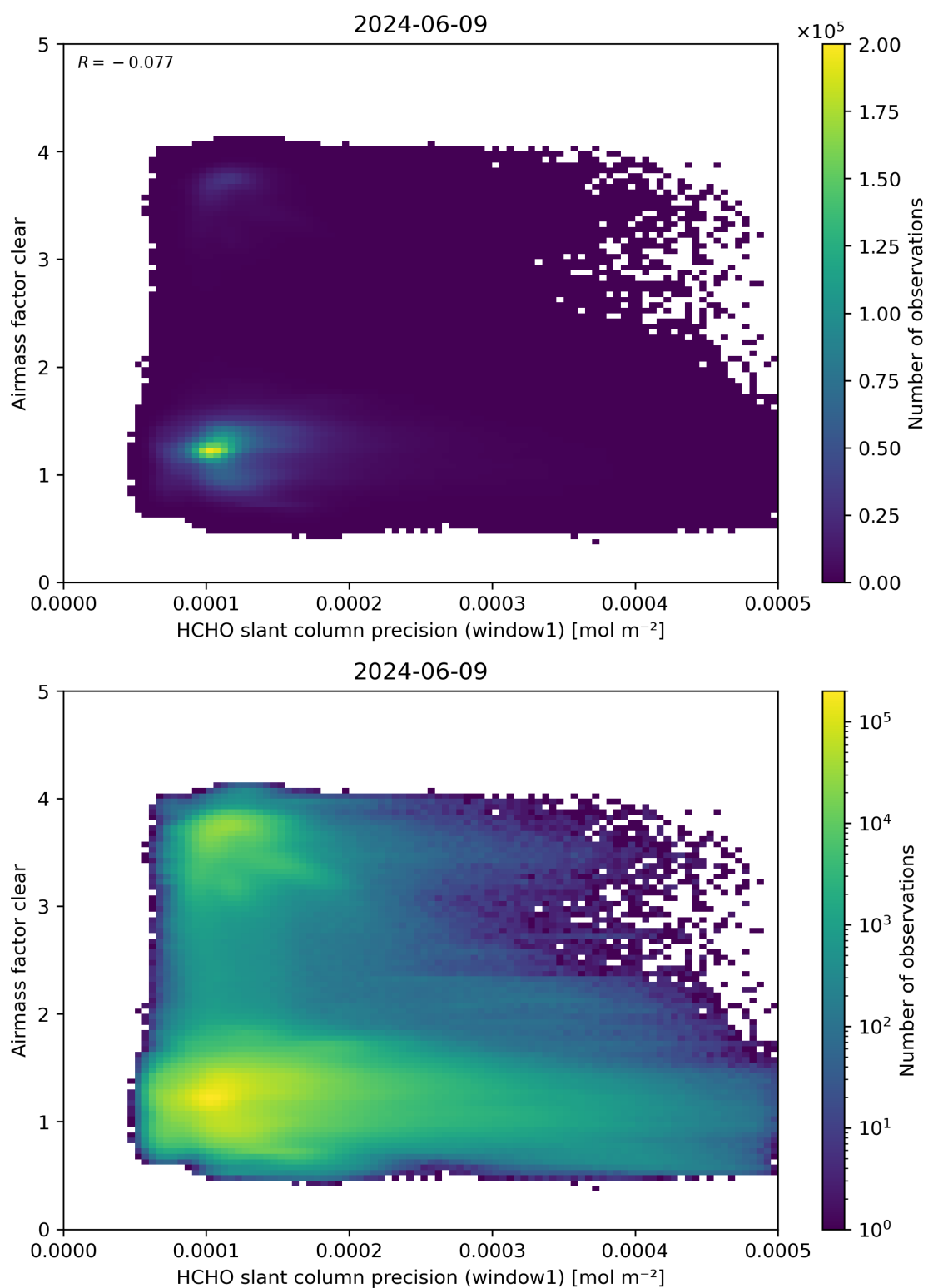
Figure 91: Scatter density plot of “HCHO slant column precision (window1)” against “Airmass factor clear” for 2024-06-08 to 2024-06-10.
