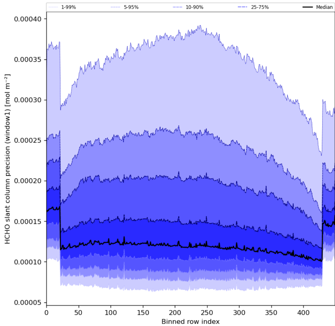
Figure 53: Along track statistics of “HCHO slant column precision (window1)” for 2024-06-08 to 2024-06-10
