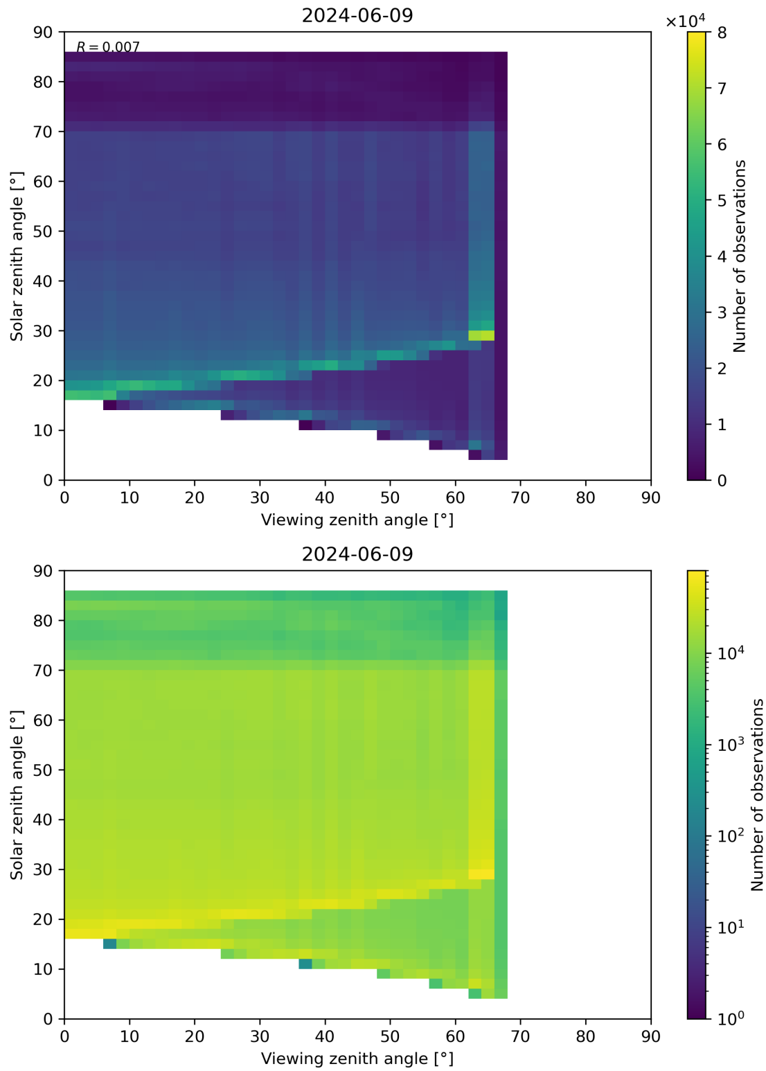
Figure 197: Scatter density plot of “Viewing zenith angle” against “Solar zenith angle” for 2024-06-08 to 2024-06-10.
