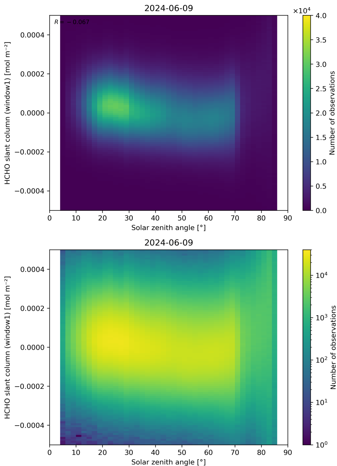
Figure 173: Scatter density plot of “Solar zenith angle” against “HCHO slant column (window1)” for 2024-06-08 to 2024-06-10.
