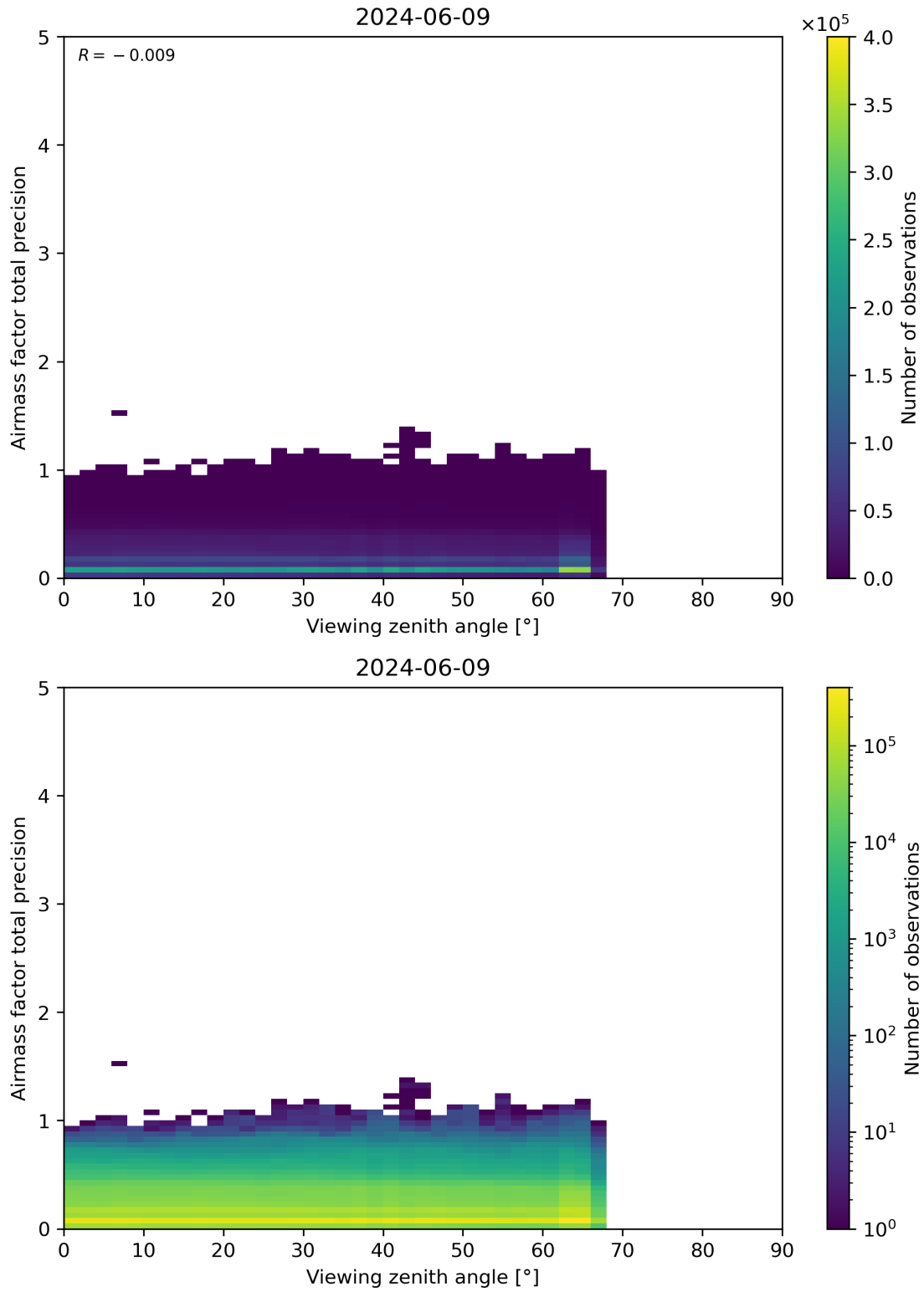
Figure 191: Scatter density plot of “Viewing zenith angle” against “Airmass factor total precision” for 2024-06-08 to 2024-06-10.
