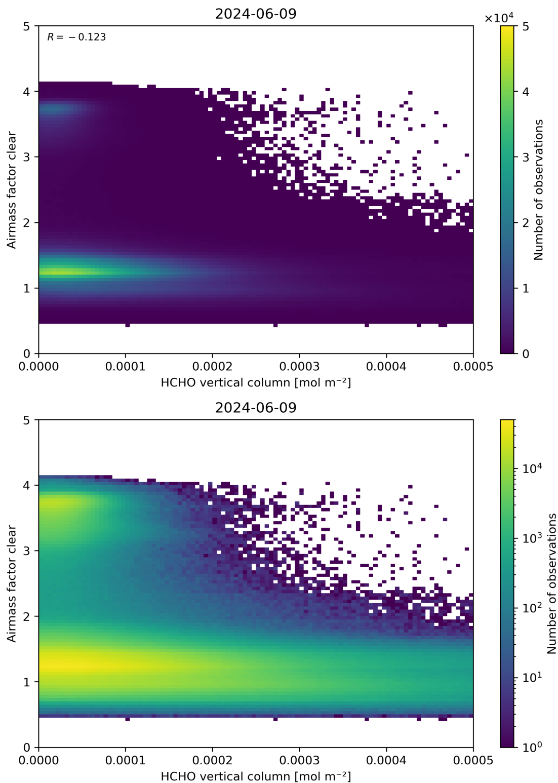
Figure 126: Scatter density plot of “HCHO vertical column” against “Airmass factor clear” for 2024-06-08 to 2024-06-10.
