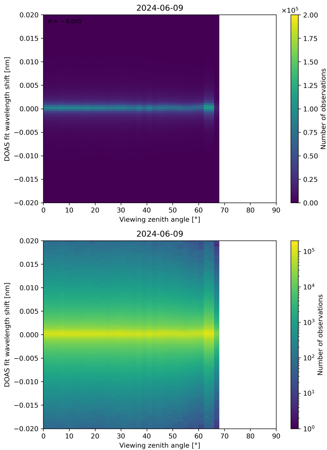
Figure 183: Scatter density plot of “Viewing zenith angle” against “DOAS fit wavelength shift” for 2024-06-08 to 2024-06-10.
