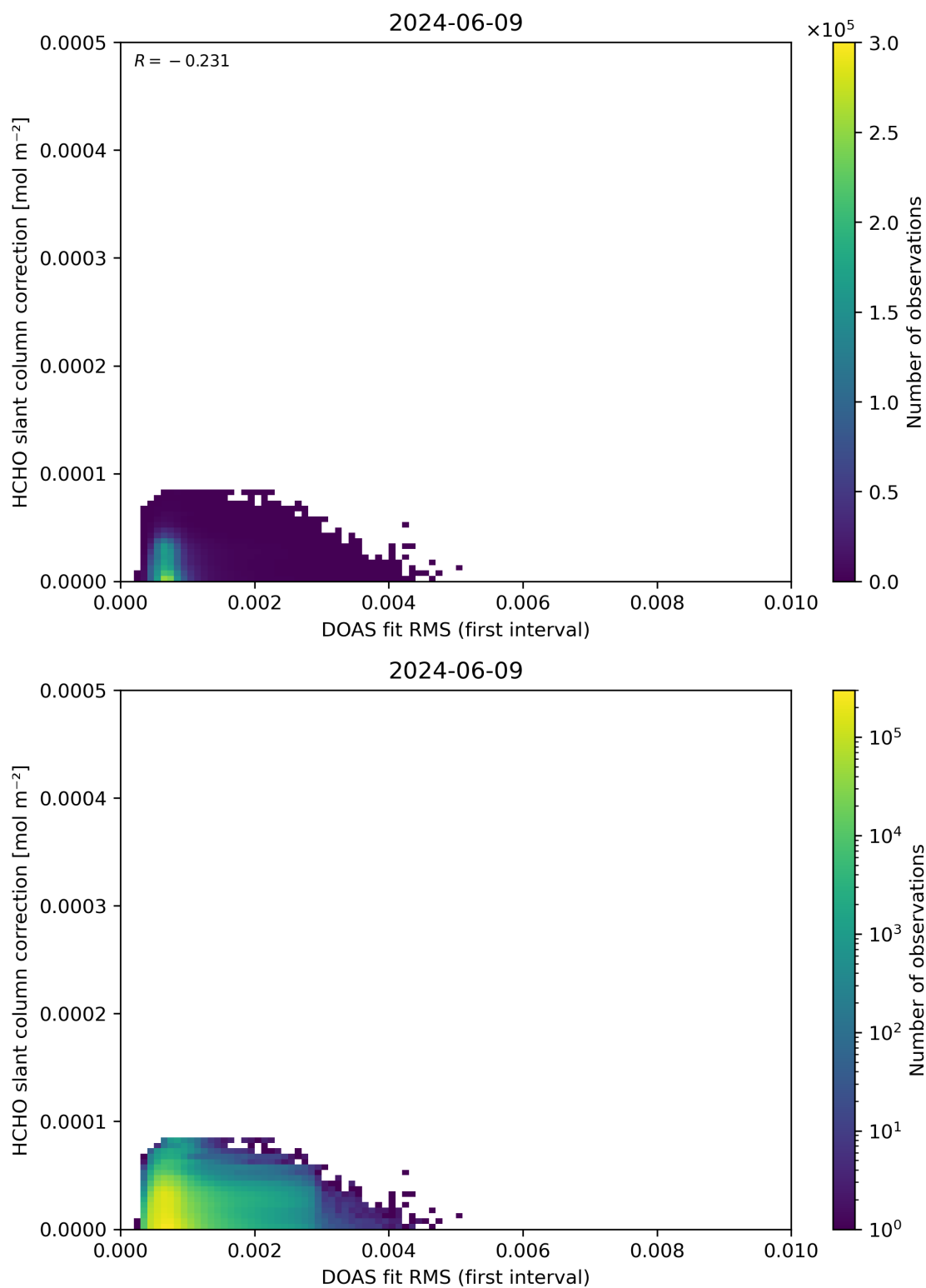
Figure 63: Scatter density plot of “DOAS fit RMS (first interval)” against “HCHO slant column correction” for 2024-06-08 to 2024-06-10.
