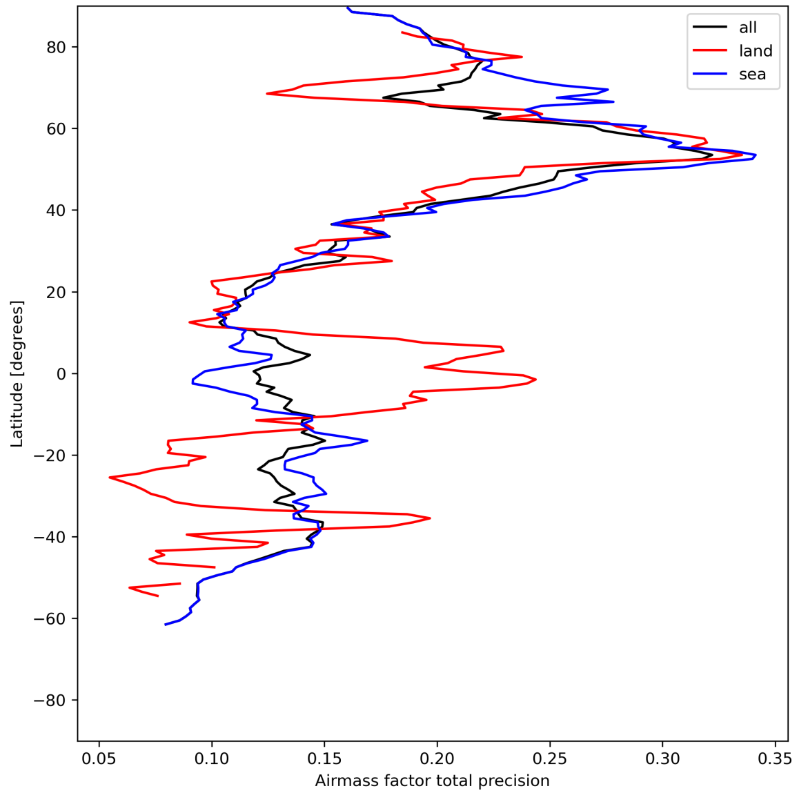
Figure 27: Zonal average of “Airmass factor total precision” for 2024-06-08 to 2024-06-10.
