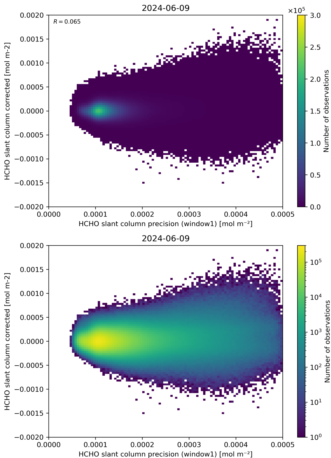
Figure 92: Scatter density plot of “HCHO slant column precision (window1)” against “HCHO slant column corrected” for 2024-06-08 to 2024-06-10.
