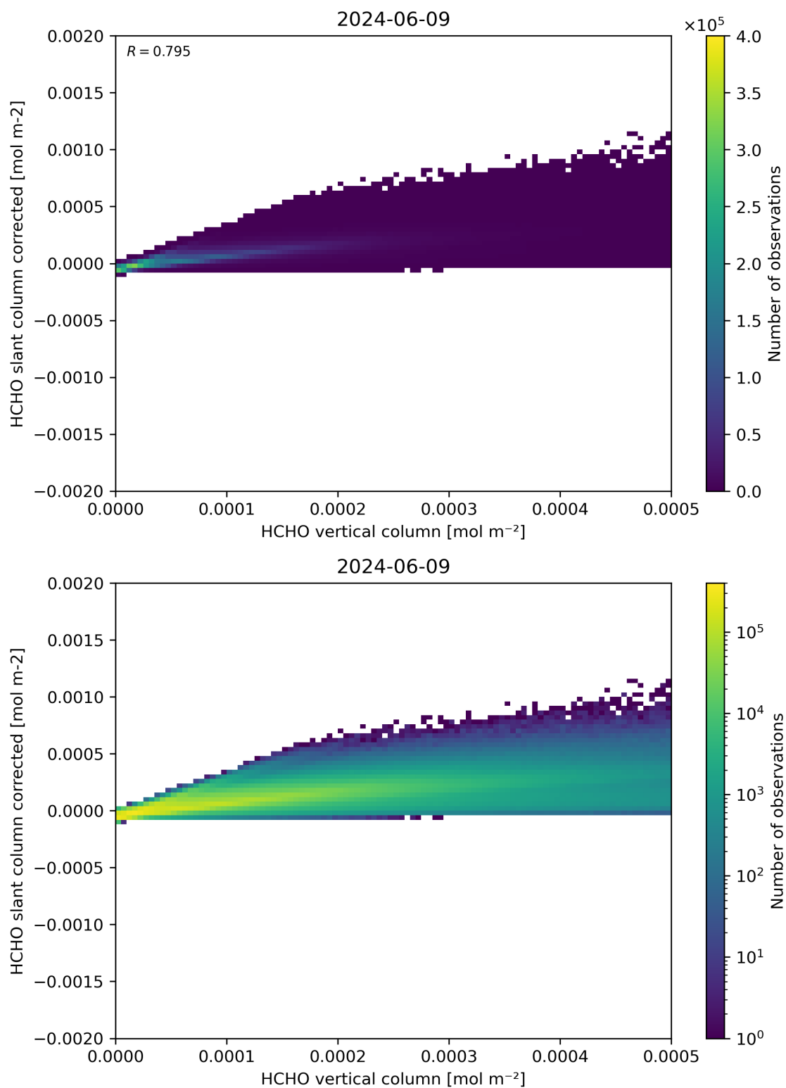
Figure 127: Scatter density plot of “HCHO vertical column” against “HCHO slant column corrected” for 2024-06-08 to 2024-06-10.
