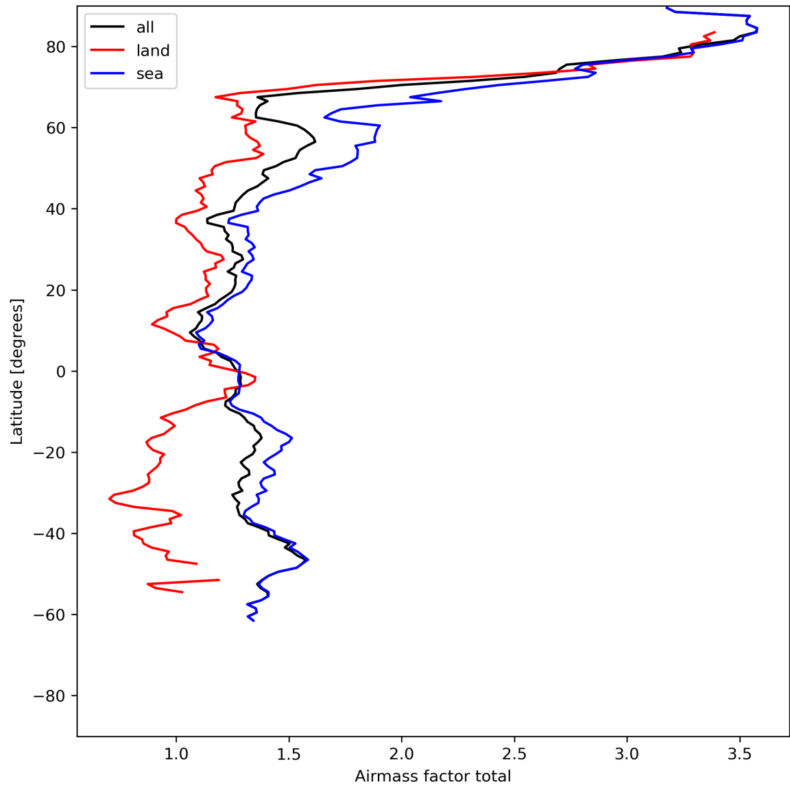
Figure 26: Zonal average of “Airmass factor total” for 2024-06-08 to 2024-06-10.
