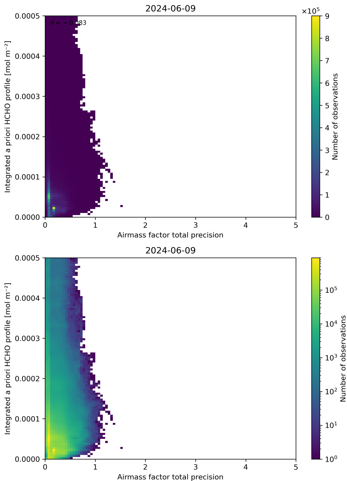
Figure 111: Scatter density plot of “Airmass factor total precision” against “Integrated a priori HCHO profile” for 2024-06-08 to 2024-06-10.
