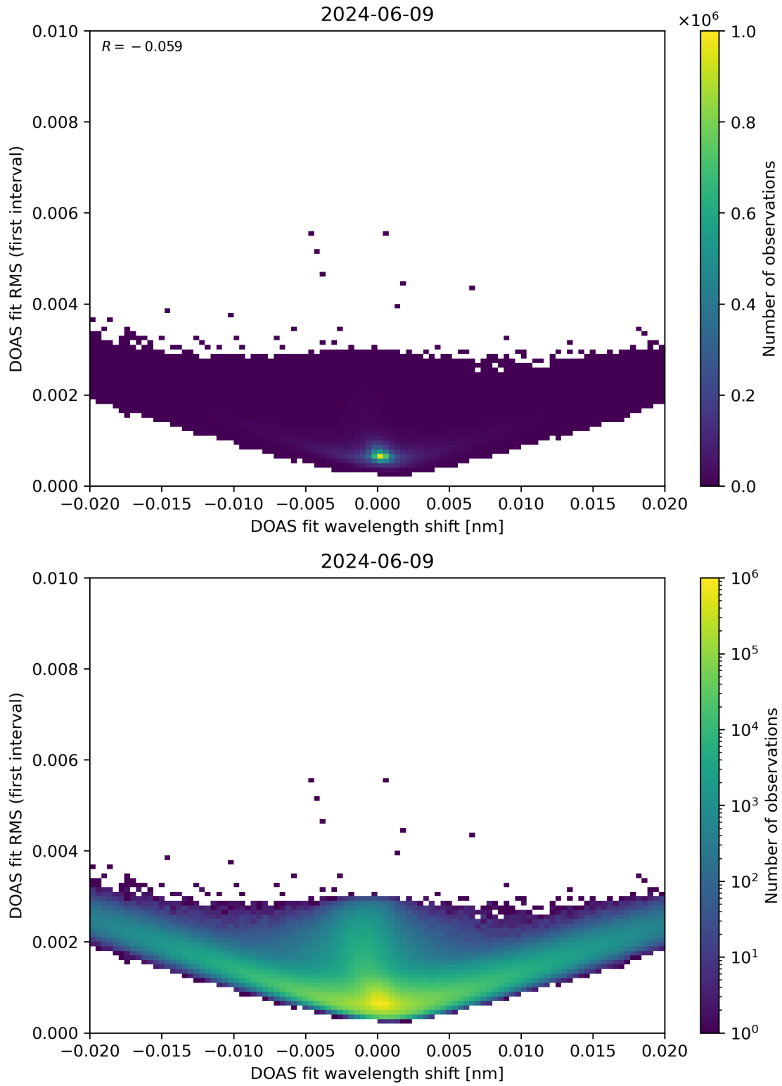
Figure 64: Scatter density plot of “DOAS fit wavelength shift” against “DOAS fit RMS (first interval)” for 2024-06-08 to 2024-06-10.
