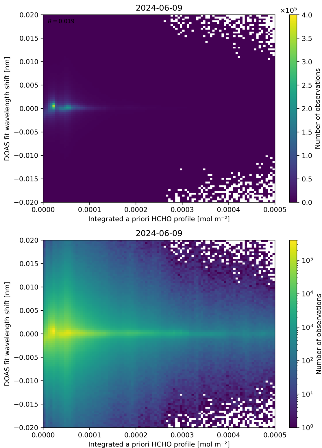
Figure 149: Scatter density plot of “Integrated a priori HCHO profile” against “DOAS fit wavelength shift” for 2024-06-08 to 2024-06-10.
