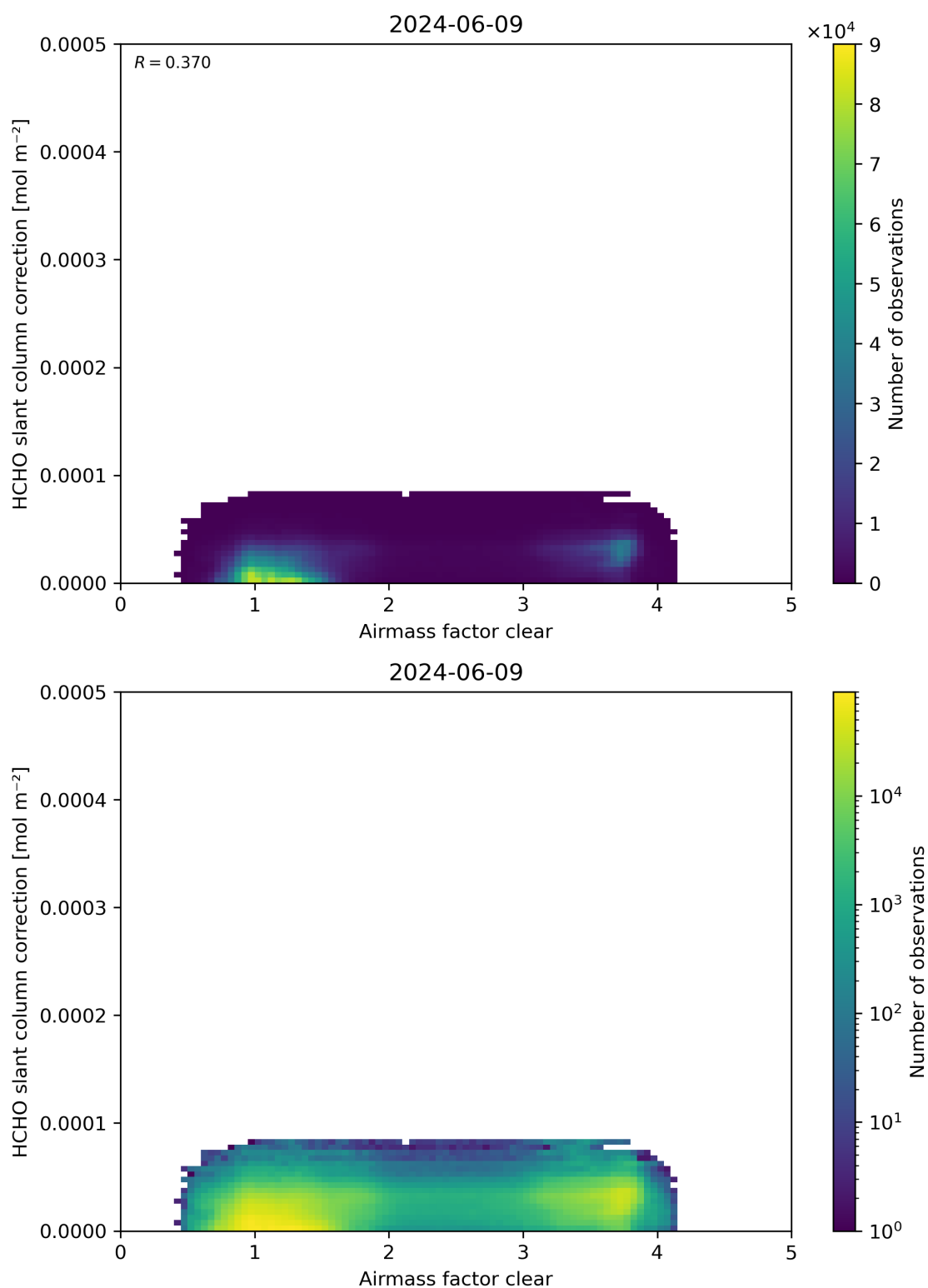
Figure 75: Scatter density plot of “Airmass factor clear” against “HCHO slant column correction” for 2024-06-08 to 2024-06-10.
