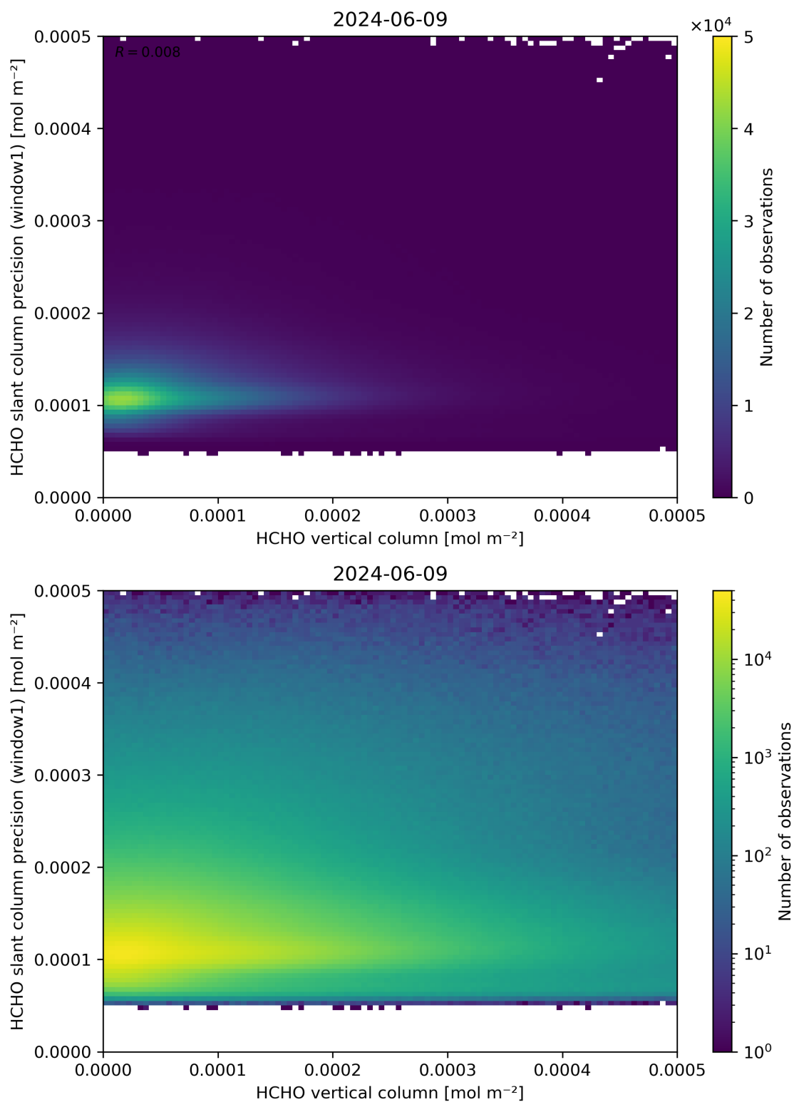
Figure 130: Scatter density plot of “HCHO vertical column” against “HCHO slant column precision (window1)” for 2024-06-08 to 2024-06-10.
