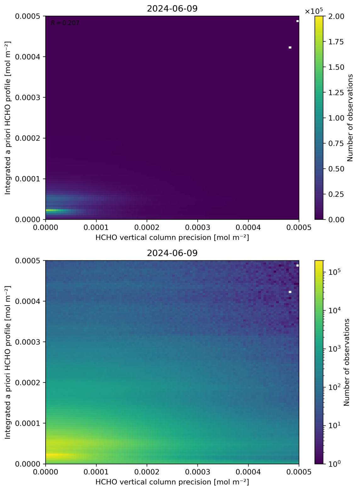
Figure 147: Scatter density plot of “HCHO vertical column precision” against “Integrated a priori HCHO profile” for 2024-06-08 to 2024-06-10.
