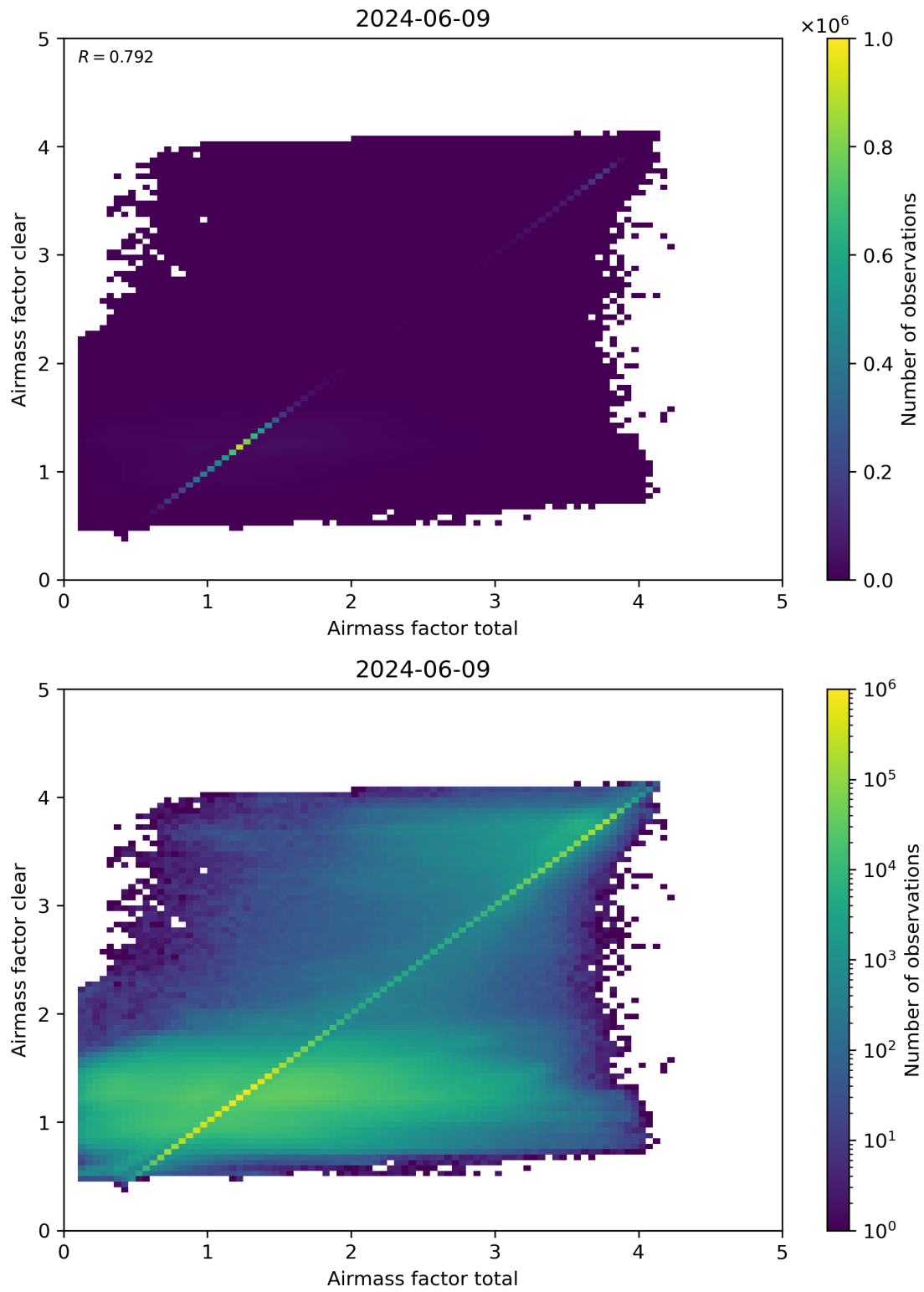
Figure 100: Scatter density plot of “Airmass factor total” against “Airmass factor clear” for 2024-06-08 to 2024-06-10.
