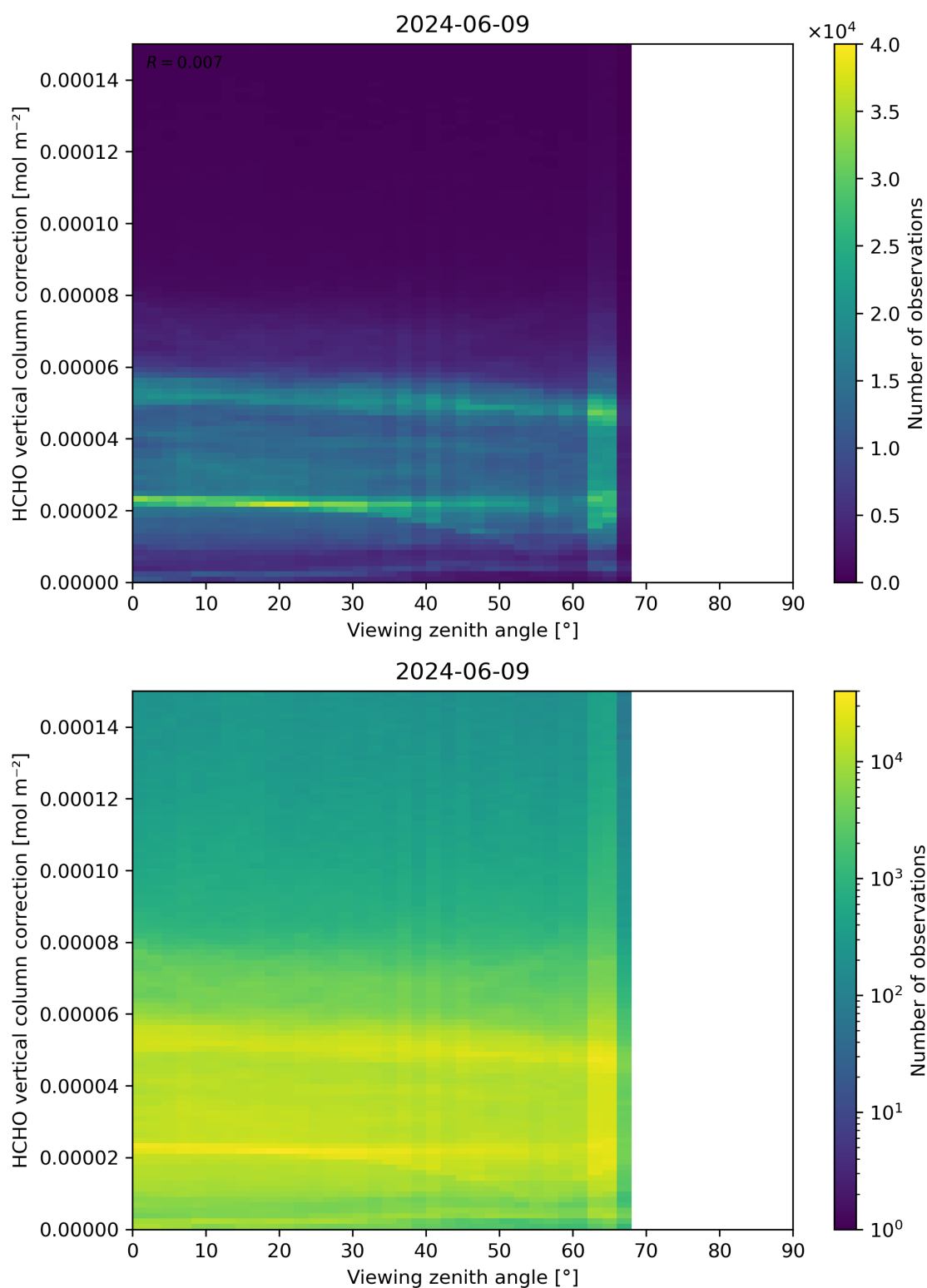
Figure 193: Scatter density plot of “Viewing zenith angle” against “HCHO vertical column correction” for 2024-06-08 to 2024-06-10.
