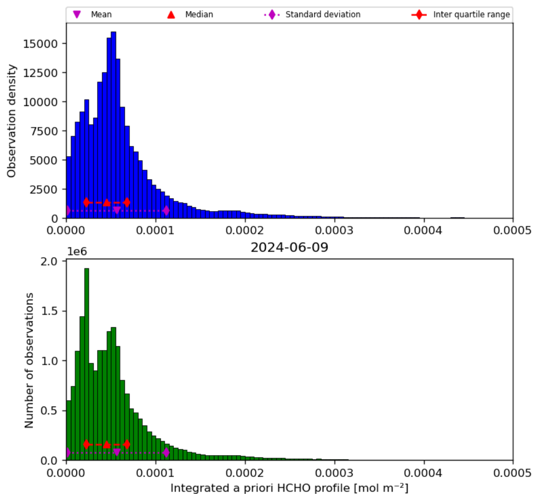
Figure 43: Histogram of “Integrated a priori HCHO profile” for 2024-06-08 to 2024-06-10
