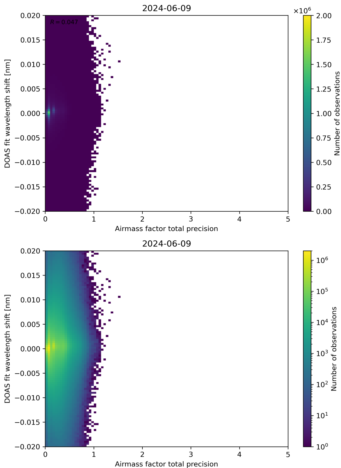
Figure 106: Scatter density plot of “Airmass factor total precision” against “DOAS fit wavelength shift” for 2024-06-08 to 2024-06-10.
