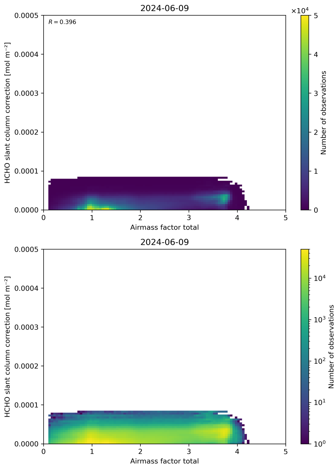
Figure 102: Scatter density plot of “Airmass factor total” against “HCHO slant column correction” for 2024-06-08 to 2024-06-10.
