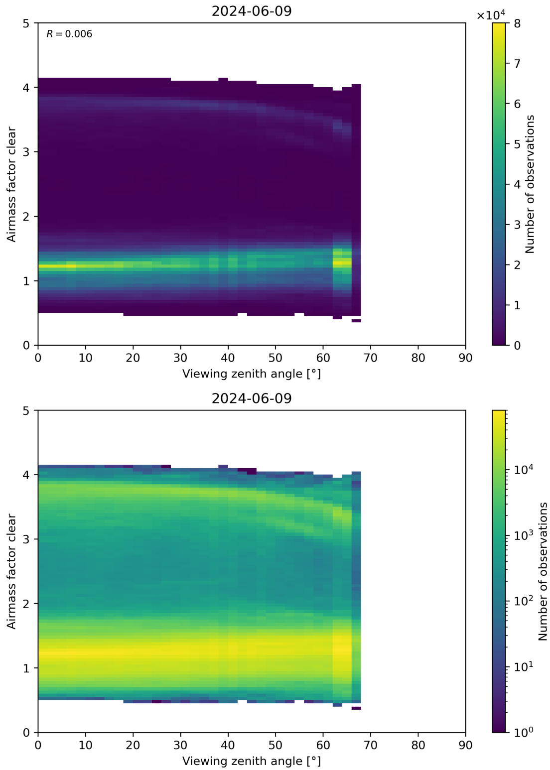
Figure 185: Scatter density plot of “Viewing zenith angle” against “Airmass factor clear” for 2024-06-08 to 2024-06-10.
