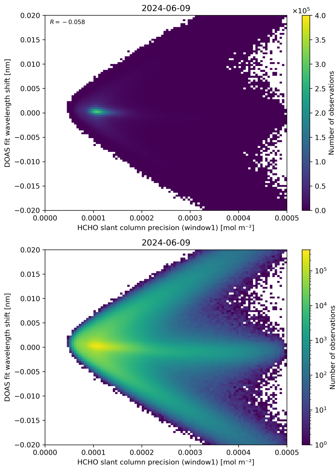
Figure 89: Scatter density plot of “HCHO slant column precision (window1)” against “DOAS fit wavelength shift” for 2024-06-08 to 2024-06-10.
