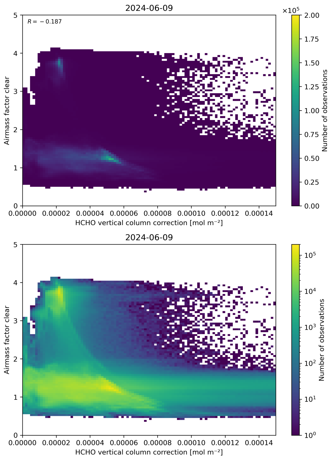
Figure 115: Scatter density plot of “HCHO vertical column correction” against “Airmass factor clear” for 2024-06-08 to 2024-06-10.
