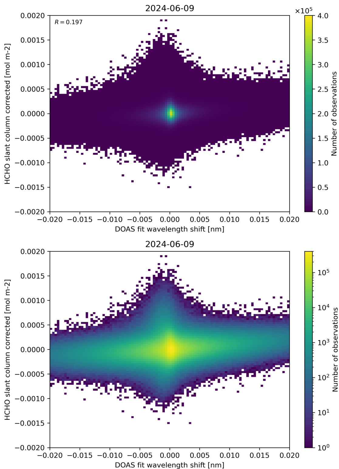
Figure 66: Scatter density plot of “DOAS fit wavelength shift” against “HCHO slant column corrected” for 2024-06-08 to 2024-06-10.
