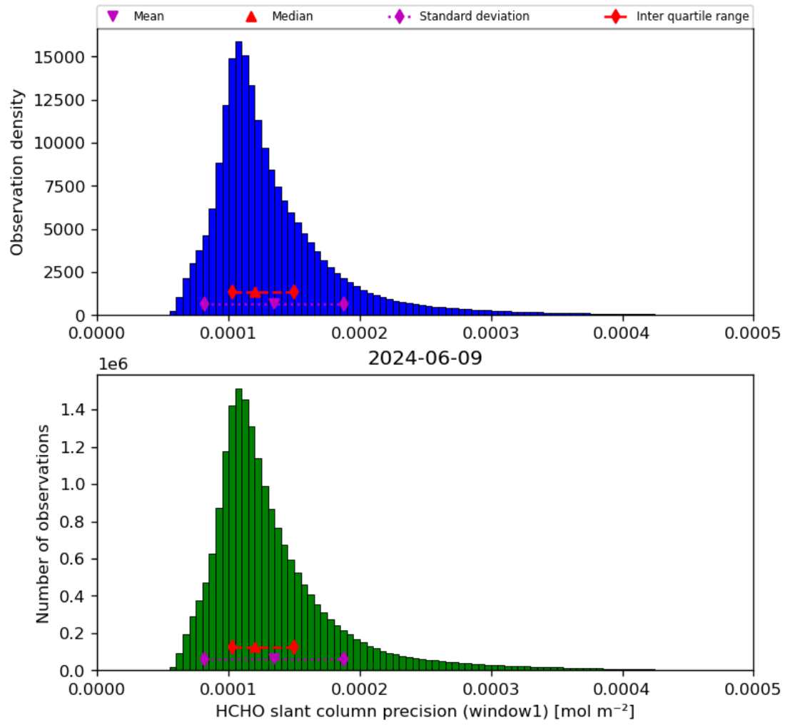
Figure 39: Histogram of “HCHO slant column precision (window1)” for 2024-06-08 to 2024-06-10
