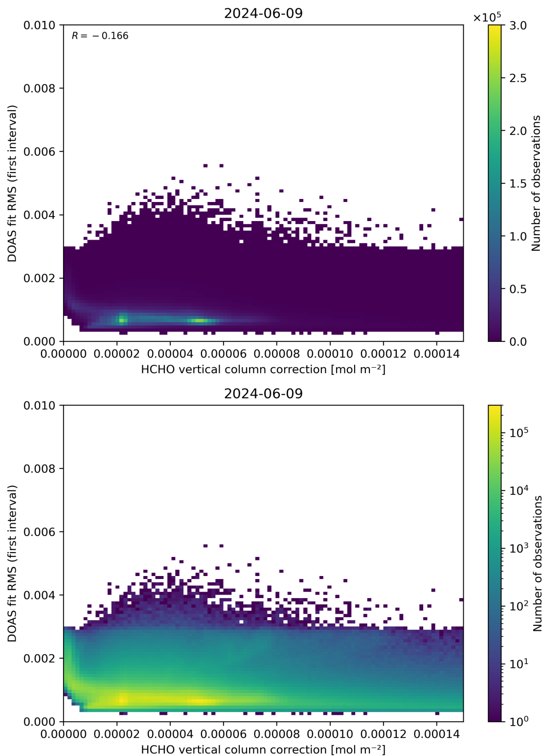
Figure 112: Scatter density plot of “HCHO vertical column correction” against “DOAS fit RMS (first interval)” for 2024-06-08 to 2024-06-10.
