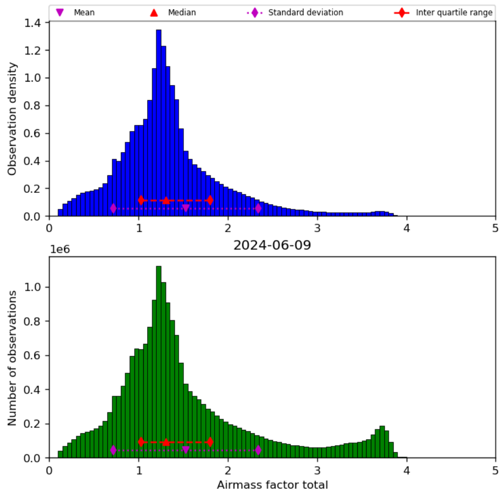
Figure 40: Histogram of “Airmass factor total” for 2024-06-08 to 2024-06-10
