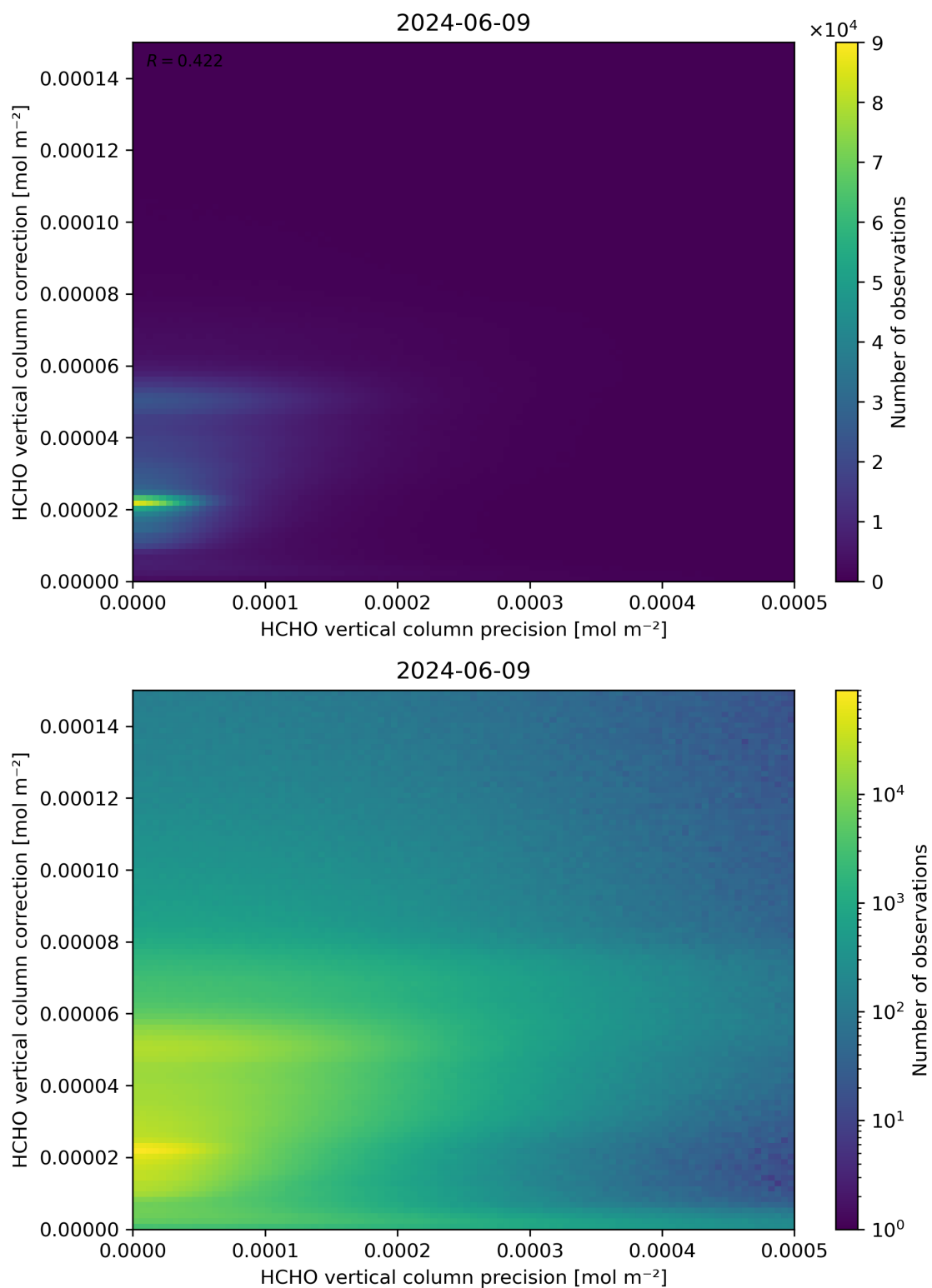
Figure 146: Scatter density plot of “HCHO vertical column precision” against “HCHO vertical column correction” for 2024-06-08 to 2024-06-10.
