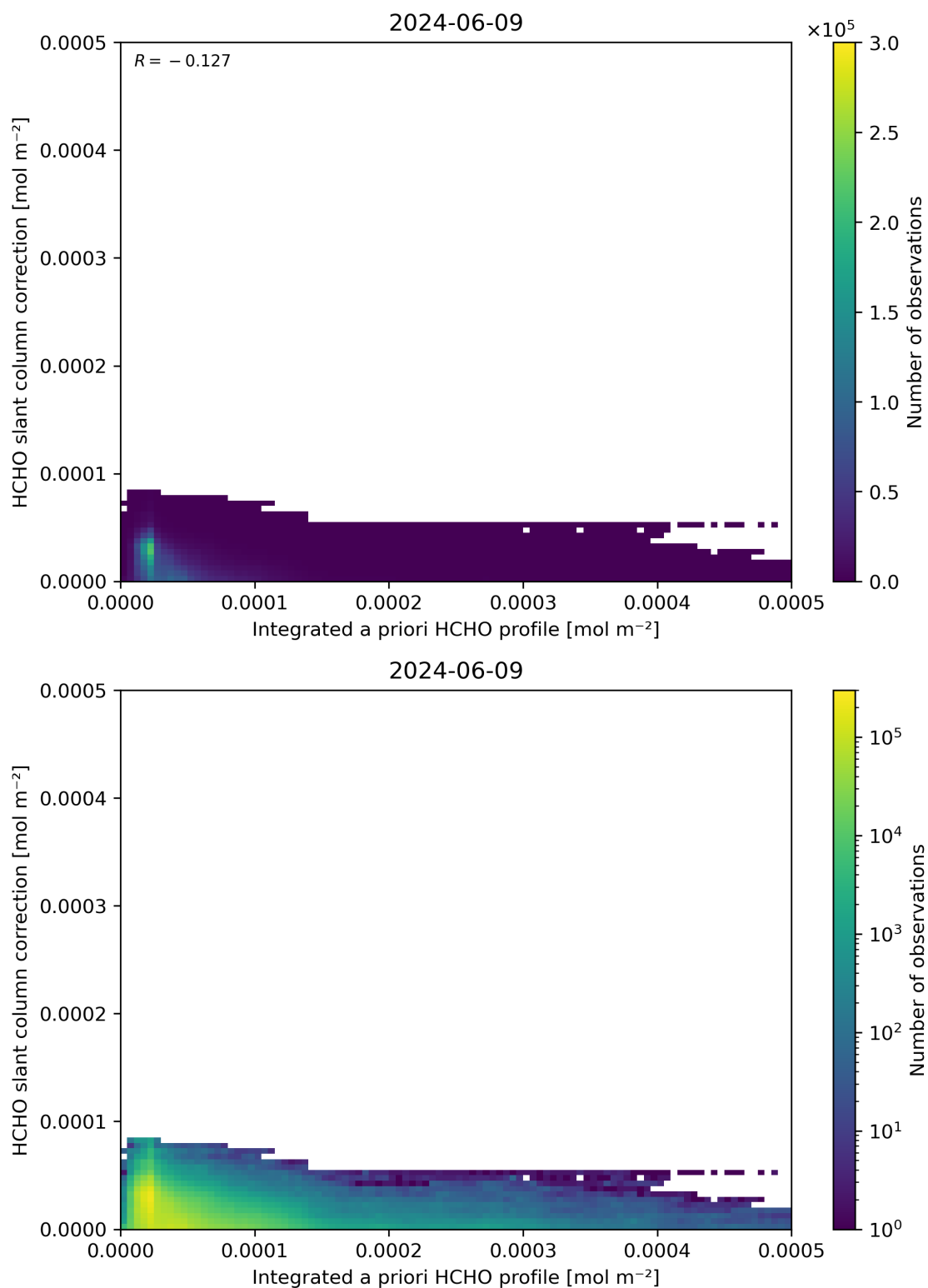
Figure 152: Scatter density plot of “Integrated a priori HCHO profile” against “HCHO slant column correction” for 2024-06-08 to 2024-06-10.
