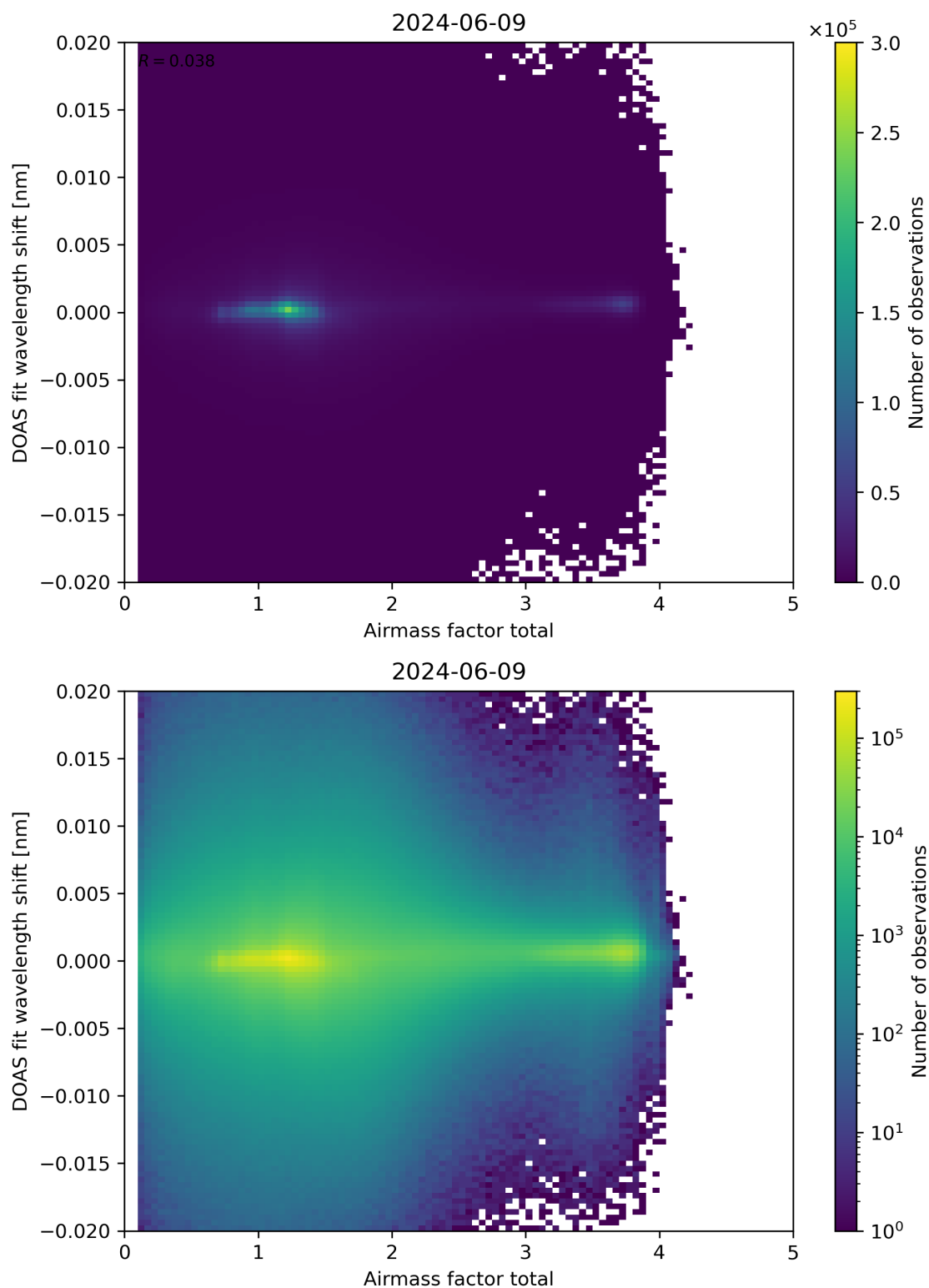
Figure 98: Scatter density plot of “Airmass factor total” against “DOAS fit wavelength shift” for 2024-06-08 to 2024-06-10.
