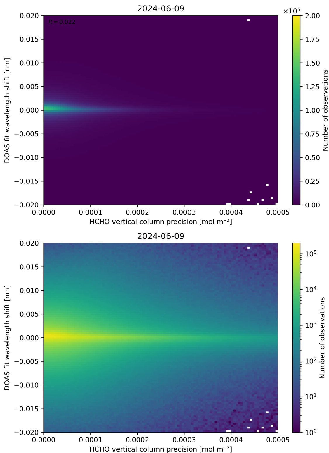
Figure 137: Scatter density plot of “HCHO vertical column precision” against “DOAS fit wavelength shift” for 2024-06-08 to 2024-06-10.
