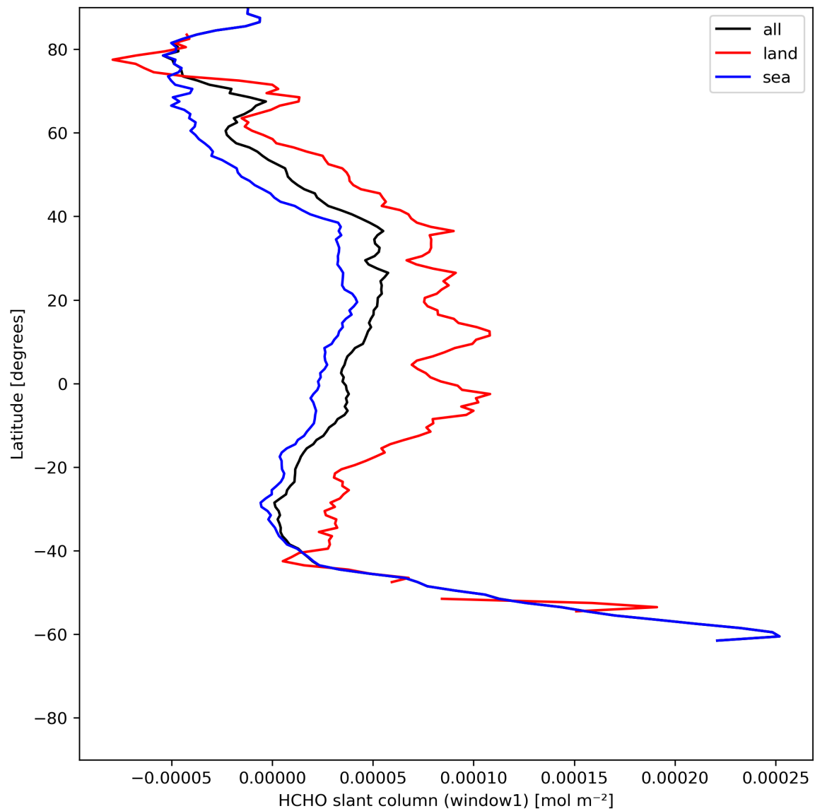
Figure 24: Zonal average of “HCHO slant column (window1)” for 2024-06-08 to 2024-06-10.
