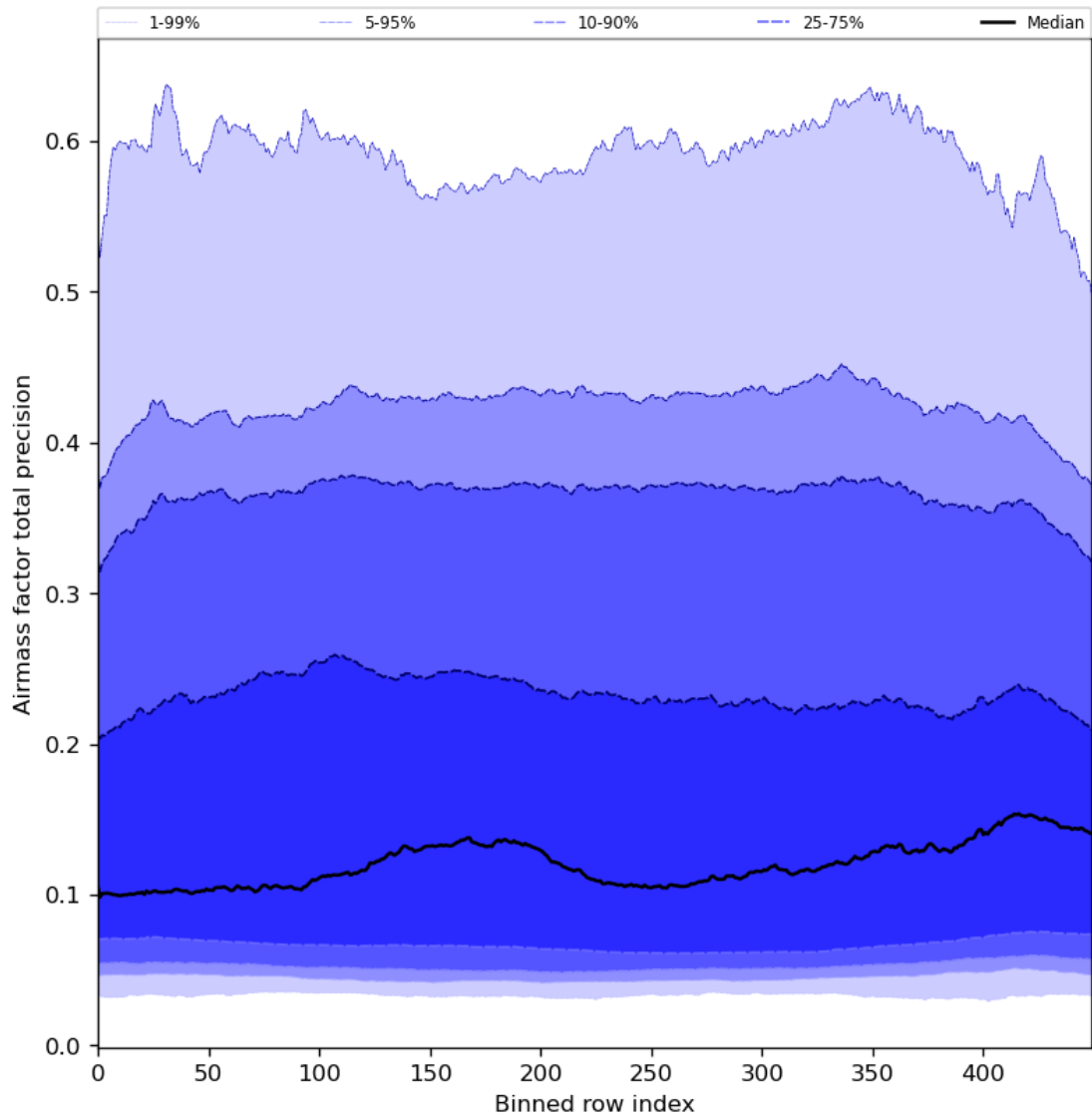
Figure 55: Along track statistics of “Airmass factor total precision” for 2024-06-08 to 2024-06-10
