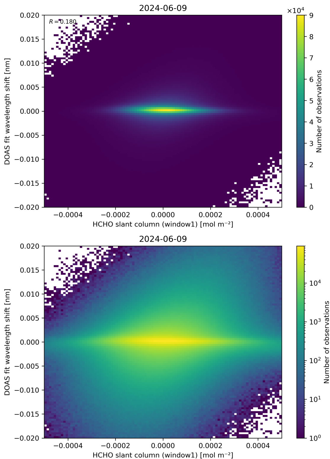
Figure 79: Scatter density plot of “HCHO slant column (window1)” against “DOAS fit wavelength shift” for 2024-06-08 to 2024-06-10.
