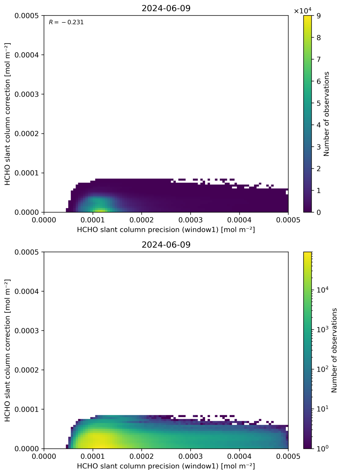
Figure 93: Scatter density plot of “HCHO slant column precision (window1)” against “HCHO slant column correction” for 2024-06-08 to 2024-06-10.
