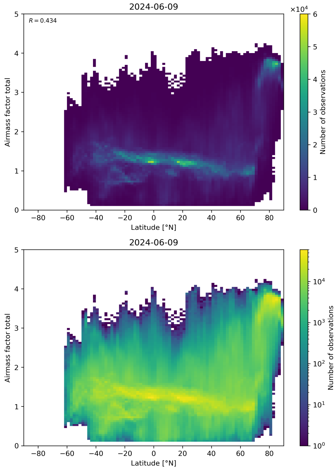
Figure 161: Scatter density plot of “Latitude” against “Airmass factor total” for 2024-06-08 to 2024-06-10.
