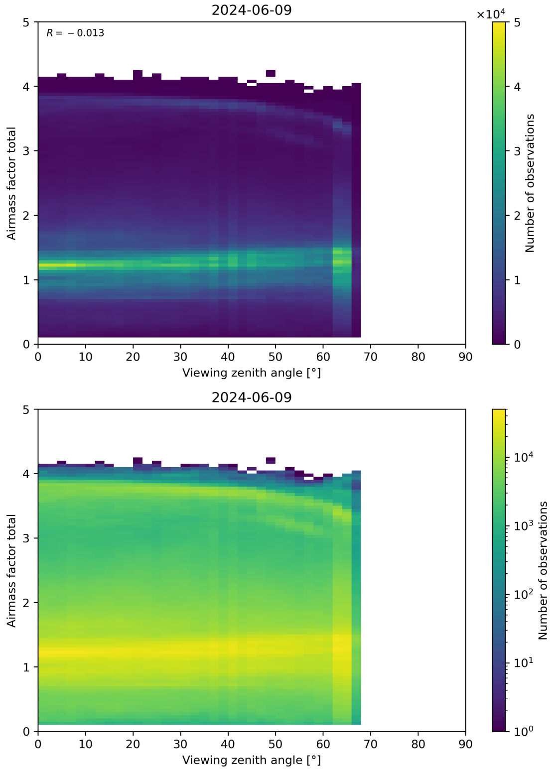
Figure 190: Scatter density plot of “Viewing zenith angle” against “Airmass factor total” for 2024-06-08 to 2024-06-10.
