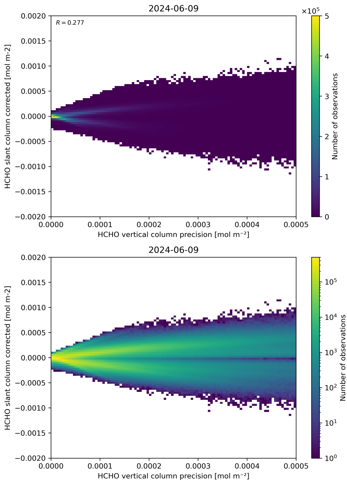
Figure 140: Scatter density plot of “HCHO vertical column precision” against “HCHO slant column corrected” for 2024-06-08 to 2024-06-10.
