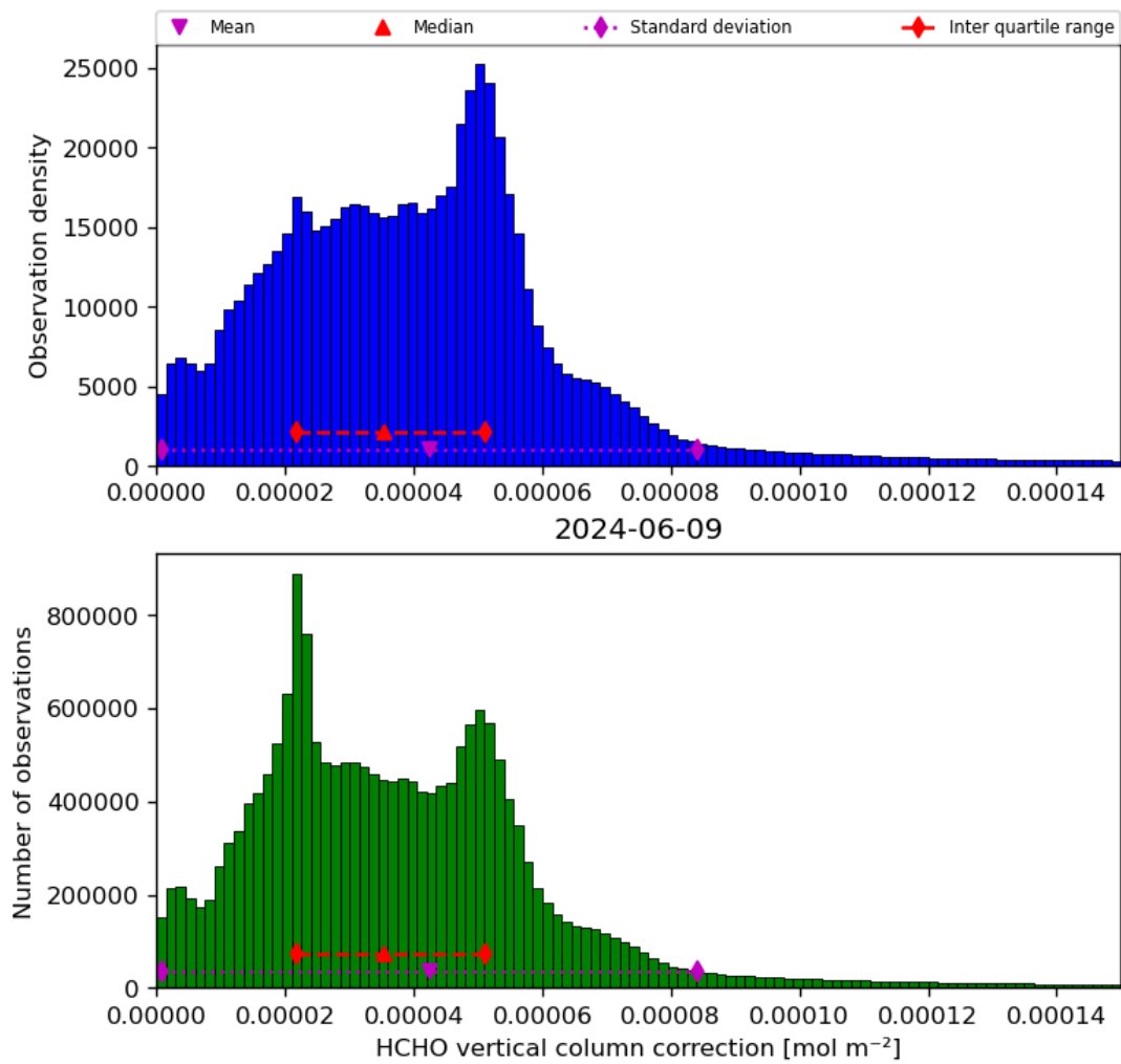
Figure 37: Histogram of “HCHO vertical column correction” for 2024-06-08 to 2024-06-10
