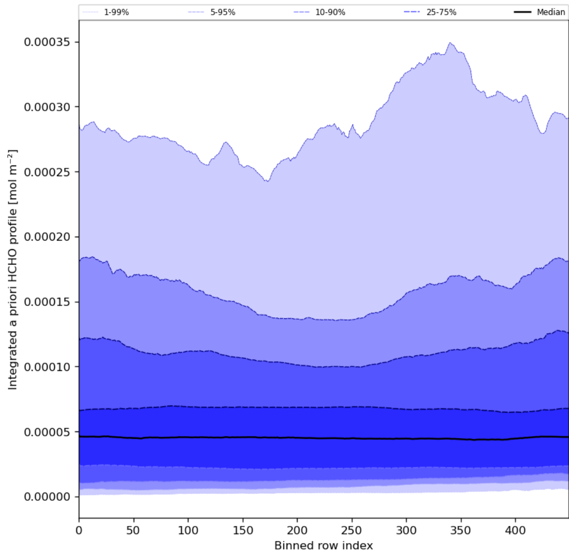
Figure 57: Along track statistics of “Integrated a priori HCHO profile” for 2024-06-08 to 2024-06-10
