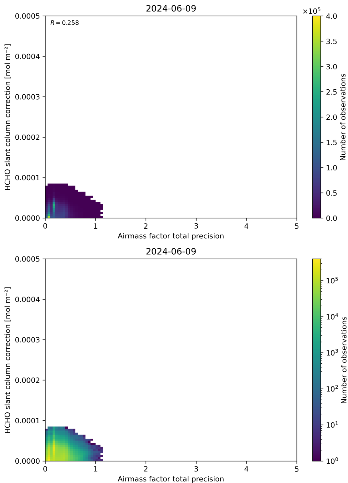
Figure 110: Scatter density plot of “Airmass factor total precision” against “HCHO slant column correction” for 2024-06-08 to 2024-06-10.
