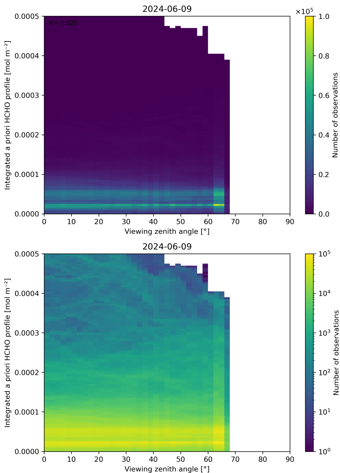
Figure 195: Scatter density plot of “Viewing zenith angle” against “Integrated a priori HCHO profile” for 2024-06-08 to 2024-06-10.
