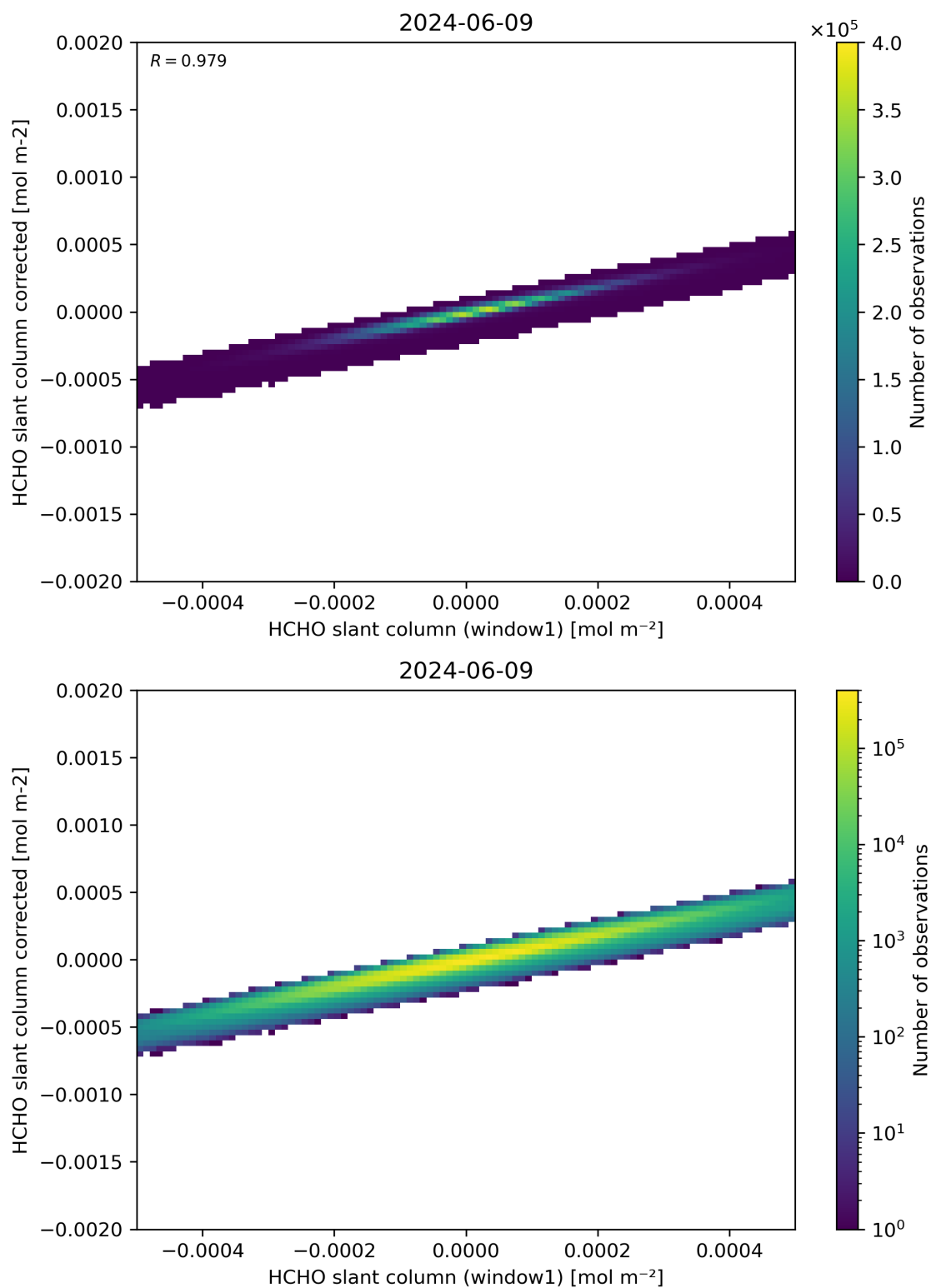
Figure 82: Scatter density plot of “HCHO slant column (window1)” against “HCHO slant column corrected” for 2024-06-08 to 2024-06-10.
