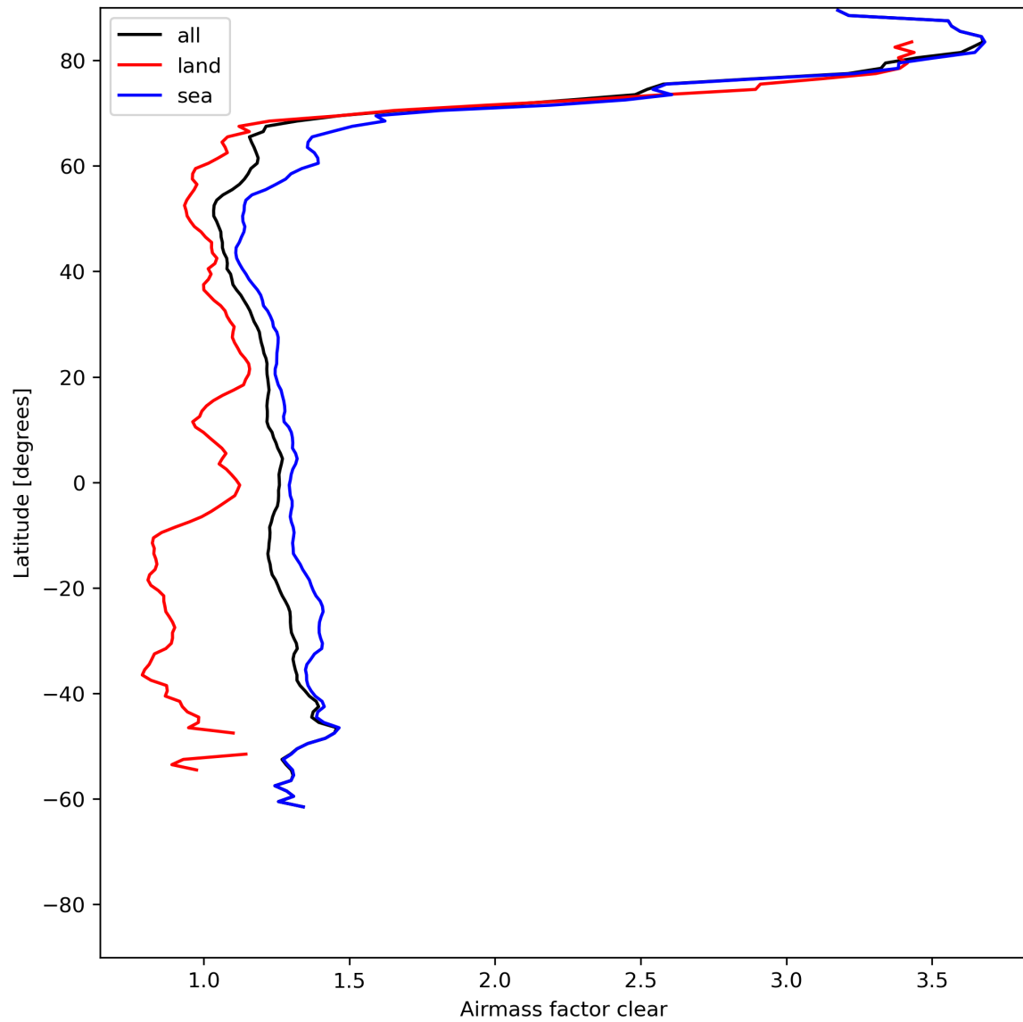
Figure 28: Zonal average of “Airmass factor clear” for 2024-06-08 to 2024-06-10.
