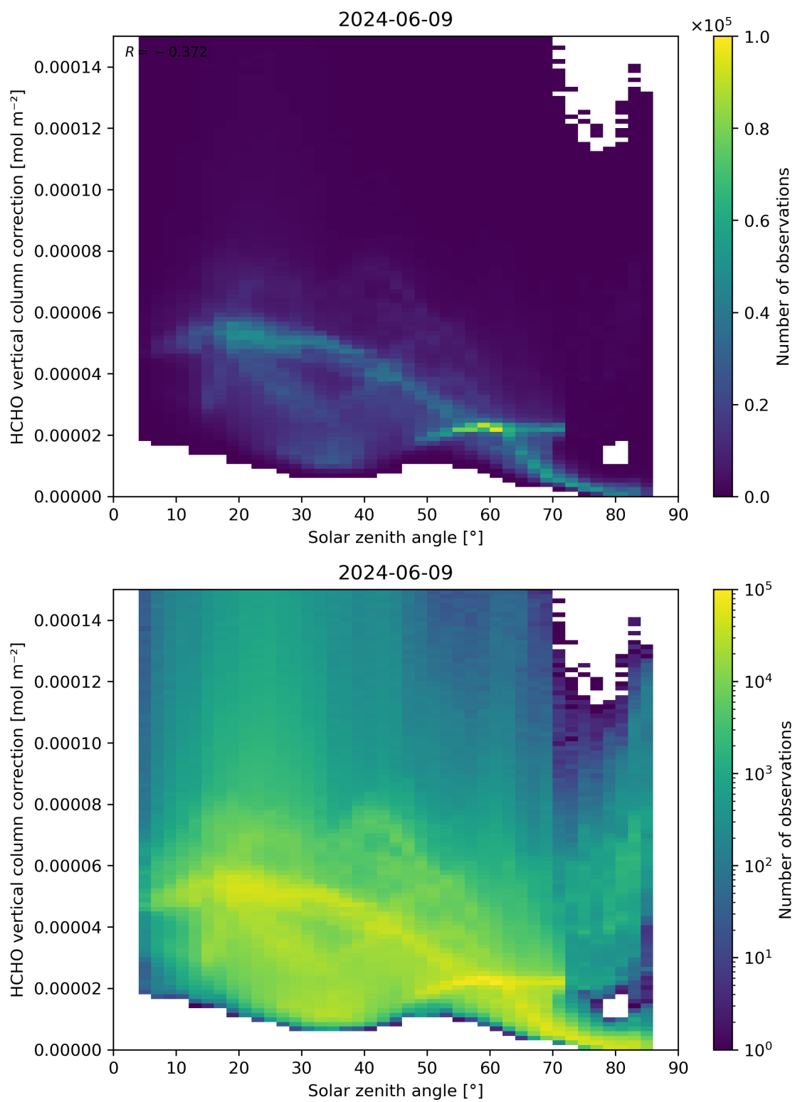
Figure 178: Scatter density plot of “Solar zenith angle” against “HCHO vertical column correction” for 2024-06-08 to 2024-06-10.
