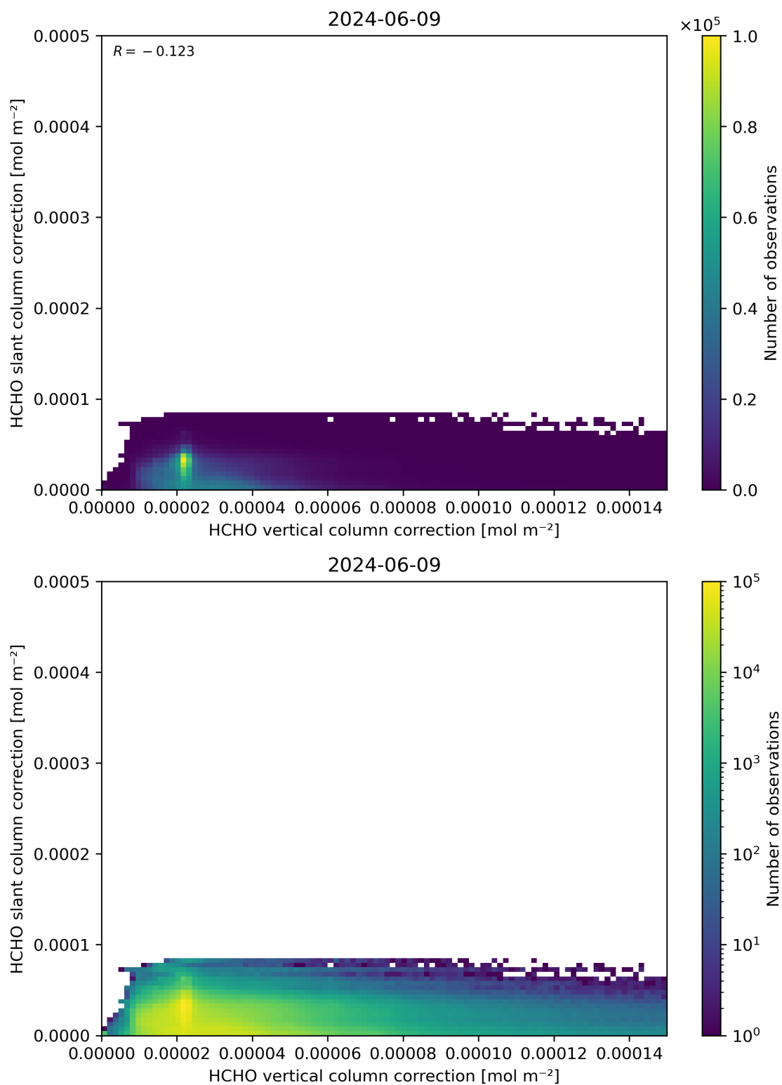
Figure 117: Scatter density plot of “HCHO vertical column correction” against “HCHO slant column correction” for 2024-06-08 to 2024-06-10.
