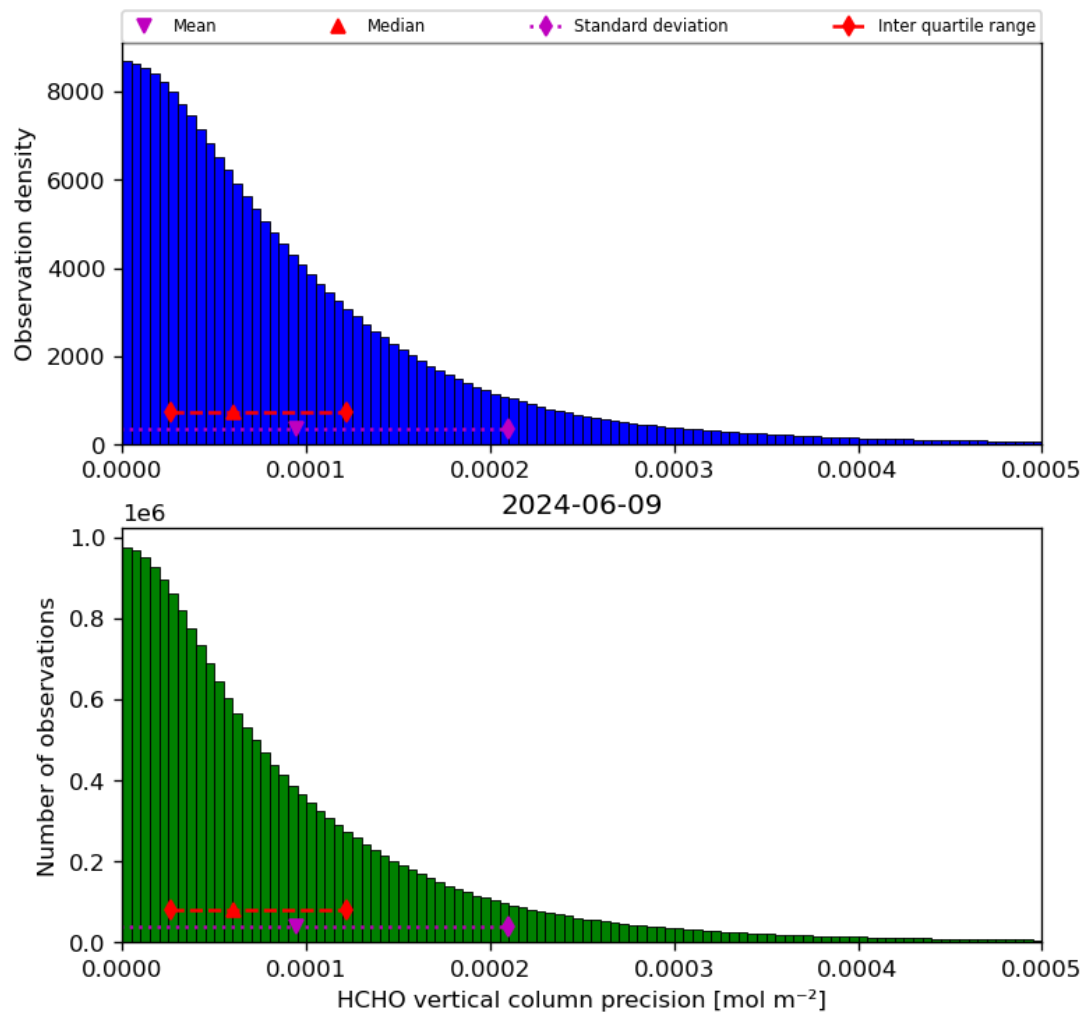
Figure 36: Histogram of “HCHO vertical column precision” for 2024-06-08 to 2024-06-10
