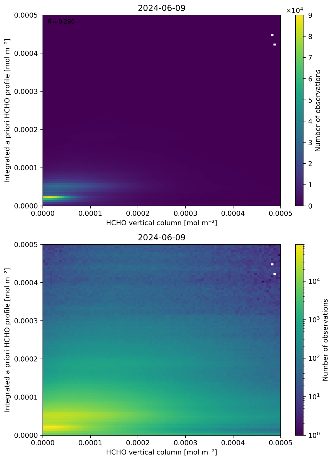
Figure 135: Scatter density plot of “HCHO vertical column” against “Integrated a priori HCHO profile” for 2024-06-08 to 2024-06-10.
