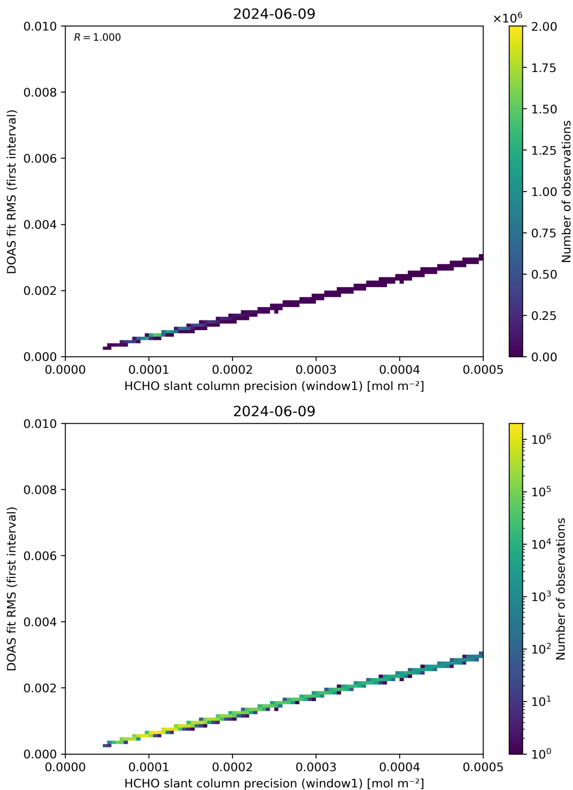
Figure 88: Scatter density plot of “HCHO slant column precision (window1)” against “DOAS fit RMS (first interval)” for 2024-06-08 to 2024-06-10.
