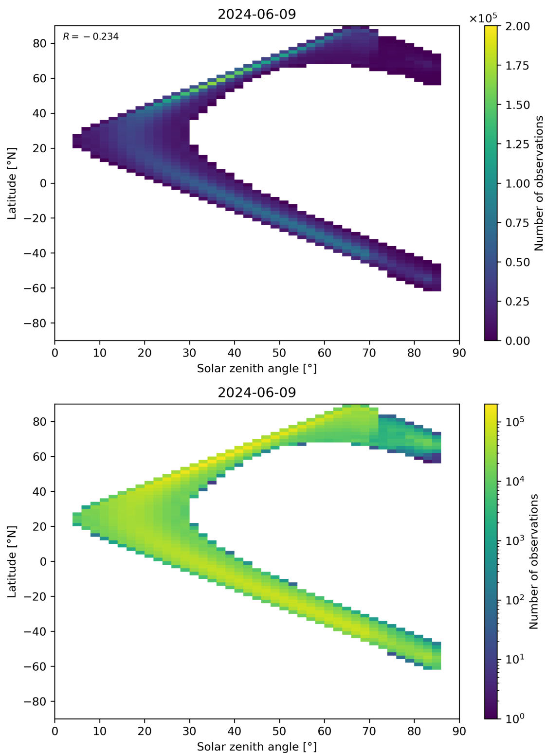
Figure 181: Scatter density plot of “Solar zenith angle” against “Latitude” for 2024-06-08 to 2024-06-10.
