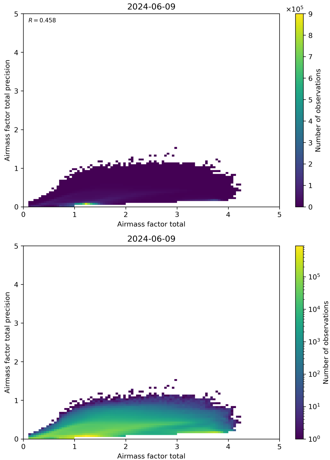
Figure 103: Scatter density plot of “Airmass factor total” against “Airmass factor total precision” for 2024-06-08 to 2024-06-10.
