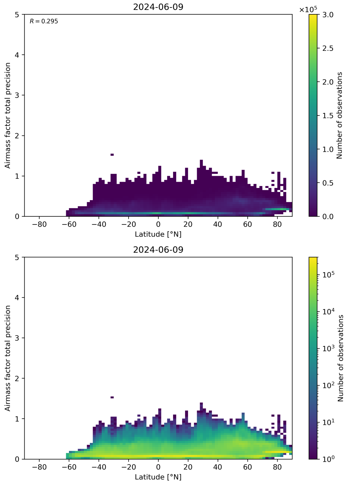
Figure 162: Scatter density plot of “Latitude” against “Airmass factor total precision” for 2024-06-08 to 2024-06-10.
