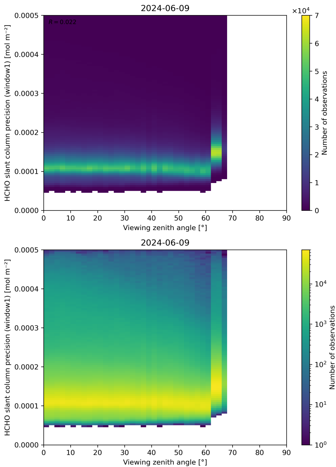
Figure 189: Scatter density plot of “Viewing zenith angle” against “HCHO slant column precision (window1)” for 2024-06-08 to 2024-06-10.
