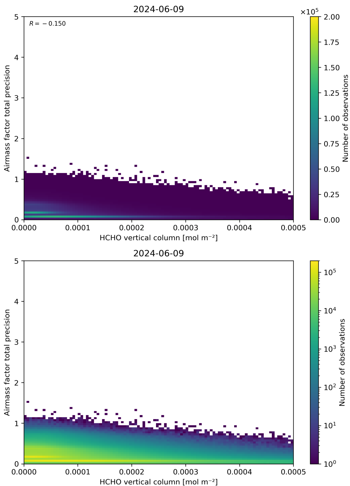
Figure 132: Scatter density plot of “HCHO vertical column” against “Airmass factor total precision” for 2024-06-08 to 2024-06-10.
