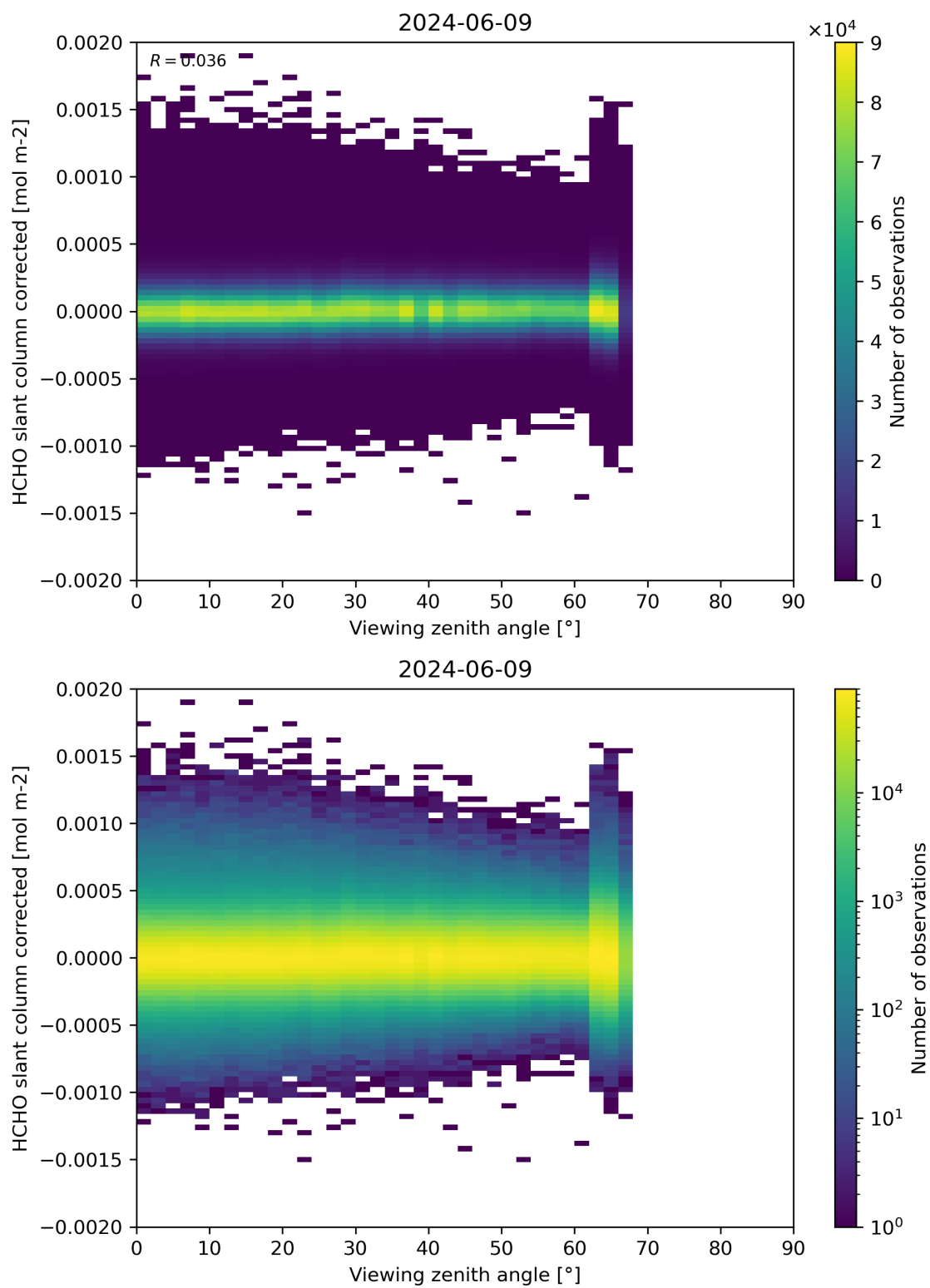
Figure 186: Scatter density plot of “Viewing zenith angle” against “HCHO slant column corrected” for 2024-06-08 to 2024-06-10.
