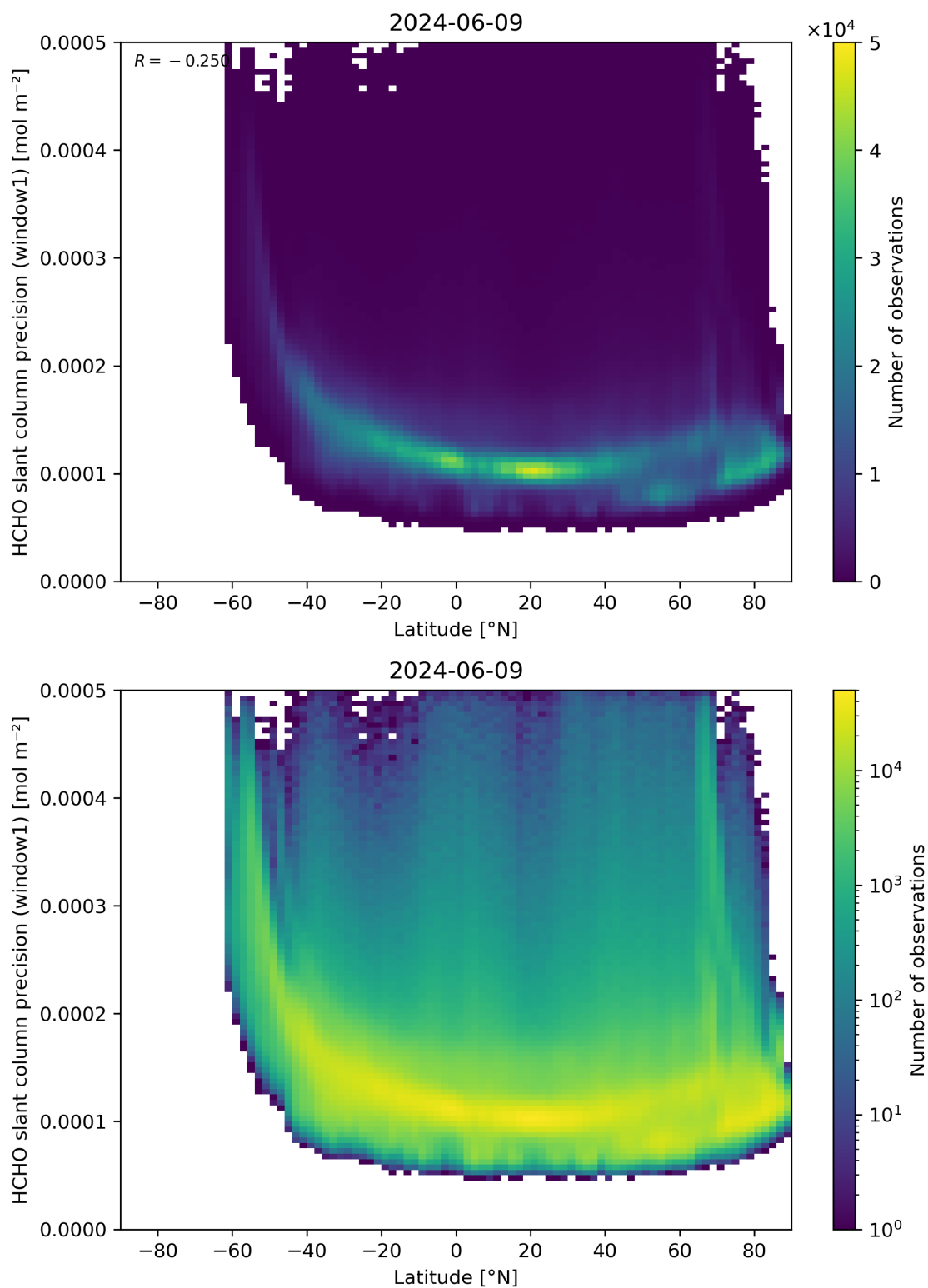
Figure 160: Scatter density plot of “Latitude” against “HCHO slant column precision (window1)” for 2024-06-08 to 2024-06-10.
