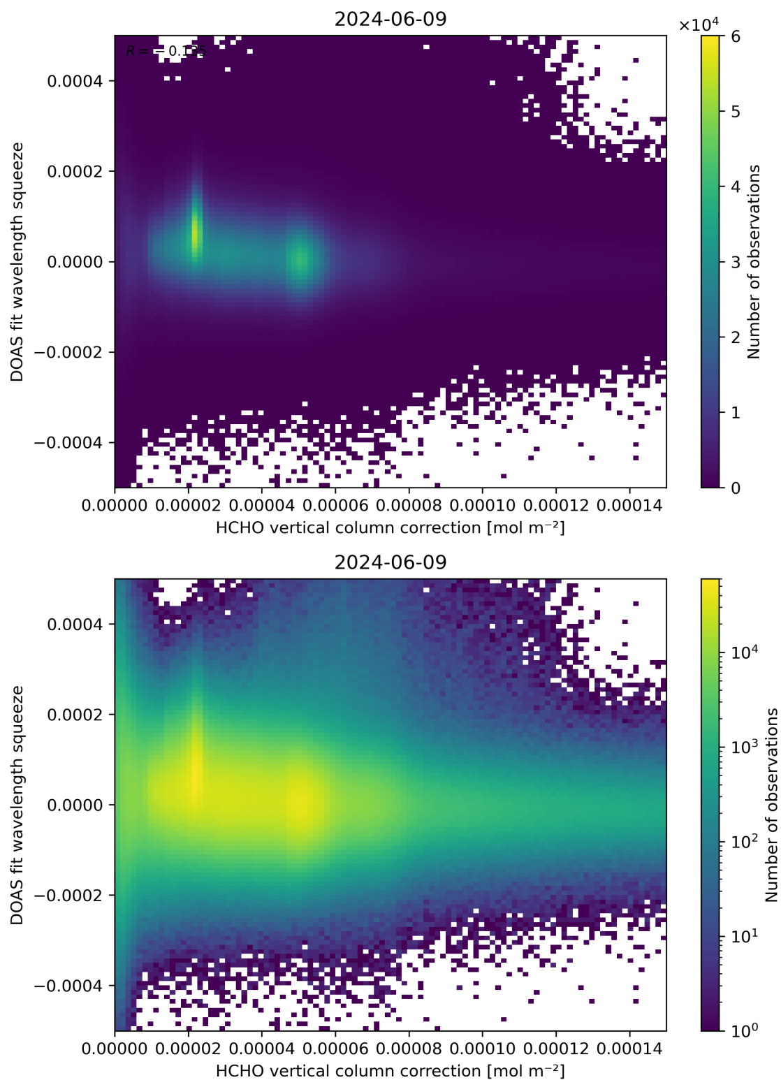
Figure 114: Scatter density plot of “HCHO vertical column correction” against “DOAS fit wavelength squeeze” for 2024-06-08 to 2024-06-10.
