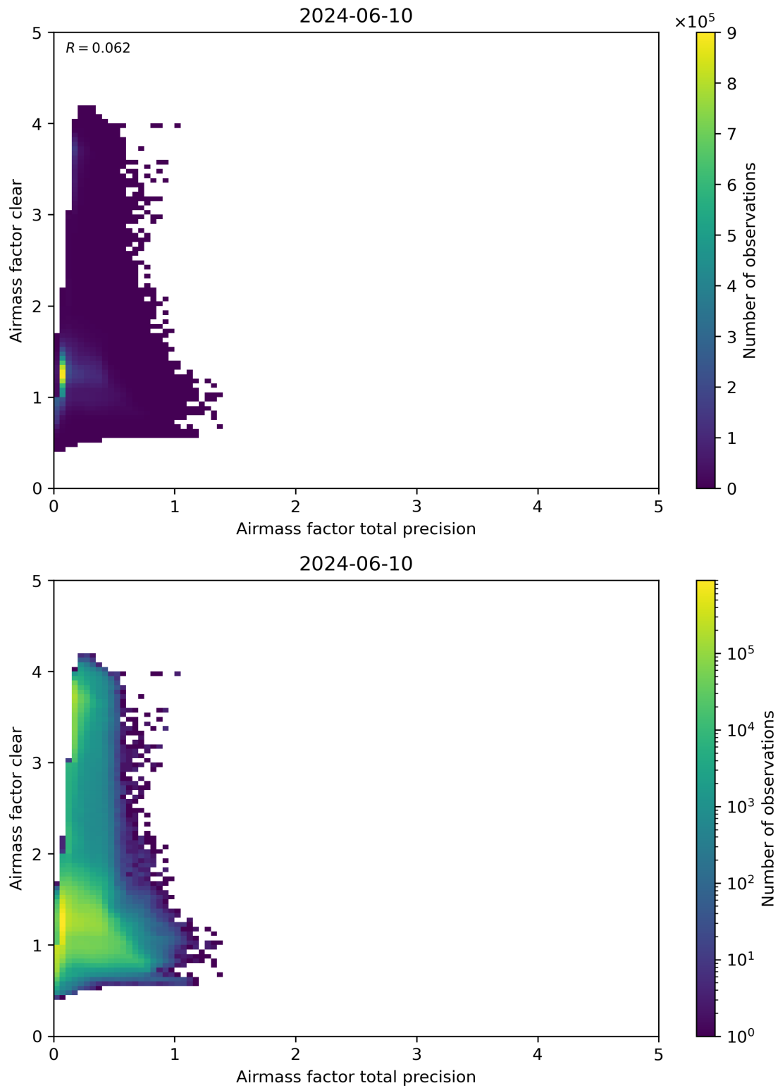
Figure 108: Scatter density plot of “Airmass factor total precision” against “Airmass factor clear” for 2024-06-09 to 2024-06-11.
