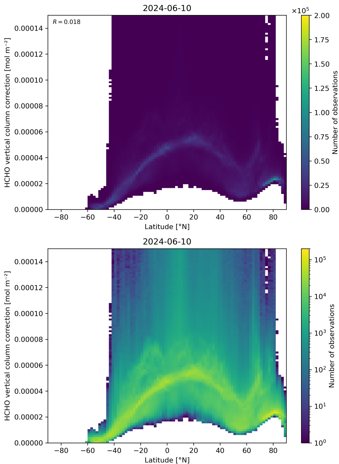
Figure 164: Scatter density plot of “Latitude” against “HCHO vertical column correction” for 2024-06-09 to 2024-06-11.
