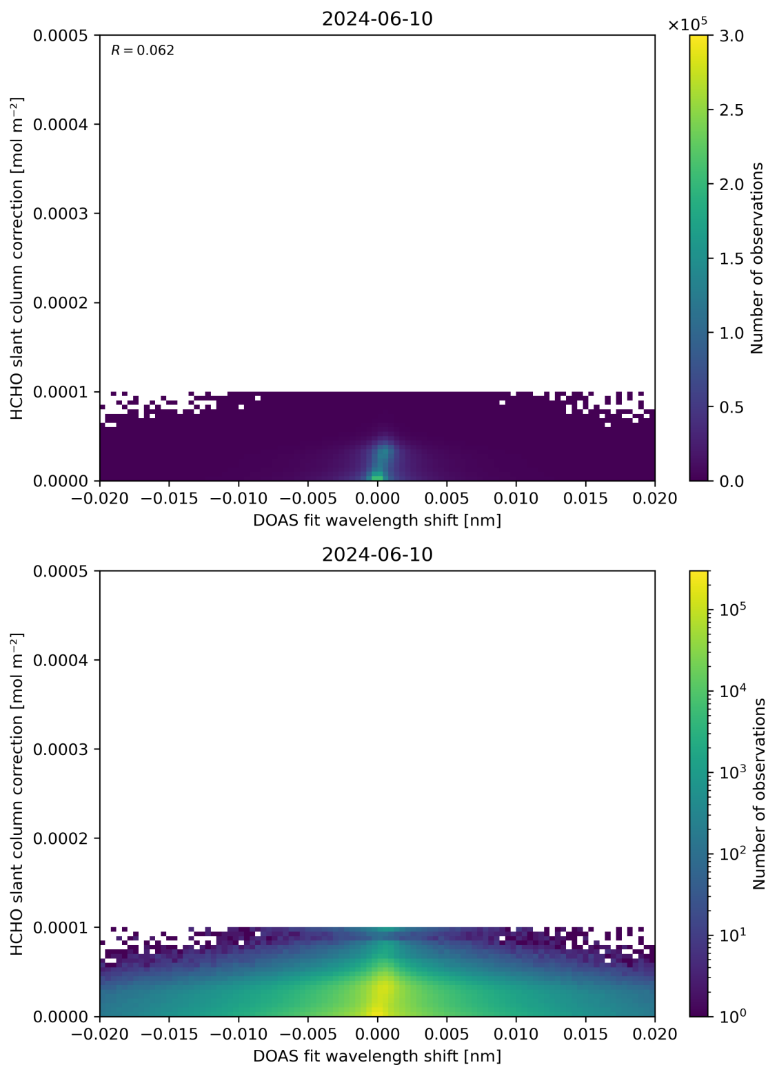
Figure 67: Scatter density plot of “DOAS fit wavelength shift” against “HCHO slant column correction” for 2024-06-09 to 2024-06-11.
