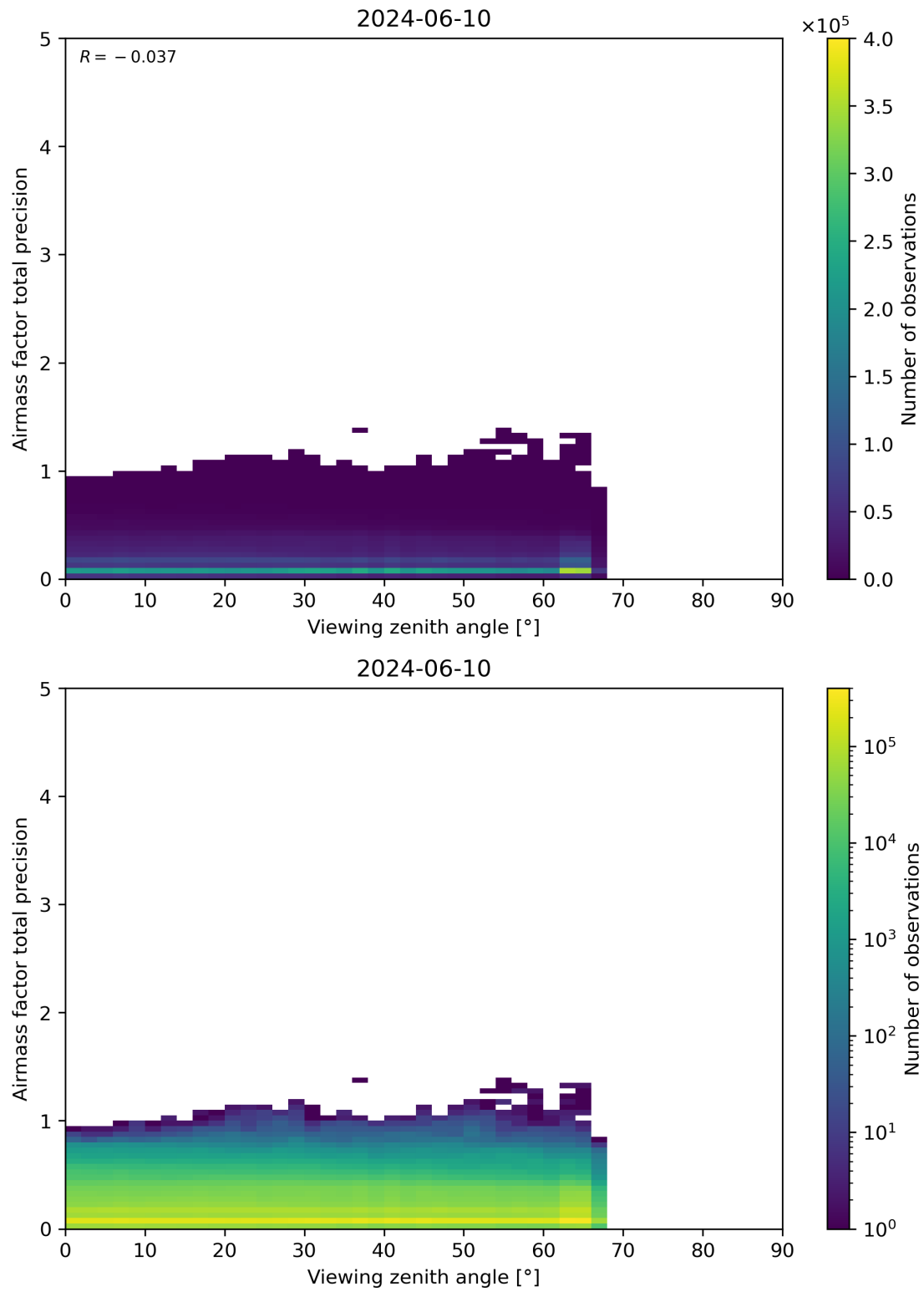
Figure 191: Scatter density plot of “Viewing zenith angle” against “Airmass factor total precision” for 2024-06-09 to 2024-06-11.
