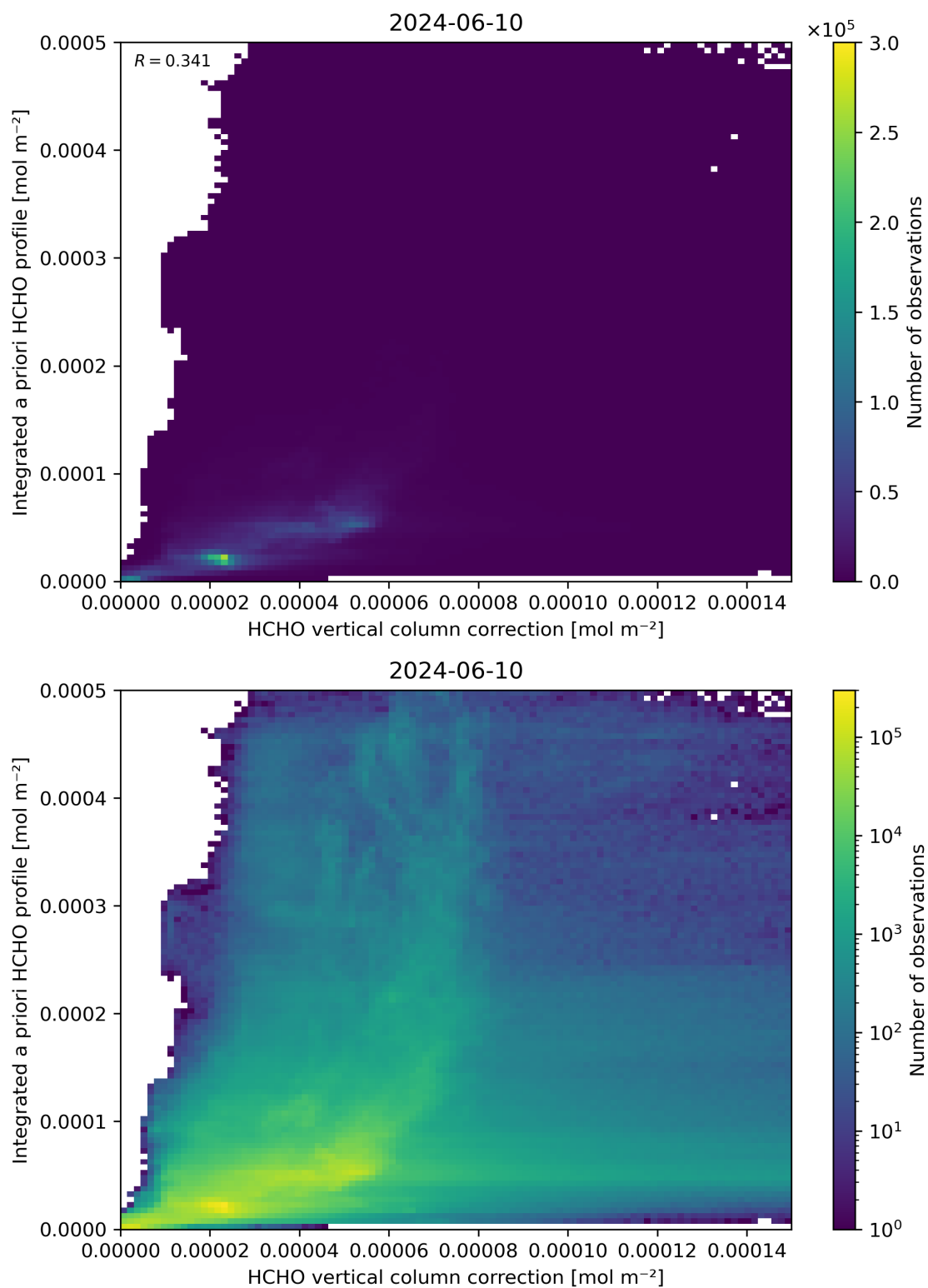
Figure 122: Scatter density plot of “HCHO vertical column correction” against “Integrated a priori HCHO profile” for 2024-06-09 to 2024-06-11.
