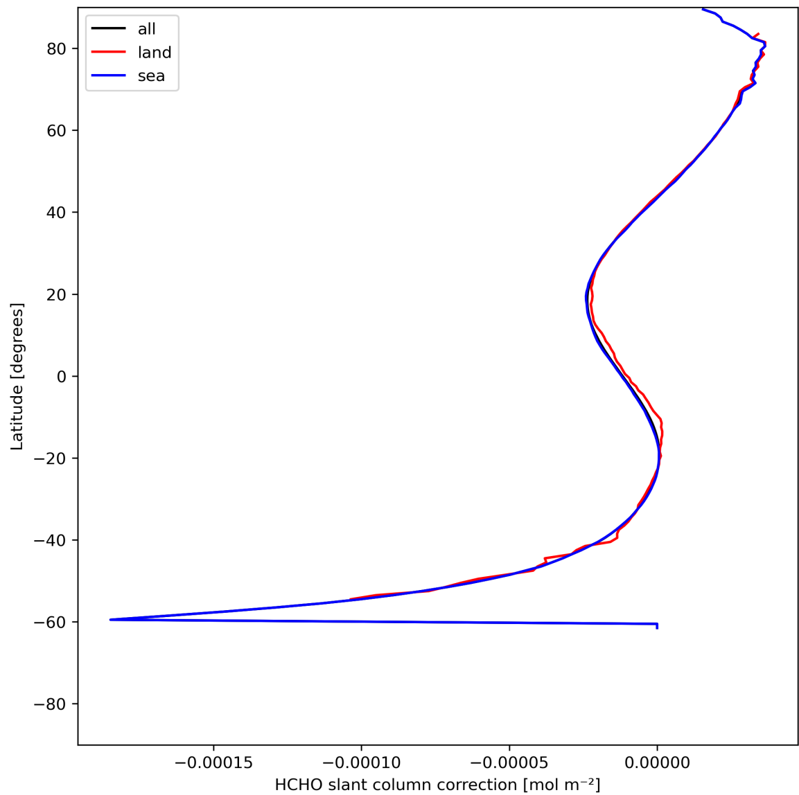
Figure 33: Zonal average of “HCHO slant column correction” for 2024-06-09 to 2024-06-11.
