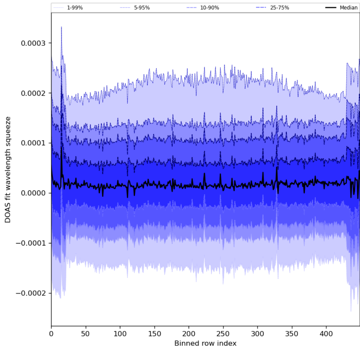
Figure 59: Along track statistics of “DOAS fit wavelength squeeze” for 2024-06-09 to 2024-06-11
