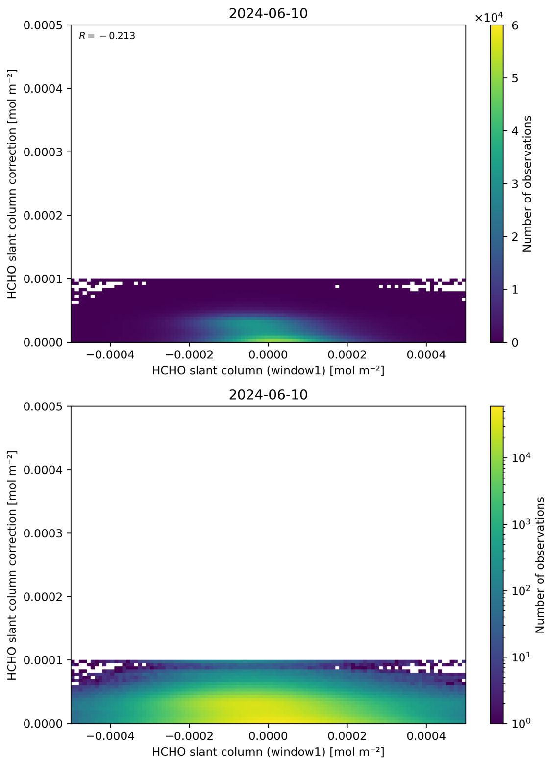
Figure 83: Scatter density plot of “HCHO slant column (window1)” against “HCHO slant column correction” for 2024-06-09 to 2024-06-11.
