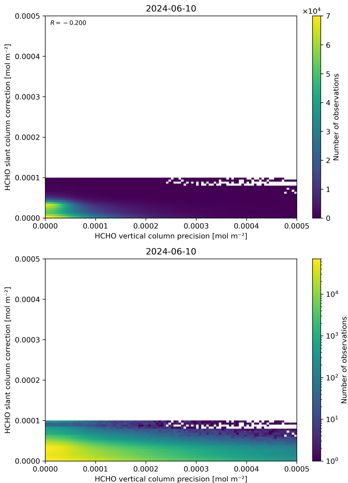
Figure 141: Scatter density plot of “HCHO vertical column precision” against “HCHO slant column correction” for 2024-06-09 to 2024-06-11.
