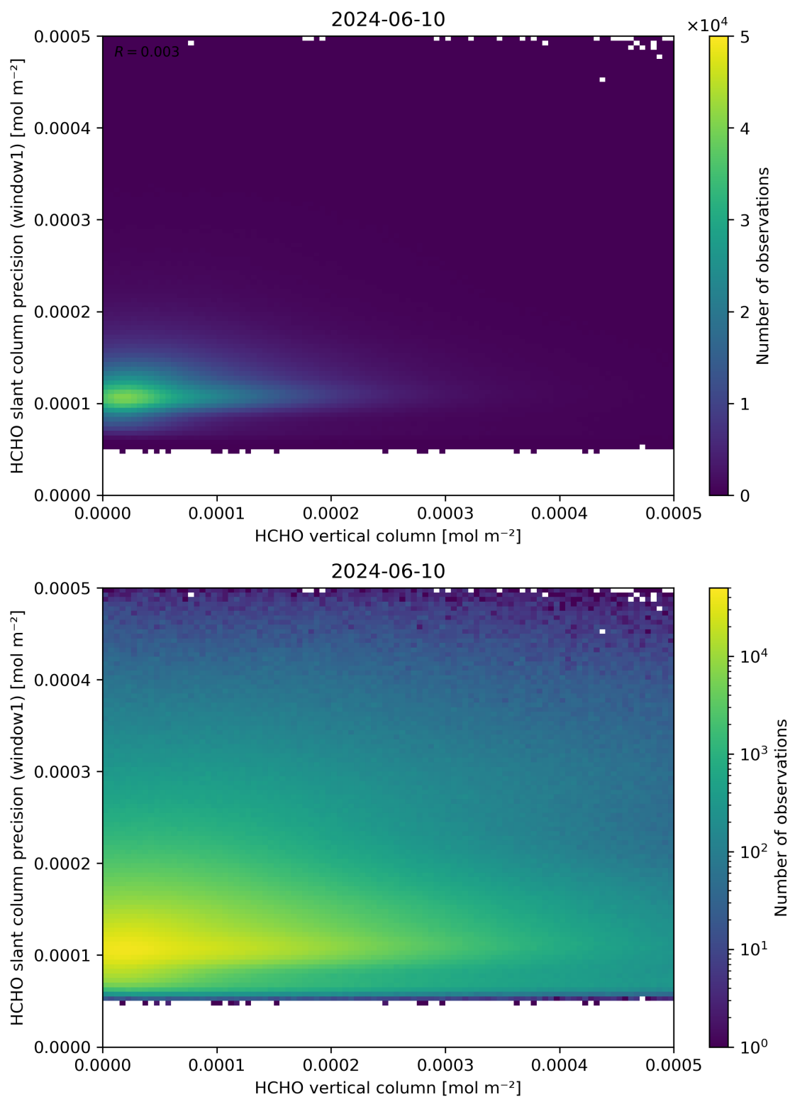
Figure 130: Scatter density plot of “HCHO vertical column” against “HCHO slant column precision (window1)” for 2024-06-09 to 2024-06-11.
