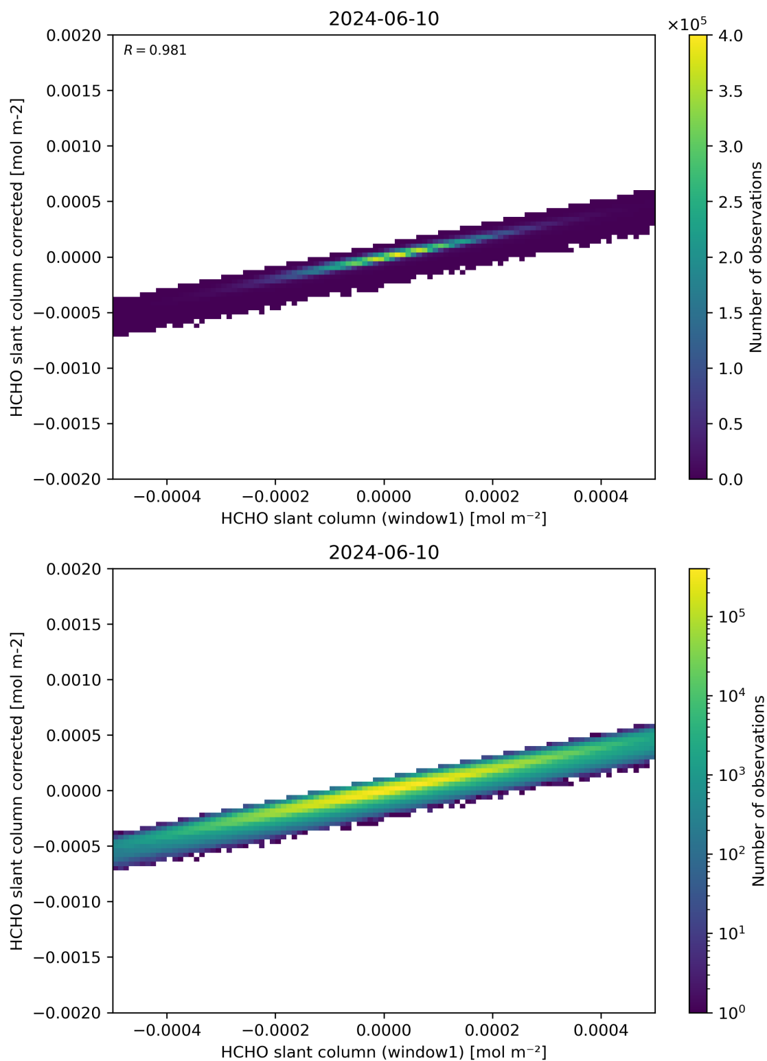
Figure 82: Scatter density plot of “HCHO slant column (window1)” against “HCHO slant column corrected” for 2024-06-09 to 2024-06-11.
