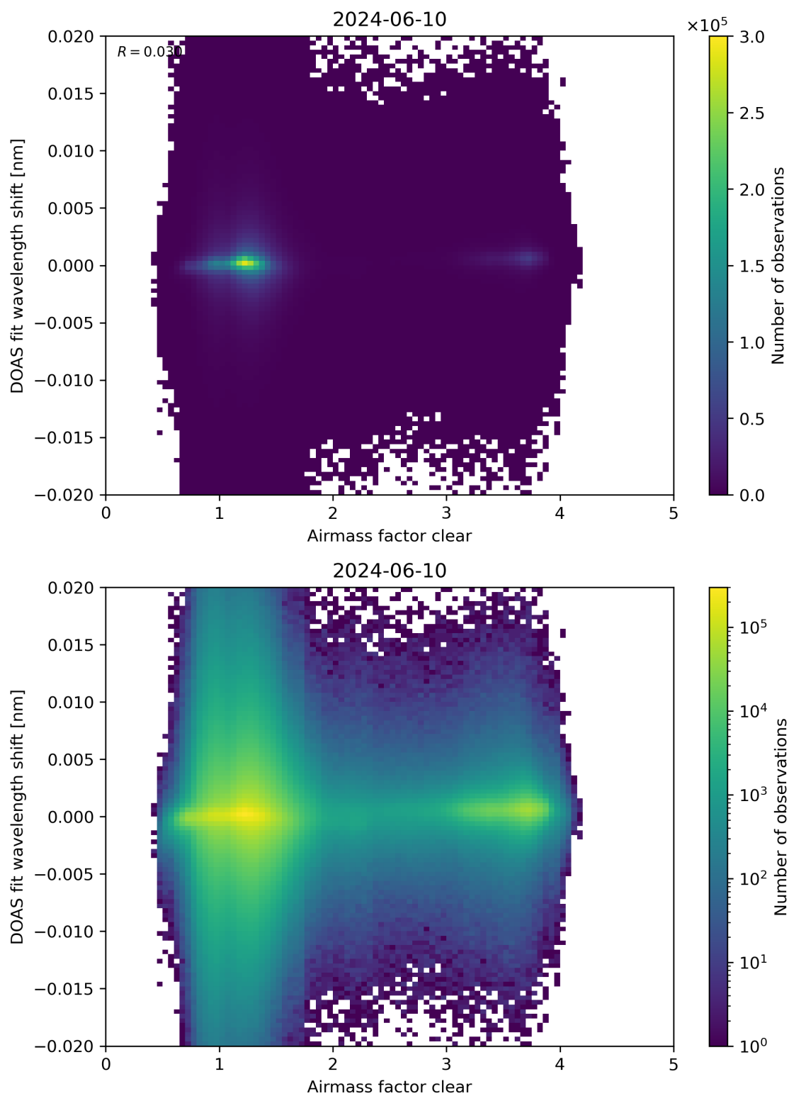
Figure 72: Scatter density plot of “Airmass factor clear” against “DOAS fit wavelength shift” for 2024-06-09 to 2024-06-11.
