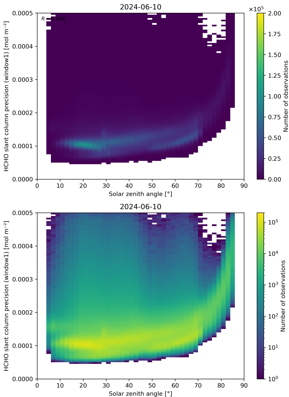
Figure 174: Scatter density plot of “Solar zenith angle” against “HCHO slant column precision (window1)” for 2024-06-09 to 2024-06-11.
