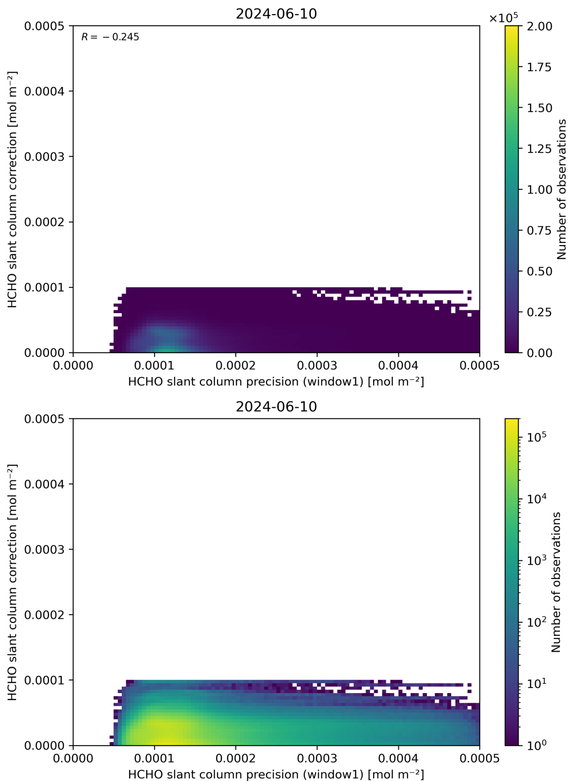
Figure 93: Scatter density plot of “HCHO slant column precision (window1)” against “HCHO slant column correction” for 2024-06-09 to 2024-06-11.
