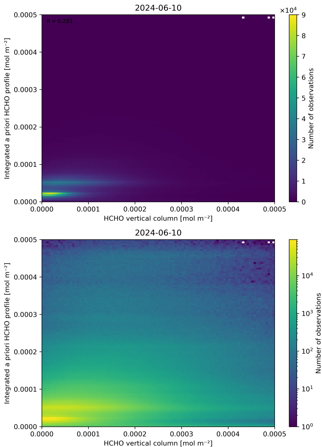
Figure 135: Scatter density plot of “HCHO vertical column” against “Integrated a priori HCHO profile” for 2024-06-09 to 2024-06-11.
