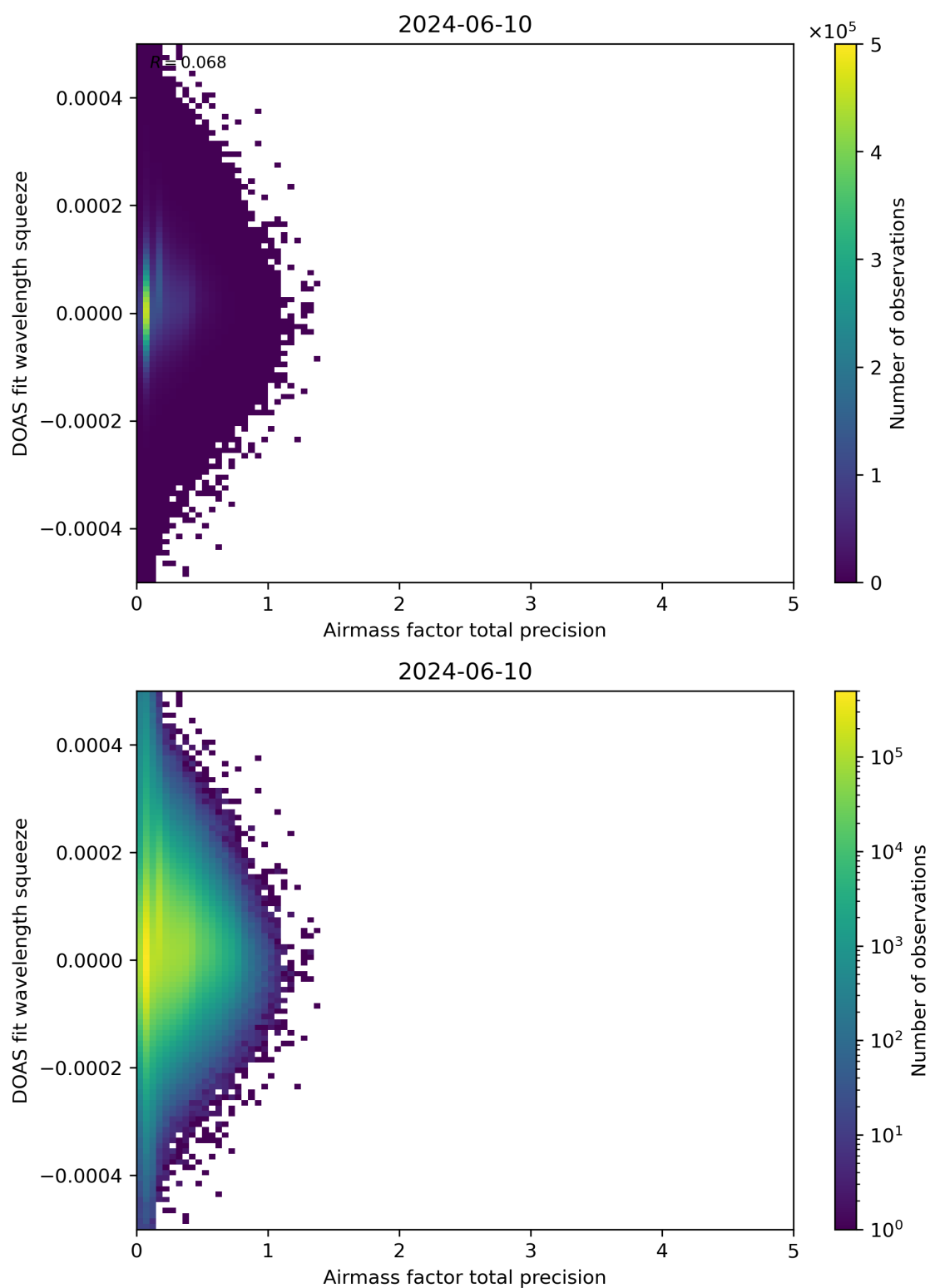
Figure 107: Scatter density plot of “Airmass factor total precision” against “DOAS fit wavelength squeeze” for 2024-06-09 to 2024-06-11.
