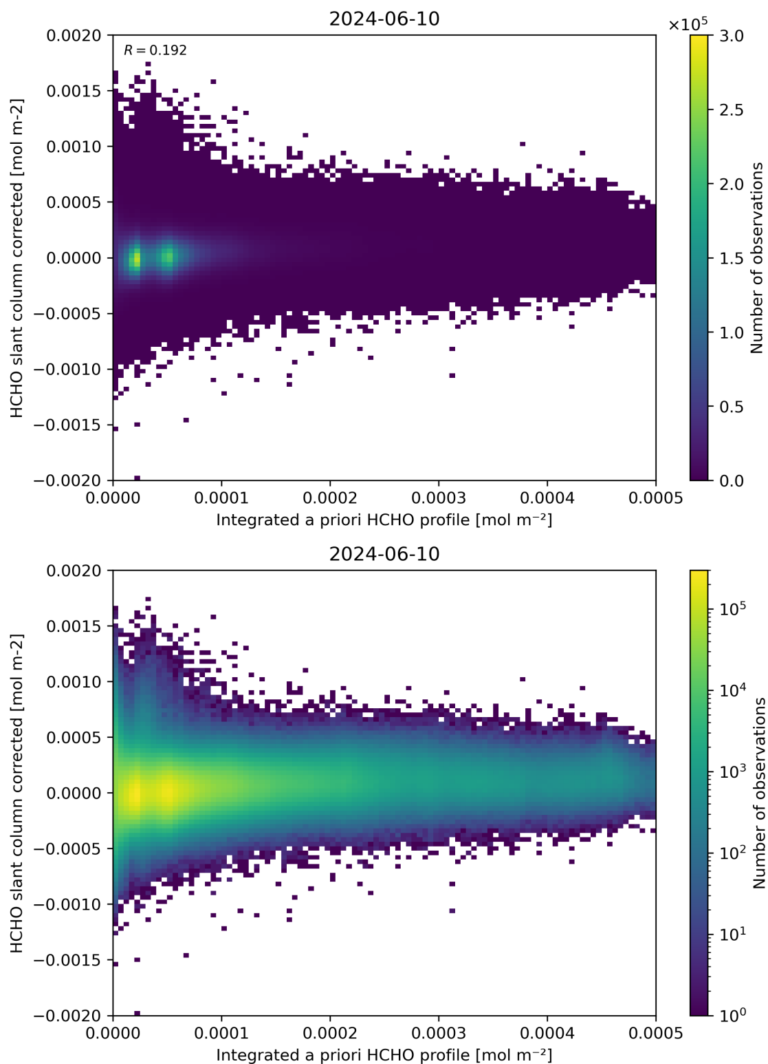
Figure 151: Scatter density plot of “Integrated a priori HCHO profile” against “HCHO slant column corrected” for 2024-06-09 to 2024-06-11.
