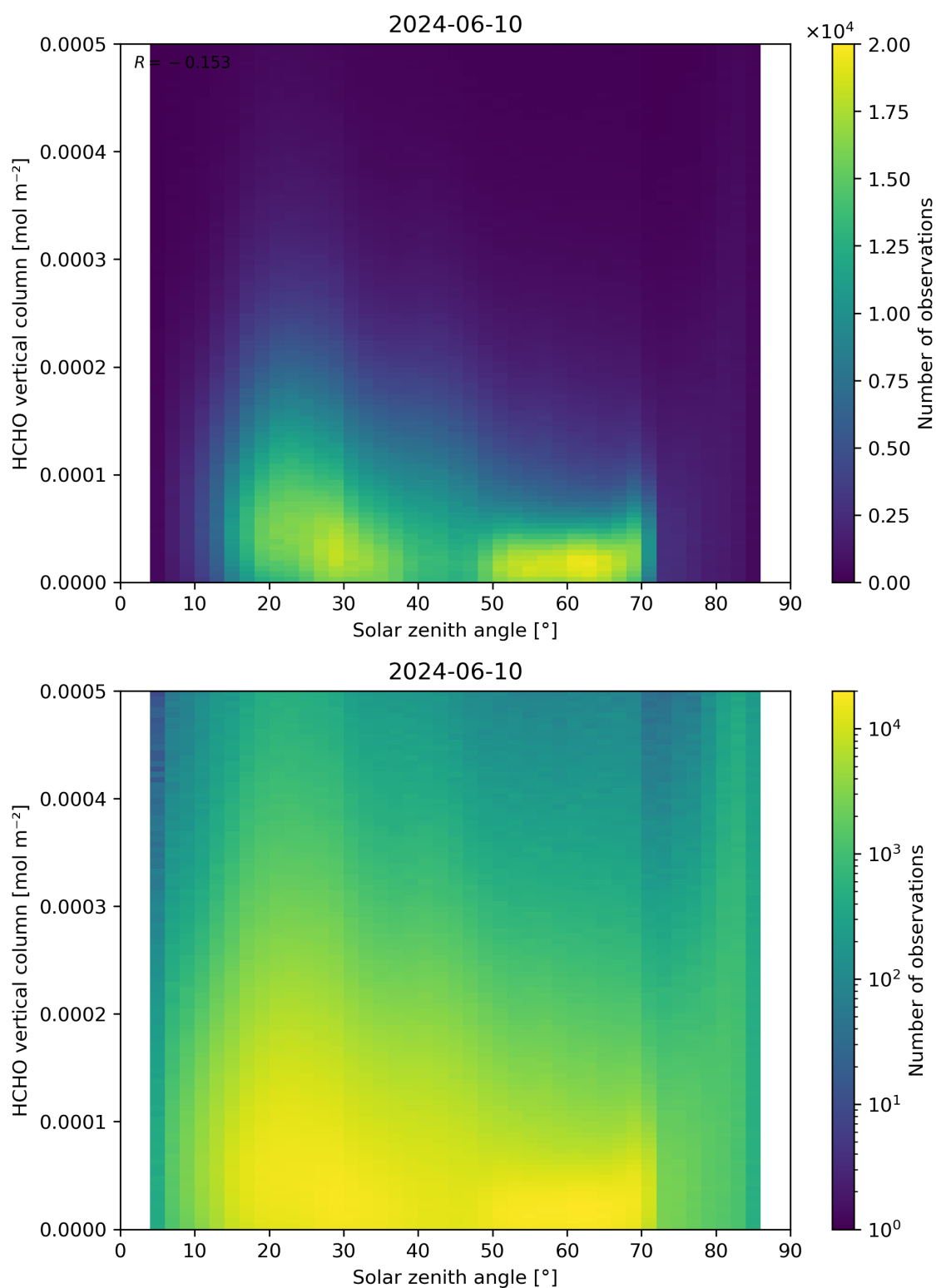
Figure 177: Scatter density plot of “Solar zenith angle” against “HCHO vertical column” for 2024-06-09 to 2024-06-11.
