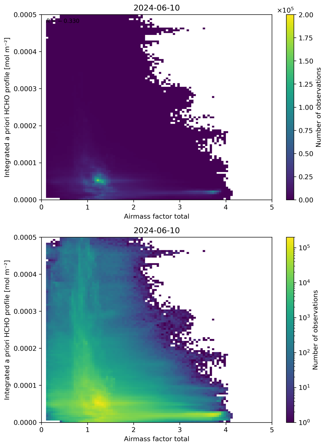
Figure 104: Scatter density plot of “Airmass factor total” against “Integrated a priori HCHO profile” for 2024-06-09 to 2024-06-11.
