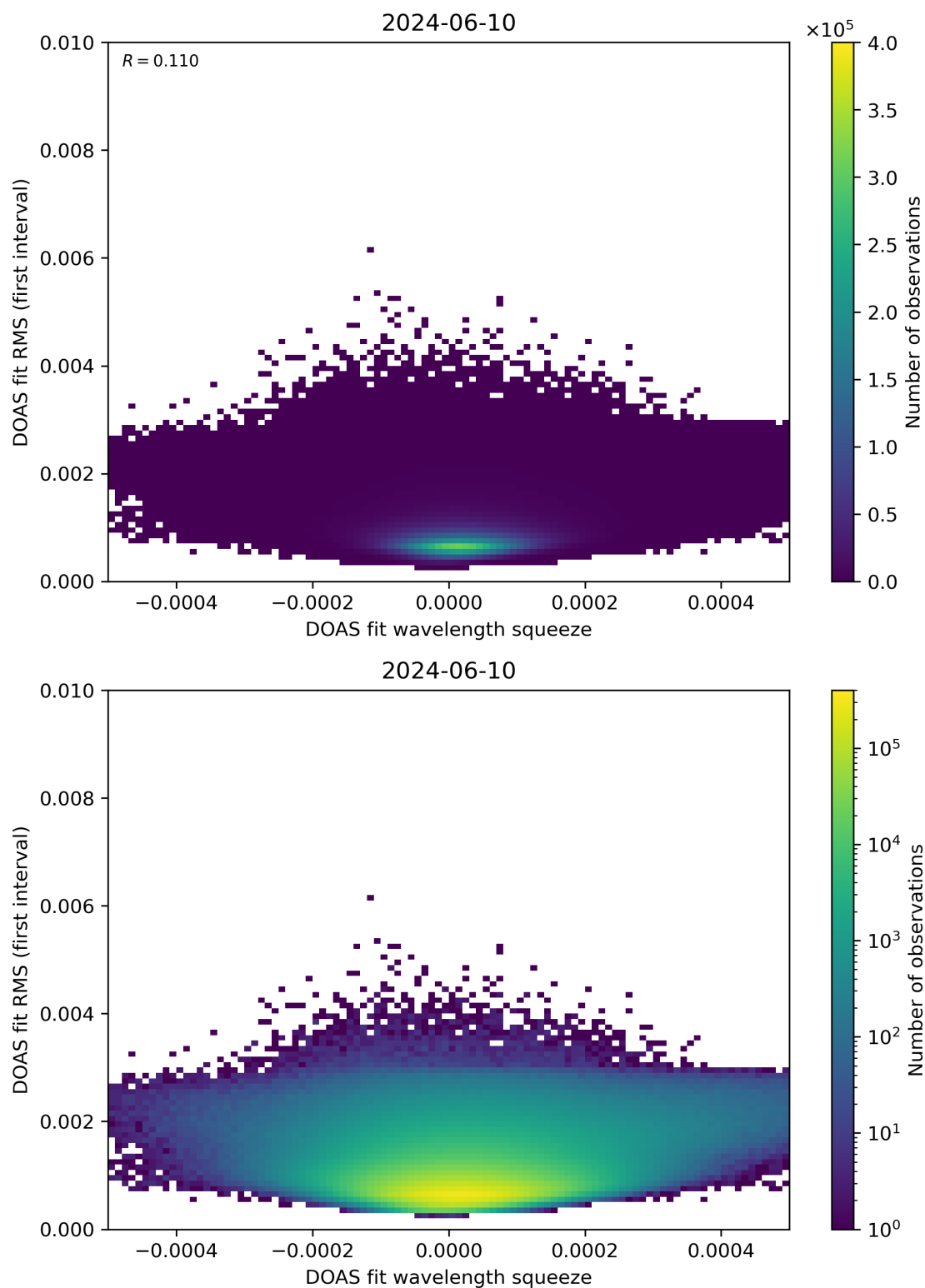
Figure 68: Scatter density plot of “DOAS fit wavelength squeeze” against “DOAS fit RMS (first interval)” for 2024-06-09 to 2024-06-11.
