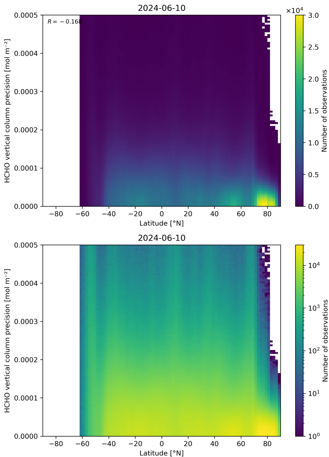
Figure 165: Scatter density plot of “Latitude” against “HCHO vertical column precision” for 2024-06-09 to 2024-06-11.
