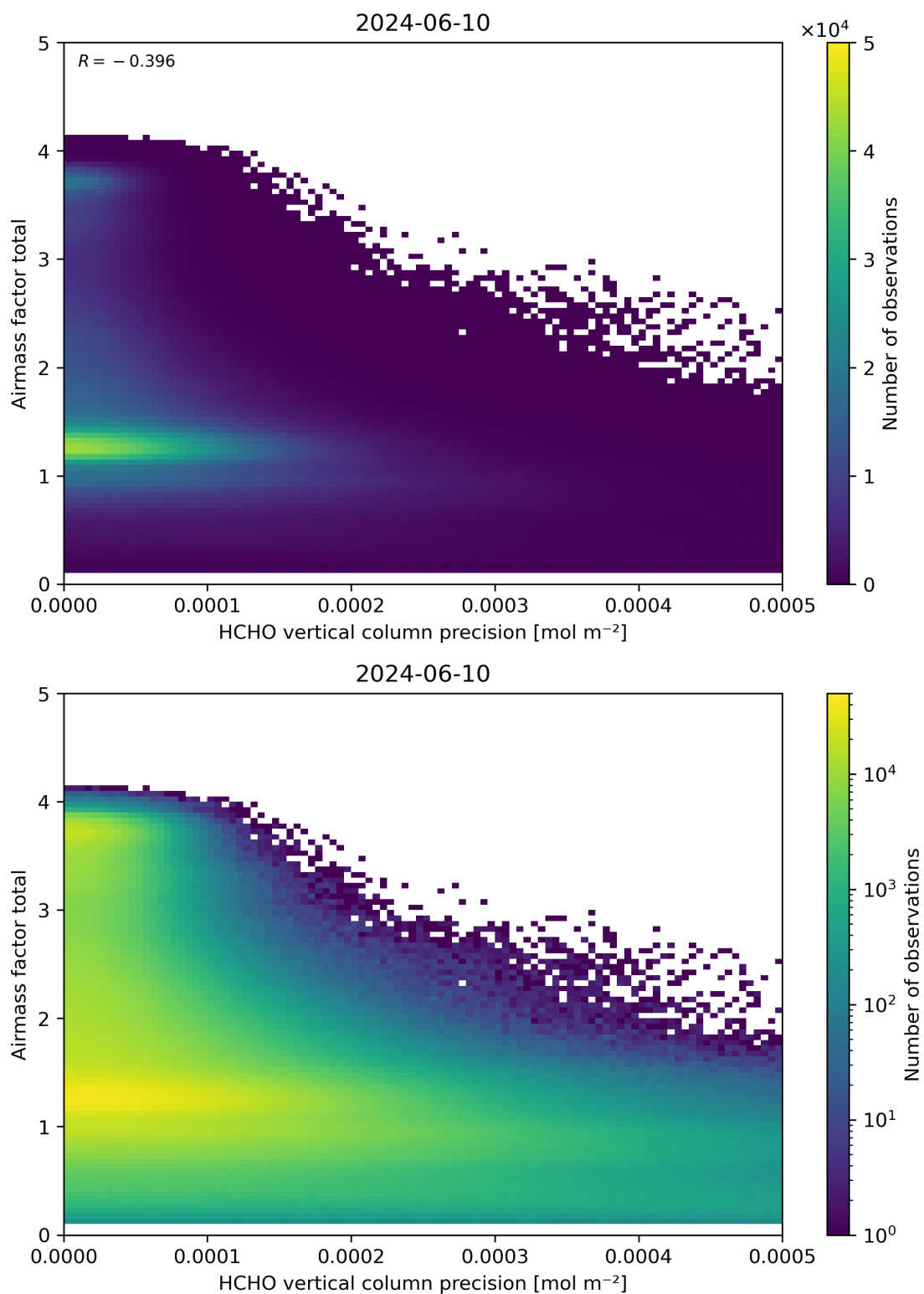
Figure 144: Scatter density plot of “HCHO vertical column precision” against “Airmass factor total” for 2024-06-09 to 2024-06-11.
