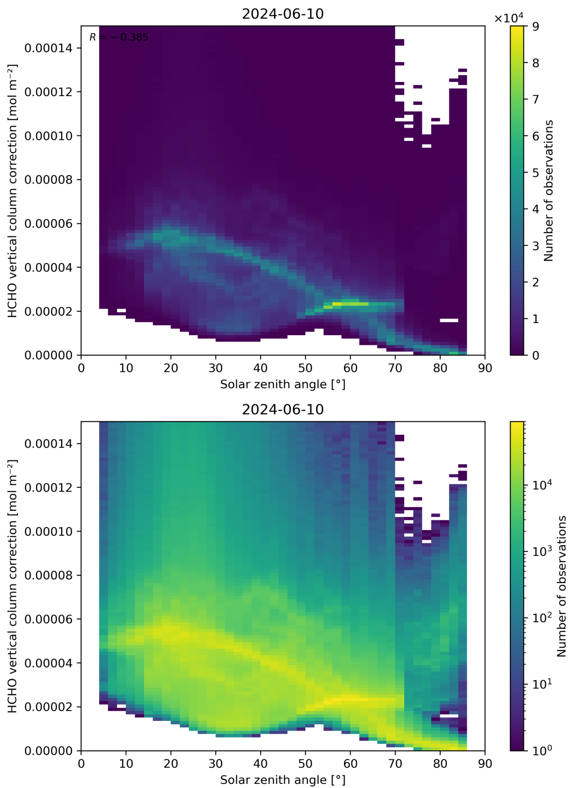
Figure 178: Scatter density plot of “Solar zenith angle” against “HCHO vertical column correction” for 2024-06-09 to 2024-06-11.
