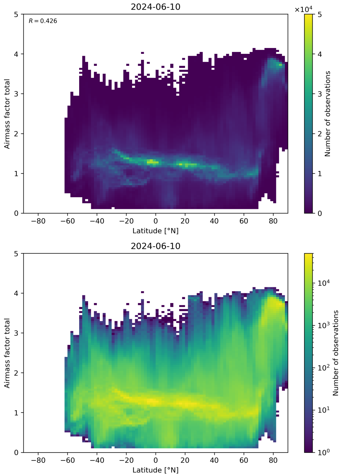
Figure 161: Scatter density plot of “Latitude” against “Airmass factor total” for 2024-06-09 to 2024-06-11.
