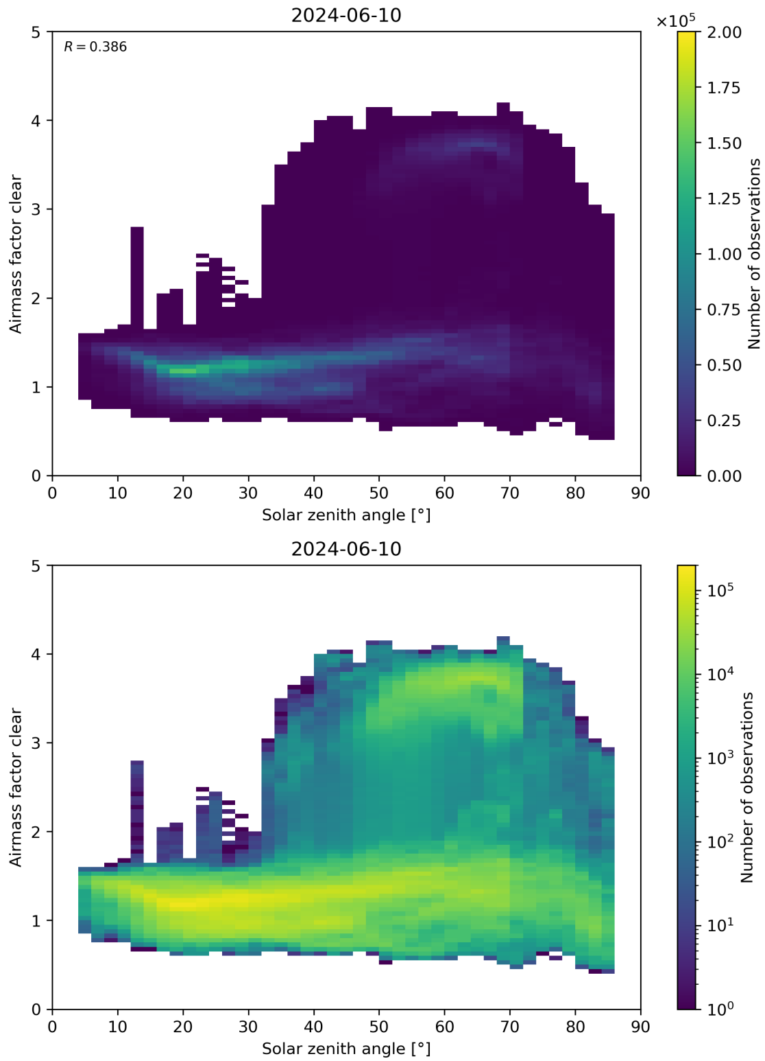
Figure 170: Scatter density plot of “Solar zenith angle” against “Airmass factor clear” for 2024-06-09 to 2024-06-11.
