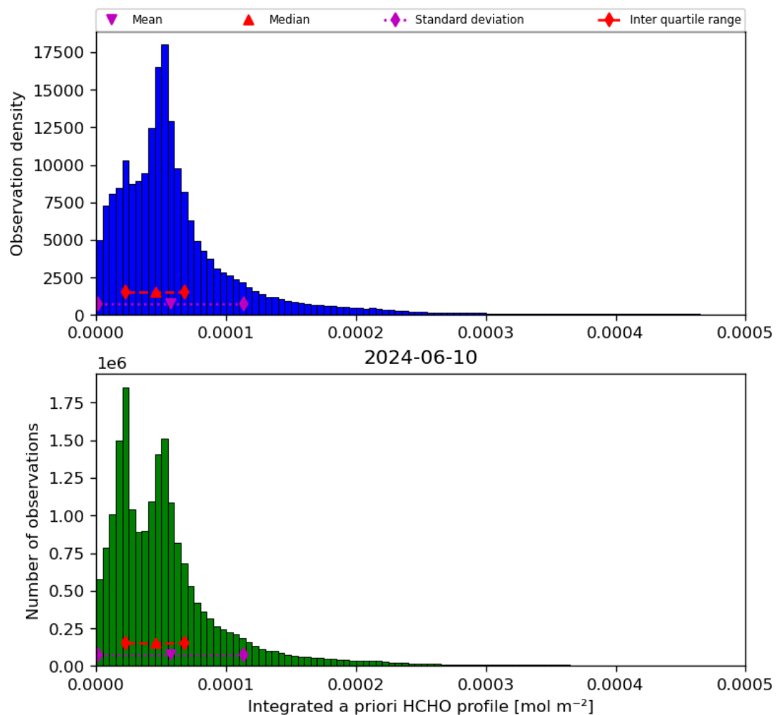
Figure 43: Histogram of “Integrated a priori HCHO profile” for 2024-06-09 to 2024-06-11
