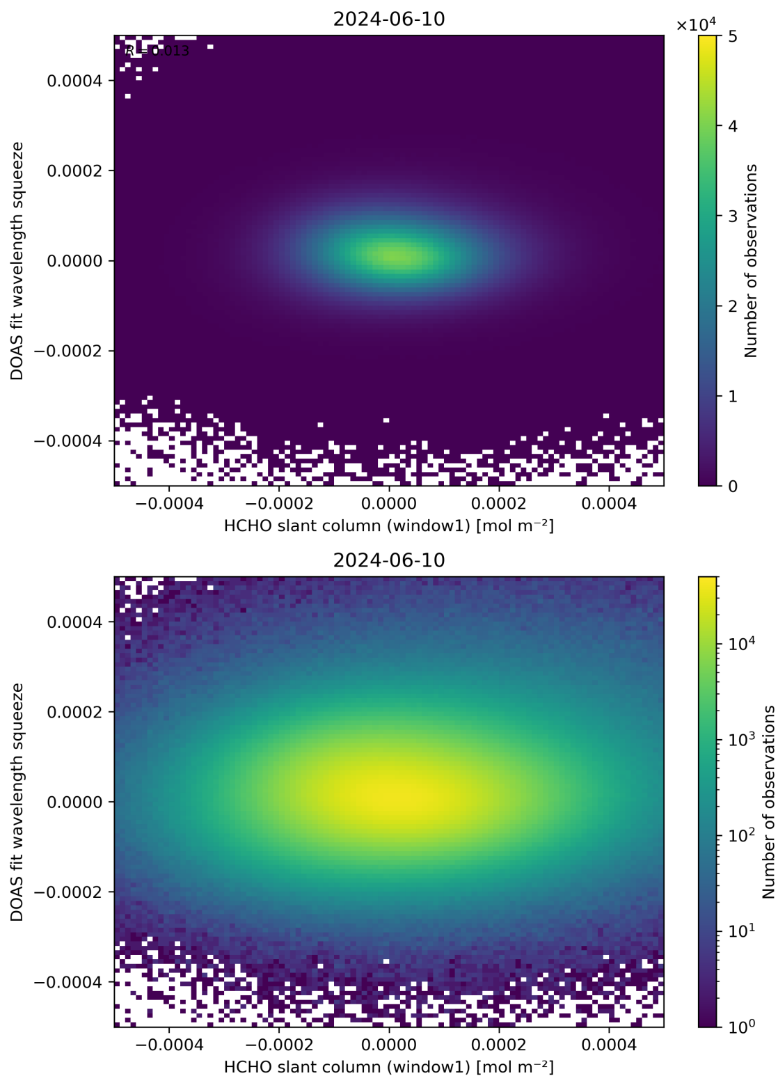
Figure 80: Scatter density plot of “HCHO slant column (window1)” against “DOAS fit wavelength squeeze” for 2024-06-09 to 2024-06-11.
