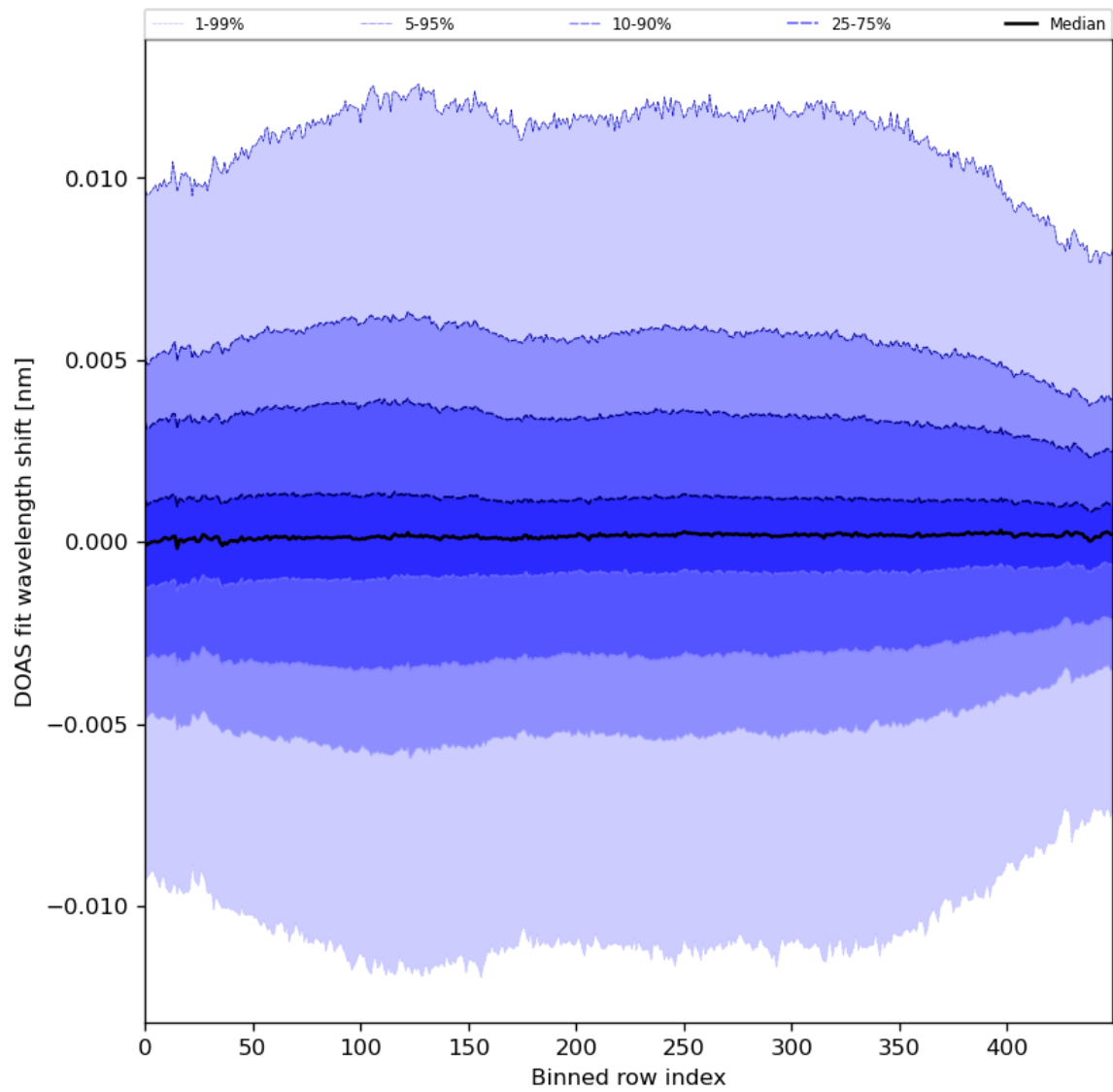
Figure 58: Along track statistics of “DOAS fit wavelength shift” for 2024-06-09 to 2024-06-11
