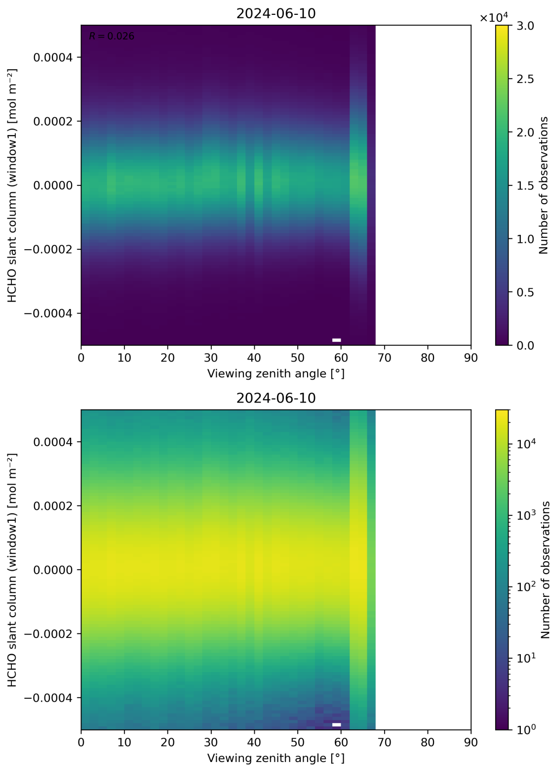
Figure 188: Scatter density plot of “Viewing zenith angle” against “HCHO slant column (window1)” for 2024-06-09 to 2024-06-11.
