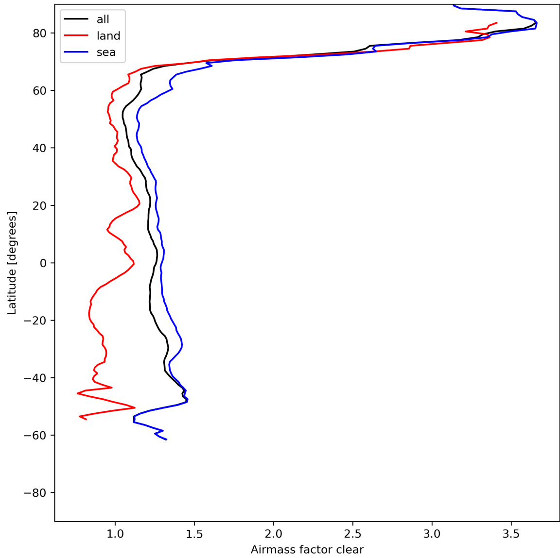
Figure 28: Zonal average of “Airmass factor clear” for 2024-06-09 to 2024-06-11.
