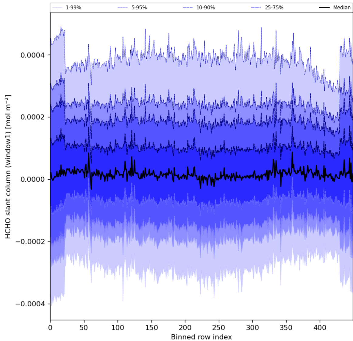
Figure 52: Along track statistics of “HCHO slant column (window1)” for 2024-06-09 to 2024-06-11
