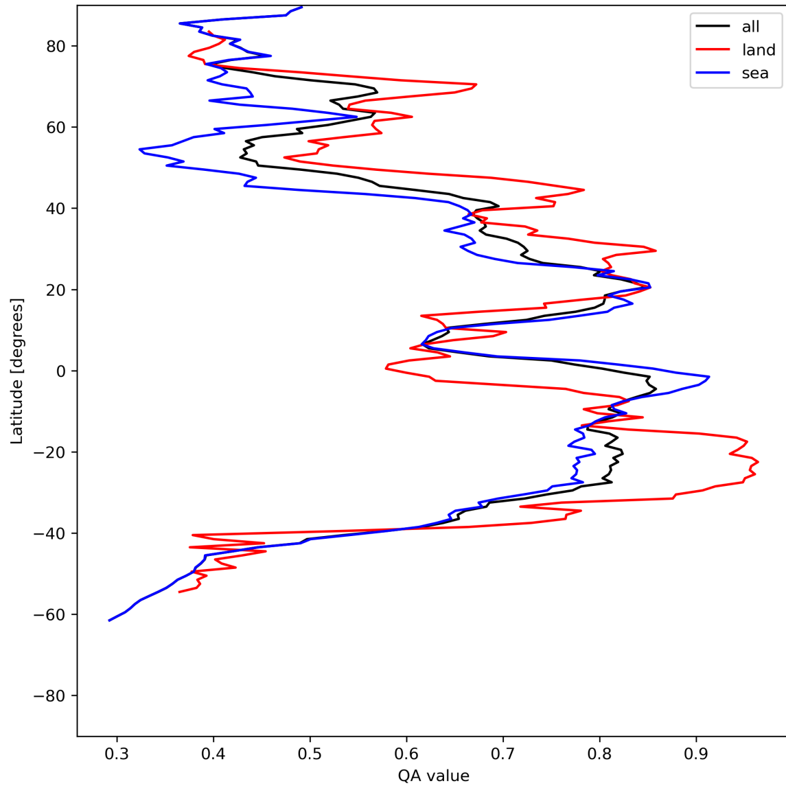
Figure 20: Zonal average of “QA value” for 2024-06-09 to 2024-06-11.
