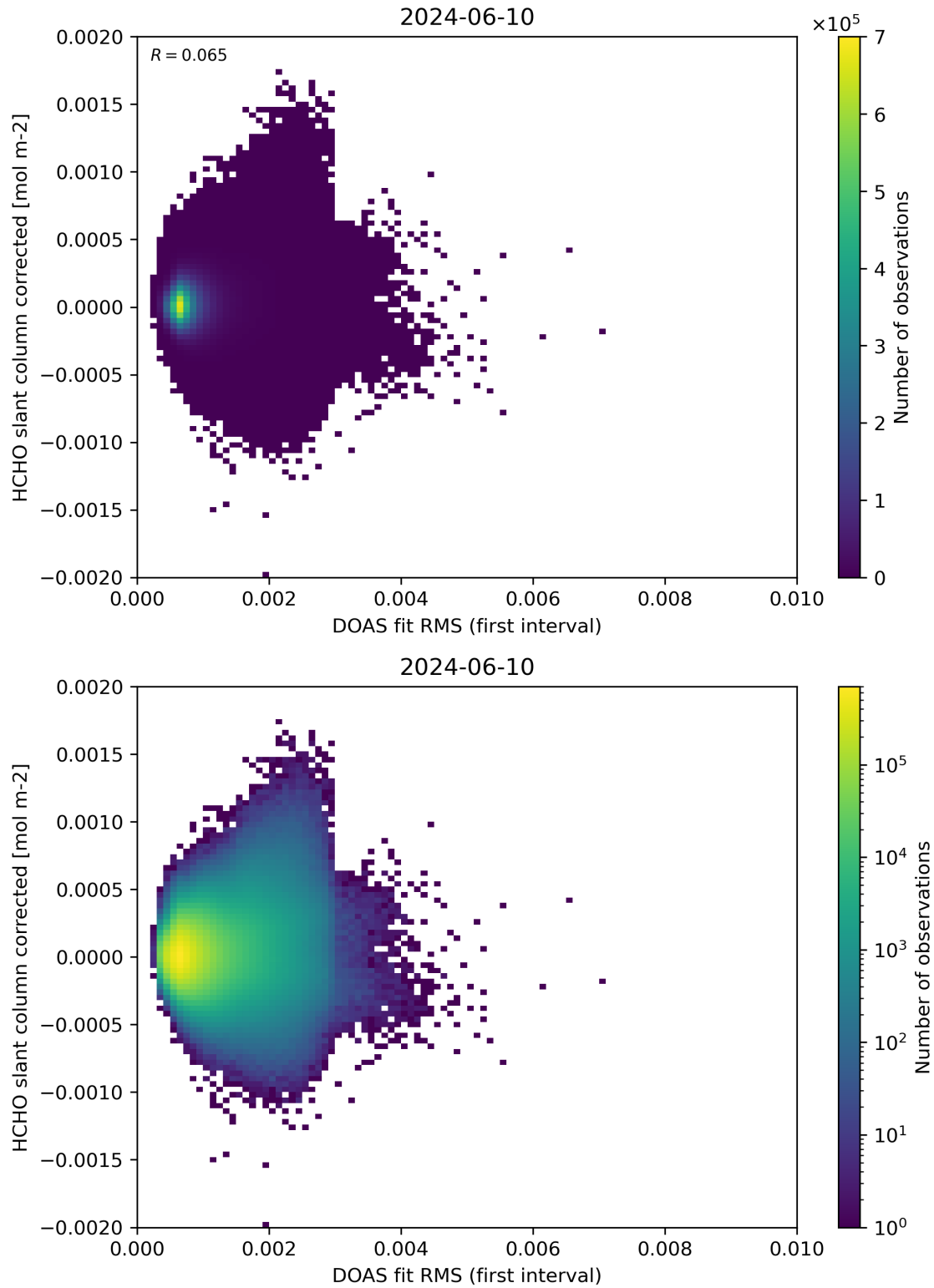
Figure 62: Scatter density plot of “DOAS fit RMS (first interval)” against “HCHO slant column corrected” for 2024-06-09 to 2024-06-11.
