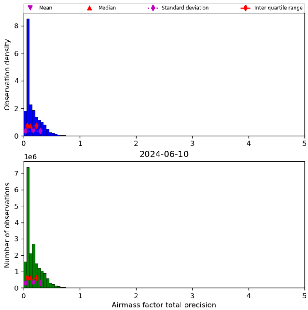
Figure 41: Histogram of “Airmass factor total precision” for 2024-06-09 to 2024-06-11
