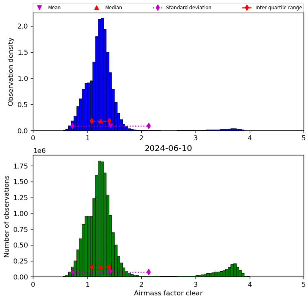
Figure 42: Histogram of “Airmass factor clear” for 2024-06-09 to 2024-06-11
