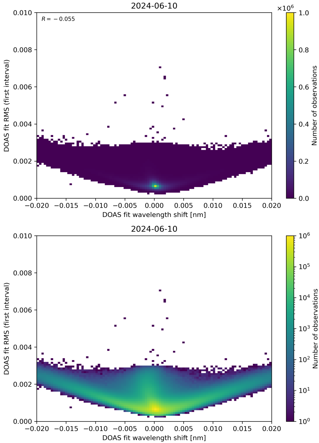
Figure 64: Scatter density plot of “DOAS fit wavelength shift” against “DOAS fit RMS (first interval)” for 2024-06-09 to 2024-06-11.
