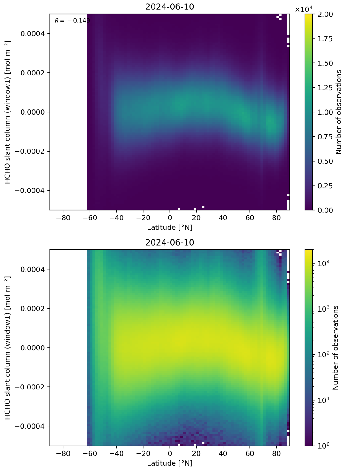
Figure 159: Scatter density plot of “Latitude” against “HCHO slant column (window1)” for 2024-06-09 to 2024-06-11.
