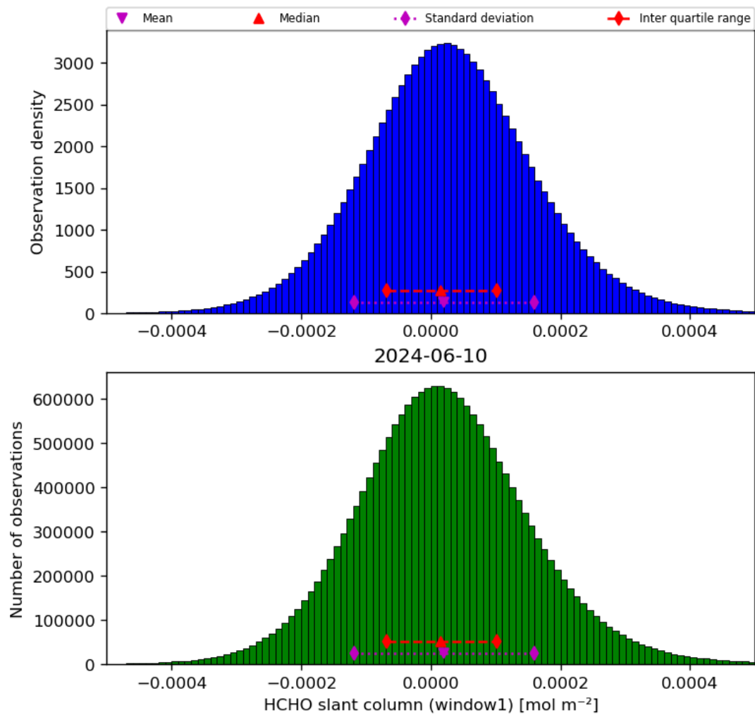
Figure 38: Histogram of “HCHO slant column (window1)” for 2024-06-09 to 2024-06-11
