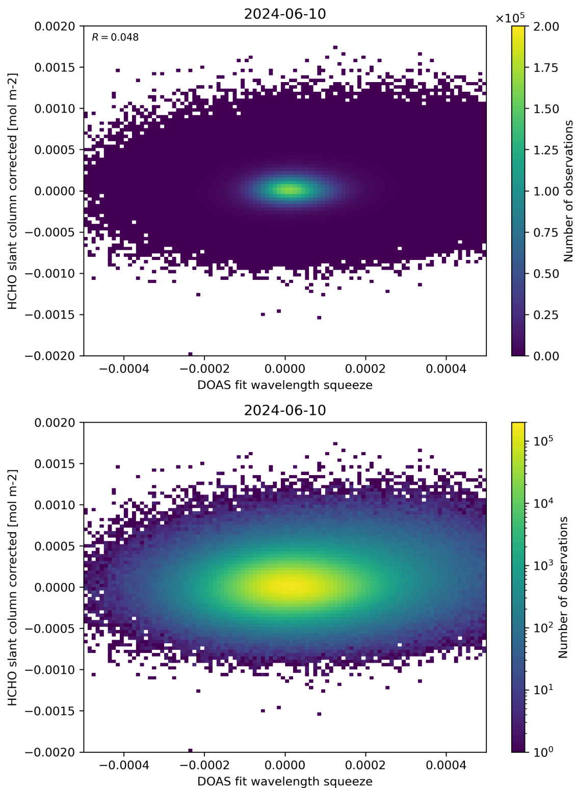
Figure 69: Scatter density plot of “DOAS fit wavelength squeeze” against “HCHO slant column corrected” for 2024-06-09 to 2024-06-11.
