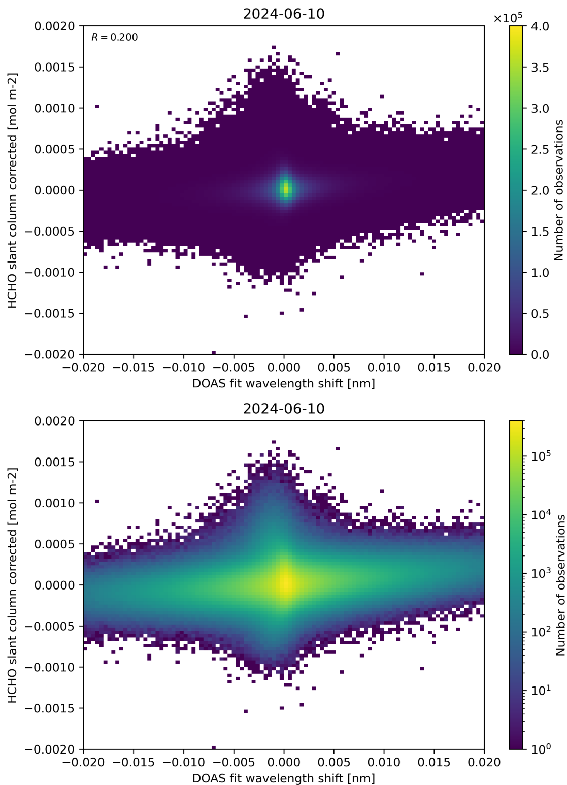
Figure 66: Scatter density plot of “DOAS fit wavelength shift” against “HCHO slant column corrected” for 2024-06-09 to 2024-06-11.
