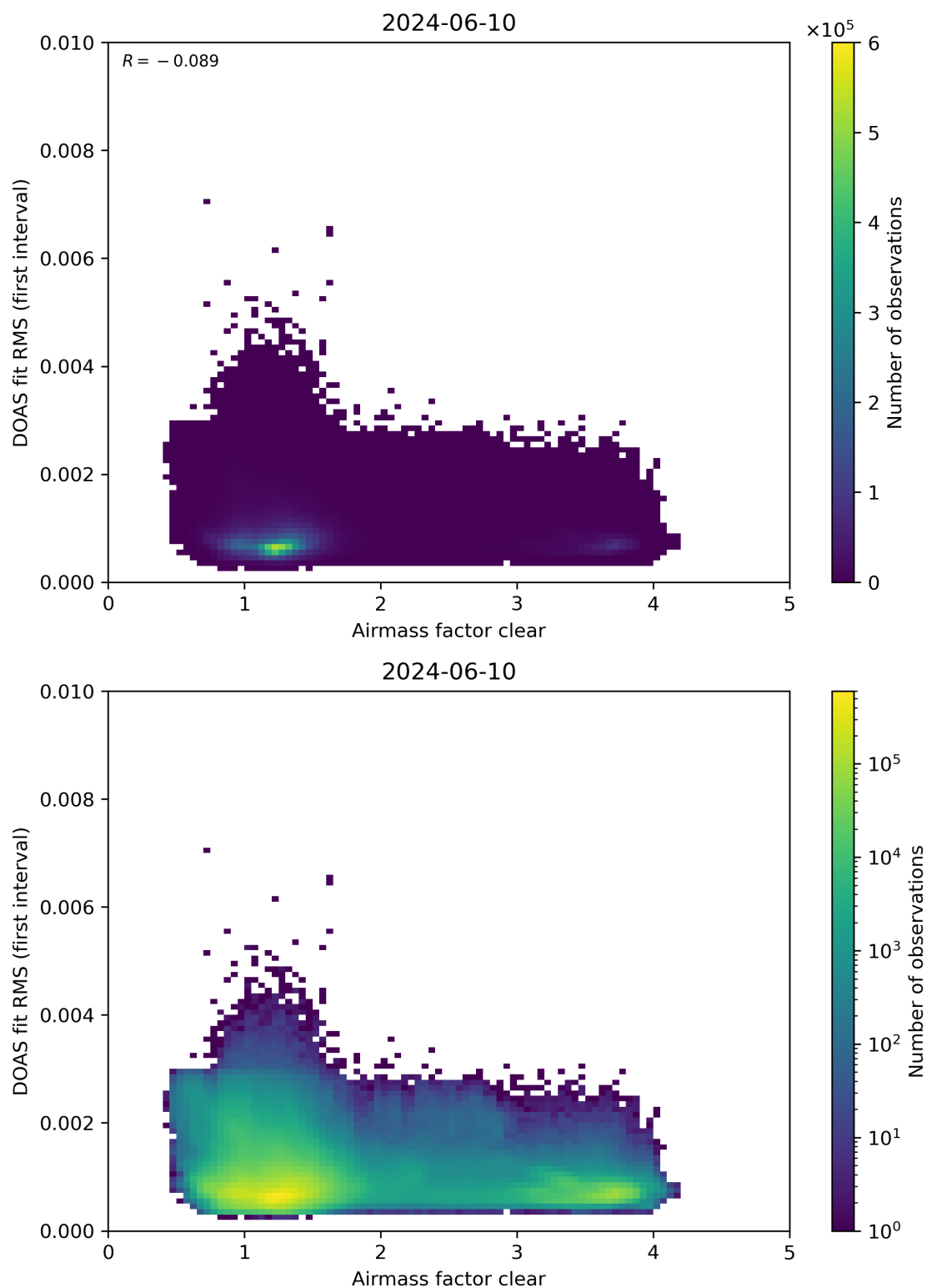
Figure 71: Scatter density plot of “Airmass factor clear” against “DOAS fit RMS (first interval)” for 2024-06-09 to 2024-06-11.
