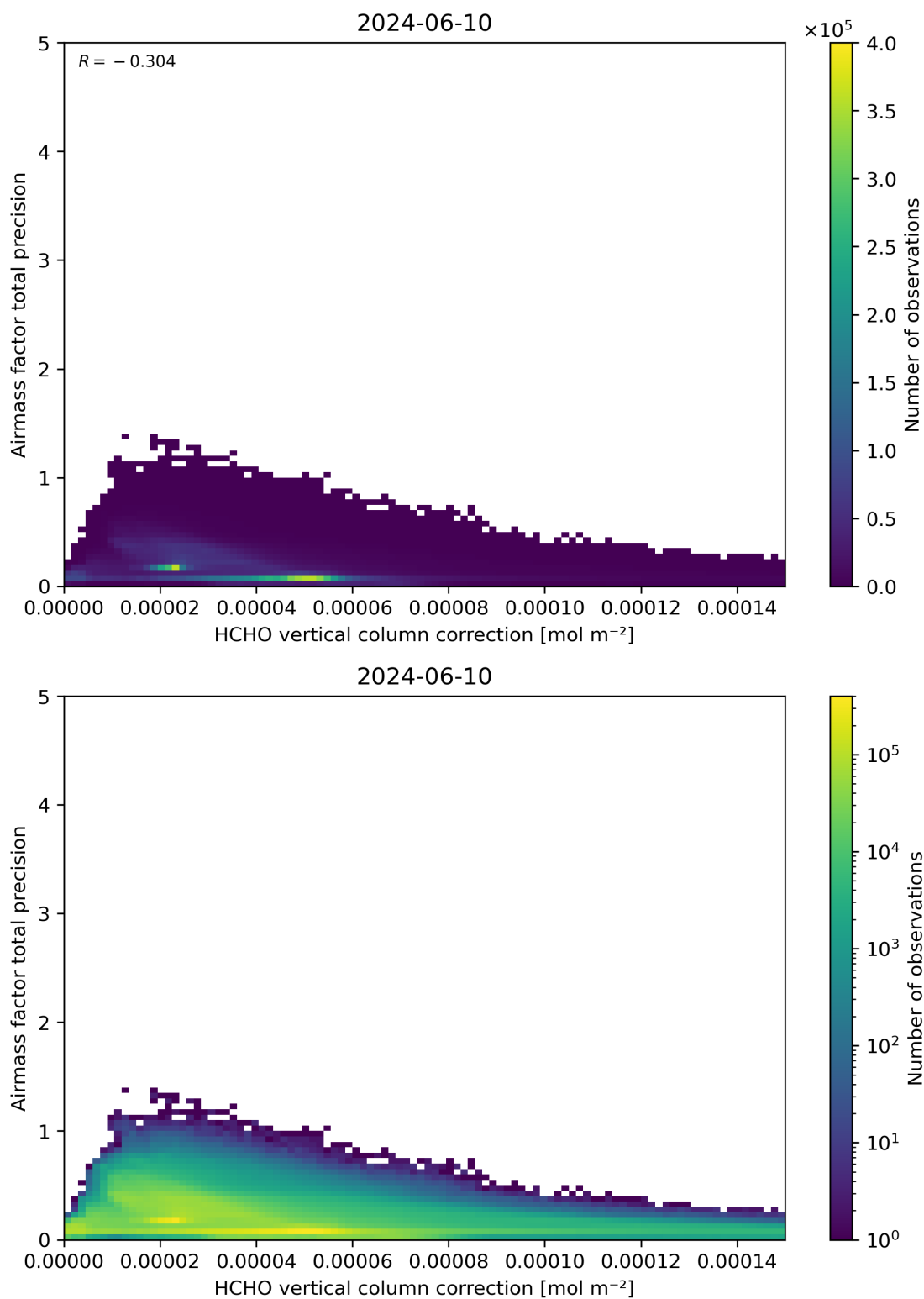
Figure 121: Scatter density plot of “HCHO vertical column correction” against “Airmass factor total precision” for 2024-06-09 to 2024-06-11.
