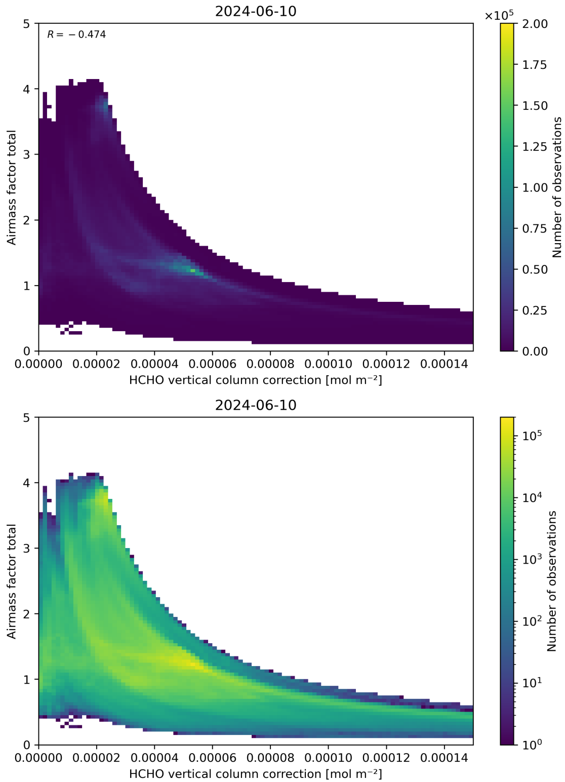
Figure 120: Scatter density plot of “HCHO vertical column correction” against “Airmass factor total” for 2024-06-09 to 2024-06-11.
