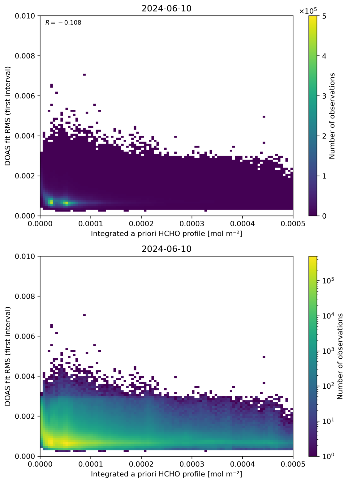
Figure 148: Scatter density plot of “Integrated a priori HCHO profile” against “DOAS fit RMS (first interval)” for 2024-06-09 to 2024-06-11.
