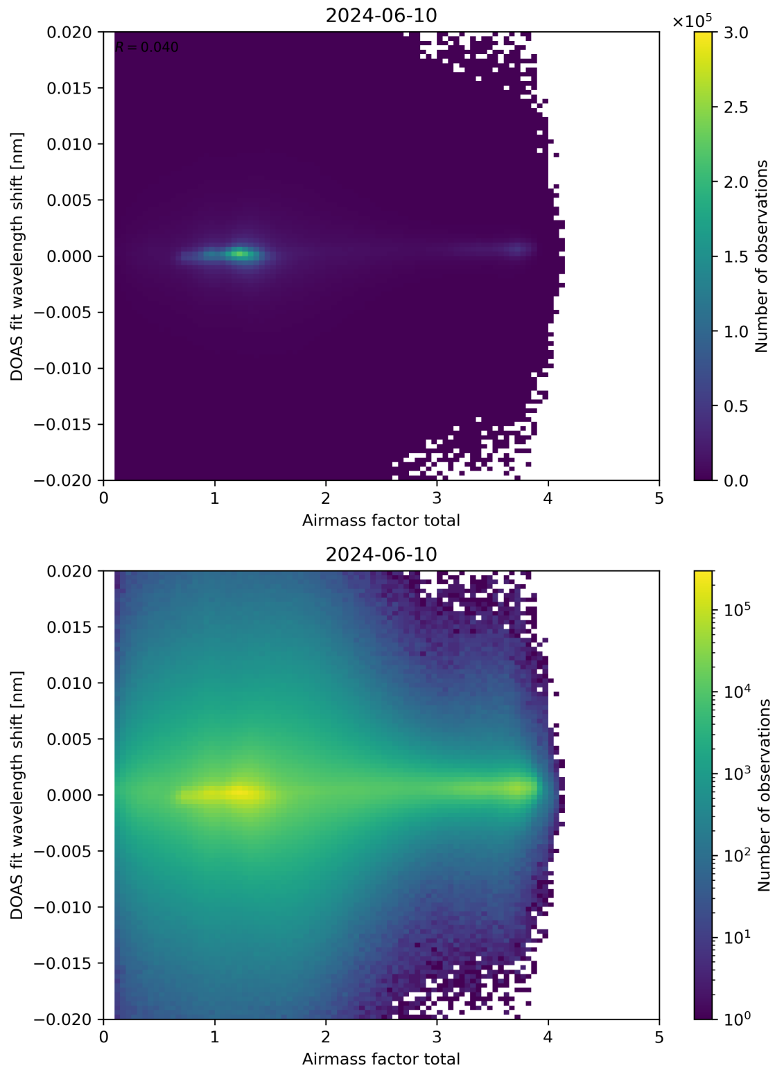
Figure 98: Scatter density plot of “Airmass factor total” against “DOAS fit wavelength shift” for 2024-06-09 to 2024-06-11.
