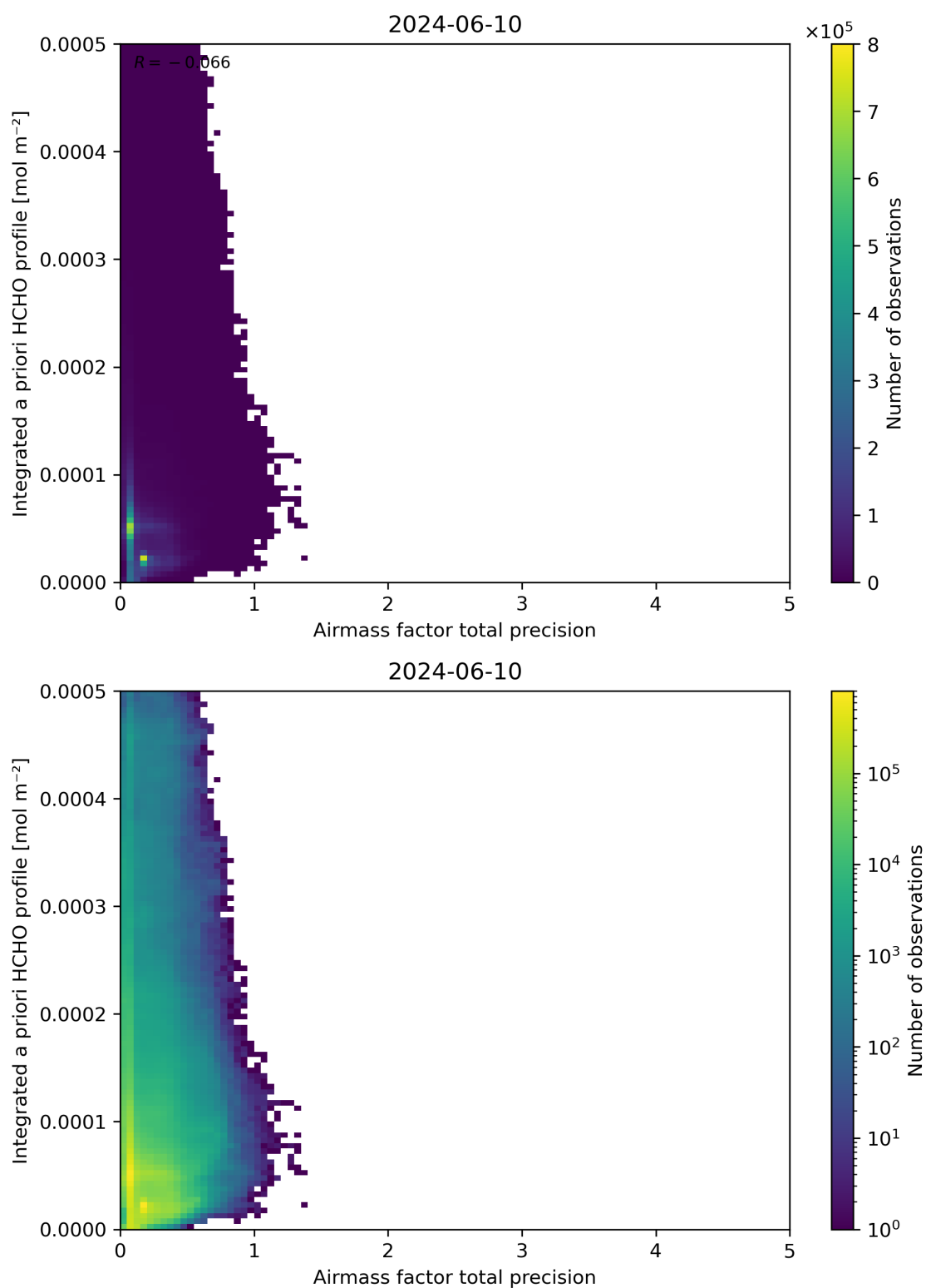
Figure 111: Scatter density plot of “Airmass factor total precision” against “Integrated a priori HCHO profile” for 2024-06-09 to 2024-06-11.
