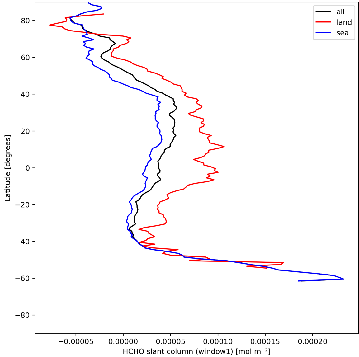
Figure 24: Zonal average of “HCHO slant column (window1)” for 2024-06-09 to 2024-06-11.
