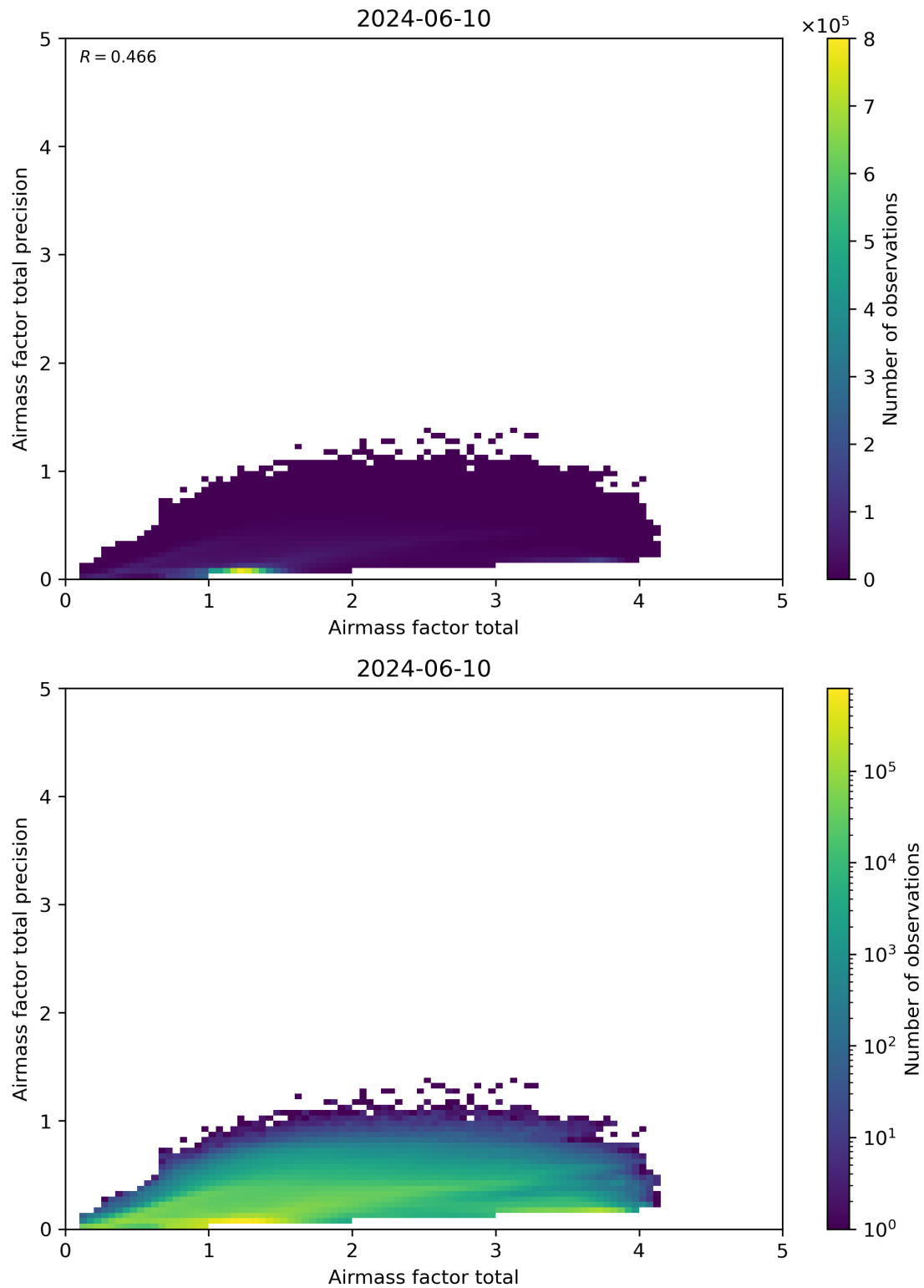
Figure 103: Scatter density plot of “Airmass factor total” against “Airmass factor total precision” for 2024-06-09 to 2024-06-11.
