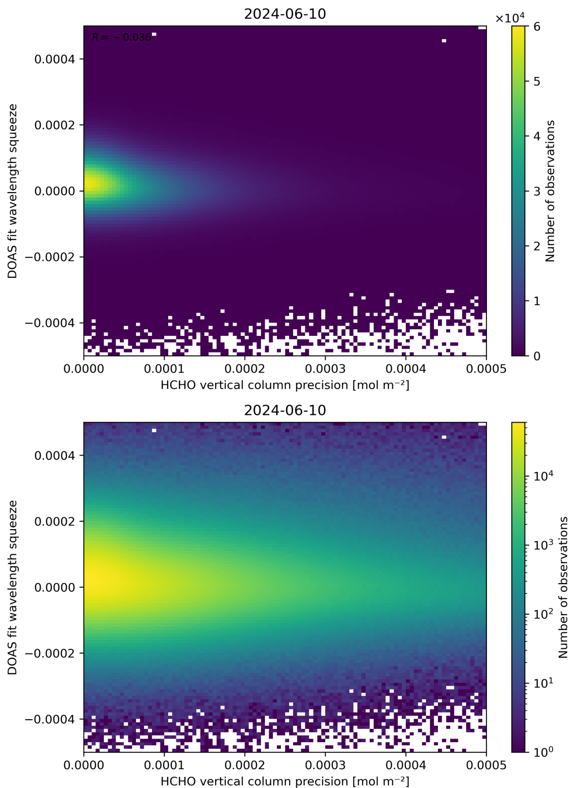
Figure 138: Scatter density plot of “HCHO vertical column precision” against “DOAS fit wavelength squeeze” for 2024-06-09 to 2024-06-11.
