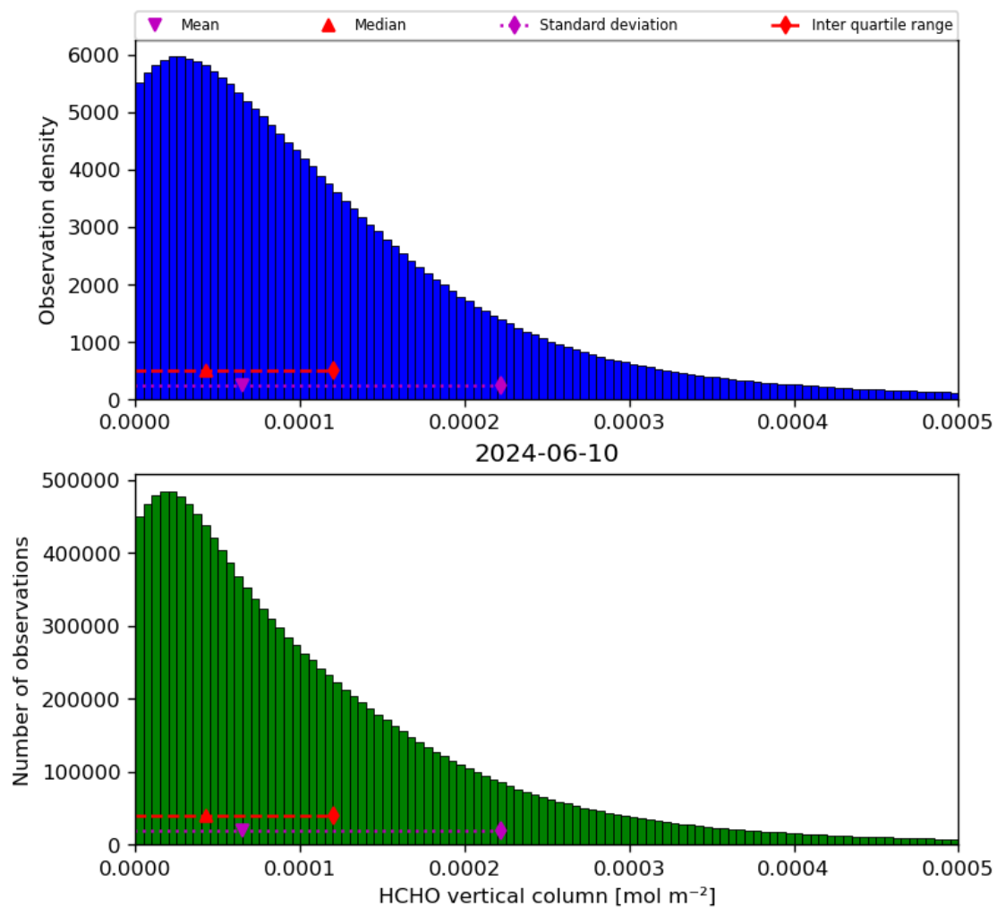
Figure 35: Histogram of “HCHO vertical column” for 2024-06-09 to 2024-06-11
