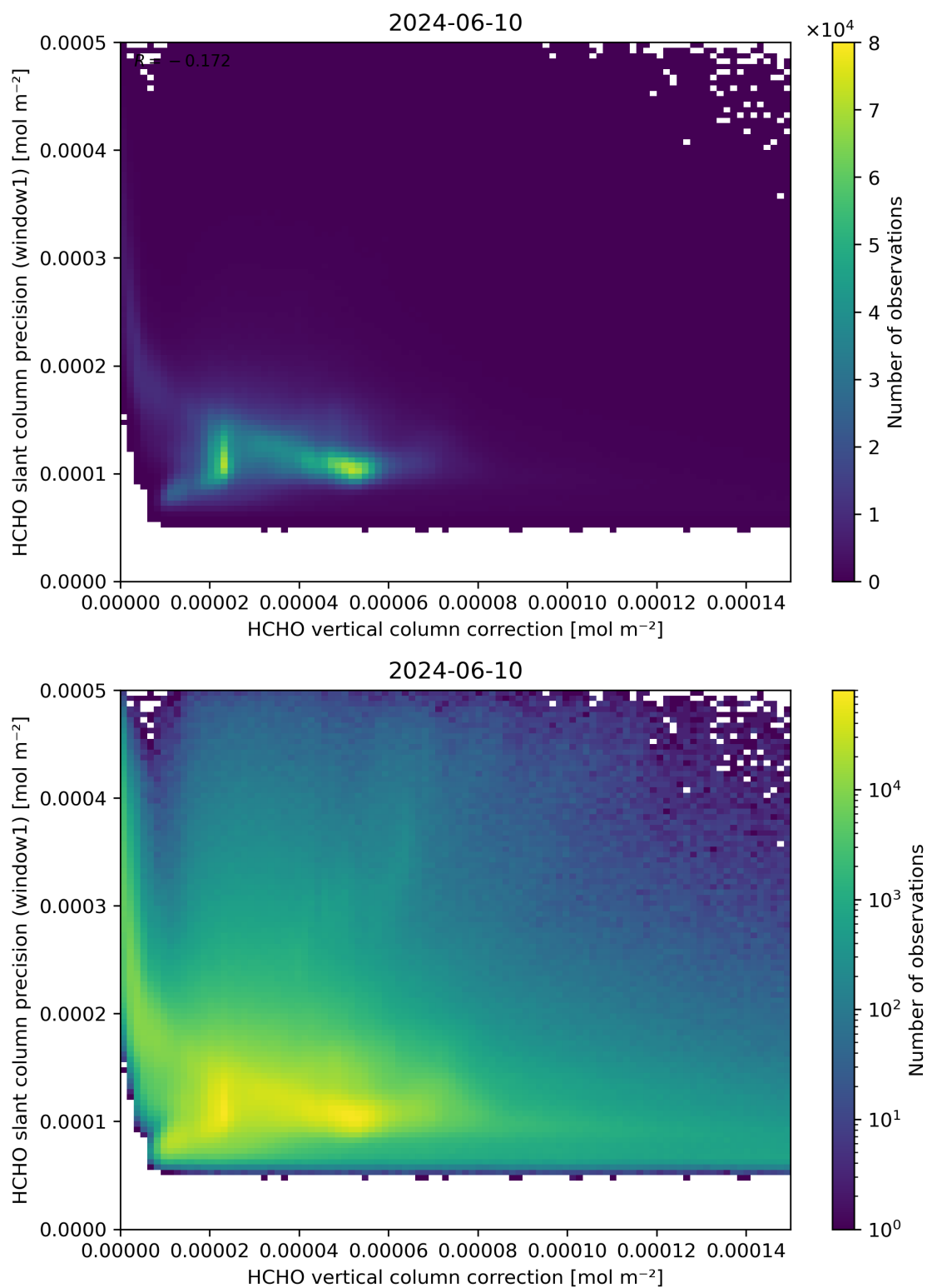
Figure 119: Scatter density plot of “HCHO vertical column correction” against “HCHO slant column precision (window1)” for 2024-06-09 to 2024-06-11.
