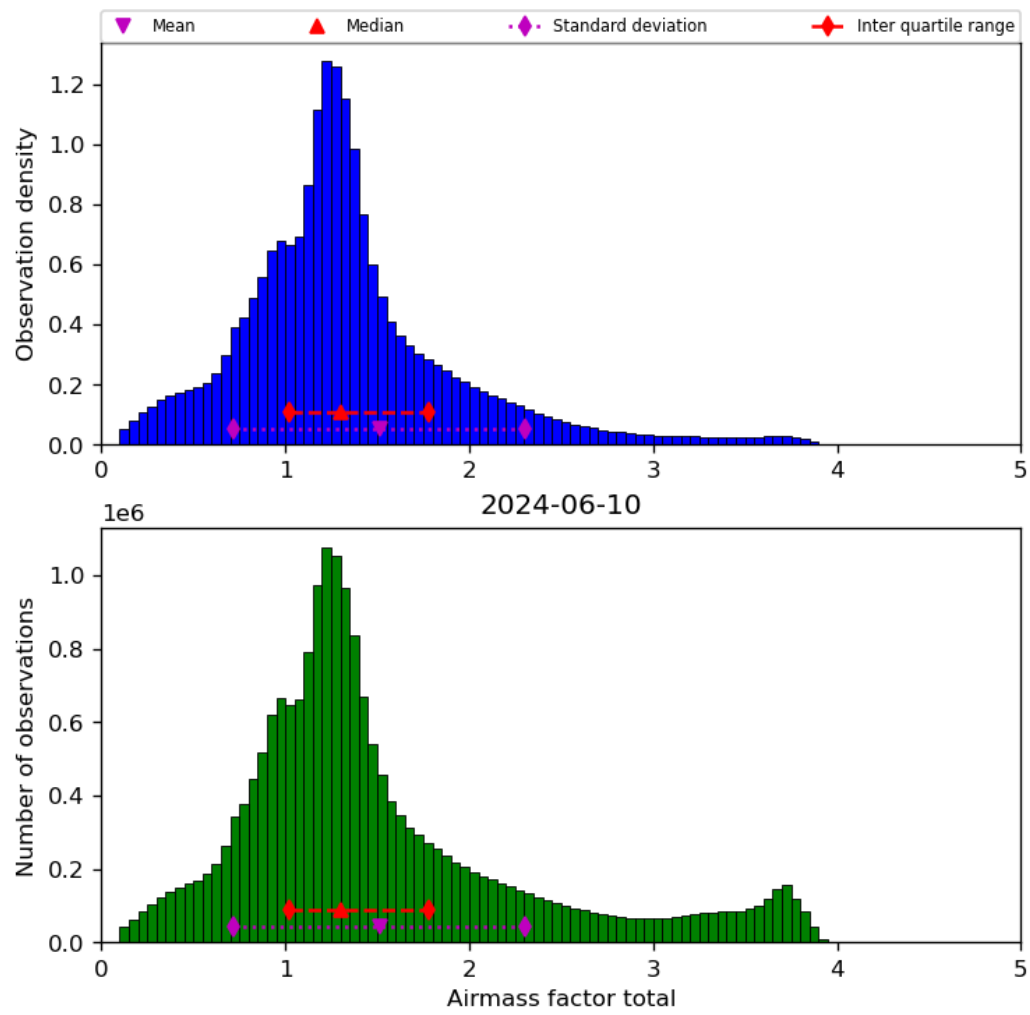
Figure 40: Histogram of “Airmass factor total” for 2024-06-09 to 2024-06-11
