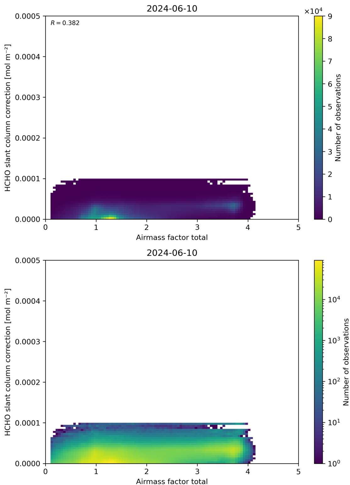
Figure 102: Scatter density plot of “Airmass factor total” against “HCHO slant column correction” for 2024-06-09 to 2024-06-11.
