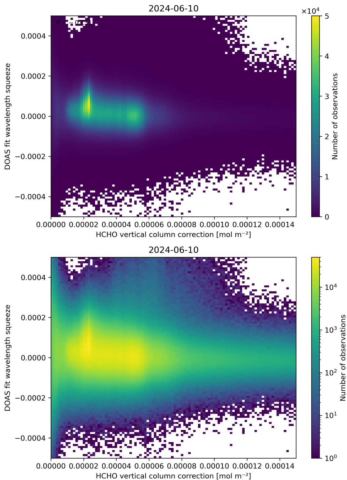
Figure 114: Scatter density plot of “HCHO vertical column correction” against “DOAS fit wavelength squeeze” for 2024-06-09 to 2024-06-11.
