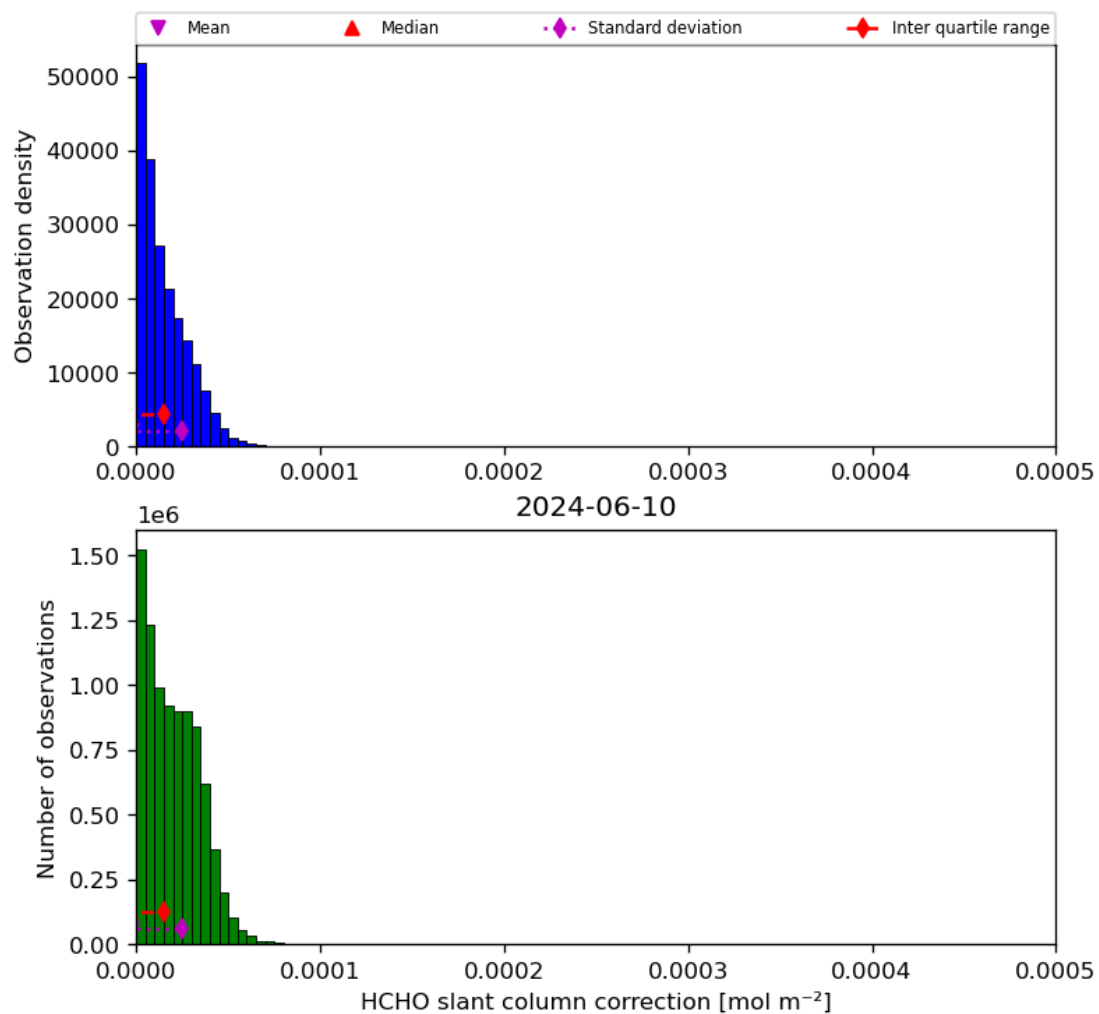
Figure 47: Histogram of “HCHO slant column correction” for 2024-06-09 to 2024-06-11
