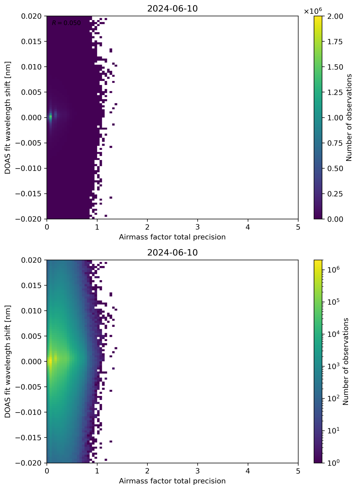
Figure 106: Scatter density plot of “Airmass factor total precision” against “DOAS fit wavelength shift” for 2024-06-09 to 2024-06-11.
