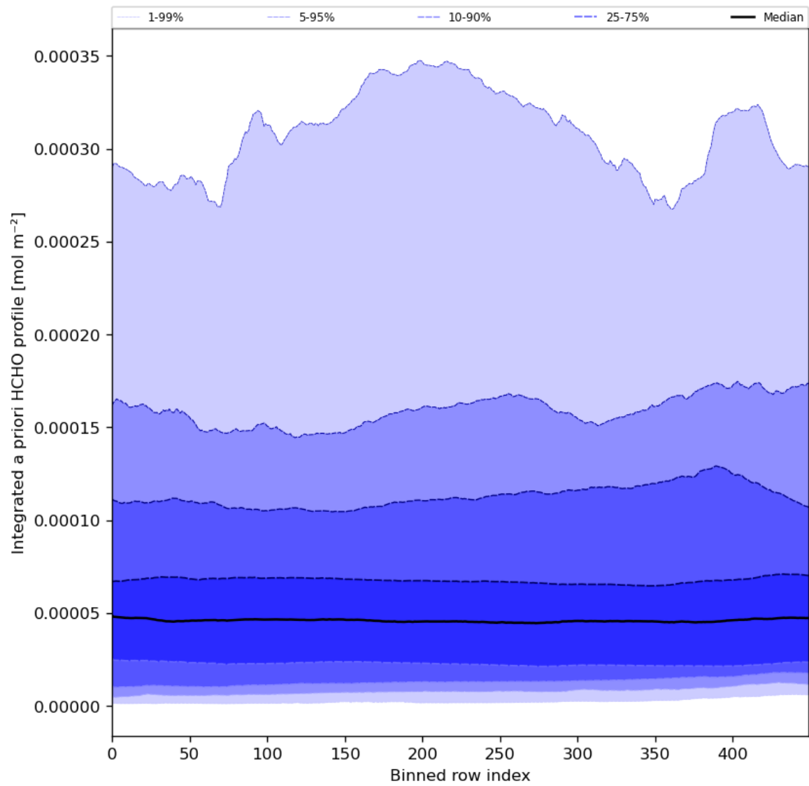
Figure 57: Along track statistics of "Integrated a priori HCHO profile" for 2024-06-09 to 2024-06-11
