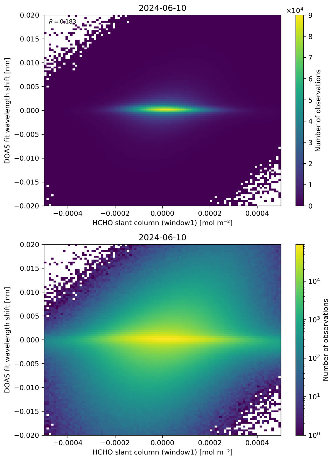
Figure 79: Scatter density plot of “HCHO slant column (window1)” against “DOAS fit wavelength shift” for 2024-06-09 to 2024-06-11.
