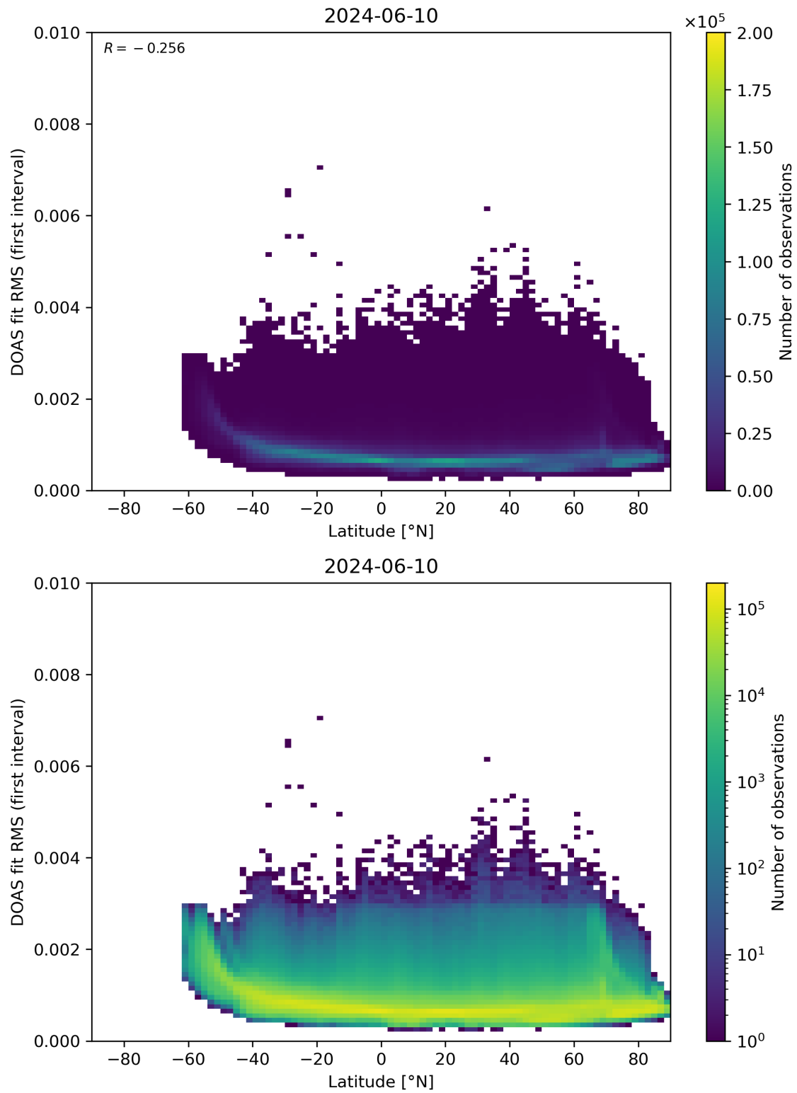
Figure 153: Scatter density plot of “Latitude” against “DOAS fit RMS (first interval)” for 2024-06-09 to 2024-06-11.
