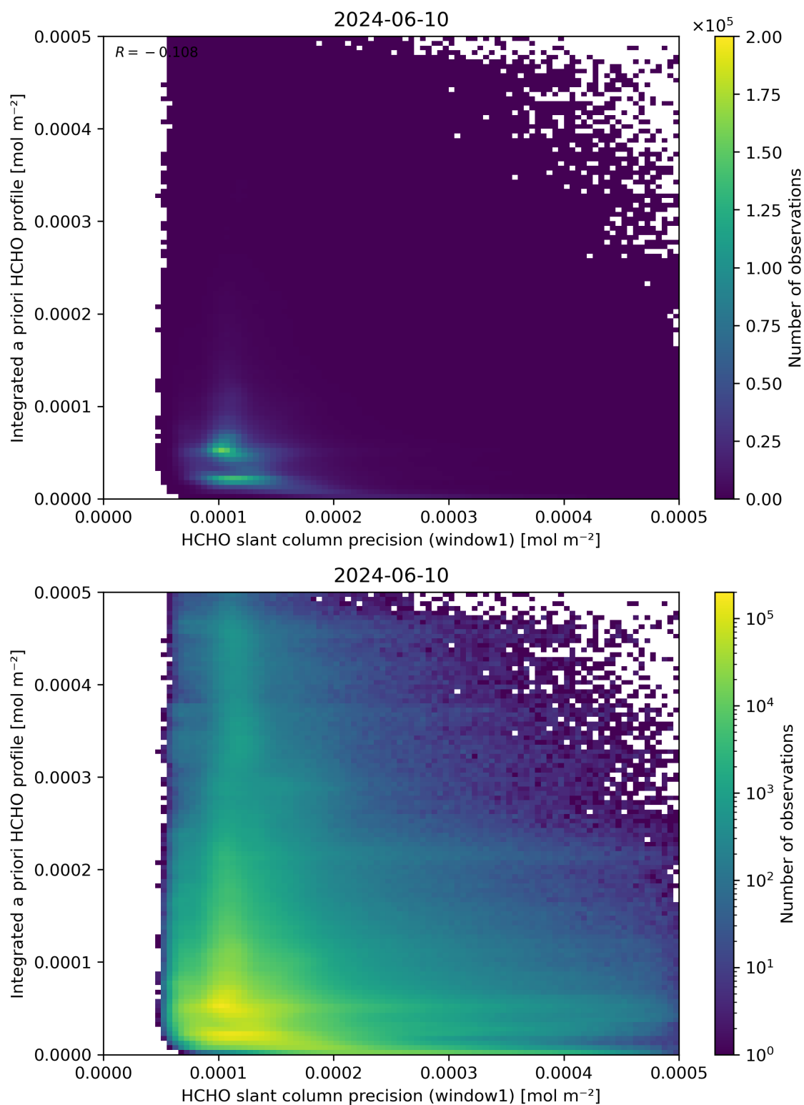
Figure 96: Scatter density plot of “HCHO slant column precision (window1)” against “Integrated a priori HCHO profile” for 2024-06-09 to 2024-06-11.
