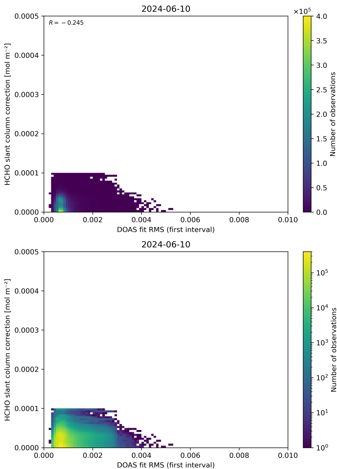
Figure 63: Scatter density plot of “DOAS fit RMS (first interval)” against “HCHO slant column correction” for 2024-06-09 to 2024-06-11.
