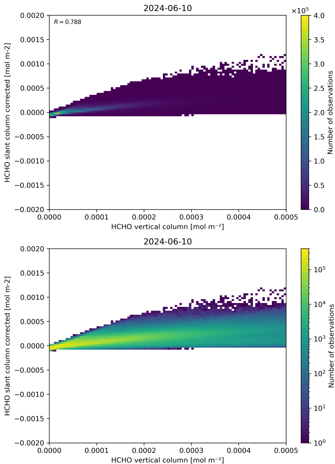
Figure 127: Scatter density plot of “HCHO vertical column” against “HCHO slant column corrected” for 2024-06-09 to 2024-06-11.
