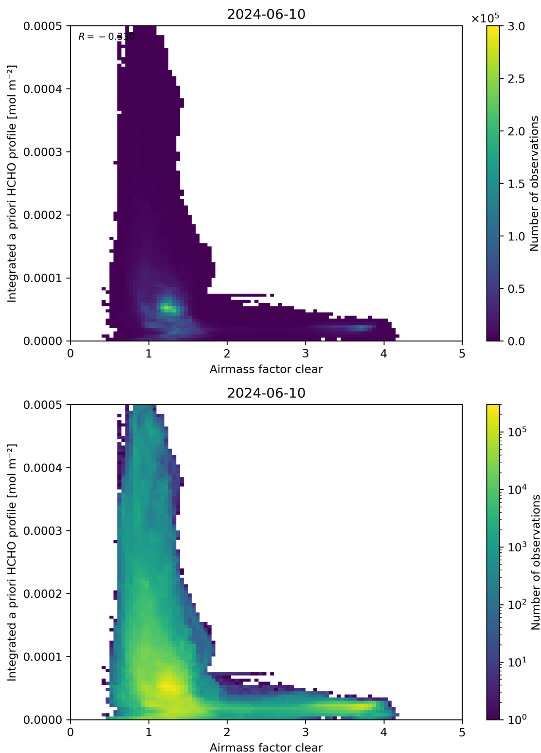
Figure 76: Scatter density plot of “Airmass factor clear” against “Integrated a priori HCHO profile” for 2024-06-09 to 2024-06-11.
