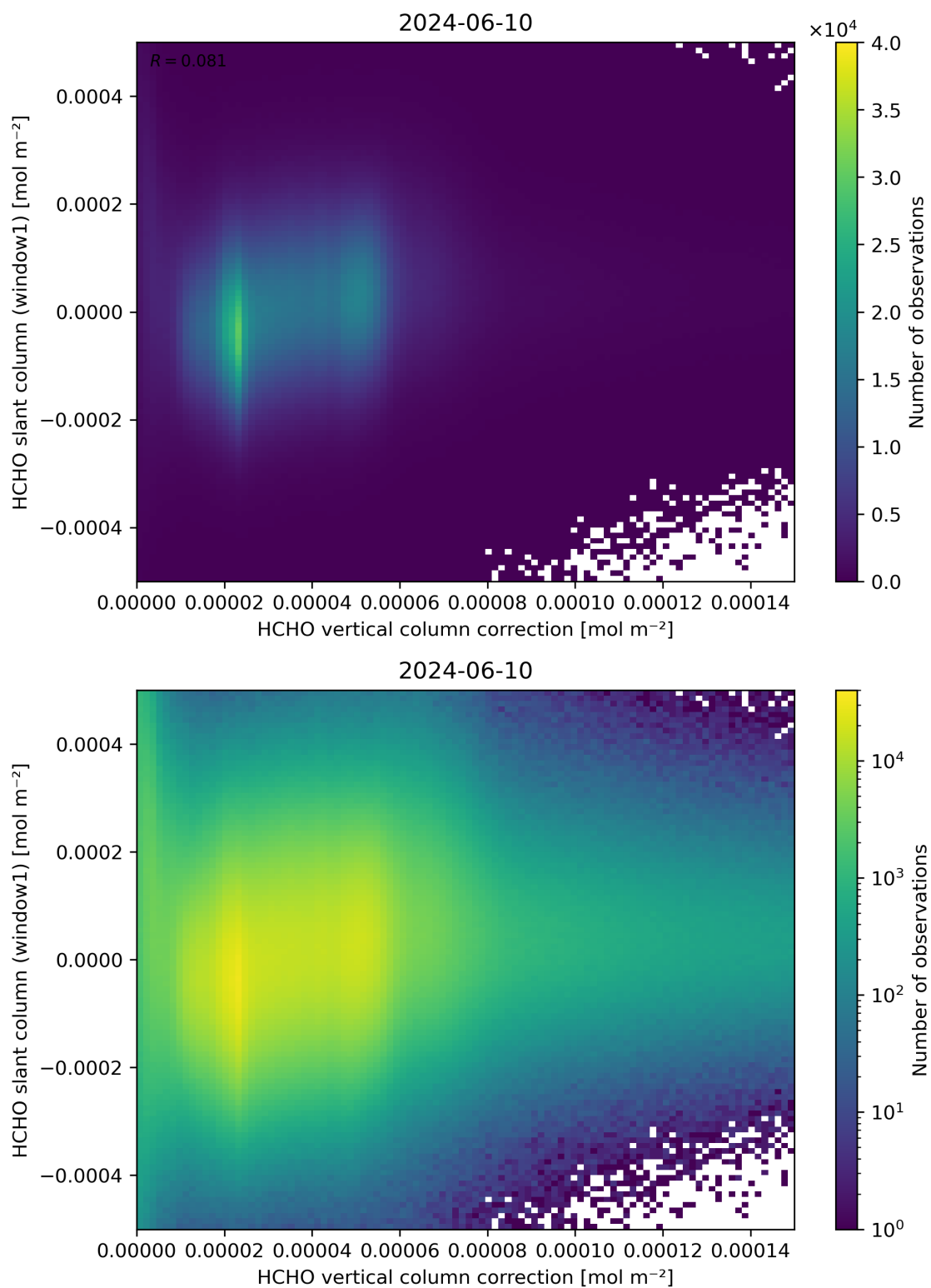
Figure 118: Scatter density plot of “HCHO vertical column correction” against “HCHO slant column (window1)” for 2024-06-09 to 2024-06-11.
