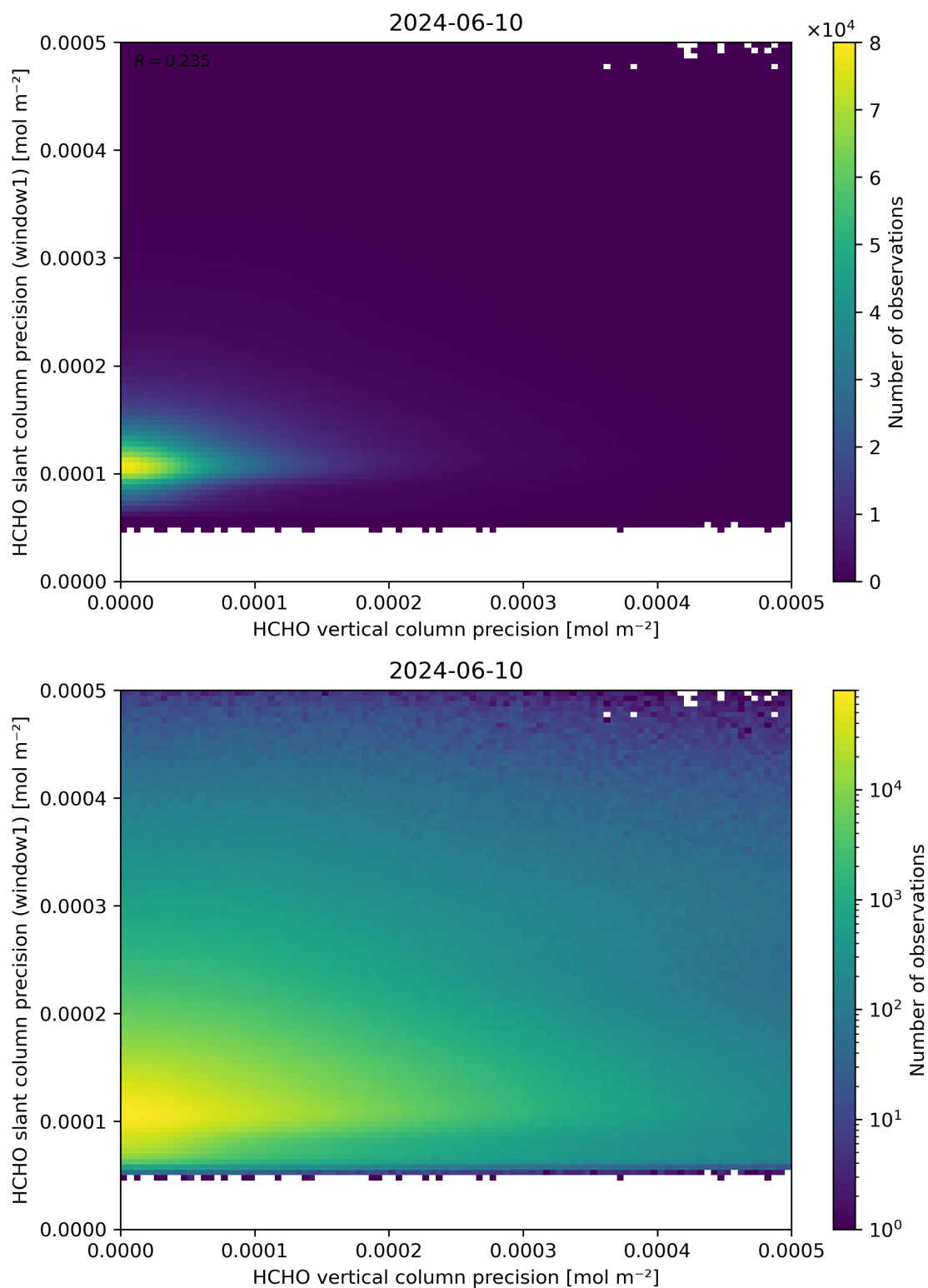
Figure 143: Scatter density plot of “HCHO vertical column precision” against “HCHO slant column precision (window1)” for 2024-06-09 to 2024-06-11.
