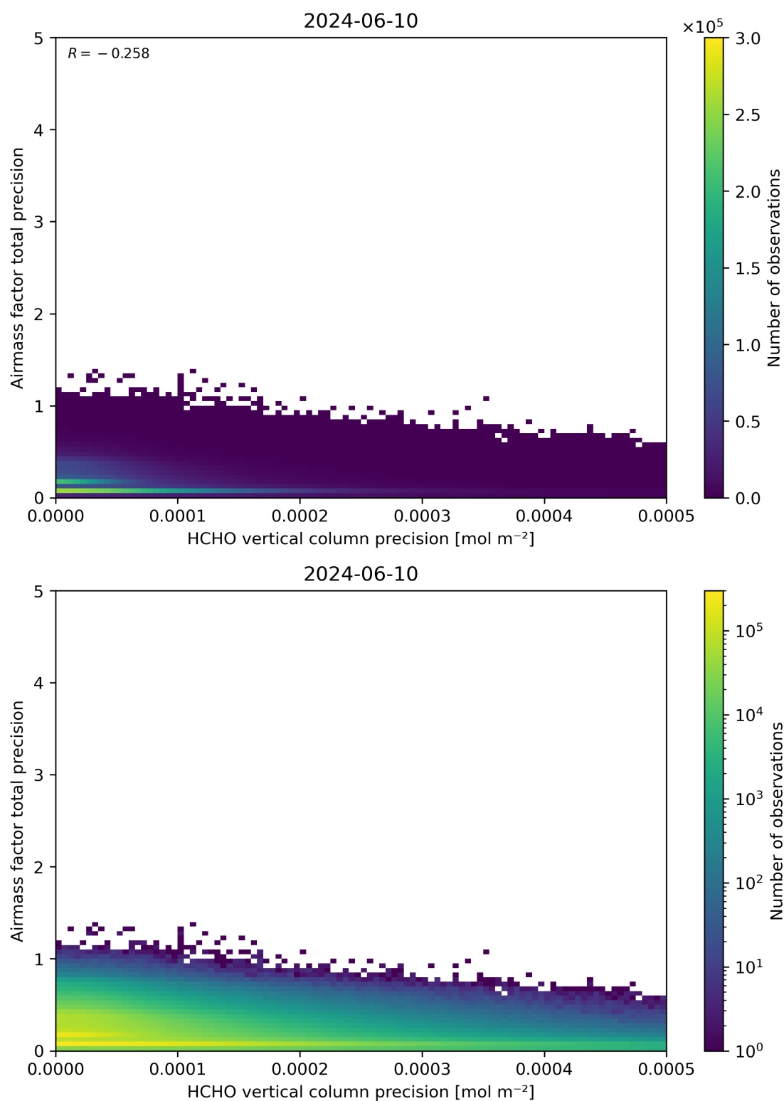
Figure 145: Scatter density plot of “HCHO vertical column precision” against “Airmass factor total precision” for 2024-06-09 to 2024-06-11.
