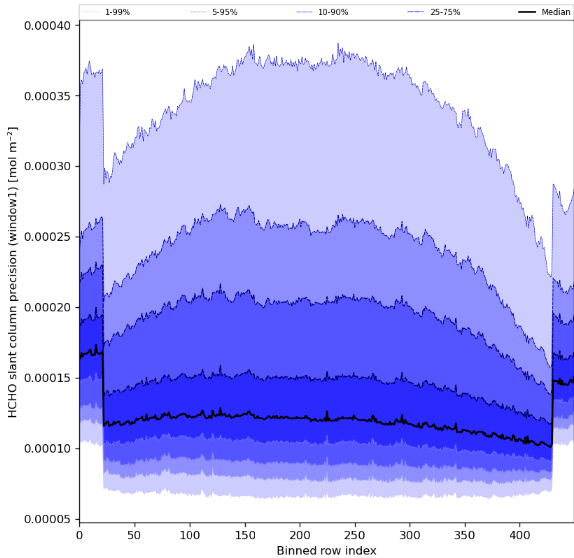
Figure 53: Along track statistics of “HCHO slant column precision (window1)” for 2024-06-09 to 2024-06-11
