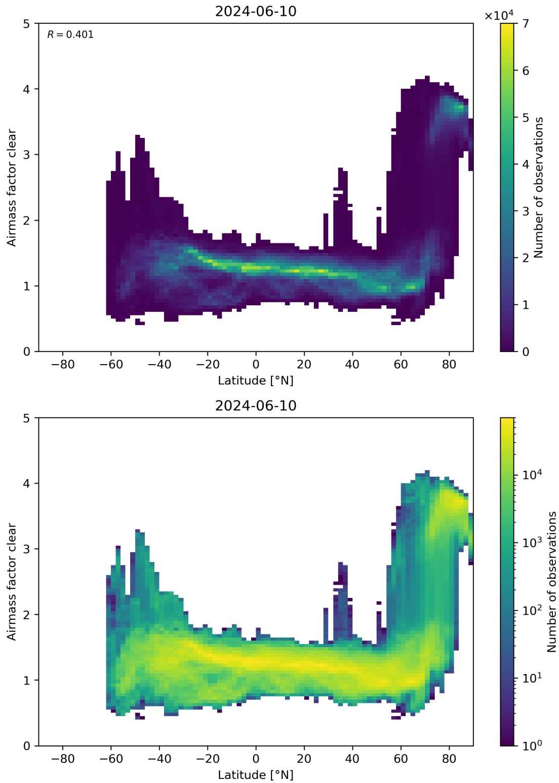
Figure 156: Scatter density plot of “Latitude” against “Airmass factor clear” for 2024-06-09 to 2024-06-11.
