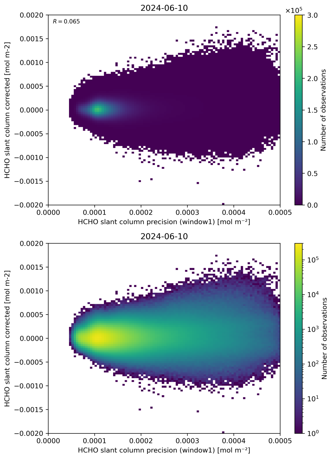
Figure 92: Scatter density plot of “HCHO slant column precision (window1)” against “HCHO slant column corrected” for 2024-06-09 to 2024-06-11.
