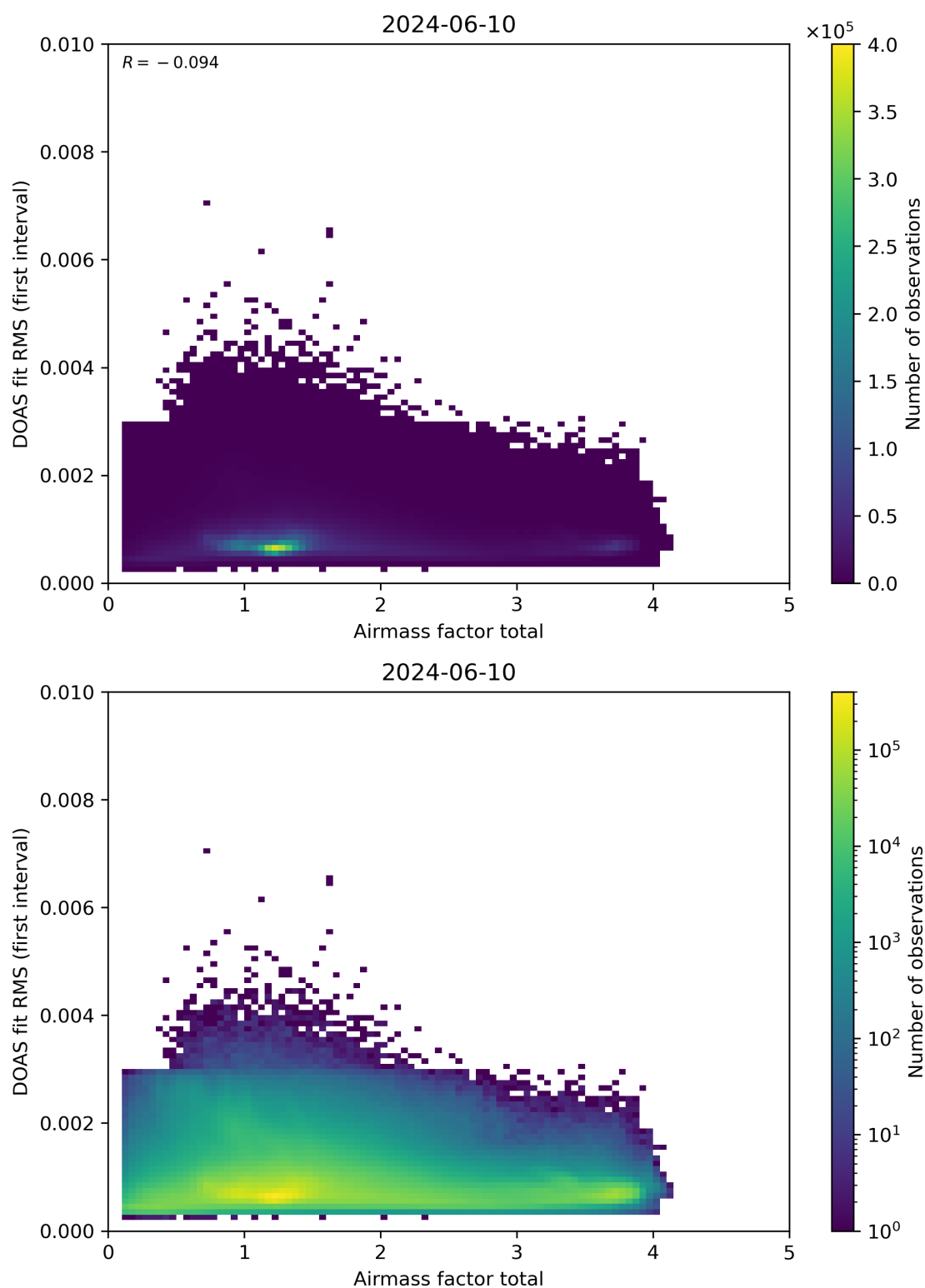
Figure 97: Scatter density plot of “Airmass factor total” against “DOAS fit RMS (first interval)” for 2024-06-09 to 2024-06-11.
