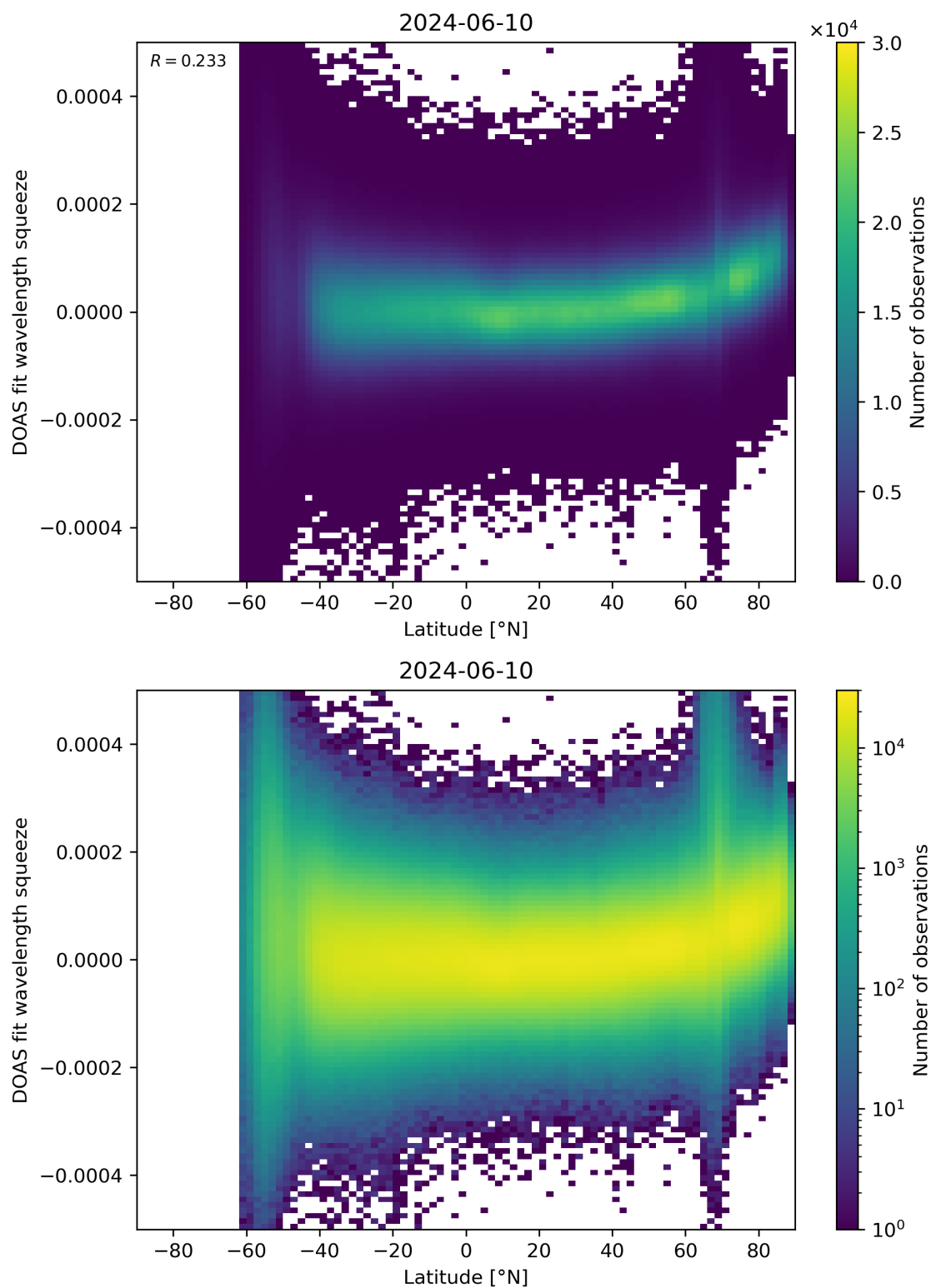
Figure 155: Scatter density plot of “Latitude” against “DOAS fit wavelength squeeze” for 2024-06-09 to 2024-06-11.
