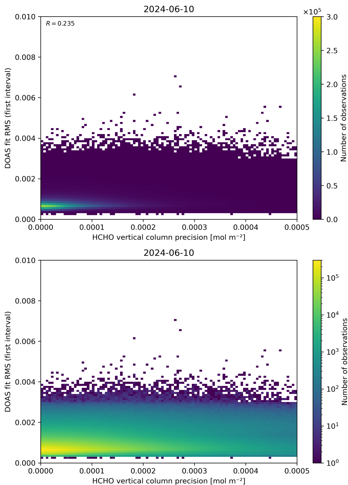
Figure 136: Scatter density plot of “HCHO vertical column precision” against “DOAS fit RMS (first interval)” for 2024-06-09 to 2024-06-11.
