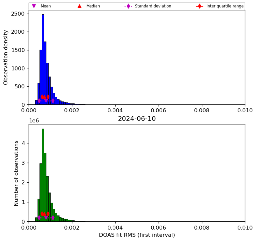
Figure 46: Histogram of “DOAS fit RMS (first interval)” for 2024-06-09 to 2024-06-11
