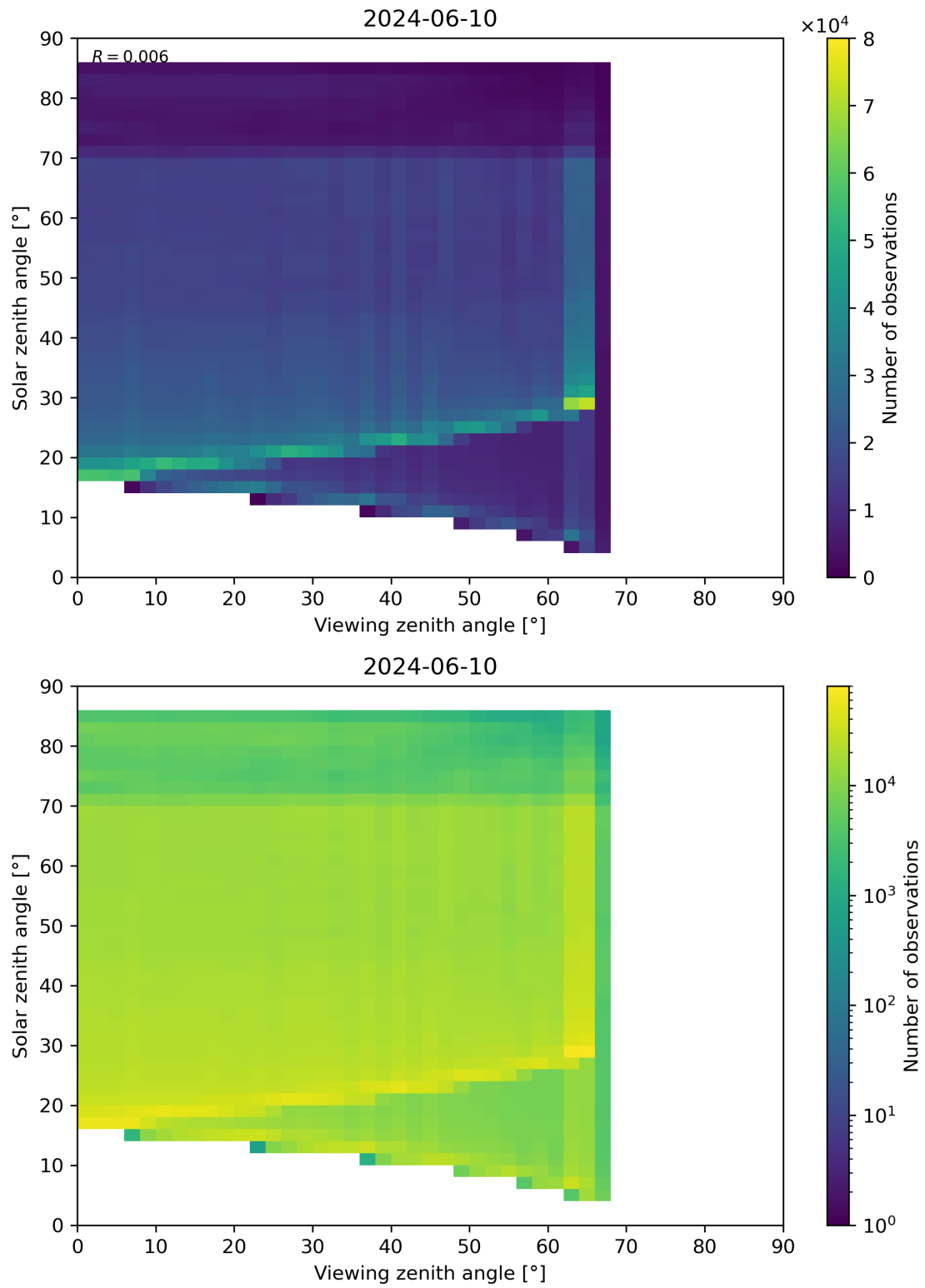
Figure 197: Scatter density plot of “Viewing zenith angle” against “Solar zenith angle” for 2024-06-09 to 2024-06-11.
