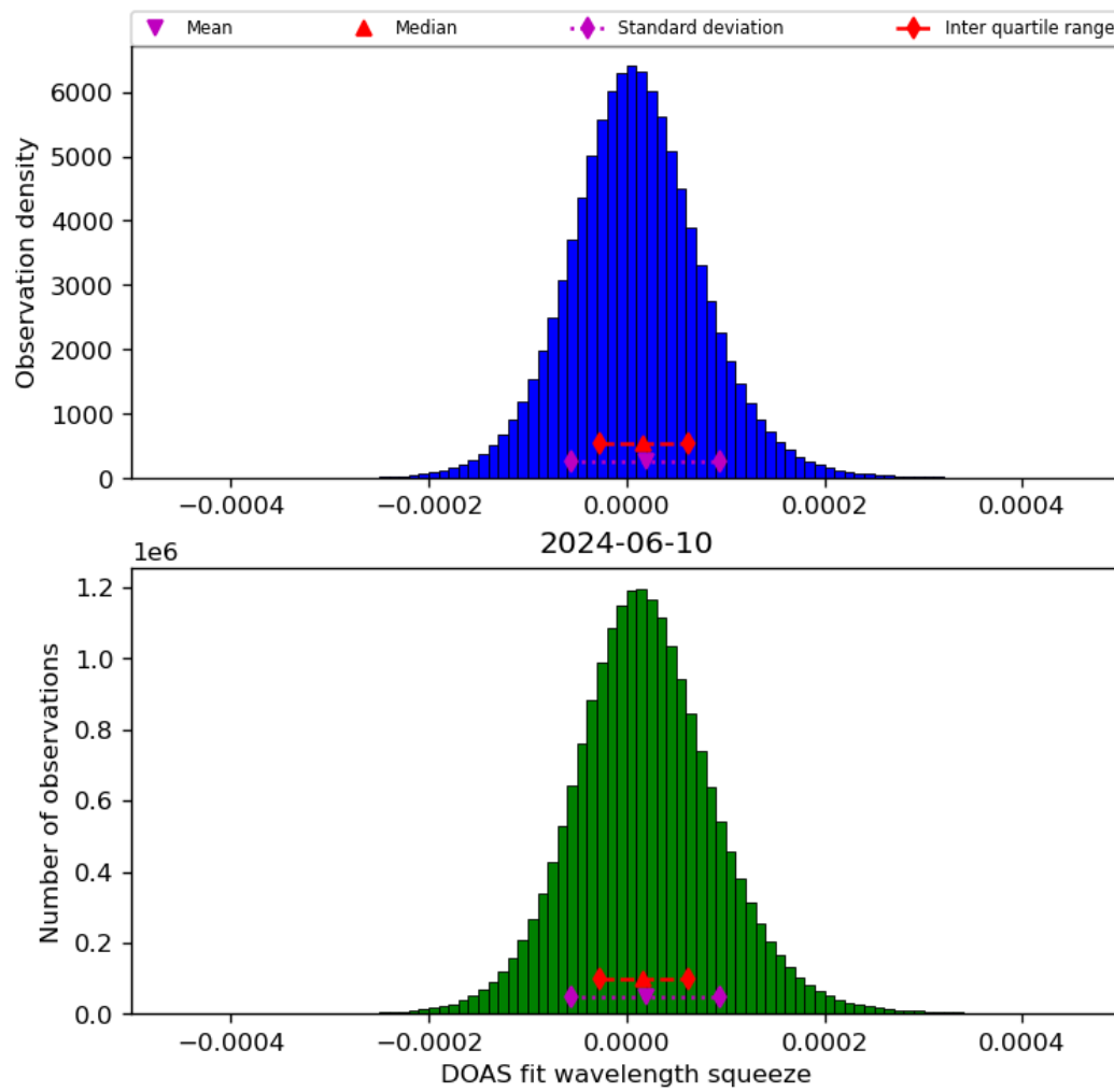
Figure 45: Histogram of “DOAS fit wavelength squeeze” for 2024-06-09 to 2024-06-11
