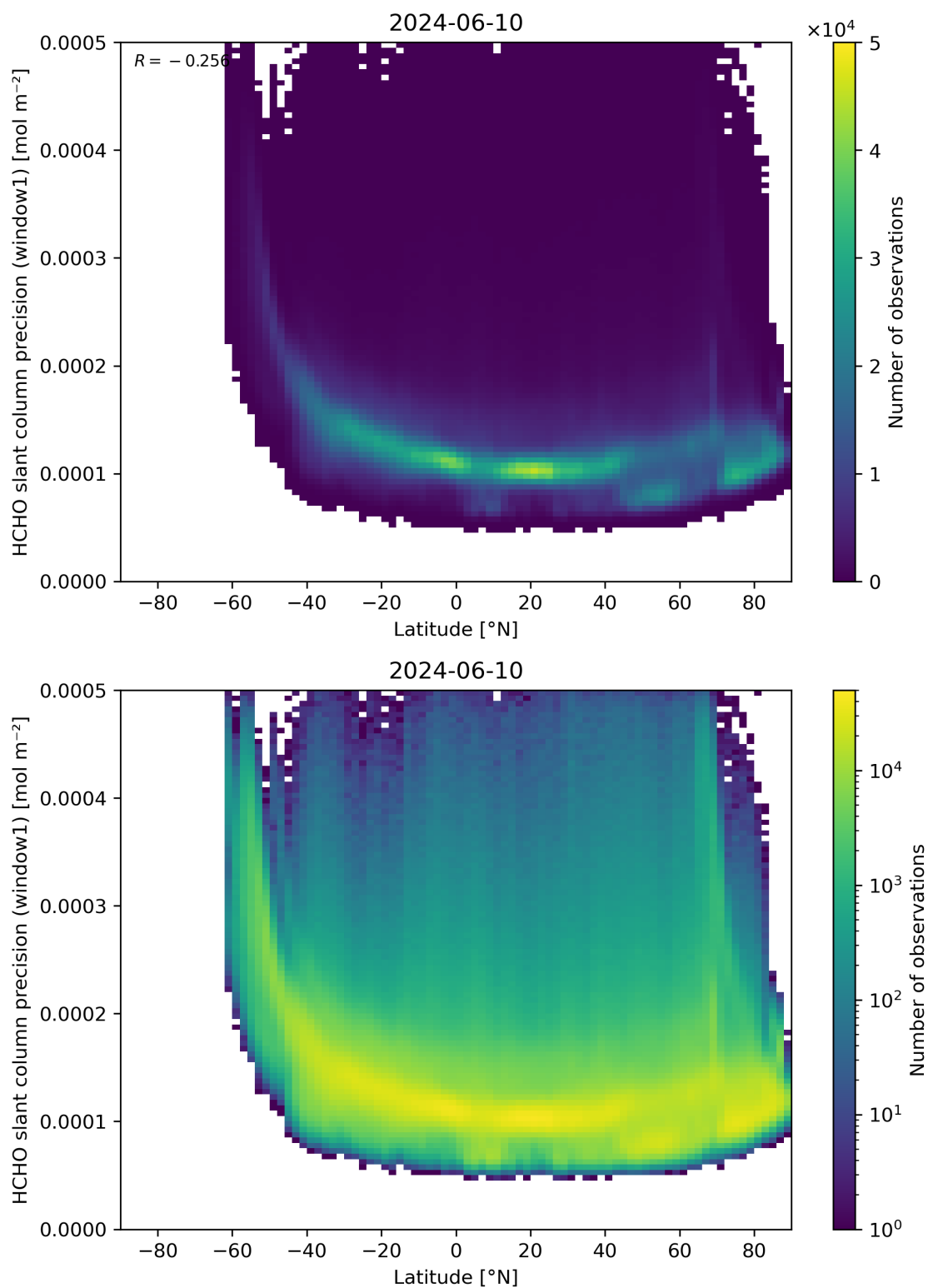
Figure 160: Scatter density plot of “Latitude” against “HCHO slant column precision (window1)” for 2024-06-09 to 2024-06-11.
