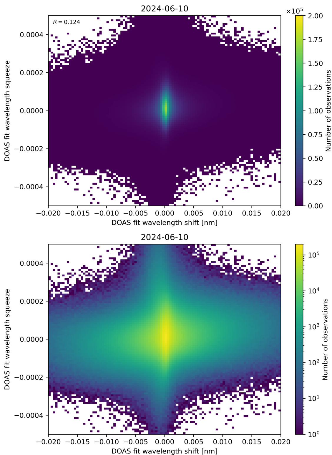
Figure 65: Scatter density plot of “DOAS fit wavelength shift” against “DOAS fit wavelength squeeze” for 2024-06-09 to 2024-06-11.
