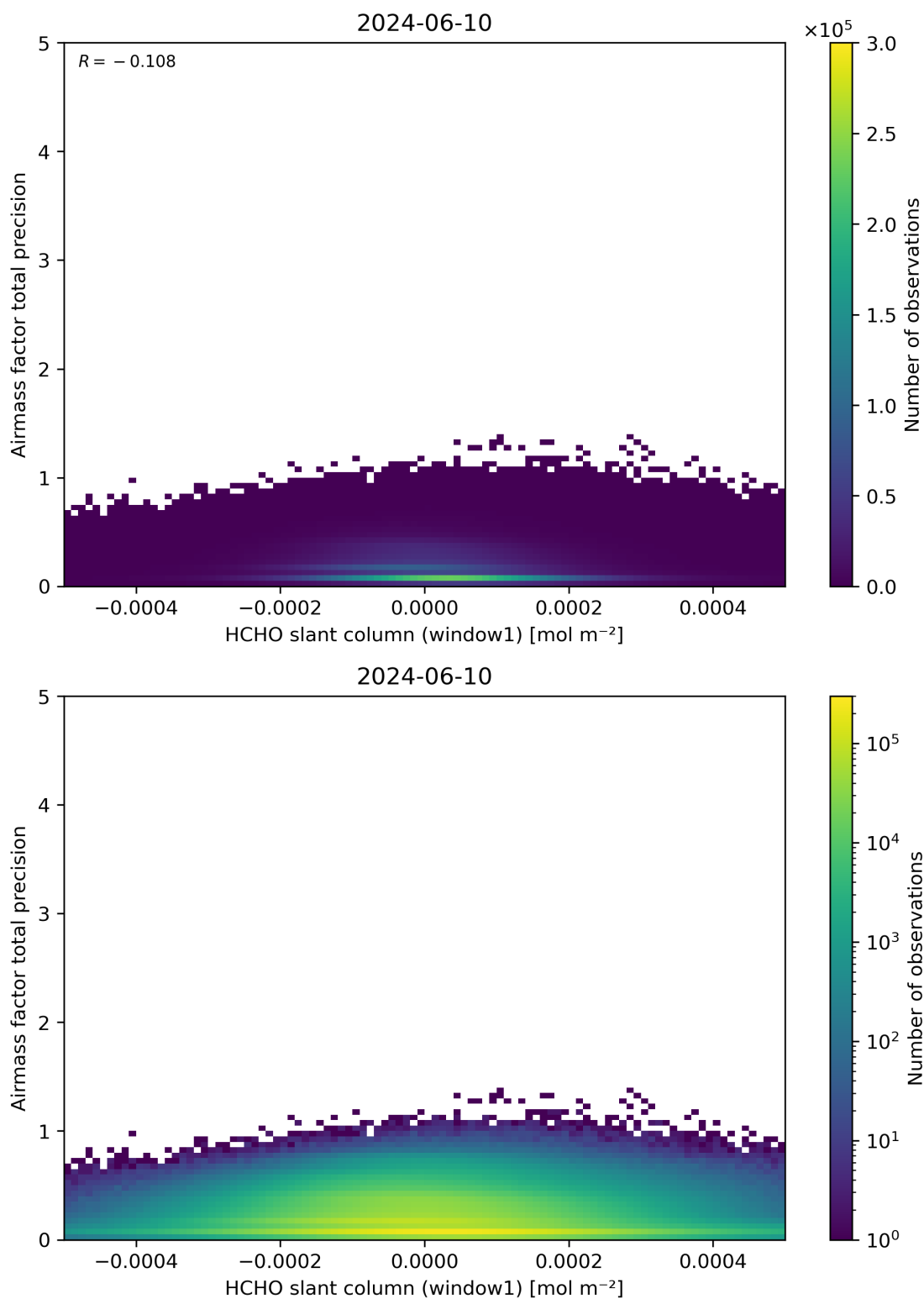
Figure 86: Scatter density plot of “HCHO slant column (window1)” against “Airmass factor total precision” for 2024-06-09 to 2024-06-11.
