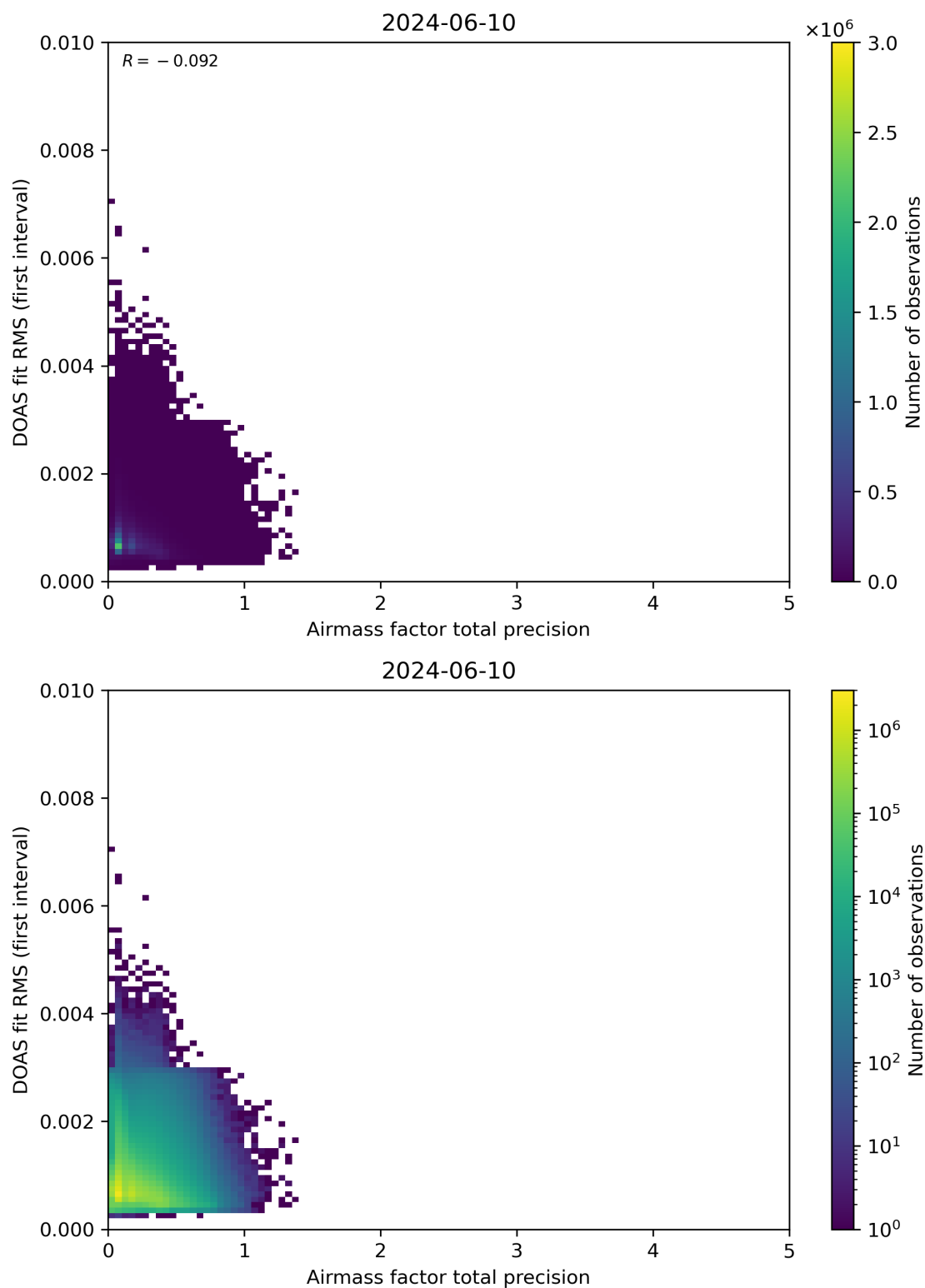
Figure 105: Scatter density plot of “Airmass factor total precision” against “DOAS fit RMS (first interval)” for 2024-06-09 to 2024-06-11.
