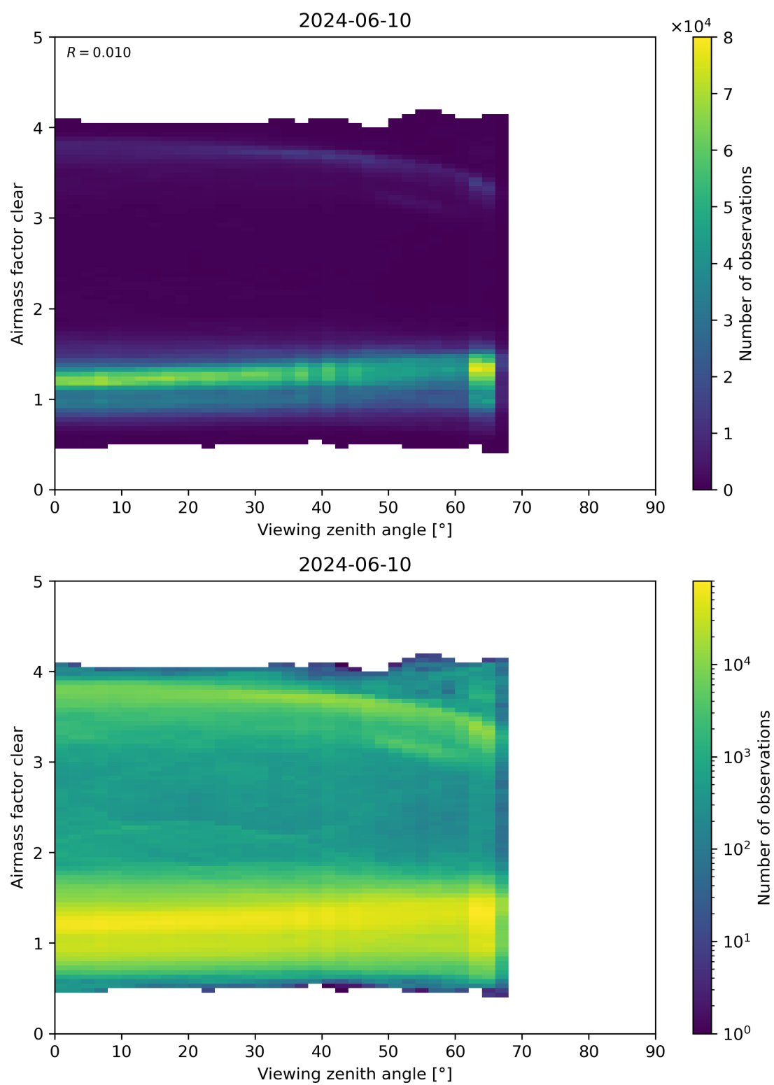
Figure 185: Scatter density plot of “Viewing zenith angle” against “Airmass factor clear” for 2024-06-09 to 2024-06-11.
