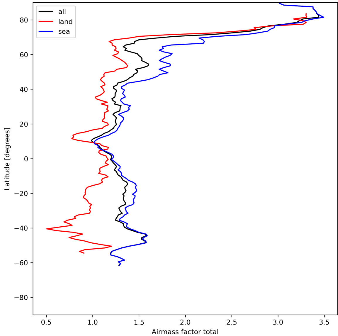
Figure 26: Zonal average of “Airmass factor total” for 2024-06-09 to 2024-06-11.
