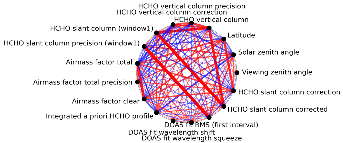
Figure 1: Map of correlation graph for 2024-06-09 to 2024-06-11.
