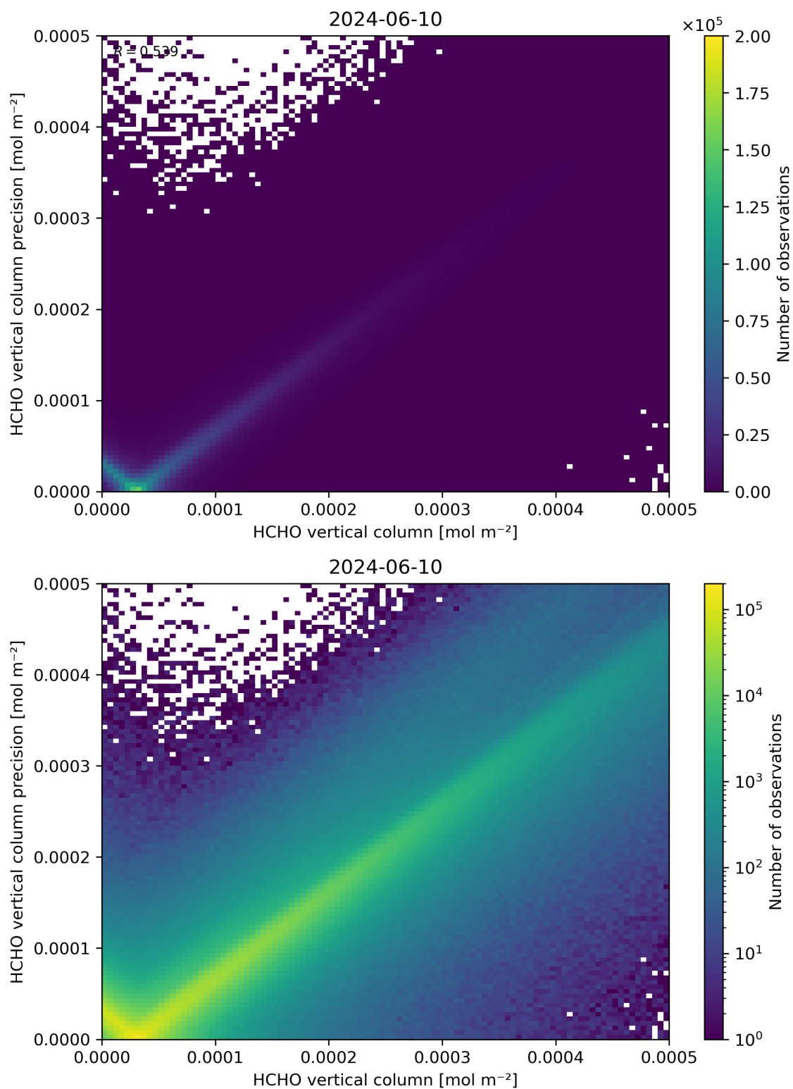
Figure 134: Scatter density plot of “HCHO vertical column” against “HCHO vertical column precision” for 2024-06-09 to 2024-06-11.
