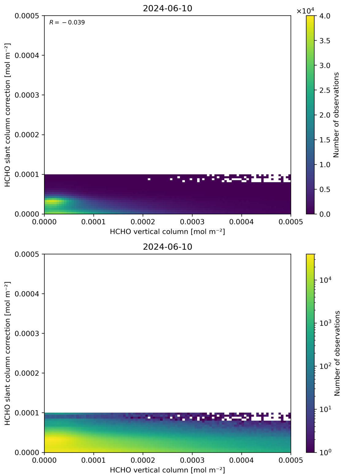
Figure 128: Scatter density plot of “HCHO vertical column” against “HCHO slant column correction” for 2024-06-09 to 2024-06-11.
