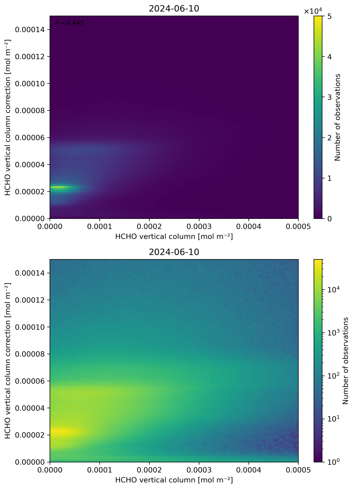
Figure 133: Scatter density plot of “HCHO vertical column” against “HCHO vertical column correction” for 2024-06-09 to 2024-06-11.
