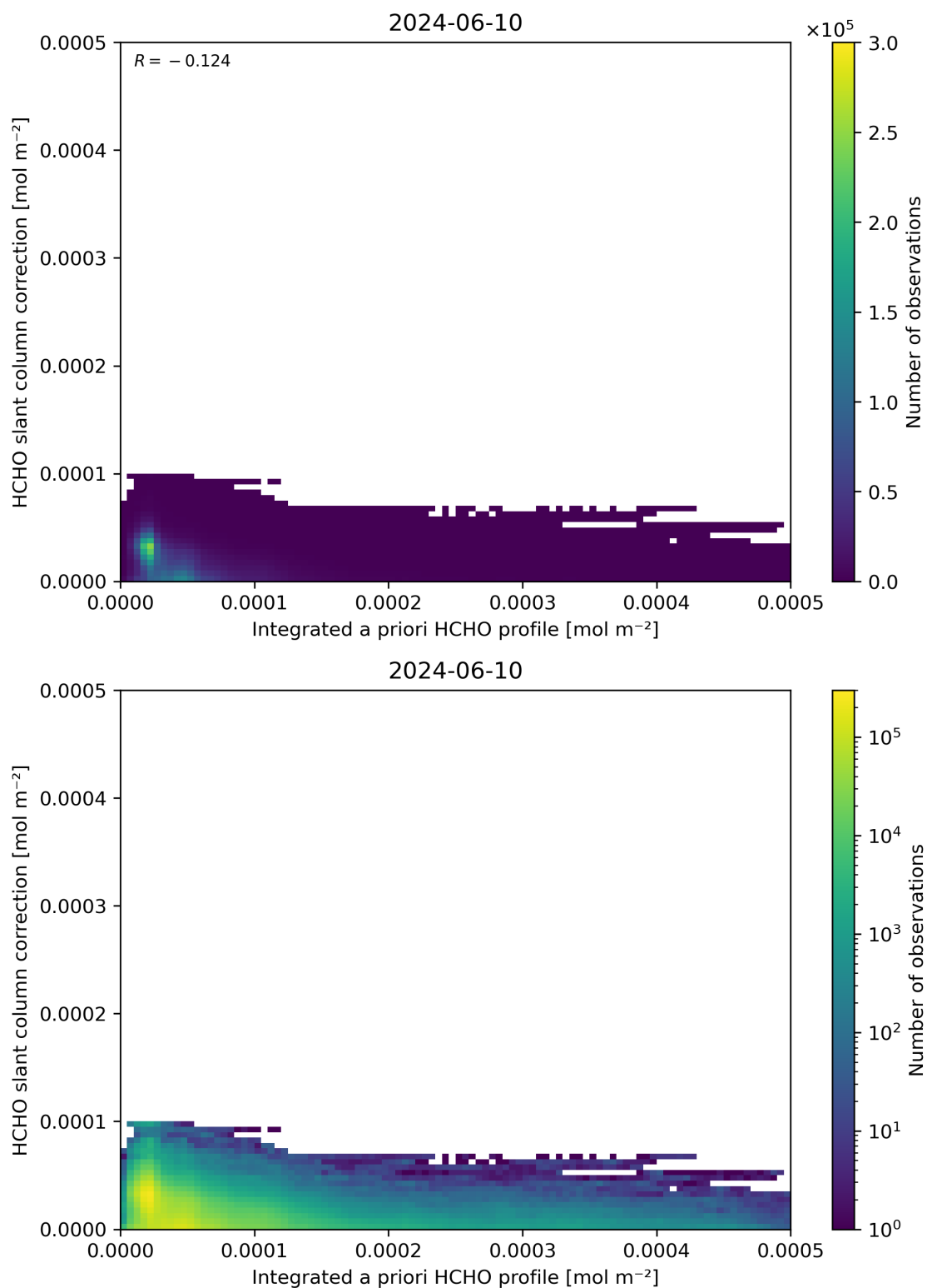
Figure 152: Scatter density plot of “Integrated a priori HCHO profile” against “HCHO slant column correction” for 2024-06-09 to 2024-06-11.
