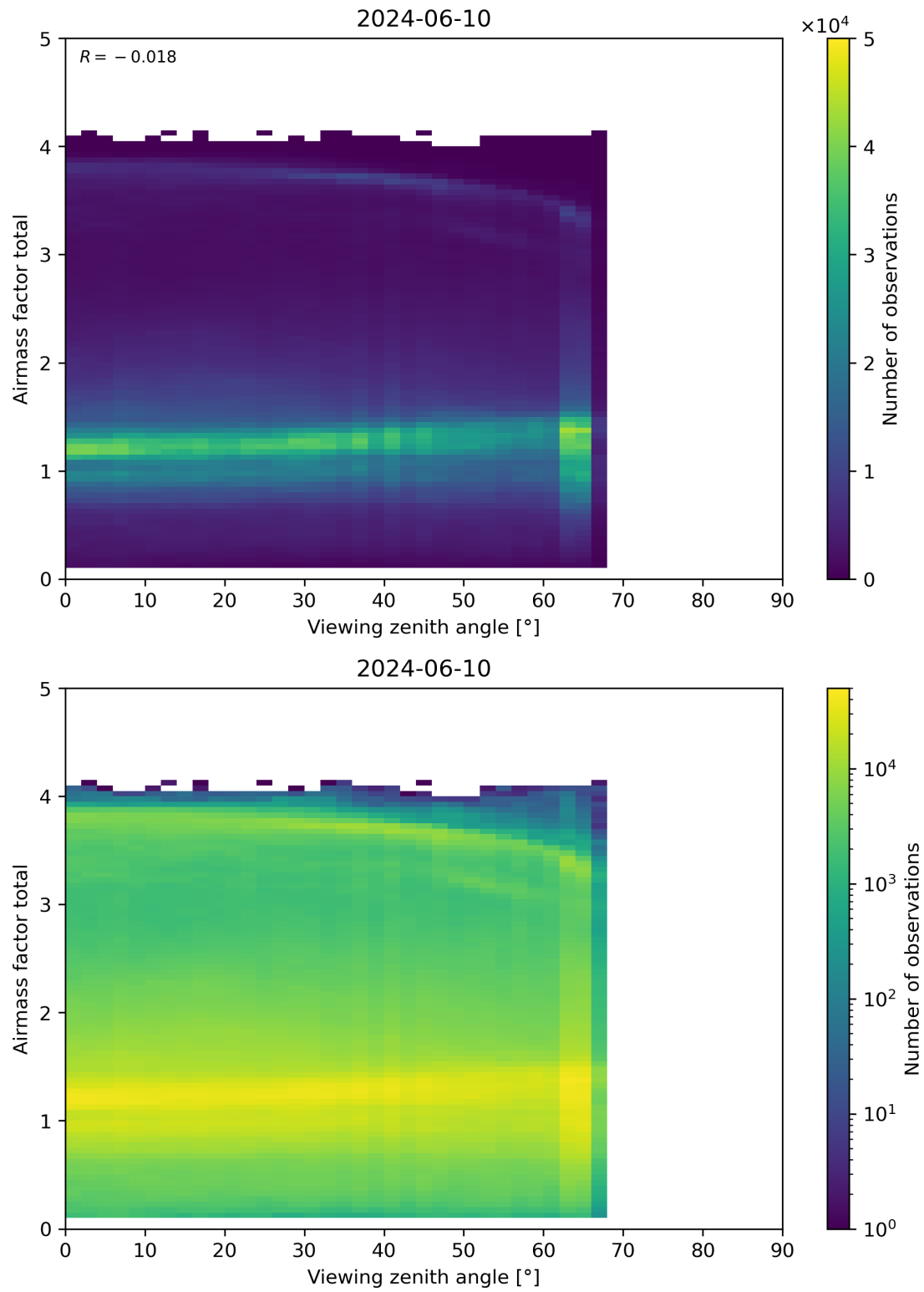
Figure 190: Scatter density plot of “Viewing zenith angle” against “Airmass factor total” for 2024-06-09 to 2024-06-11.
