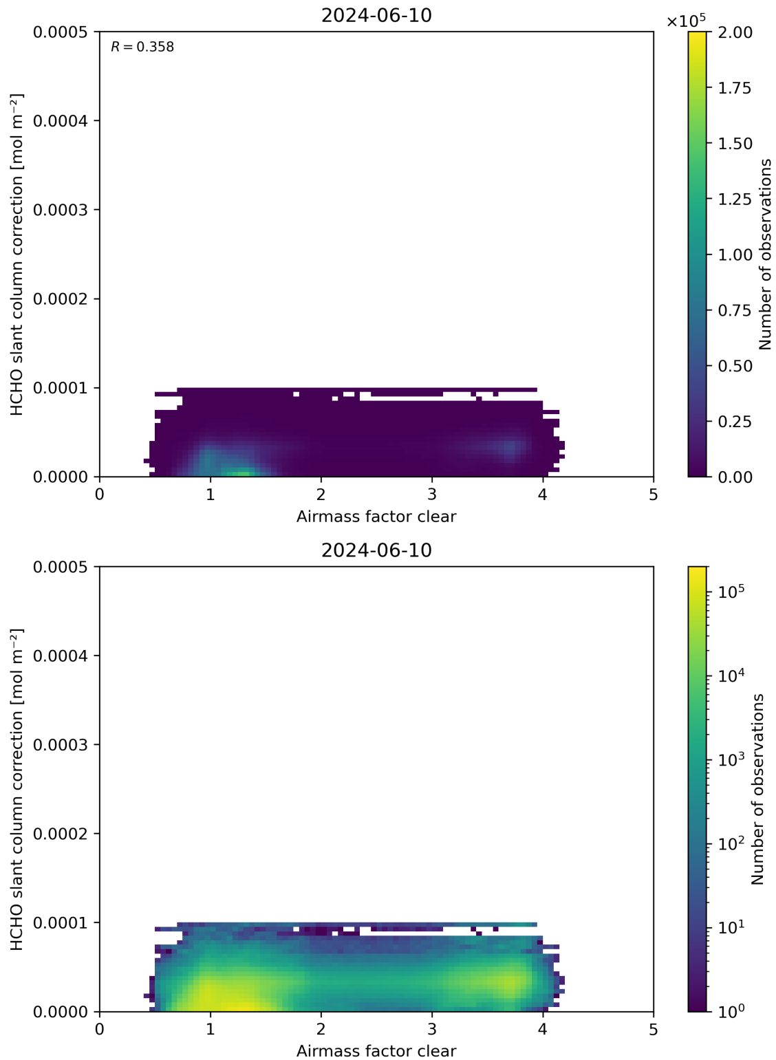
Figure 75: Scatter density plot of “Airmass factor clear” against “HCHO slant column correction” for 2024-06-09 to 2024-06-11.
