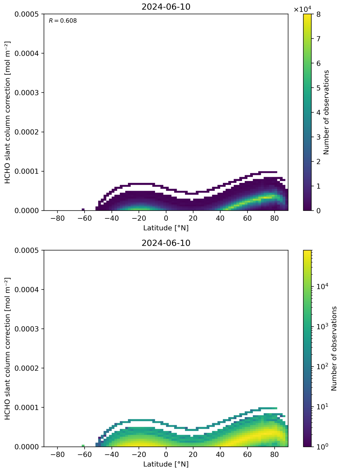
Figure 158: Scatter density plot of “Latitude” against “HCHO slant column correction” for 2024-06-09 to 2024-06-11.
