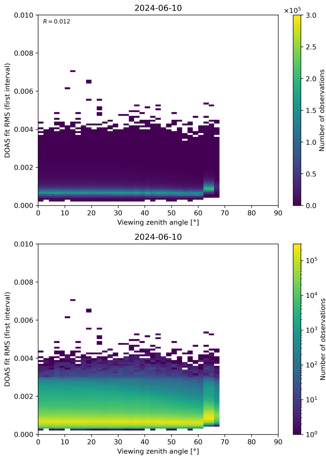
Figure 182: Scatter density plot of “Viewing zenith angle” against “DOAS fit RMS (first interval)” for 2024-06-09 to 2024-06-11.
