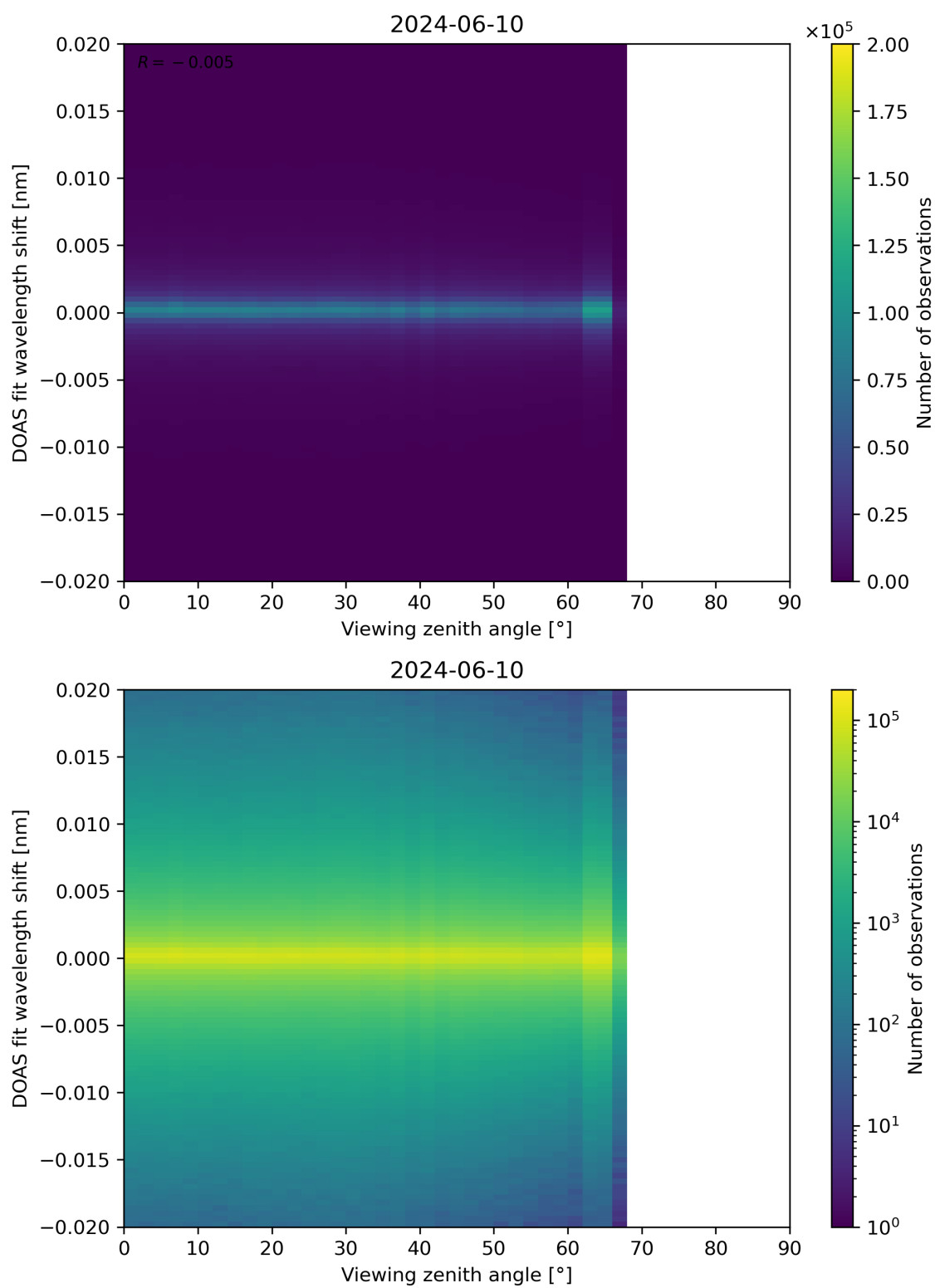
Figure 183: Scatter density plot of “Viewing zenith angle” against “DOAS fit wavelength shift” for 2024-06-09 to 2024-06-11.
