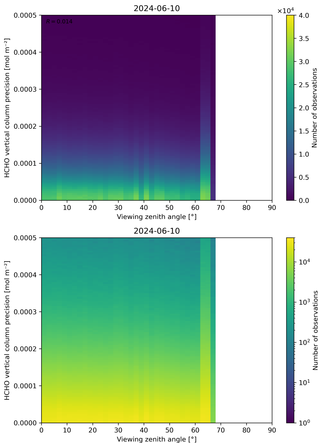
Figure 194: Scatter density plot of “Viewing zenith angle” against “HCHO vertical column precision” for 2024-06-09 to 2024-06-11.
