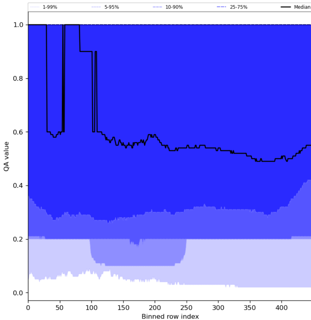
Figure 48: Along track statistics of “QA value” for 2024-06-09 to 2024-06-11
