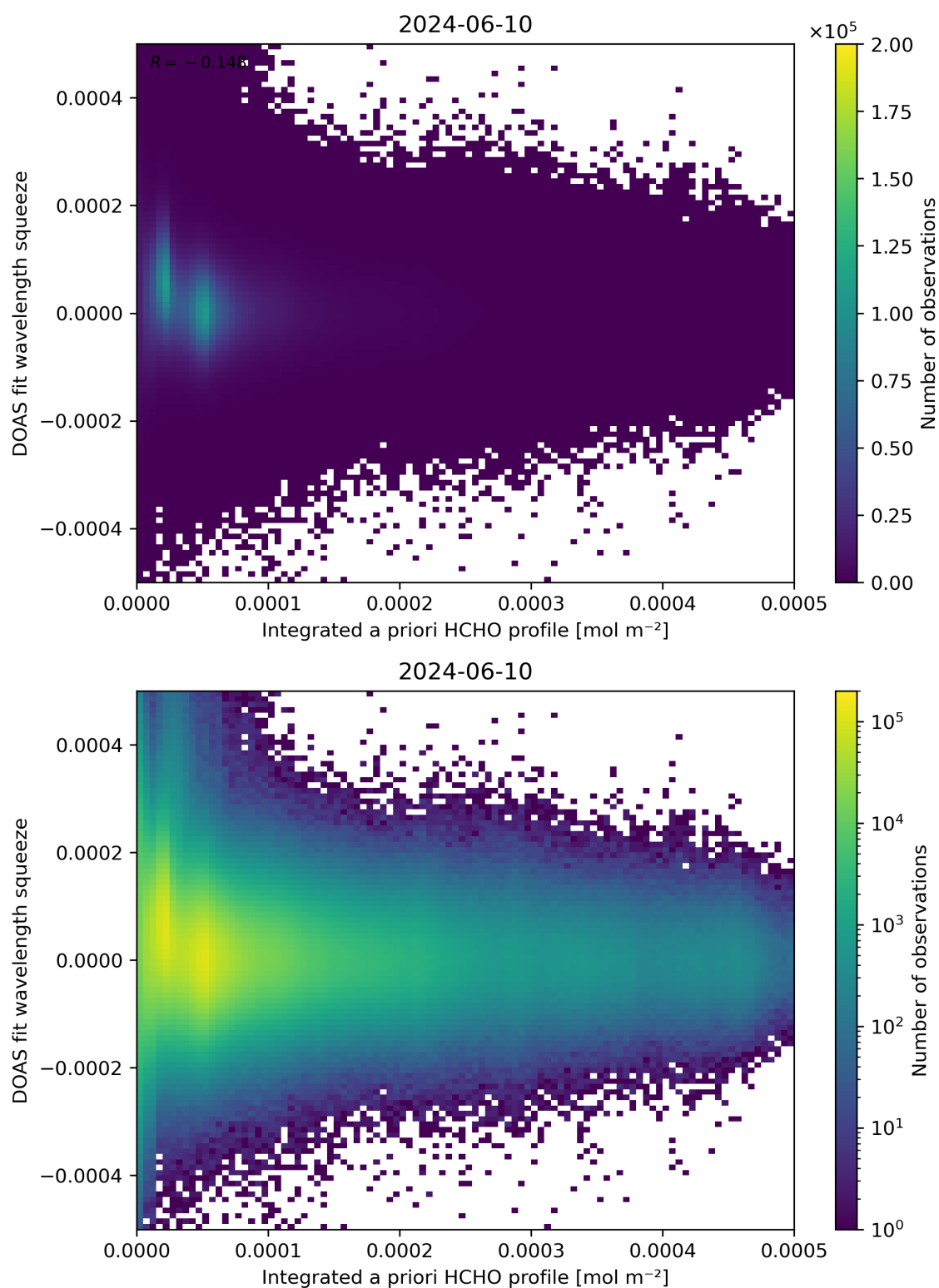
Figure 150: Scatter density plot of “Integrated a priori HCHO profile” against “DOAS fit wavelength squeeze” for 2024-06-09 to 2024-06-11.
