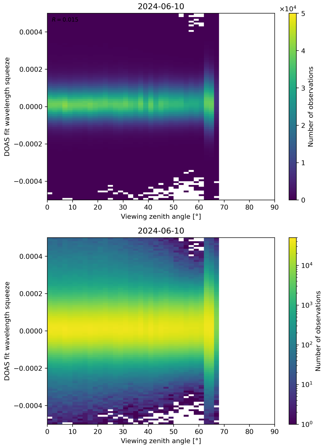
Figure 184: Scatter density plot of “Viewing zenith angle” against “DOAS fit wavelength squeeze” for 2024-06-09 to 2024-06-11.
