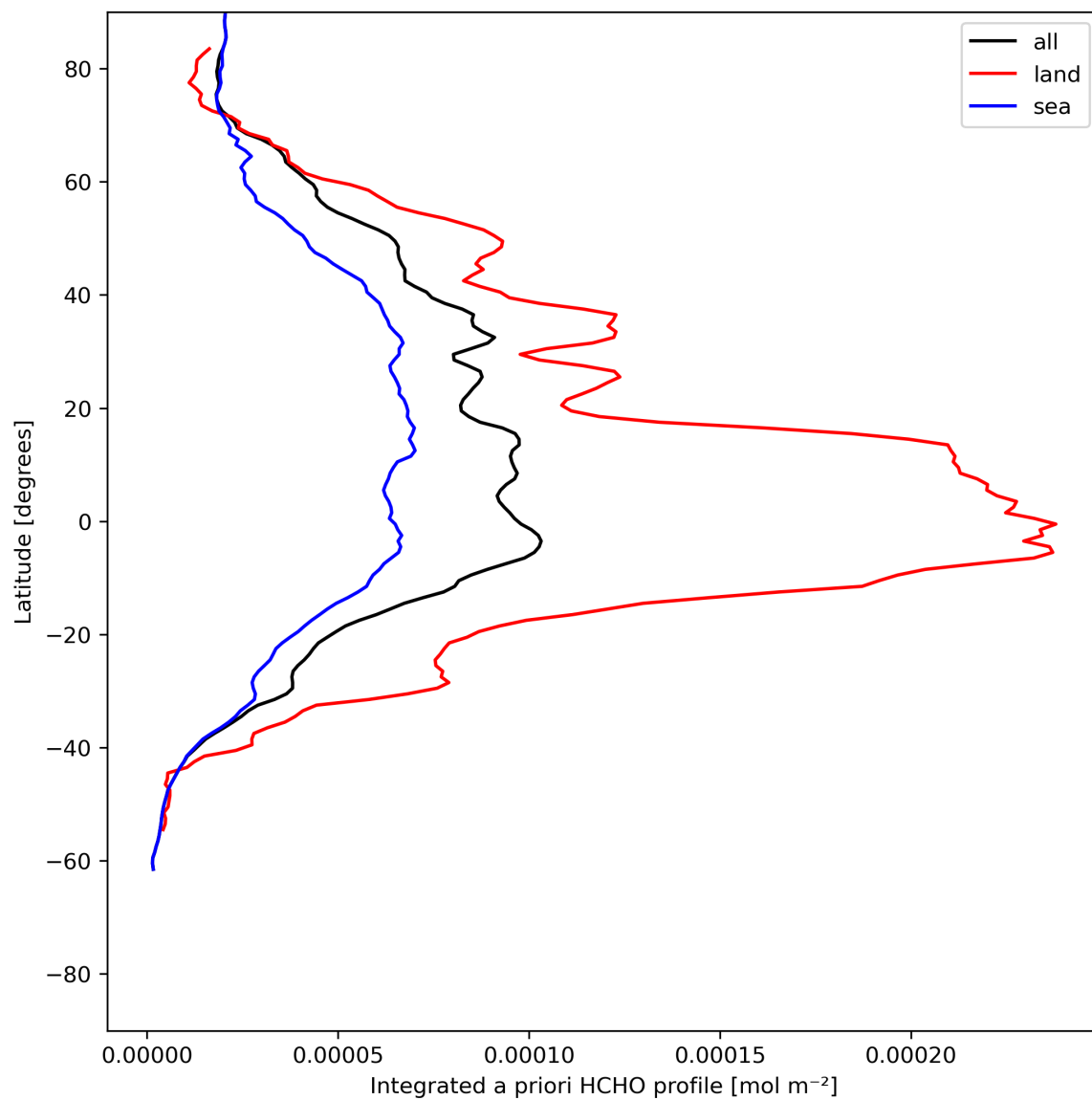
Figure 29: Zonal average of “Integrated a priori HCHO profile” for 2024-06-09 to 2024-06-11.
