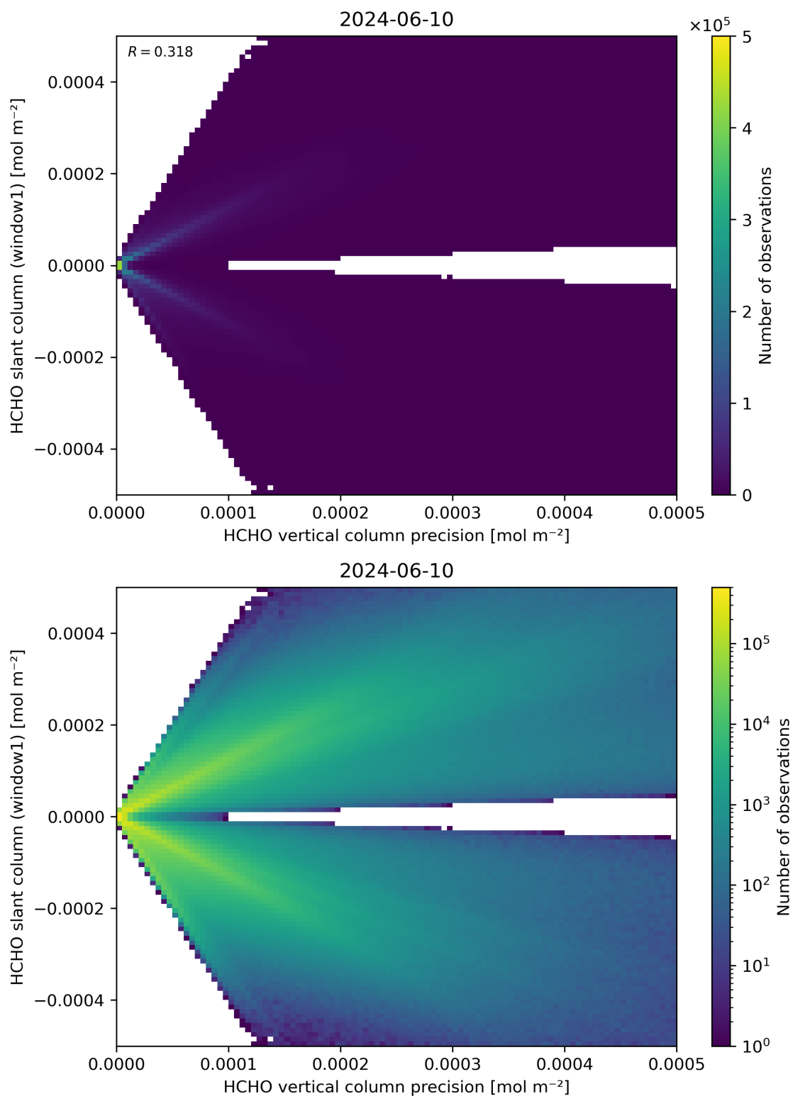
Figure 142: Scatter density plot of “HCHO vertical column precision” against “HCHO slant column (window1)” for 2024-06-09 to 2024-06-11.
