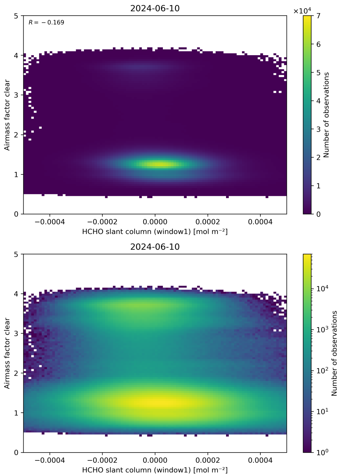
Figure 81: Scatter density plot of “HCHO slant column (window1)” against “Airmass factor clear” for 2024-06-09 to 2024-06-11.
