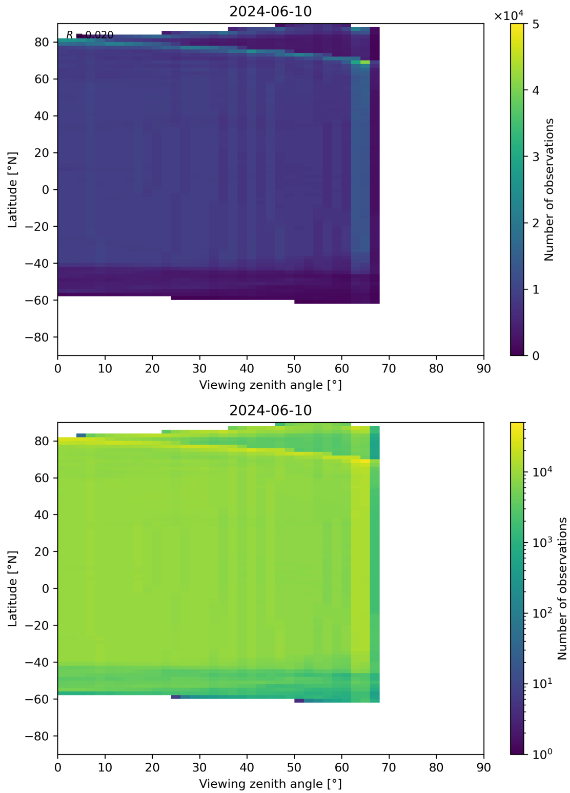
Figure 196: Scatter density plot of “Viewing zenith angle” against “Latitude” for 2024-06-09 to 2024-06-11.
