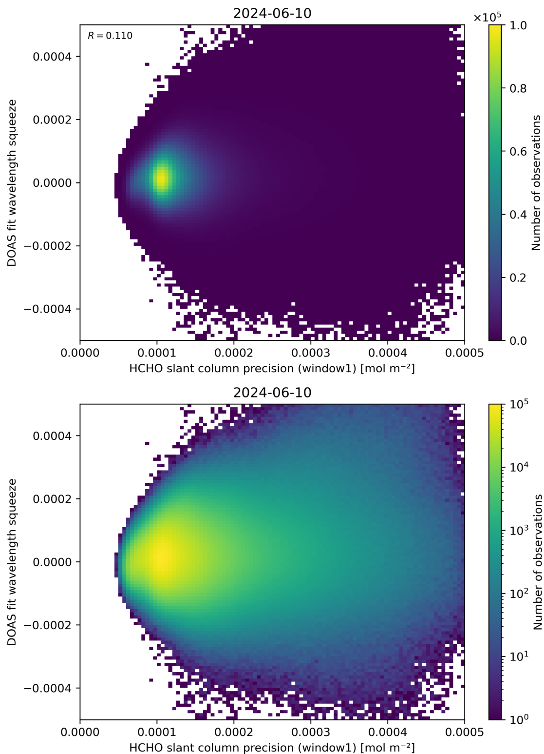
Figure 90: Scatter density plot of “HCHO slant column precision (window1)” against “DOAS fit wavelength squeeze” for 2024-06-09 to 2024-06-11.
