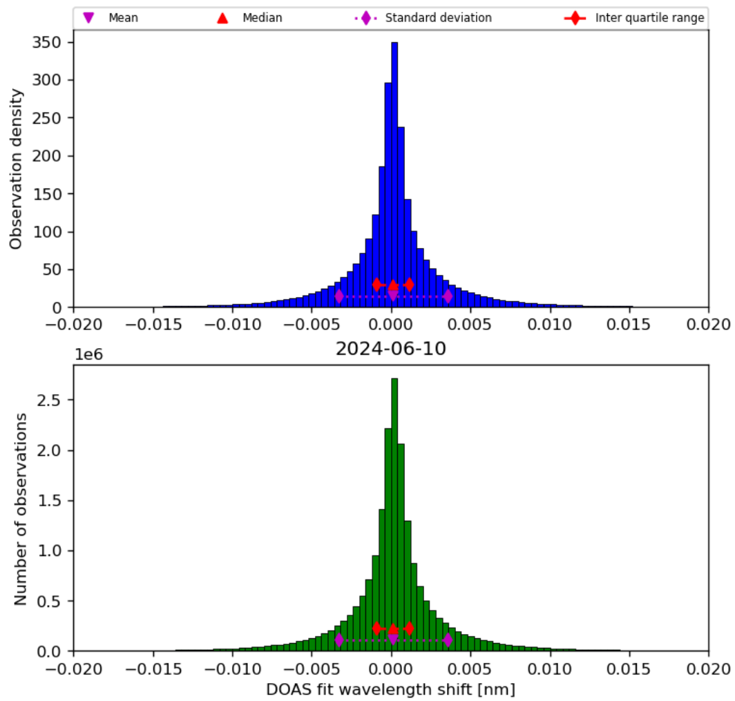
Figure 44: Histogram of “DOAS fit wavelength shift” for 2024-06-09 to 2024-06-11
