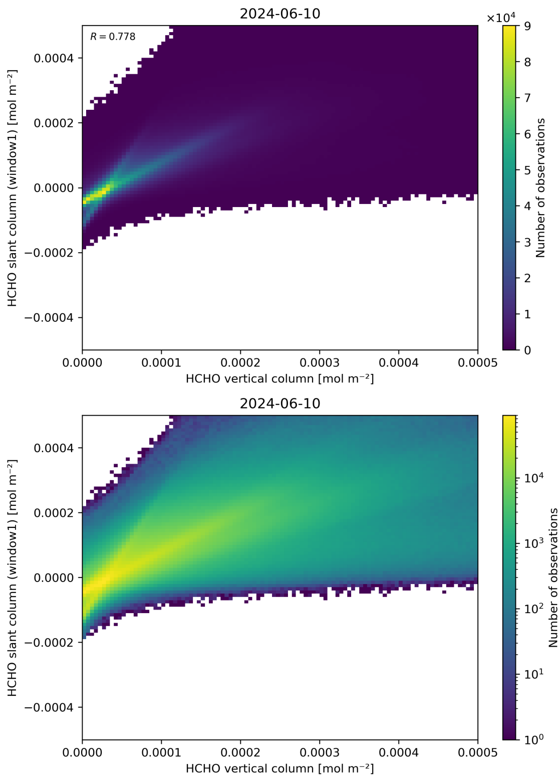
Figure 129: Scatter density plot of “HCHO vertical column” against “HCHO slant column (window1)” for 2024-06-09 to 2024-06-11.
