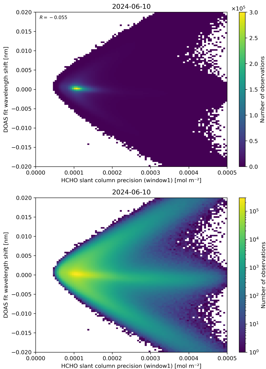
Figure 89: Scatter density plot of “HCHO slant column precision (window1)” against “DOAS fit wavelength shift” for 2024-06-09 to 2024-06-11.
