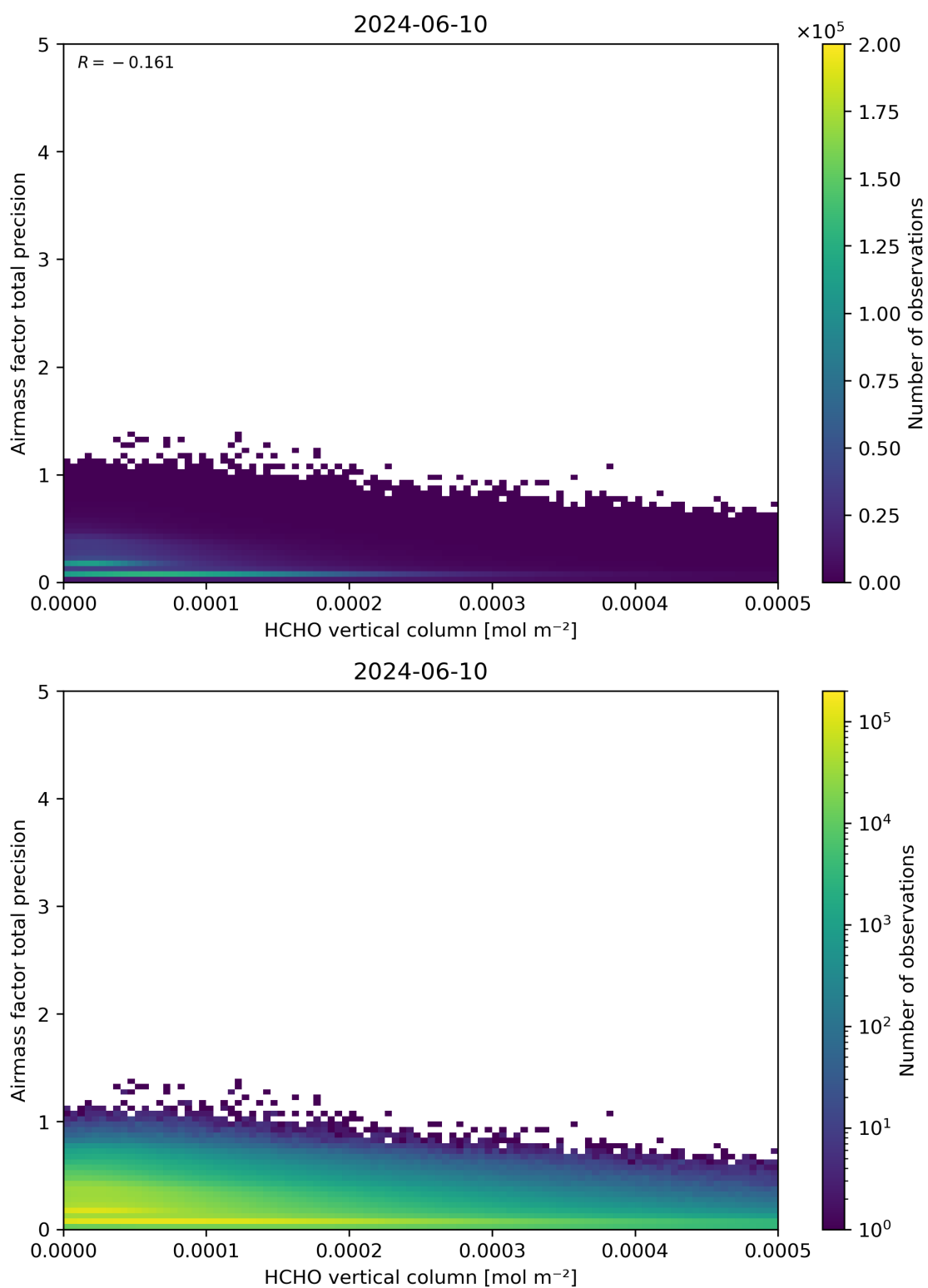
Figure 132: Scatter density plot of “HCHO vertical column” against “Airmass factor total precision” for 2024-06-09 to 2024-06-11.
