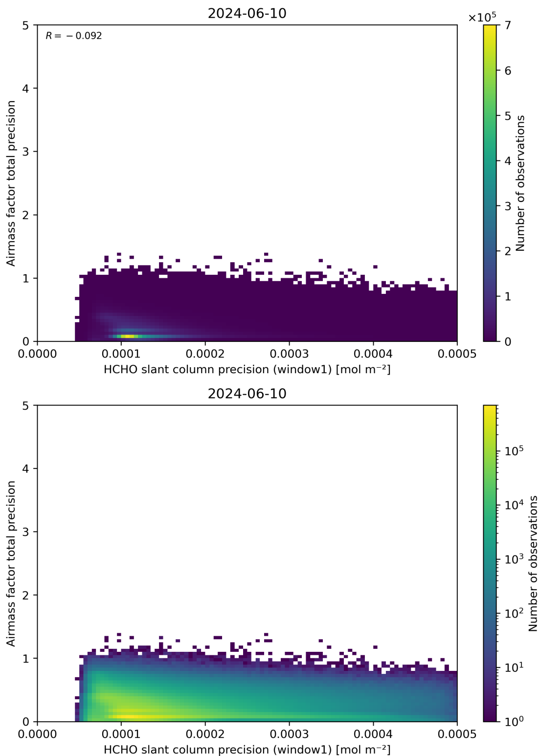
Figure 95: Scatter density plot of “HCHO slant column precision (window1)” against “Airmass factor total precision” for 2024-06-09 to 2024-06-11.
