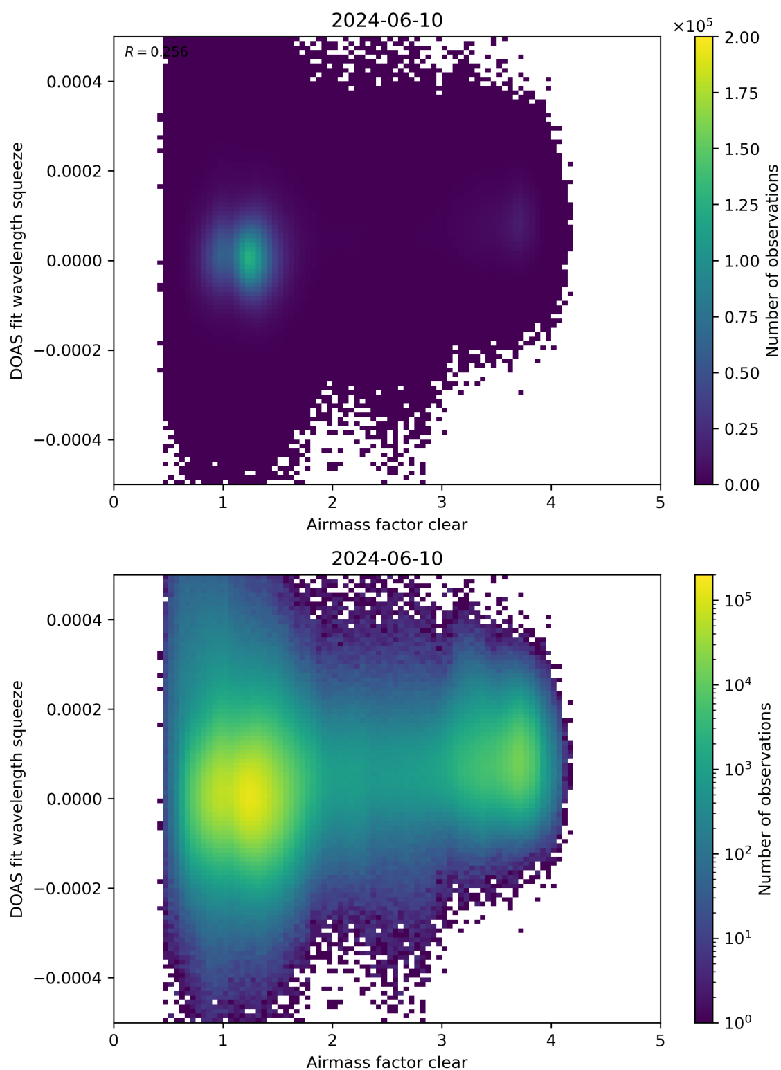
Figure 73: Scatter density plot of “Airmass factor clear” against “DOAS fit wavelength squeeze” for 2024-06-09 to 2024-06-11.
