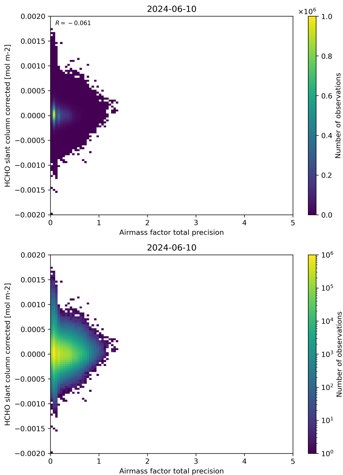
Figure 109: Scatter density plot of “Airmass factor total precision” against “HCHO slant column corrected” for 2024-06-09 to 2024-06-11.
