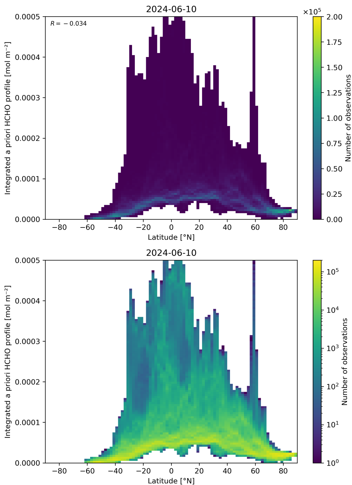
Figure 166: Scatter density plot of “Latitude” against “Integrated a priori HCHO profile” for 2024-06-09 to 2024-06-11.
