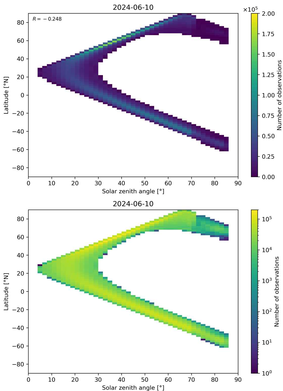
Figure 181: Scatter density plot of “Solar zenith angle” against “Latitude” for 2024-06-09 to 2024-06-11.
