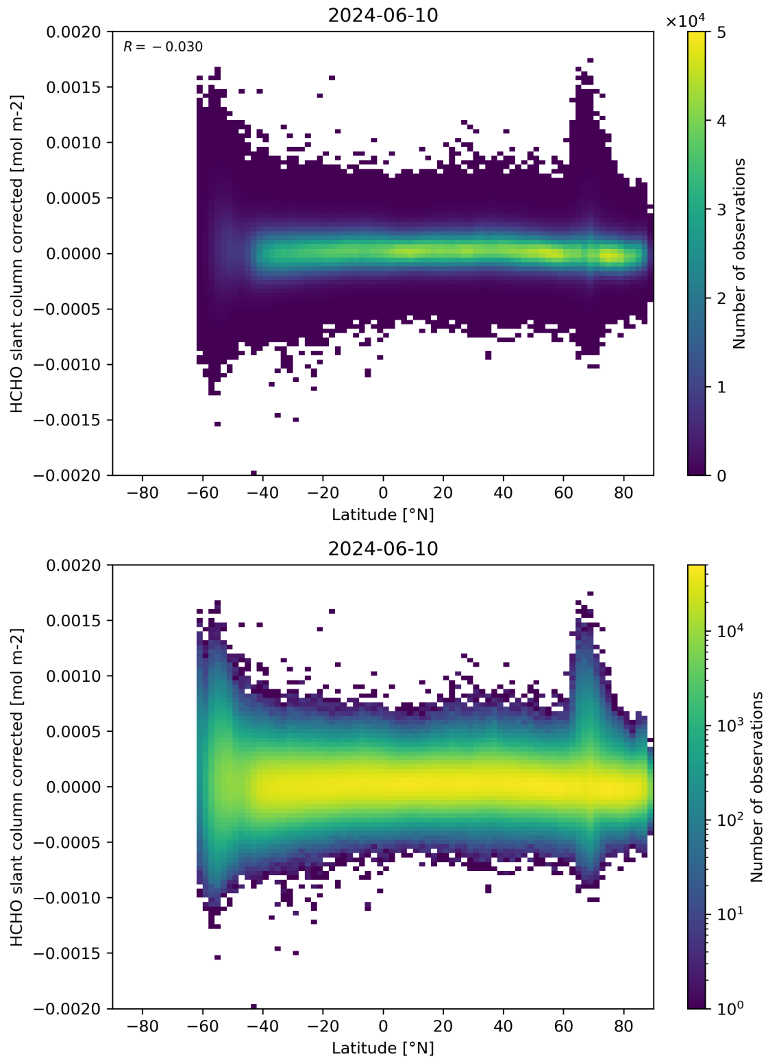
Figure 157: Scatter density plot of “Latitude” against “HCHO slant column corrected” for 2024-06-09 to 2024-06-11.
