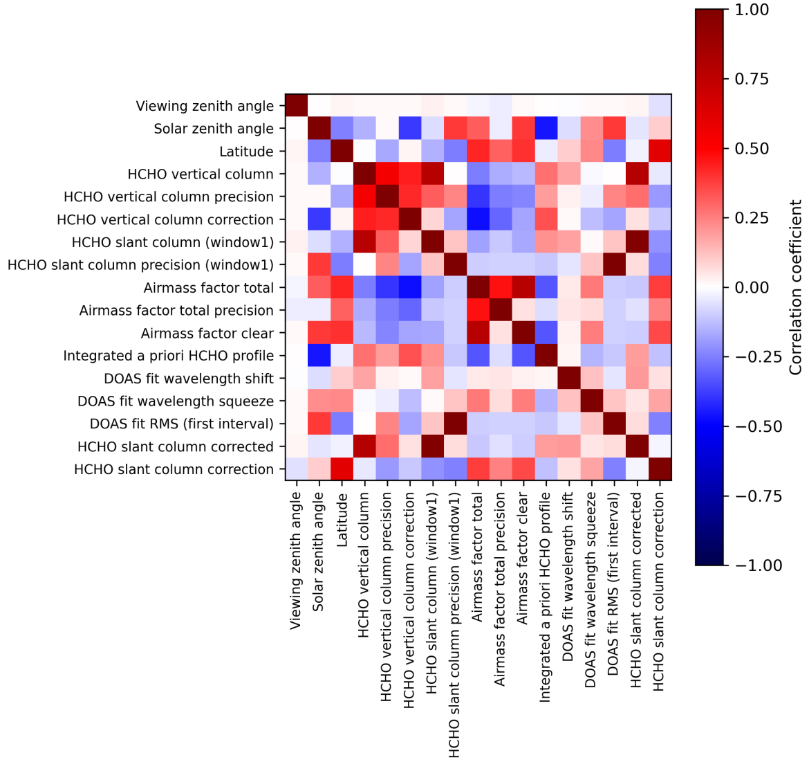
Figure 2: Map of correlation matrix for 2024-06-09 to 2024-06-11.
