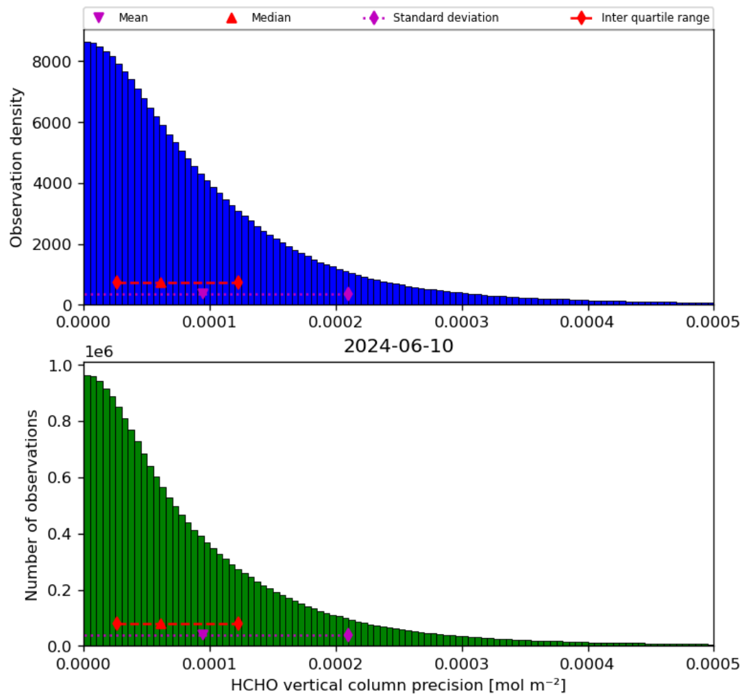
Figure 36: Histogram of “HCHO vertical column precision” for 2024-06-09 to 2024-06-11
