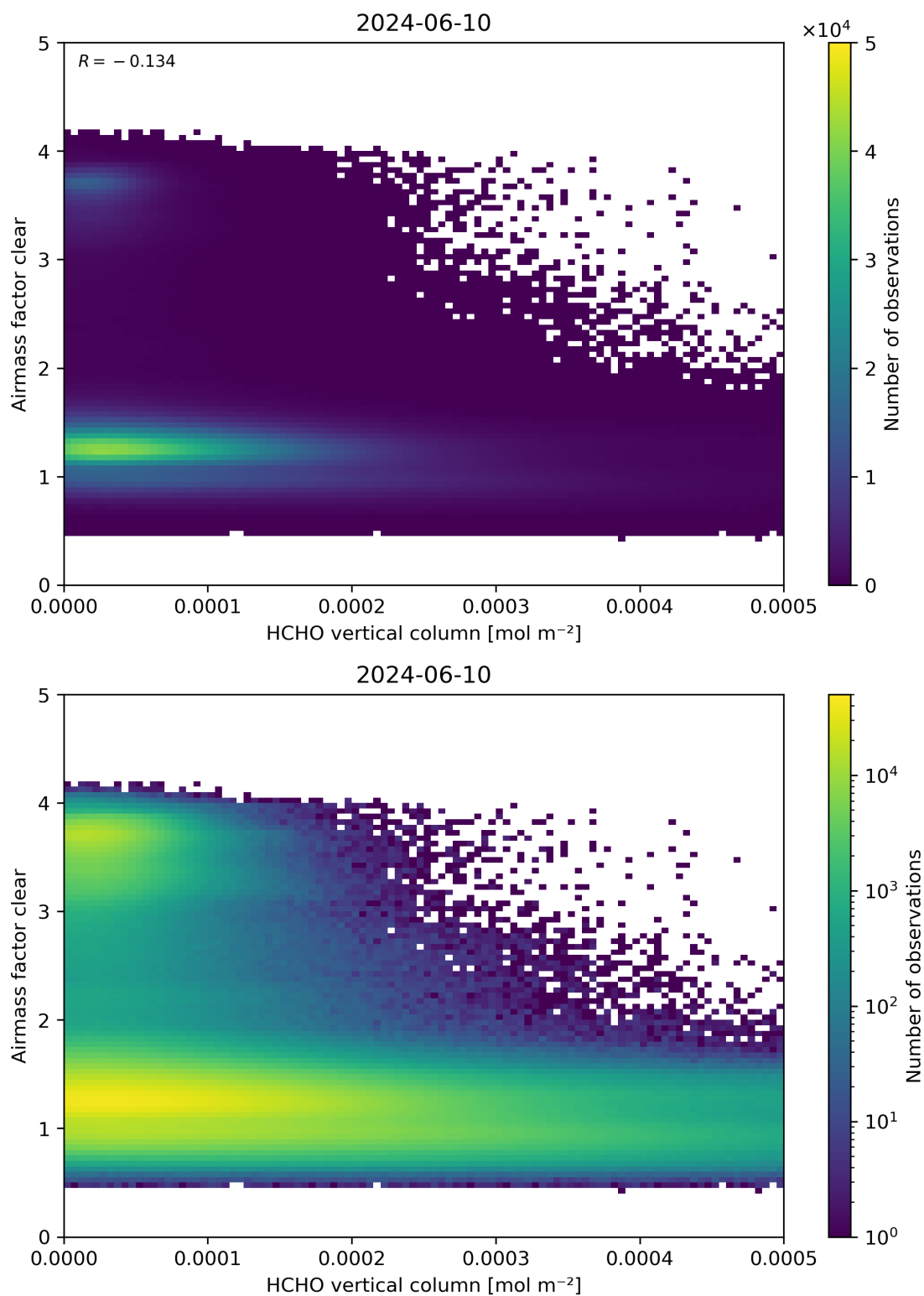
Figure 126: Scatter density plot of “HCHO vertical column” against “Airmass factor clear” for 2024-06-09 to 2024-06-11.
