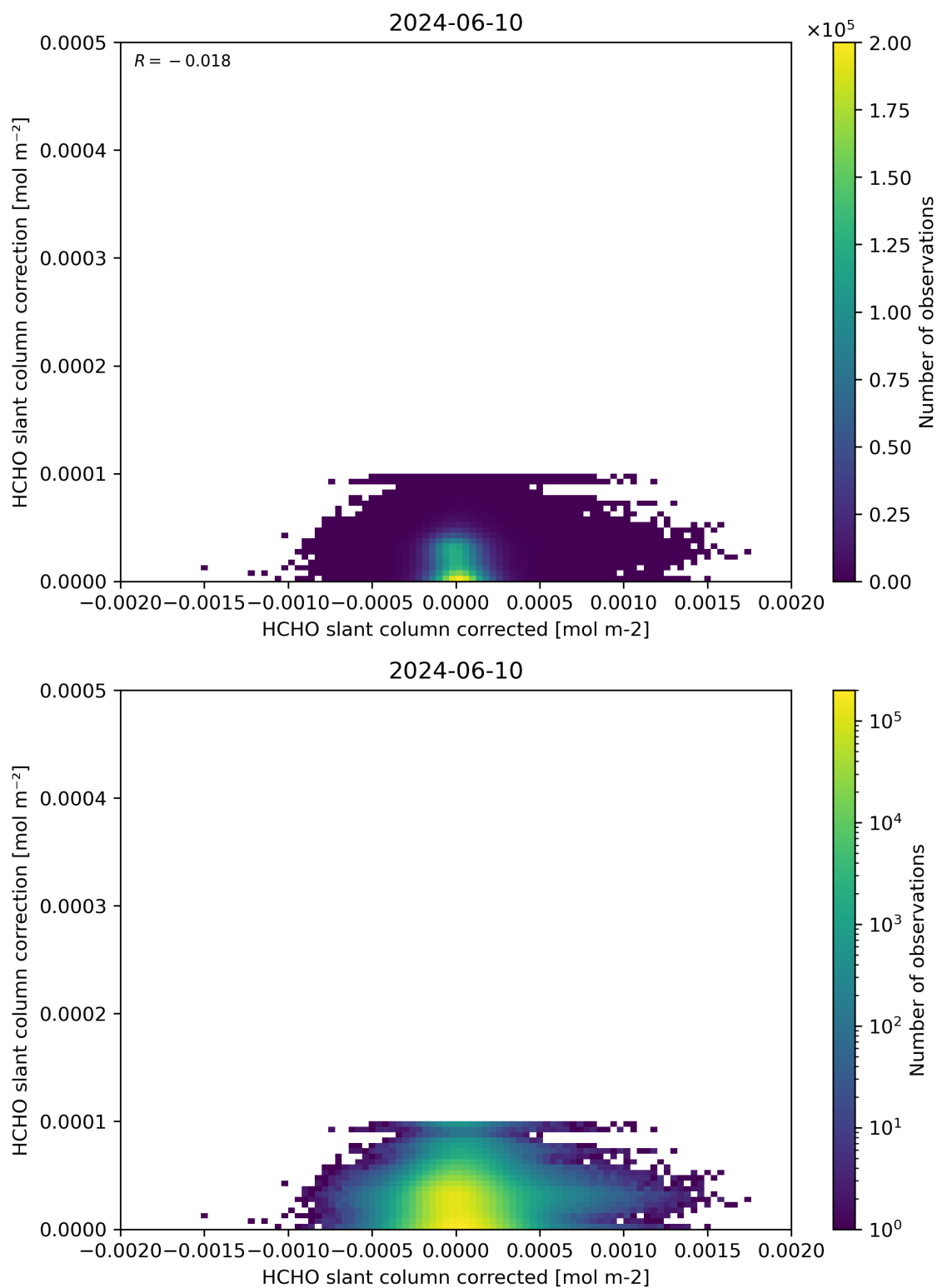
Figure 77: Scatter density plot of “HCHO slant column corrected” against “HCHO slant column correction” for 2024-06-09 to 2024-06-11.
