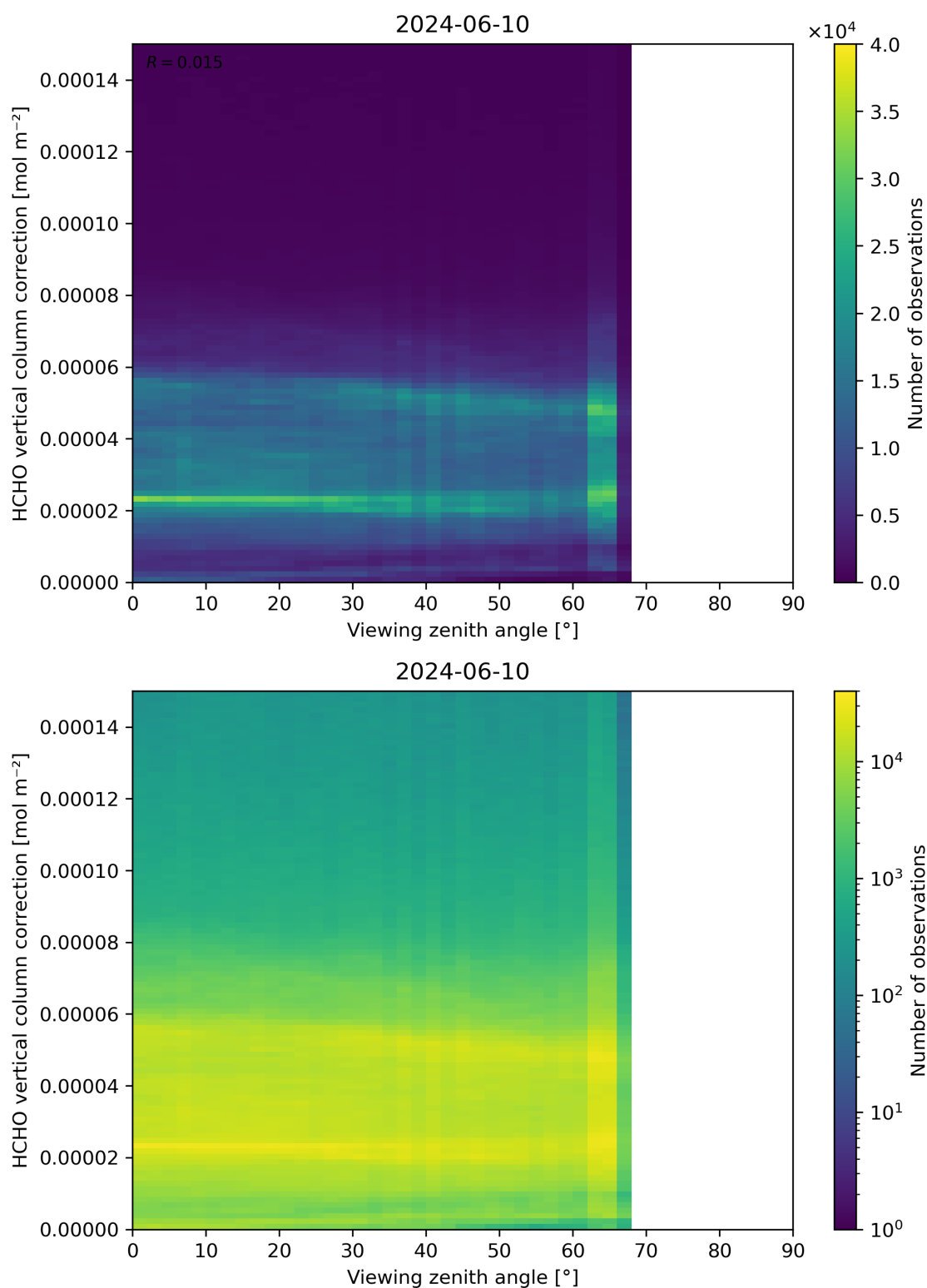
Figure 193: Scatter density plot of “Viewing zenith angle” against “HCHO vertical column correction” for 2024-06-09 to 2024-06-11.
