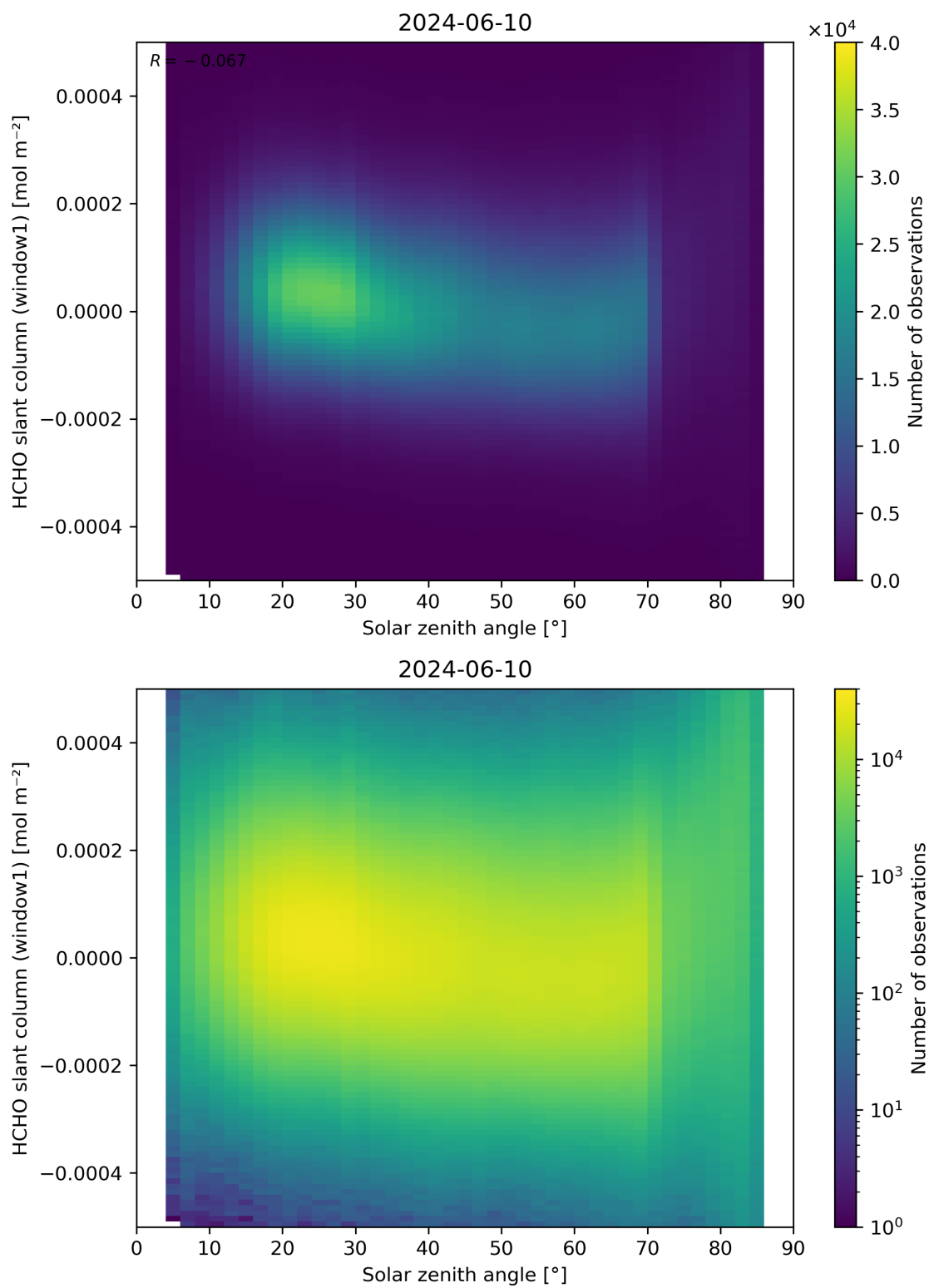
Figure 173: Scatter density plot of “Solar zenith angle” against “HCHO slant column (window1)” for 2024-06-09 to 2024-06-11.
