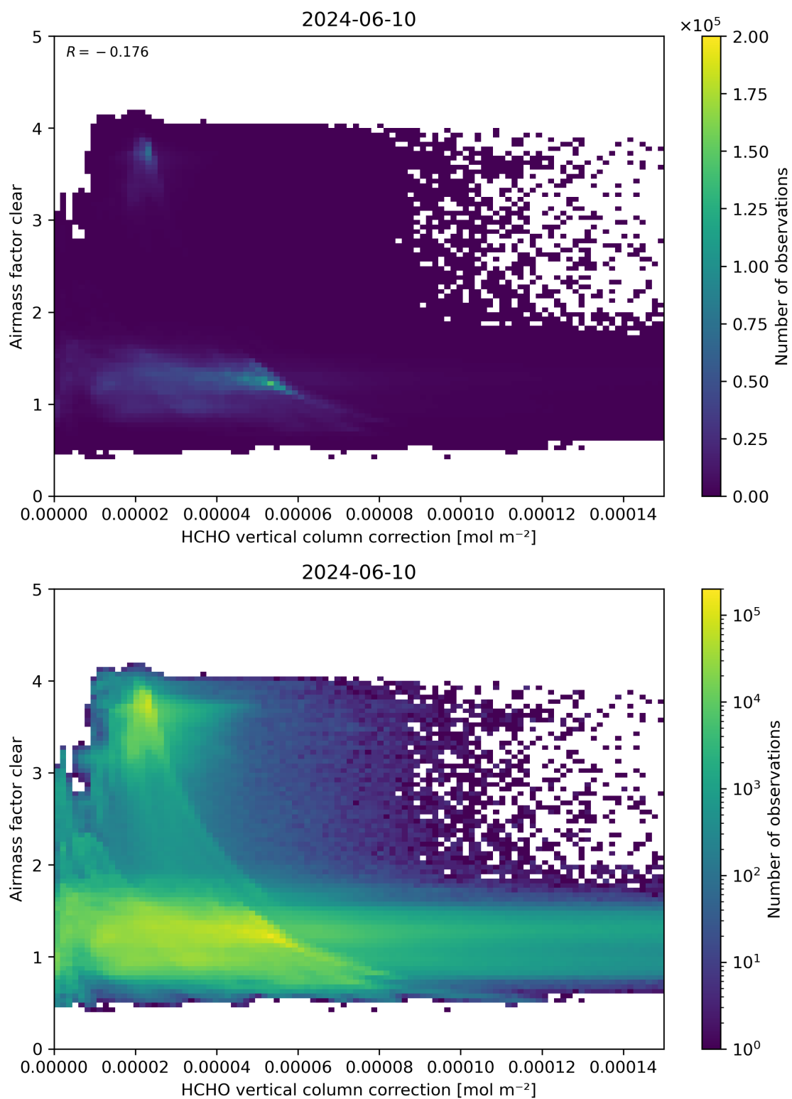
Figure 115: Scatter density plot of “HCHO vertical column correction” against “Airmass factor clear” for 2024-06-09 to 2024-06-11.
