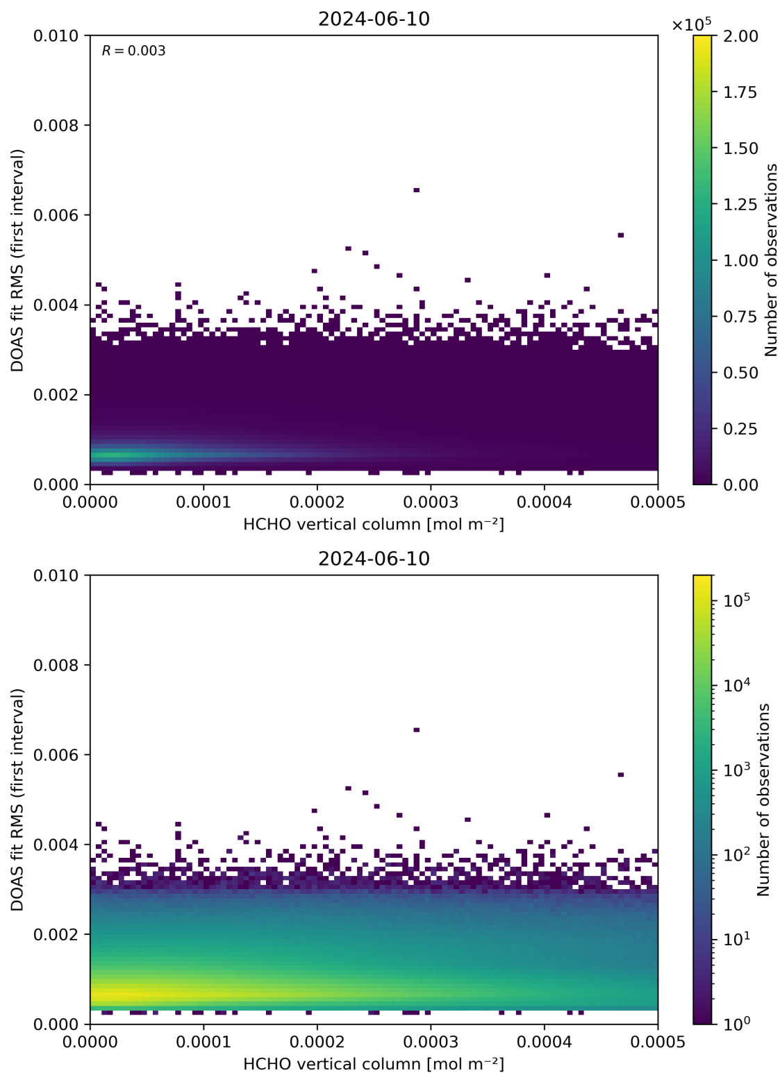
Figure 123: Scatter density plot of “HCHO vertical column” against “DOAS fit RMS (first interval)” for 2024-06-09 to 2024-06-11.
