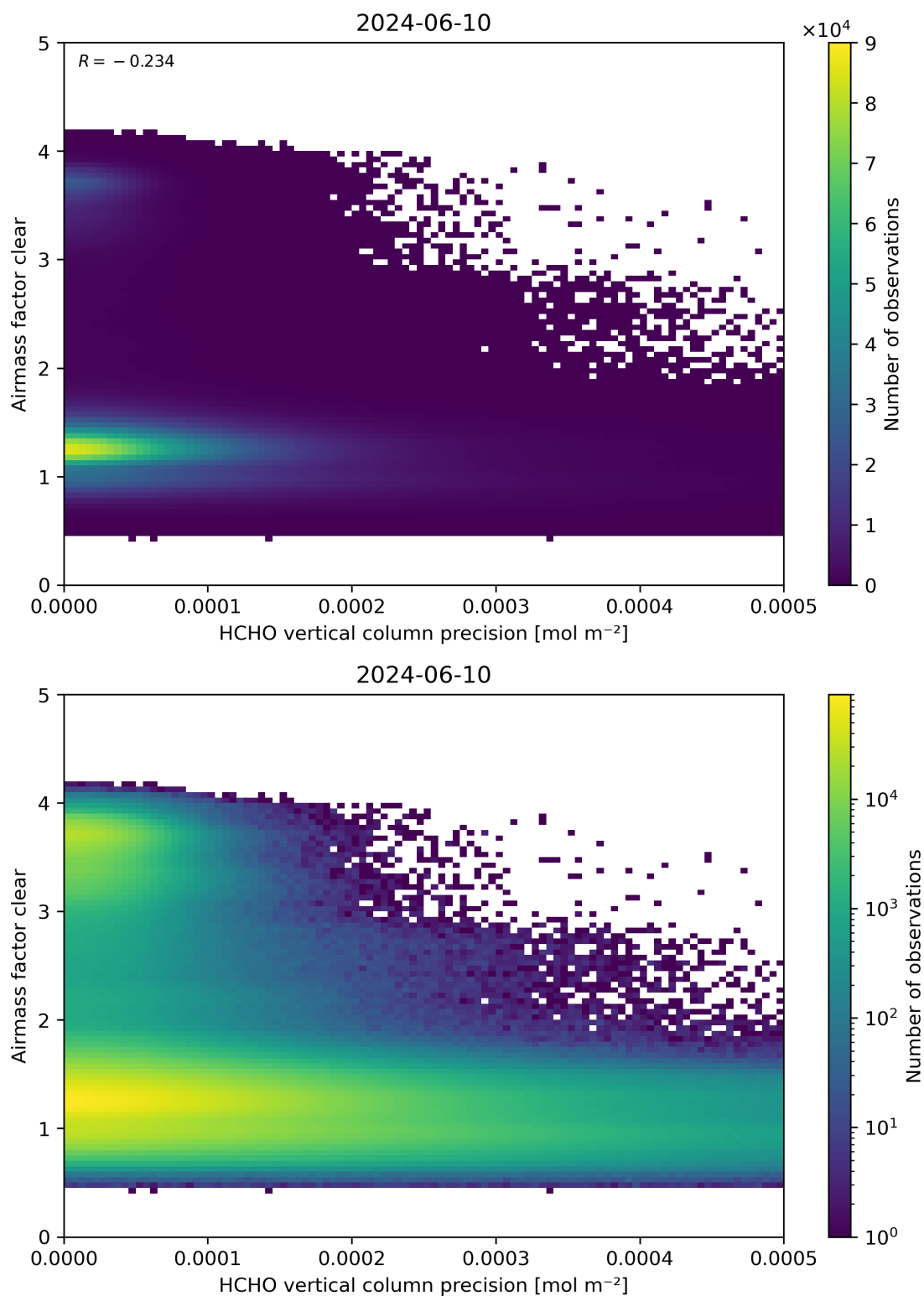
Figure 139: Scatter density plot of “HCHO vertical column precision” against “Airmass factor clear” for 2024-06-09 to 2024-06-11.
