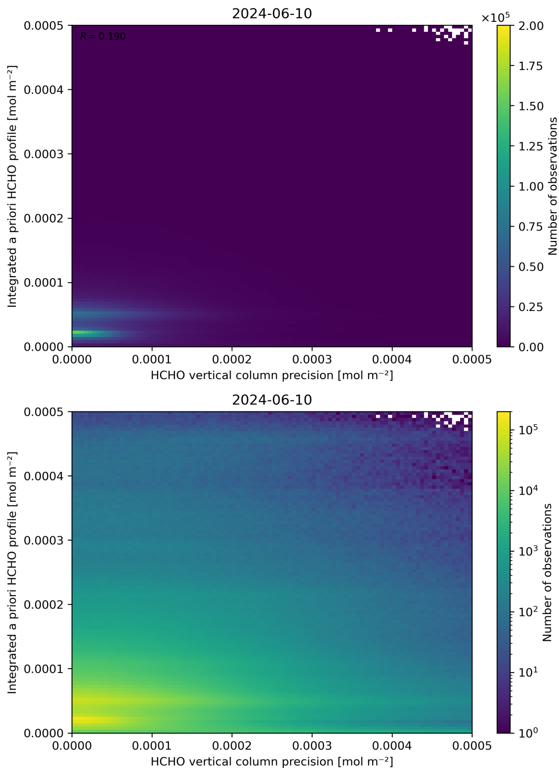
Figure 147: Scatter density plot of “HCHO vertical column precision” against “Integrated a priori HCHO profile” for 2024-06-09 to 2024-06-11.
