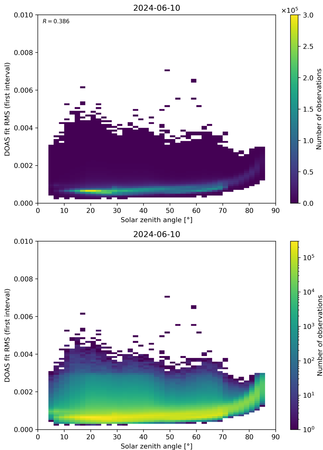
Figure 167: Scatter density plot of “Solar zenith angle” against “DOAS fit RMS (first interval)” for 2024-06-09 to 2024-06-11.
