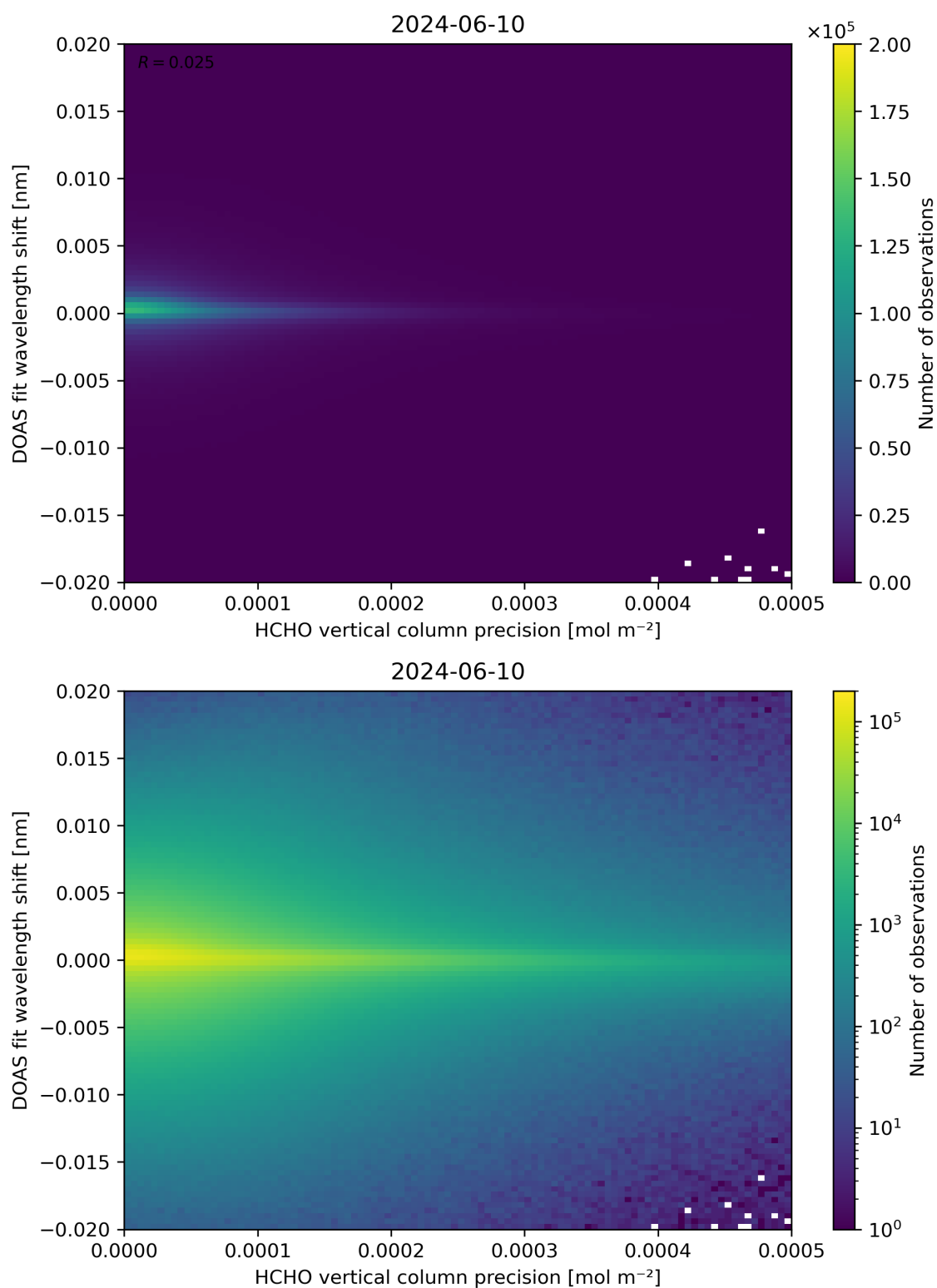
Figure 137: Scatter density plot of “HCHO vertical column precision” against “DOAS fit wavelength shift” for 2024-06-09 to 2024-06-11.
