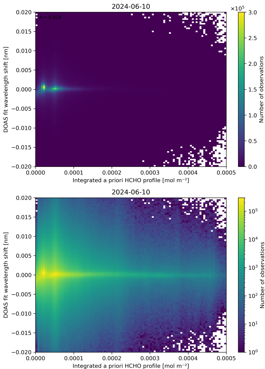
Figure 149: Scatter density plot of “Integrated a priori HCHO profile” against “DOAS fit wavelength shift” for 2024-06-09 to 2024-06-11.
