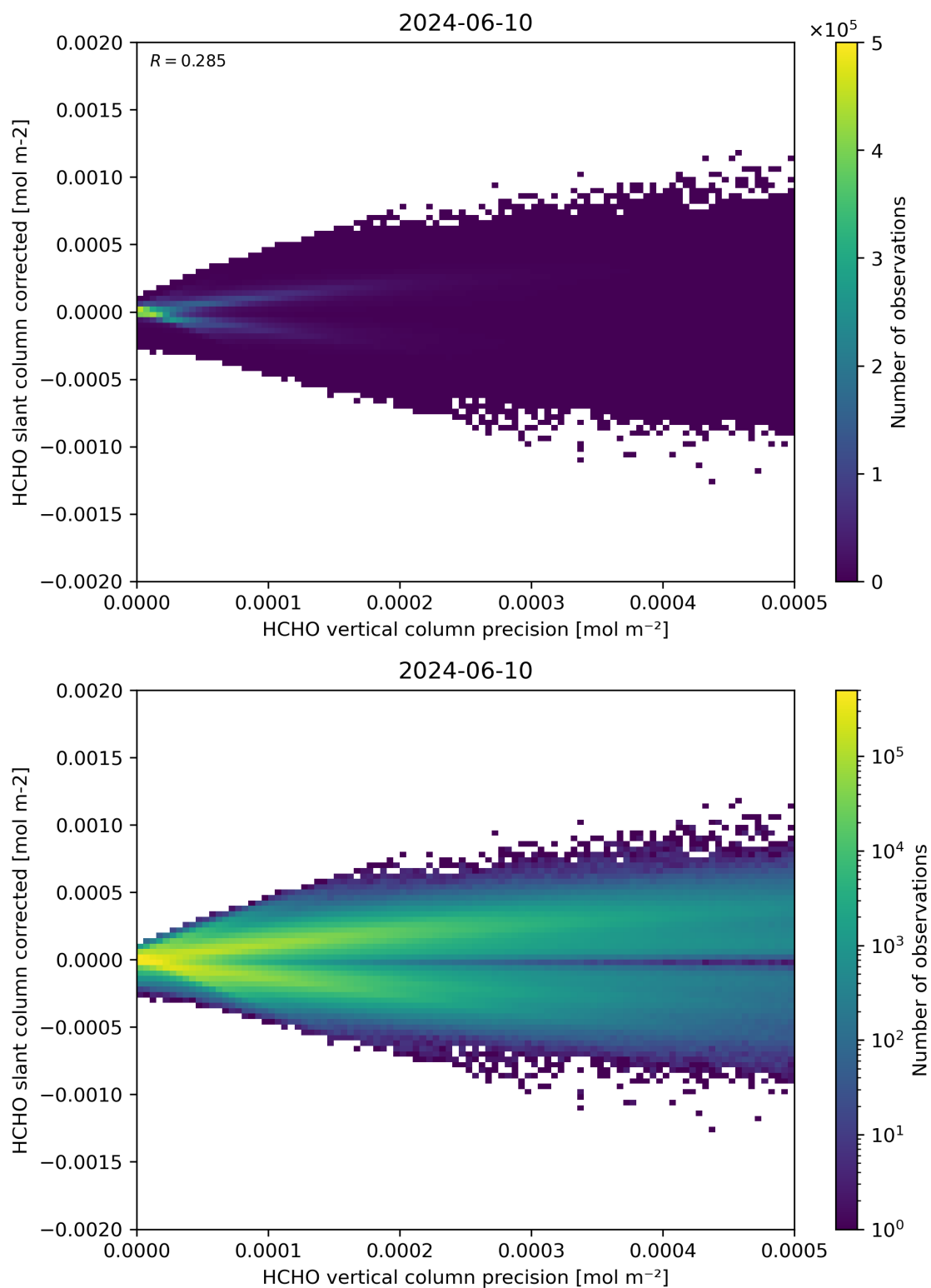
Figure 140: Scatter density plot of “HCHO vertical column precision” against “HCHO slant column corrected” for 2024-06-09 to 2024-06-11.
