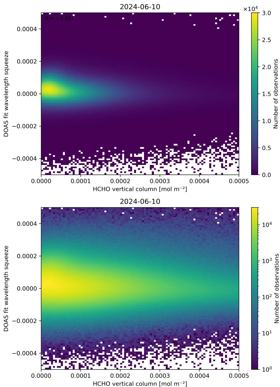
Figure 125: Scatter density plot of “HCHO vertical column” against “DOAS fit wavelength squeeze” for 2024-06-09 to 2024-06-11.
