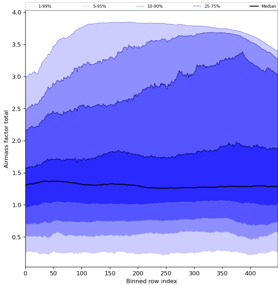
Figure 54: Along track statistics of “Airmass factor total” for 2024-06-09 to 2024-06-11
