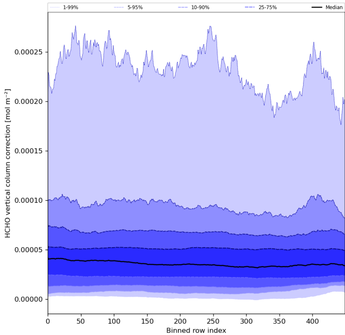
Figure 51: Along track statistics of “HCHO vertical column correction” for 2024-06-09 to 2024-06-11
