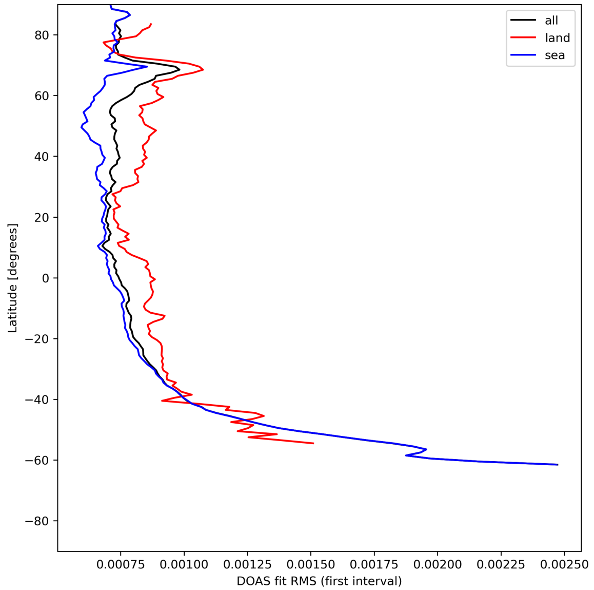
Figure 32: Zonal average of “DOAS fit RMS (first interval)” for 2024-06-09 to 2024-06-11.
