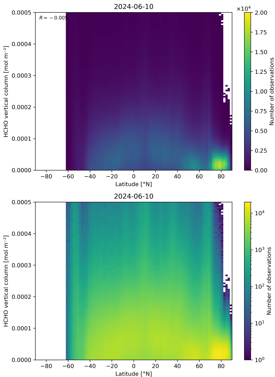
Figure 163: Scatter density plot of “Latitude” against “HCHO vertical column” for 2024-06-09 to 2024-06-11.
