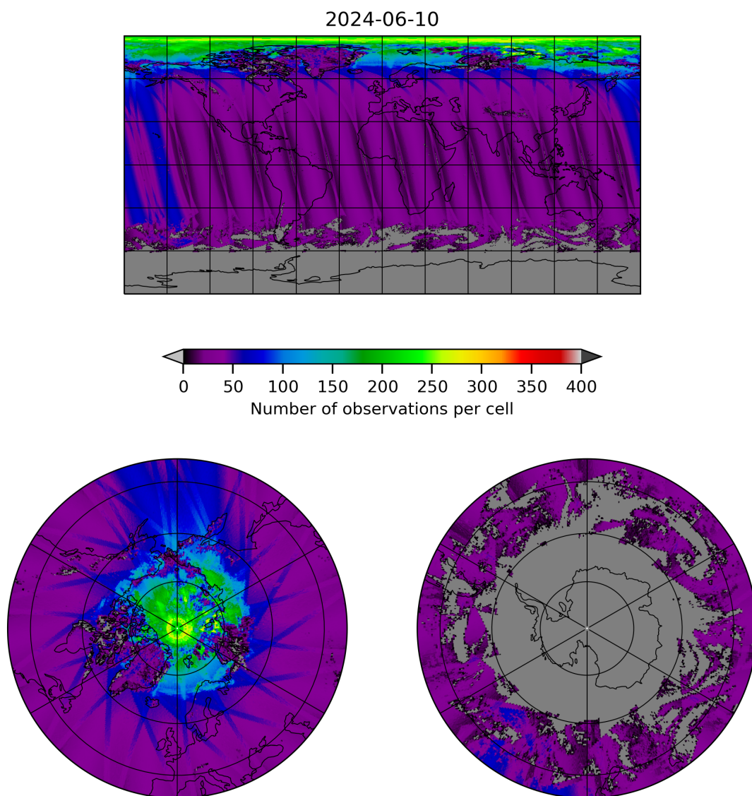
Figure 19: Map of the number of observations for 2024-06-09 to 2024-06-11
