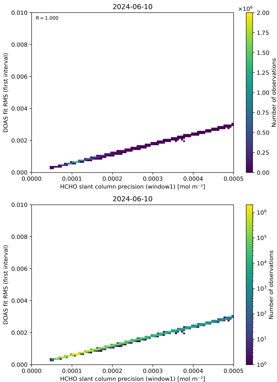
Figure 88: Scatter density plot of “HCHO slant column precision (window1)” against “DOAS fit RMS (first interval)” for 2024-06-09 to 2024-06-11.
