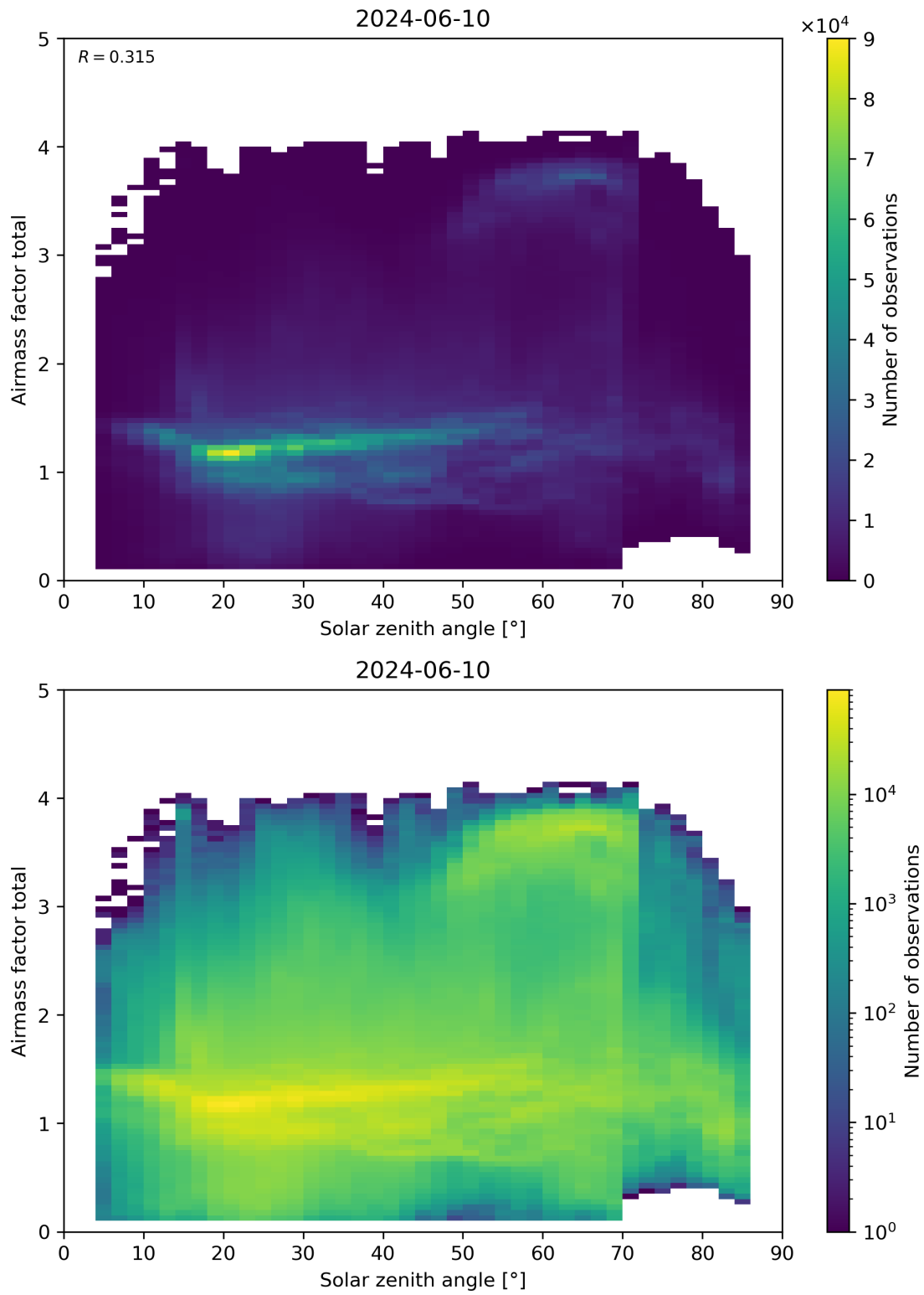
Figure 175: Scatter density plot of “Solar zenith angle” against “Airmass factor total” for 2024-06-09 to 2024-06-11.
