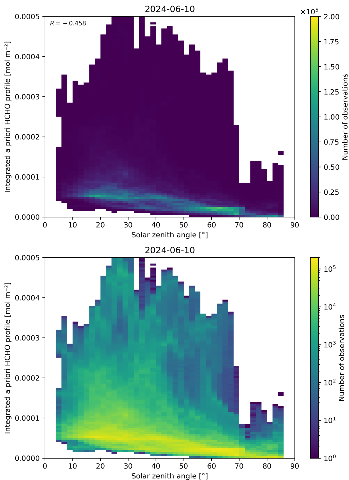
Figure 180: Scatter density plot of “Solar zenith angle” against “Integrated a priori HCHO profile” for 2024-06-09 to 2024-06-11.
