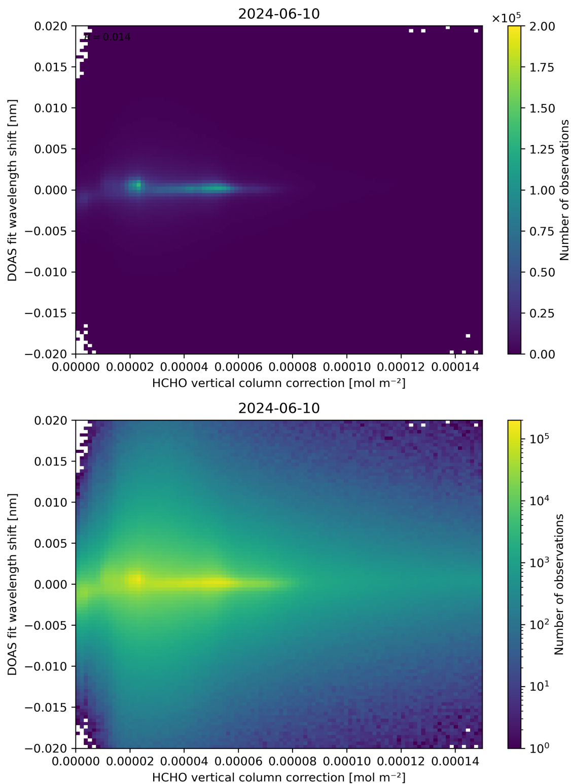
Figure 113: Scatter density plot of “HCHO vertical column correction” against “DOAS fit wavelength shift” for 2024-06-09 to 2024-06-11.
