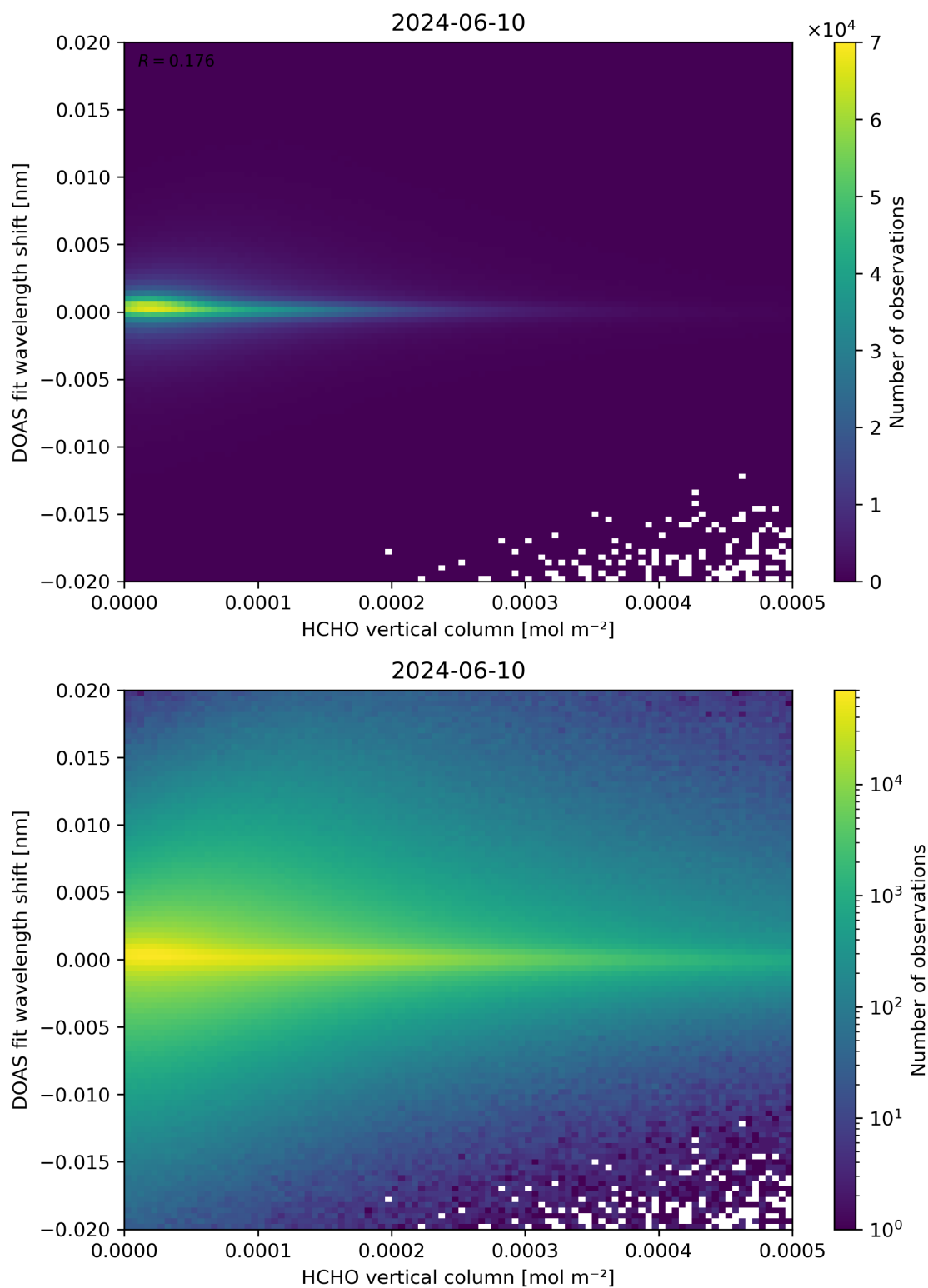
Figure 124: Scatter density plot of “HCHO vertical column” against “DOAS fit wavelength shift” for 2024-06-09 to 2024-06-11.
