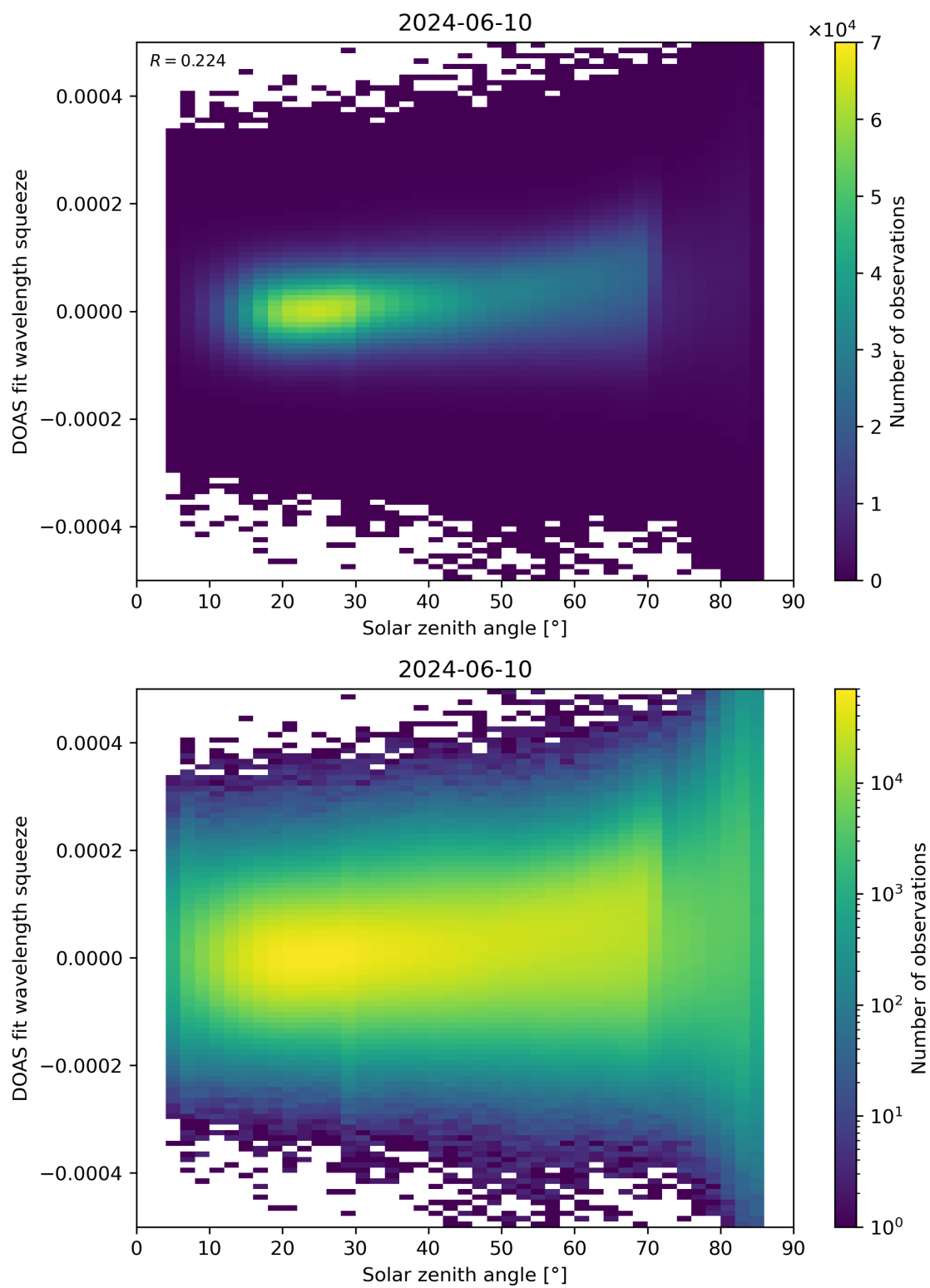
Figure 169: Scatter density plot of “Solar zenith angle” against “DOAS fit wavelength squeeze” for 2024-06-09 to 2024-06-11.
