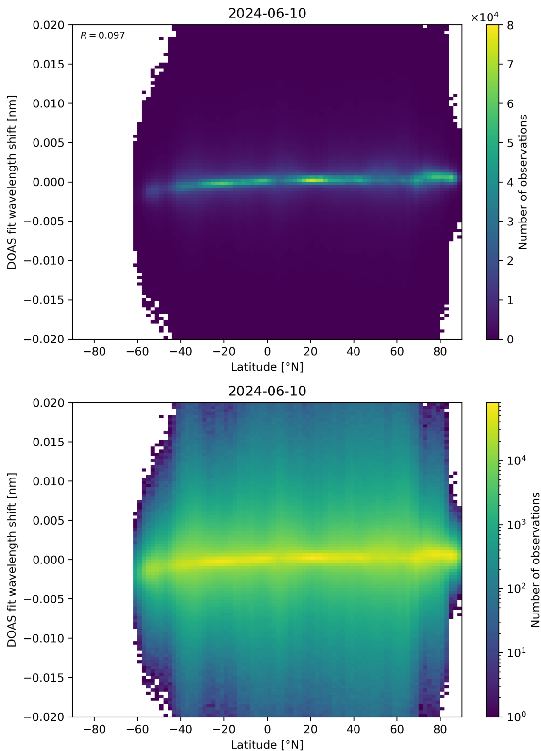
Figure 154: Scatter density plot of “Latitude” against “DOAS fit wavelength shift” for 2024-06-09 to 2024-06-11.
