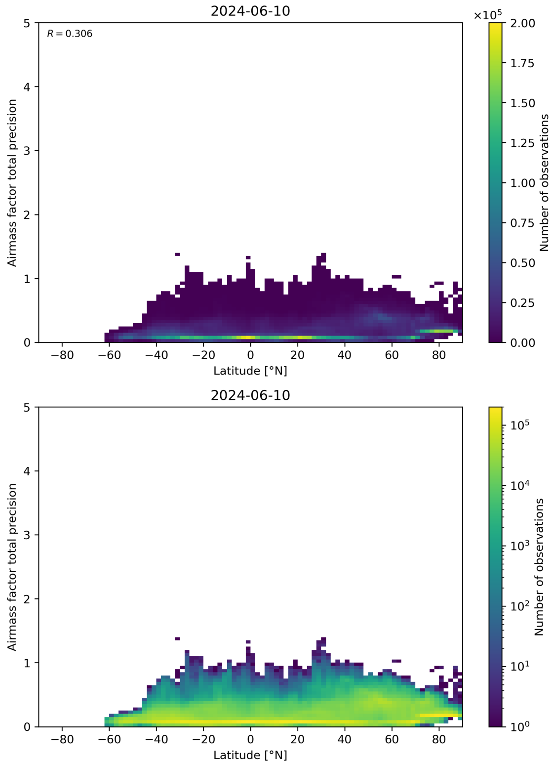
Figure 162: Scatter density plot of “Latitude” against “Airmass factor total precision” for 2024-06-09 to 2024-06-11.
