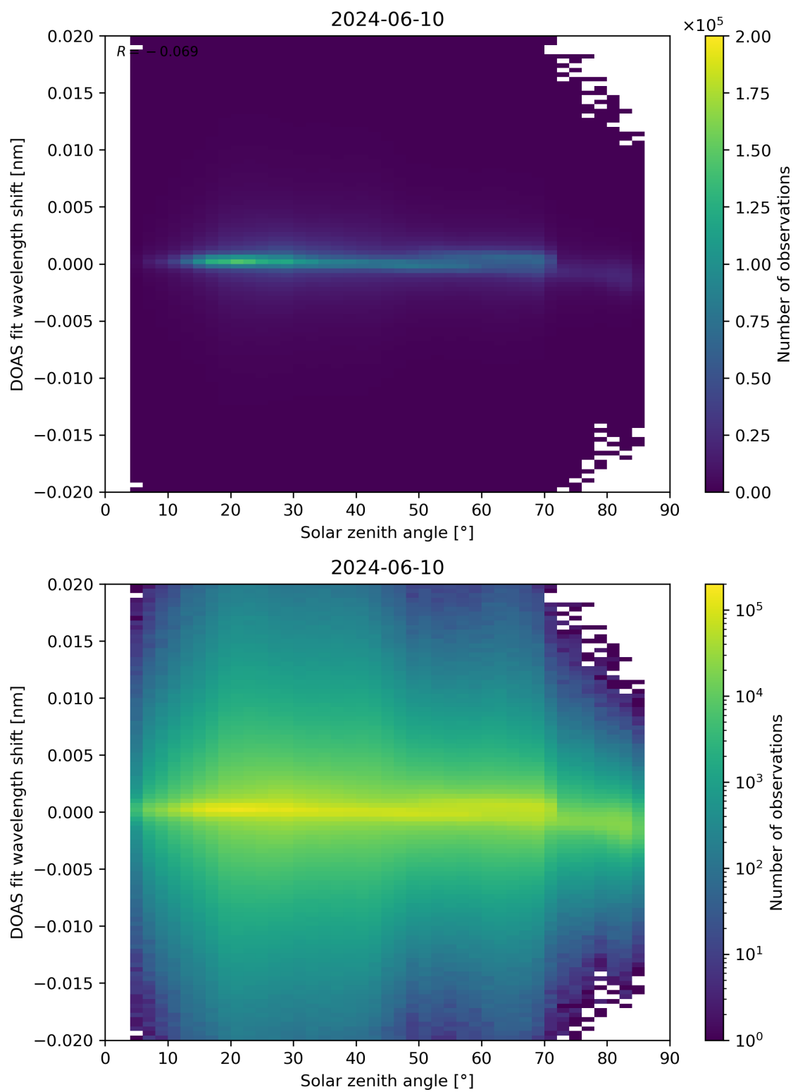
Figure 168: Scatter density plot of “Solar zenith angle” against “DOAS fit wavelength shift” for 2024-06-09 to 2024-06-11.
