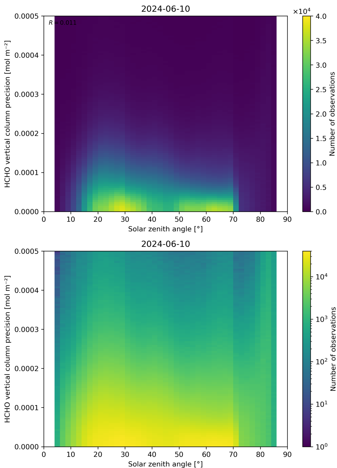
Figure 179: Scatter density plot of “Solar zenith angle” against “HCHO vertical column precision” for 2024-06-09 to 2024-06-11.
