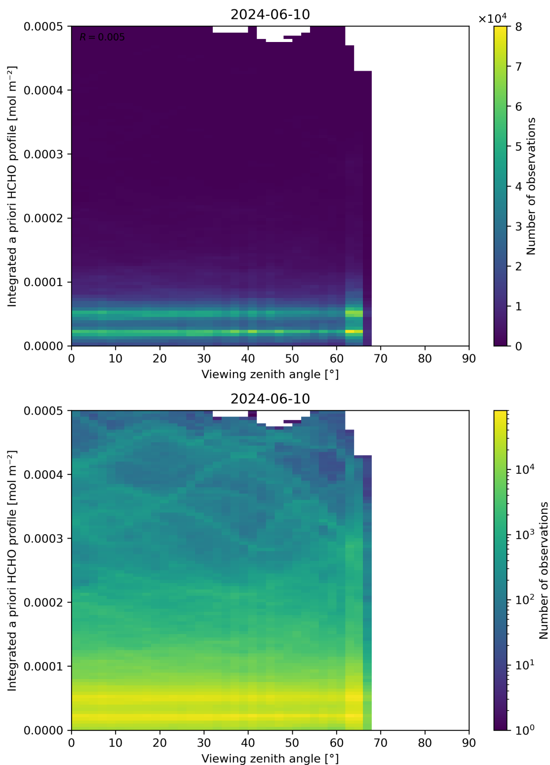
Figure 195: Scatter density plot of “Viewing zenith angle” against “Integrated a priori HCHO profile” for 2024-06-09 to 2024-06-11.
