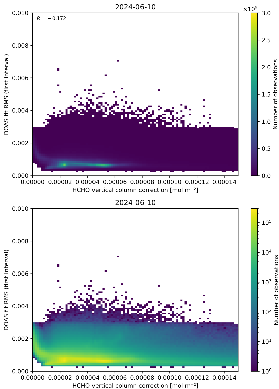
Figure 112: Scatter density plot of “HCHO vertical column correction” against “DOAS fit RMS (first interval)” for 2024-06-09 to 2024-06-11.
