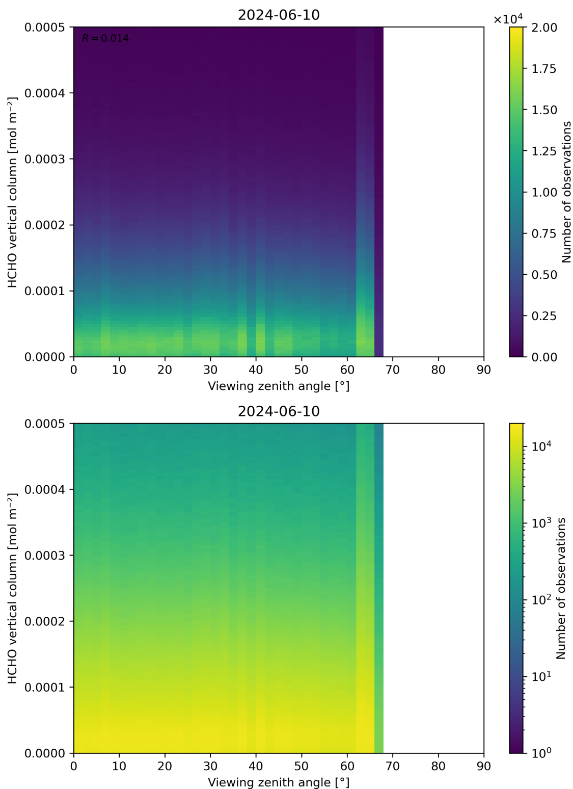
Figure 192: Scatter density plot of “Viewing zenith angle” against “HCHO vertical column” for 2024-06-09 to 2024-06-11.
