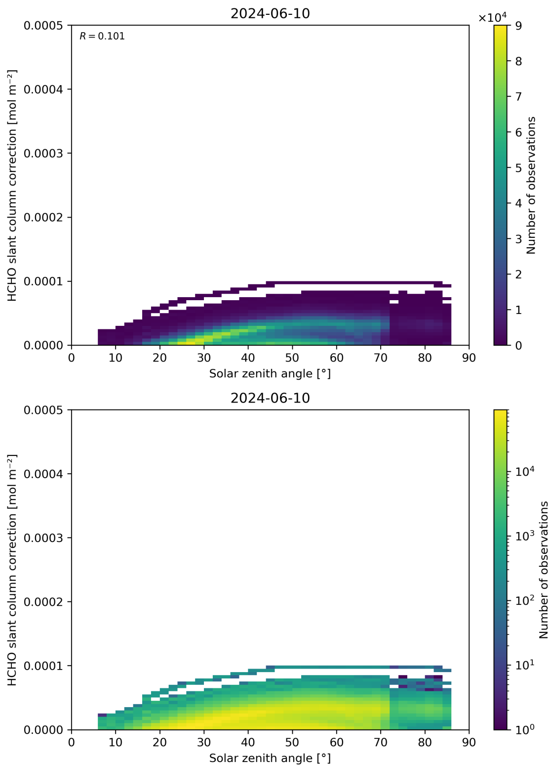
Figure 172: Scatter density plot of “Solar zenith angle” against “HCHO slant column correction” for 2024-06-09 to 2024-06-11.
