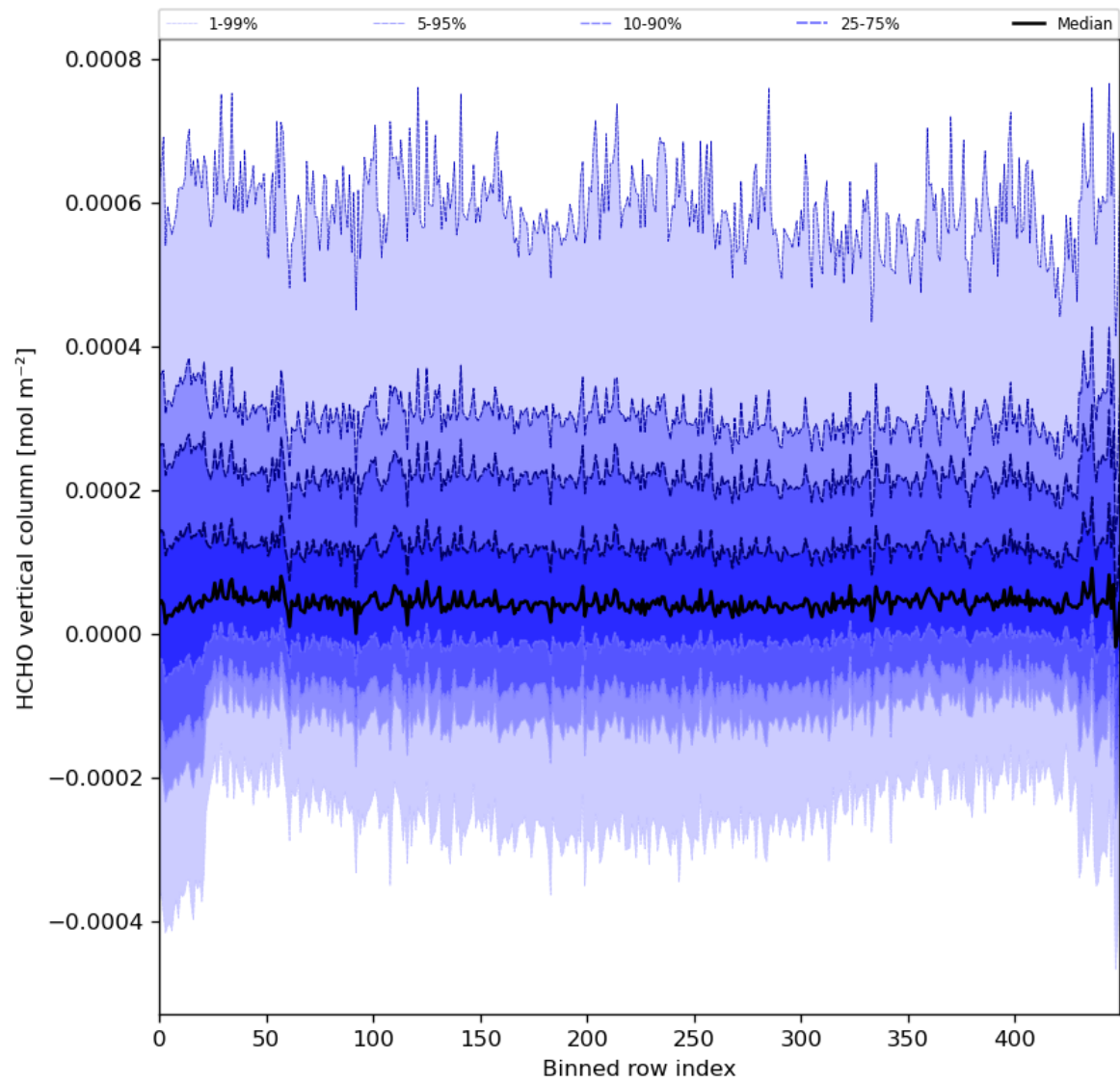
Figure 49: Along track statistics of “HCHO vertical column” for 2024-06-09 to 2024-06-11
