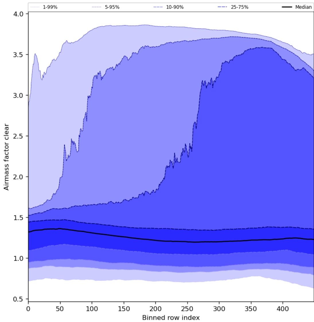
Figure 56: Along track statistics of “Airmass factor clear” for 2024-06-09 to 2024-06-11
