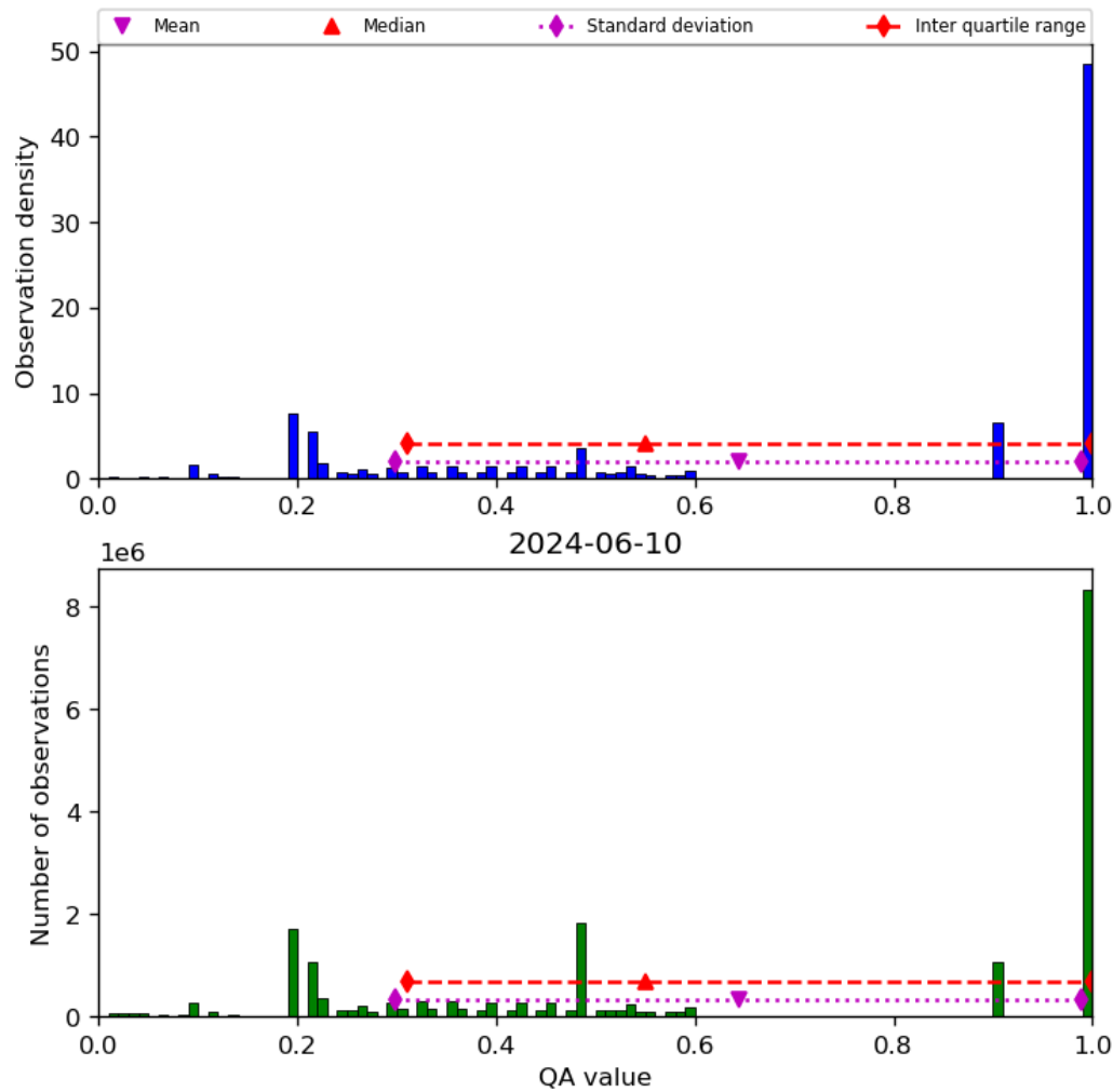
Figure 34: Histogram of “QA value” for 2024-06-09 to 2024-06-11
