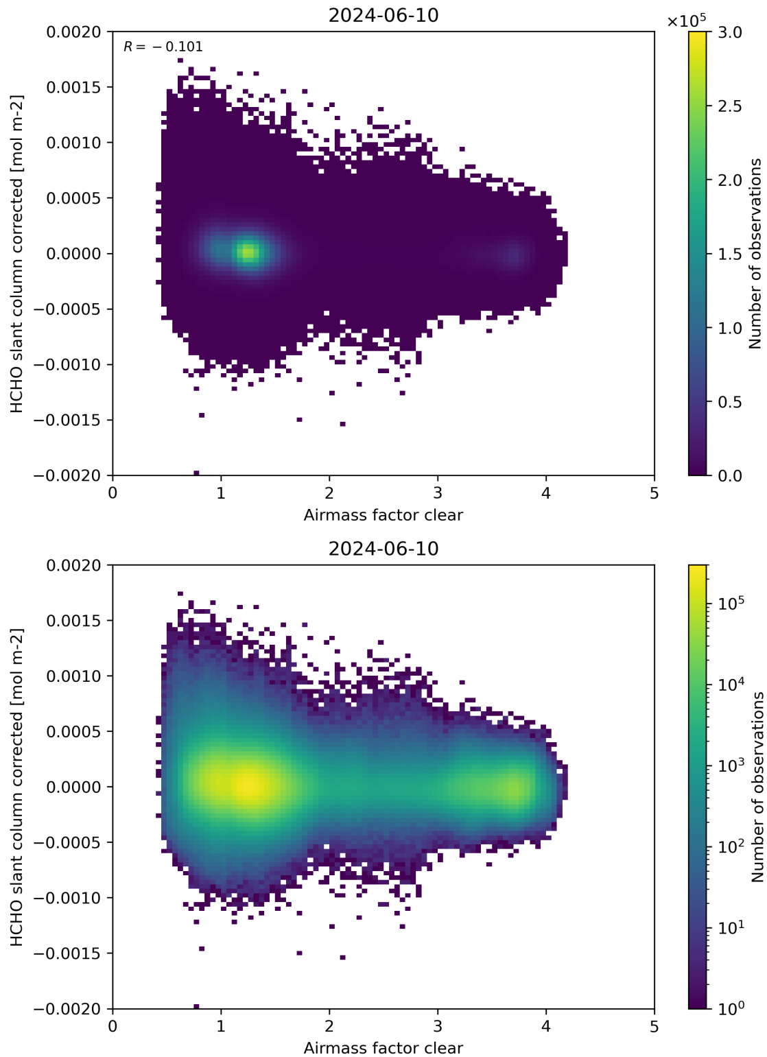
Figure 74: Scatter density plot of “Airmass factor clear” against “HCHO slant column corrected” for 2024-06-09 to 2024-06-11.
