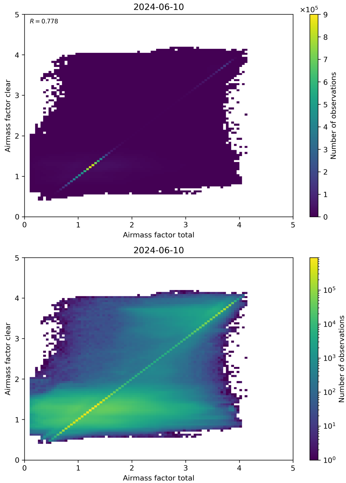
Figure 100: Scatter density plot of “Airmass factor total” against “Airmass factor clear” for 2024-06-09 to 2024-06-11.
