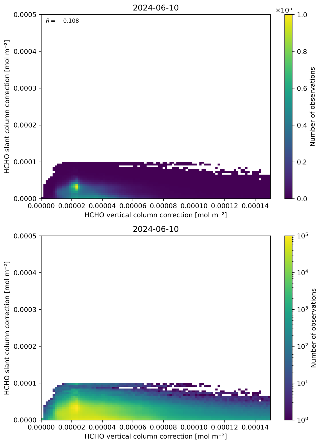
Figure 117: Scatter density plot of “HCHO vertical column correction” against “HCHO slant column correction” for 2024-06-09 to 2024-06-11.
