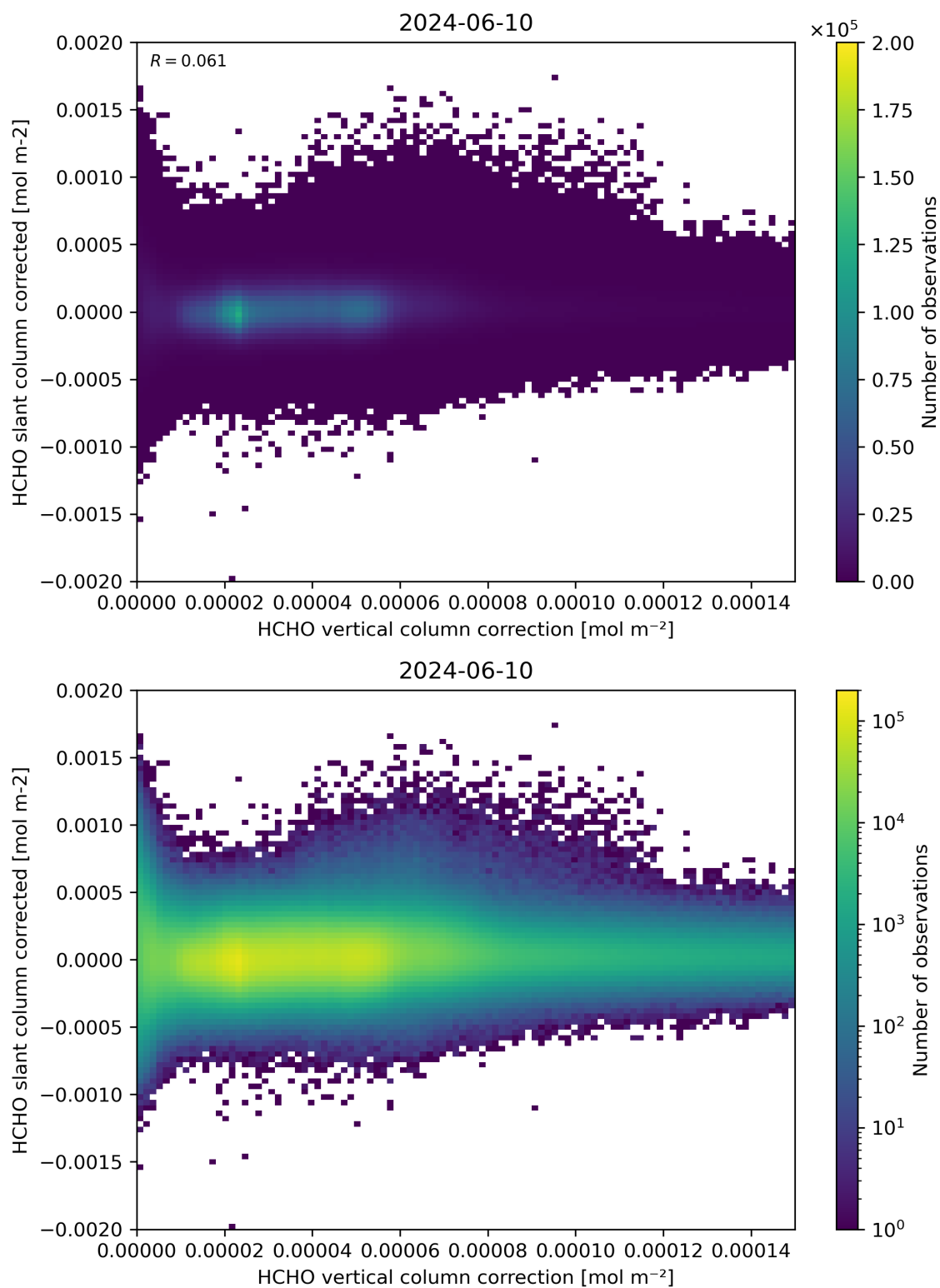
Figure 116: Scatter density plot of “HCHO vertical column correction” against “HCHO slant column corrected” for 2024-06-09 to 2024-06-11.
