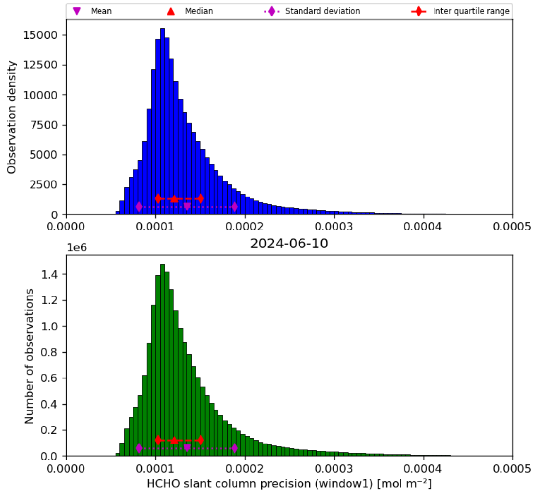
Figure 39: Histogram of “HCHO slant column precision (window1)” for 2024-06-09 to 2024-06-11
