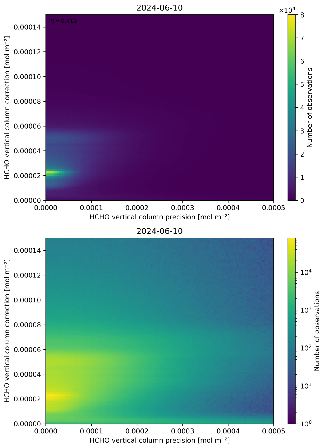
Figure 146: Scatter density plot of “HCHO vertical column precision” against “HCHO vertical column correction” for 2024-06-09 to 2024-06-11.
