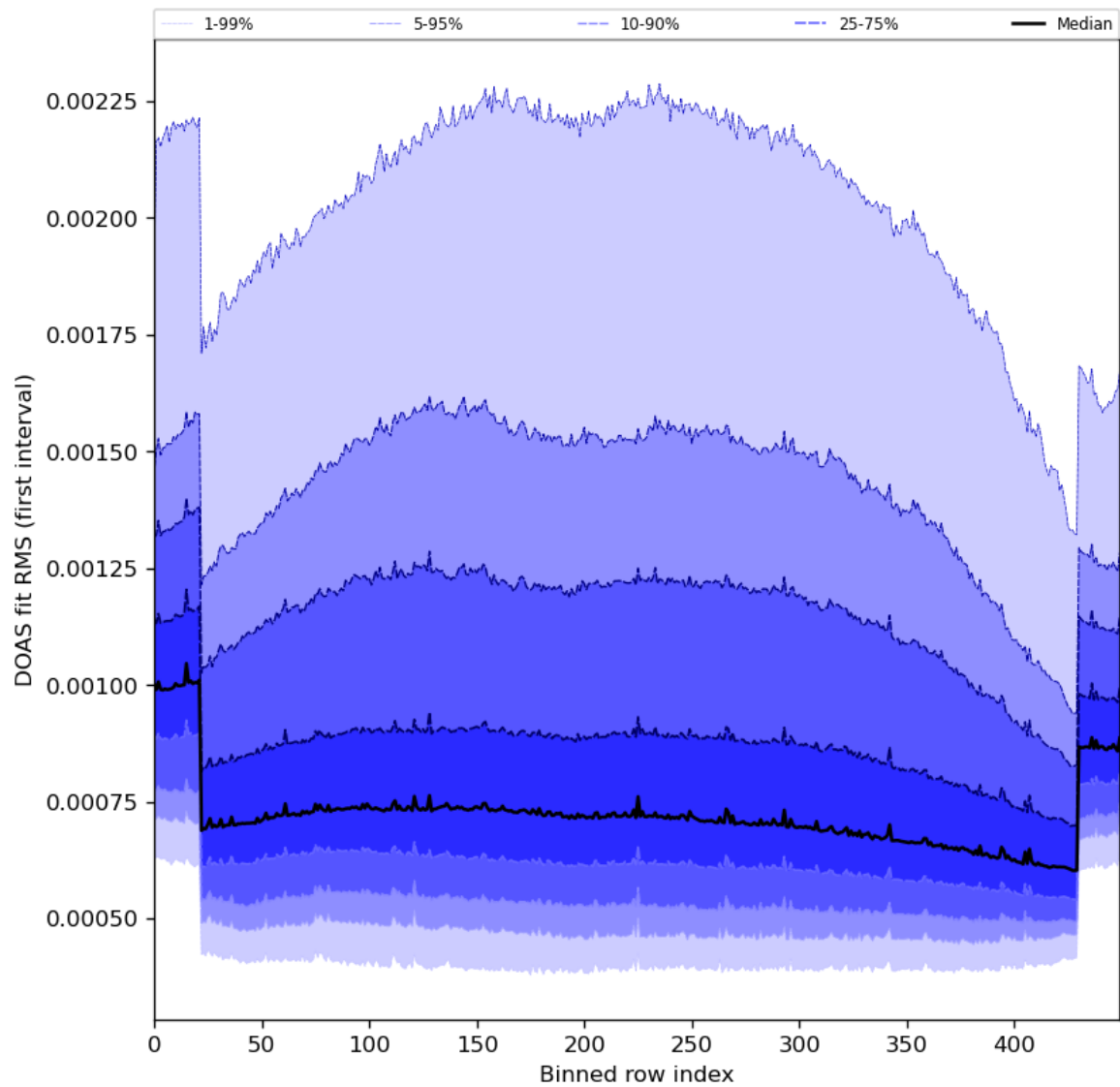
Figure 60: Along track statistics of “DOAS fit RMS (first interval)” for 2024-06-09 to 2024-06-11
