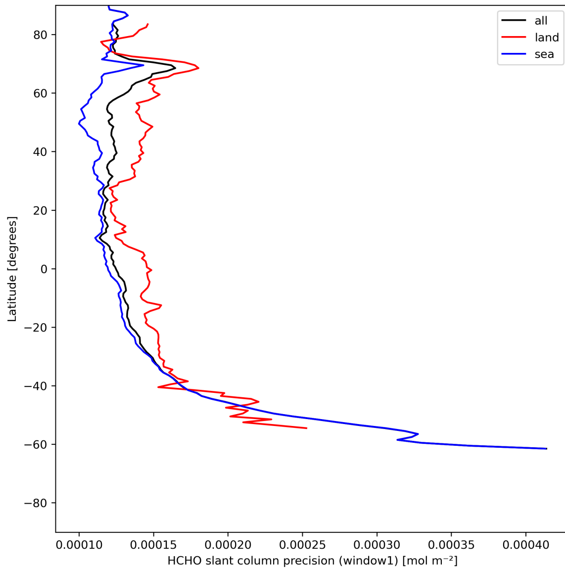
Figure 25: Zonal average of “HCHO slant column precision (window1)” for 2024-06-09 to 2024-06-11.
