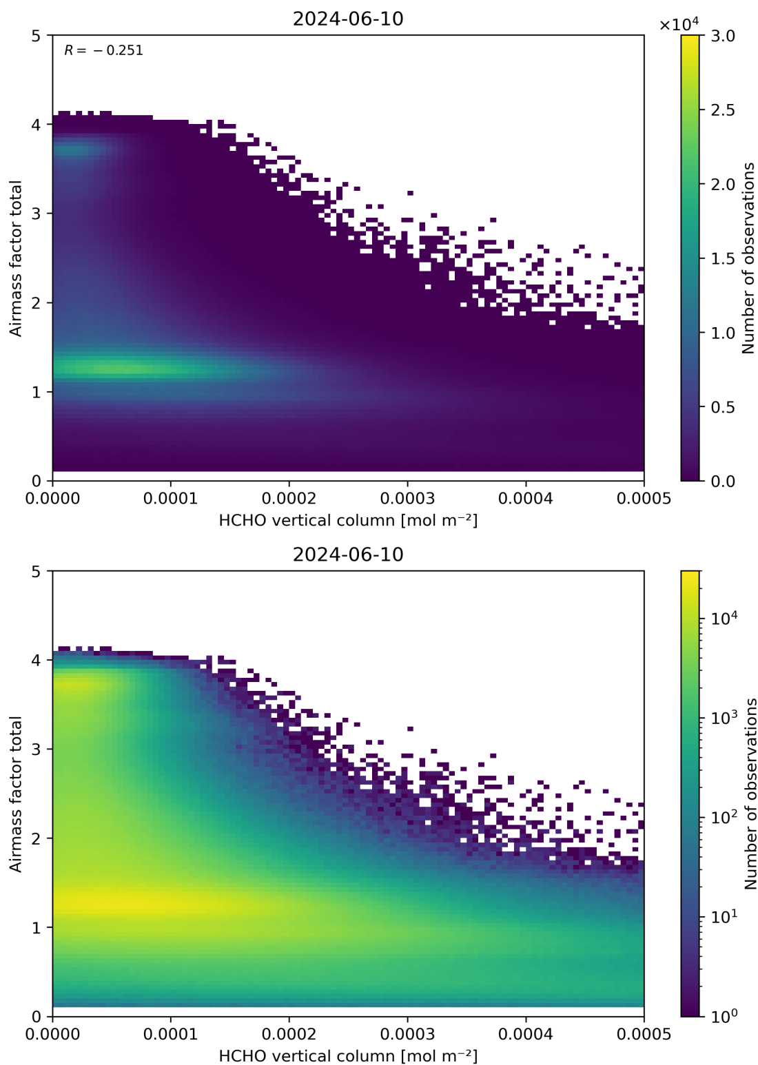
Figure 131: Scatter density plot of “HCHO vertical column” against “Airmass factor total” for 2024-06-09 to 2024-06-11.
