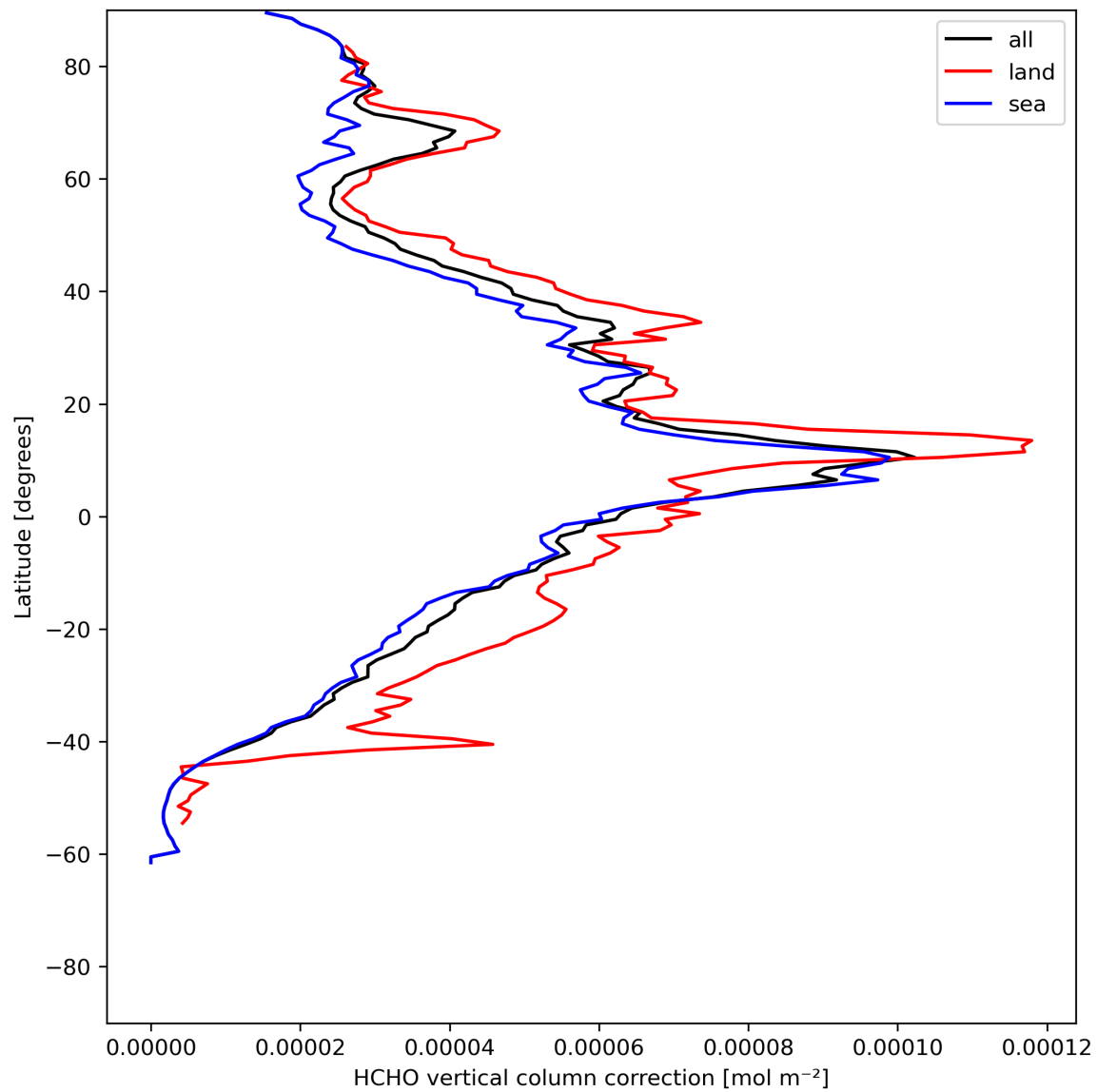
Figure 23: Zonal average of “HCHO vertical column correction” for 2024-06-09 to 2024-06-11.
