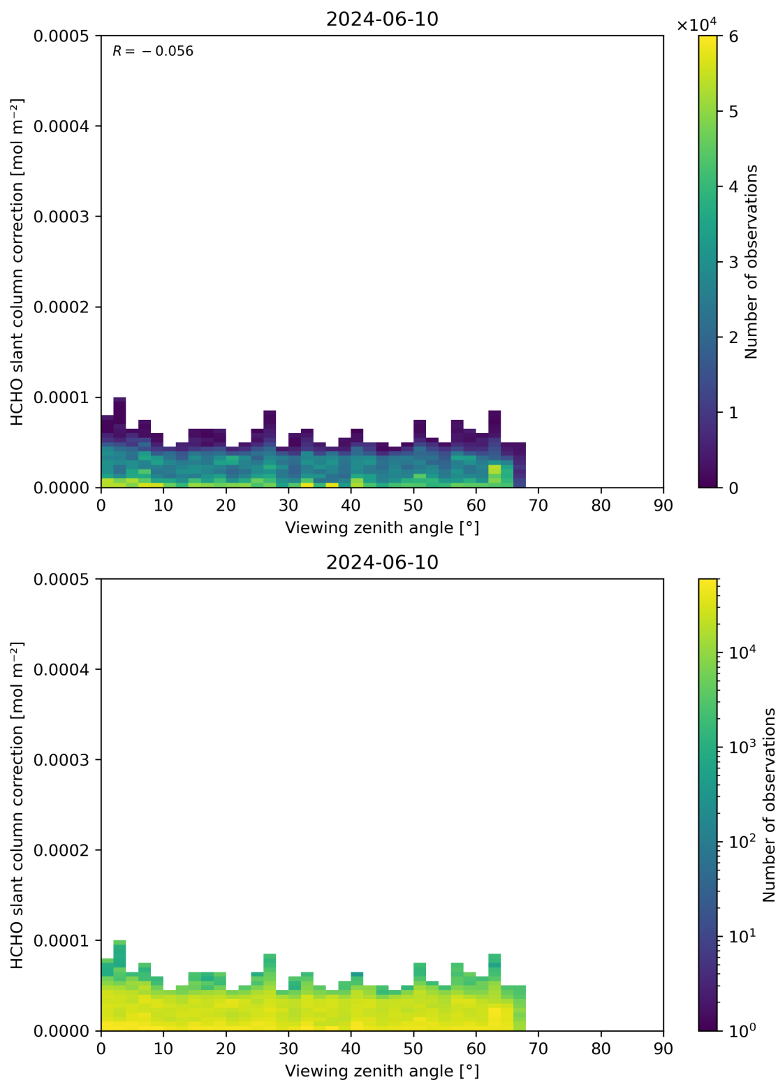
Figure 187: Scatter density plot of “Viewing zenith angle” against “HCHO slant column correction” for 2024-06-09 to 2024-06-11.
