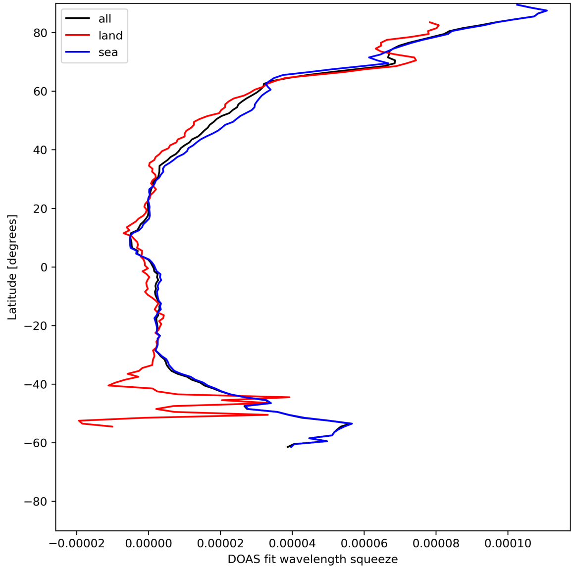
Figure 31: Zonal average of “DOAS fit wavelength squeeze” for 2024-06-09 to 2024-06-11.
