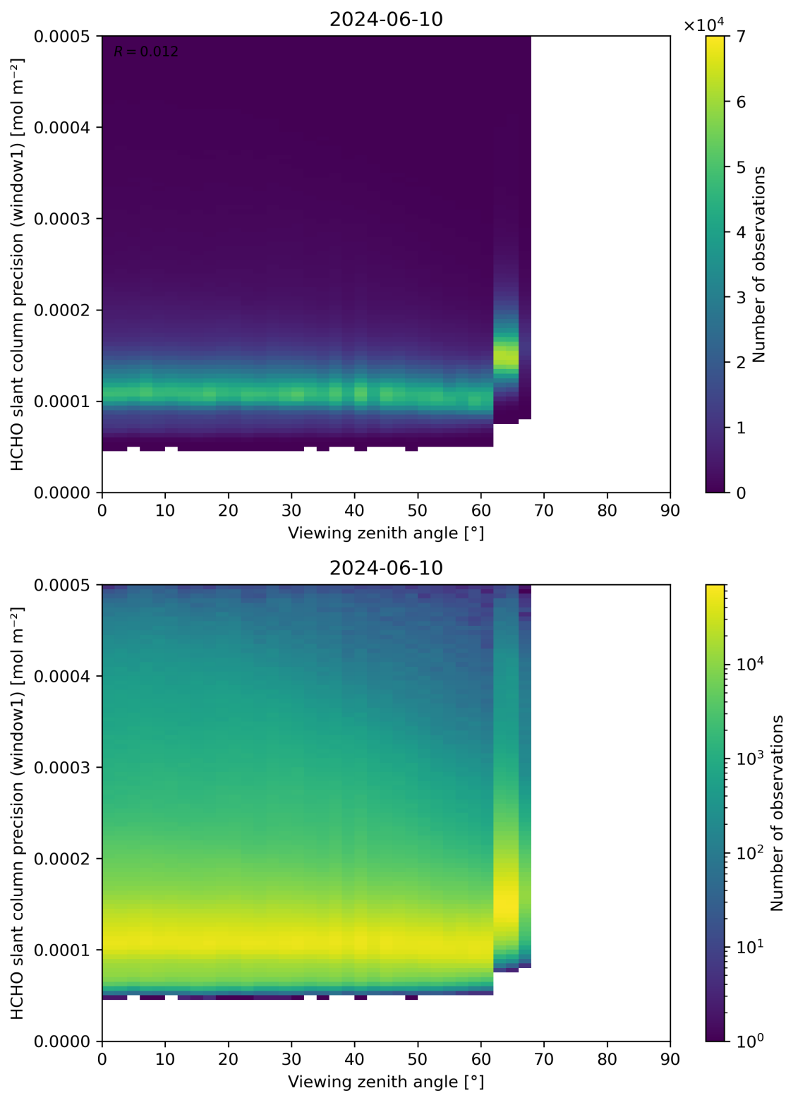
Figure 189: Scatter density plot of “Viewing zenith angle” against “HCHO slant column precision (window1)” for 2024-06-09 to 2024-06-11.
