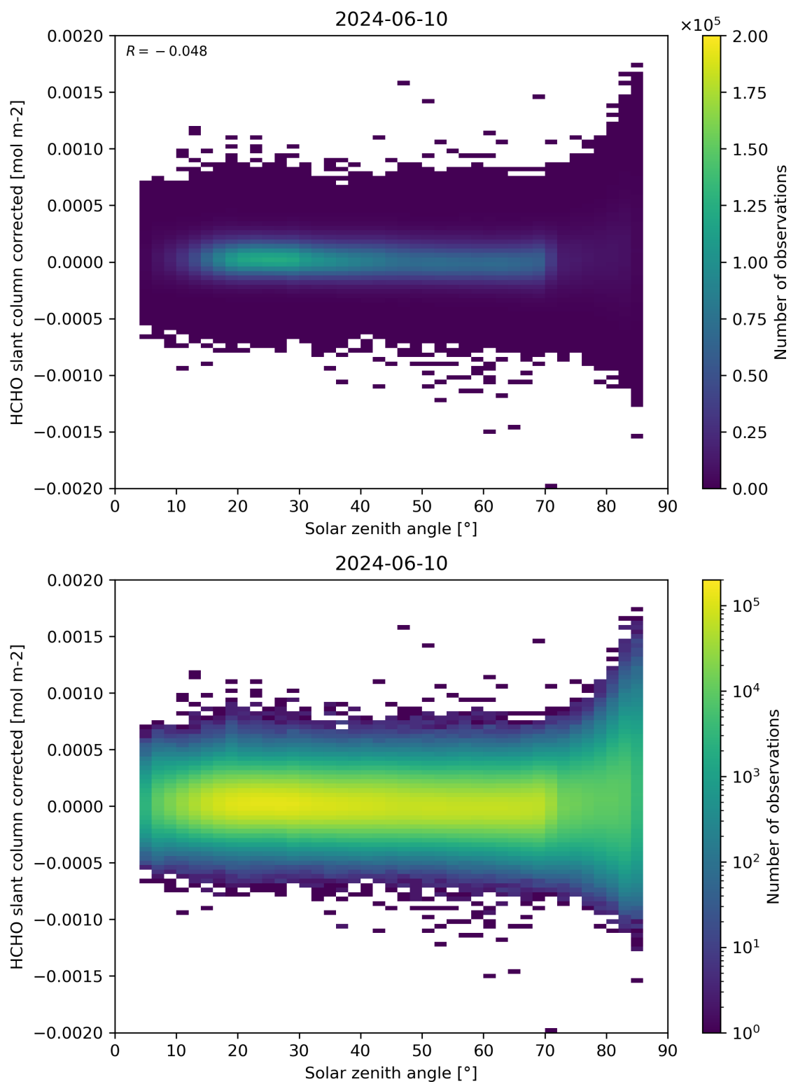
Figure 171: Scatter density plot of “Solar zenith angle” against “HCHO slant column corrected” for 2024-06-09 to 2024-06-11.
