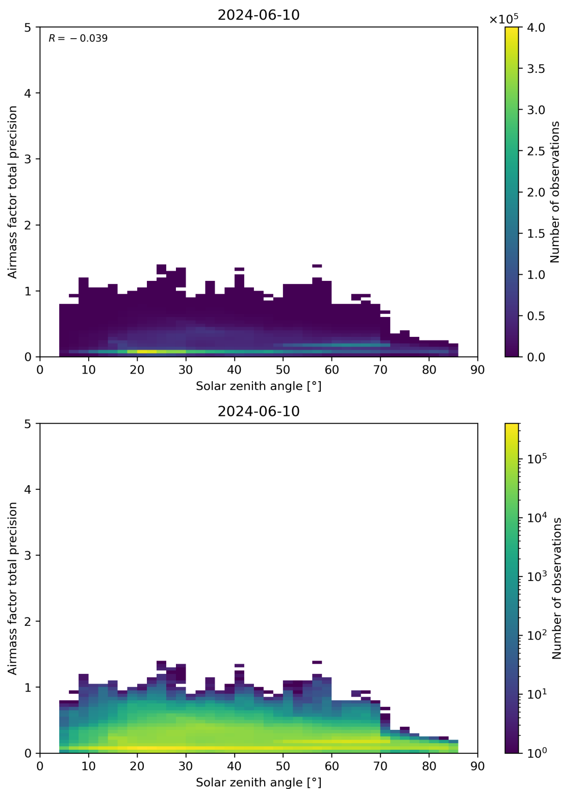
Figure 176: Scatter density plot of “Solar zenith angle” against “Airmass factor total precision” for 2024-06-09 to 2024-06-11.
