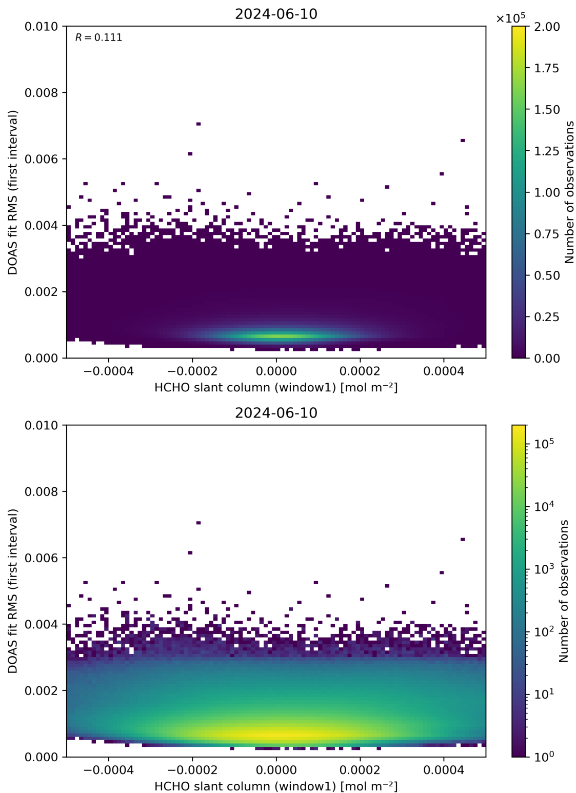
Figure 78: Scatter density plot of “HCHO slant column (window1)” against “DOAS fit RMS (first interval)” for 2024-06-09 to 2024-06-11.
