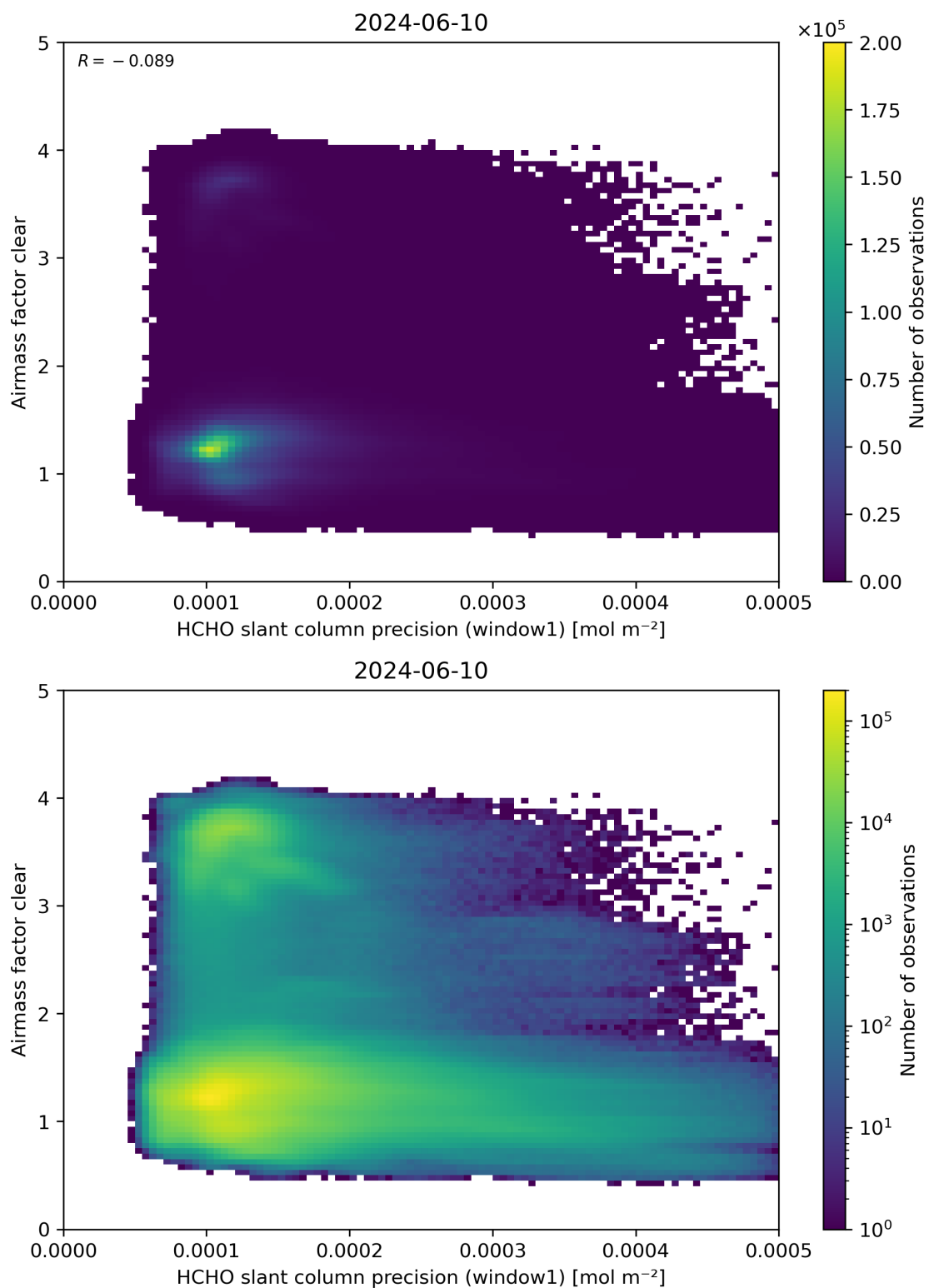
Figure 91: Scatter density plot of “HCHO slant column precision (window1)” against “Airmass factor clear” for 2024-06-09 to 2024-06-11.
