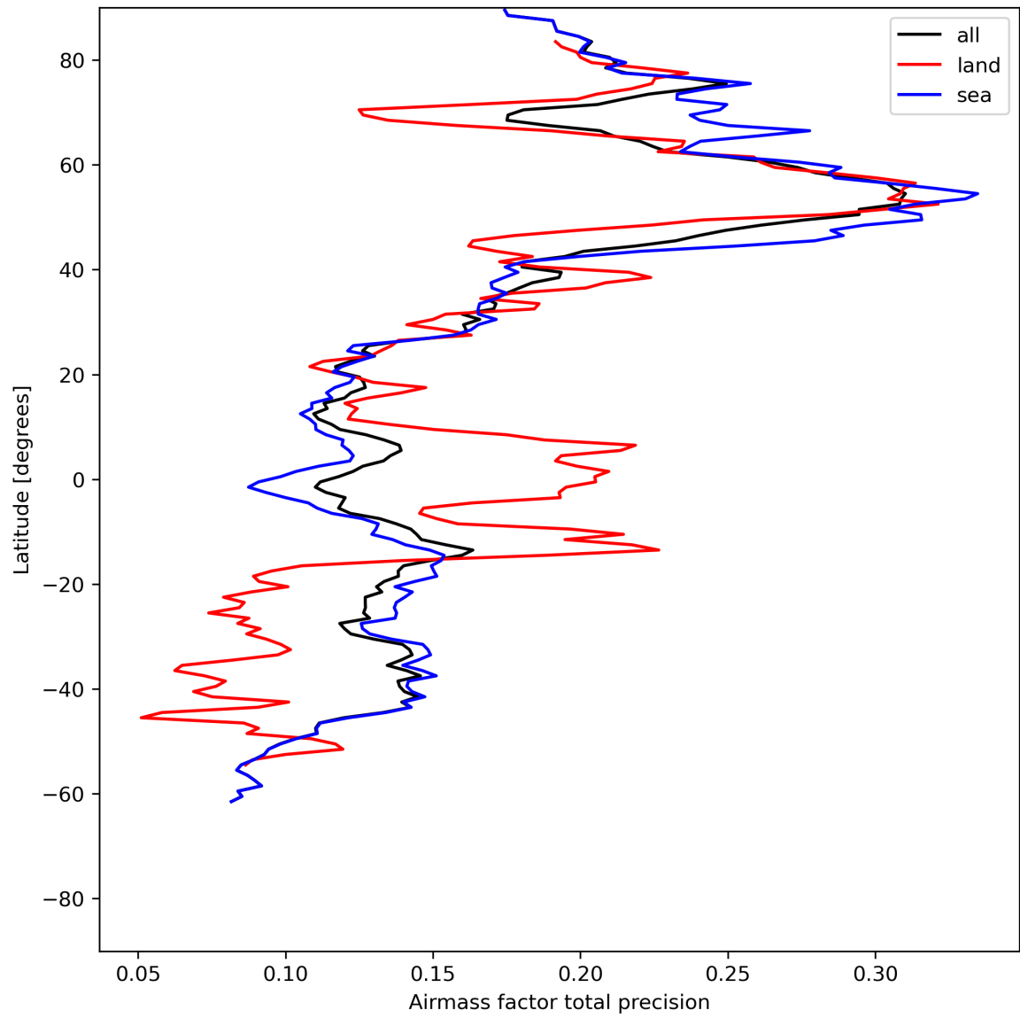
Figure 27: Zonal average of “Airmass factor total precision” for 2024-06-09 to 2024-06-11.
