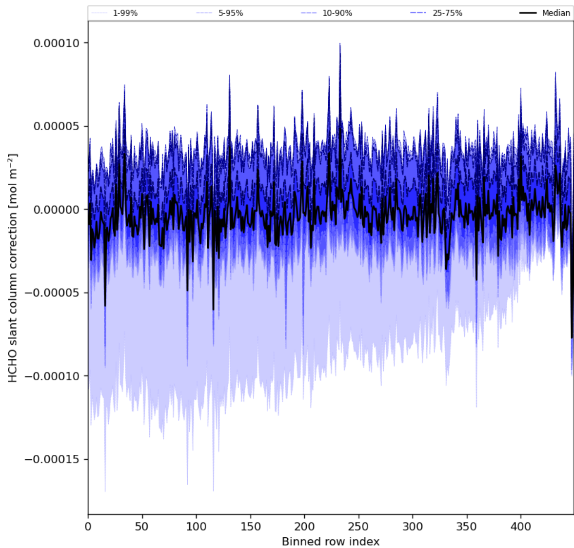
Figure 61: Along track statistics of “HCHO slant column correction” for 2024-06-09 to 2024-06-11
