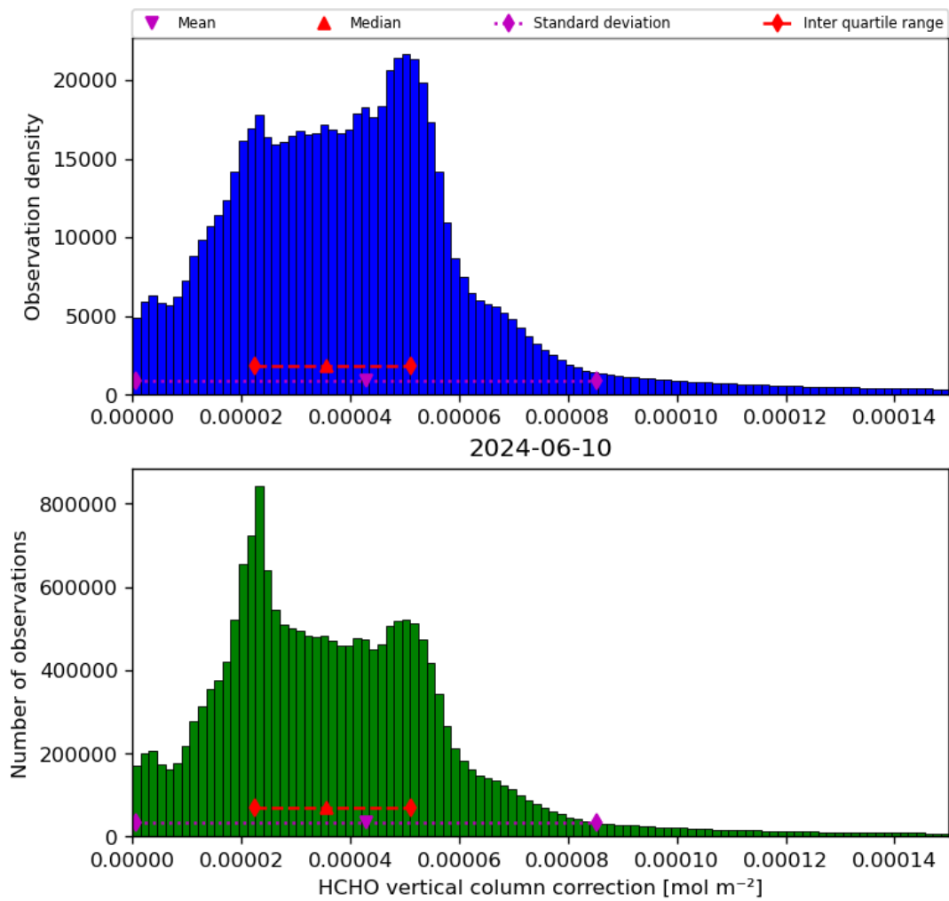
Figure 37: Histogram of “HCHO vertical column correction” for 2024-06-09 to 2024-06-11
