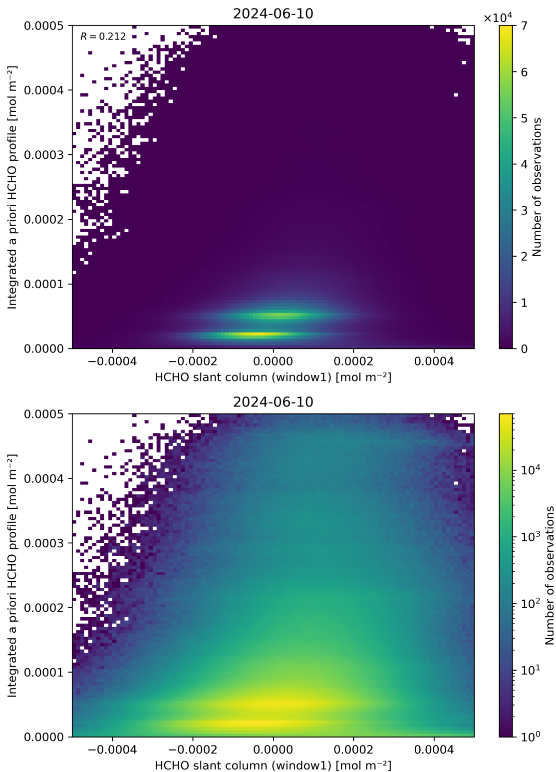
Figure 87: Scatter density plot of “HCHO slant column (window1)” against “Integrated a priori HCHO profile” for 2024-06-09 to 2024-06-11.
