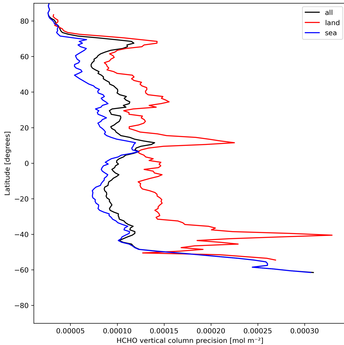
Figure 22: Zonal average of “HCHO vertical column precision” for 2024-06-09 to 2024-06-11.
