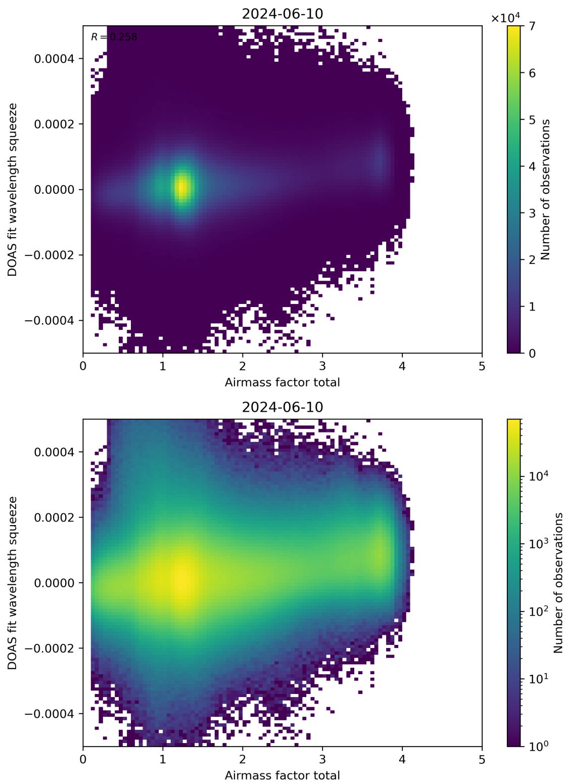
Figure 99: Scatter density plot of “Airmass factor total” against “DOAS fit wavelength squeeze” for 2024-06-09 to 2024-06-11.
