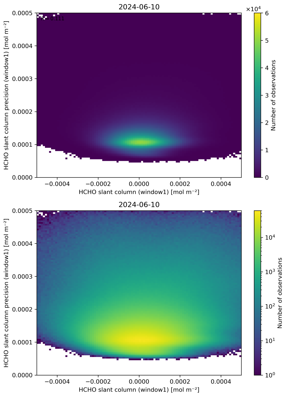
Figure 84: Scatter density plot of “HCHO slant column (window1)” against “HCHO slant column precision (window1)” for 2024-06-09 to 2024-06-11.
