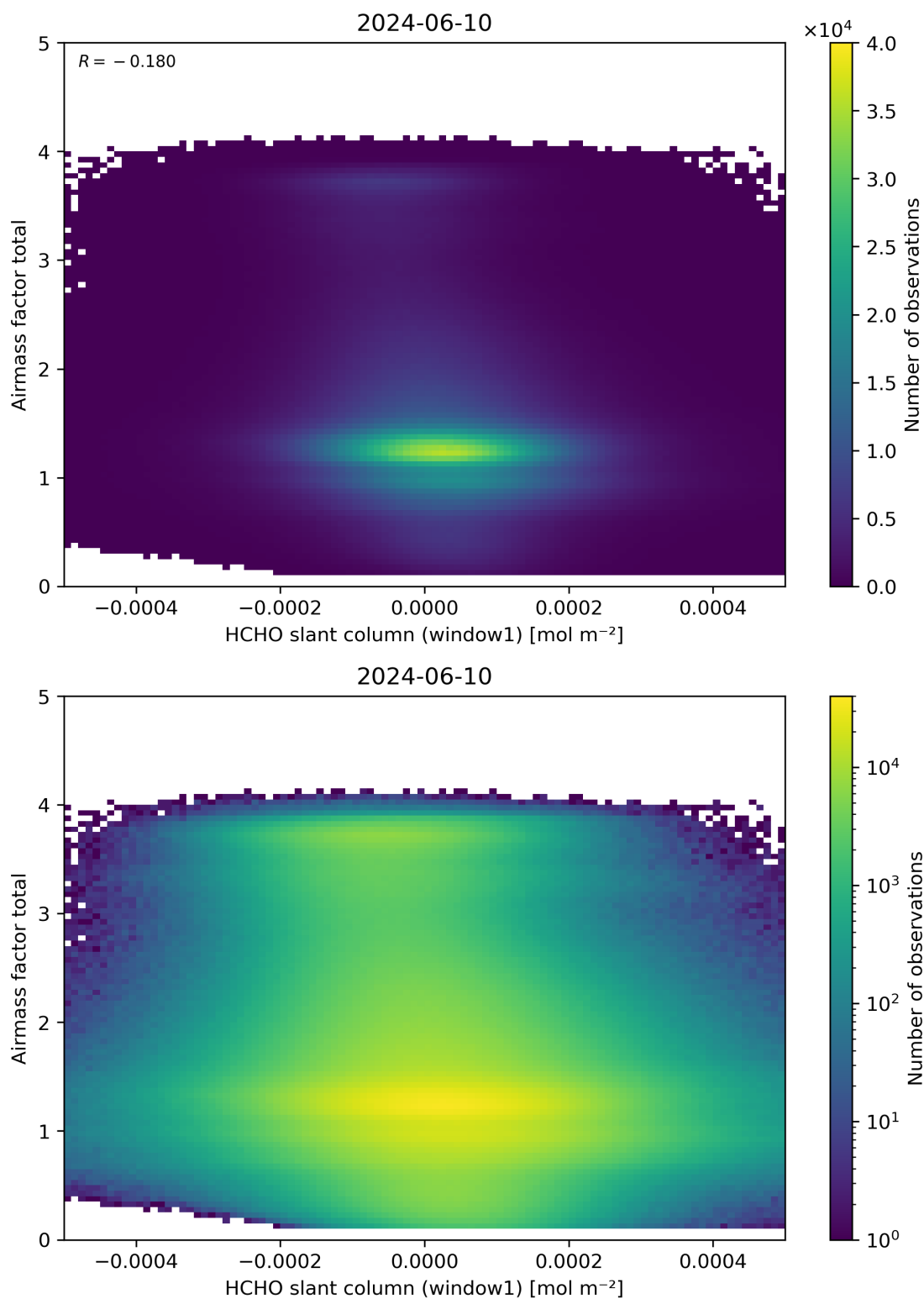
Figure 85: Scatter density plot of “HCHO slant column (window1)” against “Airmass factor total” for 2024-06-09 to 2024-06-11.
