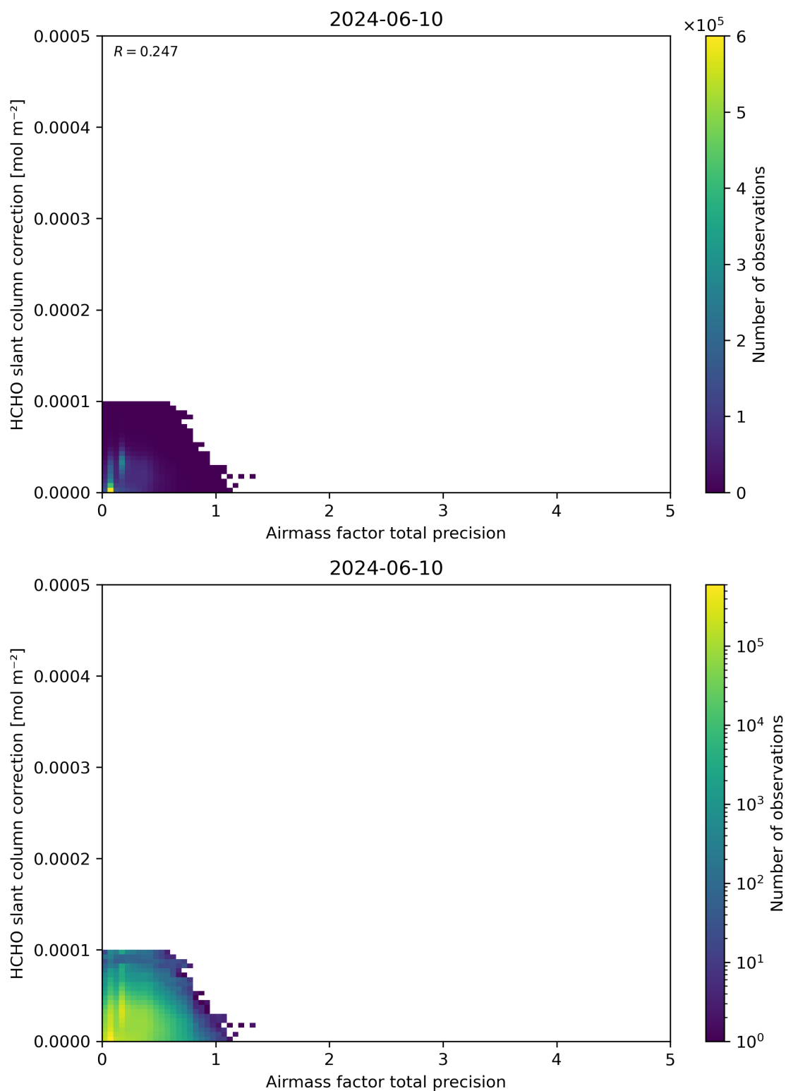
Figure 110: Scatter density plot of “Airmass factor total precision” against “HCHO slant column correction” for 2024-06-09 to 2024-06-11.
