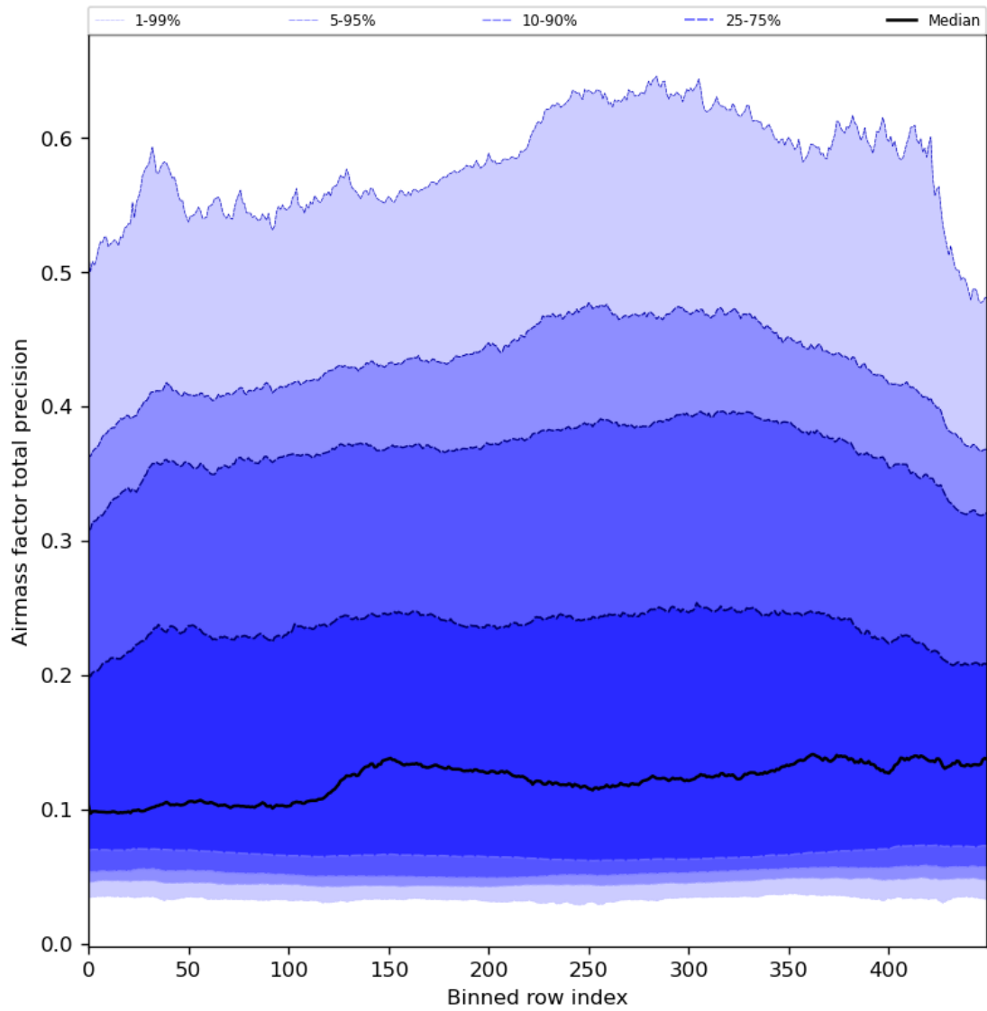
Figure 55: Along track statistics of “Airmass factor total precision” for 2024-06-09 to 2024-06-11
