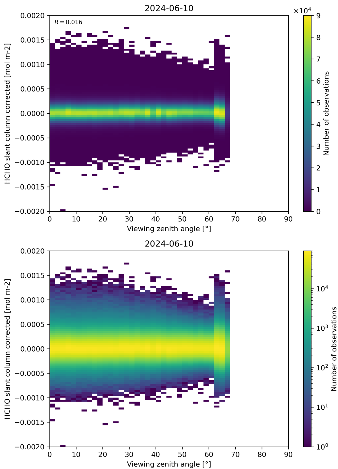
Figure 186: Scatter density plot of “Viewing zenith angle” against “HCHO slant column corrected” for 2024-06-09 to 2024-06-11.
