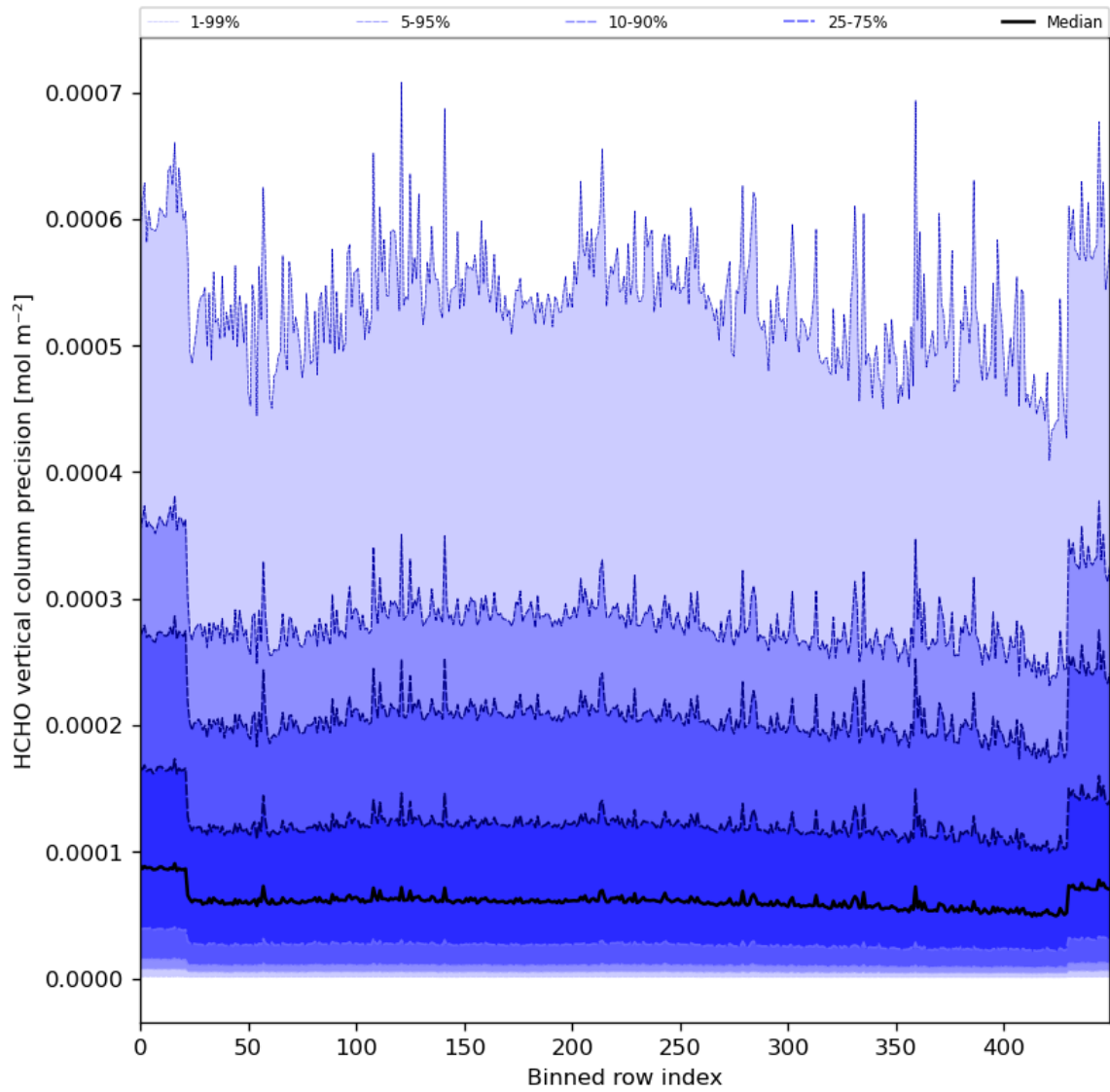
Figure 50: Along track statistics of “HCHO vertical column precision” for 2024-06-09 to 2024-06-11
