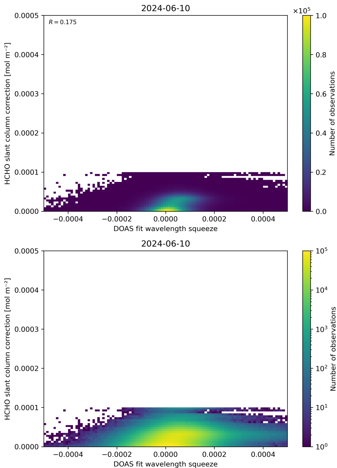
Figure 70: Scatter density plot of “DOAS fit wavelength squeeze” against “HCHO slant column correction” for 2024-06-09 to 2024-06-11.
