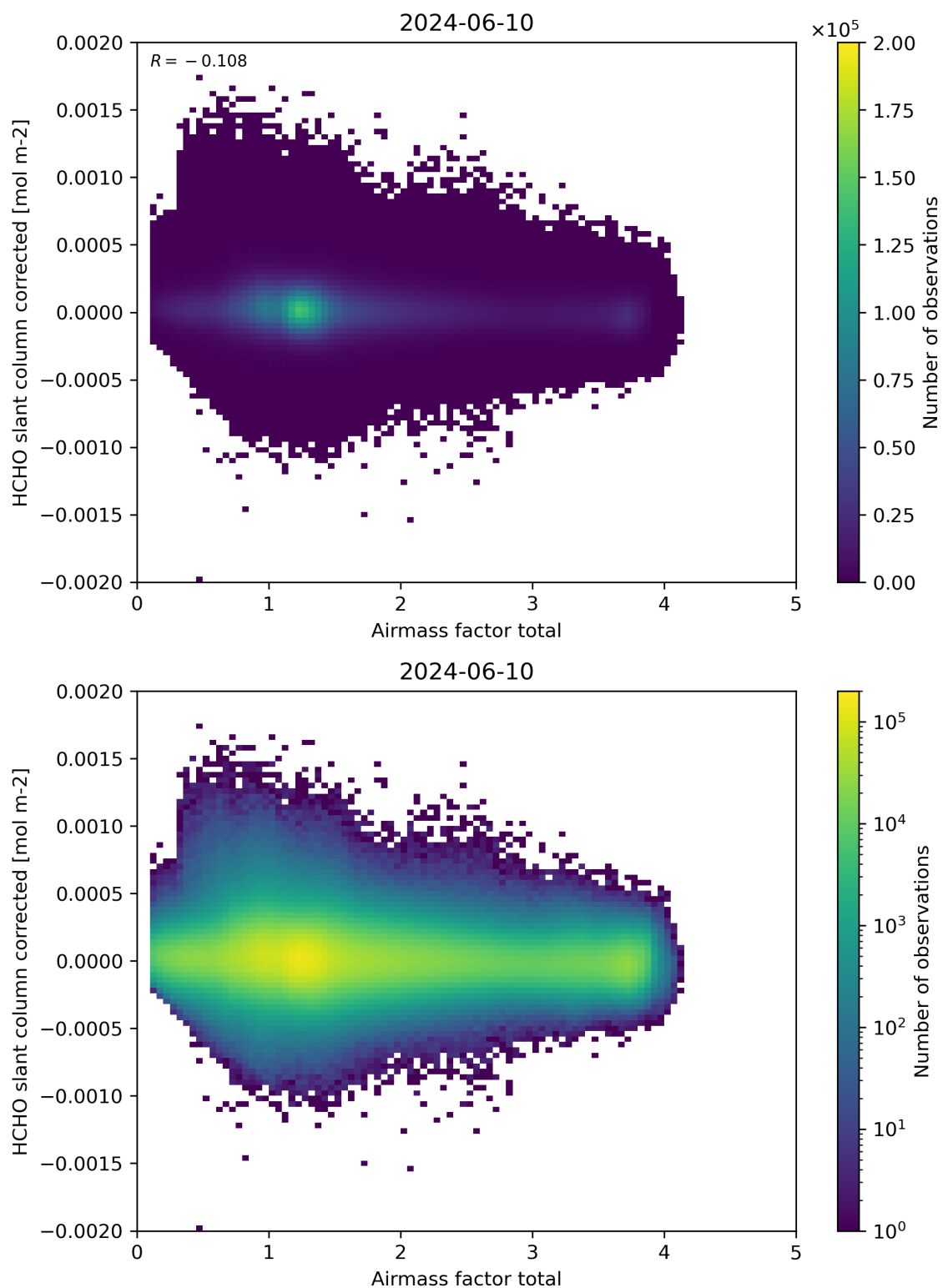
Figure 101: Scatter density plot of “Airmass factor total” against “HCHO slant column corrected” for 2024-06-09 to 2024-06-11.
