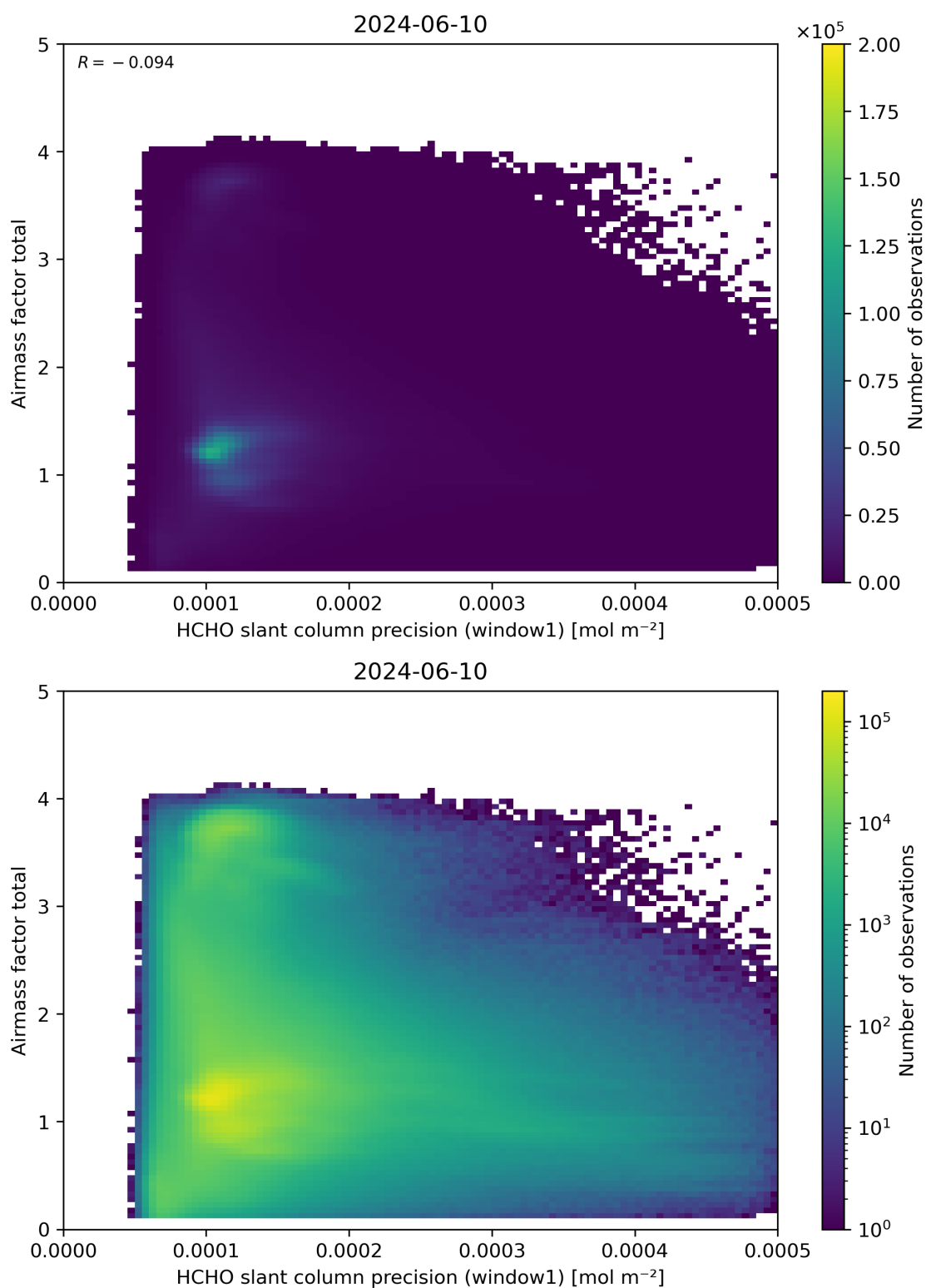
Figure 94: Scatter density plot of “HCHO slant column precision (window1)” against “Airmass factor total” for 2024-06-09 to 2024-06-11.
