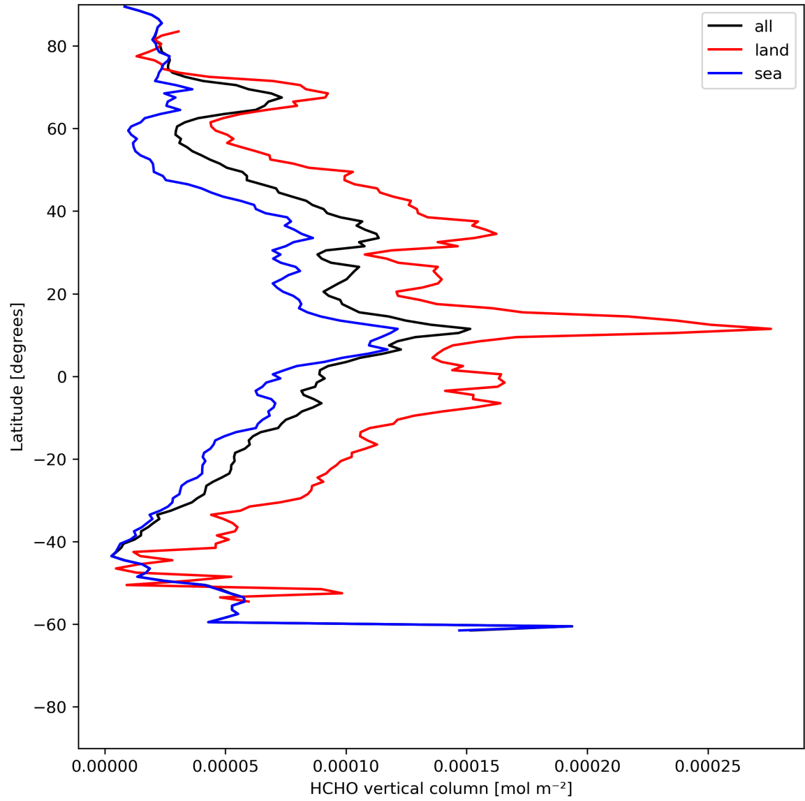
Figure 21: Zonal average of “HCHO vertical column” for 2024-06-09 to 2024-06-11.
