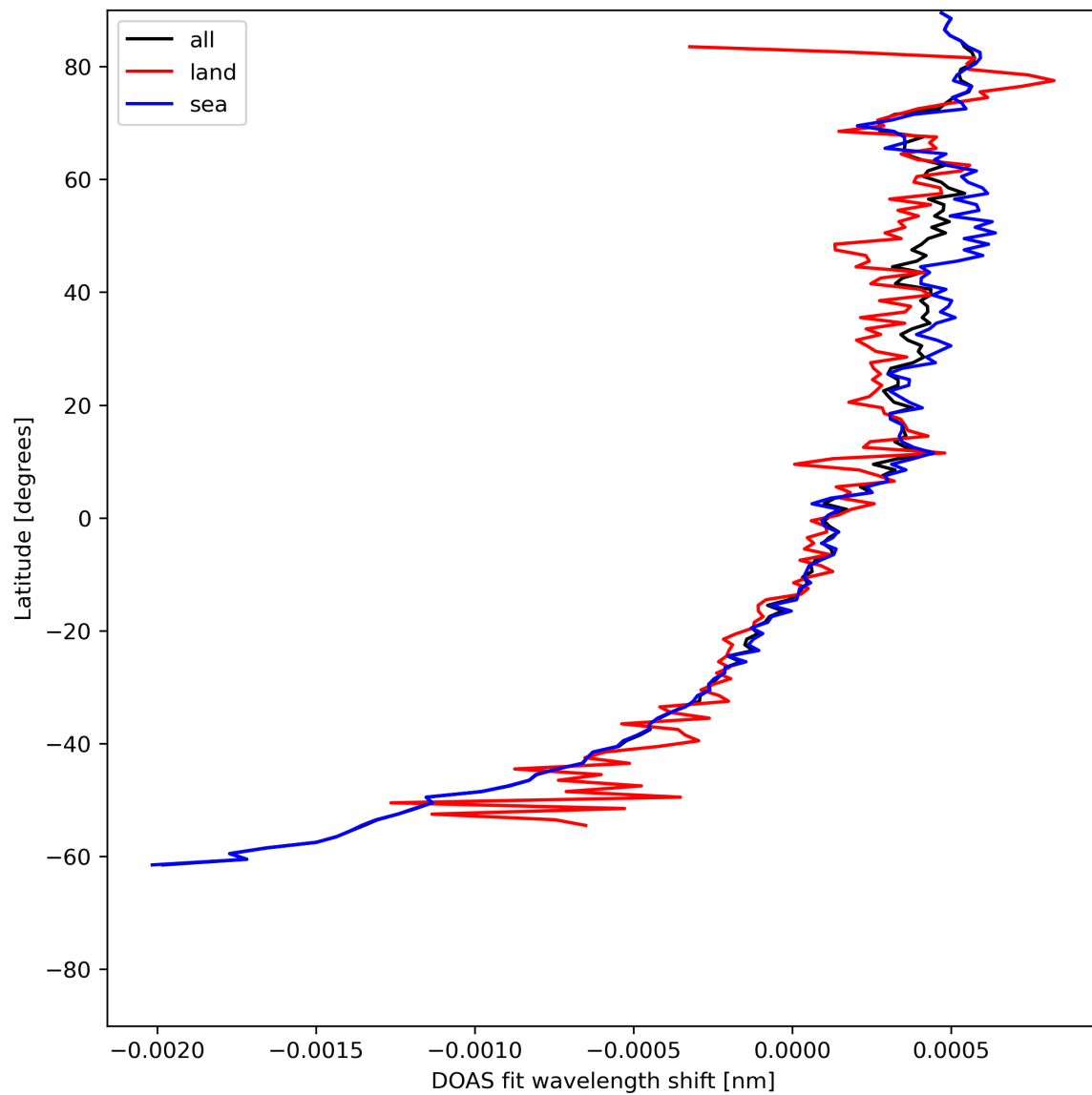
Figure 30: Zonal average of “DOAS fit wavelength shift” for 2024-06-09 to 2024-06-11.
